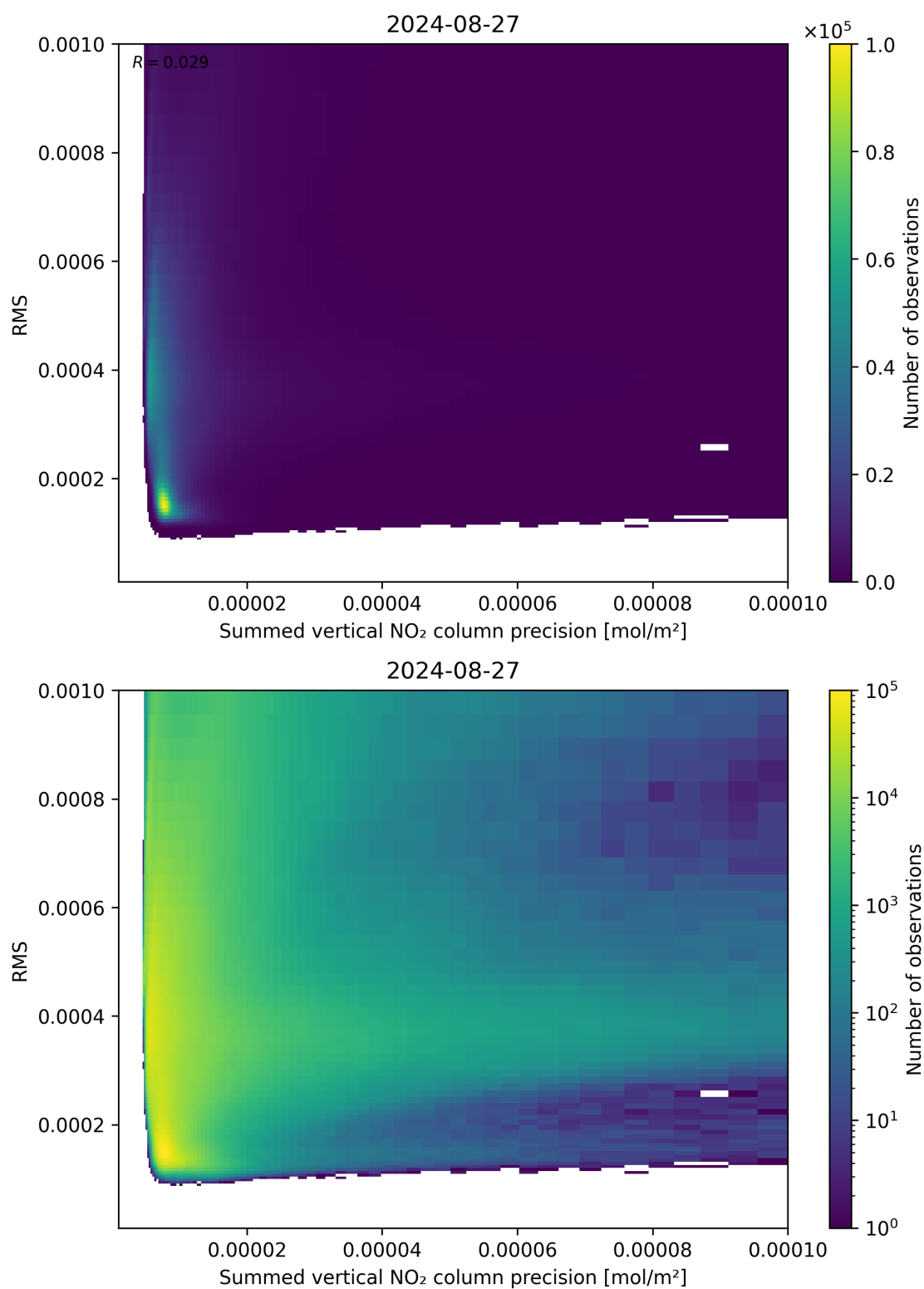
Figure 108: Scatter density plot of “Summed vertical NO 2 column precision” against “RMS” for 2024-08-27 to 2024-08-28.
