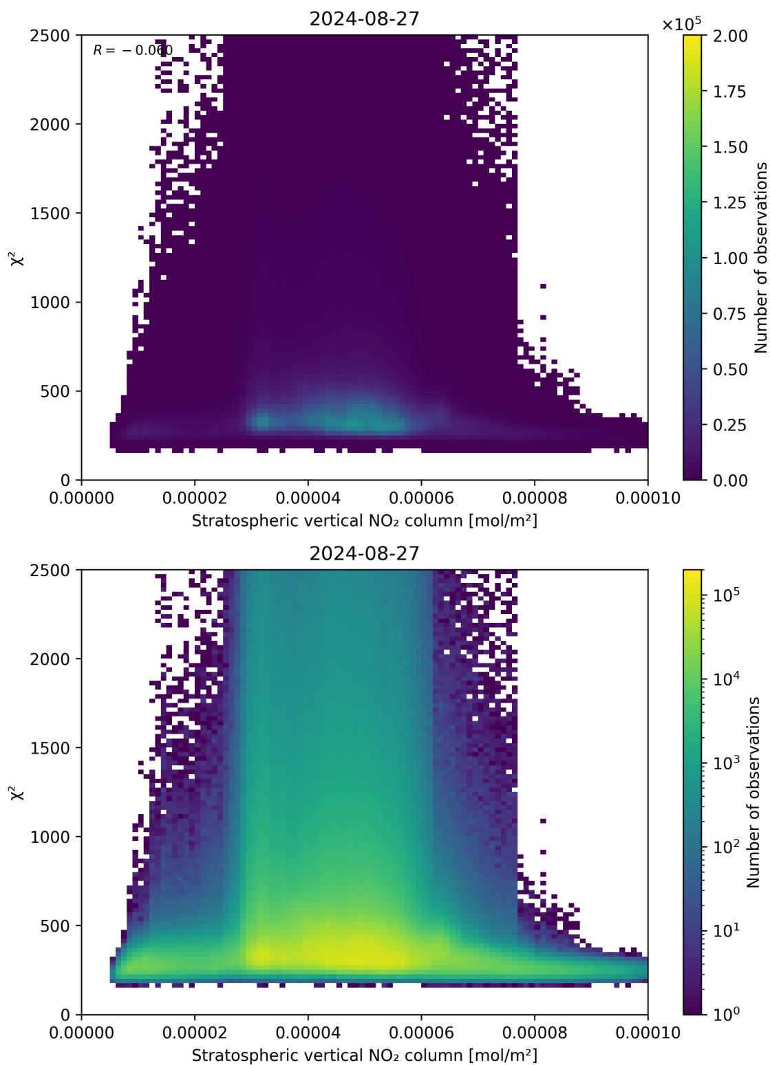
Figure 97: Scatter density plot of “Stratospheric vertical NO 2 column” against “ \chi^2 ” for 2024-08-27 to 2024-08-28.
