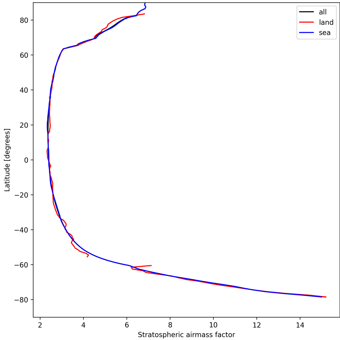
Figure 27: Zonal average of “Stratospheric airmass factor” for 2024-08-27 to 2024-08-28.
