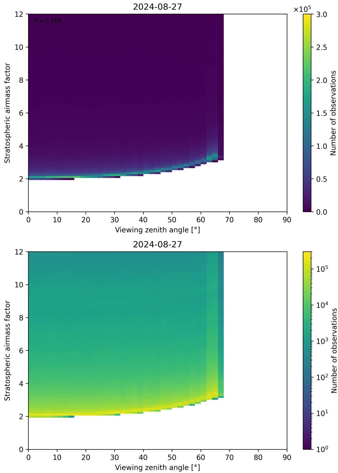
Figure 159: Scatter density plot of “Viewing zenith angle” against “Stratospheric airmass factor” for 2024-08-27 to 2024-08-28.
