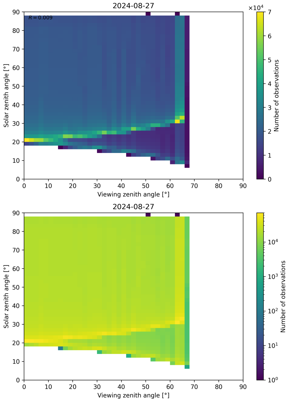
Figure 172: Scatter density plot of “Viewing zenith angle” against “Solar zenith angle” for 2024-08-27 to 2024-08-28.
