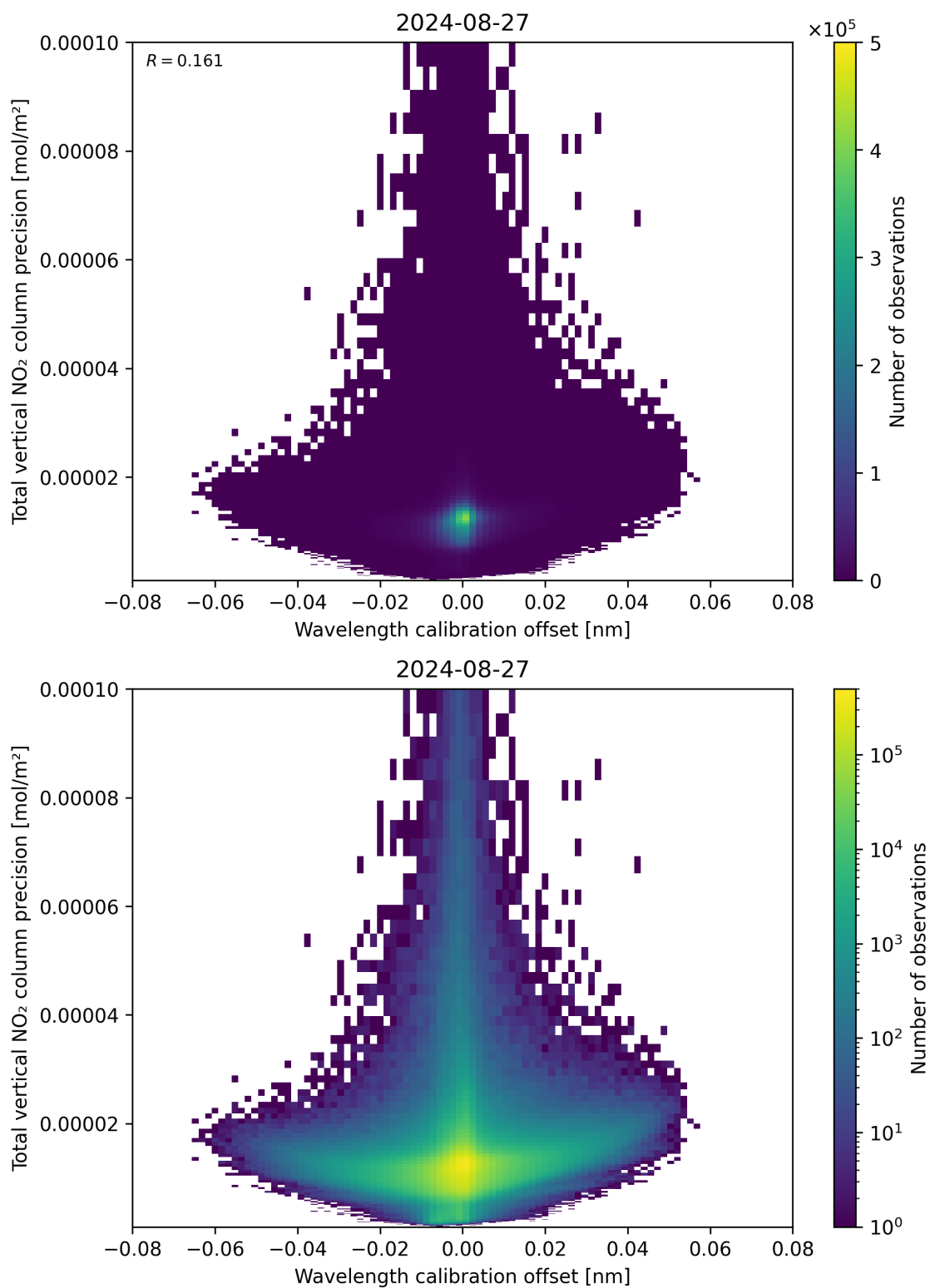
Figure 180: Scatter density plot of “Wavelength calibration offset” against “Total vertical NO 2 column precision” for 2024-08-27 to 2024-08-28.
