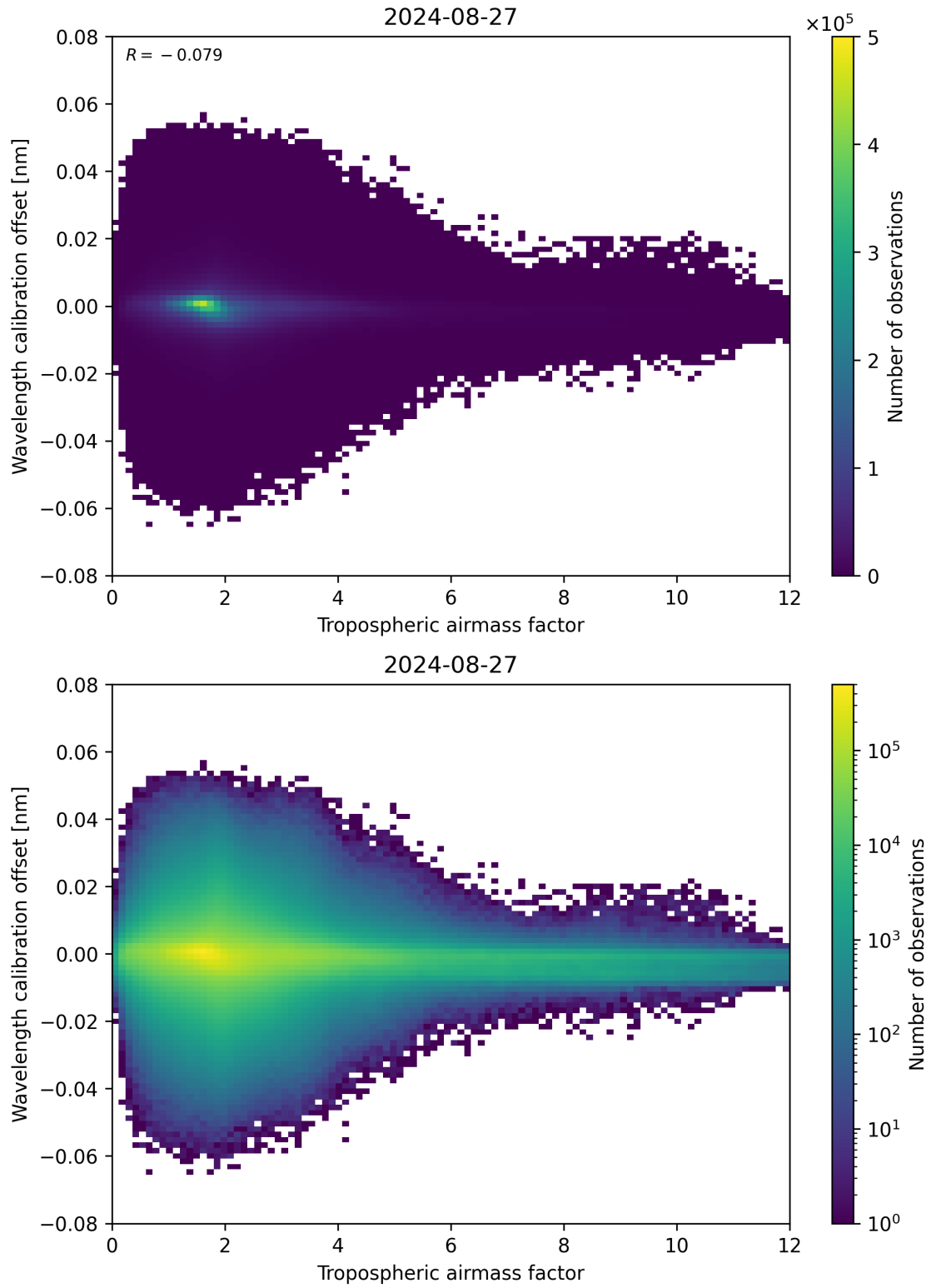
Figure 80: Scatter density plot of “Tropospheric airmass factor” against “Wavelength calibration offset” for 2024-08-27 to 2024-08-28.
