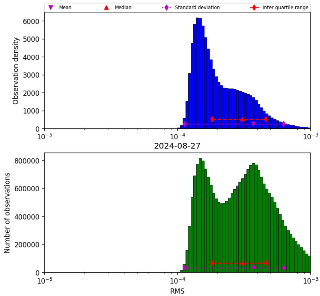
Figure 43: Histogram of “RMS” for 2024-08-27 to 2024-08-28
