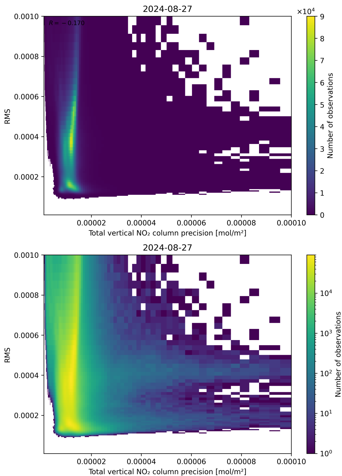
Figure 119: Scatter density plot of “Total vertical NO 2 column precision” against “RMS” for 2024-08-27 to 2024-08-28.
