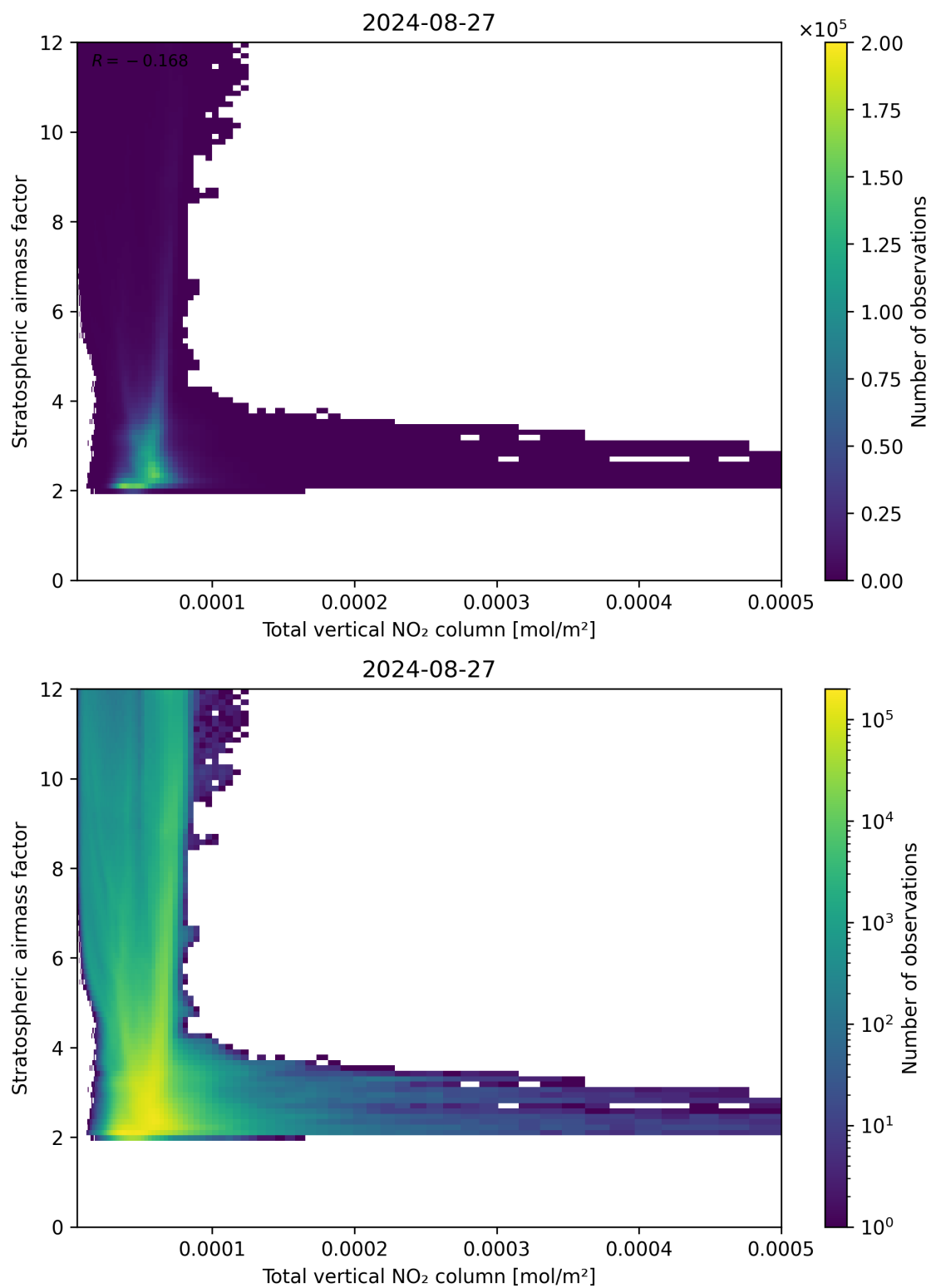
Figure 110: Scatter density plot of “Total vertical NO 2 column” against “Stratospheric airmass factor” for 2024-08-27 to 2024-08-28.
