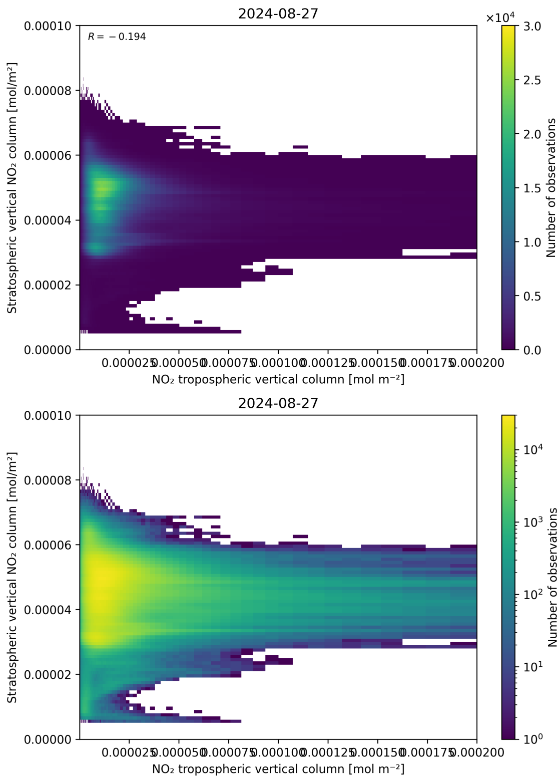
Figure 125: Scatter density plot of “NO 2 tropospheric vertical column” against “Stratospheric vertical NO 2 column” for 2024-08-27 to 2024-08-28.
