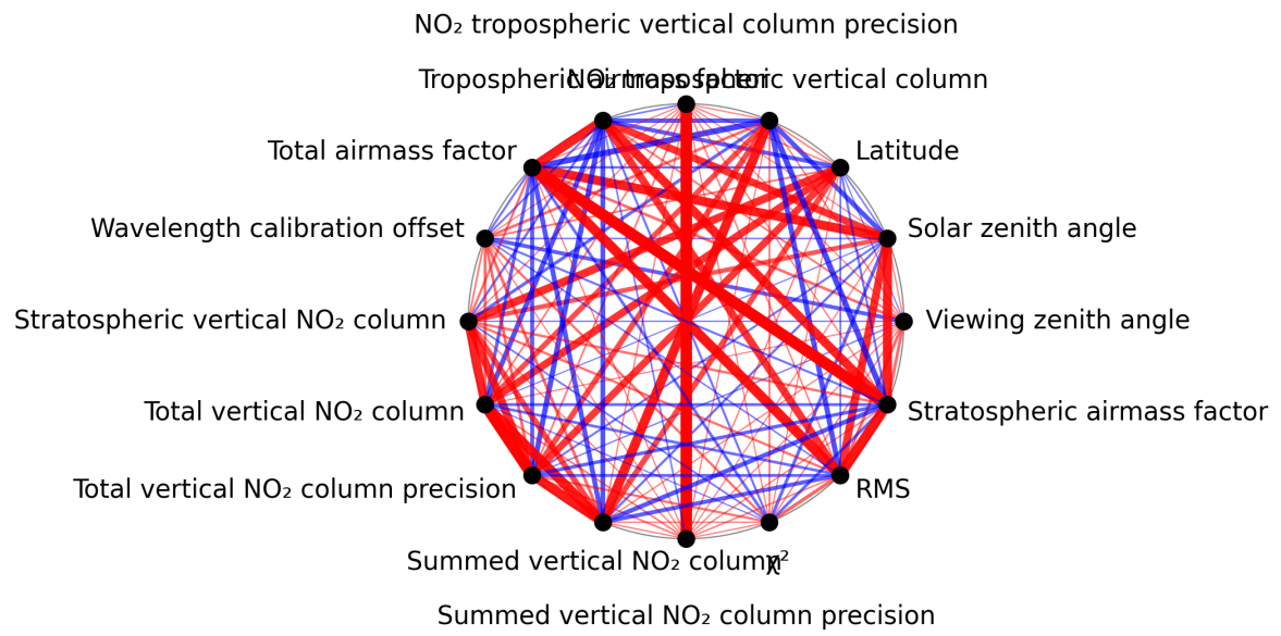
Figure 1: Map of correlation graph for 2024-08-27 to 2024-08-28.
