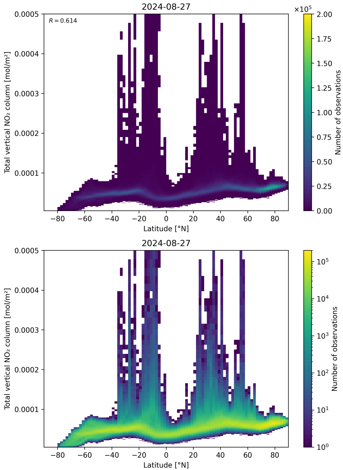
Figure 90: Scatter density plot of “Latitude” against “Total vertical NO 2 column” for 2024-08-27 to 2024-08-28.
