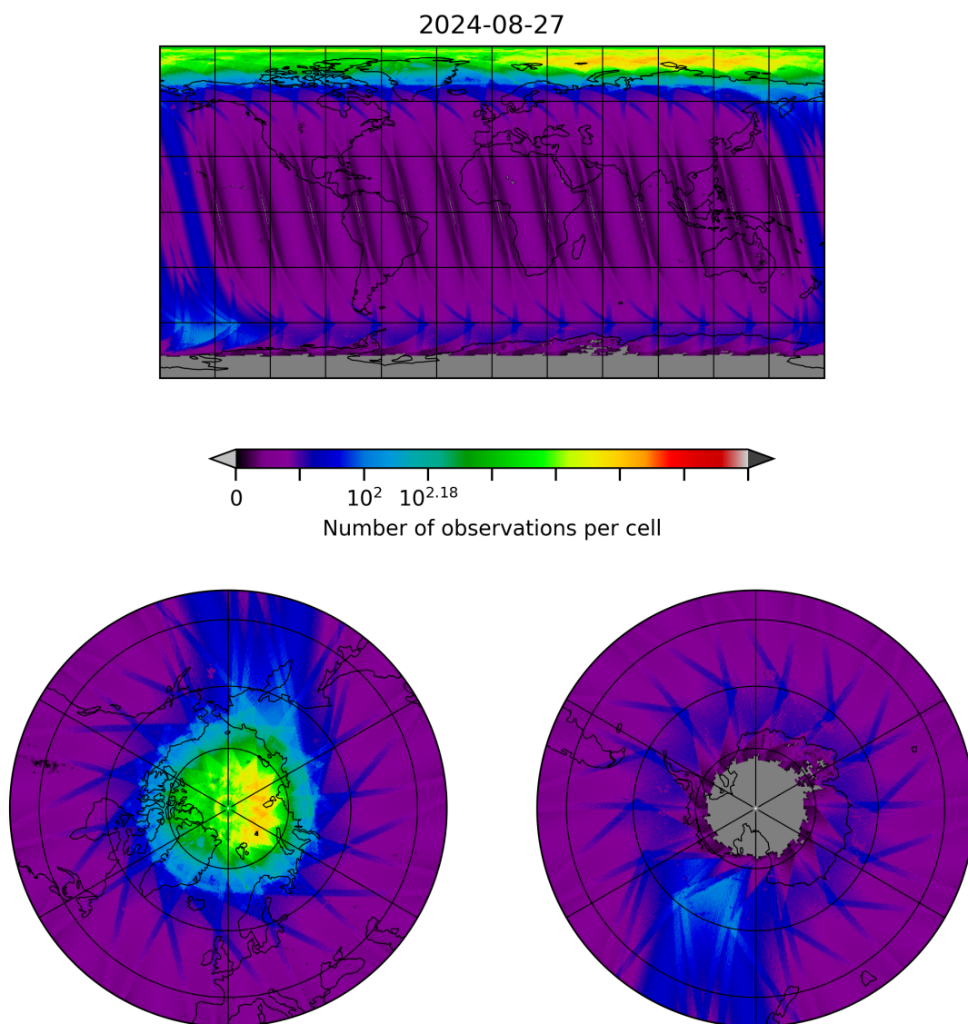
Figure 10: Map of the number of observations for 2024-08-27 to 2024-08-28
