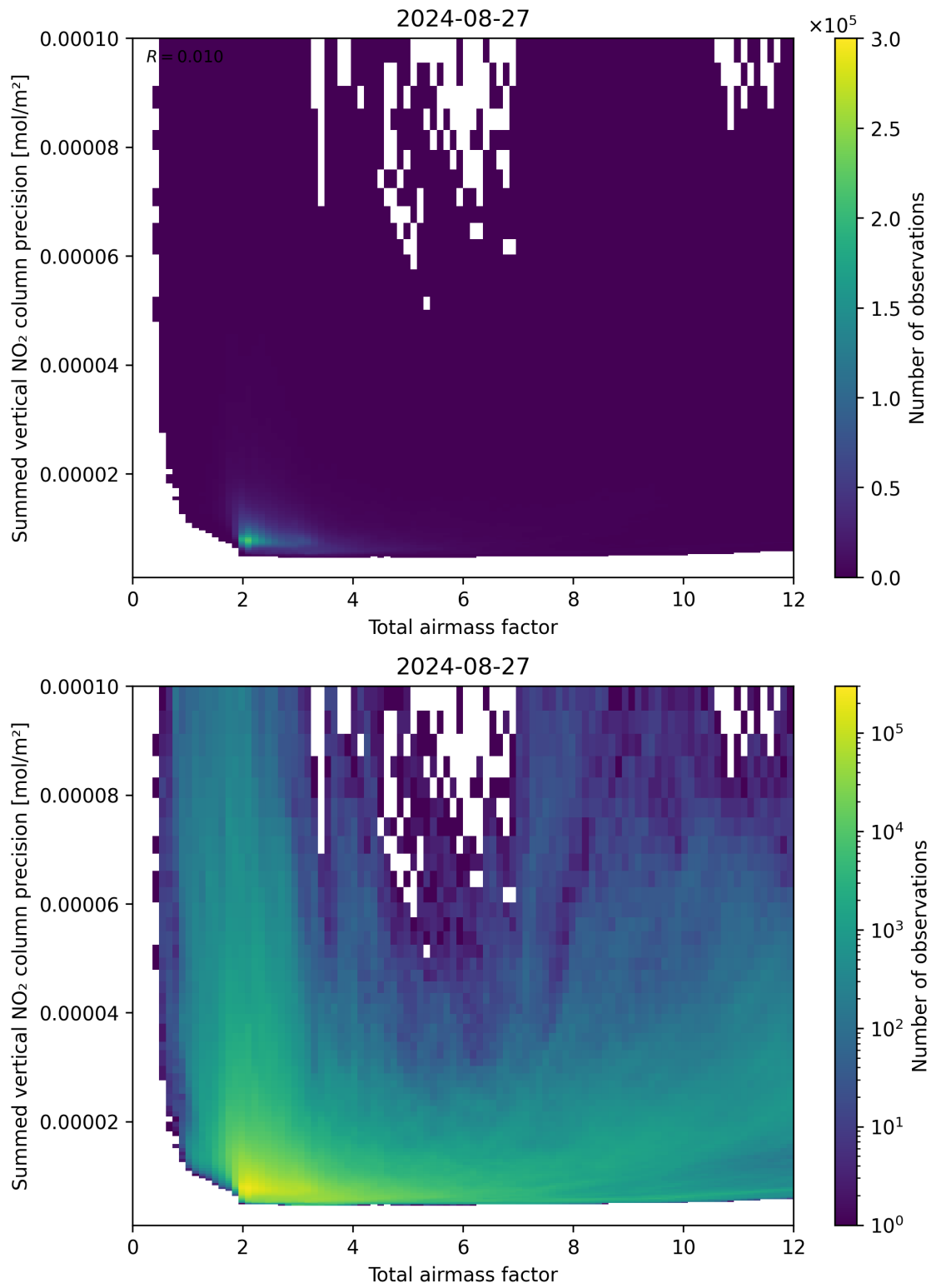
Figure 66: Scatter density plot of “Total airmass factor” against “Summed vertical NO 2 column precision” for 2024-08-27 to 2024-08-28.
