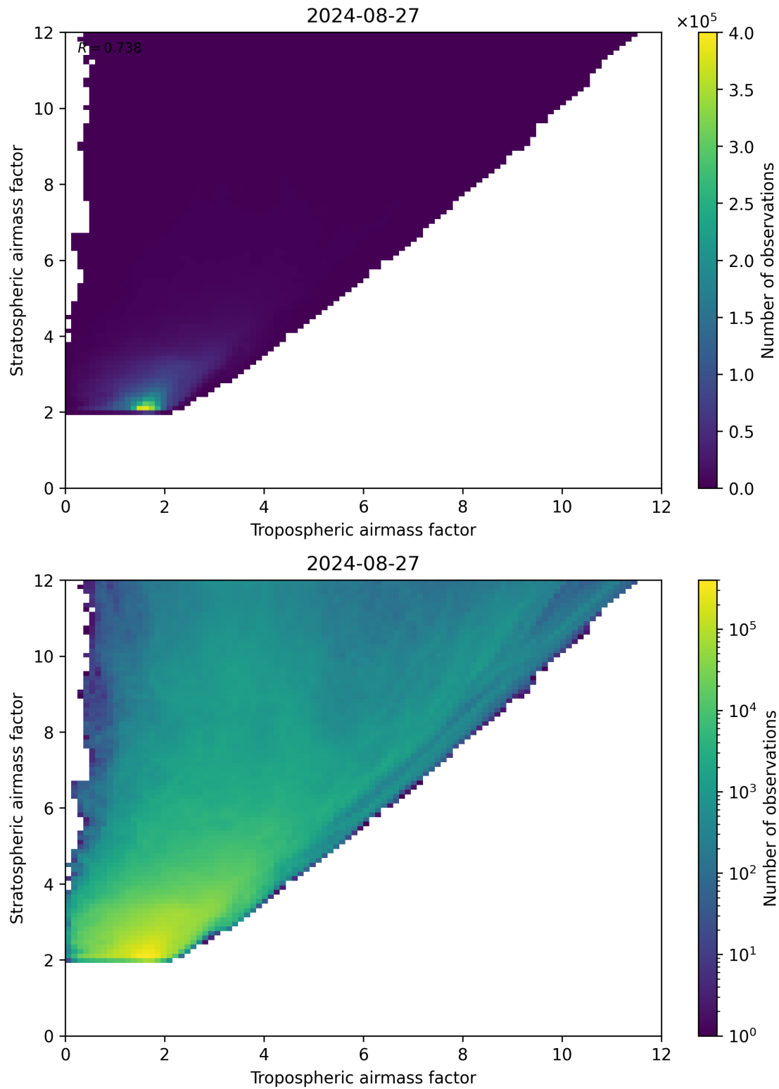
Figure 71: Scatter density plot of “Tropospheric airmass factor” against “Stratospheric airmass factor” for 2024-08-27 to 2024-08-28.
