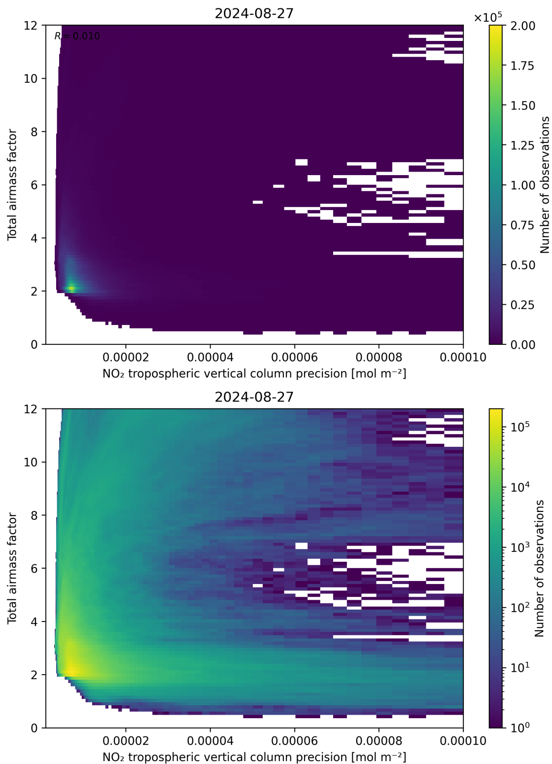
Figure 132: Scatter density plot of “NO 2 tropospheric vertical column precision” against “Total air mass factor” for 2024-08-27 to 2024-08-28.
