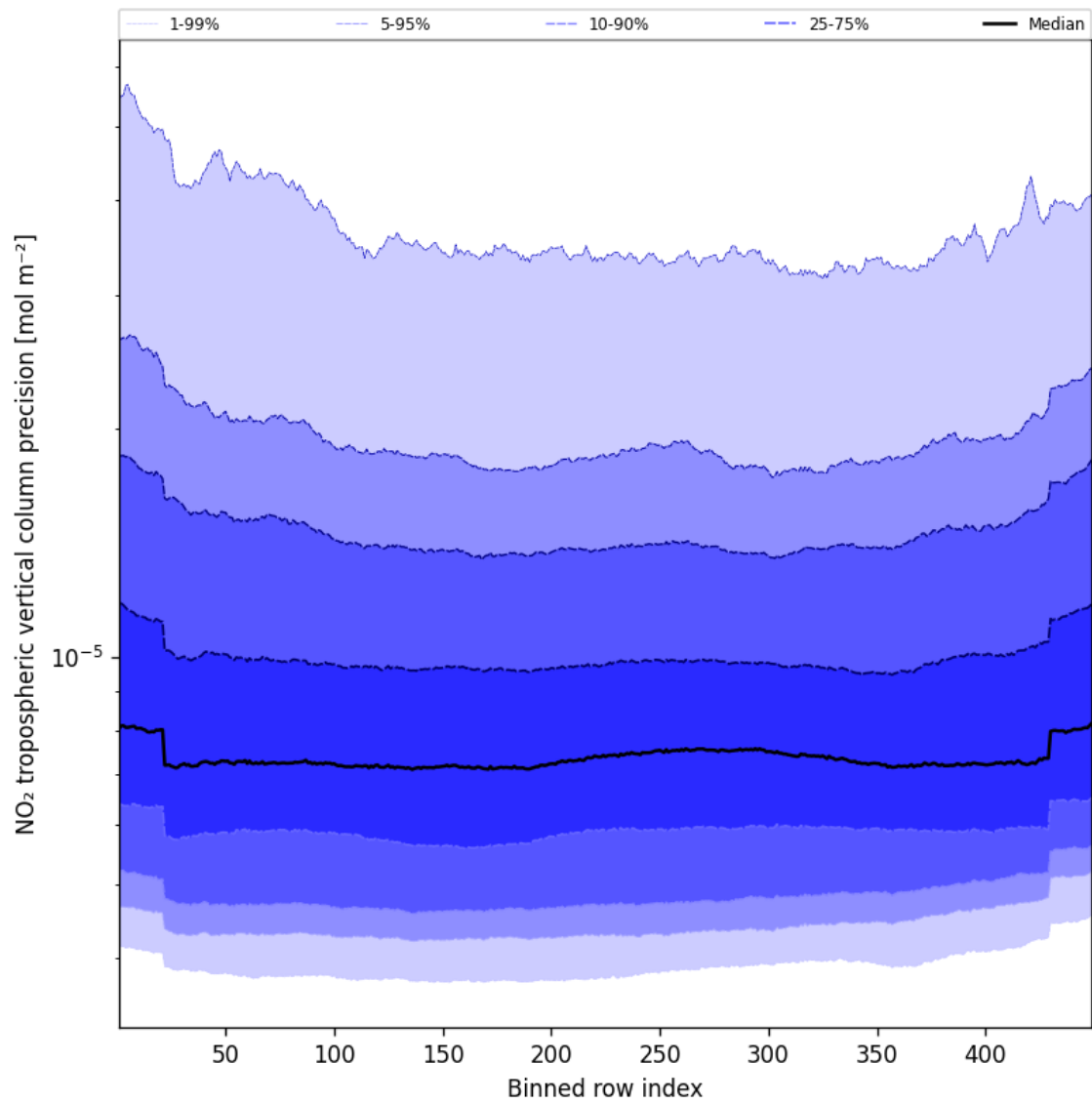
Figure 47: Along track statistics of “NO 2 tropospheric vertical column precision” for 2024-08-27 to 2024-08-28
