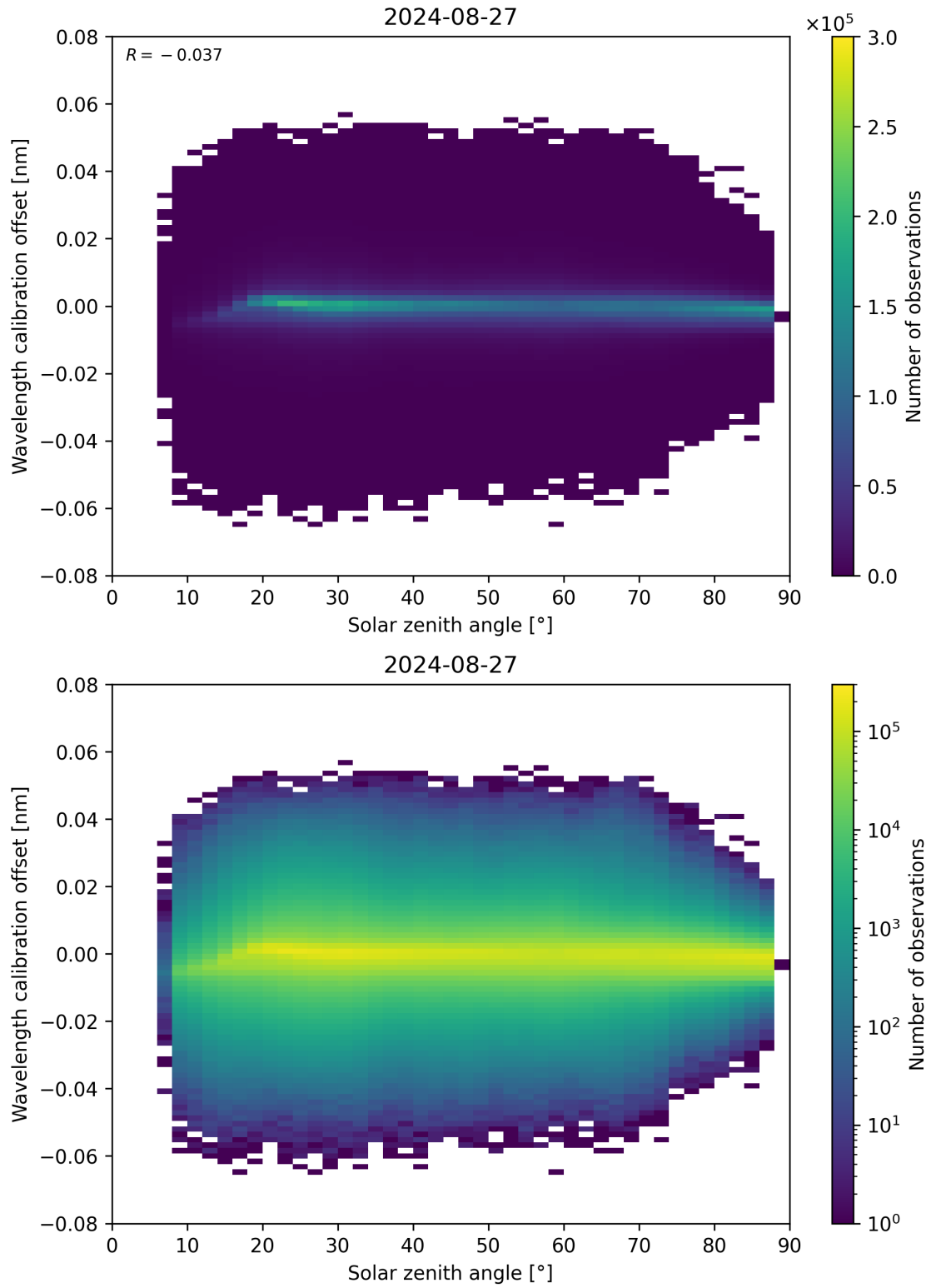
Figure 158: Scatter density plot of “Solar zenith angle” against “Wavelength calibration offset” for 2024-08-27 to 2024-08-28.
