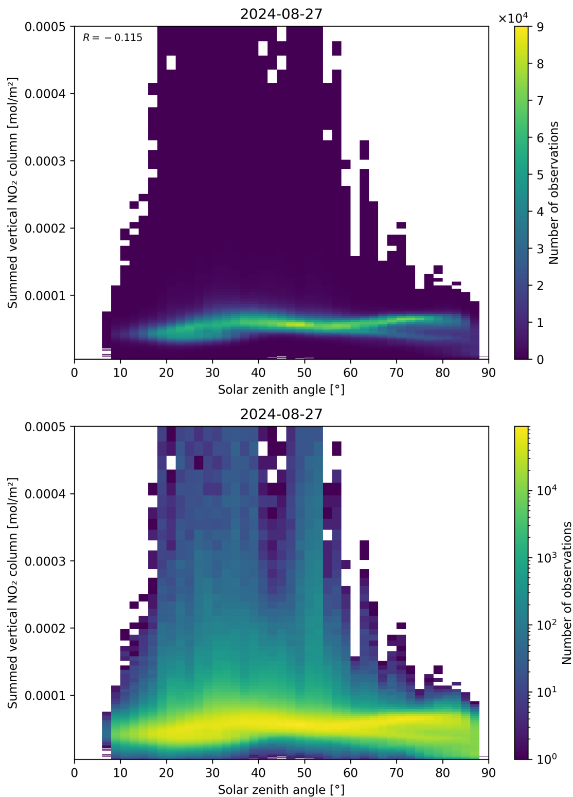
Figure 151: Scatter density plot of “Solar zenith angle” against “Summed vertical NO 2 column” for 2024-08-27 to 2024-08-28.
