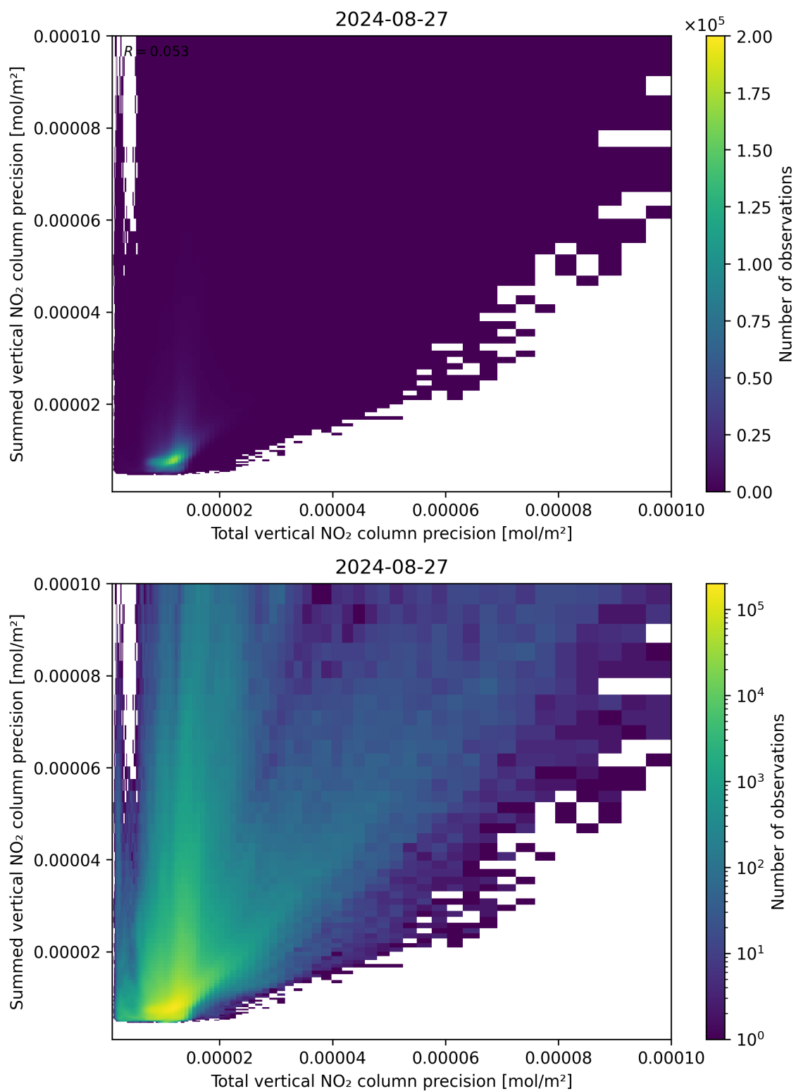
Figure 118: Scatter density plot of “Total vertical NO 2 column precision” against “Summed vertical NO 2 column precision” for 2024-08-27 to 2024-08-28.
