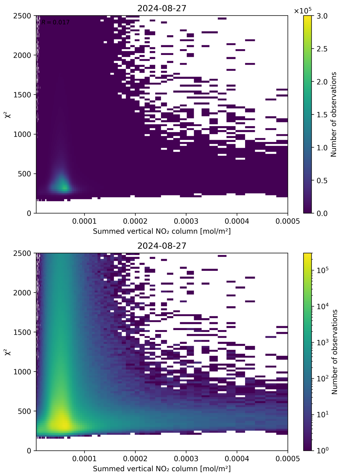
Figure 104: Scatter density plot of “Summed vertical NO 2 column” against “ \chi^2 ” for 2024-08-27 to 2024-08-28.
