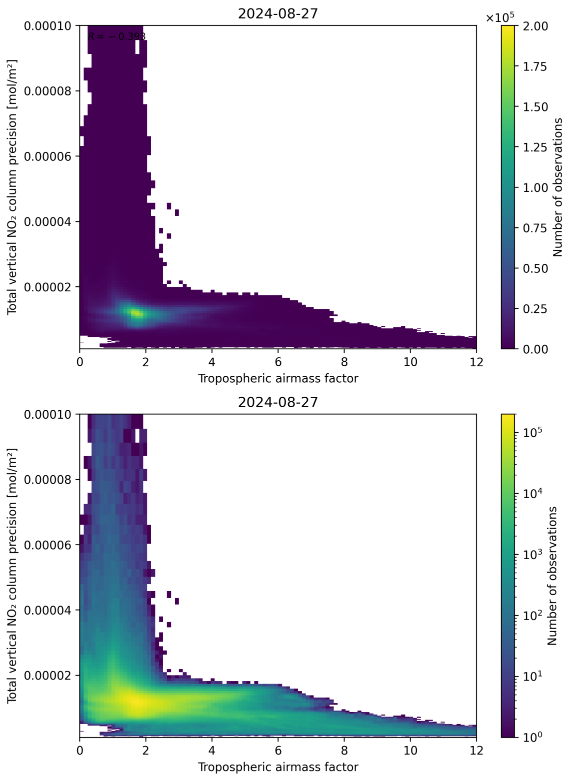
Figure 78: Scatter density plot of “Tropospheric air mass factor” against “Total vertical NO 2 column precision” for 2024-08-27 to 2024-08-28.
