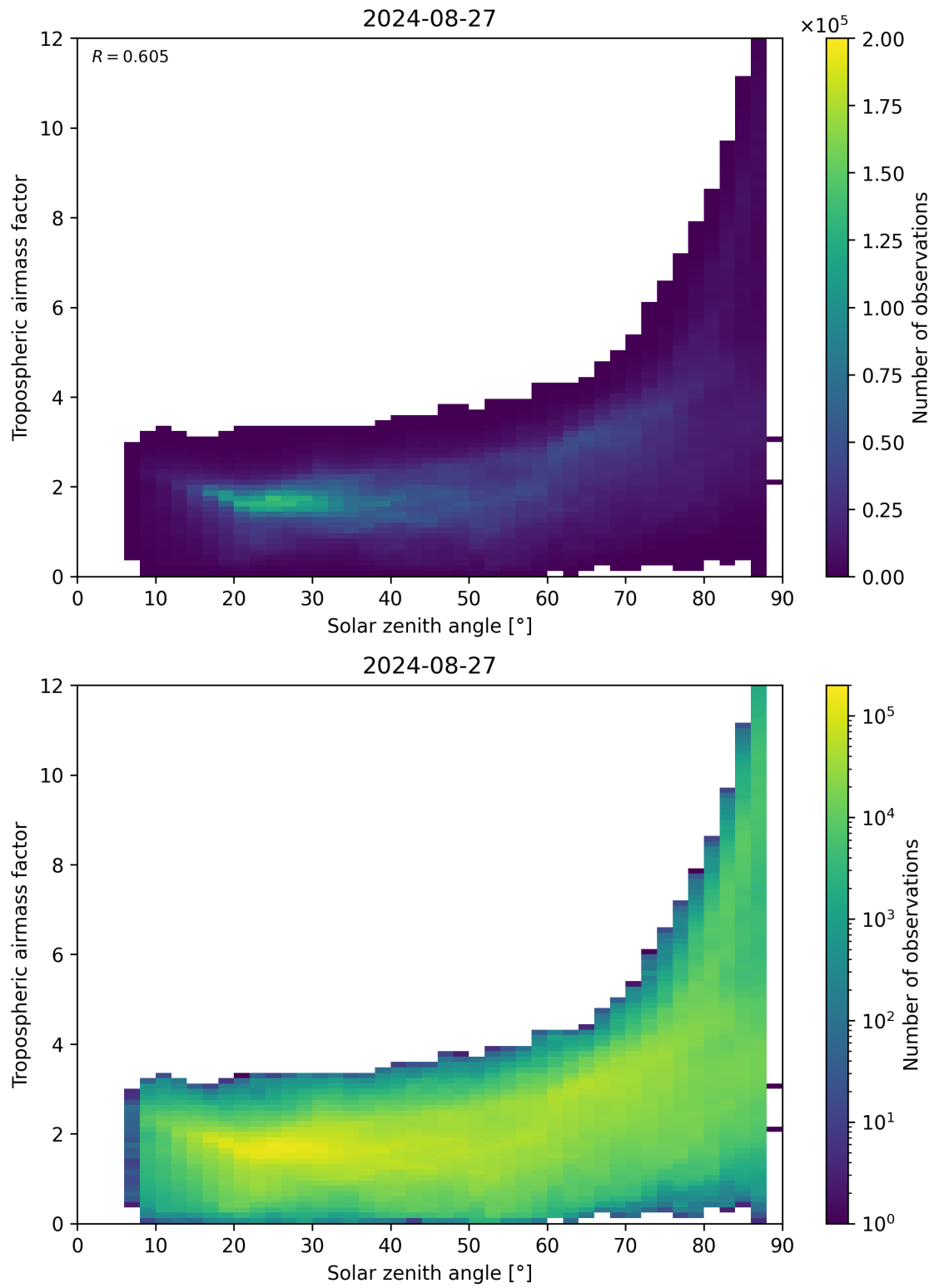
Figure 147: Scatter density plot of “Solar zenith angle” against “Tropospheric airmass factor” for 2024-08-27 to 2024-08-28.
