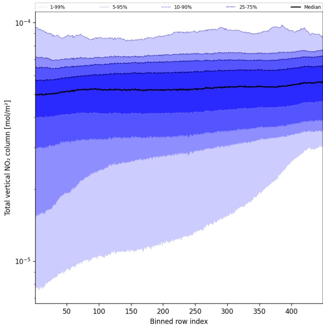
Figure 55: Along track statistics of “Total vertical NO 2 column” for 2024-08-27 to 2024-08-28
