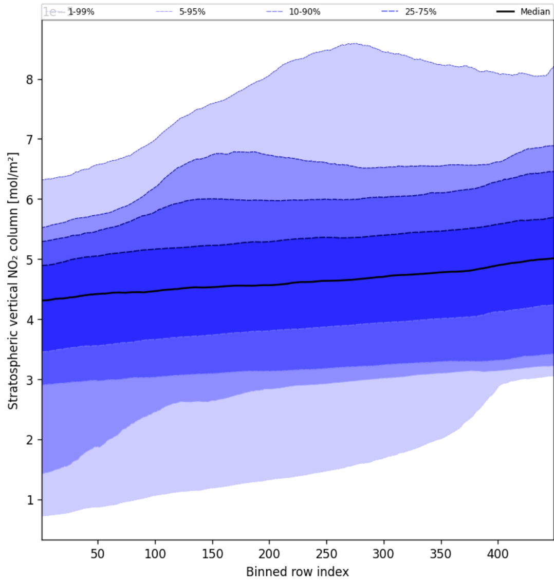
Figure 53: Along track statistics of “Stratospheric vertical NO 2 column” for 2024-08-27 to 2024-08-28
