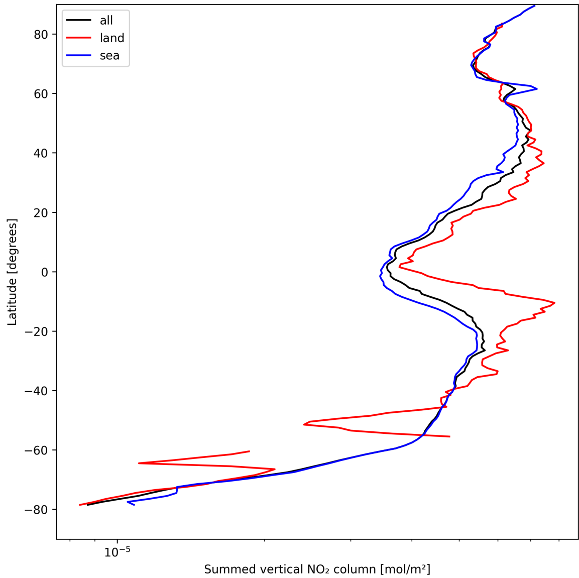
Figure 23: Zonal average of “Summed vertical NO 2 column” for 2024-08-27 to 2024-08-28.
