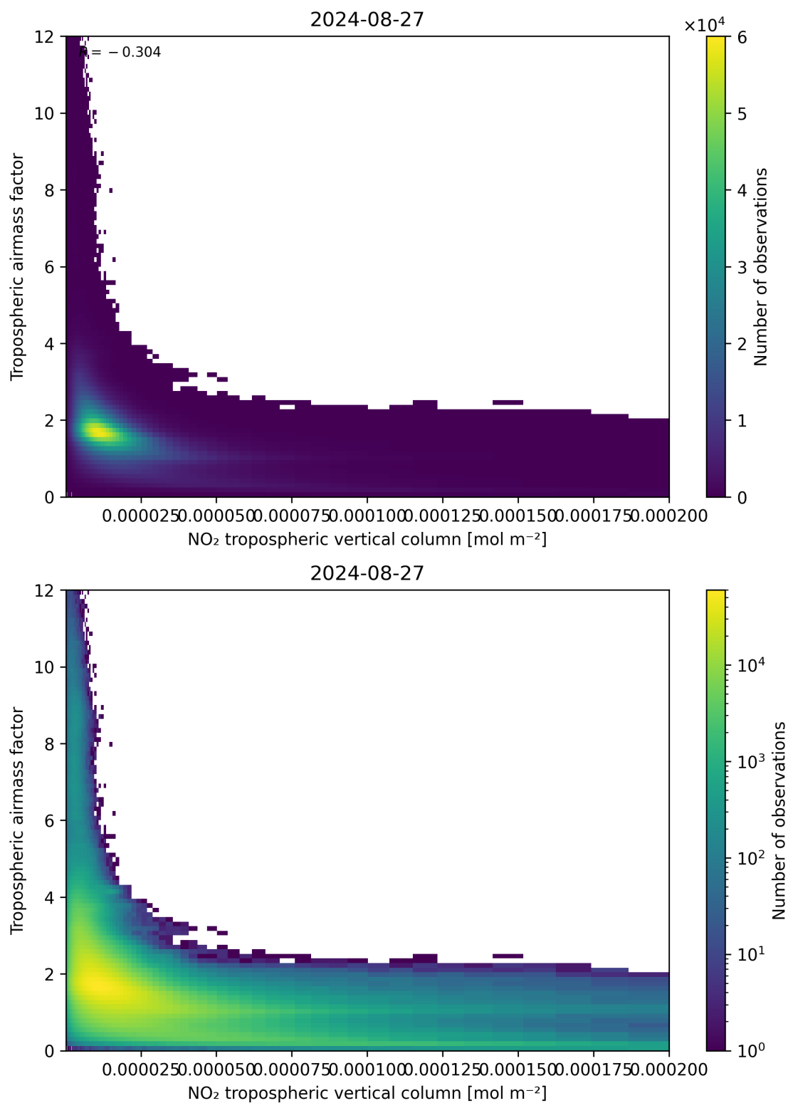
Figure 123: Scatter density plot of “NO 2 tropospheric vertical column” against “Tropospheric air mass factor” for 2024-08-27 to 2024-08-28.
