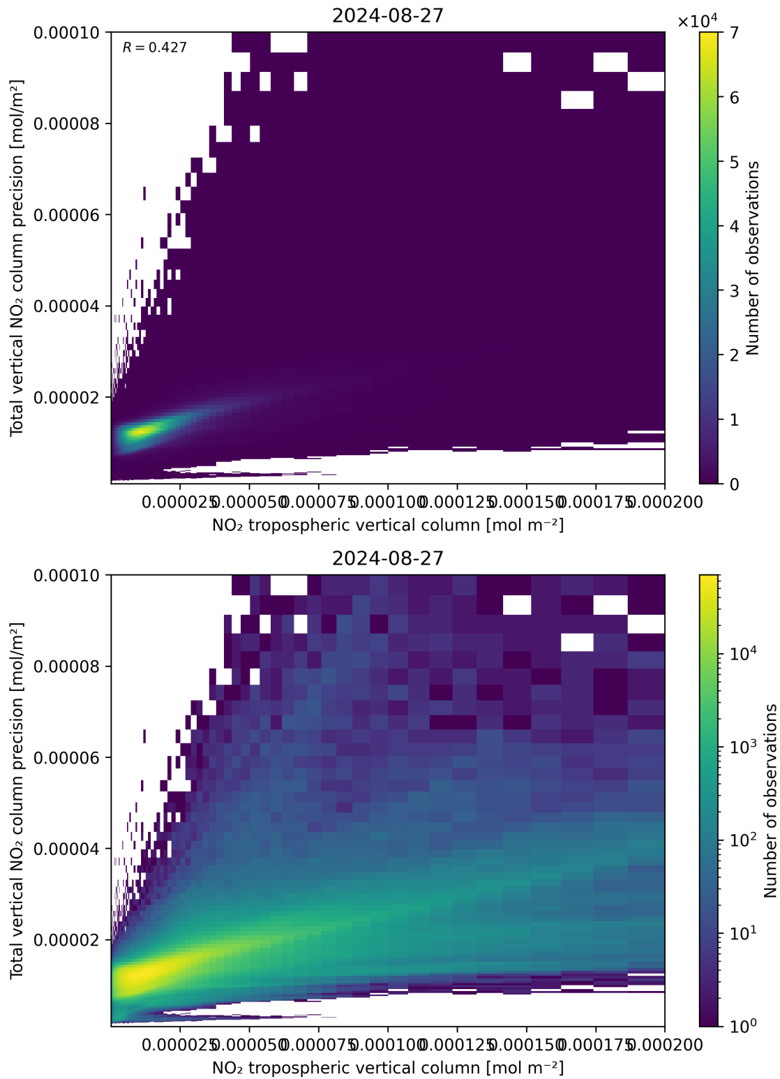
Figure 129: Scatter density plot of “NO 2 tropospheric vertical column” against “Total vertical NO 2 column precision” for 2024-08-27 to 2024-08-28.
