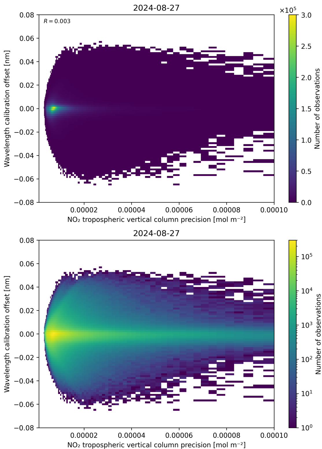
Figure 141: Scatter density plot of “NO 2 tropospheric vertical column precision” against “Wavelength calibration offset” for 2024-08-27 to 2024-08-28.
