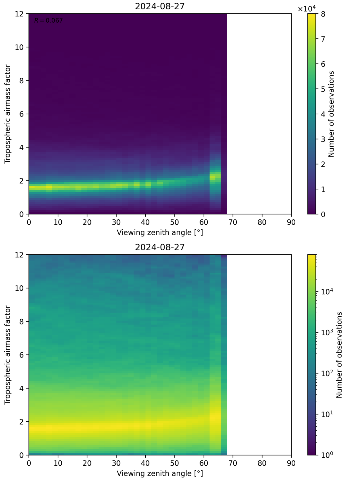
Figure 161: Scatter density plot of “Viewing zenith angle” against “Tropospheric airmass factor” for 2024-08-27 to 2024-08-28.
