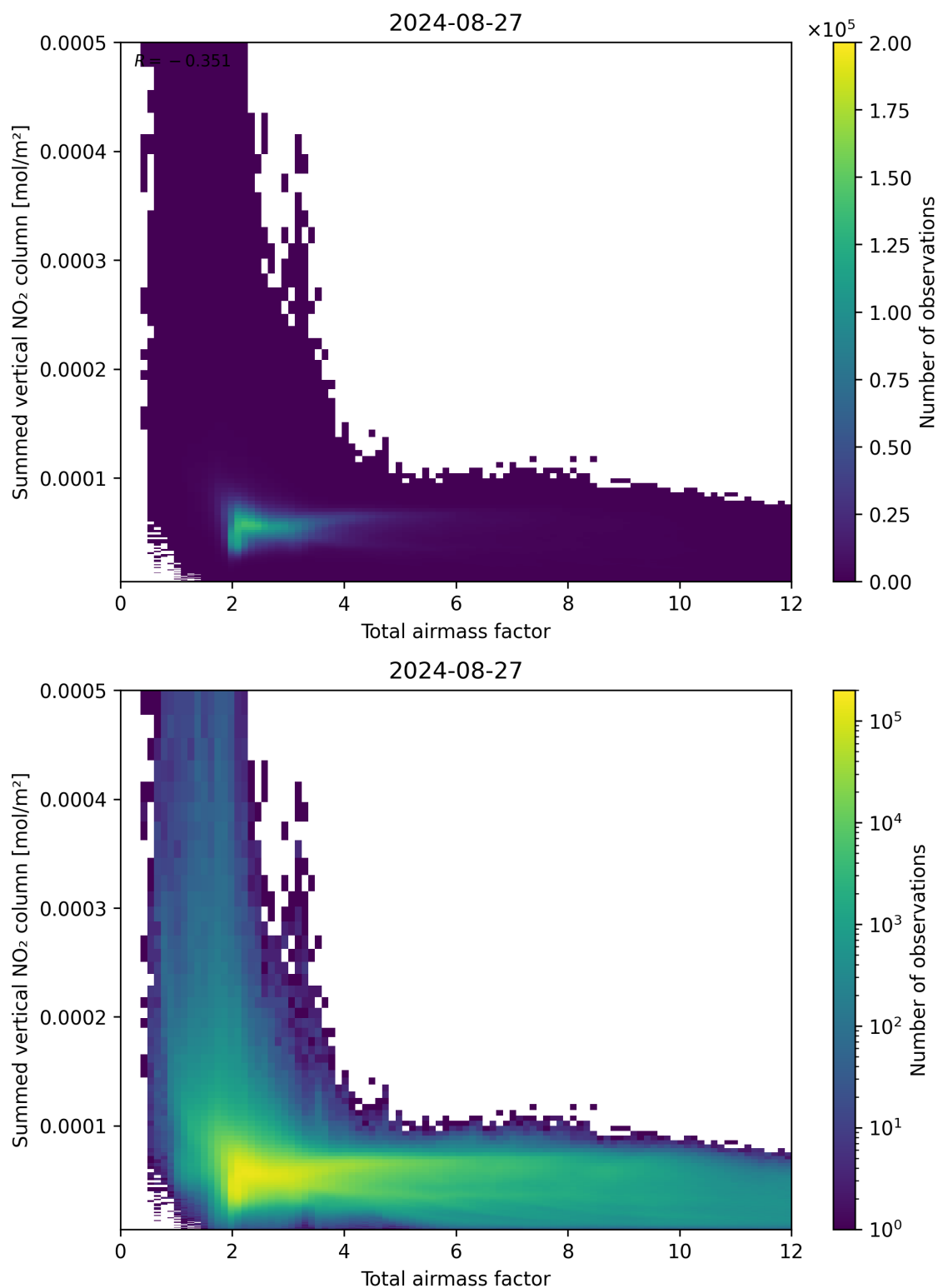
Figure 65: Scatter density plot of “Total airmass factor” against “Summed vertical NO 2 column” for 2024-08-27 to 2024-08-28.
