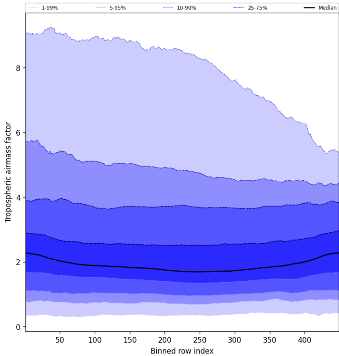
Figure 48: Along track statistics of “Tropospheric air mass factor” for 2024-08-27 to 2024-08-28
