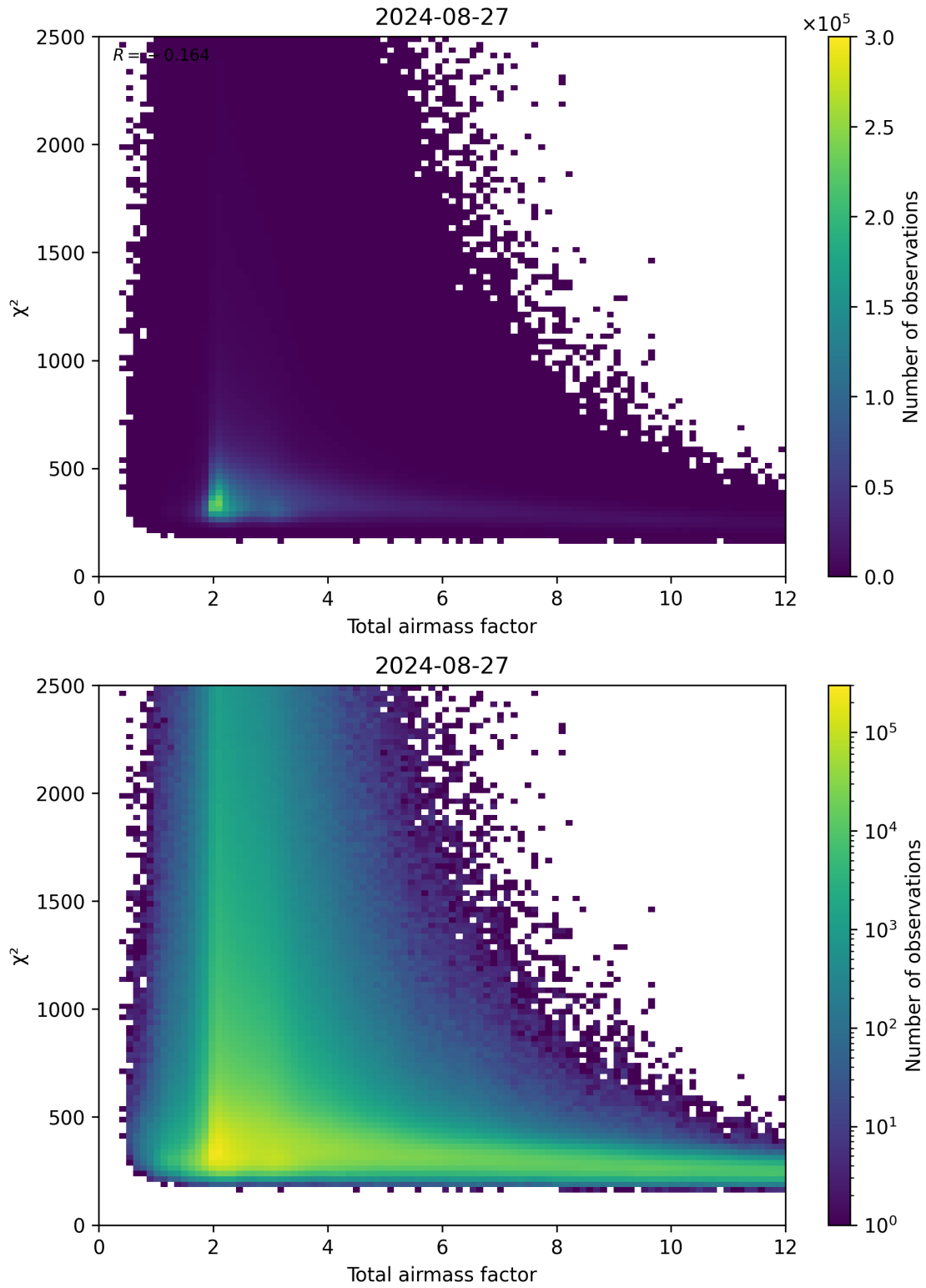
Figure 63: Scatter density plot of “Total airmass factor” against “ \chi^2 ” for 2024-08-27 to 2024-08-28.
