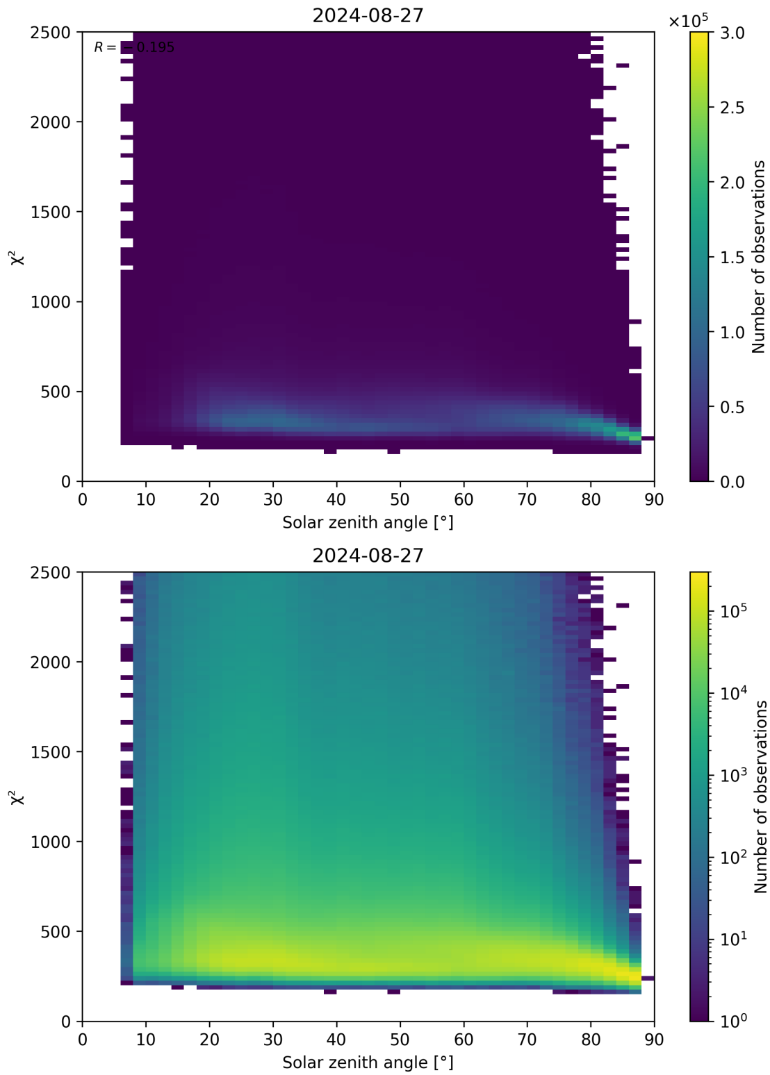
Figure 148: Scatter density plot of “Solar zenith angle” against “ \chi^2 ” for 2024-08-27 to 2024-08-28.
