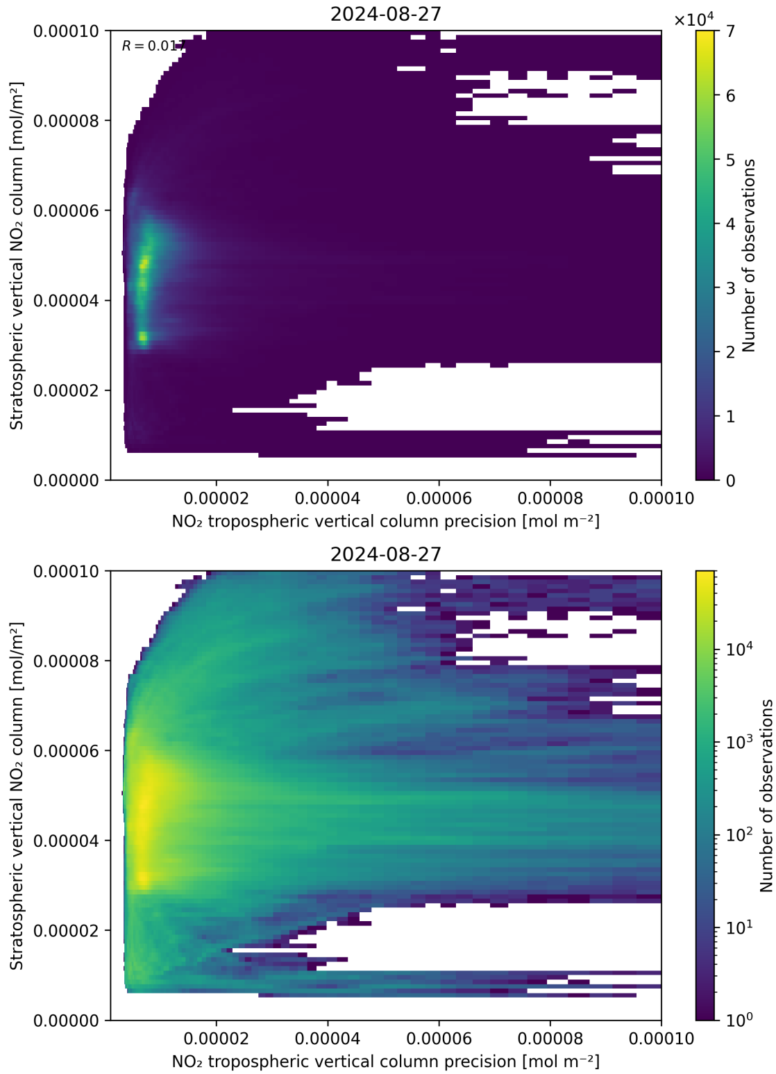
Figure 135: Scatter density plot of “NO 2 tropospheric vertical column precision” against “Stratospheric vertical NO 2 column” for 2024-08-27 to 2024-08-28.
