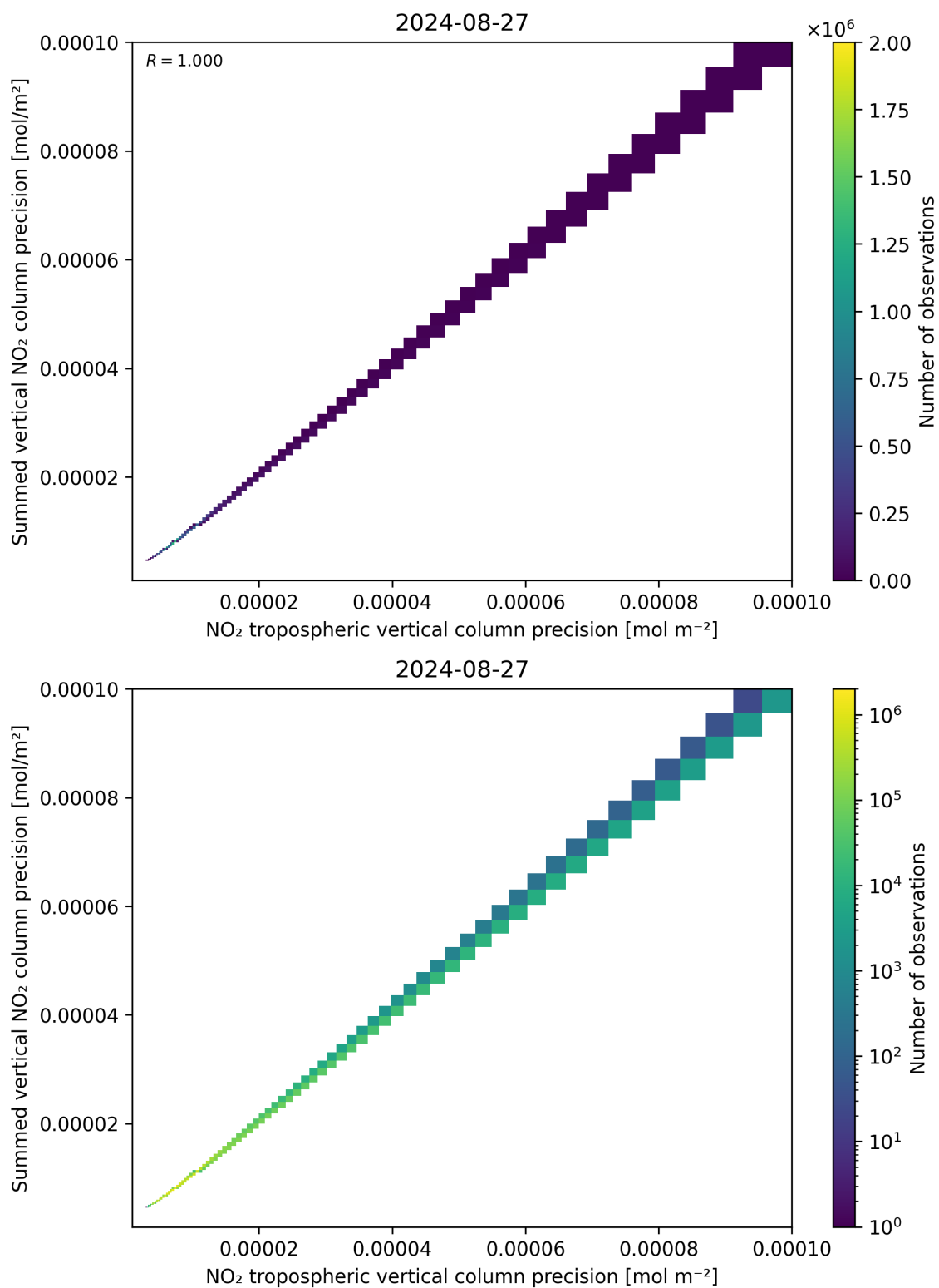
Figure 137: Scatter density plot of “NO 2 tropospheric vertical column precision” against “Summed vertical NO 2 column precision” for 2024-08-27 to 2024-08-28.
