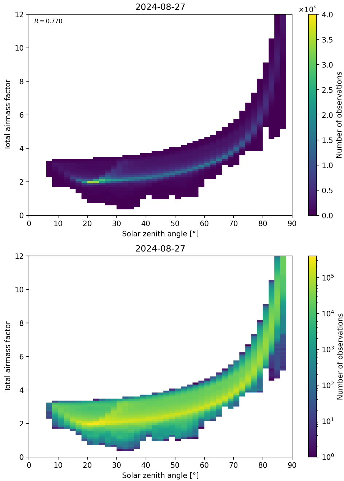
Figure 146: Scatter density plot of “Solar zenith angle” against “Total air mass factor” for 2024-08-27 to 2024-08-28.
