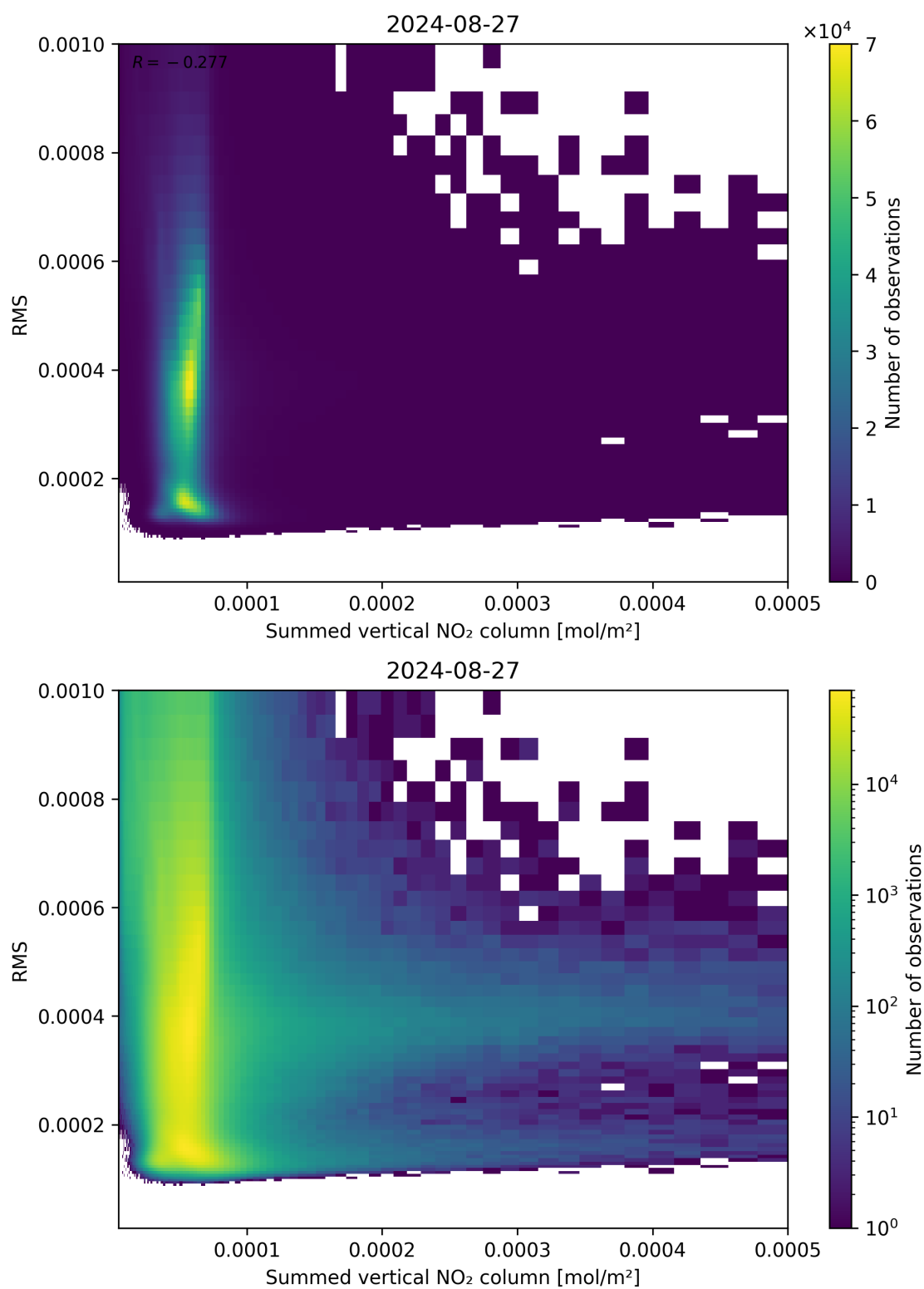
Figure 109: Scatter density plot of “Summed vertical NO 2 column” against “RMS” for 2024-08-27 to 2024-08-28.
