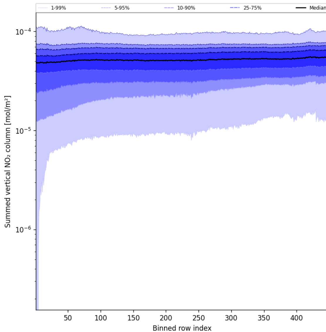
Figure 57: Along track statistics of “Summed vertical NO 2 column” for 2024-08-27 to 2024-08-28
