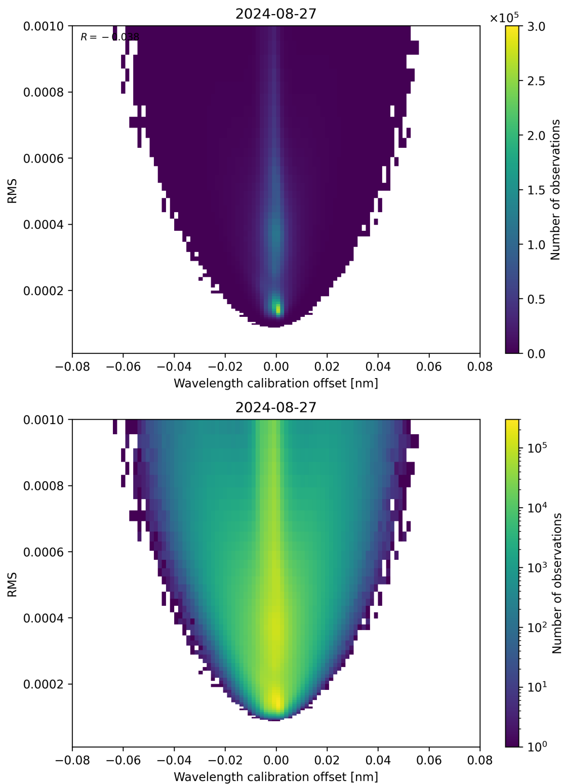
Figure 181: Scatter density plot of “Wavelength calibration offset” against “RMS” for 2024-08-27 to 2024-08-28.
