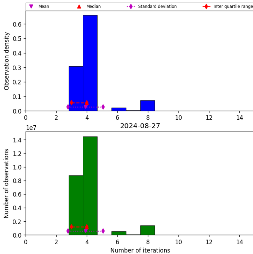
Figure 34: Histogram of “Number of iterations” for 2024-08-27 to 2024-08-28
