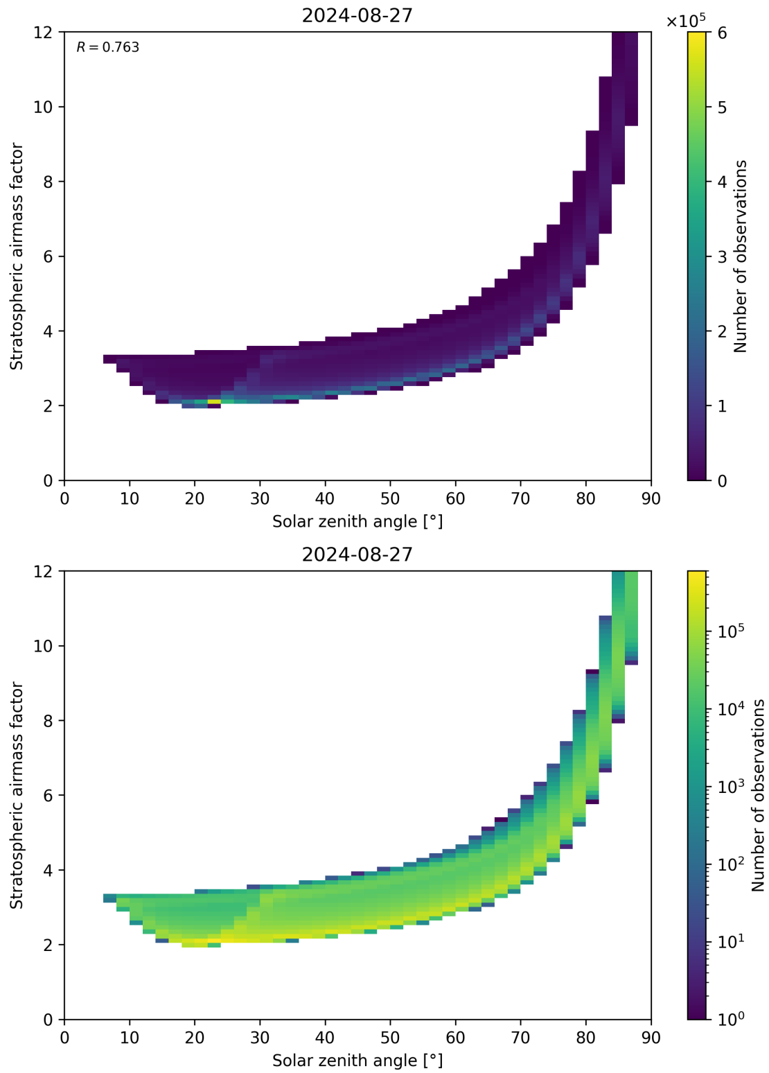
Figure 145: Scatter density plot of “Solar zenith angle” against “Stratospheric airmass factor” for 2024-08-27 to 2024-08-28.
