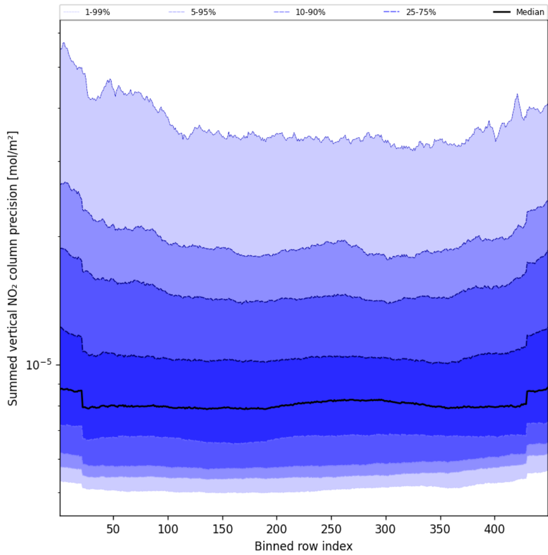
Figure 58: Along track statistics of “Summed vertical NO 2 column precision” for 2024-08-27 to 2024-08-28
