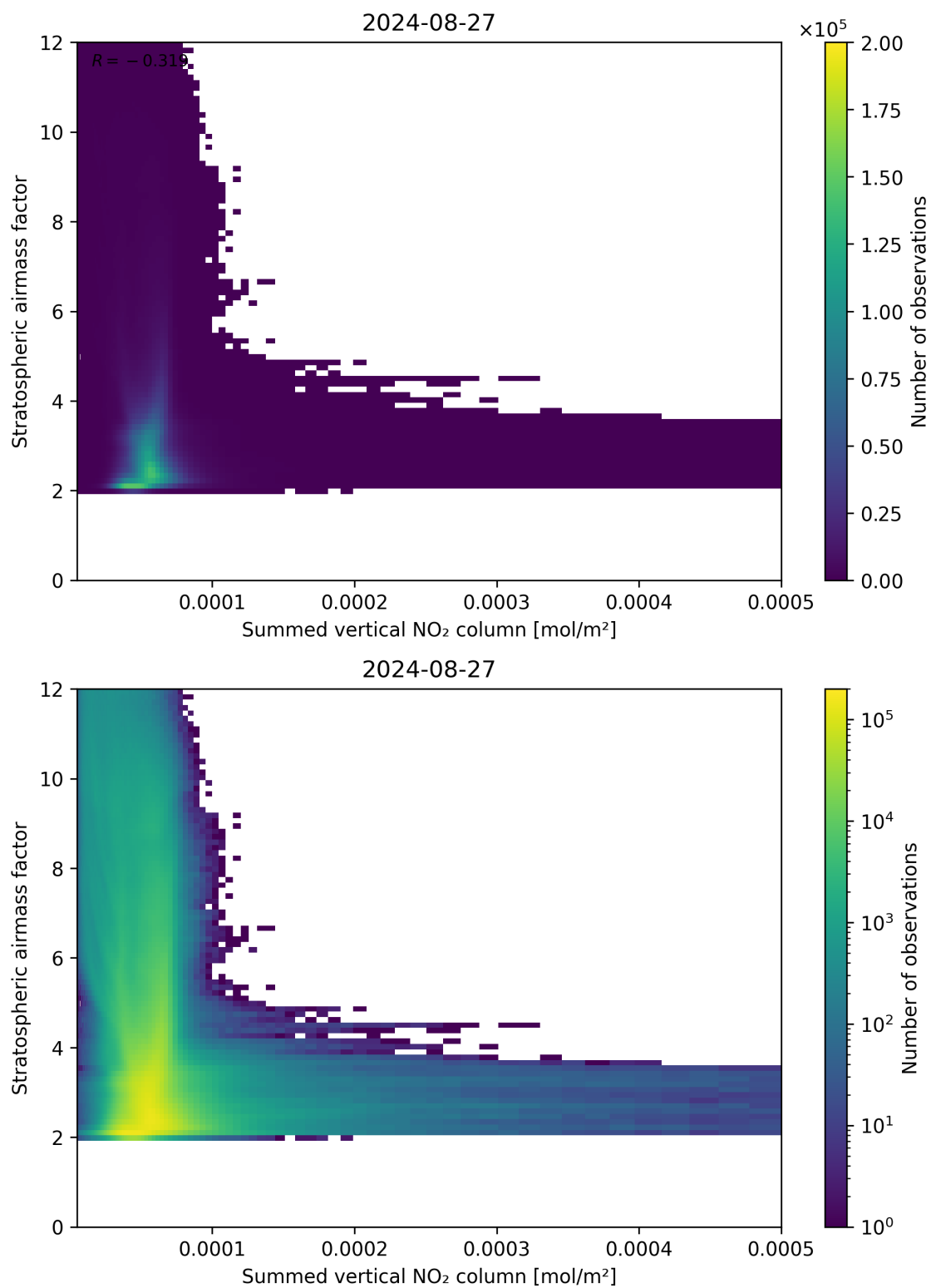
Figure 103: Scatter density plot of “Summed vertical NO 2 column” against “Stratospheric air mass factor” for 2024-08-27 to 2024-08-28.
