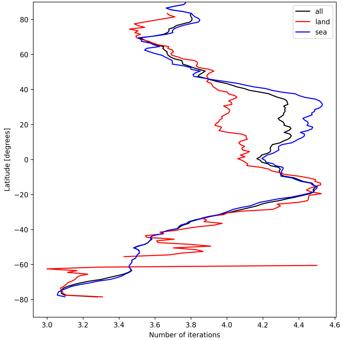
Figure 17: Zonal average of “Number of iterations” for 2024-08-27 to 2024-08-28.
