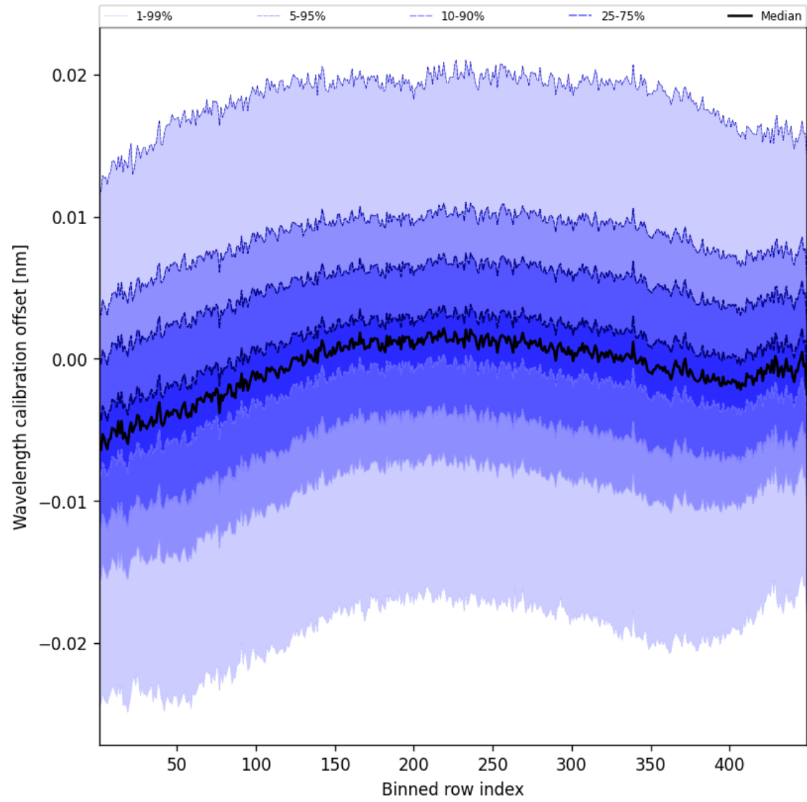
Figure 52: Along track statistics of “Wavelength calibration offset” for 2024-08-27 to 2024-08-28
