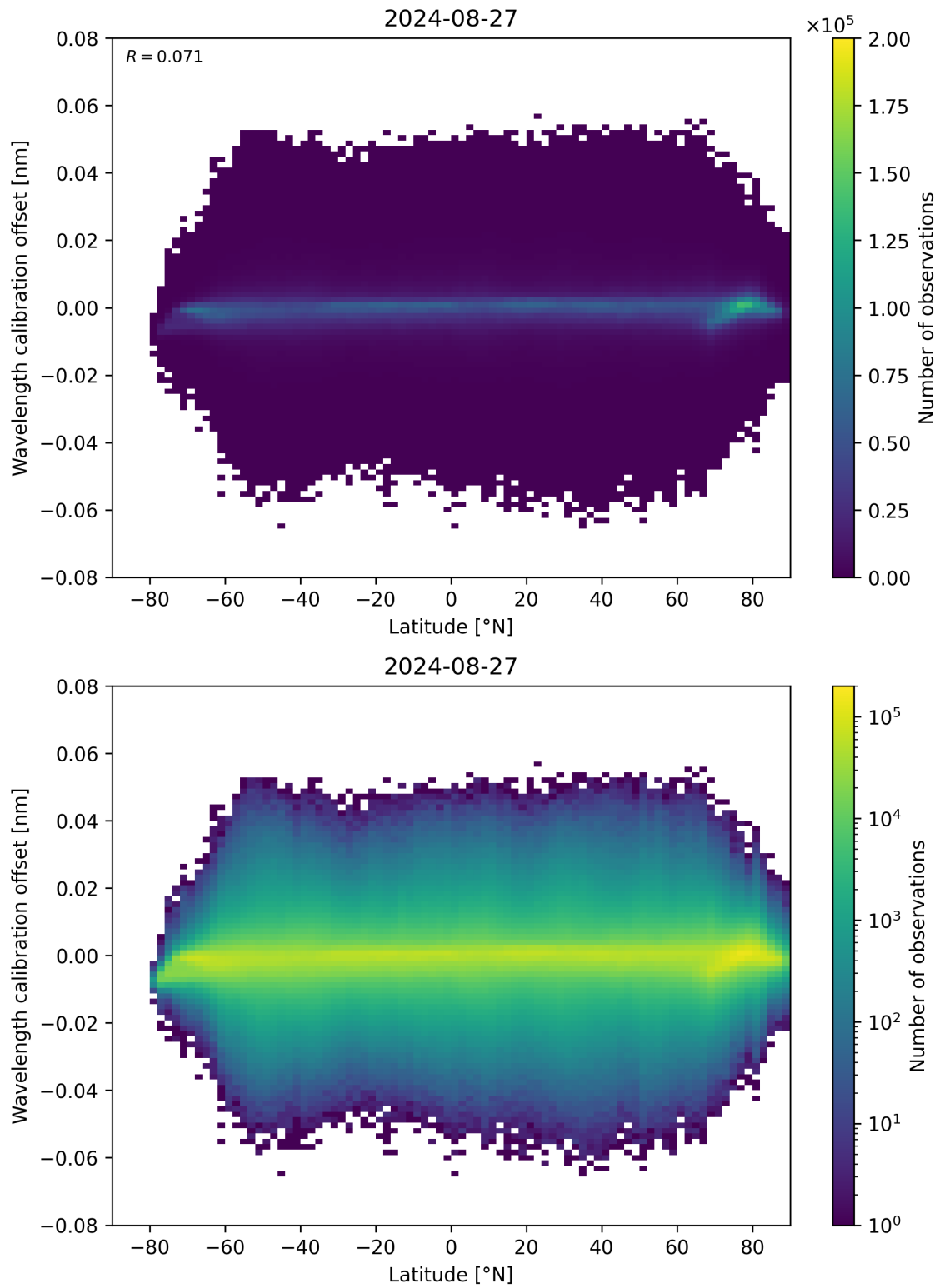
Figure 95: Scatter density plot of “Latitude” against “Wavelength calibration offset” for 2024-08-27 to 2024-08-28.
