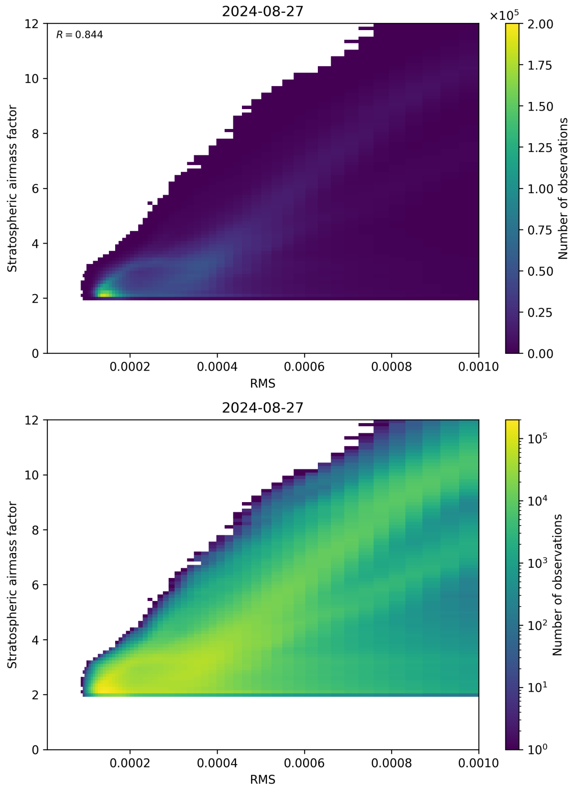
Figure 144: Scatter density plot of “RMS” against “Stratospheric airmass factor” for 2024-08-27 to 2024-08-28.
