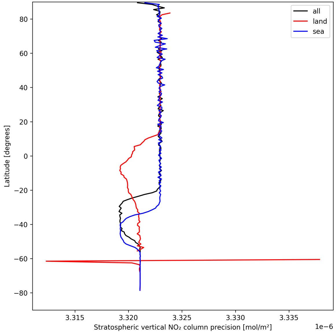
Figure 20: Zonal average of “Stratospheric vertical NO 2 column precision” for 2024-08-27 to 2024-08-28.
