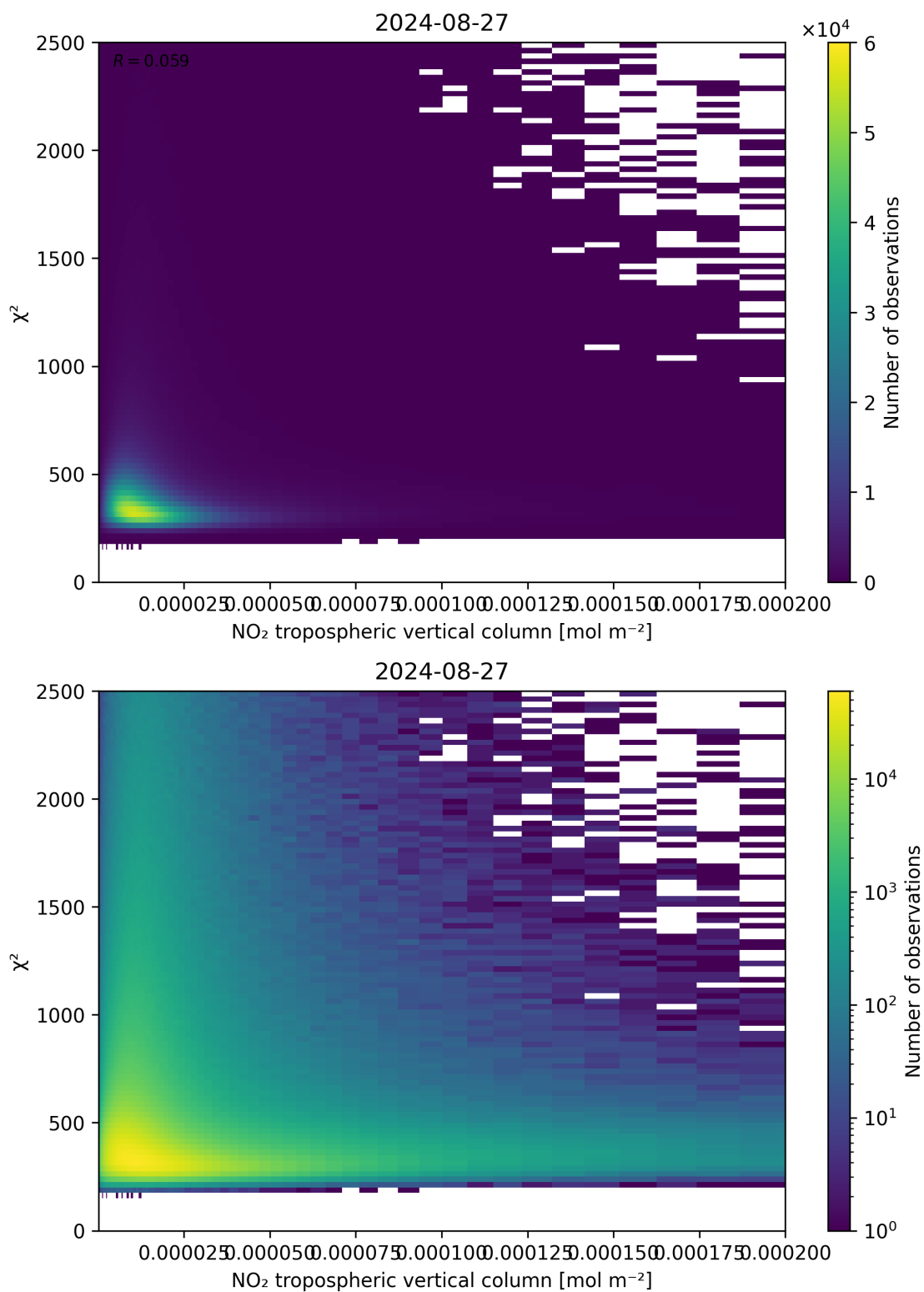
Figure 124: Scatter density plot of “NO 2 tropospheric vertical column” against “ \chi^2 ” for 2024-08-27 to 2024-08-28.
