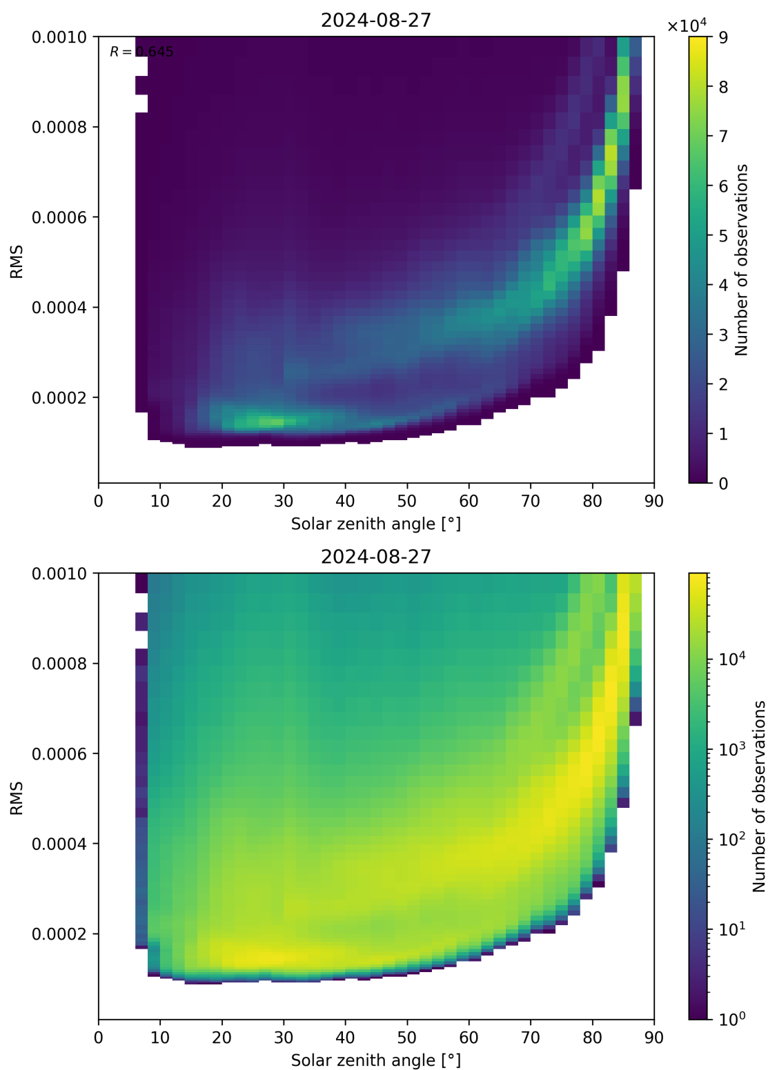
Figure 157: Scatter density plot of “Solar zenith angle” against “RMS” for 2024-08-27 to 2024-08-28.
