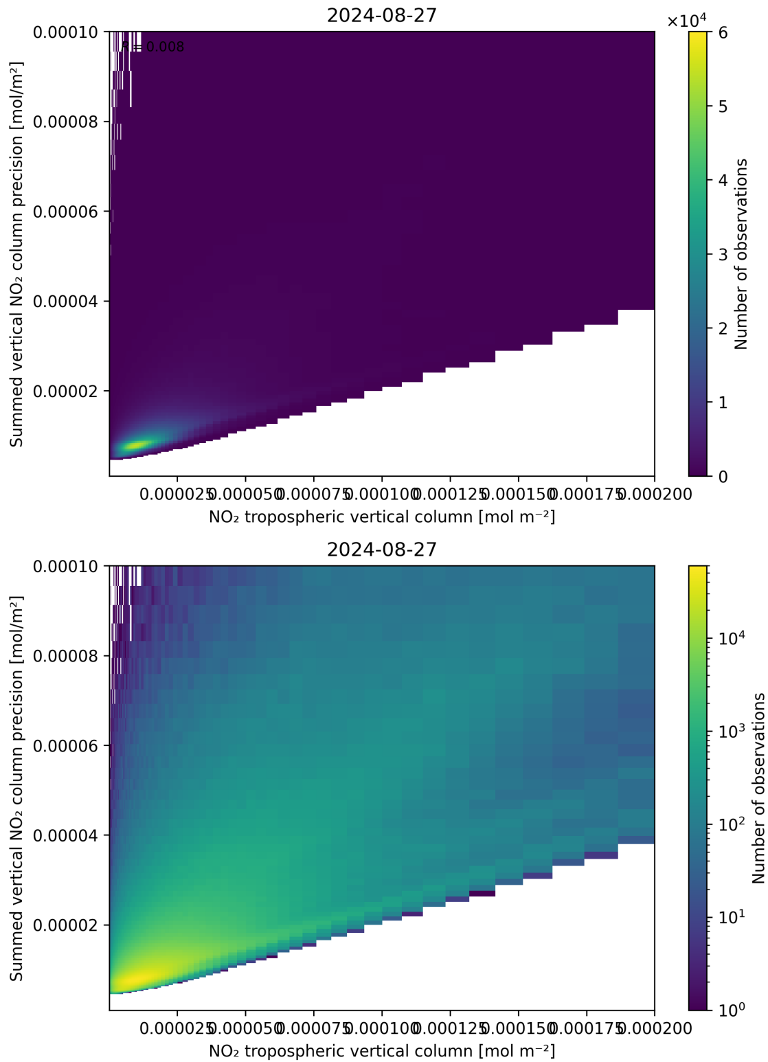
Figure 127: Scatter density plot of “NO 2 tropospheric vertical column” against “Summed vertical NO 2 column precision” for 2024-08-27 to 2024-08-28.
