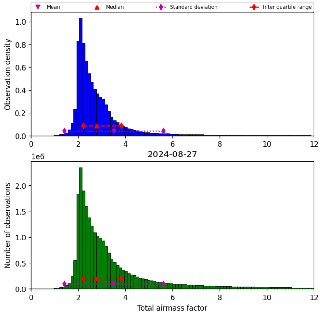
Figure 32: Histogram of “Total airmass factor” for 2024-08-27 to 2024-08-28
