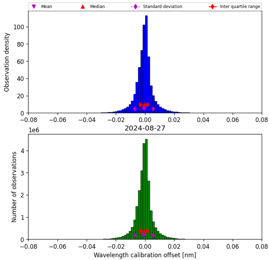
Figure 35: Histogram of “Wavelength calibration offset” for 2024-08-27 to 2024-08-28
