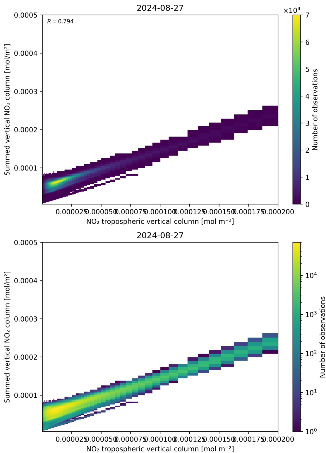
Figure 126: Scatter density plot of “NO 2 tropospheric vertical column” against “Summed vertical NO 2 column” for 2024-08-27 to 2024-08-28.
