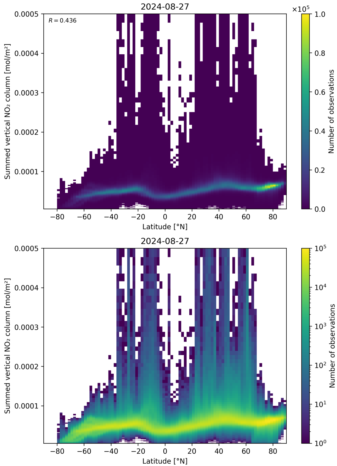
Figure 88: Scatter density plot of “Latitude” against “Summed vertical NO 2 column” for 2024-08-27 to 2024-08-28.
