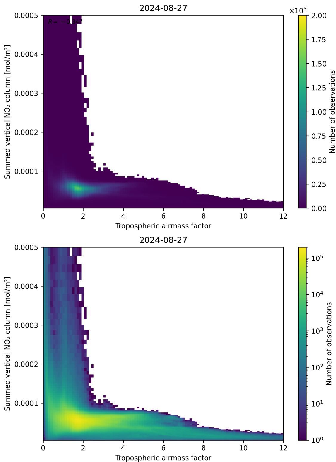
Figure 75: Scatter density plot of “Tropospheric airmass factor” against “Summed vertical NO 2 column” for 2024-08-27 to 2024-08-28.
