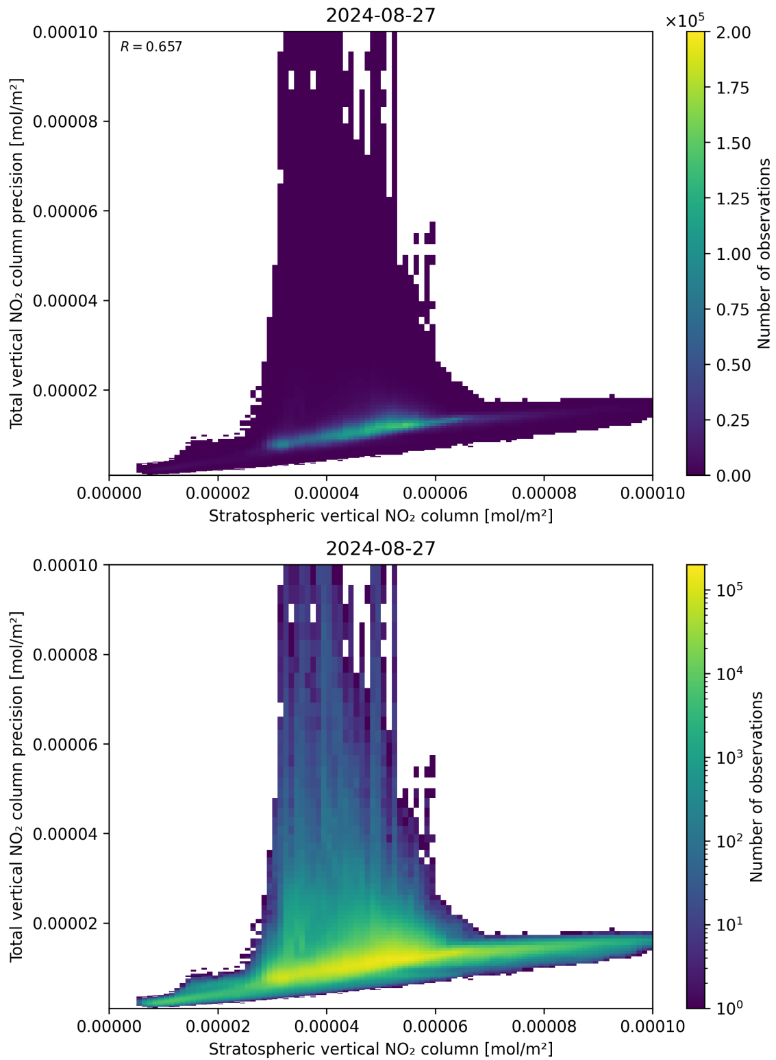
Figure 101: Scatter density plot of “Stratospheric vertical NO 2 column” against “Total vertical NO 2 column precision” for 2024-08-27 to 2024-08-28.
