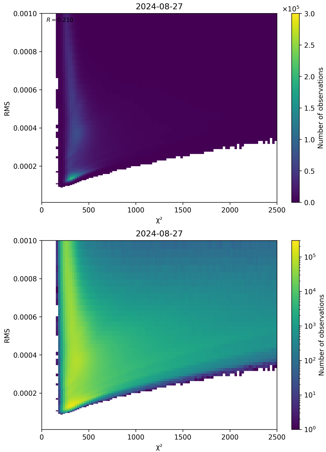
Figure 82: Scatter density plot of “ \chi^2 ” against “RMS” for 2024-08-27 to 2024-08-28.
