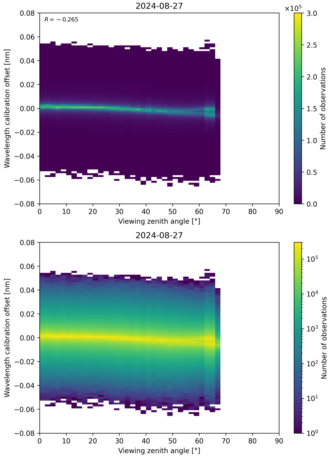
Figure 173: Scatter density plot of “Viewing zenith angle” against “Wavelength calibration offset” for 2024-08-27 to 2024-08-28.
