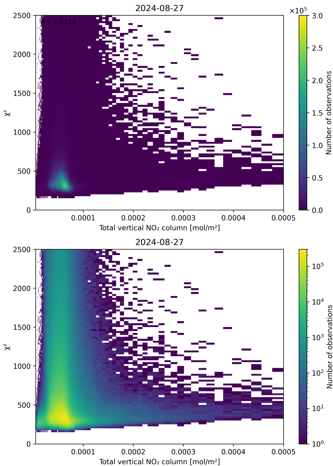
Figure 111: Scatter density plot of “Total vertical NO 2 column” against “ \chi^2 ” for 2024-08-27 to 2024-08-28.
