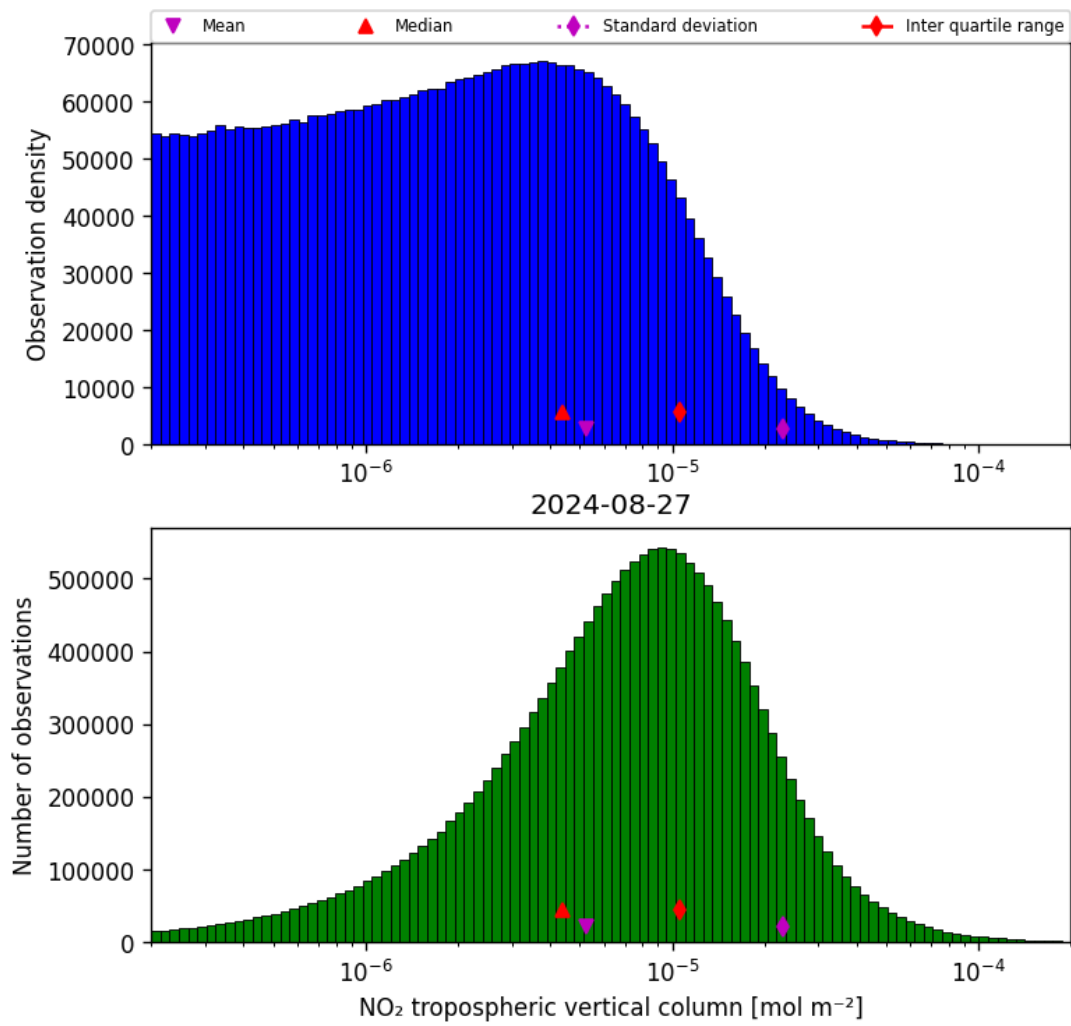
Figure 29: Histogram of “NO 2 tropospheric vertical column” for 2024-08-27 to 2024-08-28
