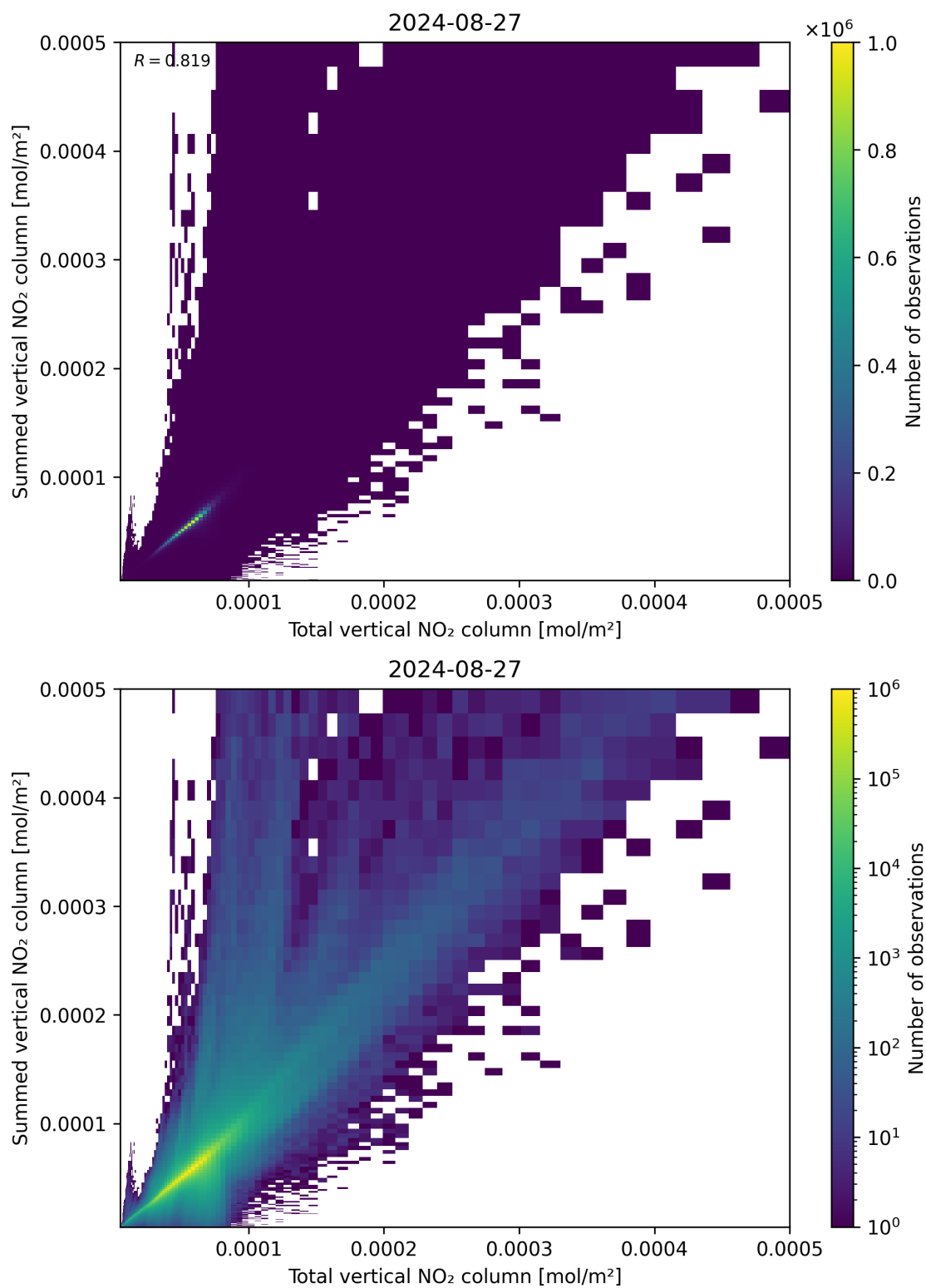
Figure 112: Scatter density plot of “Total vertical NO 2 column” against “Summed vertical NO 2 column” for 2024-08-27 to 2024-08-28.
