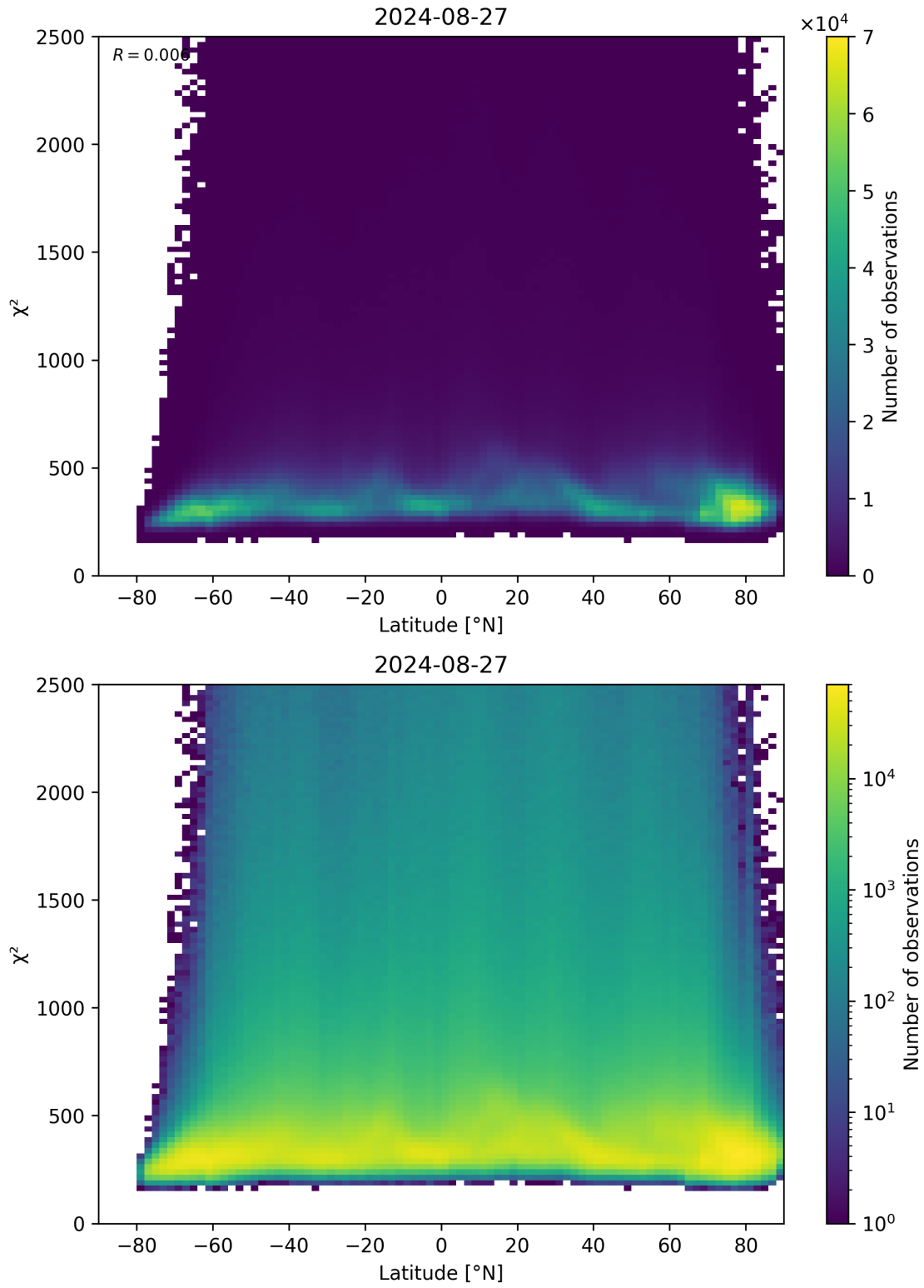
Figure 86: Scatter density plot of “Latitude” against “ \chi^2 ” for 2024-08-27 to 2024-08-28.
