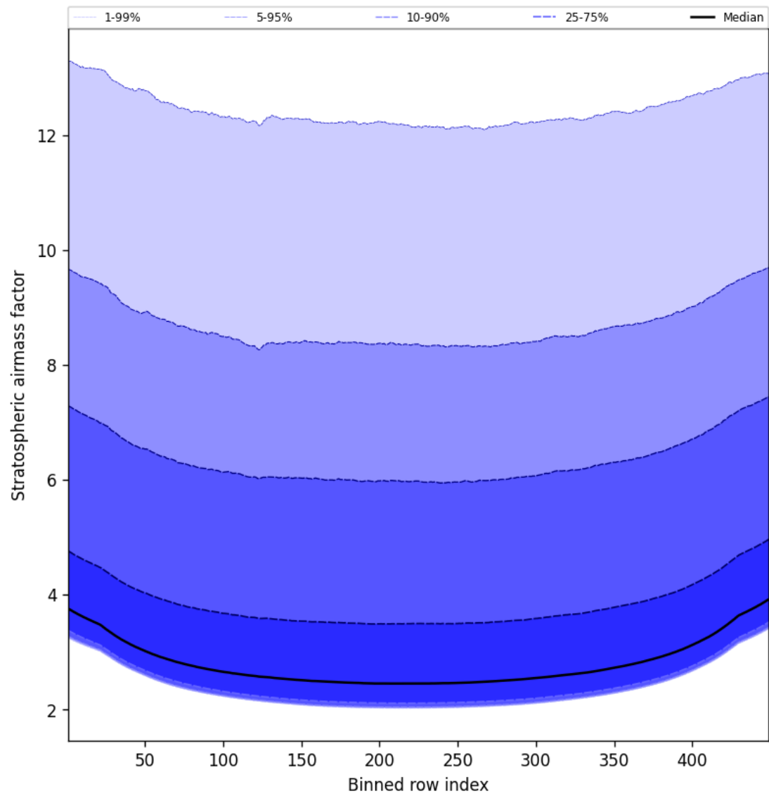
Figure 61: Along track statistics of “Stratospheric airmass factor” for 2024-08-27 to 2024-08-28
