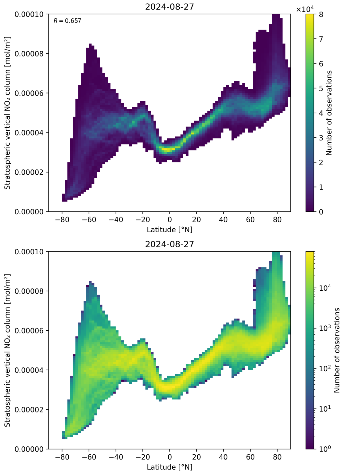
Figure 87: Scatter density plot of “Latitude” against “Stratospheric vertical \text{NO}_2 column” for 2024-08-27 to 2024-08-28.
