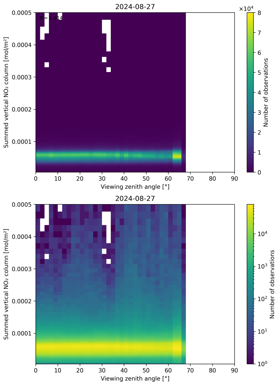
Figure 165: Scatter density plot of “Viewing zenith angle” against “Summed vertical NO 2 column” for 2024-08-27 to 2024-08-28.
