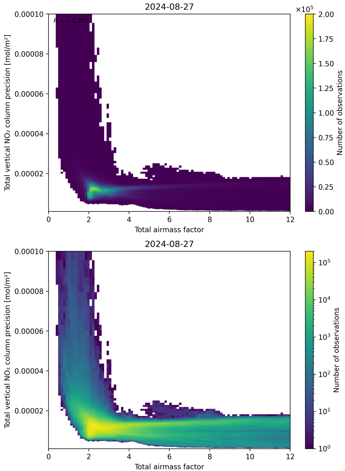
Figure 68: Scatter density plot of “Total airmass factor” against “Total vertical NO 2 column precision” for 2024-08-27 to 2024-08-28.
