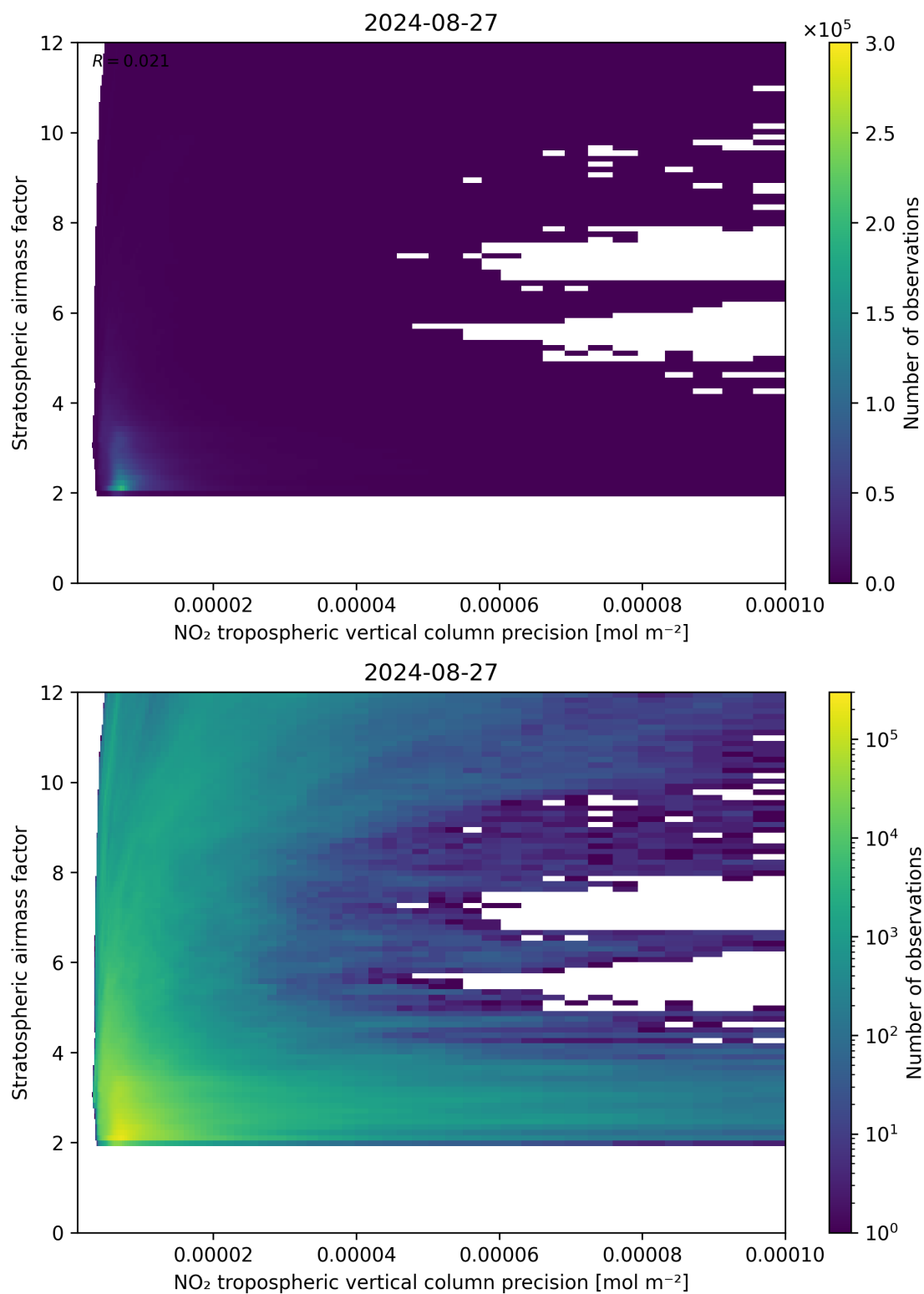
Figure 131: Scatter density plot of “NO 2 tropospheric vertical column precision” against “Stratospheric airmass factor” for 2024-08-27 to 2024-08-28.
