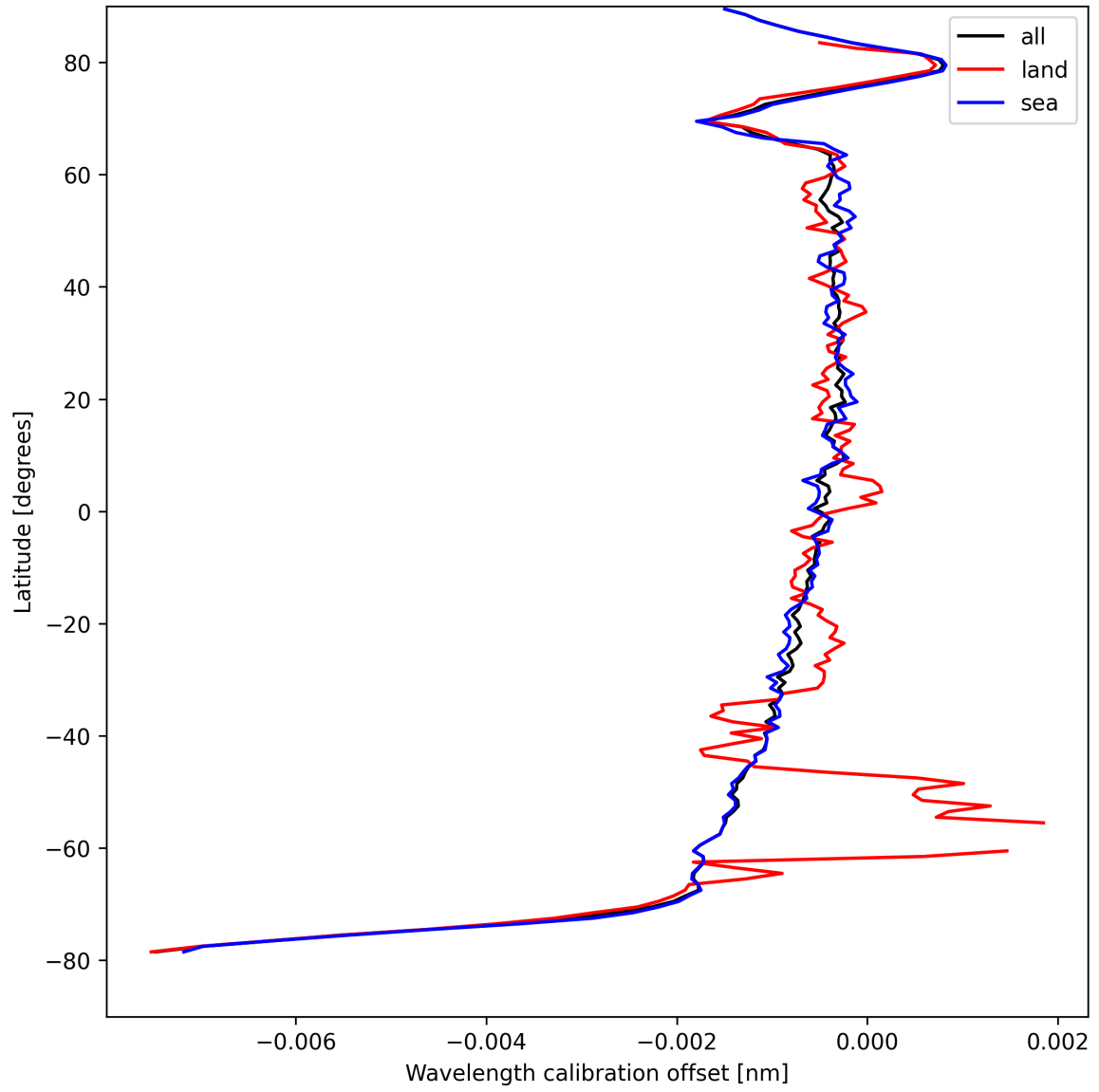
Figure 18: Zonal average of “Wavelength calibration offset” for 2024-08-27 to 2024-08-28.
