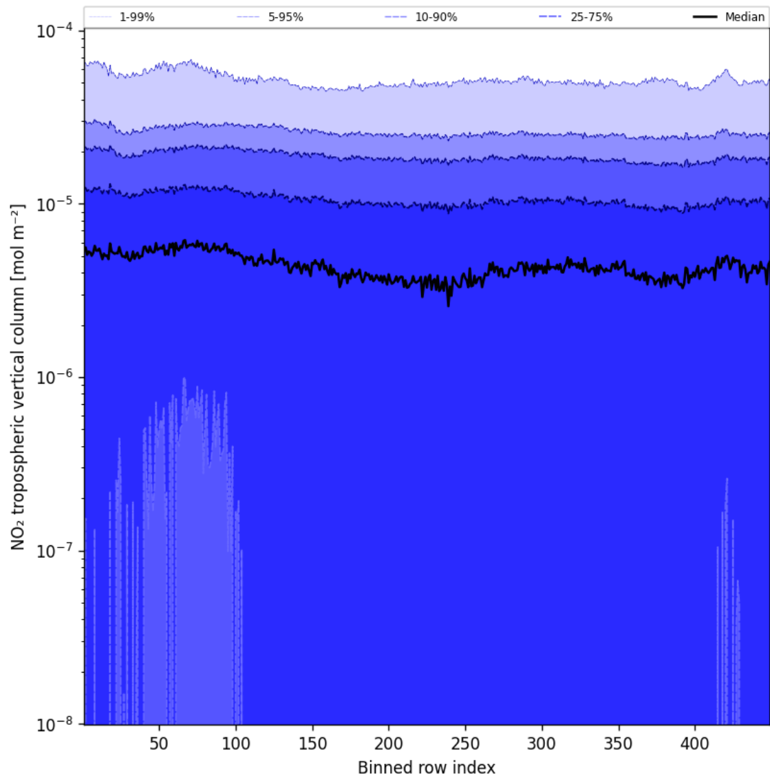
Figure 46: Along track statistics of “NO 2 tropospheric vertical column” for 2024-08-27 to 2024-08-28
