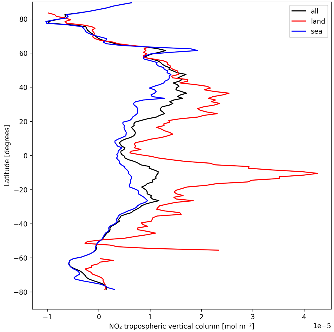
Figure 12: Zonal average of “NO 2 tropospheric vertical column” for 2024-08-27 to 2024-08-28.
