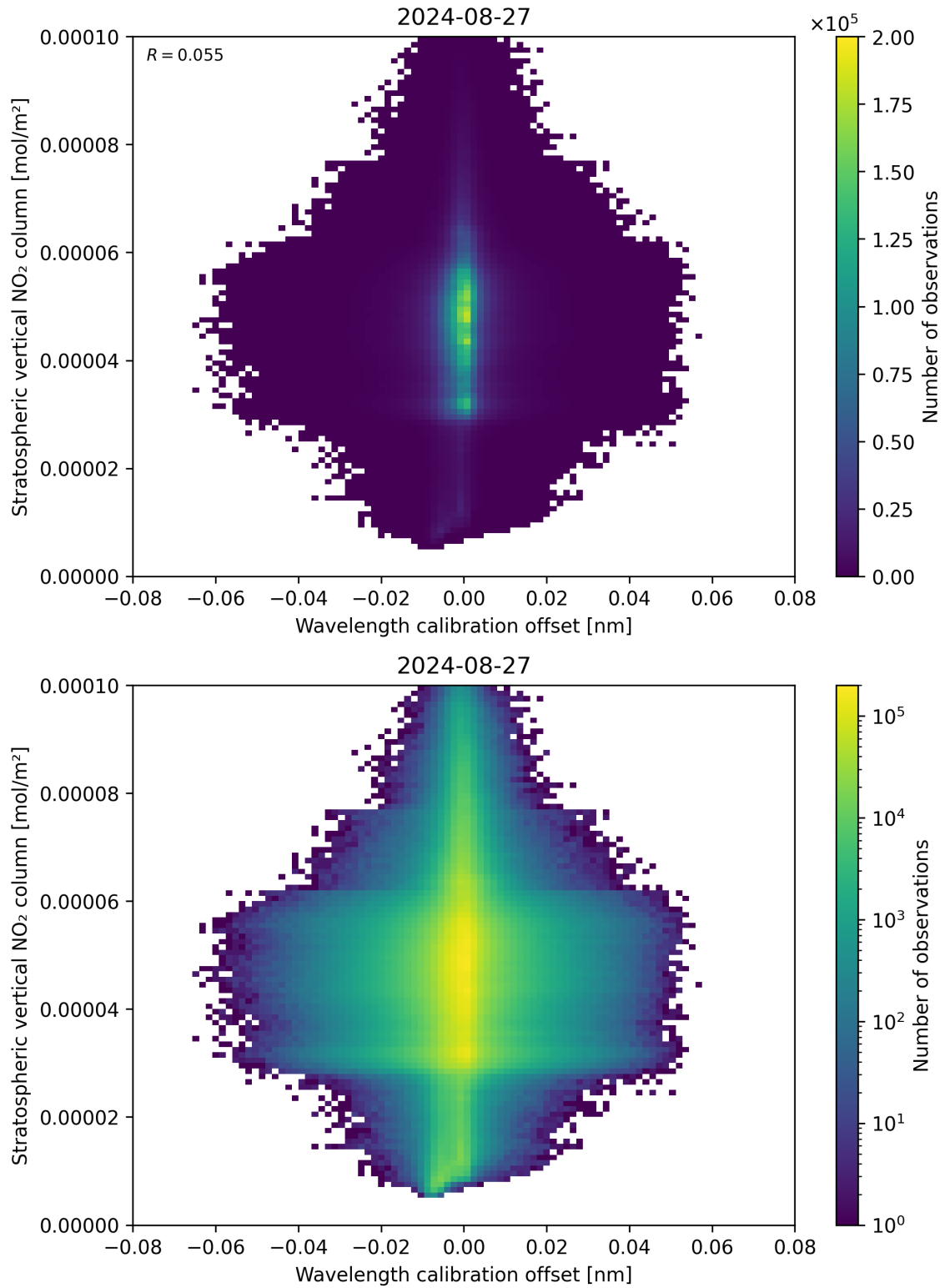
Figure 176: Scatter density plot of “Wavelength calibration offset” against “Stratospheric vertical NO 2 column” for 2024-08-27 to 2024-08-28.
