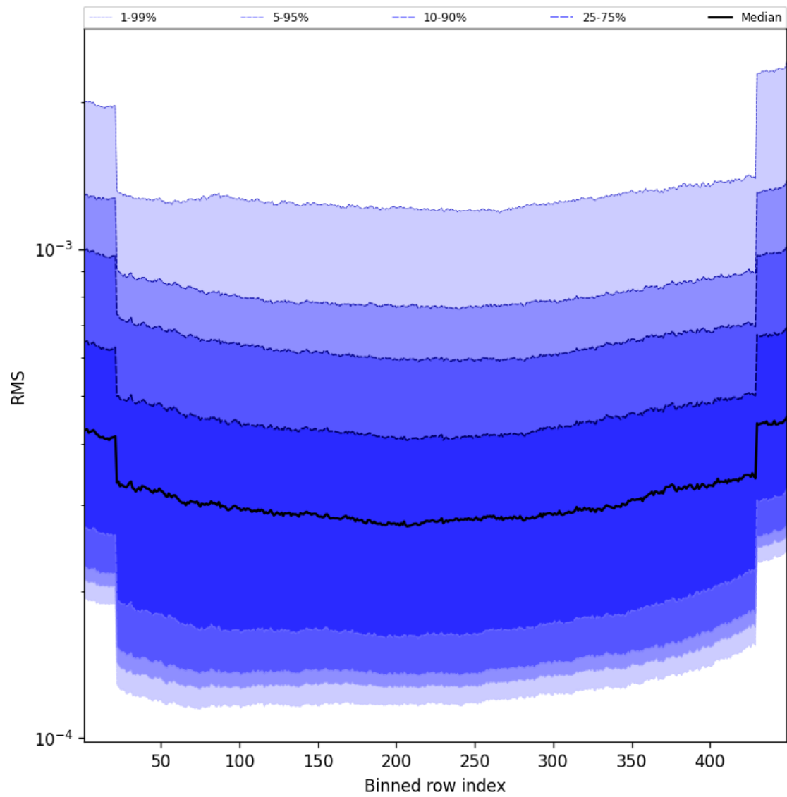
Figure 60: Along track statistics of “RMS” for 2024-08-27 to 2024-08-28
