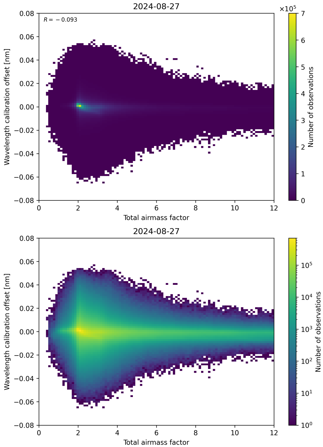
Figure 70: Scatter density plot of “Total airmass factor” against “Wavelength calibration offset” for 2024-08-27 to 2024-08-28.
