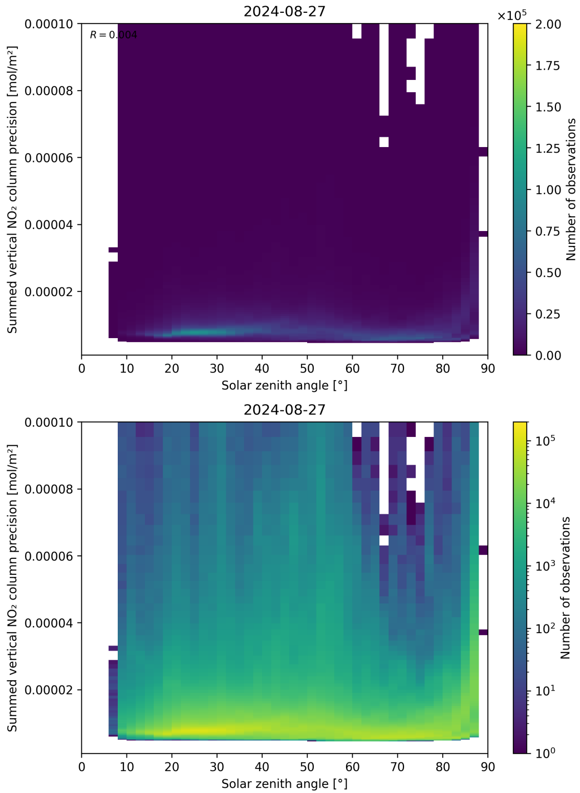
Figure 152: Scatter density plot of “Solar zenith angle” against “Summed vertical NO 2 column precision” for 2024-08-27 to 2024-08-28.
