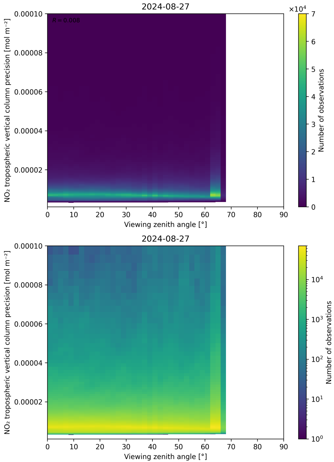
Figure 170: Scatter density plot of “Viewing zenith angle” against “NO 2 tropospheric vertical column precision” for 2024-08-27 to 2024-08-28.
