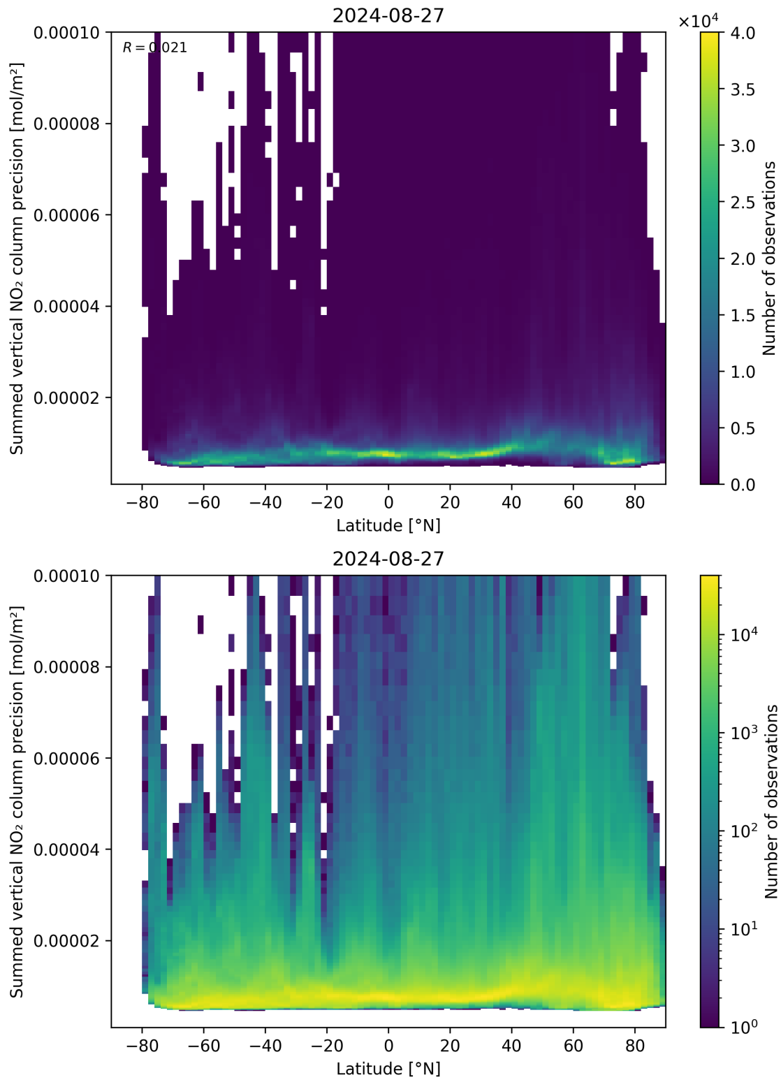
Figure 89: Scatter density plot of “Latitude” against “Summed vertical NO 2 column precision” for 2024-08-27 to 2024-08-28.
