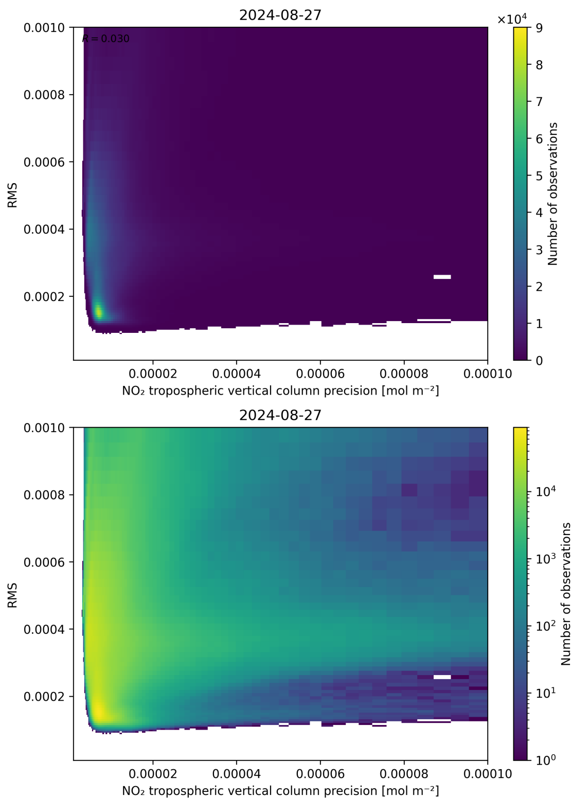
Figure 140: Scatter density plot of “NO 2 tropospheric vertical column precision” against “RMS” for 2024-08-27 to 2024-08-28.
