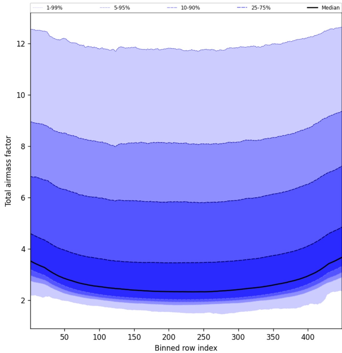
Figure 49: Along track statistics of “Total airmass factor” for 2024-08-27 to 2024-08-28
