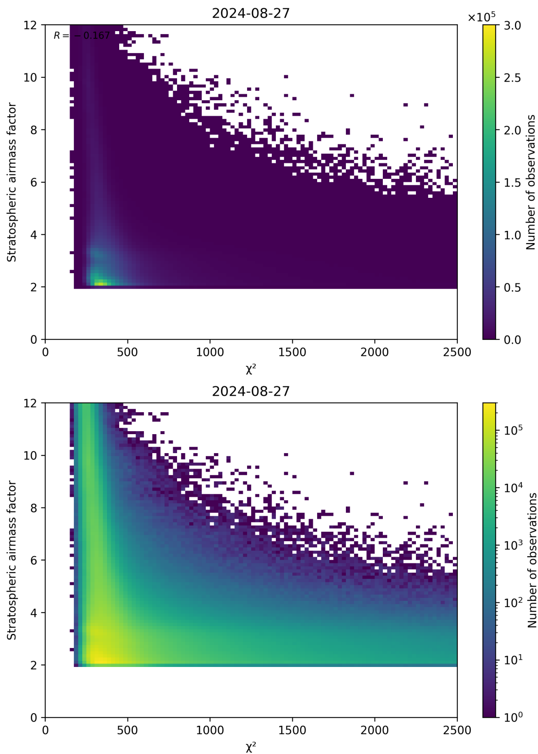
Figure 81: Scatter density plot of “ \chi^2 ” against “Stratospheric airmass factor” for 2024-08-27 to 2024-08-28.
