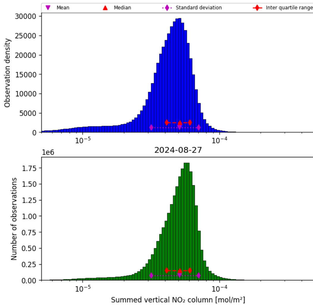
Figure 40: Histogram of “Summed vertical NO 2 column” for 2024-08-27 to 2024-08-28
