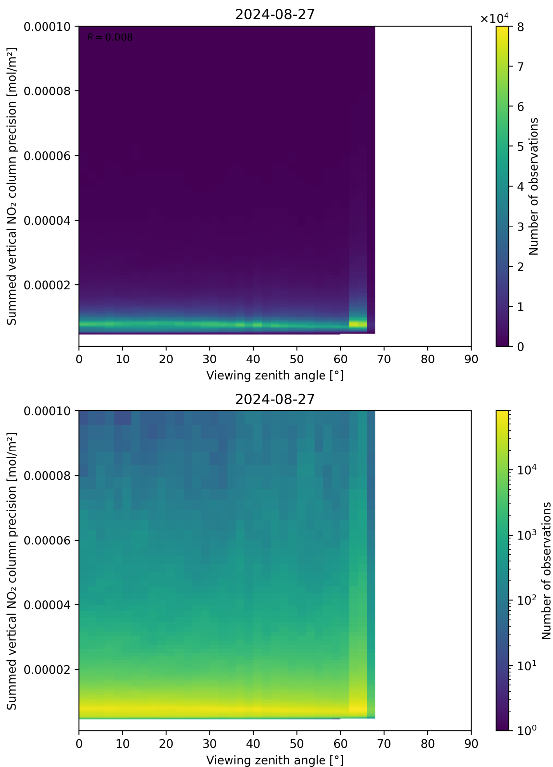
Figure 166: Scatter density plot of “Viewing zenith angle” against “Summed vertical NO 2 column precision” for 2024-08-27 to 2024-08-28.
