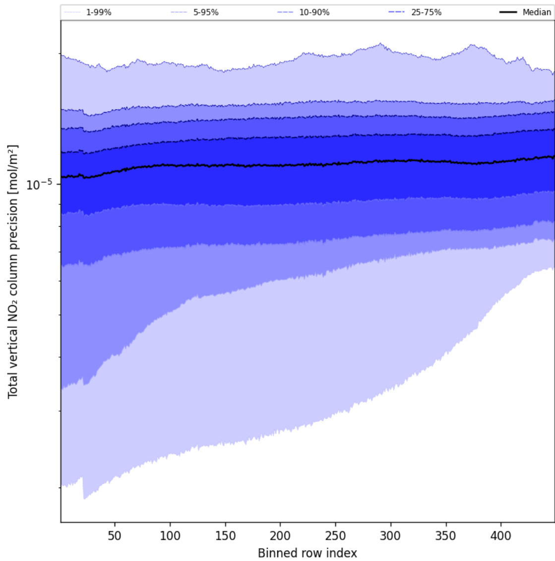
Figure 56: Along track statistics of “Total vertical NO 2 column precision” for 2024-08-27 to 2024-08-28
