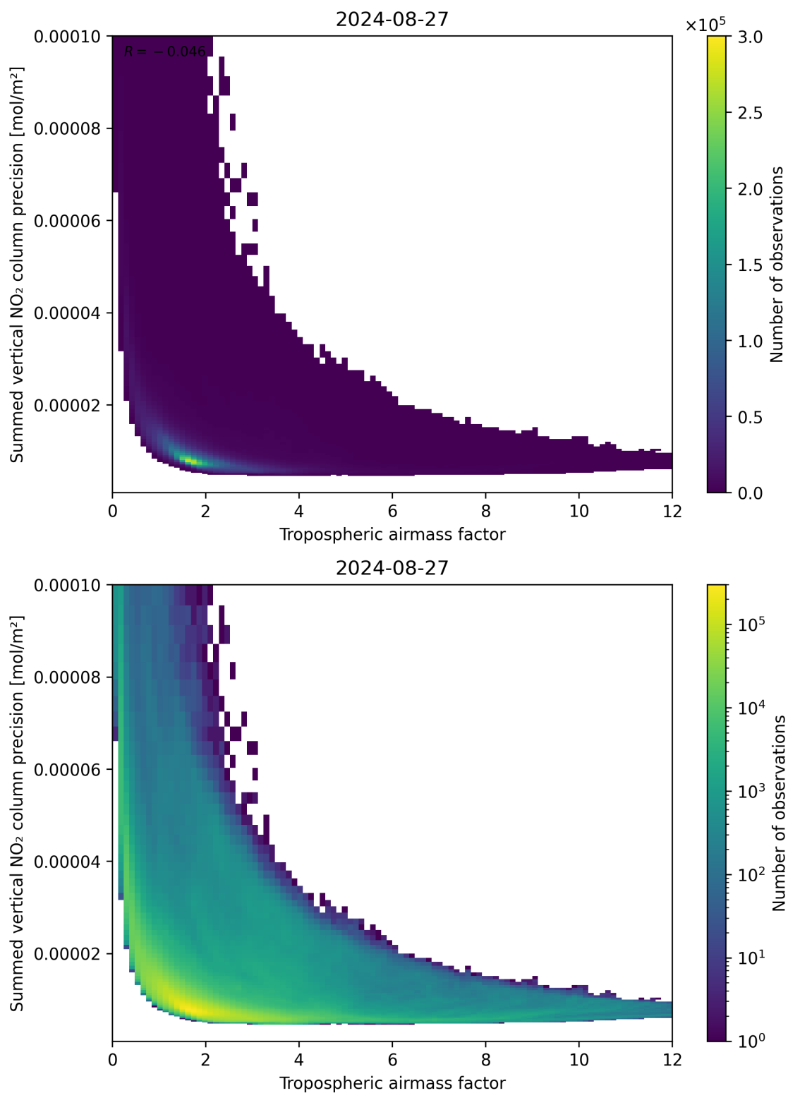
Figure 76: Scatter density plot of “Tropospheric airmass factor” against “Summed vertical NO 2 column precision” for 2024-08-27 to 2024-08-28.
