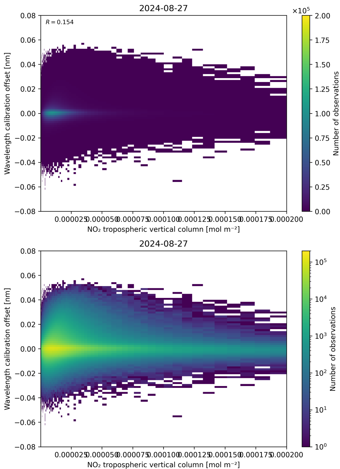
Figure 143: Scatter density plot of “NO 2 tropospheric vertical column” against “Wavelength calibration offset” for 2024-08-27 to 2024-08-28.
