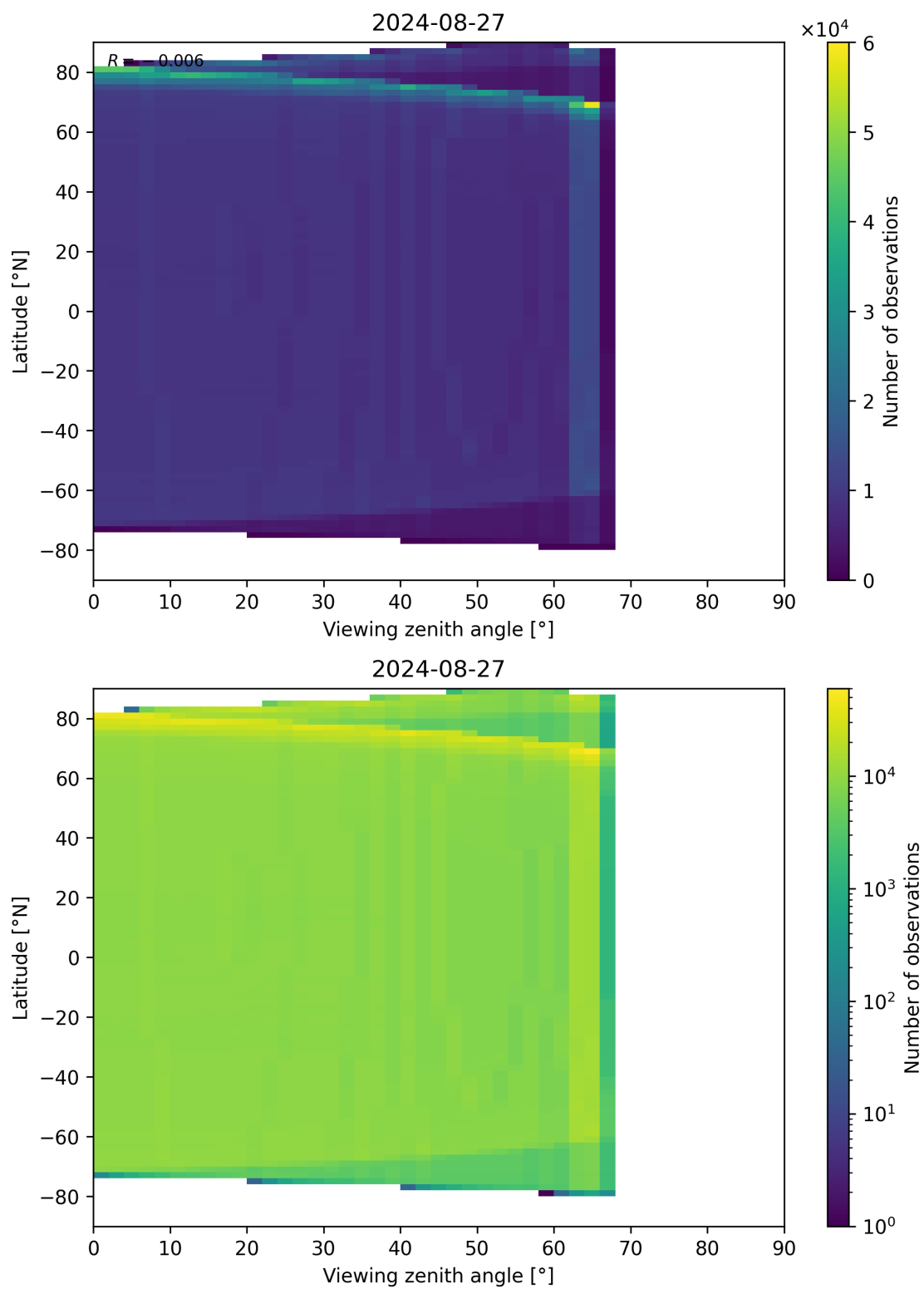
Figure 163: Scatter density plot of “Viewing zenith angle” against “Latitude” for 2024-08-27 to 2024-08-28.
