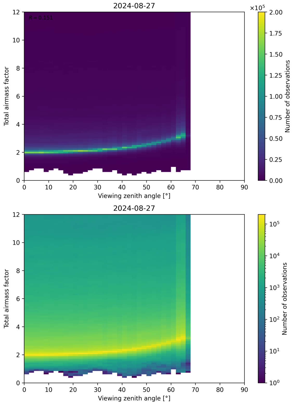
Figure 160: Scatter density plot of “Viewing zenith angle” against “Total airmass factor” for 2024-08-27 to 2024-08-28.
