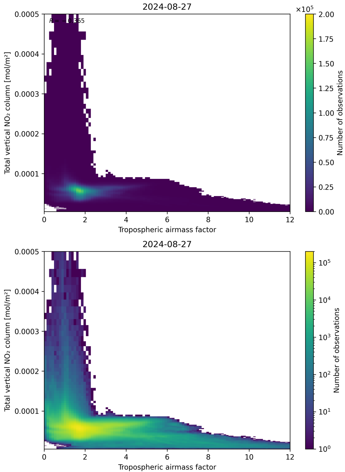
Figure 77: Scatter density plot of “Tropospheric airmass factor” against “Total vertical NO 2 column” for 2024-08-27 to 2024-08-28.
