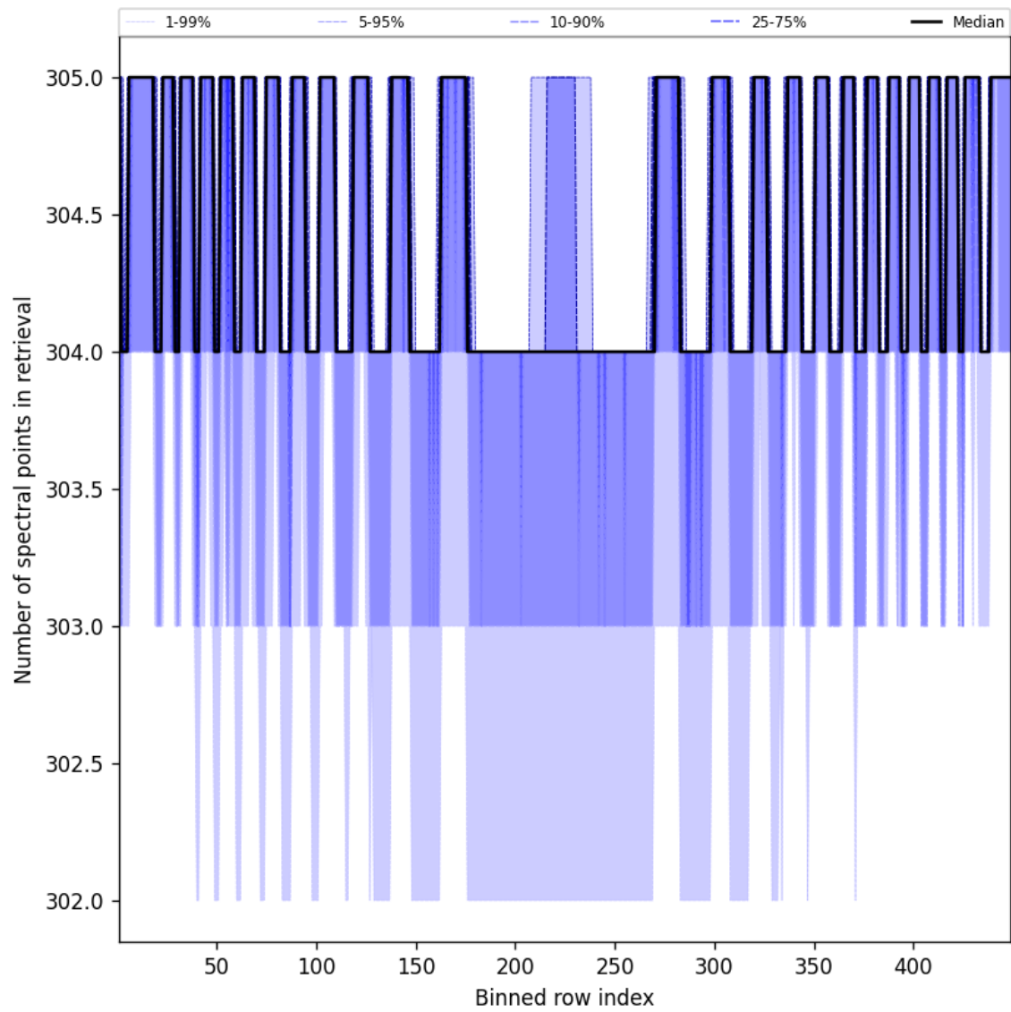
Figure 50: Along track statistics of “Number of spectral points in retrieval” for 2024-08-27 to 2024-08-28
