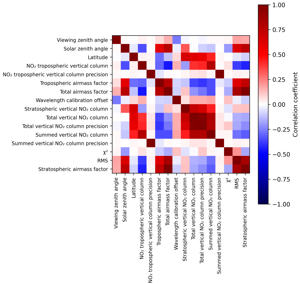
Figure 2: Map of correlation matrix for 2024-08-27 to 2024-08-28.
