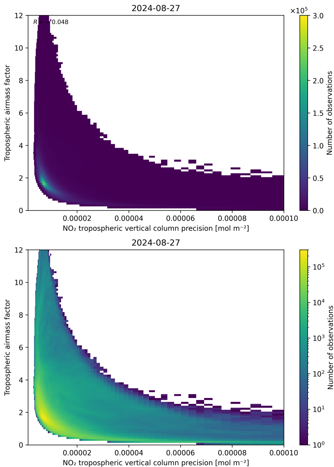
Figure 133: Scatter density plot of “NO 2 tropospheric vertical column precision” against “Tropospheric airmass factor” for 2024-08-27 to 2024-08-28.
