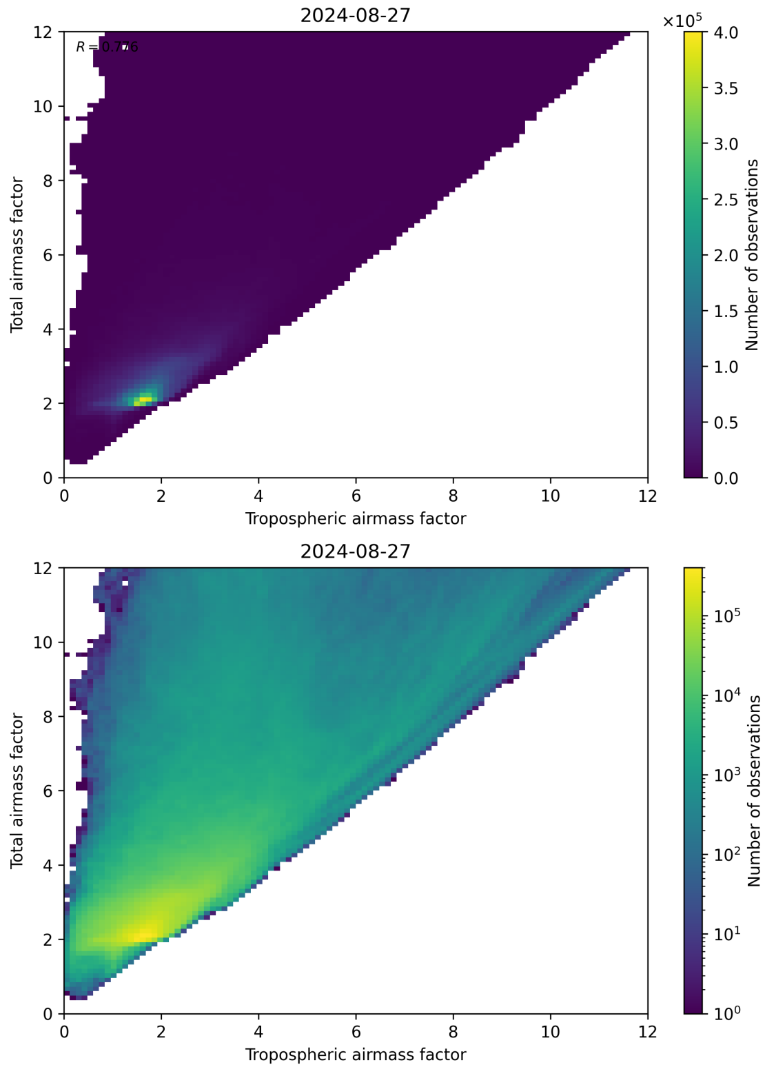
Figure 72: Scatter density plot of “Tropospheric airmass factor” against “Total airmass factor” for 2024-08-27 to 2024-08-28.
