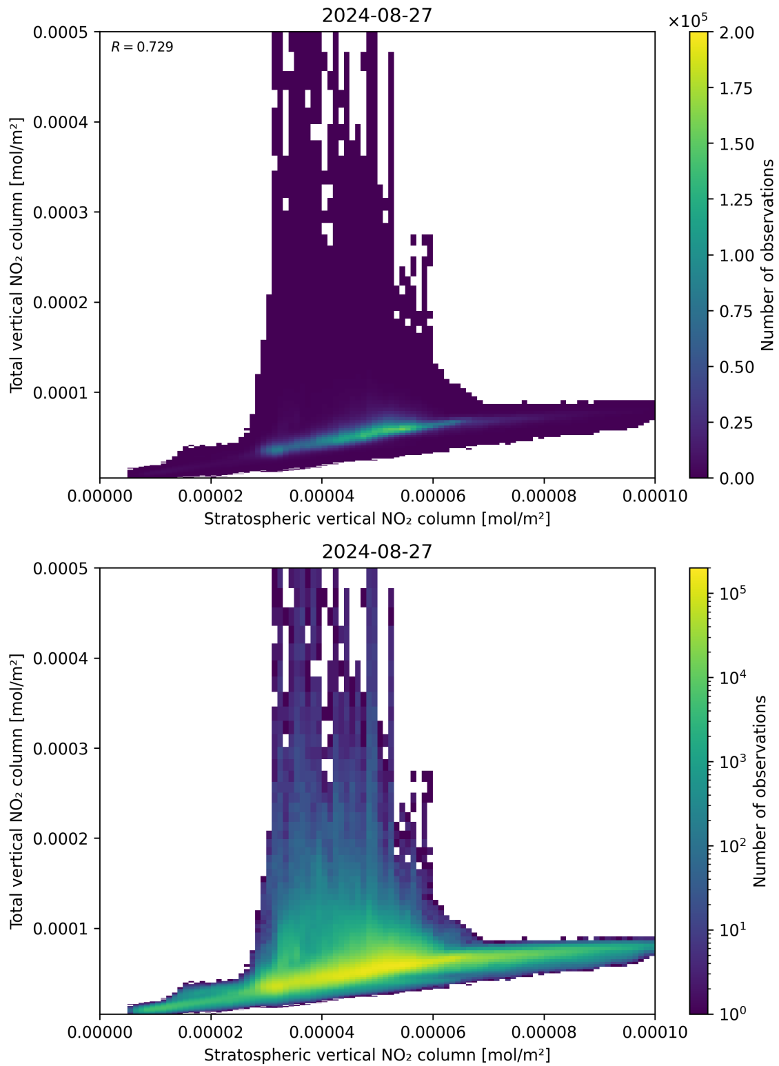
Figure 100: Scatter density plot of “Stratospheric vertical NO 2 column” against “Total vertical NO 2 column” for 2024-08-27 to 2024-08-28.
