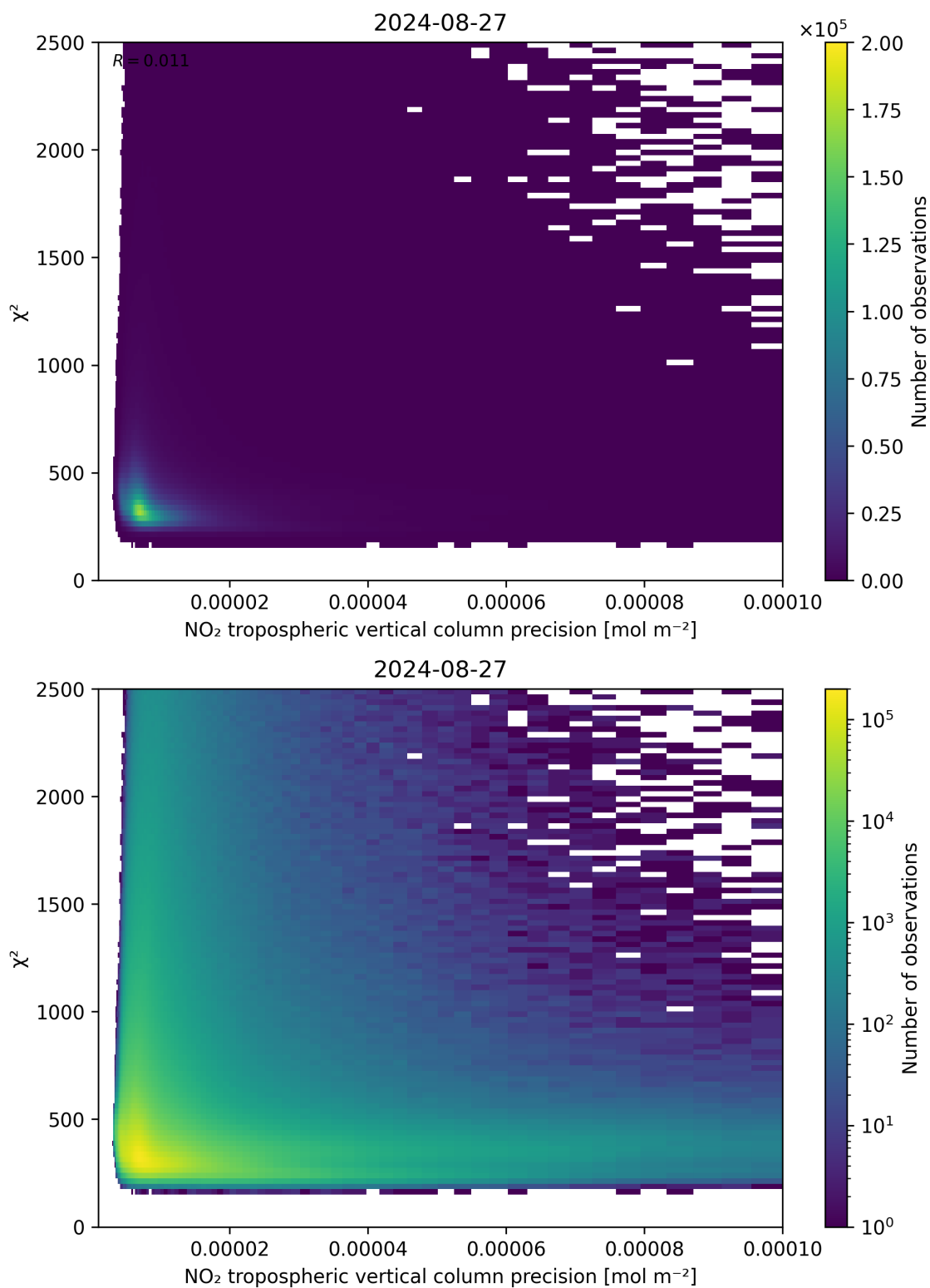
Figure 134: Scatter density plot of “NO 2 tropospheric vertical column precision” against “ \chi^2 ” for 2024-08-27 to 2024-08-28.
