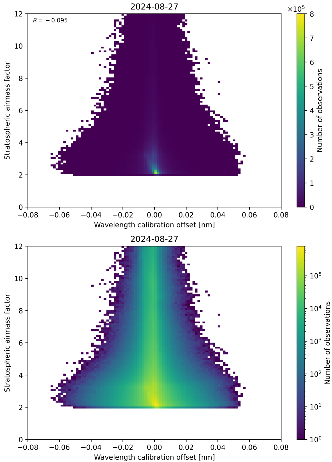
Figure 174: Scatter density plot of “Wavelength calibration offset” against “Stratospheric air mass factor” for 2024-08-27 to 2024-08-28.
