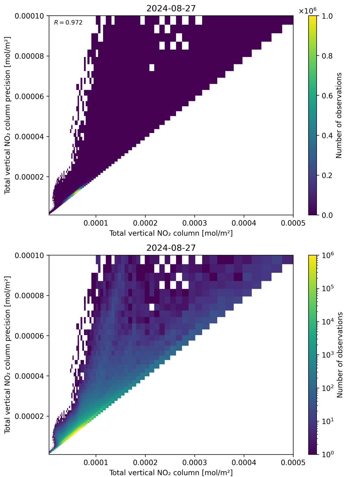
Figure 114: Scatter density plot of “Total vertical NO 2 column” against “Total vertical NO 2 column precision” for 2024-08-27 to 2024-08-28.
