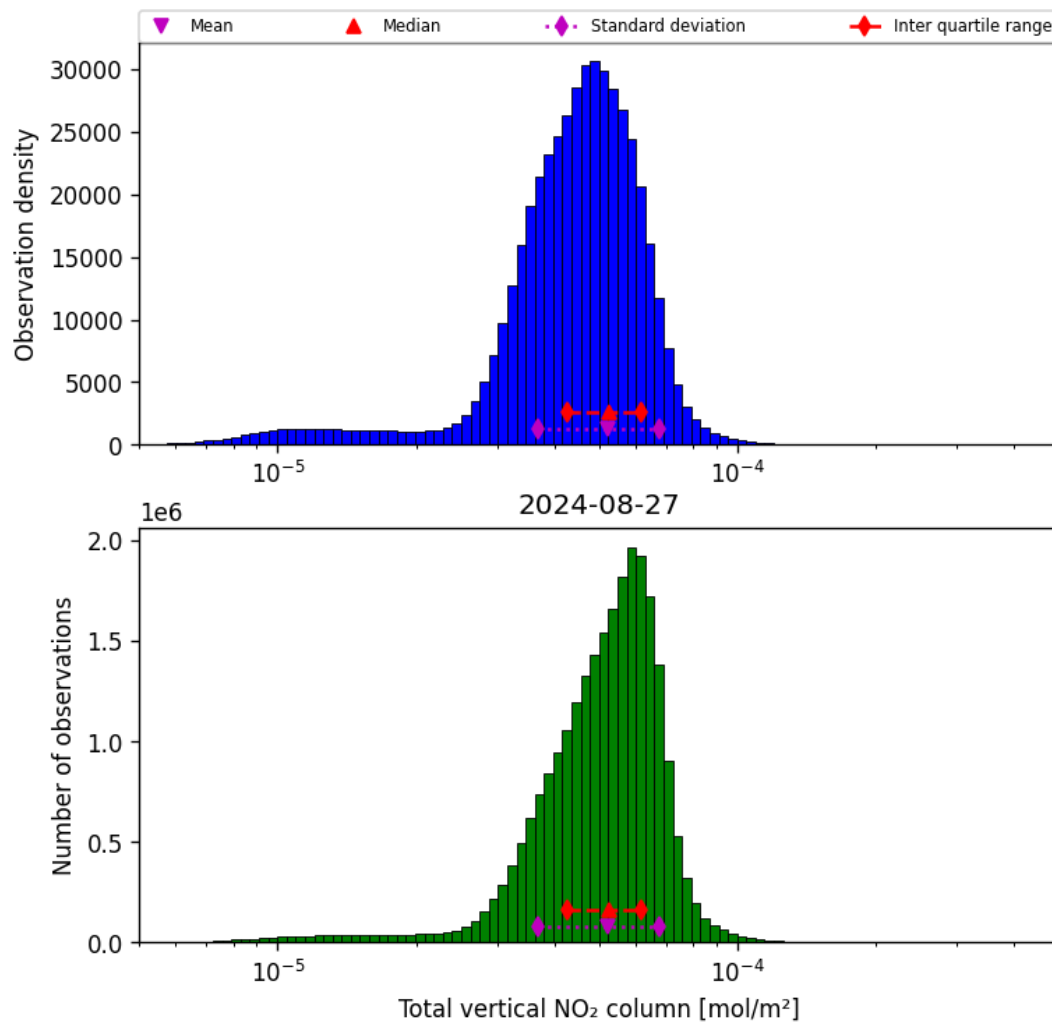
Figure 38: Histogram of “Total vertical NO 2 column” for 2024-08-27 to 2024-08-28
