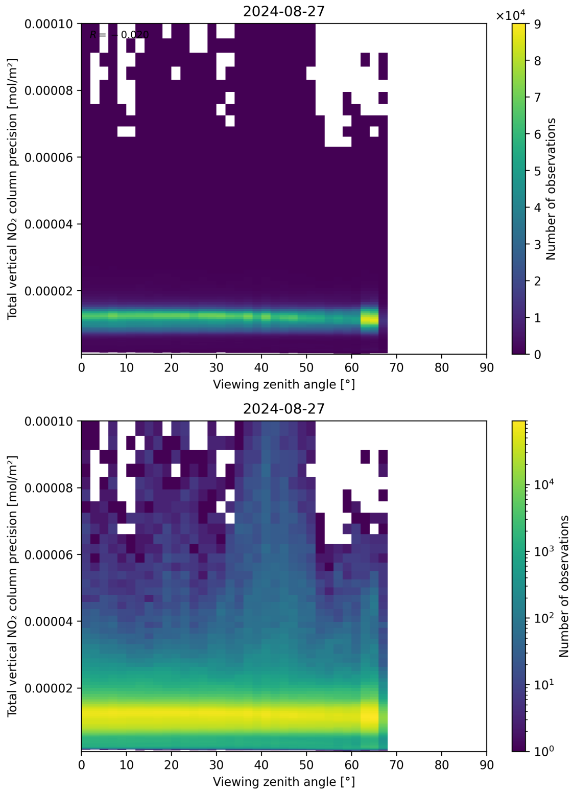
Figure 168: Scatter density plot of “Viewing zenith angle” against “Total vertical NO 2 column precision” for 2024-08-27 to 2024-08-28.
