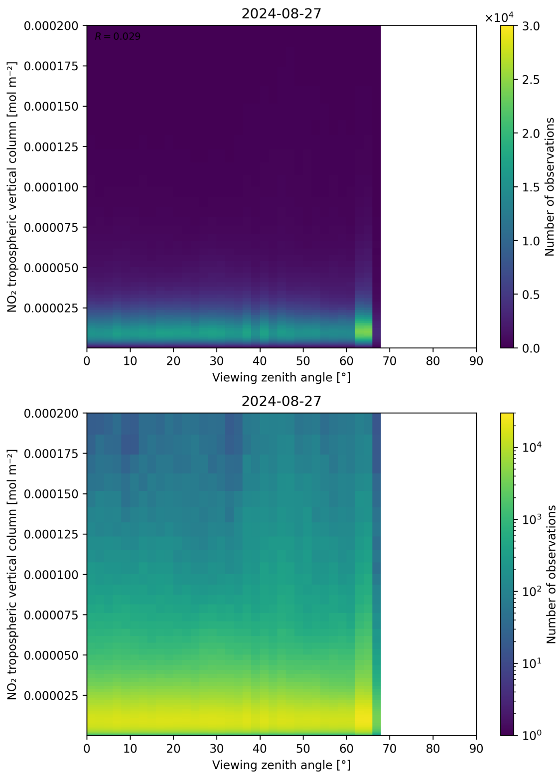
Figure 169: Scatter density plot of “Viewing zenith angle” against “NO 2 tropospheric vertical column” for 2024-08-27 to 2024-08-28.
