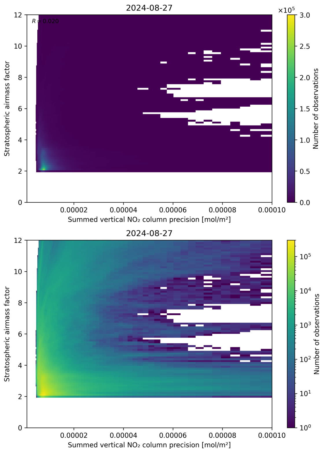
Figure 106: Scatter density plot of “Summed vertical NO 2 column precision” against “Stratospheric airmass factor” for 2024-08-27 to 2024-08-28.
