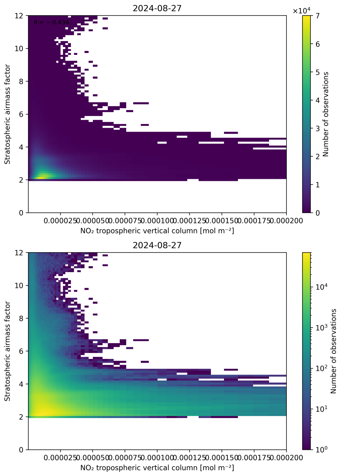
Figure 121: Scatter density plot of “NO 2 tropospheric vertical column” against “Stratospheric air mass factor” for 2024-08-27 to 2024-08-28.
