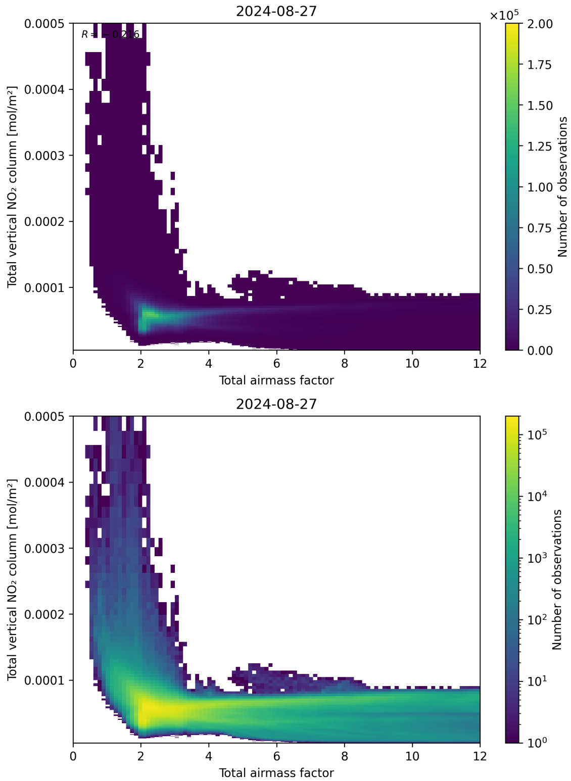
Figure 67: Scatter density plot of “Total airmass factor” against “Total vertical NO 2 column” for 2024-08-27 to 2024-08-28.
