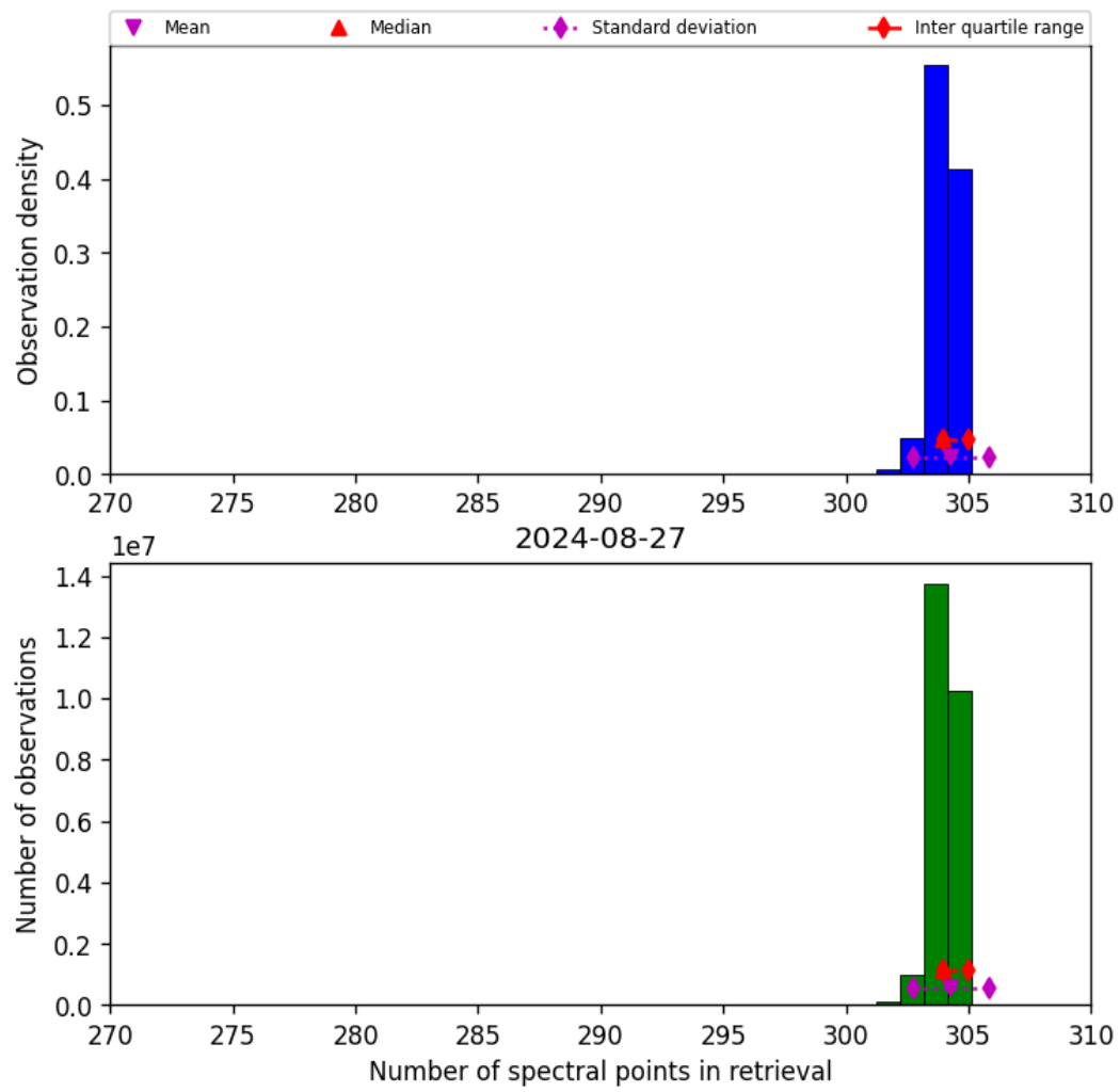
Figure 33: Histogram of “Number of spectral points in retrieval” for 2024-08-27 to 2024-08-28
