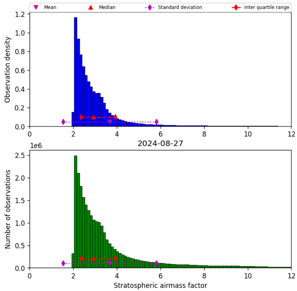
Figure 44: Histogram of “Stratospheric airmass factor” for 2024-08-27 to 2024-08-28
