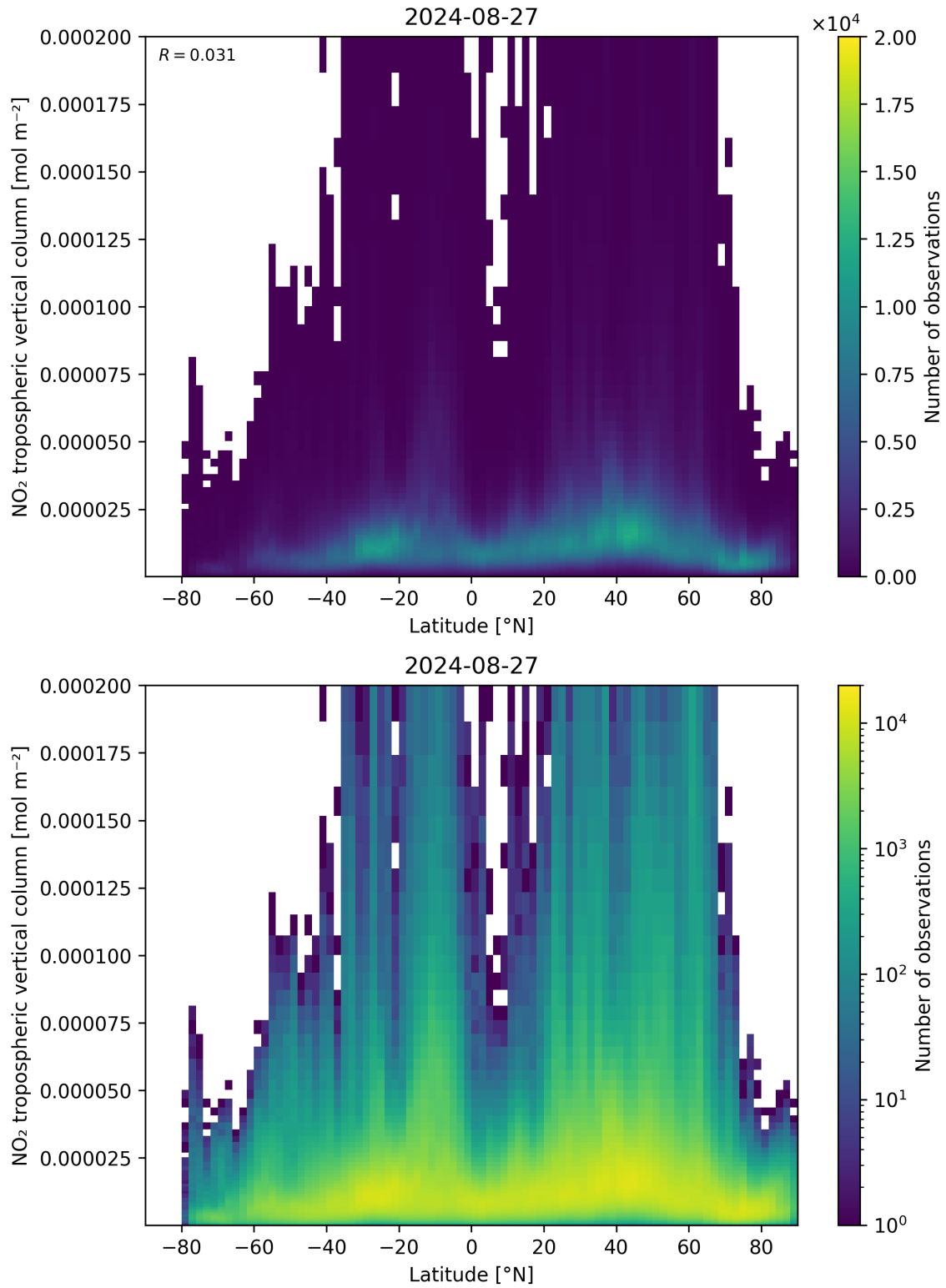
Figure 92: Scatter density plot of “Latitude” against “NO 2 tropospheric vertical column” for 2024-08-27 to 2024-08-28.
