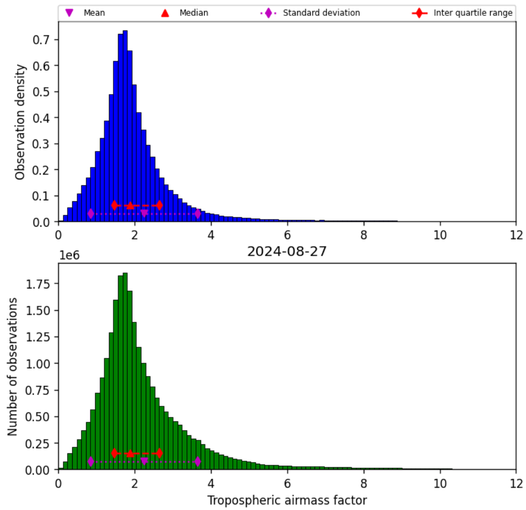
Figure 31: Histogram of “Tropospheric airmass factor” for 2024-08-27 to 2024-08-28
