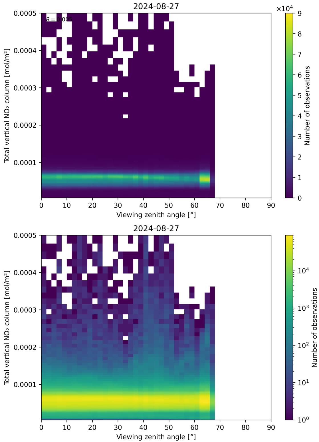
Figure 167: Scatter density plot of “Viewing zenith angle” against “Total vertical NO 2 column” for 2024-08-27 to 2024-08-28.
