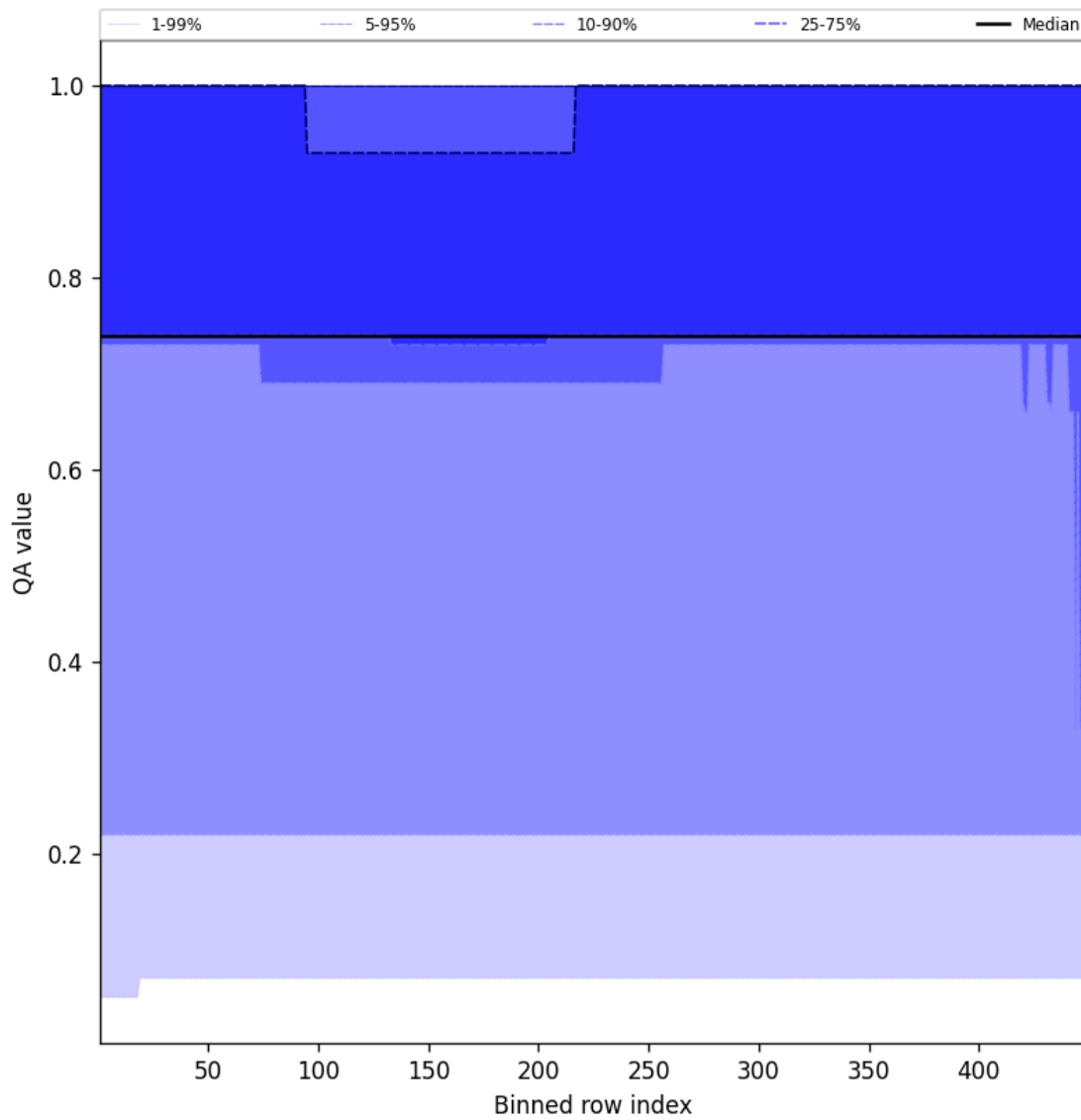
Figure 45: Along track statistics of “QA value” for 2024-08-27 to 2024-08-28
