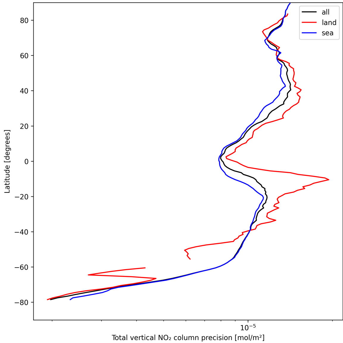
Figure 22: Zonal average of “Total vertical NO 2 column precision” for 2024-08-27 to 2024-08-28.
