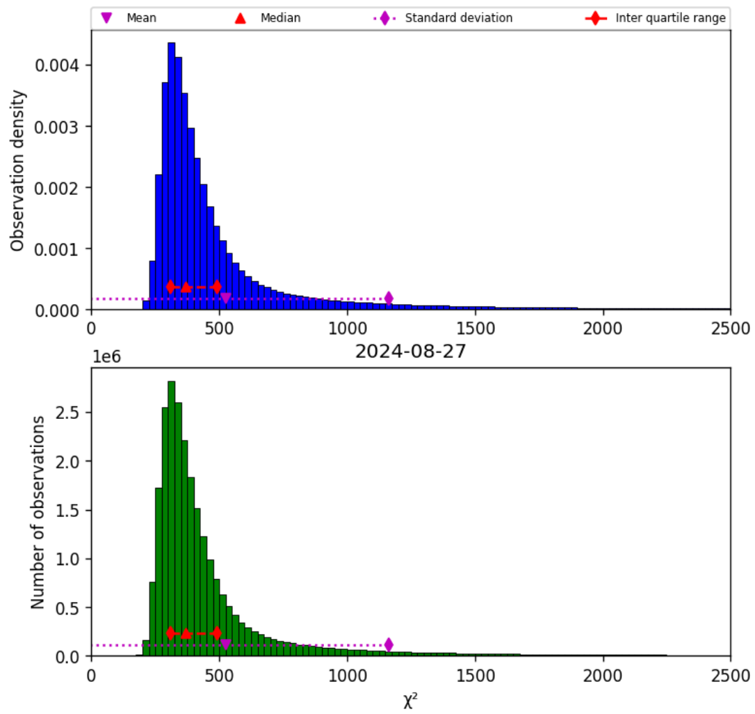
Figure 42: Histogram of “ \chi^2 ” for 2024-08-27 to 2024-08-28
