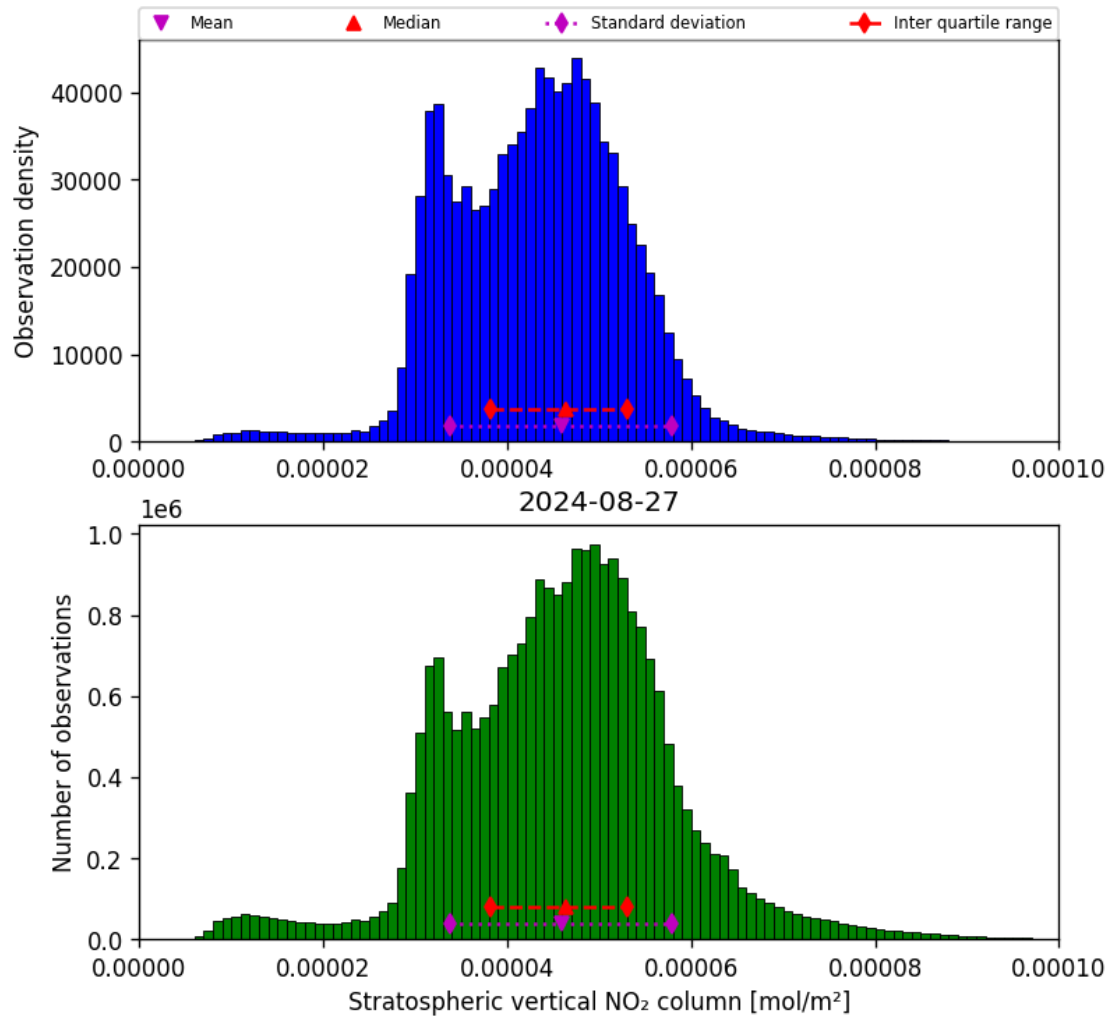
Figure 36: Histogram of “Stratospheric vertical NO 2 column” for 2024-08-27 to 2024-08-28
