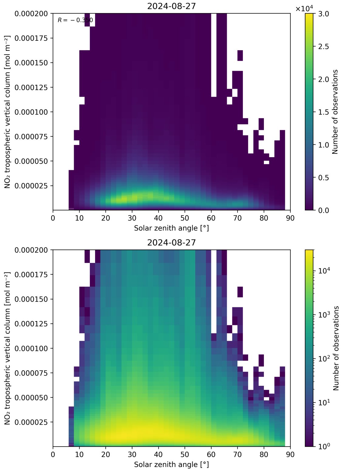
Figure 155: Scatter density plot of “Solar zenith angle” against “NO 2 tropospheric vertical column” for 2024-08-27 to 2024-08-28.
