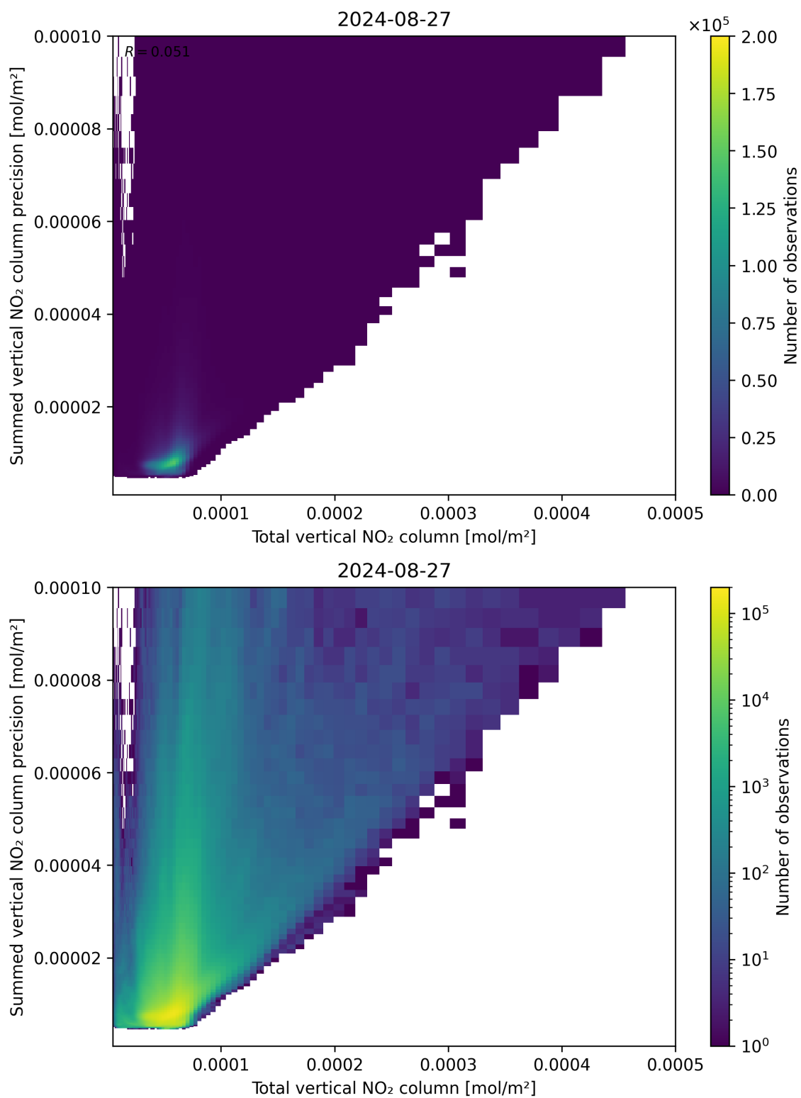
Figure 113: Scatter density plot of “Total vertical NO 2 column” against “Summed vertical NO 2 column precision” for 2024-08-27 to 2024-08-28.
