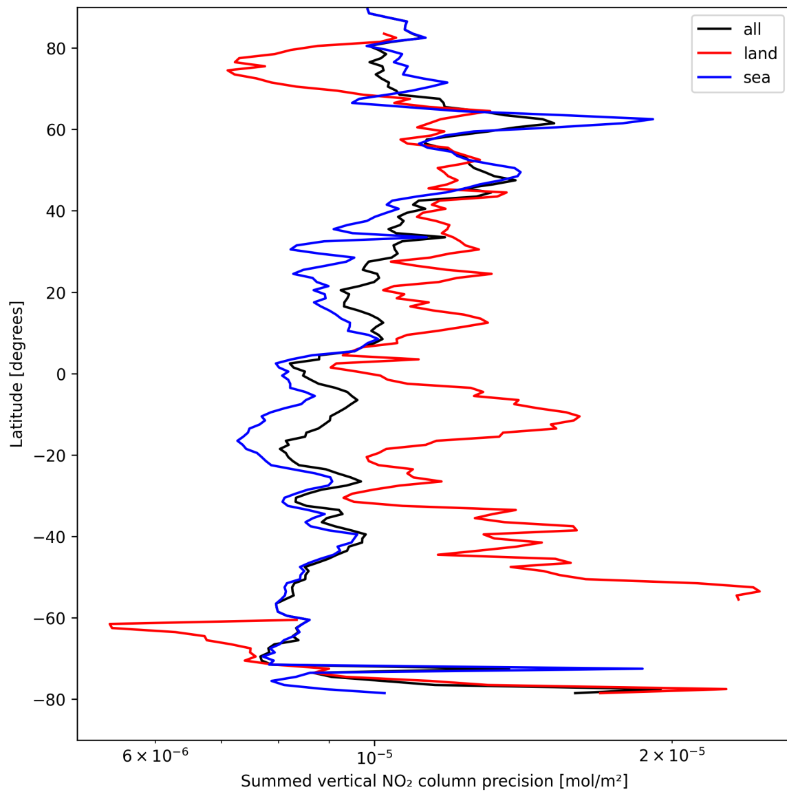
Figure 24: Zonal average of “Summed vertical NO 2 column precision” for 2024-08-27 to 2024-08-28.
