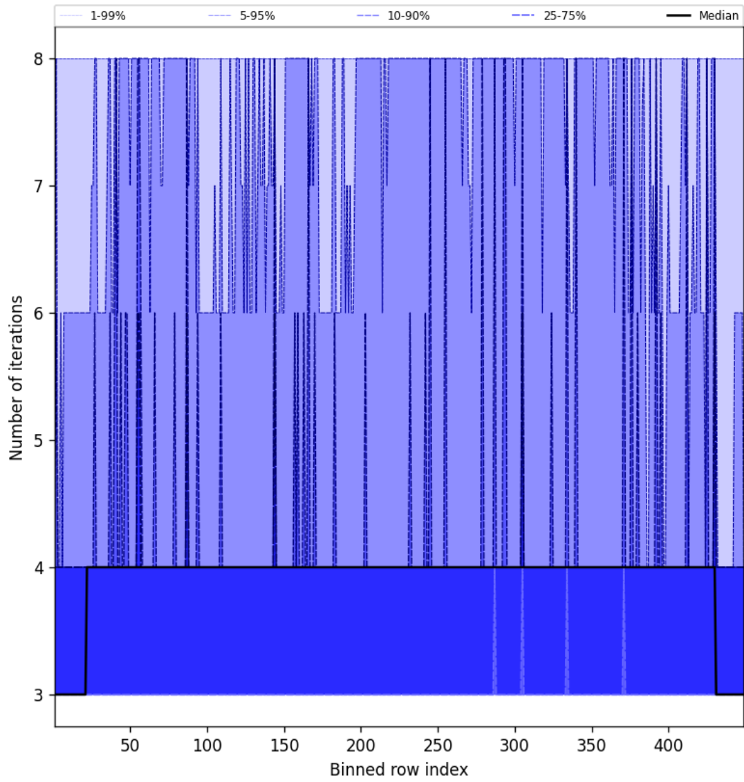
Figure 51: Along track statistics of “Number of iterations” for 2024-08-27 to 2024-08-28
