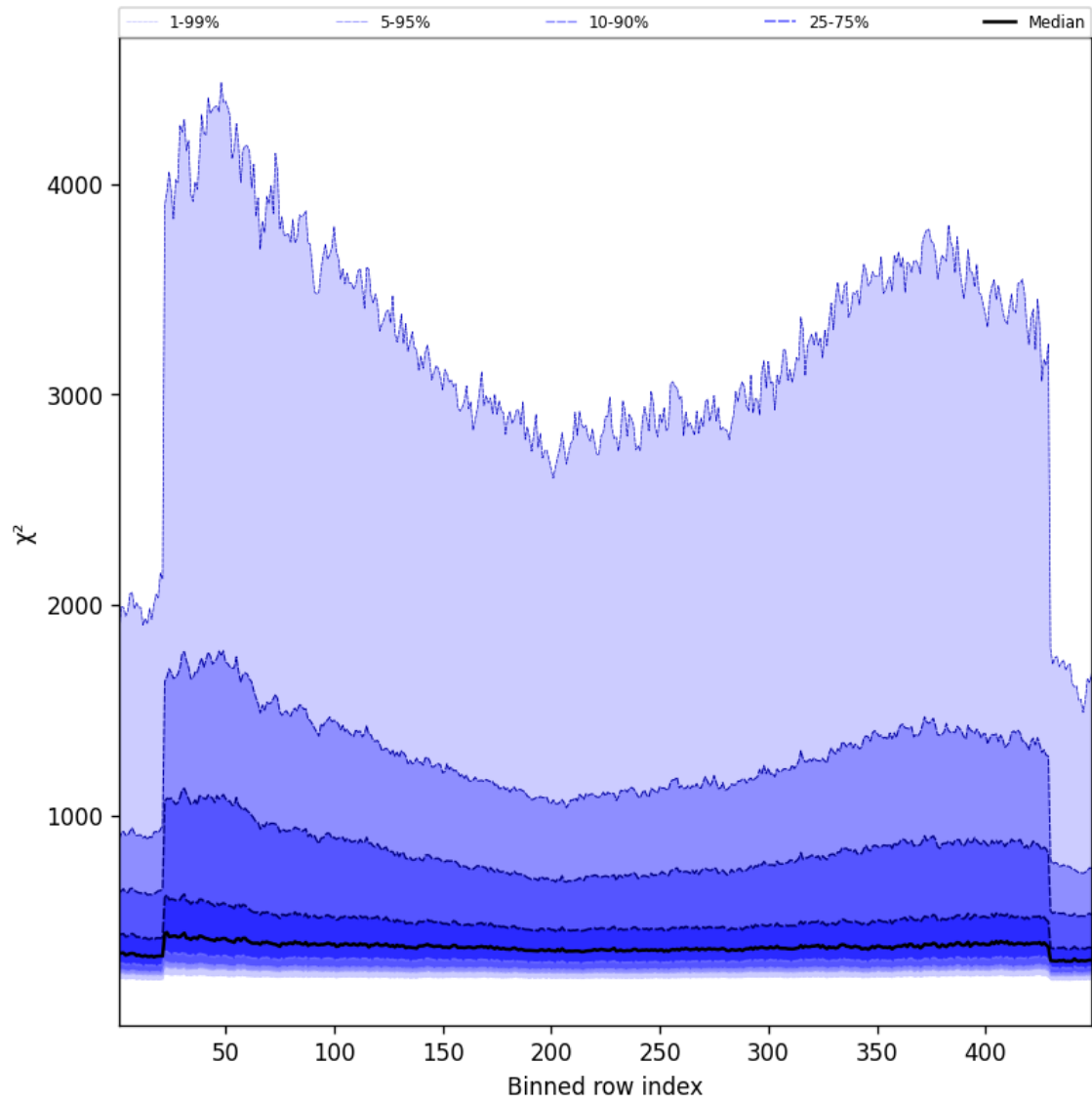
Figure 59: Along track statistics of “ \chi^2 ” for 2024-08-27 to 2024-08-28
