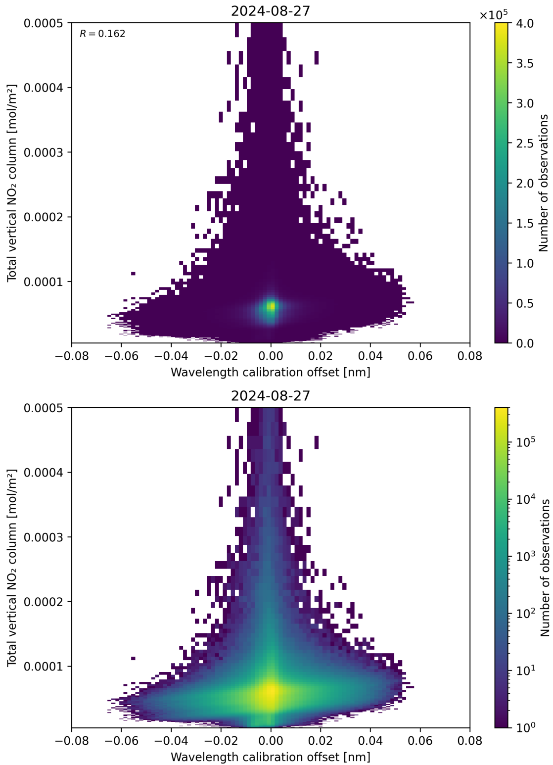
Figure 179: Scatter density plot of “Wavelength calibration offset” against “Total vertical NO 2 column” for 2024-08-27 to 2024-08-28.
