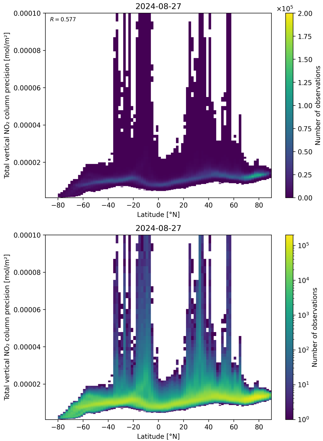
Figure 91: Scatter density plot of “Latitude” against “Total vertical NO 2 column precision” for 2024-08-27 to 2024-08-28.
