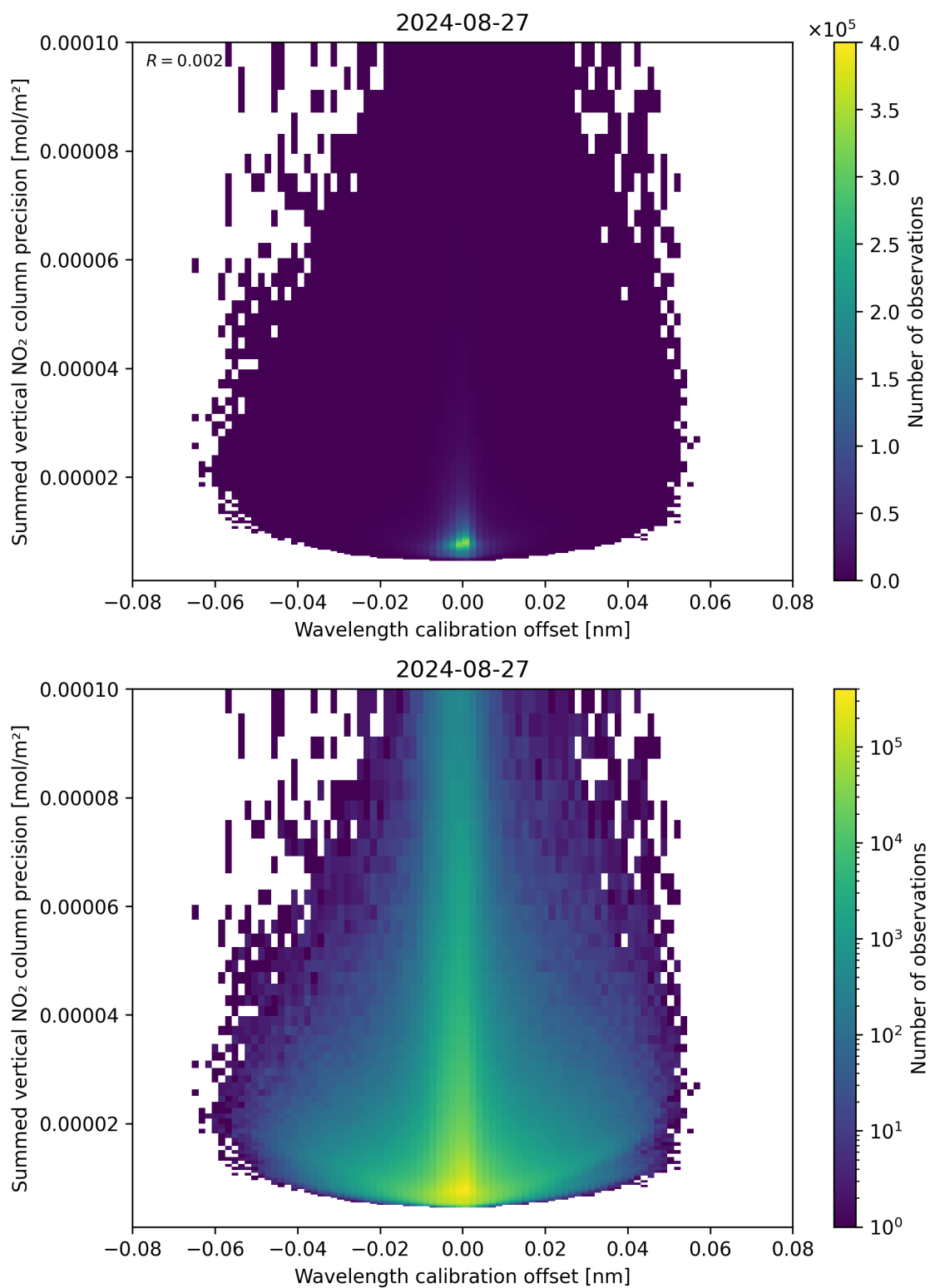
Figure 178: Scatter density plot of “Wavelength calibration offset” against “Summed vertical NO 2 column precision” for 2024-08-27 to 2024-08-28.
