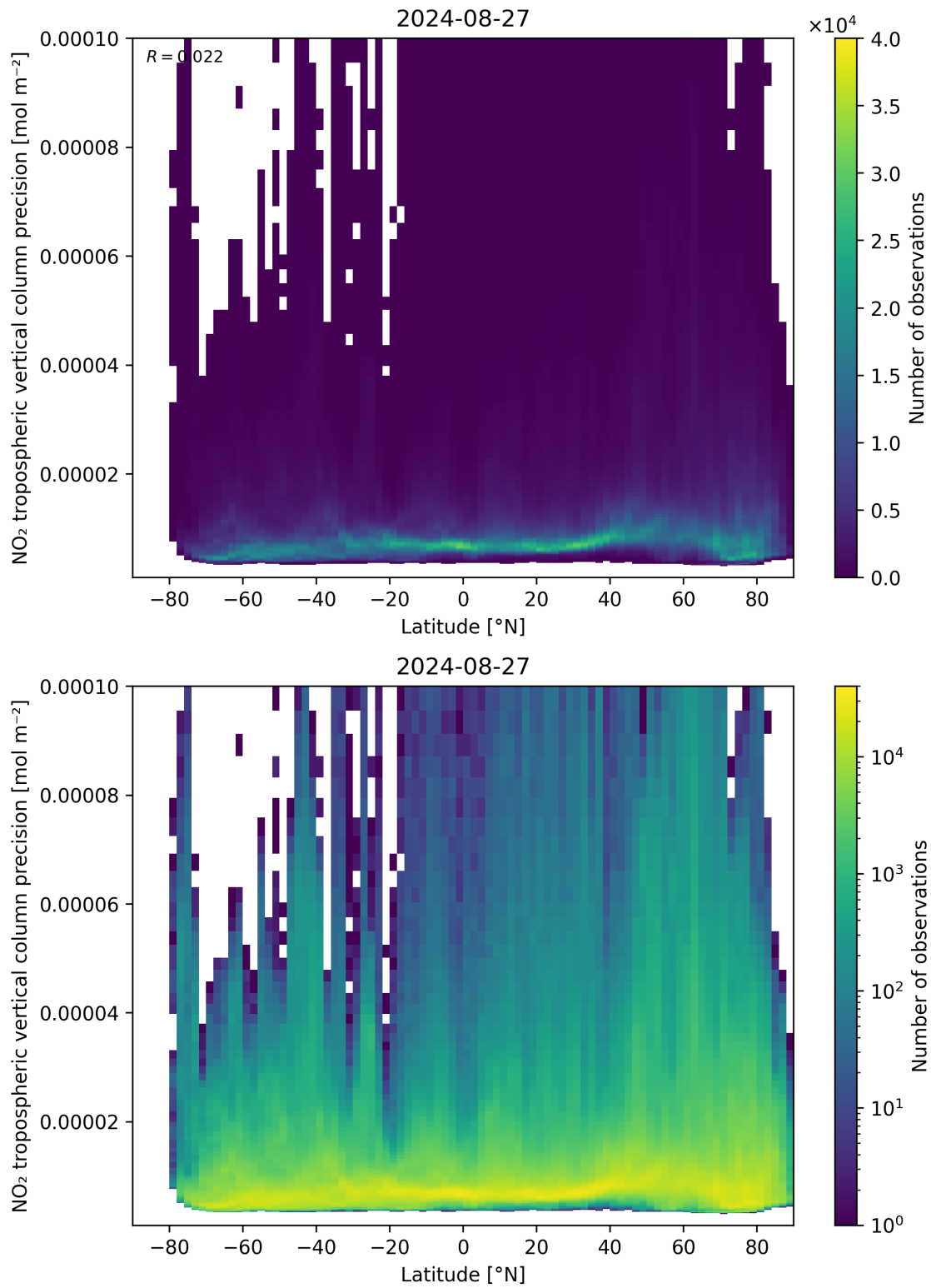
Figure 93: Scatter density plot of “Latitude” against “NO 2 tropospheric vertical column precision” for 2024-08-27 to 2024-08-28.
