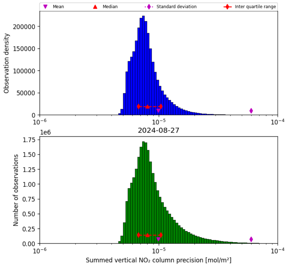
Figure 41: Histogram of “Summed vertical NO 2 column precision” for 2024-08-27 to 2024-08-28
