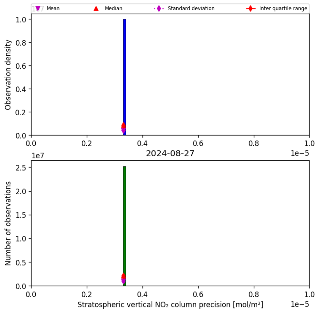
Figure 37: Histogram of “Stratospheric vertical NO 2 column precision” for 2024-08-27 to 2024-08-28
