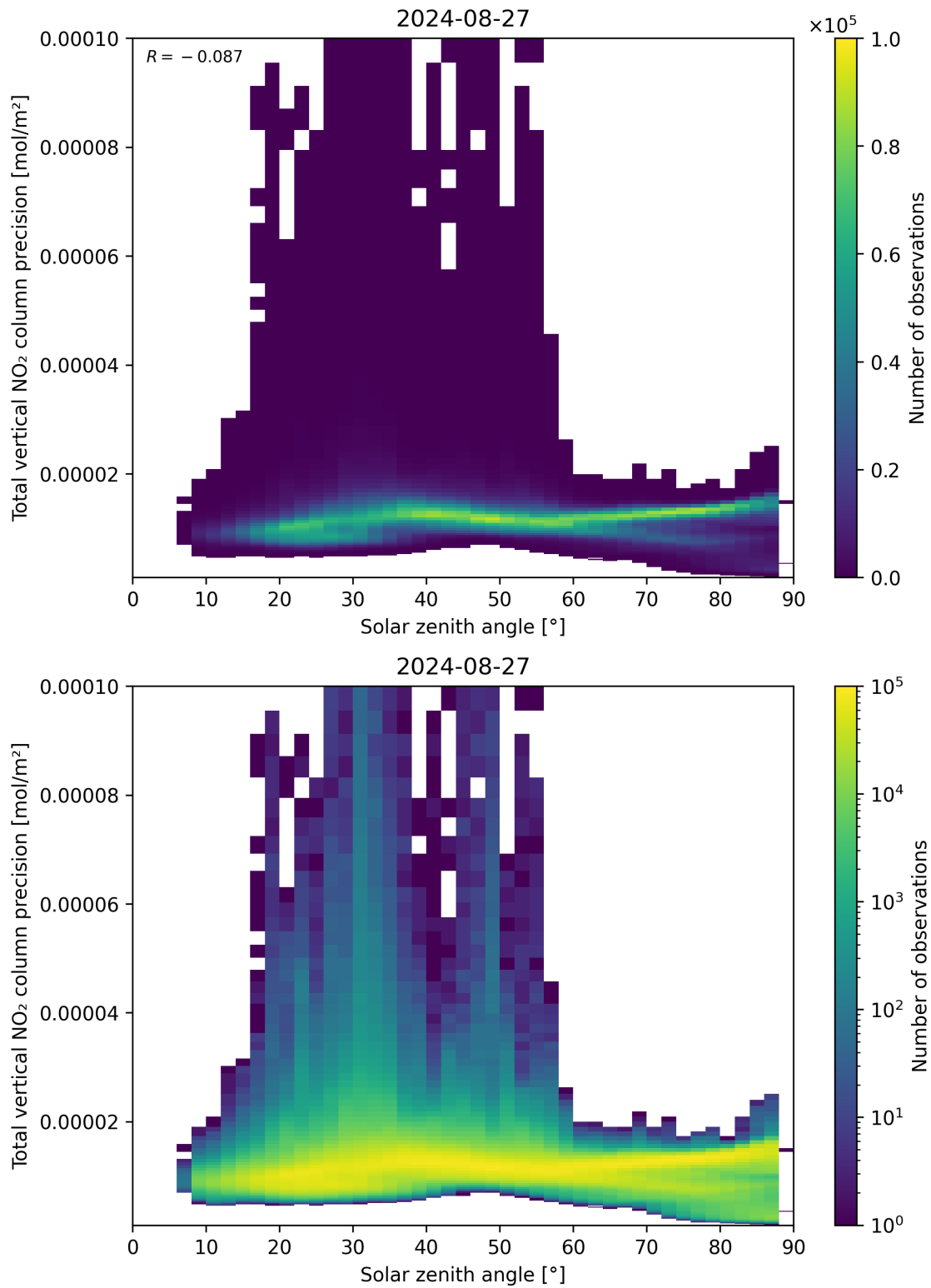
Figure 154: Scatter density plot of “Solar zenith angle” against “Total vertical NO 2 column precision” for 2024-08-27 to 2024-08-28.
