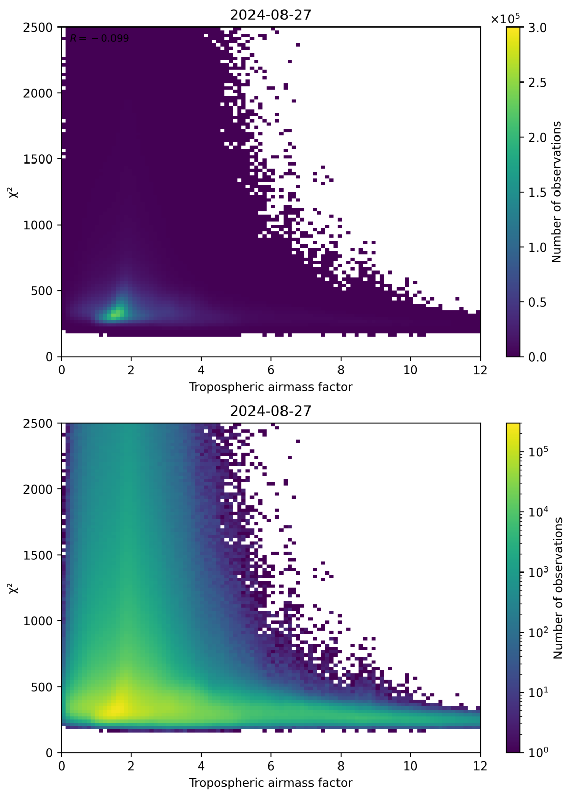
Figure 73: Scatter density plot of “Tropospheric airmass factor” against “ \chi^2 ” for 2024-08-27 to 2024-08-28.
