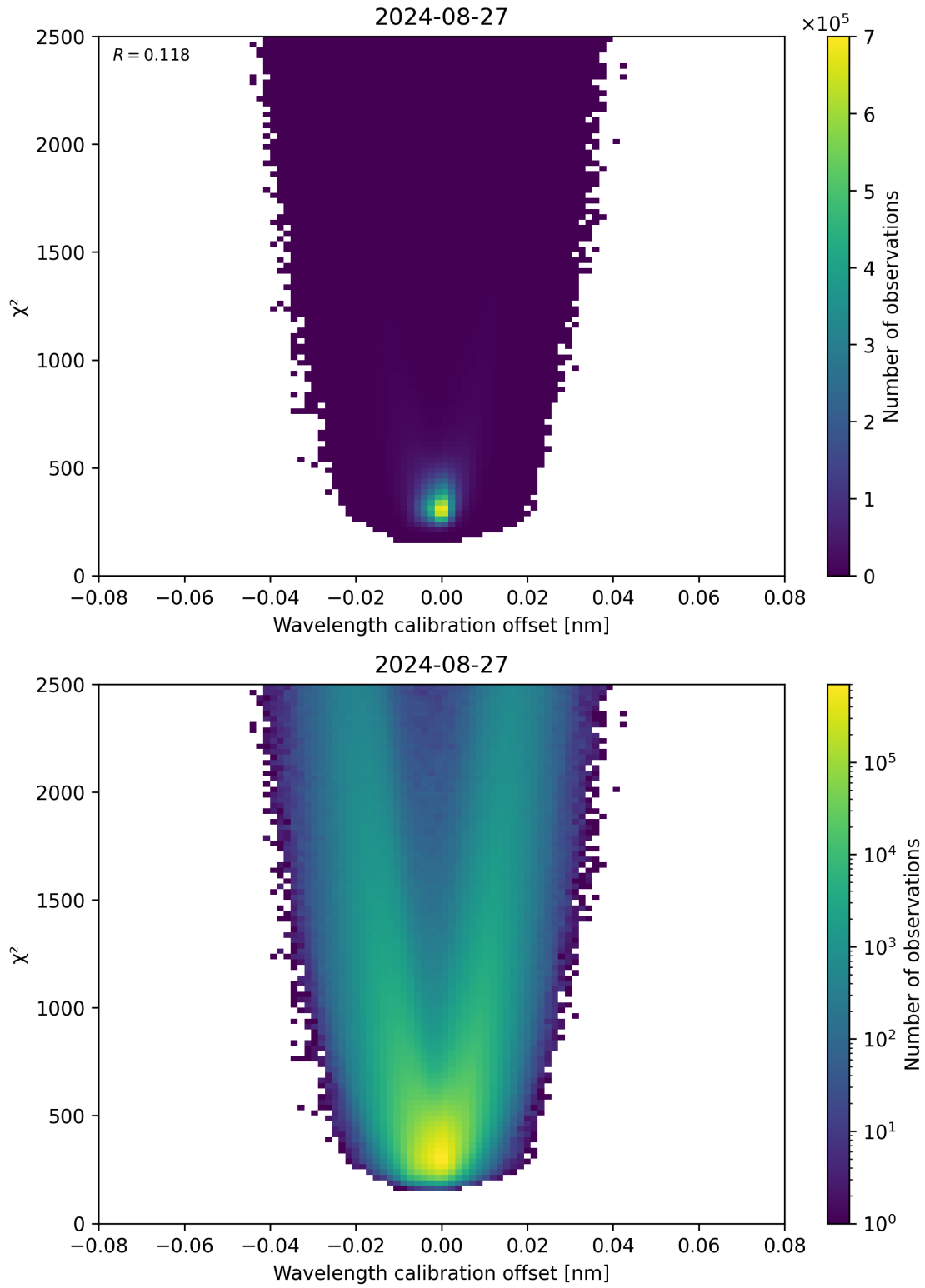
Figure 175: Scatter density plot of “Wavelength calibration offset” against “ \chi^2 ” for 2024-08-27 to 2024-08-28.
