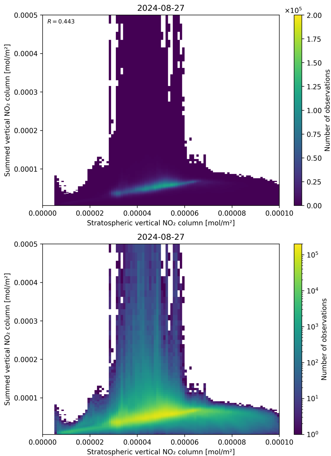
Figure 98: Scatter density plot of “Stratospheric vertical NO 2 column” against “Summed vertical NO 2 column” for 2024-08-27 to 2024-08-28.
