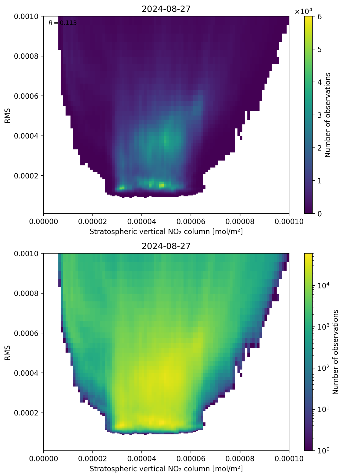
Figure 102: Scatter density plot of “Stratospheric vertical NO 2 column” against “RMS” for 2024-08-27 to 2024-08-28.
