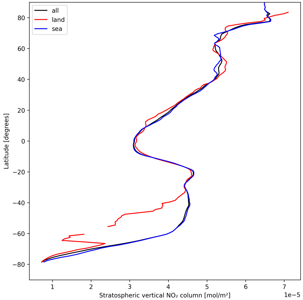
Figure 19: Zonal average of “Stratospheric vertical NO 2 column” for 2024-08-27 to 2024-08-28.
