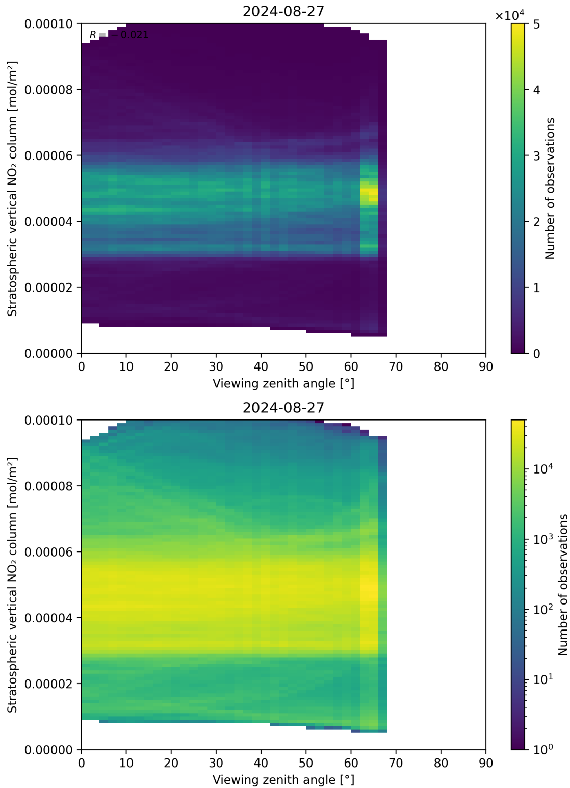
Figure 164: Scatter density plot of “Viewing zenith angle” against “Stratospheric vertical NO 2 column” for 2024-08-27 to 2024-08-28.
