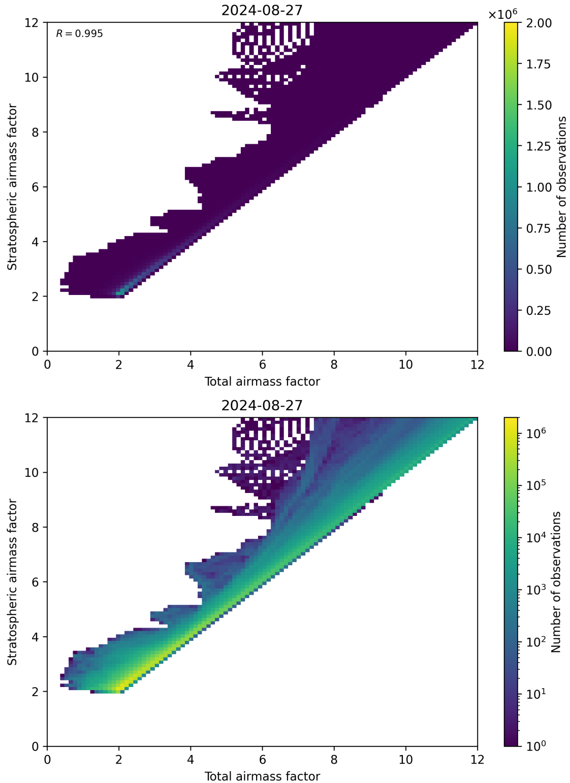
Figure 62: Scatter density plot of “Total airmass factor” against “Stratospheric airmass factor” for 2024-08-27 to 2024-08-28.
