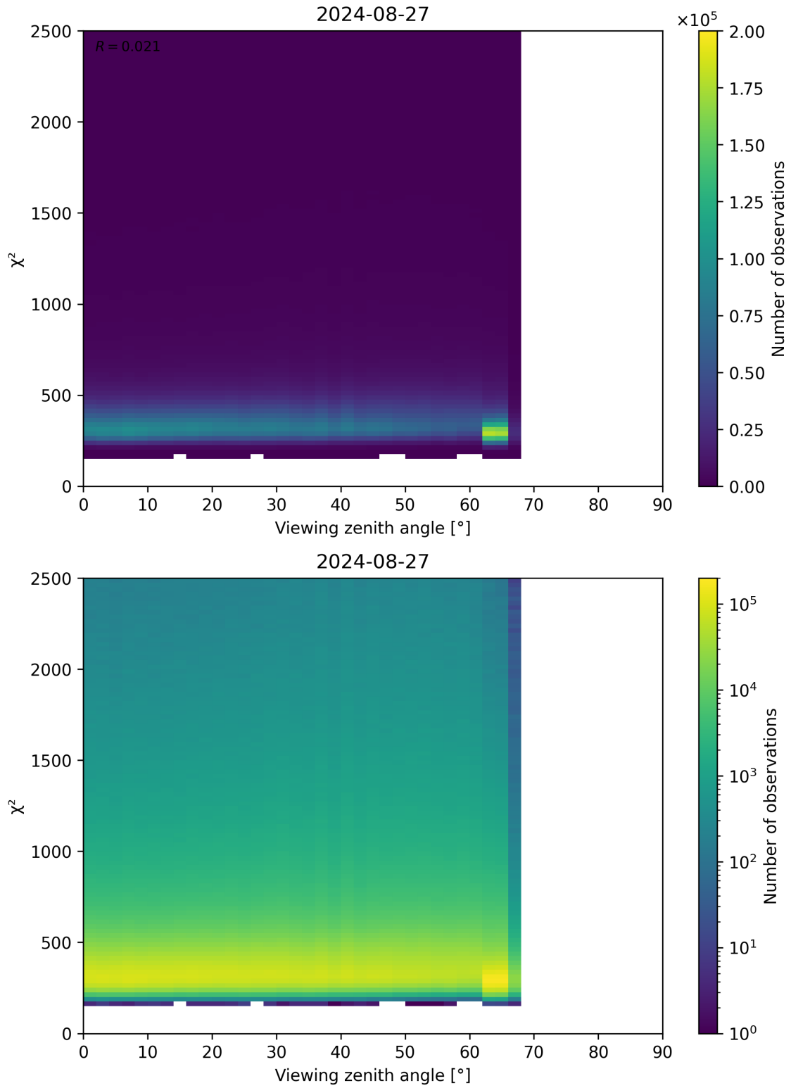
Figure 162: Scatter density plot of “Viewing zenith angle” against “ \chi^2 ” for 2024-08-27 to 2024-08-28.
