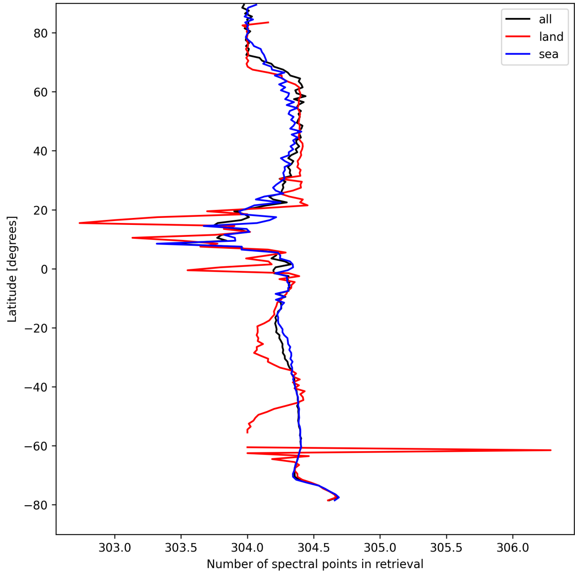
Figure 16: Zonal average of “Number of spectral points in retrieval” for 2024-08-27 to 2024-08-28.
