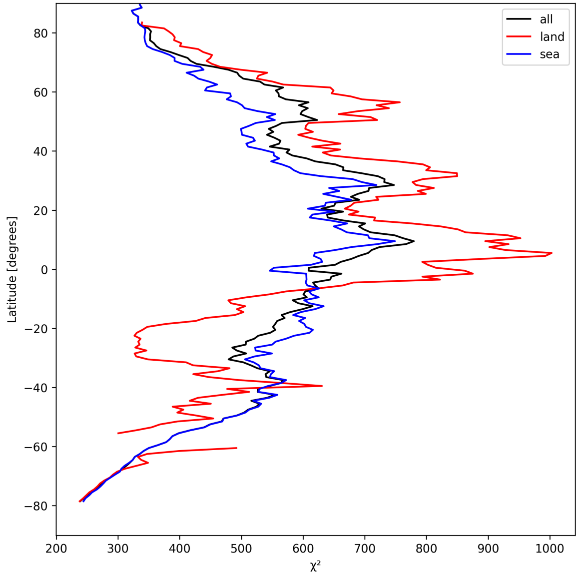
Figure 25: Zonal average of “ \chi^2 ” for 2024-08-27 to 2024-08-28.
