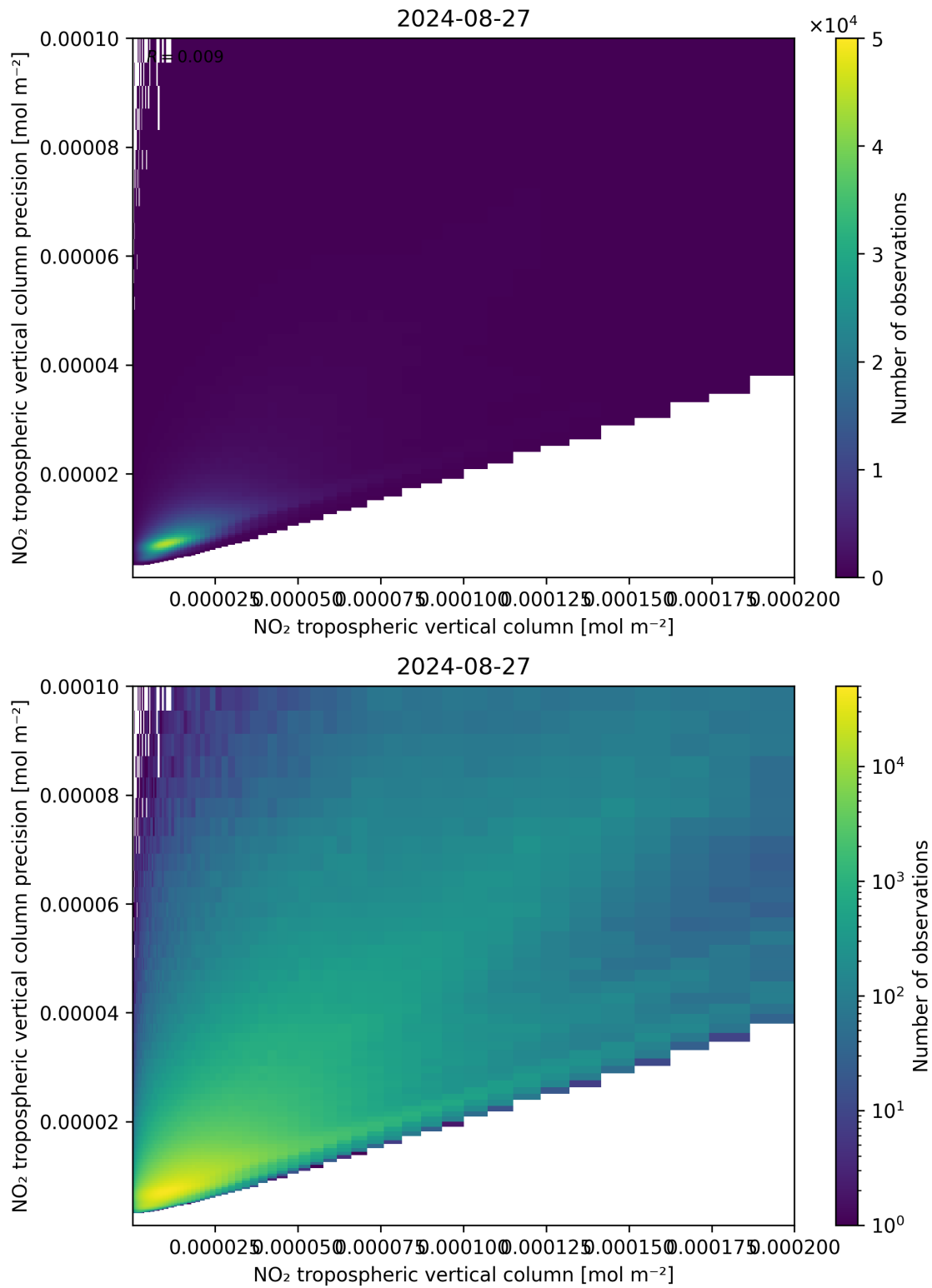
Figure 130: Scatter density plot of “NO 2 tropospheric vertical column” against “NO 2 tropospheric vertical column precision” for 2024-08-27 to 2024-08-28.
