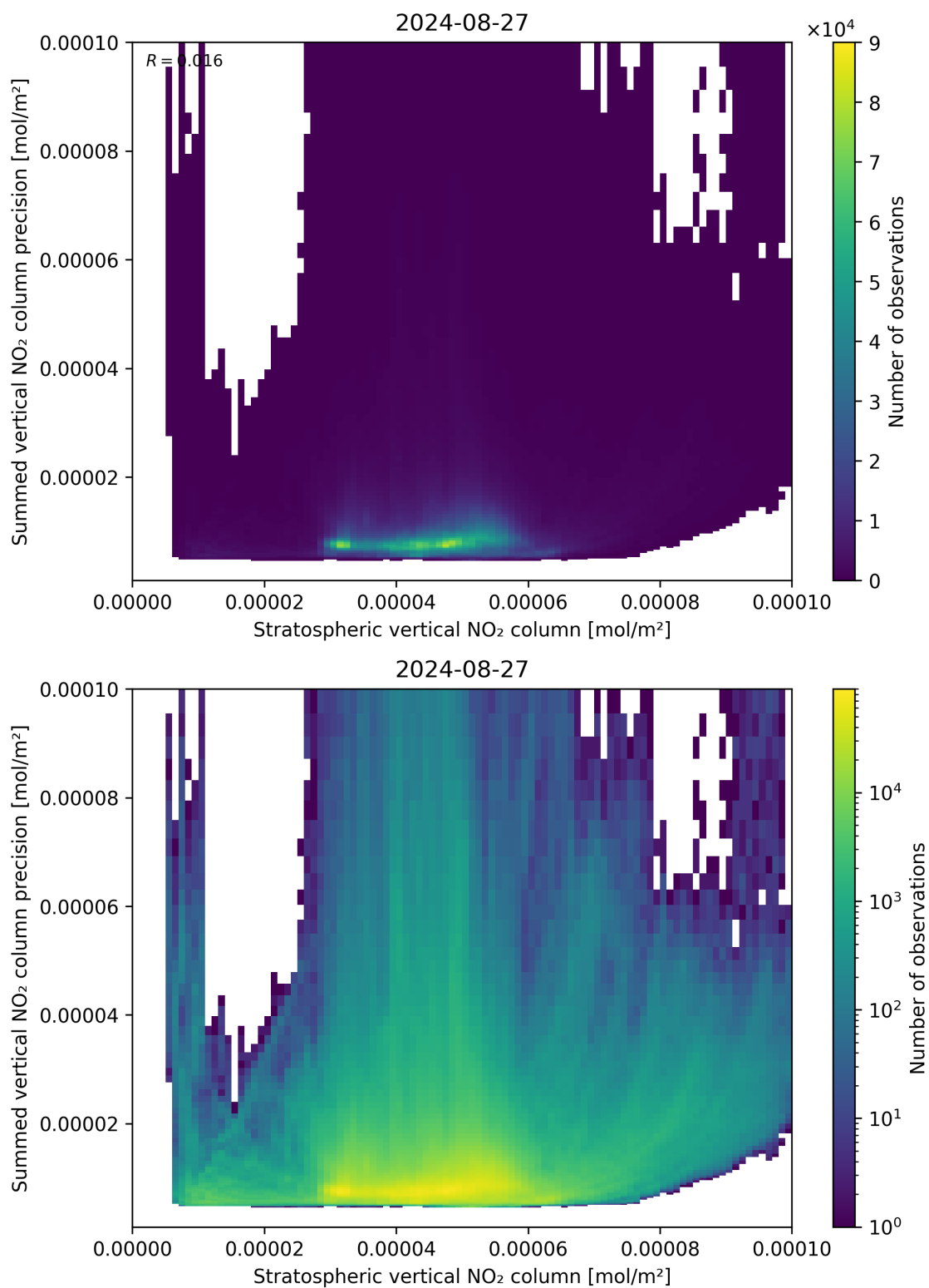
Figure 99: Scatter density plot of “Stratospheric vertical NO 2 column” against “Summed vertical NO 2 column precision” for 2024-08-27 to 2024-08-28.
