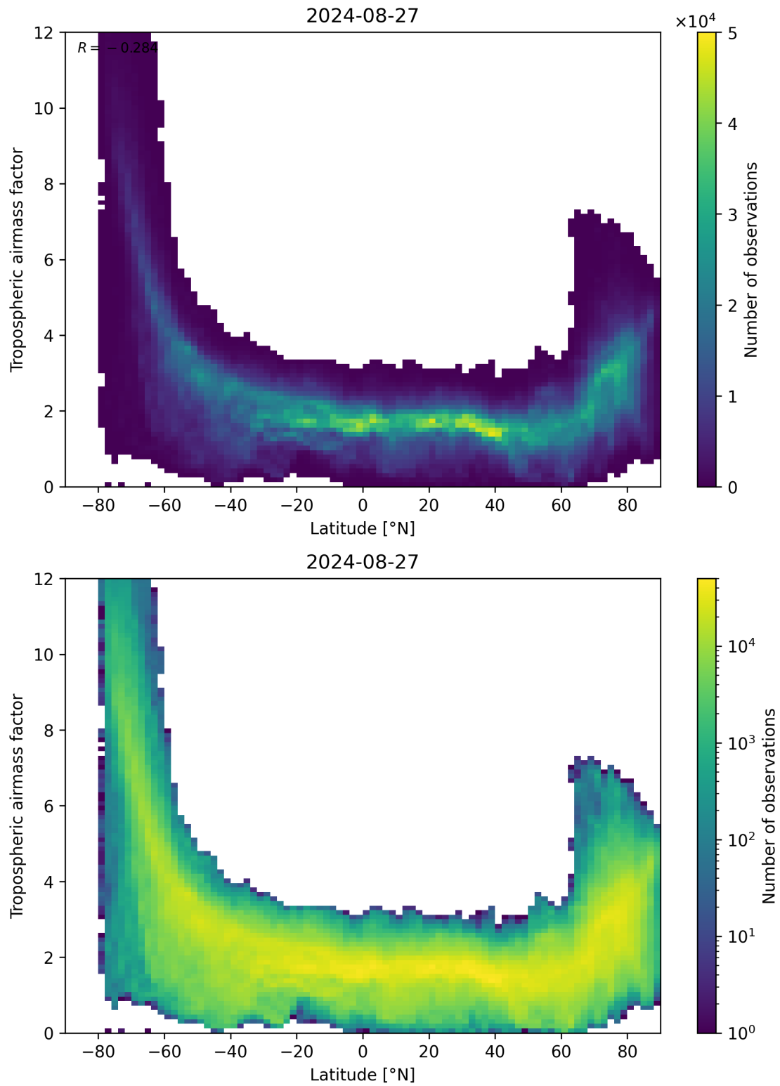
Figure 85: Scatter density plot of “Latitude” against “Tropospheric airmass factor” for 2024-08-27 to 2024-08-28.
