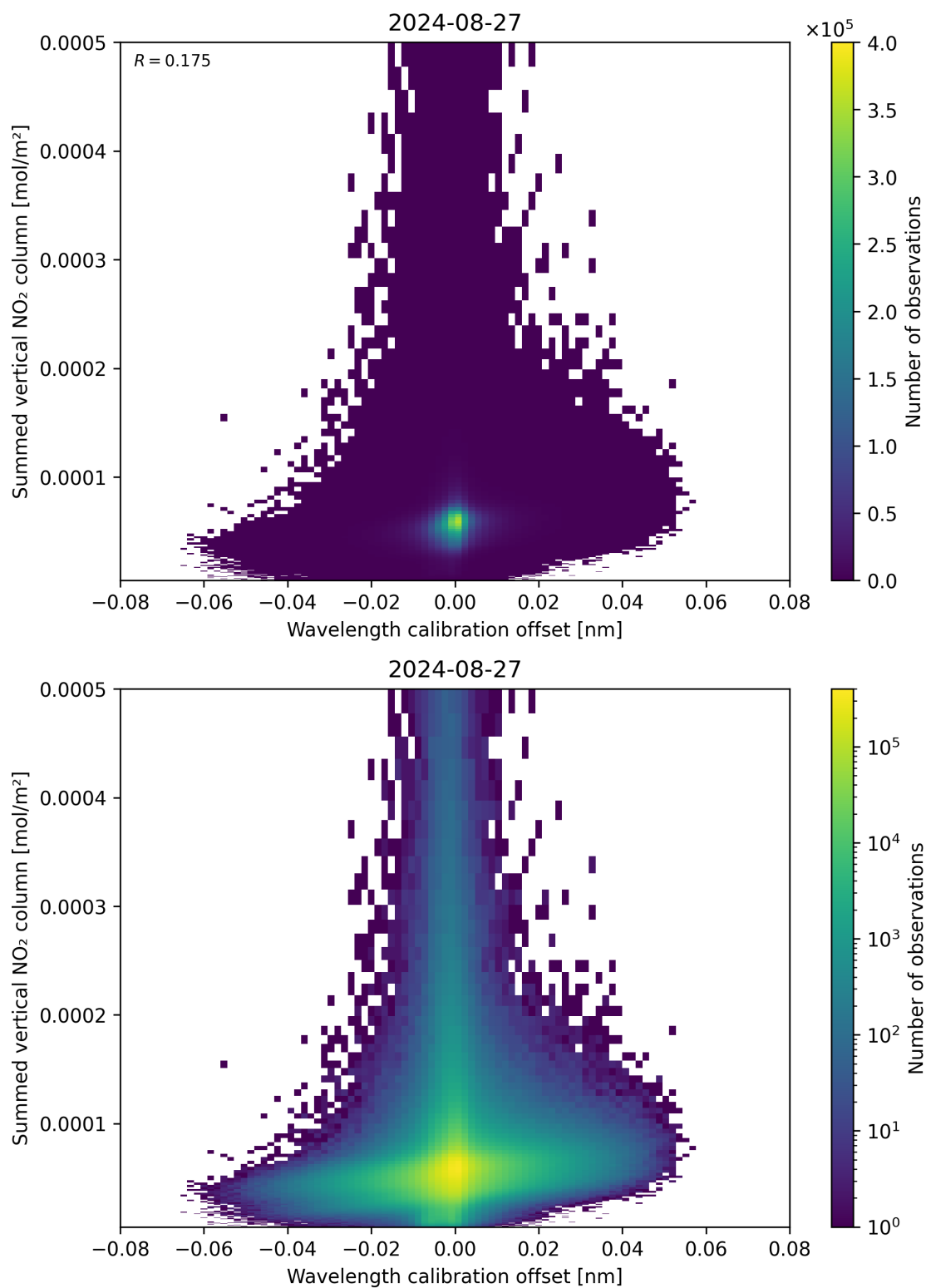
Figure 177: Scatter density plot of “Wavelength calibration offset” against “Summed vertical NO 2 column” for 2024-08-27 to 2024-08-28.
