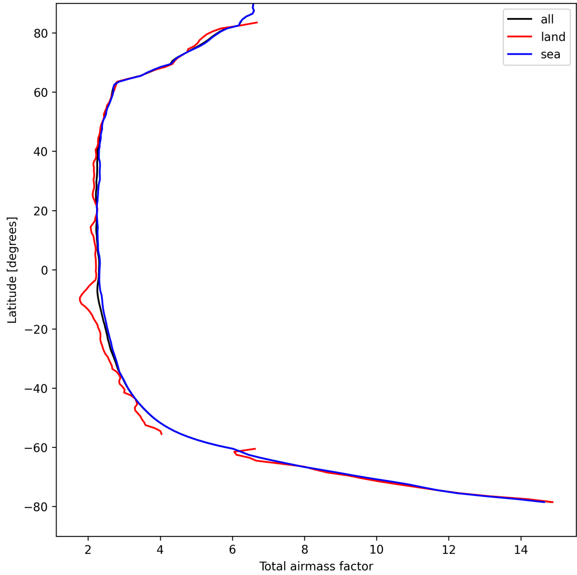
Figure 15: Zonal average of “Total airmass factor” for 2024-08-27 to 2024-08-28.
