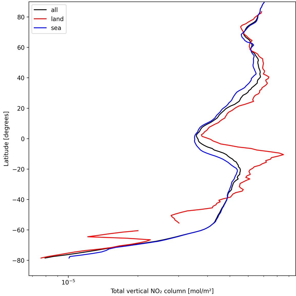
Figure 21: Zonal average of “Total vertical NO 2 column” for 2024-08-27 to 2024-08-28.
