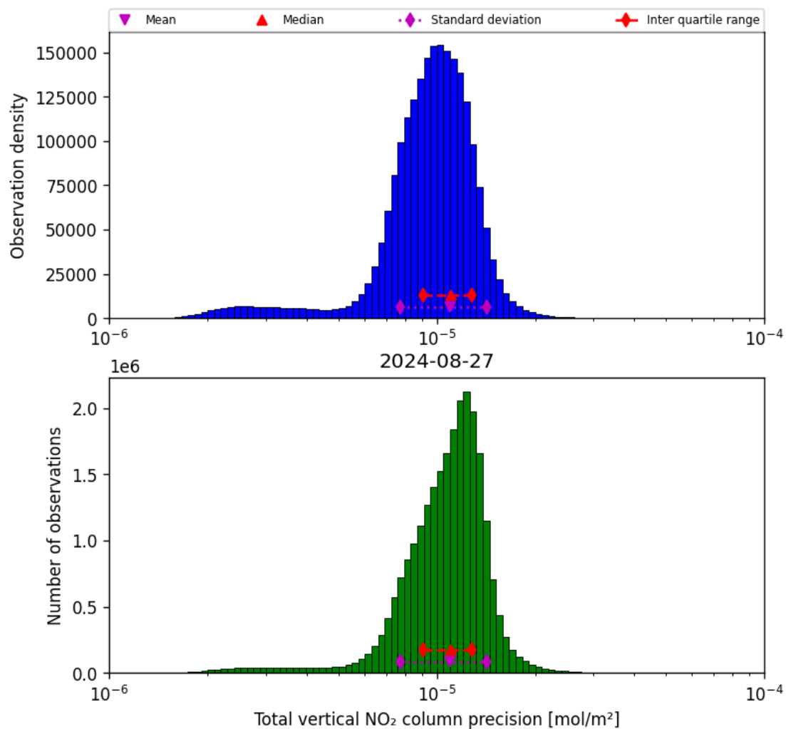
Figure 39: Histogram of “Total vertical NO 2 column precision” for 2024-08-27 to 2024-08-28
