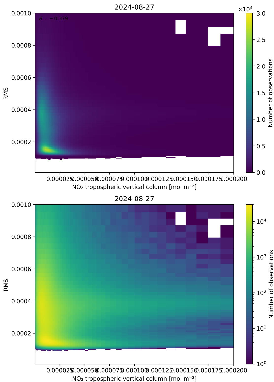
Figure 142: Scatter density plot of “NO 2 tropospheric vertical column” against “RMS” for 2024-08-27 to 2024-08-28.
