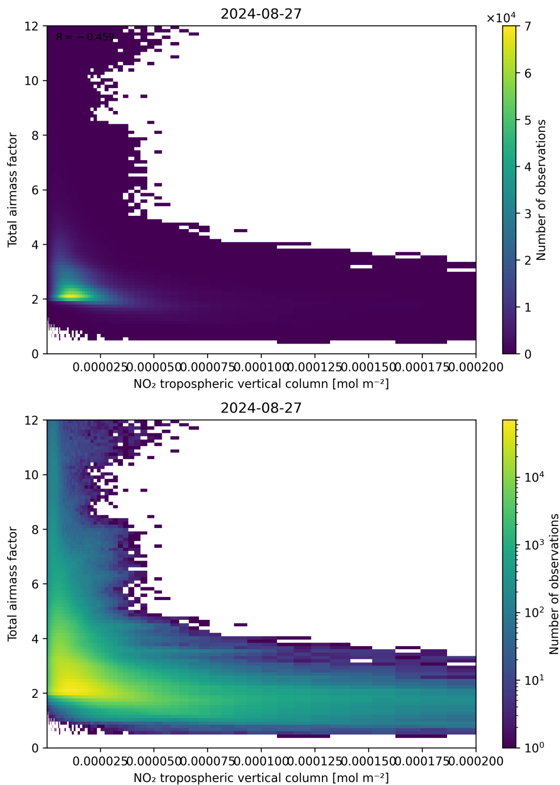
Figure 122: Scatter density plot of “NO 2 tropospheric vertical column” against “Total air mass factor” for 2024-08-27 to 2024-08-28.
