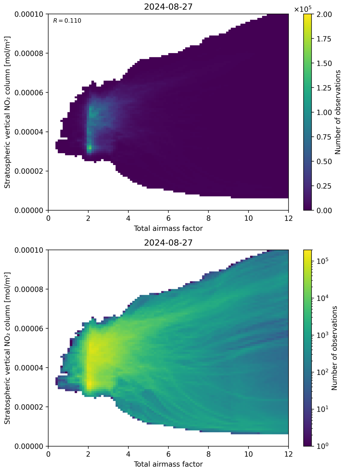
Figure 64: Scatter density plot of “Total airmass factor” against “Stratospheric vertical NO 2 column” for 2024-08-27 to 2024-08-28.
