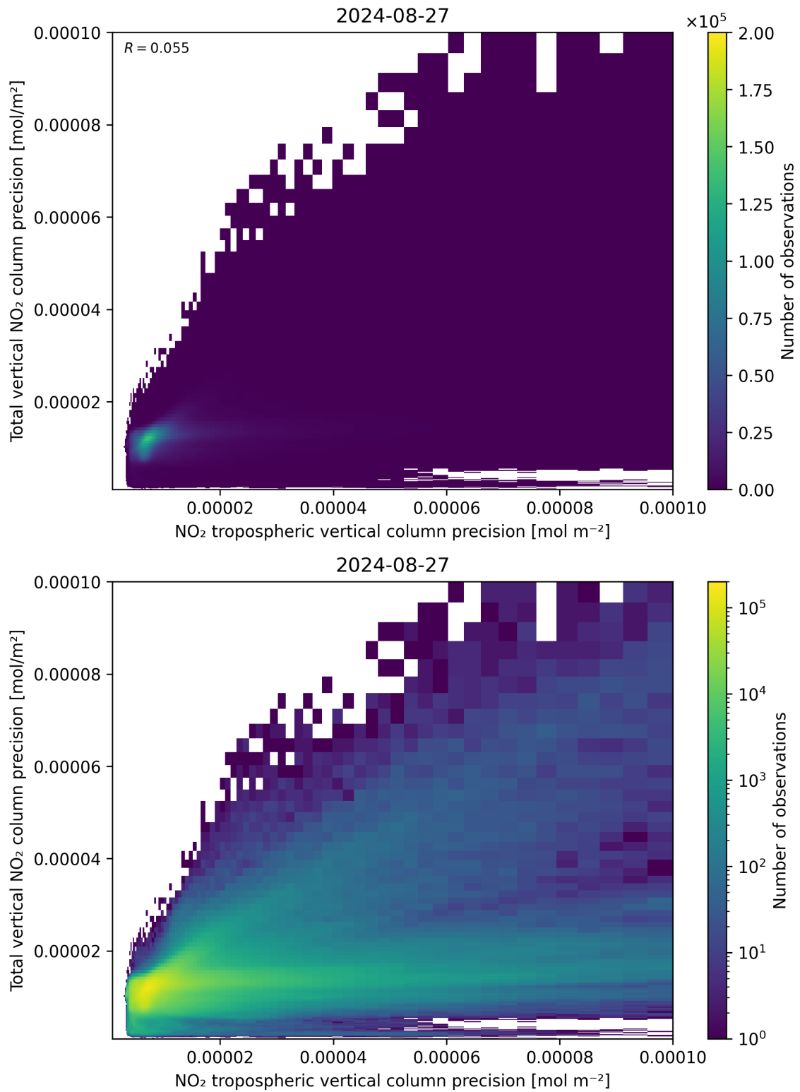
Figure 139: Scatter density plot of “NO 2 tropospheric vertical column precision” against “Total vertical NO 2 column precision” for 2024-08-27 to 2024-08-28.
