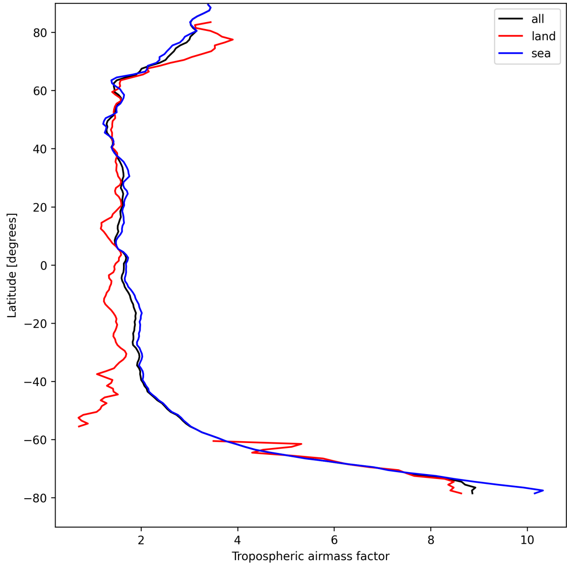
Figure 14: Zonal average of “Tropospheric airmass factor” for 2024-08-27 to 2024-08-28.
