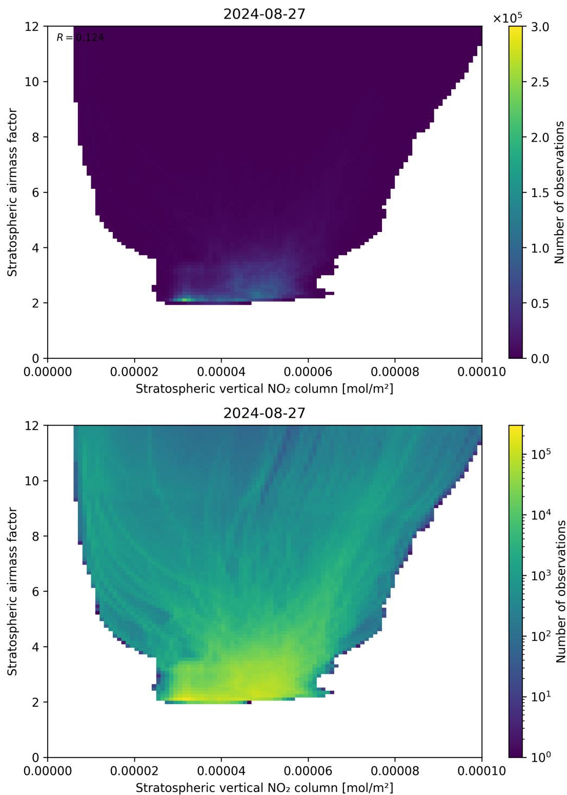
Figure 96: Scatter density plot of “Stratospheric vertical NO 2 column” against “Stratospheric airmass factor” for 2024-08-27 to 2024-08-28.
