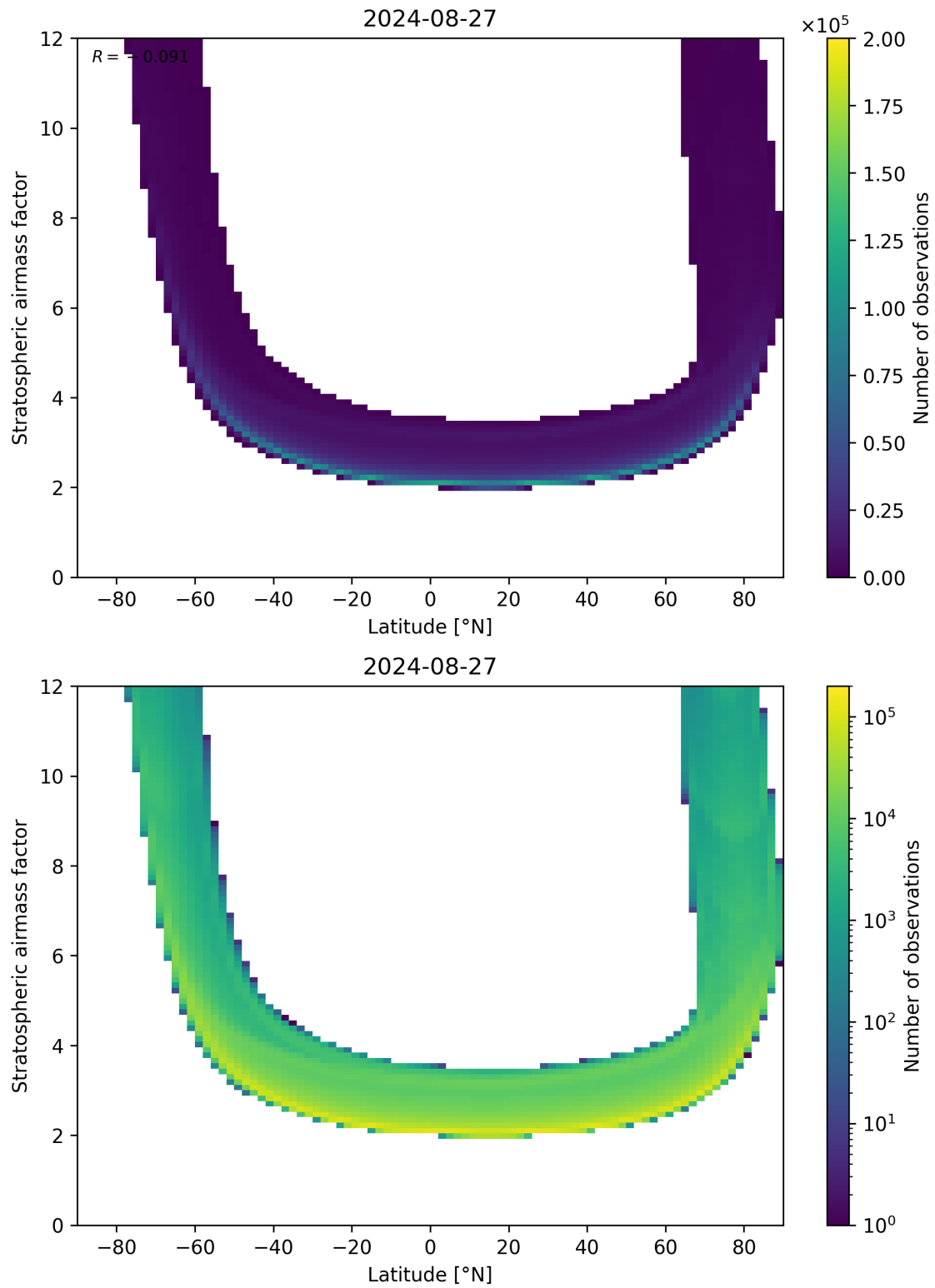
Figure 83: Scatter density plot of “Latitude” against “Stratospheric air mass factor” for 2024-08-27 to 2024-08-28.
