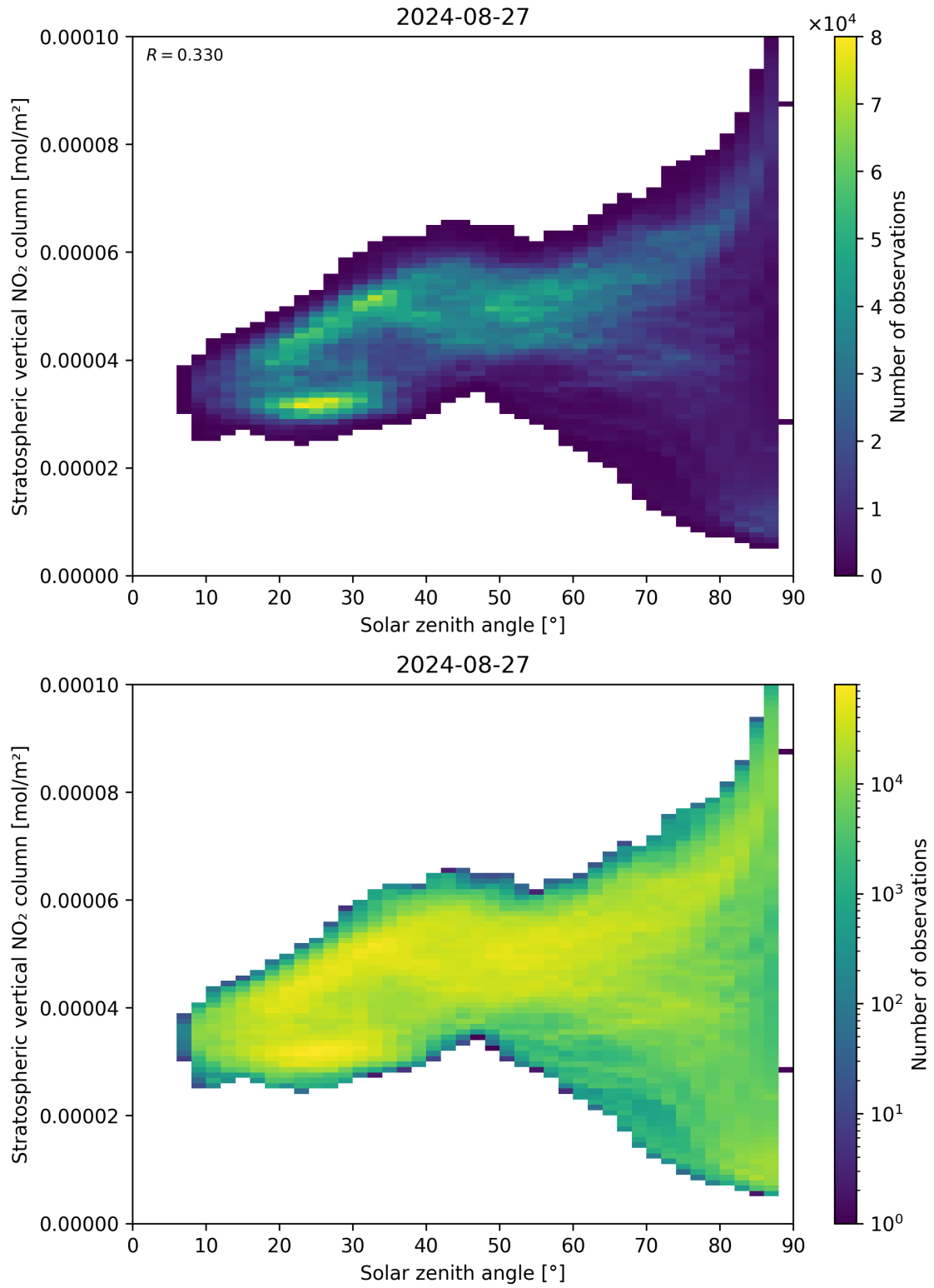
Figure 150: Scatter density plot of “Solar zenith angle” against “Stratospheric vertical NO 2 column” for 2024-08-27 to 2024-08-28.
