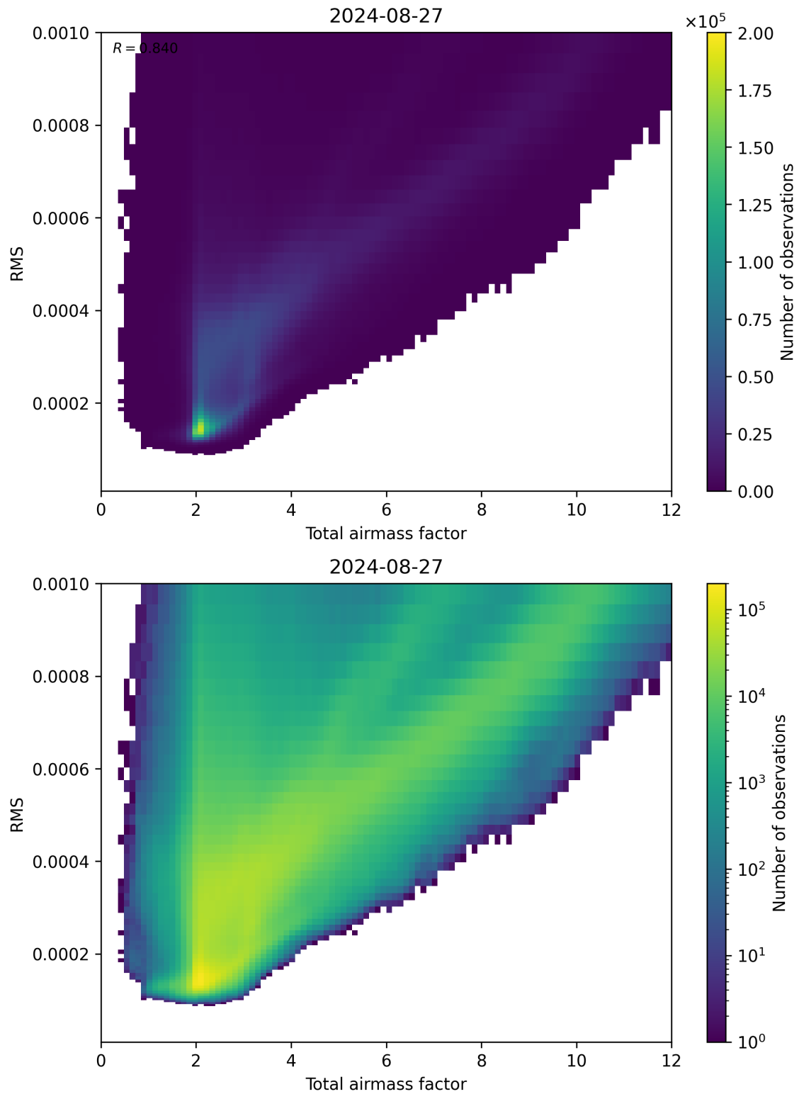
Figure 69: Scatter density plot of “Total airmass factor” against “RMS” for 2024-08-27 to 2024-08-28.
