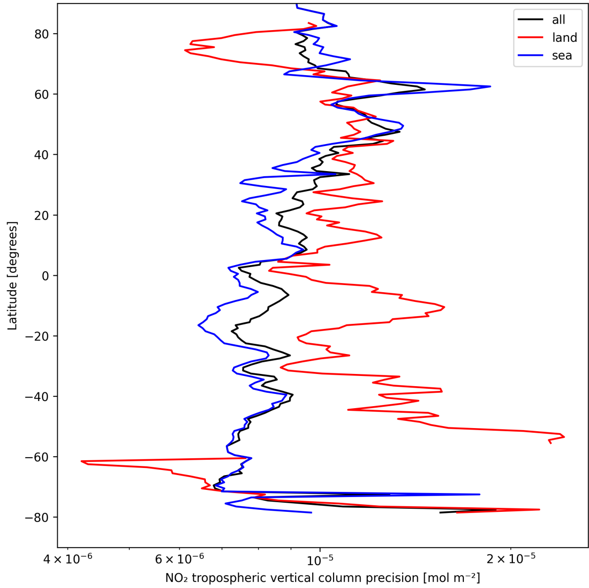
Figure 13: Zonal average of “NO 2 tropospheric vertical column precision” for 2024-08-27 to 2024-08-28.
