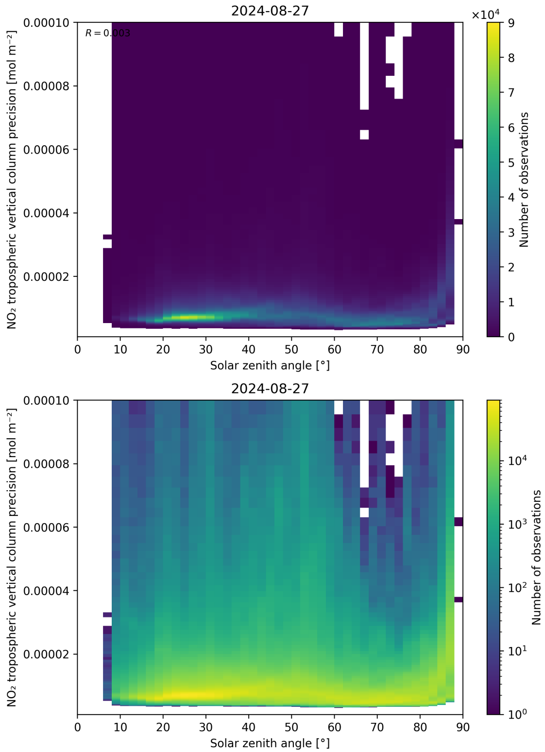
Figure 156: Scatter density plot of “Solar zenith angle” against “NO 2 tropospheric vertical column precision” for 2024-08-27 to 2024-08-28.
