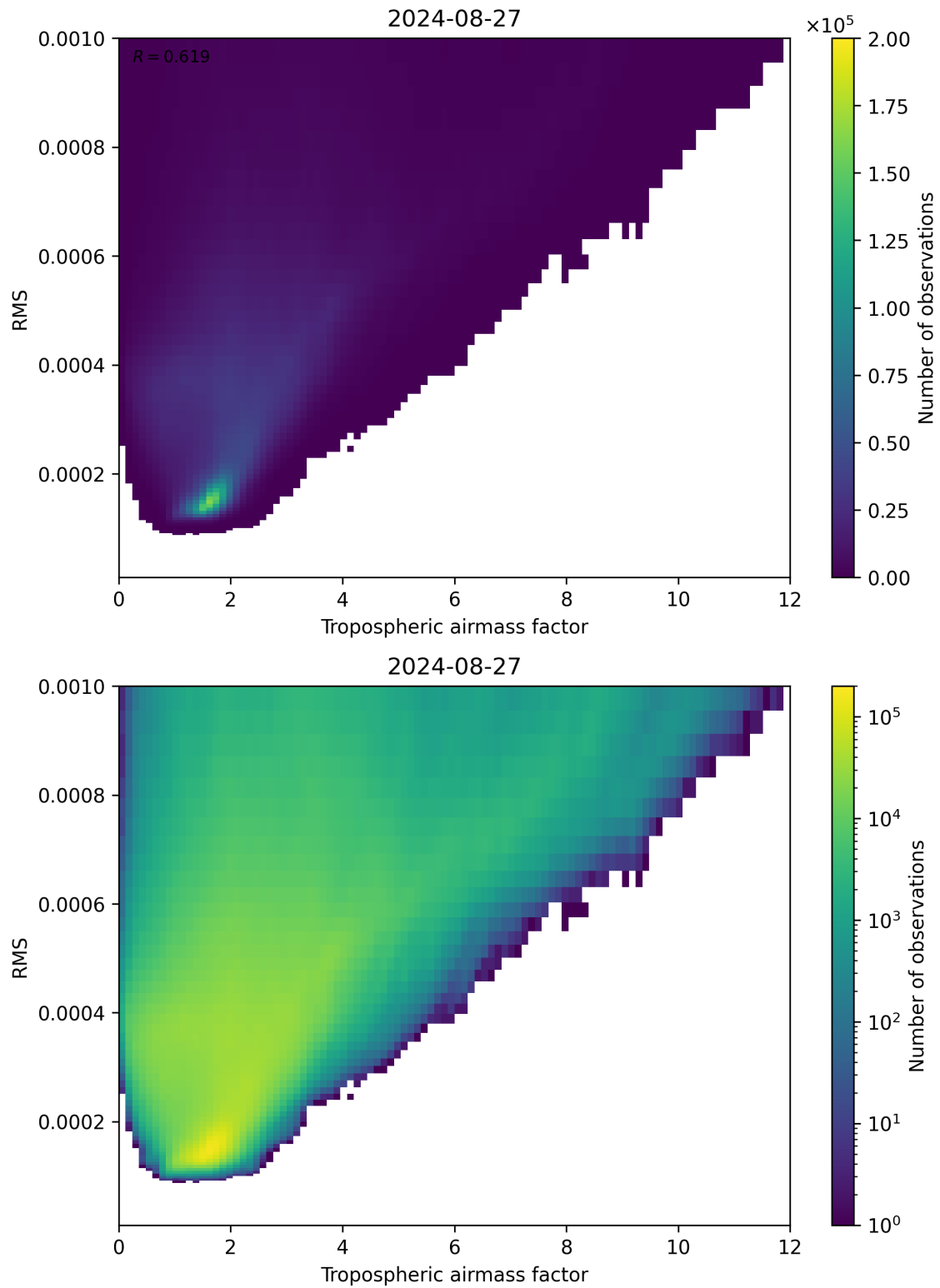
Figure 79: Scatter density plot of “Tropospheric airmass factor” against “RMS” for 2024-08-27 to 2024-08-28.
