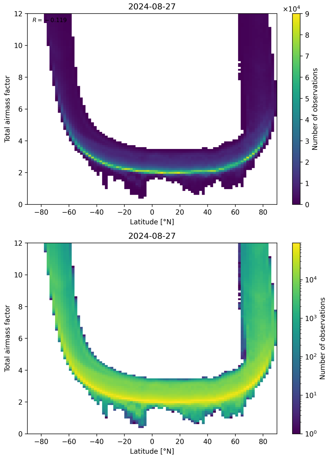
Figure 84: Scatter density plot of “Latitude” against “Total airmass factor” for 2024-08-27 to 2024-08-28.
