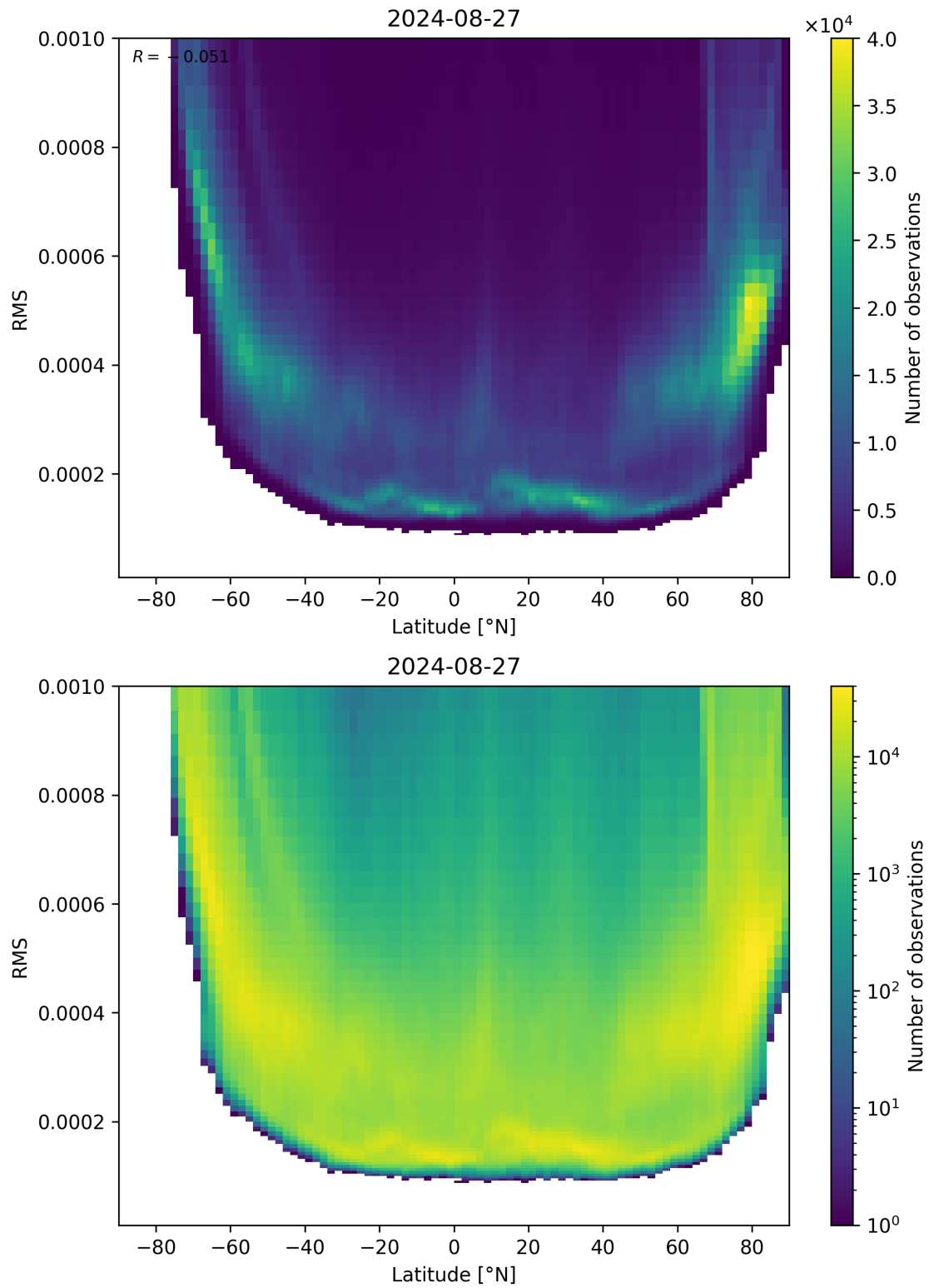
Figure 94: Scatter density plot of “Latitude” against “RMS” for 2024-08-27 to 2024-08-28.
