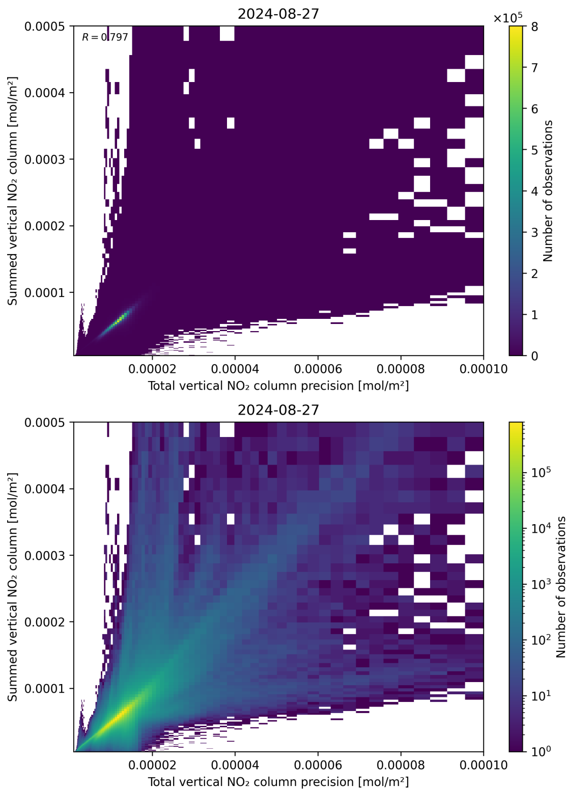
Figure 117: Scatter density plot of “Total vertical NO 2 column precision” against “Summed vertical NO 2 column” for 2024-08-27 to 2024-08-28.
