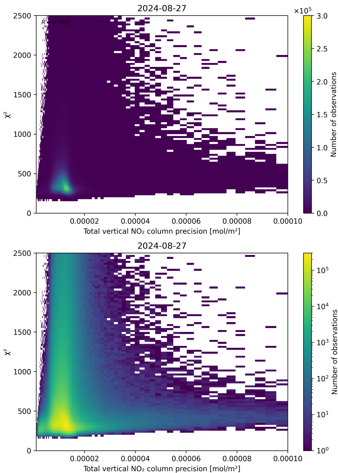
Figure 116: Scatter density plot of “Total vertical NO 2 column precision” against “ \chi^2 ” for 2024-08-27 to 2024-08-28.
