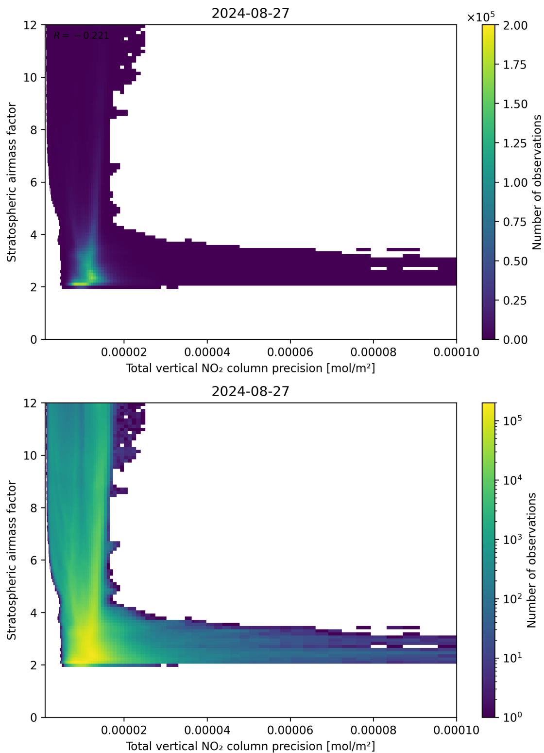
Figure 115: Scatter density plot of “Total vertical NO 2 column precision” against “Stratospheric air mass factor” for 2024-08-27 to 2024-08-28.
