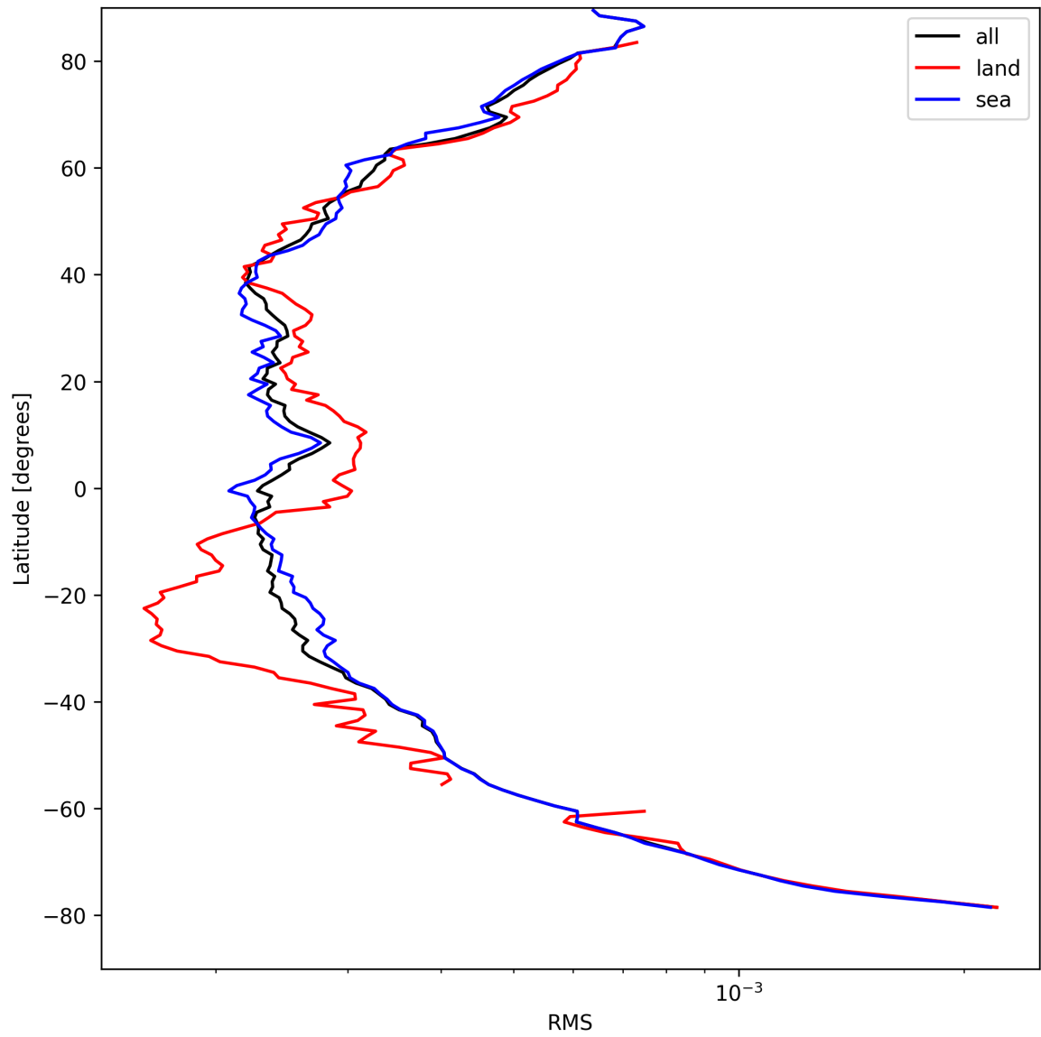
Figure 26: Zonal average of “RMS” for 2024-08-27 to 2024-08-28.
