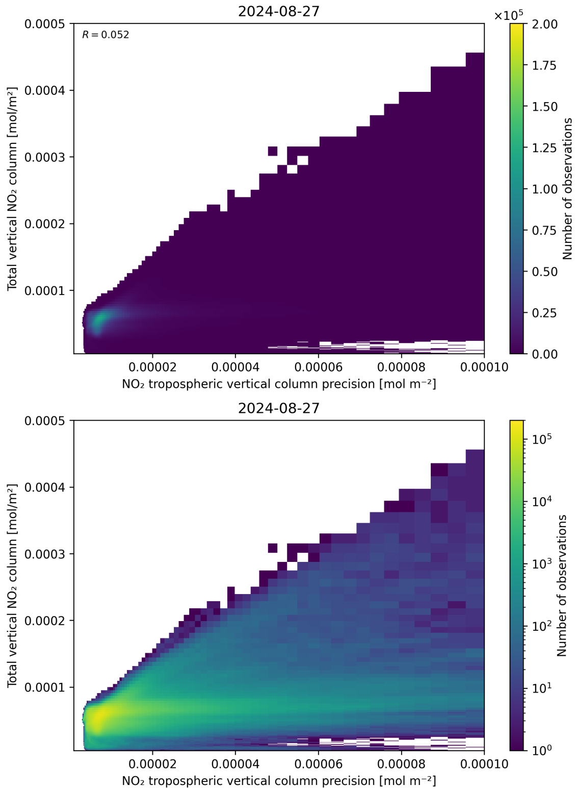
Figure 138: Scatter density plot of “NO 2 tropospheric vertical column precision” against “Total vertical NO 2 column” for 2024-08-27 to 2024-08-28.
