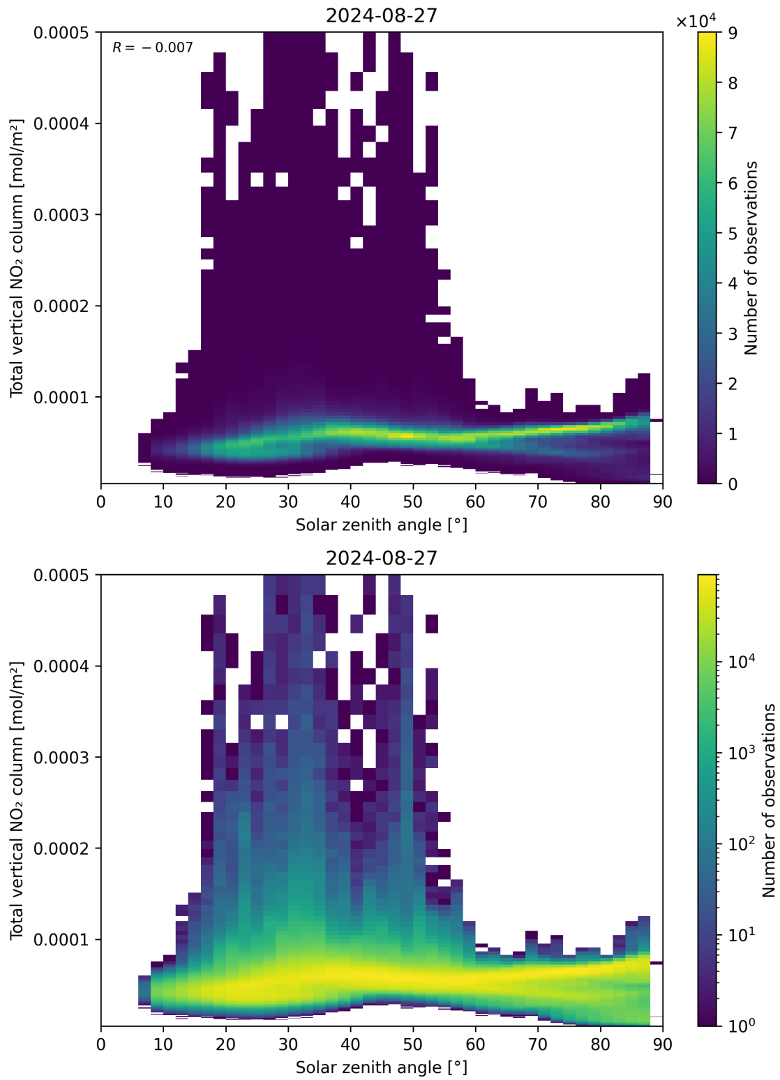
Figure 153: Scatter density plot of “Solar zenith angle” against “Total vertical NO 2 column” for 2024-08-27 to 2024-08-28.
