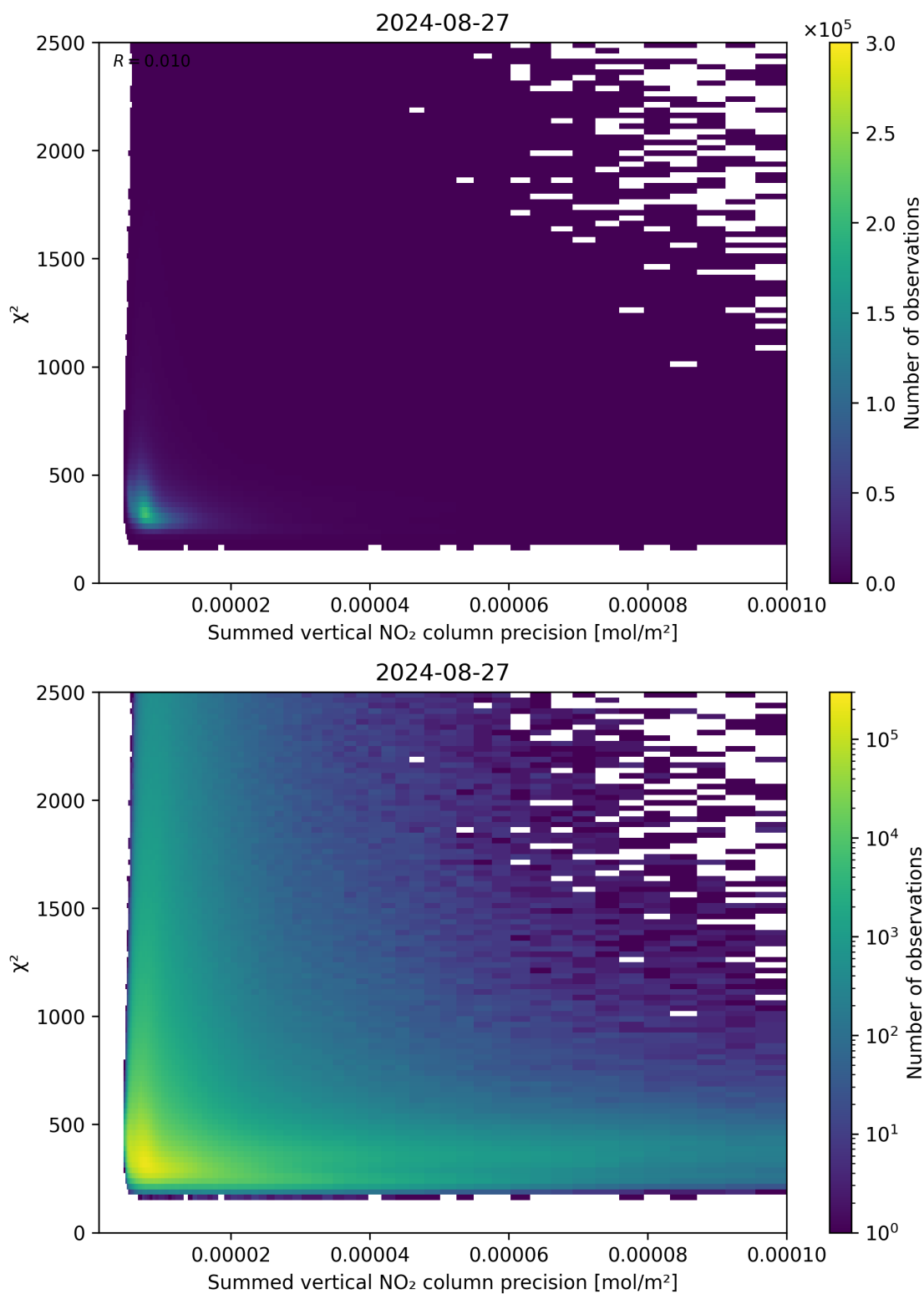
Figure 107: Scatter density plot of “Summed vertical NO 2 column precision” against “ \chi^2 ” for 2024-08-27 to 2024-08-28.
