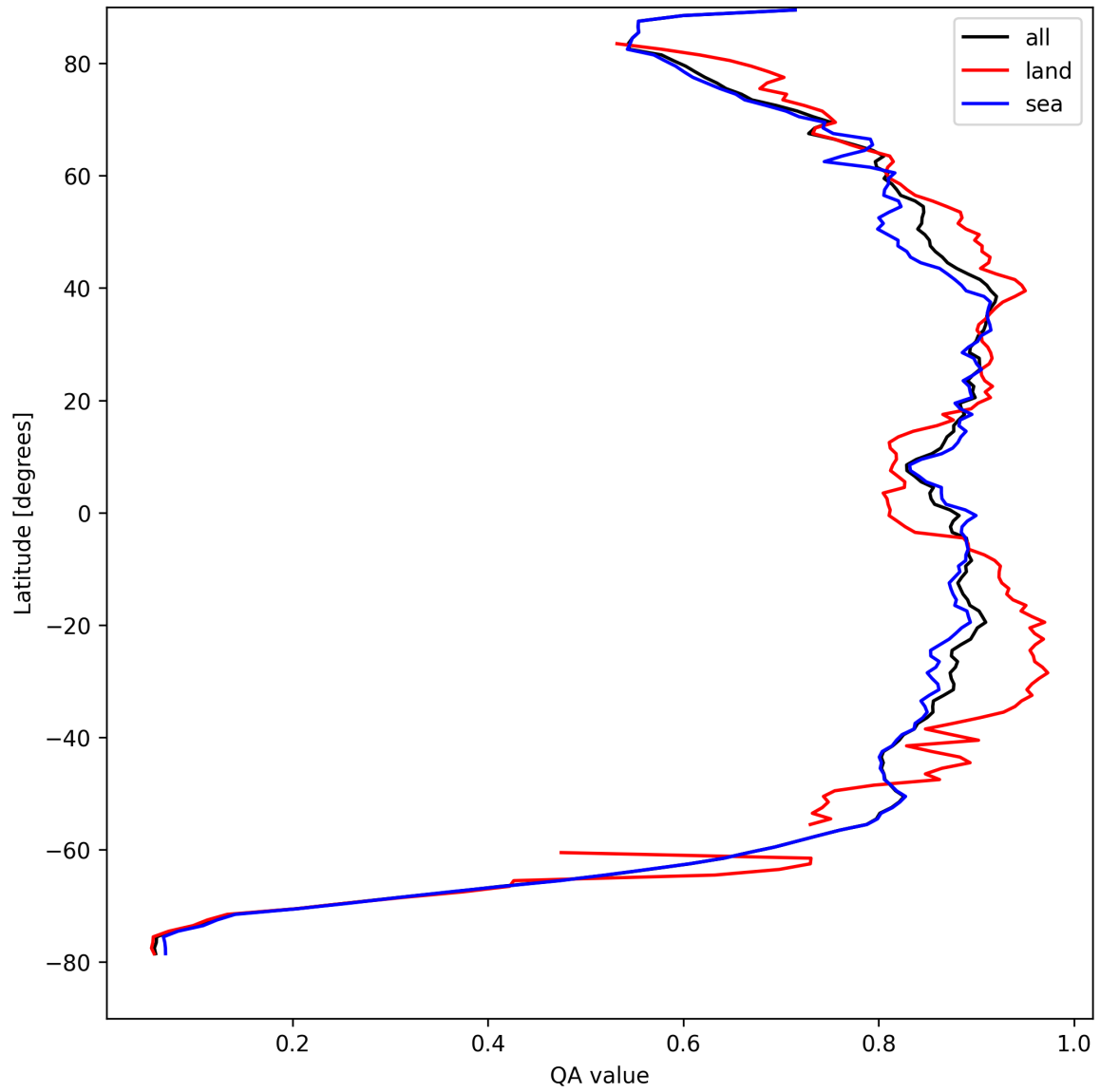
Figure 11: Zonal average of “QA value” for 2024-08-27 to 2024-08-28.
