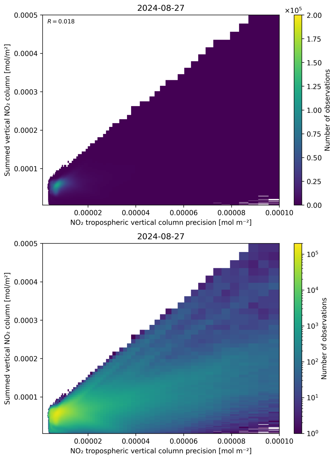
Figure 136: Scatter density plot of “NO 2 tropospheric vertical column precision” against “Summed vertical NO 2 column” for 2024-08-27 to 2024-08-28.
