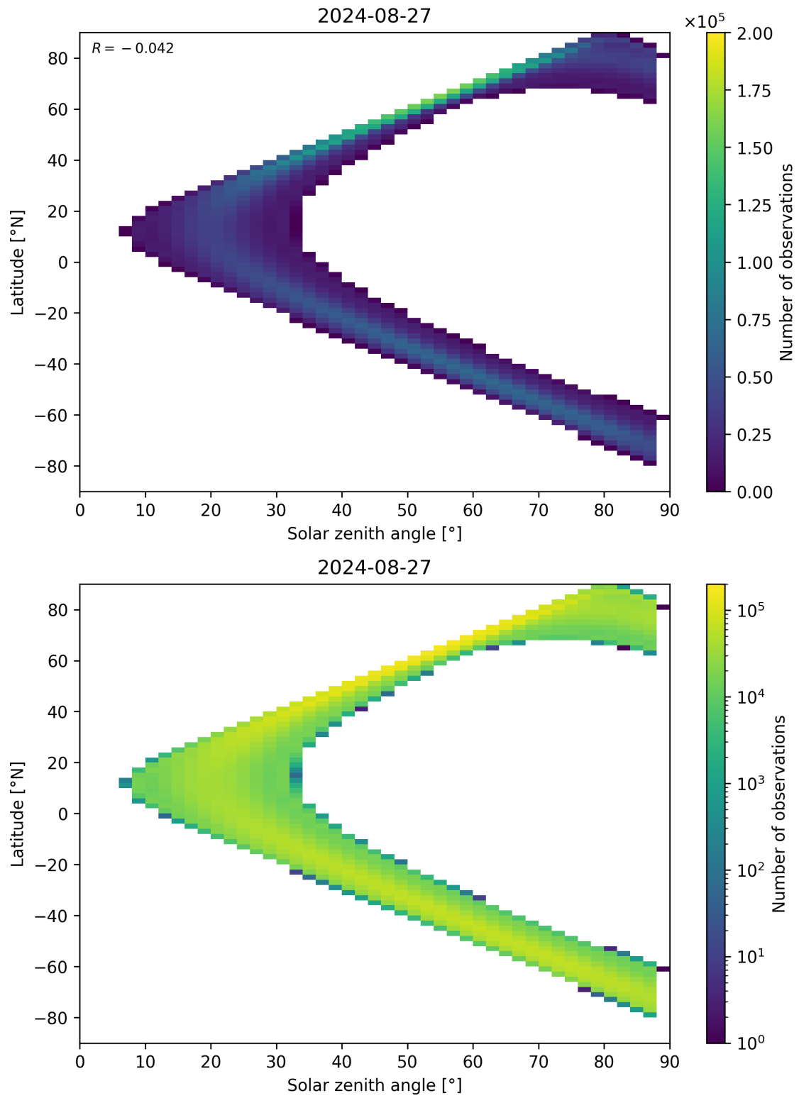
Figure 149: Scatter density plot of “Solar zenith angle” against “Latitude” for 2024-08-27 to 2024-08-28.
