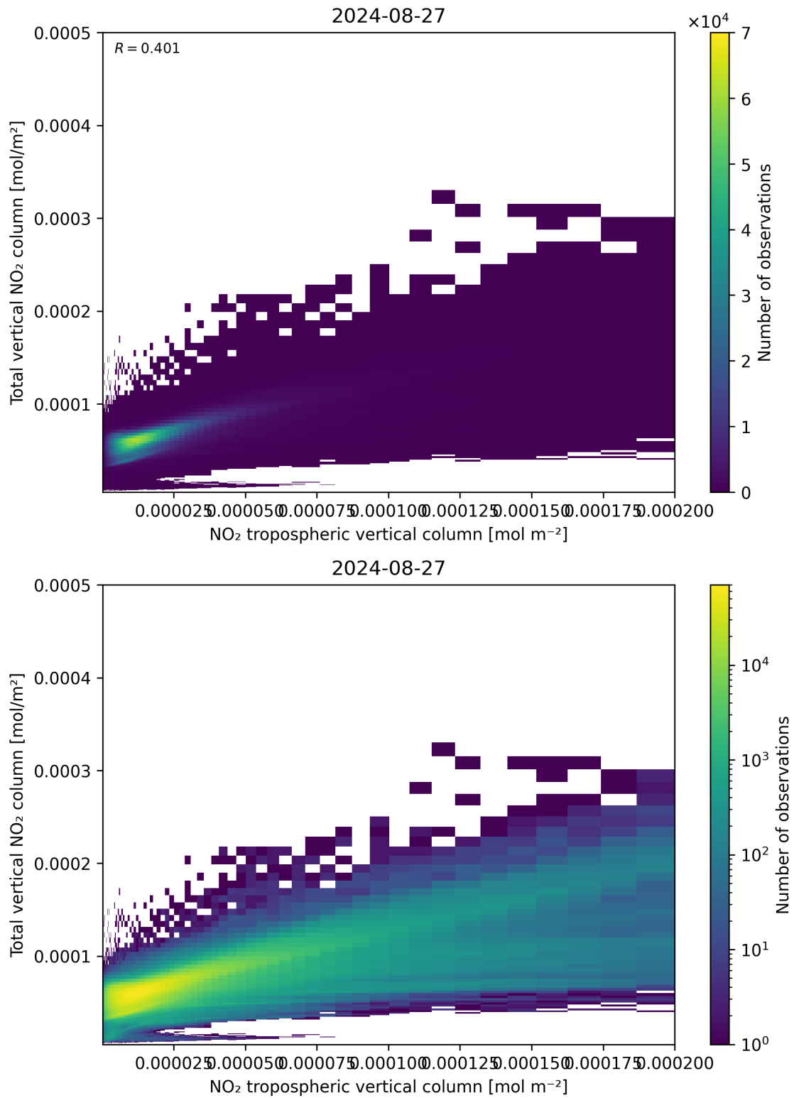
Figure 128: Scatter density plot of “NO 2 tropospheric vertical column” against “Total vertical NO 2 column” for 2024-08-27 to 2024-08-28.
