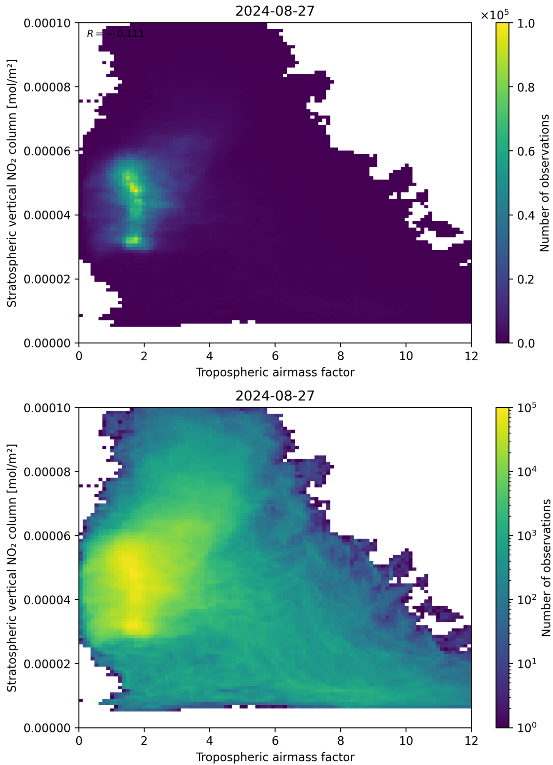
Figure 74: Scatter density plot of “Tropospheric airmass factor” against “Stratospheric vertical NO 2 column” for 2024-08-27 to 2024-08-28.
