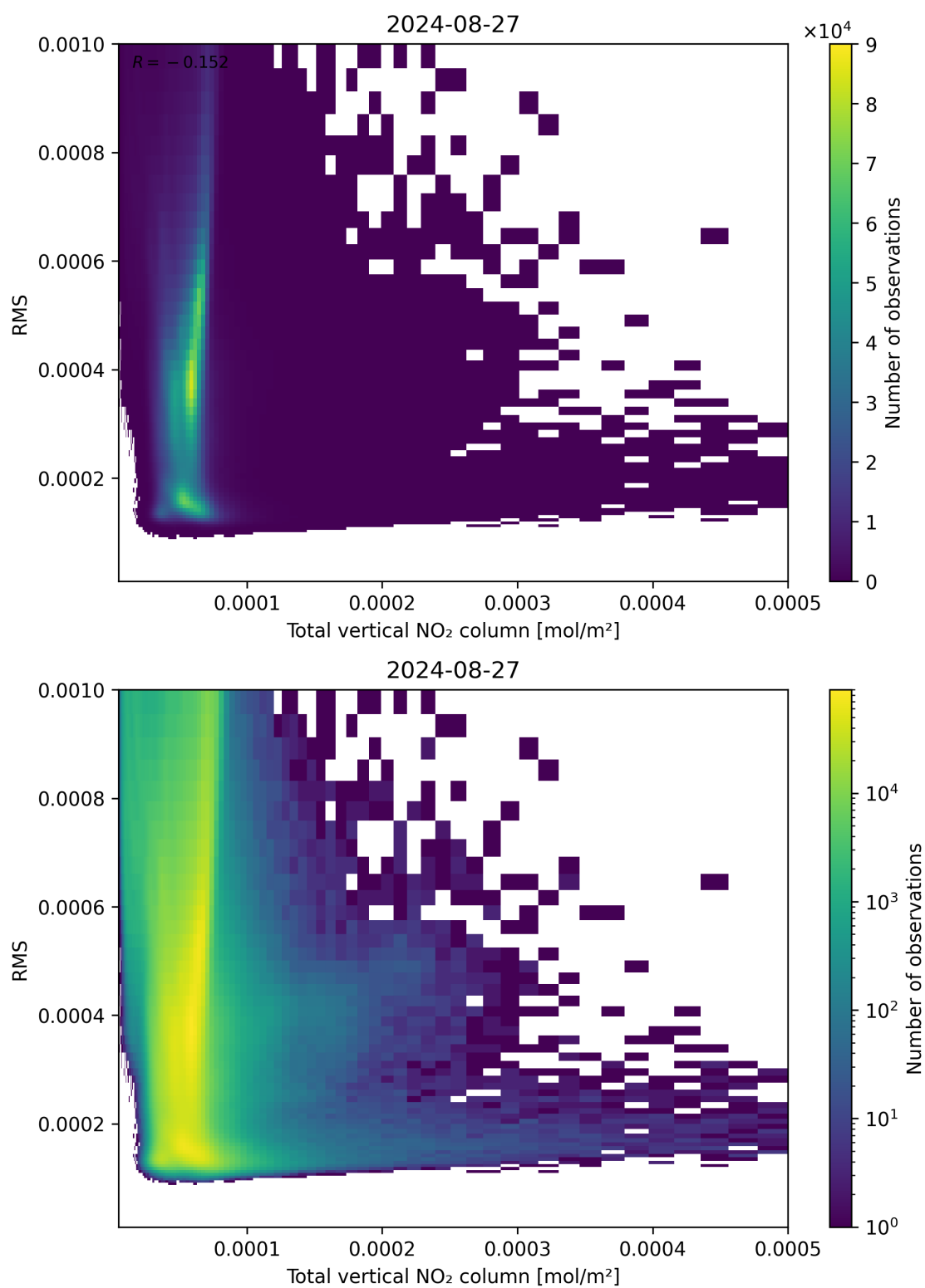
Figure 120: Scatter density plot of “Total vertical NO 2 column” against “RMS” for 2024-08-27 to 2024-08-28.
