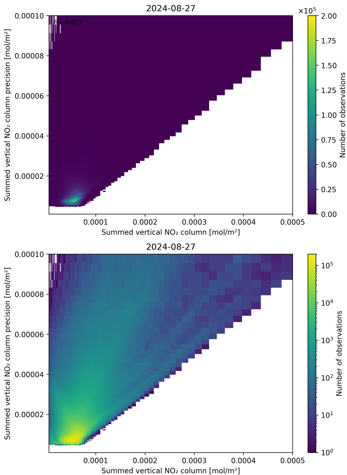
Figure 105: Scatter density plot of “Summed vertical NO 2 column” against “Summed vertical NO 2 column precision” for 2024-08-27 to 2024-08-28.
