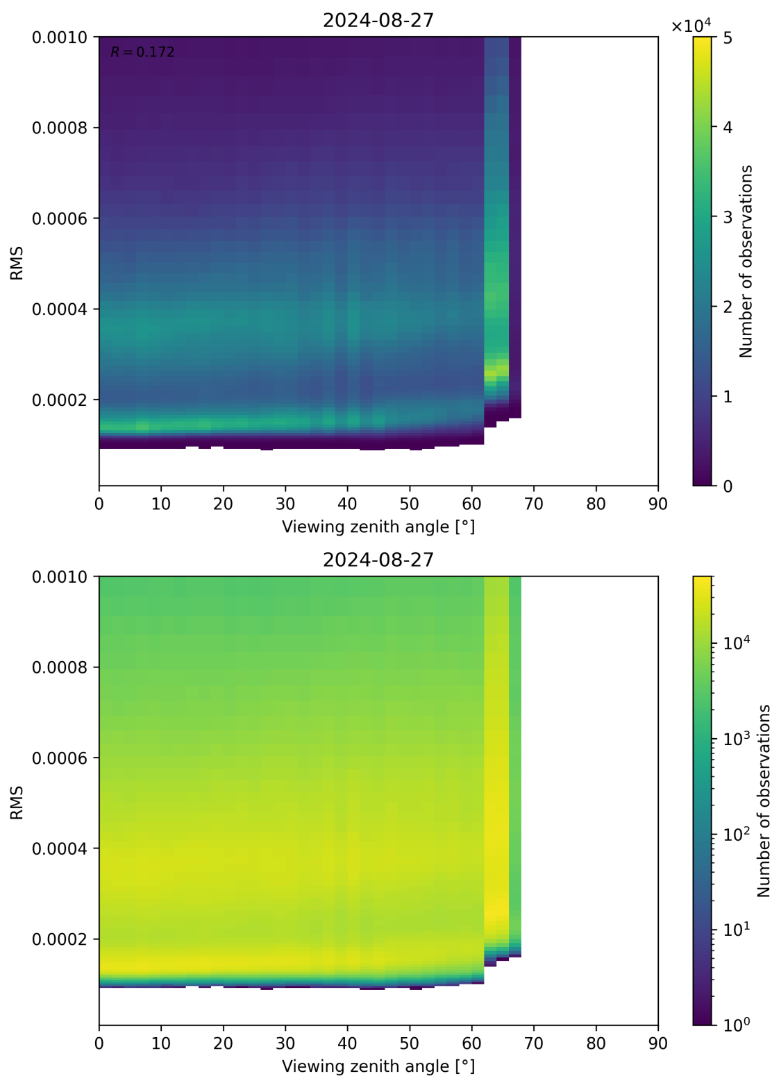
Figure 171: Scatter density plot of “Viewing zenith angle” against “RMS” for 2024-08-27 to 2024-08-28.
