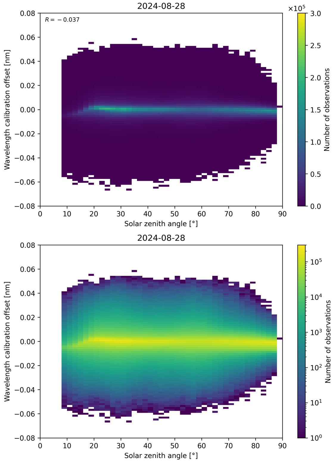
Figure 158: Scatter density plot of “Solar zenith angle” against “Wavelength calibration offset” for 2024-08-27 to 2024-08-29.
