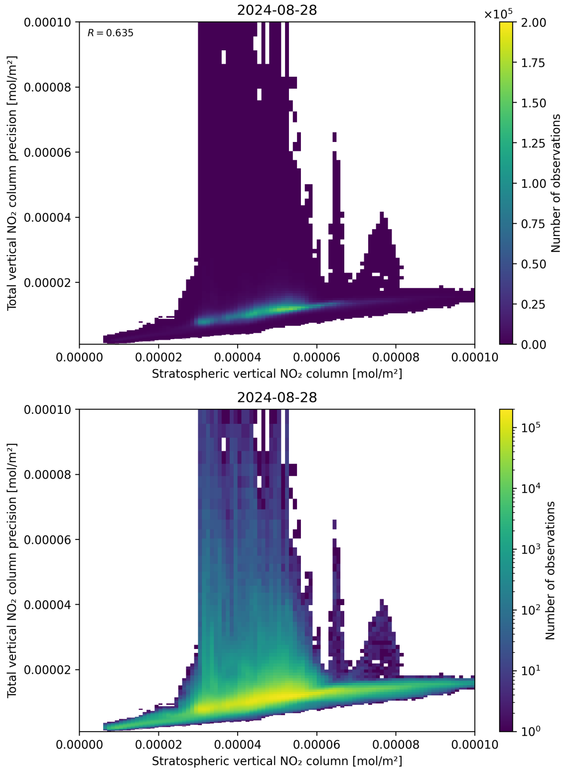
Figure 101: Scatter density plot of “Stratospheric vertical NO 2 column” against “Total vertical NO 2 column precision” for 2024-08-27 to 2024-08-29.
