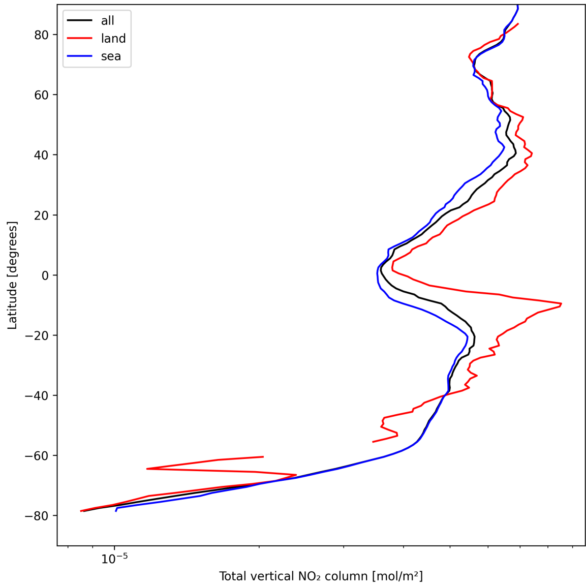
Figure 21: Zonal average of “Total vertical NO 2 column” for 2024-08-27 to 2024-08-29.
