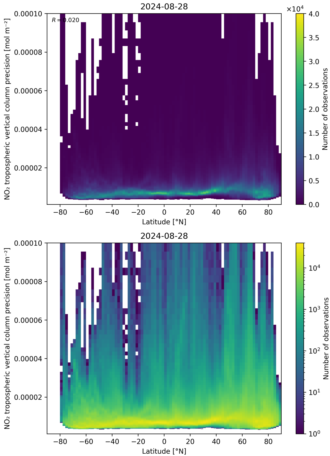
Figure 93: Scatter density plot of “Latitude” against “NO 2 tropospheric vertical column precision” for 2024-08-27 to 2024-08-29.
