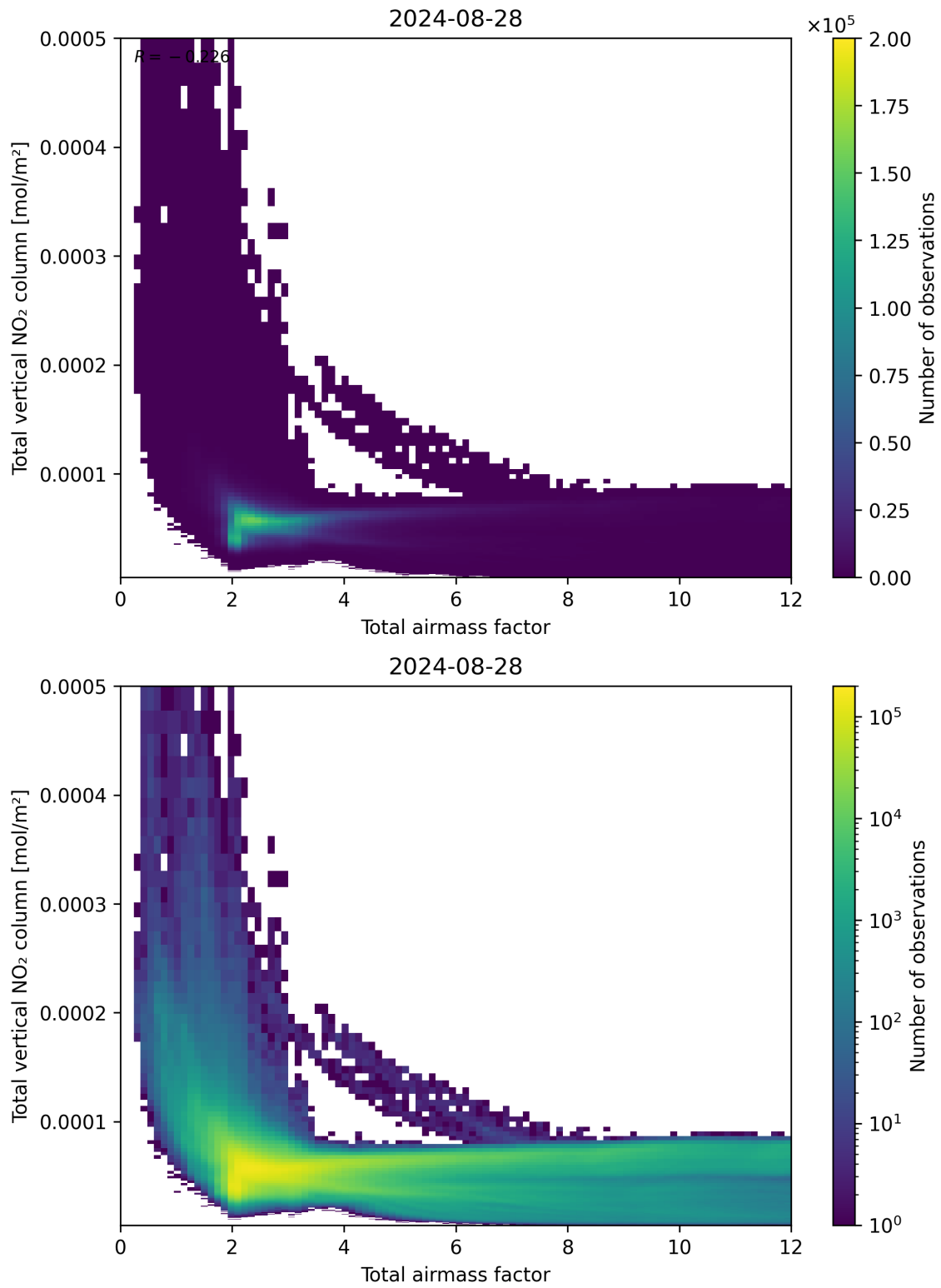
Figure 67: Scatter density plot of “Total airmass factor” against “Total vertical NO 2 column” for 2024-08-27 to 2024-08-29.
