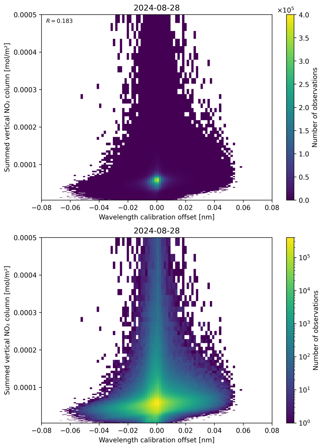
Figure 177: Scatter density plot of “Wavelength calibration offset” against “Summed vertical NO 2 column” for 2024-08-27 to 2024-08-29.
