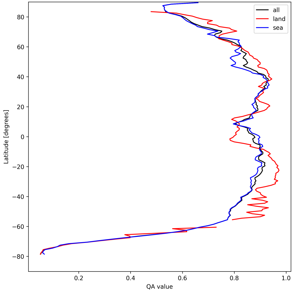
Figure 11: Zonal average of “QA value” for 2024-08-27 to 2024-08-29.
