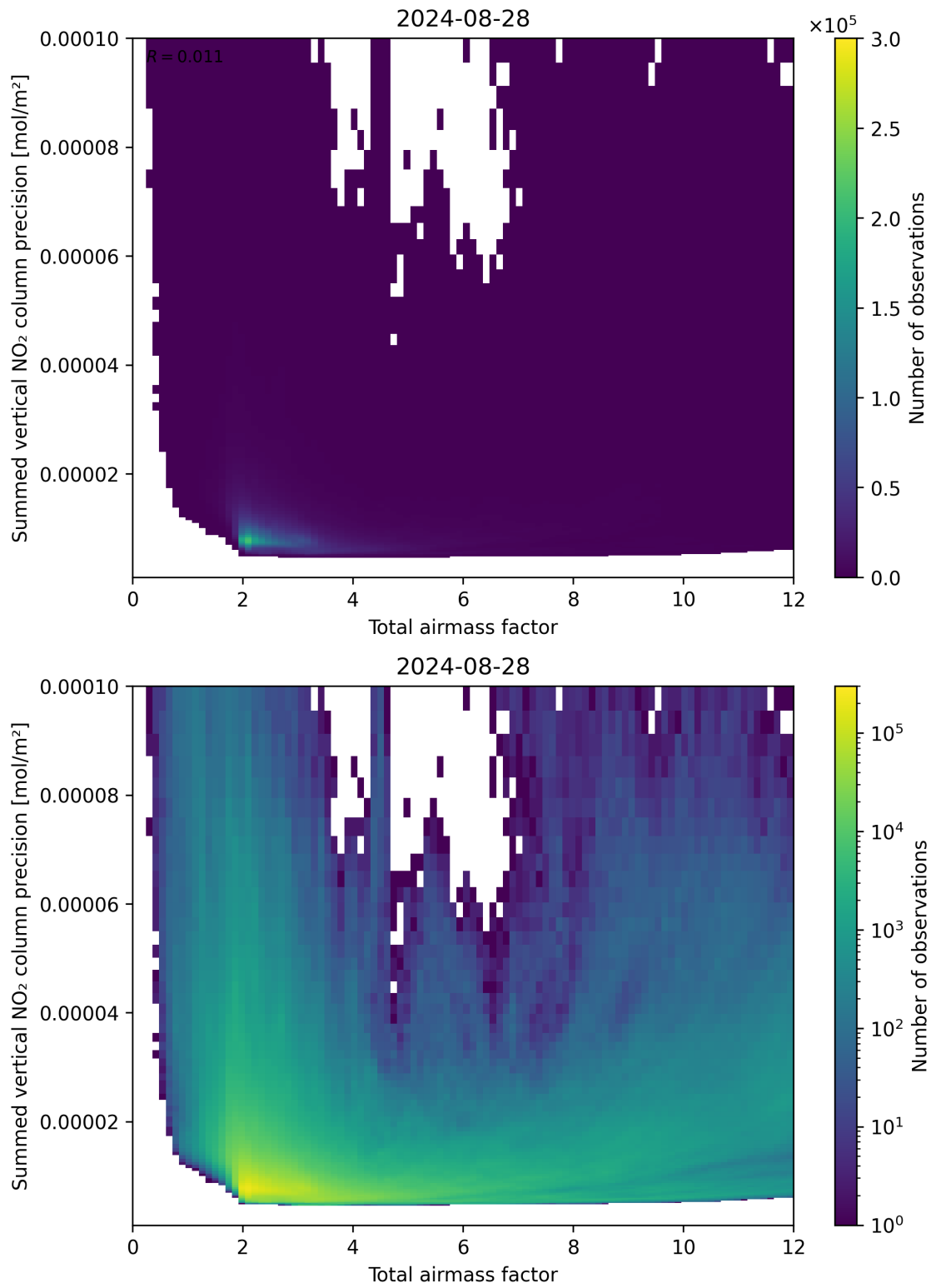
Figure 66: Scatter density plot of “Total airmass factor” against “Summed vertical NO 2 column precision” for 2024-08-27 to 2024-08-29.
