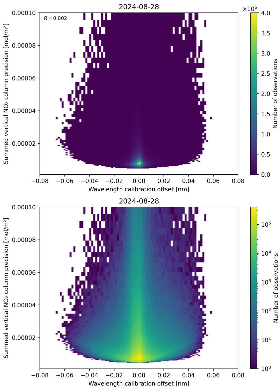
Figure 178: Scatter density plot of “Wavelength calibration offset” against “Summed vertical NO 2 column precision” for 2024-08-27 to 2024-08-29.
