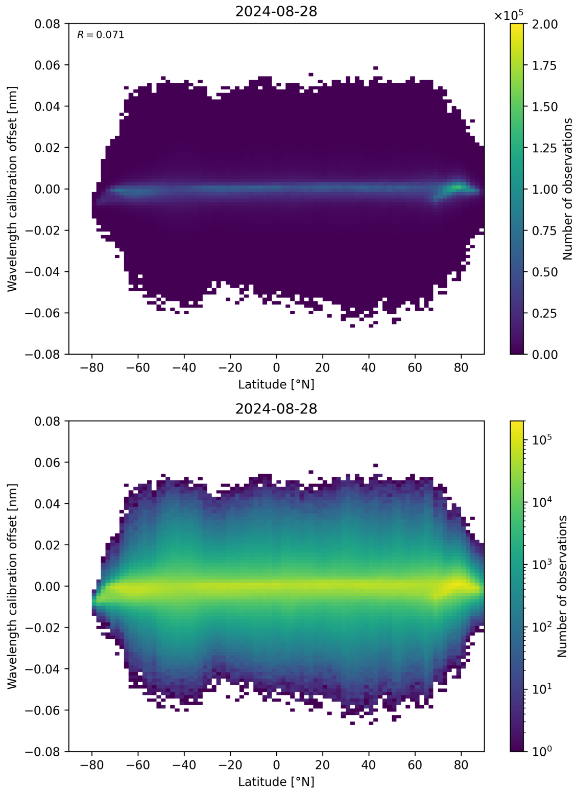
Figure 95: Scatter density plot of “Latitude” against “Wavelength calibration offset” for 2024-08-27 to 2024-08-29.
