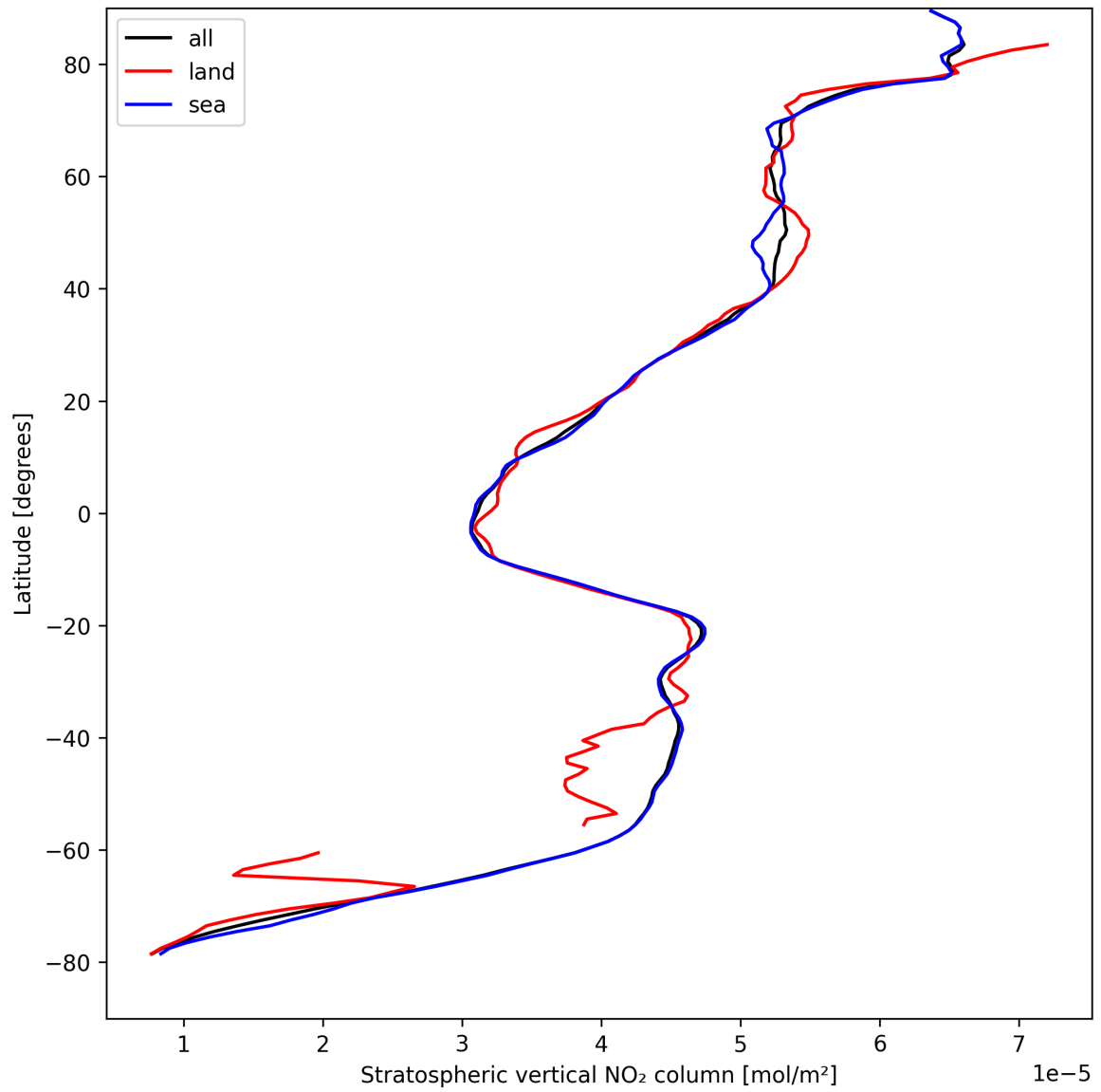
Figure 19: Zonal average of “Stratospheric vertical NO 2 column” for 2024-08-27 to 2024-08-29.
