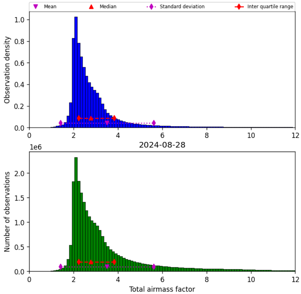
Figure 32: Histogram of “Total airmass factor” for 2024-08-27 to 2024-08-29
