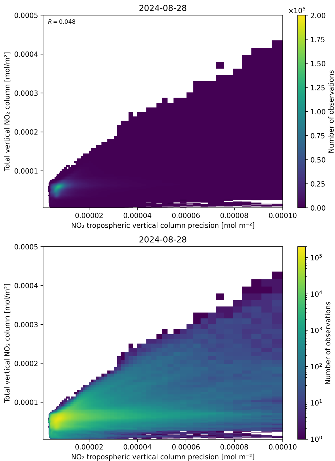
Figure 138: Scatter density plot of “NO 2 tropospheric vertical column precision” against “Total vertical NO 2 column” for 2024-08-27 to 2024-08-29.
