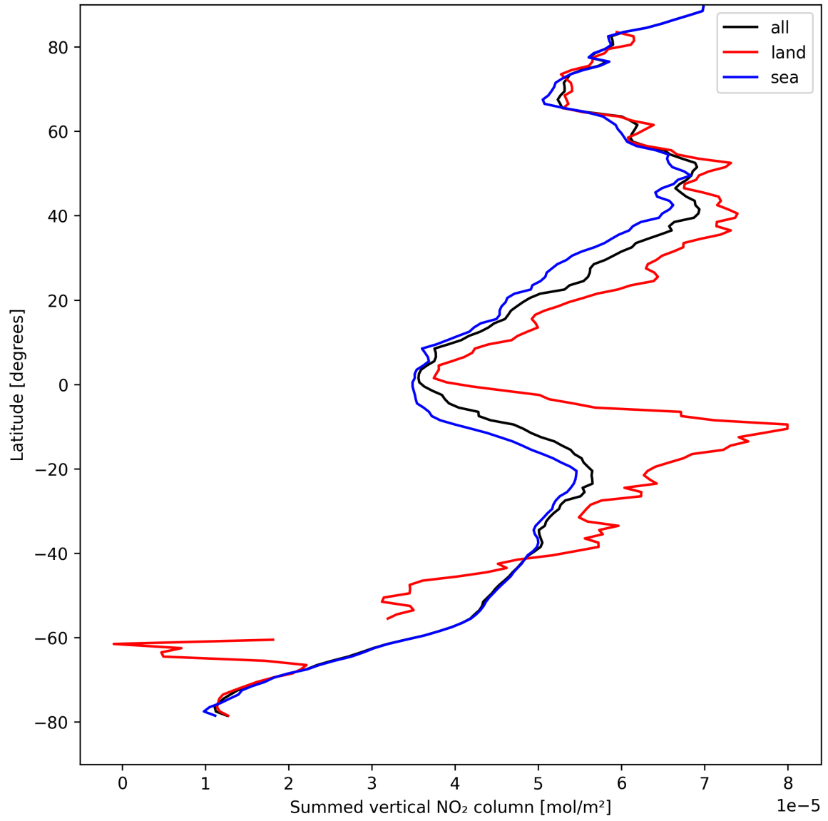
Figure 23: Zonal average of “Summed vertical NO 2 column” for 2024-08-27 to 2024-08-29.
