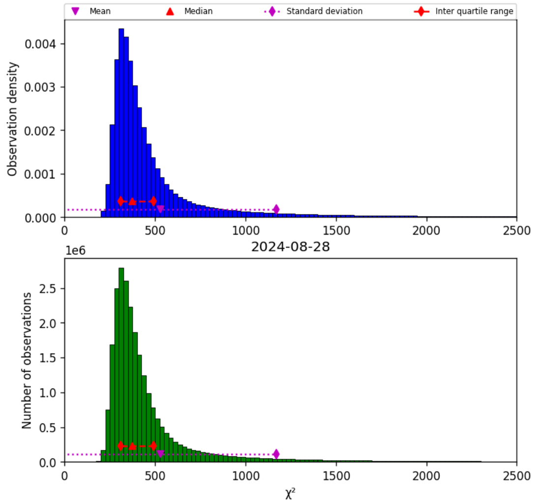
Figure 42: Histogram of “ \chi^2 ” for 2024-08-27 to 2024-08-29
