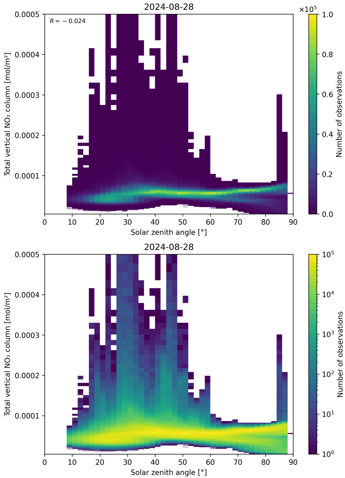
Figure 153: Scatter density plot of “Solar zenith angle” against “Total vertical NO 2 column” for 2024-08-27 to 2024-08-29.
