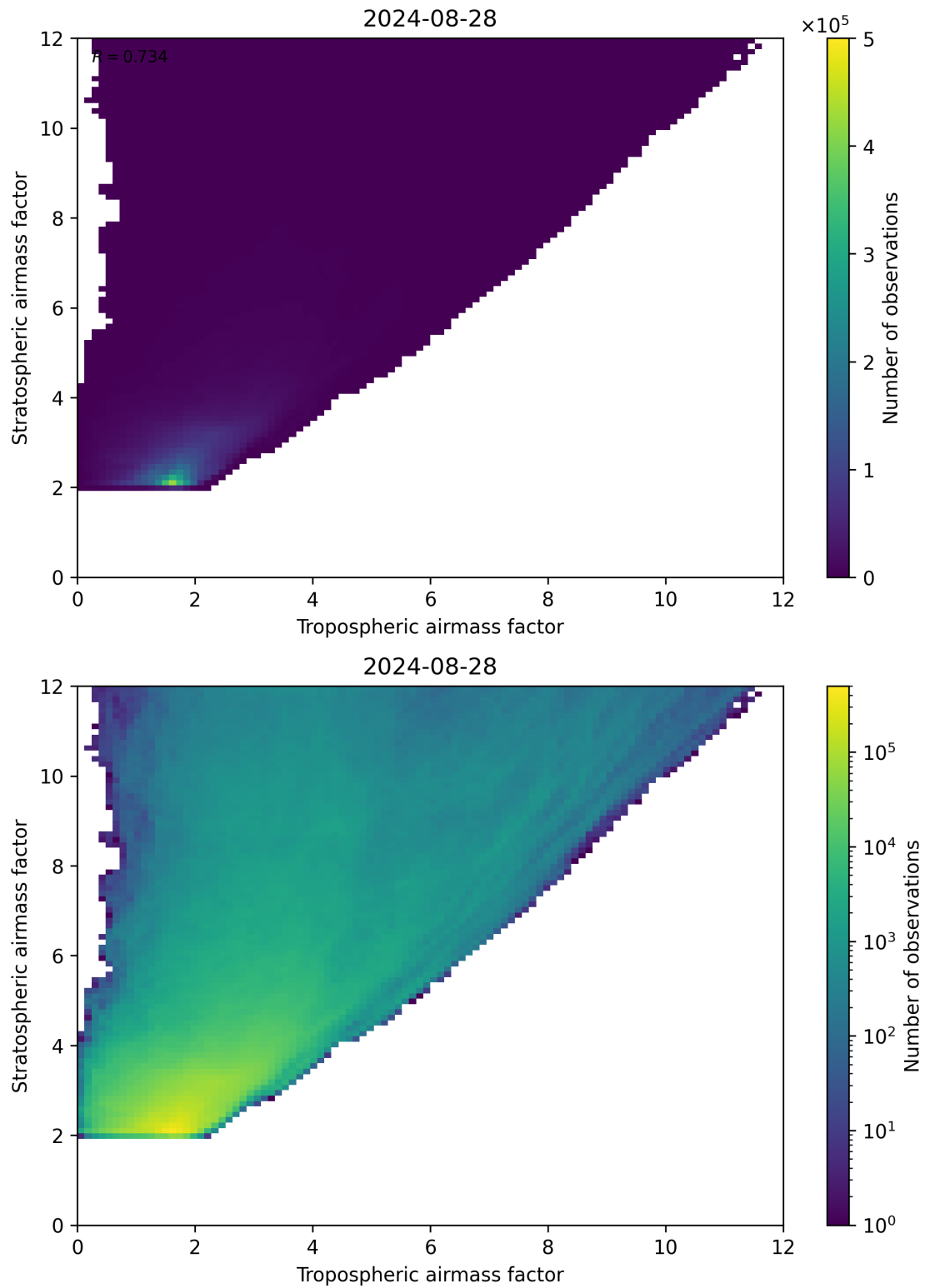
Figure 71: Scatter density plot of “Tropospheric airmass factor” against “Stratospheric airmass factor” for 2024-08-27 to 2024-08-29.
