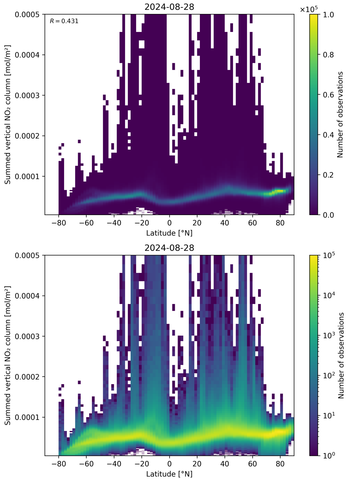
Figure 88: Scatter density plot of “Latitude” against “Summed vertical NO 2 column” for 2024-08-27 to 2024-08-29.
