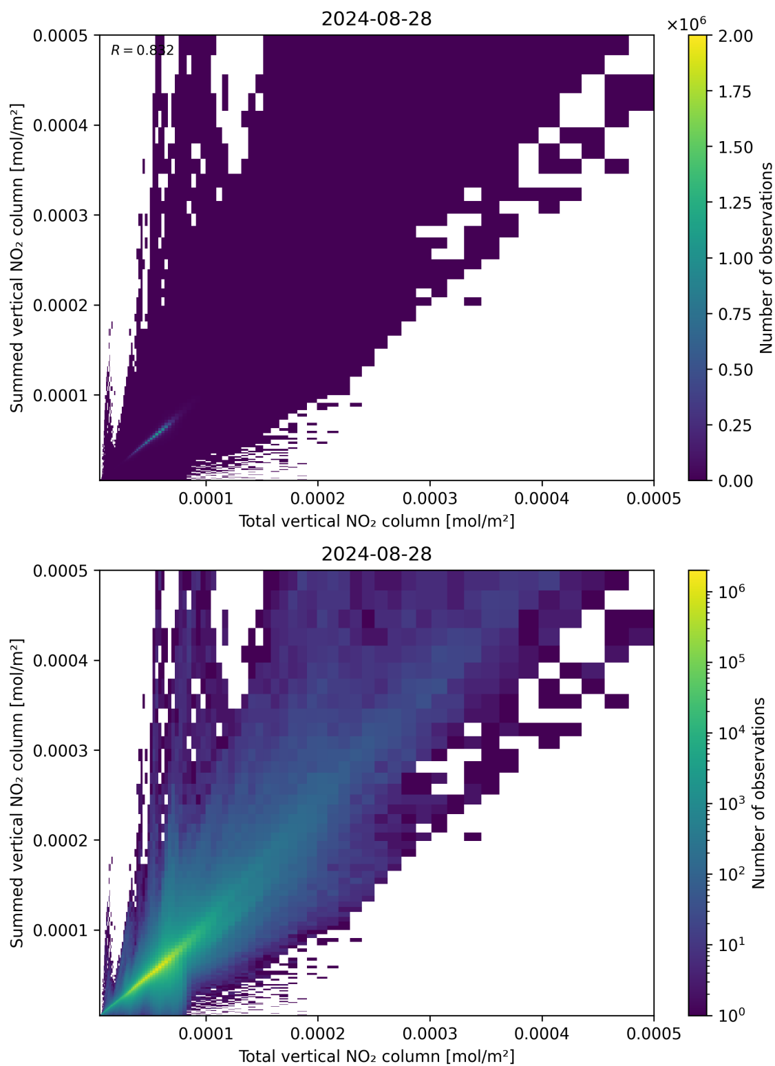
Figure 112: Scatter density plot of “Total vertical NO 2 column” against “Summed vertical NO 2 column” for 2024-08-27 to 2024-08-29.
