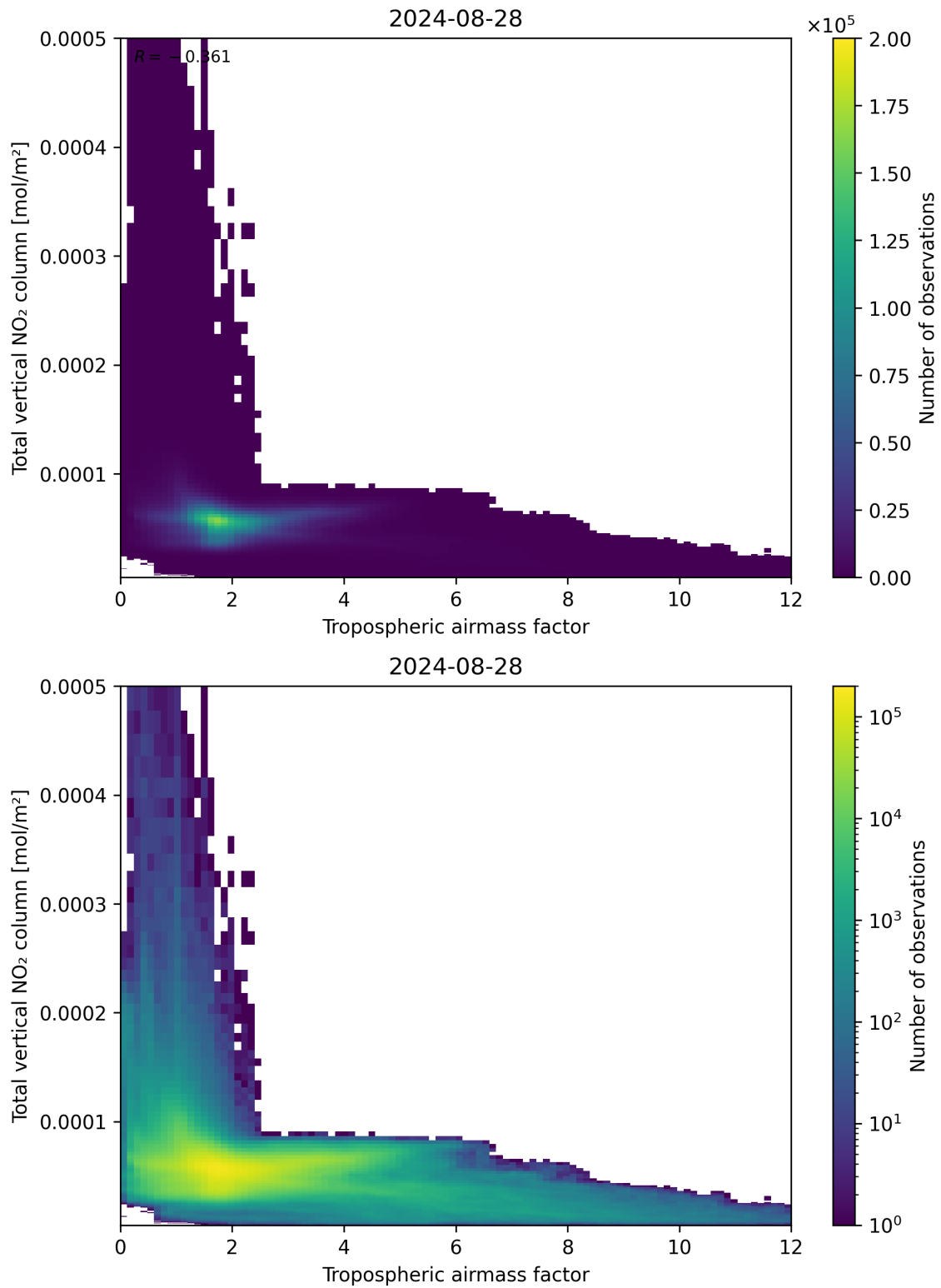
Figure 77: Scatter density plot of “Tropospheric airmass factor” against “Total vertical NO 2 column” for 2024-08-27 to 2024-08-29.
