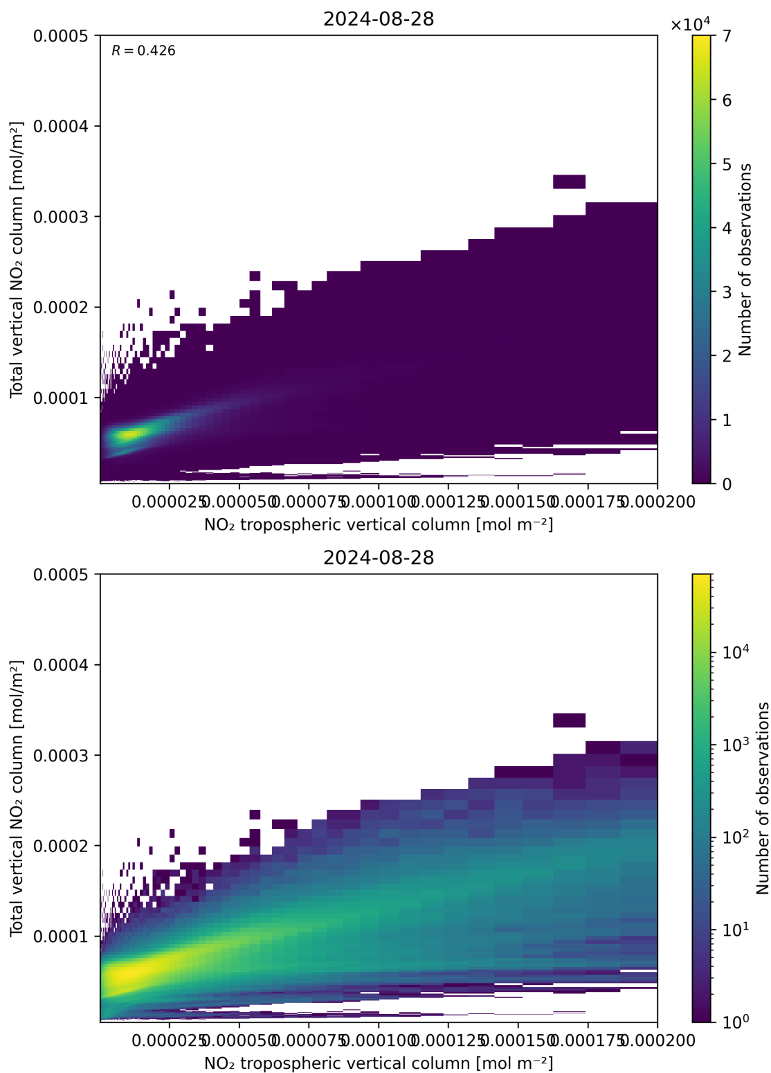
Figure 128: Scatter density plot of “NO 2 tropospheric vertical column” against “Total vertical NO 2 column” for 2024-08-27 to 2024-08-29.
