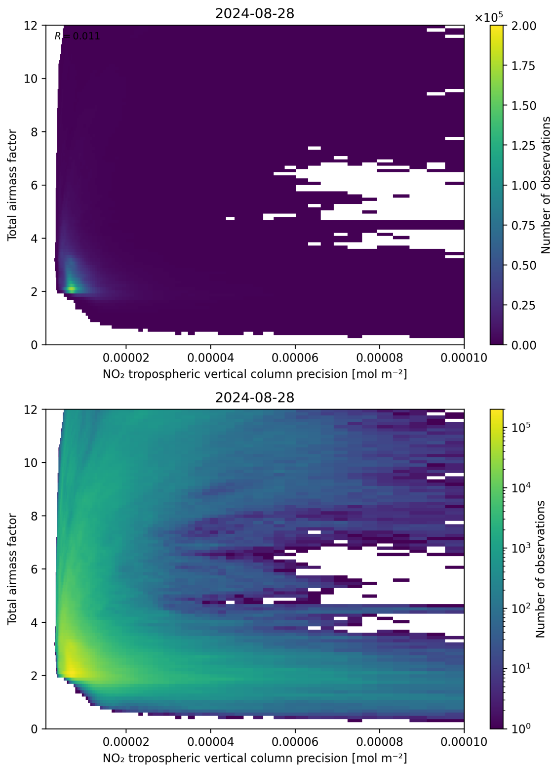
Figure 132: Scatter density plot of “NO 2 tropospheric vertical column precision” against “Total air mass factor” for 2024-08-27 to 2024-08-29.
