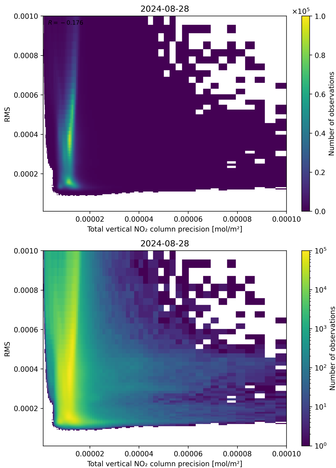
Figure 119: Scatter density plot of “Total vertical NO 2 column precision” against “RMS” for 2024-08-27 to 2024-08-29.
