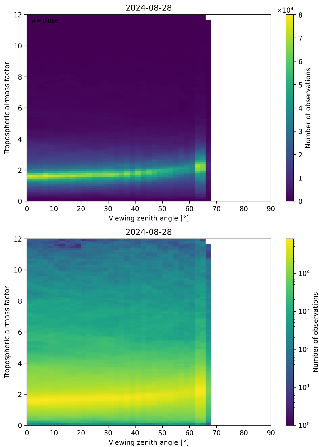
Figure 161: Scatter density plot of “Viewing zenith angle” against “Tropospheric airmass factor” for 2024-08-27 to 2024-08-29.
