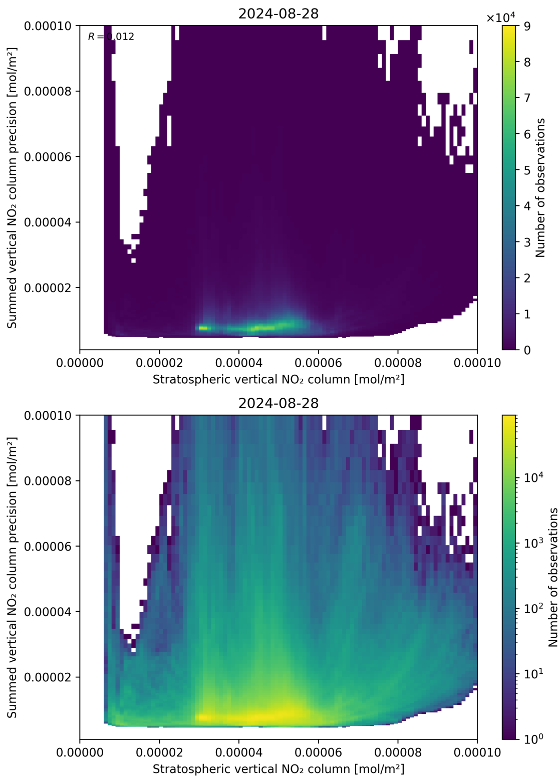
Figure 99: Scatter density plot of “Stratospheric vertical NO 2 column” against “Summed vertical NO 2 column precision” for 2024-08-27 to 2024-08-29.
