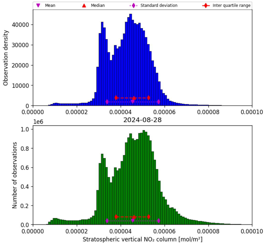
Figure 36: Histogram of “Stratospheric vertical NO 2 column” for 2024-08-27 to 2024-08-29
