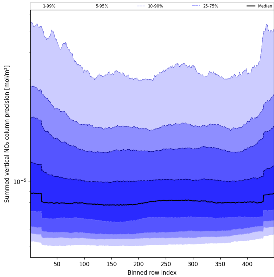
Figure 58: Along track statistics of “Summed vertical NO 2 column precision” for 2024-08-27 to 2024-08-29
