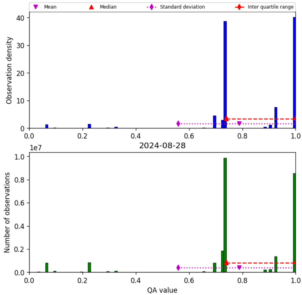
Figure 28: Histogram of “QA value” for 2024-08-27 to 2024-08-29
