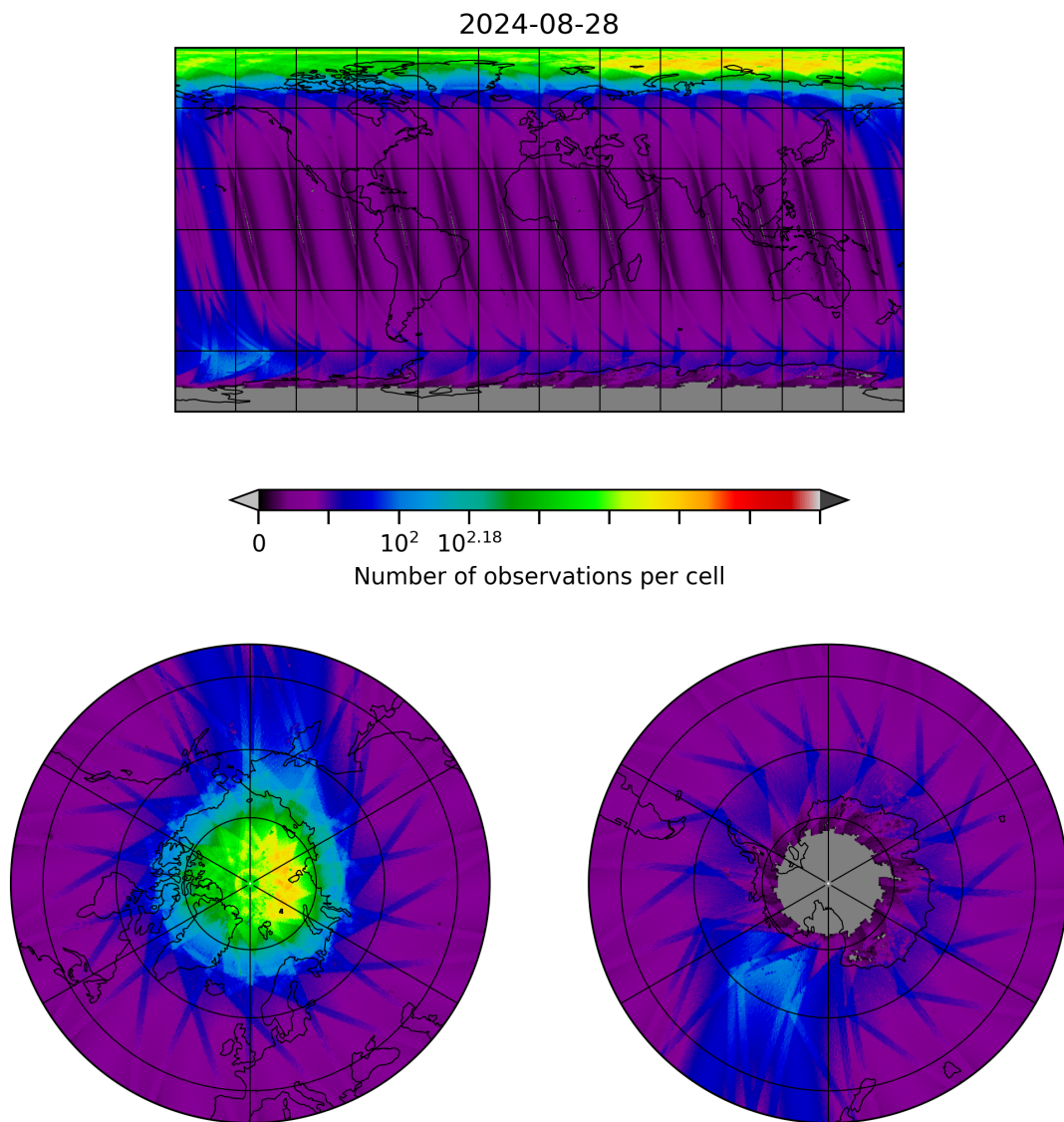
Figure 10: Map of the number of observations for 2024-08-27 to 2024-08-29
