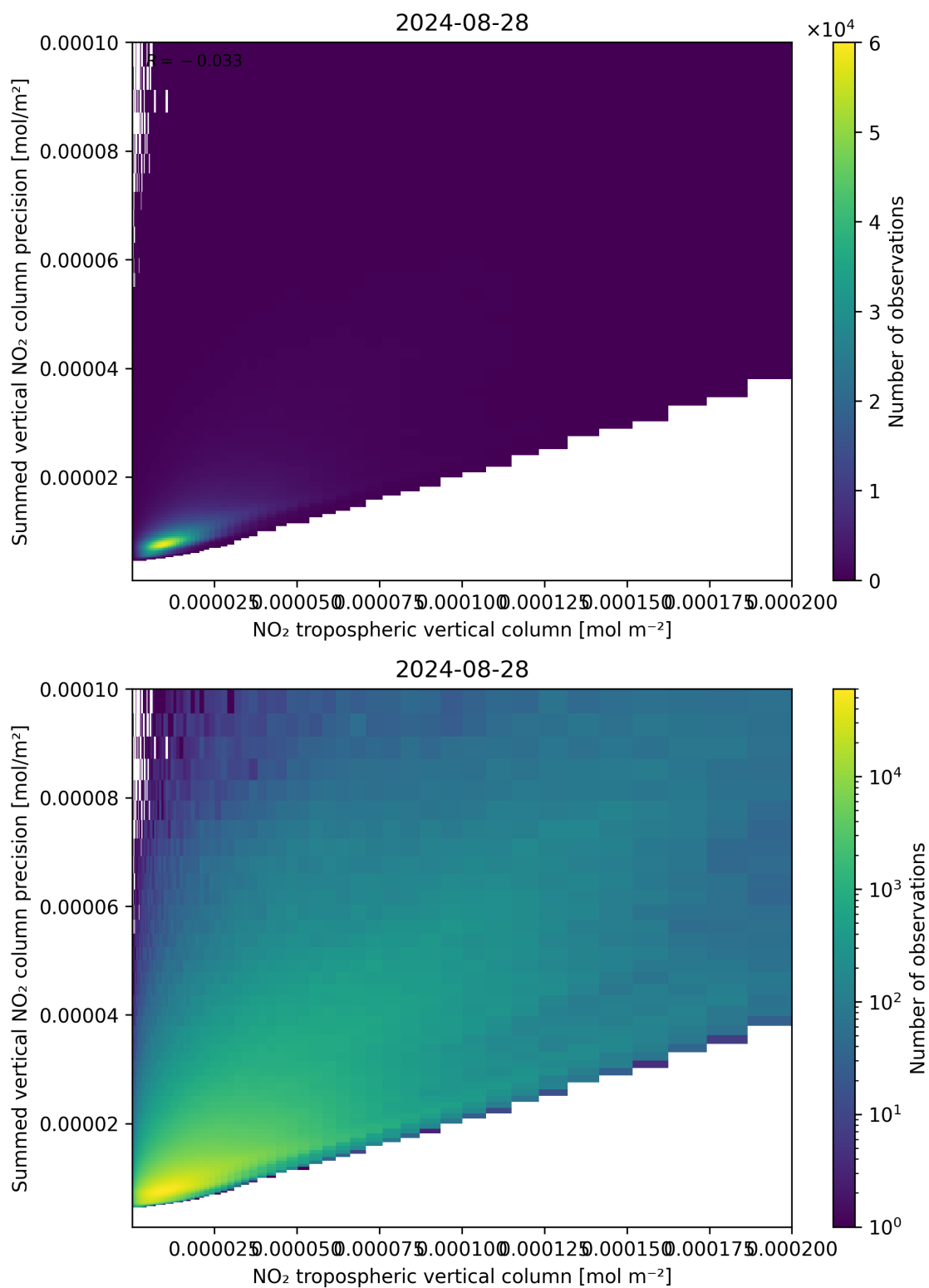
Figure 127: Scatter density plot of “NO 2 tropospheric vertical column” against “Summed vertical NO 2 column precision” for 2024-08-27 to 2024-08-29.
