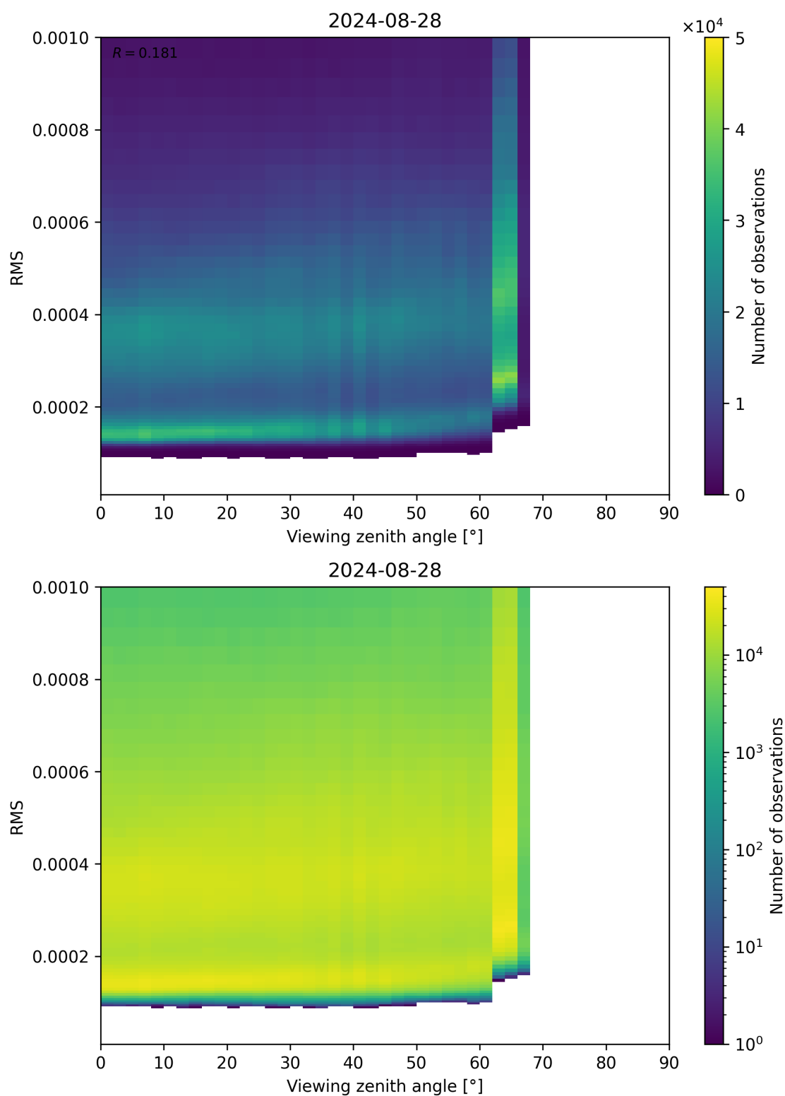
Figure 171: Scatter density plot of “Viewing zenith angle” against “RMS” for 2024-08-27 to 2024-08-29.
