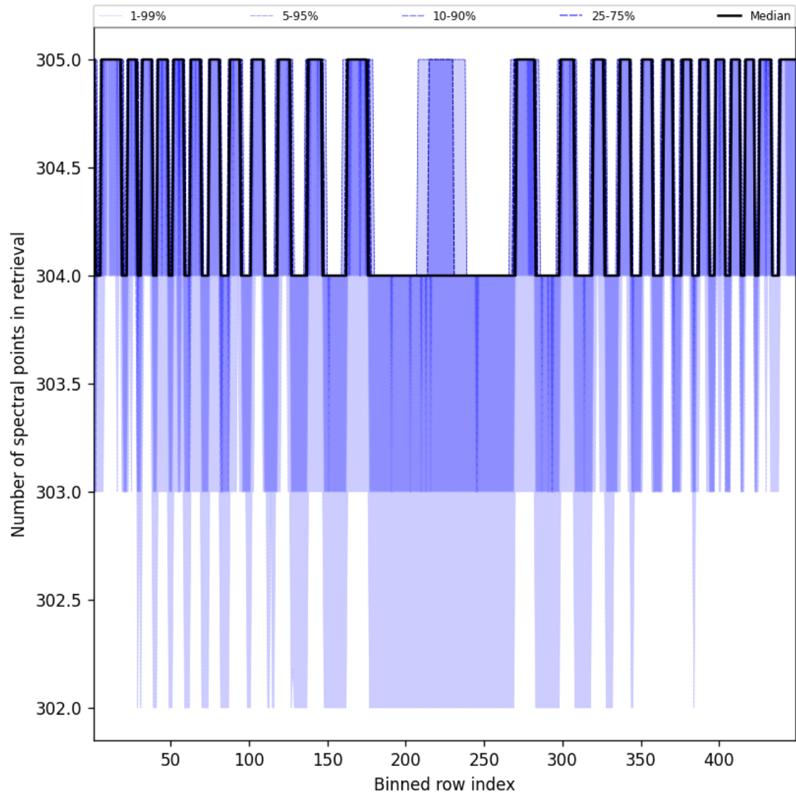
Figure 50: Along track statistics of “Number of spectral points in retrieval” for 2024-08-27 to 2024-08-29
