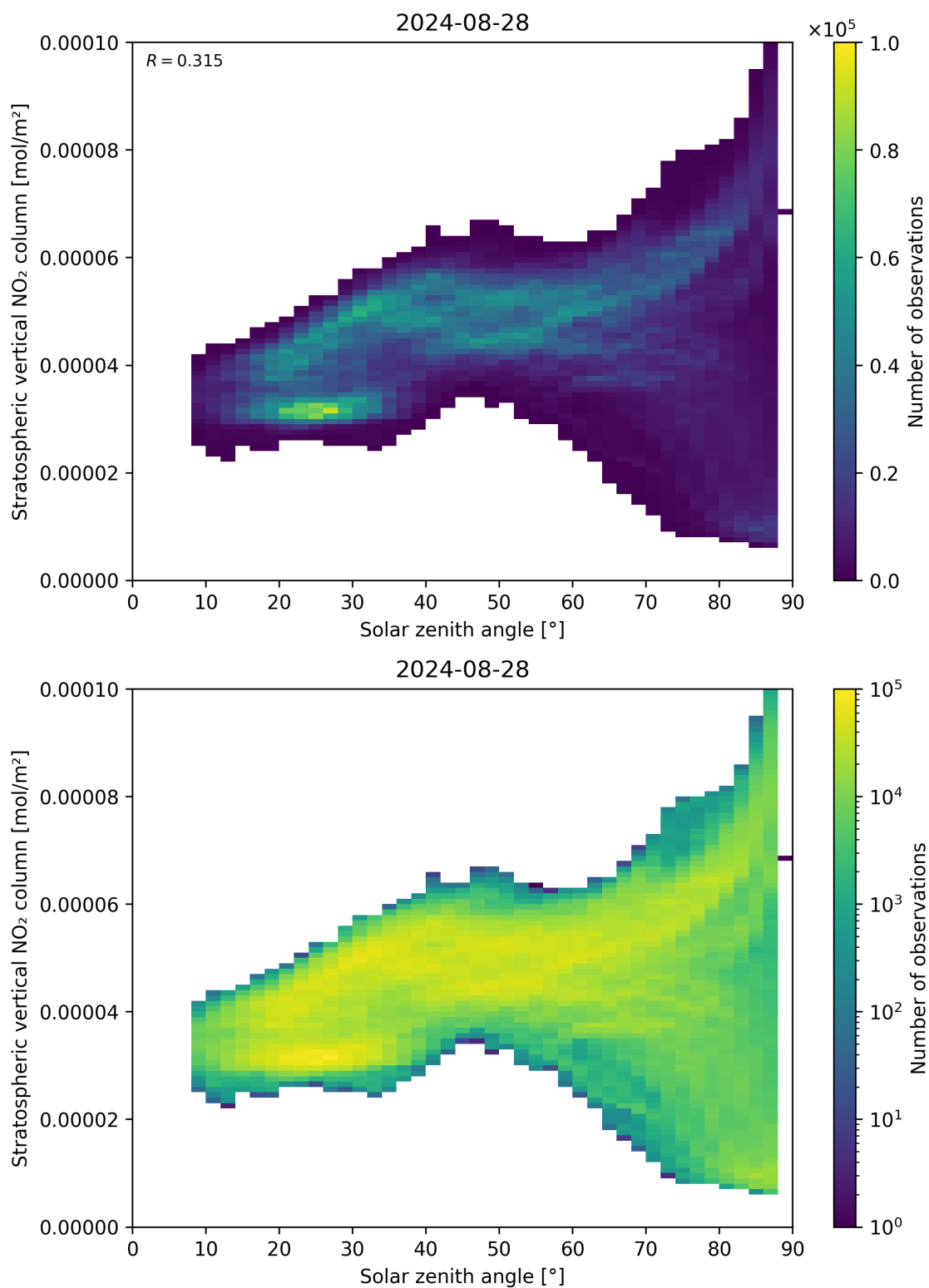
Figure 150: Scatter density plot of “Solar zenith angle” against “Stratospheric vertical NO 2 column” for 2024-08-27 to 2024-08-29.
