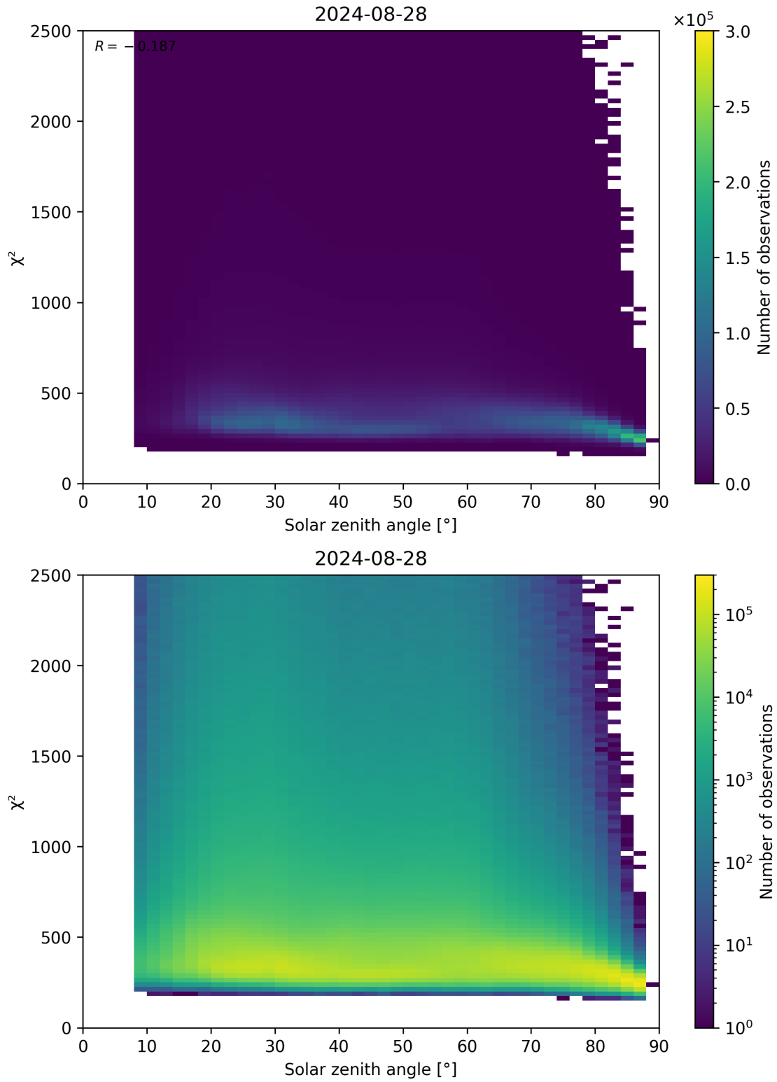
Figure 148: Scatter density plot of “Solar zenith angle” against “ \chi^2 ” for 2024-08-27 to 2024-08-29.
