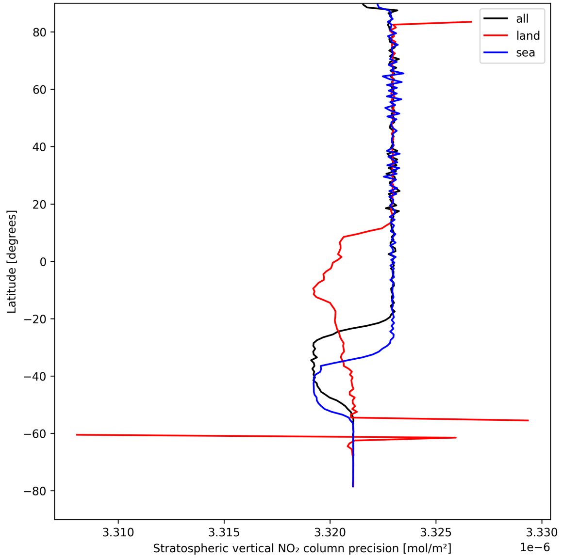
Figure 20: Zonal average of “Stratospheric vertical NO 2 column precision” for 2024-08-27 to 2024-08-29.
