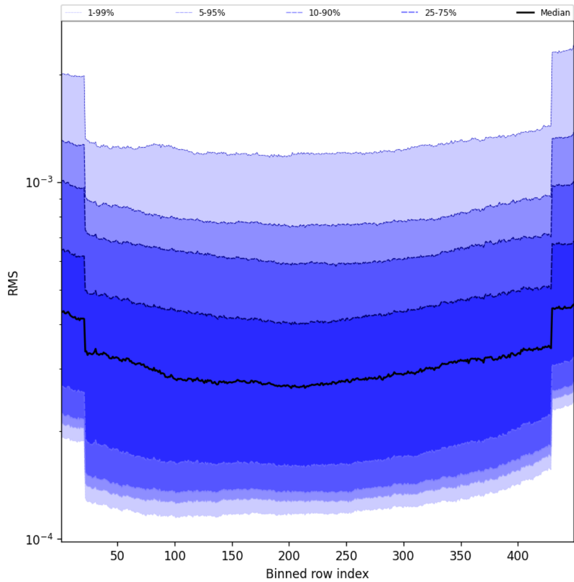
Figure 60: Along track statistics of “RMS” for 2024-08-27 to 2024-08-29
