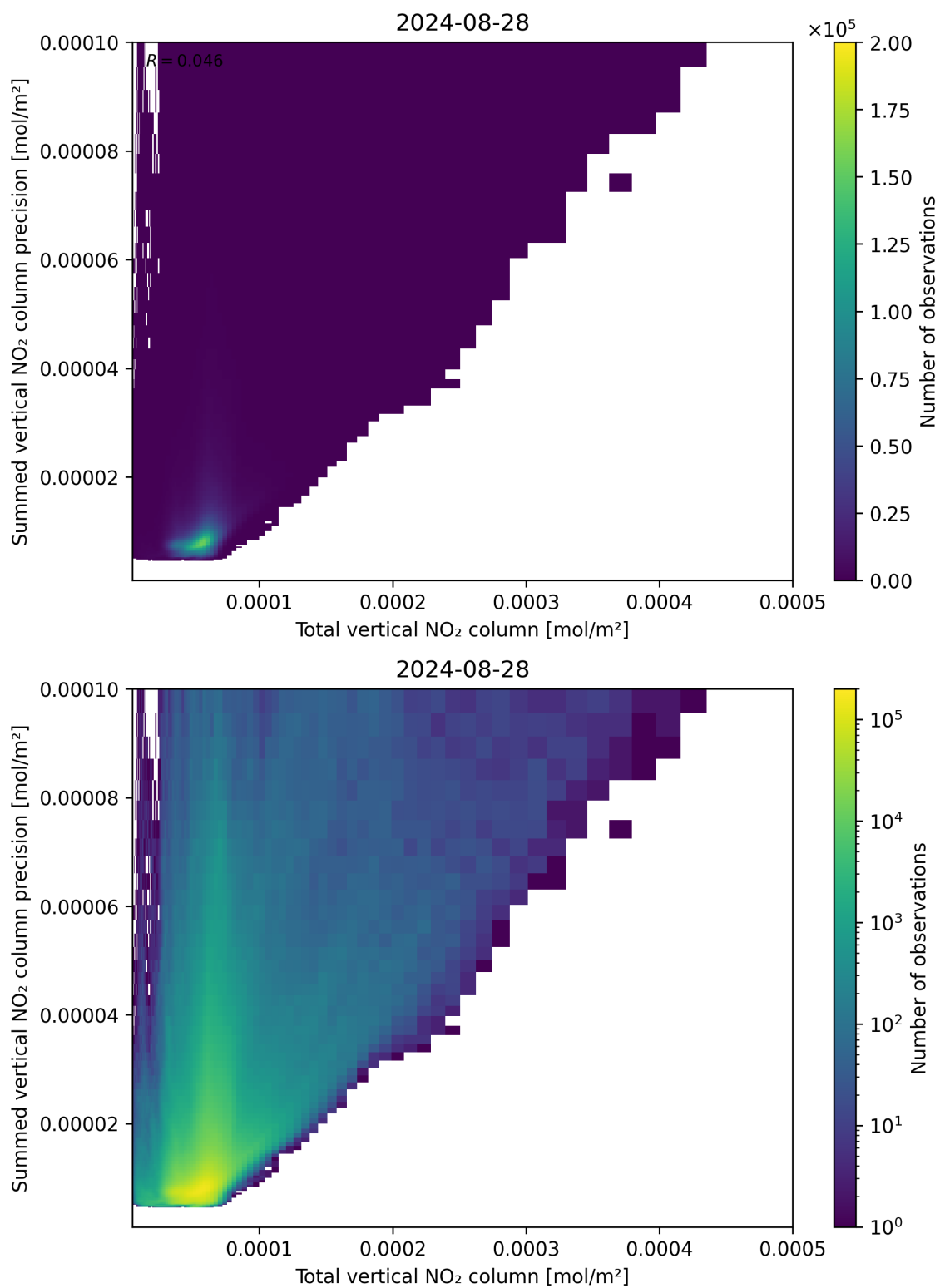
Figure 113: Scatter density plot of “Total vertical NO 2 column” against “Summed vertical NO 2 column precision” for 2024-08-27 to 2024-08-29.
