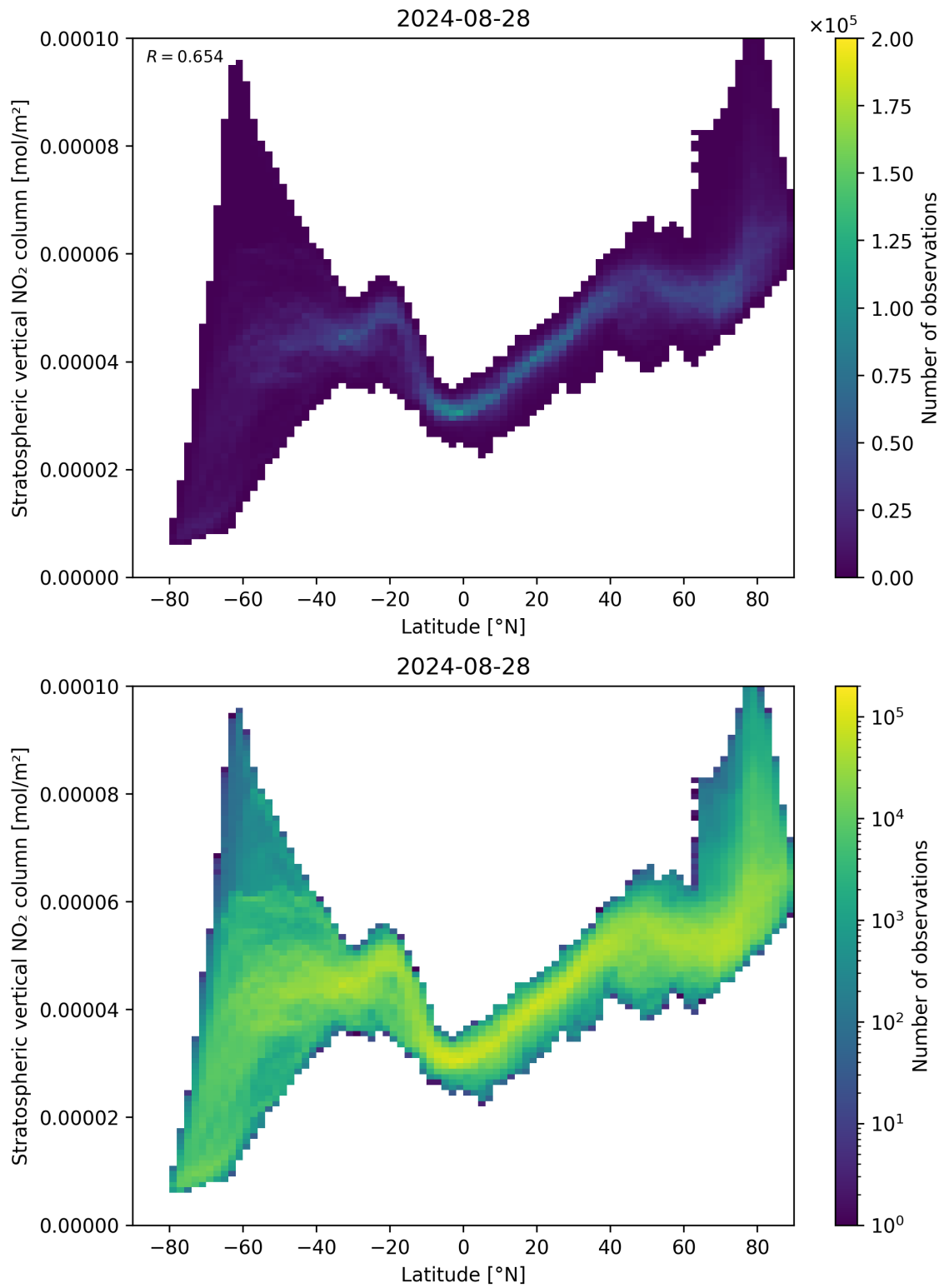
Figure 87: Scatter density plot of “Latitude” against “Stratospheric vertical NO 2 column” for 2024-08-27 to 2024-08-29.
