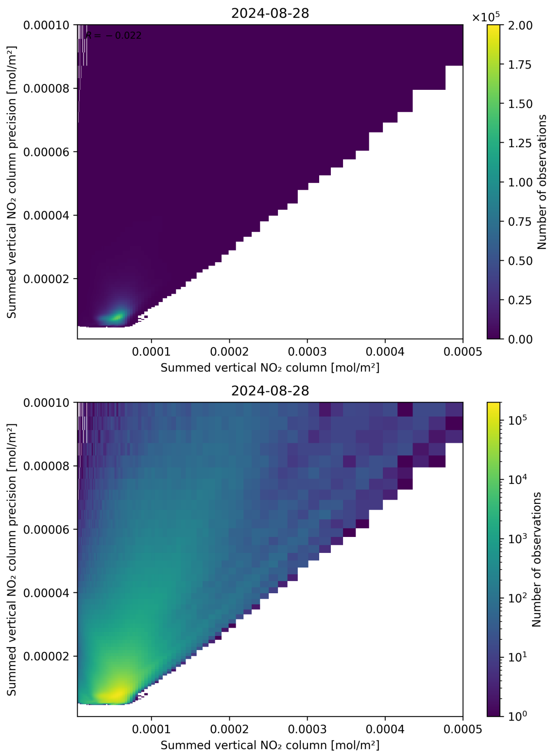
Figure 105: Scatter density plot of “Summed vertical NO 2 column” against “Summed vertical NO 2 column precision” for 2024-08-27 to 2024-08-29.
