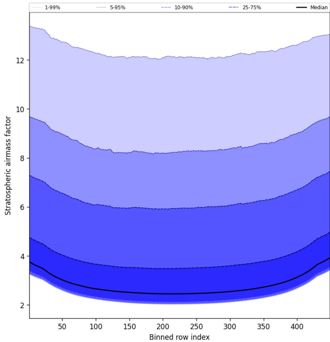
Figure 61: Along track statistics of “Stratospheric airmass factor” for 2024-08-27 to 2024-08-29
