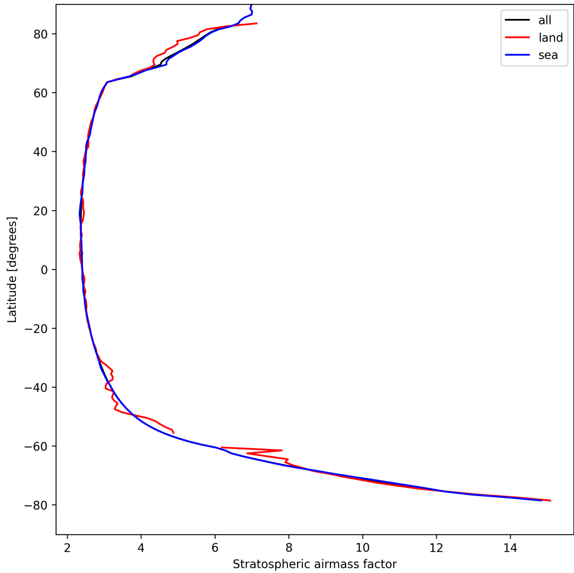
Figure 27: Zonal average of “Stratospheric airmass factor” for 2024-08-27 to 2024-08-29.
