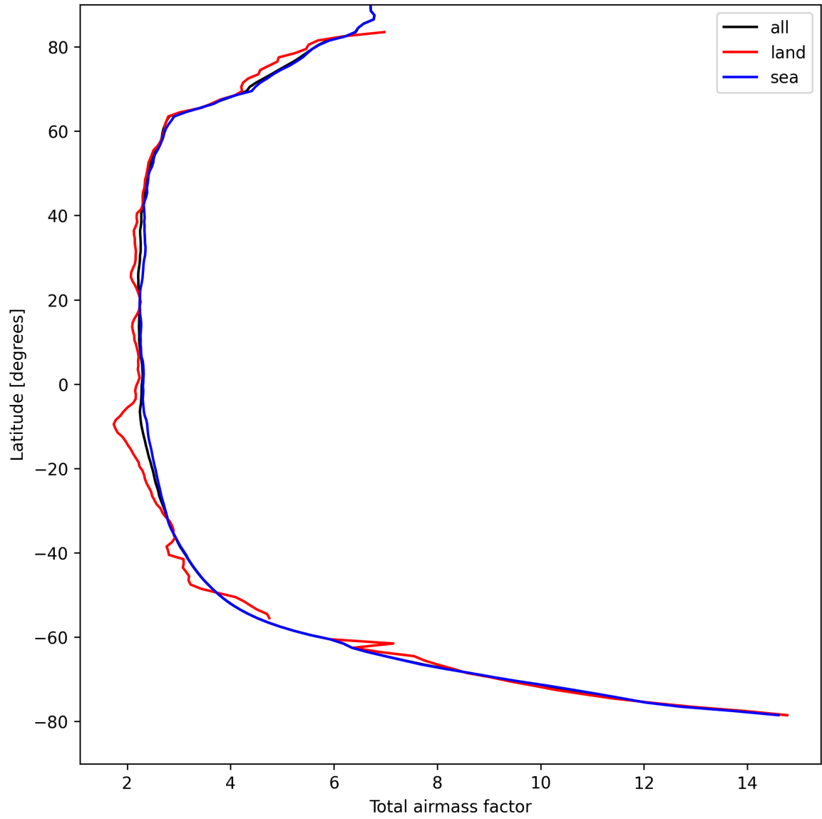
Figure 15: Zonal average of “Total airmass factor” for 2024-08-27 to 2024-08-29.
