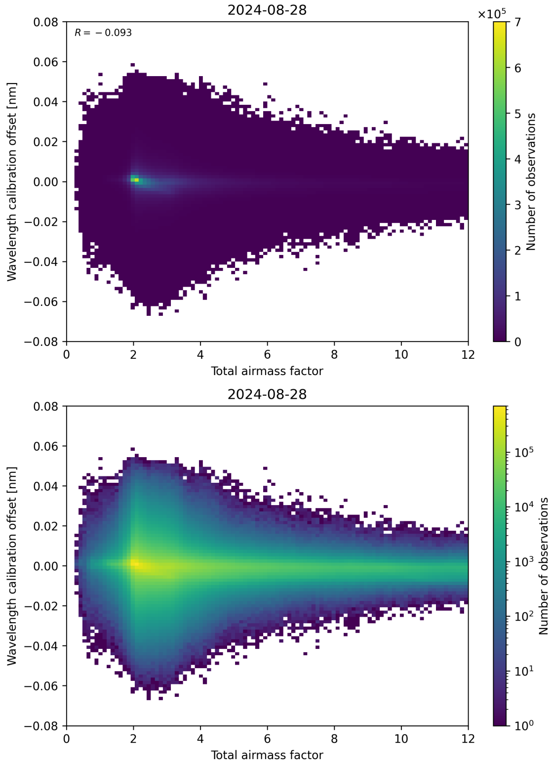
Figure 70: Scatter density plot of “Total airmass factor” against “Wavelength calibration offset” for 2024-08-27 to 2024-08-29.
