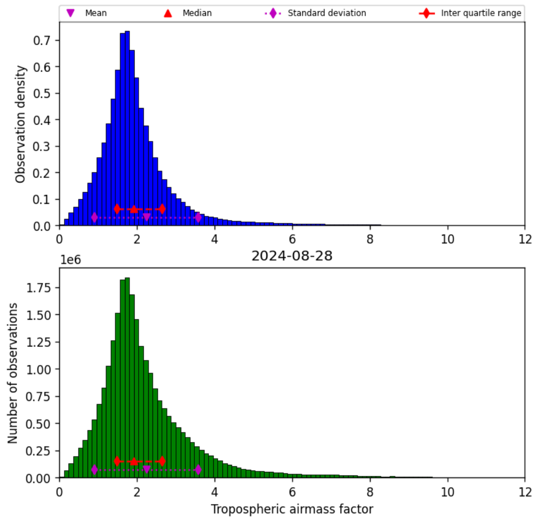
Figure 31: Histogram of “Tropospheric airmass factor” for 2024-08-27 to 2024-08-29
