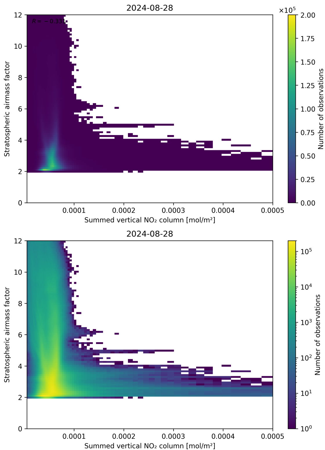
Figure 103: Scatter density plot of “Summed vertical NO 2 column” against “Stratospheric airmass factor” for 2024-08-27 to 2024-08-29.
