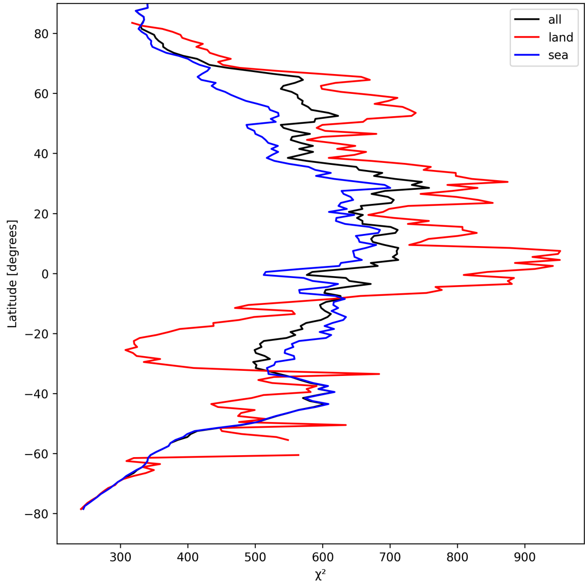
Figure 25: Zonal average of “ \chi^2 ” for 2024-08-27 to 2024-08-29.
