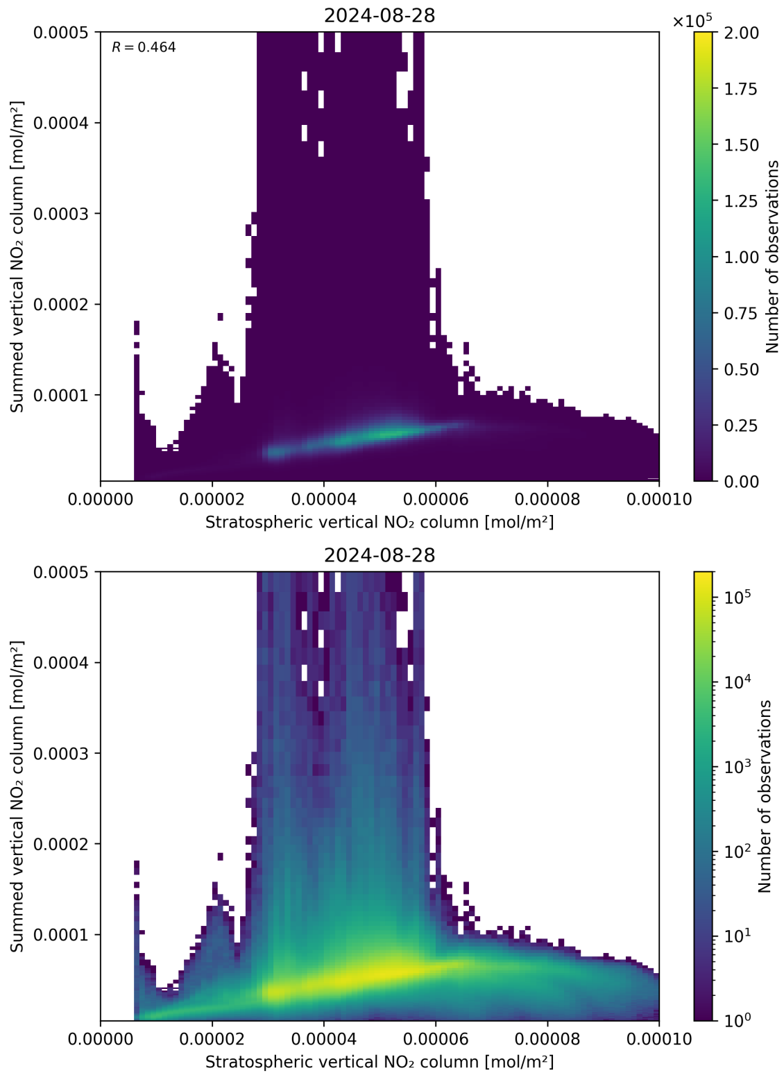
Figure 98: Scatter density plot of “Stratospheric vertical NO 2 column” against “Summed vertical NO 2 column” for 2024-08-27 to 2024-08-29.
