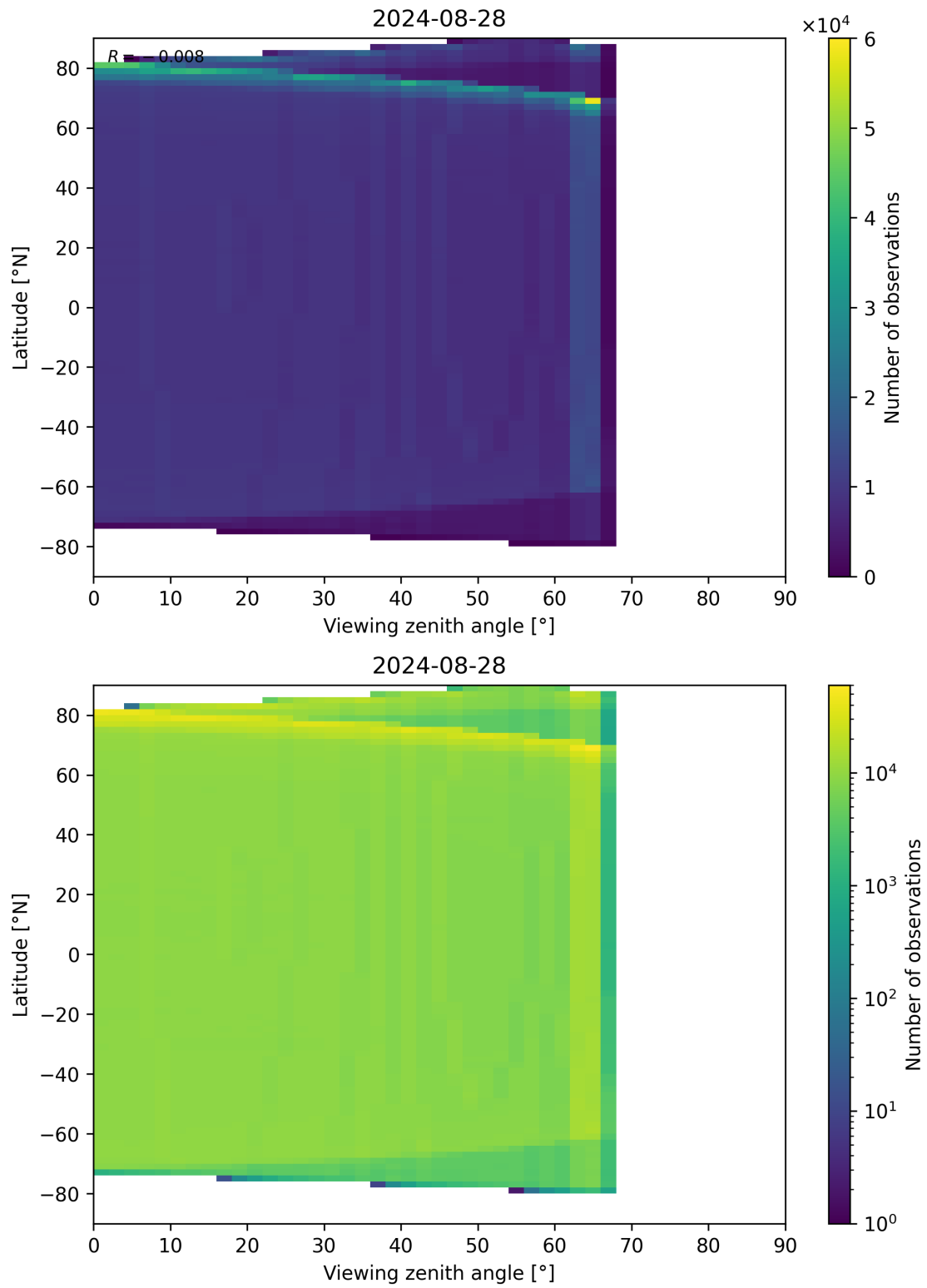
Figure 163: Scatter density plot of “Viewing zenith angle” against “Latitude” for 2024-08-27 to 2024-08-29.
