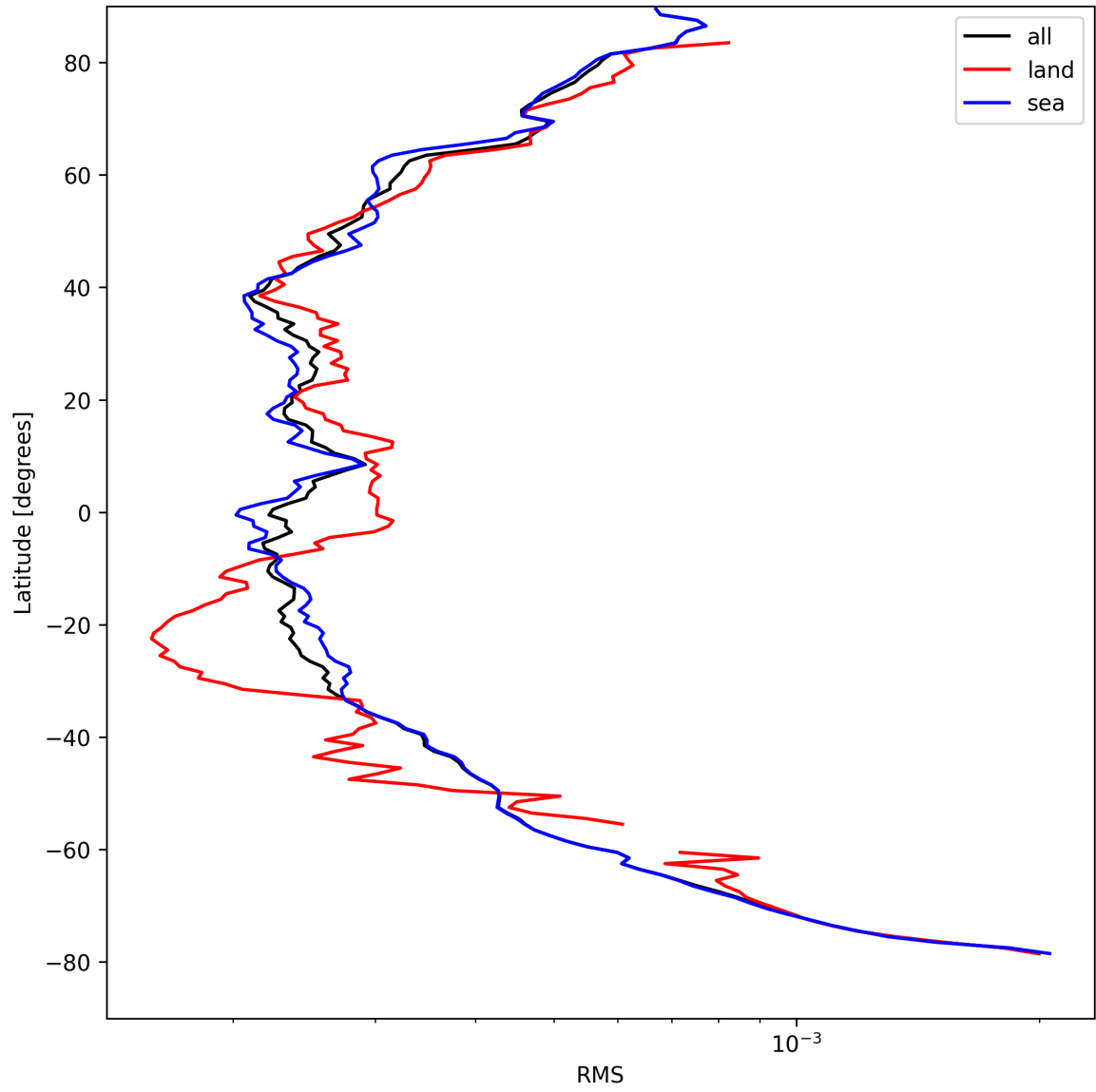
Figure 26: Zonal average of “RMS” for 2024-08-27 to 2024-08-29.
