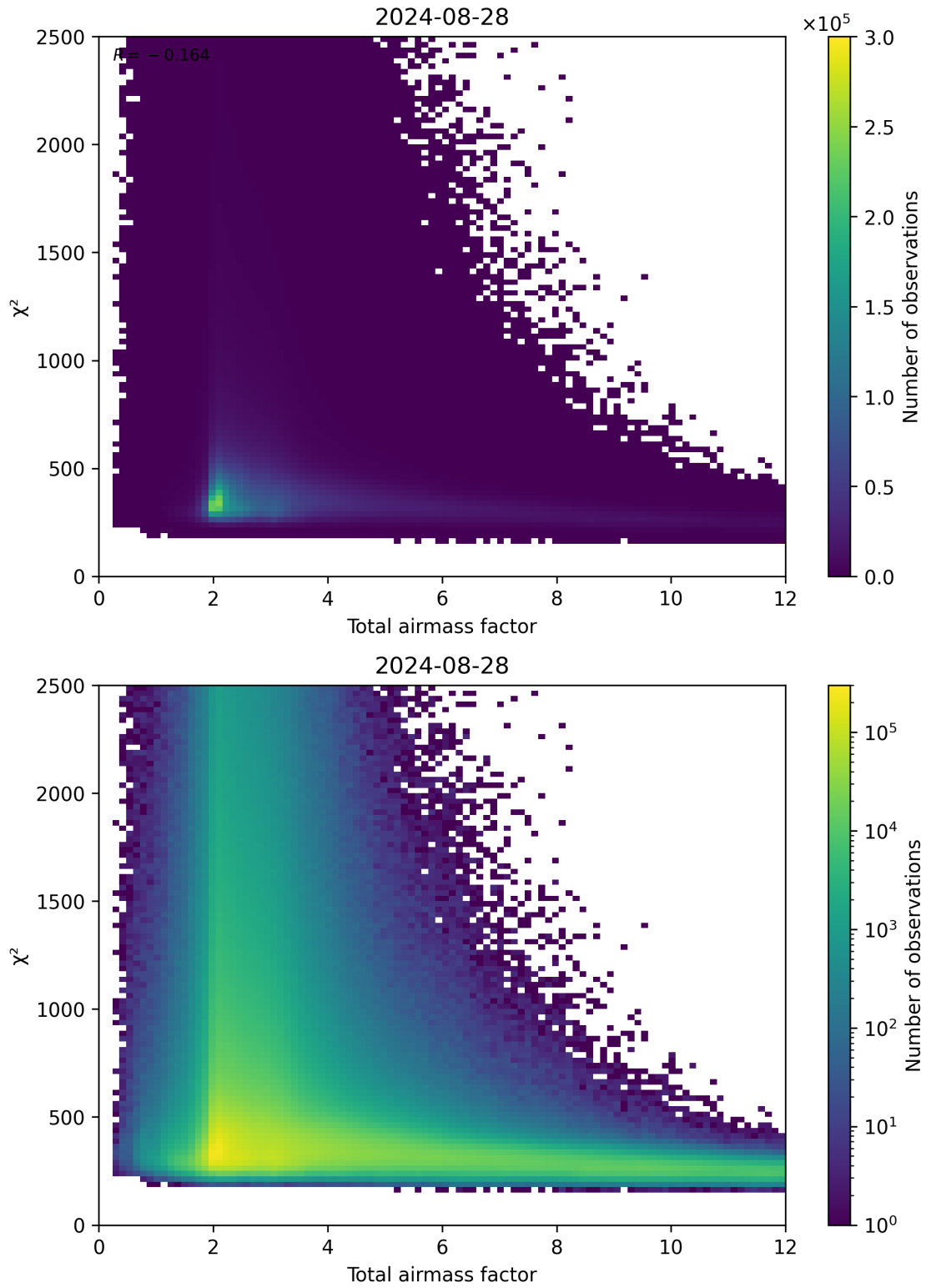
Figure 63: Scatter density plot of “Total airmass factor” against “ \chi^2 ” for 2024-08-27 to 2024-08-29.
