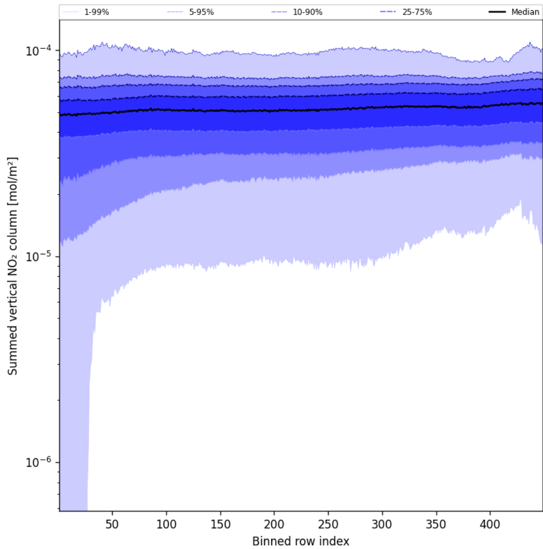
Figure 57: Along track statistics of “Summed vertical NO 2 column” for 2024-08-27 to 2024-08-29
