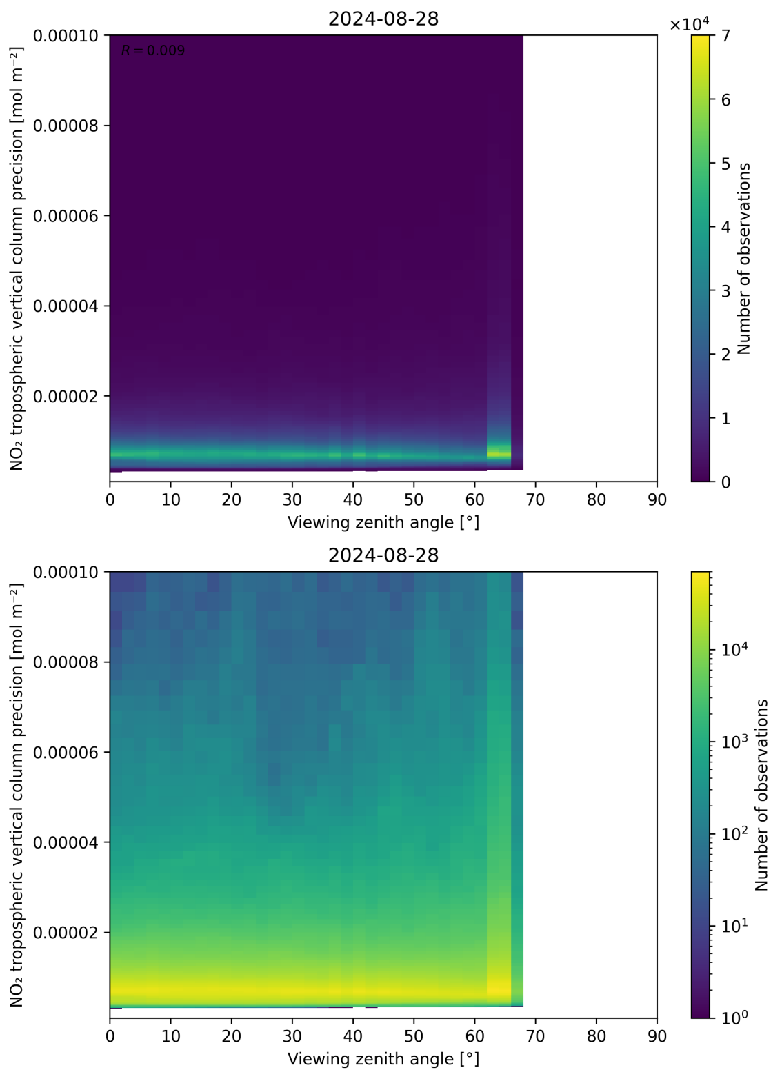
Figure 170: Scatter density plot of “Viewing zenith angle” against “NO 2 tropospheric vertical column precision” for 2024-08-27 to 2024-08-29.
