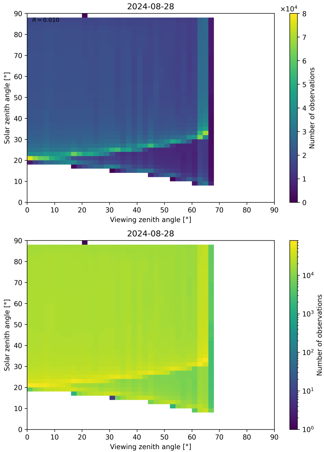
Figure 172: Scatter density plot of “Viewing zenith angle” against “Solar zenith angle” for 2024-08-27 to 2024-08-29.
