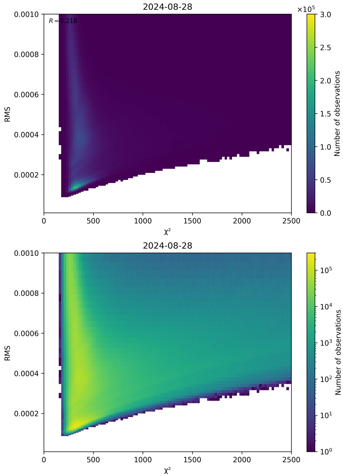
Figure 82: Scatter density plot of “ \chi^2 ” against “RMS” for 2024-08-27 to 2024-08-29.
