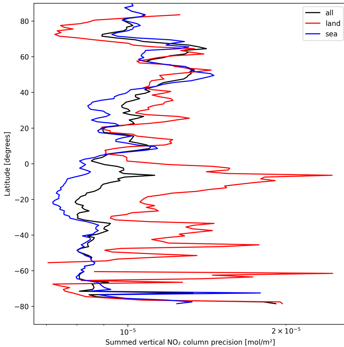
Figure 24: Zonal average of “Summed vertical NO 2 column precision” for 2024-08-27 to 2024-08-29.
