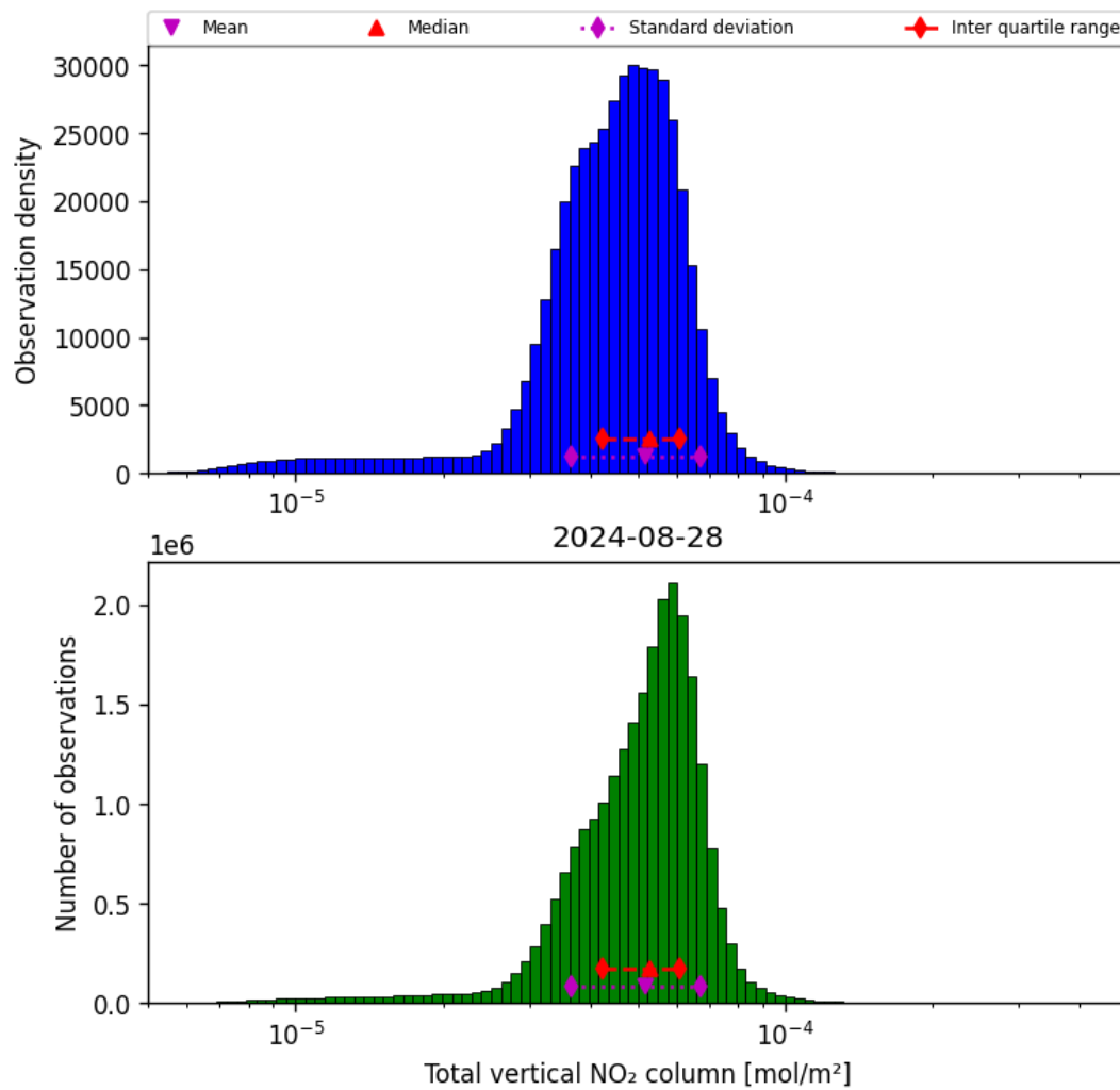
Figure 38: Histogram of "Total vertical NO 2 column" for 2024-08-27 to 2024-08-29
