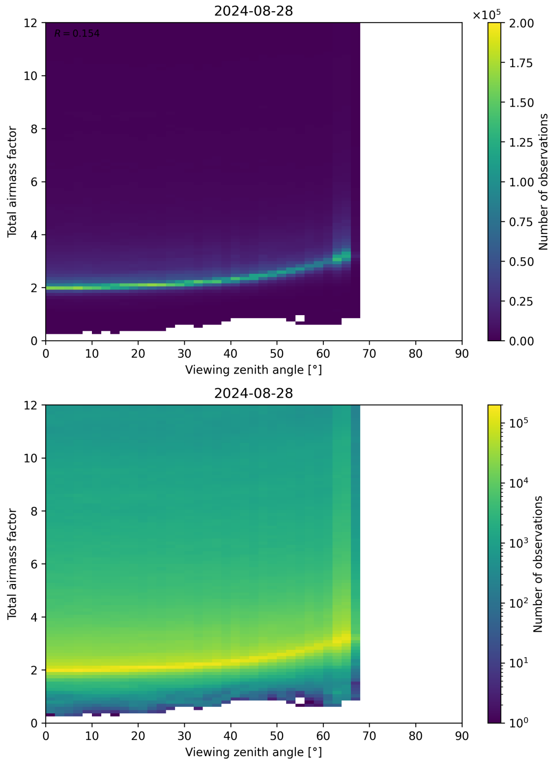
Figure 160: Scatter density plot of “Viewing zenith angle” against “Total airmass factor” for 2024-08-27 to 2024-08-29.
