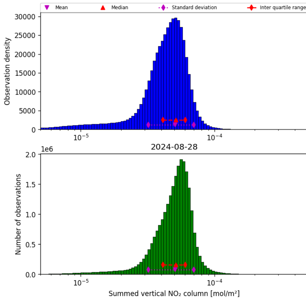
Figure 40: Histogram of “Summed vertical NO 2 column” for 2024-08-27 to 2024-08-29
