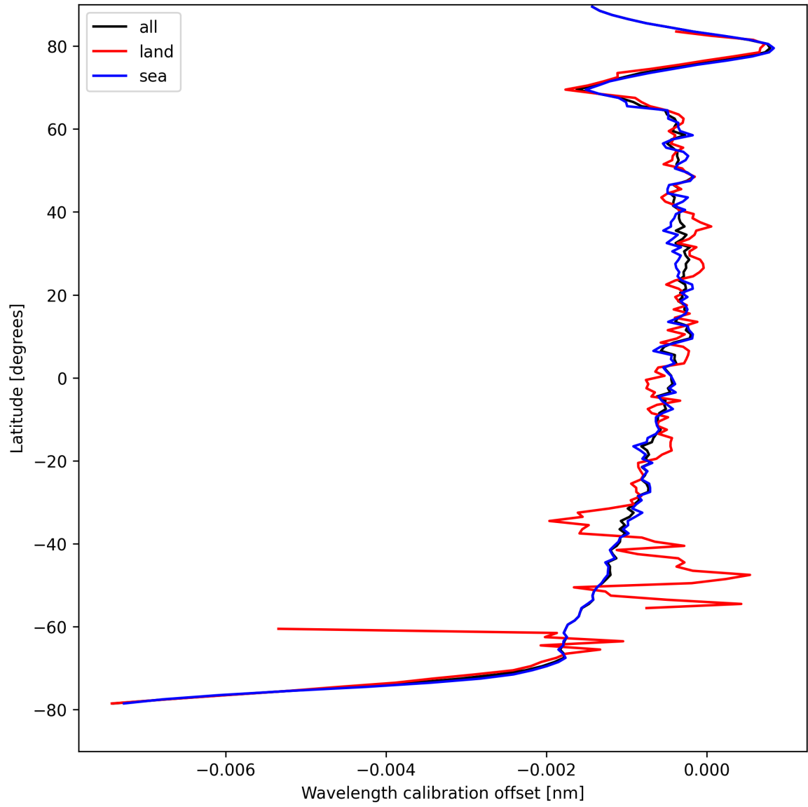
Figure 18: Zonal average of “Wavelength calibration offset” for 2024-08-27 to 2024-08-29.
