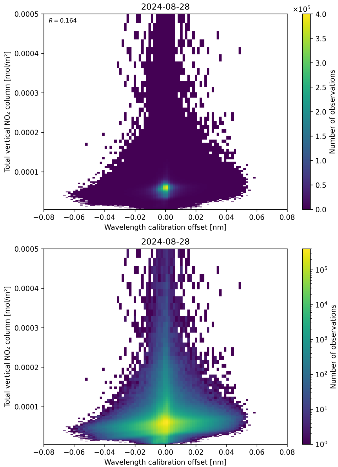
Figure 179: Scatter density plot of “Wavelength calibration offset” against “Total vertical NO 2 column” for 2024-08-27 to 2024-08-29.
