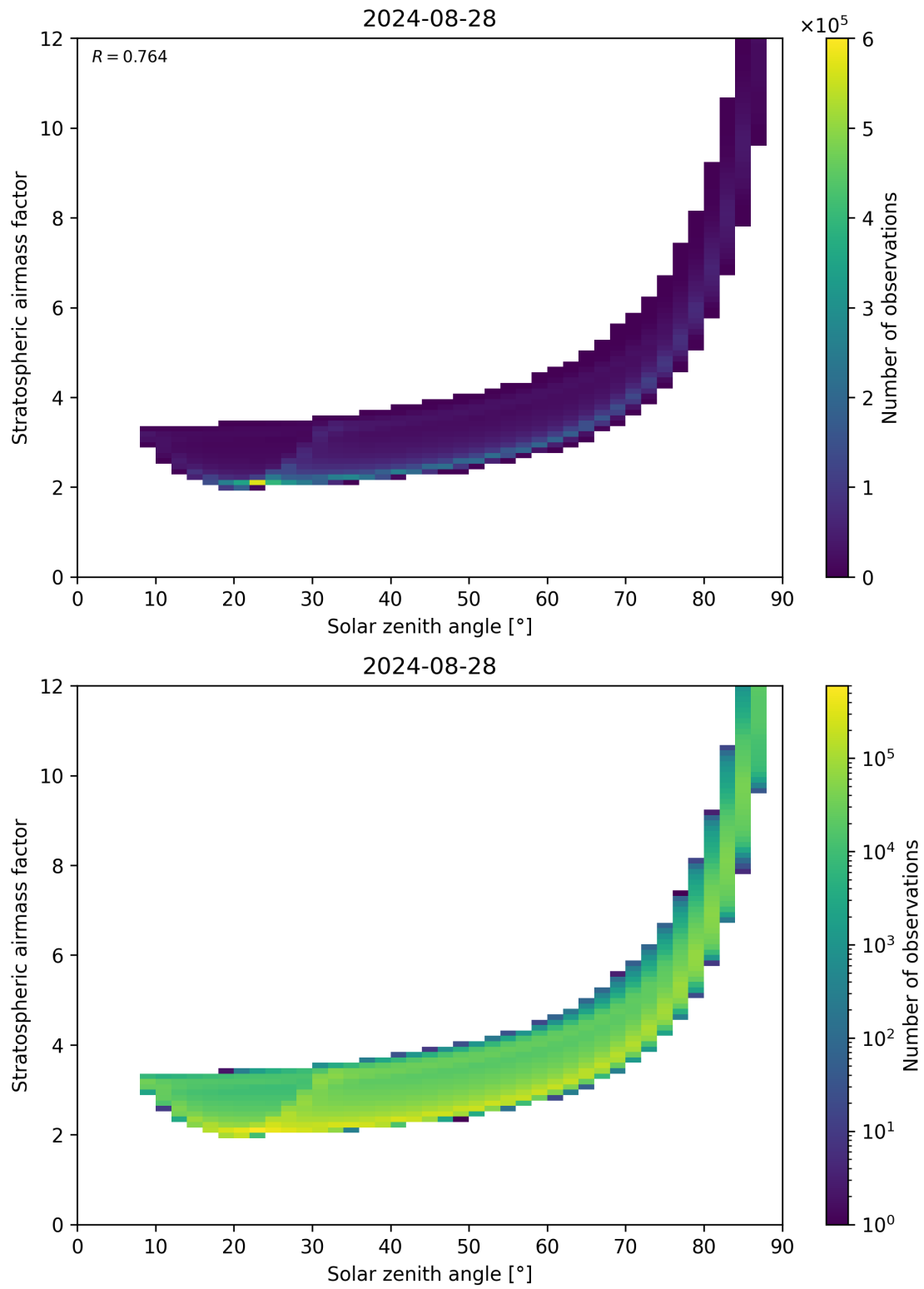
Figure 145: Scatter density plot of “Solar zenith angle” against “Stratospheric airmass factor” for 2024-08-27 to 2024-08-29.
