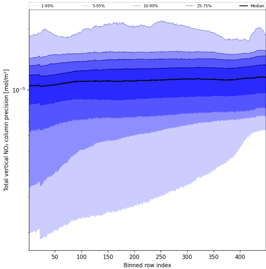
Figure 56: Along track statistics of “Total vertical NO 2 column precision” for 2024-08-27 to 2024-08-29
