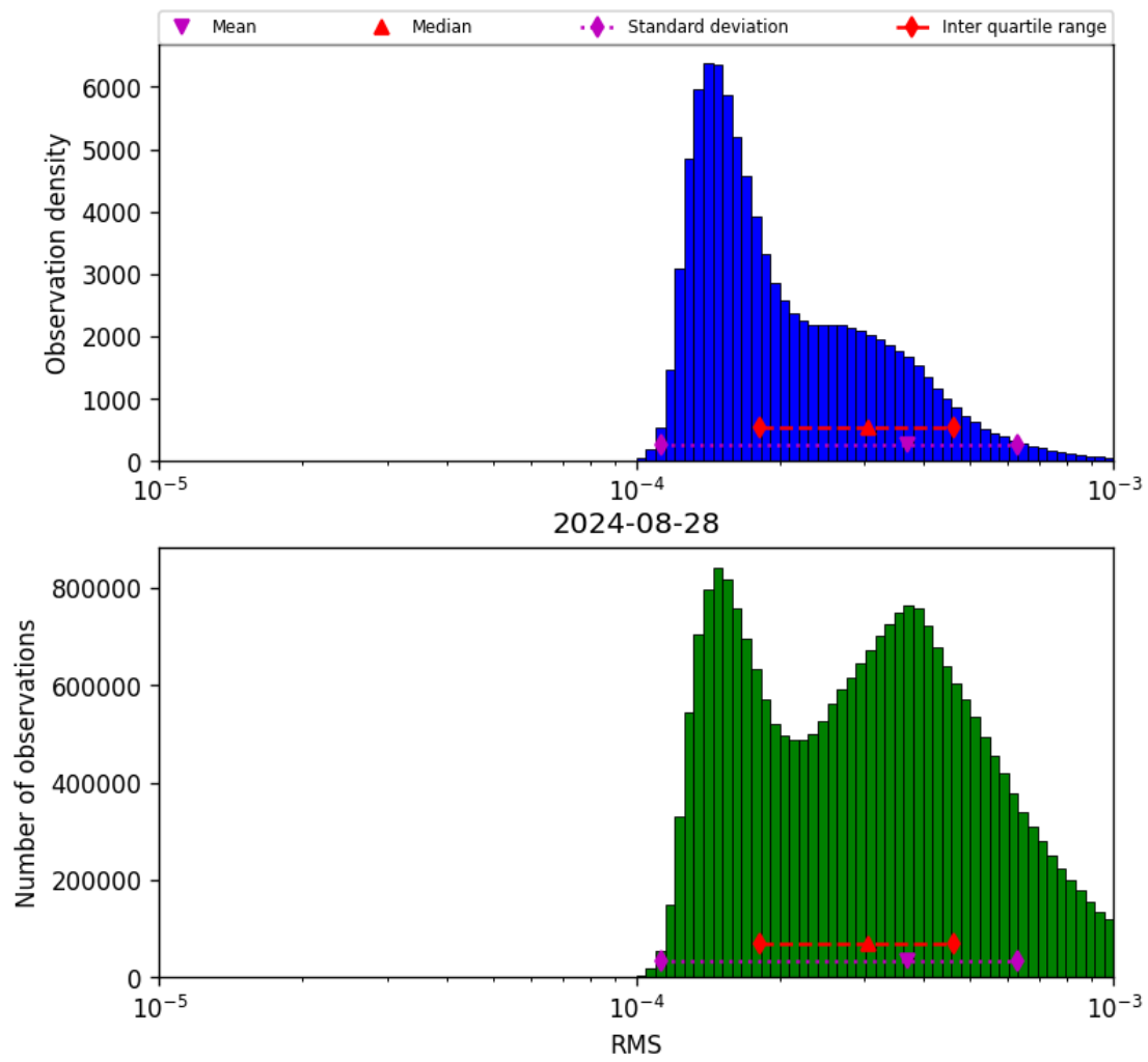
Figure 43: Histogram of “RMS” for 2024-08-27 to 2024-08-29
