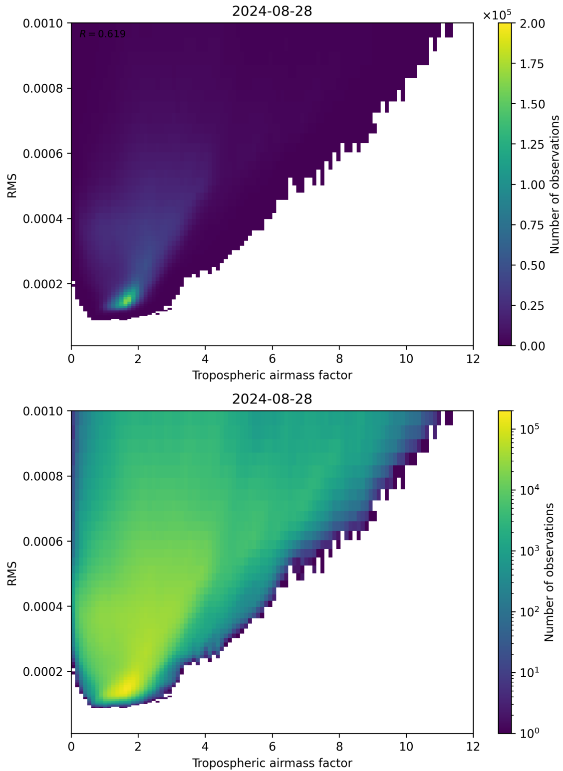
Figure 79: Scatter density plot of “Tropospheric airmass factor” against “RMS” for 2024-08-27 to 2024-08-29.
