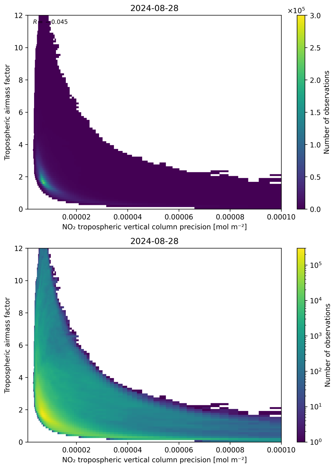
Figure 133: Scatter density plot of “NO 2 tropospheric vertical column precision” against “Tropospheric airmass factor” for 2024-08-27 to 2024-08-29.
