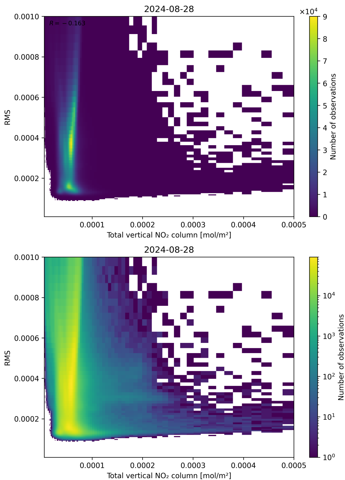
Figure 120: Scatter density plot of “Total vertical NO 2 column” against “RMS” for 2024-08-27 to 2024-08-29.
