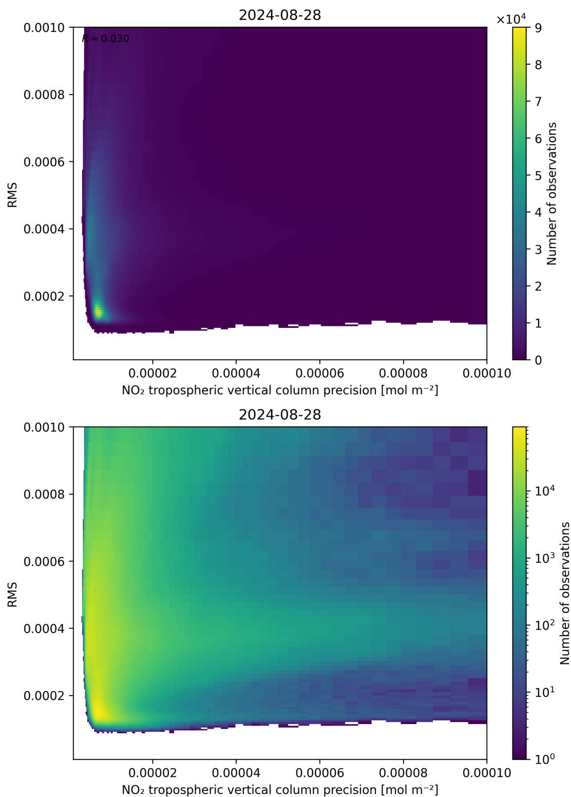
Figure 140: Scatter density plot of “NO 2 tropospheric vertical column precision” against “RMS” for 2024-08-27 to 2024-08-29.
