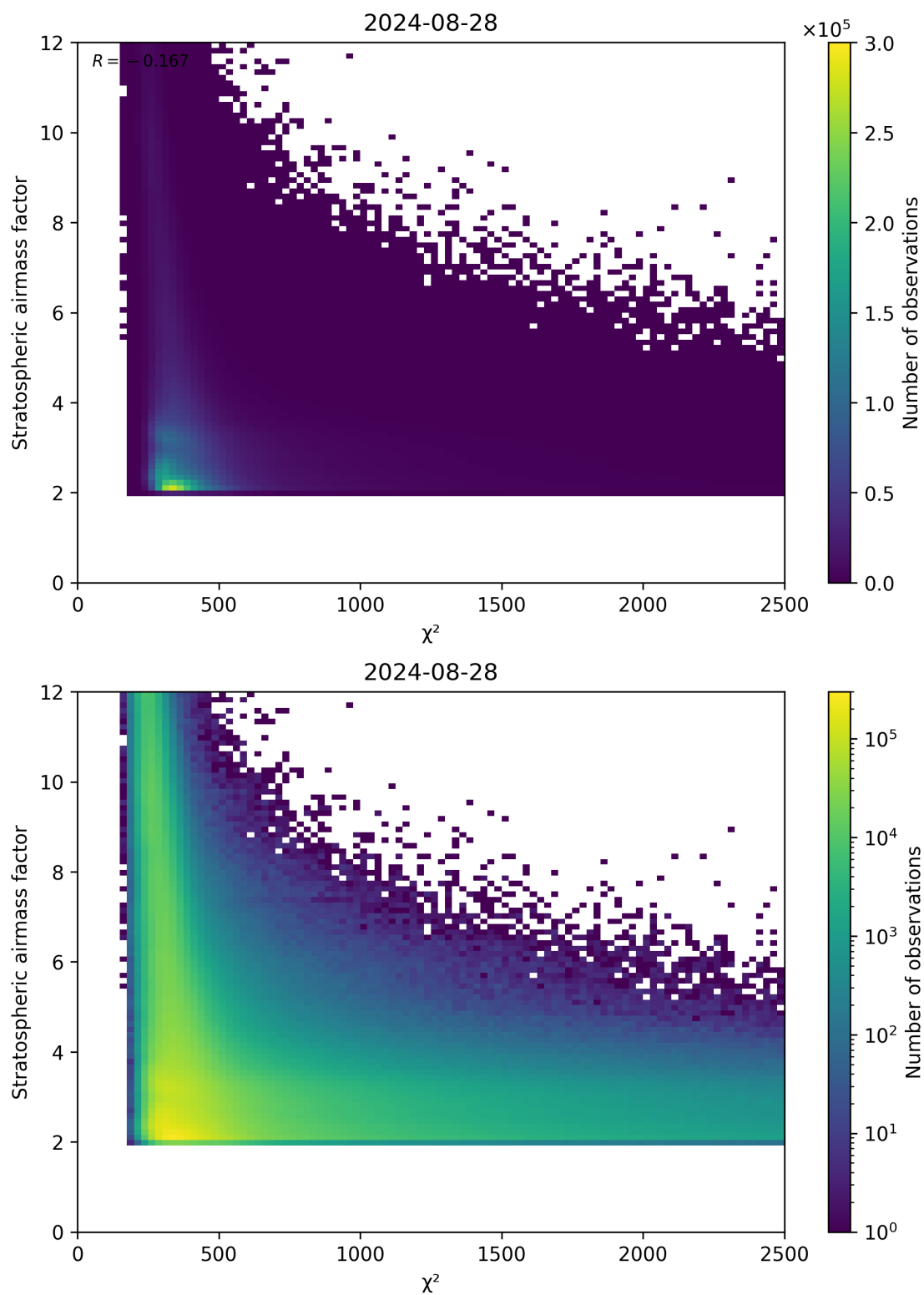
Figure 81: Scatter density plot of “ \chi^2 ” against “Stratospheric airmass factor” for 2024-08-27 to 2024-08-29.
