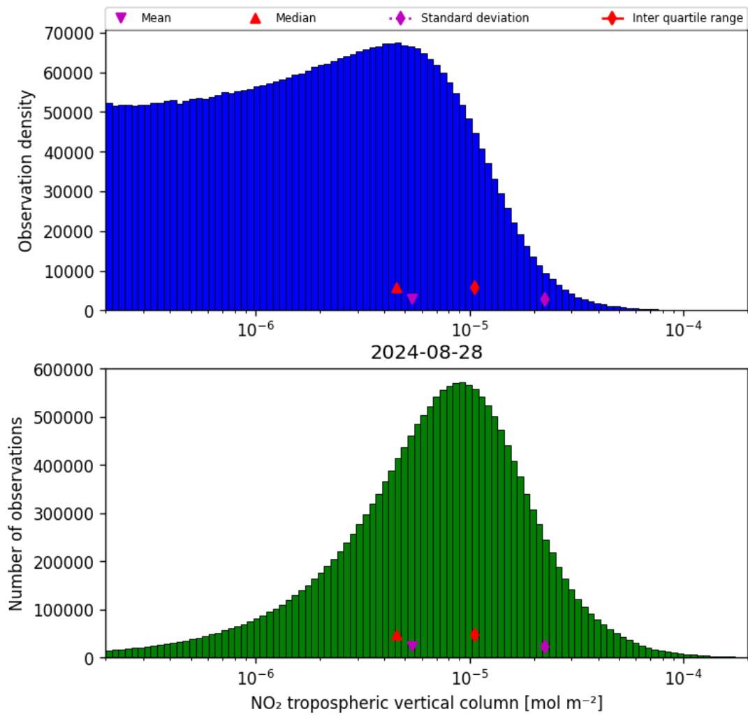
Figure 29: Histogram of “NO 2 tropospheric vertical column” for 2024-08-27 to 2024-08-29
