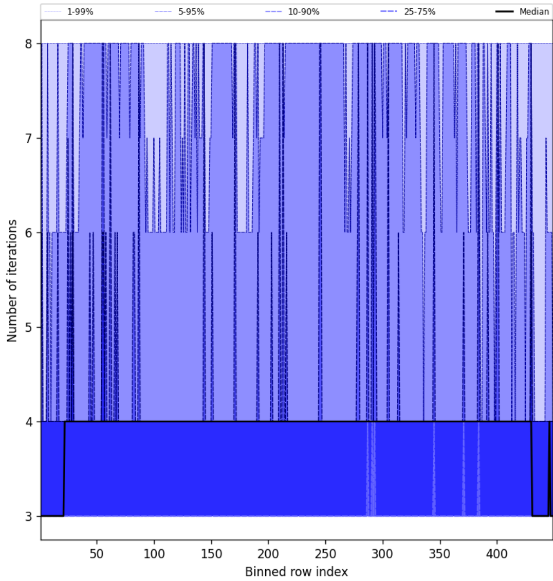
Figure 51: Along track statistics of “Number of iterations” for 2024-08-27 to 2024-08-29
