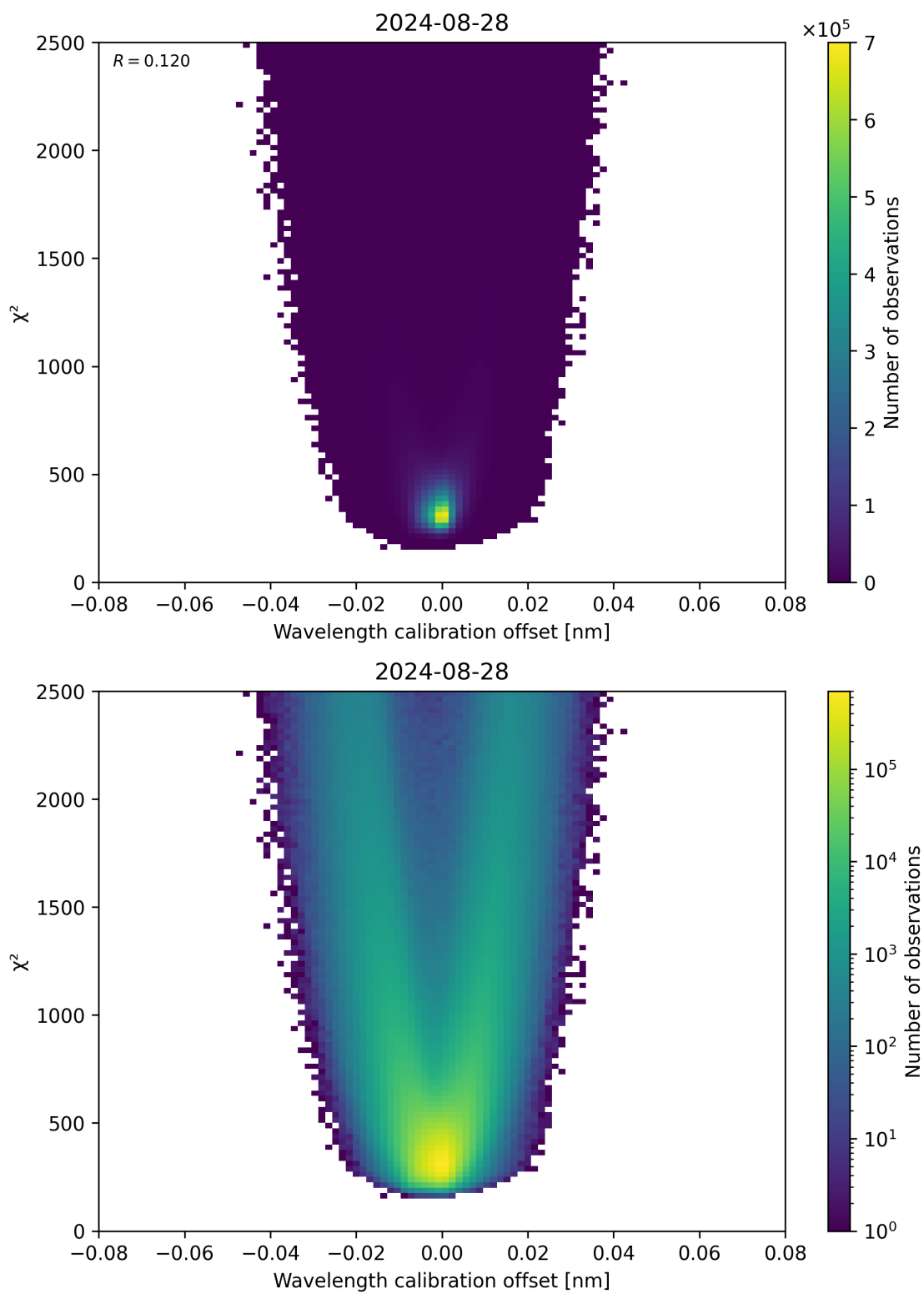
Figure 175: Scatter density plot of “Wavelength calibration offset” against “ \chi^2 ” for 2024-08-27 to 2024-08-29.
