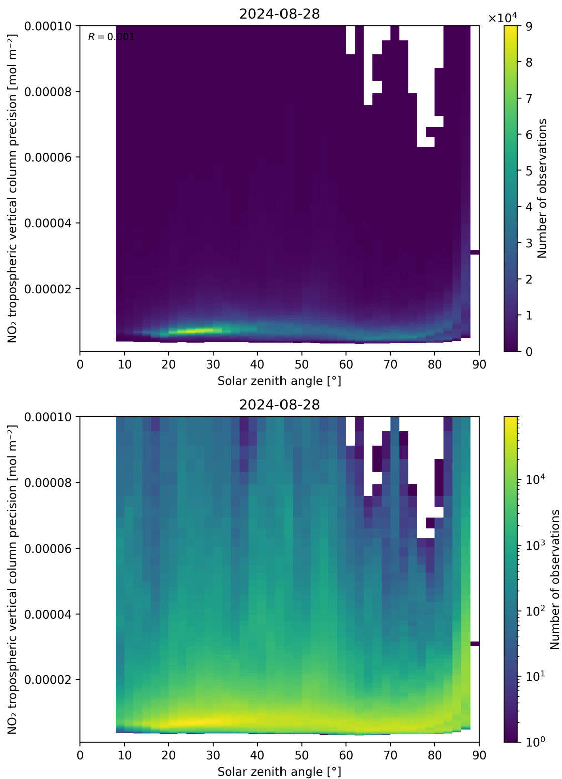
Figure 156: Scatter density plot of “Solar zenith angle” against “NO 2 tropospheric vertical column precision” for 2024-08-27 to 2024-08-29.
