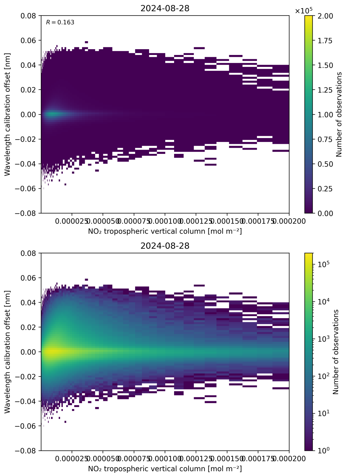
Figure 143: Scatter density plot of “NO 2 tropospheric vertical column” against “Wavelength calibration offset” for 2024-08-27 to 2024-08-29.
