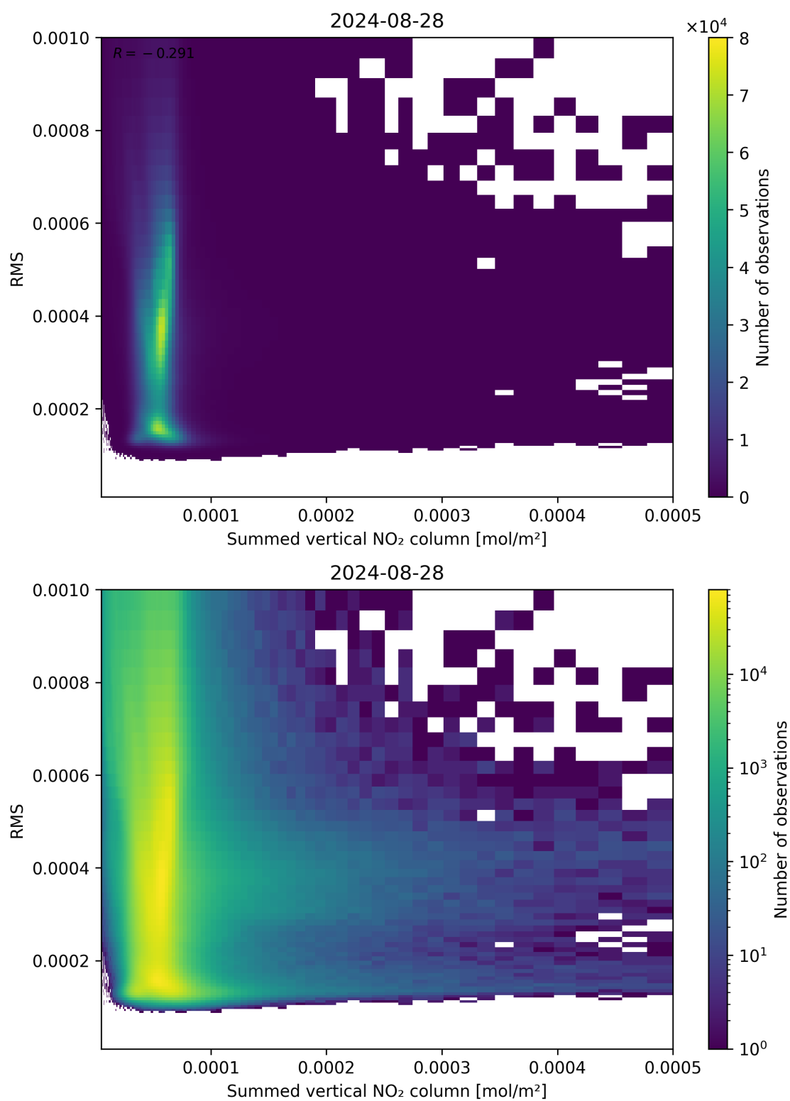
Figure 109: Scatter density plot of “Summed vertical NO 2 column” against “RMS” for 2024-08-27 to 2024-08-29.
