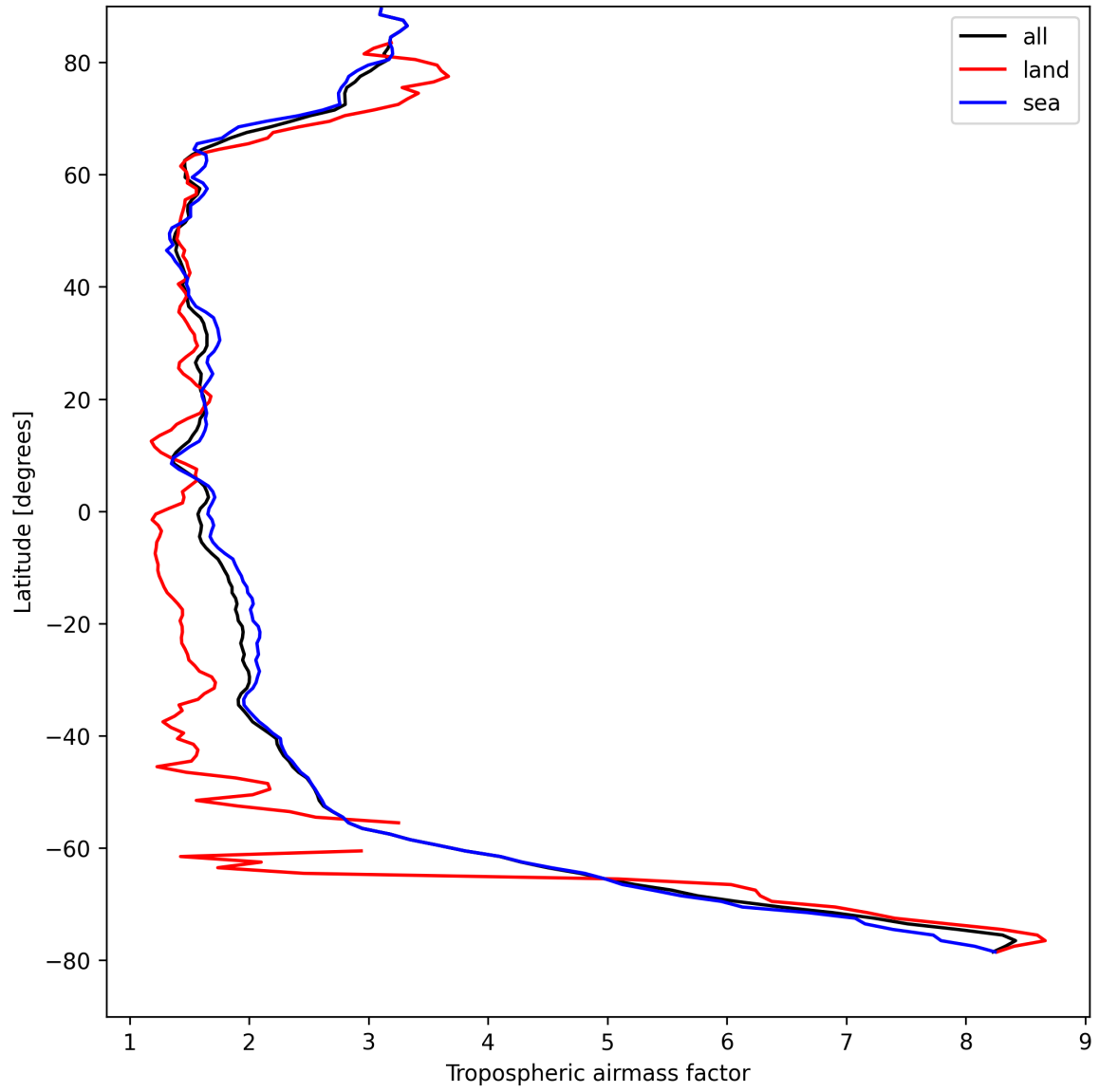
Figure 14: Zonal average of “Tropospheric air mass factor” for 2024-08-27 to 2024-08-29.
