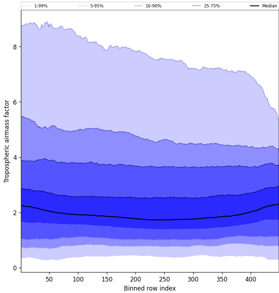
Figure 48: Along track statistics of “Tropospheric air mass factor” for 2024-08-27 to 2024-08-29
