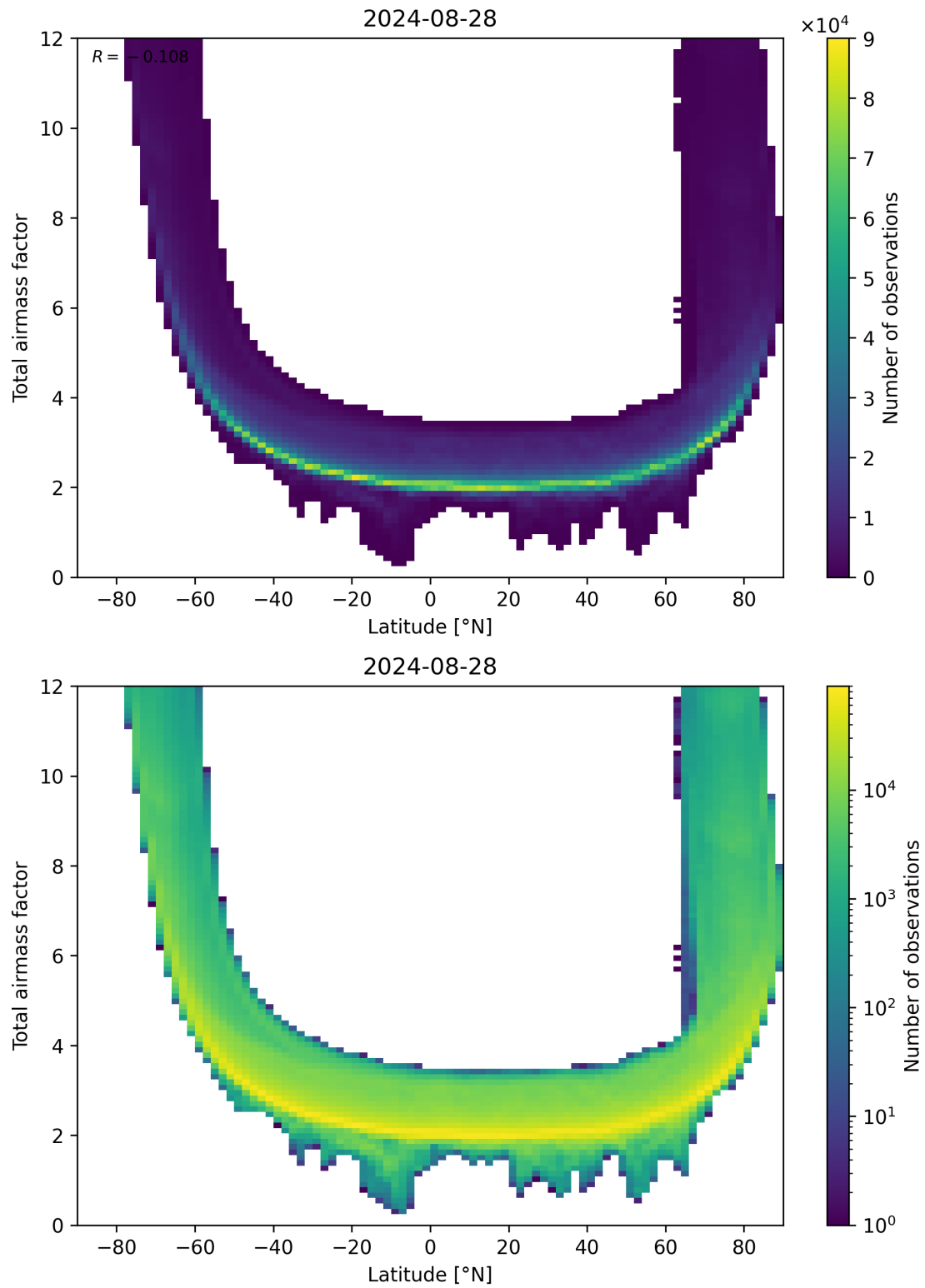
Figure 84: Scatter density plot of “Latitude” against “Total air mass factor” for 2024-08-27 to 2024-08-29.
