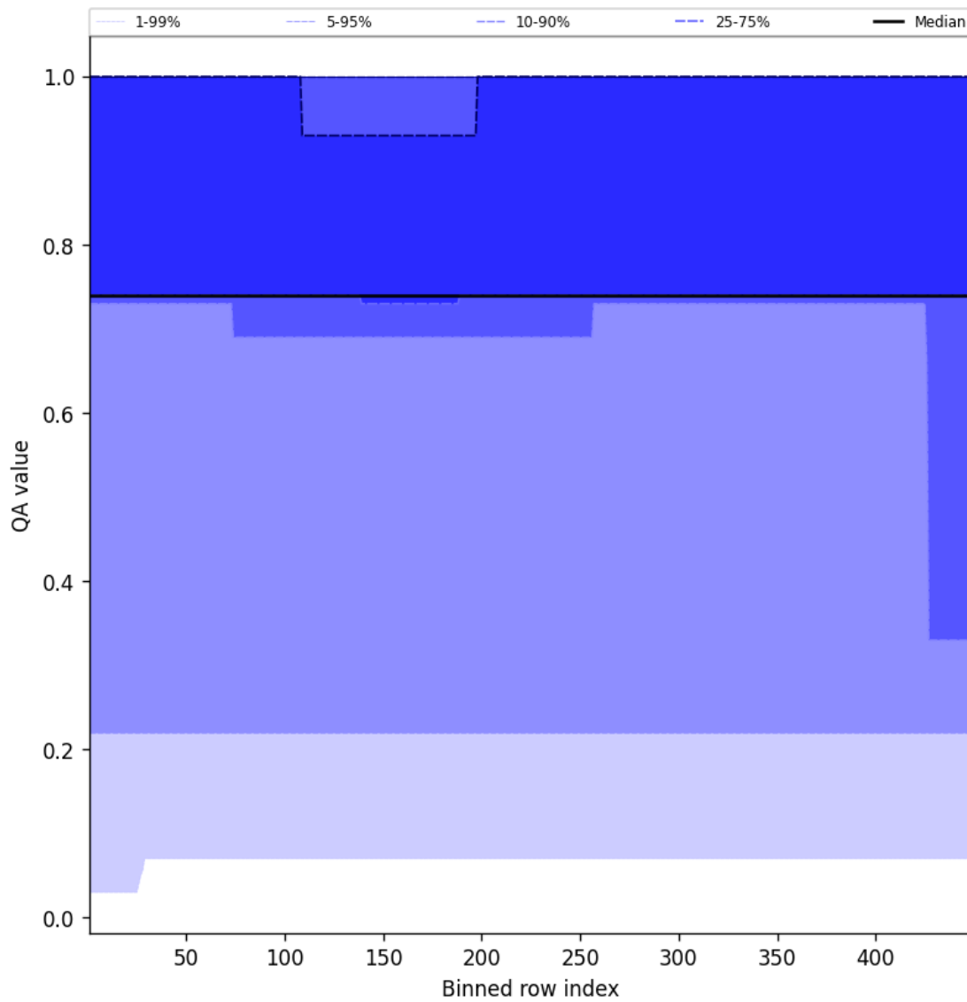
Figure 45: Along track statistics of “QA value” for 2024-08-27 to 2024-08-29
