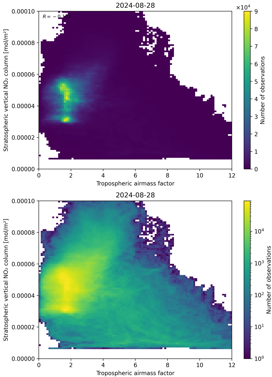
Figure 74: Scatter density plot of “Tropospheric air mass factor” against “Stratospheric vertical NO 2 column” for 2024-08-27 to 2024-08-29.
