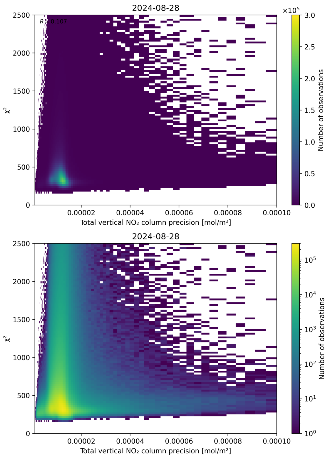
Figure 116: Scatter density plot of “Total vertical NO 2 column precision” against “ \chi^2 ” for 2024-08-27 to 2024-08-29.
