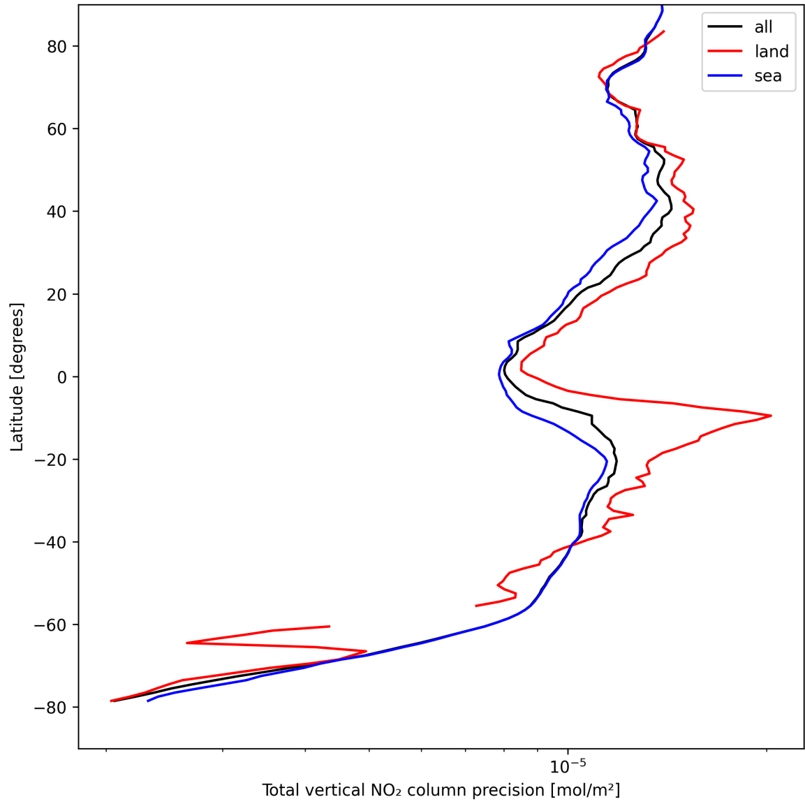
Figure 22: Zonal average of “Total vertical NO 2 column precision” for 2024-08-27 to 2024-08-29.
