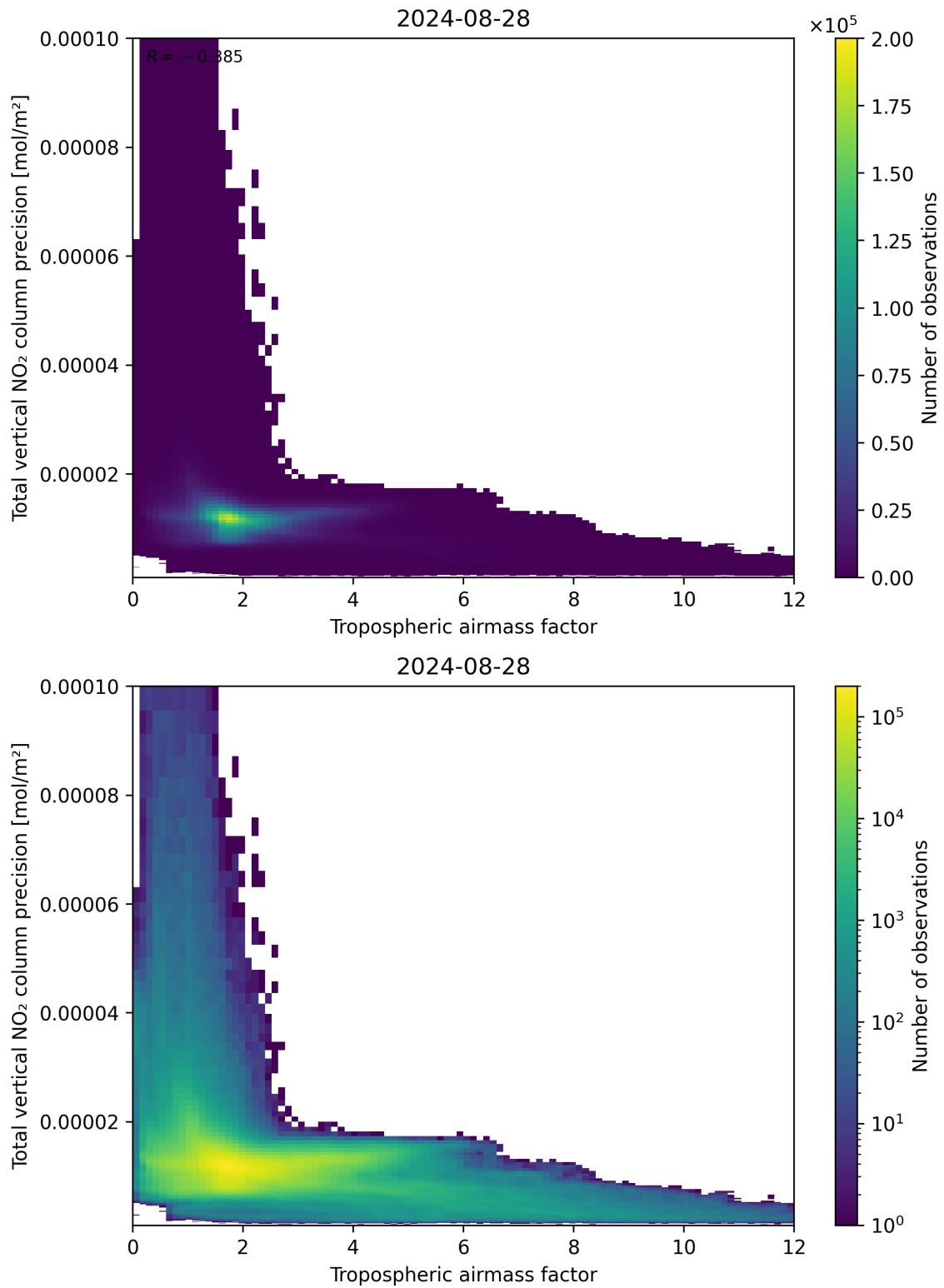
Figure 78: Scatter density plot of “Tropospheric air mass factor” against “Total vertical NO 2 column precision” for 2024-08-27 to 2024-08-29.
