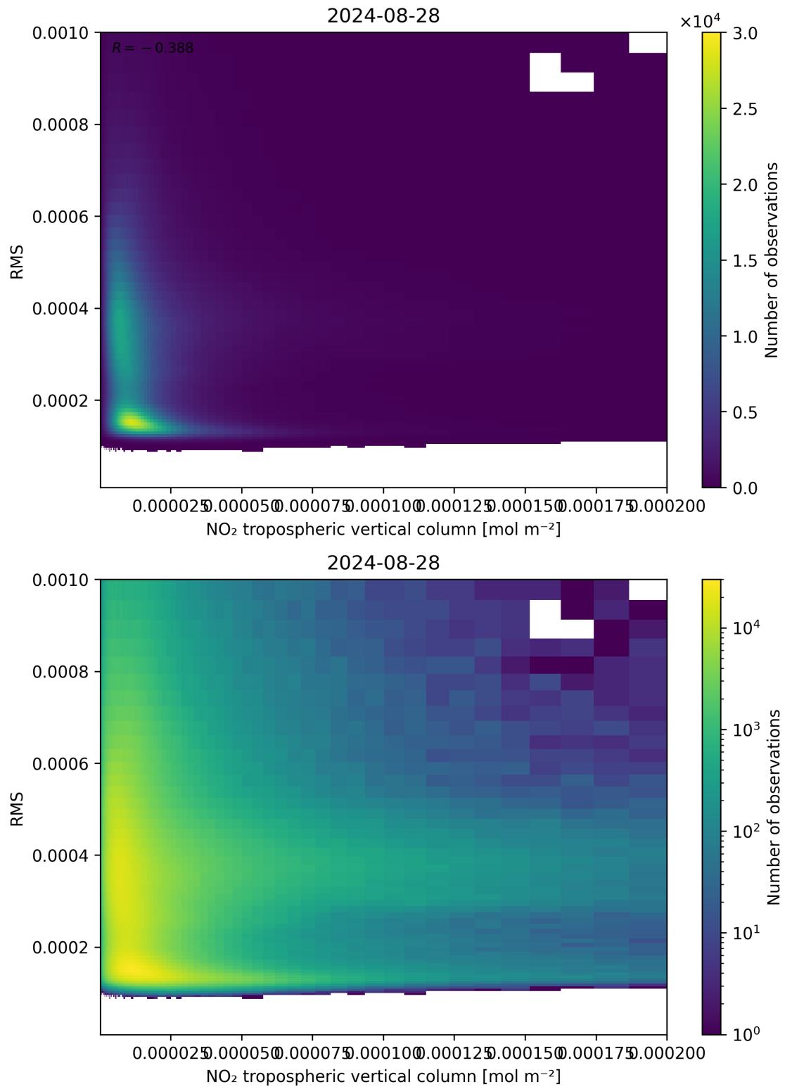
Figure 142: Scatter density plot of “NO 2 tropospheric vertical column” against “RMS” for 2024-08-27 to 2024-08-29.
