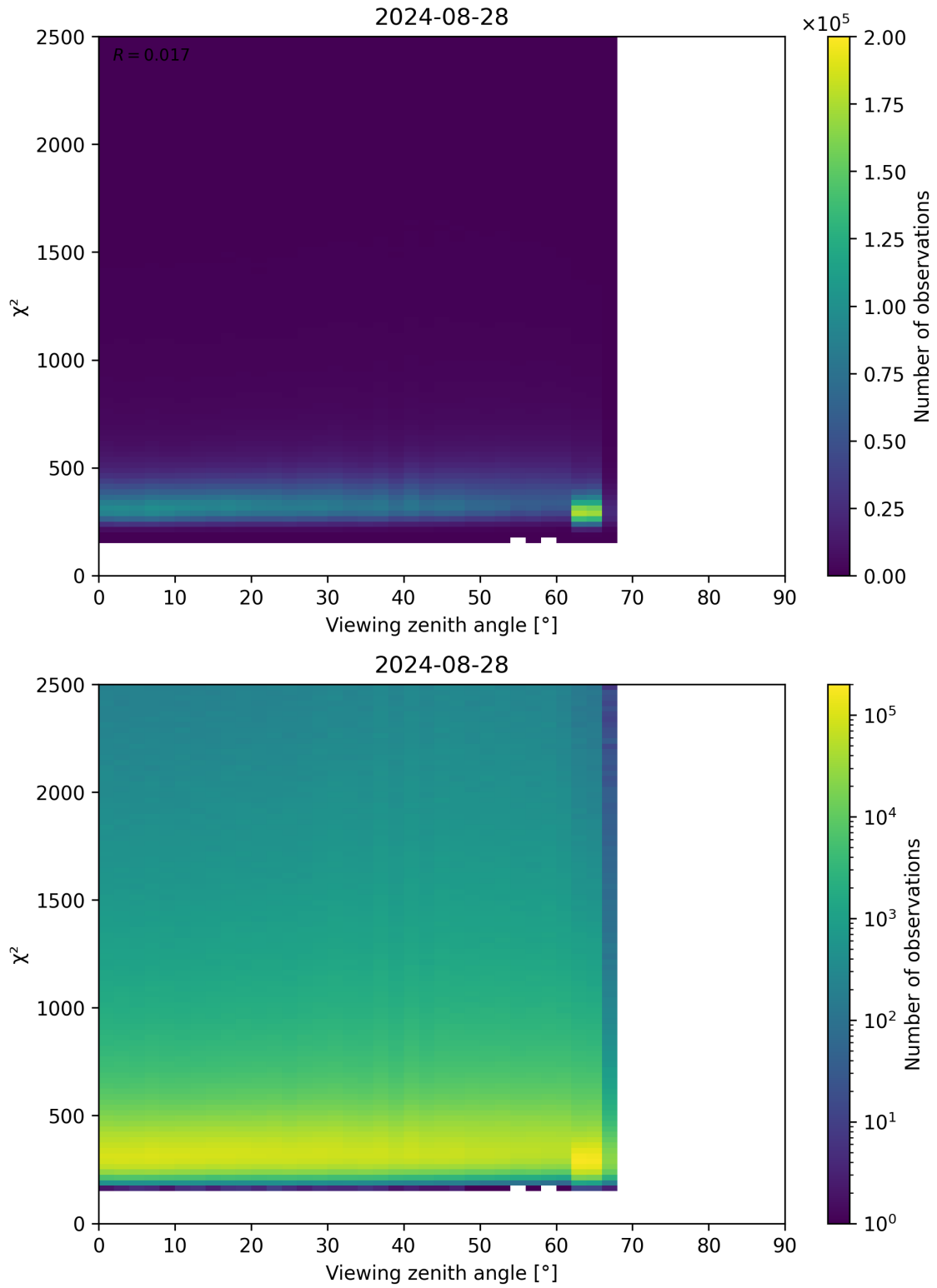
Figure 162: Scatter density plot of “Viewing zenith angle” against “ \chi^2 ” for 2024-08-27 to 2024-08-29.
