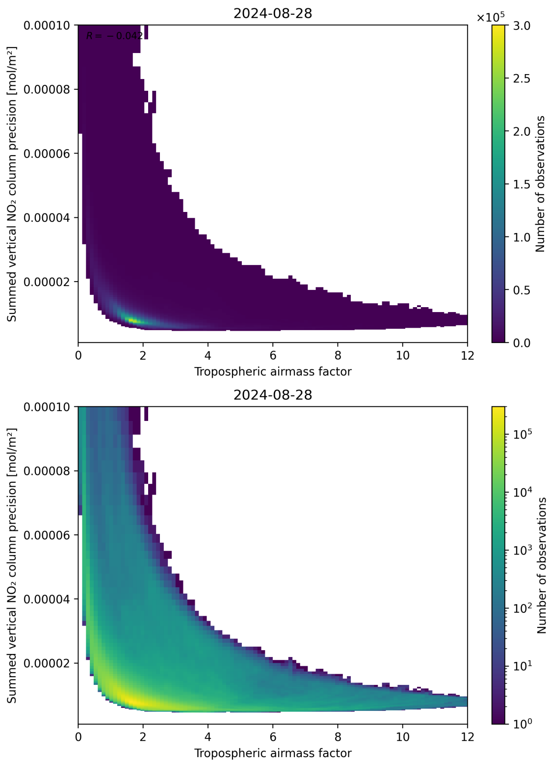
Figure 76: Scatter density plot of “Tropospheric airmass factor” against “Summed vertical NO 2 column precision” for 2024-08-27 to 2024-08-29.
