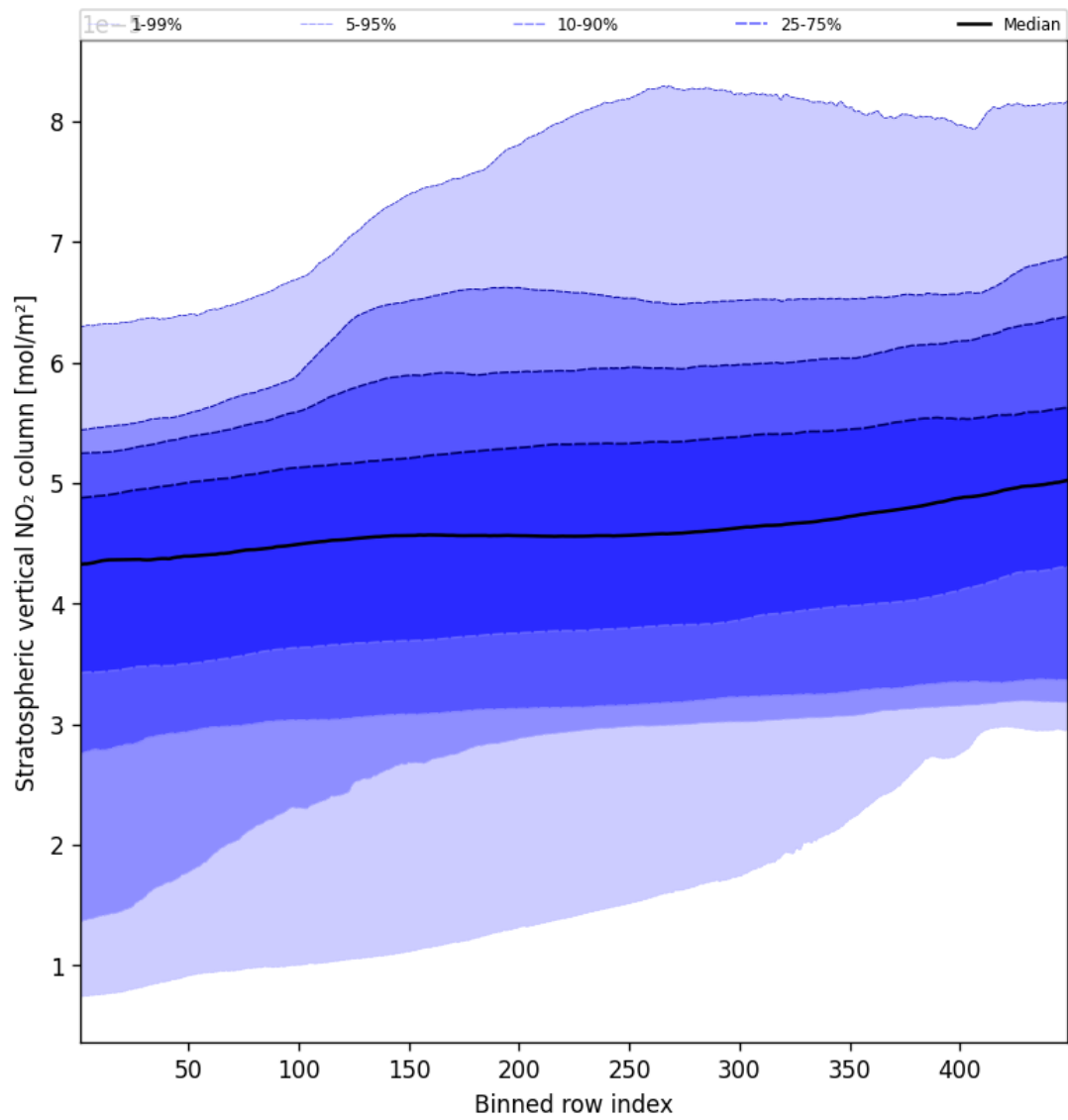
Figure 53: Along track statistics of “Stratospheric vertical NO 2 column” for 2024-08-27 to 2024-08-29
