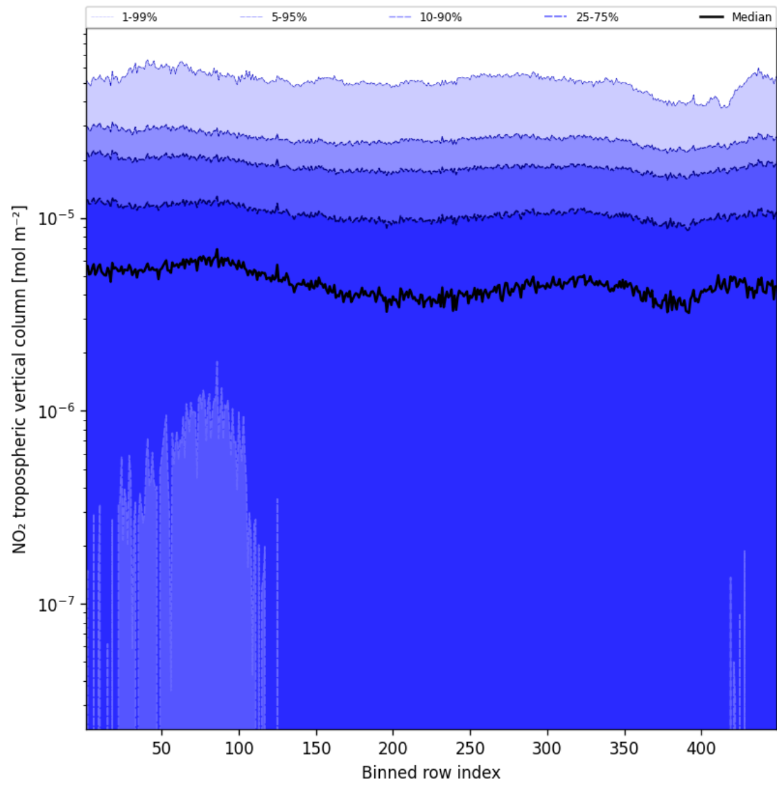
Figure 46: Along track statistics of “NO 2 tropospheric vertical column” for 2024-08-27 to 2024-08-29
