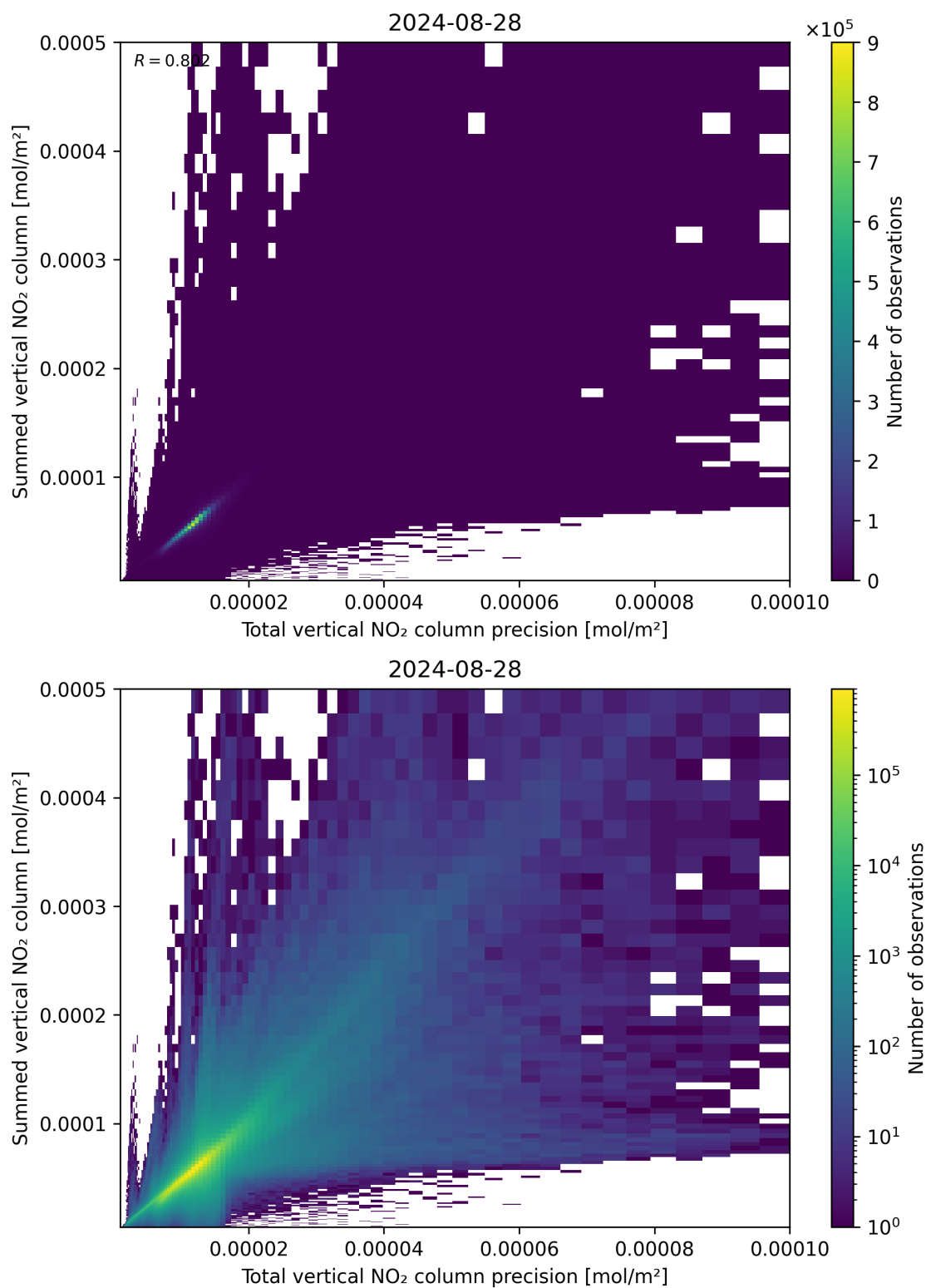
Figure 117: Scatter density plot of “Total vertical NO 2 column precision” against “Summed vertical NO 2 column” for 2024-08-27 to 2024-08-29.
