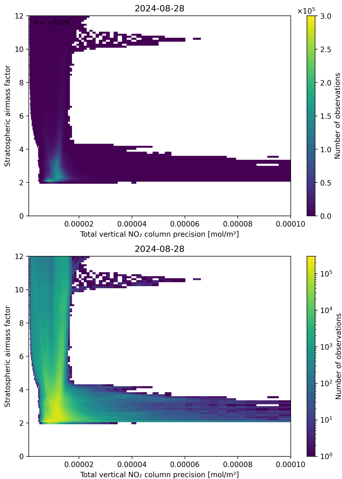
Figure 115: Scatter density plot of “Total vertical NO 2 column precision” against “Stratospheric airmass factor” for 2024-08-27 to 2024-08-29.
