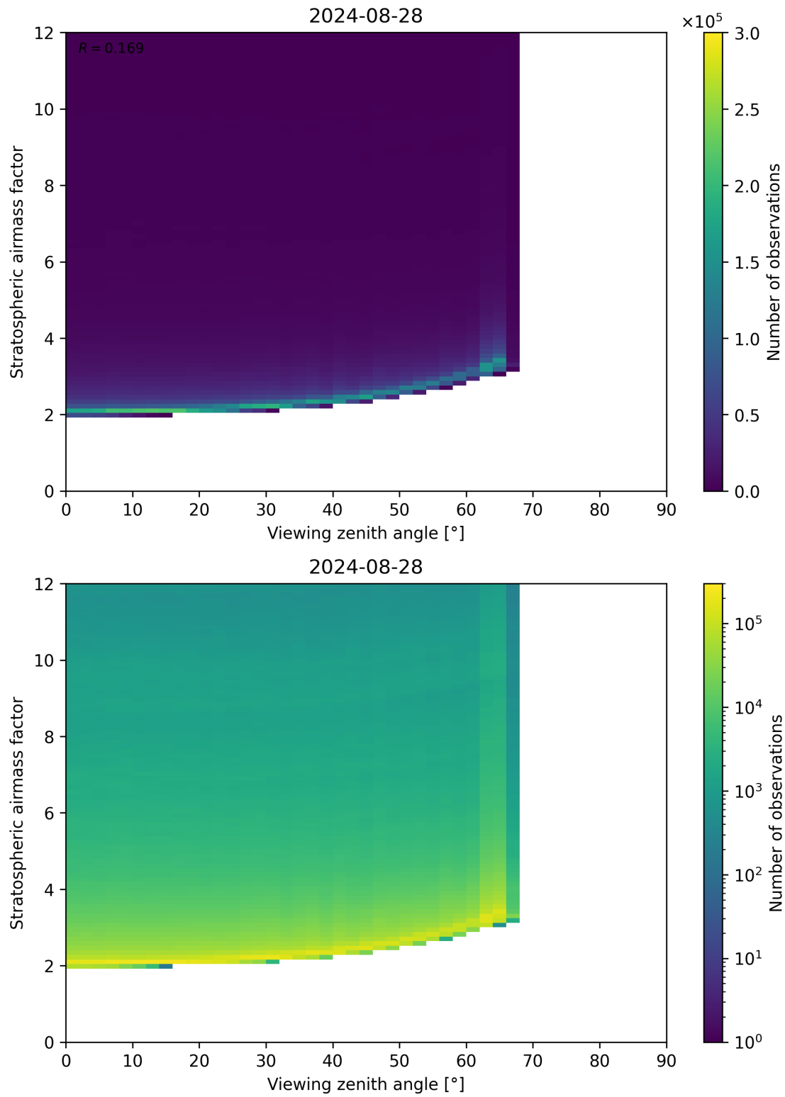
Figure 159: Scatter density plot of “Viewing zenith angle” against “Stratospheric airmass factor” for 2024-08-27 to 2024-08-29.
