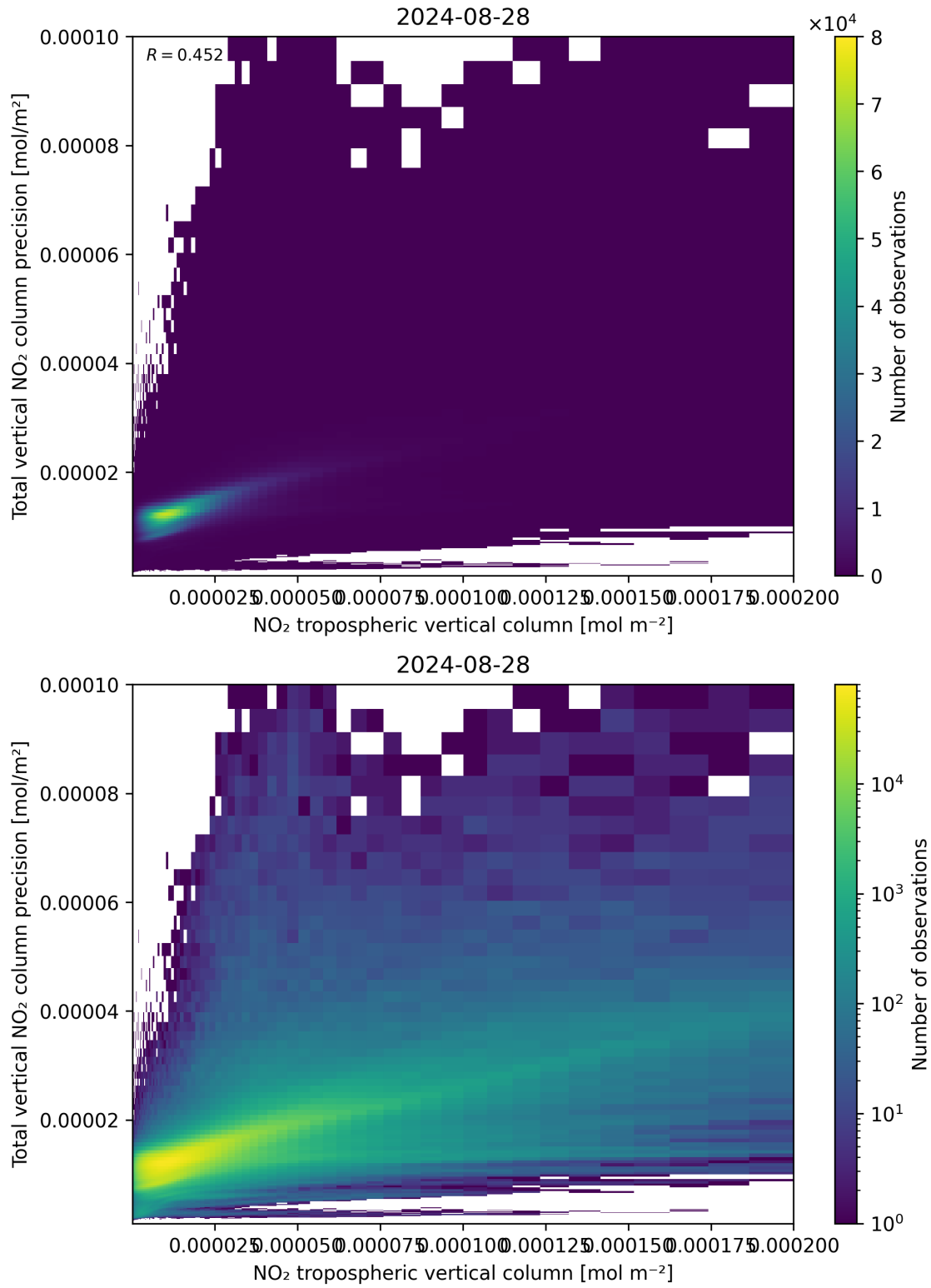
Figure 129: Scatter density plot of “NO 2 tropospheric vertical column” against “Total vertical NO 2 column precision” for 2024-08-27 to 2024-08-29.
