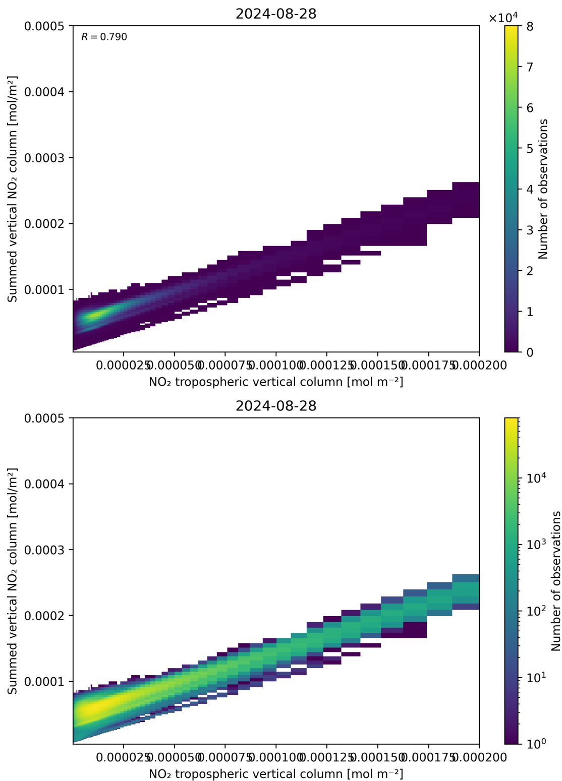
Figure 126: Scatter density plot of “NO 2 tropospheric vertical column” against “Summed vertical NO 2 column” for 2024-08-27 to 2024-08-29.
