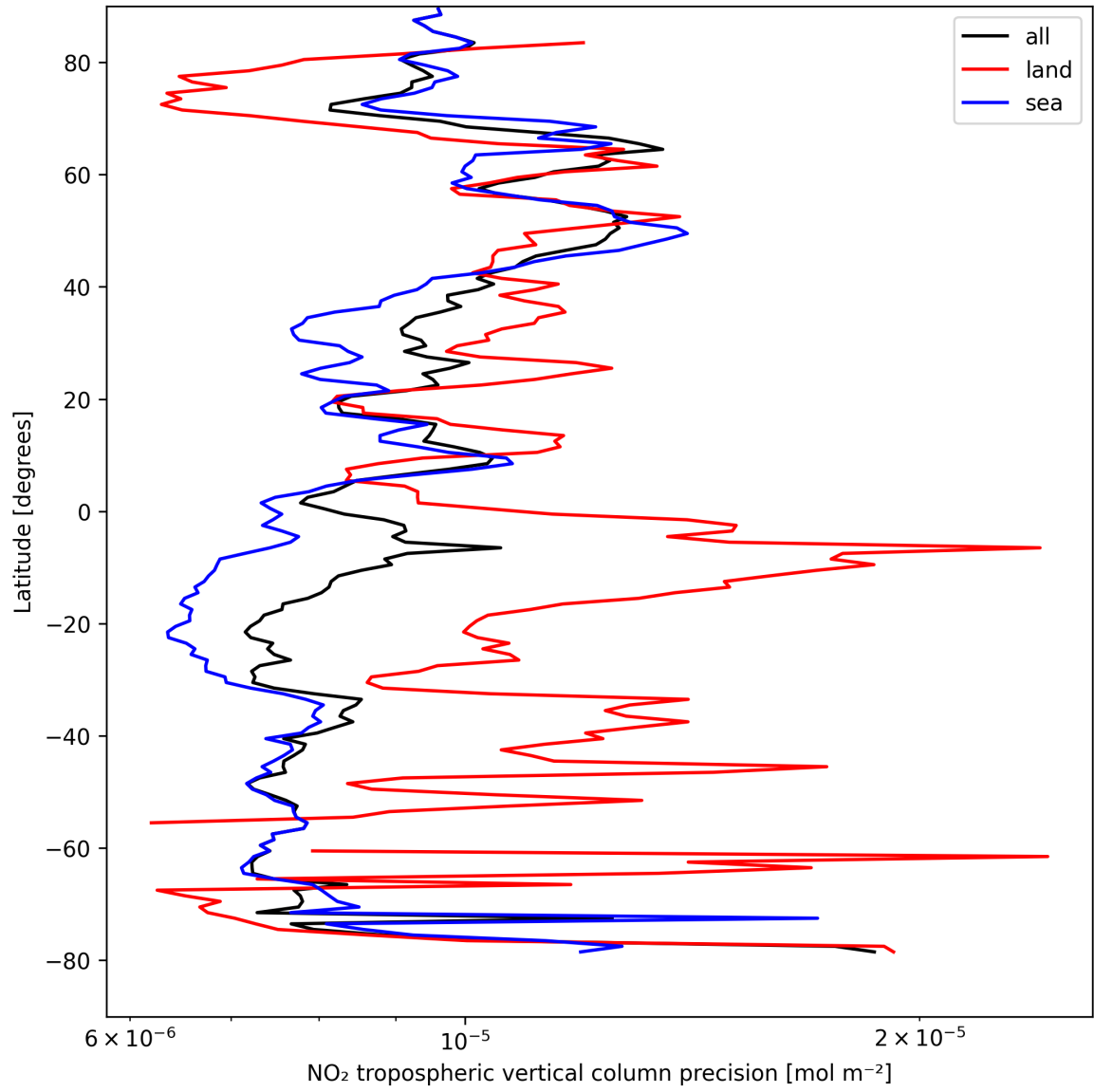
Figure 13: Zonal average of “NO 2 tropospheric vertical column precision” for 2024-08-27 to 2024-08-29.
