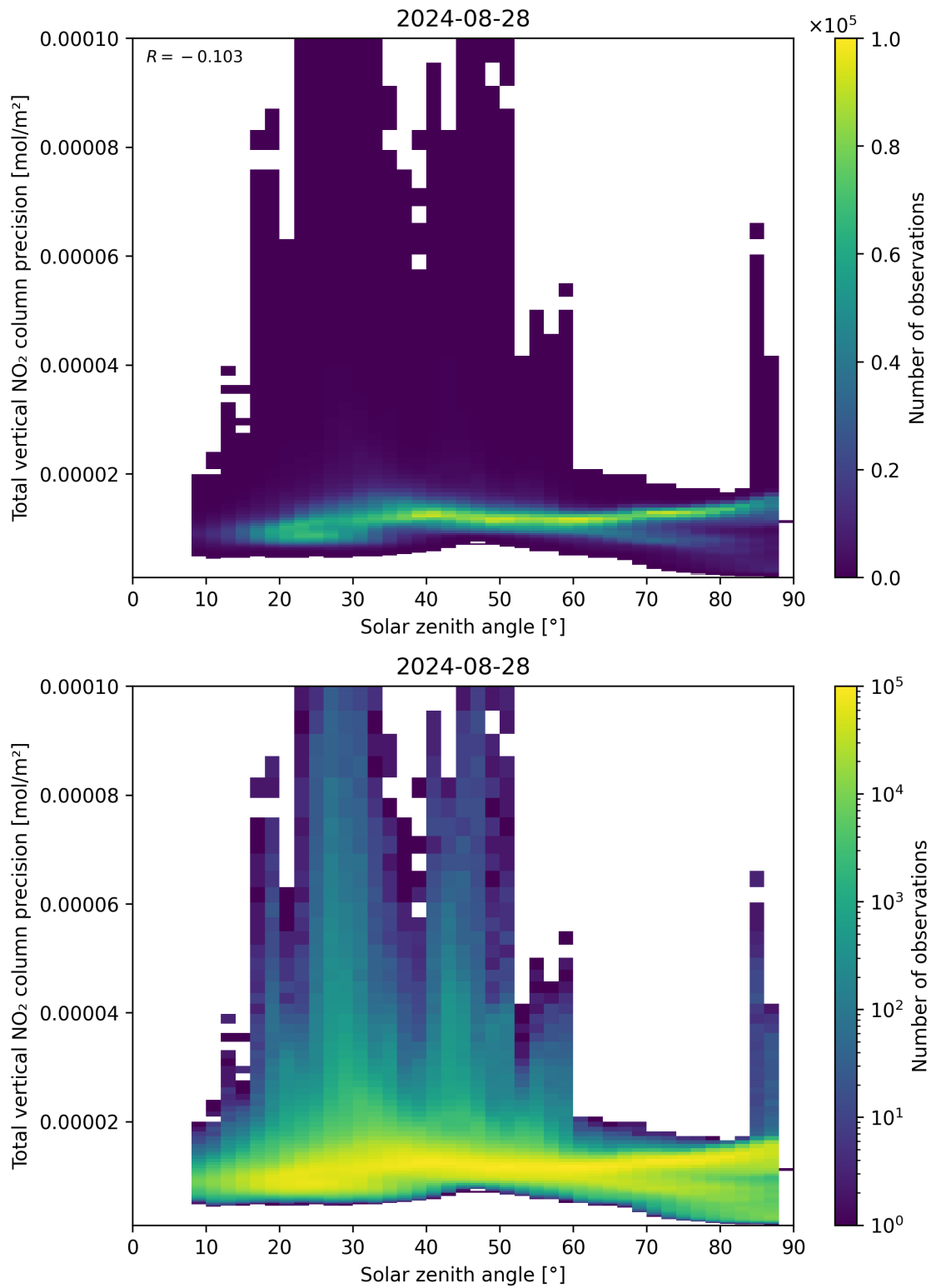
Figure 154: Scatter density plot of “Solar zenith angle” against “Total vertical NO 2 column precision” for 2024-08-27 to 2024-08-29.
