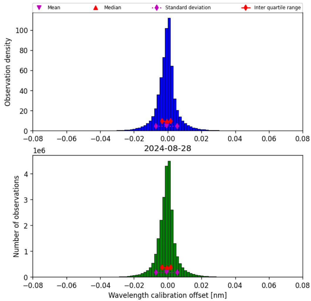
Figure 35: Histogram of “Wavelength calibration offset” for 2024-08-27 to 2024-08-29
