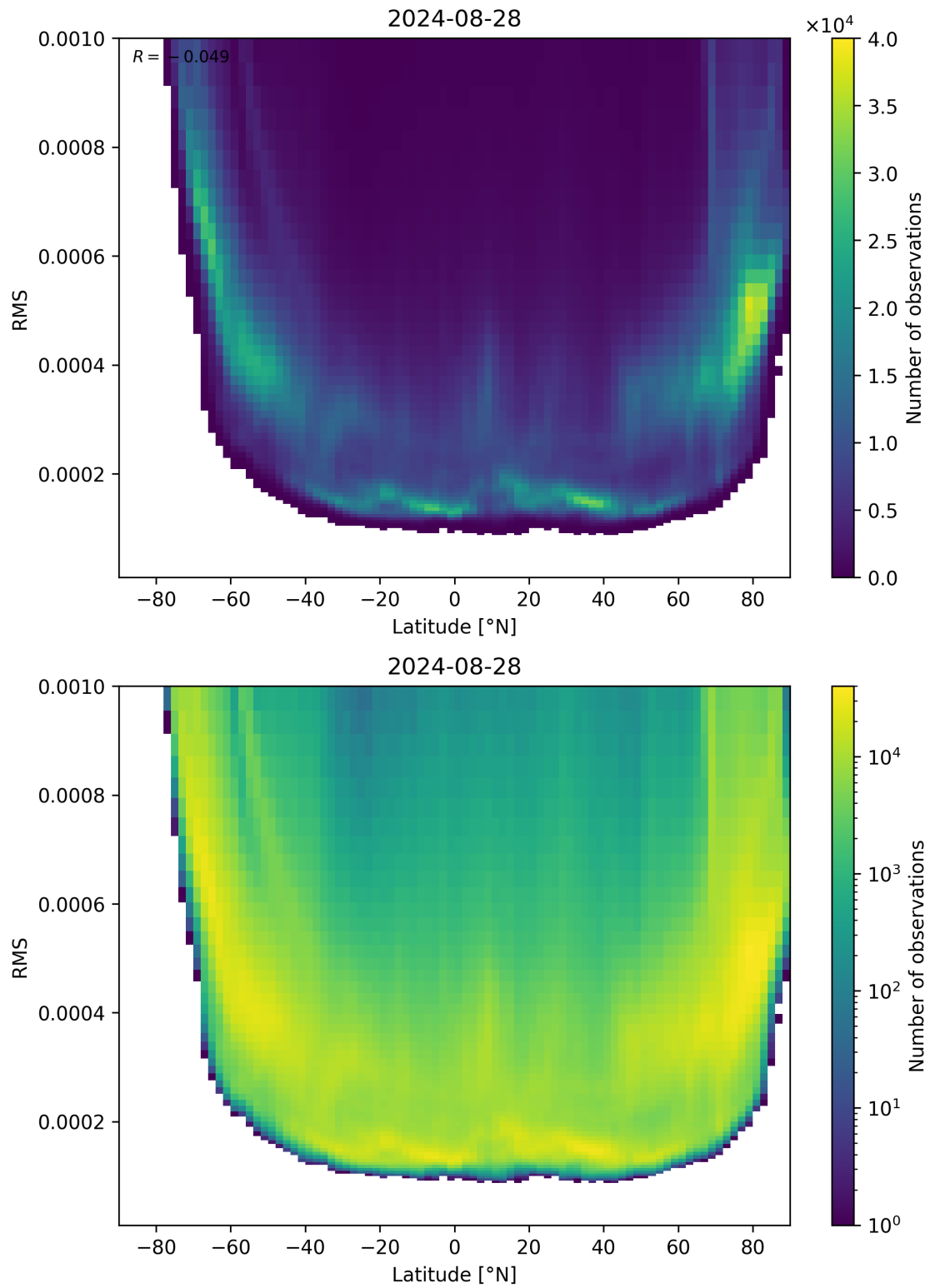
Figure 94: Scatter density plot of “Latitude” against “RMS” for 2024-08-27 to 2024-08-29.
