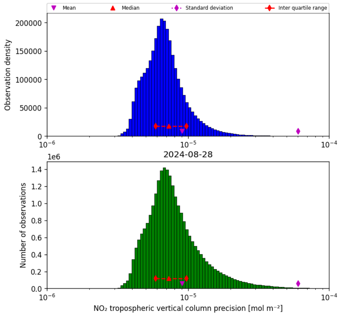
Figure 30: Histogram of “NO 2 tropospheric vertical column precision” for 2024-08-27 to 2024-08-29
