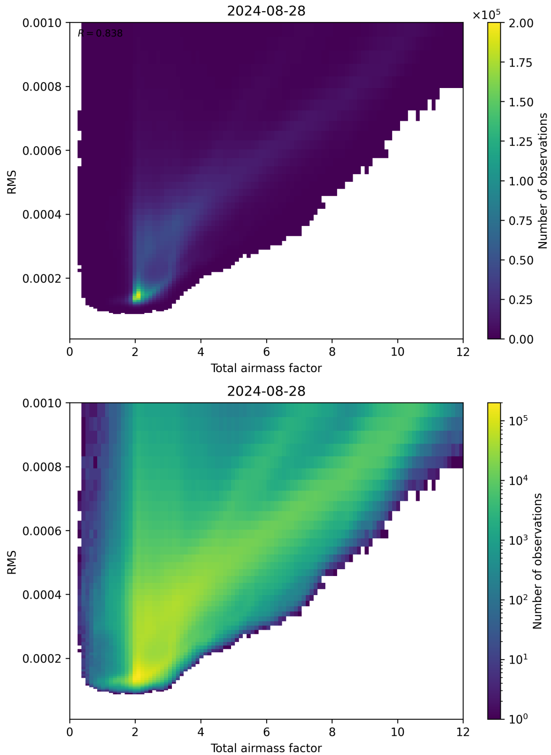
Figure 69: Scatter density plot of “Total airmass factor” against “RMS” for 2024-08-27 to 2024-08-29.
