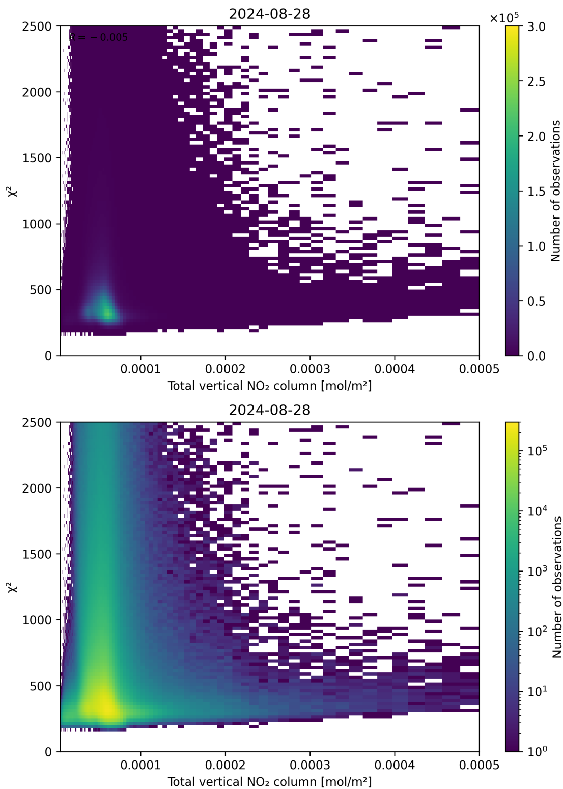
Figure 111: Scatter density plot of “Total vertical NO 2 column” against “ \chi^2 ” for 2024-08-27 to 2024-08-29.
