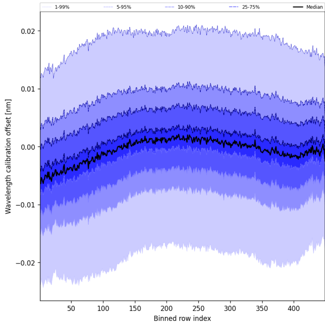
Figure 52: Along track statistics of “Wavelength calibration offset” for 2024-08-27 to 2024-08-29
