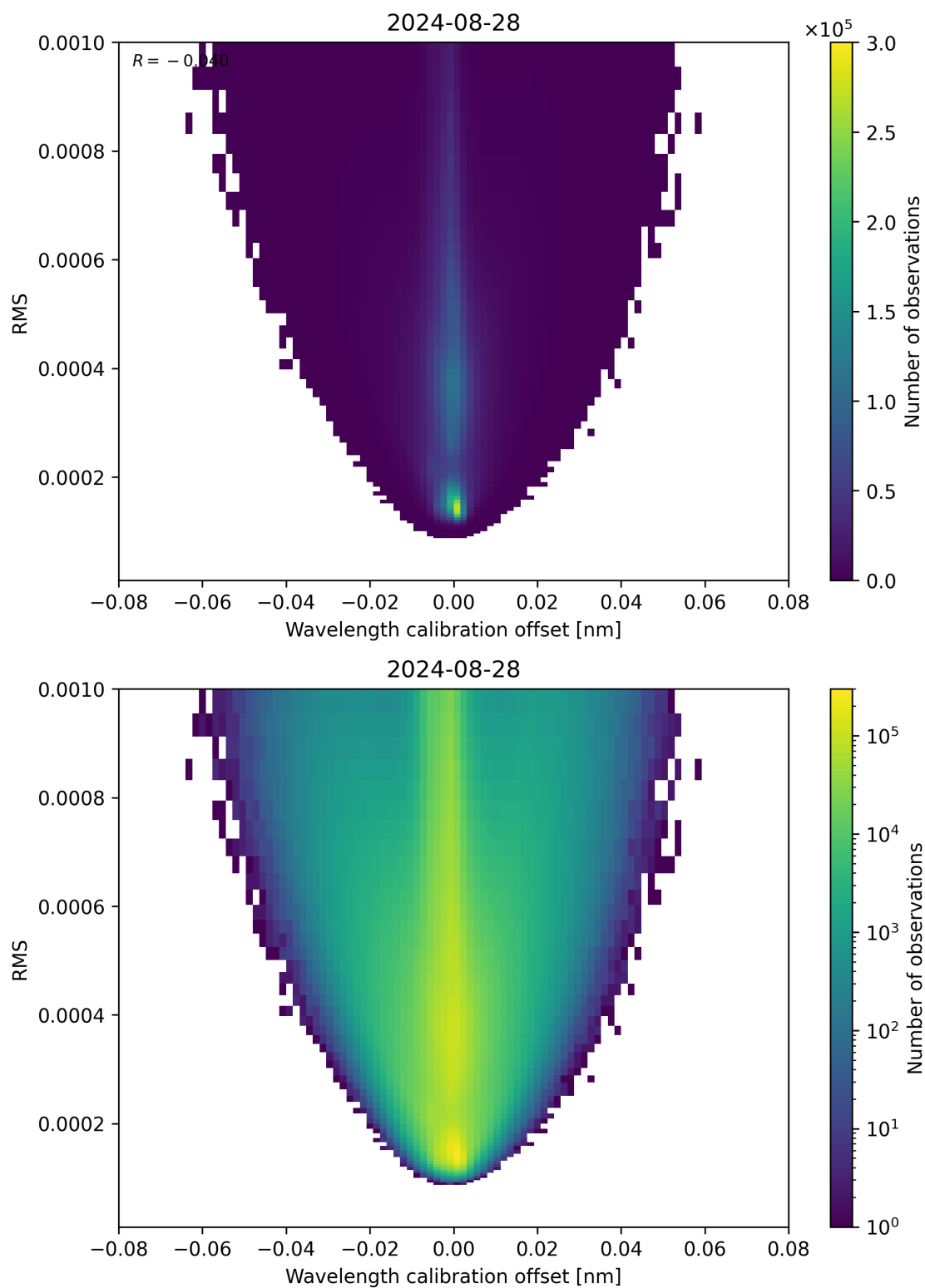
Figure 181: Scatter density plot of “Wavelength calibration offset” against “RMS” for 2024-08-27 to 2024-08-29.
