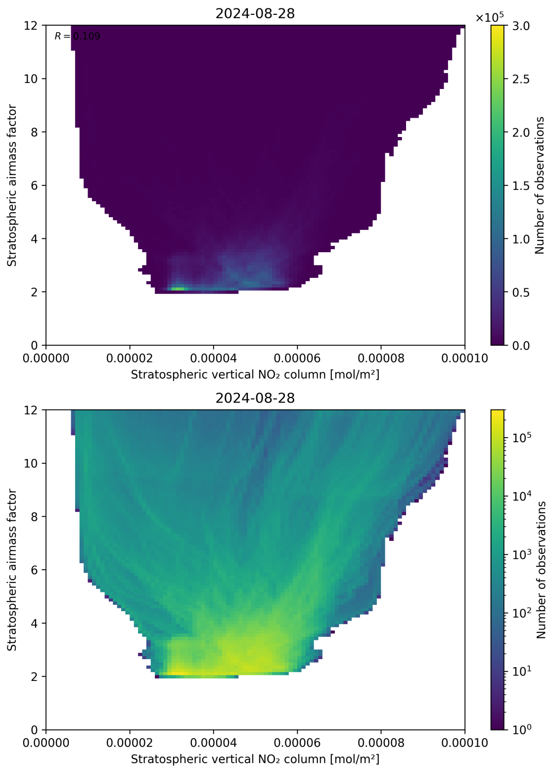
Figure 96: Scatter density plot of “Stratospheric vertical NO 2 column” against “Stratospheric airmass factor” for 2024-08-27 to 2024-08-29.
