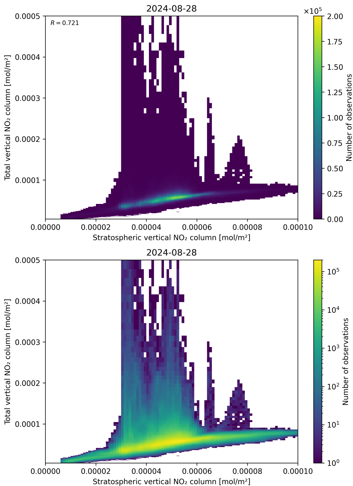
Figure 100: Scatter density plot of “Stratospheric vertical NO 2 column” against “Total vertical NO 2 column” for 2024-08-27 to 2024-08-29.
