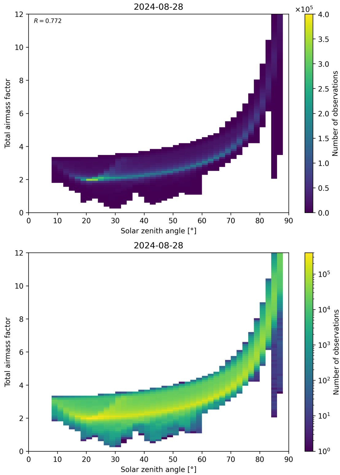
Figure 146: Scatter density plot of “Solar zenith angle” against “Total air mass factor” for 2024-08-27 to 2024-08-29.
