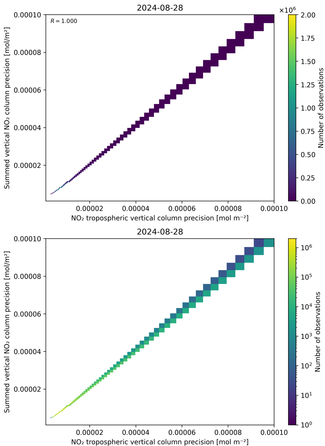
Figure 137: Scatter density plot of “NO 2 tropospheric vertical column precision” against “Summed vertical NO 2 column precision” for 2024-08-27 to 2024-08-29.
