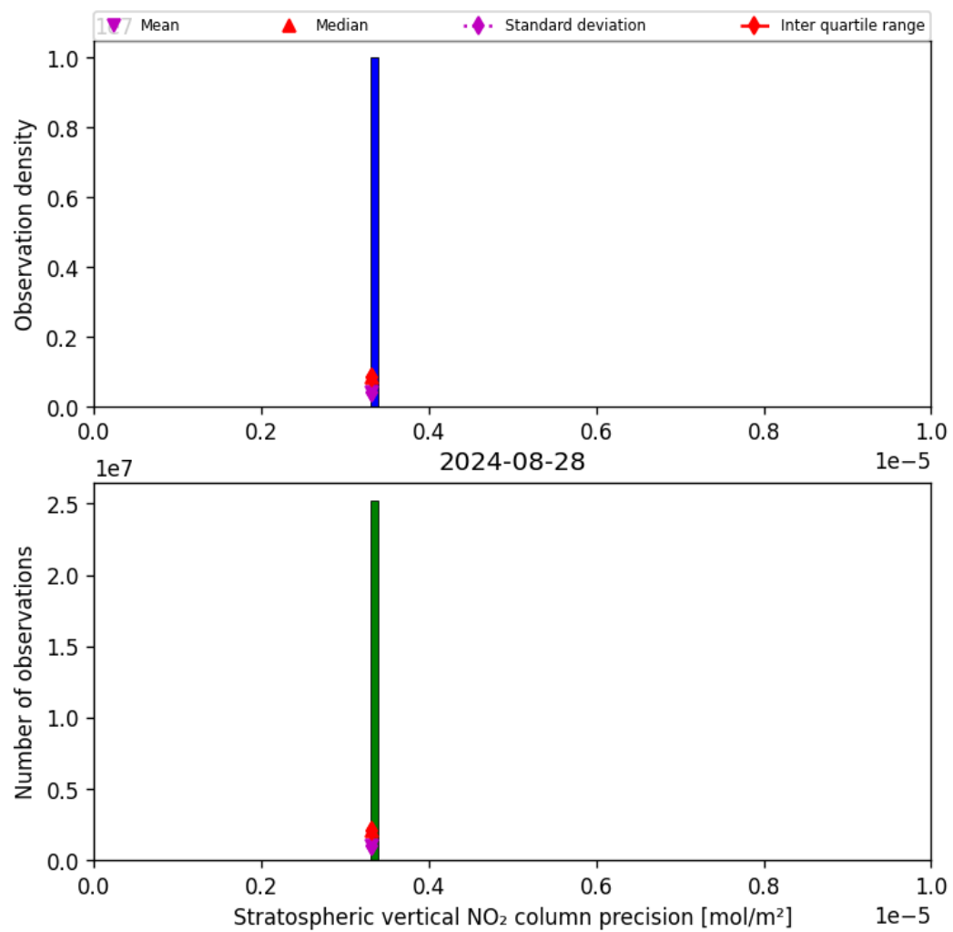
Figure 37: Histogram of “Stratospheric vertical NO 2 column precision” for 2024-08-27 to 2024-08-29
