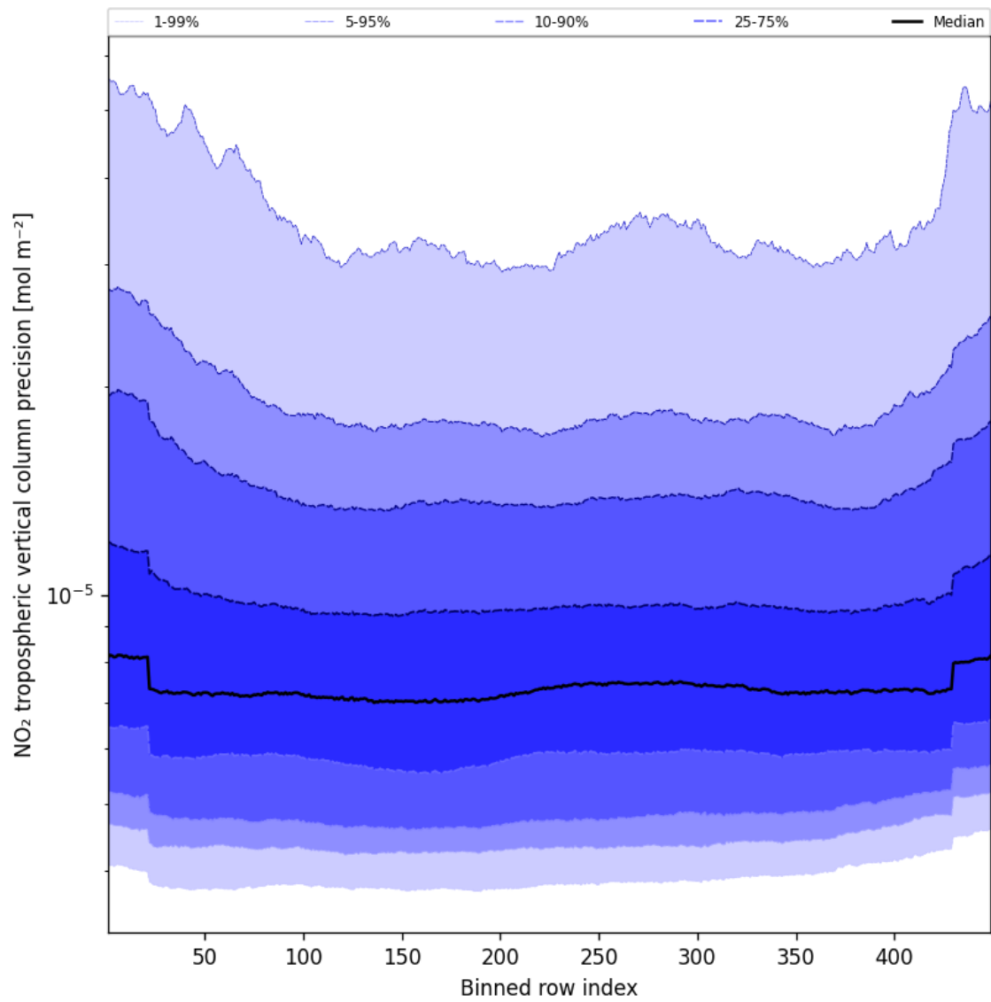
Figure 47: Along track statistics of “NO 2 tropospheric vertical column precision” for 2024-08-27 to 2024-08-29
