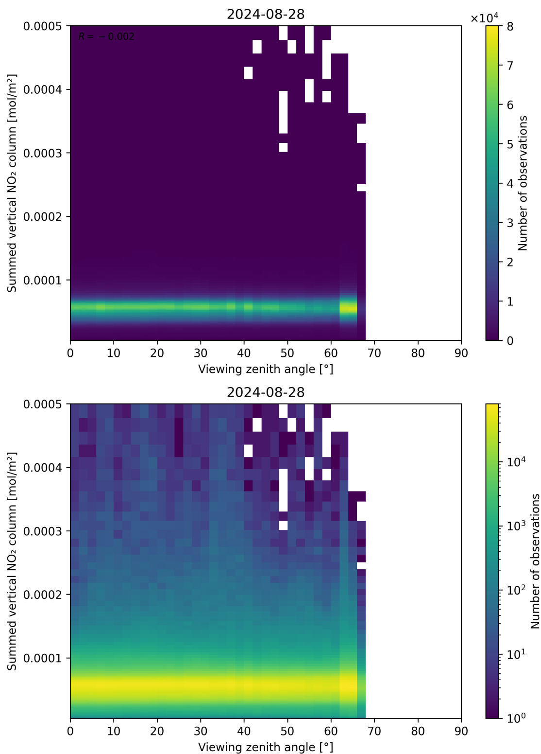
Figure 165: Scatter density plot of “Viewing zenith angle” against “Summed vertical NO 2 column” for 2024-08-27 to 2024-08-29.
