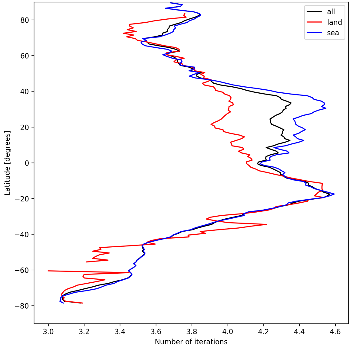
Figure 17: Zonal average of “Number of iterations” for 2024-08-27 to 2024-08-29.
