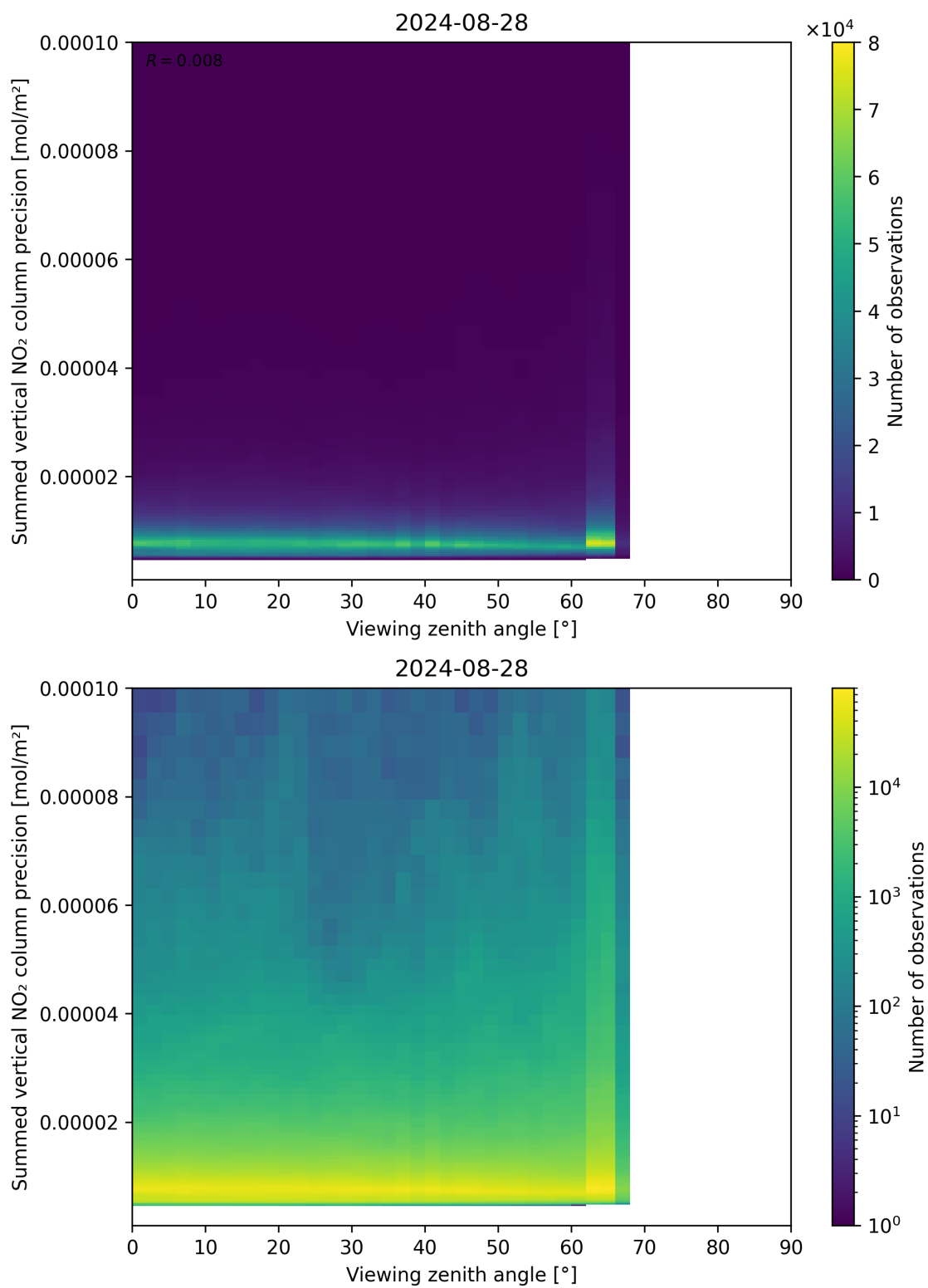
Figure 166: Scatter density plot of “Viewing zenith angle” against “Summed vertical NO 2 column precision” for 2024-08-27 to 2024-08-29.
