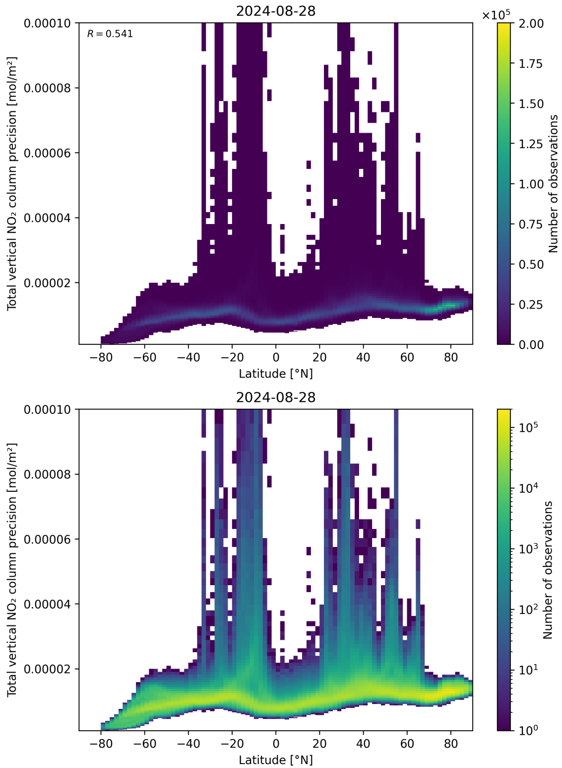
Figure 91: Scatter density plot of “Latitude” against “Total vertical NO 2 column precision” for 2024-08-27 to 2024-08-29.
