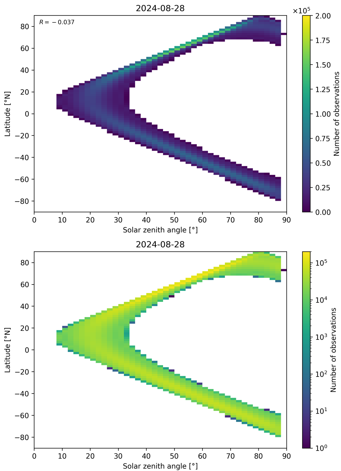
Figure 149: Scatter density plot of “Solar zenith angle” against “Latitude” for 2024-08-27 to 2024-08-29.
