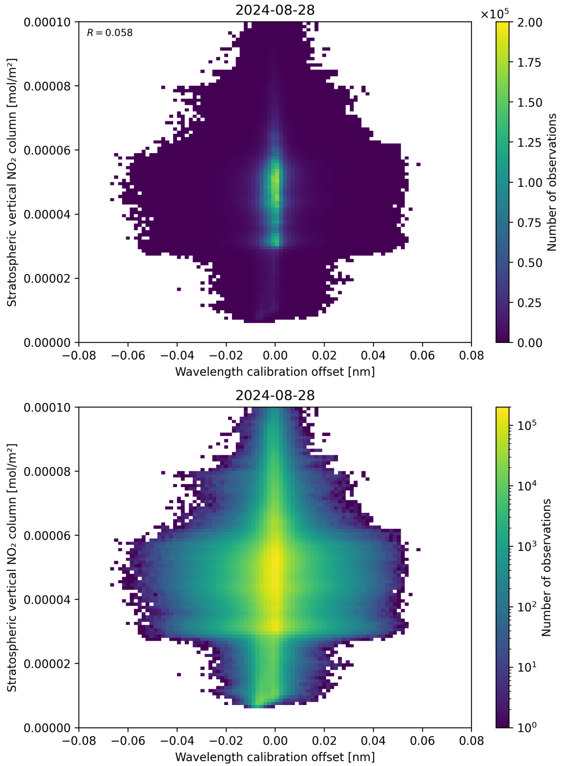
Figure 176: Scatter density plot of “Wavelength calibration offset” against “Stratospheric vertical NO 2 column” for 2024-08-27 to 2024-08-29.
