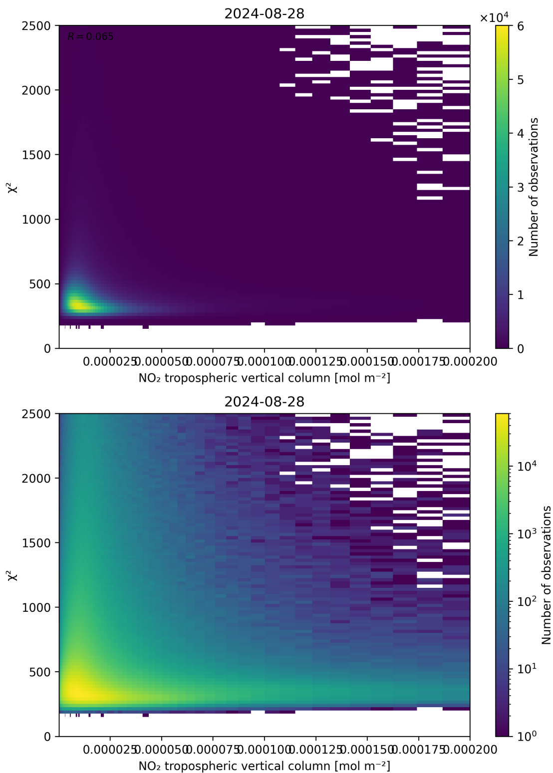
Figure 124: Scatter density plot of “NO 2 tropospheric vertical column” against “ \chi^2 ” for 2024-08-27 to 2024-08-29.
