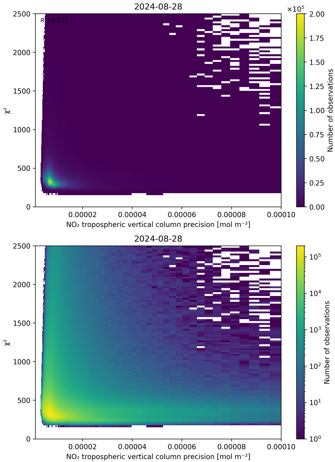
Figure 134: Scatter density plot of “NO 2 tropospheric vertical column precision” against “ \chi^2 ” for 2024-08-27 to 2024-08-29.
