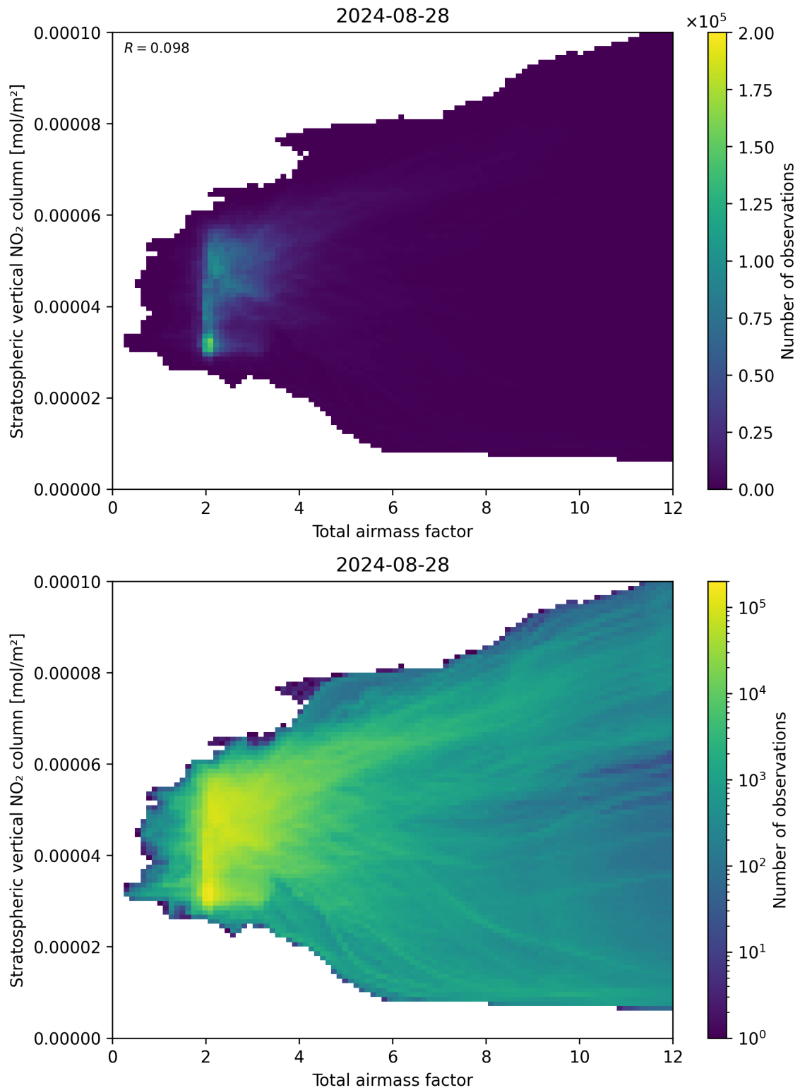
Figure 64: Scatter density plot of “Total airmass factor” against “Stratospheric vertical NO 2 column” for 2024-08-27 to 2024-08-29.
