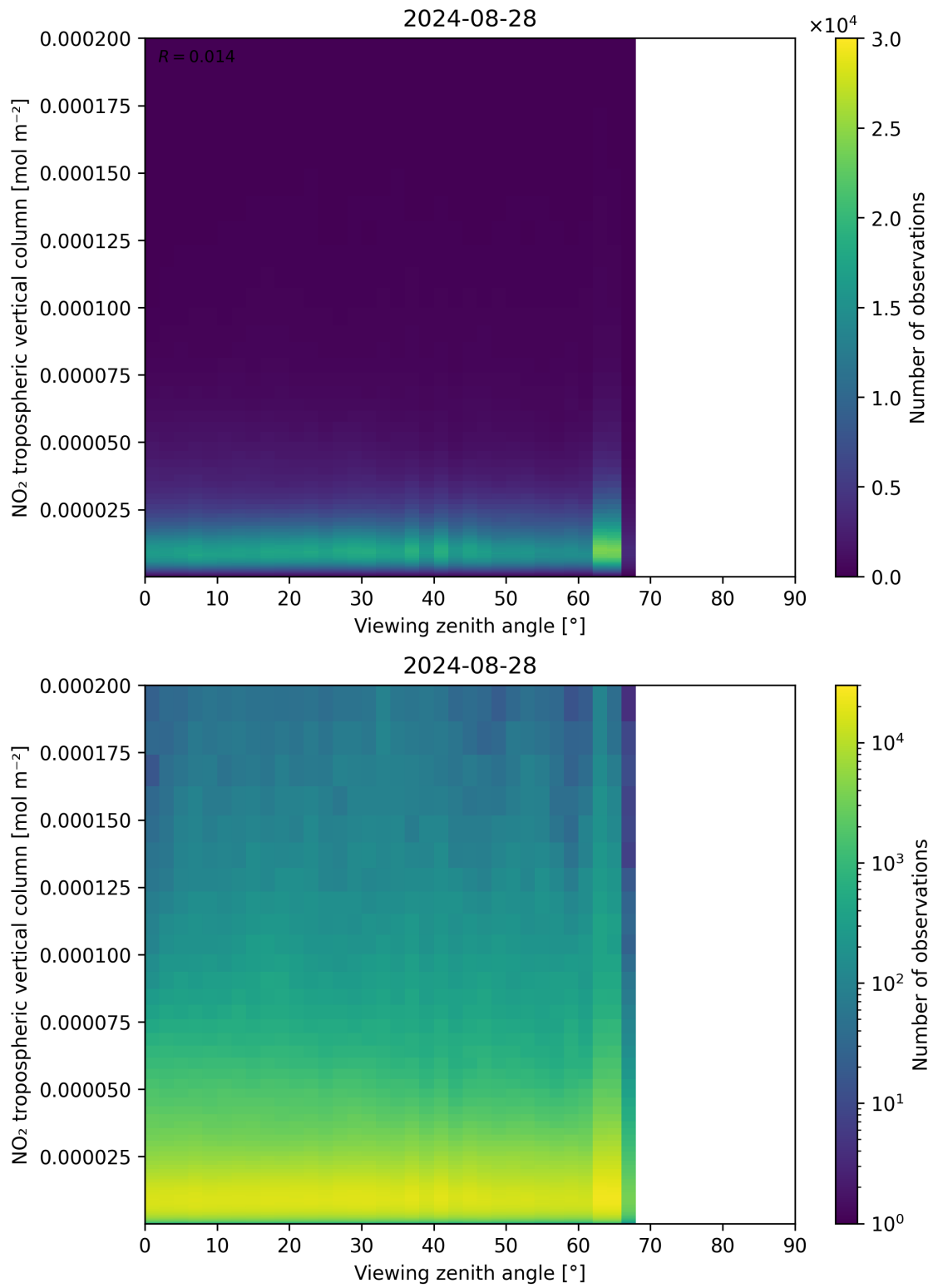
Figure 169: Scatter density plot of “Viewing zenith angle” against “NO 2 tropospheric vertical column” for 2024-08-27 to 2024-08-29.
