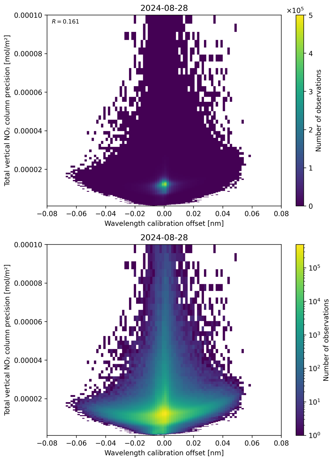
Figure 180: Scatter density plot of “Wavelength calibration offset” against “Total vertical NO 2 column precision” for 2024-08-27 to 2024-08-29.
