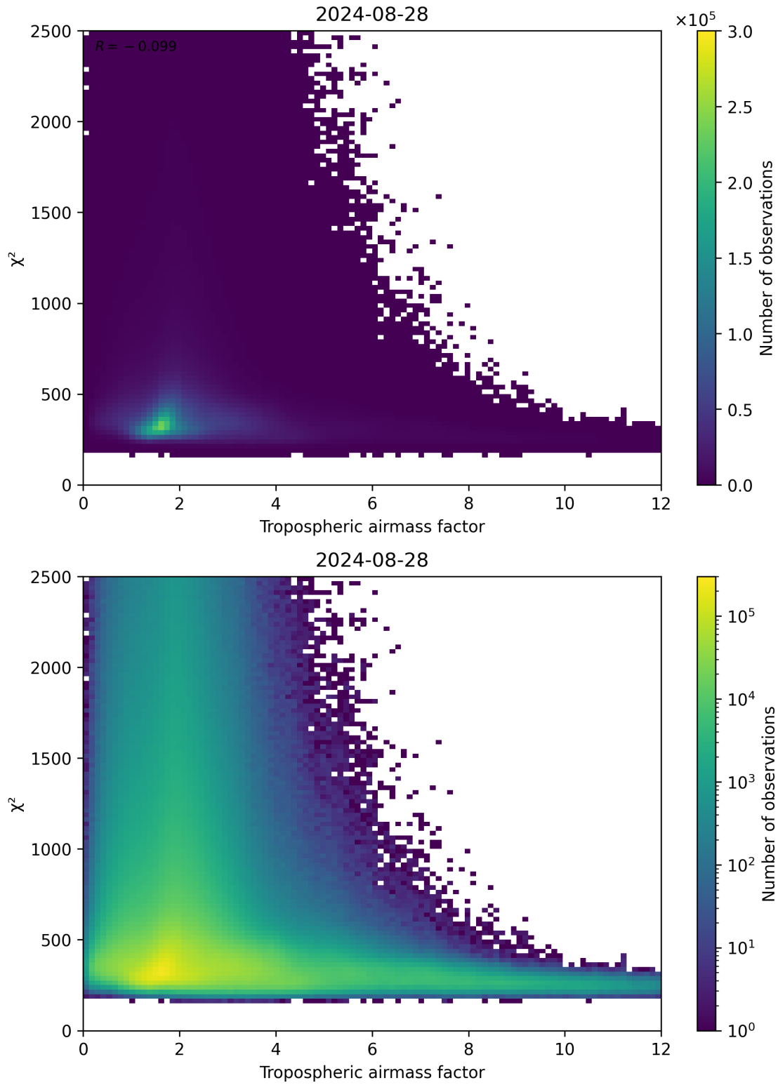
Figure 73: Scatter density plot of “Tropospheric airmass factor” against “ \chi^2 ” for 2024-08-27 to 2024-08-29.
