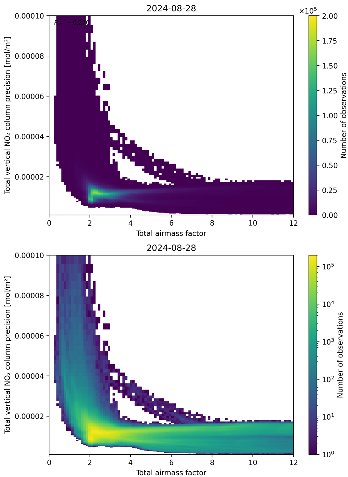
Figure 68: Scatter density plot of “Total airmass factor” against “Total vertical NO 2 column precision” for 2024-08-27 to 2024-08-29.
