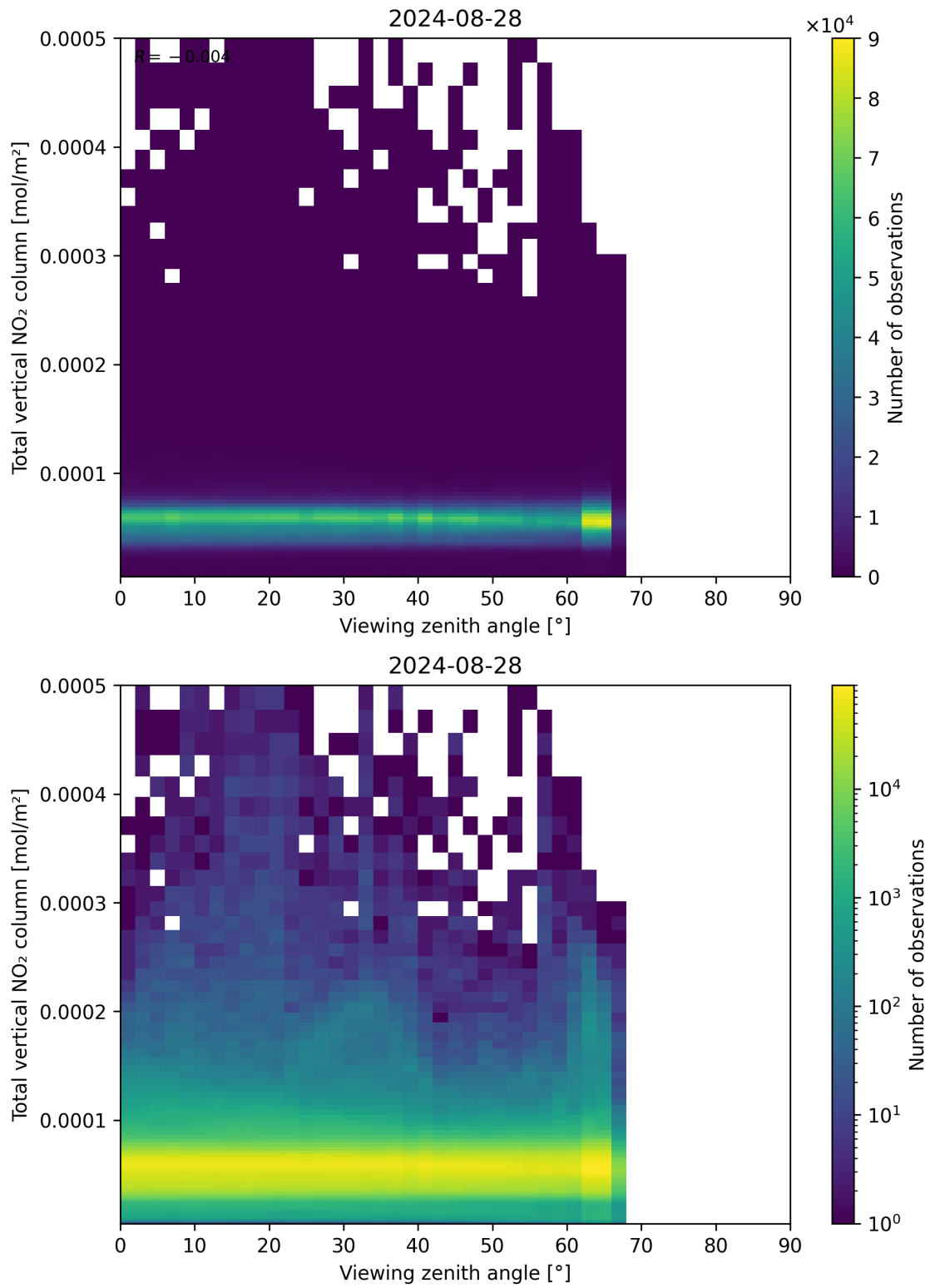
Figure 167: Scatter density plot of “Viewing zenith angle” against “Total vertical NO 2 column” for 2024-08-27 to 2024-08-29.
