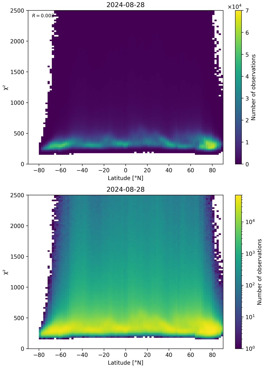
Figure 86: Scatter density plot of “Latitude” against “ \chi^2 ” for 2024-08-27 to 2024-08-29.
