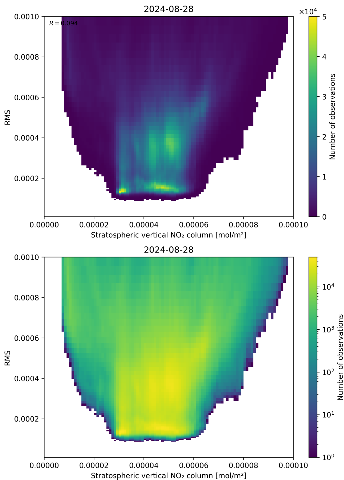
Figure 102: Scatter density plot of “Stratospheric vertical NO 2 column” against “RMS” for 2024-08-27 to 2024-08-29.
