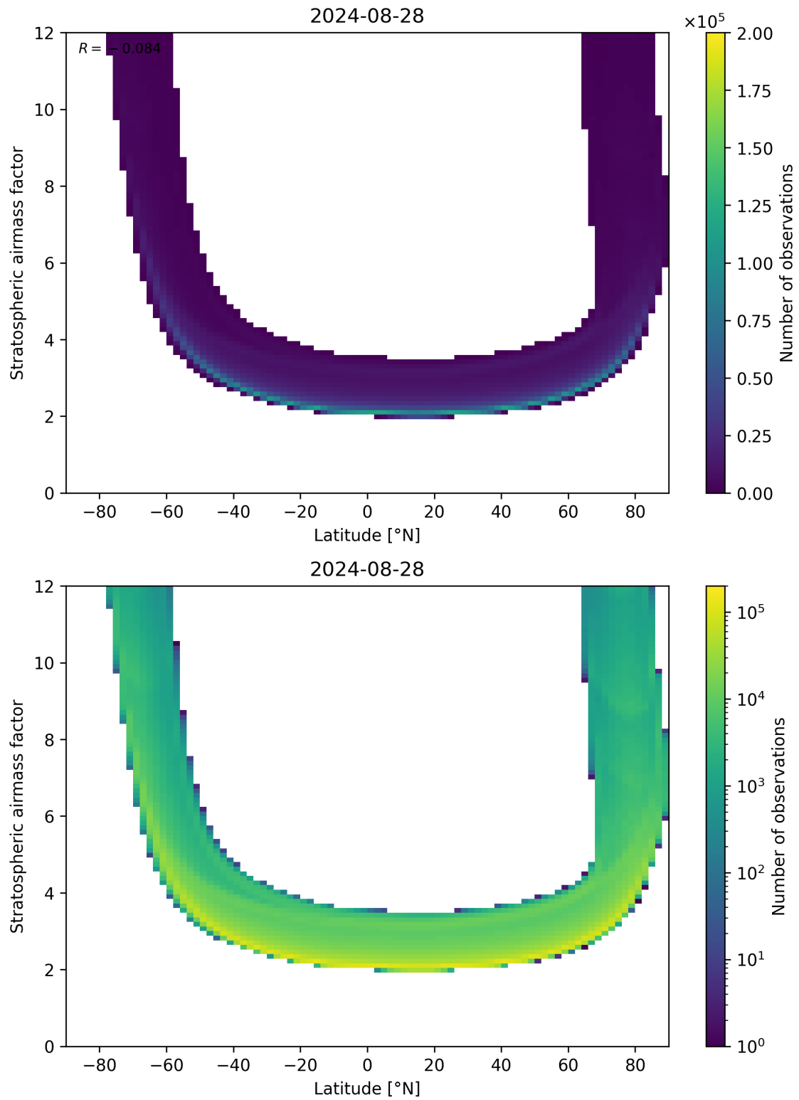
Figure 83: Scatter density plot of “Latitude” against “Stratospheric air mass factor” for 2024-08-27 to 2024-08-29.
