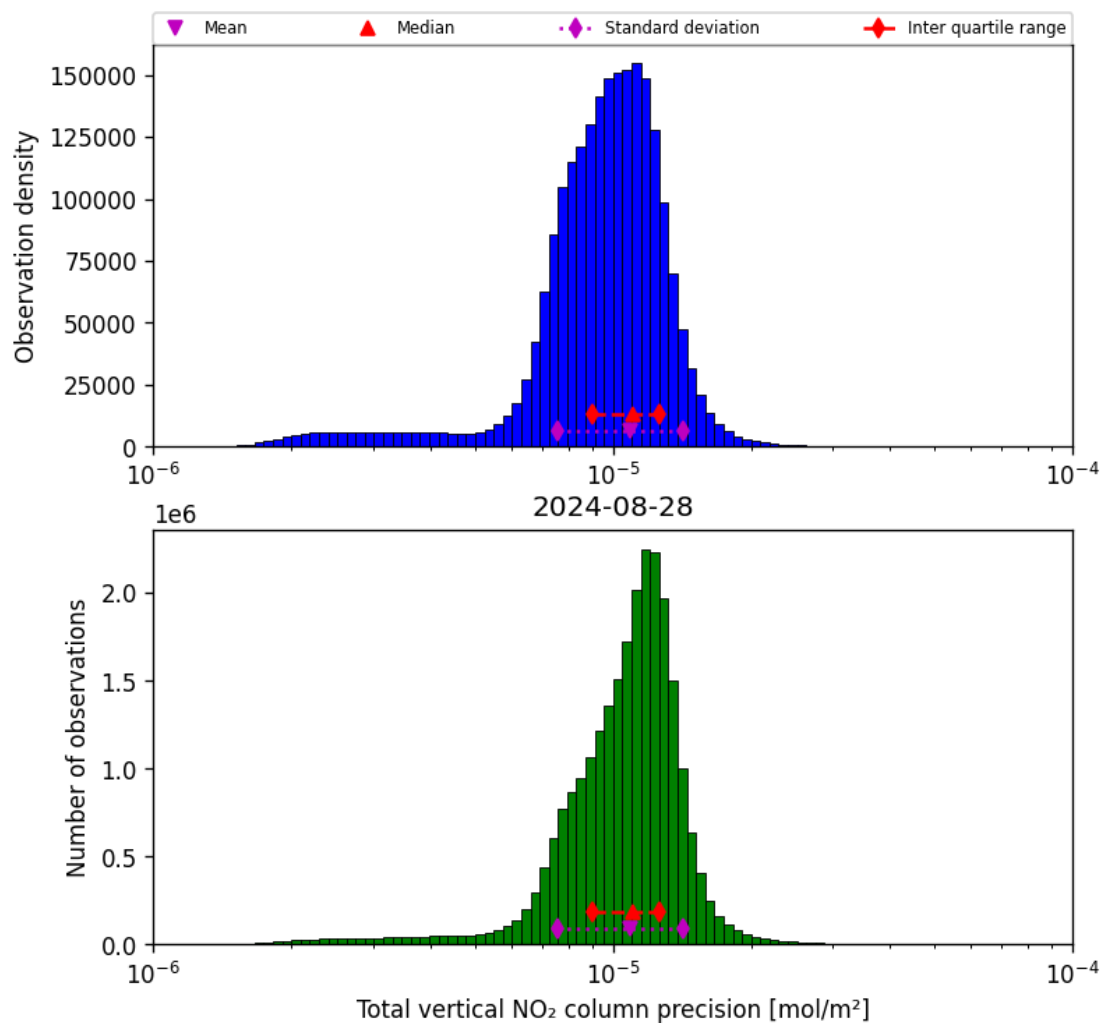
Figure 39: Histogram of “Total vertical NO 2 column precision” for 2024-08-27 to 2024-08-29
