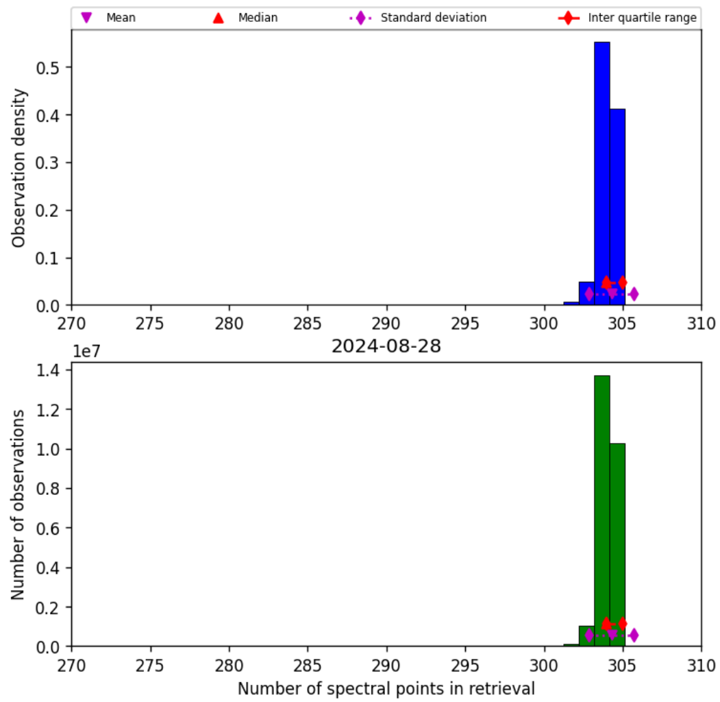
Figure 33: Histogram of “Number of spectral points in retrieval” for 2024-08-27 to 2024-08-29
