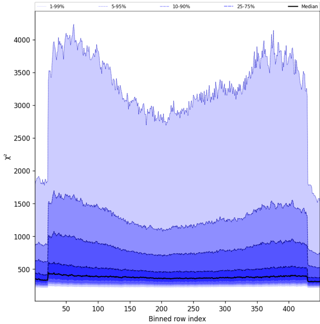
Figure 59: Along track statistics of “ \chi^2 ” for 2024-08-27 to 2024-08-29
