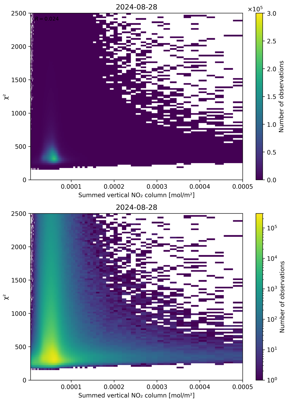
Figure 104: Scatter density plot of “Summed vertical NO 2 column” against “ \chi^2 ” for 2024-08-27 to 2024-08-29.
