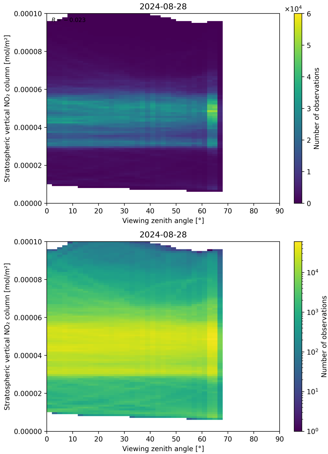
Figure 164: Scatter density plot of “Viewing zenith angle” against “Stratospheric vertical NO 2 column” for 2024-08-27 to 2024-08-29.
