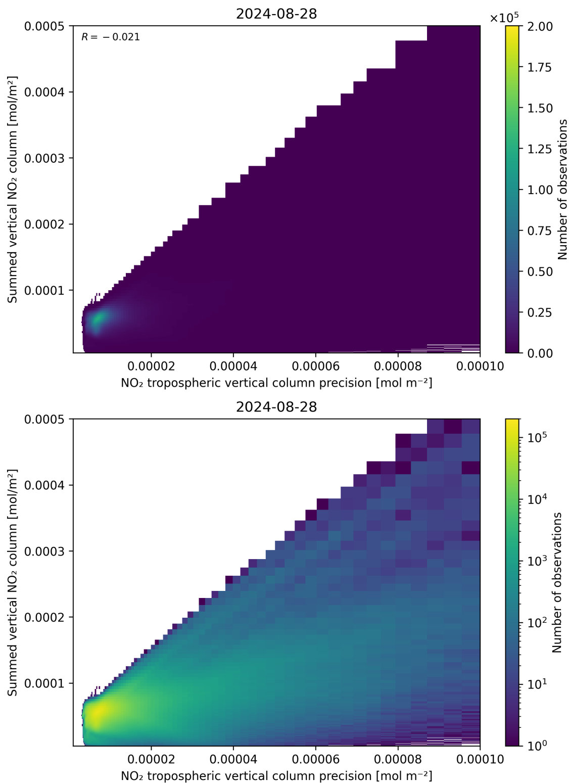
Figure 136: Scatter density plot of “NO 2 tropospheric vertical column precision” against “Summed vertical NO 2 column” for 2024-08-27 to 2024-08-29.
