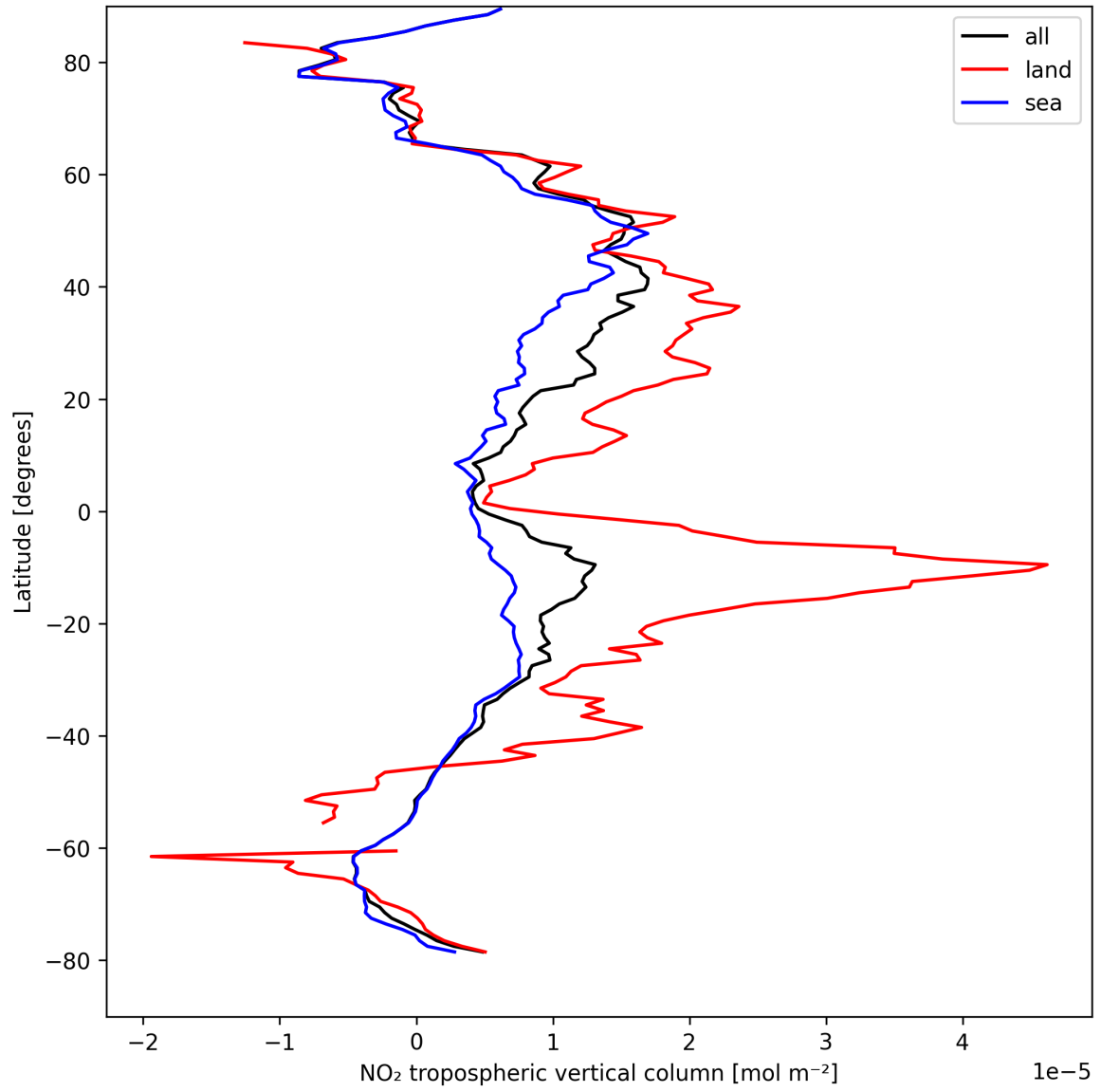
Figure 12: Zonal average of “NO 2 tropospheric vertical column” for 2024-08-27 to 2024-08-29.
