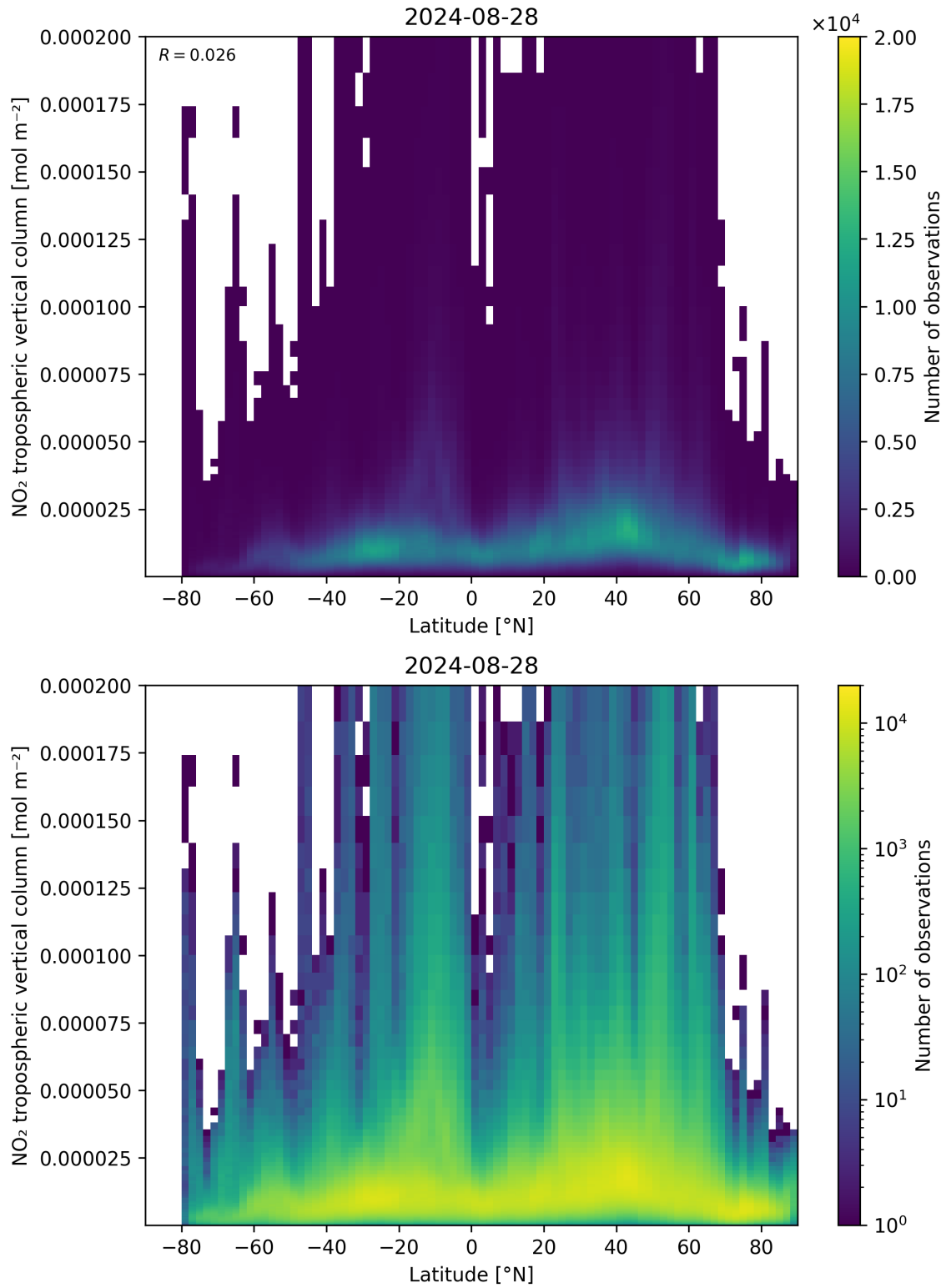
Figure 92: Scatter density plot of “Latitude” against “NO 2 tropospheric vertical column” for 2024-08-27 to 2024-08-29.
