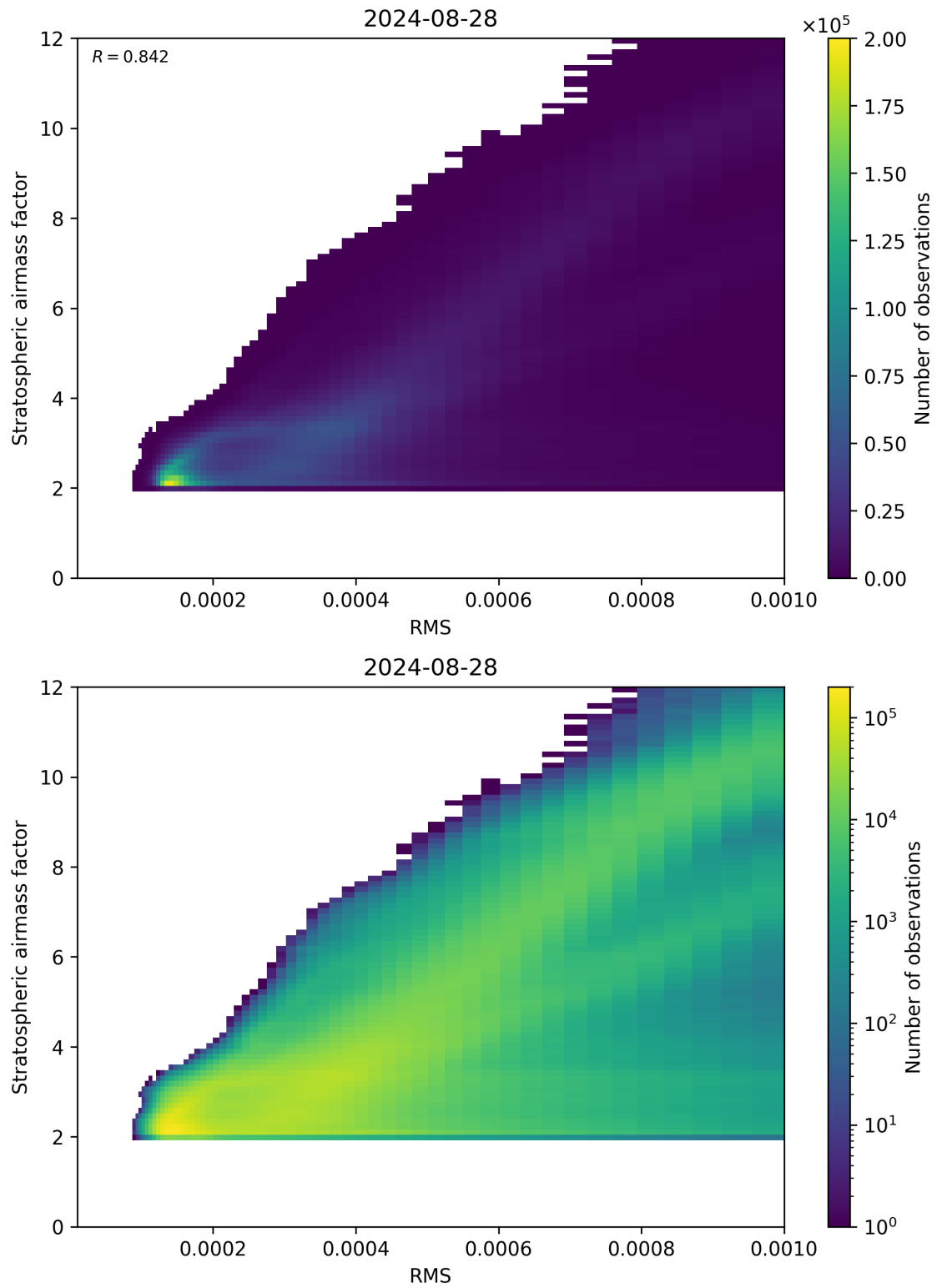
Figure 144: Scatter density plot of “RMS” against “Stratospheric airmass factor” for 2024-08-27 to 2024-08-29.
