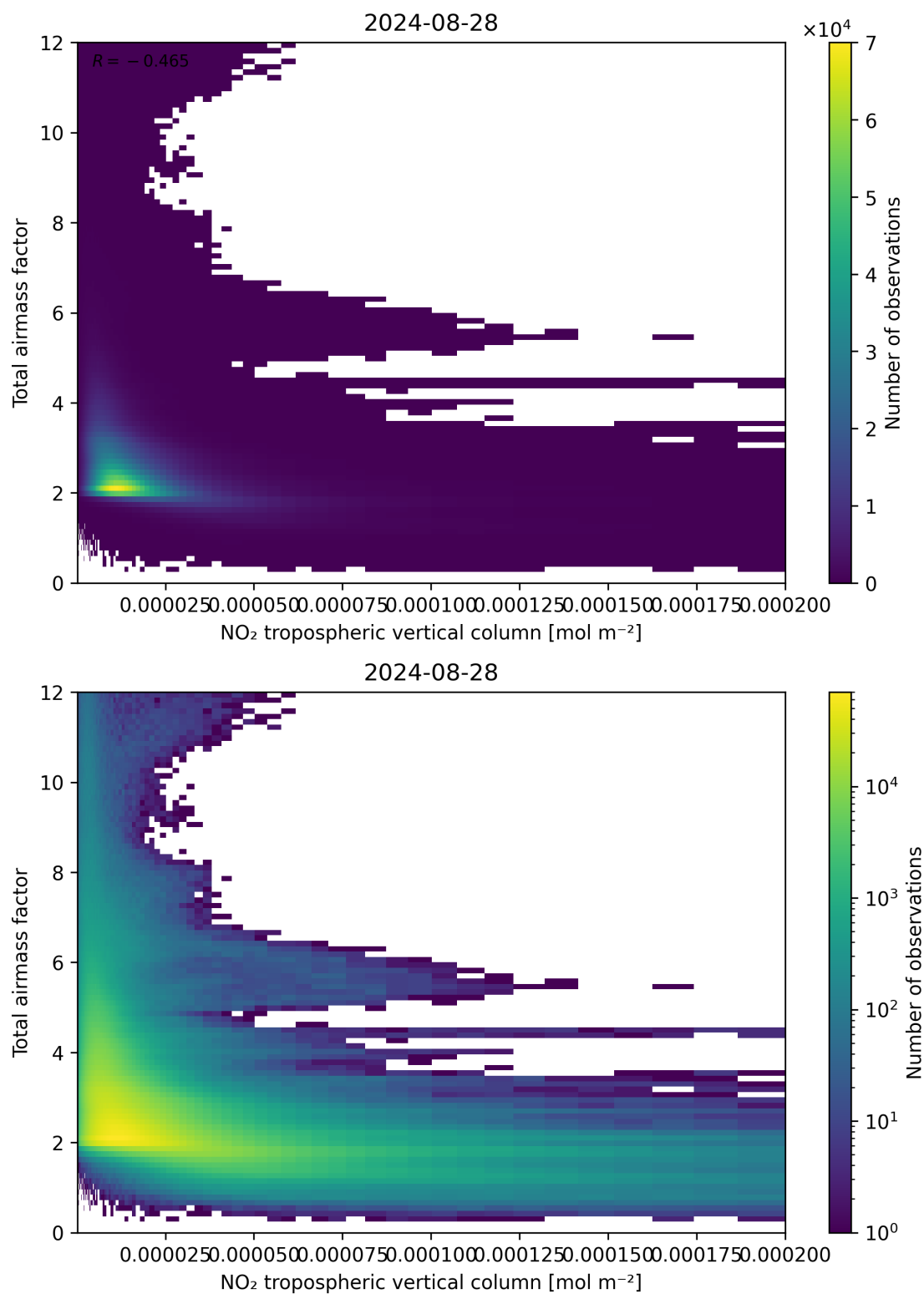
Figure 122: Scatter density plot of “NO 2 tropospheric vertical column” against “Total air mass factor” for 2024-08-27 to 2024-08-29.
