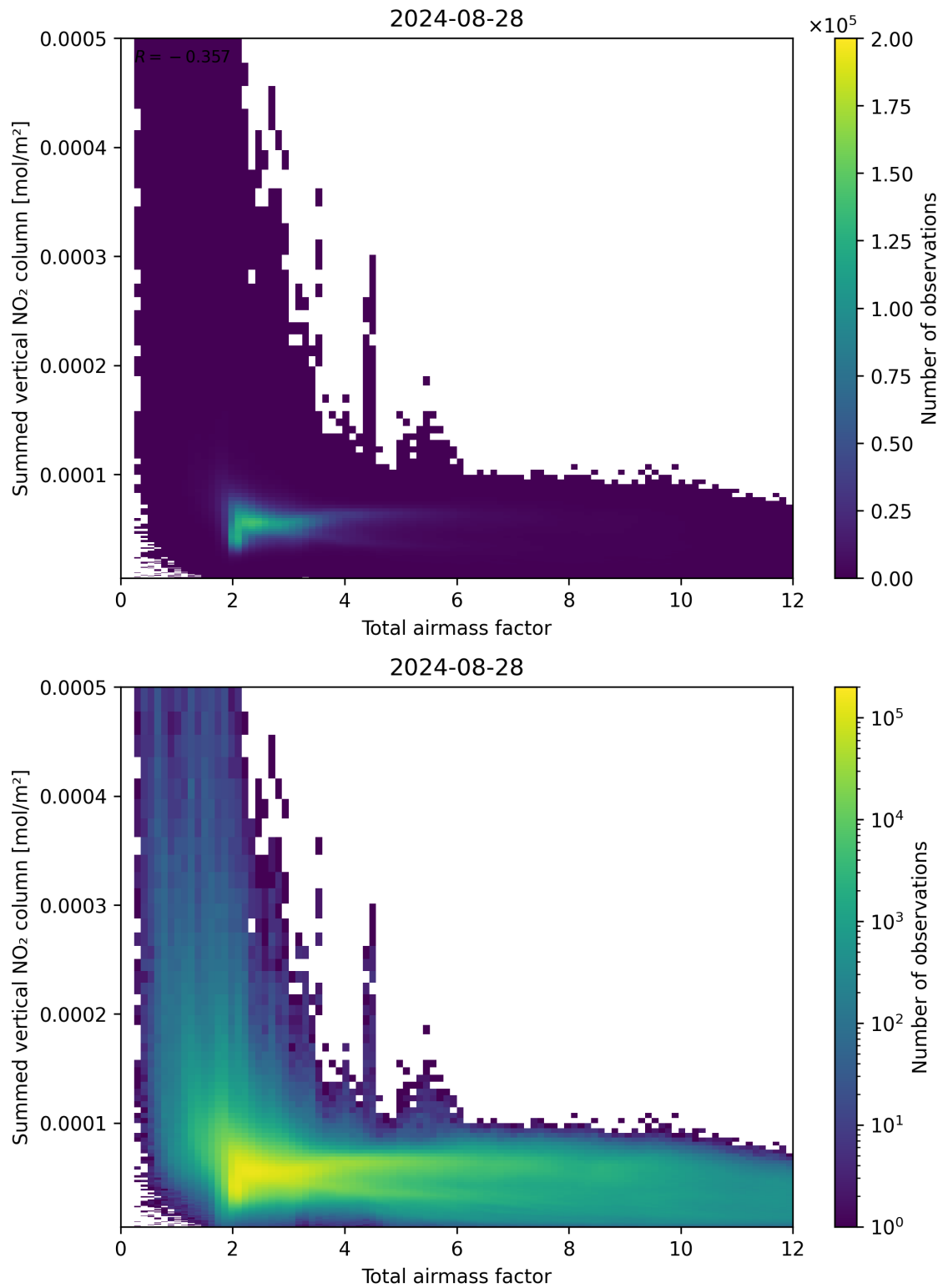
Figure 65: Scatter density plot of “Total airmass factor” against “Summed vertical NO 2 column” for 2024-08-27 to 2024-08-29.
