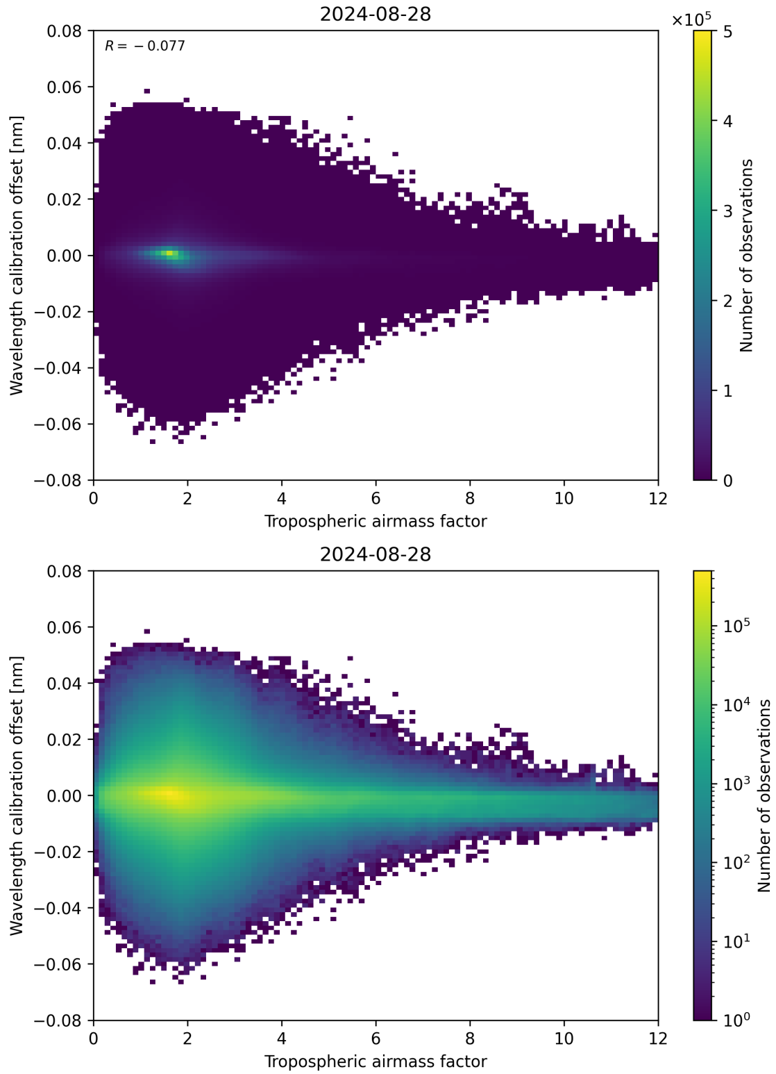
Figure 80: Scatter density plot of “Tropospheric airmass factor” against “Wavelength calibration offset” for 2024-08-27 to 2024-08-29.
