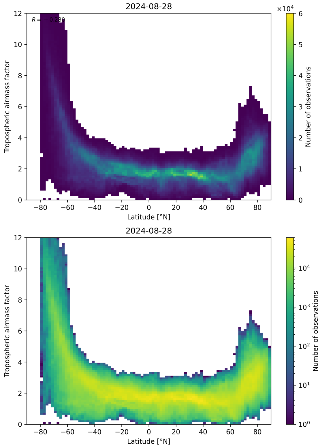
Figure 85: Scatter density plot of “Latitude” against “Tropospheric air mass factor” for 2024-08-27 to 2024-08-29.
