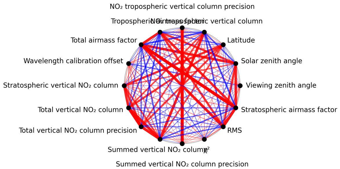
Figure 1: Map of correlation graph for 2024-08-27 to 2024-08-29.
