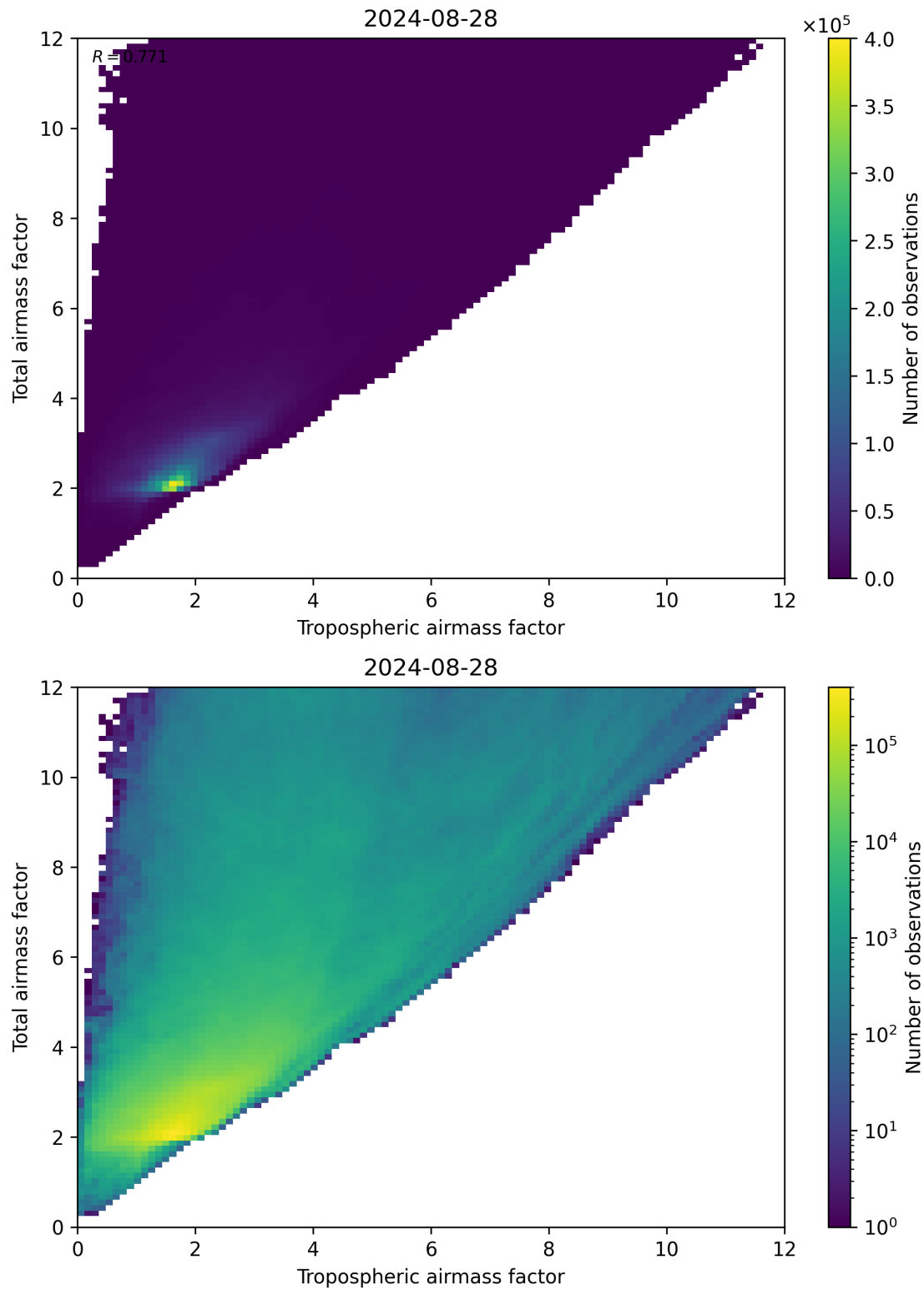
Figure 72: Scatter density plot of “Tropospheric airmass factor” against “Total airmass factor” for 2024-08-27 to 2024-08-29.
