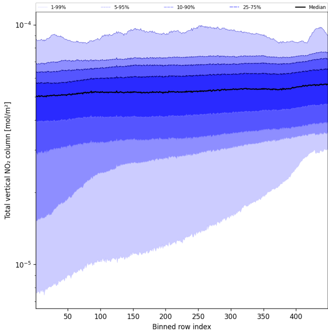
Figure 55: Along track statistics of “Total vertical NO 2 column” for 2024-08-27 to 2024-08-29
