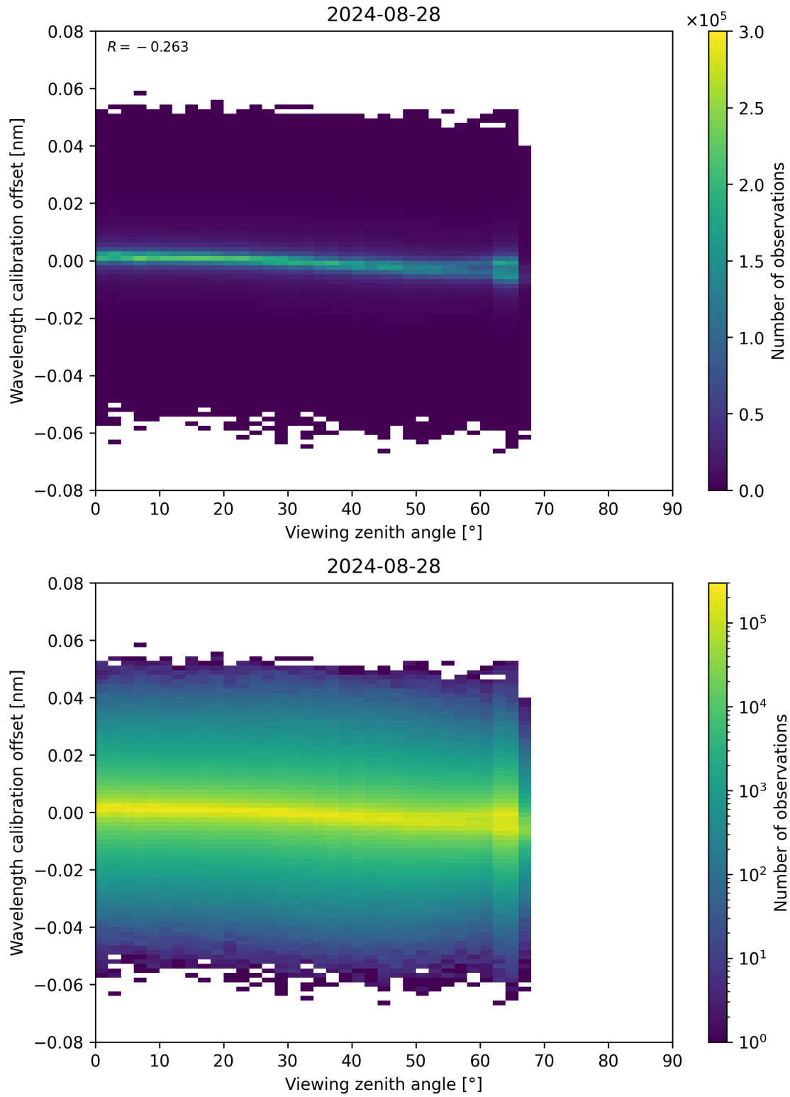
Figure 173: Scatter density plot of “Viewing zenith angle” against “Wavelength calibration offset” for 2024-08-27 to 2024-08-29.
