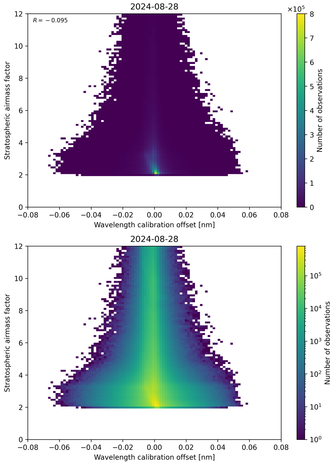
Figure 174: Scatter density plot of “Wavelength calibration offset” against “Stratospheric airmass factor” for 2024-08-27 to 2024-08-29.
