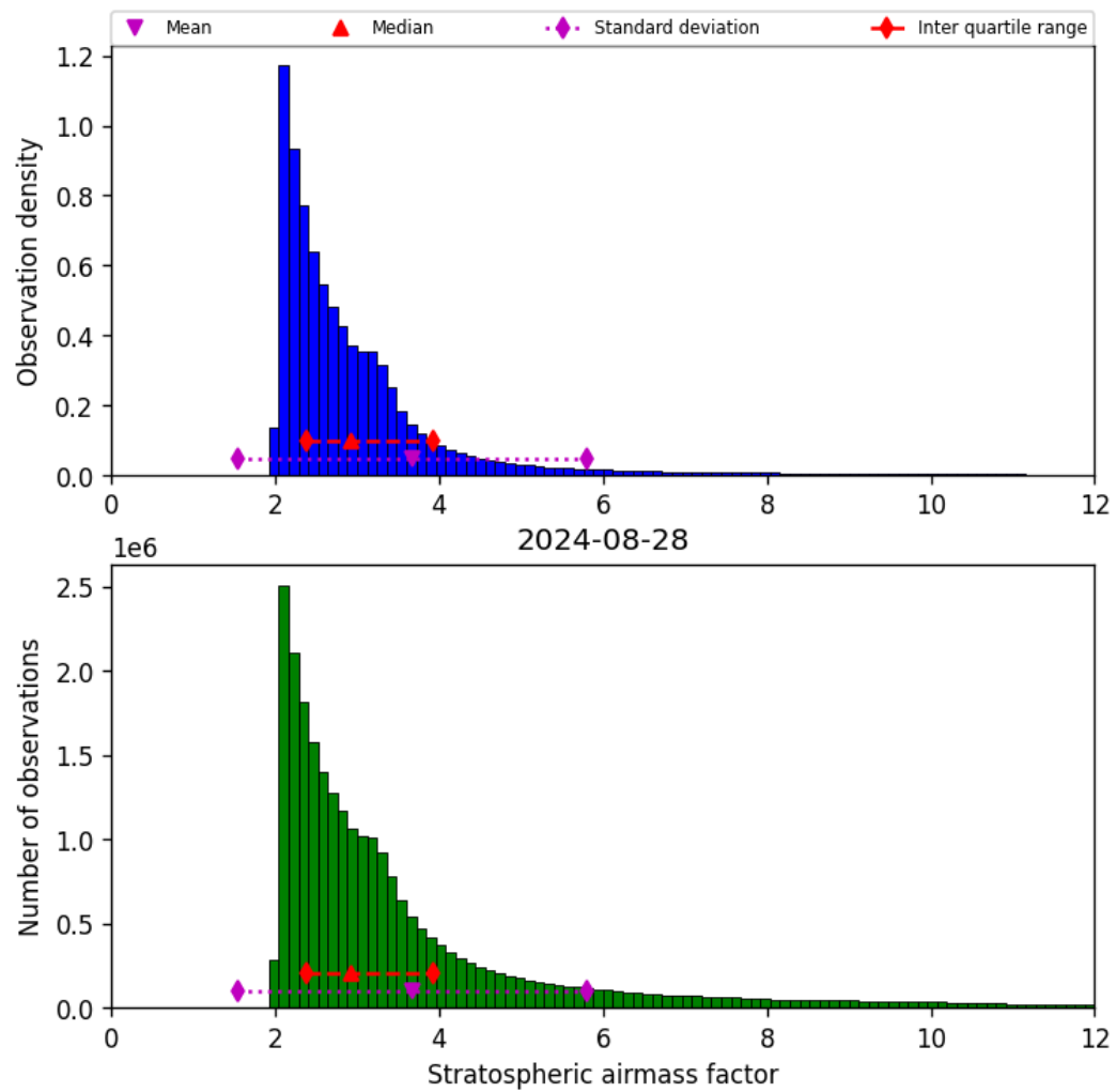
Figure 44: Histogram of “Stratospheric airmass factor” for 2024-08-27 to 2024-08-29
