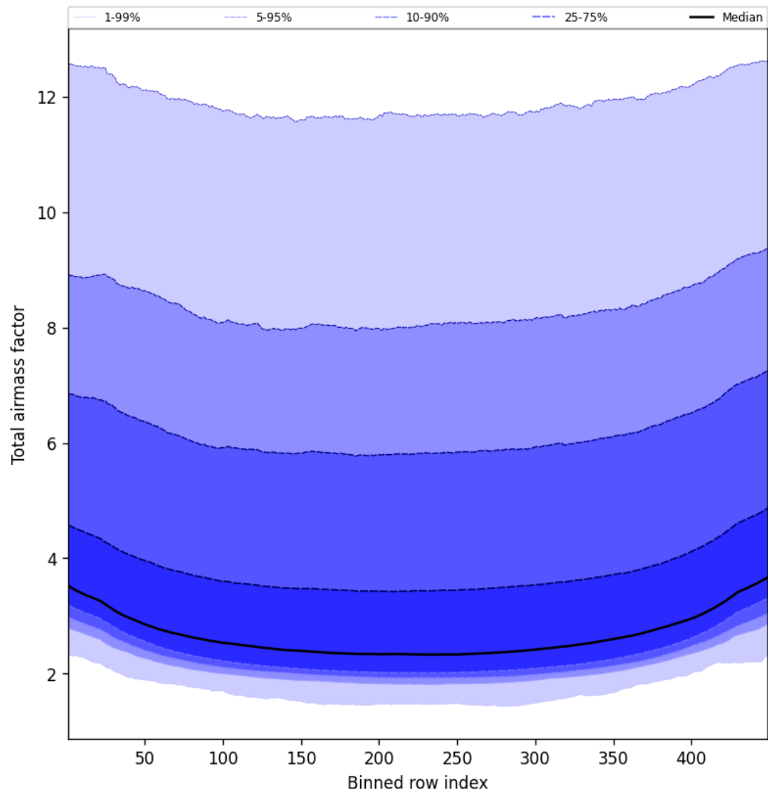
Figure 49: Along track statistics of “Total airmass factor” for 2024-08-27 to 2024-08-29
