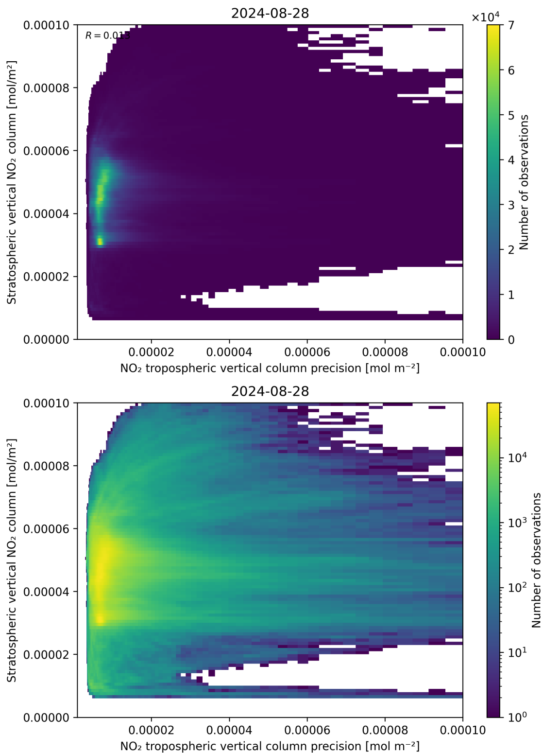
Figure 135: Scatter density plot of “NO 2 tropospheric vertical column precision” against “Stratospheric vertical NO 2 column” for 2024-08-27 to 2024-08-29.
