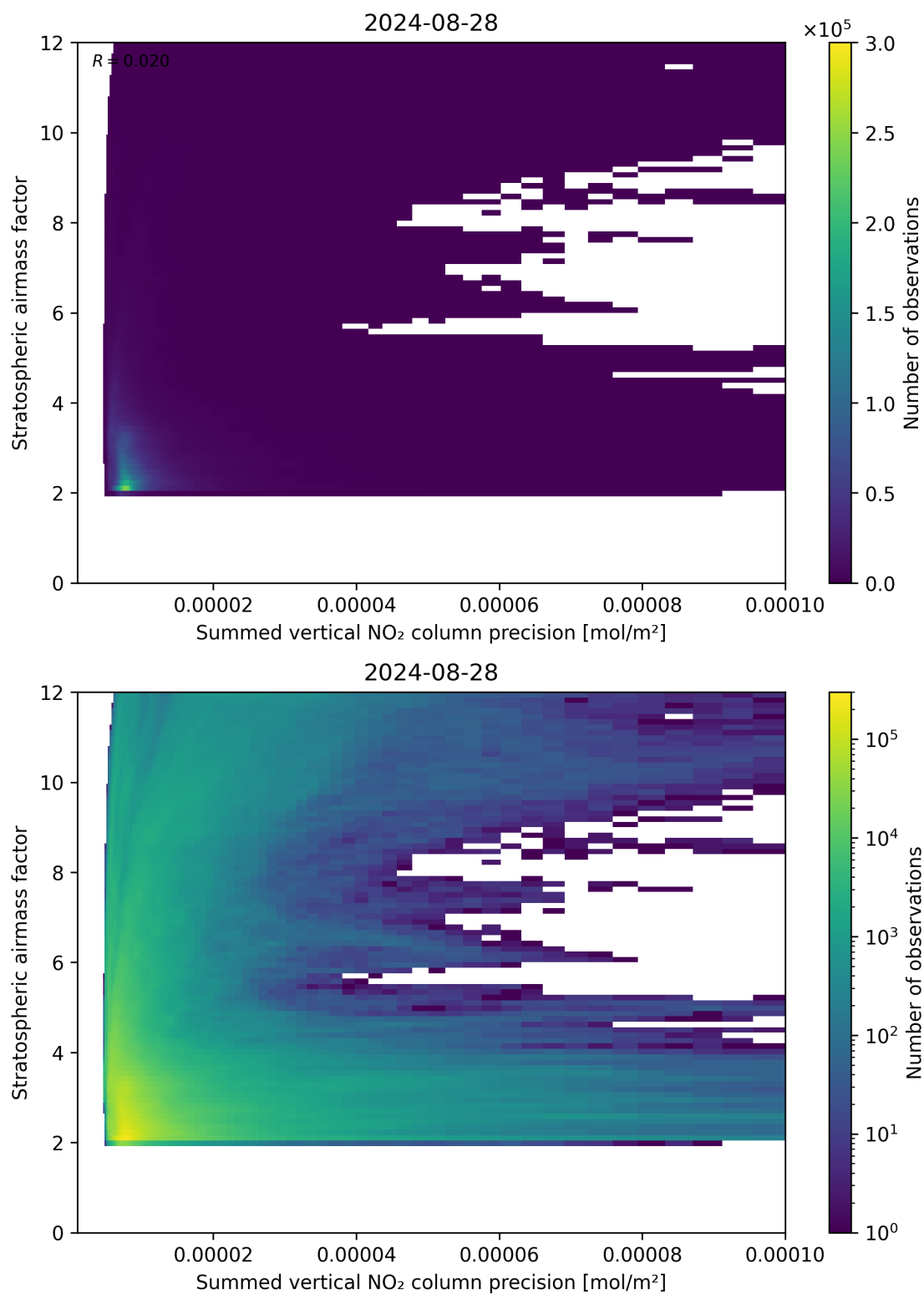
Figure 106: Scatter density plot of “Summed vertical NO 2 column precision” against “Stratospheric airmass factor” for 2024-08-27 to 2024-08-29.
