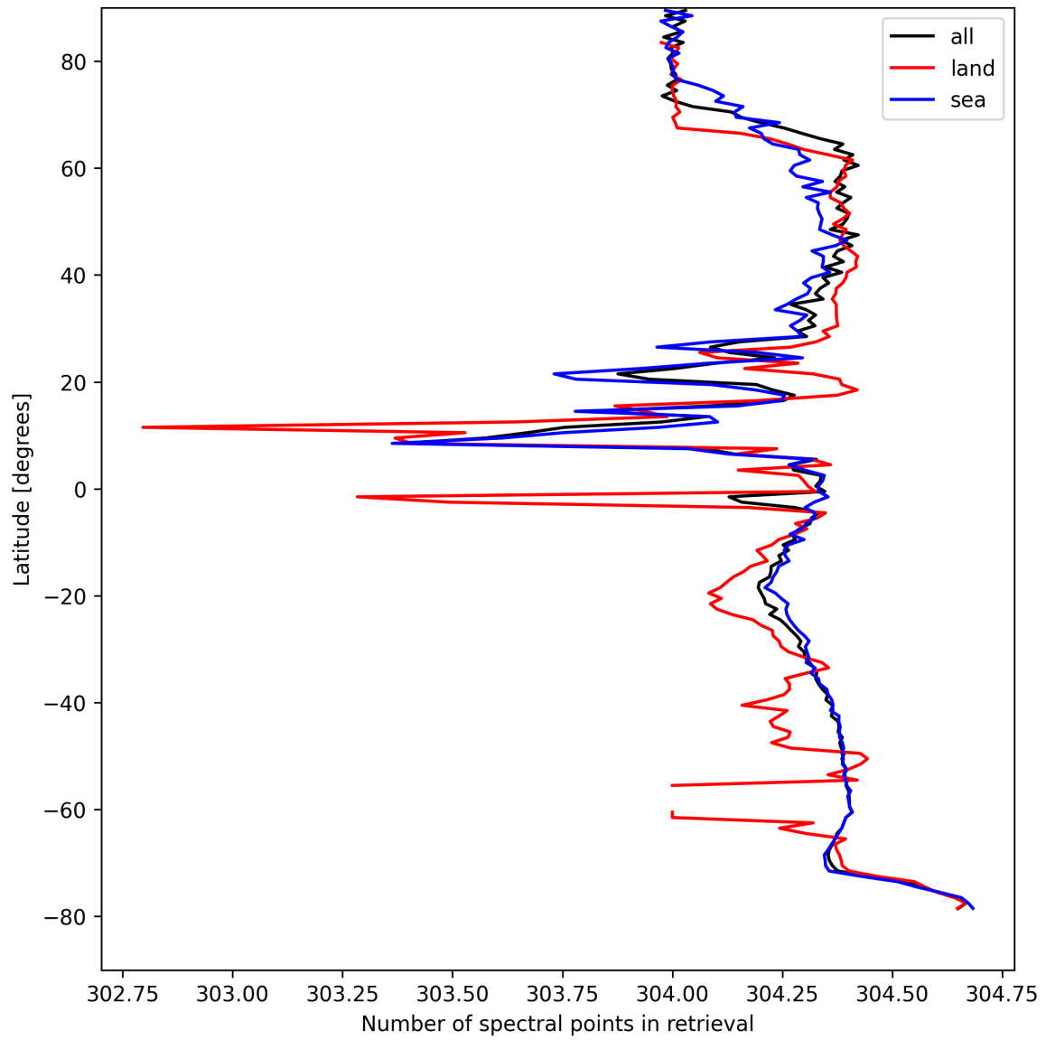
Figure 16: Zonal average of “Number of spectral points in retrieval” for 2024-08-27 to 2024-08-29.
