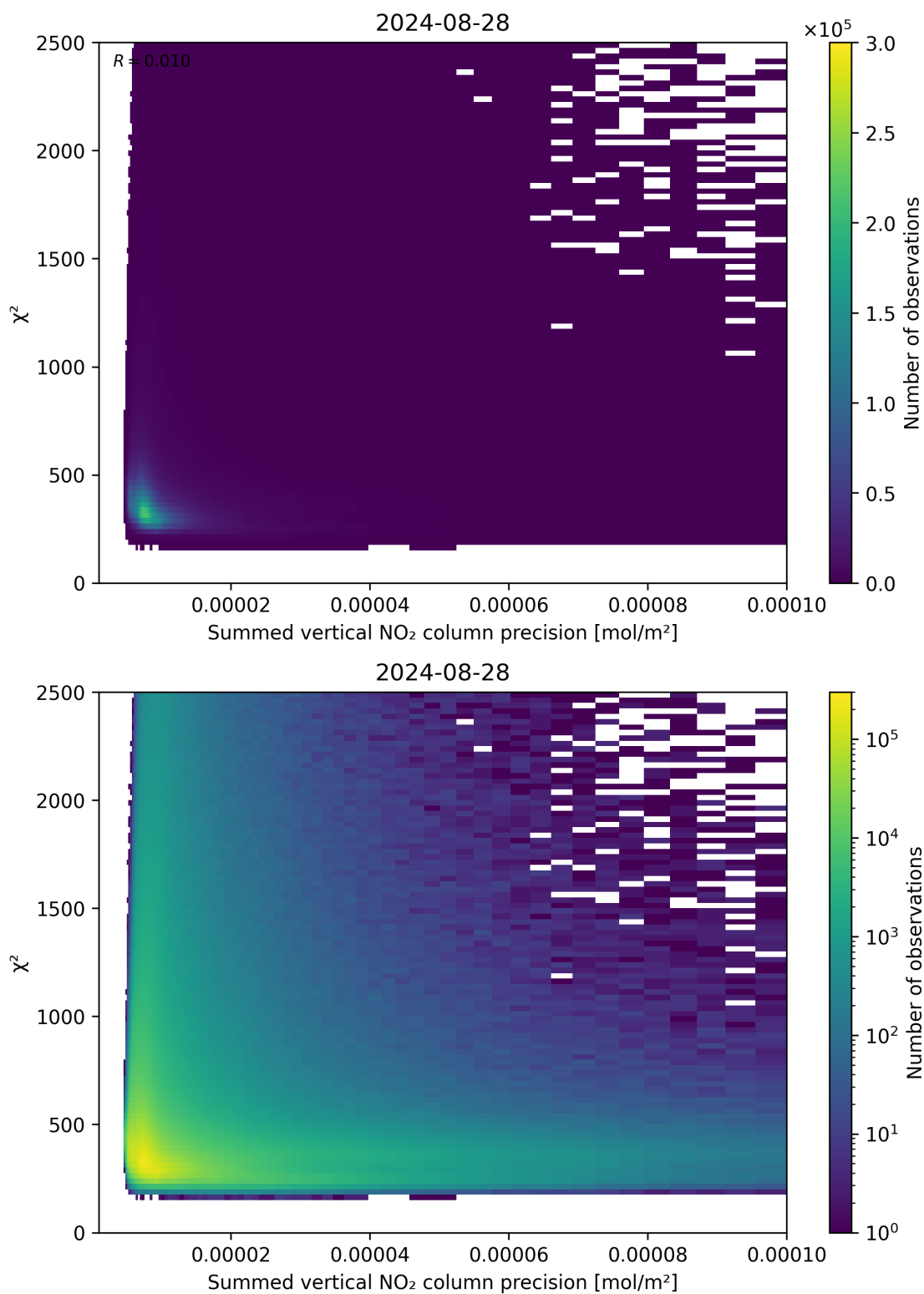
Figure 107: Scatter density plot of “Summed vertical NO 2 column precision” against “ \chi^2 ” for 2024-08-27 to 2024-08-29.
