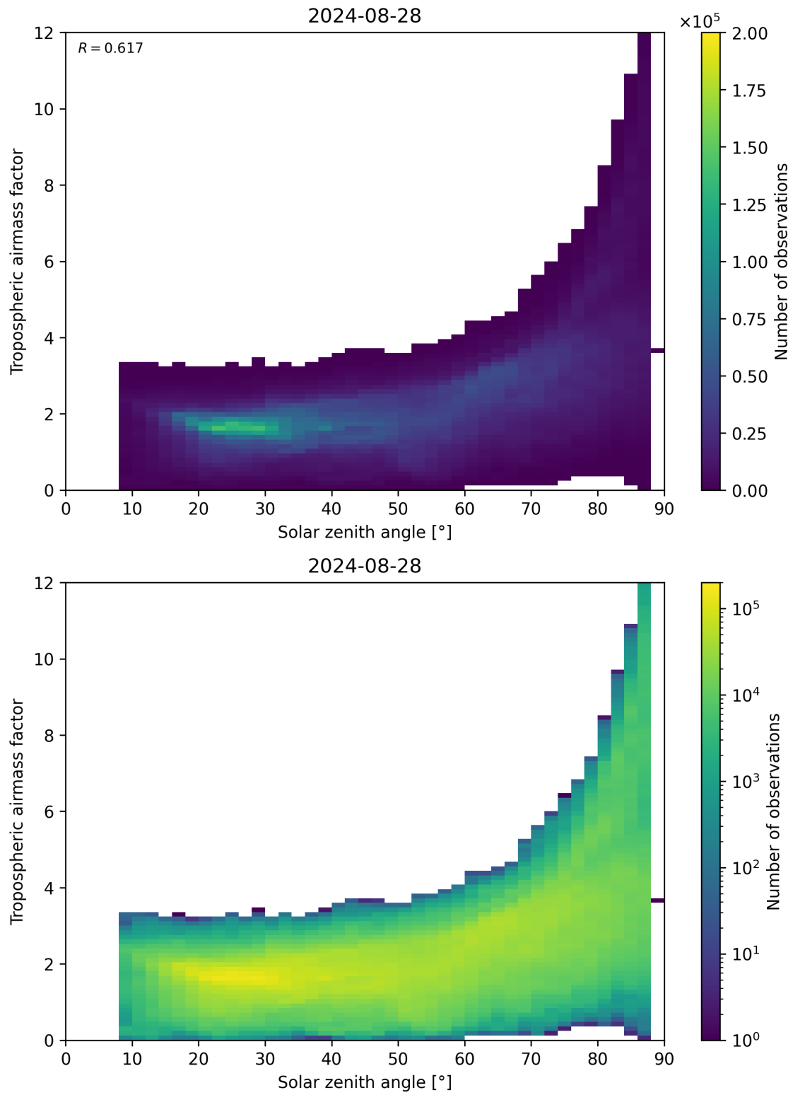
Figure 147: Scatter density plot of “Solar zenith angle” against “Tropospheric airmass factor” for 2024-08-27 to 2024-08-29.
