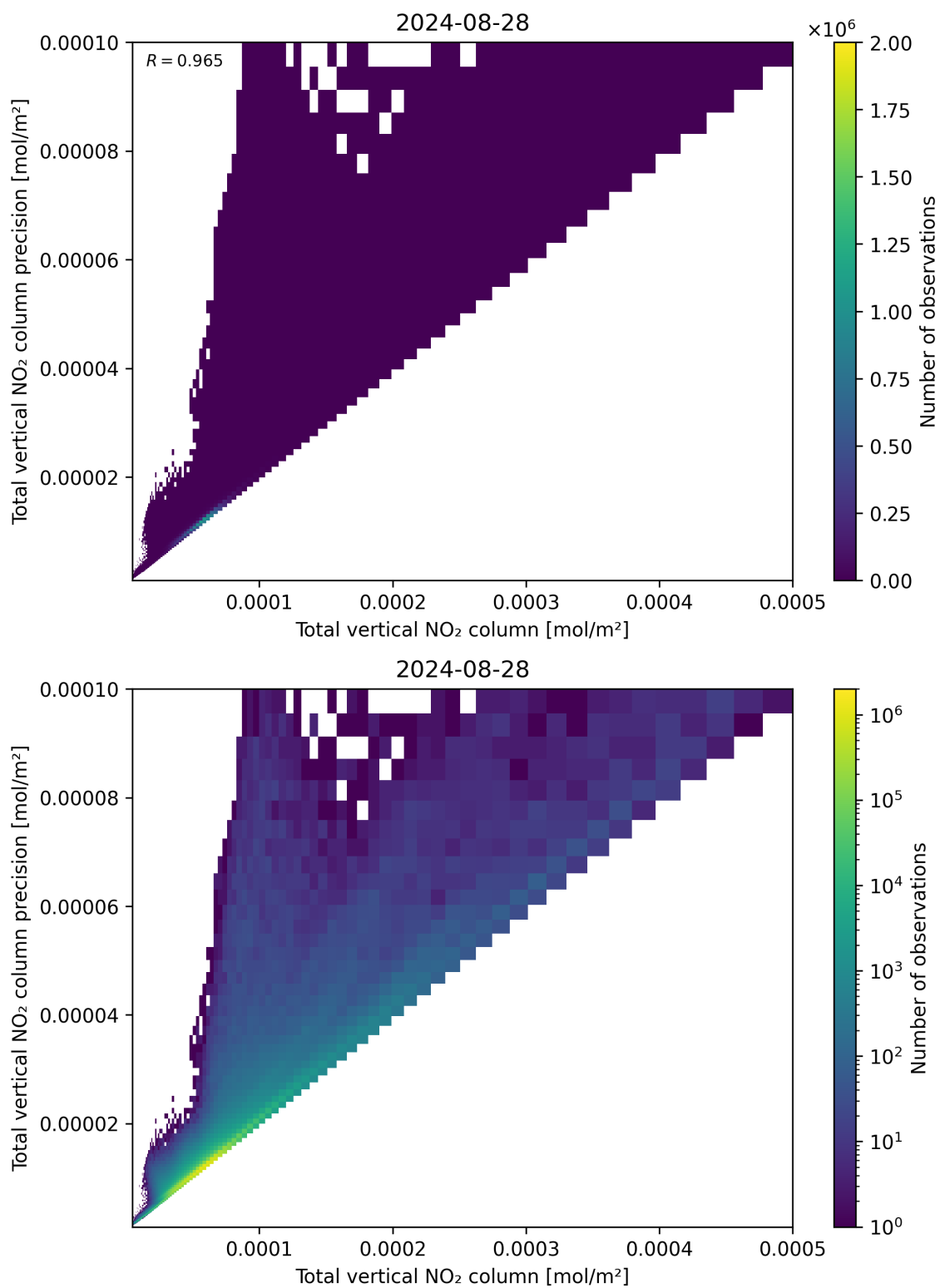
Figure 114: Scatter density plot of “Total vertical NO 2 column” against “Total vertical NO 2 column precision” for 2024-08-27 to 2024-08-29.
