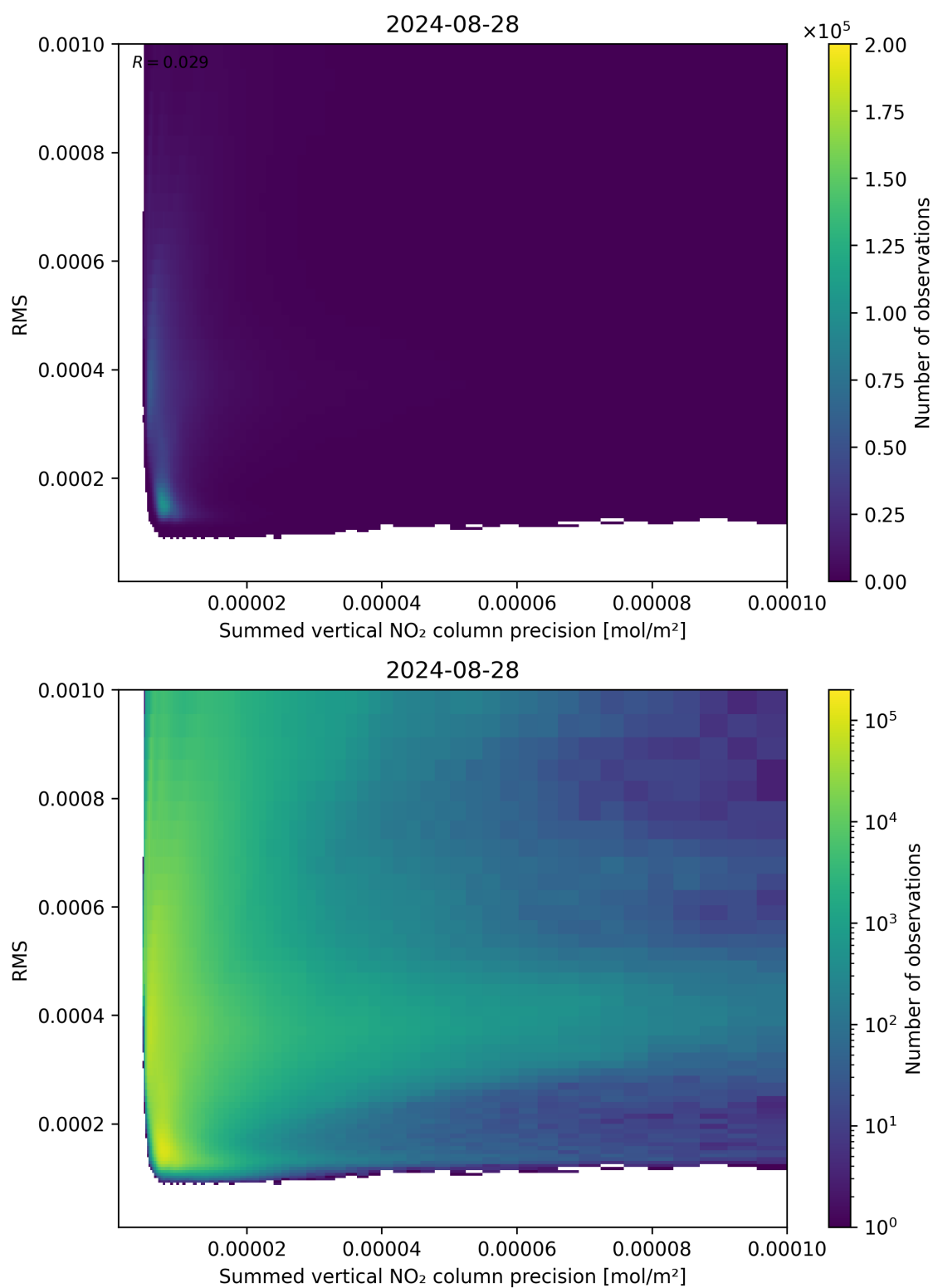
Figure 108: Scatter density plot of “Summed vertical NO 2 column precision” against “RMS” for 2024-08-27 to 2024-08-29.
