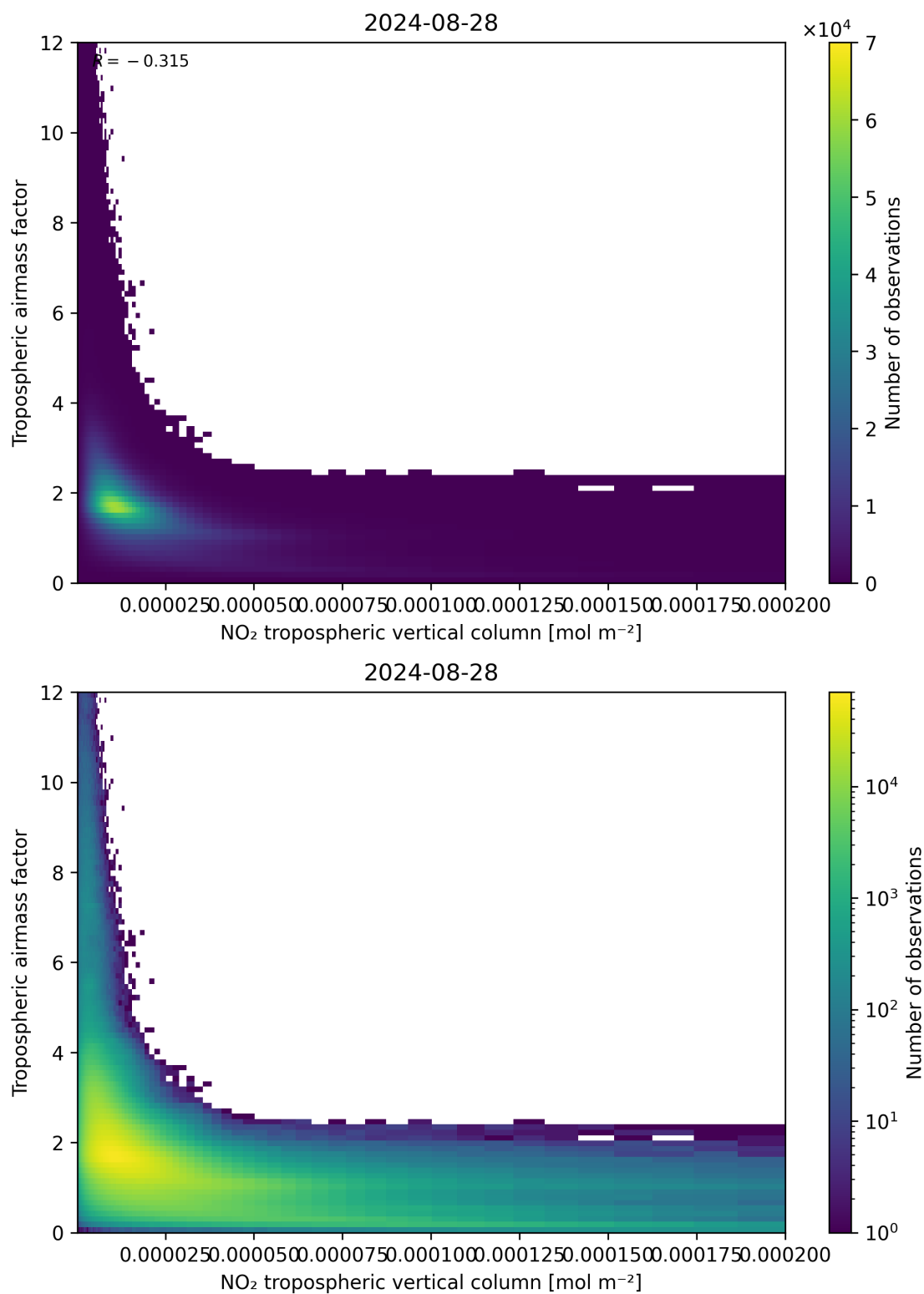
Figure 123: Scatter density plot of “NO 2 tropospheric vertical column” against “Tropospheric air mass factor” for 2024-08-27 to 2024-08-29.
