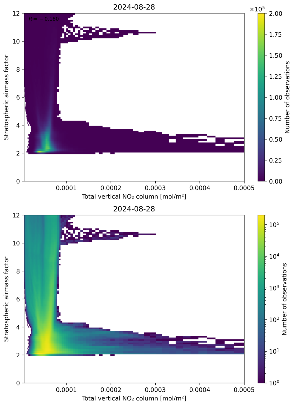
Figure 110: Scatter density plot of “Total vertical NO 2 column” against “Stratospheric airmass factor” for 2024-08-27 to 2024-08-29.
