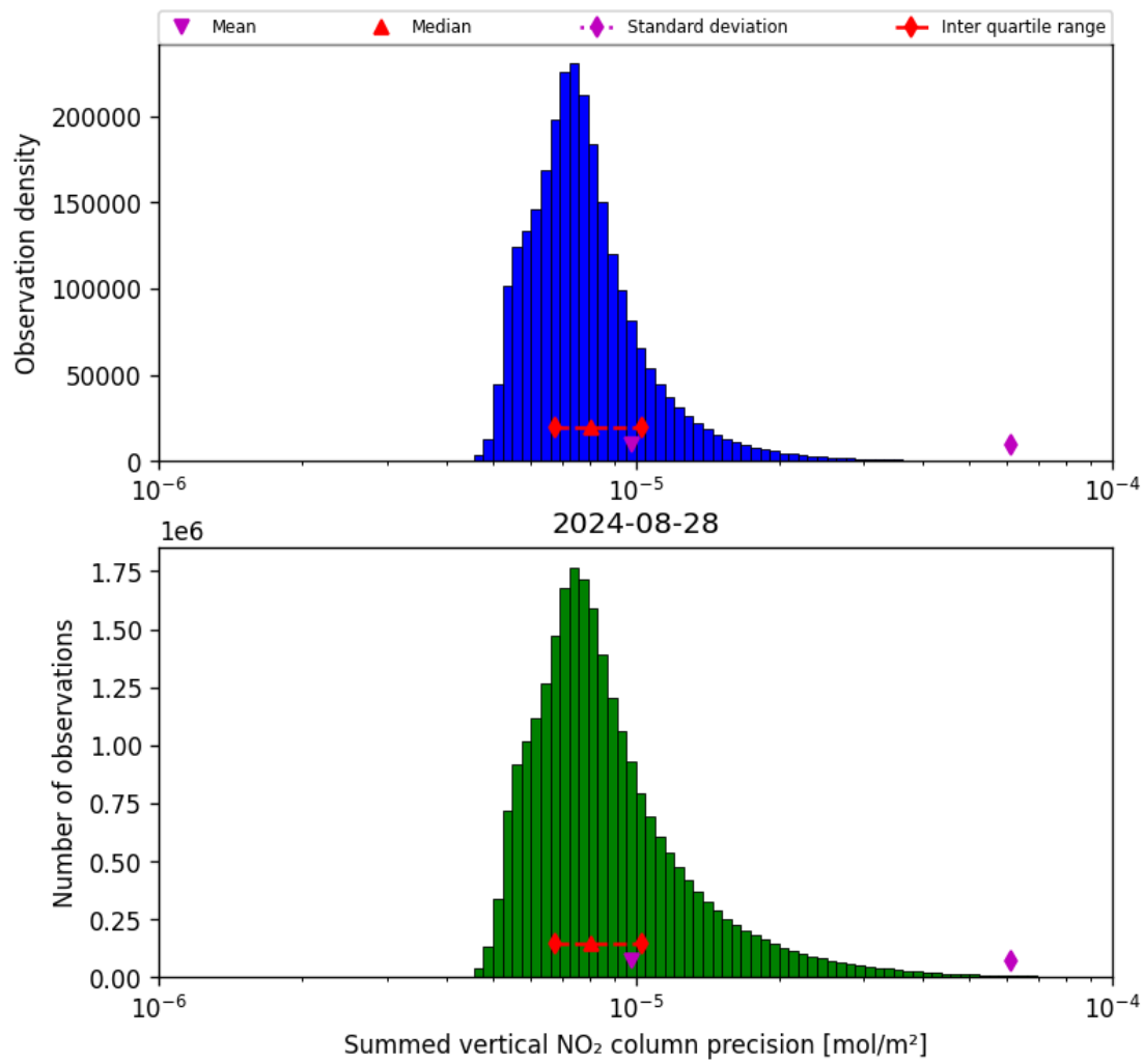
Figure 41: Histogram of “Summed vertical NO 2 column precision” for 2024-08-27 to 2024-08-29
