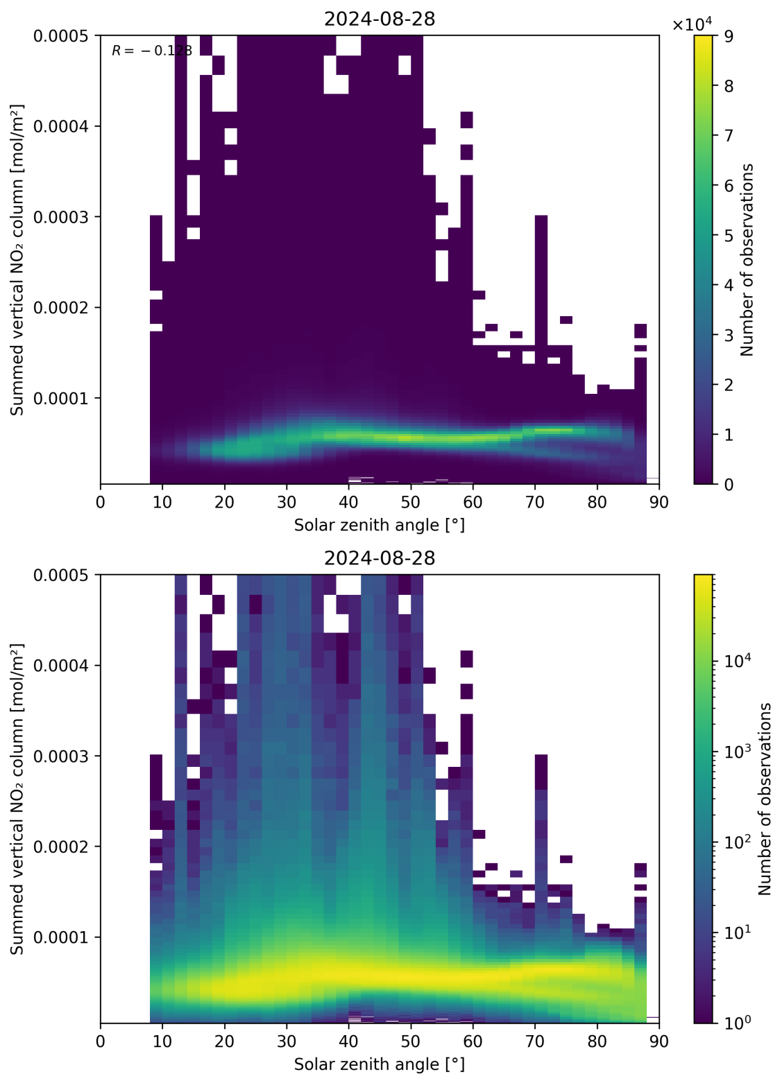
Figure 151: Scatter density plot of “Solar zenith angle” against “Summed vertical NO 2 column” for 2024-08-27 to 2024-08-29.
