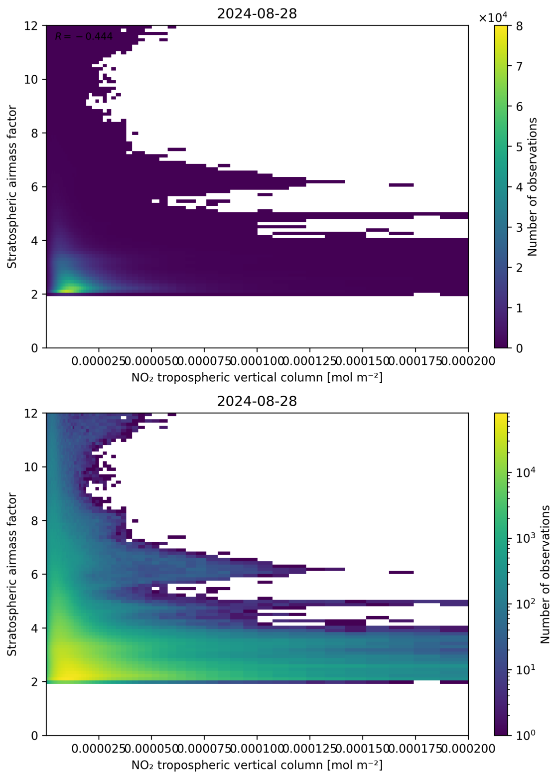
Figure 121: Scatter density plot of “NO 2 tropospheric vertical column” against “Stratospheric air mass factor” for 2024-08-27 to 2024-08-29.
