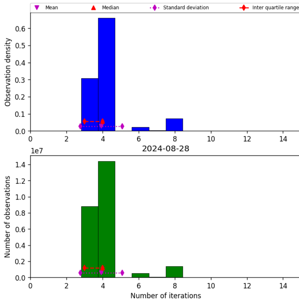
Figure 34: Histogram of “Number of iterations” for 2024-08-27 to 2024-08-29
