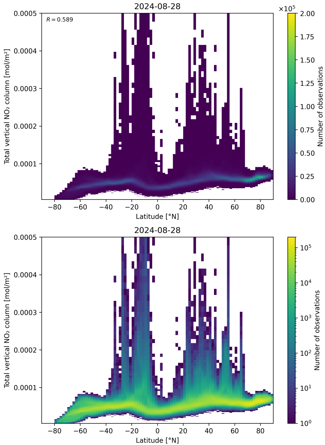
Figure 90: Scatter density plot of “Latitude” against “Total vertical NO 2 column” for 2024-08-27 to 2024-08-29.
