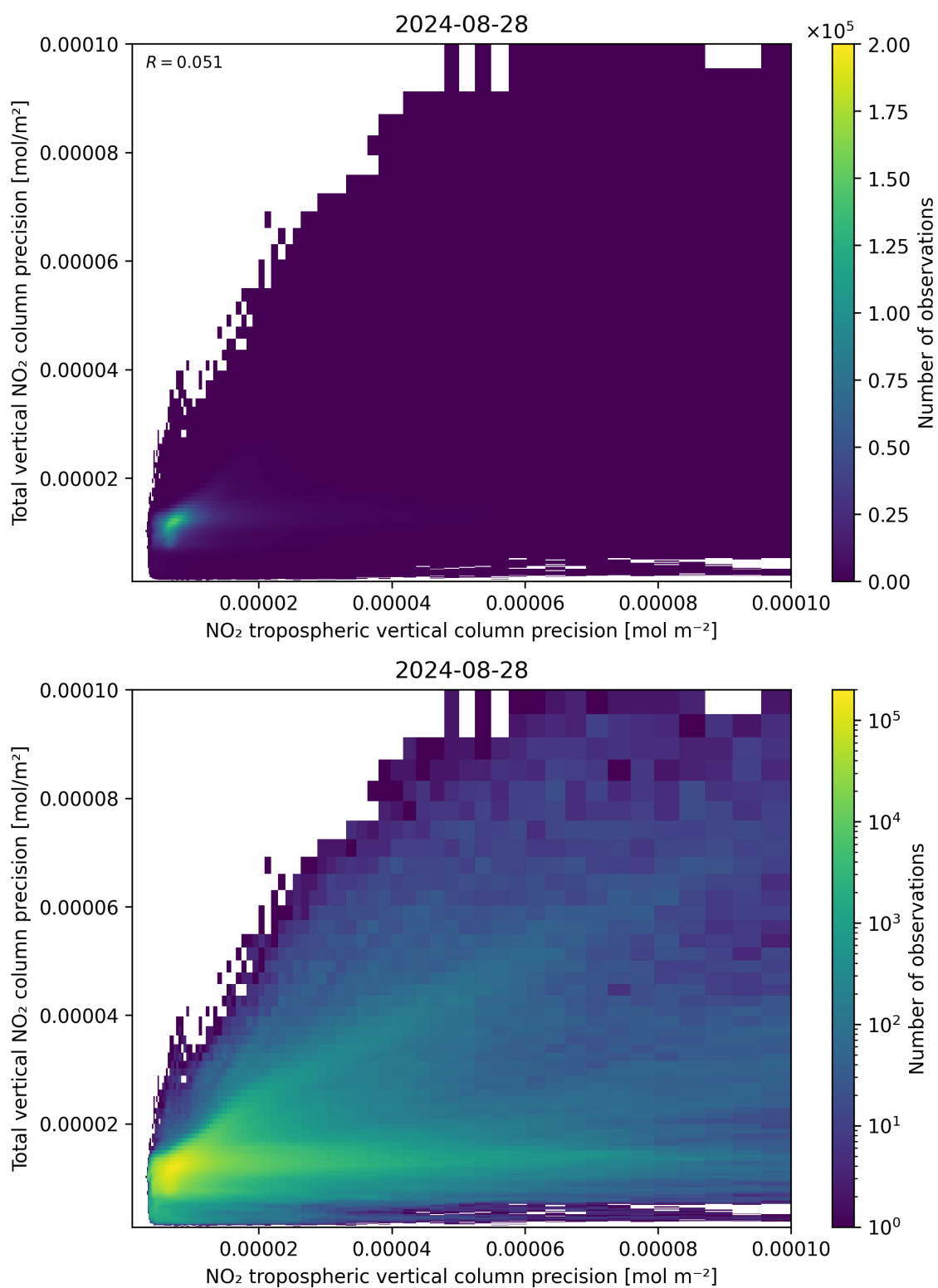
Figure 139: Scatter density plot of “NO 2 tropospheric vertical column precision” against “Total vertical NO 2 column precision” for 2024-08-27 to 2024-08-29.
