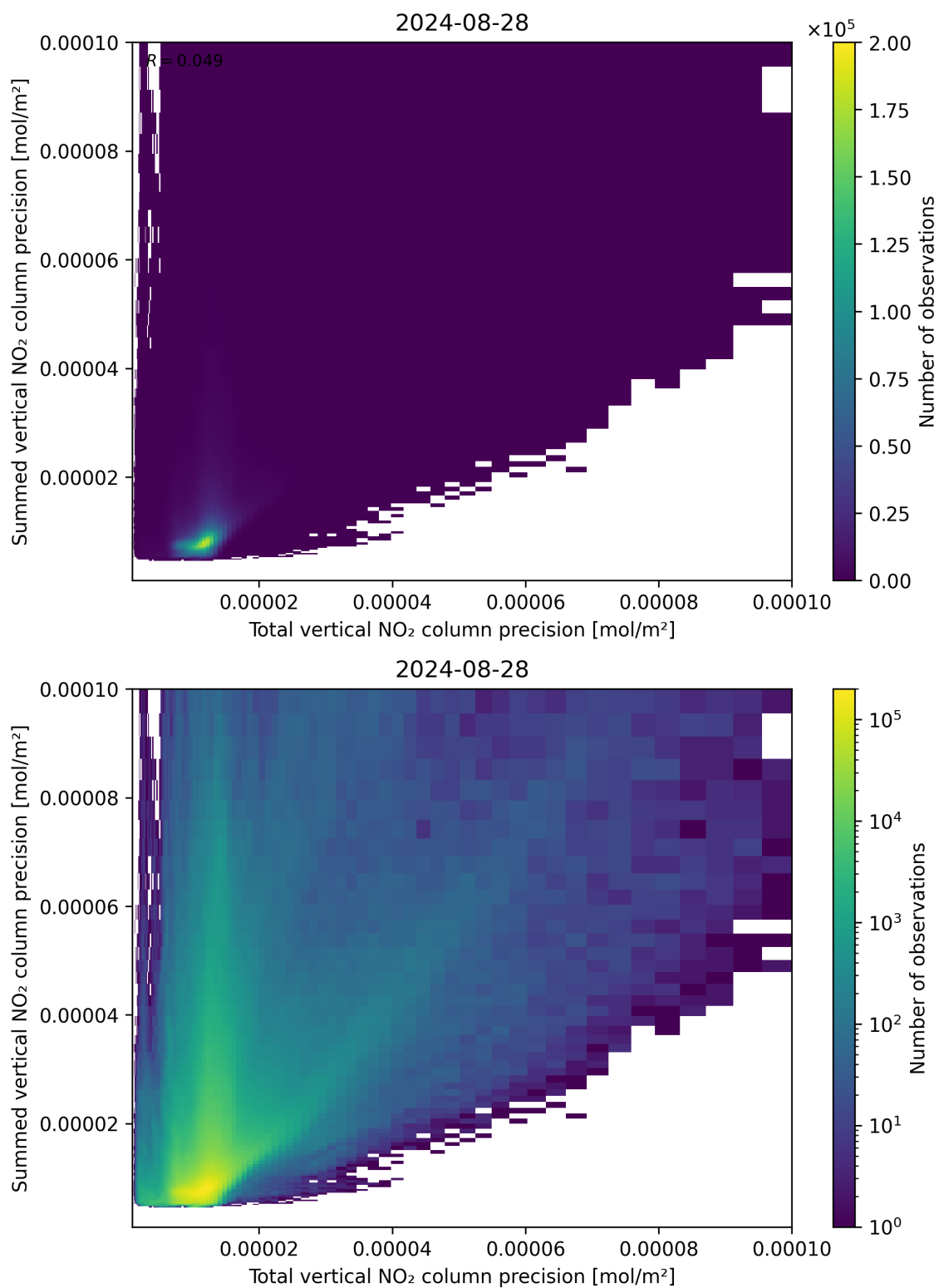
Figure 118: Scatter density plot of “Total vertical NO 2 column precision” against “Summed vertical NO 2 column precision” for 2024-08-27 to 2024-08-29.
