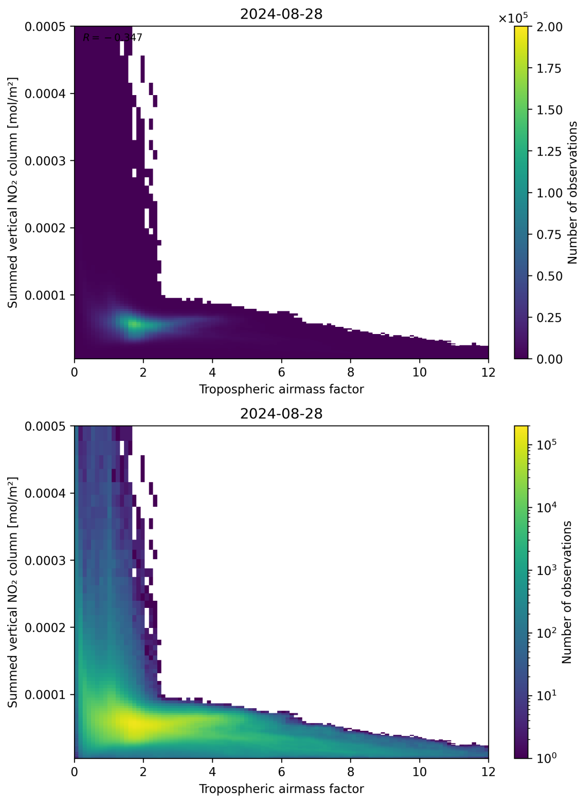
Figure 75: Scatter density plot of “Tropospheric air mass factor” against “Summed vertical NO 2 column” for 2024-08-27 to 2024-08-29.
