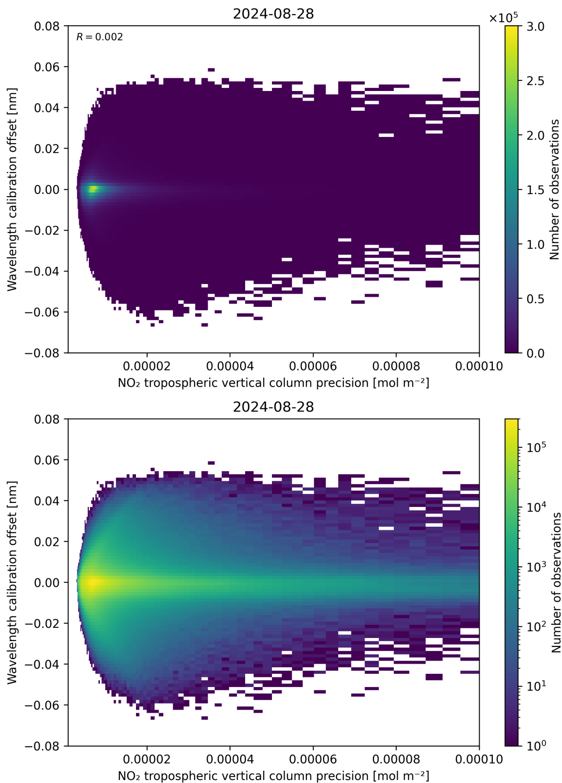
Figure 141: Scatter density plot of “NO 2 tropospheric vertical column precision” against “Wavelength calibration offset” for 2024-08-27 to 2024-08-29.
