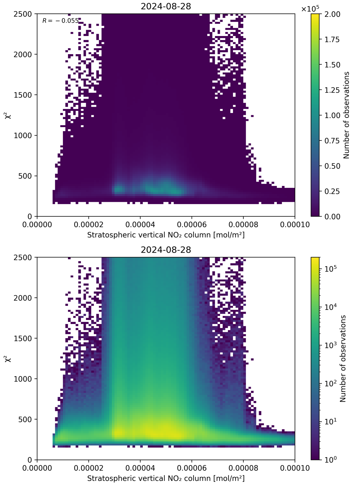
Figure 97: Scatter density plot of “Stratospheric vertical NO 2 column” against “ \chi^2 ” for 2024-08-27 to 2024-08-29.
