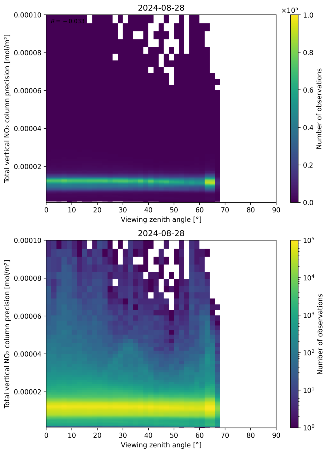
Figure 168: Scatter density plot of “Viewing zenith angle” against “Total vertical NO 2 column precision” for 2024-08-27 to 2024-08-29.
