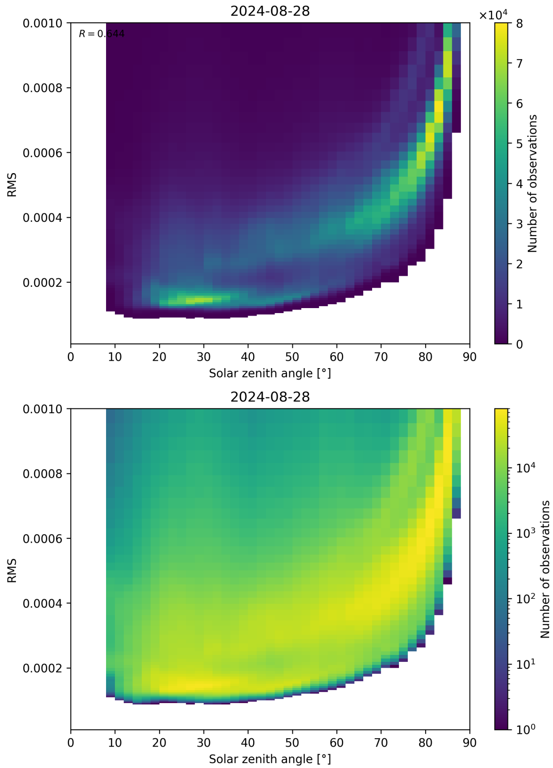
Figure 157: Scatter density plot of “Solar zenith angle” against “RMS” for 2024-08-27 to 2024-08-29.
