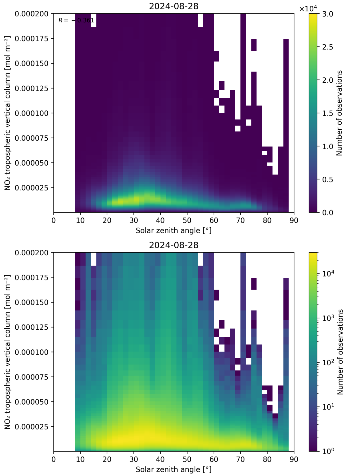
Figure 155: Scatter density plot of “Solar zenith angle” against “NO 2 tropospheric vertical column” for 2024-08-27 to 2024-08-29.
