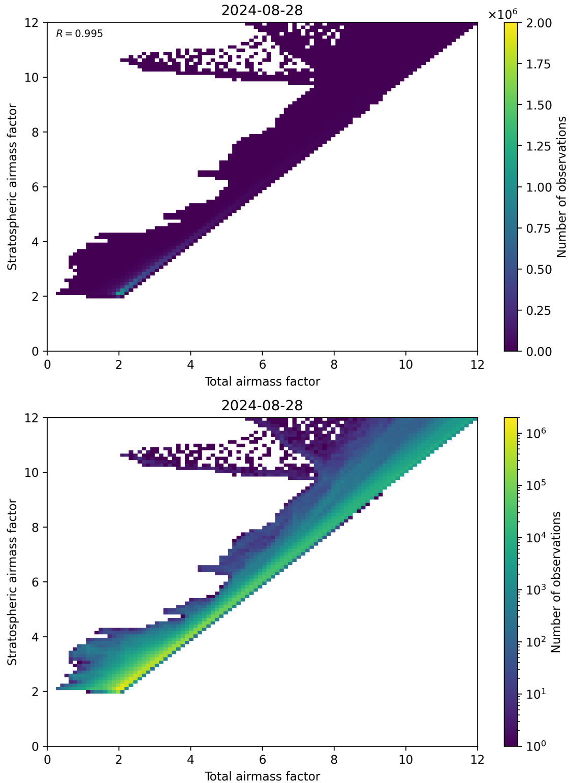
Figure 62: Scatter density plot of “Total airmass factor” against “Stratospheric airmass factor” for 2024-08-27 to 2024-08-29.
