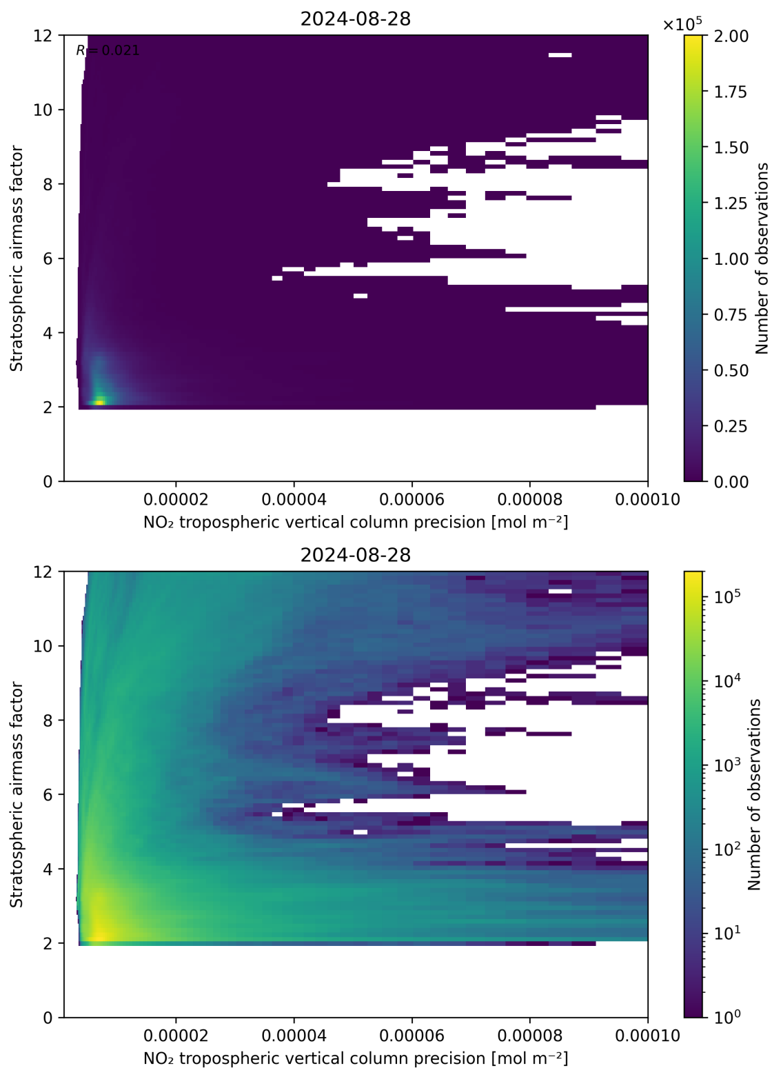
Figure 131: Scatter density plot of “NO 2 tropospheric vertical column precision” against “Stratospheric airmass factor” for 2024-08-27 to 2024-08-29.
