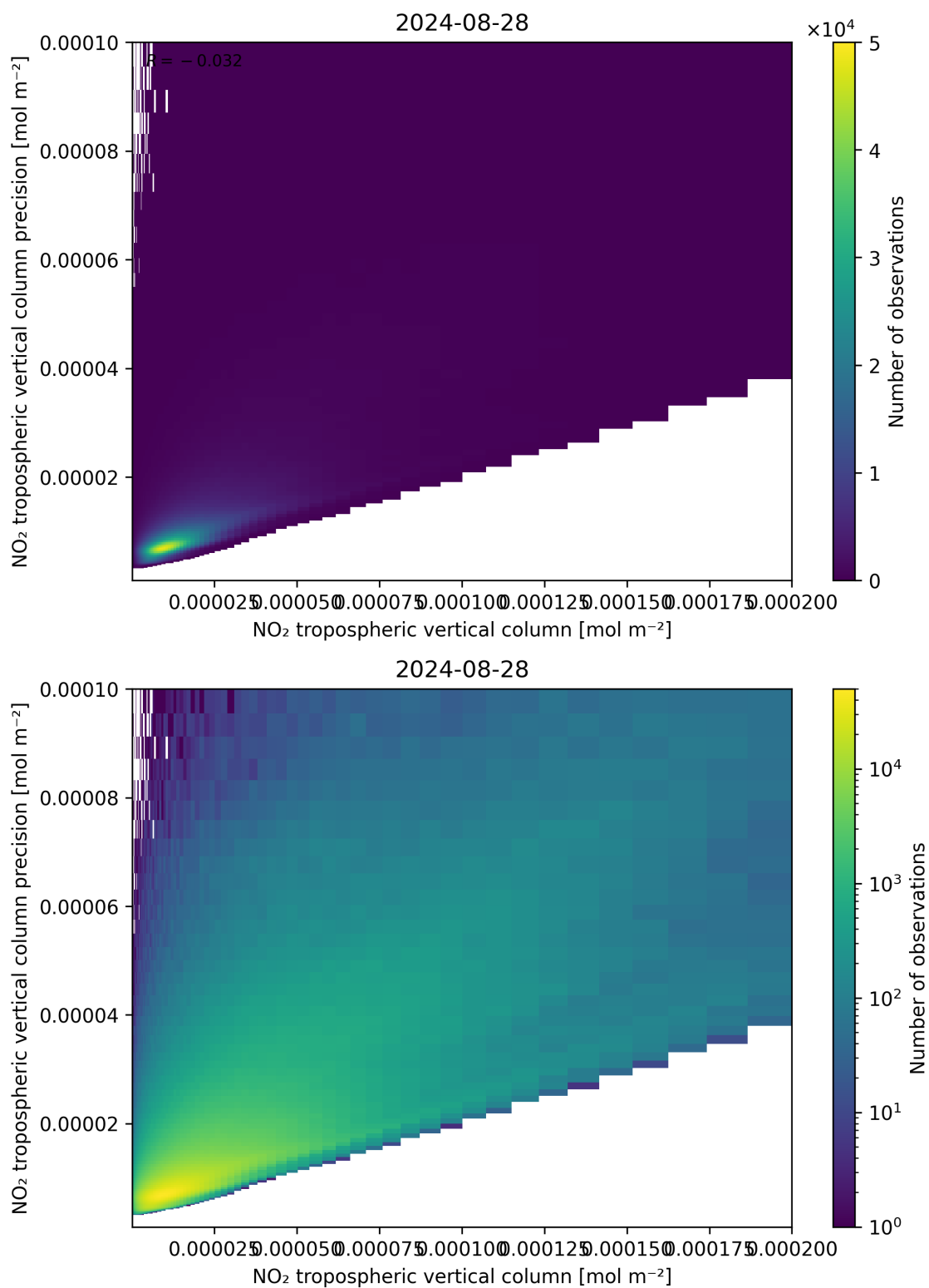
Figure 130: Scatter density plot of “NO 2 tropospheric vertical column” against “NO 2 tropospheric vertical column precision” for 2024-08-27 to 2024-08-29.
