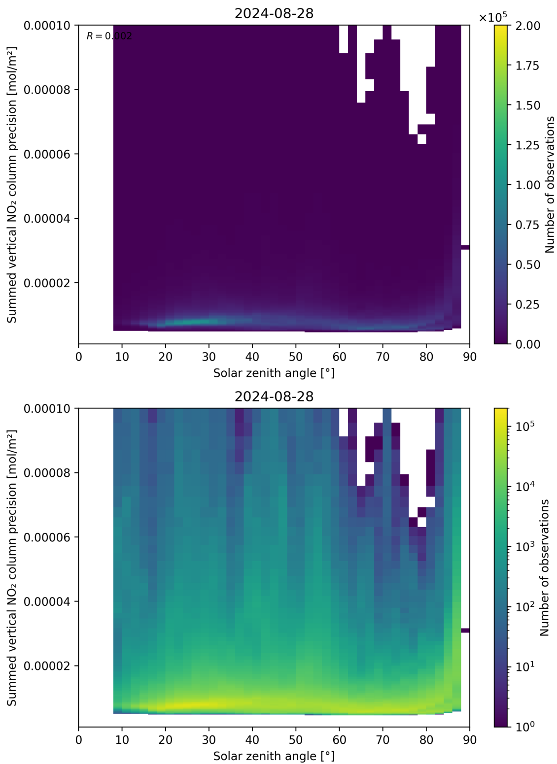
Figure 152: Scatter density plot of “Solar zenith angle” against “Summed vertical NO 2 column precision” for 2024-08-27 to 2024-08-29.
