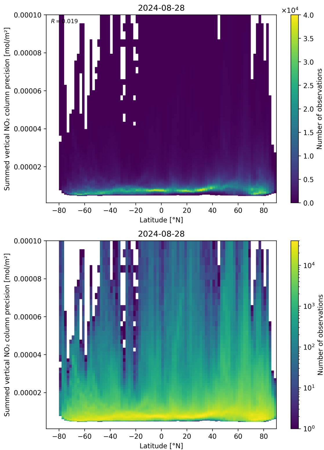
Figure 89: Scatter density plot of “Latitude” against “Summed vertical NO 2 column precision” for 2024-08-27 to 2024-08-29.
