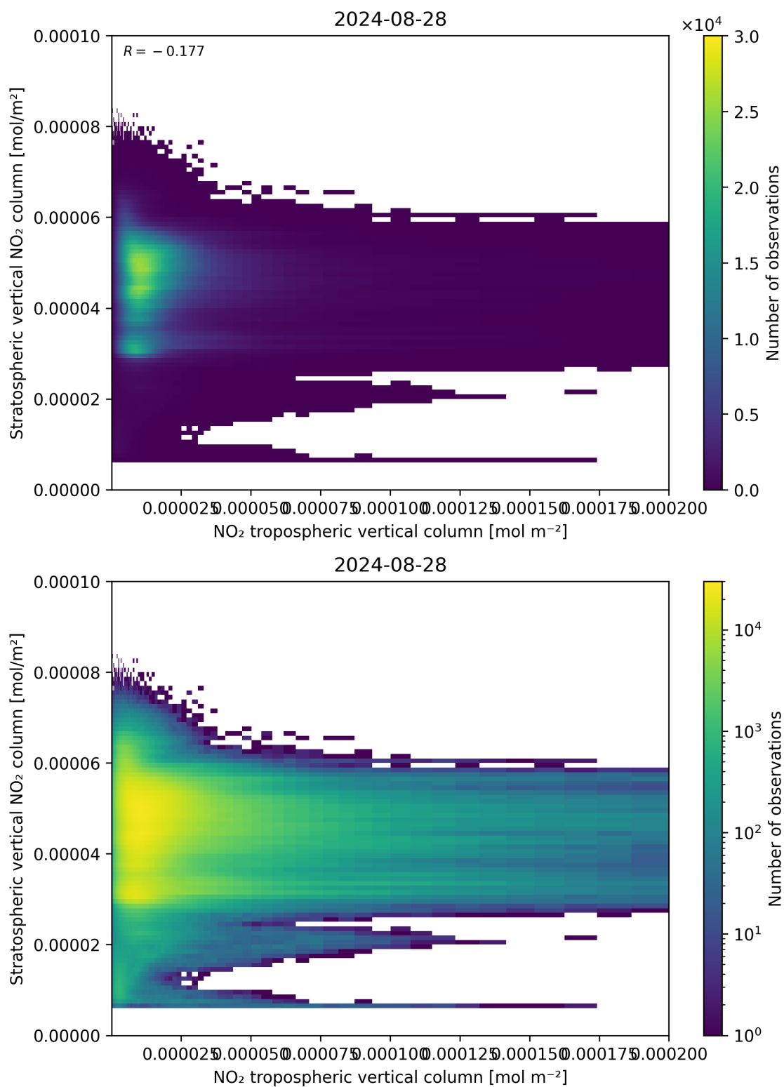
Figure 125: Scatter density plot of “NO 2 tropospheric vertical column” against “Stratospheric vertical NO 2 column” for 2024-08-27 to 2024-08-29.
