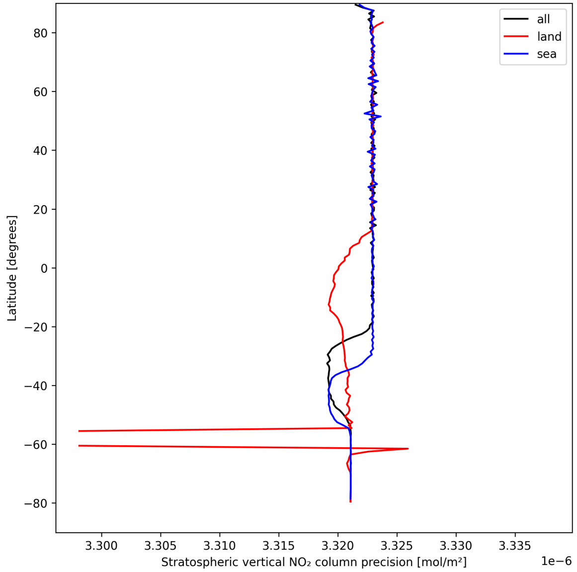
Figure 20: Zonal average of “Stratospheric vertical NO 2 column precision” for 2024-08-28 to 2024-08-30.
