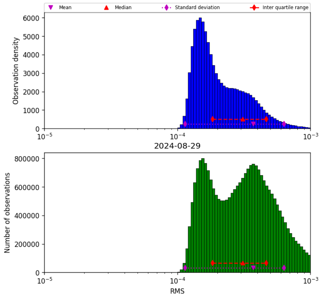
Figure 43: Histogram of “RMS” for 2024-08-28 to 2024-08-30
