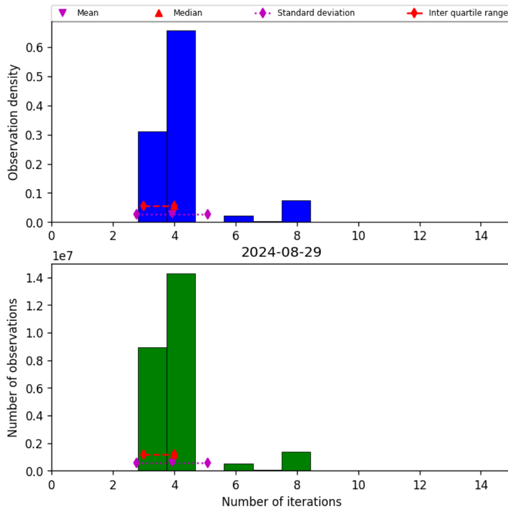
Figure 34: Histogram of “Number of iterations” for 2024-08-28 to 2024-08-30
