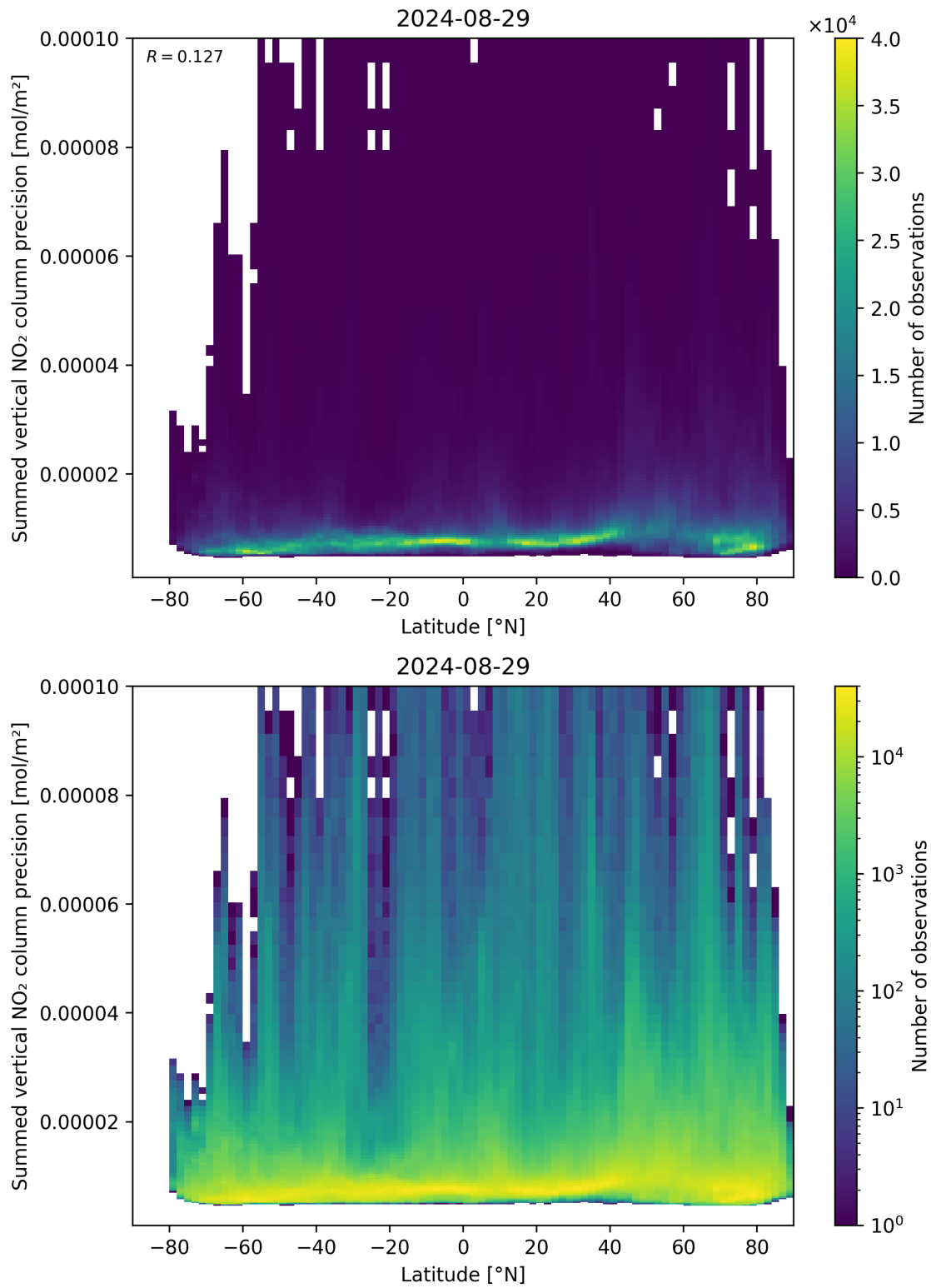
Figure 89: Scatter density plot of “Latitude” against “Summed vertical NO 2 column precision” for 2024-08-28 to 2024-08-30.
