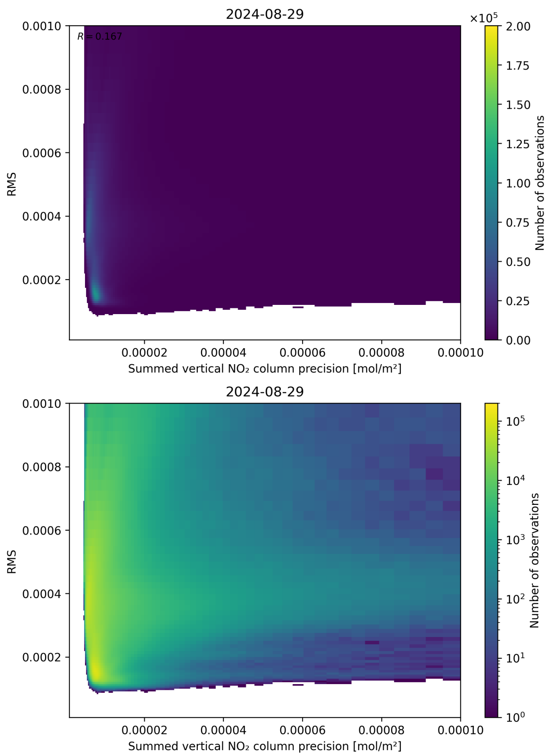
Figure 108: Scatter density plot of “Summed vertical NO 2 column precision” against “RMS” for 2024-08-28 to 2024-08-30.
