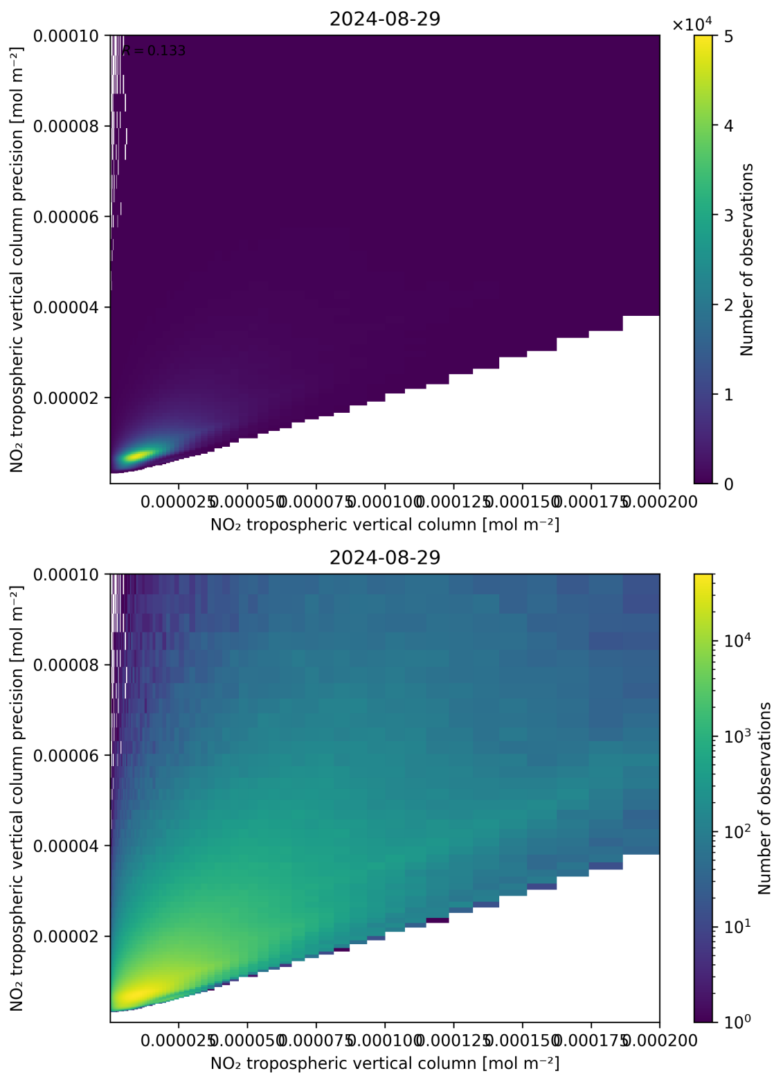
Figure 130: Scatter density plot of “NO 2 tropospheric vertical column” against “NO 2 tropospheric vertical column precision” for 2024-08-28 to 2024-08-30.
