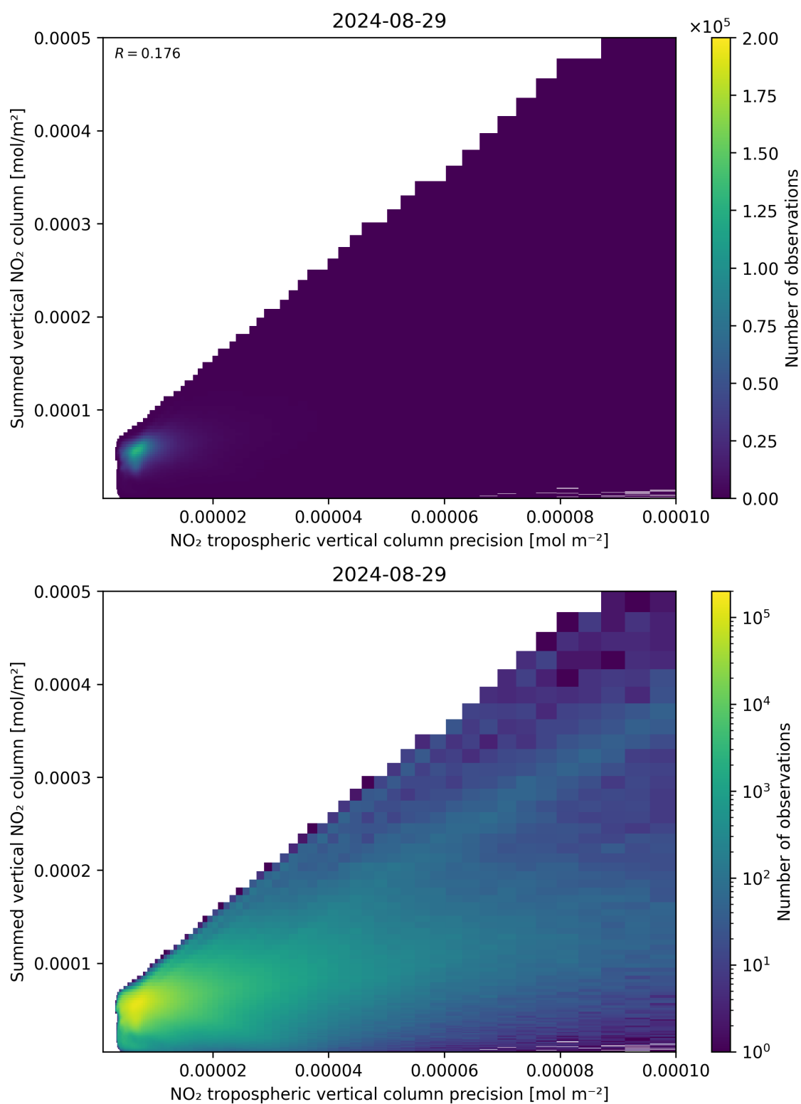
Figure 136: Scatter density plot of “NO 2 tropospheric vertical column precision” against “Summed vertical NO 2 column” for 2024-08-28 to 2024-08-30.
