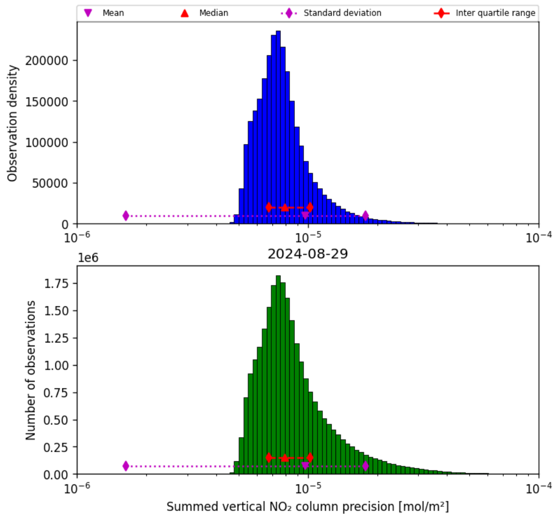
Figure 41: Histogram of “Summed vertical NO 2 column precision” for 2024-08-28 to 2024-08-30
