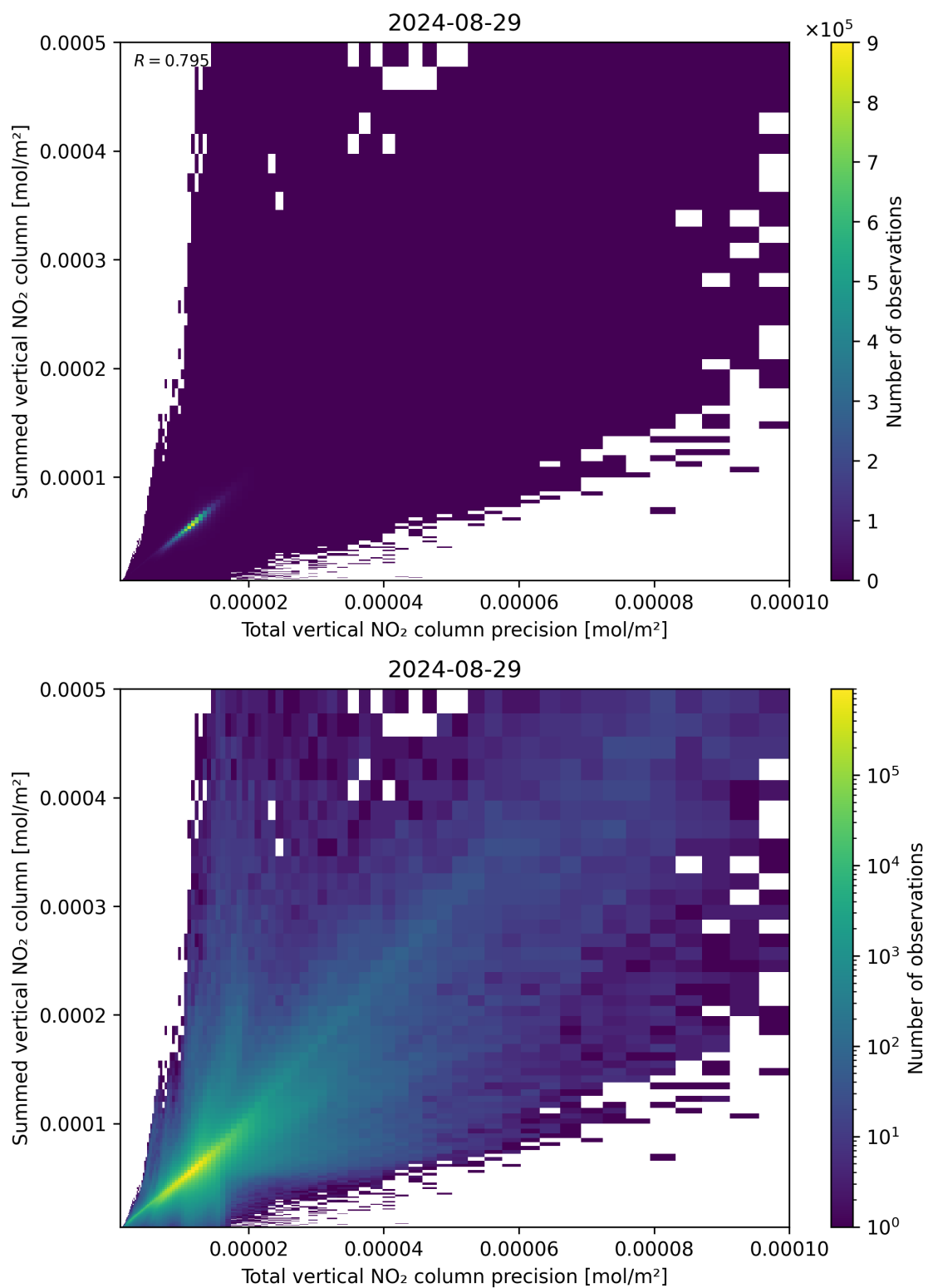
Figure 117: Scatter density plot of “Total vertical NO 2 column precision” against “Summed vertical NO 2 column” for 2024-08-28 to 2024-08-30.
