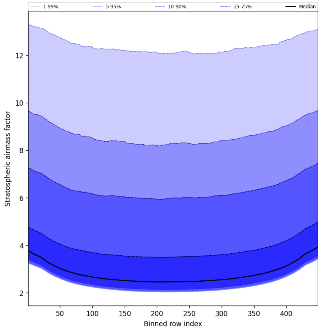
Figure 61: Along track statistics of “Stratospheric airmass factor” for 2024-08-28 to 2024-08-30
