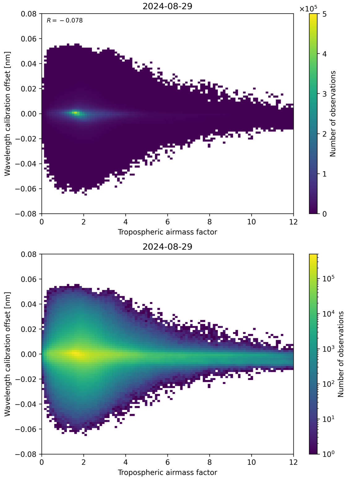
Figure 80: Scatter density plot of “Tropospheric airmass factor” against “Wavelength calibration offset” for 2024-08-28 to 2024-08-30.
