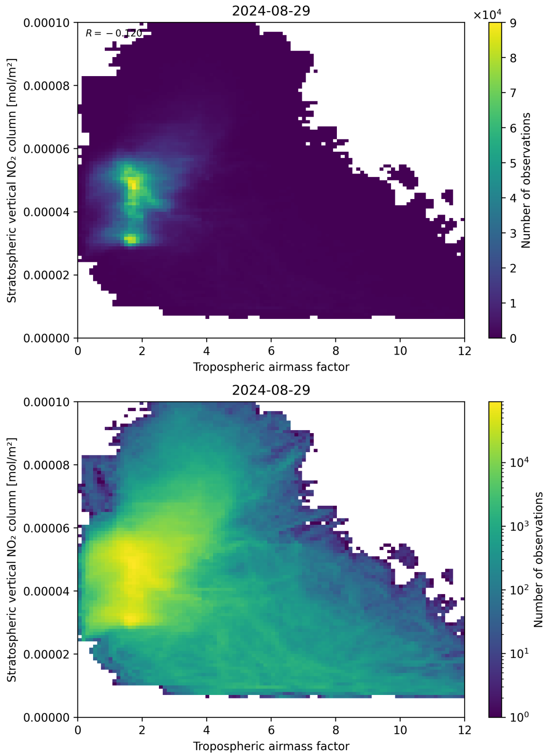
Figure 74: Scatter density plot of “Tropospheric air mass factor” against “Stratospheric vertical NO 2 column” for 2024-08-28 to 2024-08-30.
