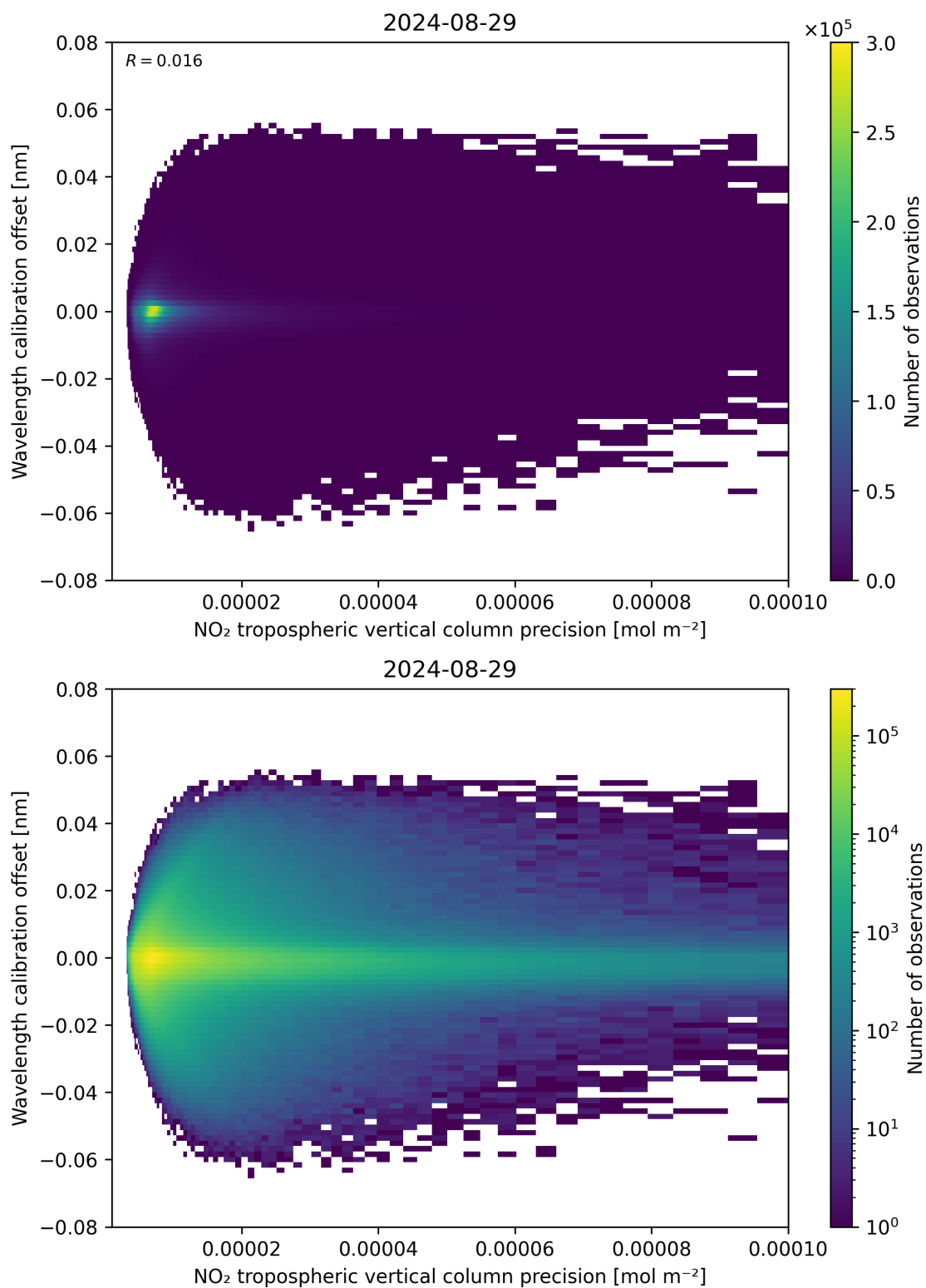
Figure 141: Scatter density plot of “NO 2 tropospheric vertical column precision” against “Wavelength calibration offset” for 2024-08-28 to 2024-08-30.
