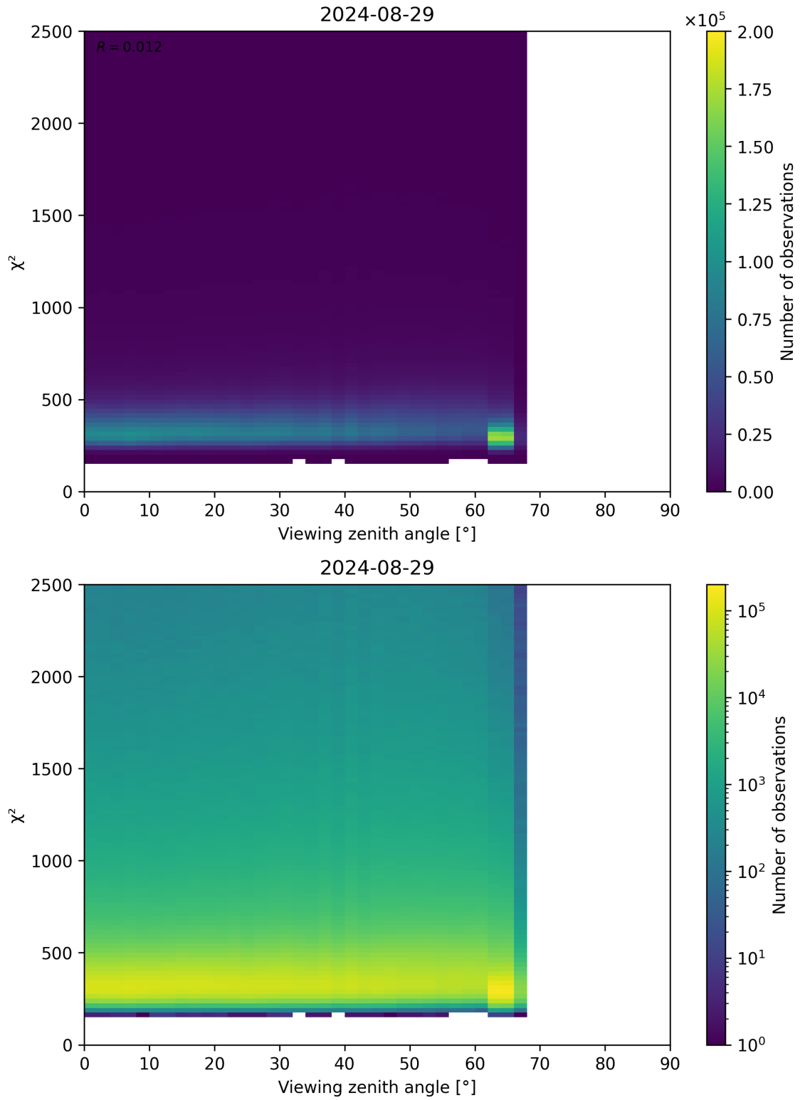
Figure 162: Scatter density plot of “Viewing zenith angle” against “ \chi^2 ” for 2024-08-28 to 2024-08-30.
