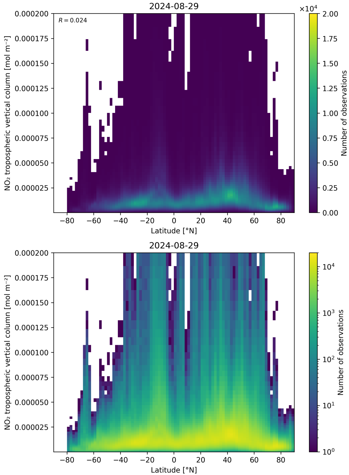
Figure 92: Scatter density plot of “Latitude” against “NO 2 tropospheric vertical column” for 2024-08-28 to 2024-08-30.
