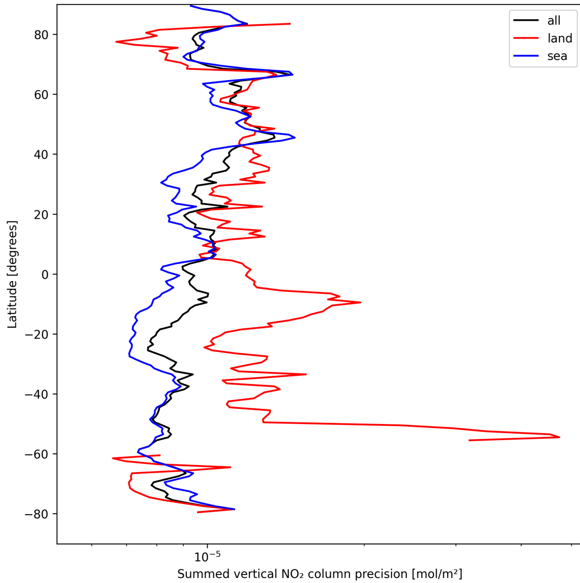
Figure 24: Zonal average of “Summed vertical NO 2 column precision” for 2024-08-28 to 2024-08-30.
