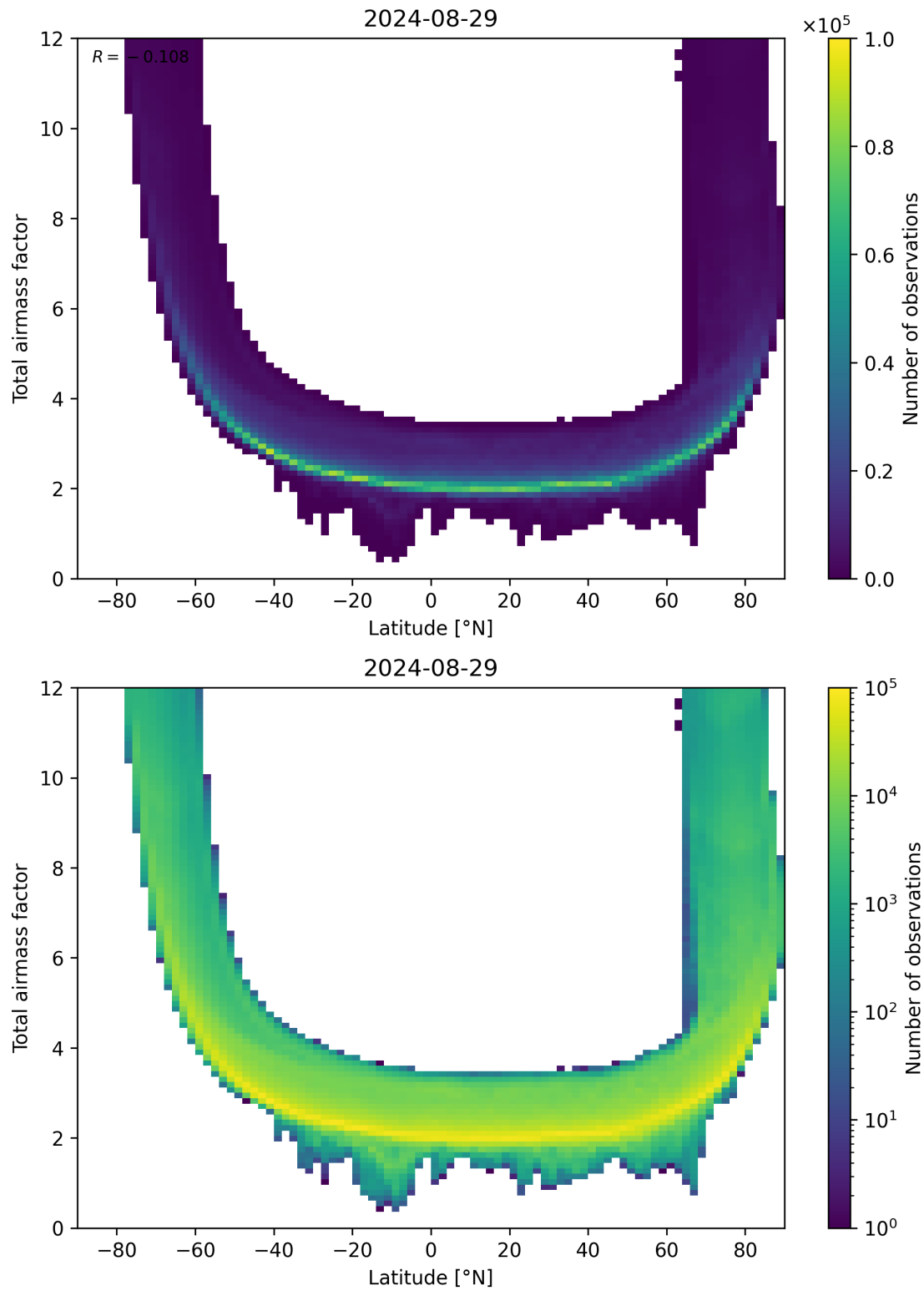
Figure 84: Scatter density plot of “Latitude” against “Total airmass factor” for 2024-08-28 to 2024-08-30.
