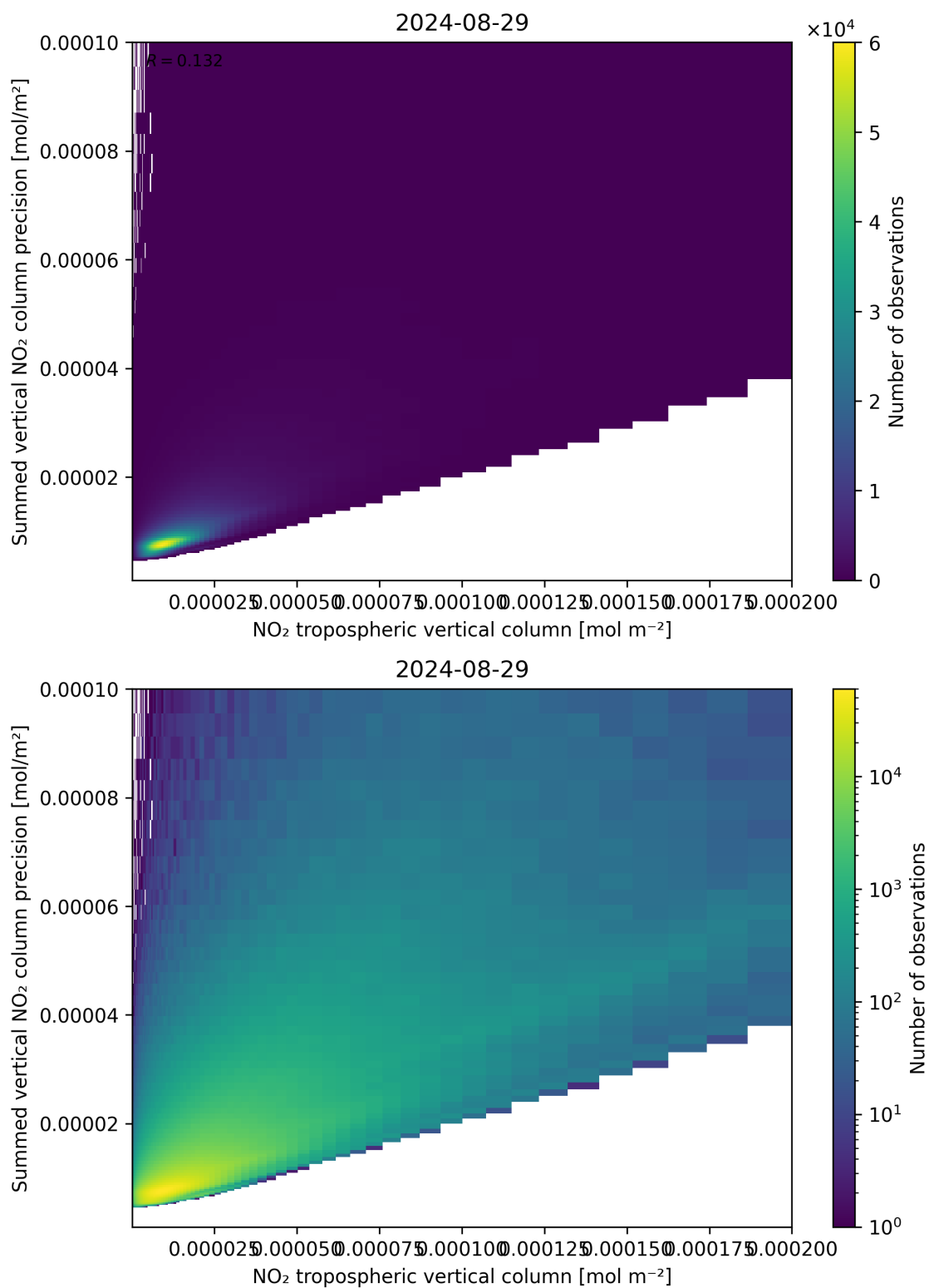
Figure 127: Scatter density plot of “NO 2 tropospheric vertical column” against “Summed vertical NO 2 column precision” for 2024-08-28 to 2024-08-30.
