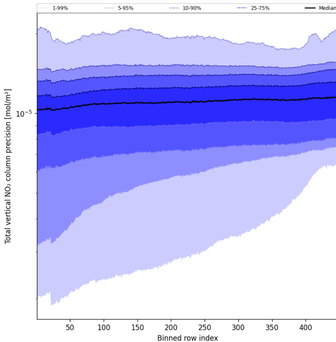
Figure 56: Along track statistics of “Total vertical NO 2 column precision” for 2024-08-28 to 2024-08-30
