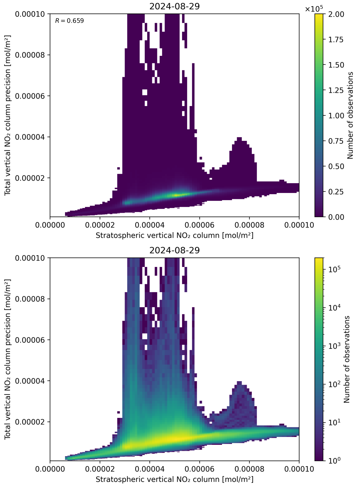
Figure 101: Scatter density plot of “Stratospheric vertical NO 2 column” against “Total vertical NO 2 column precision” for 2024-08-28 to 2024-08-30.
