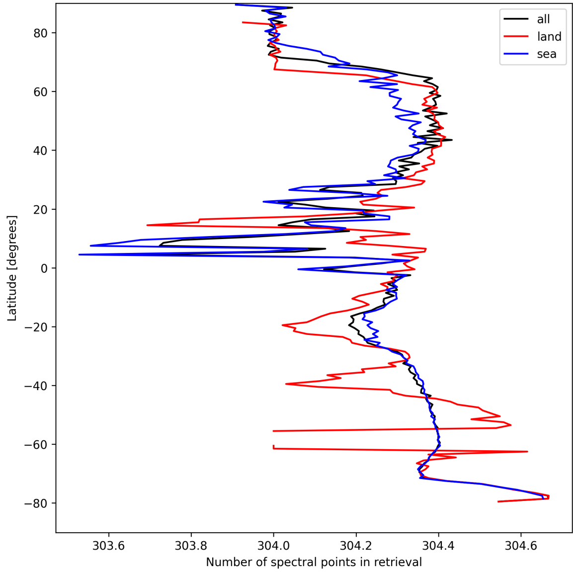
Figure 16: Zonal average of “Number of spectral points in retrieval” for 2024-08-28 to 2024-08-30.
