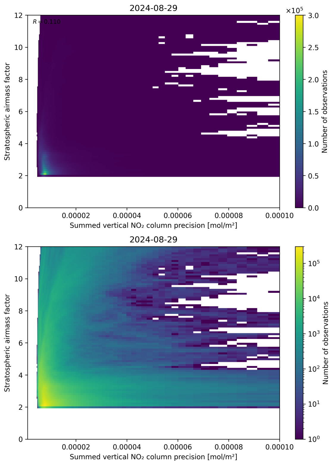
Figure 106: Scatter density plot of “Summed vertical NO 2 column precision” against “Stratospheric airmass factor” for 2024-08-28 to 2024-08-30.
