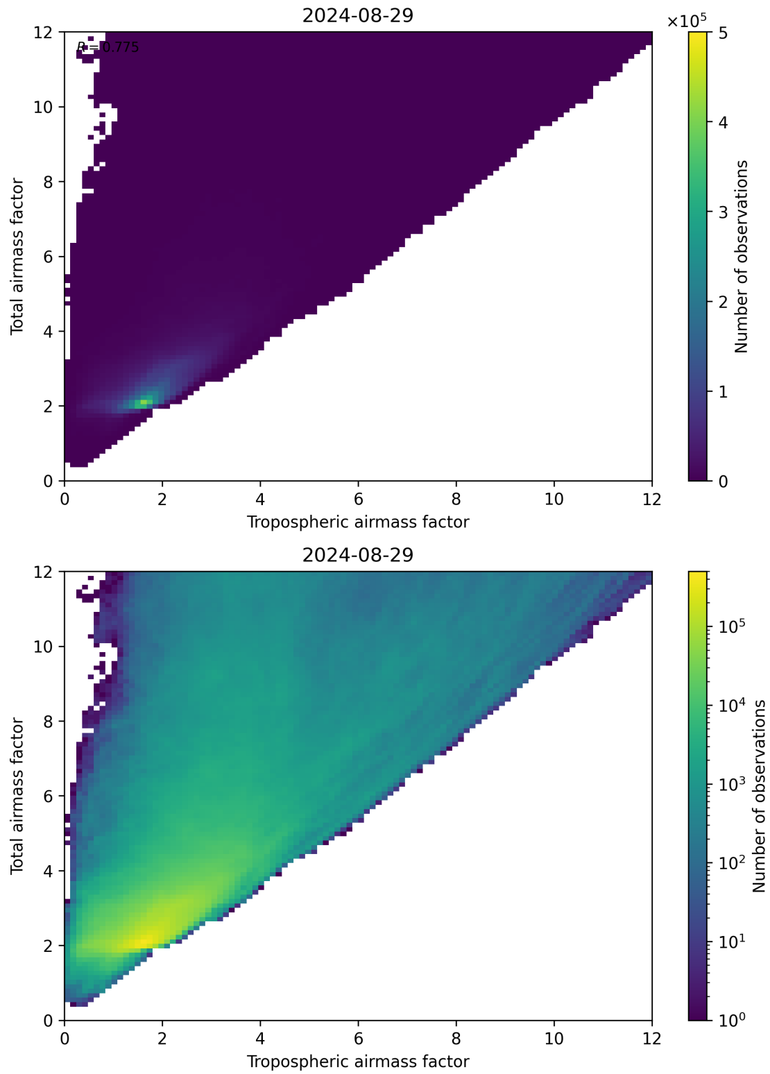
Figure 72: Scatter density plot of “Tropospheric airmass factor” against “Total airmass factor” for 2024-08-28 to 2024-08-30.
