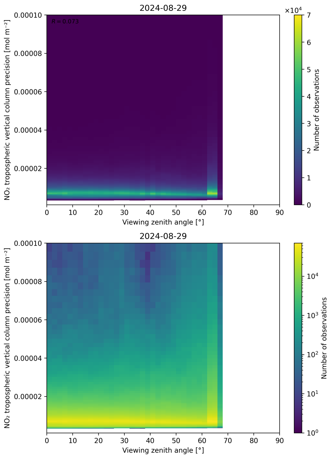
Figure 170: Scatter density plot of “Viewing zenith angle” against “NO 2 tropospheric vertical column precision” for 2024-08-28 to 2024-08-30.
