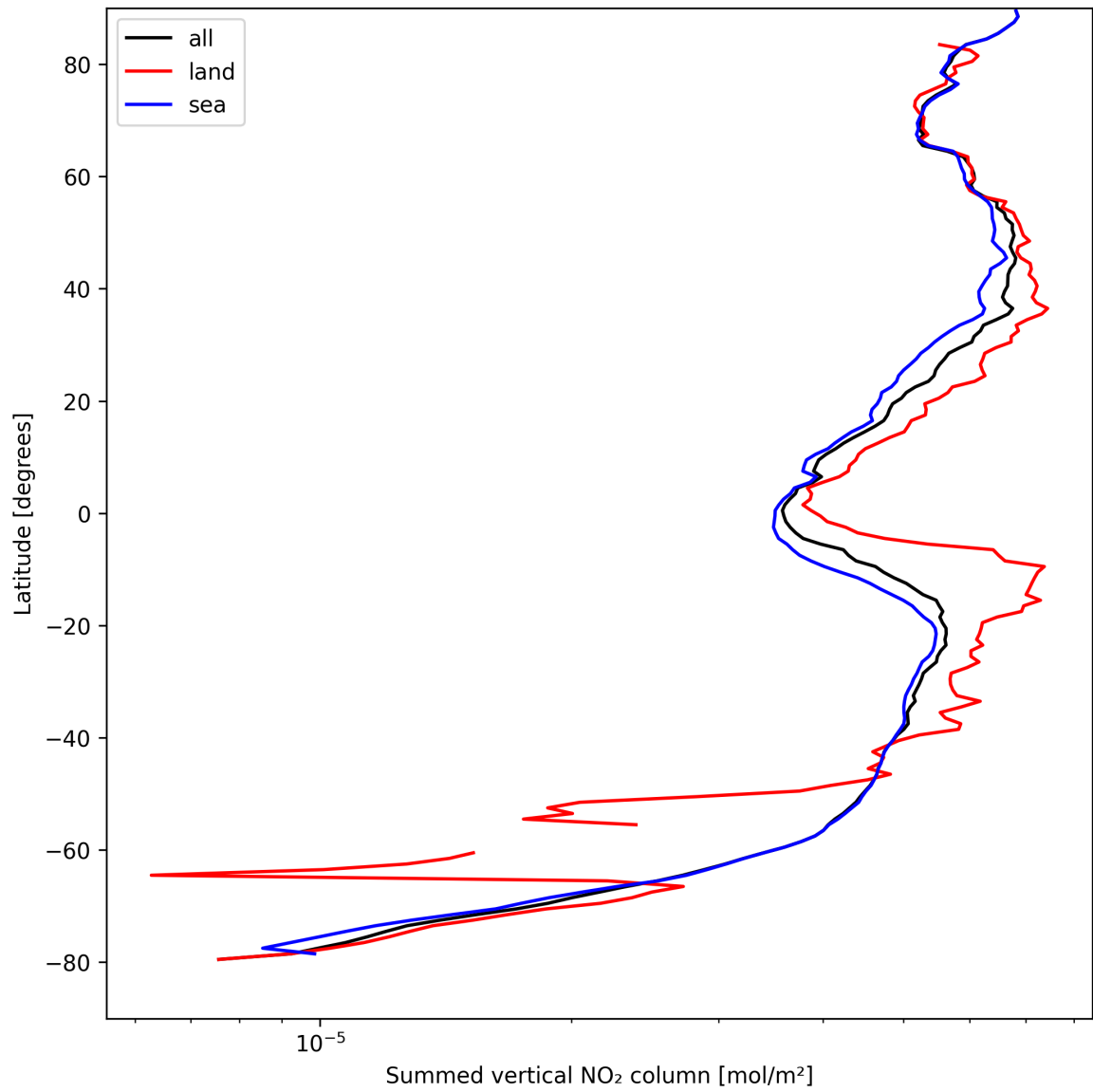
Figure 23: Zonal average of “Summed vertical NO 2 column” for 2024-08-28 to 2024-08-30.
