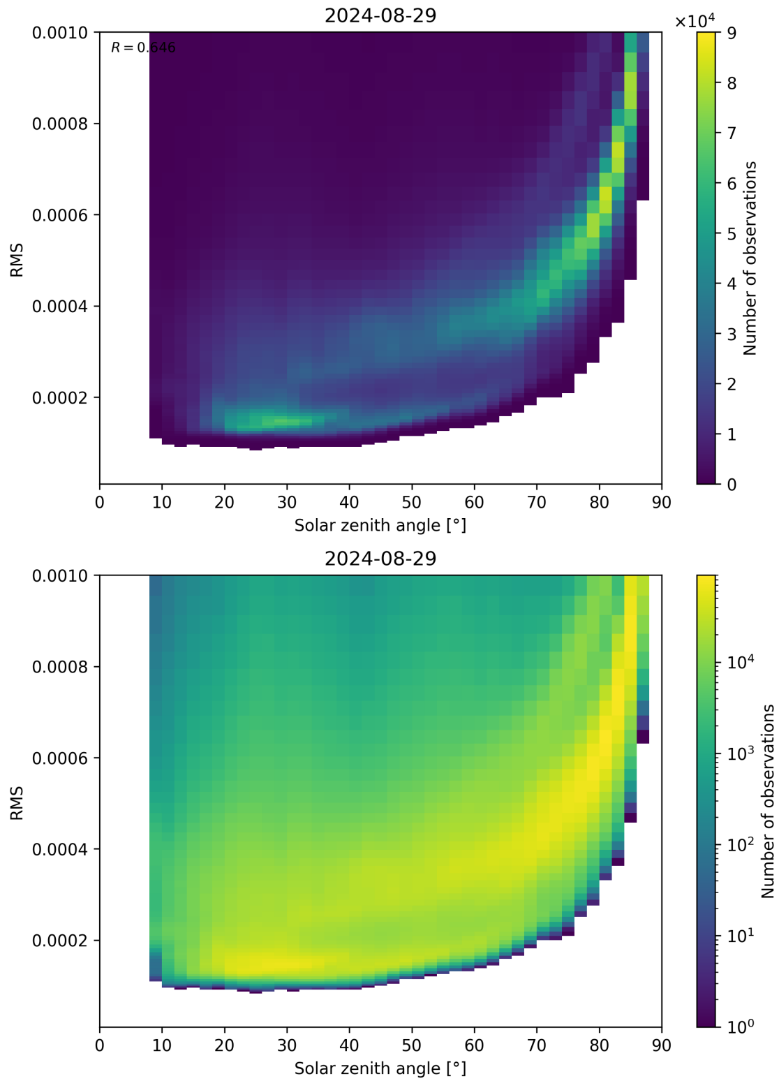
Figure 157: Scatter density plot of “Solar zenith angle” against “RMS” for 2024-08-28 to 2024-08-30.
