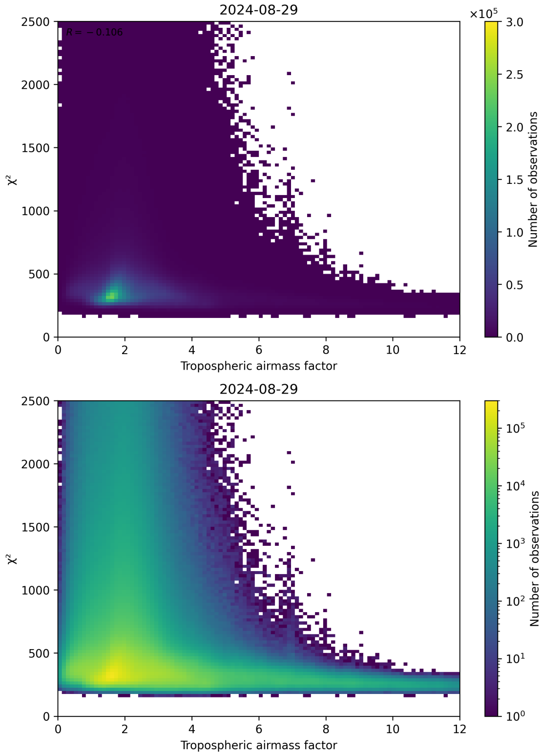
Figure 73: Scatter density plot of “Tropospheric airmass factor” against “ \chi^2 ” for 2024-08-28 to 2024-08-30.
