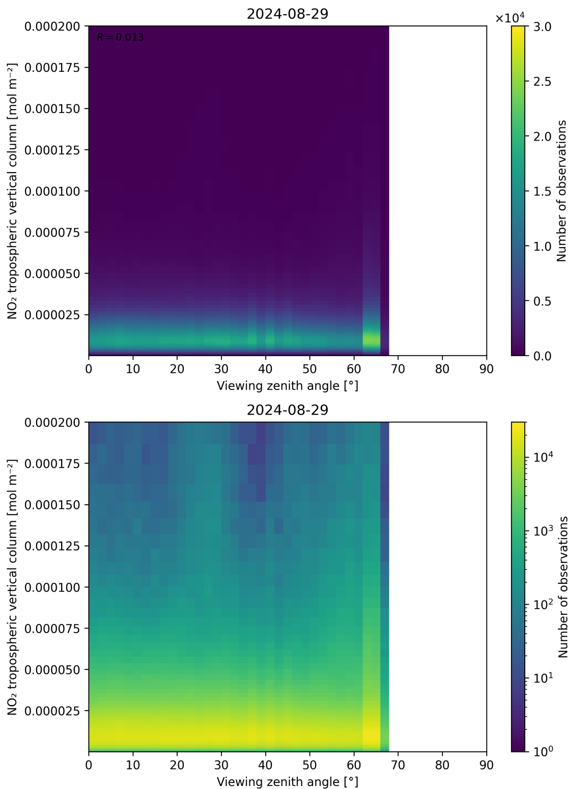
Figure 169: Scatter density plot of “Viewing zenith angle” against “NO 2 tropospheric vertical column” for 2024-08-28 to 2024-08-30.
