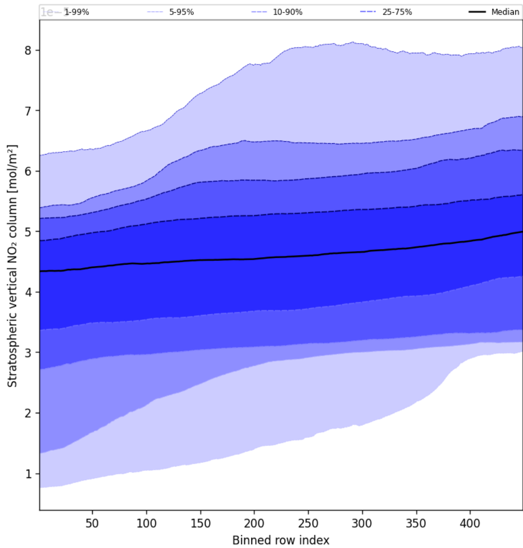
Figure 53: Along track statistics of “Stratospheric vertical NO 2 column” for 2024-08-28 to 2024-08-30
