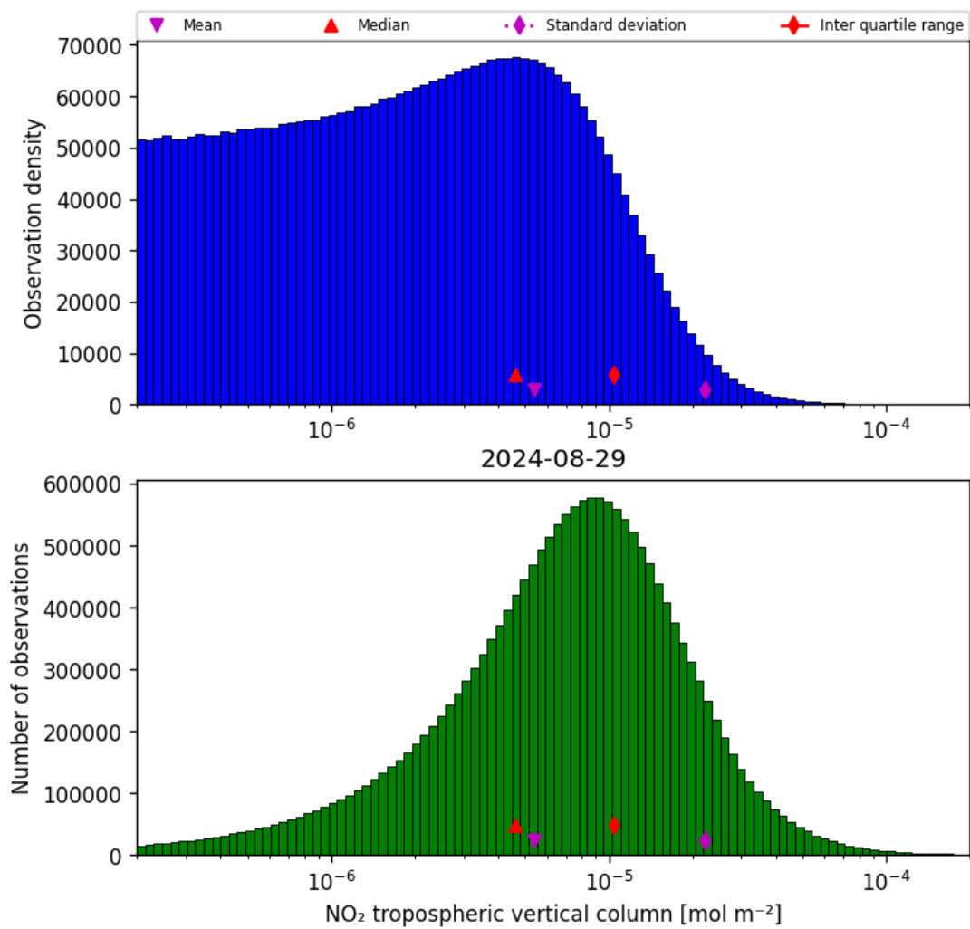
Figure 29: Histogram of “NO 2 tropospheric vertical column” for 2024-08-28 to 2024-08-30
