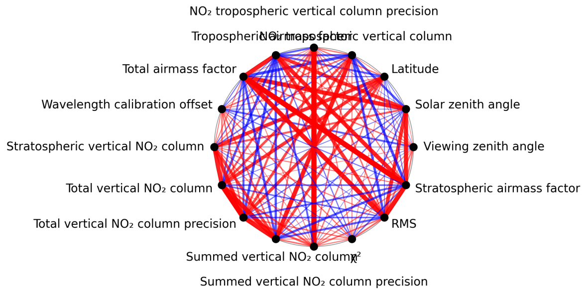
Figure 1: Map of correlation graph for 2024-08-28 to 2024-08-30.
