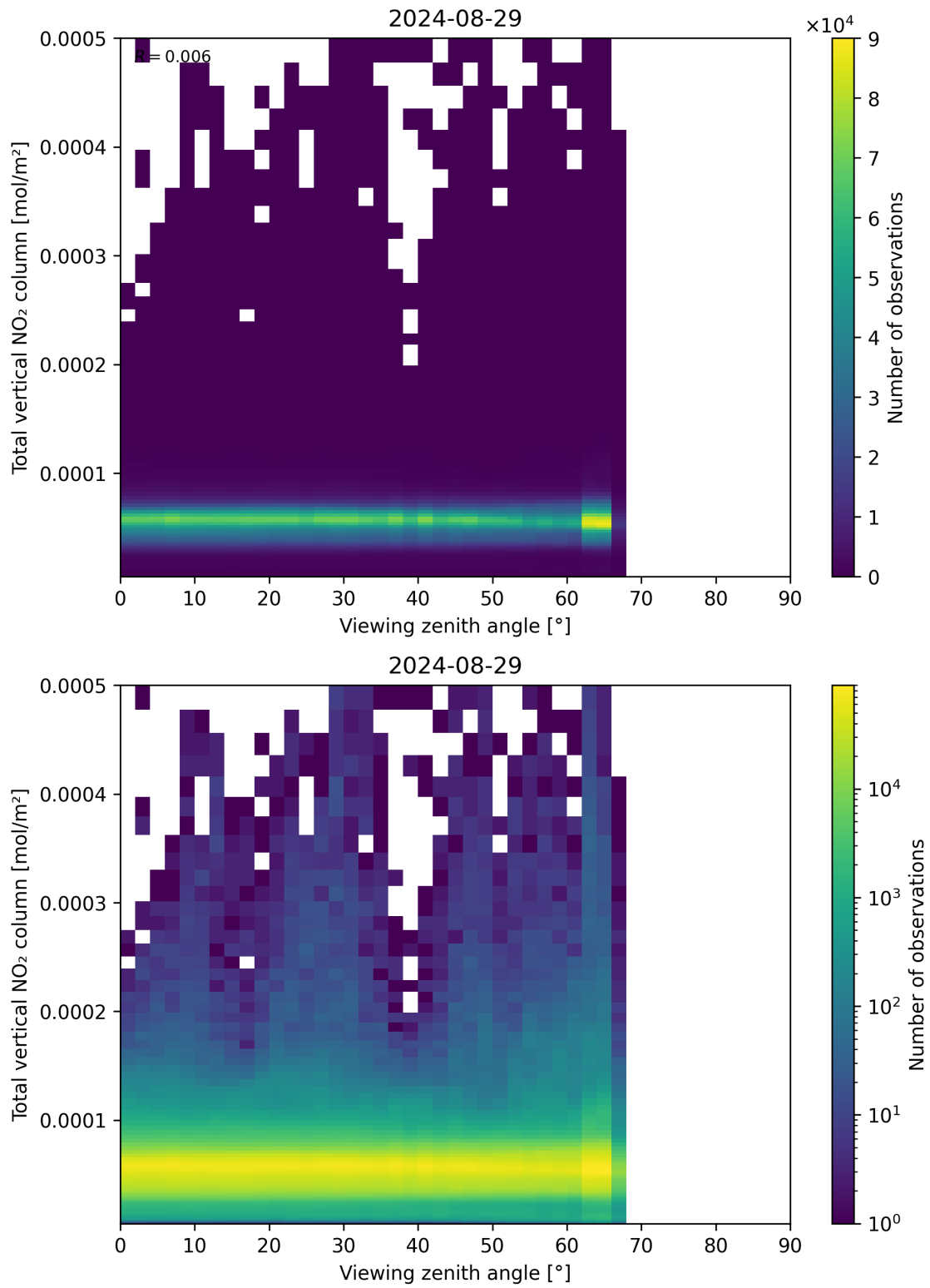
Figure 167: Scatter density plot of “Viewing zenith angle” against “Total vertical NO 2 column” for 2024-08-28 to 2024-08-30.
