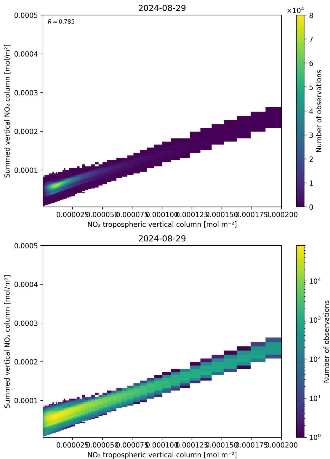
Figure 126: Scatter density plot of “NO 2 tropospheric vertical column” against “Summed vertical NO 2 column” for 2024-08-28 to 2024-08-30.
