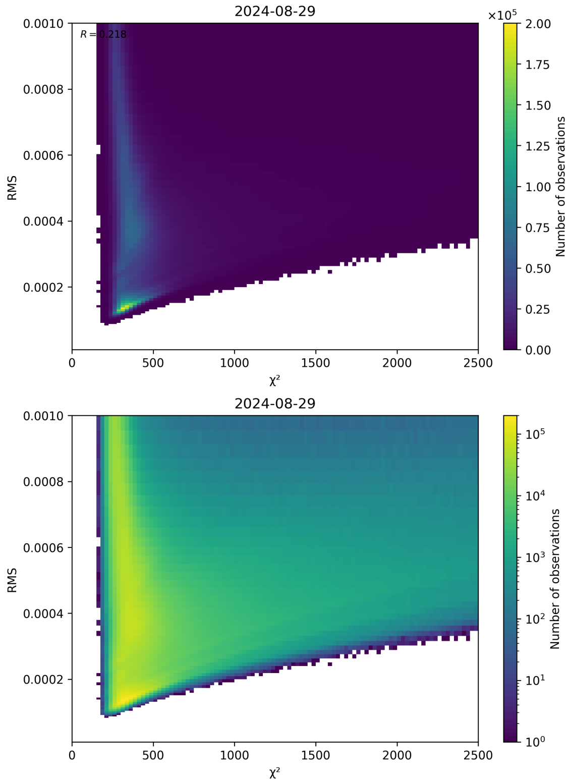
Figure 82: Scatter density plot of “ \chi^2 ” against “RMS” for 2024-08-28 to 2024-08-30.
