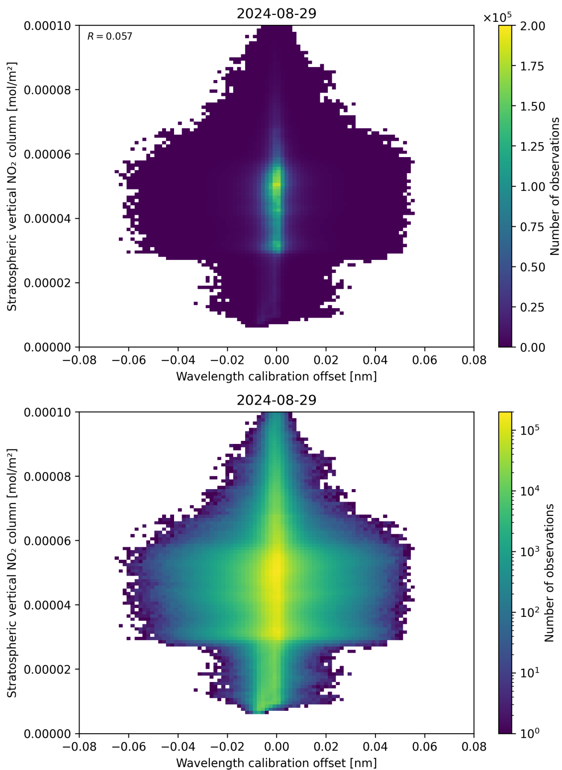
Figure 176: Scatter density plot of “Wavelength calibration offset” against “Stratospheric vertical NO 2 column” for 2024-08-28 to 2024-08-30.
