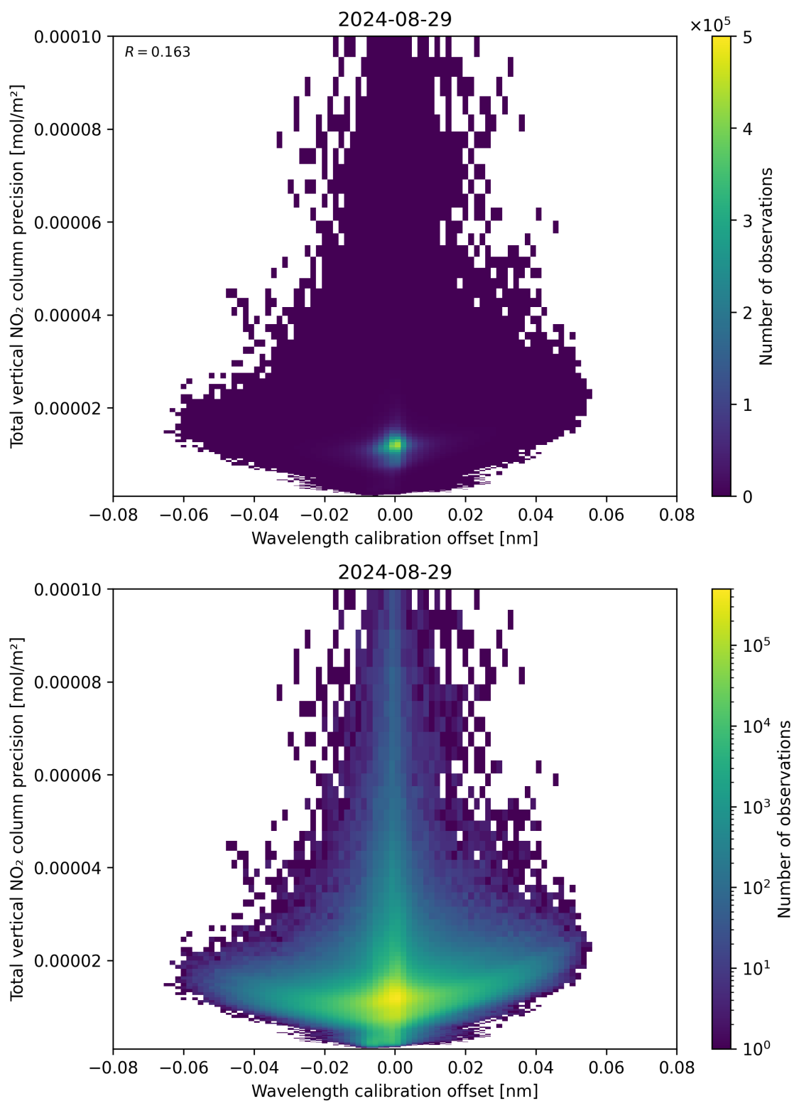
Figure 180: Scatter density plot of “Wavelength calibration offset” against “Total vertical NO 2 column precision” for 2024-08-28 to 2024-08-30.
