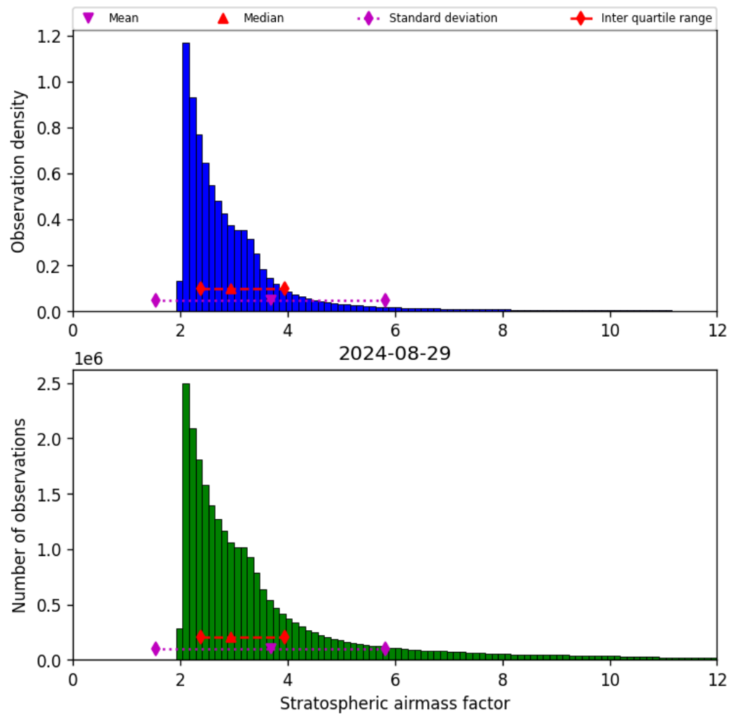
Figure 44: Histogram of “Stratospheric airmass factor” for 2024-08-28 to 2024-08-30
