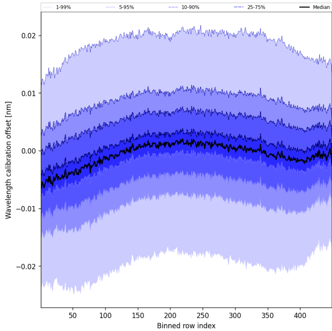
Figure 52: Along track statistics of “Wavelength calibration offset” for 2024-08-28 to 2024-08-30
