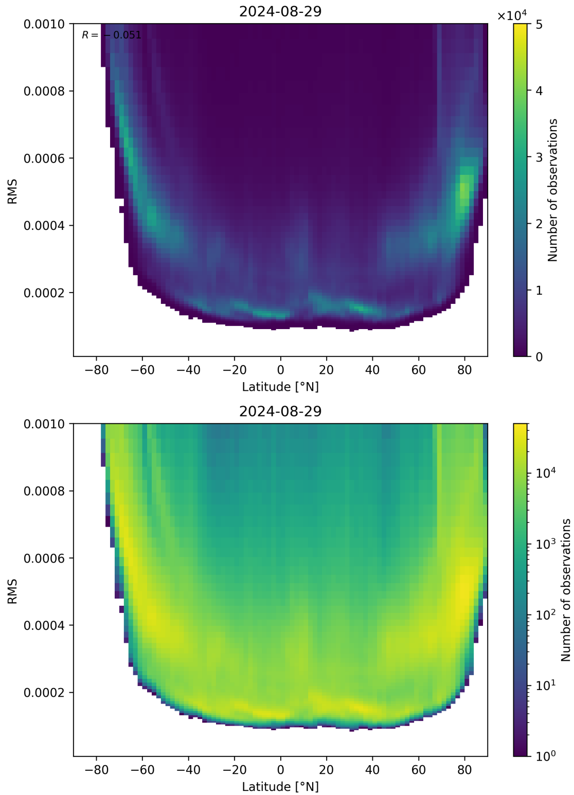
Figure 94: Scatter density plot of “Latitude” against “RMS” for 2024-08-28 to 2024-08-30.
