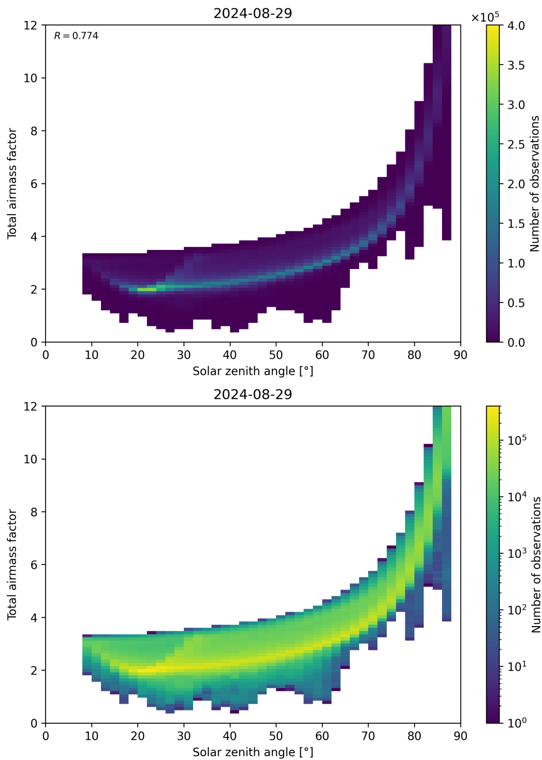
Figure 146: Scatter density plot of “Solar zenith angle” against “Total air mass factor” for 2024-08-28 to 2024-08-30.
