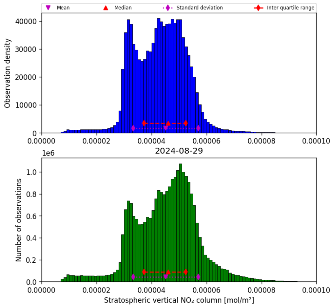
Figure 36: Histogram of “Stratospheric vertical NO 2 column” for 2024-08-28 to 2024-08-30
