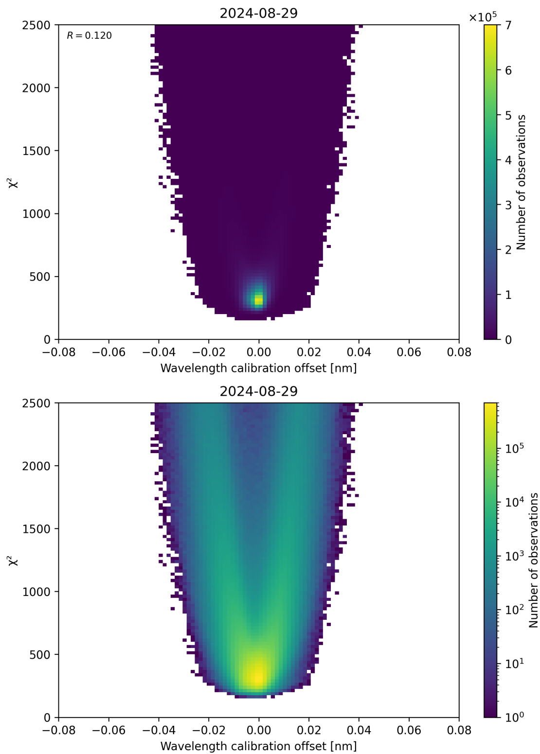
Figure 175: Scatter density plot of “Wavelength calibration offset” against “ \chi^2 ” for 2024-08-28 to 2024-08-30.
