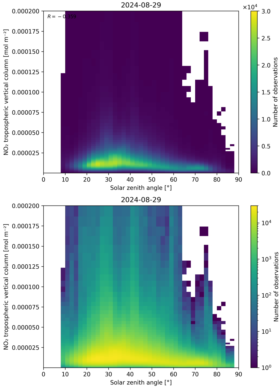
Figure 155: Scatter density plot of “Solar zenith angle” against “NO 2 tropospheric vertical column” for 2024-08-28 to 2024-08-30.
