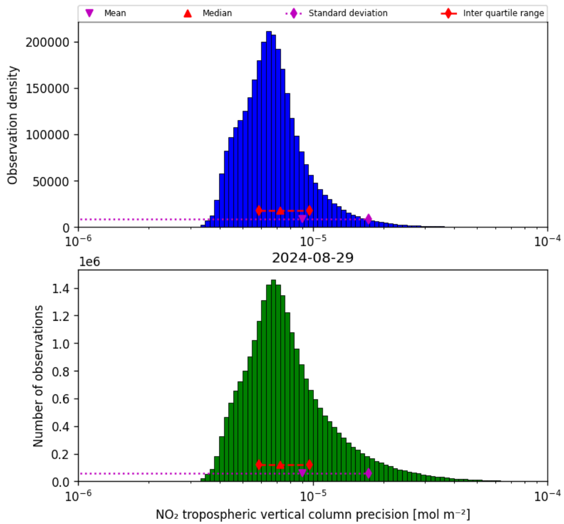
Figure 30: Histogram of “NO 2 tropospheric vertical column precision” for 2024-08-28 to 2024-08-30
