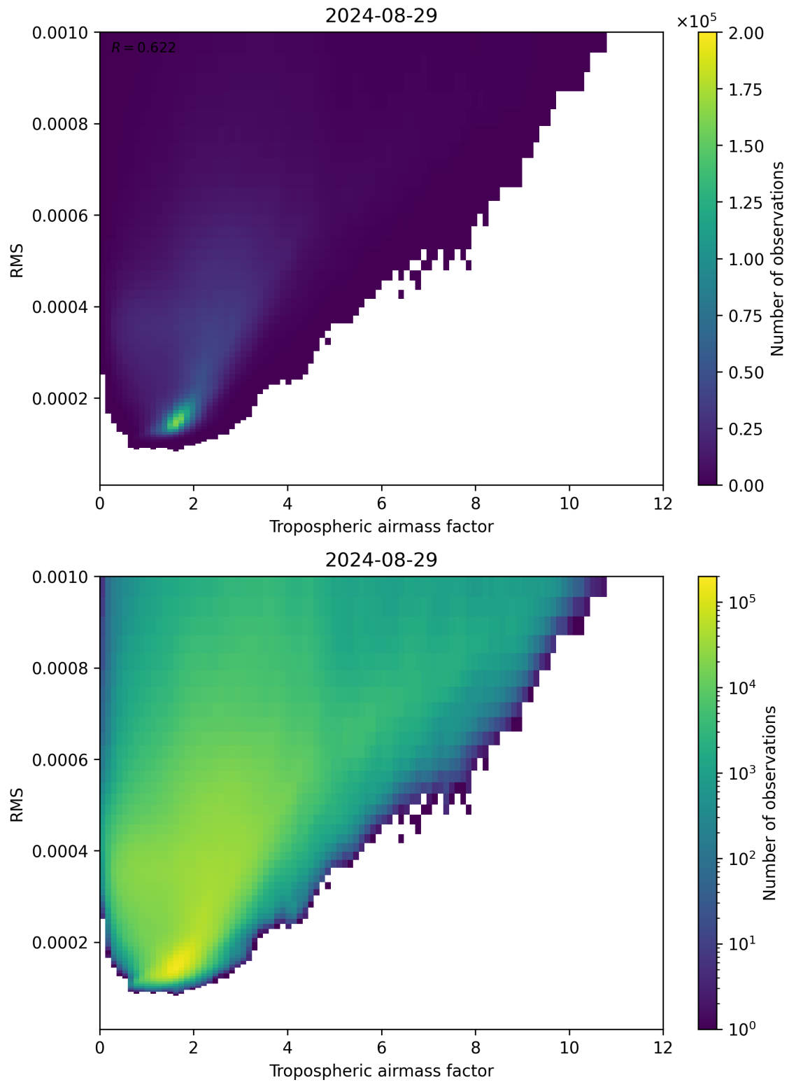
Figure 79: Scatter density plot of “Tropospheric airmass factor” against “RMS” for 2024-08-28 to 2024-08-30.
