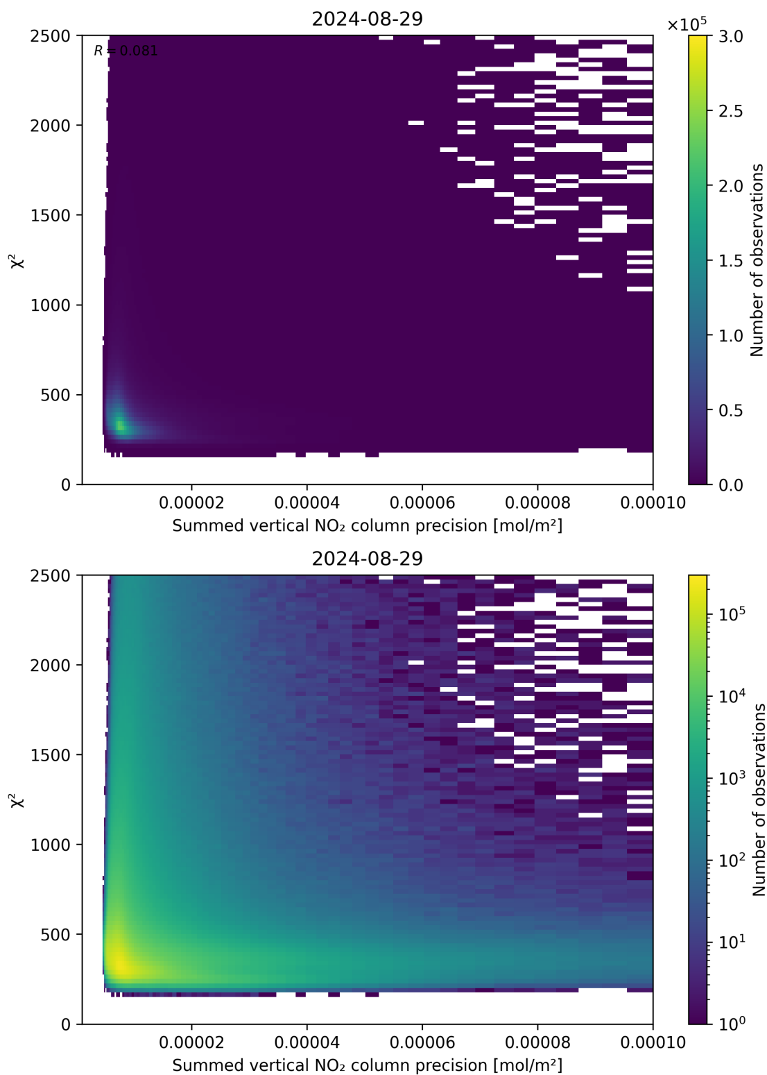
Figure 107: Scatter density plot of “Summed vertical NO 2 column precision” against “ \chi^2 ” for 2024-08-28 to 2024-08-30.
