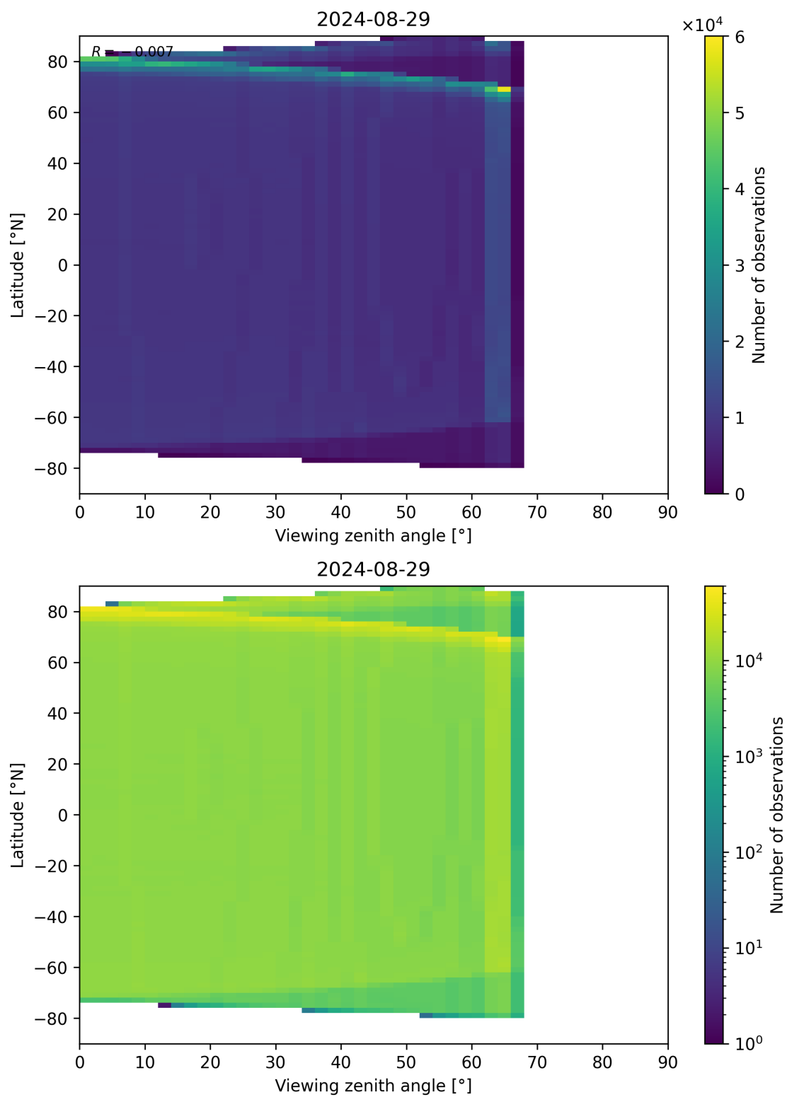
Figure 163: Scatter density plot of “Viewing zenith angle” against “Latitude” for 2024-08-28 to 2024-08-30.
