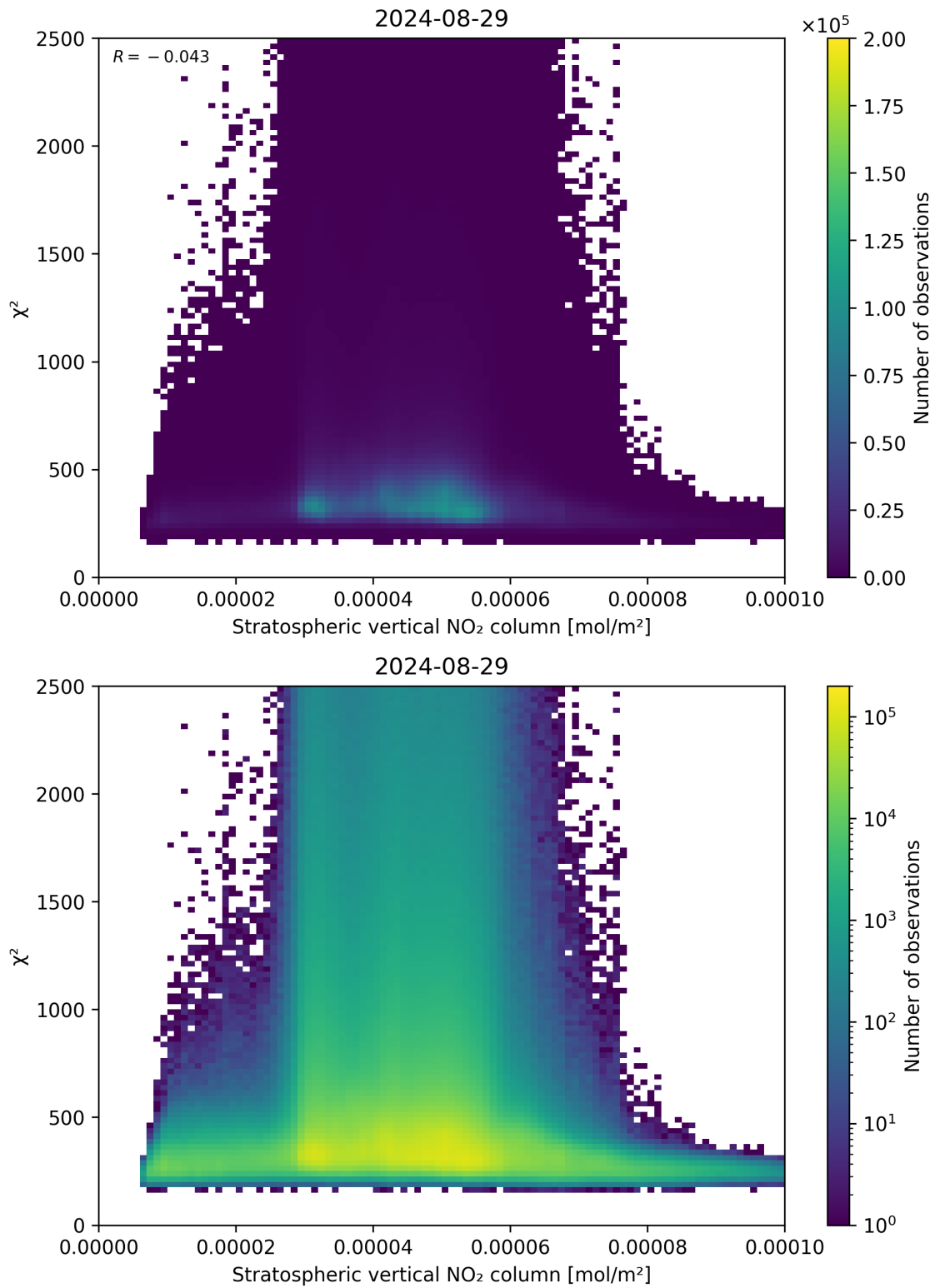
Figure 97: Scatter density plot of “Stratospheric vertical NO 2 column” against “ \chi^2 ” for 2024-08-28 to 2024-08-30.
