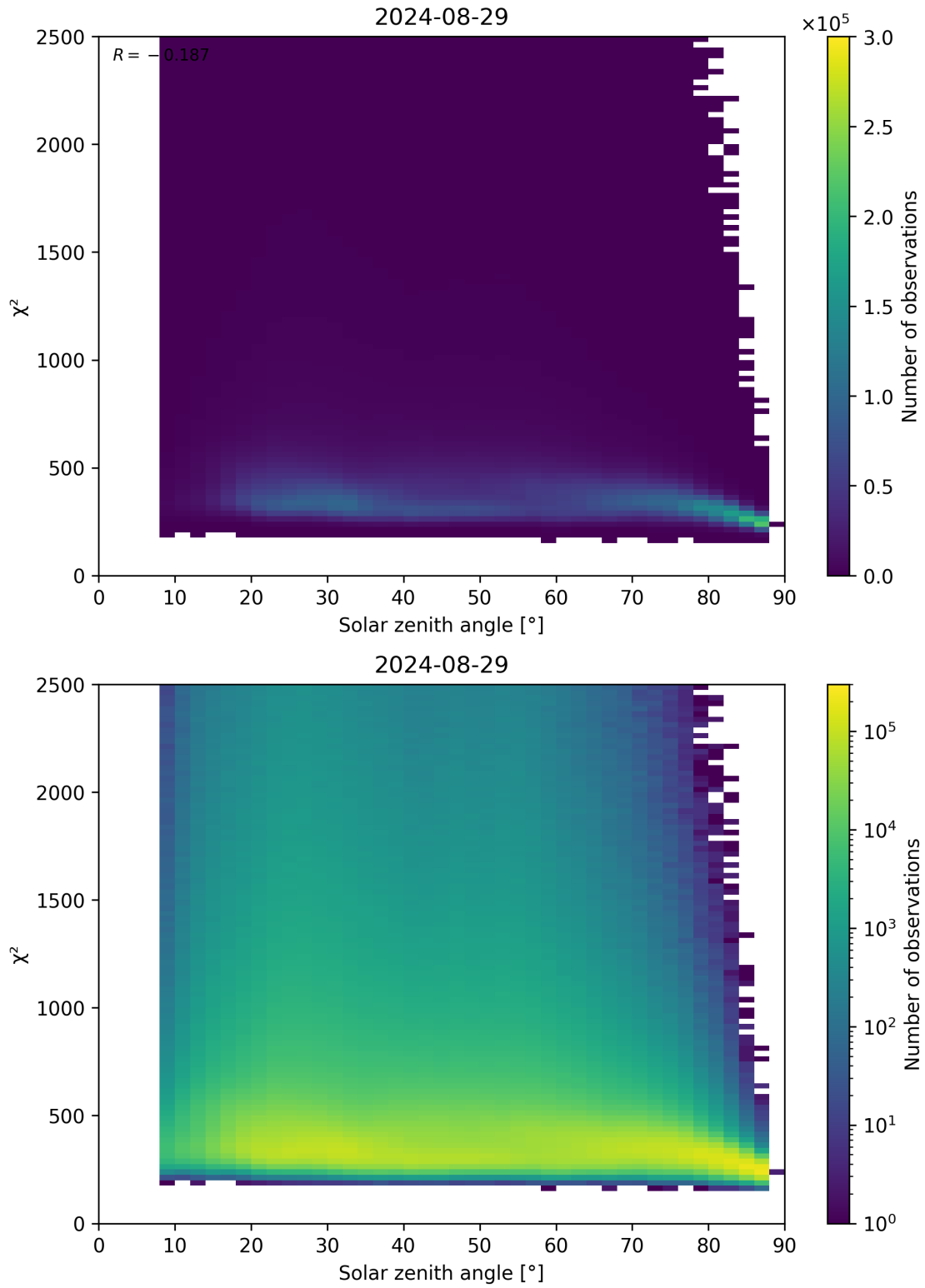
Figure 148: Scatter density plot of “Solar zenith angle” against “ \chi^2 ” for 2024-08-28 to 2024-08-30.
