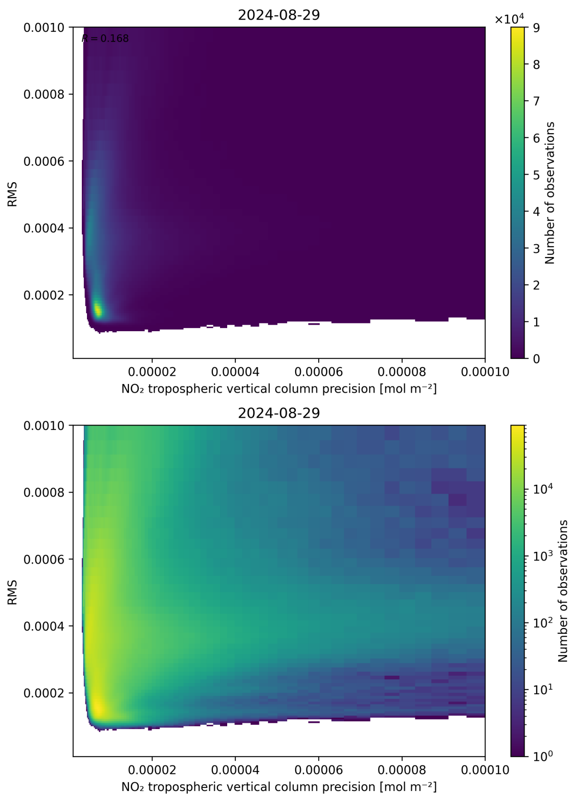
Figure 140: Scatter density plot of “NO 2 tropospheric vertical column precision” against “RMS” for 2024-08-28 to 2024-08-30.
