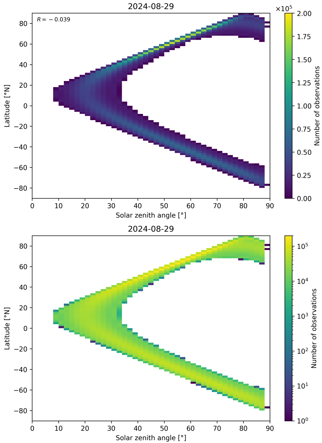
Figure 149: Scatter density plot of “Solar zenith angle” against “Latitude” for 2024-08-28 to 2024-08-30.
