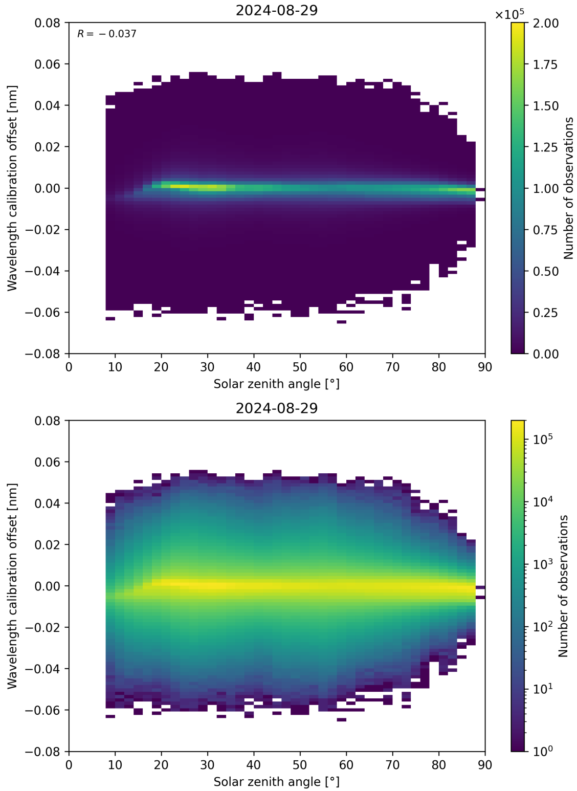
Figure 158: Scatter density plot of “Solar zenith angle” against “Wavelength calibration offset” for 2024-08-28 to 2024-08-30.
