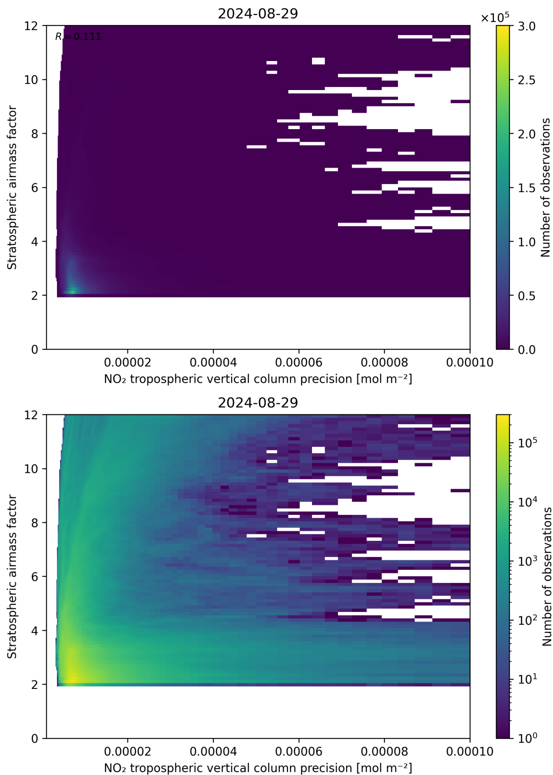
Figure 131: Scatter density plot of “NO 2 tropospheric vertical column precision” against “Stratospheric airmass factor” for 2024-08-28 to 2024-08-30.
