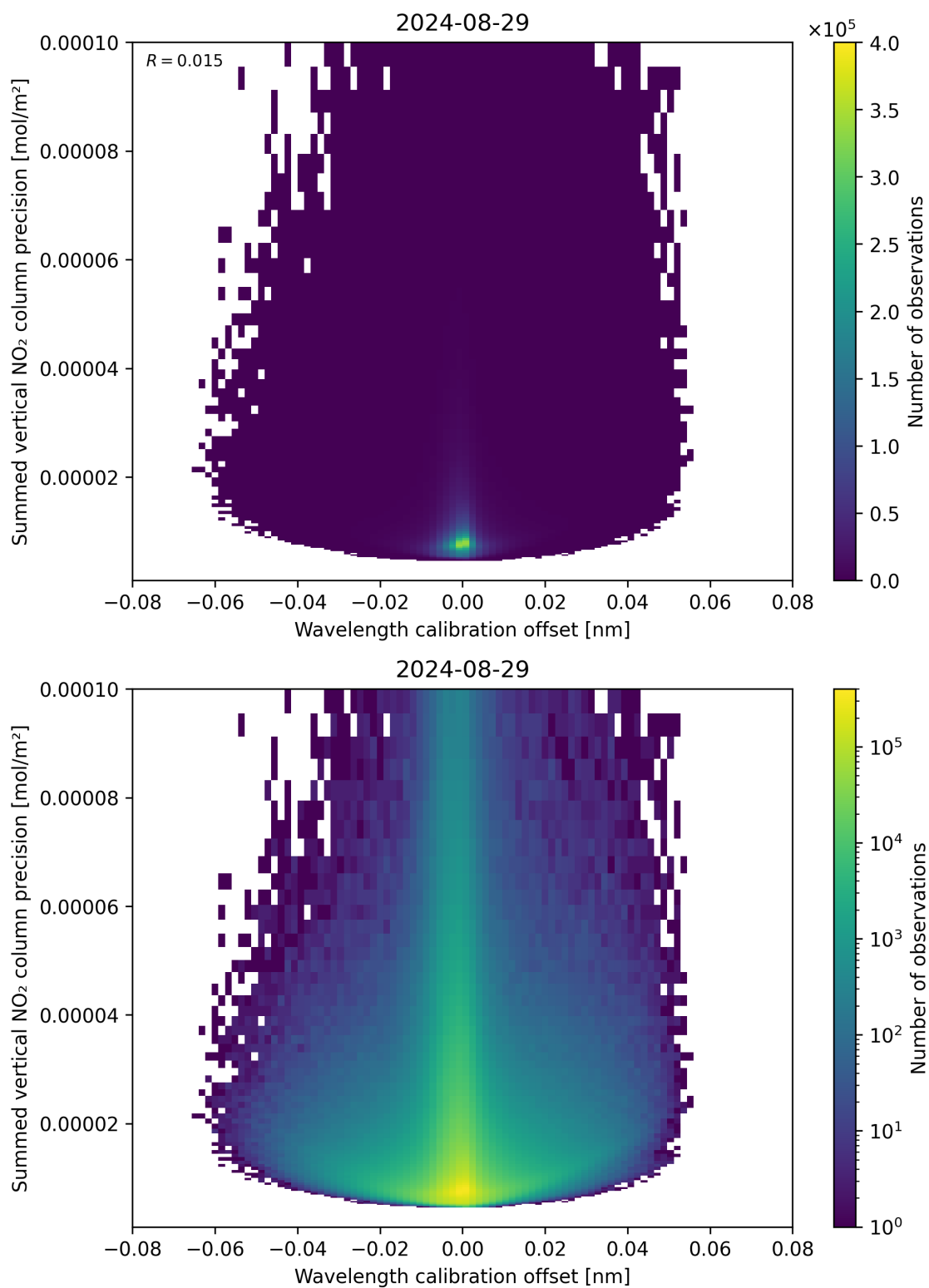
Figure 178: Scatter density plot of “Wavelength calibration offset” against “Summed vertical NO 2 column precision” for 2024-08-28 to 2024-08-30.
