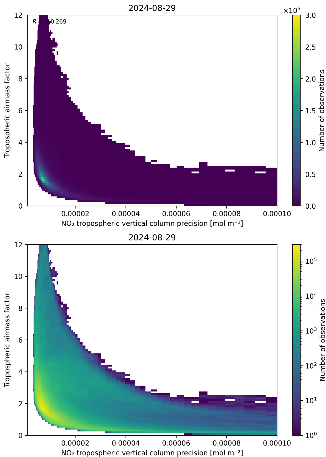
Figure 133: Scatter density plot of “NO 2 tropospheric vertical column precision” against “Tropospheric air mass factor” for 2024-08-28 to 2024-08-30.
