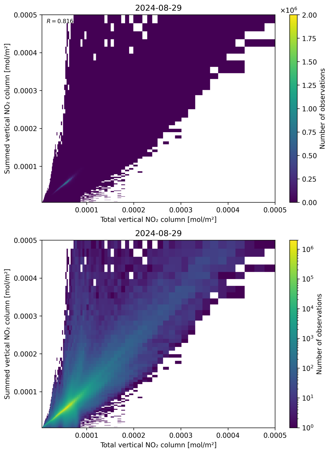
Figure 112: Scatter density plot of “Total vertical NO 2 column” against “Summed vertical NO 2 column” for 2024-08-28 to 2024-08-30.
