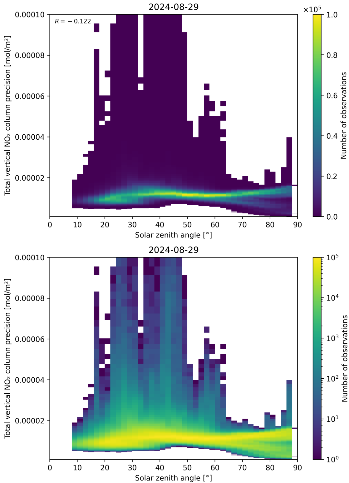
Figure 154: Scatter density plot of “Solar zenith angle” against “Total vertical NO 2 column precision” for 2024-08-28 to 2024-08-30.
