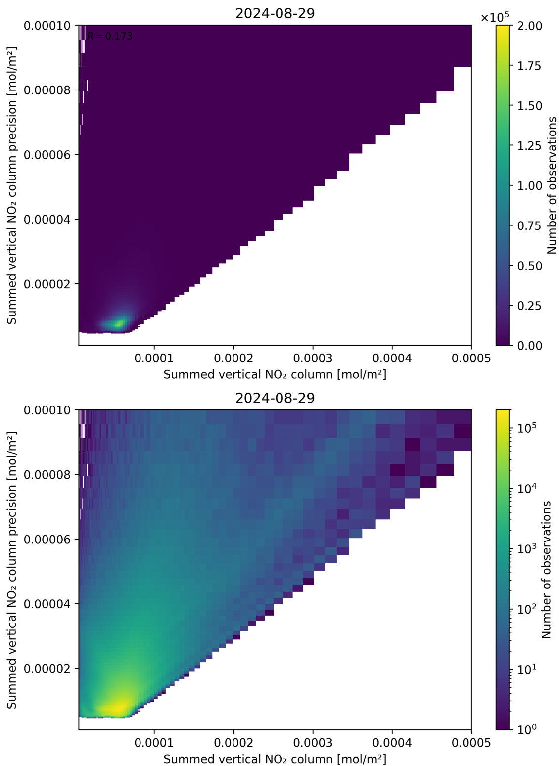
Figure 105: Scatter density plot of “Summed vertical NO 2 column” against “Summed vertical NO 2 column precision” for 2024-08-28 to 2024-08-30.
