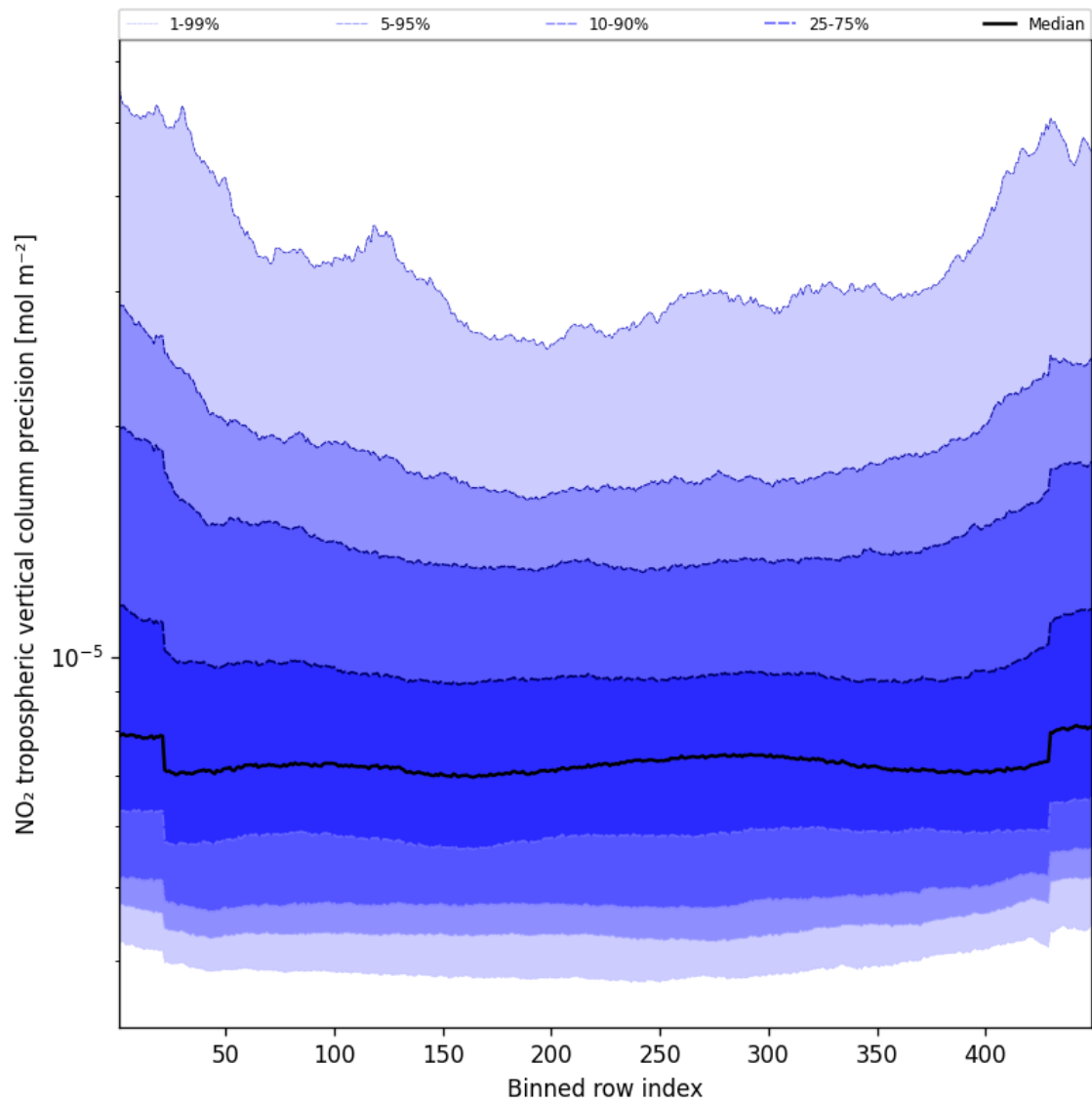
Figure 47: Along track statistics of “NO 2 tropospheric vertical column precision” for 2024-08-28 to 2024-08-30
