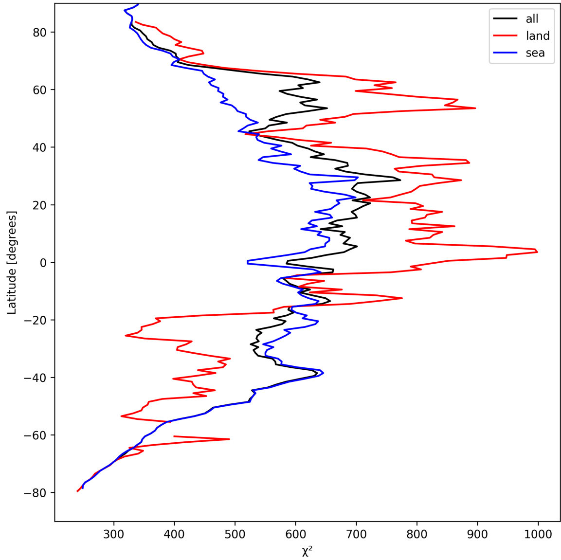
Figure 25: Zonal average of “ \chi^2 ” for 2024-08-28 to 2024-08-30.
