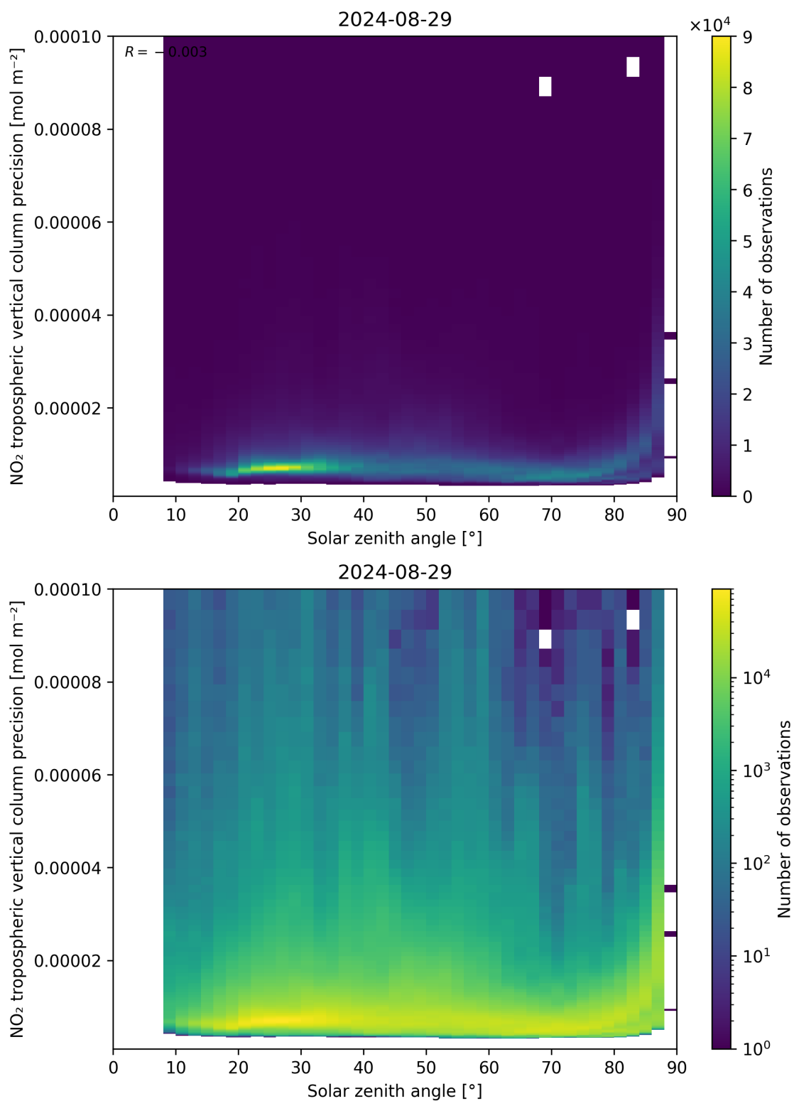
Figure 156: Scatter density plot of “Solar zenith angle” against “NO 2 tropospheric vertical column precision” for 2024-08-28 to 2024-08-30.
