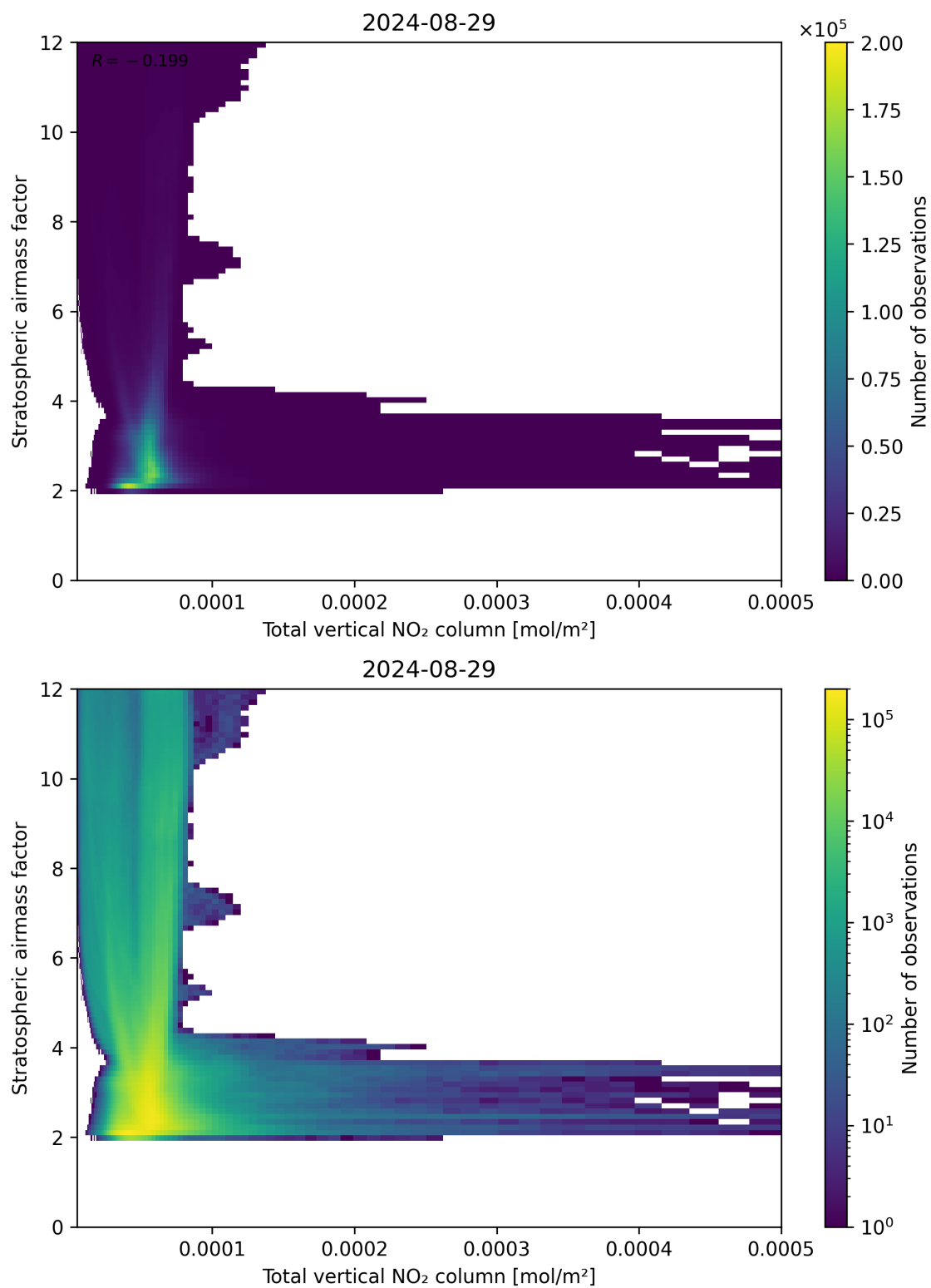
Figure 110: Scatter density plot of “Total vertical NO 2 column” against “Stratospheric airmass factor” for 2024-08-28 to 2024-08-30.
