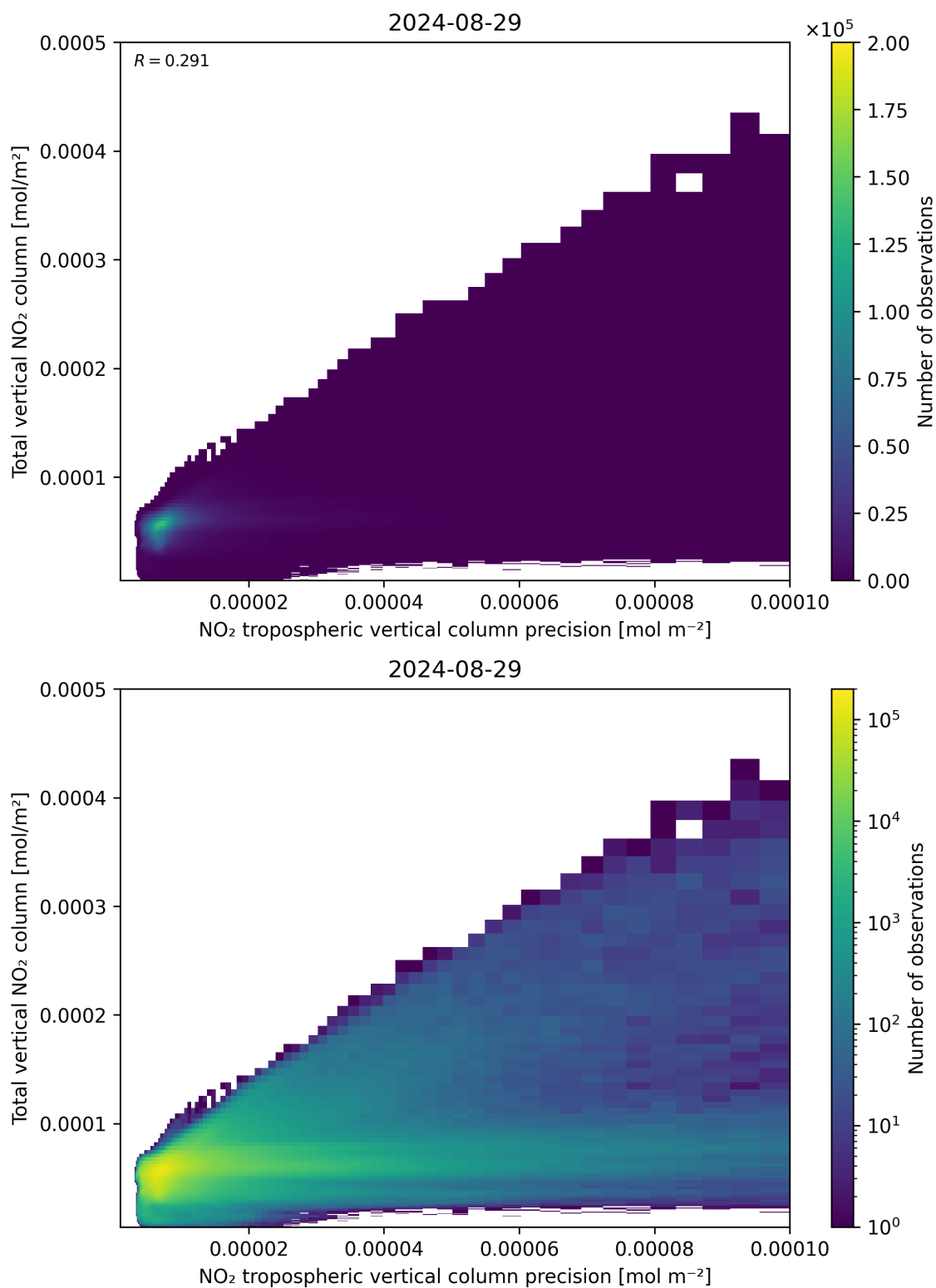
Figure 138: Scatter density plot of “NO 2 tropospheric vertical column precision” against “Total vertical NO 2 column” for 2024-08-28 to 2024-08-30.
