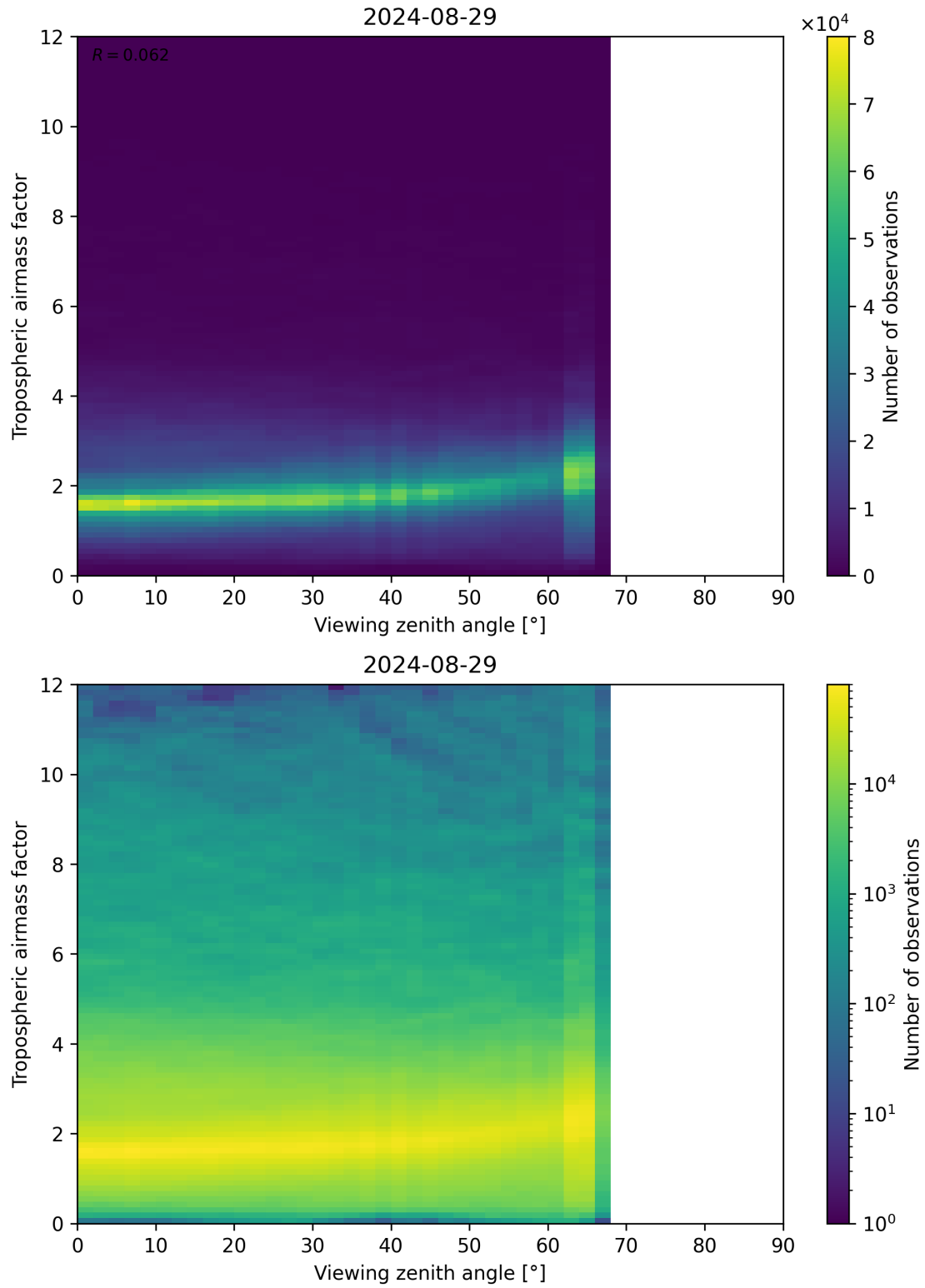
Figure 161: Scatter density plot of “Viewing zenith angle” against “Tropospheric airmass factor” for 2024-08-28 to 2024-08-30.
