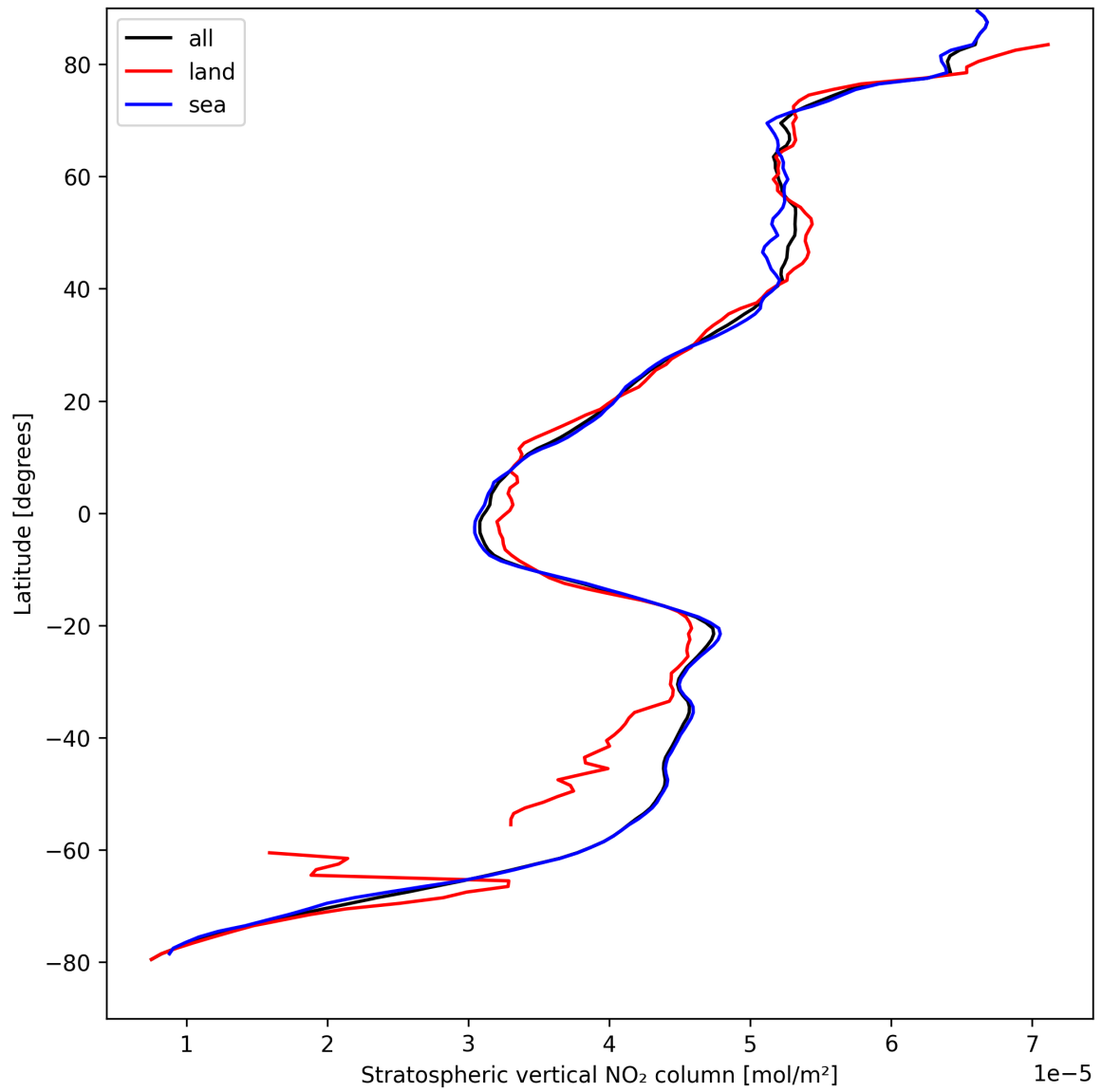
Figure 19: Zonal average of “Stratospheric vertical NO 2 column” for 2024-08-28 to 2024-08-30.
