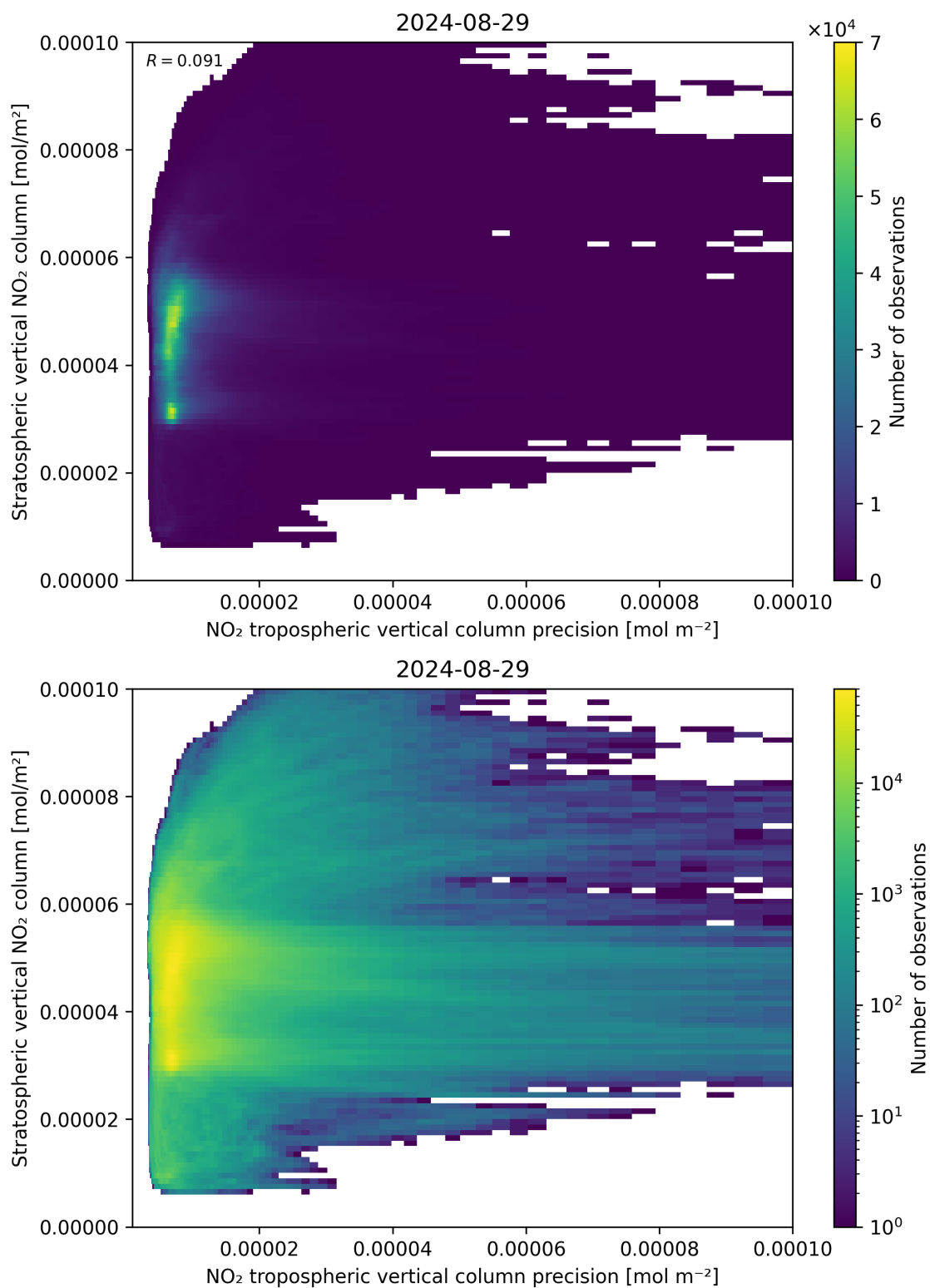
Figure 135: Scatter density plot of “NO 2 tropospheric vertical column precision” against “Stratospheric vertical NO 2 column” for 2024-08-28 to 2024-08-30.
