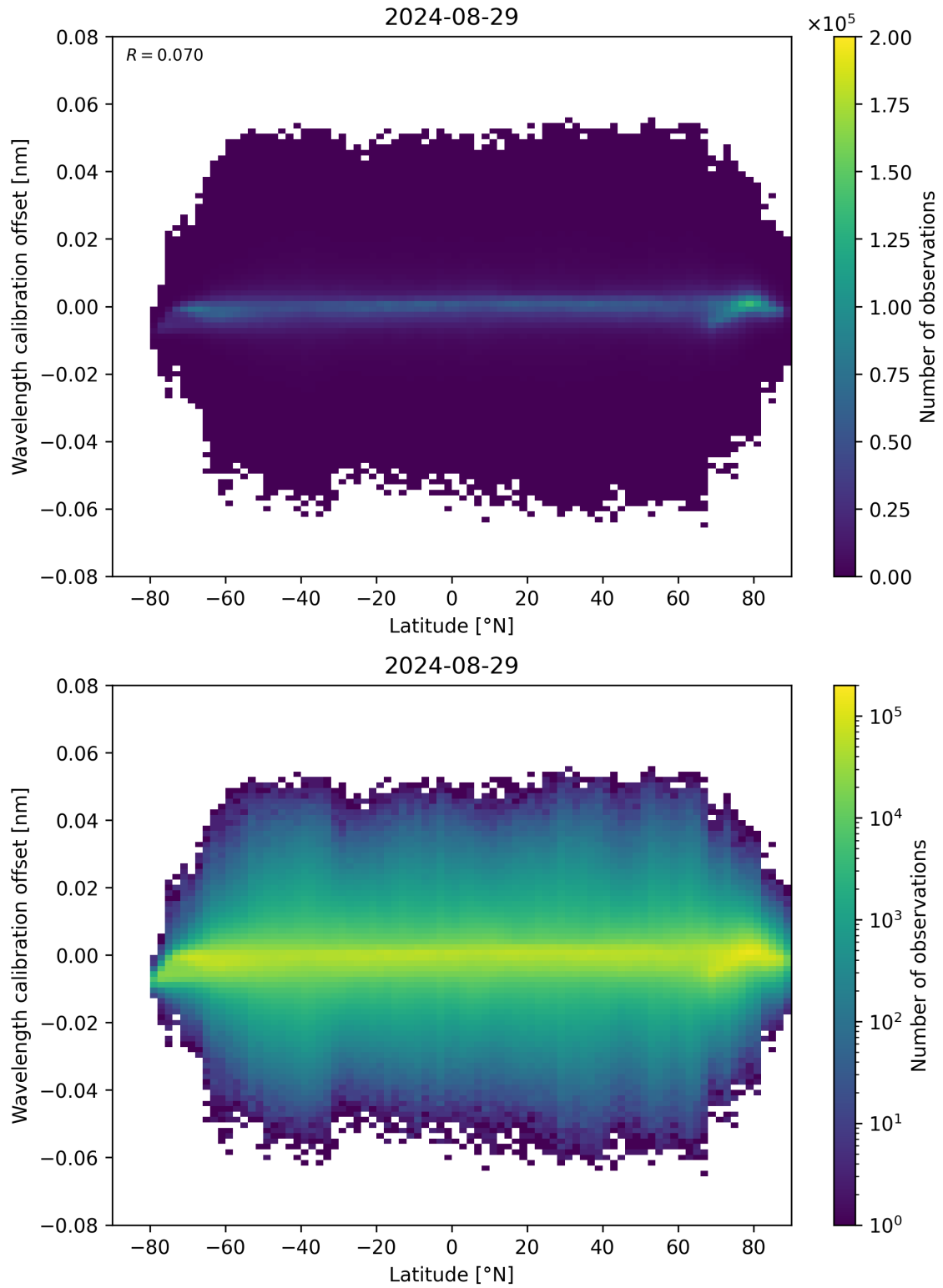
Figure 95: Scatter density plot of “Latitude” against “Wavelength calibration offset” for 2024-08-28 to 2024-08-30.
