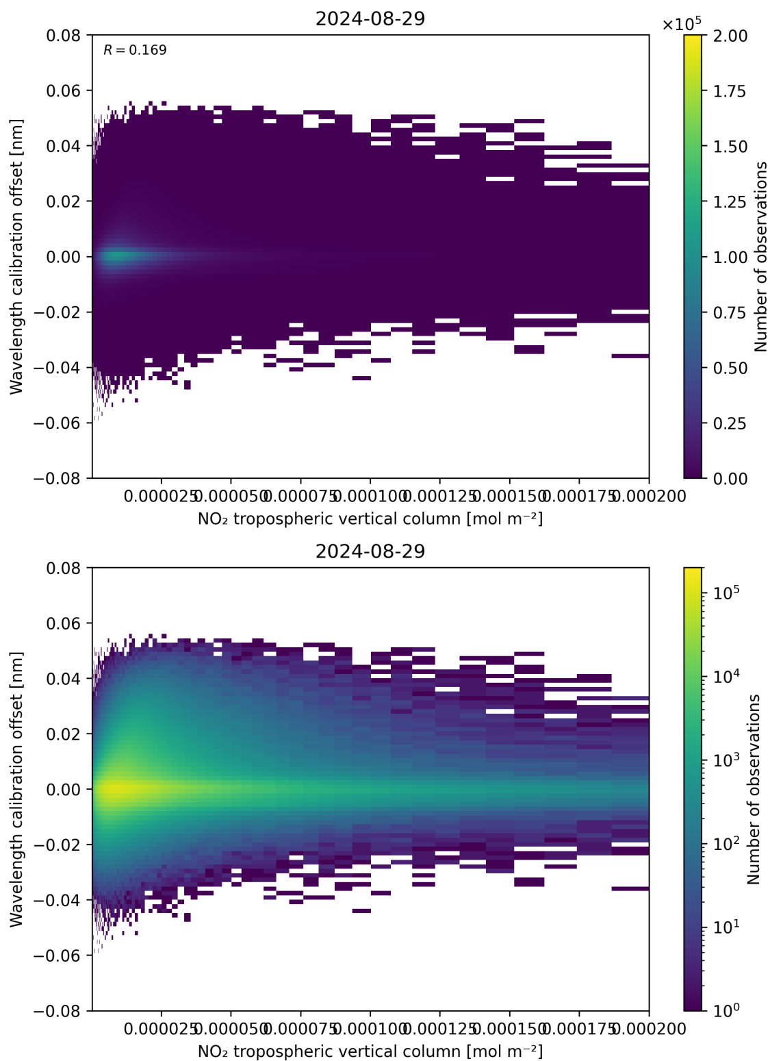
Figure 143: Scatter density plot of “NO 2 tropospheric vertical column” against “Wavelength calibration offset” for 2024-08-28 to 2024-08-30.
