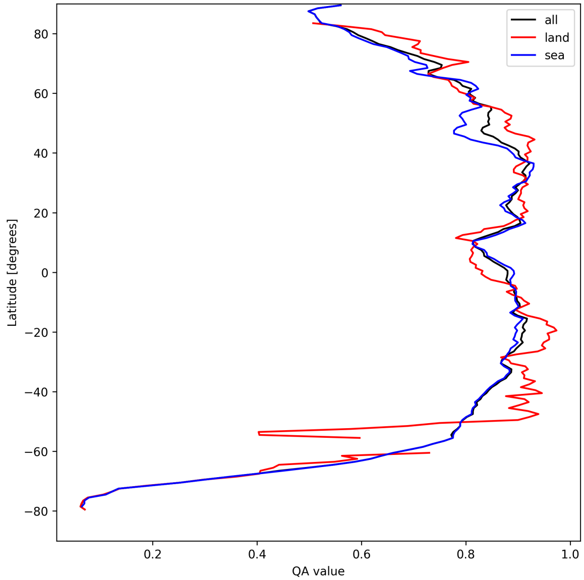
Figure 11: Zonal average of “QA value” for 2024-08-28 to 2024-08-30.
