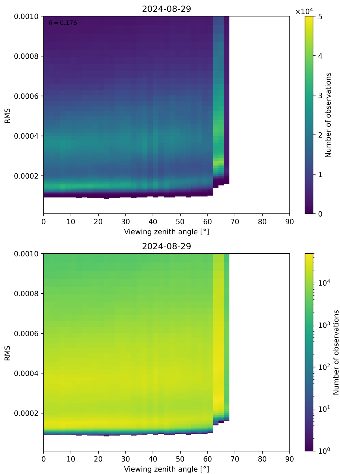
Figure 171: Scatter density plot of “Viewing zenith angle” against “RMS” for 2024-08-28 to 2024-08-30.
