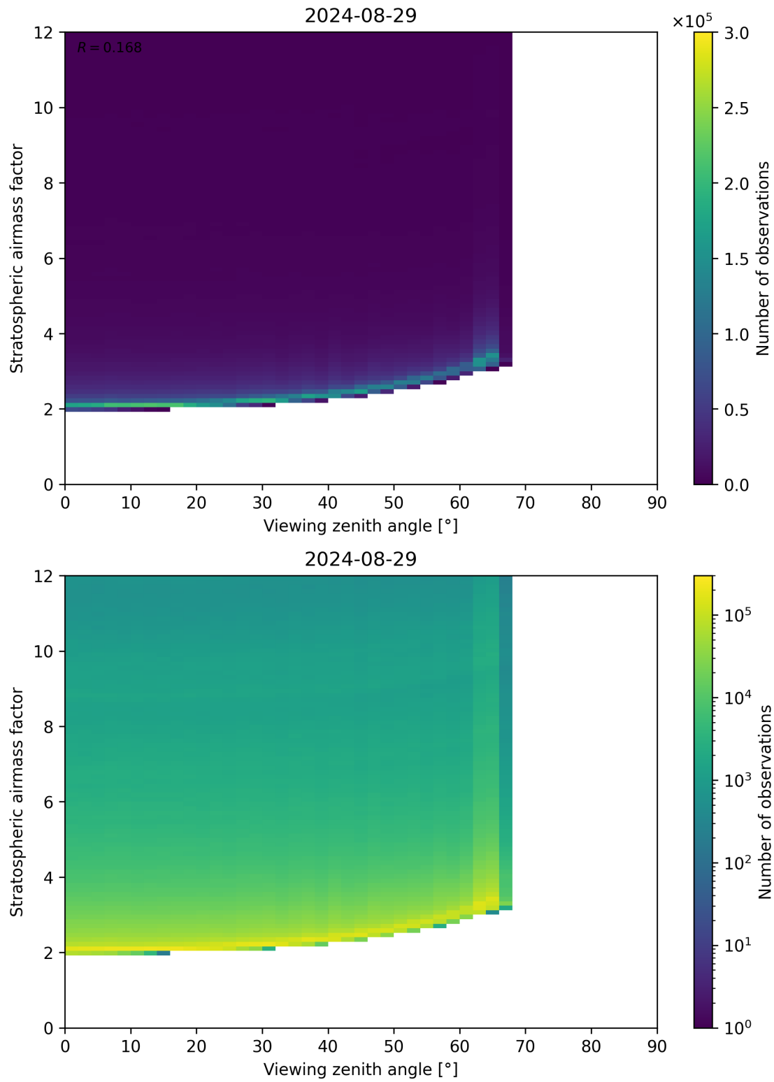
Figure 159: Scatter density plot of “Viewing zenith angle” against “Stratospheric airmass factor” for 2024-08-28 to 2024-08-30.
