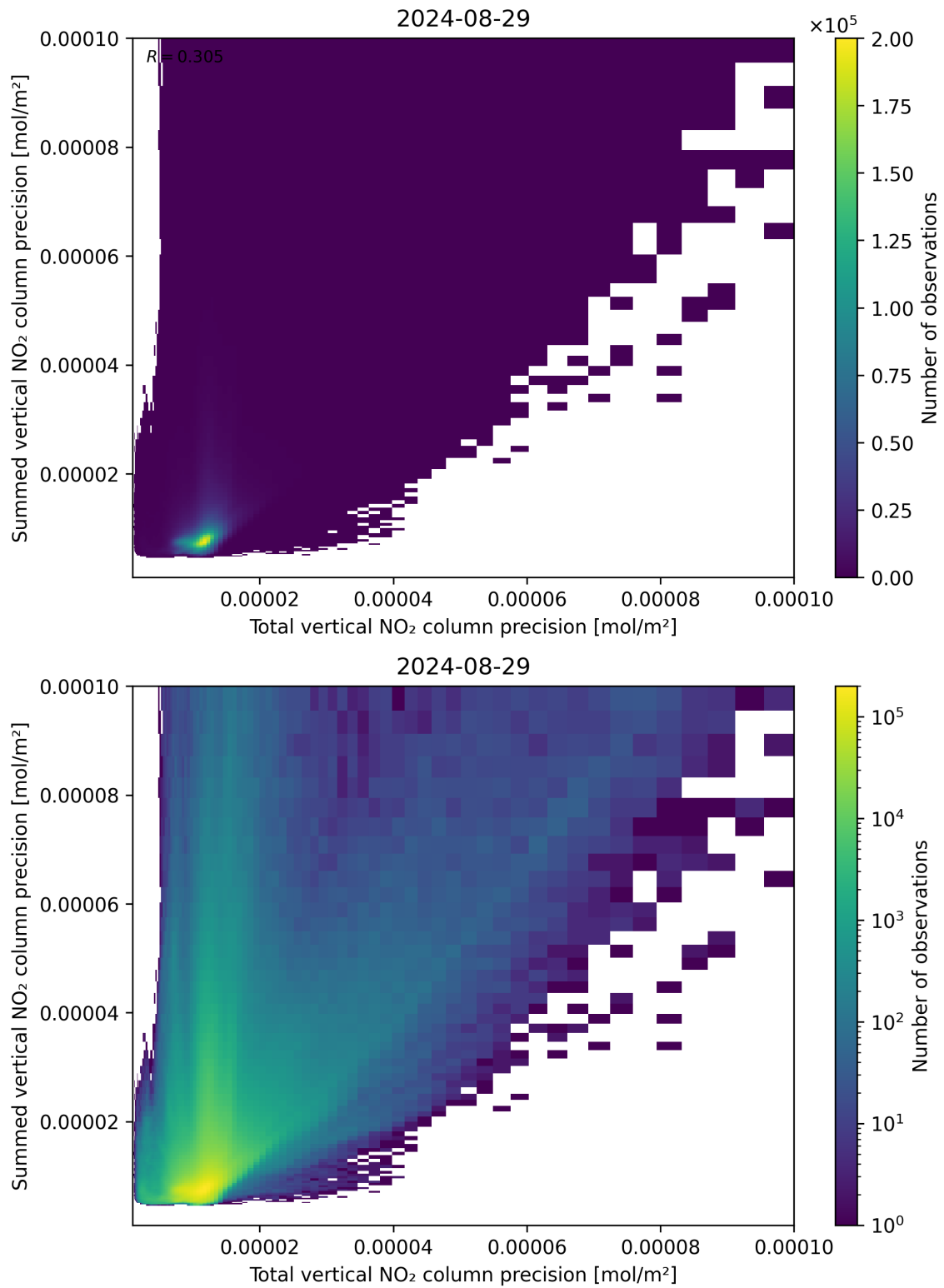
Figure 118: Scatter density plot of “Total vertical NO 2 column precision” against “Summed vertical NO 2 column precision” for 2024-08-28 to 2024-08-30.
