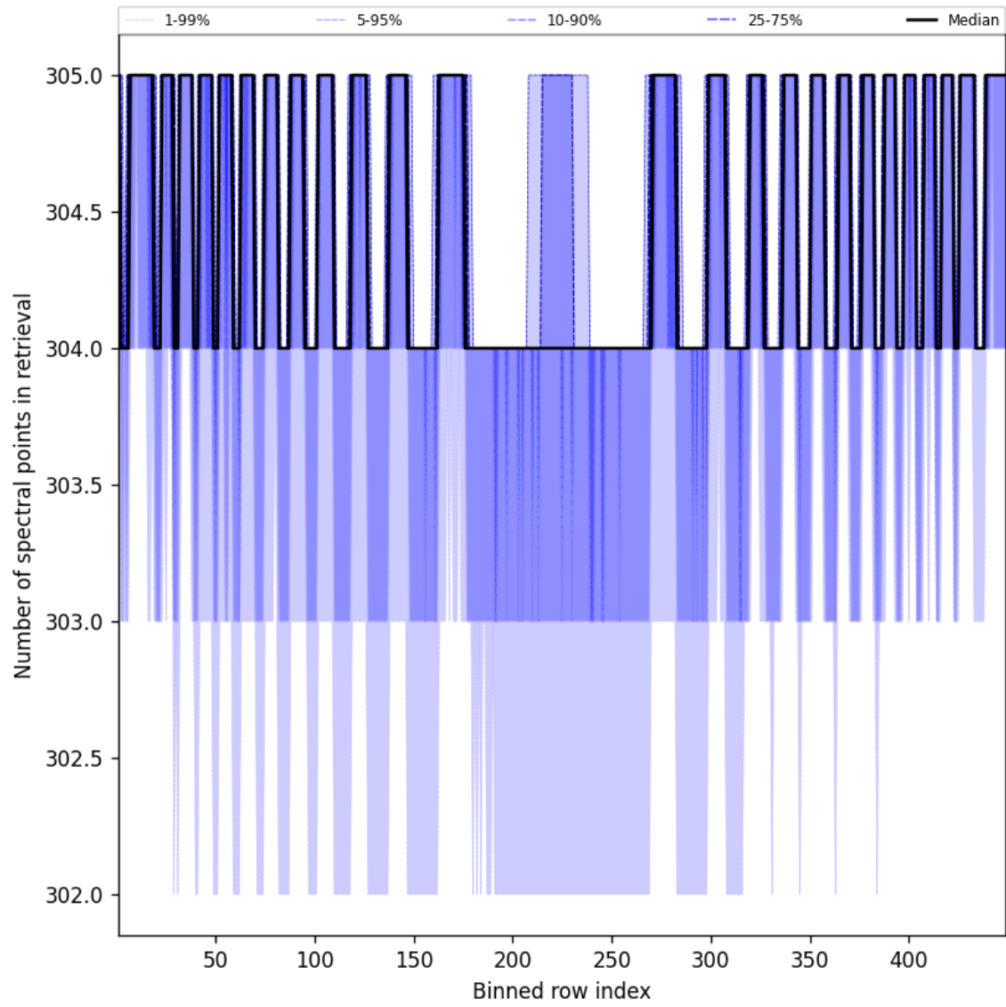
Figure 50: Along track statistics of “Number of spectral points in retrieval” for 2024-08-28 to 2024-08-30
