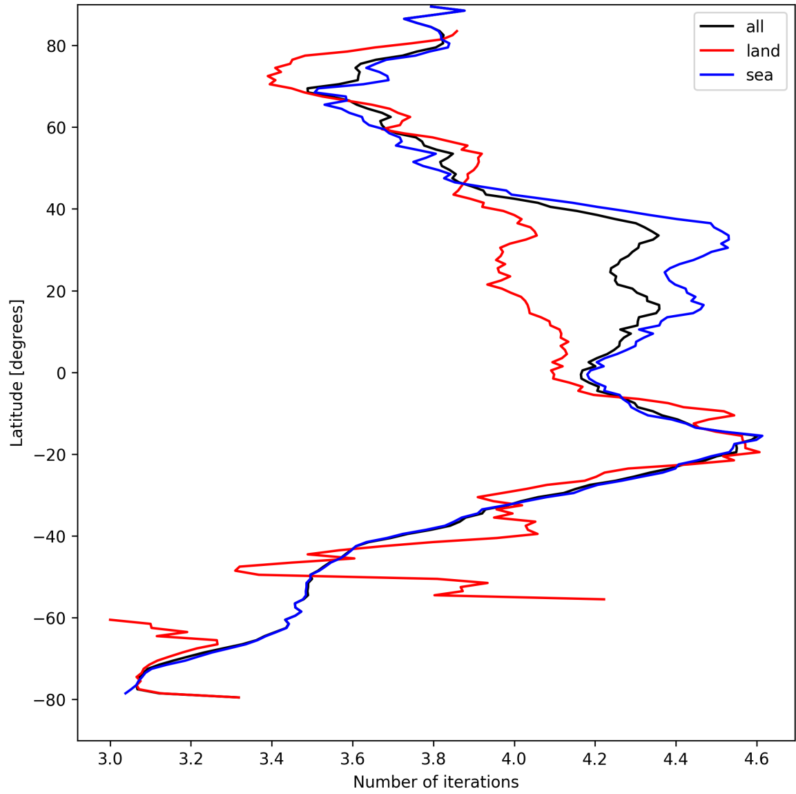
Figure 17: Zonal average of “Number of iterations” for 2024-08-28 to 2024-08-30.
