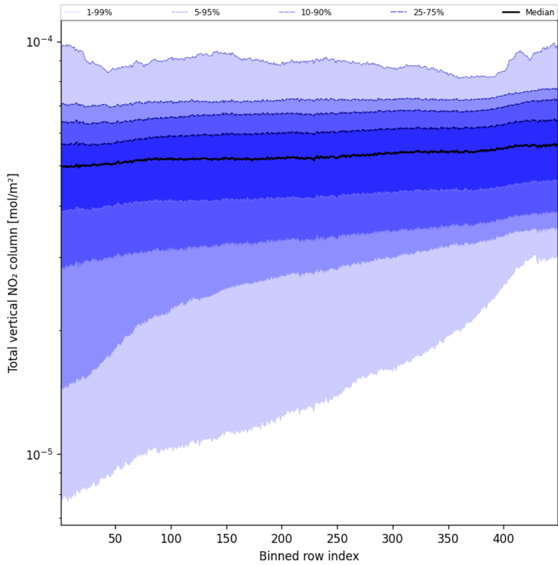
Figure 55: Along track statistics of “Total vertical NO 2 column” for 2024-08-28 to 2024-08-30
