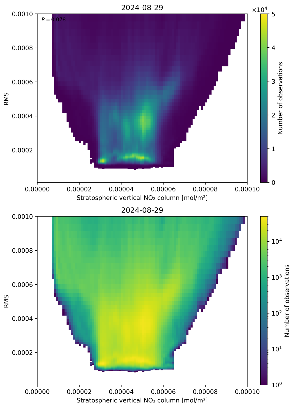
Figure 102: Scatter density plot of “Stratospheric vertical NO 2 column” against “RMS” for 2024-08-28 to 2024-08-30.
