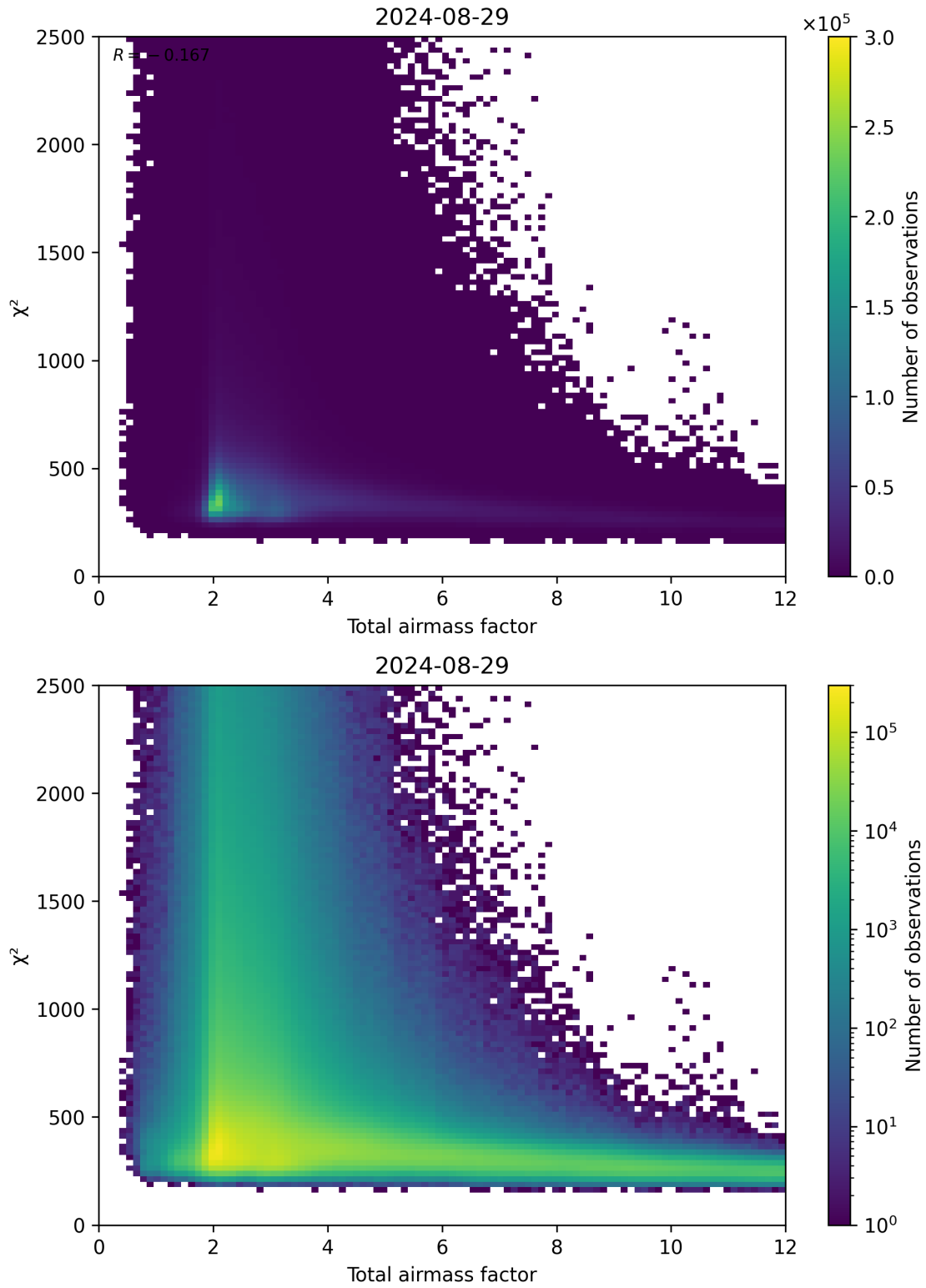
Figure 63: Scatter density plot of “Total airmass factor” against “ \chi^2 ” for 2024-08-28 to 2024-08-30.
