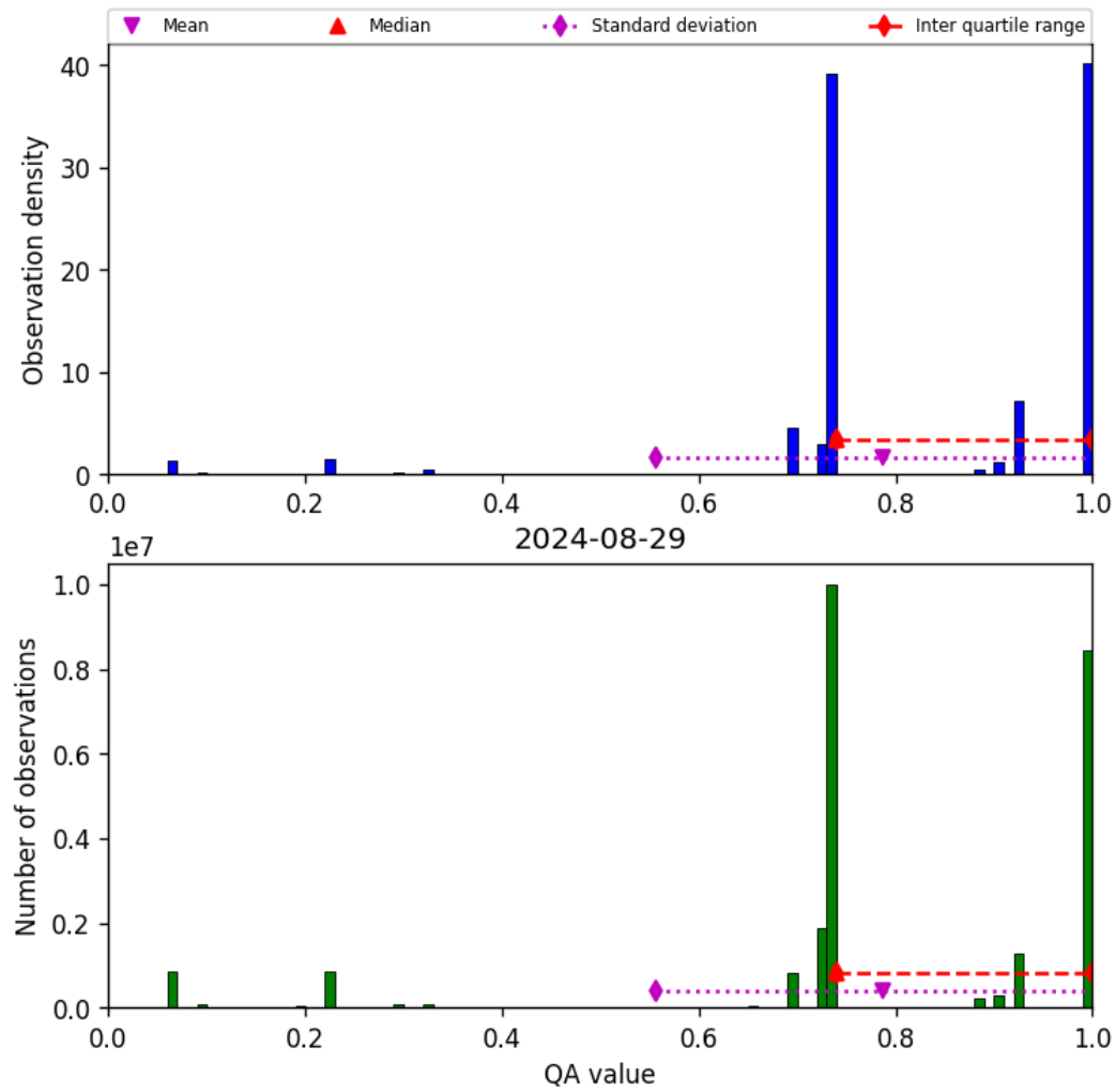
Figure 28: Histogram of “QA value” for 2024-08-28 to 2024-08-30
