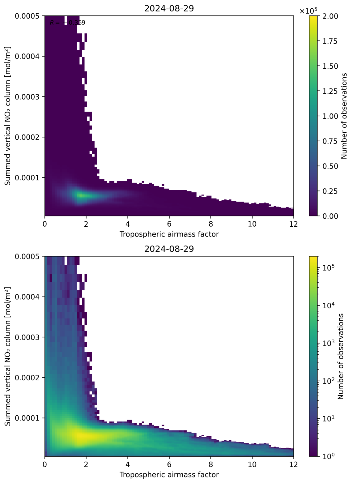
Figure 75: Scatter density plot of “Tropospheric airmass factor” against “Summed vertical NO 2 column” for 2024-08-28 to 2024-08-30.
