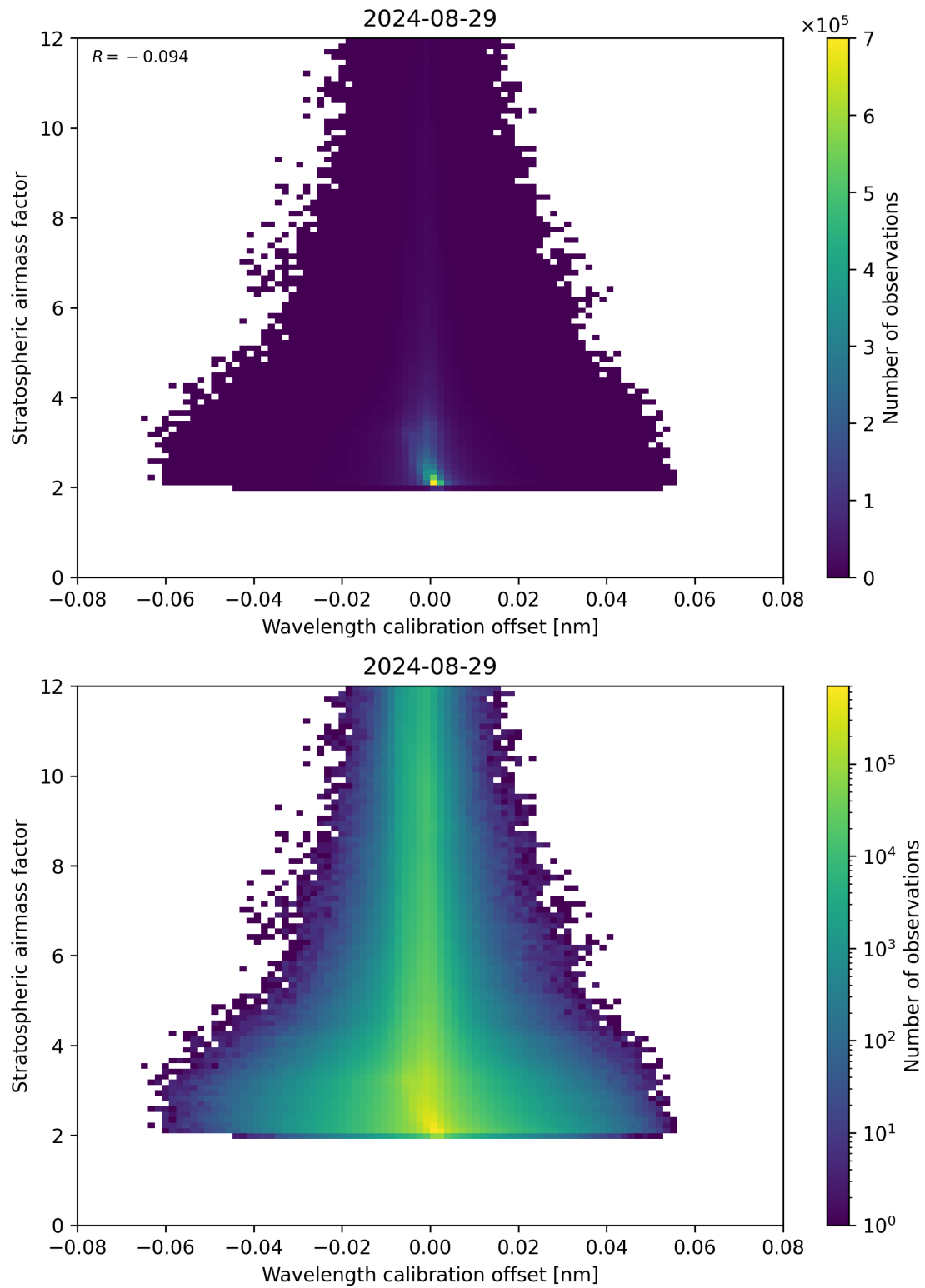
Figure 174: Scatter density plot of “Wavelength calibration offset” against “Stratospheric airmass factor” for 2024-08-28 to 2024-08-30.
