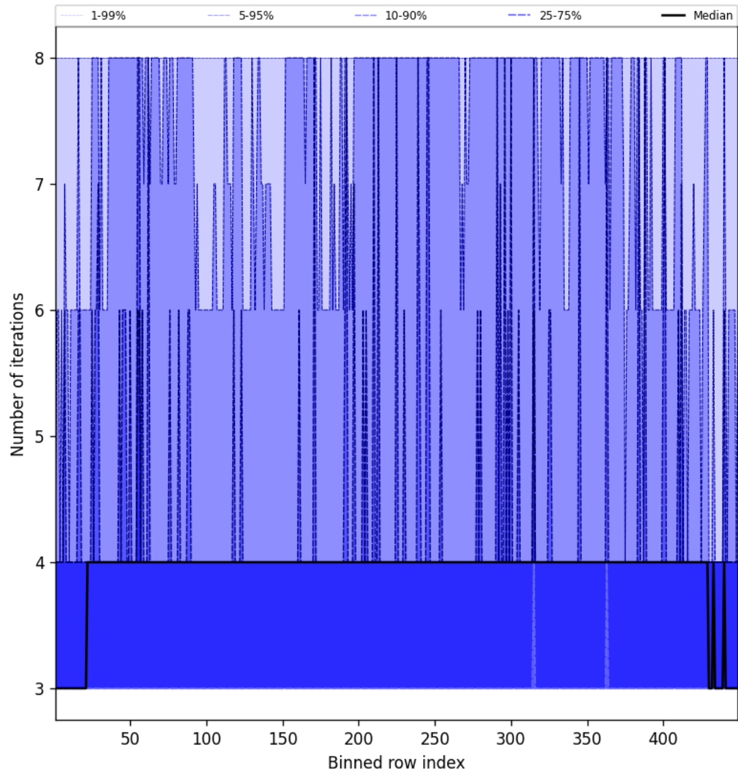
Figure 51: Along track statistics of “Number of iterations” for 2024-08-28 to 2024-08-30
