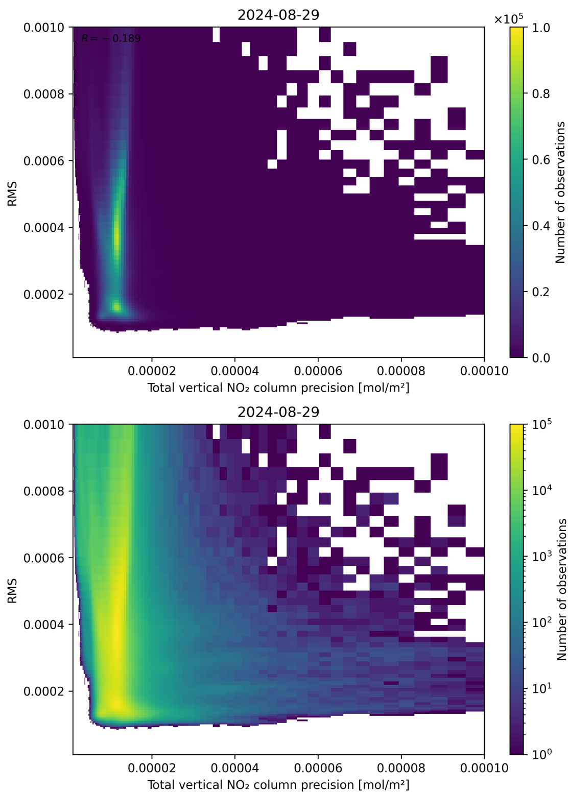
Figure 119: Scatter density plot of “Total vertical NO 2 column precision” against “RMS” for 2024-08-28 to 2024-08-30.
