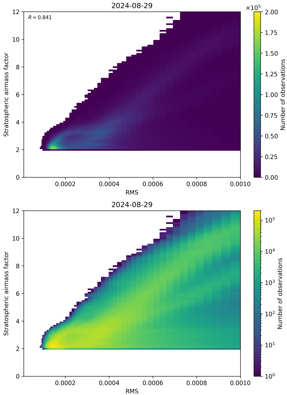
Figure 144: Scatter density plot of “RMS” against “Stratospheric airmass factor” for 2024-08-28 to 2024-08-30.
