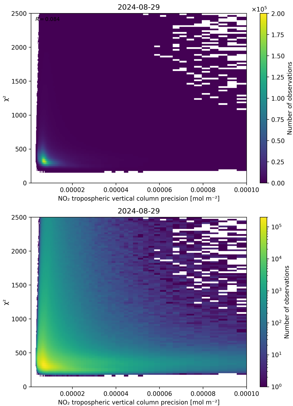
Figure 134: Scatter density plot of “NO 2 tropospheric vertical column precision” against “ \chi^2 ” for 2024-08-28 to 2024-08-30.
