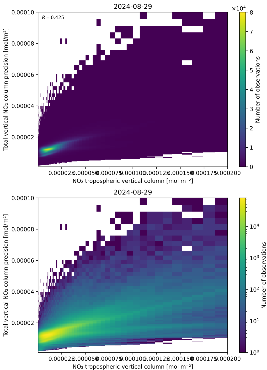
Figure 129: Scatter density plot of “NO 2 tropospheric vertical column” against “Total vertical NO 2 column precision” for 2024-08-28 to 2024-08-30.
