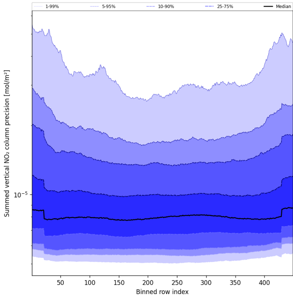
Figure 58: Along track statistics of “Summed vertical NO 2 column precision” for 2024-08-28 to 2024-08-30
