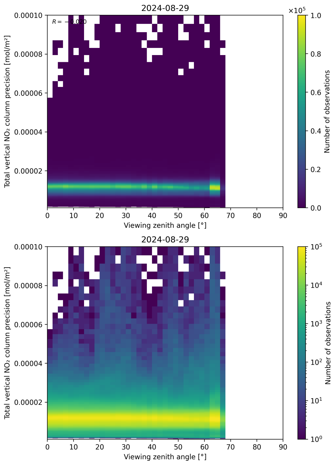
Figure 168: Scatter density plot of “Viewing zenith angle” against “Total vertical NO 2 column precision” for 2024-08-28 to 2024-08-30.
