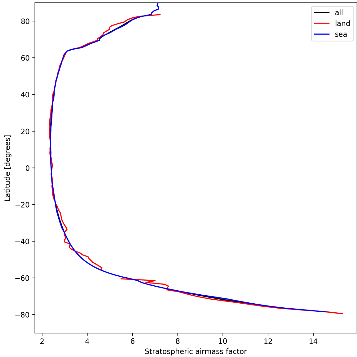
Figure 27: Zonal average of “Stratospheric airmass factor” for 2024-08-28 to 2024-08-30.
