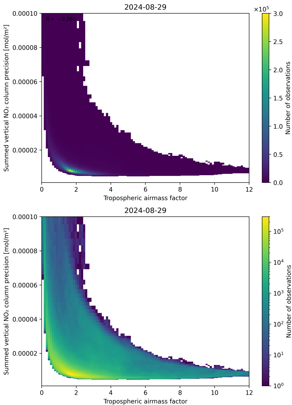
Figure 76: Scatter density plot of “Tropospheric air mass factor” against “Summed vertical NO 2 column precision” for 2024-08-28 to 2024-08-30.
