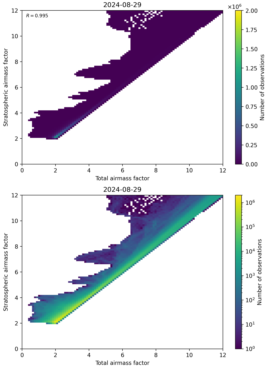
Figure 62: Scatter density plot of “Total airmass factor” against “Stratospheric airmass factor” for 2024-08-28 to 2024-08-30.
