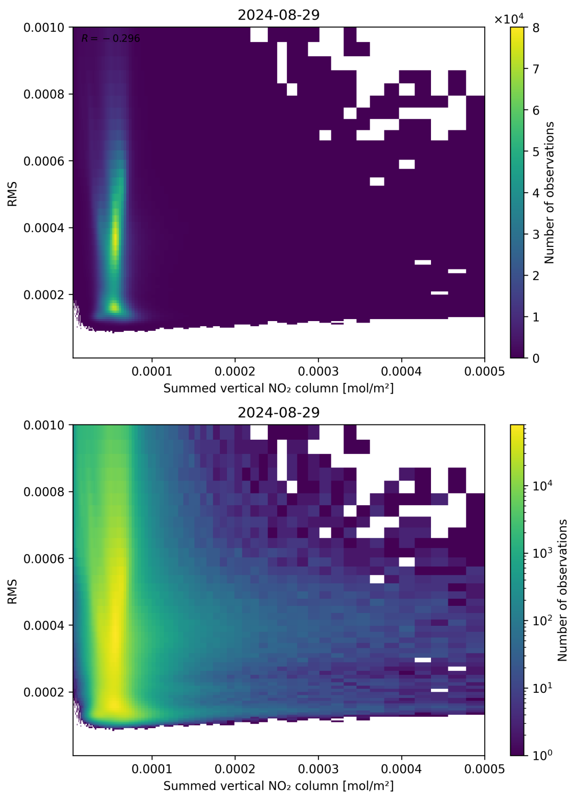
Figure 109: Scatter density plot of “Summed vertical NO 2 column” against “RMS” for 2024-08-28 to 2024-08-30.
