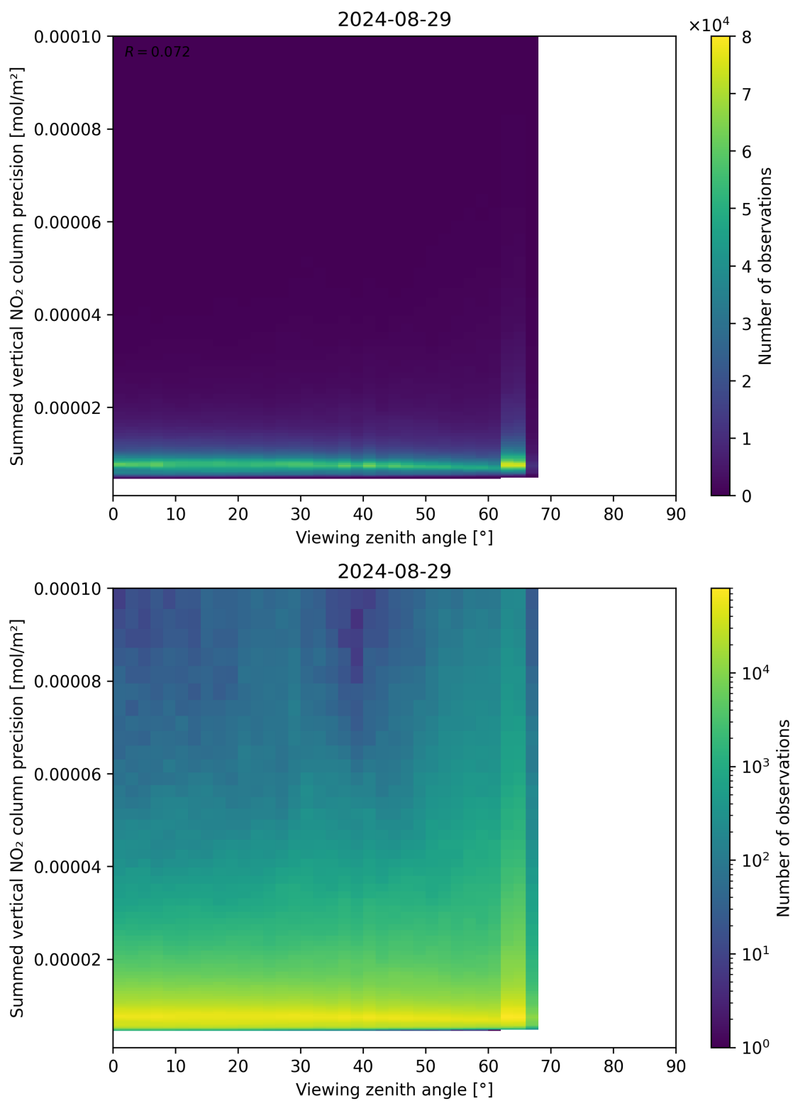
Figure 166: Scatter density plot of “Viewing zenith angle” against “Summed vertical NO 2 column precision” for 2024-08-28 to 2024-08-30.
