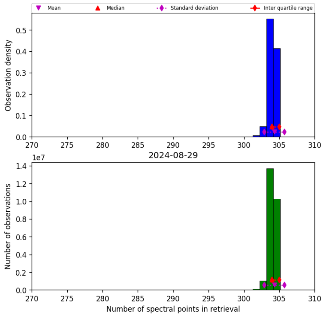
Figure 33: Histogram of “Number of spectral points in retrieval” for 2024-08-28 to 2024-08-30
