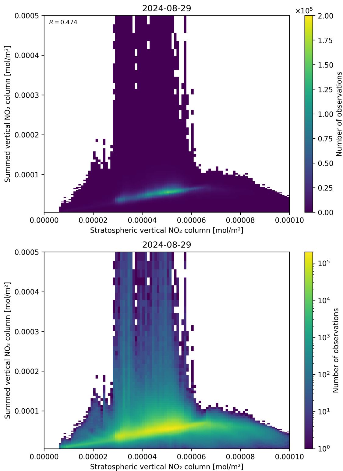
Figure 98: Scatter density plot of “Stratospheric vertical NO 2 column” against “Summed vertical NO 2 column” for 2024-08-28 to 2024-08-30.
