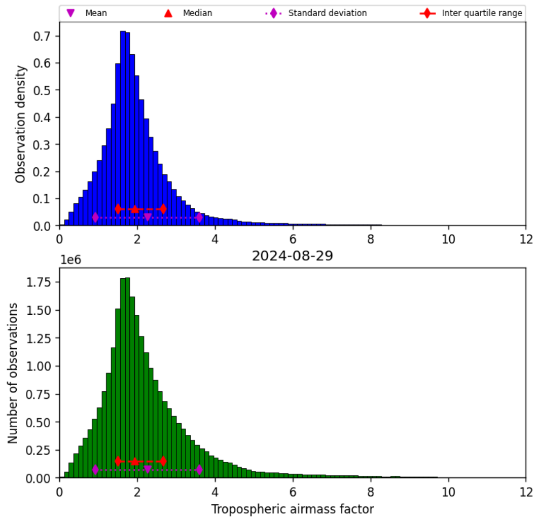
Figure 31: Histogram of “Tropospheric airmass factor” for 2024-08-28 to 2024-08-30
