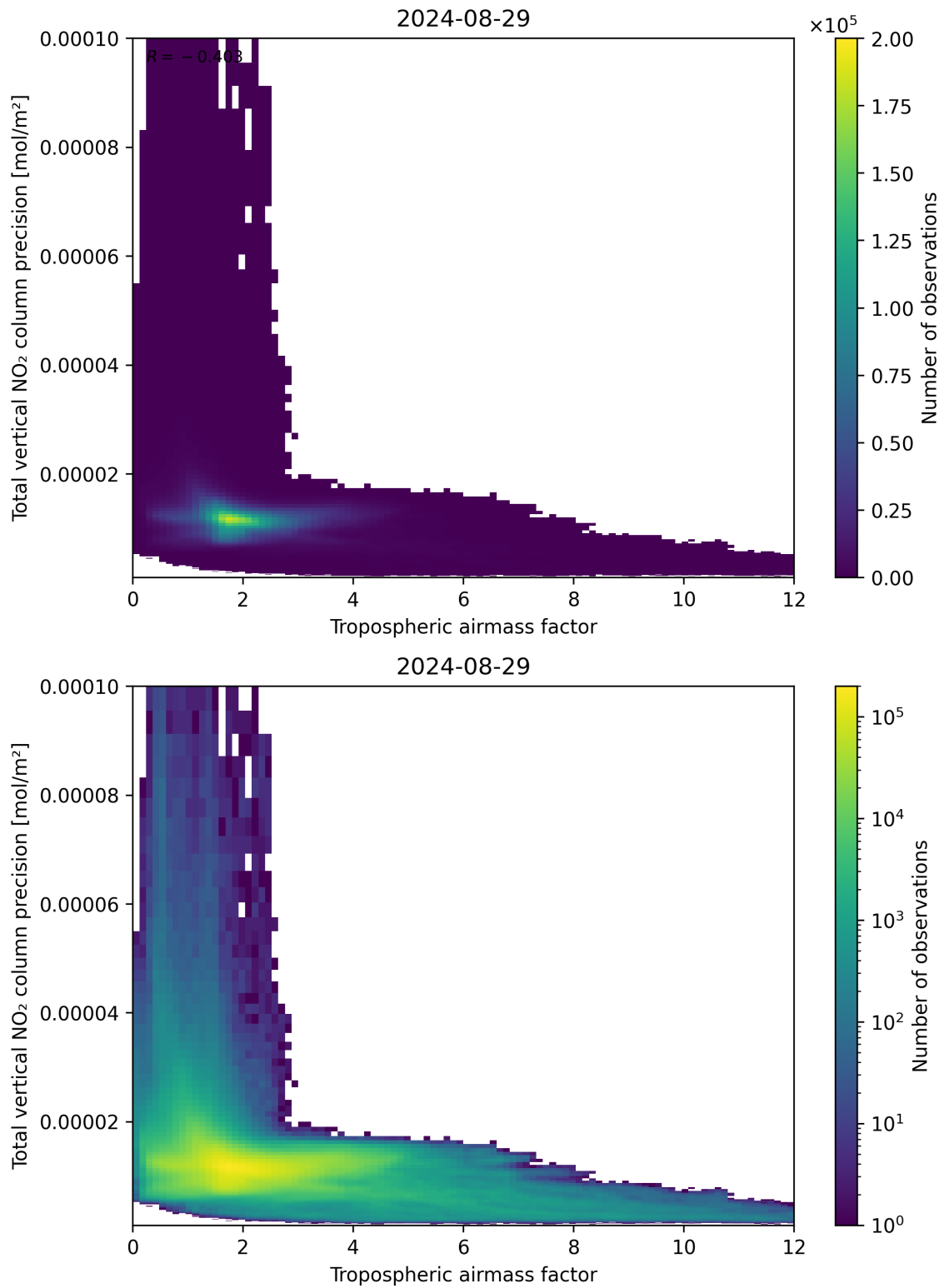
Figure 78: Scatter density plot of “Tropospheric airmass factor” against “Total vertical NO 2 column precision” for 2024-08-28 to 2024-08-30.
