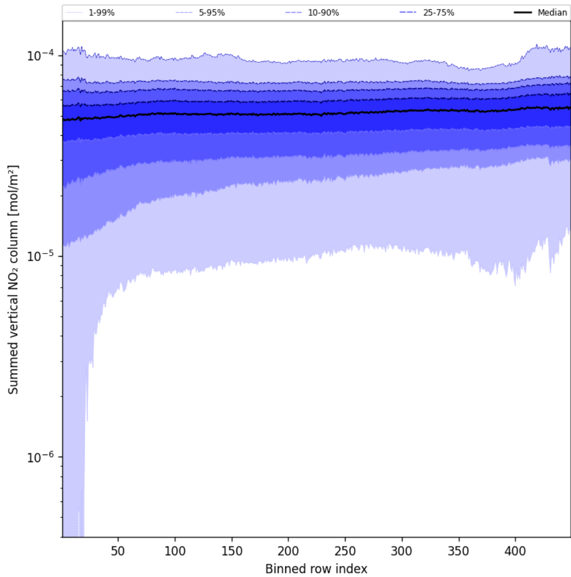
Figure 57: Along track statistics of “Summed vertical NO 2 column” for 2024-08-28 to 2024-08-30
