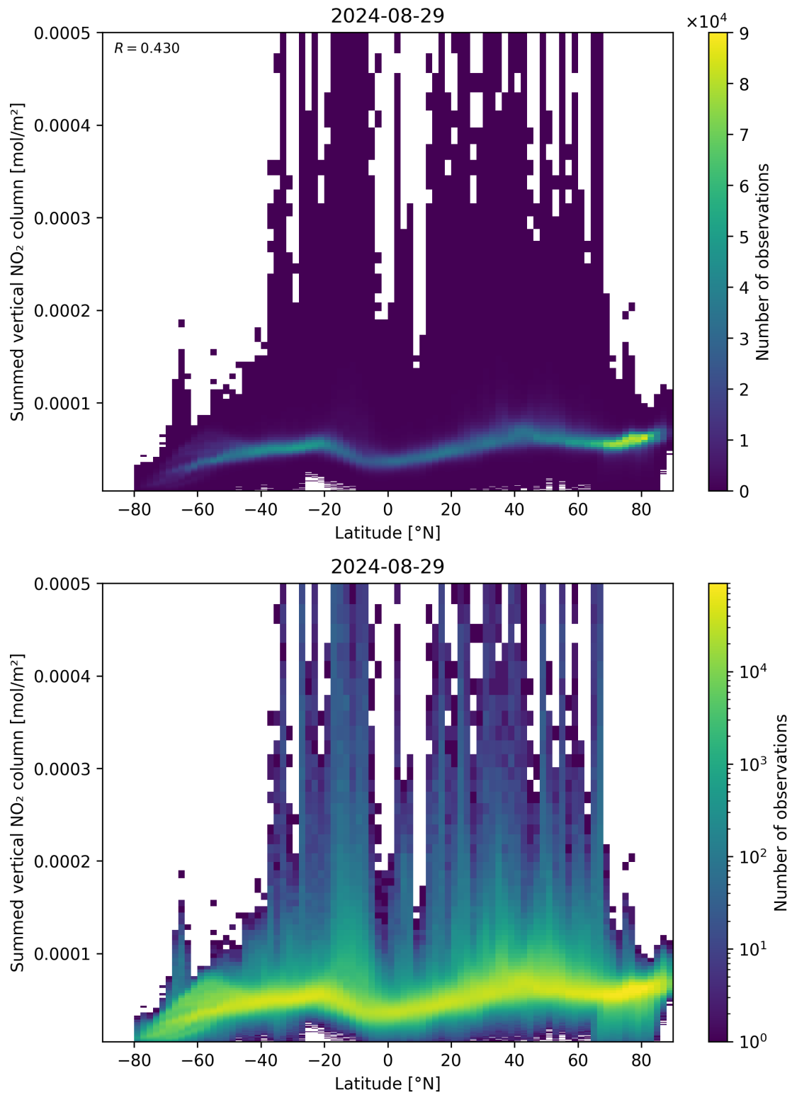
Figure 88: Scatter density plot of “Latitude” against “Summed vertical NO 2 column” for 2024-08-28 to 2024-08-30.
