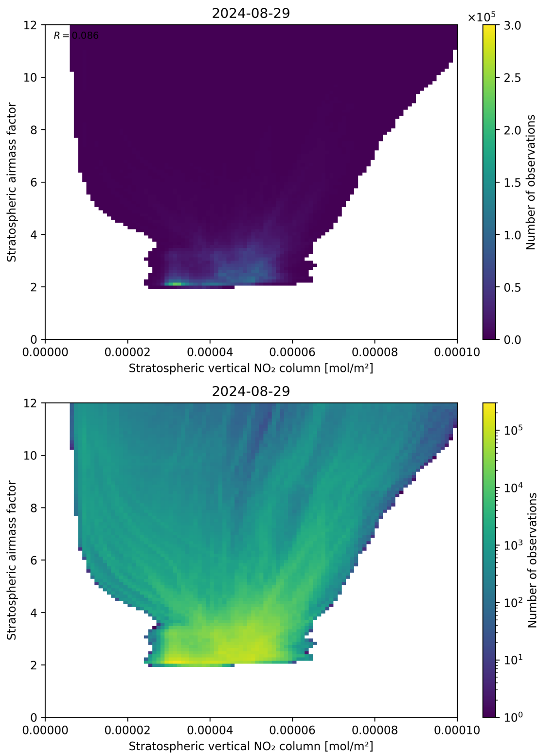
Figure 96: Scatter density plot of “Stratospheric vertical NO 2 column” against “Stratospheric airmass factor” for 2024-08-28 to 2024-08-30.
