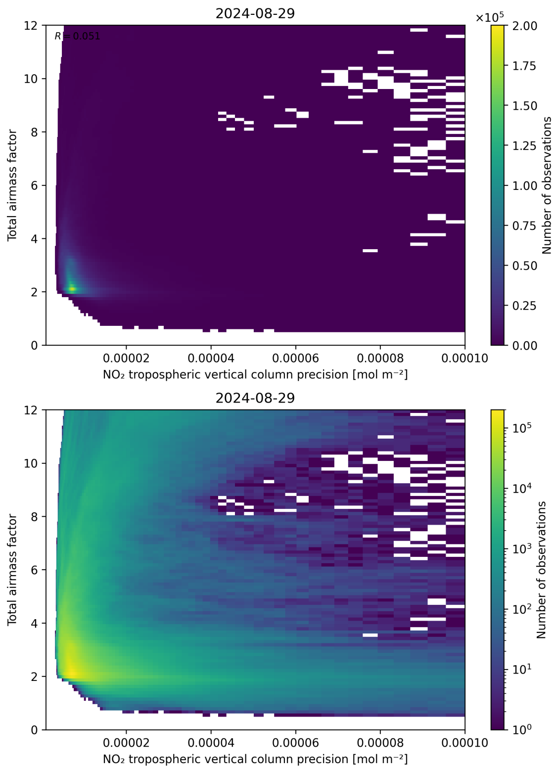
Figure 132: Scatter density plot of “NO 2 tropospheric vertical column precision” against “Total air mass factor” for 2024-08-28 to 2024-08-30.
