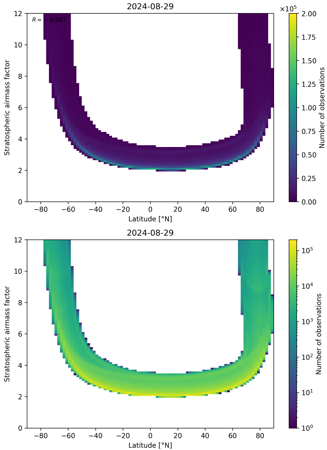
Figure 83: Scatter density plot of “Latitude” against “Stratospheric air mass factor” for 2024-08-28 to 2024-08-30.
