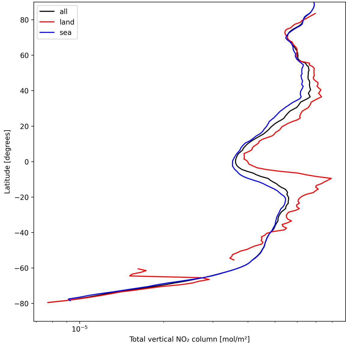
Figure 21: Zonal average of “Total vertical NO 2 column” for 2024-08-28 to 2024-08-30.
