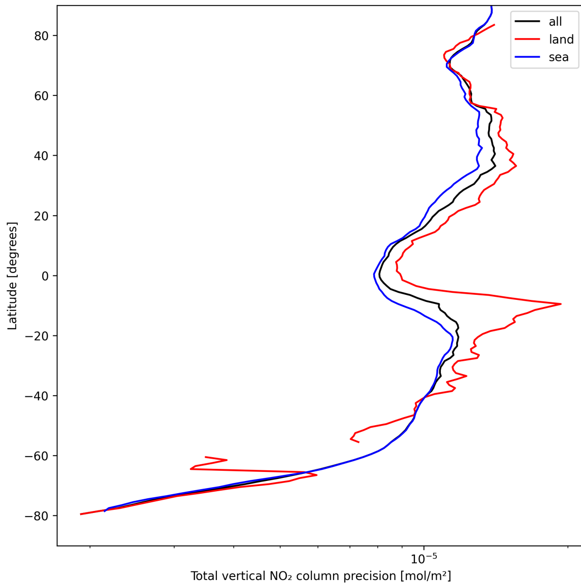
Figure 22: Zonal average of “Total vertical NO 2 column precision” for 2024-08-28 to 2024-08-30.
