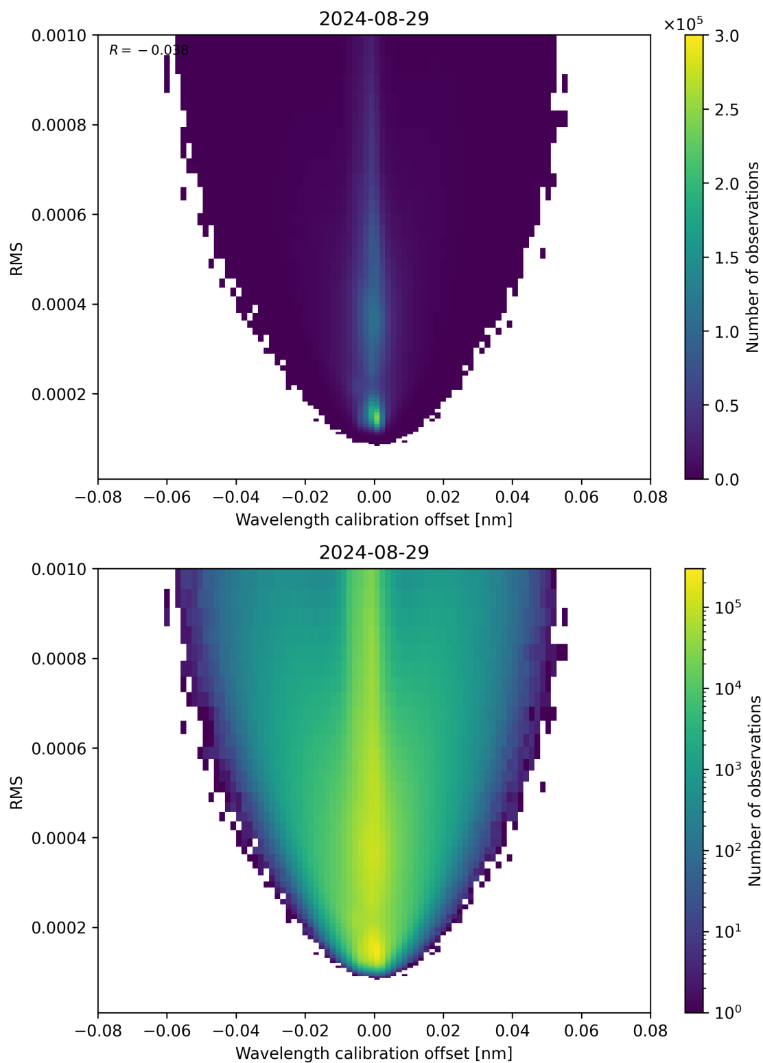
Figure 181: Scatter density plot of “Wavelength calibration offset” against “RMS” for 2024-08-28 to 2024-08-30.
