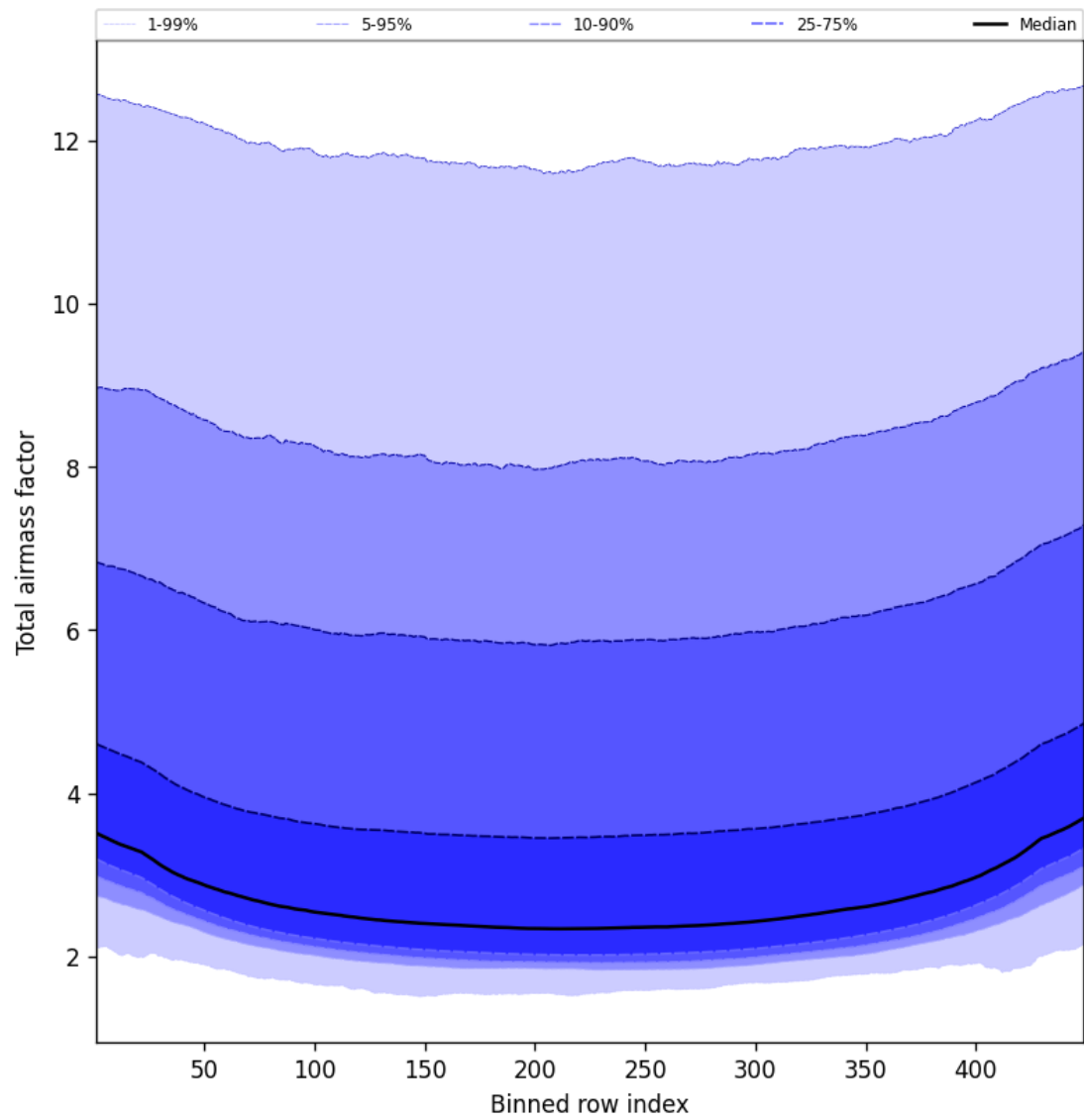
Figure 49: Along track statistics of “Total airmass factor” for 2024-08-28 to 2024-08-30
