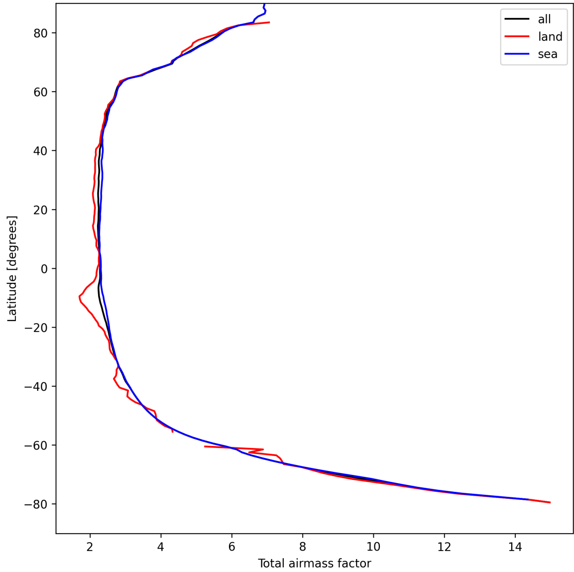
Figure 15: Zonal average of “Total airmass factor” for 2024-08-28 to 2024-08-30.
