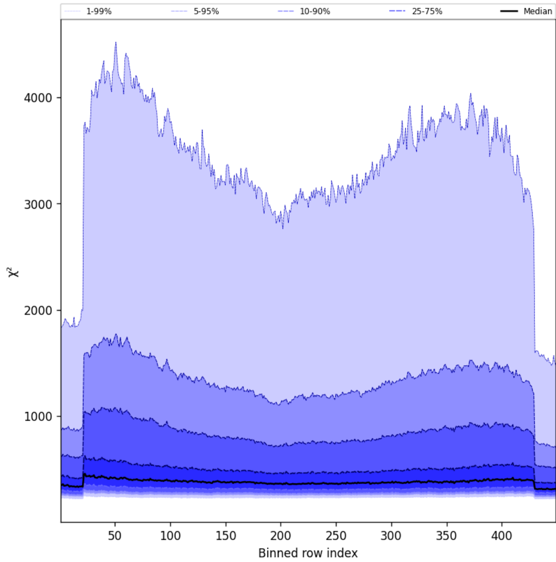
Figure 59: Along track statistics of “ \chi^2 ” for 2024-08-28 to 2024-08-30
