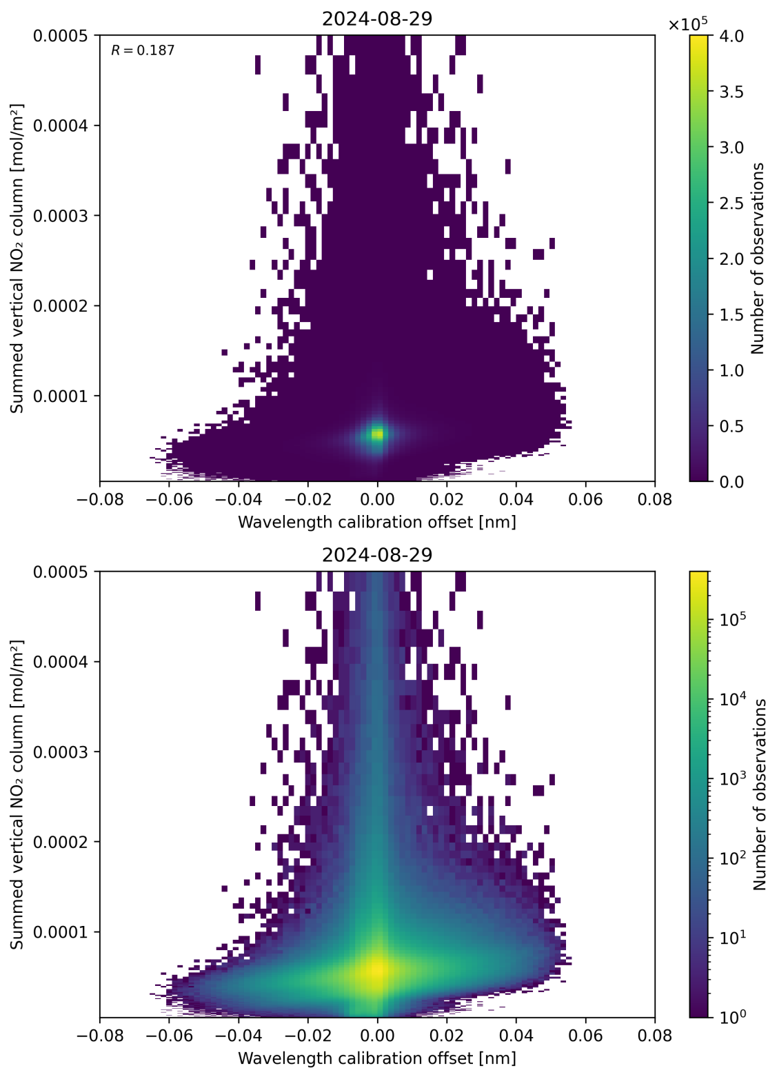
Figure 177: Scatter density plot of “Wavelength calibration offset” against “Summed vertical NO 2 column” for 2024-08-28 to 2024-08-30.
