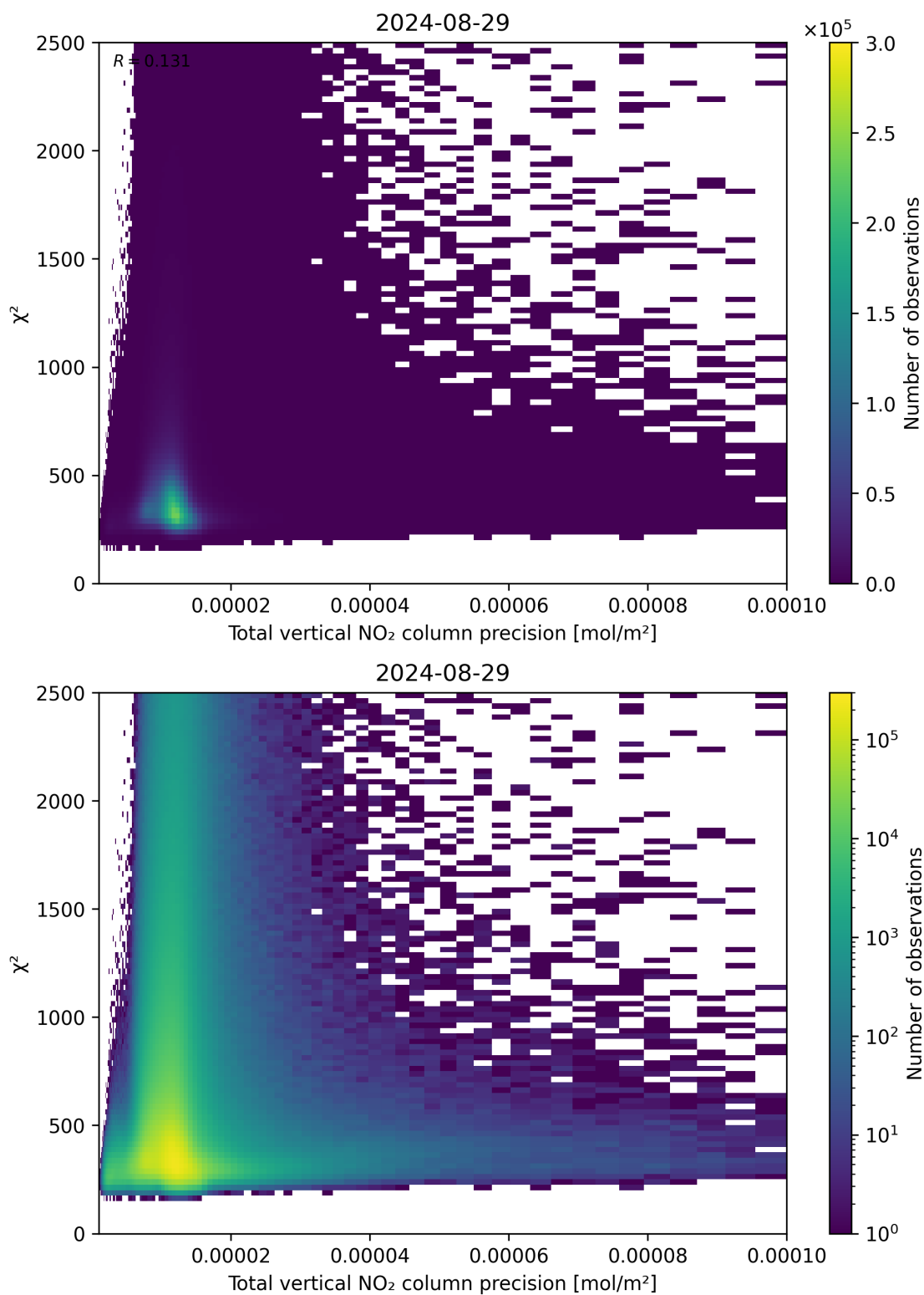
Figure 116: Scatter density plot of “Total vertical NO 2 column precision” against “ \chi^2 ” for 2024-08-28 to 2024-08-30.
