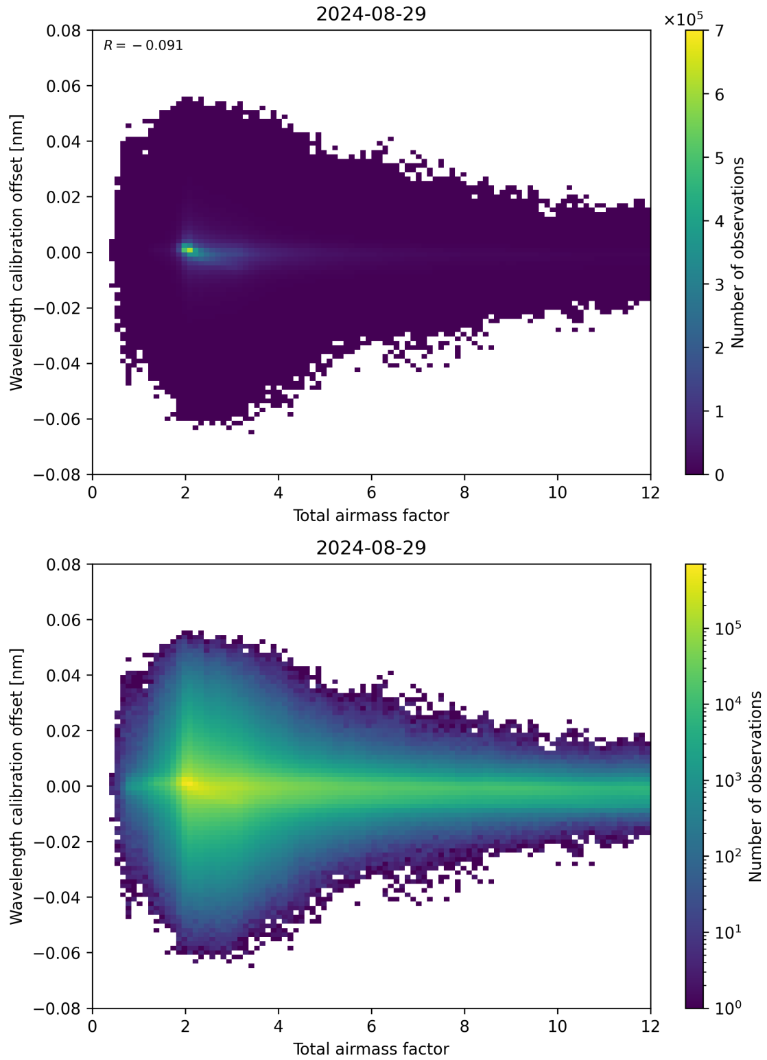
Figure 70: Scatter density plot of “Total airmass factor” against “Wavelength calibration offset” for 2024-08-28 to 2024-08-30.
