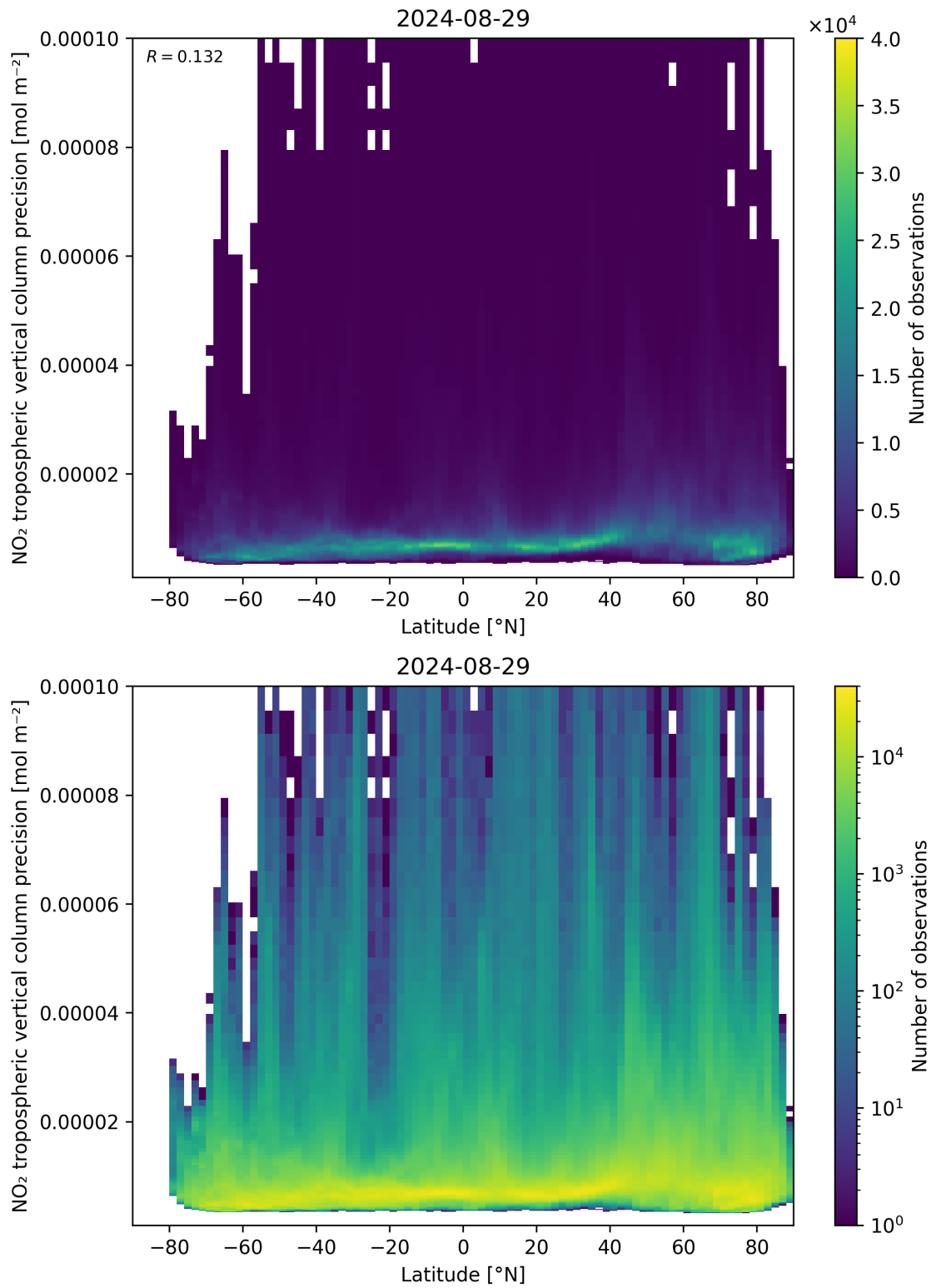
Figure 93: Scatter density plot of “Latitude” against “NO 2 tropospheric vertical column precision” for 2024-08-28 to 2024-08-30.
