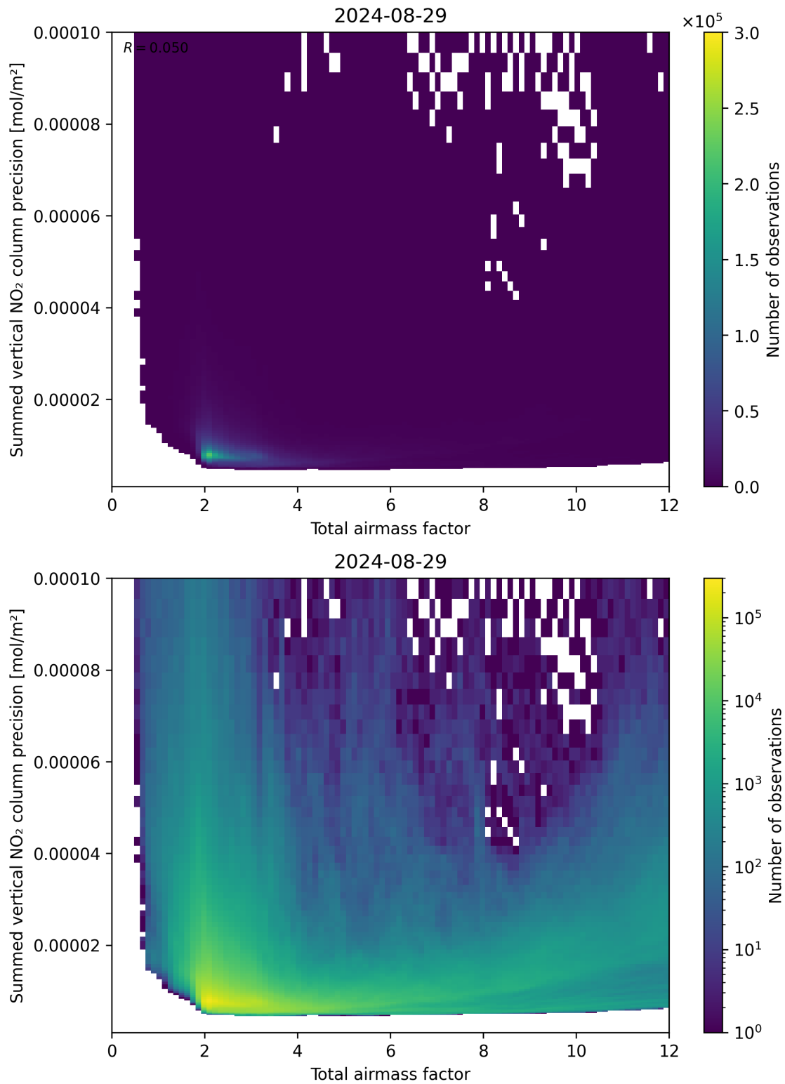
Figure 66: Scatter density plot of “Total airmass factor” against “Summed vertical NO 2 column precision” for 2024-08-28 to 2024-08-30.
