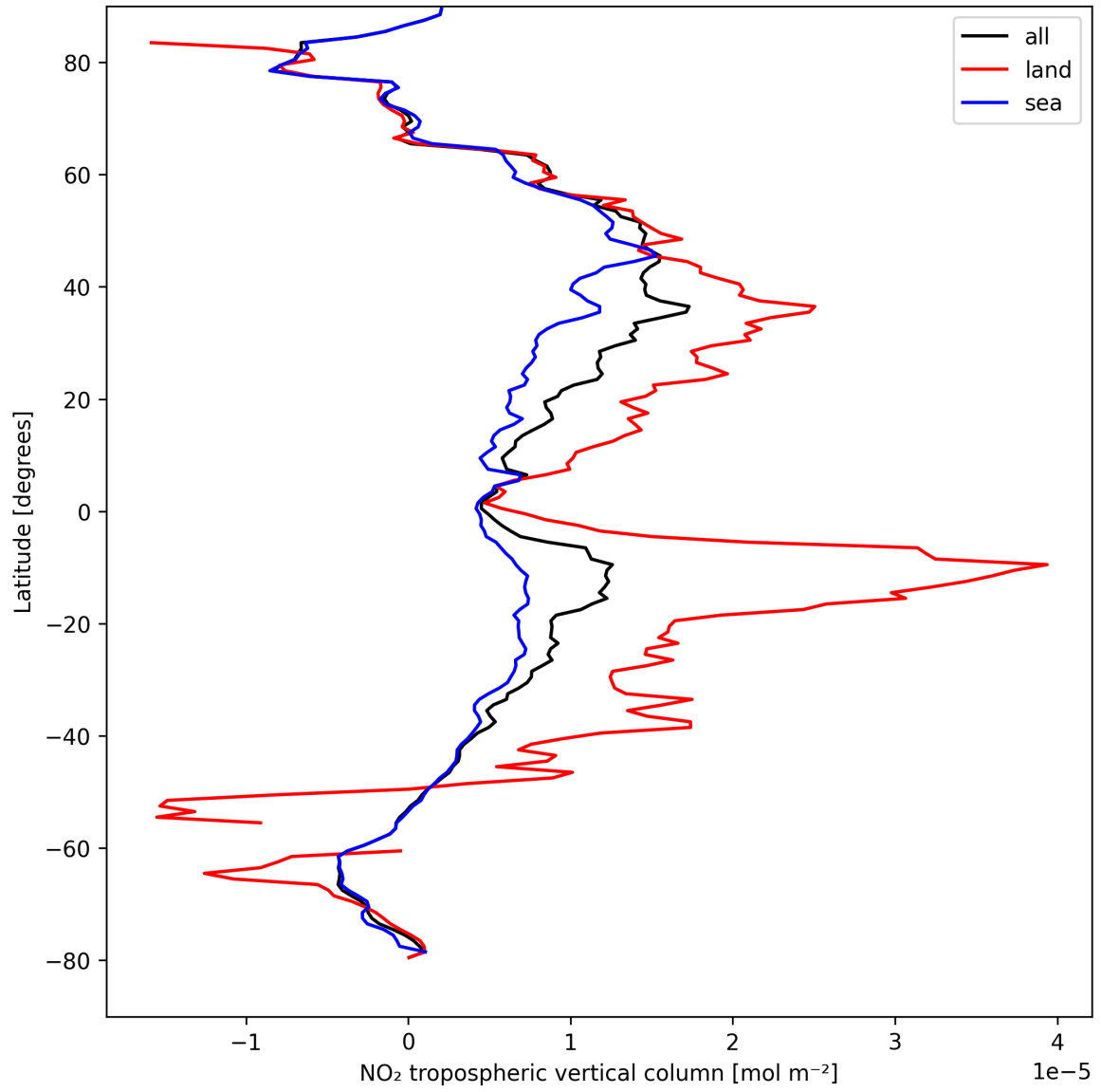
Figure 12: Zonal average of “NO 2 tropospheric vertical column” for 2024-08-28 to 2024-08-30.
