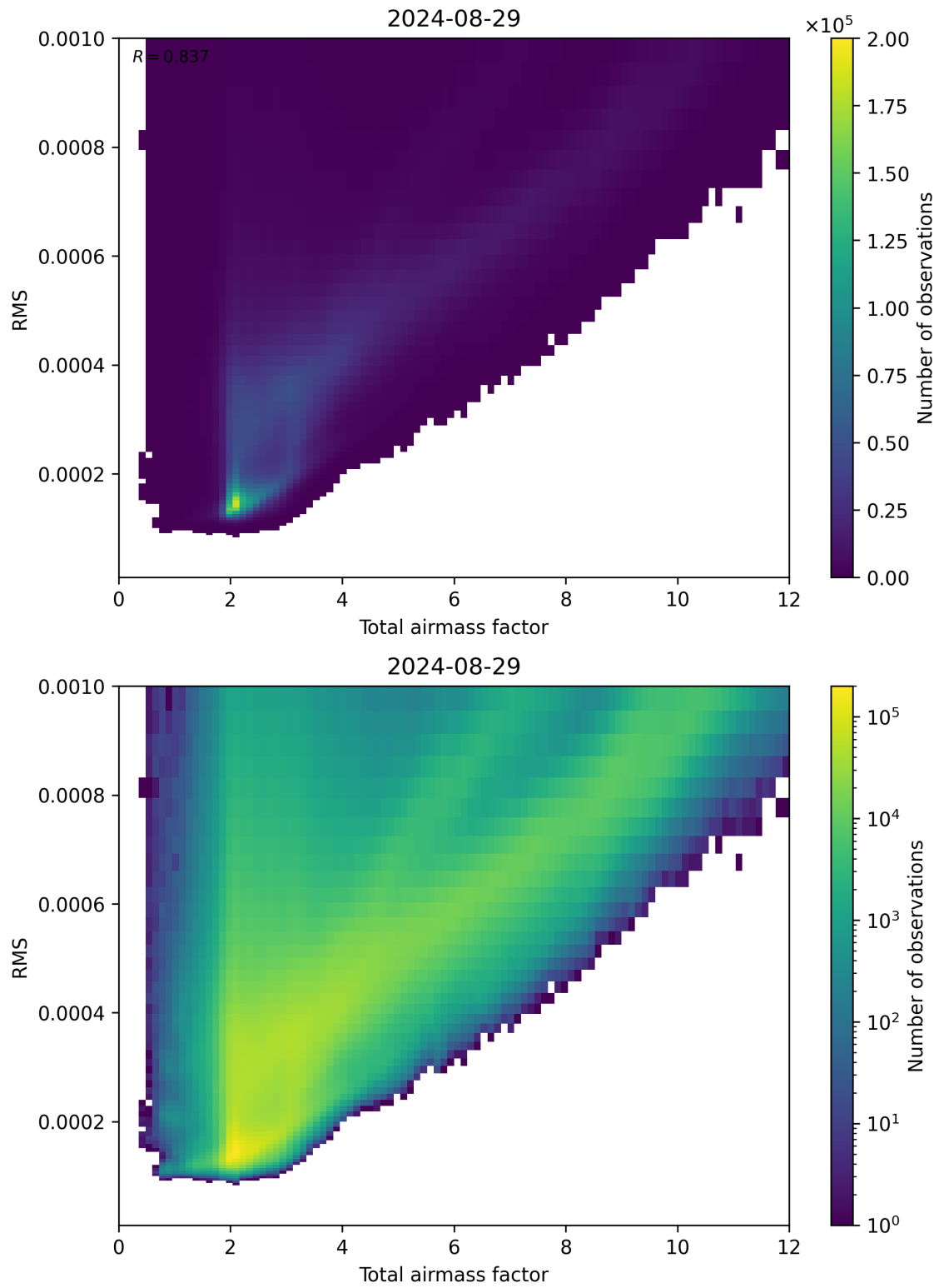
Figure 69: Scatter density plot of “Total airmass factor” against “RMS” for 2024-08-28 to 2024-08-30.
