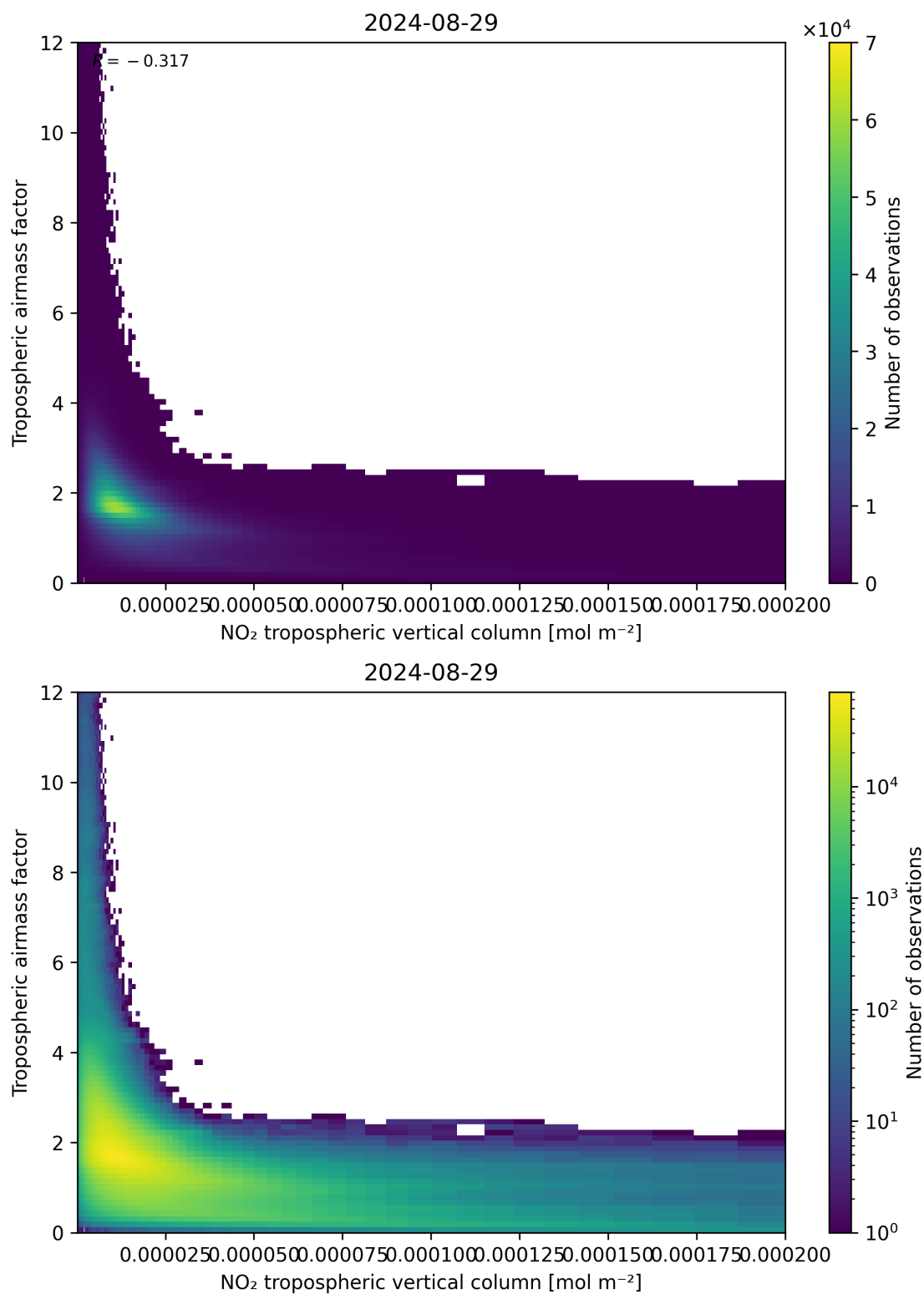
Figure 123: Scatter density plot of “NO 2 tropospheric vertical column” against “Tropospheric air mass factor” for 2024-08-28 to 2024-08-30.
