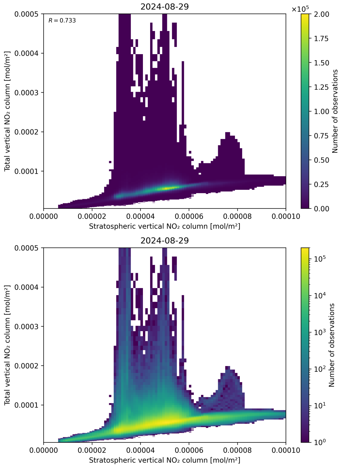
Figure 100: Scatter density plot of “Stratospheric vertical NO 2 column” against “Total vertical NO 2 column” for 2024-08-28 to 2024-08-30.
