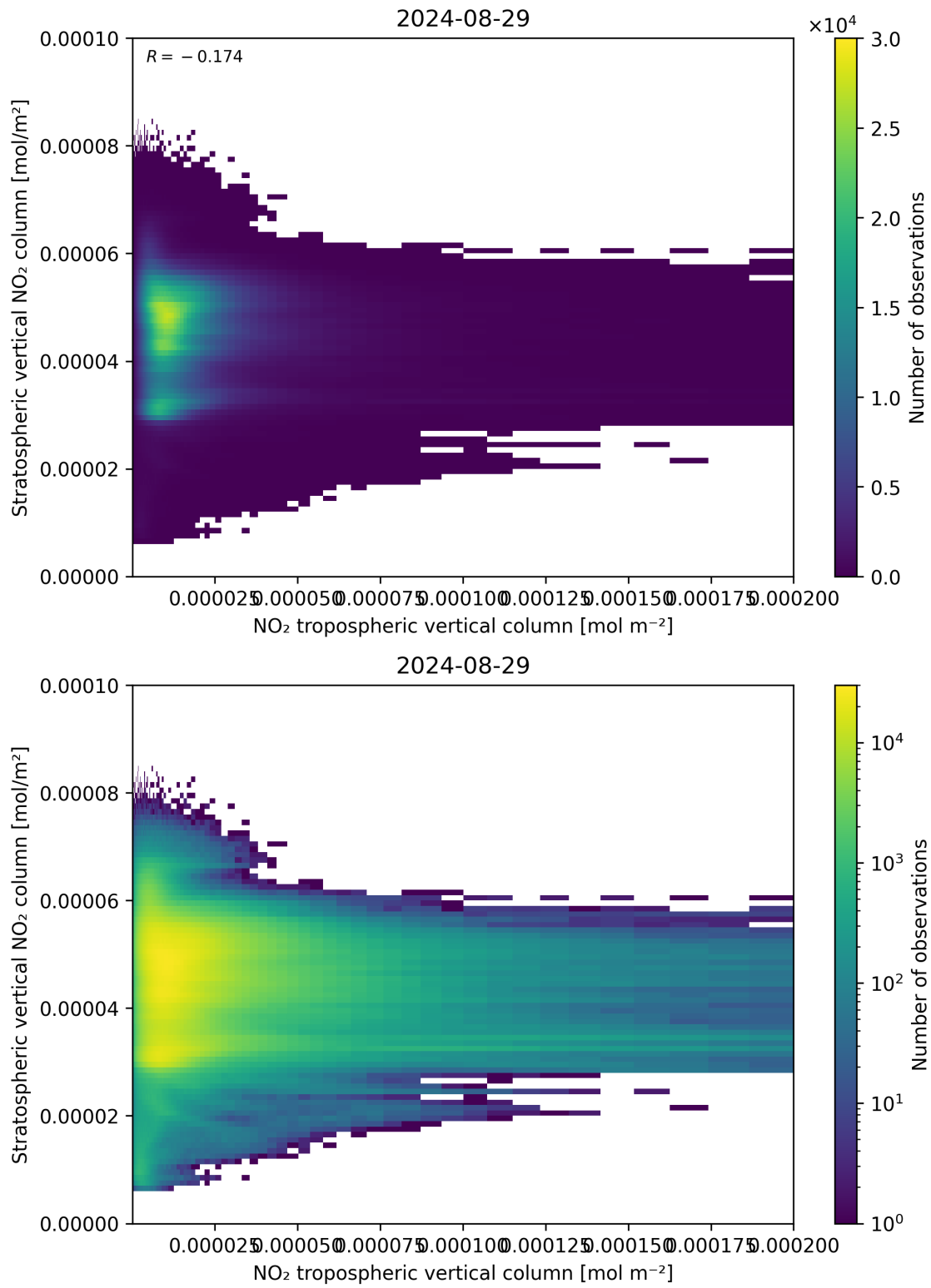
Figure 125: Scatter density plot of “NO 2 tropospheric vertical column” against “Stratospheric vertical NO 2 column” for 2024-08-28 to 2024-08-30.
