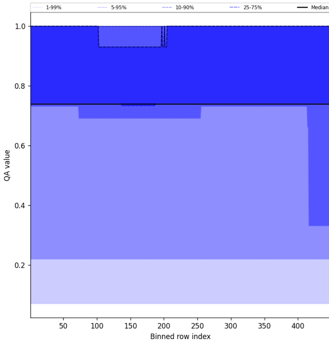
Figure 45: Along track statistics of “QA value” for 2024-08-28 to 2024-08-30
