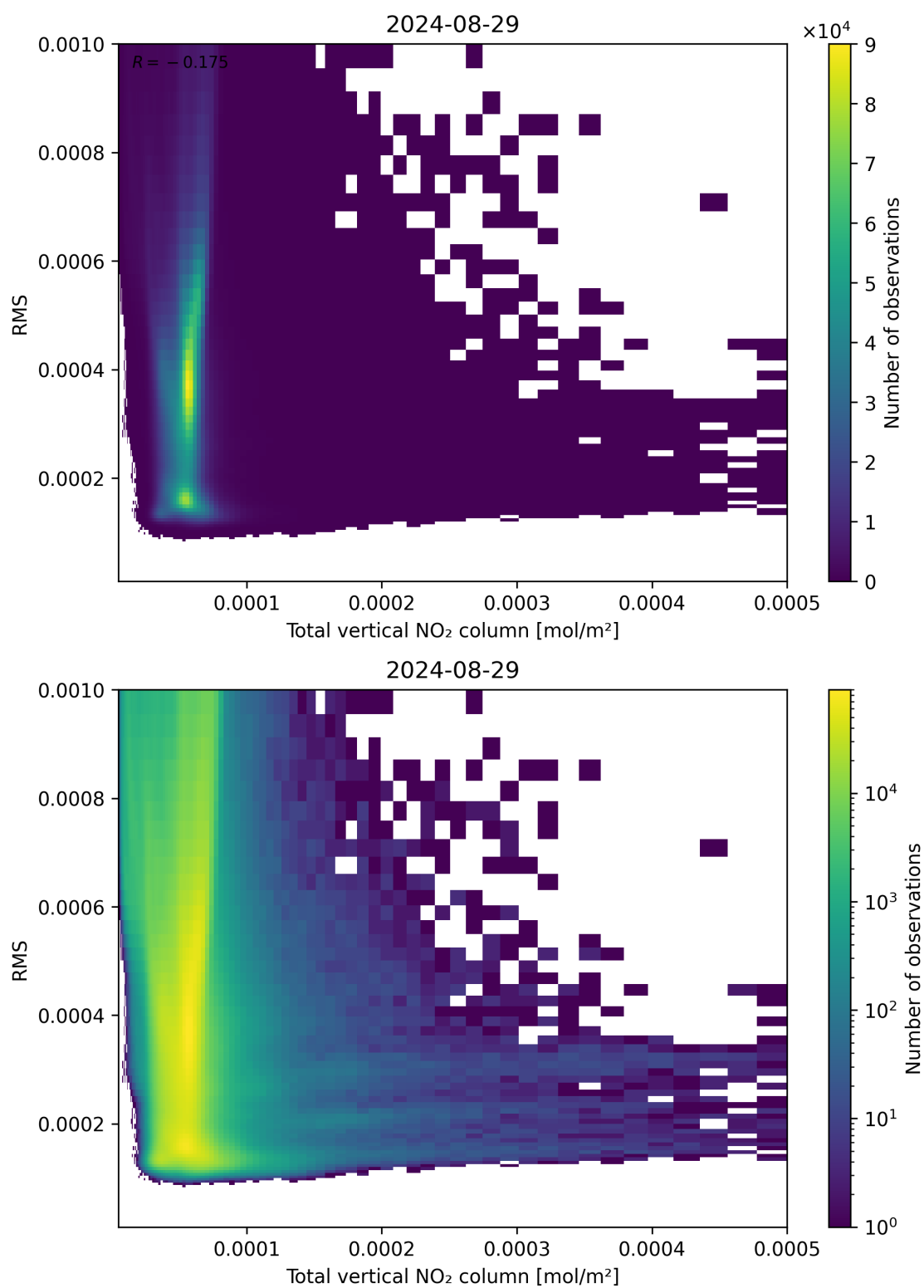
Figure 120: Scatter density plot of “Total vertical NO 2 column” against “RMS” for 2024-08-28 to 2024-08-30.
