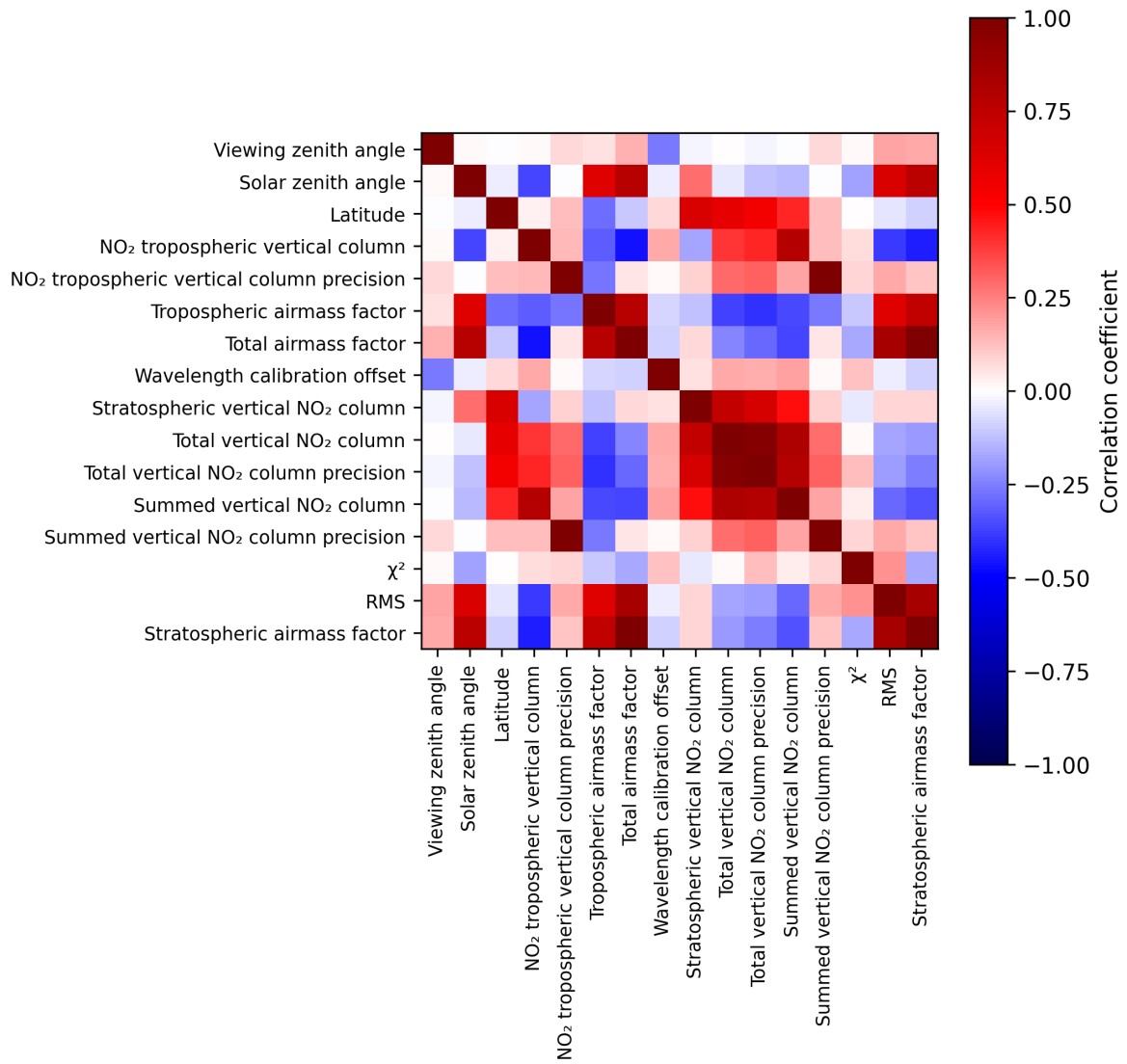
Figure 2: Map of correlation matrix for 2024-08-28 to 2024-08-30.
