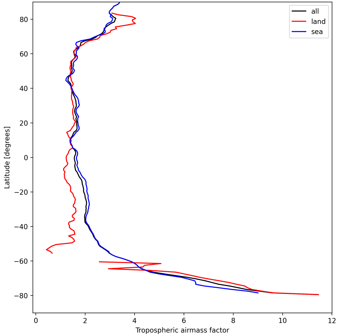
Figure 14: Zonal average of “Tropospheric airmass factor” for 2024-08-28 to 2024-08-30.
