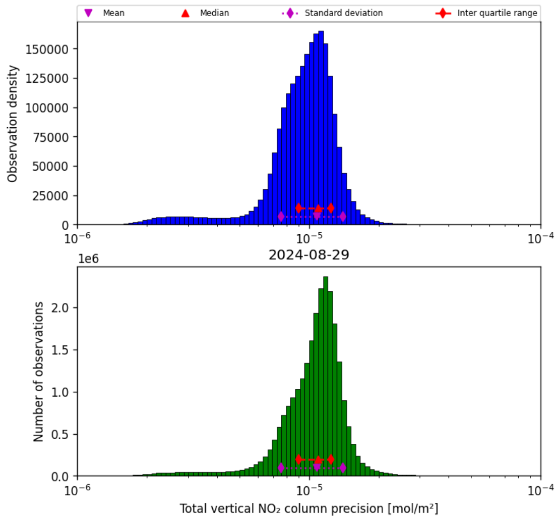
Figure 39: Histogram of “Total vertical NO 2 column precision” for 2024-08-28 to 2024-08-30
