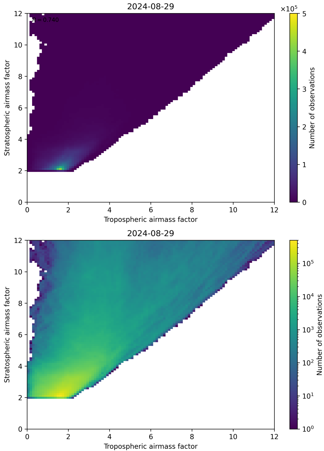
Figure 71: Scatter density plot of “Tropospheric airmass factor” against “Stratospheric airmass factor” for 2024-08-28 to 2024-08-30.
