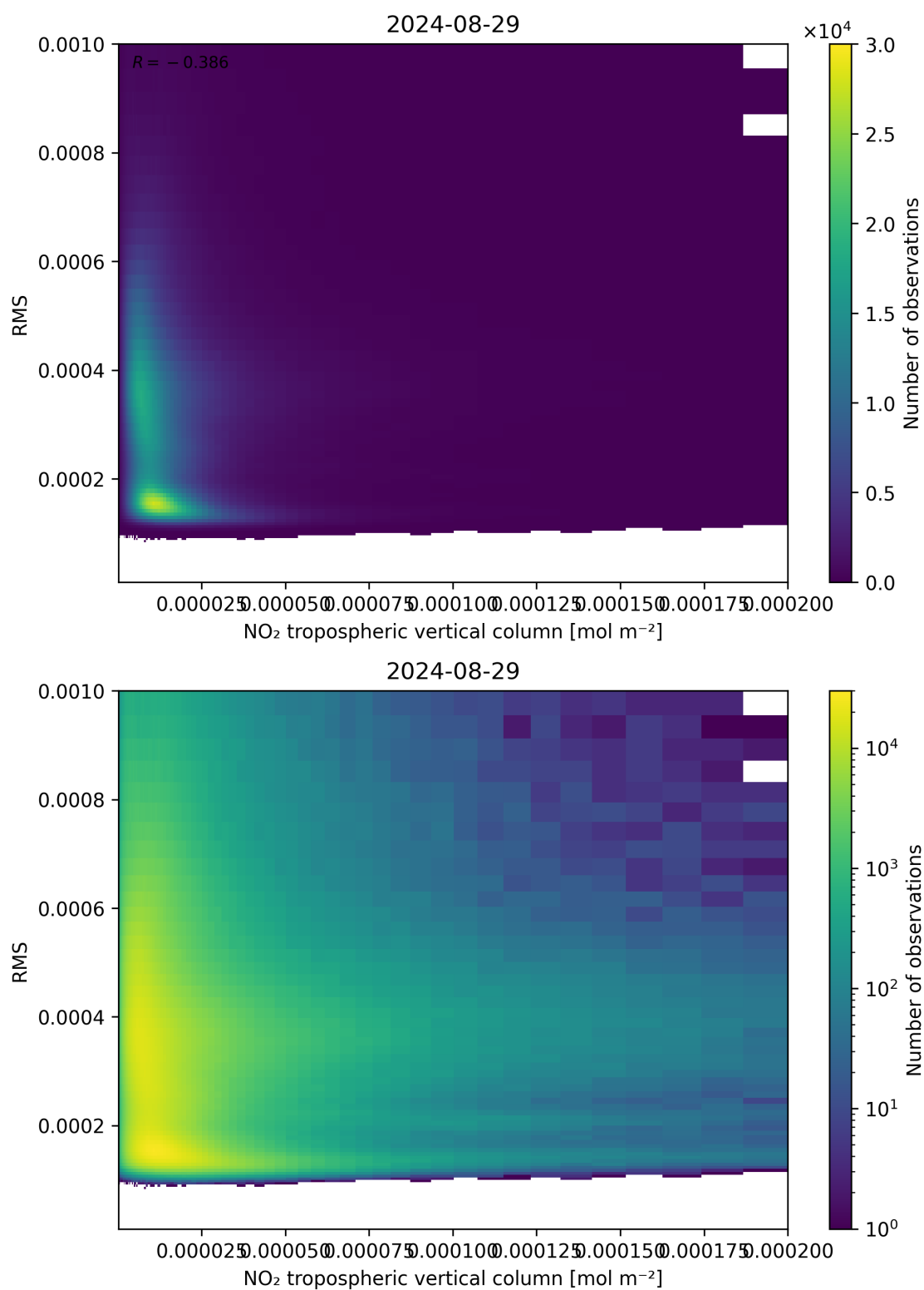
Figure 142: Scatter density plot of “NO 2 tropospheric vertical column” against “RMS” for 2024-08-28 to 2024-08-30.
