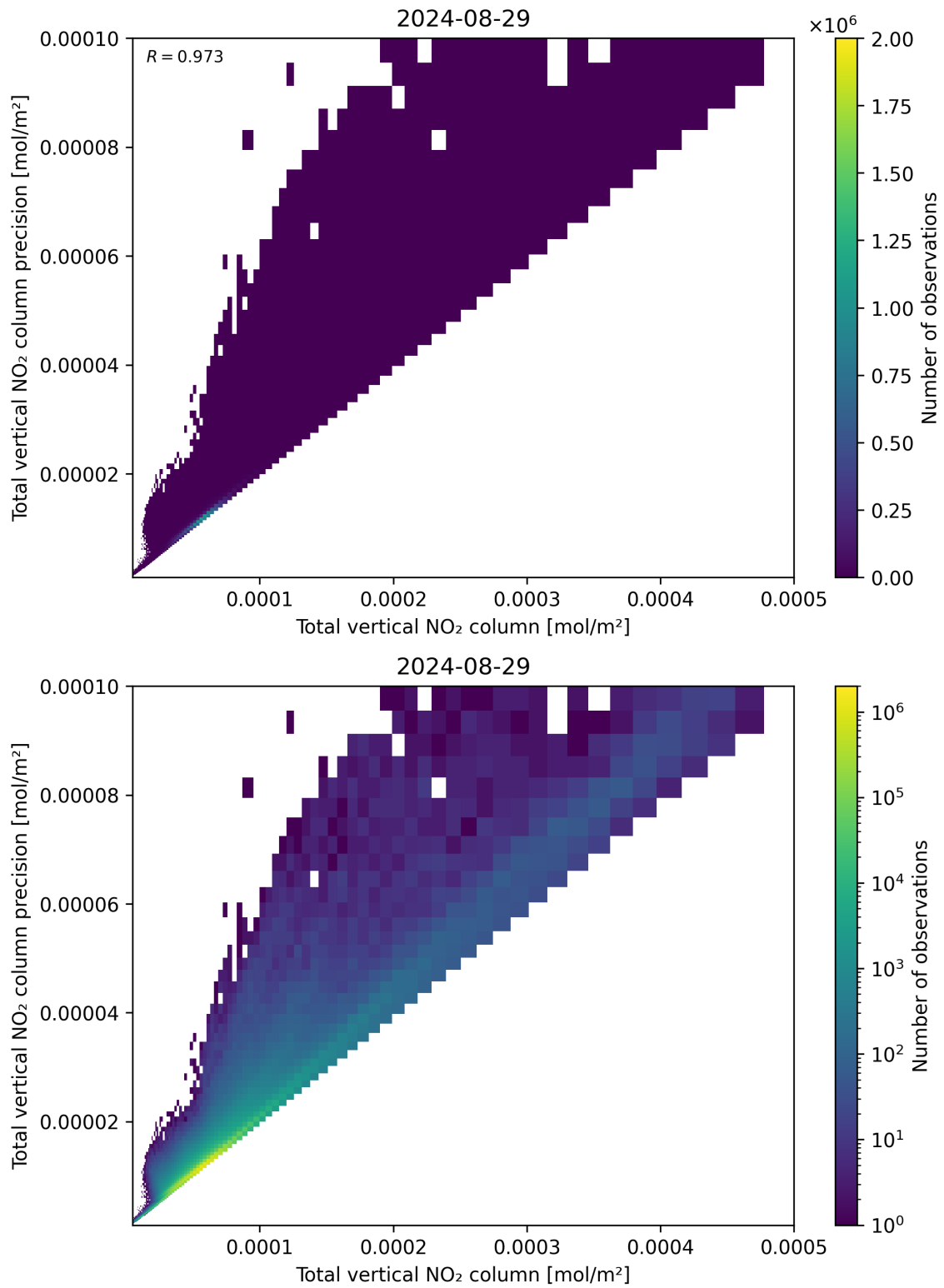
Figure 114: Scatter density plot of “Total vertical NO 2 column” against “Total vertical NO 2 column precision” for 2024-08-28 to 2024-08-30.
