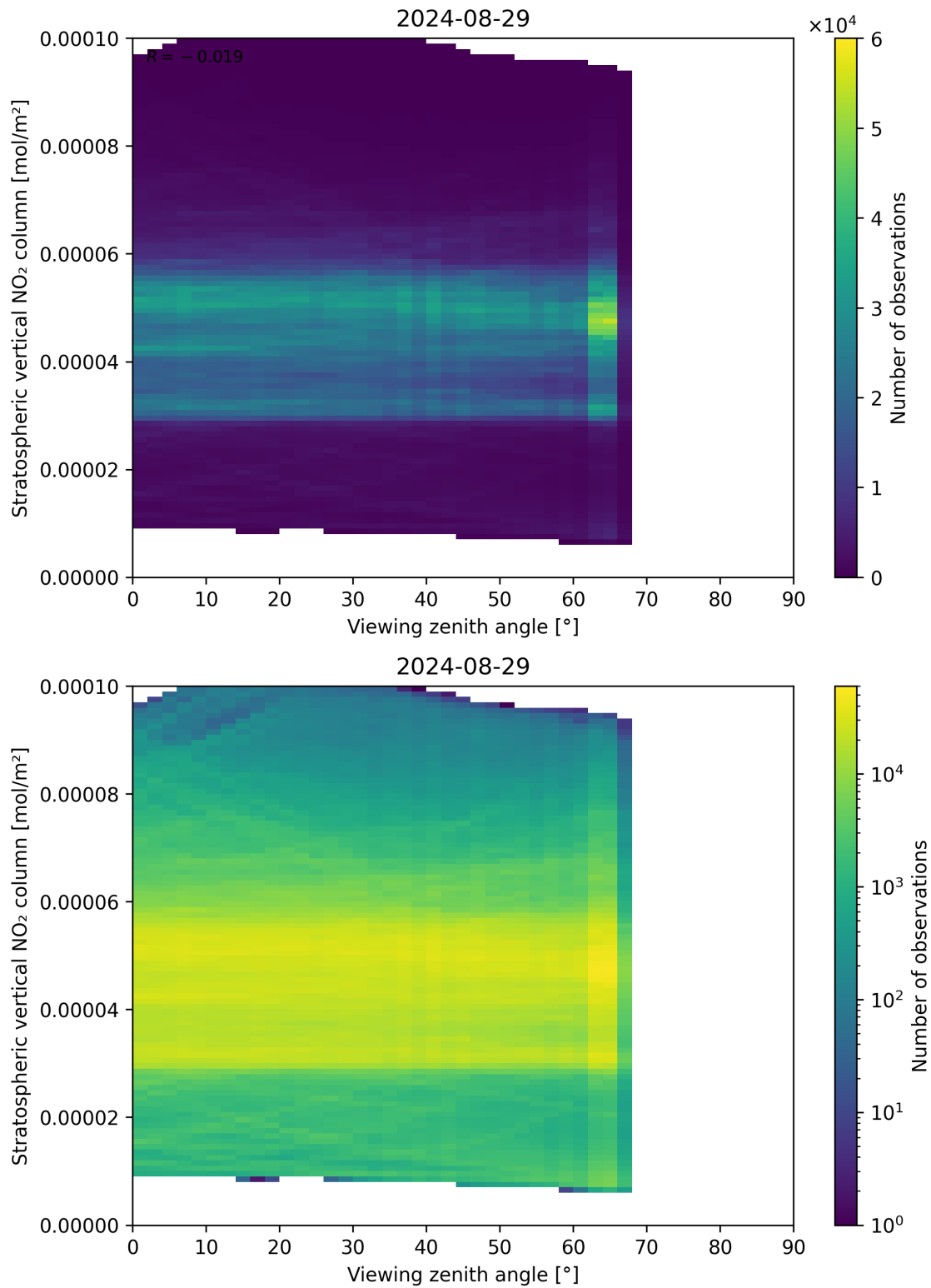
Figure 164: Scatter density plot of “Viewing zenith angle” against “Stratospheric vertical NO 2 column” for 2024-08-28 to 2024-08-30.
