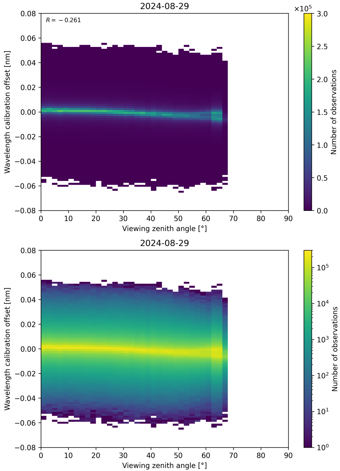
Figure 173: Scatter density plot of “Viewing zenith angle” against “Wavelength calibration offset” for 2024-08-28 to 2024-08-30.
