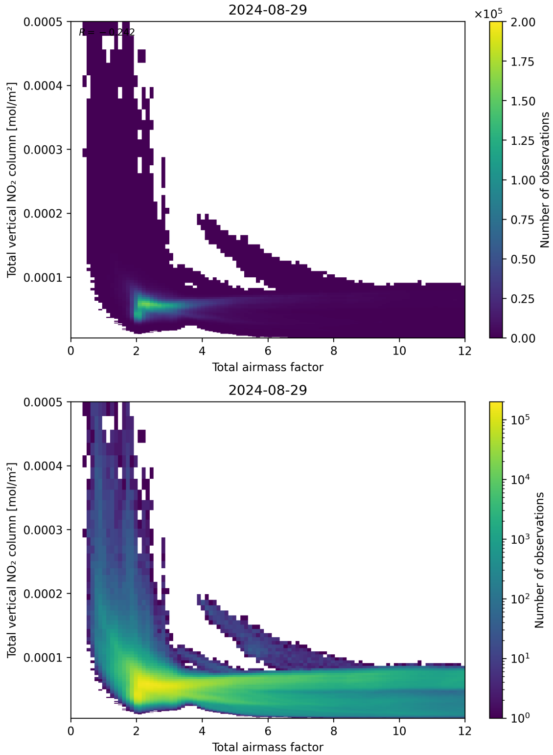
Figure 67: Scatter density plot of “Total airmass factor” against “Total vertical NO 2 column” for 2024-08-28 to 2024-08-30.
