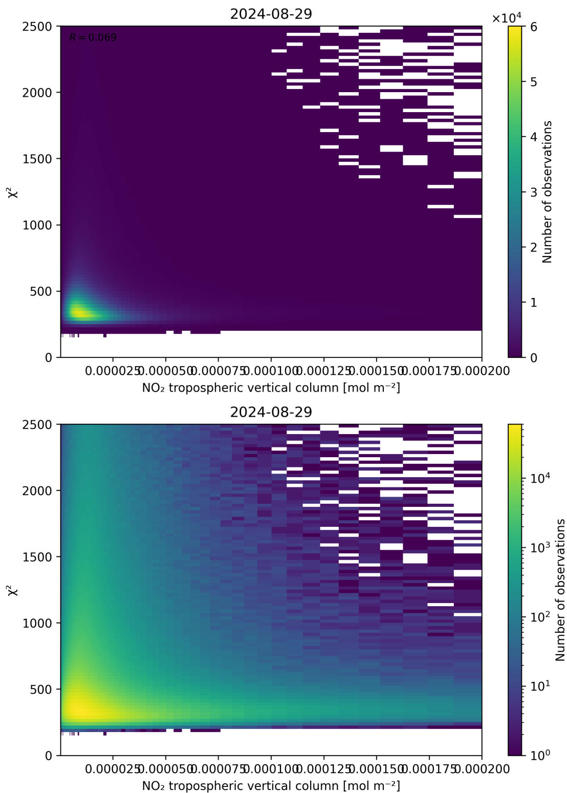
Figure 124: Scatter density plot of “NO 2 tropospheric vertical column” against “ \chi^2 ” for 2024-08-28 to 2024-08-30.
