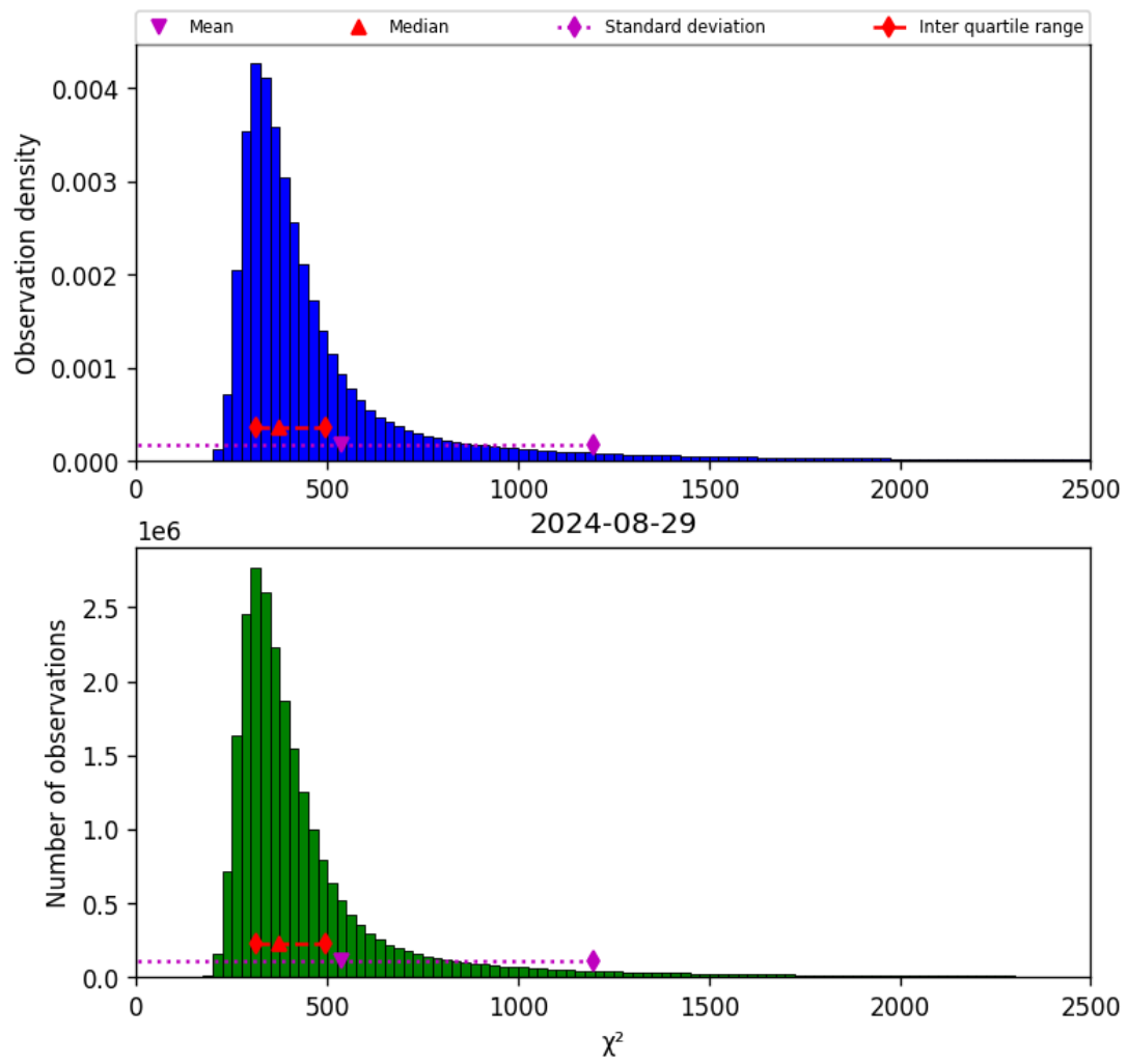
Figure 42: Histogram of “ \chi^2 ” for 2024-08-28 to 2024-08-30
