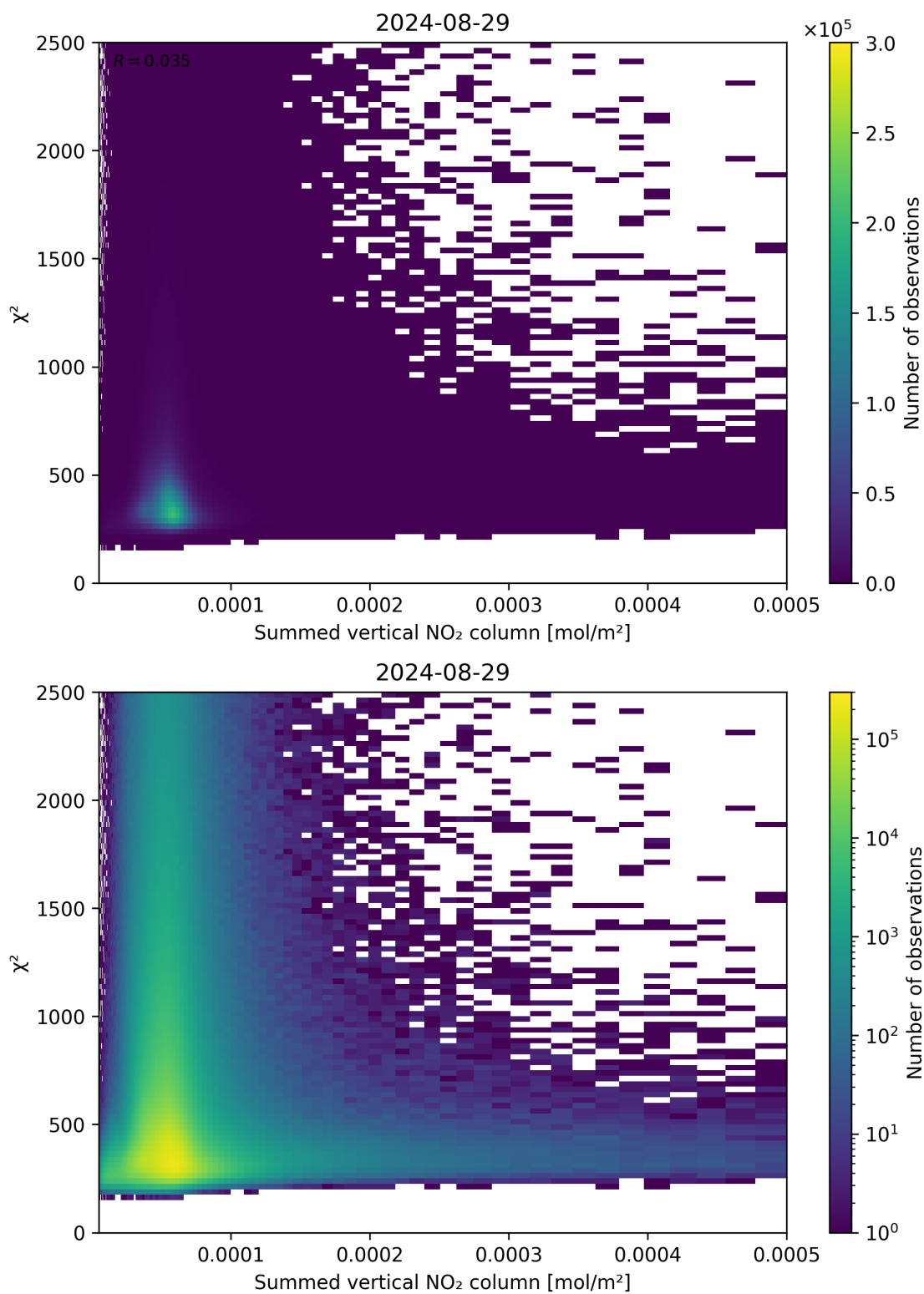
Figure 104: Scatter density plot of “Summed vertical NO 2 column” against “ \chi^2 ” for 2024-08-28 to 2024-08-30.
