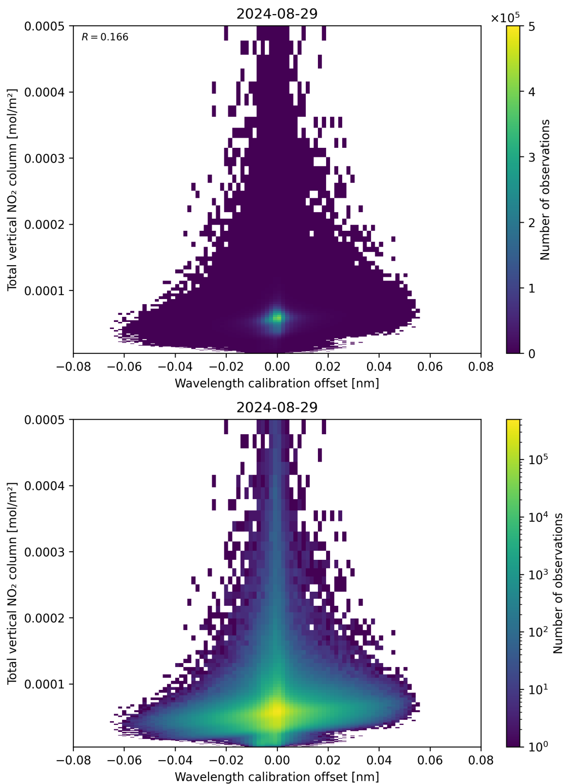
Figure 179: Scatter density plot of “Wavelength calibration offset” against “Total vertical NO 2 column” for 2024-08-28 to 2024-08-30.
