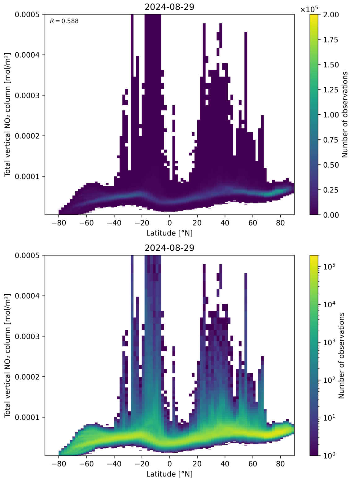
Figure 90: Scatter density plot of “Latitude” against “Total vertical NO 2 column” for 2024-08-28 to 2024-08-30.
