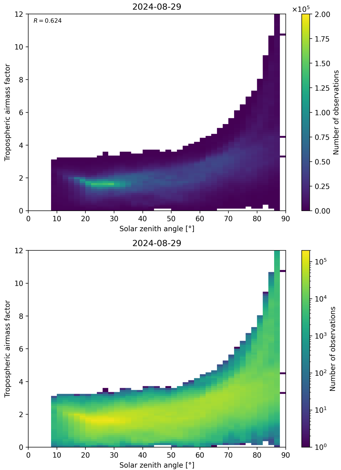
Figure 147: Scatter density plot of “Solar zenith angle” against “Tropospheric airmass factor” for 2024-08-28 to 2024-08-30.
