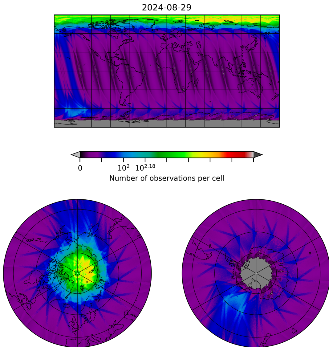
Figure 10: Map of the number of observations for 2024-08-28 to 2024-08-30
