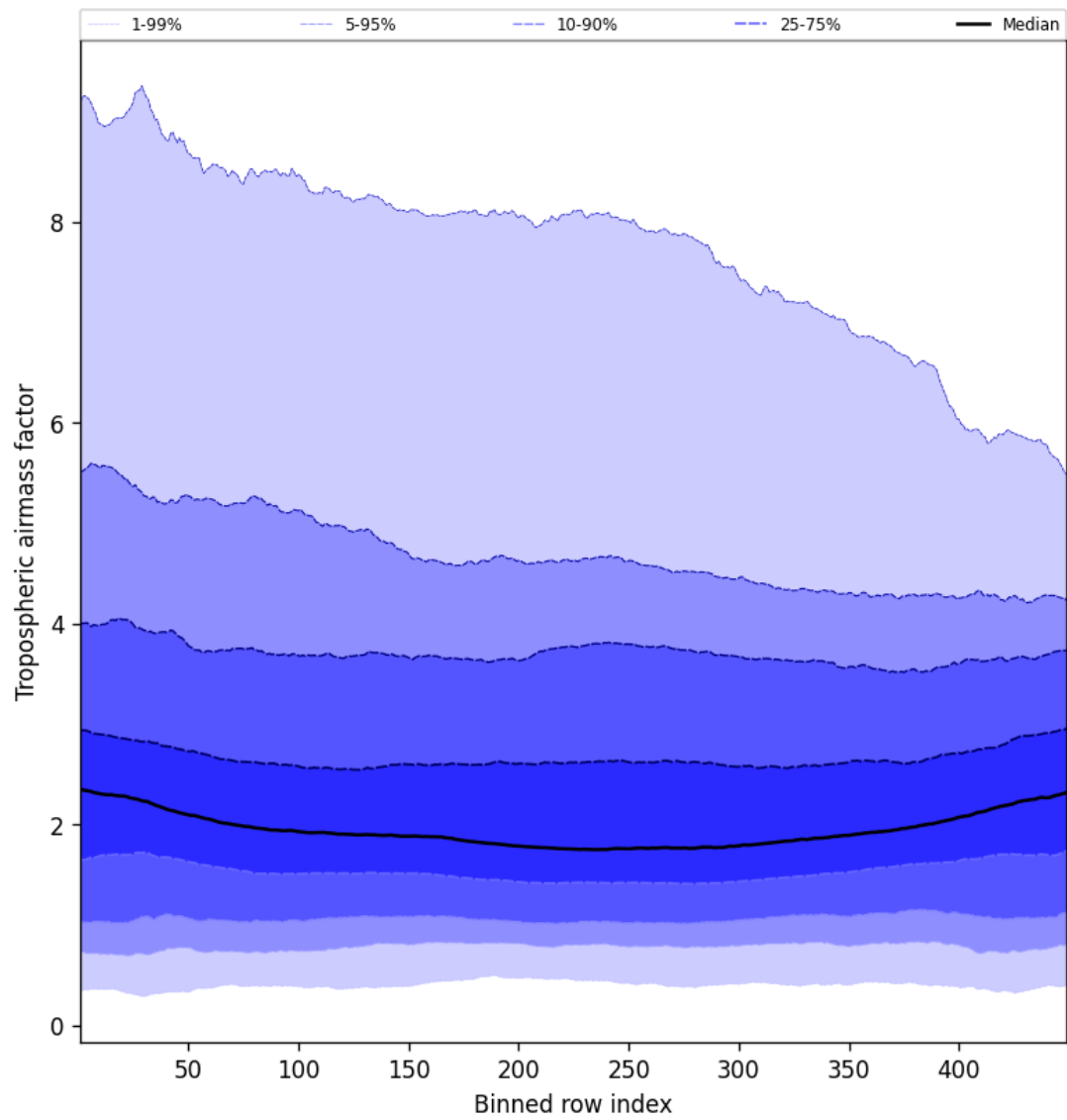
Figure 48: Along track statistics of “Tropospheric air mass factor” for 2024-08-28 to 2024-08-30
