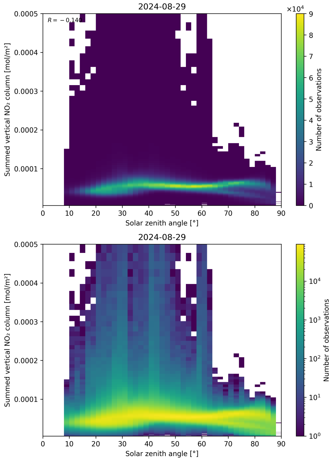
Figure 151: Scatter density plot of “Solar zenith angle” against “Summed vertical NO 2 column” for 2024-08-28 to 2024-08-30.
