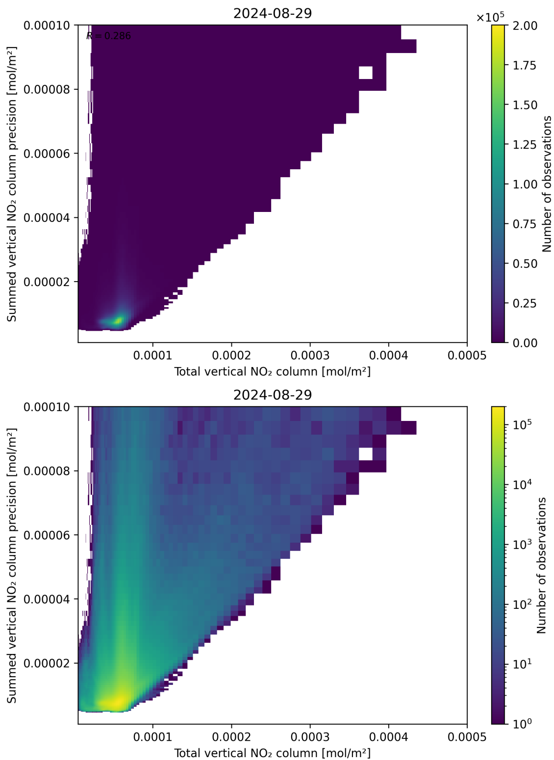
Figure 113: Scatter density plot of “Total vertical NO 2 column” against “Summed vertical NO 2 column precision” for 2024-08-28 to 2024-08-30.
