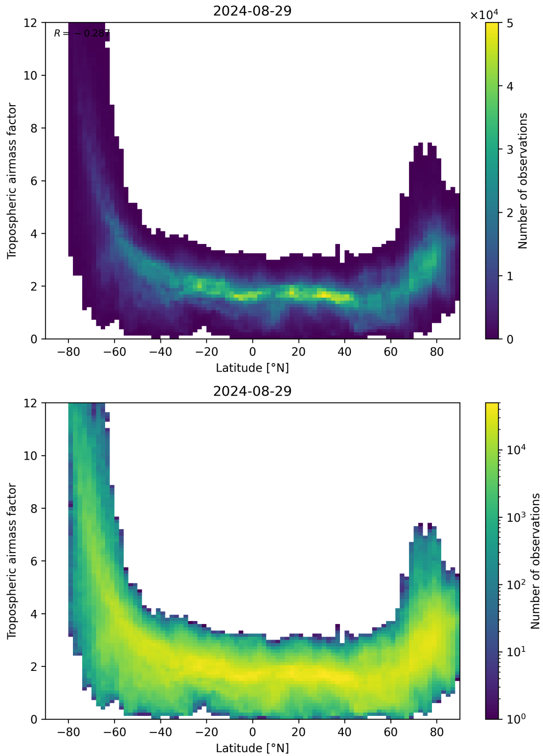
Figure 85: Scatter density plot of “Latitude” against “Tropospheric airmass factor” for 2024-08-28 to 2024-08-30.
