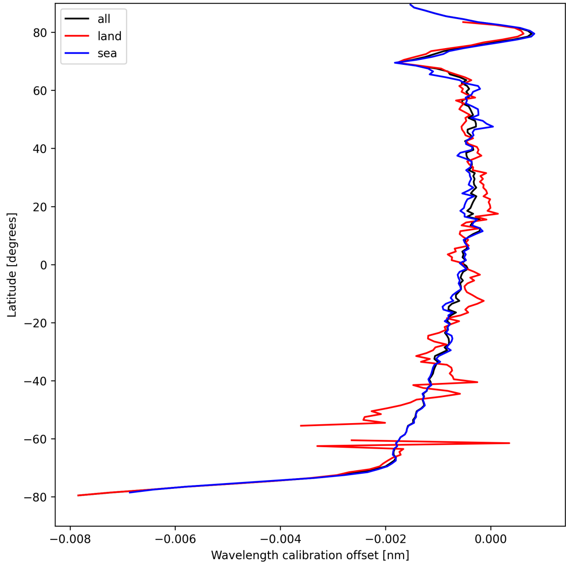
Figure 18: Zonal average of “Wavelength calibration offset” for 2024-08-28 to 2024-08-30.
