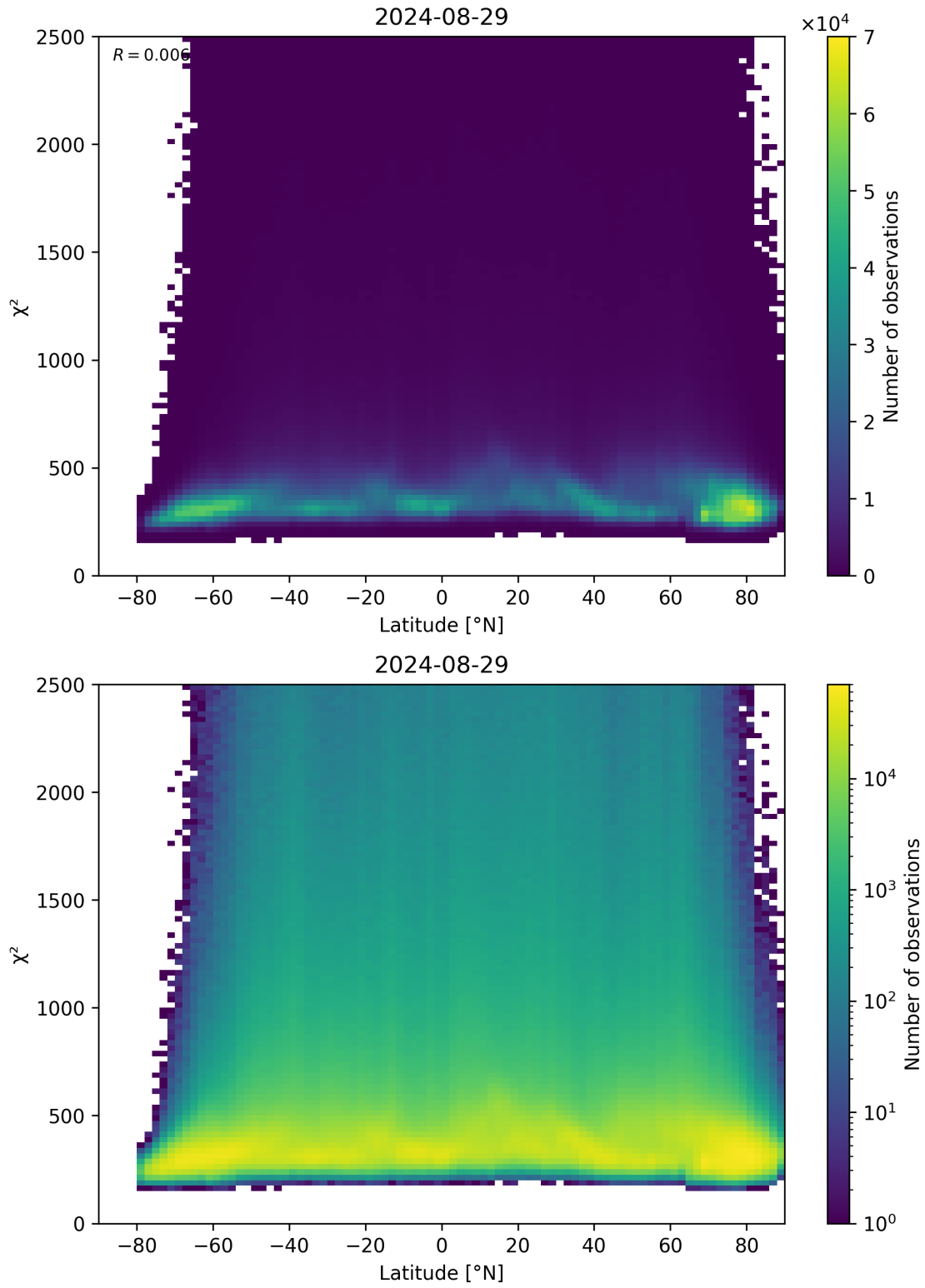
Figure 86: Scatter density plot of “Latitude” against “ \chi^2 ” for 2024-08-28 to 2024-08-30.
