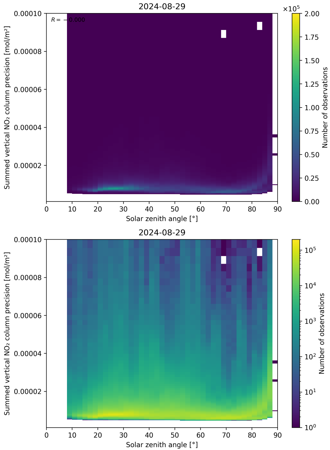
Figure 152: Scatter density plot of “Solar zenith angle” against “Summed vertical NO 2 column precision” for 2024-08-28 to 2024-08-30.
