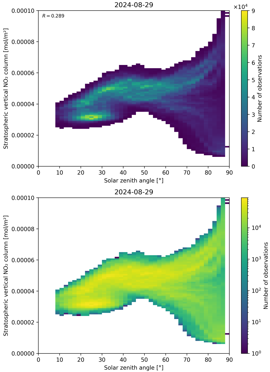
Figure 150: Scatter density plot of “Solar zenith angle” against “Stratospheric vertical NO 2 column” for 2024-08-28 to 2024-08-30.
