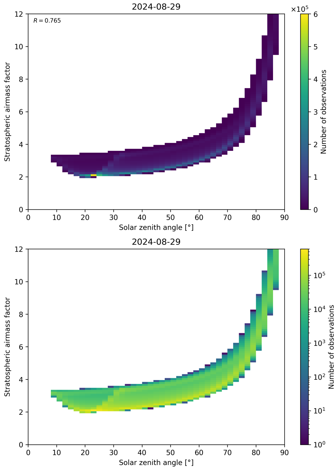
Figure 145: Scatter density plot of “Solar zenith angle” against “Stratospheric airmass factor” for 2024-08-28 to 2024-08-30.
