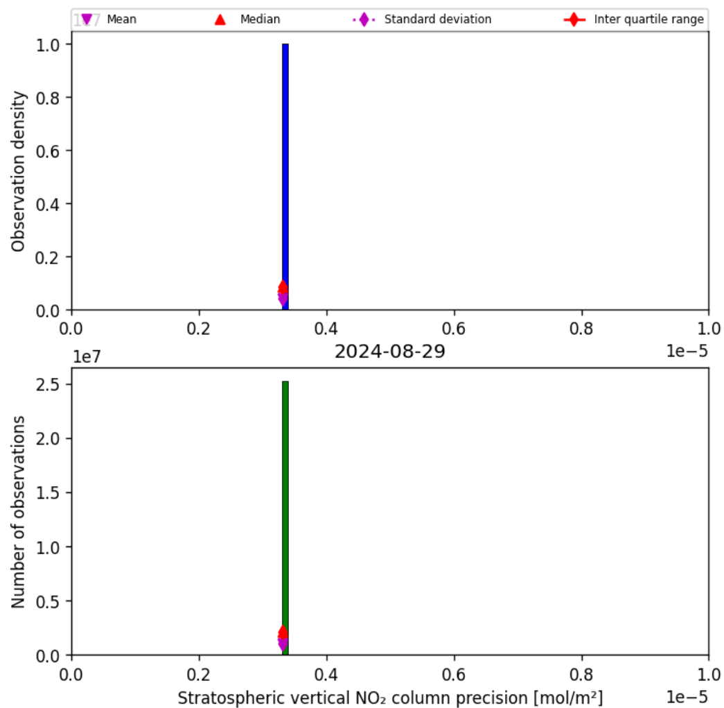
Figure 37: Histogram of “Stratospheric vertical NO 2 column precision” for 2024-08-28 to 2024-08-30
