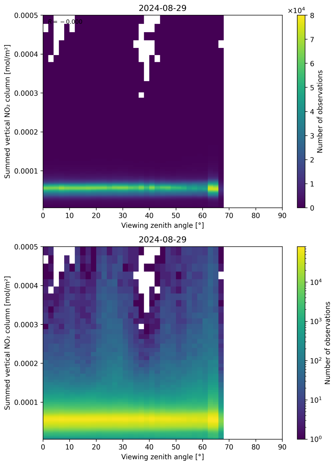
Figure 165: Scatter density plot of “Viewing zenith angle” against “Summed vertical NO 2 column” for 2024-08-28 to 2024-08-30.
