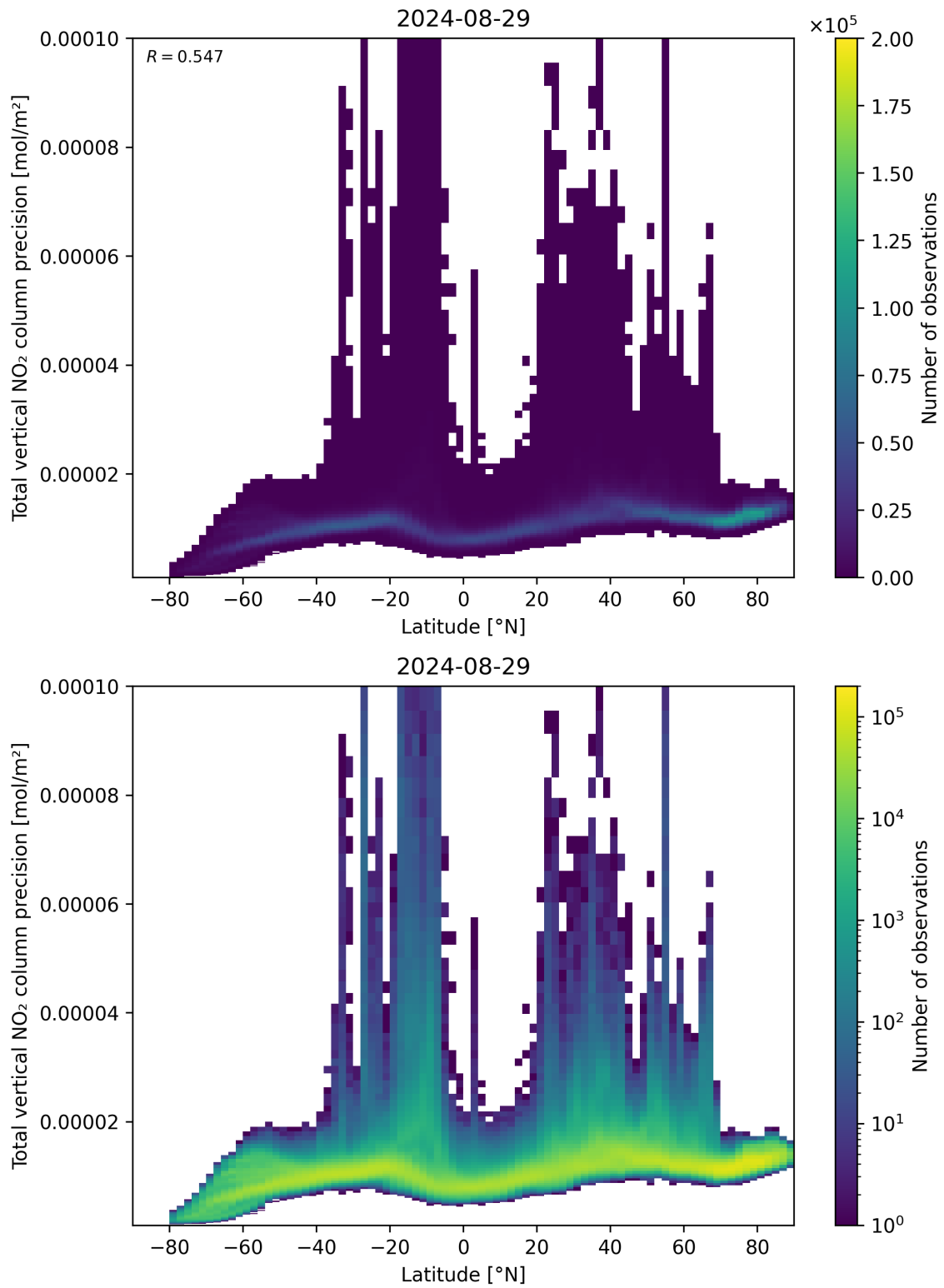
Figure 91: Scatter density plot of “Latitude” against “Total vertical NO 2 column precision” for 2024-08-28 to 2024-08-30.
