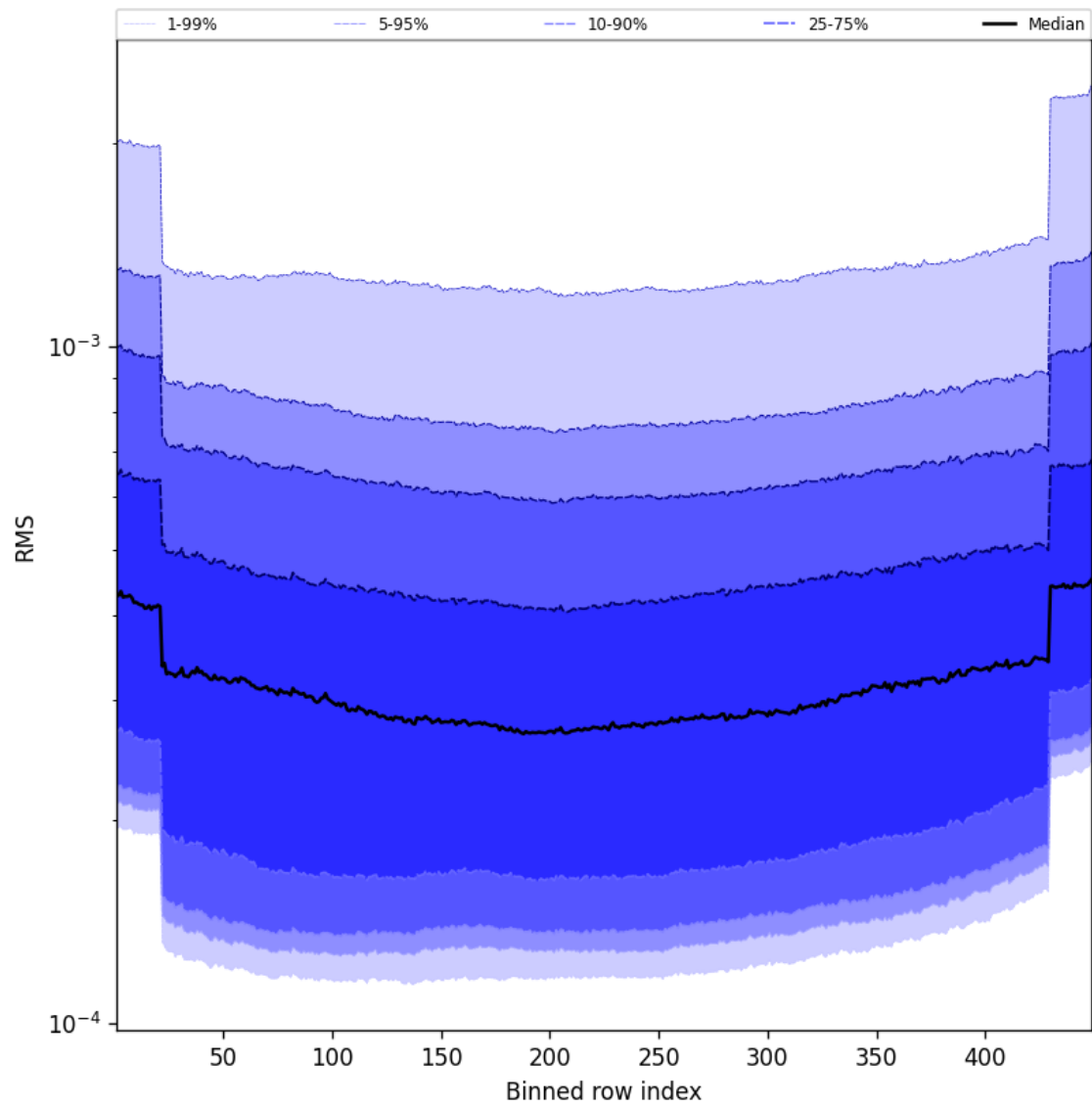
Figure 60: Along track statistics of “RMS” for 2024-08-28 to 2024-08-30
