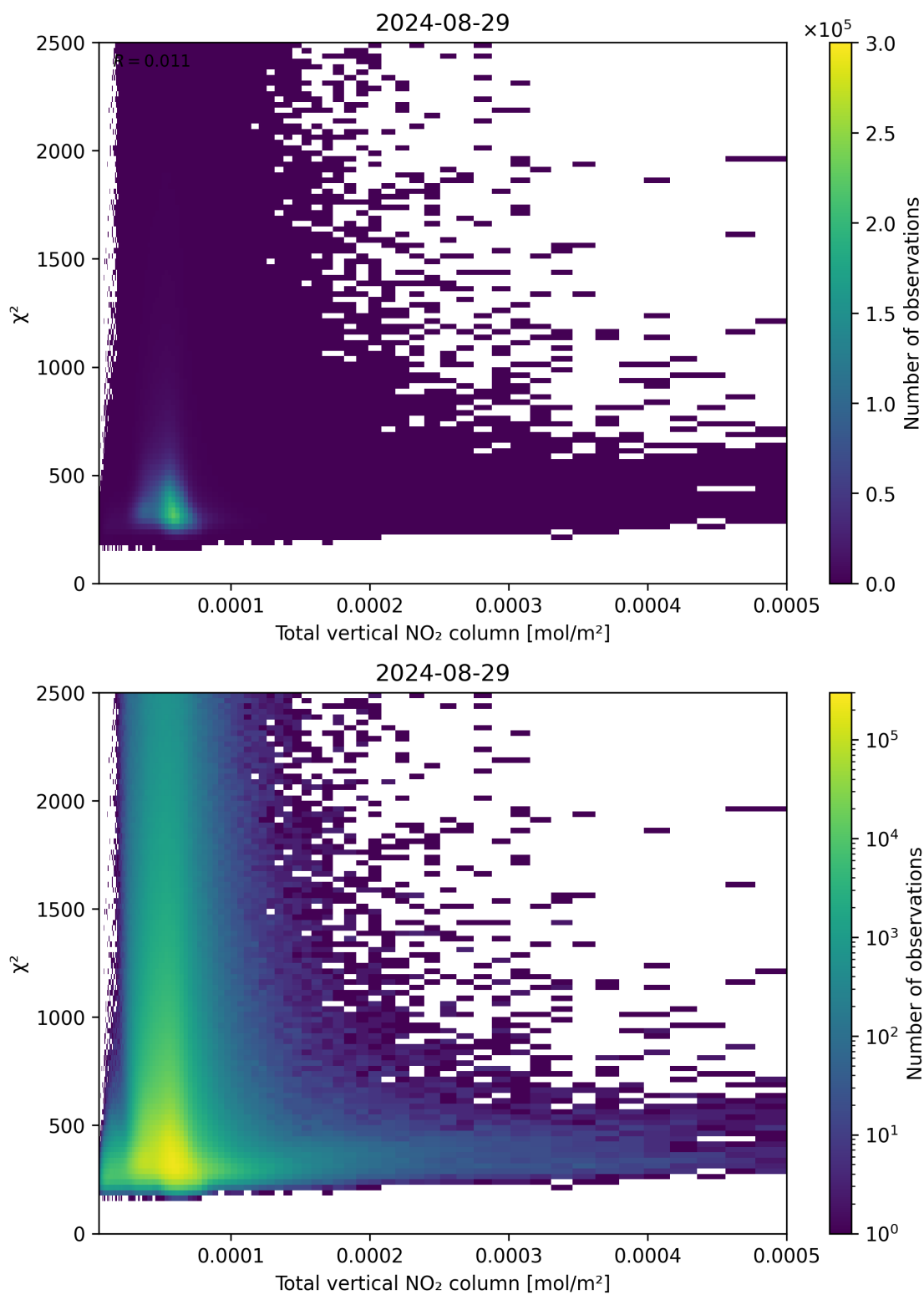
Figure 111: Scatter density plot of “Total vertical NO 2 column” against “ \chi^2 ” for 2024-08-28 to 2024-08-30.
