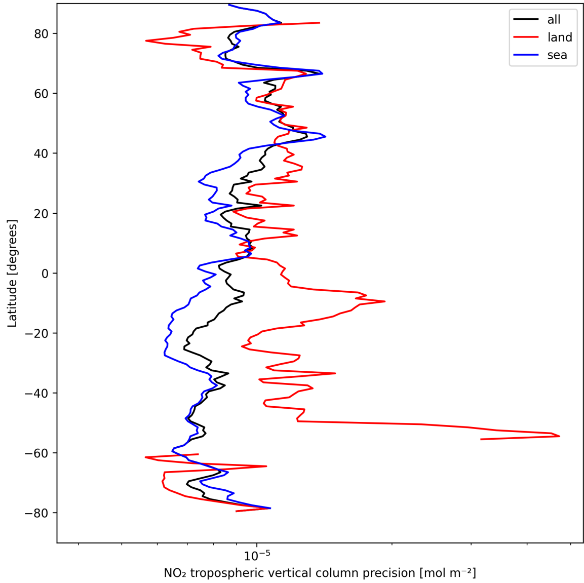
Figure 13: Zonal average of “NO 2 tropospheric vertical column precision” for 2024-08-28 to 2024-08-30.
