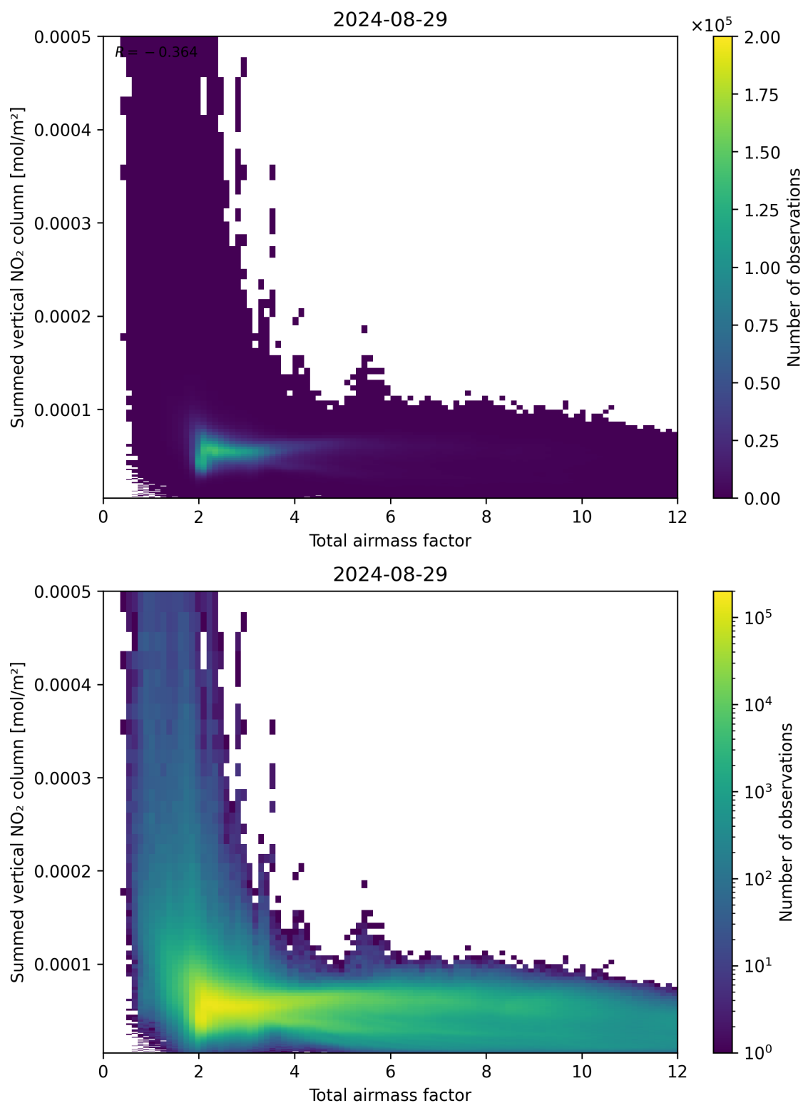
Figure 65: Scatter density plot of “Total airmass factor” against “Summed vertical NO 2 column” for 2024-08-28 to 2024-08-30.
