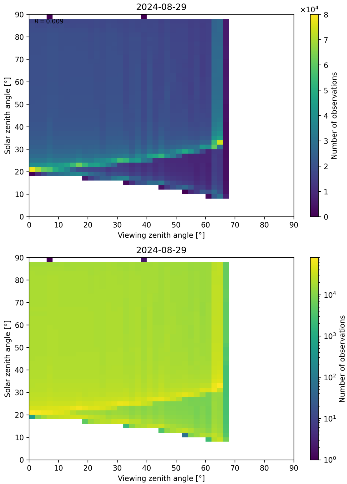
Figure 172: Scatter density plot of “Viewing zenith angle” against “Solar zenith angle” for 2024-08-28 to 2024-08-30.
