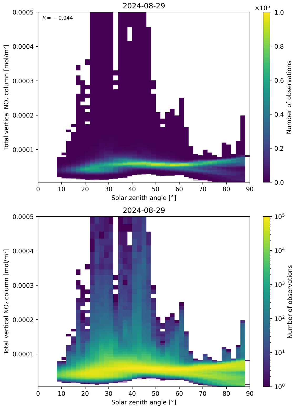
Figure 153: Scatter density plot of “Solar zenith angle” against “Total vertical NO 2 column” for 2024-08-28 to 2024-08-30.
