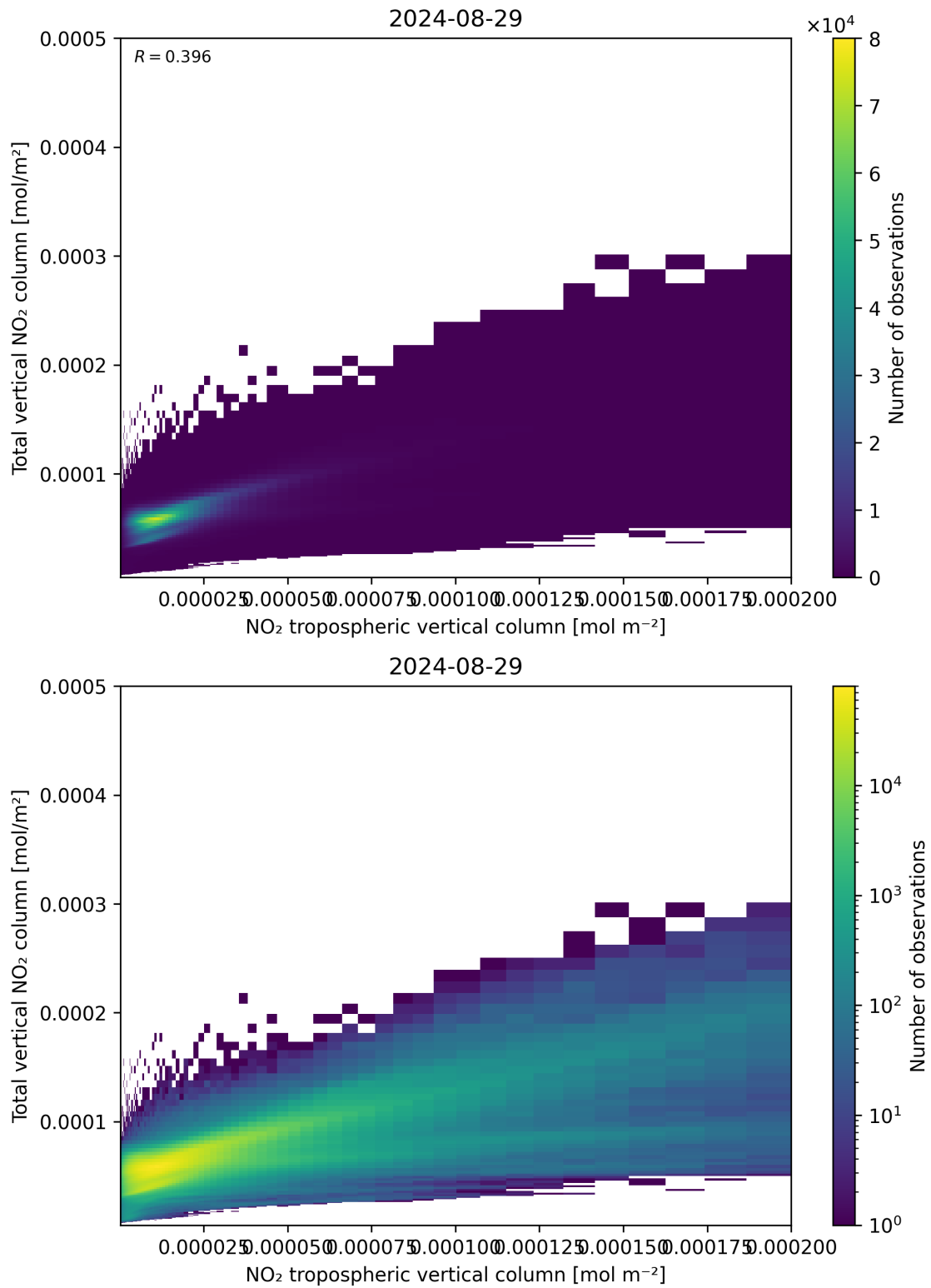
Figure 128: Scatter density plot of “NO 2 tropospheric vertical column” against “Total vertical NO 2 column” for 2024-08-28 to 2024-08-30.
