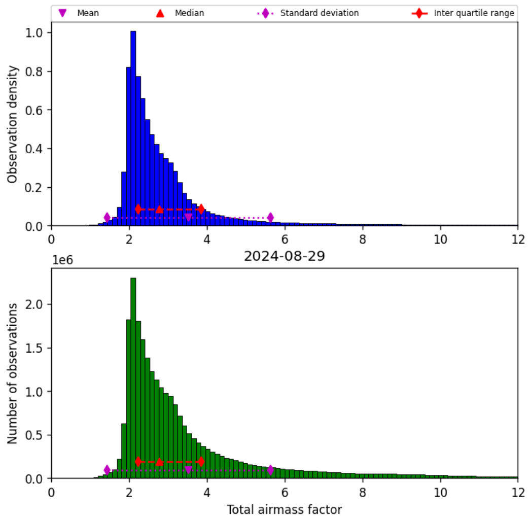
Figure 32: Histogram of “Total airmass factor” for 2024-08-28 to 2024-08-30
