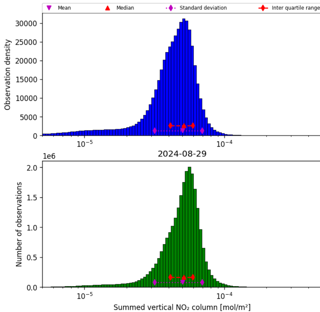
Figure 40: Histogram of “Summed vertical NO 2 column” for 2024-08-28 to 2024-08-30
