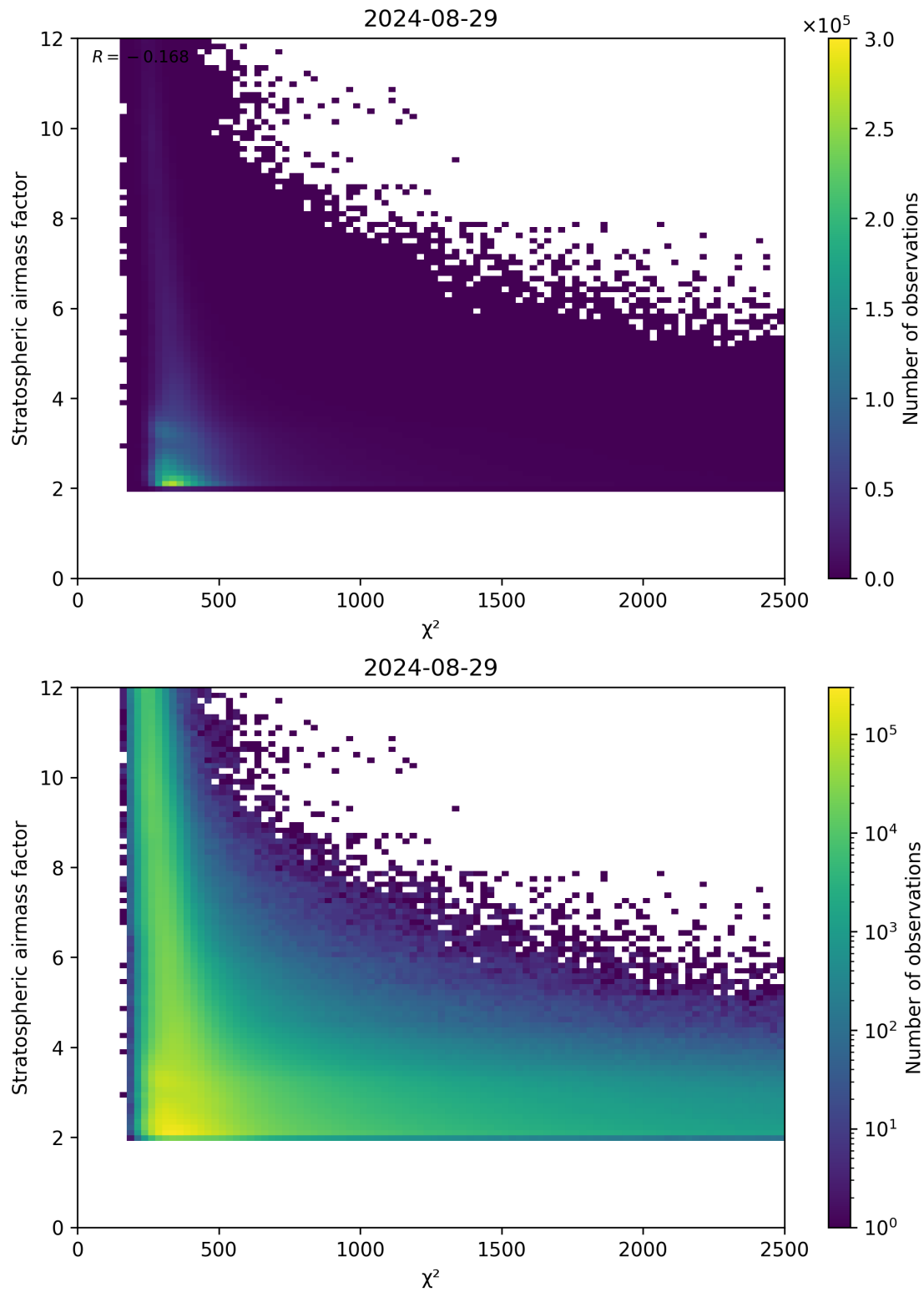
Figure 81: Scatter density plot of “ \chi^2 ” against “Stratospheric airmass factor” for 2024-08-28 to 2024-08-30.
