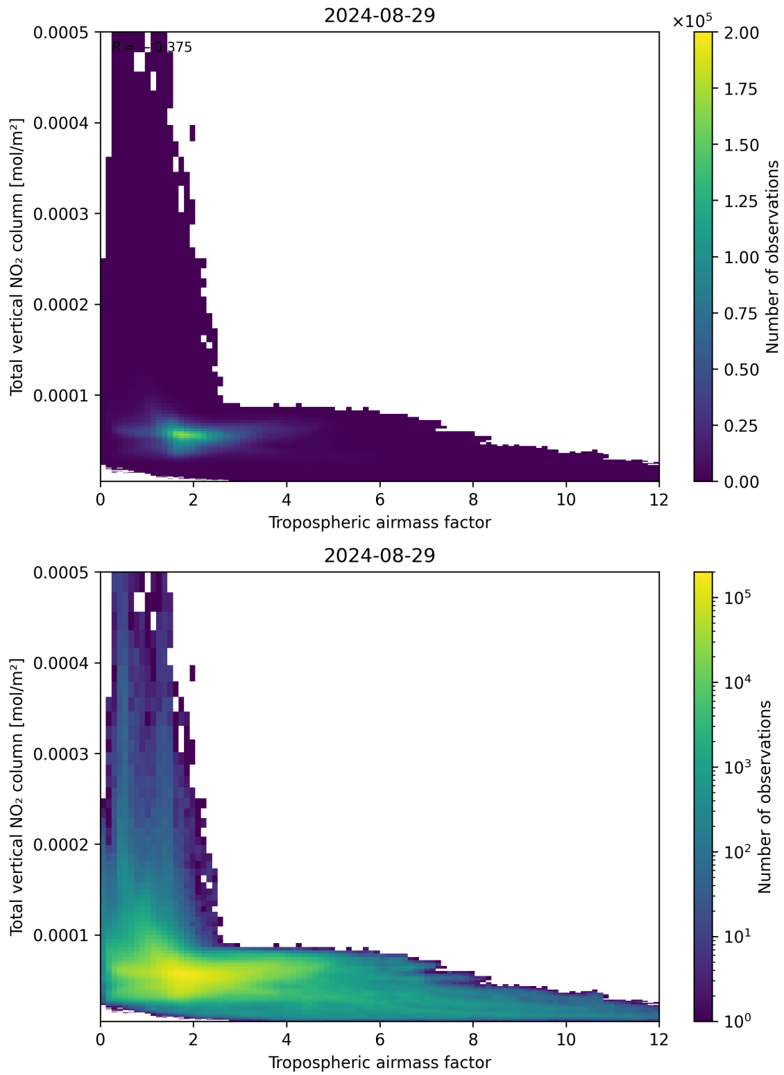
Figure 77: Scatter density plot of “Tropospheric airmass factor” against “Total vertical NO 2 column” for 2024-08-28 to 2024-08-30.
