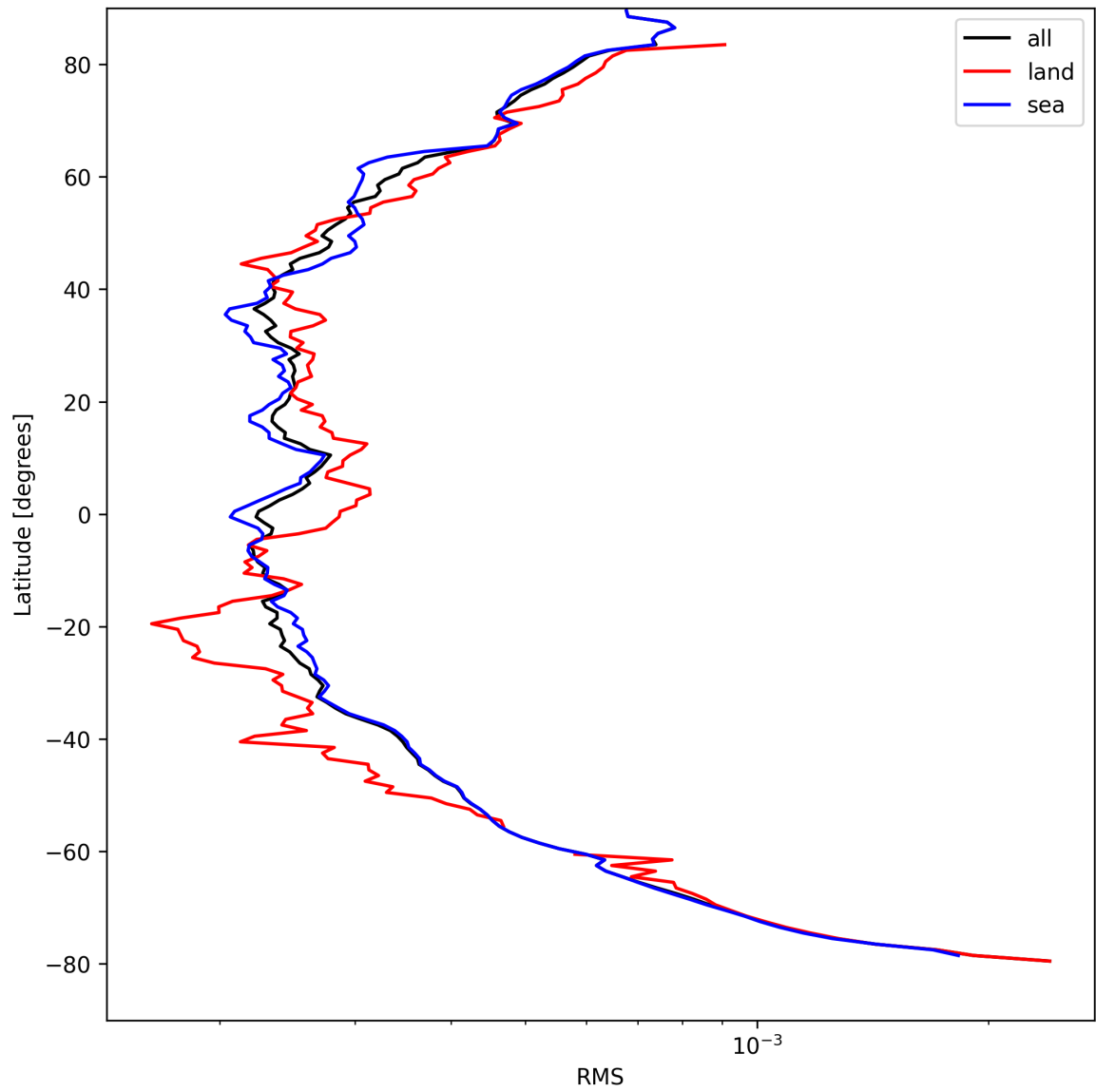
Figure 26: Zonal average of “RMS” for 2024-08-28 to 2024-08-30.
