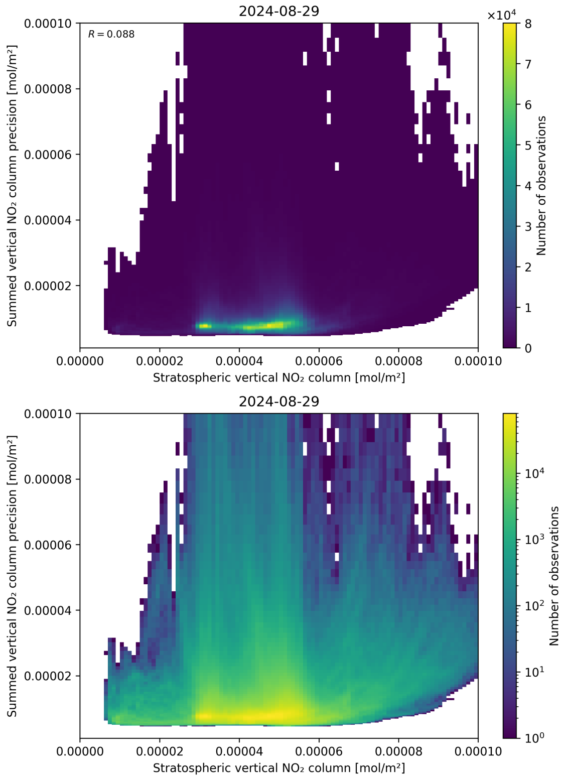
Figure 99: Scatter density plot of “Stratospheric vertical NO 2 column” against “Summed vertical NO 2 column precision” for 2024-08-28 to 2024-08-30.
