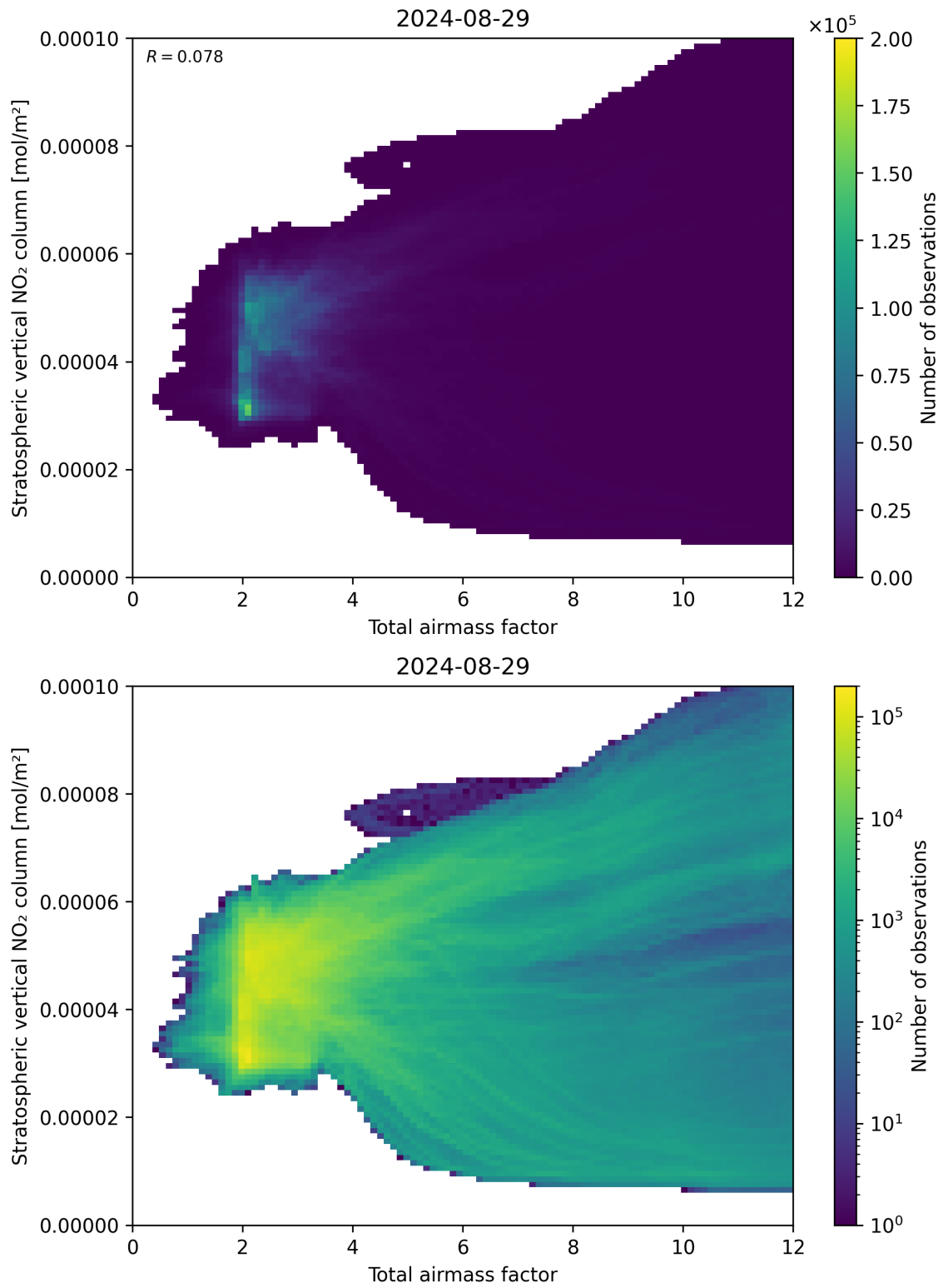
Figure 64: Scatter density plot of “Total airmass factor” against “Stratospheric vertical \text{NO}_2 column” for 2024-08-28 to 2024-08-30.
