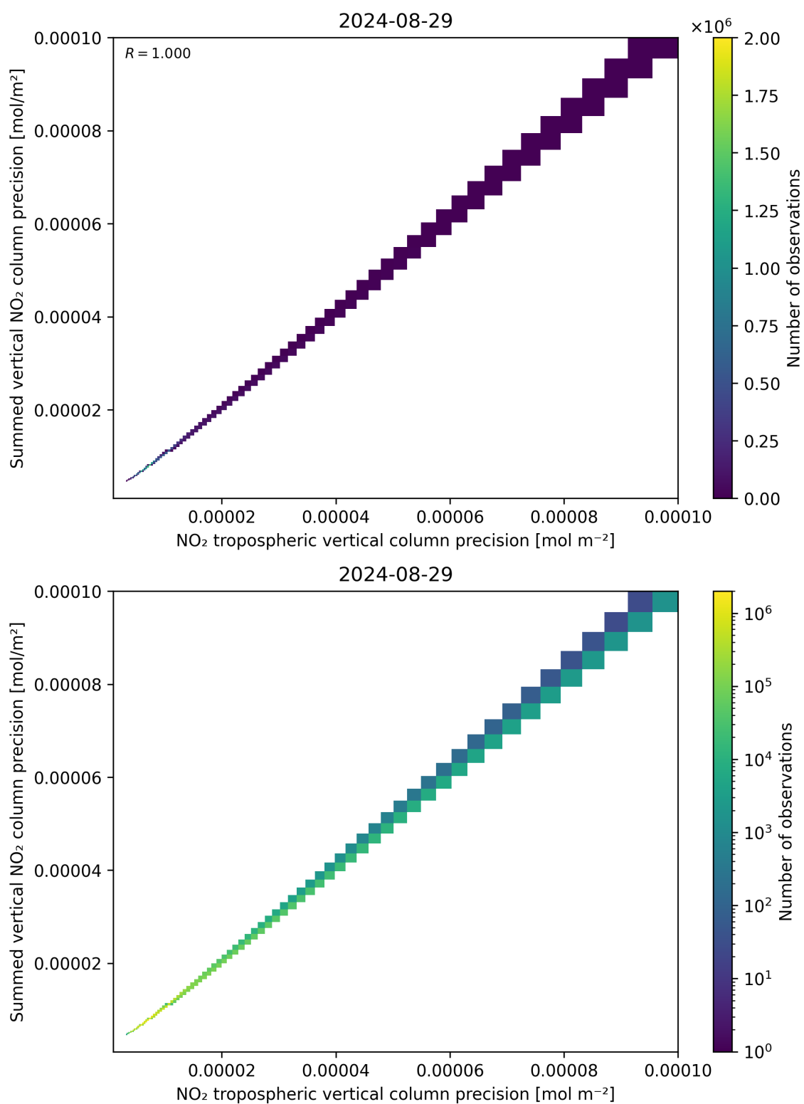
Figure 137: Scatter density plot of “NO 2 tropospheric vertical column precision” against “Summed vertical NO 2 column precision” for 2024-08-28 to 2024-08-30.
