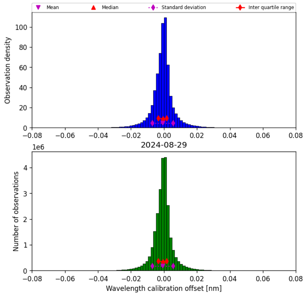
Figure 35: Histogram of “Wavelength calibration offset” for 2024-08-28 to 2024-08-30
