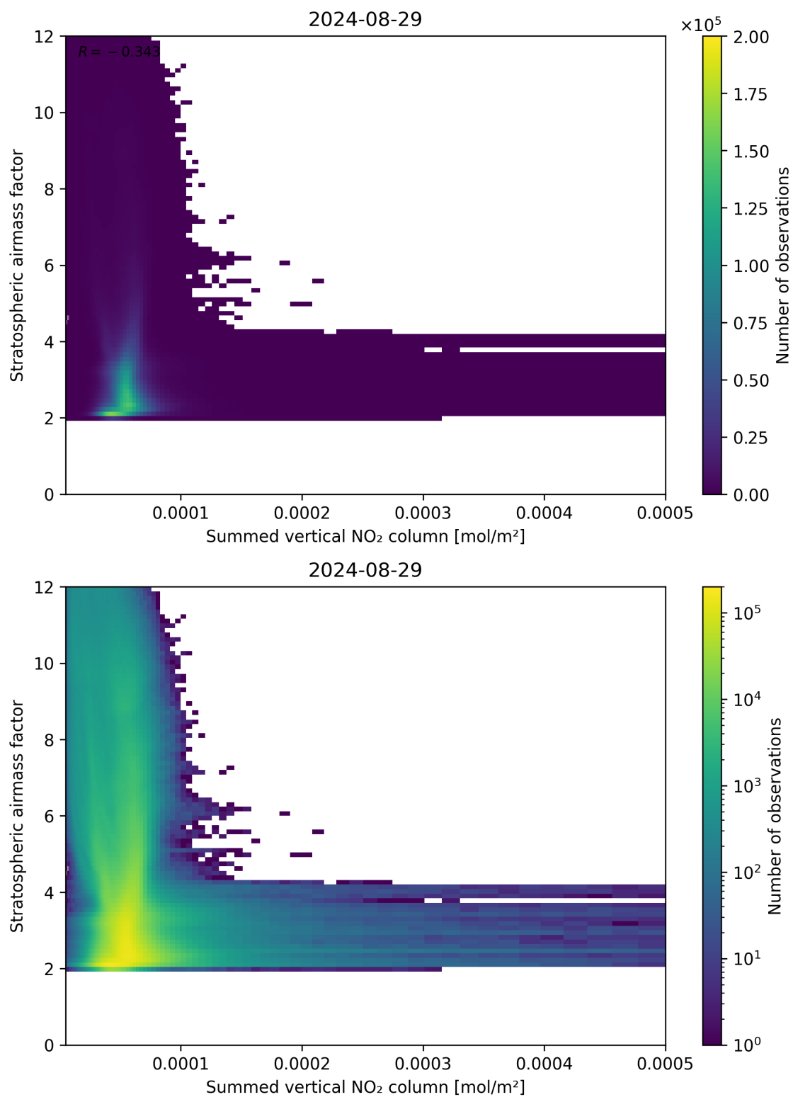
Figure 103: Scatter density plot of “Summed vertical NO 2 column” against “Stratospheric airmass factor” for 2024-08-28 to 2024-08-30.
