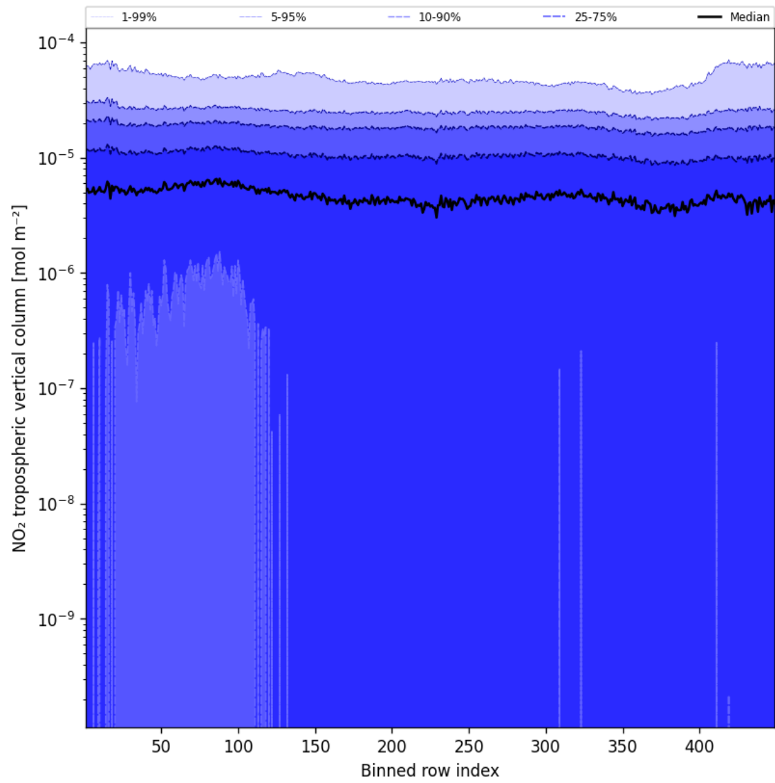
Figure 46: Along track statistics of “NO 2 tropospheric vertical column” for 2024-08-28 to 2024-08-30
