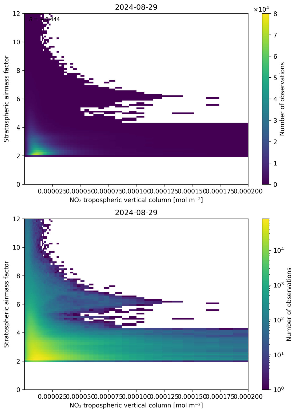
Figure 121: Scatter density plot of “NO 2 tropospheric vertical column” against “Stratospheric air mass factor” for 2024-08-28 to 2024-08-30.
