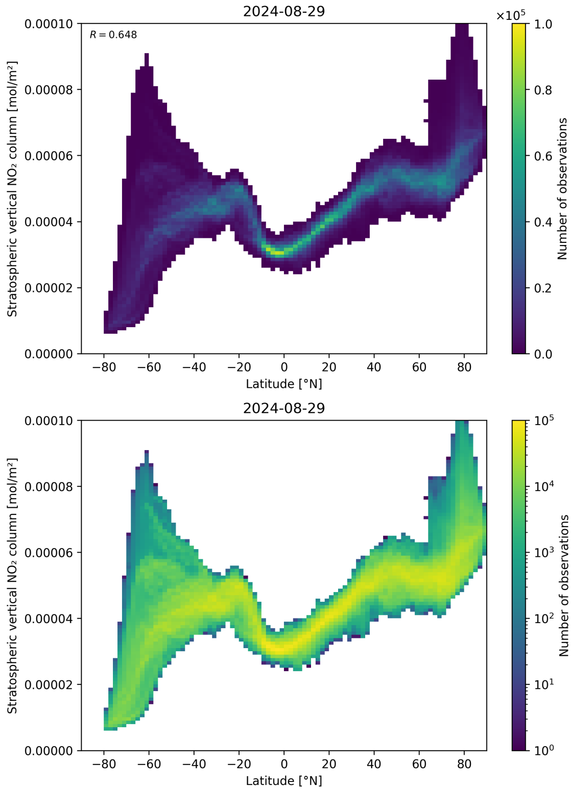
Figure 87: Scatter density plot of “Latitude” against “Stratospheric vertical NO 2 column” for 2024-08-28 to 2024-08-30.
