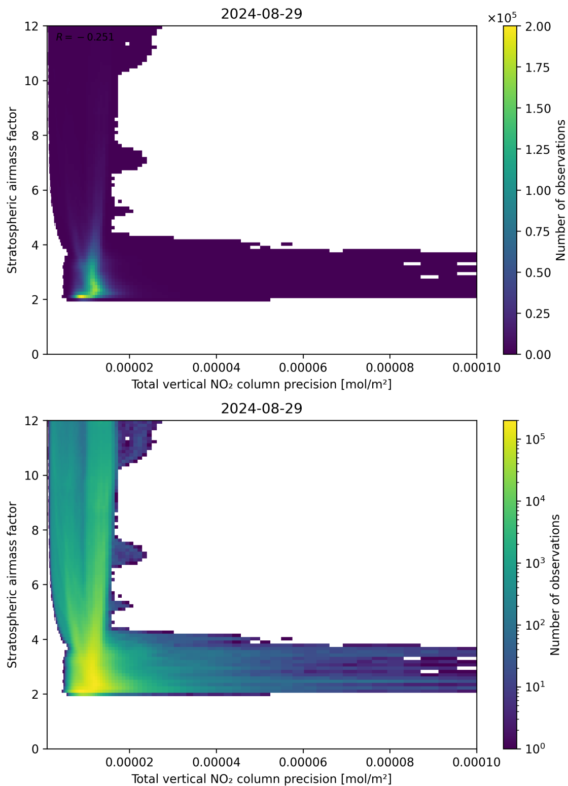
Figure 115: Scatter density plot of “Total vertical NO 2 column precision” against “Stratospheric air mass factor” for 2024-08-28 to 2024-08-30.
