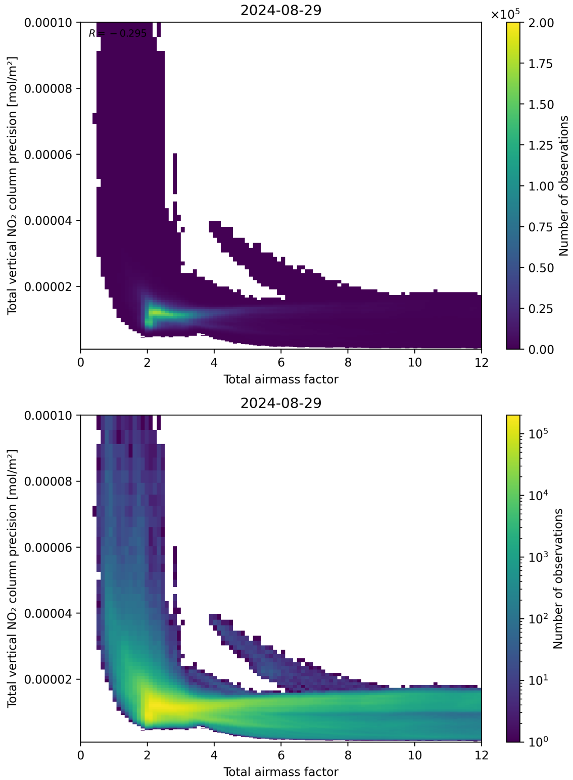
Figure 68: Scatter density plot of “Total airmass factor” against “Total vertical NO 2 column precision” for 2024-08-28 to 2024-08-30.
