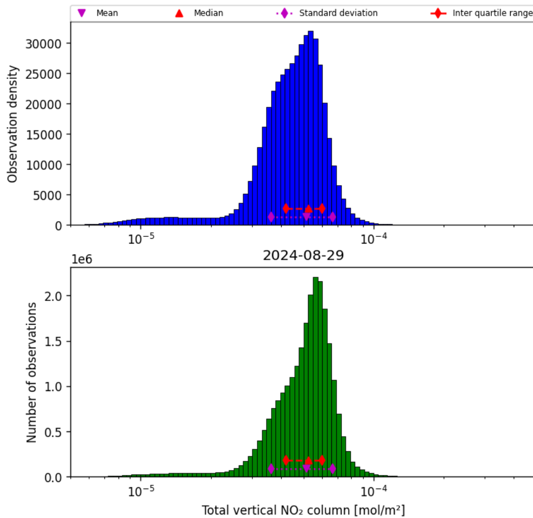
Figure 38: Histogram of "Total vertical NO 2 column" for 2024-08-28 to 2024-08-30
