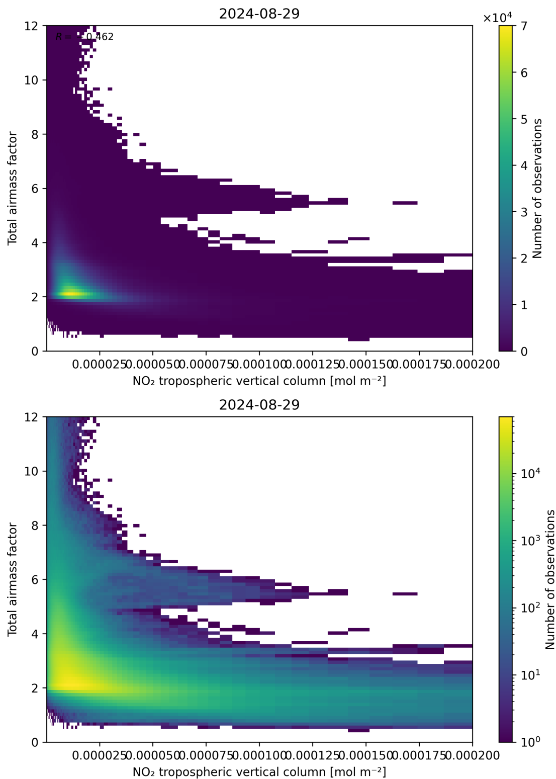
Figure 122: Scatter density plot of “NO 2 tropospheric vertical column” against “Total air mass factor” for 2024-08-28 to 2024-08-30.
