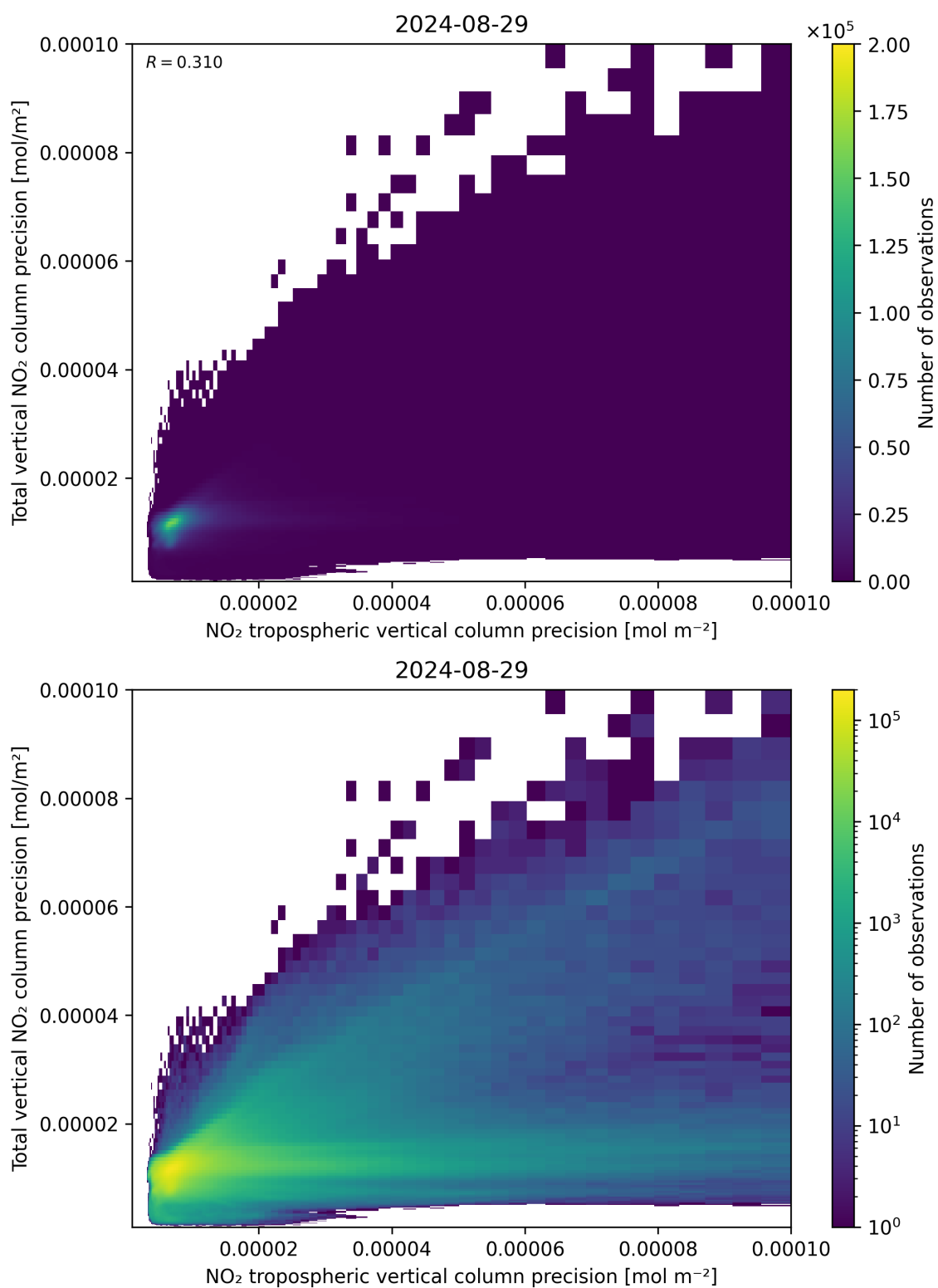
Figure 139: Scatter density plot of “NO 2 tropospheric vertical column precision” against “Total vertical NO 2 column precision” for 2024-08-28 to 2024-08-30.
