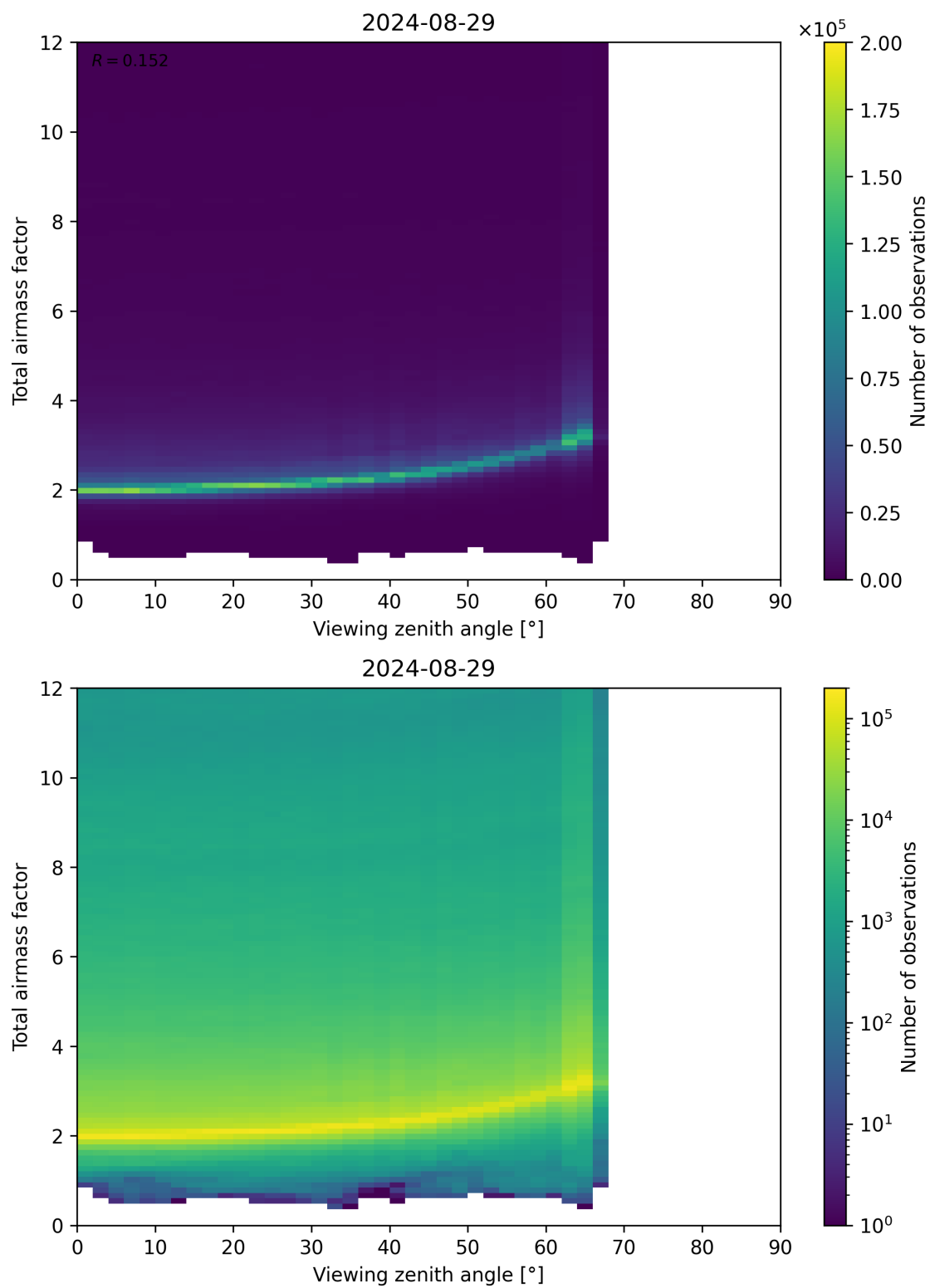
Figure 160: Scatter density plot of “Viewing zenith angle” against “Total airmass factor” for 2024-08-28 to 2024-08-30.
