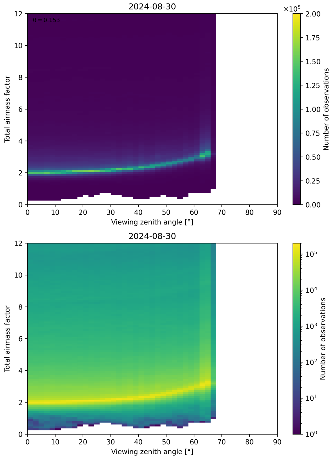
Figure 160: Scatter density plot of “Viewing zenith angle” against “Total airmass factor” for 2024-08-29 to 2024-08-31.
