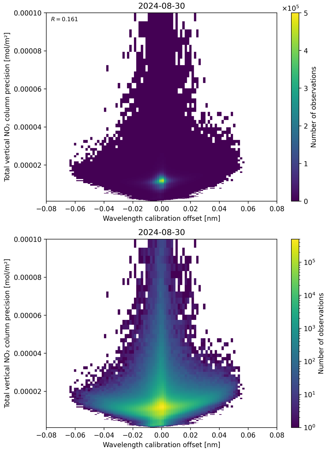
Figure 180: Scatter density plot of “Wavelength calibration offset” against “Total vertical NO 2 column precision” for 2024-08-29 to 2024-08-31.
