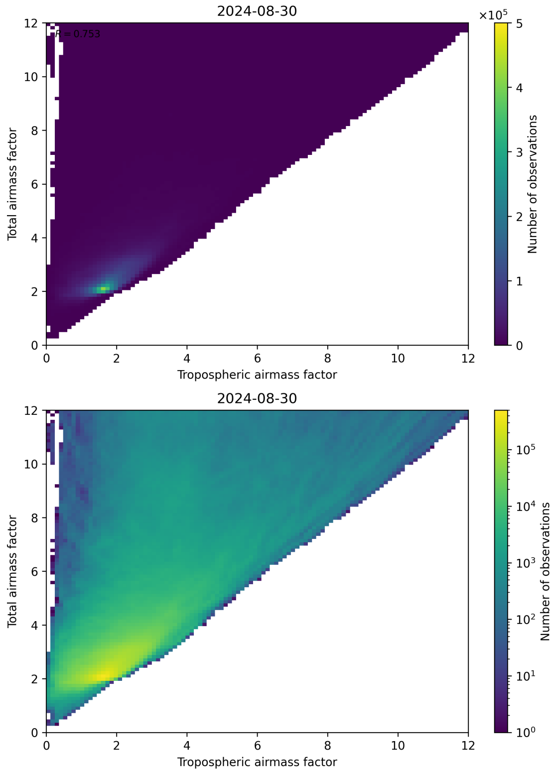
Figure 72: Scatter density plot of “Tropospheric airmass factor” against “Total airmass factor” for 2024-08-29 to 2024-08-31.
