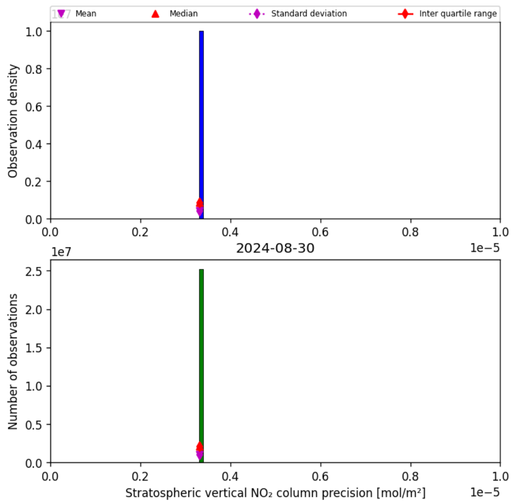
Figure 37: Histogram of “Stratospheric vertical NO 2 column precision” for 2024-08-29 to 2024-08-31
