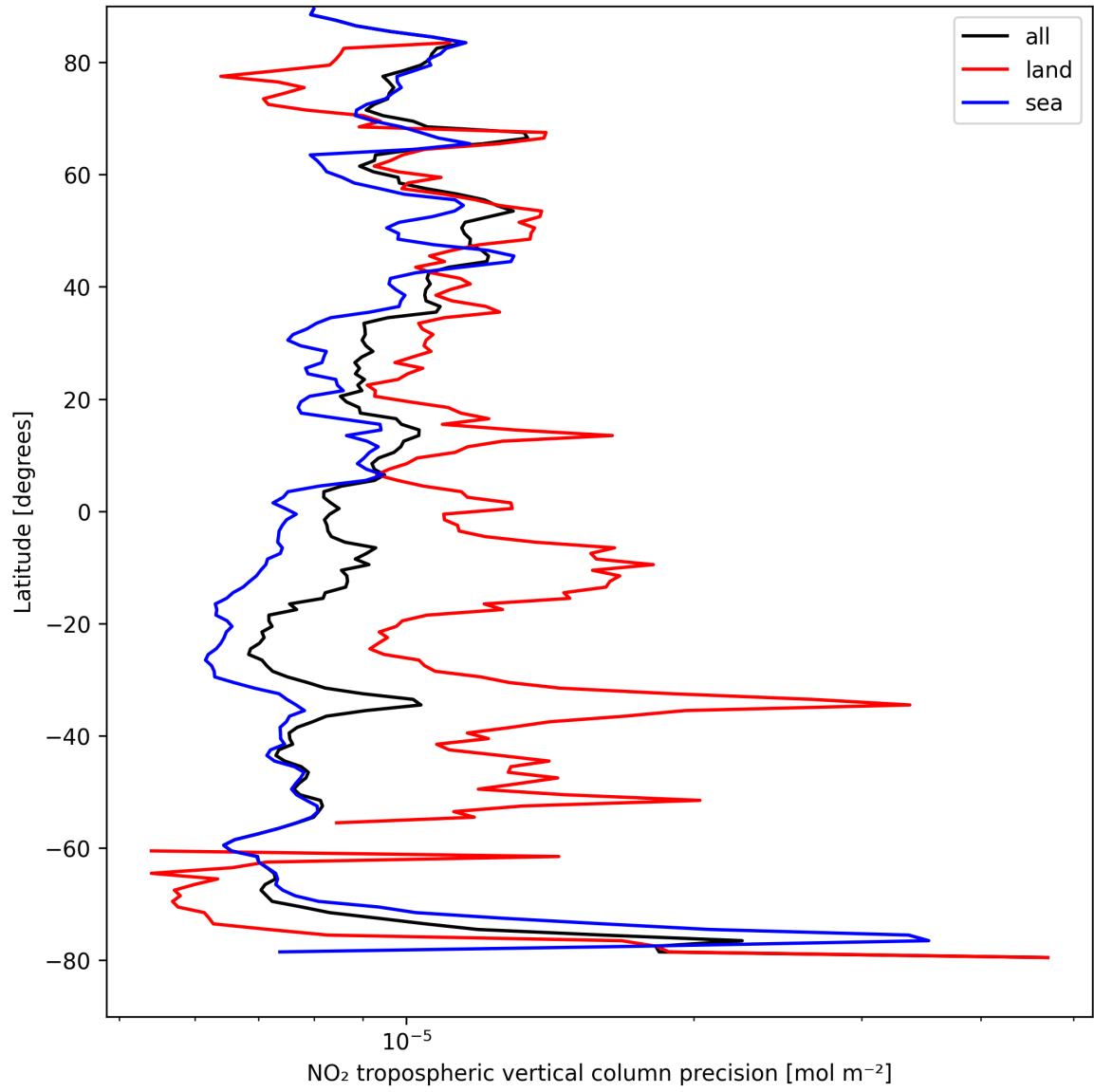
Figure 13: Zonal average of “NO 2 tropospheric vertical column precision” for 2024-08-29 to 2024-08-31.
