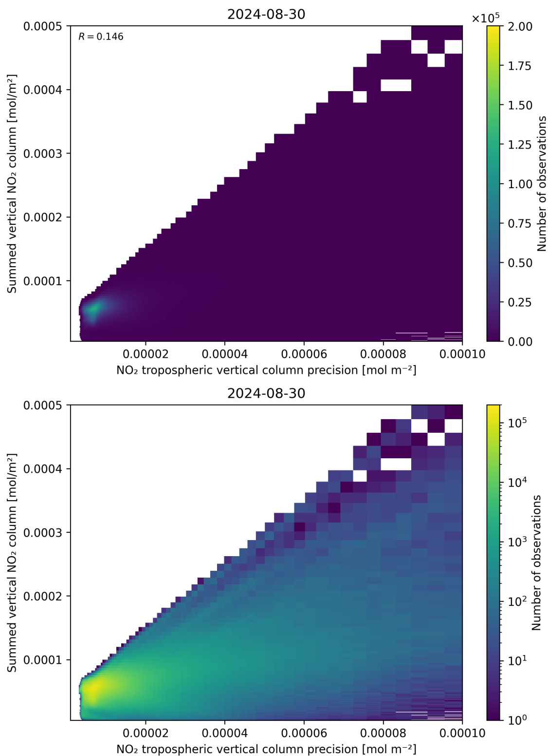
Figure 136: Scatter density plot of “NO 2 tropospheric vertical column precision” against “Summed vertical NO 2 column” for 2024-08-29 to 2024-08-31.
