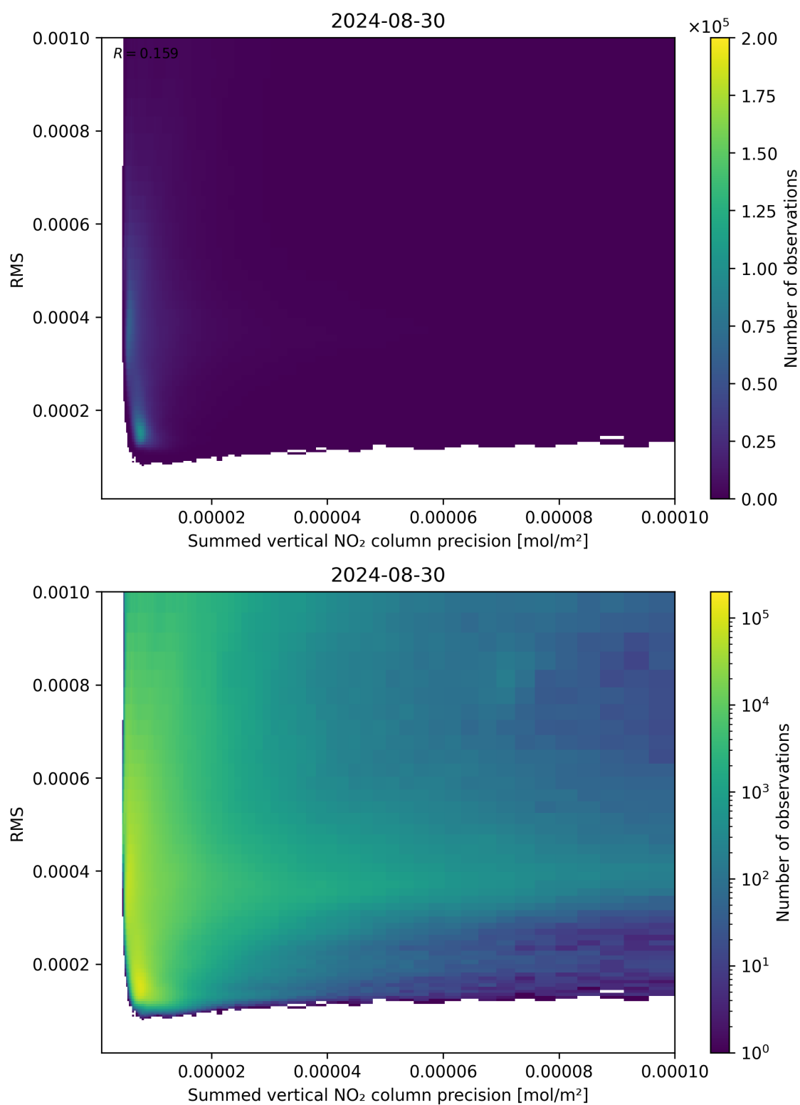
Figure 108: Scatter density plot of “Summed vertical NO 2 column precision” against “RMS” for 2024-08-29 to 2024-08-31.
