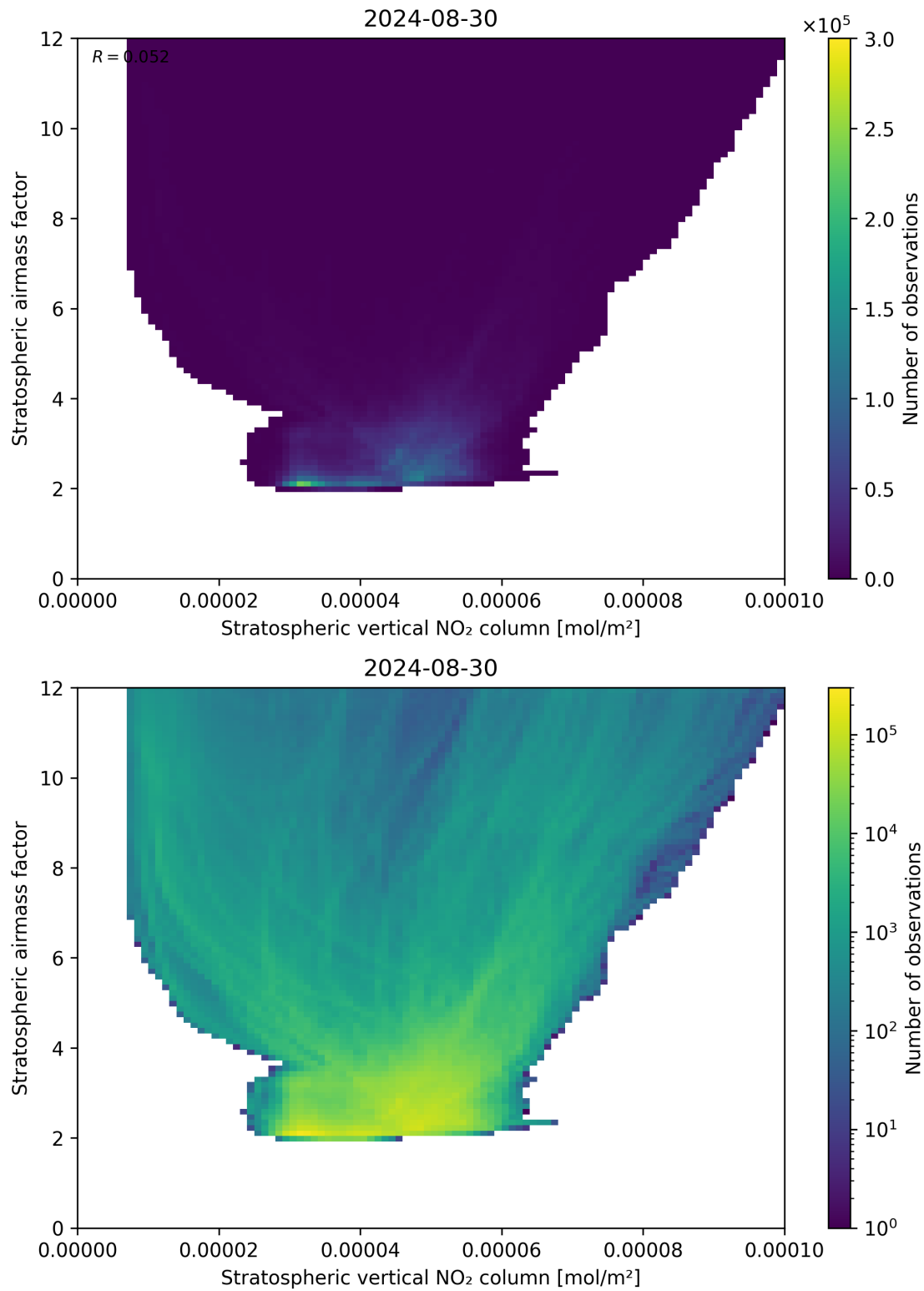
Figure 96: Scatter density plot of “Stratospheric vertical NO 2 column” against “Stratospheric airmass factor” for 2024-08-29 to 2024-08-31.
