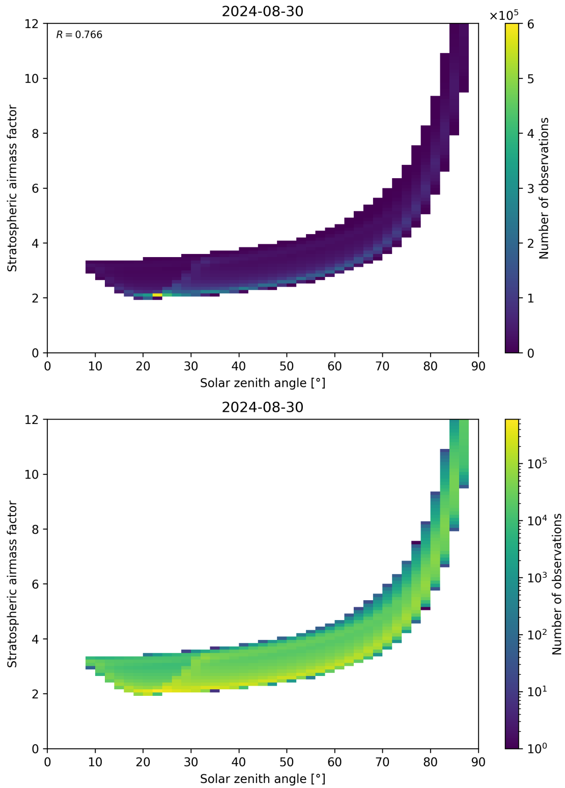
Figure 145: Scatter density plot of “Solar zenith angle” against “Stratospheric airmass factor” for 2024-08-29 to 2024-08-31.
