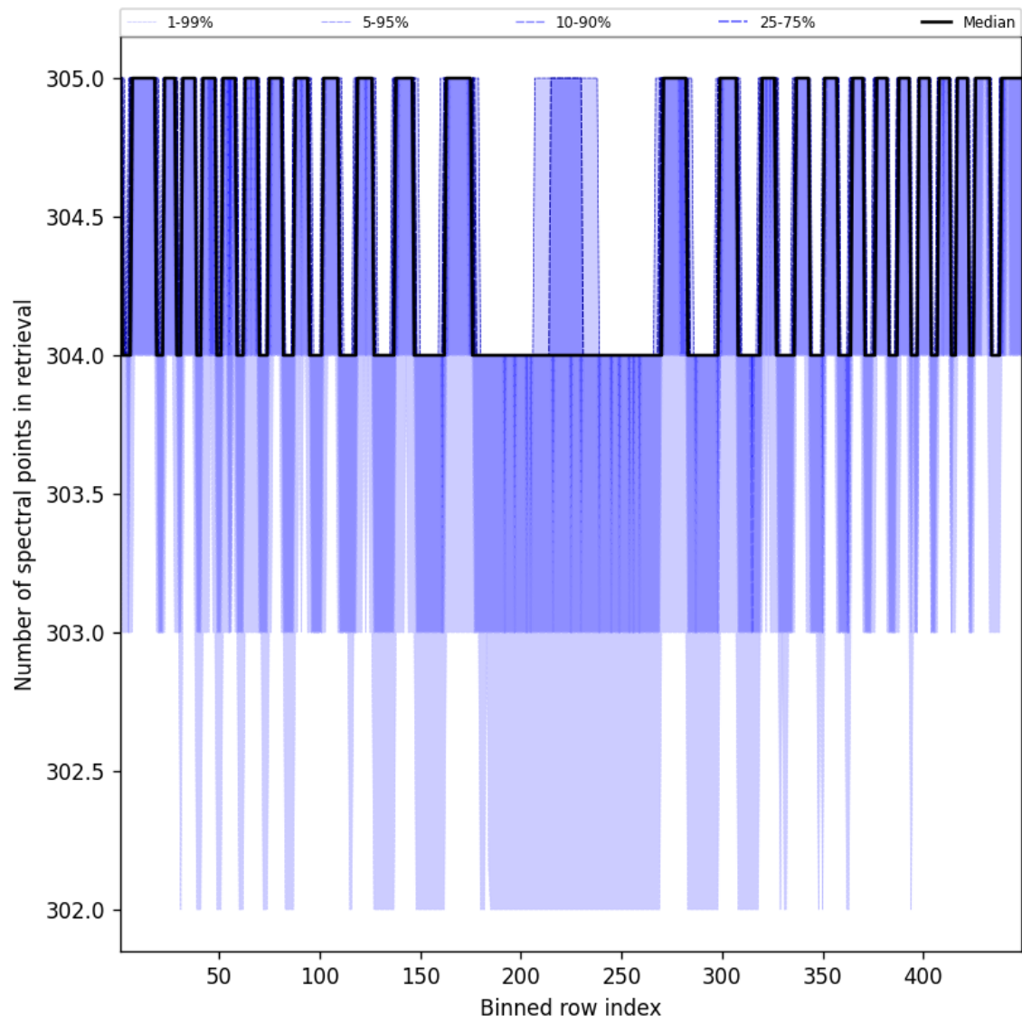
Figure 50: Along track statistics of “Number of spectral points in retrieval” for 2024-08-29 to 2024-08-31
