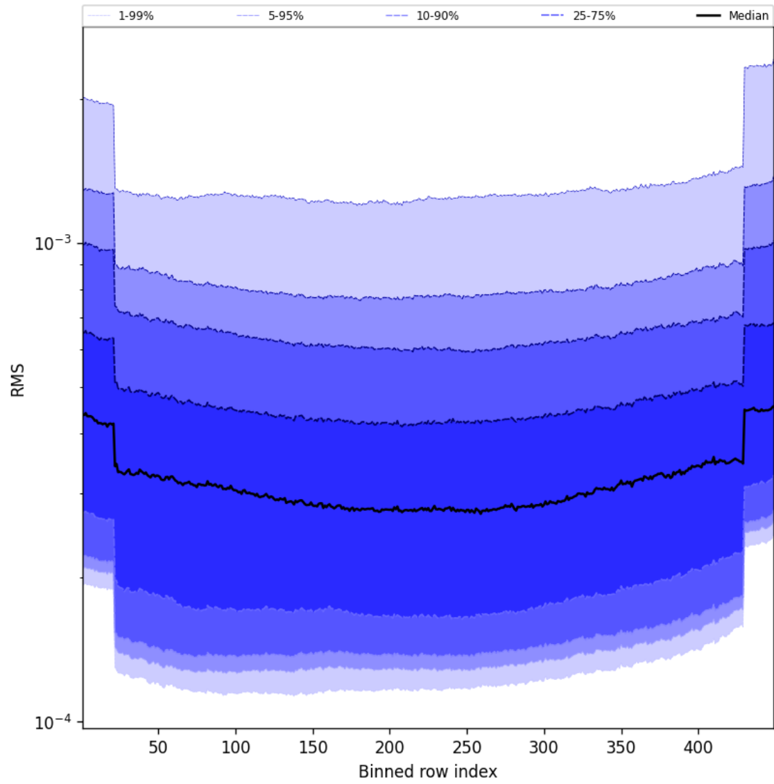
Figure 60: Along track statistics of “RMS” for 2024-08-29 to 2024-08-31
