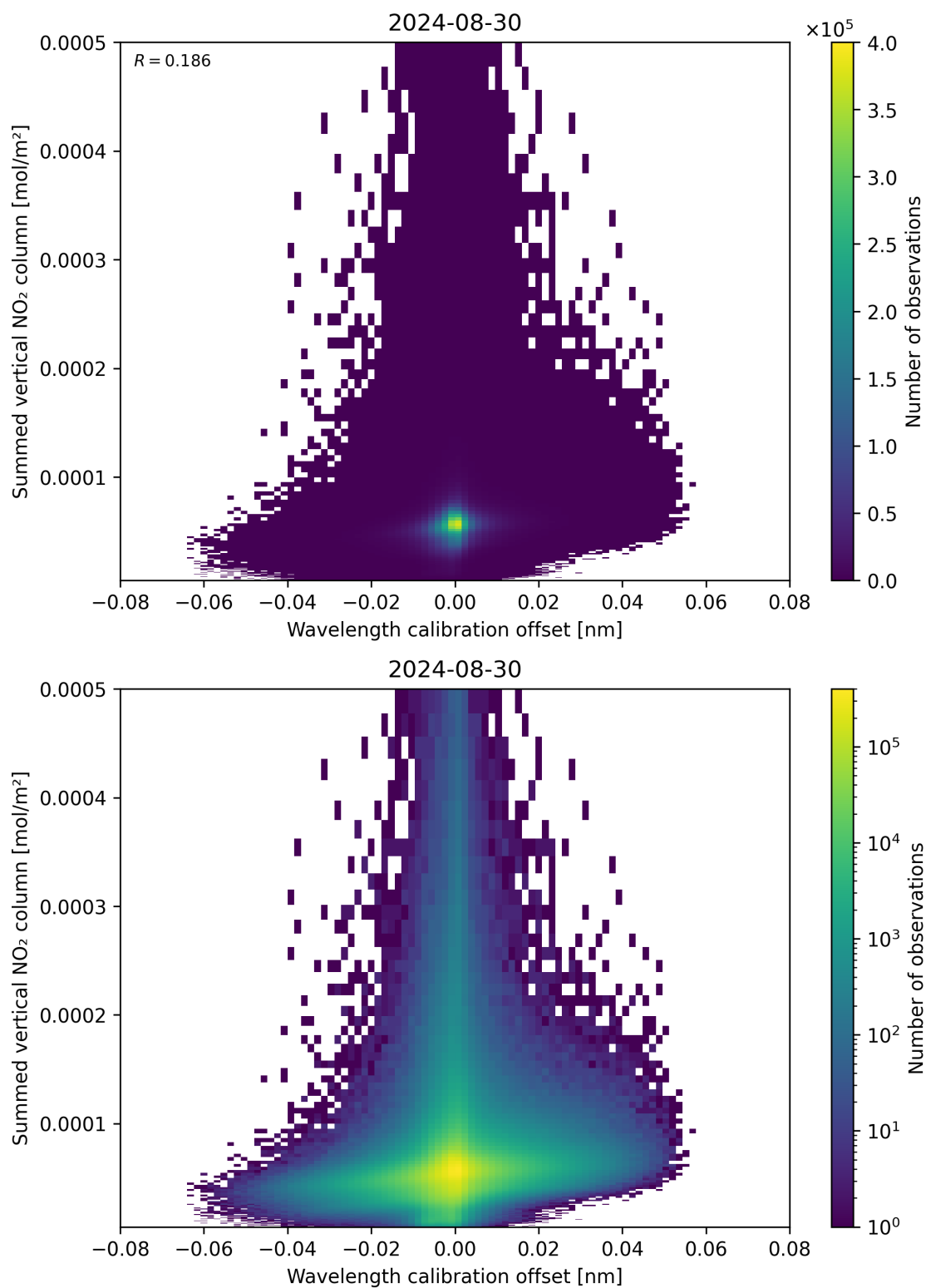
Figure 177: Scatter density plot of “Wavelength calibration offset” against “Summed vertical NO 2 column” for 2024-08-29 to 2024-08-31.
