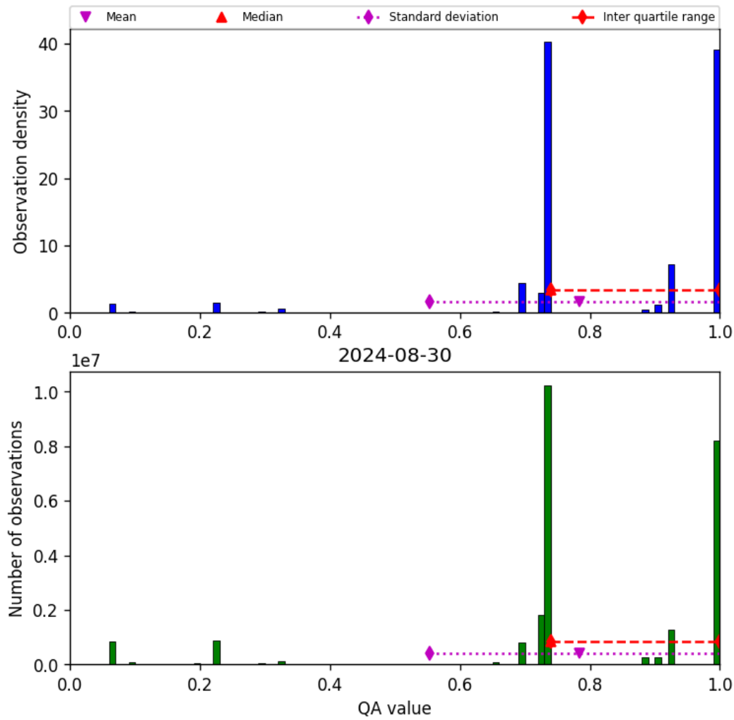
Figure 28: Histogram of “QA value” for 2024-08-29 to 2024-08-31
