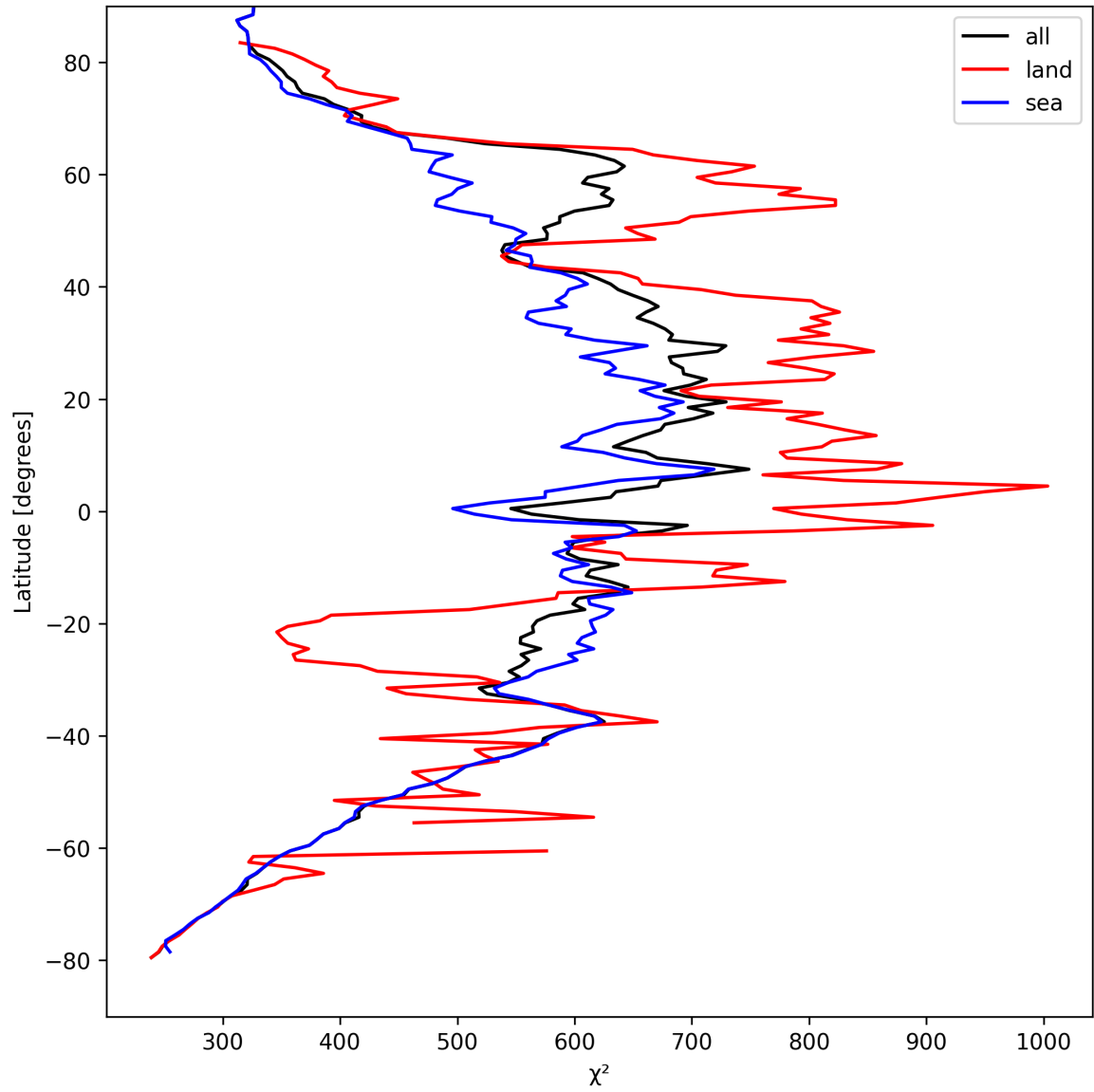
Figure 25: Zonal average of “ \chi^2 ” for 2024-08-29 to 2024-08-31.
