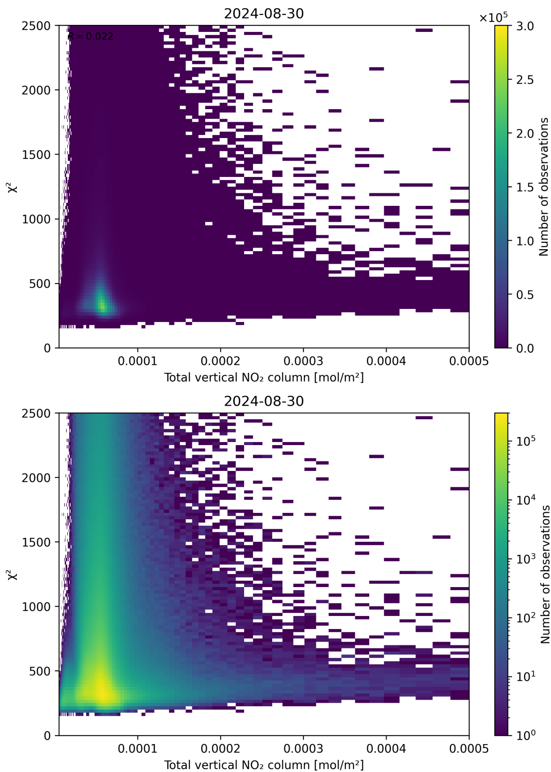
Figure 111: Scatter density plot of “Total vertical NO 2 column” against “ \chi^2 ” for 2024-08-29 to 2024-08-31.
