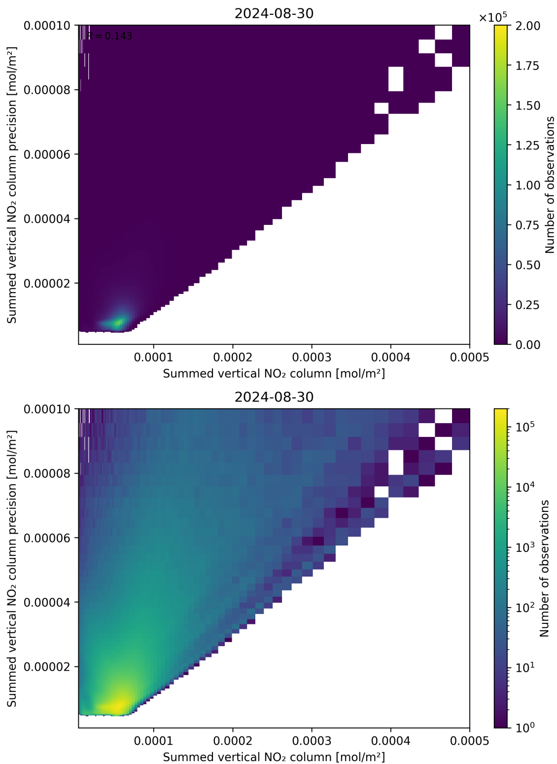
Figure 105: Scatter density plot of “Summed vertical NO 2 column” against “Summed vertical NO 2 column precision” for 2024-08-29 to 2024-08-31.
