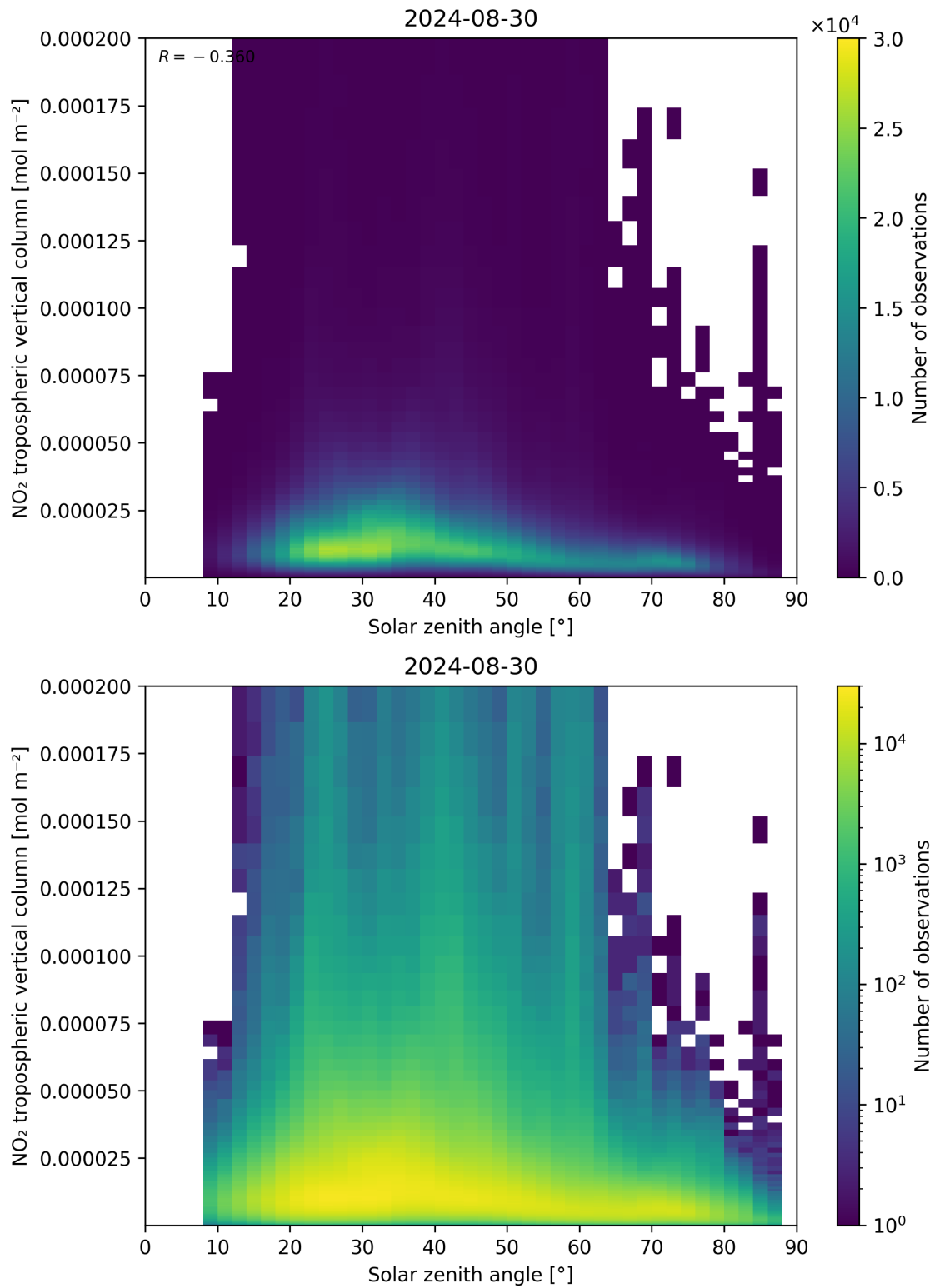
Figure 155: Scatter density plot of “Solar zenith angle” against “NO 2 tropospheric vertical column” for 2024-08-29 to 2024-08-31.
