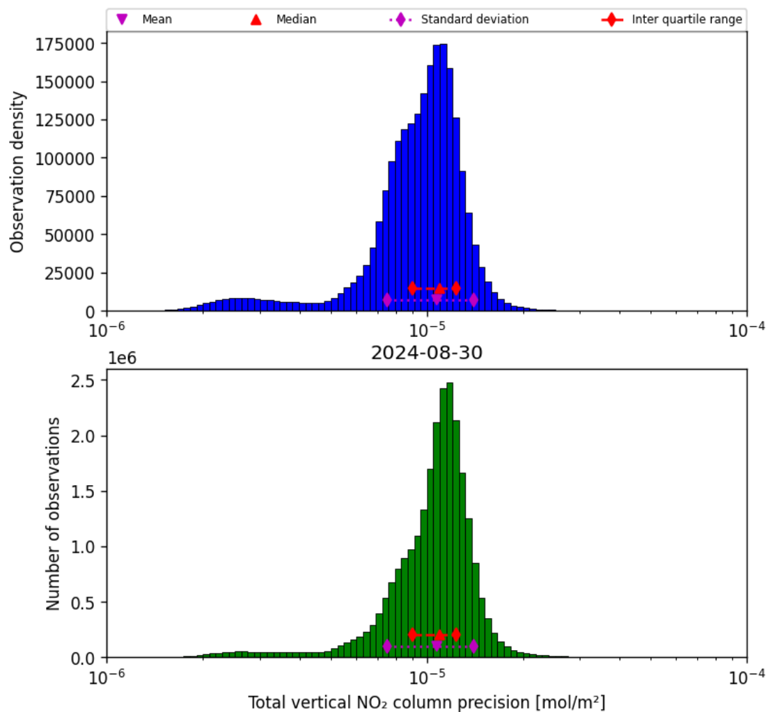
Figure 39: Histogram of "Total vertical NO 2 column precision" for 2024-08-29 to 2024-08-31
