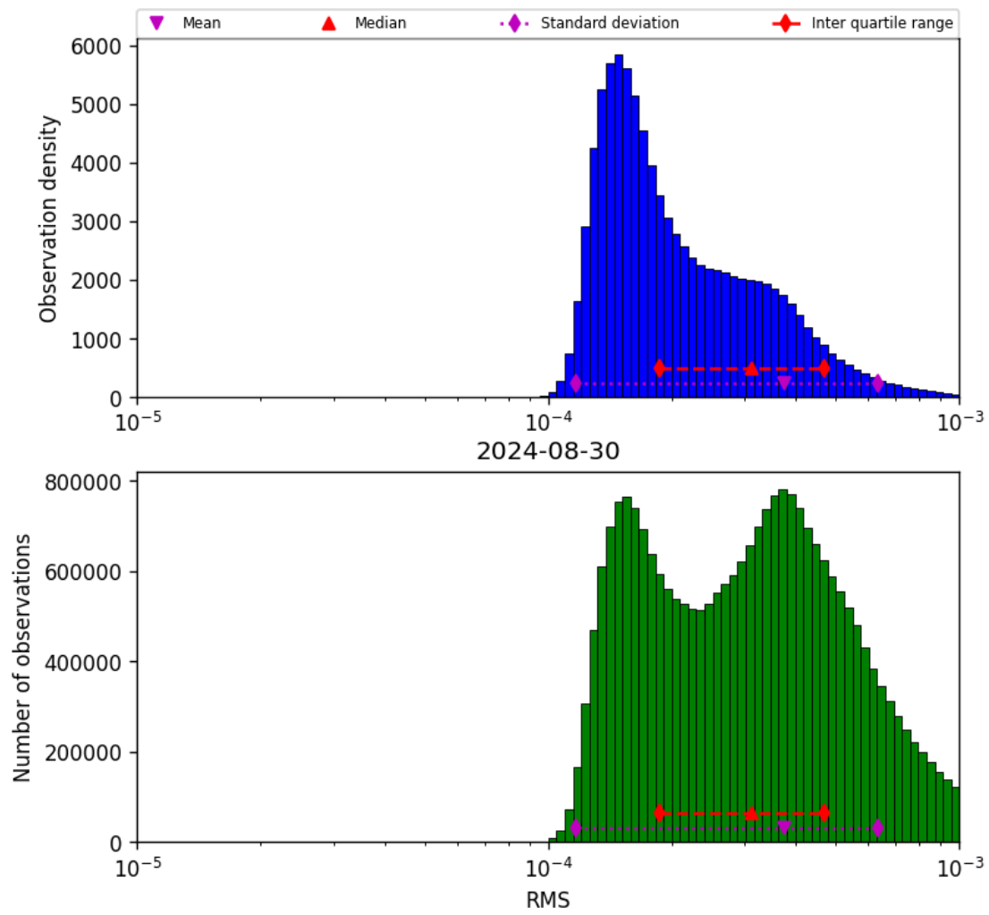
Figure 43: Histogram of “RMS” for 2024-08-29 to 2024-08-31
