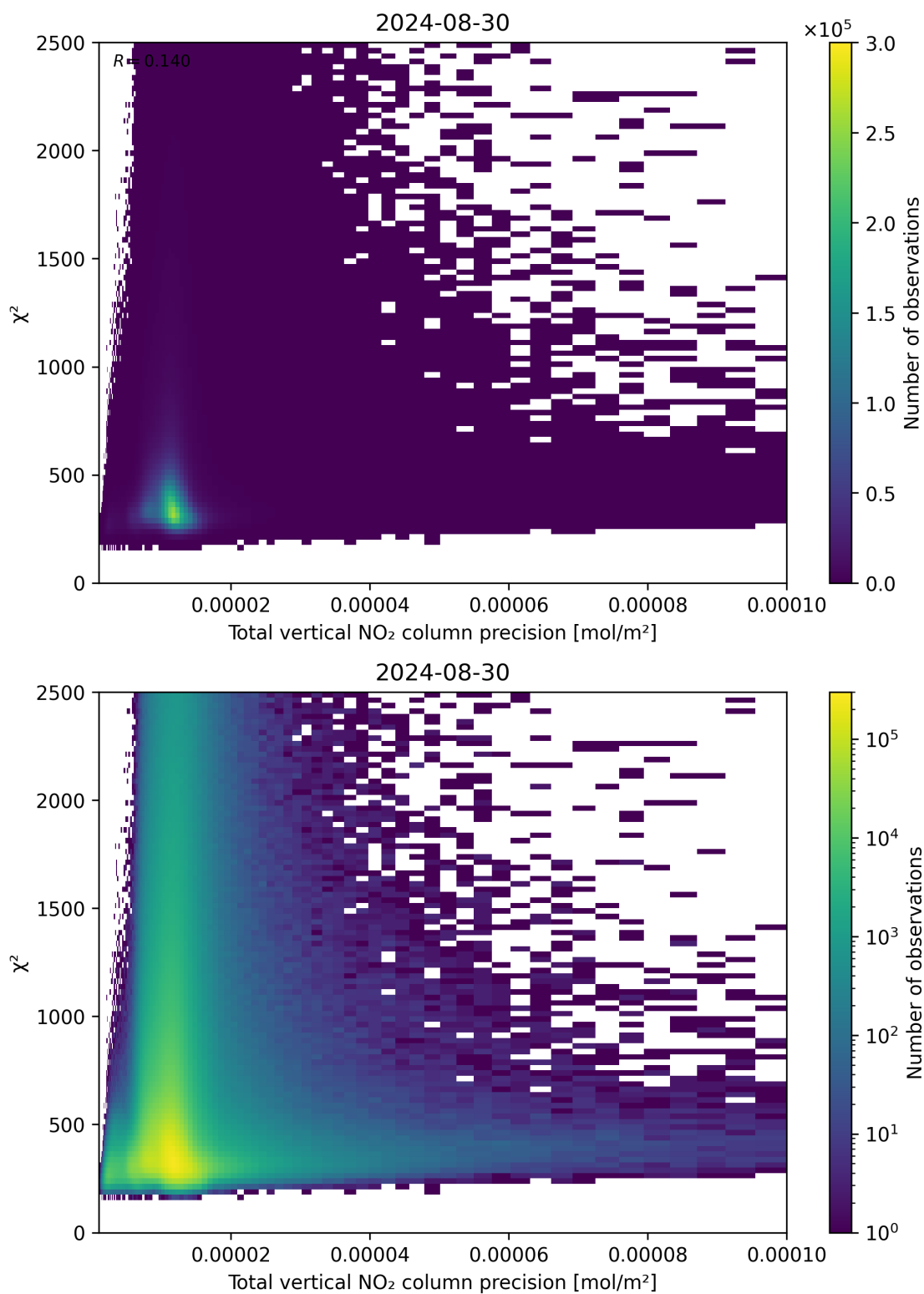
Figure 116: Scatter density plot of “Total vertical NO 2 column precision” against “ \chi^2 ” for 2024-08-29 to 2024-08-31.
