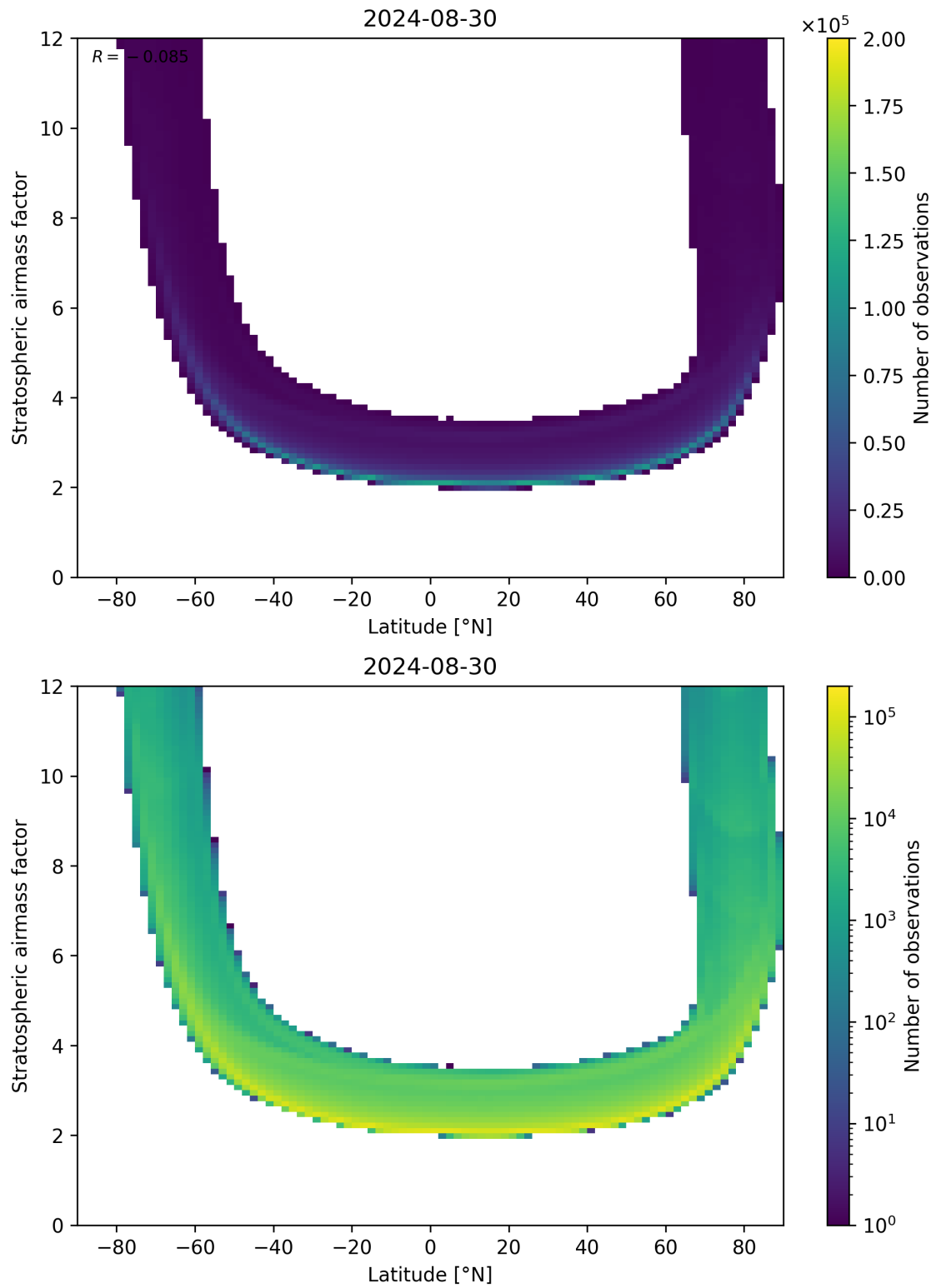
Figure 83: Scatter density plot of “Latitude” against “Stratospheric airmass factor” for 2024-08-29 to 2024-08-31.
