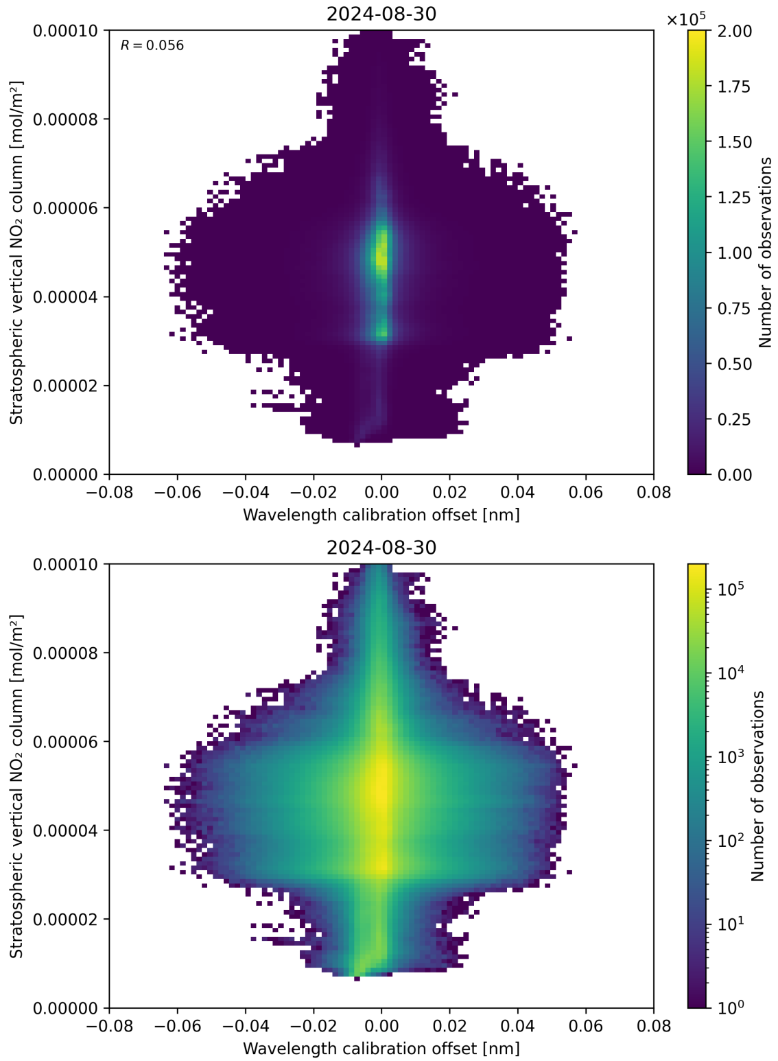
Figure 176: Scatter density plot of “Wavelength calibration offset” against “Stratospheric vertical NO 2 column” for 2024-08-29 to 2024-08-31.
