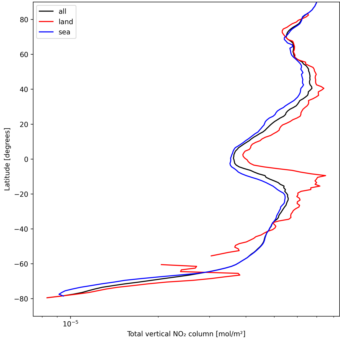
Figure 21: Zonal average of “Total vertical NO 2 column” for 2024-08-29 to 2024-08-31.
