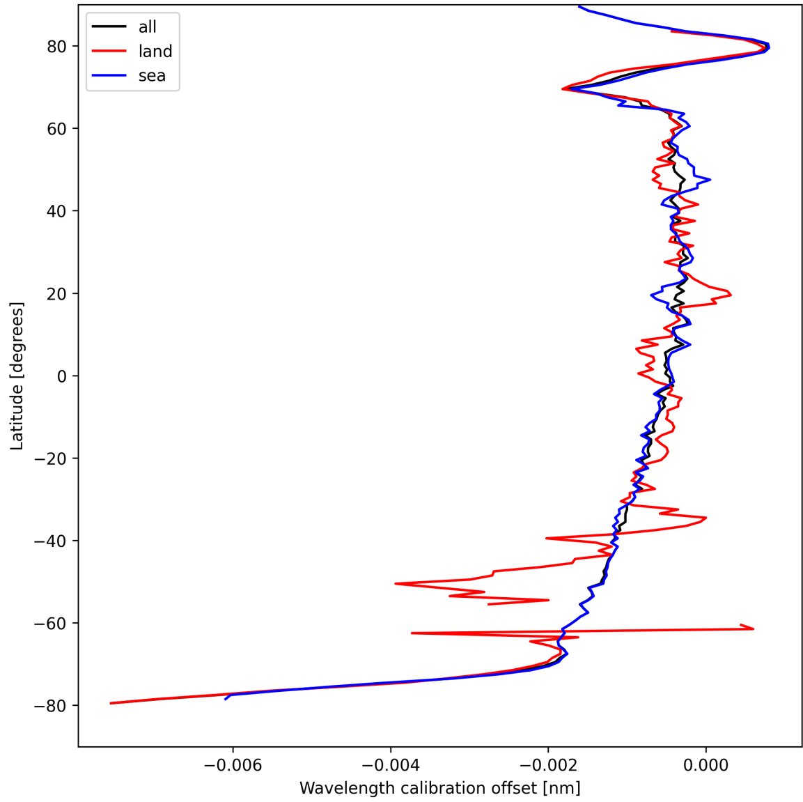
Figure 18: Zonal average of “Wavelength calibration offset” for 2024-08-29 to 2024-08-31.
