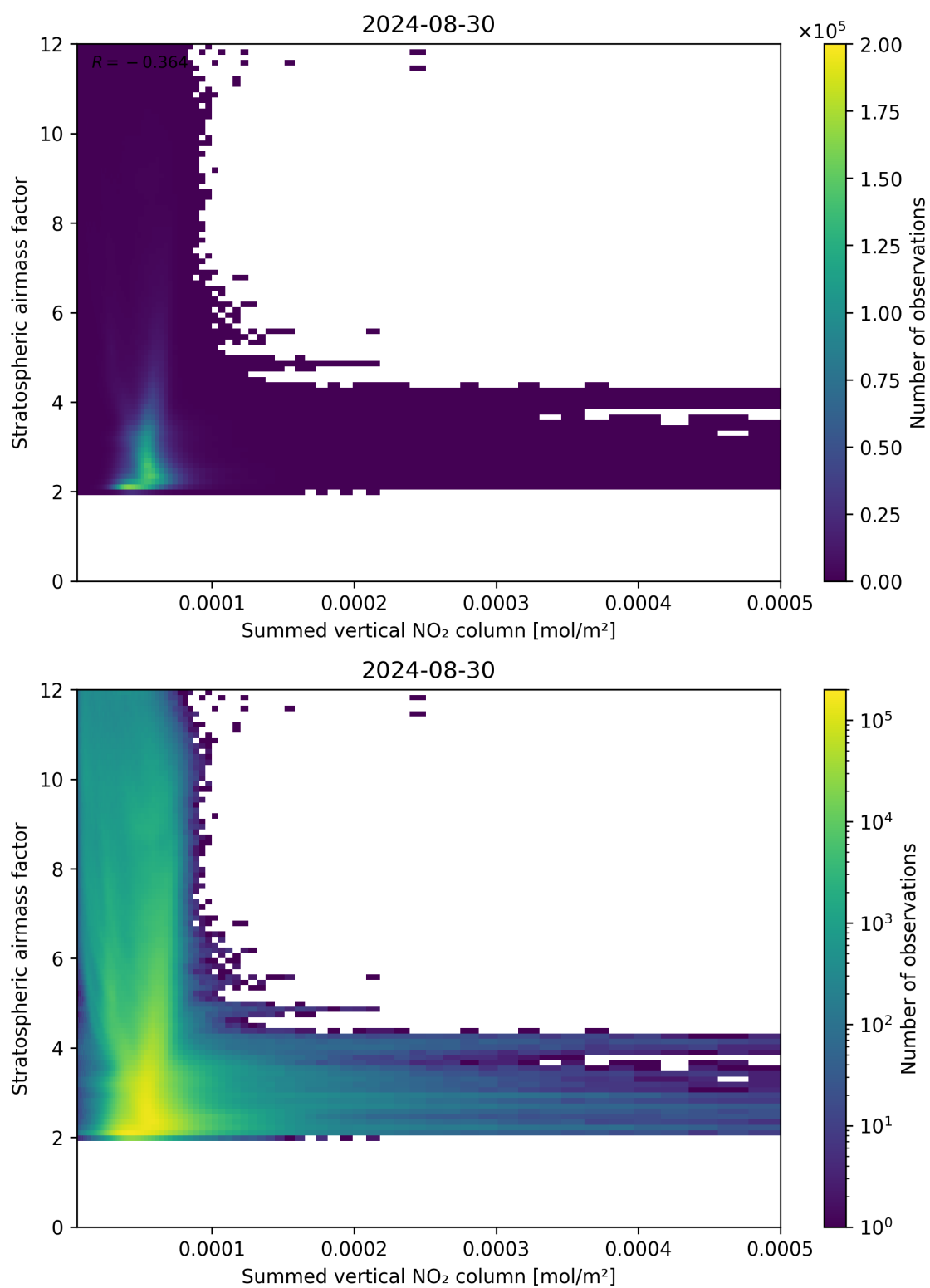
Figure 103: Scatter density plot of “Summed vertical NO 2 column” against “Stratospheric airmass factor” for 2024-08-29 to 2024-08-31.
