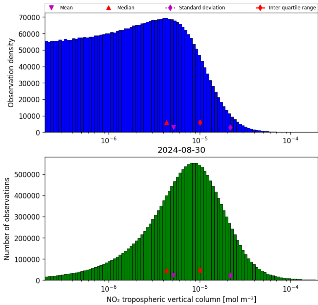
Figure 29: Histogram of “ \text{NO}_2 tropospheric vertical column” for 2024-08-29 to 2024-08-31
