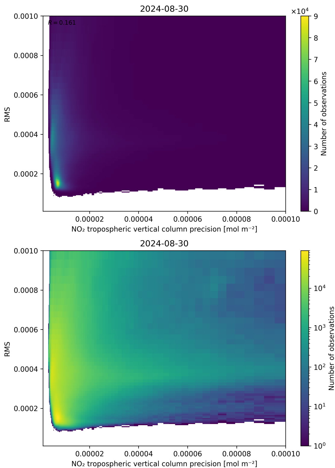
Figure 140: Scatter density plot of “NO 2 tropospheric vertical column precision” against “RMS” for 2024-08-29 to 2024-08-31.
