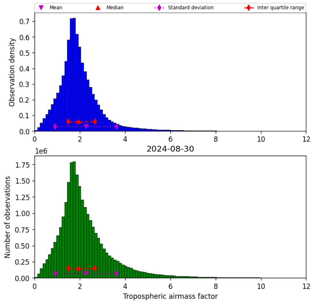
Figure 31: Histogram of “Tropospheric airmass factor” for 2024-08-29 to 2024-08-31
