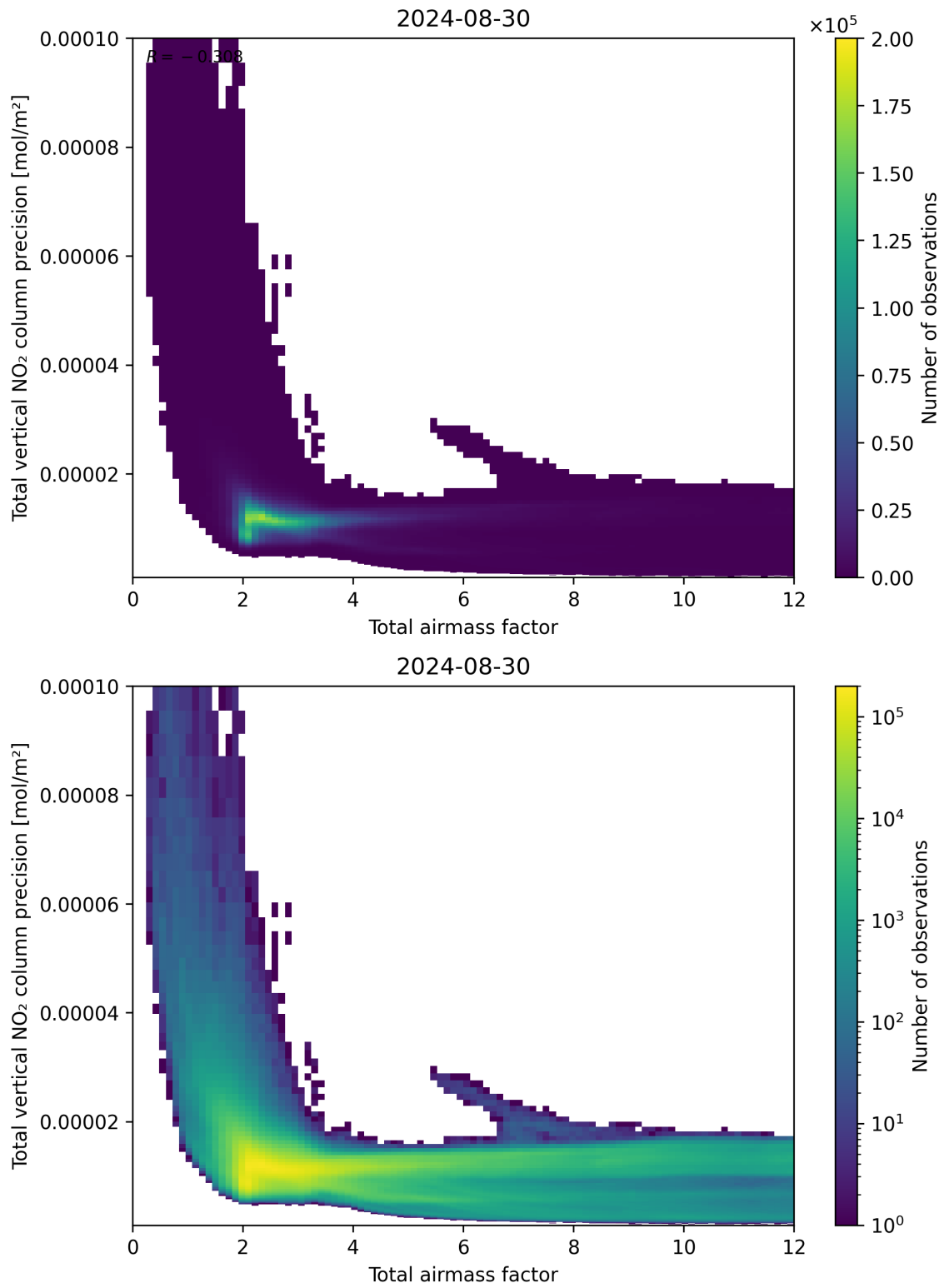
Figure 68: Scatter density plot of “Total airmass factor” against “Total vertical NO 2 column precision” for 2024-08-29 to 2024-08-31.
