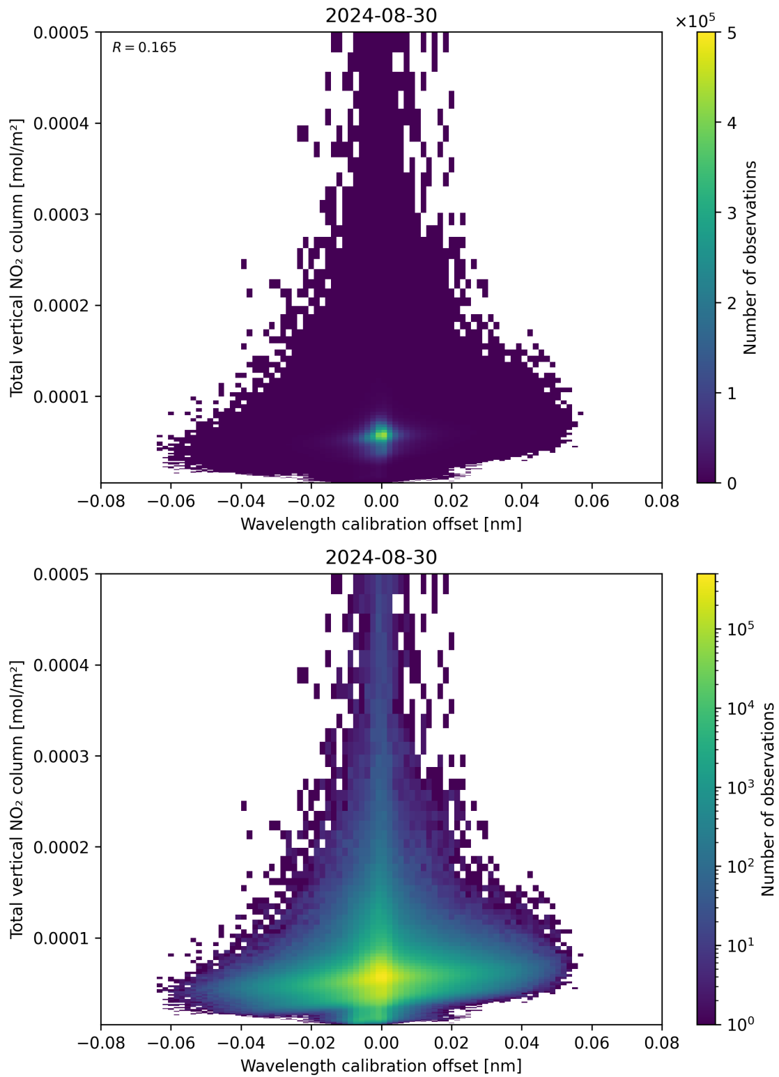
Figure 179: Scatter density plot of “Wavelength calibration offset” against “Total vertical NO 2 column” for 2024-08-29 to 2024-08-31.
