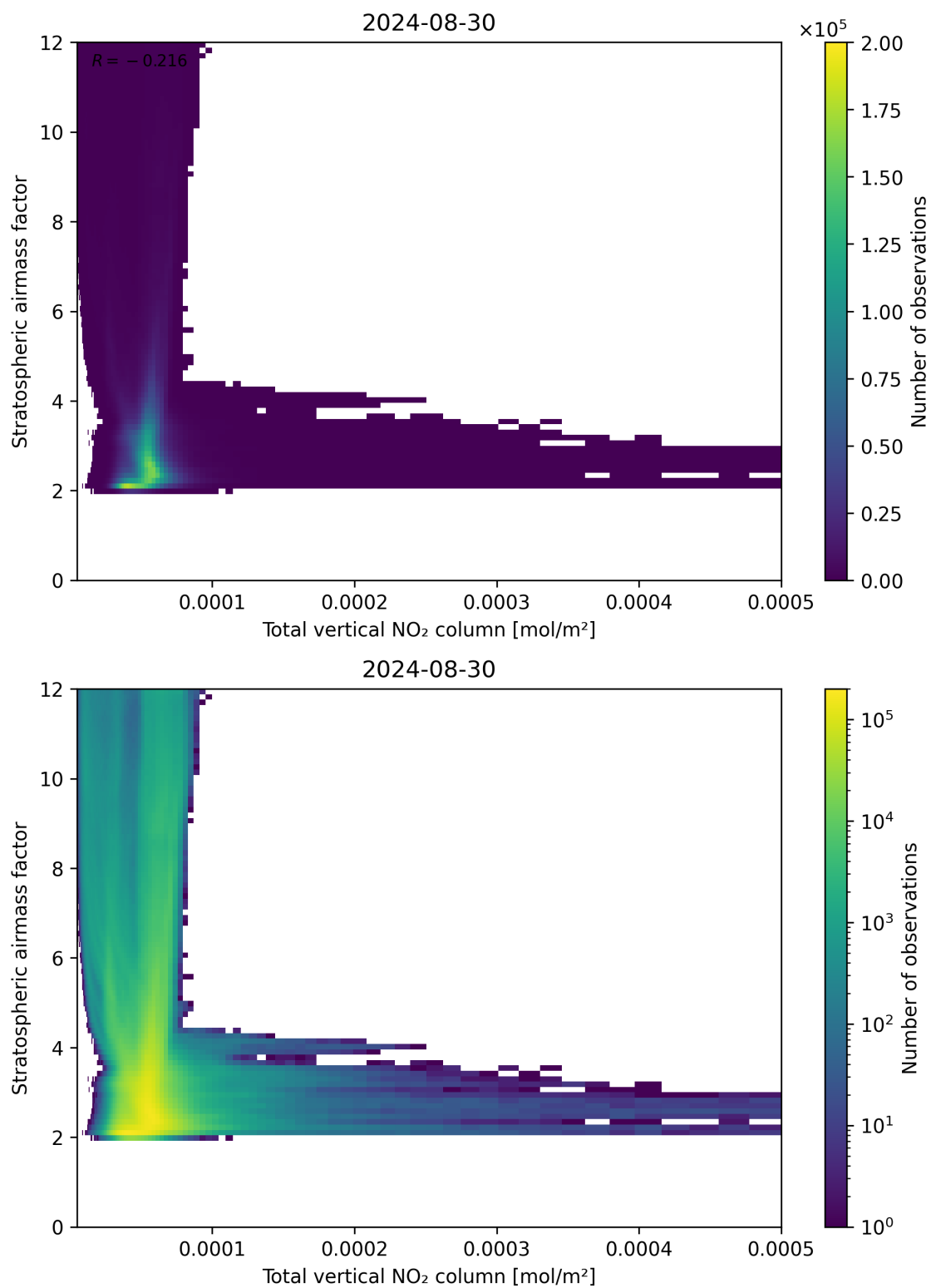
Figure 110: Scatter density plot of “Total vertical NO 2 column” against “Stratospheric airmass factor” for 2024-08-29 to 2024-08-31.
