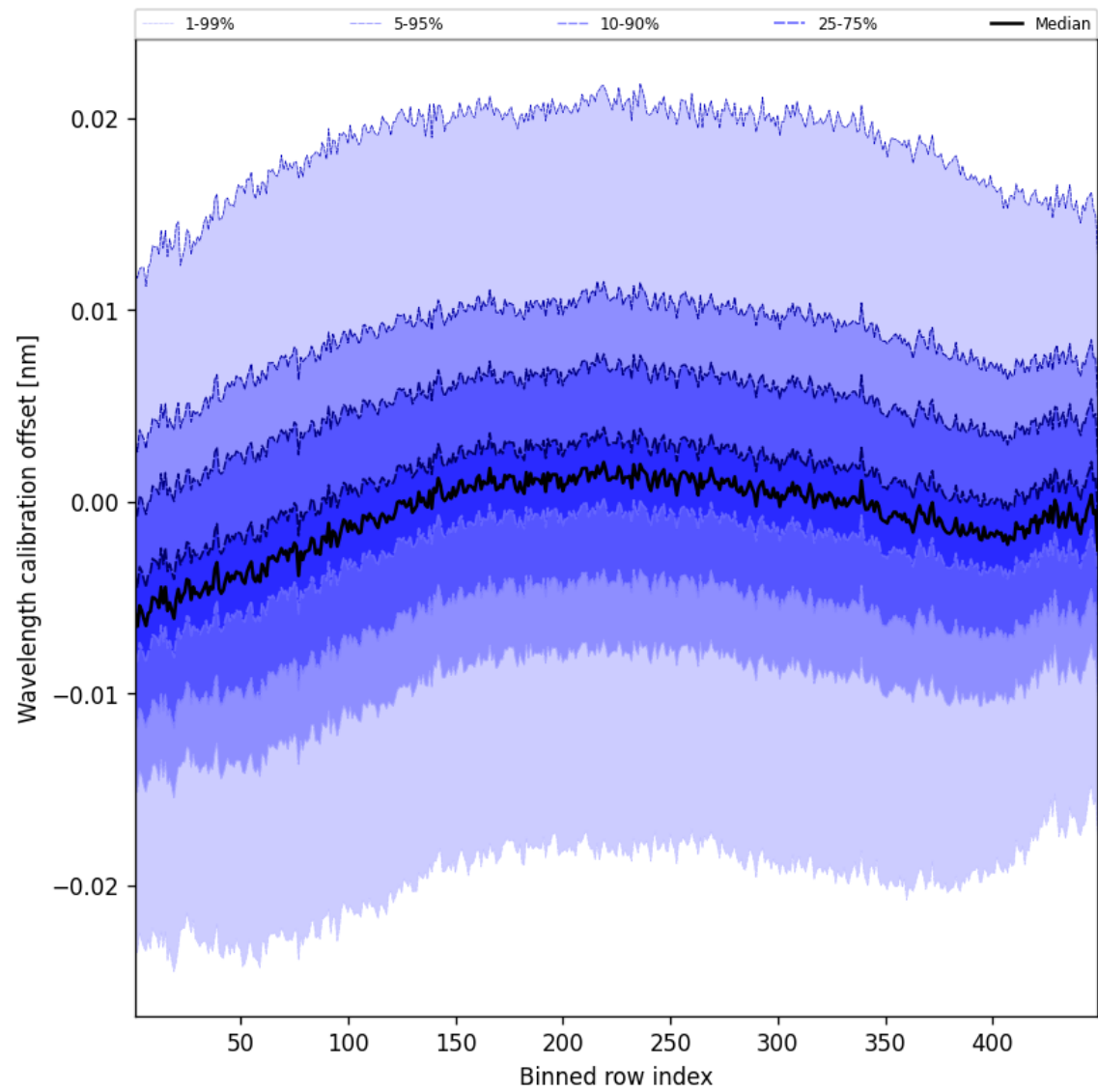
Figure 52: Along track statistics of “Wavelength calibration offset” for 2024-08-29 to 2024-08-31
