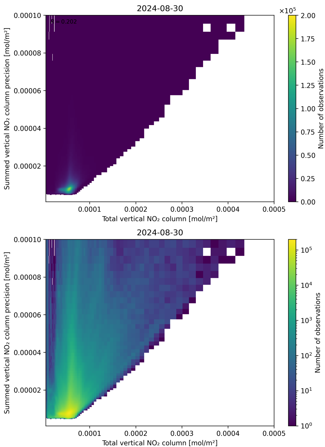
Figure 113: Scatter density plot of “Total vertical NO 2 column” against “Summed vertical NO 2 column precision” for 2024-08-29 to 2024-08-31.
