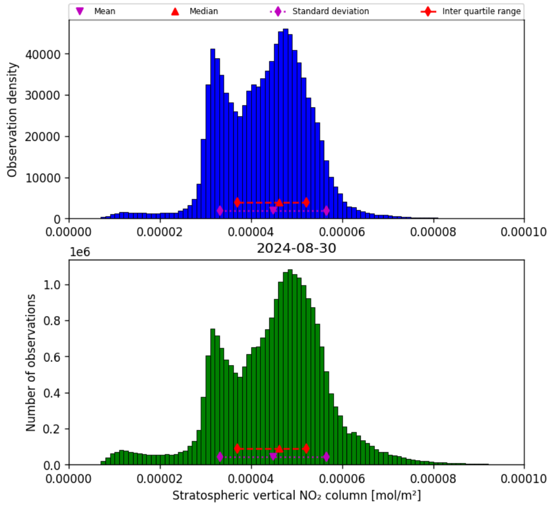
Figure 36: Histogram of “Stratospheric vertical NO 2 column” for 2024-08-29 to 2024-08-31
