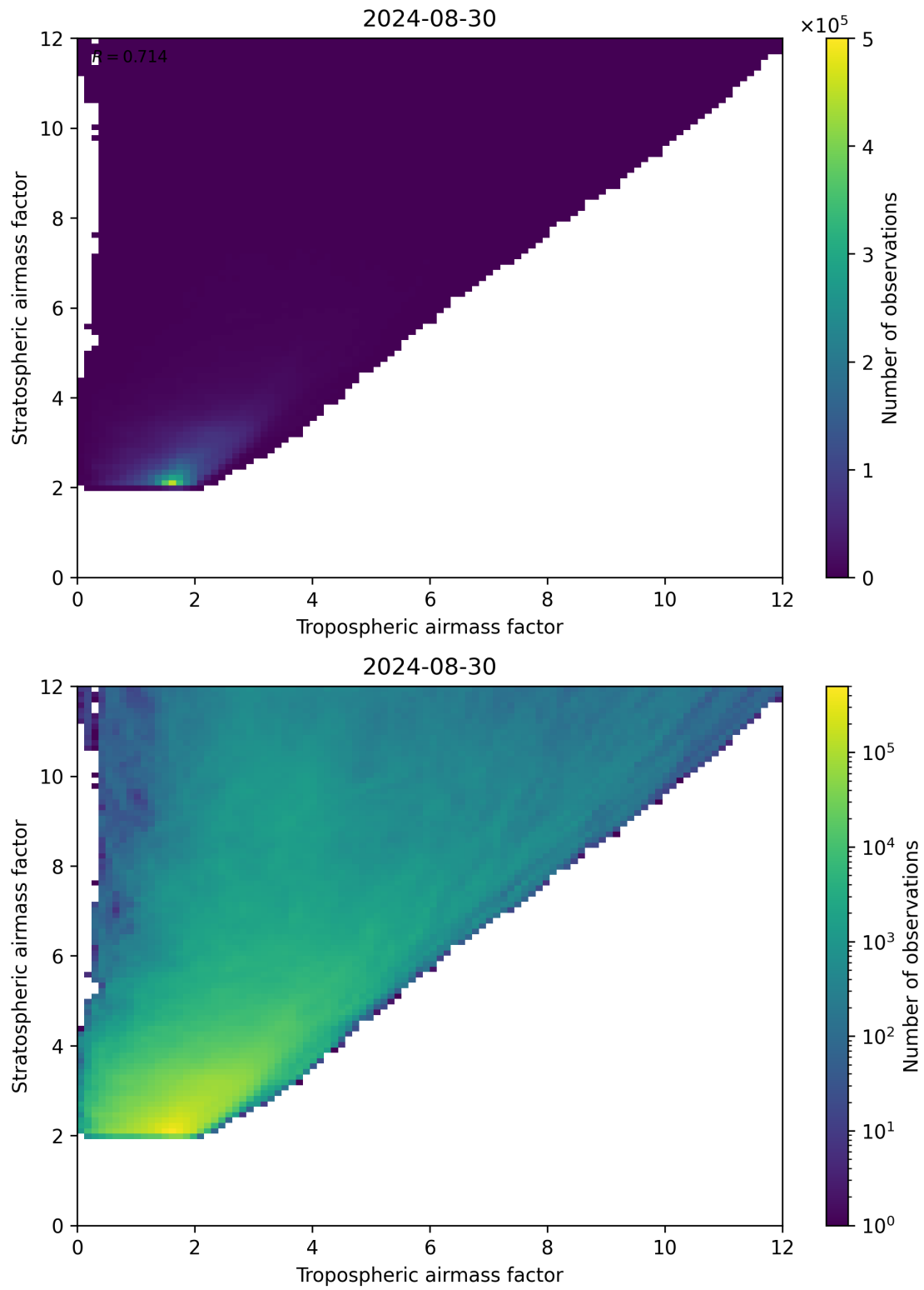
Figure 71: Scatter density plot of “Tropospheric airmass factor” against “Stratospheric airmass factor” for 2024-08-29 to 2024-08-31.
