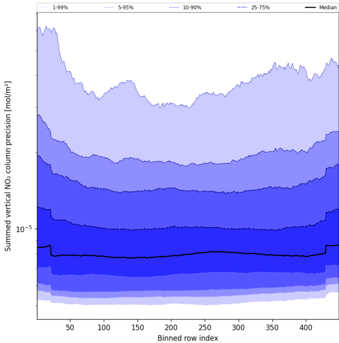
Figure 58: Along track statistics of “Summed vertical NO 2 column precision” for 2024-08-29 to 2024-08-31
