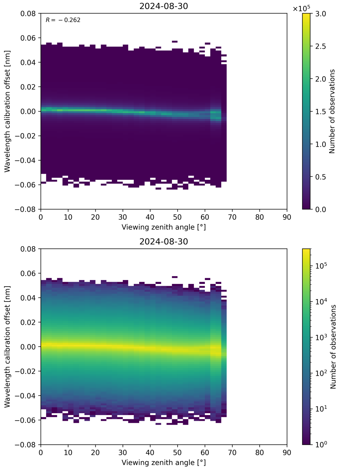
Figure 173: Scatter density plot of “Viewing zenith angle” against “Wavelength calibration offset” for 2024-08-29 to 2024-08-31.
