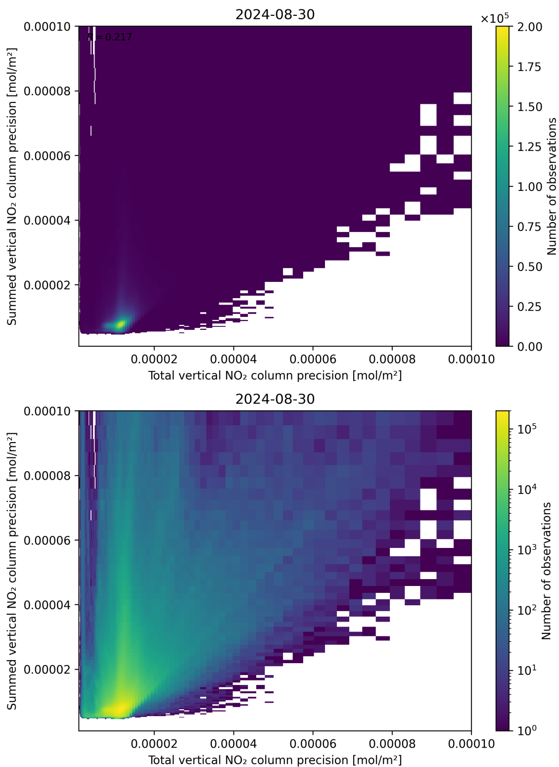
Figure 118: Scatter density plot of “Total vertical NO 2 column precision” against “Summed vertical NO 2 column precision” for 2024-08-29 to 2024-08-31.
