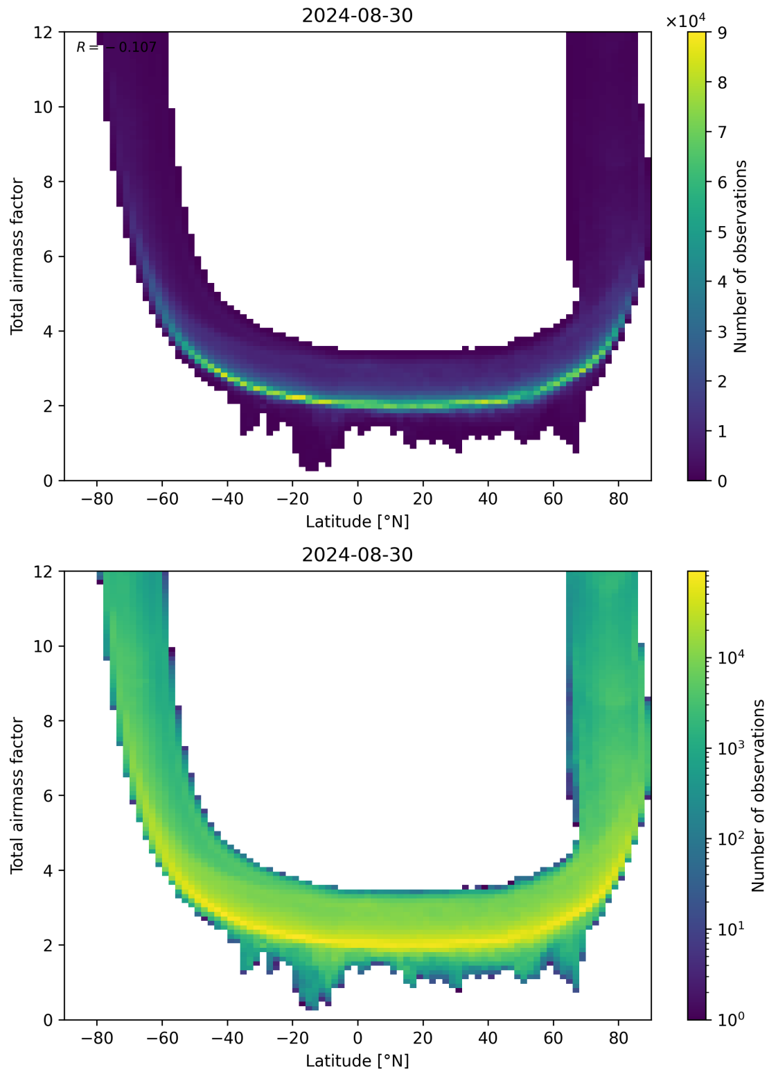
Figure 84: Scatter density plot of “Latitude” against “Total airmass factor” for 2024-08-29 to 2024-08-31.
