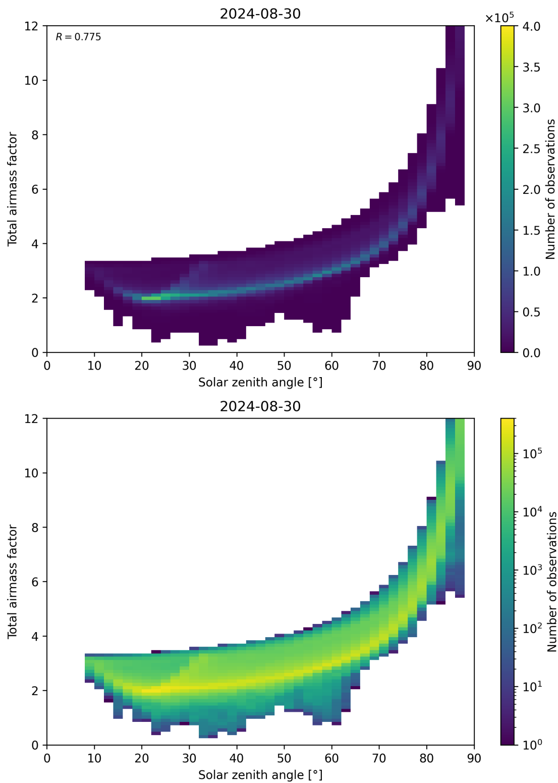
Figure 146: Scatter density plot of “Solar zenith angle” against “Total air mass factor” for 2024-08-29 to 2024-08-31.
