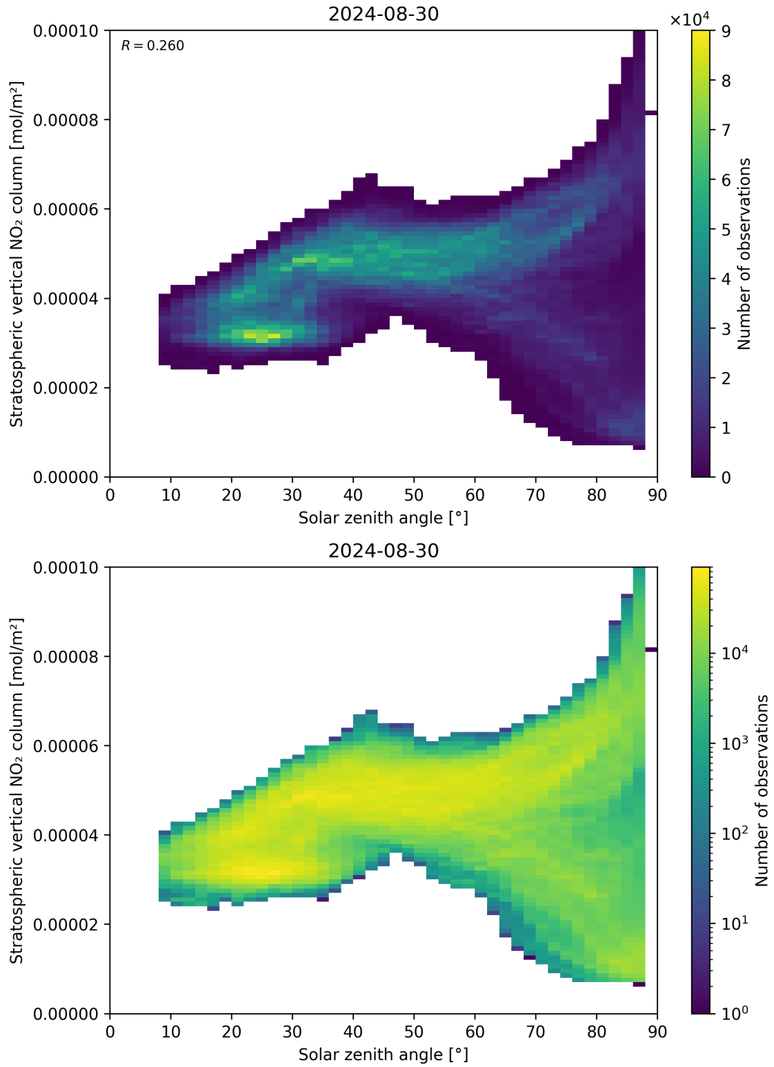
Figure 150: Scatter density plot of “Solar zenith angle” against “Stratospheric vertical NO 2 column” for 2024-08-29 to 2024-08-31.
