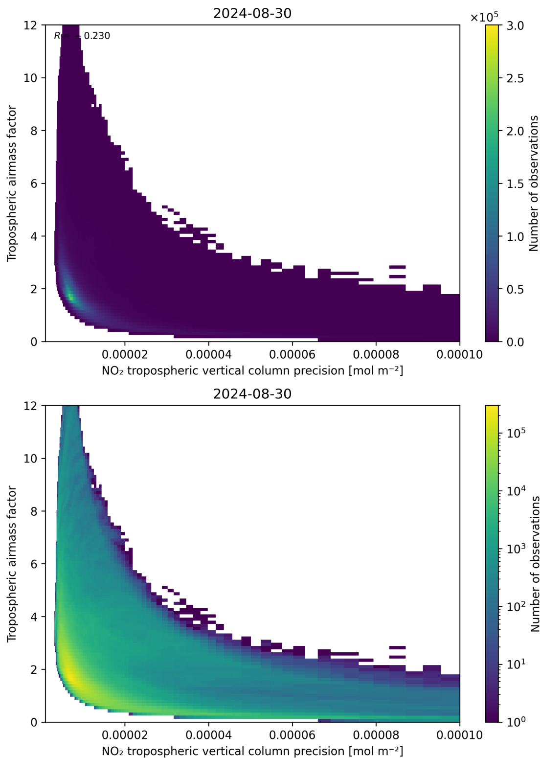
Figure 133: Scatter density plot of “NO 2 tropospheric vertical column precision” against “Tropospheric airmass factor” for 2024-08-29 to 2024-08-31.
