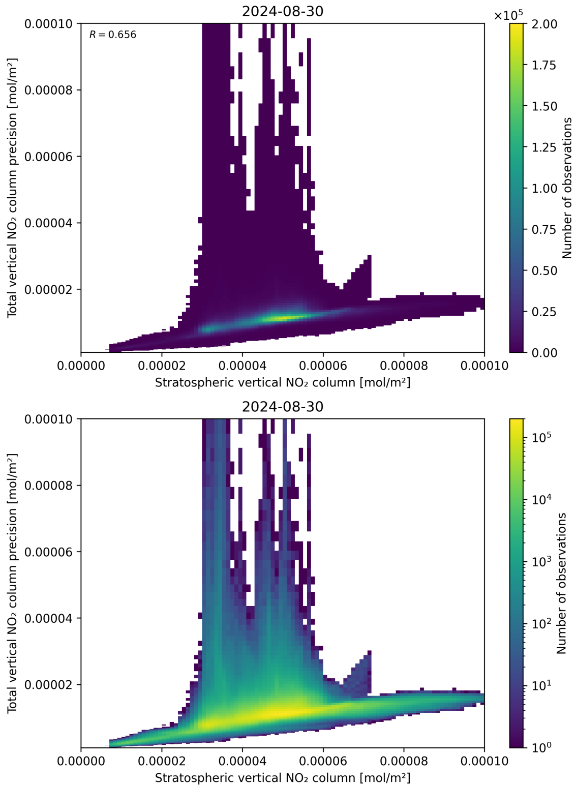
Figure 101: Scatter density plot of “Stratospheric vertical NO 2 column” against “Total vertical NO 2 column precision” for 2024-08-29 to 2024-08-31.
