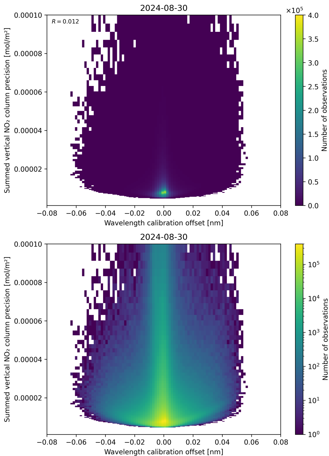
Figure 178: Scatter density plot of “Wavelength calibration offset” against “Summed vertical NO 2 column precision” for 2024-08-29 to 2024-08-31.
