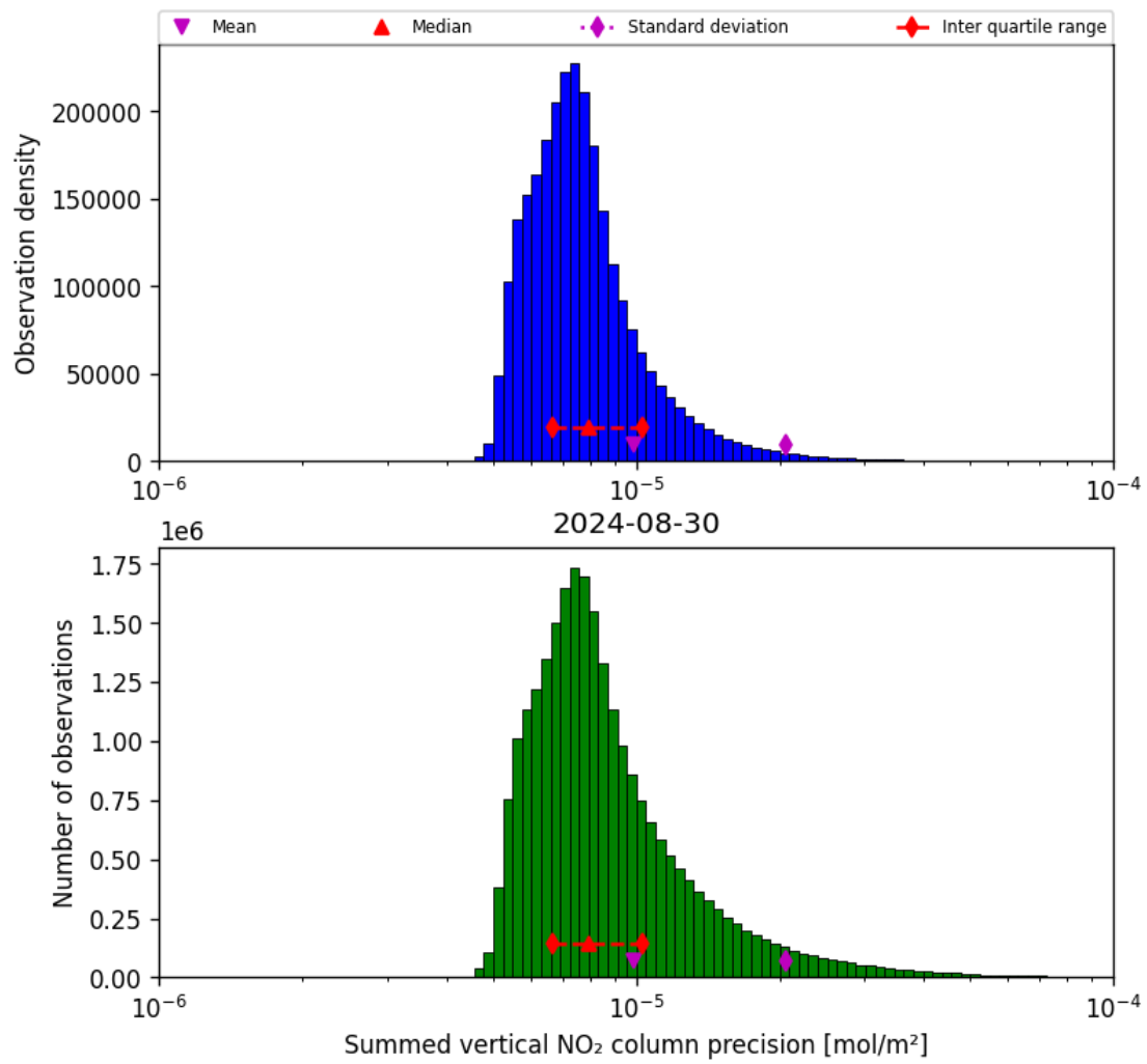
Figure 41: Histogram of “Summed vertical NO 2 column precision” for 2024-08-29 to 2024-08-31
