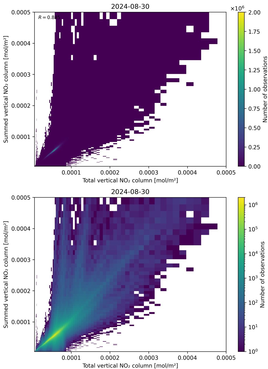
Figure 112: Scatter density plot of “Total vertical NO 2 column” against “Summed vertical NO 2 column” for 2024-08-29 to 2024-08-31.
