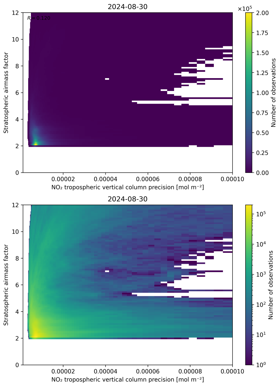
Figure 131: Scatter density plot of “NO 2 tropospheric vertical column precision” against “Stratospheric airmass factor” for 2024-08-29 to 2024-08-31.
