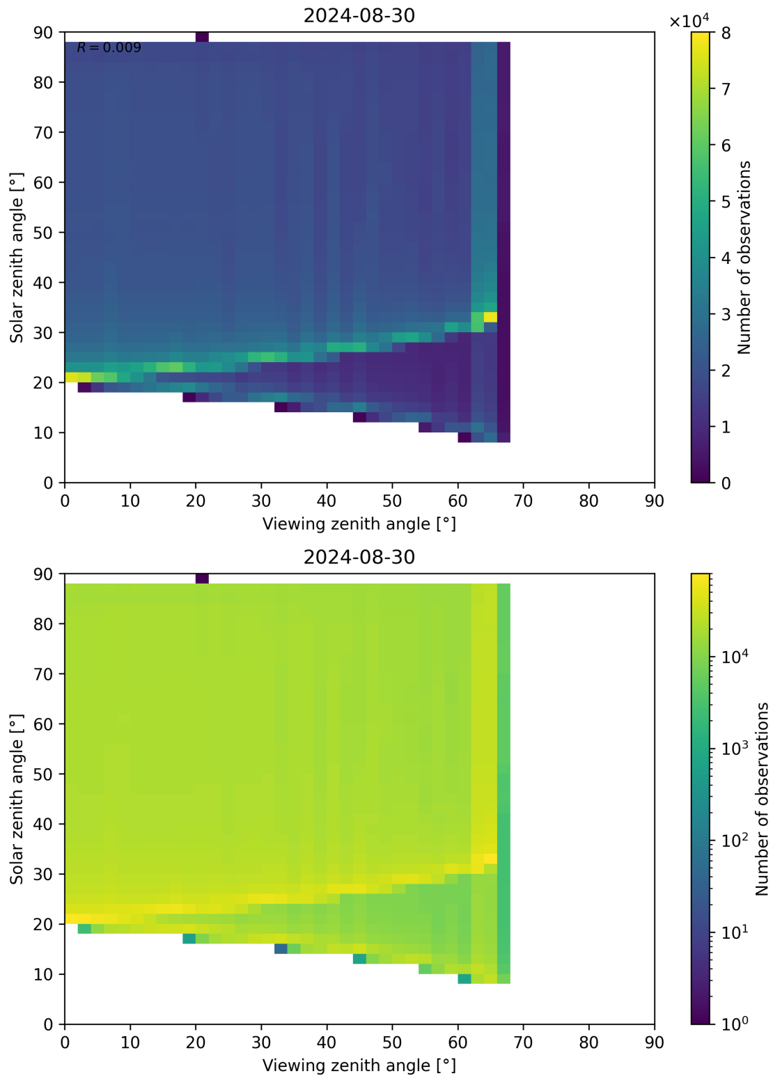
Figure 172: Scatter density plot of “Viewing zenith angle” against “Solar zenith angle” for 2024-08-29 to 2024-08-31.
