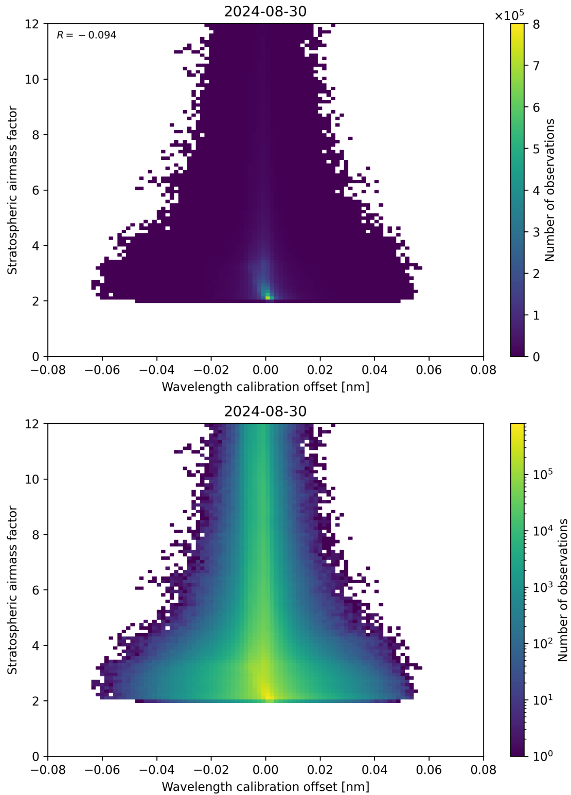
Figure 174: Scatter density plot of “Wavelength calibration offset” against “Stratospheric airmass factor” for 2024-08-29 to 2024-08-31.
