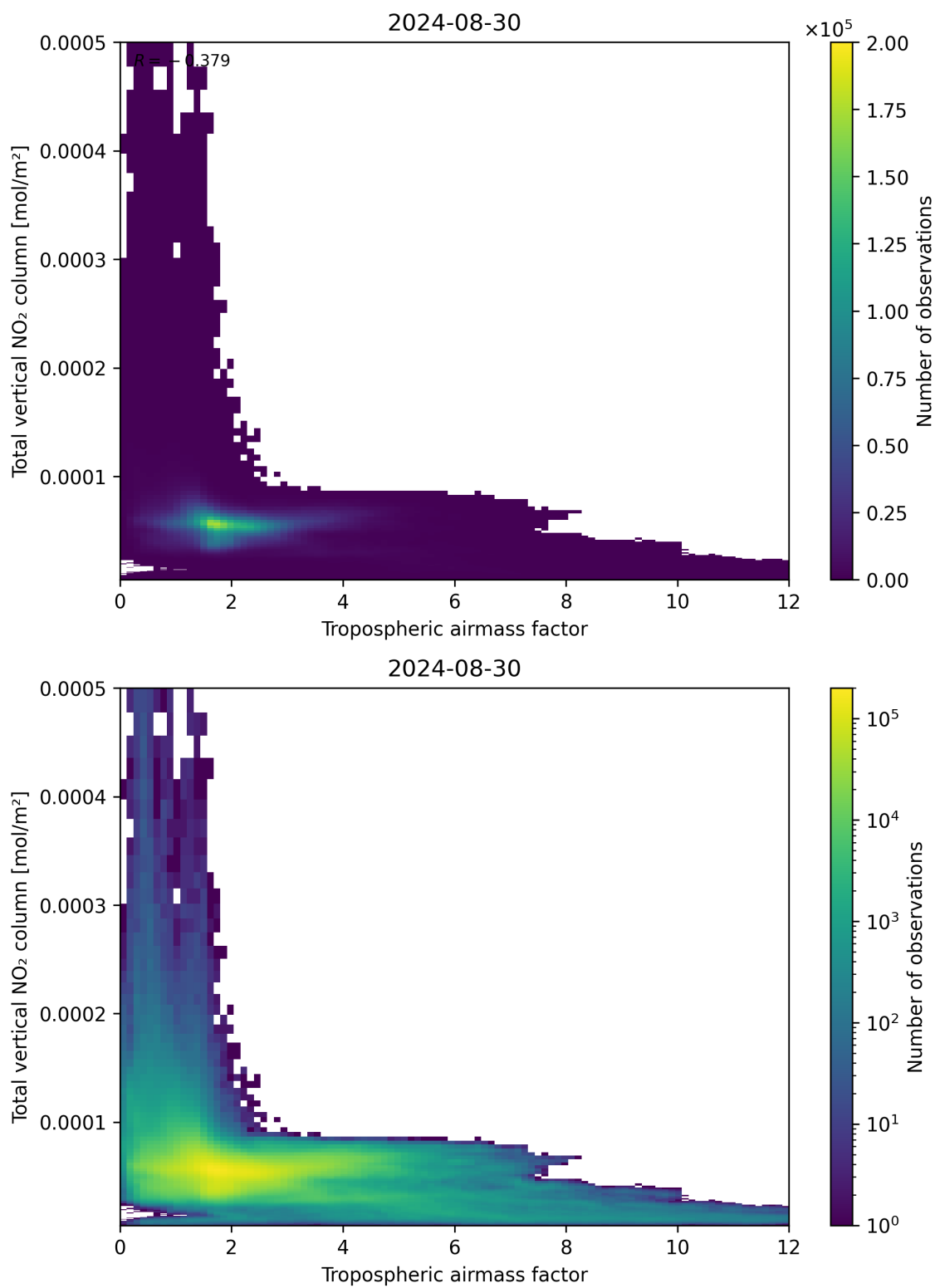
Figure 77: Scatter density plot of “Tropospheric airmass factor” against “Total vertical NO 2 column” for 2024-08-29 to 2024-08-31.
