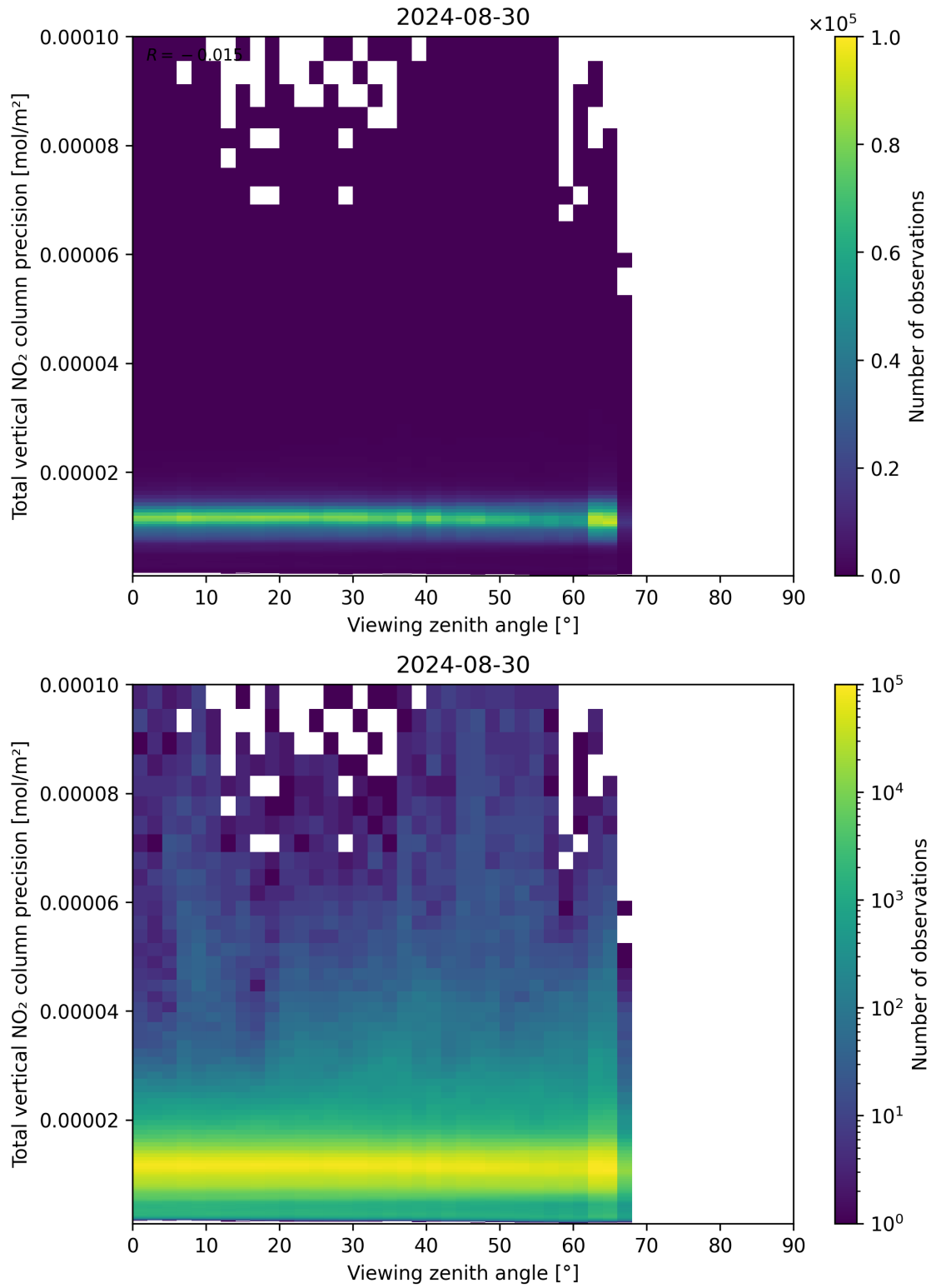
Figure 168: Scatter density plot of “Viewing zenith angle” against “Total vertical NO 2 column precision” for 2024-08-29 to 2024-08-31.
