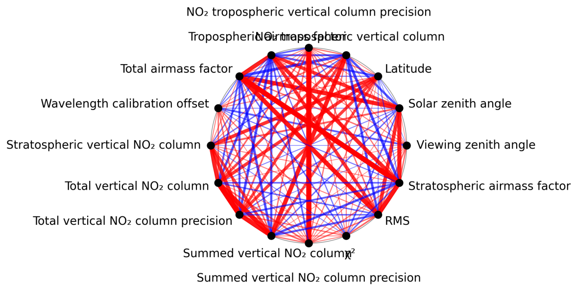
Figure 1: Map of correlation graph for 2024-08-29 to 2024-08-31.
