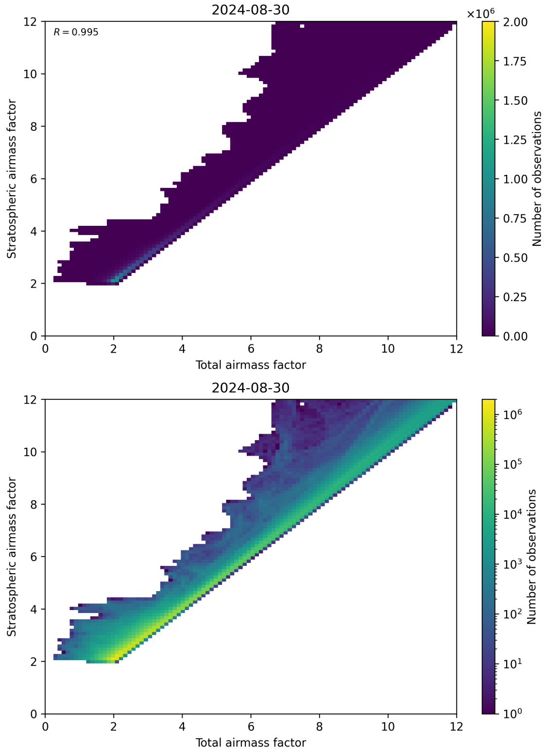
Figure 62: Scatter density plot of “Total air mass factor” against “Stratospheric air mass factor” for 2024-08-29 to 2024-08-31.
