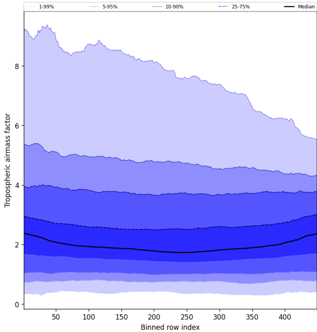
Figure 48: Along track statistics of “Tropospheric air mass factor” for 2024-08-29 to 2024-08-31
