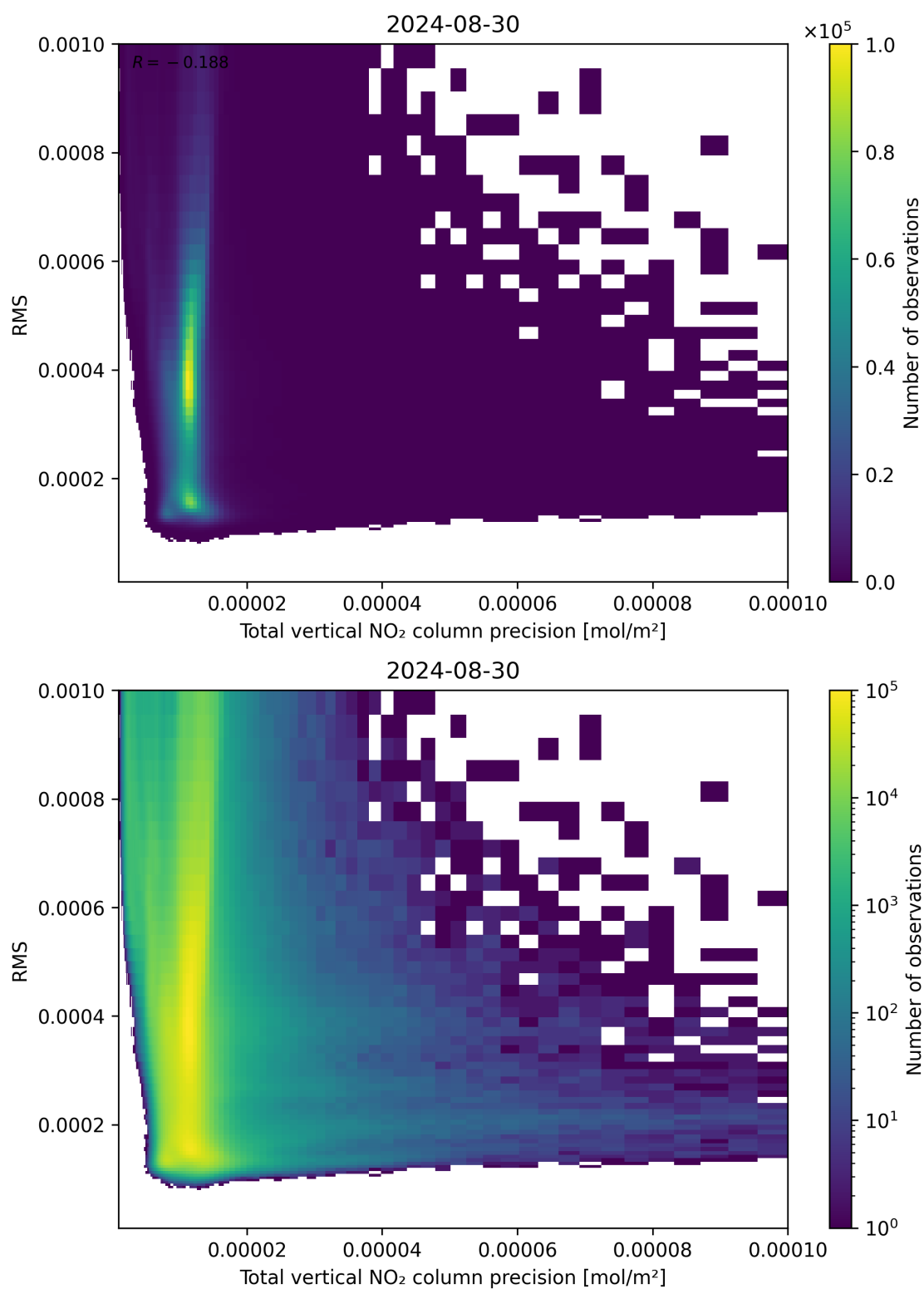
Figure 119: Scatter density plot of “Total vertical NO 2 column precision” against “RMS” for 2024-08-29 to 2024-08-31.
