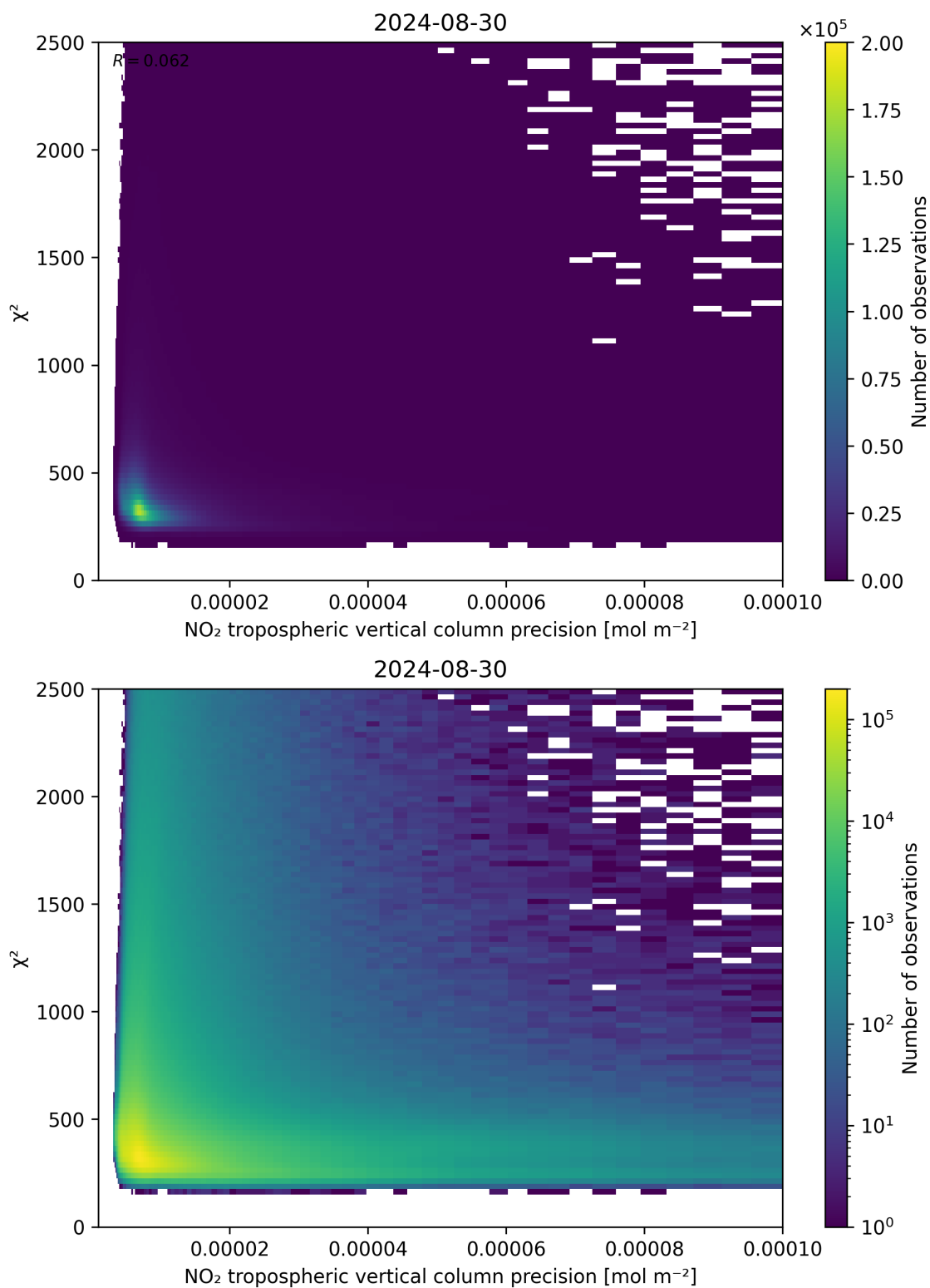
Figure 134: Scatter density plot of “NO 2 tropospheric vertical column precision” against “ \chi^2 ” for 2024-08-29 to 2024-08-31.
