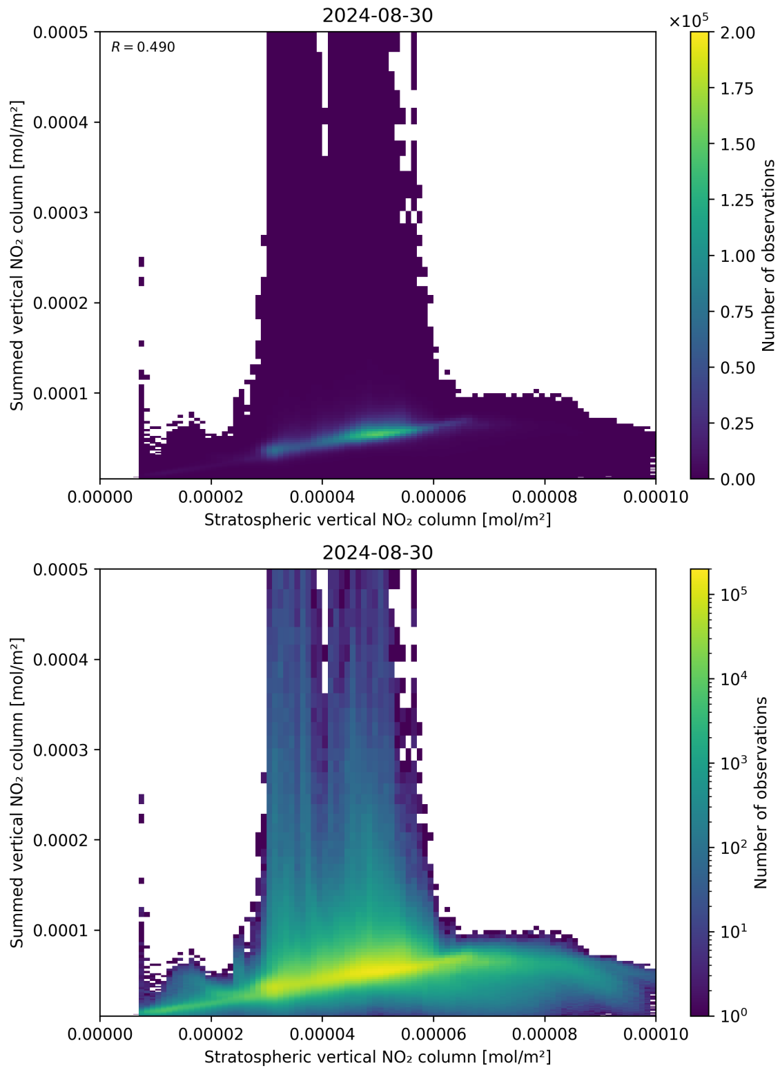
Figure 98: Scatter density plot of “Stratospheric vertical NO 2 column” against “Summed vertical NO 2 column” for 2024-08-29 to 2024-08-31.
