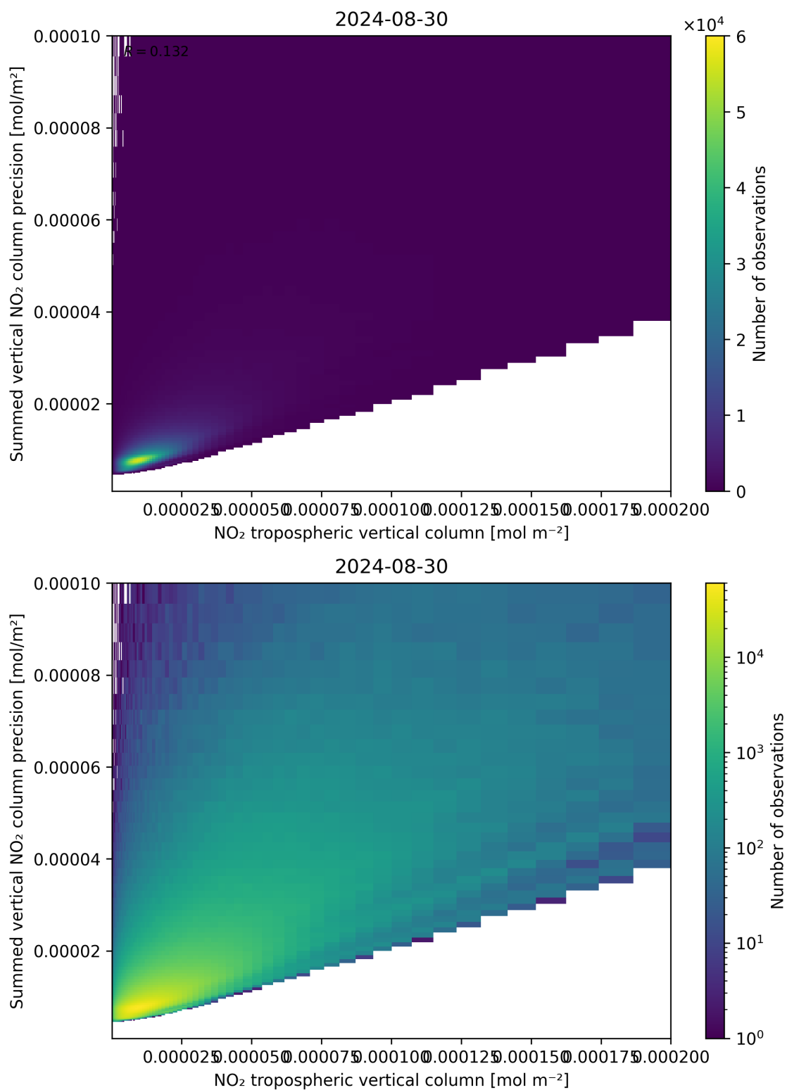
Figure 127: Scatter density plot of “NO 2 tropospheric vertical column” against “Summed vertical NO 2 column precision” for 2024-08-29 to 2024-08-31.
