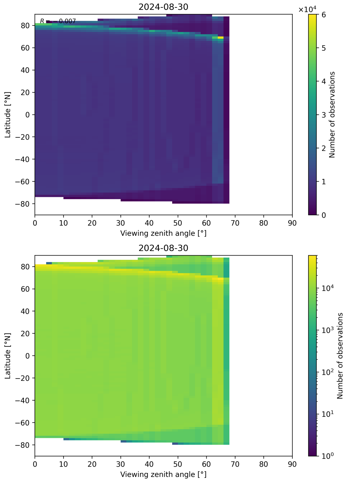
Figure 163: Scatter density plot of “Viewing zenith angle” against “Latitude” for 2024-08-29 to 2024-08-31.
