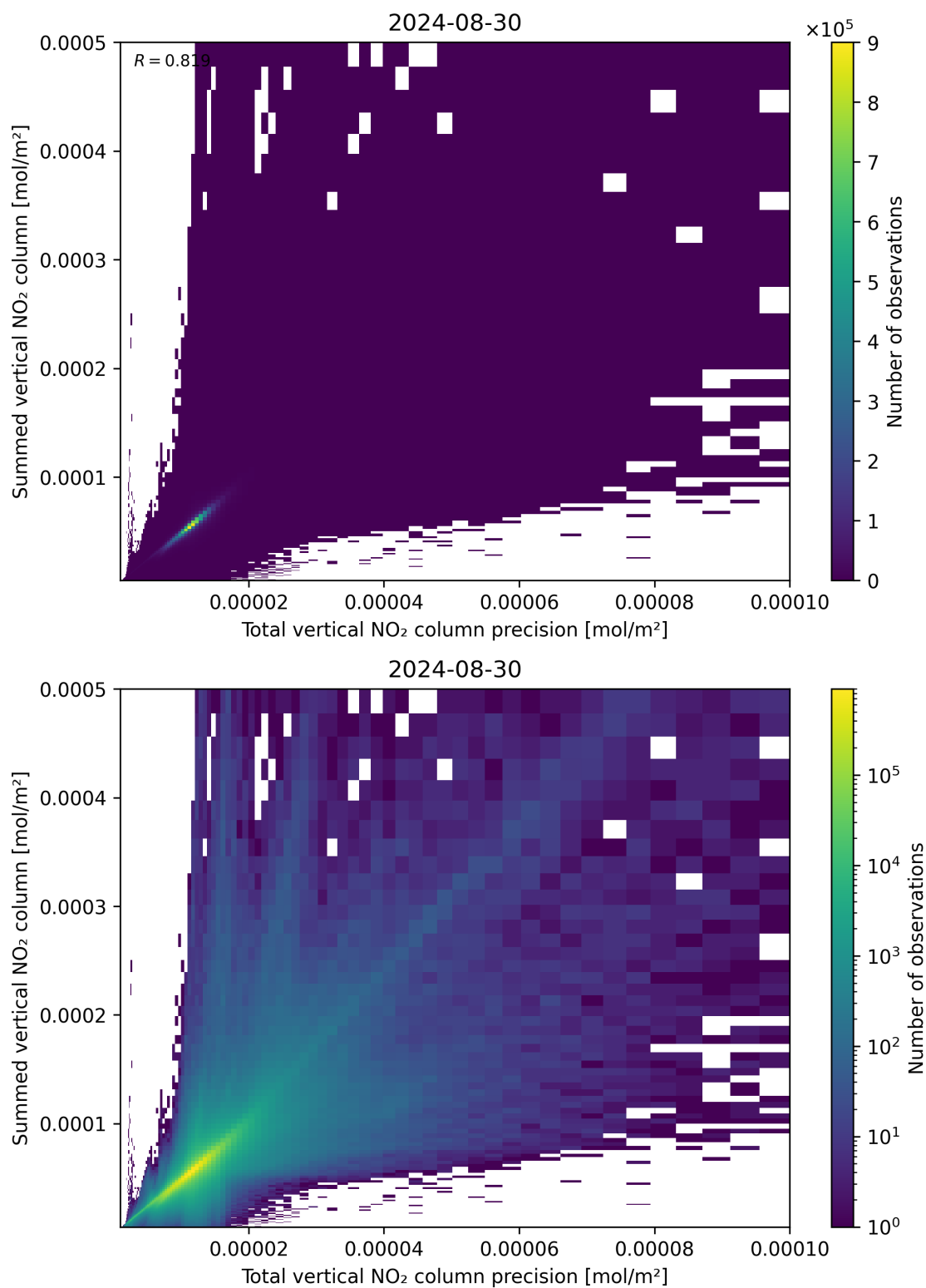
Figure 117: Scatter density plot of “Total vertical NO 2 column precision” against “Summed vertical NO 2 column” for 2024-08-29 to 2024-08-31.
