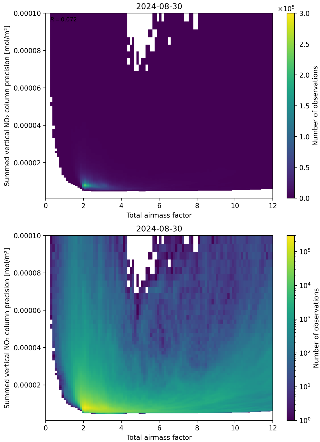
Figure 66: Scatter density plot of “Total airmass factor” against “Summed vertical NO 2 column precision” for 2024-08-29 to 2024-08-31.
