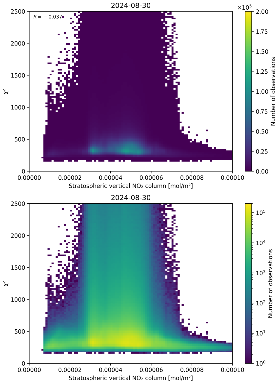
Figure 97: Scatter density plot of “Stratospheric vertical NO 2 column” against “ \chi^2 ” for 2024-08-29 to 2024-08-31.
