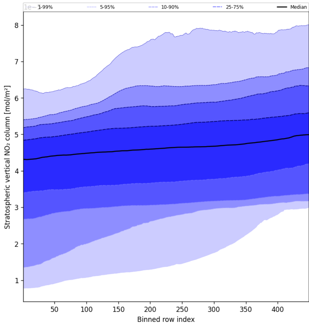
Figure 53: Along track statistics of “Stratospheric vertical NO 2 column” for 2024-08-29 to 2024-08-31
