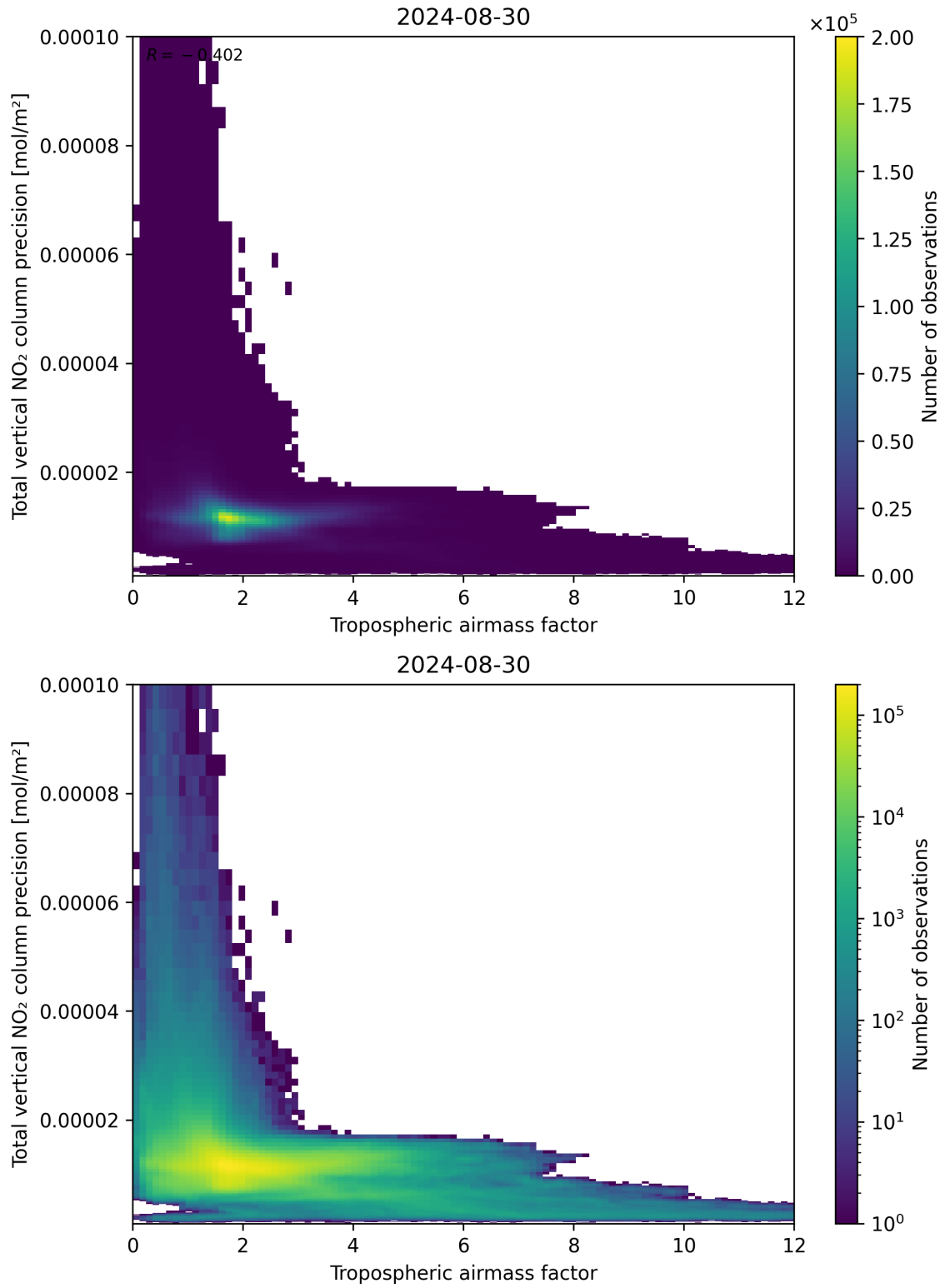
Figure 78: Scatter density plot of “Tropospheric airmass factor” against “Total vertical NO 2 column precision” for 2024-08-29 to 2024-08-31.
