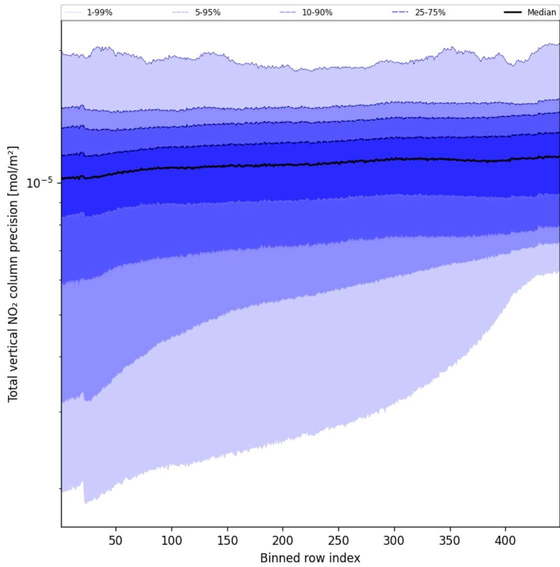
Figure 56: Along track statistics of “Total vertical NO 2 column precision” for 2024-08-29 to 2024-08-31
