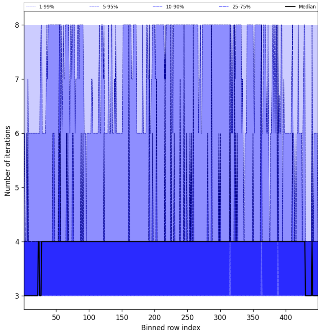
Figure 51: Along track statistics of “Number of iterations” for 2024-08-29 to 2024-08-31
