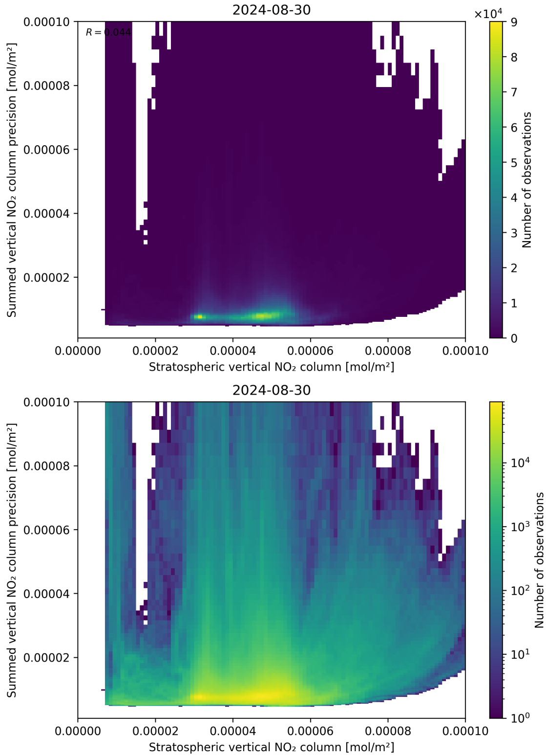
Figure 99: Scatter density plot of “Stratospheric vertical NO 2 column” against “Summed vertical NO 2 column precision” for 2024-08-29 to 2024-08-31.
