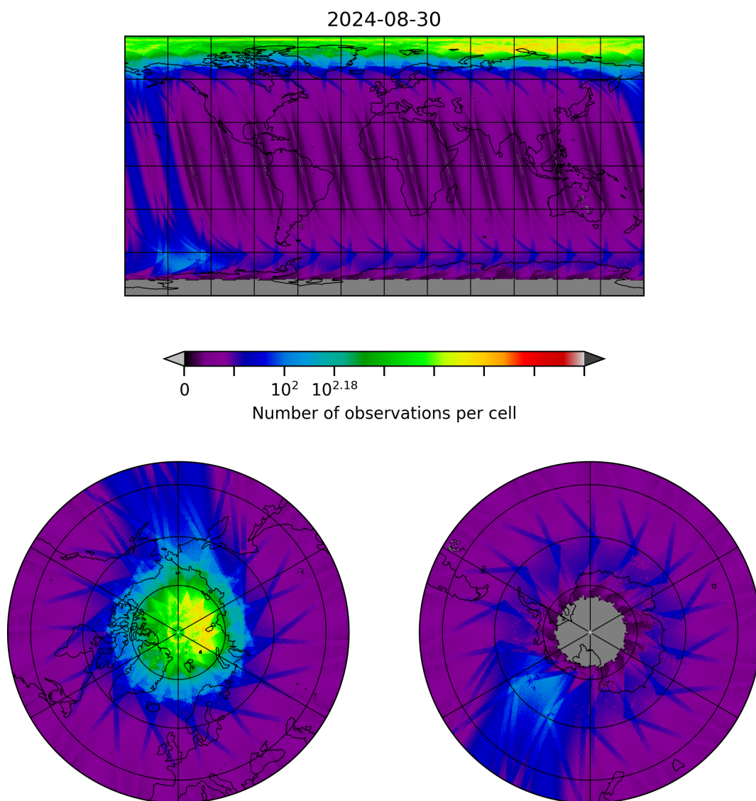
Figure 10: Map of the number of observations for 2024-08-29 to 2024-08-31
