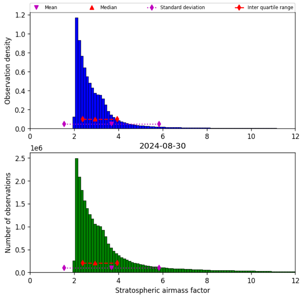
Figure 44: Histogram of “Stratospheric airmass factor” for 2024-08-29 to 2024-08-31
