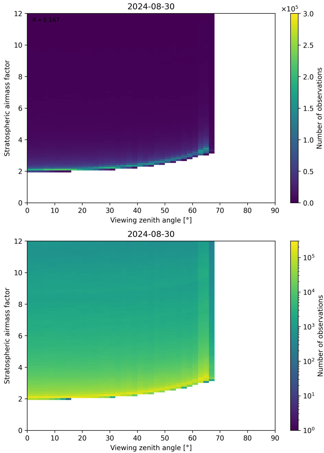
Figure 159: Scatter density plot of “Viewing zenith angle” against “Stratospheric airmass factor” for 2024-08-29 to 2024-08-31.
