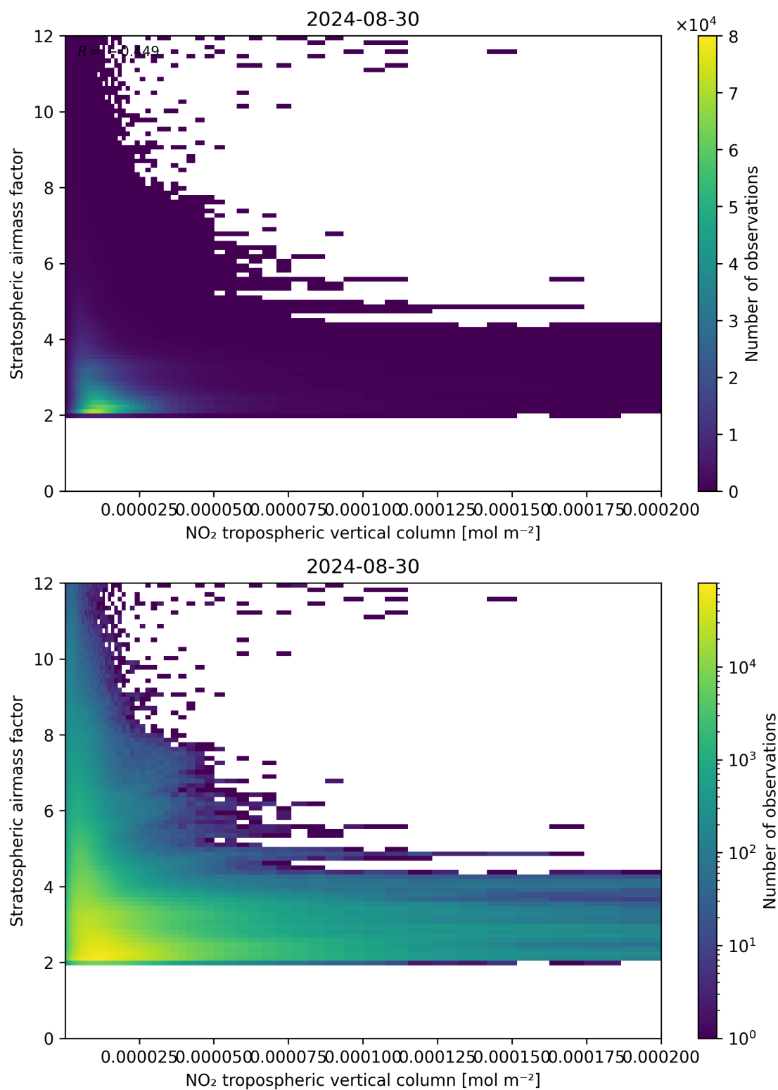
Figure 121: Scatter density plot of “NO 2 tropospheric vertical column” against “Stratospheric air mass factor” for 2024-08-29 to 2024-08-31.
