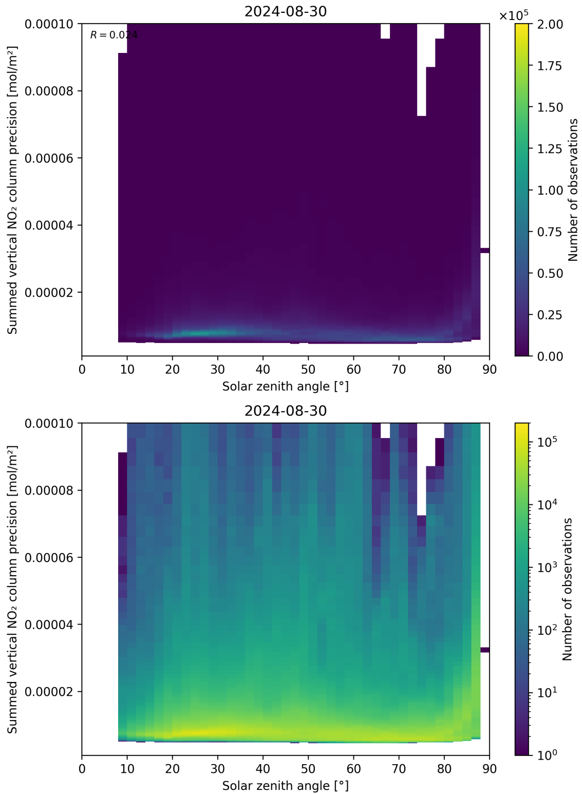
Figure 152: Scatter density plot of “Solar zenith angle” against “Summed vertical NO 2 column precision” for 2024-08-29 to 2024-08-31.
