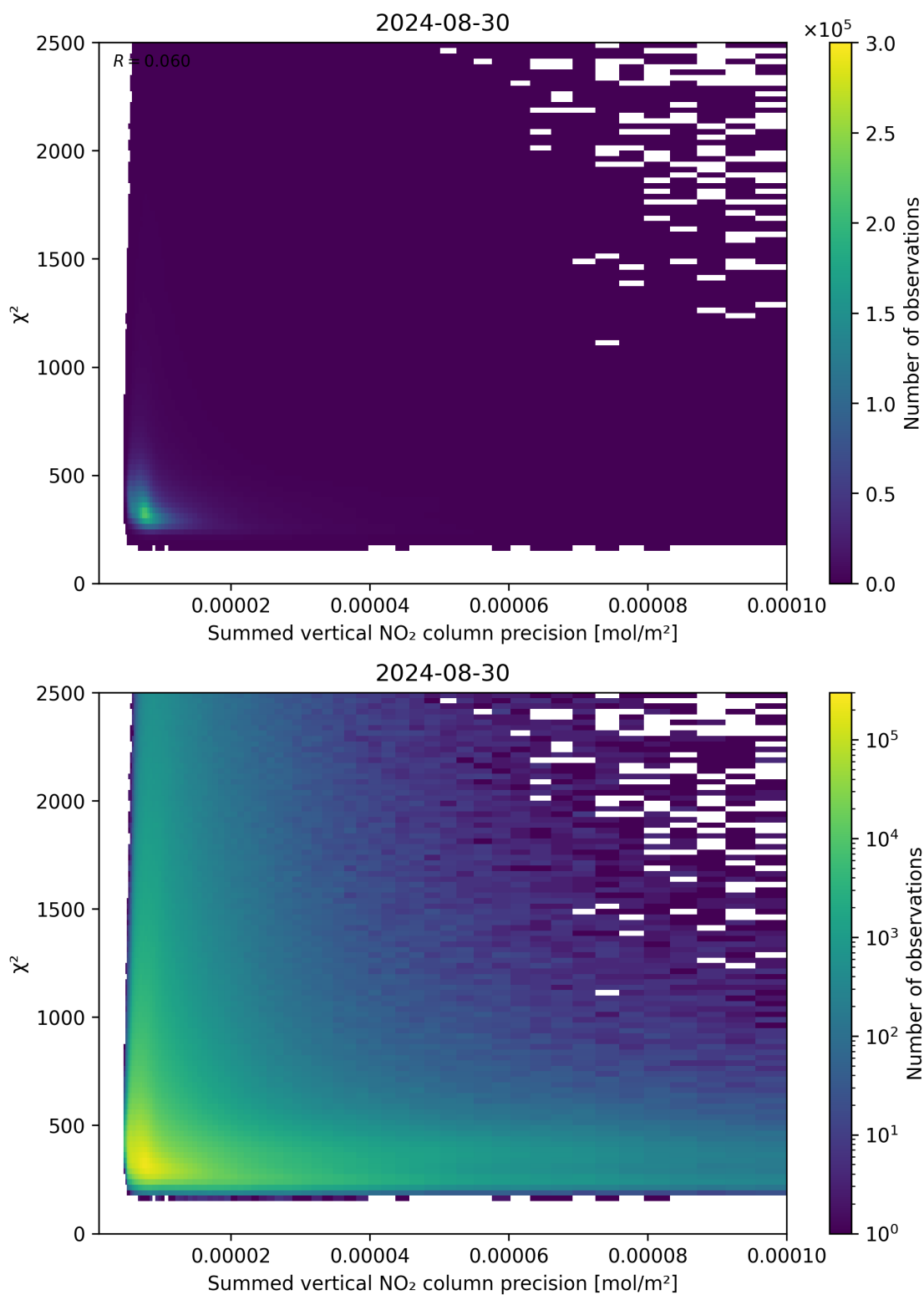
Figure 107: Scatter density plot of “Summed vertical NO 2 column precision” against “ \chi^2 ” for 2024-08-29 to 2024-08-31.
