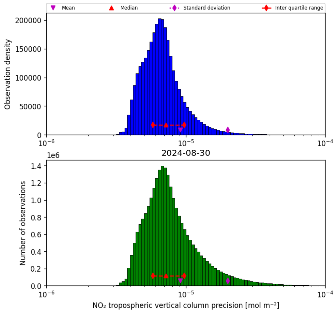
Figure 30: Histogram of “NO 2 tropospheric vertical column precision” for 2024-08-29 to 2024-08-31
