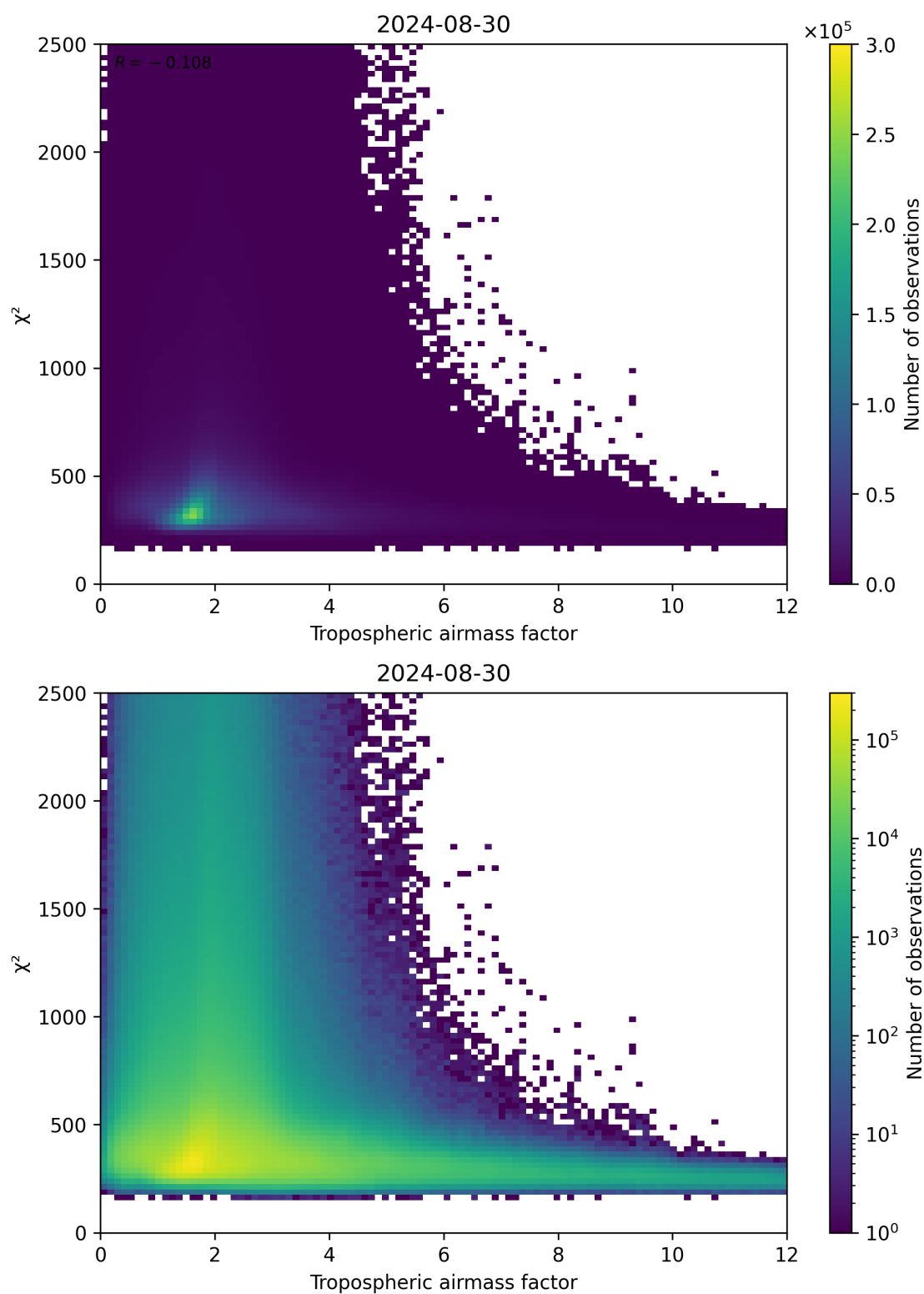
Figure 73: Scatter density plot of “Tropospheric airmass factor” against “ \chi^2 ” for 2024-08-29 to 2024-08-31.
