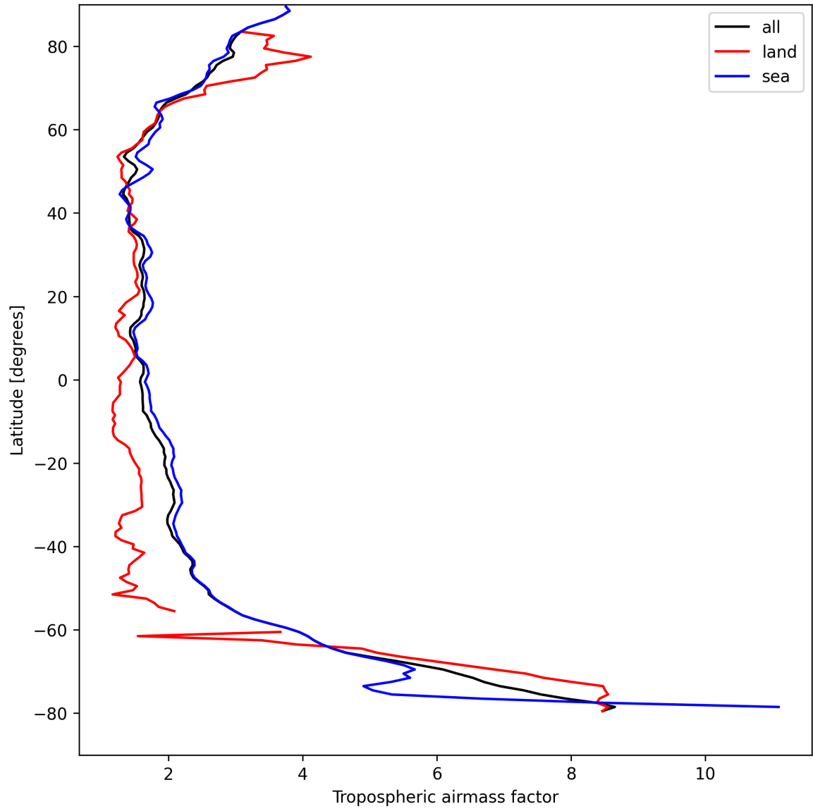
Figure 14: Zonal average of “Tropospheric airmass factor” for 2024-08-29 to 2024-08-31.
