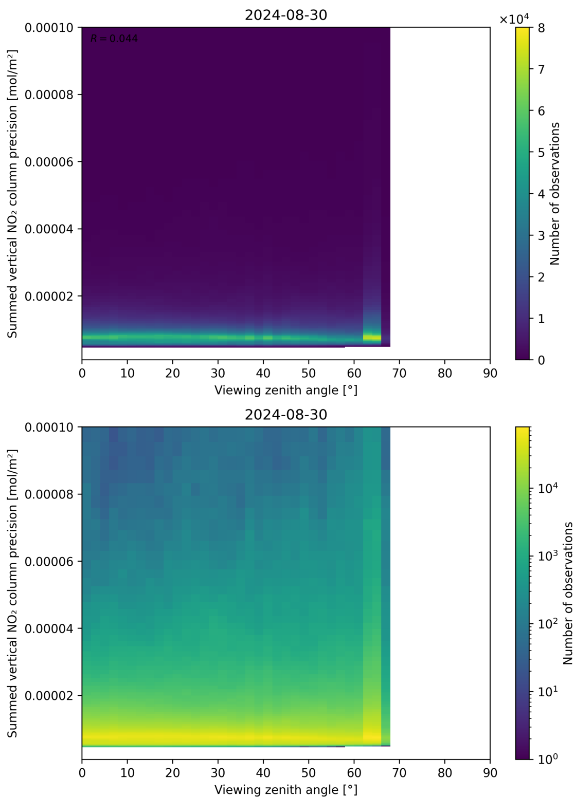
Figure 166: Scatter density plot of “Viewing zenith angle” against “Summed vertical NO 2 column precision” for 2024-08-29 to 2024-08-31.
