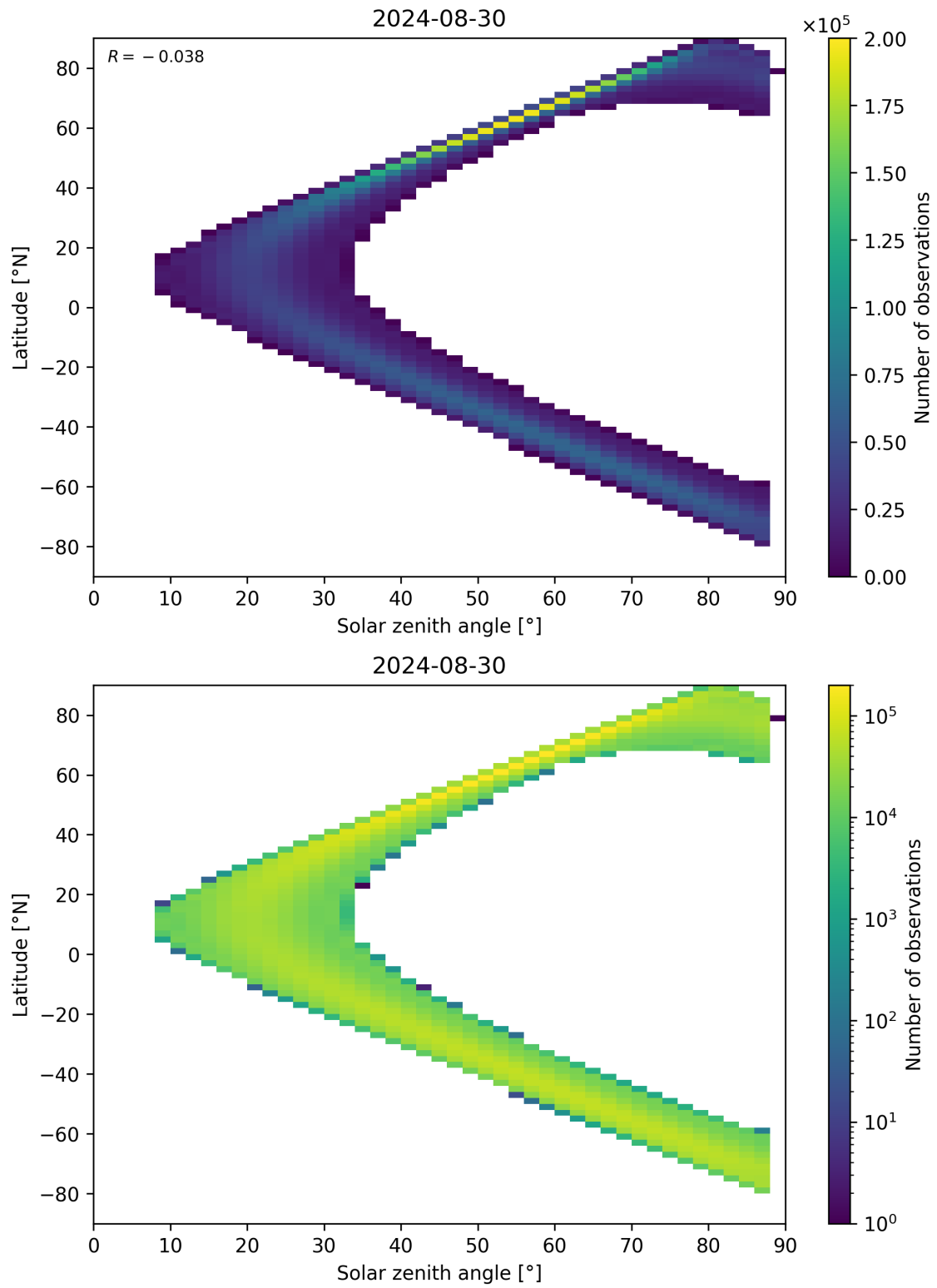
Figure 149: Scatter density plot of “Solar zenith angle” against “Latitude” for 2024-08-29 to 2024-08-31.
