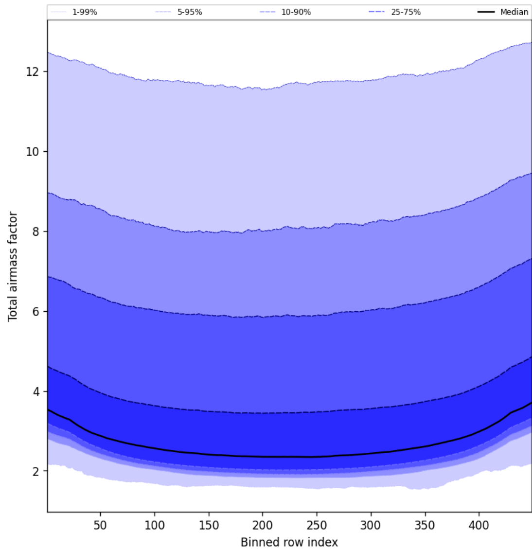
Figure 49: Along track statistics of “Total airmass factor” for 2024-08-29 to 2024-08-31
