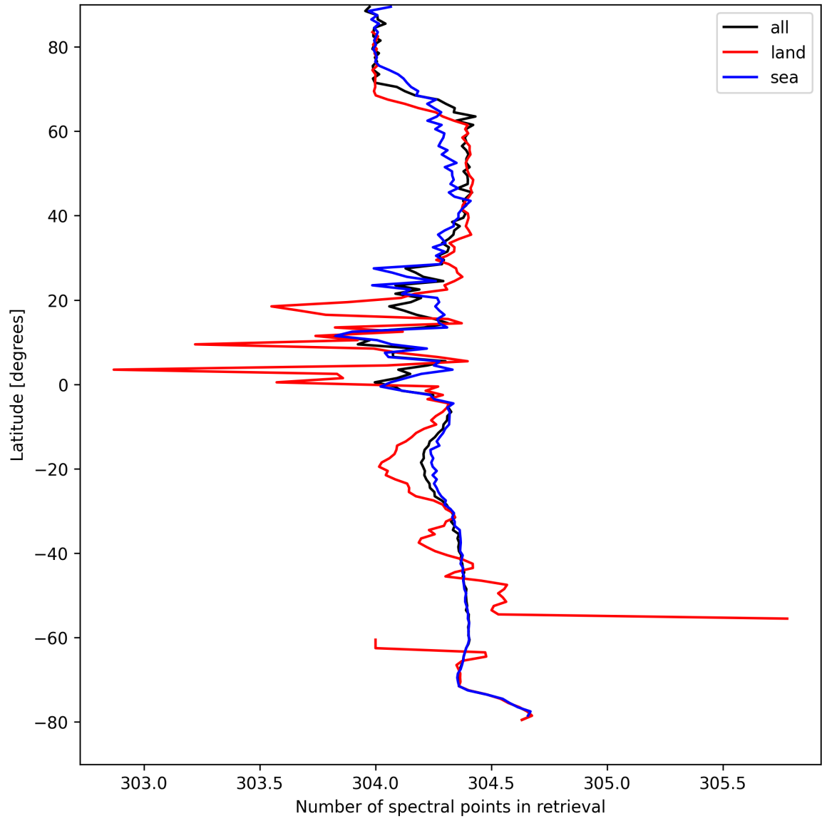
Figure 16: Zonal average of “Number of spectral points in retrieval” for 2024-08-29 to 2024-08-31.
