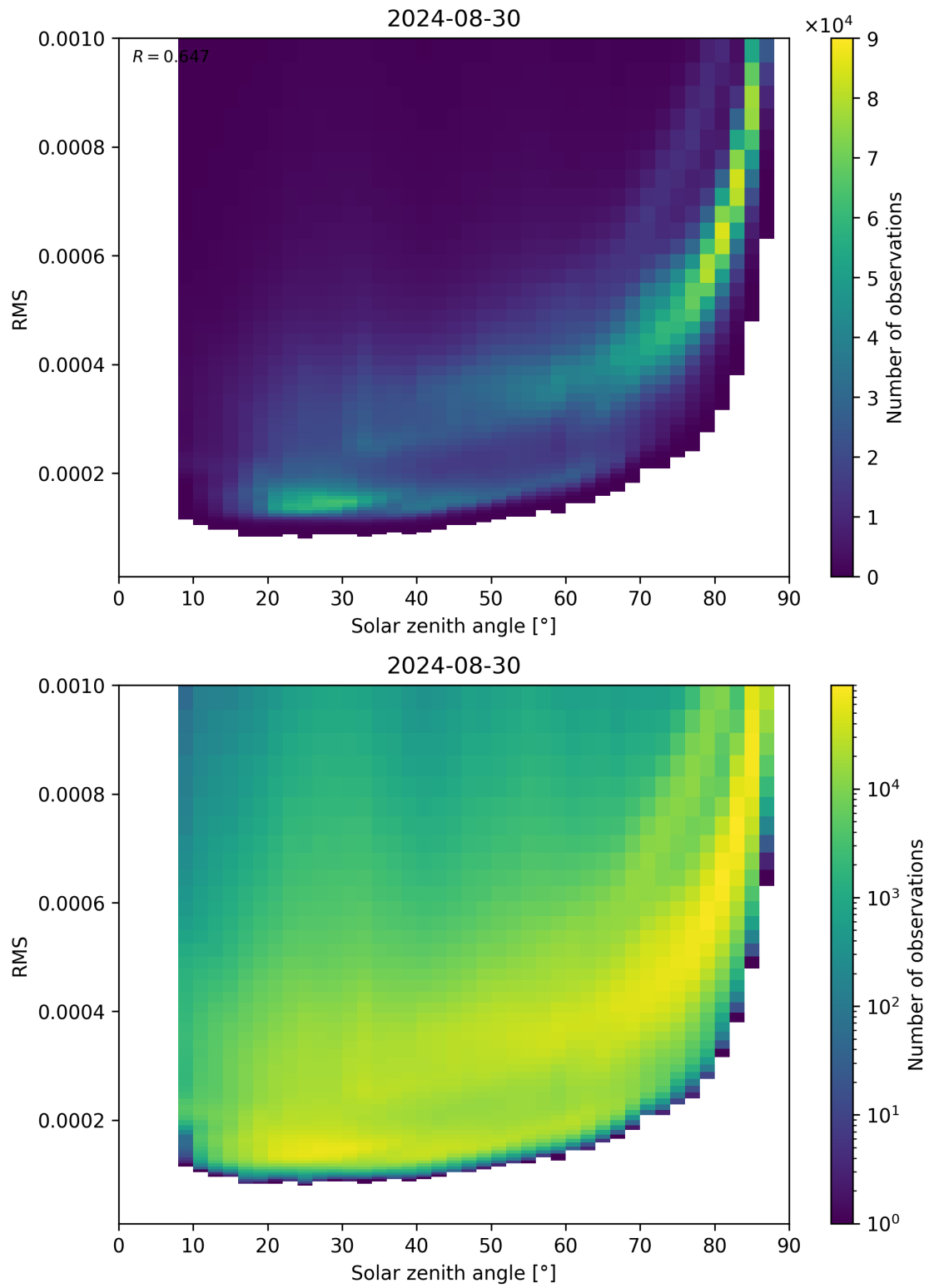
Figure 157: Scatter density plot of “Solar zenith angle” against “RMS” for 2024-08-29 to 2024-08-31.
