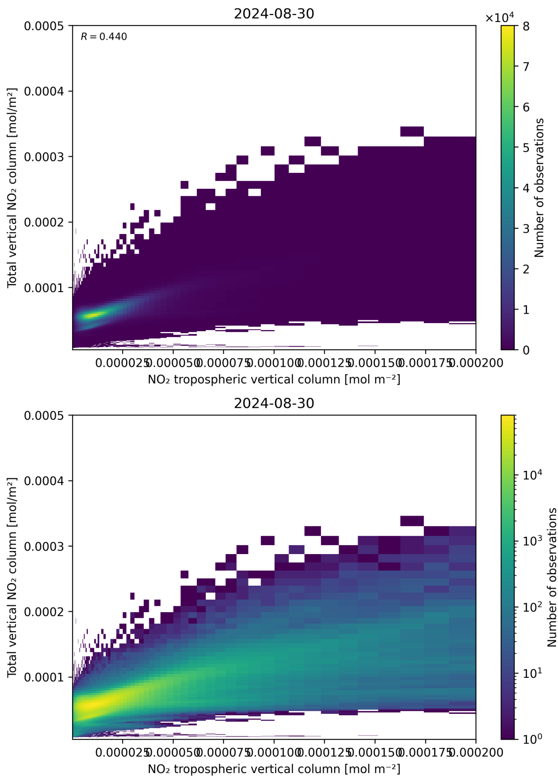
Figure 128: Scatter density plot of “NO 2 tropospheric vertical column” against “Total vertical NO 2 column” for 2024-08-29 to 2024-08-31.
