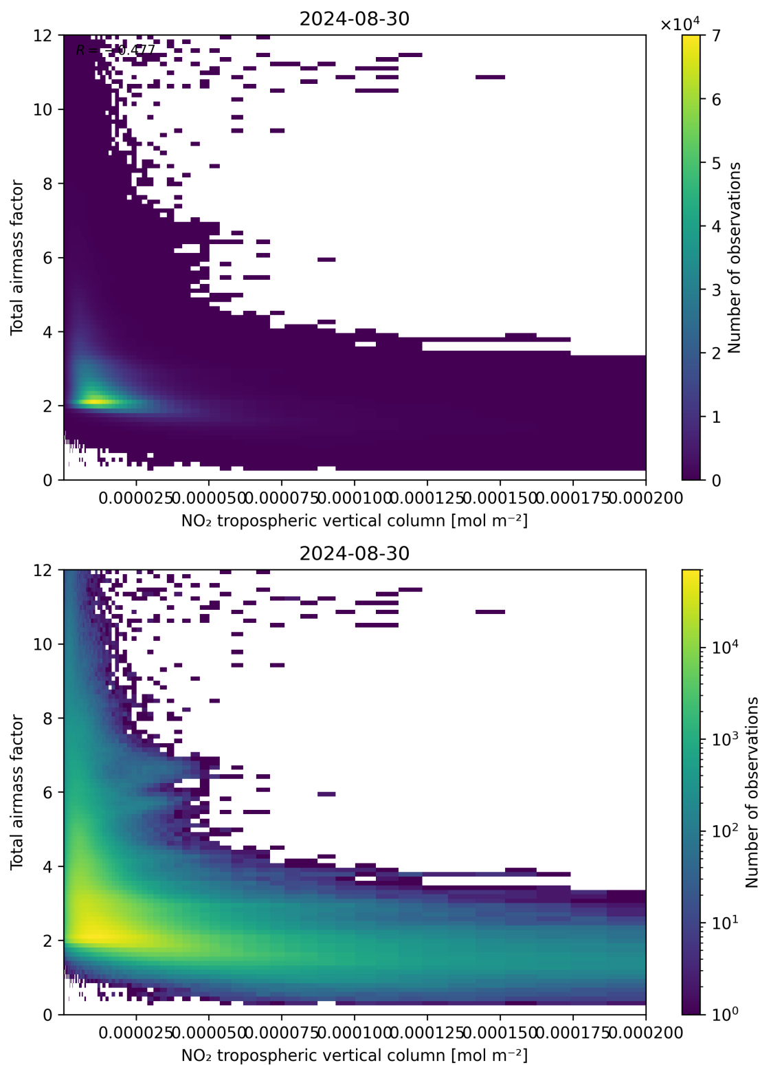
Figure 122: Scatter density plot of “NO 2 tropospheric vertical column” against “Total airmass factor” for 2024-08-29 to 2024-08-31.
