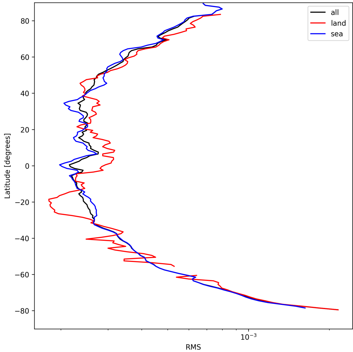
Figure 26: Zonal average of “RMS” for 2024-08-29 to 2024-08-31.
