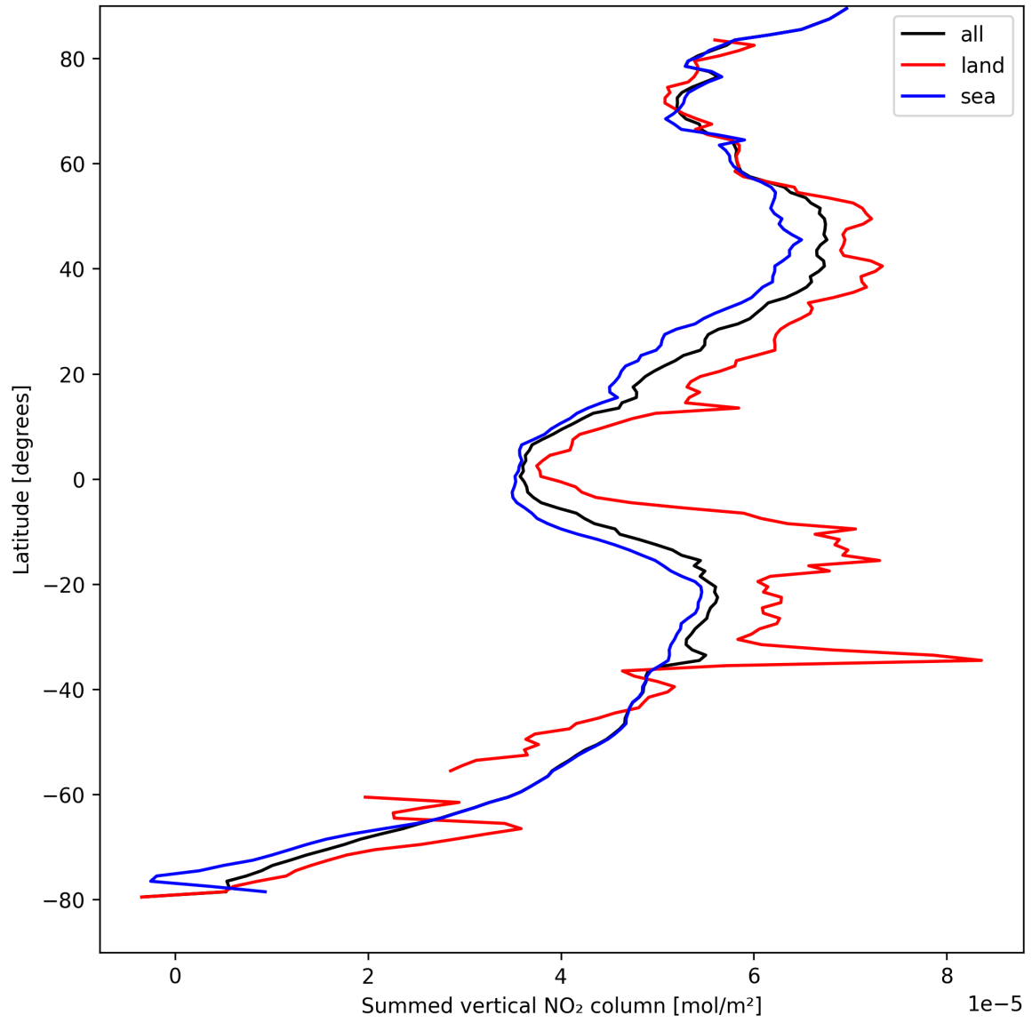
Figure 23: Zonal average of “Summed vertical NO 2 column” for 2024-08-29 to 2024-08-31.
