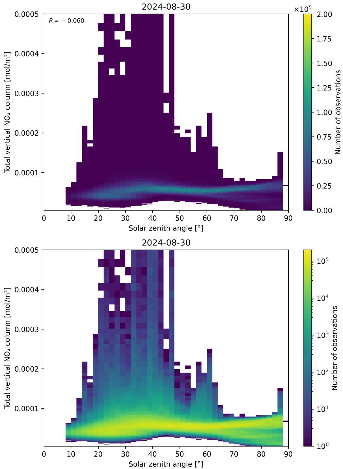
Figure 153: Scatter density plot of “Solar zenith angle” against “Total vertical NO 2 column” for 2024-08-29 to 2024-08-31.
