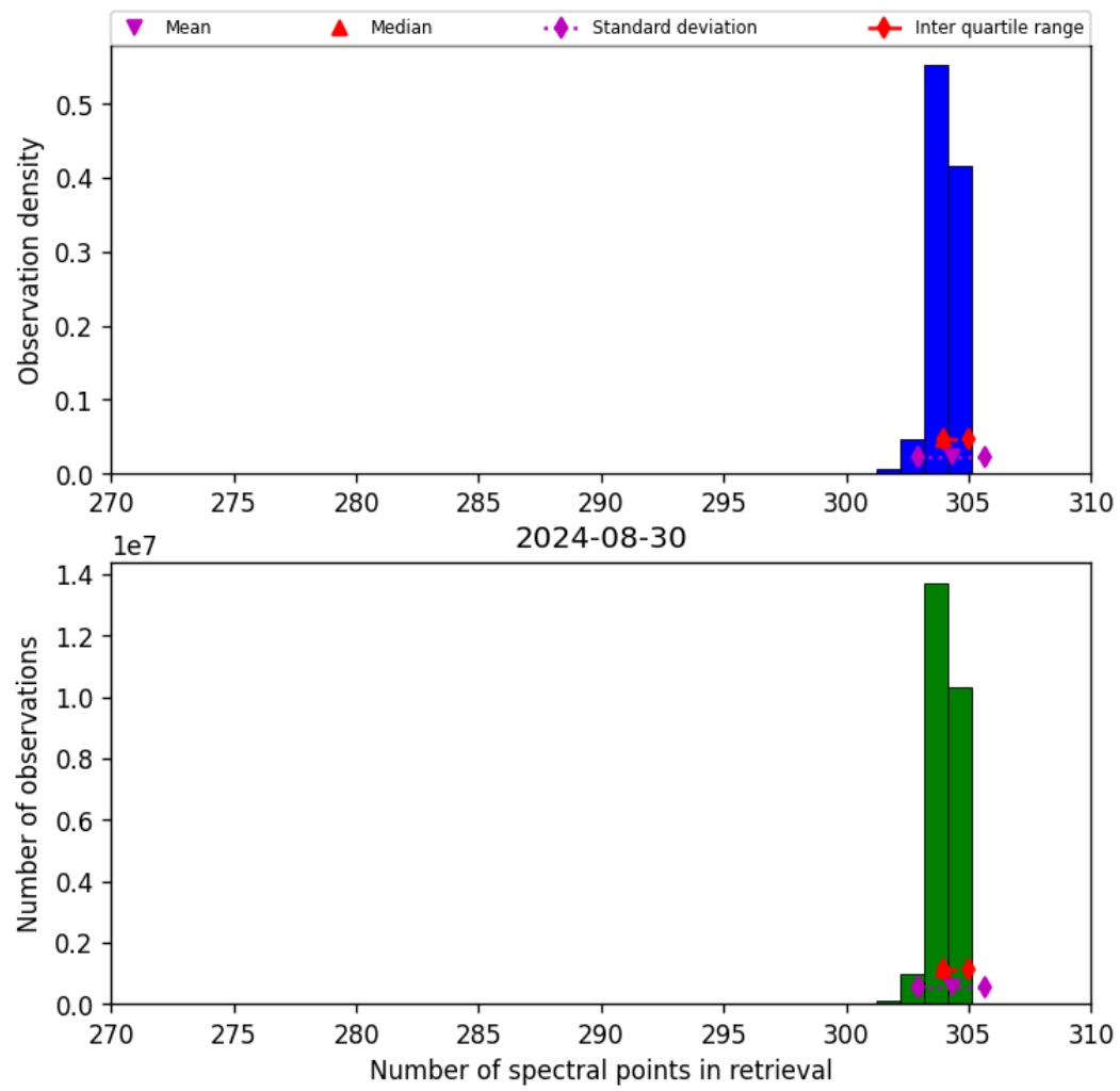
Figure 33: Histogram of “Number of spectral points in retrieval” for 2024-08-29 to 2024-08-31
