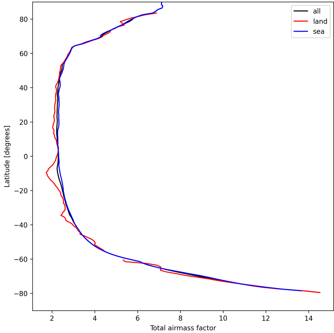
Figure 15: Zonal average of “Total airmass factor” for 2024-08-29 to 2024-08-31.
