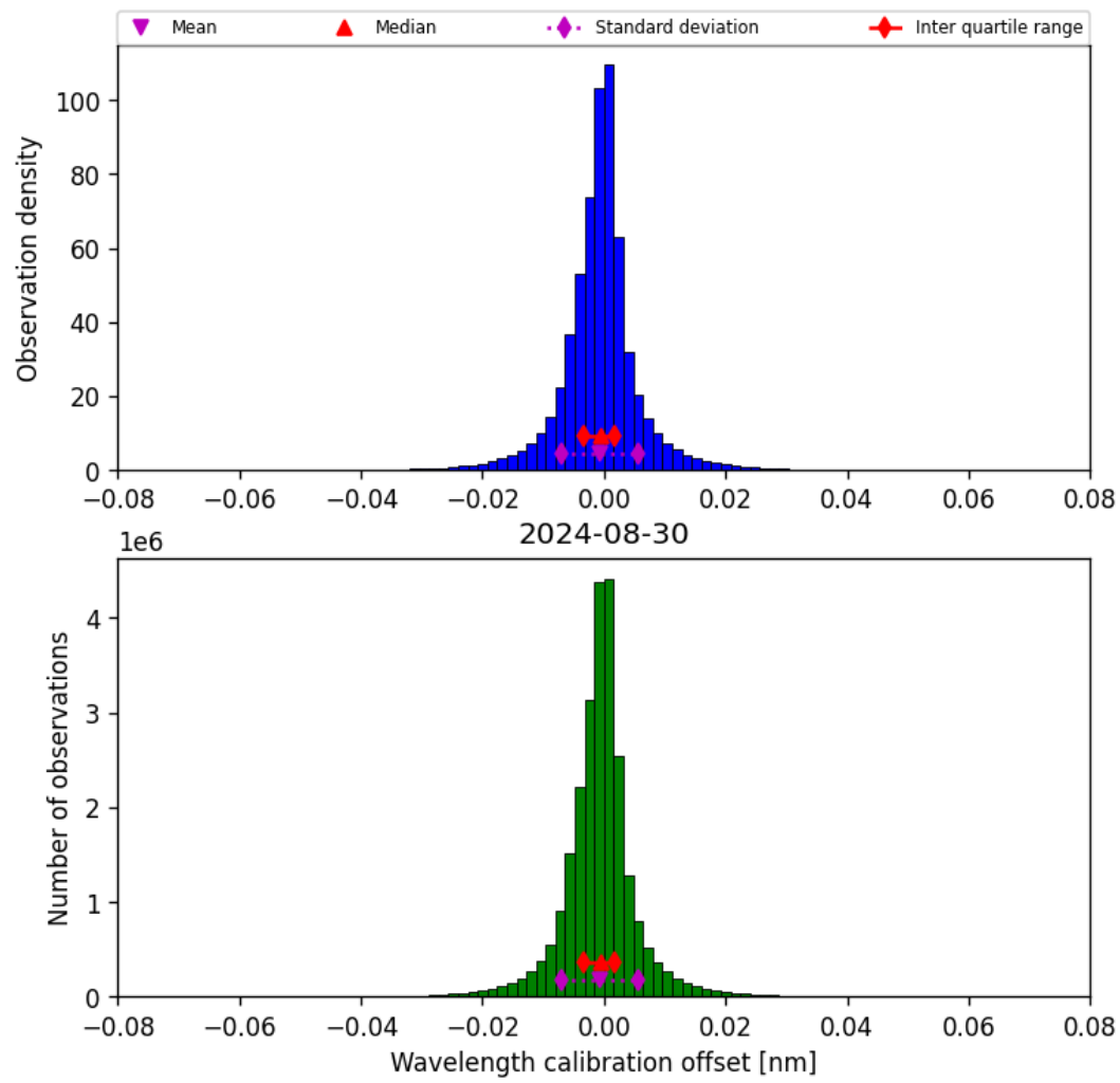
Figure 35: Histogram of “Wavelength calibration offset” for 2024-08-29 to 2024-08-31
