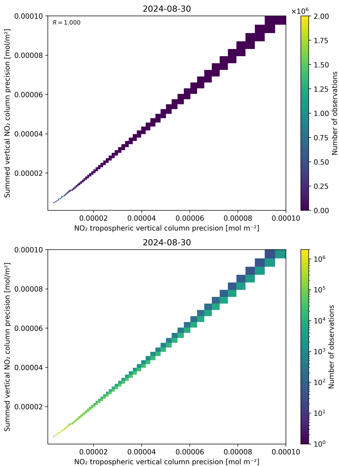
Figure 137: Scatter density plot of “NO 2 tropospheric vertical column precision” against “Summed vertical NO 2 column precision” for 2024-08-29 to 2024-08-31.
