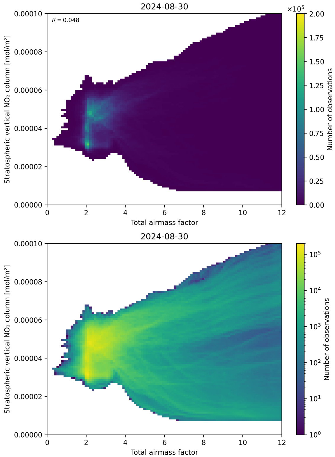
Figure 64: Scatter density plot of “Total airmass factor” against “Stratospheric vertical \text{NO}_2 column” for 2024-08-29 to 2024-08-31.
