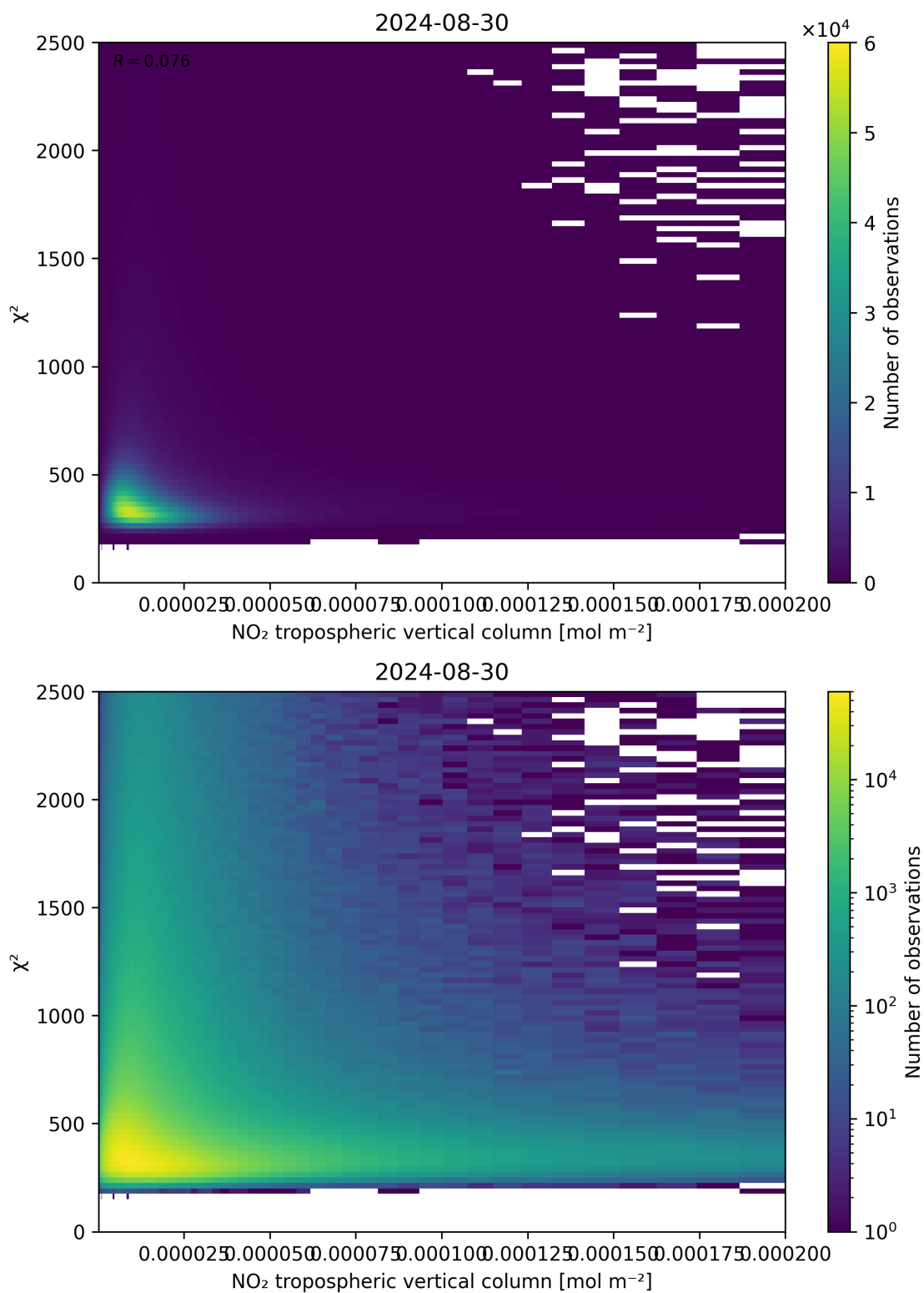
Figure 124: Scatter density plot of “NO 2 tropospheric vertical column” against “ \chi^2 ” for 2024-08-29 to 2024-08-31.
