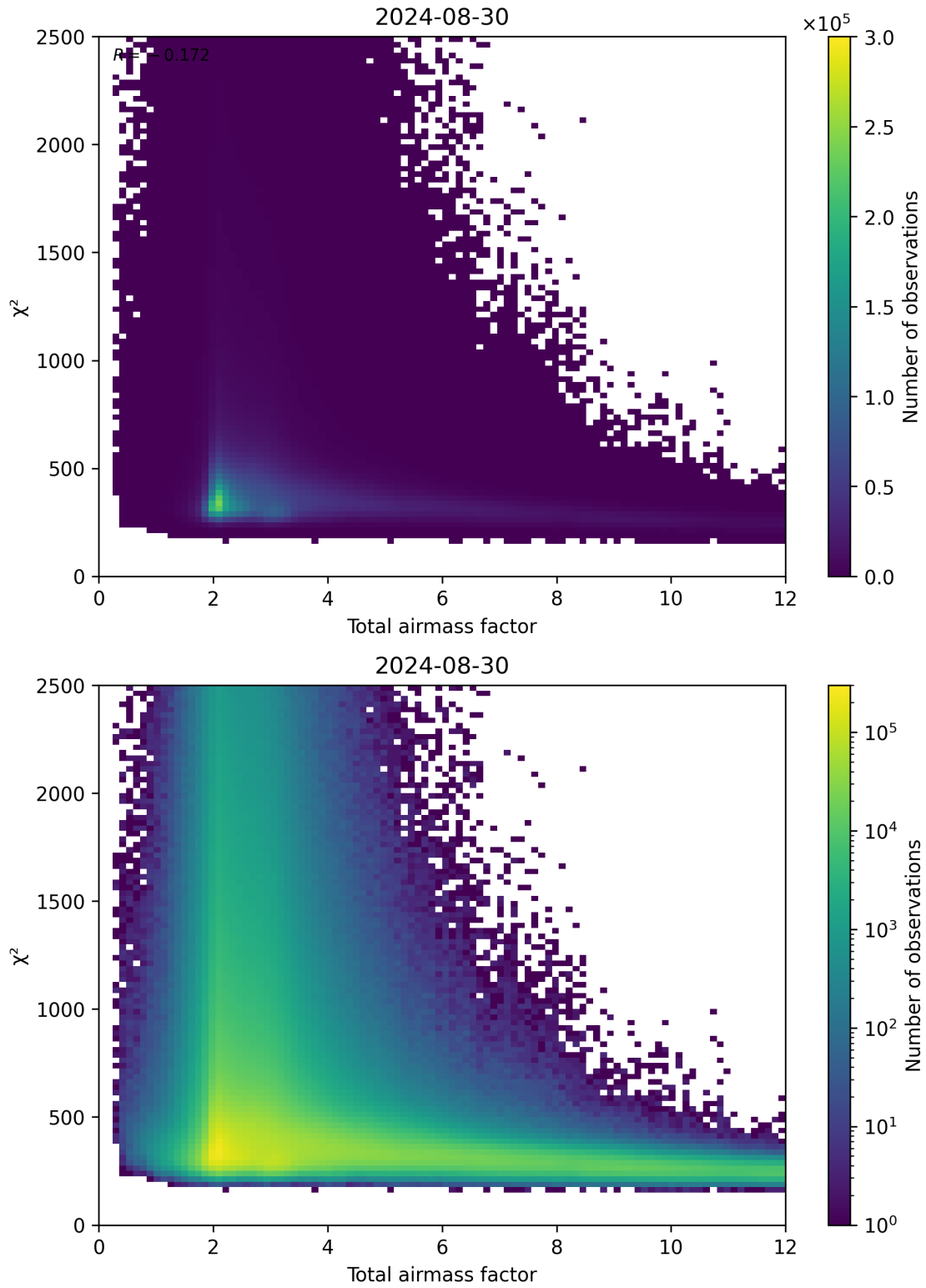
Figure 63: Scatter density plot of “Total airmass factor” against “ \chi^2 ” for 2024-08-29 to 2024-08-31.
