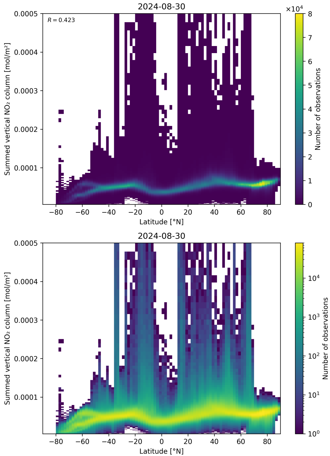
Figure 88: Scatter density plot of “Latitude” against “Summed vertical NO 2 column” for 2024-08-29 to 2024-08-31.
