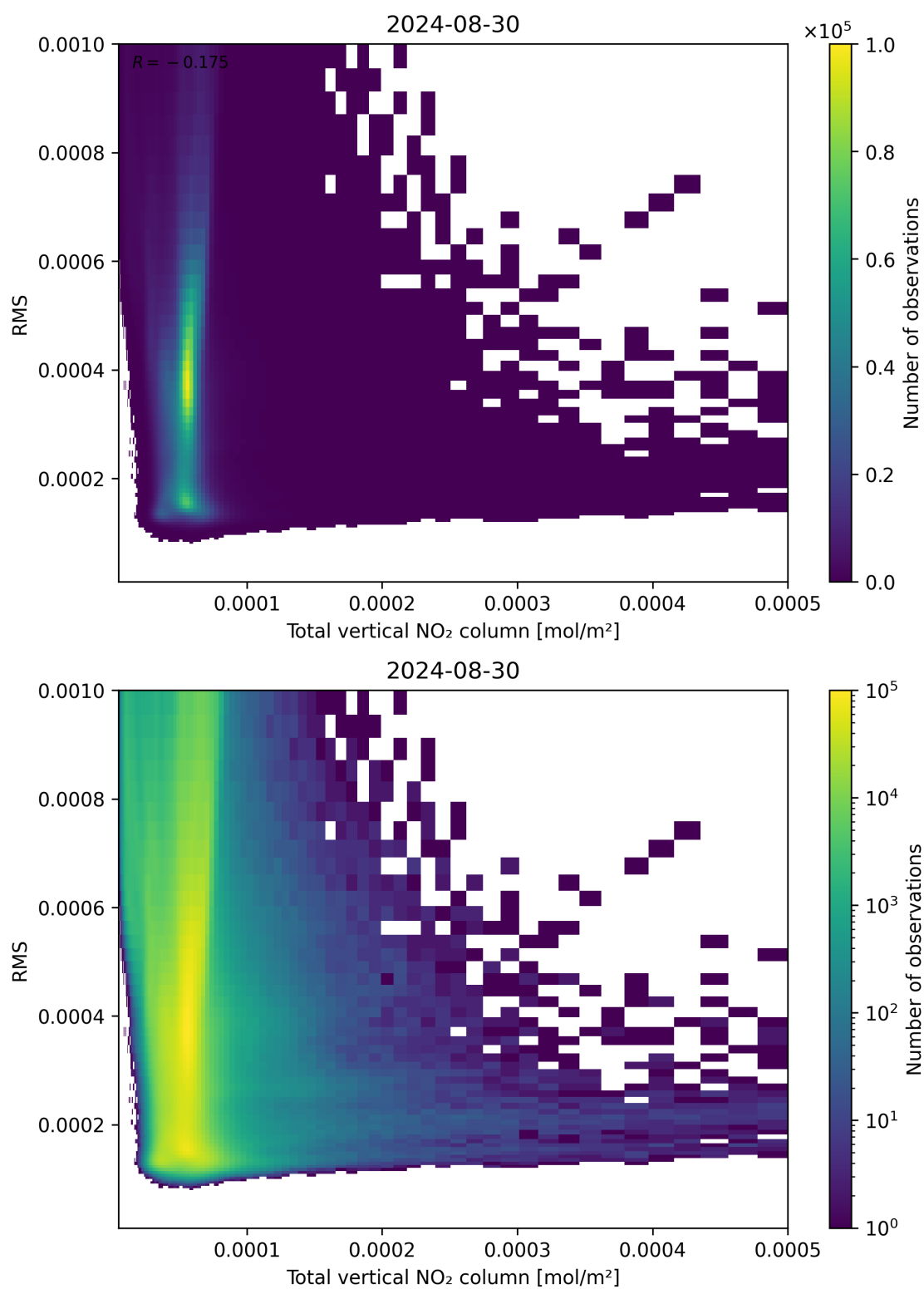
Figure 120: Scatter density plot of “Total vertical NO 2 column” against “RMS” for 2024-08-29 to 2024-08-31.
