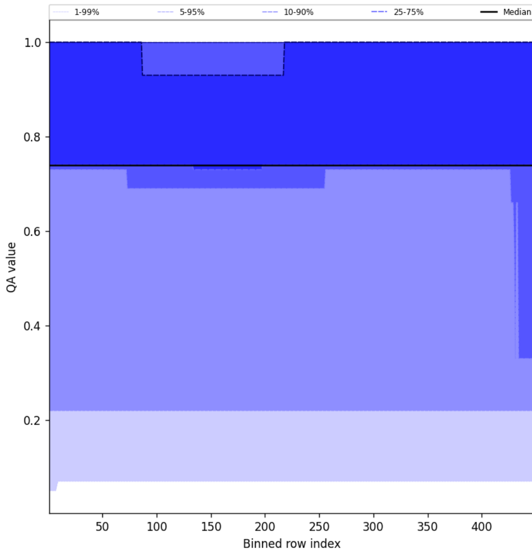
Figure 45: Along track statistics of “QA value” for 2024-08-29 to 2024-08-31
