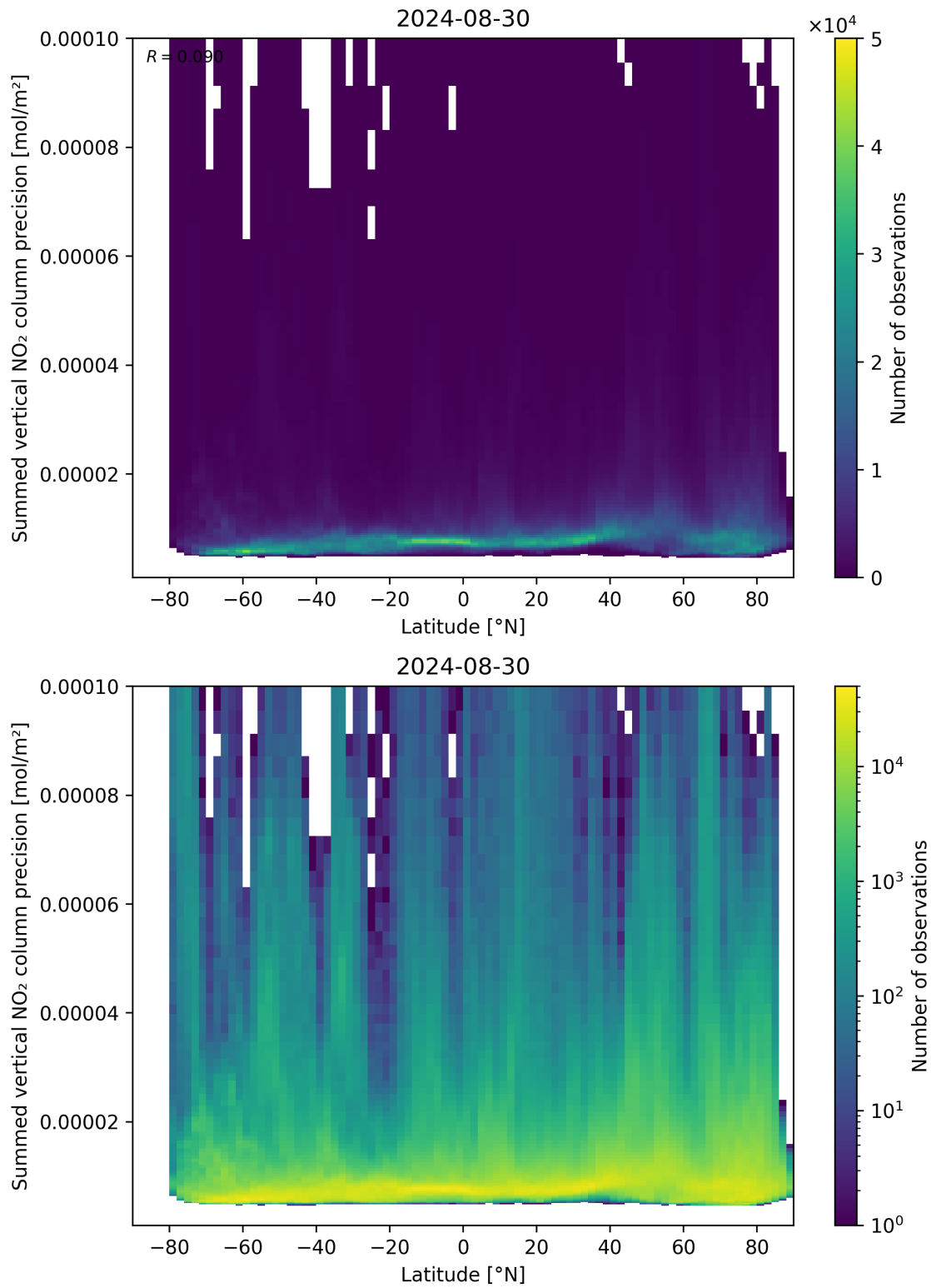
Figure 89: Scatter density plot of “Latitude” against “Summed vertical NO 2 column precision” for 2024-08-29 to 2024-08-31.
