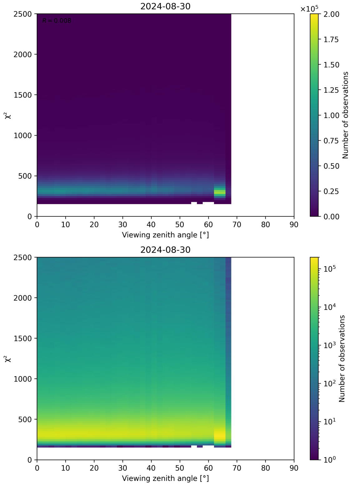
Figure 162: Scatter density plot of “Viewing zenith angle” against “ \chi^2 ” for 2024-08-29 to 2024-08-31.
