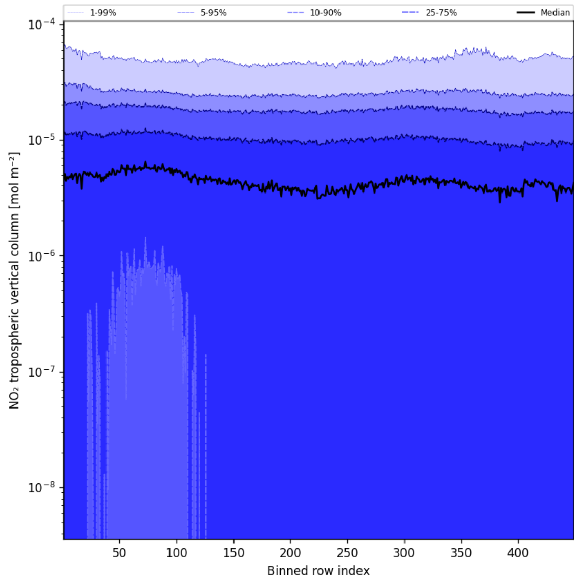
Figure 46: Along track statistics of “NO 2 tropospheric vertical column” for 2024-08-29 to 2024-08-31
