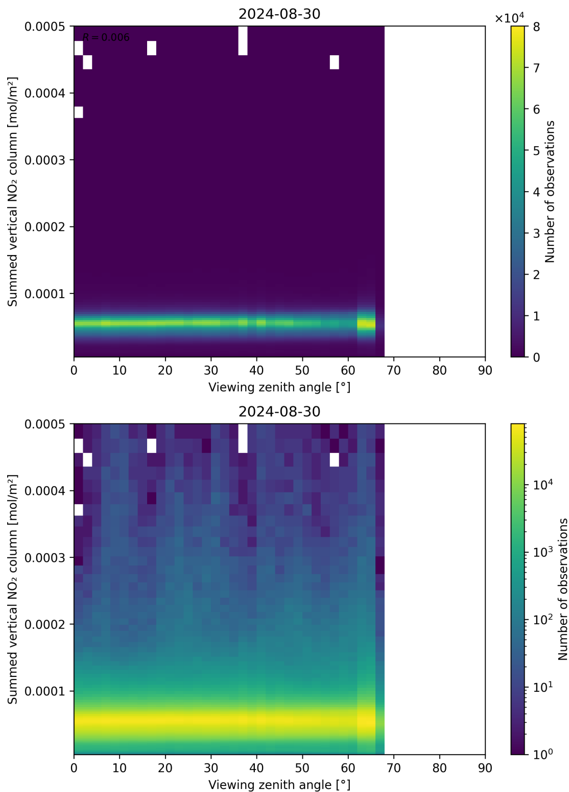
Figure 165: Scatter density plot of “Viewing zenith angle” against “Summed vertical NO 2 column” for 2024-08-29 to 2024-08-31.
