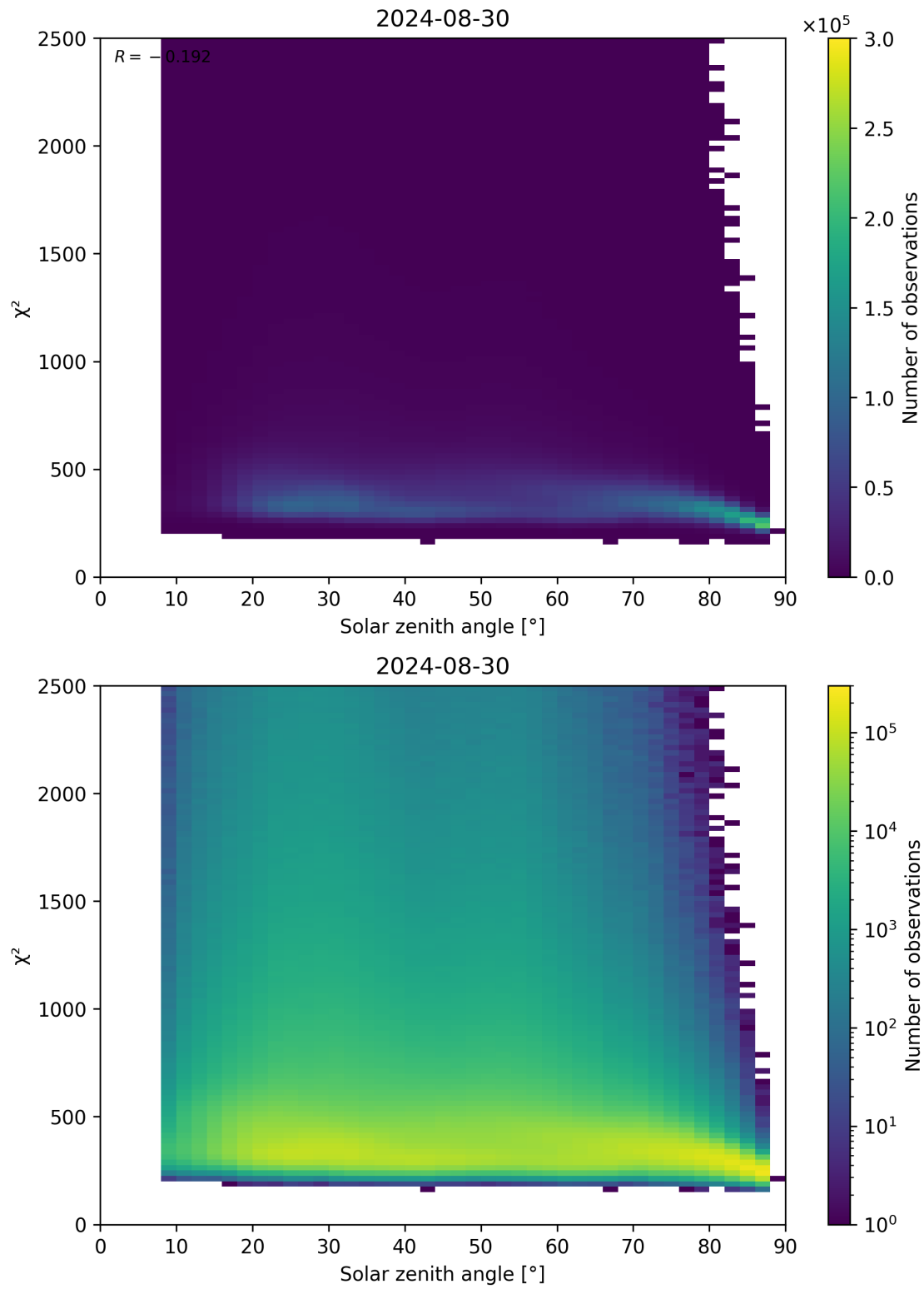
Figure 148: Scatter density plot of “Solar zenith angle” against “ \chi^2 ” for 2024-08-29 to 2024-08-31.
