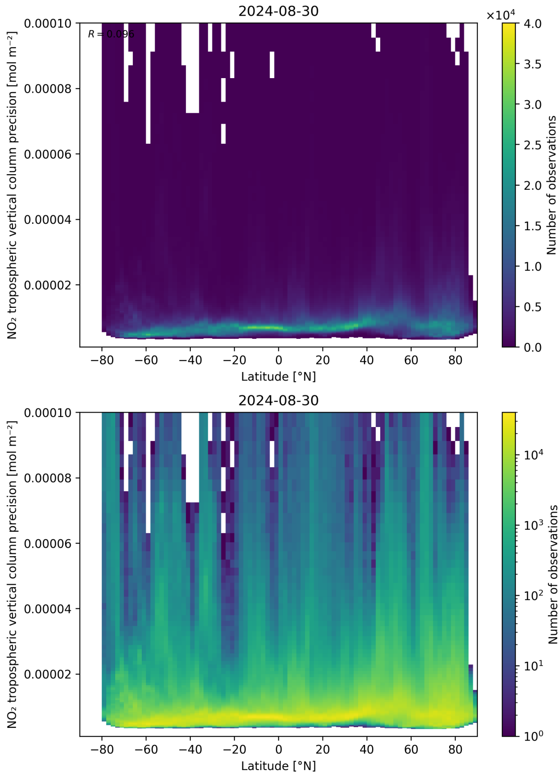
Figure 93: Scatter density plot of “Latitude” against “NO 2 tropospheric vertical column precision” for 2024-08-29 to 2024-08-31.
