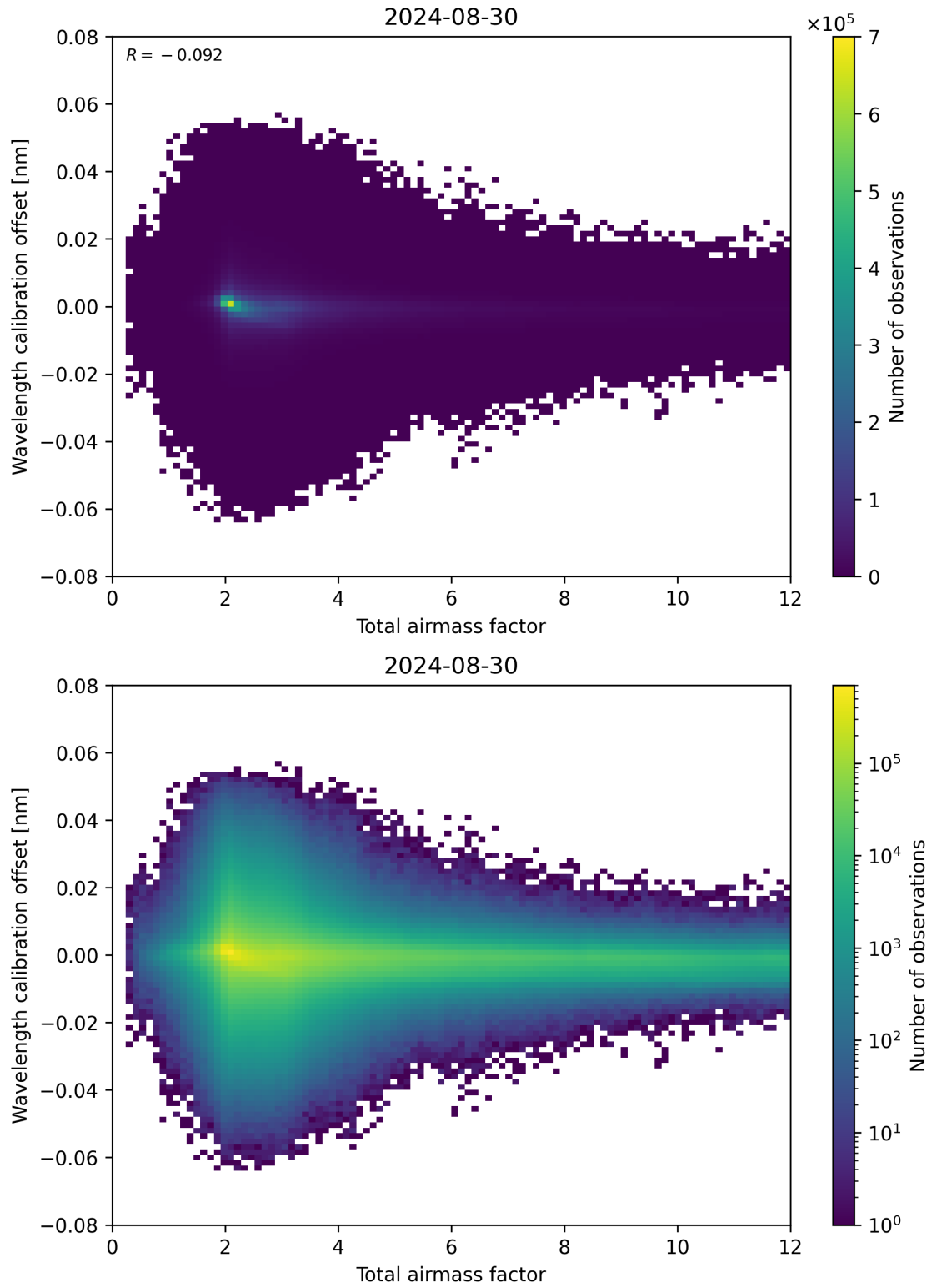
Figure 70: Scatter density plot of “Total airmass factor” against “Wavelength calibration offset” for 2024-08-29 to 2024-08-31.
