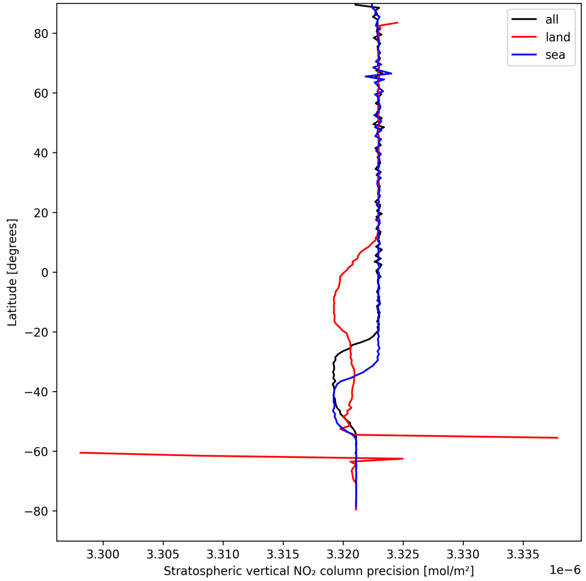
Figure 20: Zonal average of “Stratospheric vertical NO 2 column precision” for 2024-08-29 to 2024-08-31.
