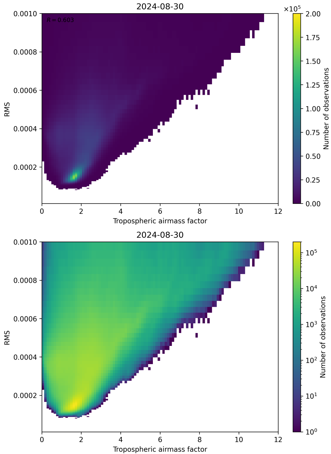
Figure 79: Scatter density plot of “Tropospheric airmass factor” against “RMS” for 2024-08-29 to 2024-08-31.
