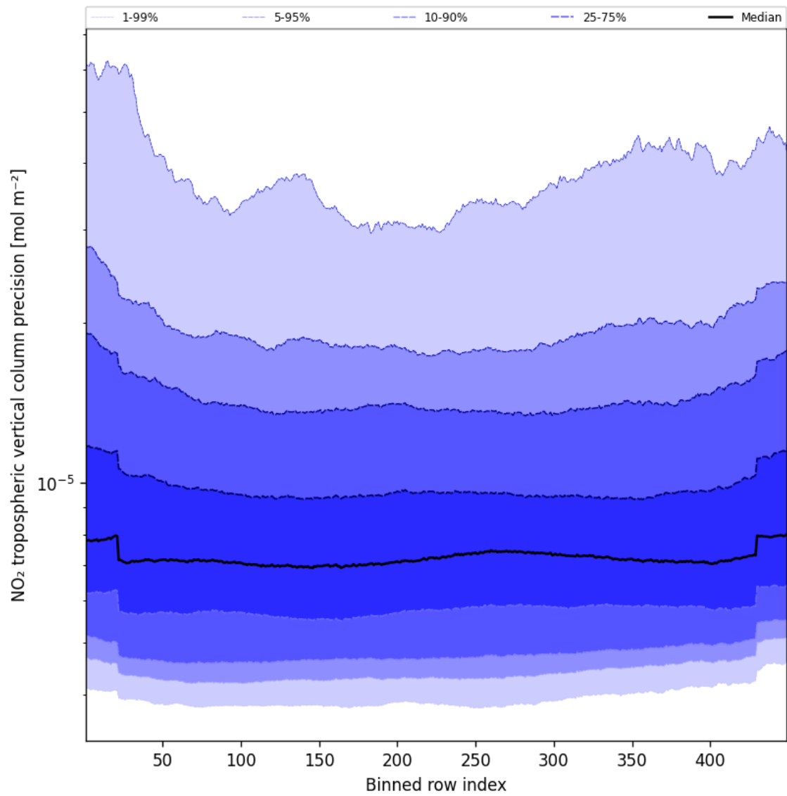
Figure 47: Along track statistics of “NO 2 tropospheric vertical column precision” for 2024-08-29 to 2024-08-31
