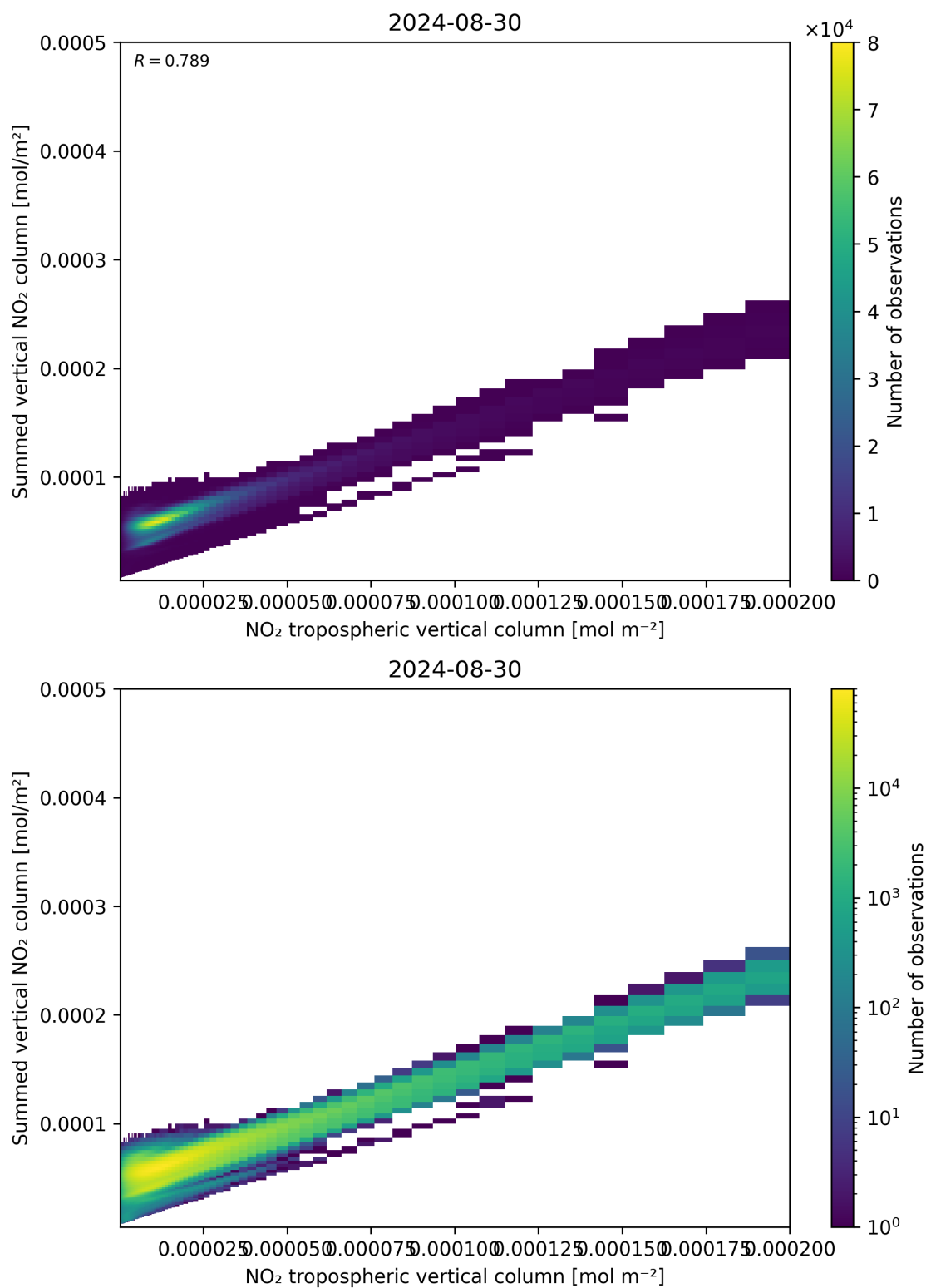
Figure 126: Scatter density plot of “NO 2 tropospheric vertical column” against “Summed vertical NO 2 column” for 2024-08-29 to 2024-08-31.
