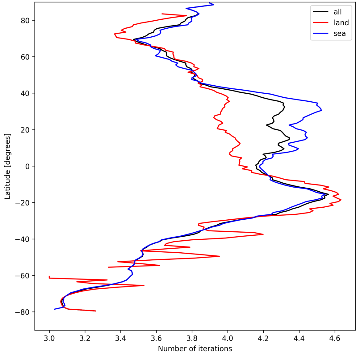
Figure 17: Zonal average of “Number of iterations” for 2024-08-29 to 2024-08-31.
