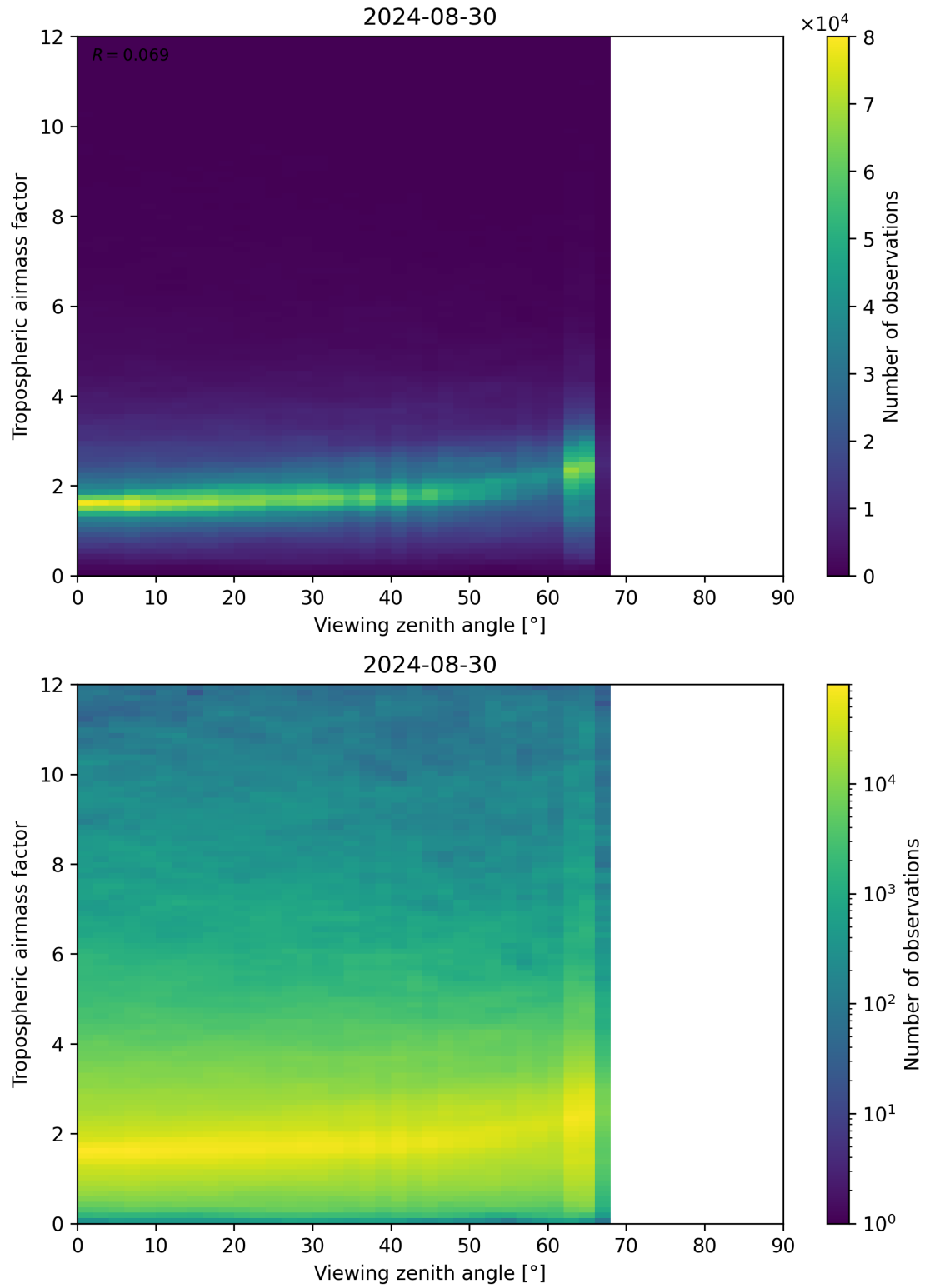
Figure 161: Scatter density plot of “Viewing zenith angle” against “Tropospheric airmass factor” for 2024-08-29 to 2024-08-31.
