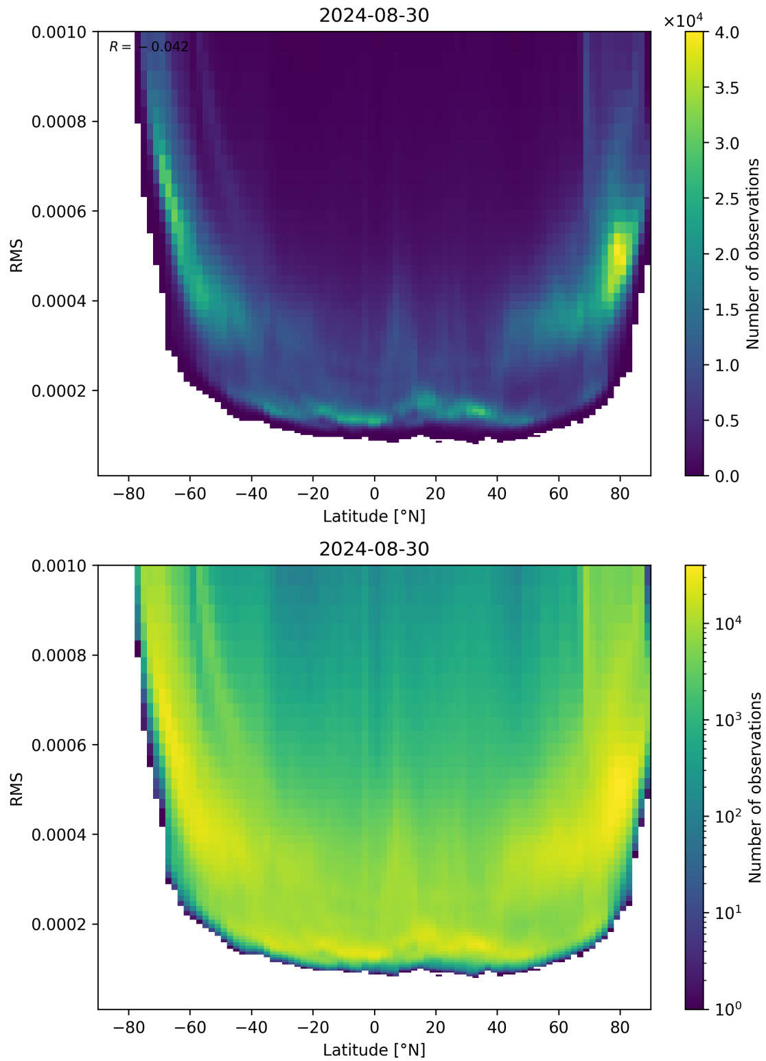
Figure 94: Scatter density plot of “Latitude” against “RMS” for 2024-08-29 to 2024-08-31.
