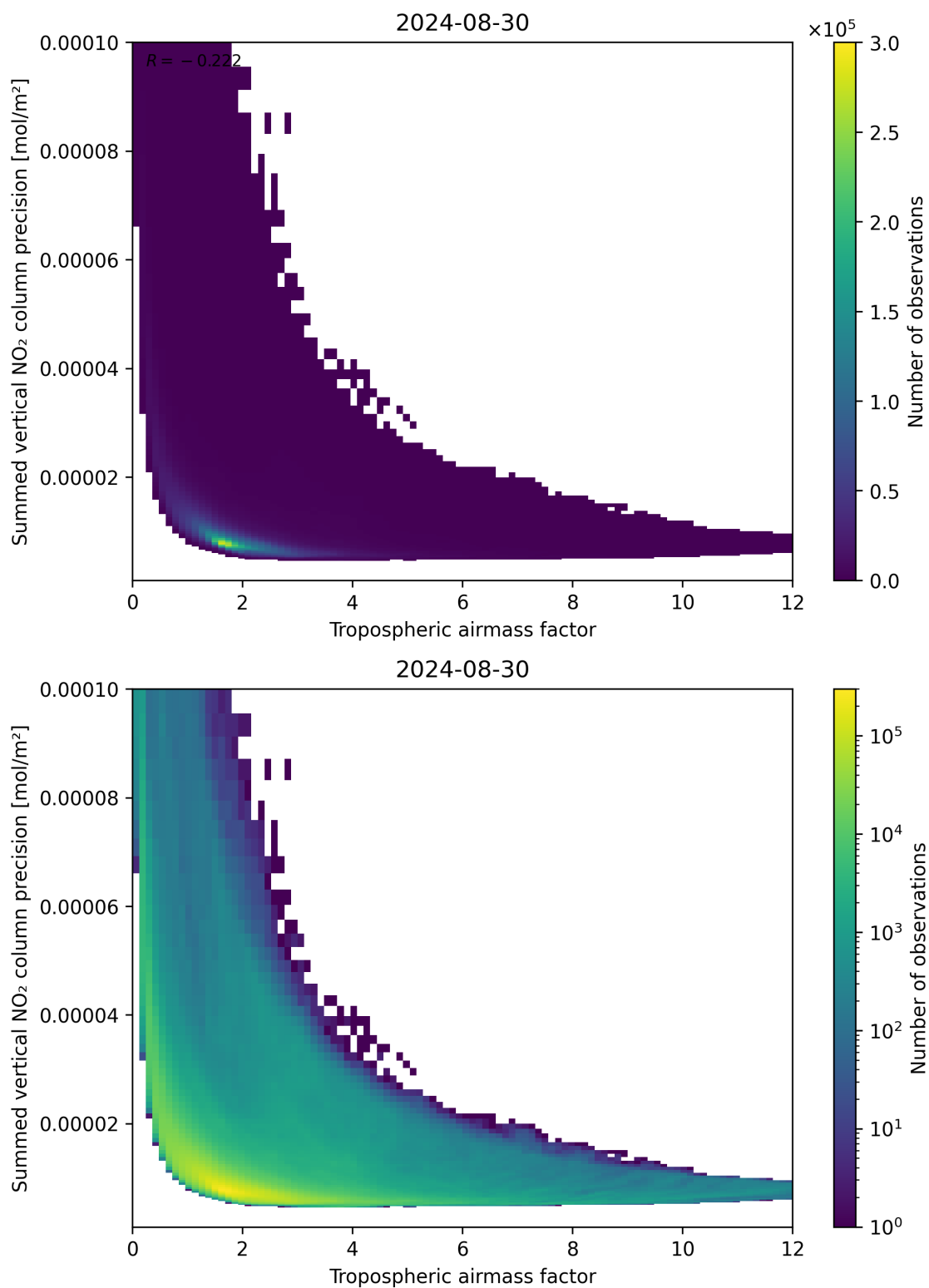
Figure 76: Scatter density plot of “Tropospheric air mass factor” against “Summed vertical NO 2 column precision” for 2024-08-29 to 2024-08-31.
