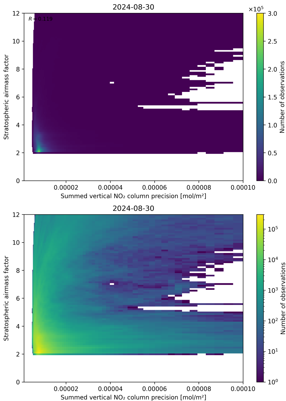
Figure 106: Scatter density plot of “Summed vertical NO 2 column precision” against “Stratospheric airmass factor” for 2024-08-29 to 2024-08-31.
