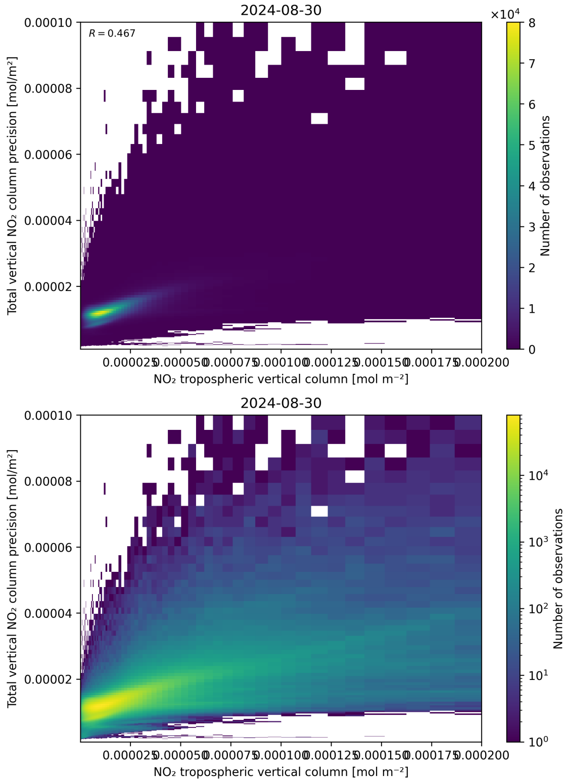
Figure 129: Scatter density plot of “NO 2 tropospheric vertical column” against “Total vertical NO 2 column precision” for 2024-08-29 to 2024-08-31.
