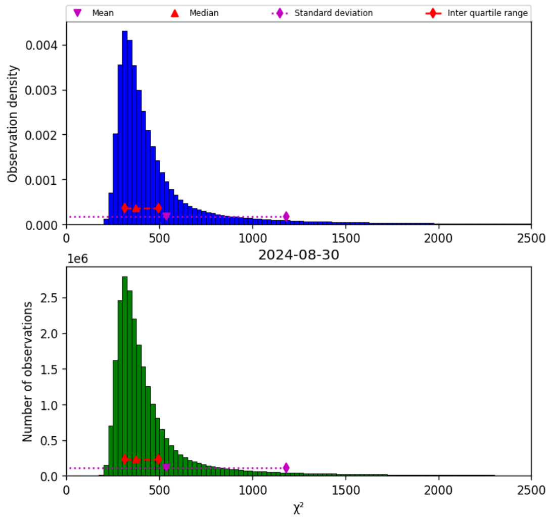
Figure 42: Histogram of “ \chi^2 ” for 2024-08-29 to 2024-08-31
