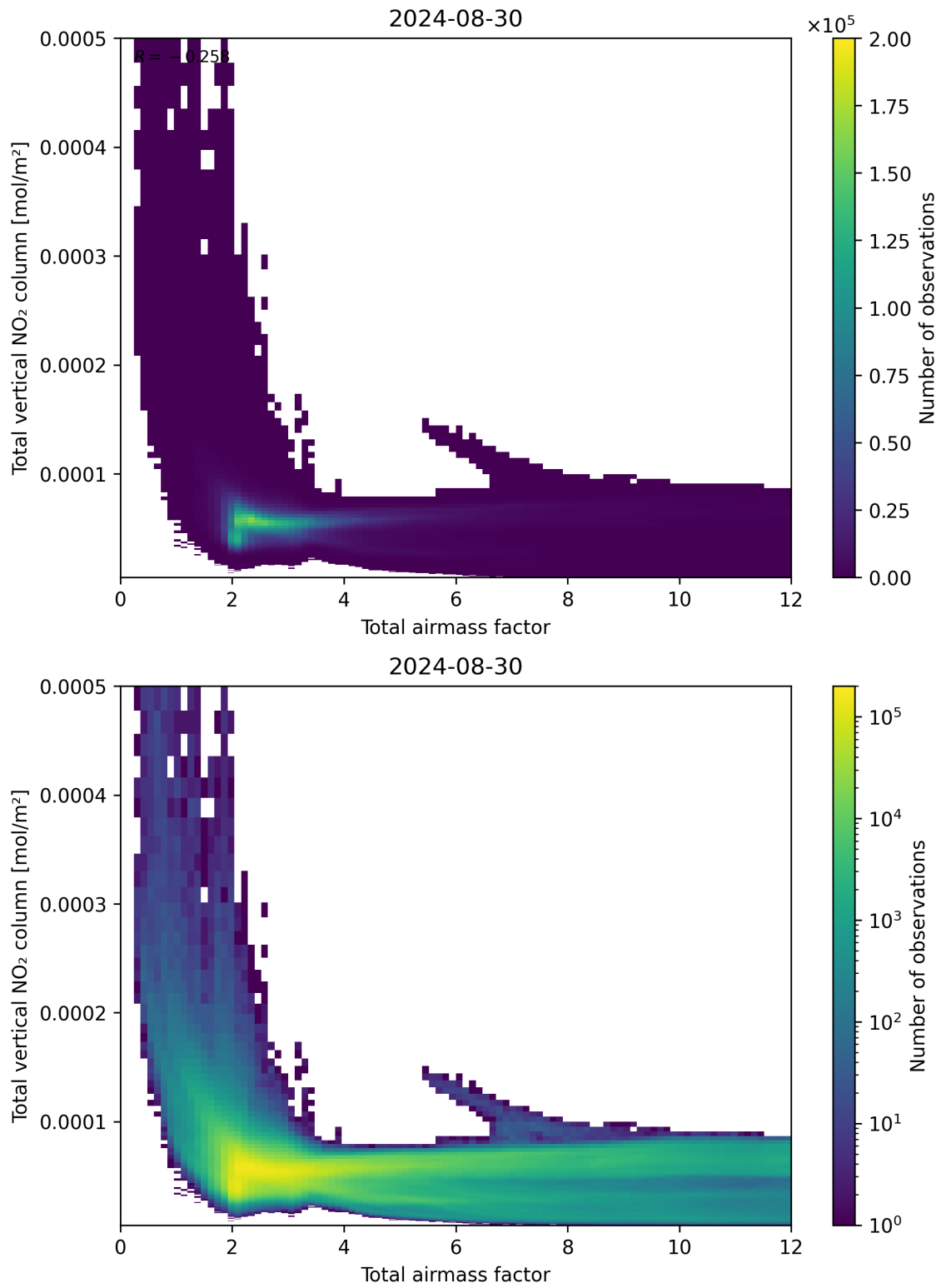
Figure 67: Scatter density plot of “Total airmass factor” against “Total vertical NO 2 column” for 2024-08-29 to 2024-08-31.
