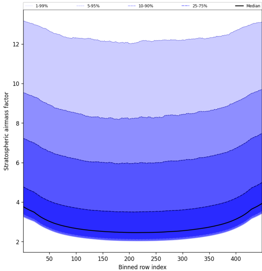
Figure 61: Along track statistics of “Stratospheric airmass factor” for 2024-08-29 to 2024-08-31
