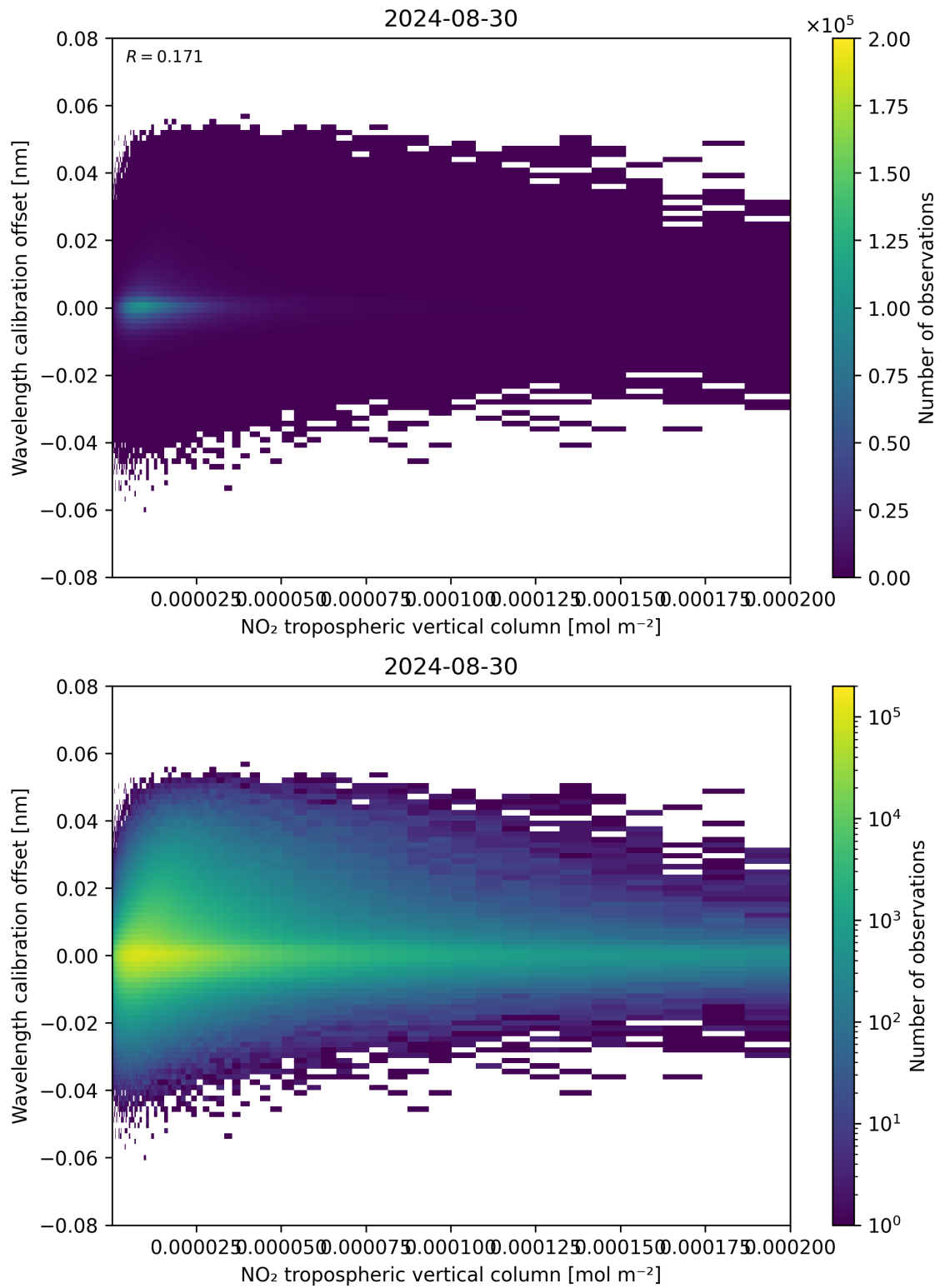
Figure 143: Scatter density plot of “NO 2 tropospheric vertical column” against “Wavelength calibration offset” for 2024-08-29 to 2024-08-31.
