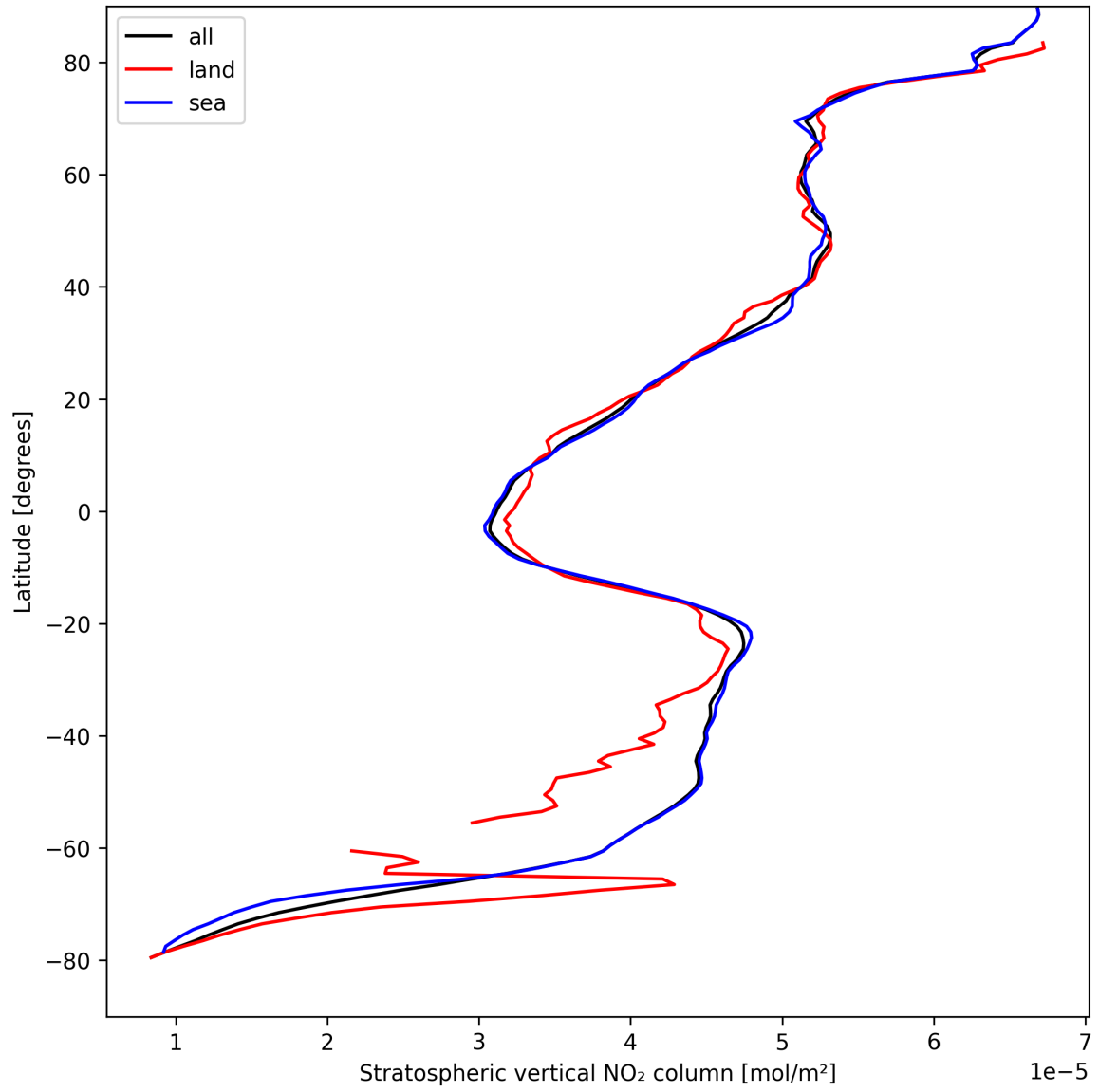
Figure 19: Zonal average of “Stratospheric vertical NO 2 column” for 2024-08-29 to 2024-08-31.
