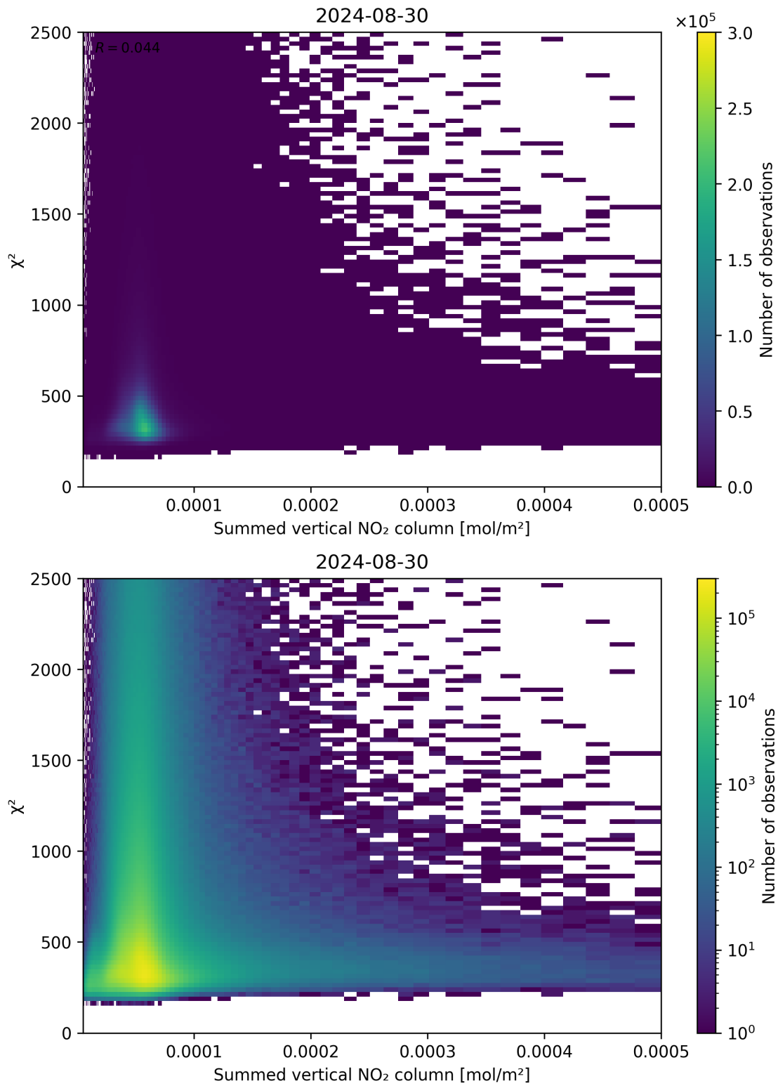
Figure 104: Scatter density plot of “Summed vertical NO 2 column” against “ \chi^2 ” for 2024-08-29 to 2024-08-31.
