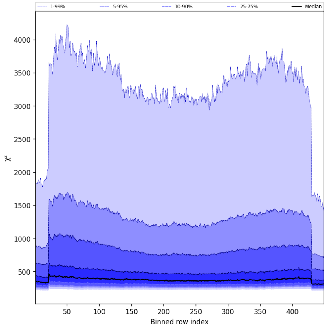
Figure 59: Along track statistics of “ \chi^2 ” for 2024-08-29 to 2024-08-31
