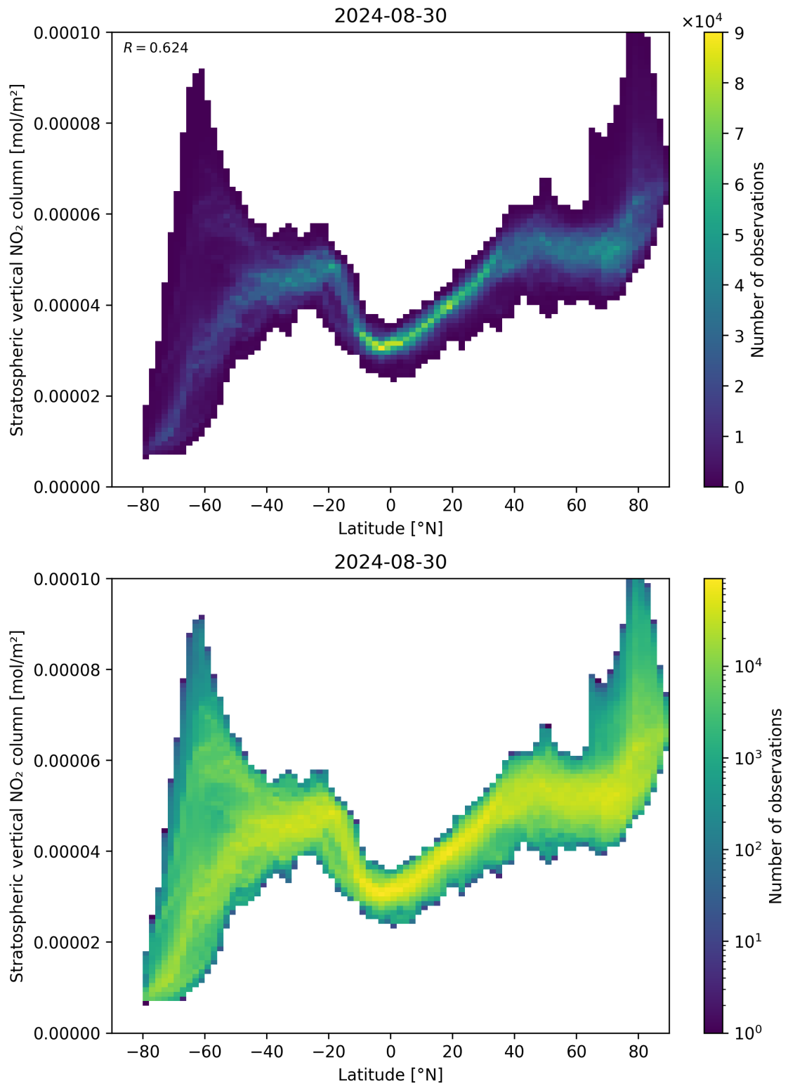
Figure 87: Scatter density plot of “Latitude” against “Stratospheric vertical NO 2 column” for 2024-08-29 to 2024-08-31.
