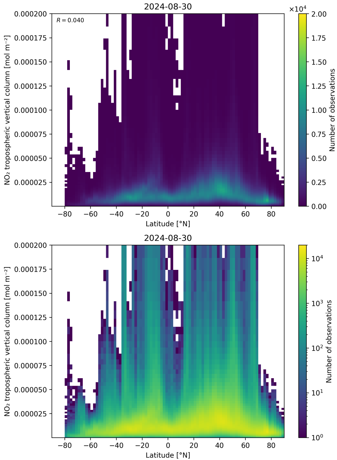
Figure 92: Scatter density plot of “Latitude” against “NO 2 tropospheric vertical column” for 2024-08-29 to 2024-08-31.
