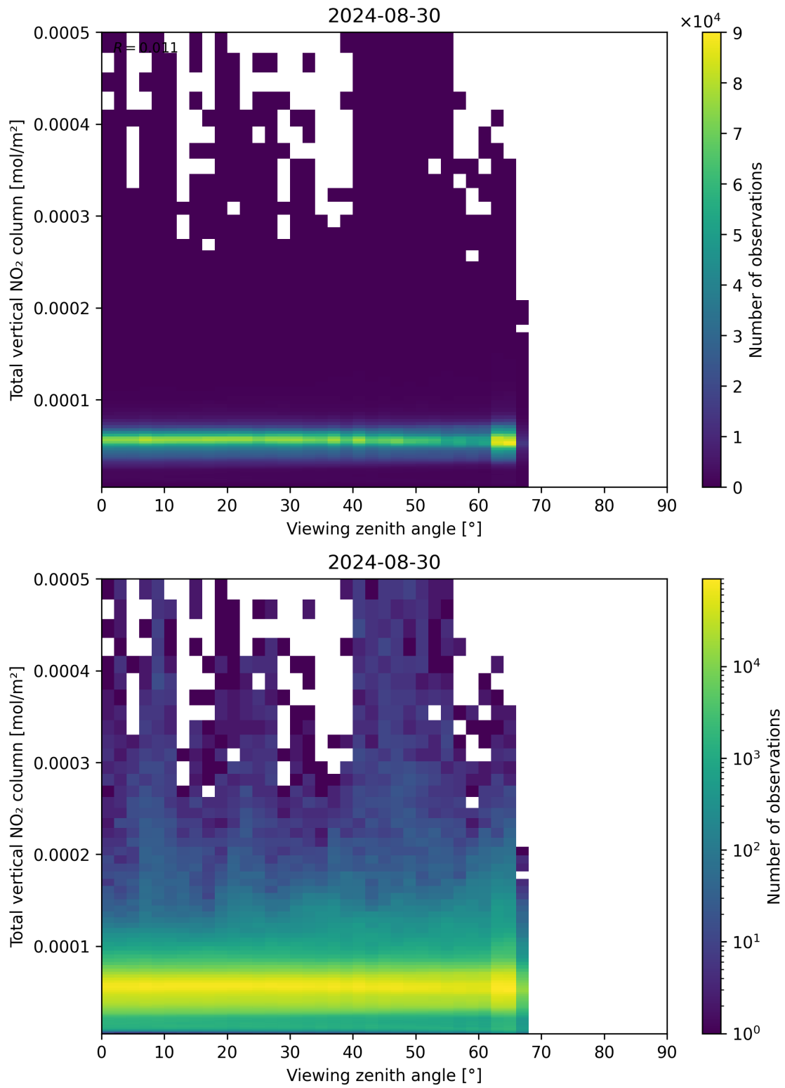
Figure 167: Scatter density plot of “Viewing zenith angle” against “Total vertical NO 2 column” for 2024-08-29 to 2024-08-31.
