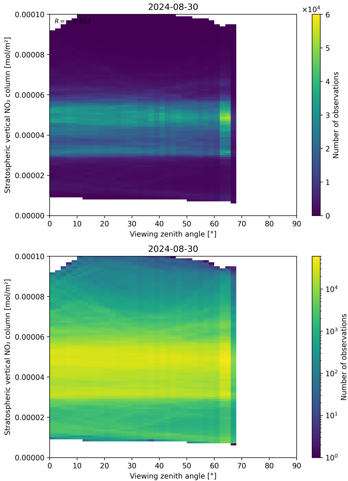
Figure 164: Scatter density plot of “Viewing zenith angle” against “Stratospheric vertical NO 2 column” for 2024-08-29 to 2024-08-31.
