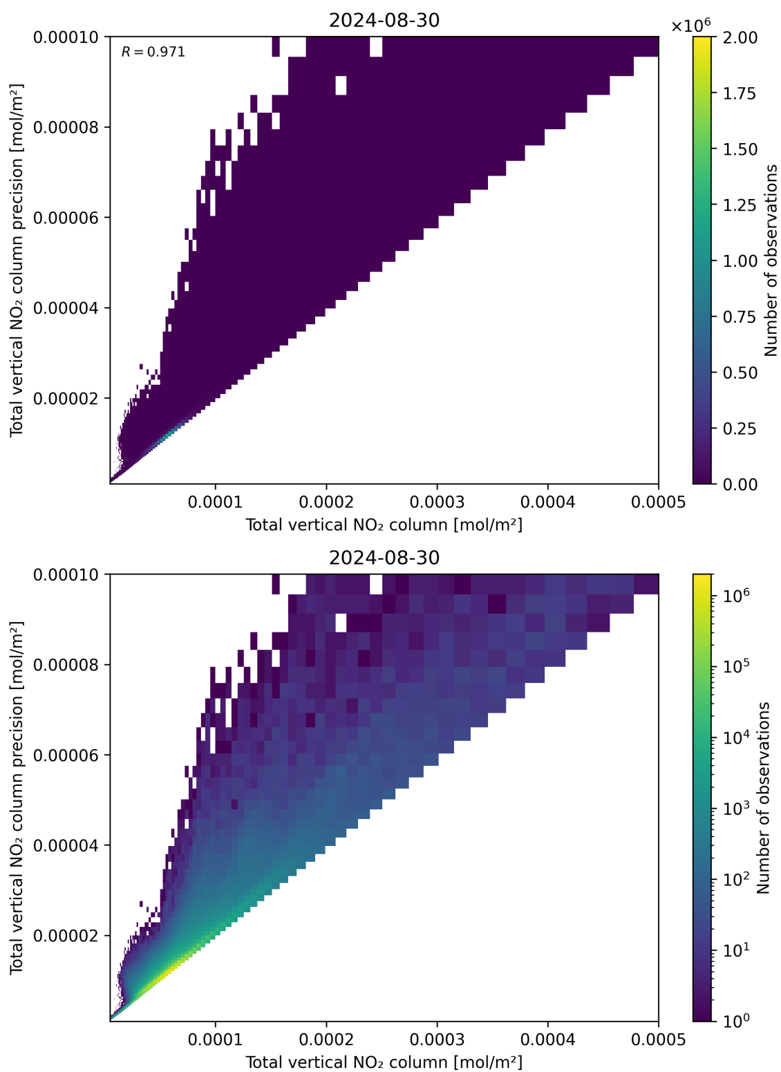
Figure 114: Scatter density plot of “Total vertical NO 2 column” against “Total vertical NO 2 column precision” for 2024-08-29 to 2024-08-31.
