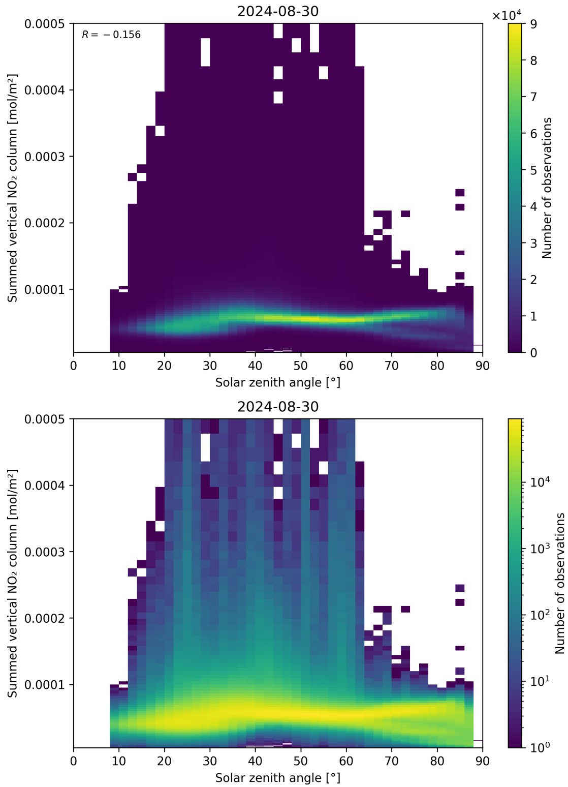
Figure 151: Scatter density plot of “Solar zenith angle” against “Summed vertical NO 2 column” for 2024-08-29 to 2024-08-31.
