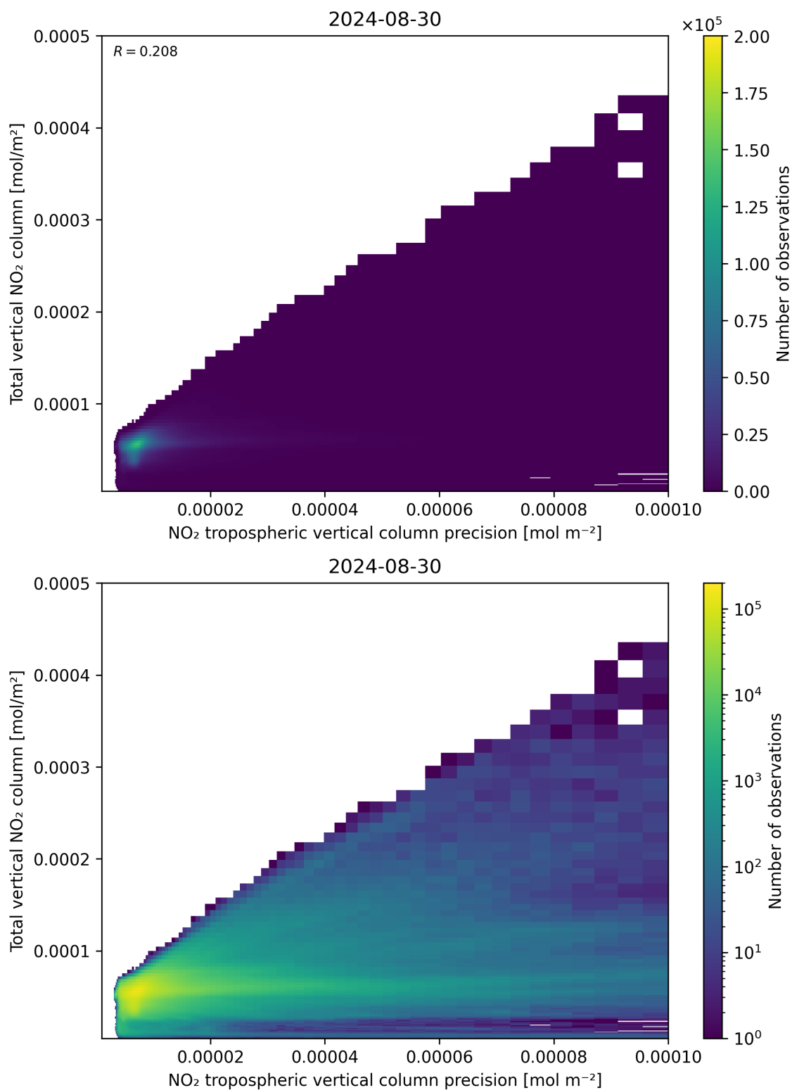
Figure 138: Scatter density plot of “NO 2 tropospheric vertical column precision” against “Total vertical NO 2 column” for 2024-08-29 to 2024-08-31.
