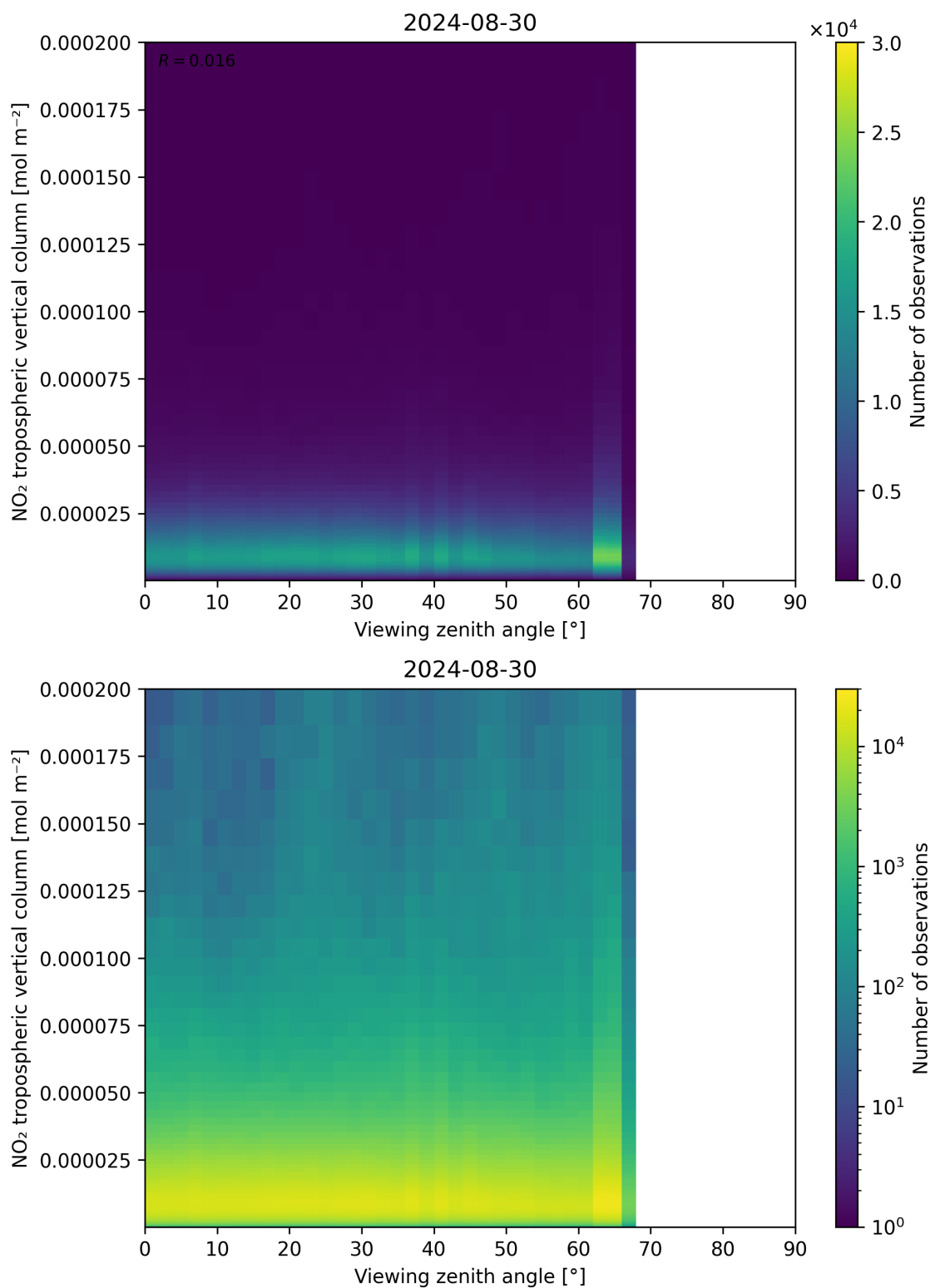
Figure 169: Scatter density plot of “Viewing zenith angle” against “NO 2 tropospheric vertical column” for 2024-08-29 to 2024-08-31.
