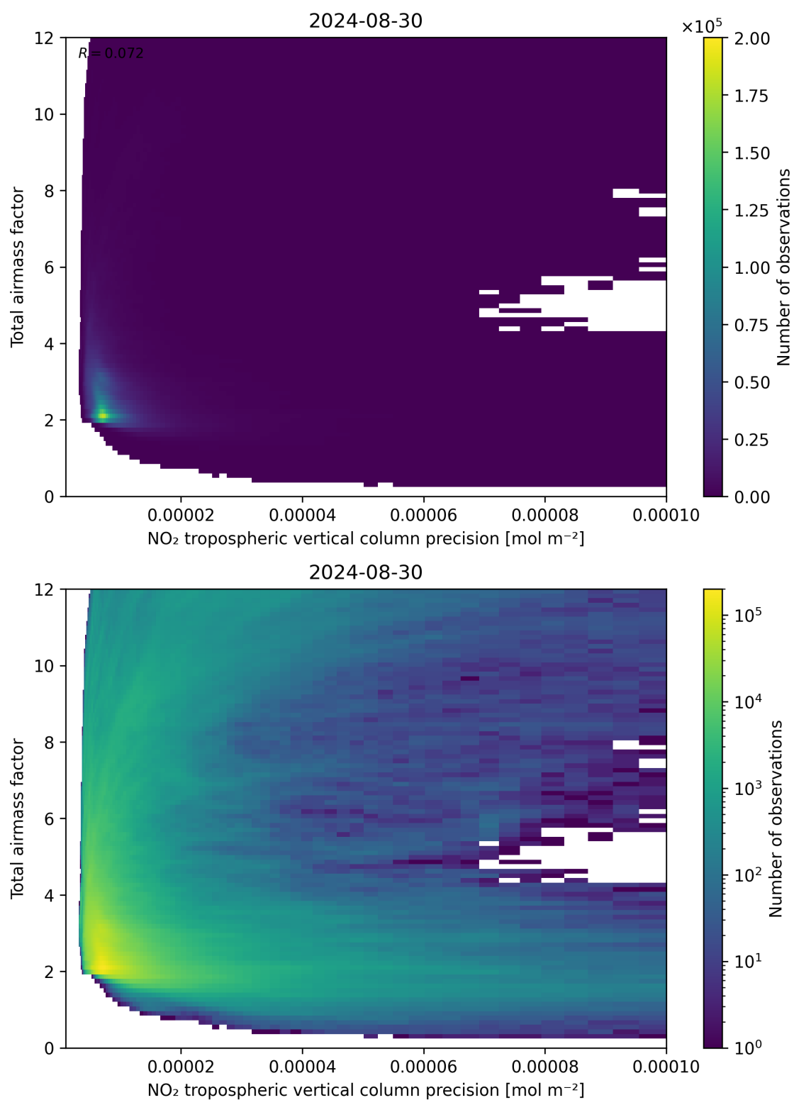
Figure 132: Scatter density plot of “NO 2 tropospheric vertical column precision” against “Total air mass factor” for 2024-08-29 to 2024-08-31.
