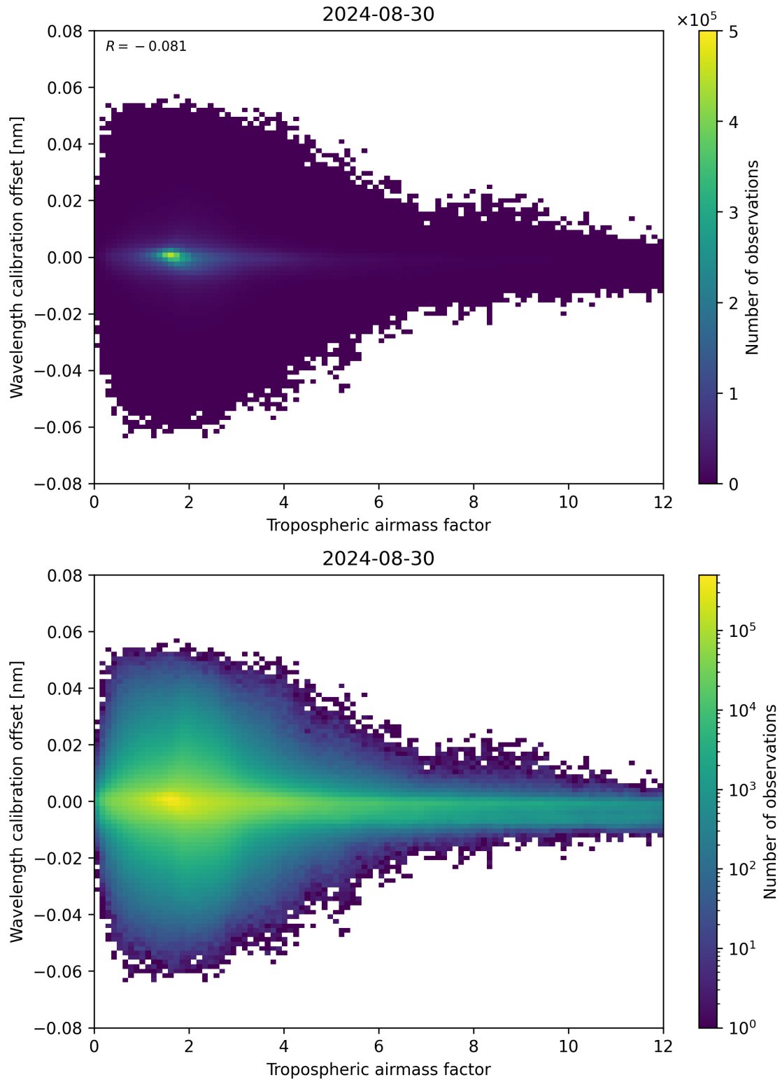
Figure 80: Scatter density plot of “Tropospheric airmass factor” against “Wavelength calibration offset” for 2024-08-29 to 2024-08-31.
