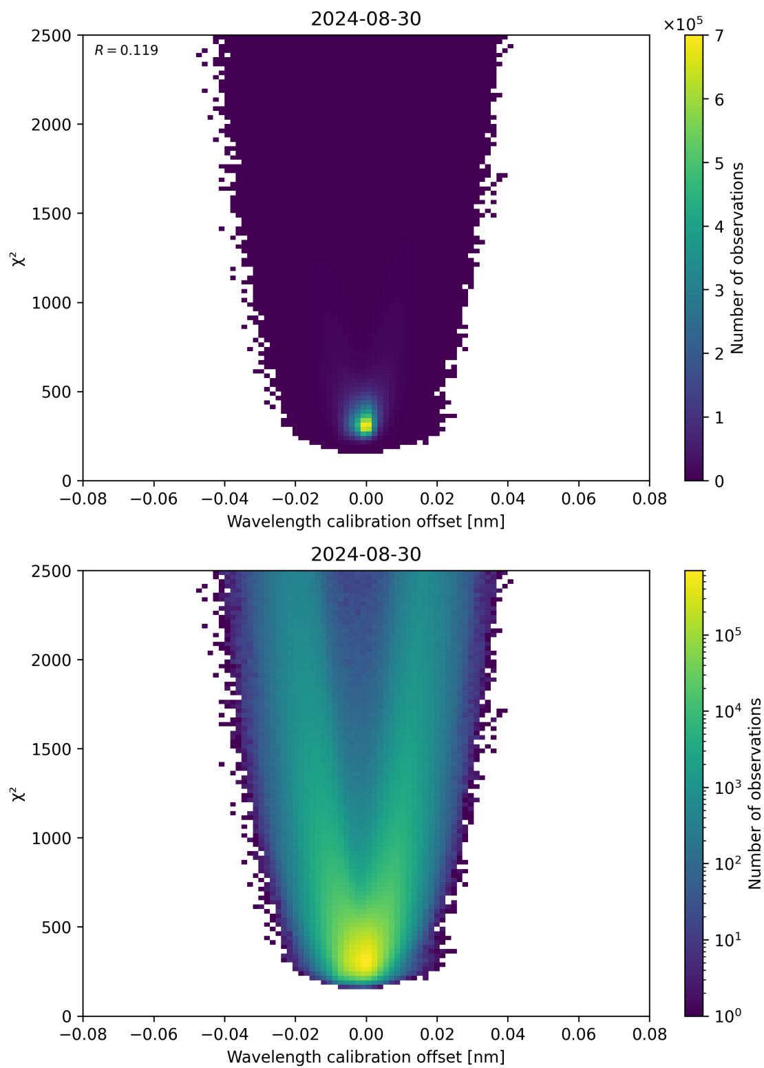
Figure 175: Scatter density plot of “Wavelength calibration offset” against “ \chi^2 ” for 2024-08-29 to 2024-08-31.
