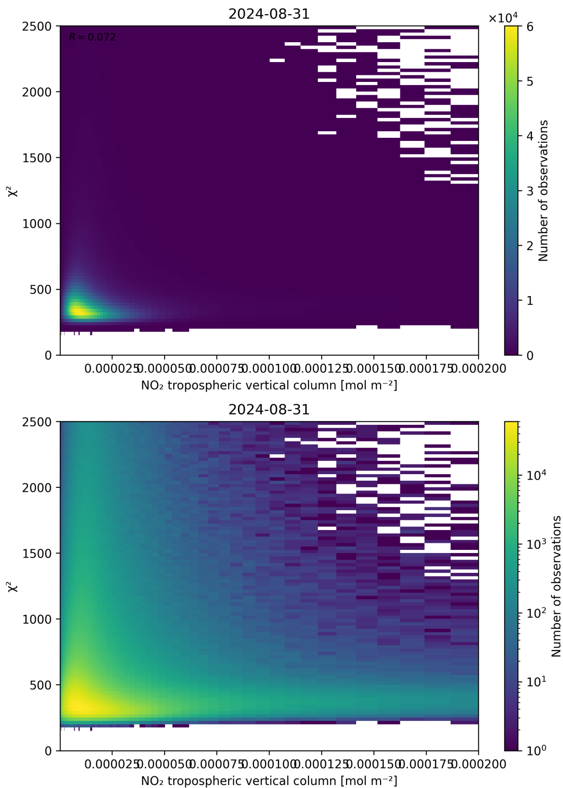
Figure 124: Scatter density plot of “NO 2 tropospheric vertical column” against “ \chi^2 ” for 2024-08-30 to 2024-09-01.
