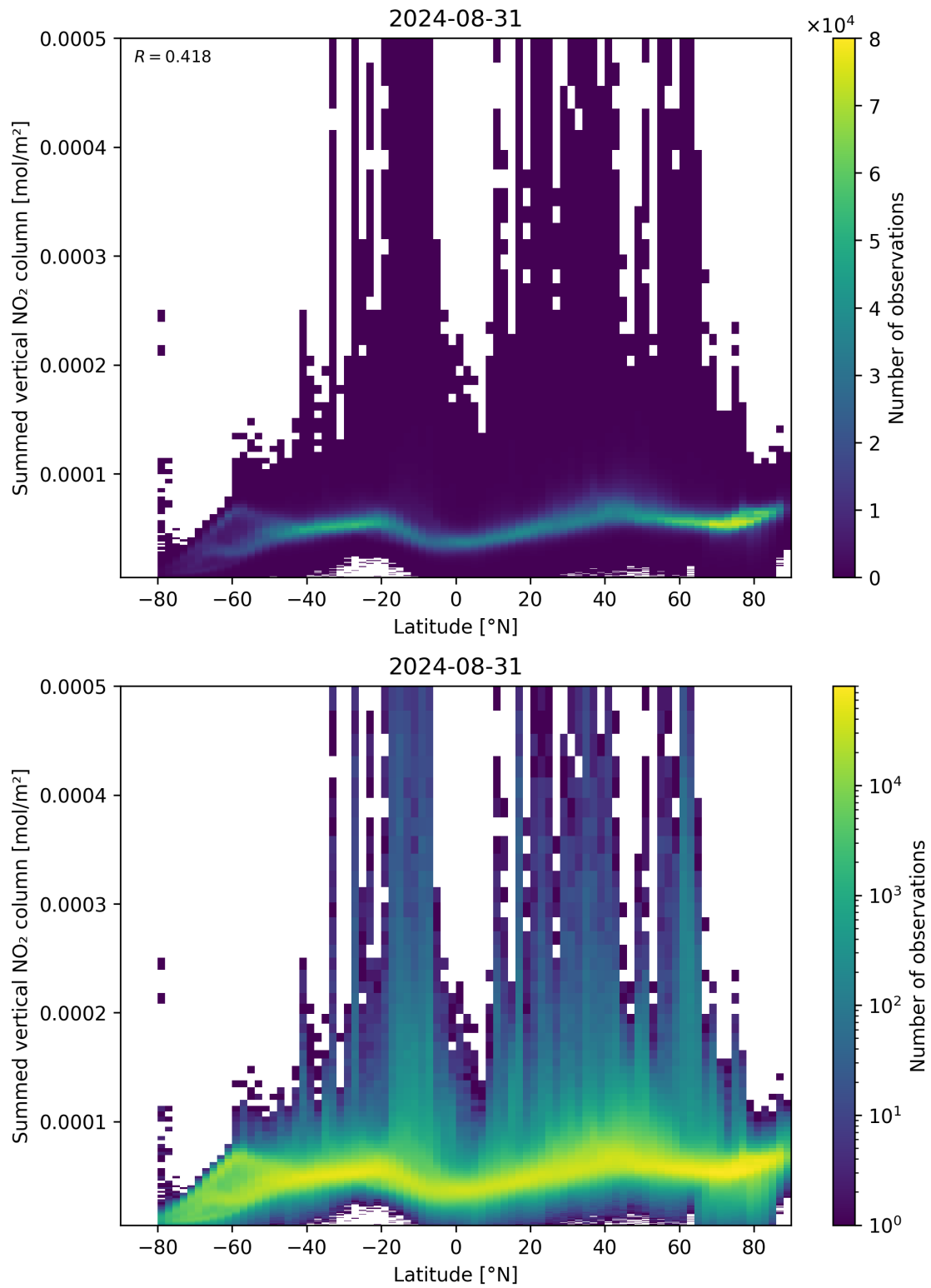
Figure 88: Scatter density plot of “Latitude” against “Summed vertical NO 2 column” for 2024-08-30 to 2024-09-01.
