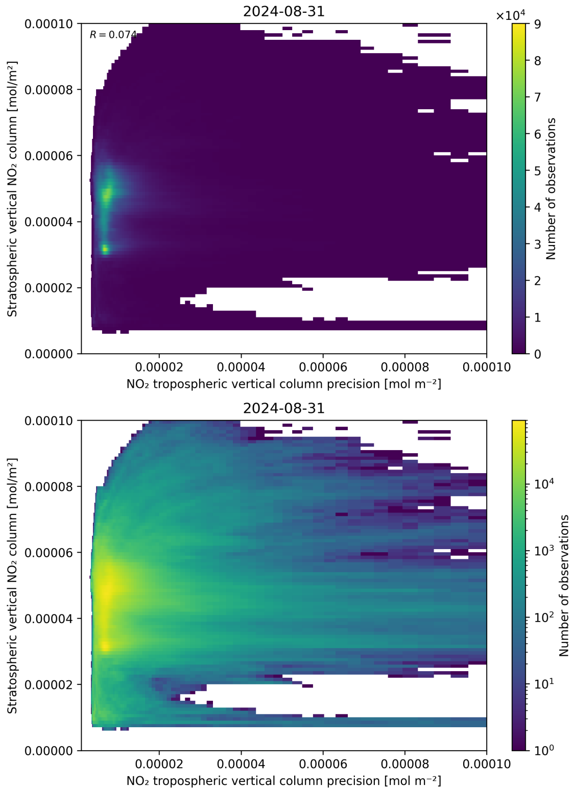
Figure 135: Scatter density plot of “NO 2 tropospheric vertical column precision” against “Stratospheric vertical NO 2 column” for 2024-08-30 to 2024-09-01.
