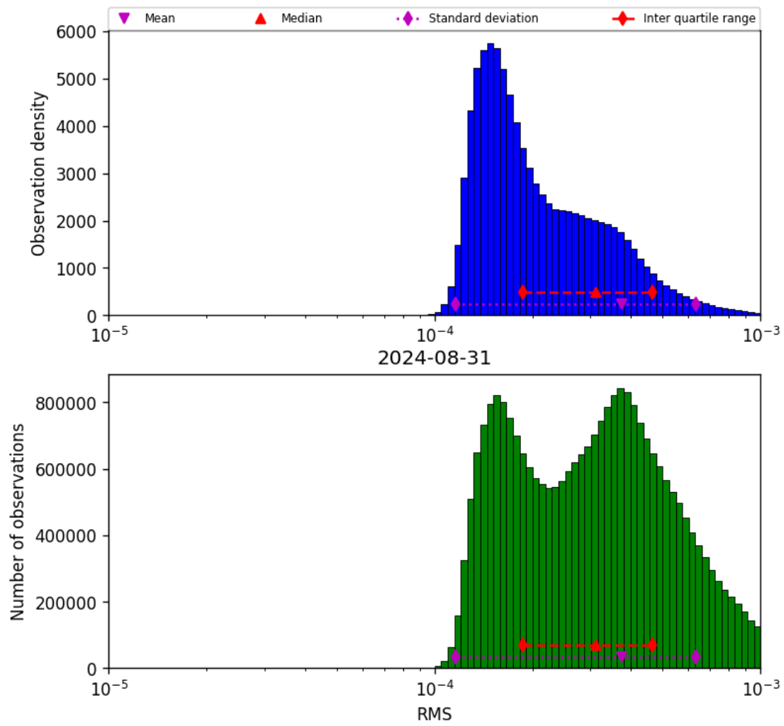
Figure 43: Histogram of “RMS” for 2024-08-30 to 2024-09-01
