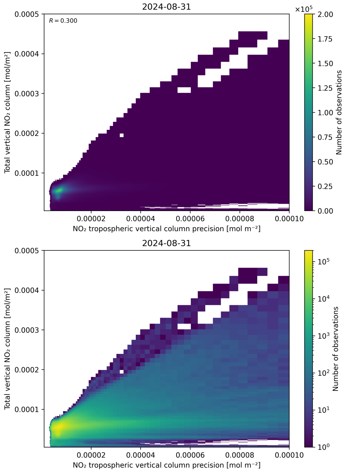
Figure 138: Scatter density plot of “NO 2 tropospheric vertical column precision” against “Total vertical NO 2 column” for 2024-08-30 to 2024-09-01.
