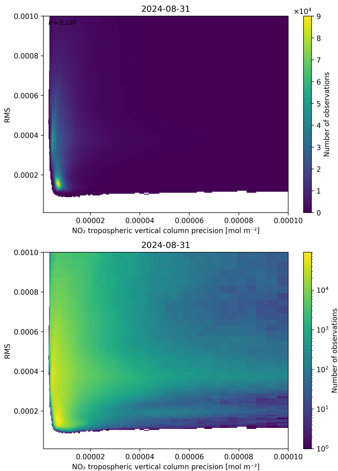
Figure 140: Scatter density plot of “NO 2 tropospheric vertical column precision” against “RMS” for 2024-08-30 to 2024-09-01.
