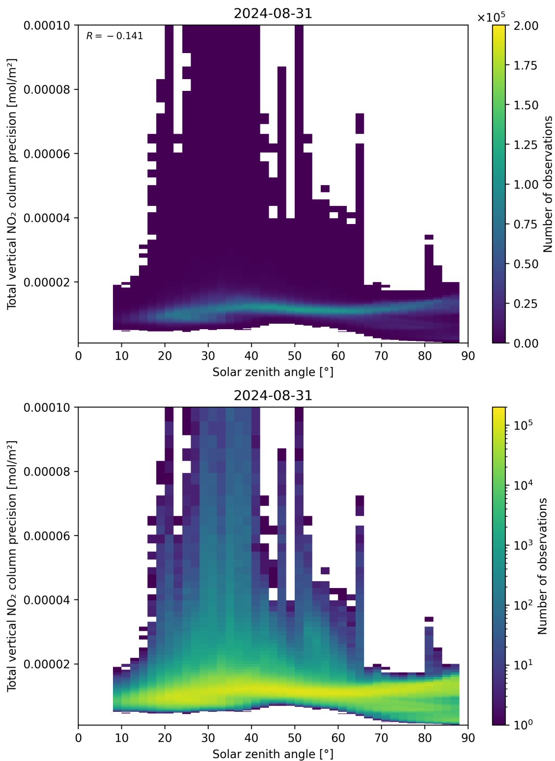
Figure 154: Scatter density plot of “Solar zenith angle” against “Total vertical NO 2 column precision” for 2024-08-30 to 2024-09-01.
