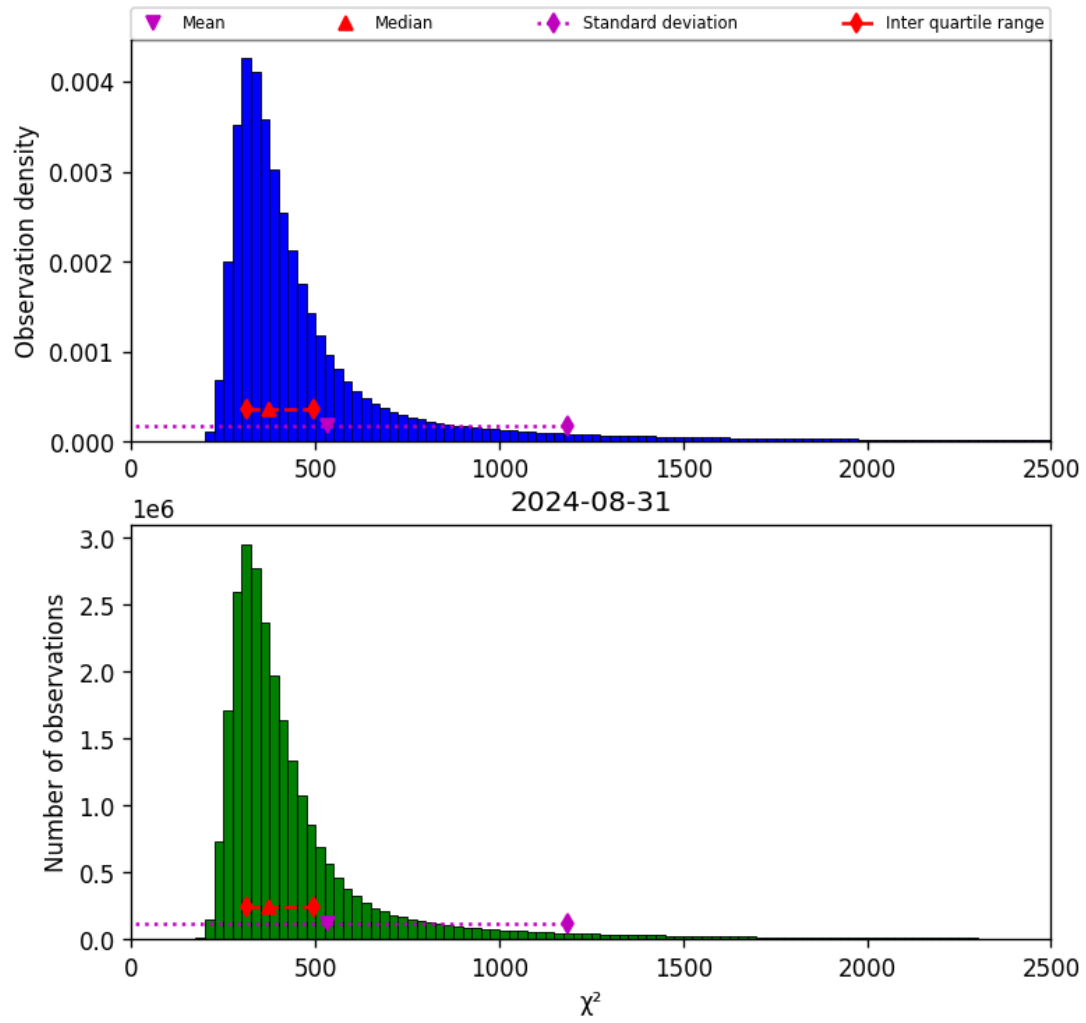
Figure 42: Histogram of " \chi^2 " for 2024-08-30 to 2024-09-01
