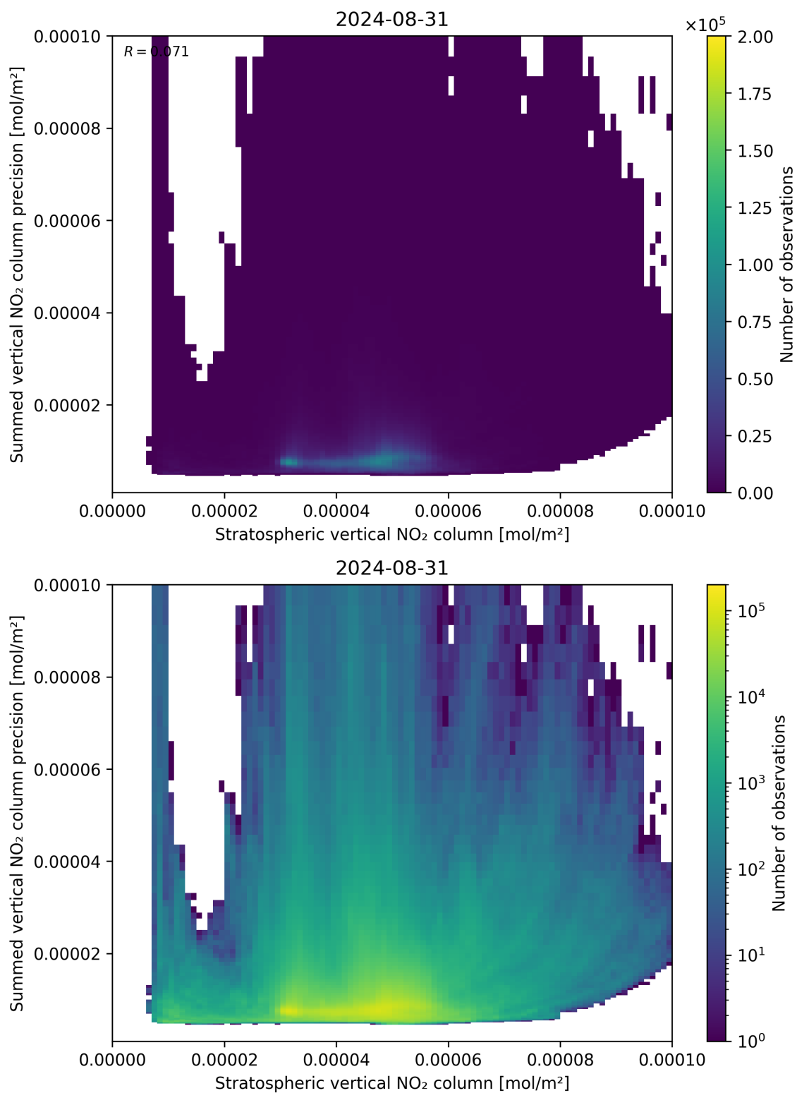
Figure 99: Scatter density plot of “Stratospheric vertical NO 2 column” against “Summed vertical NO 2 column precision” for 2024-08-30 to 2024-09-01.
