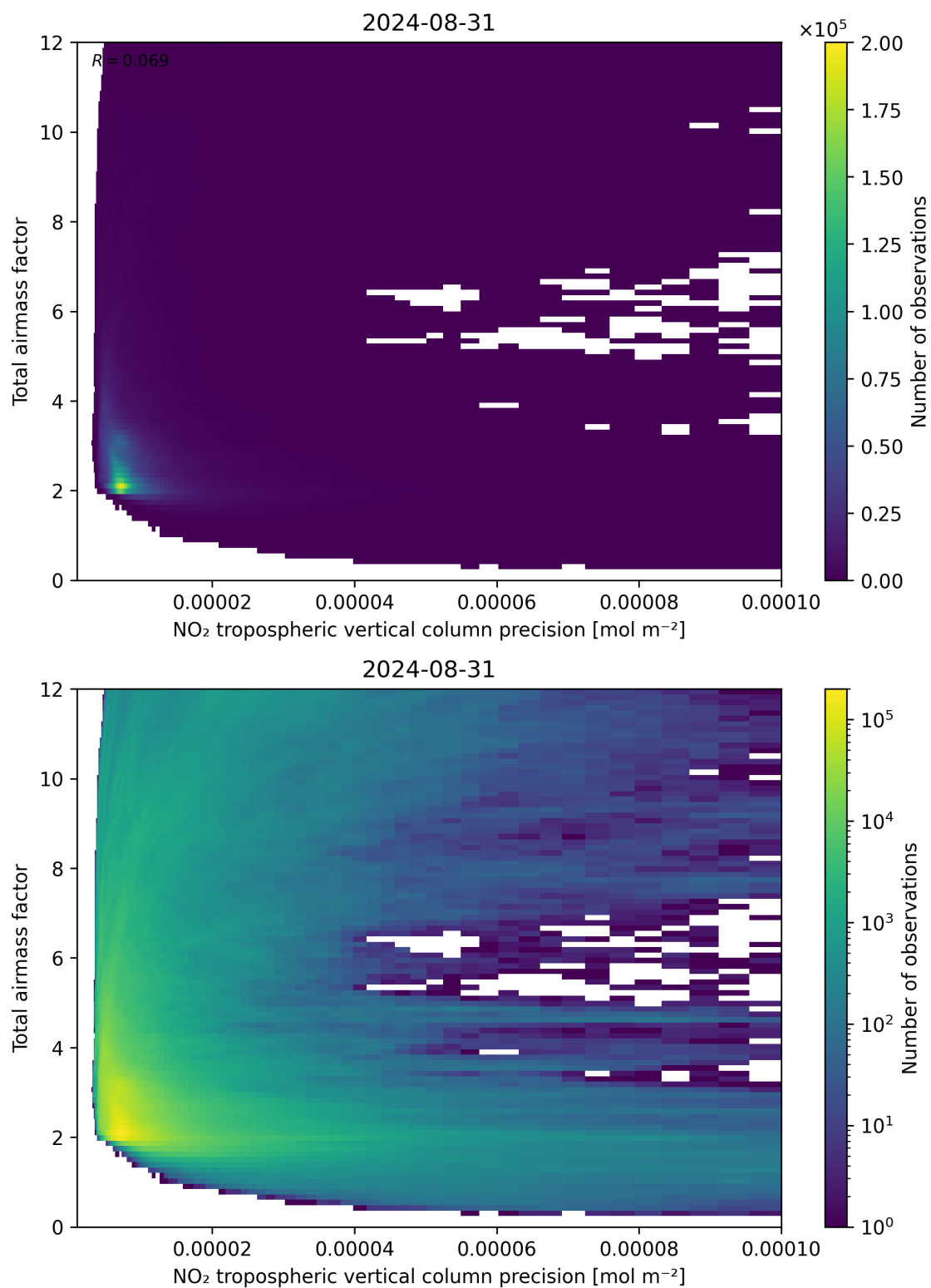
Figure 132: Scatter density plot of “NO 2 tropospheric vertical column precision” against “Total air mass factor” for 2024-08-30 to 2024-09-01.
