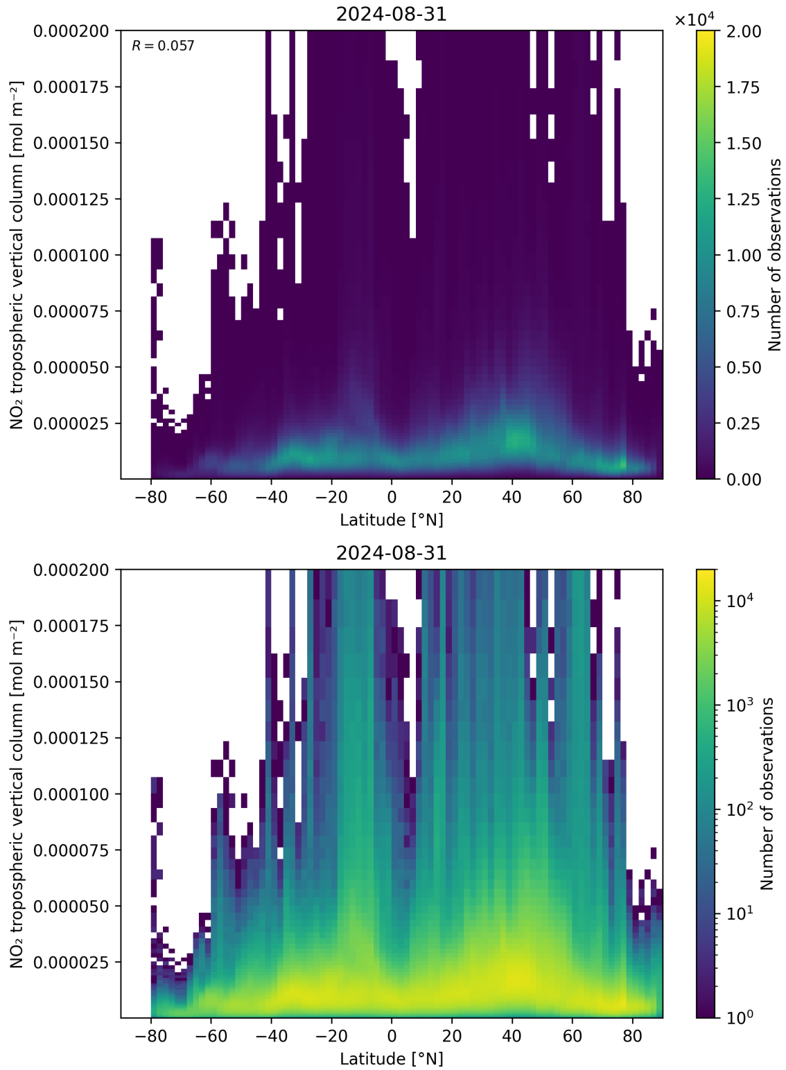
Figure 92: Scatter density plot of “Latitude” against “NO 2 tropospheric vertical column” for 2024-08-30 to 2024-09-01.
