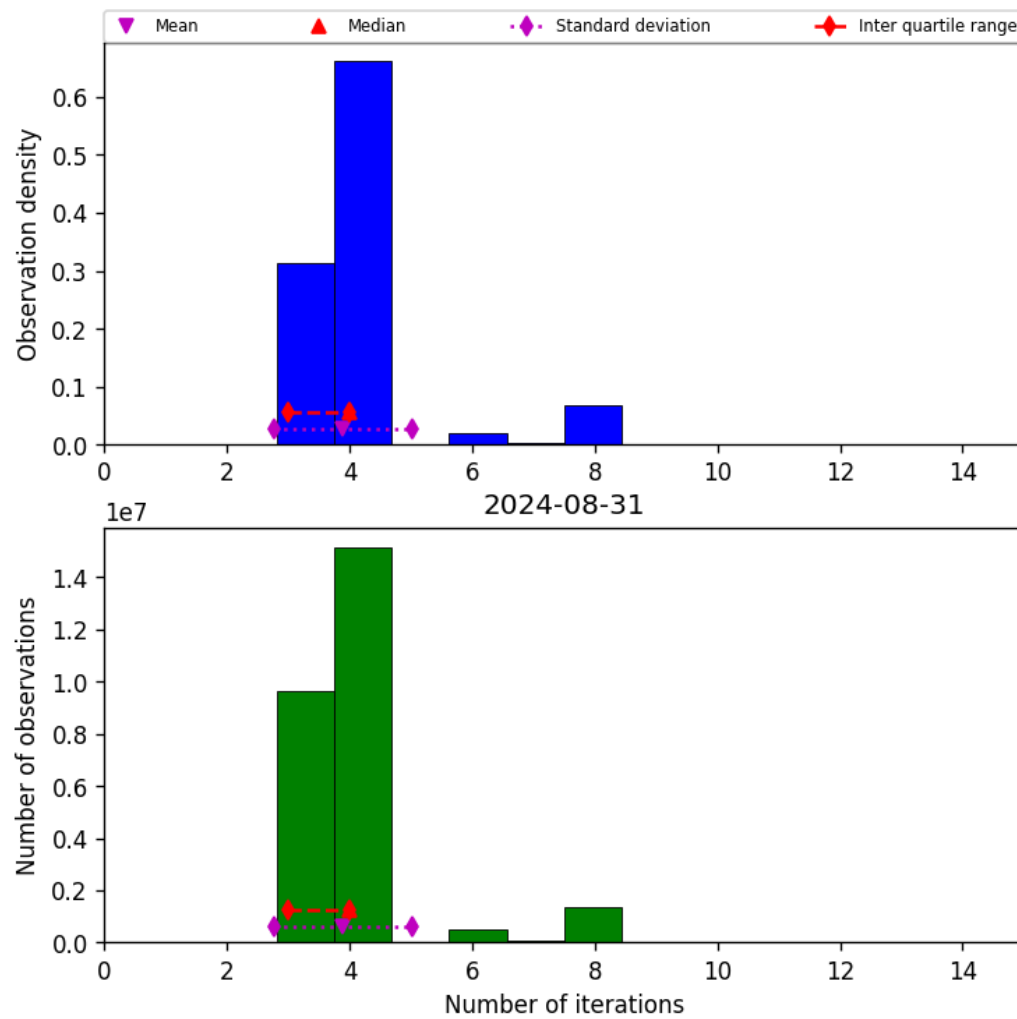
Figure 34: Histogram of "Number of iterations" for 2024-08-30 to 2024-09-01
