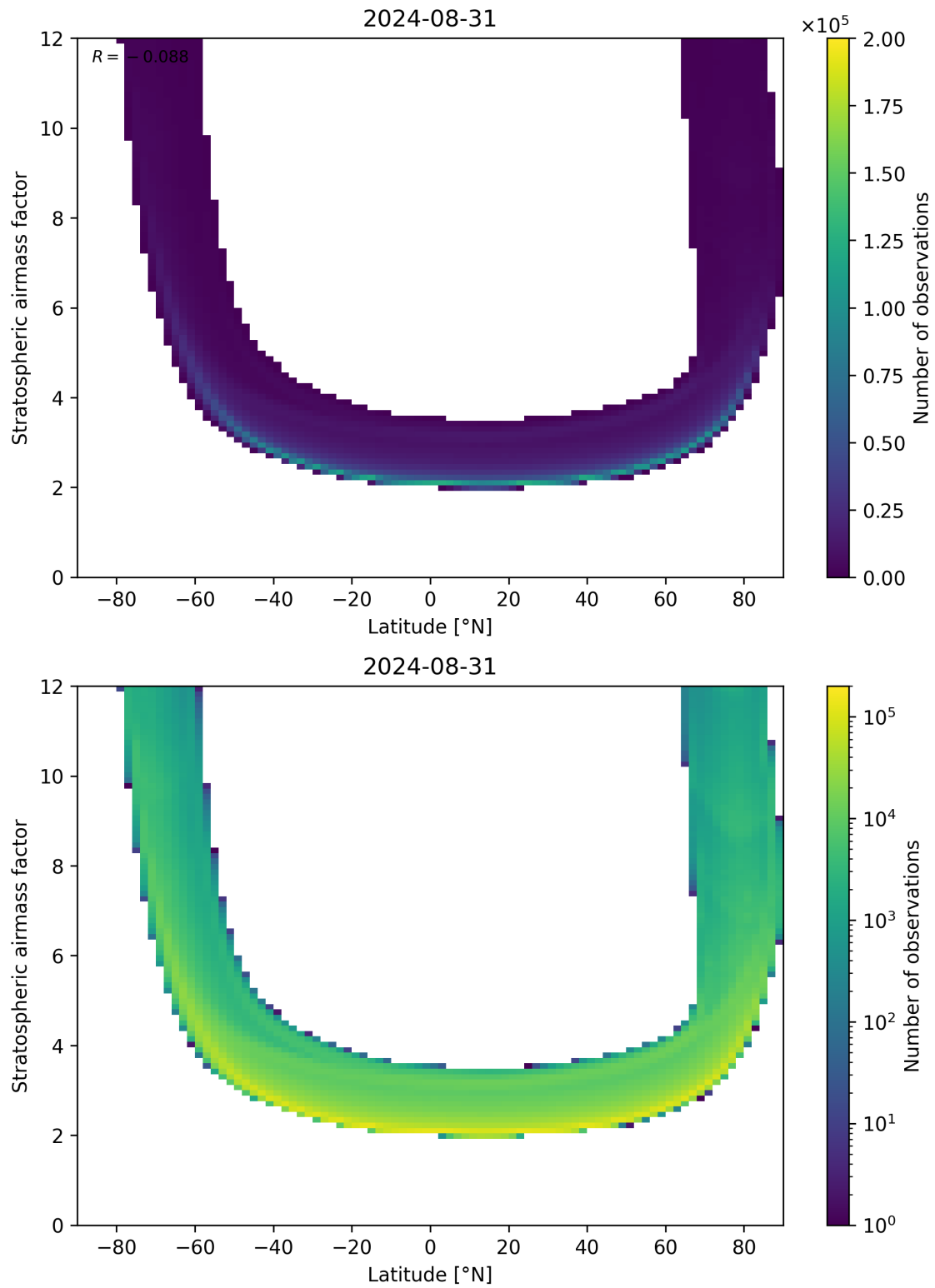
Figure 83: Scatter density plot of “Latitude” against “Stratospheric air mass factor” for 2024-08-30 to 2024-09-01.
