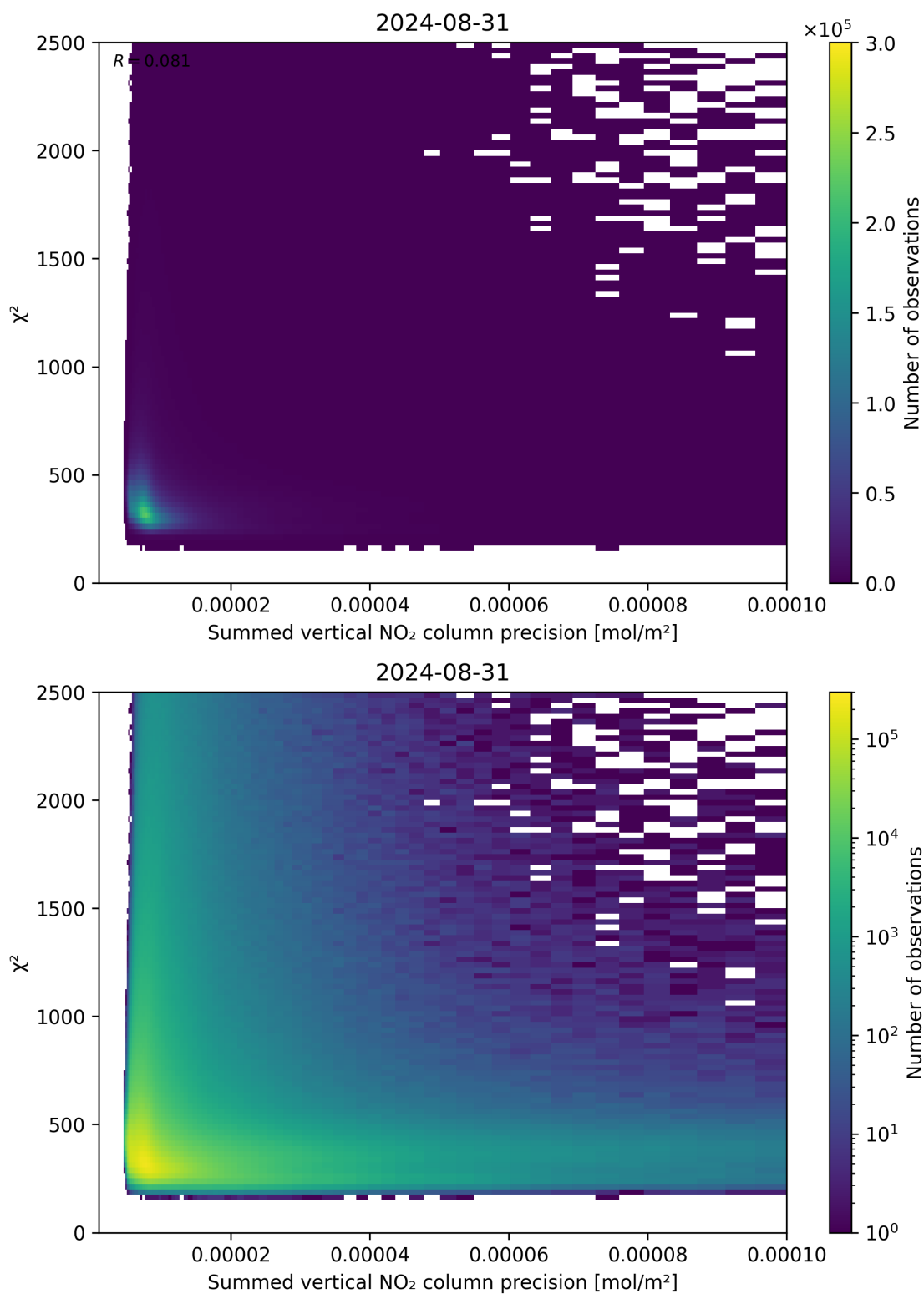
Figure 107: Scatter density plot of “Summed vertical NO 2 column precision” against “ \chi^2 ” for 2024-08-30 to 2024-09-01.
