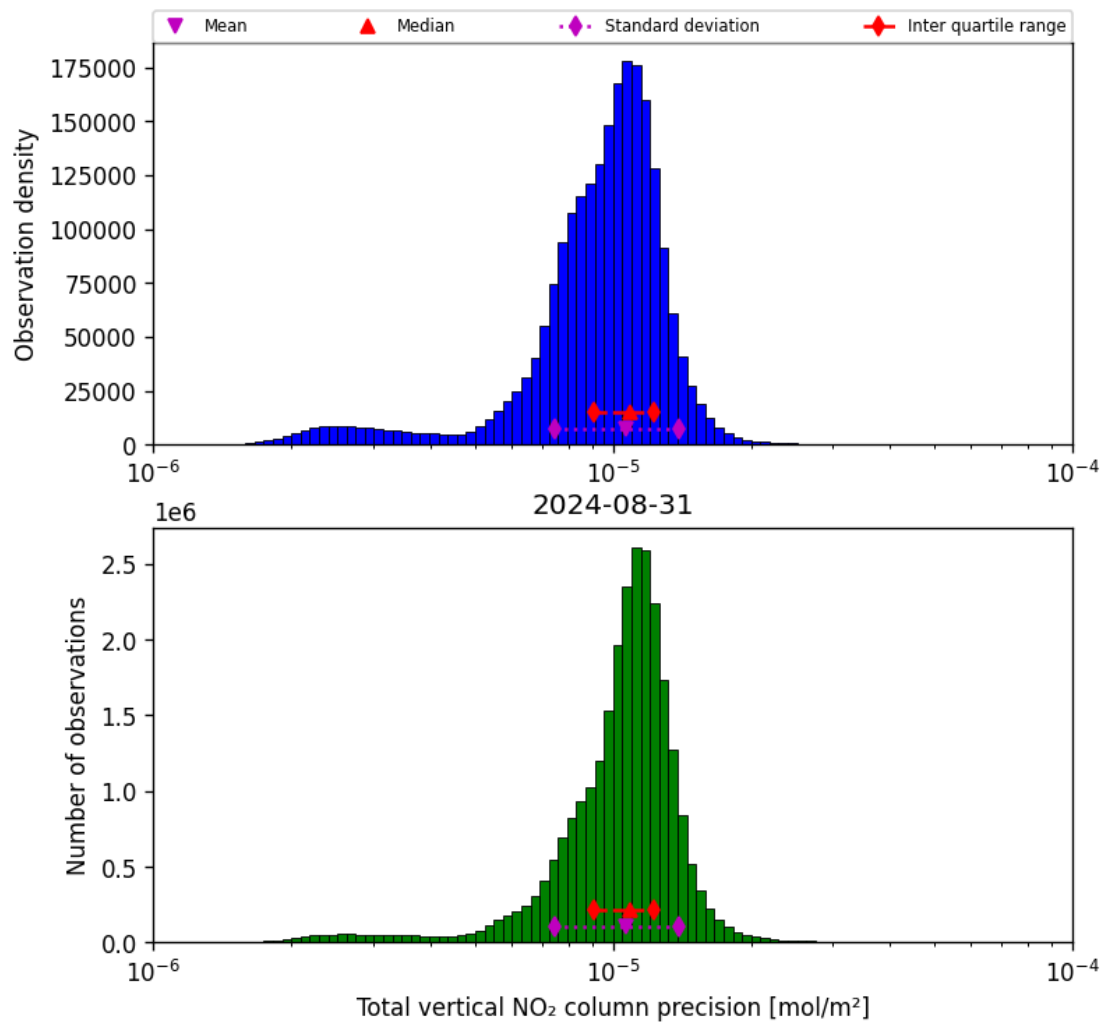
Figure 39: Histogram of “Total vertical NO 2 column precision” for 2024-08-30 to 2024-09-01
