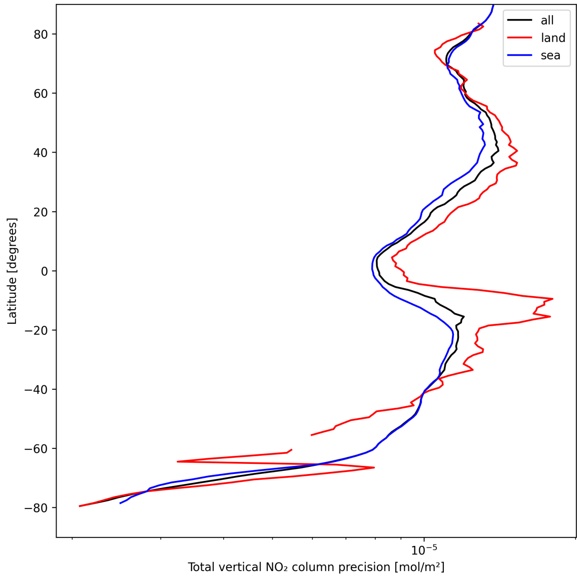
Figure 22: Zonal average of “Total vertical NO 2 column precision” for 2024-08-30 to 2024-09-01.
