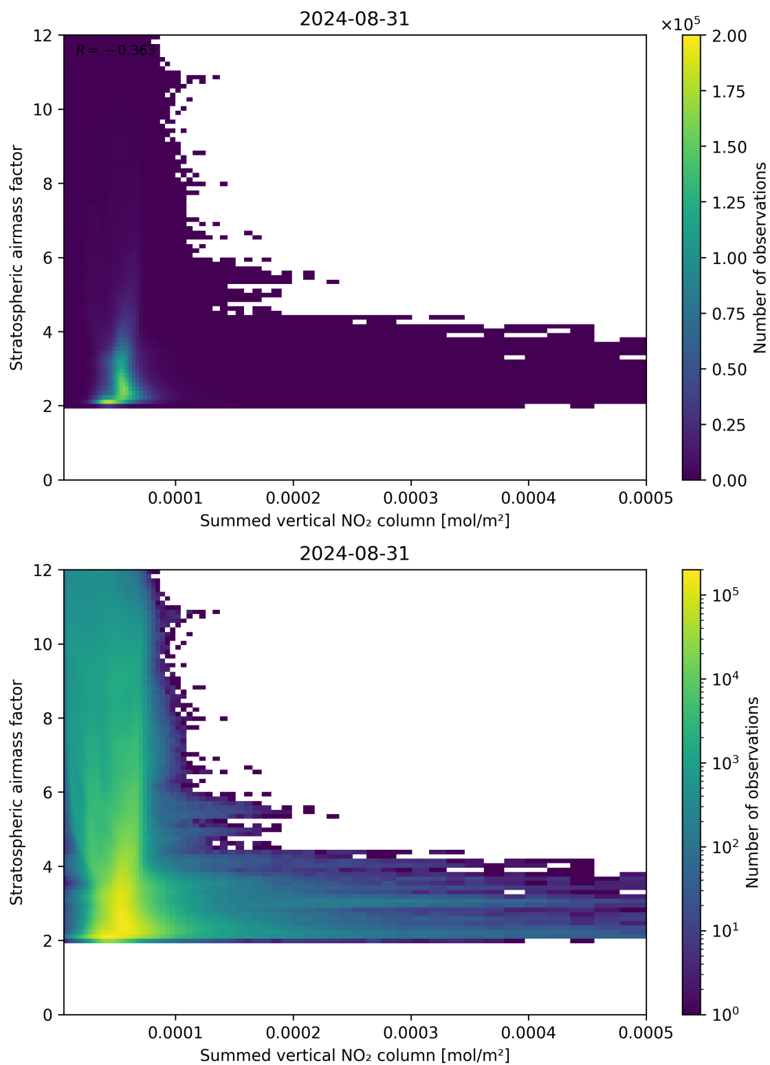
Figure 103: Scatter density plot of “Summed vertical NO 2 column” against “Stratospheric air mass factor” for 2024-08-30 to 2024-09-01.
