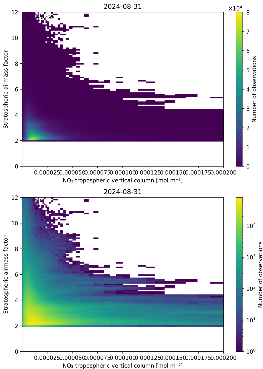
Figure 121: Scatter density plot of “NO 2 tropospheric vertical column” against “Stratospheric air mass factor” for 2024-08-30 to 2024-09-01.
