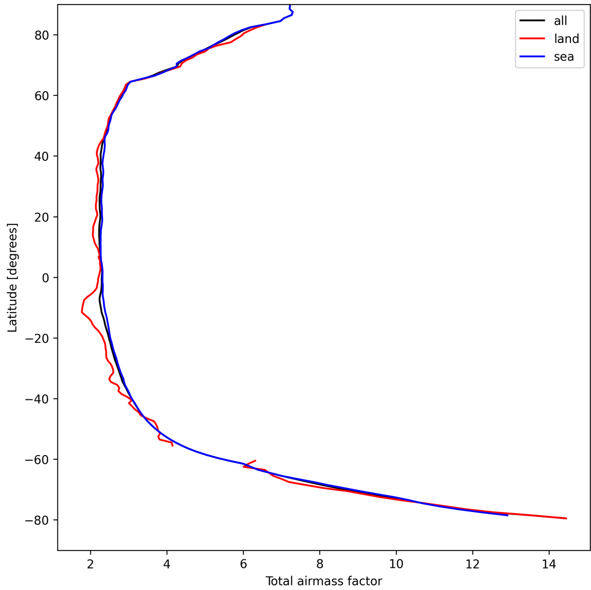
Figure 15: Zonal average of “Total airmass factor” for 2024-08-30 to 2024-09-01.
