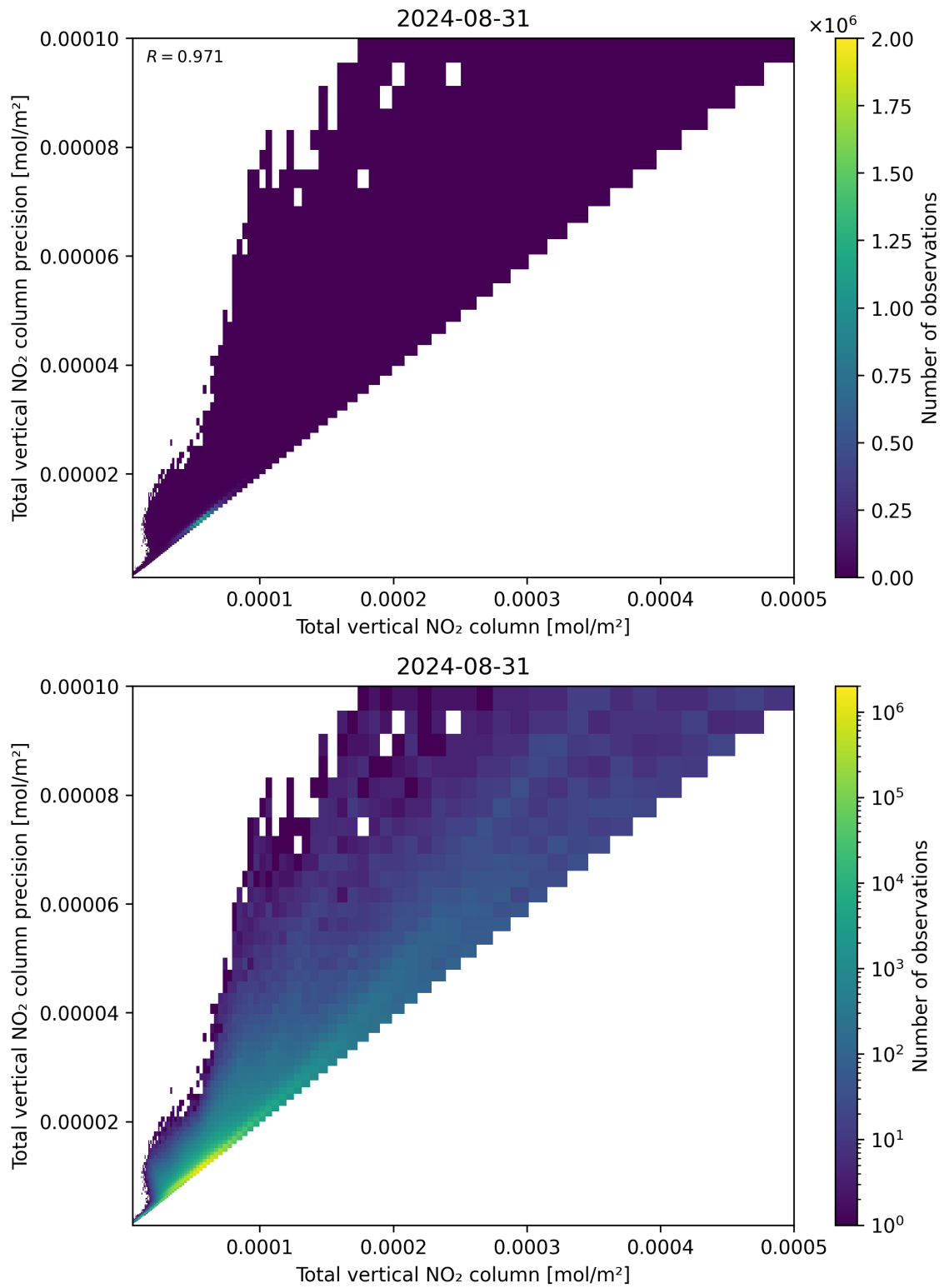
Figure 114: Scatter density plot of “Total vertical NO 2 column” against “Total vertical NO 2 column precision” for 2024-08-30 to 2024-09-01.
