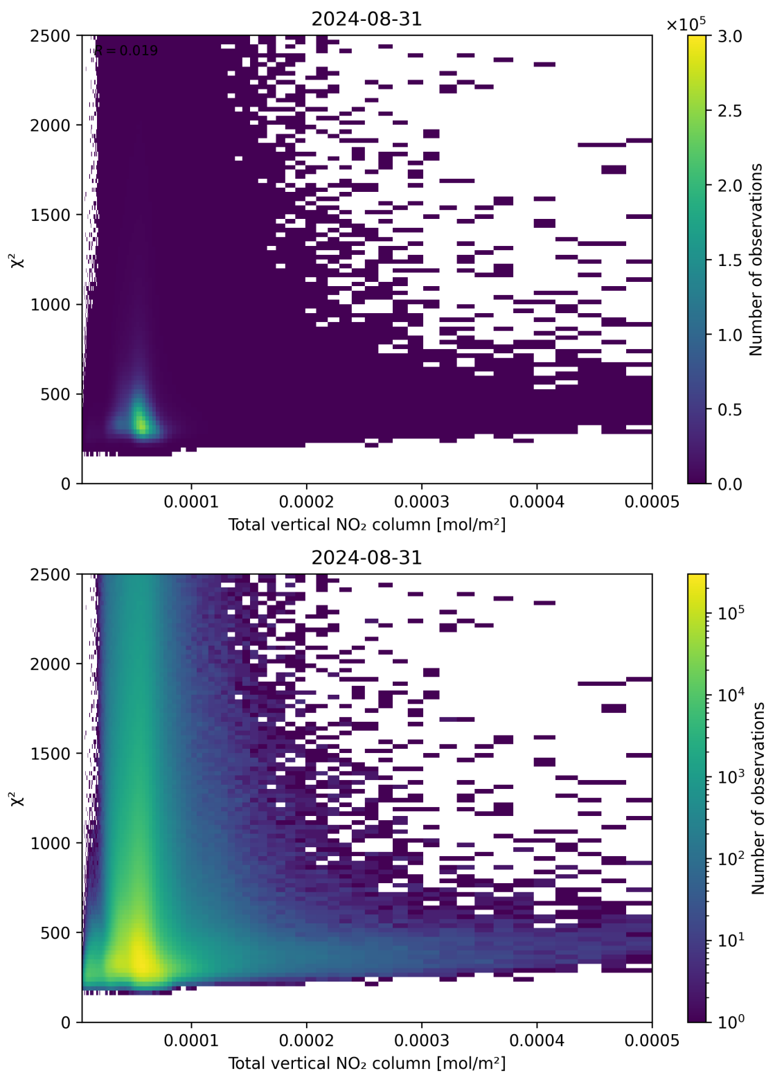
Figure 111: Scatter density plot of “Total vertical NO 2 column” against “ \chi^2 ” for 2024-08-30 to 2024-09-01.
