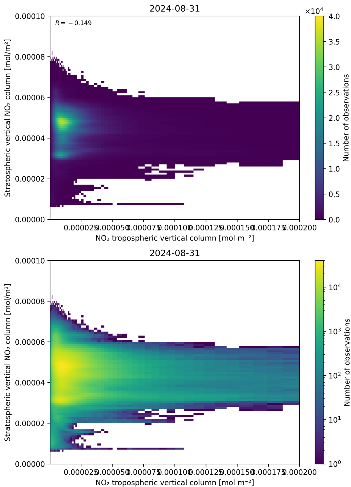
Figure 125: Scatter density plot of “NO 2 tropospheric vertical column” against “Stratospheric vertical NO 2 column” for 2024-08-30 to 2024-09-01.
