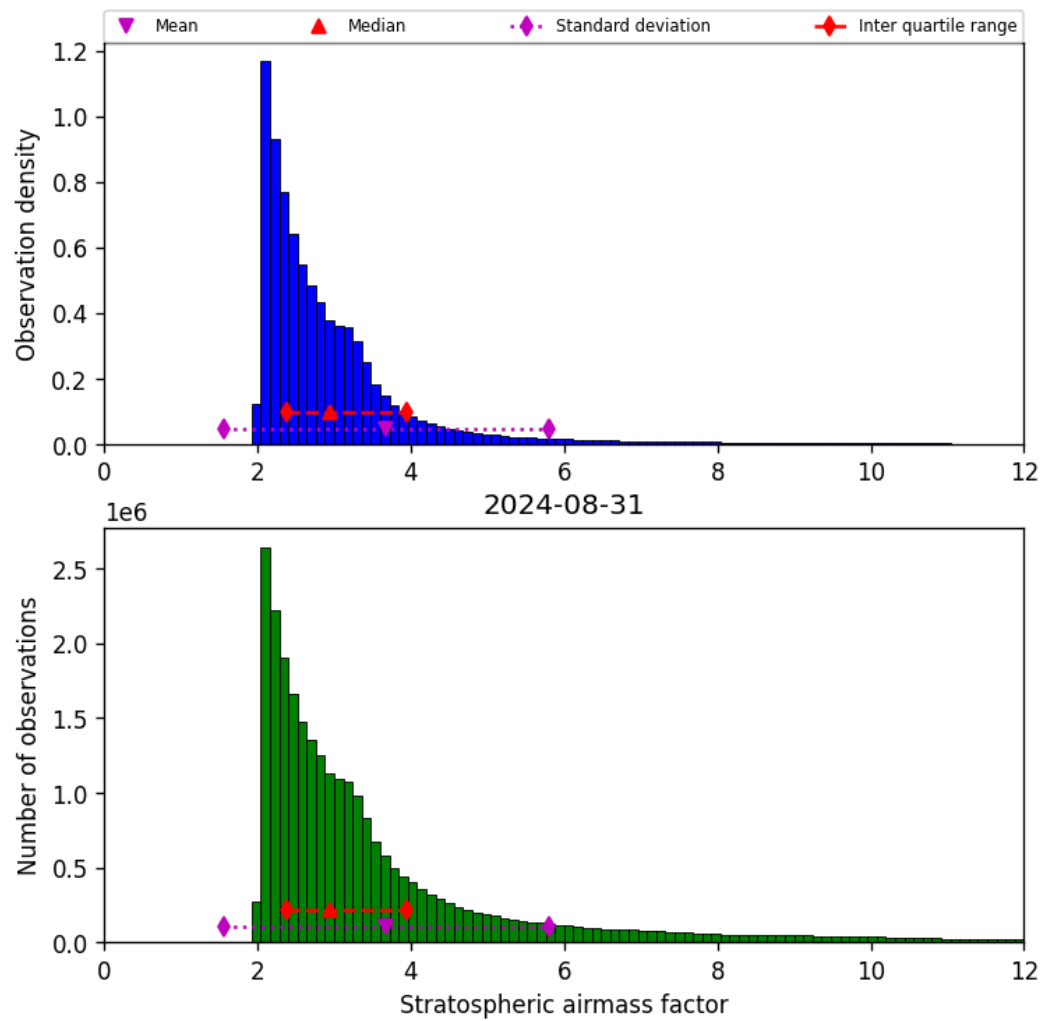
Figure 44: Histogram of “Stratospheric airmass factor” for 2024-08-30 to 2024-09-01
