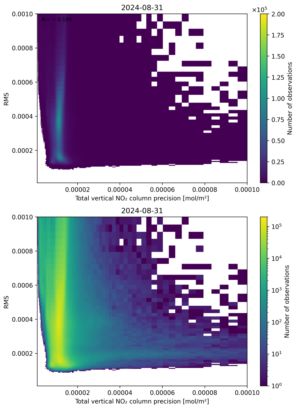
Figure 119: Scatter density plot of “Total vertical NO 2 column precision” against “RMS” for 2024-08-30 to 2024-09-01.
