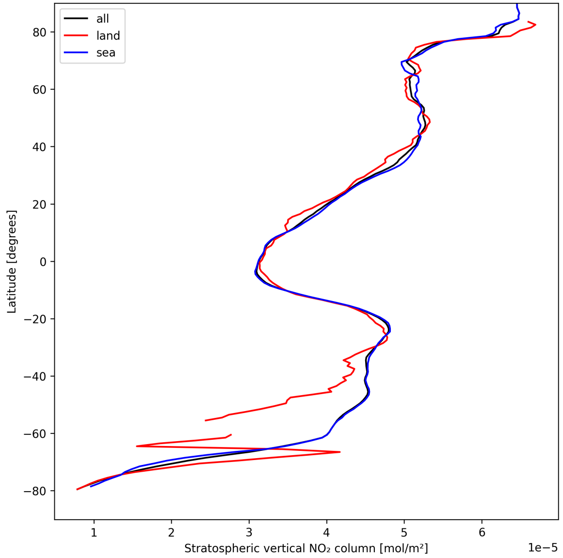
Figure 19: Zonal average of “Stratospheric vertical NO 2 column” for 2024-08-30 to 2024-09-01.
