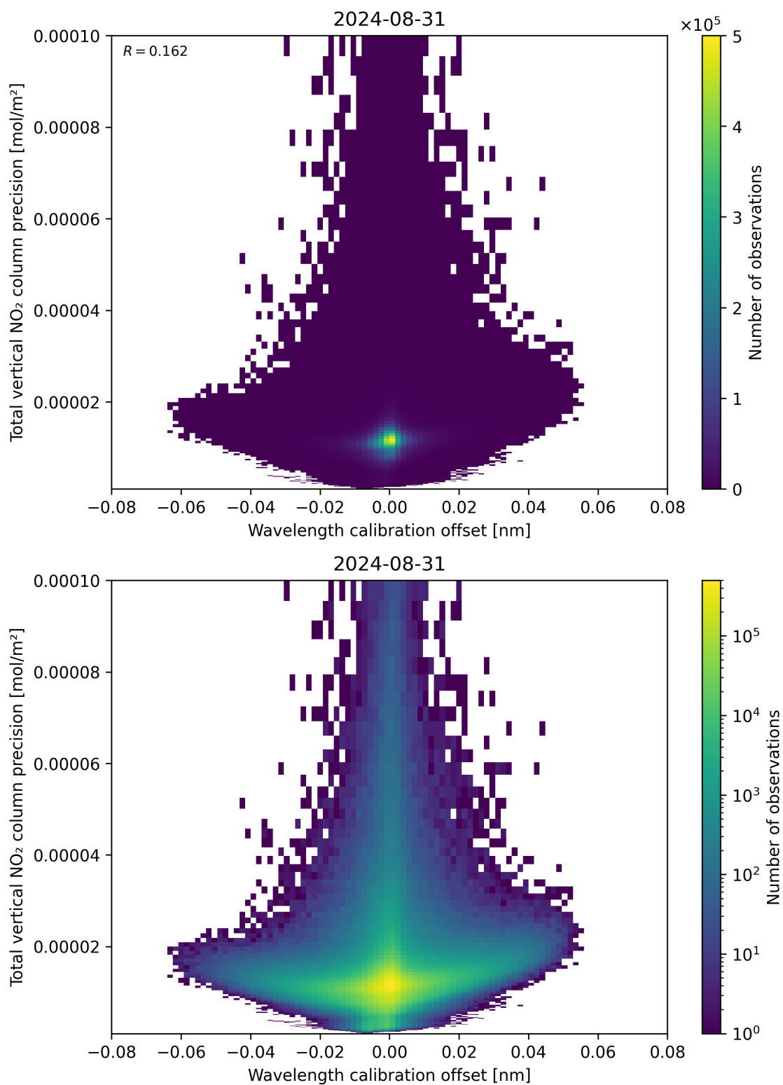
Figure 180: Scatter density plot of “Wavelength calibration offset” against “Total vertical NO 2 column precision” for 2024-08-30 to 2024-09-01.
