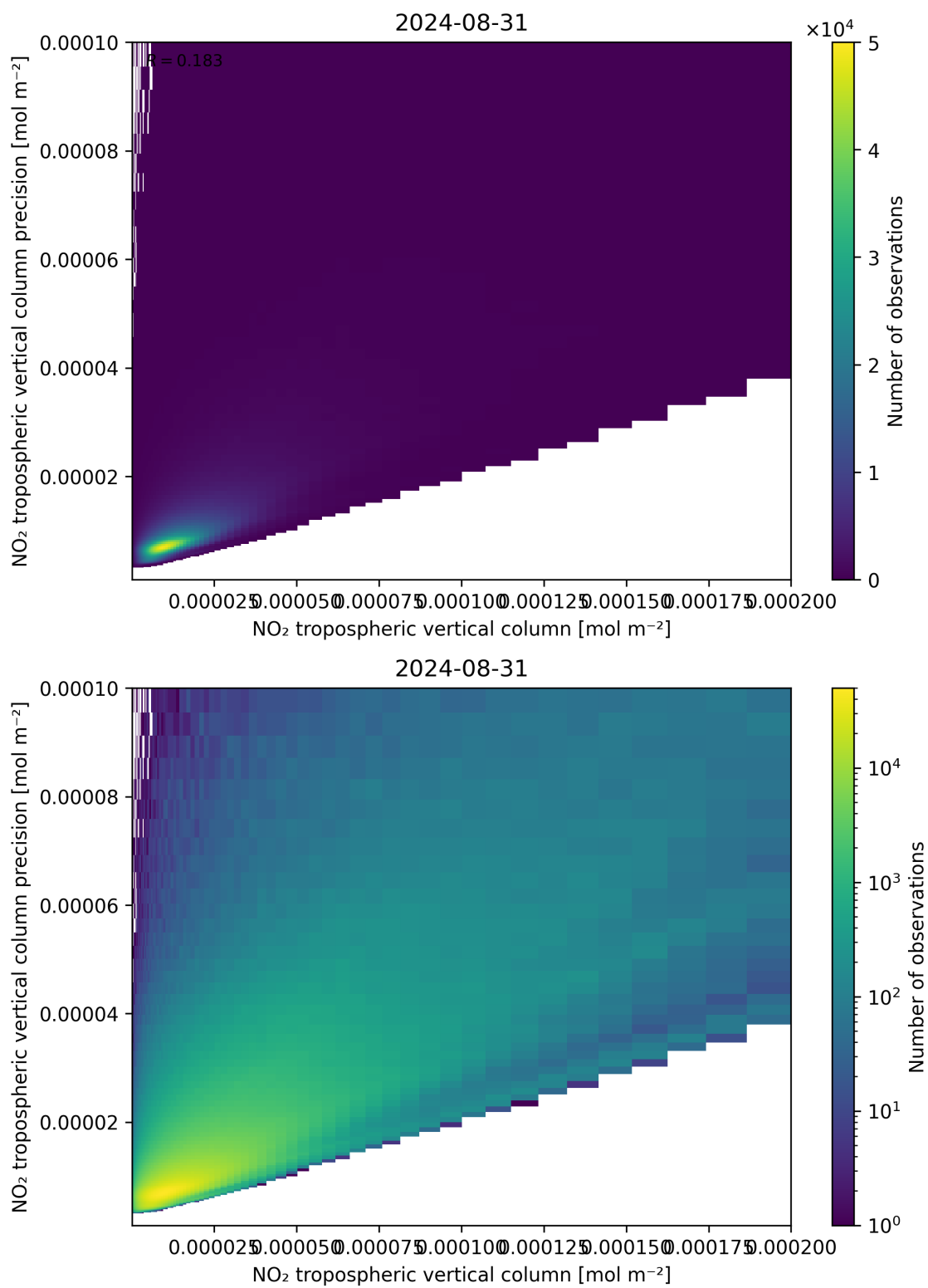
Figure 130: Scatter density plot of “NO 2 tropospheric vertical column” against “NO 2 tropospheric vertical column precision” for 2024-08-30 to 2024-09-01.
