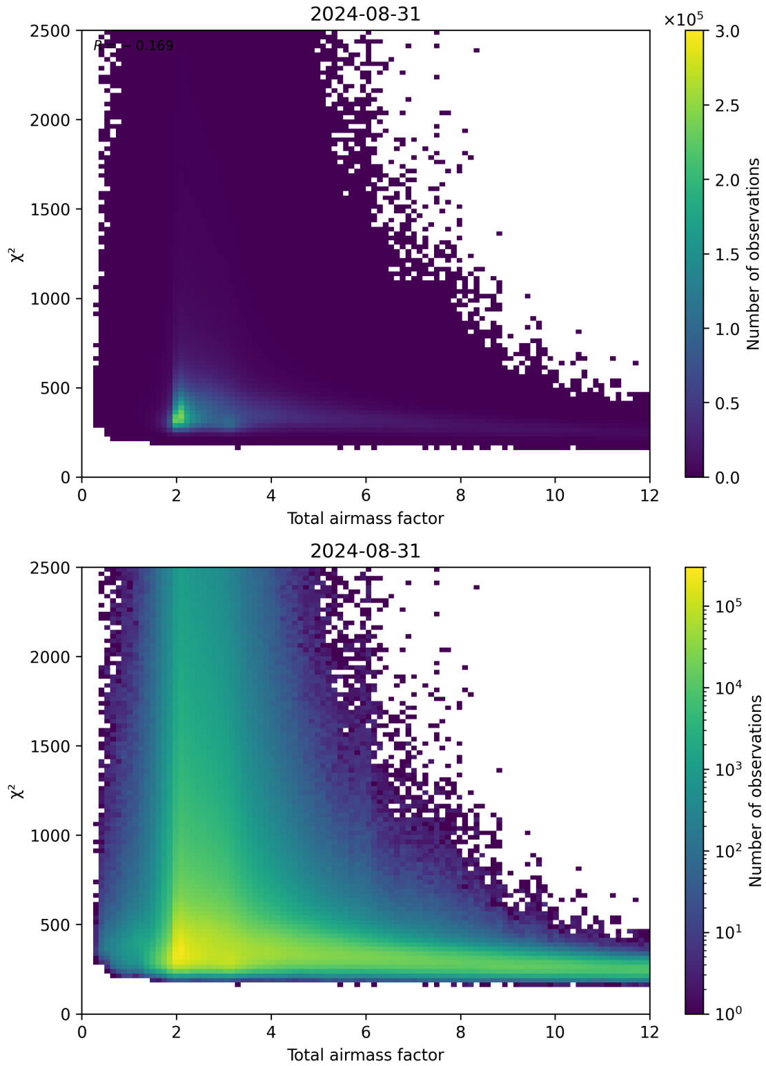
Figure 63: Scatter density plot of “Total airmass factor” against “ \chi^2 ” for 2024-08-30 to 2024-09-01.
