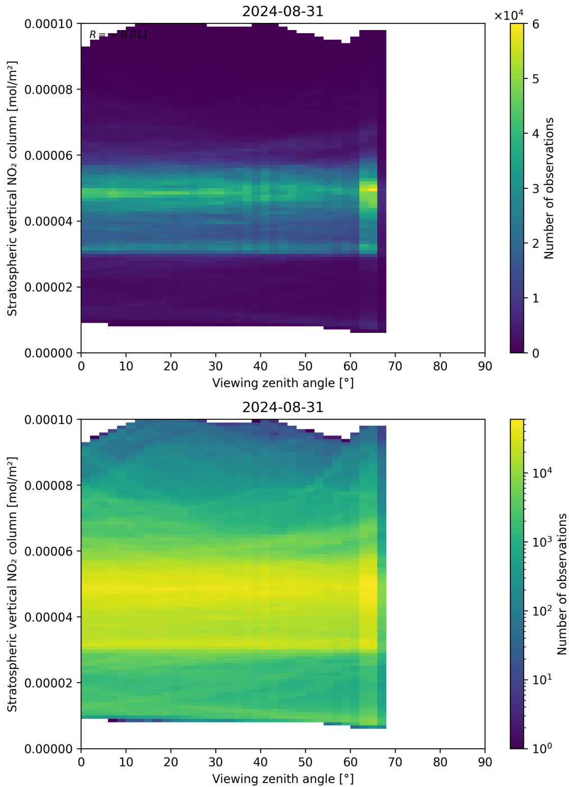
Figure 164: Scatter density plot of “Viewing zenith angle” against “Stratospheric vertical NO 2 column” for 2024-08-30 to 2024-09-01.
