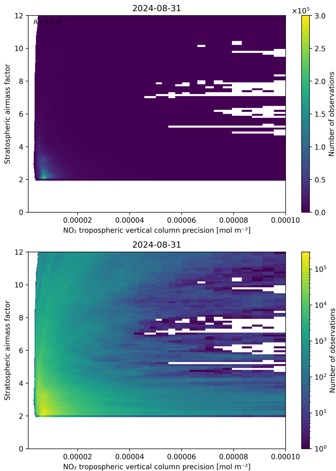
Figure 131: Scatter density plot of “NO 2 tropospheric vertical column precision” against “Stratospheric airmass factor” for 2024-08-30 to 2024-09-01.
