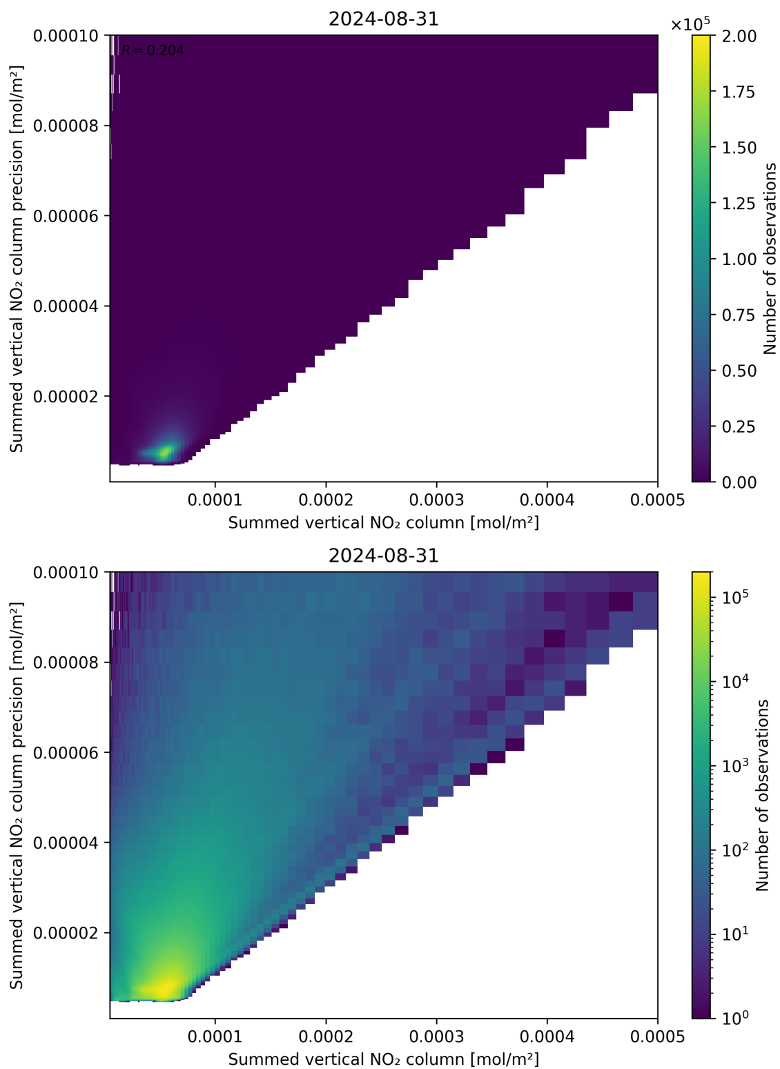
Figure 105: Scatter density plot of “Summed vertical NO 2 column” against “Summed vertical NO 2 column precision” for 2024-08-30 to 2024-09-01.
