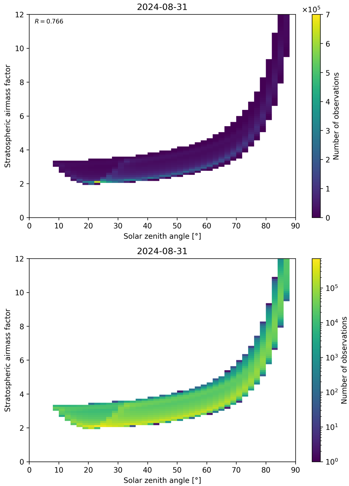
Figure 145: Scatter density plot of “Solar zenith angle” against “Stratospheric airmass factor” for 2024-08-30 to 2024-09-01.
