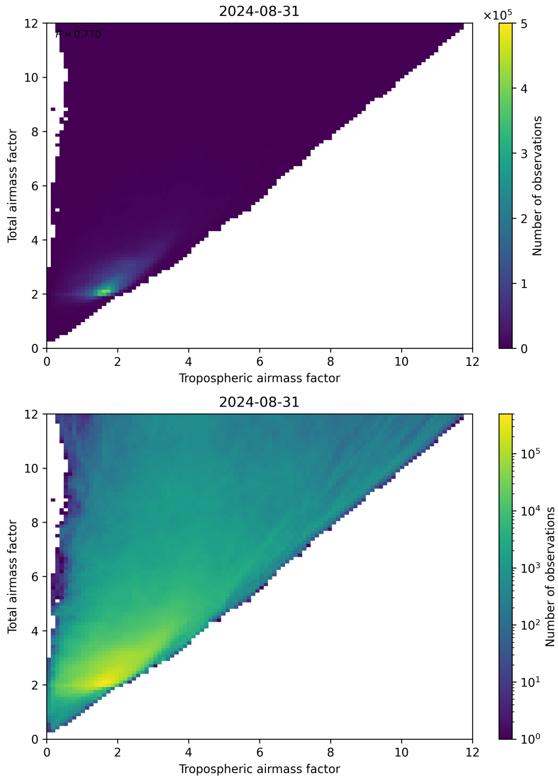
Figure 72: Scatter density plot of “Tropospheric airmass factor” against “Total airmass factor” for 2024-08-30 to 2024-09-01.
