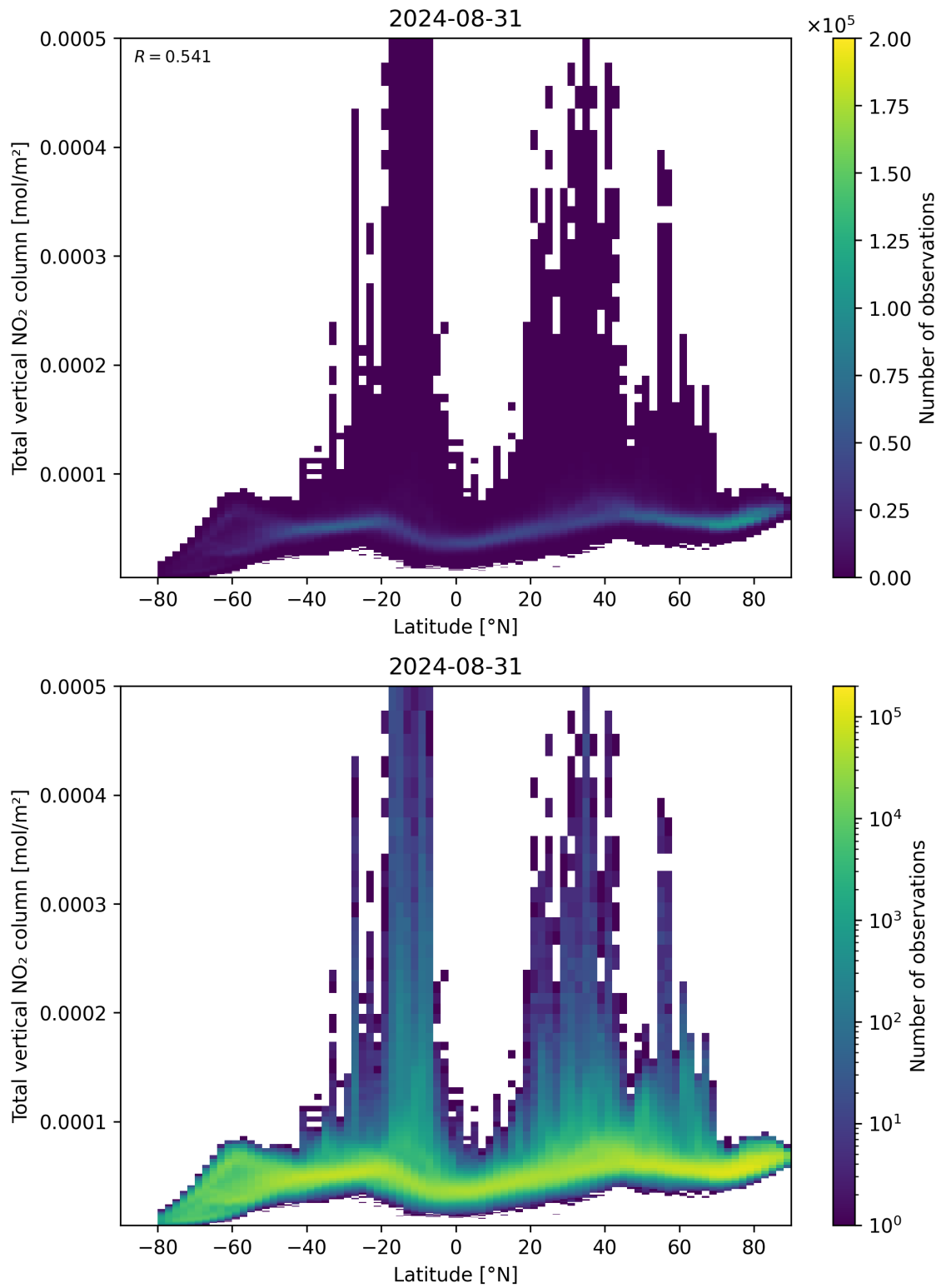
Figure 90: Scatter density plot of “Latitude” against “Total vertical NO 2 column” for 2024-08-30 to 2024-09-01.
