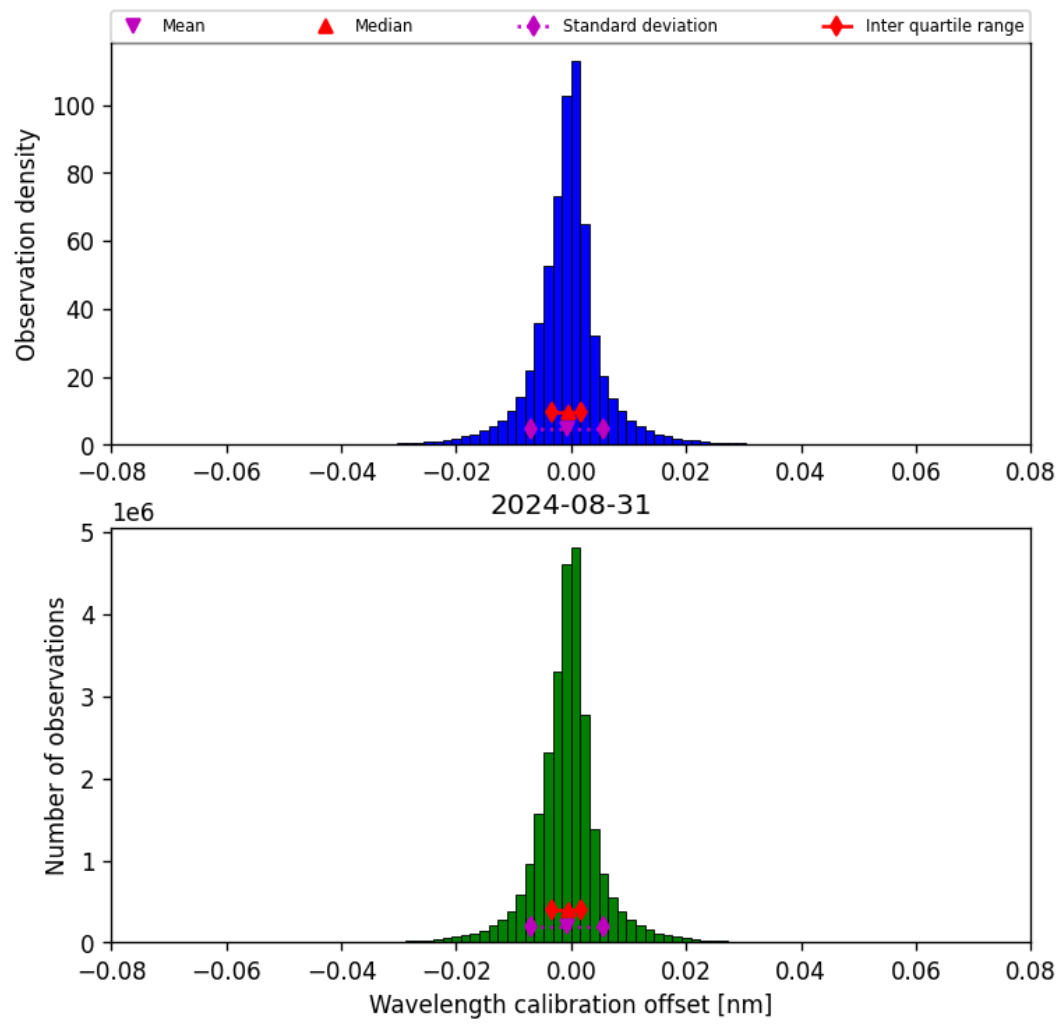
Figure 35: Histogram of “Wavelength calibration offset” for 2024-08-30 to 2024-09-01
