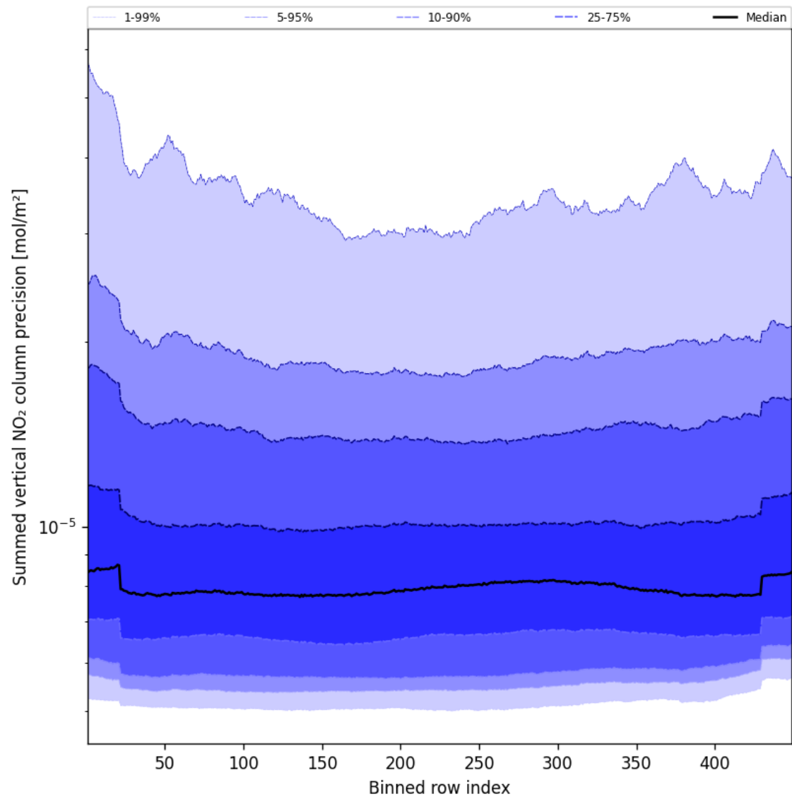
Figure 58: Along track statistics of “Summed vertical NO 2 column precision” for 2024-08-30 to 2024-09-01
