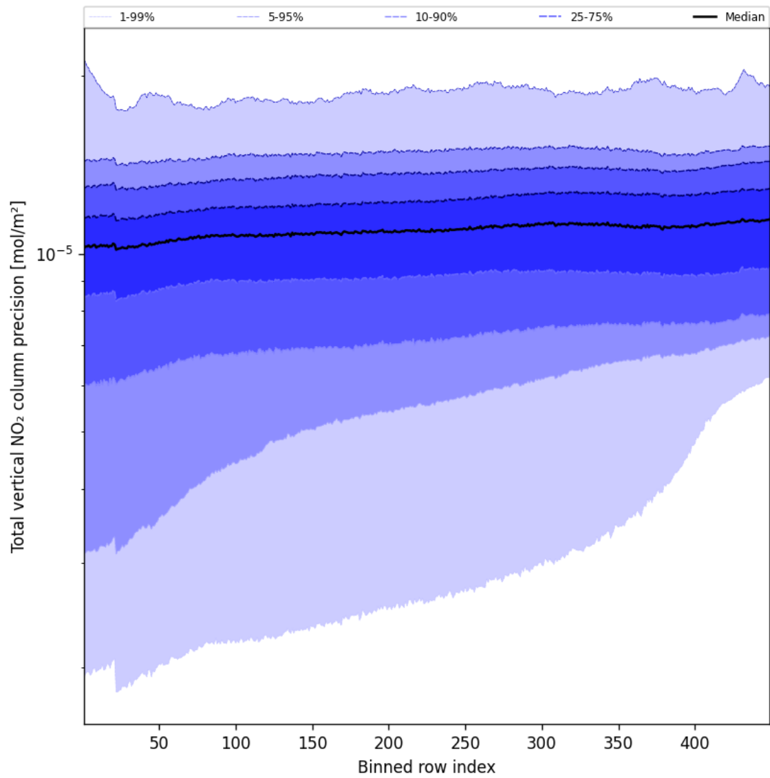
Figure 56: Along track statistics of "Total vertical NO 2 column precision" for 2024-08-30 to 2024-09-01
