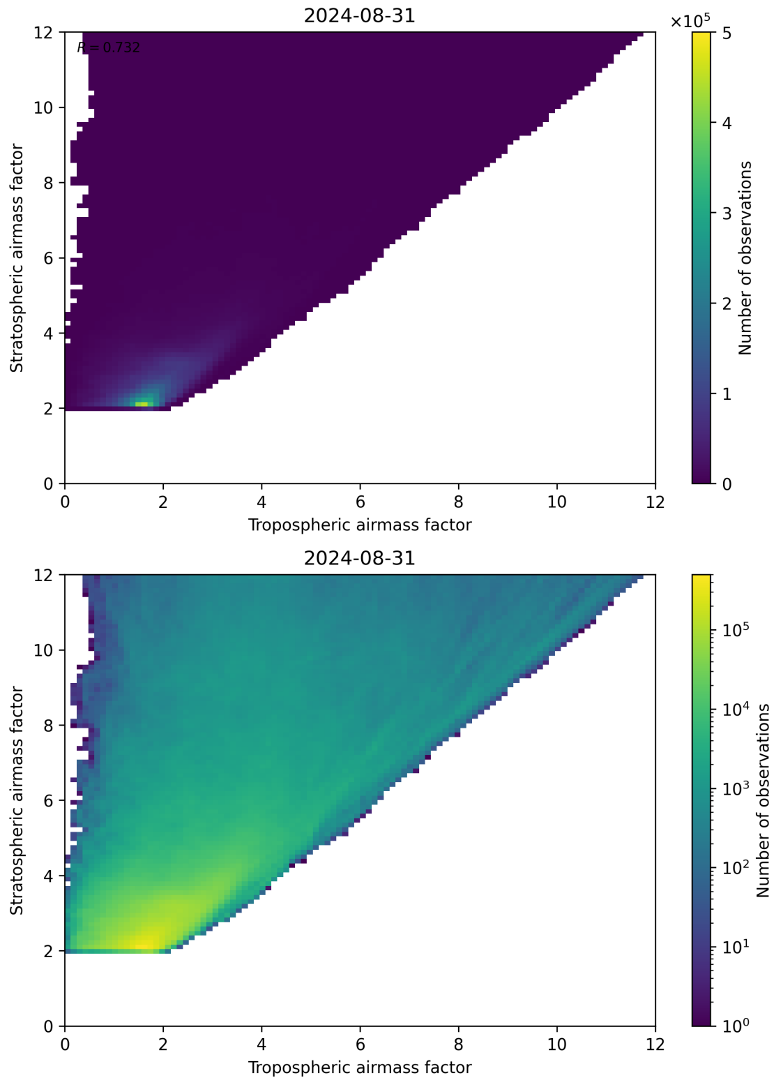
Figure 71: Scatter density plot of “Tropospheric airmass factor” against “Stratospheric airmass factor” for 2024-08-30 to 2024-09-01.
