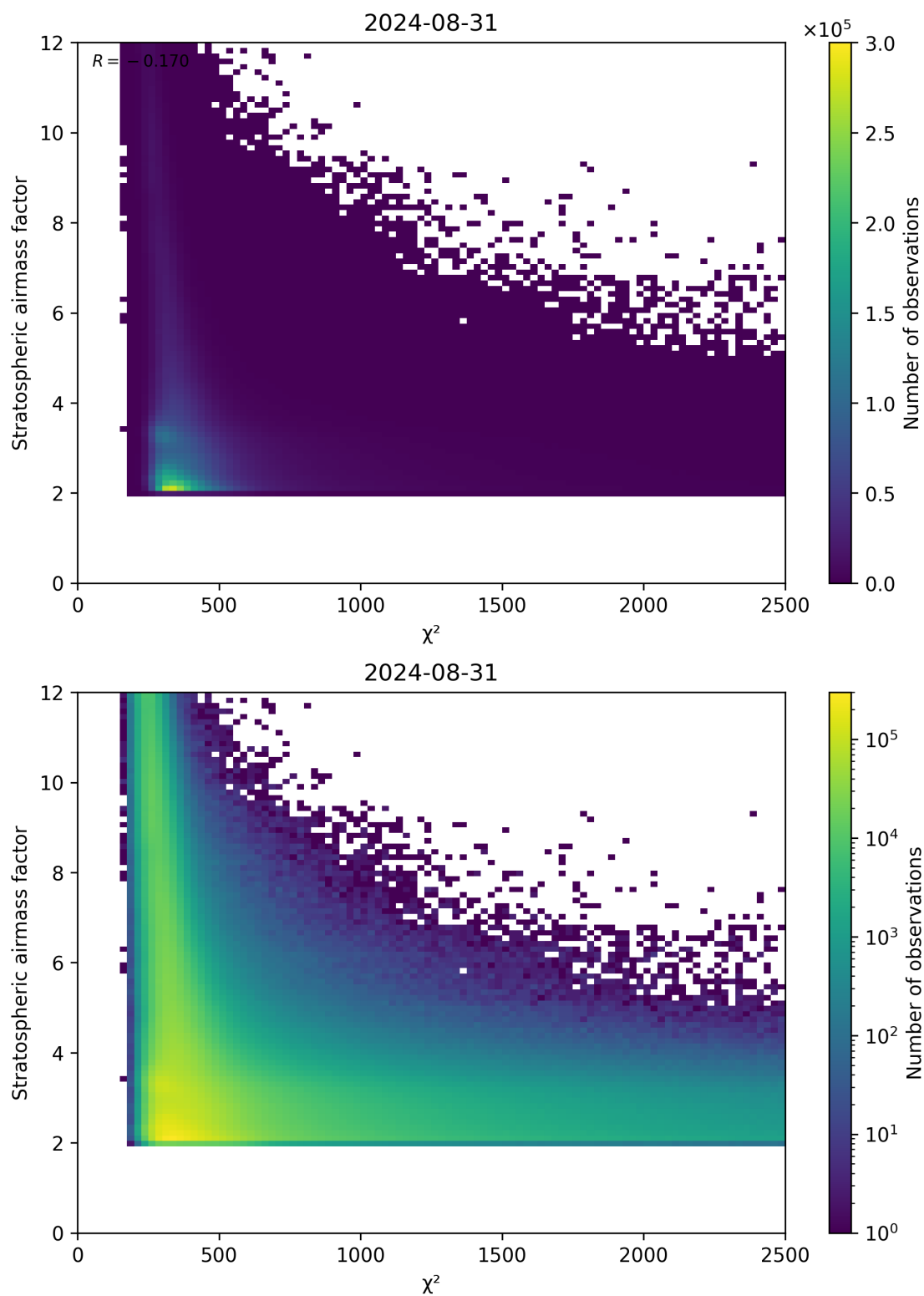
Figure 81: Scatter density plot of “ \chi^2 ” against “Stratospheric airmass factor” for 2024-08-30 to 2024-09-01.
