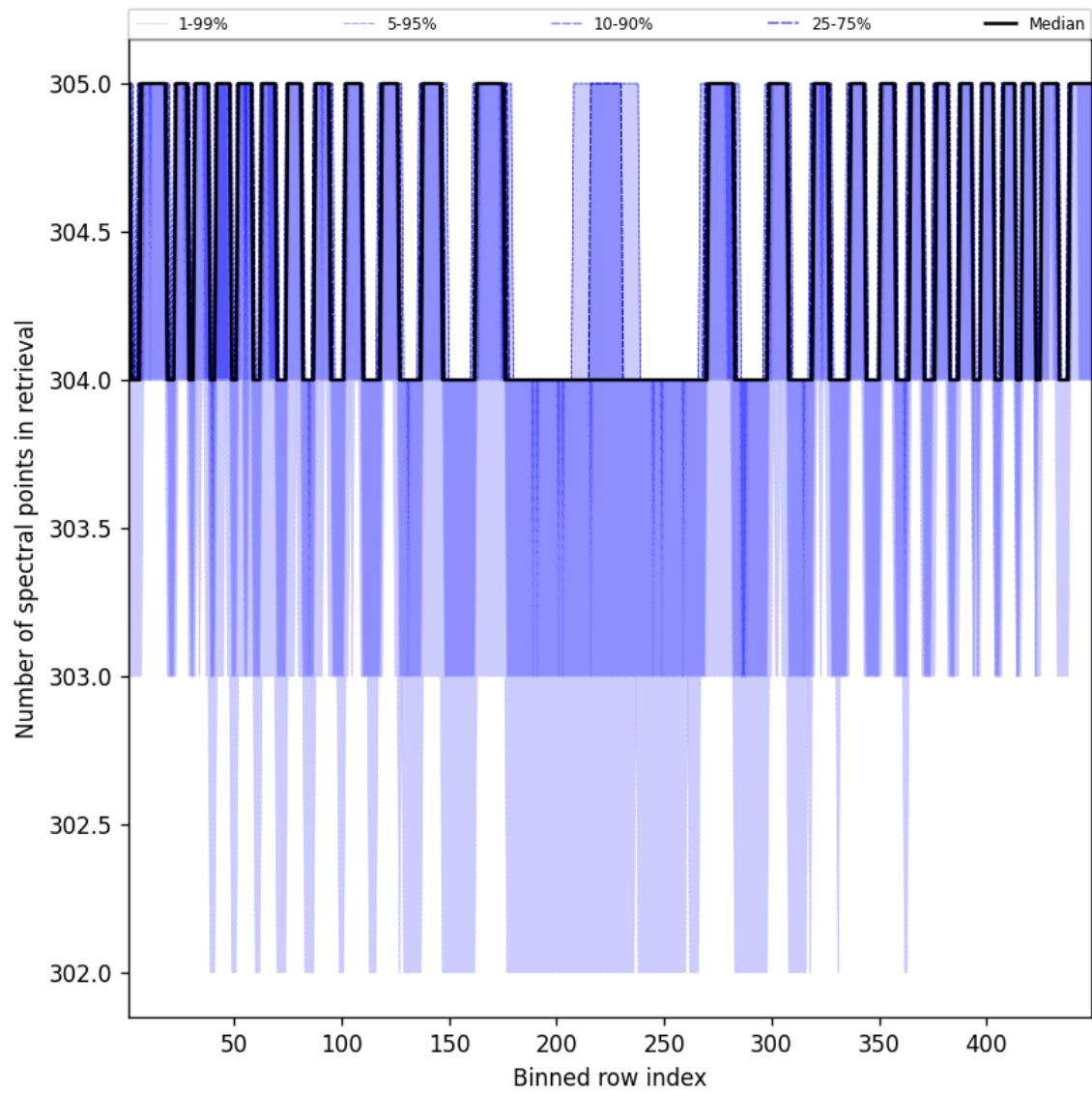
Figure 50: Along track statistics of “Number of spectral points in retrieval” for 2024-08-30 to 2024-09-01
