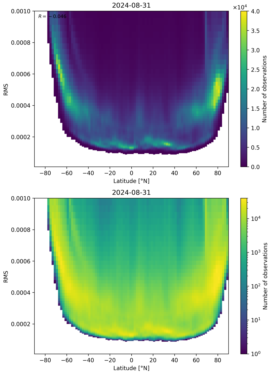
Figure 94: Scatter density plot of “Latitude” against “RMS” for 2024-08-30 to 2024-09-01.
