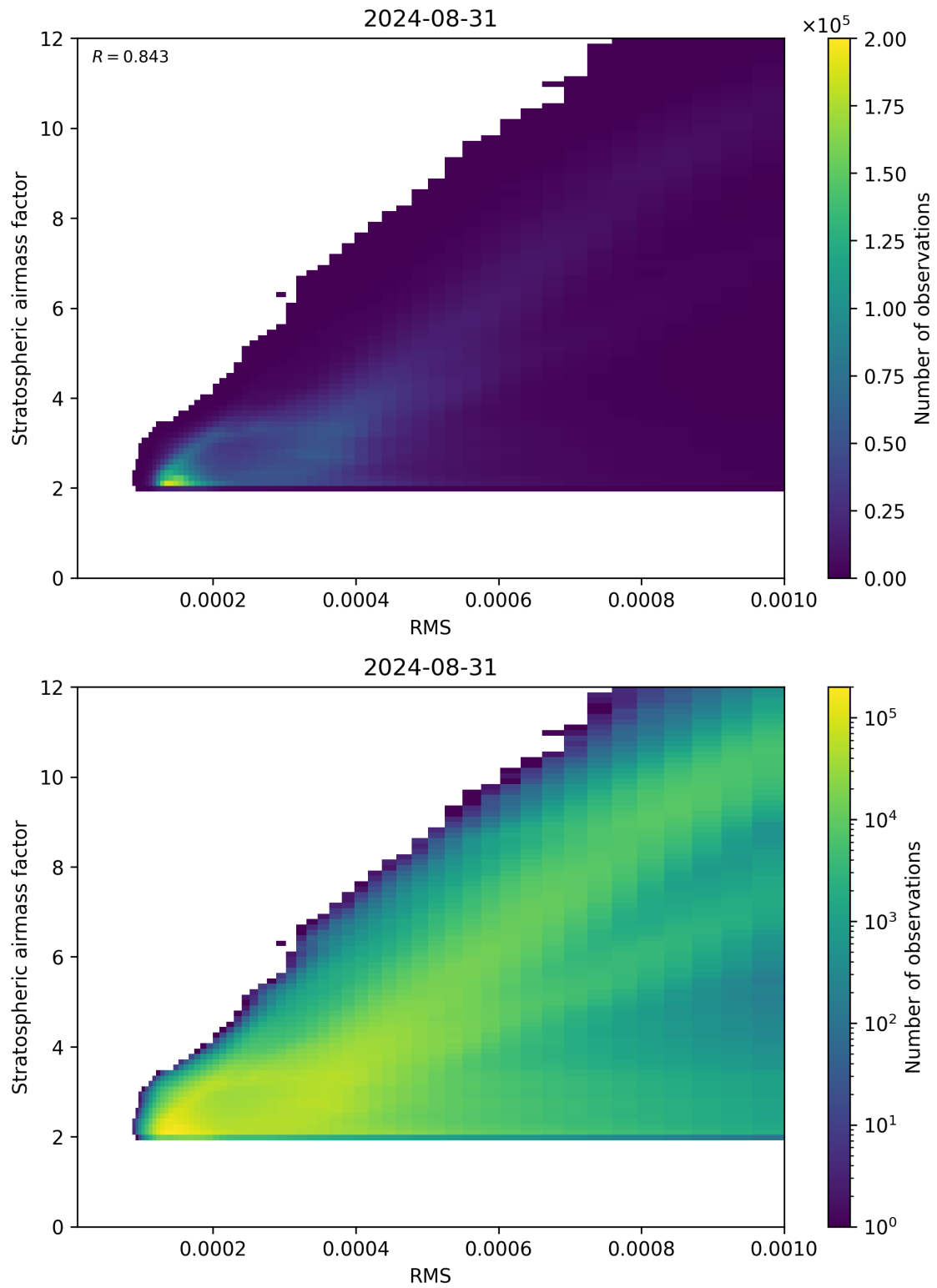
Figure 144: Scatter density plot of “RMS” against “Stratospheric airmass factor” for 2024-08-30 to 2024-09-01.
