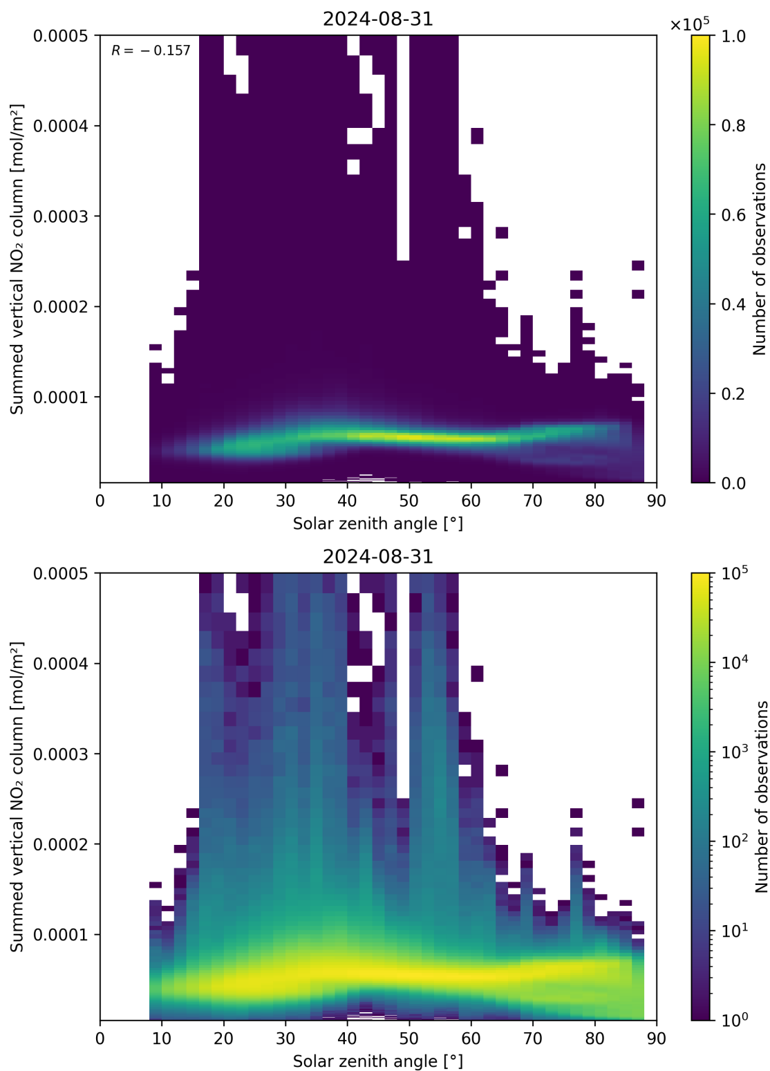
Figure 151: Scatter density plot of “Solar zenith angle” against “Summed vertical NO 2 column” for 2024-08-30 to 2024-09-01.
