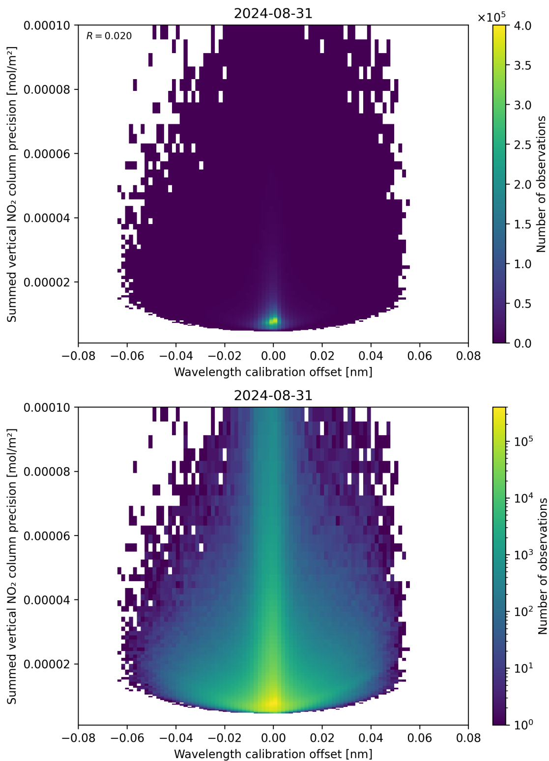
Figure 178: Scatter density plot of “Wavelength calibration offset” against “Summed vertical NO 2 column precision” for 2024-08-30 to 2024-09-01.
