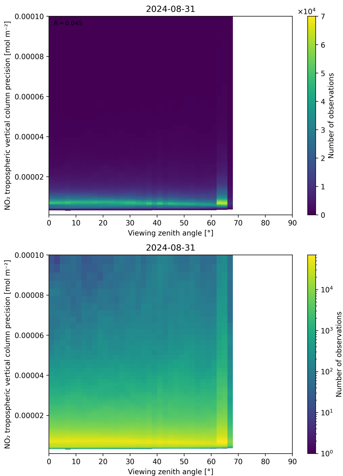
Figure 170: Scatter density plot of “Viewing zenith angle” against “NO 2 tropospheric vertical column precision” for 2024-08-30 to 2024-09-01.
