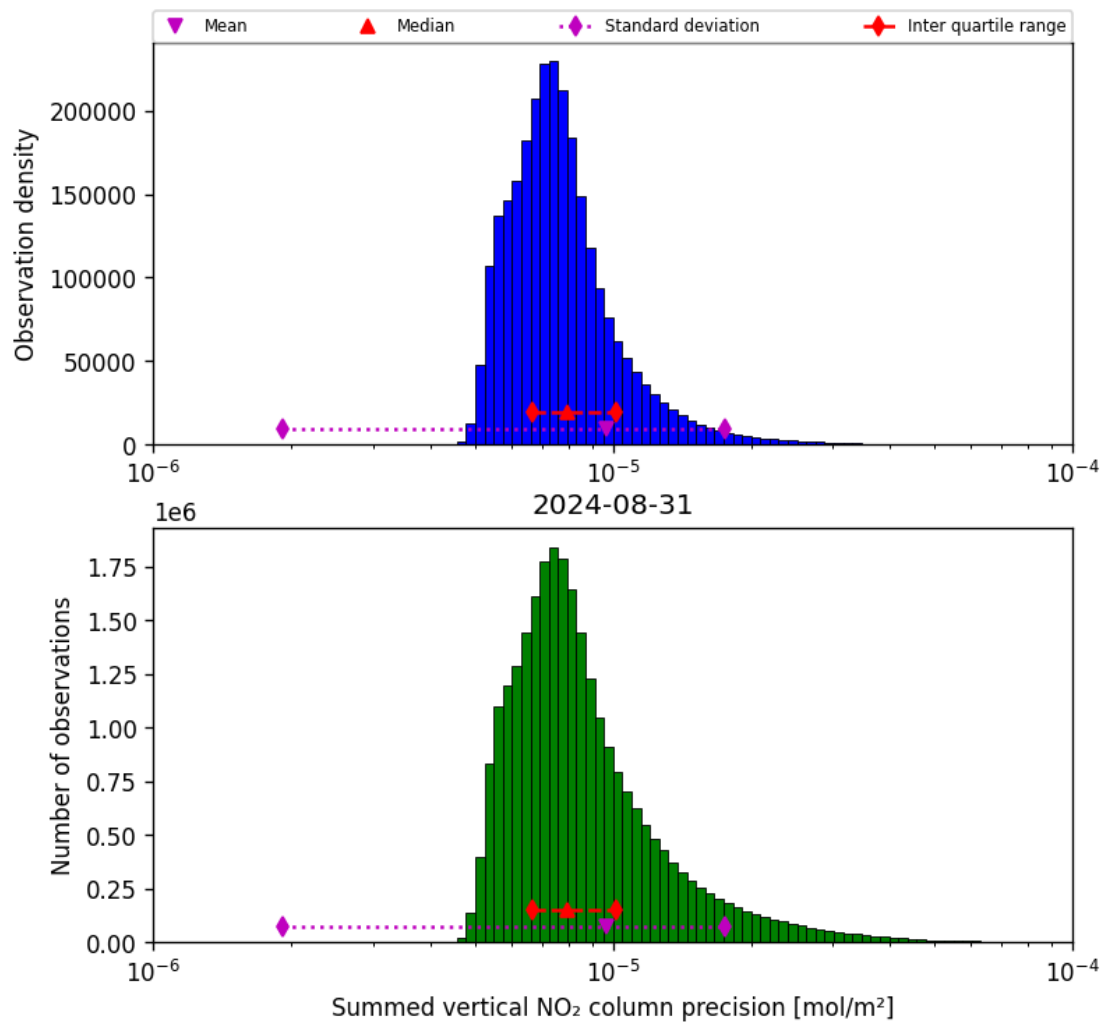
Figure 41: Histogram of "Summed vertical NO 2 column precision" for 2024-08-30 to 2024-09-01
