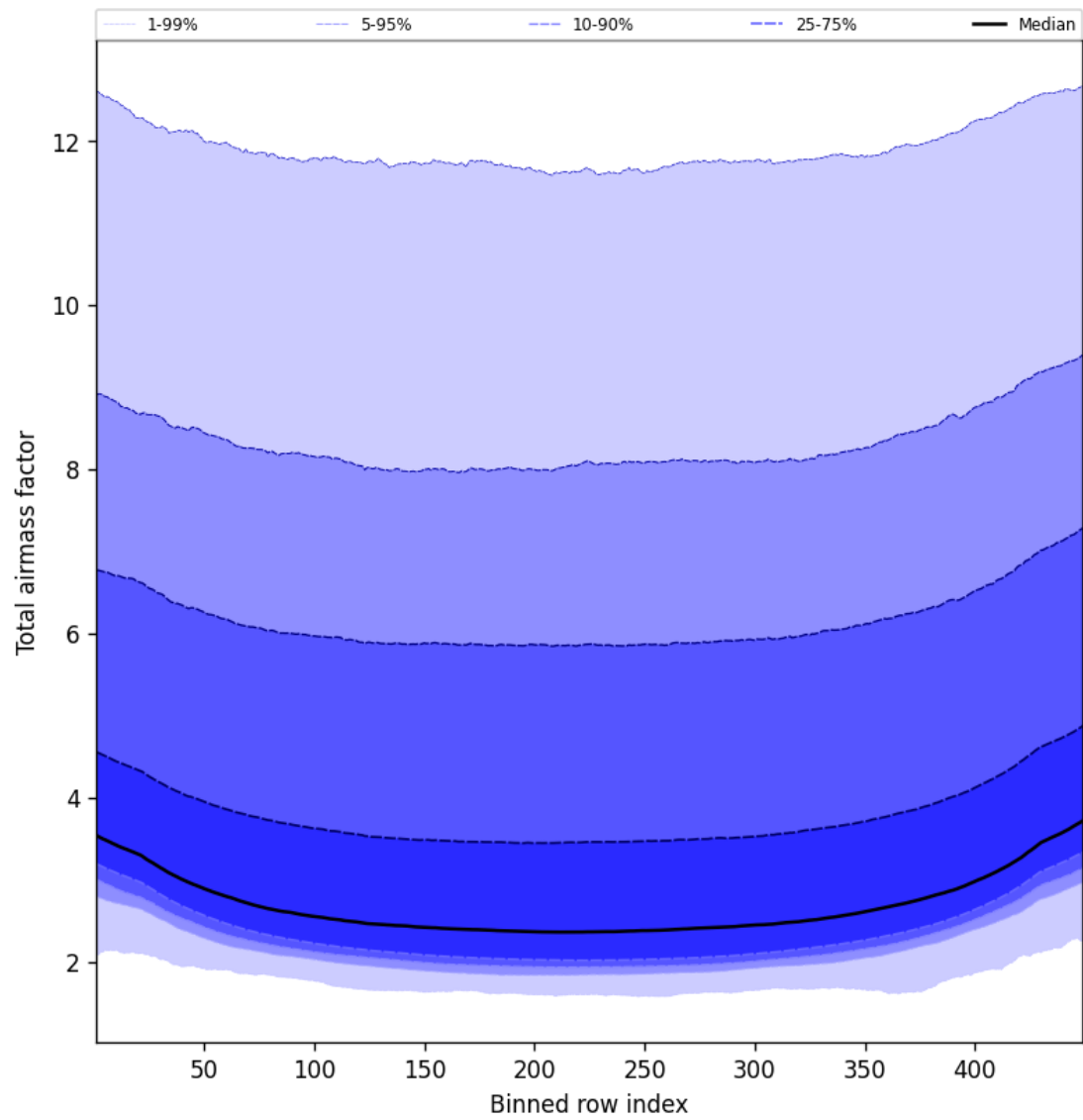
Figure 49: Along track statistics of “Total airmass factor” for 2024-08-30 to 2024-09-01
