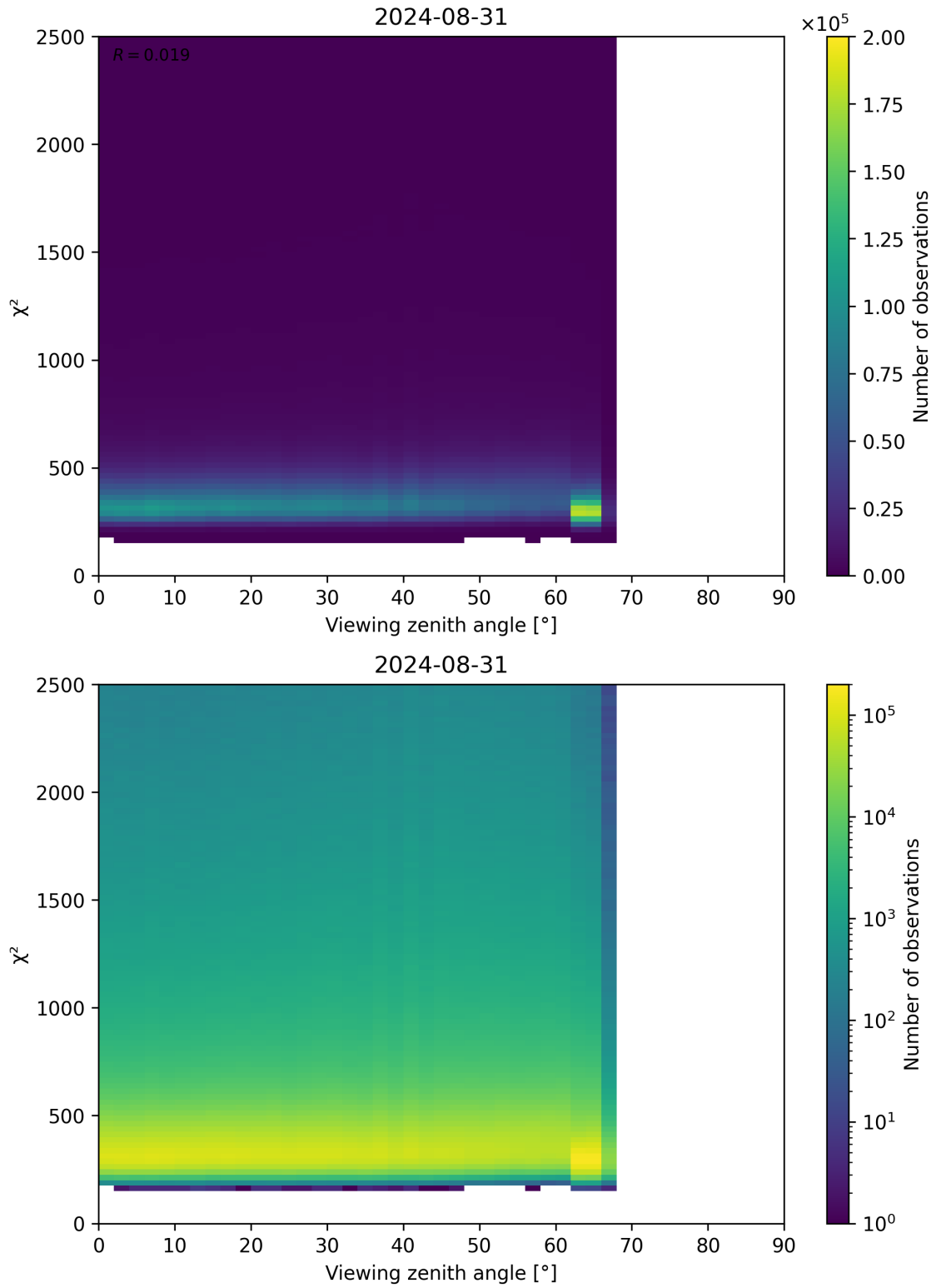
Figure 162: Scatter density plot of “Viewing zenith angle” against “ \chi^2 ” for 2024-08-30 to 2024-09-01.
