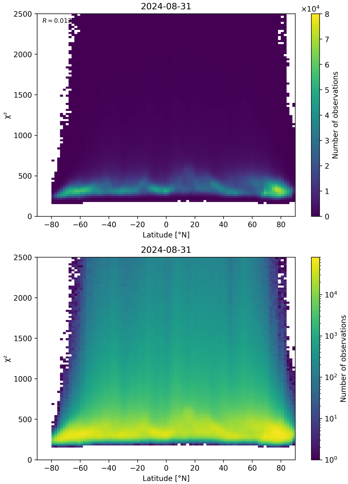
Figure 86: Scatter density plot of “Latitude” against “ \chi^2 ” for 2024-08-30 to 2024-09-01.
