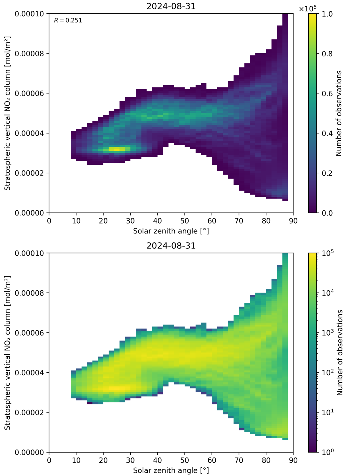
Figure 150: Scatter density plot of “Solar zenith angle” against “Stratospheric vertical NO 2 column” for 2024-08-30 to 2024-09-01.
