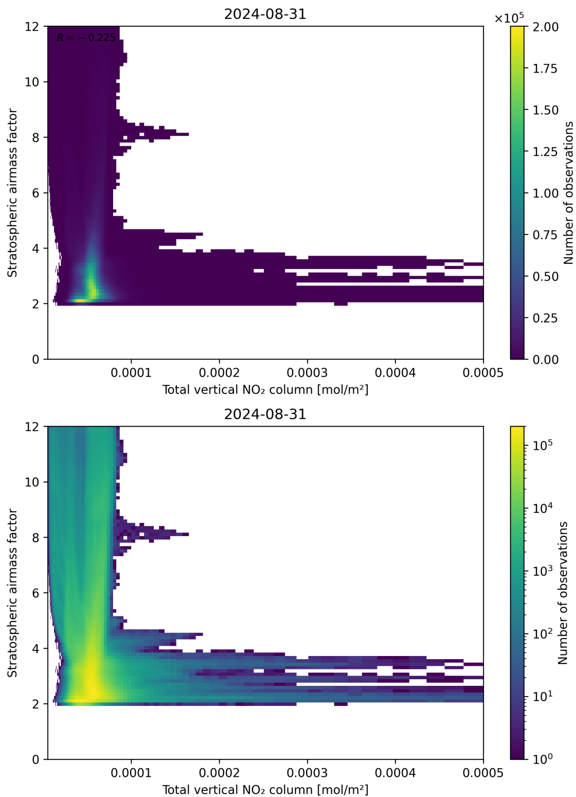
Figure 110: Scatter density plot of “Total vertical NO 2 column” against “Stratospheric airmass factor” for 2024-08-30 to 2024-09-01.
