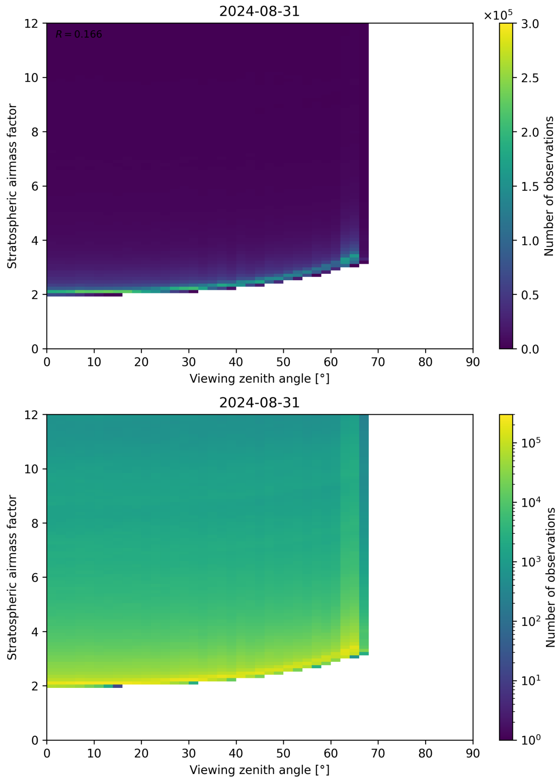
Figure 159: Scatter density plot of “Viewing zenith angle” against “Stratospheric airmass factor” for 2024-08-30 to 2024-09-01.
