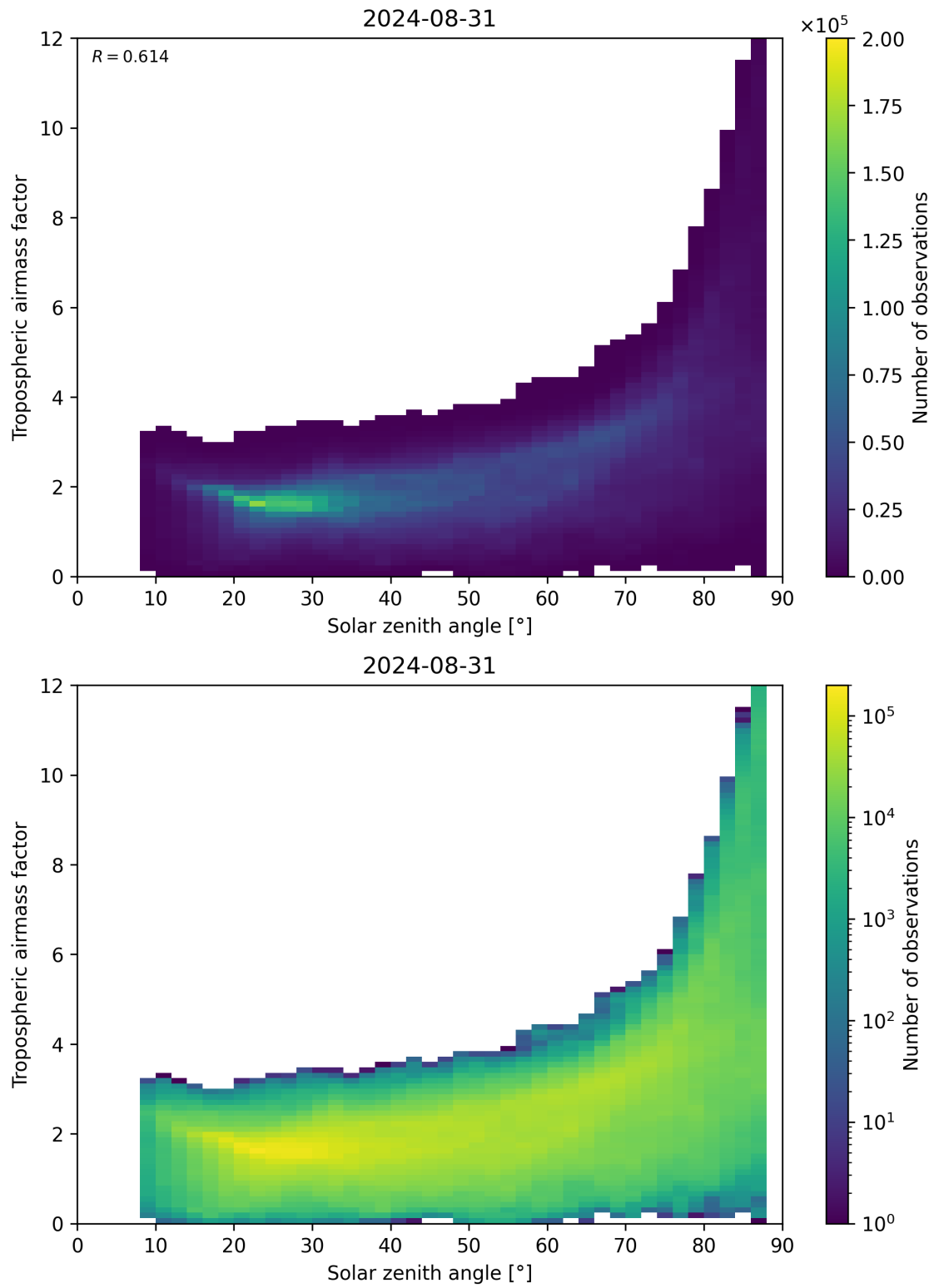
Figure 147: Scatter density plot of “Solar zenith angle” against “Tropospheric airmass factor” for 2024-08-30 to 2024-09-01.
