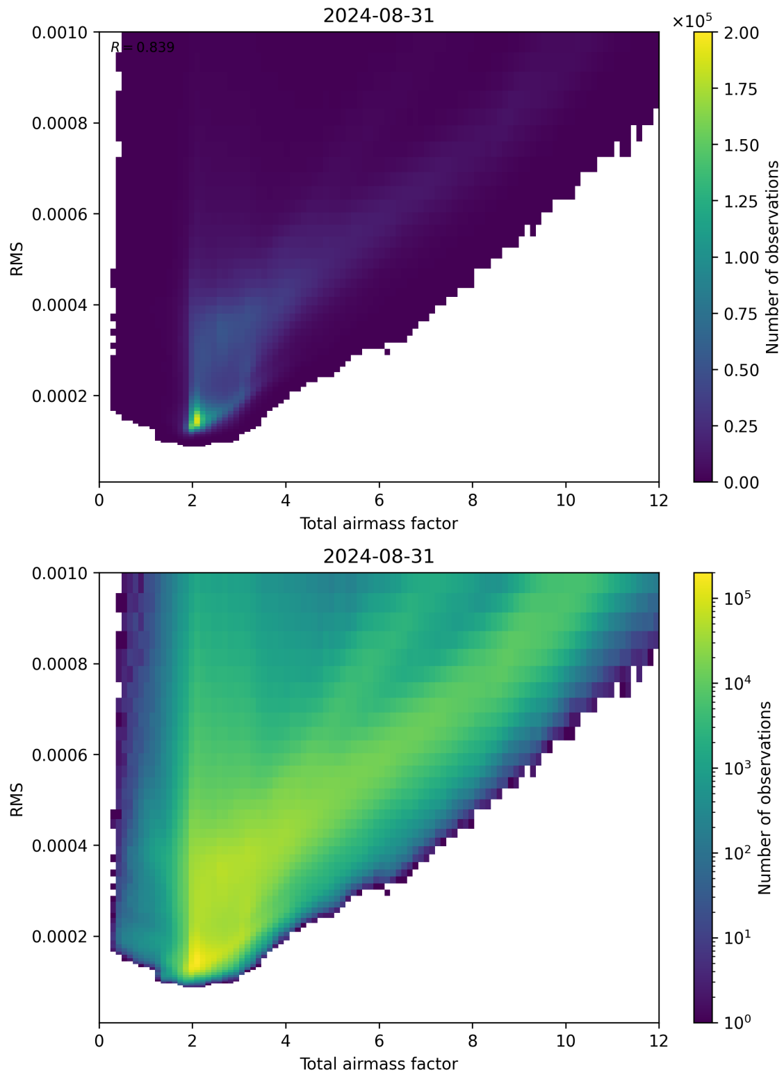
Figure 69: Scatter density plot of “Total airmass factor” against “RMS” for 2024-08-30 to 2024-09-01.
