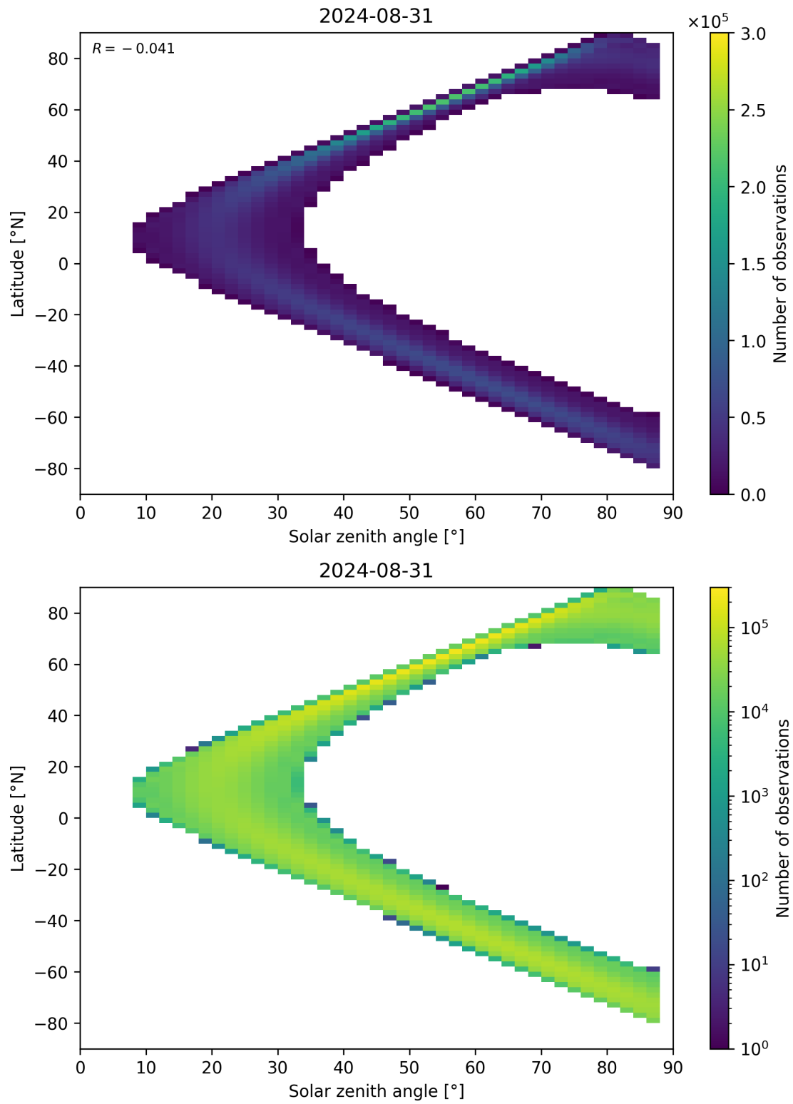
Figure 149: Scatter density plot of “Solar zenith angle” against “Latitude” for 2024-08-30 to 2024-09-01.
