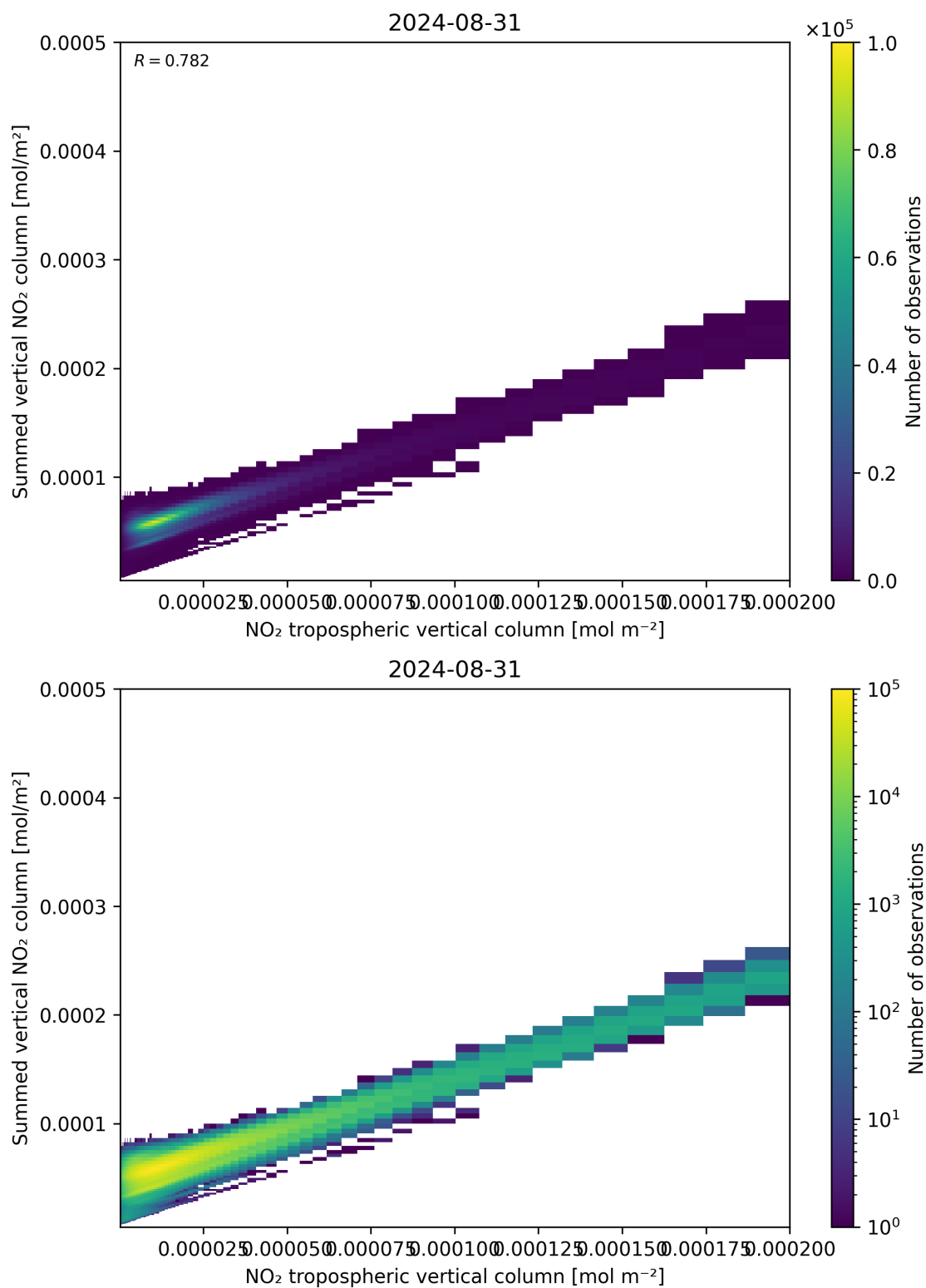
Figure 126: Scatter density plot of “NO 2 tropospheric vertical column” against “Summed vertical NO 2 column” for 2024-08-30 to 2024-09-01.
