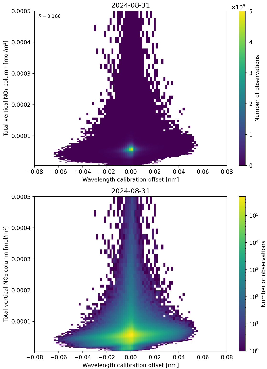
Figure 179: Scatter density plot of “Wavelength calibration offset” against “Total vertical NO 2 column” for 2024-08-30 to 2024-09-01.
