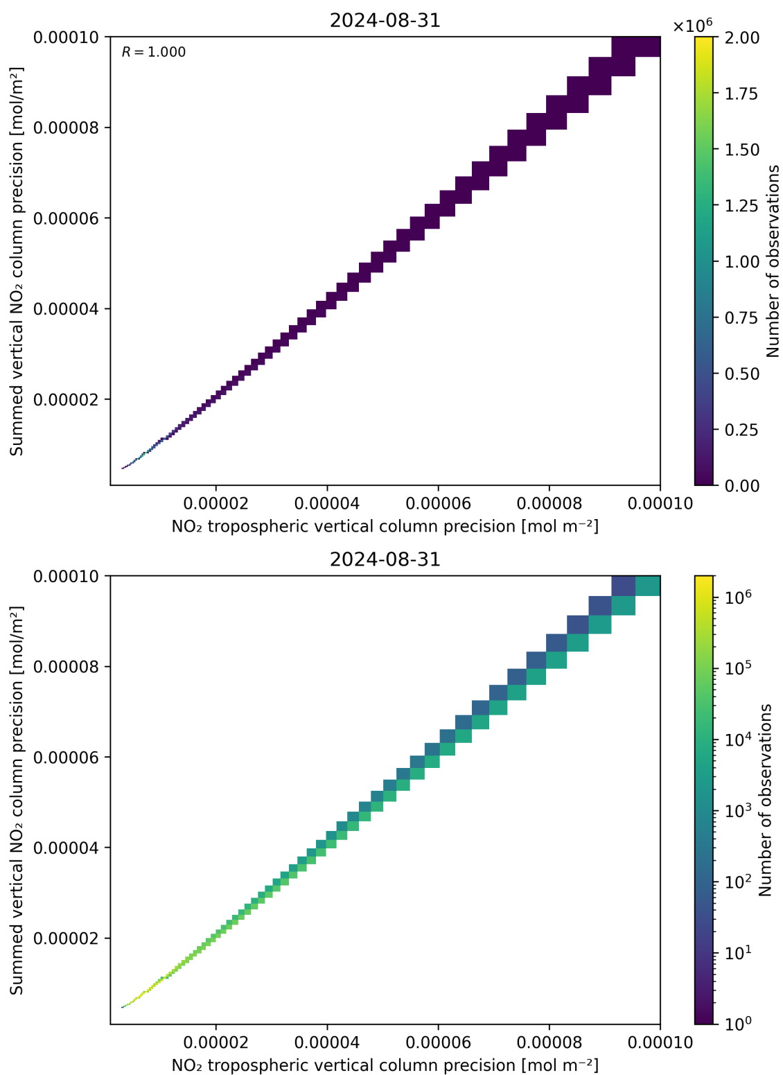
Figure 137: Scatter density plot of “NO 2 tropospheric vertical column precision” against “Summed vertical NO 2 column precision” for 2024-08-30 to 2024-09-01.
