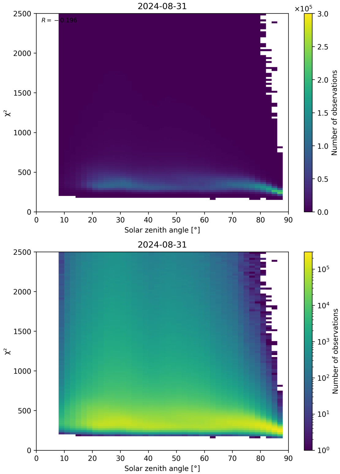
Figure 148: Scatter density plot of “Solar zenith angle” against “ \chi^2 ” for 2024-08-30 to 2024-09-01.
