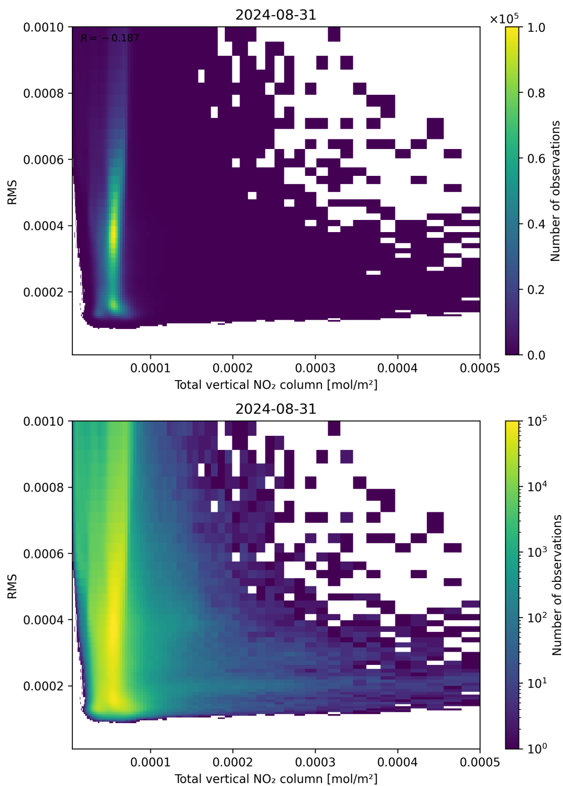
Figure 120: Scatter density plot of “Total vertical NO 2 column” against “RMS” for 2024-08-30 to 2024-09-01.
