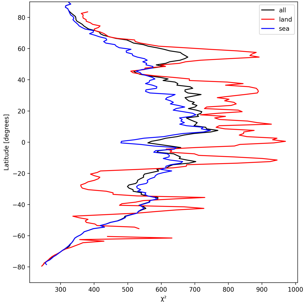
Figure 25: Zonal average of “ \chi^2 ” for 2024-08-30 to 2024-09-01.
