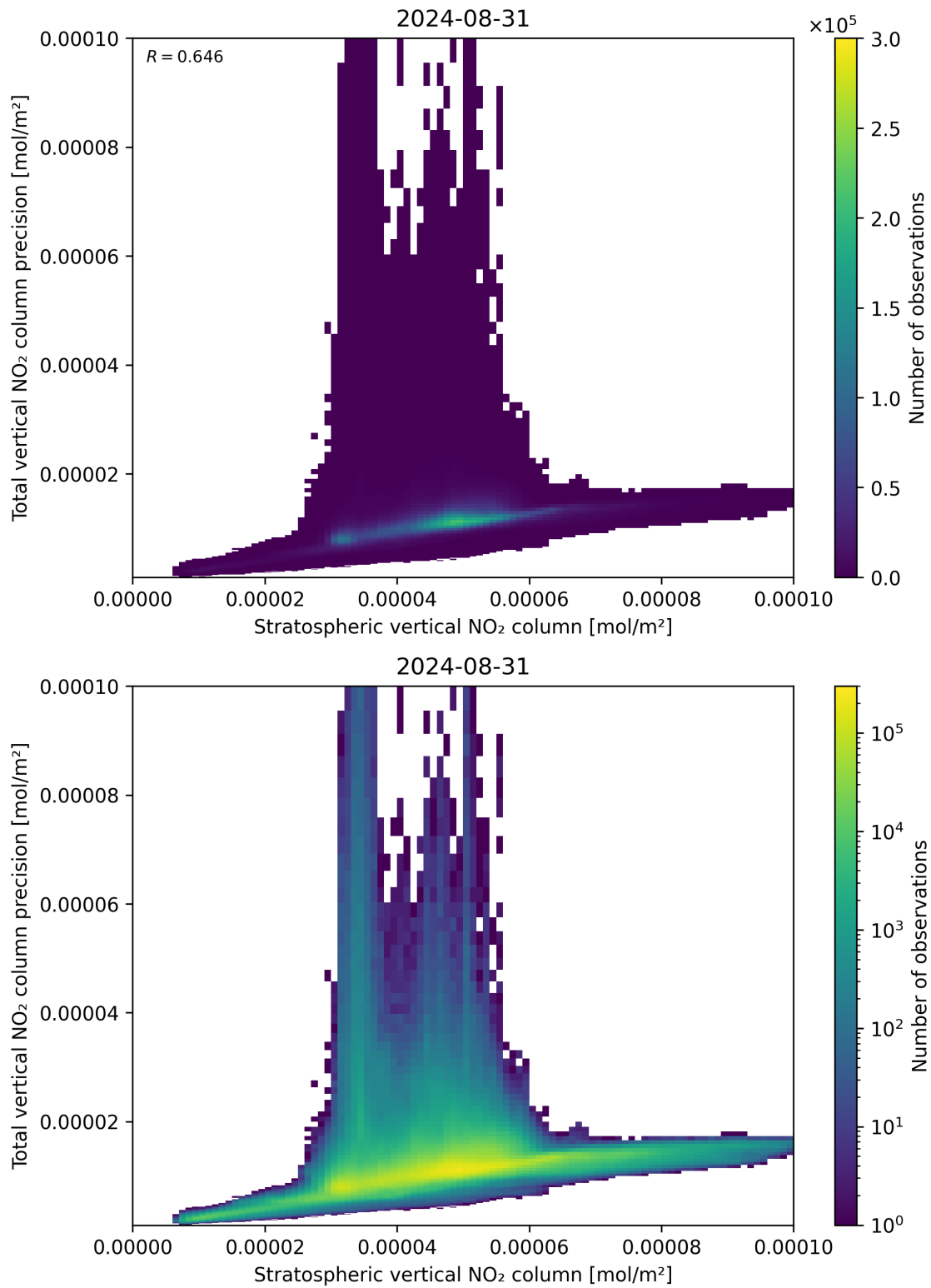
Figure 101: Scatter density plot of “Stratospheric vertical NO 2 column” against “Total vertical NO 2 column precision” for 2024-08-30 to 2024-09-01.
