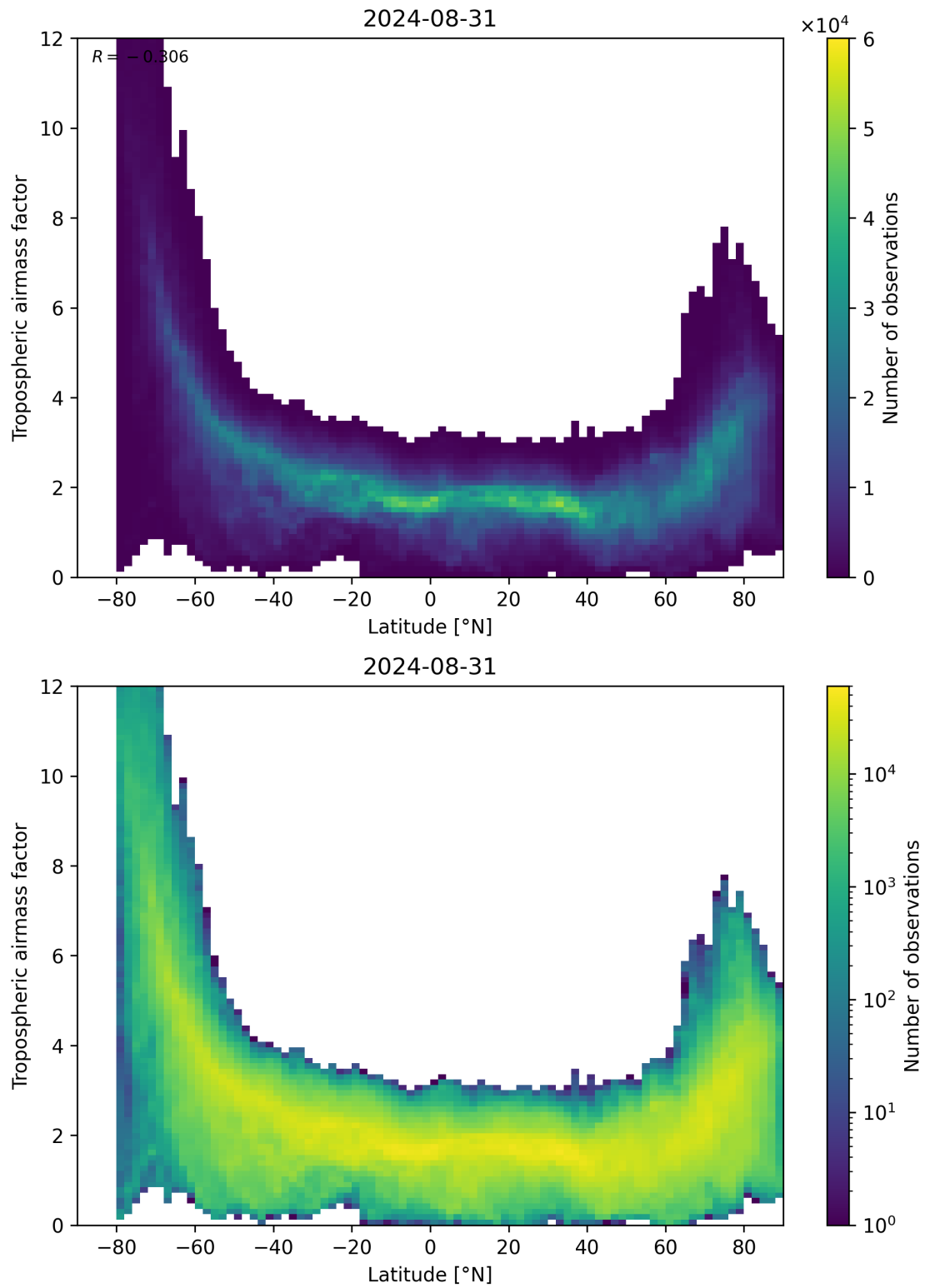
Figure 85: Scatter density plot of “Latitude” against “Tropospheric airmass factor” for 2024-08-30 to 2024-09-01.
