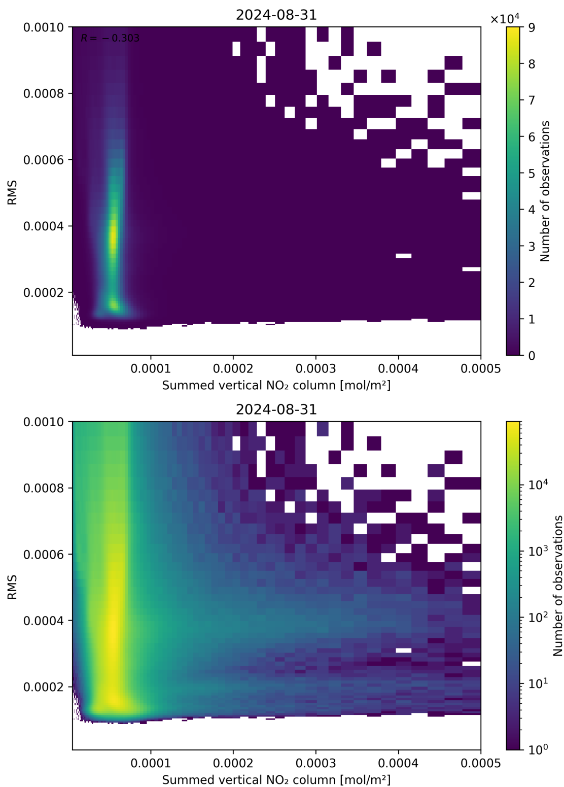
Figure 109: Scatter density plot of “Summed vertical NO 2 column” against “RMS” for 2024-08-30 to 2024-09-01.
