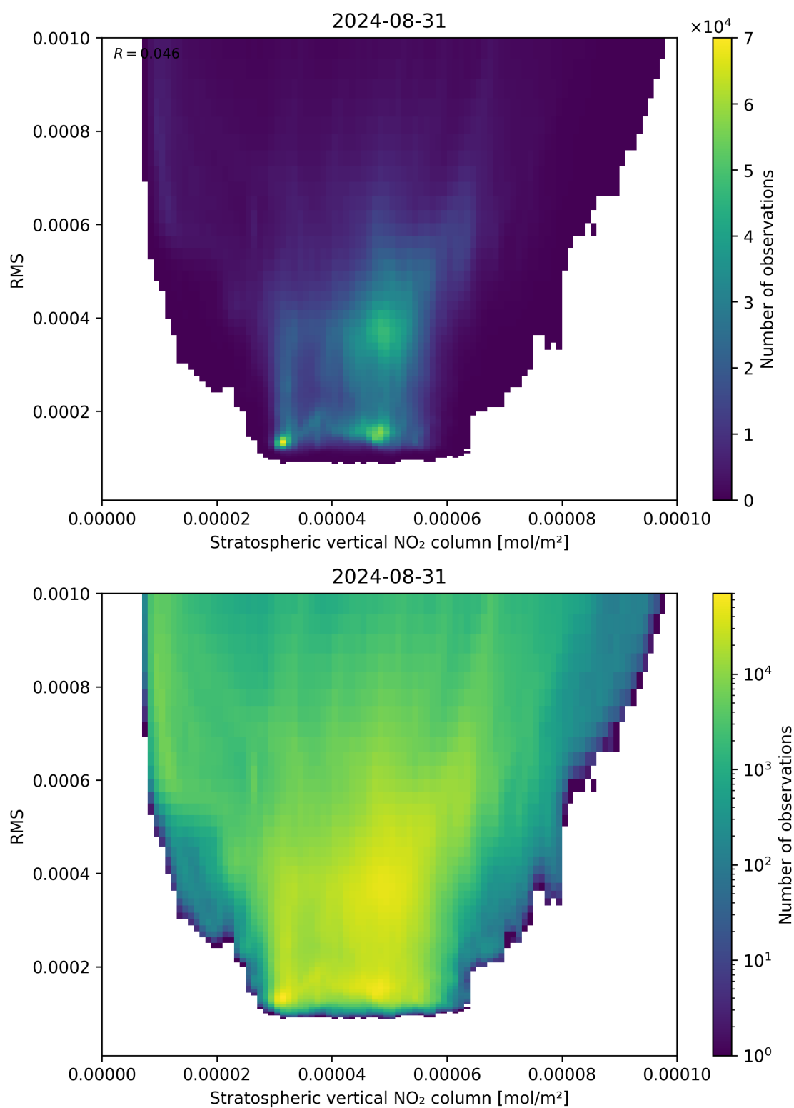
Figure 102: Scatter density plot of “Stratospheric vertical NO 2 column” against “RMS” for 2024-08-30 to 2024-09-01.
