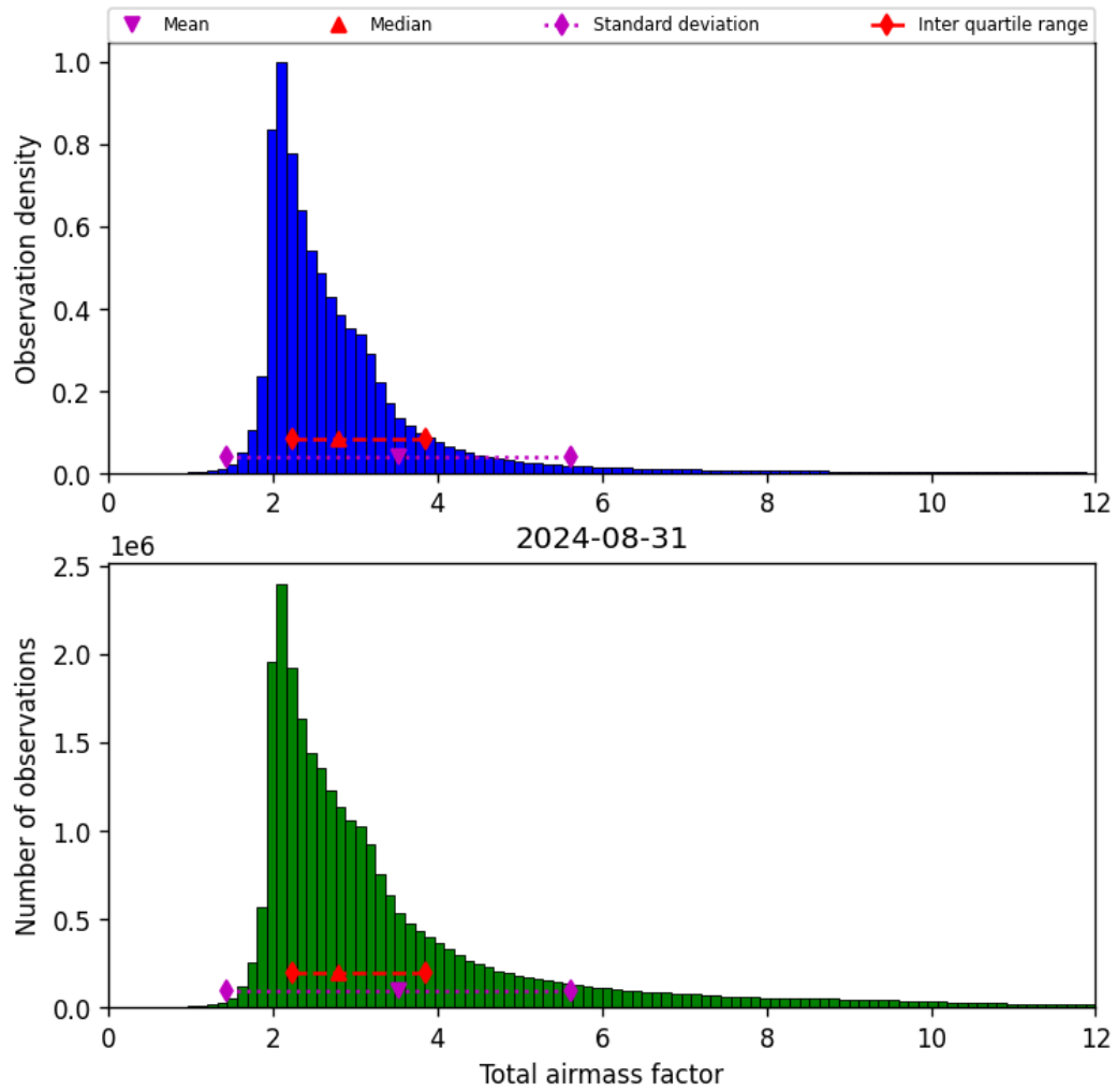
Figure 32: Histogram of “Total airmass factor” for 2024-08-30 to 2024-09-01
