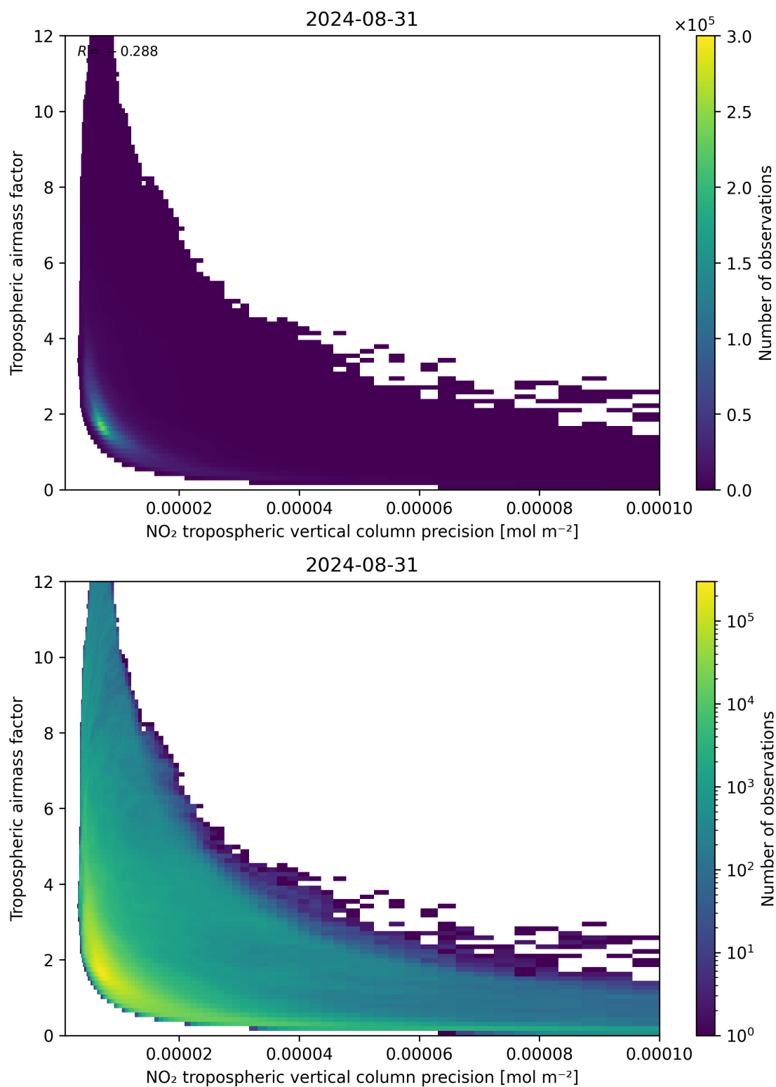
Figure 133: Scatter density plot of “NO 2 tropospheric vertical column precision” against “Tropospheric airmass factor” for 2024-08-30 to 2024-09-01.
