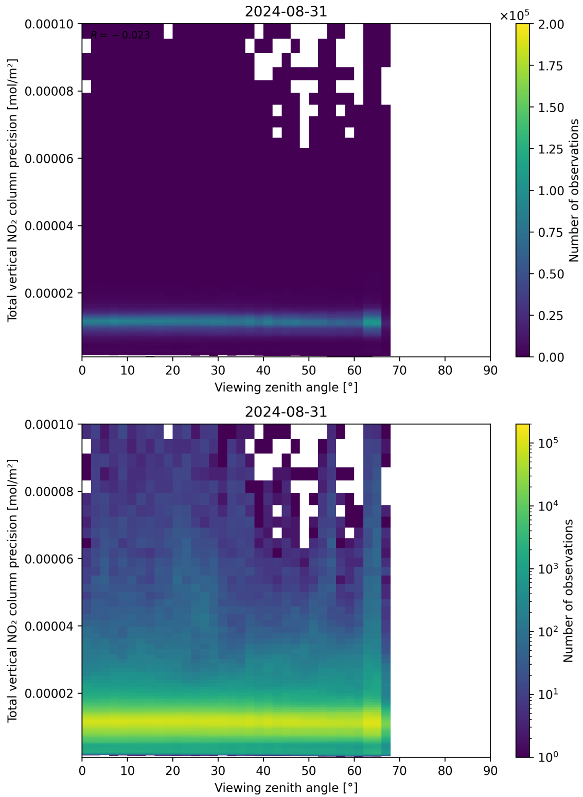
Figure 168: Scatter density plot of “Viewing zenith angle” against “Total vertical NO 2 column precision” for 2024-08-30 to 2024-09-01.
