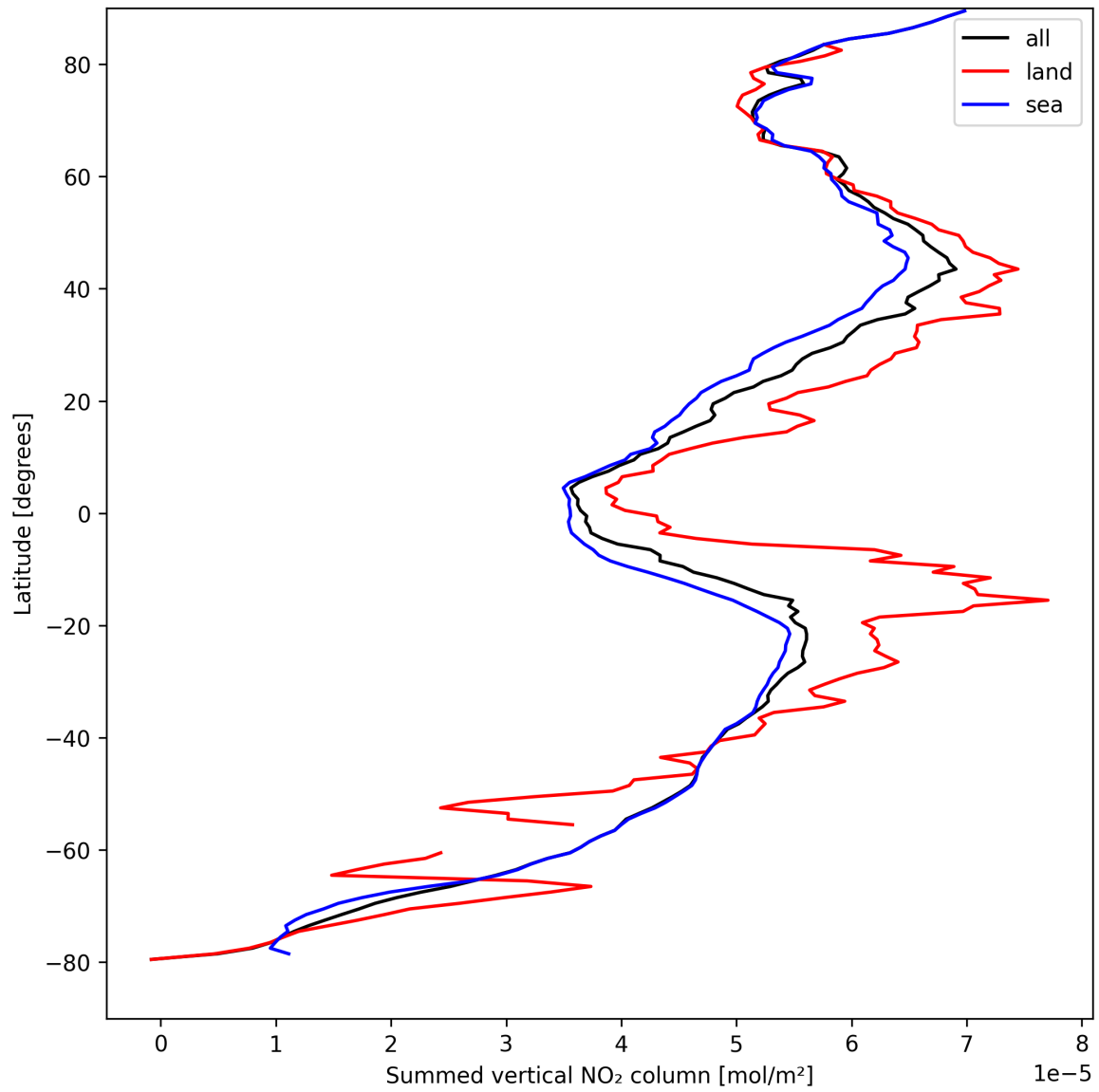
Figure 23: Zonal average of “Summed vertical NO 2 column” for 2024-08-30 to 2024-09-01.
