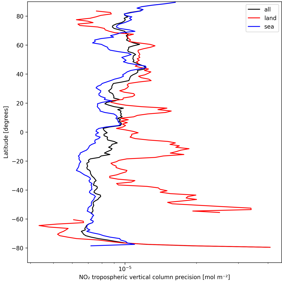
Figure 13: Zonal average of “NO 2 tropospheric vertical column precision” for 2024-08-30 to 2024-09-01.
