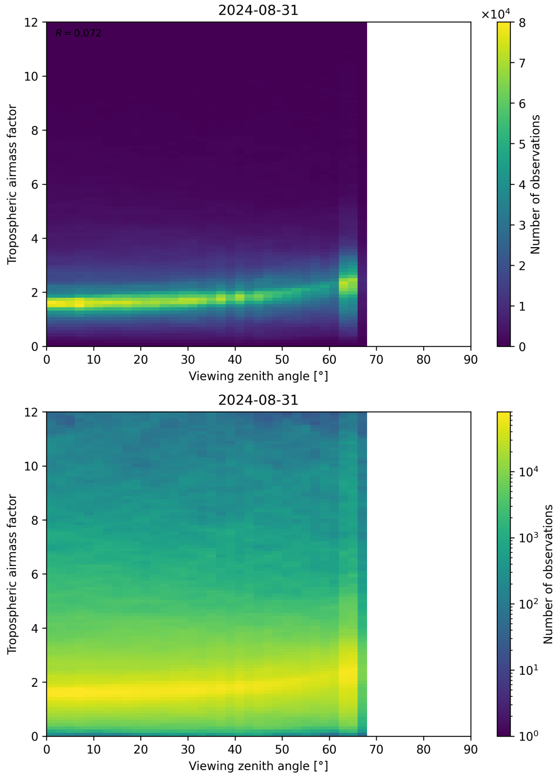
Figure 161: Scatter density plot of “Viewing zenith angle” against “Tropospheric air mass factor” for 2024-08-30 to 2024-09-01.
