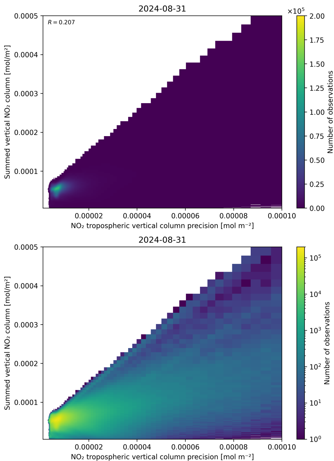
Figure 136: Scatter density plot of “NO 2 tropospheric vertical column precision” against “Summed vertical NO 2 column” for 2024-08-30 to 2024-09-01.
