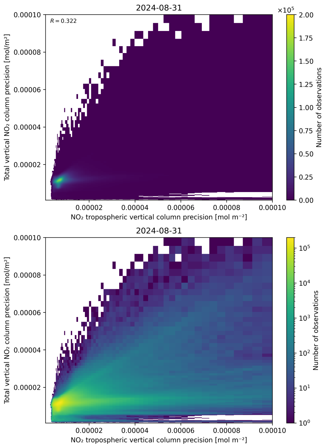
Figure 139: Scatter density plot of “NO 2 tropospheric vertical column precision” against “Total vertical NO 2 column precision” for 2024-08-30 to 2024-09-01.
