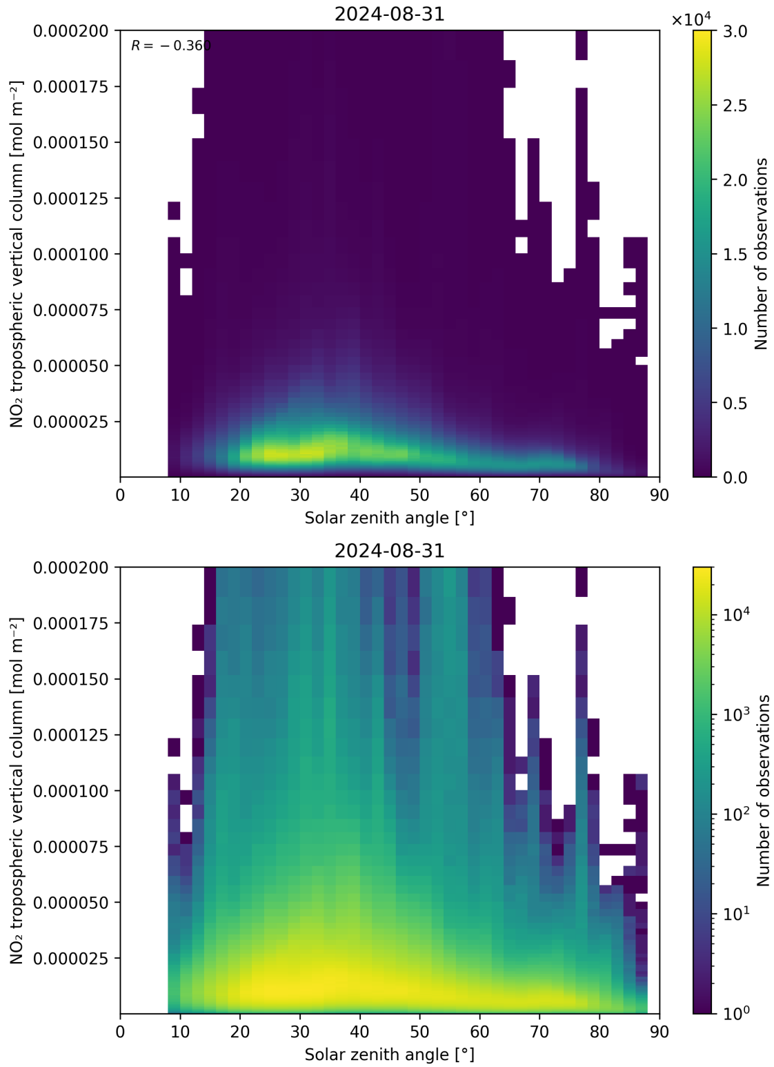
Figure 155: Scatter density plot of “Solar zenith angle” against “NO 2 tropospheric vertical column” for 2024-08-30 to 2024-09-01.
