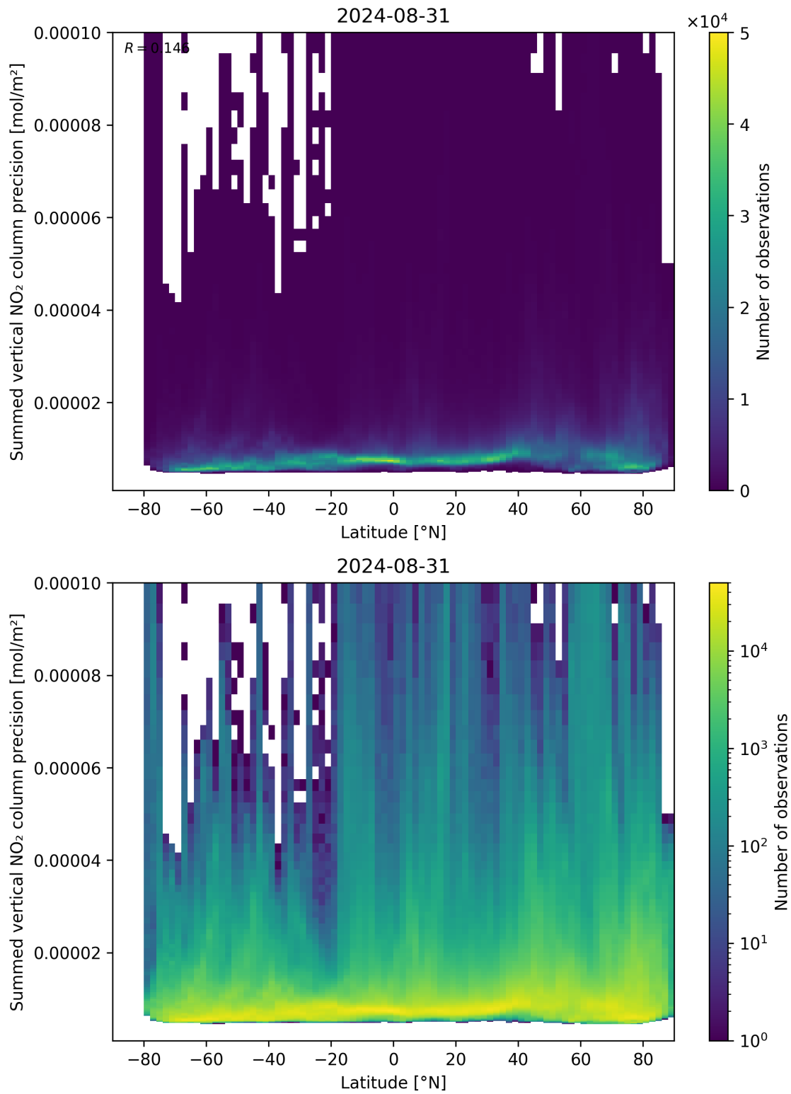
Figure 89: Scatter density plot of “Latitude” against “Summed vertical NO 2 column precision” for 2024-08-30 to 2024-09-01.
