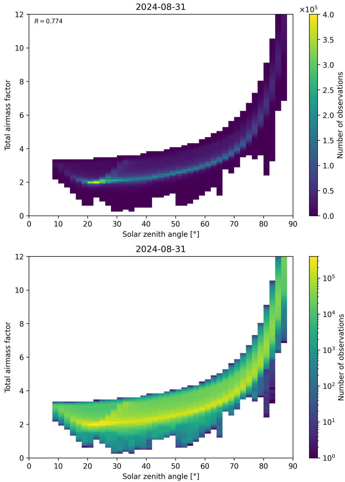
Figure 146: Scatter density plot of “Solar zenith angle” against “Total air mass factor” for 2024-08-30 to 2024-09-01.
