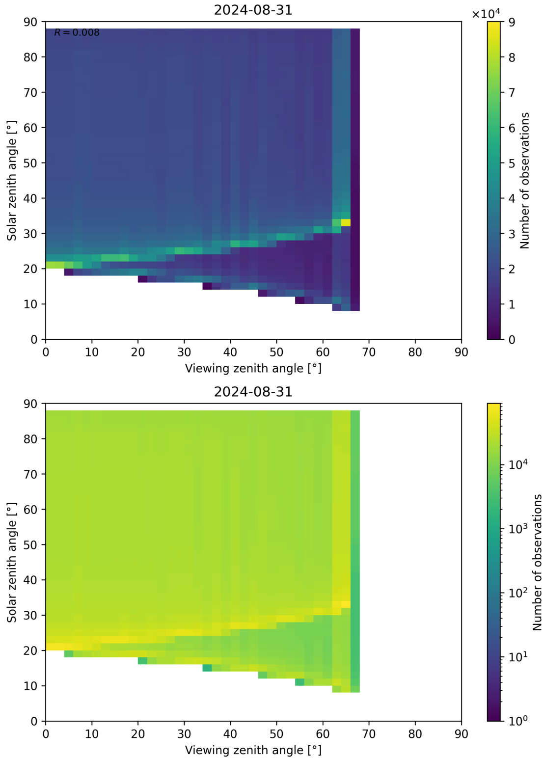
Figure 172: Scatter density plot of “Viewing zenith angle” against “Solar zenith angle” for 2024-08-30 to 2024-09-01.
