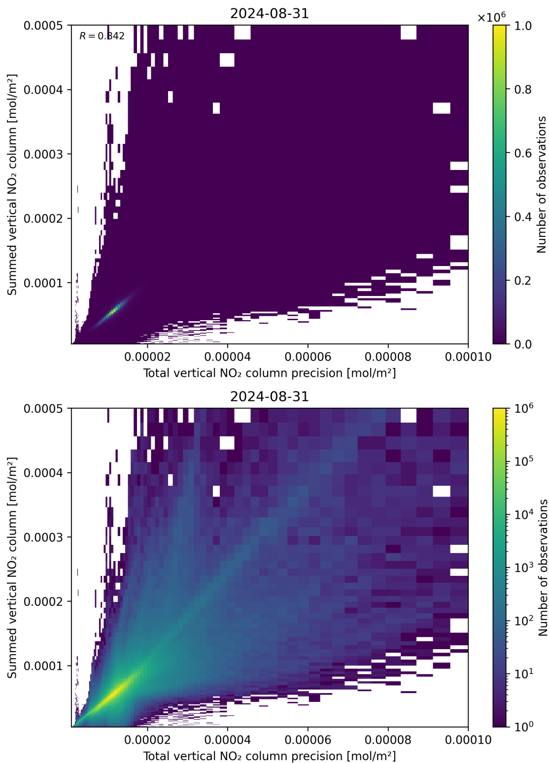
Figure 117: Scatter density plot of “Total vertical NO 2 column precision” against “Summed vertical NO 2 column” for 2024-08-30 to 2024-09-01.
