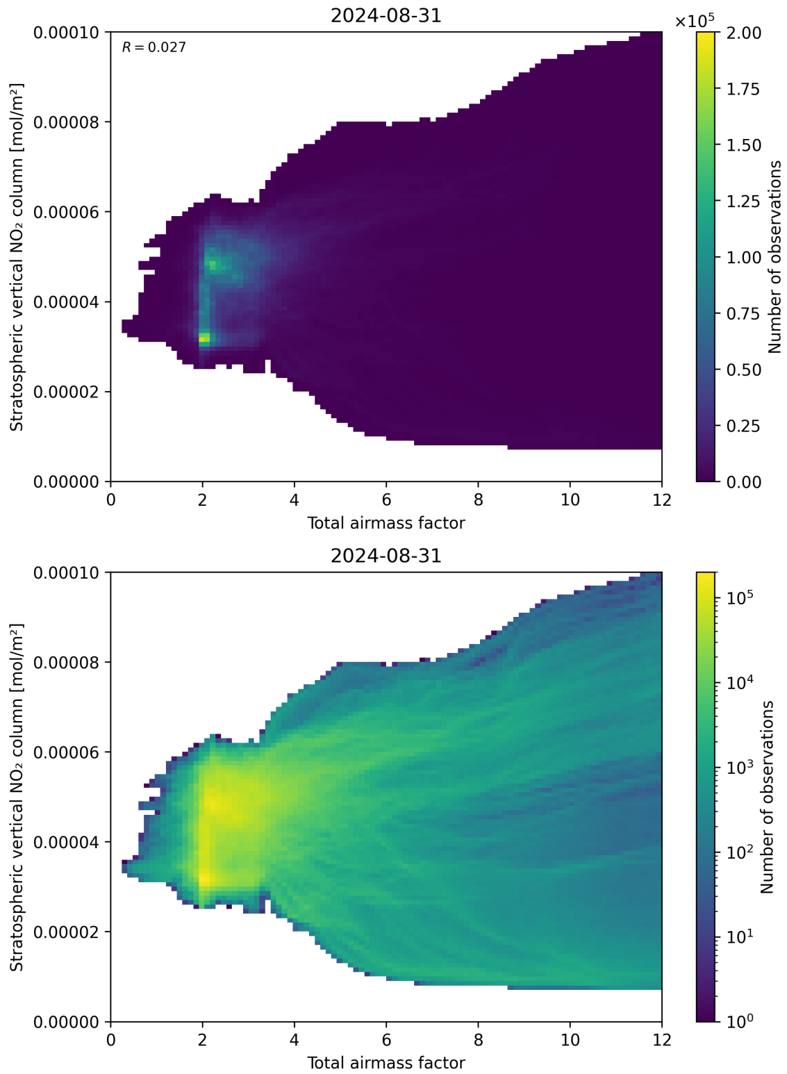
Figure 64: Scatter density plot of “Total airmass factor” against “Stratospheric vertical \text{NO}_2 column” for 2024-08-30 to 2024-09-01.
