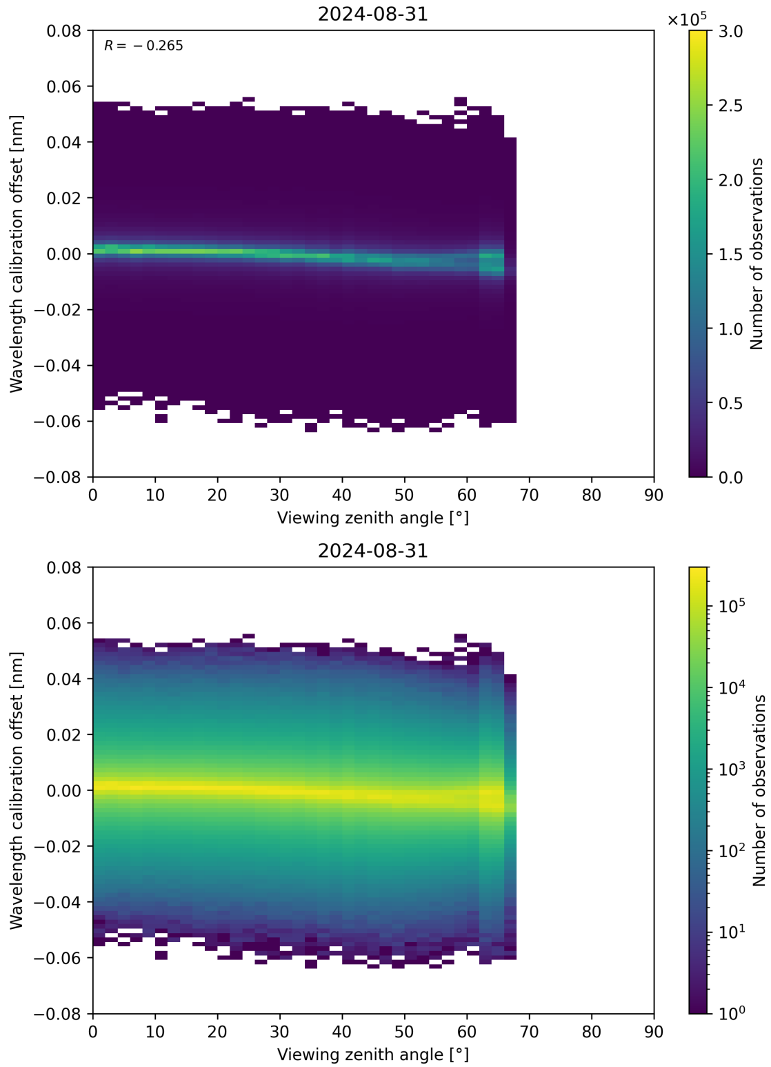
Figure 173: Scatter density plot of “Viewing zenith angle” against “Wavelength calibration offset” for 2024-08-30 to 2024-09-01.
