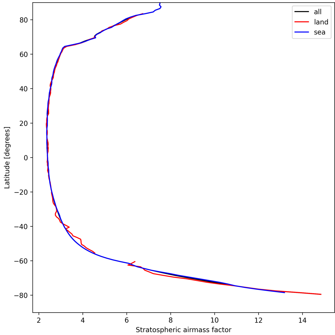
Figure 27: Zonal average of “Stratospheric airmass factor” for 2024-08-30 to 2024-09-01.
