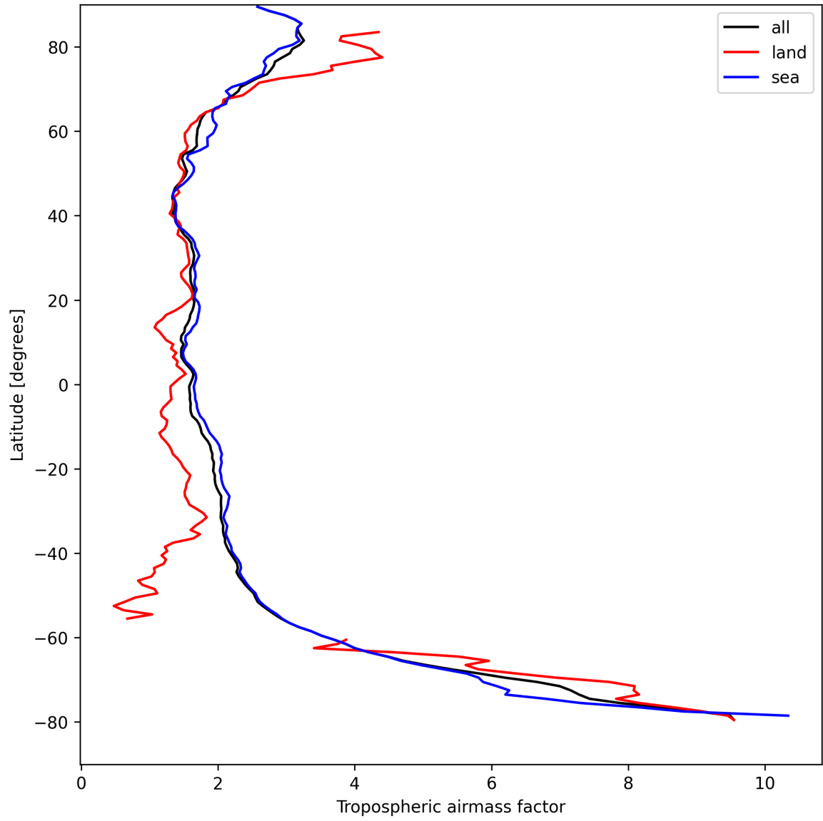
Figure 14: Zonal average of “Tropospheric airmass factor” for 2024-08-30 to 2024-09-01.
