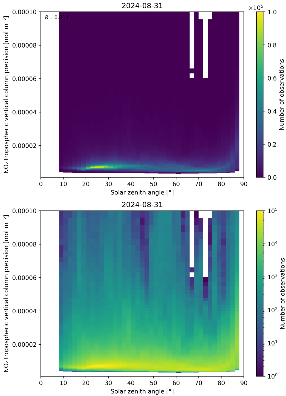
Figure 156: Scatter density plot of “Solar zenith angle” against “NO 2 tropospheric vertical column precision” for 2024-08-30 to 2024-09-01.
