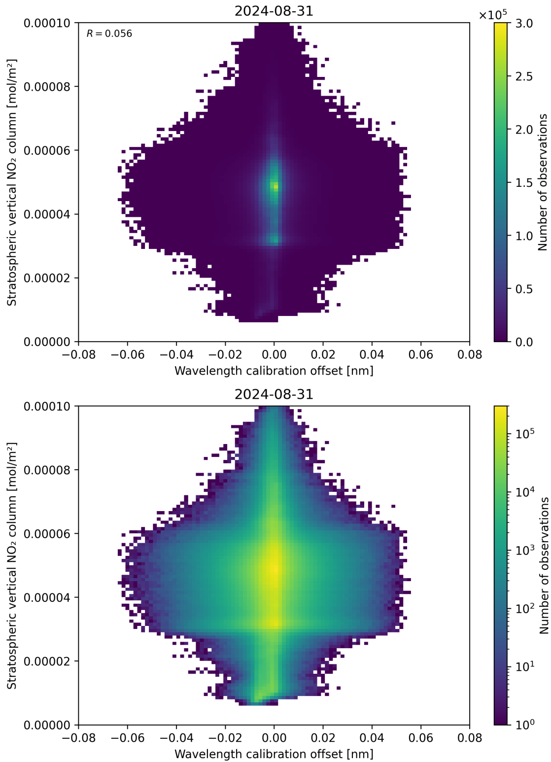
Figure 176: Scatter density plot of “Wavelength calibration offset” against “Stratospheric vertical NO 2 column” for 2024-08-30 to 2024-09-01.
