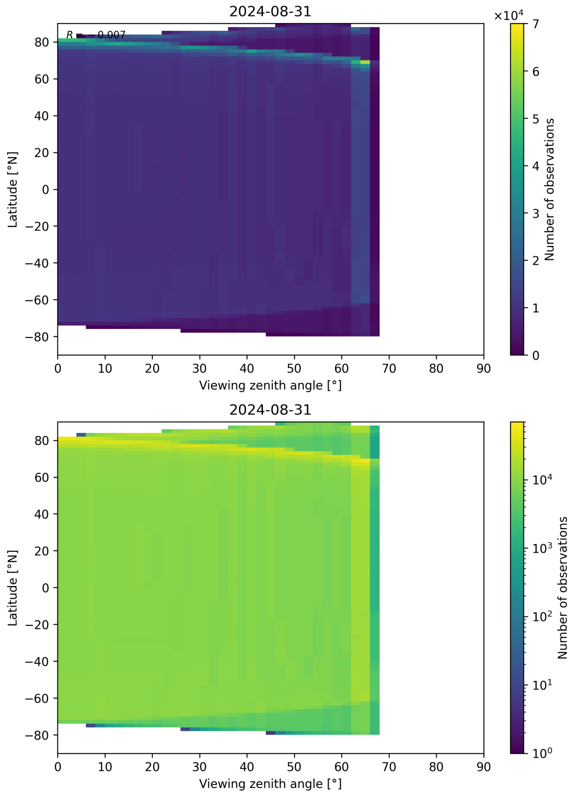
Figure 163: Scatter density plot of “Viewing zenith angle” against “Latitude” for 2024-08-30 to 2024-09-01.
