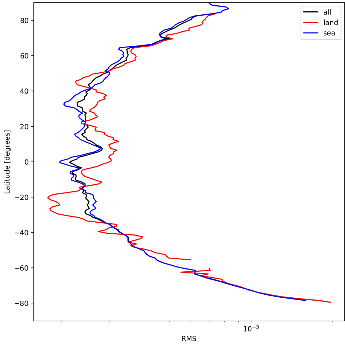
Figure 26: Zonal average of “RMS” for 2024-08-30 to 2024-09-01.
