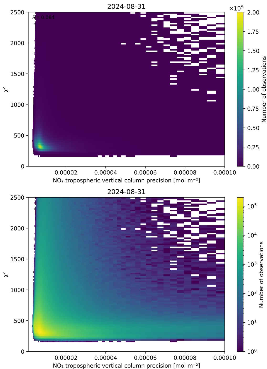
Figure 134: Scatter density plot of “NO 2 tropospheric vertical column precision” against “ \chi^2 ” for 2024-08-30 to 2024-09-01.
