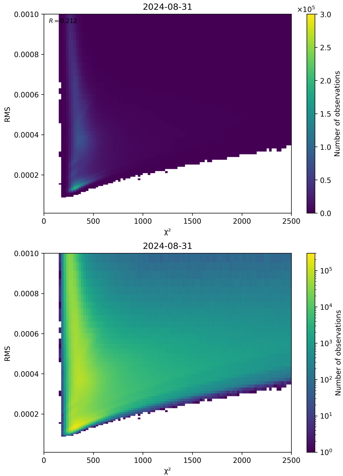
Figure 82: Scatter density plot of “ \chi^2 ” against “RMS” for 2024-08-30 to 2024-09-01.
