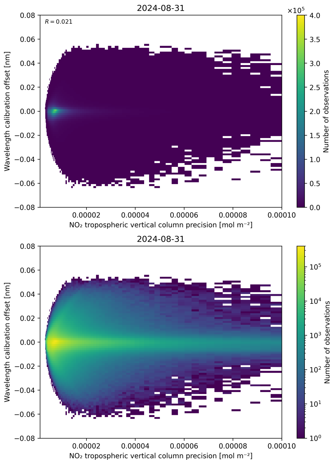
Figure 141: Scatter density plot of “NO 2 tropospheric vertical column precision” against “Wavelength calibration offset” for 2024-08-30 to 2024-09-01.
