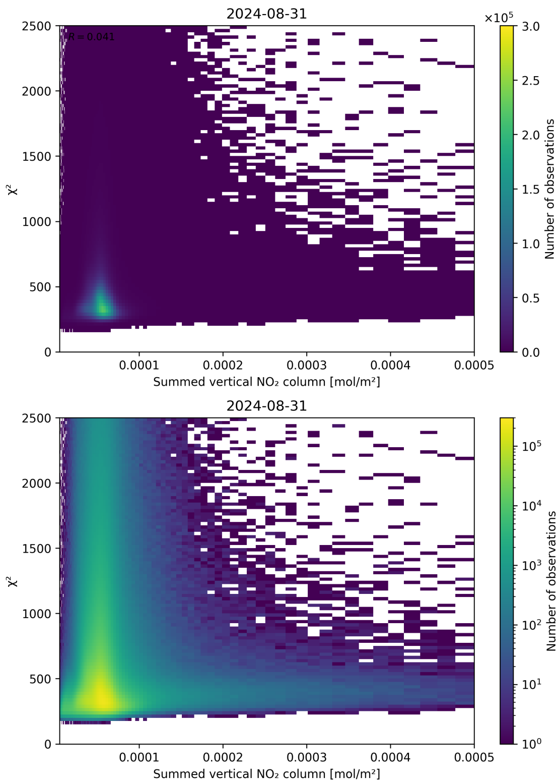
Figure 104: Scatter density plot of “Summed vertical NO 2 column” against “ \chi^2 ” for 2024-08-30 to 2024-09-01.
