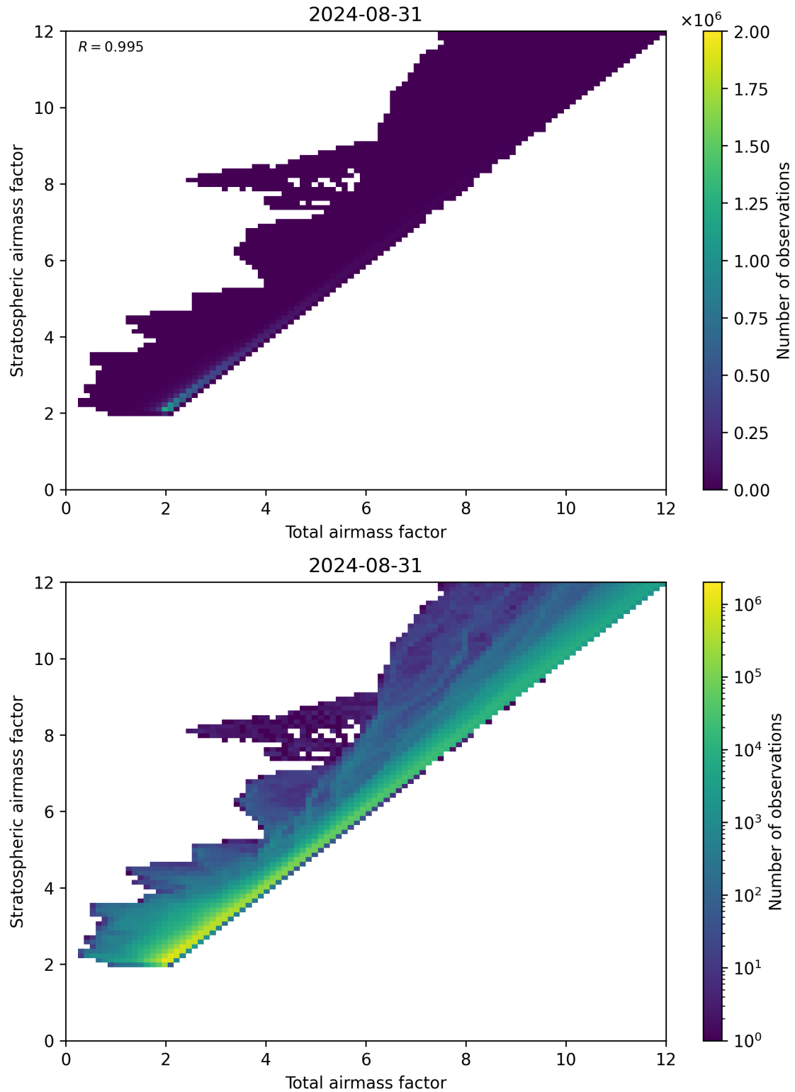
Figure 62: Scatter density plot of “Total airmass factor” against “Stratospheric airmass factor” for 2024-08-30 to 2024-09-01.
