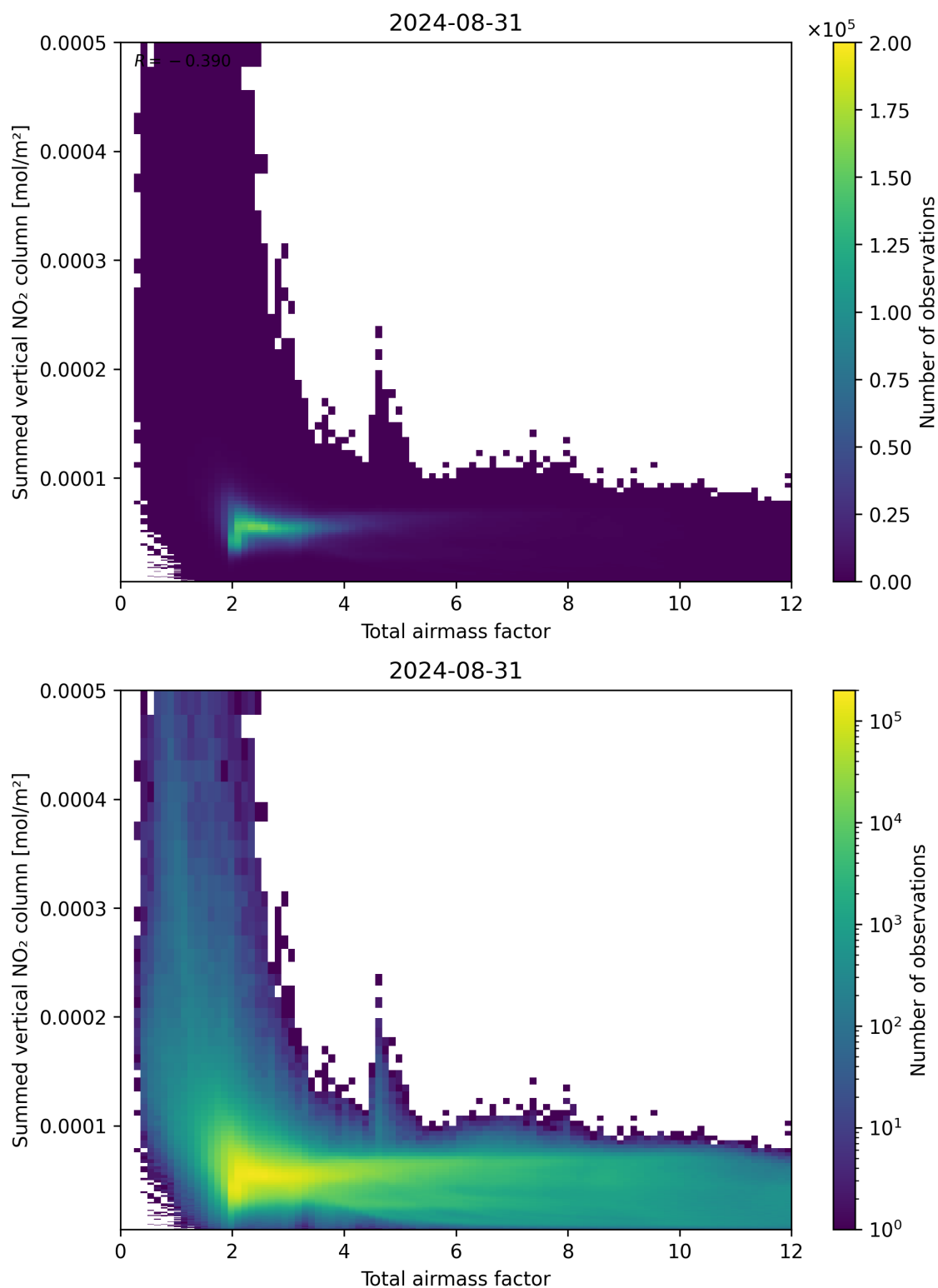
Figure 65: Scatter density plot of “Total airmass factor” against “Summed vertical NO 2 column” for 2024-08-30 to 2024-09-01.
