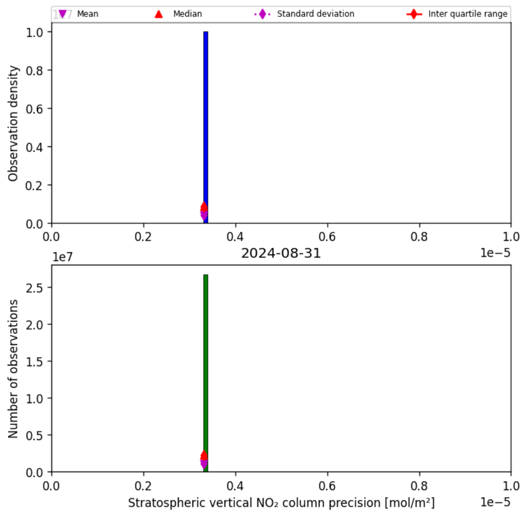
Figure 37: Histogram of “Stratospheric vertical NO 2 column precision” for 2024-08-30 to 2024-09-01
