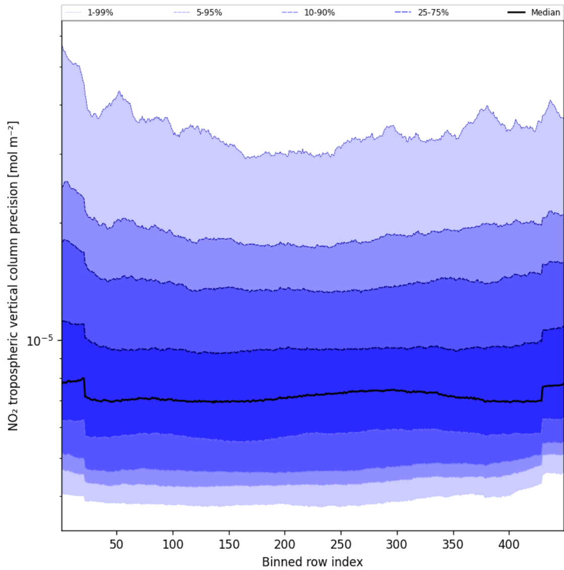
Figure 47: Along track statistics of “NO 2 tropospheric vertical column precision” for 2024-08-30 to 2024-09-01
