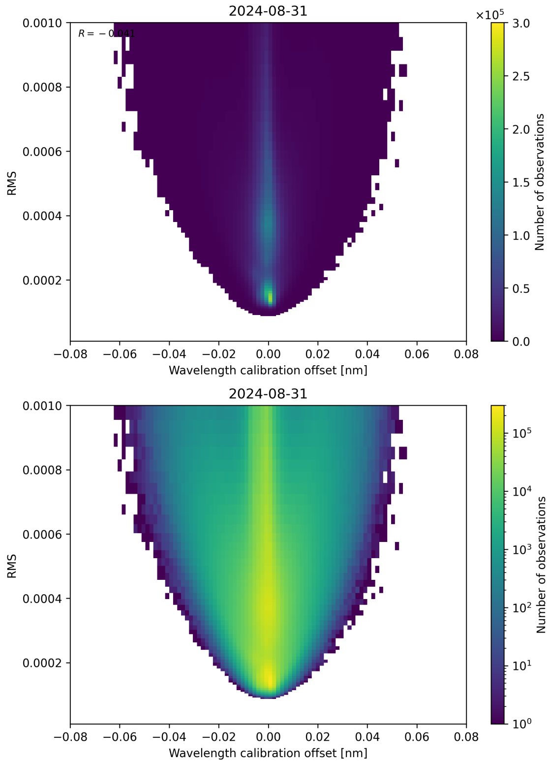
Figure 181: Scatter density plot of “Wavelength calibration offset” against “RMS” for 2024-08-30 to 2024-09-01.
