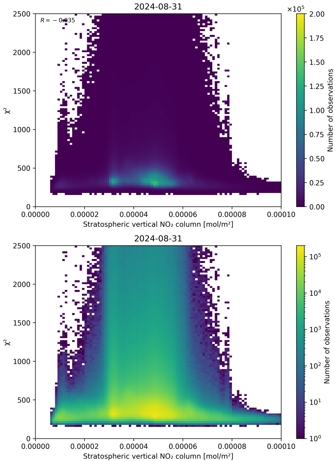
Figure 97: Scatter density plot of “Stratospheric vertical NO 2 column” against “ \chi^2 ” for 2024-08-30 to 2024-09-01.
