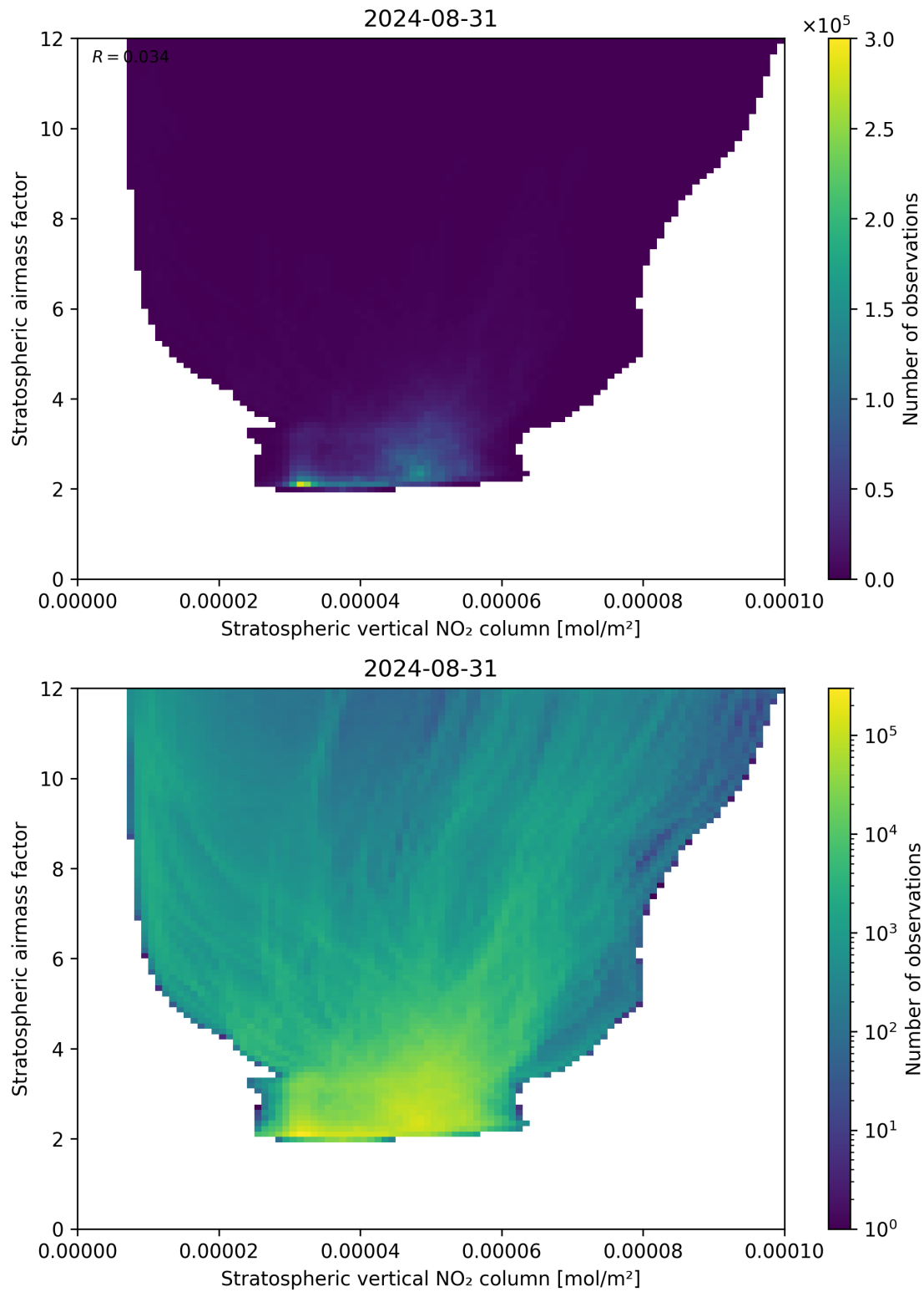
Figure 96: Scatter density plot of “Stratospheric vertical NO 2 column” against “Stratospheric airmass factor” for 2024-08-30 to 2024-09-01.
