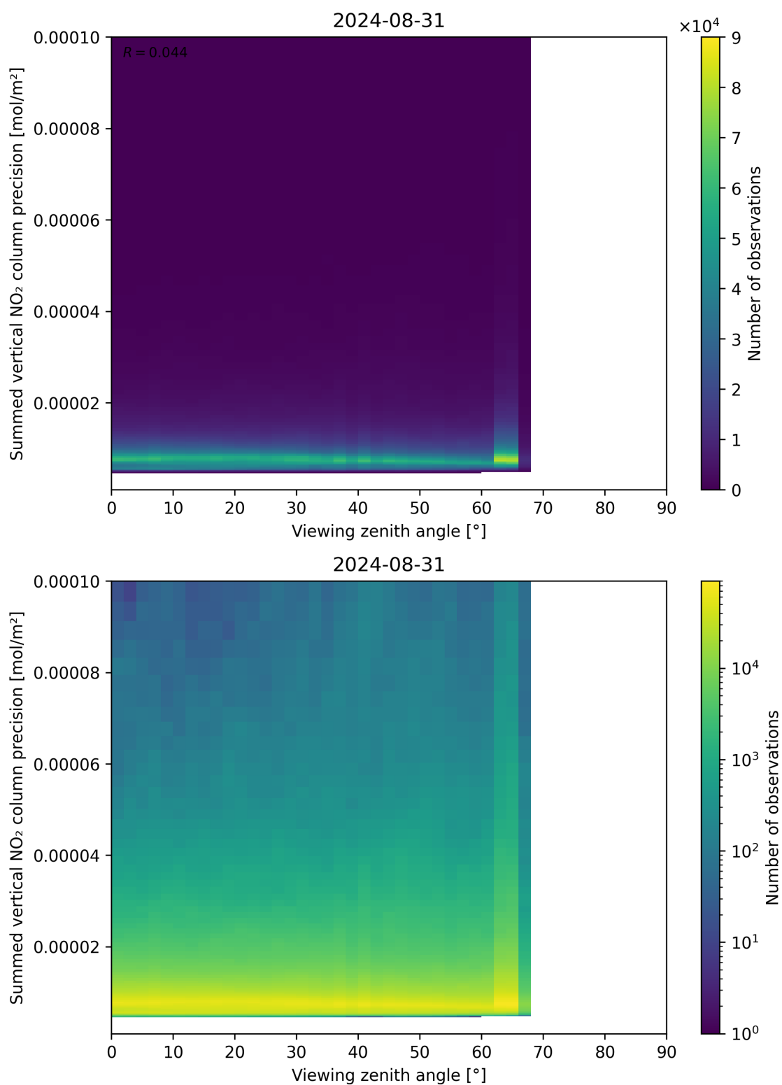
Figure 166: Scatter density plot of “Viewing zenith angle” against “Summed vertical NO 2 column precision” for 2024-08-30 to 2024-09-01.
