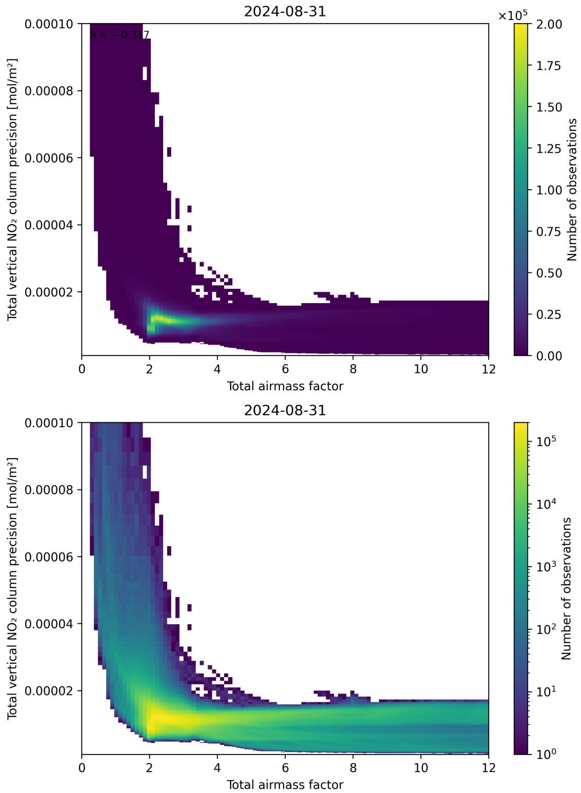
Figure 68: Scatter density plot of “Total airmass factor” against “Total vertical NO 2 column precision” for 2024-08-30 to 2024-09-01.
