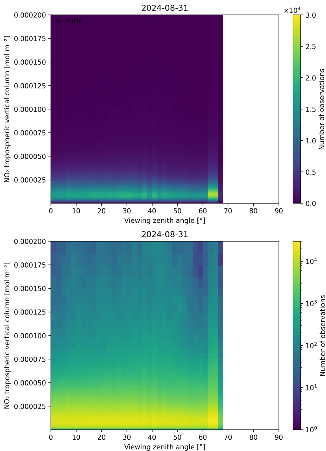
Figure 169: Scatter density plot of “Viewing zenith angle” against “NO 2 tropospheric vertical column” for 2024-08-30 to 2024-09-01.
