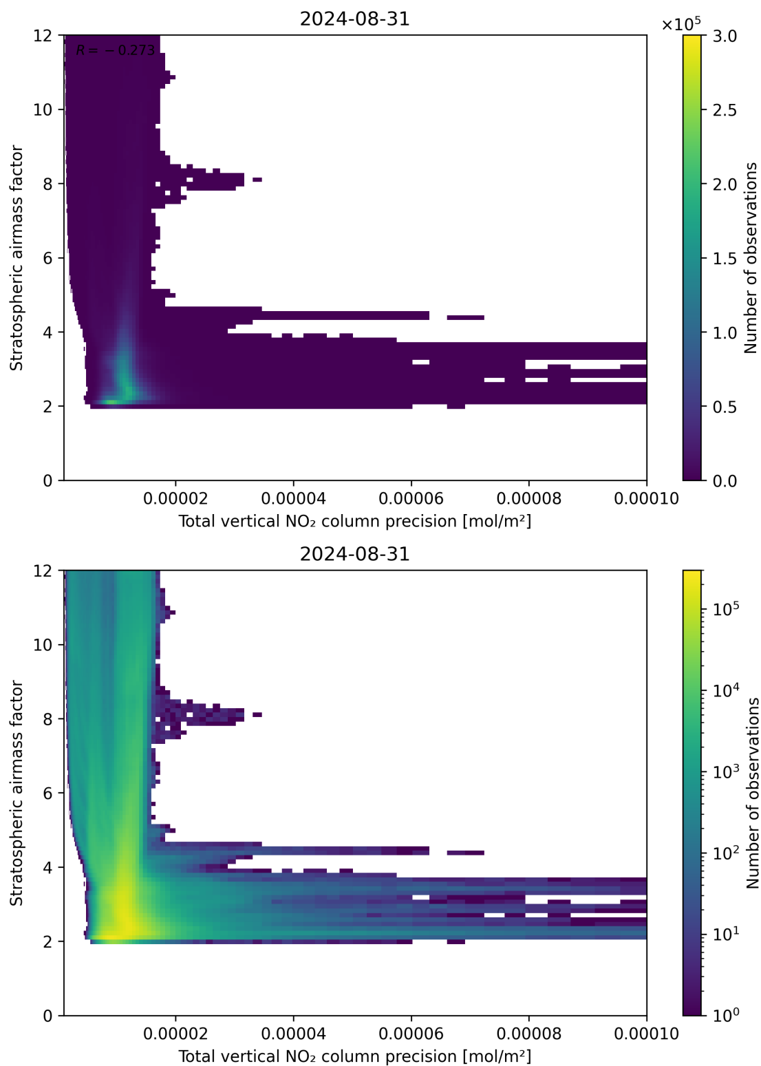
Figure 115: Scatter density plot of “Total vertical NO 2 column precision” against “Stratospheric air mass factor” for 2024-08-30 to 2024-09-01.
