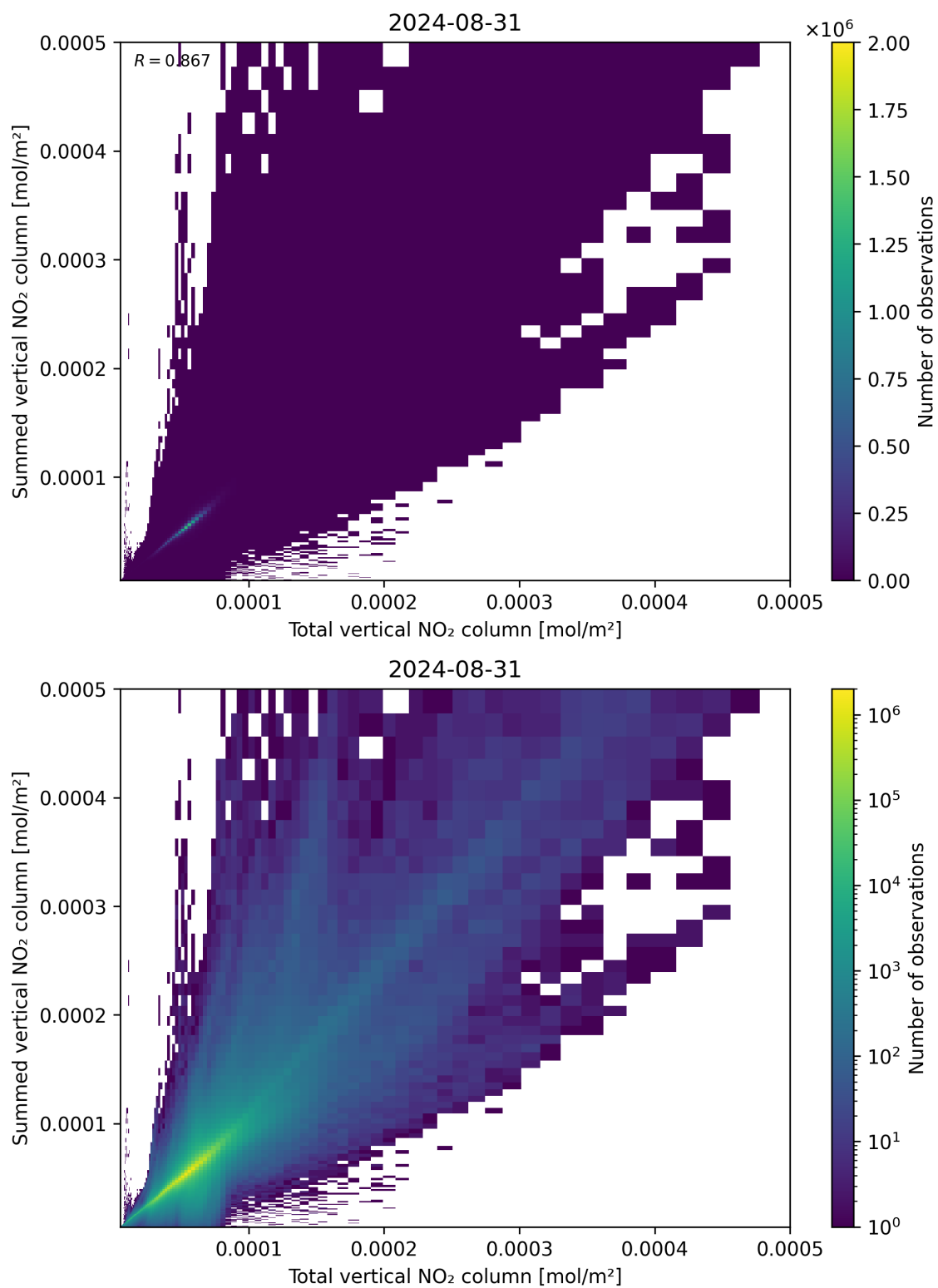
Figure 112: Scatter density plot of “Total vertical NO 2 column” against “Summed vertical NO 2 column” for 2024-08-30 to 2024-09-01.
