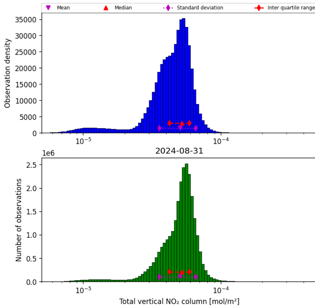
Figure 38: Histogram of “Total vertical NO 2 column” for 2024-08-30 to 2024-09-01
