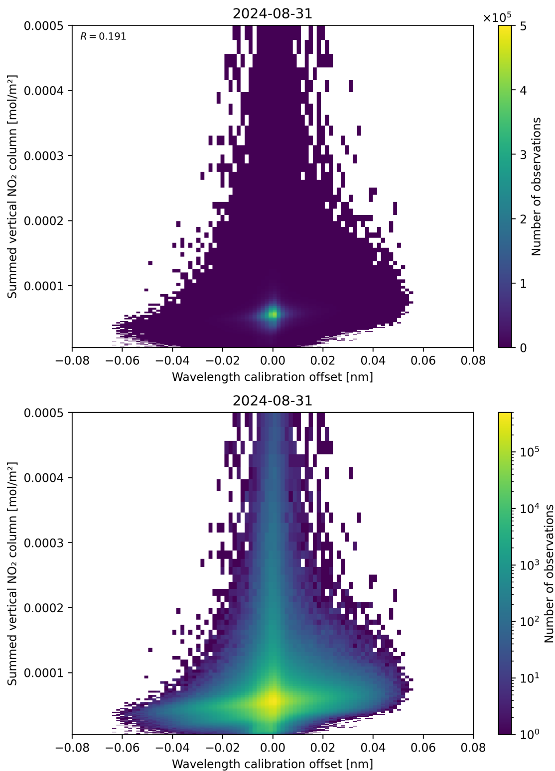
Figure 177: Scatter density plot of “Wavelength calibration offset” against “Summed vertical NO 2 column” for 2024-08-30 to 2024-09-01.
