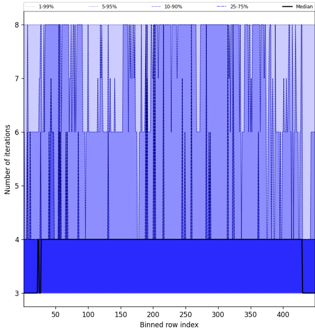
Figure 51: Along track statistics of “Number of iterations” for 2024-08-30 to 2024-09-01
