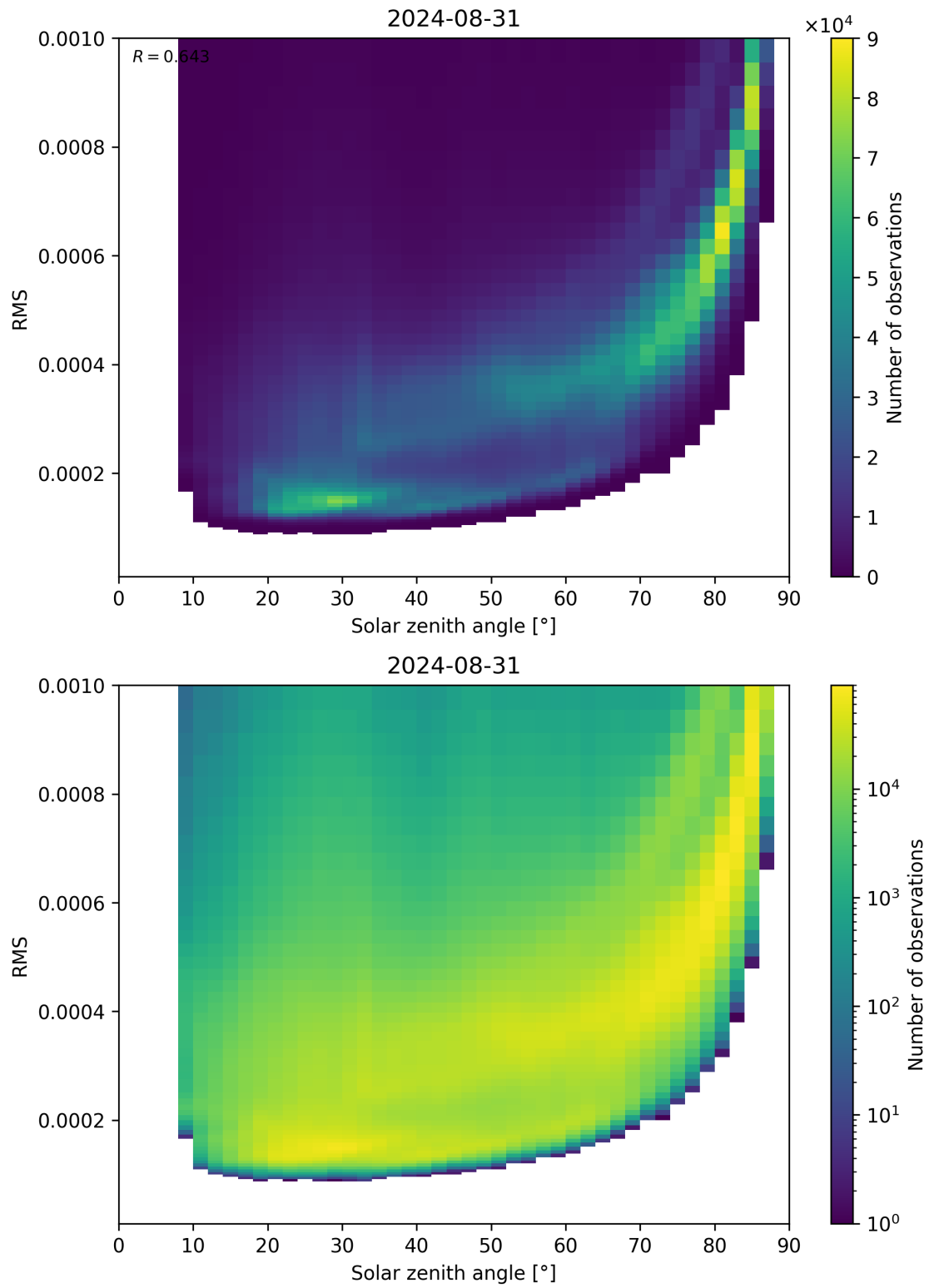
Figure 157: Scatter density plot of “Solar zenith angle” against “RMS” for 2024-08-30 to 2024-09-01.
