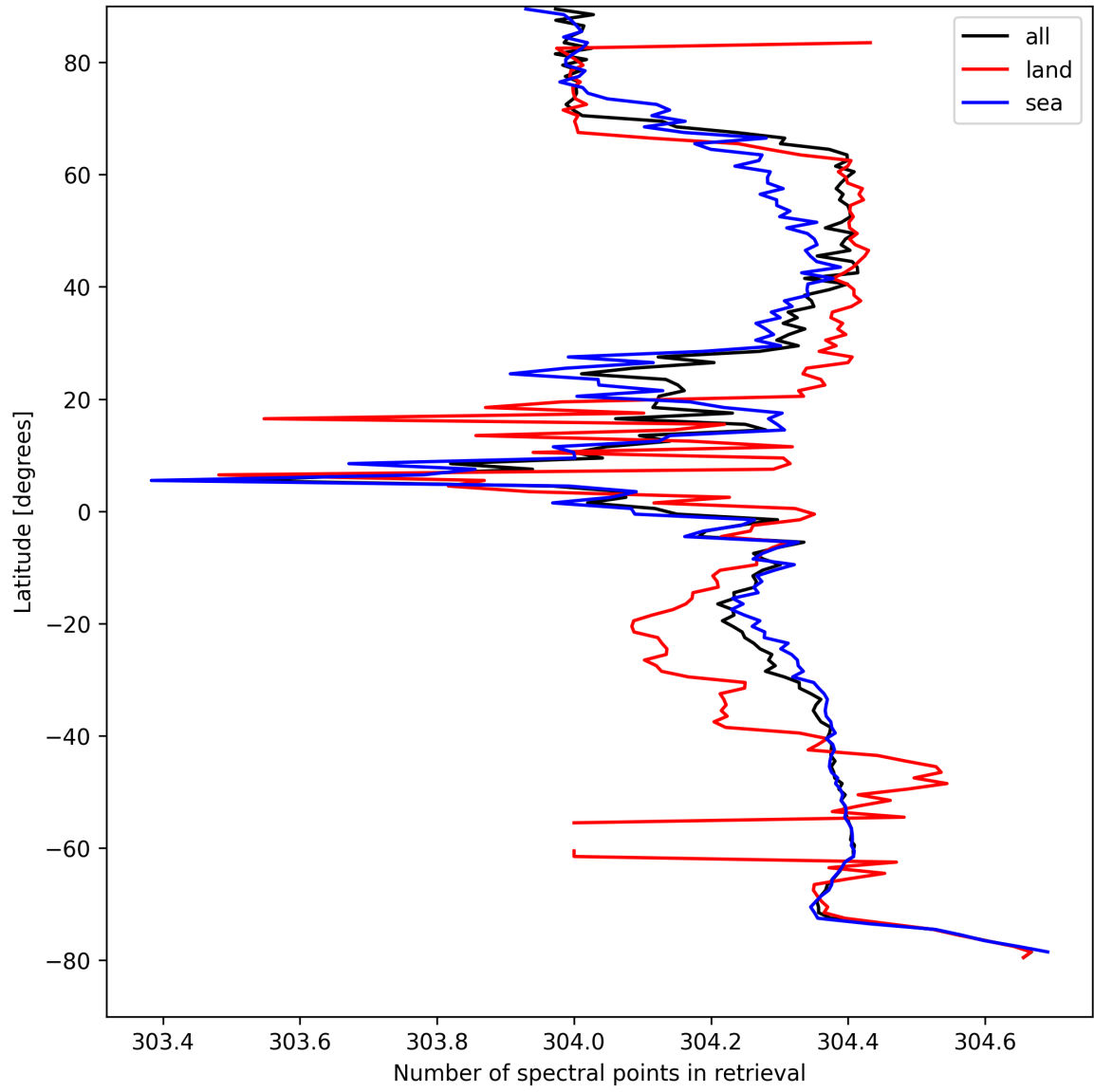
Figure 16: Zonal average of “Number of spectral points in retrieval” for 2024-08-30 to 2024-09-01.
