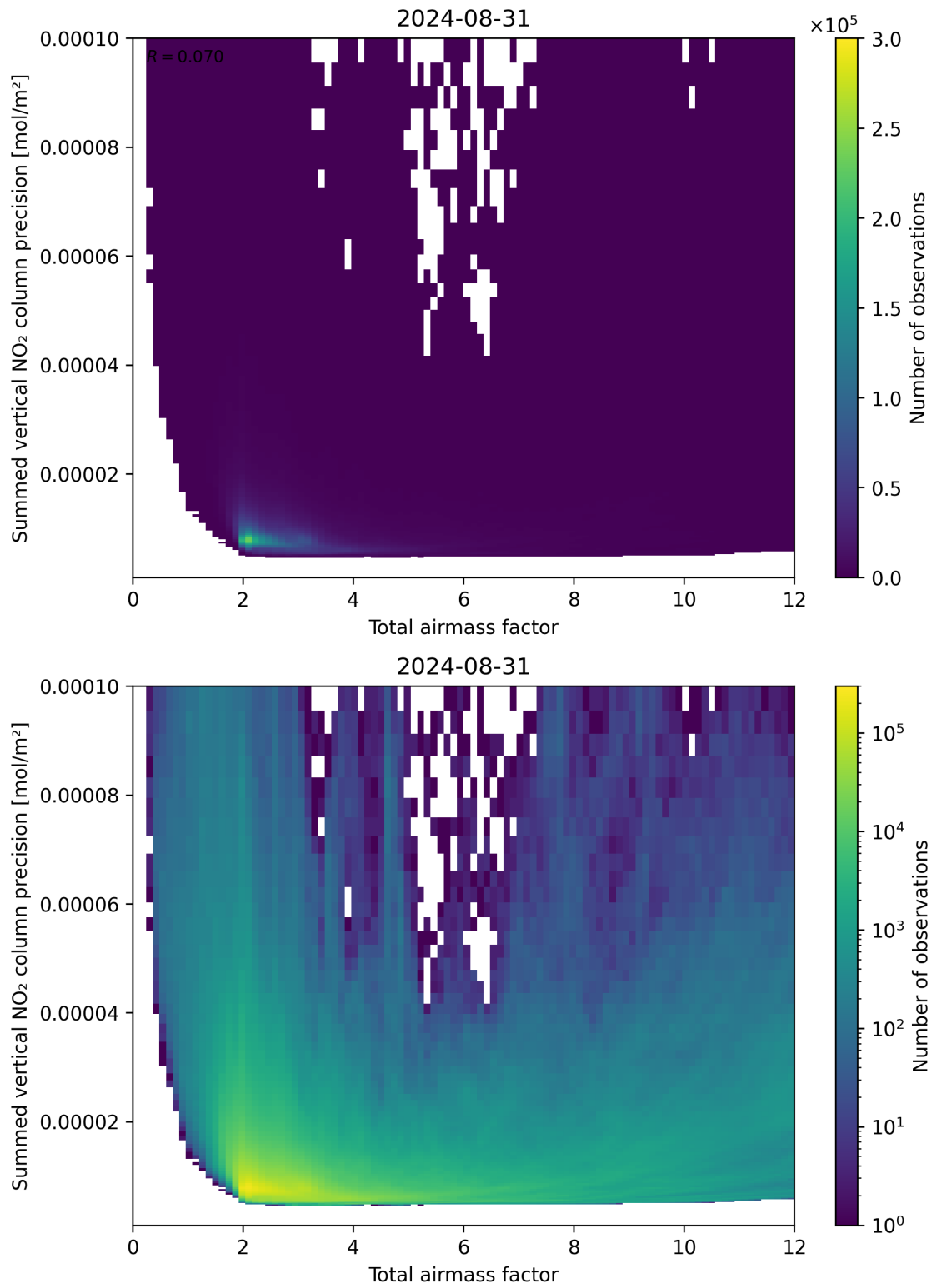
Figure 66: Scatter density plot of “Total airmass factor” against “Summed vertical NO 2 column precision” for 2024-08-30 to 2024-09-01.
