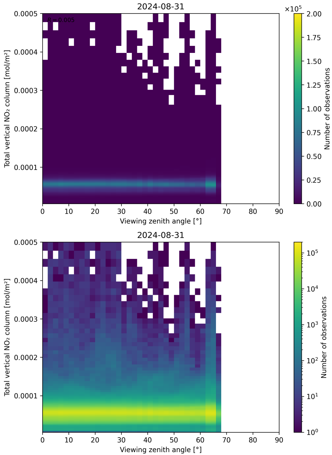
Figure 167: Scatter density plot of “Viewing zenith angle” against “Total vertical NO 2 column” for 2024-08-30 to 2024-09-01.
