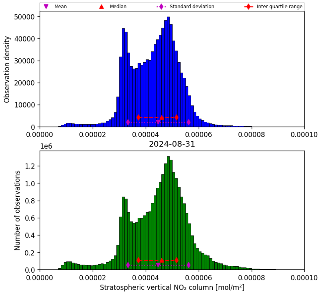
Figure 36: Histogram of “Stratospheric vertical NO 2 column” for 2024-08-30 to 2024-09-01
