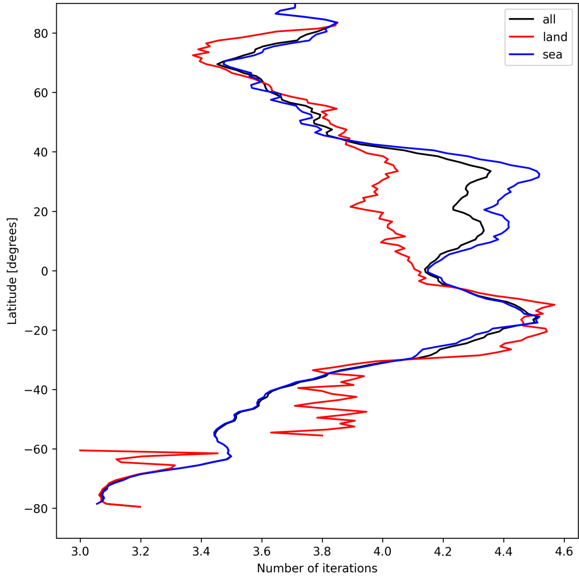
Figure 17: Zonal average of “Number of iterations” for 2024-08-30 to 2024-09-01.
