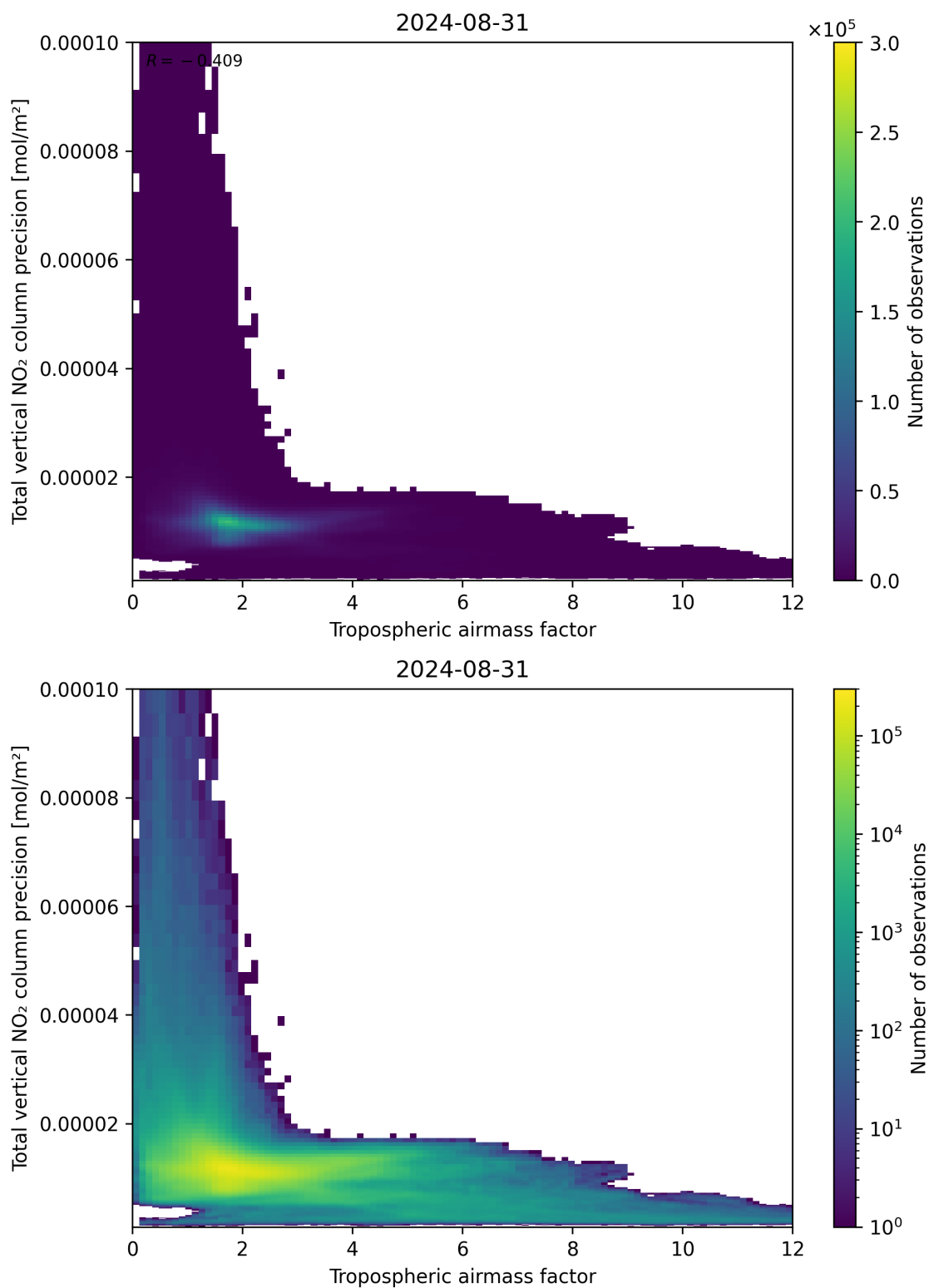
Figure 78: Scatter density plot of “Tropospheric air mass factor” against “Total vertical NO 2 column precision” for 2024-08-30 to 2024-09-01.
