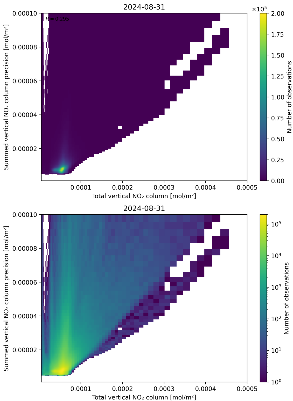
Figure 113: Scatter density plot of “Total vertical NO 2 column” against “Summed vertical NO 2 column precision” for 2024-08-30 to 2024-09-01.
