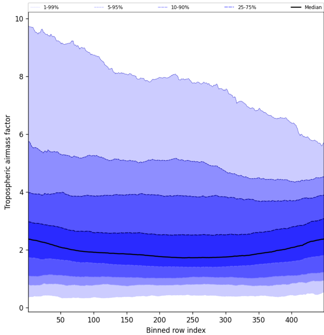
Figure 48: Along track statistics of “Tropospheric air mass factor” for 2024-08-30 to 2024-09-01
