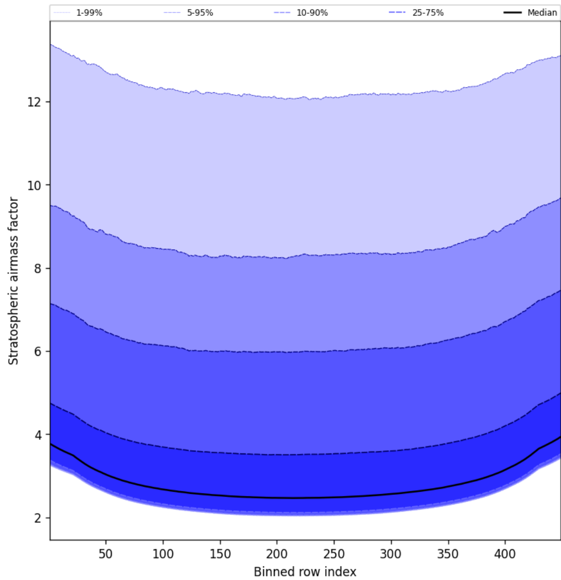
Figure 61: Along track statistics of “Stratospheric airmass factor” for 2024-08-30 to 2024-09-01
