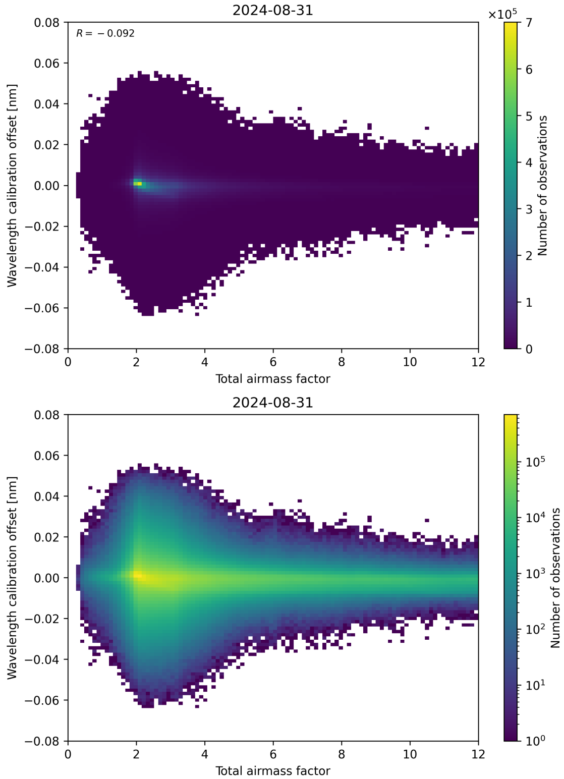
Figure 70: Scatter density plot of “Total airmass factor” against “Wavelength calibration offset” for 2024-08-30 to 2024-09-01.
