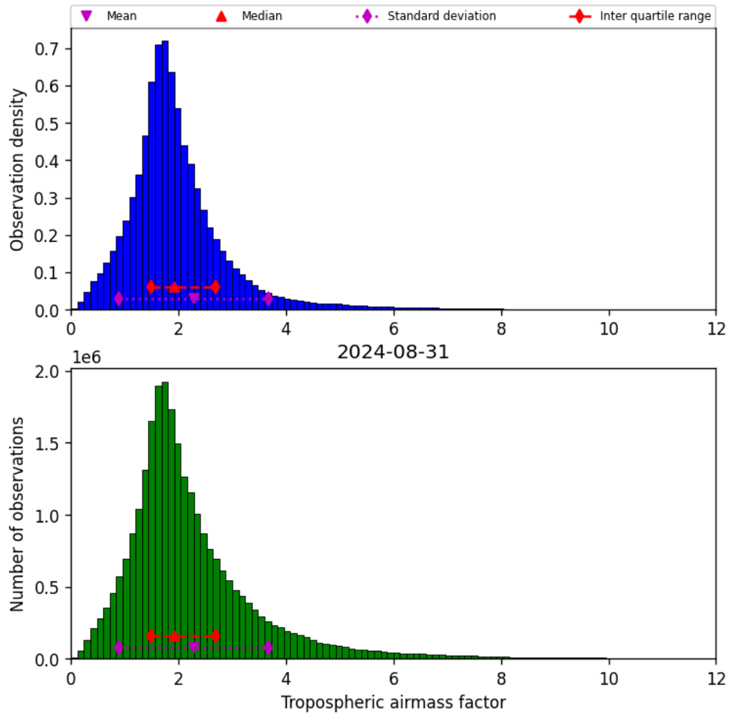
Figure 31: Histogram of “Tropospheric airmass factor” for 2024-08-30 to 2024-09-01
