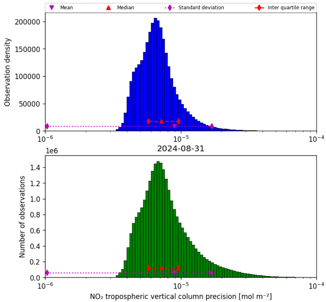
Figure 30: Histogram of “NO 2 tropospheric vertical column precision” for 2024-08-30 to 2024-09-01
