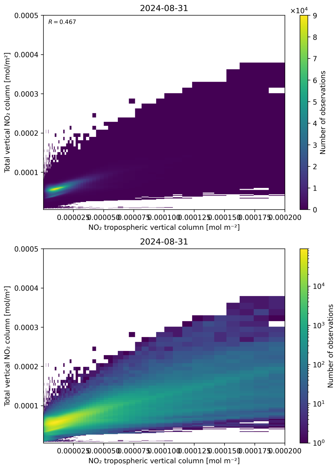
Figure 128: Scatter density plot of “NO 2 tropospheric vertical column” against “Total vertical NO 2 column” for 2024-08-30 to 2024-09-01.
