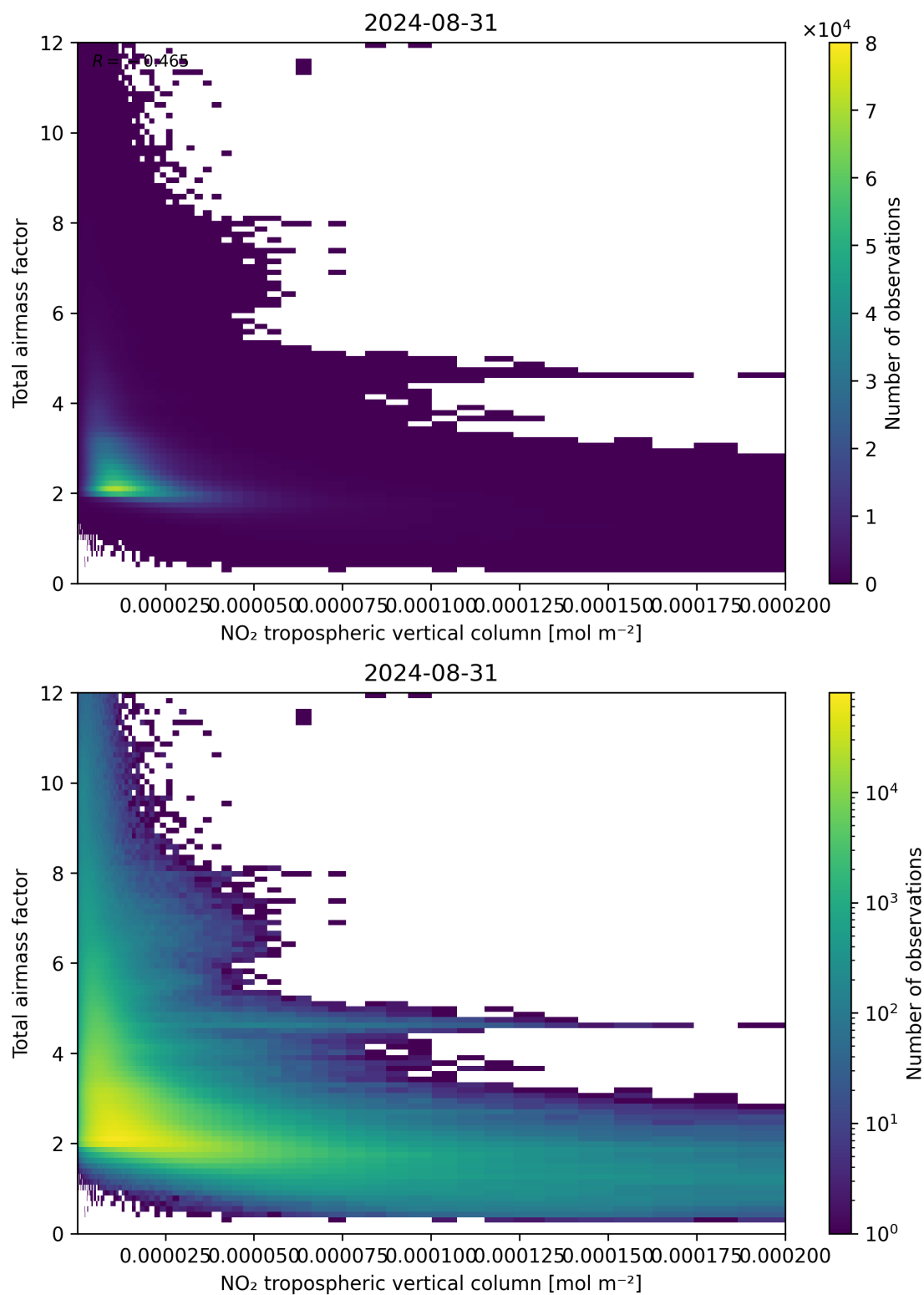
Figure 122: Scatter density plot of “NO 2 tropospheric vertical column” against “Total air mass factor” for 2024-08-30 to 2024-09-01.
