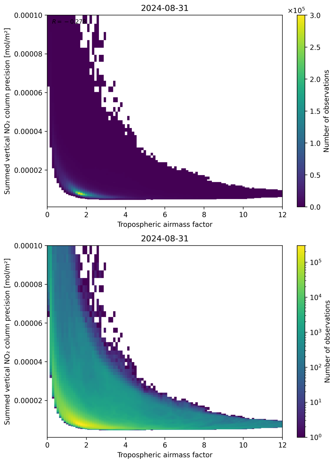
Figure 76: Scatter density plot of “Tropospheric air mass factor” against “Summed vertical NO 2 column precision” for 2024-08-30 to 2024-09-01.
