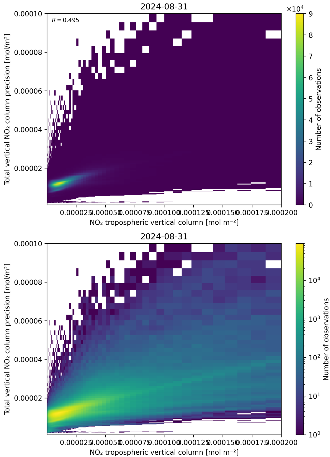
Figure 129: Scatter density plot of “NO 2 tropospheric vertical column” against “Total vertical NO 2 column precision” for 2024-08-30 to 2024-09-01.
