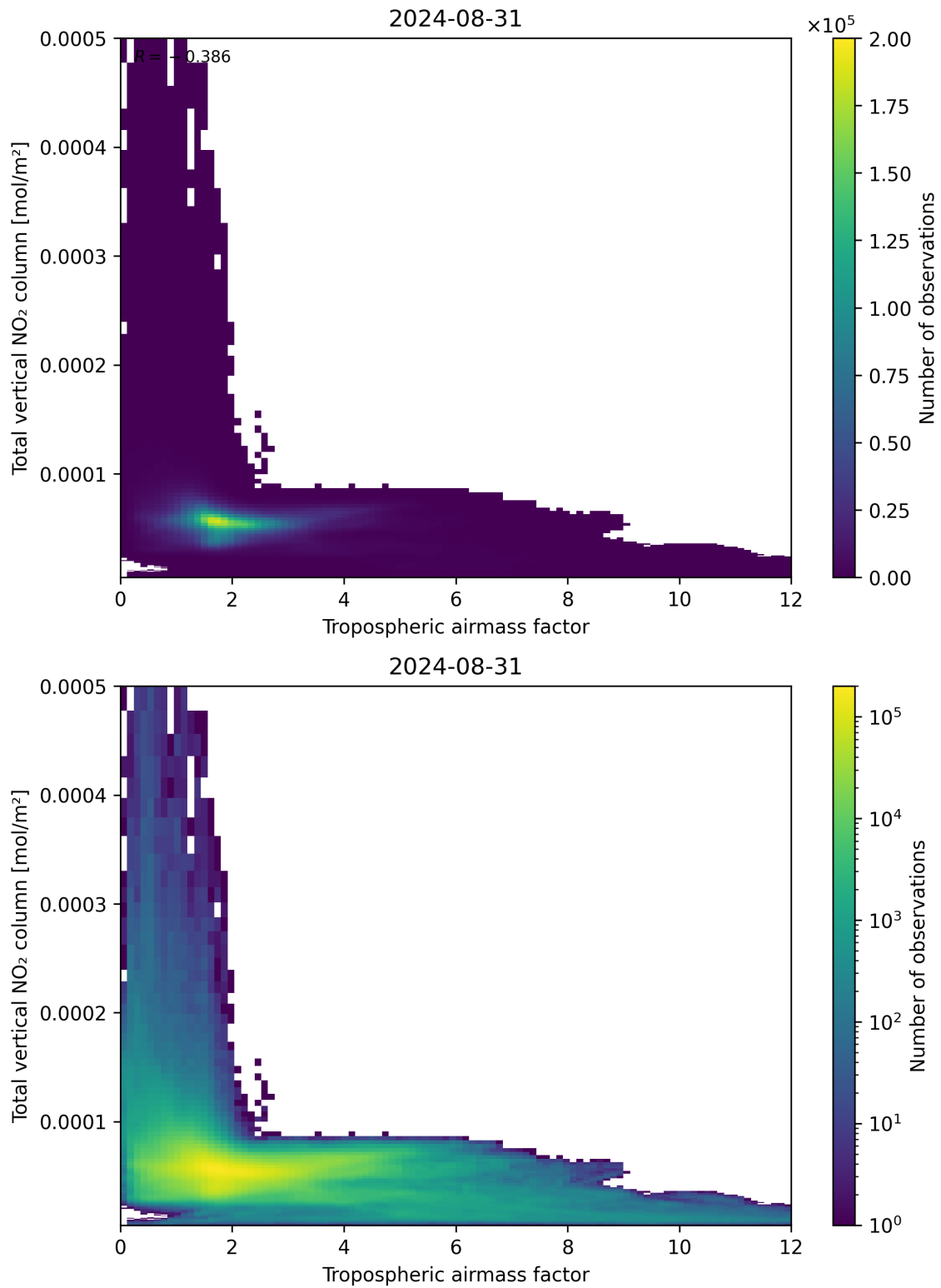
Figure 77: Scatter density plot of “Tropospheric airmass factor” against “Total vertical \text{NO}_2 column” for 2024-08-30 to 2024-09-01.
