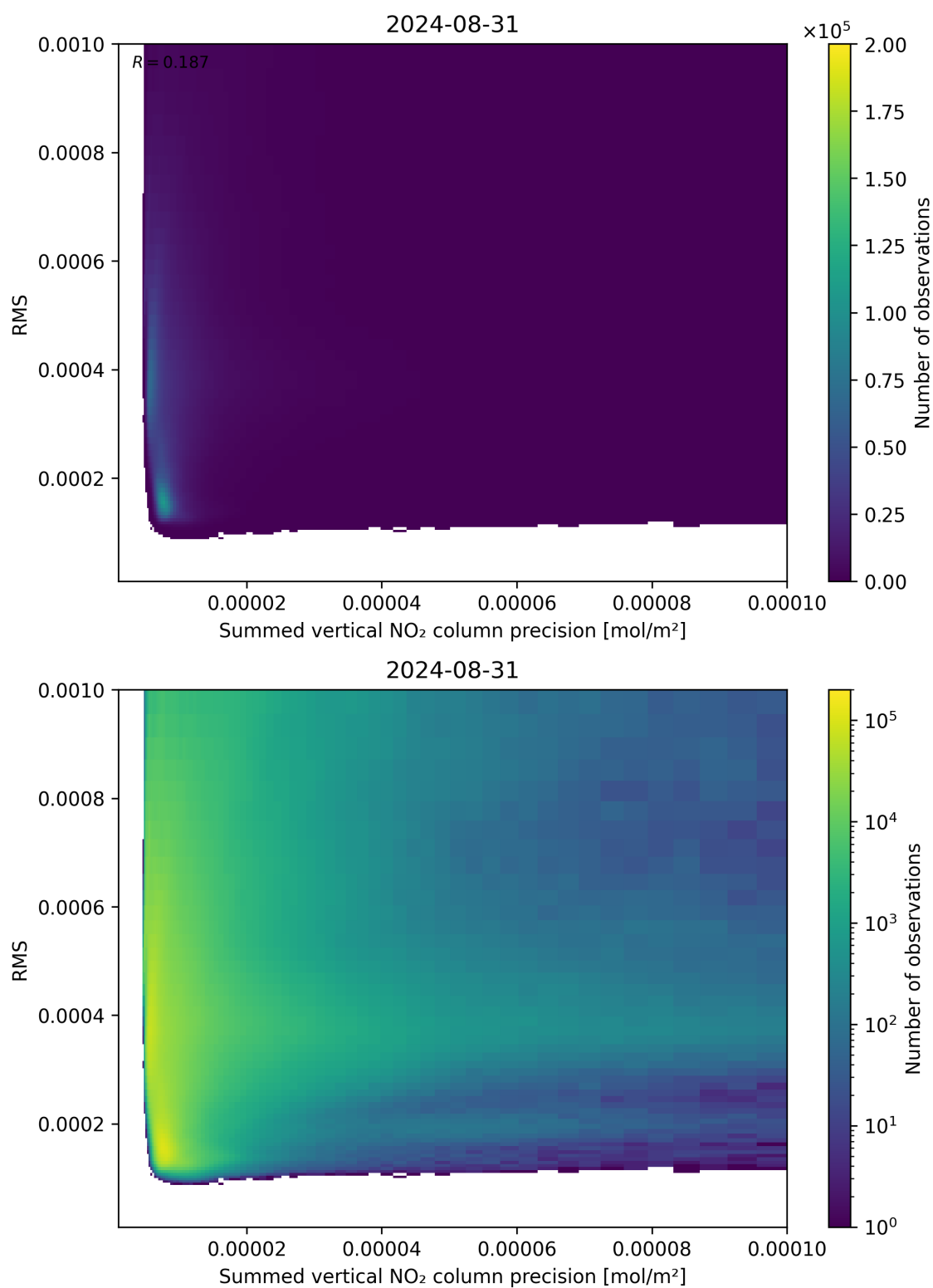
Figure 108: Scatter density plot of “Summed vertical NO 2 column precision” against “RMS” for 2024-08-30 to 2024-09-01.
