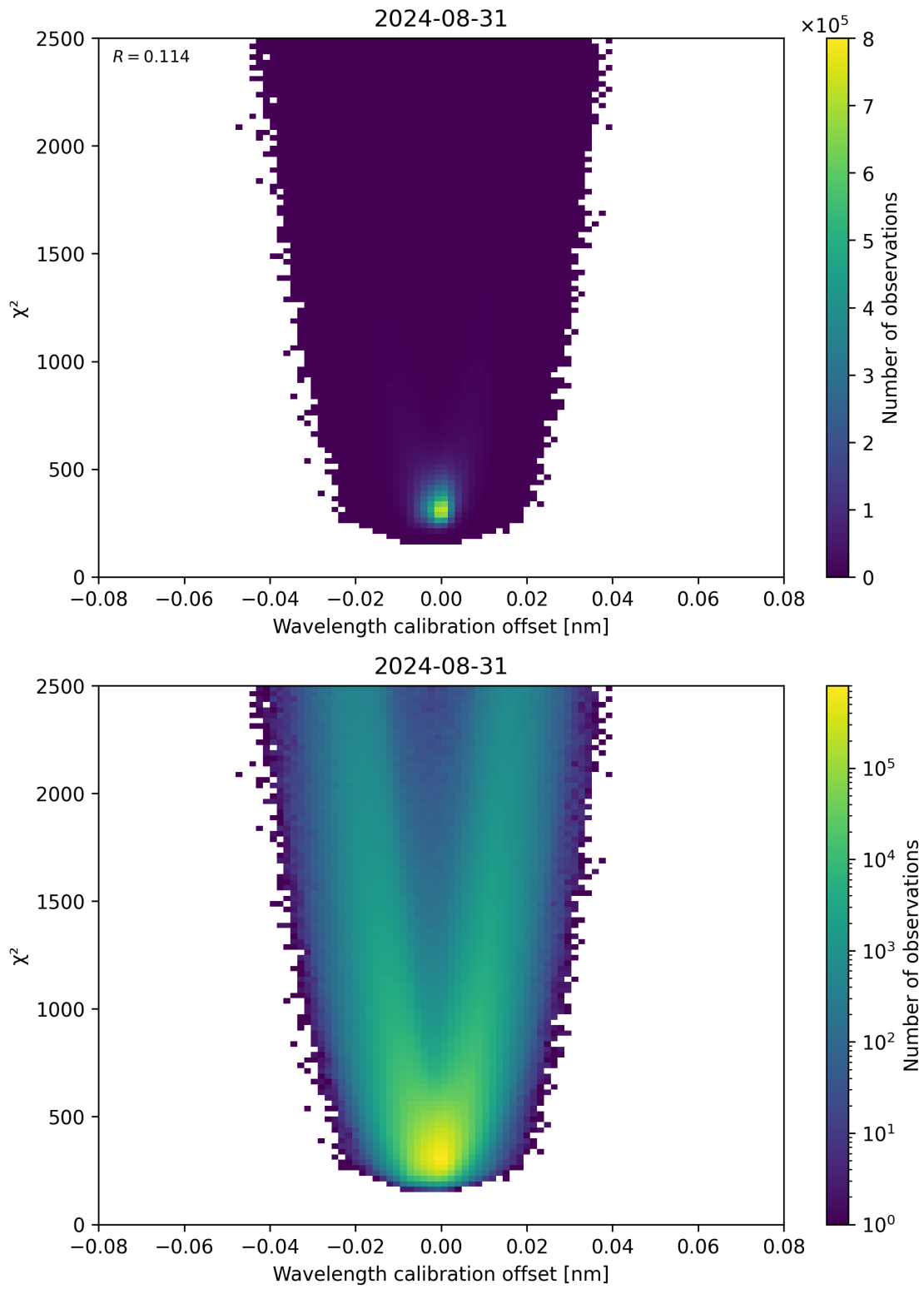
Figure 175: Scatter density plot of “Wavelength calibration offset” against “ \chi^2 ” for 2024-08-30 to 2024-09-01.
