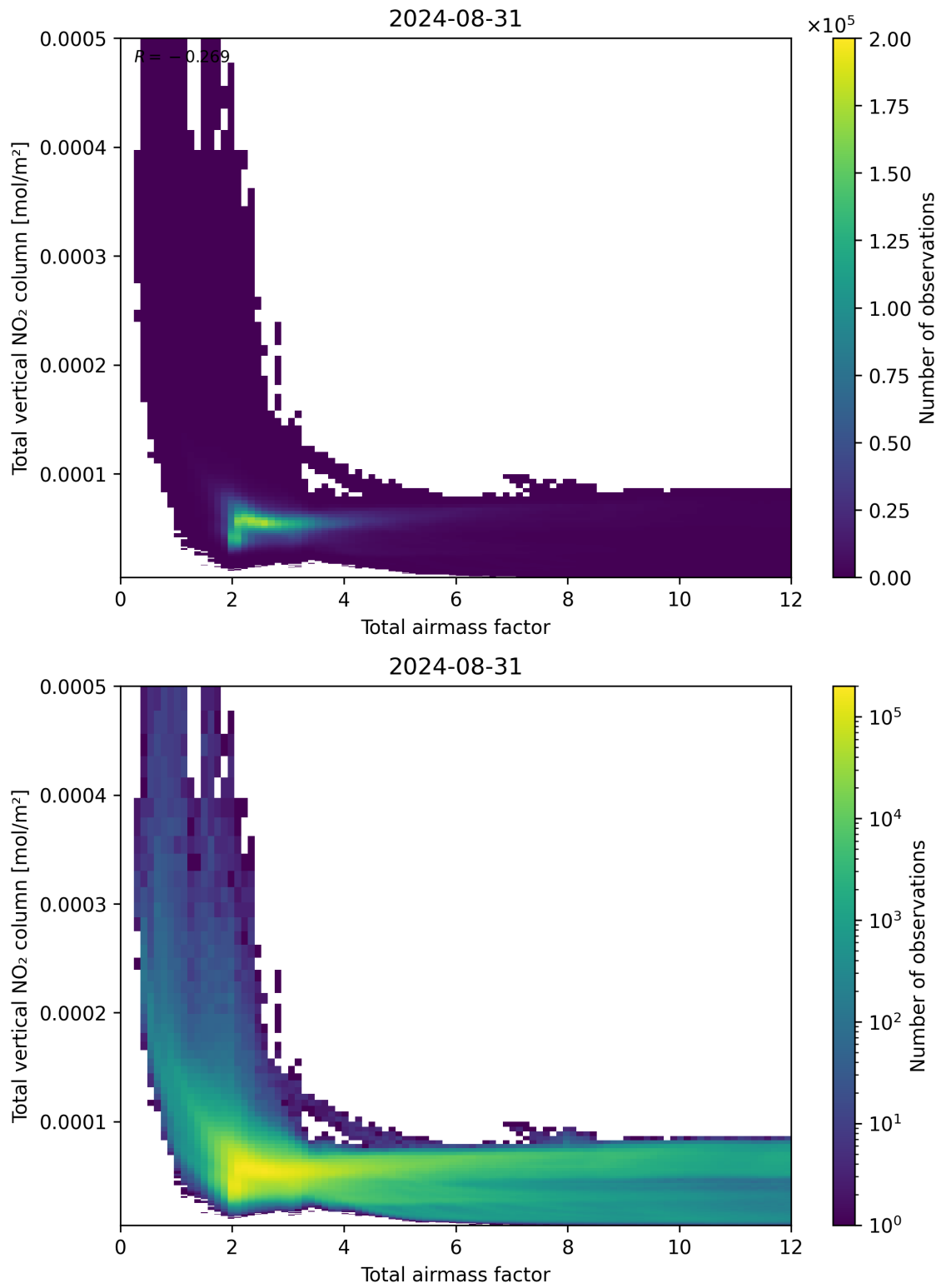
Figure 67: Scatter density plot of “Total airmass factor” against “Total vertical NO 2 column” for 2024-08-30 to 2024-09-01.
