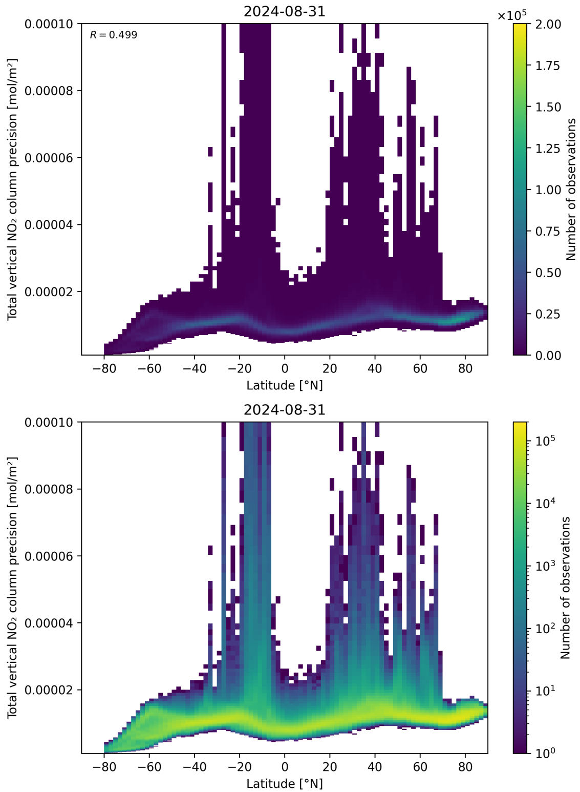
Figure 91: Scatter density plot of “Latitude” against “Total vertical NO 2 column precision” for 2024-08-30 to 2024-09-01.
