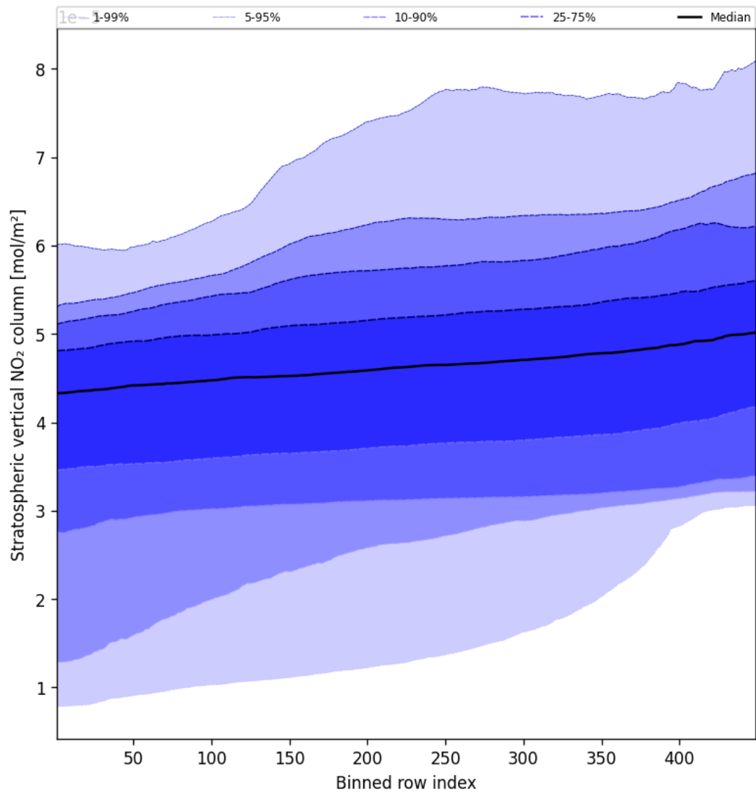
Figure 53: Along track statistics of “Stratospheric vertical NO 2 column” for 2024-08-30 to 2024-09-01
