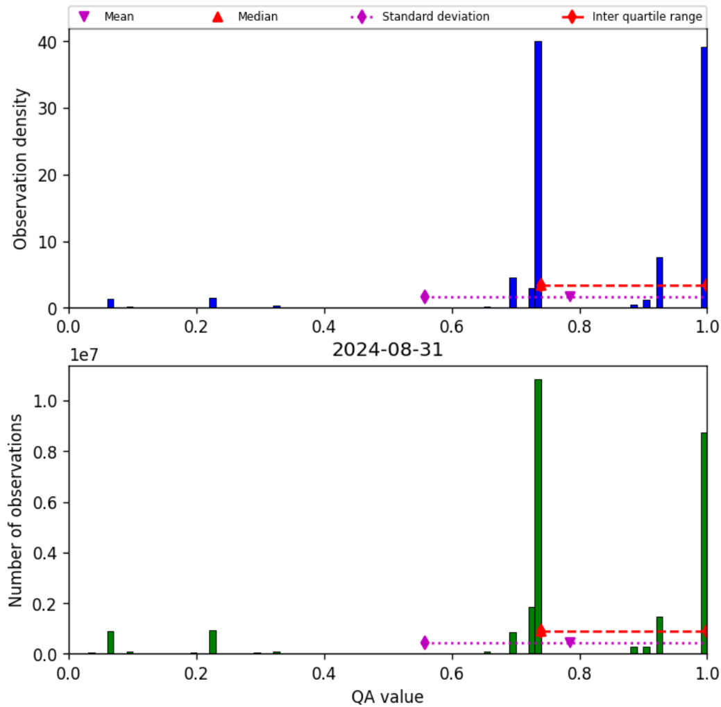
Figure 28: Histogram of “QA value” for 2024-08-30 to 2024-09-01
