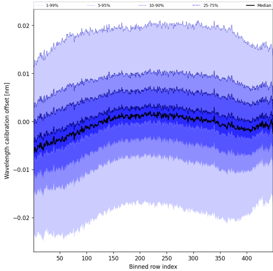
Figure 52: Along track statistics of “Wavelength calibration offset” for 2024-08-30 to 2024-09-01
