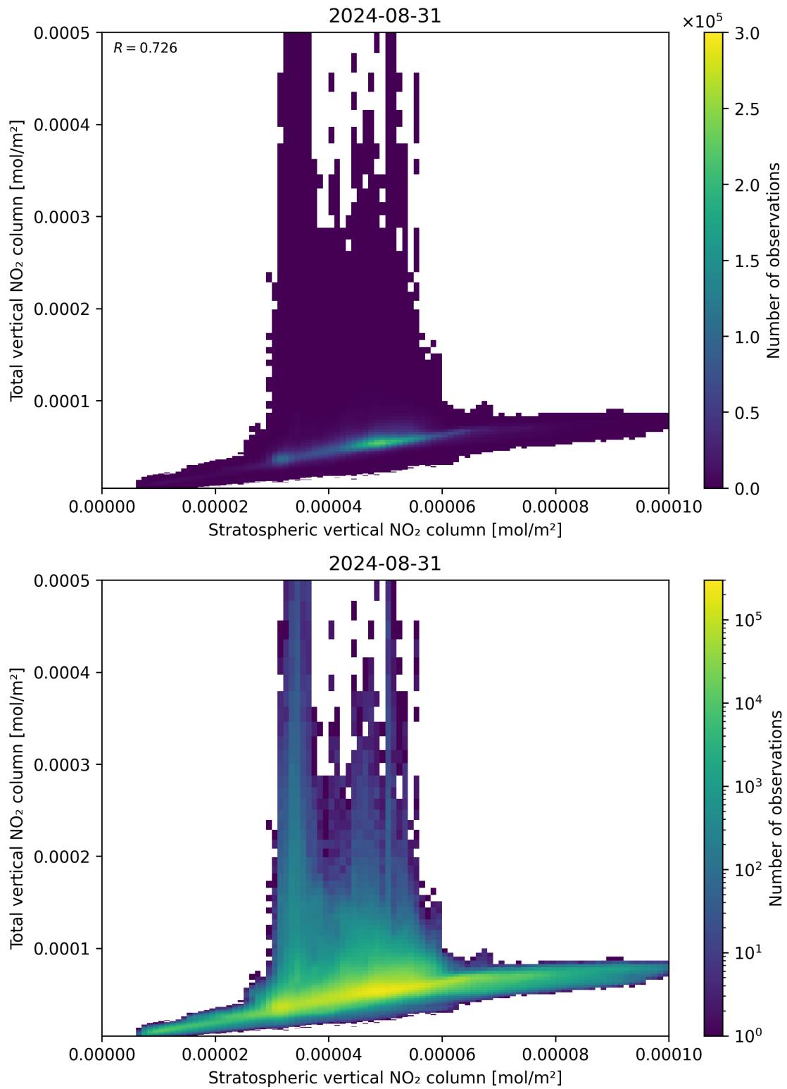
Figure 100: Scatter density plot of “Stratospheric vertical NO 2 column” against “Total vertical NO 2 column” for 2024-08-30 to 2024-09-01.
