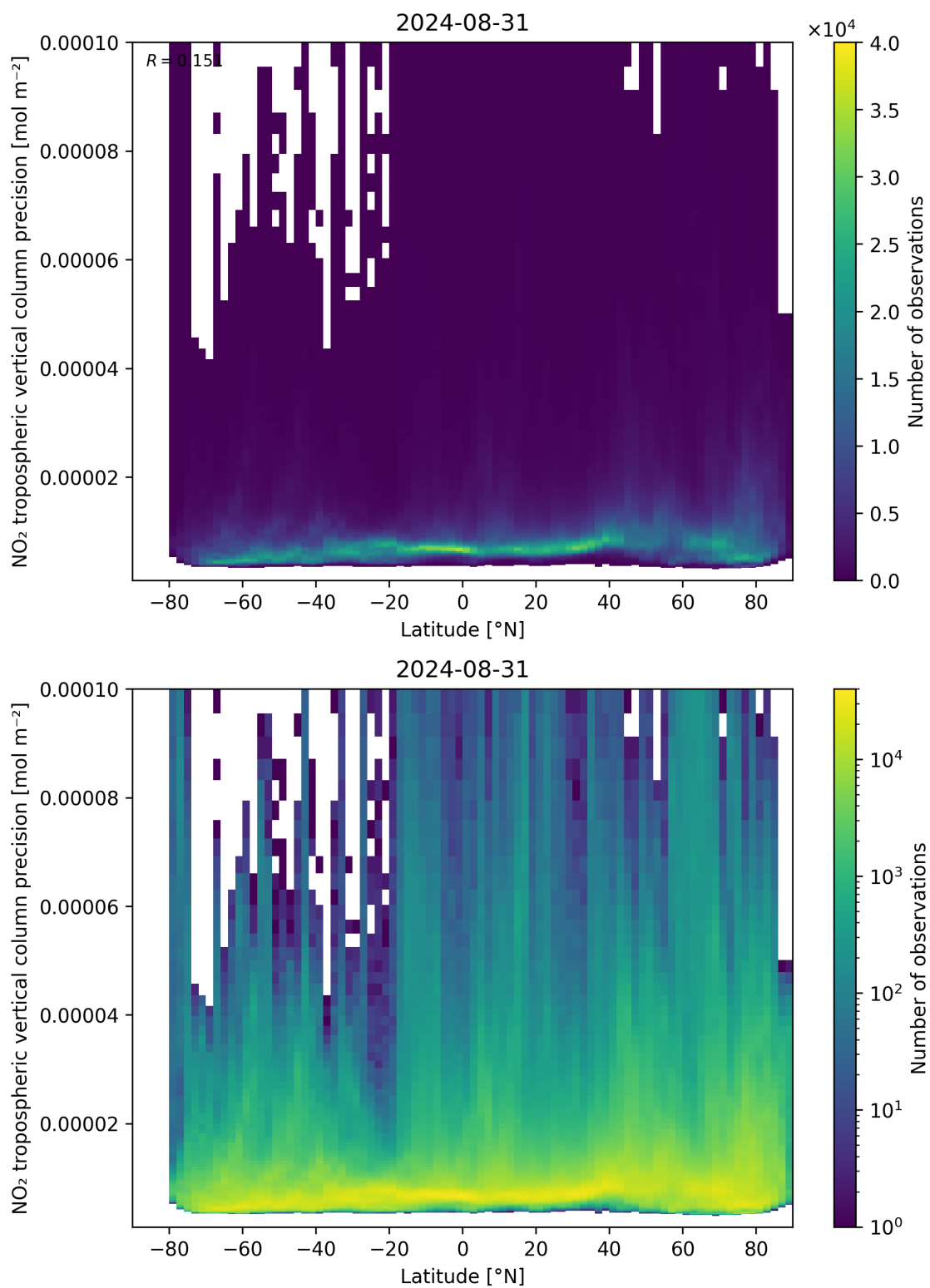
Figure 93: Scatter density plot of “Latitude” against “NO 2 tropospheric vertical column precision” for 2024-08-30 to 2024-09-01.
