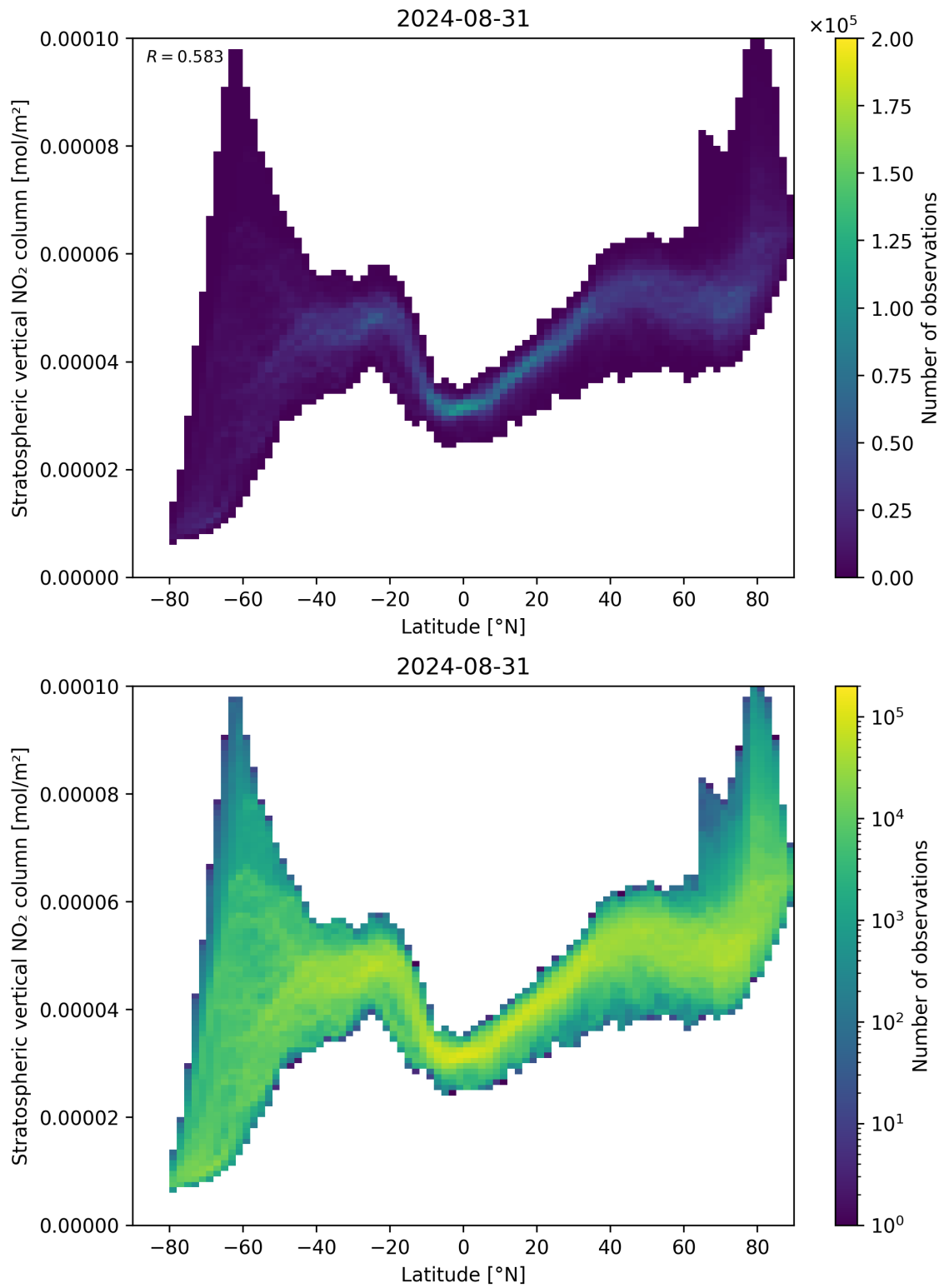
Figure 87: Scatter density plot of “Latitude” against “Stratospheric vertical NO 2 column” for 2024-08-30 to 2024-09-01.
