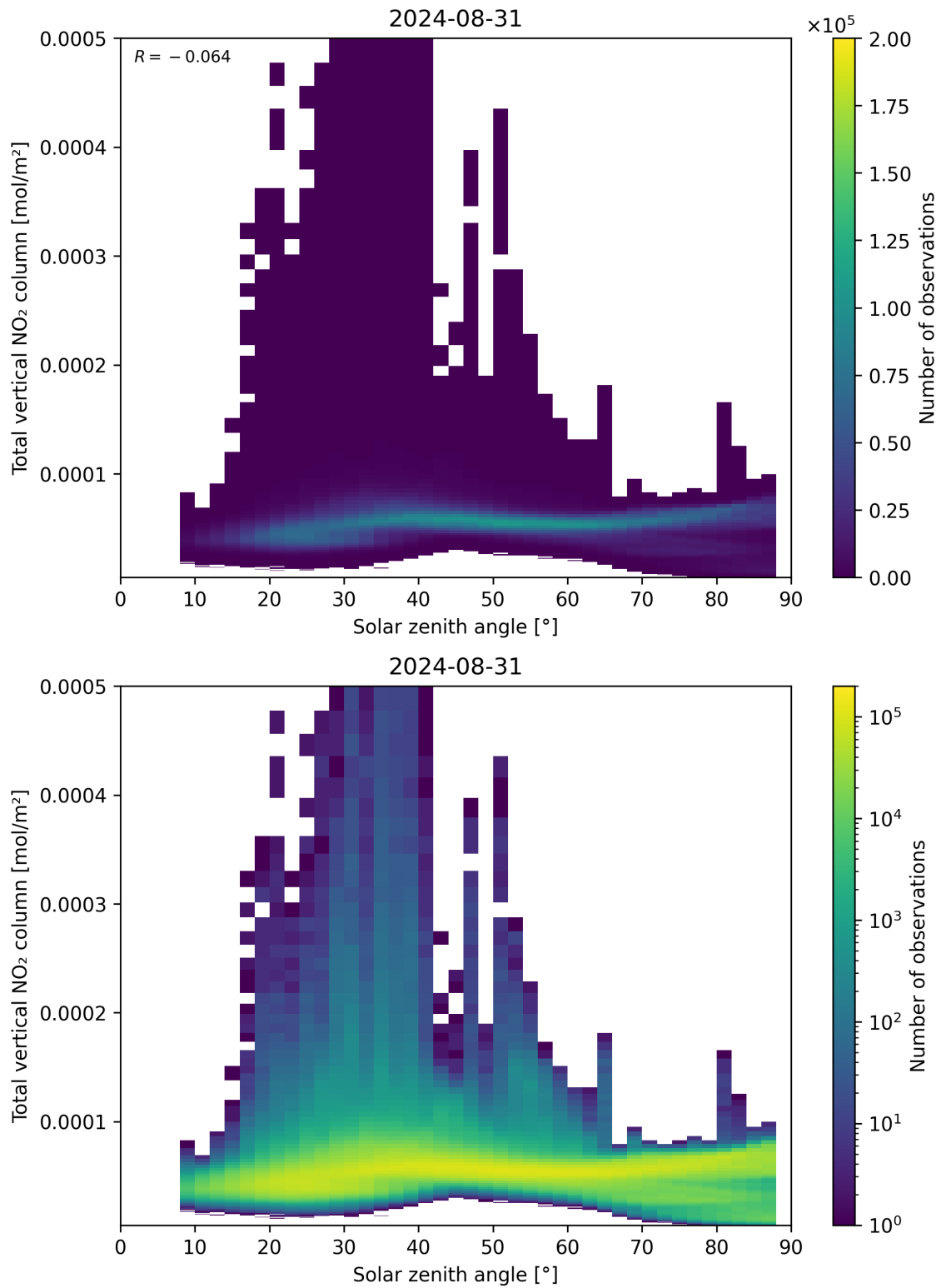
Figure 153: Scatter density plot of “Solar zenith angle” against “Total vertical NO 2 column” for 2024-08-30 to 2024-09-01.
