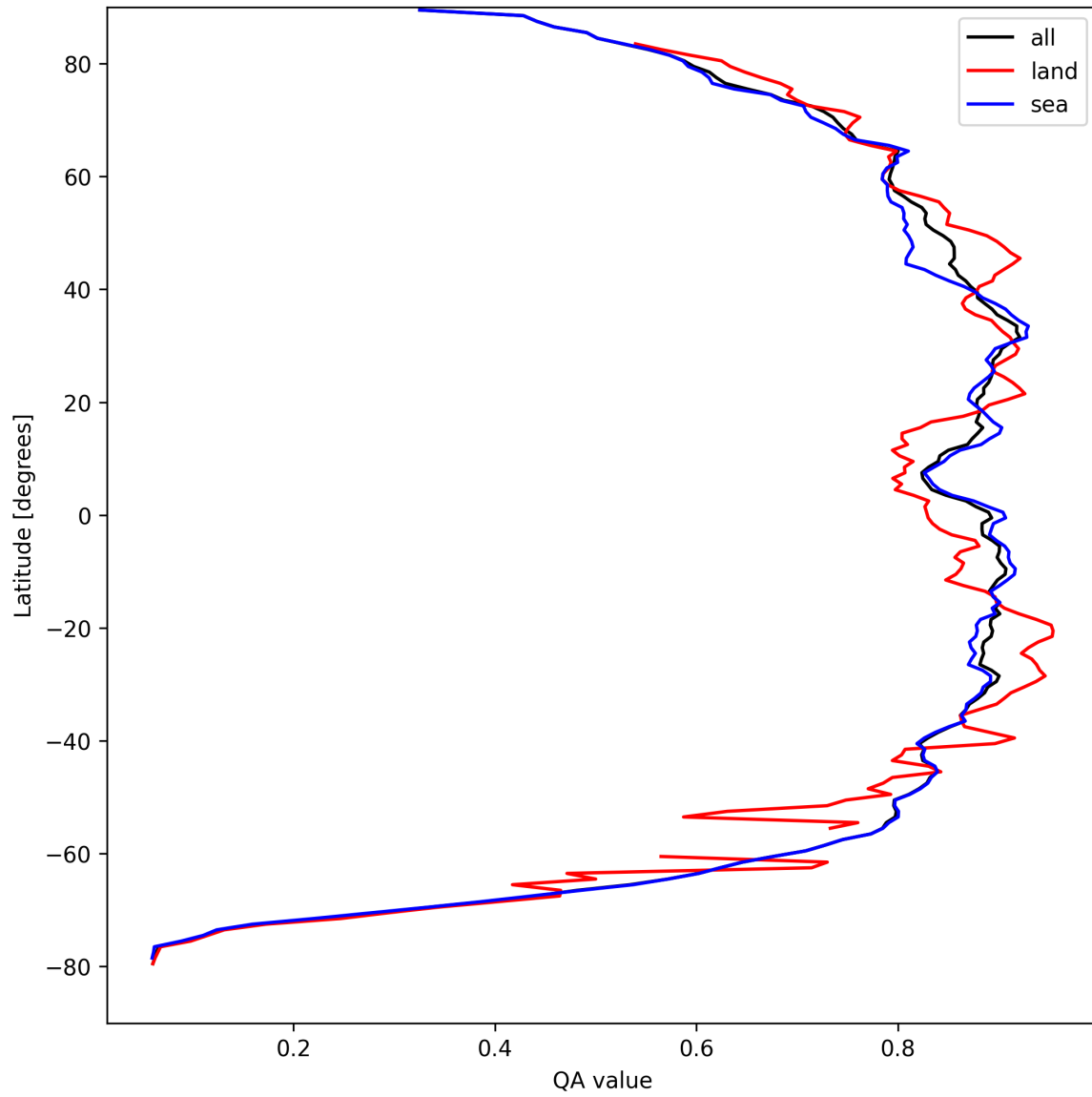
Figure 11: Zonal average of “QA value” for 2024-08-30 to 2024-09-01.
