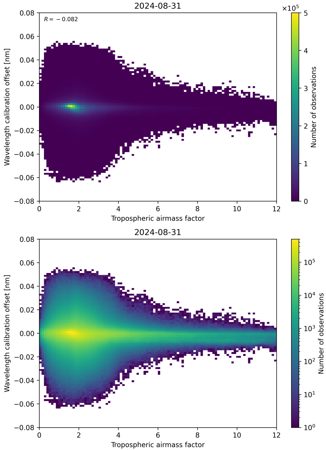
Figure 80: Scatter density plot of “Tropospheric air mass factor” against “Wavelength calibration offset” for 2024-08-30 to 2024-09-01.
