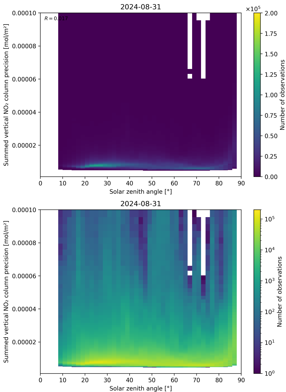
Figure 152: Scatter density plot of “Solar zenith angle” against “Summed vertical NO 2 column precision” for 2024-08-30 to 2024-09-01.
