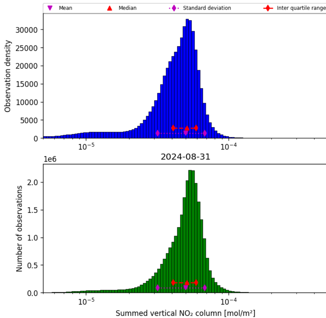
Figure 40: Histogram of "Summed vertical NO 2 column" for 2024-08-30 to 2024-09-01
