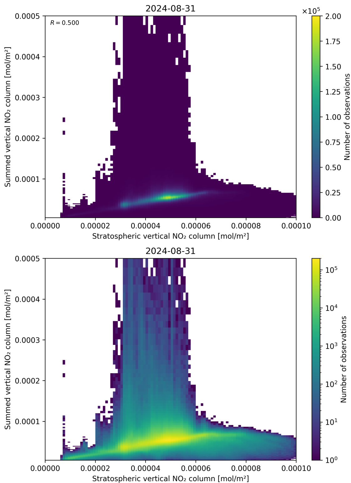
Figure 98: Scatter density plot of “Stratospheric vertical NO 2 column” against “Summed vertical NO 2 column” for 2024-08-30 to 2024-09-01.
