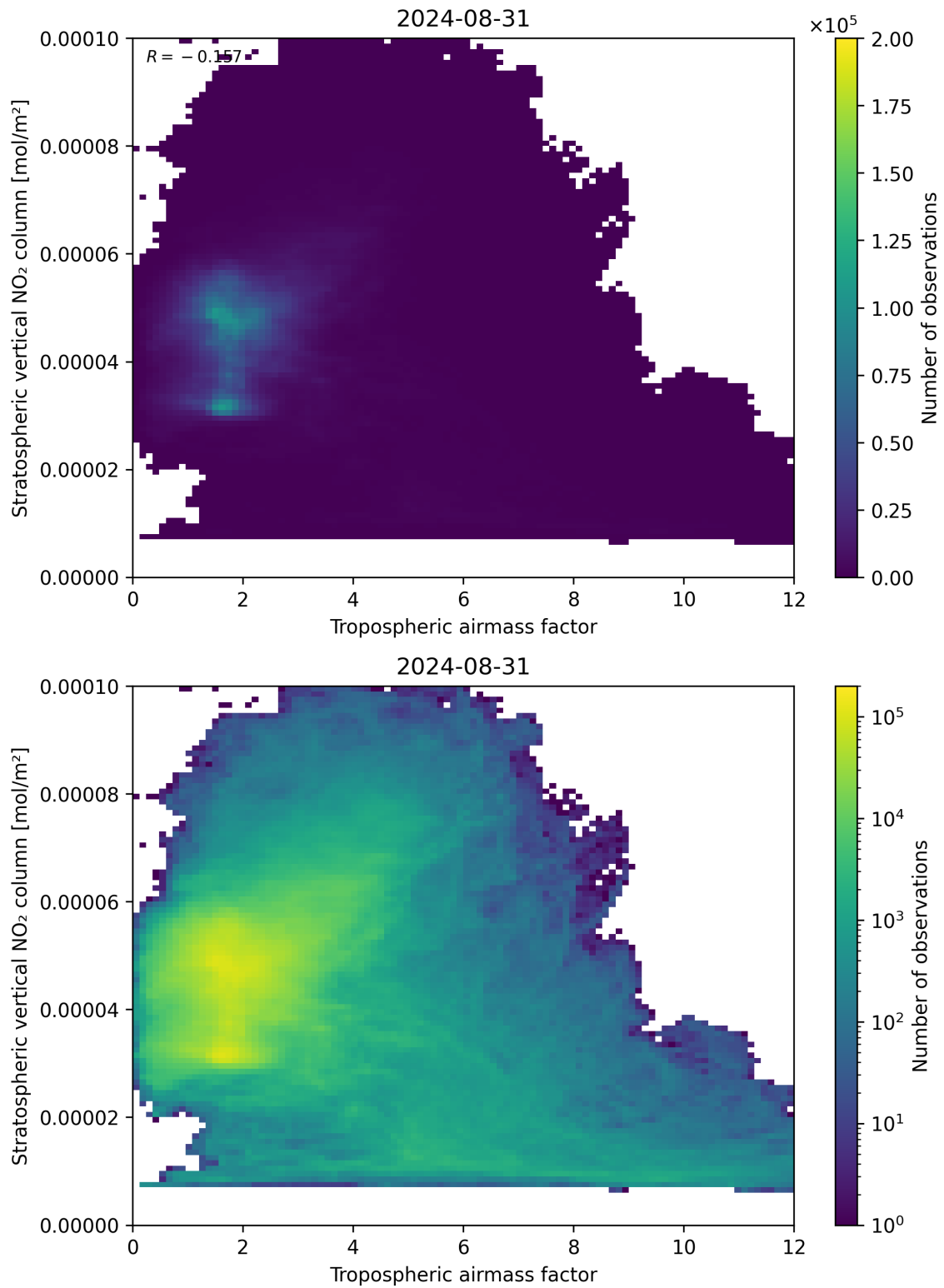
Figure 74: Scatter density plot of “Tropospheric air mass factor” against “Stratospheric vertical NO 2 column” for 2024-08-30 to 2024-09-01.
