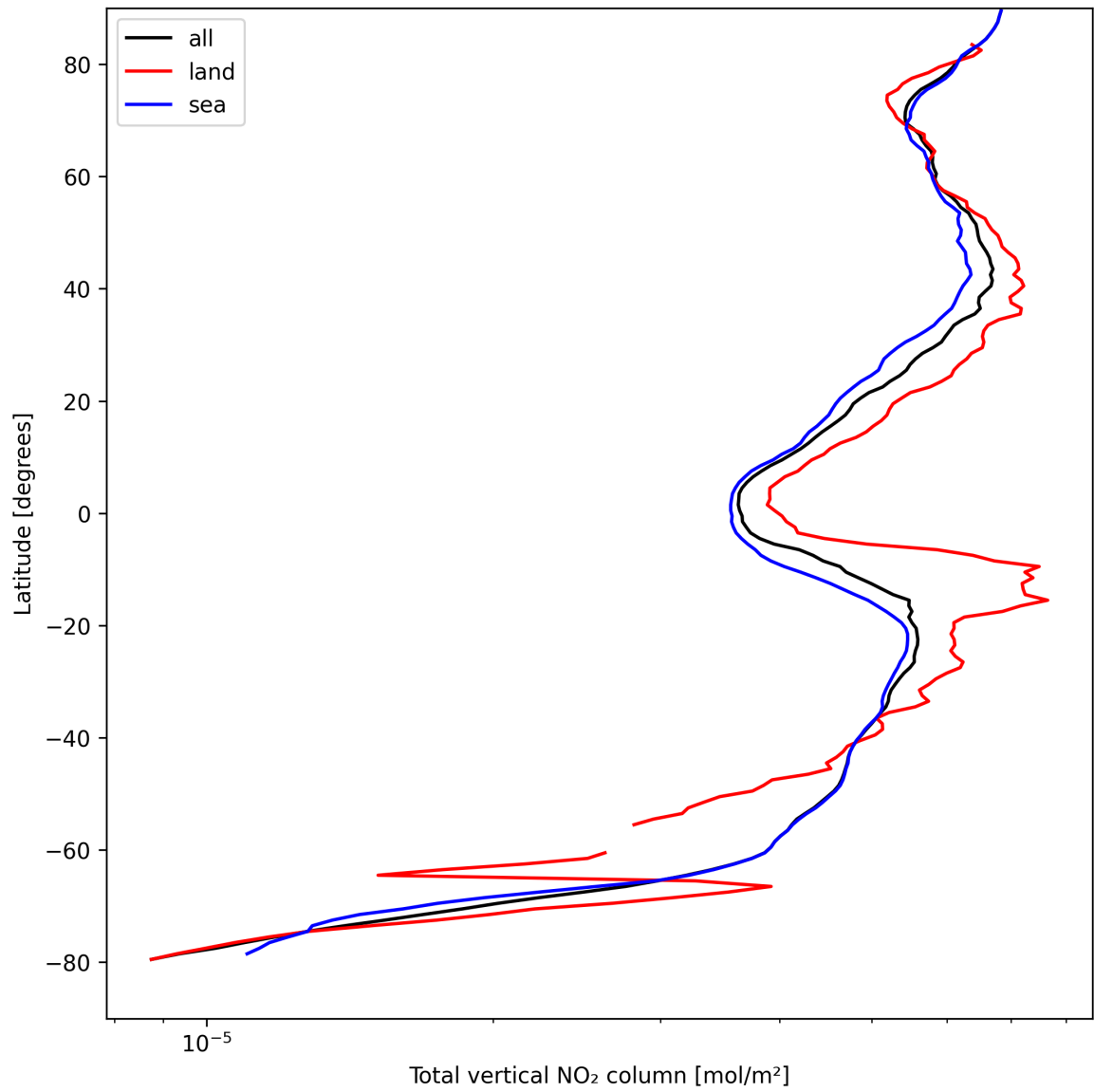
Figure 21: Zonal average of “Total vertical NO 2 column” for 2024-08-30 to 2024-09-01.
