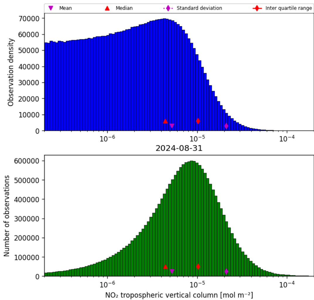
Figure 29: Histogram of “NO 2 tropospheric vertical column” for 2024-08-30 to 2024-09-01
