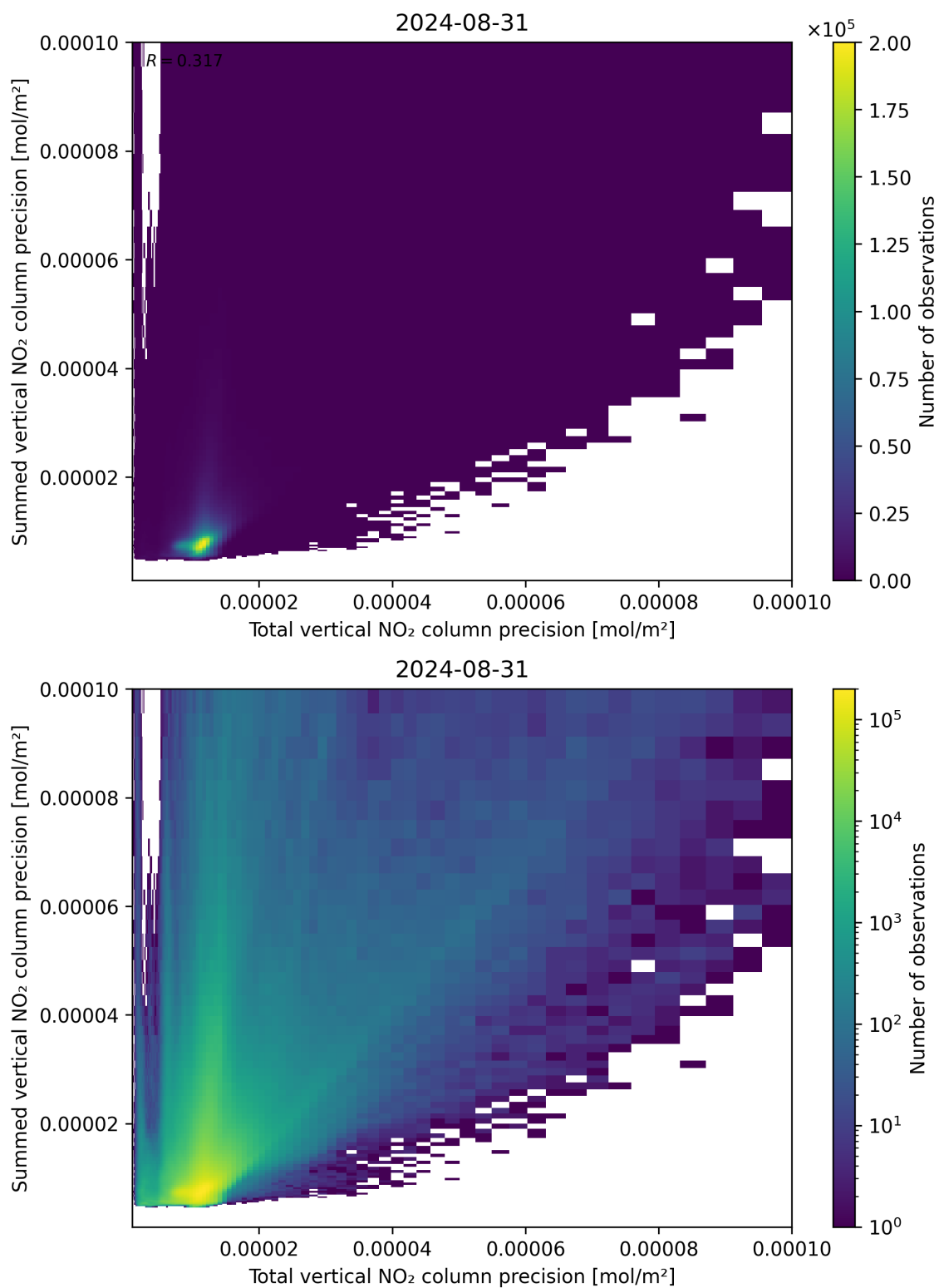
Figure 118: Scatter density plot of “Total vertical NO 2 column precision” against “Summed vertical NO 2 column precision” for 2024-08-30 to 2024-09-01.
