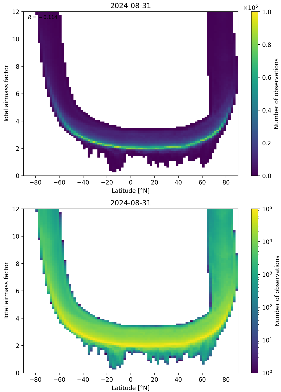
Figure 84: Scatter density plot of “Latitude” against “Total airmass factor” for 2024-08-30 to 2024-09-01.
