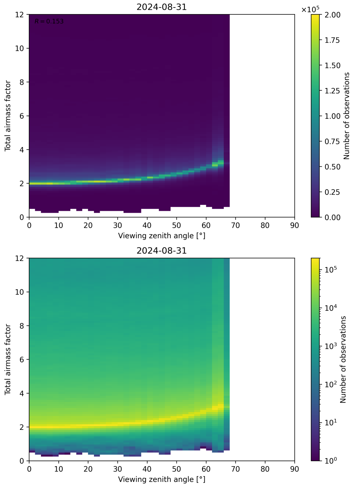
Figure 160: Scatter density plot of “Viewing zenith angle” against “Total airmass factor” for 2024-08-30 to 2024-09-01.
