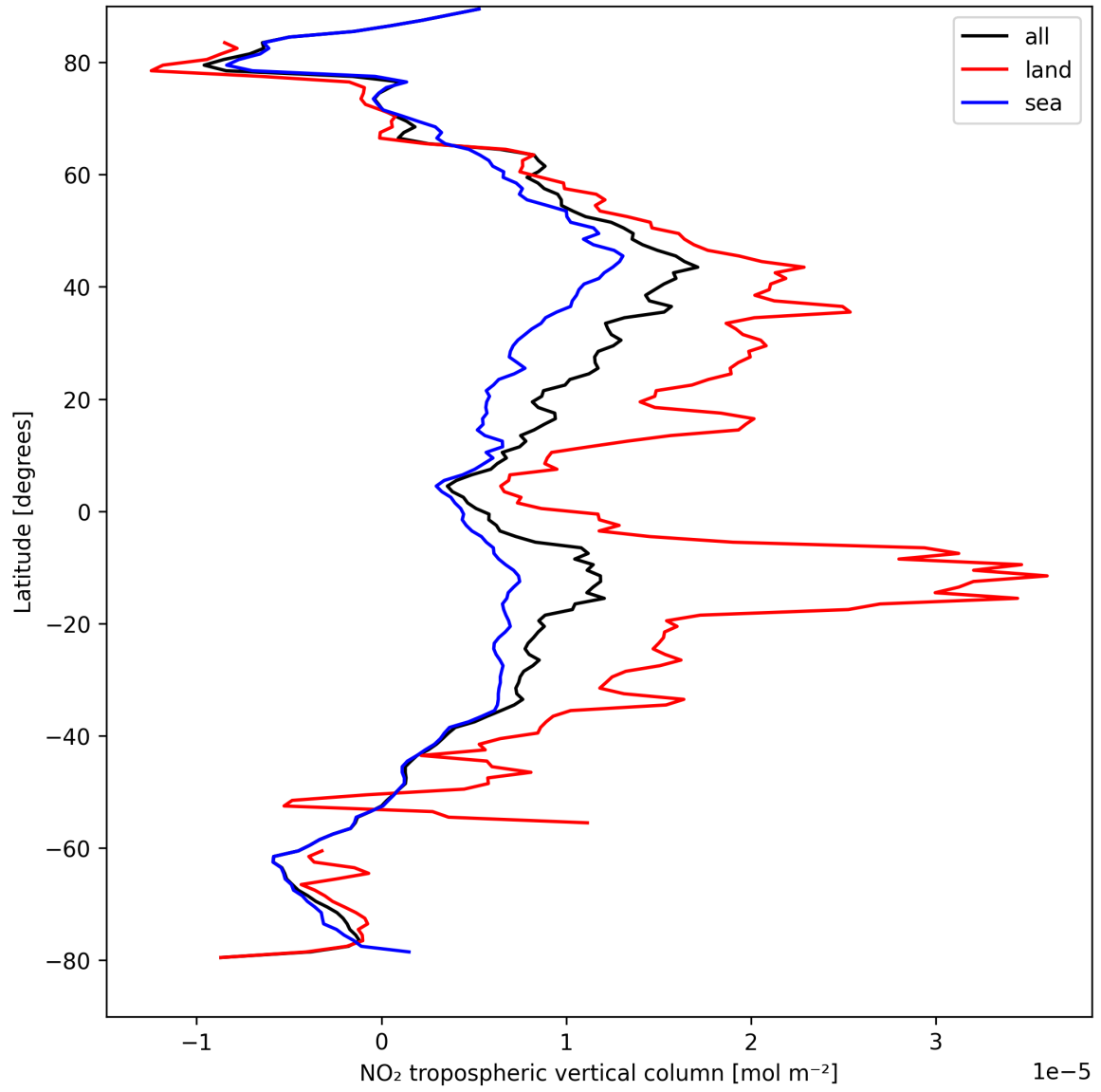
Figure 12: Zonal average of “NO 2 tropospheric vertical column” for 2024-08-30 to 2024-09-01.
