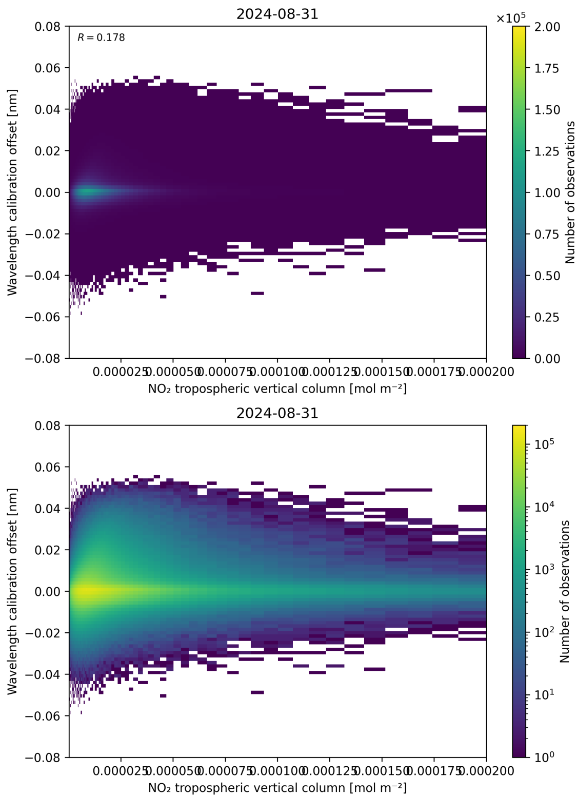
Figure 143: Scatter density plot of “NO 2 tropospheric vertical column” against “Wavelength calibration offset” for 2024-08-30 to 2024-09-01.
