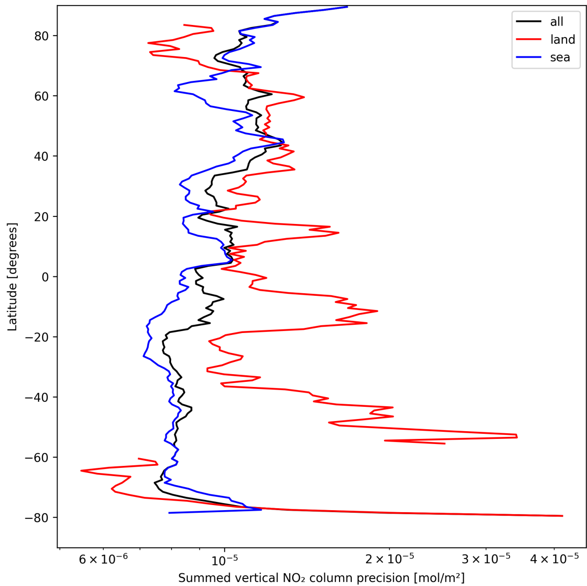
Figure 24: Zonal average of “Summed vertical NO 2 column precision” for 2024-08-30 to 2024-09-01.
