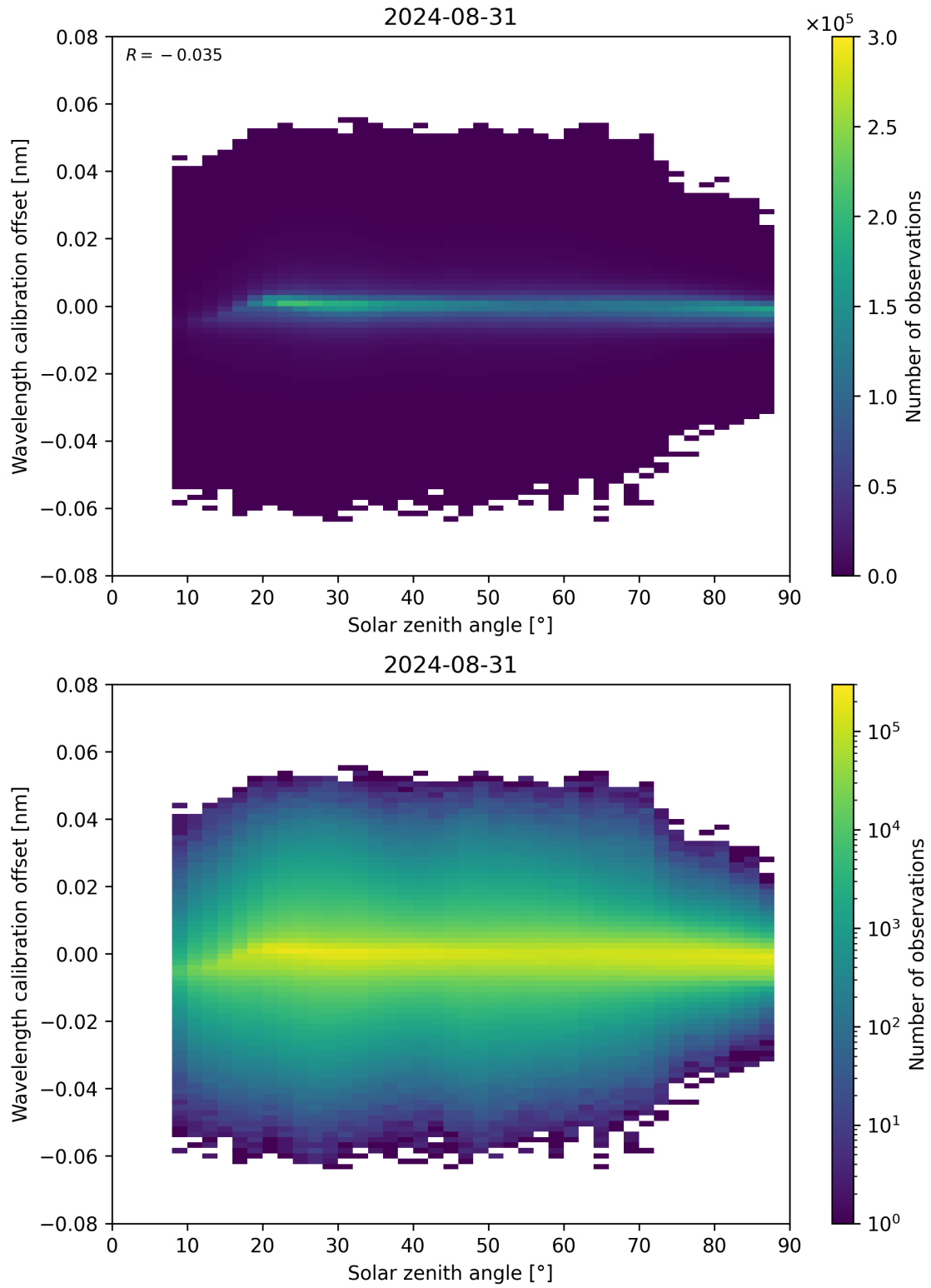
Figure 158: Scatter density plot of “Solar zenith angle” against “Wavelength calibration offset” for 2024-08-30 to 2024-09-01.
