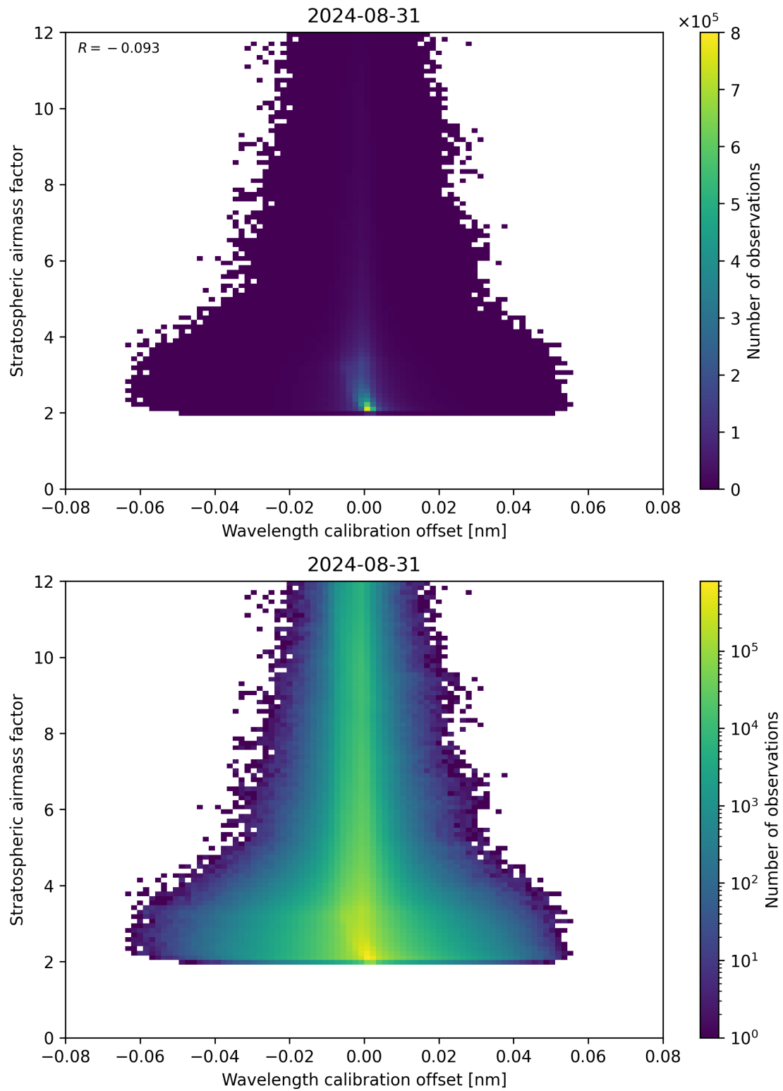
Figure 174: Scatter density plot of “Wavelength calibration offset” against “Stratospheric airmass factor” for 2024-08-30 to 2024-09-01.
