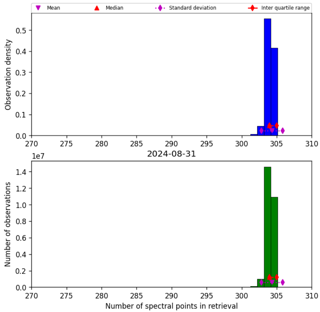
Figure 33: Histogram of “Number of spectral points in retrieval” for 2024-08-30 to 2024-09-01
