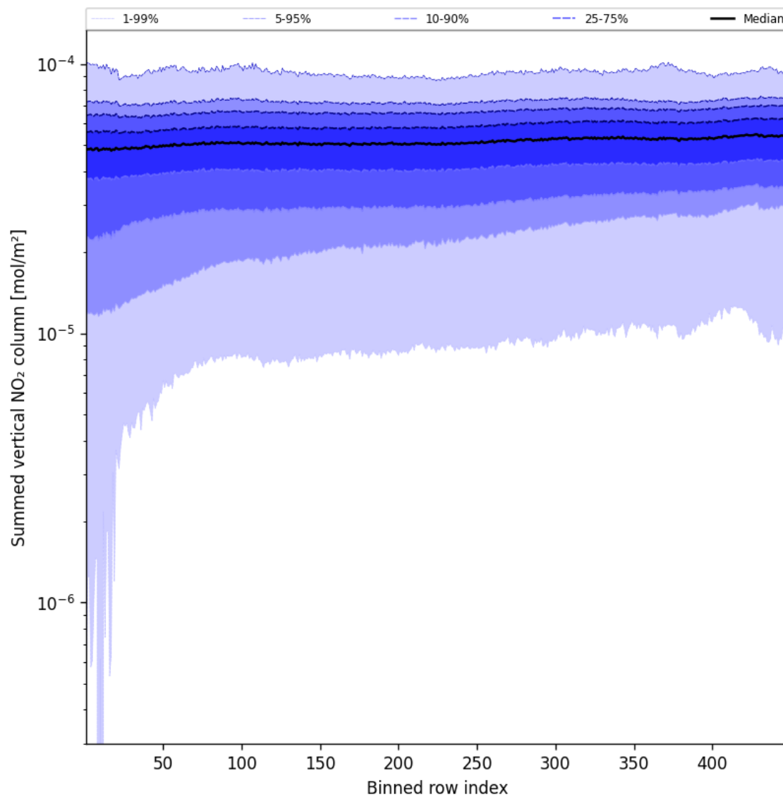
Figure 57: Along track statistics of “Summed vertical NO 2 column” for 2024-08-30 to 2024-09-01
