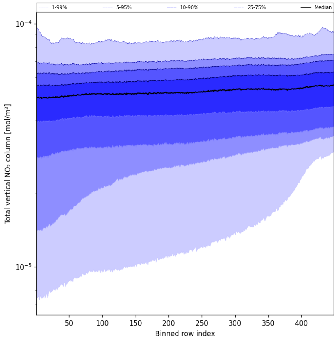
Figure 55: Along track statistics of “Total vertical NO 2 column” for 2024-08-30 to 2024-09-01
