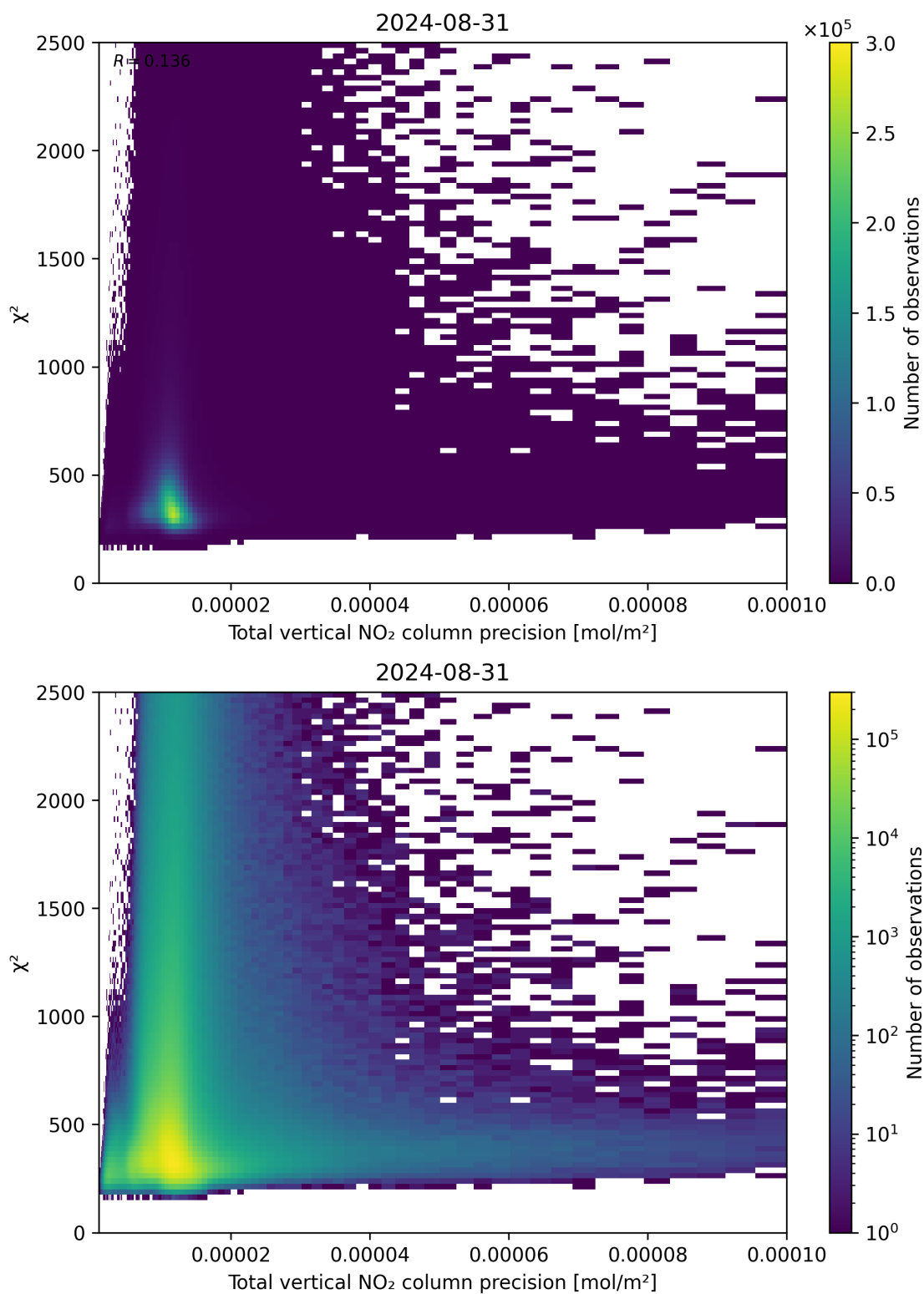
Figure 116: Scatter density plot of “Total vertical NO 2 column precision” against “ \chi^2 ” for 2024-08-30 to 2024-09-01.
