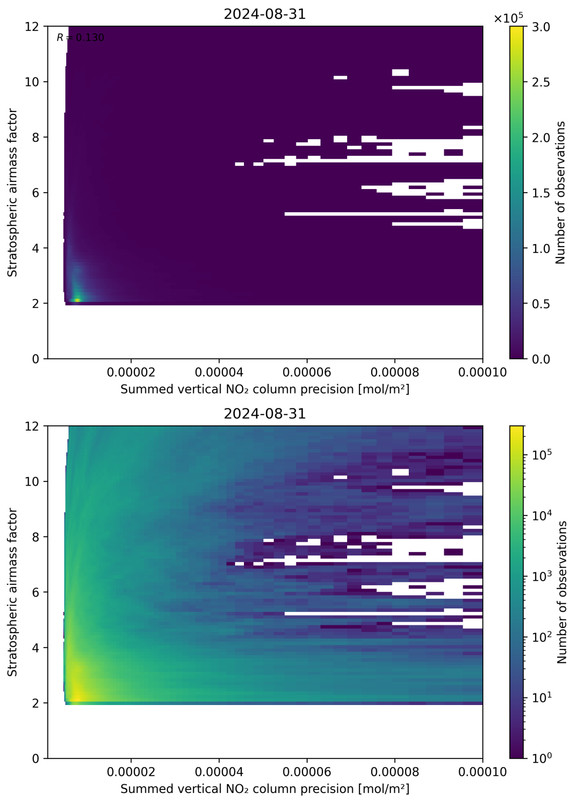
Figure 106: Scatter density plot of “Summed vertical NO 2 column precision” against “Stratospheric airmass factor” for 2024-08-30 to 2024-09-01.
