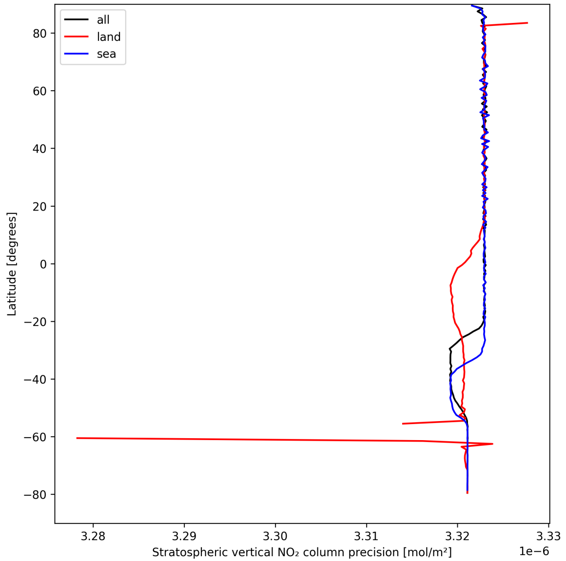
Figure 20: Zonal average of “Stratospheric vertical NO 2 column precision” for 2024-08-30 to 2024-09-01.
