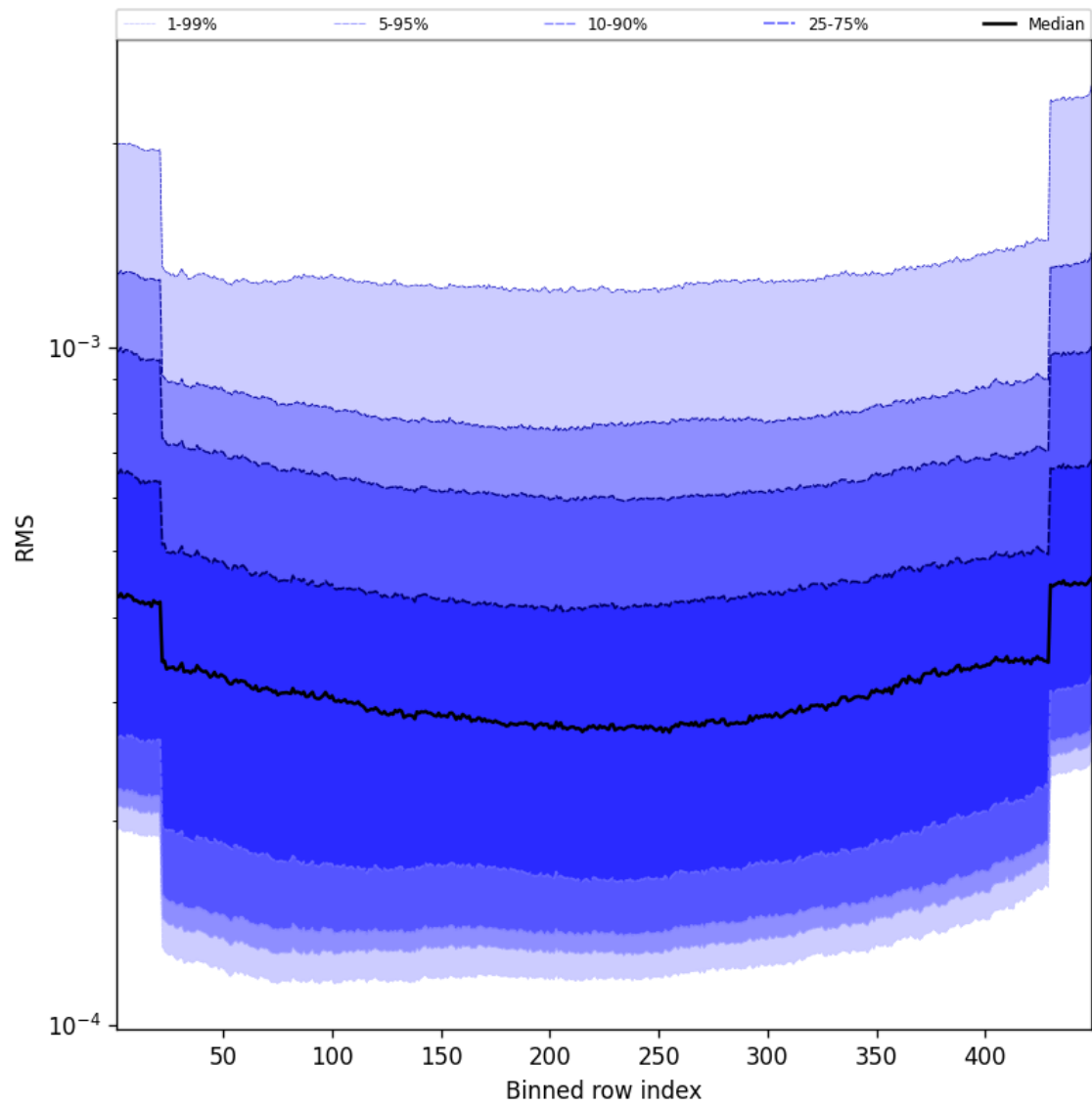
Figure 60: Along track statistics of “RMS” for 2024-08-30 to 2024-09-01
