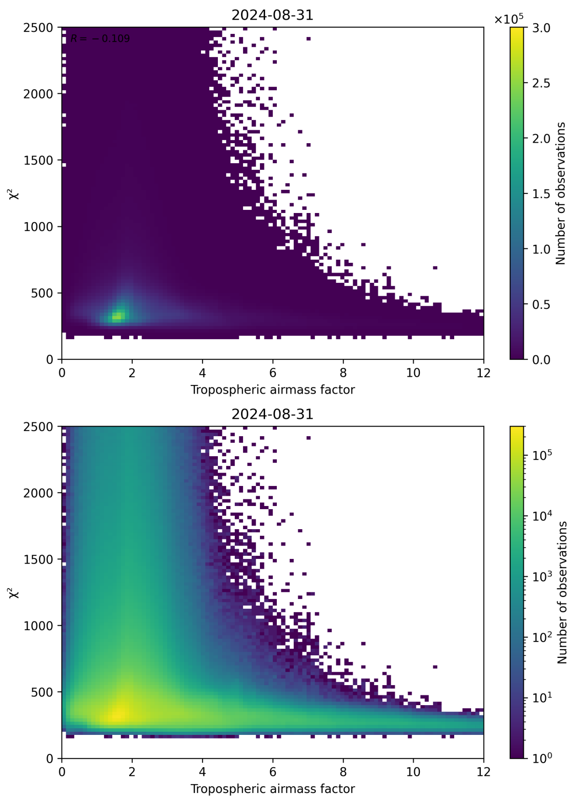
Figure 73: Scatter density plot of “Tropospheric airmass factor” against “ \chi^2 ” for 2024-08-30 to 2024-09-01.
