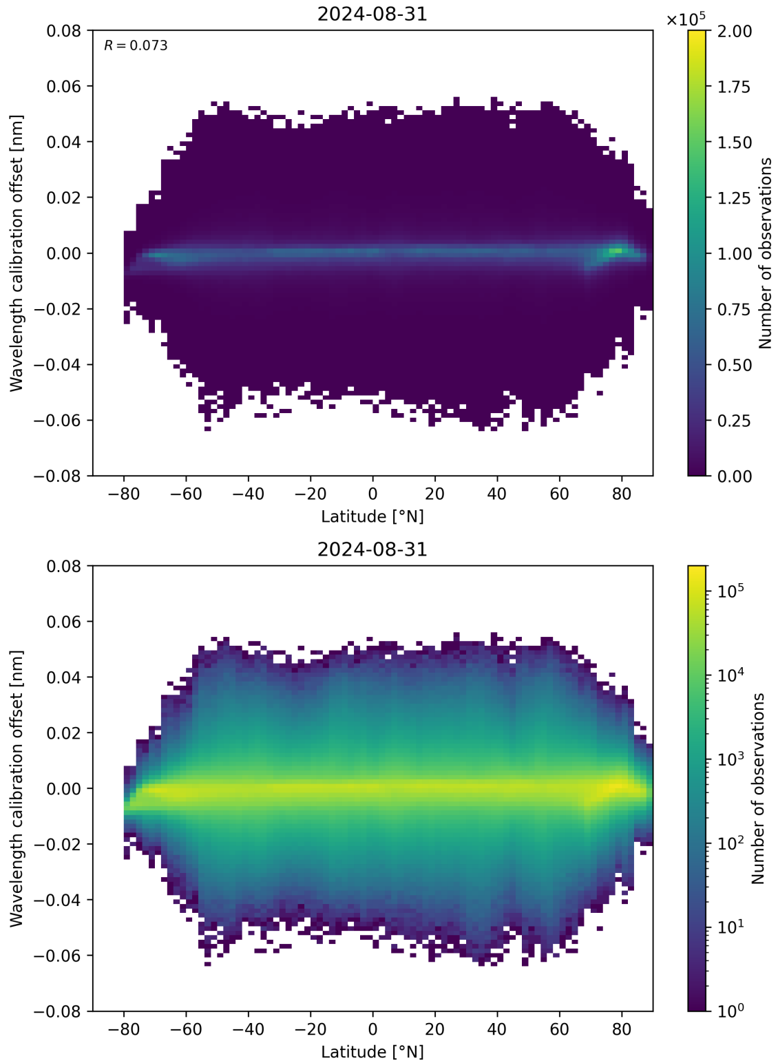
Figure 95: Scatter density plot of “Latitude” against “Wavelength calibration offset” for 2024-08-30 to 2024-09-01.
