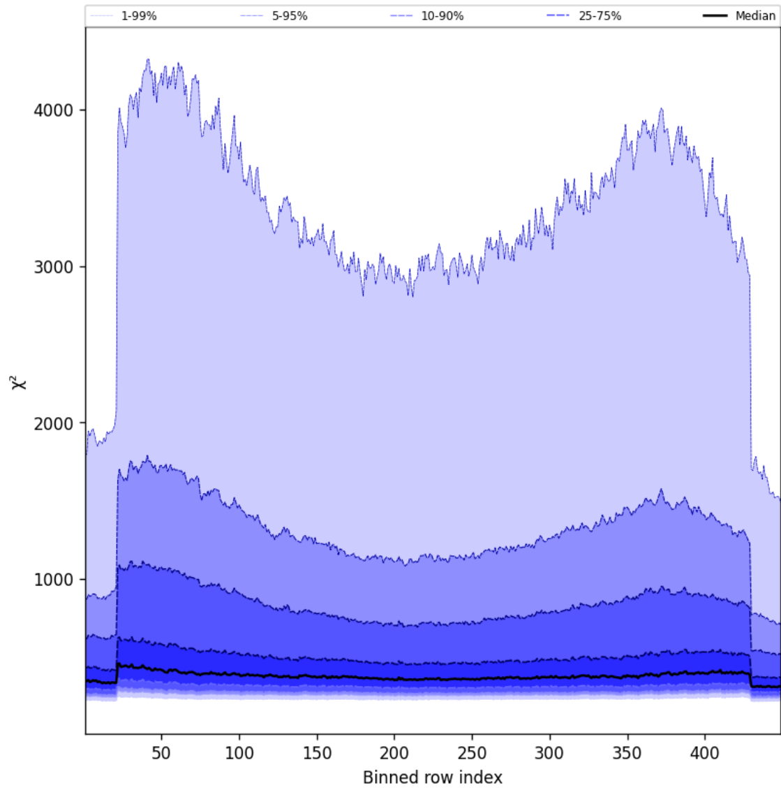
Figure 59: Along track statistics of “ \chi^2 ” for 2024-08-30 to 2024-09-01
