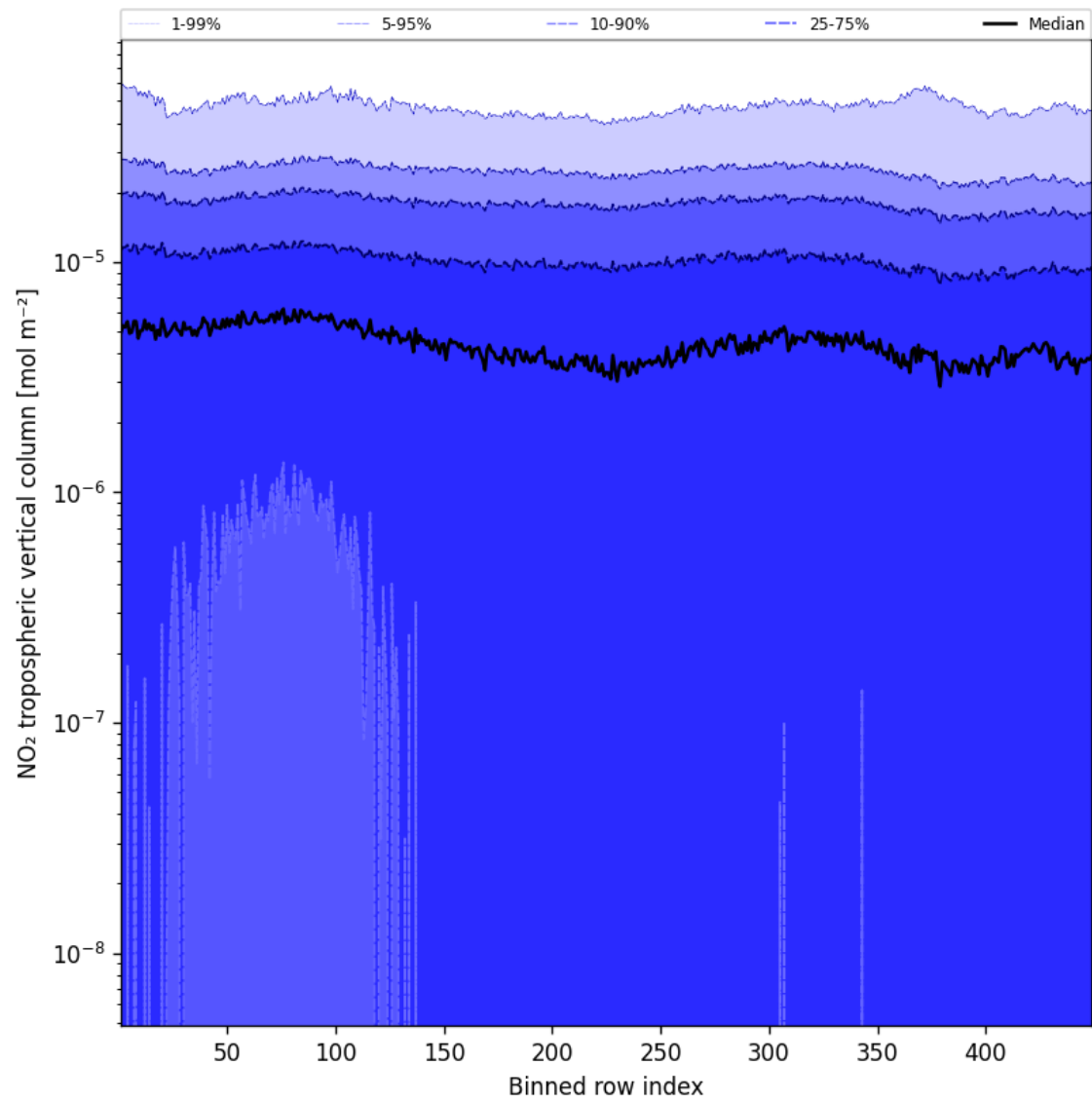
Figure 46: Along track statistics of “NO 2 tropospheric vertical column” for 2024-08-30 to 2024-09-01
