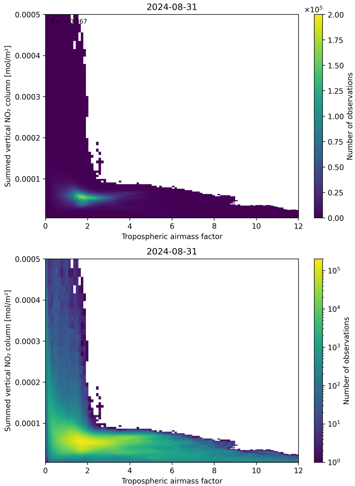
Figure 75: Scatter density plot of “Tropospheric airmass factor” against “Summed vertical NO 2 column” for 2024-08-30 to 2024-09-01.
