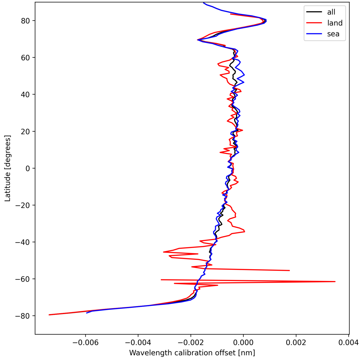
Figure 18: Zonal average of “Wavelength calibration offset” for 2024-08-30 to 2024-09-01.
