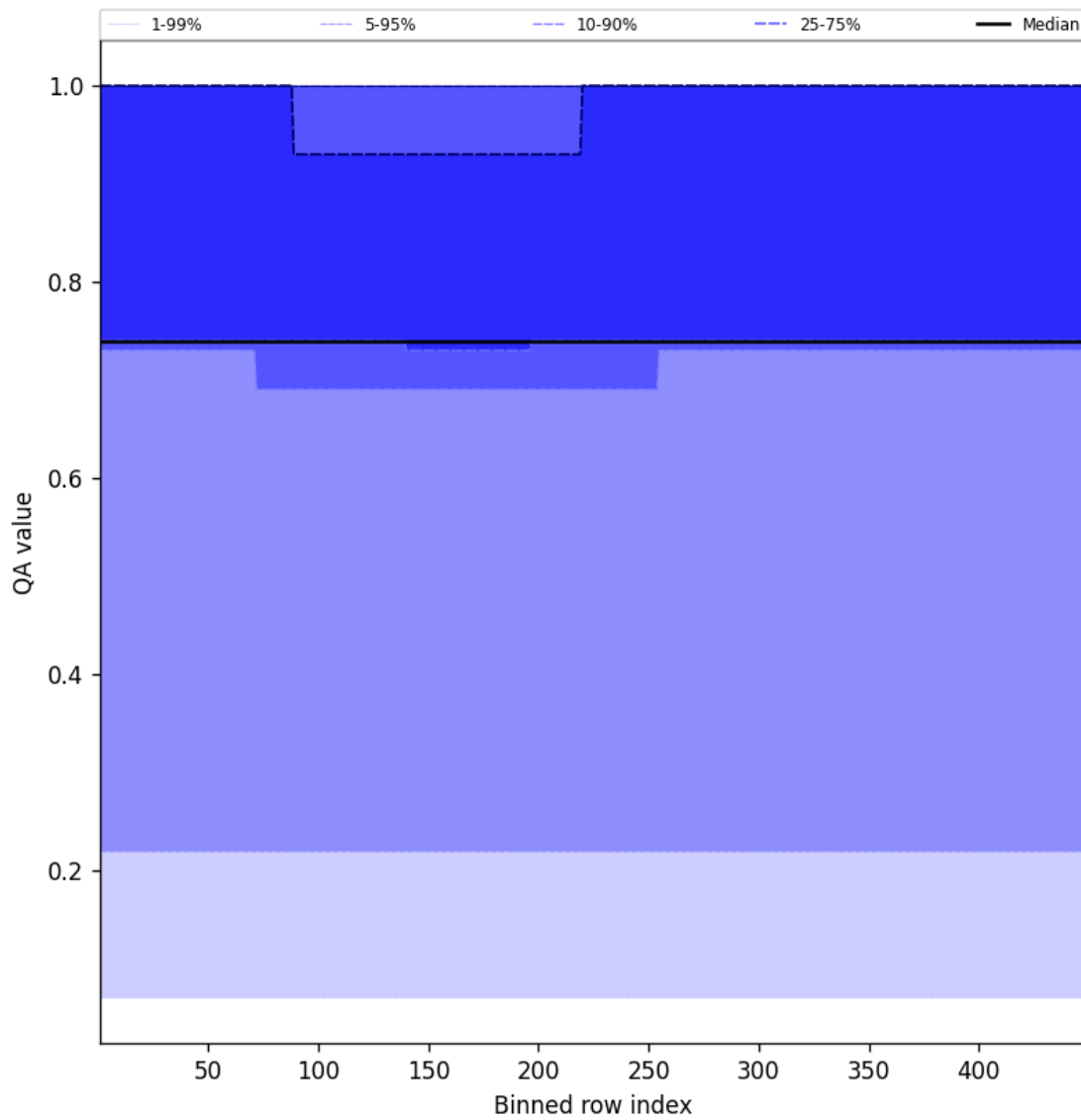
Figure 45: Along track statistics of “QA value” for 2024-08-30 to 2024-09-01
