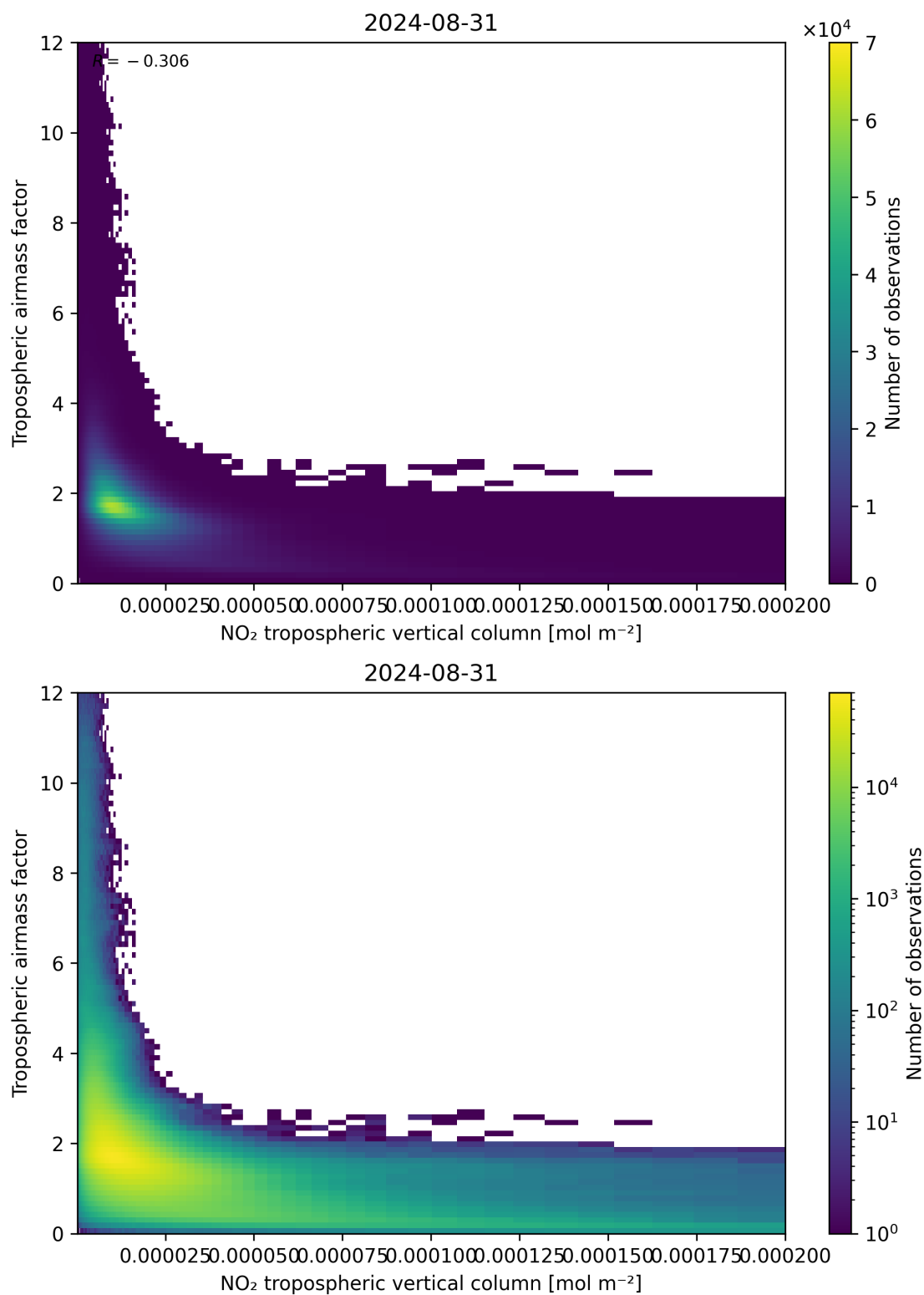
Figure 123: Scatter density plot of “NO 2 tropospheric vertical column” against “Tropospheric air mass factor” for 2024-08-30 to 2024-09-01.
