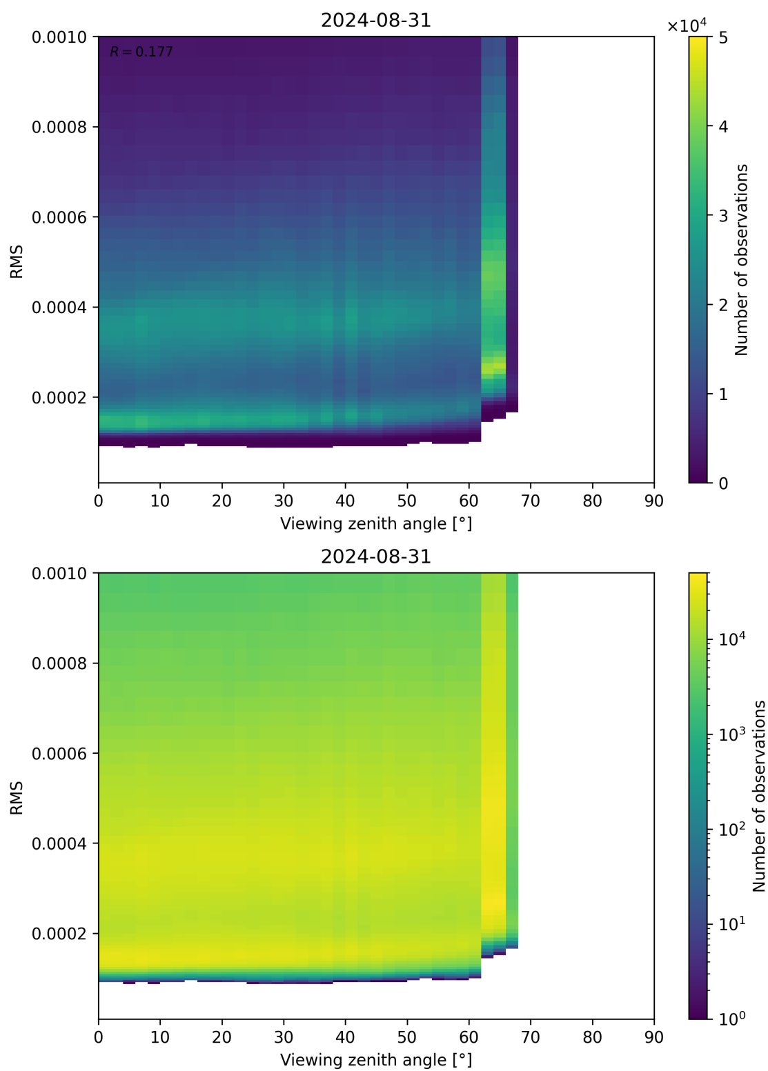
Figure 171: Scatter density plot of “Viewing zenith angle” against “RMS” for 2024-08-30 to 2024-09-01.
