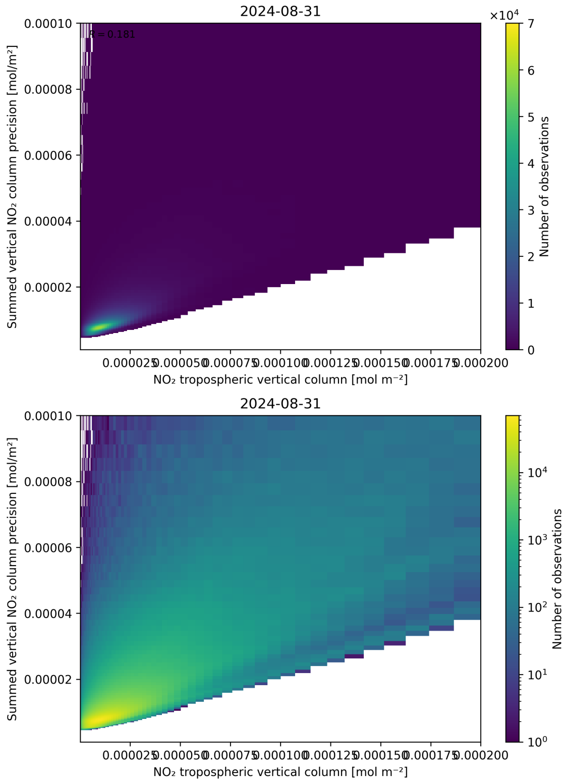
Figure 127: Scatter density plot of “NO 2 tropospheric vertical column” against “Summed vertical NO 2 column precision” for 2024-08-30 to 2024-09-01.
