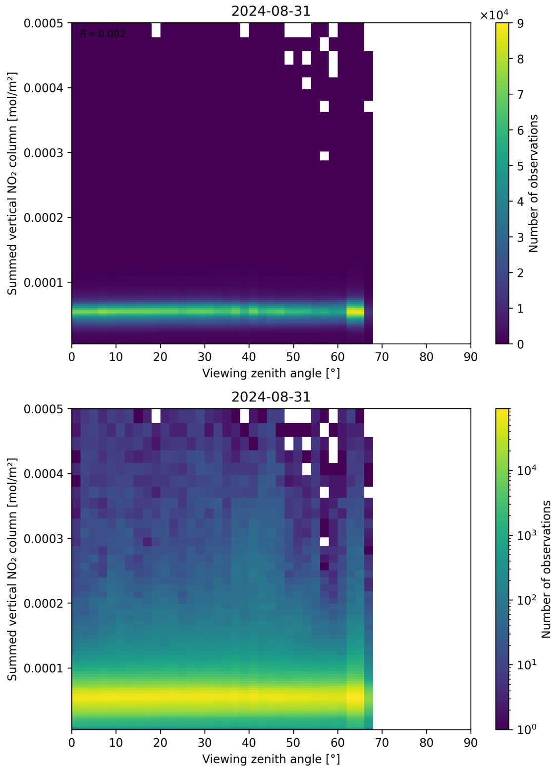
Figure 165: Scatter density plot of “Viewing zenith angle” against “Summed vertical NO 2 column” for 2024-08-30 to 2024-09-01.
