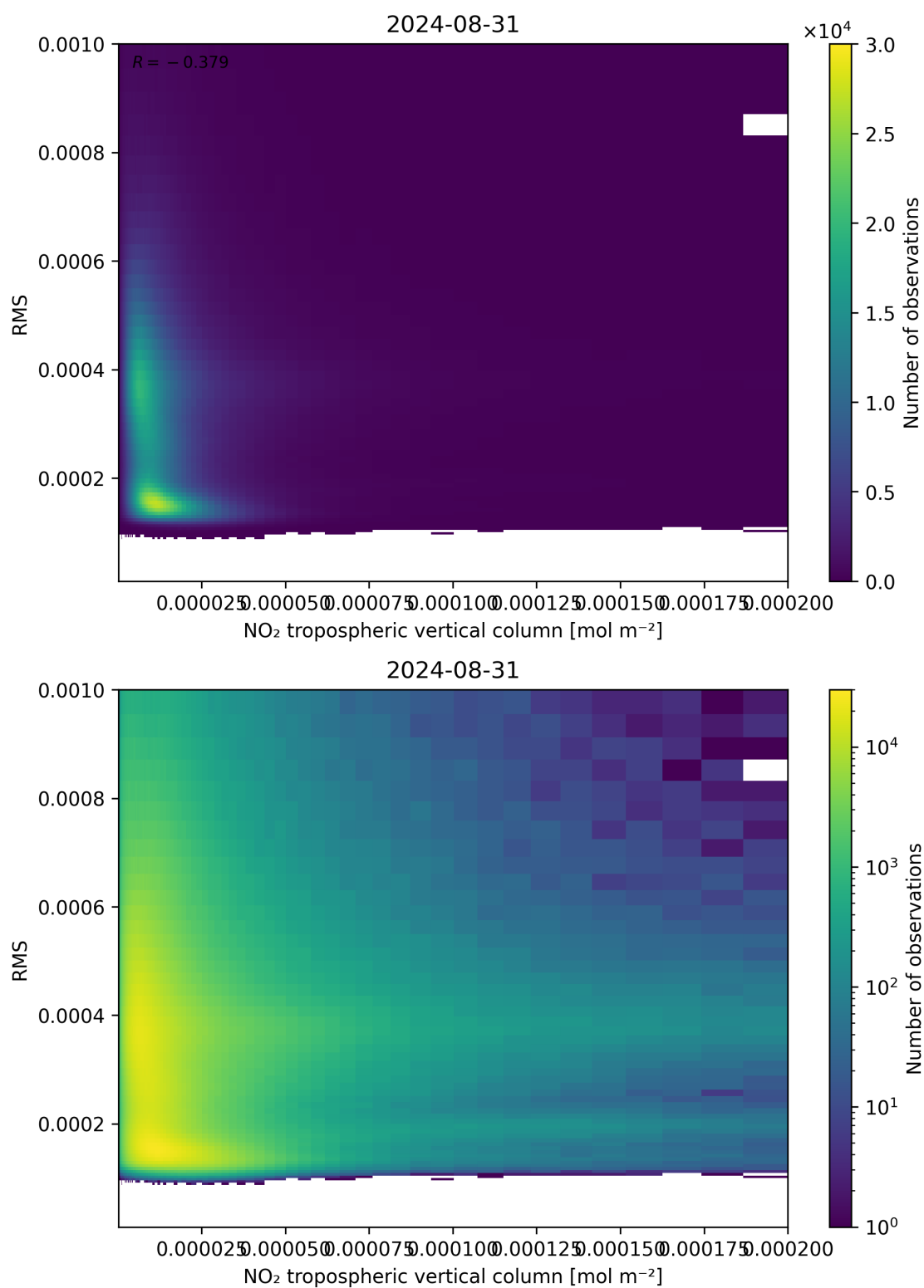
Figure 142: Scatter density plot of “NO 2 tropospheric vertical column” against “RMS” for 2024-08-30 to 2024-09-01.
