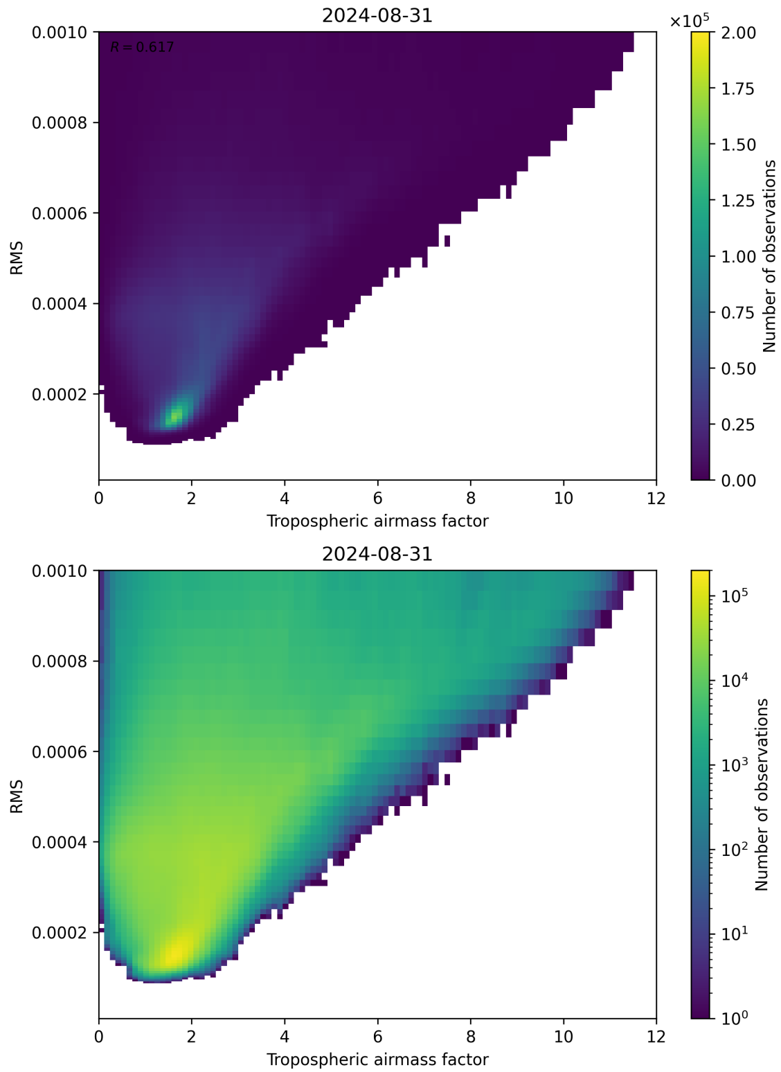
Figure 79: Scatter density plot of “Tropospheric airmass factor” against “RMS” for 2024-08-30 to 2024-09-01.
