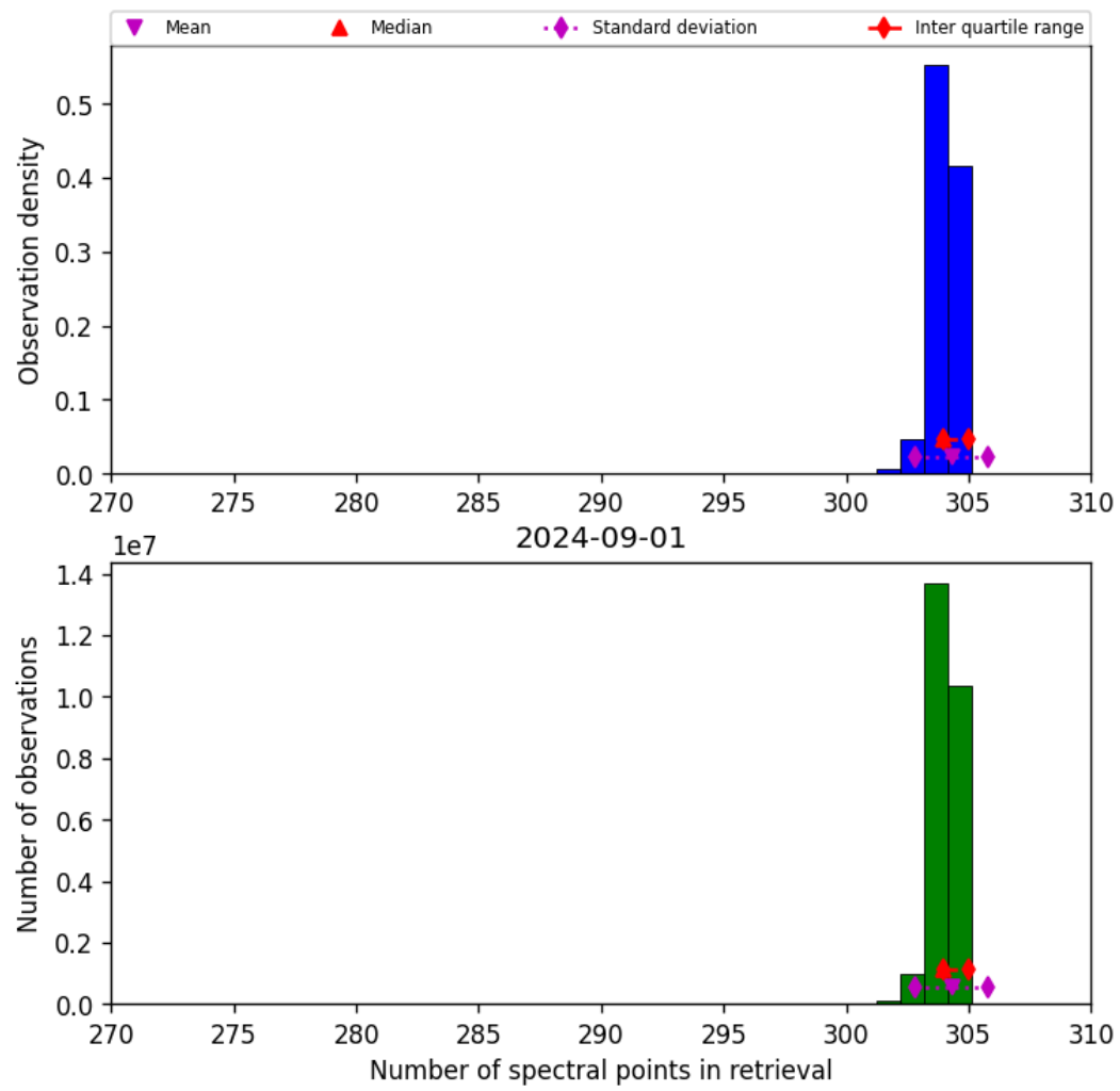
Figure 33: Histogram of “Number of spectral points in retrieval” for 2024-09-01 to 2024-09-02
