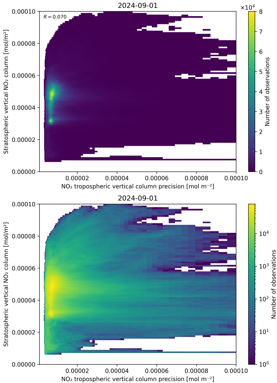
Figure 135: Scatter density plot of “NO 2 tropospheric vertical column precision” against “Stratospheric vertical NO 2 column” for 2024-09-01 to 2024-09-02.
