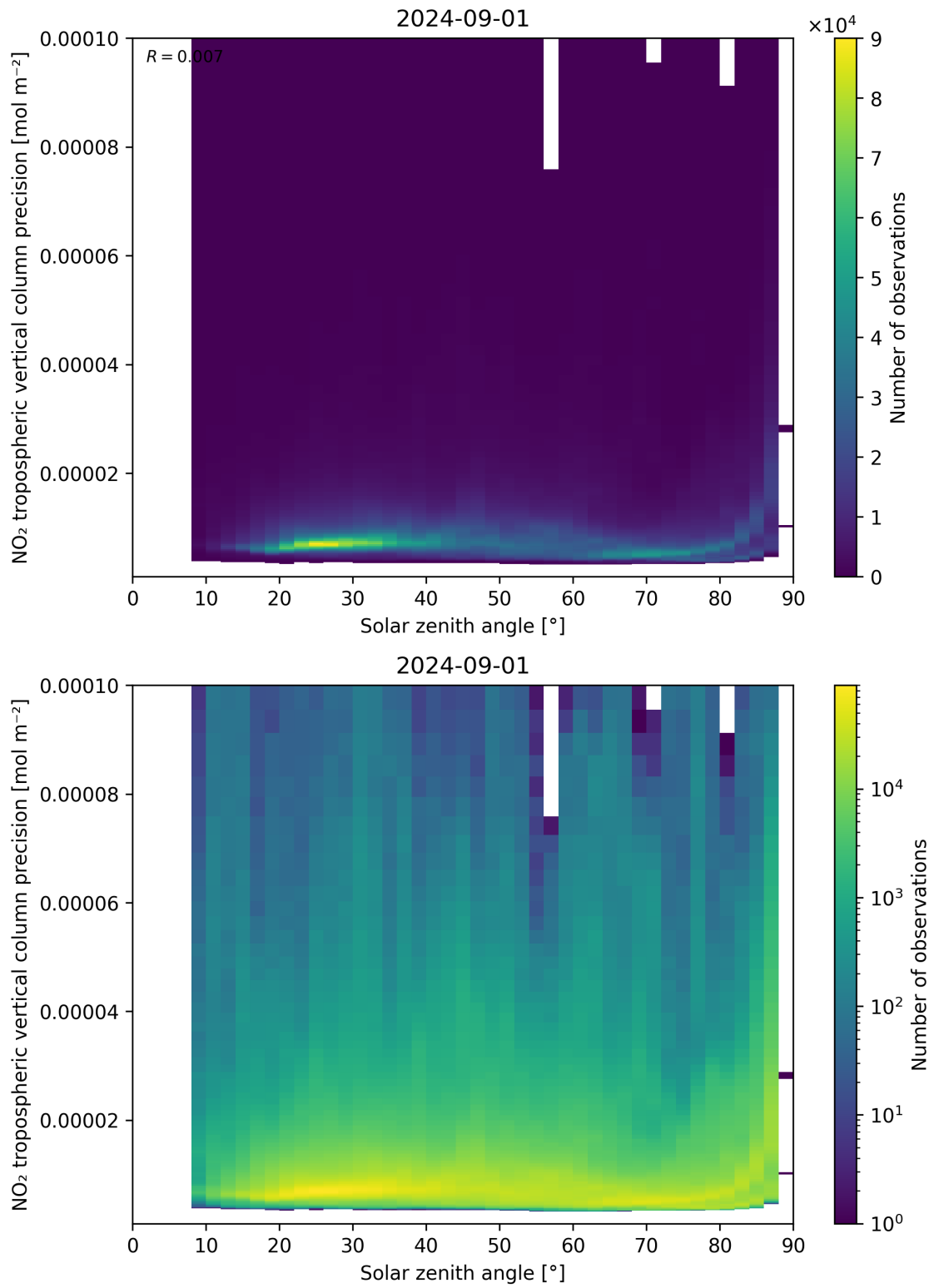
Figure 156: Scatter density plot of “Solar zenith angle” against “NO 2 tropospheric vertical column precision” for 2024-09-01 to 2024-09-02.
