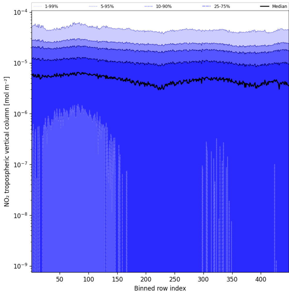
Figure 46: Along track statistics of “NO 2 tropospheric vertical column” for 2024-09-01 to 2024-09-02
