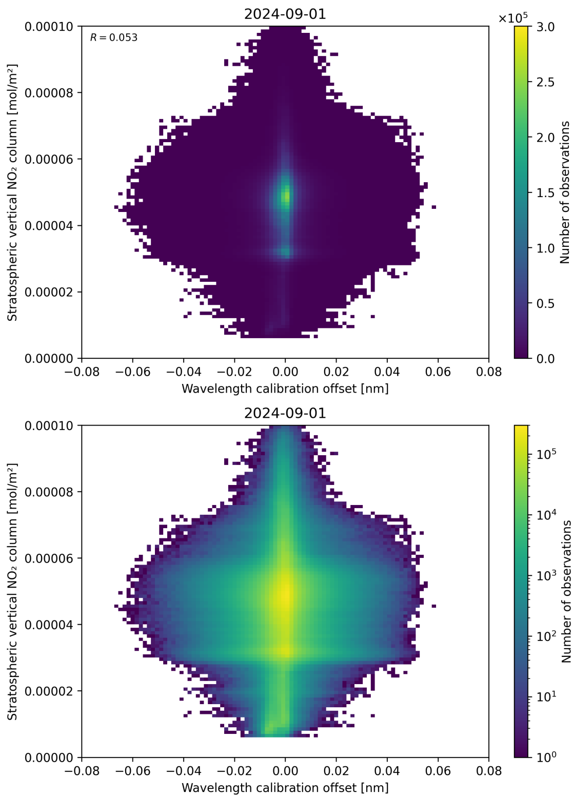
Figure 176: Scatter density plot of “Wavelength calibration offset” against “Stratospheric vertical NO 2 column” for 2024-09-01 to 2024-09-02.
