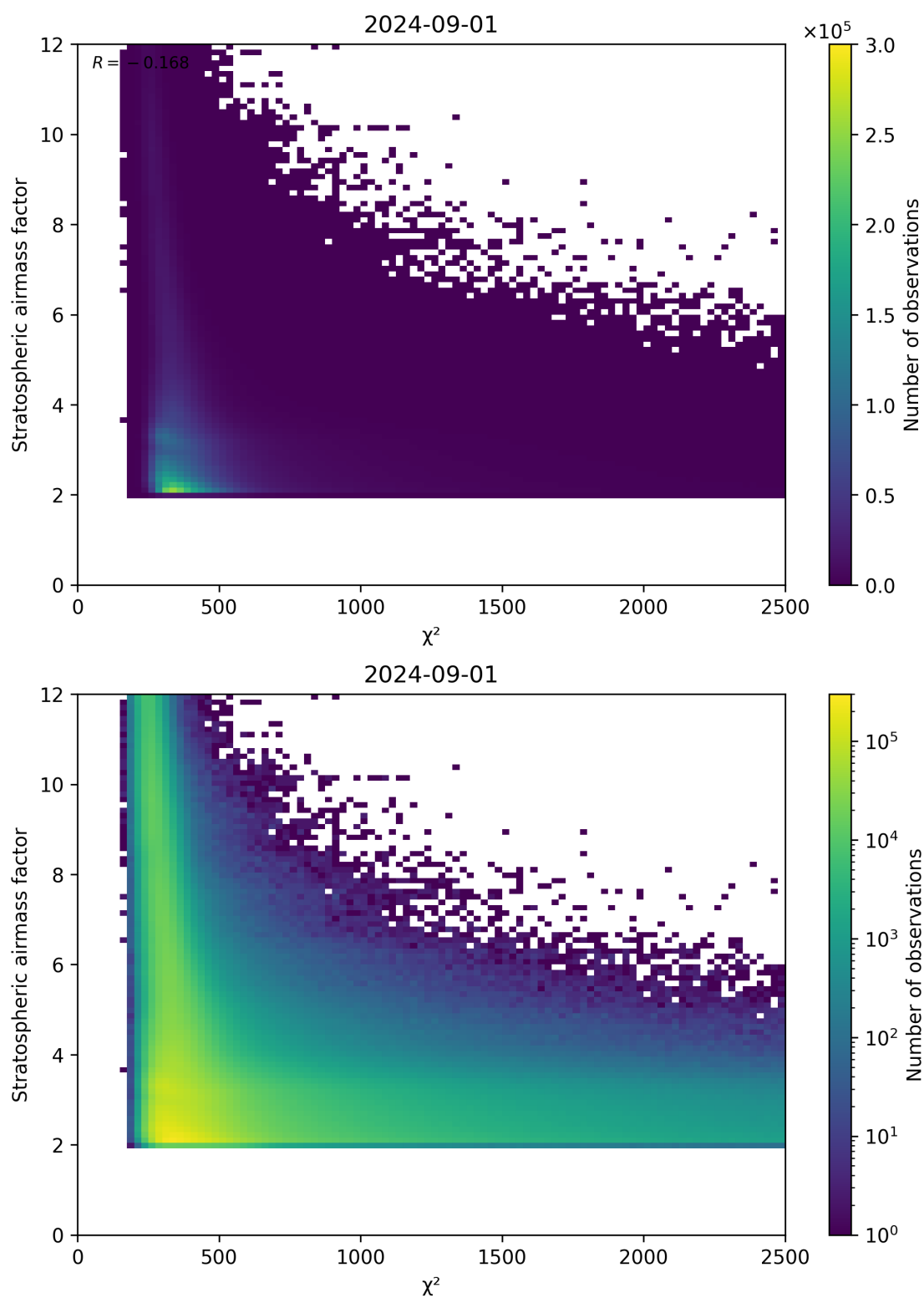
Figure 81: Scatter density plot of “ \chi^2 ” against “Stratospheric airmass factor” for 2024-09-01 to 2024-09-02.
