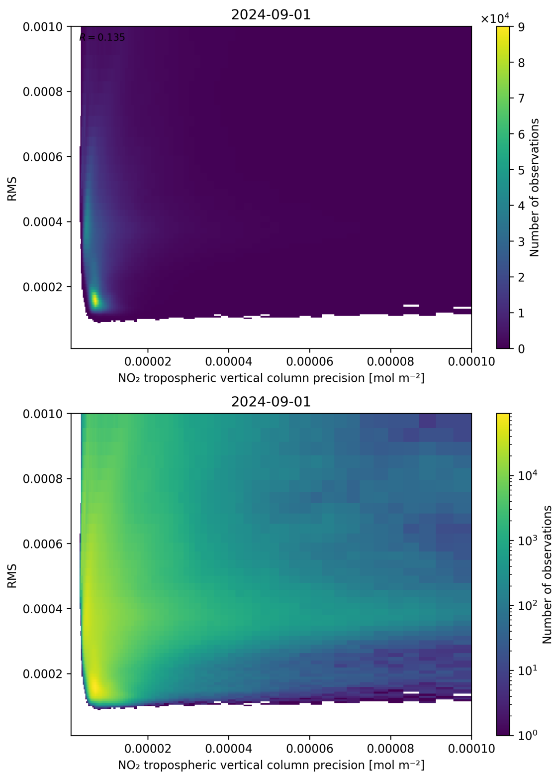
Figure 140: Scatter density plot of “NO 2 tropospheric vertical column precision” against “RMS” for 2024-09-01 to 2024-09-02.
