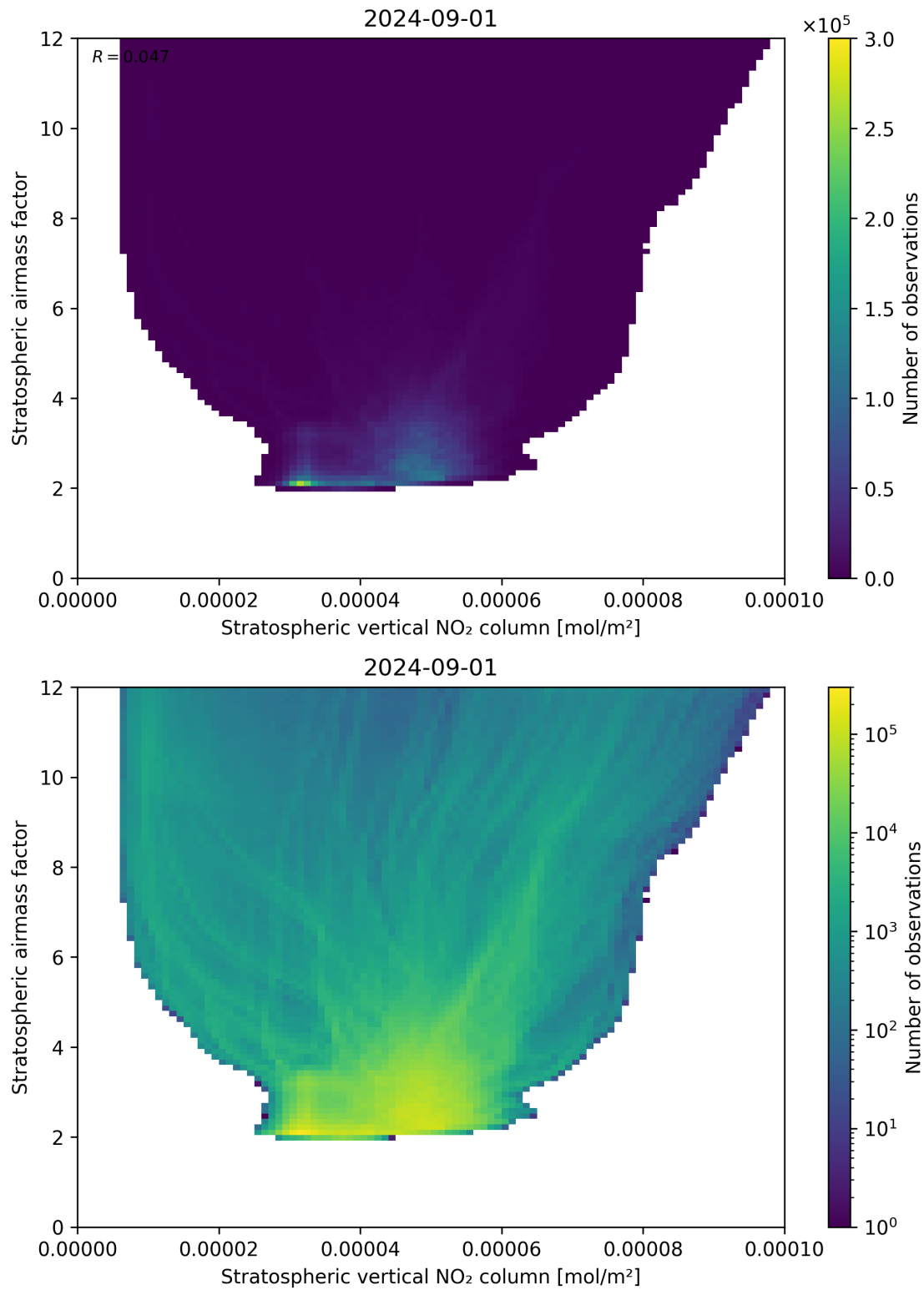
Figure 96: Scatter density plot of “Stratospheric vertical NO 2 column” against “Stratospheric airmass factor” for 2024-09-01 to 2024-09-02.
