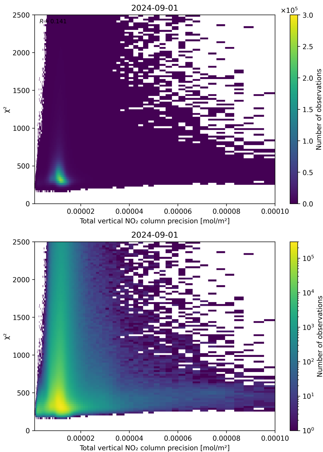
Figure 116: Scatter density plot of “Total vertical NO 2 column precision” against “ \chi^2 ” for 2024-09-01 to 2024-09-02.
