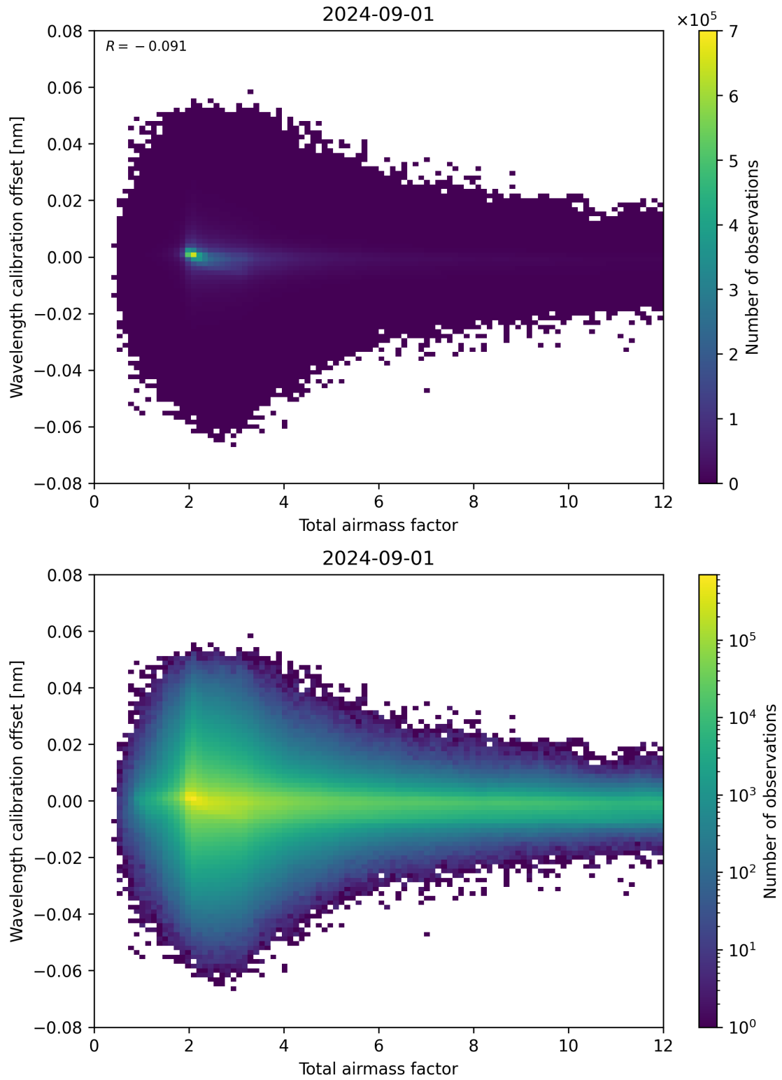
Figure 70: Scatter density plot of “Total airmass factor” against “Wavelength calibration offset” for 2024-09-01 to 2024-09-02.
