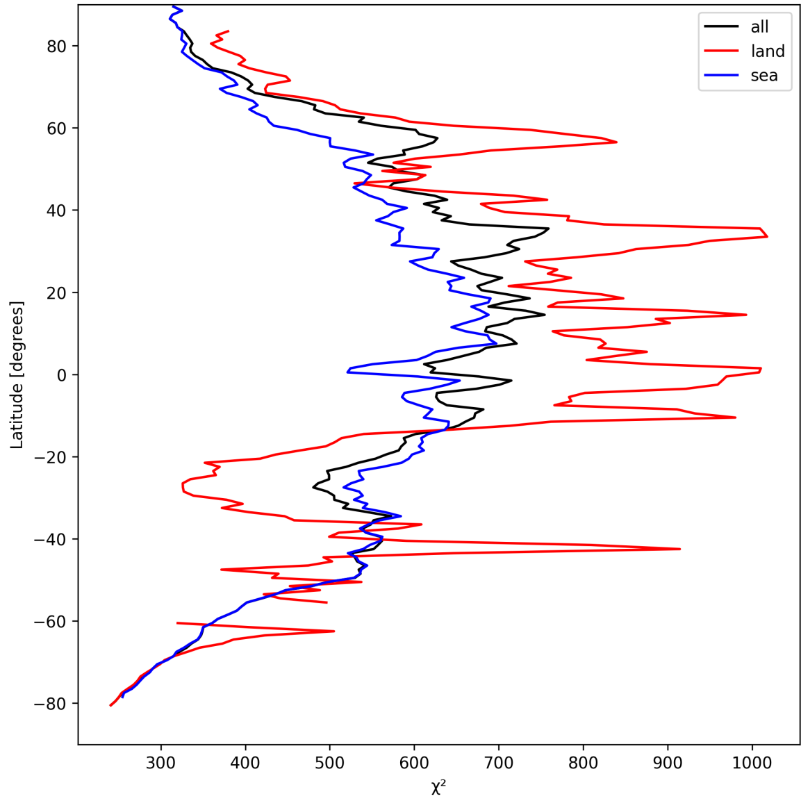
Figure 25: Zonal average of “ \chi^2 ” for 2024-09-01 to 2024-09-02.
