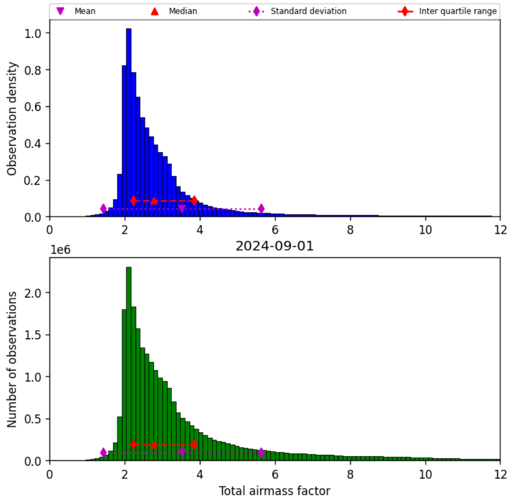
Figure 32: Histogram of “Total airmass factor” for 2024-09-01 to 2024-09-02
