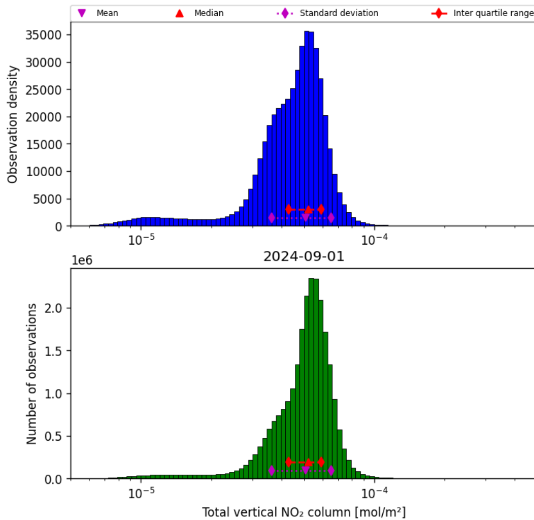
Figure 38: Histogram of “Total vertical NO 2 column” for 2024-09-01 to 2024-09-02
