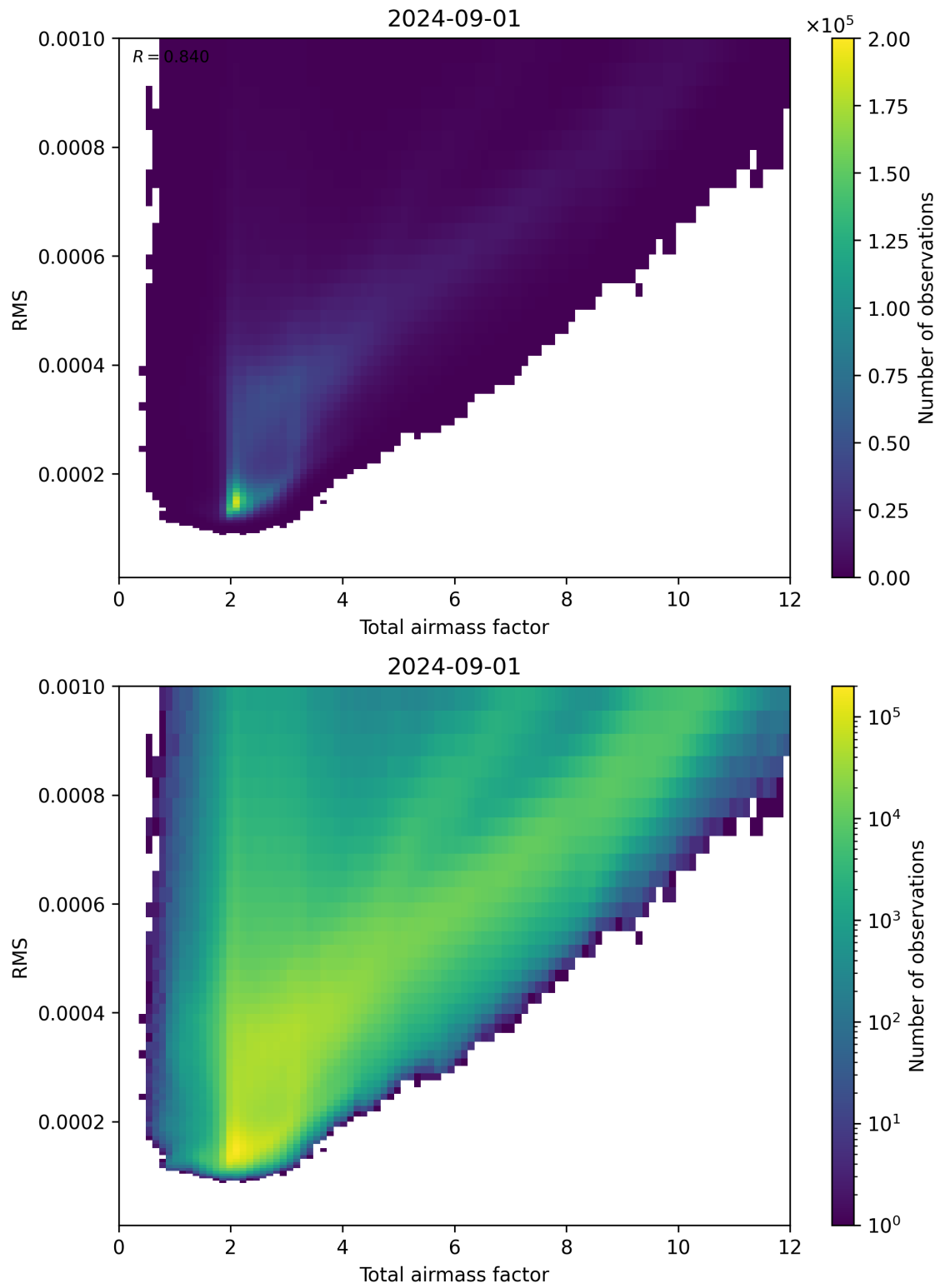
Figure 69: Scatter density plot of “Total airmass factor” against “RMS” for 2024-09-01 to 2024-09-02.
