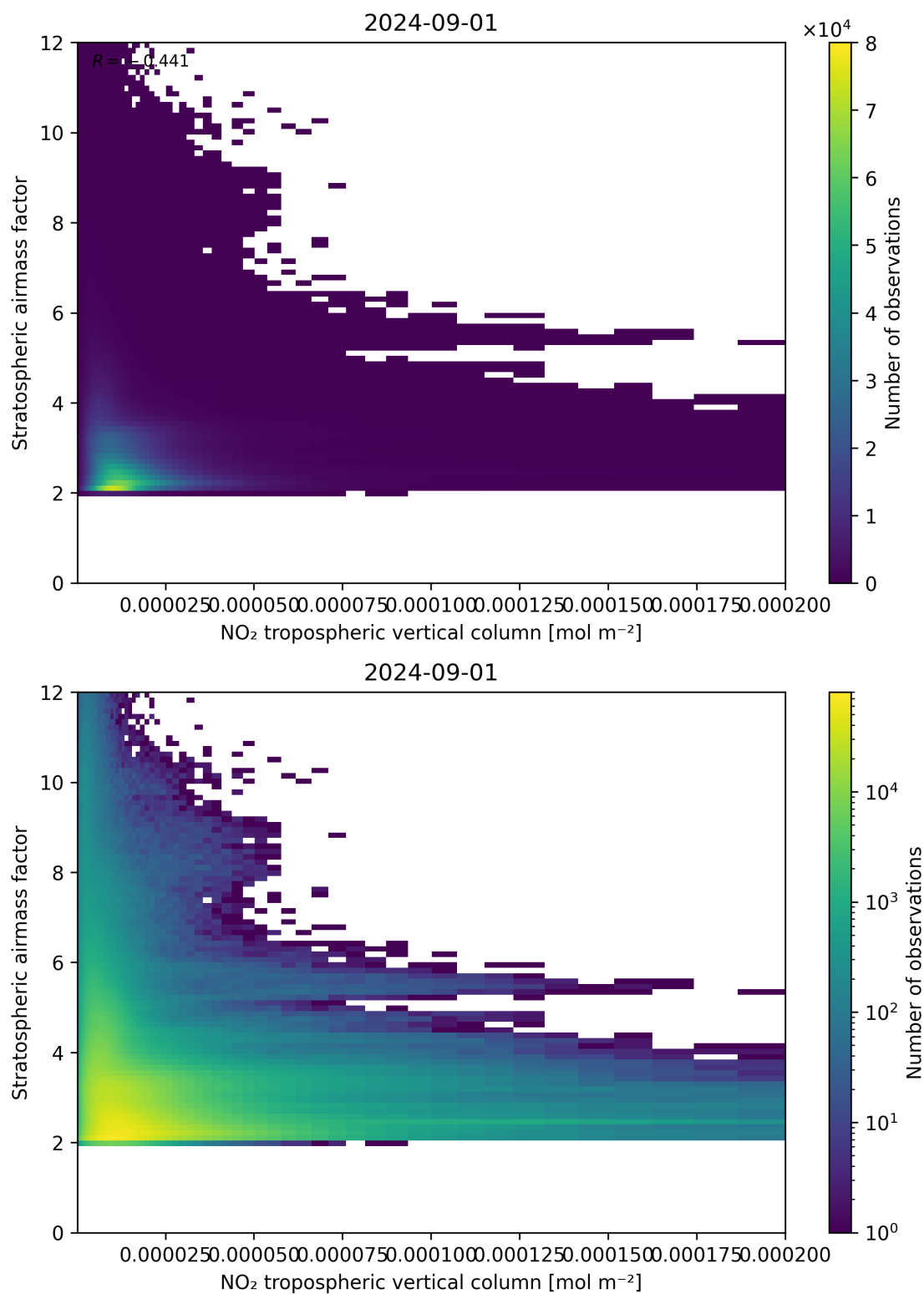
Figure 121: Scatter density plot of “NO 2 tropospheric vertical column” against “Stratospheric air mass factor” for 2024-09-01 to 2024-09-02.
