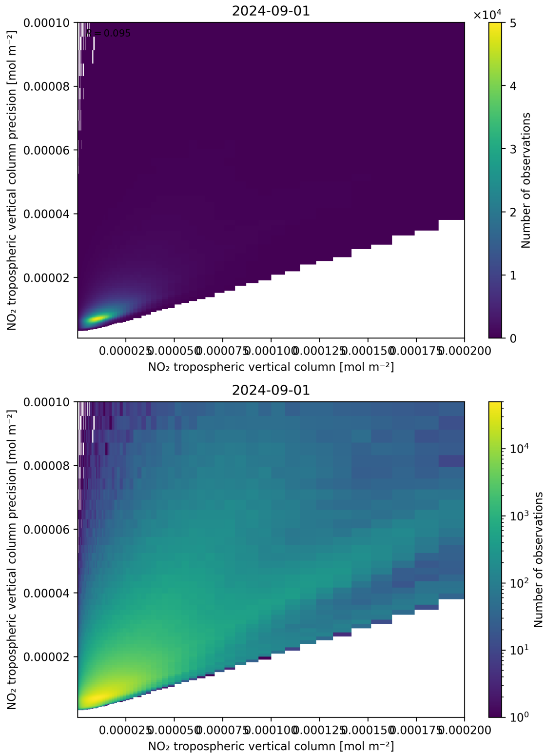
Figure 130: Scatter density plot of “NO 2 tropospheric vertical column” against “NO 2 tropospheric vertical column precision” for 2024-09-01 to 2024-09-02.
