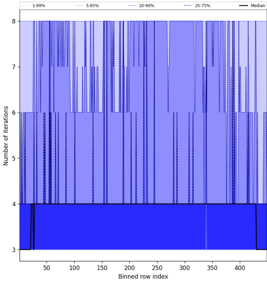
Figure 51: Along track statistics of “Number of iterations” for 2024-09-01 to 2024-09-02
