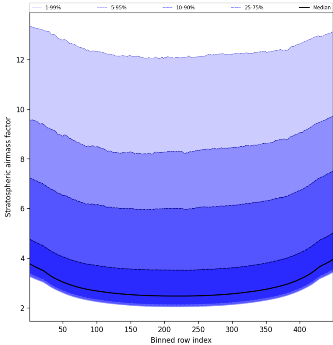
Figure 61: Along track statistics of “Stratospheric airmass factor” for 2024-09-01 to 2024-09-02
