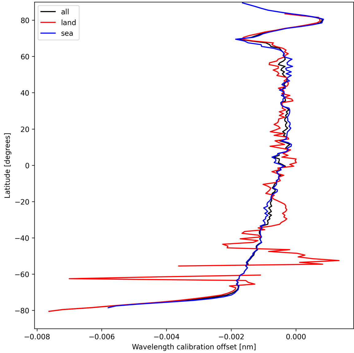
Figure 18: Zonal average of “Wavelength calibration offset” for 2024-09-01 to 2024-09-02.
