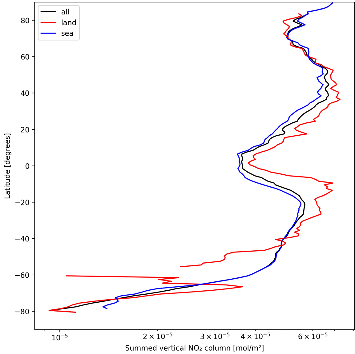
Figure 23: Zonal average of “Summed vertical NO 2 column” for 2024-09-01 to 2024-09-02.
