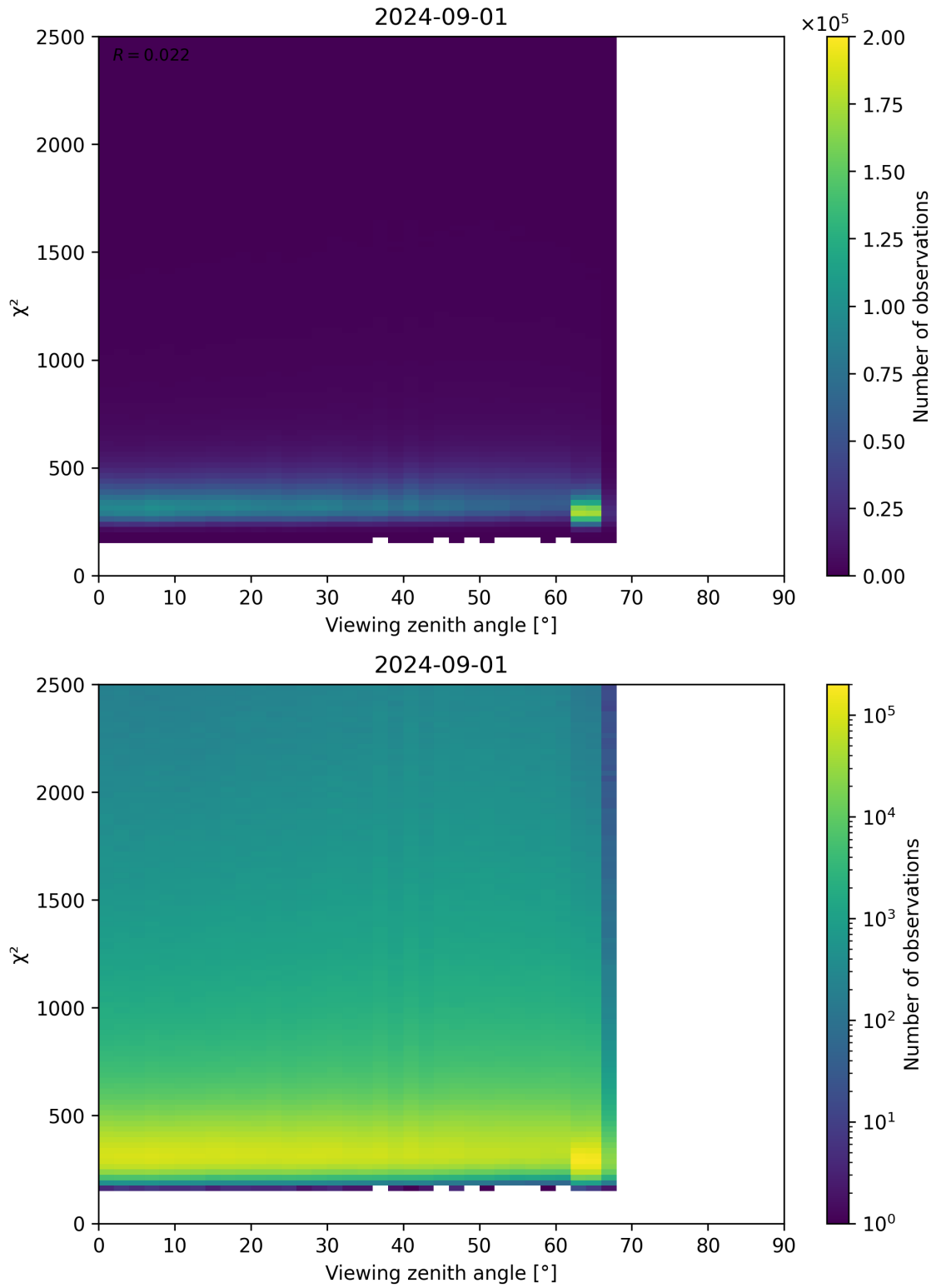
Figure 162: Scatter density plot of “Viewing zenith angle” against “ \chi^2 ” for 2024-09-01 to 2024-09-02.
