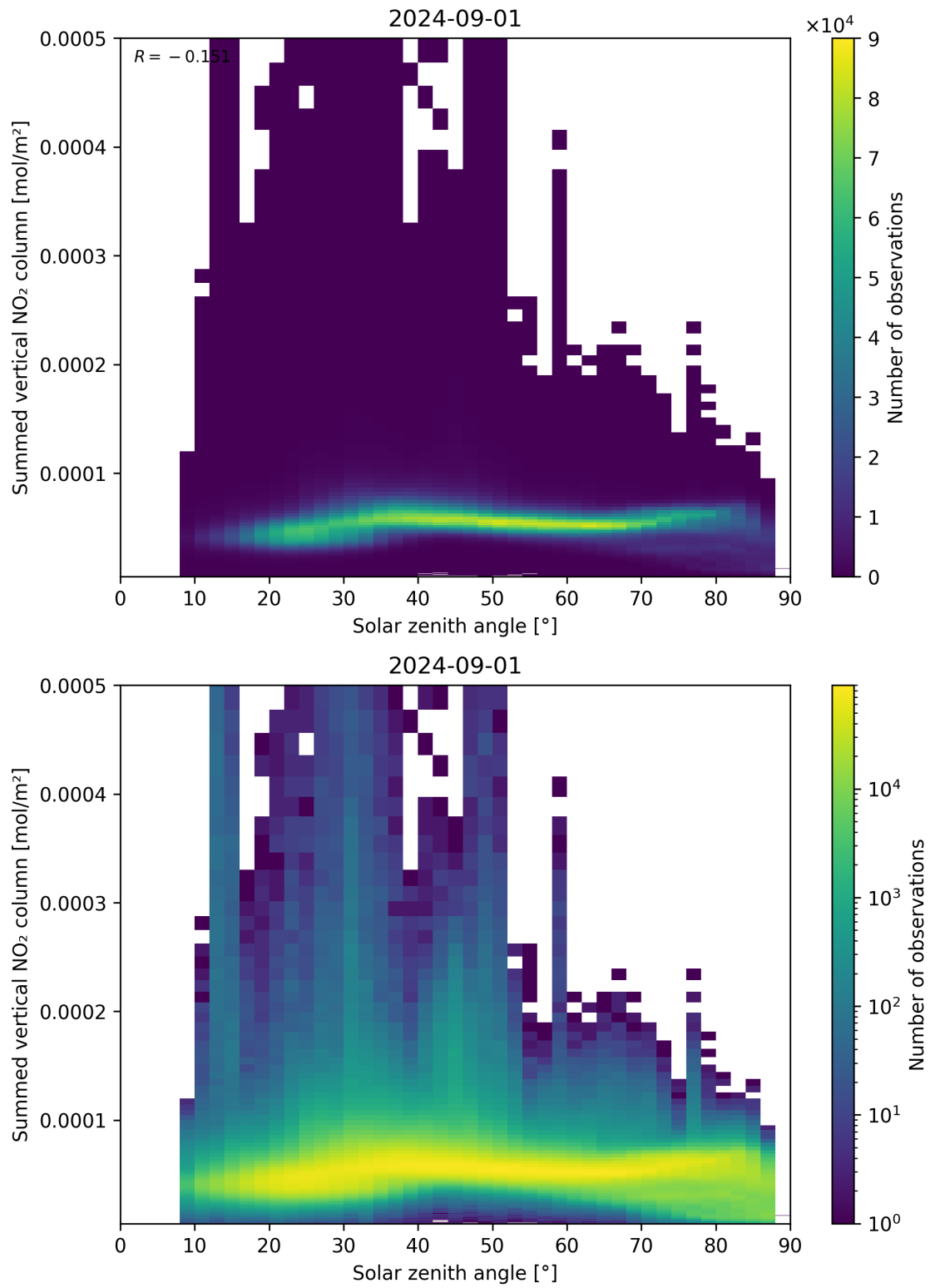
Figure 151: Scatter density plot of “Solar zenith angle” against “Summed vertical NO 2 column” for 2024-09-01 to 2024-09-02.
