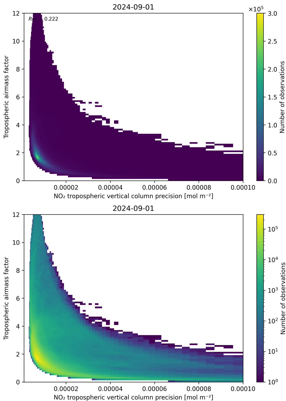
Figure 133: Scatter density plot of “NO 2 tropospheric vertical column precision” against “Tropospheric air mass factor” for 2024-09-01 to 2024-09-02.
