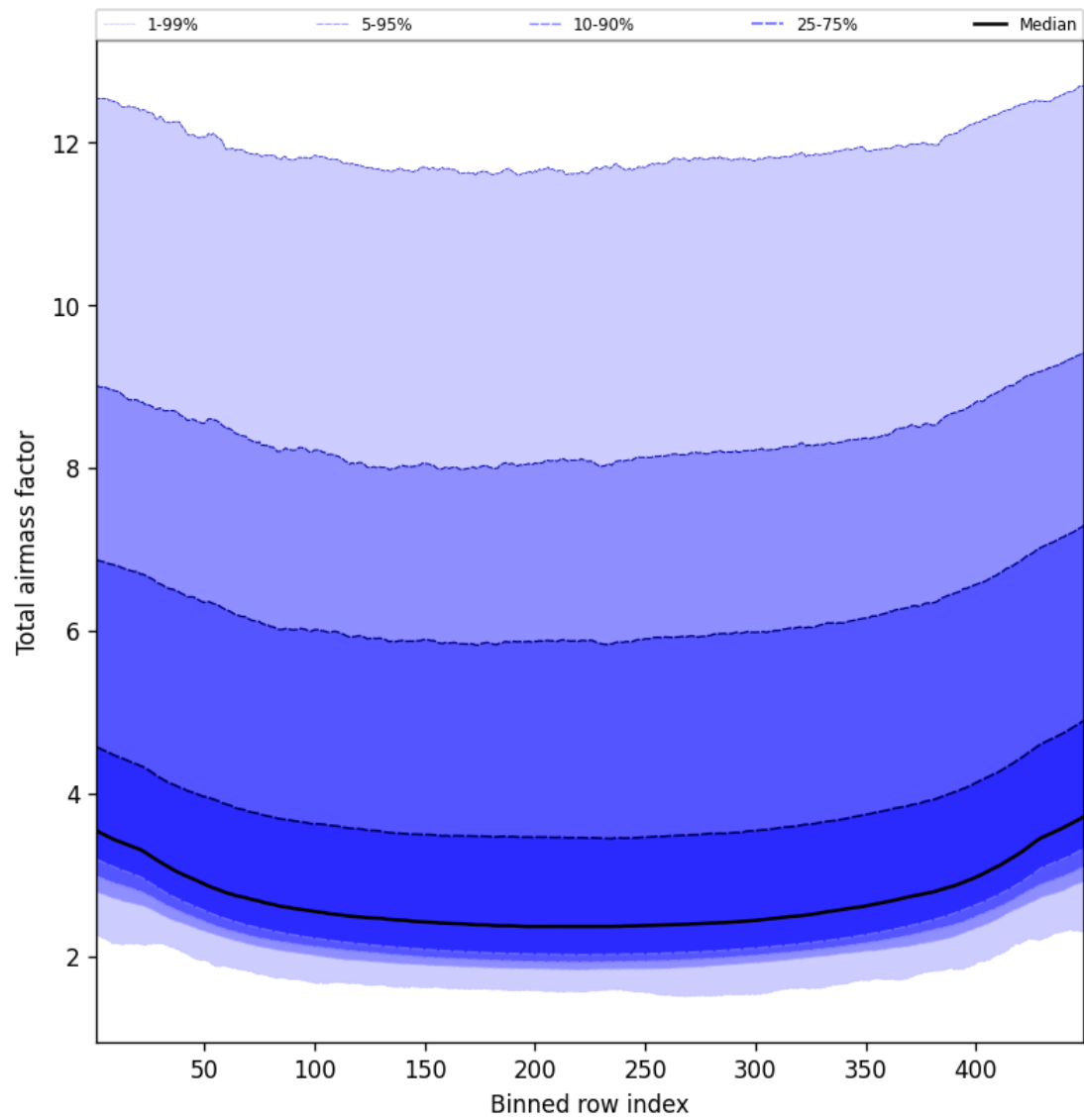
Figure 49: Along track statistics of “Total airmass factor” for 2024-09-01 to 2024-09-02
