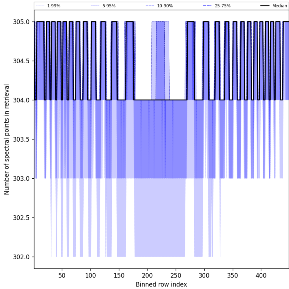
Figure 50: Along track statistics of “Number of spectral points in retrieval” for 2024-09-01 to 2024-09-02
