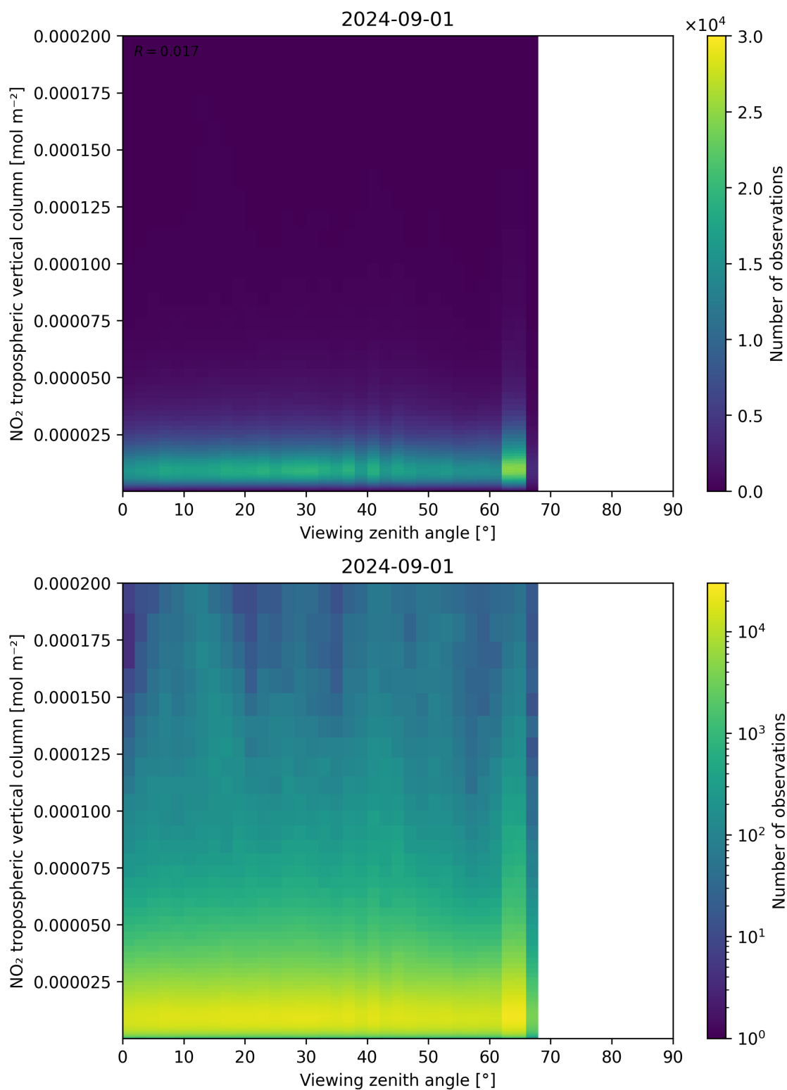
Figure 169: Scatter density plot of “Viewing zenith angle” against “NO 2 tropospheric vertical column” for 2024-09-01 to 2024-09-02.
