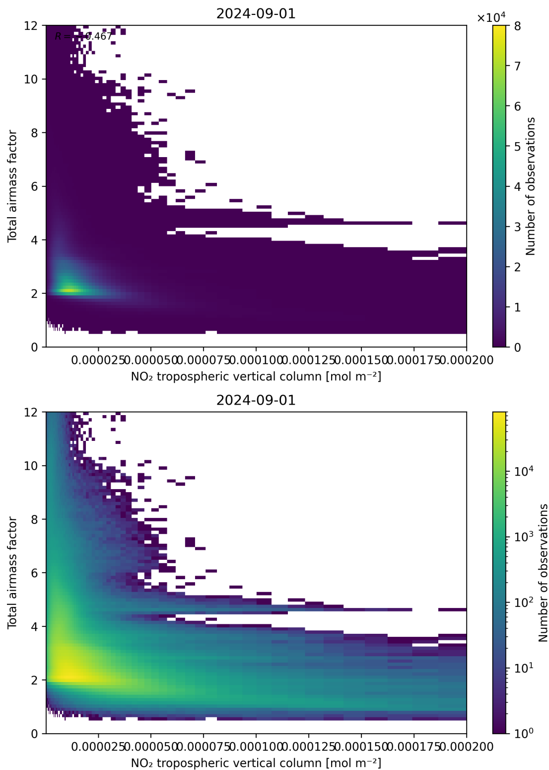
Figure 122: Scatter density plot of “NO 2 tropospheric vertical column” against “Total air mass factor” for 2024-09-01 to 2024-09-02.
