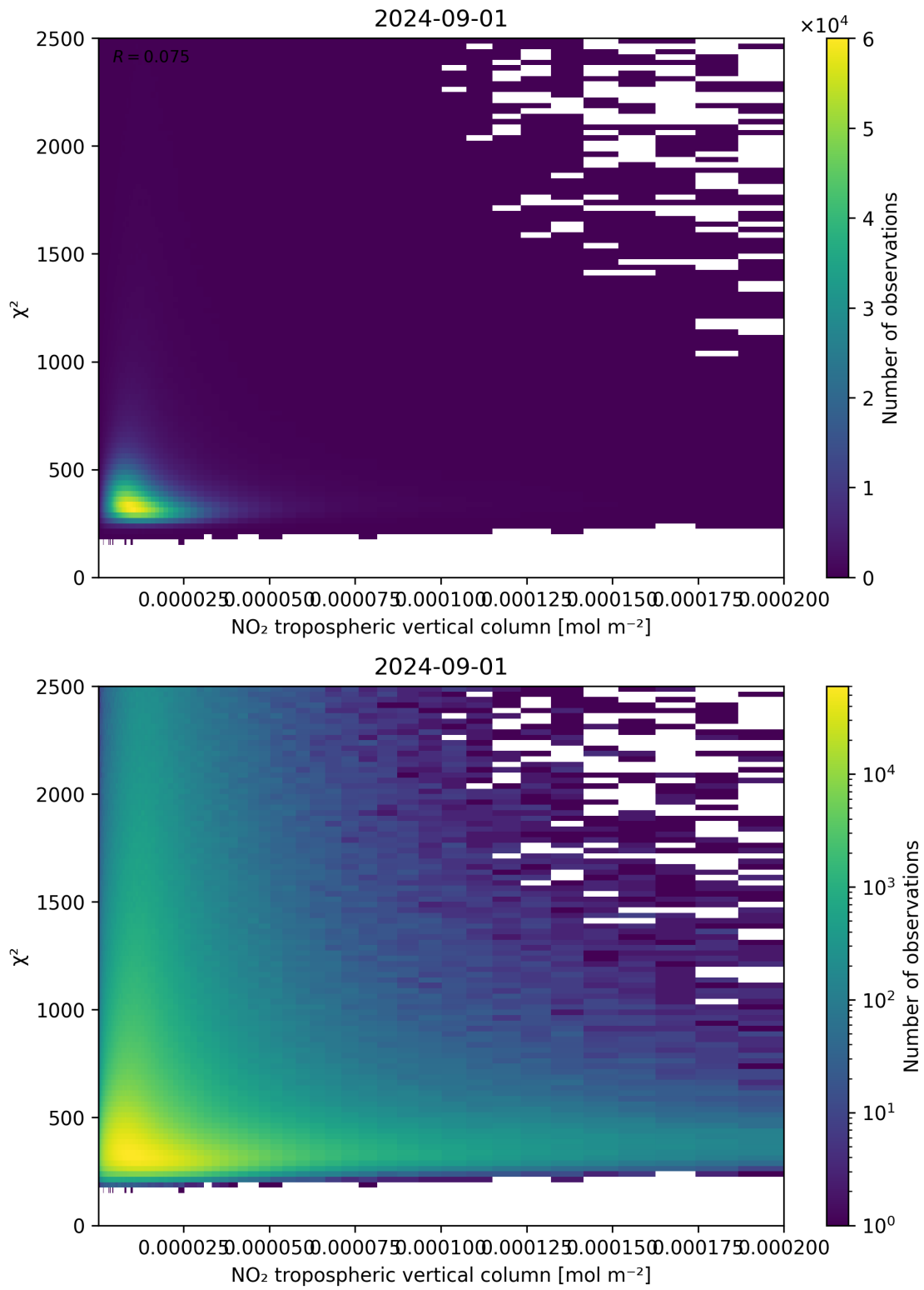
Figure 124: Scatter density plot of “NO 2 tropospheric vertical column” against “ \chi^2 ” for 2024-09-01 to 2024-09-02.
