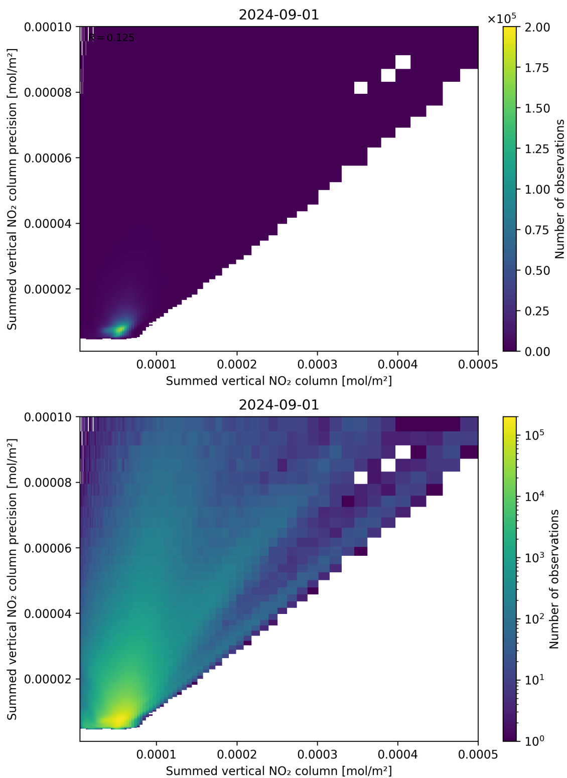
Figure 105: Scatter density plot of “Summed vertical NO 2 column” against “Summed vertical NO 2 column precision” for 2024-09-01 to 2024-09-02.
