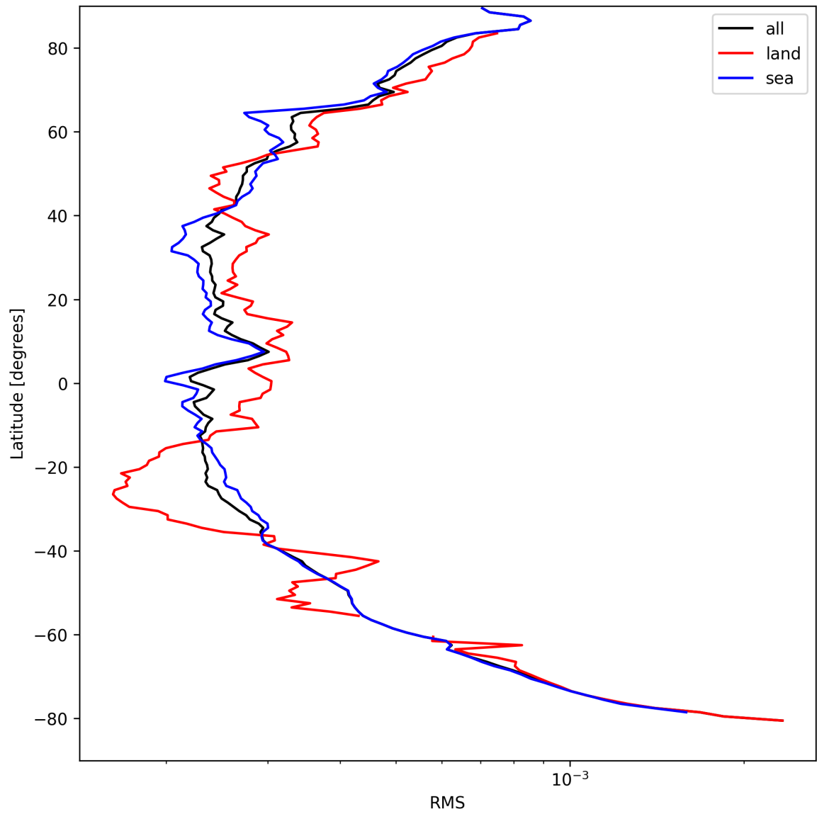
Figure 26: Zonal average of “RMS” for 2024-09-01 to 2024-09-02.
