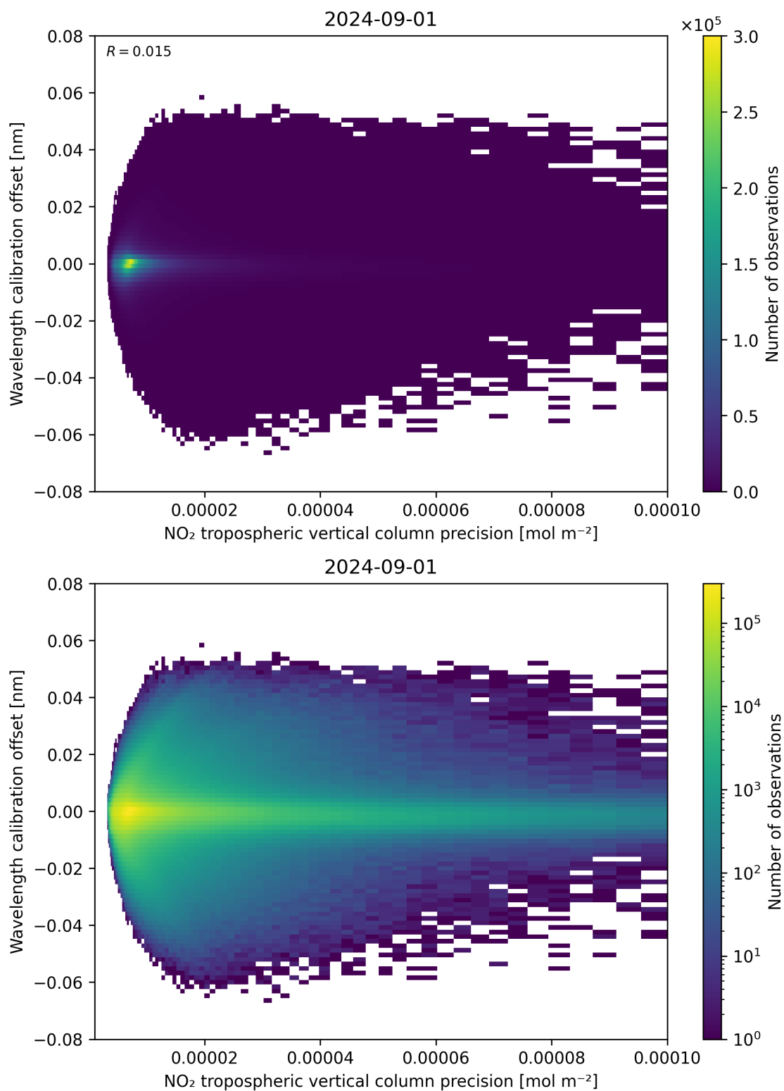
Figure 141: Scatter density plot of “NO 2 tropospheric vertical column precision” against “Wavelength calibration offset” for 2024-09-01 to 2024-09-02.
