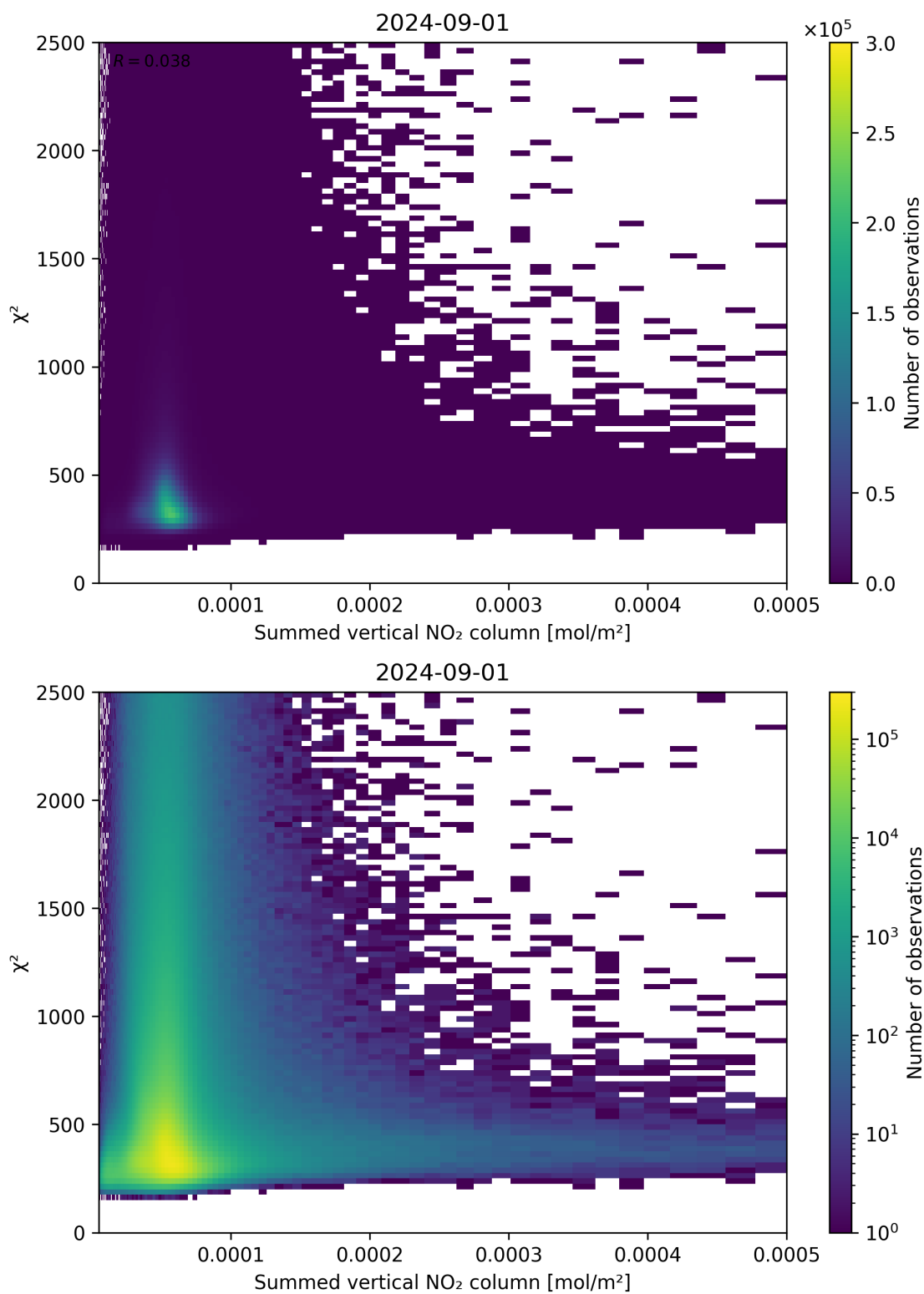
Figure 104: Scatter density plot of “Summed vertical NO 2 column” against “ \chi^2 ” for 2024-09-01 to 2024-09-02.
