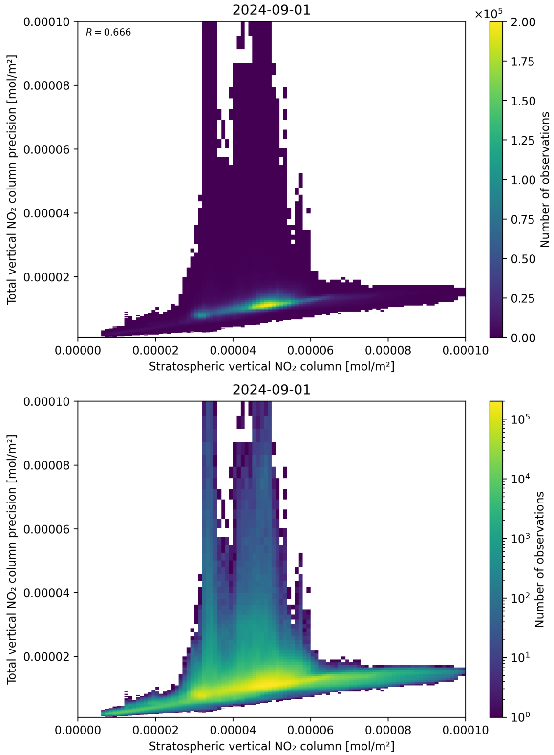
Figure 101: Scatter density plot of “Stratospheric vertical NO 2 column” against “Total vertical NO 2 column precision” for 2024-09-01 to 2024-09-02.
