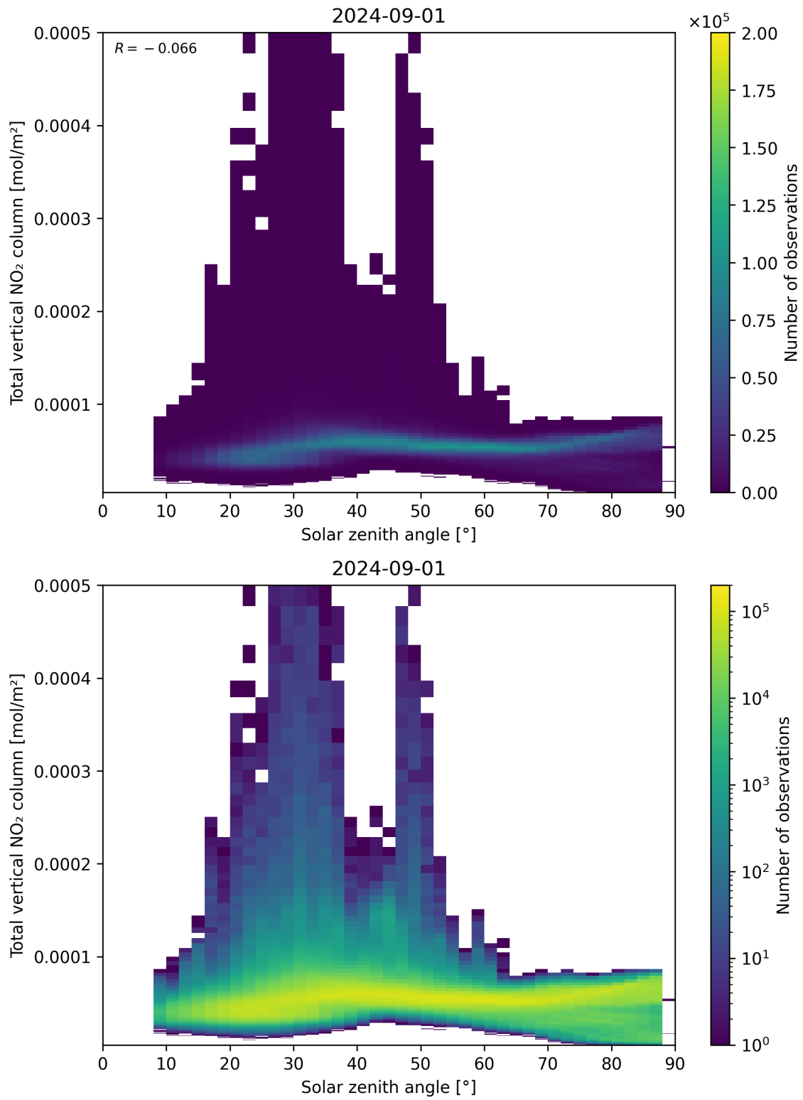
Figure 153: Scatter density plot of “Solar zenith angle” against “Total vertical NO 2 column” for 2024-09-01 to 2024-09-02.
