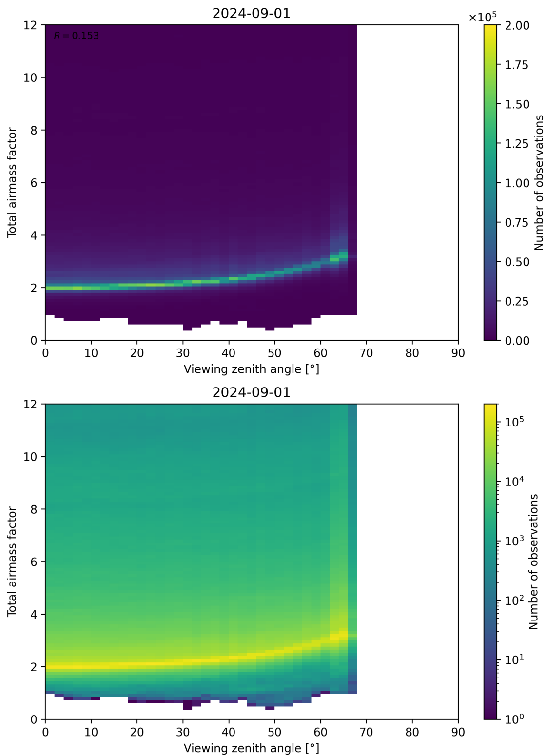
Figure 160: Scatter density plot of “Viewing zenith angle” against “Total airmass factor” for 2024-09-01 to 2024-09-02.
