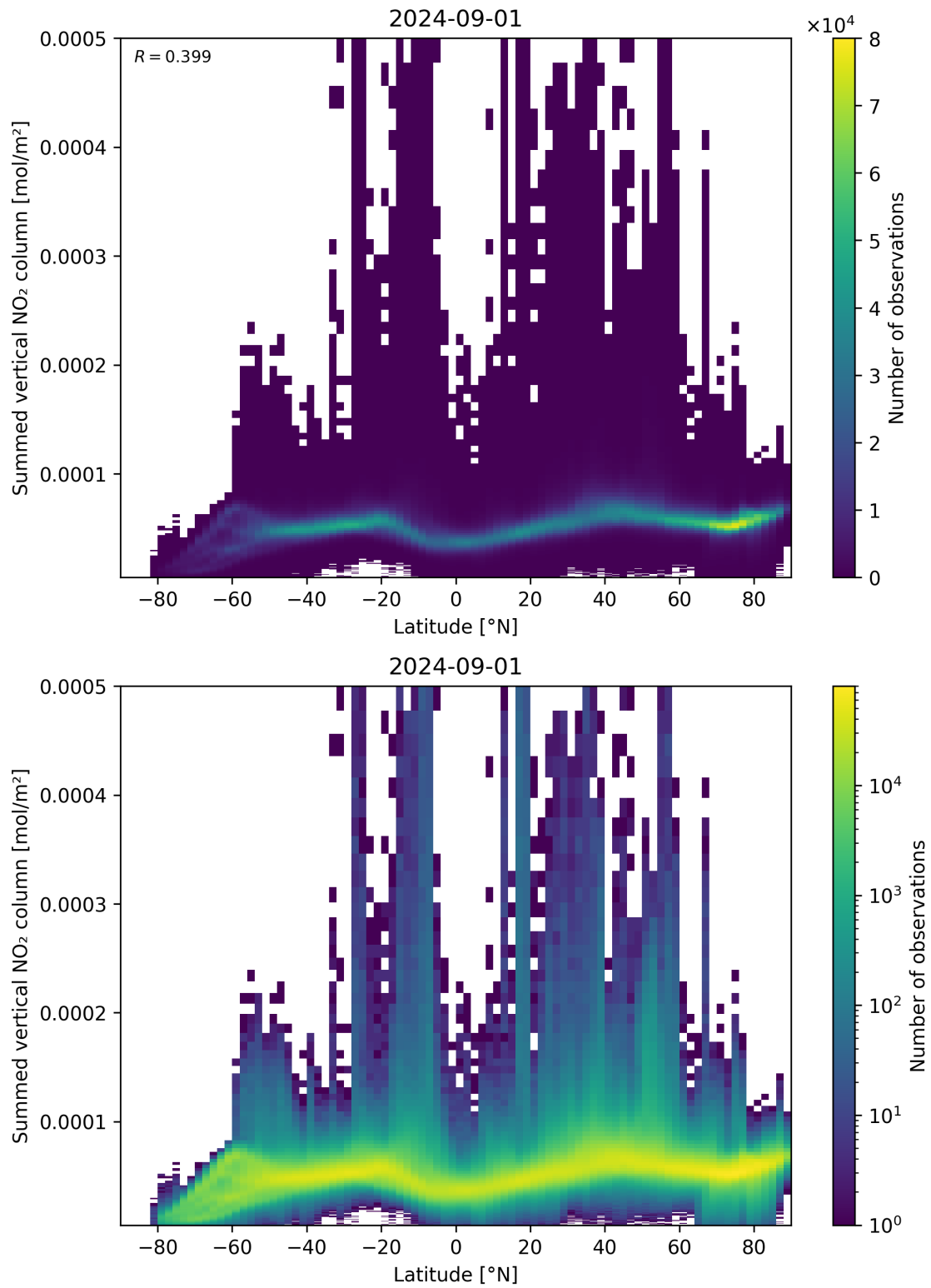
Figure 88: Scatter density plot of “Latitude” against “Summed vertical NO 2 column” for 2024-09-01 to 2024-09-02.
