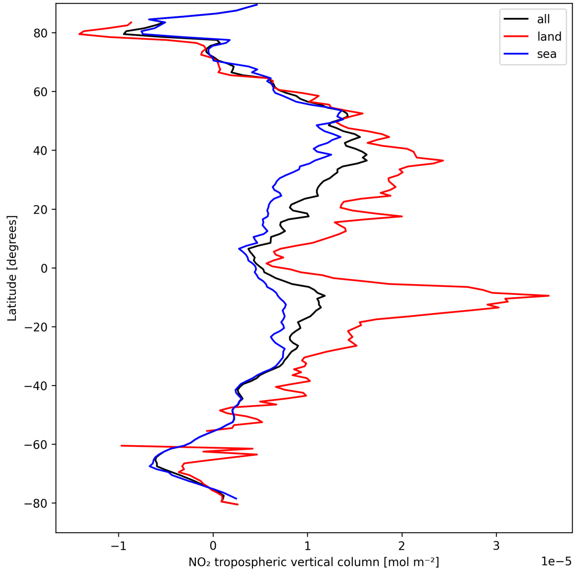
Figure 12: Zonal average of “NO 2 tropospheric vertical column” for 2024-09-01 to 2024-09-02.
