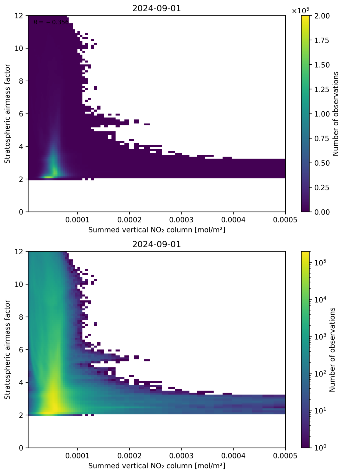
Figure 103: Scatter density plot of “Summed vertical NO 2 column” against “Stratospheric airmass factor” for 2024-09-01 to 2024-09-02.
