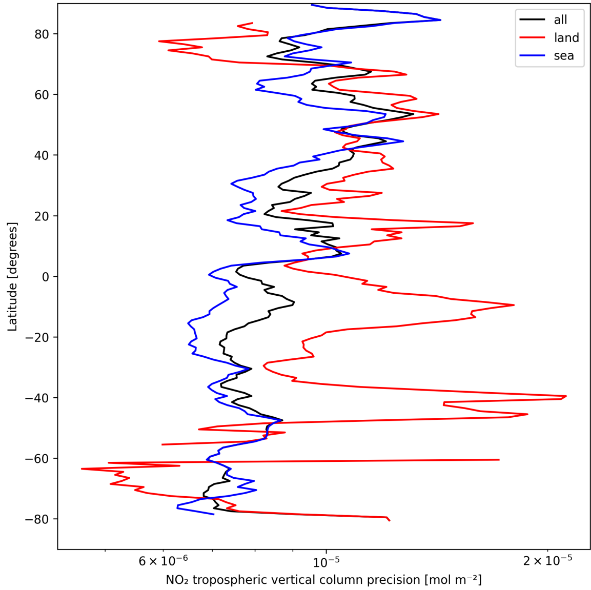
Figure 13: Zonal average of “NO 2 tropospheric vertical column precision” for 2024-09-01 to 2024-09-02.
