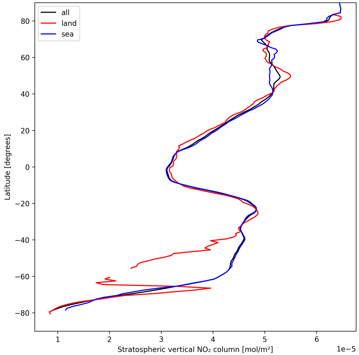
Figure 19: Zonal average of “Stratospheric vertical NO 2 column” for 2024-09-01 to 2024-09-02.
