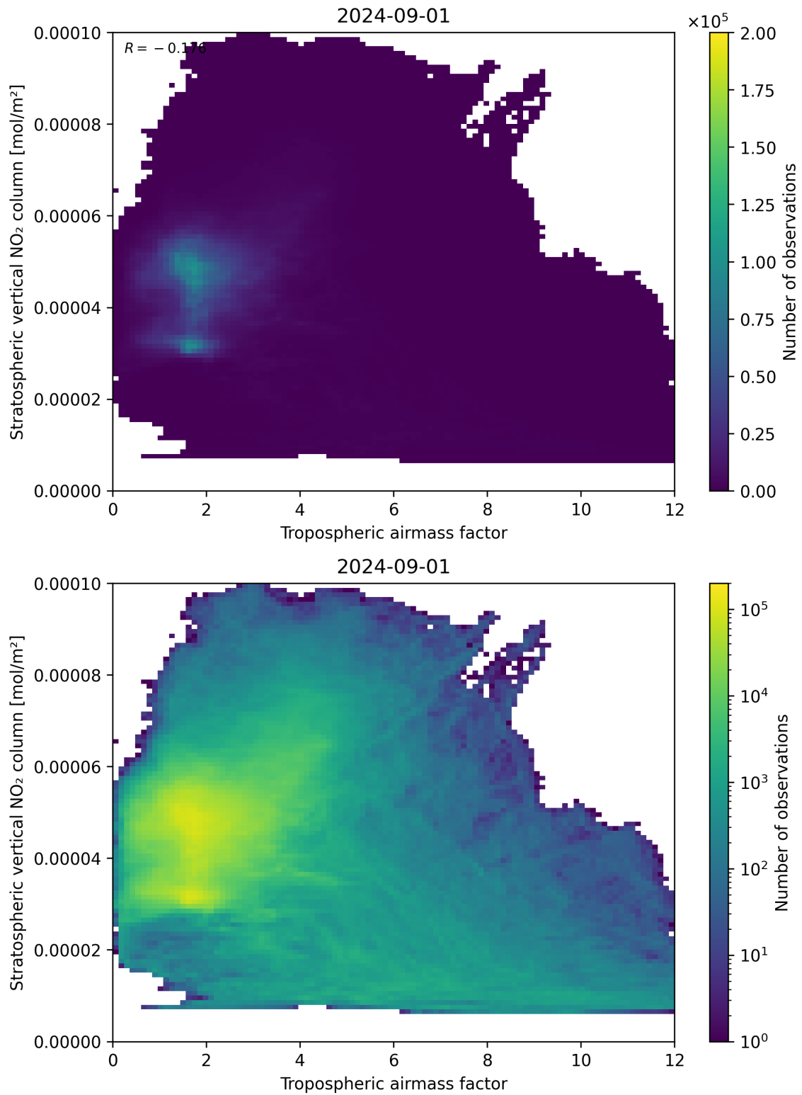
Figure 74: Scatter density plot of “Tropospheric air mass factor” against “Stratospheric vertical NO 2 column” for 2024-09-01 to 2024-09-02.
