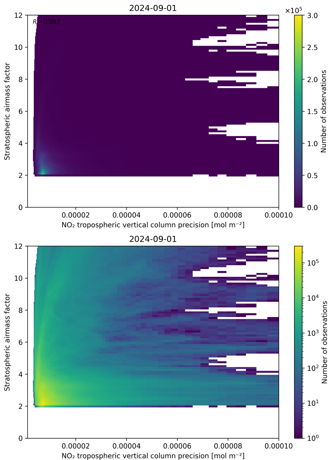
Figure 131: Scatter density plot of “NO 2 tropospheric vertical column precision” against “Stratospheric airmass factor” for 2024-09-01 to 2024-09-02.
