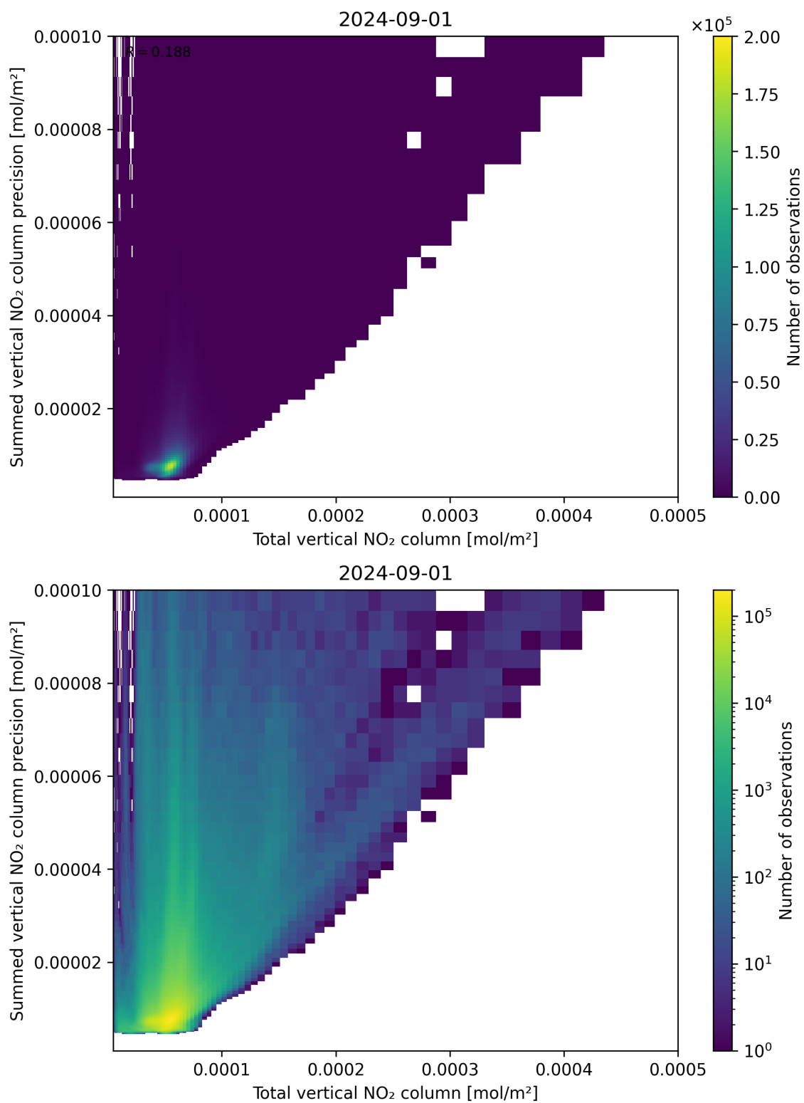
Figure 113: Scatter density plot of “Total vertical NO 2 column” against “Summed vertical NO 2 column precision” for 2024-09-01 to 2024-09-02.
