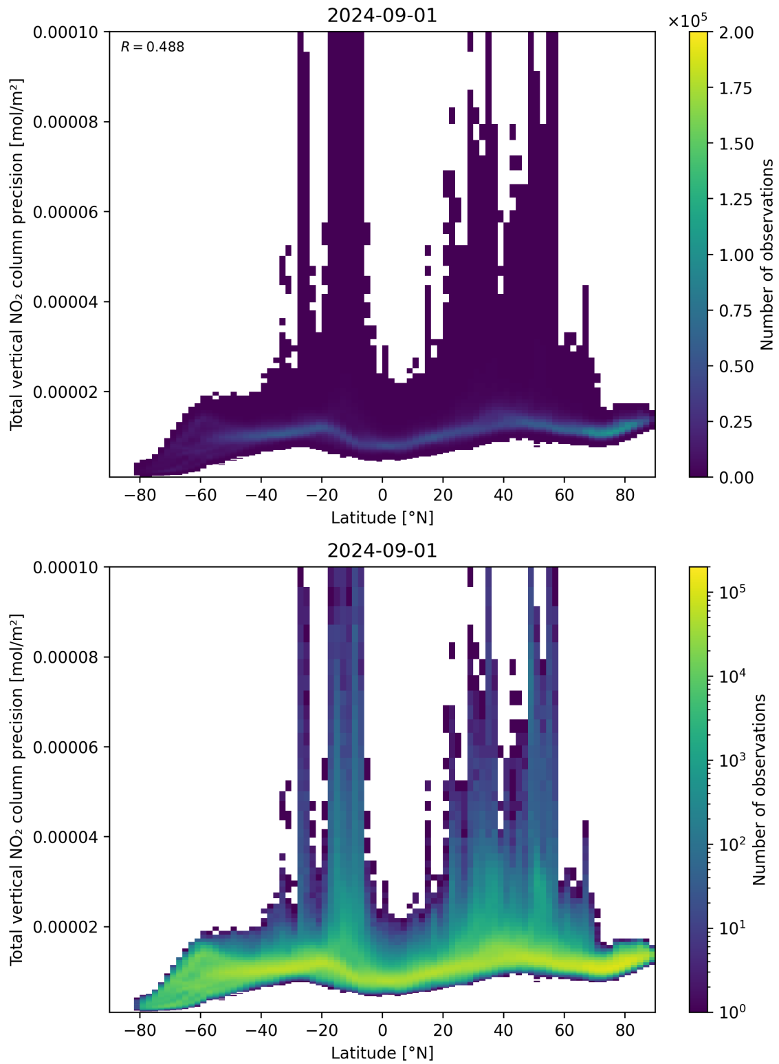
Figure 91: Scatter density plot of “Latitude” against “Total vertical NO 2 column precision” for 2024-09-01 to 2024-09-02.
