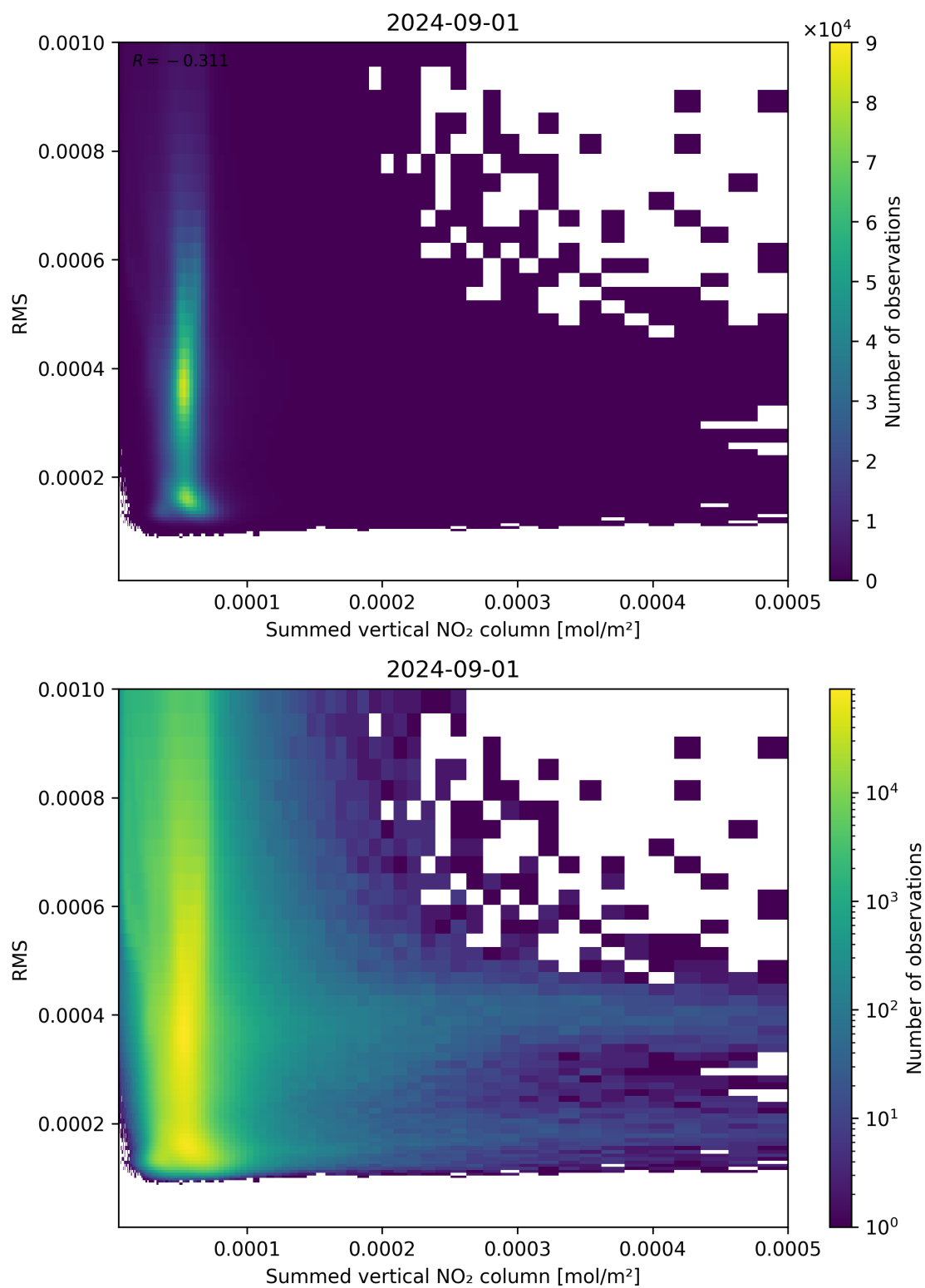
Figure 109: Scatter density plot of “Summed vertical NO 2 column” against “RMS” for 2024-09-01 to 2024-09-02.
