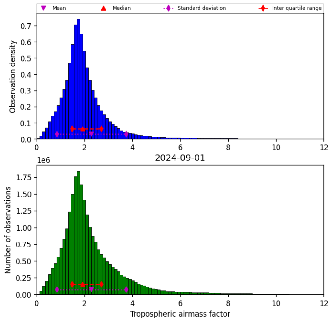
Figure 31: Histogram of “Tropospheric airmass factor” for 2024-09-01 to 2024-09-02
