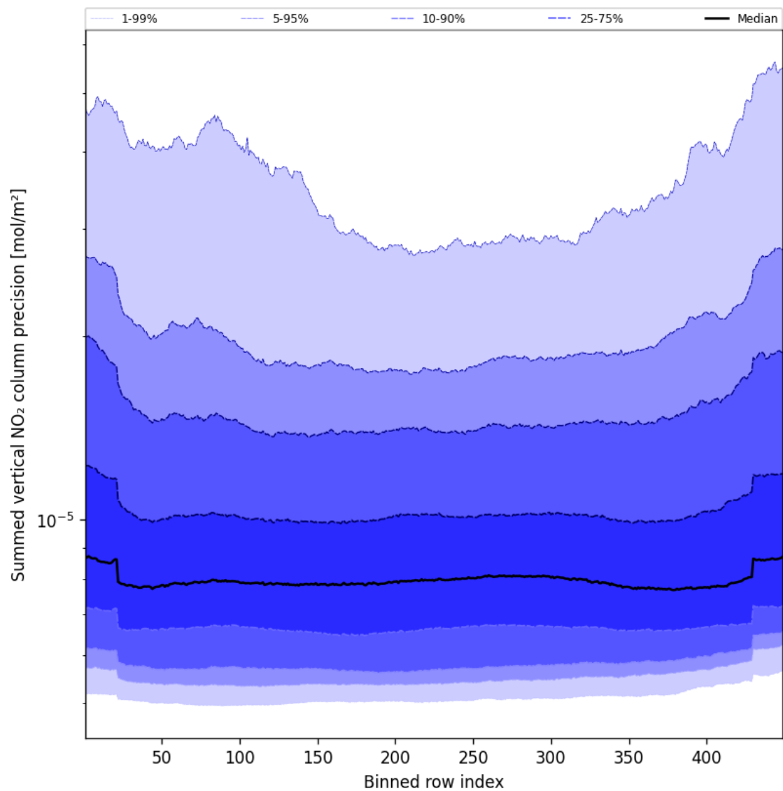
Figure 58: Along track statistics of “Summed vertical NO 2 column precision” for 2024-09-01 to 2024-09-02
