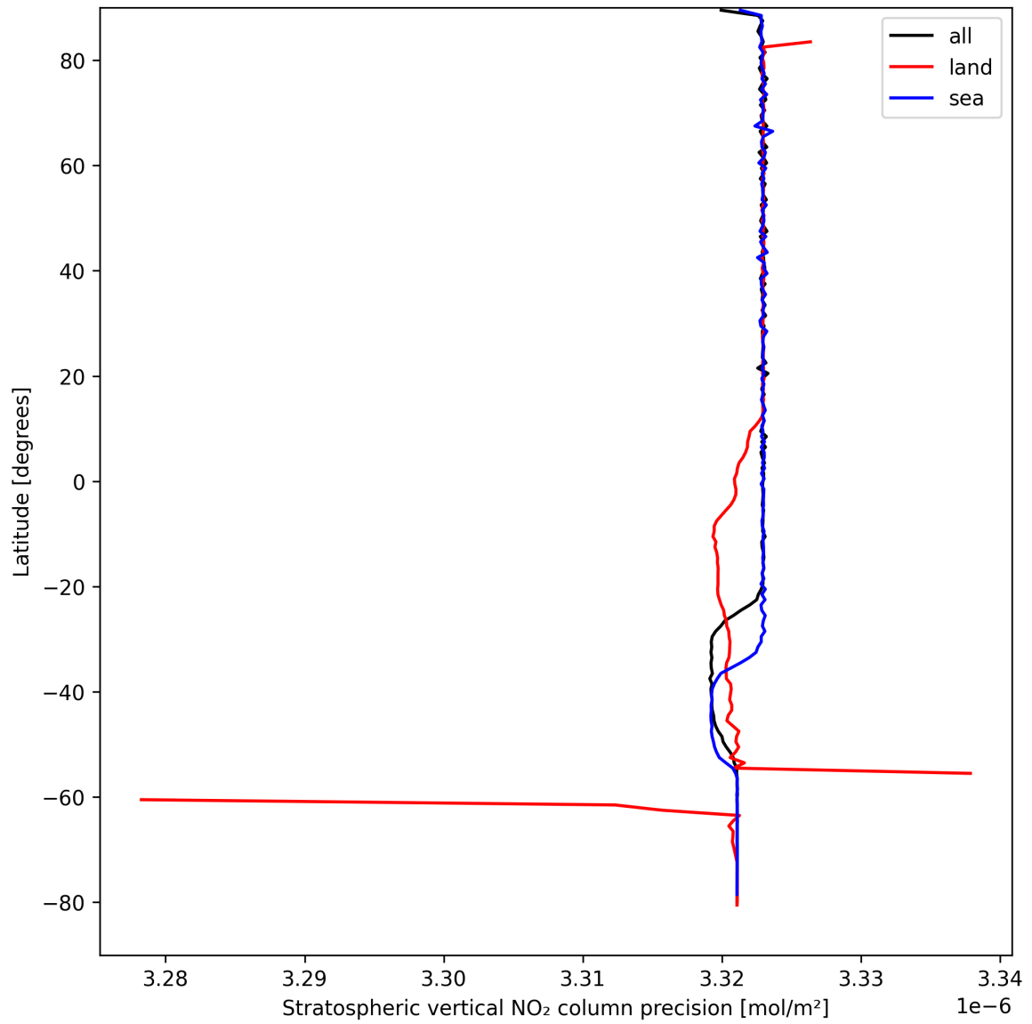
Figure 20: Zonal average of “Stratospheric vertical NO 2 column precision” for 2024-09-01 to 2024-09-02.
