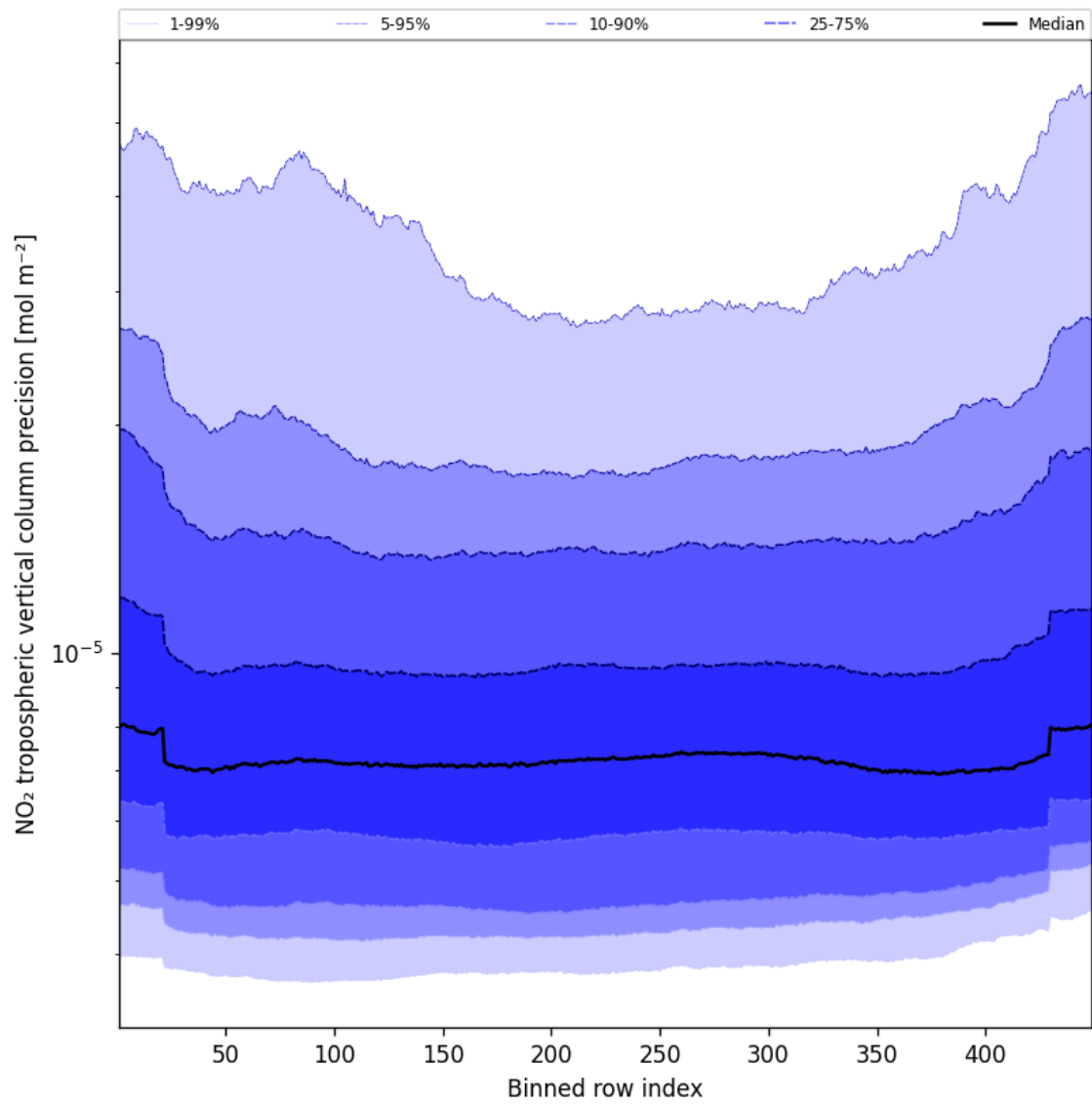
Figure 47: Along track statistics of “NO 2 tropospheric vertical column precision” for 2024-09-01 to 2024-09-02
