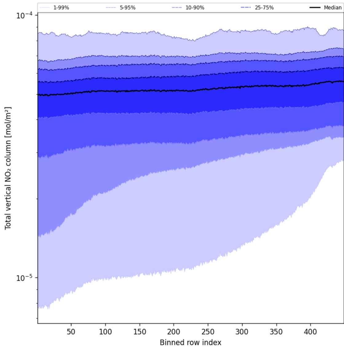
Figure 55: Along track statistics of “Total vertical NO 2 column” for 2024-09-01 to 2024-09-02
