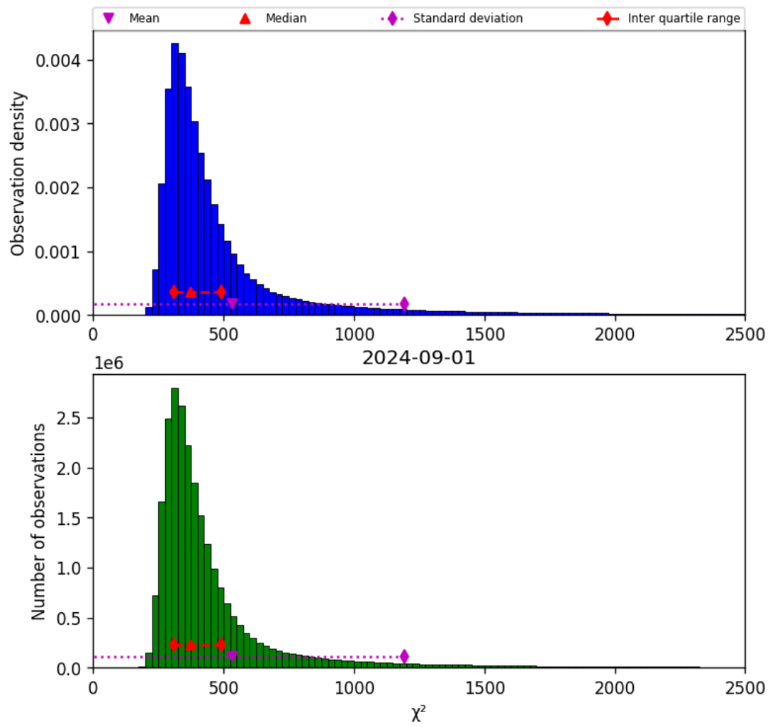
Figure 42: Histogram of " \chi^2 " for 2024-09-01 to 2024-09-02
