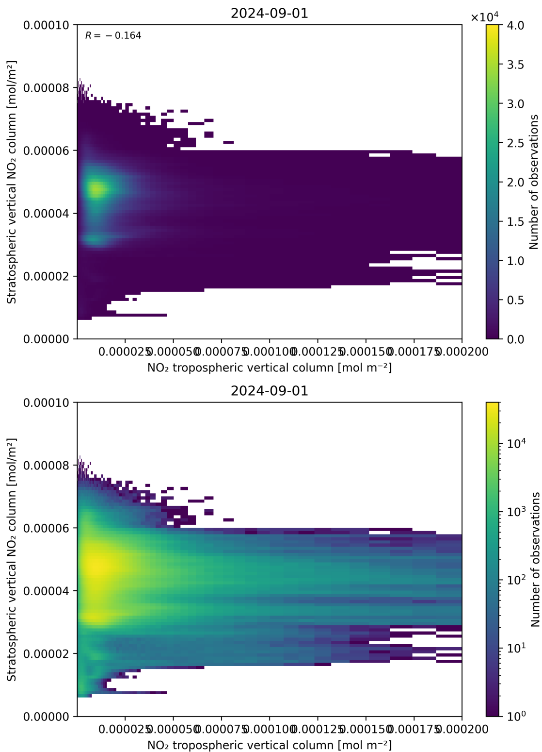
Figure 125: Scatter density plot of “NO 2 tropospheric vertical column” against “Stratospheric vertical NO 2 column” for 2024-09-01 to 2024-09-02.
