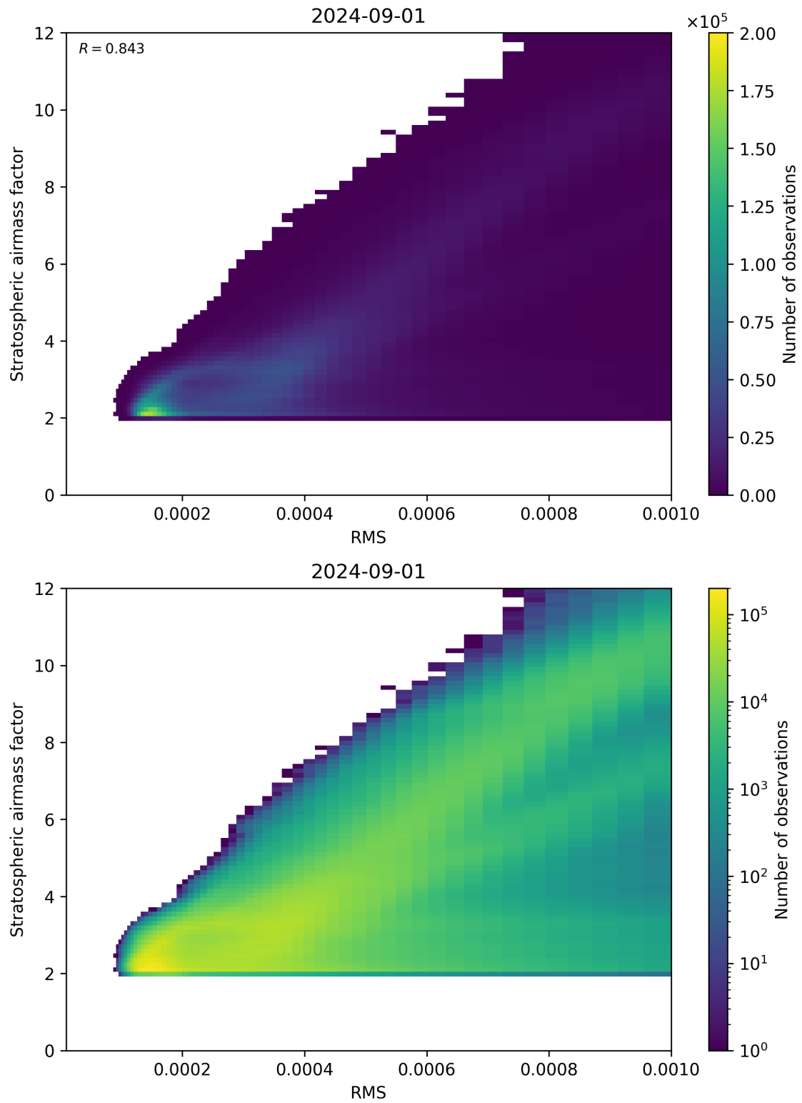
Figure 144: Scatter density plot of “RMS” against “Stratospheric airmass factor” for 2024-09-01 to 2024-09-02.
