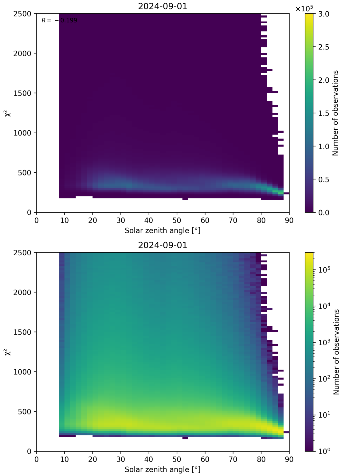
Figure 148: Scatter density plot of “Solar zenith angle” against “ \chi^2 ” for 2024-09-01 to 2024-09-02.
