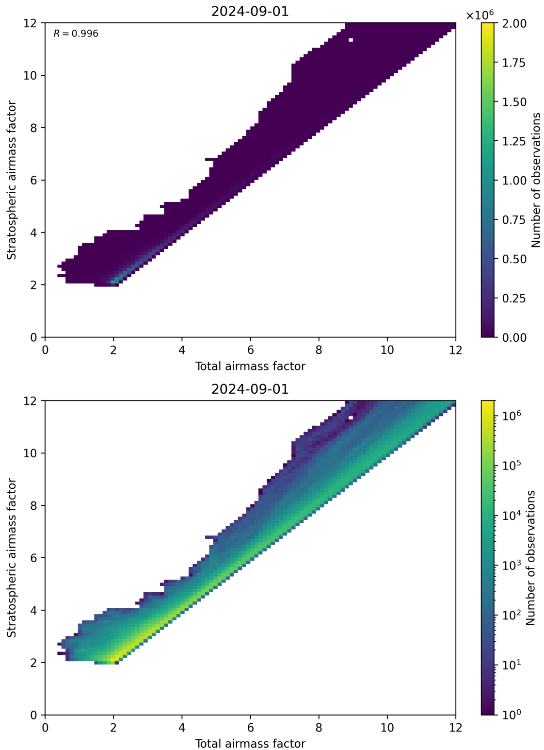
Figure 62: Scatter density plot of “Total airmass factor” against “Stratospheric airmass factor” for 2024-09-01 to 2024-09-02.
