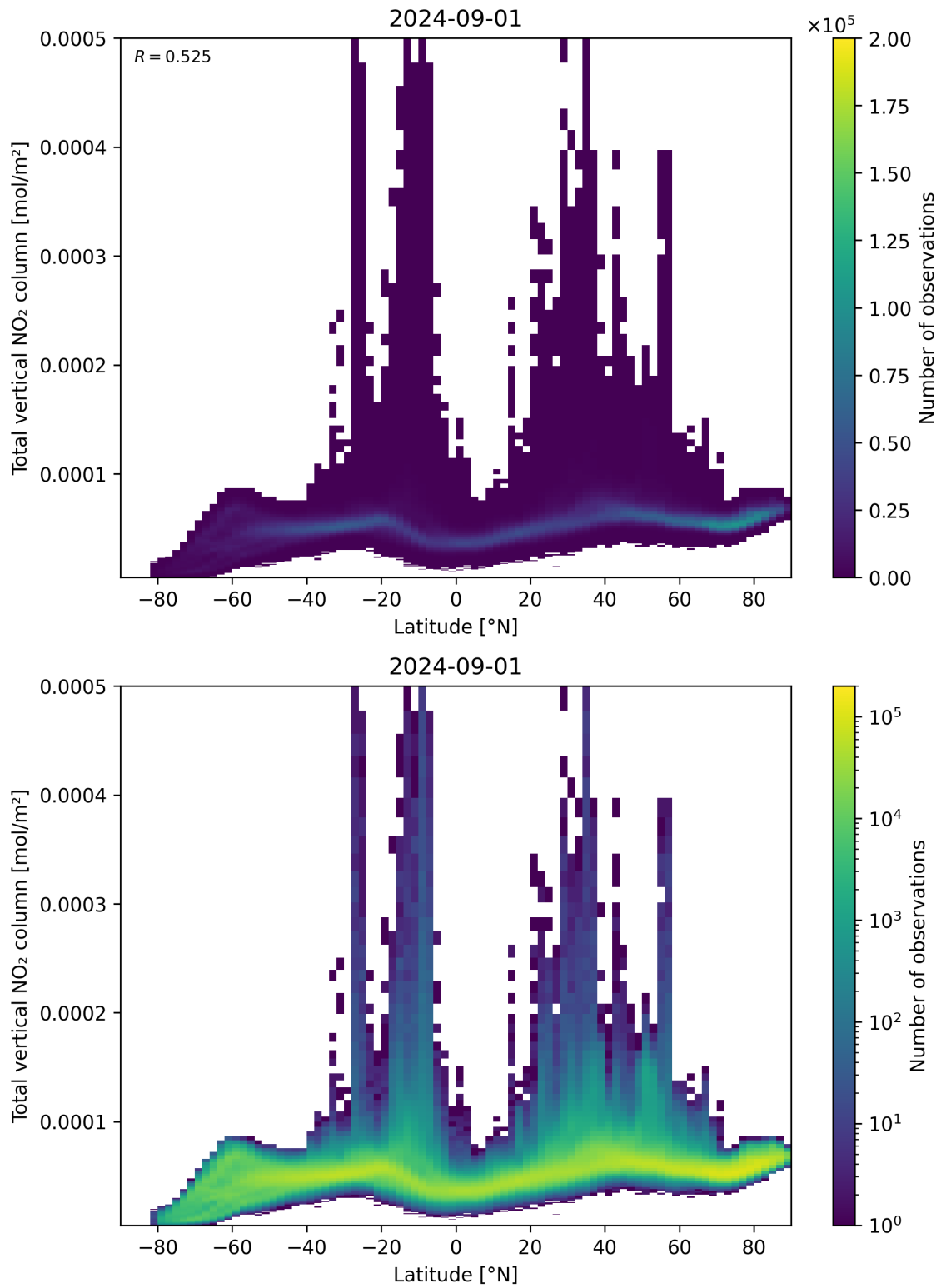
Figure 90: Scatter density plot of “Latitude” against “Total vertical NO 2 column” for 2024-09-01 to 2024-09-02.
