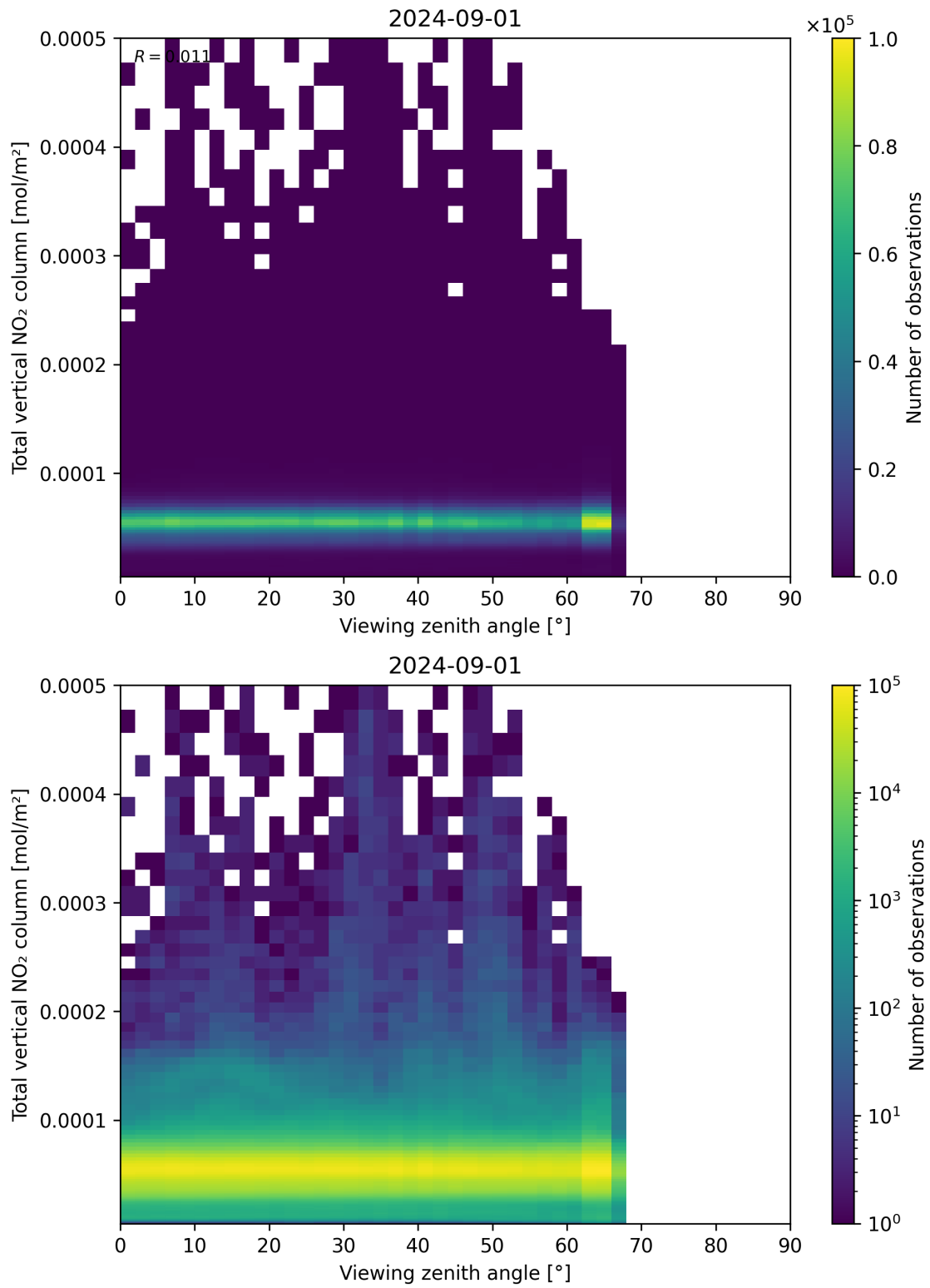
Figure 167: Scatter density plot of “Viewing zenith angle” against “Total vertical NO 2 column” for 2024-09-01 to 2024-09-02.
