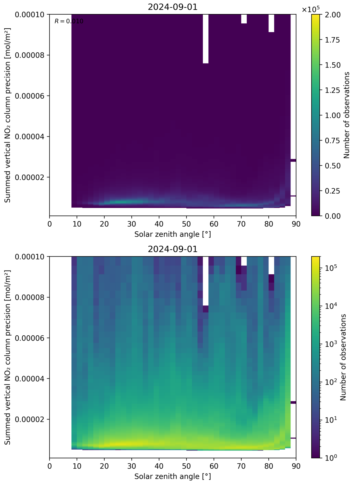
Figure 152: Scatter density plot of “Solar zenith angle” against “Summed vertical NO 2 column precision” for 2024-09-01 to 2024-09-02.
