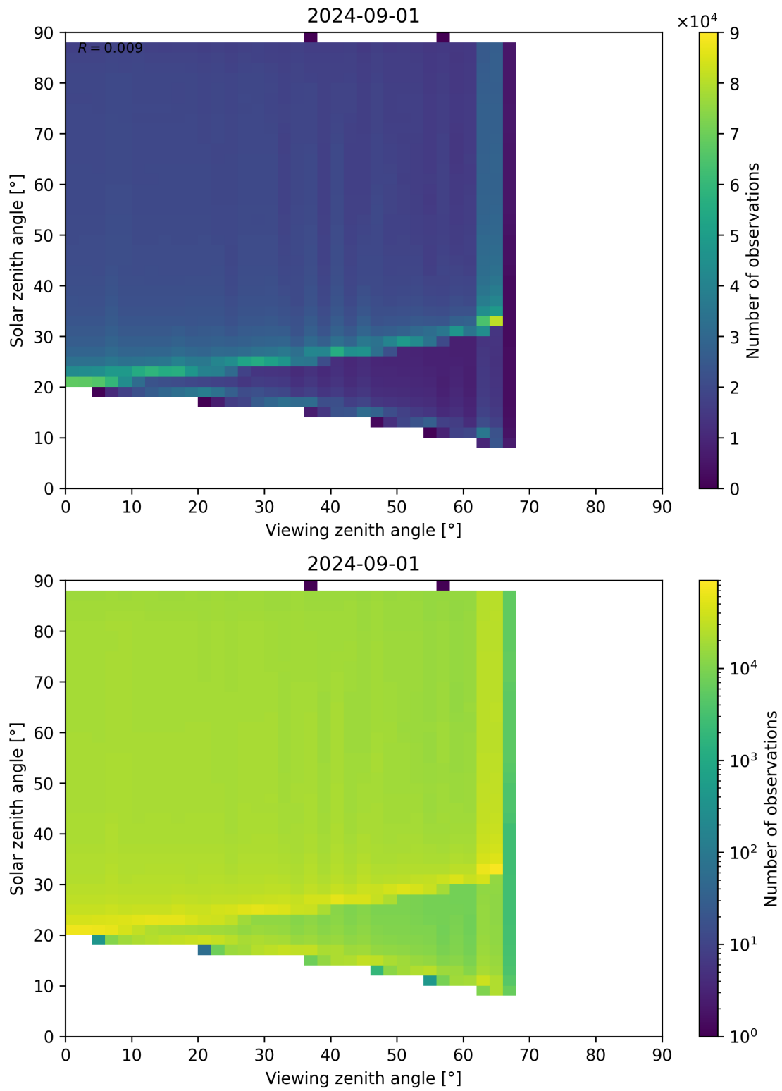
Figure 172: Scatter density plot of “Viewing zenith angle” against “Solar zenith angle” for 2024-09-01 to 2024-09-02.
