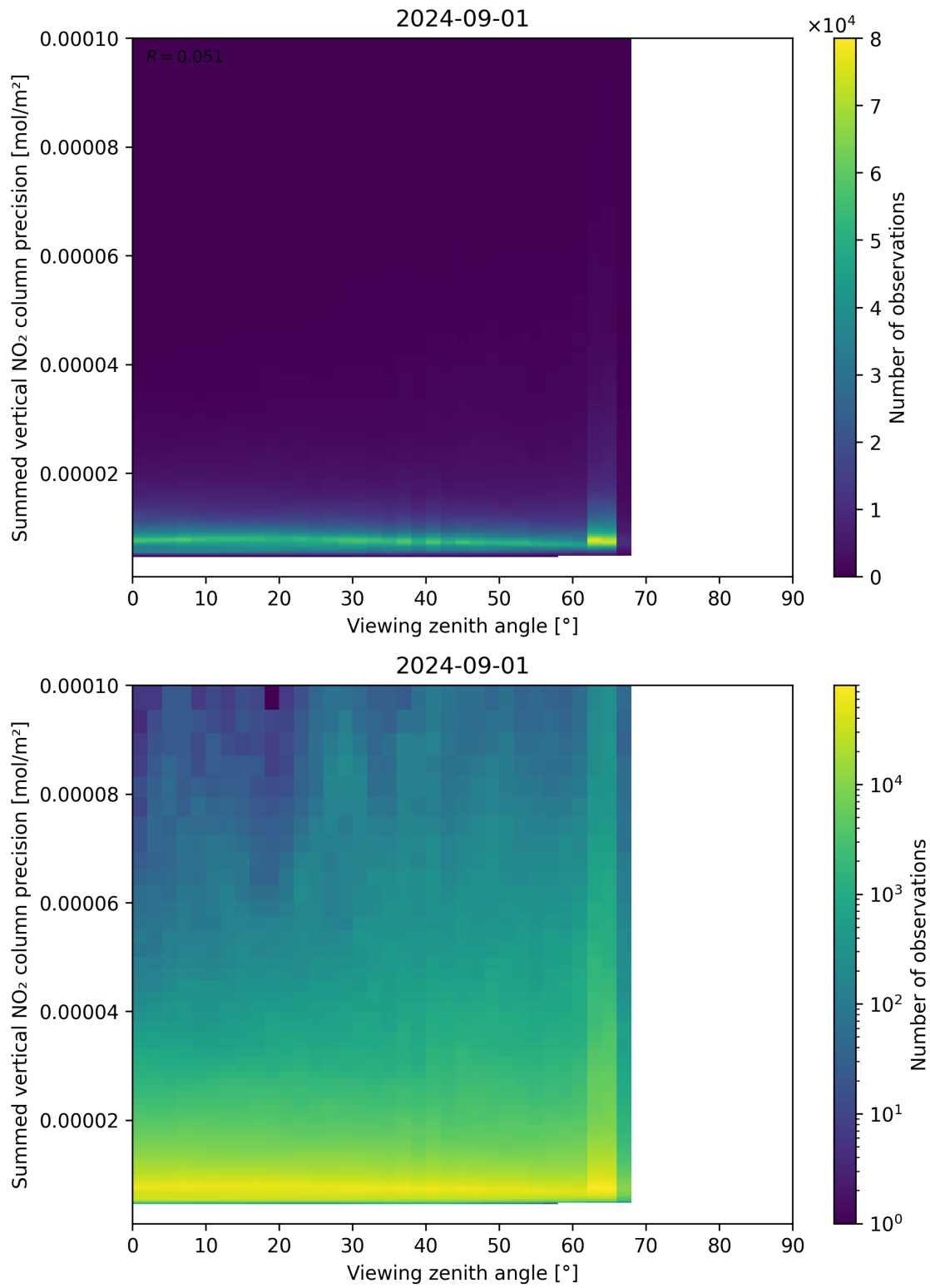
Figure 166: Scatter density plot of “Viewing zenith angle” against “Summed vertical NO 2 column precision” for 2024-09-01 to 2024-09-02.
