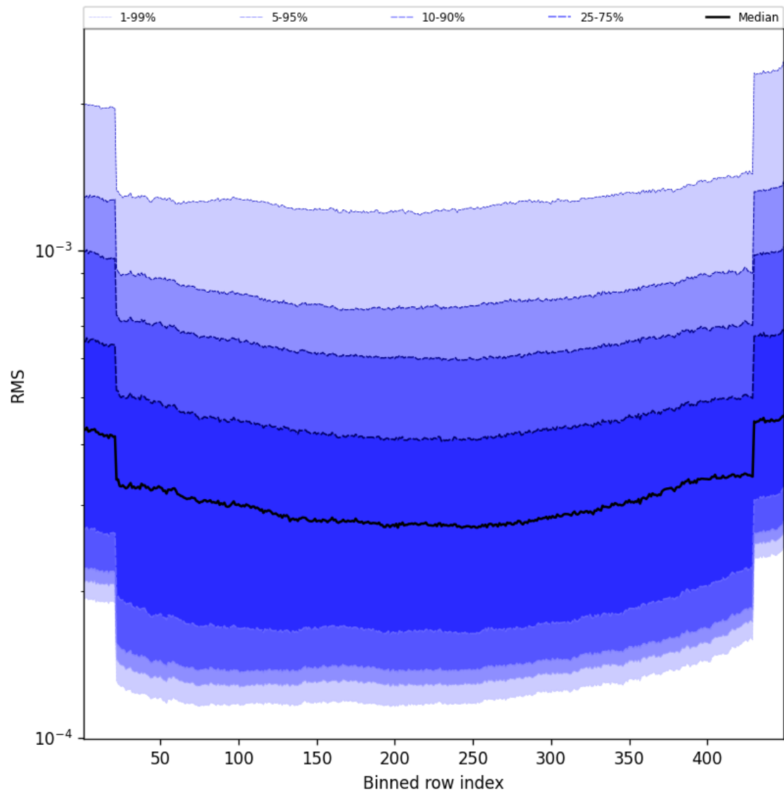
Figure 60: Along track statistics of “RMS” for 2024-09-01 to 2024-09-02
