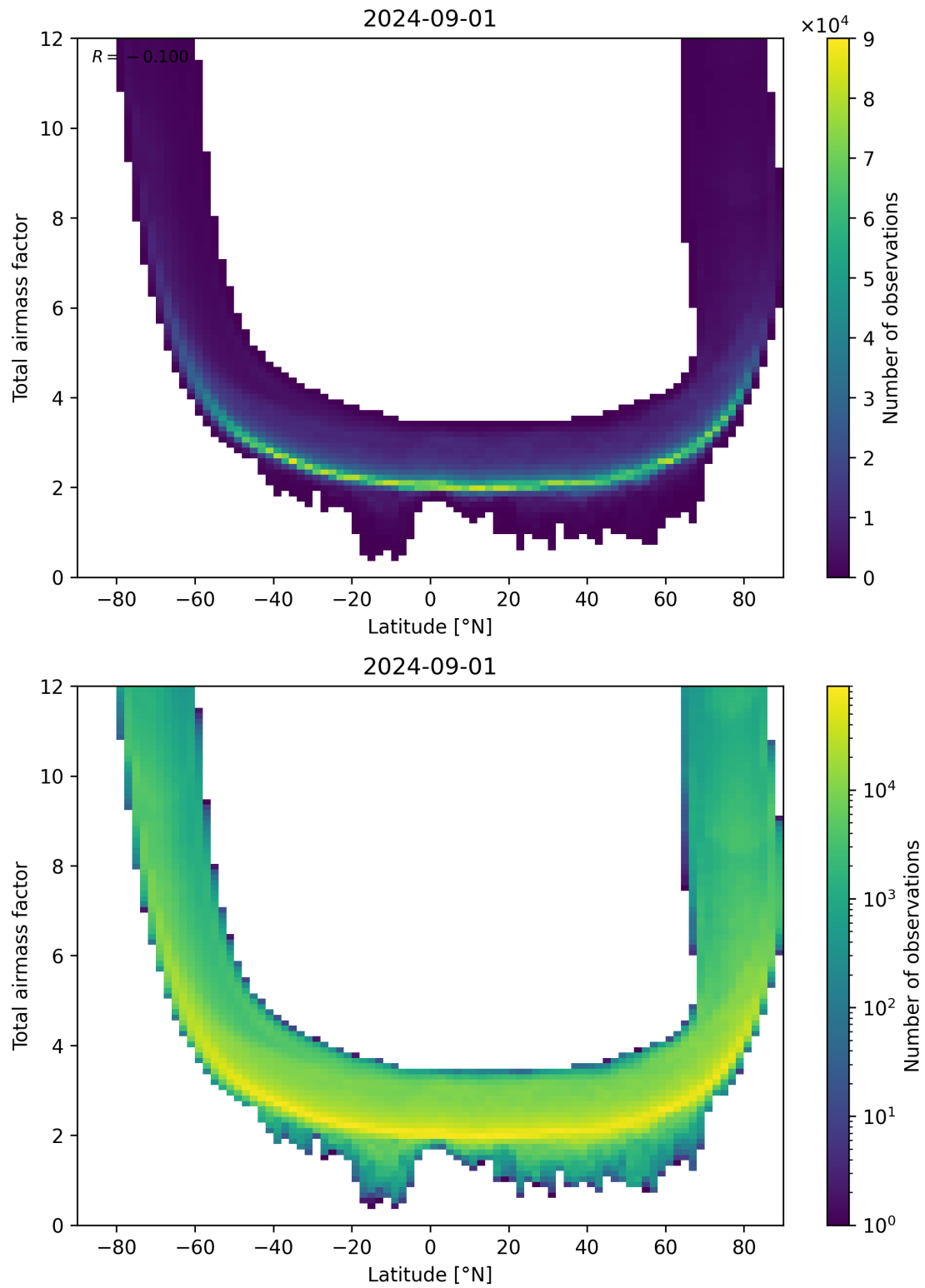
Figure 84: Scatter density plot of “Latitude” against “Total airmass factor” for 2024-09-01 to 2024-09-02.
