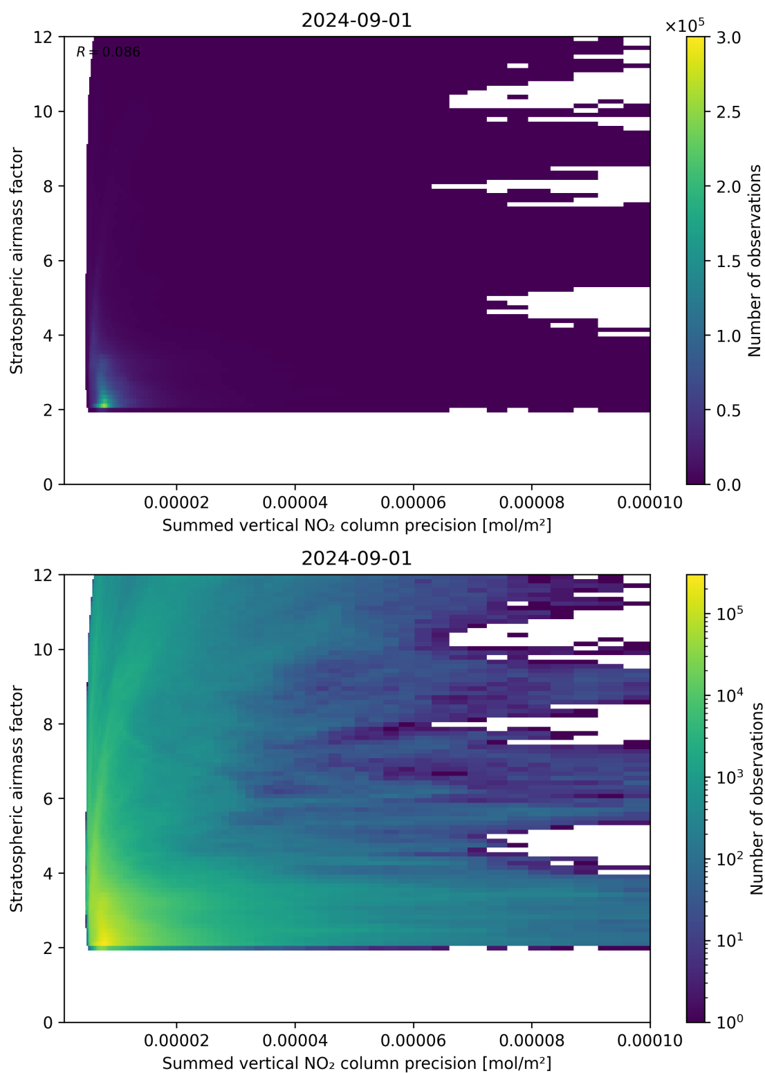
Figure 106: Scatter density plot of “Summed vertical NO 2 column precision” against “Stratospheric airmass factor” for 2024-09-01 to 2024-09-02.
