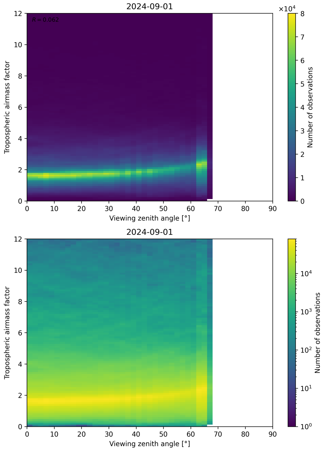
Figure 161: Scatter density plot of “Viewing zenith angle” against “Tropospheric airmass factor” for 2024-09-01 to 2024-09-02.
