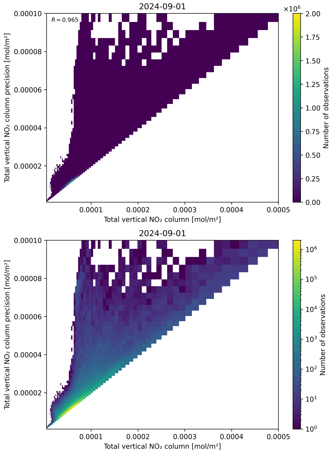
Figure 114: Scatter density plot of “Total vertical NO 2 column” against “Total vertical NO 2 column precision” for 2024-09-01 to 2024-09-02.
