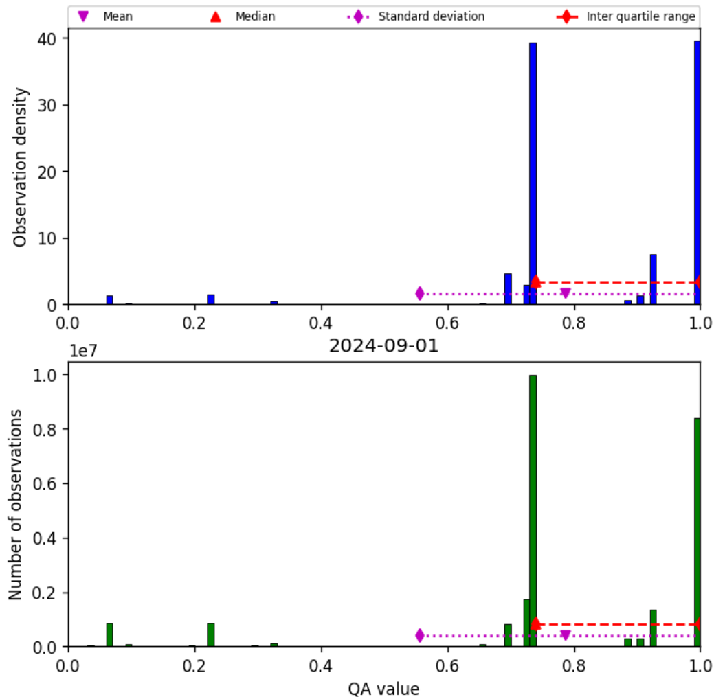
Figure 28: Histogram of “QA value” for 2024-09-01 to 2024-09-02
