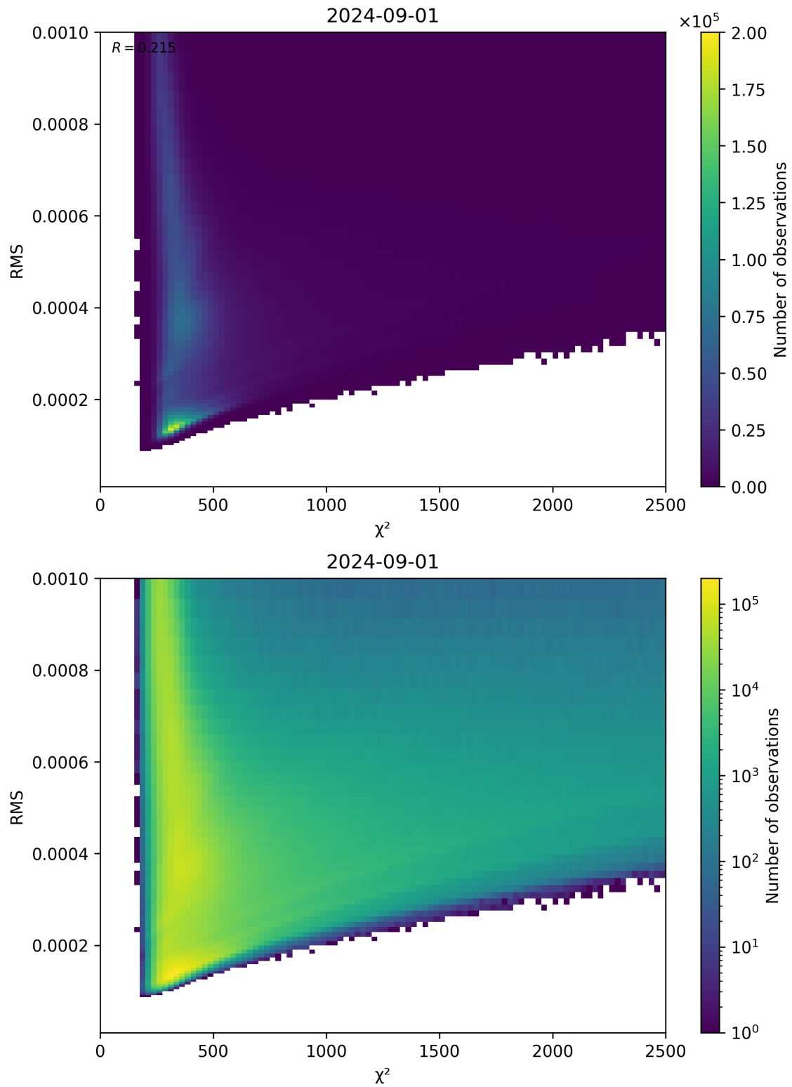
Figure 82: Scatter density plot of “ \chi^2 ” against “RMS” for 2024-09-01 to 2024-09-02.
