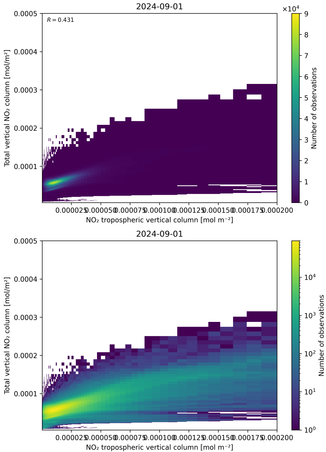
Figure 128: Scatter density plot of “NO 2 tropospheric vertical column” against “Total vertical NO 2 column” for 2024-09-01 to 2024-09-02.
