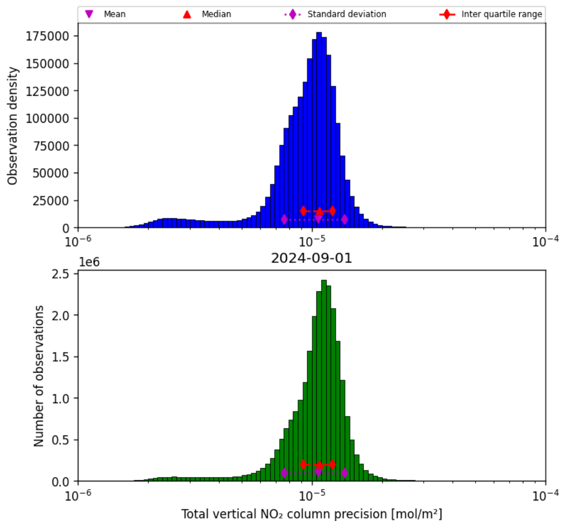
Figure 39: Histogram of “Total vertical NO 2 column precision” for 2024-09-01 to 2024-09-02
