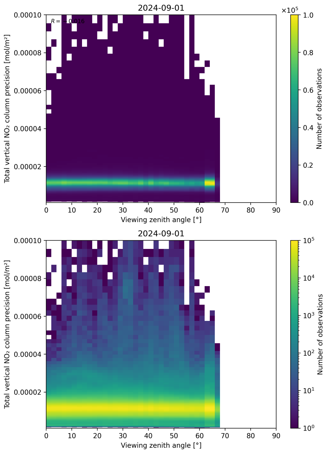
Figure 168: Scatter density plot of “Viewing zenith angle” against “Total vertical NO 2 column precision” for 2024-09-01 to 2024-09-02.
