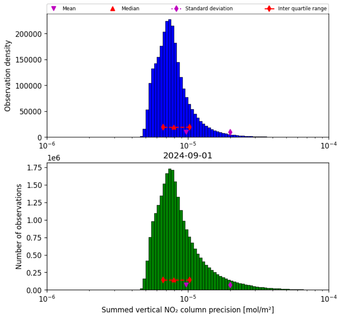
Figure 41: Histogram of "Summed vertical NO 2 column precision" for 2024-09-01 to 2024-09-02
