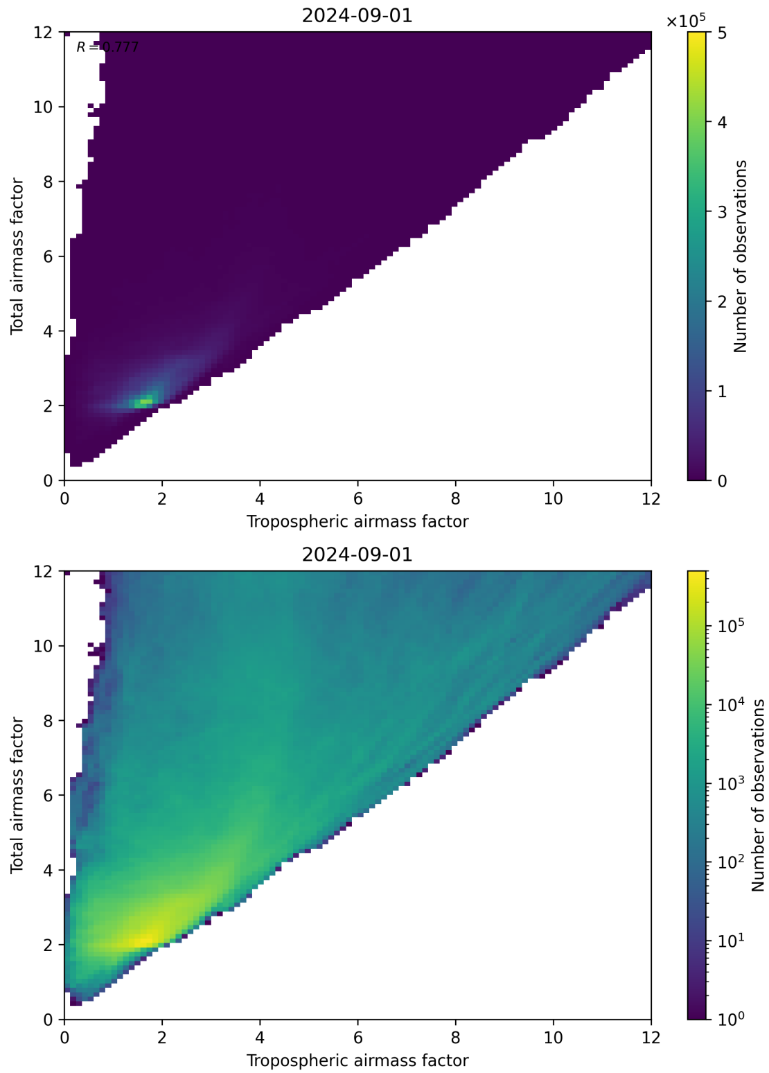
Figure 72: Scatter density plot of “Tropospheric airmass factor” against “Total airmass factor” for 2024-09-01 to 2024-09-02.
