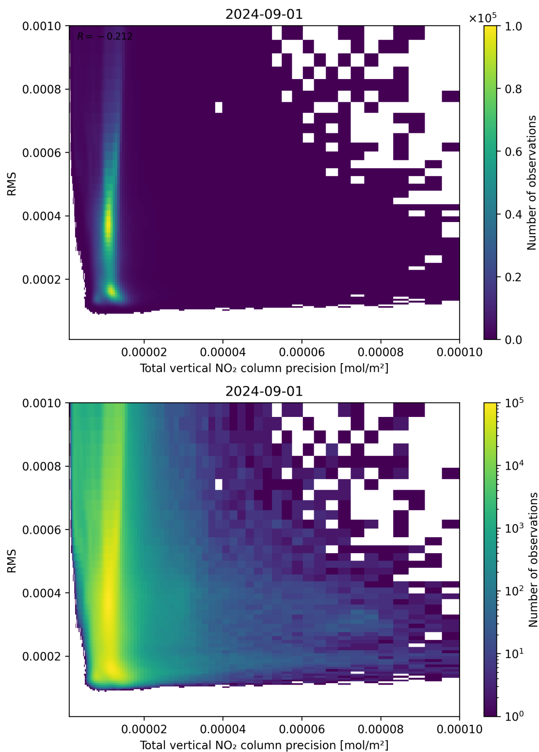
Figure 119: Scatter density plot of “Total vertical NO 2 column precision” against “RMS” for 2024-09-01 to 2024-09-02.
