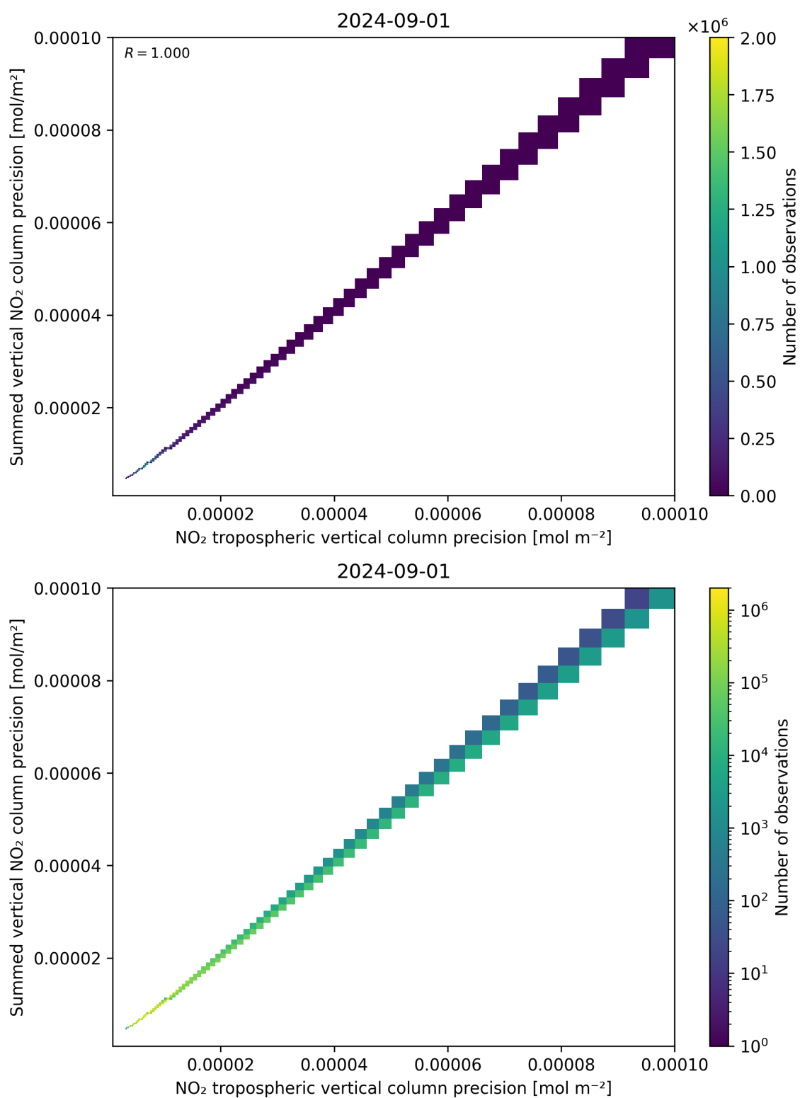
Figure 137: Scatter density plot of “NO 2 tropospheric vertical column precision” against “Summed vertical NO 2 column precision” for 2024-09-01 to 2024-09-02.
