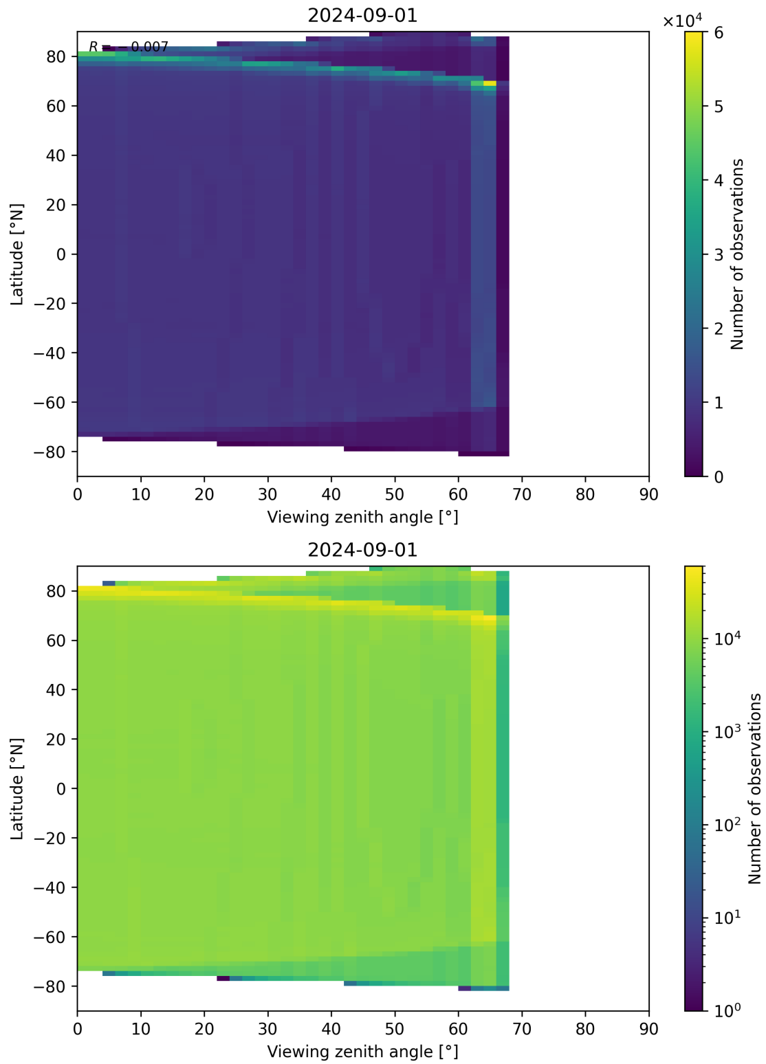
Figure 163: Scatter density plot of “Viewing zenith angle” against “Latitude” for 2024-09-01 to 2024-09-02.
