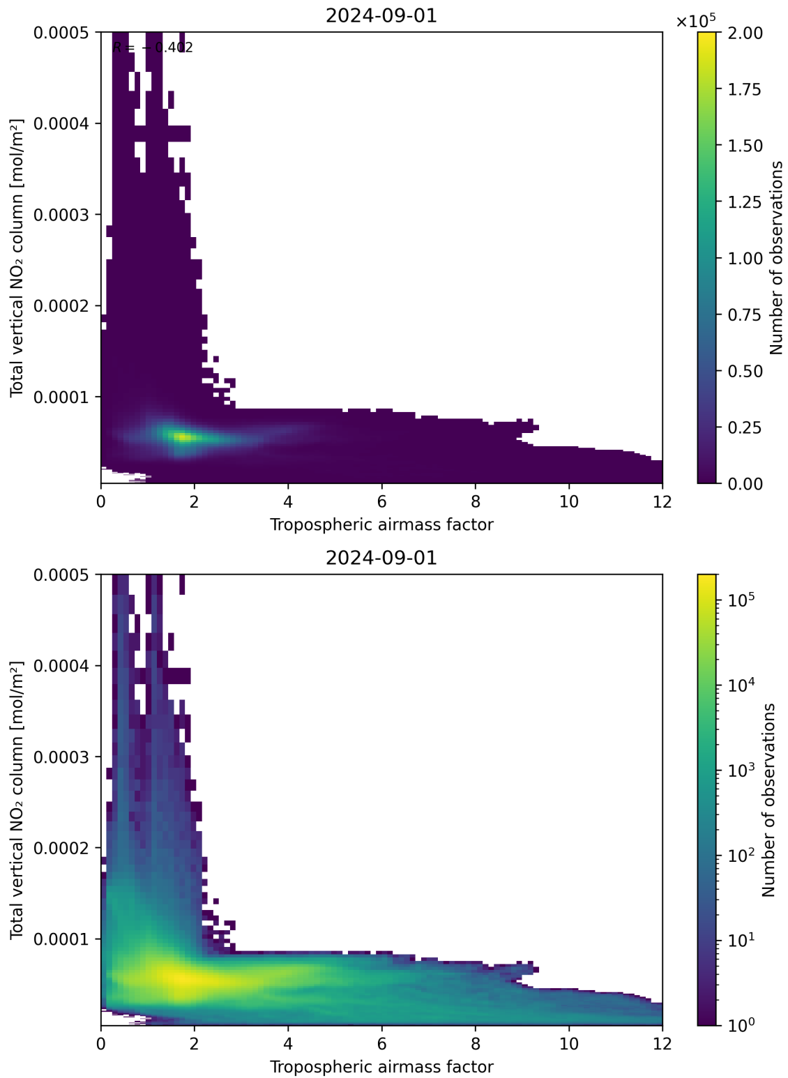
Figure 77: Scatter density plot of “Tropospheric airmass factor” against “Total vertical NO 2 column” for 2024-09-01 to 2024-09-02.
