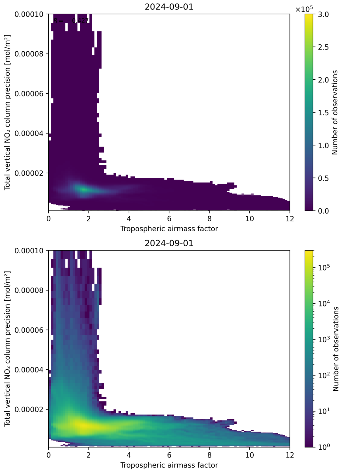
Figure 78: Scatter density plot of “Tropospheric air mass factor” against “Total vertical NO 2 column precision” for 2024-09-01 to 2024-09-02.
