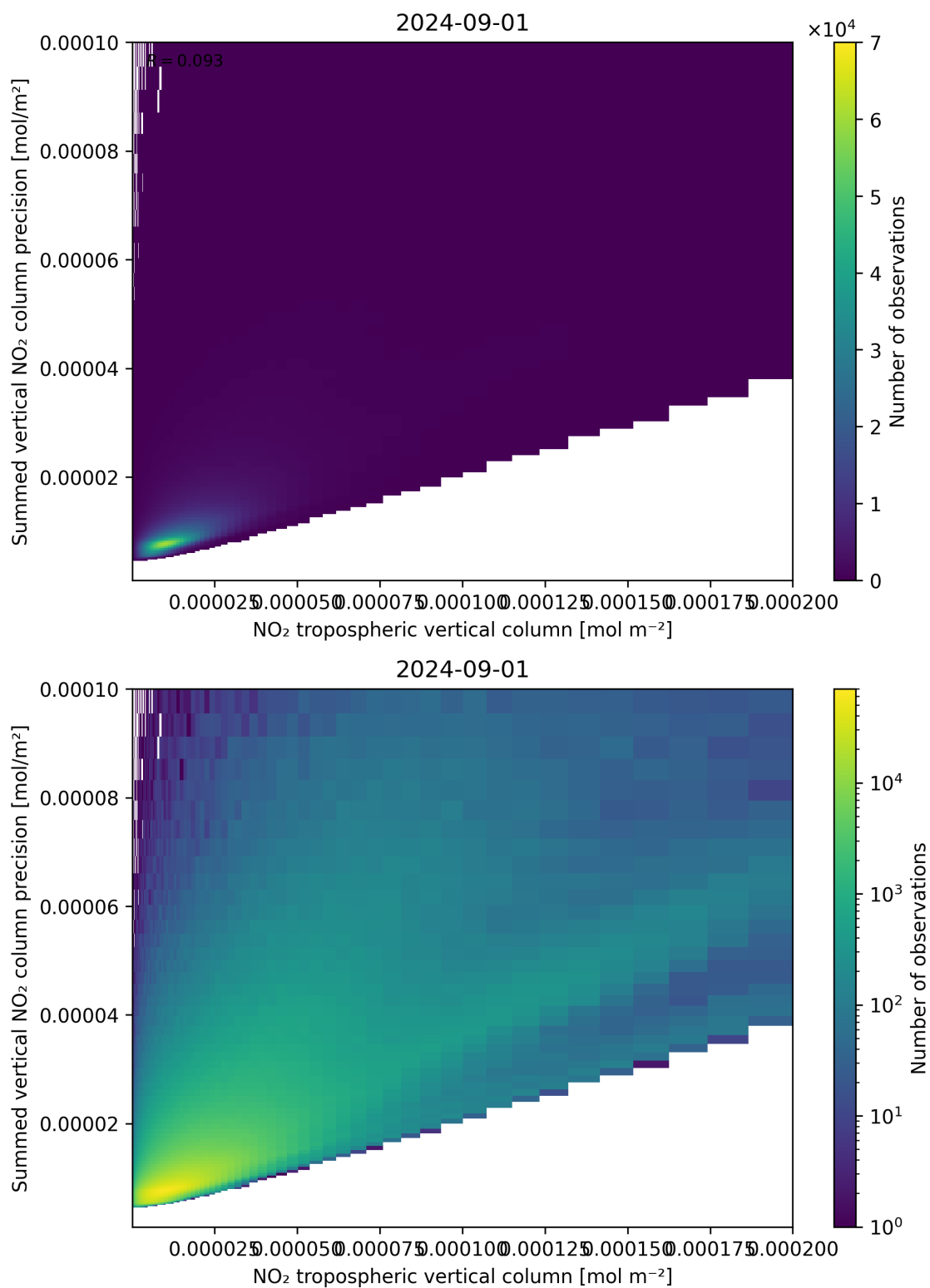
Figure 127: Scatter density plot of “NO 2 tropospheric vertical column” against “Summed vertical NO 2 column precision” for 2024-09-01 to 2024-09-02.
