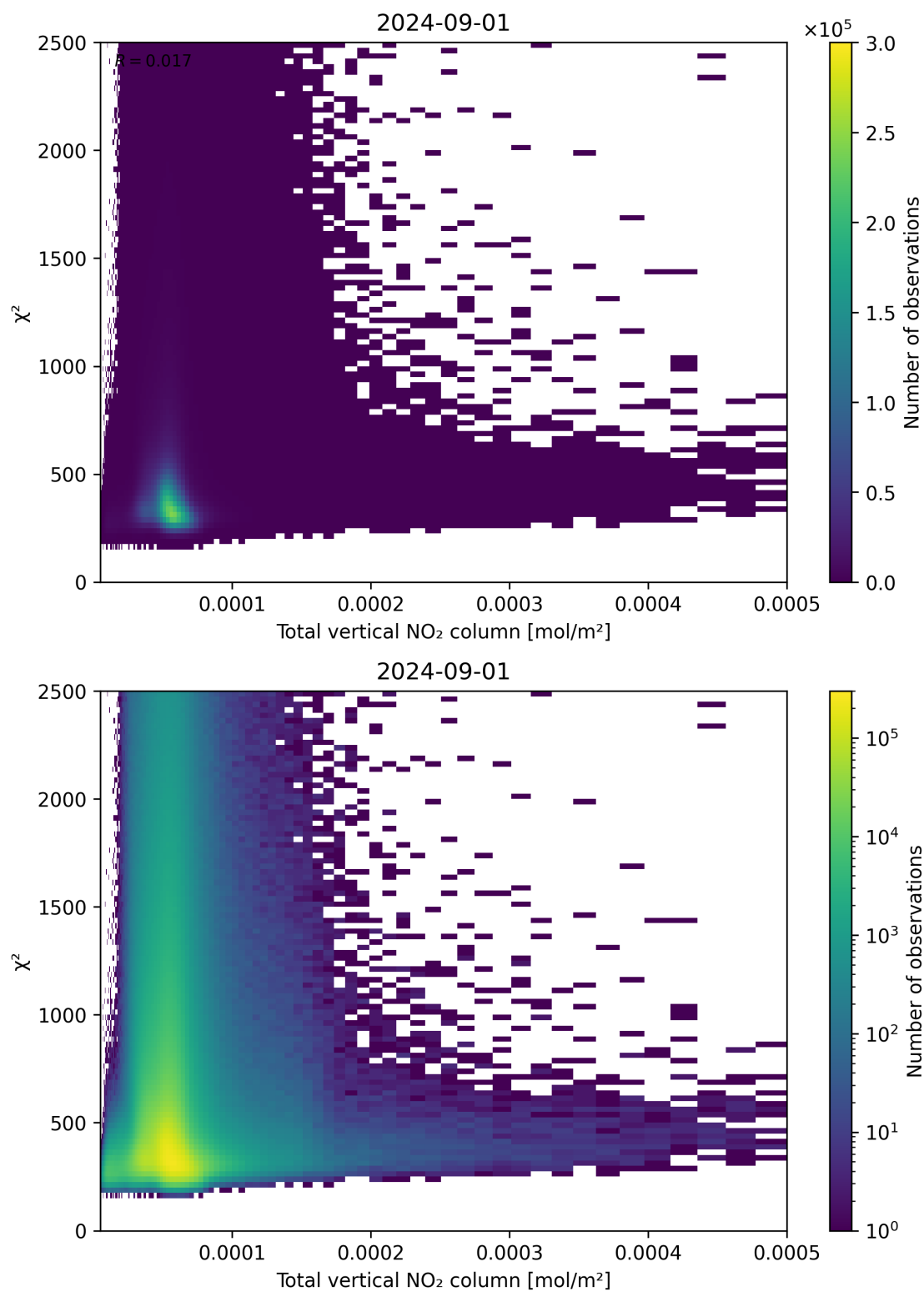
Figure 111: Scatter density plot of “Total vertical NO 2 column” against “ \chi^2 ” for 2024-09-01 to 2024-09-02.
