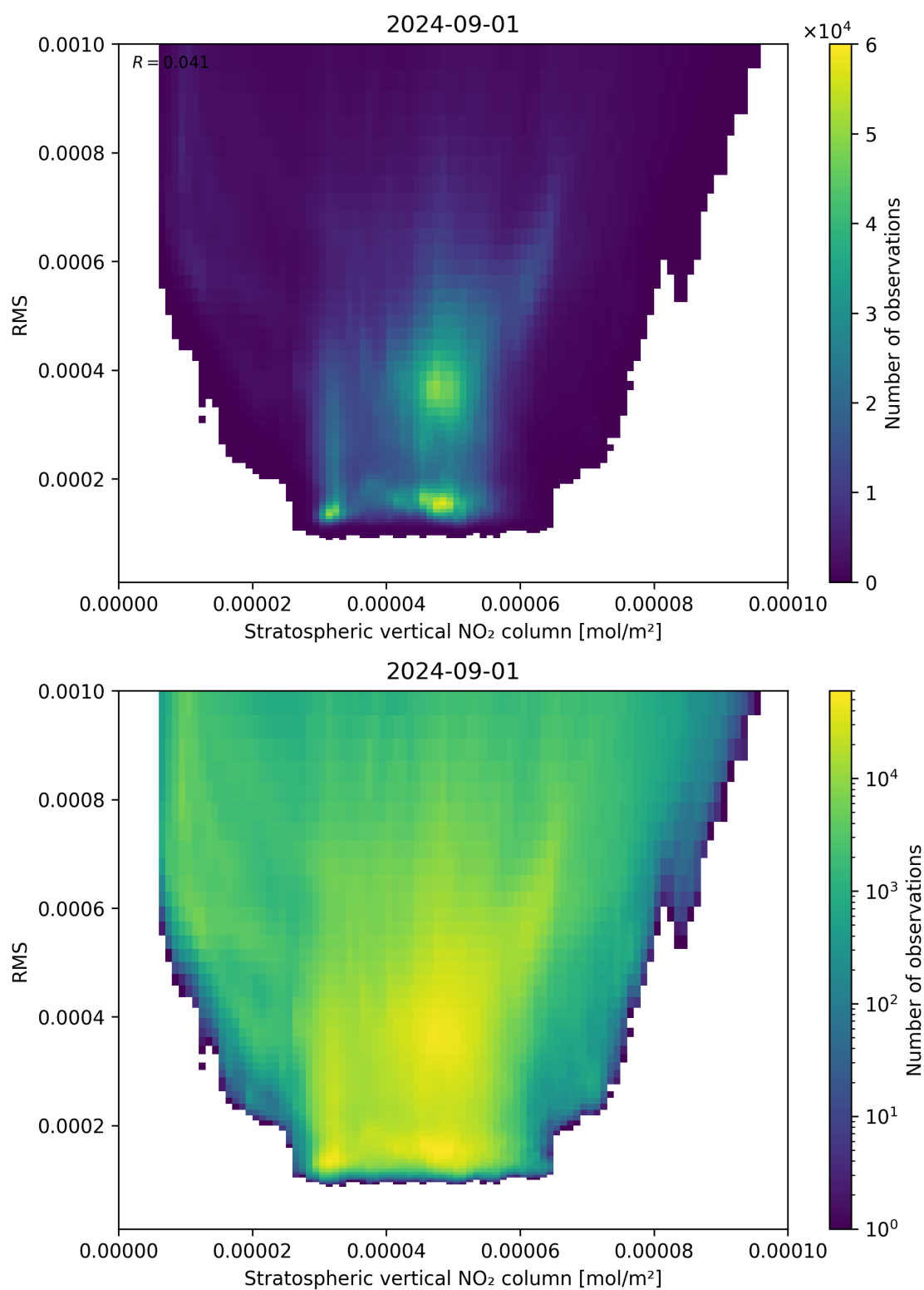
Figure 102: Scatter density plot of “Stratospheric vertical NO 2 column” against “RMS” for 2024-09-01 to 2024-09-02.
