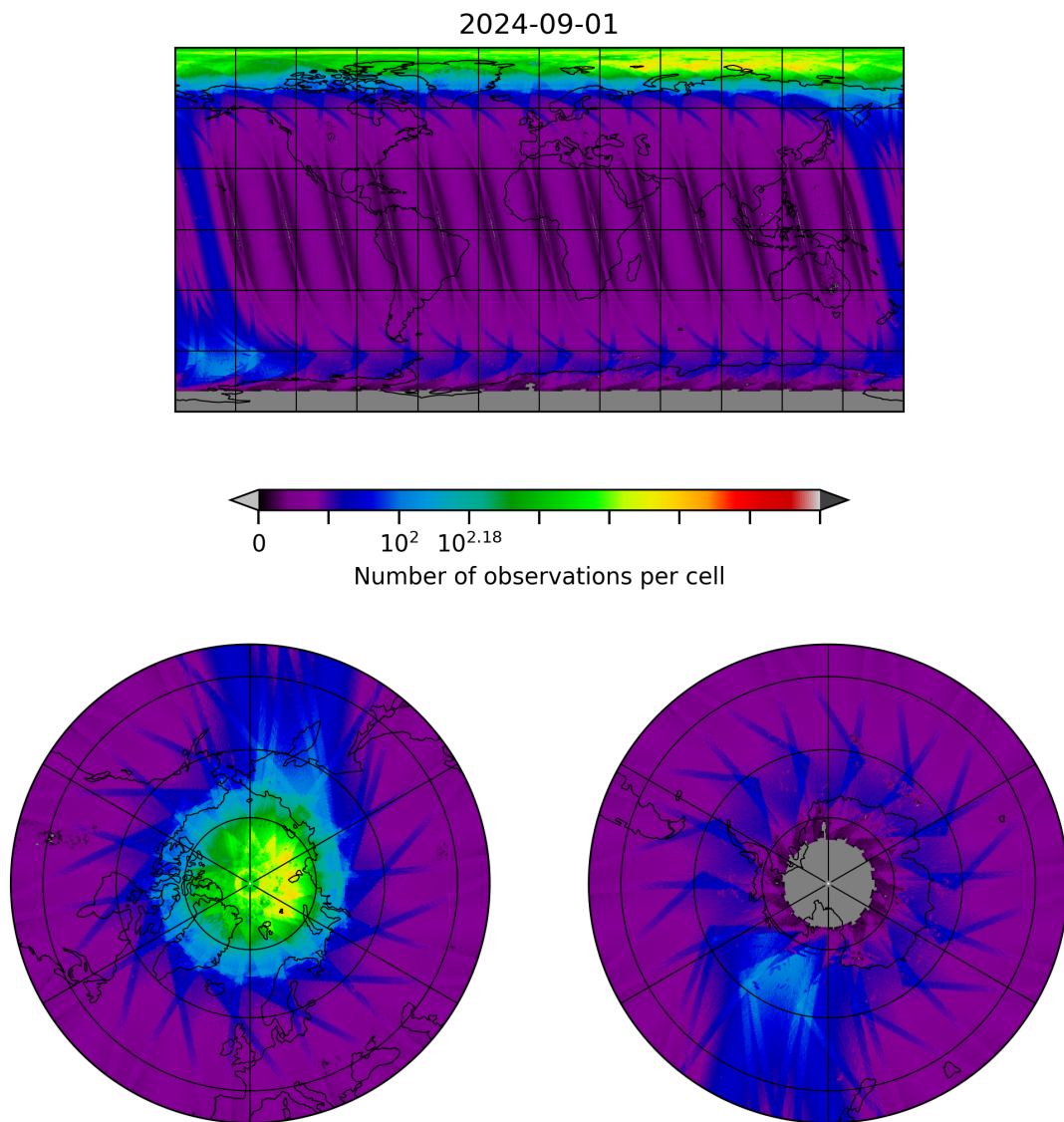
Figure 10: Map of the number of observations for 2024-09-01 to 2024-09-02
