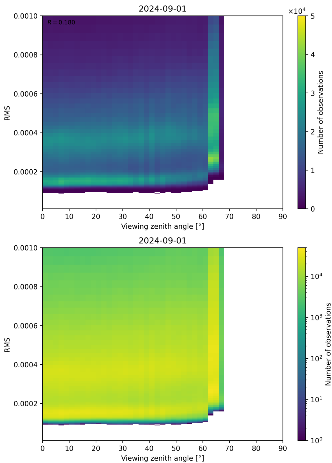
Figure 171: Scatter density plot of “Viewing zenith angle” against “RMS” for 2024-09-01 to 2024-09-02.
