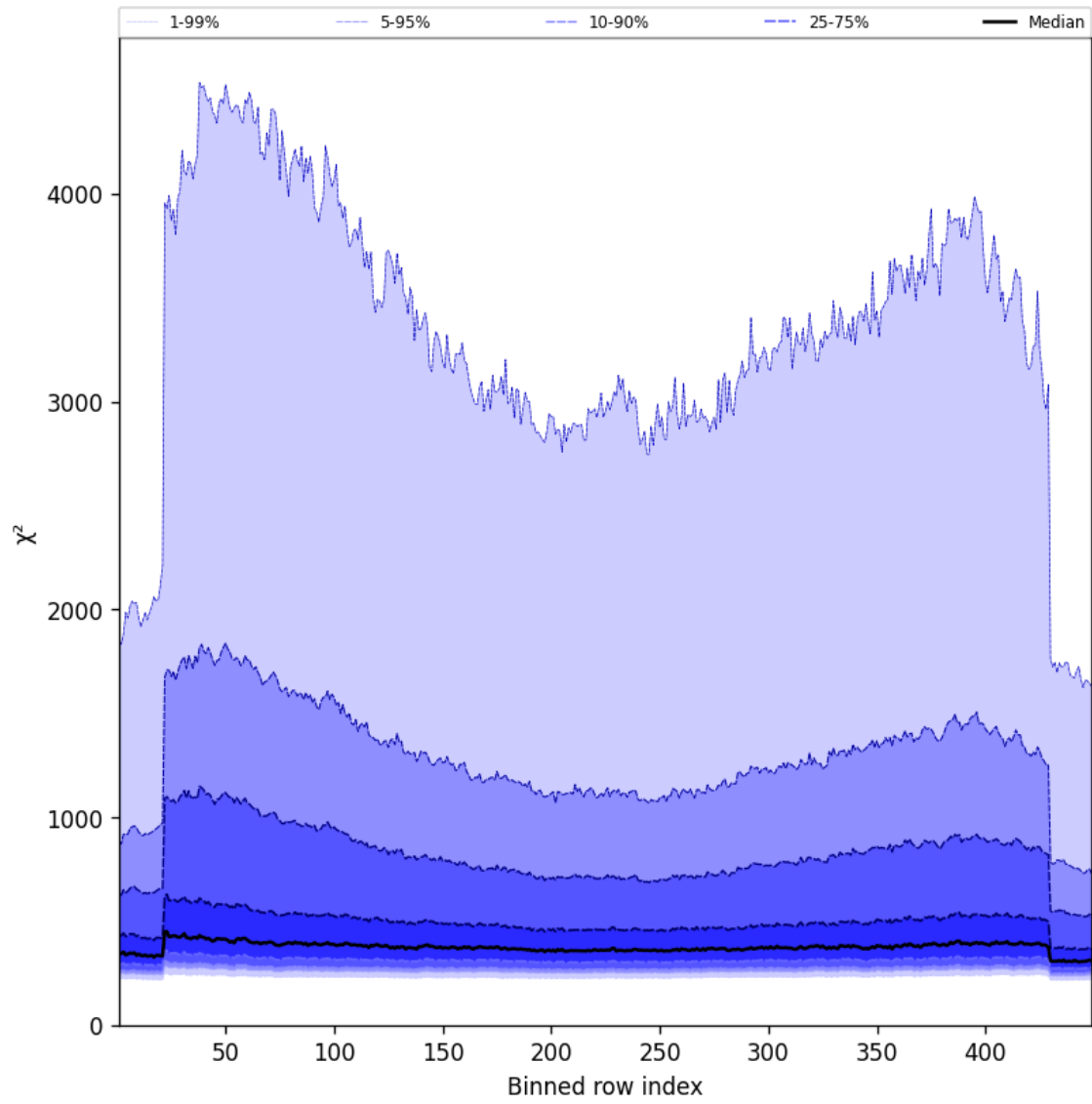
Figure 59: Along track statistics of “ \chi^2 ” for 2024-09-01 to 2024-09-02
