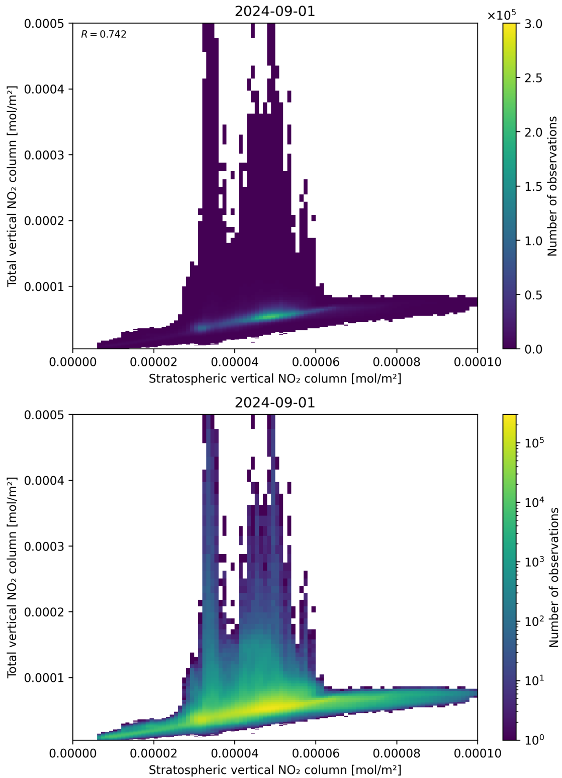
Figure 100: Scatter density plot of “Stratospheric vertical NO 2 column” against “Total vertical NO 2 column” for 2024-09-01 to 2024-09-02.
