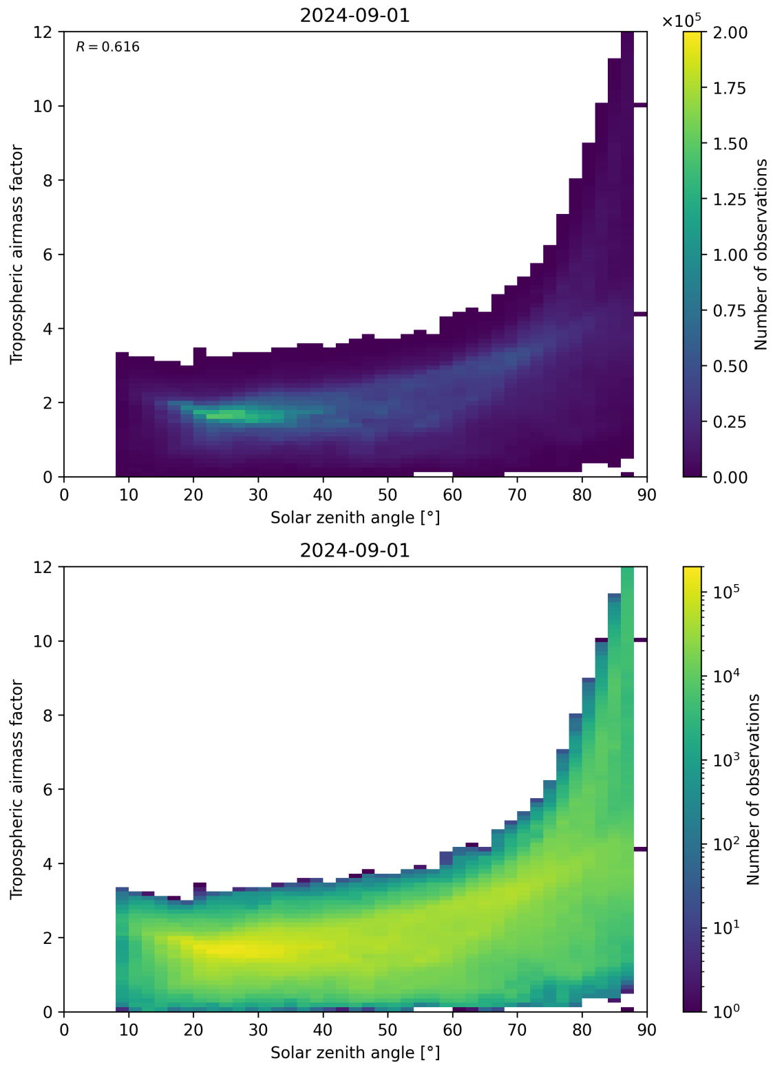
Figure 147: Scatter density plot of “Solar zenith angle” against “Tropospheric airmass factor” for 2024-09-01 to 2024-09-02.
