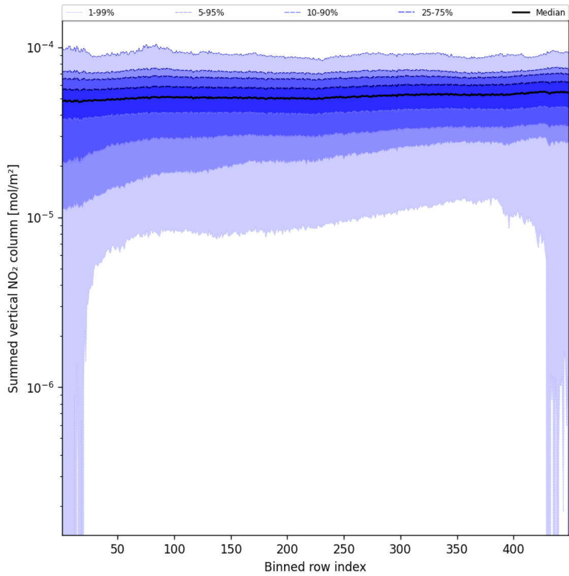
Figure 57: Along track statistics of “Summed vertical NO 2 column” for 2024-09-01 to 2024-09-02
