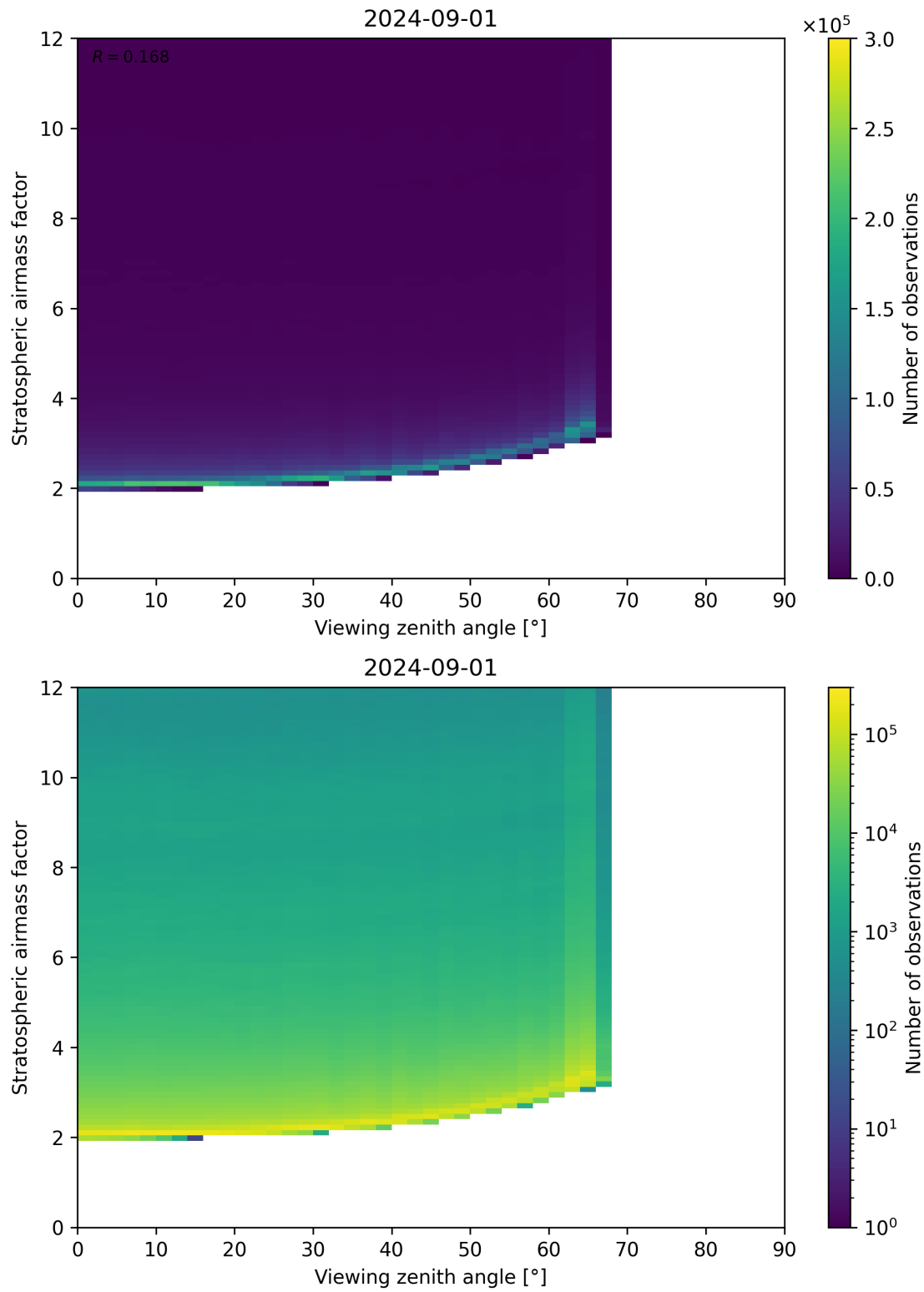
Figure 159: Scatter density plot of “Viewing zenith angle” against “Stratospheric airmass factor” for 2024-09-01 to 2024-09-02.
