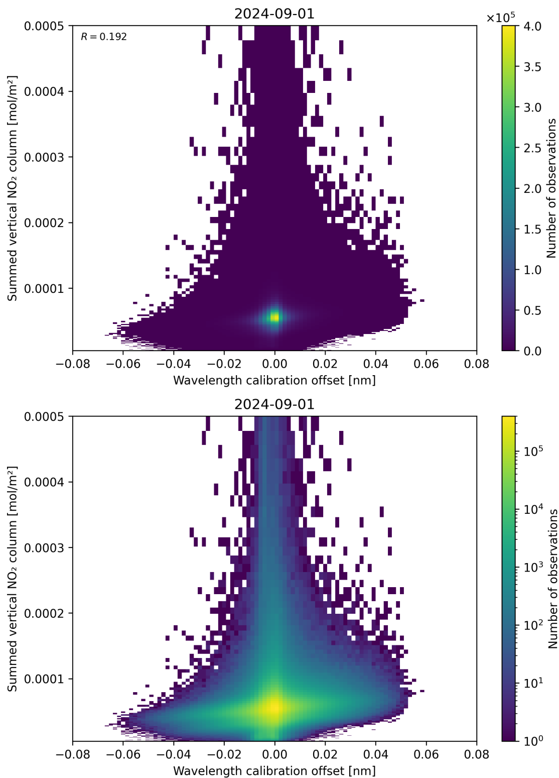
Figure 177: Scatter density plot of “Wavelength calibration offset” against “Summed vertical NO 2 column” for 2024-09-01 to 2024-09-02.
