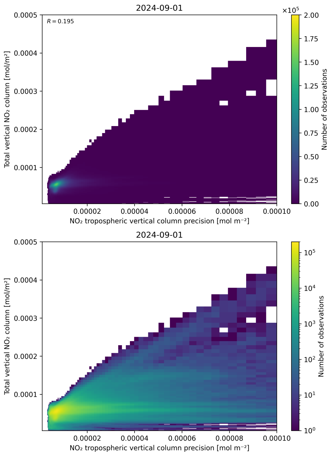
Figure 138: Scatter density plot of “NO 2 tropospheric vertical column precision” against “Total vertical NO 2 column” for 2024-09-01 to 2024-09-02.
