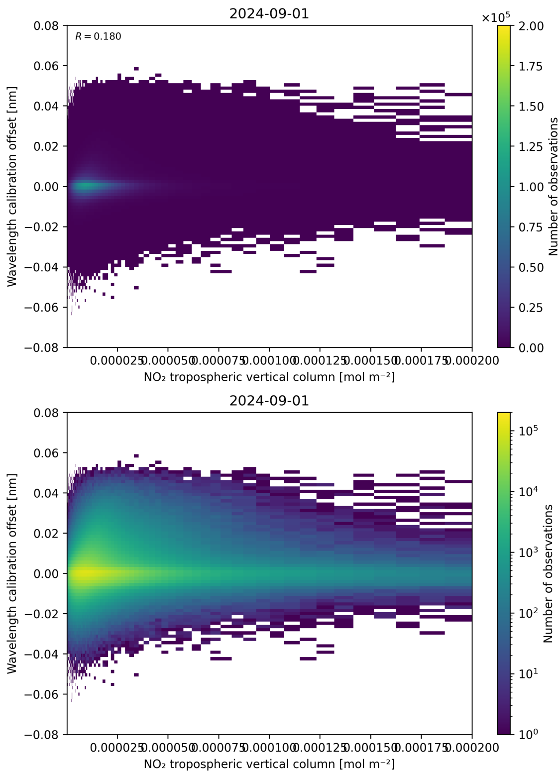
Figure 143: Scatter density plot of “NO 2 tropospheric vertical column” against “Wavelength calibration offset” for 2024-09-01 to 2024-09-02.
