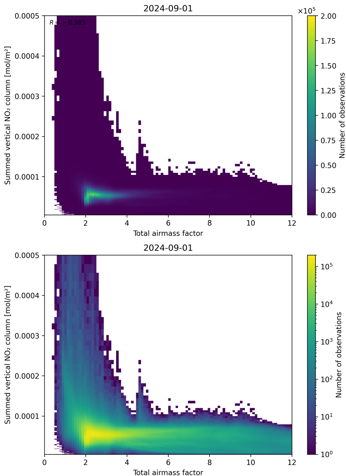
Figure 65: Scatter density plot of “Total airmass factor” against “Summed vertical NO 2 column” for 2024-09-01 to 2024-09-02.
