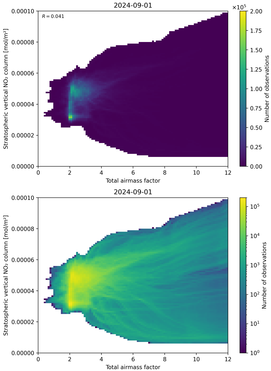
Figure 64: Scatter density plot of “Total airmass factor” against “Stratospheric vertical NO 2 column” for 2024-09-01 to 2024-09-02.
