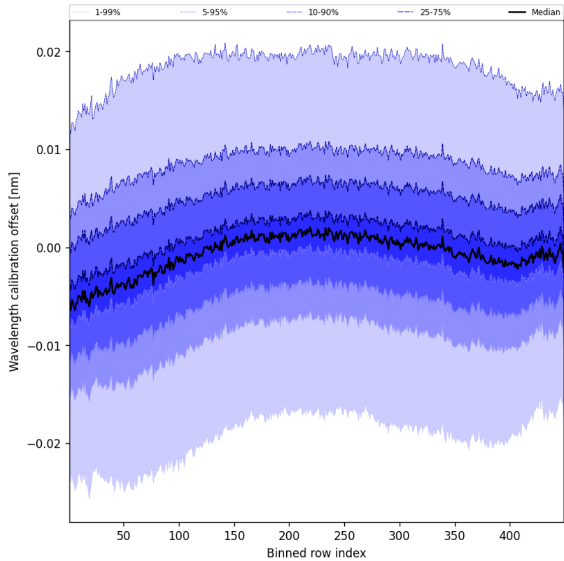
Figure 52: Along track statistics of “Wavelength calibration offset” for 2024-09-01 to 2024-09-02
