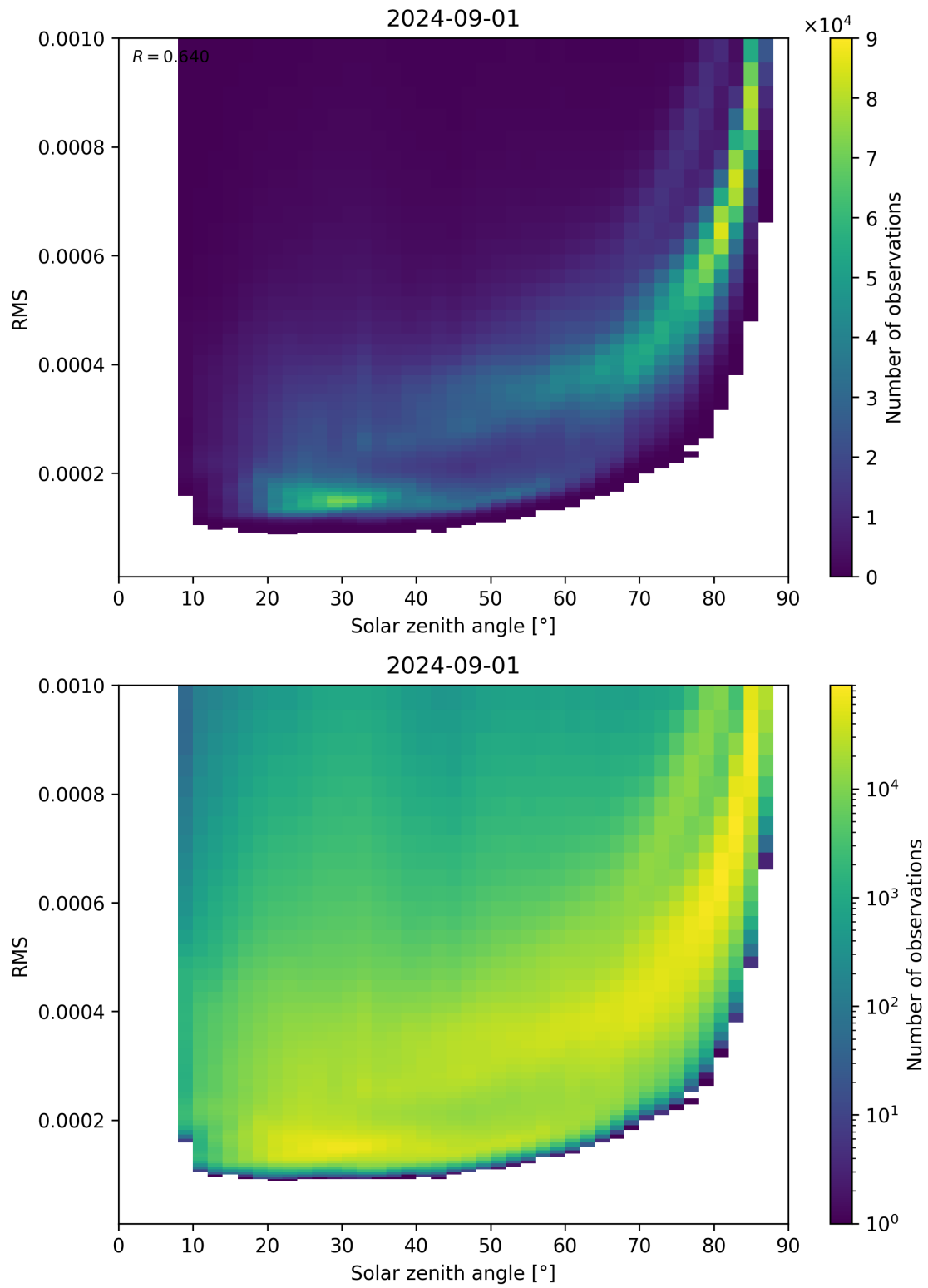
Figure 157: Scatter density plot of “Solar zenith angle” against “RMS” for 2024-09-01 to 2024-09-02.
