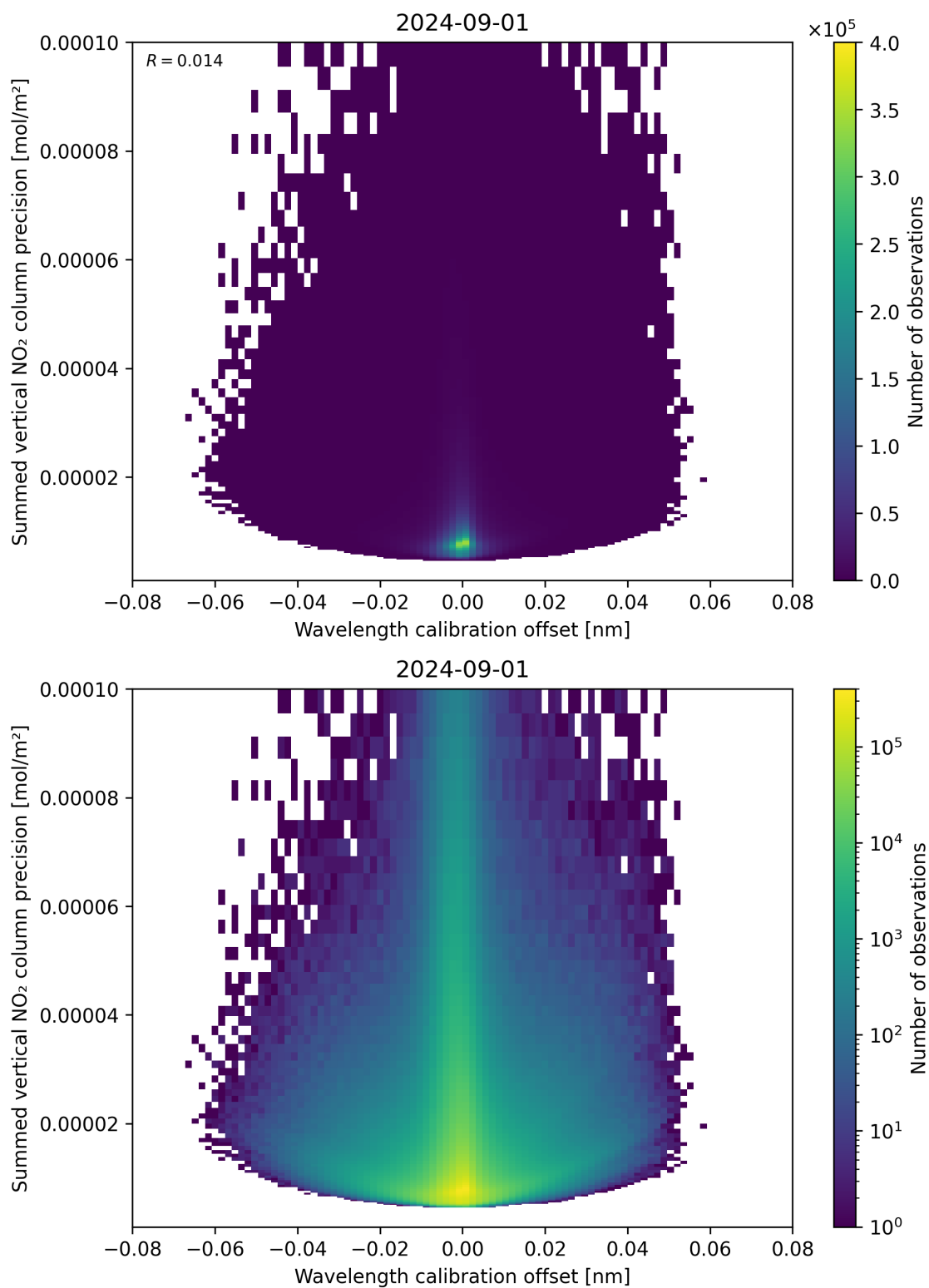
Figure 178: Scatter density plot of “Wavelength calibration offset” against “Summed vertical NO 2 column precision” for 2024-09-01 to 2024-09-02.
