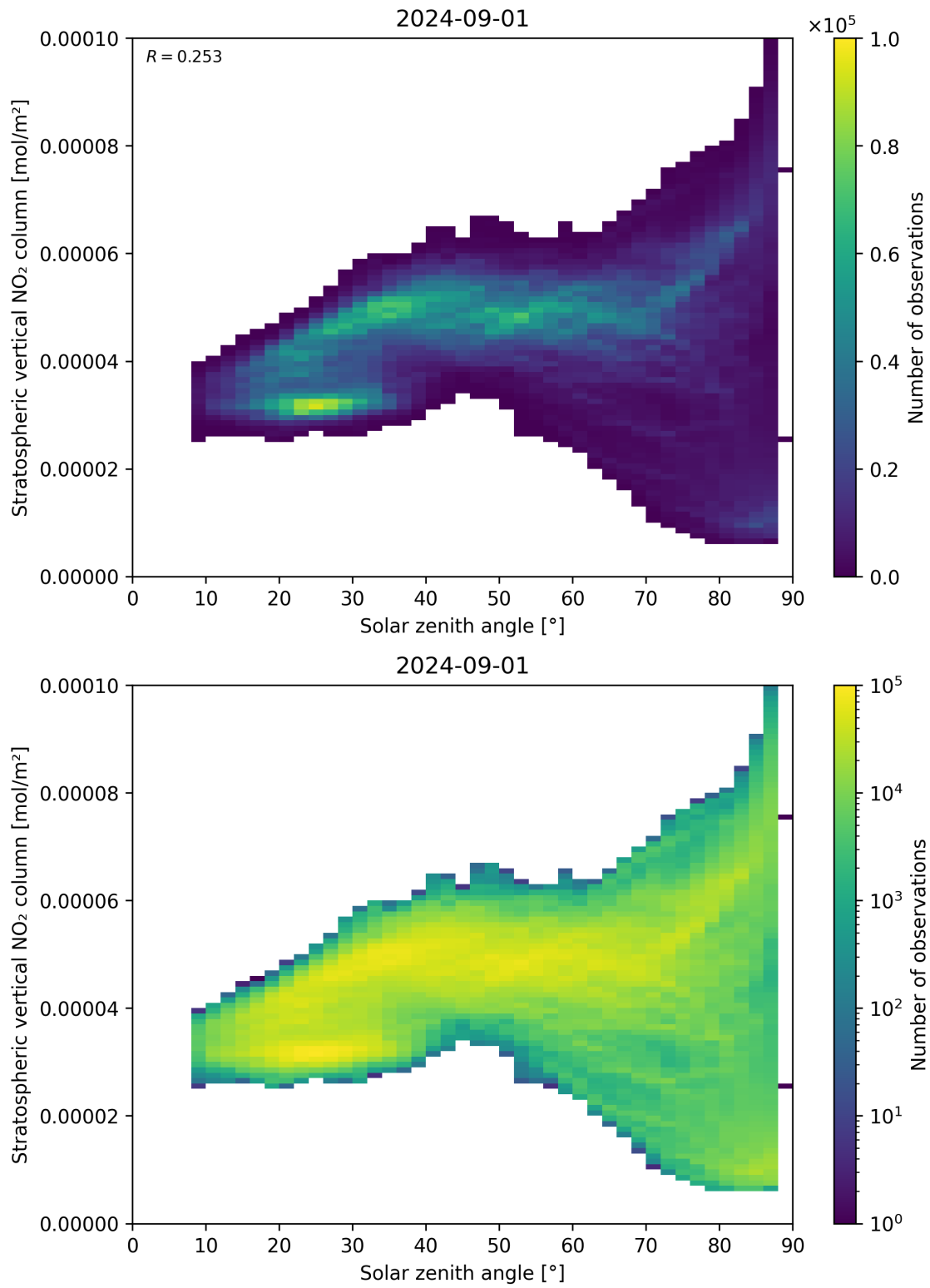
Figure 150: Scatter density plot of “Solar zenith angle” against “Stratospheric vertical NO 2 column” for 2024-09-01 to 2024-09-02.
