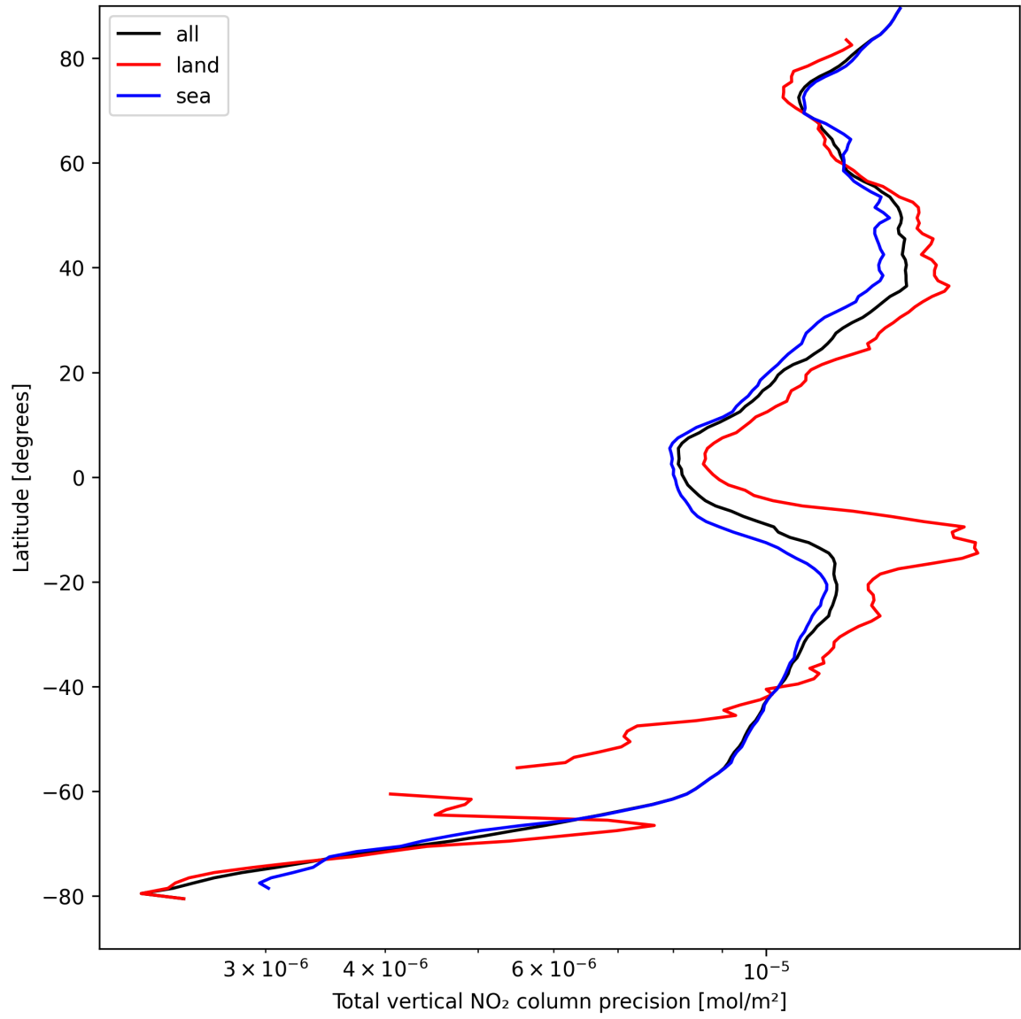
Figure 22: Zonal average of “Total vertical NO 2 column precision” for 2024-09-01 to 2024-09-02.
