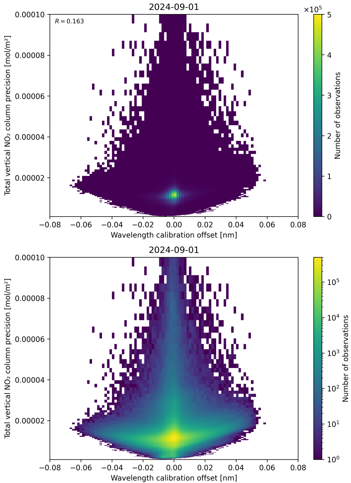
Figure 180: Scatter density plot of “Wavelength calibration offset” against “Total vertical NO 2 column precision” for 2024-09-01 to 2024-09-02.
