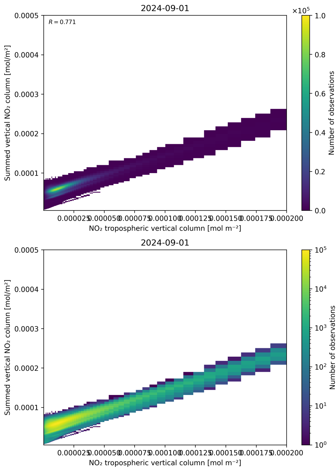
Figure 126: Scatter density plot of “NO 2 tropospheric vertical column” against “Summed vertical NO 2 column” for 2024-09-01 to 2024-09-02.
