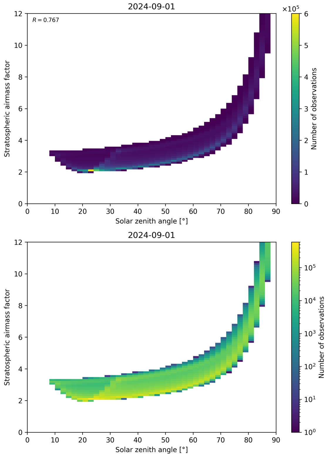
Figure 145: Scatter density plot of “Solar zenith angle” against “Stratospheric airmass factor” for 2024-09-01 to 2024-09-02.
