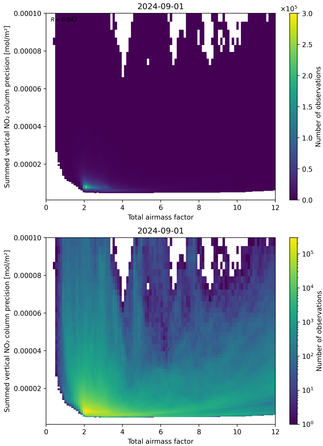
Figure 66: Scatter density plot of “Total airmass factor” against “Summed vertical NO 2 column precision” for 2024-09-01 to 2024-09-02.
