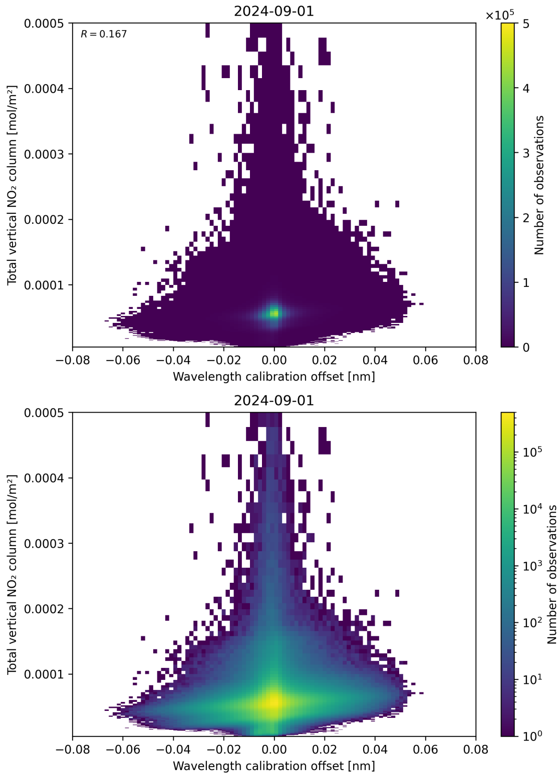
Figure 179: Scatter density plot of “Wavelength calibration offset” against “Total vertical NO 2 column” for 2024-09-01 to 2024-09-02.
