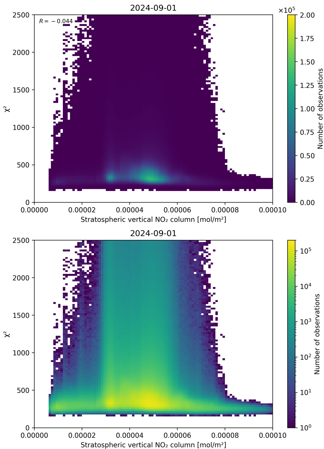
Figure 97: Scatter density plot of “Stratospheric vertical NO 2 column” against “ \chi^2 ” for 2024-09-01 to 2024-09-02.
