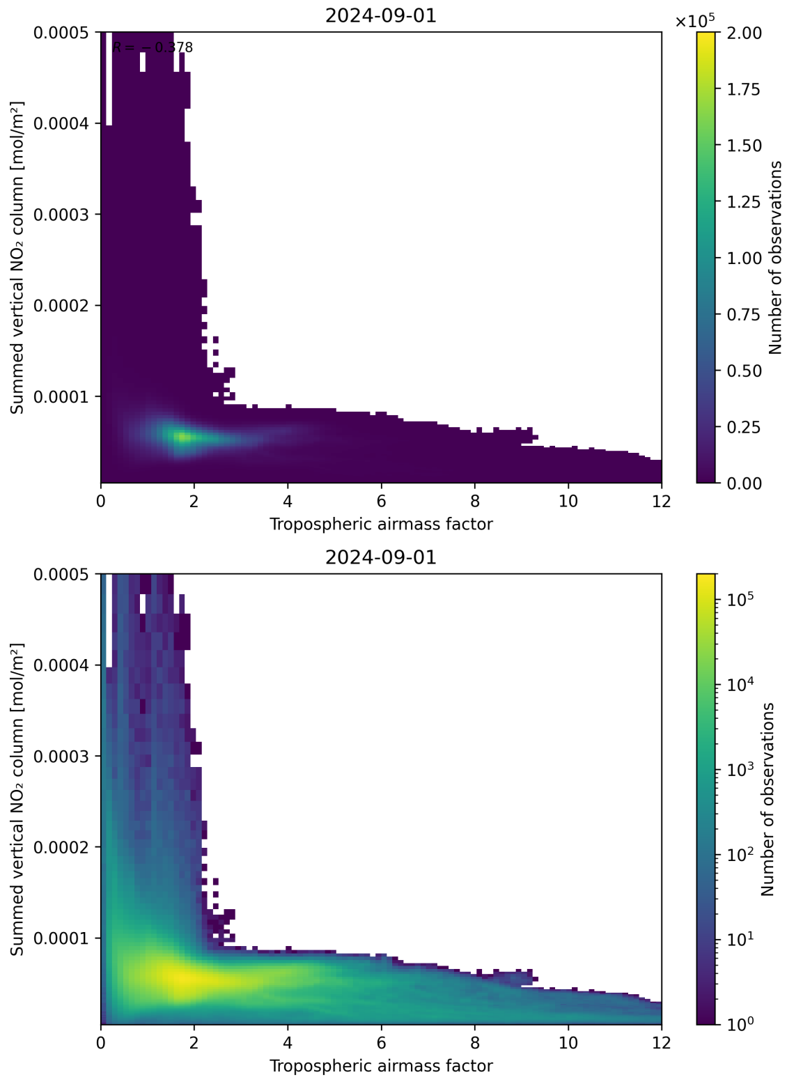
Figure 75: Scatter density plot of “Tropospheric airmass factor” against “Summed vertical NO 2 column” for 2024-09-01 to 2024-09-02.
