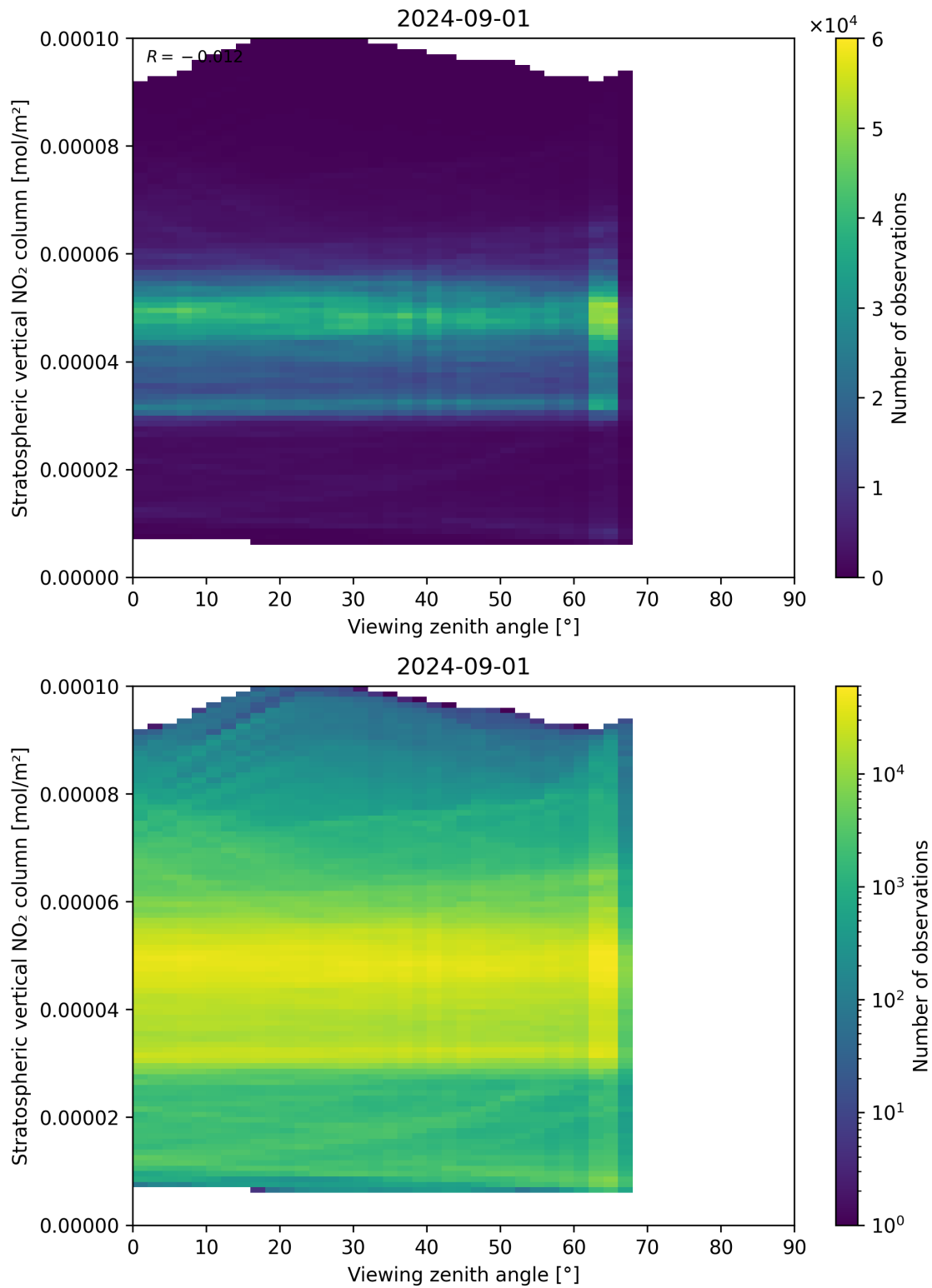
Figure 164: Scatter density plot of “Viewing zenith angle” against “Stratospheric vertical NO 2 column” for 2024-09-01 to 2024-09-02.
