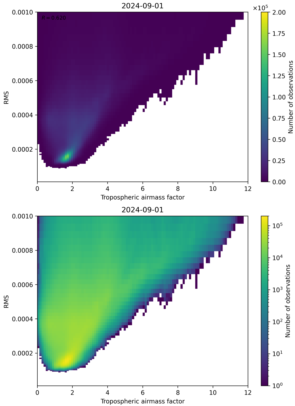
Figure 79: Scatter density plot of “Tropospheric airmass factor” against “RMS” for 2024-09-01 to 2024-09-02.
