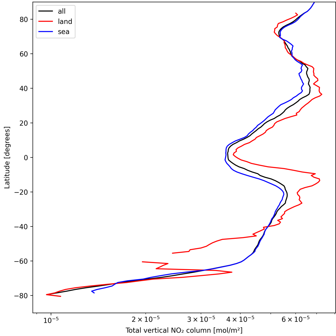
Figure 21: Zonal average of “Total vertical NO 2 column” for 2024-09-01 to 2024-09-02.
