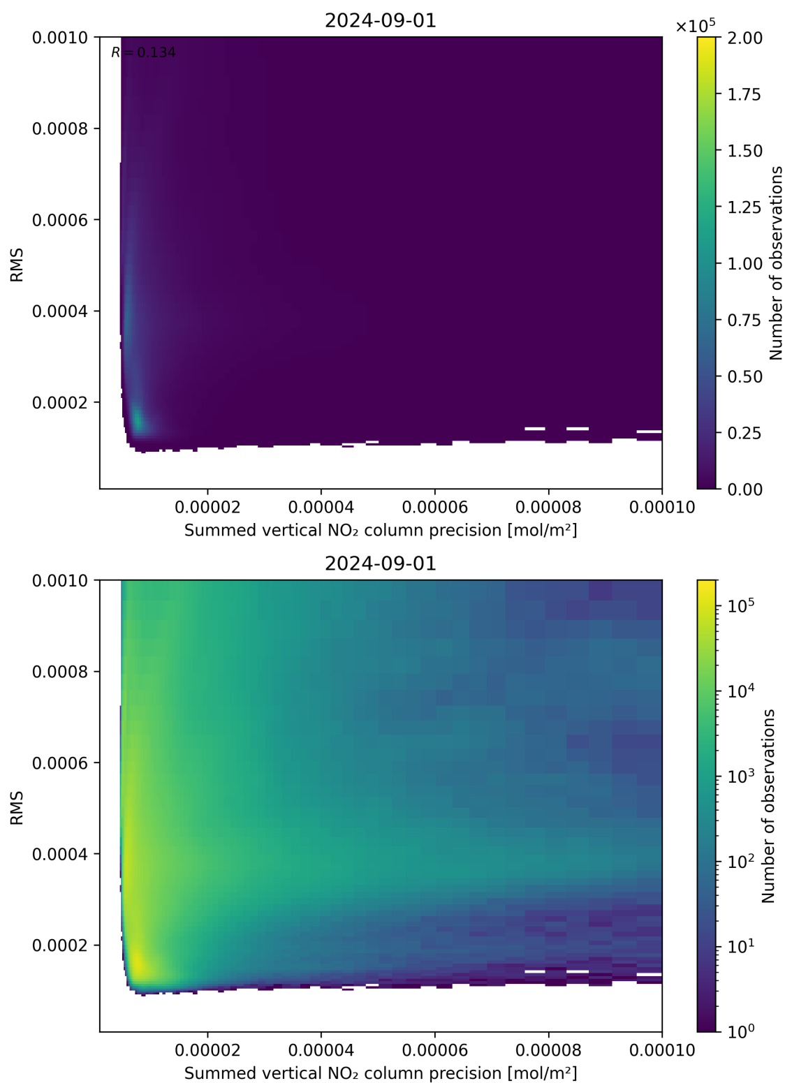
Figure 108: Scatter density plot of “Summed vertical NO 2 column precision” against “RMS” for 2024-09-01 to 2024-09-02.
