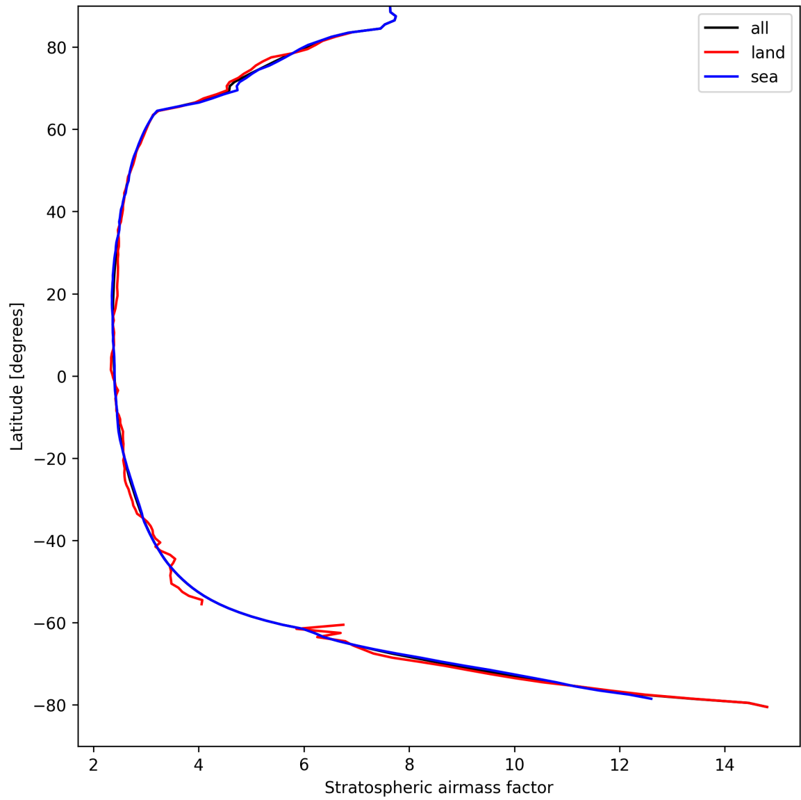
Figure 27: Zonal average of “Stratospheric air mass factor” for 2024-09-01 to 2024-09-02.
