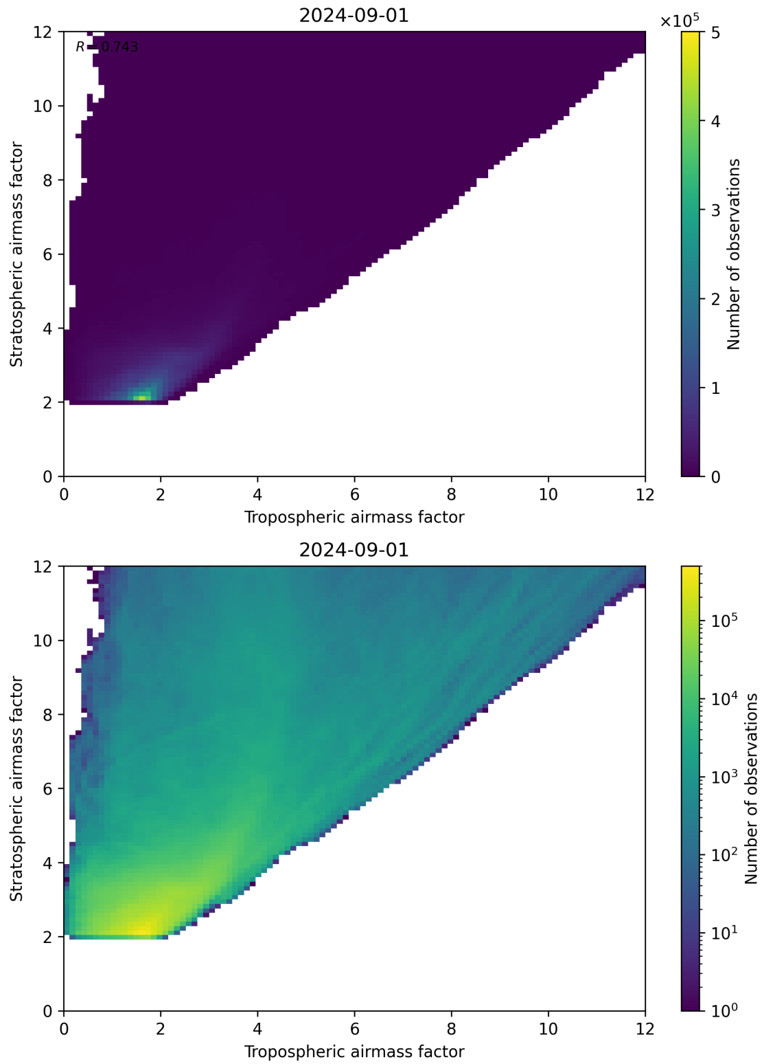
Figure 71: Scatter density plot of “Tropospheric airmass factor” against “Stratospheric airmass factor” for 2024-09-01 to 2024-09-02.
