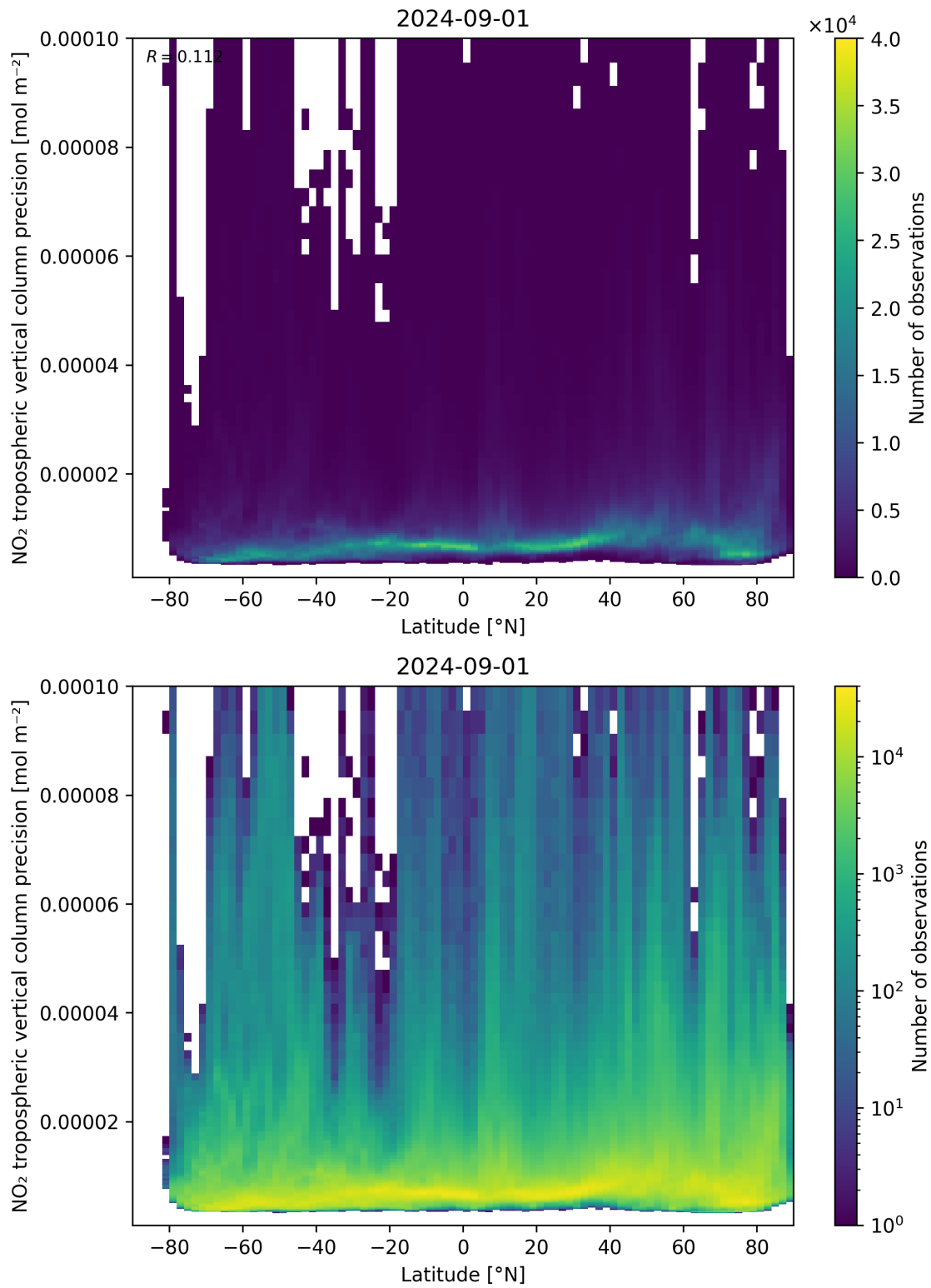
Figure 93: Scatter density plot of “Latitude” against “NO 2 tropospheric vertical column precision” for 2024-09-01 to 2024-09-02.
