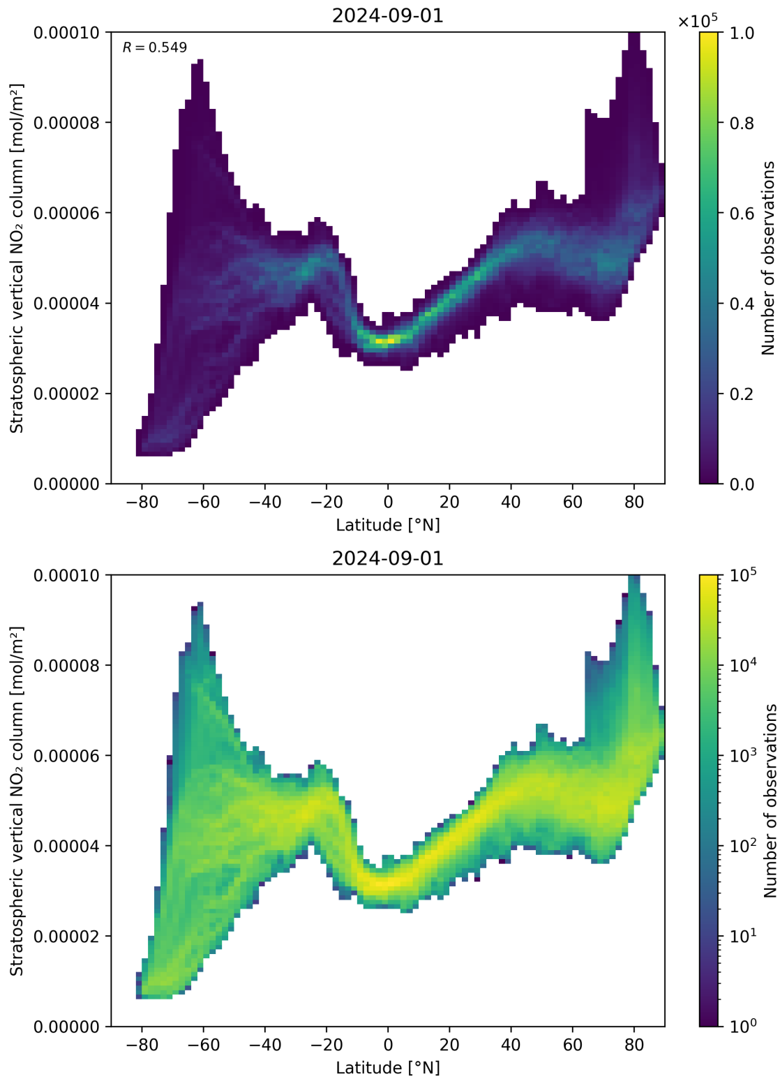
Figure 87: Scatter density plot of “Latitude” against “Stratospheric vertical NO 2 column” for 2024-09-01 to 2024-09-02.
