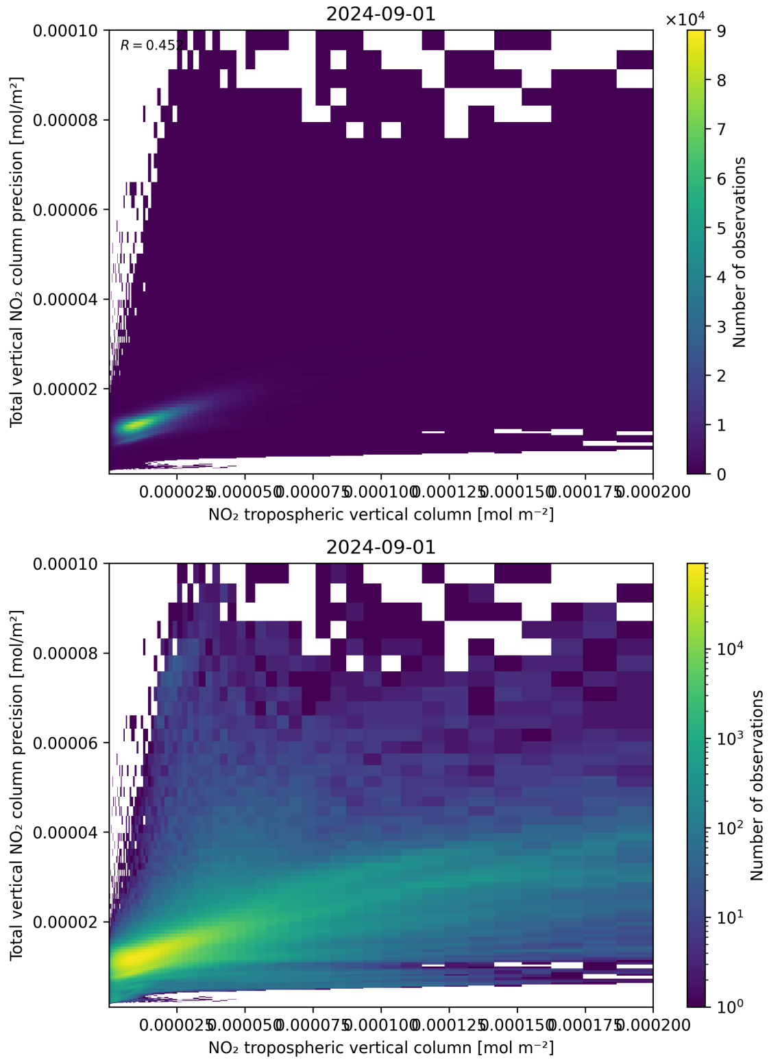
Figure 129: Scatter density plot of “NO 2 tropospheric vertical column” against “Total vertical NO 2 column precision” for 2024-09-01 to 2024-09-02.
