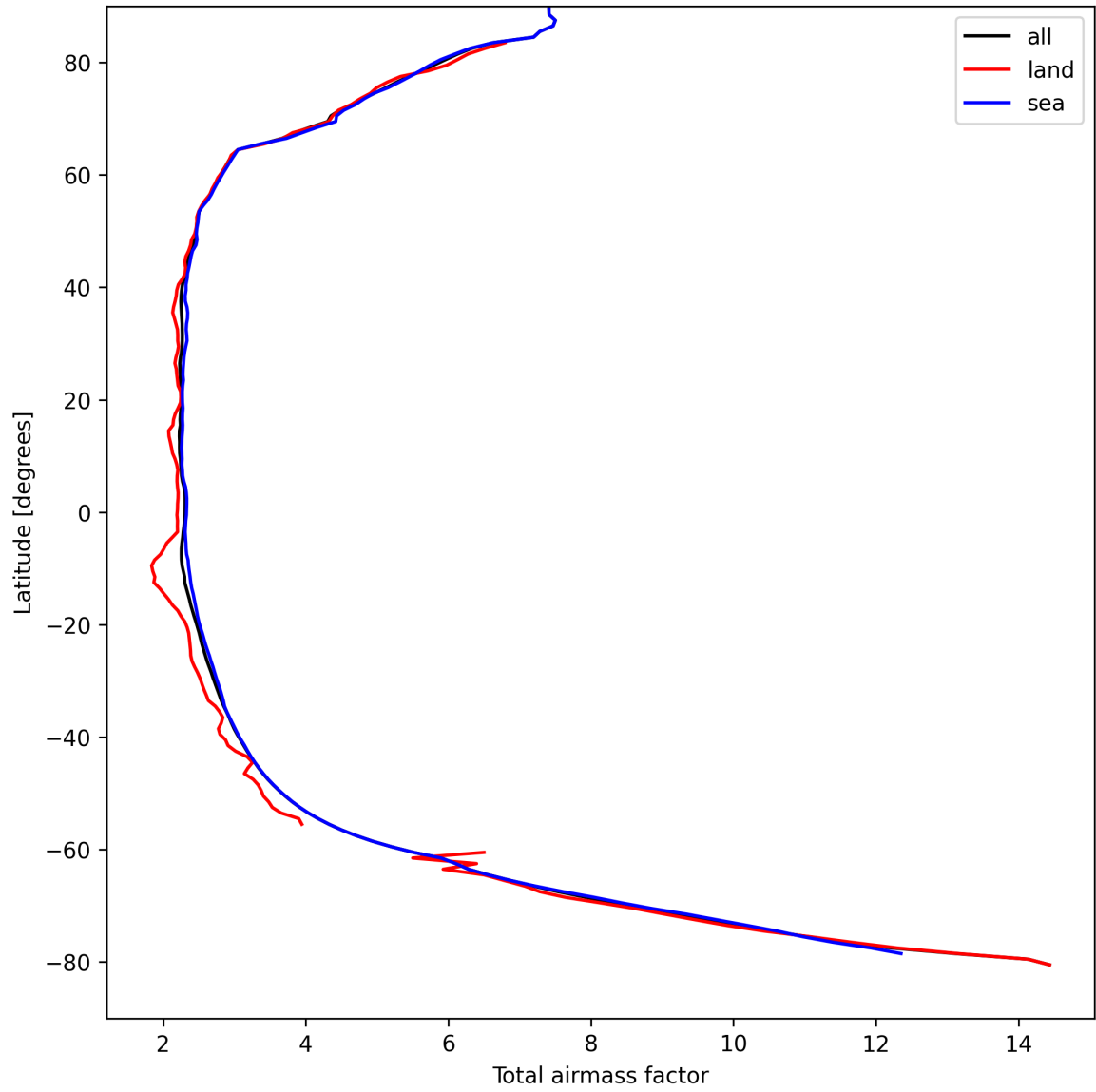
Figure 15: Zonal average of “Total airmass factor” for 2024-09-01 to 2024-09-02.
