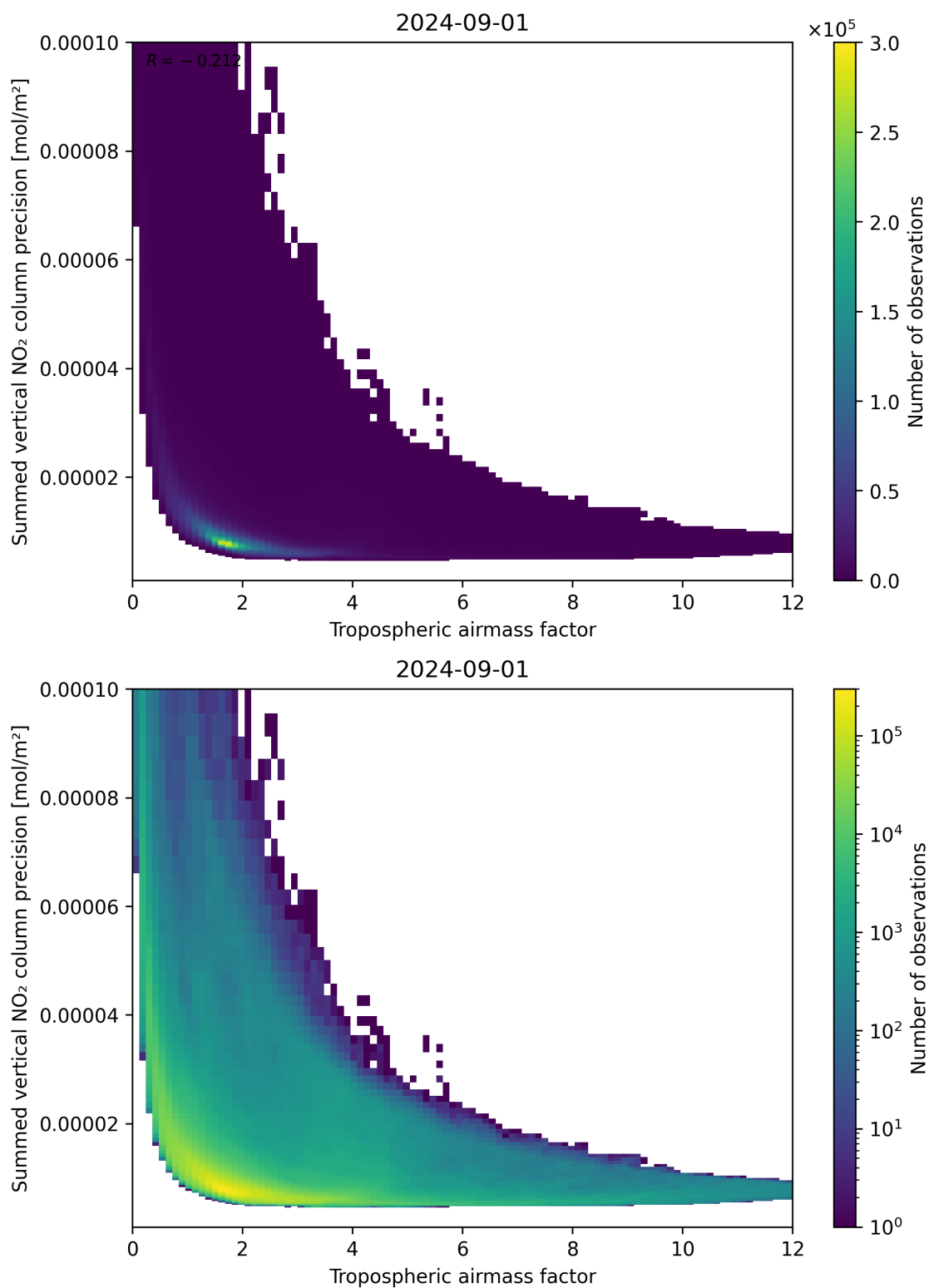
Figure 76: Scatter density plot of “Tropospheric air mass factor” against “Summed vertical NO 2 column precision” for 2024-09-01 to 2024-09-02.
