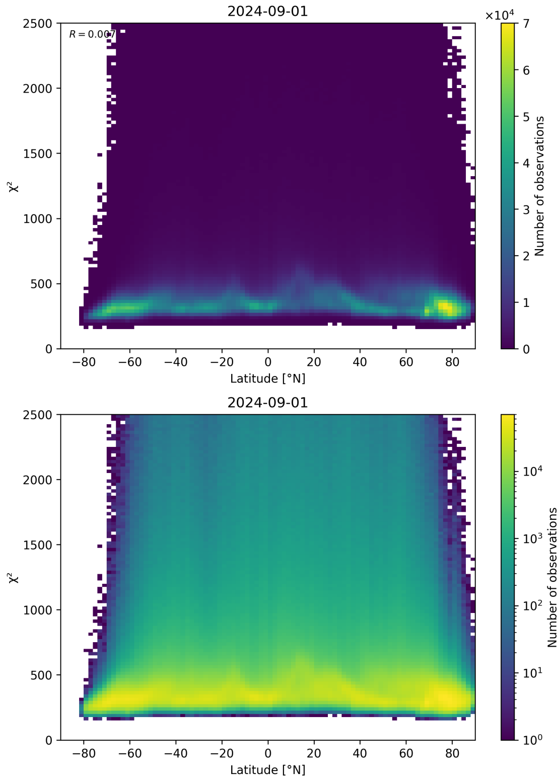
Figure 86: Scatter density plot of “Latitude” against “ \chi^2 ” for 2024-09-01 to 2024-09-02.
