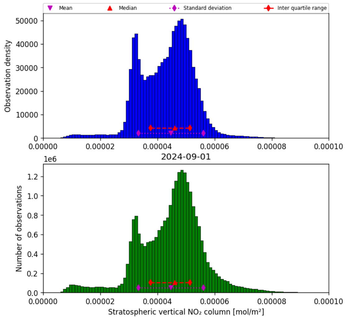
Figure 36: Histogram of “Stratospheric vertical NO 2 column” for 2024-09-01 to 2024-09-02
