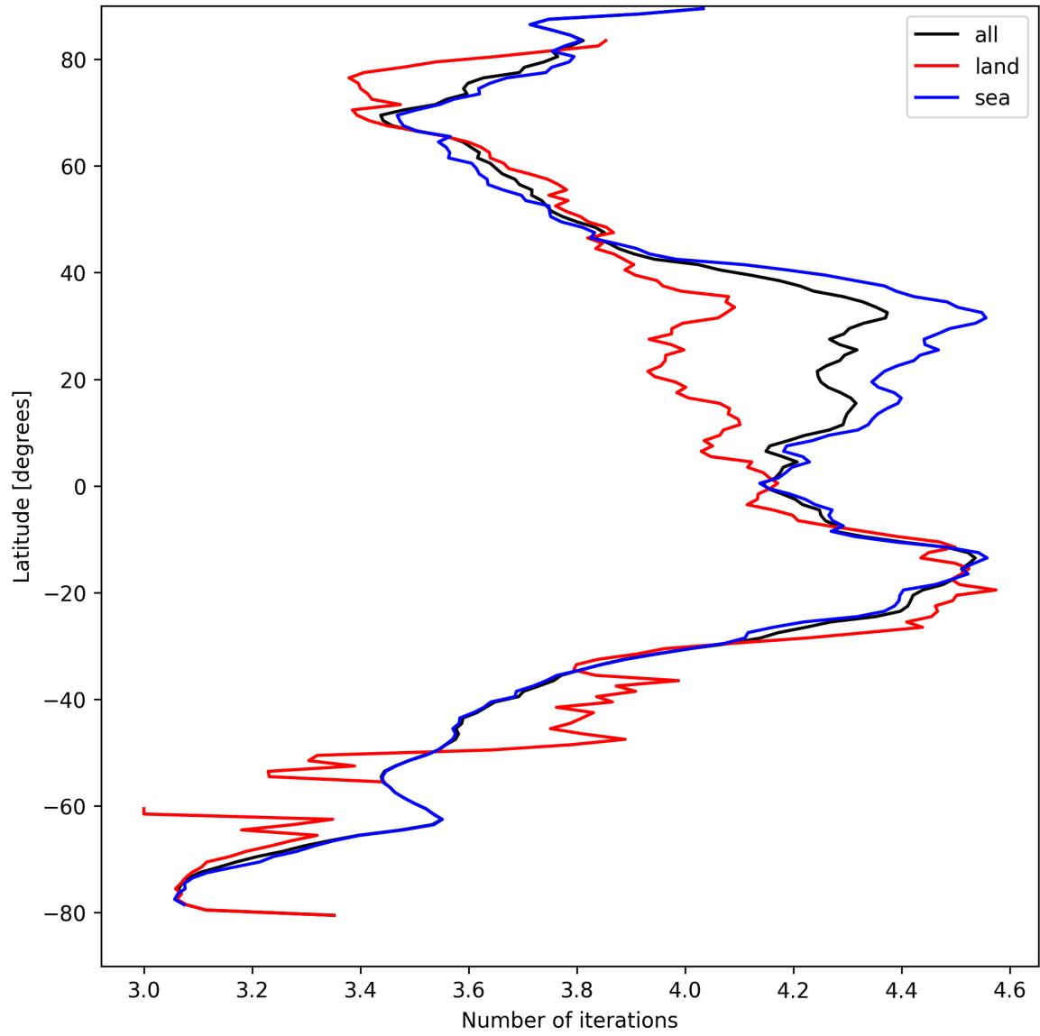
Figure 17: Zonal average of “Number of iterations” for 2024-09-01 to 2024-09-02.
