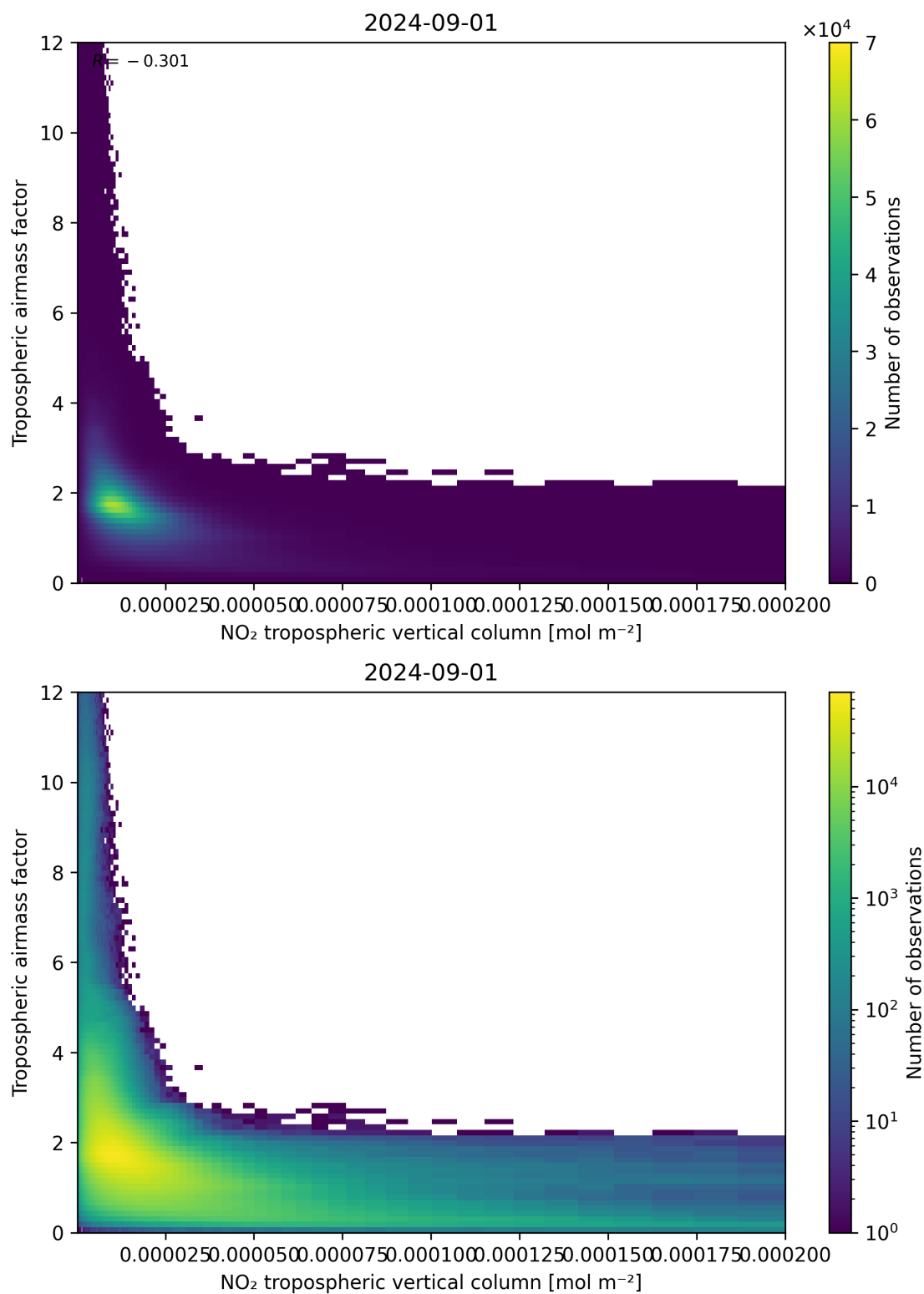
Figure 123: Scatter density plot of “NO 2 tropospheric vertical column” against “Tropospheric air mass factor” for 2024-09-01 to 2024-09-02.
