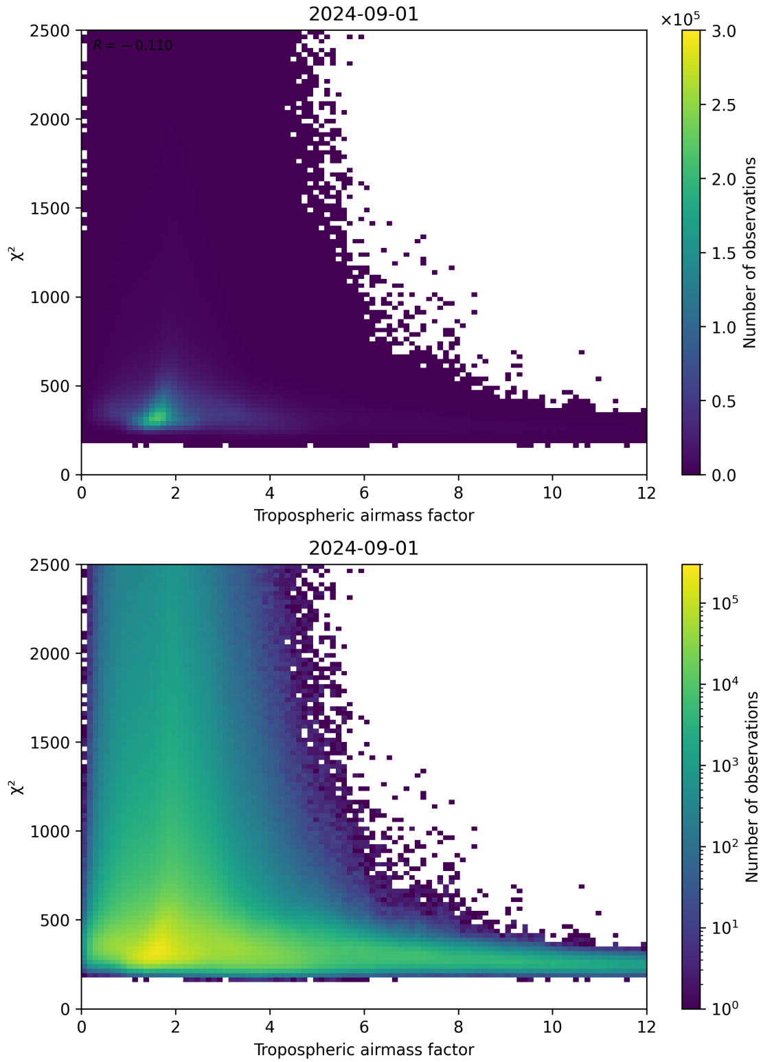
Figure 73: Scatter density plot of “Tropospheric airmass factor” against “ \chi^2 ” for 2024-09-01 to 2024-09-02.
