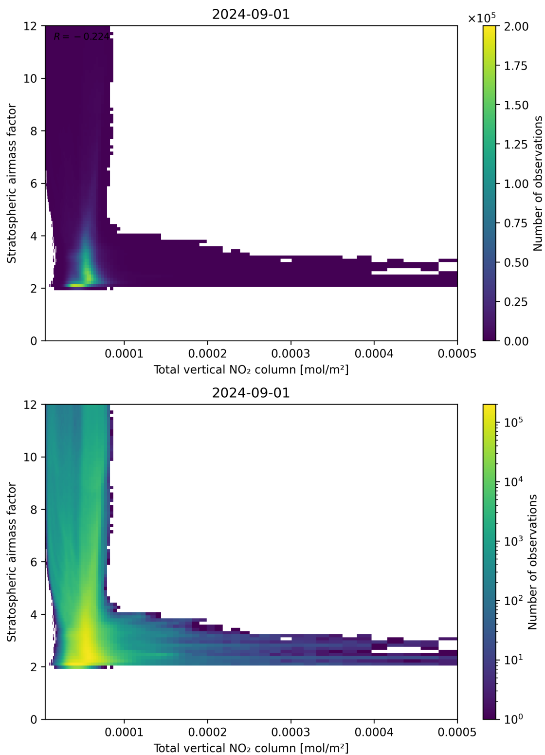
Figure 110: Scatter density plot of “Total vertical NO 2 column” against “Stratospheric airmass factor” for 2024-09-01 to 2024-09-02.
