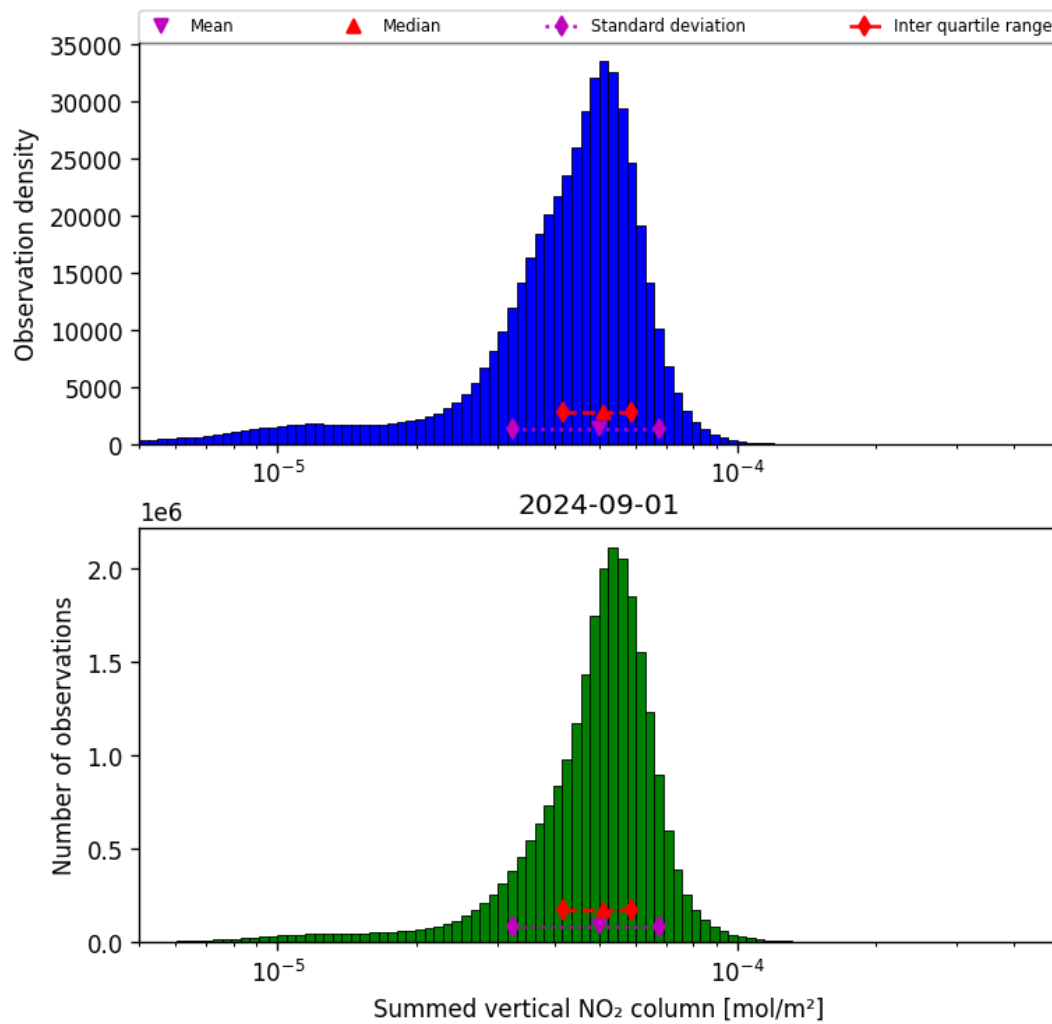
Figure 40: Histogram of “Summed vertical NO 2 column” for 2024-09-01 to 2024-09-02
