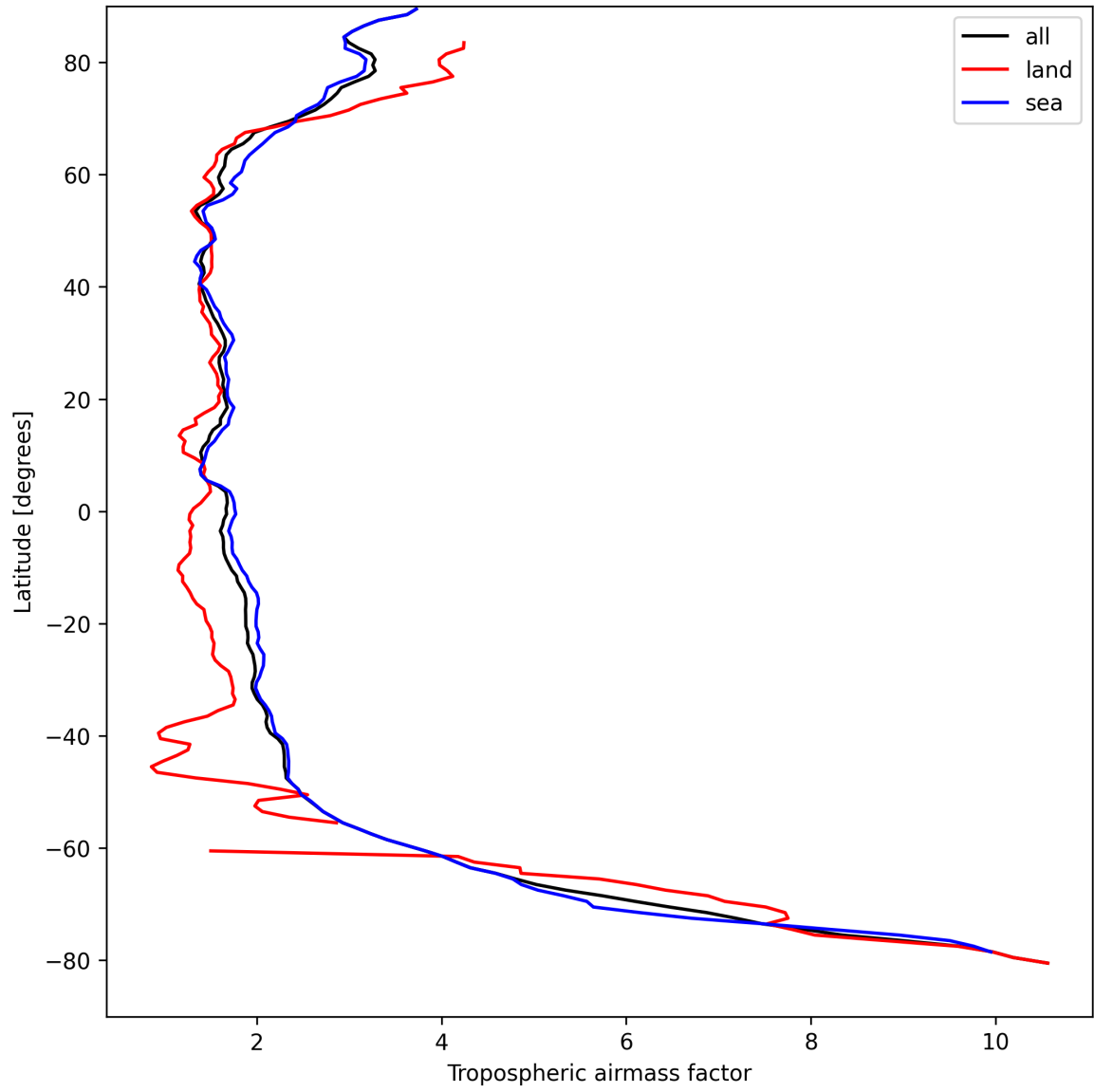
Figure 14: Zonal average of “Tropospheric airmass factor” for 2024-09-01 to 2024-09-02.
