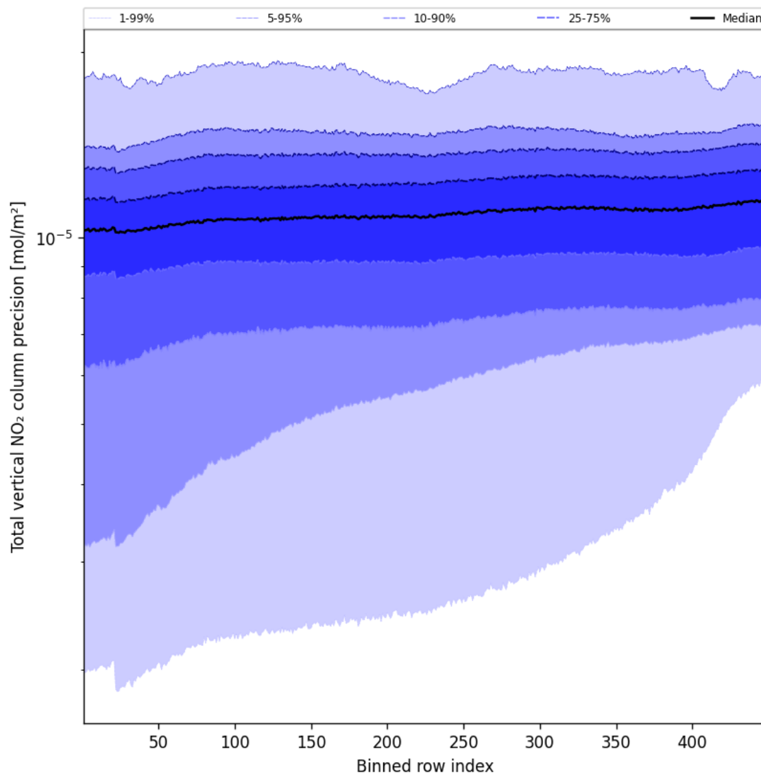
Figure 56: Along track statistics of “Total vertical NO 2 column precision” for 2024-09-01 to 2024-09-02
