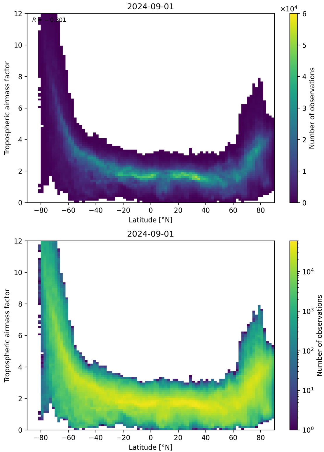
Figure 85: Scatter density plot of “Latitude” against “Tropospheric air mass factor” for 2024-09-01 to 2024-09-02.
