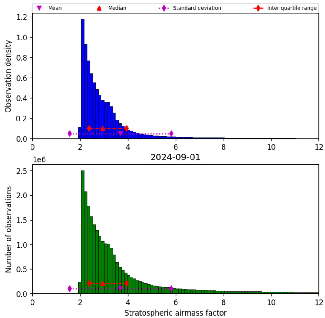
Figure 44: Histogram of “Stratospheric airmass factor” for 2024-09-01 to 2024-09-02
