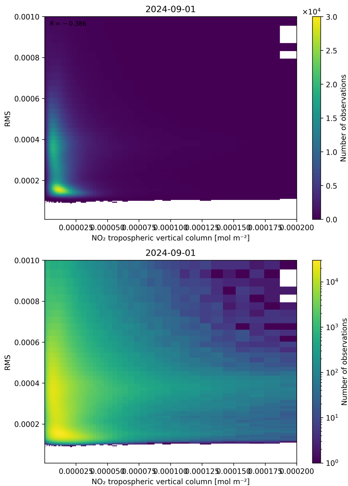
Figure 142: Scatter density plot of “NO 2 tropospheric vertical column” against “RMS” for 2024-09-01 to 2024-09-02.
