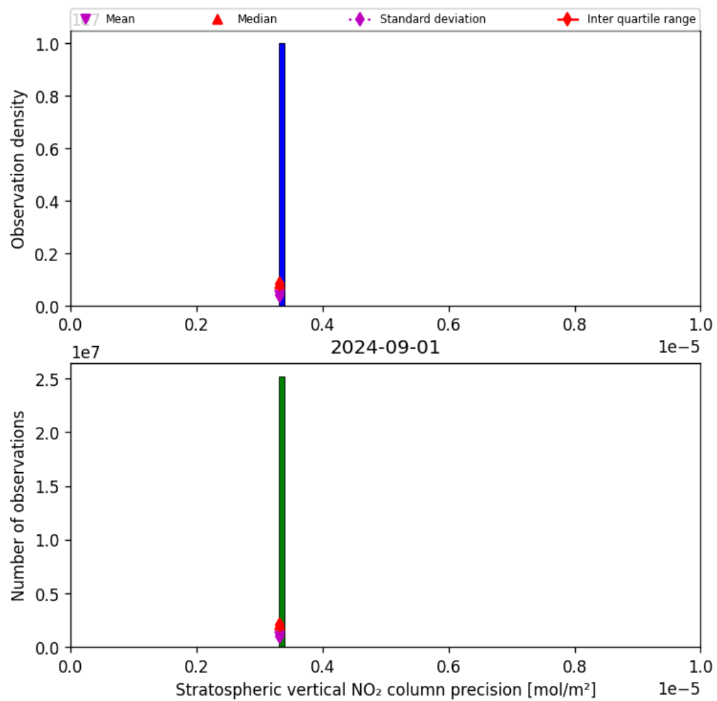
Figure 37: Histogram of “Stratospheric vertical NO 2 column precision” for 2024-09-01 to 2024-09-02
