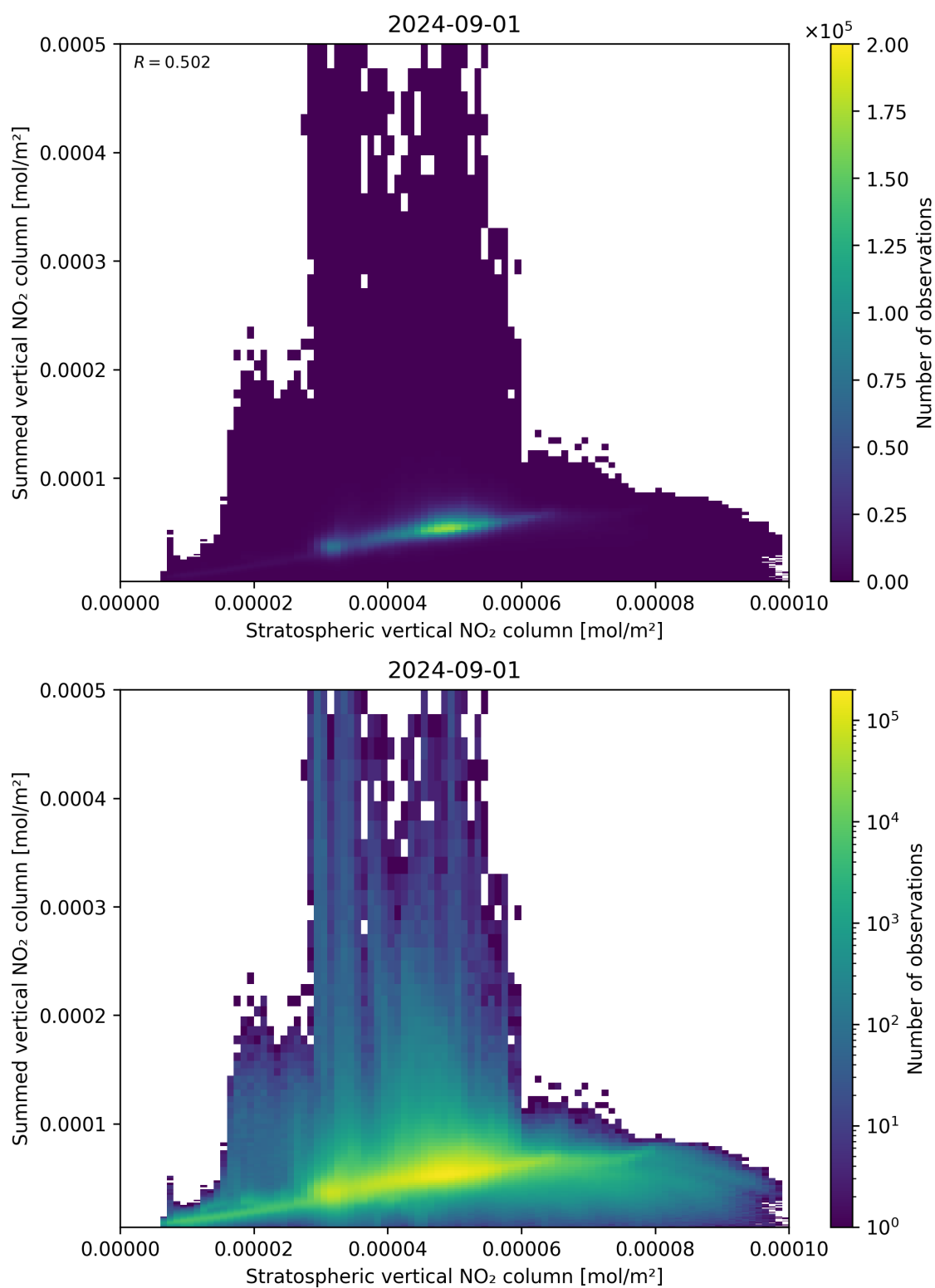
Figure 98: Scatter density plot of “Stratospheric vertical NO 2 column” against “Summed vertical NO 2 column” for 2024-09-01 to 2024-09-02.
