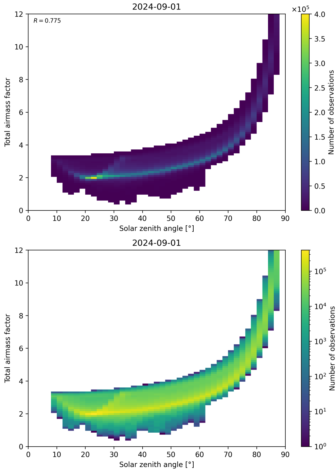
Figure 146: Scatter density plot of “Solar zenith angle” against “Total air mass factor” for 2024-09-01 to 2024-09-02.
