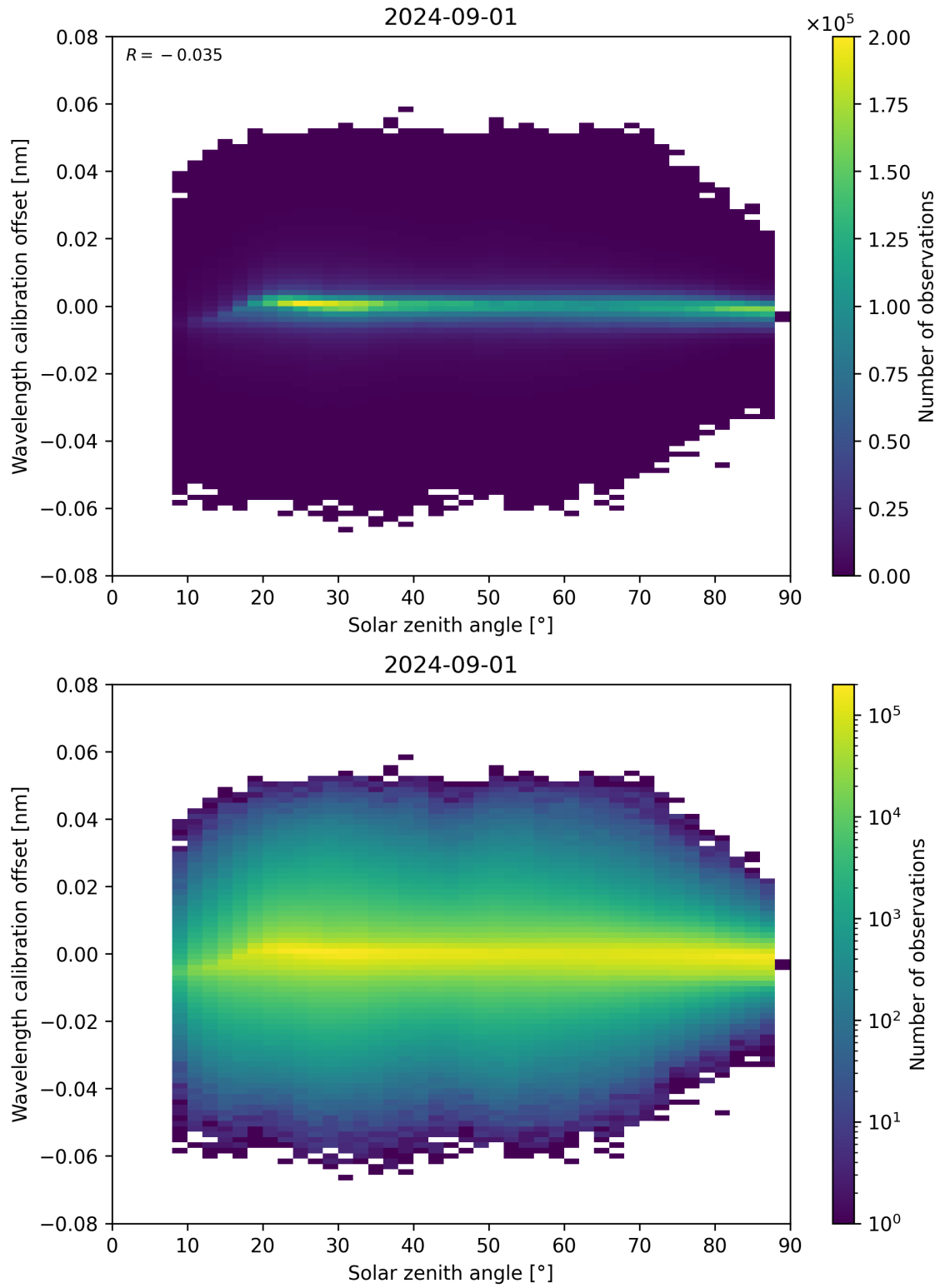
Figure 158: Scatter density plot of “Solar zenith angle” against “Wavelength calibration offset” for 2024-09-01 to 2024-09-02.
