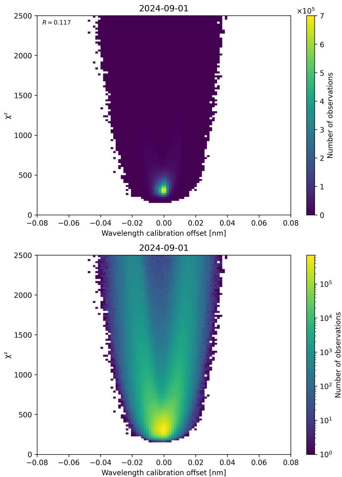
Figure 175: Scatter density plot of “Wavelength calibration offset” against “ \chi^2 ” for 2024-09-01 to 2024-09-02.
