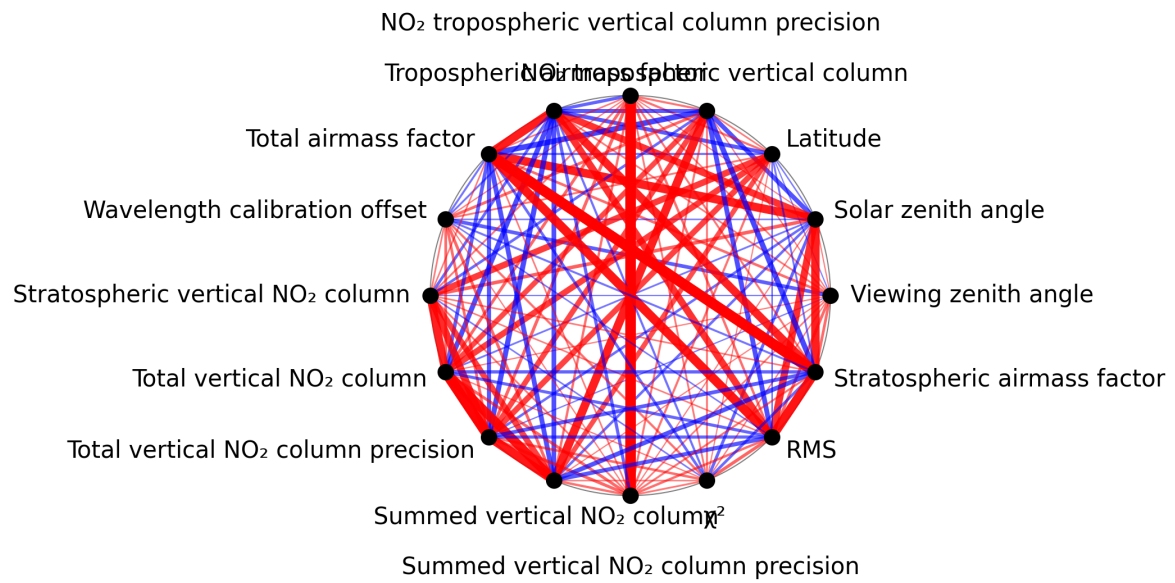
Figure 1: Map of correlation graph for 2024-09-01 to 2024-09-02.
