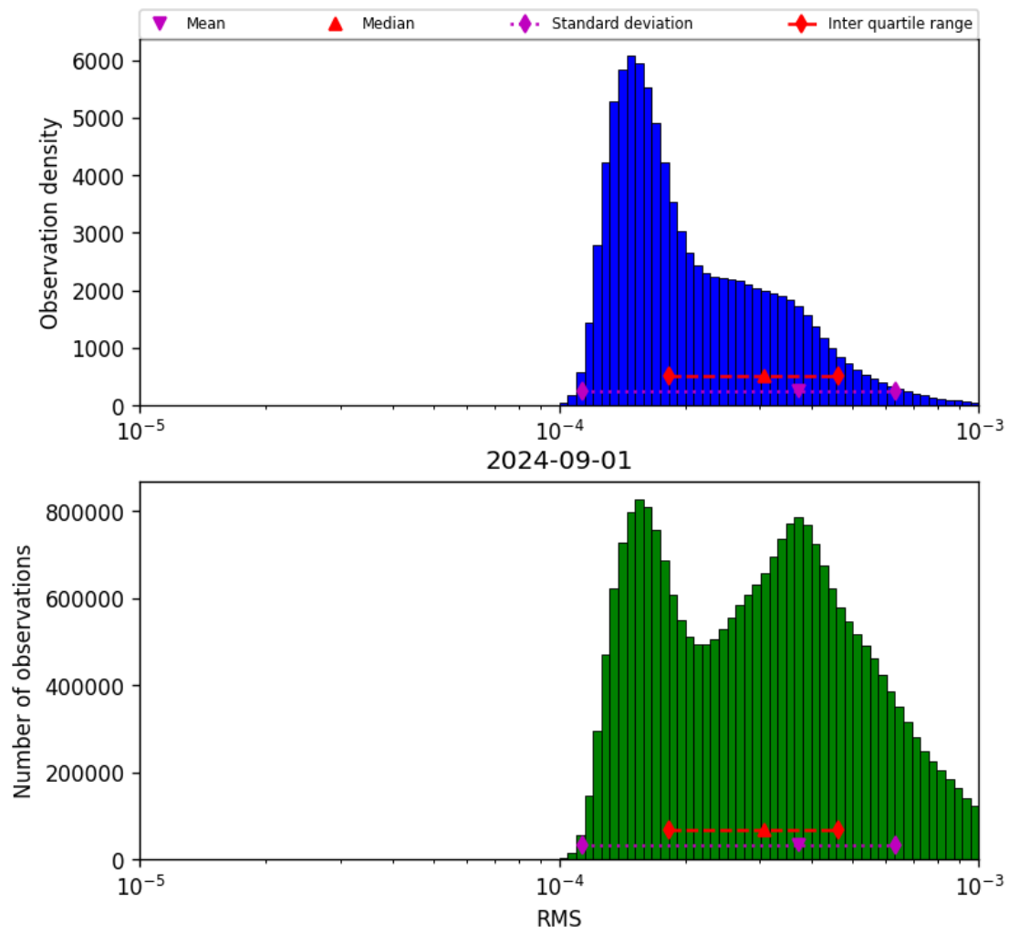
Figure 43: Histogram of “RMS” for 2024-09-01 to 2024-09-02
