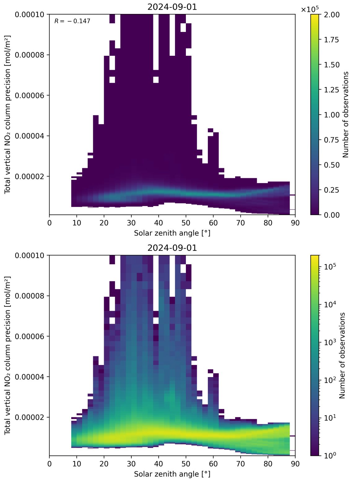
Figure 154: Scatter density plot of “Solar zenith angle” against “Total vertical NO 2 column precision” for 2024-09-01 to 2024-09-02.
