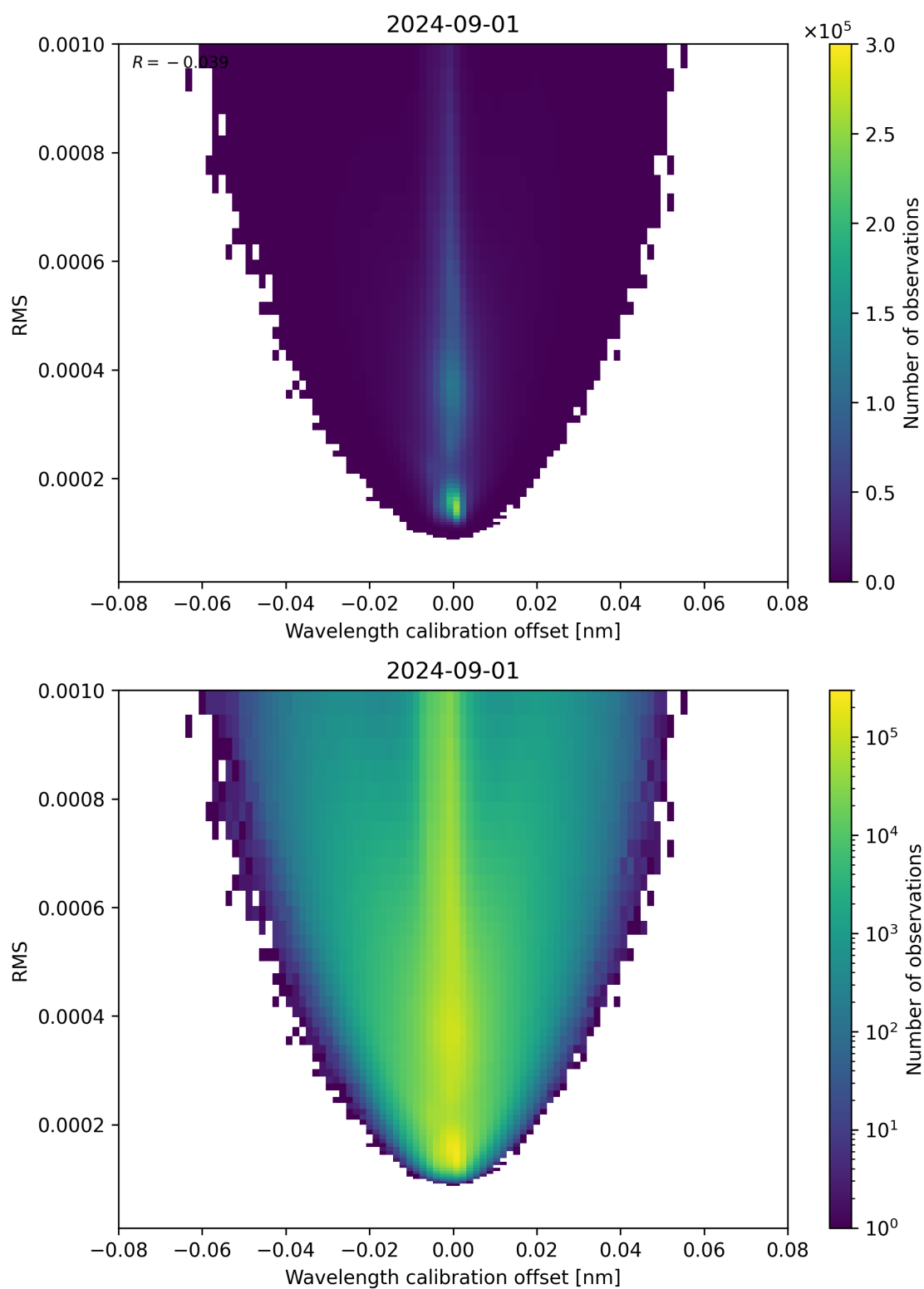
Figure 181: Scatter density plot of “Wavelength calibration offset” against “RMS” for 2024-09-01 to 2024-09-02.
