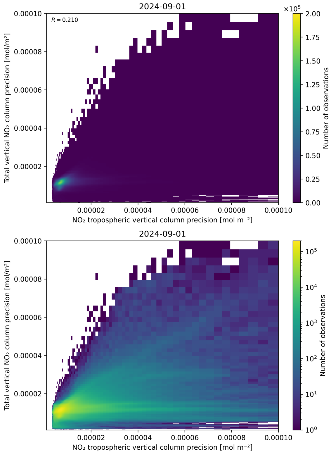
Figure 139: Scatter density plot of “NO 2 tropospheric vertical column precision” against “Total vertical NO 2 column precision” for 2024-09-01 to 2024-09-02.
