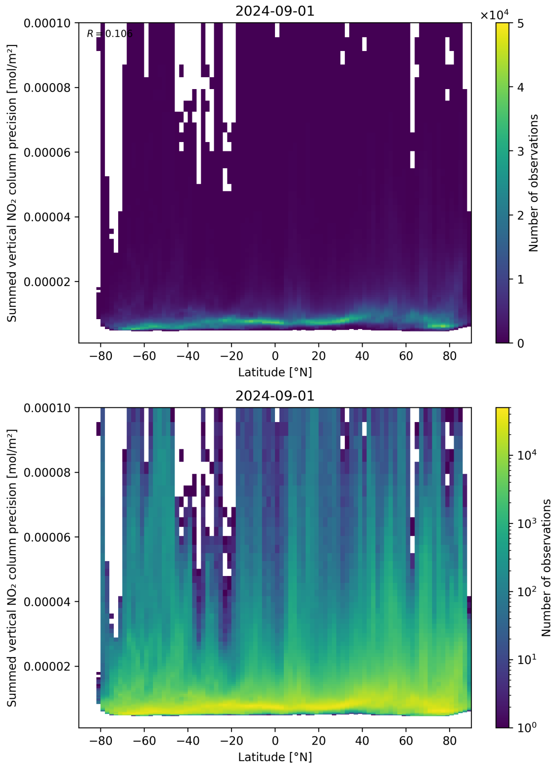
Figure 89: Scatter density plot of “Latitude” against “Summed vertical NO 2 column precision” for 2024-09-01 to 2024-09-02.
