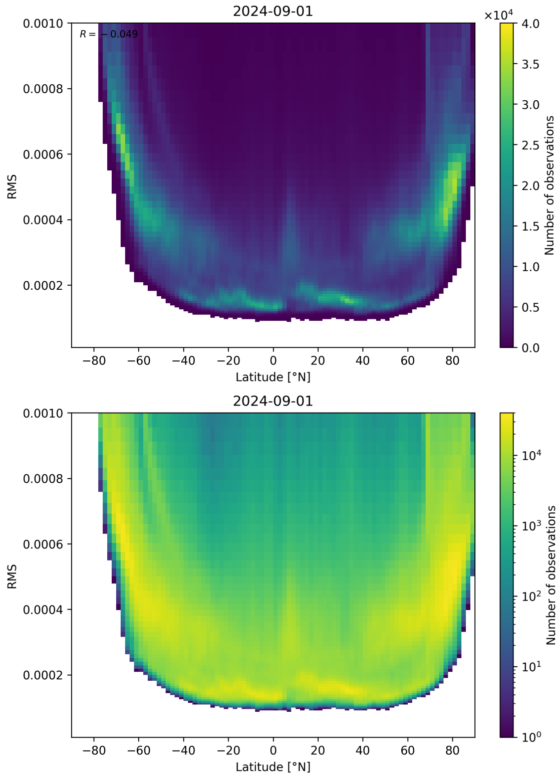
Figure 94: Scatter density plot of “Latitude” against “RMS” for 2024-09-01 to 2024-09-02.
