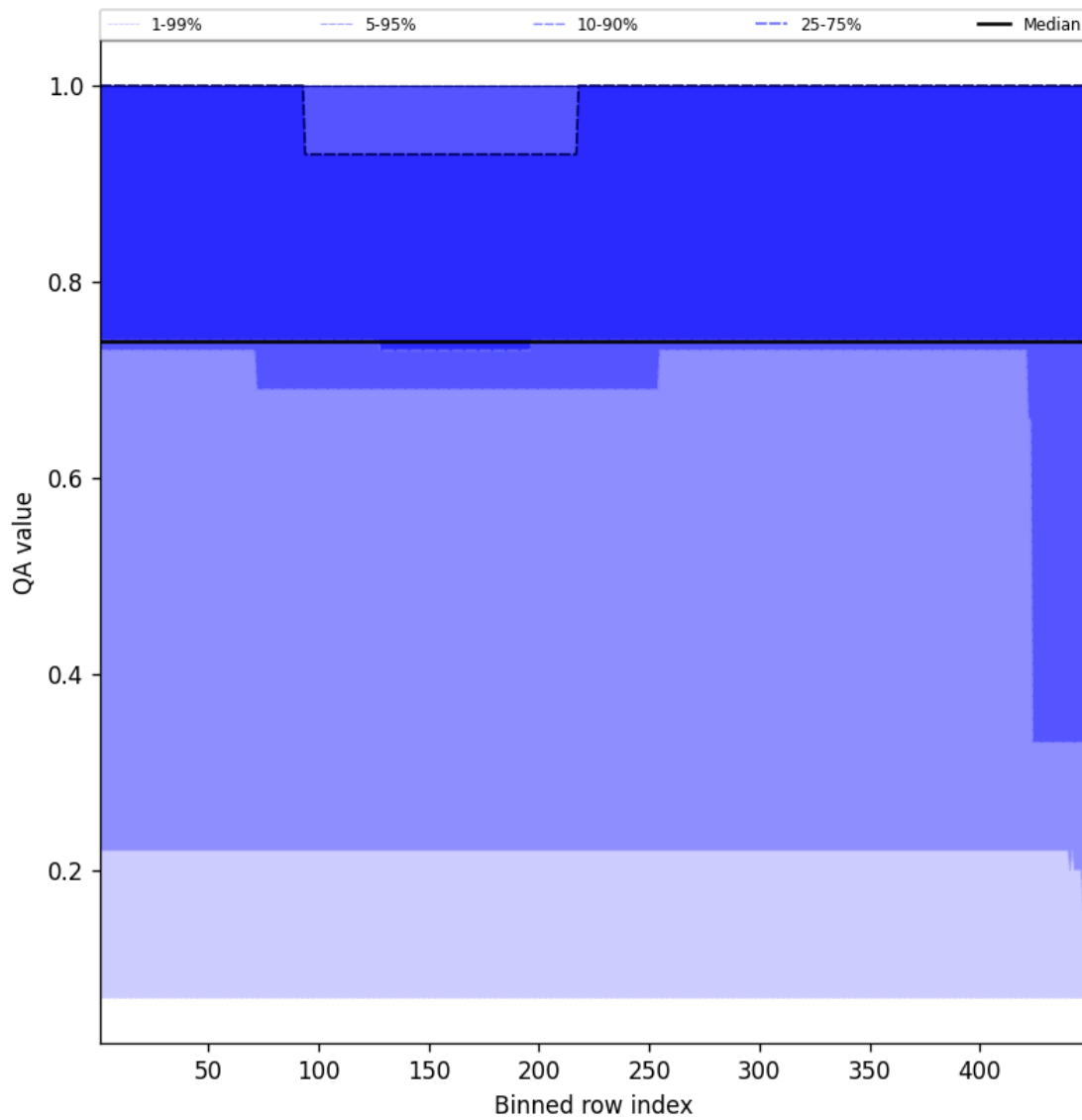
Figure 45: Along track statistics of “QA value” for 2024-09-01 to 2024-09-02
