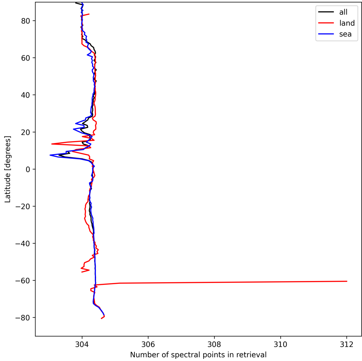
Figure 16: Zonal average of “Number of spectral points in retrieval” for 2024-09-01 to 2024-09-02.
