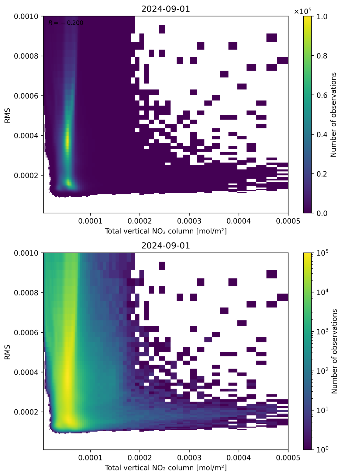
Figure 120: Scatter density plot of “Total vertical NO 2 column” against “RMS” for 2024-09-01 to 2024-09-02.
