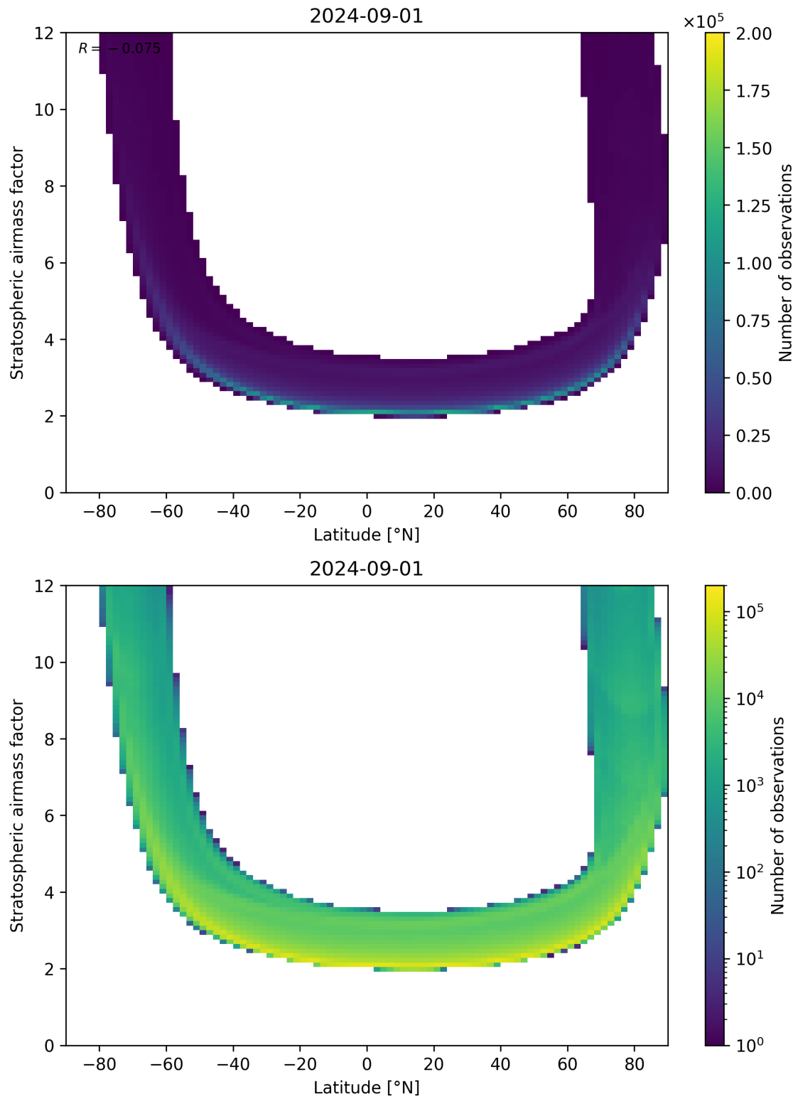
Figure 83: Scatter density plot of “Latitude” against “Stratospheric airmass factor” for 2024-09-01 to 2024-09-02.
