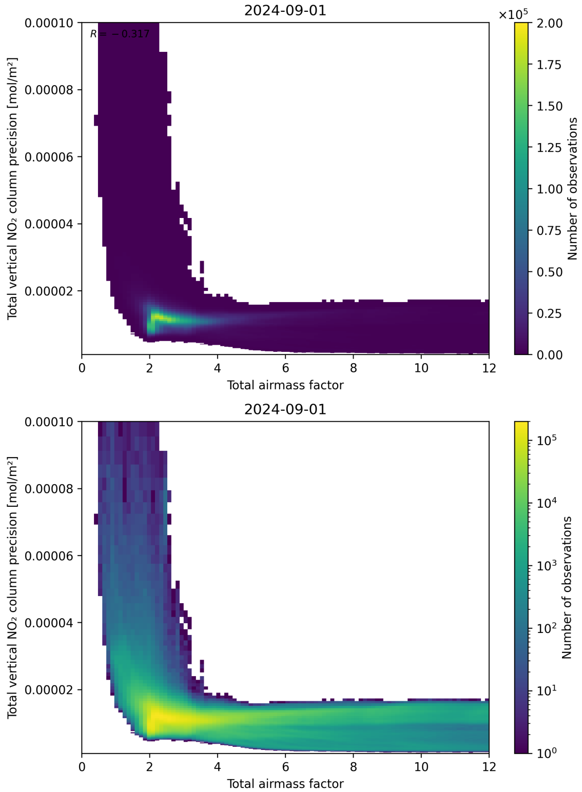
Figure 68: Scatter density plot of “Total airmass factor” against “Total vertical NO 2 column precision” for 2024-09-01 to 2024-09-02.
