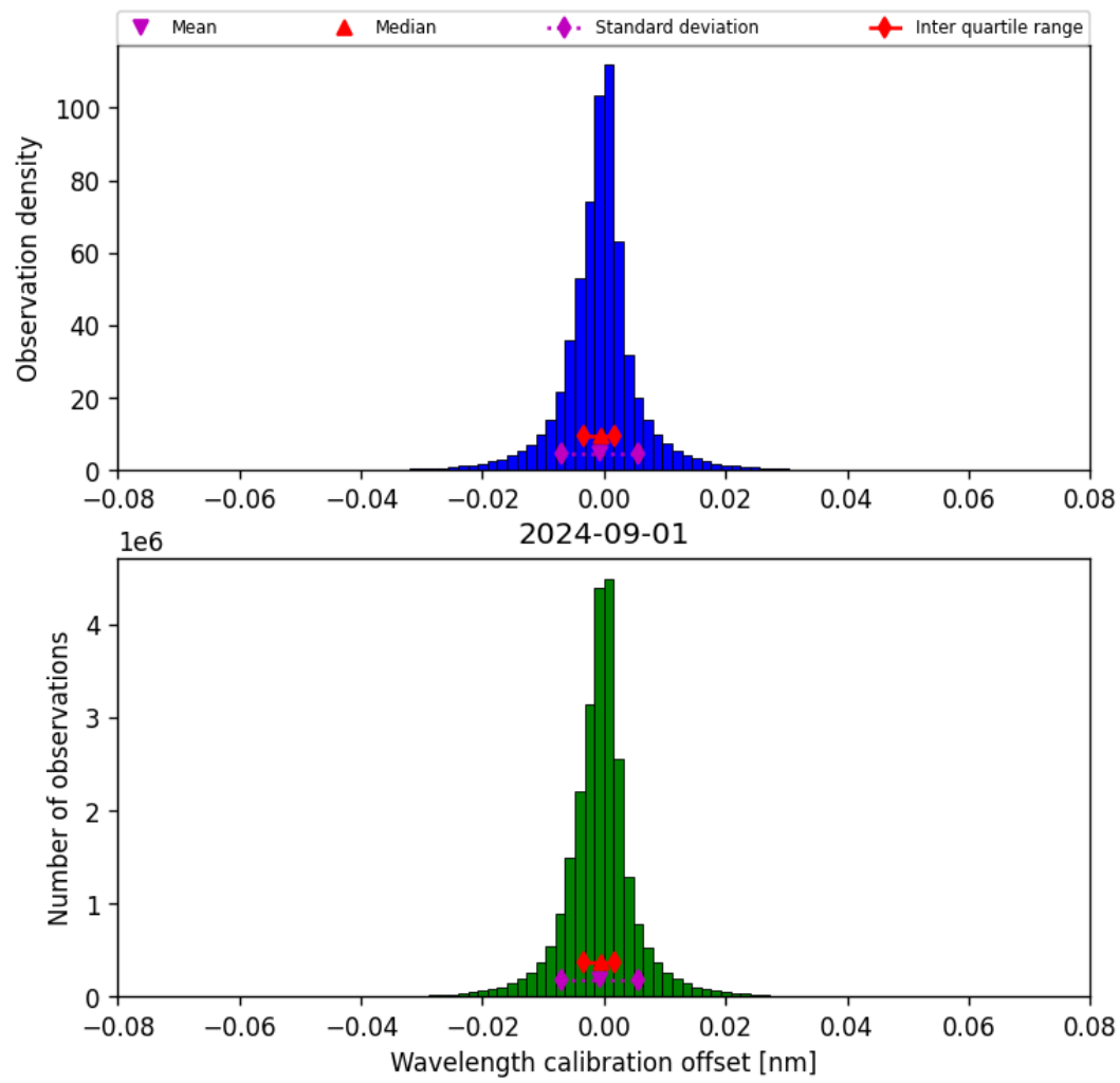
Figure 35: Histogram of “Wavelength calibration offset” for 2024-09-01 to 2024-09-02
