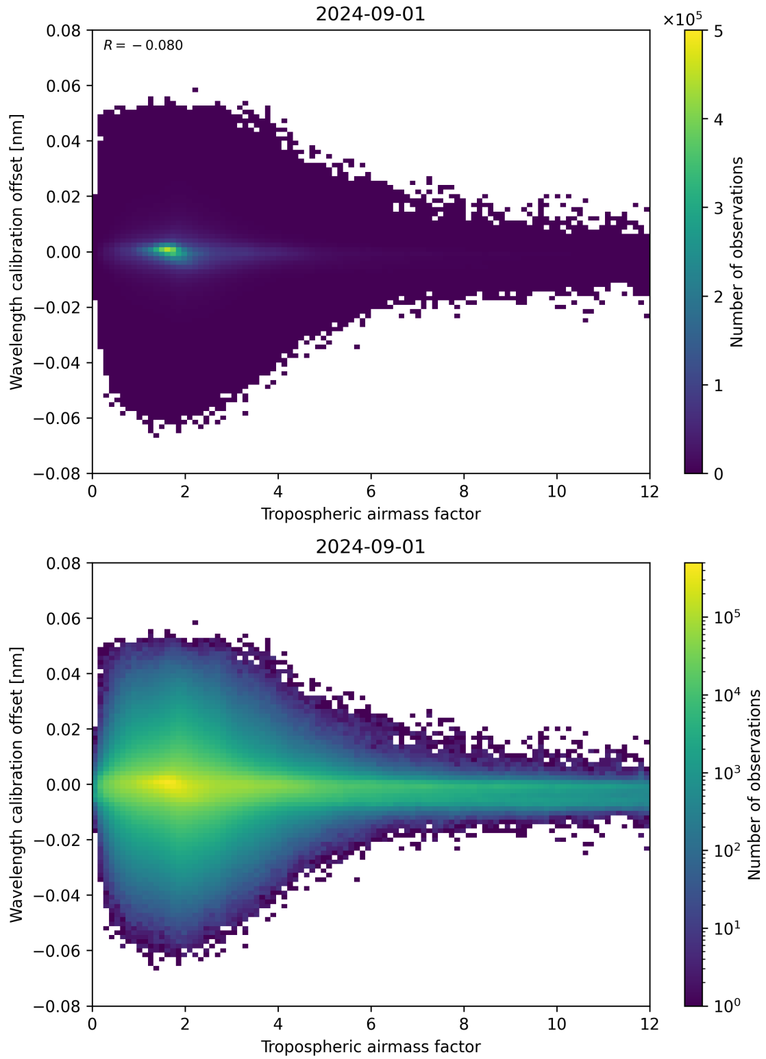
Figure 80: Scatter density plot of “Tropospheric airmass factor” against “Wavelength calibration offset” for 2024-09-01 to 2024-09-02.
