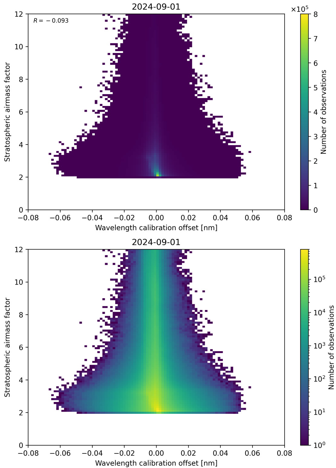
Figure 174: Scatter density plot of “Wavelength calibration offset” against “Stratospheric airmass factor” for 2024-09-01 to 2024-09-02.
