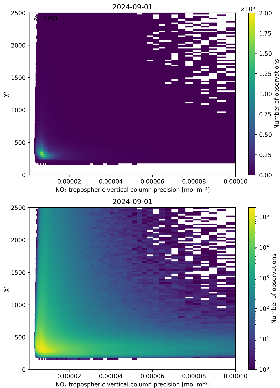
Figure 134: Scatter density plot of “NO 2 tropospheric vertical column precision” against “ \chi^2 ” for 2024-09-01 to 2024-09-02.
