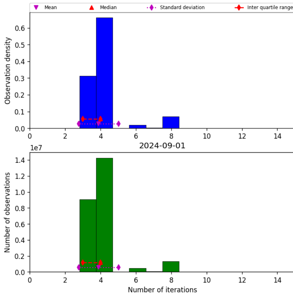
Figure 34: Histogram of “Number of iterations” for 2024-09-01 to 2024-09-02
