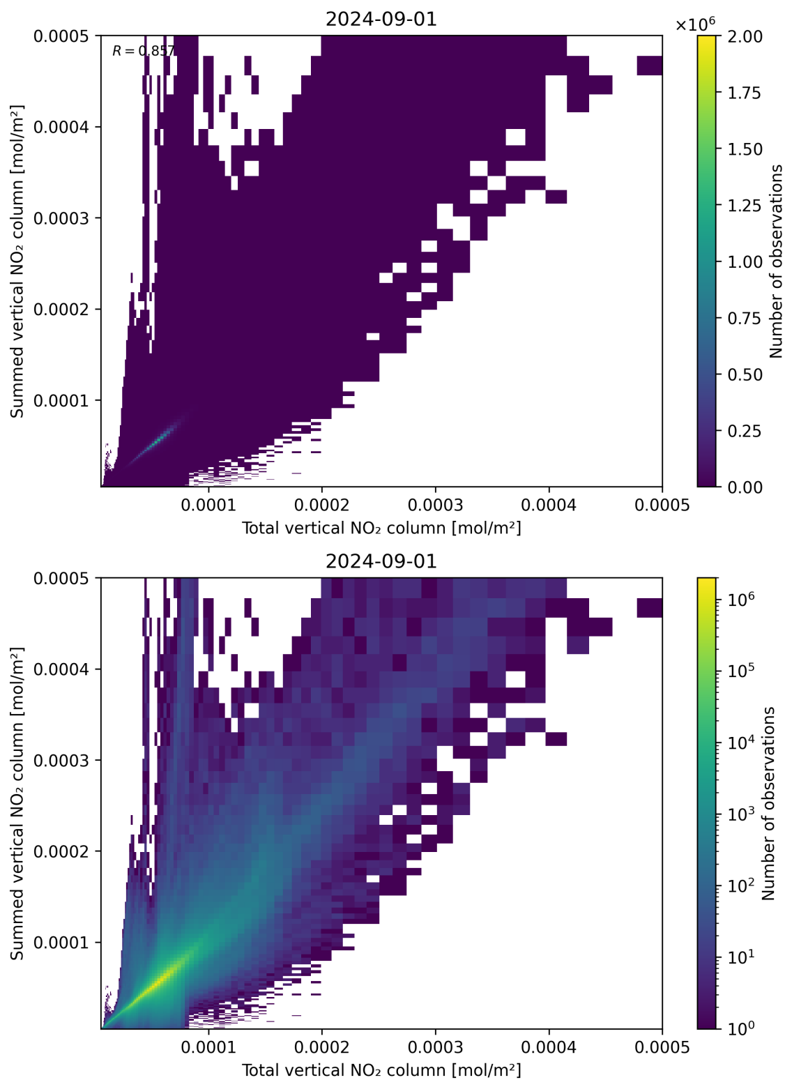
Figure 112: Scatter density plot of “Total vertical NO 2 column” against “Summed vertical NO 2 column” for 2024-09-01 to 2024-09-02.
