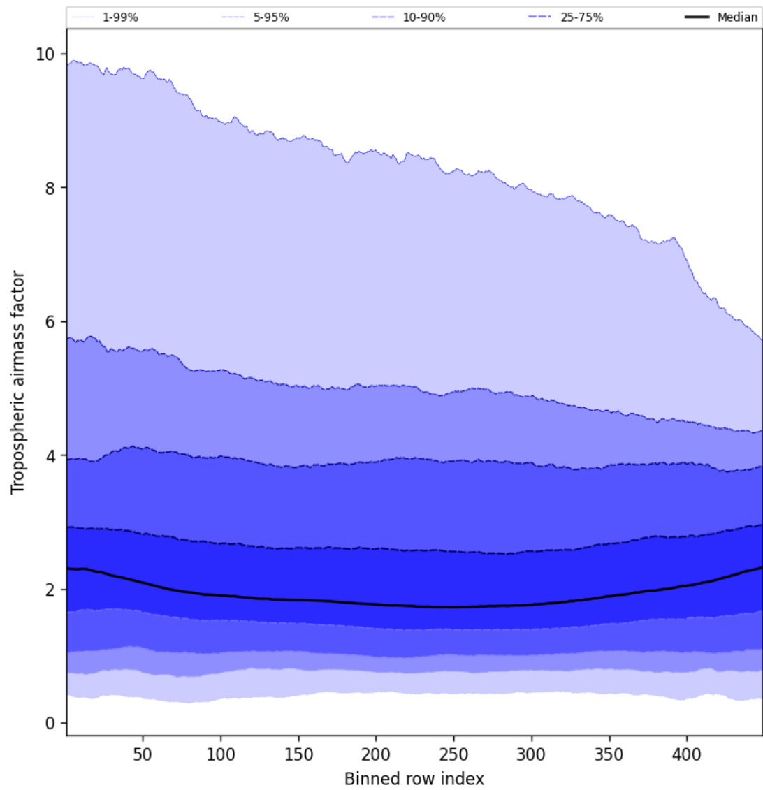
Figure 48: Along track statistics of “Tropospheric airmass factor” for 2024-09-01 to 2024-09-02
