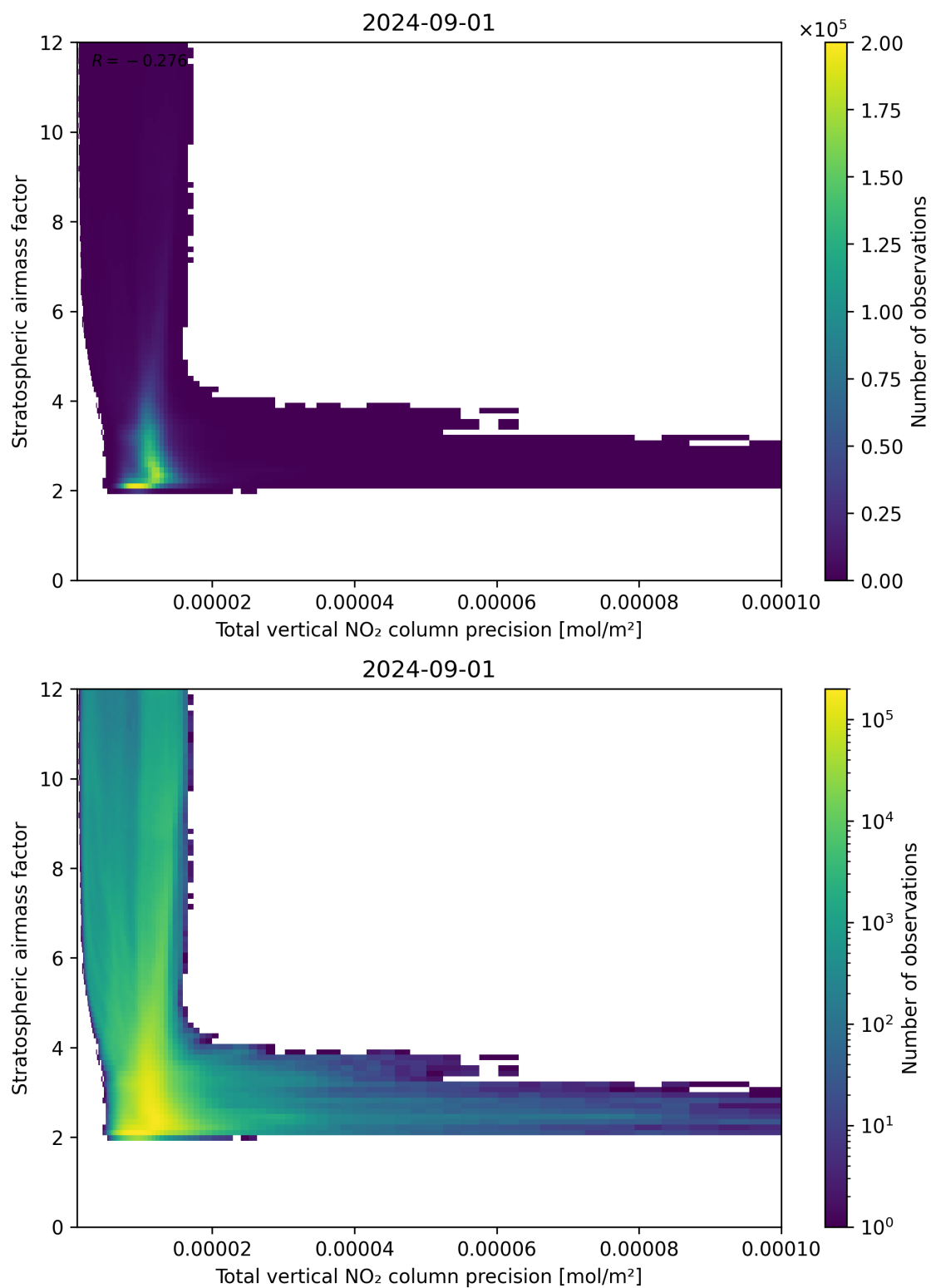
Figure 115: Scatter density plot of “Total vertical NO 2 column precision” against “Stratospheric airmass factor” for 2024-09-01 to 2024-09-02.
