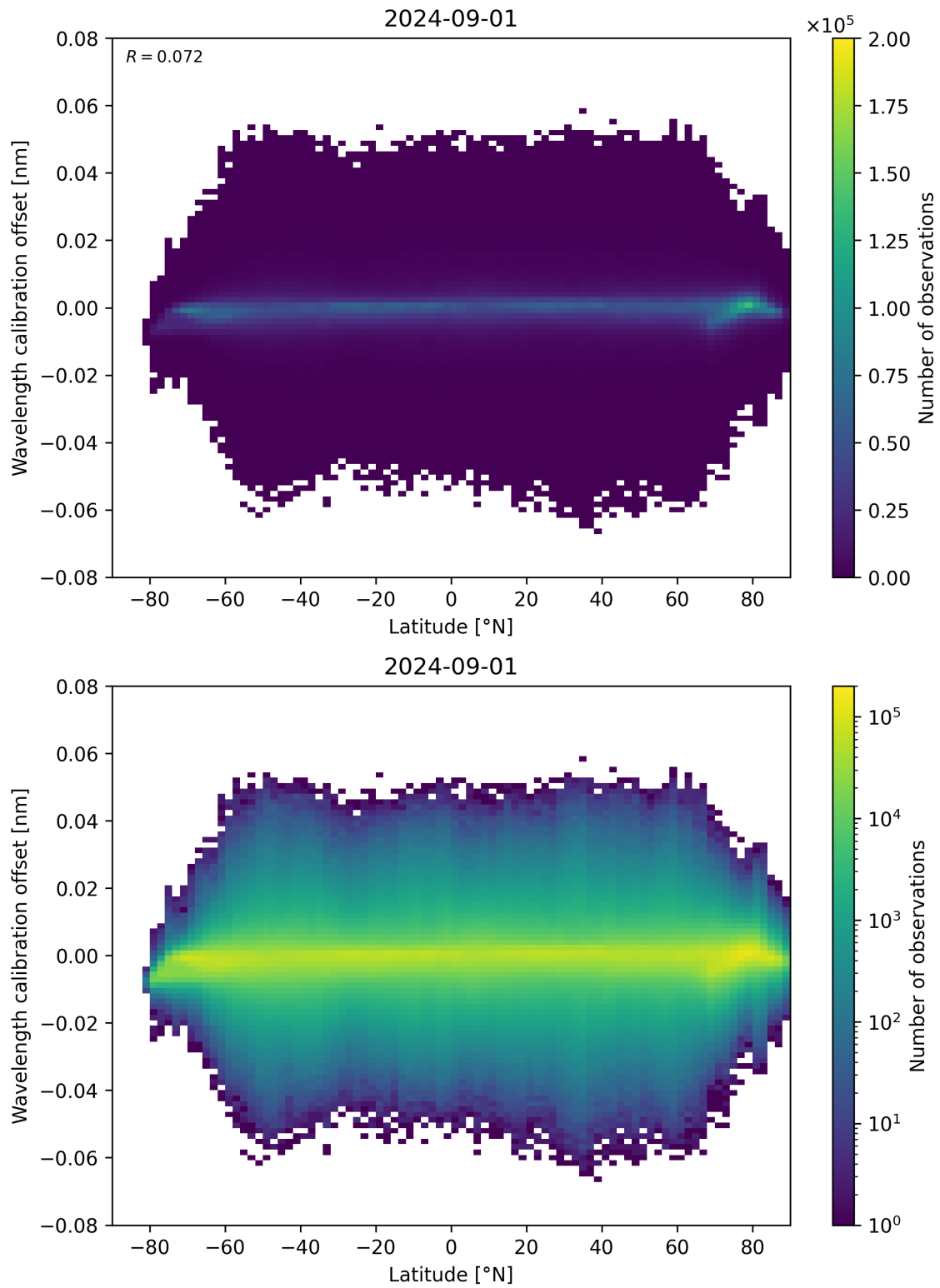
Figure 95: Scatter density plot of “Latitude” against “Wavelength calibration offset” for 2024-09-01 to 2024-09-02.
