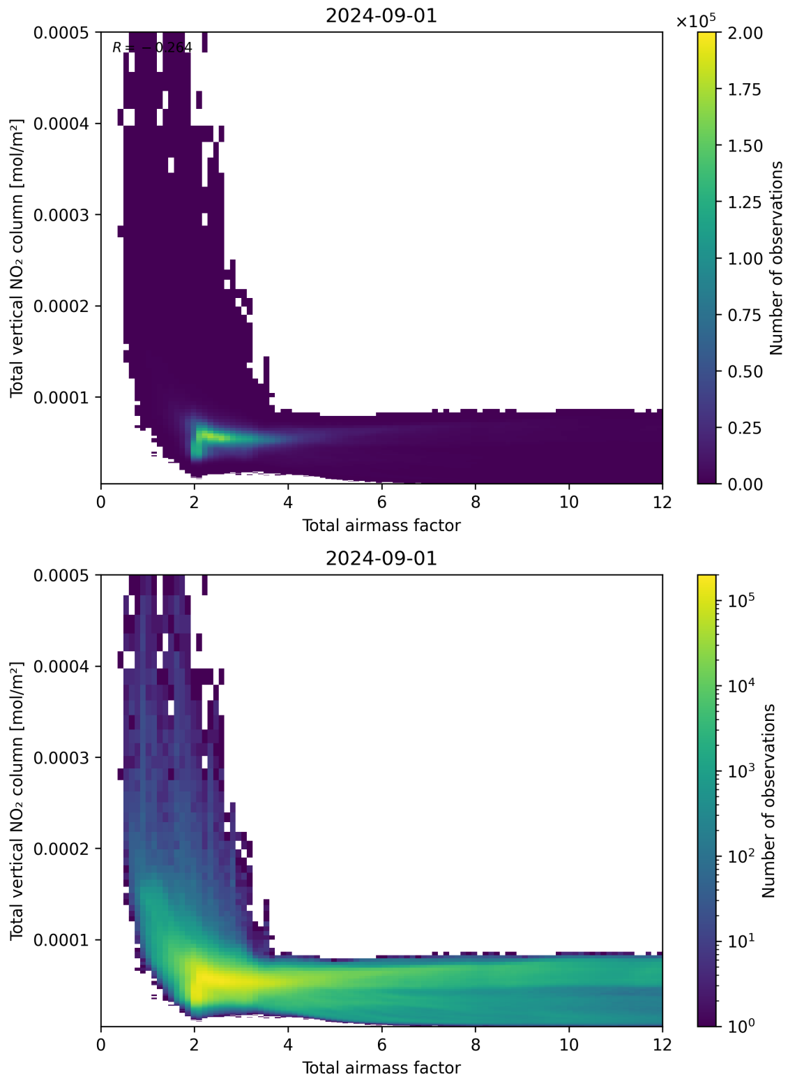
Figure 67: Scatter density plot of “Total airmass factor” against “Total vertical NO 2 column” for 2024-09-01 to 2024-09-02.
