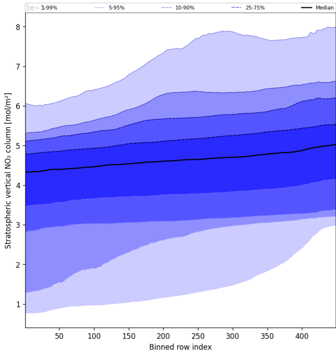
Figure 53: Along track statistics of “Stratospheric vertical NO 2 column” for 2024-09-01 to 2024-09-02
