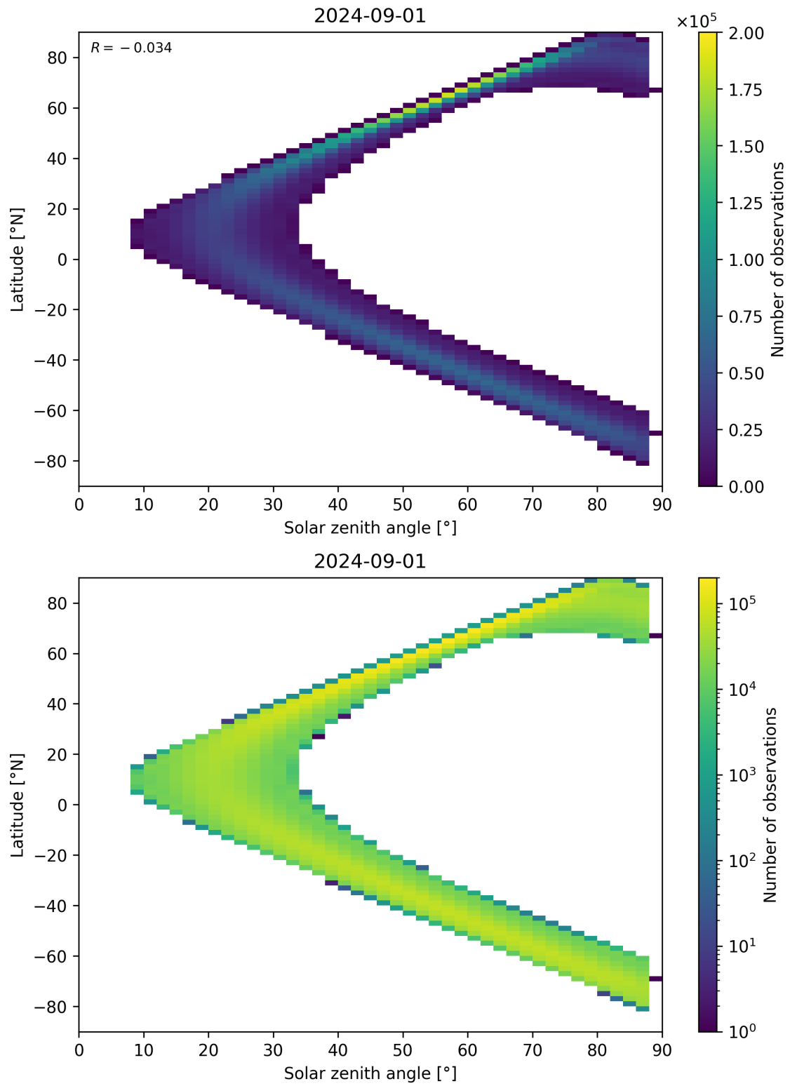
Figure 149: Scatter density plot of “Solar zenith angle” against “Latitude” for 2024-09-01 to 2024-09-02.
