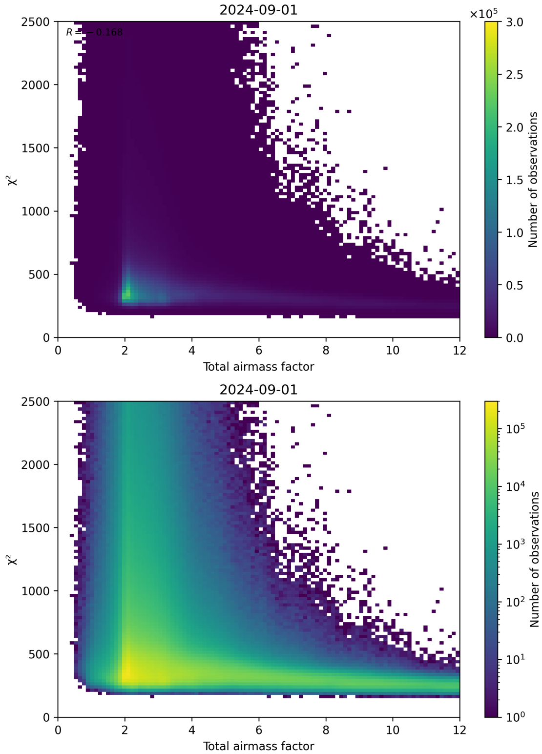
Figure 63: Scatter density plot of “Total airmass factor” against “ \chi^2 ” for 2024-09-01 to 2024-09-02.
