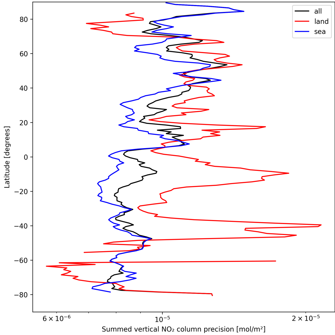
Figure 24: Zonal average of “Summed vertical NO 2 column precision” for 2024-09-01 to 2024-09-02.
