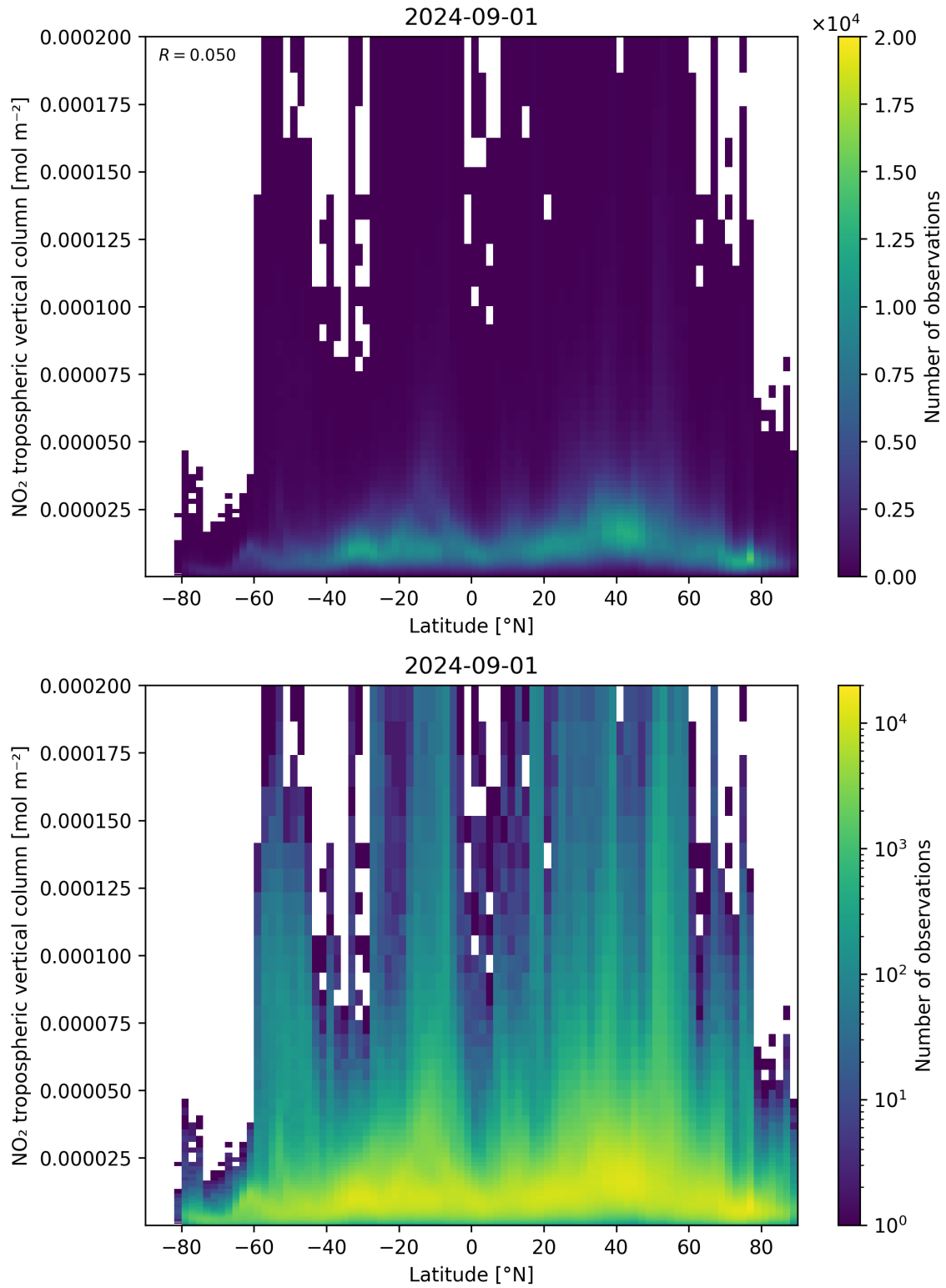
Figure 92: Scatter density plot of “Latitude” against “NO 2 tropospheric vertical column” for 2024-09-01 to 2024-09-02.
