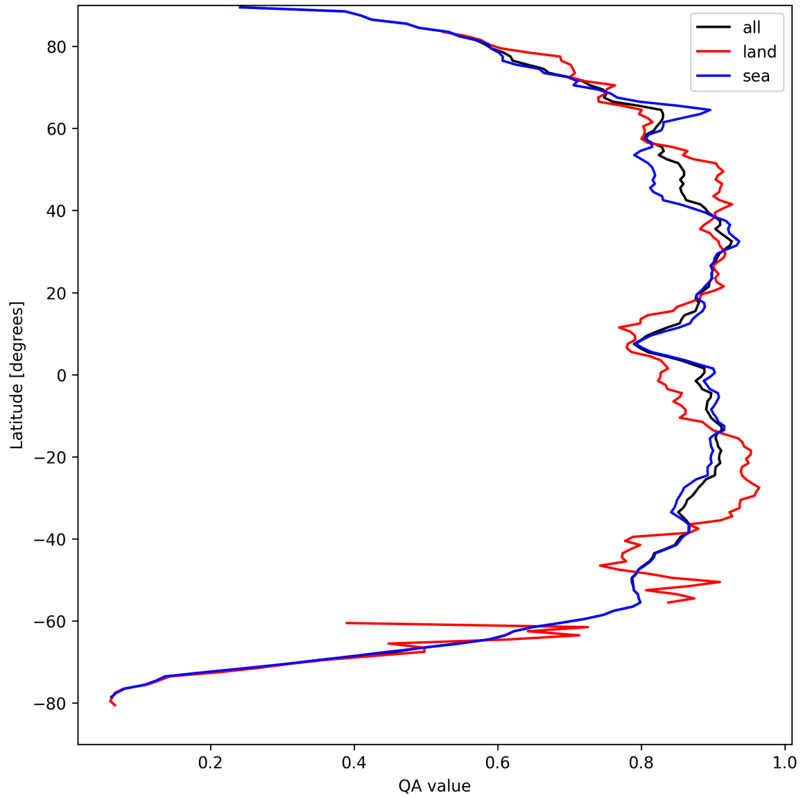
Figure 11: Zonal average of “QA value” for 2024-09-01 to 2024-09-02.
