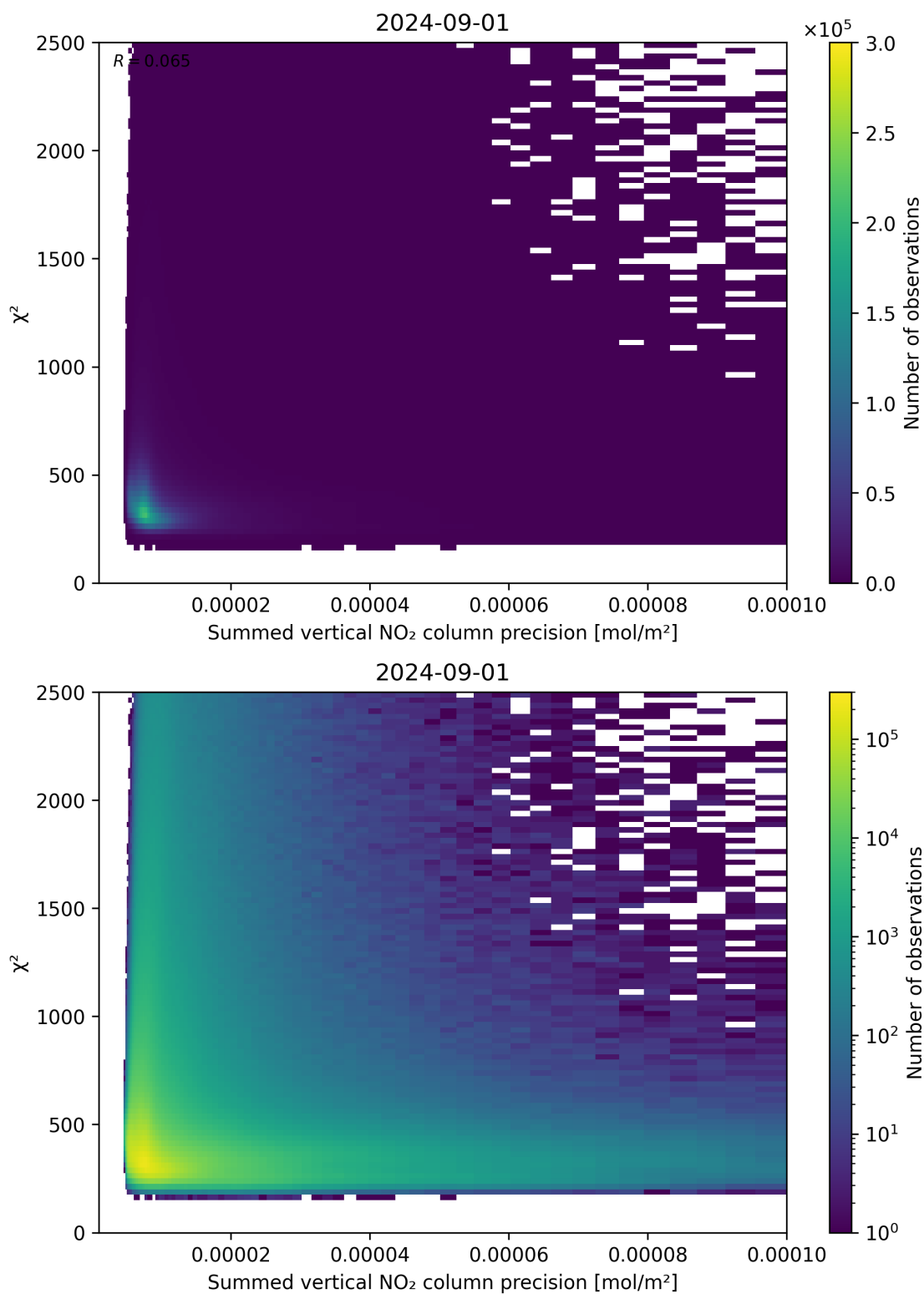
Figure 107: Scatter density plot of “Summed vertical NO 2 column precision” against “ \chi^2 ” for 2024-09-01 to 2024-09-02.
