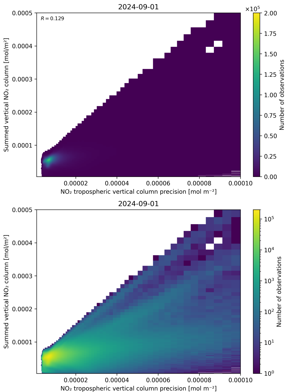
Figure 136: Scatter density plot of “NO 2 tropospheric vertical column precision” against “Summed vertical NO 2 column” for 2024-09-01 to 2024-09-02.
