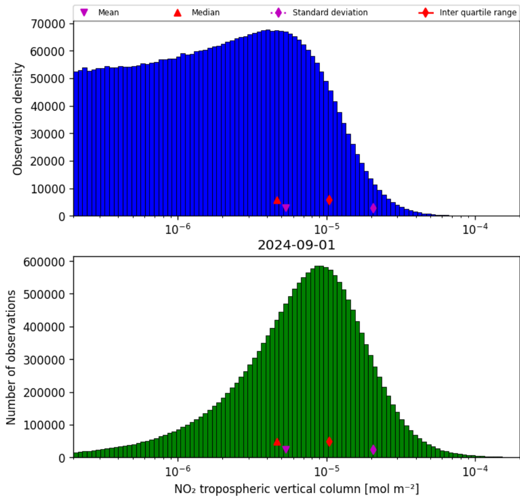
Figure 29: Histogram of “NO 2 tropospheric vertical column” for 2024-09-01 to 2024-09-02
