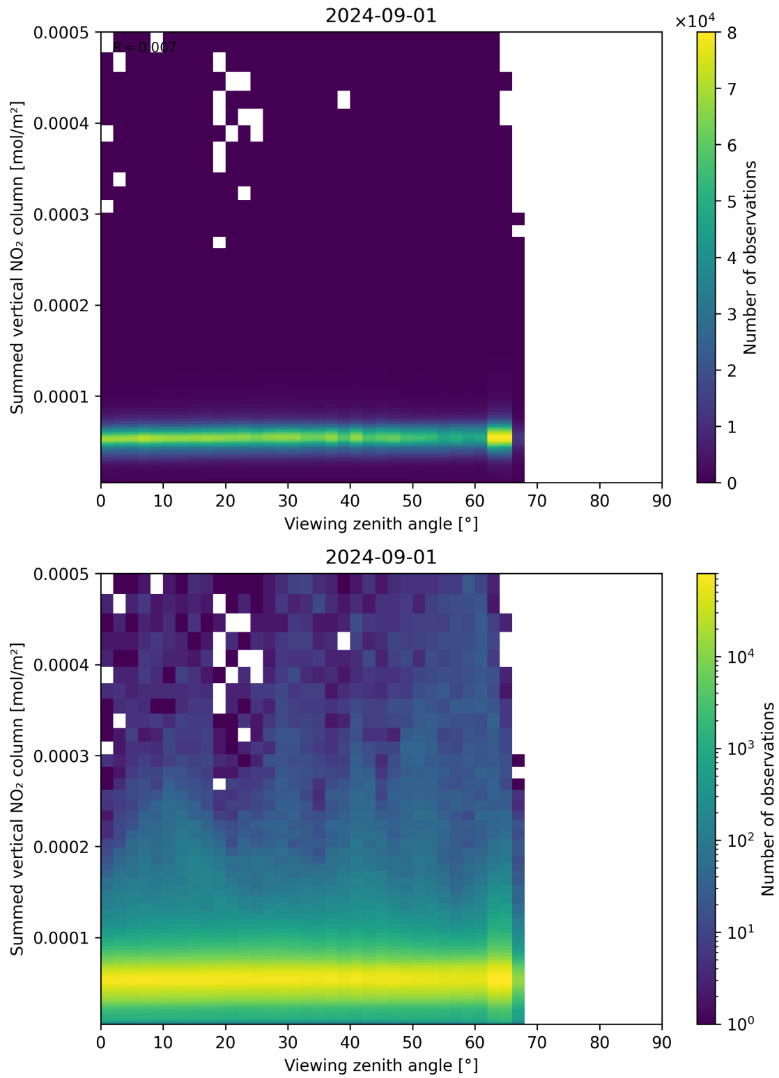
Figure 165: Scatter density plot of “Viewing zenith angle” against “Summed vertical NO 2 column” for 2024-09-01 to 2024-09-02.
