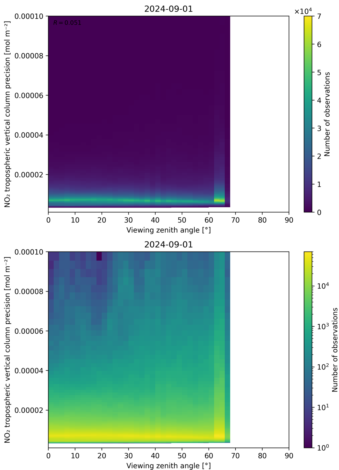
Figure 170: Scatter density plot of “Viewing zenith angle” against “NO 2 tropospheric vertical column precision” for 2024-09-01 to 2024-09-02.
