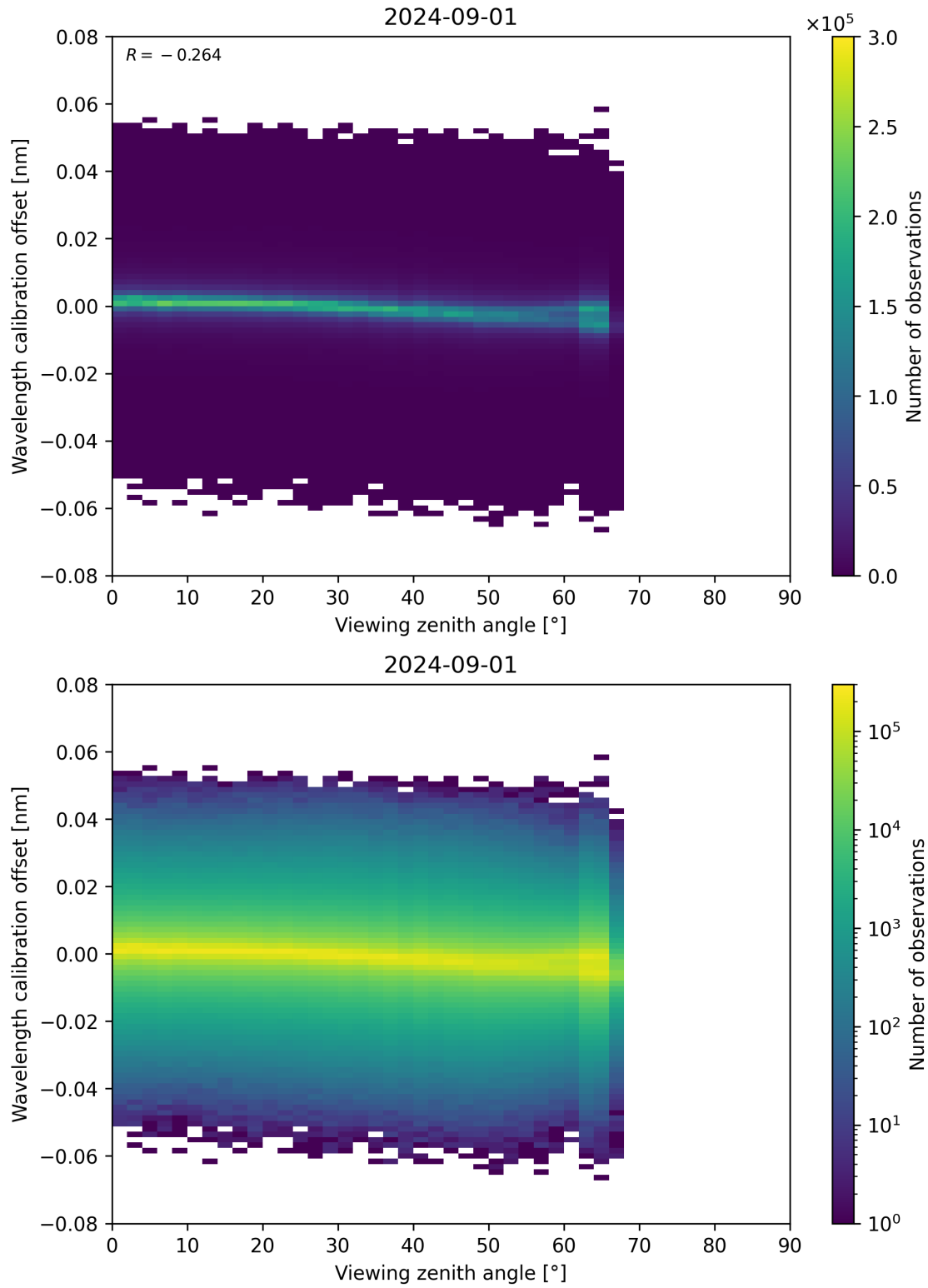
Figure 173: Scatter density plot of “Viewing zenith angle” against “Wavelength calibration offset” for 2024-09-01 to 2024-09-02.
