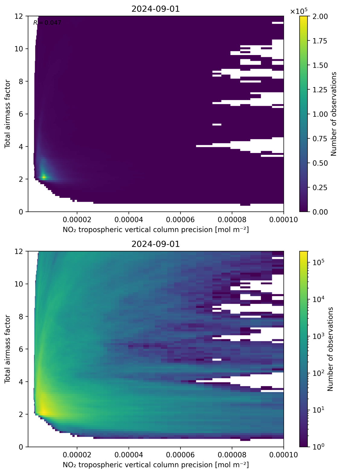
Figure 132: Scatter density plot of “NO 2 tropospheric vertical column precision” against “Total air mass factor” for 2024-09-01 to 2024-09-02.
