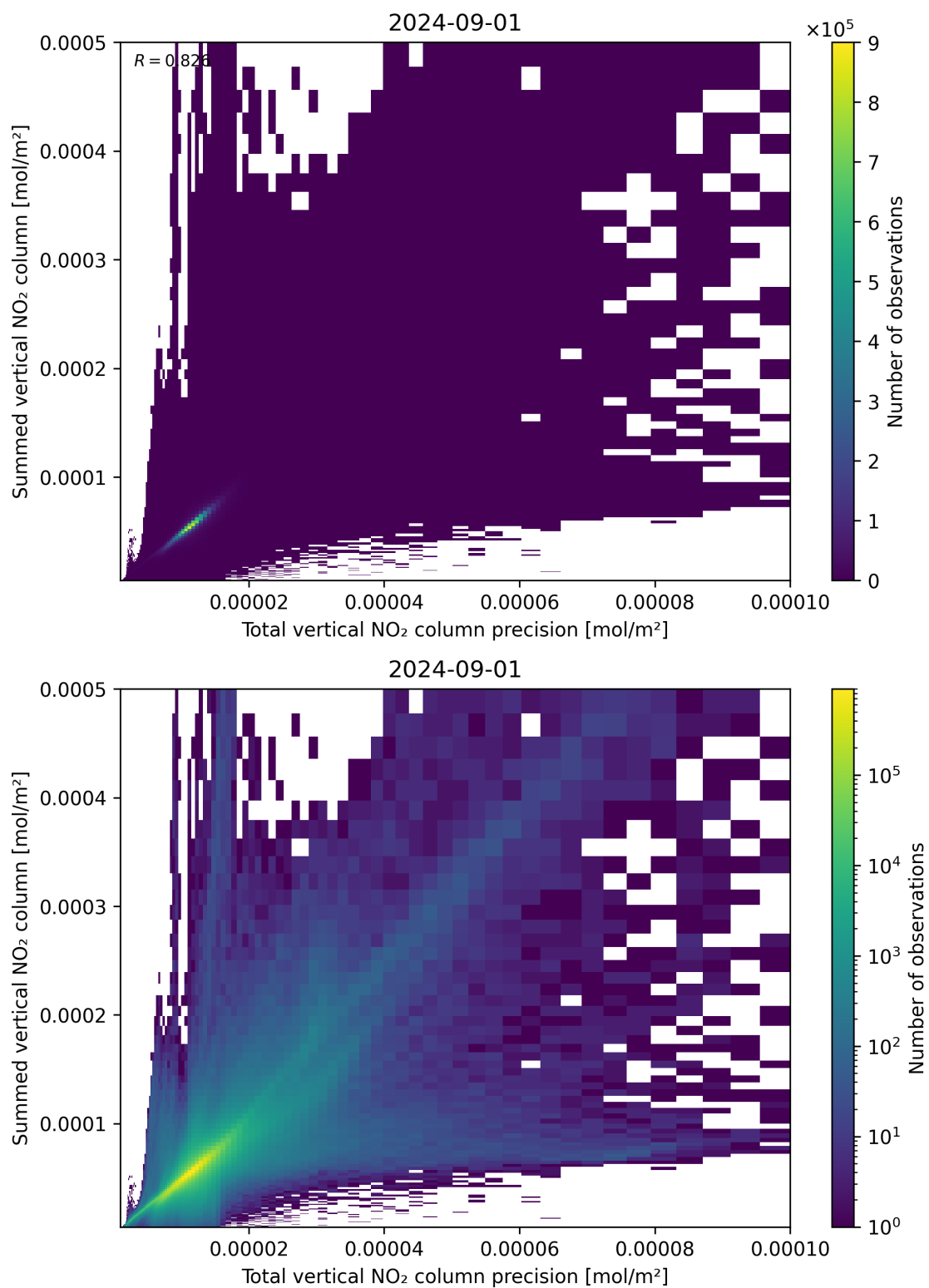
Figure 117: Scatter density plot of “Total vertical NO 2 column precision” against “Summed vertical NO 2 column” for 2024-09-01 to 2024-09-02.
