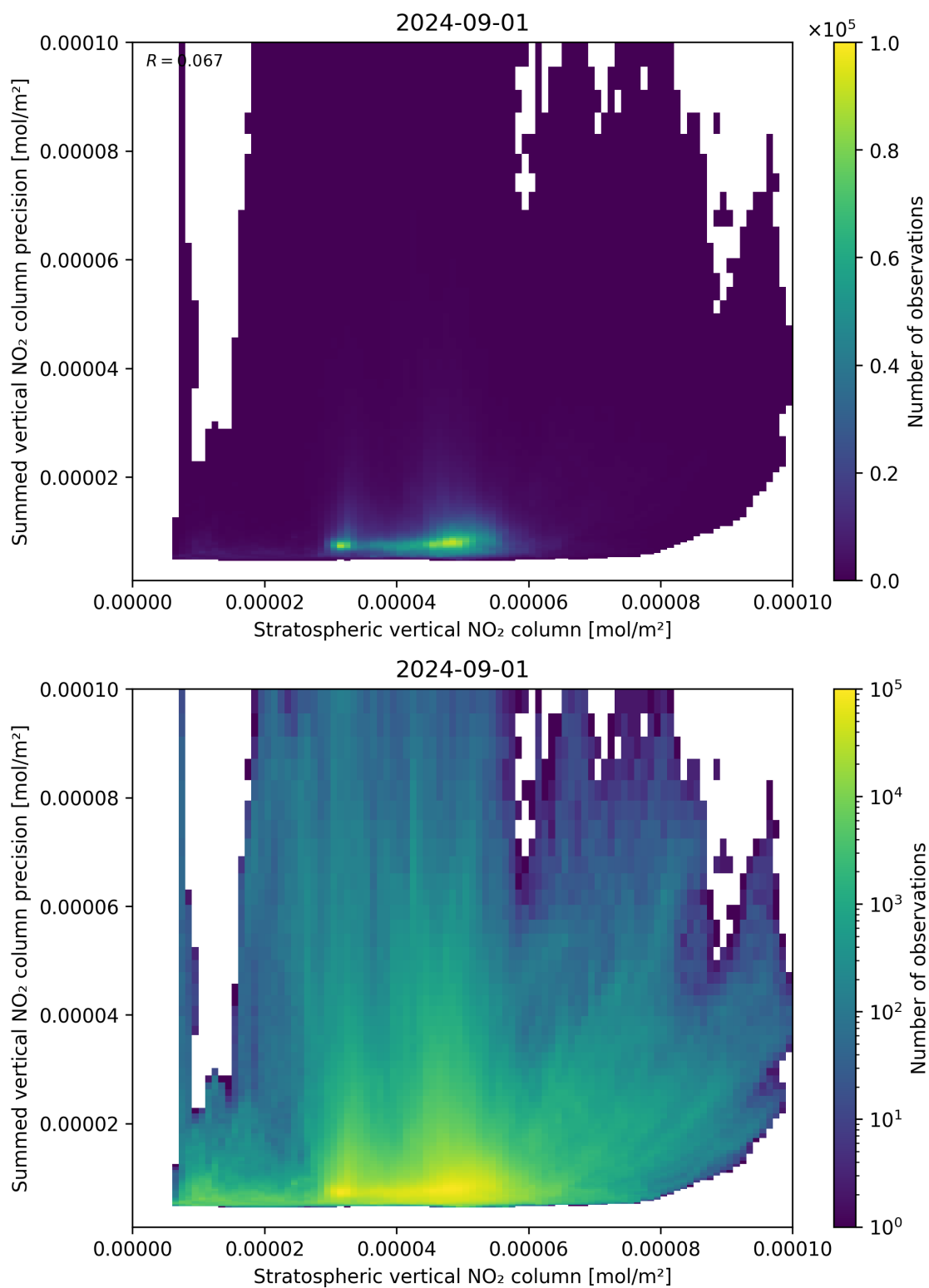
Figure 99: Scatter density plot of “Stratospheric vertical NO 2 column” against “Summed vertical NO 2 column precision” for 2024-09-01 to 2024-09-02.
