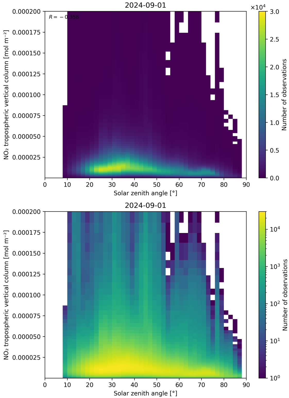
Figure 155: Scatter density plot of “Solar zenith angle” against “NO 2 tropospheric vertical column” for 2024-09-01 to 2024-09-02.
