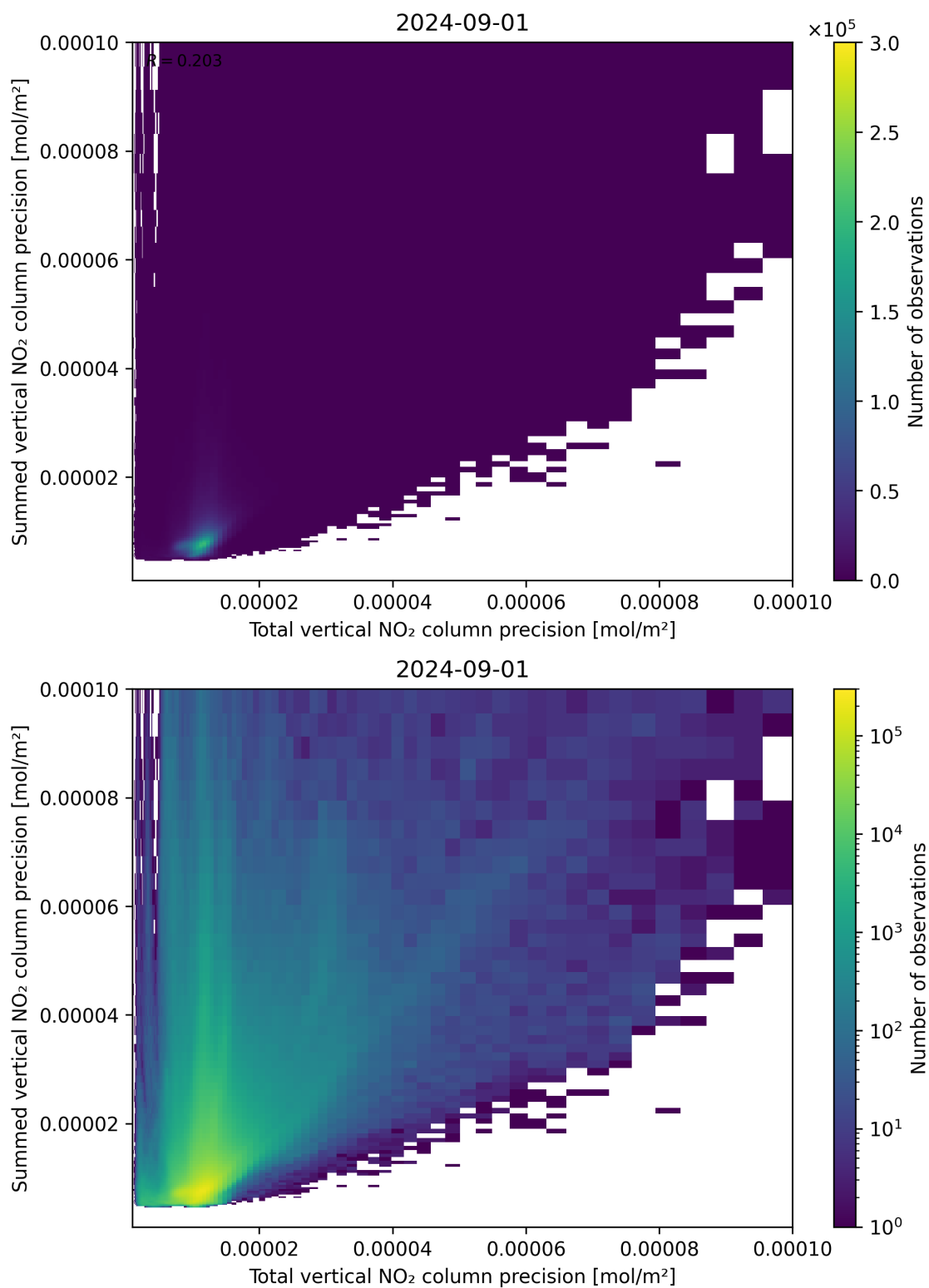
Figure 118: Scatter density plot of “Total vertical NO 2 column precision” against “Summed vertical NO 2 column precision” for 2024-09-01 to 2024-09-02.
