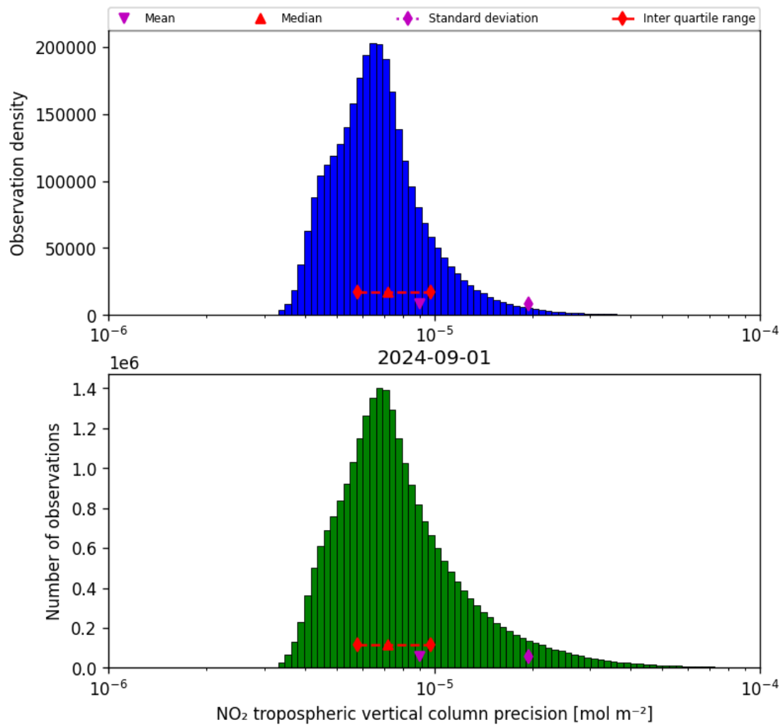
Figure 30: Histogram of "NO 2 tropospheric vertical column precision" for 2024-09-01 to 2024-09-02
