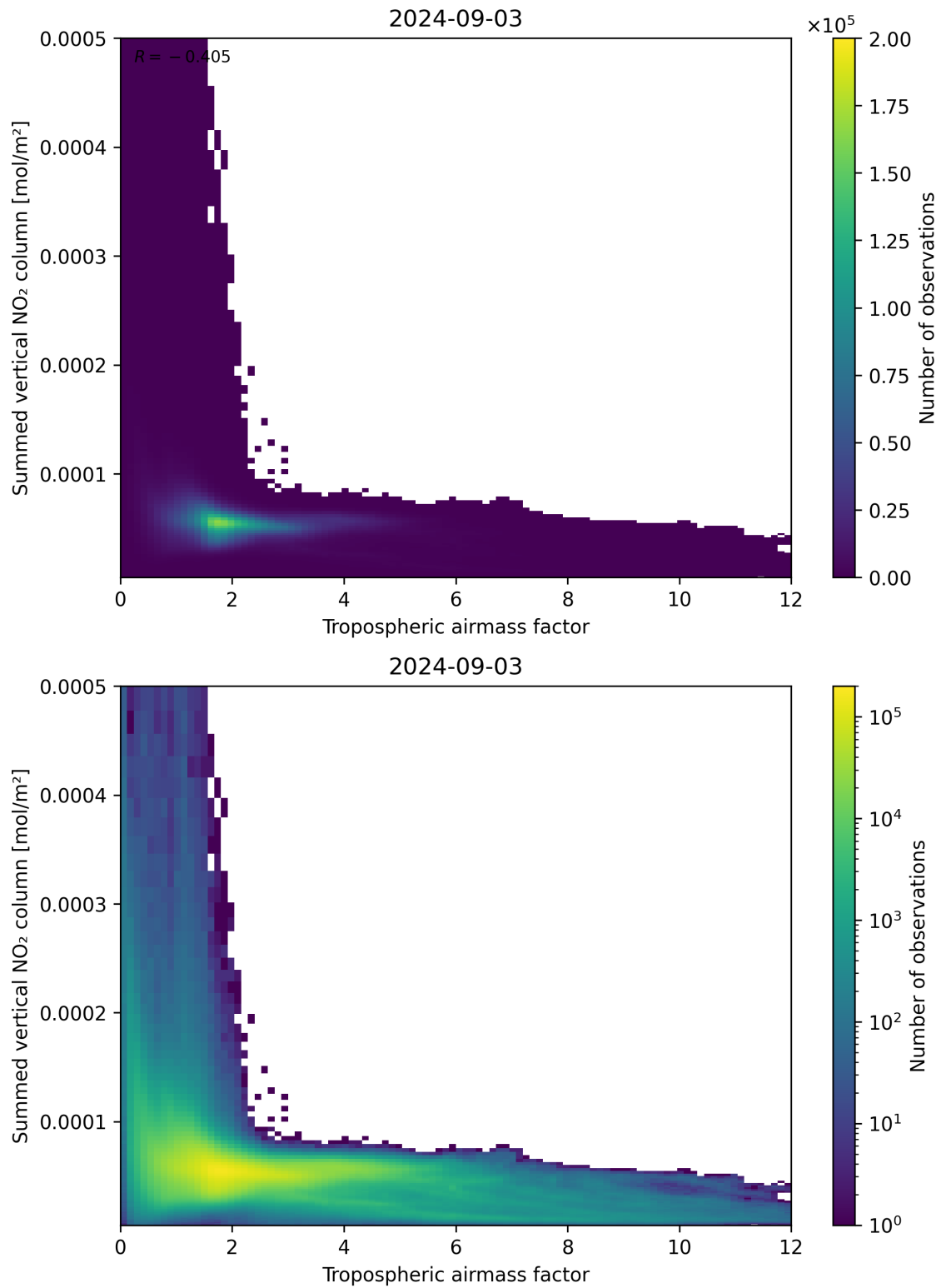
Figure 75: Scatter density plot of “Tropospheric airmass factor” against “Summed vertical NO 2 column” for 2024-09-02 to 2024-09-04.
