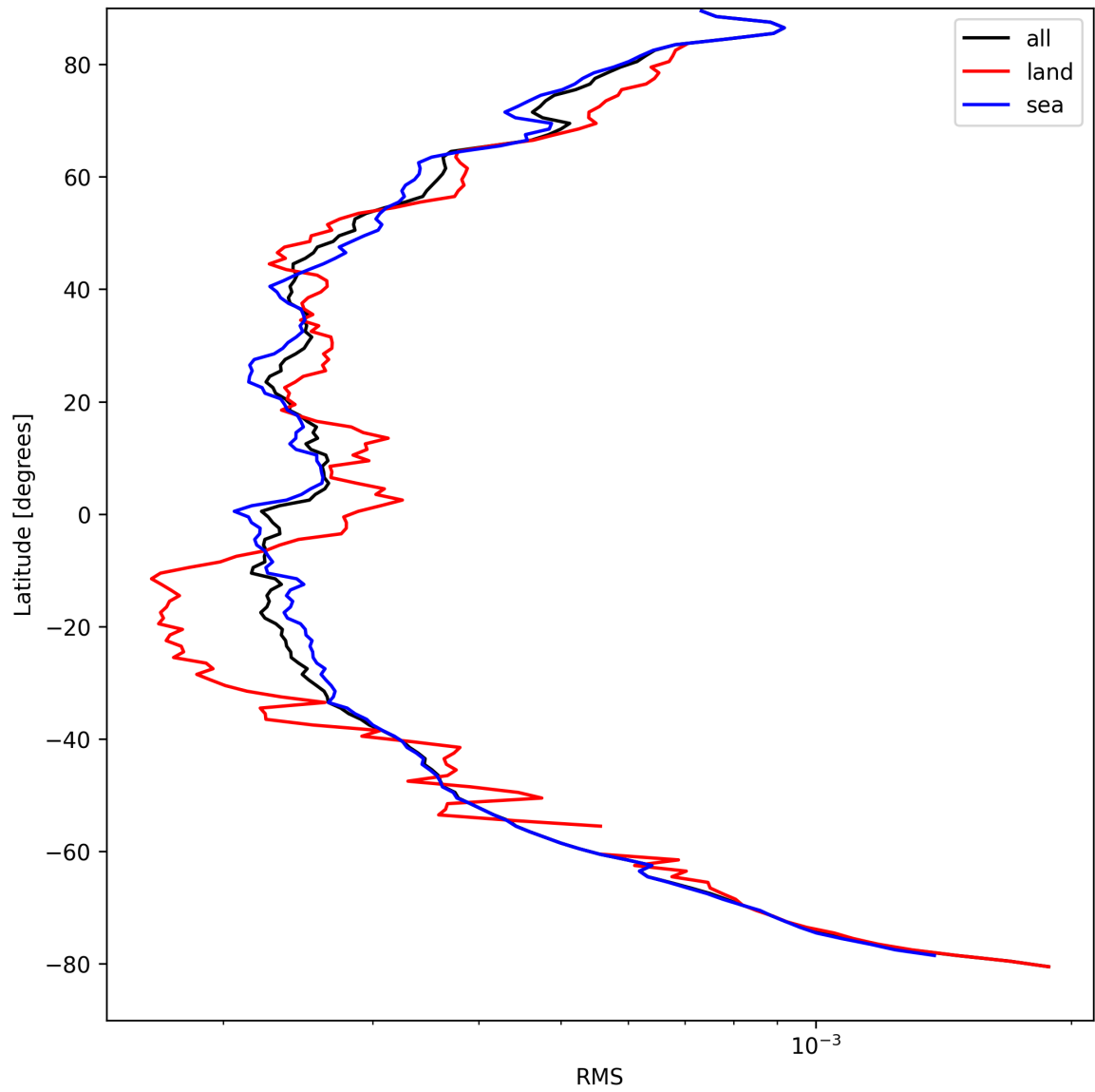
Figure 26: Zonal average of “RMS” for 2024-09-02 to 2024-09-04.
