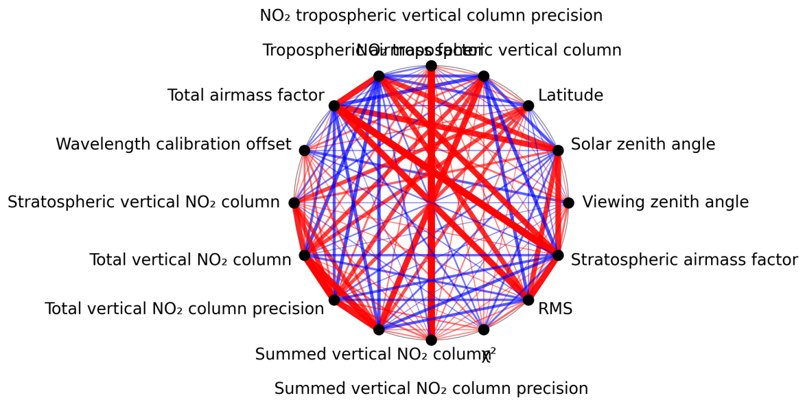
Figure 1: Map of correlation graph for 2024-09-02 to 2024-09-04.
