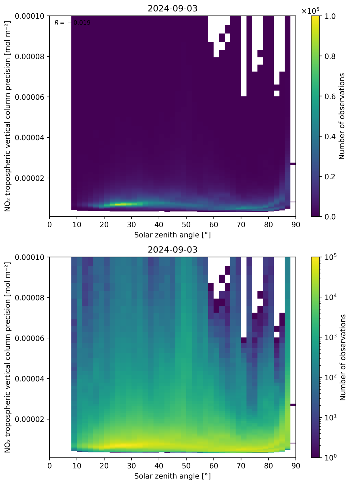
Figure 156: Scatter density plot of “Solar zenith angle” against “NO 2 tropospheric vertical column precision” for 2024-09-02 to 2024-09-04.
