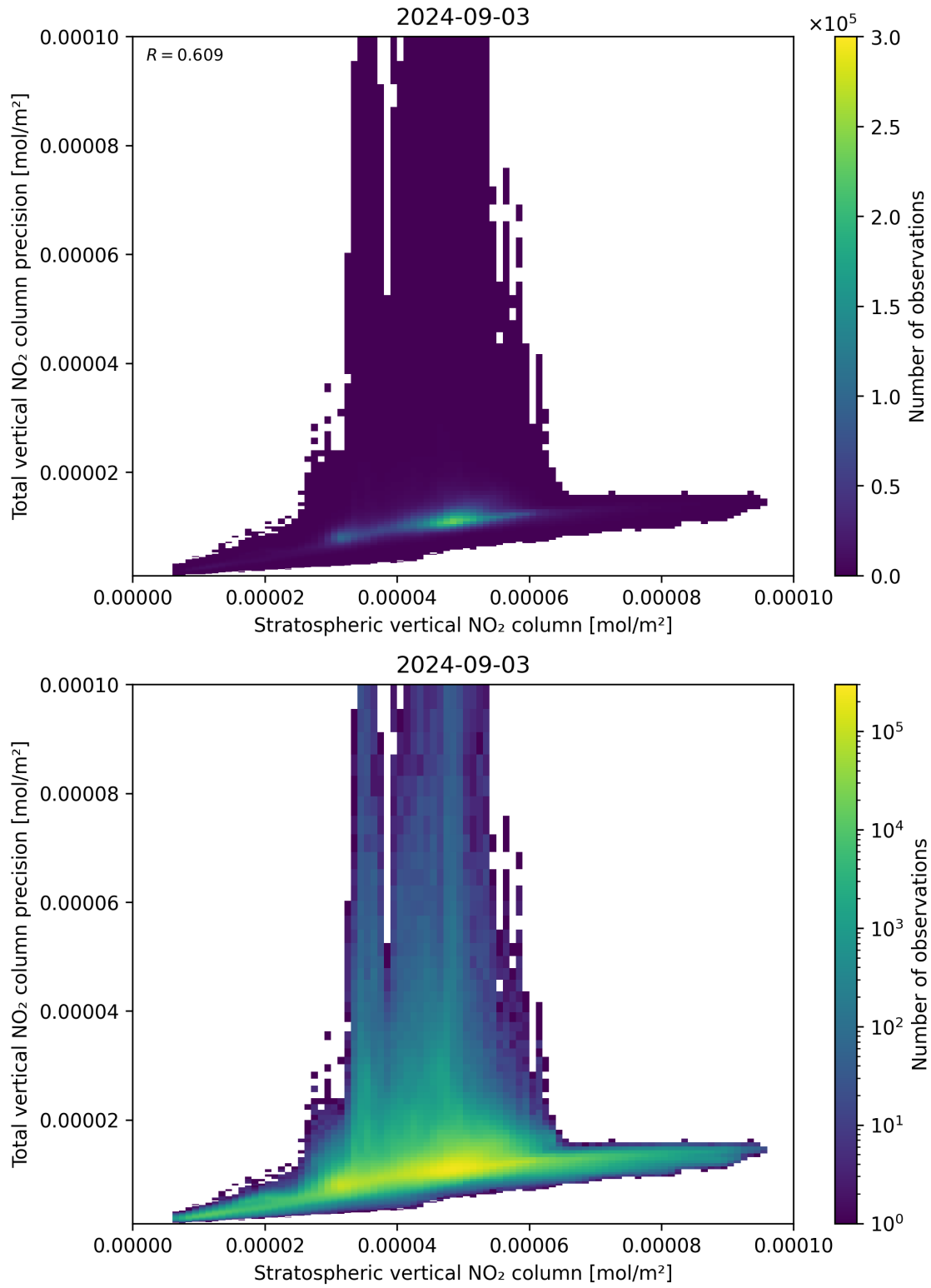
Figure 101: Scatter density plot of “Stratospheric vertical NO 2 column” against “Total vertical NO 2 column precision” for 2024-09-02 to 2024-09-04.
