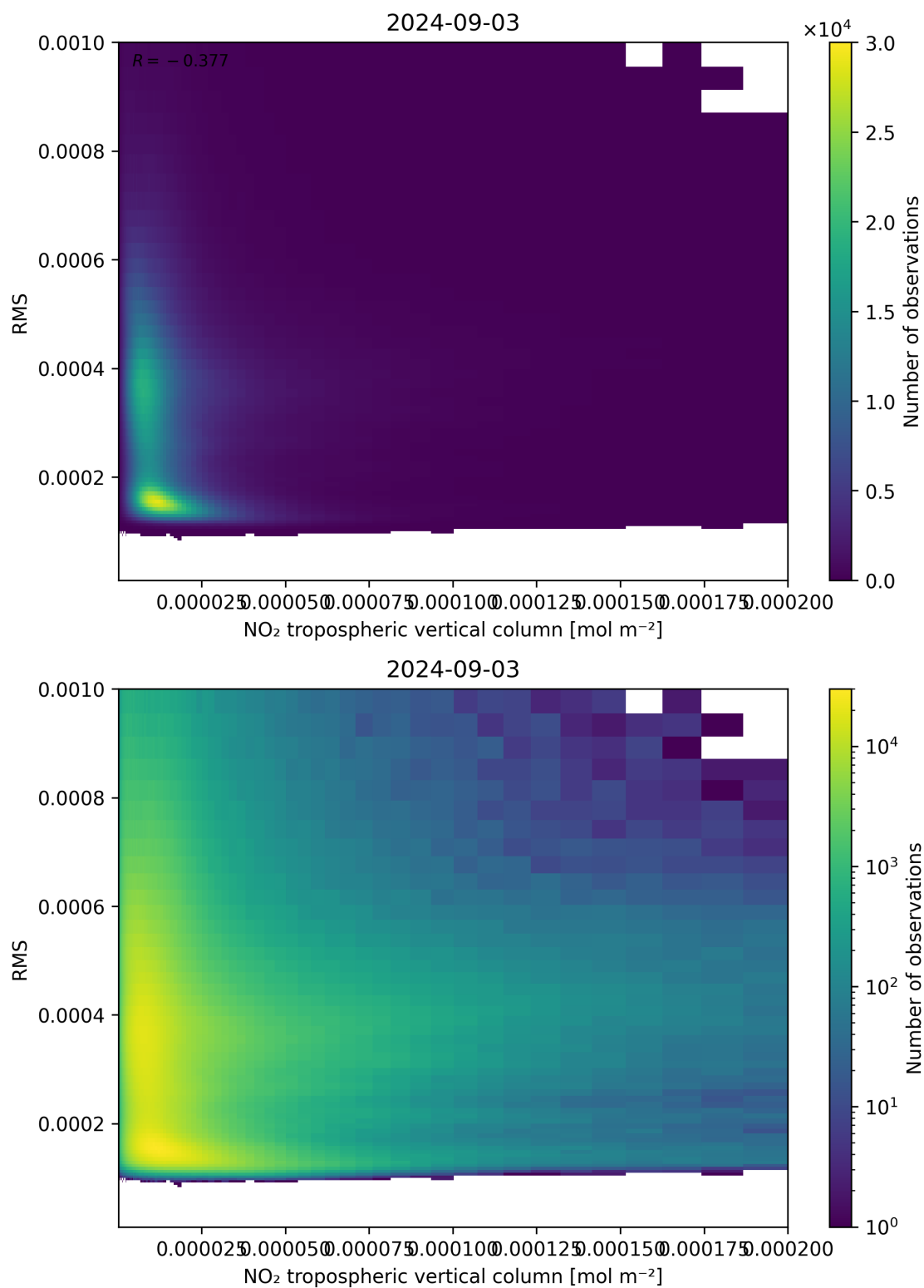
Figure 142: Scatter density plot of “NO 2 tropospheric vertical column” against “RMS” for 2024-09-02 to 2024-09-04.
