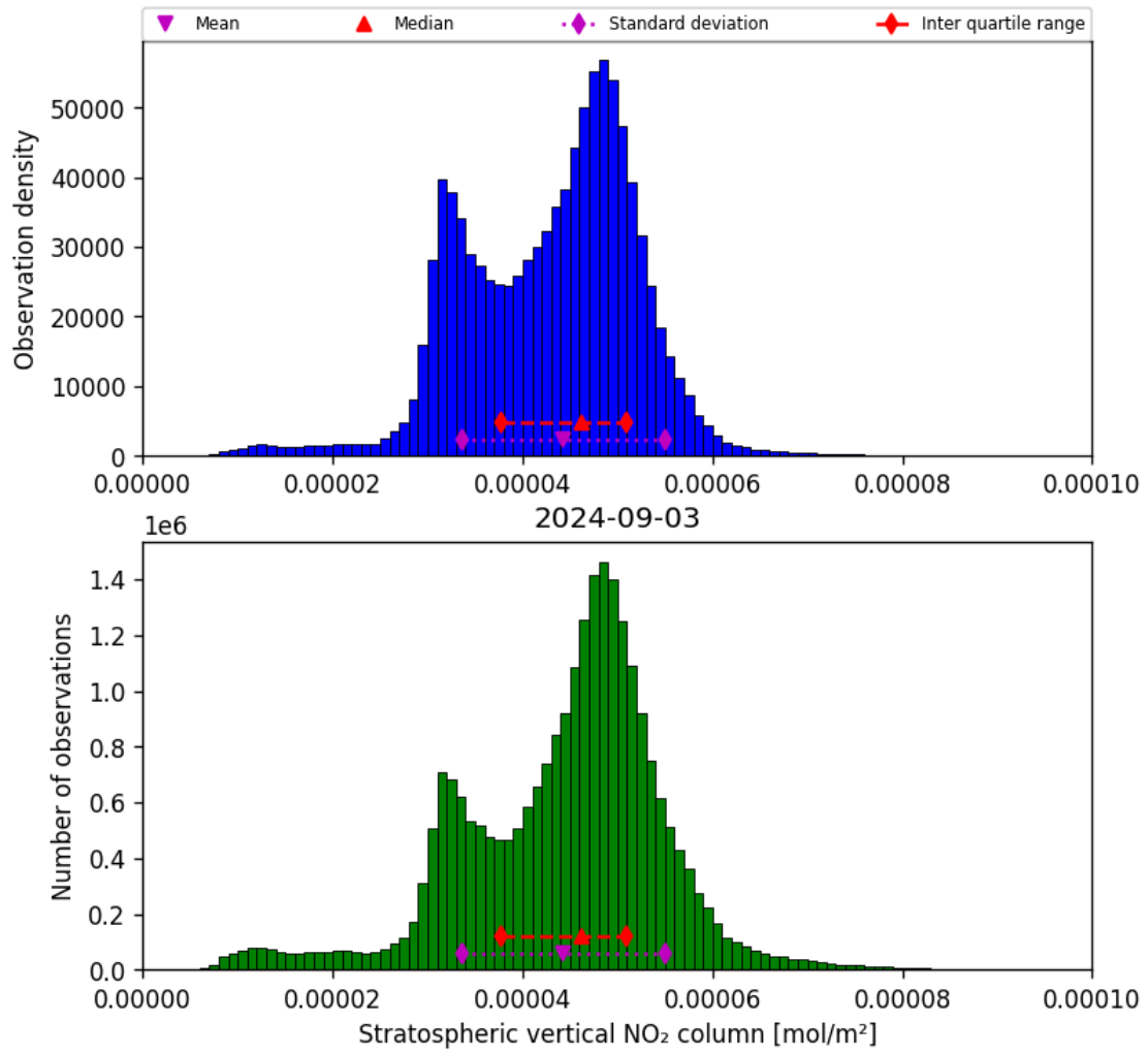
Figure 36: Histogram of “Stratospheric vertical NO 2 column” for 2024-09-02 to 2024-09-04
