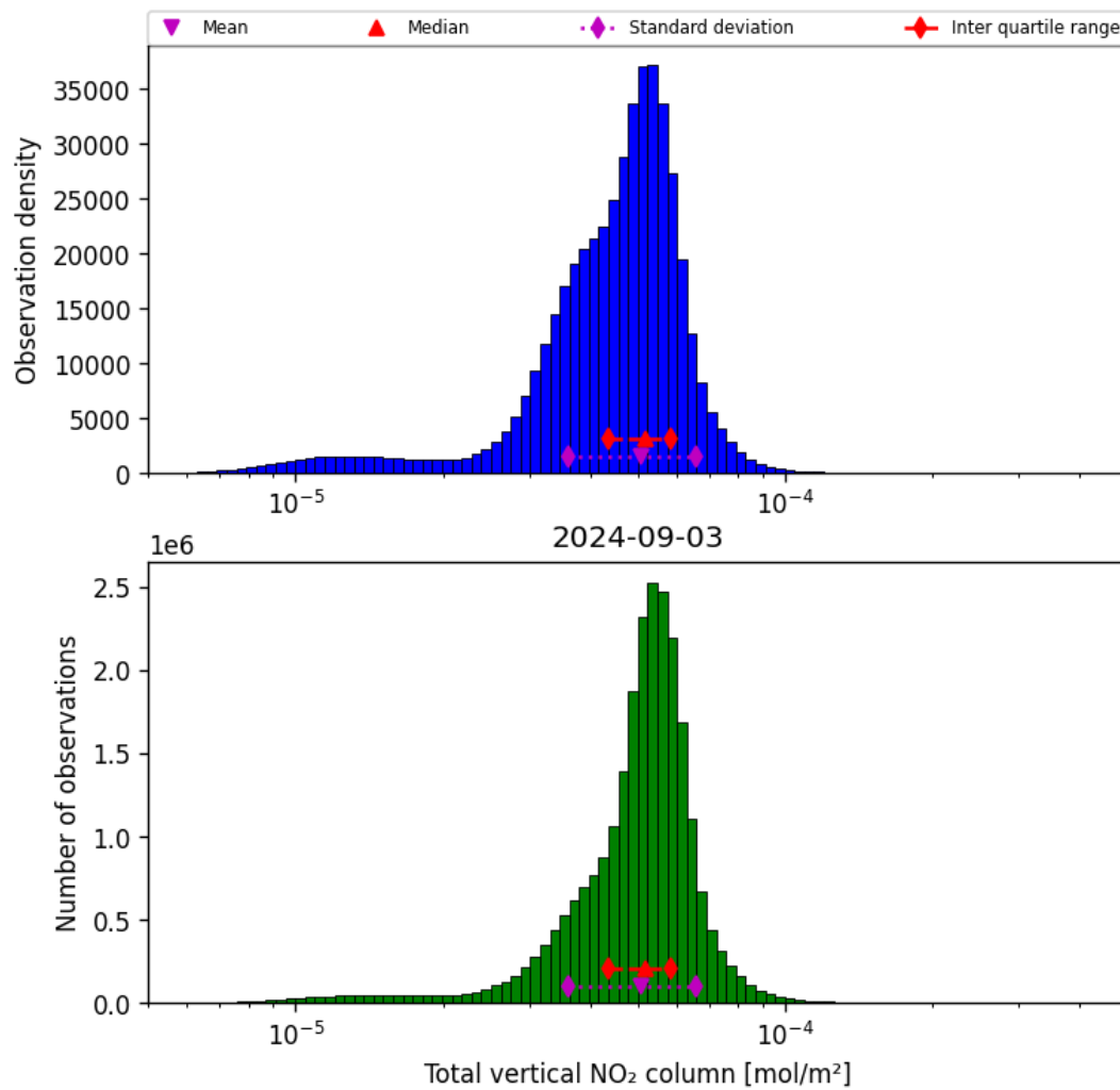
Figure 38: Histogram of “Total vertical NO 2 column” for 2024-09-02 to 2024-09-04
