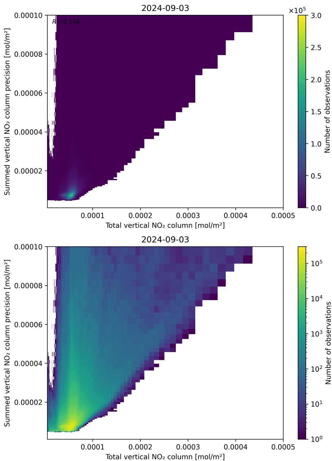
Figure 113: Scatter density plot of “Total vertical NO 2 column” against “Summed vertical NO 2 column precision” for 2024-09-02 to 2024-09-04.
