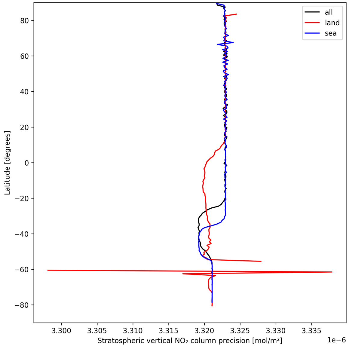
Figure 20: Zonal average of “Stratospheric vertical NO 2 column precision” for 2024-09-02 to 2024-09-04.
