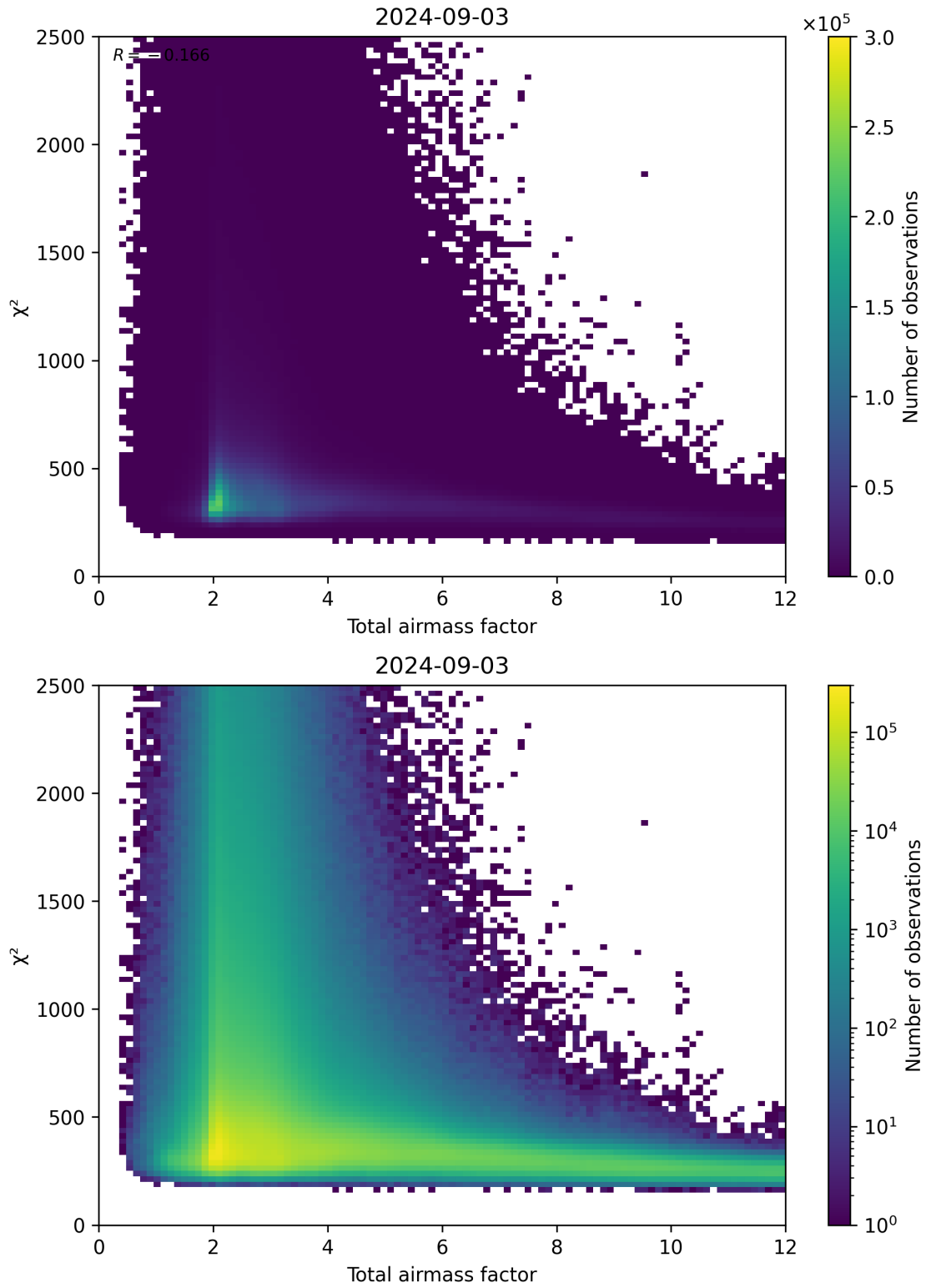
Figure 63: Scatter density plot of “Total airmass factor” against “ \chi^2 ” for 2024-09-02 to 2024-09-04.
