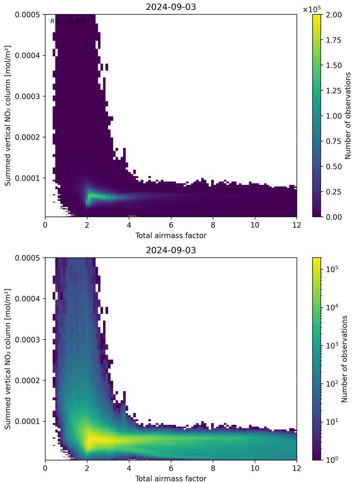
Figure 65: Scatter density plot of “Total airmass factor” against “Summed vertical NO 2 column” for 2024-09-02 to 2024-09-04.
