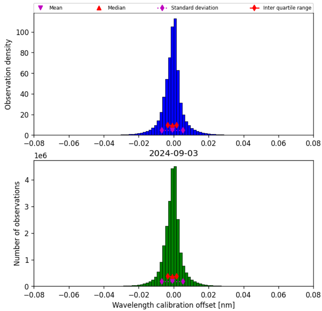
Figure 35: Histogram of “Wavelength calibration offset” for 2024-09-02 to 2024-09-04
