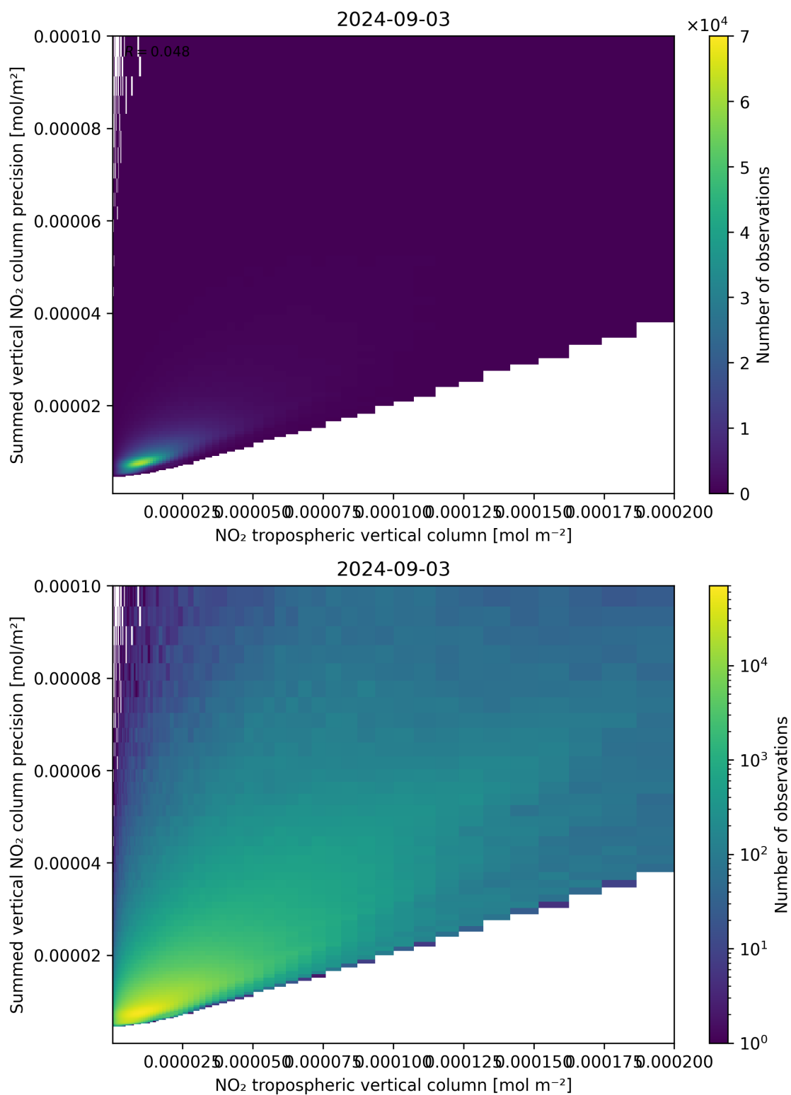
Figure 127: Scatter density plot of “NO 2 tropospheric vertical column” against “Summed vertical NO 2 column precision” for 2024-09-02 to 2024-09-04.
