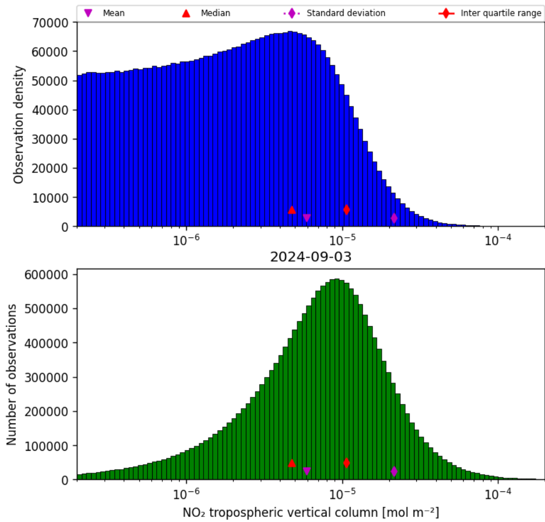
Figure 29: Histogram of “NO 2 tropospheric vertical column” for 2024-09-02 to 2024-09-04
