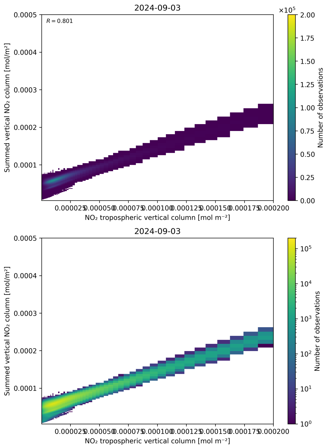
Figure 126: Scatter density plot of “NO 2 tropospheric vertical column” against “Summed vertical NO 2 column” for 2024-09-02 to 2024-09-04.
