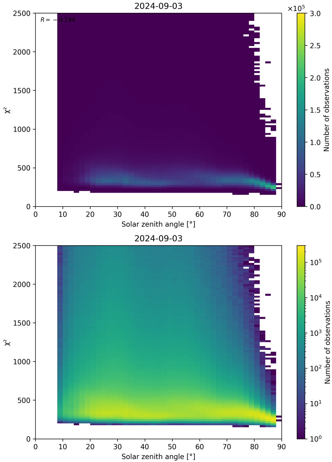
Figure 148: Scatter density plot of “Solar zenith angle” against “ \chi^2 ” for 2024-09-02 to 2024-09-04.
