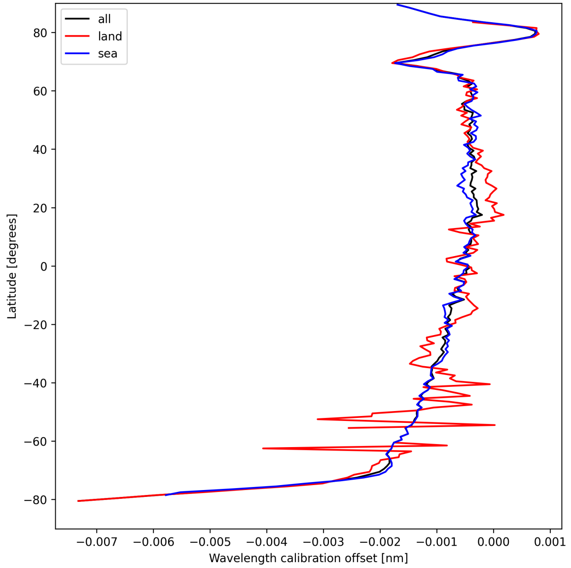
Figure 18: Zonal average of “Wavelength calibration offset” for 2024-09-02 to 2024-09-04.
