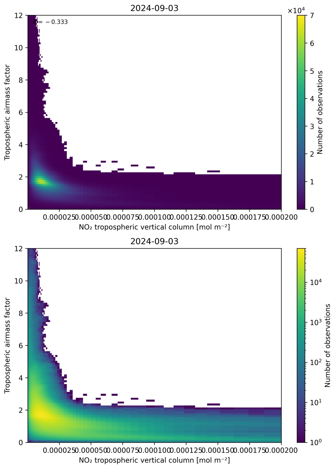
Figure 123: Scatter density plot of “NO 2 tropospheric vertical column” against “Tropospheric air mass factor” for 2024-09-02 to 2024-09-04.
