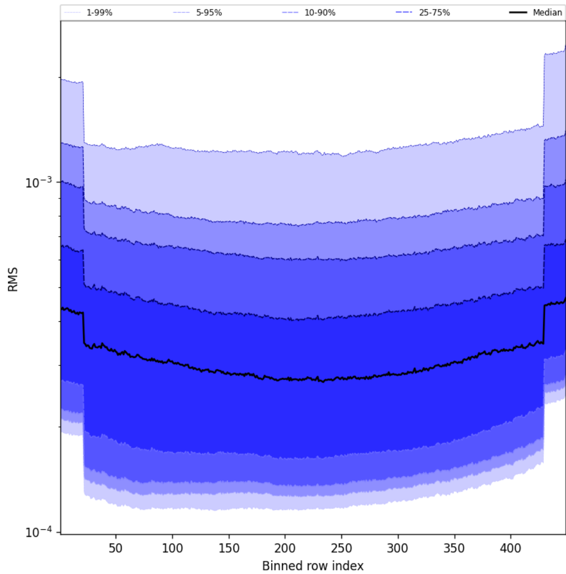
Figure 60: Along track statistics of “RMS” for 2024-09-02 to 2024-09-04
