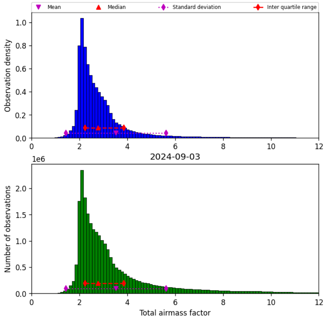
Figure 32: Histogram of “Total airmass factor” for 2024-09-02 to 2024-09-04
