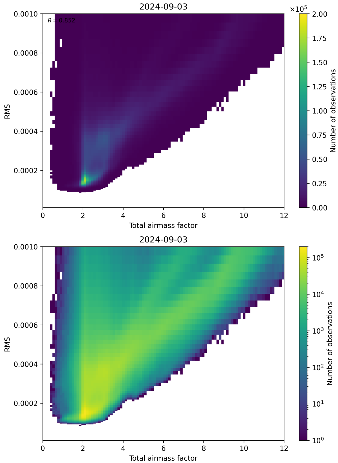
Figure 69: Scatter density plot of “Total airmass factor” against “RMS” for 2024-09-02 to 2024-09-04.
