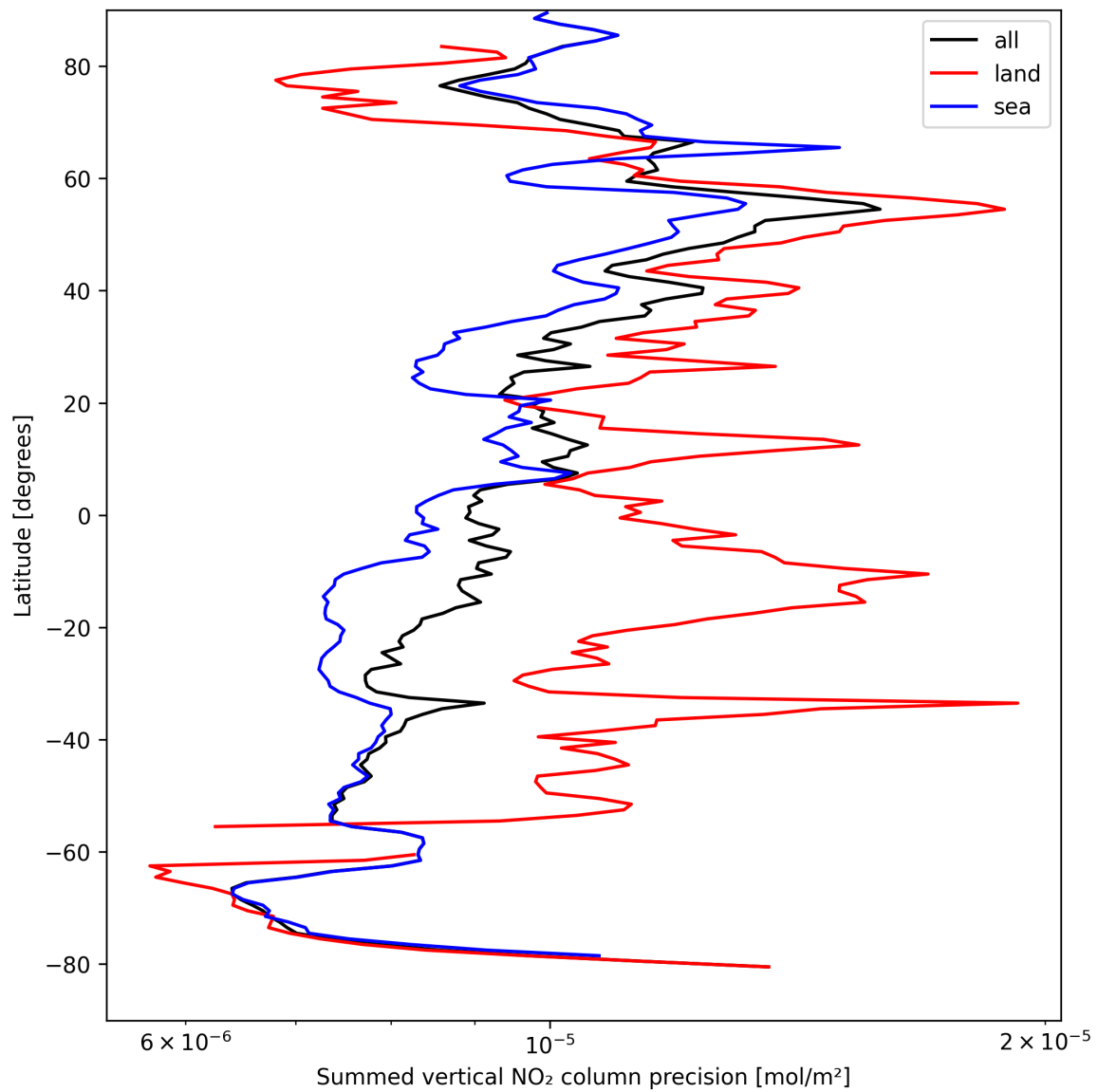
Figure 24: Zonal average of “Summed vertical NO 2 column precision” for 2024-09-02 to 2024-09-04.
