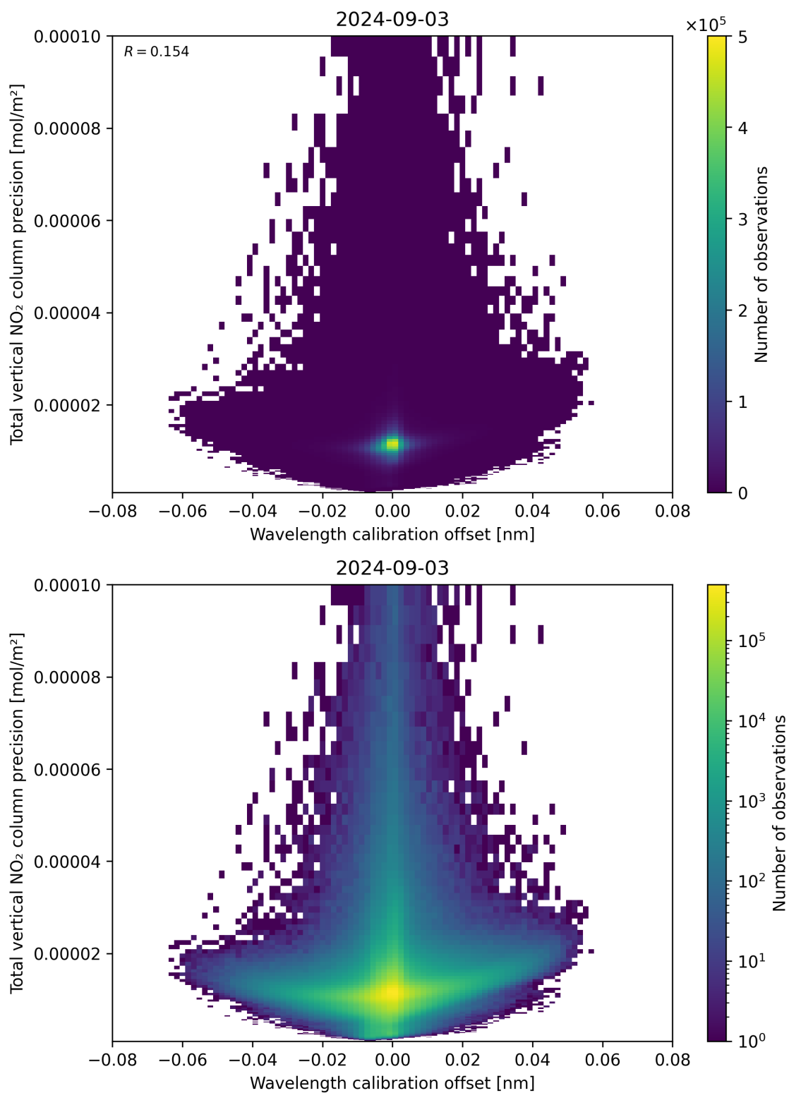
Figure 180: Scatter density plot of “Wavelength calibration offset” against “Total vertical NO 2 column precision” for 2024-09-02 to 2024-09-04.
