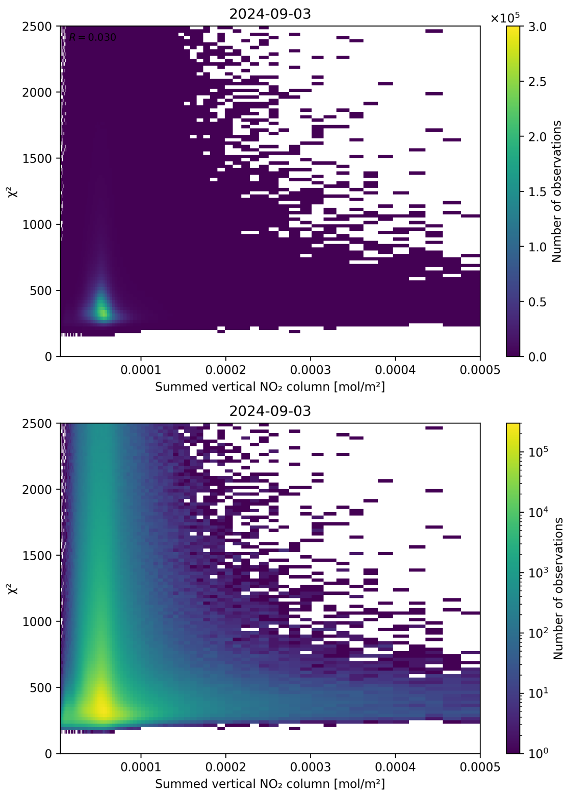
Figure 104: Scatter density plot of “Summed vertical NO 2 column” against “ \chi^2 ” for 2024-09-02 to 2024-09-04.
