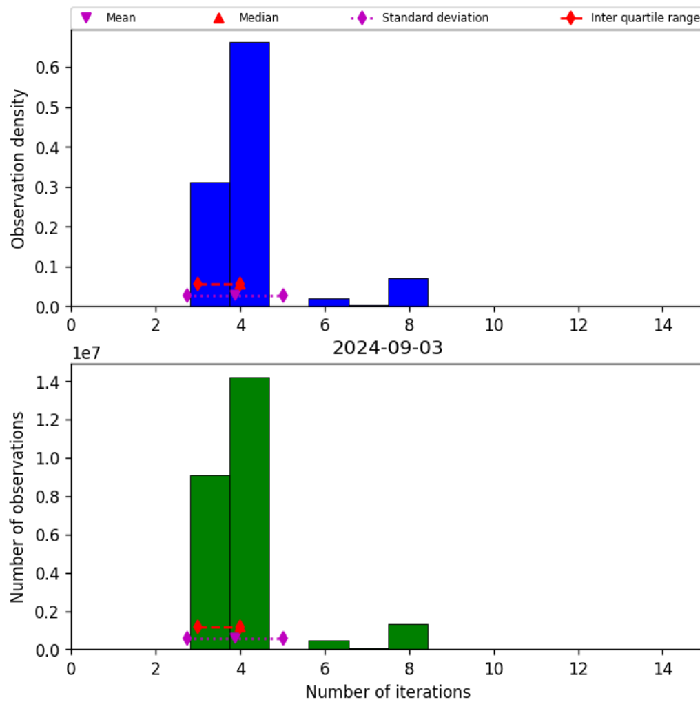
Figure 34: Histogram of “Number of iterations” for 2024-09-02 to 2024-09-04
