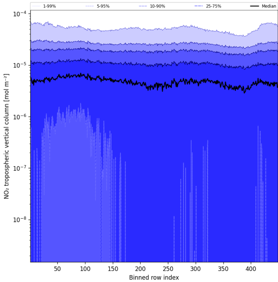
Figure 46: Along track statistics of “NO 2 tropospheric vertical column” for 2024-09-02 to 2024-09-04
