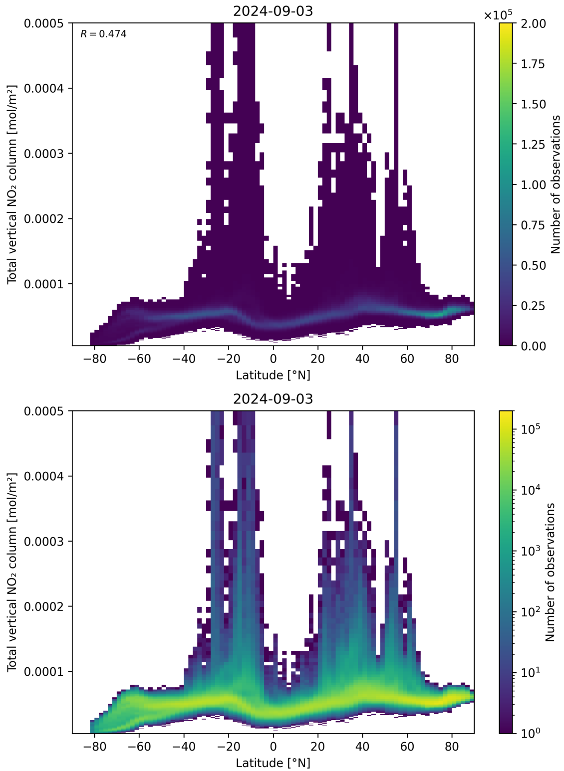
Figure 90: Scatter density plot of “Latitude” against “Total vertical NO 2 column” for 2024-09-02 to 2024-09-04.
