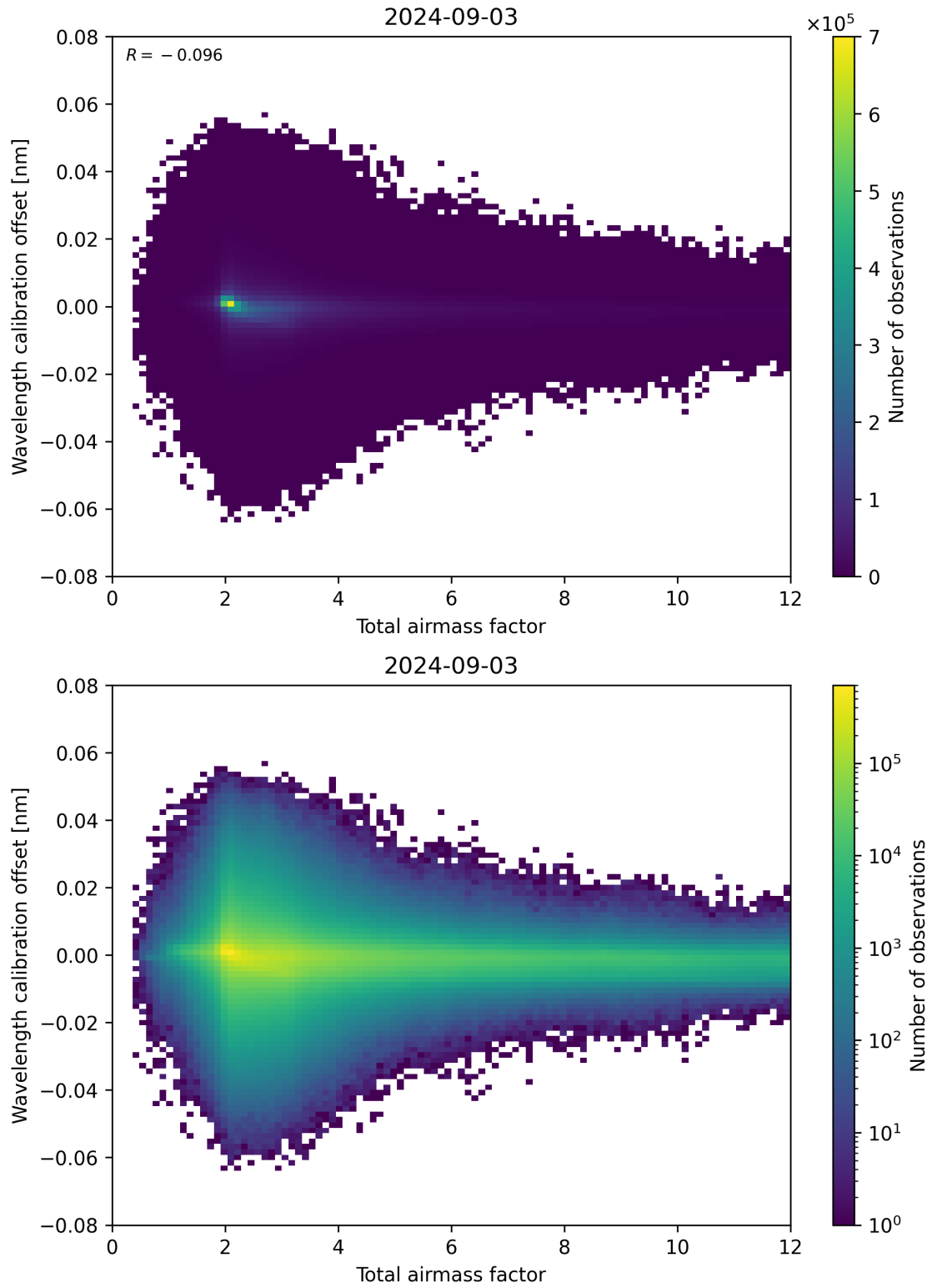
Figure 70: Scatter density plot of “Total airmass factor” against “Wavelength calibration offset” for 2024-09-02 to 2024-09-04.
