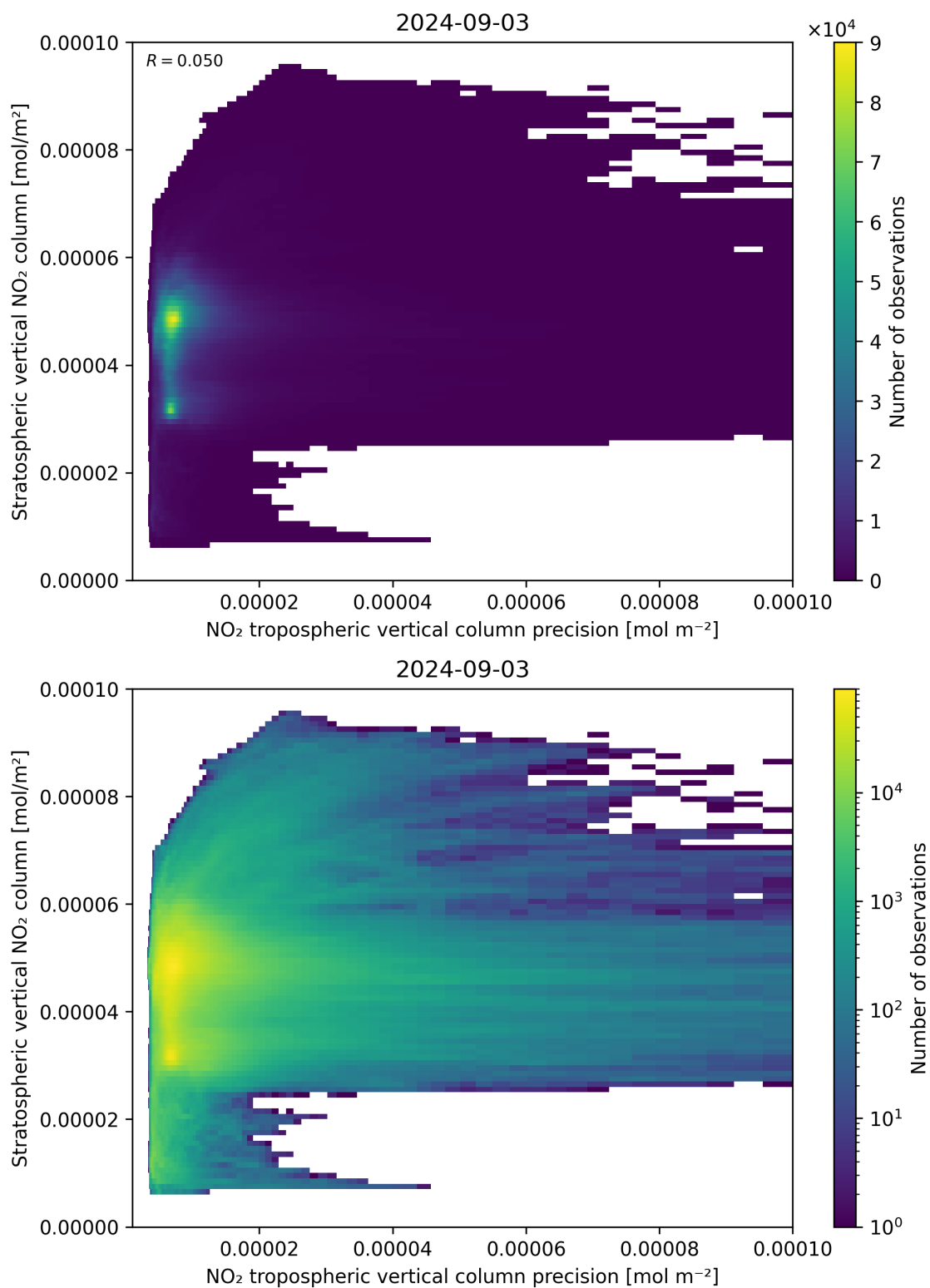
Figure 135: Scatter density plot of “NO 2 tropospheric vertical column precision” against “Stratospheric vertical NO 2 column” for 2024-09-02 to 2024-09-04.
