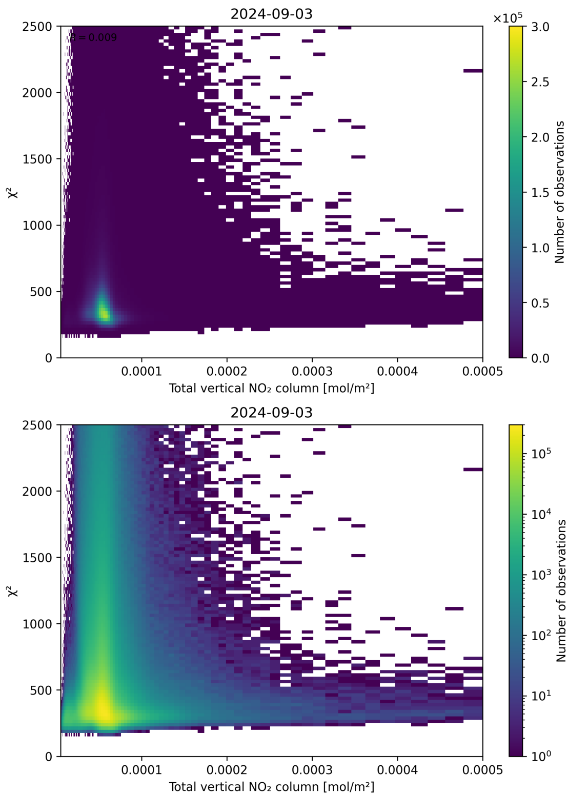
Figure 111: Scatter density plot of “Total vertical NO 2 column” against “ \chi^2 ” for 2024-09-02 to 2024-09-04.
