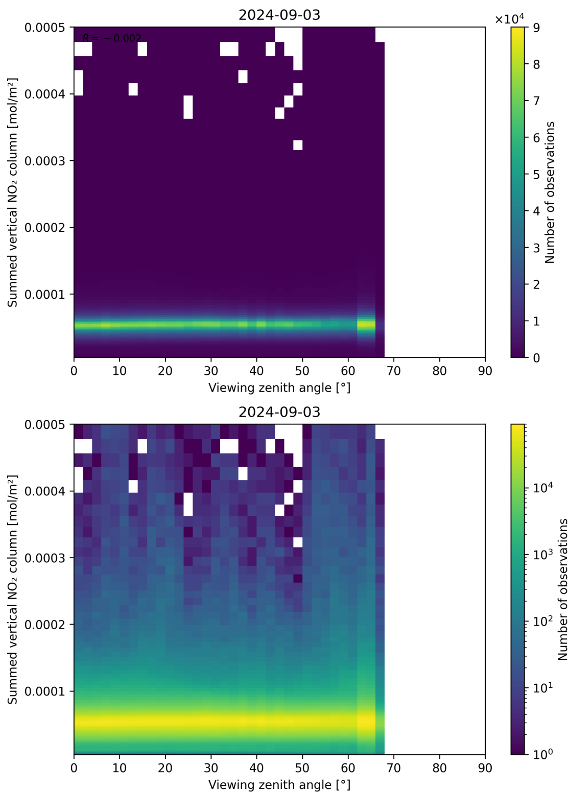
Figure 165: Scatter density plot of “Viewing zenith angle” against “Summed vertical NO 2 column” for 2024-09-02 to 2024-09-04.
