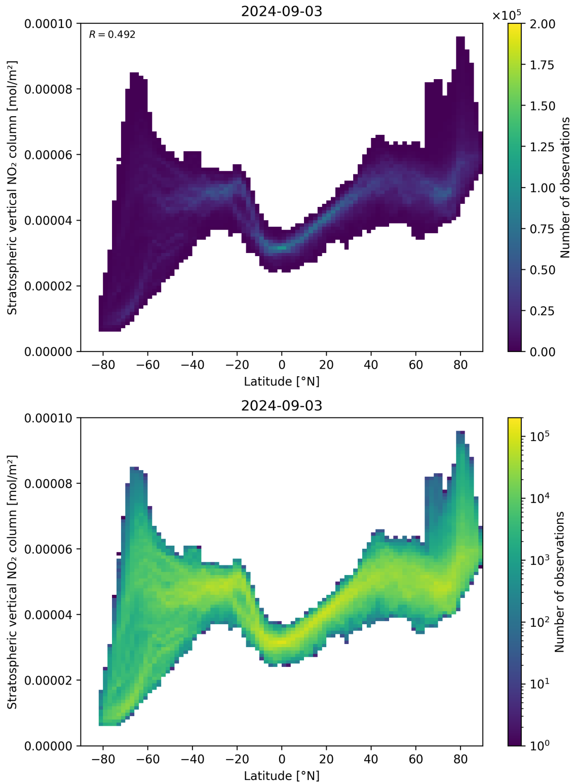
Figure 87: Scatter density plot of “Latitude” against “Stratospheric vertical NO 2 column” for 2024-09-02 to 2024-09-04.
