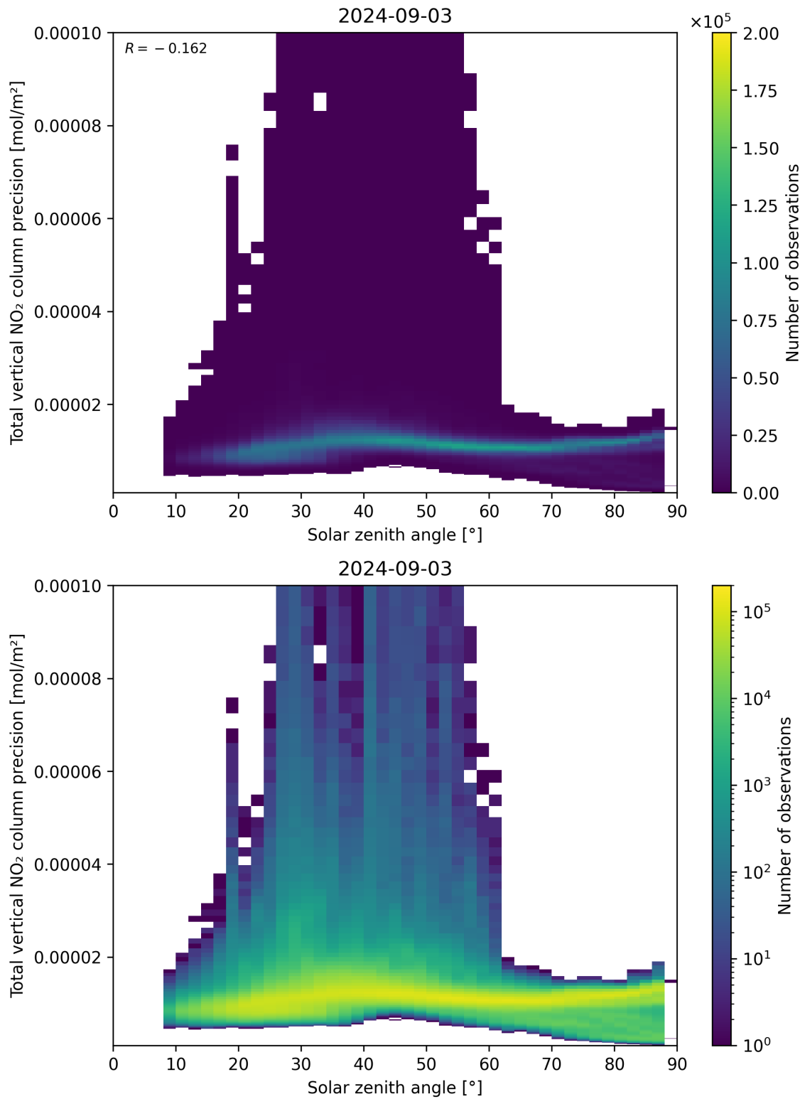
Figure 154: Scatter density plot of “Solar zenith angle” against “Total vertical NO 2 column precision” for 2024-09-02 to 2024-09-04.
