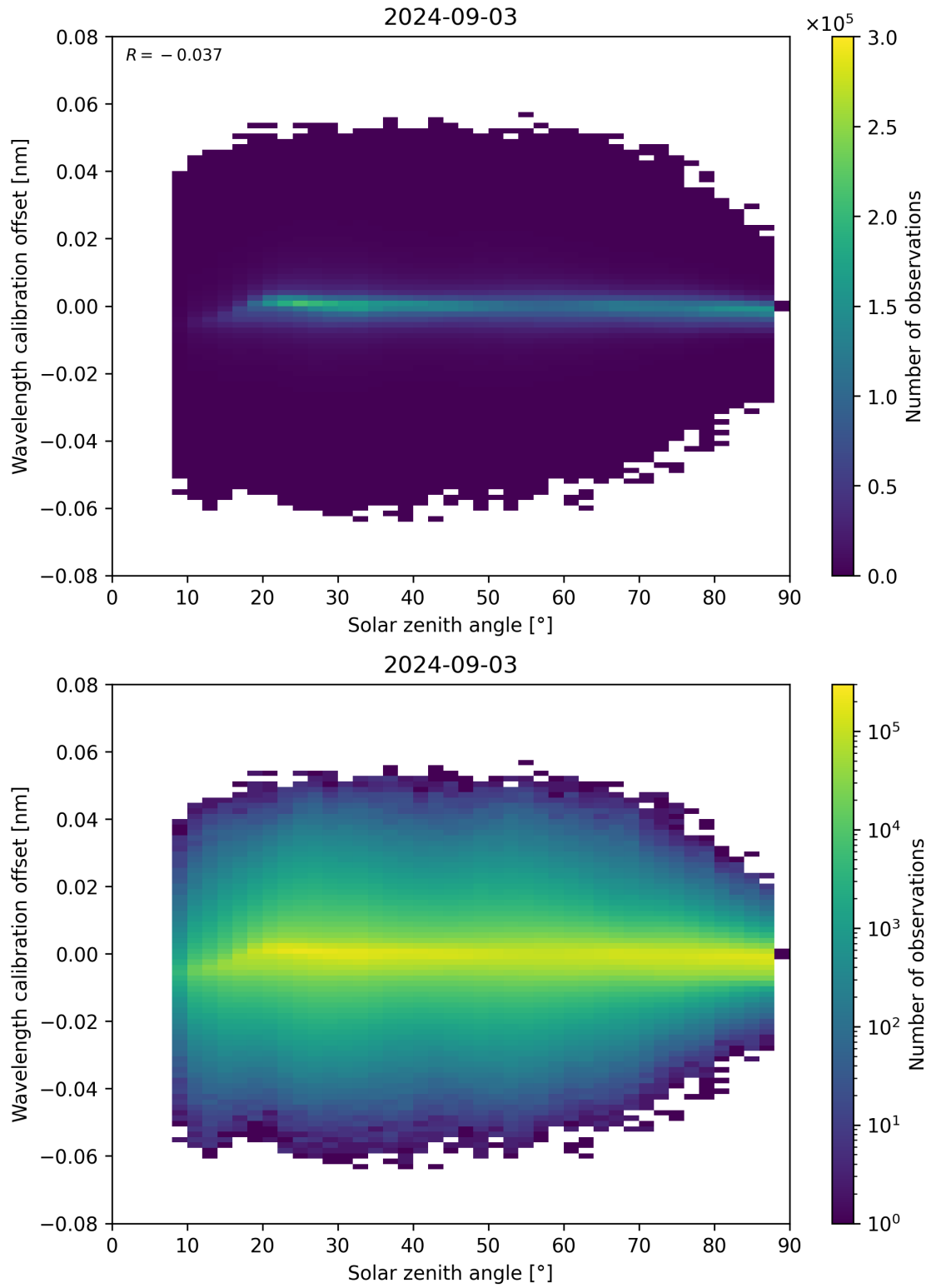
Figure 158: Scatter density plot of “Solar zenith angle” against “Wavelength calibration offset” for 2024-09-02 to 2024-09-04.
