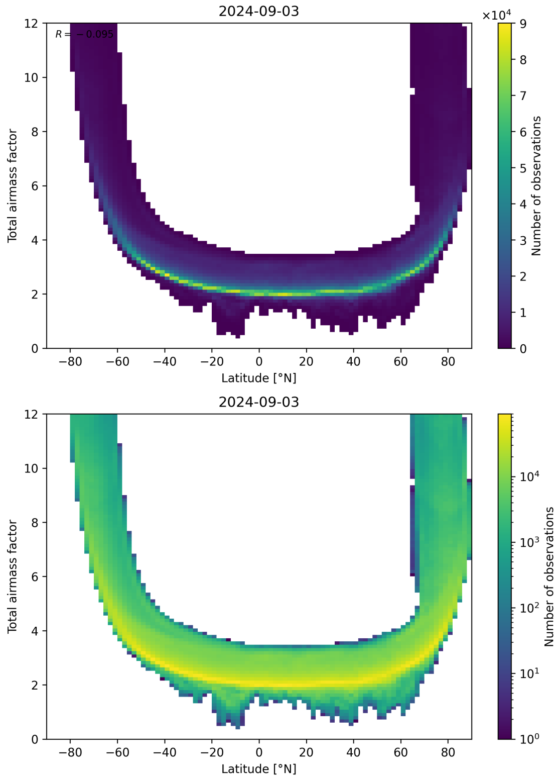
Figure 84: Scatter density plot of “Latitude” against “Total airmass factor” for 2024-09-02 to 2024-09-04.
