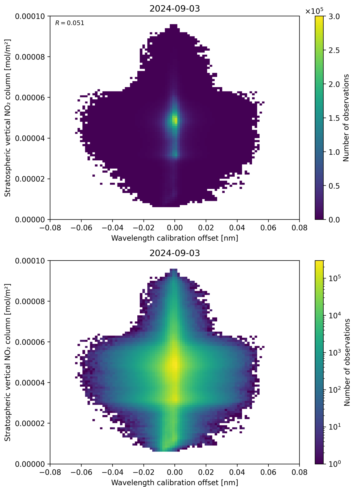
Figure 176: Scatter density plot of “Wavelength calibration offset” against “Stratospheric vertical NO 2 column” for 2024-09-02 to 2024-09-04.
