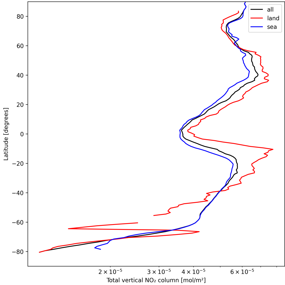
Figure 21: Zonal average of “Total vertical NO 2 column” for 2024-09-02 to 2024-09-04.
