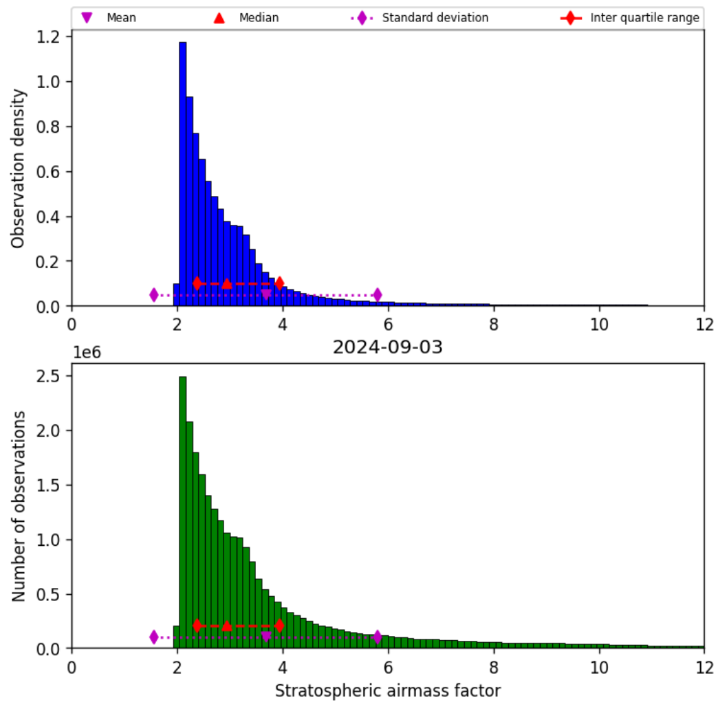
Figure 44: Histogram of “Stratospheric airmass factor” for 2024-09-02 to 2024-09-04
