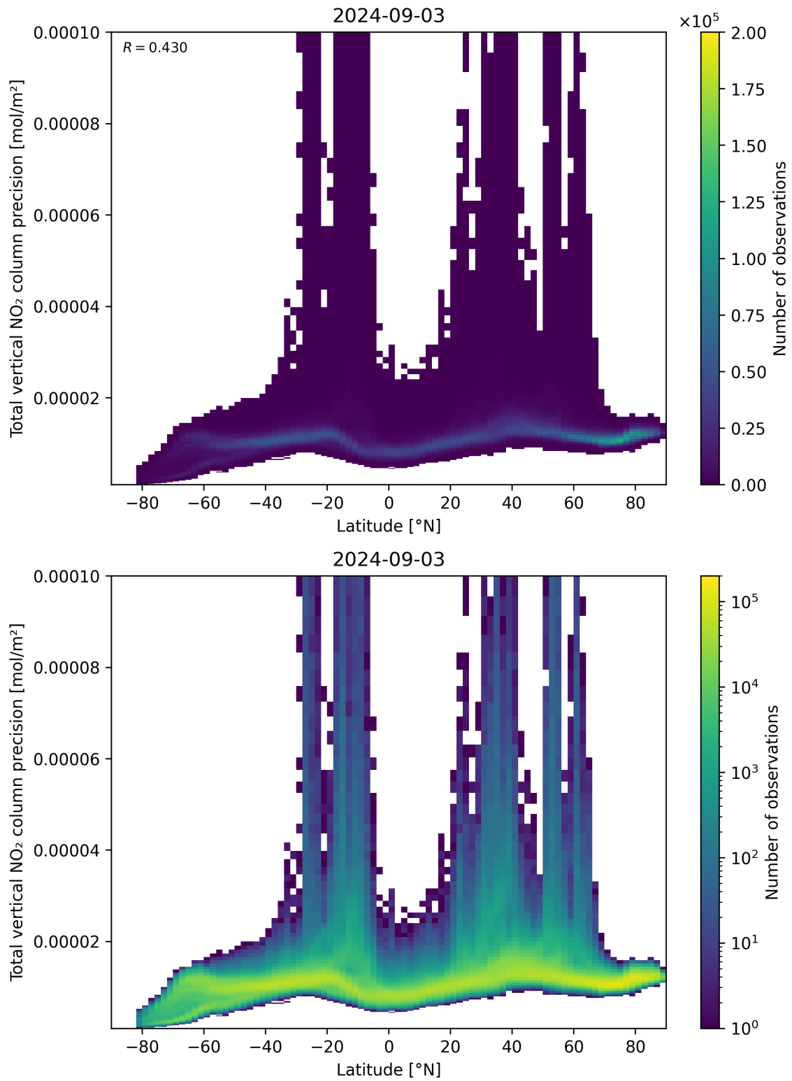
Figure 91: Scatter density plot of “Latitude” against “Total vertical NO 2 column precision” for 2024-09-02 to 2024-09-04.
