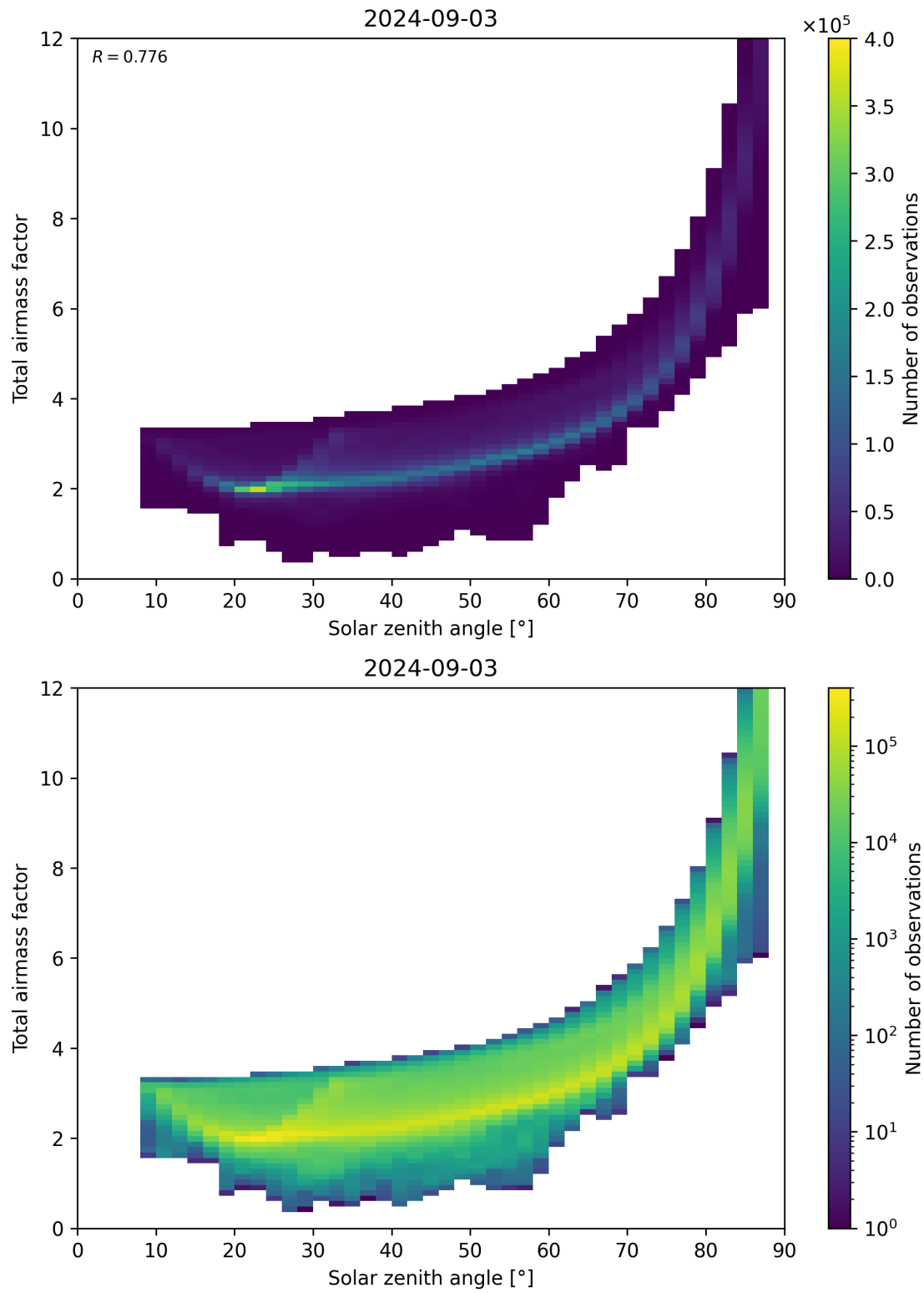
Figure 146: Scatter density plot of “Solar zenith angle” against “Total air mass factor” for 2024-09-02 to 2024-09-04.
