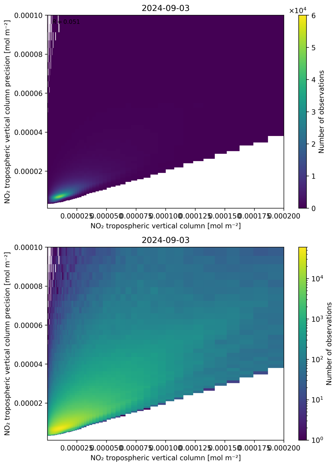
Figure 130: Scatter density plot of “NO 2 tropospheric vertical column” against “NO 2 tropospheric vertical column precision” for 2024-09-02 to 2024-09-04.
