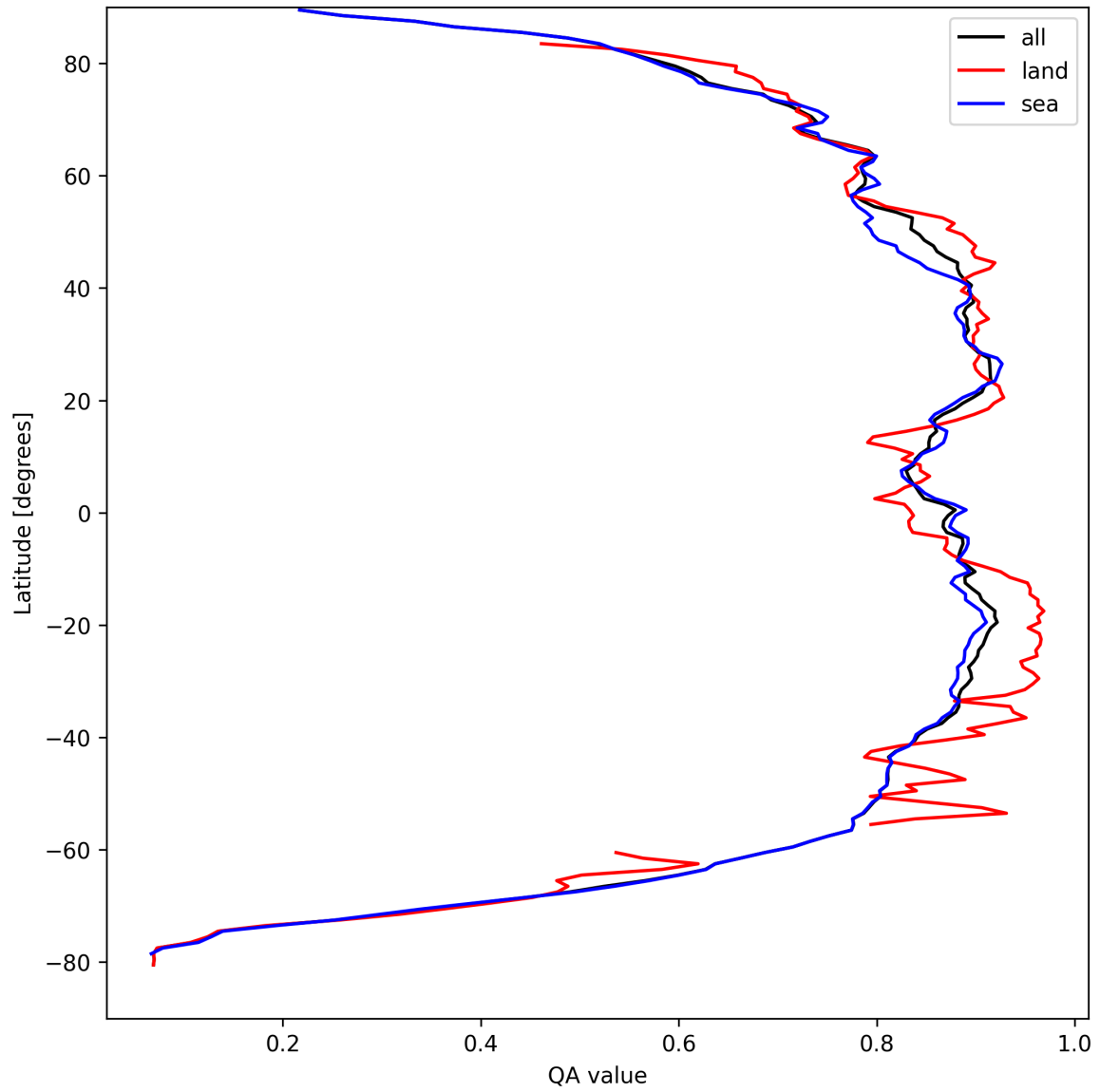
Figure 11: Zonal average of “QA value” for 2024-09-02 to 2024-09-04.
