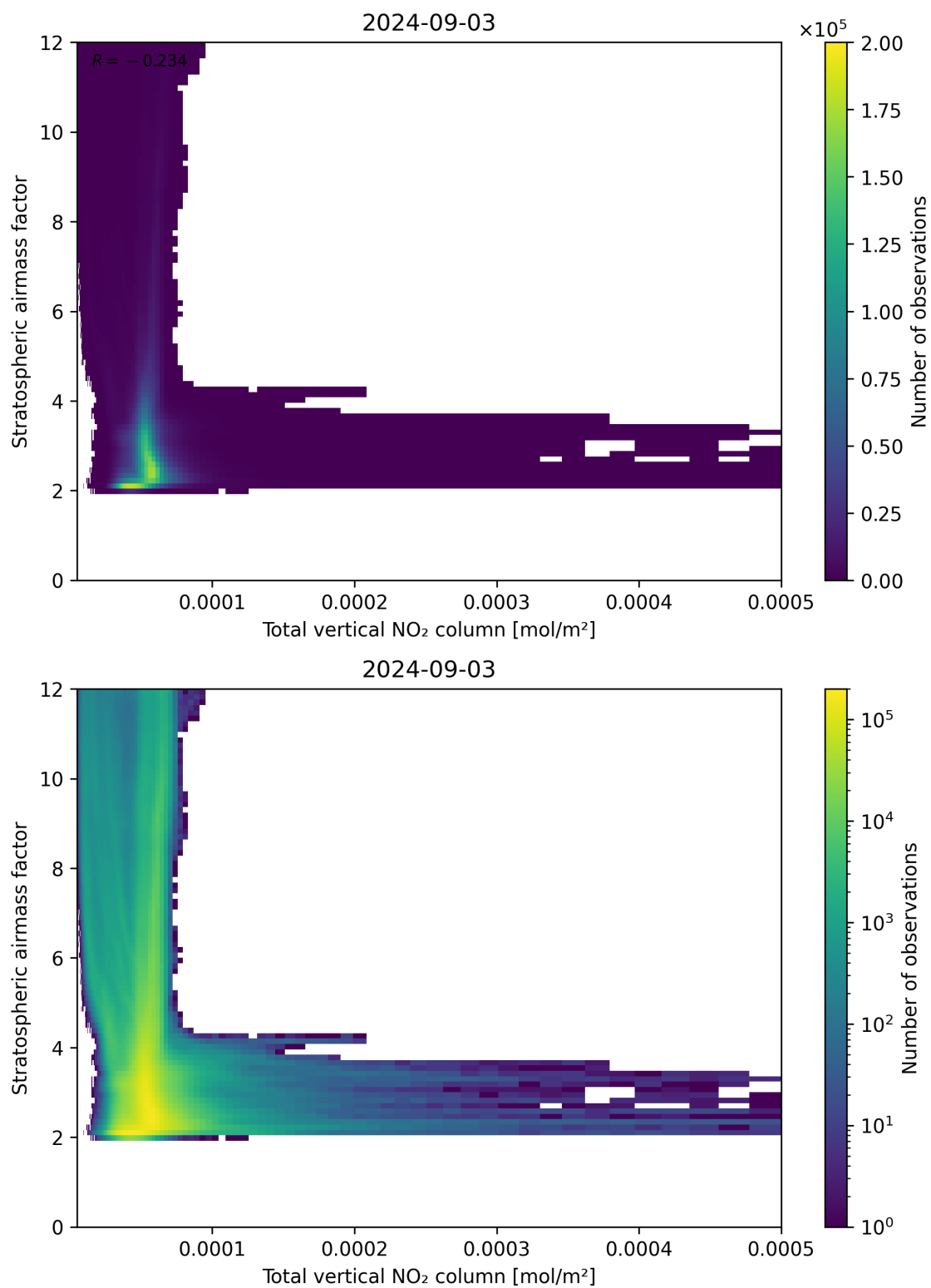
Figure 110: Scatter density plot of “Total vertical NO 2 column” against “Stratospheric airmass factor” for 2024-09-02 to 2024-09-04.
