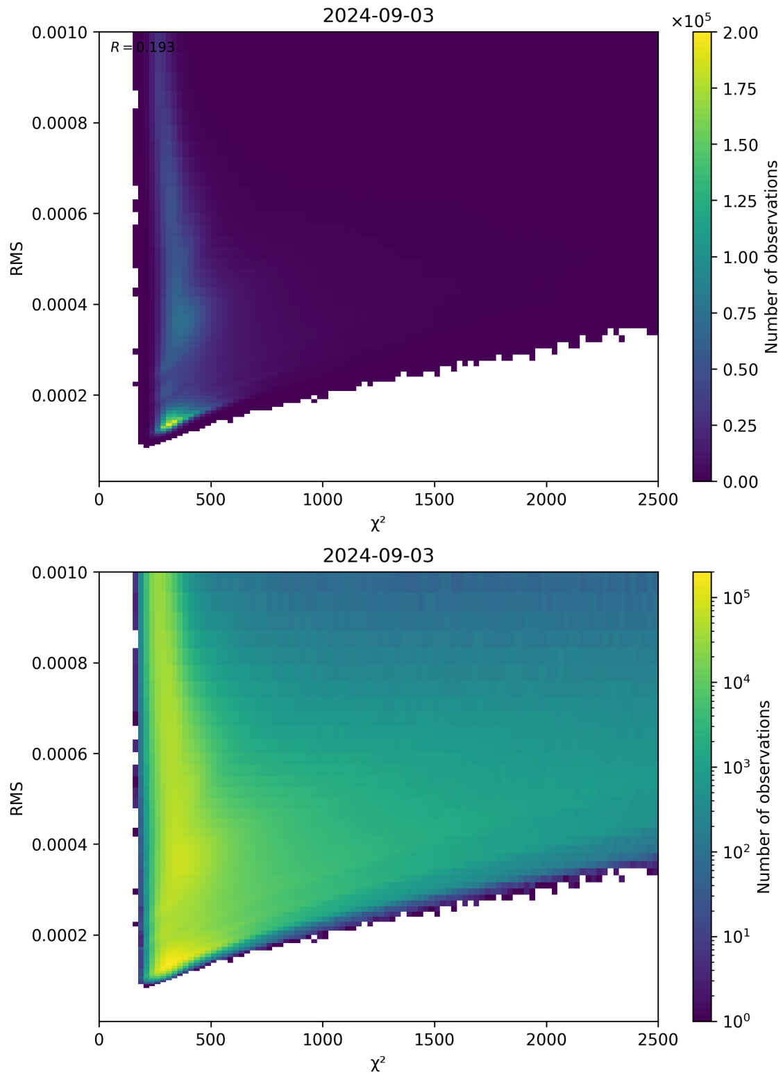
Figure 82: Scatter density plot of “ \chi^2 ” against “RMS” for 2024-09-02 to 2024-09-04.
