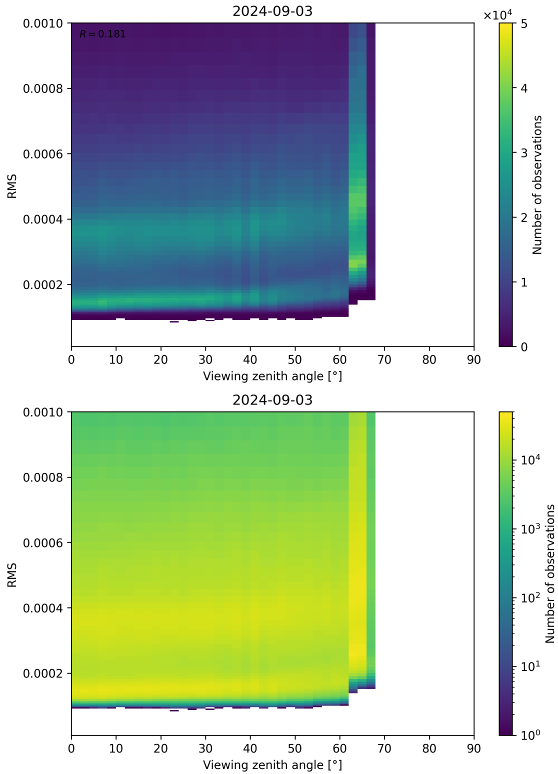
Figure 171: Scatter density plot of “Viewing zenith angle” against “RMS” for 2024-09-02 to 2024-09-04.
