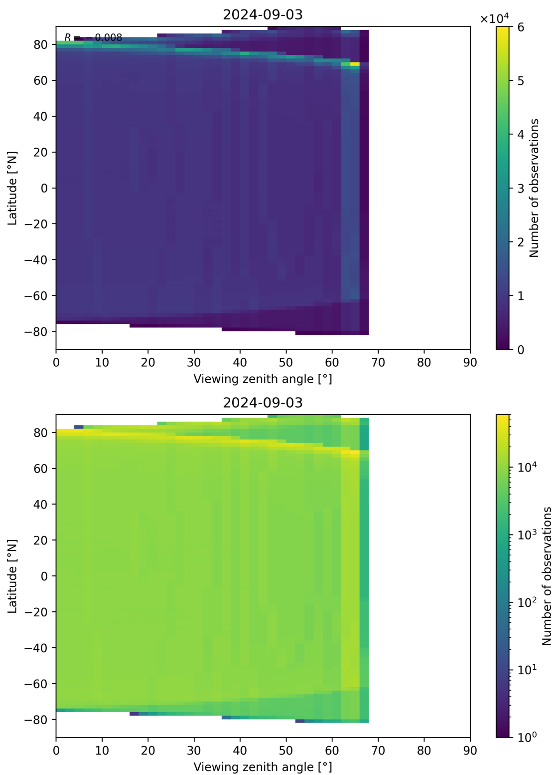
Figure 163: Scatter density plot of “Viewing zenith angle” against “Latitude” for 2024-09-02 to 2024-09-04.
