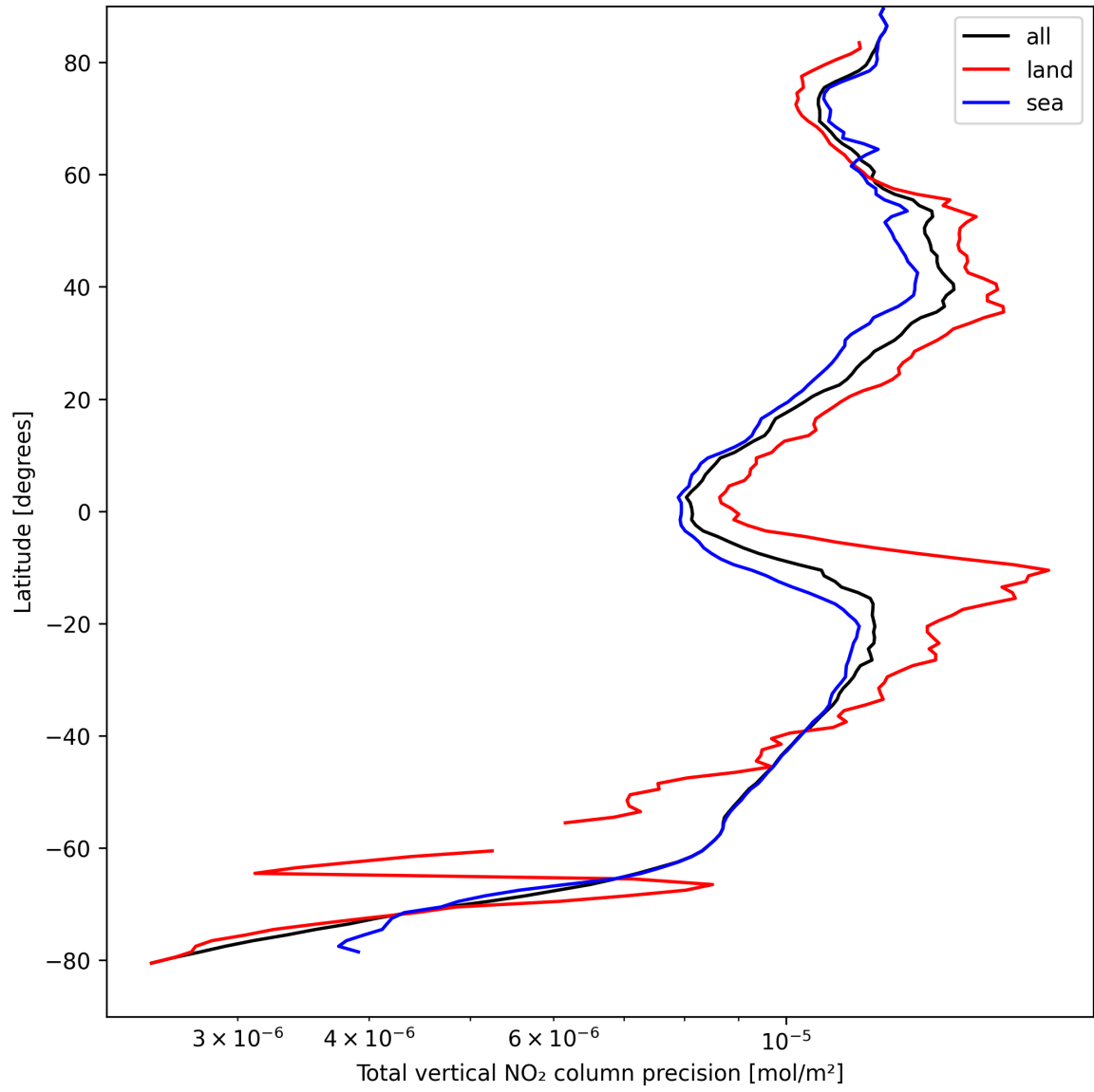
Figure 22: Zonal average of “Total vertical NO 2 column precision” for 2024-09-02 to 2024-09-04.
