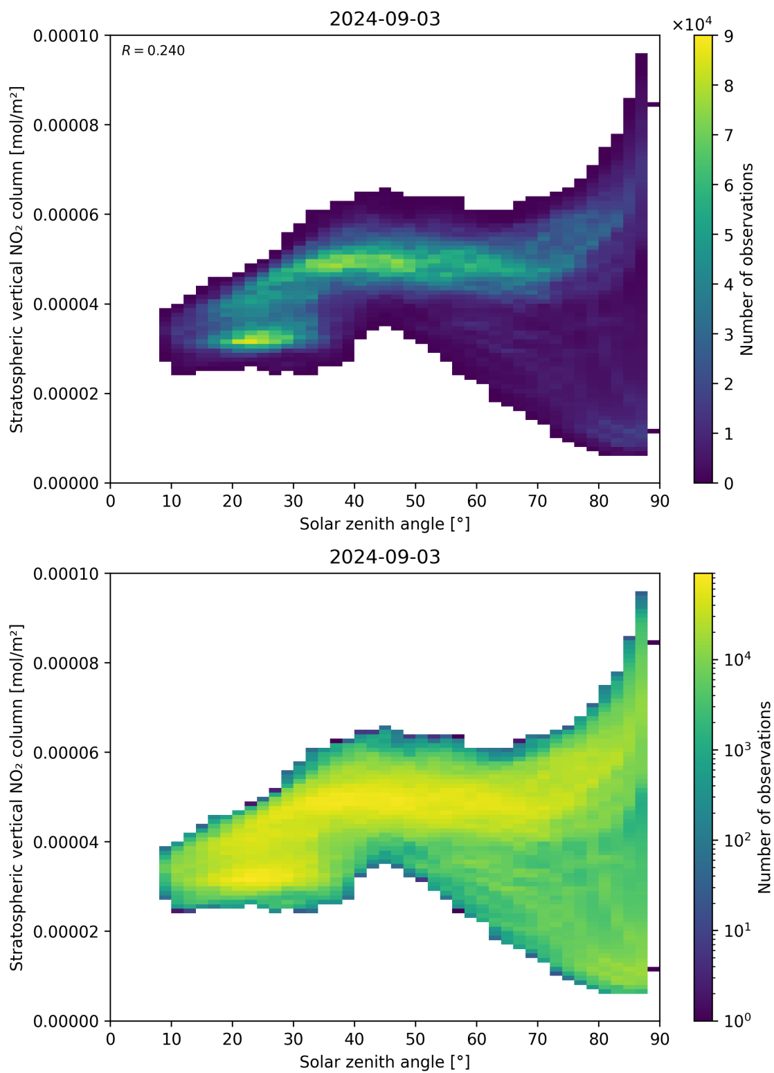
Figure 150: Scatter density plot of “Solar zenith angle” against “Stratospheric vertical NO 2 column” for 2024-09-02 to 2024-09-04.
