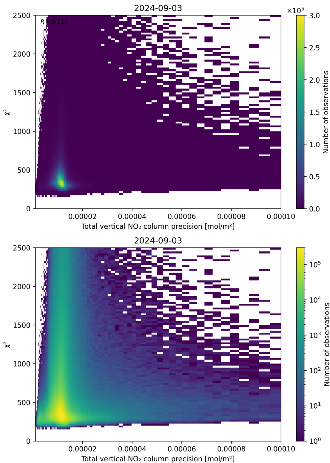
Figure 116: Scatter density plot of “Total vertical NO 2 column precision” against “ \chi^2 ” for 2024-09-02 to 2024-09-04.
