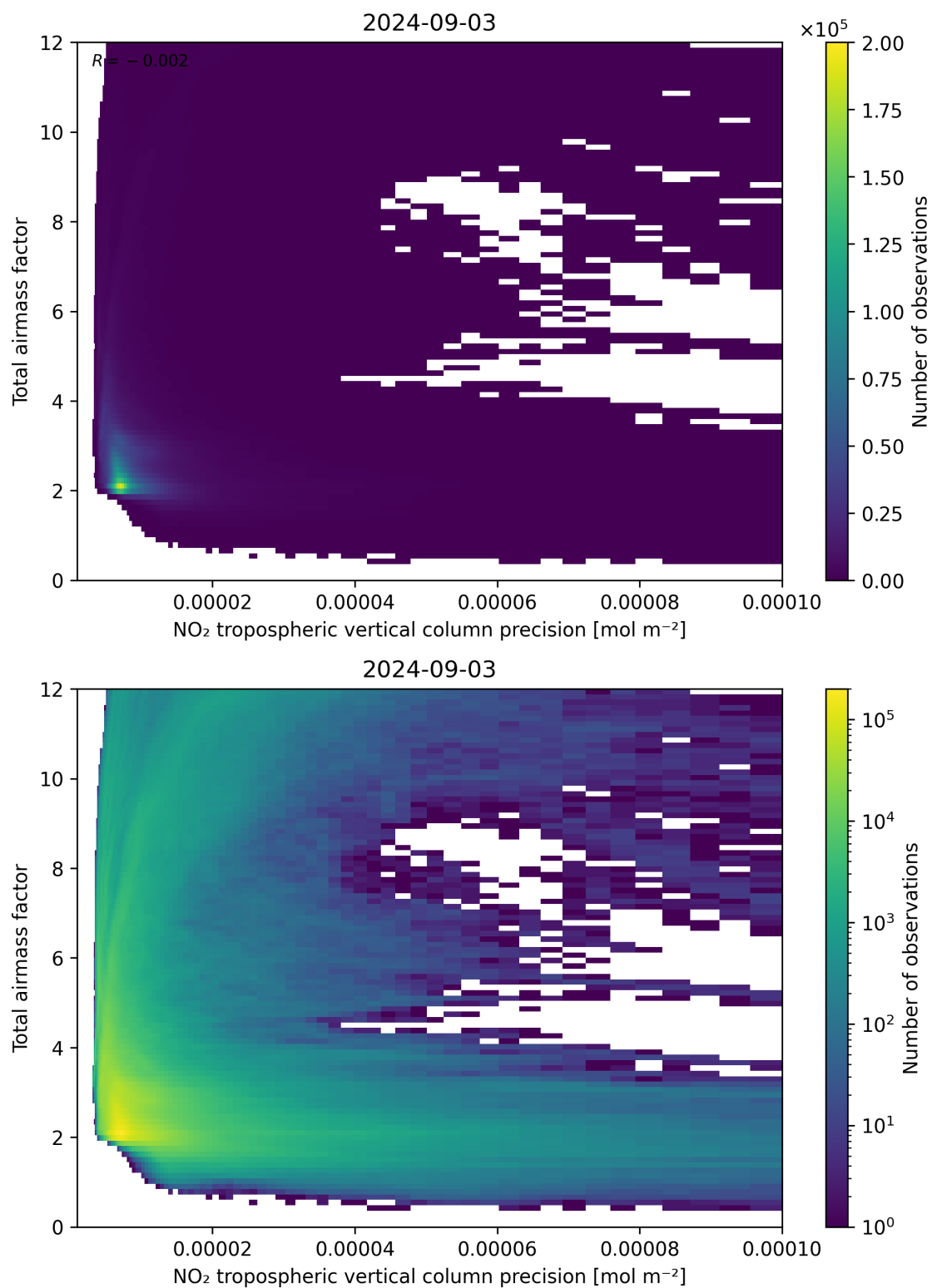
Figure 132: Scatter density plot of “NO 2 tropospheric vertical column precision” against “Total air mass factor” for 2024-09-02 to 2024-09-04.
