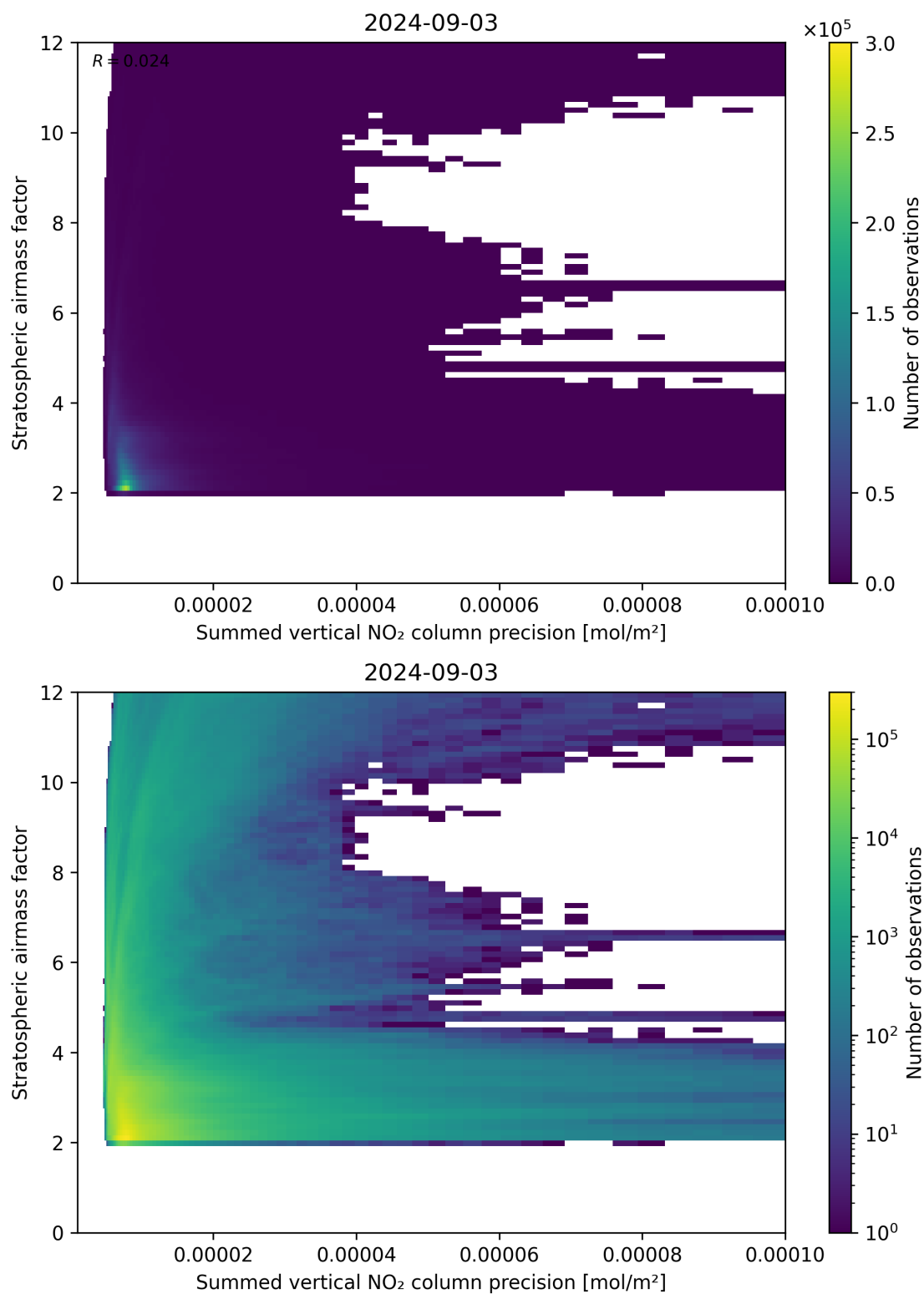
Figure 106: Scatter density plot of “Summed vertical NO 2 column precision” against “Stratospheric airmass factor” for 2024-09-02 to 2024-09-04.
