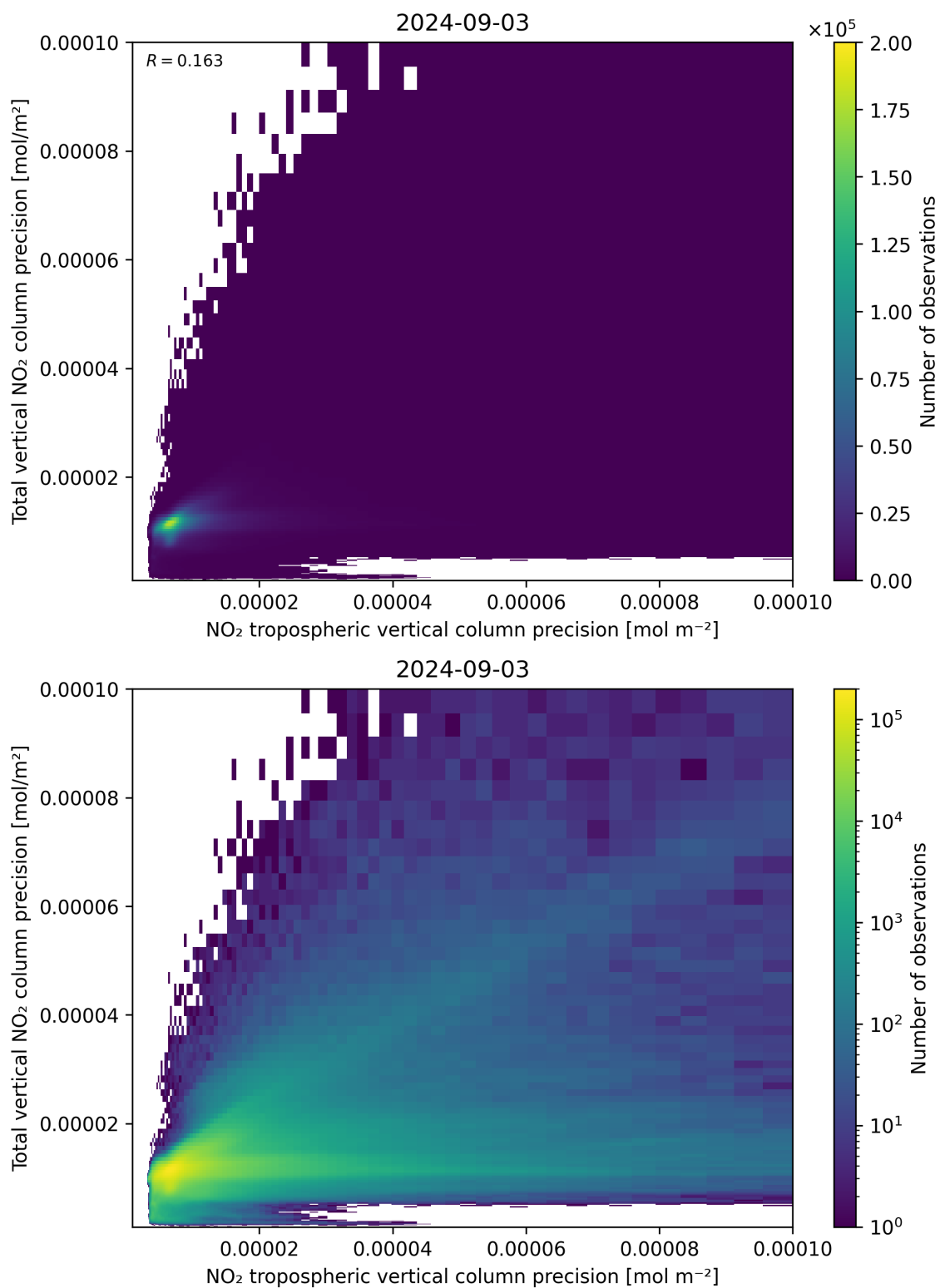
Figure 139: Scatter density plot of “NO 2 tropospheric vertical column precision” against “Total vertical NO 2 column precision” for 2024-09-02 to 2024-09-04.
