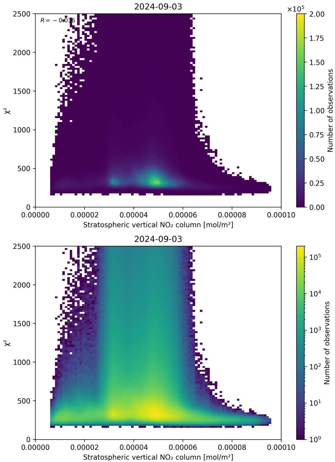
Figure 97: Scatter density plot of “Stratospheric vertical NO 2 column” against “ \chi^2 ” for 2024-09-02 to 2024-09-04.
