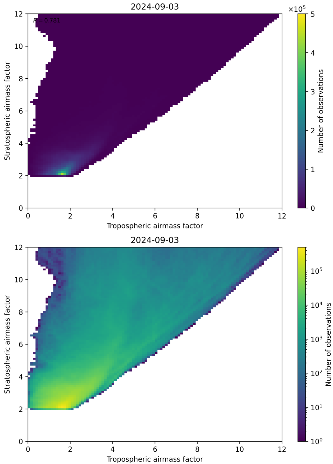
Figure 71: Scatter density plot of “Tropospheric airmass factor” against “Stratospheric airmass factor” for 2024-09-02 to 2024-09-04.
