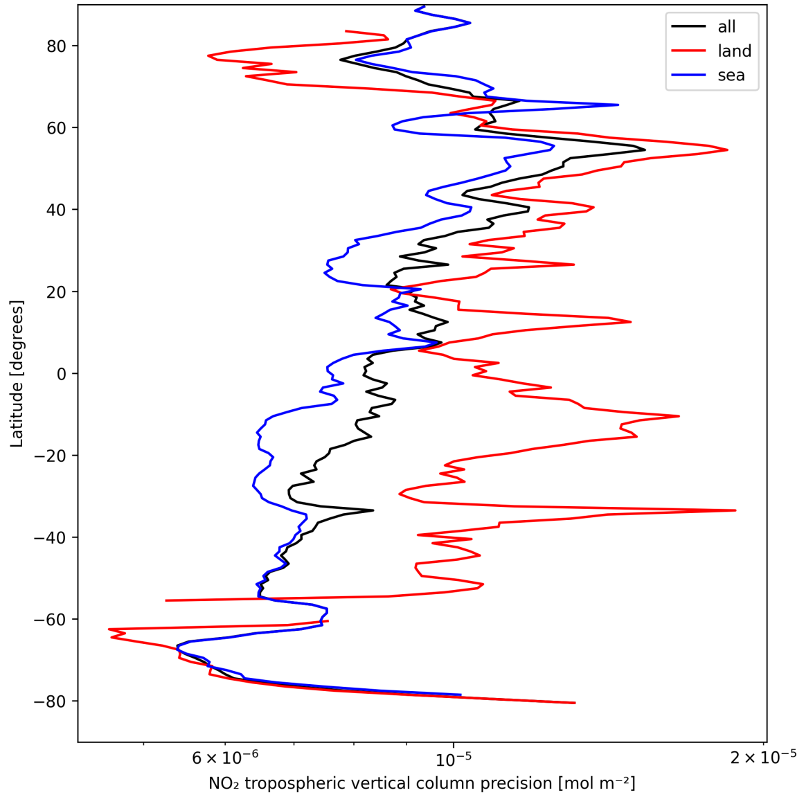
Figure 13: Zonal average of “NO 2 tropospheric vertical column precision” for 2024-09-02 to 2024-09-04.
