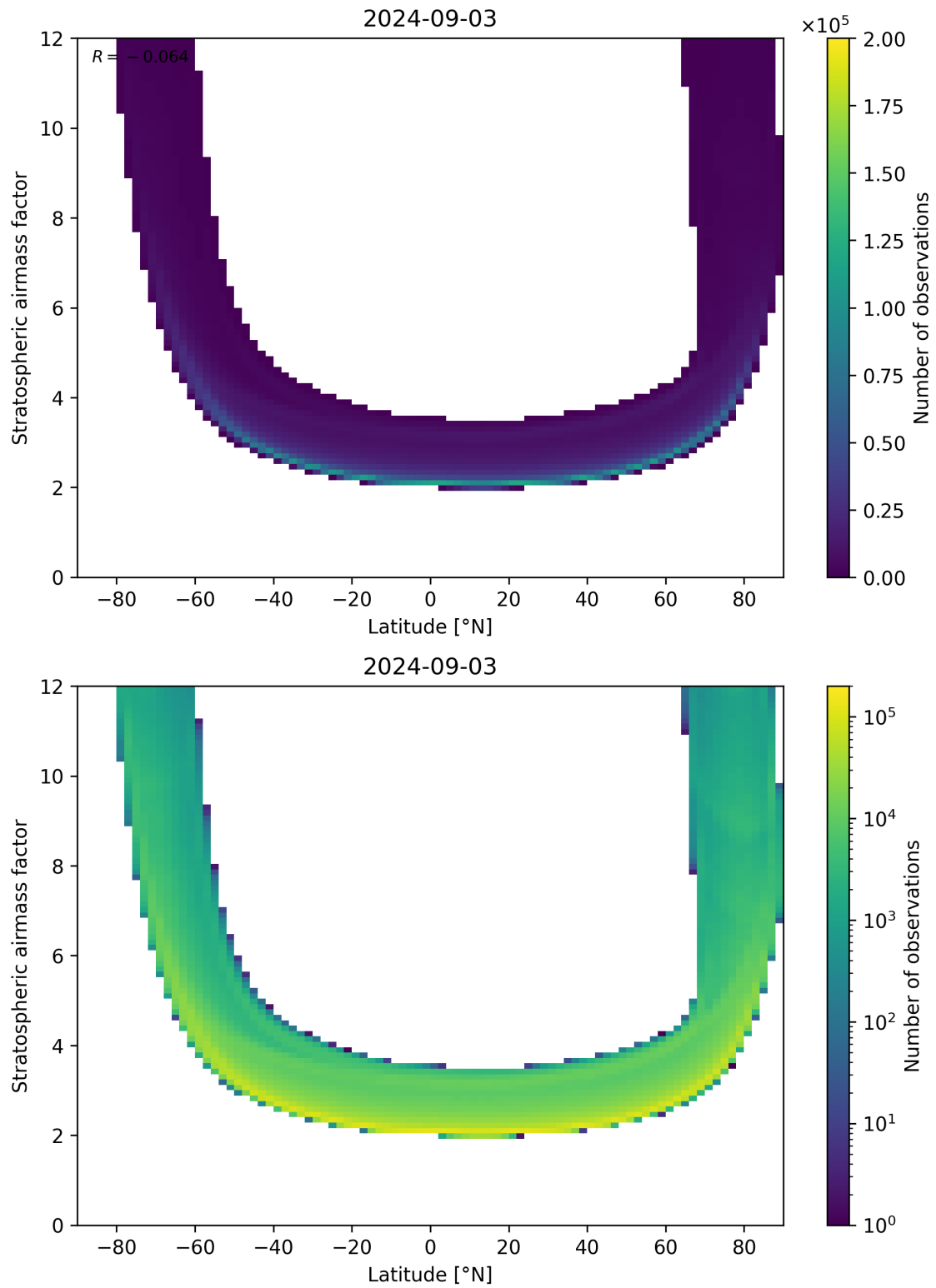
Figure 83: Scatter density plot of “Latitude” against “Stratospheric air mass factor” for 2024-09-02 to 2024-09-04.
