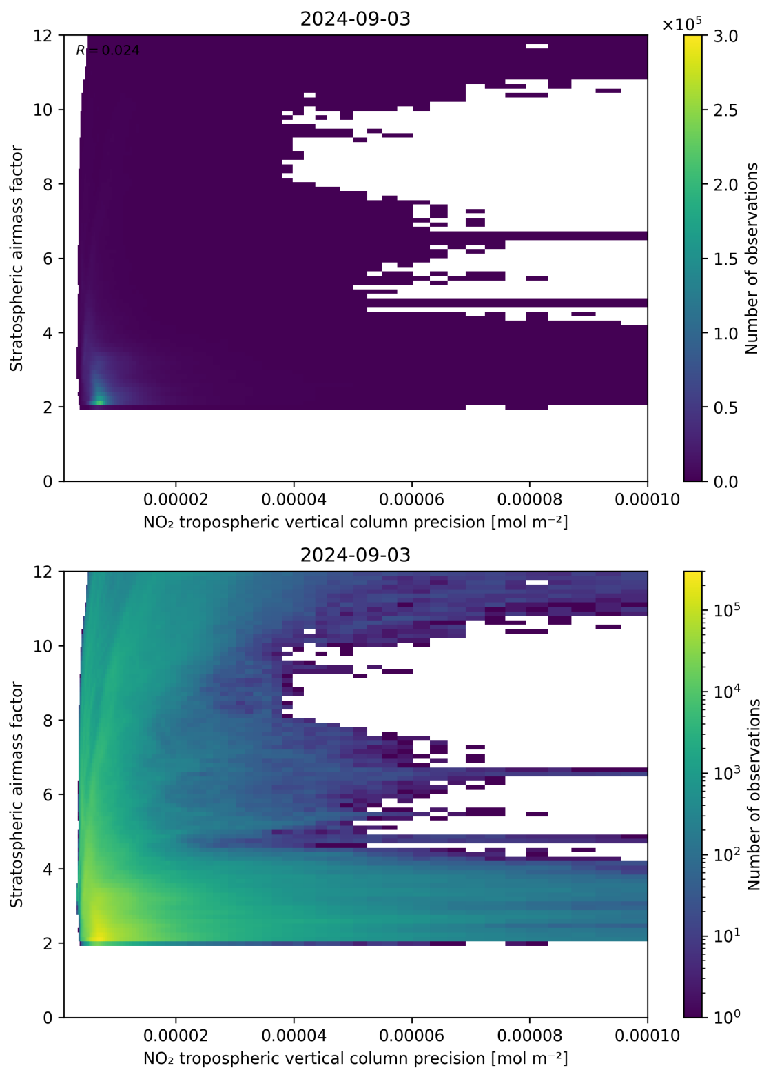
Figure 131: Scatter density plot of “NO 2 tropospheric vertical column precision” against “Stratospheric airmass factor” for 2024-09-02 to 2024-09-04.
