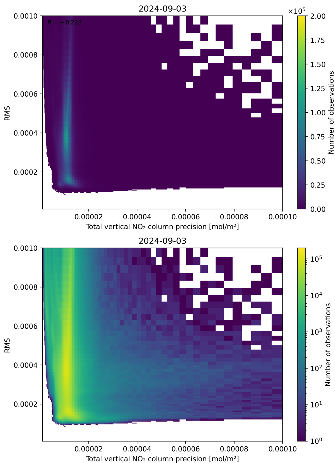
Figure 119: Scatter density plot of “Total vertical NO 2 column precision” against “RMS” for 2024-09-02 to 2024-09-04.
