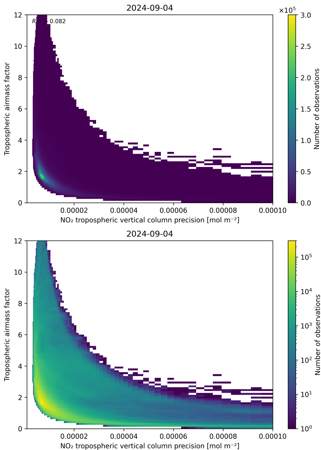
Figure 133: Scatter density plot of “NO 2 tropospheric vertical column precision” against “Tropospheric airmass factor” for 2024-09-03 to 2024-09-05.
