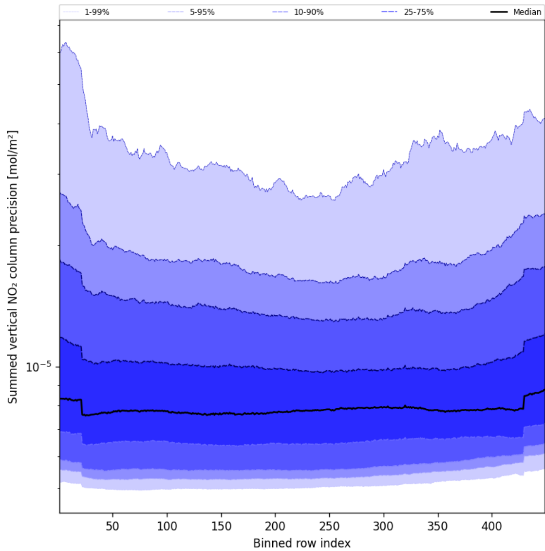
Figure 58: Along track statistics of “Summed vertical NO 2 column precision” for 2024-09-03 to 2024-09-05
