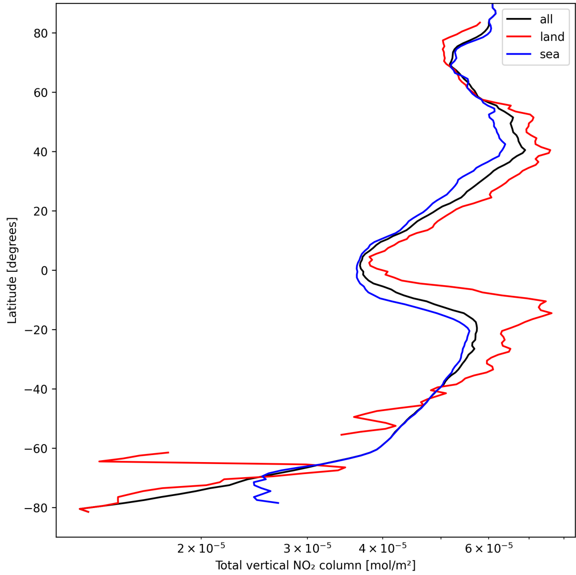
Figure 21: Zonal average of “Total vertical NO 2 column” for 2024-09-03 to 2024-09-05.
