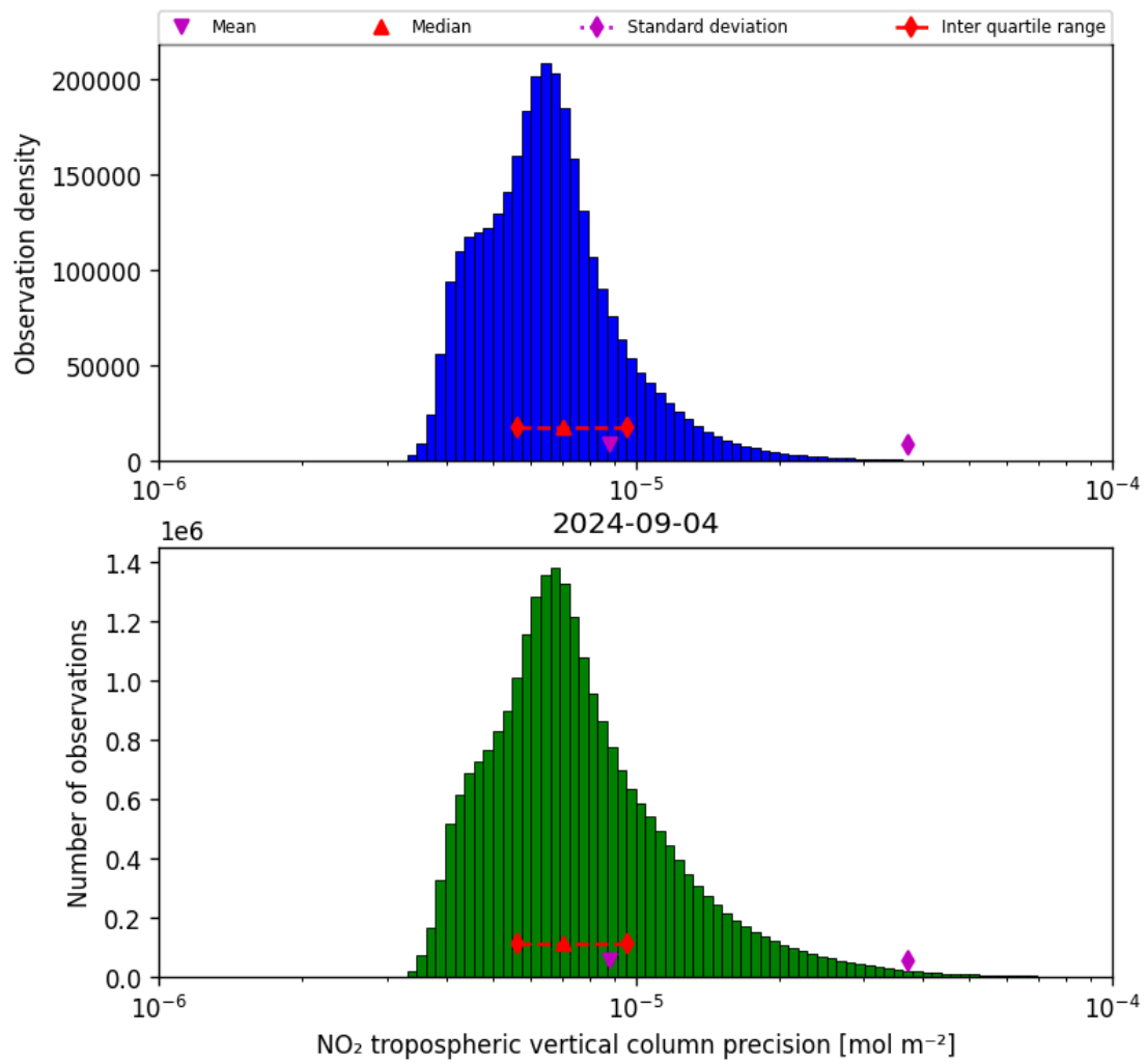
Figure 30: Histogram of “NO 2 tropospheric vertical column precision” for 2024-09-03 to 2024-09-05
