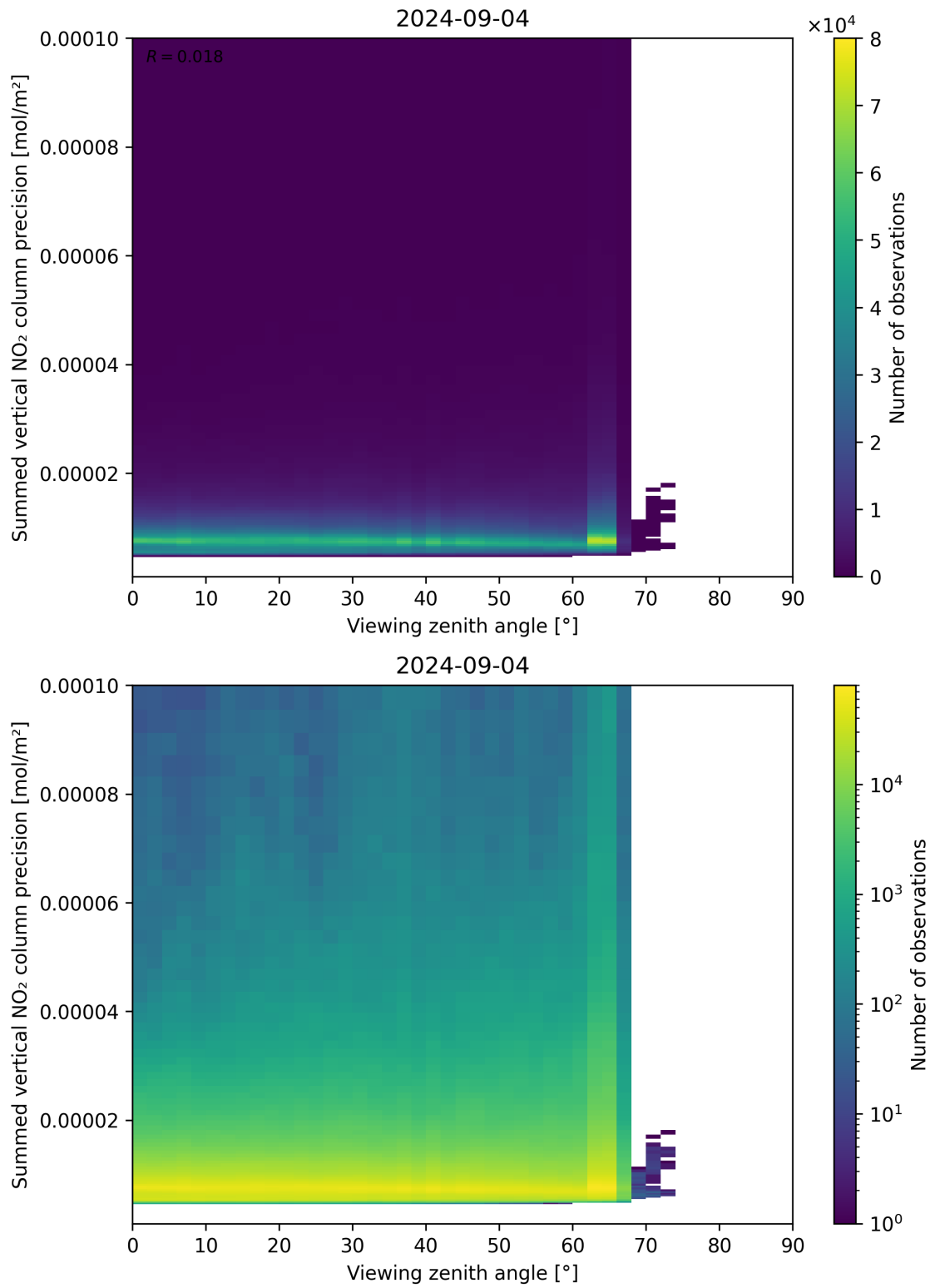
Figure 166: Scatter density plot of “Viewing zenith angle” against “Summed vertical NO 2 column precision” for 2024-09-03 to 2024-09-05.
