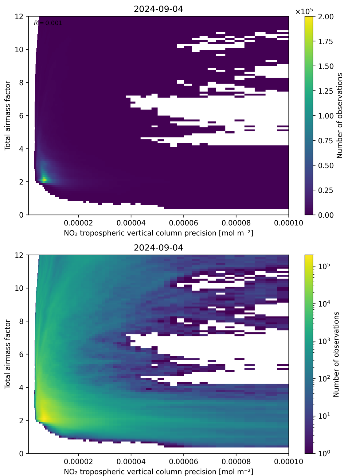
Figure 132: Scatter density plot of “NO 2 tropospheric vertical column precision” against “Total air mass factor” for 2024-09-03 to 2024-09-05.
