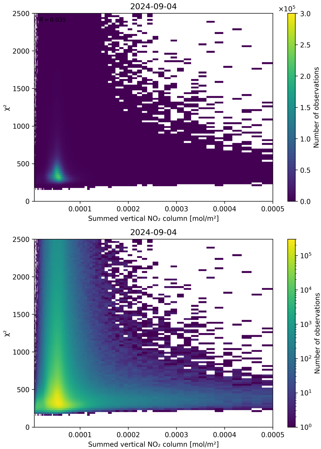
Figure 104: Scatter density plot of “Summed vertical NO 2 column” against “ \chi^2 ” for 2024-09-03 to 2024-09-05.
