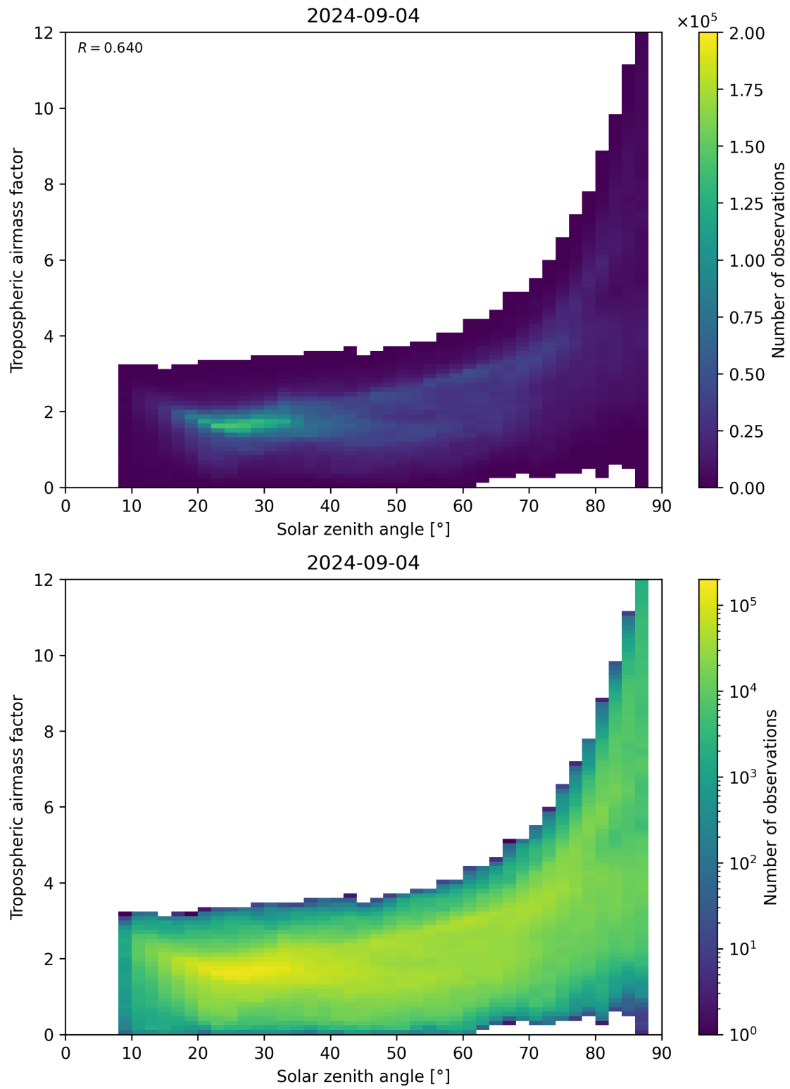
Figure 147: Scatter density plot of “Solar zenith angle” against “Tropospheric airmass factor” for 2024-09-03 to 2024-09-05.
