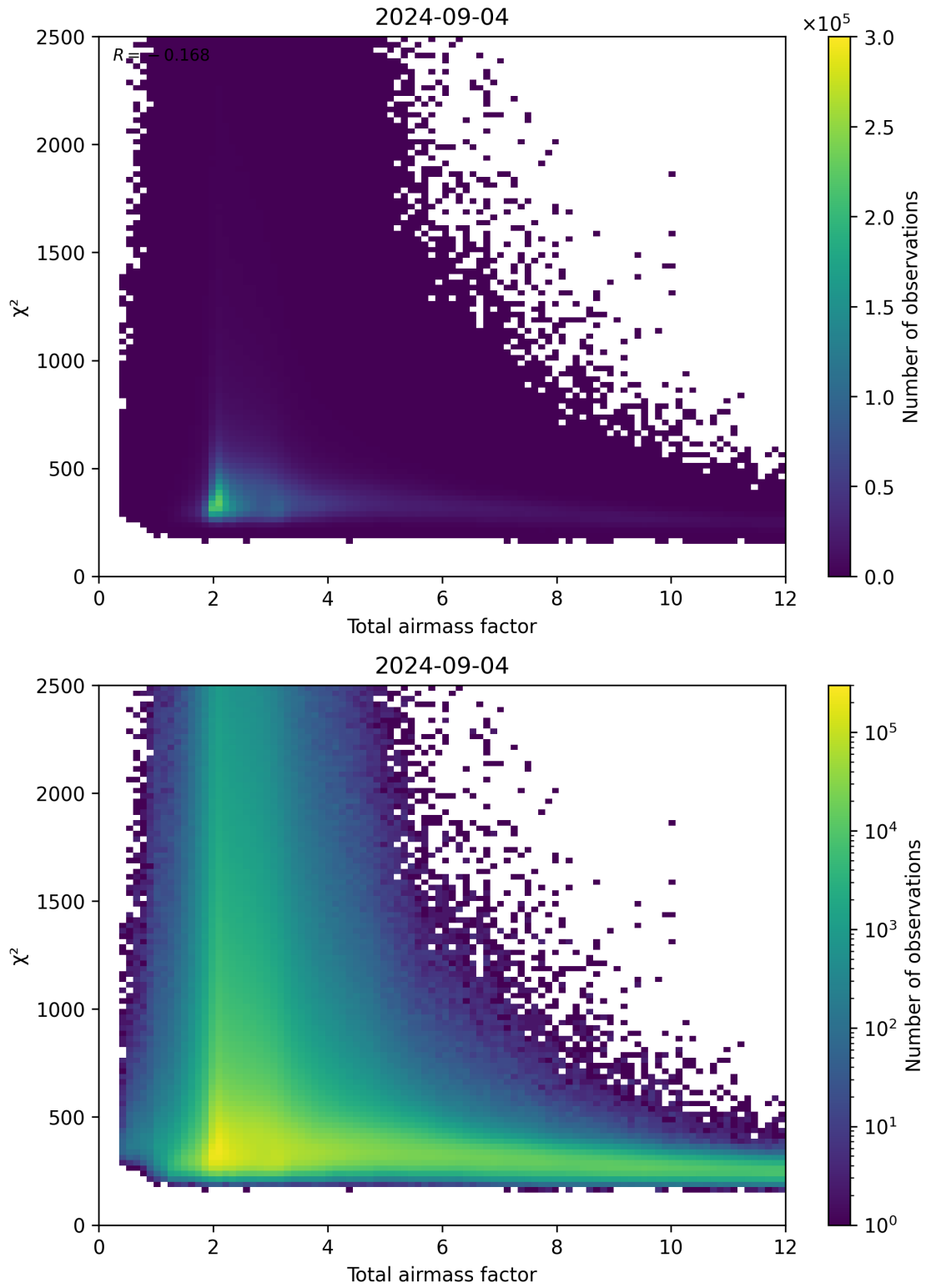
Figure 63: Scatter density plot of “Total airmass factor” against “ \chi^2 ” for 2024-09-03 to 2024-09-05.
