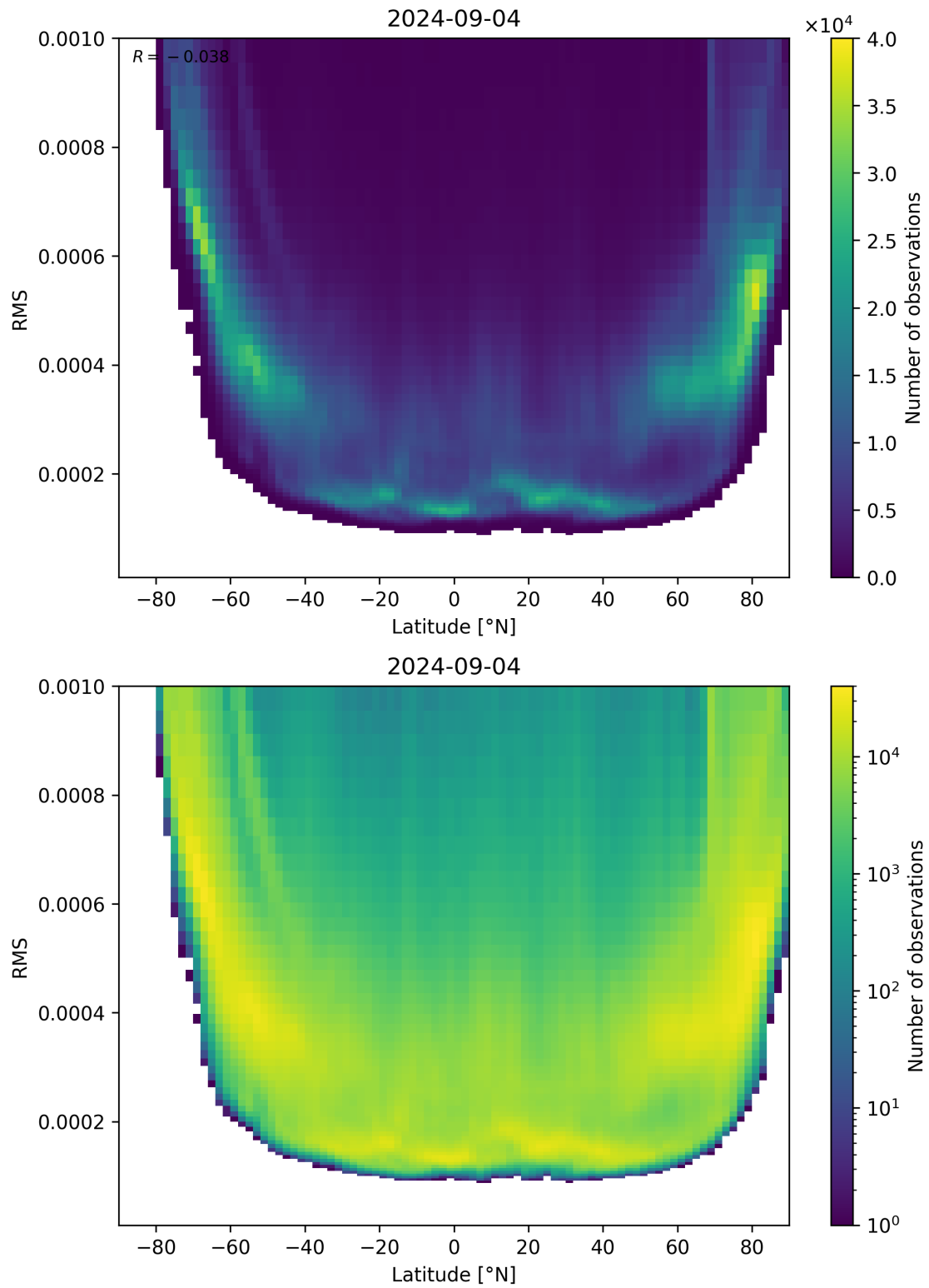
Figure 94: Scatter density plot of “Latitude” against “RMS” for 2024-09-03 to 2024-09-05.
