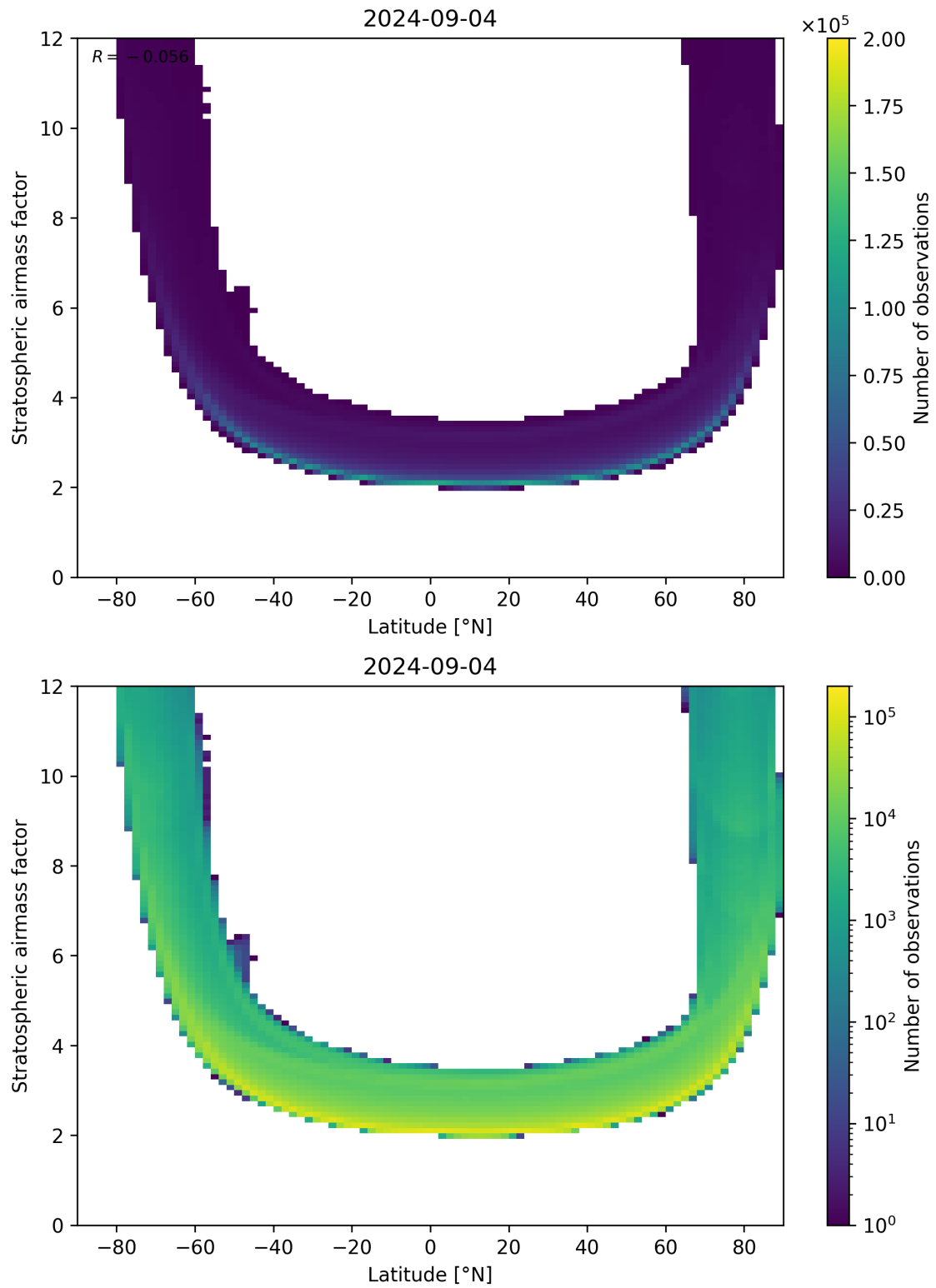
Figure 83: Scatter density plot of “Latitude” against “Stratospheric air mass factor” for 2024-09-03 to 2024-09-05.
