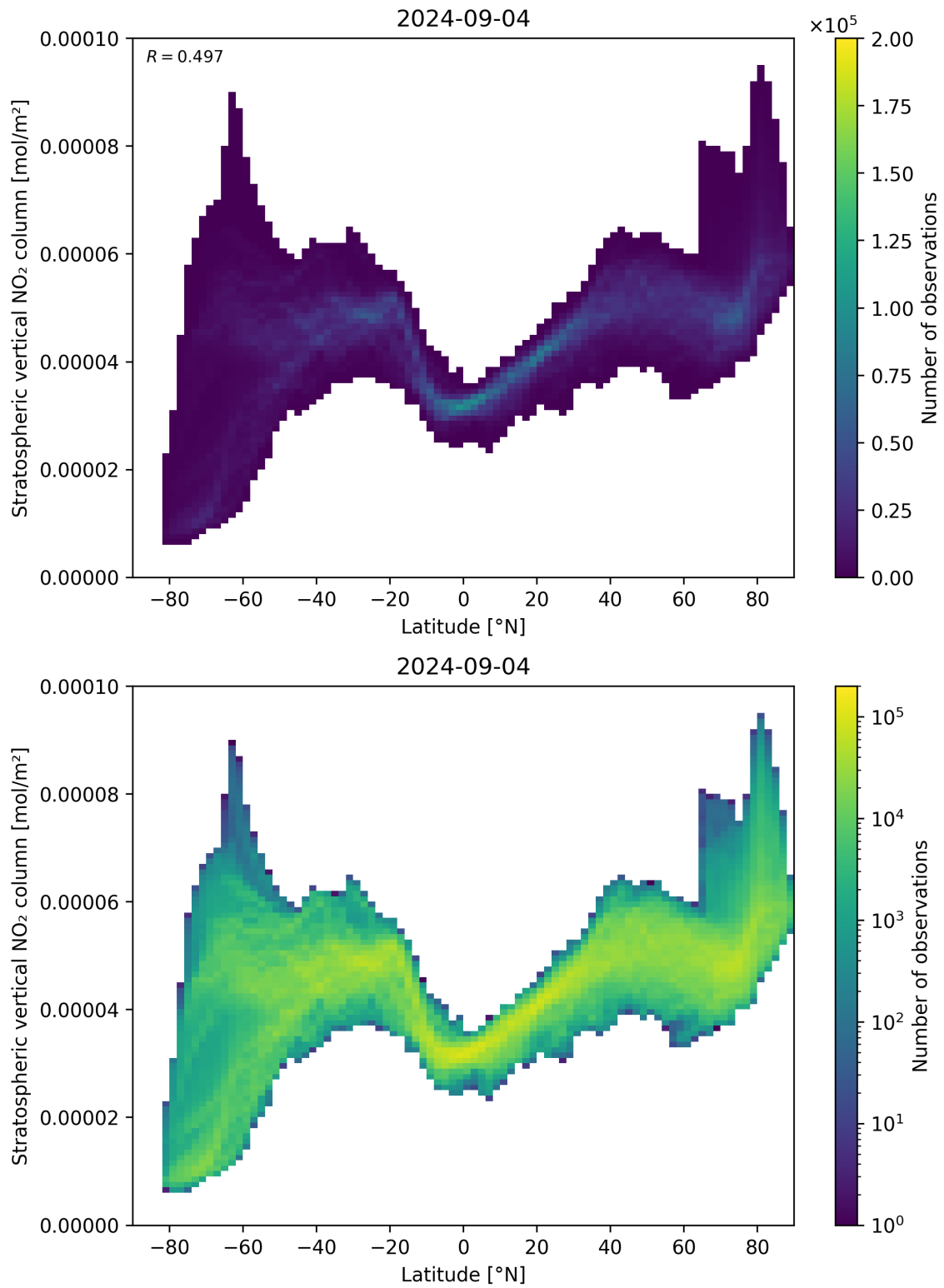
Figure 87: Scatter density plot of “Latitude” against “Stratospheric vertical NO 2 column” for 2024-09-03 to 2024-09-05.
