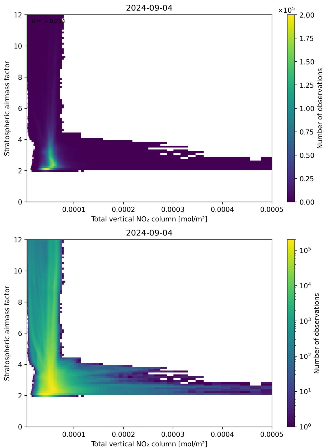
Figure 110: Scatter density plot of “Total vertical NO 2 column” against “Stratospheric airmass factor” for 2024-09-03 to 2024-09-05.
