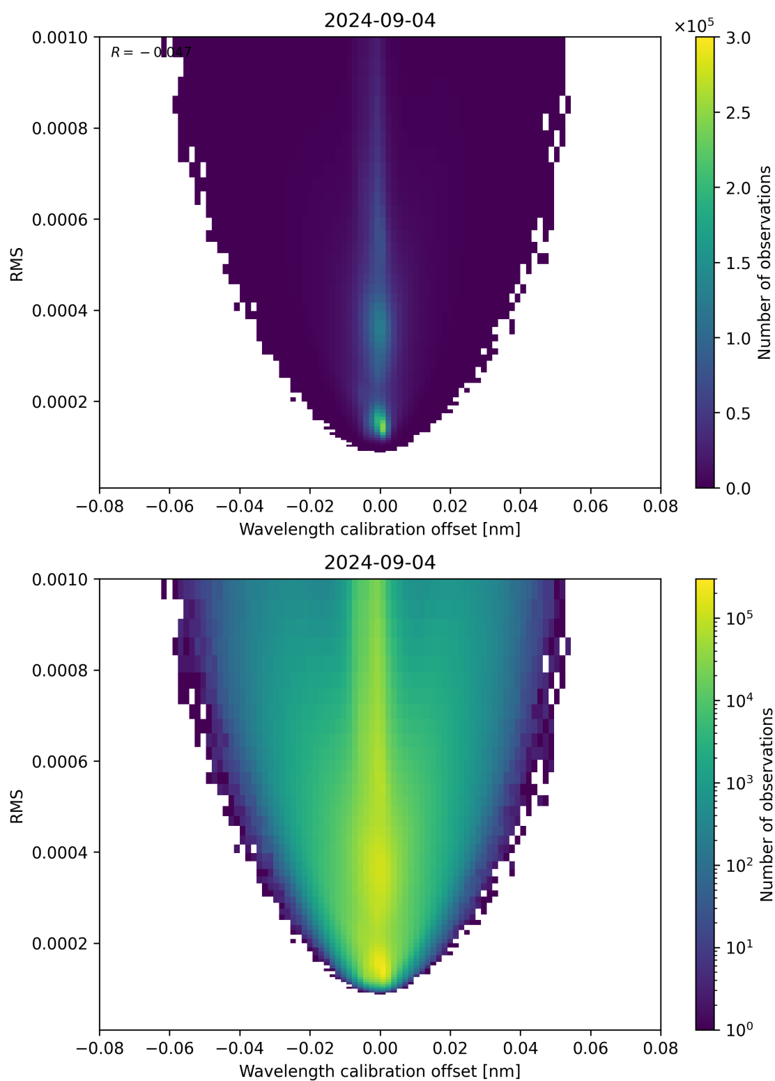
Figure 181: Scatter density plot of “Wavelength calibration offset” against “RMS” for 2024-09-03 to 2024-09-05.
