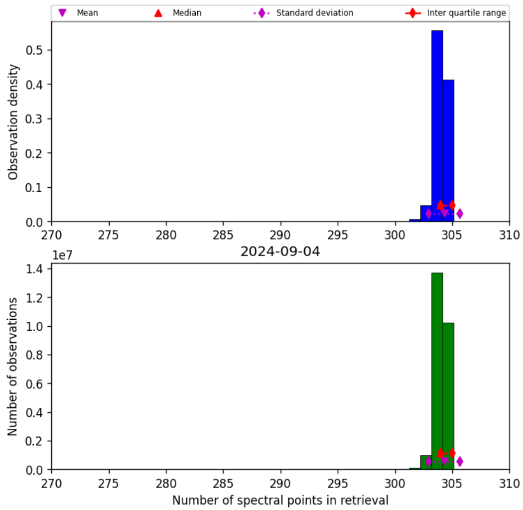
Figure 33: Histogram of “Number of spectral points in retrieval” for 2024-09-03 to 2024-09-05
