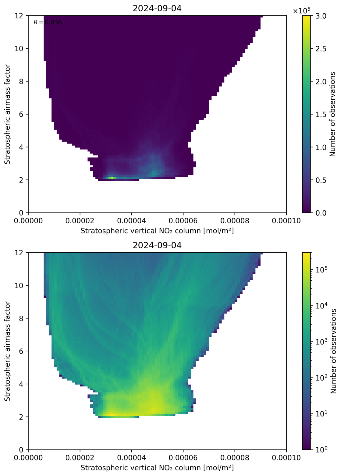
Figure 96: Scatter density plot of “Stratospheric vertical NO 2 column” against “Stratospheric airmass factor” for 2024-09-03 to 2024-09-05.
