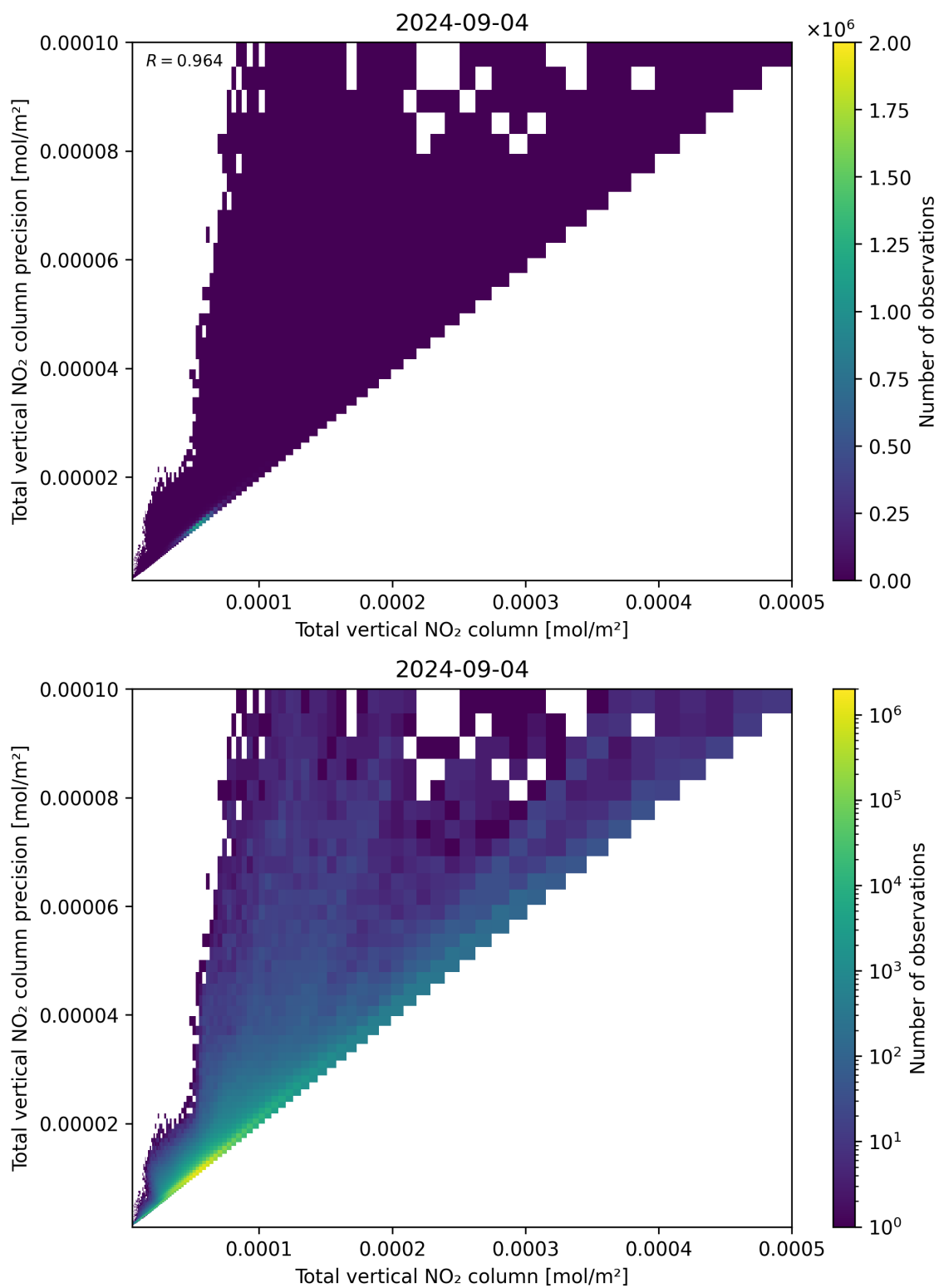
Figure 114: Scatter density plot of “Total vertical NO 2 column” against “Total vertical NO 2 column precision” for 2024-09-03 to 2024-09-05.
