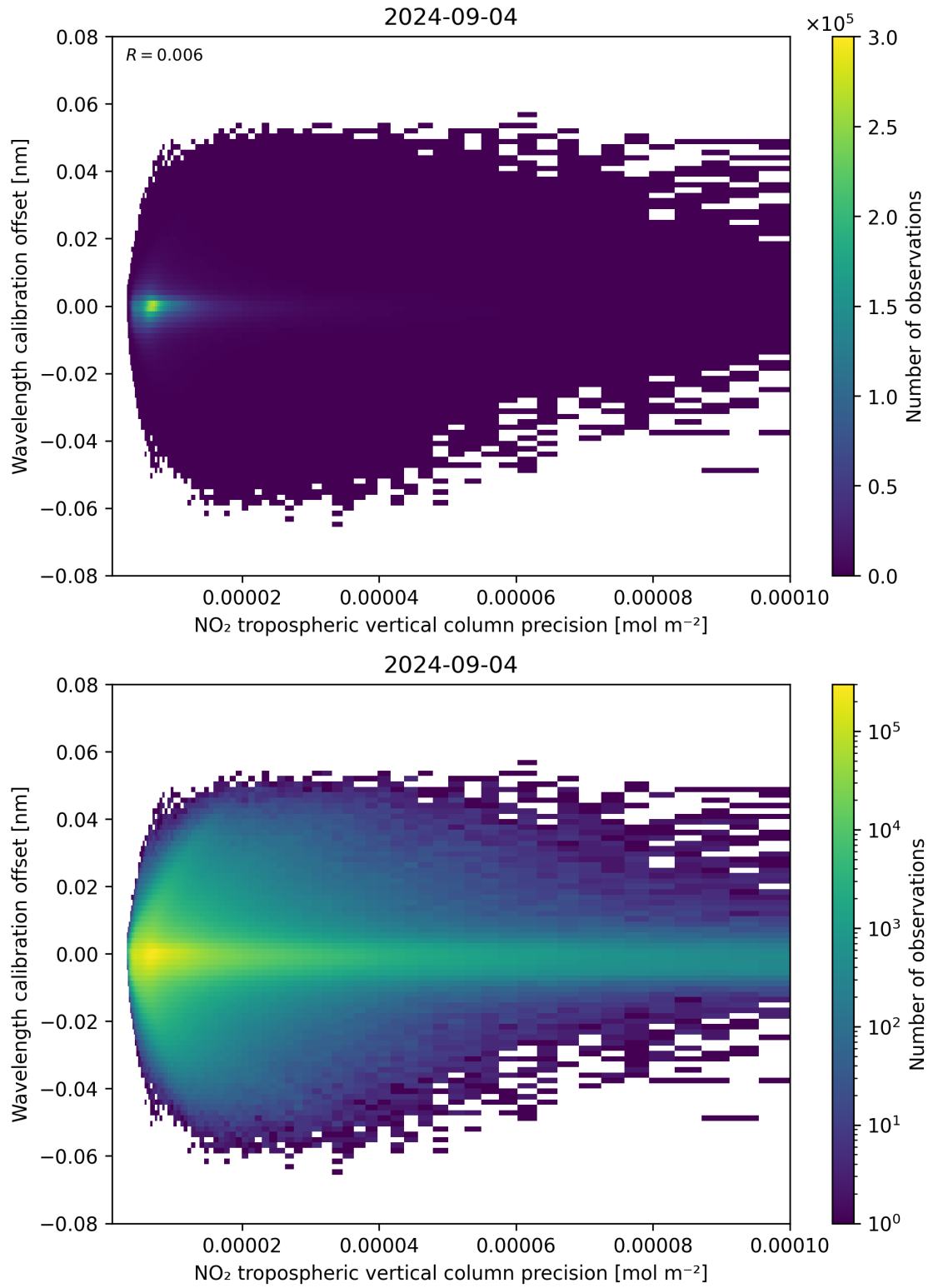
Figure 141: Scatter density plot of “NO 2 tropospheric vertical column precision” against “Wavelength calibration offset” for 2024-09-03 to 2024-09-05.
