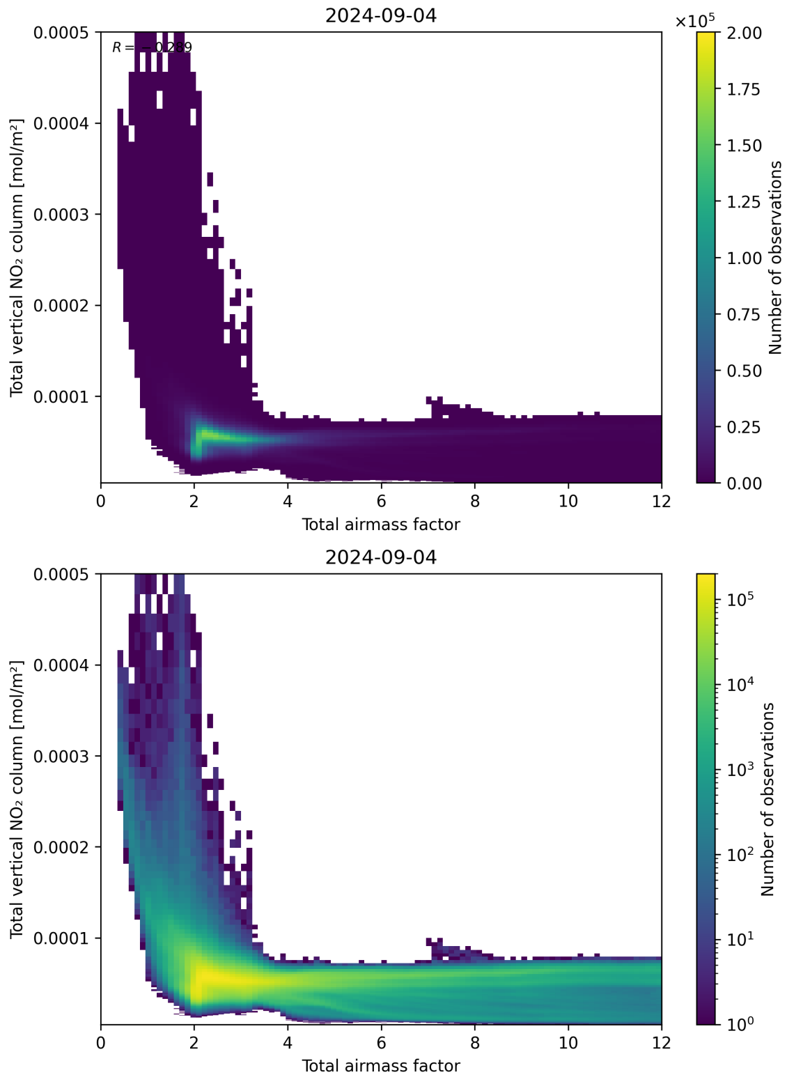
Figure 67: Scatter density plot of “Total airmass factor” against “Total vertical NO 2 column” for 2024-09-03 to 2024-09-05.
