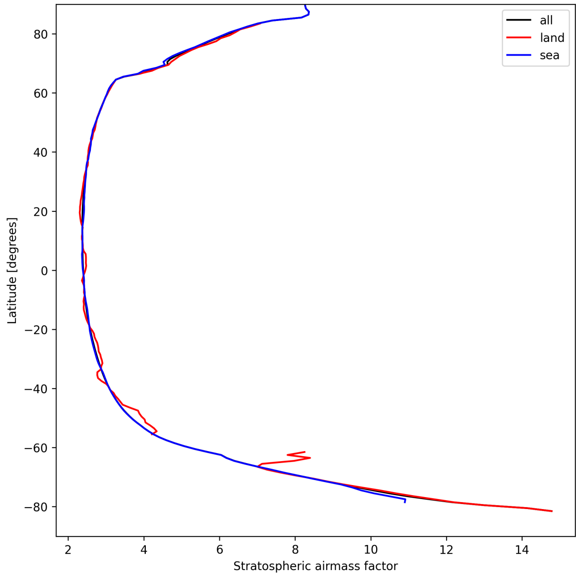
Figure 27: Zonal average of “Stratospheric airmass factor” for 2024-09-03 to 2024-09-05.
