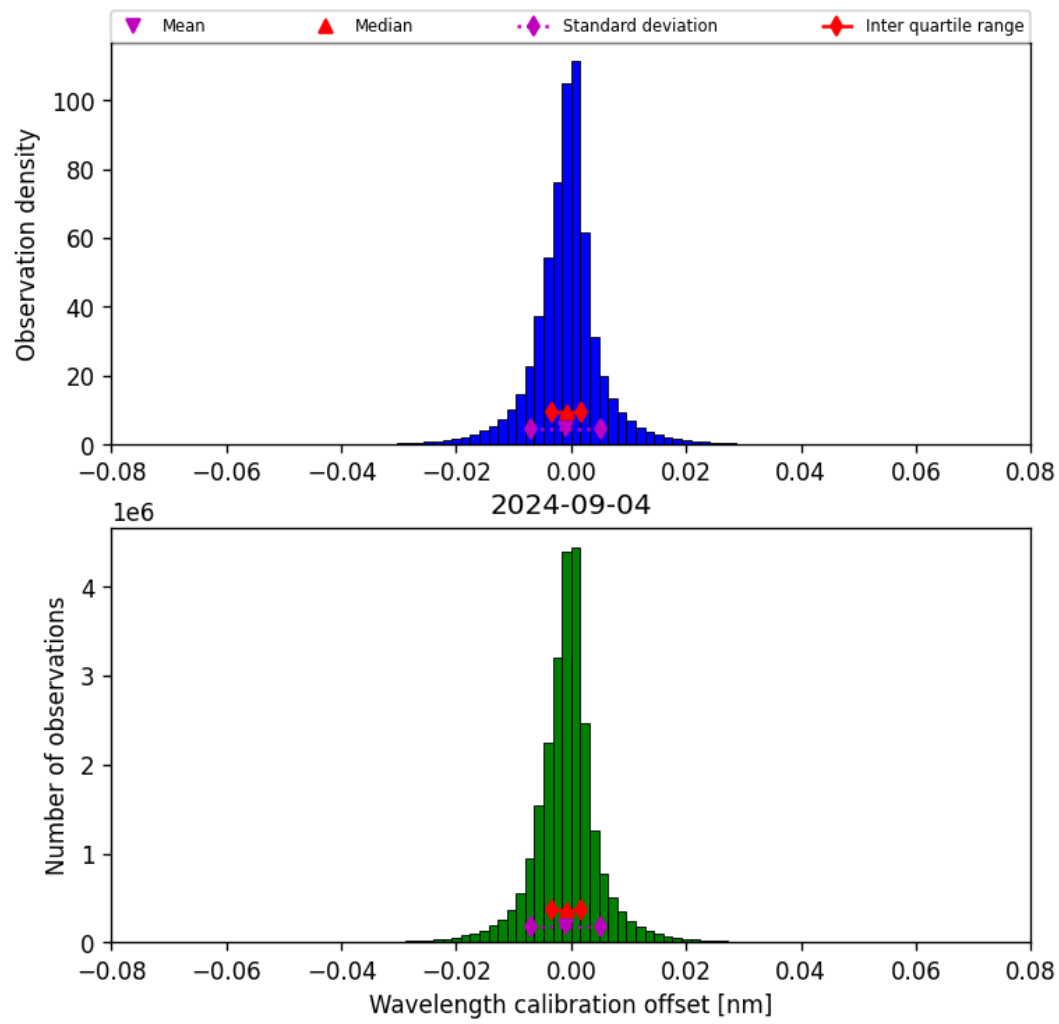
Figure 35: Histogram of “Wavelength calibration offset” for 2024-09-03 to 2024-09-05
