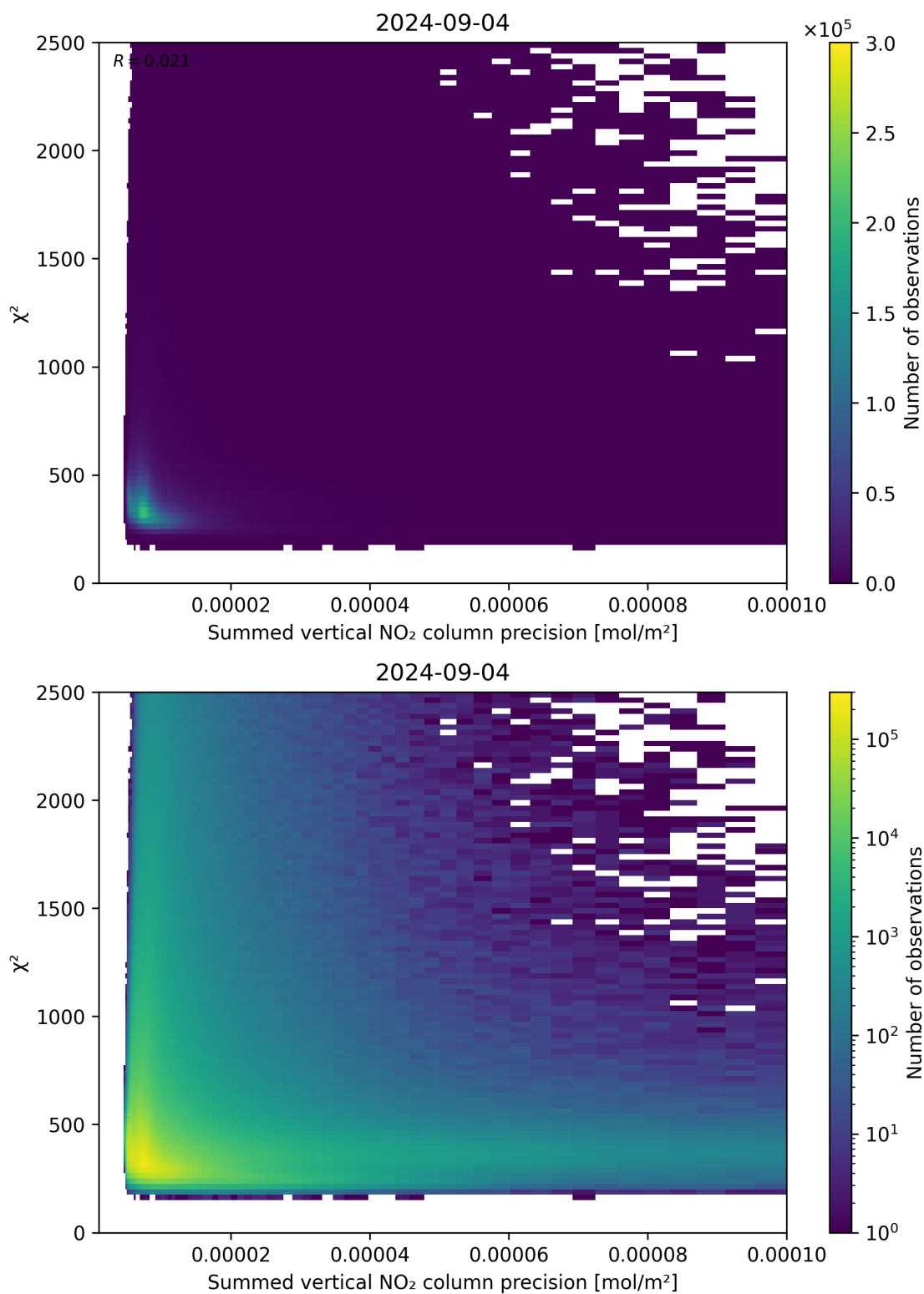
Figure 107: Scatter density plot of “Summed vertical NO 2 column precision” against “ \chi^2 ” for 2024-09-03 to 2024-09-05.
