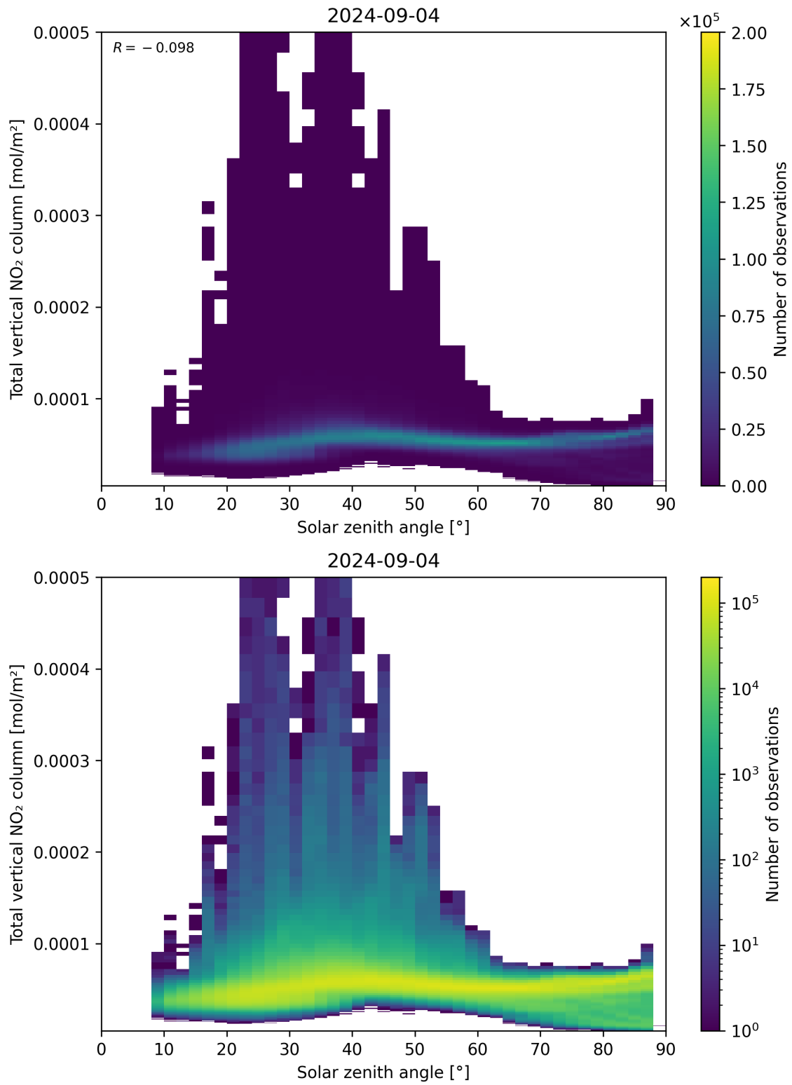
Figure 153: Scatter density plot of “Solar zenith angle” against “Total vertical NO 2 column” for 2024-09-03 to 2024-09-05.
