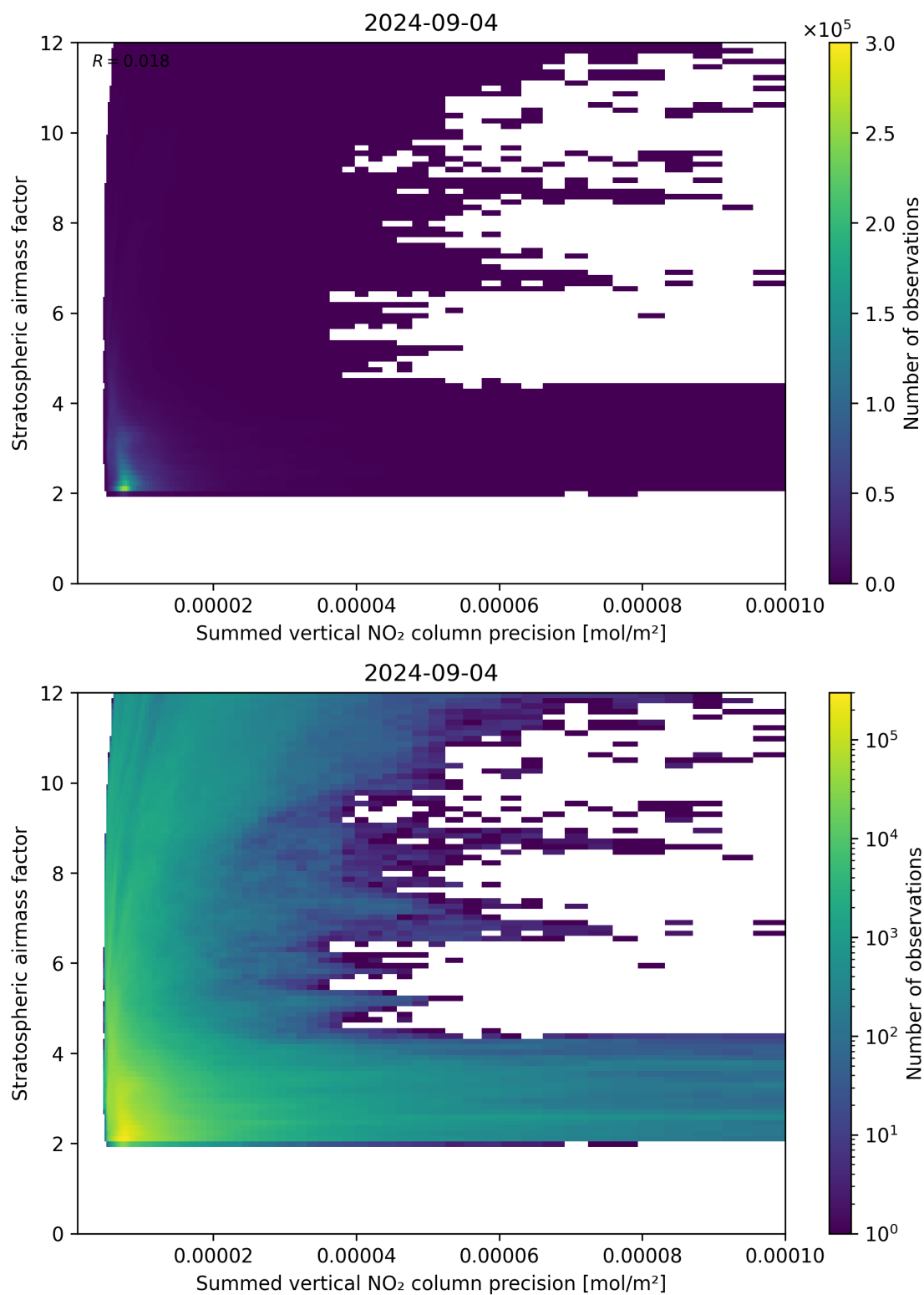
Figure 106: Scatter density plot of “Summed vertical NO 2 column precision” against “Stratospheric airmass factor” for 2024-09-03 to 2024-09-05.
