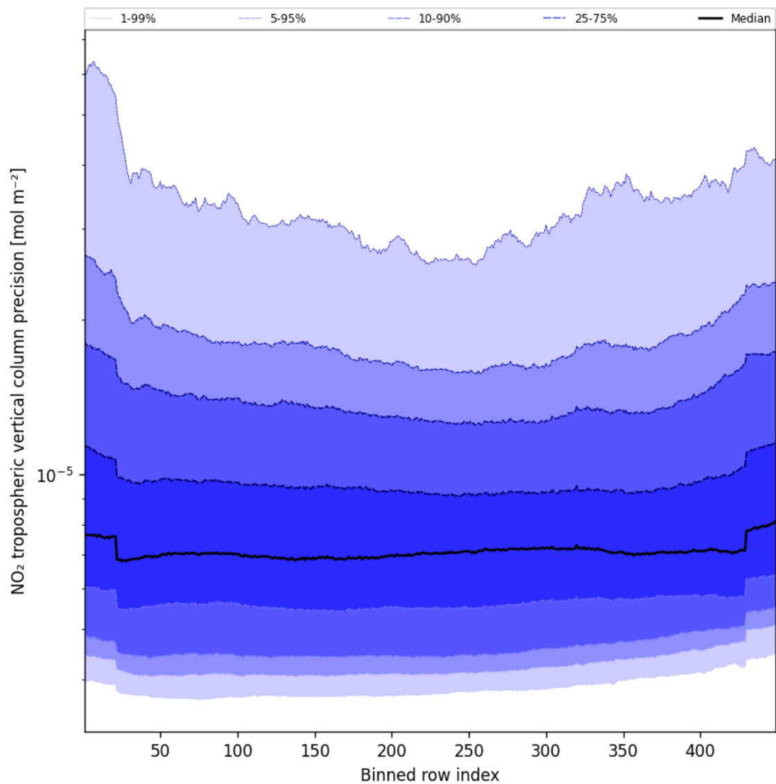
Figure 47: Along track statistics of “NO 2 tropospheric vertical column precision” for 2024-09-03 to 2024-09-05
