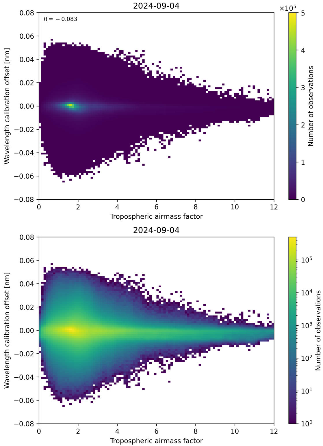
Figure 80: Scatter density plot of “Tropospheric airmass factor” against “Wavelength calibration offset” for 2024-09-03 to 2024-09-05.
