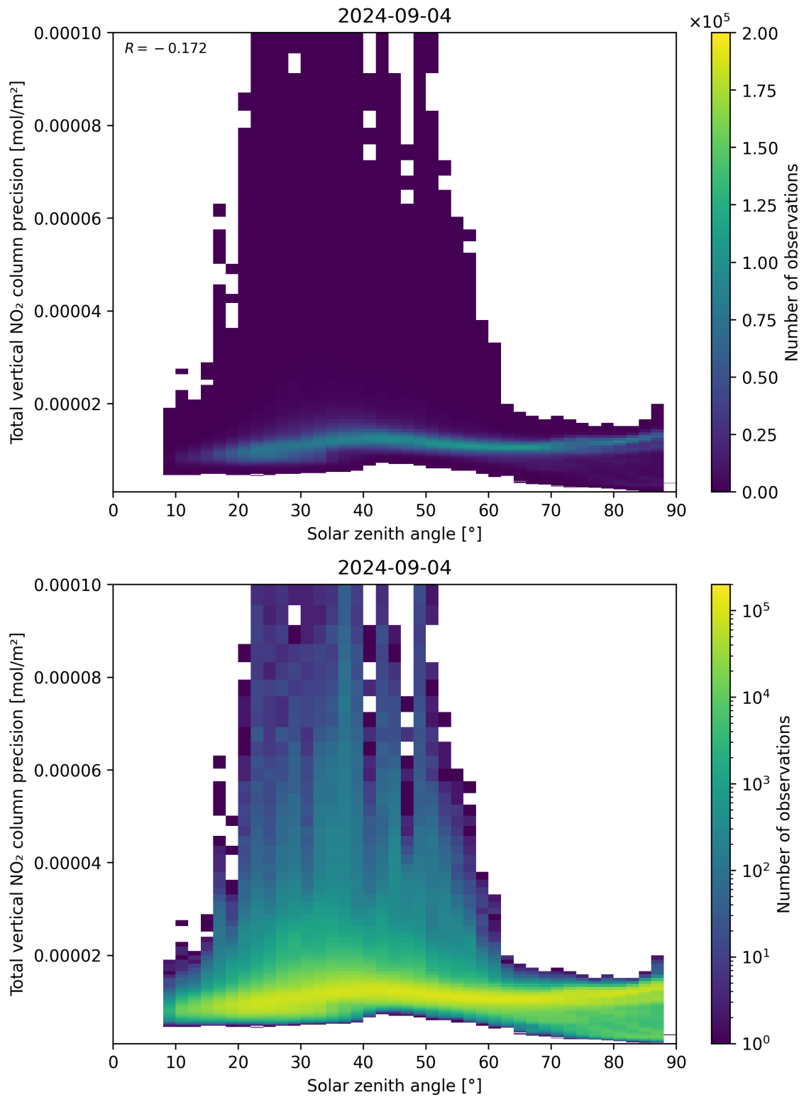
Figure 154: Scatter density plot of “Solar zenith angle” against “Total vertical NO 2 column precision” for 2024-09-03 to 2024-09-05.
