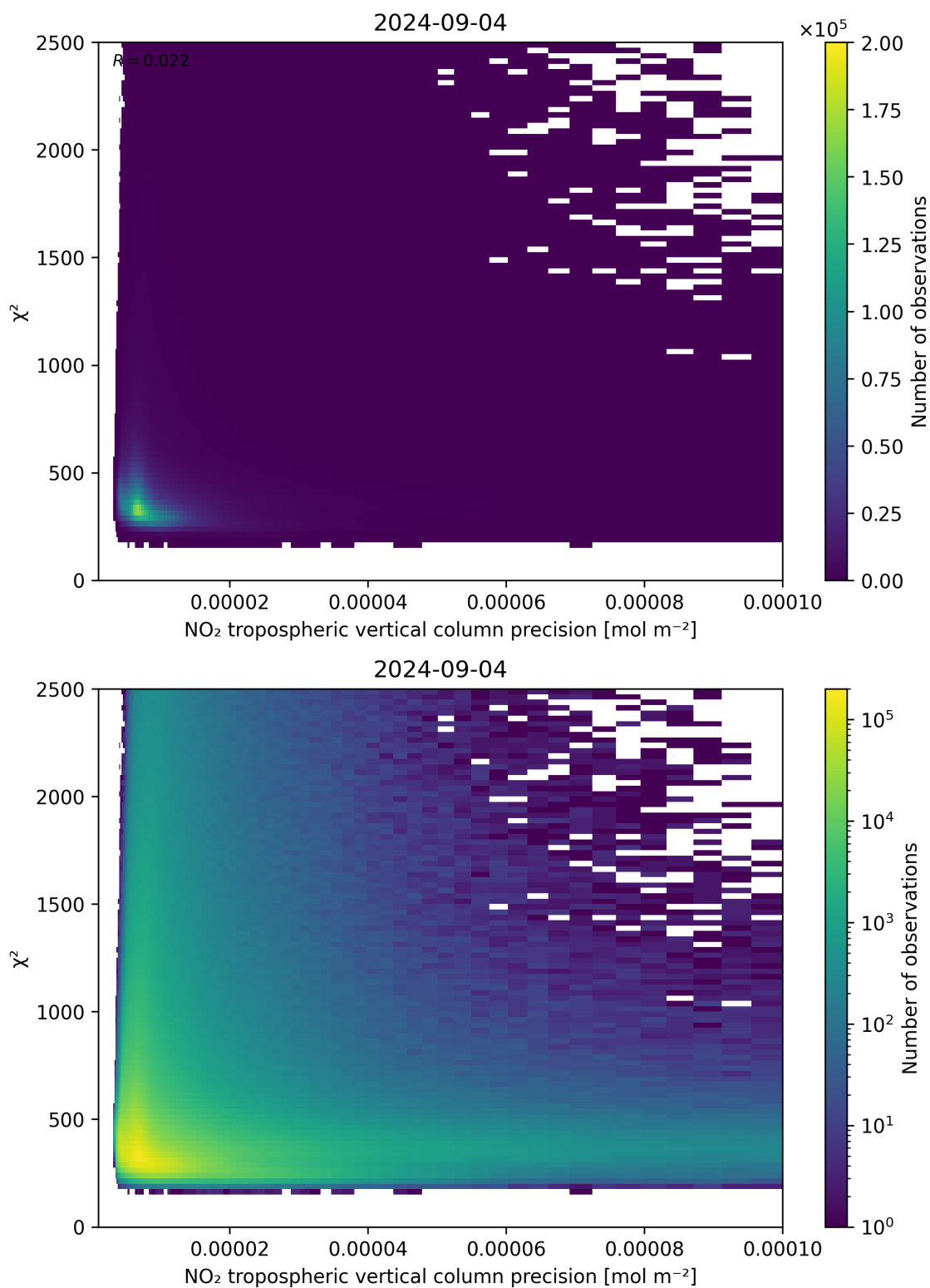
Figure 134: Scatter density plot of “NO 2 tropospheric vertical column precision” against “ \chi^2 ” for 2024-09-03 to 2024-09-05.
