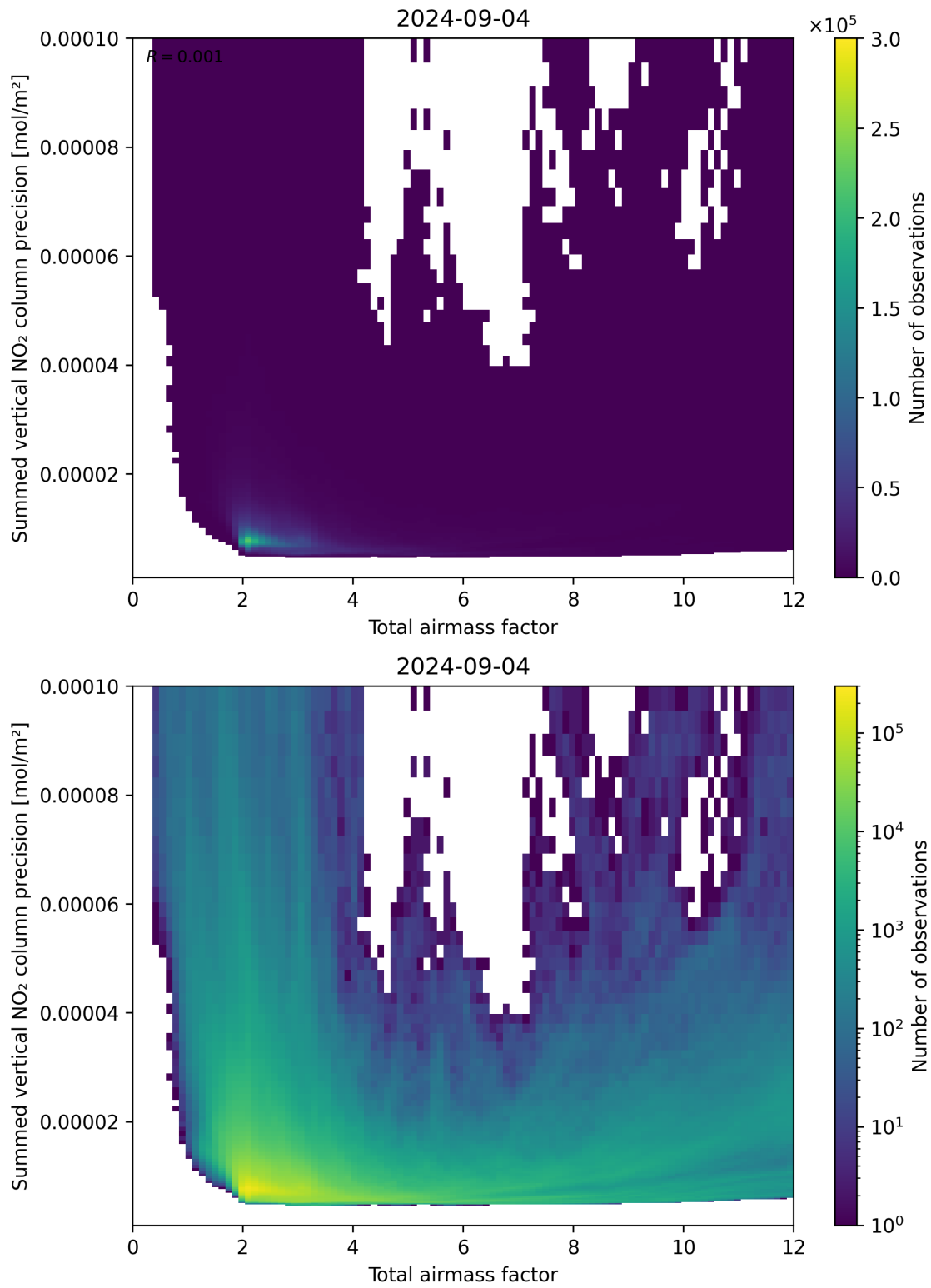
Figure 66: Scatter density plot of “Total airmass factor” against “Summed vertical NO 2 column precision” for 2024-09-03 to 2024-09-05.
