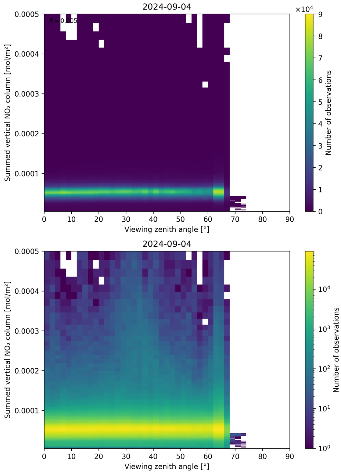
Figure 165: Scatter density plot of “Viewing zenith angle” against “Summed vertical NO 2 column” for 2024-09-03 to 2024-09-05.
