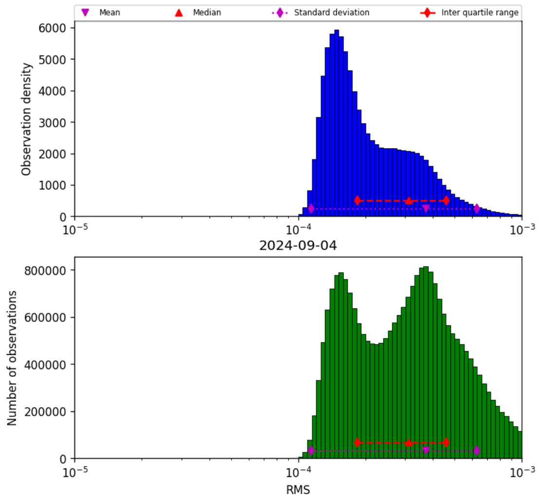
Figure 43: Histogram of “RMS” for 2024-09-03 to 2024-09-05
