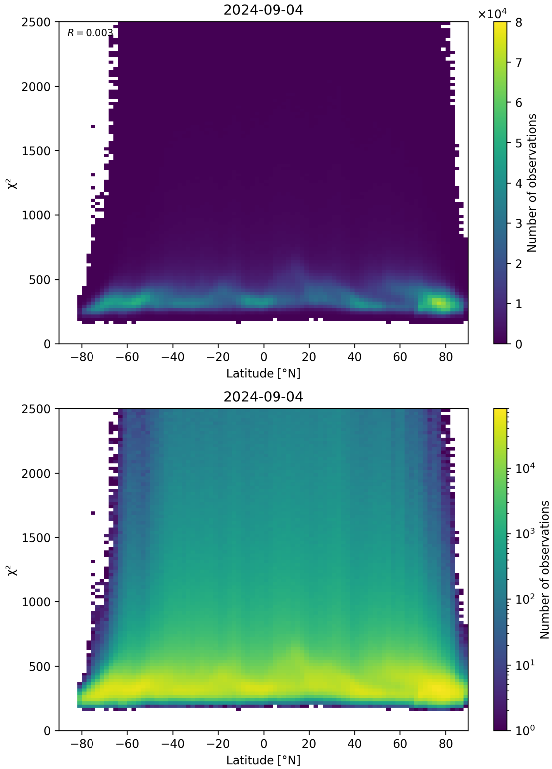
Figure 86: Scatter density plot of “Latitude” against “ \chi^2 ” for 2024-09-03 to 2024-09-05.
