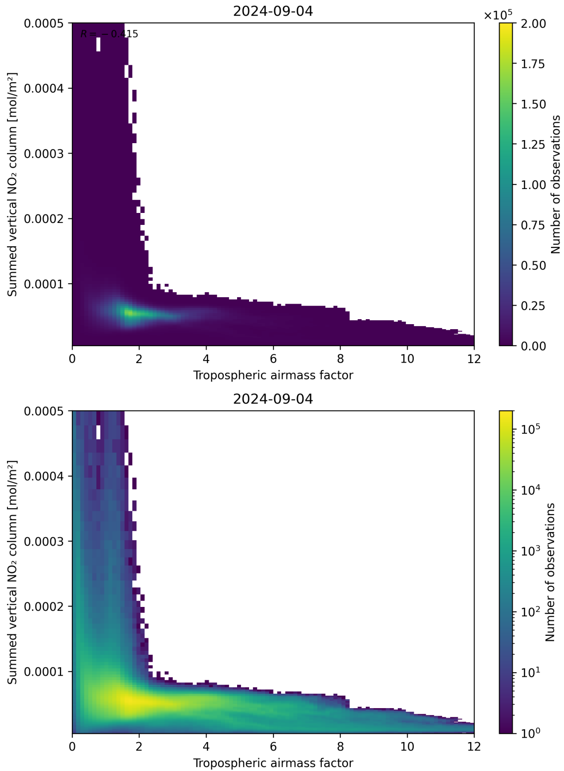
Figure 75: Scatter density plot of “Tropospheric airmass factor” against “Summed vertical NO 2 column” for 2024-09-03 to 2024-09-05.
