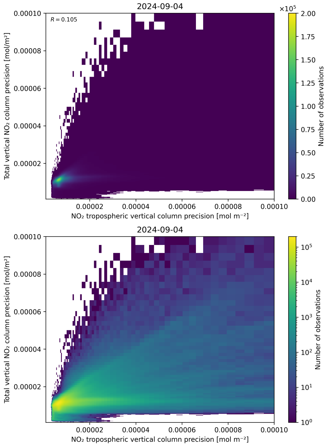
Figure 139: Scatter density plot of “NO 2 tropospheric vertical column precision” against “Total vertical NO 2 column precision” for 2024-09-03 to 2024-09-05.
