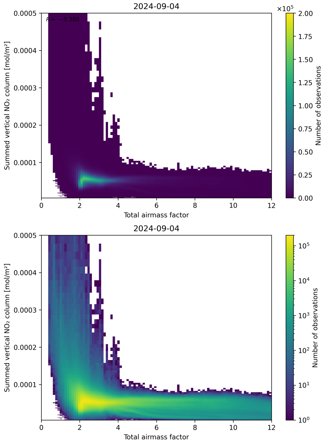
Figure 65: Scatter density plot of “Total airmass factor” against “Summed vertical NO 2 column” for 2024-09-03 to 2024-09-05.
