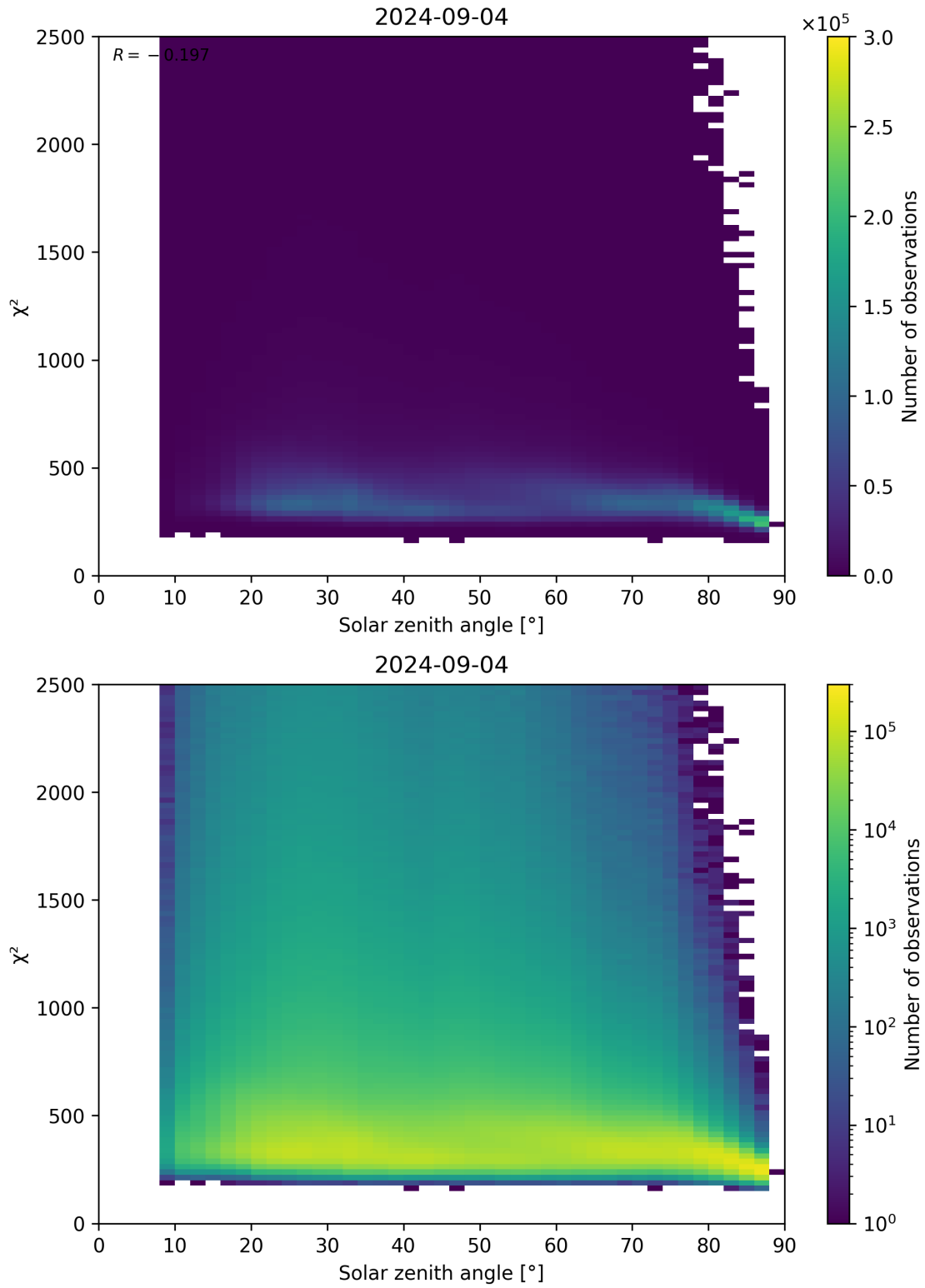
Figure 148: Scatter density plot of “Solar zenith angle” against “ \chi^2 ” for 2024-09-03 to 2024-09-05.
