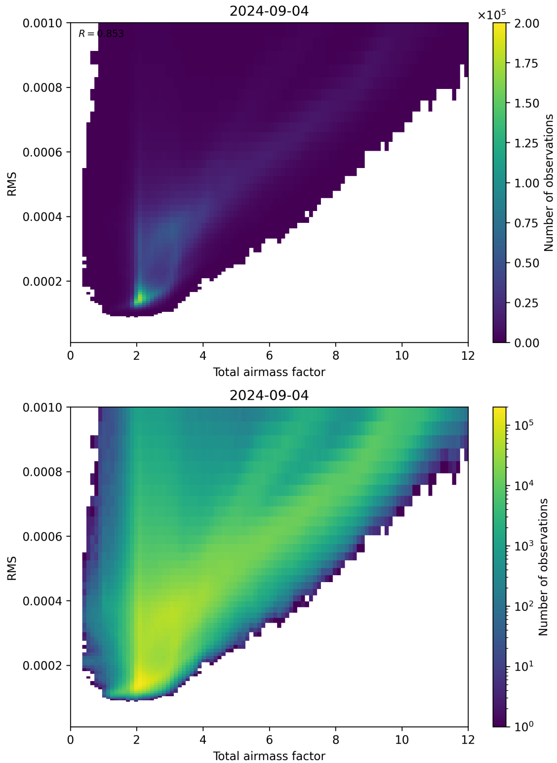
Figure 69: Scatter density plot of “Total airmass factor” against “RMS” for 2024-09-03 to 2024-09-05.
