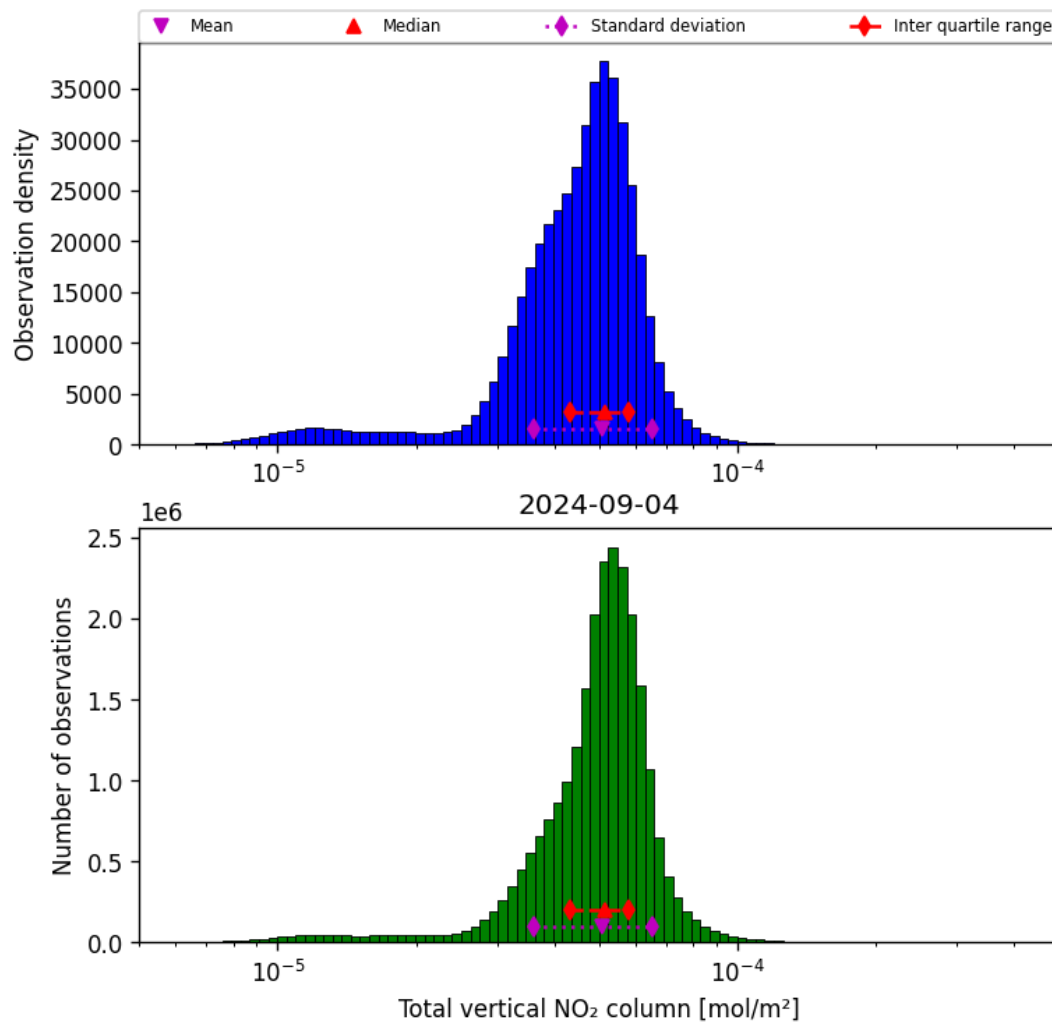
Figure 38: Histogram of “Total vertical NO 2 column” for 2024-09-03 to 2024-09-05
