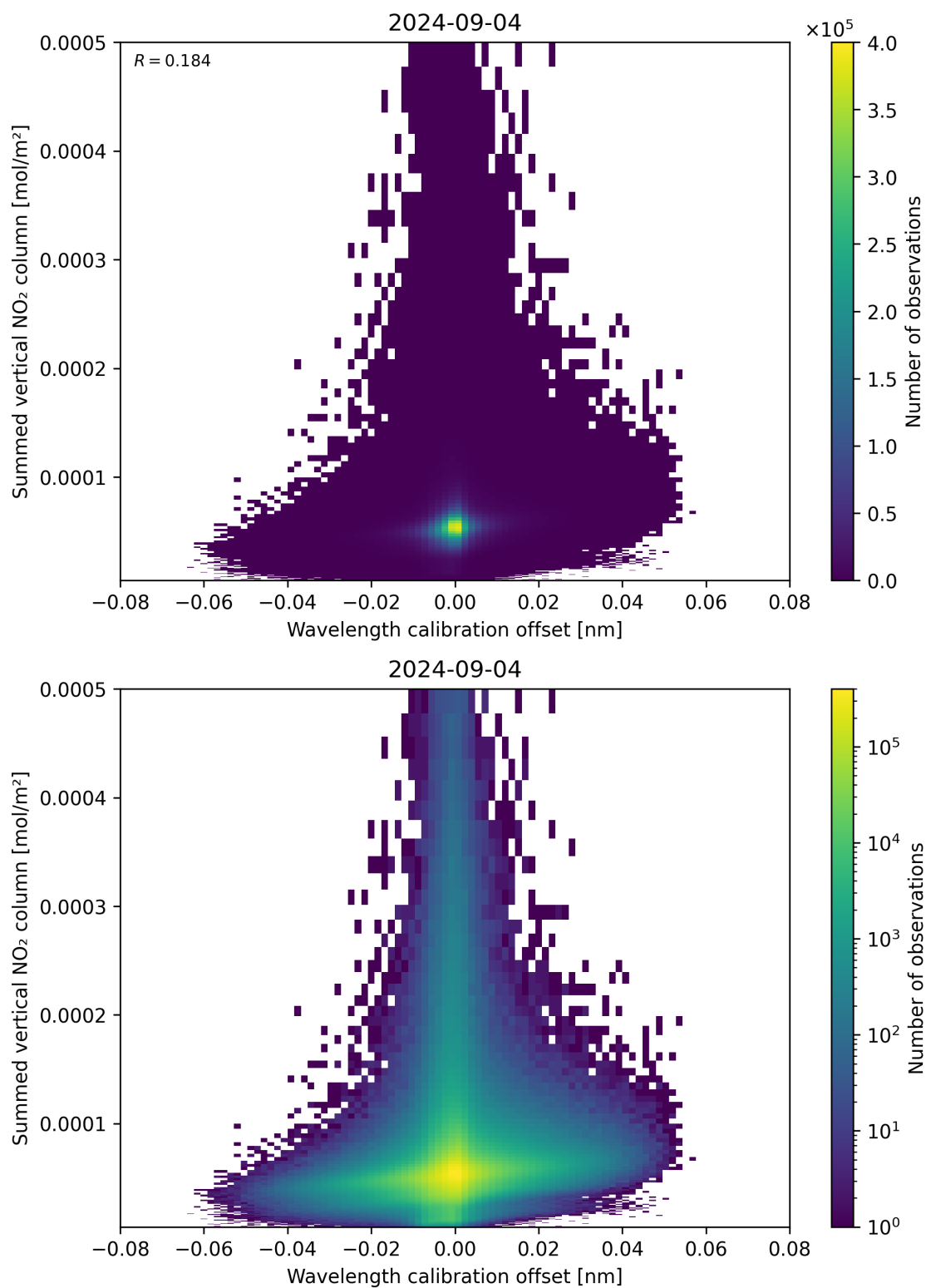
Figure 177: Scatter density plot of “Wavelength calibration offset” against “Summed vertical NO 2 column” for 2024-09-03 to 2024-09-05.
