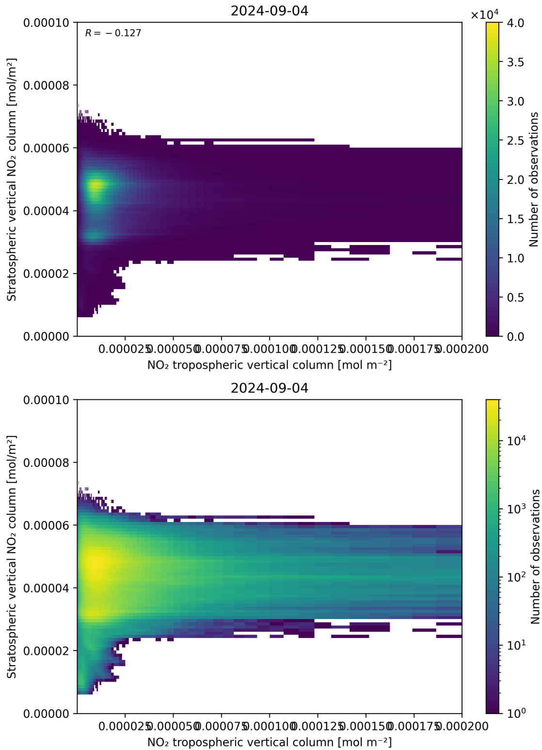
Figure 125: Scatter density plot of “NO 2 tropospheric vertical column” against “Stratospheric vertical NO 2 column” for 2024-09-03 to 2024-09-05.
