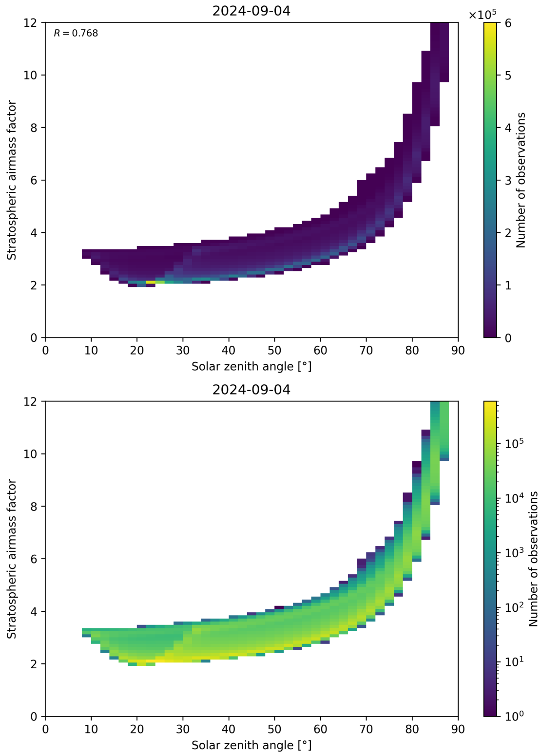
Figure 145: Scatter density plot of “Solar zenith angle” against “Stratospheric airmass factor” for 2024-09-03 to 2024-09-05.
