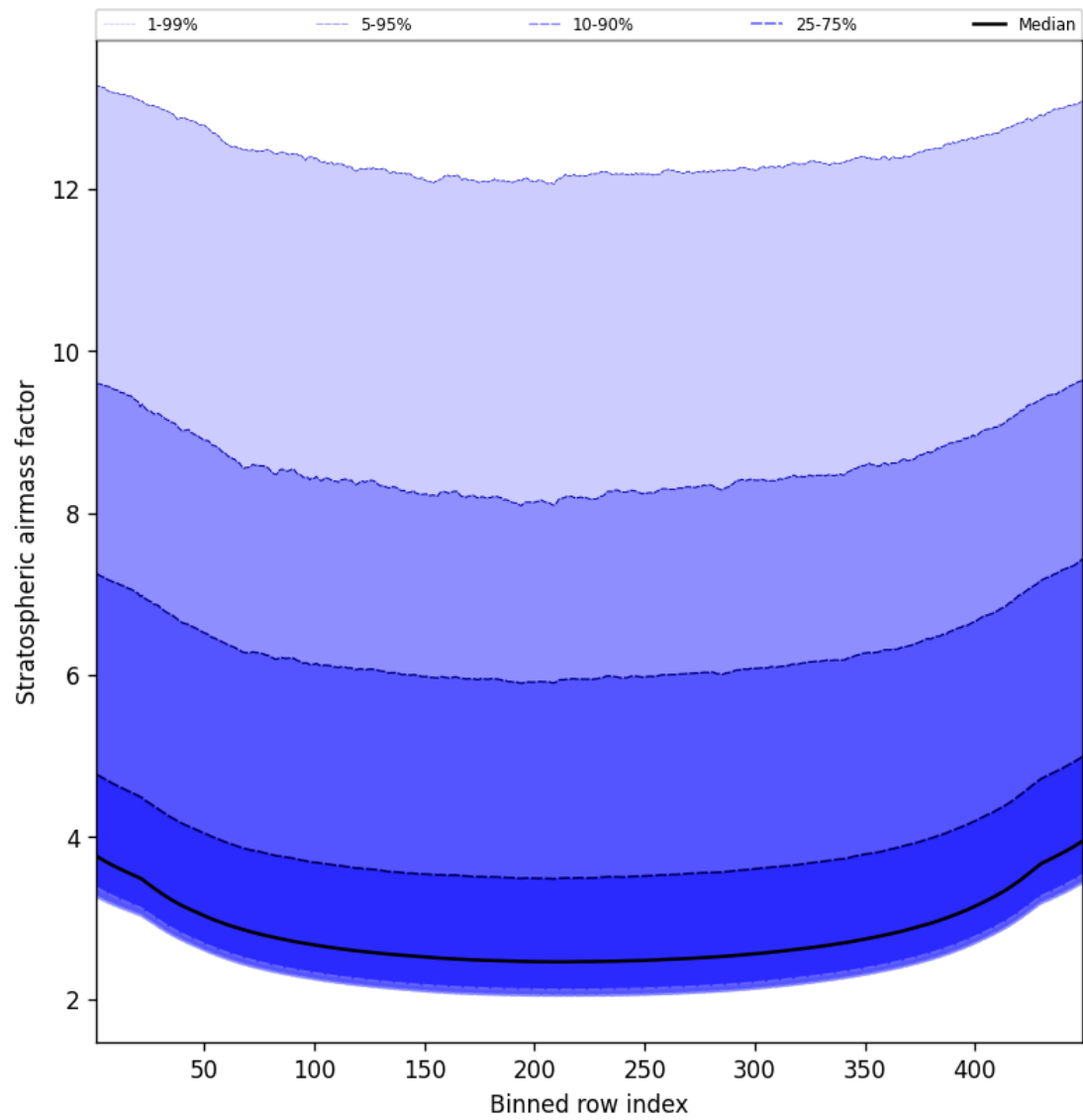
Figure 61: Along track statistics of “Stratospheric airmass factor” for 2024-09-03 to 2024-09-05
