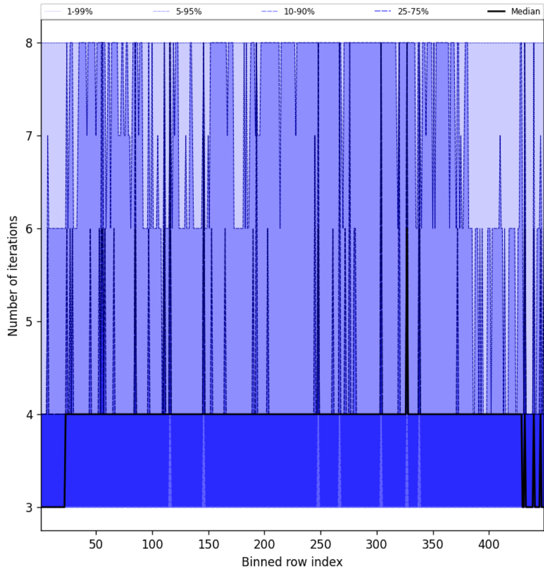
Figure 51: Along track statistics of “Number of iterations” for 2024-09-03 to 2024-09-05
