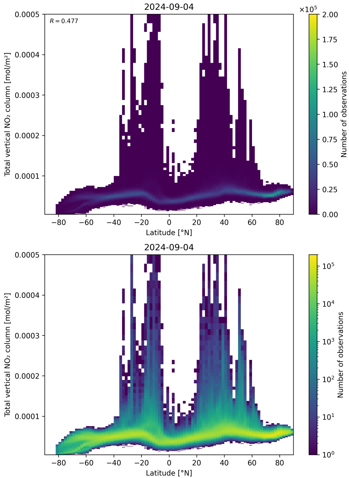
Figure 90: Scatter density plot of “Latitude” against “Total vertical NO 2 column” for 2024-09-03 to 2024-09-05.
