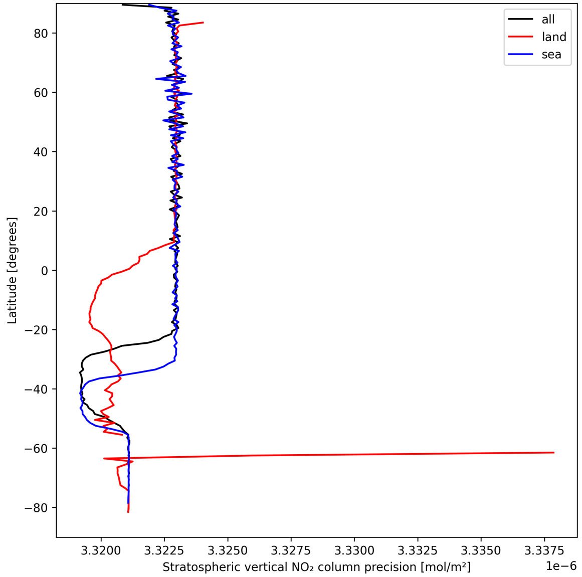
Figure 20: Zonal average of “Stratospheric vertical NO 2 column precision” for 2024-09-03 to 2024-09-05.
