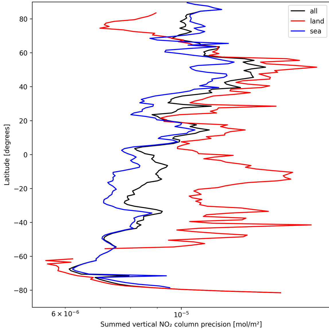
Figure 24: Zonal average of “Summed vertical NO 2 column precision” for 2024-09-03 to 2024-09-05.
