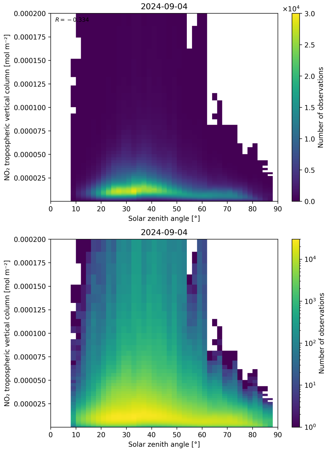
Figure 155: Scatter density plot of “Solar zenith angle” against “NO 2 tropospheric vertical column” for 2024-09-03 to 2024-09-05.
