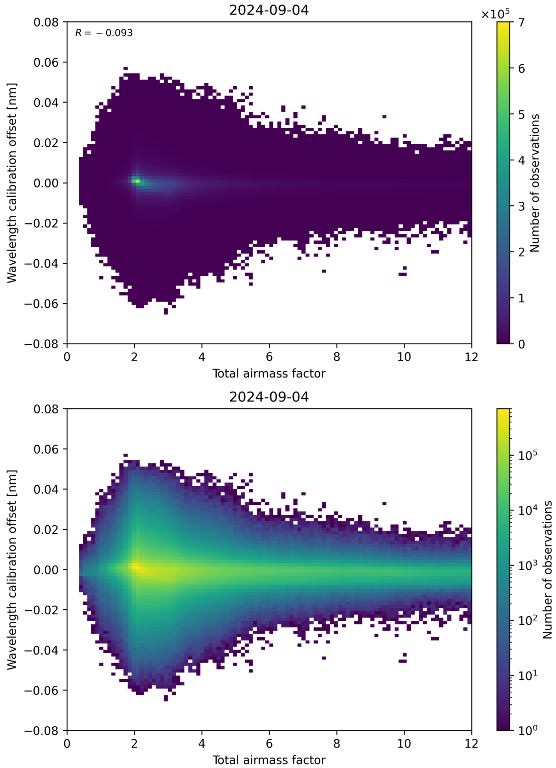
Figure 70: Scatter density plot of “Total airmass factor” against “Wavelength calibration offset” for 2024-09-03 to 2024-09-05.
