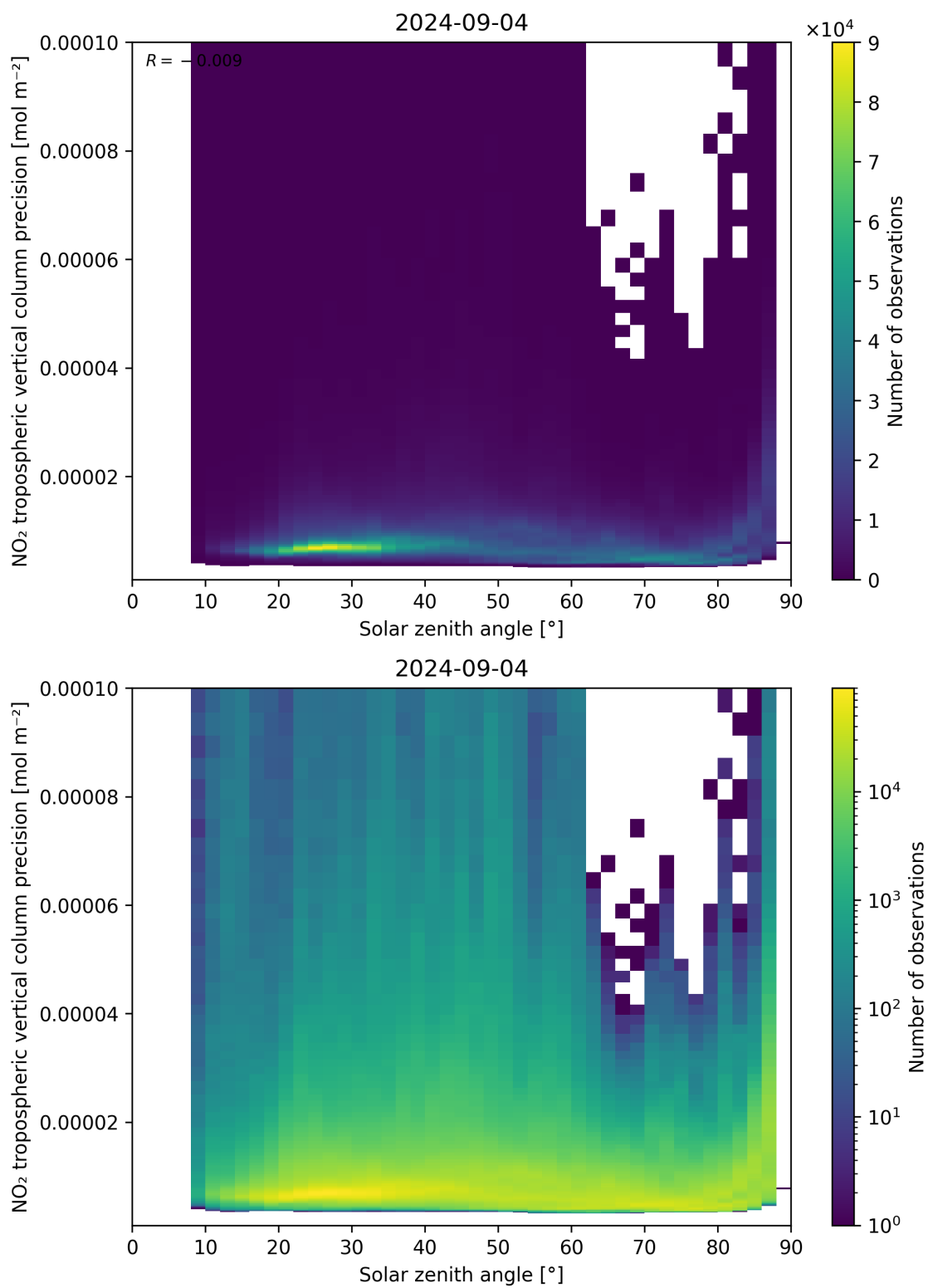
Figure 156: Scatter density plot of “Solar zenith angle” against “NO 2 tropospheric vertical column precision” for 2024-09-03 to 2024-09-05.
