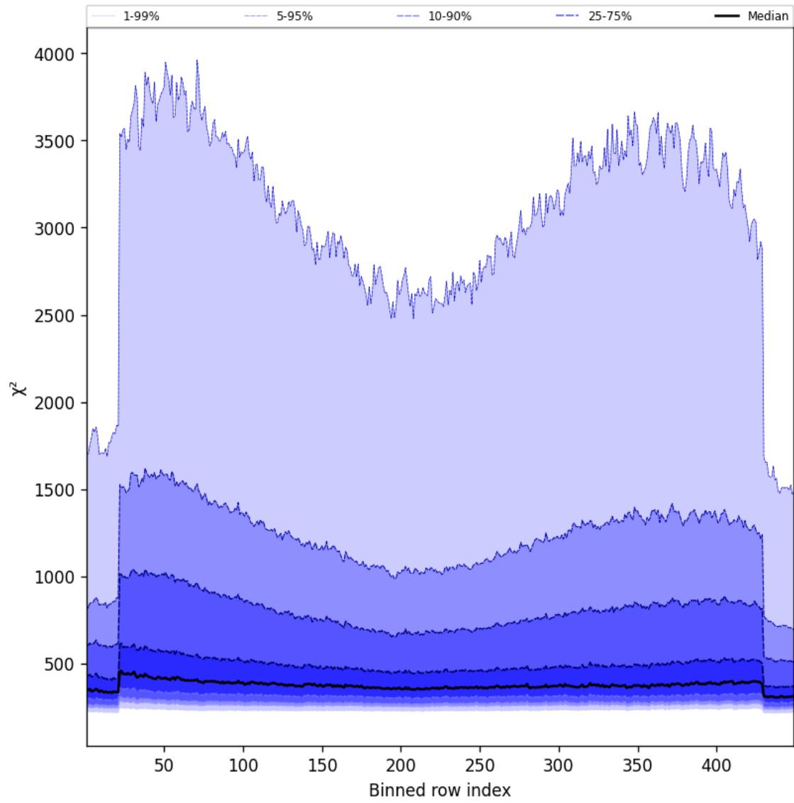
Figure 59: Along track statistics of “ \chi^2 ” for 2024-09-03 to 2024-09-05
