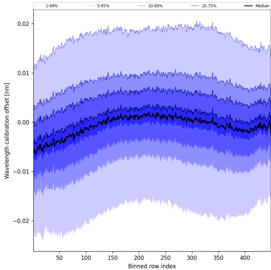
Figure 52: Along track statistics of “Wavelength calibration offset” for 2024-09-03 to 2024-09-05
