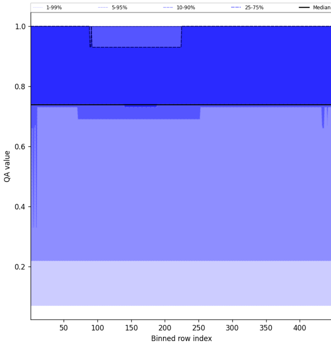
Figure 45: Along track statistics of “QA value” for 2024-09-03 to 2024-09-05
