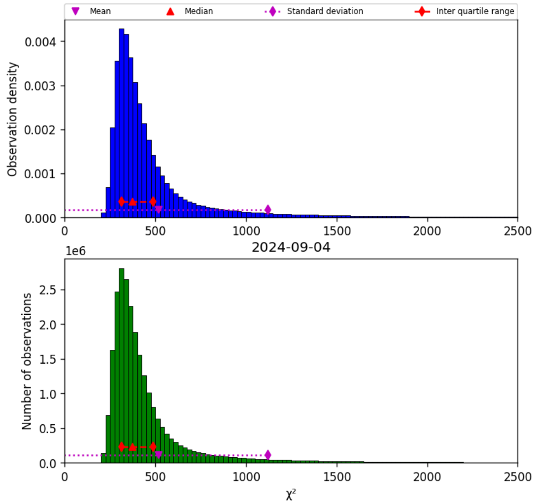
Figure 42: Histogram of " \chi^2 " for 2024-09-03 to 2024-09-05
