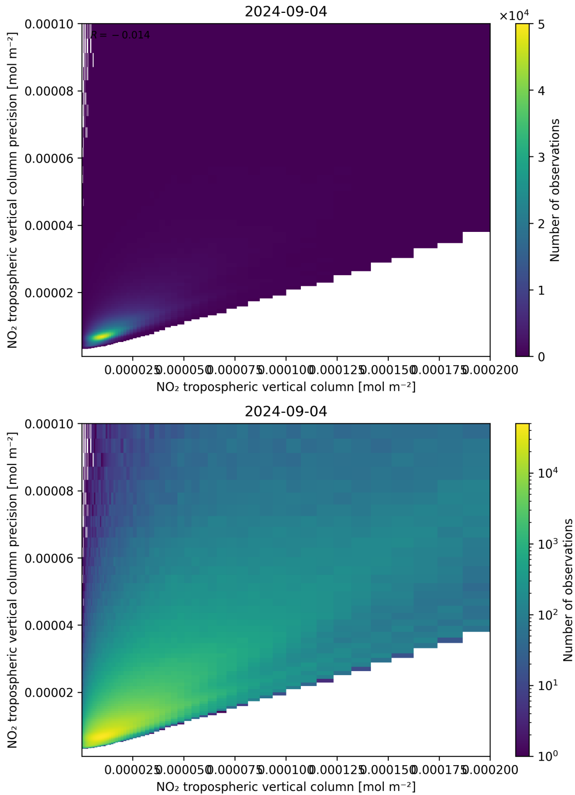
Figure 130: Scatter density plot of “NO 2 tropospheric vertical column” against “NO 2 tropospheric vertical column precision” for 2024-09-03 to 2024-09-05.
