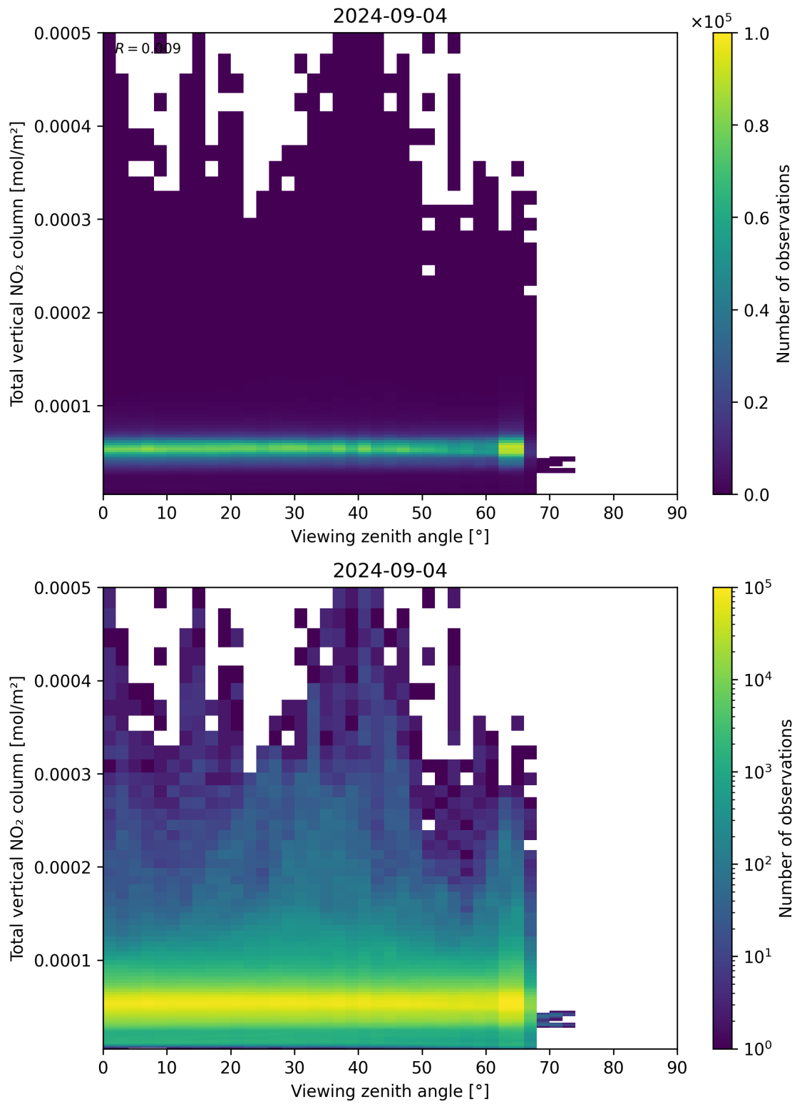
Figure 167: Scatter density plot of “Viewing zenith angle” against “Total vertical NO 2 column” for 2024-09-03 to 2024-09-05.
