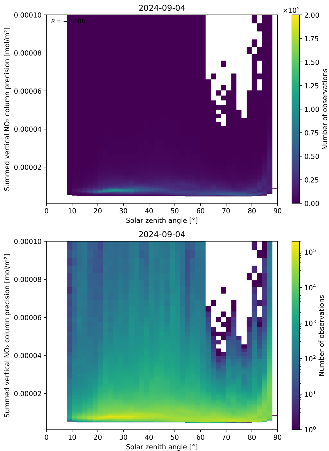
Figure 152: Scatter density plot of “Solar zenith angle” against “Summed vertical NO 2 column precision” for 2024-09-03 to 2024-09-05.
