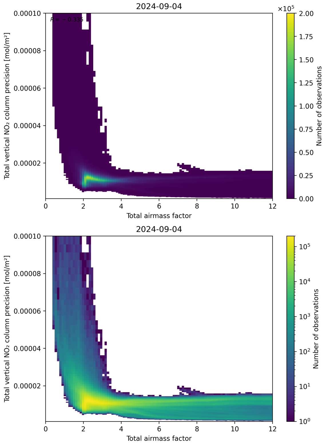
Figure 68: Scatter density plot of “Total airmass factor” against “Total vertical NO 2 column precision” for 2024-09-03 to 2024-09-05.
