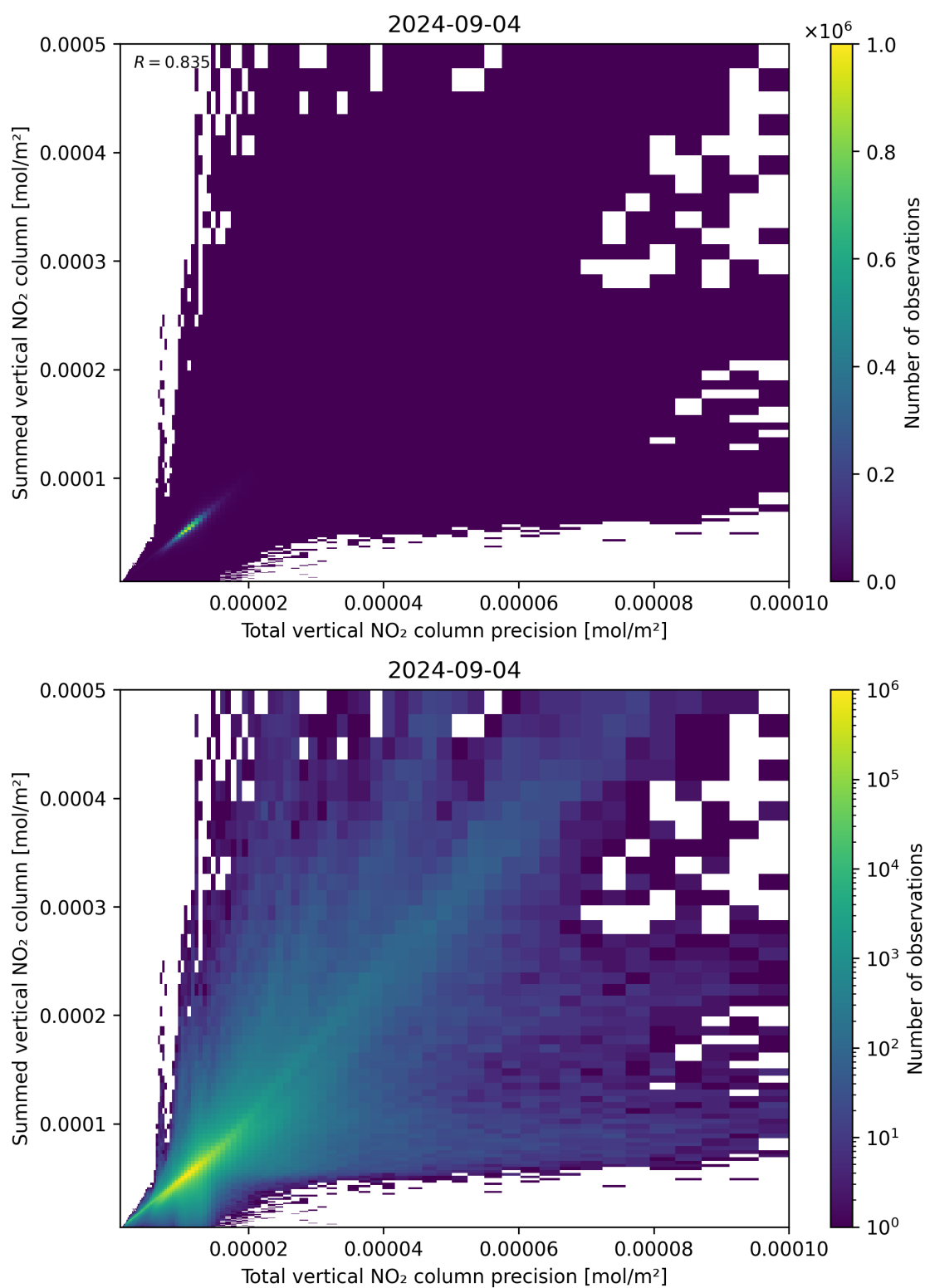
Figure 117: Scatter density plot of “Total vertical NO 2 column precision” against “Summed vertical NO 2 column” for 2024-09-03 to 2024-09-05.
