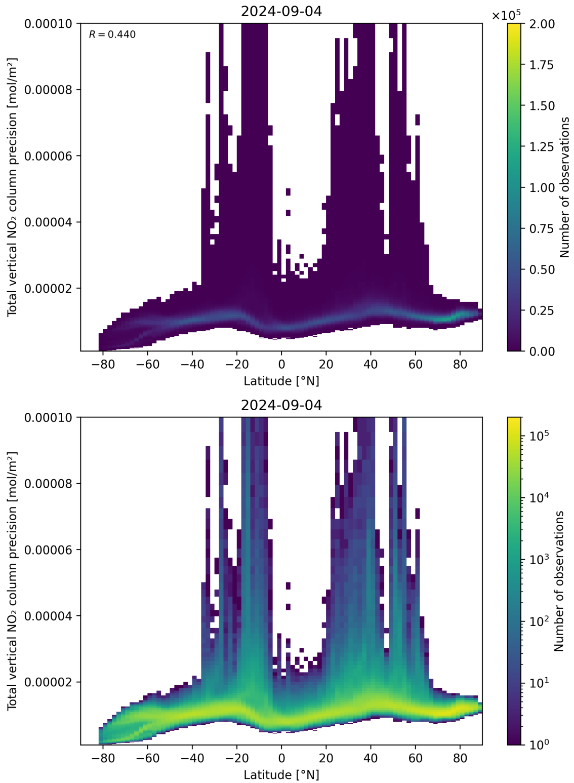
Figure 91: Scatter density plot of “Latitude” against “Total vertical NO 2 column precision” for 2024-09-03 to 2024-09-05.
