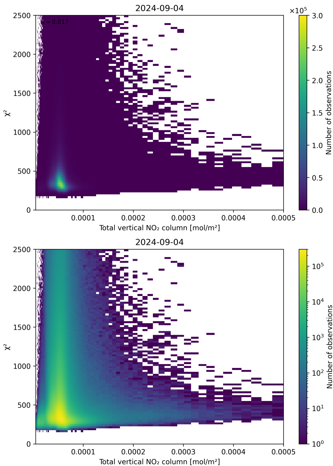
Figure 111: Scatter density plot of “Total vertical NO 2 column” against “ \chi^2 ” for 2024-09-03 to 2024-09-05.
