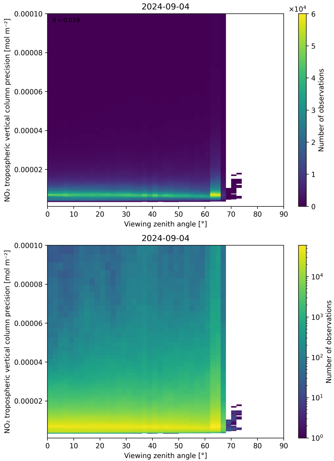
Figure 170: Scatter density plot of “Viewing zenith angle” against “NO 2 tropospheric vertical column precision” for 2024-09-03 to 2024-09-05.
