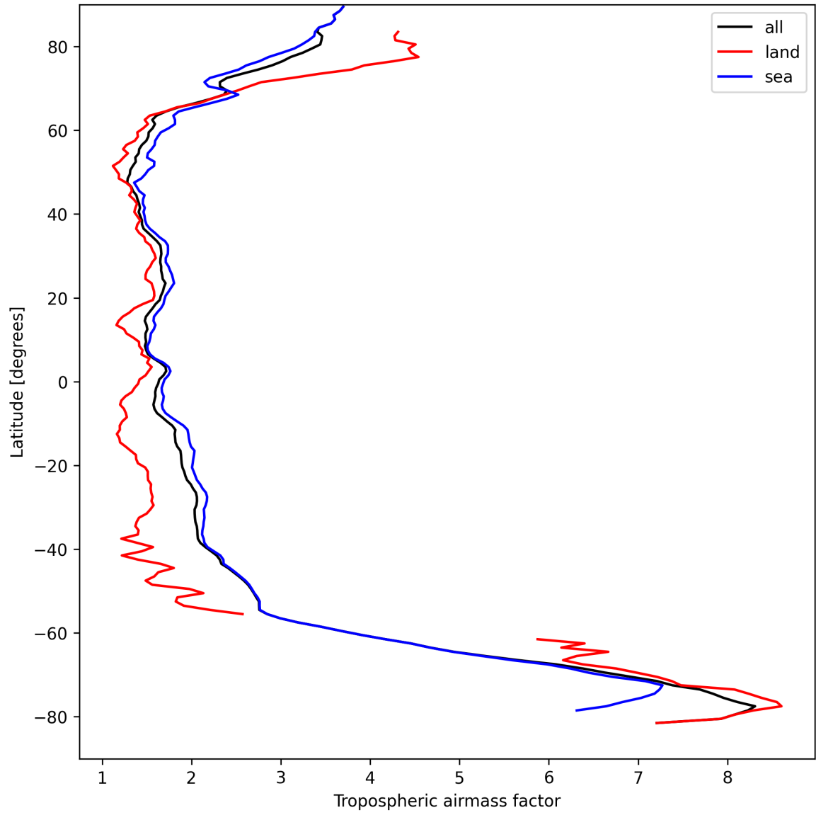
Figure 14: Zonal average of “Tropospheric airmass factor” for 2024-09-03 to 2024-09-05.
