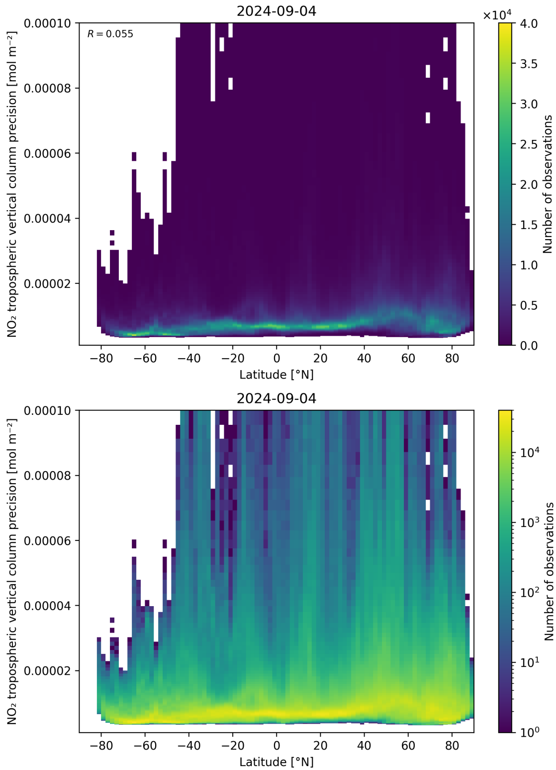
Figure 93: Scatter density plot of “Latitude” against “NO 2 tropospheric vertical column precision” for 2024-09-03 to 2024-09-05.
