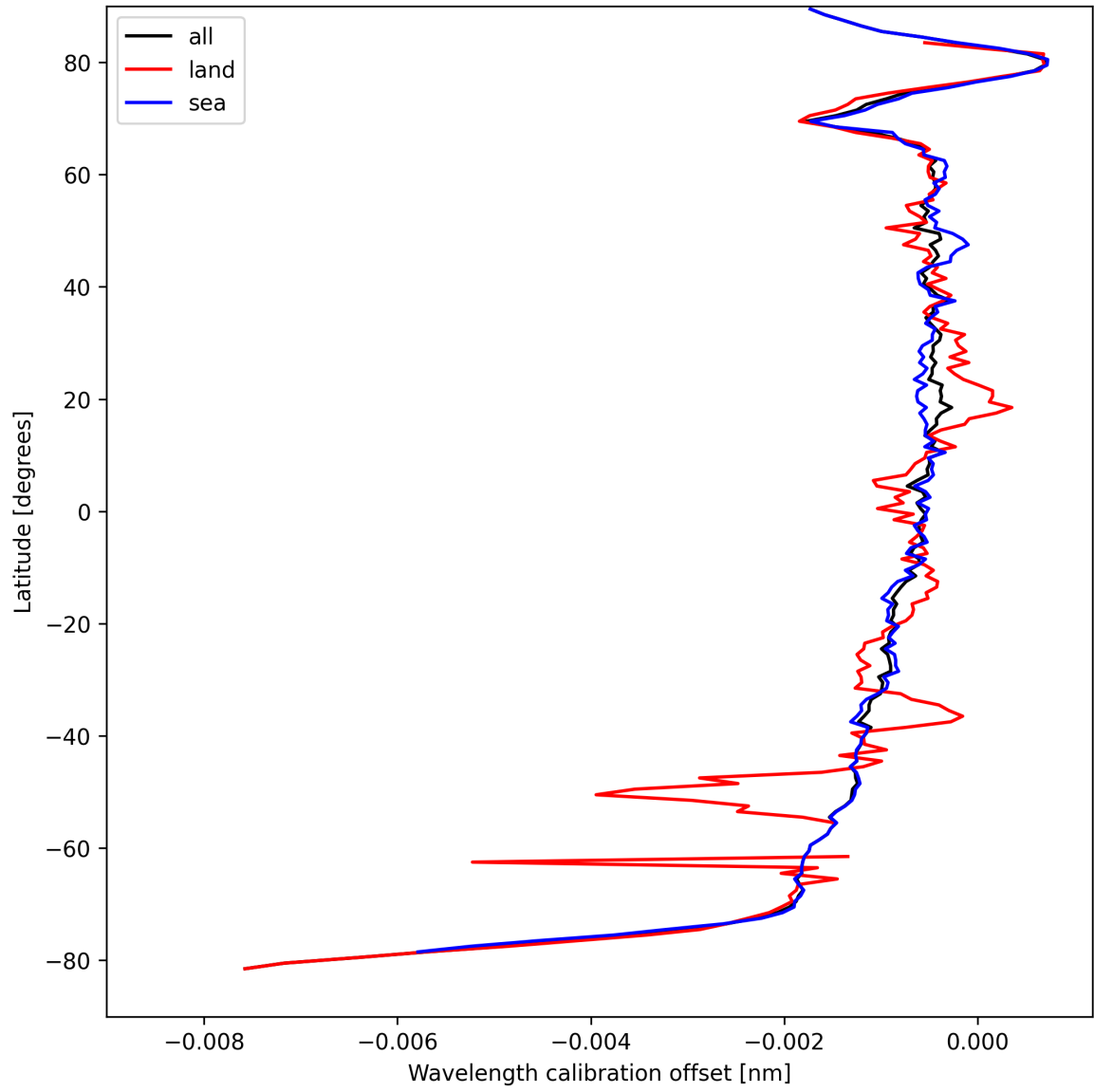
Figure 18: Zonal average of “Wavelength calibration offset” for 2024-09-03 to 2024-09-05.
