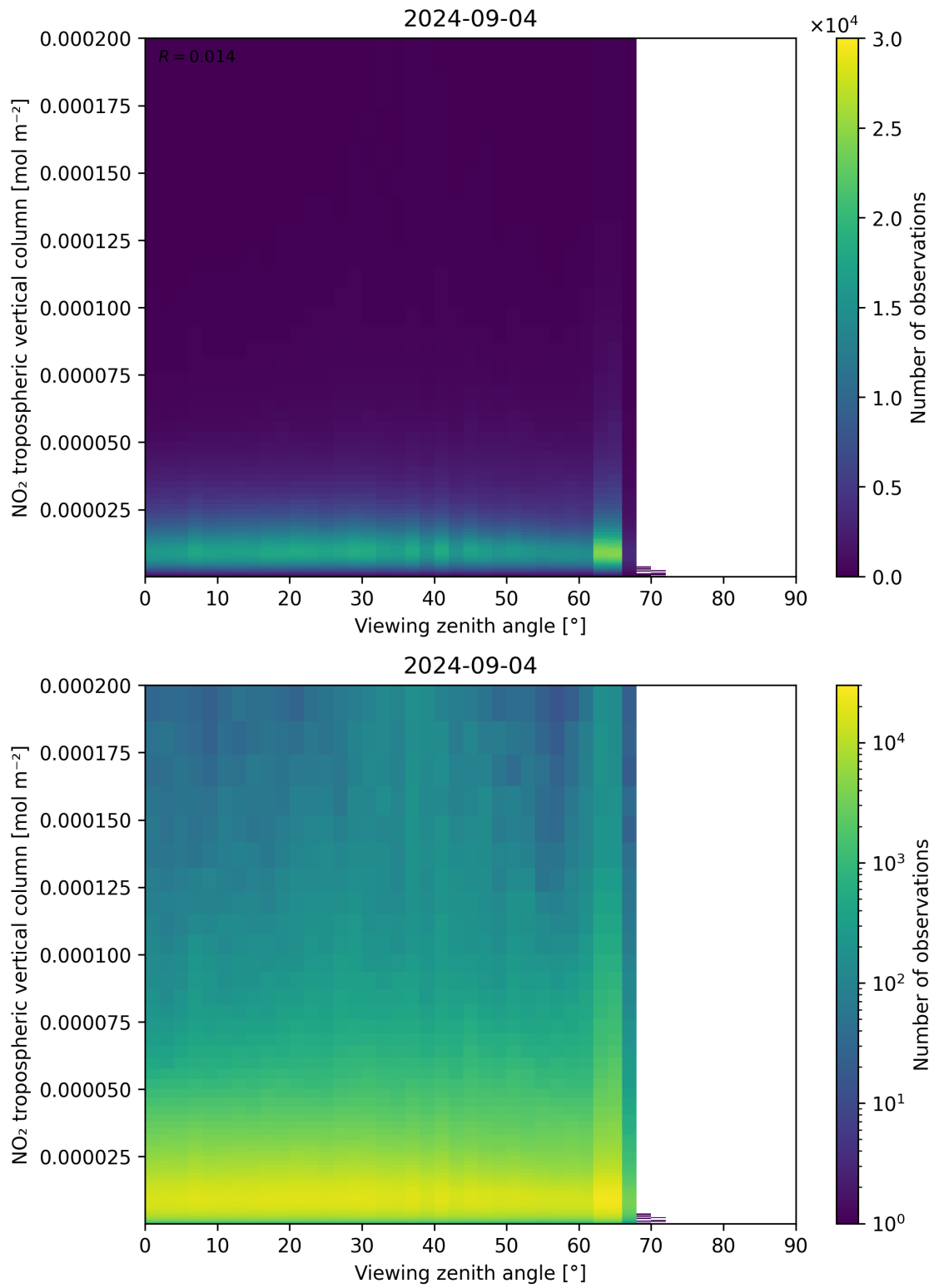
Figure 169: Scatter density plot of “Viewing zenith angle” against “NO 2 tropospheric vertical column” for 2024-09-03 to 2024-09-05.
