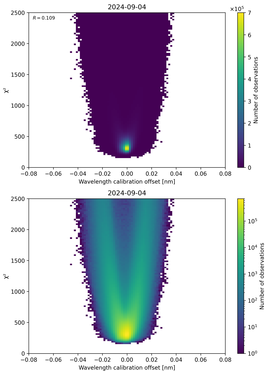
Figure 175: Scatter density plot of “Wavelength calibration offset” against “ \chi^2 ” for 2024-09-03 to 2024-09-05.
