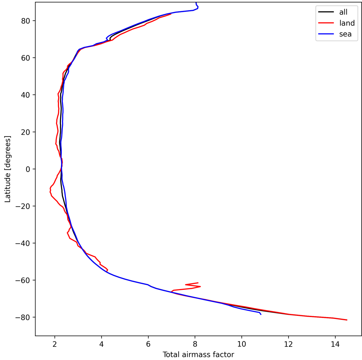
Figure 15: Zonal average of “Total airmass factor” for 2024-09-03 to 2024-09-05.
