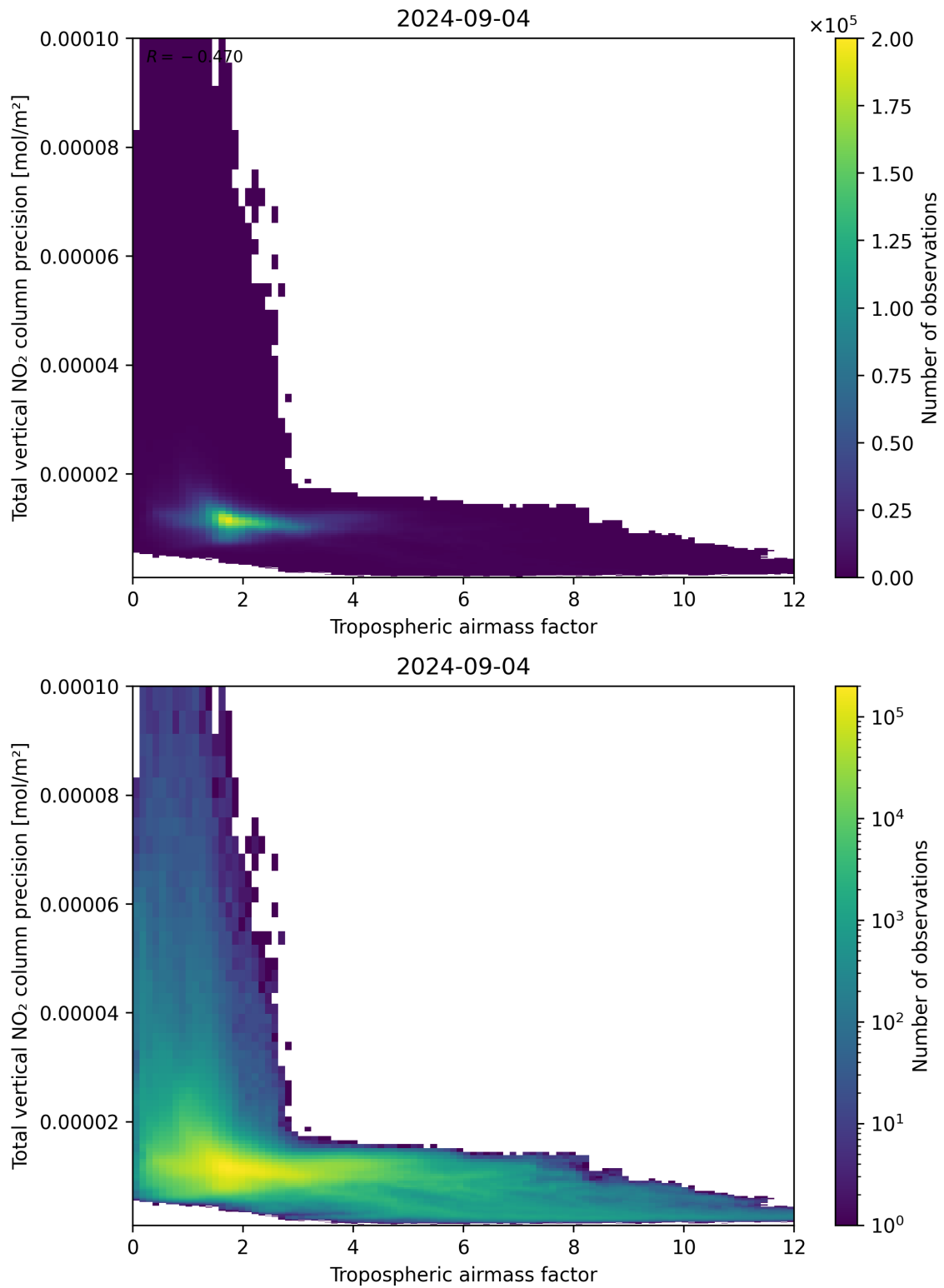
Figure 78: Scatter density plot of “Tropospheric air mass factor” against “Total vertical NO 2 column precision” for 2024-09-03 to 2024-09-05.
