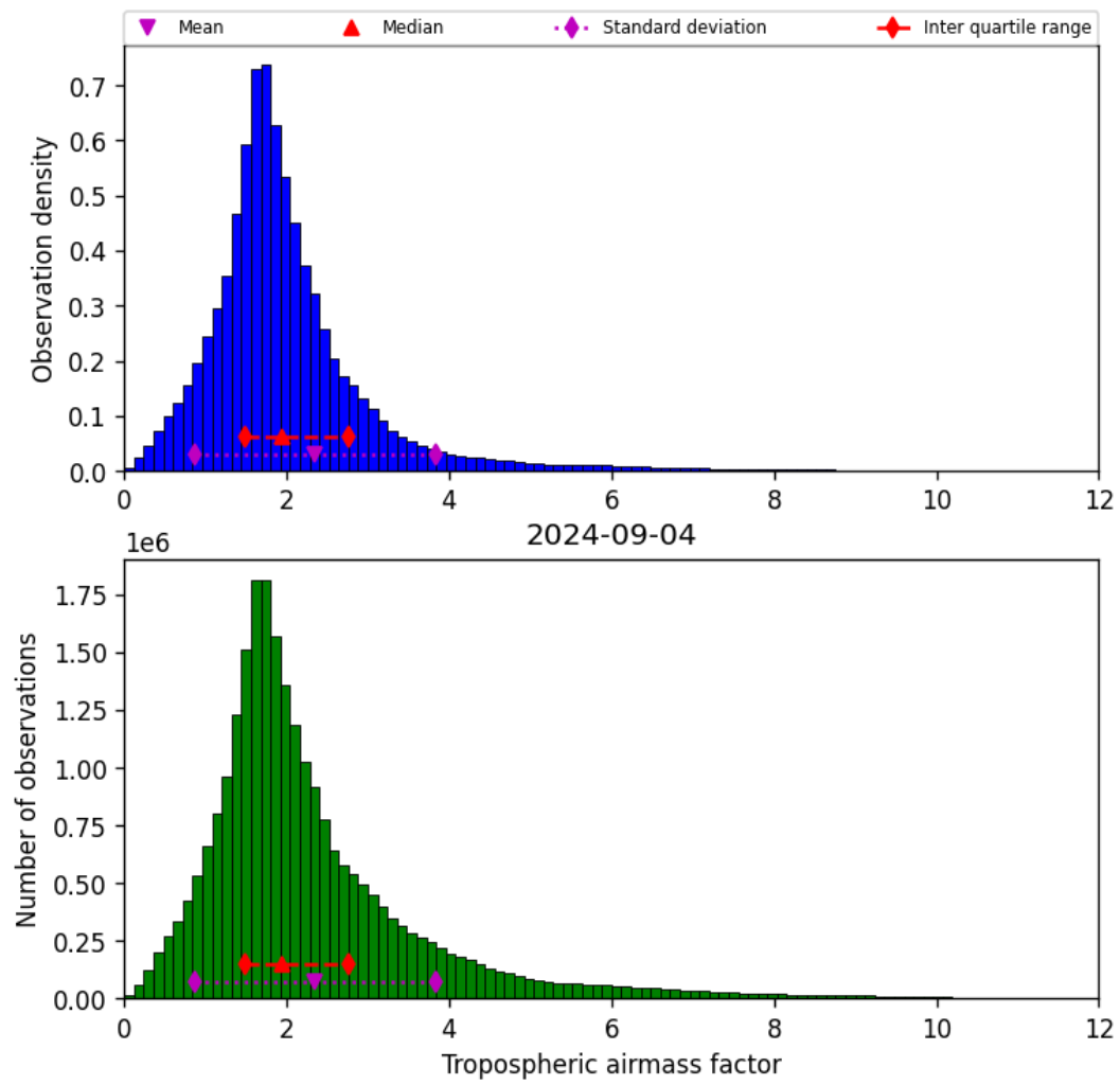
Figure 31: Histogram of “Tropospheric air mass factor” for 2024-09-03 to 2024-09-05
