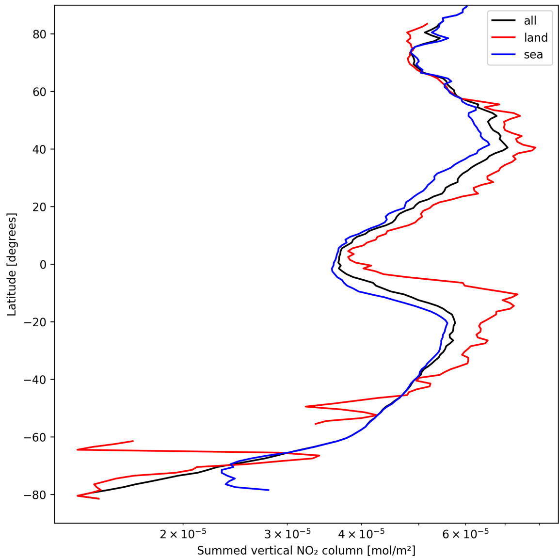
Figure 23: Zonal average of “Summed vertical NO 2 column” for 2024-09-03 to 2024-09-05.
