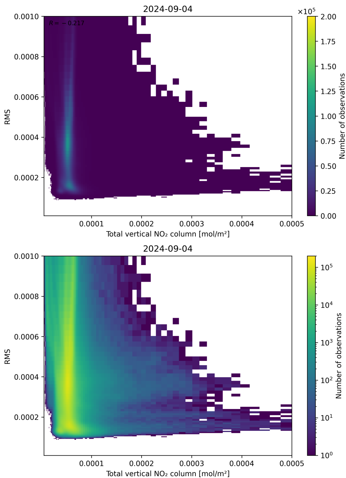
Figure 120: Scatter density plot of “Total vertical NO 2 column” against “RMS” for 2024-09-03 to 2024-09-05.
