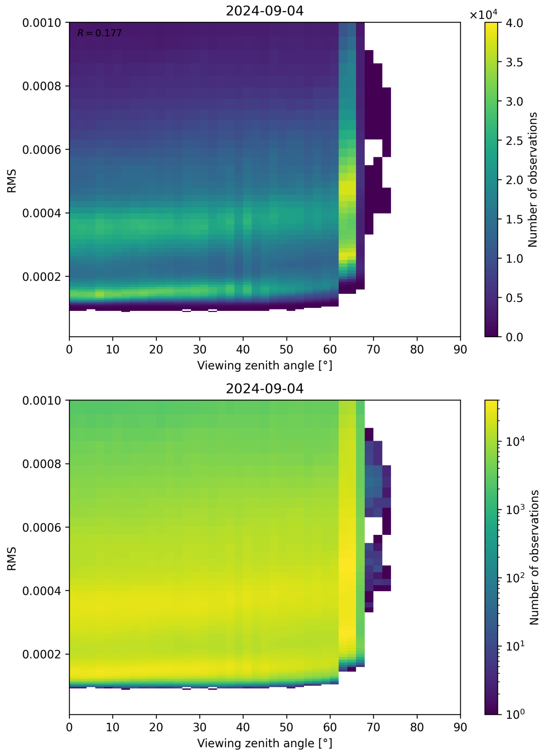
Figure 171: Scatter density plot of “Viewing zenith angle” against “RMS” for 2024-09-03 to 2024-09-05.
