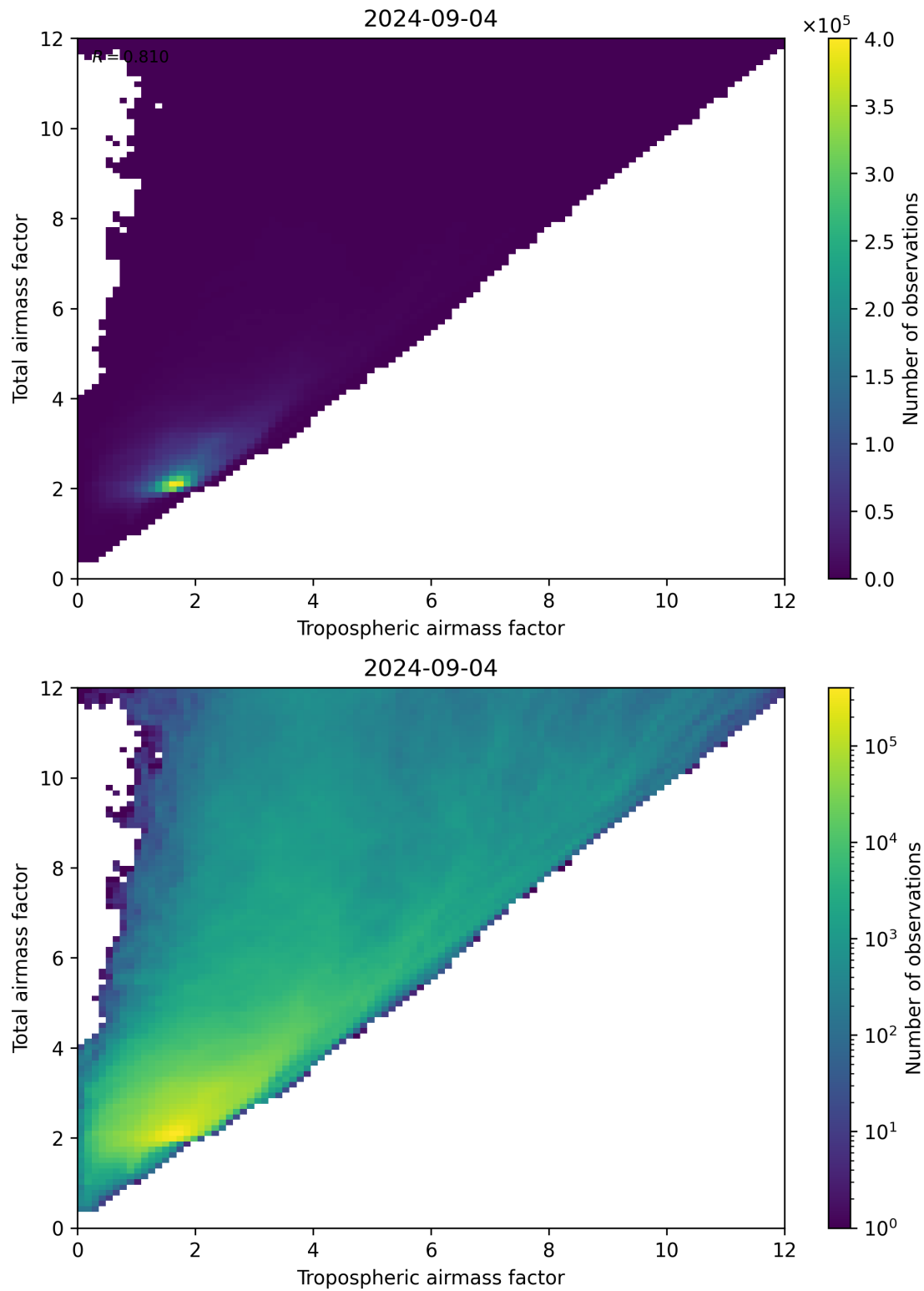
Figure 72: Scatter density plot of “Tropospheric airmass factor” against “Total airmass factor” for 2024-09-03 to 2024-09-05.
