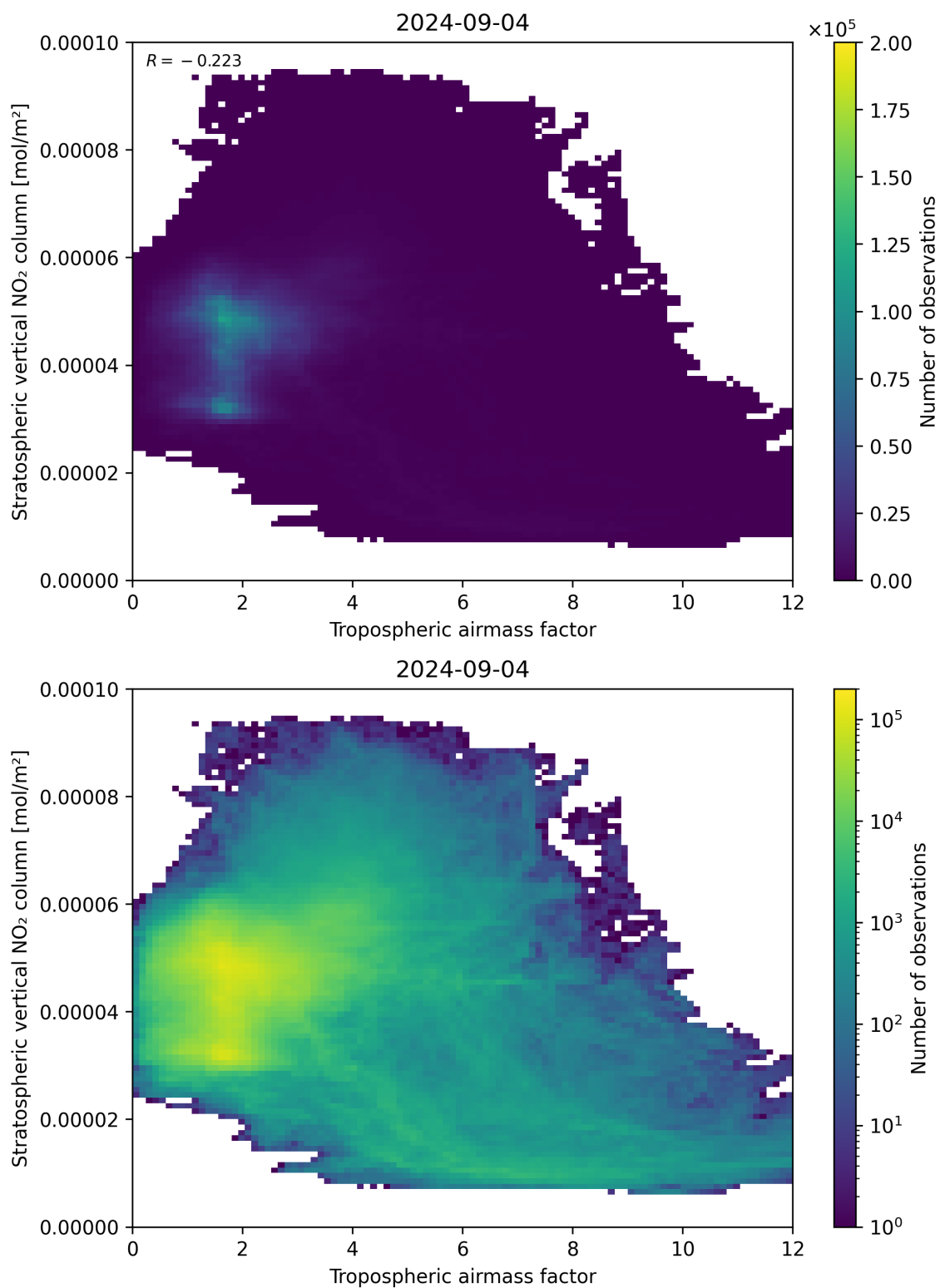
Figure 74: Scatter density plot of “Tropospheric air mass factor” against “Stratospheric vertical NO 2 column” for 2024-09-03 to 2024-09-05.
