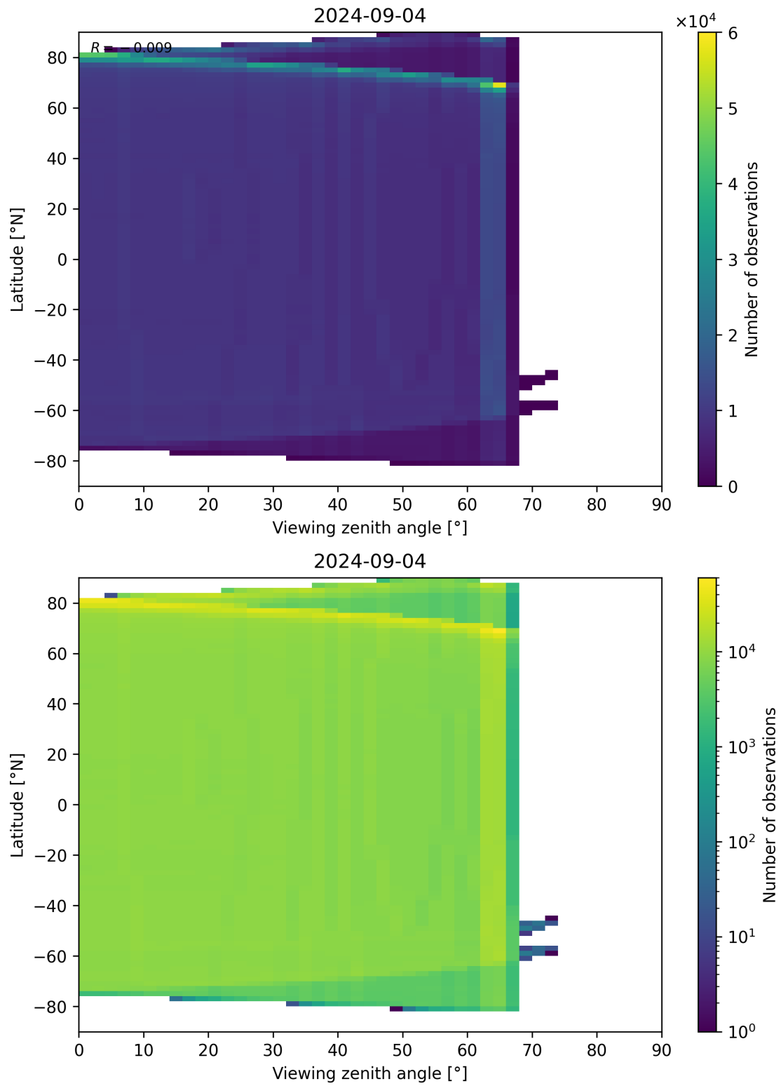
Figure 163: Scatter density plot of “Viewing zenith angle” against “Latitude” for 2024-09-03 to 2024-09-05.
