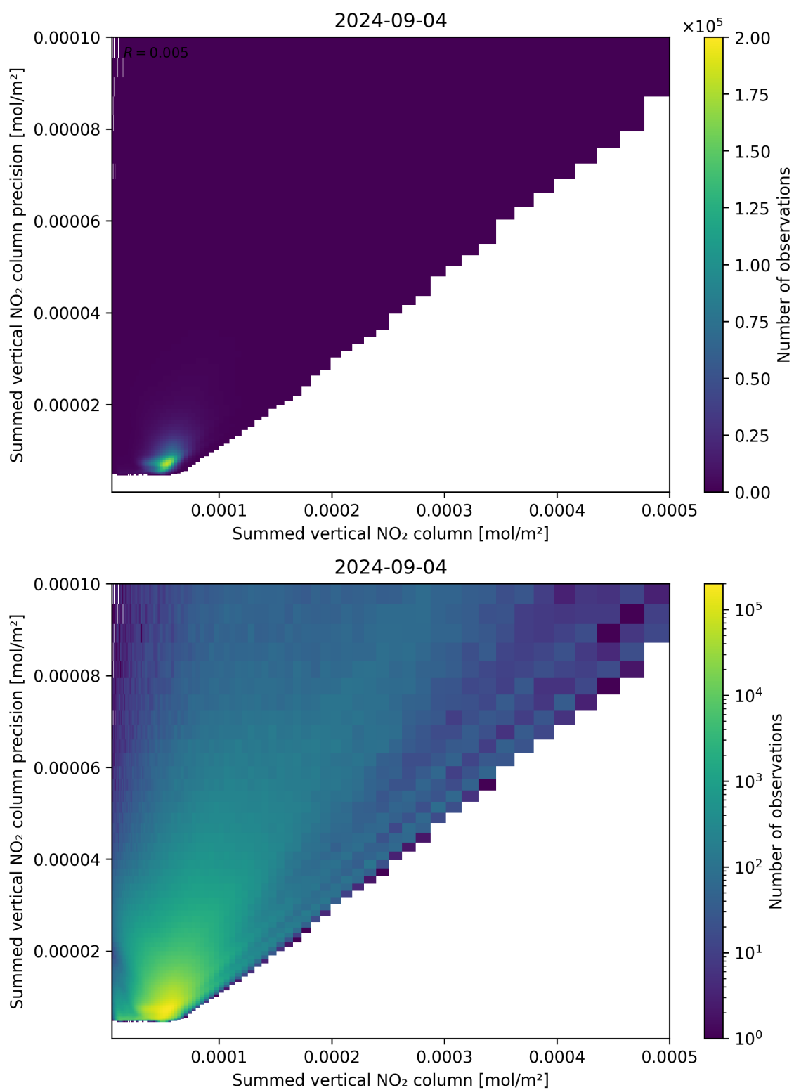
Figure 105: Scatter density plot of “Summed vertical NO 2 column” against “Summed vertical NO 2 column precision” for 2024-09-03 to 2024-09-05.
