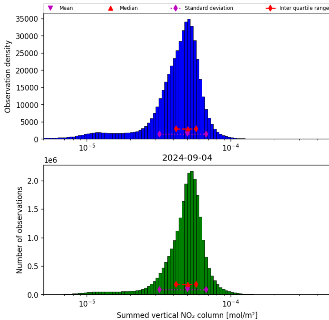
Figure 40: Histogram of “Summed vertical NO 2 column” for 2024-09-03 to 2024-09-05
