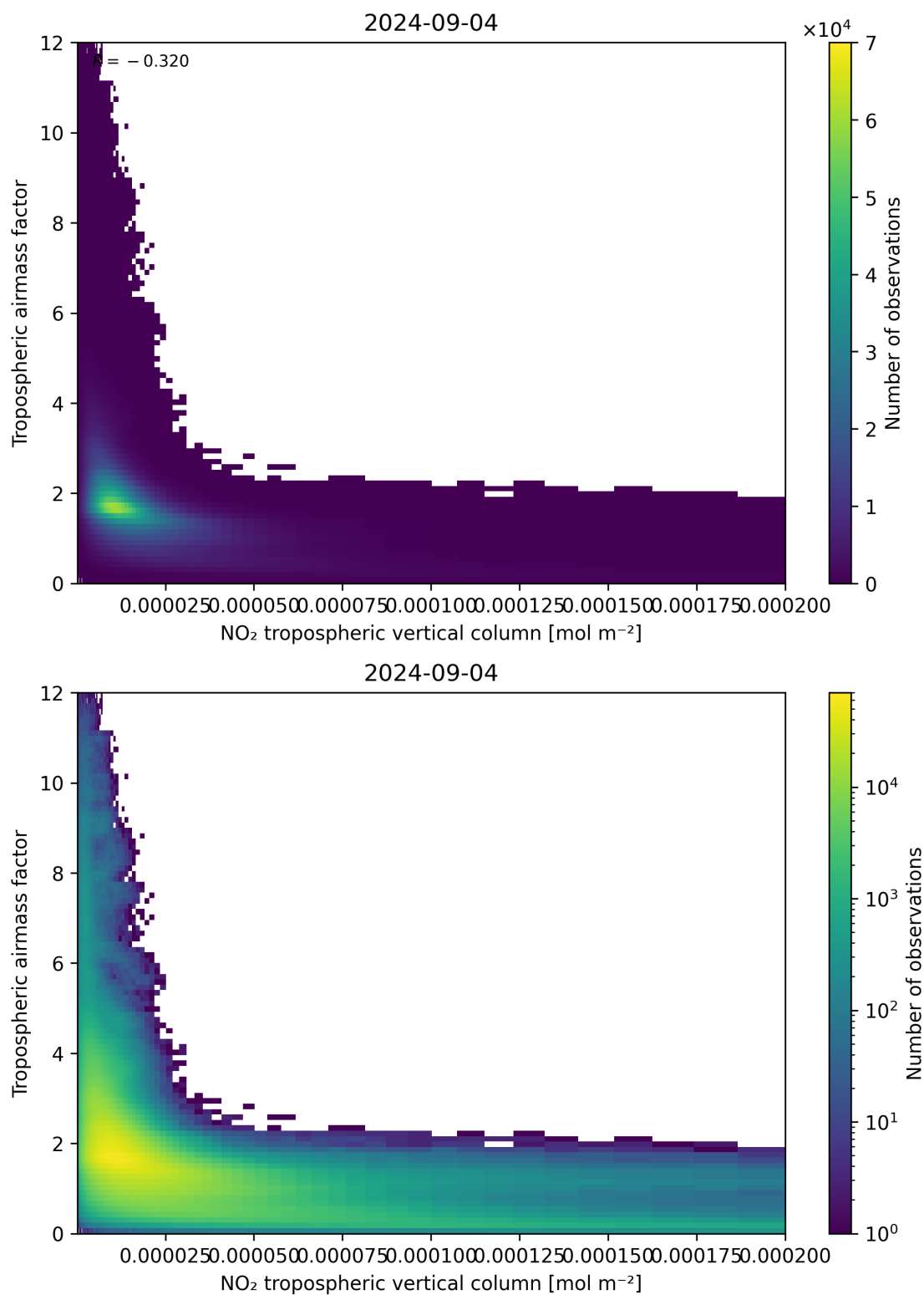
Figure 123: Scatter density plot of “NO 2 tropospheric vertical column” against “Tropospheric air mass factor” for 2024-09-03 to 2024-09-05.
