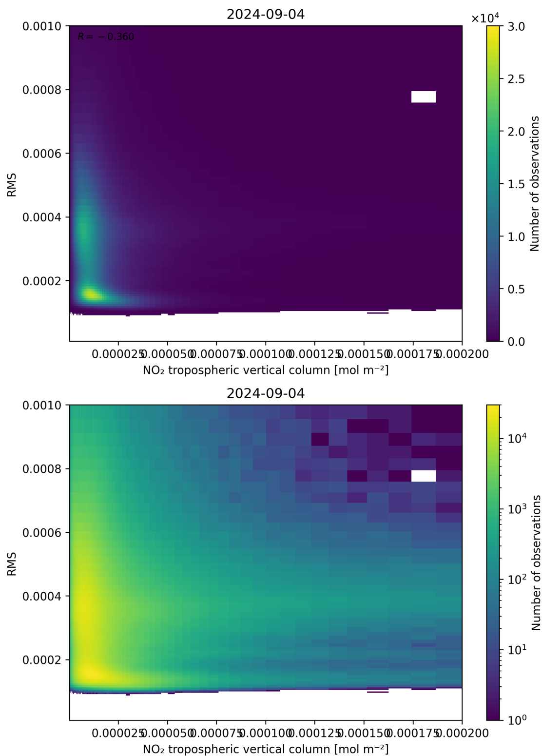
Figure 142: Scatter density plot of “NO 2 tropospheric vertical column” against “RMS” for 2024-09-03 to 2024-09-05.
