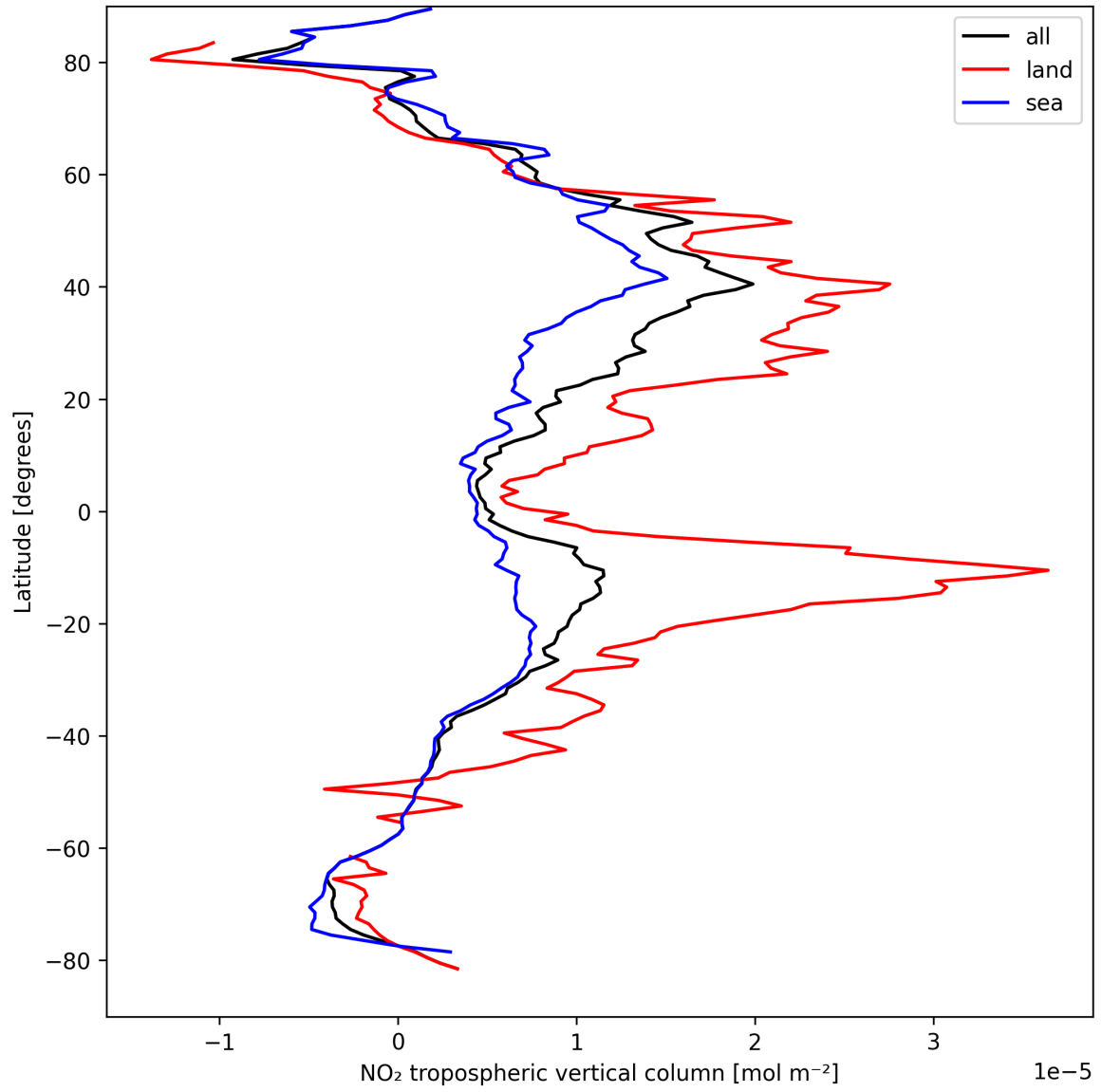
Figure 12: Zonal average of “NO 2 tropospheric vertical column” for 2024-09-03 to 2024-09-05.
