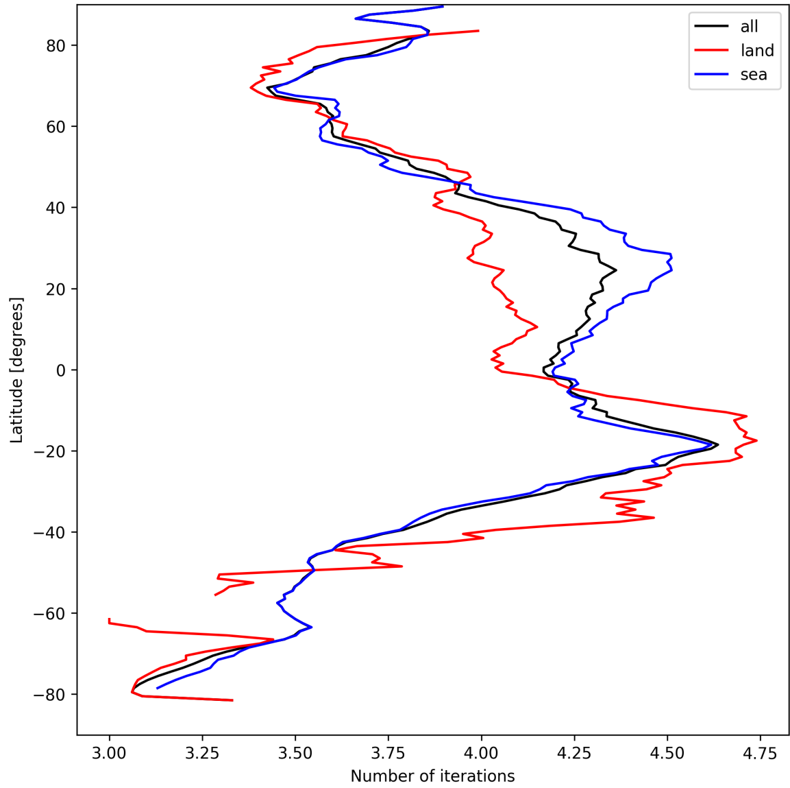
Figure 17: Zonal average of “Number of iterations” for 2024-09-03 to 2024-09-05.
