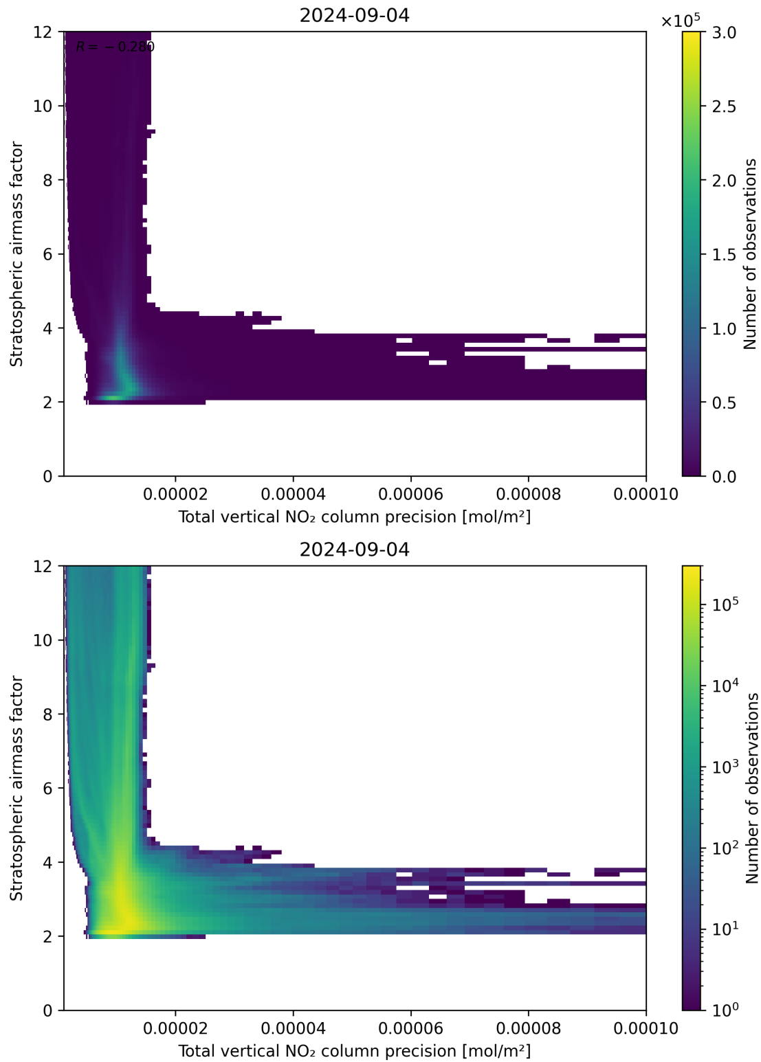
Figure 115: Scatter density plot of “Total vertical NO 2 column precision” against “Stratospheric air mass factor” for 2024-09-03 to 2024-09-05.
