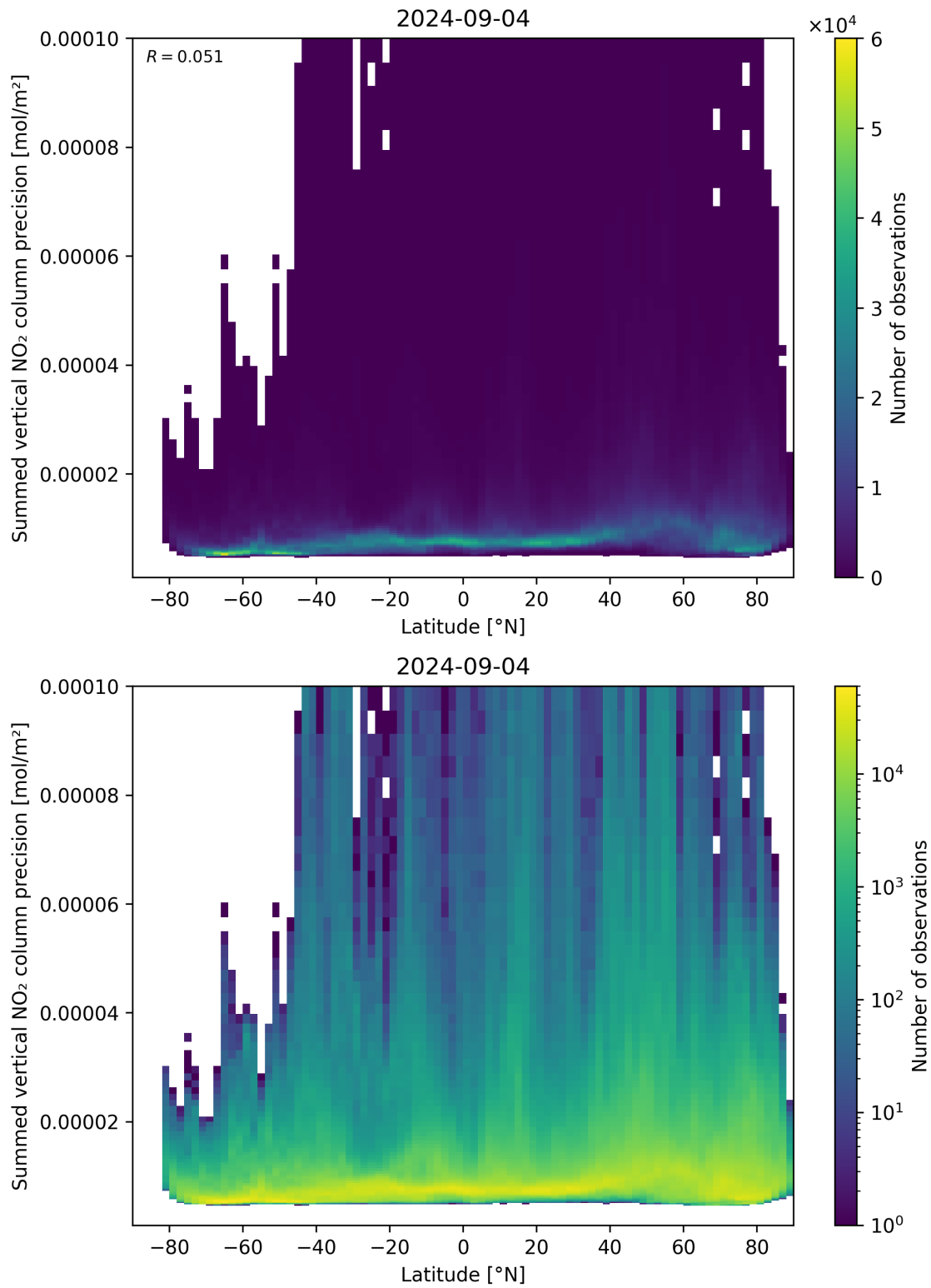
Figure 89: Scatter density plot of “Latitude” against “Summed vertical NO 2 column precision” for 2024-09-03 to 2024-09-05.
