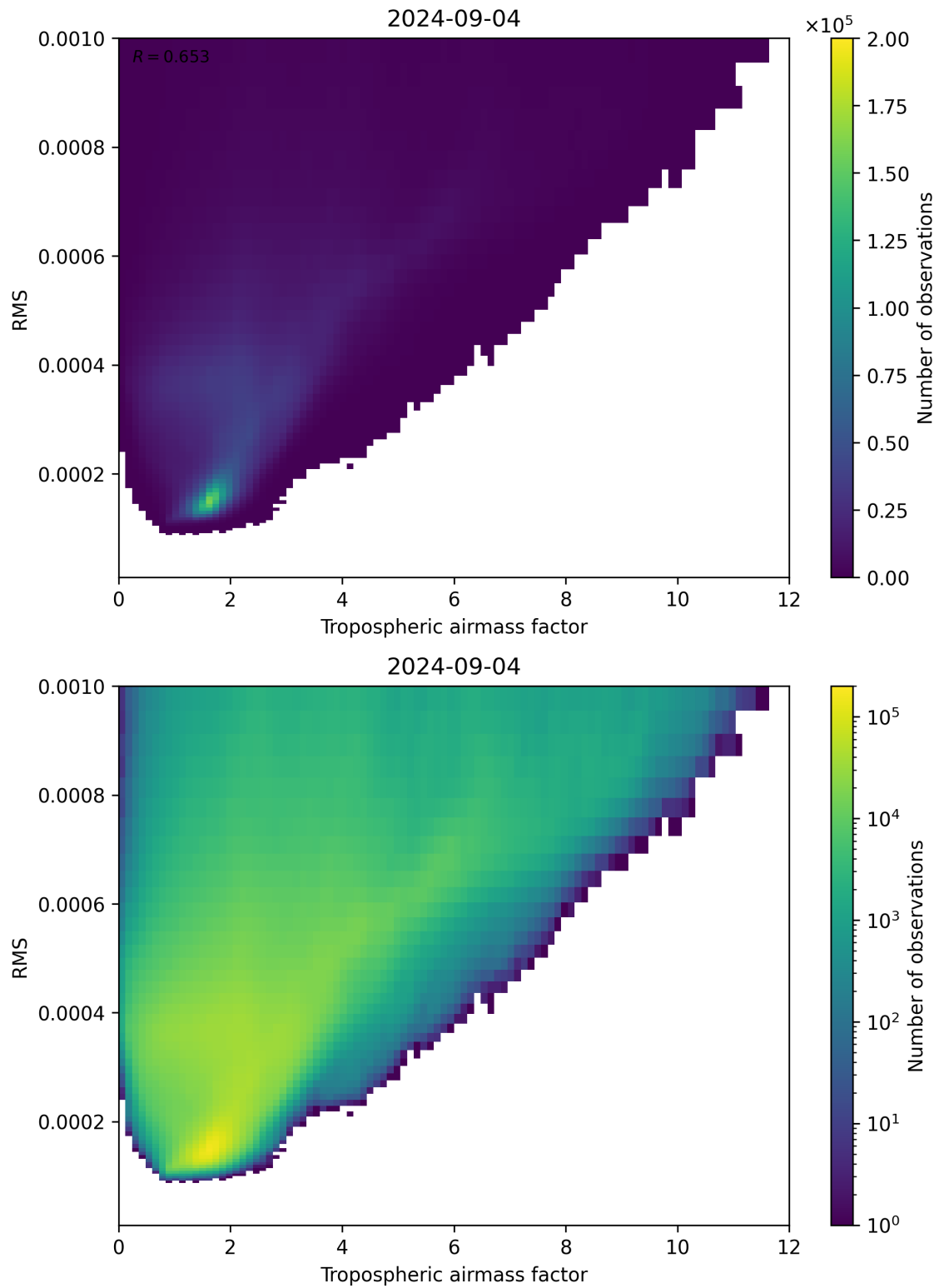
Figure 79: Scatter density plot of “Tropospheric airmass factor” against “RMS” for 2024-09-03 to 2024-09-05.
