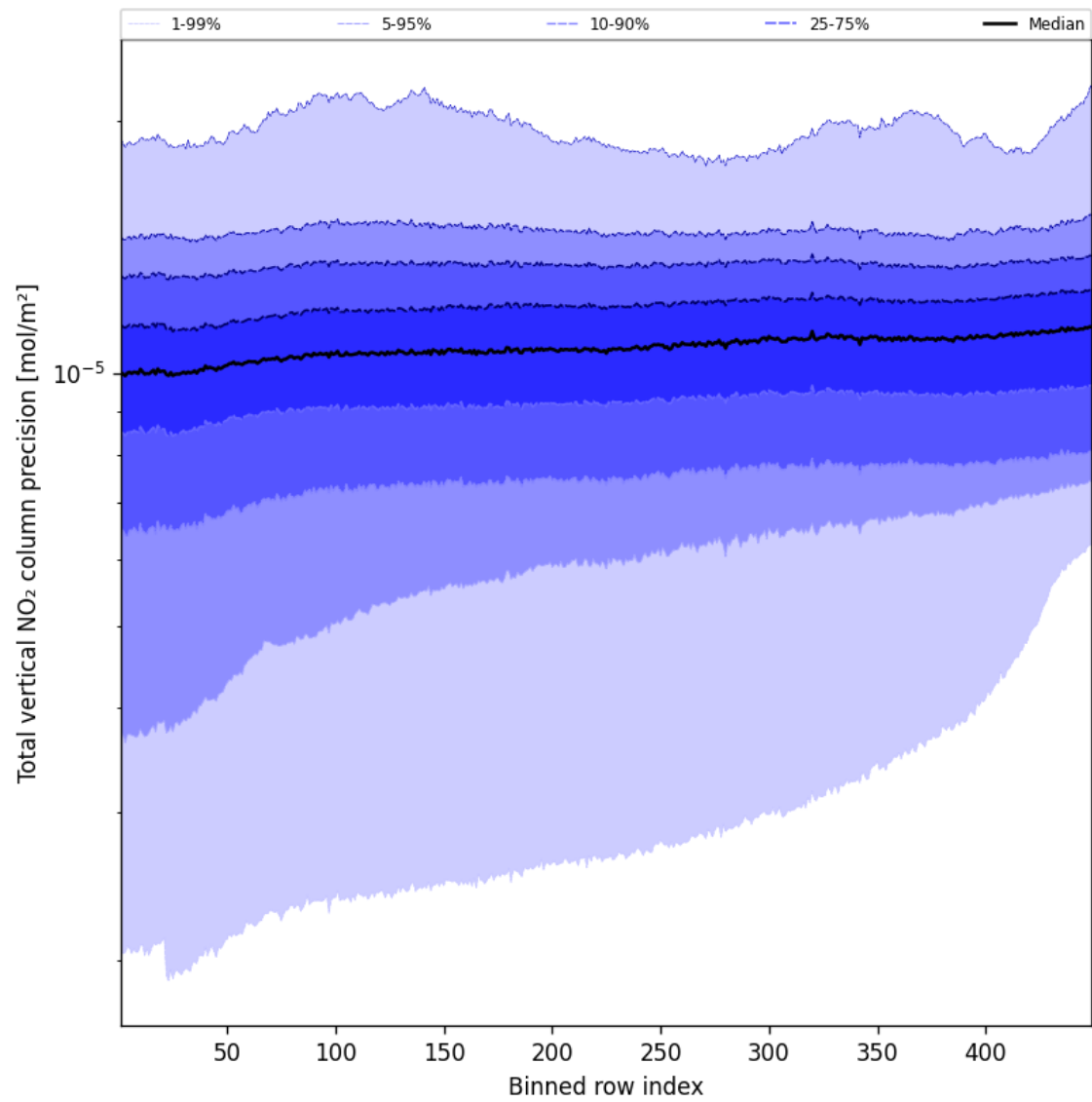
Figure 56: Along track statistics of “Total vertical NO 2 column precision” for 2024-09-03 to 2024-09-05
