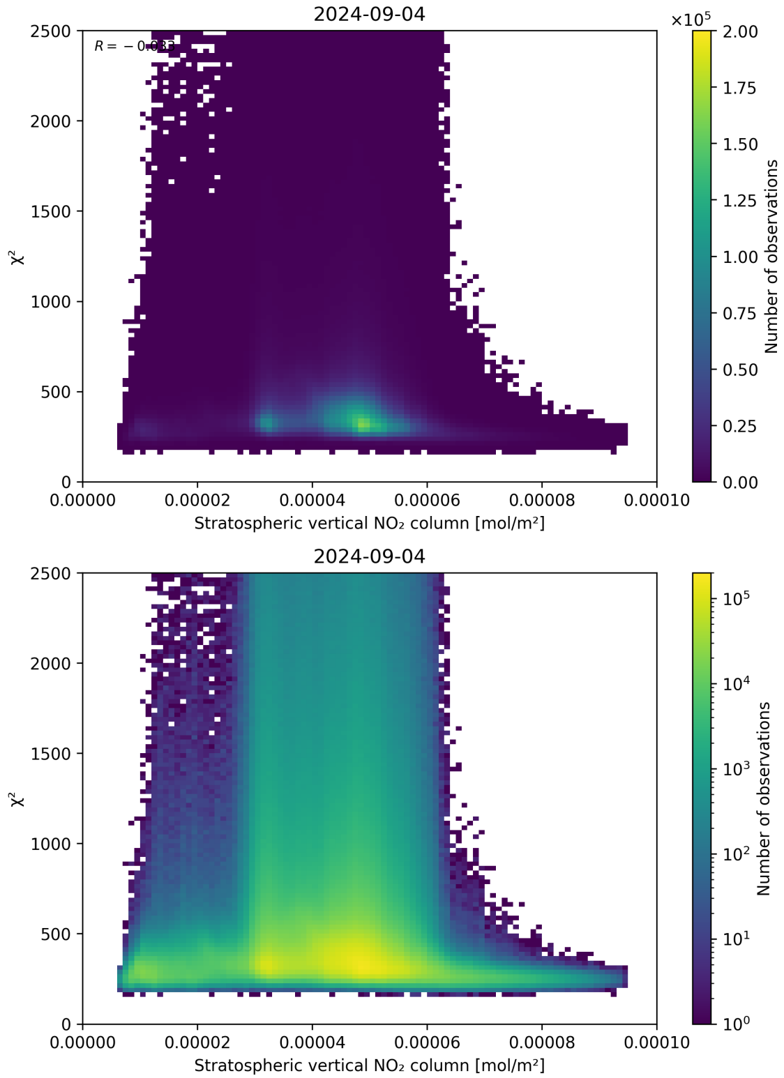
Figure 97: Scatter density plot of “Stratospheric vertical NO 2 column” against “ \chi^2 ” for 2024-09-03 to 2024-09-05.
