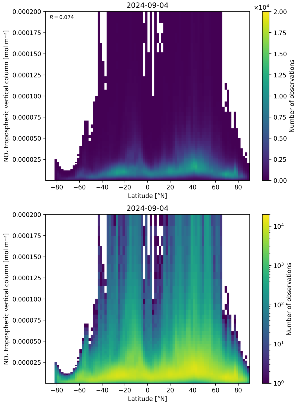
Figure 92: Scatter density plot of “Latitude” against “NO 2 tropospheric vertical column” for 2024-09-03 to 2024-09-05.
