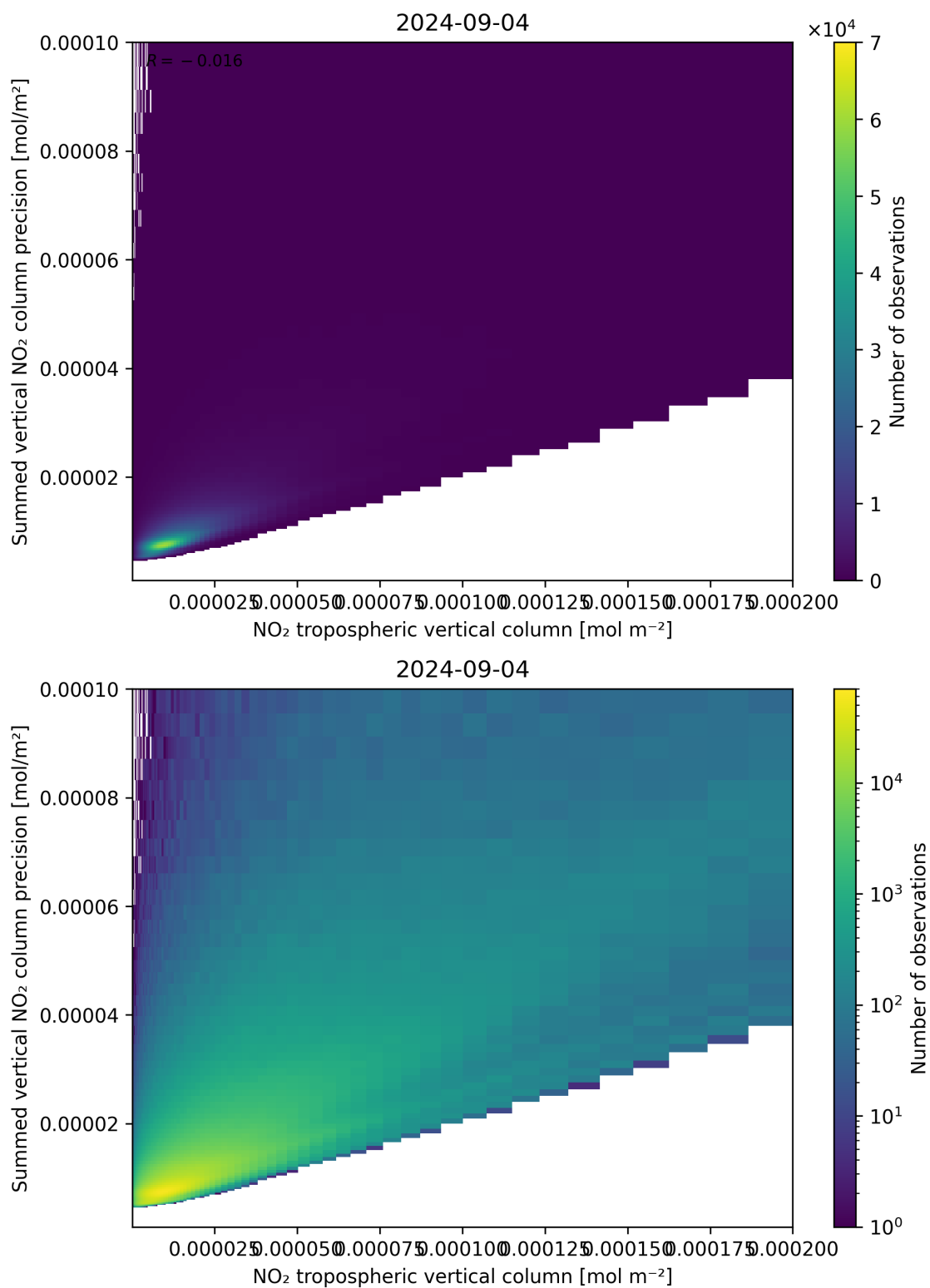
Figure 127: Scatter density plot of “NO 2 tropospheric vertical column” against “Summed vertical NO 2 column precision” for 2024-09-03 to 2024-09-05.
