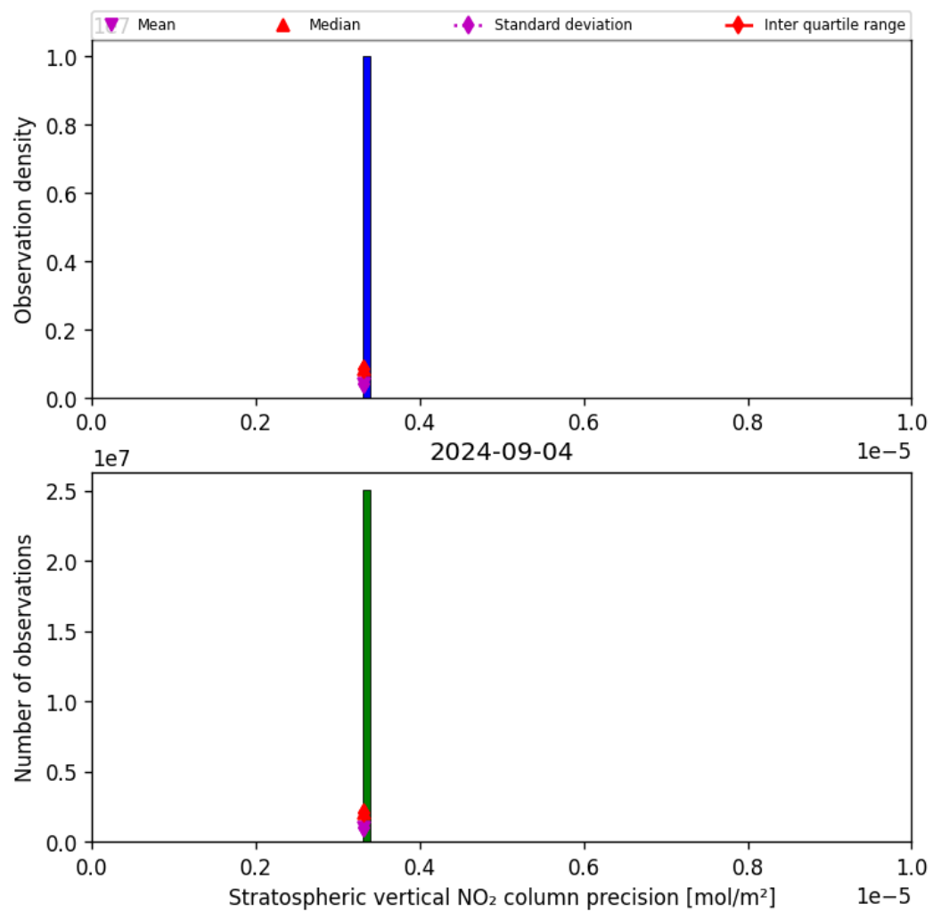
Figure 37: Histogram of “Stratospheric vertical NO 2 column precision” for 2024-09-03 to 2024-09-05
