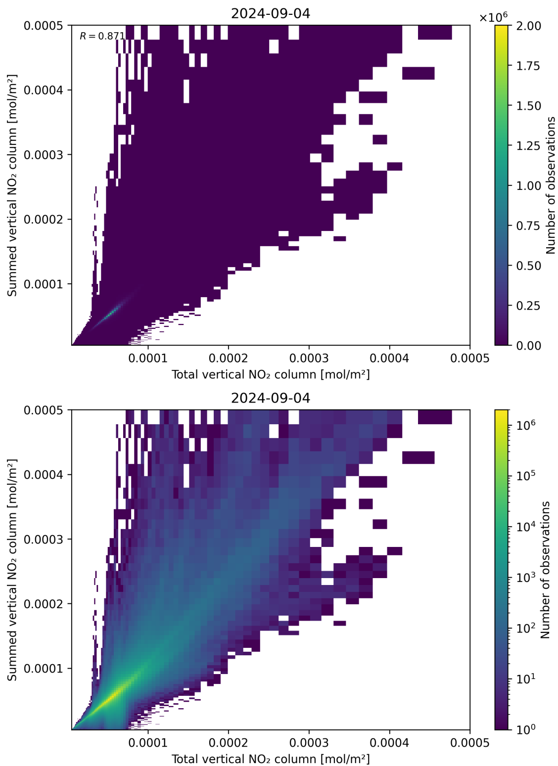
Figure 112: Scatter density plot of “Total vertical NO 2 column” against “Summed vertical NO 2 column” for 2024-09-03 to 2024-09-05.
