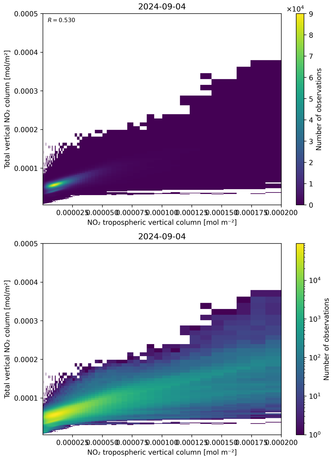
Figure 128: Scatter density plot of “NO 2 tropospheric vertical column” against “Total vertical NO 2 column” for 2024-09-03 to 2024-09-05.
