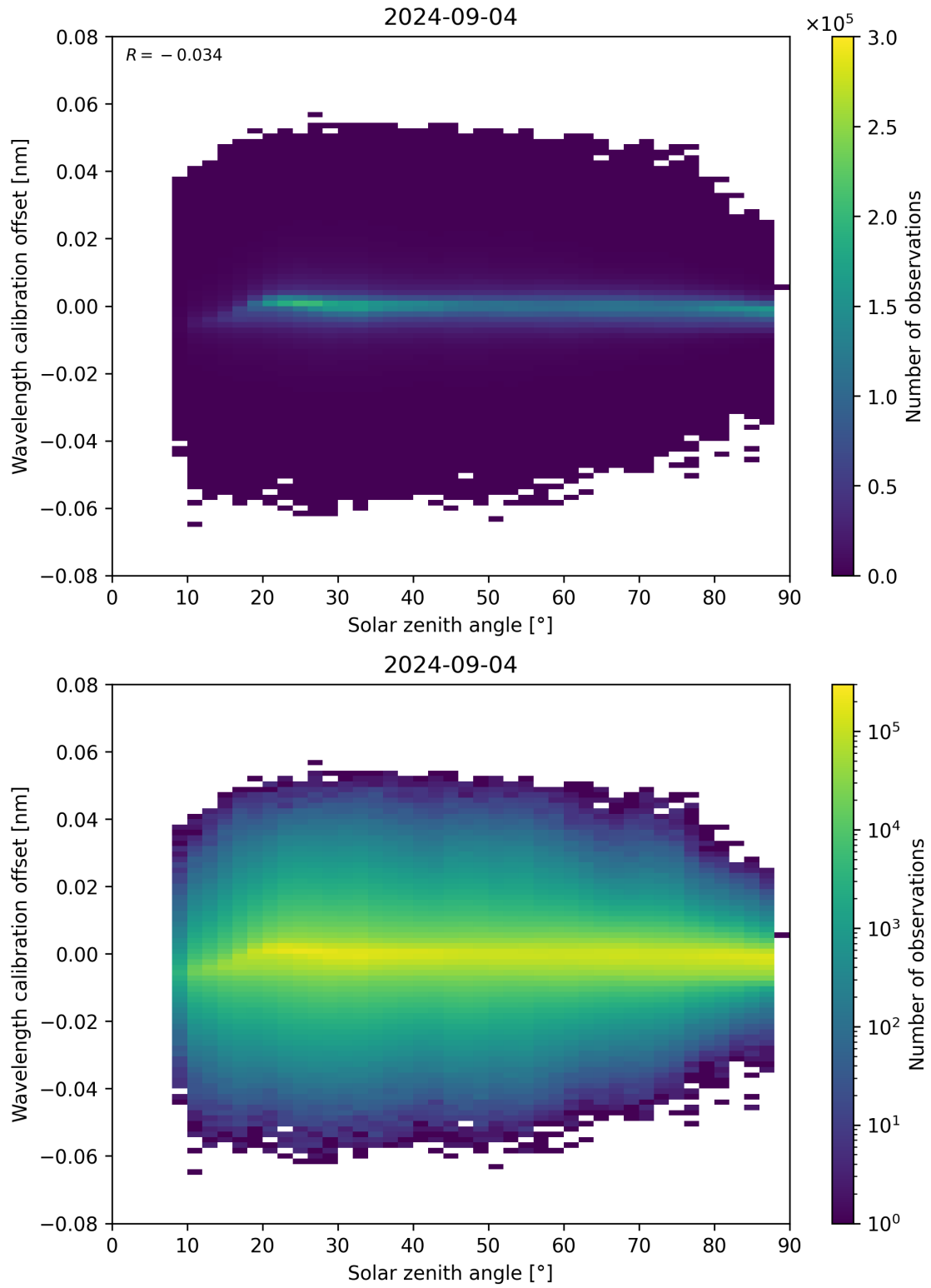
Figure 158: Scatter density plot of “Solar zenith angle” against “Wavelength calibration offset” for 2024-09-03 to 2024-09-05.
