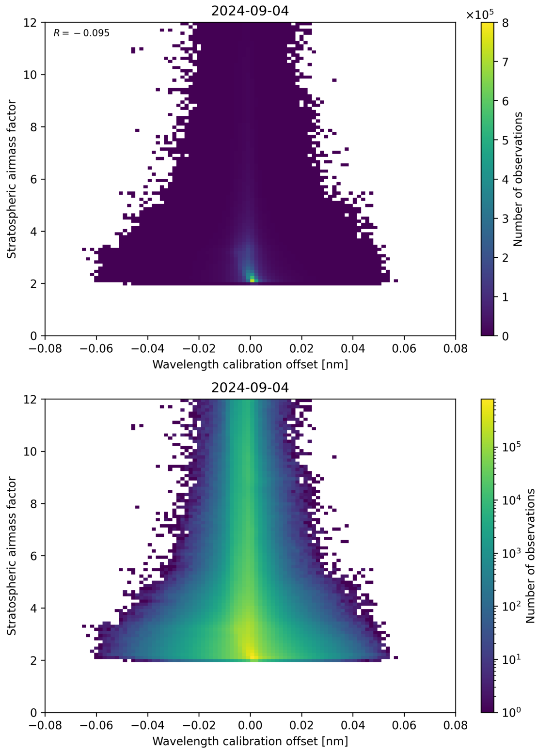
Figure 174: Scatter density plot of “Wavelength calibration offset” against “Stratospheric airmass factor” for 2024-09-03 to 2024-09-05.
