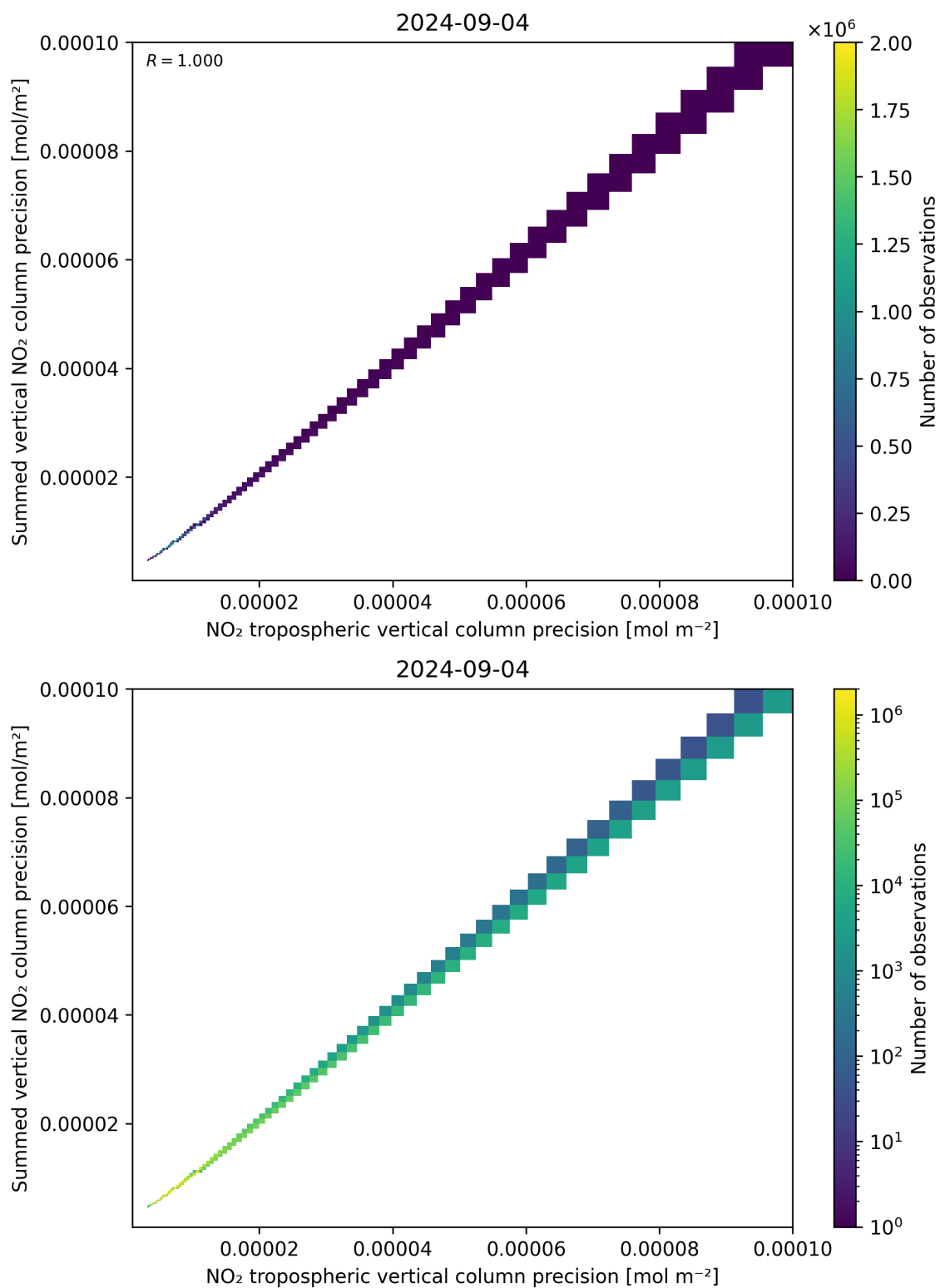
Figure 137: Scatter density plot of “NO 2 tropospheric vertical column precision” against “Summed vertical NO 2 column precision” for 2024-09-03 to 2024-09-05.
