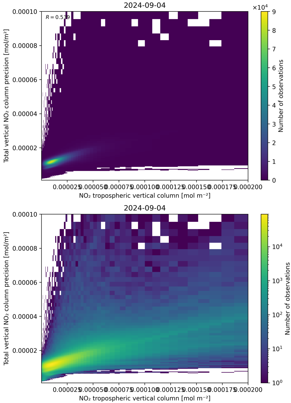
Figure 129: Scatter density plot of “NO 2 tropospheric vertical column” against “Total vertical NO 2 column precision” for 2024-09-03 to 2024-09-05.
