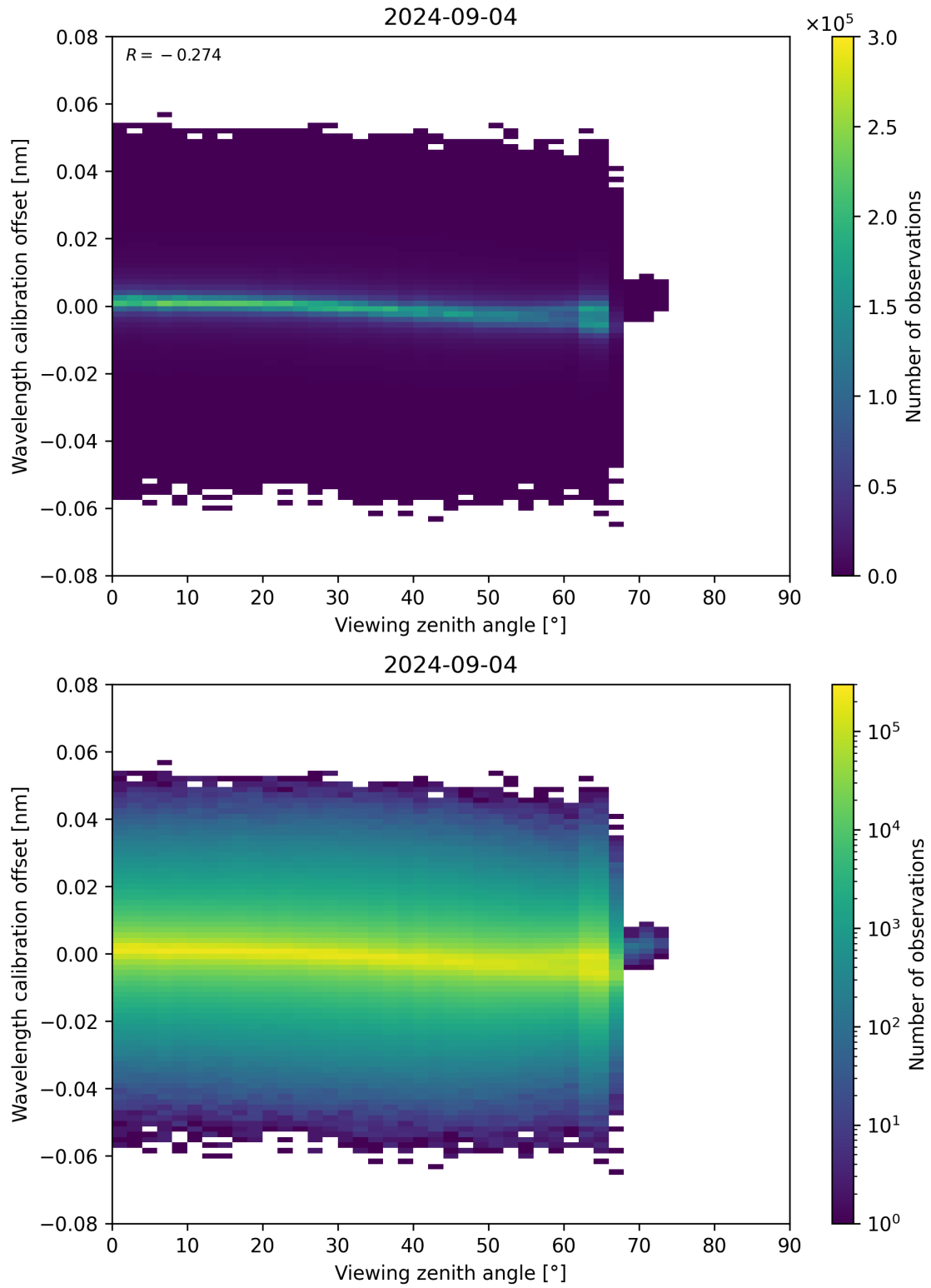
Figure 173: Scatter density plot of “Viewing zenith angle” against “Wavelength calibration offset” for 2024-09-03 to 2024-09-05.
