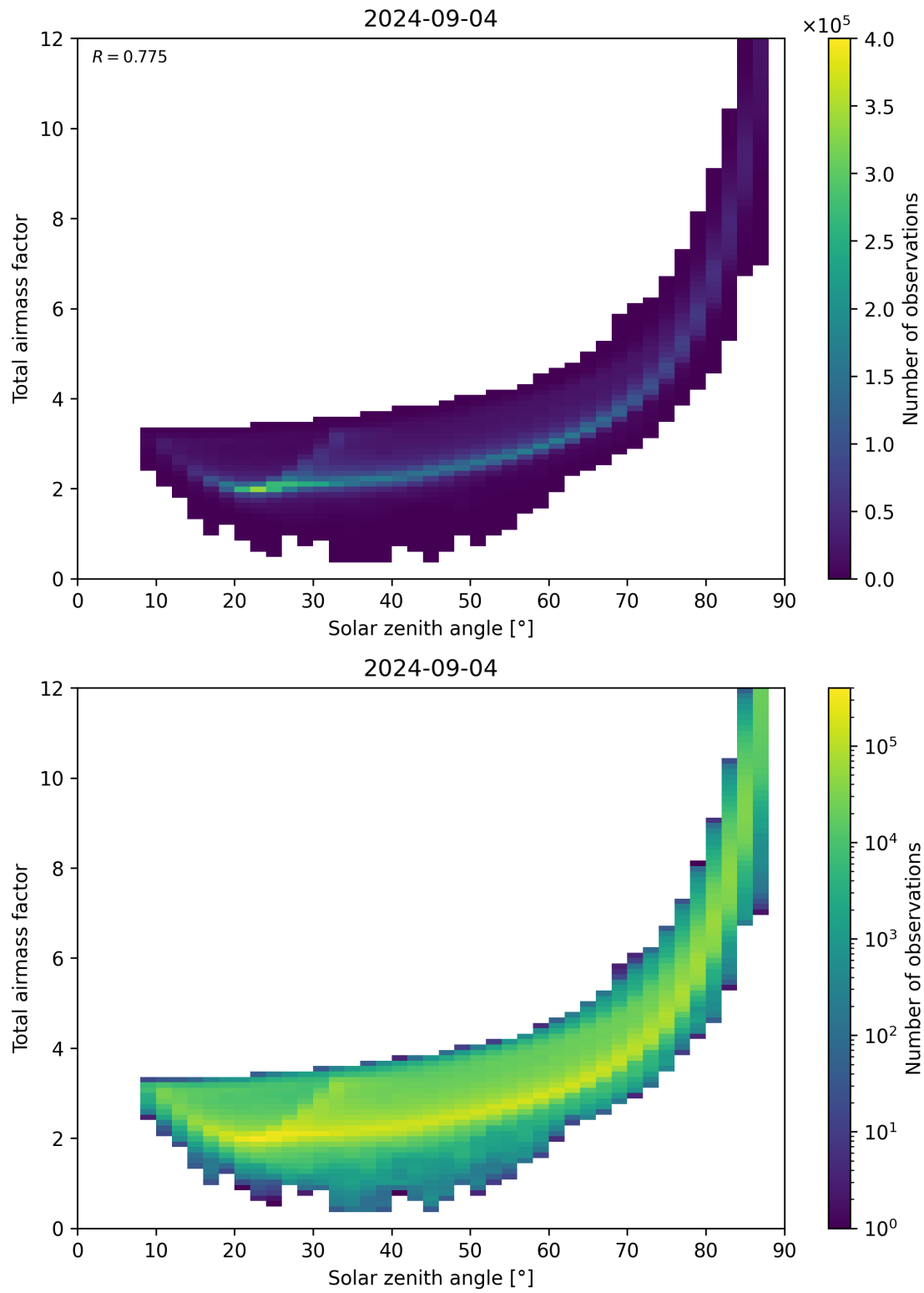
Figure 146: Scatter density plot of “Solar zenith angle” against “Total air mass factor” for 2024-09-03 to 2024-09-05.
