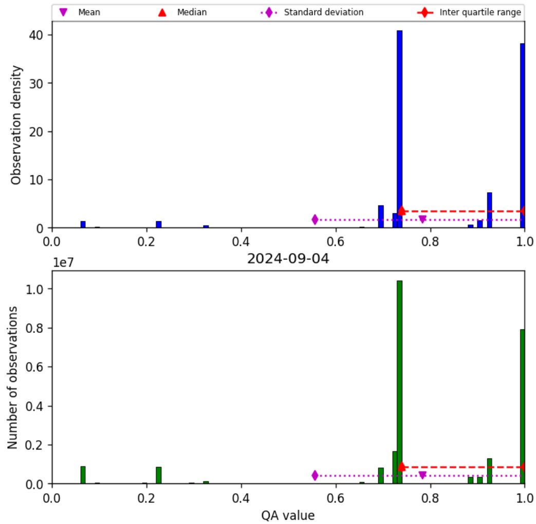
Figure 28: Histogram of “QA value” for 2024-09-03 to 2024-09-05
