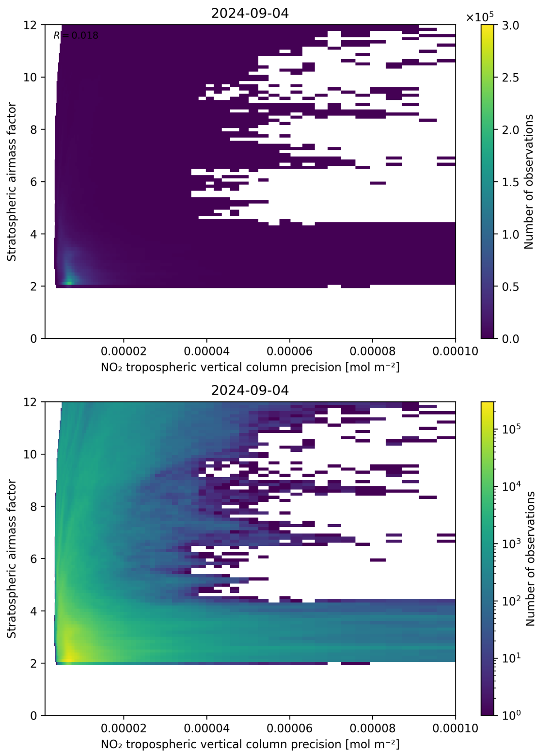
Figure 131: Scatter density plot of “NO 2 tropospheric vertical column precision” against “Stratospheric airmass factor” for 2024-09-03 to 2024-09-05.
