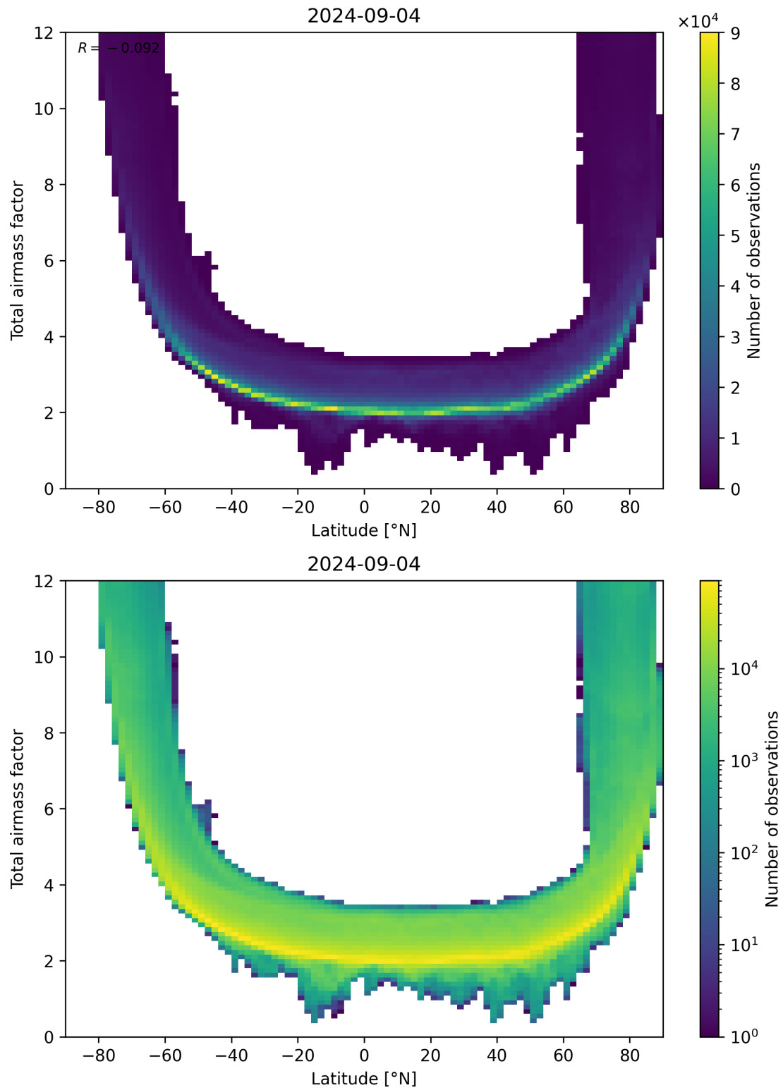
Figure 84: Scatter density plot of “Latitude” against “Total airmass factor” for 2024-09-03 to 2024-09-05.
