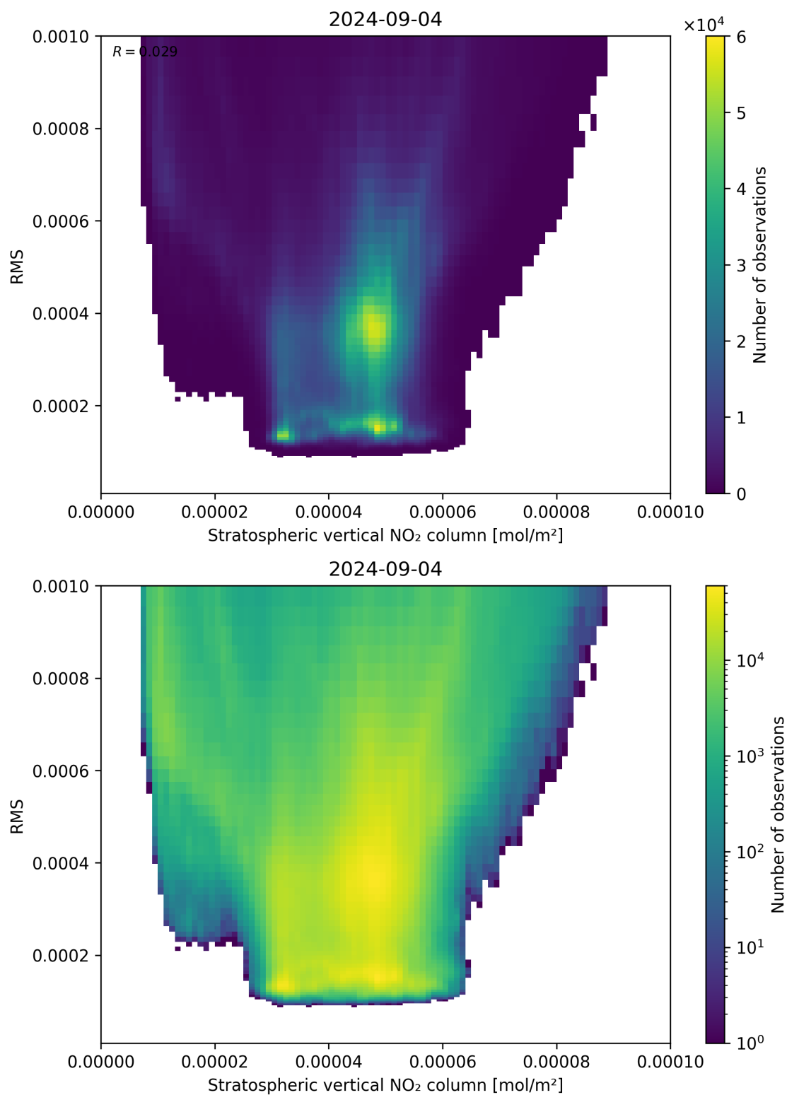
Figure 102: Scatter density plot of “Stratospheric vertical NO 2 column” against “RMS” for 2024-09-03 to 2024-09-05.
