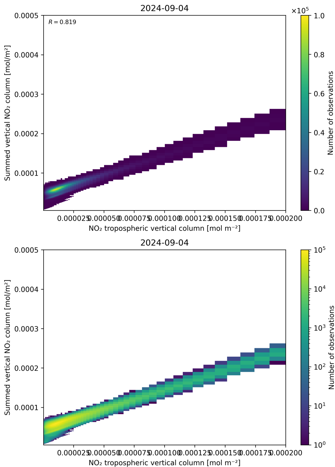
Figure 126: Scatter density plot of “NO 2 tropospheric vertical column” against “Summed vertical NO 2 column” for 2024-09-03 to 2024-09-05.
