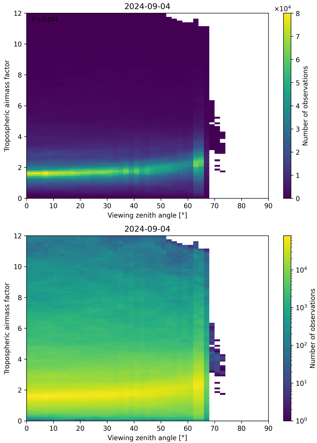
Figure 161: Scatter density plot of “Viewing zenith angle” against “Tropospheric airmass factor” for 2024-09-03 to 2024-09-05.
