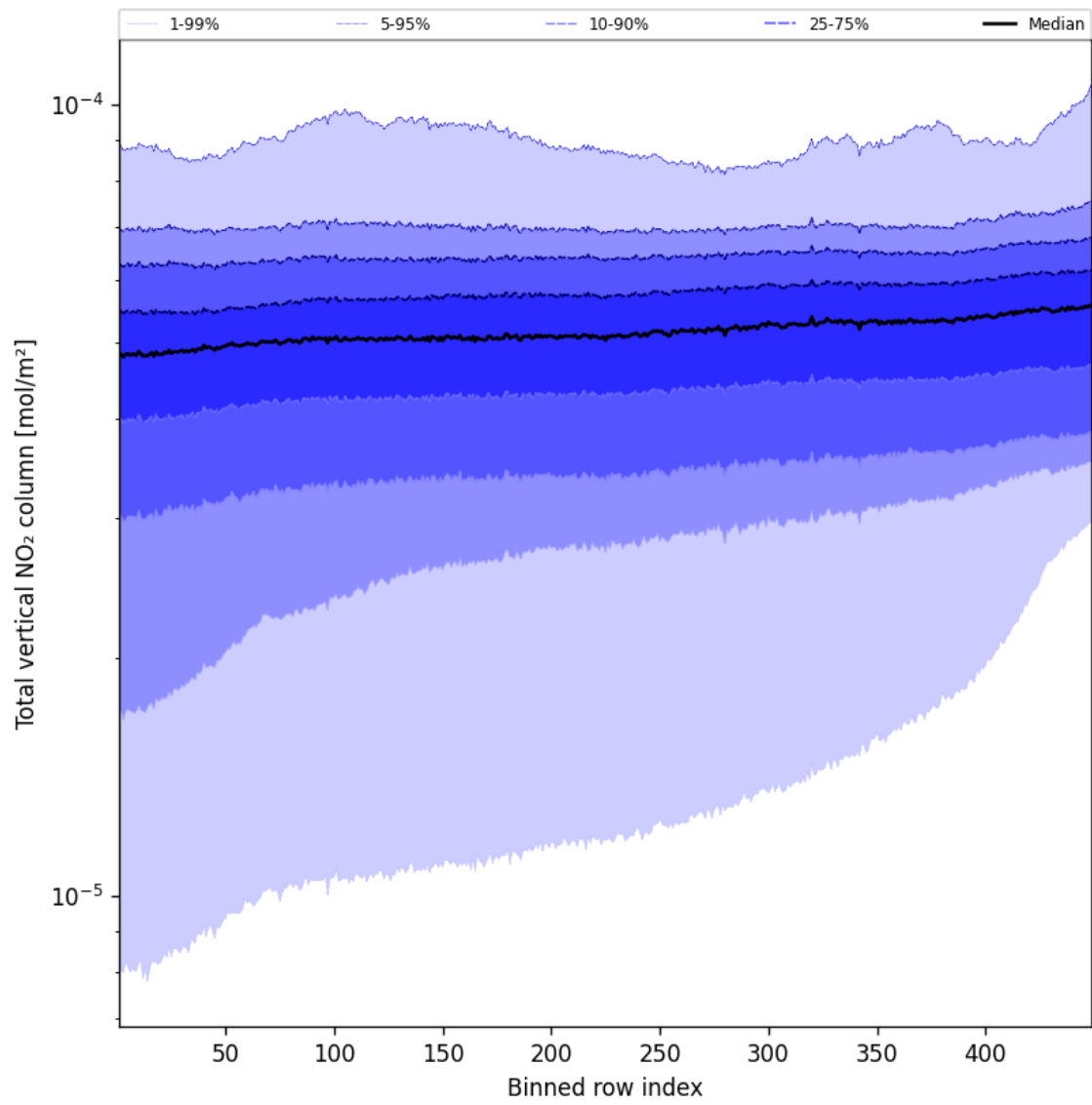
Figure 55: Along track statistics of “Total vertical NO 2 column” for 2024-09-03 to 2024-09-05
