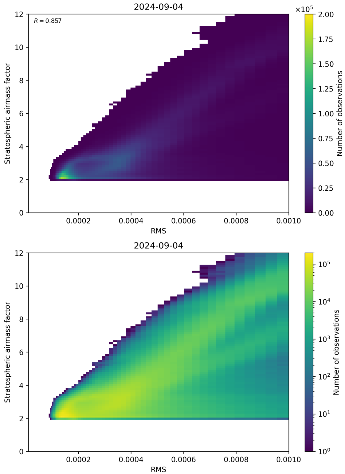
Figure 144: Scatter density plot of “RMS” against “Stratospheric airmass factor” for 2024-09-03 to 2024-09-05.
