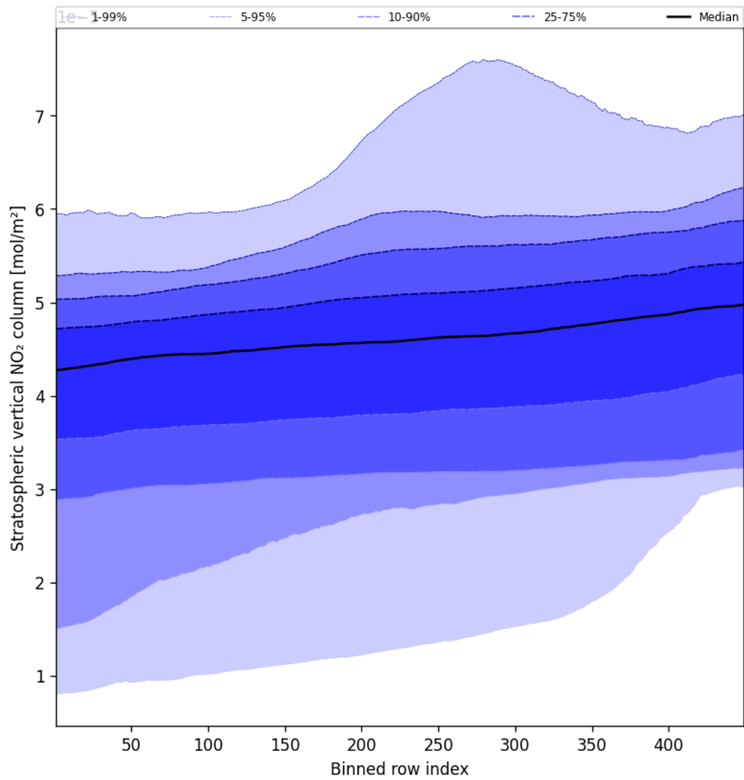
Figure 53: Along track statistics of “Stratospheric vertical NO 2 column” for 2024-09-03 to 2024-09-05
