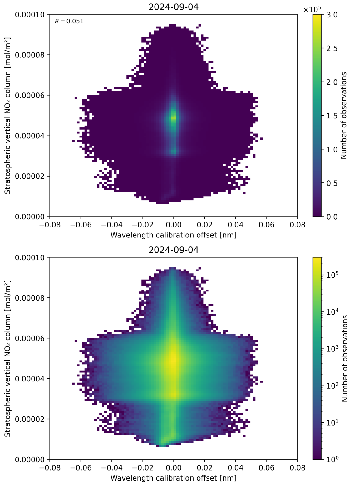
Figure 176: Scatter density plot of “Wavelength calibration offset” against “Stratospheric vertical NO 2 column” for 2024-09-03 to 2024-09-05.
