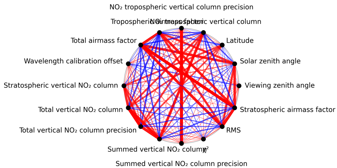
Figure 1: Map of correlation graph for 2024-09-03 to 2024-09-05.
