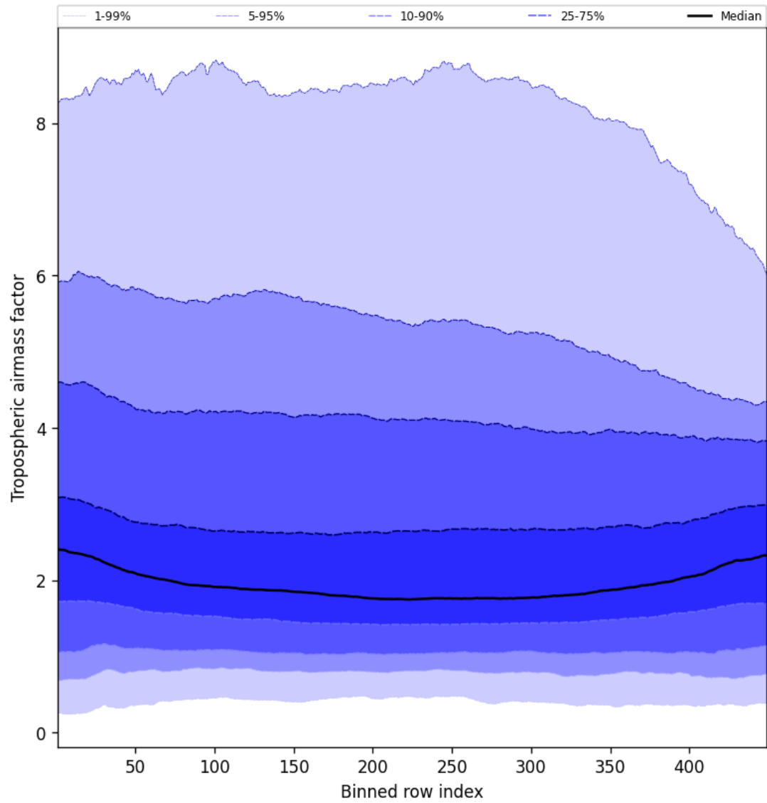
Figure 48: Along track statistics of “Tropospheric airmass factor” for 2024-09-03 to 2024-09-05
