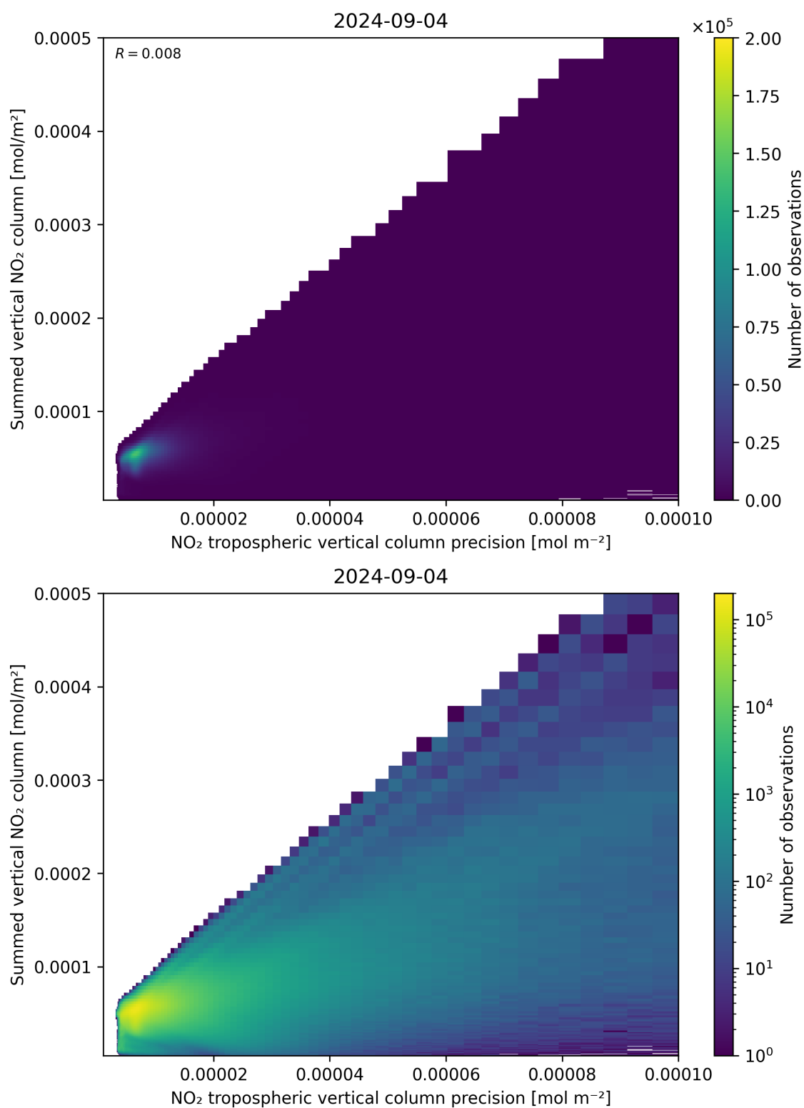
Figure 136: Scatter density plot of “NO 2 tropospheric vertical column precision” against “Summed vertical NO 2 column” for 2024-09-03 to 2024-09-05.
