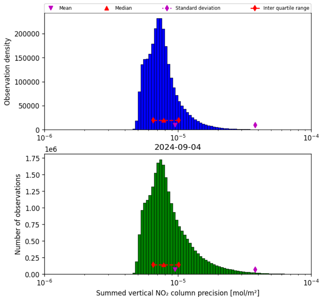
Figure 41: Histogram of "Summed vertical NO 2 column precision" for 2024-09-03 to 2024-09-05
