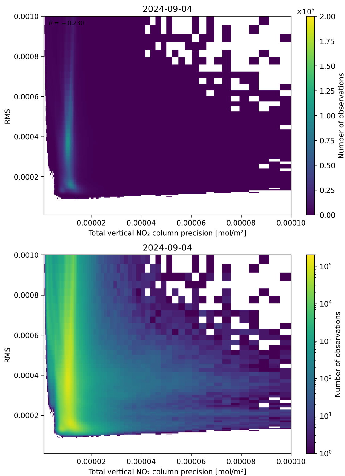
Figure 119: Scatter density plot of “Total vertical NO 2 column precision” against “RMS” for 2024-09-03 to 2024-09-05.
