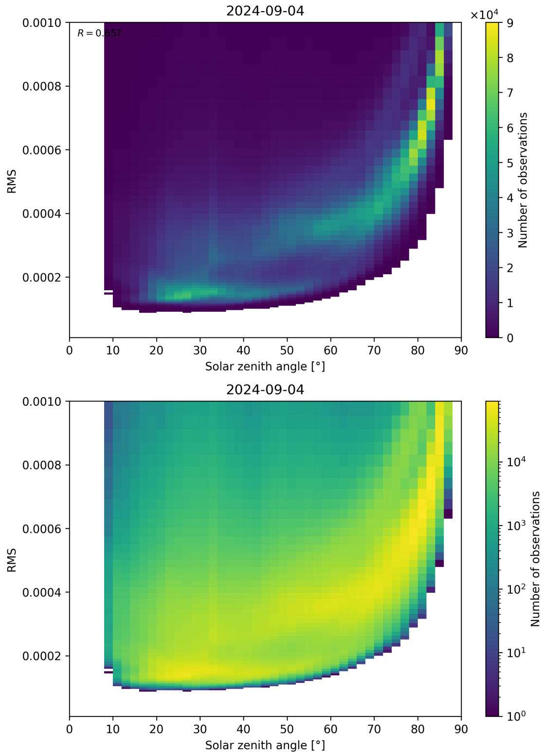
Figure 157: Scatter density plot of “Solar zenith angle” against “RMS” for 2024-09-03 to 2024-09-05.
