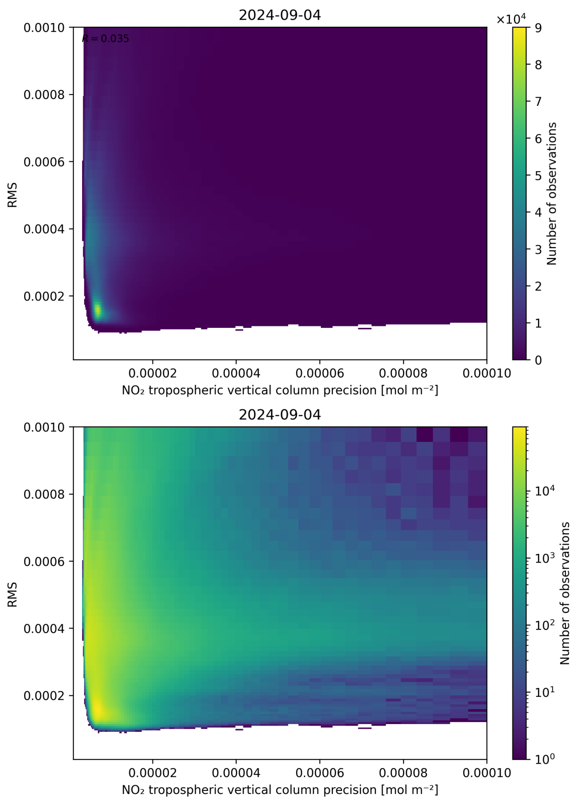
Figure 140: Scatter density plot of “NO 2 tropospheric vertical column precision” against “RMS” for 2024-09-03 to 2024-09-05.
