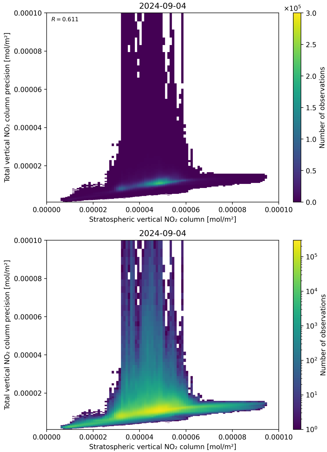
Figure 101: Scatter density plot of “Stratospheric vertical NO 2 column” against “Total vertical NO 2 column precision” for 2024-09-03 to 2024-09-05.
