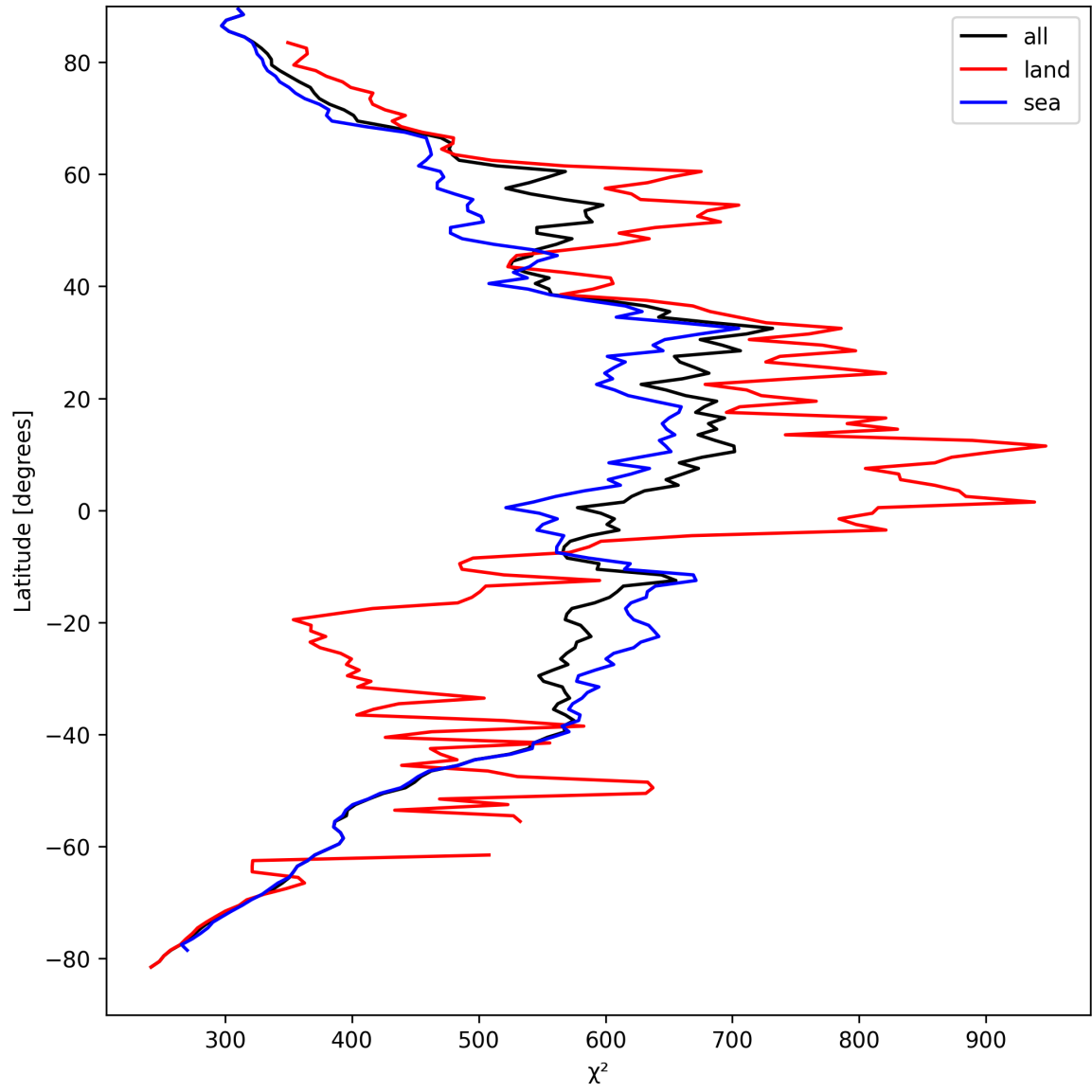
Figure 25: Zonal average of “ \chi^2 ” for 2024-09-03 to 2024-09-05.
