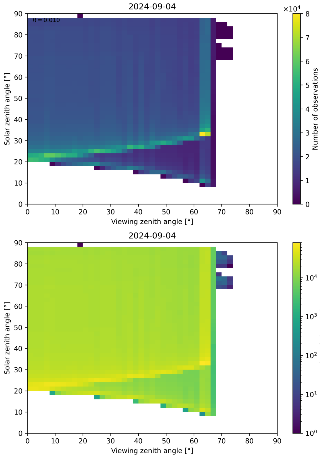
Figure 172: Scatter density plot of “Viewing zenith angle” against “Solar zenith angle” for 2024-09-03 to 2024-09-05.
