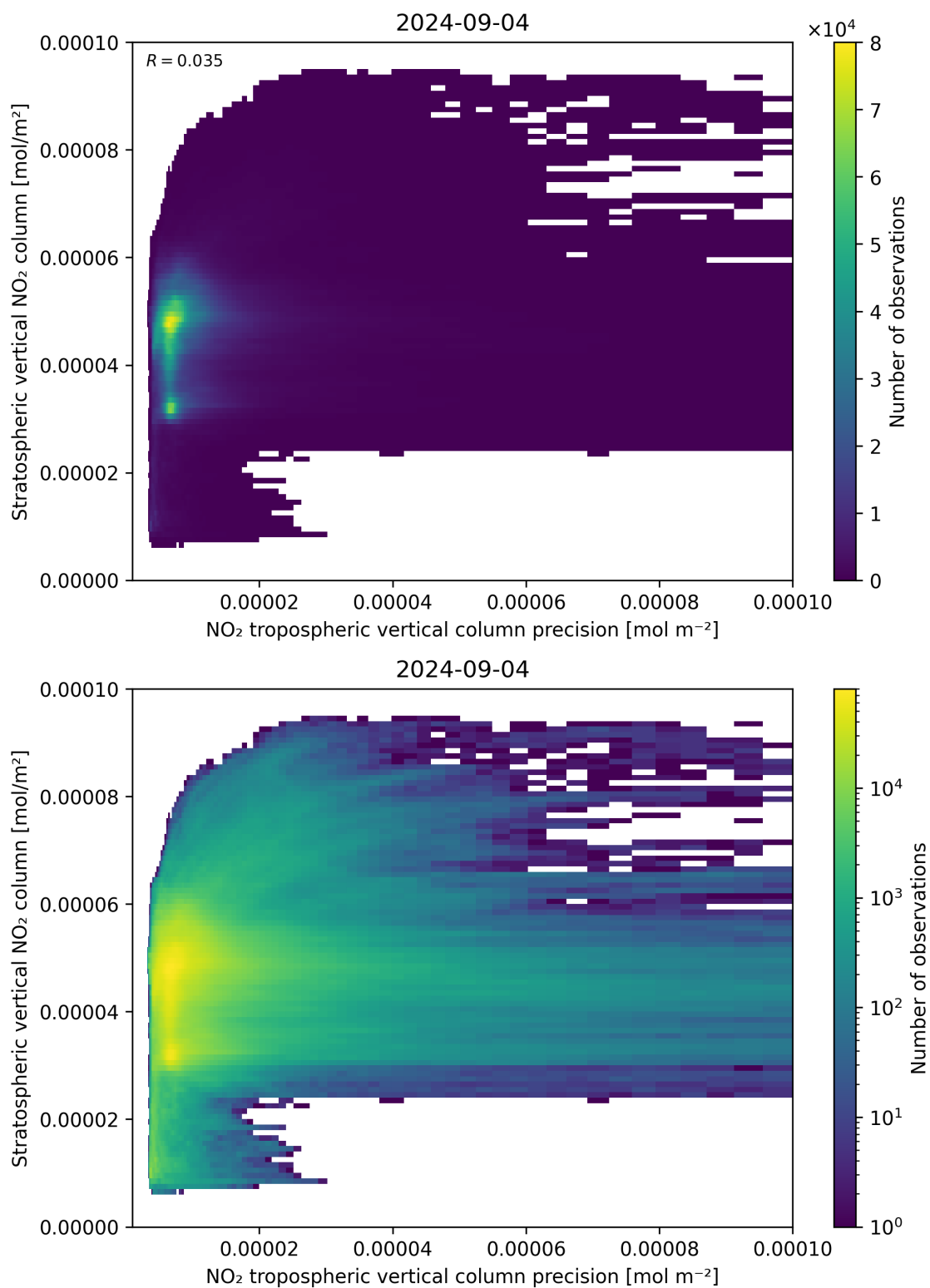
Figure 135: Scatter density plot of “NO 2 tropospheric vertical column precision” against “Stratospheric vertical NO 2 column” for 2024-09-03 to 2024-09-05.
