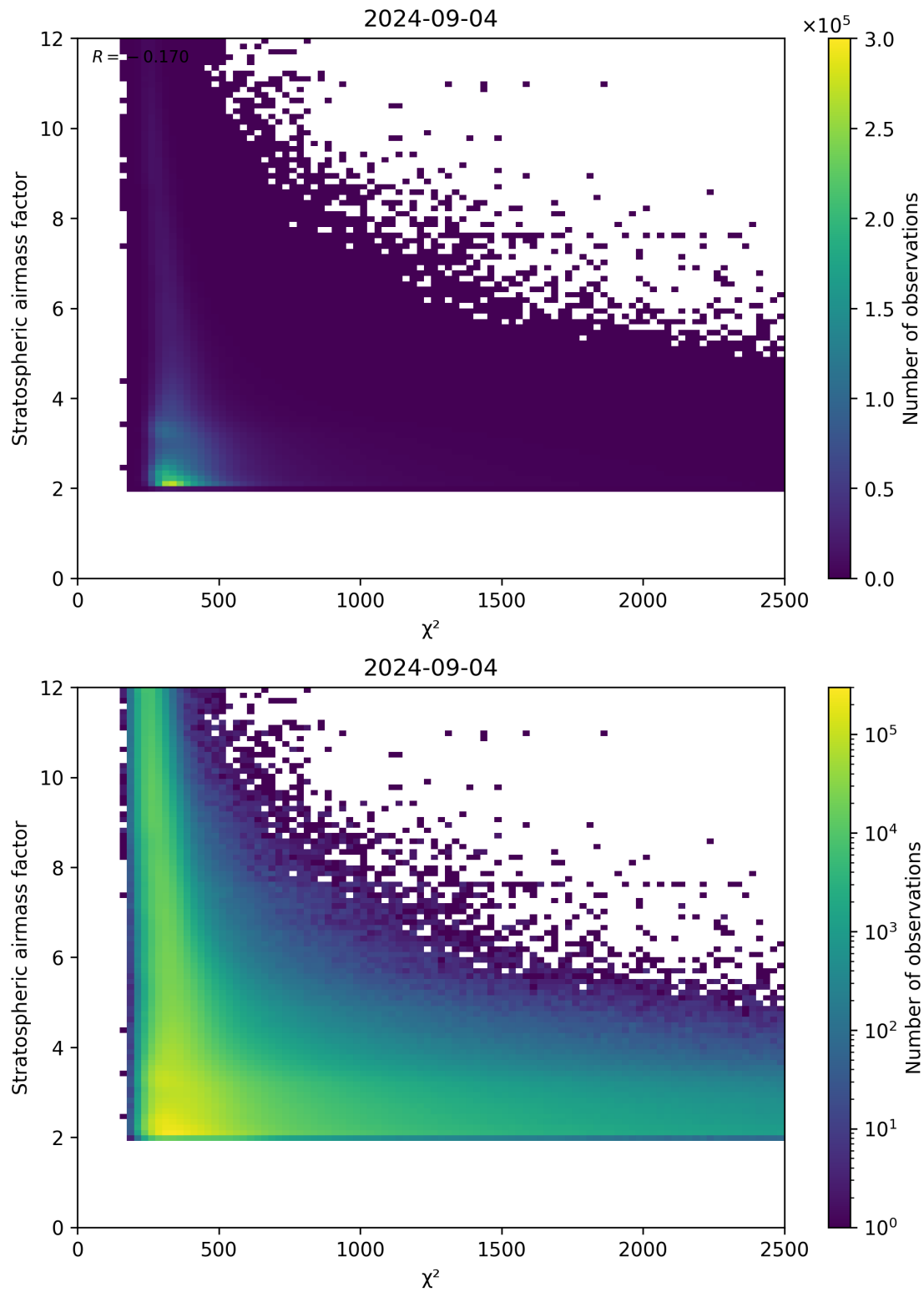
Figure 81: Scatter density plot of “ \chi^2 ” against “Stratospheric airmass factor” for 2024-09-03 to 2024-09-05.
