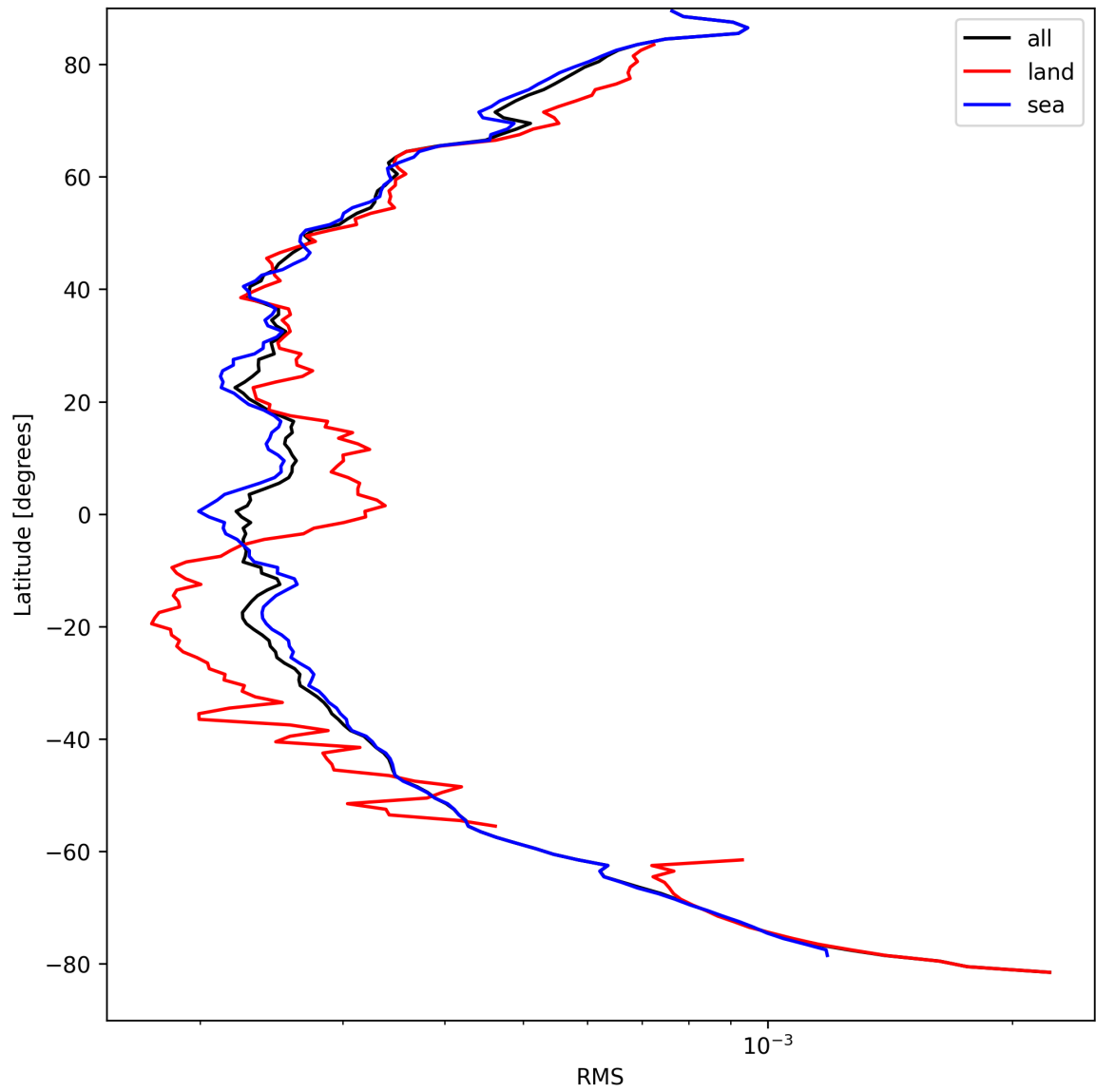
Figure 26: Zonal average of “RMS” for 2024-09-03 to 2024-09-05.
