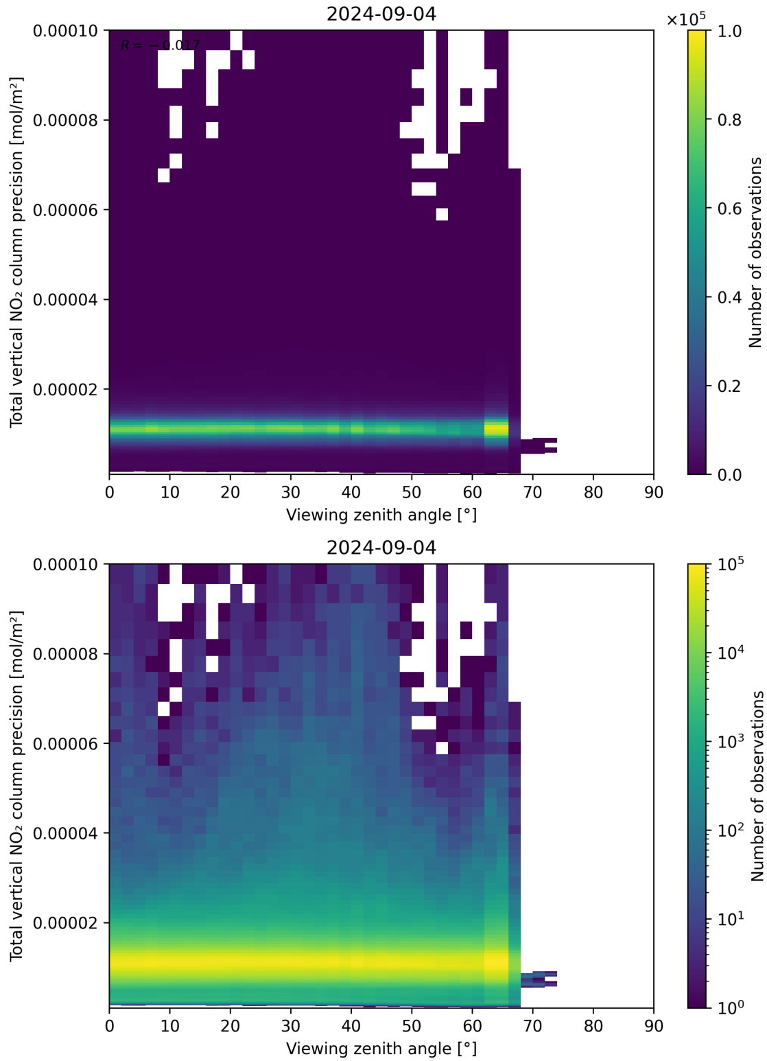
Figure 168: Scatter density plot of “Viewing zenith angle” against “Total vertical NO 2 column precision” for 2024-09-03 to 2024-09-05.
