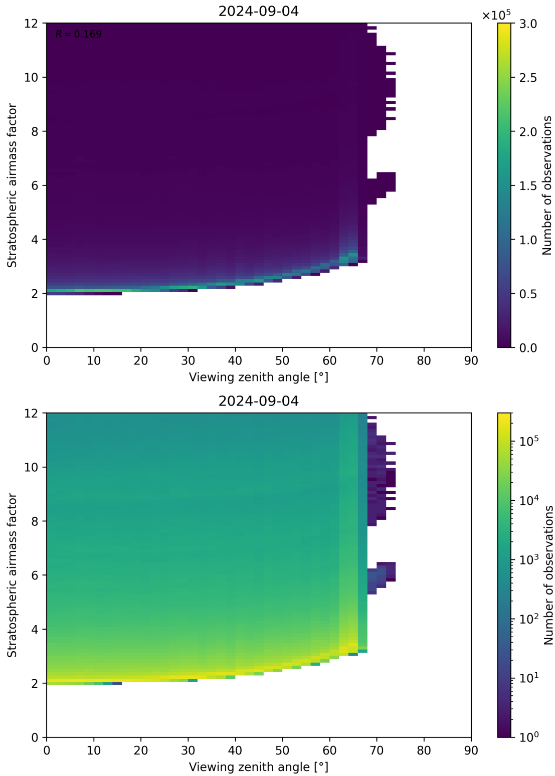
Figure 159: Scatter density plot of “Viewing zenith angle” against “Stratospheric airmass factor” for 2024-09-03 to 2024-09-05.
