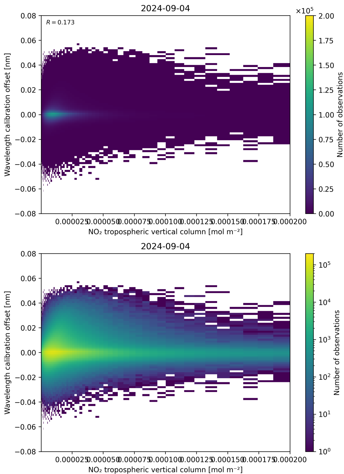
Figure 143: Scatter density plot of “NO 2 tropospheric vertical column” against “Wavelength calibration offset” for 2024-09-03 to 2024-09-05.
