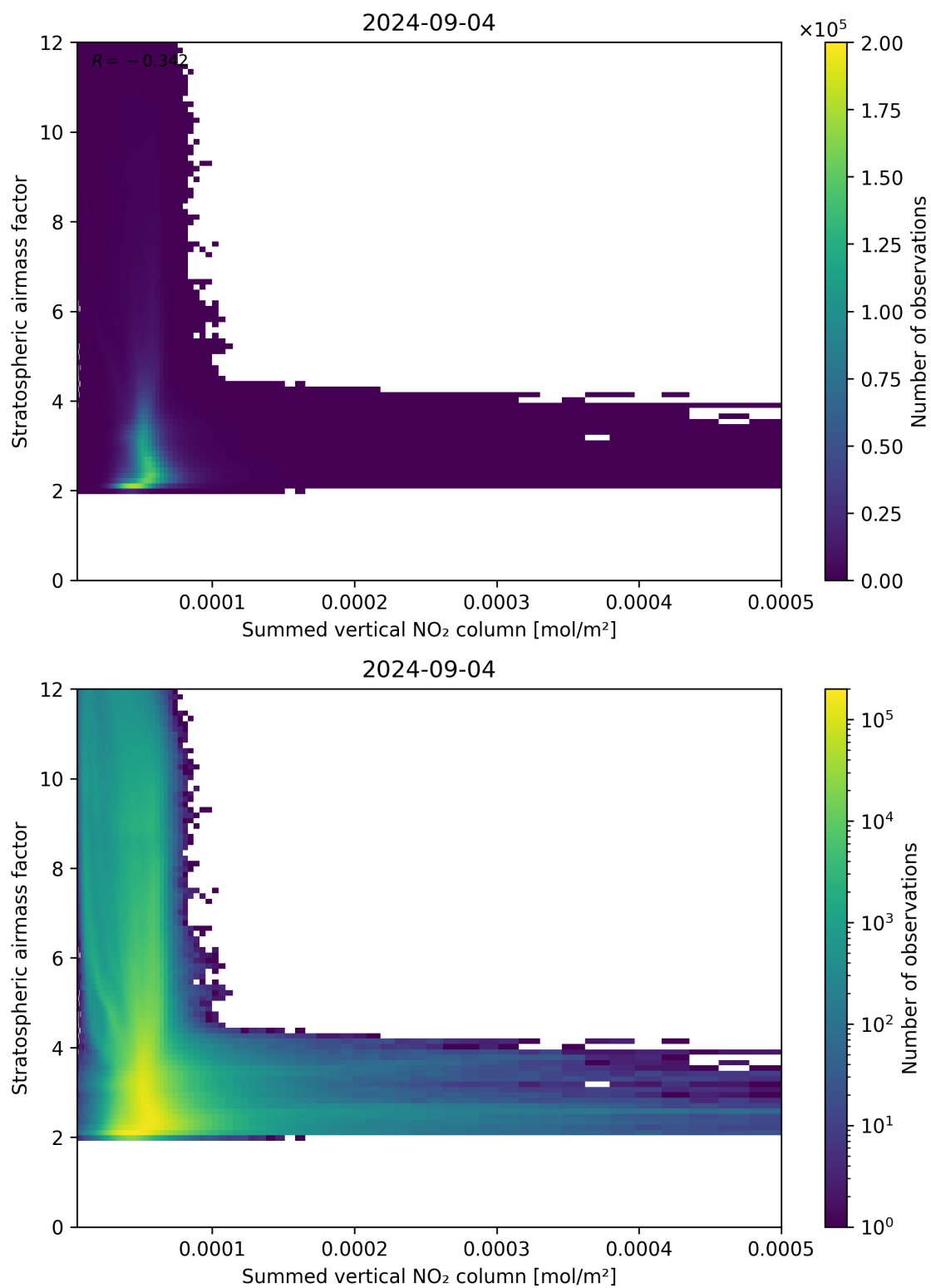
Figure 103: Scatter density plot of “Summed vertical NO 2 column” against “Stratospheric airmass factor” for 2024-09-03 to 2024-09-05.
