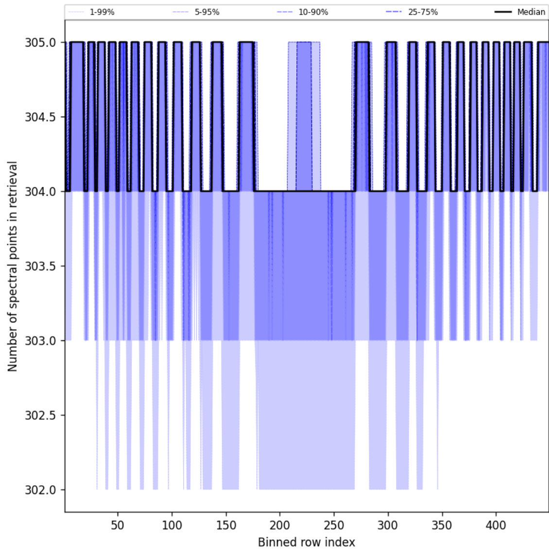
Figure 50: Along track statistics of “Number of spectral points in retrieval” for 2024-09-03 to 2024-09-05
