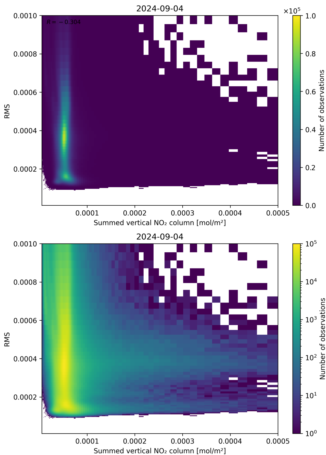
Figure 109: Scatter density plot of “Summed vertical NO 2 column” against “RMS” for 2024-09-03 to 2024-09-05.
