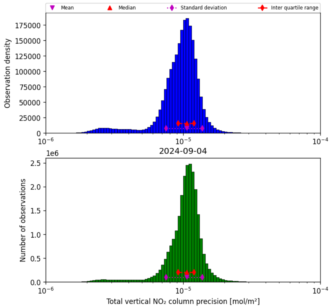
Figure 39: Histogram of “Total vertical NO 2 column precision” for 2024-09-03 to 2024-09-05
