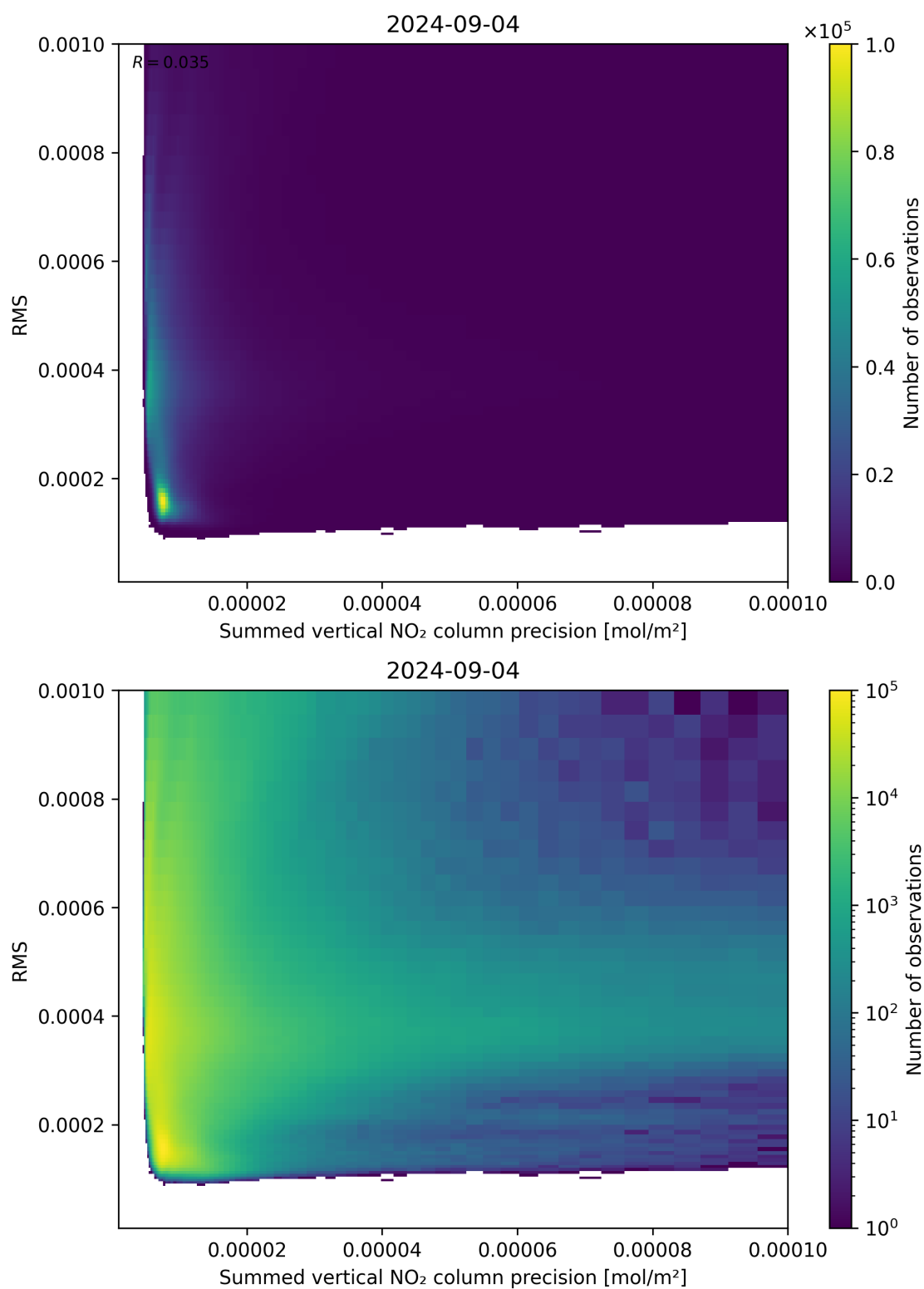
Figure 108: Scatter density plot of “Summed vertical NO 2 column precision” against “RMS” for 2024-09-03 to 2024-09-05.
