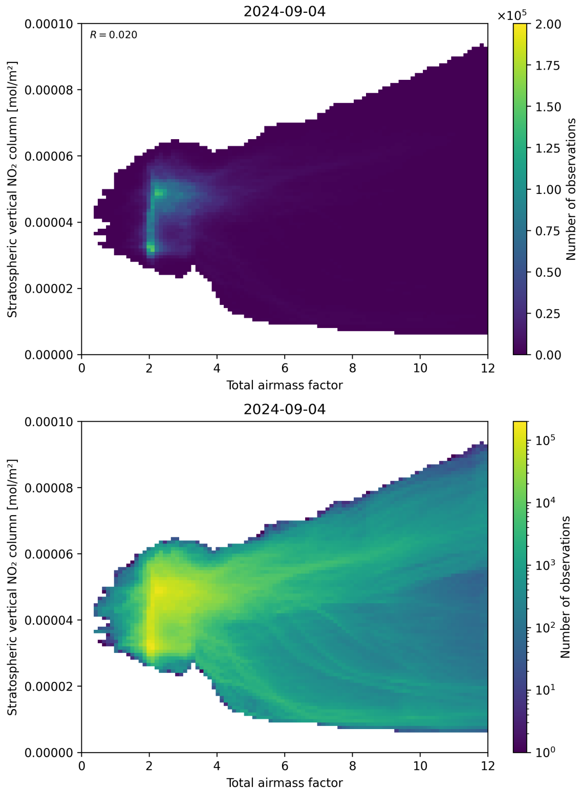
Figure 64: Scatter density plot of “Total airmass factor” against “Stratospheric vertical \text{NO}_2 column” for 2024-09-03 to 2024-09-05.
