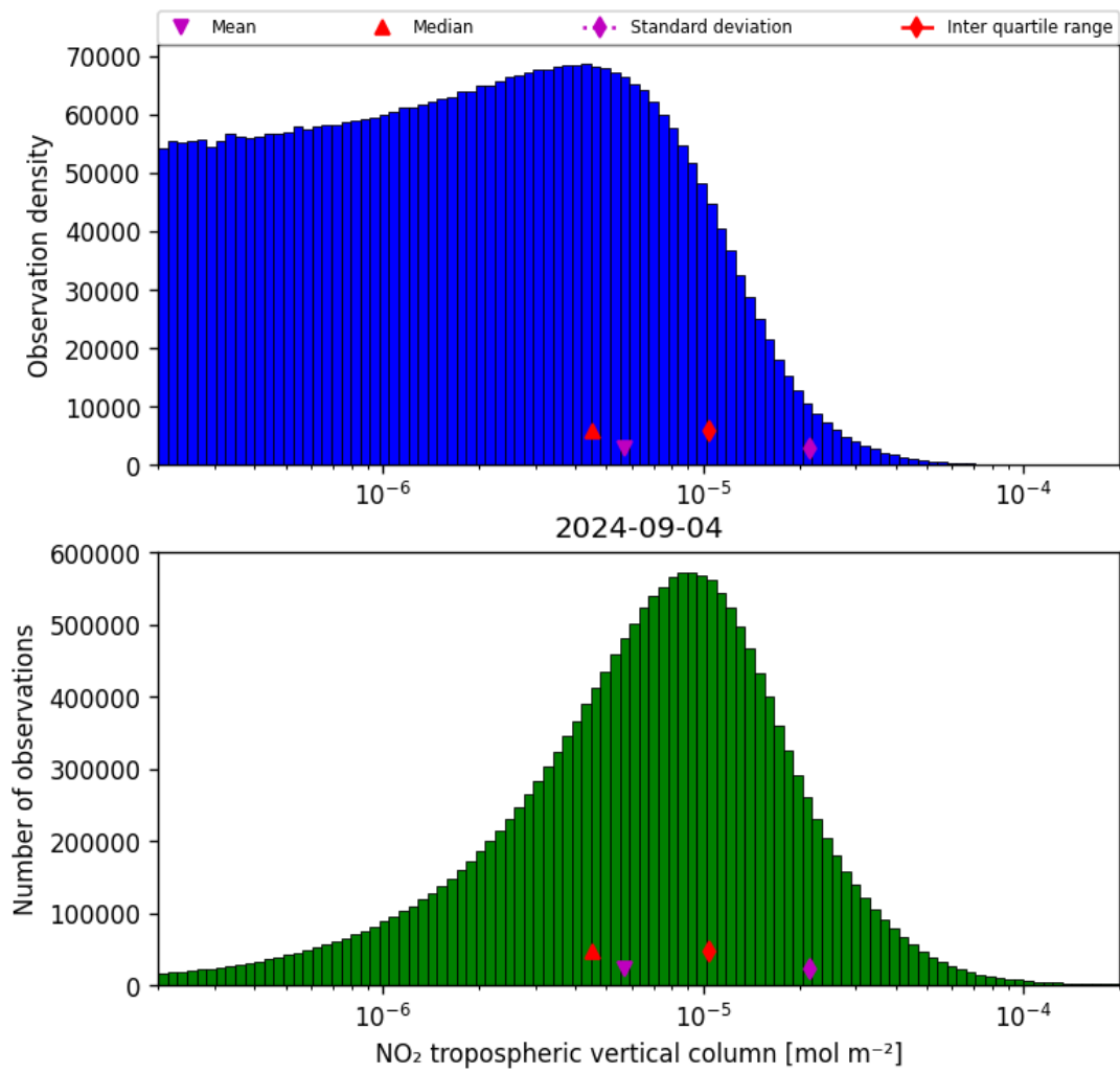
Figure 29: Histogram of “NO 2 tropospheric vertical column” for 2024-09-03 to 2024-09-05
