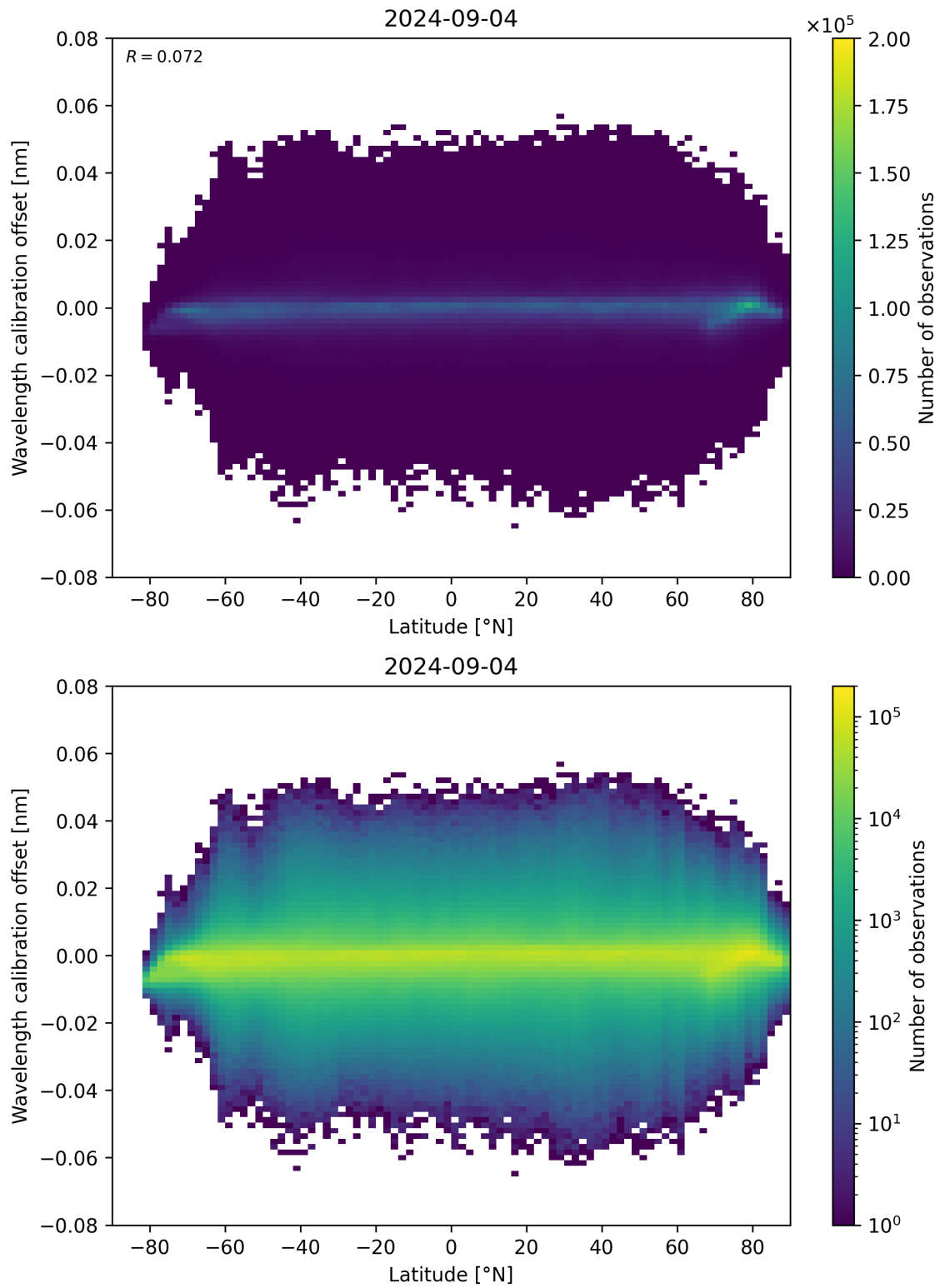
Figure 95: Scatter density plot of “Latitude” against “Wavelength calibration offset” for 2024-09-03 to 2024-09-05.
