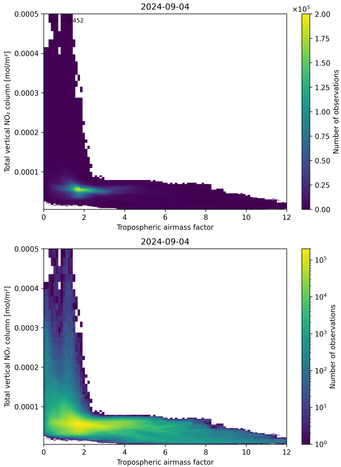
Figure 77: Scatter density plot of “Tropospheric airmass factor” against “Total vertical NO 2 column” for 2024-09-03 to 2024-09-05.
