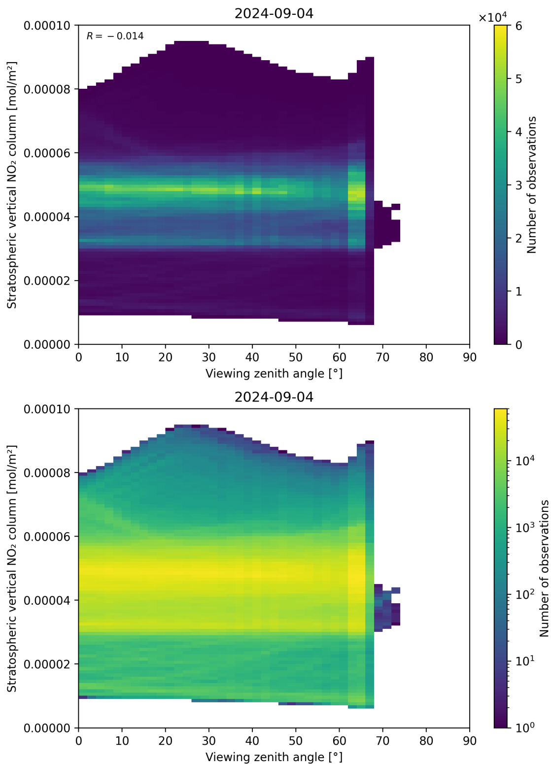
Figure 164: Scatter density plot of “Viewing zenith angle” against “Stratospheric vertical NO 2 column” for 2024-09-03 to 2024-09-05.
