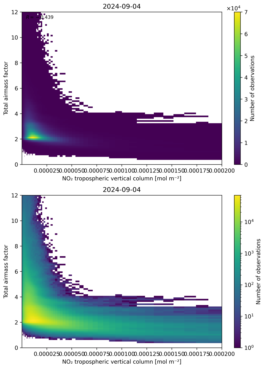
Figure 122: Scatter density plot of “NO 2 tropospheric vertical column” against “Total airmass factor” for 2024-09-03 to 2024-09-05.
