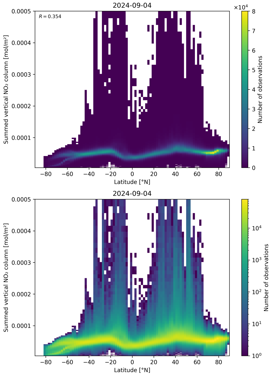
Figure 88: Scatter density plot of “Latitude” against “Summed vertical NO 2 column” for 2024-09-03 to 2024-09-05.
