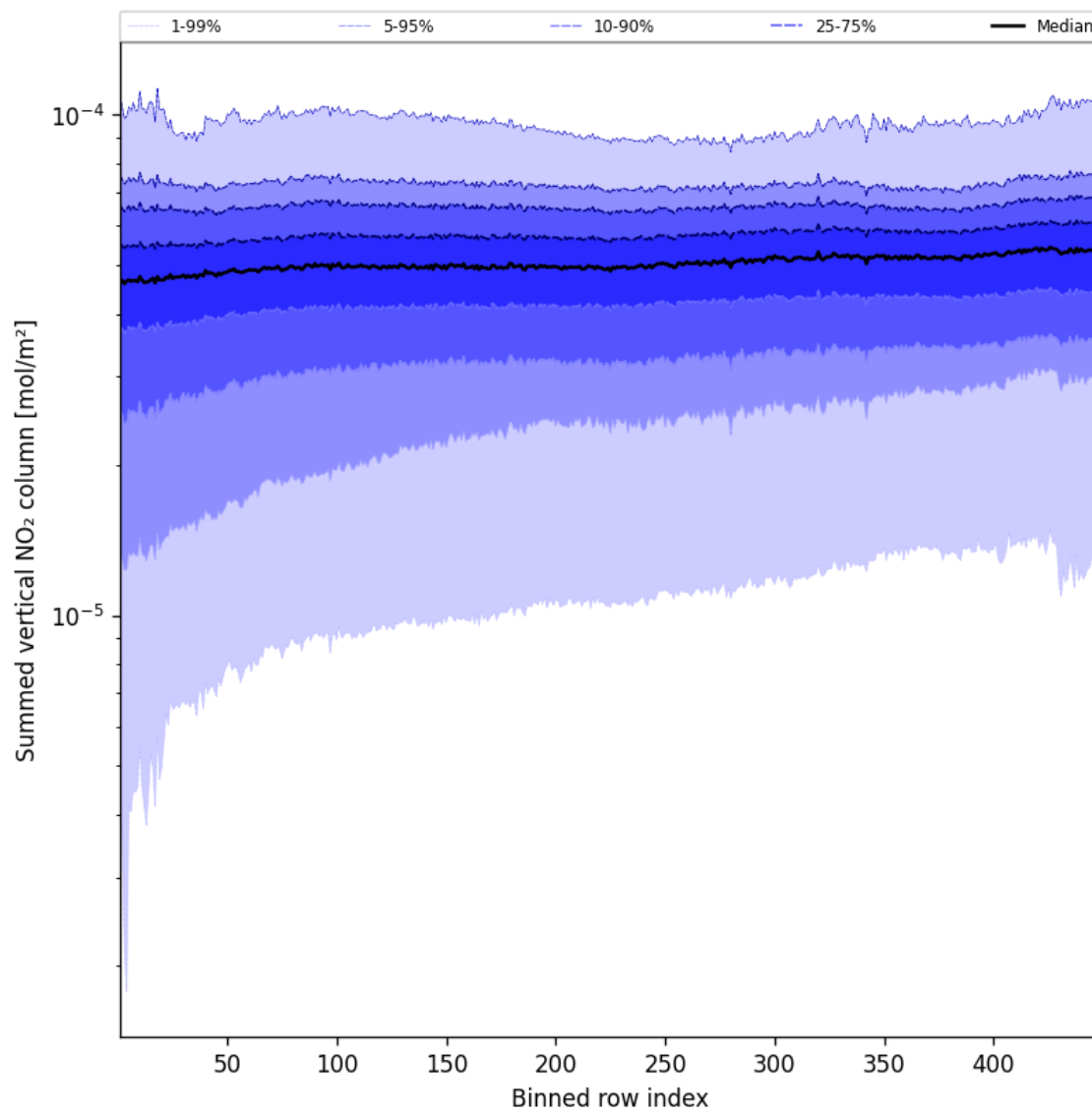
Figure 57: Along track statistics of “Summed vertical NO 2 column” for 2024-09-03 to 2024-09-05
