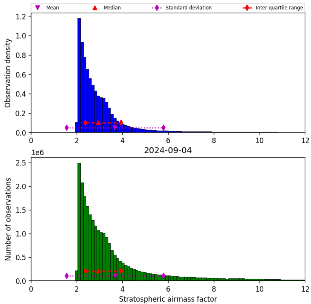
Figure 44: Histogram of “Stratospheric airmass factor” for 2024-09-03 to 2024-09-05
