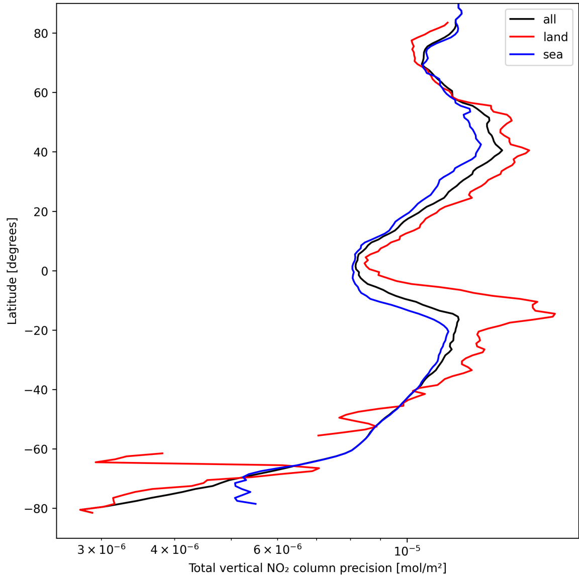
Figure 22: Zonal average of “Total vertical NO 2 column precision” for 2024-09-03 to 2024-09-05.
