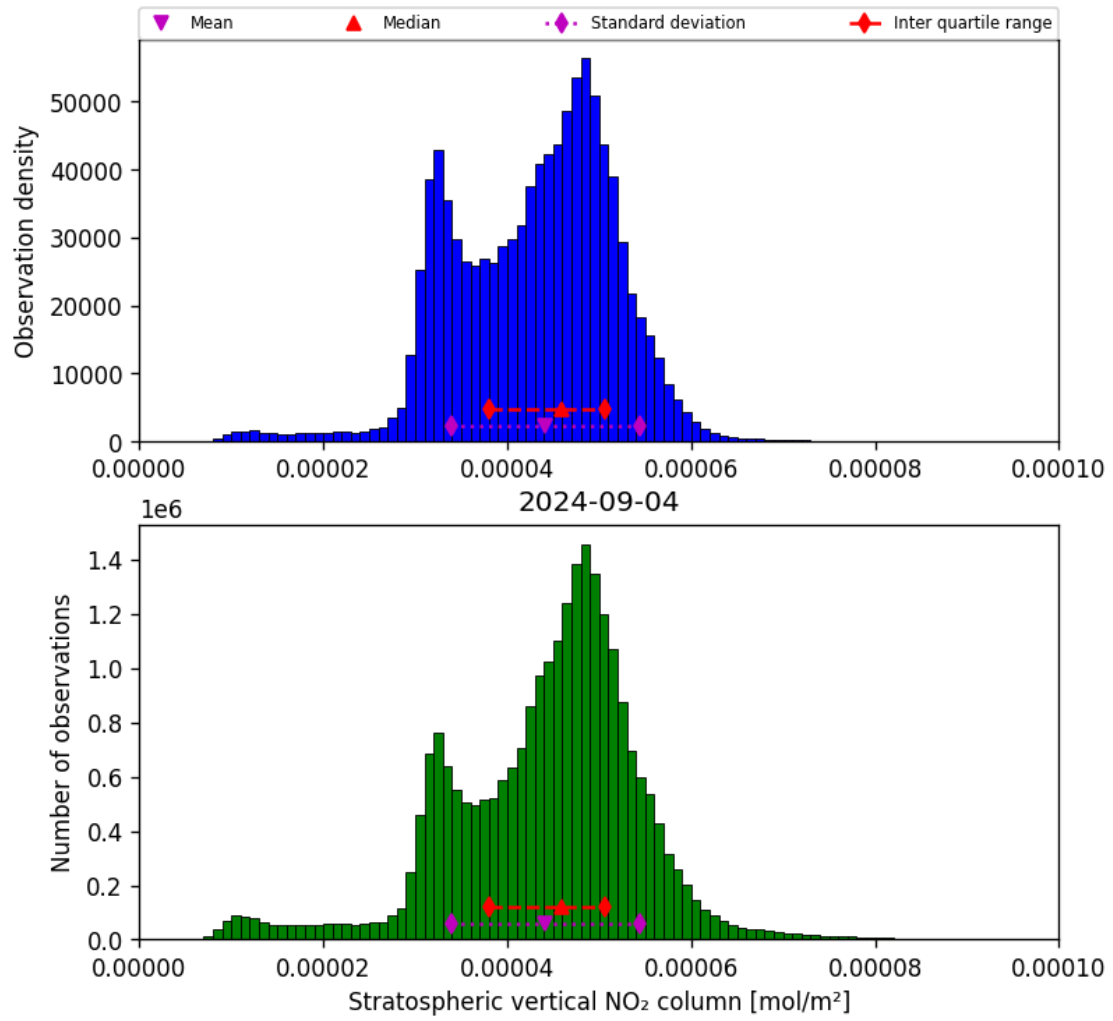
Figure 36: Histogram of “Stratospheric vertical NO 2 column” for 2024-09-03 to 2024-09-05
