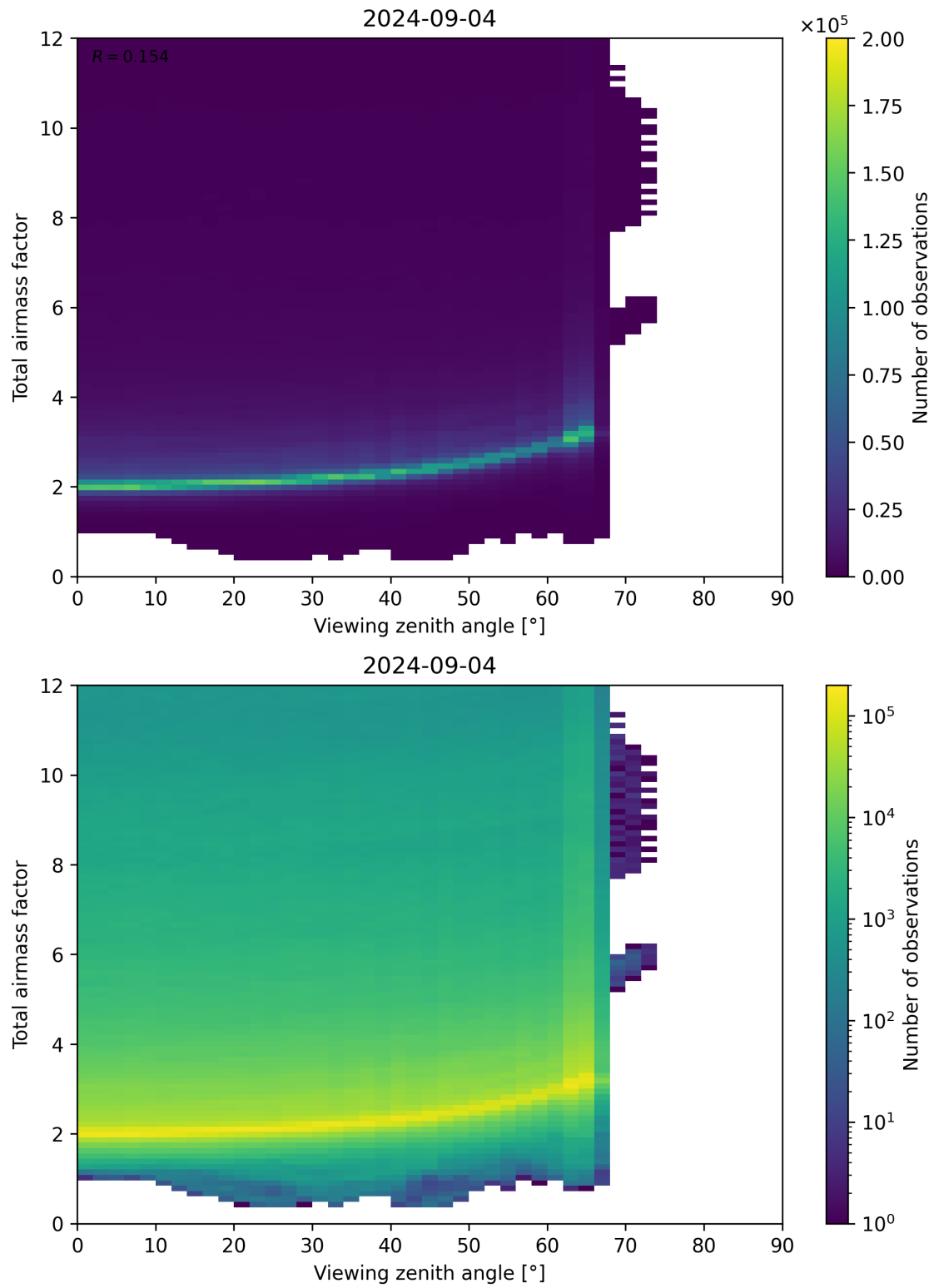
Figure 160: Scatter density plot of “Viewing zenith angle” against “Total airmass factor” for 2024-09-03 to 2024-09-05.
