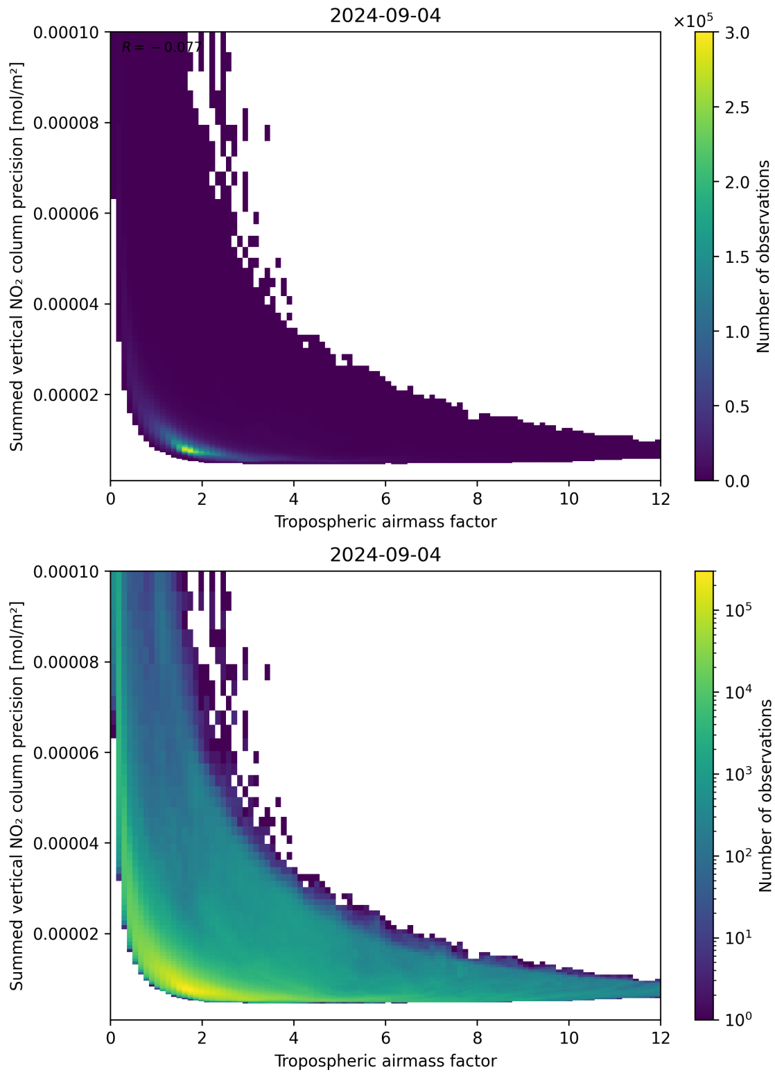
Figure 76: Scatter density plot of “Tropospheric air mass factor” against “Summed vertical NO 2 column precision” for 2024-09-03 to 2024-09-05.
