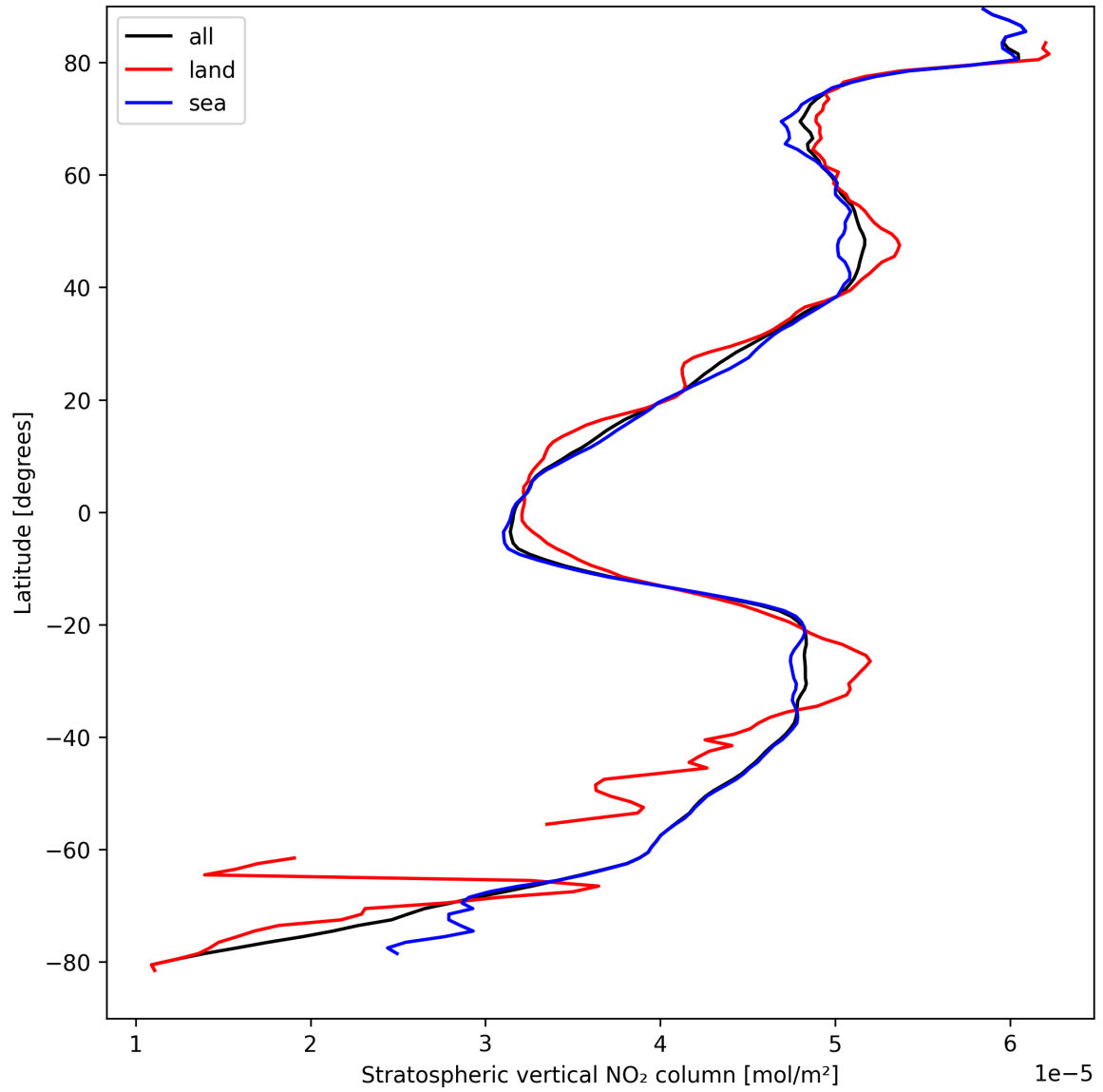
Figure 19: Zonal average of “Stratospheric vertical NO 2 column” for 2024-09-03 to 2024-09-05.
