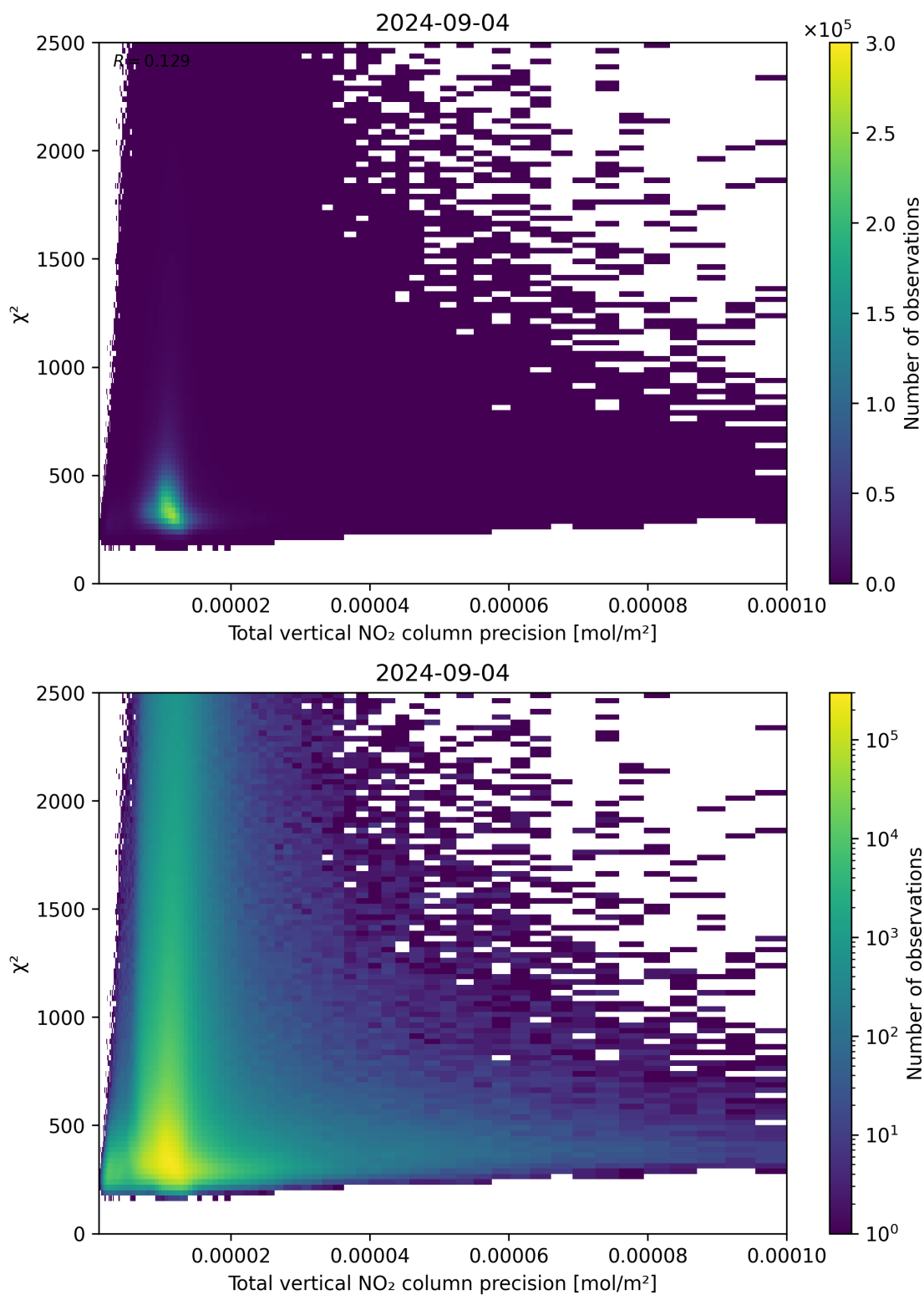
Figure 116: Scatter density plot of “Total vertical NO 2 column precision” against “ \chi^2 ” for 2024-09-03 to 2024-09-05.
