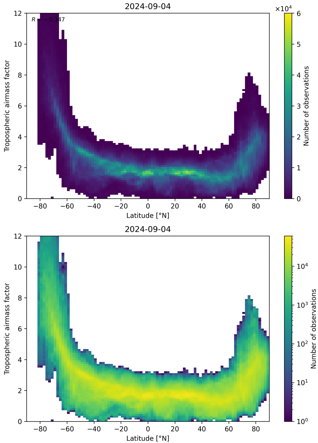
Figure 85: Scatter density plot of “Latitude” against “Tropospheric air mass factor” for 2024-09-03 to 2024-09-05.
