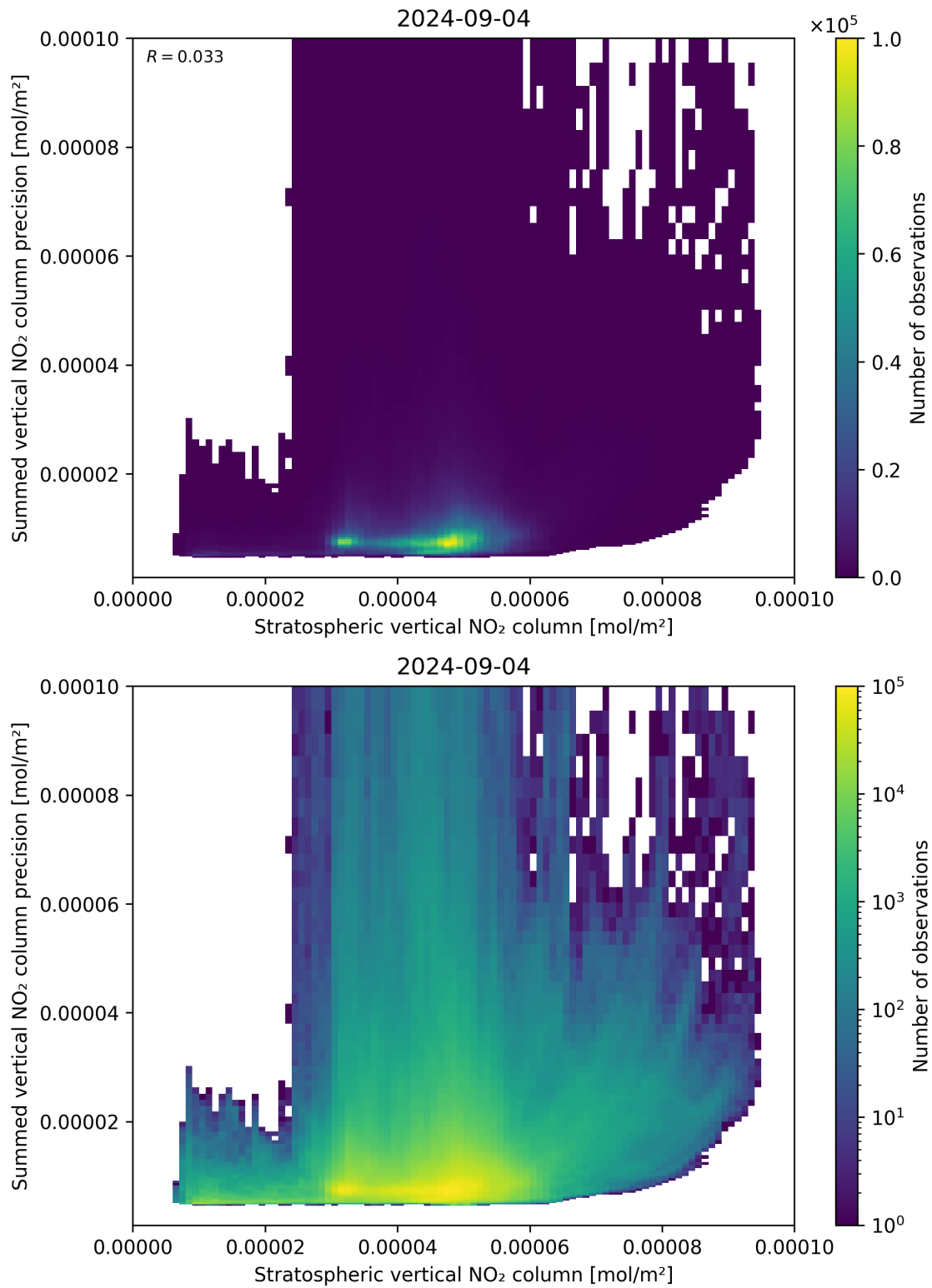
Figure 99: Scatter density plot of “Stratospheric vertical NO 2 column” against “Summed vertical NO 2 column precision” for 2024-09-03 to 2024-09-05.
