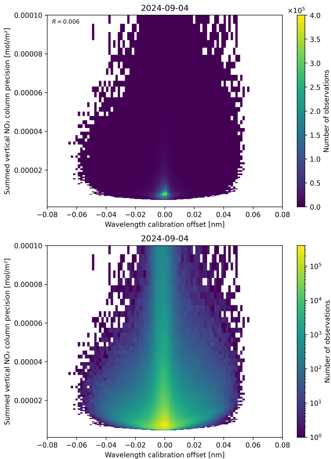
Figure 178: Scatter density plot of “Wavelength calibration offset” against “Summed vertical NO 2 column precision” for 2024-09-03 to 2024-09-05.
