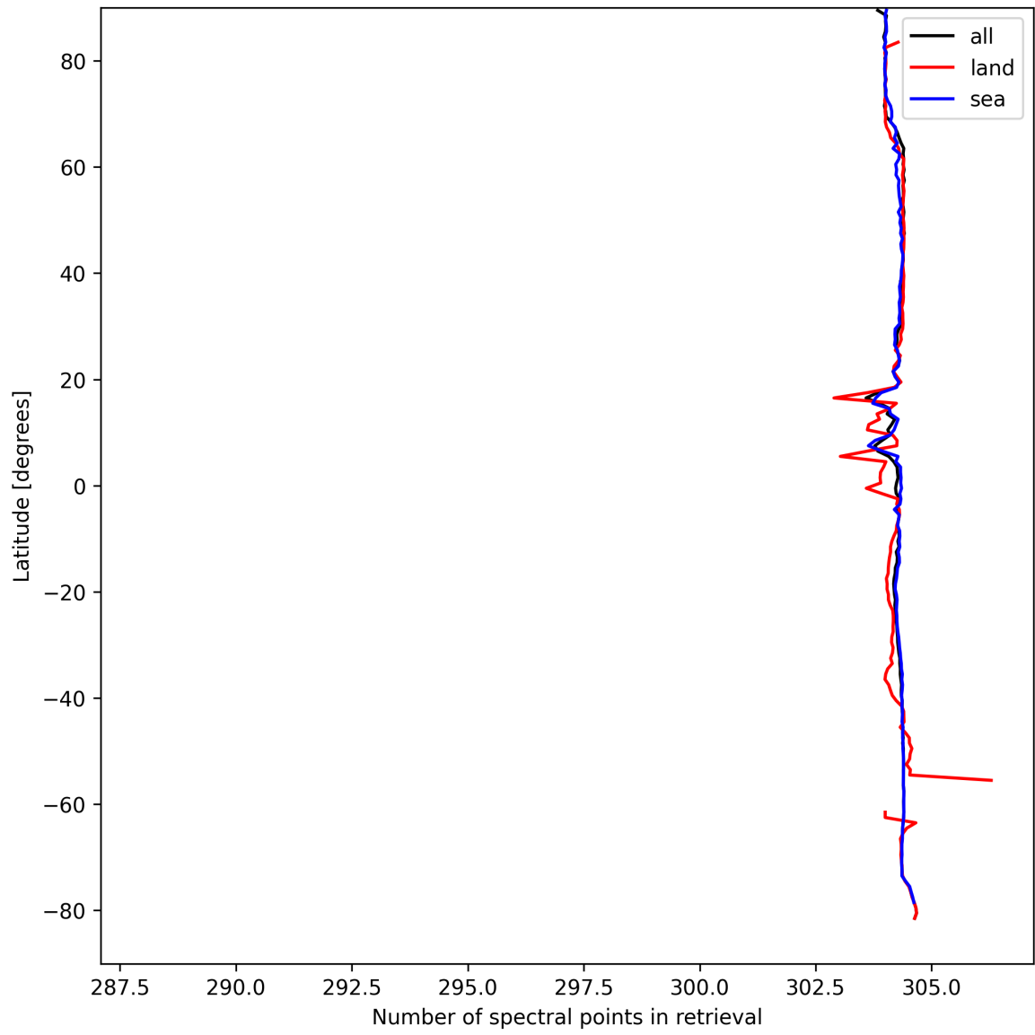
Figure 16: Zonal average of “Number of spectral points in retrieval” for 2024-09-03 to 2024-09-05.
