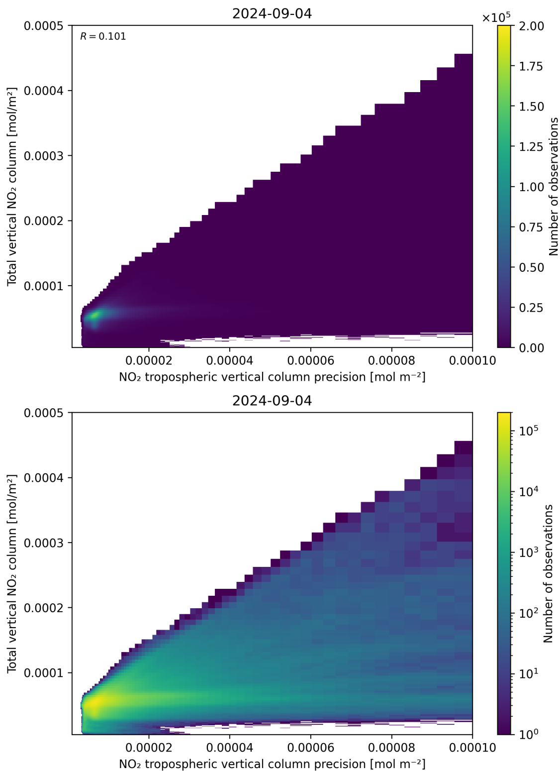
Figure 138: Scatter density plot of “NO 2 tropospheric vertical column precision” against “Total vertical NO 2 column” for 2024-09-03 to 2024-09-05.
