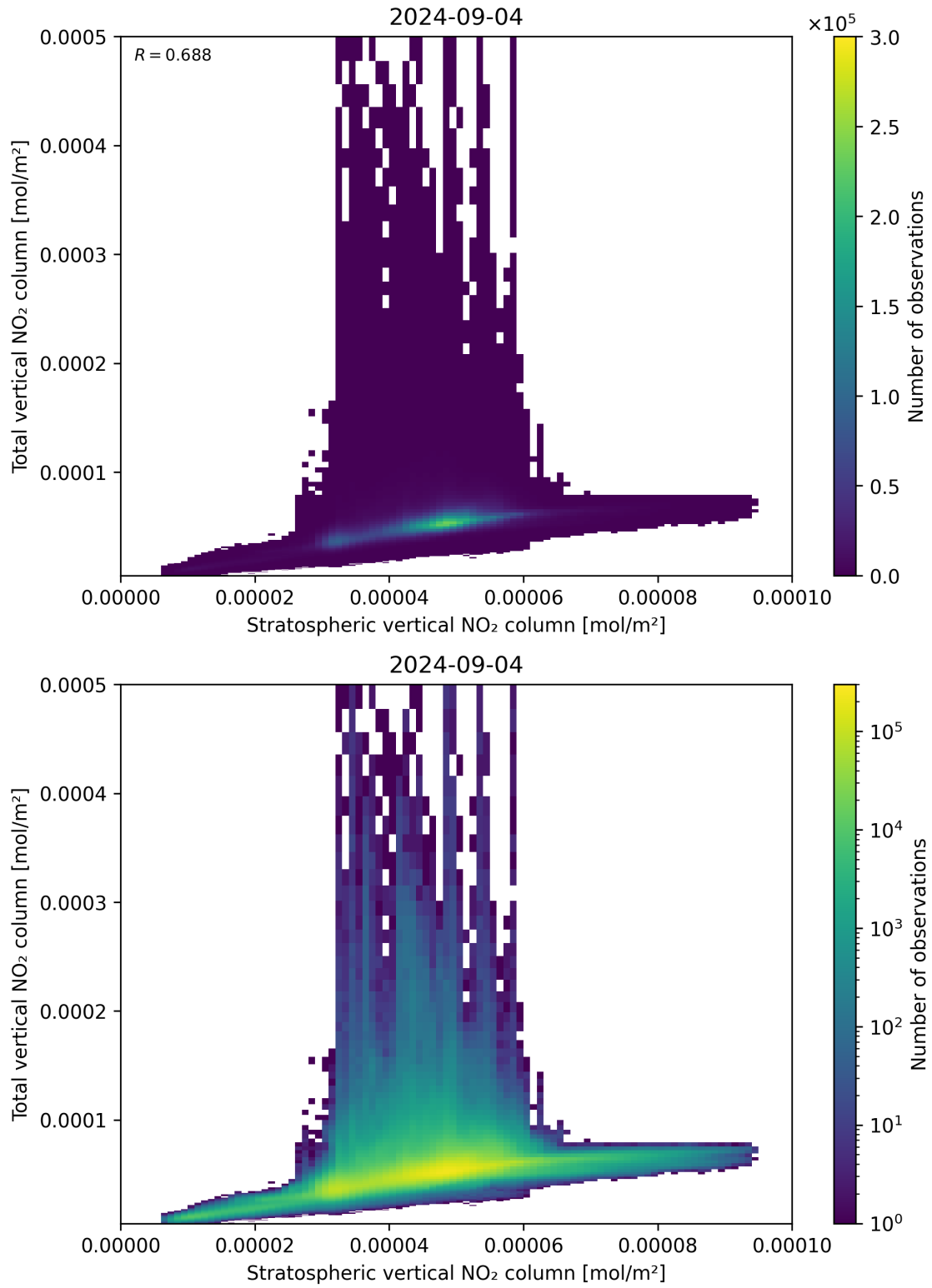
Figure 100: Scatter density plot of “Stratospheric vertical NO 2 column” against “Total vertical NO 2 column” for 2024-09-03 to 2024-09-05.
