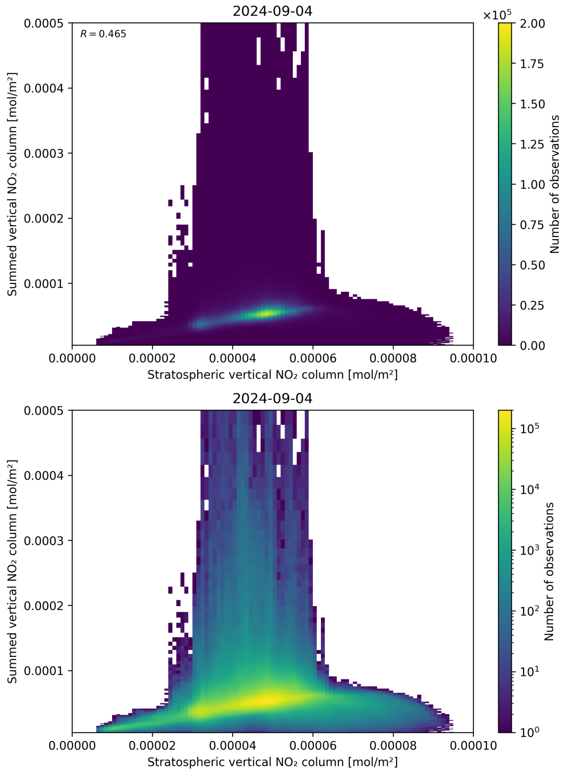
Figure 98: Scatter density plot of “Stratospheric vertical NO 2 column” against “Summed vertical NO 2 column” for 2024-09-03 to 2024-09-05.
