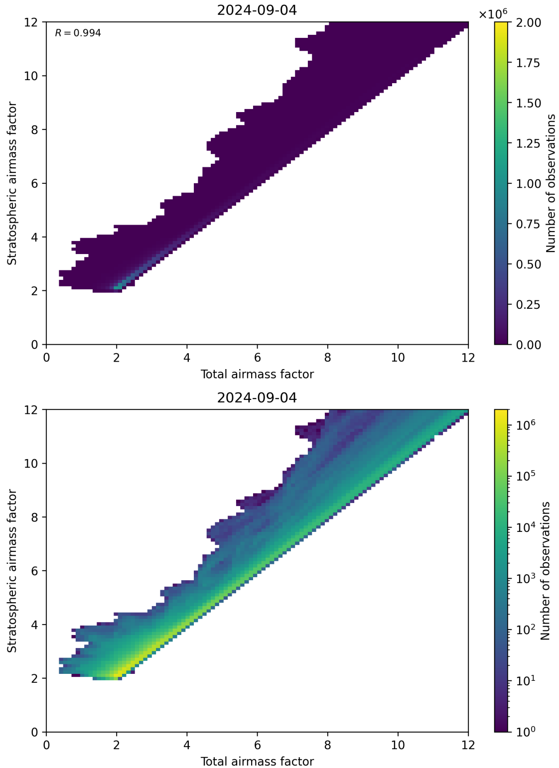
Figure 62: Scatter density plot of “Total airmass factor” against “Stratospheric airmass factor” for 2024-09-03 to 2024-09-05.
