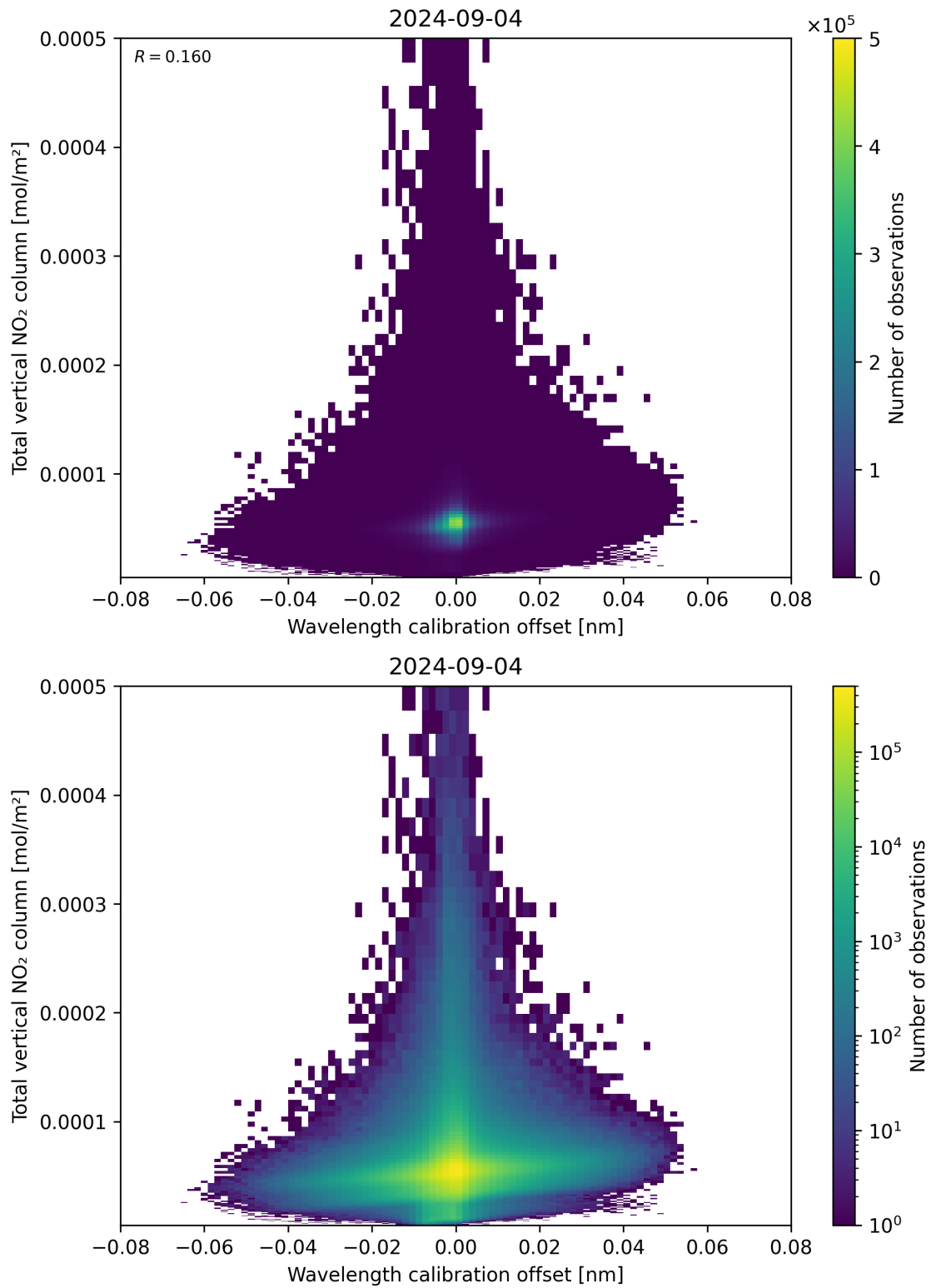
Figure 179: Scatter density plot of “Wavelength calibration offset” against “Total vertical NO 2 column” for 2024-09-03 to 2024-09-05.
