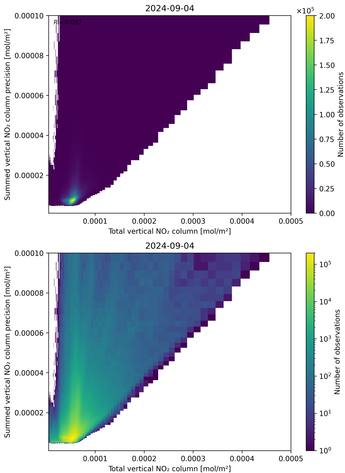
Figure 113: Scatter density plot of “Total vertical NO 2 column” against “Summed vertical NO 2 column precision” for 2024-09-03 to 2024-09-05.
