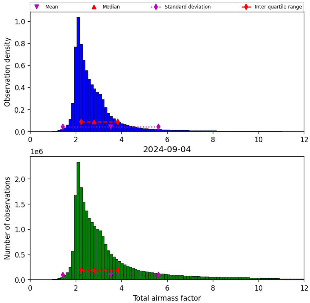
Figure 32: Histogram of “Total airmass factor” for 2024-09-03 to 2024-09-05
