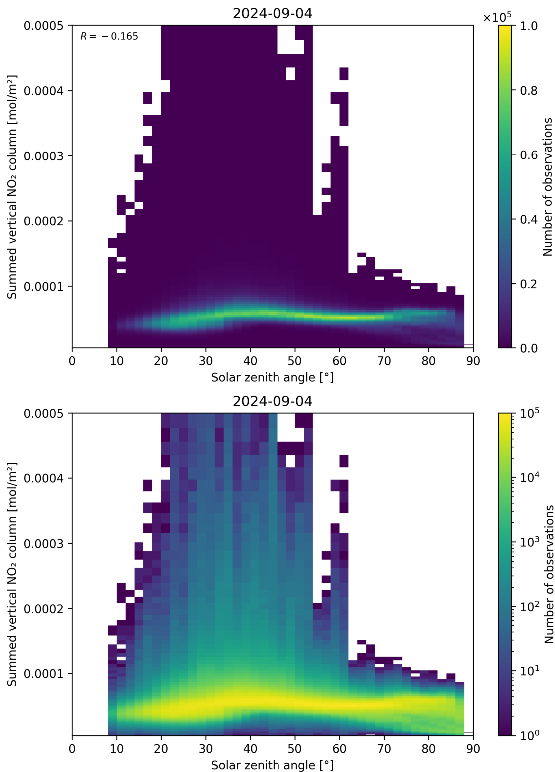
Figure 151: Scatter density plot of “Solar zenith angle” against “Summed vertical NO 2 column” for 2024-09-03 to 2024-09-05.
