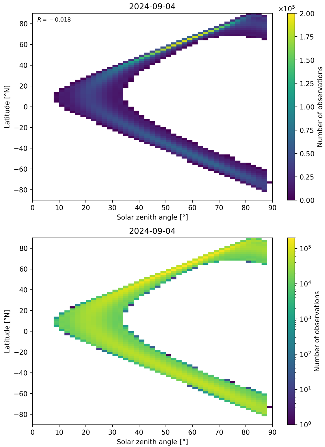
Figure 149: Scatter density plot of “Solar zenith angle” against “Latitude” for 2024-09-03 to 2024-09-05.
