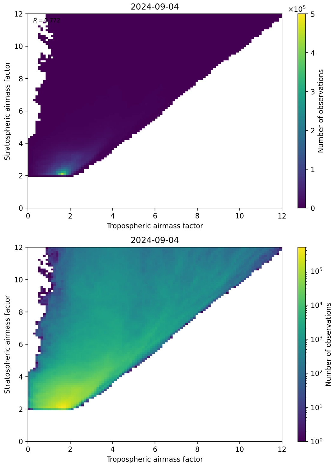
Figure 71: Scatter density plot of “Tropospheric airmass factor” against “Stratospheric airmass factor” for 2024-09-03 to 2024-09-05.
