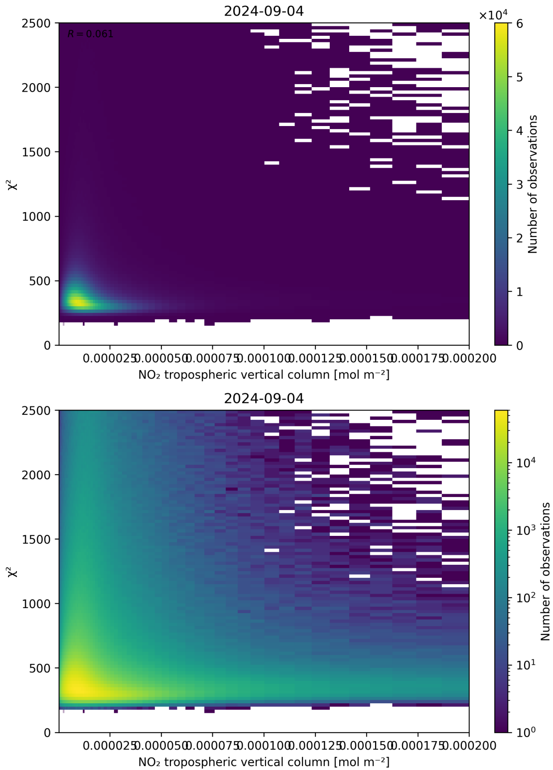
Figure 124: Scatter density plot of “NO 2 tropospheric vertical column” against “ \chi^2 ” for 2024-09-03 to 2024-09-05.
