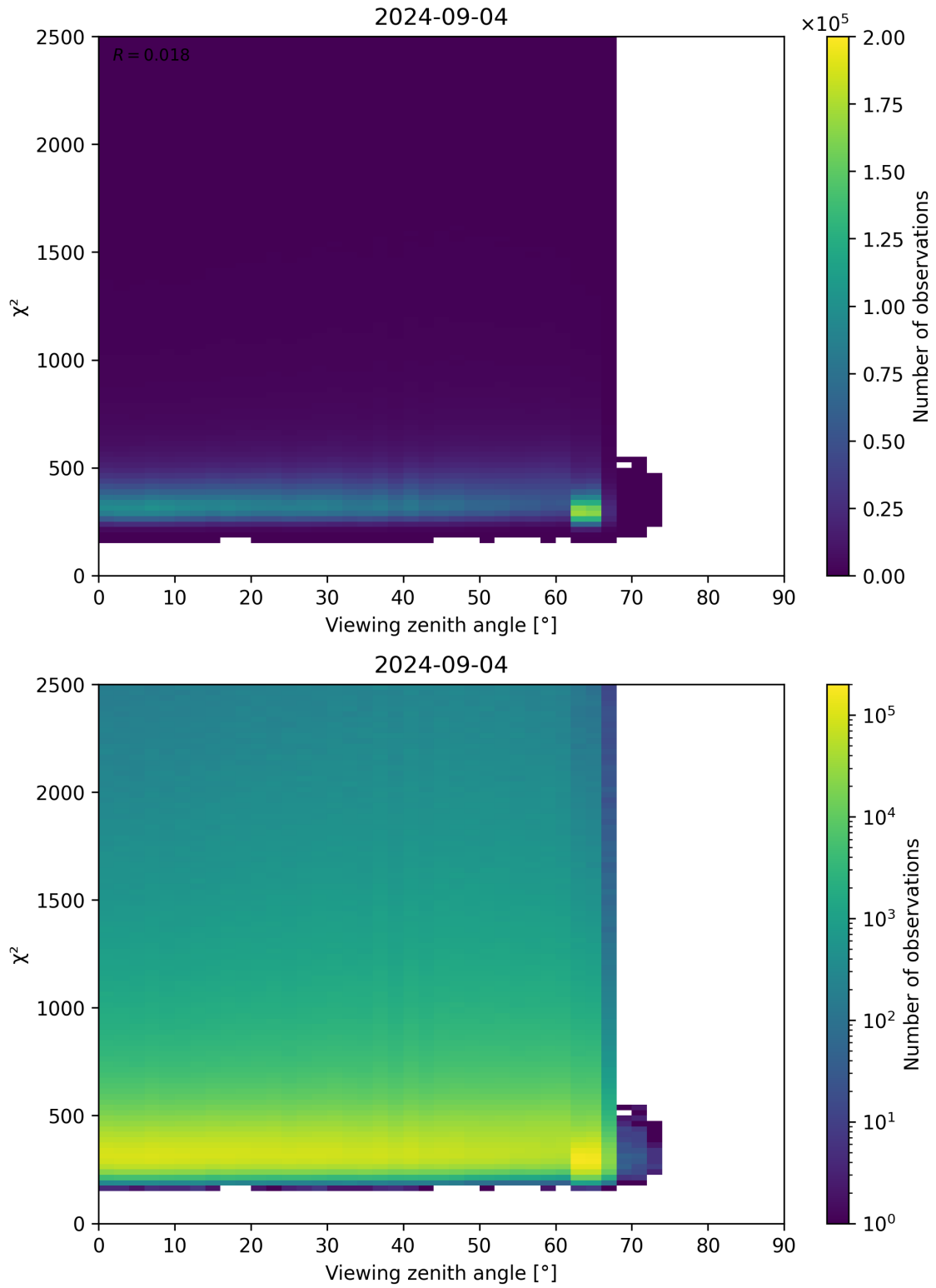
Figure 162: Scatter density plot of “Viewing zenith angle” against “ \chi^2 ” for 2024-09-03 to 2024-09-05.
