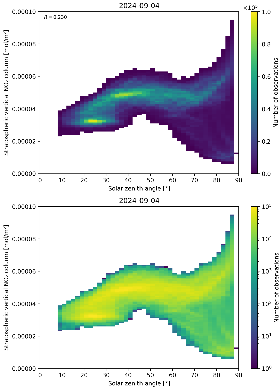
Figure 150: Scatter density plot of “Solar zenith angle” against “Stratospheric vertical NO 2 column” for 2024-09-03 to 2024-09-05.
