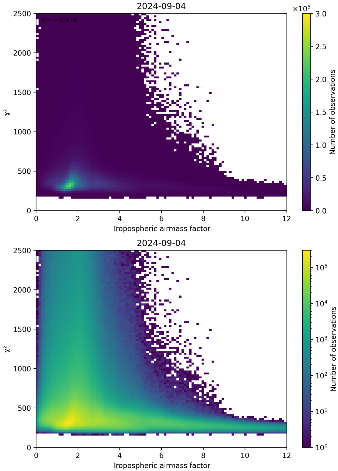
Figure 73: Scatter density plot of “Tropospheric airmass factor” against “ \chi^2 ” for 2024-09-03 to 2024-09-05.
