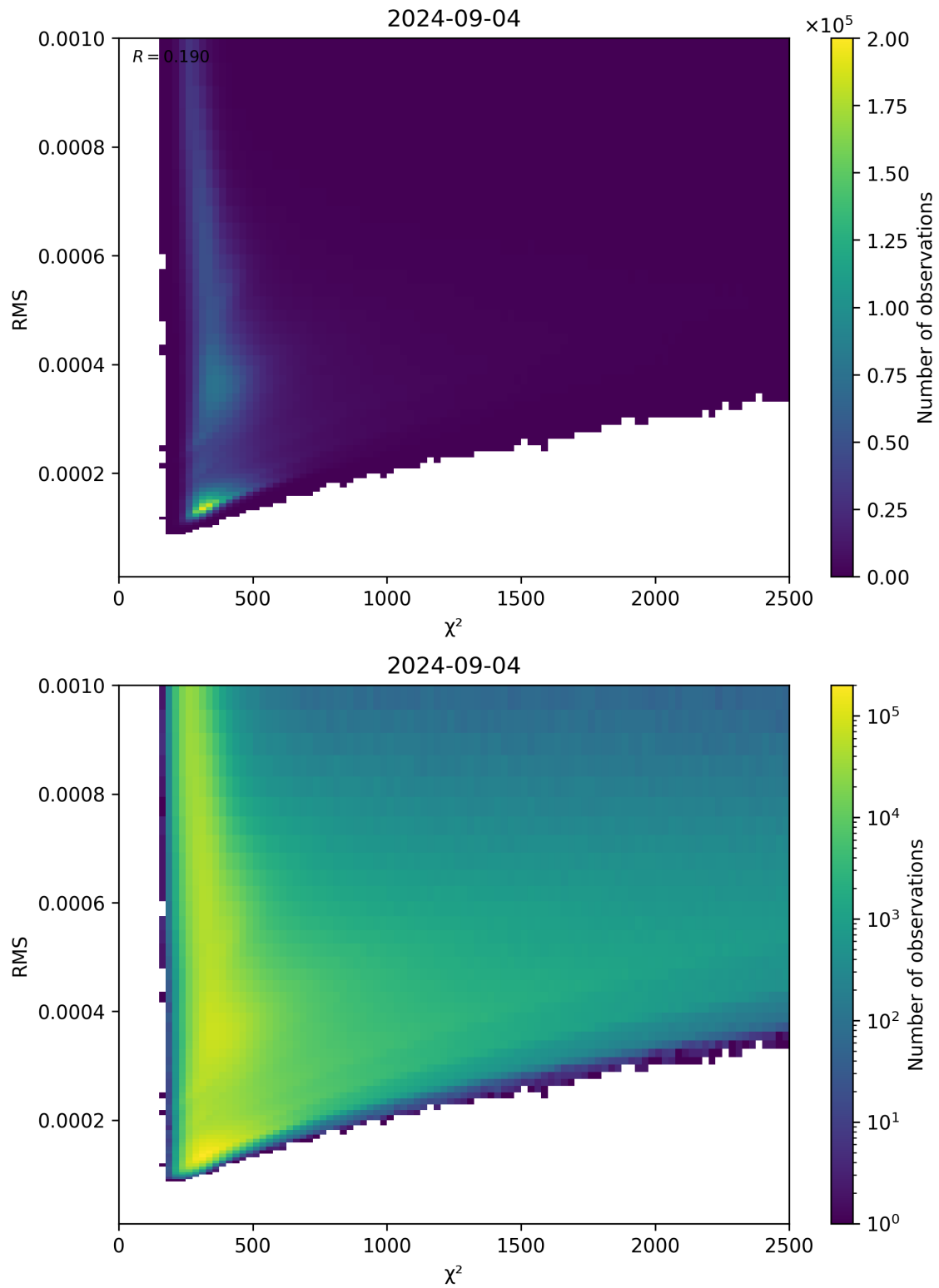
Figure 82: Scatter density plot of “ \chi^2 ” against “RMS” for 2024-09-03 to 2024-09-05.
