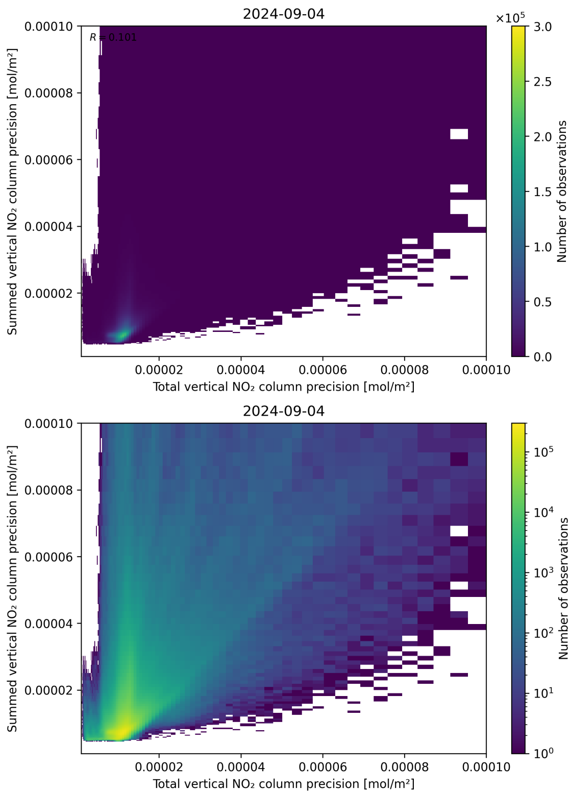
Figure 118: Scatter density plot of “Total vertical NO 2 column precision” against “Summed vertical NO 2 column precision” for 2024-09-03 to 2024-09-05.
