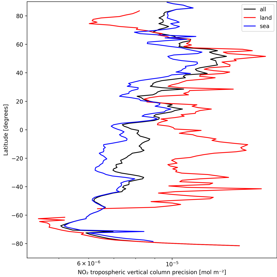
Figure 13: Zonal average of "NO 2 tropospheric vertical column precision" for 2024-09-03 to 2024-09-05.
