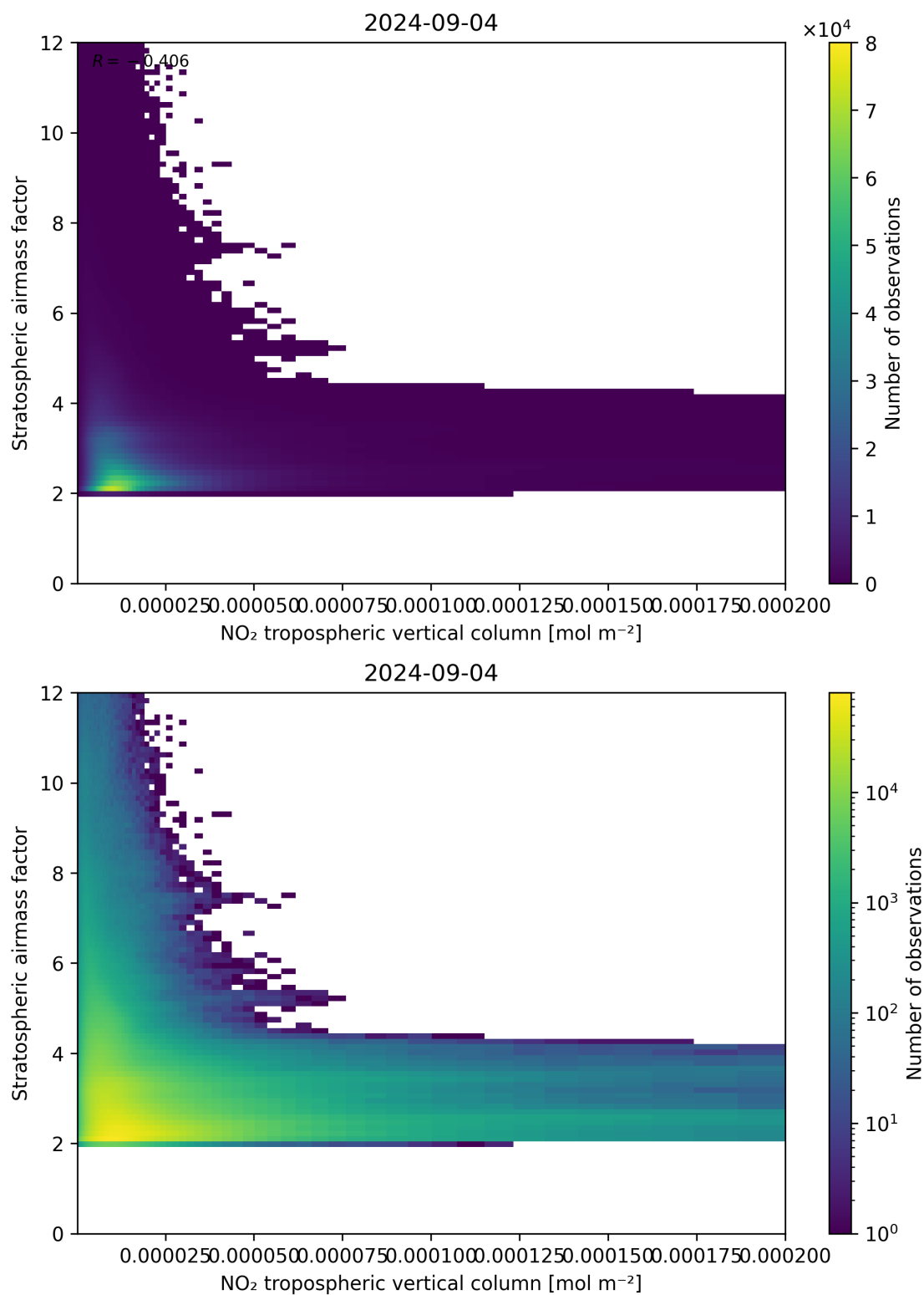
Figure 121: Scatter density plot of “NO 2 tropospheric vertical column” against “Stratospheric air mass factor” for 2024-09-03 to 2024-09-05.
