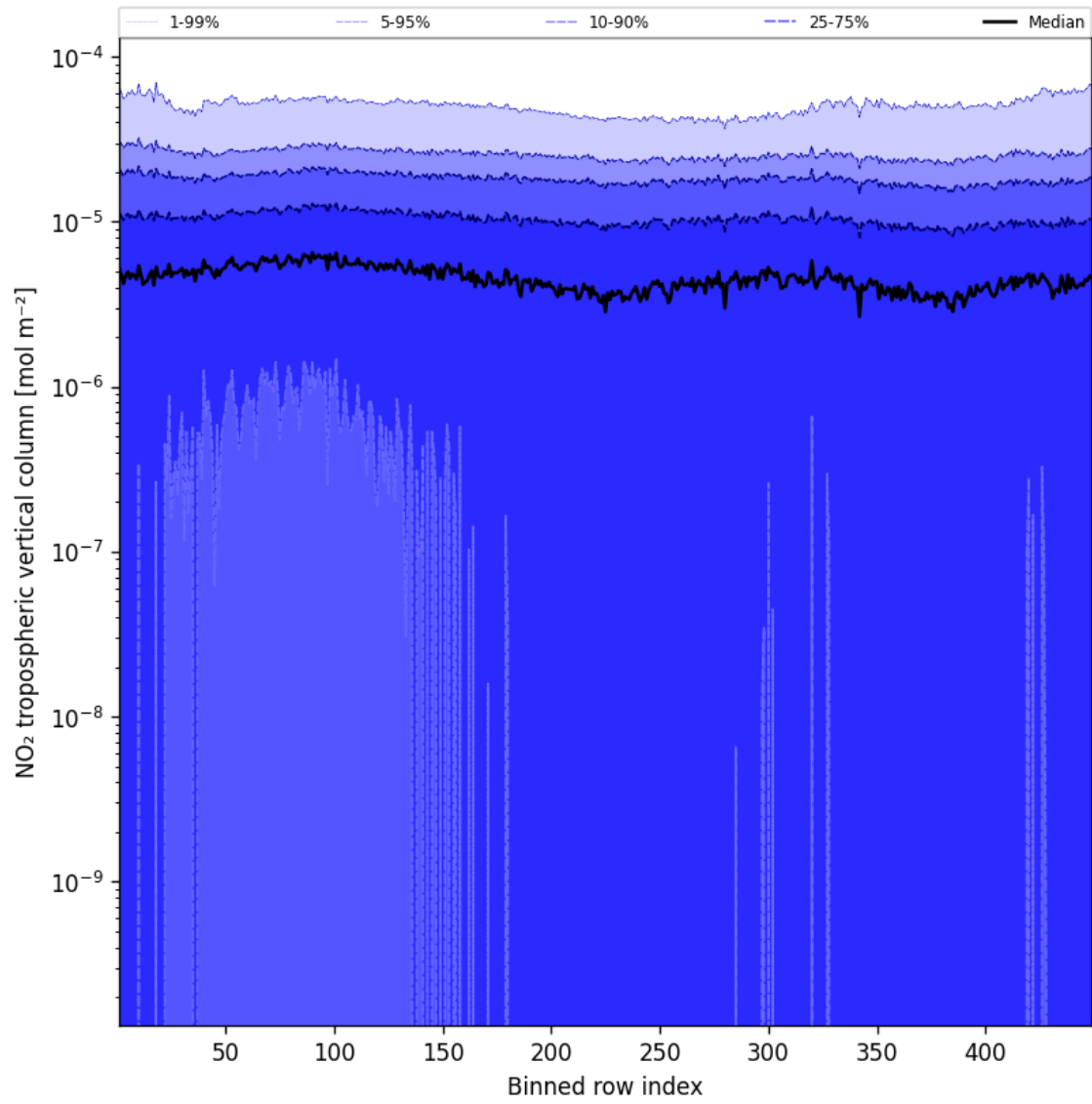
Figure 46: Along track statistics of “NO 2 tropospheric vertical column” for 2024-09-03 to 2024-09-05
