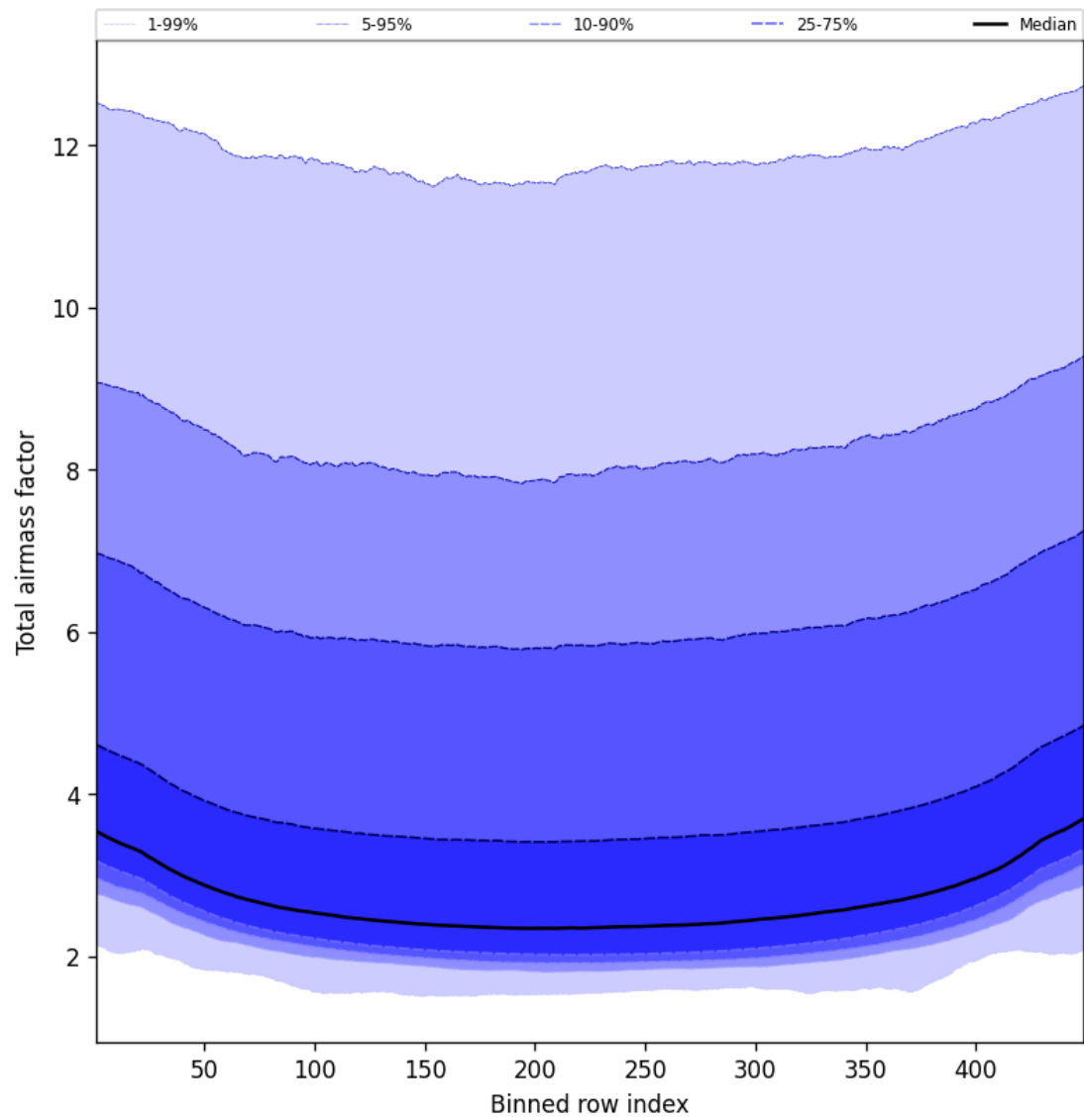
Figure 49: Along track statistics of “Total airmass factor” for 2024-09-03 to 2024-09-05
