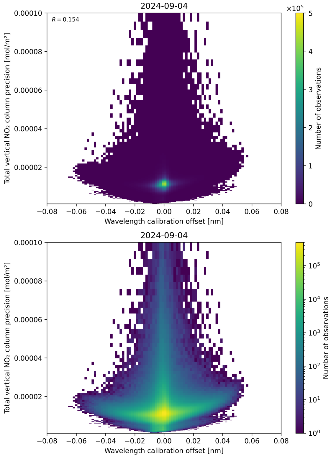
Figure 180: Scatter density plot of “Wavelength calibration offset” against “Total vertical NO 2 column precision” for 2024-09-03 to 2024-09-05.
