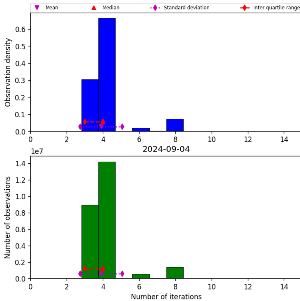
Figure 34: Histogram of “Number of iterations” for 2024-09-03 to 2024-09-05
