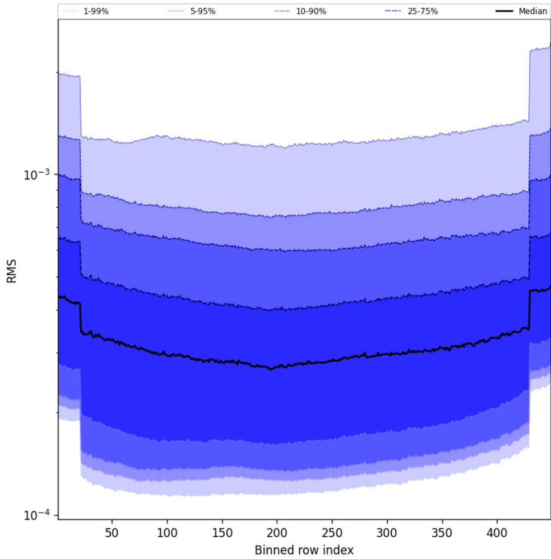
Figure 60: Along track statistics of “RMS” for 2024-09-03 to 2024-09-05
