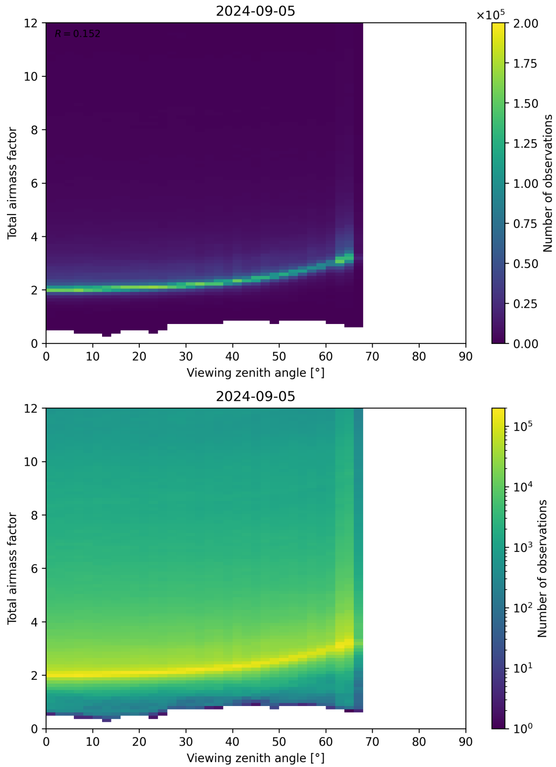
Figure 160: Scatter density plot of “Viewing zenith angle” against “Total airmass factor” for 2024-09-04 to 2024-09-06.
