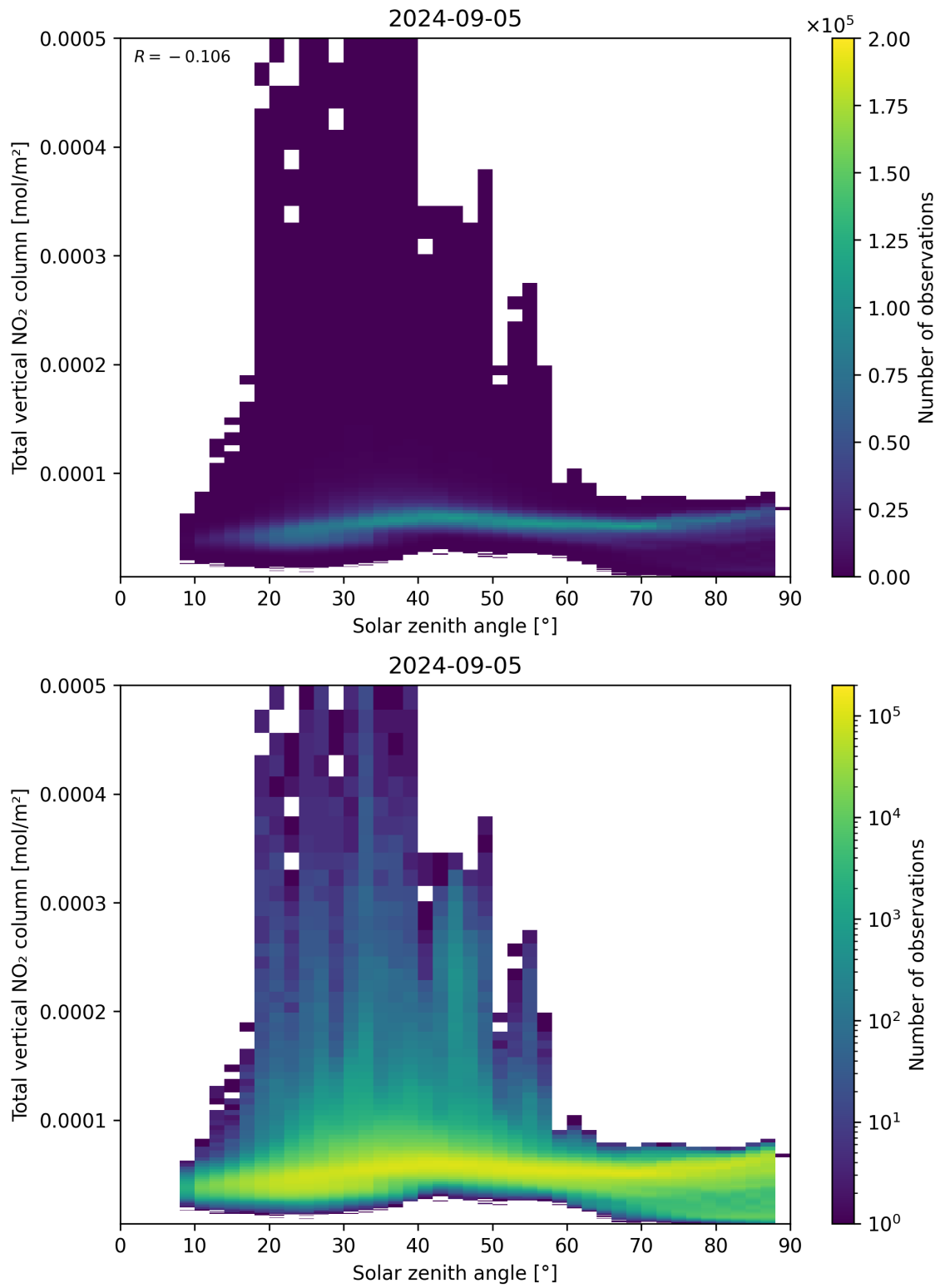
Figure 153: Scatter density plot of “Solar zenith angle” against “Total vertical NO 2 column” for 2024-09-04 to 2024-09-06.
