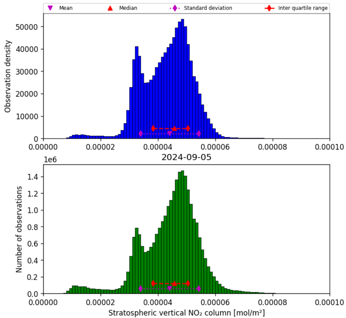
Figure 36: Histogram of “Stratospheric vertical NO 2 column” for 2024-09-04 to 2024-09-06
