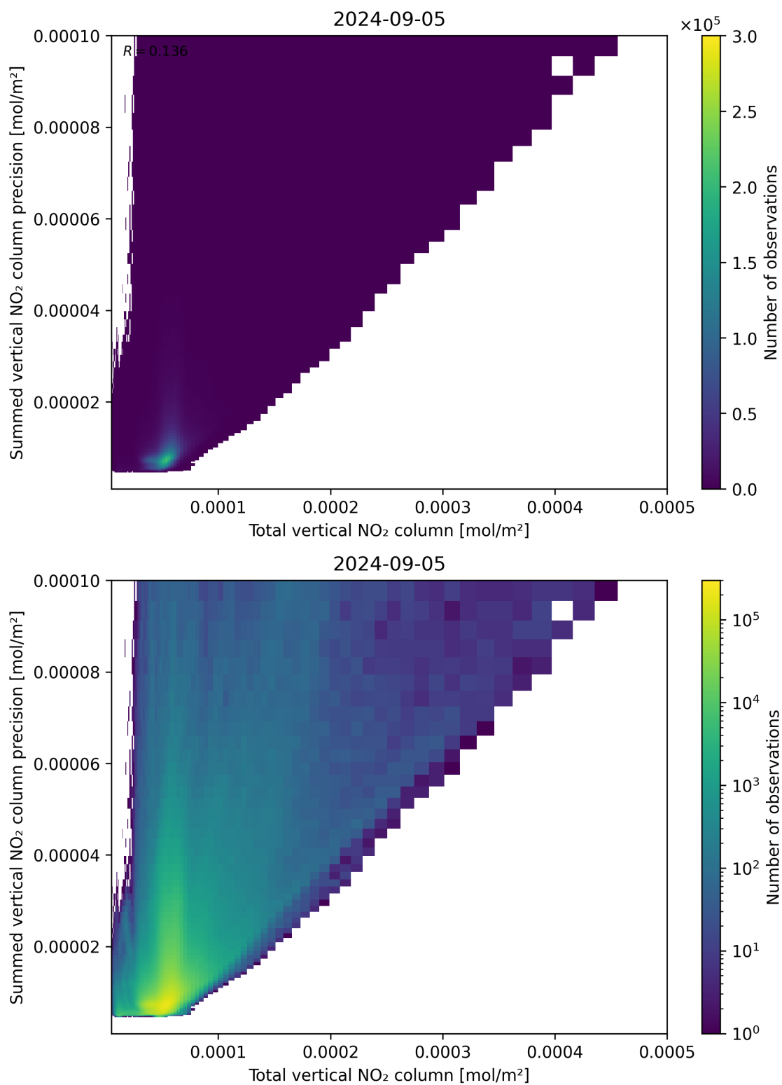
Figure 113: Scatter density plot of “Total vertical NO 2 column” against “Summed vertical NO 2 column precision” for 2024-09-04 to 2024-09-06.
