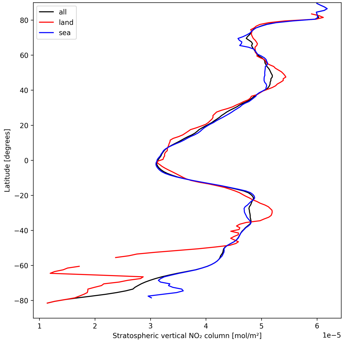
Figure 19: Zonal average of “Stratospheric vertical NO 2 column” for 2024-09-04 to 2024-09-06.
