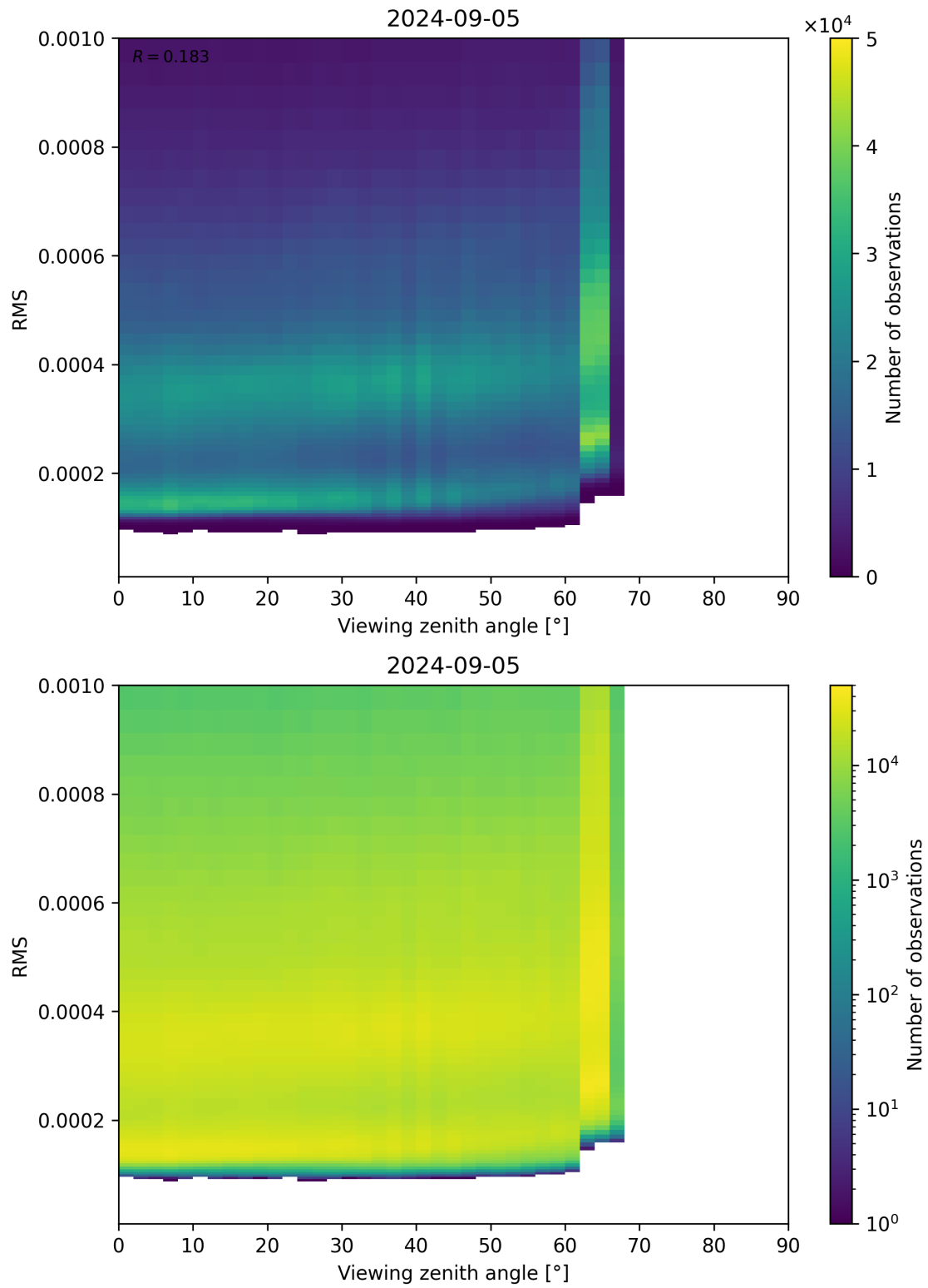
Figure 171: Scatter density plot of “Viewing zenith angle” against “RMS” for 2024-09-04 to 2024-09-06.
