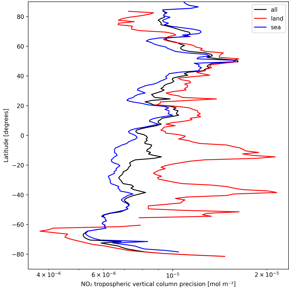
Figure 13: Zonal average of “NO 2 tropospheric vertical column precision” for 2024-09-04 to 2024-09-06.
