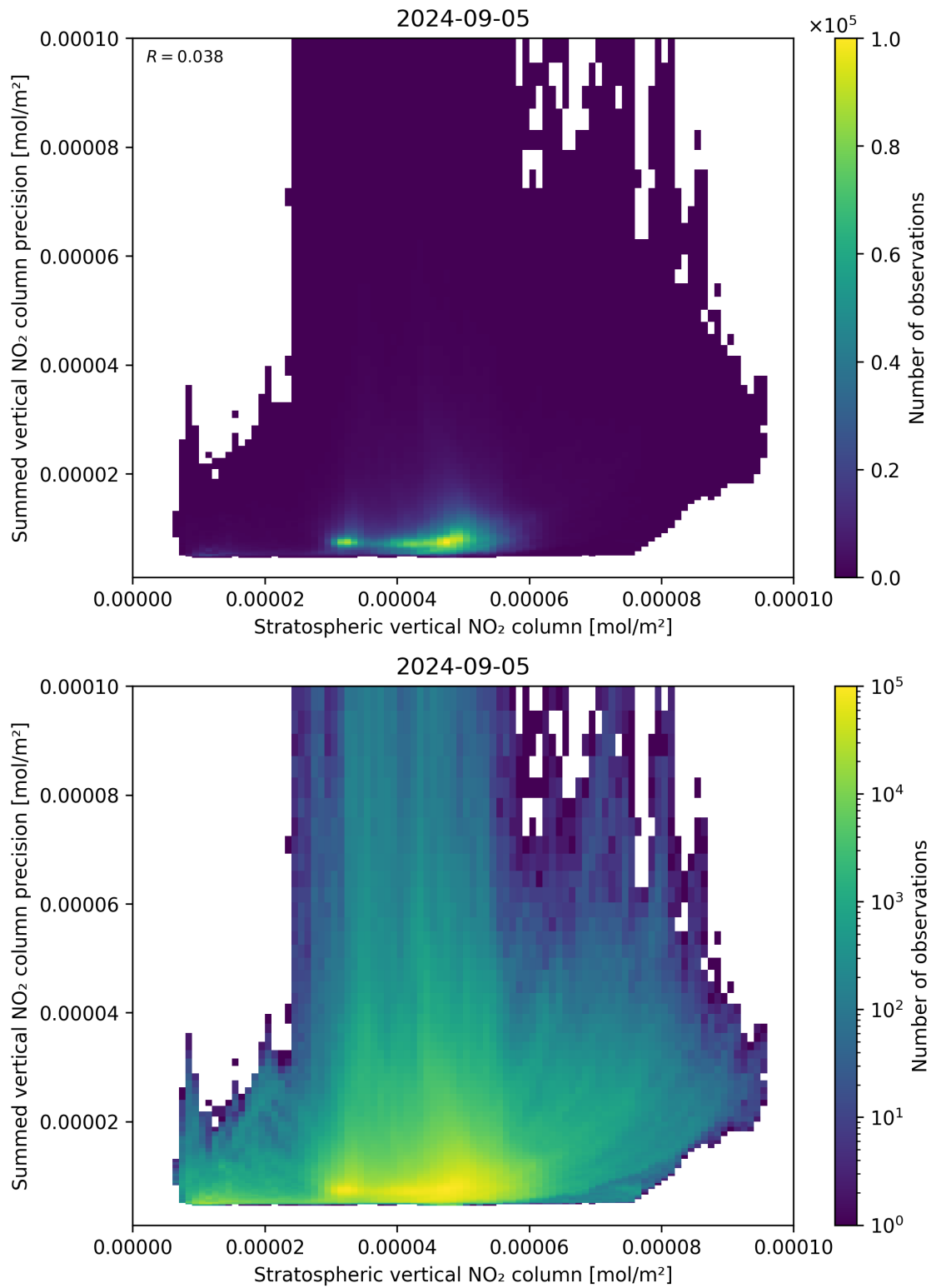
Figure 99: Scatter density plot of “Stratospheric vertical NO 2 column” against “Summed vertical NO 2 column precision” for 2024-09-04 to 2024-09-06.
