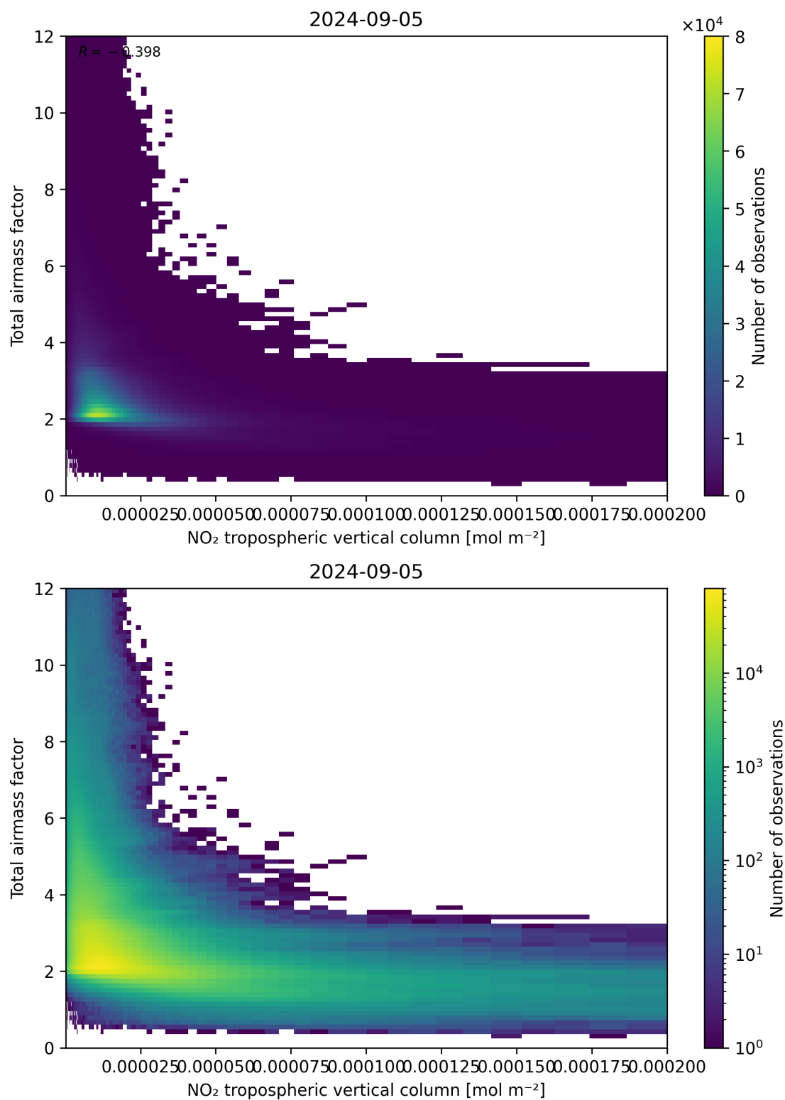
Figure 122: Scatter density plot of “NO 2 tropospheric vertical column” against “Total air mass factor” for 2024-09-04 to 2024-09-06.
