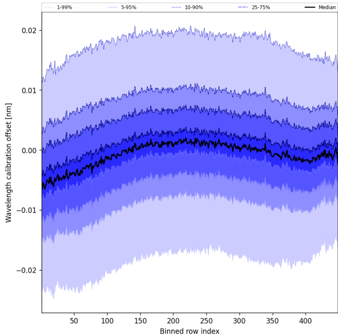
Figure 52: Along track statistics of “Wavelength calibration offset” for 2024-09-04 to 2024-09-06
