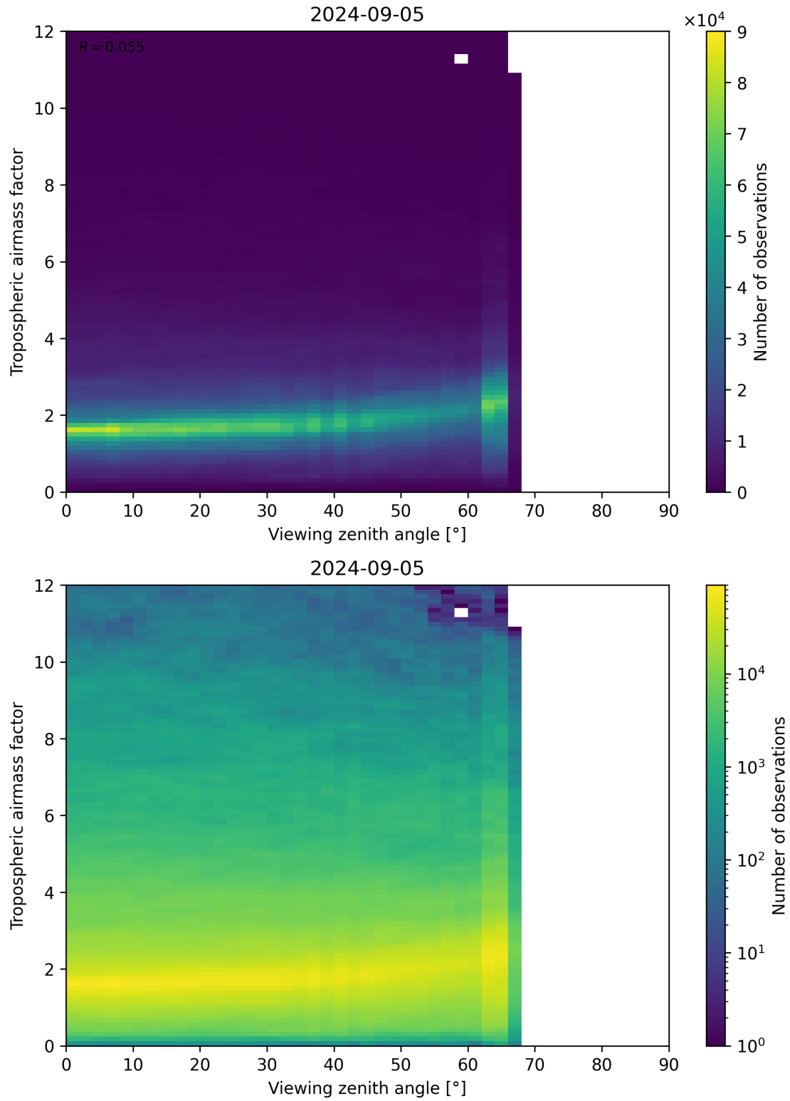
Figure 161: Scatter density plot of “Viewing zenith angle” against “Tropospheric airmass factor” for 2024-09-04 to 2024-09-06.
