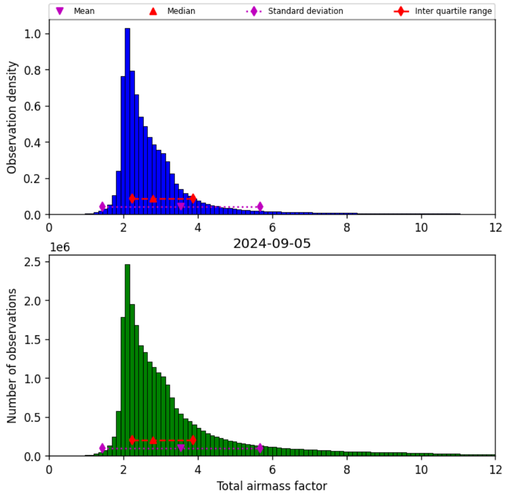
Figure 32: Histogram of “Total airmass factor” for 2024-09-04 to 2024-09-06
