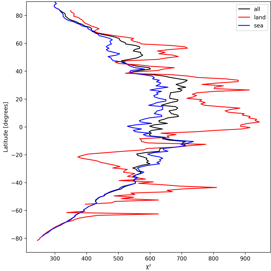
Figure 25: Zonal average of “ \chi^2 ” for 2024-09-04 to 2024-09-06.
