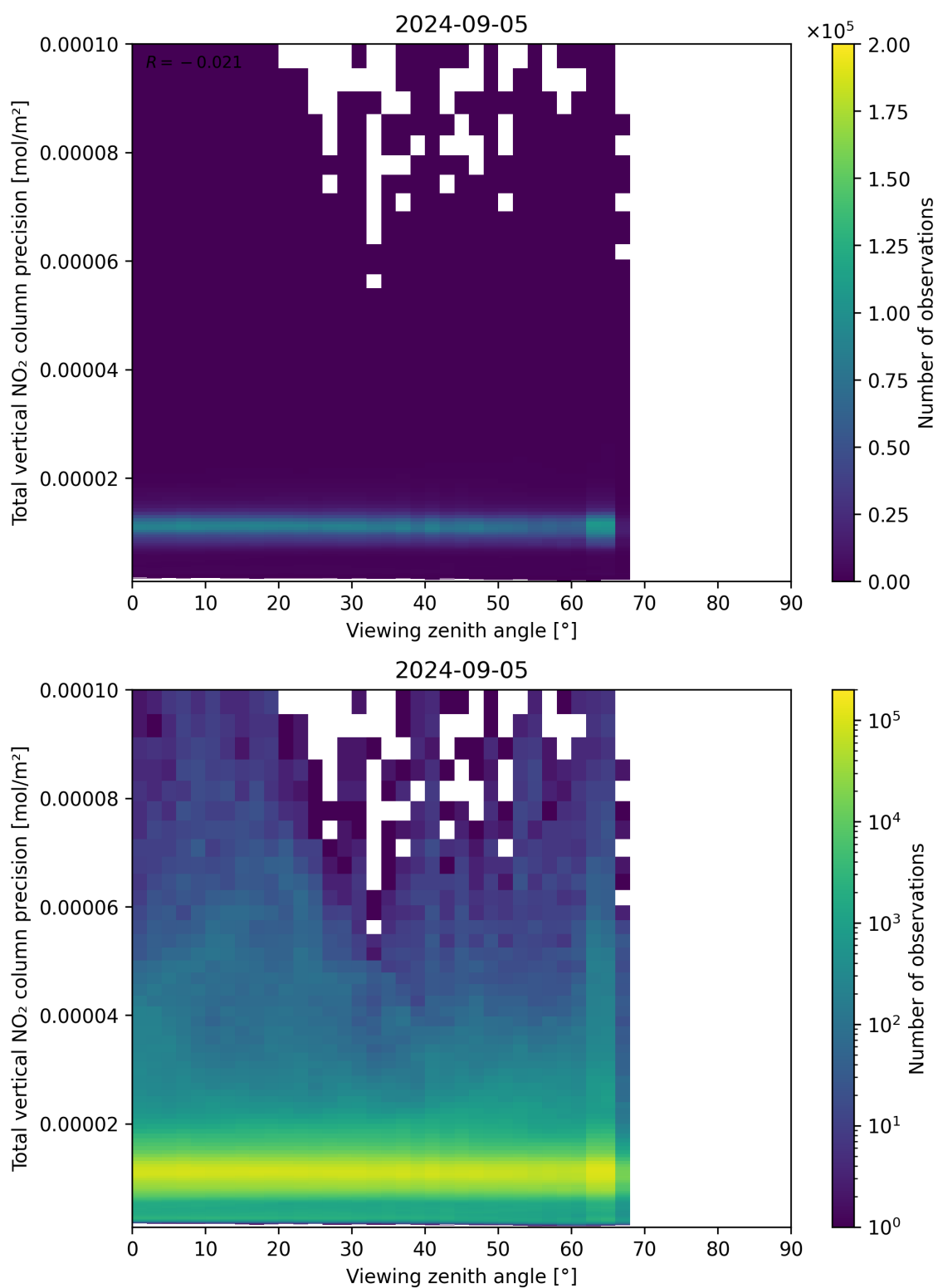
Figure 168: Scatter density plot of “Viewing zenith angle” against “Total vertical NO 2 column precision” for 2024-09-04 to 2024-09-06.
