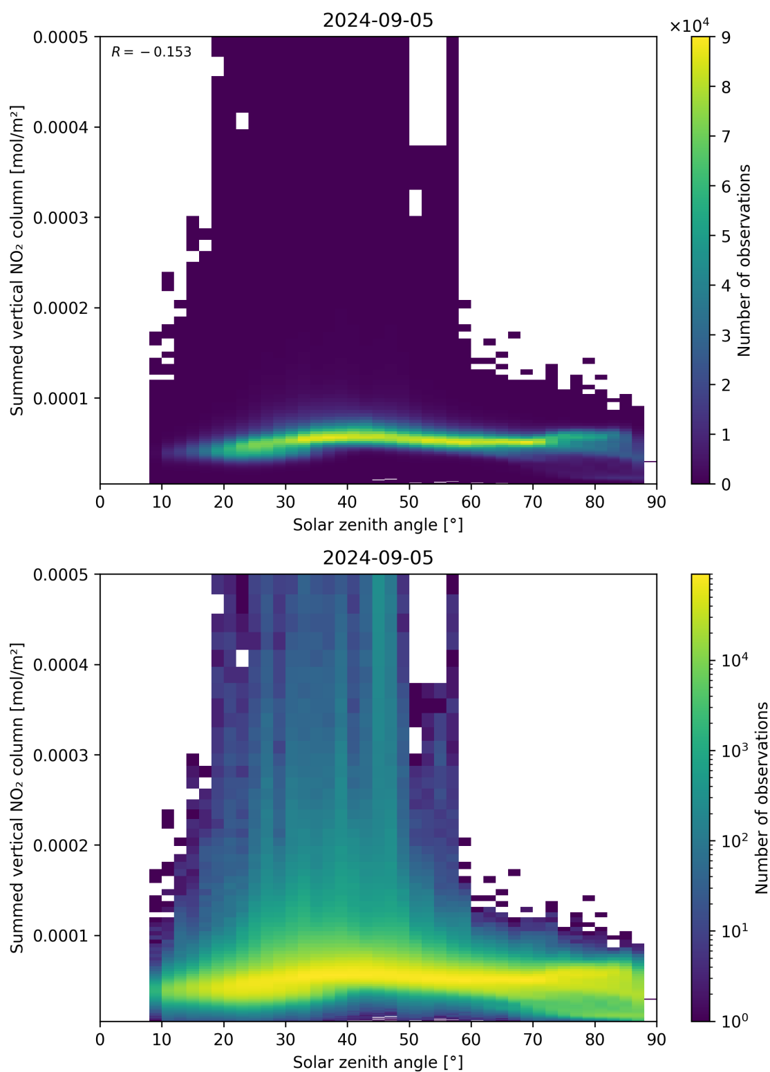
Figure 151: Scatter density plot of “Solar zenith angle” against “Summed vertical NO 2 column” for 2024-09-04 to 2024-09-06.
