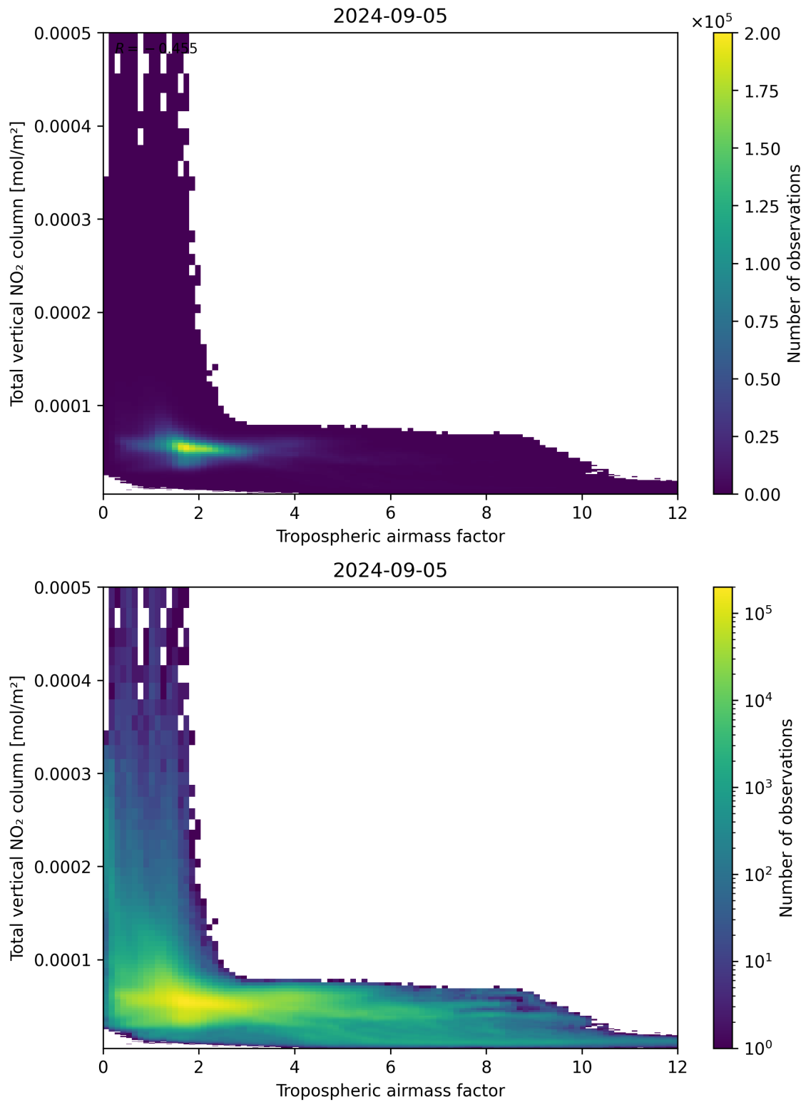
Figure 77: Scatter density plot of “Tropospheric airmass factor” against “Total vertical NO 2 column” for 2024-09-04 to 2024-09-06.
