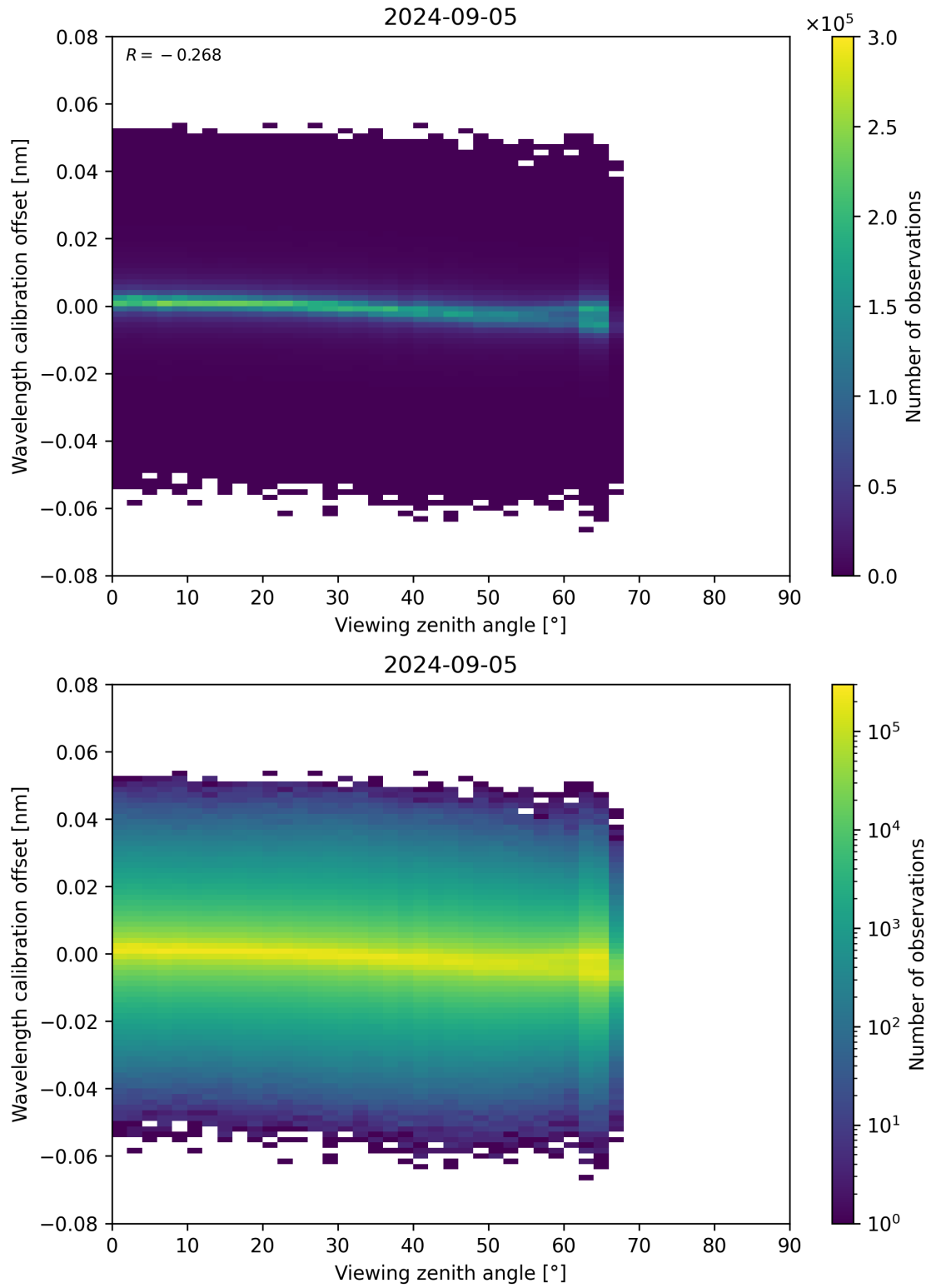
Figure 173: Scatter density plot of “Viewing zenith angle” against “Wavelength calibration offset” for 2024-09-04 to 2024-09-06.
