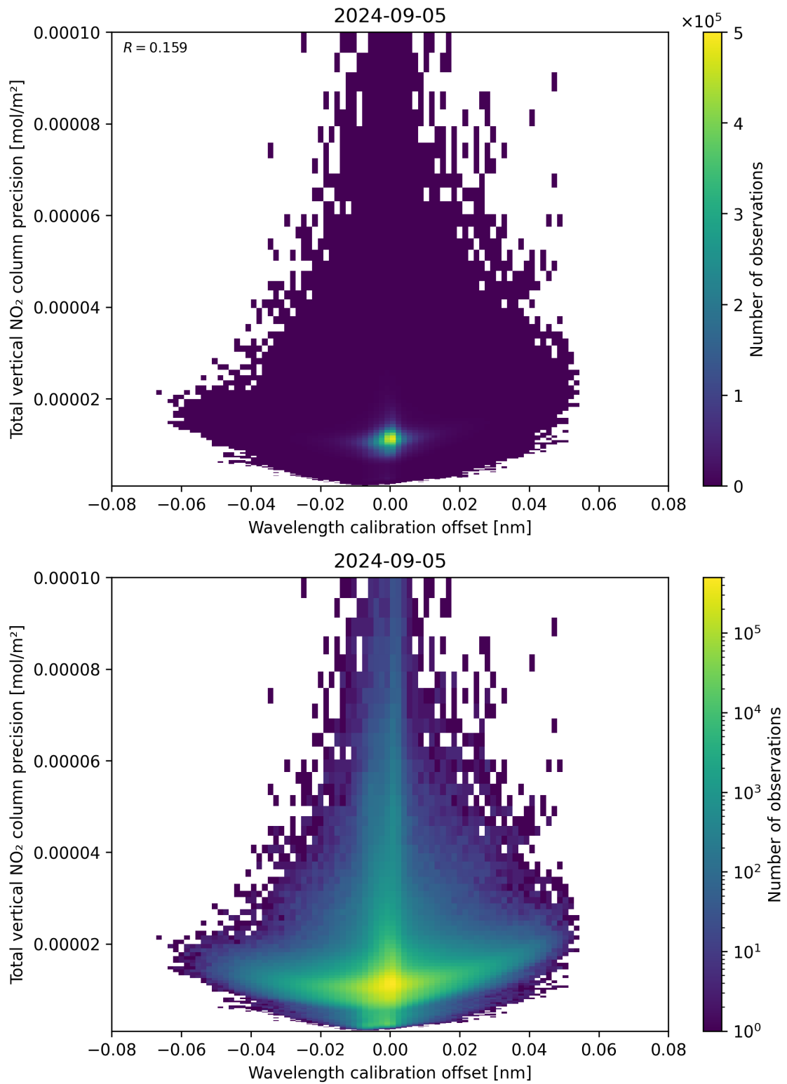
Figure 180: Scatter density plot of “Wavelength calibration offset” against “Total vertical NO 2 column precision” for 2024-09-04 to 2024-09-06.
