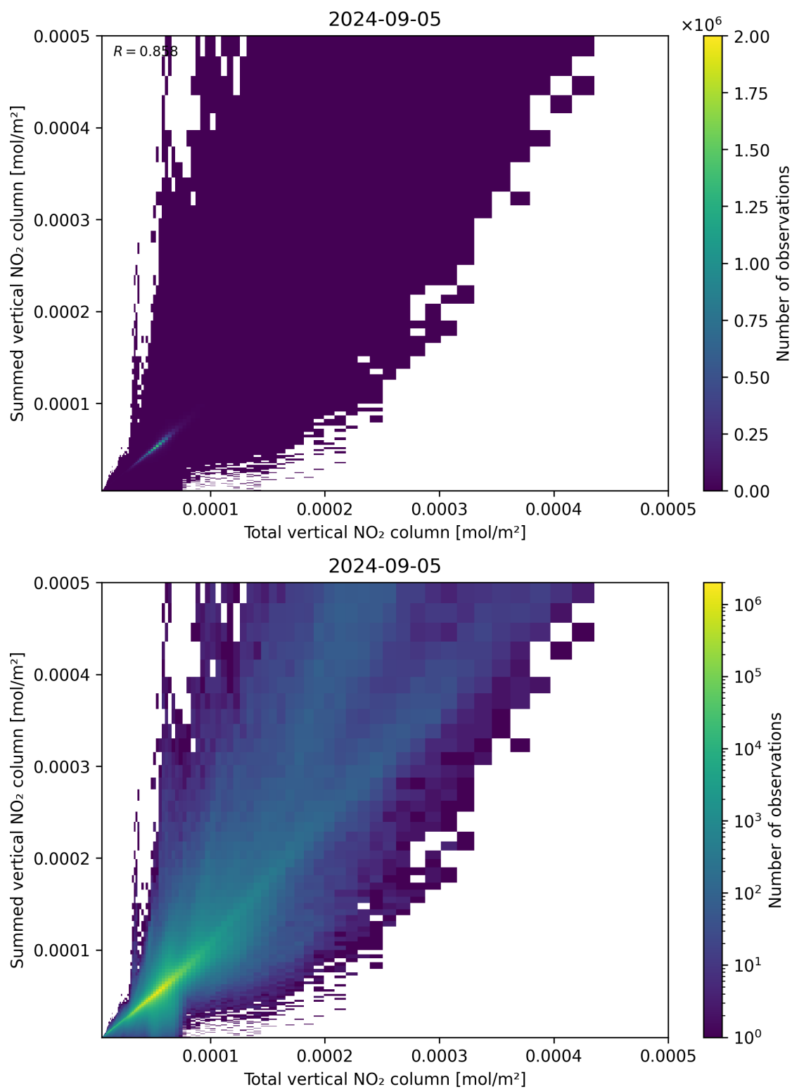
Figure 112: Scatter density plot of “Total vertical NO 2 column” against “Summed vertical NO 2 column” for 2024-09-04 to 2024-09-06.
