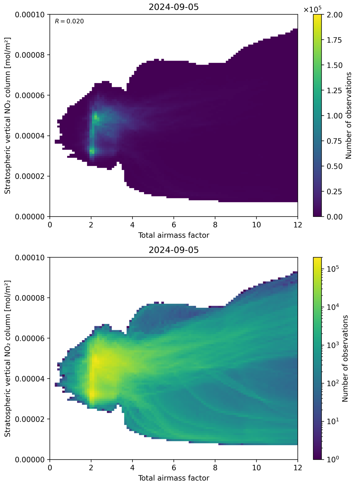
Figure 64: Scatter density plot of “Total airmass factor” against “Stratospheric vertical NO 2 column” for 2024-09-04 to 2024-09-06.
