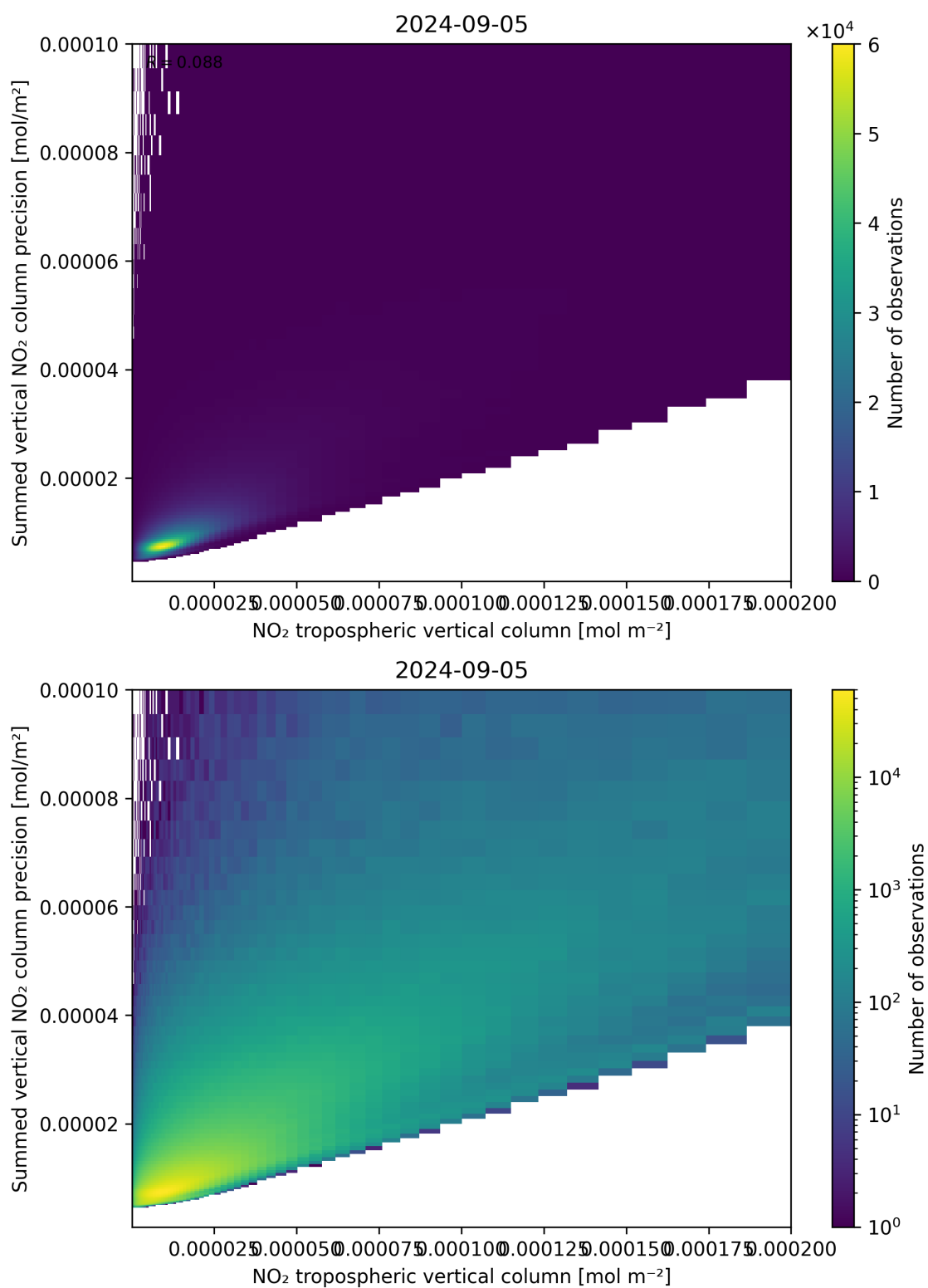
Figure 127: Scatter density plot of “NO 2 tropospheric vertical column” against “Summed vertical NO 2 column precision” for 2024-09-04 to 2024-09-06.
