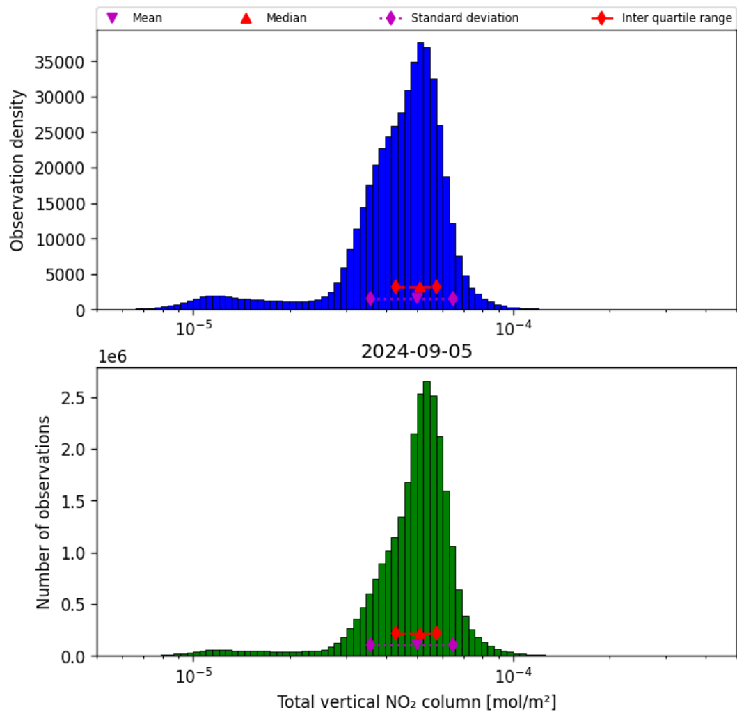
Figure 38: Histogram of “Total vertical NO 2 column” for 2024-09-04 to 2024-09-06
