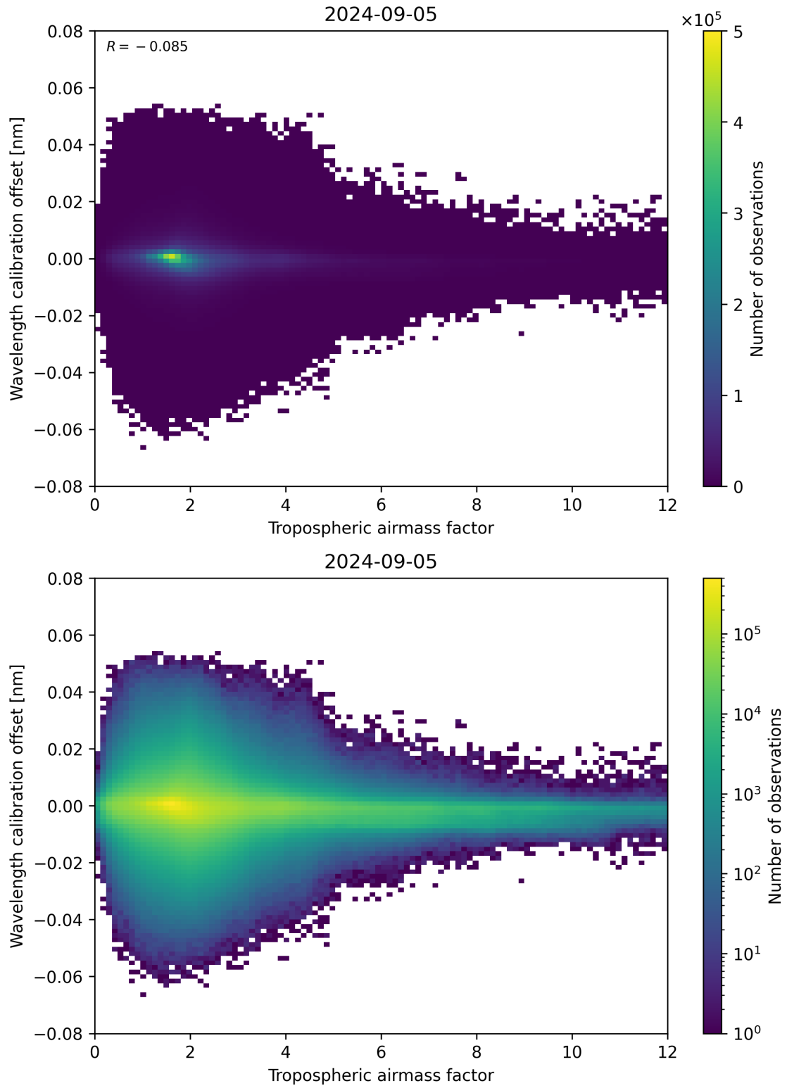
Figure 80: Scatter density plot of “Tropospheric airmass factor” against “Wavelength calibration offset” for 2024-09-04 to 2024-09-06.
