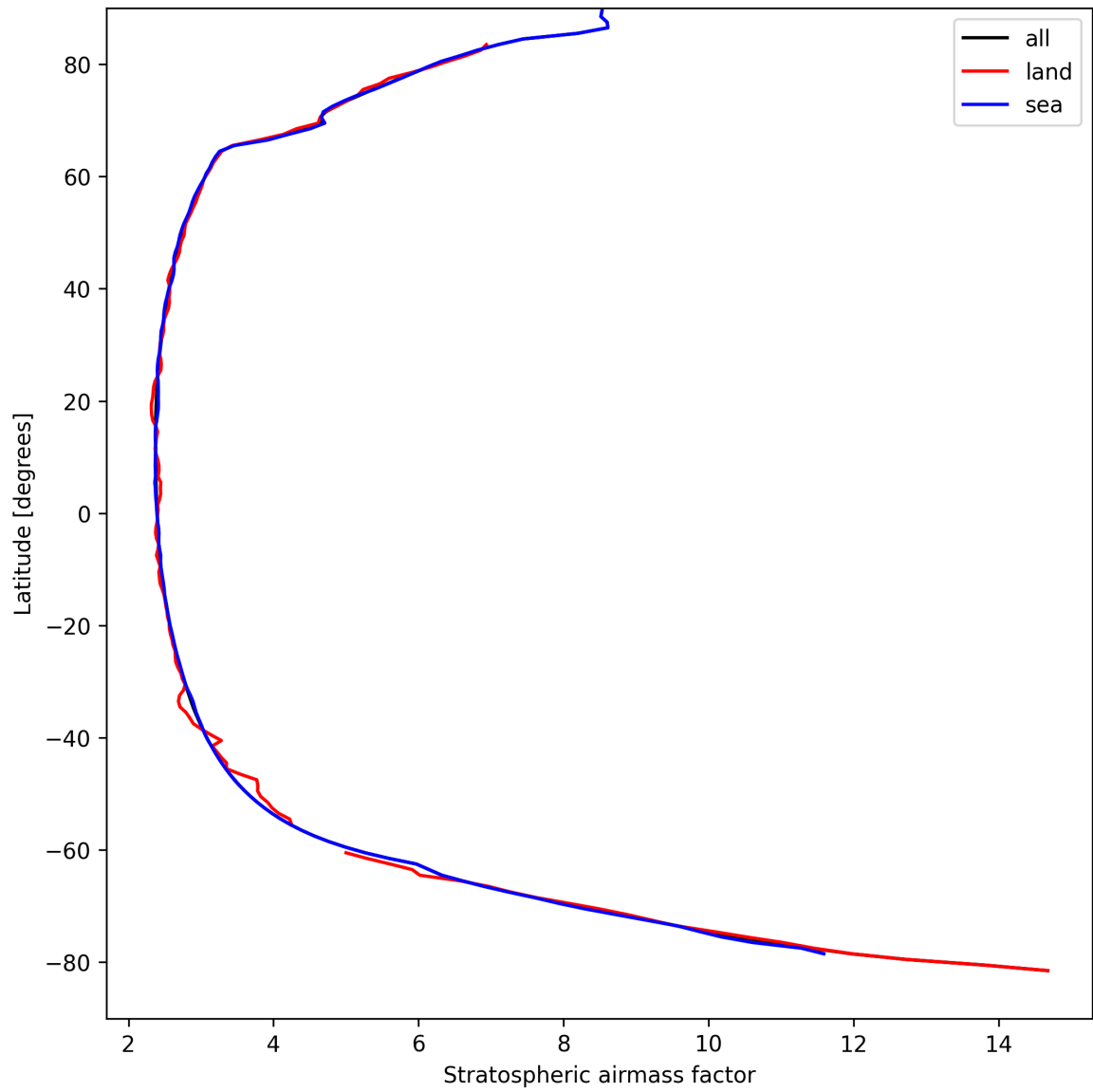
Figure 27: Zonal average of “Stratospheric air mass factor” for 2024-09-04 to 2024-09-06.
