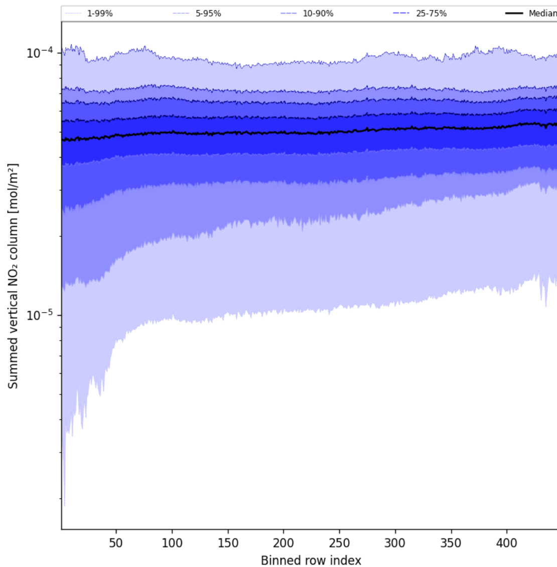
Figure 57: Along track statistics of “Summed vertical NO 2 column” for 2024-09-04 to 2024-09-06
