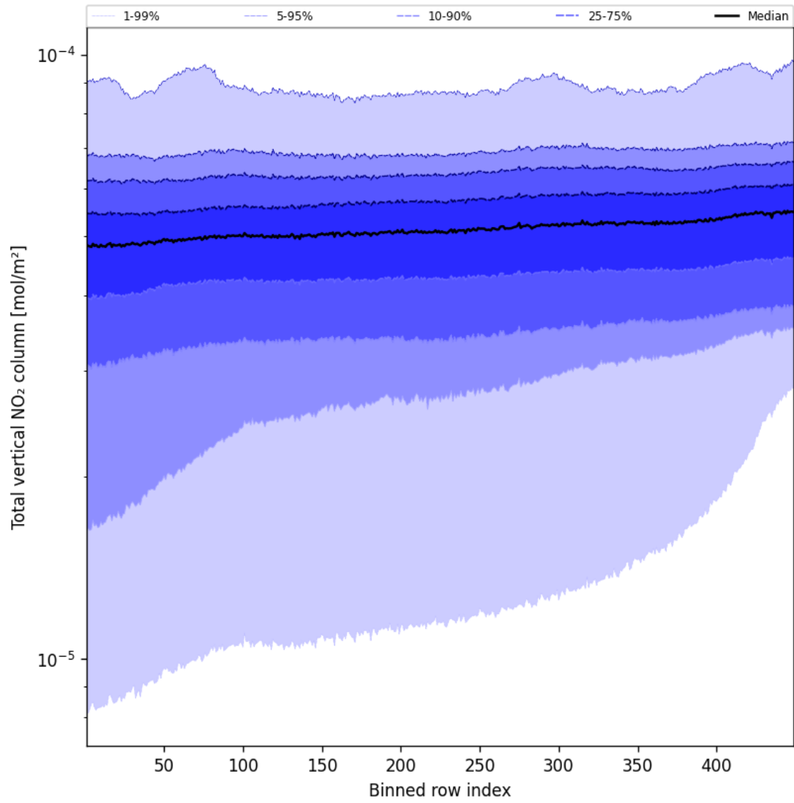
Figure 55: Along track statistics of “Total vertical NO 2 column” for 2024-09-04 to 2024-09-06
