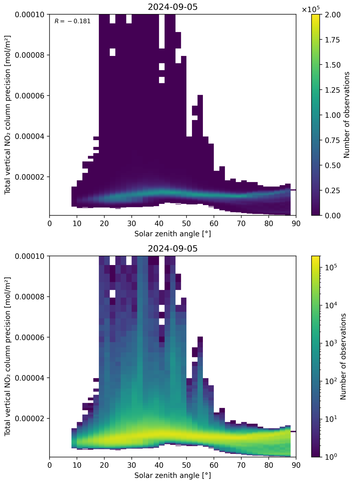
Figure 154: Scatter density plot of “Solar zenith angle” against “Total vertical NO 2 column precision” for 2024-09-04 to 2024-09-06.
