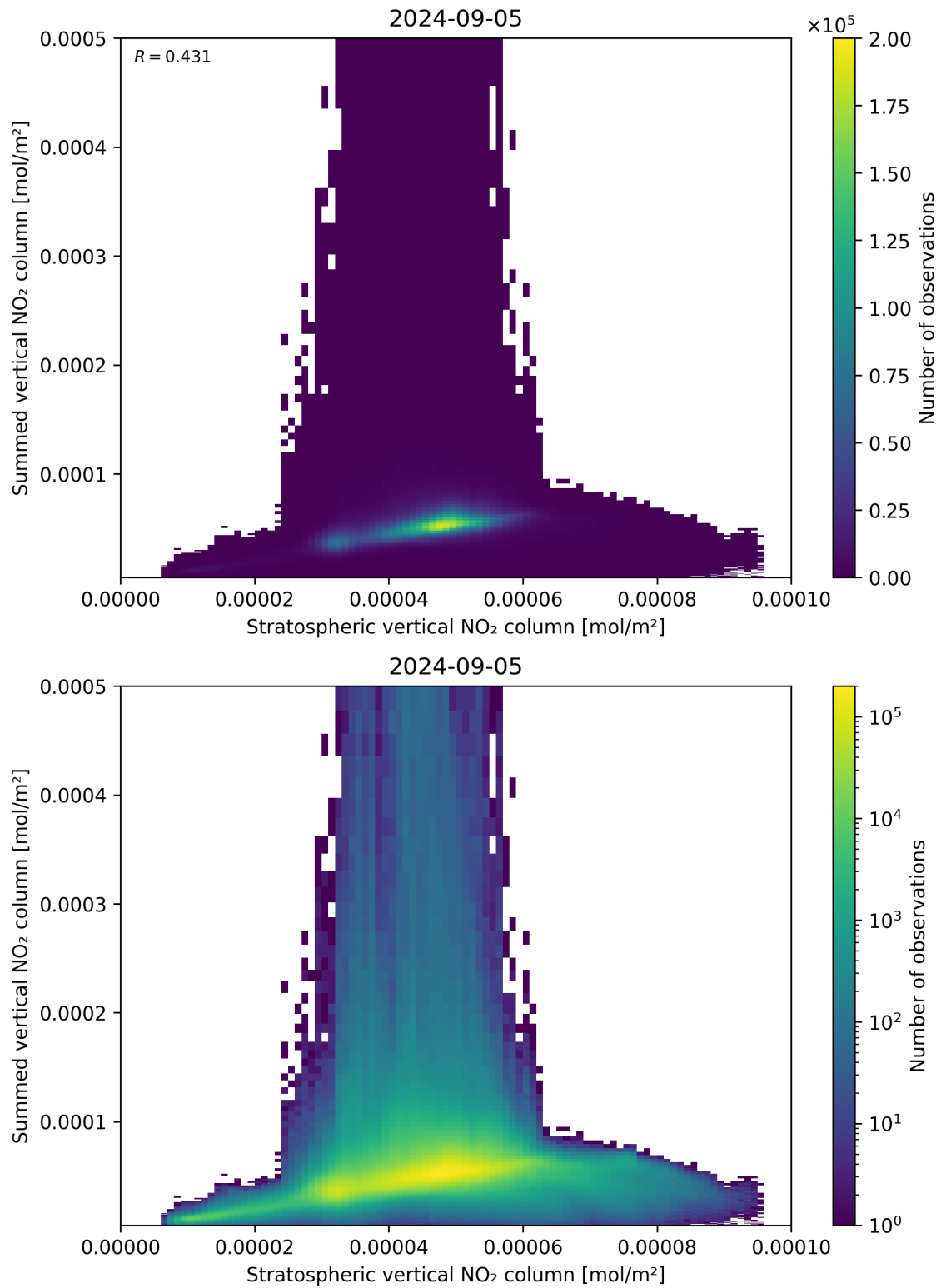
Figure 98: Scatter density plot of “Stratospheric vertical NO 2 column” against “Summed vertical NO 2 column” for 2024-09-04 to 2024-09-06.
