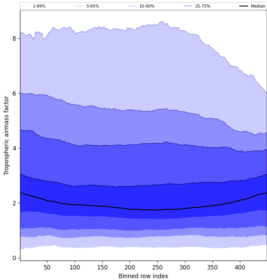
Figure 48: Along track statistics of “Tropospheric air mass factor” for 2024-09-04 to 2024-09-06
