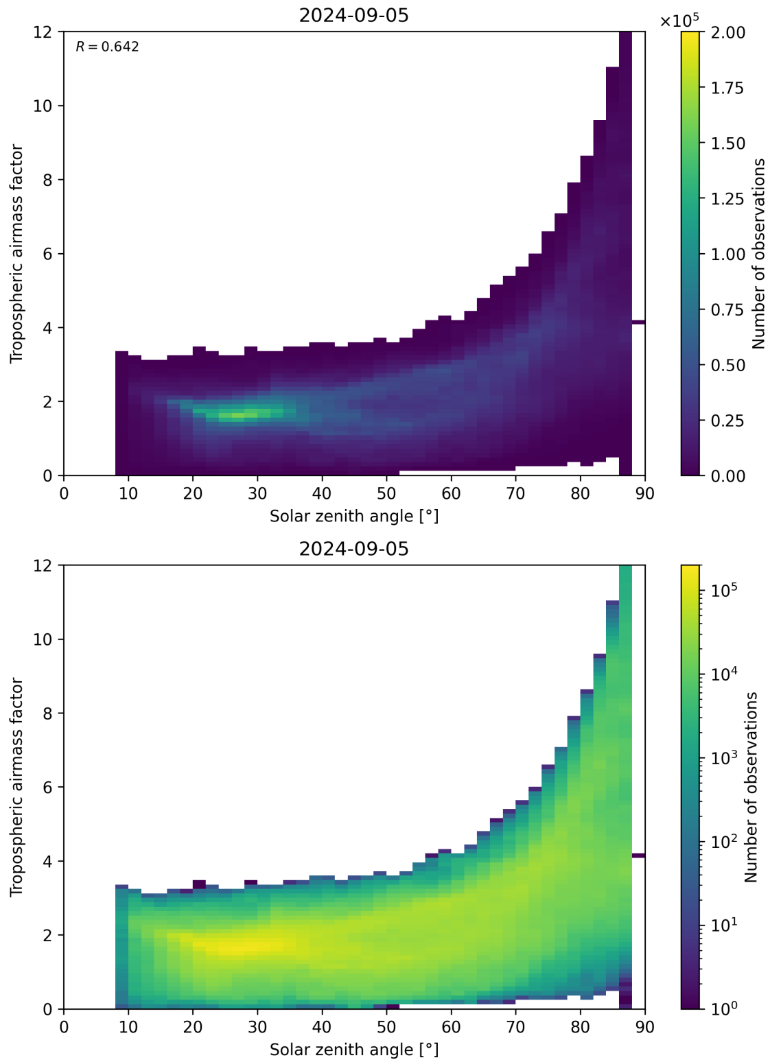
Figure 147: Scatter density plot of “Solar zenith angle” against “Tropospheric airmass factor” for 2024-09-04 to 2024-09-06.
