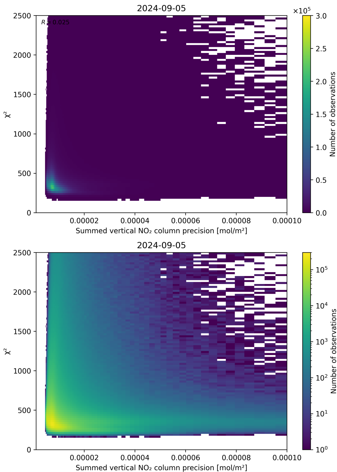
Figure 107: Scatter density plot of “Summed vertical NO 2 column precision” against “ \chi^2 ” for 2024-09-04 to 2024-09-06.
