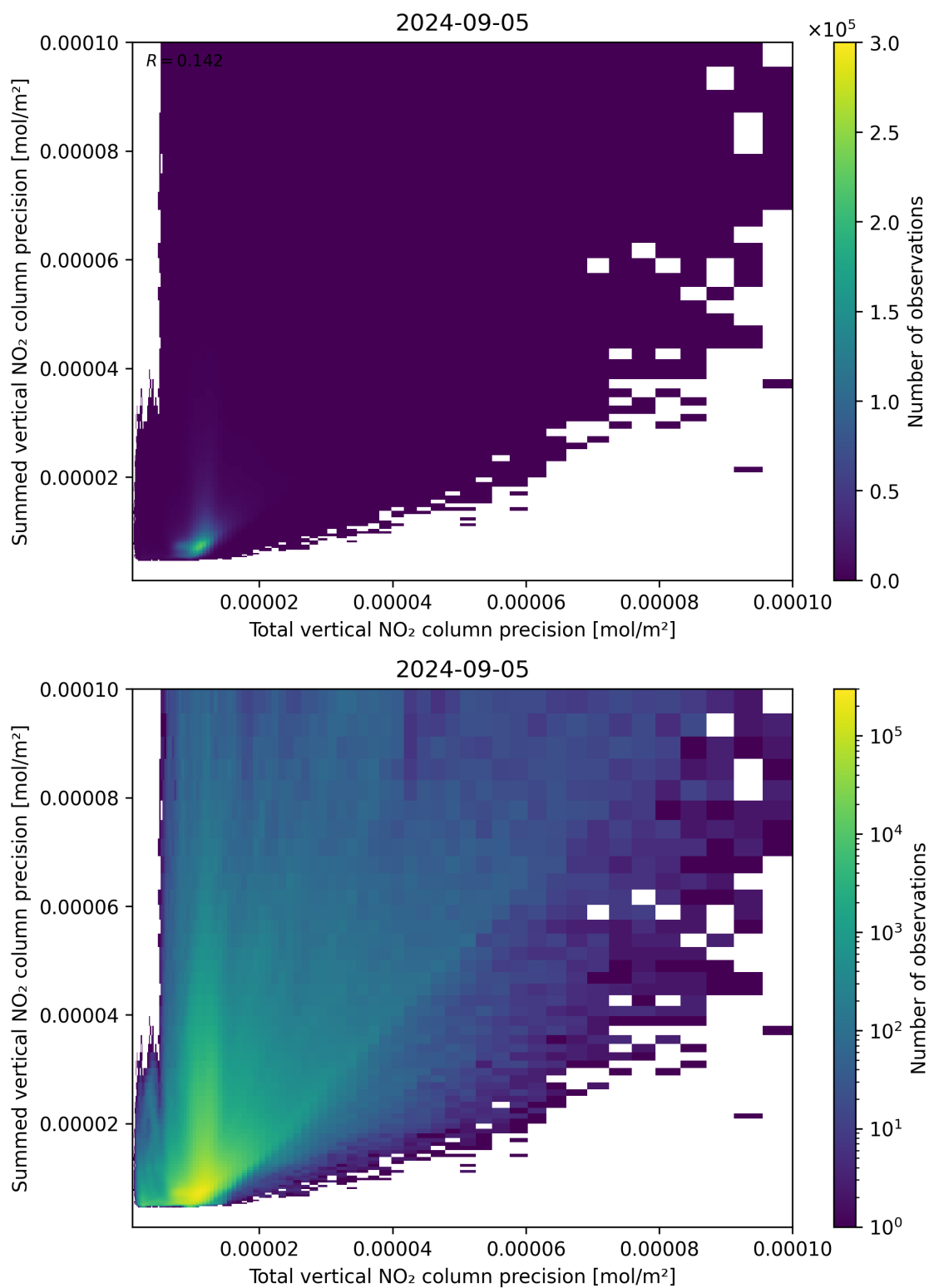
Figure 118: Scatter density plot of “Total vertical NO 2 column precision” against “Summed vertical NO 2 column precision” for 2024-09-04 to 2024-09-06.
