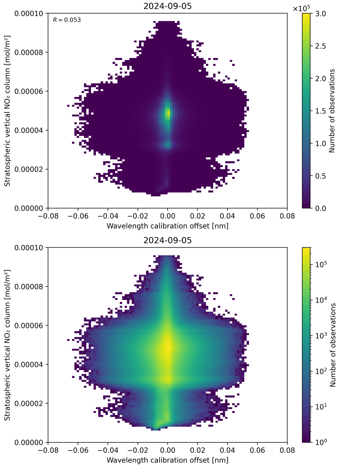
Figure 176: Scatter density plot of “Wavelength calibration offset” against “Stratospheric vertical NO 2 column” for 2024-09-04 to 2024-09-06.
