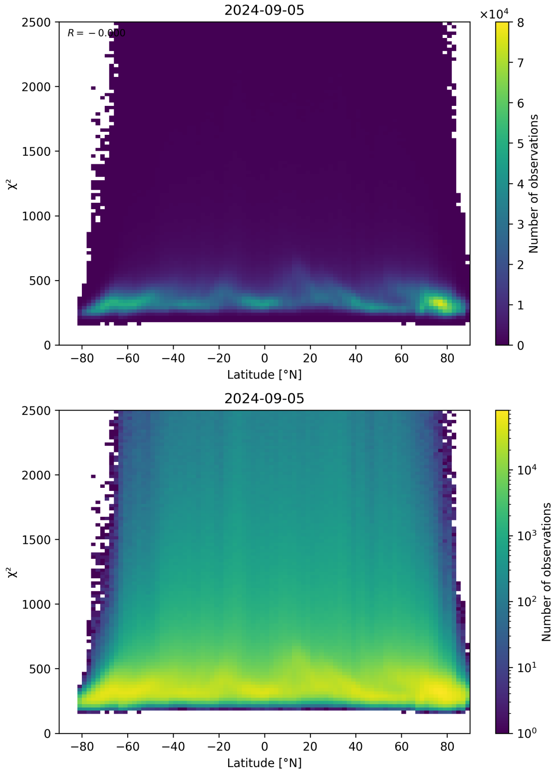
Figure 86: Scatter density plot of “Latitude” against “ \chi^2 ” for 2024-09-04 to 2024-09-06.
