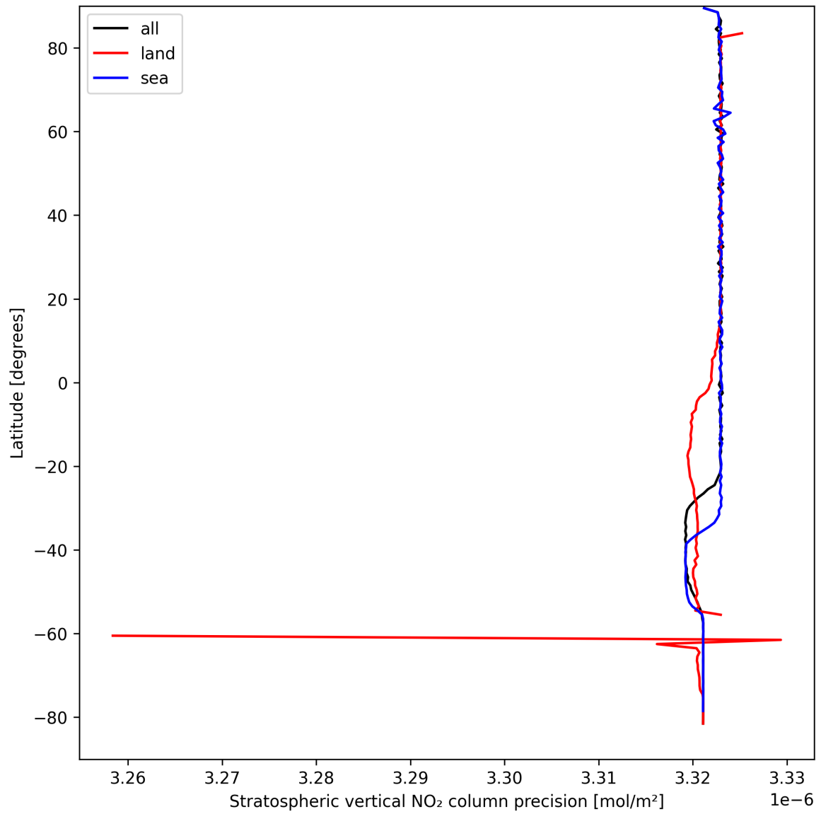
Figure 20: Zonal average of “Stratospheric vertical NO 2 column precision” for 2024-09-04 to 2024-09-06.
