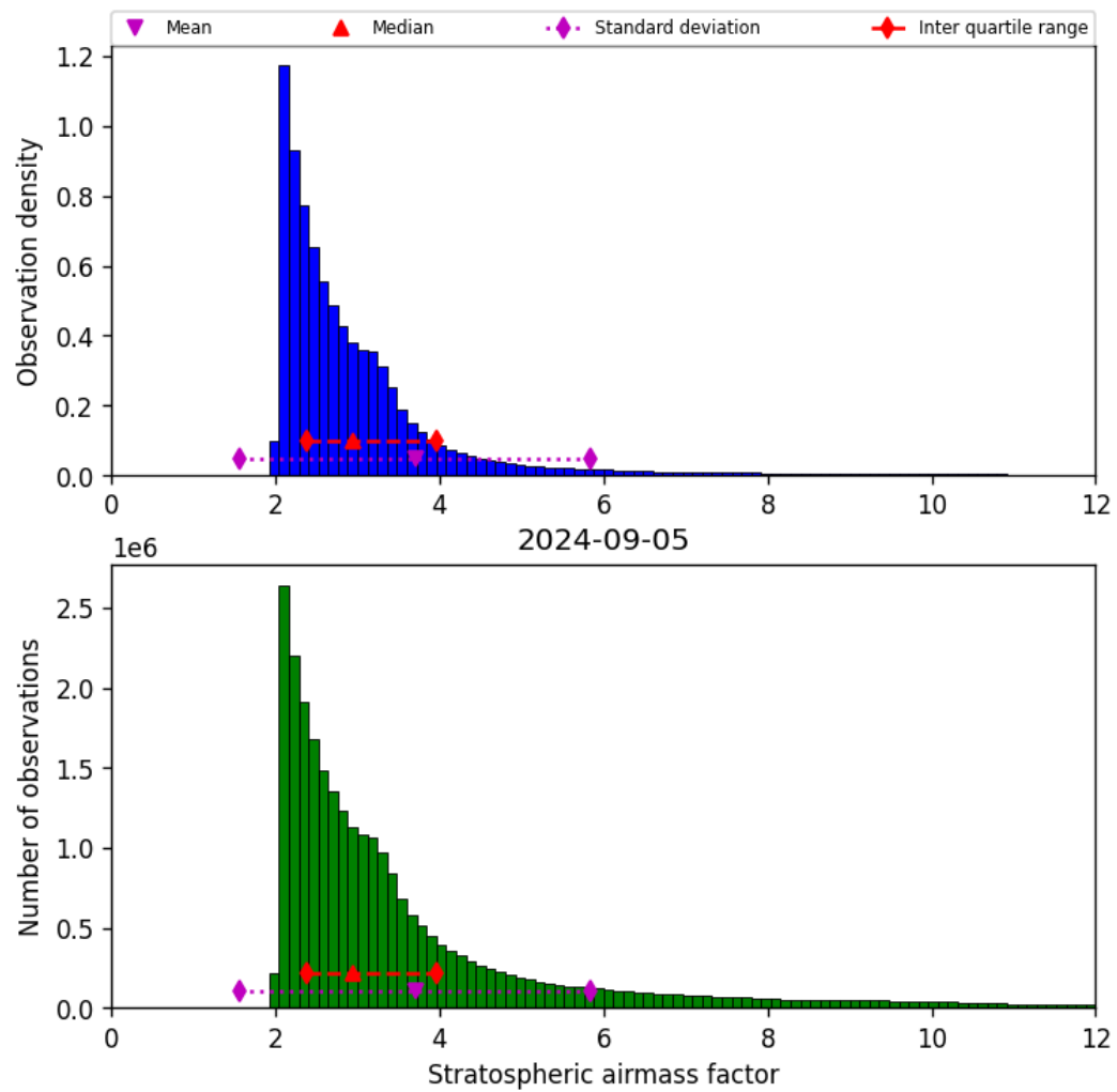
Figure 44: Histogram of “Stratospheric airmass factor” for 2024-09-04 to 2024-09-06
