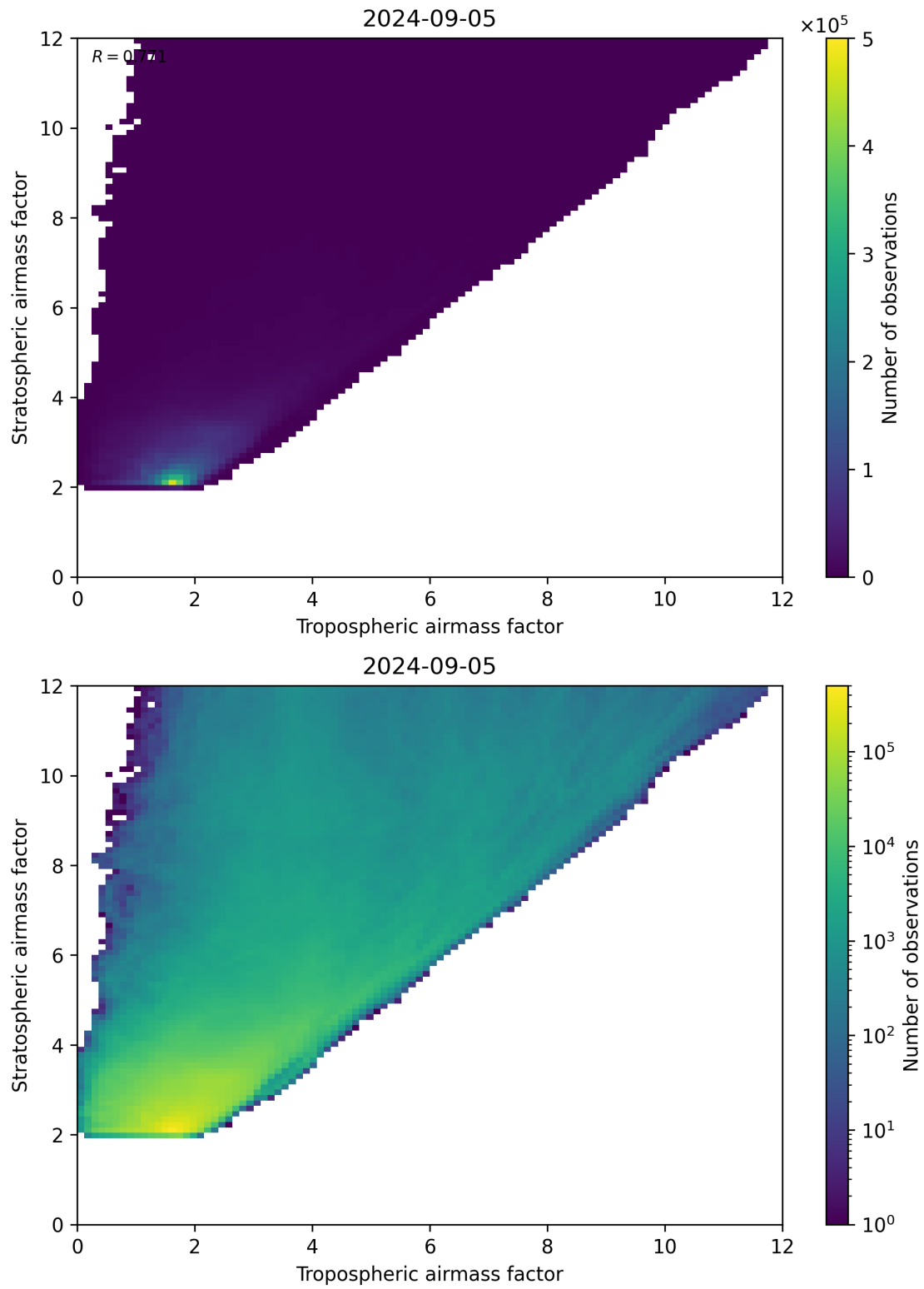
Figure 71: Scatter density plot of “Tropospheric airmass factor” against “Stratospheric airmass factor” for 2024-09-04 to 2024-09-06.
