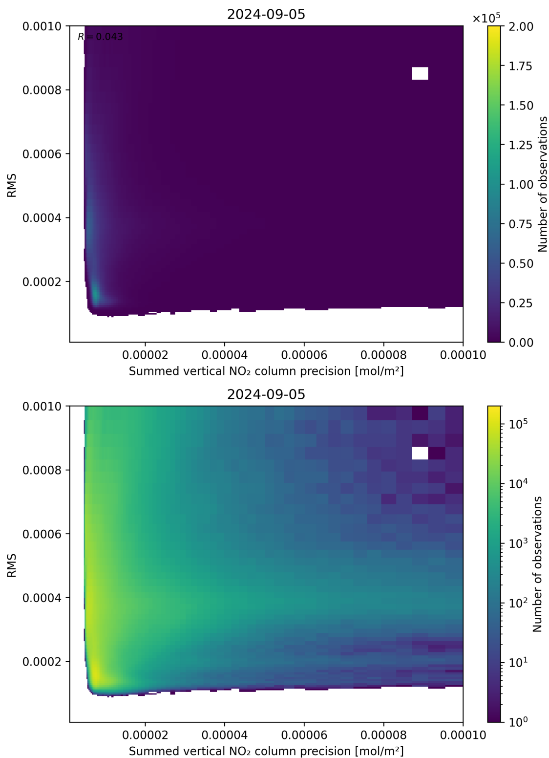
Figure 108: Scatter density plot of “Summed vertical NO 2 column precision” against “RMS” for 2024-09-04 to 2024-09-06.
