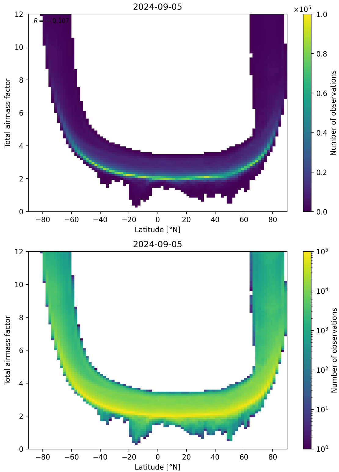
Figure 84: Scatter density plot of “Latitude” against “Total airmass factor” for 2024-09-04 to 2024-09-06.
