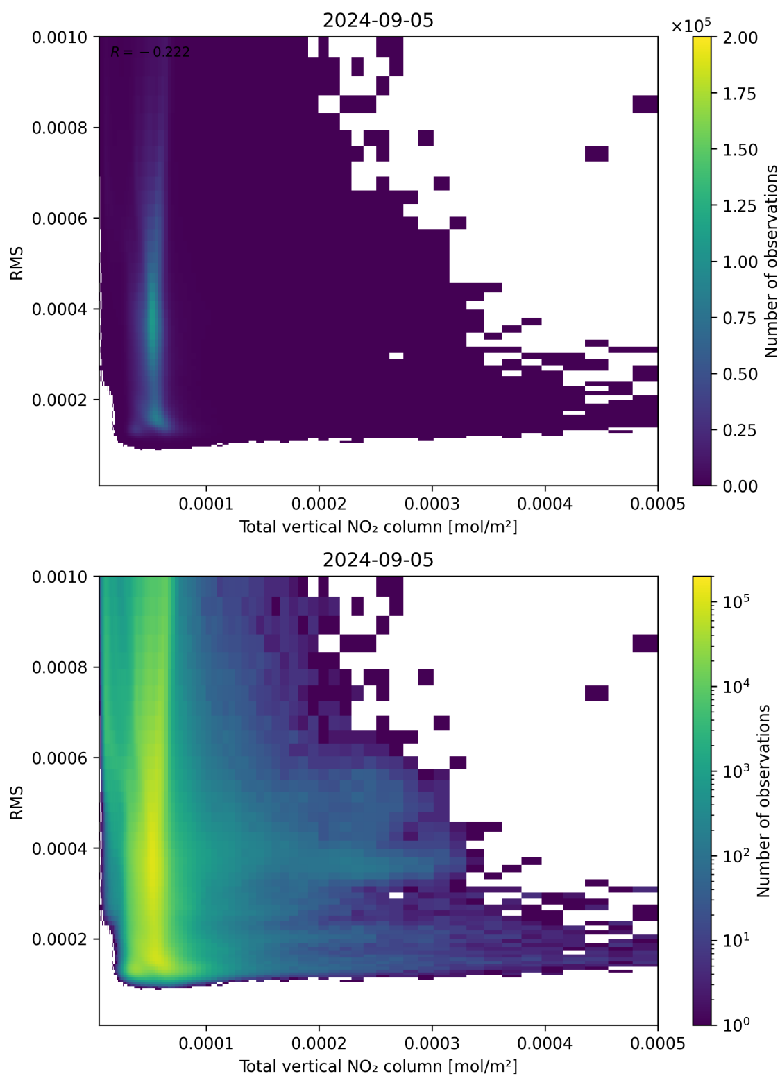
Figure 120: Scatter density plot of “Total vertical NO 2 column” against “RMS” for 2024-09-04 to 2024-09-06.
