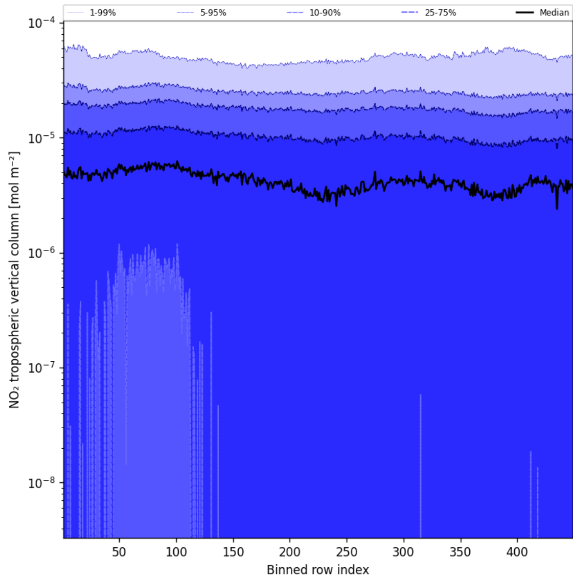
Figure 46: Along track statistics of “NO 2 tropospheric vertical column” for 2024-09-04 to 2024-09-06
