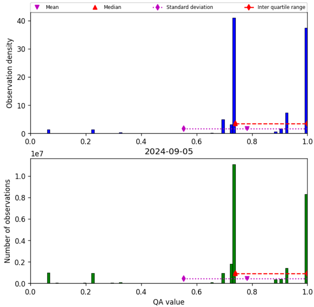
Figure 28: Histogram of “QA value” for 2024-09-04 to 2024-09-06
