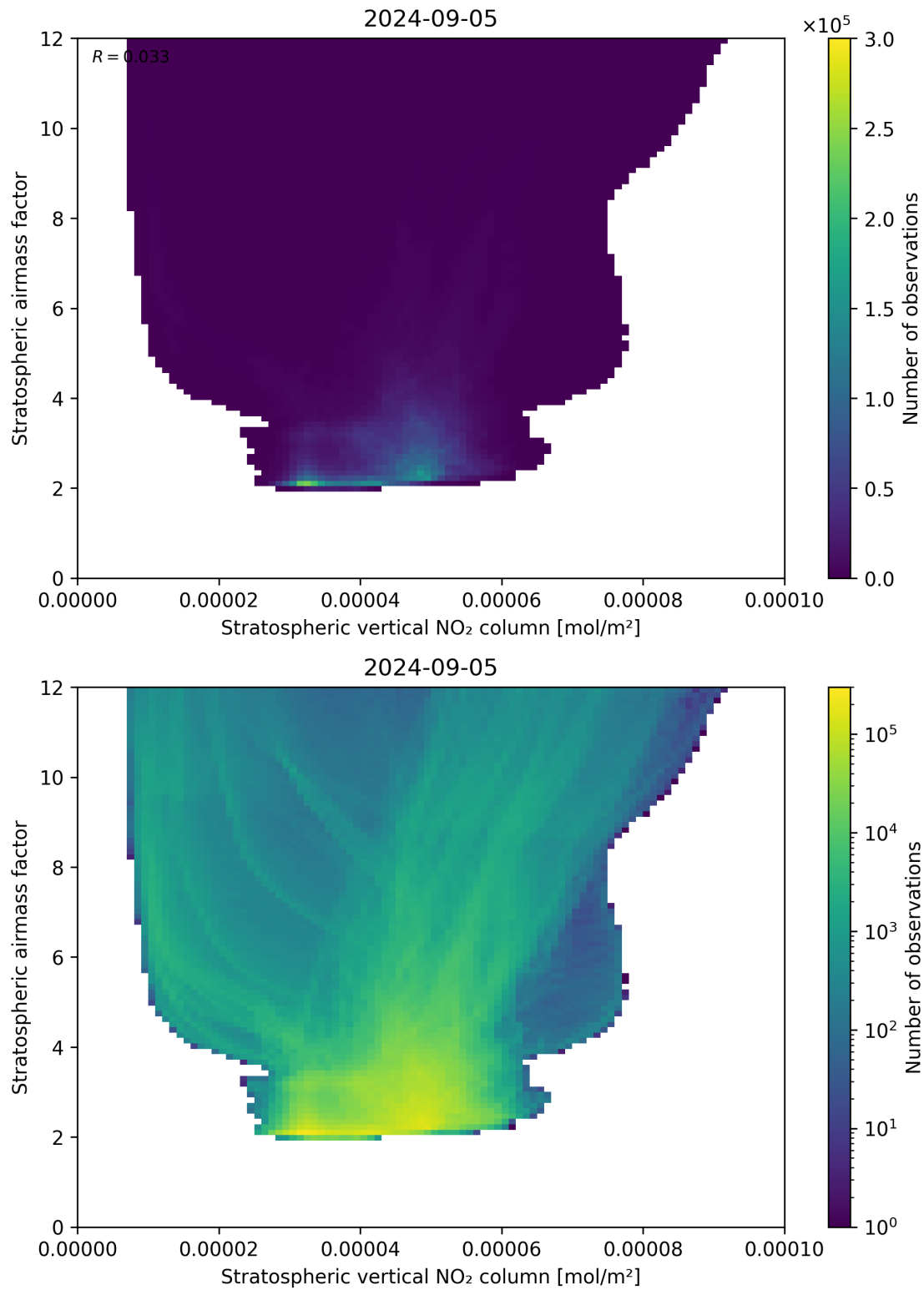
Figure 96: Scatter density plot of “Stratospheric vertical NO 2 column” against “Stratospheric airmass factor” for 2024-09-04 to 2024-09-06.
