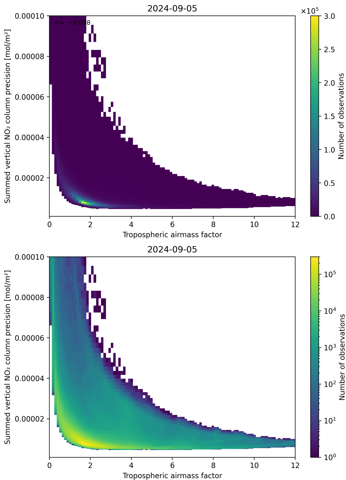
Figure 76: Scatter density plot of “Tropospheric air mass factor” against “Summed vertical NO 2 column precision” for 2024-09-04 to 2024-09-06.
