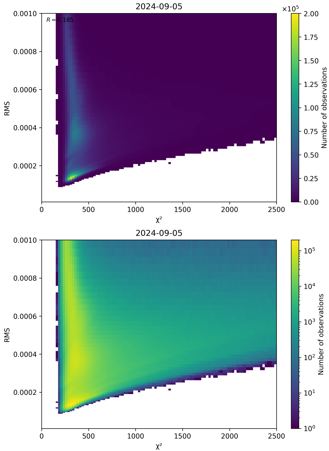
Figure 82: Scatter density plot of “ \chi^2 ” against “RMS” for 2024-09-04 to 2024-09-06.
