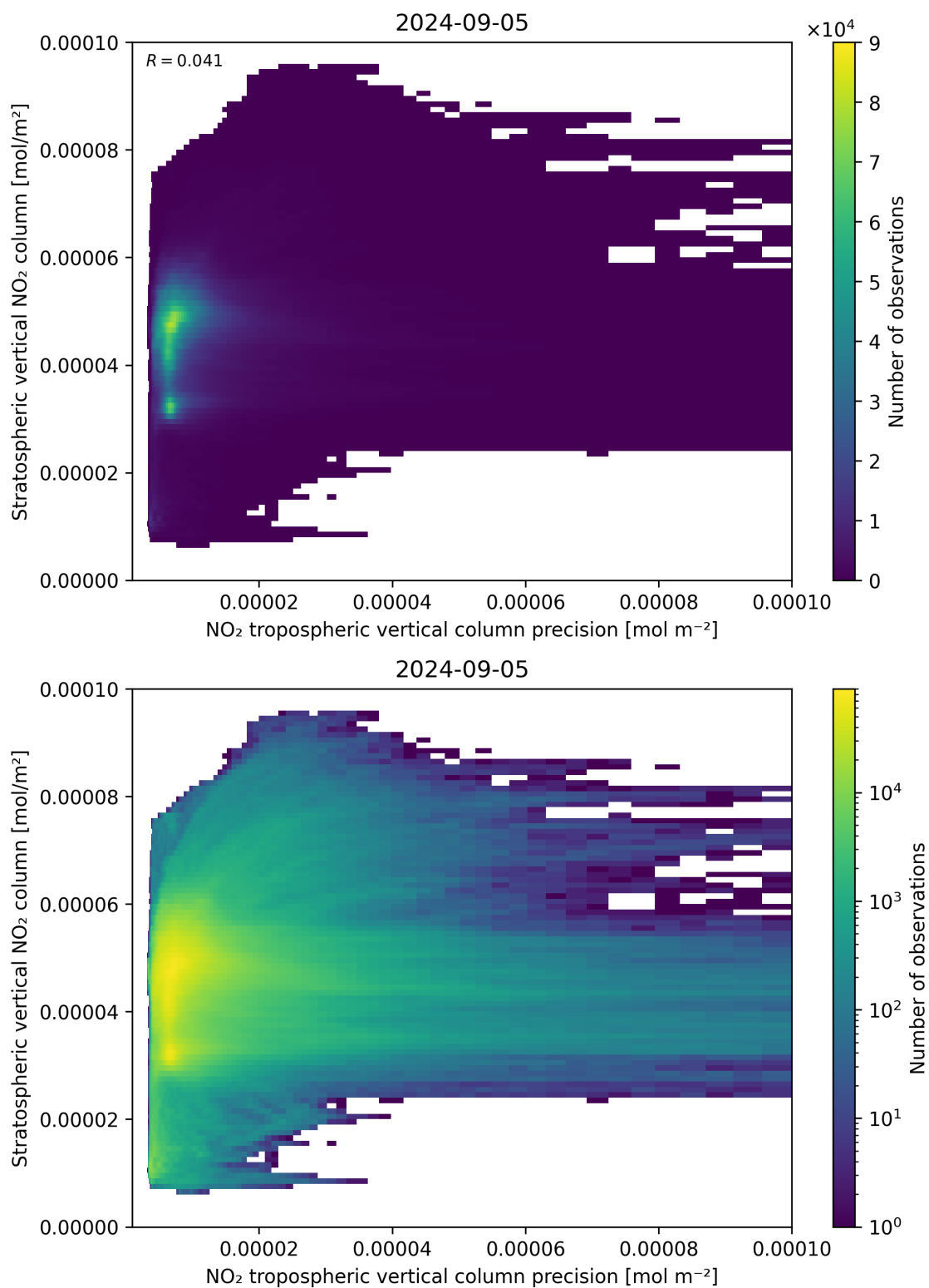
Figure 135: Scatter density plot of “NO 2 tropospheric vertical column precision” against “Stratospheric vertical NO 2 column” for 2024-09-04 to 2024-09-06.
