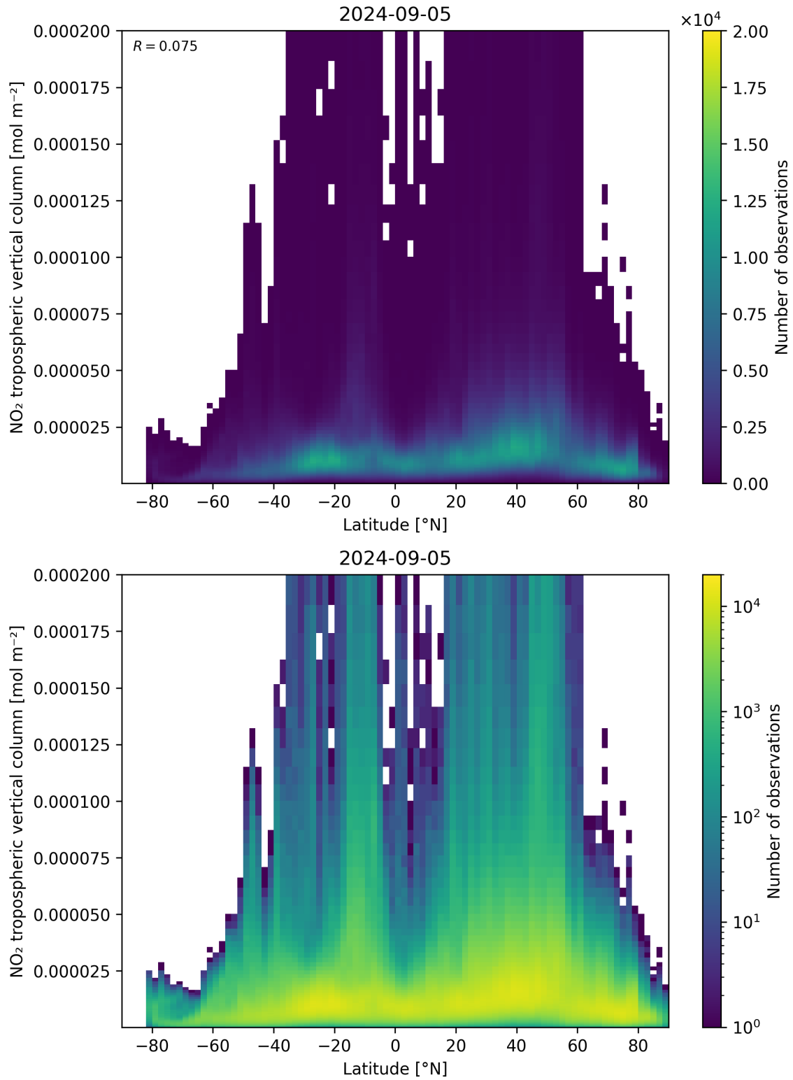
Figure 92: Scatter density plot of “Latitude” against “NO 2 tropospheric vertical column” for 2024-09-04 to 2024-09-06.
