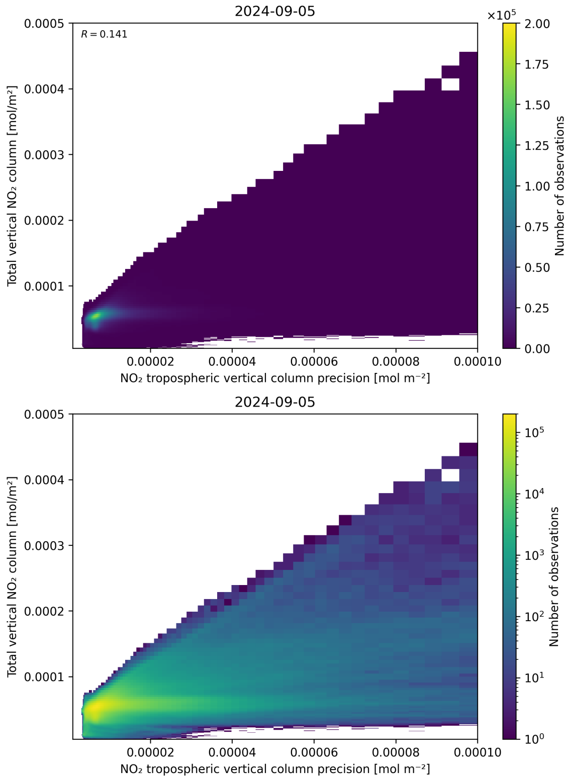
Figure 138: Scatter density plot of “NO 2 tropospheric vertical column precision” against “Total vertical NO 2 column” for 2024-09-04 to 2024-09-06.
