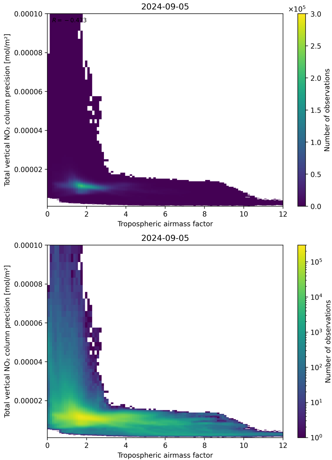
Figure 78: Scatter density plot of “Tropospheric air mass factor” against “Total vertical NO 2 column precision” for 2024-09-04 to 2024-09-06.
