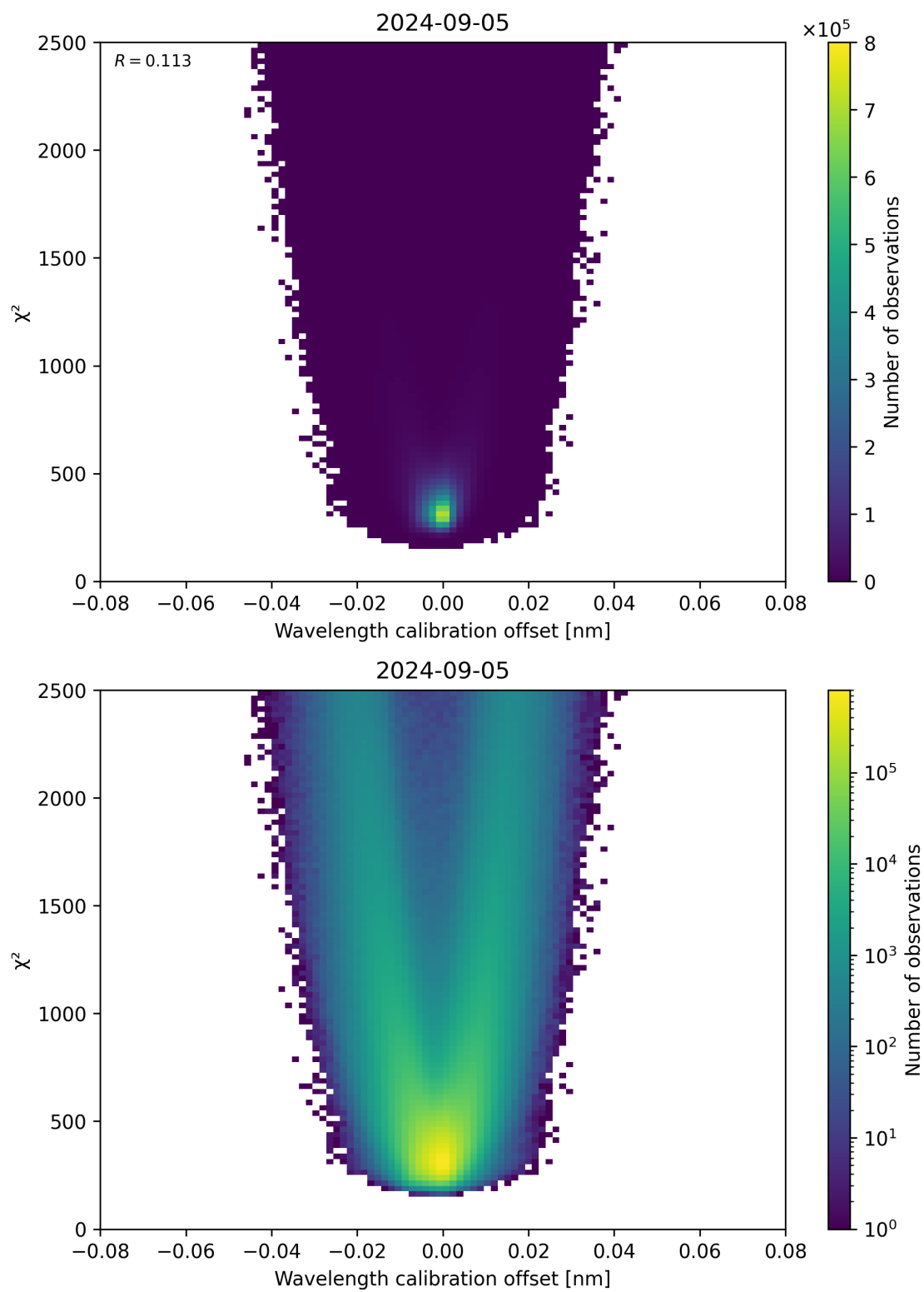
Figure 175: Scatter density plot of “Wavelength calibration offset” against “ \chi^2 ” for 2024-09-04 to 2024-09-06.
