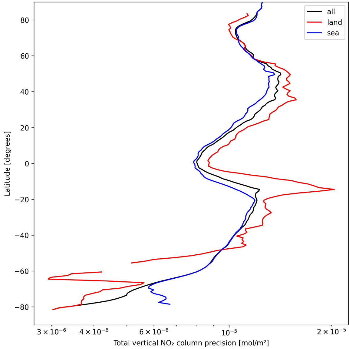
Figure 22: Zonal average of “Total vertical NO 2 column precision” for 2024-09-04 to 2024-09-06.
