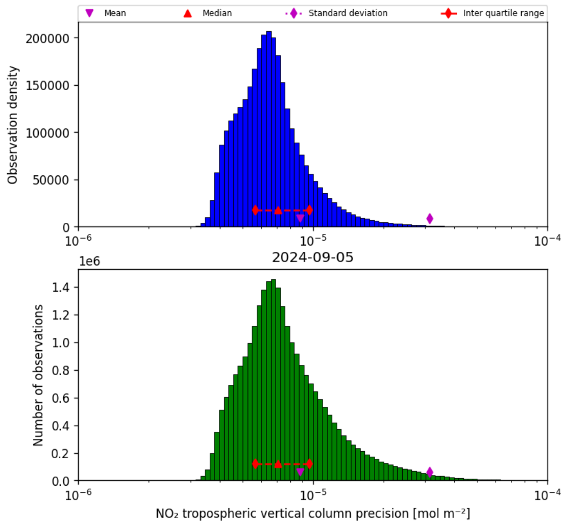
Figure 30: Histogram of “NO 2 tropospheric vertical column precision” for 2024-09-04 to 2024-09-06
