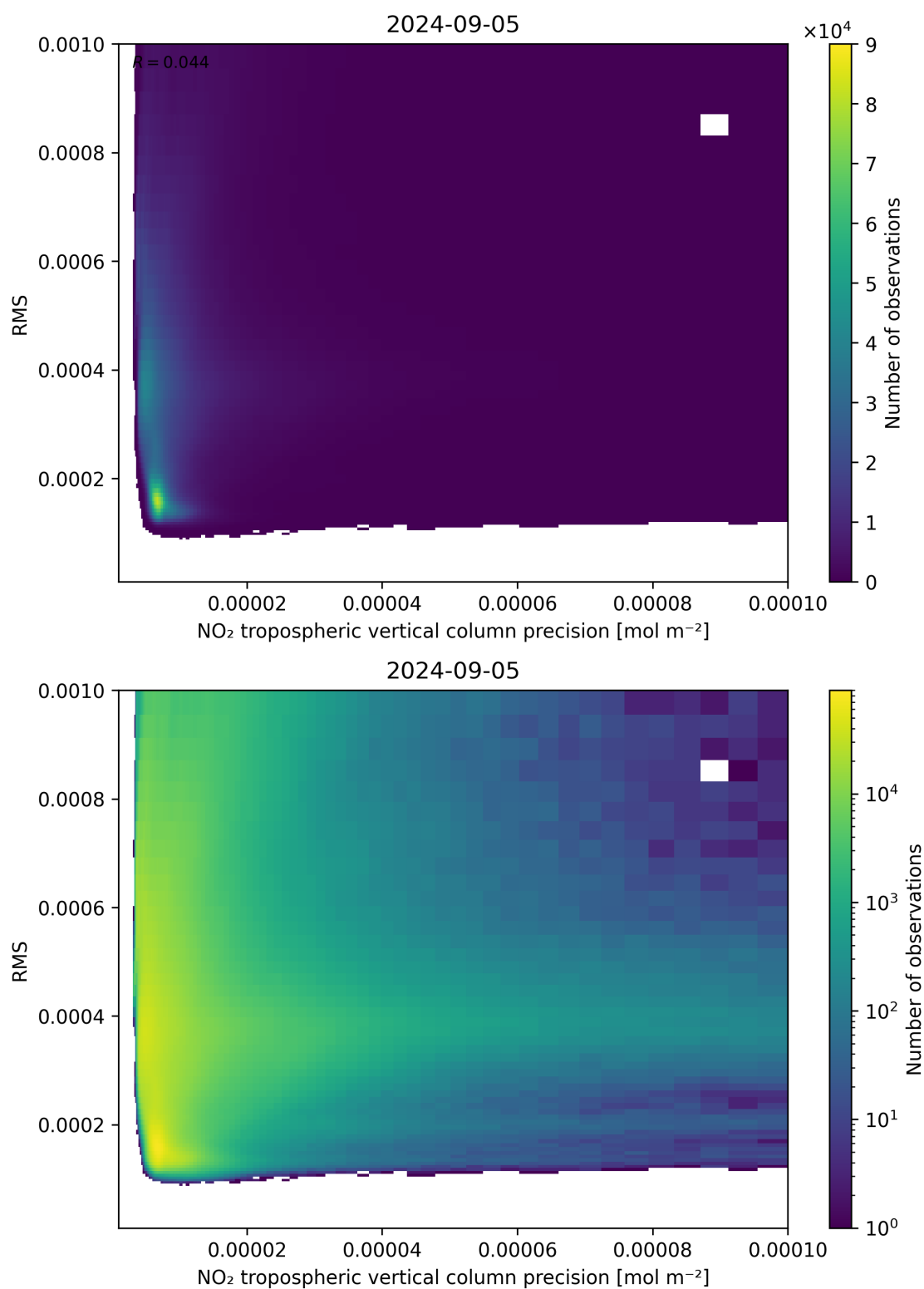
Figure 140: Scatter density plot of “NO 2 tropospheric vertical column precision” against “RMS” for 2024-09-04 to 2024-09-06.
