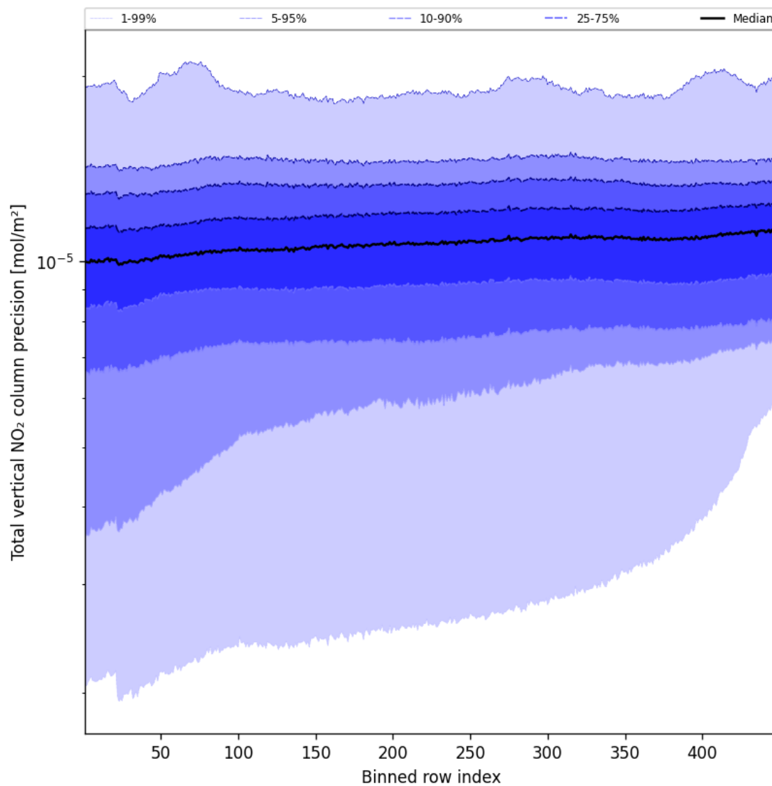
Figure 56: Along track statistics of “Total vertical NO 2 column precision” for 2024-09-04 to 2024-09-06
