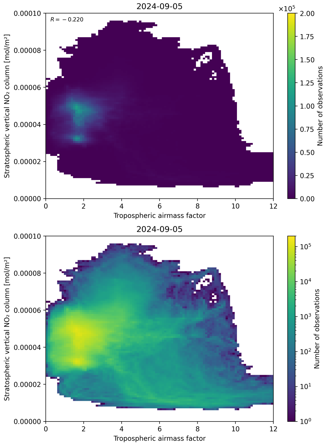
Figure 74: Scatter density plot of “Tropospheric air mass factor” against “Stratospheric vertical NO 2 column” for 2024-09-04 to 2024-09-06.
