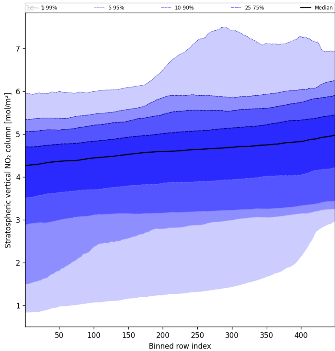
Figure 53: Along track statistics of “Stratospheric vertical NO 2 column” for 2024-09-04 to 2024-09-06
