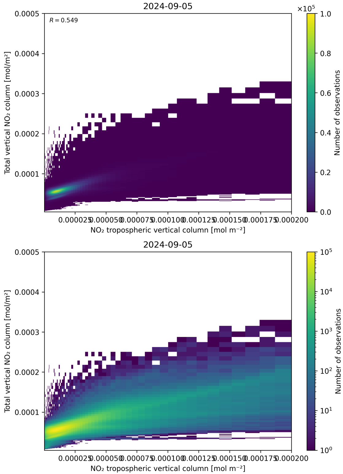
Figure 128: Scatter density plot of “NO 2 tropospheric vertical column” against “Total vertical NO 2 column” for 2024-09-04 to 2024-09-06.
