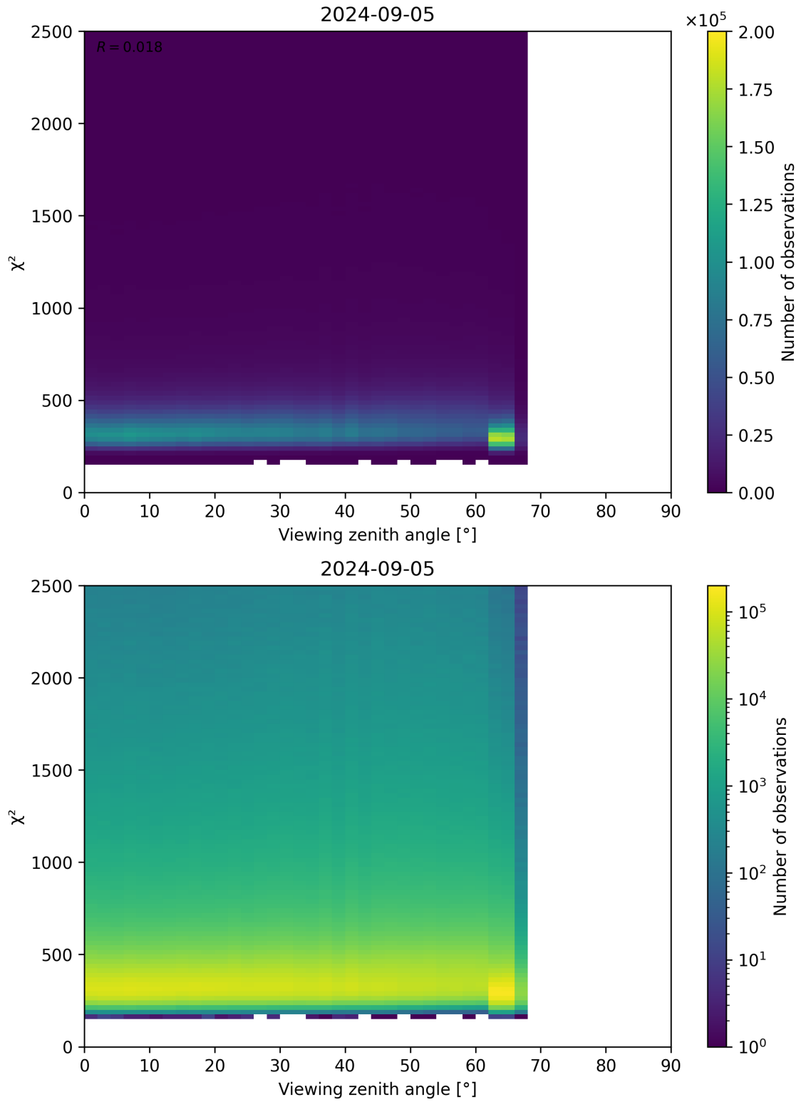
Figure 162: Scatter density plot of “Viewing zenith angle” against “ \chi^2 ” for 2024-09-04 to 2024-09-06.
