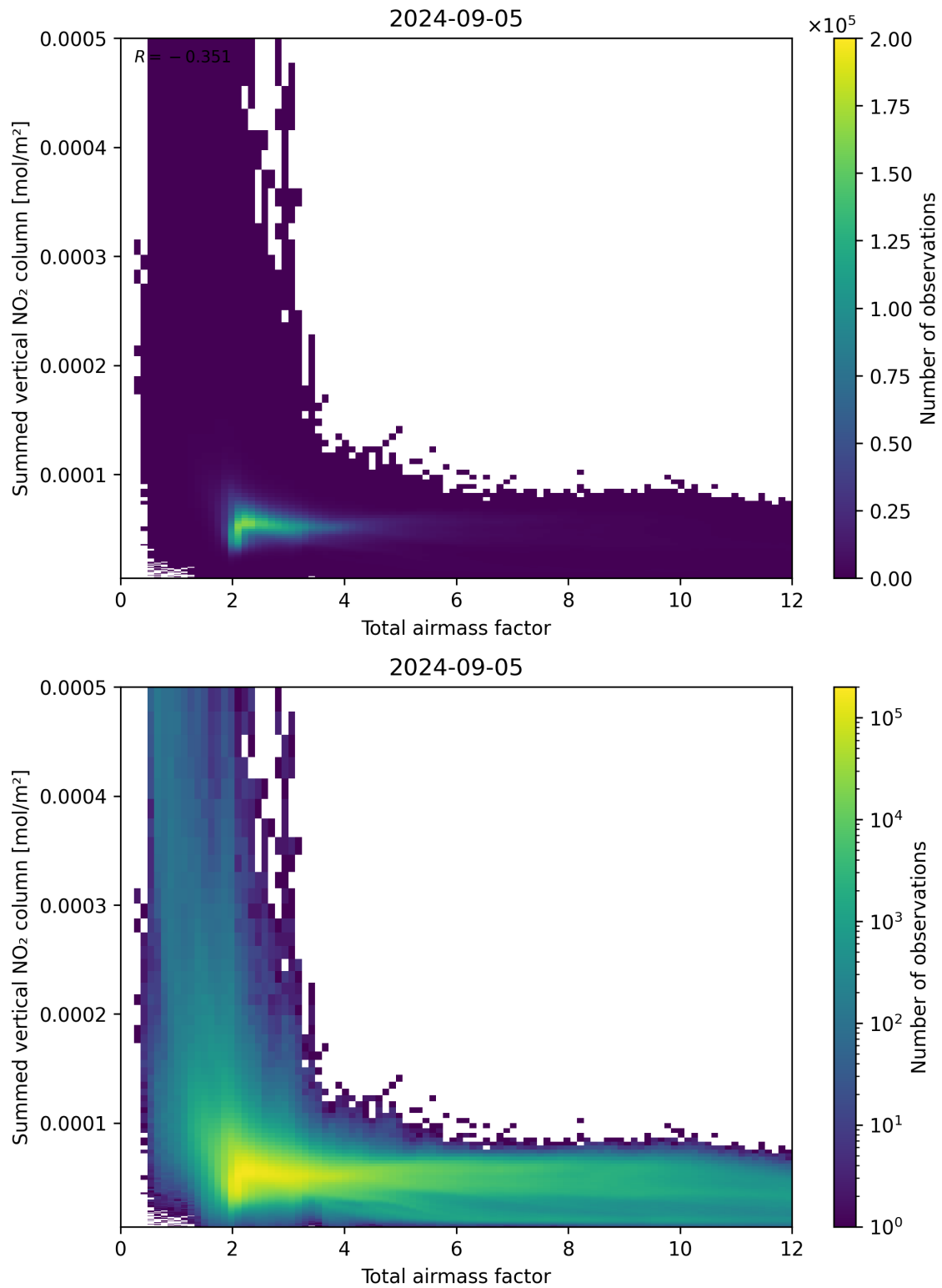
Figure 65: Scatter density plot of “Total airmass factor” against “Summed vertical NO 2 column” for 2024-09-04 to 2024-09-06.
