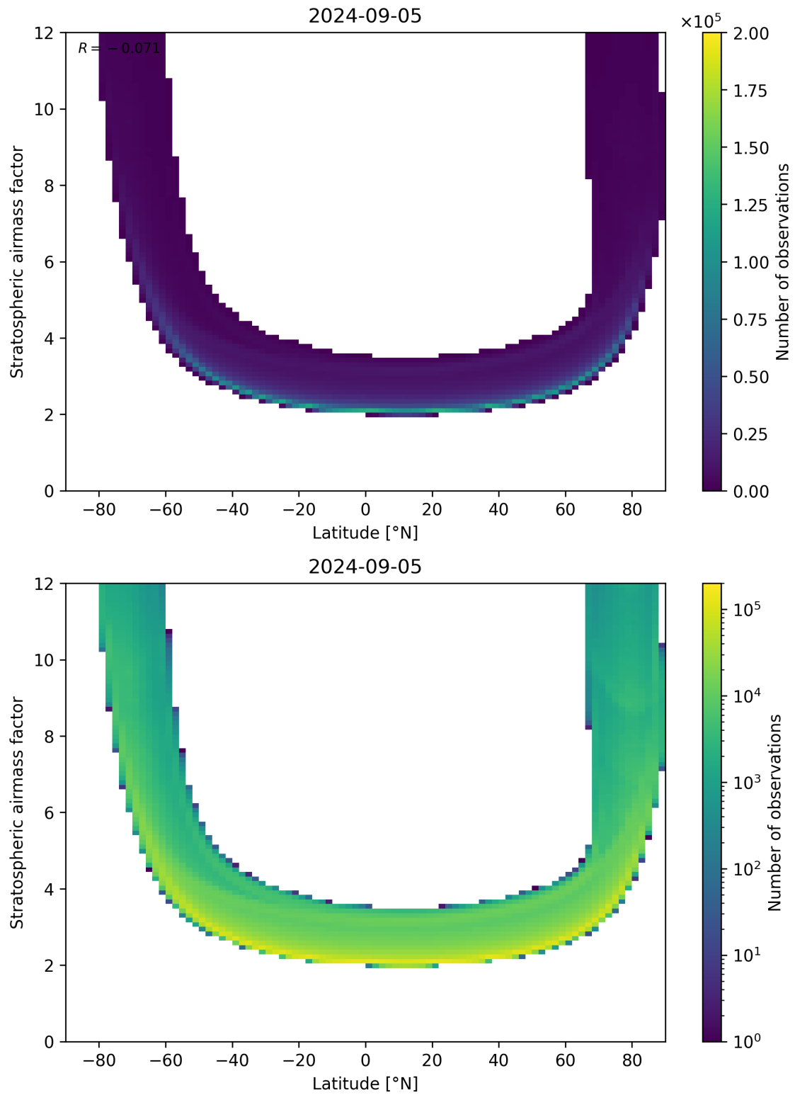
Figure 83: Scatter density plot of “Latitude” against “Stratospheric air mass factor” for 2024-09-04 to 2024-09-06.
