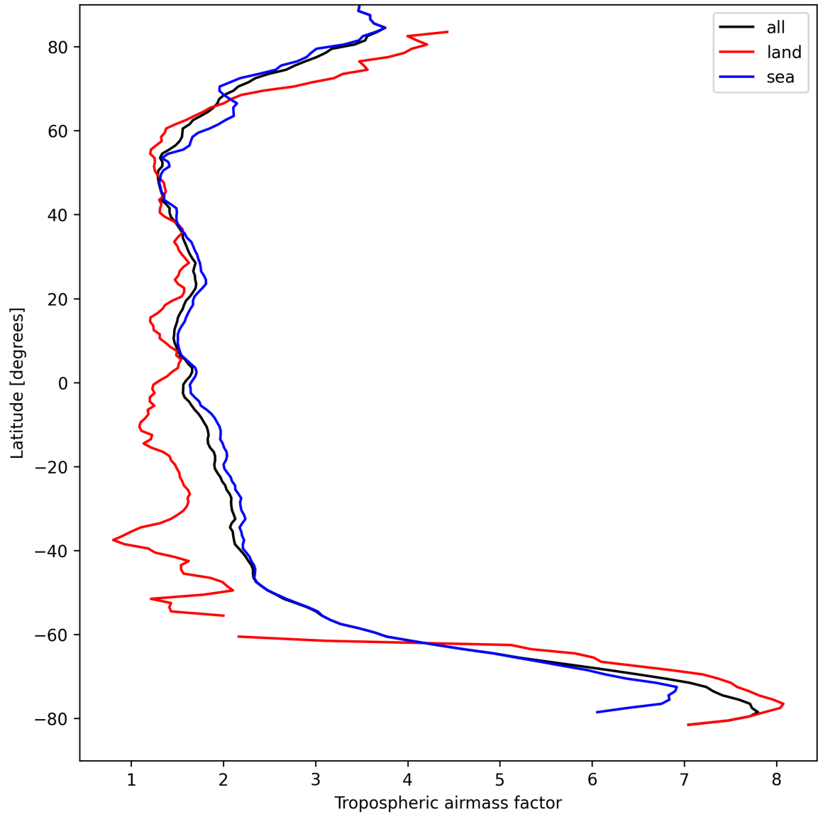
Figure 14: Zonal average of “Tropospheric air mass factor” for 2024-09-04 to 2024-09-06.
