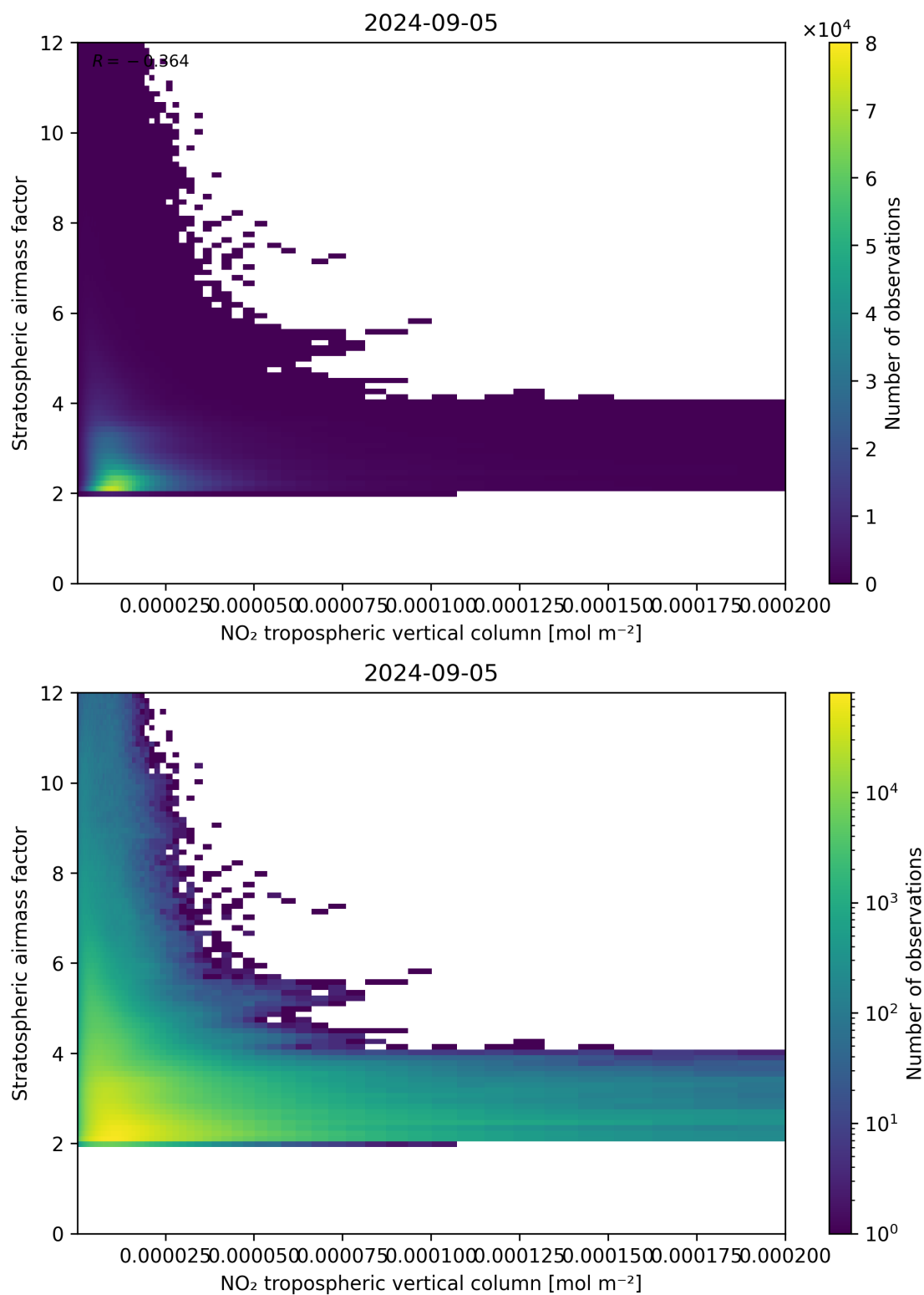
Figure 121: Scatter density plot of “NO 2 tropospheric vertical column” against “Stratospheric air mass factor” for 2024-09-04 to 2024-09-06.
