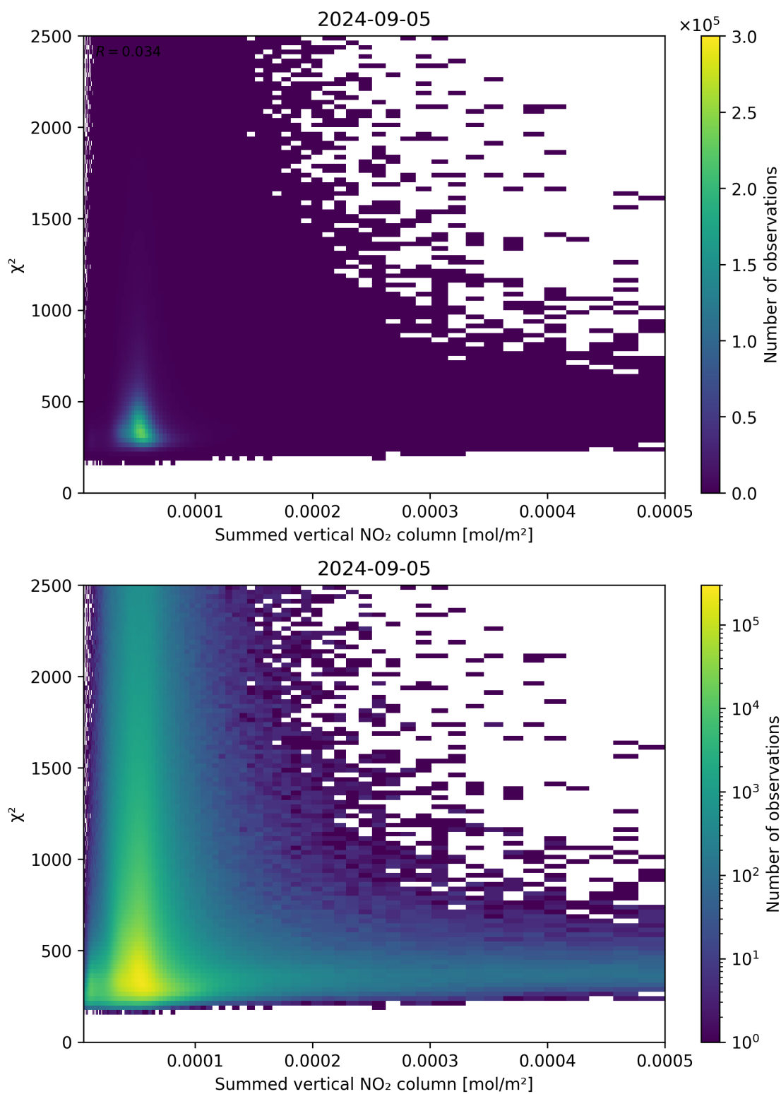
Figure 104: Scatter density plot of “Summed vertical NO 2 column” against “ \chi^2 ” for 2024-09-04 to 2024-09-06.
