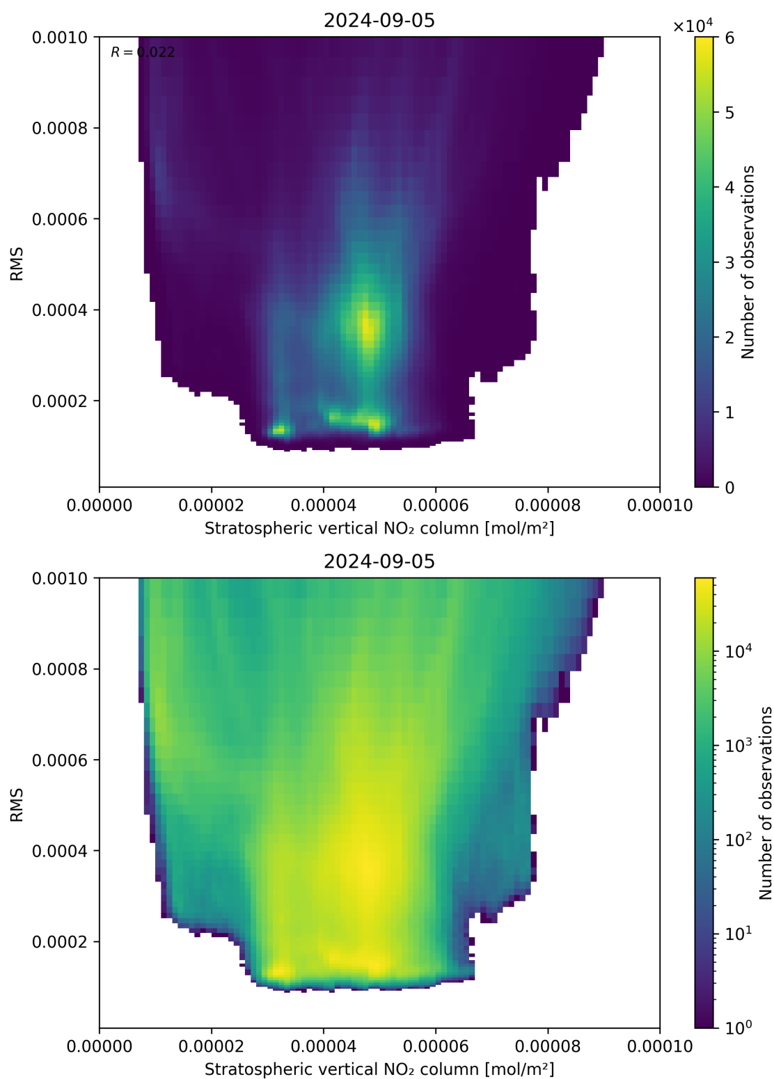
Figure 102: Scatter density plot of “Stratospheric vertical NO 2 column” against “RMS” for 2024-09-04 to 2024-09-06.
