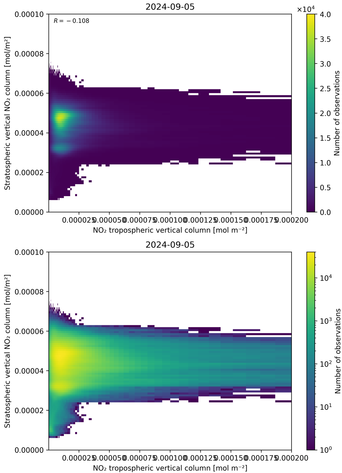
Figure 125: Scatter density plot of “NO 2 tropospheric vertical column” against “Stratospheric vertical NO 2 column” for 2024-09-04 to 2024-09-06.
