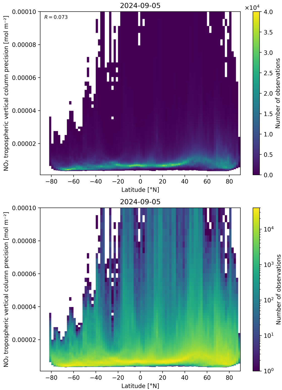
Figure 93: Scatter density plot of “Latitude” against “NO 2 tropospheric vertical column precision” for 2024-09-04 to 2024-09-06.
