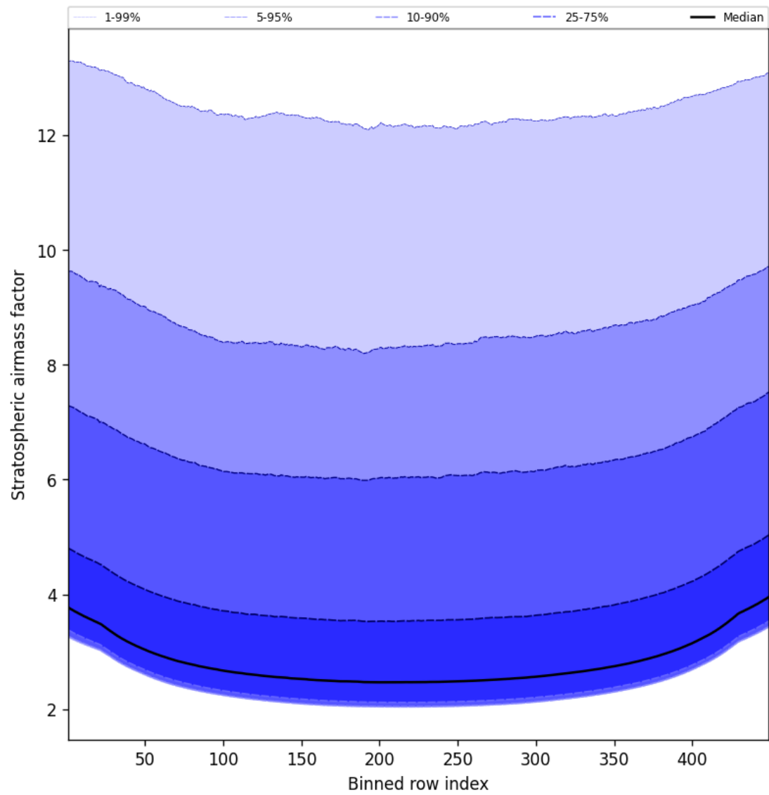
Figure 61: Along track statistics of “Stratospheric airmass factor” for 2024-09-04 to 2024-09-06
