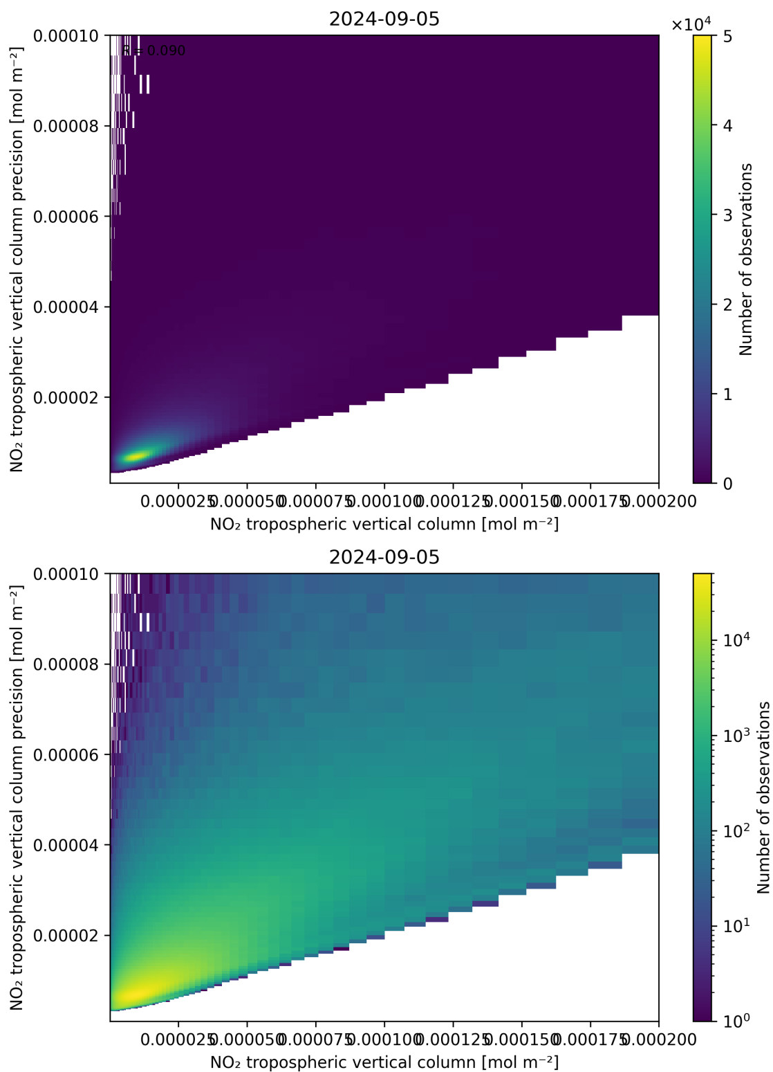
Figure 130: Scatter density plot of “NO 2 tropospheric vertical column” against “NO 2 tropospheric vertical column precision” for 2024-09-04 to 2024-09-06.
