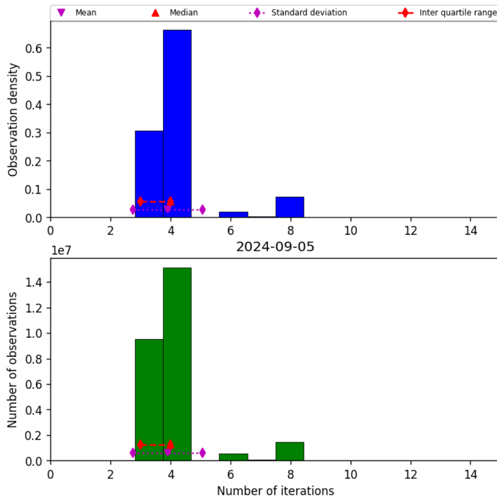
Figure 34: Histogram of “Number of iterations” for 2024-09-04 to 2024-09-06
