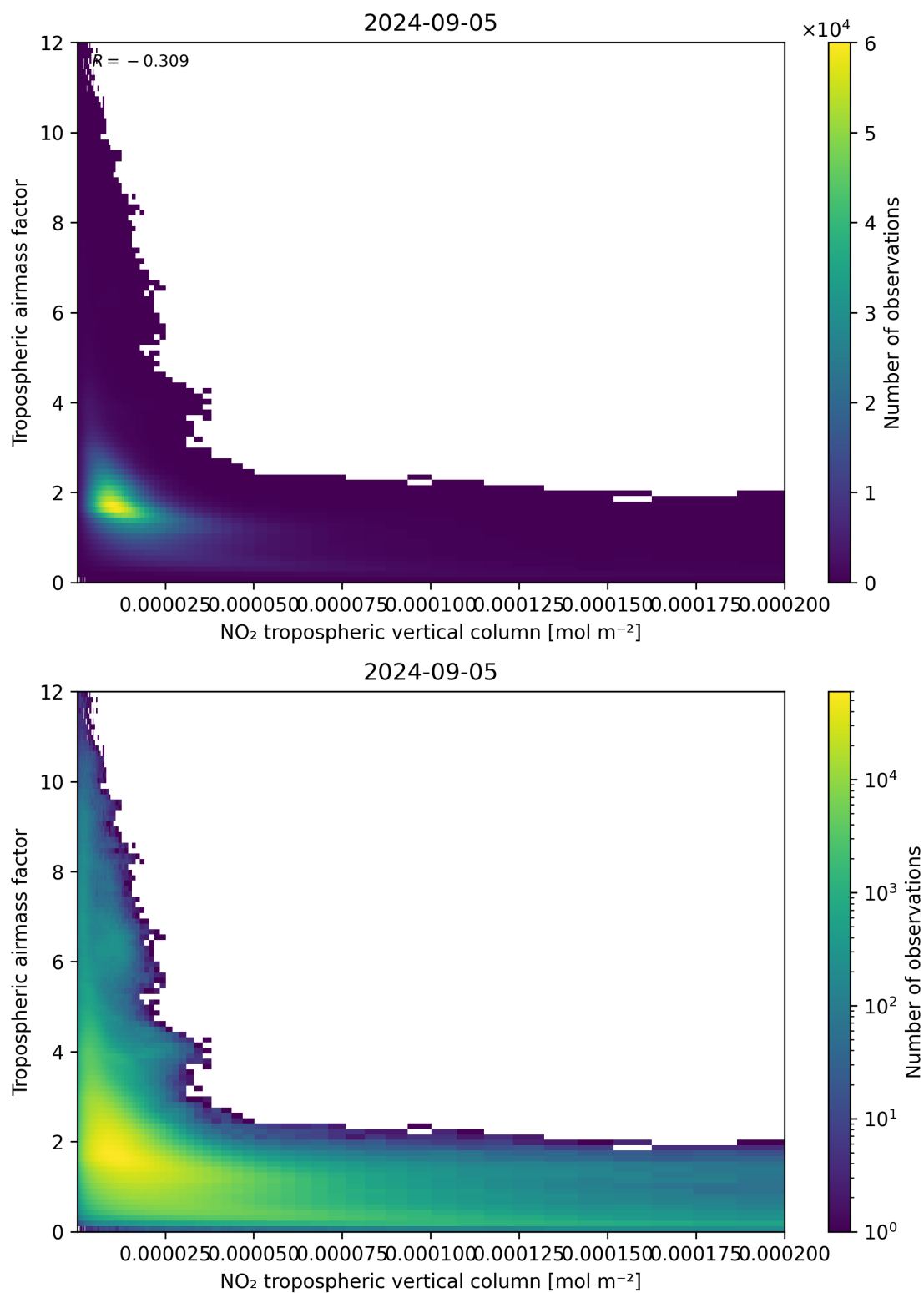
Figure 123: Scatter density plot of “NO 2 tropospheric vertical column” against “Tropospheric air mass factor” for 2024-09-04 to 2024-09-06.
