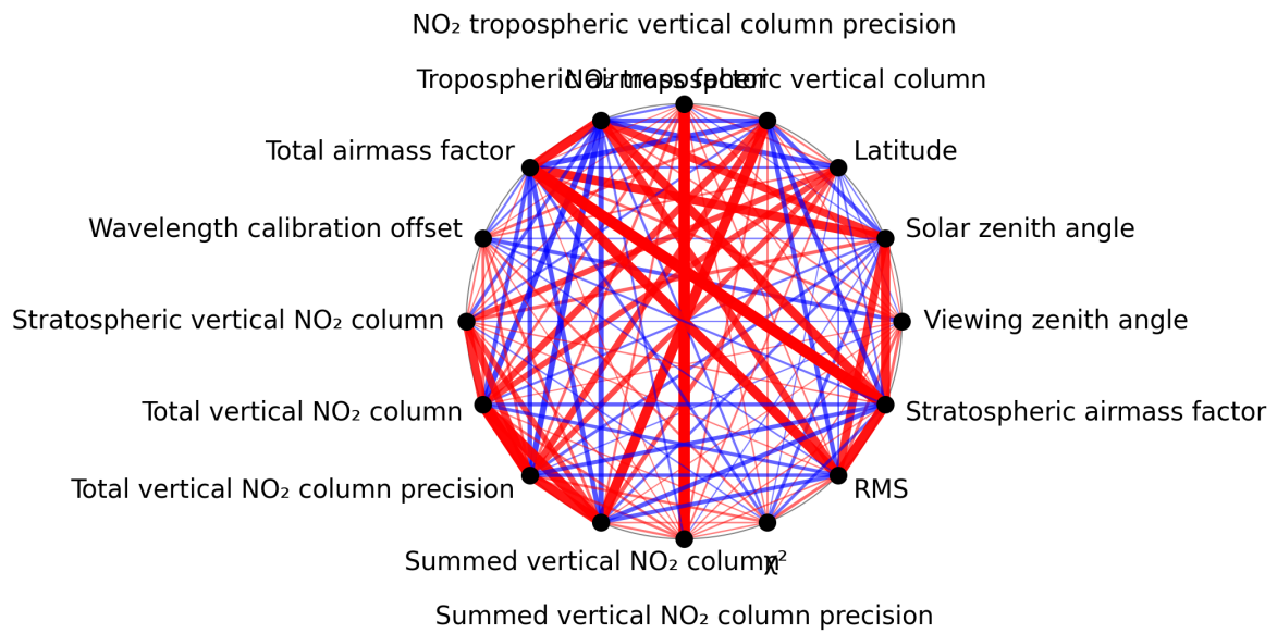
Figure 1: Map of correlation graph for 2024-09-04 to 2024-09-06.
