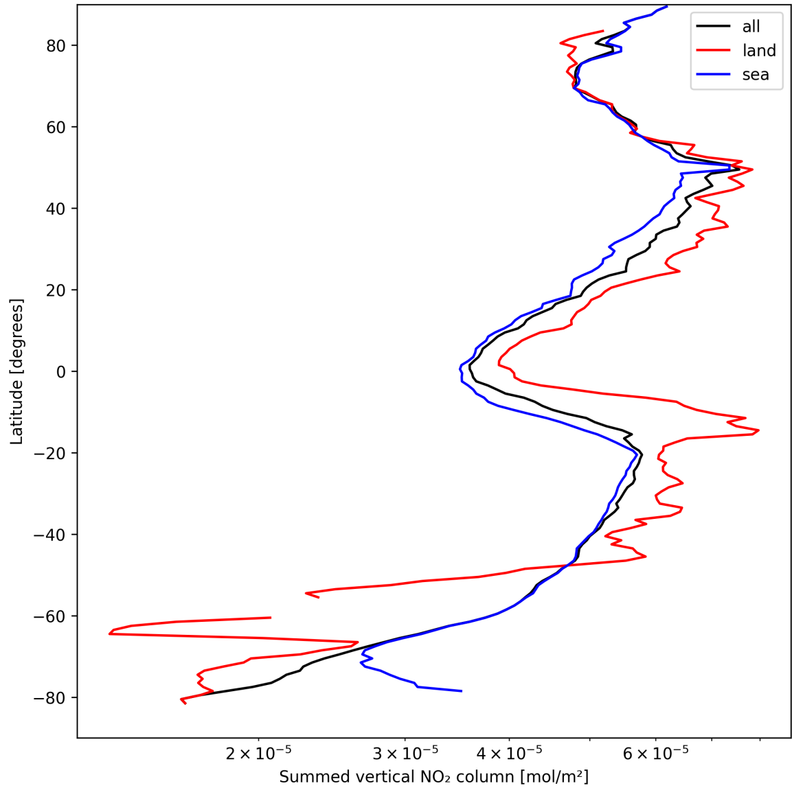
Figure 23: Zonal average of “Summed vertical NO 2 column” for 2024-09-04 to 2024-09-06.
