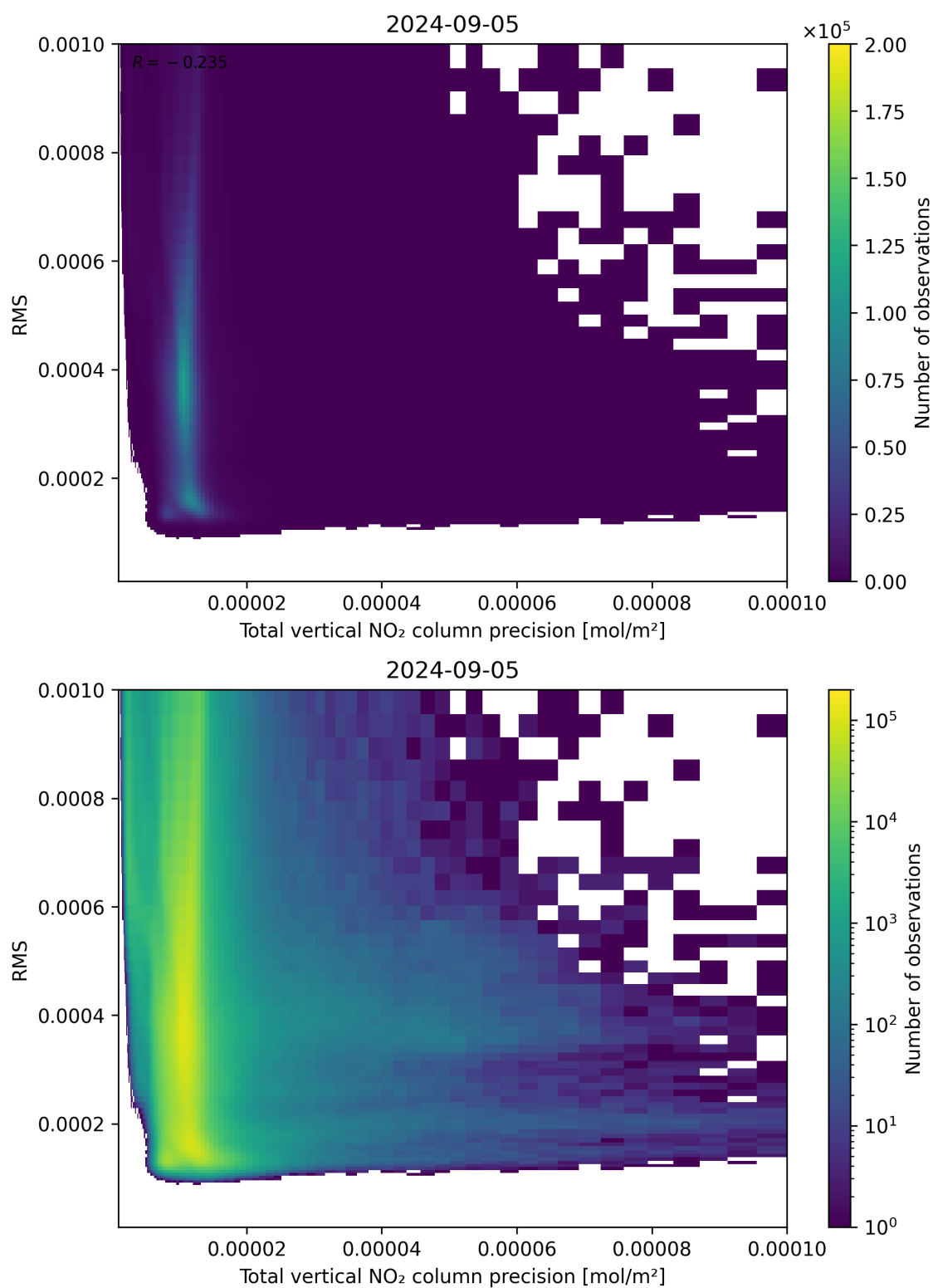
Figure 119: Scatter density plot of “Total vertical NO 2 column precision” against “RMS” for 2024-09-04 to 2024-09-06.
