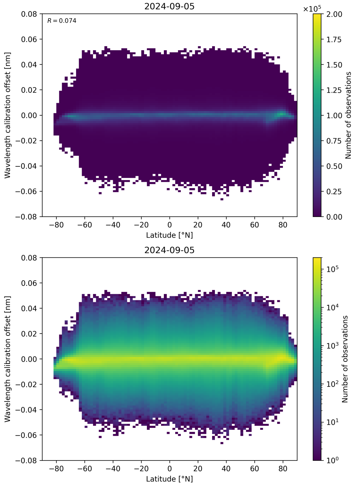
Figure 95: Scatter density plot of “Latitude” against “Wavelength calibration offset” for 2024-09-04 to 2024-09-06.
