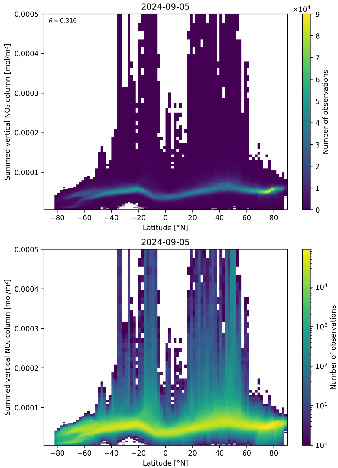
Figure 88: Scatter density plot of “Latitude” against “Summed vertical NO 2 column” for 2024-09-04 to 2024-09-06.
