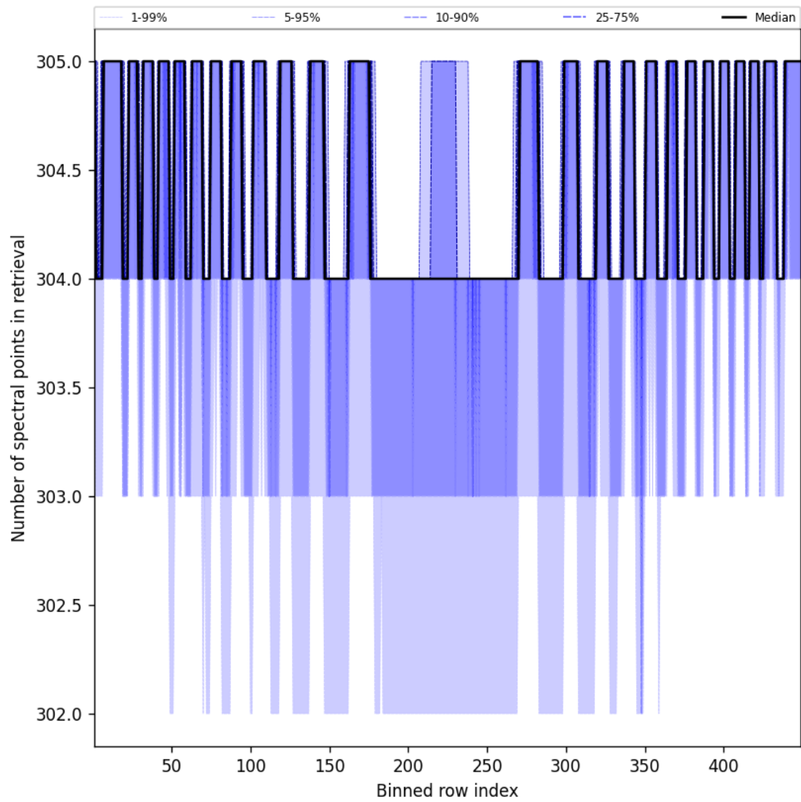
Figure 50: Along track statistics of “Number of spectral points in retrieval” for 2024-09-04 to 2024-09-06
