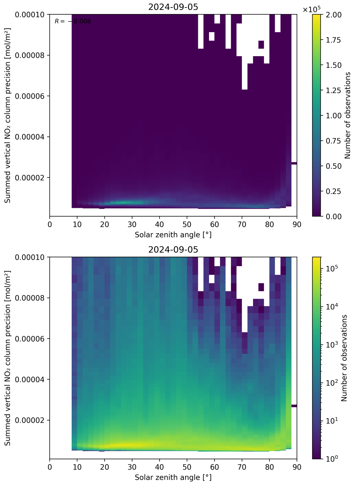
Figure 152: Scatter density plot of “Solar zenith angle” against “Summed vertical NO 2 column precision” for 2024-09-04 to 2024-09-06.
