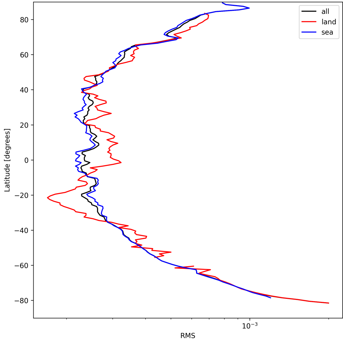
Figure 26: Zonal average of “RMS” for 2024-09-04 to 2024-09-06.
