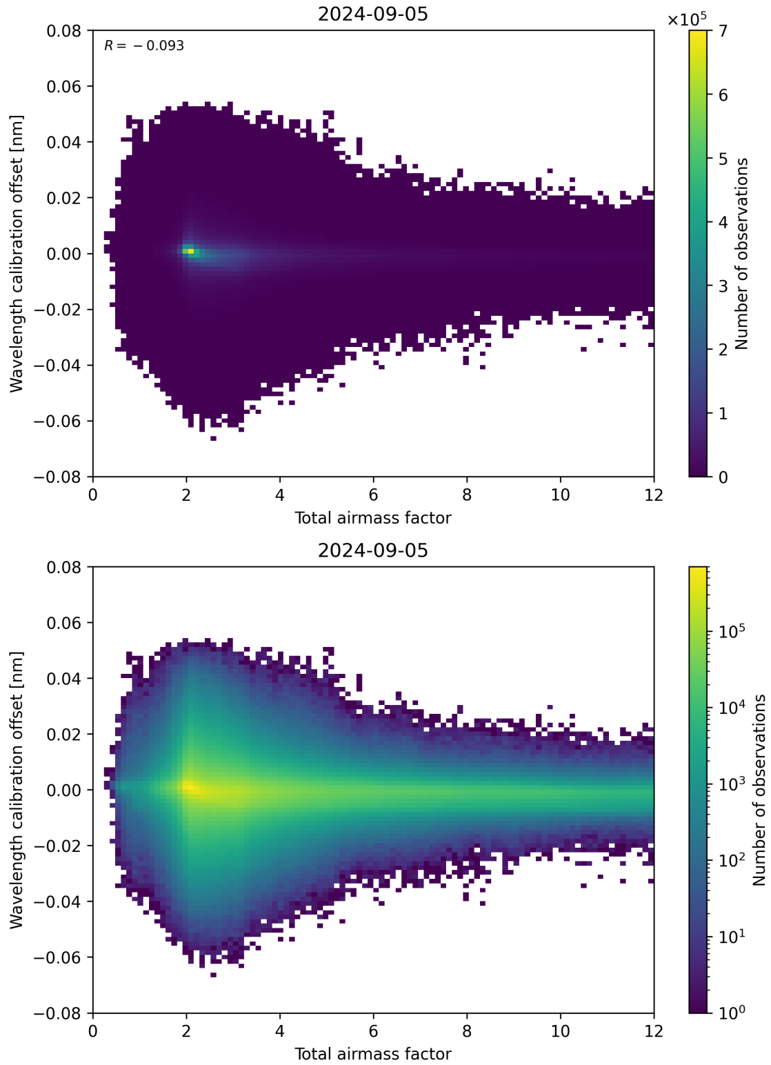
Figure 70: Scatter density plot of “Total airmass factor” against “Wavelength calibration offset” for 2024-09-04 to 2024-09-06.
