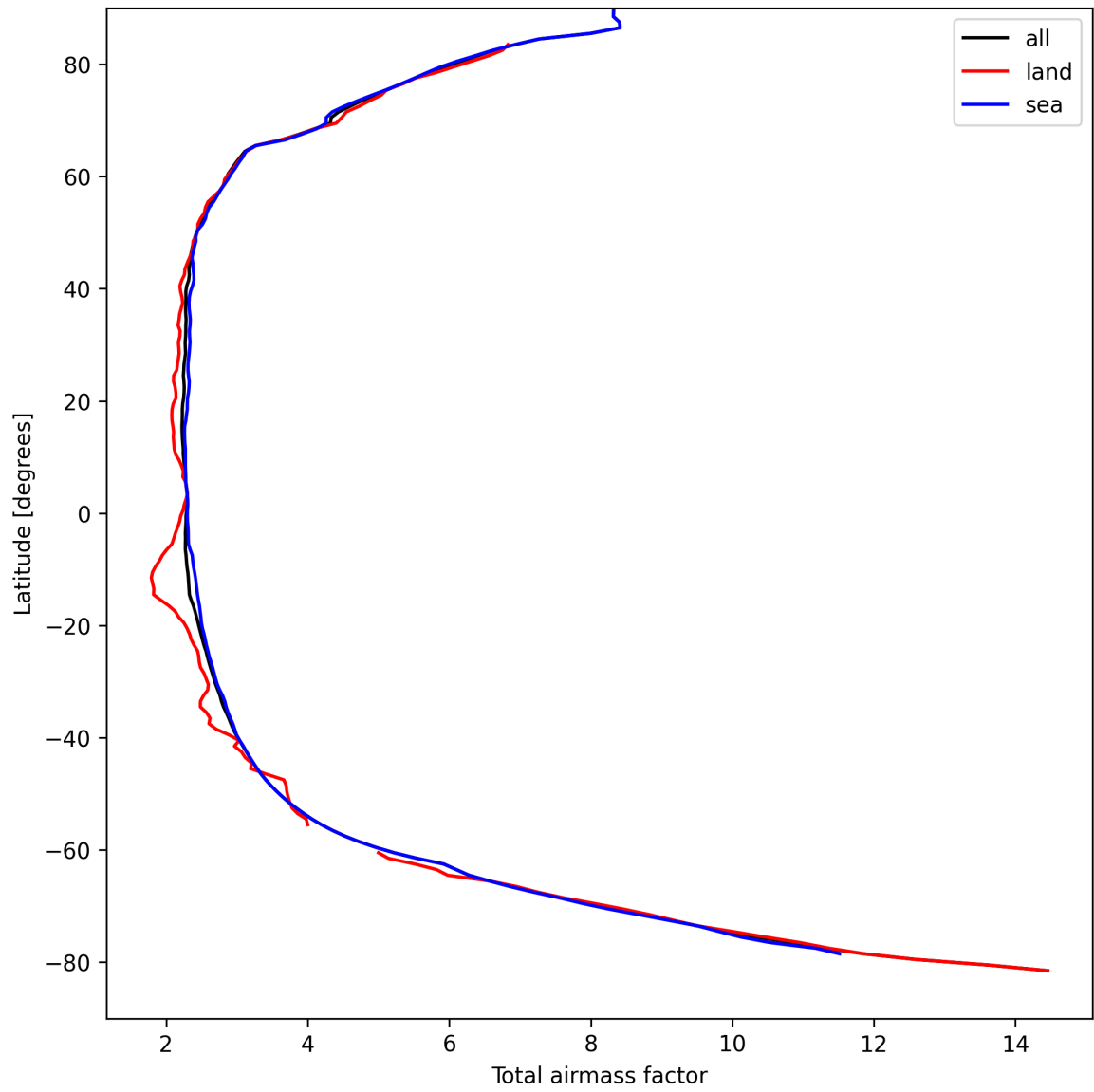
Figure 15: Zonal average of “Total airmass factor” for 2024-09-04 to 2024-09-06.
