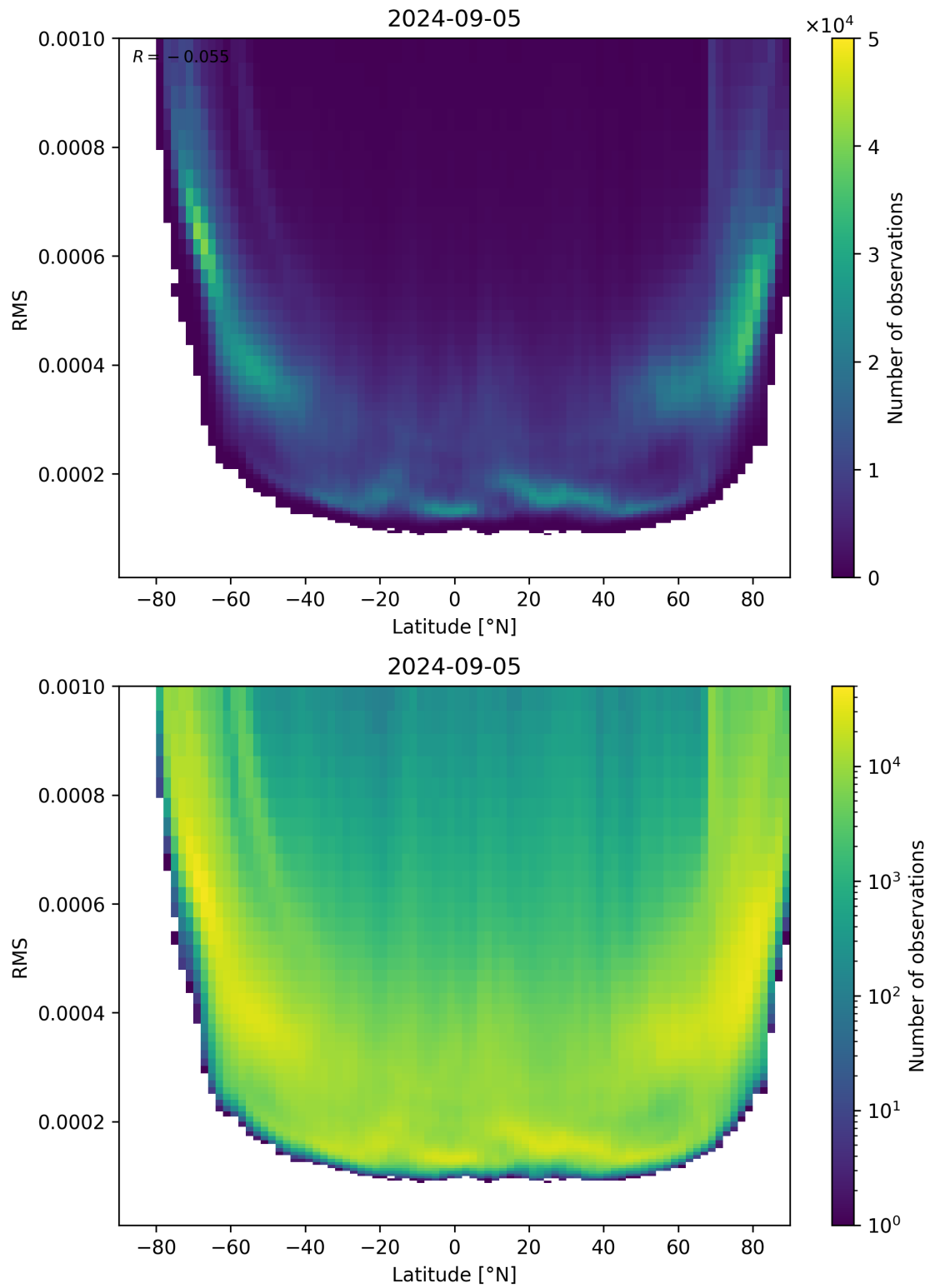
Figure 94: Scatter density plot of “Latitude” against “RMS” for 2024-09-04 to 2024-09-06.
