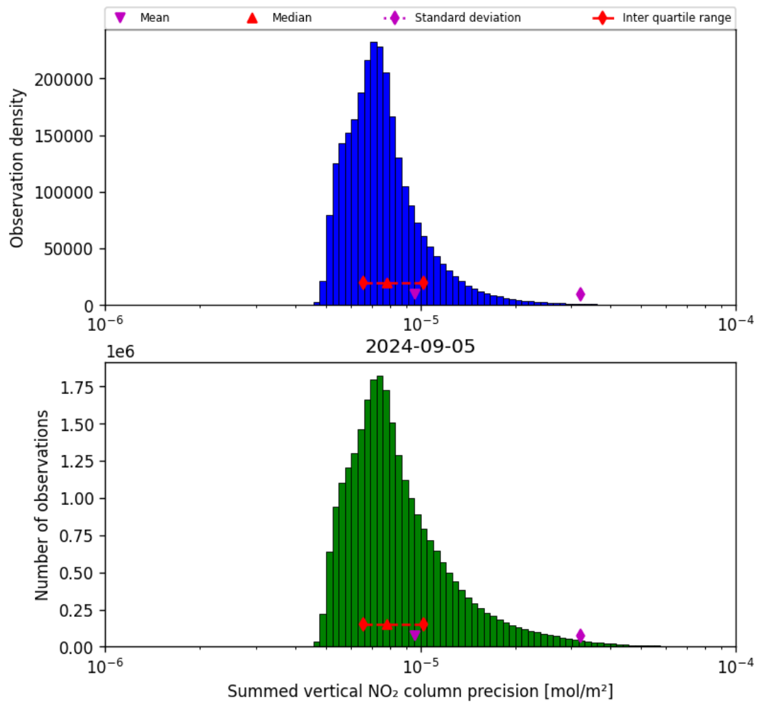
Figure 41: Histogram of “Summed vertical NO 2 column precision” for 2024-09-04 to 2024-09-06
