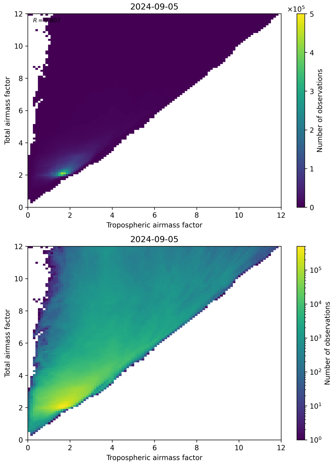
Figure 72: Scatter density plot of “Tropospheric airmass factor” against “Total airmass factor” for 2024-09-04 to 2024-09-06.
