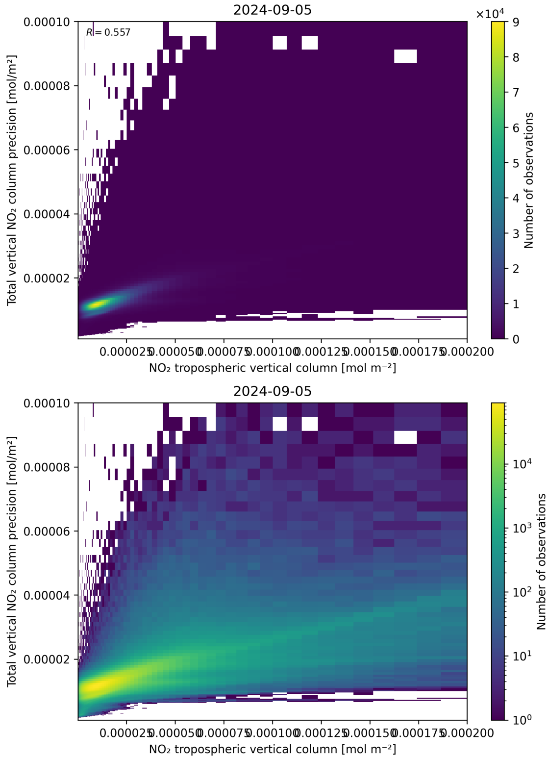
Figure 129: Scatter density plot of “NO 2 tropospheric vertical column” against “Total vertical NO 2 column precision” for 2024-09-04 to 2024-09-06.
