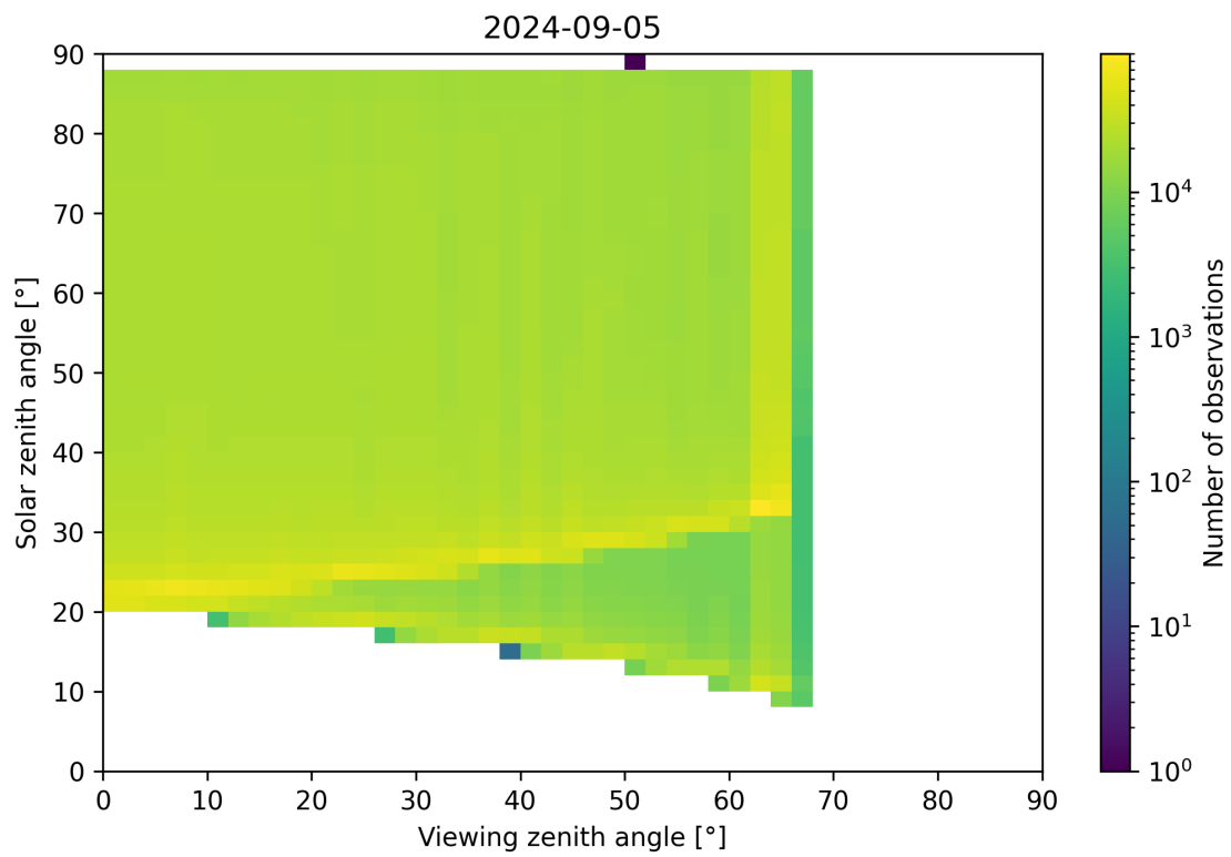
Figure 172: Scatter density plot of “Viewing zenith angle” against “Solar zenith angle” for 2024-09-04 to 2024-09-06.
