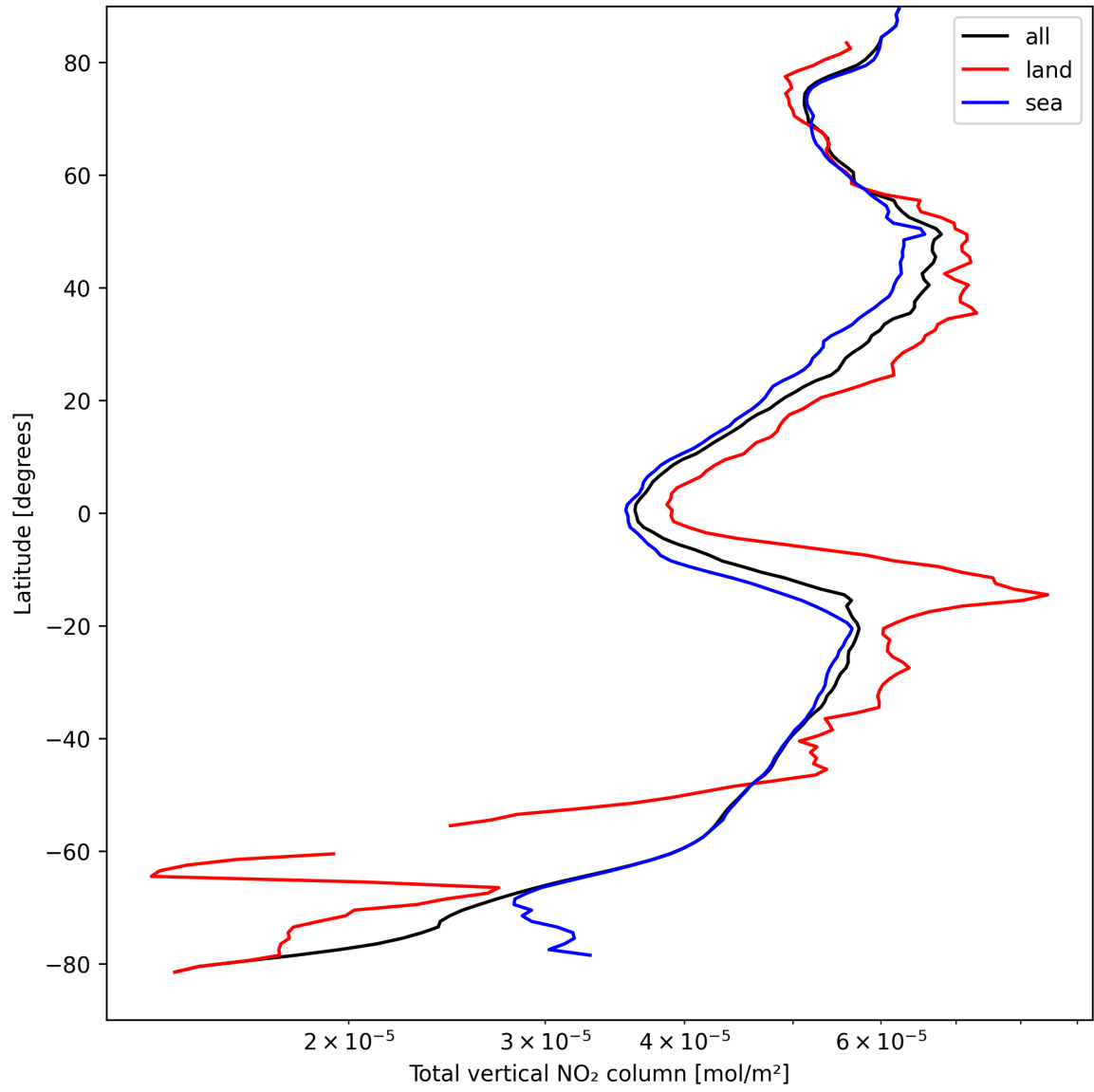
Figure 21: Zonal average of “Total vertical NO 2 column” for 2024-09-04 to 2024-09-06.
