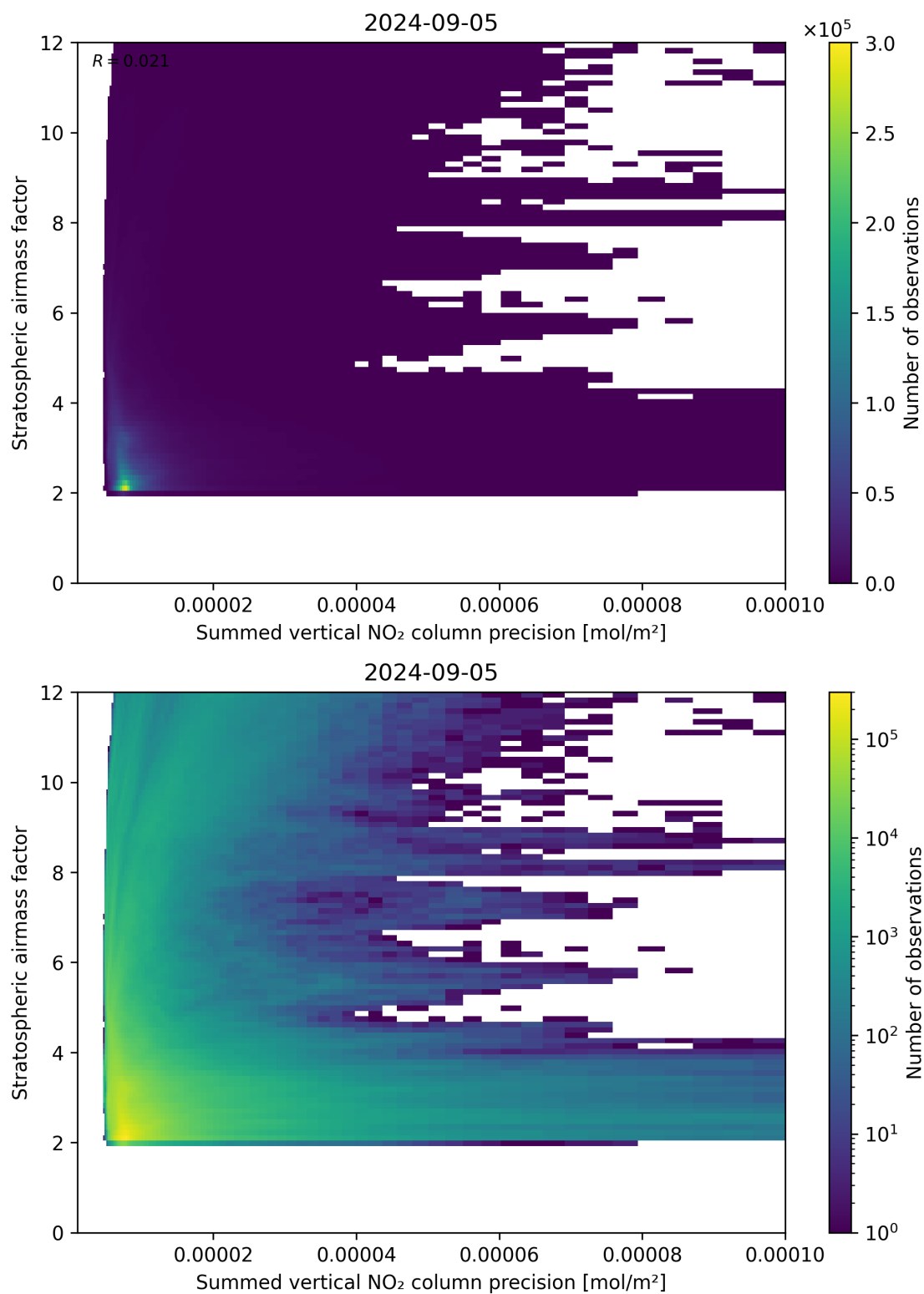
Figure 106: Scatter density plot of “Summed vertical NO 2 column precision” against “Stratospheric airmass factor” for 2024-09-04 to 2024-09-06.
