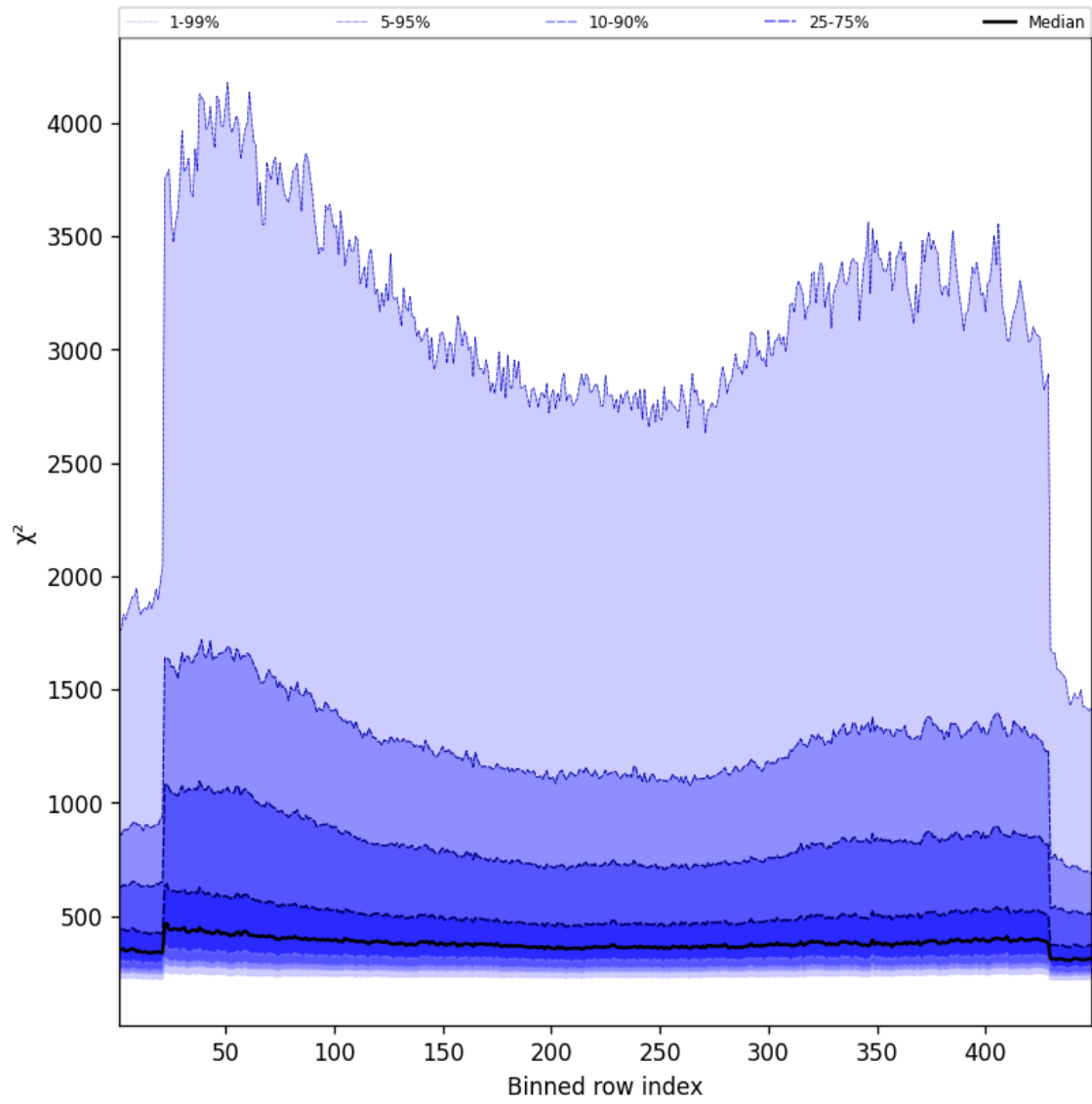
Figure 59: Along track statistics of “ \chi^2 ” for 2024-09-04 to 2024-09-06
