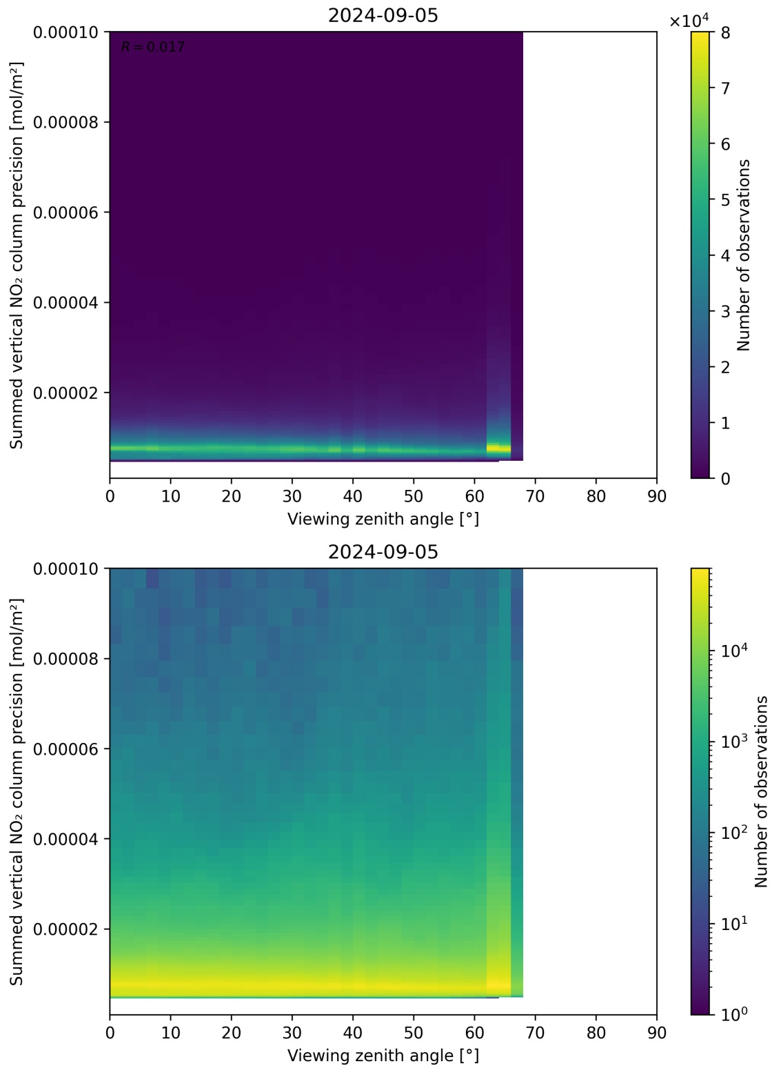
Figure 166: Scatter density plot of “Viewing zenith angle” against “Summed vertical NO 2 column precision” for 2024-09-04 to 2024-09-06.
