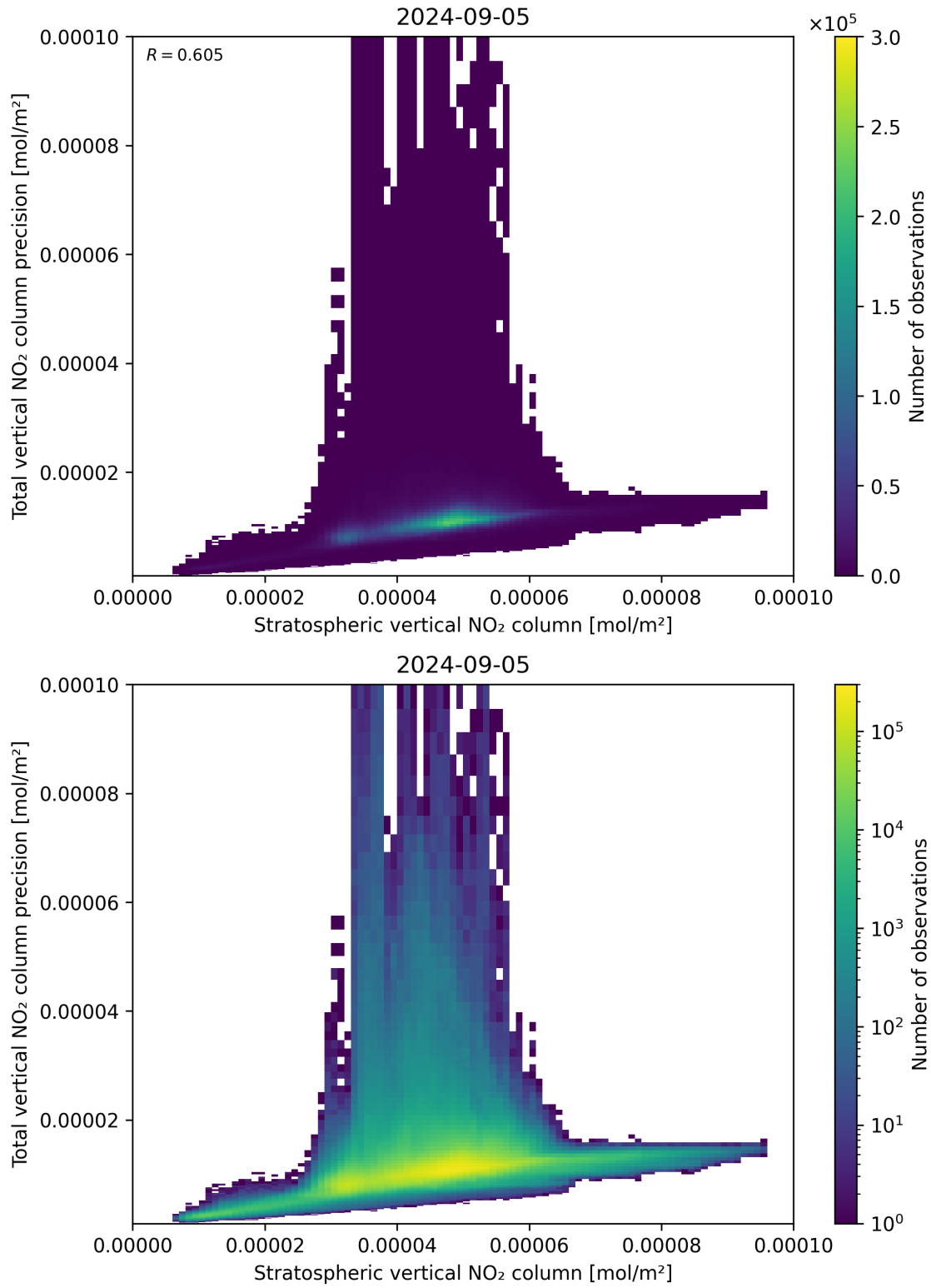
Figure 101: Scatter density plot of “Stratospheric vertical NO 2 column” against “Total vertical NO 2 column precision” for 2024-09-04 to 2024-09-06.
