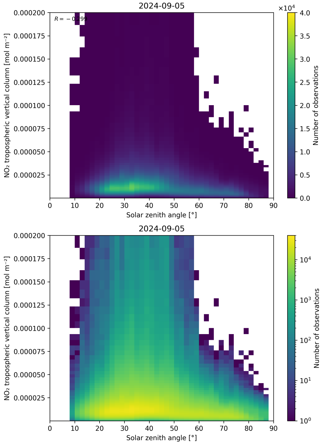
Figure 155: Scatter density plot of “Solar zenith angle” against “NO 2 tropospheric vertical column” for 2024-09-04 to 2024-09-06.
