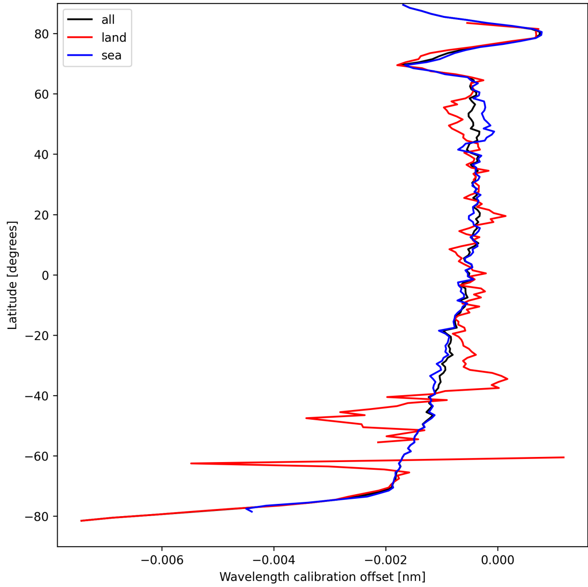
Figure 18: Zonal average of “Wavelength calibration offset” for 2024-09-04 to 2024-09-06.
