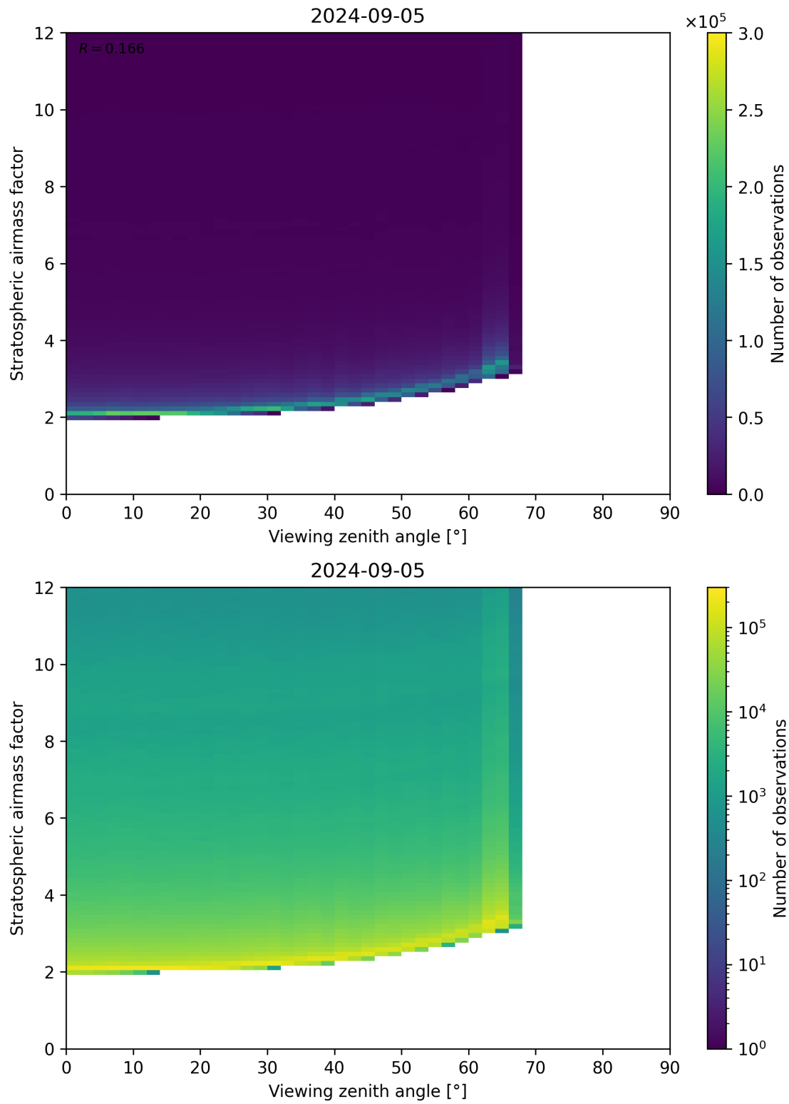
Figure 159: Scatter density plot of “Viewing zenith angle” against “Stratospheric airmass factor” for 2024-09-04 to 2024-09-06.
