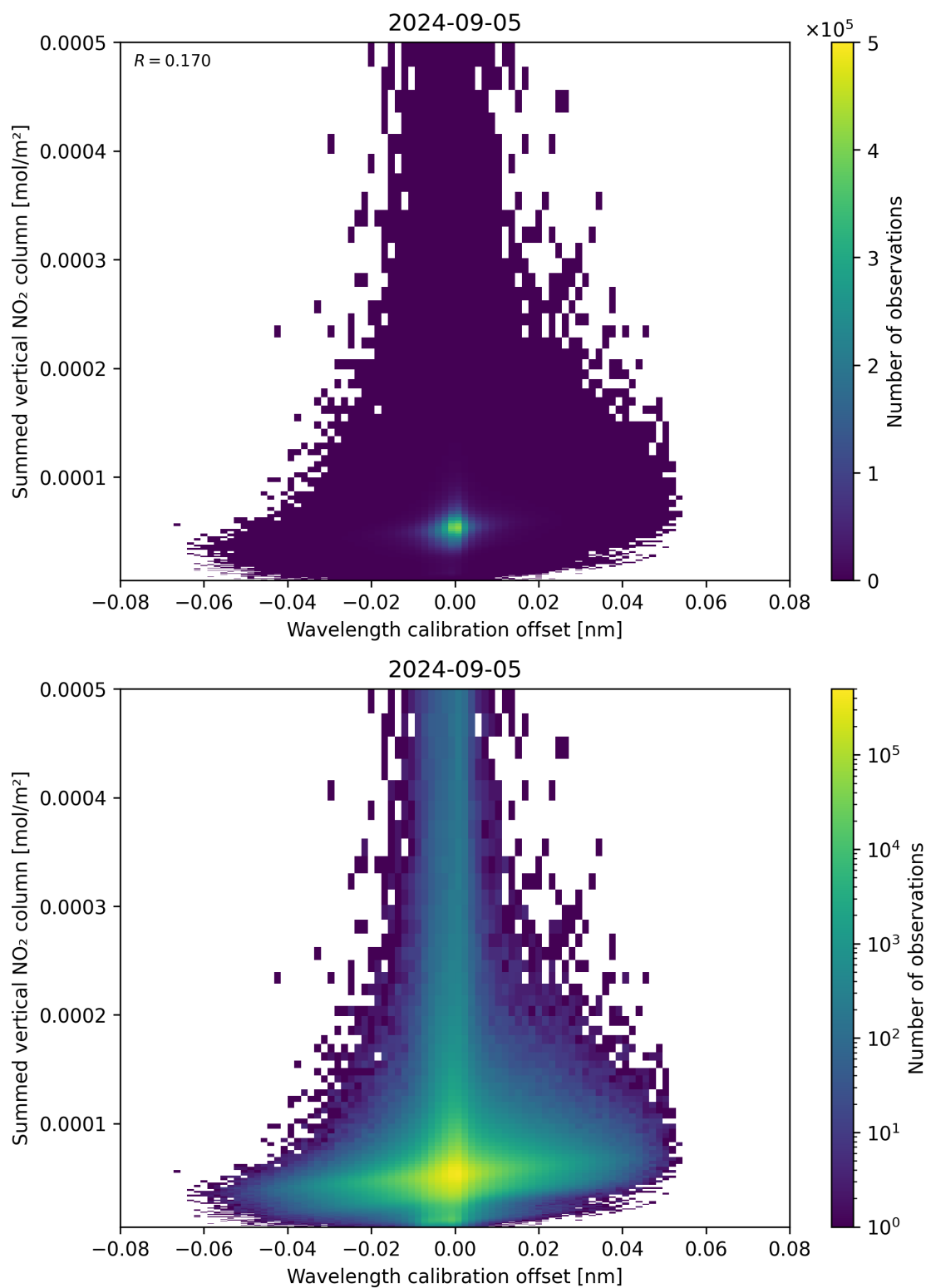
Figure 177: Scatter density plot of “Wavelength calibration offset” against “Summed vertical NO 2 column” for 2024-09-04 to 2024-09-06.
