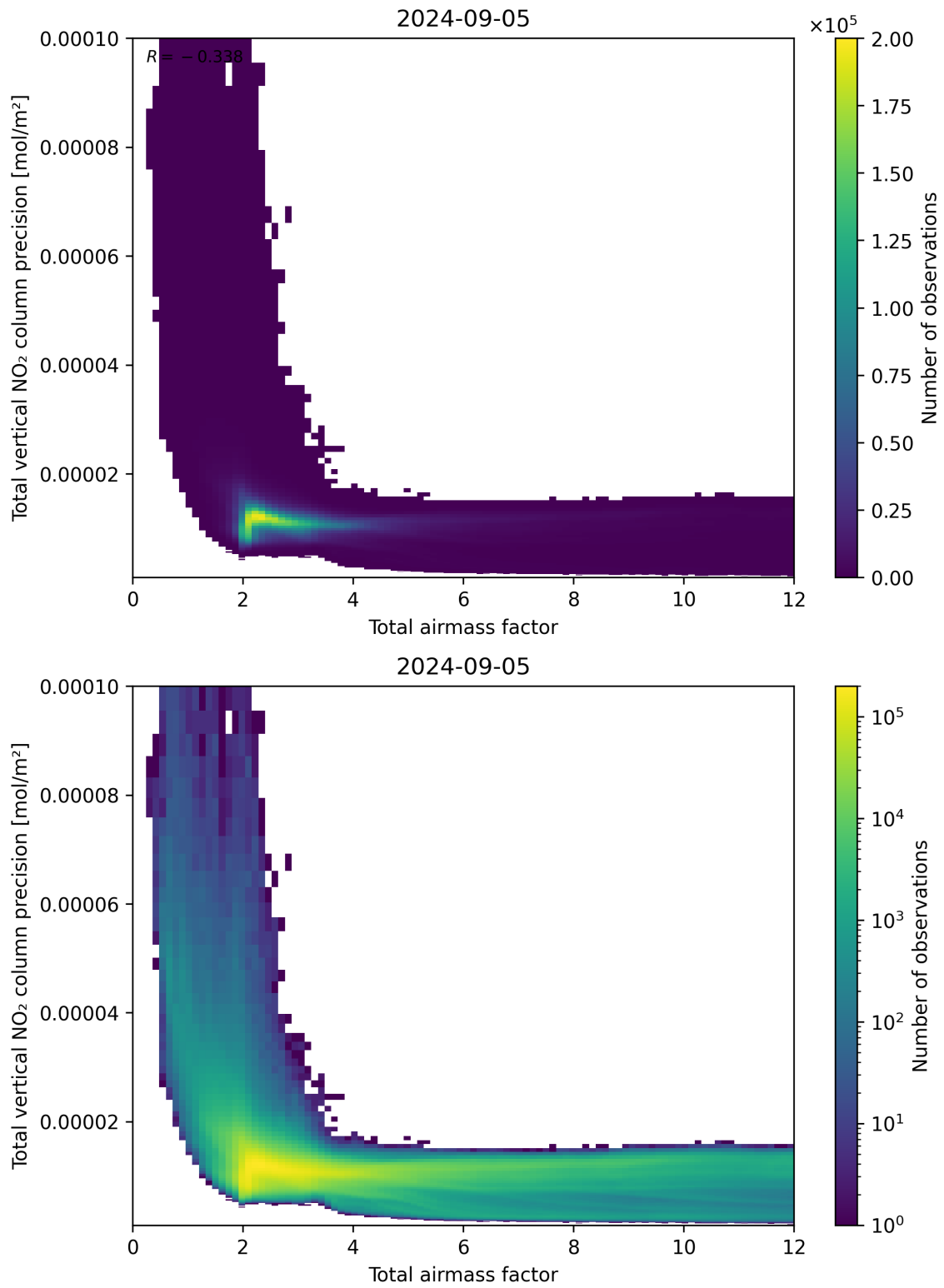
Figure 68: Scatter density plot of “Total airmass factor” against “Total vertical NO 2 column precision” for 2024-09-04 to 2024-09-06.
