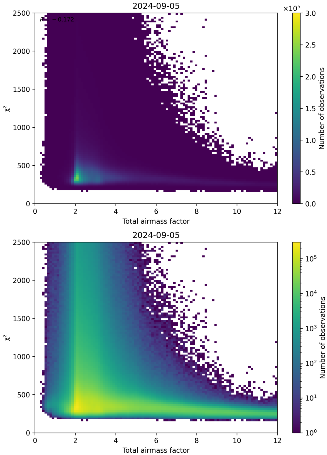
Figure 63: Scatter density plot of “Total airmass factor” against “ \chi^2 ” for 2024-09-04 to 2024-09-06.
