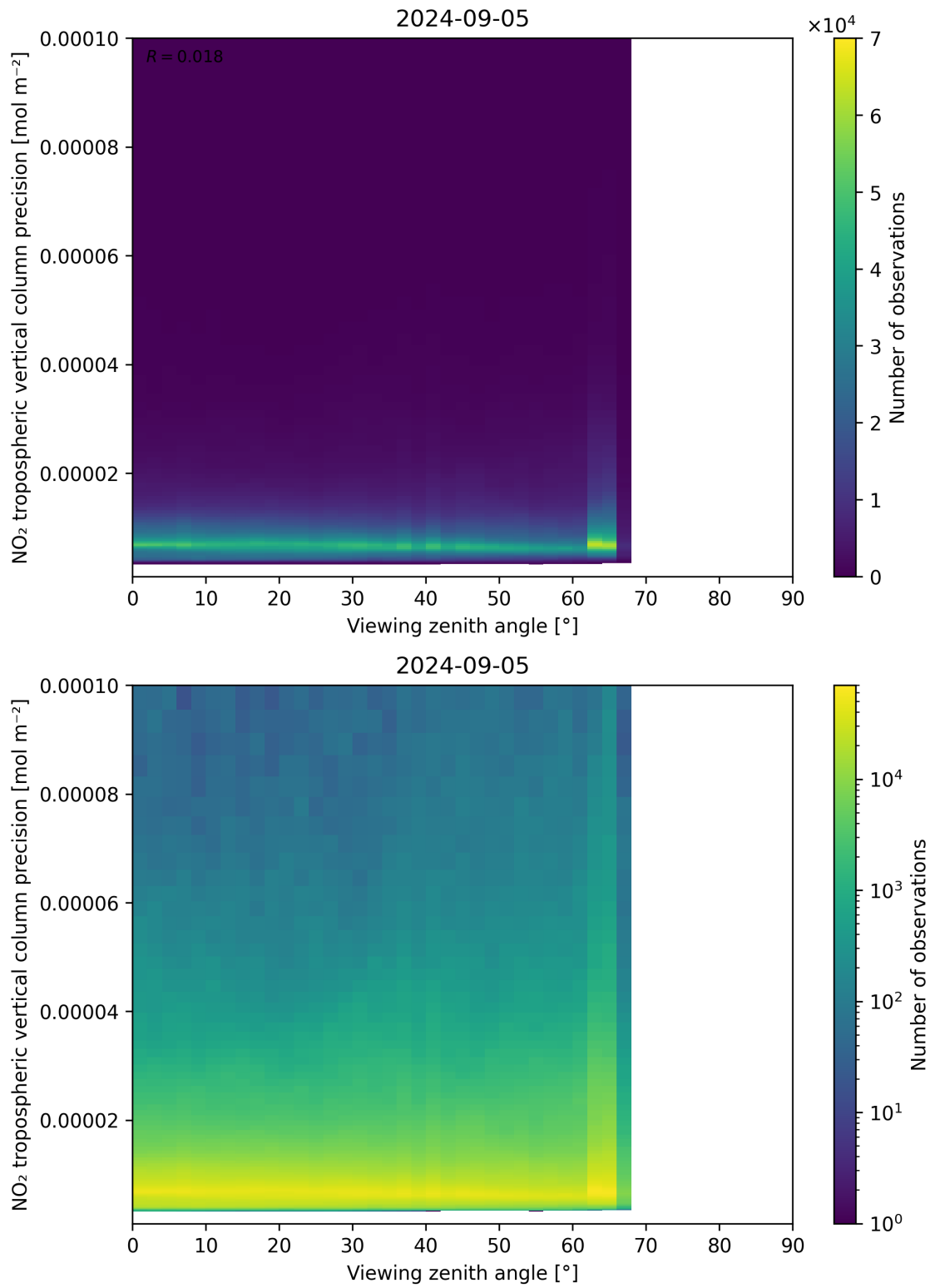
Figure 170: Scatter density plot of “Viewing zenith angle” against “NO 2 tropospheric vertical column precision” for 2024-09-04 to 2024-09-06.
