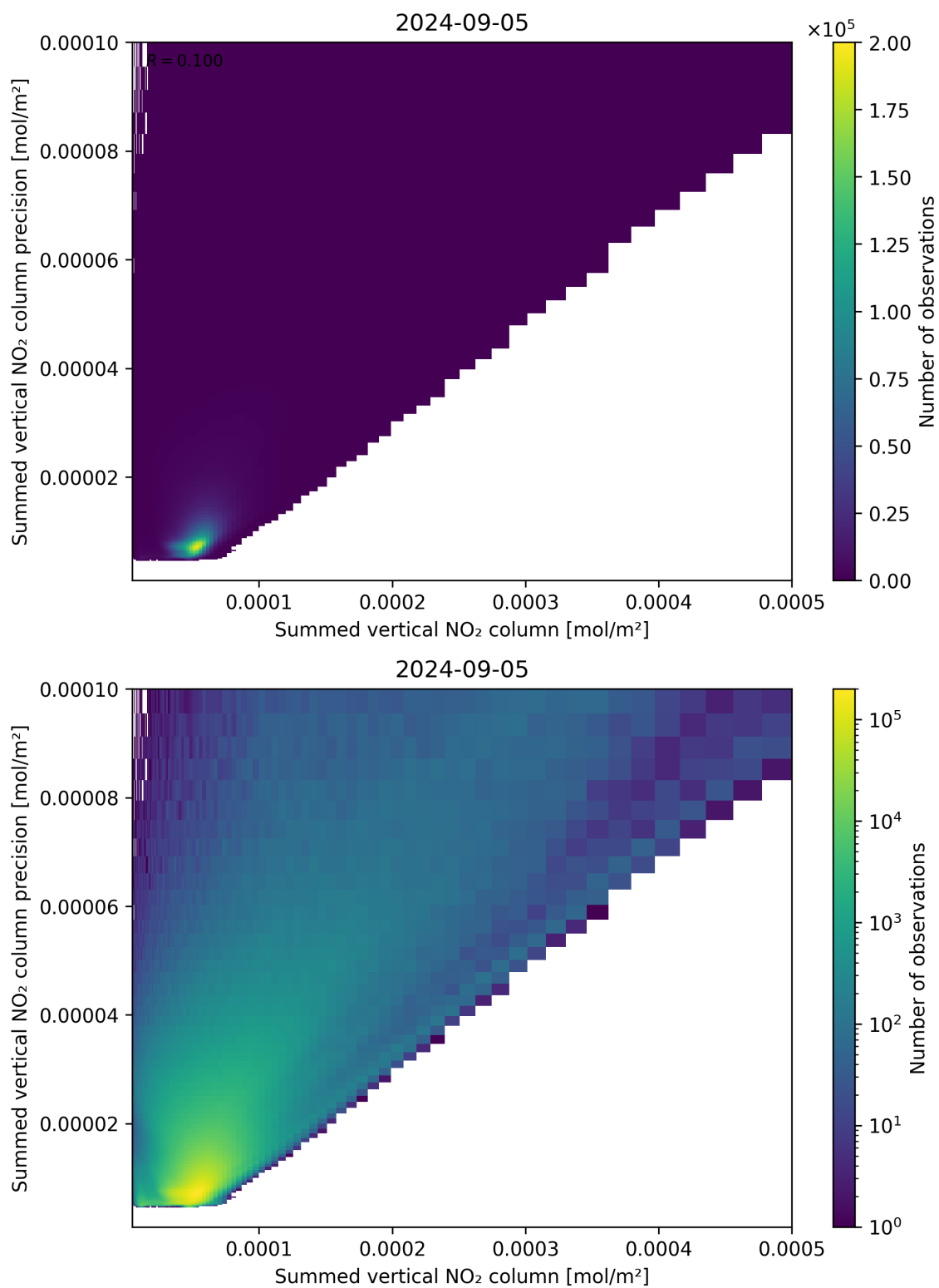
Figure 105: Scatter density plot of “Summed vertical NO 2 column” against “Summed vertical NO 2 column precision” for 2024-09-04 to 2024-09-06.
