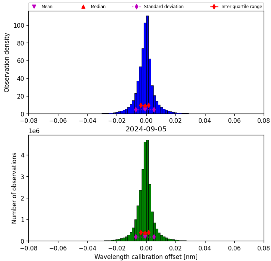
Figure 35: Histogram of “Wavelength calibration offset” for 2024-09-04 to 2024-09-06
