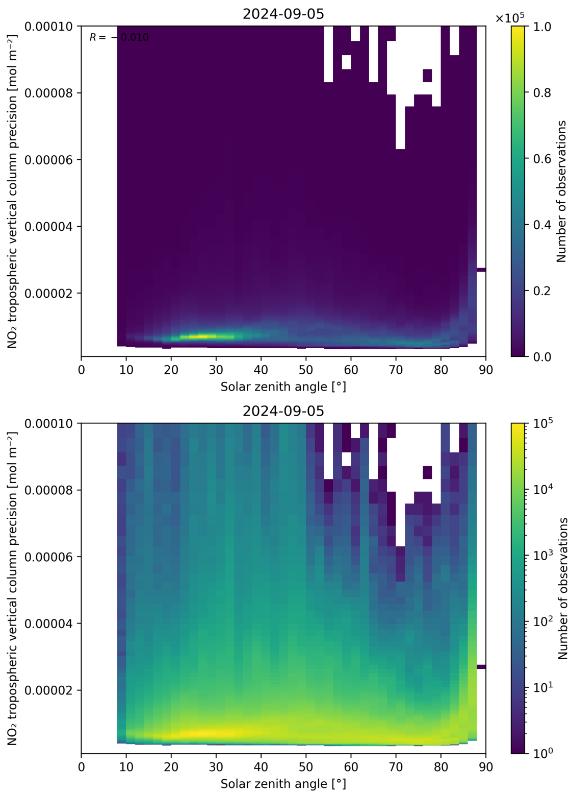
Figure 156: Scatter density plot of “Solar zenith angle” against “NO 2 tropospheric vertical column precision” for 2024-09-04 to 2024-09-06.
