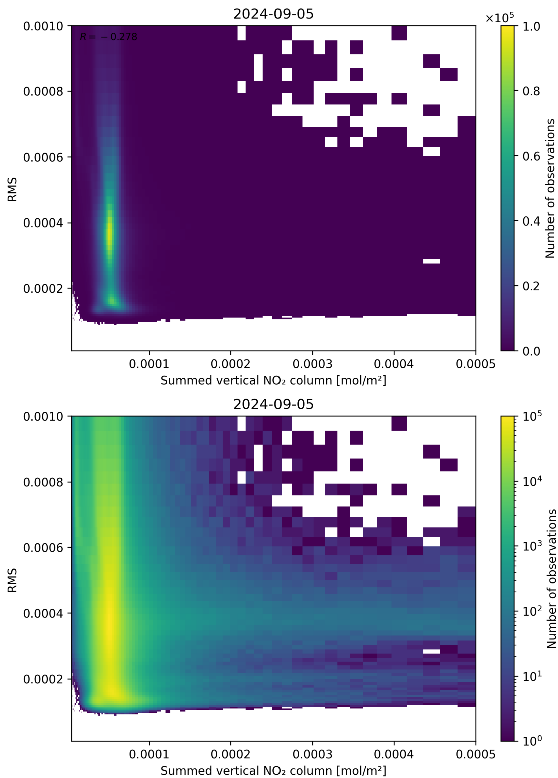
Figure 109: Scatter density plot of “Summed vertical NO 2 column” against “RMS” for 2024-09-04 to 2024-09-06.
