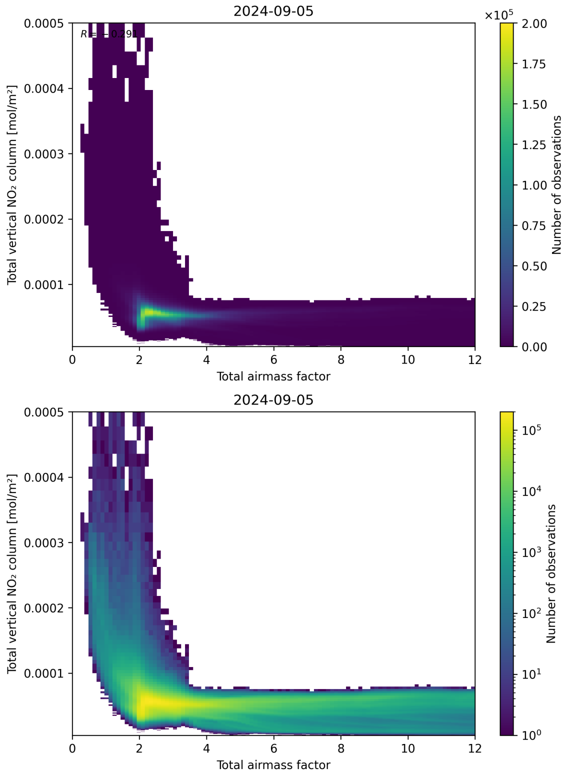
Figure 67: Scatter density plot of “Total airmass factor” against “Total vertical NO 2 column” for 2024-09-04 to 2024-09-06.
