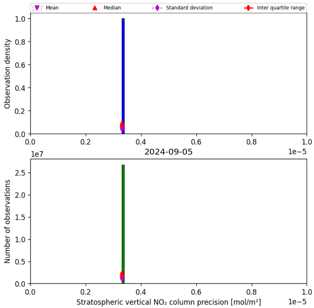
Figure 37: Histogram of “Stratospheric vertical NO 2 column precision” for 2024-09-04 to 2024-09-06
