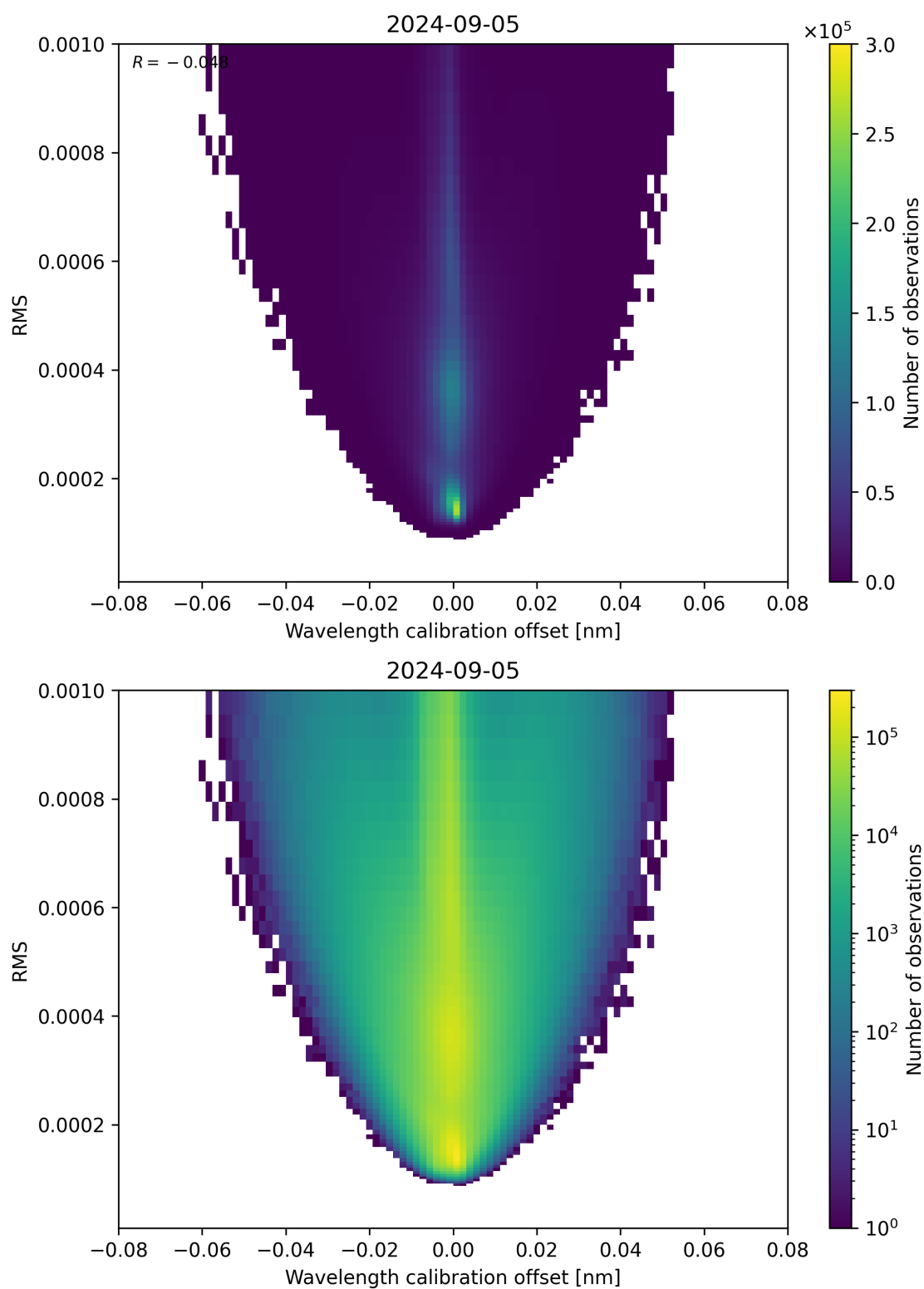
Figure 181: Scatter density plot of “Wavelength calibration offset” against “RMS” for 2024-09-04 to 2024-09-06.
