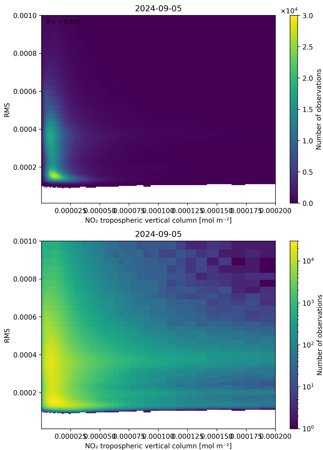
Figure 142: Scatter density plot of “NO 2 tropospheric vertical column” against “RMS” for 2024-09-04 to 2024-09-06.
