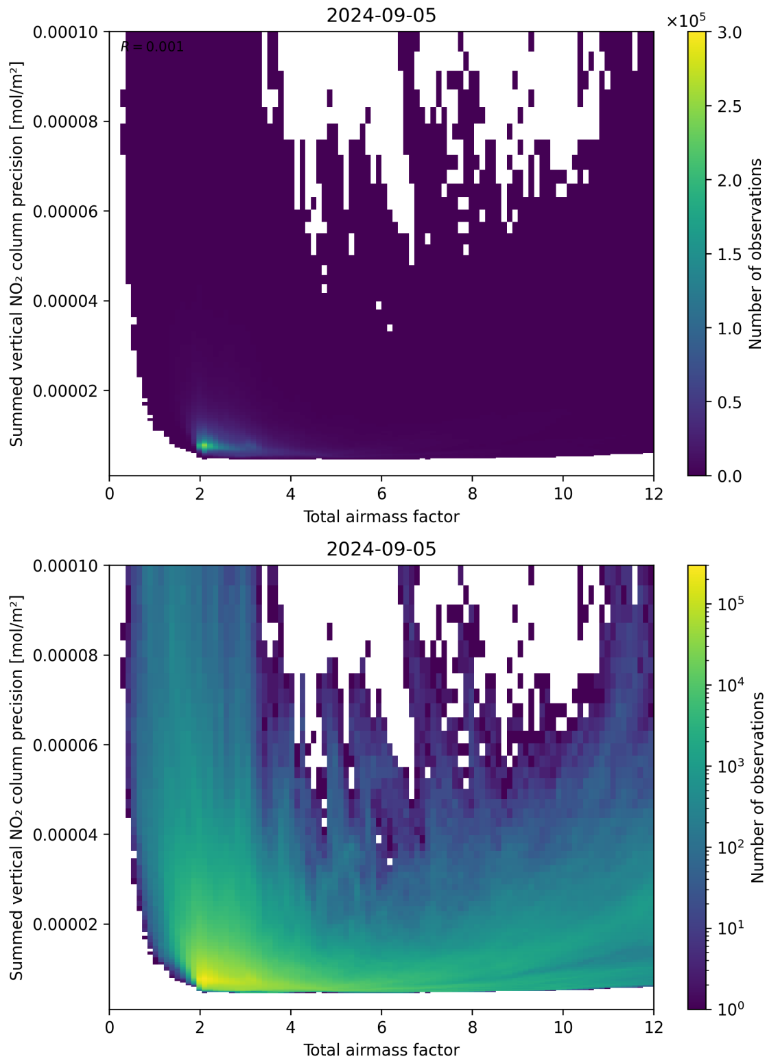
Figure 66: Scatter density plot of “Total airmass factor” against “Summed vertical NO 2 column precision” for 2024-09-04 to 2024-09-06.
