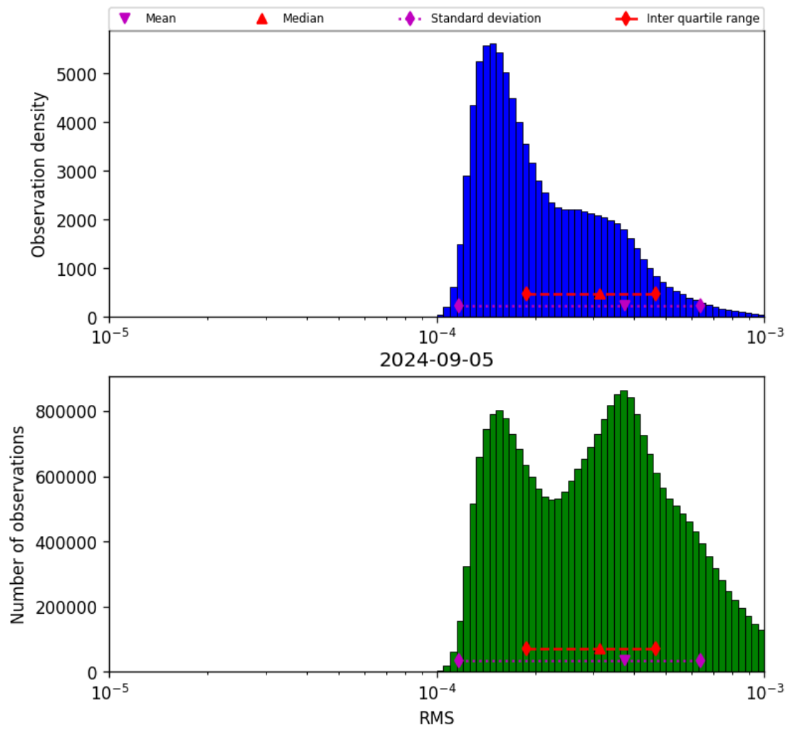
Figure 43: Histogram of “RMS” for 2024-09-04 to 2024-09-06
