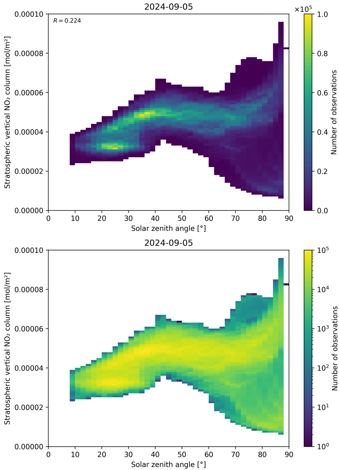
Figure 150: Scatter density plot of “Solar zenith angle” against “Stratospheric vertical NO 2 column” for 2024-09-04 to 2024-09-06.
