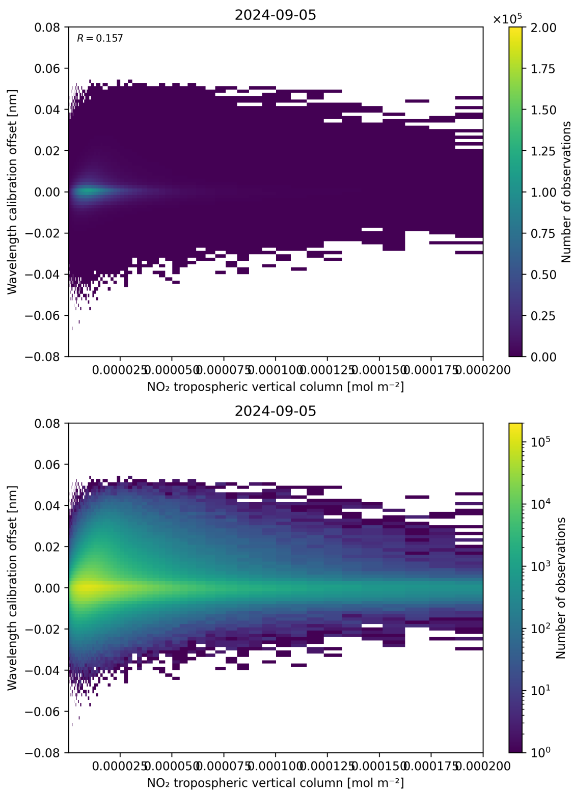
Figure 143: Scatter density plot of “NO 2 tropospheric vertical column” against “Wavelength calibration offset” for 2024-09-04 to 2024-09-06.
