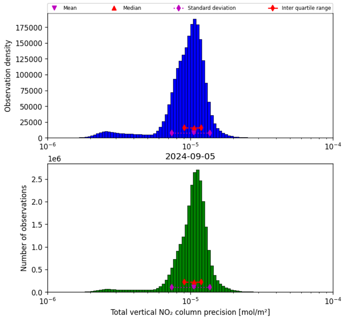
Figure 39: Histogram of “Total vertical NO 2 column precision” for 2024-09-04 to 2024-09-06
