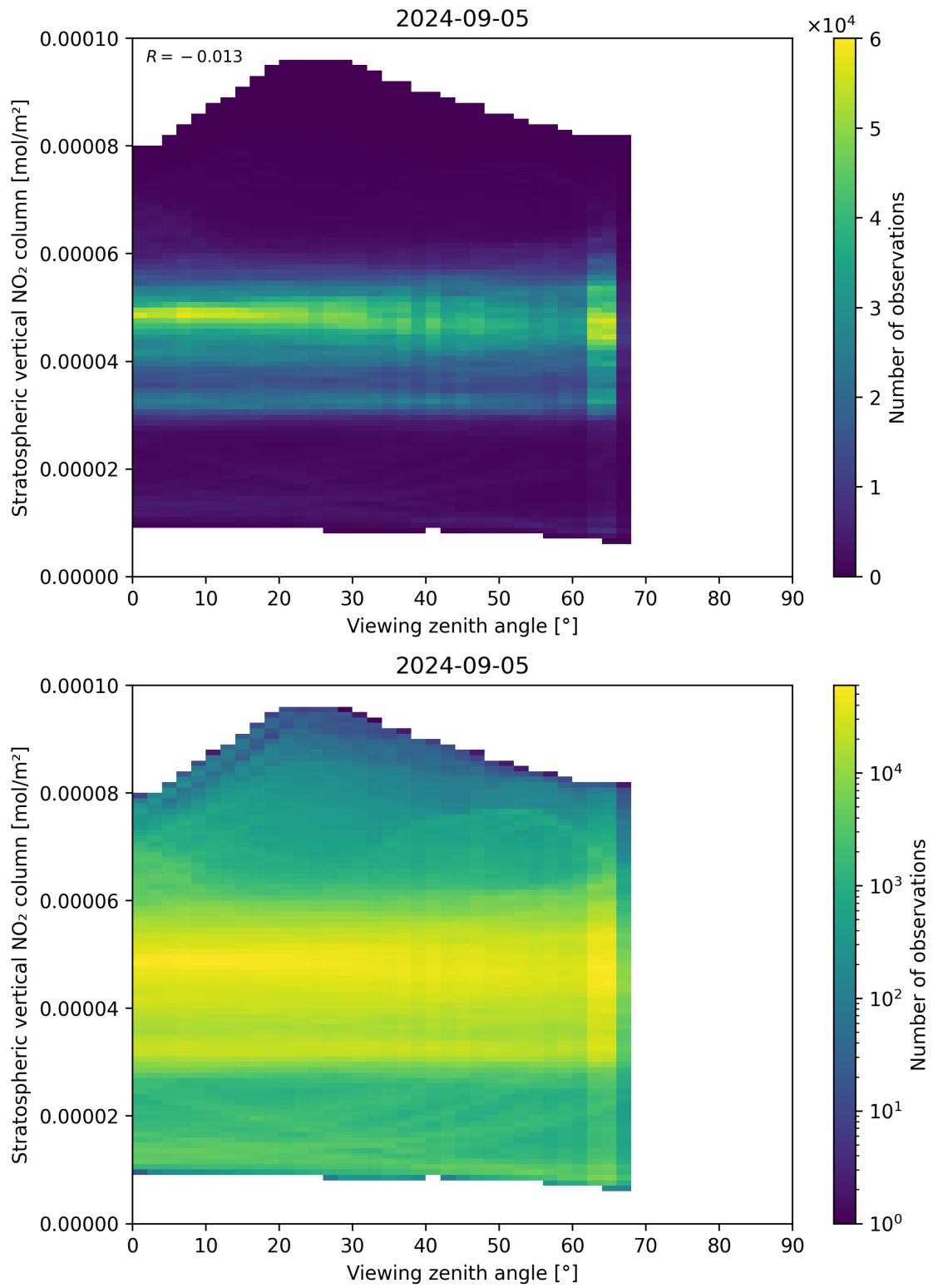
Figure 164: Scatter density plot of “Viewing zenith angle” against “Stratospheric vertical NO 2 column” for 2024-09-04 to 2024-09-06.
