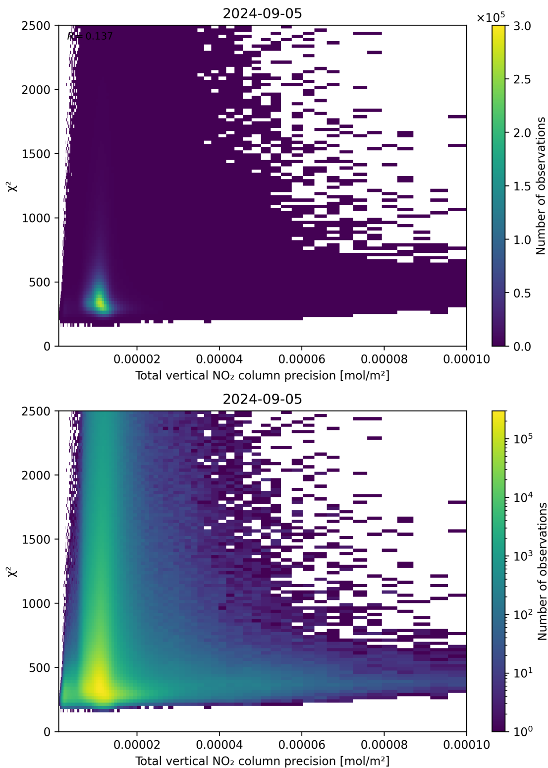
Figure 116: Scatter density plot of “Total vertical NO 2 column precision” against “ \chi^2 ” for 2024-09-04 to 2024-09-06.
