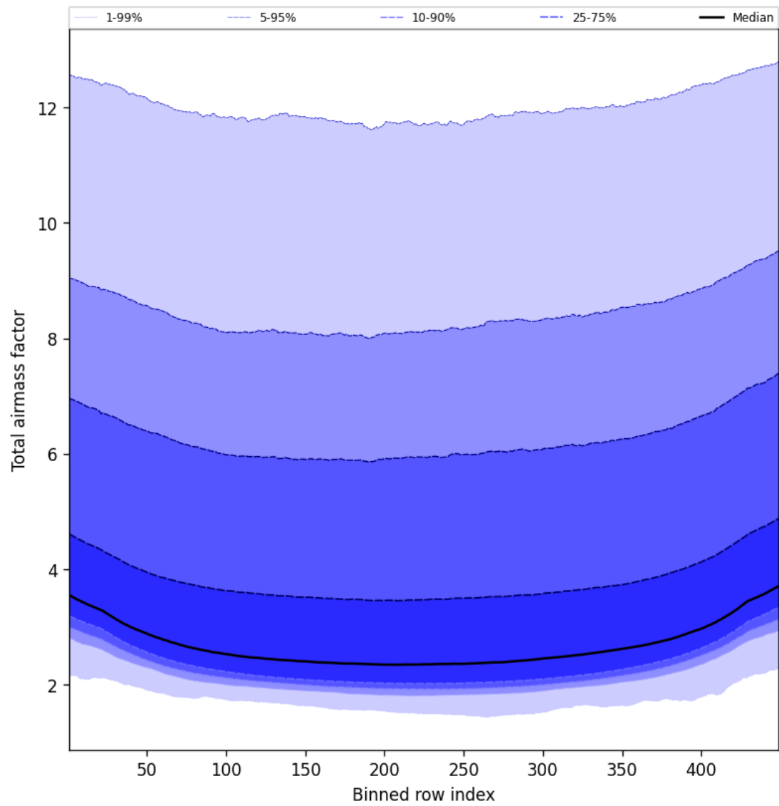
Figure 49: Along track statistics of “Total airmass factor” for 2024-09-04 to 2024-09-06
