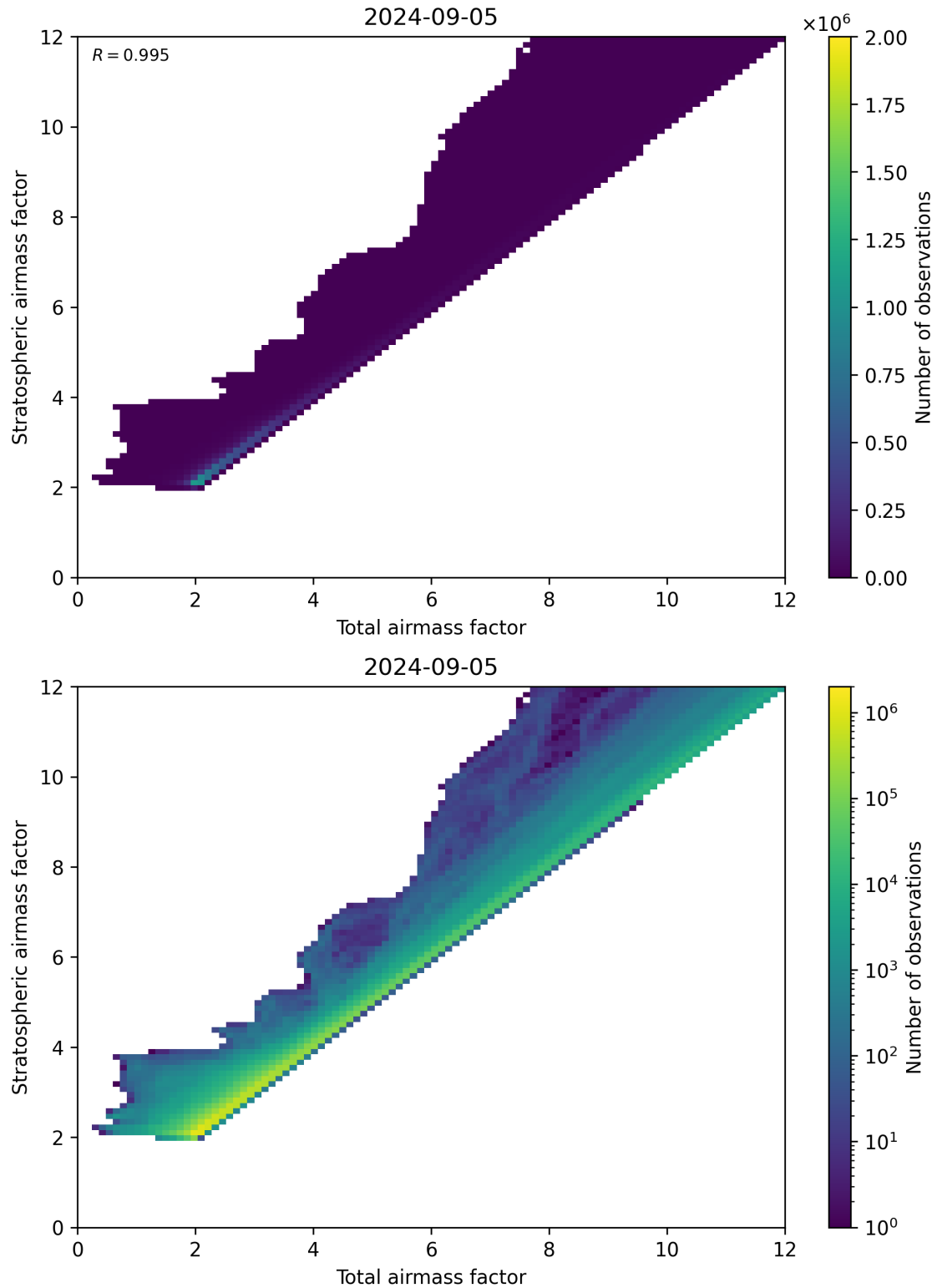
Figure 62: Scatter density plot of “Total airmass factor” against “Stratospheric airmass factor” for 2024-09-04 to 2024-09-06.
