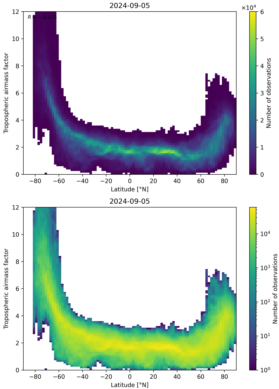
Figure 85: Scatter density plot of “Latitude” against “Tropospheric air mass factor” for 2024-09-04 to 2024-09-06.
