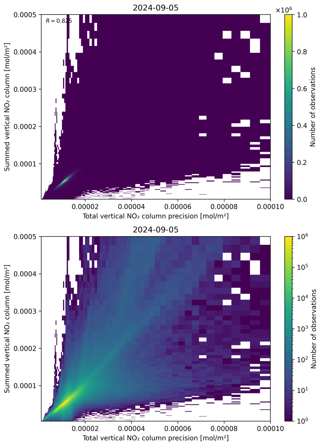
Figure 117: Scatter density plot of “Total vertical NO 2 column precision” against “Summed vertical NO 2 column” for 2024-09-04 to 2024-09-06.
