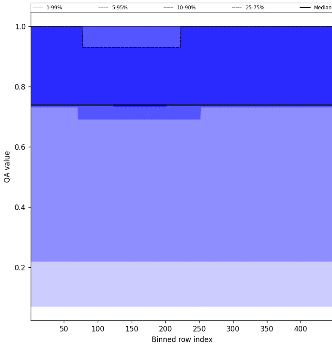
Figure 45: Along track statistics of “QA value” for 2024-09-04 to 2024-09-06
