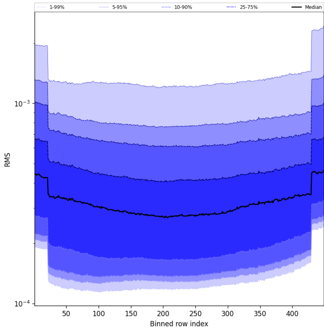
Figure 60: Along track statistics of “RMS” for 2024-09-04 to 2024-09-06
