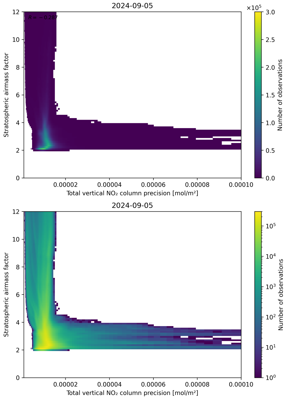
Figure 115: Scatter density plot of “Total vertical NO 2 column precision” against “Stratospheric airmass factor” for 2024-09-04 to 2024-09-06.
