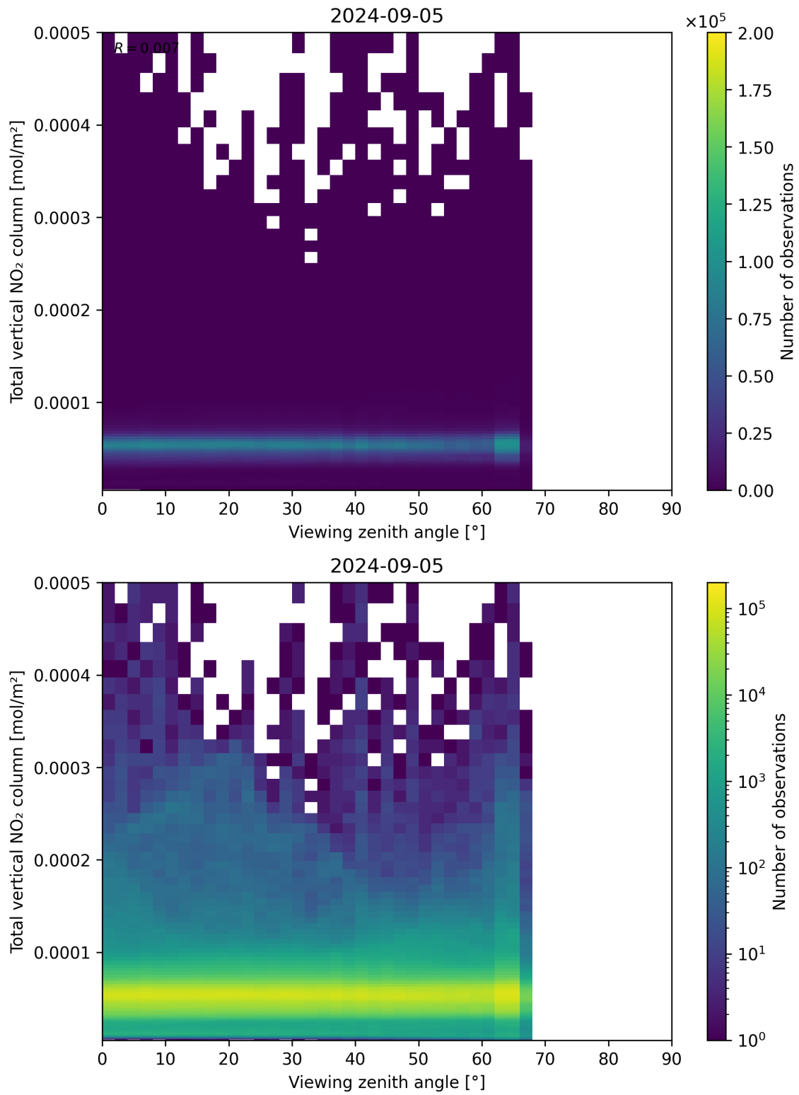
Figure 167: Scatter density plot of “Viewing zenith angle” against “Total vertical NO 2 column” for 2024-09-04 to 2024-09-06.
