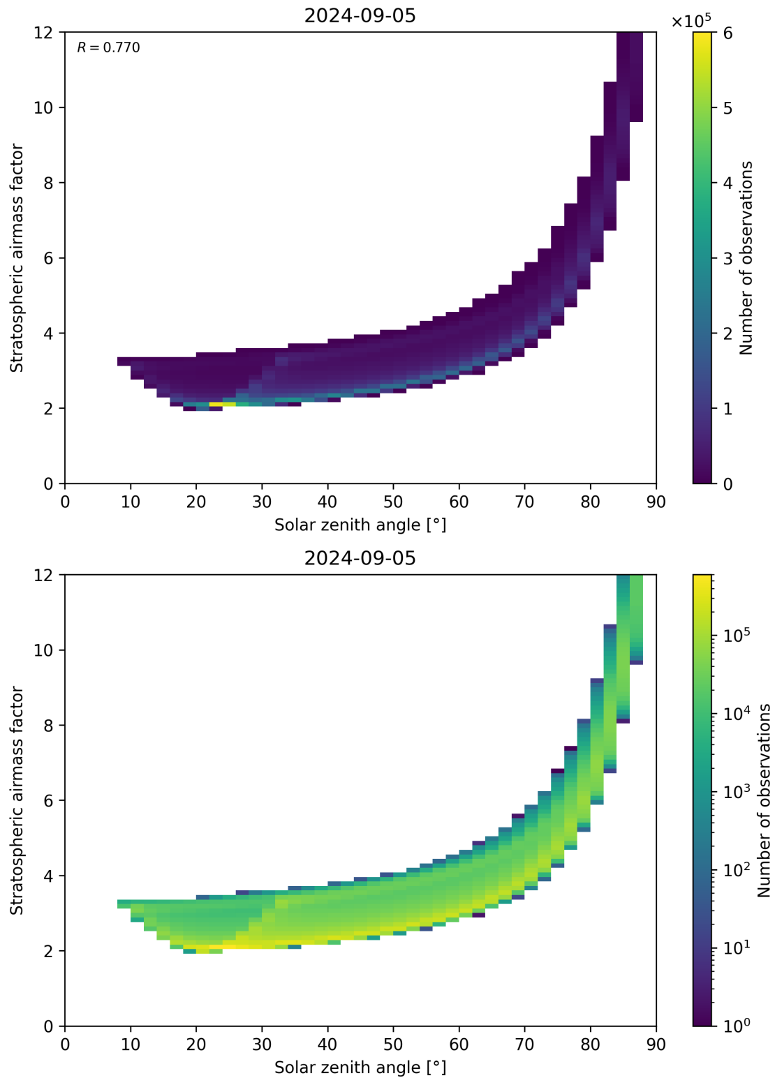
Figure 145: Scatter density plot of “Solar zenith angle” against “Stratospheric airmass factor” for 2024-09-04 to 2024-09-06.
