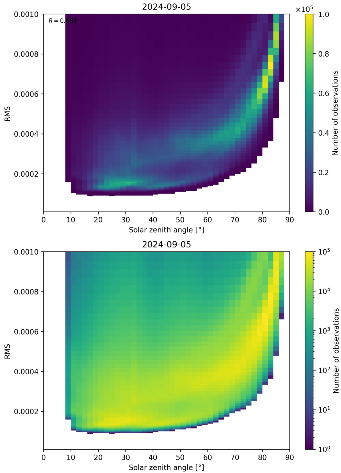
Figure 157: Scatter density plot of “Solar zenith angle” against “RMS” for 2024-09-04 to 2024-09-06.
