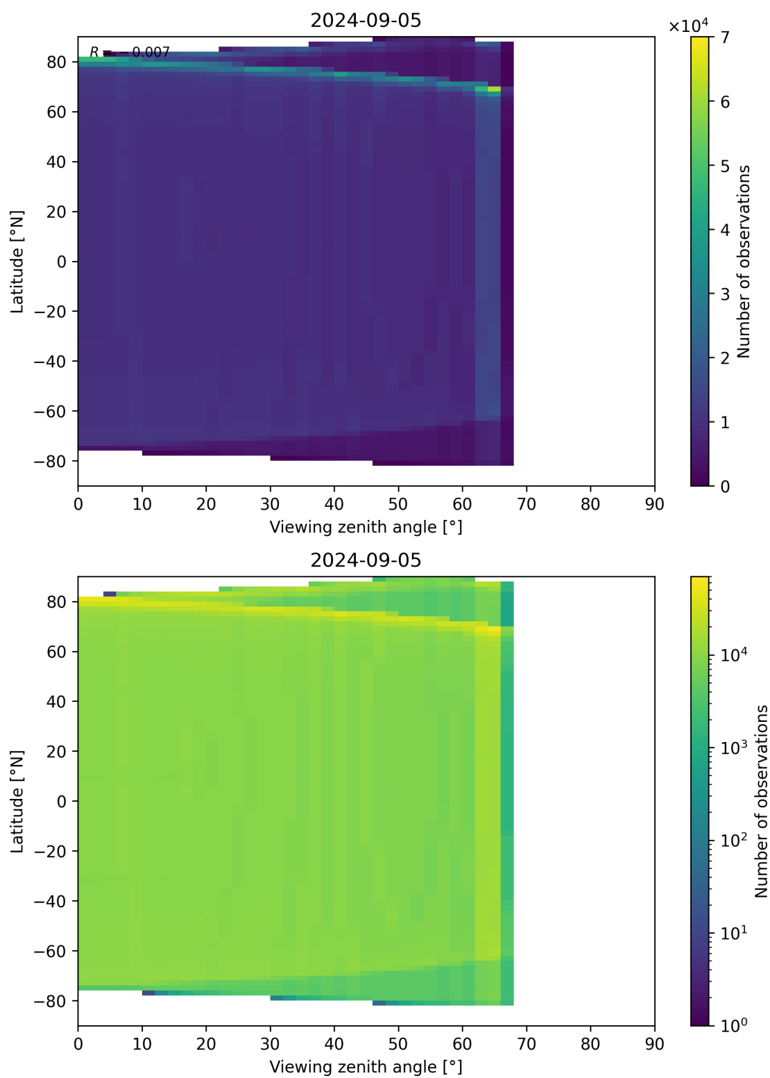
Figure 163: Scatter density plot of “Viewing zenith angle” against “Latitude” for 2024-09-04 to 2024-09-06.
