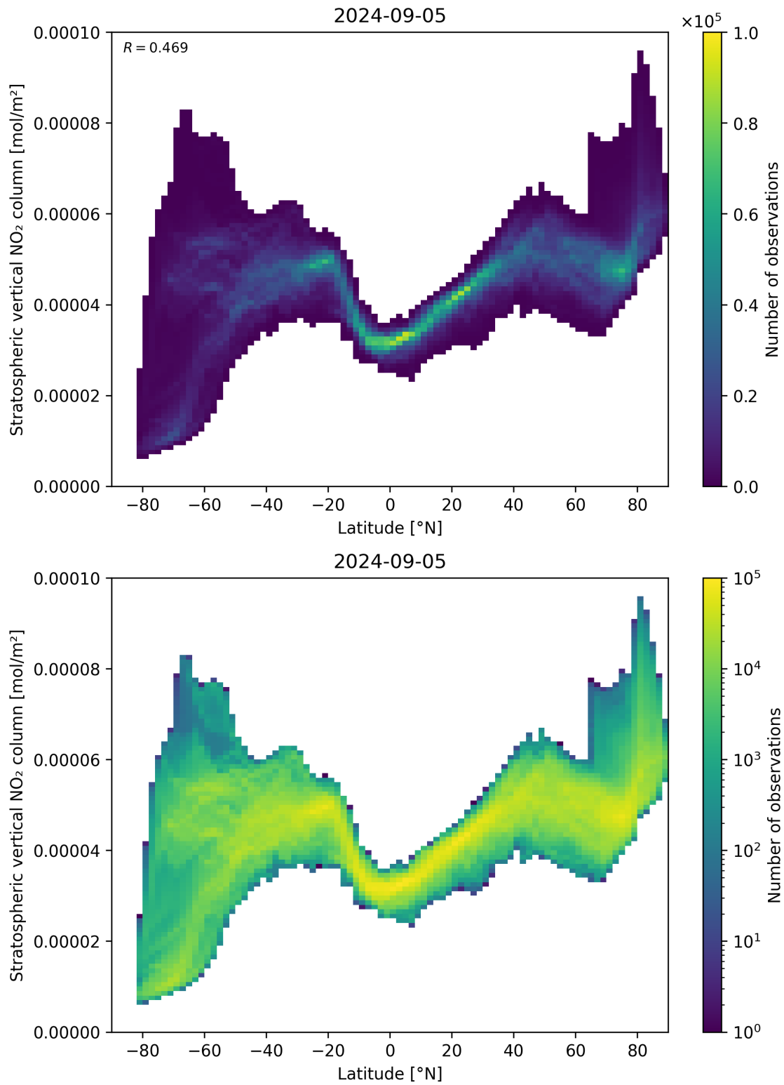
Figure 87: Scatter density plot of “Latitude” against “Stratospheric vertical NO 2 column” for 2024-09-04 to 2024-09-06.
