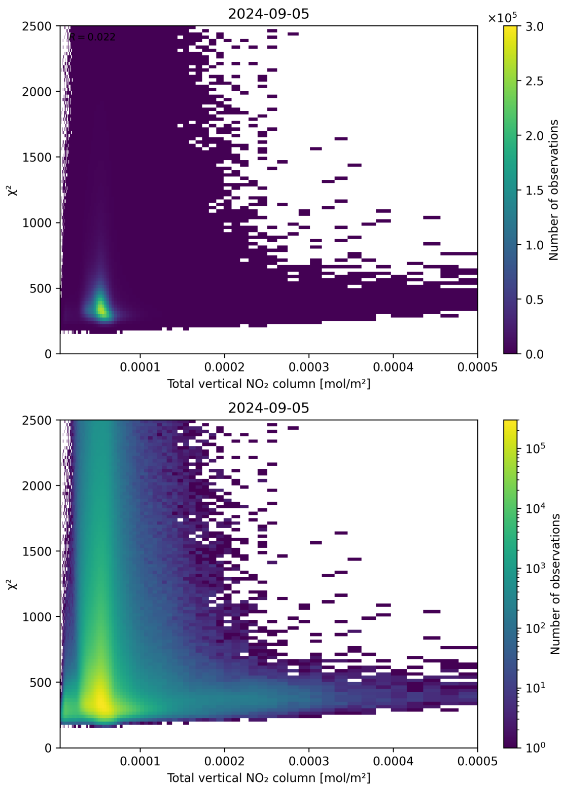
Figure 111: Scatter density plot of “Total vertical NO 2 column” against “ \chi^2 ” for 2024-09-04 to 2024-09-06.
