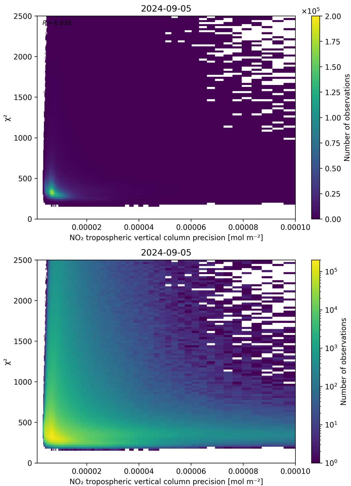
Figure 134: Scatter density plot of “NO 2 tropospheric vertical column precision” against “ \chi^2 ” for 2024-09-04 to 2024-09-06.
