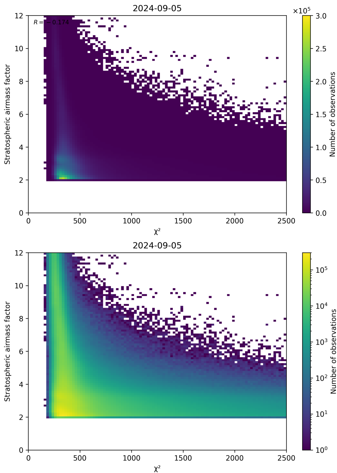
Figure 81: Scatter density plot of “ \chi^2 ” against “Stratospheric airmass factor” for 2024-09-04 to 2024-09-06.
