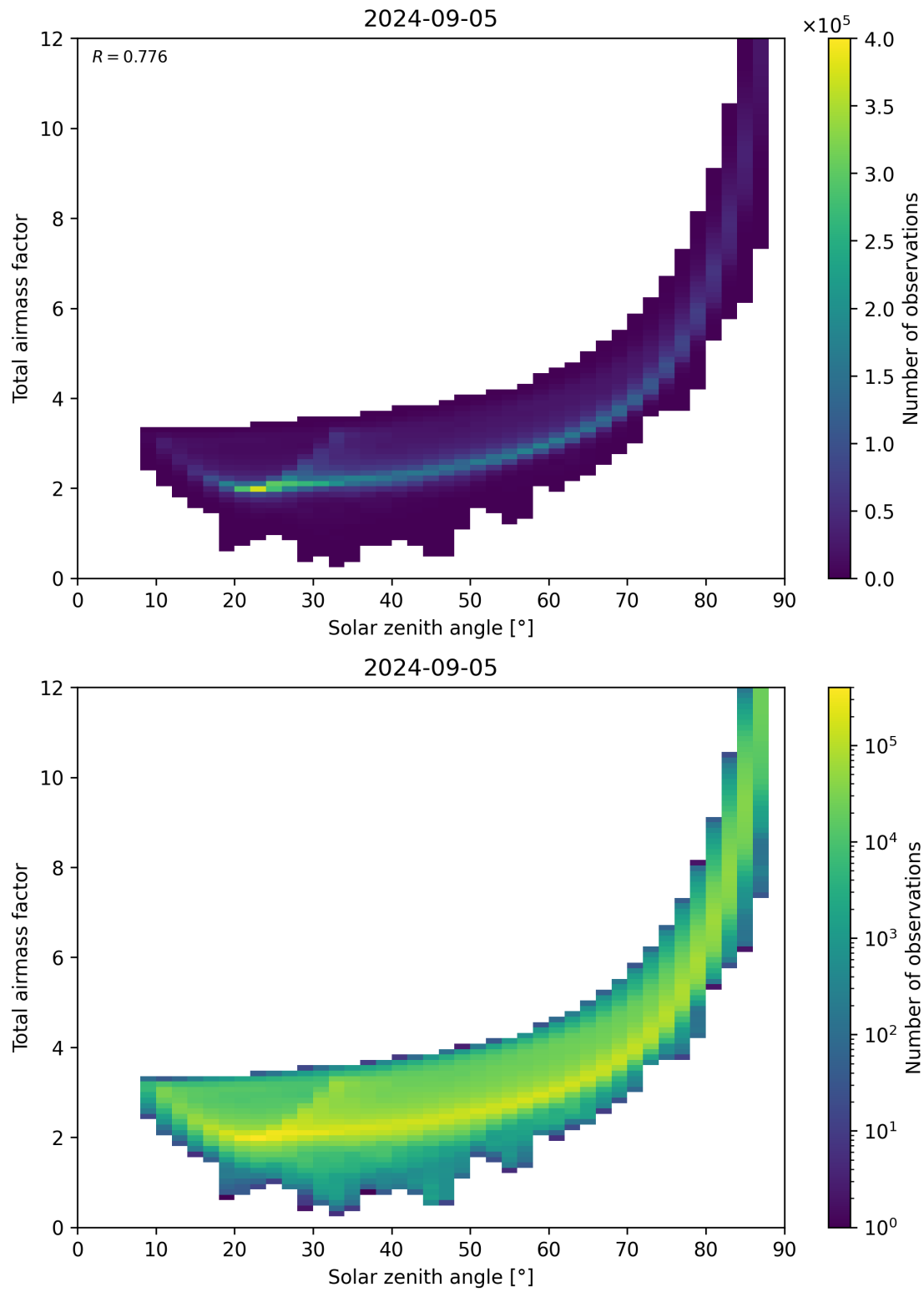
Figure 146: Scatter density plot of “Solar zenith angle” against “Total air mass factor” for 2024-09-04 to 2024-09-06.
