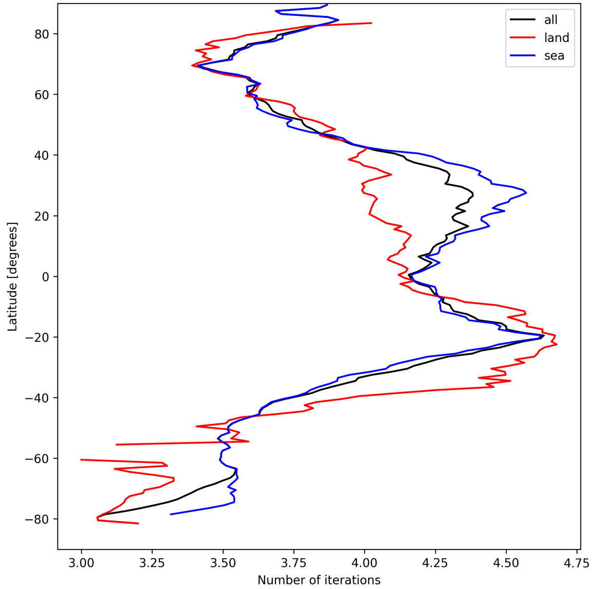
Figure 17: Zonal average of “Number of iterations” for 2024-09-04 to 2024-09-06.
