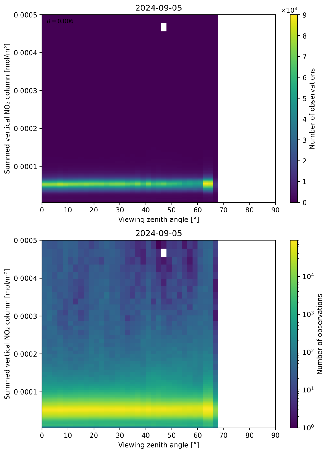
Figure 165: Scatter density plot of “Viewing zenith angle” against “Summed vertical NO 2 column” for 2024-09-04 to 2024-09-06.
