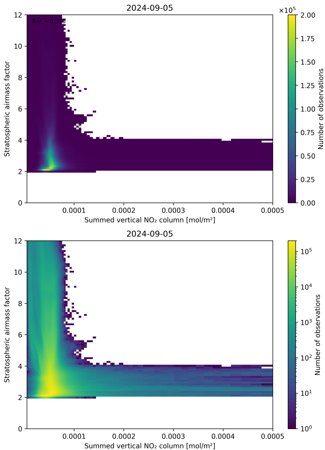
Figure 103: Scatter density plot of “Summed vertical NO 2 column” against “Stratospheric airmass factor” for 2024-09-04 to 2024-09-06.
