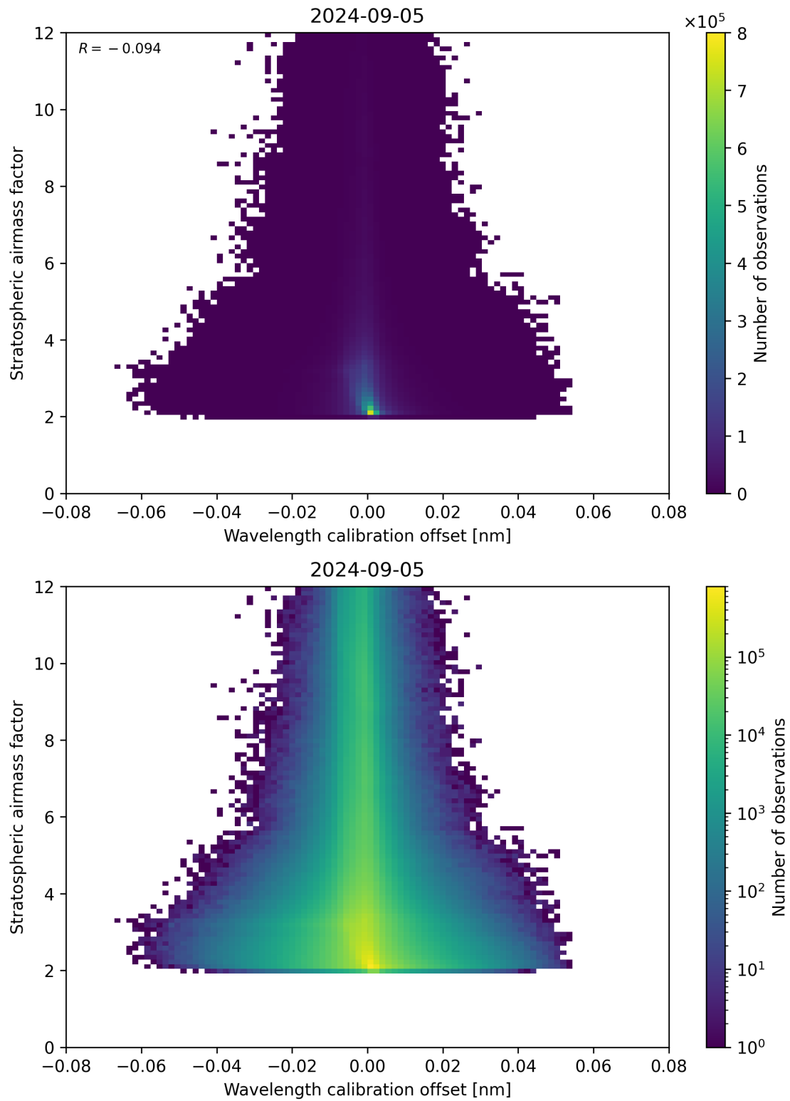
Figure 174: Scatter density plot of “Wavelength calibration offset” against “Stratospheric airmass factor” for 2024-09-04 to 2024-09-06.
