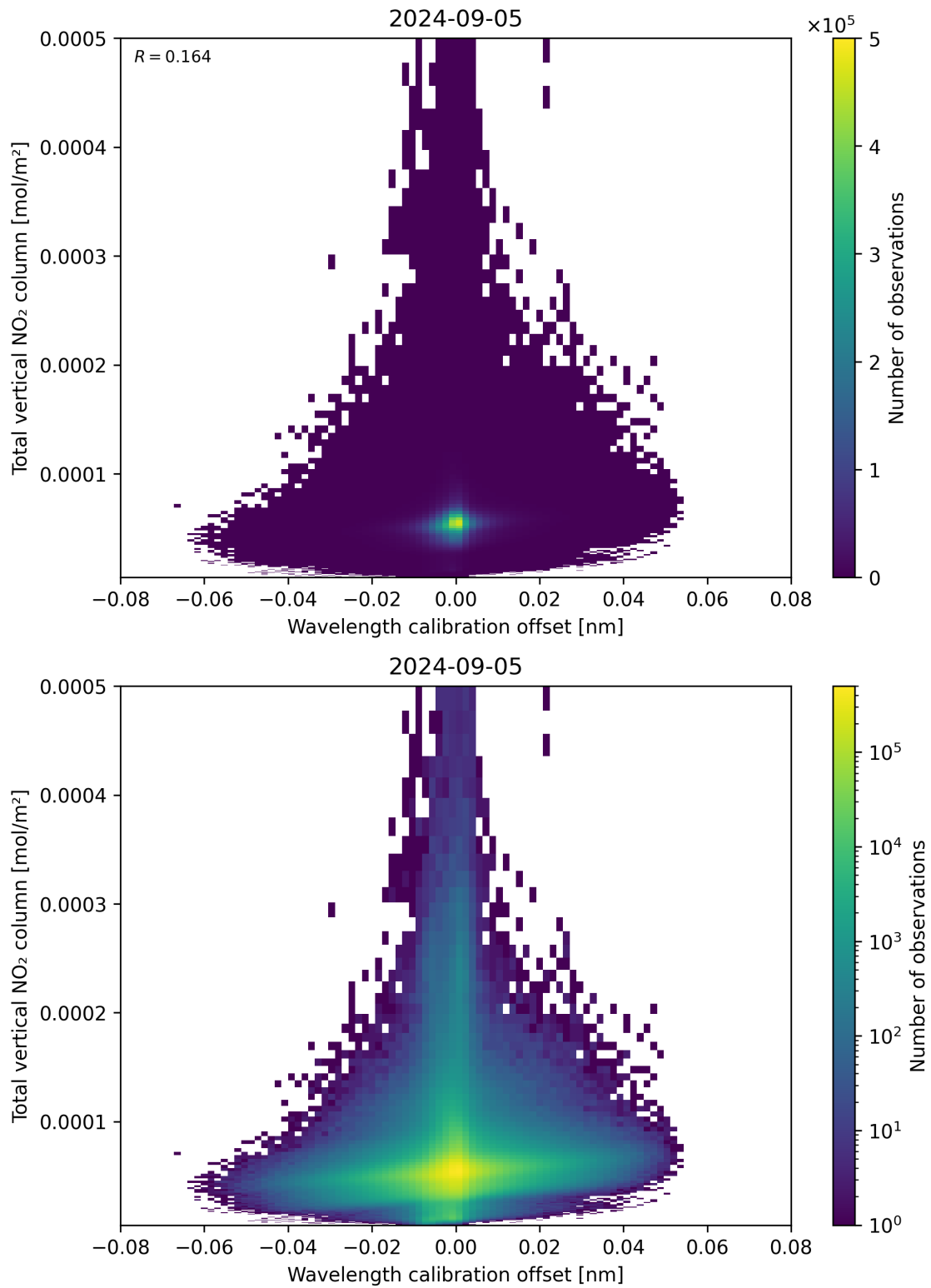
Figure 179: Scatter density plot of “Wavelength calibration offset” against “Total vertical NO 2 column” for 2024-09-04 to 2024-09-06.
