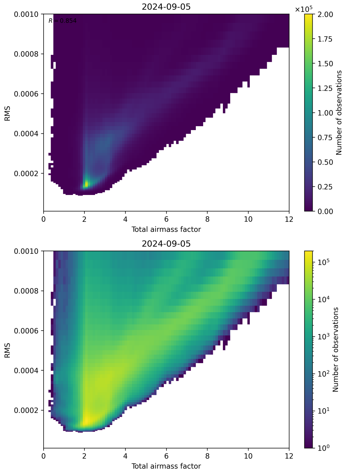
Figure 69: Scatter density plot of “Total airmass factor” against “RMS” for 2024-09-04 to 2024-09-06.
