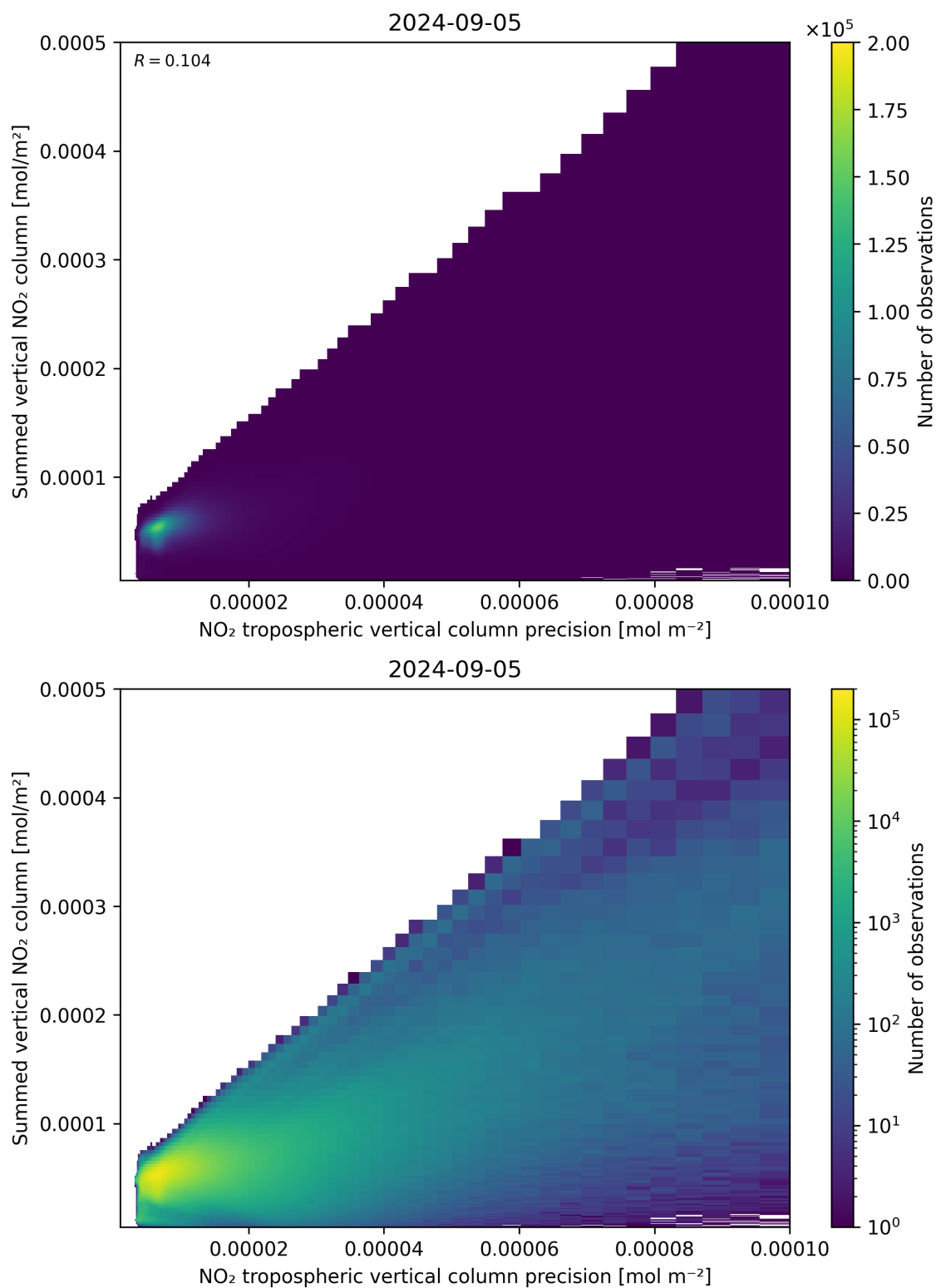
Figure 136: Scatter density plot of “NO 2 tropospheric vertical column precision” against “Summed vertical NO 2 column” for 2024-09-04 to 2024-09-06.
