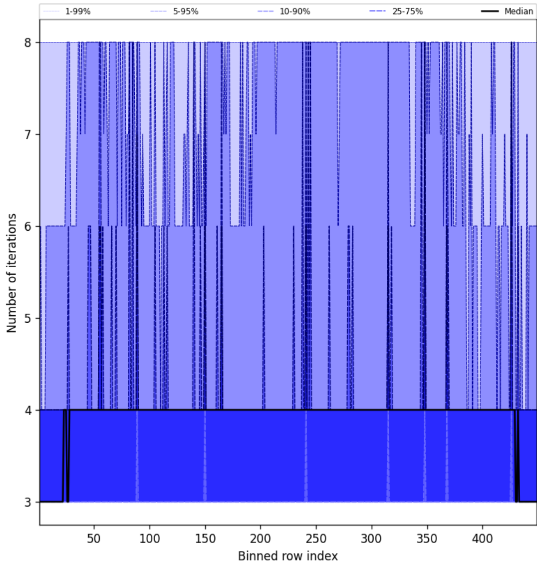
Figure 51: Along track statistics of “Number of iterations” for 2024-09-04 to 2024-09-06
