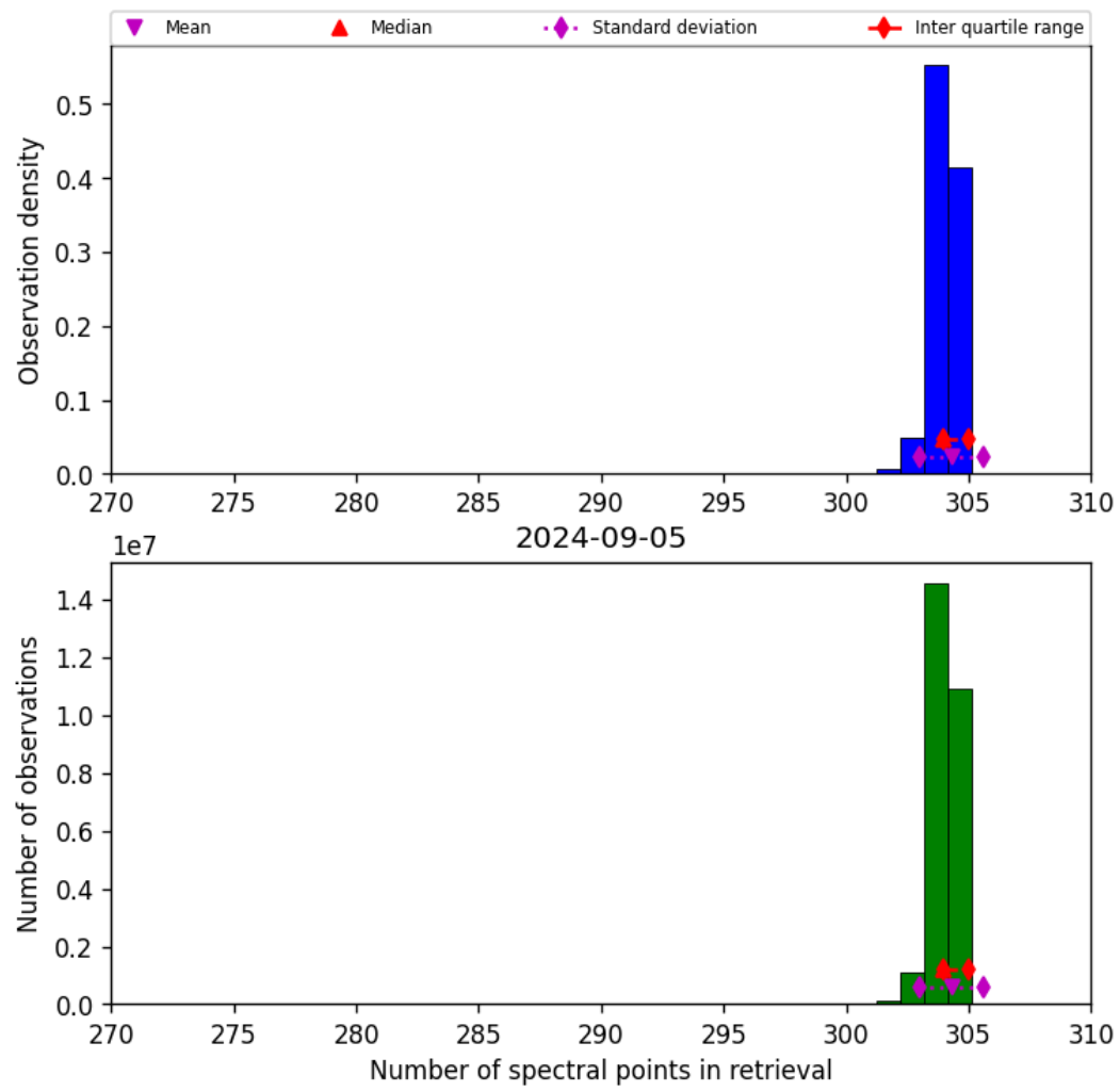
Figure 33: Histogram of “Number of spectral points in retrieval” for 2024-09-04 to 2024-09-06
