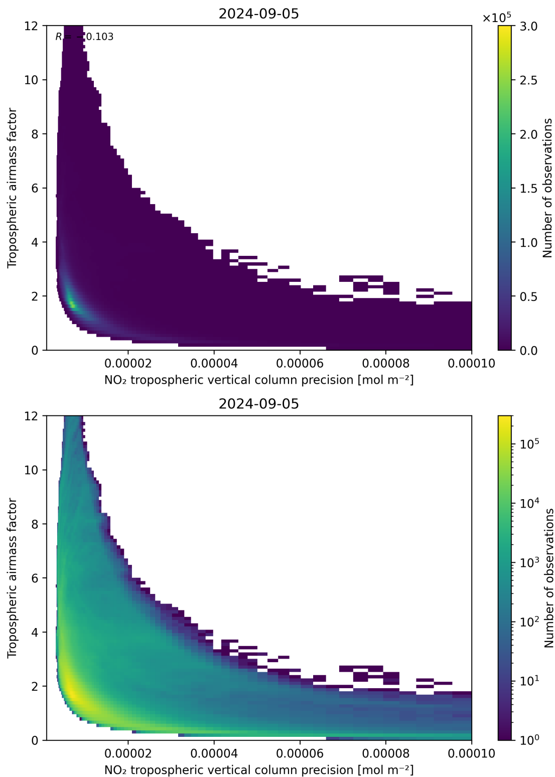
Figure 133: Scatter density plot of “NO 2 tropospheric vertical column precision” against “Tropospheric air mass factor” for 2024-09-04 to 2024-09-06.
