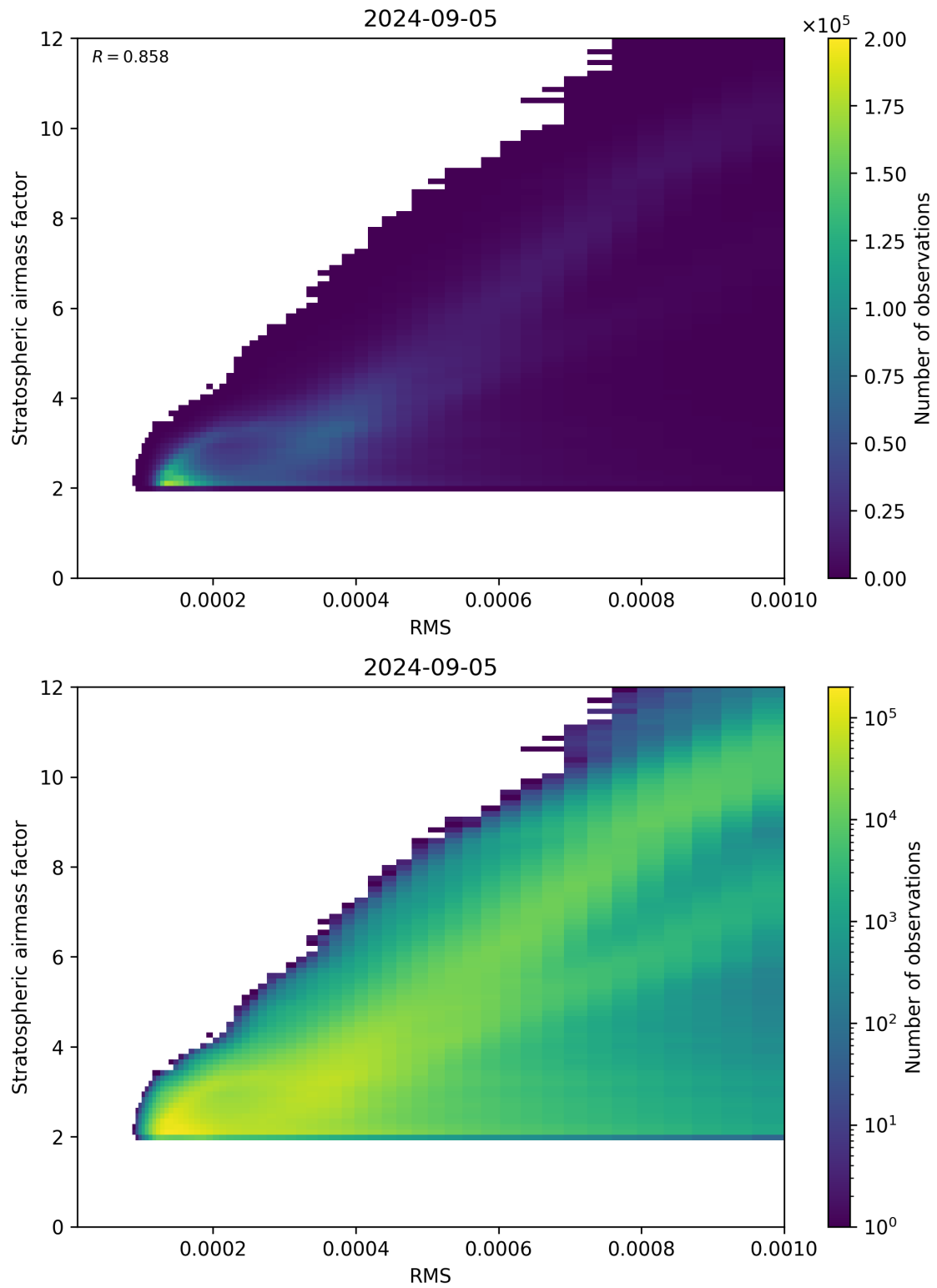
Figure 144: Scatter density plot of “RMS” against “Stratospheric airmass factor” for 2024-09-04 to 2024-09-06.
