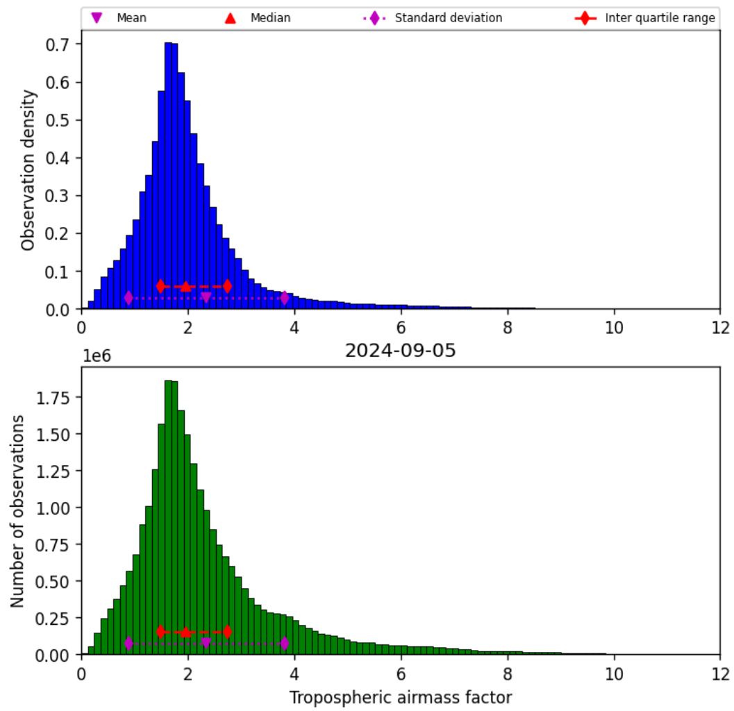
Figure 31: Histogram of “Tropospheric airmass factor” for 2024-09-04 to 2024-09-06
