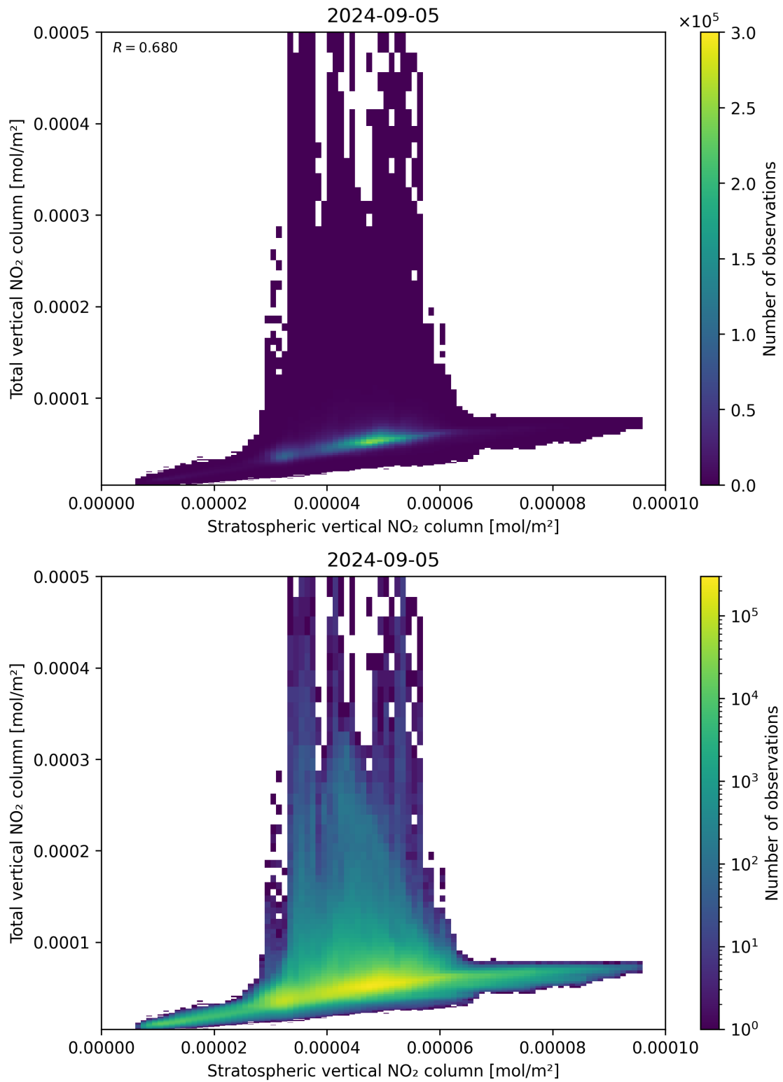
Figure 100: Scatter density plot of “Stratospheric vertical NO 2 column” against “Total vertical NO 2 column” for 2024-09-04 to 2024-09-06.
