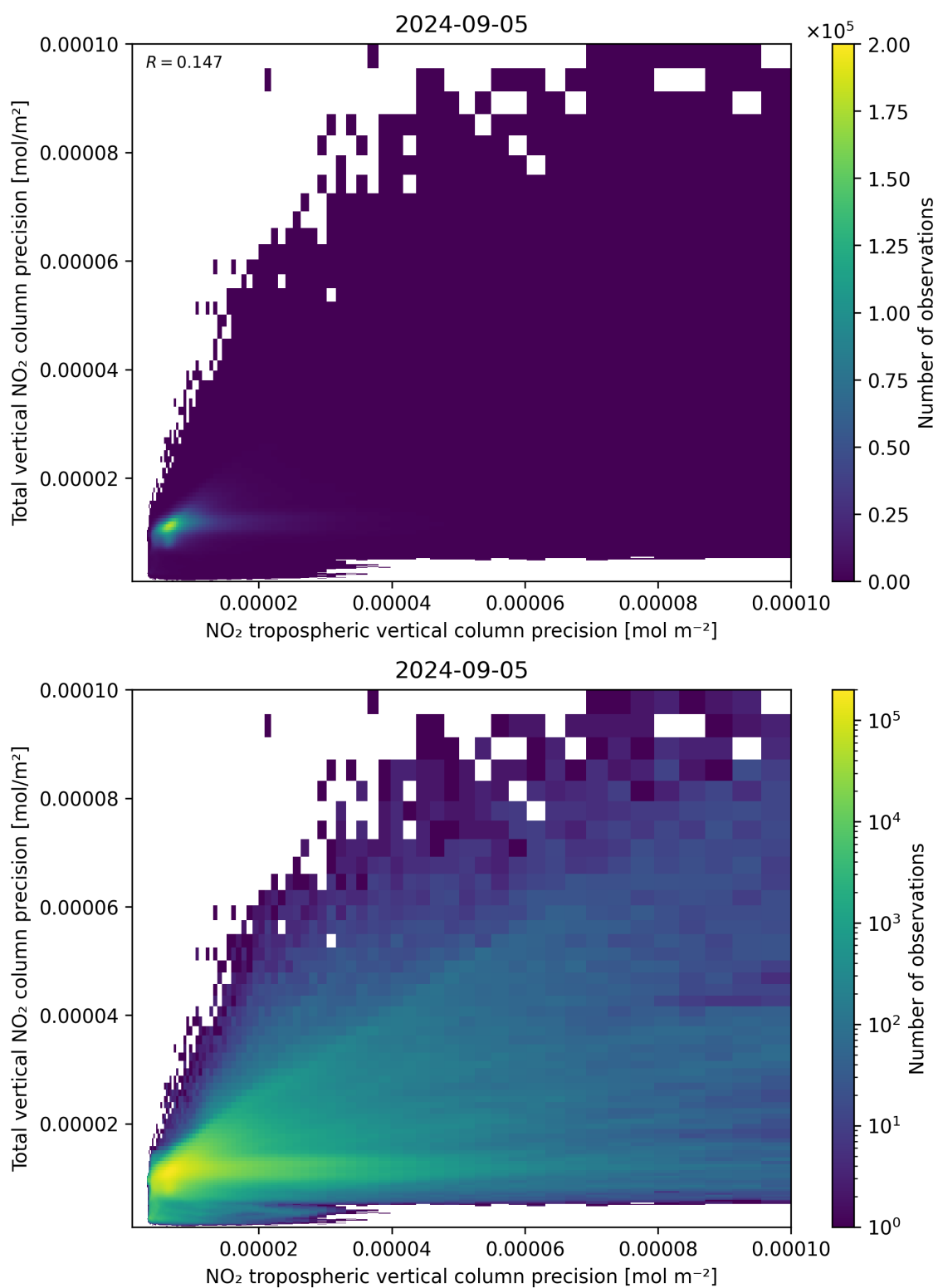
Figure 139: Scatter density plot of “NO 2 tropospheric vertical column precision” against “Total vertical NO 2 column precision” for 2024-09-04 to 2024-09-06.
