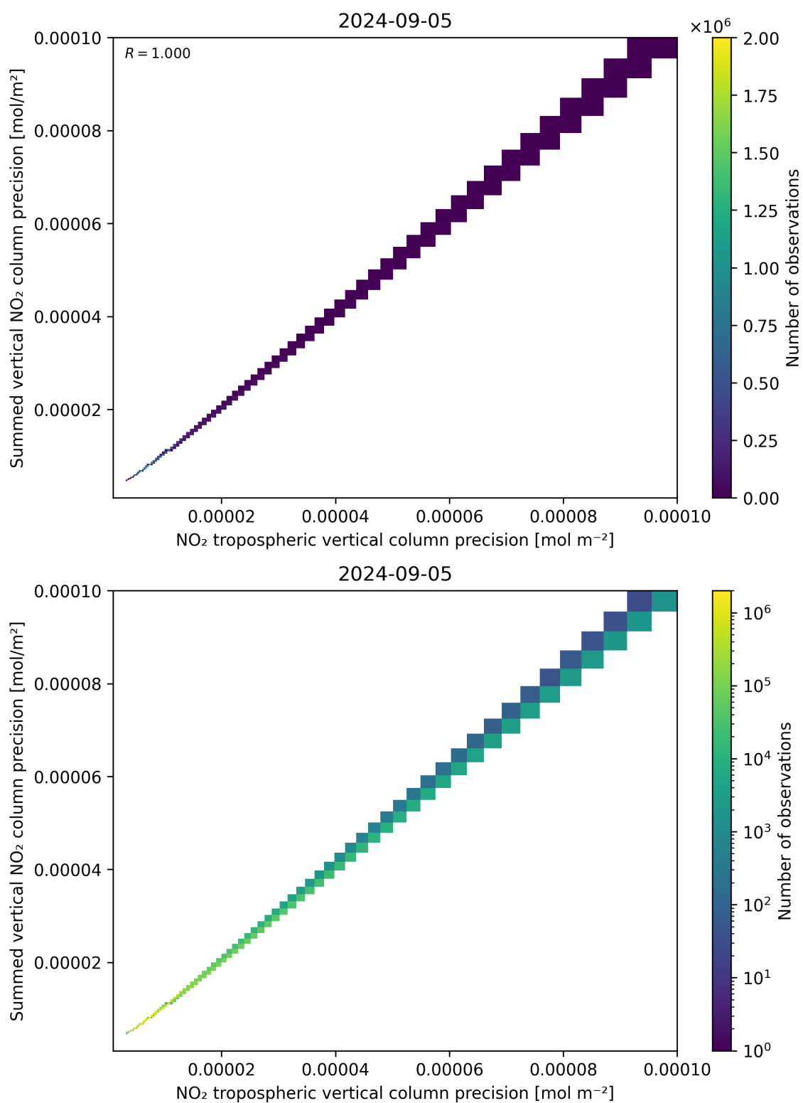
Figure 137: Scatter density plot of “NO 2 tropospheric vertical column precision” against “Summed vertical NO 2 column precision” for 2024-09-04 to 2024-09-06.
