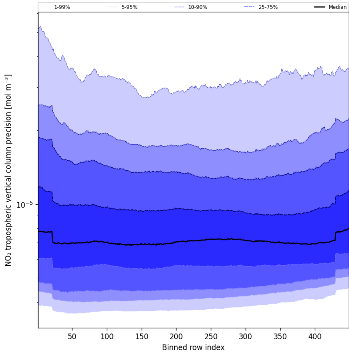
Figure 47: Along track statistics of “NO 2 tropospheric vertical column precision” for 2024-09-04 to 2024-09-06
