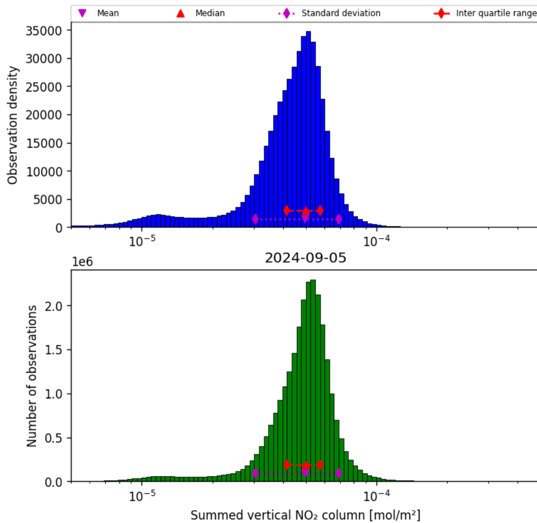
Figure 40: Histogram of “Summed vertical NO 2 column” for 2024-09-04 to 2024-09-06
