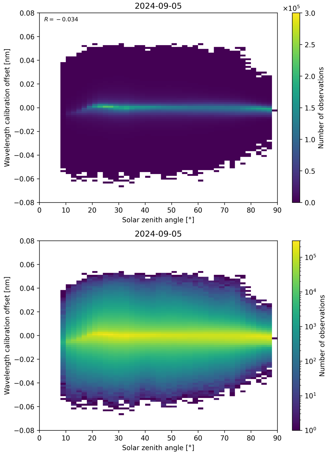
Figure 158: Scatter density plot of “Solar zenith angle” against “Wavelength calibration offset” for 2024-09-04 to 2024-09-06.
