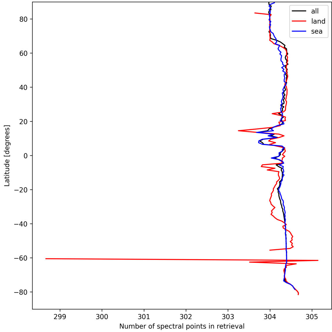
Figure 16: Zonal average of “Number of spectral points in retrieval” for 2024-09-04 to 2024-09-06.
