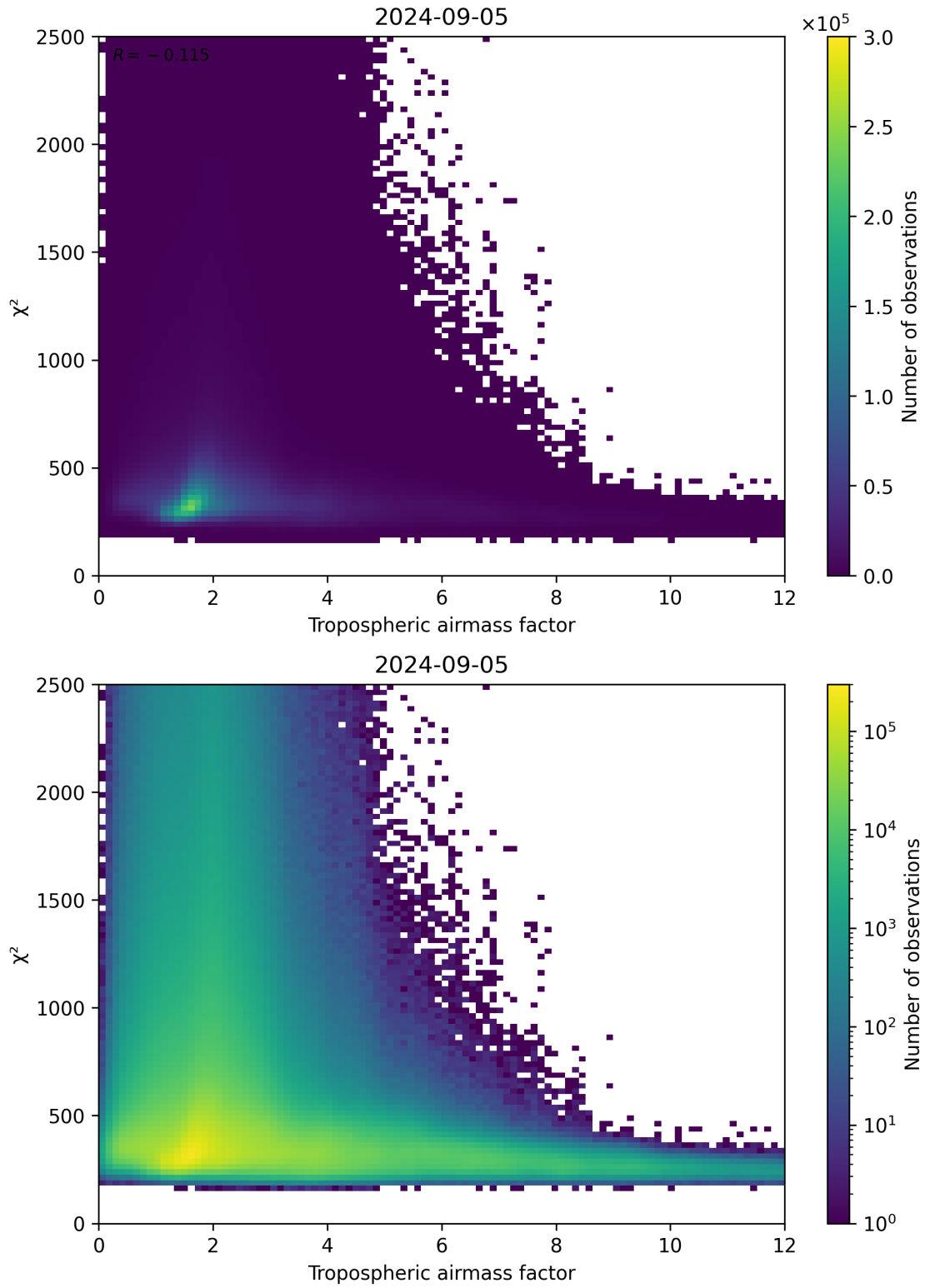
Figure 73: Scatter density plot of “Tropospheric airmass factor” against “ \chi^2 ” for 2024-09-04 to 2024-09-06.
