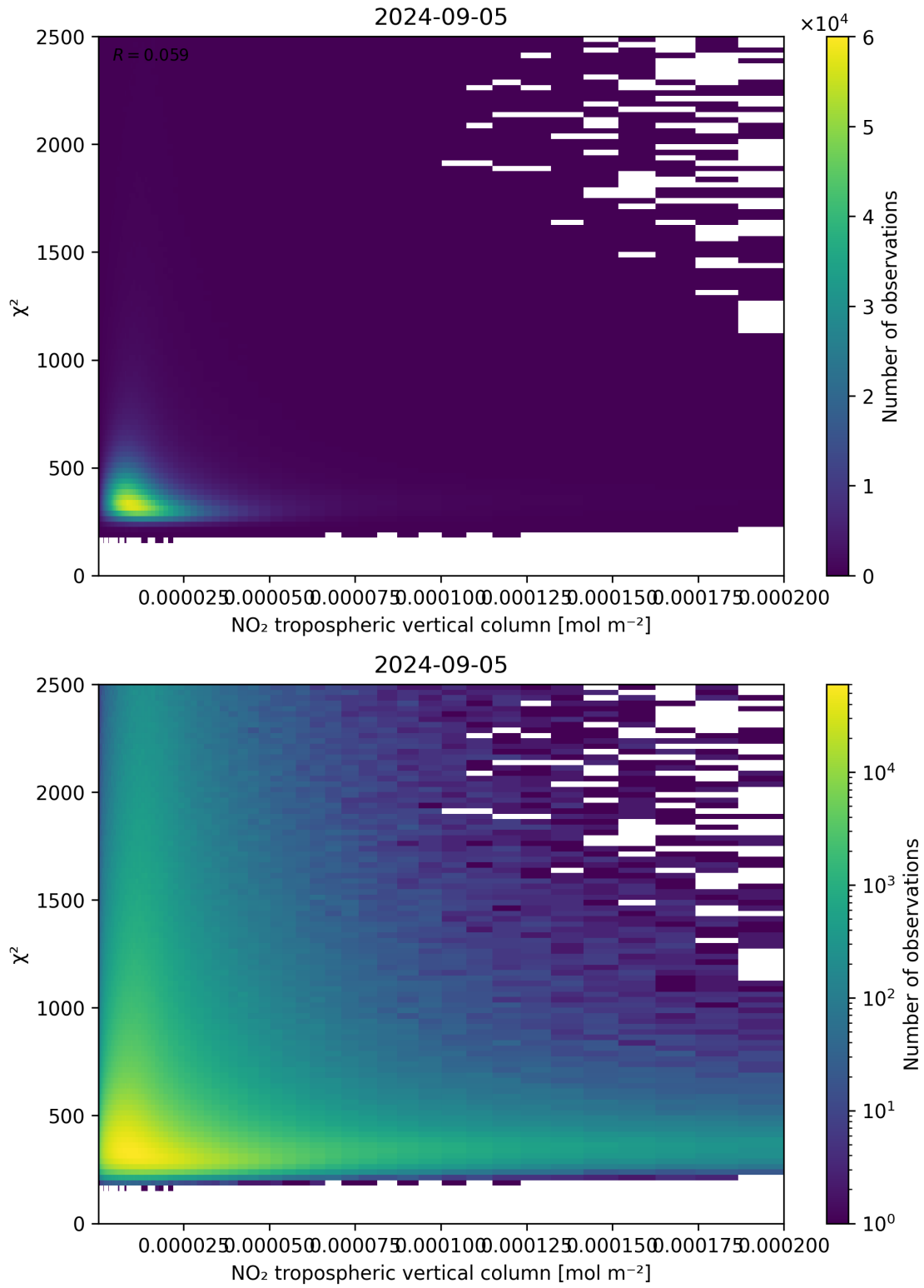
Figure 124: Scatter density plot of “NO 2 tropospheric vertical column” against “ \chi^2 ” for 2024-09-04 to 2024-09-06.
