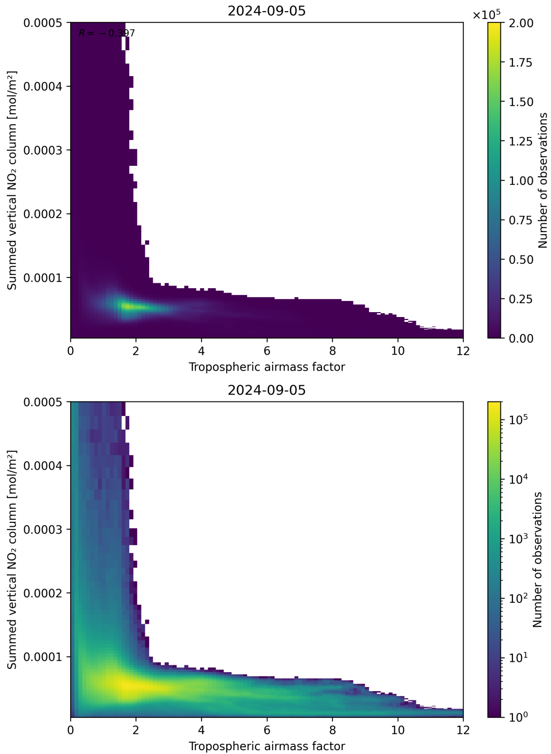
Figure 75: Scatter density plot of “Tropospheric airmass factor” against “Summed vertical NO 2 column” for 2024-09-04 to 2024-09-06.
