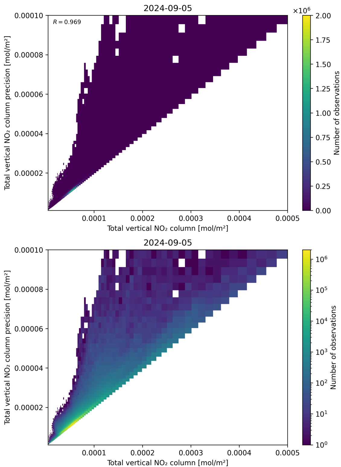
Figure 114: Scatter density plot of “Total vertical NO 2 column” against “Total vertical NO 2 column precision” for 2024-09-04 to 2024-09-06.
