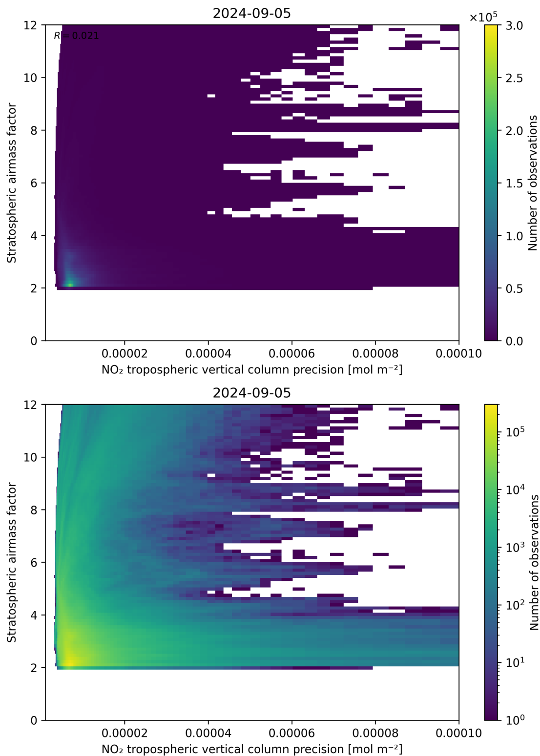
Figure 131: Scatter density plot of “NO 2 tropospheric vertical column precision” against “Stratospheric airmass factor” for 2024-09-04 to 2024-09-06.
