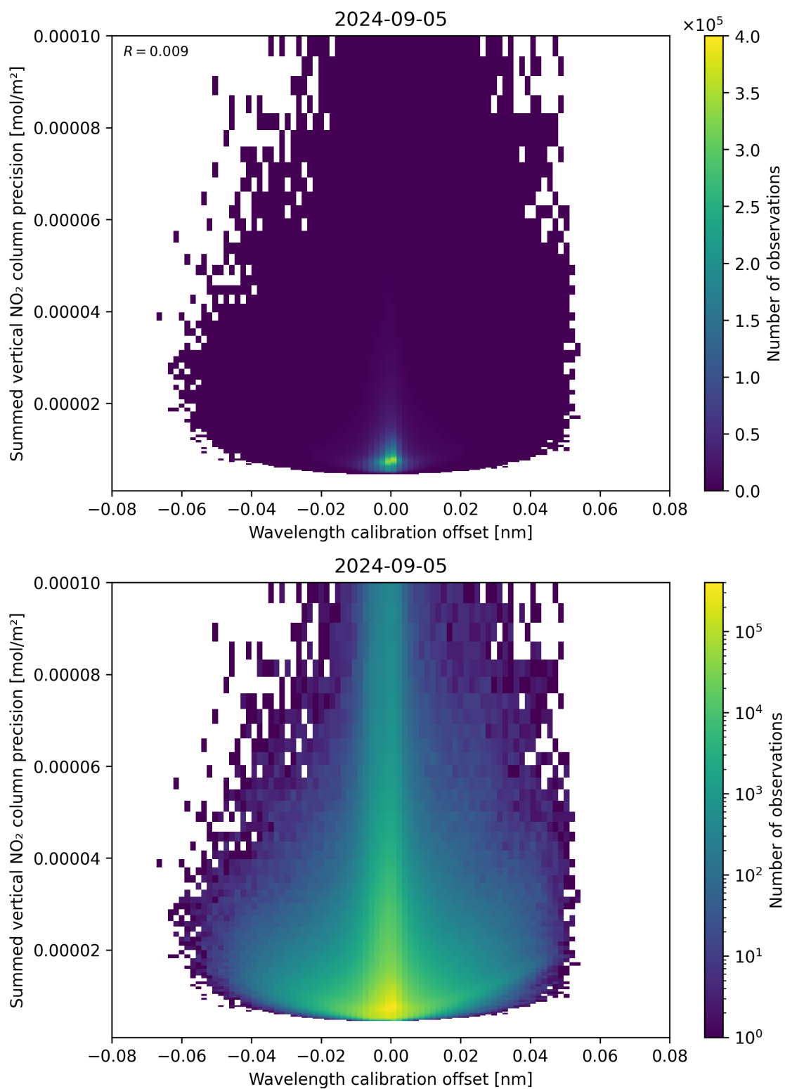
Figure 178: Scatter density plot of “Wavelength calibration offset” against “Summed vertical NO 2 column precision” for 2024-09-04 to 2024-09-06.
