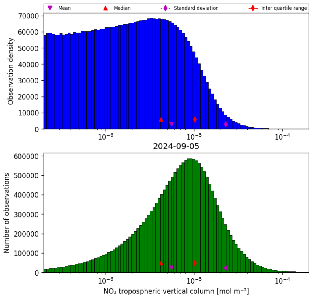
Figure 29: Histogram of “NO 2 tropospheric vertical column” for 2024-09-04 to 2024-09-06
