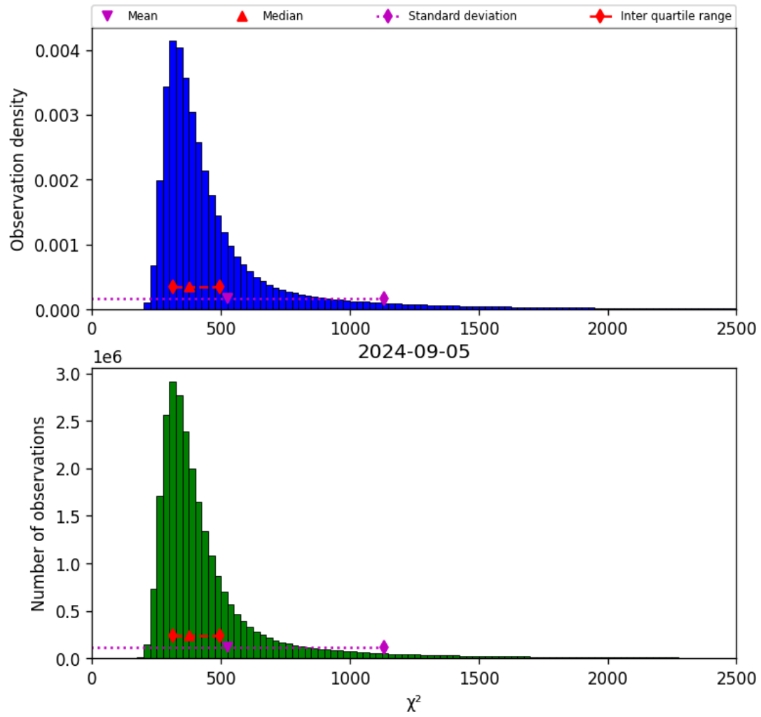
Figure 42: Histogram of " \chi^2 " for 2024-09-04 to 2024-09-06
