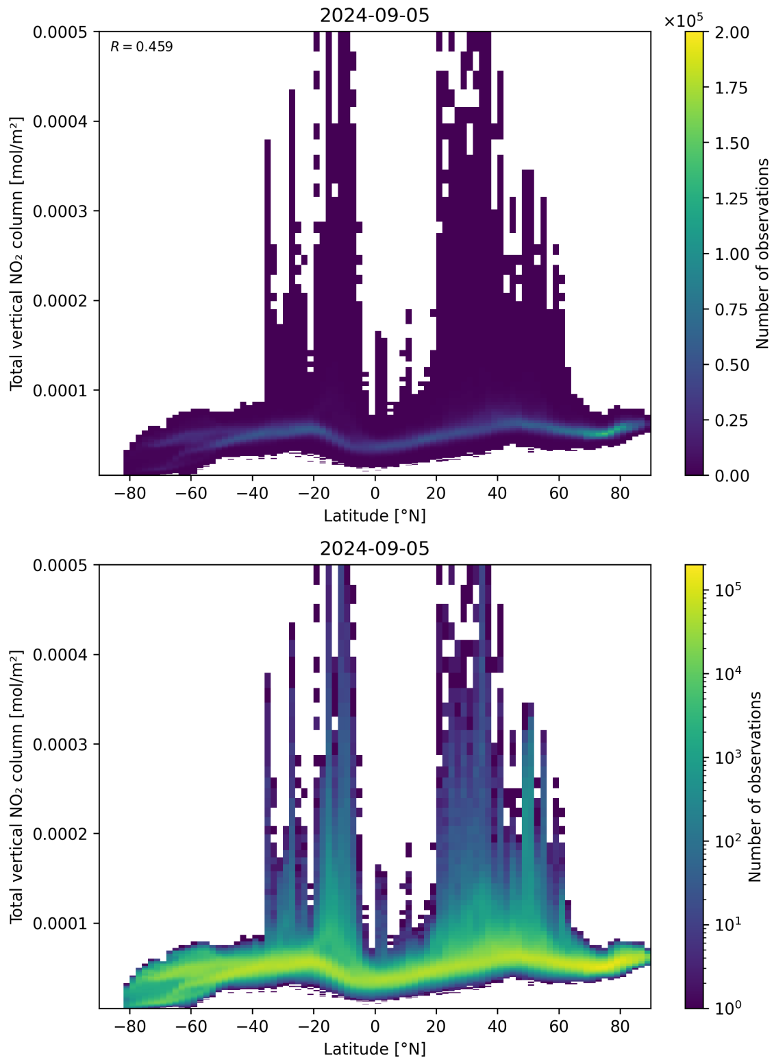
Figure 90: Scatter density plot of “Latitude” against “Total vertical NO 2 column” for 2024-09-04 to 2024-09-06.
