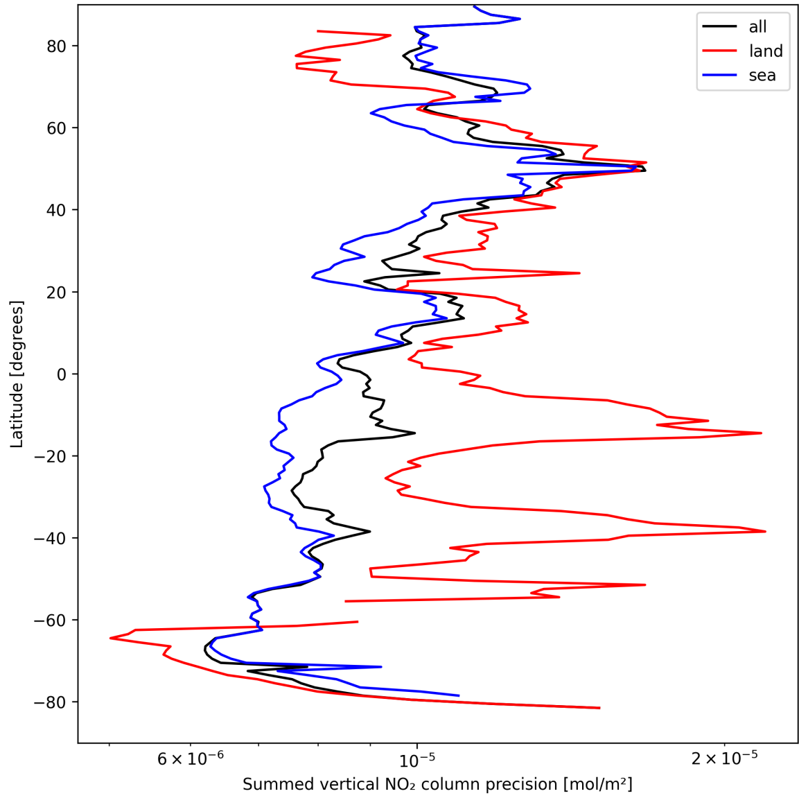
Figure 24: Zonal average of “Summed vertical NO 2 column precision” for 2024-09-04 to 2024-09-06.
