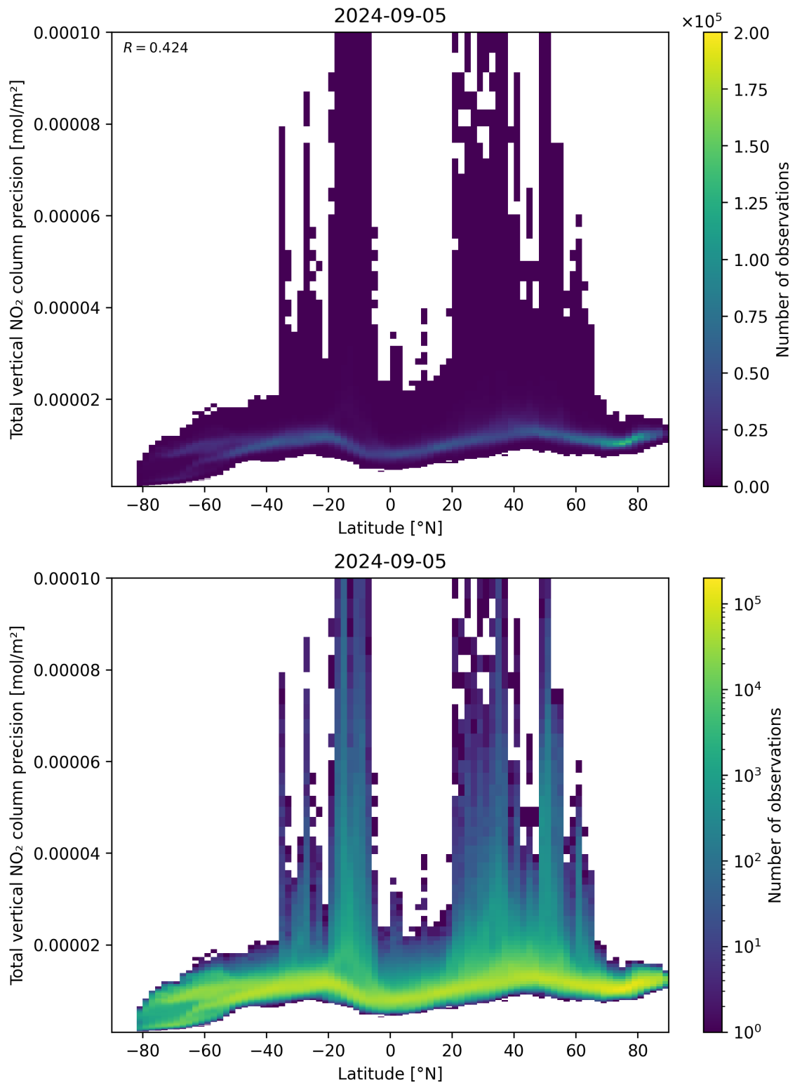
Figure 91: Scatter density plot of “Latitude” against “Total vertical NO 2 column precision” for 2024-09-04 to 2024-09-06.
