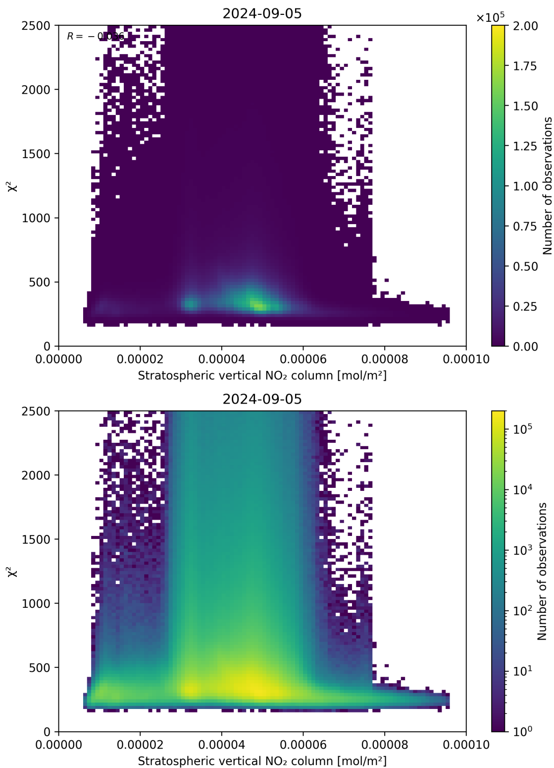
Figure 97: Scatter density plot of “Stratospheric vertical NO 2 column” against “ \chi^2 ” for 2024-09-04 to 2024-09-06.
