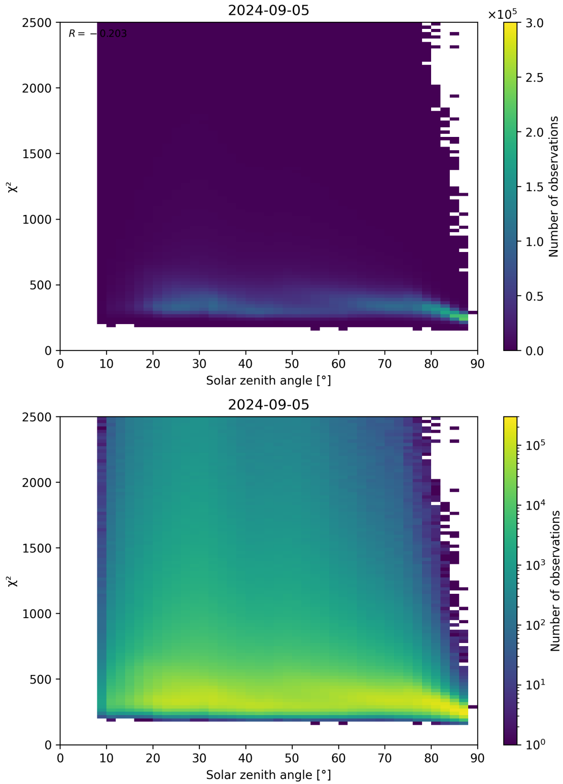
Figure 148: Scatter density plot of “Solar zenith angle” against “ \chi^2 ” for 2024-09-04 to 2024-09-06.
