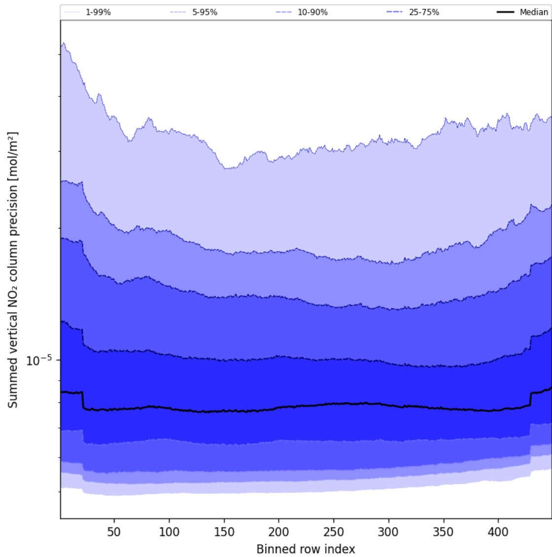
Figure 58: Along track statistics of “Summed vertical NO 2 column precision” for 2024-09-04 to 2024-09-06
