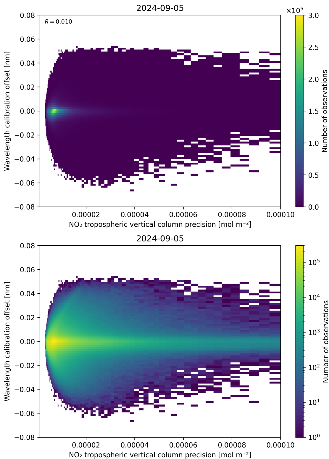
Figure 141: Scatter density plot of “NO 2 tropospheric vertical column precision” against “Wavelength calibration offset” for 2024-09-04 to 2024-09-06.
