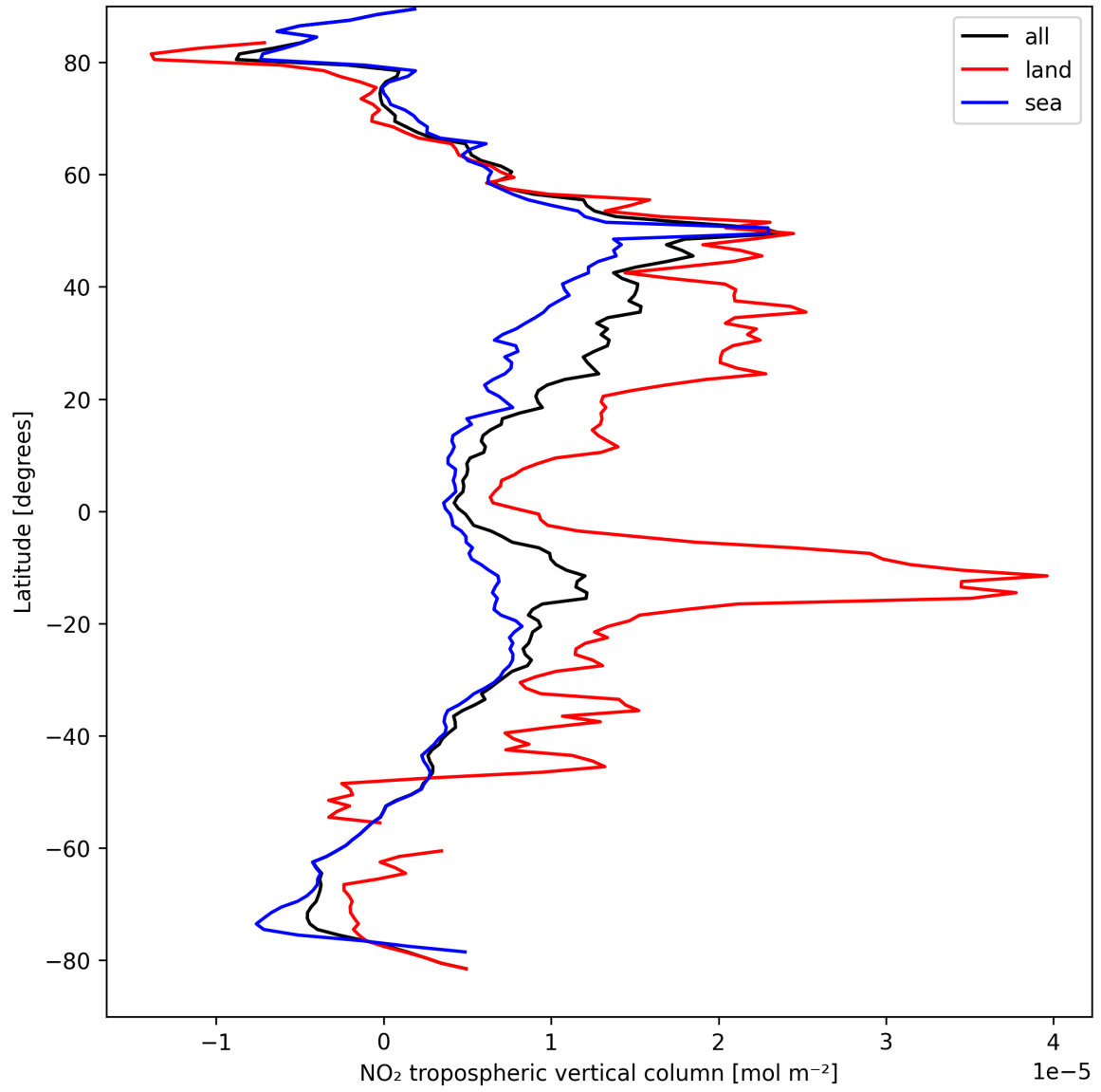
Figure 12: Zonal average of “NO 2 tropospheric vertical column” for 2024-09-04 to 2024-09-06.
