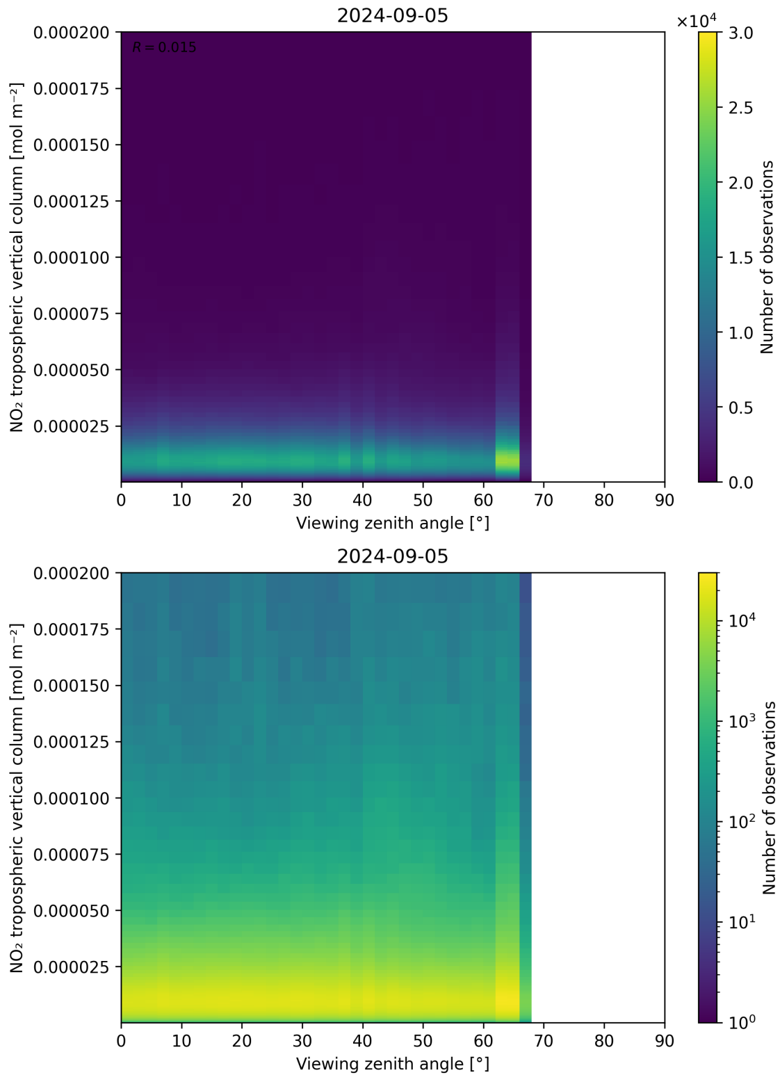
Figure 169: Scatter density plot of “Viewing zenith angle” against “NO 2 tropospheric vertical column” for 2024-09-04 to 2024-09-06.
