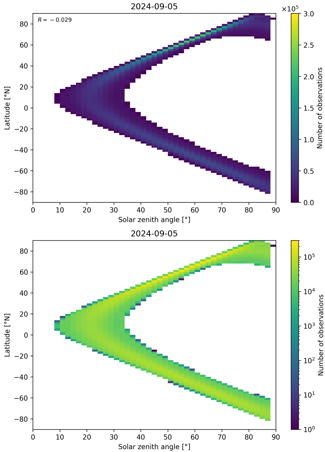
Figure 149: Scatter density plot of “Solar zenith angle” against “Latitude” for 2024-09-04 to 2024-09-06.
