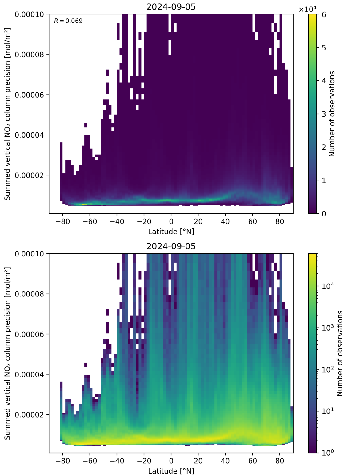
Figure 89: Scatter density plot of “Latitude” against “Summed vertical NO 2 column precision” for 2024-09-04 to 2024-09-06.
