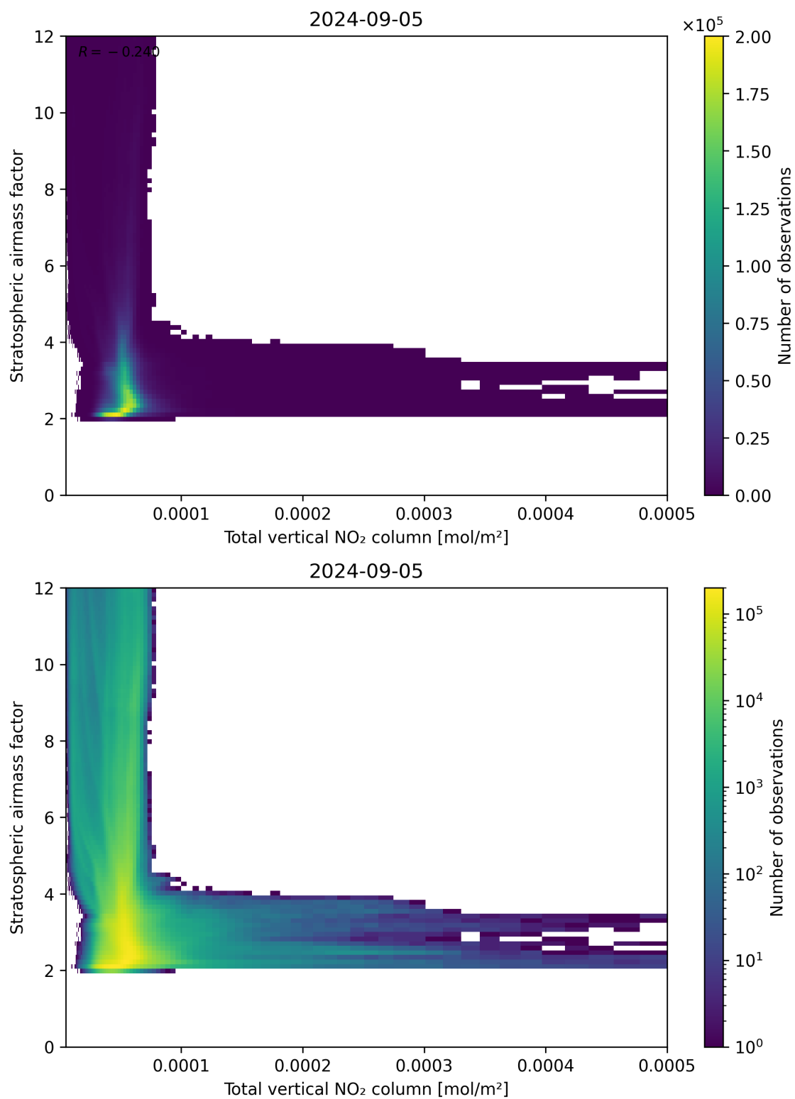
Figure 110: Scatter density plot of “Total vertical NO 2 column” against “Stratospheric airmass factor” for 2024-09-04 to 2024-09-06.
