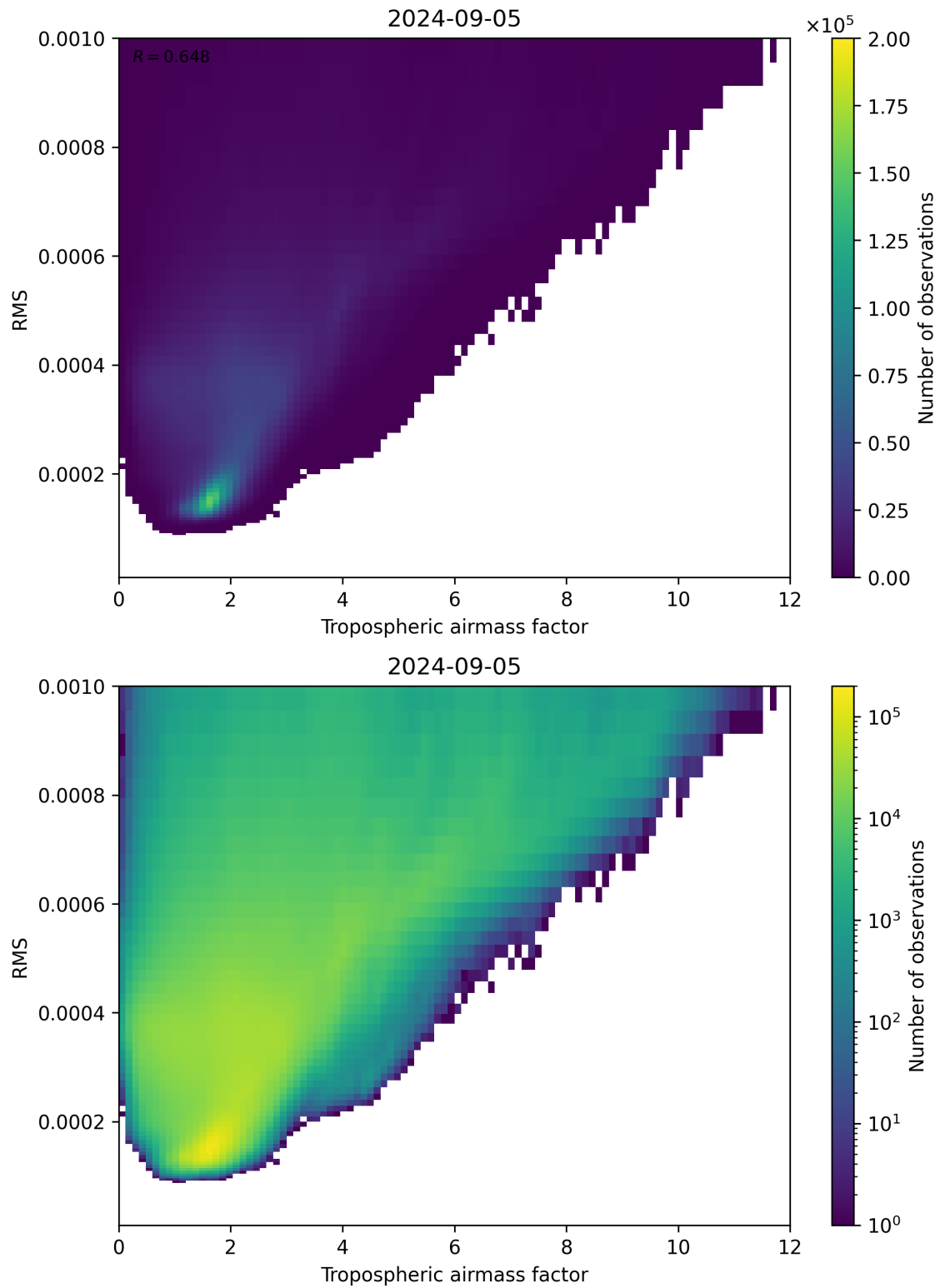
Figure 79: Scatter density plot of “Tropospheric airmass factor” against “RMS” for 2024-09-04 to 2024-09-06.
