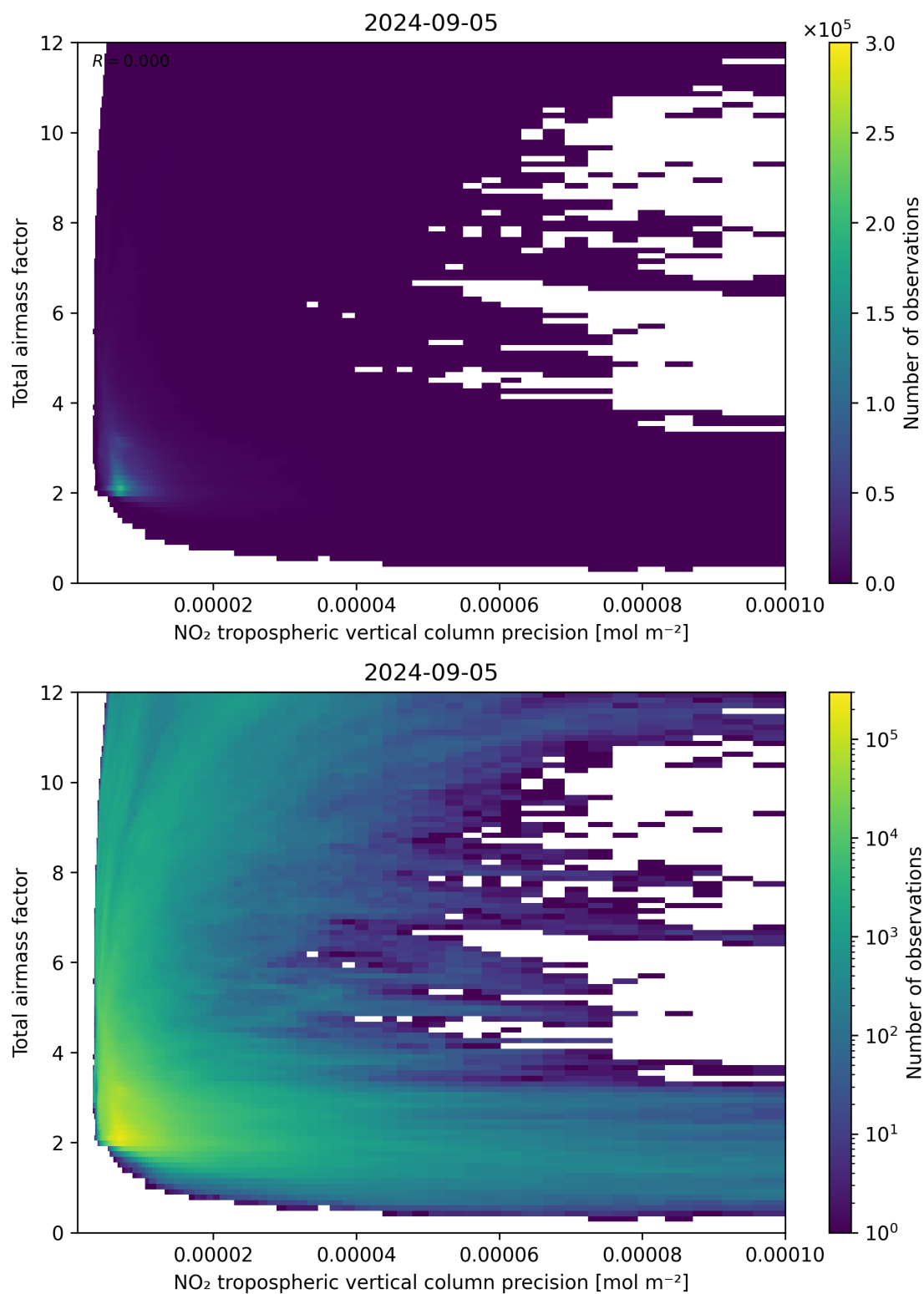
Figure 132: Scatter density plot of “NO 2 tropospheric vertical column precision” against “Total air mass factor” for 2024-09-04 to 2024-09-06.
