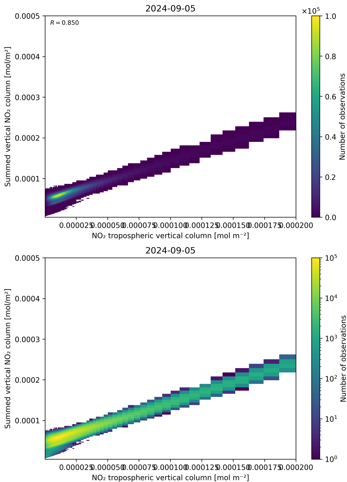
Figure 126: Scatter density plot of “NO 2 tropospheric vertical column” against “Summed vertical NO 2 column” for 2024-09-04 to 2024-09-06.
