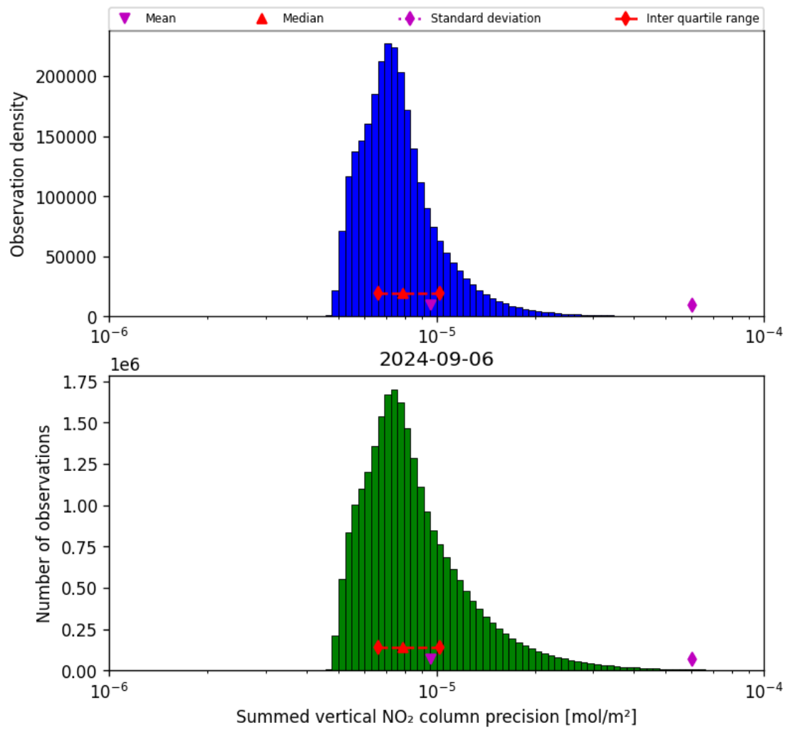
Figure 41: Histogram of “Summed vertical NO 2 column precision” for 2024-09-06 to 2024-09-07
