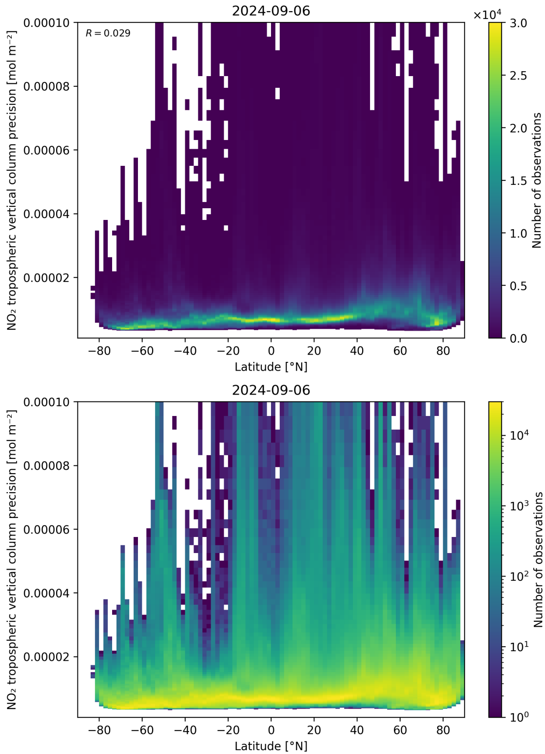
Figure 93: Scatter density plot of “Latitude” against “NO 2 tropospheric vertical column precision” for 2024-09-06 to 2024-09-07.
