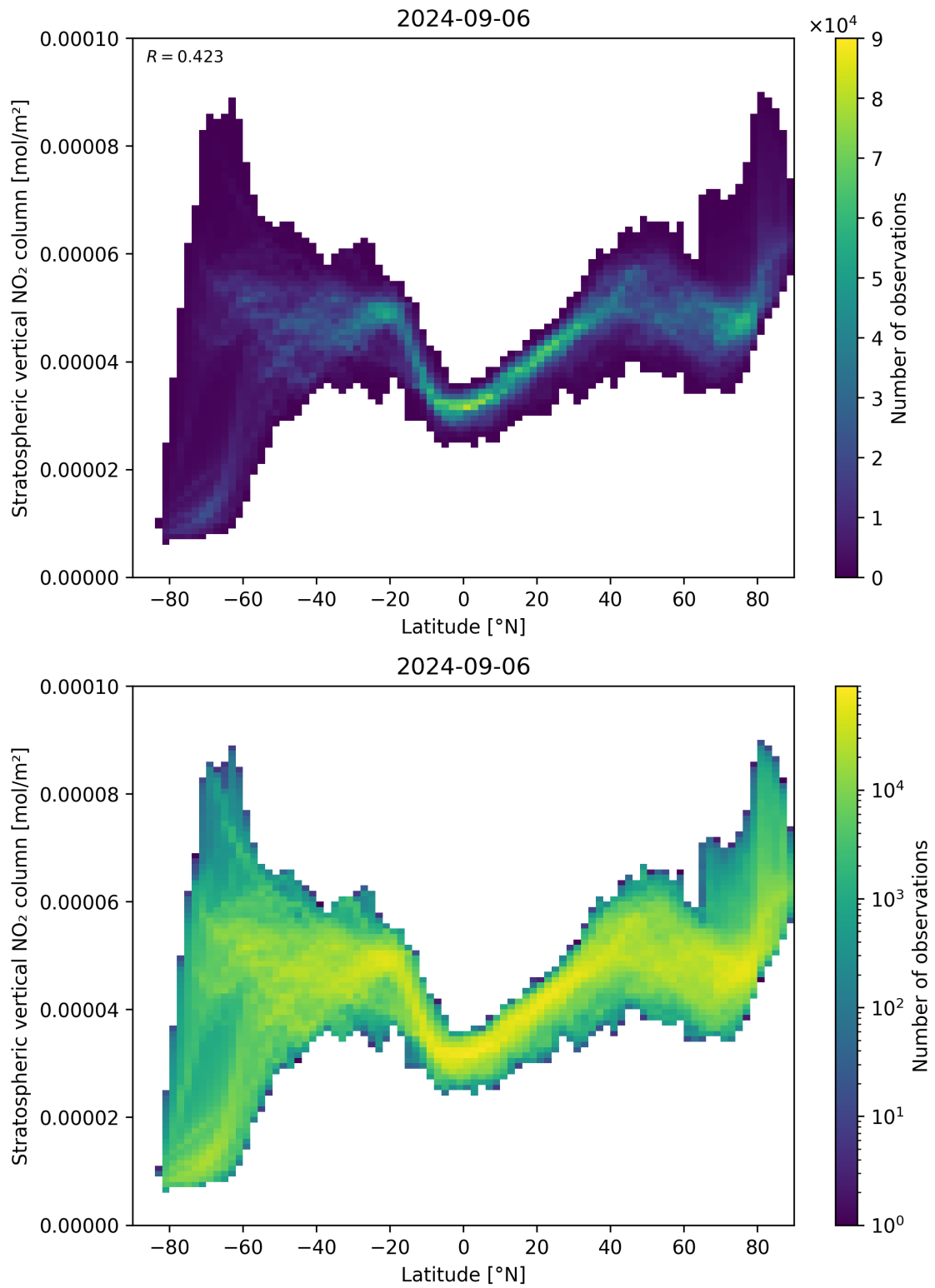
Figure 87: Scatter density plot of “Latitude” against “Stratospheric vertical NO 2 column” for 2024-09-06 to 2024-09-07.
