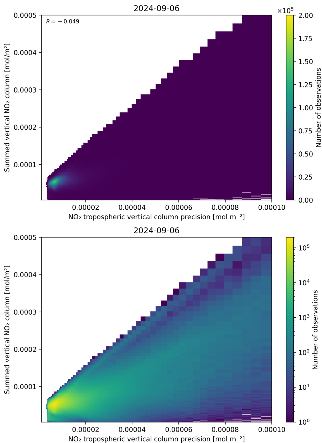
Figure 136: Scatter density plot of “NO 2 tropospheric vertical column precision” against “Summed vertical NO 2 column” for 2024-09-06 to 2024-09-07.
