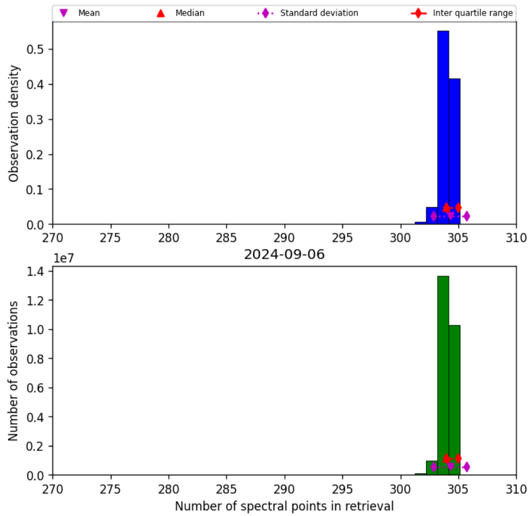
Figure 33: Histogram of “Number of spectral points in retrieval” for 2024-09-06 to 2024-09-07
