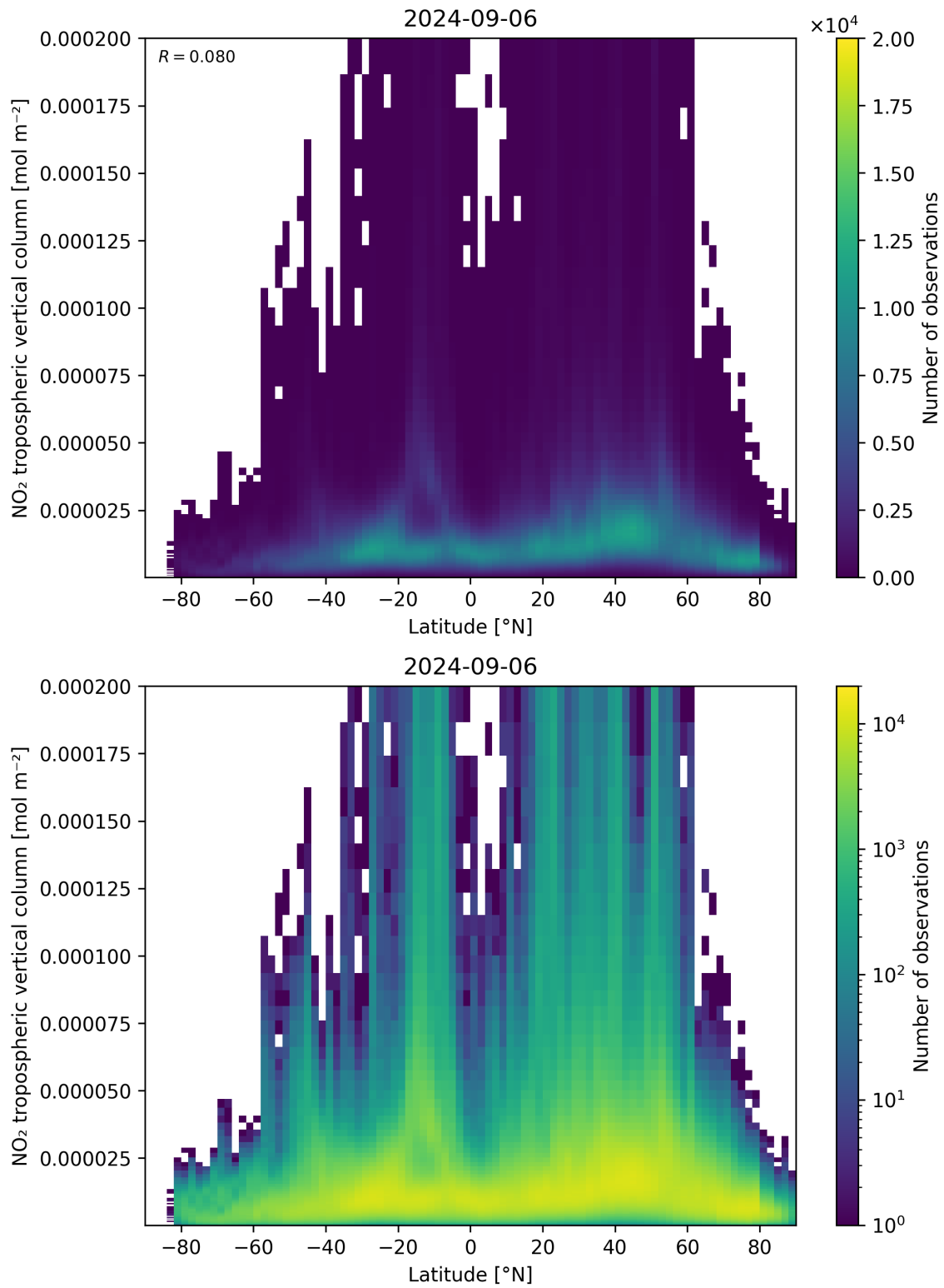
Figure 92: Scatter density plot of “Latitude” against “NO 2 tropospheric vertical column” for 2024-09-06 to 2024-09-07.
