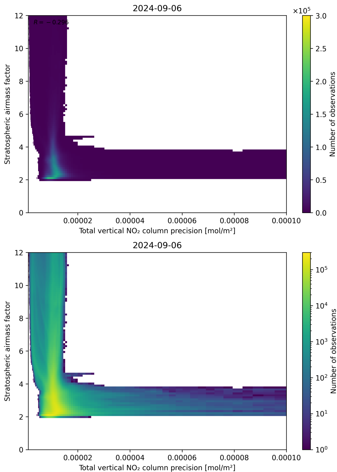
Figure 115: Scatter density plot of “Total vertical NO 2 column precision” against “Stratospheric air mass factor” for 2024-09-06 to 2024-09-07.
