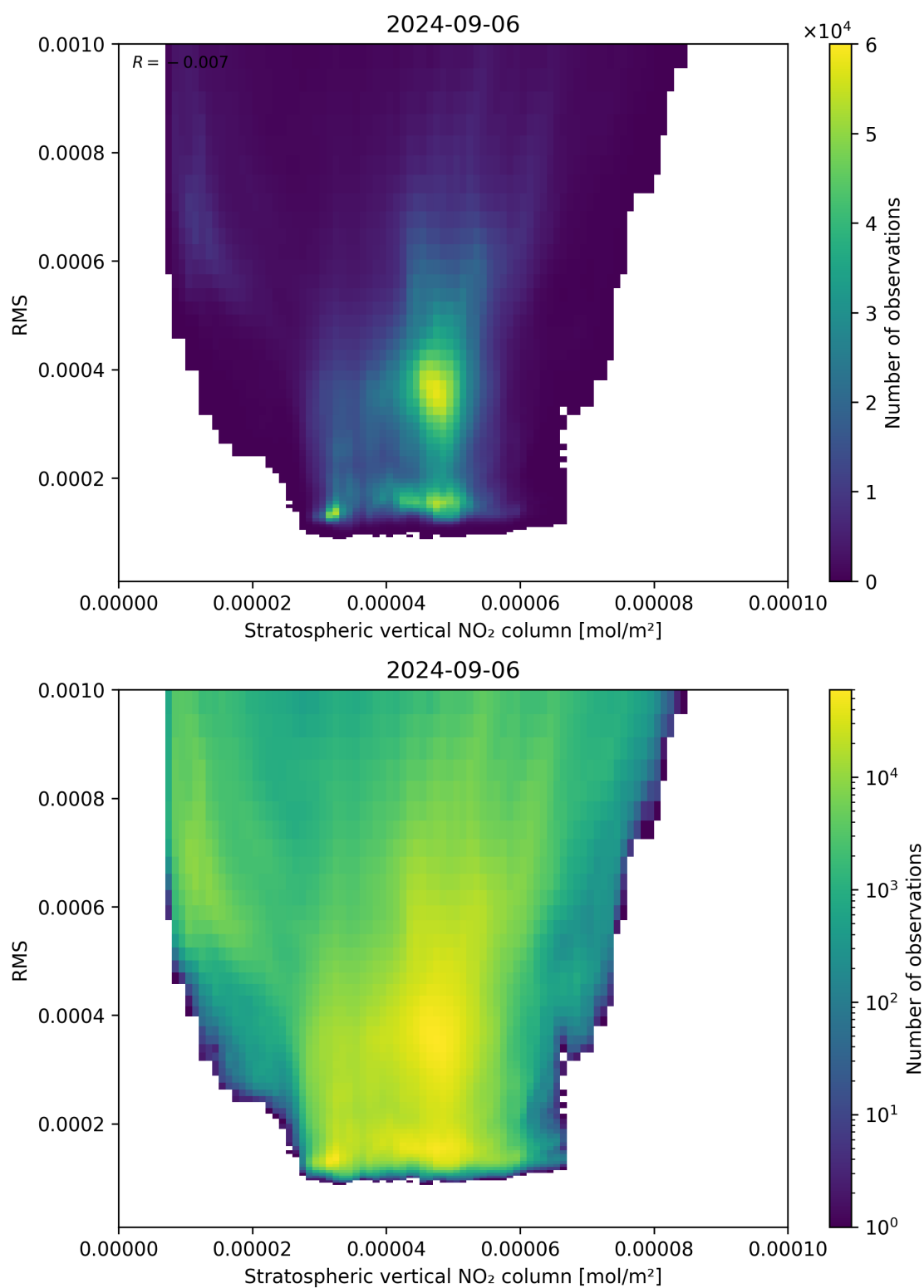
Figure 102: Scatter density plot of “Stratospheric vertical NO 2 column” against “RMS” for 2024-09-06 to 2024-09-07.
