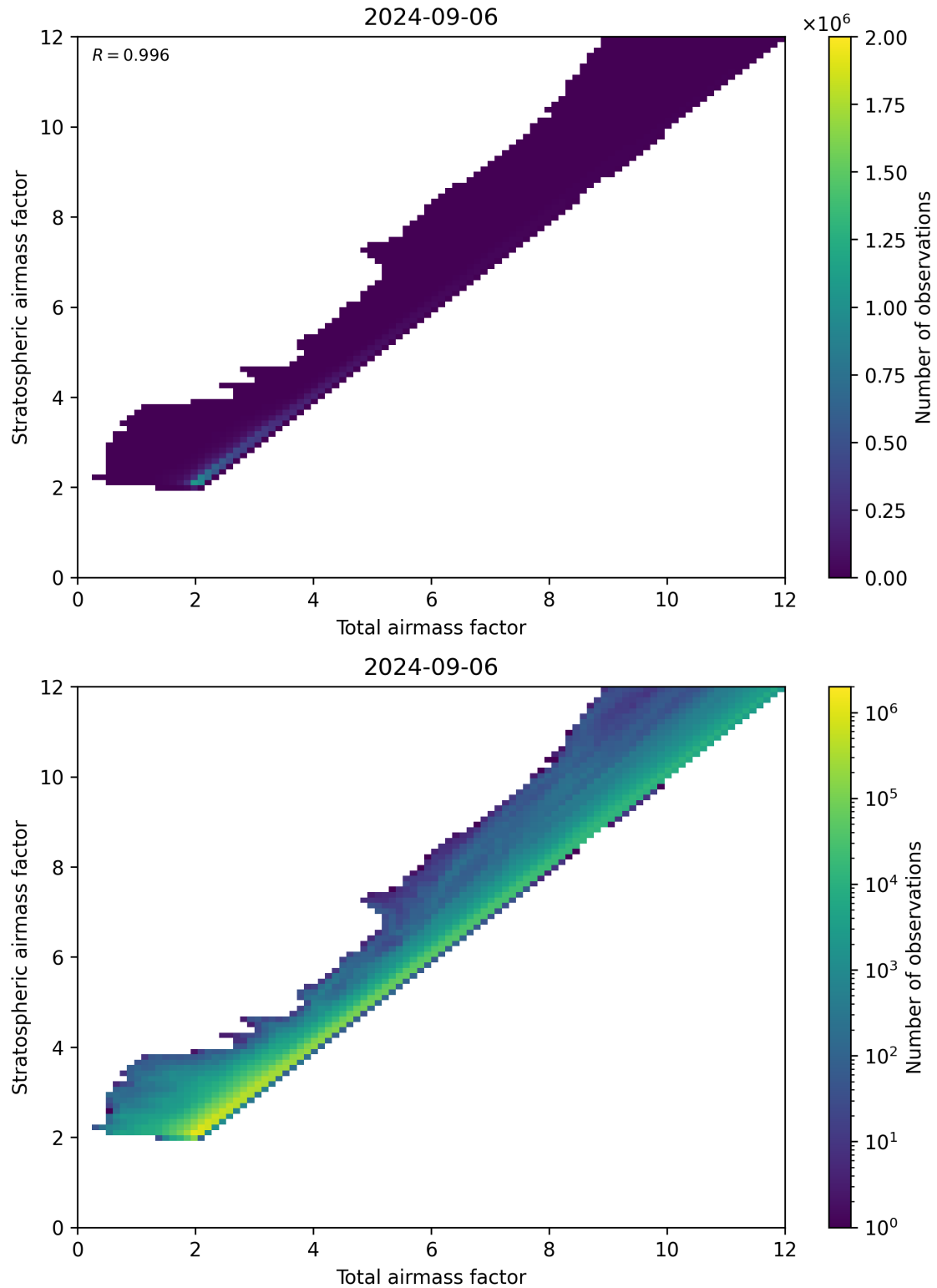
Figure 62: Scatter density plot of “Total airmass factor” against “Stratospheric airmass factor” for 2024-09-06 to 2024-09-07.
