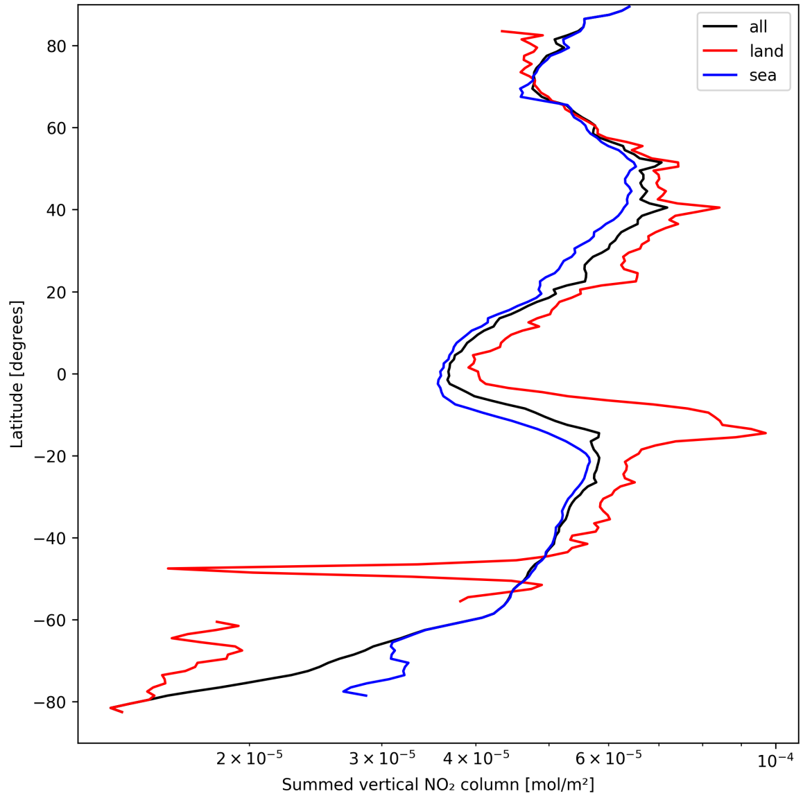
Figure 23: Zonal average of “Summed vertical NO 2 column” for 2024-09-06 to 2024-09-07.
