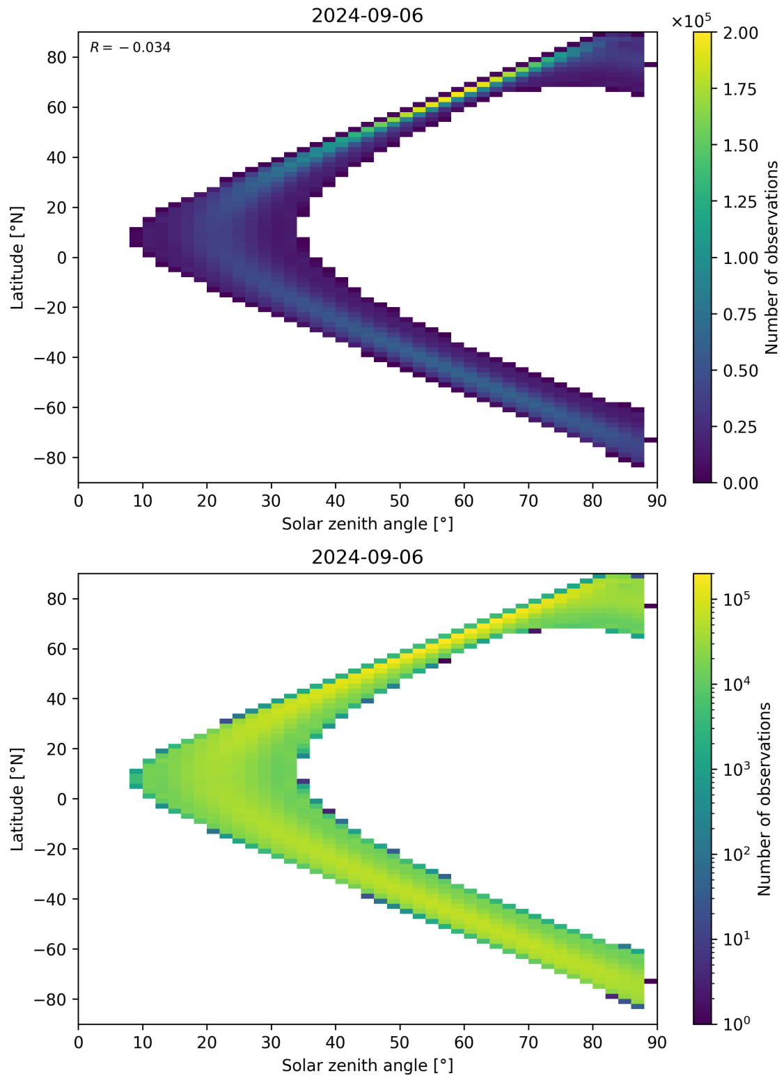
Figure 149: Scatter density plot of “Solar zenith angle” against “Latitude” for 2024-09-06 to 2024-09-07.
