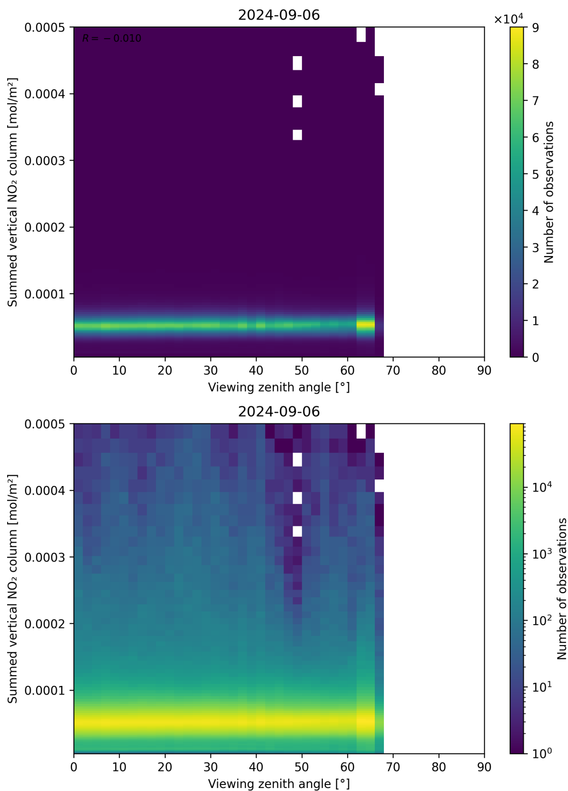
Figure 165: Scatter density plot of “Viewing zenith angle” against “Summed vertical NO 2 column” for 2024-09-06 to 2024-09-07.
