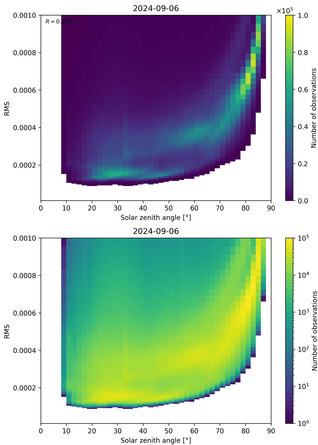
Figure 157: Scatter density plot of “Solar zenith angle” against “RMS” for 2024-09-06 to 2024-09-07.
