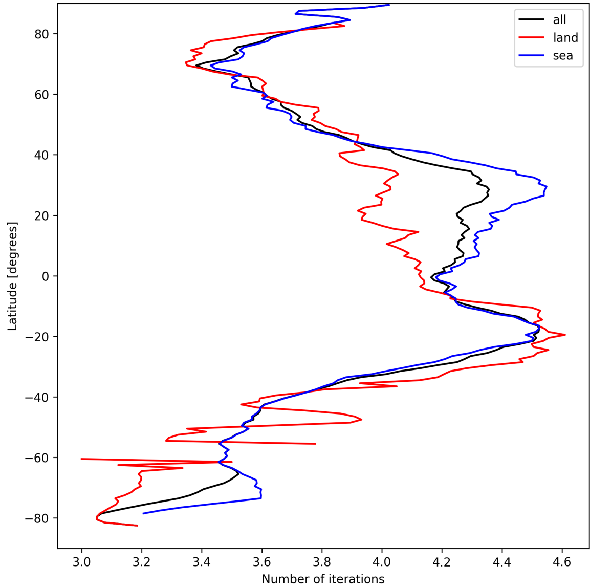
Figure 17: Zonal average of “Number of iterations” for 2024-09-06 to 2024-09-07.
