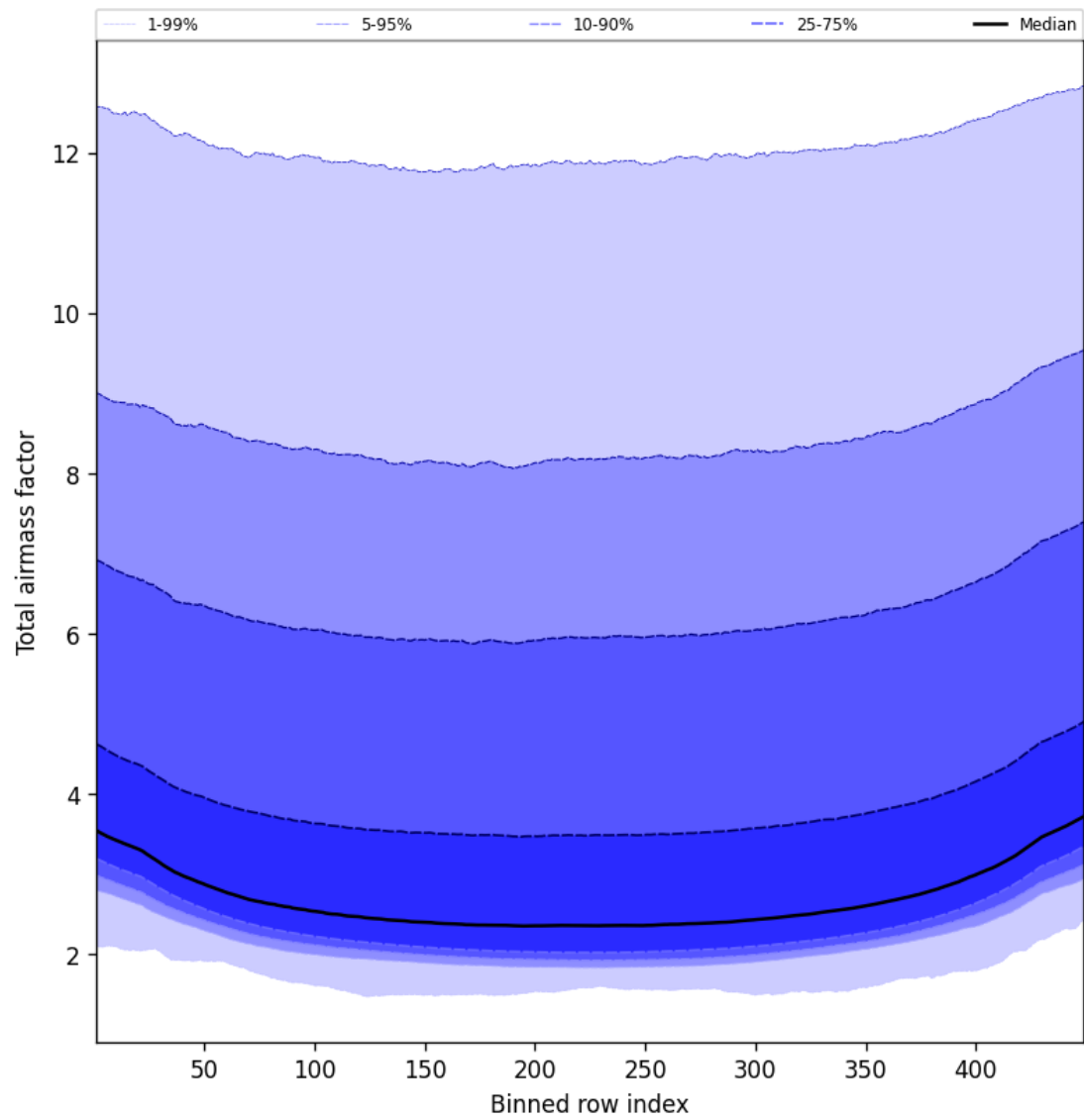
Figure 49: Along track statistics of “Total airmass factor” for 2024-09-06 to 2024-09-07
