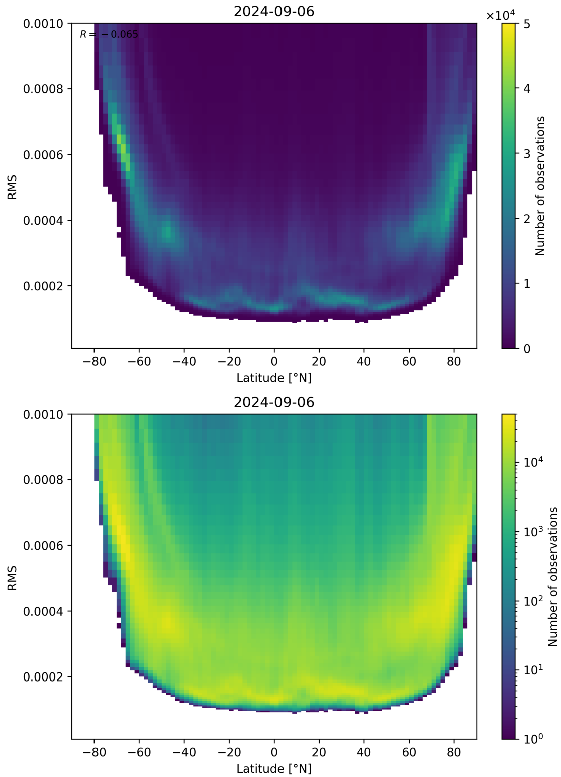
Figure 94: Scatter density plot of “Latitude” against “RMS” for 2024-09-06 to 2024-09-07.
