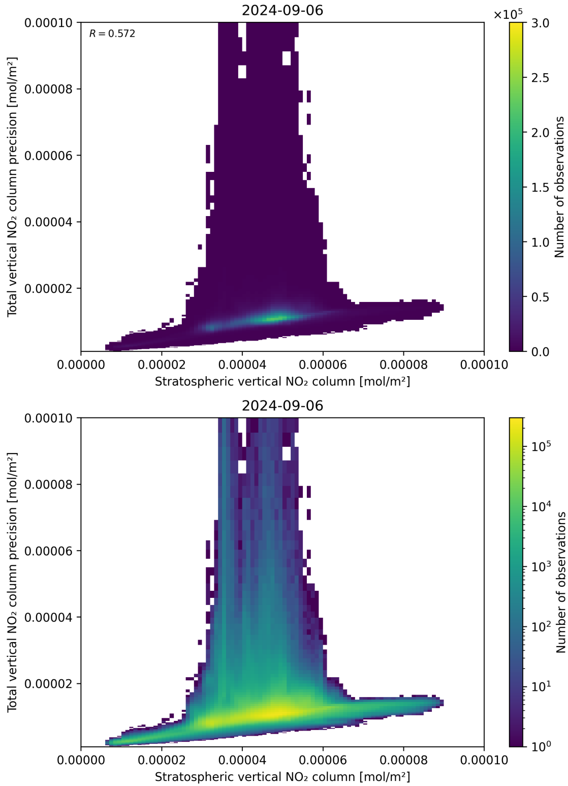
Figure 101: Scatter density plot of “Stratospheric vertical NO 2 column” against “Total vertical NO 2 column precision” for 2024-09-06 to 2024-09-07.
