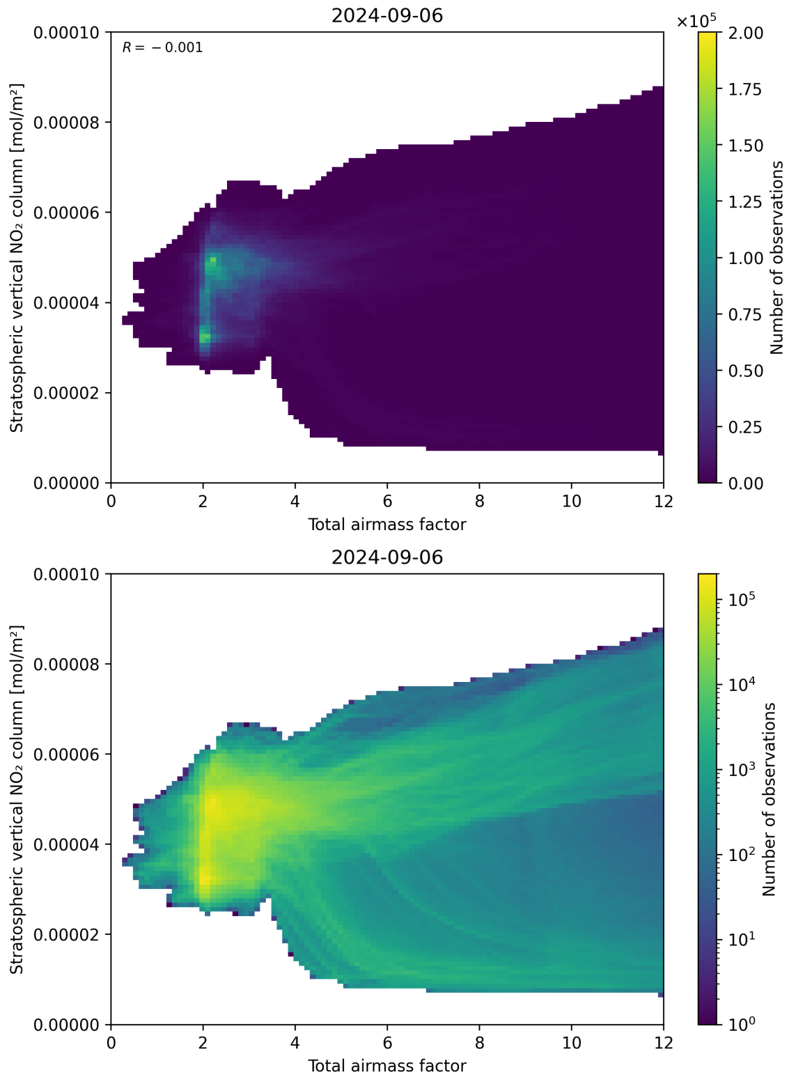
Figure 64: Scatter density plot of “Total airmass factor” against “Stratospheric vertical NO 2 column” for 2024-09-06 to 2024-09-07.
