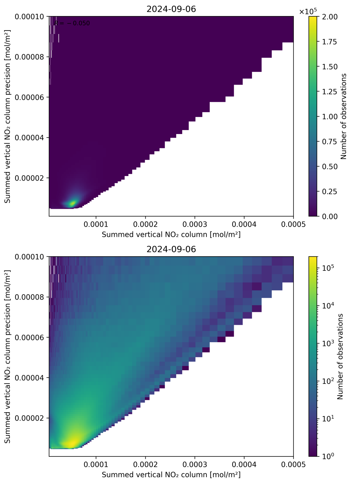
Figure 105: Scatter density plot of “Summed vertical NO 2 column” against “Summed vertical NO 2 column precision” for 2024-09-06 to 2024-09-07.
