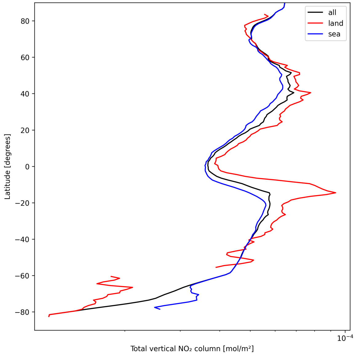
Figure 21: Zonal average of “Total vertical NO 2 column” for 2024-09-06 to 2024-09-07.
