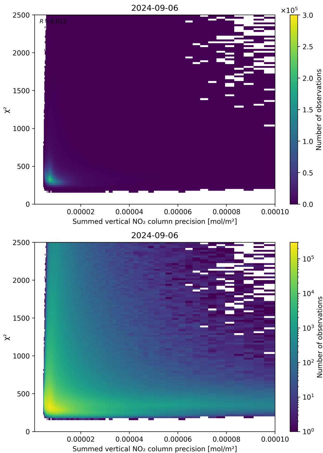
Figure 107: Scatter density plot of “Summed vertical NO 2 column precision” against “ \chi^2 ” for 2024-09-06 to 2024-09-07.
