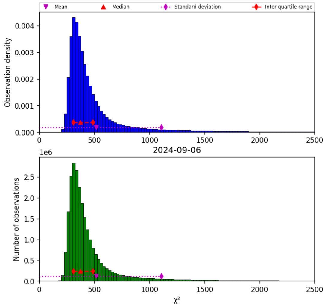
Figure 42: Histogram of “ \chi^2 ” for 2024-09-06 to 2024-09-07
