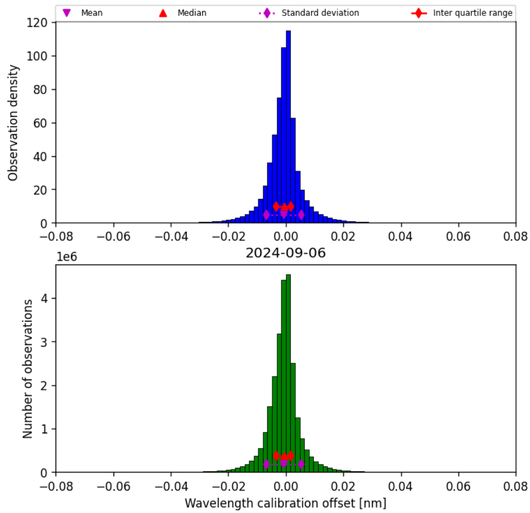
Figure 35: Histogram of “Wavelength calibration offset” for 2024-09-06 to 2024-09-07
