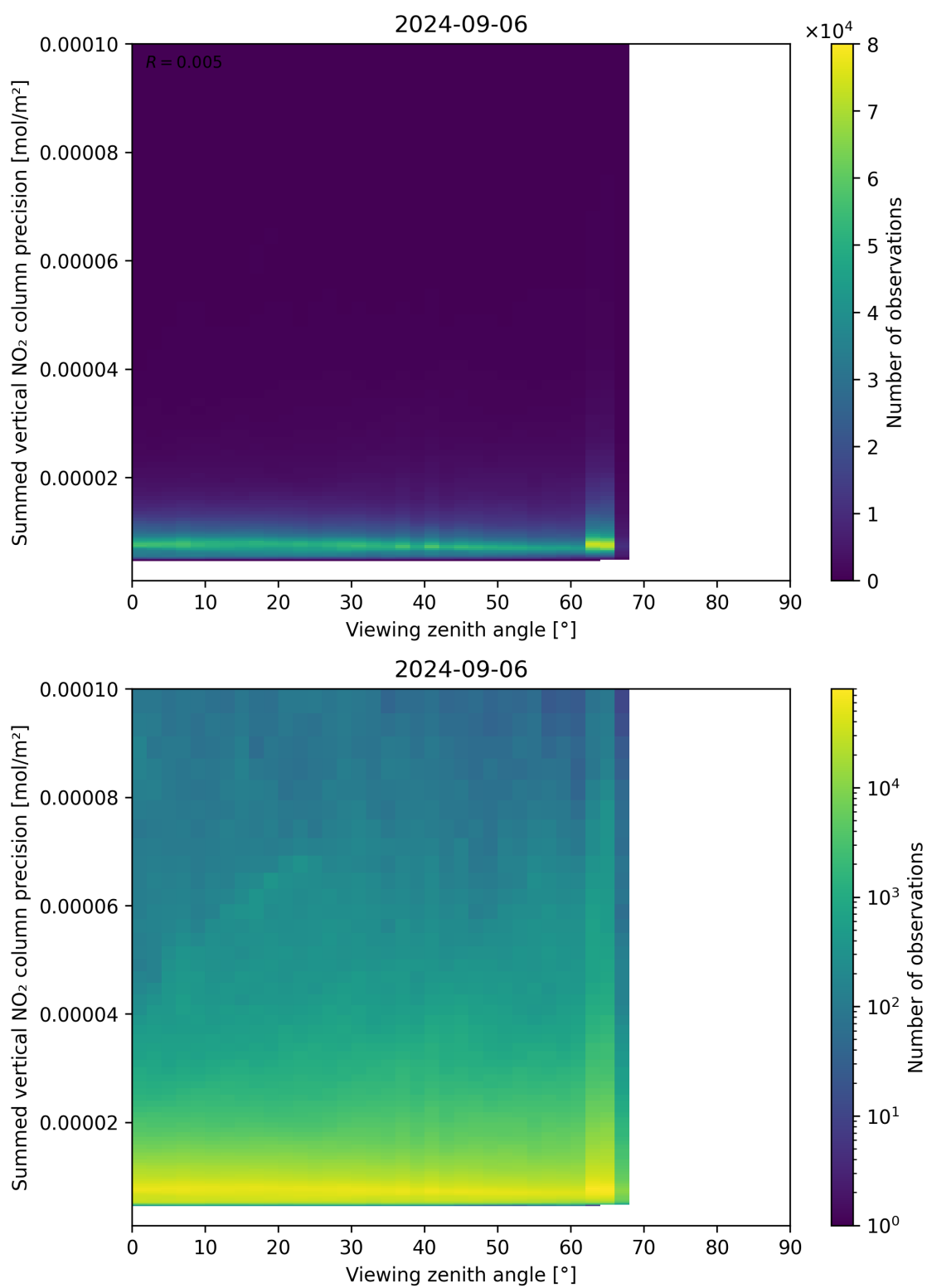
Figure 166: Scatter density plot of “Viewing zenith angle” against “Summed vertical NO 2 column precision” for 2024-09-06 to 2024-09-07.
