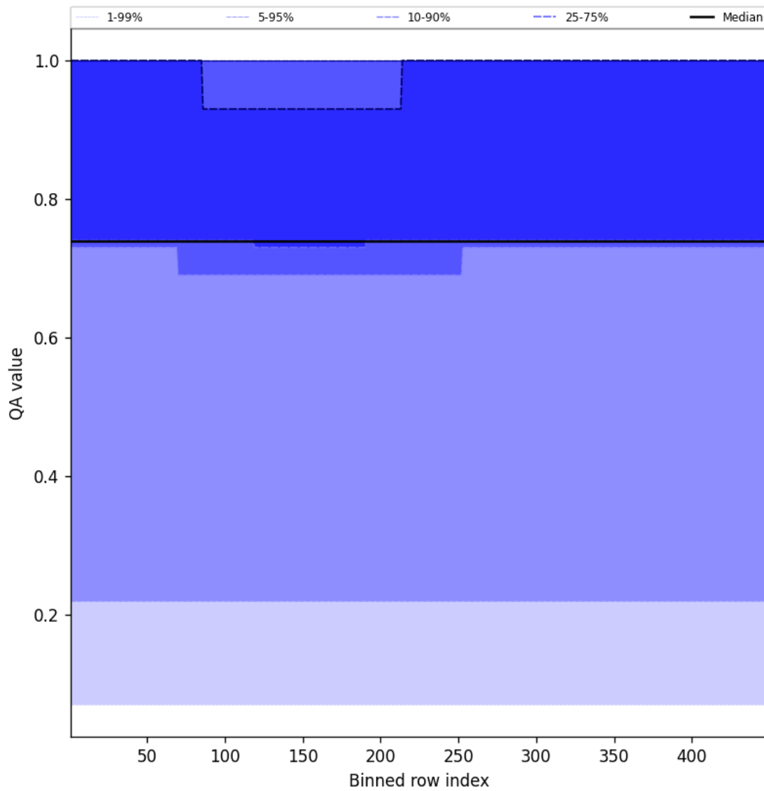
Figure 45: Along track statistics of “QA value” for 2024-09-06 to 2024-09-07
