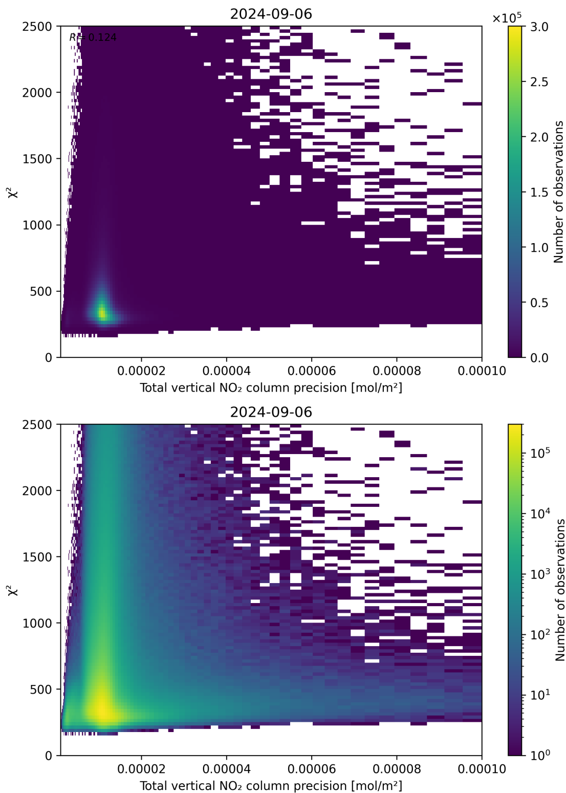
Figure 116: Scatter density plot of “Total vertical NO 2 column precision” against “ \chi^2 ” for 2024-09-06 to 2024-09-07.
