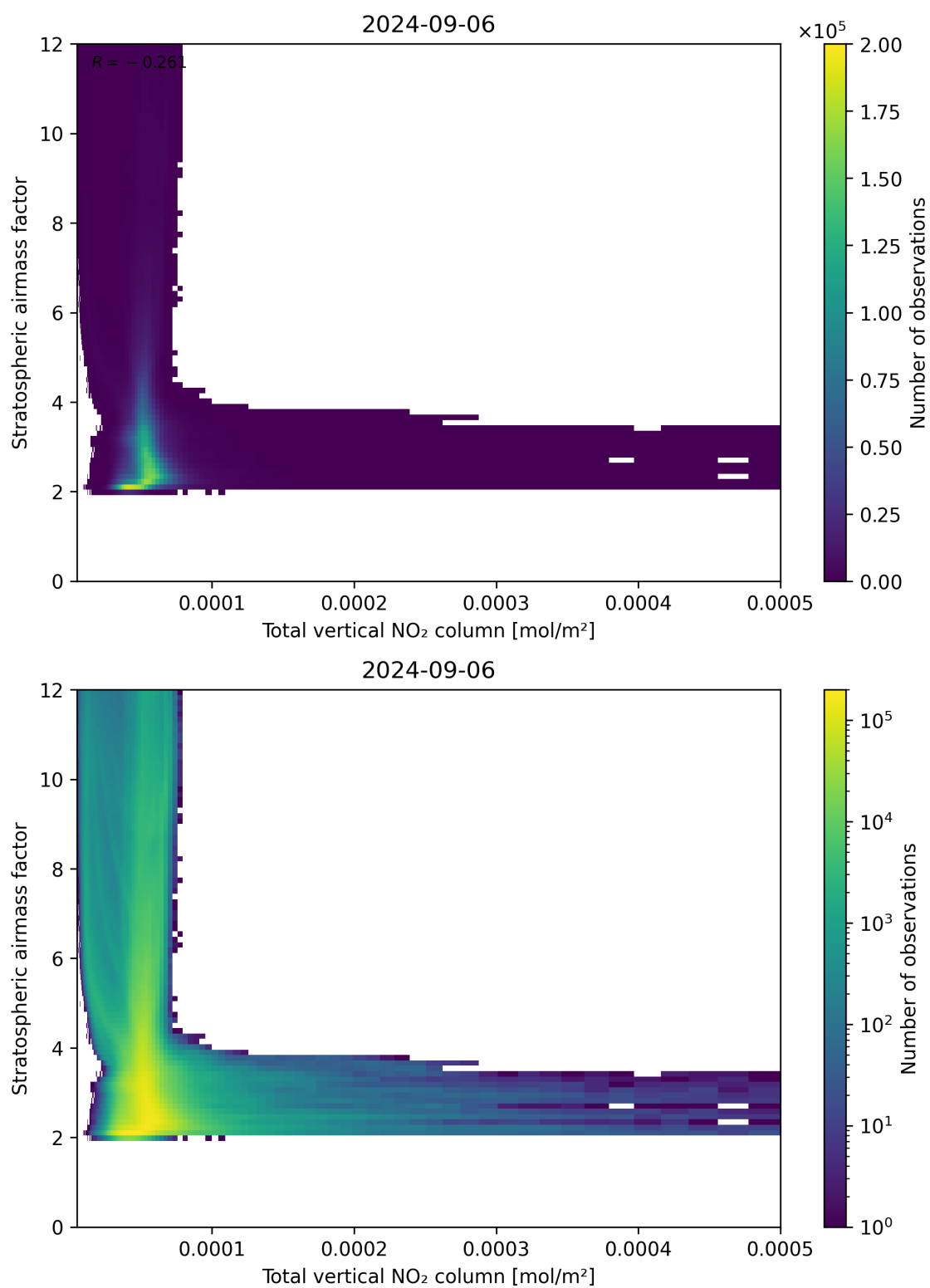
Figure 110: Scatter density plot of “Total vertical NO 2 column” against “Stratospheric airmass factor” for 2024-09-06 to 2024-09-07.
