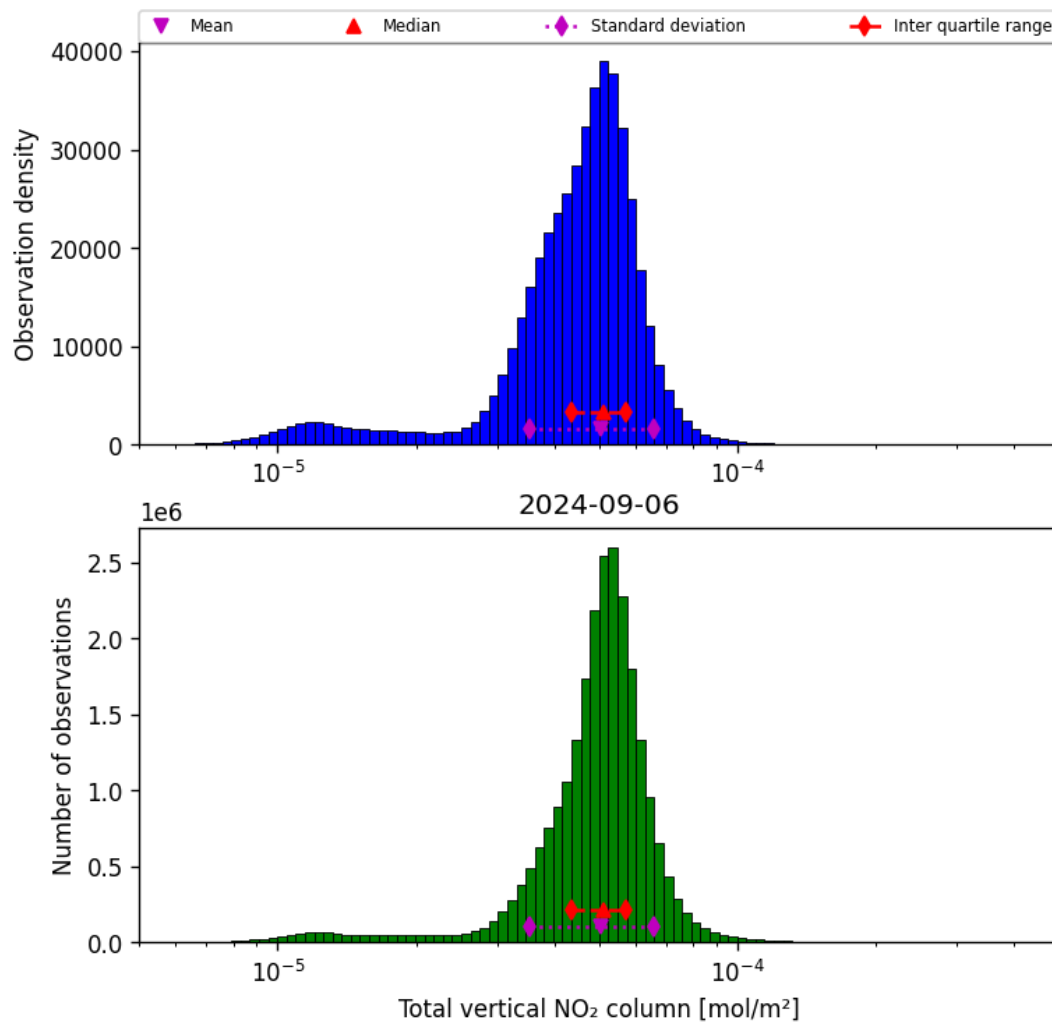
Figure 38: Histogram of “Total vertical NO 2 column” for 2024-09-06 to 2024-09-07
