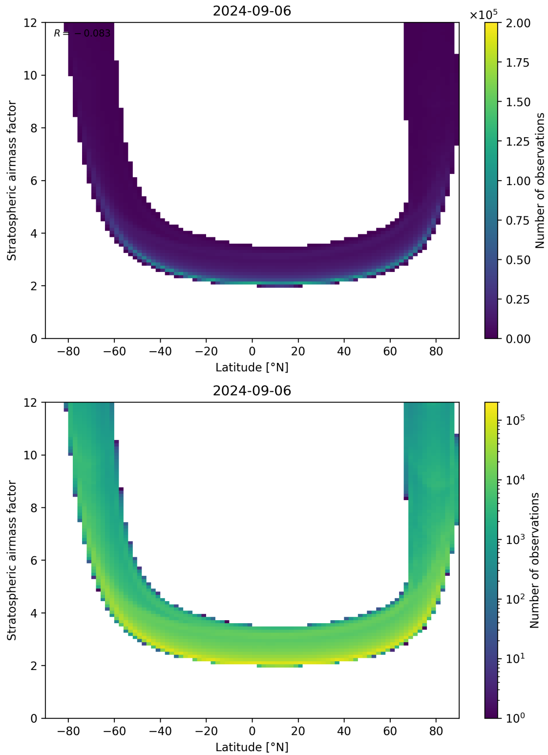
Figure 83: Scatter density plot of “Latitude” against “Stratospheric air mass factor” for 2024-09-06 to 2024-09-07.
