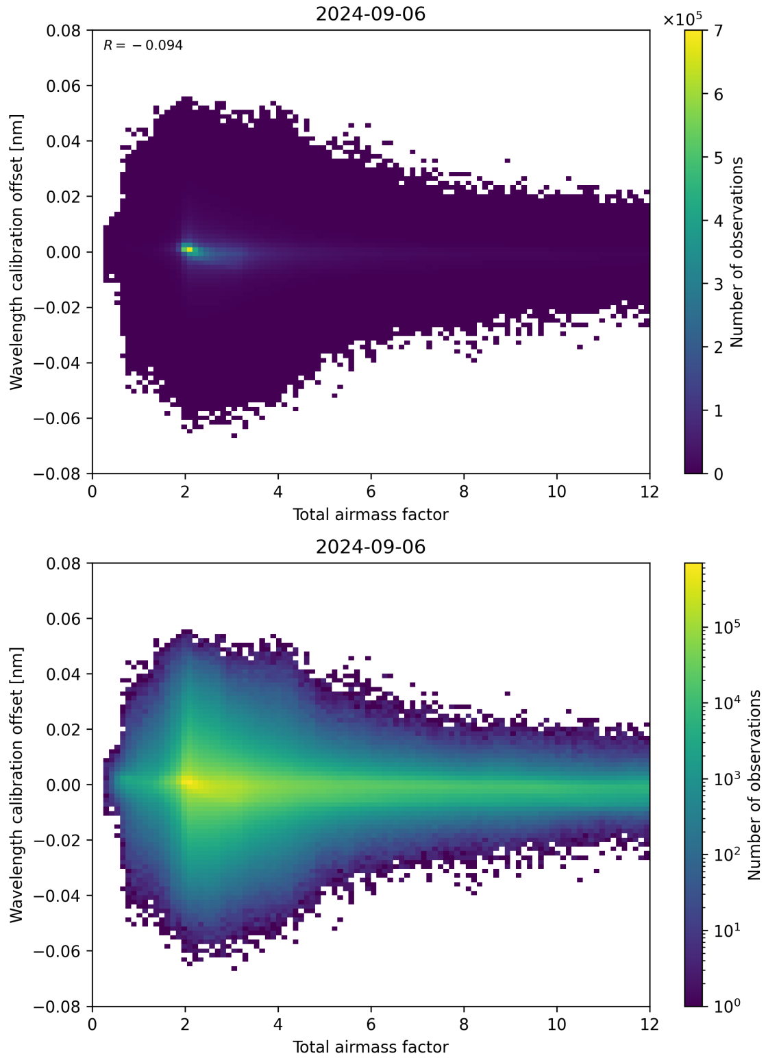
Figure 70: Scatter density plot of “Total airmass factor” against “Wavelength calibration offset” for 2024-09-06 to 2024-09-07.
