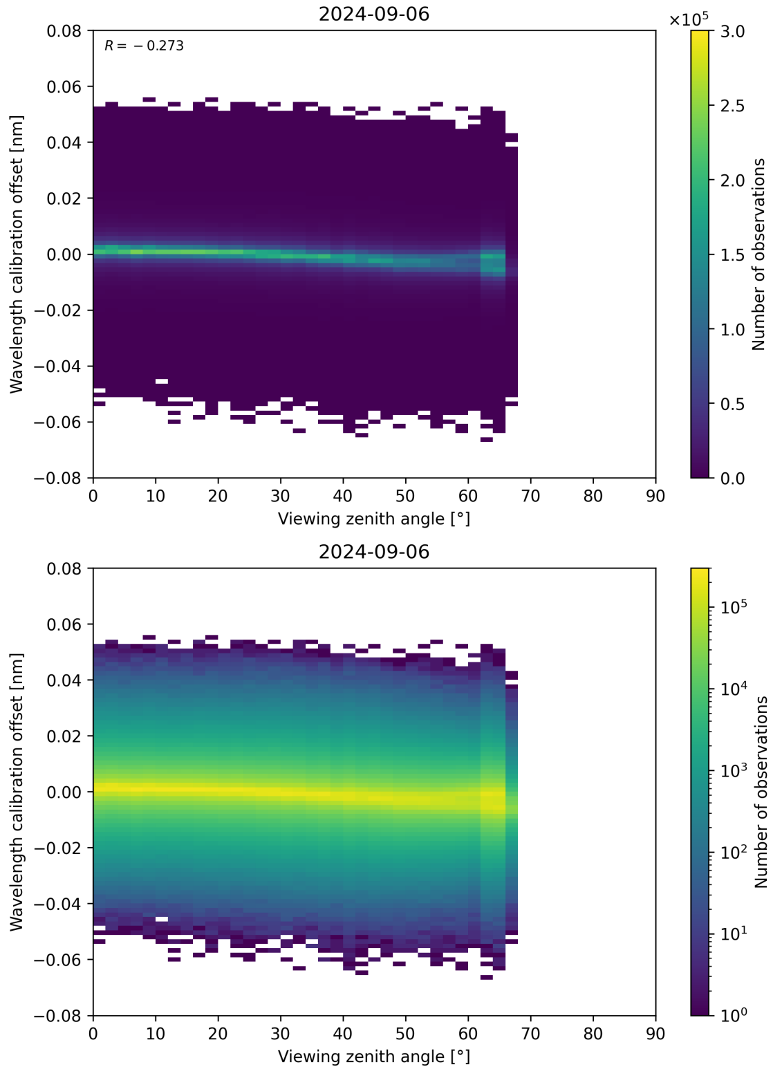
Figure 173: Scatter density plot of “Viewing zenith angle” against “Wavelength calibration offset” for 2024-09-06 to 2024-09-07.
