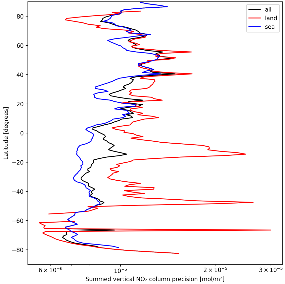
Figure 24: Zonal average of “Summed vertical NO 2 column precision” for 2024-09-06 to 2024-09-07.
