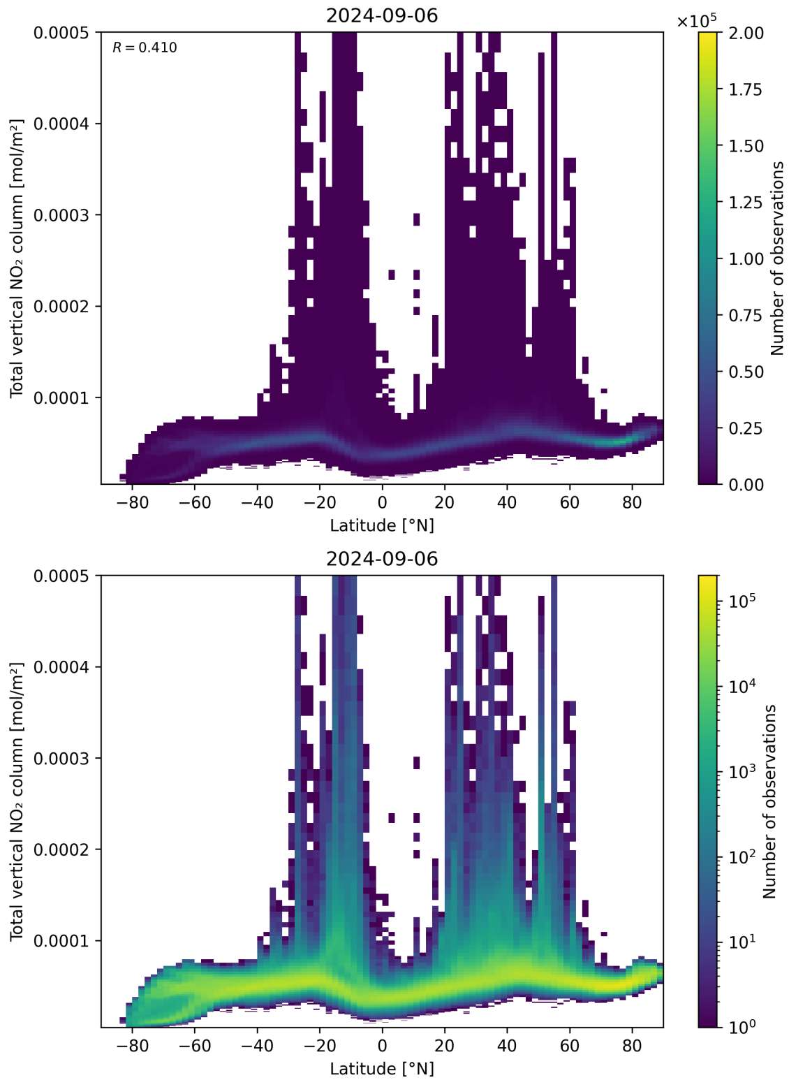
Figure 90: Scatter density plot of “Latitude” against “Total vertical NO 2 column” for 2024-09-06 to 2024-09-07.
