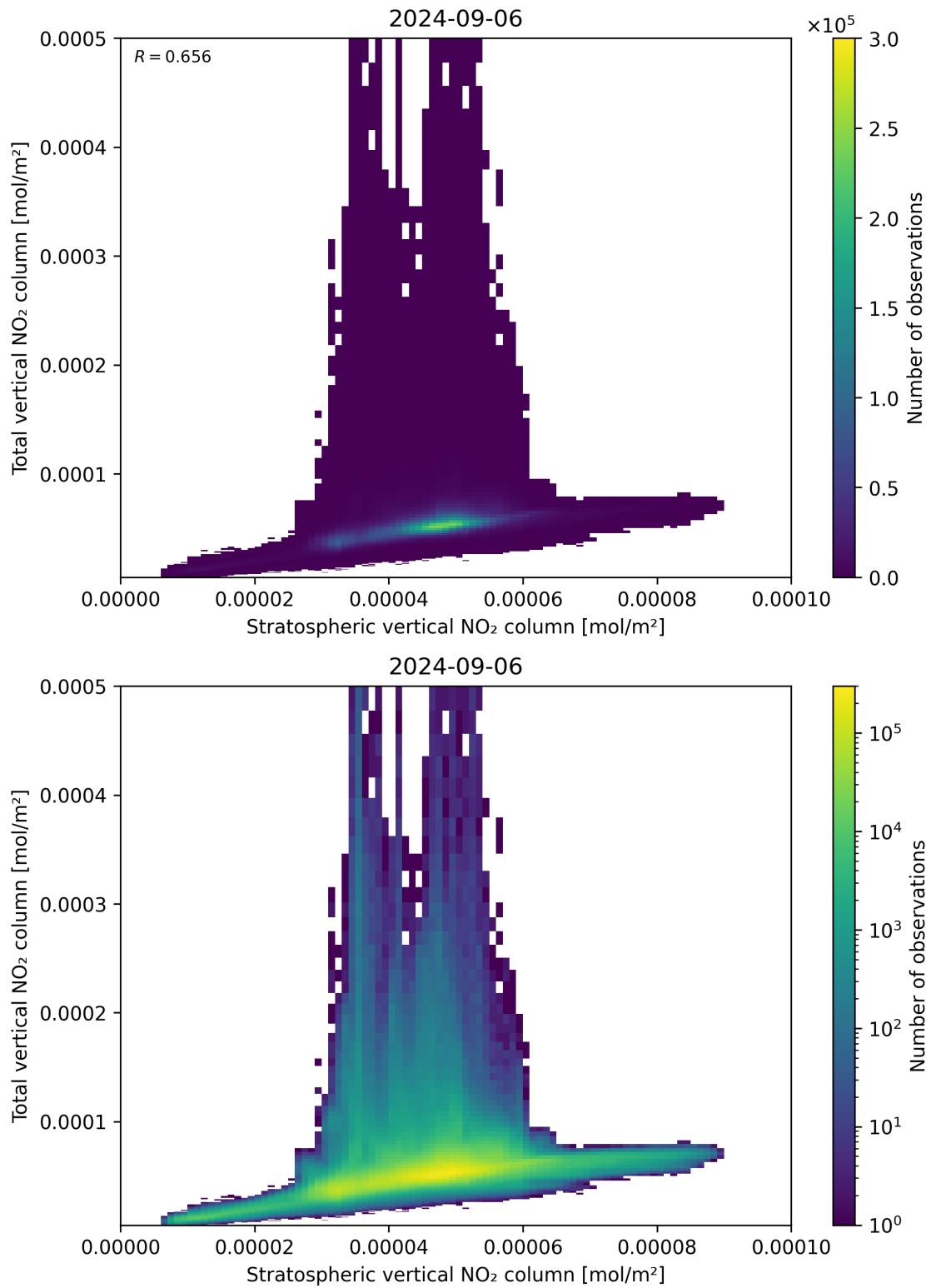
Figure 100: Scatter density plot of “Stratospheric vertical NO 2 column” against “Total vertical NO 2 column” for 2024-09-06 to 2024-09-07.
