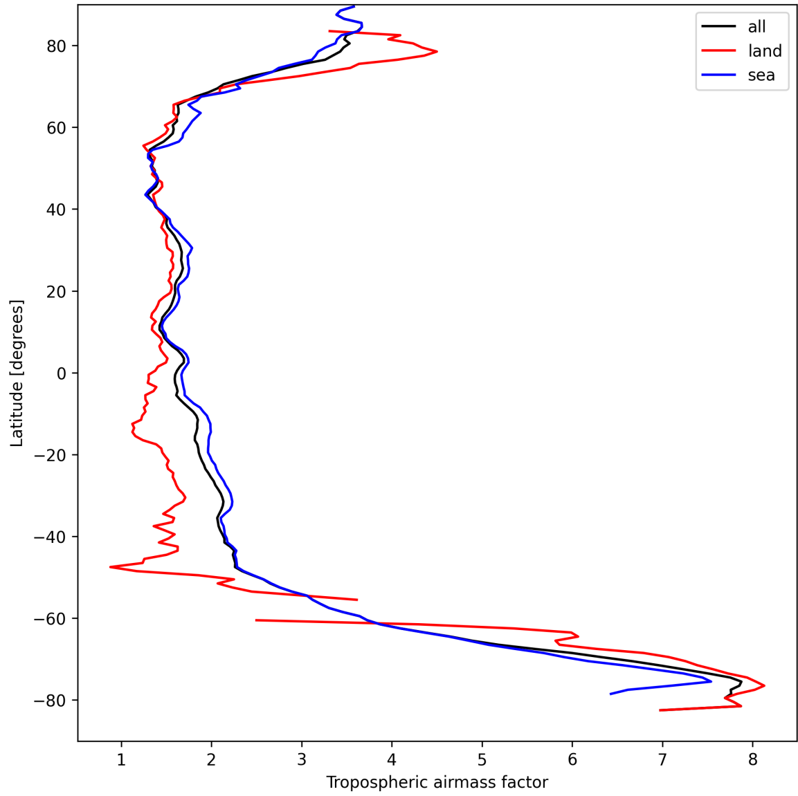
Figure 14: Zonal average of “Tropospheric airmass factor” for 2024-09-06 to 2024-09-07.
