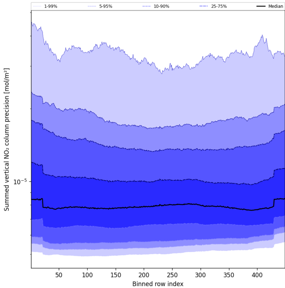
Figure 58: Along track statistics of “Summed vertical NO 2 column precision” for 2024-09-06 to 2024-09-07
