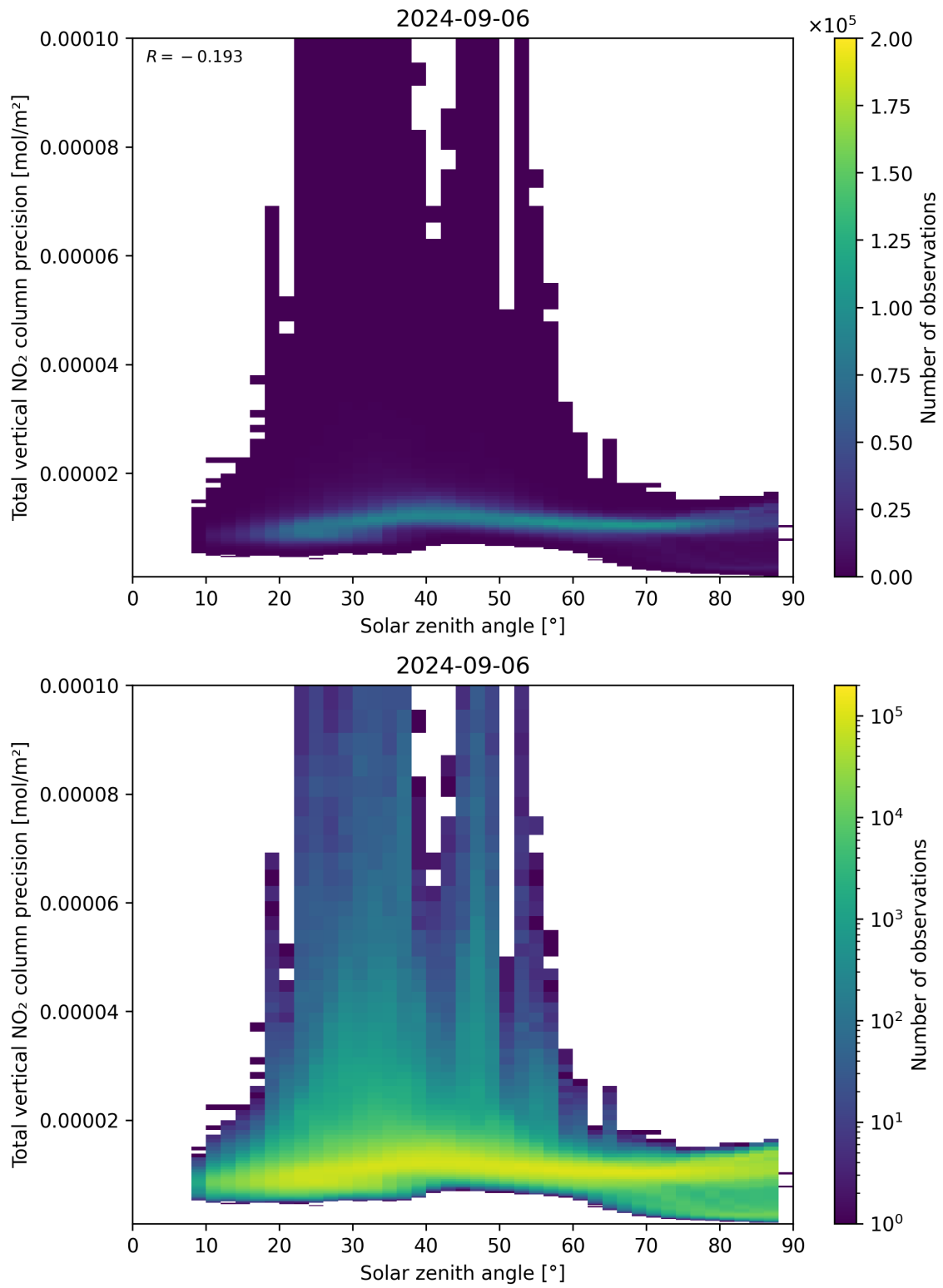
Figure 154: Scatter density plot of “Solar zenith angle” against “Total vertical NO 2 column precision” for 2024-09-06 to 2024-09-07.
