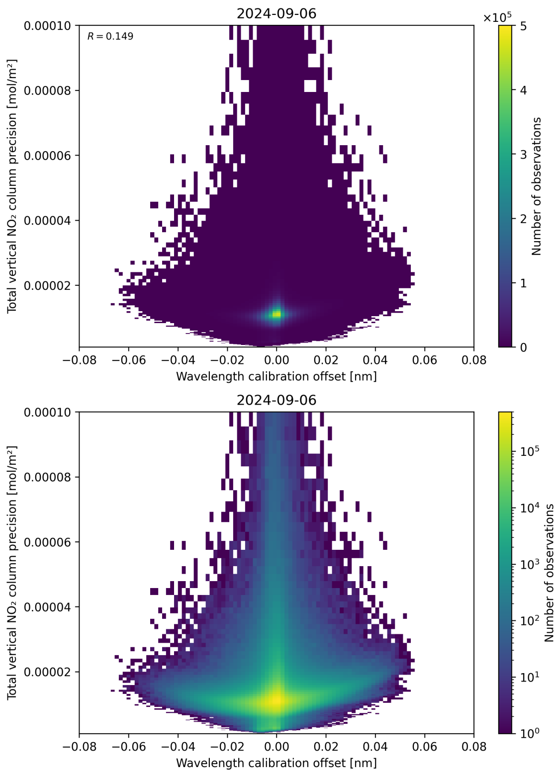
Figure 180: Scatter density plot of “Wavelength calibration offset” against “Total vertical NO 2 column precision” for 2024-09-06 to 2024-09-07.
