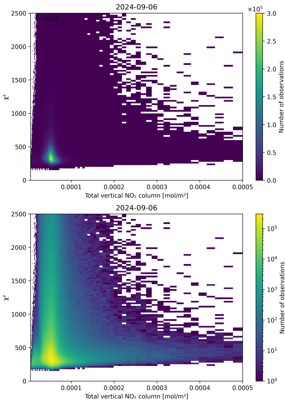
Figure 111: Scatter density plot of “Total vertical NO 2 column” against “ \chi^2 ” for 2024-09-06 to 2024-09-07.
