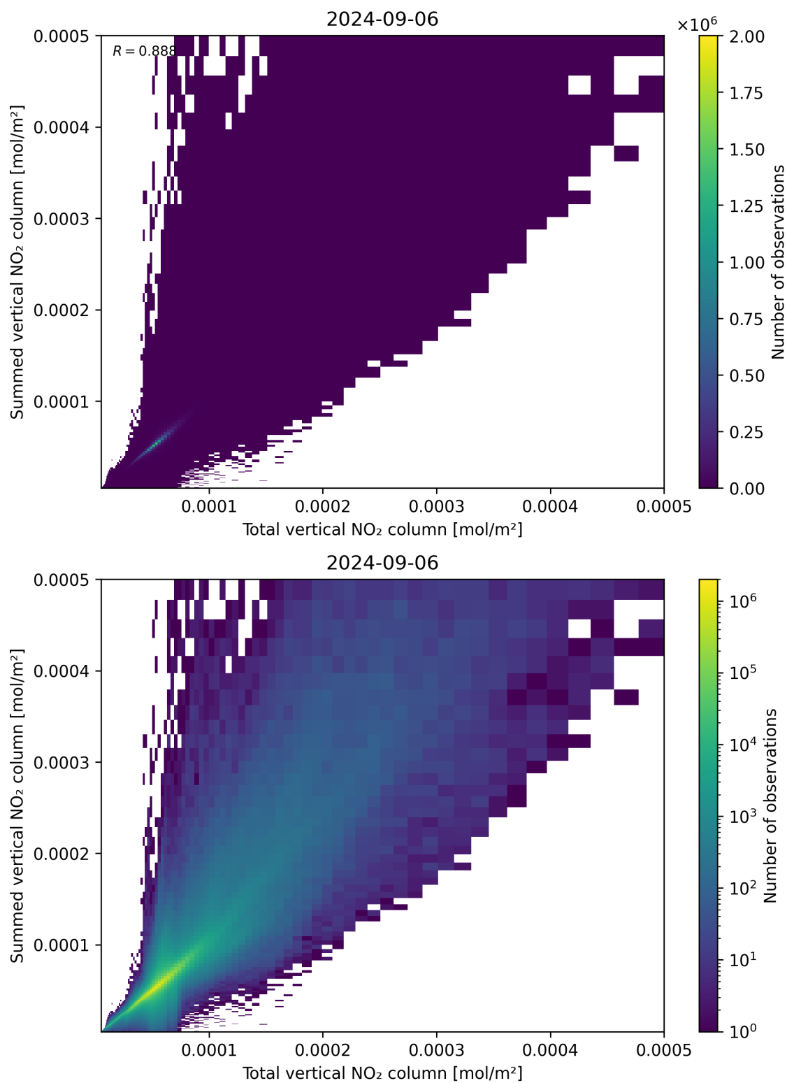
Figure 112: Scatter density plot of “Total vertical NO 2 column” against “Summed vertical NO 2 column” for 2024-09-06 to 2024-09-07.
