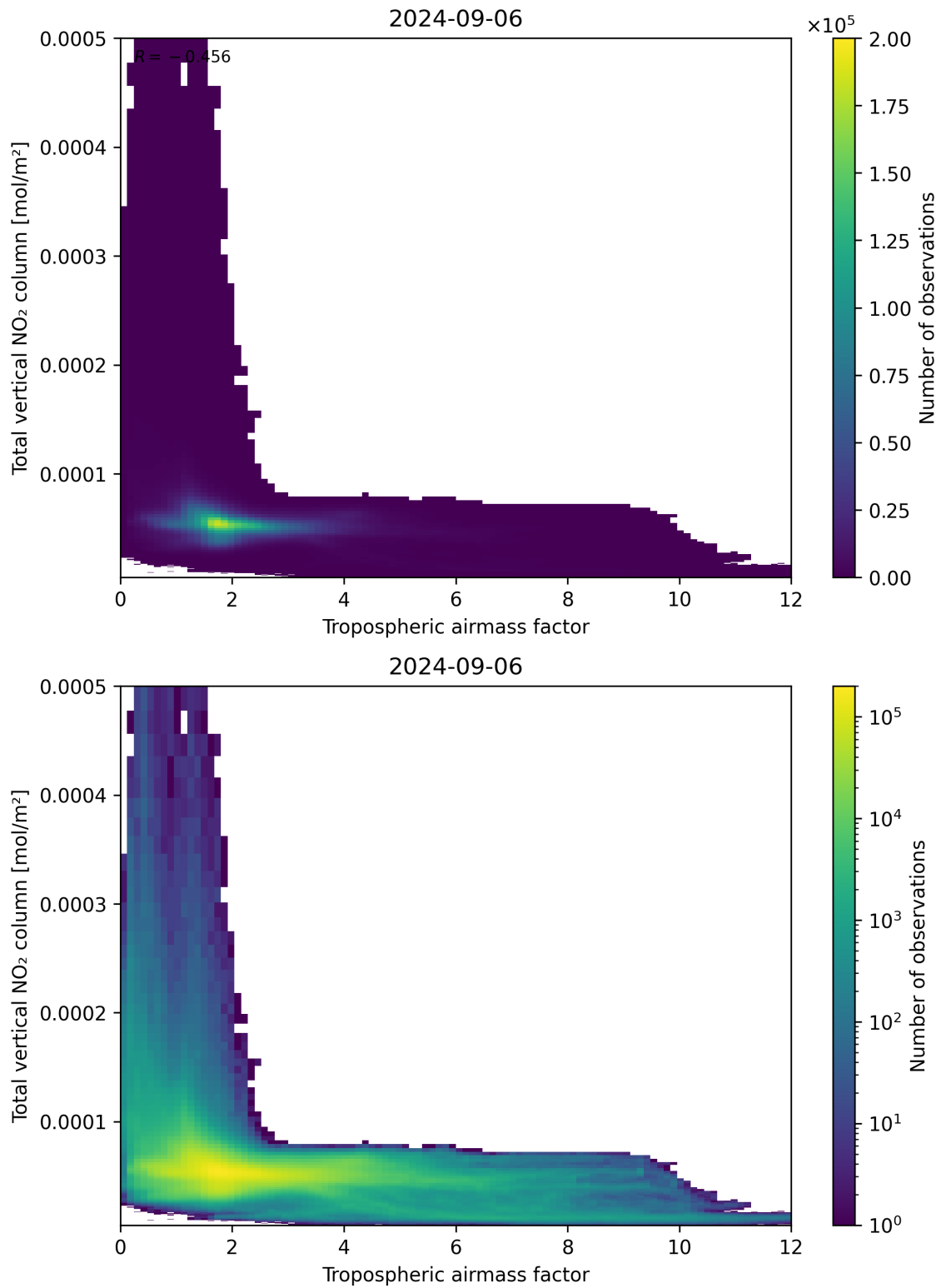
Figure 77: Scatter density plot of “Tropospheric airmass factor” against “Total vertical NO 2 column” for 2024-09-06 to 2024-09-07.
