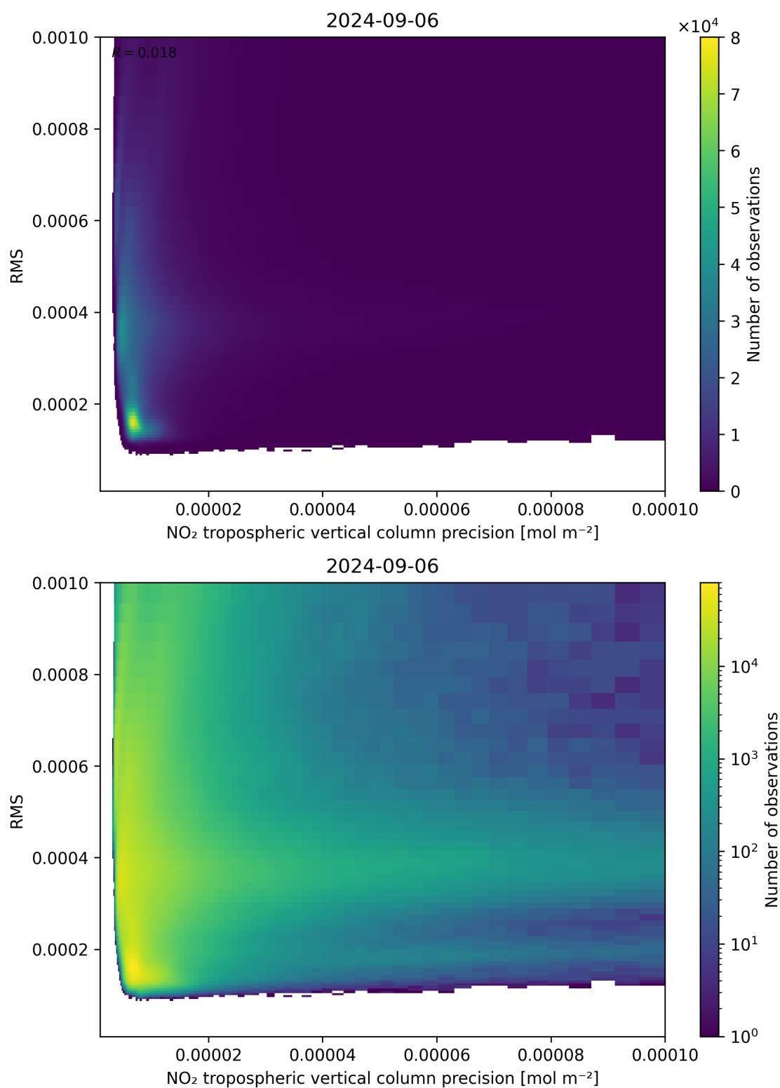
Figure 140: Scatter density plot of “NO 2 tropospheric vertical column precision” against “RMS” for 2024-09-06 to 2024-09-07.
