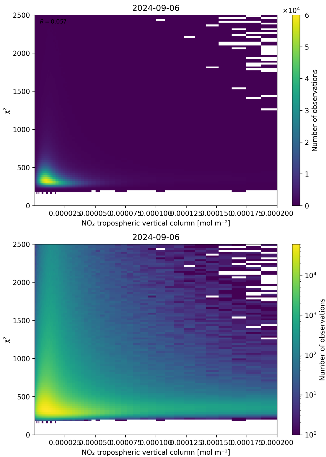
Figure 124: Scatter density plot of “NO 2 tropospheric vertical column” against “ \chi^2 ” for 2024-09-06 to 2024-09-07.
