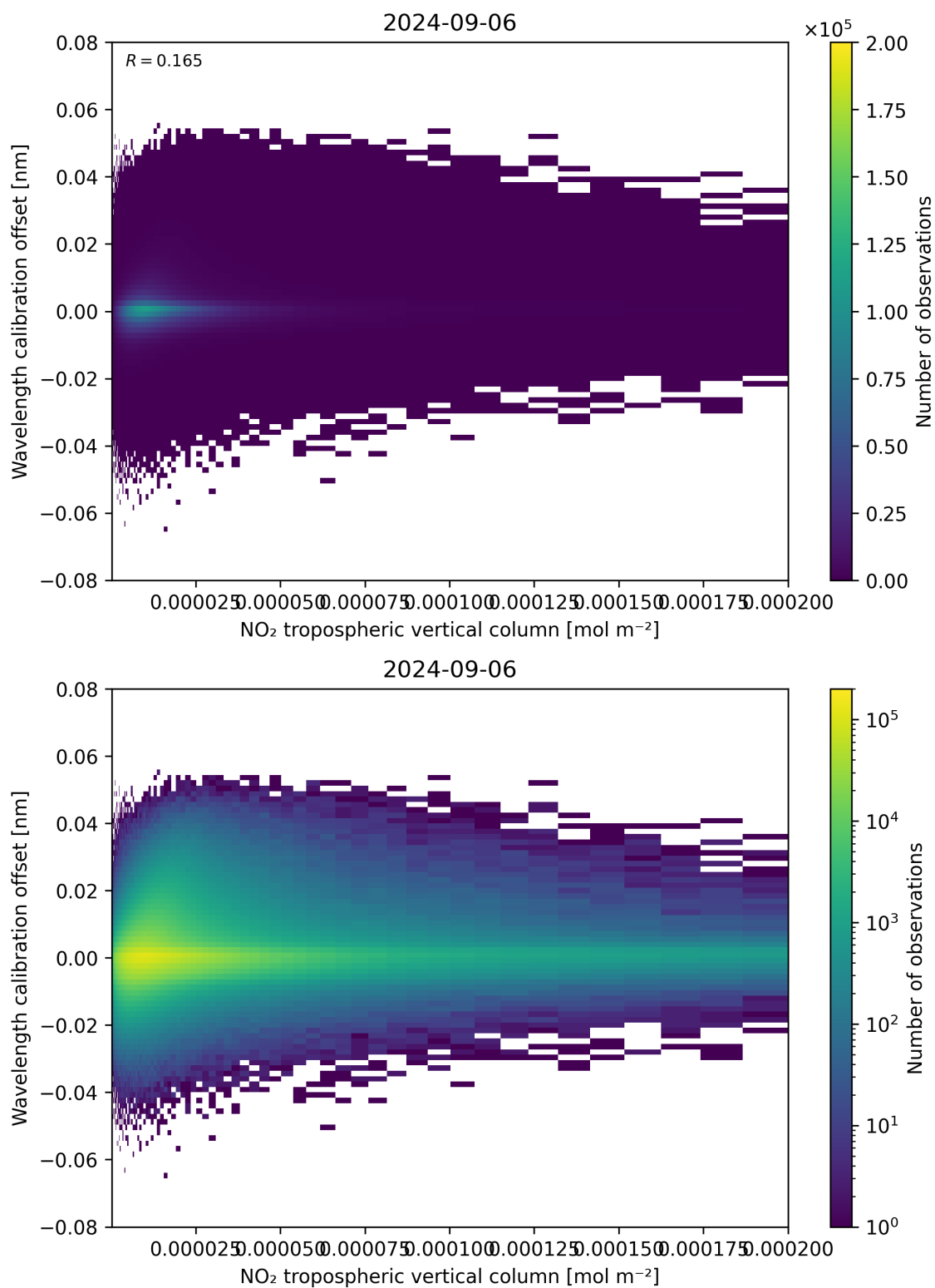
Figure 143: Scatter density plot of “NO 2 tropospheric vertical column” against “Wavelength calibration offset” for 2024-09-06 to 2024-09-07.
