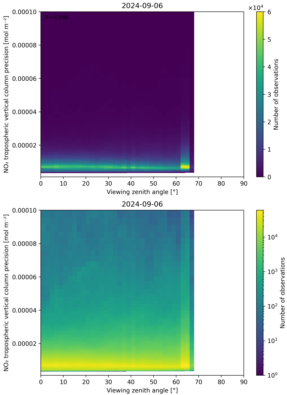
Figure 170: Scatter density plot of “Viewing zenith angle” against “NO 2 tropospheric vertical column precision” for 2024-09-06 to 2024-09-07.
