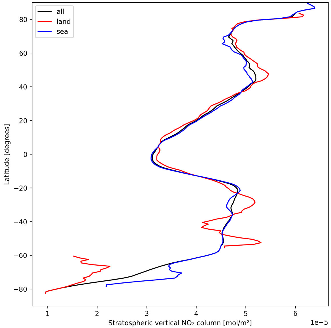
Figure 19: Zonal average of “Stratospheric vertical NO 2 column” for 2024-09-06 to 2024-09-07.
