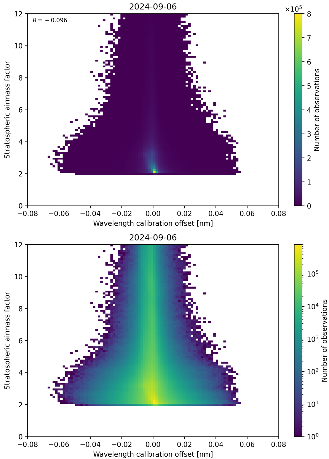
Figure 174: Scatter density plot of “Wavelength calibration offset” against “Stratospheric air mass factor” for 2024-09-06 to 2024-09-07.
