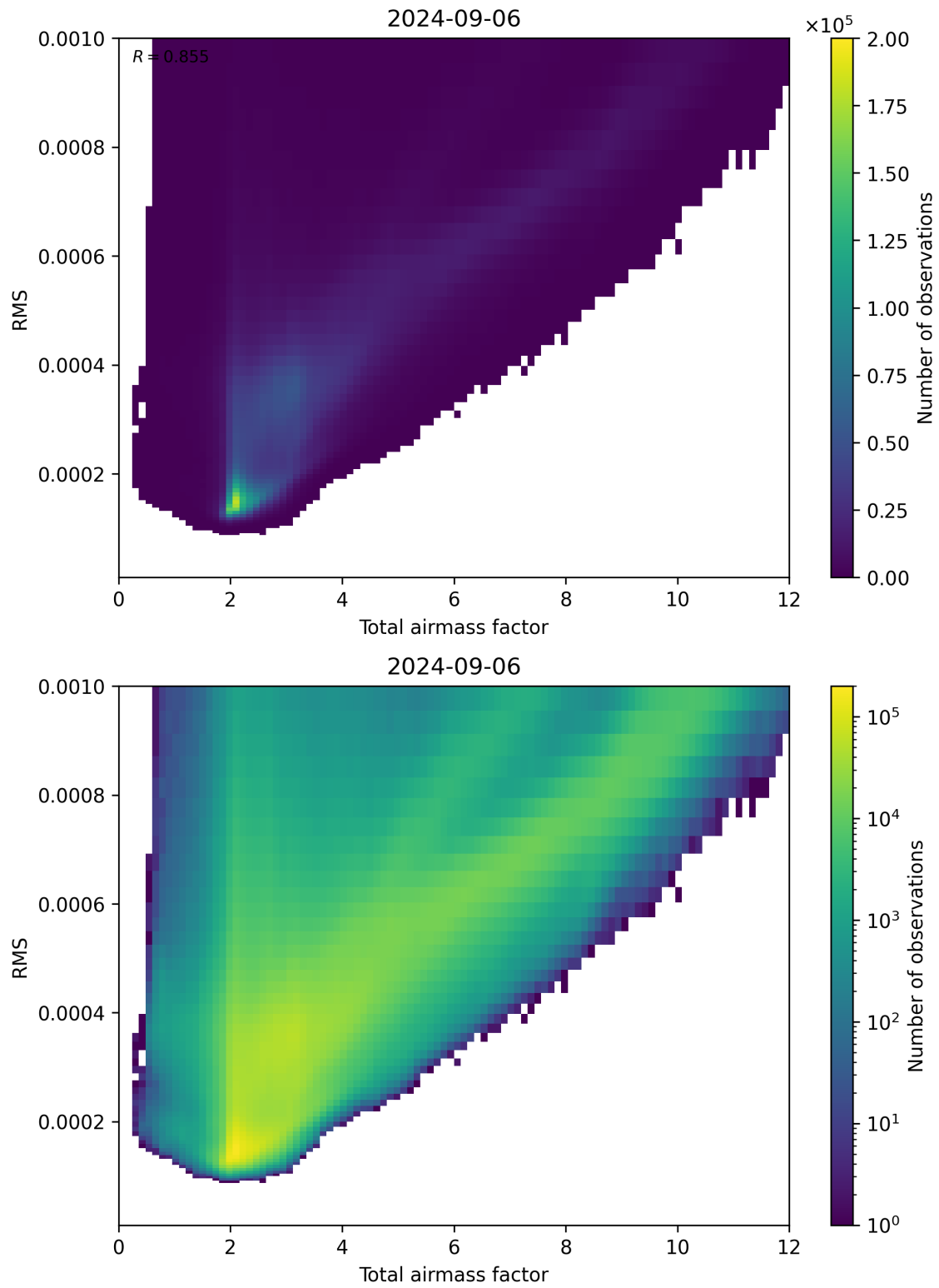
Figure 69: Scatter density plot of “Total airmass factor” against “RMS” for 2024-09-06 to 2024-09-07.
