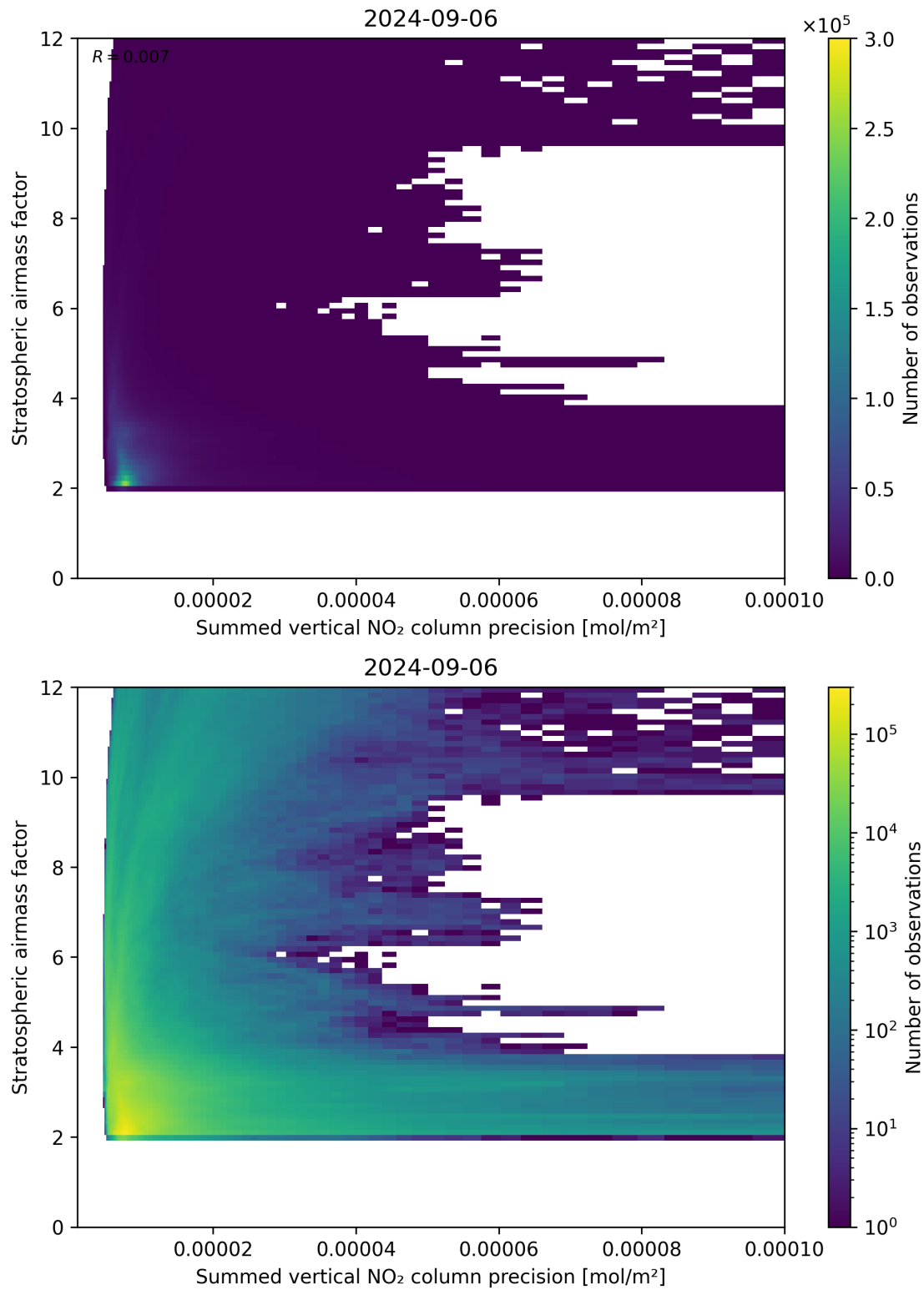
Figure 106: Scatter density plot of “Summed vertical NO 2 column precision” against “Stratospheric airmass factor” for 2024-09-06 to 2024-09-07.
