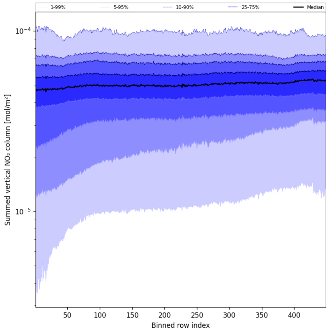
Figure 57: Along track statistics of “Summed vertical NO 2 column” for 2024-09-06 to 2024-09-07
