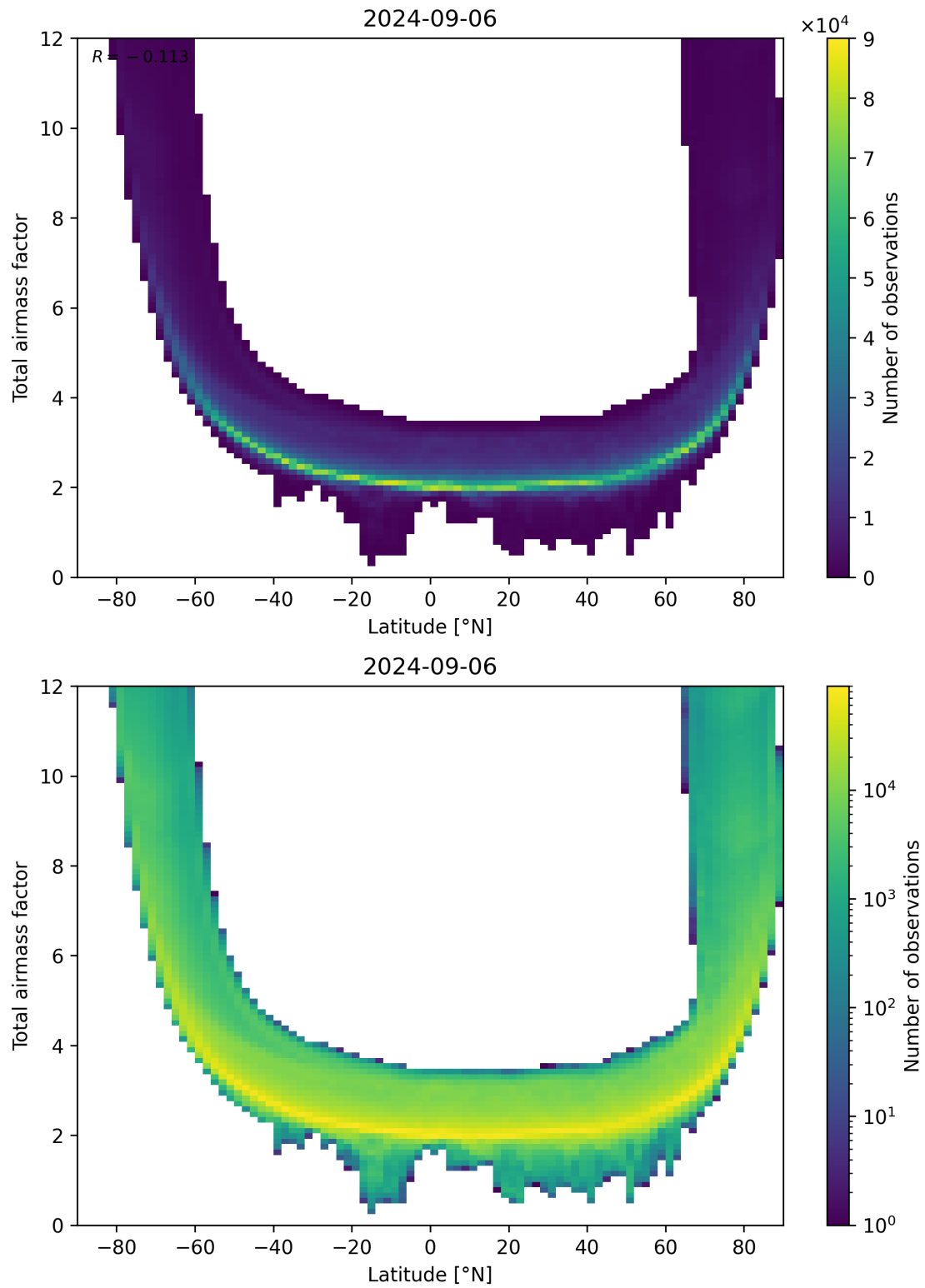
Figure 84: Scatter density plot of “Latitude” against “Total airmass factor” for 2024-09-06 to 2024-09-07.
