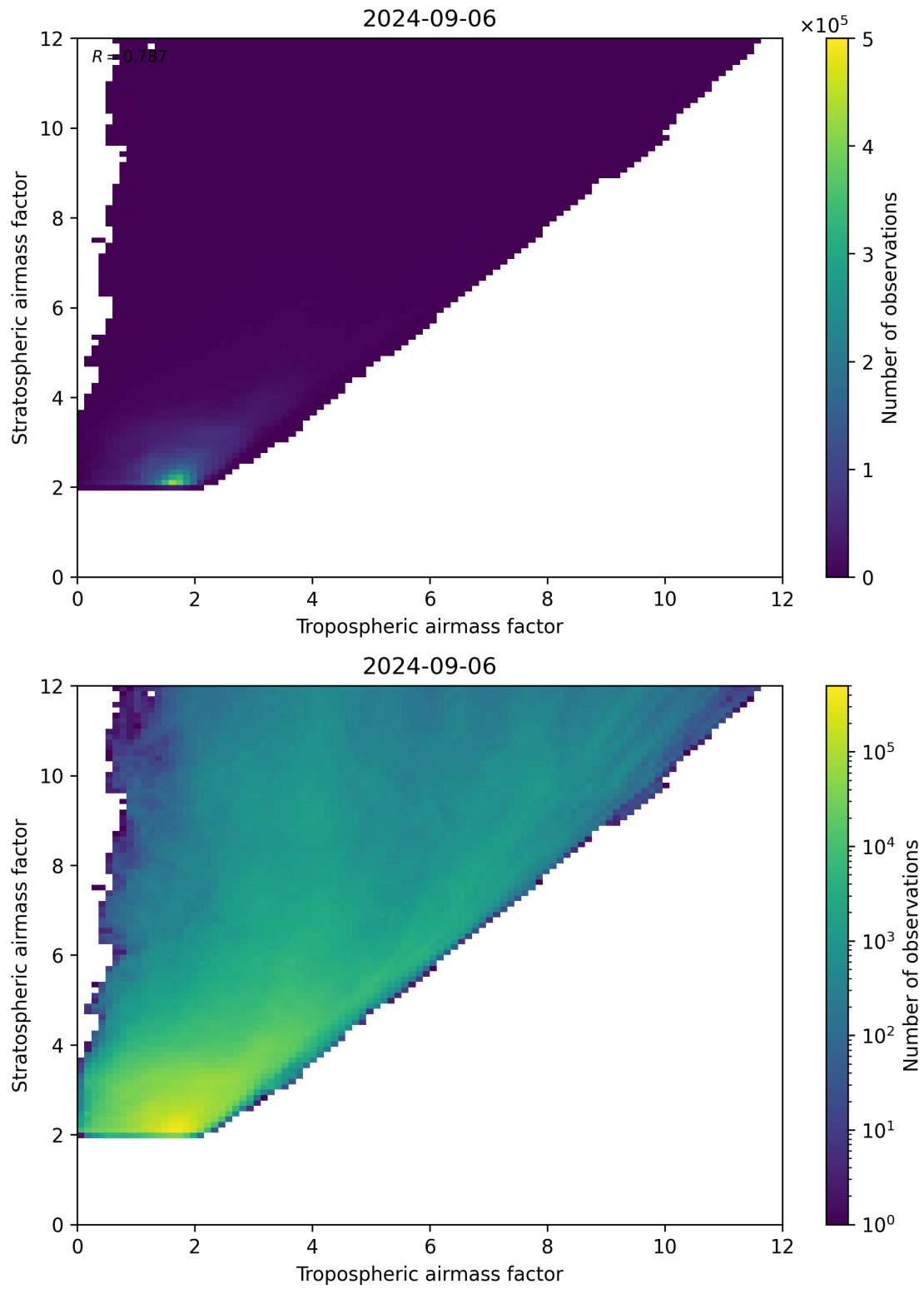
Figure 71: Scatter density plot of “Tropospheric airmass factor” against “Stratospheric airmass factor” for 2024-09-06 to 2024-09-07.
