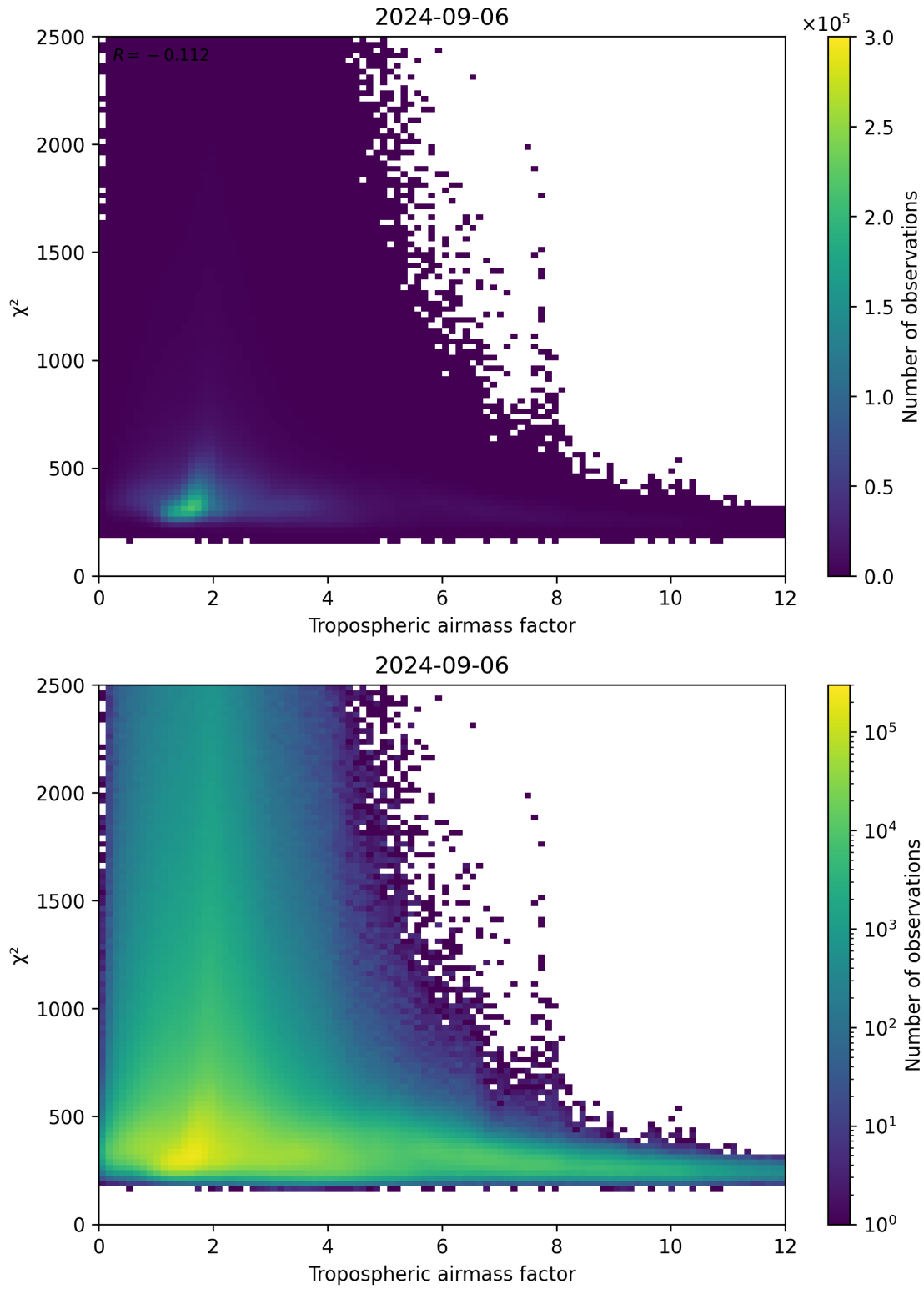
Figure 73: Scatter density plot of “Tropospheric airmass factor” against “ \chi^2 ” for 2024-09-06 to 2024-09-07.
