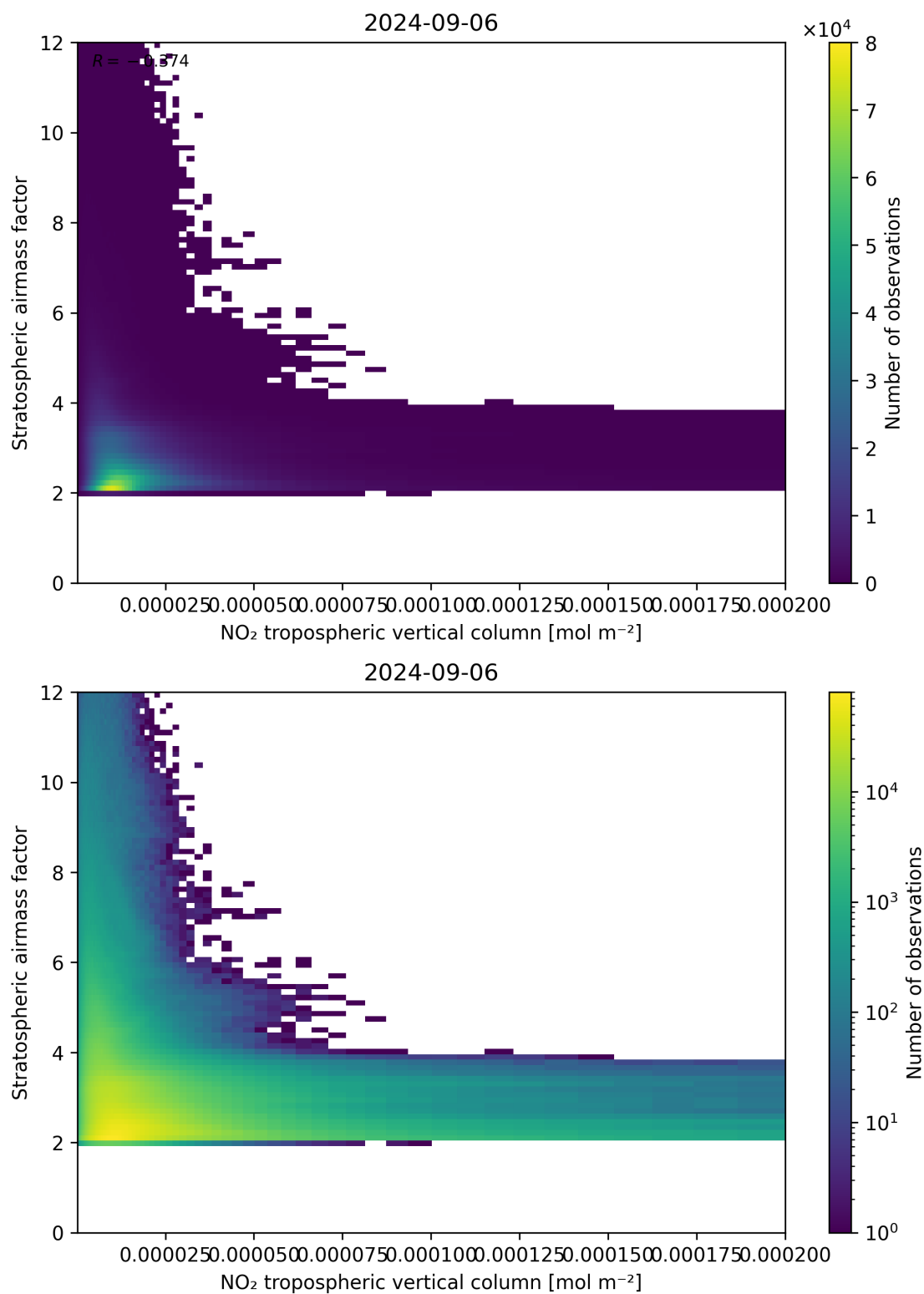
Figure 121: Scatter density plot of “NO 2 tropospheric vertical column” against “Stratospheric airmass factor” for 2024-09-06 to 2024-09-07.
