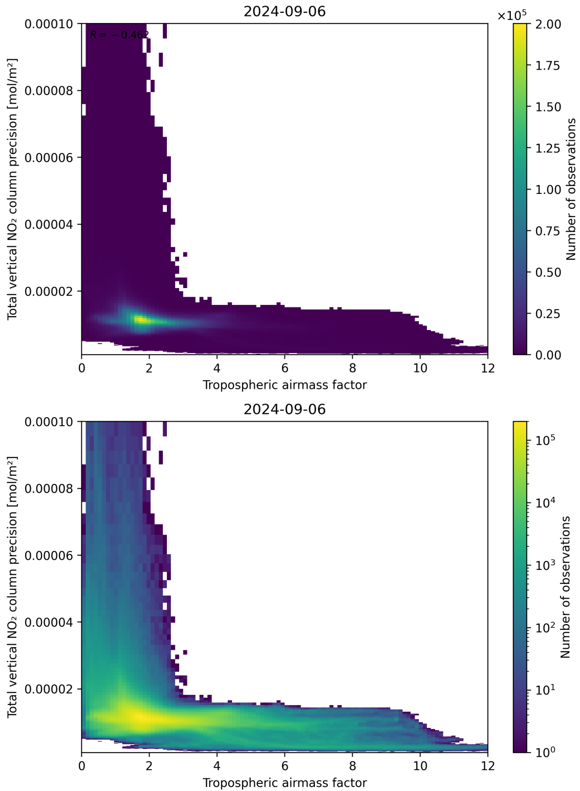
Figure 78: Scatter density plot of “Tropospheric air mass factor” against “Total vertical NO 2 column precision” for 2024-09-06 to 2024-09-07.
