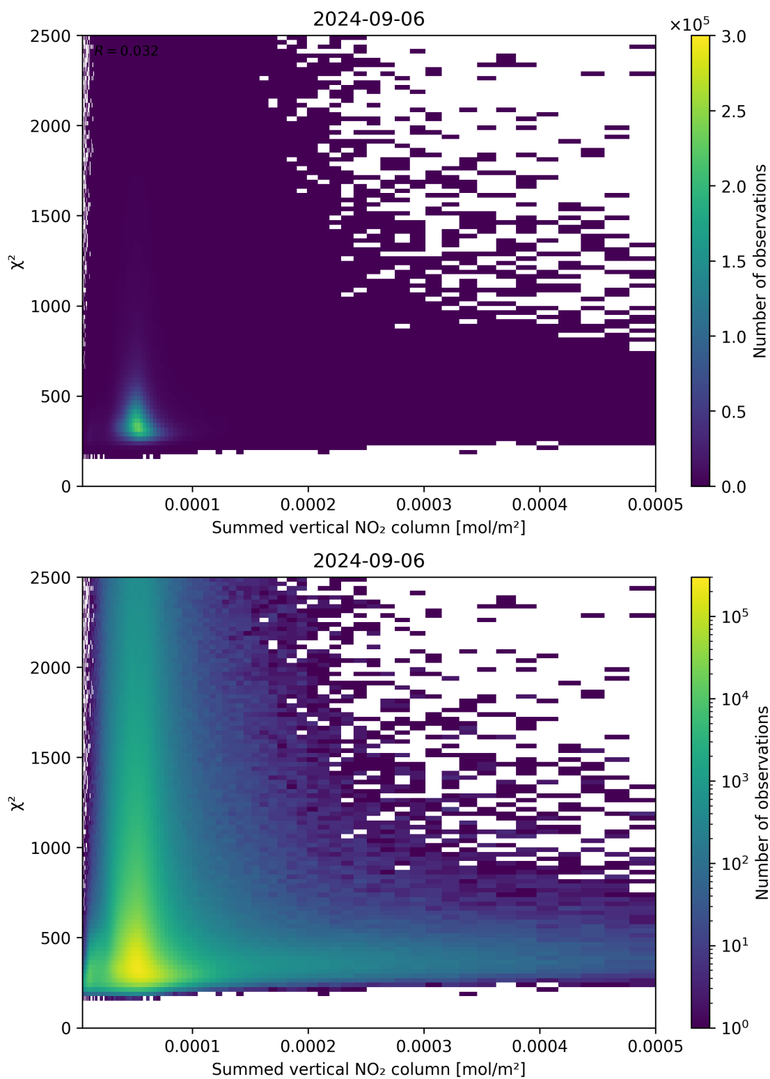
Figure 104: Scatter density plot of “Summed vertical NO 2 column” against “ \chi^2 ” for 2024-09-06 to 2024-09-07.
