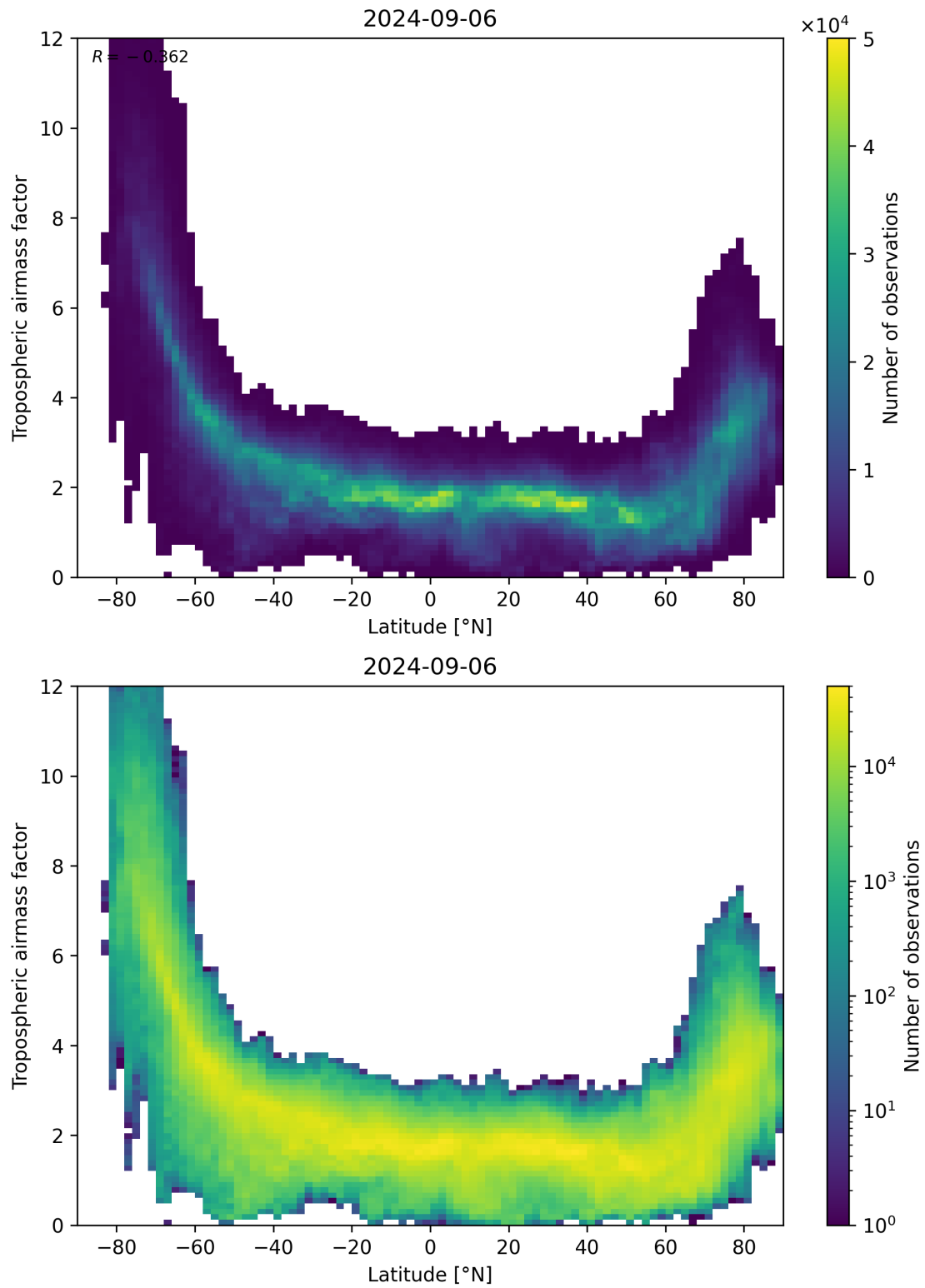
Figure 85: Scatter density plot of “Latitude” against “Tropospheric airmass factor” for 2024-09-06 to 2024-09-07.
