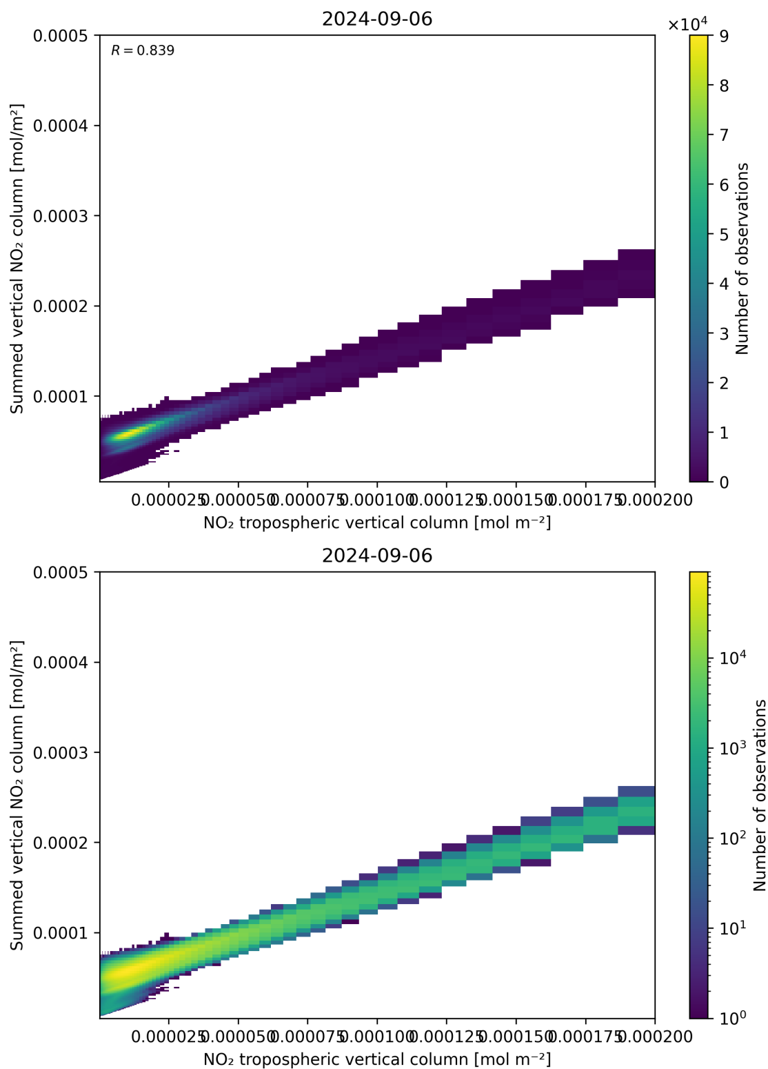
Figure 126: Scatter density plot of “NO 2 tropospheric vertical column” against “Summed vertical NO 2 column” for 2024-09-06 to 2024-09-07.
