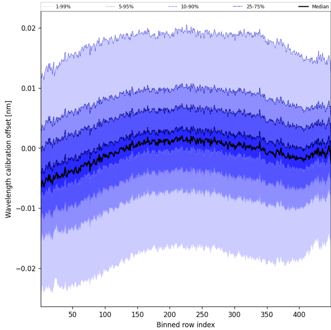
Figure 52: Along track statistics of “Wavelength calibration offset” for 2024-09-06 to 2024-09-07
