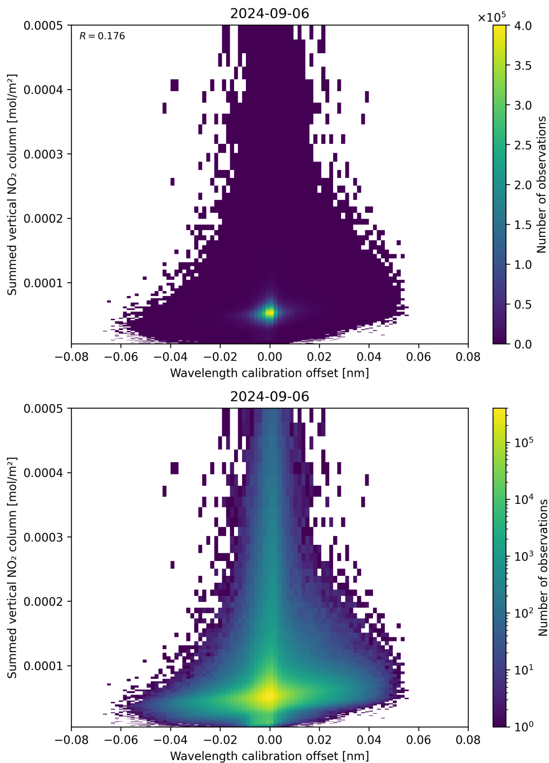
Figure 177: Scatter density plot of “Wavelength calibration offset” against “Summed vertical NO 2 column” for 2024-09-06 to 2024-09-07.
