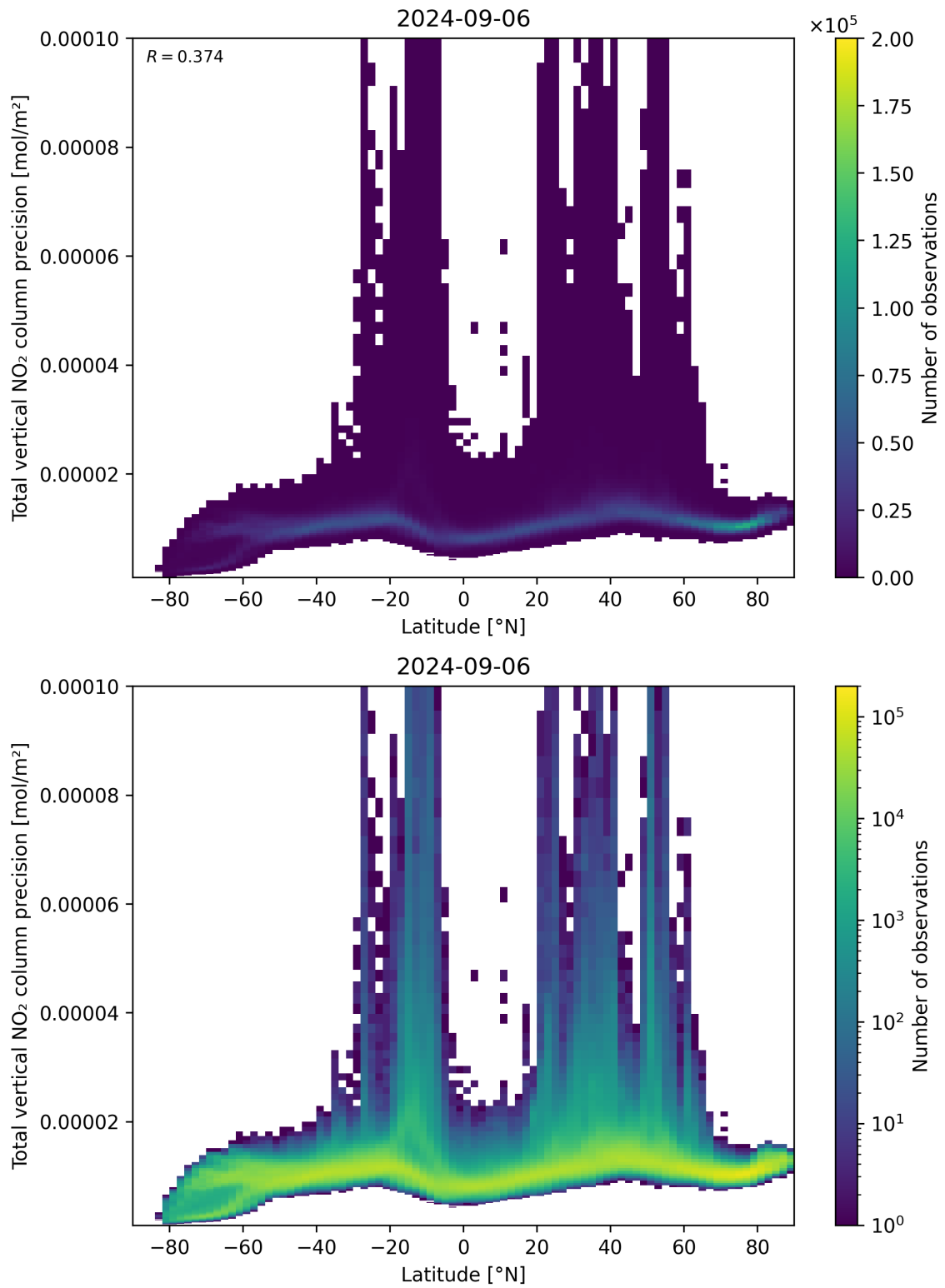
Figure 91: Scatter density plot of “Latitude” against “Total vertical NO 2 column precision” for 2024-09-06 to 2024-09-07.
