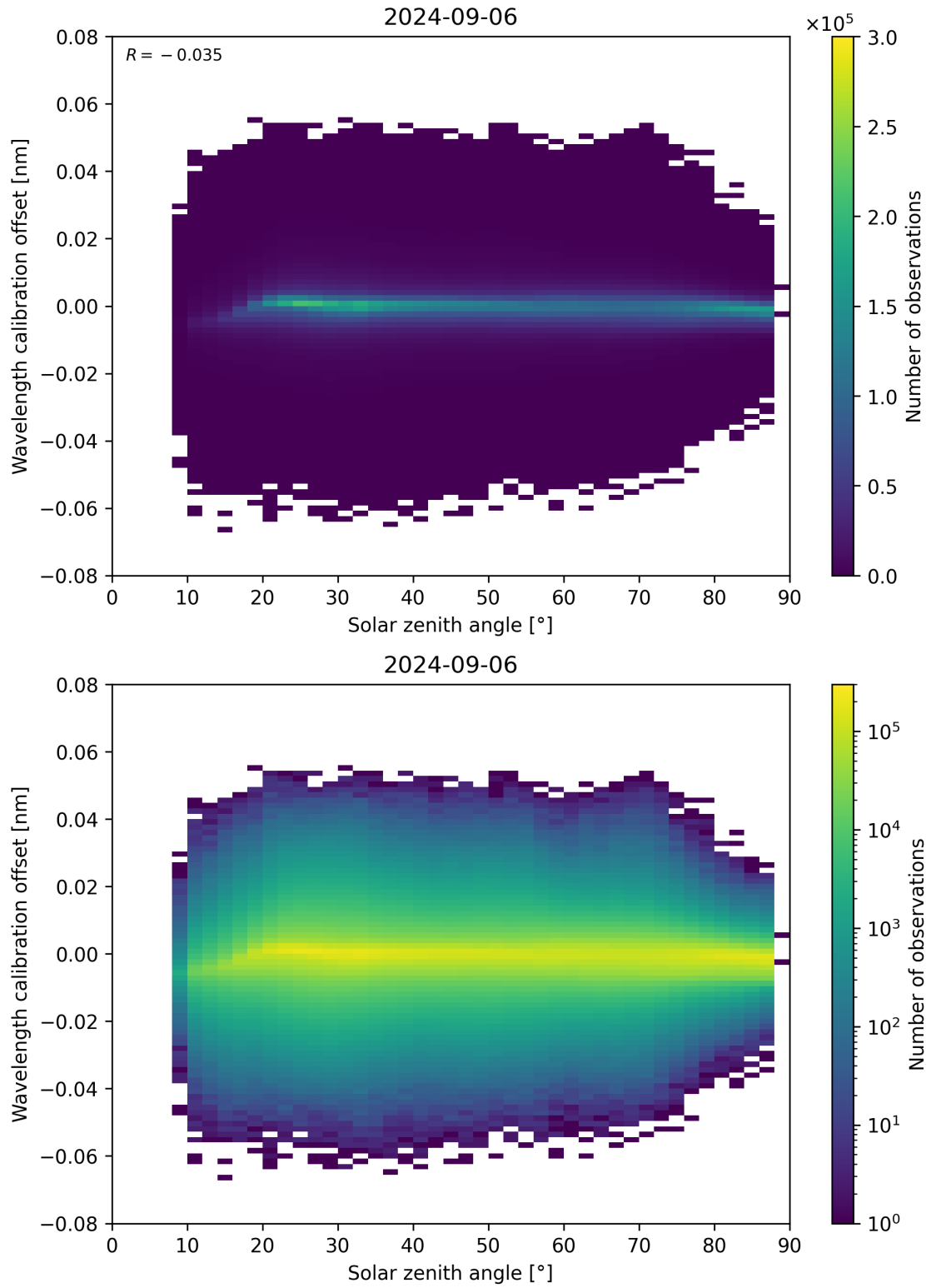
Figure 158: Scatter density plot of “Solar zenith angle” against “Wavelength calibration offset” for 2024-09-06 to 2024-09-07.
