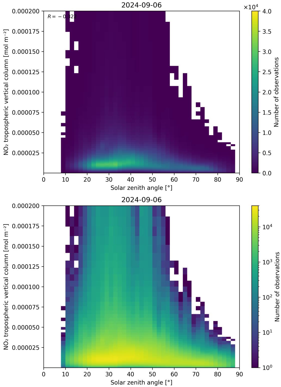
Figure 155: Scatter density plot of “Solar zenith angle” against “NO 2 tropospheric vertical column” for 2024-09-06 to 2024-09-07.
