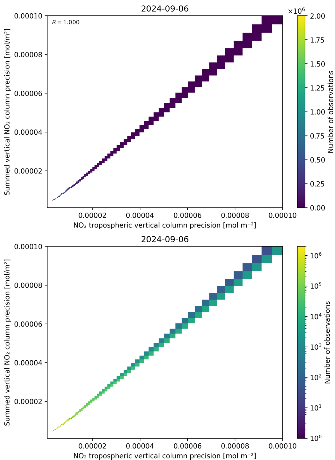
Figure 137: Scatter density plot of “NO 2 tropospheric vertical column precision” against “Summed vertical NO 2 column precision” for 2024-09-06 to 2024-09-07.
