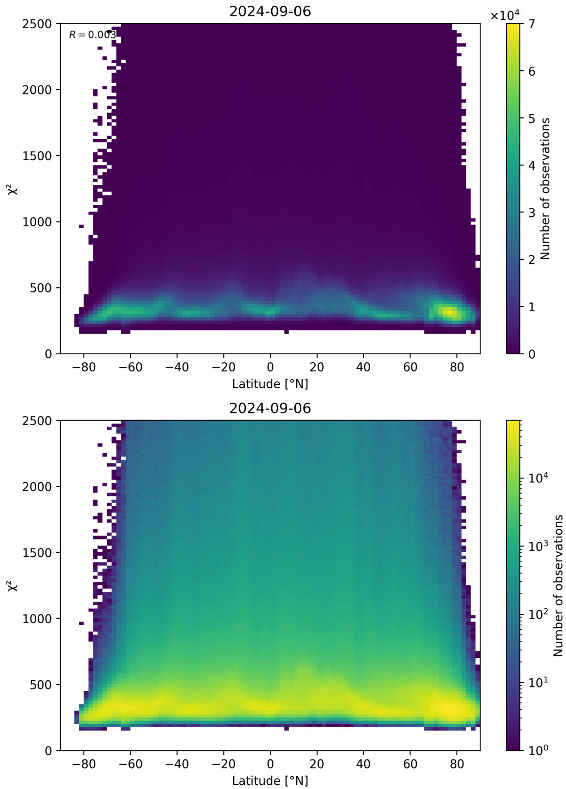
Figure 86: Scatter density plot of “Latitude” against “ \chi^2 ” for 2024-09-06 to 2024-09-07.
