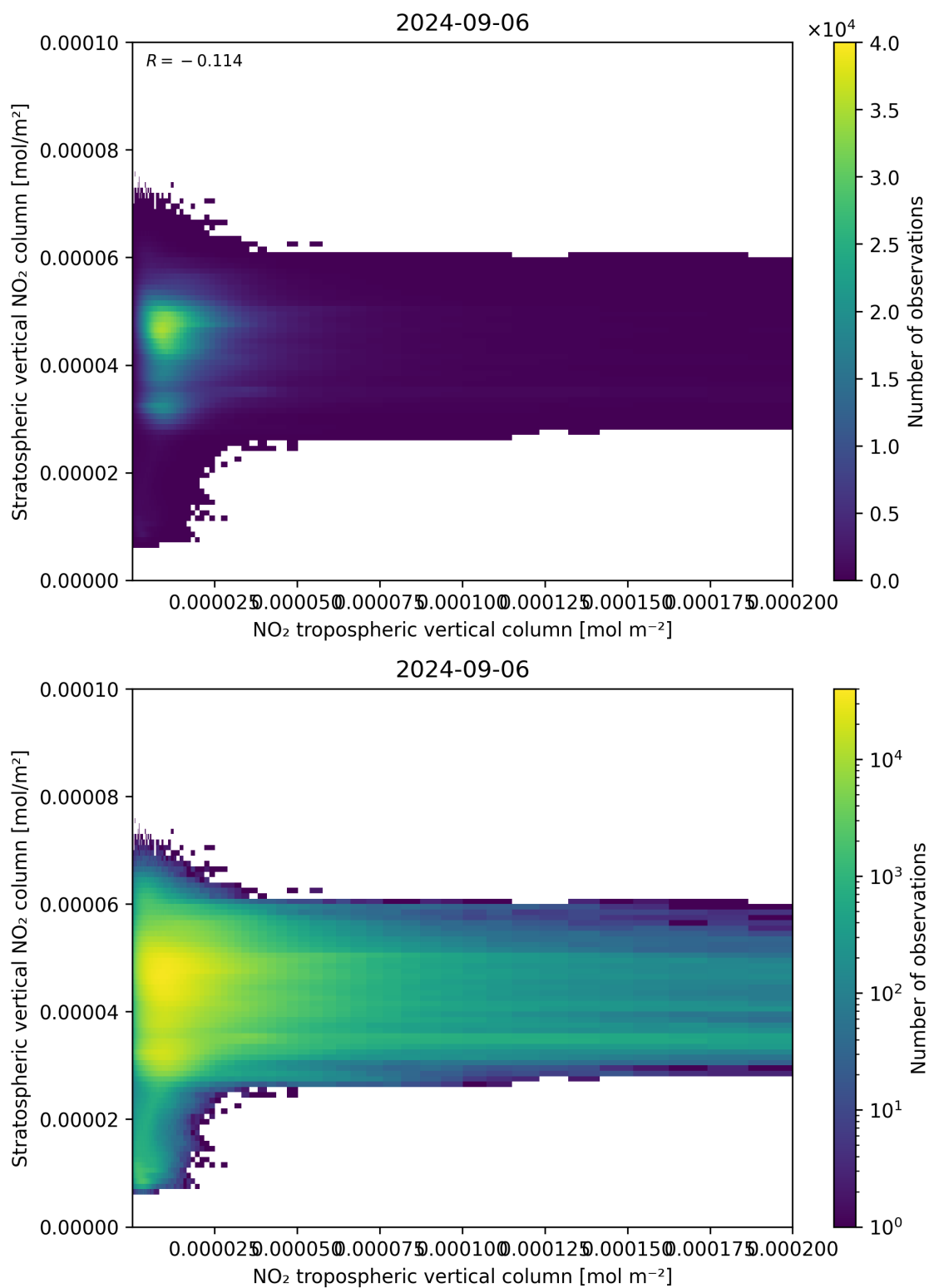
Figure 125: Scatter density plot of “NO 2 tropospheric vertical column” against “Stratospheric vertical NO 2 column” for 2024-09-06 to 2024-09-07.
