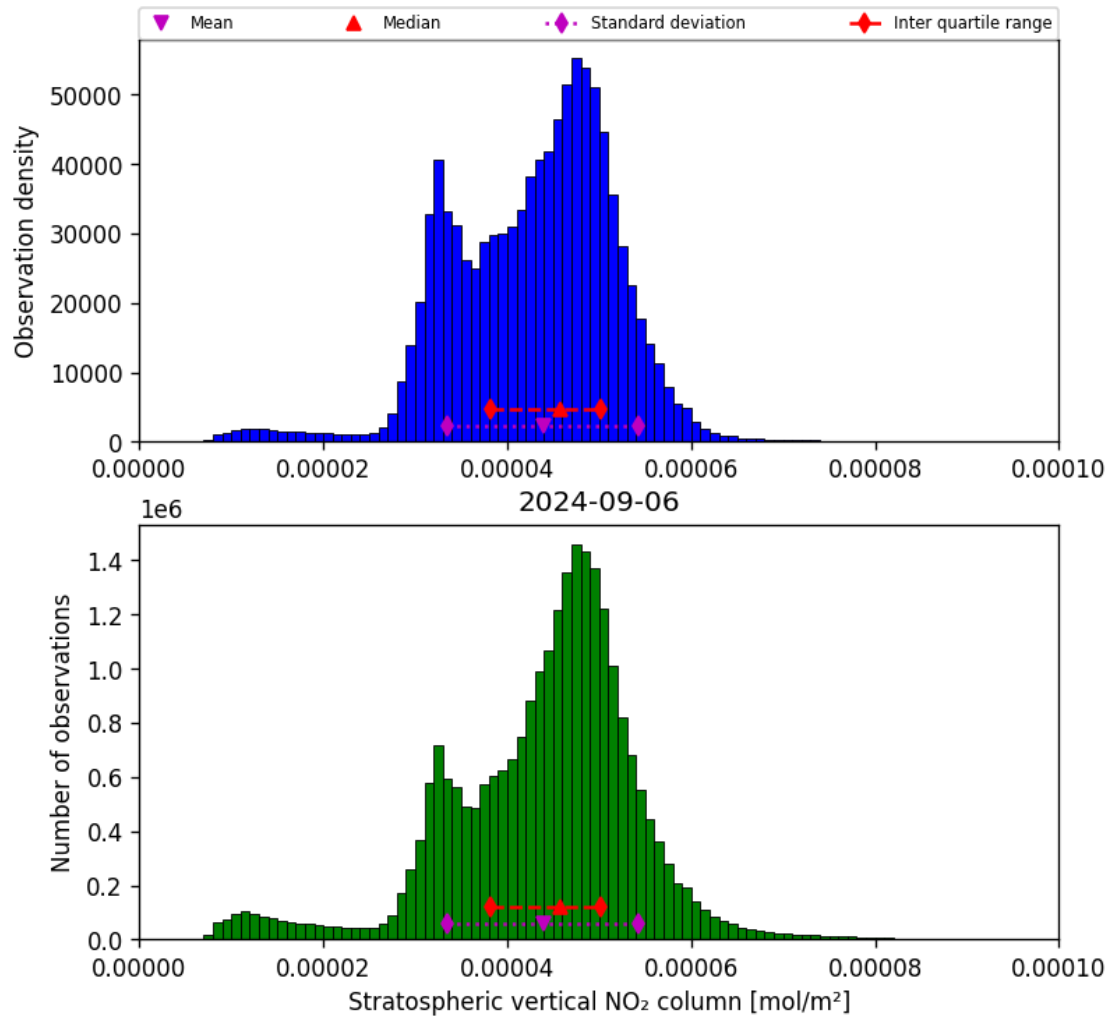
Figure 36: Histogram of “Stratospheric vertical NO 2 column” for 2024-09-06 to 2024-09-07
