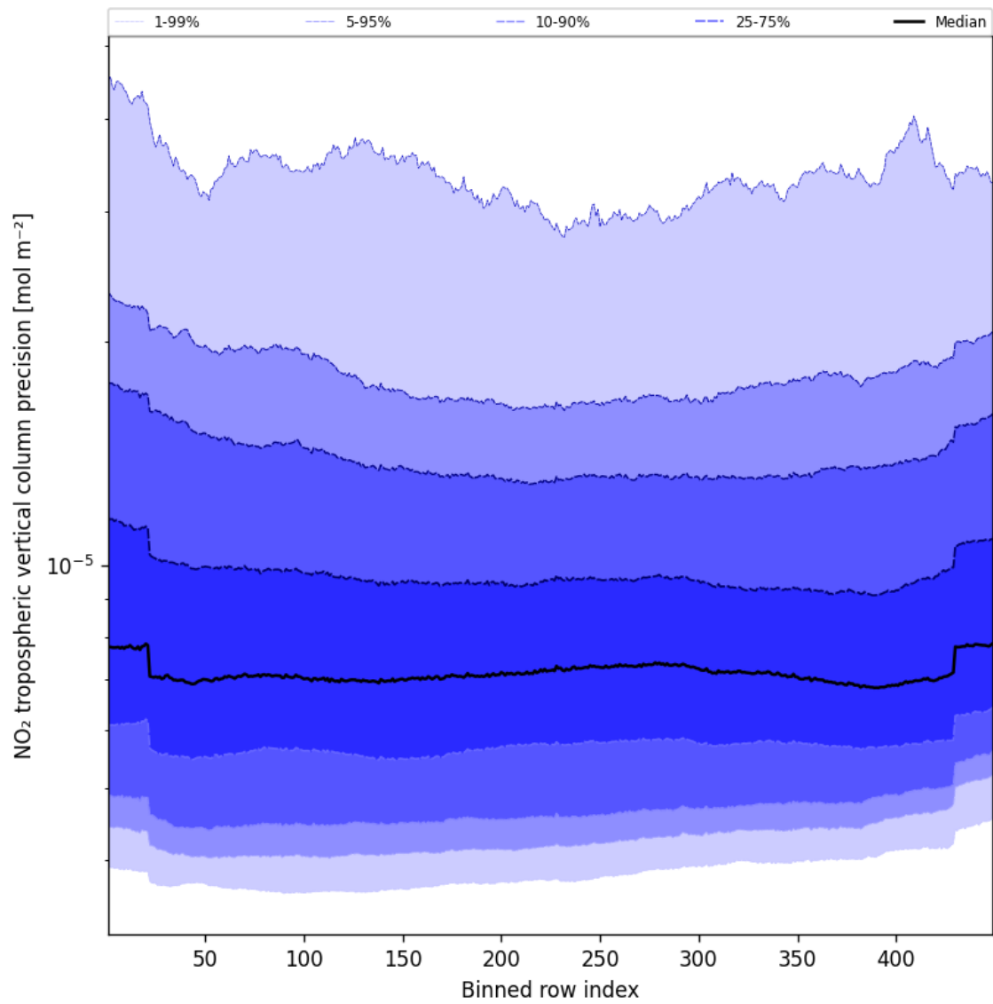
Figure 47: Along track statistics of “NO 2 tropospheric vertical column precision” for 2024-09-06 to 2024-09-07
