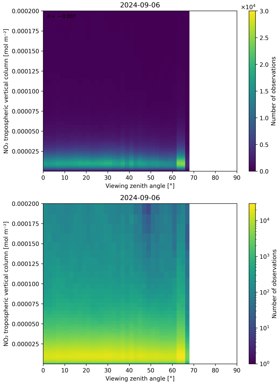
Figure 169: Scatter density plot of “Viewing zenith angle” against “NO 2 tropospheric vertical column” for 2024-09-06 to 2024-09-07.
