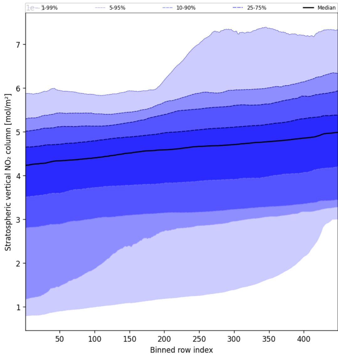
Figure 53: Along track statistics of “Stratospheric vertical NO 2 column” for 2024-09-06 to 2024-09-07
