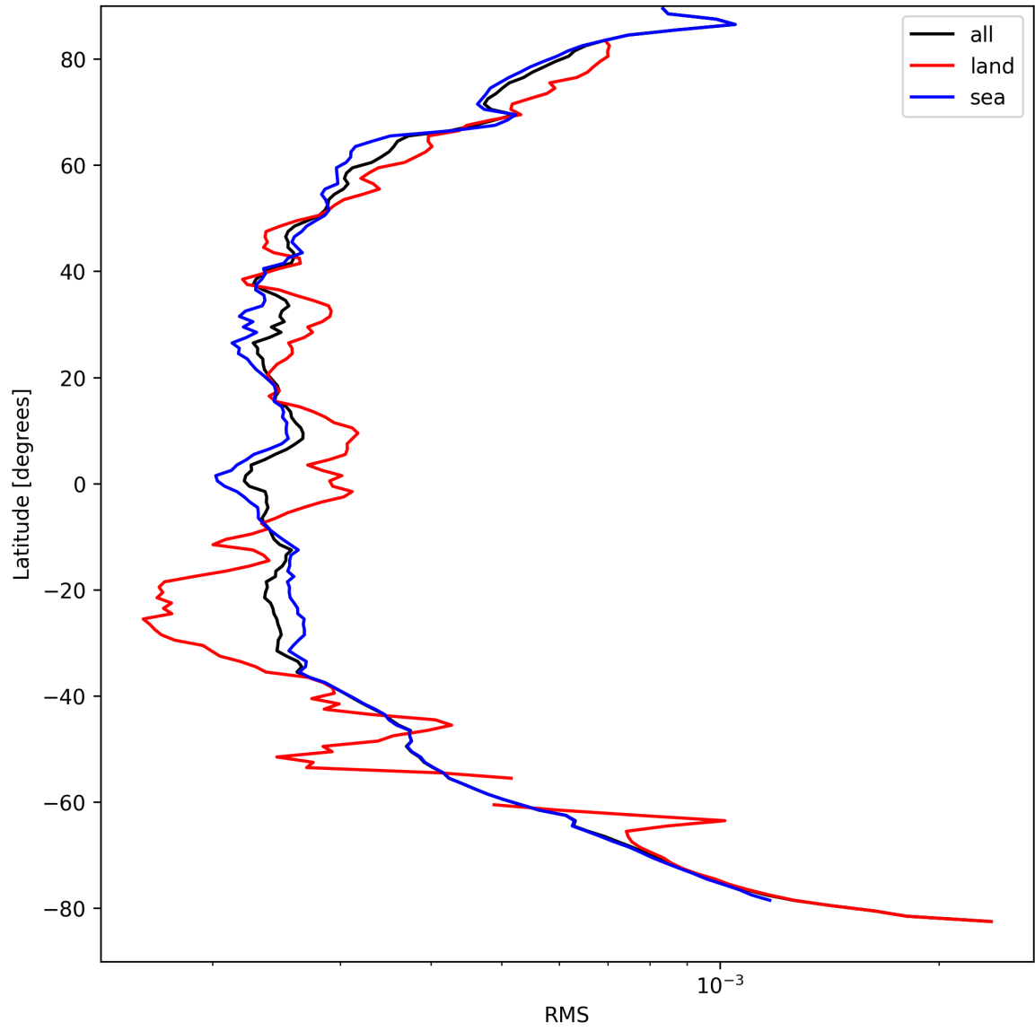
Figure 26: Zonal average of “RMS” for 2024-09-06 to 2024-09-07.
