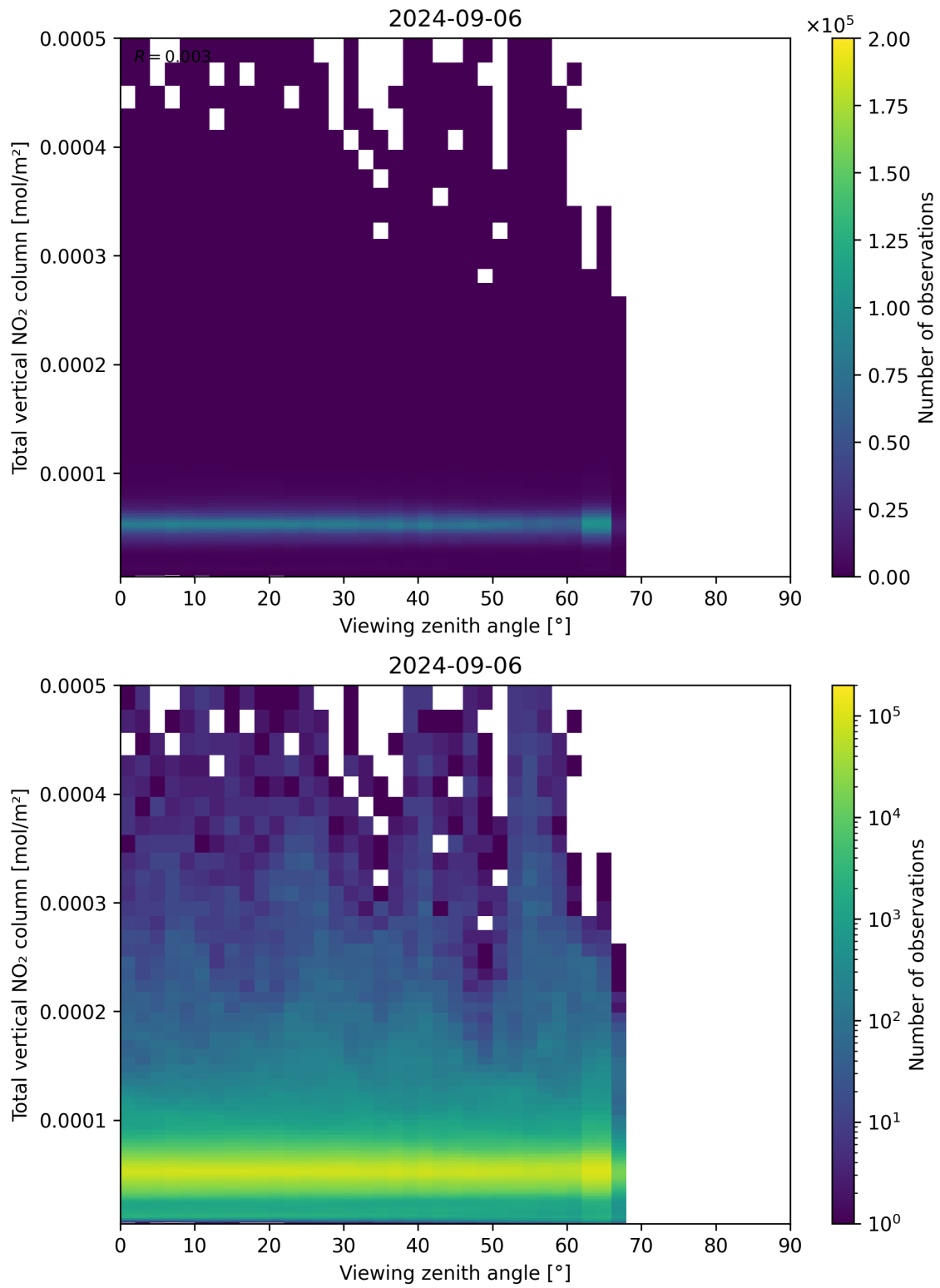
Figure 167: Scatter density plot of “Viewing zenith angle” against “Total vertical NO 2 column” for 2024-09-06 to 2024-09-07.
