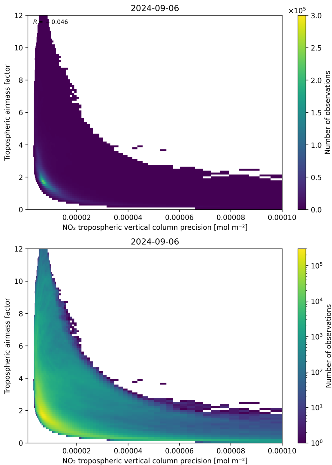
Figure 133: Scatter density plot of “NO 2 tropospheric vertical column precision” against “Tropospheric air mass factor” for 2024-09-06 to 2024-09-07.
