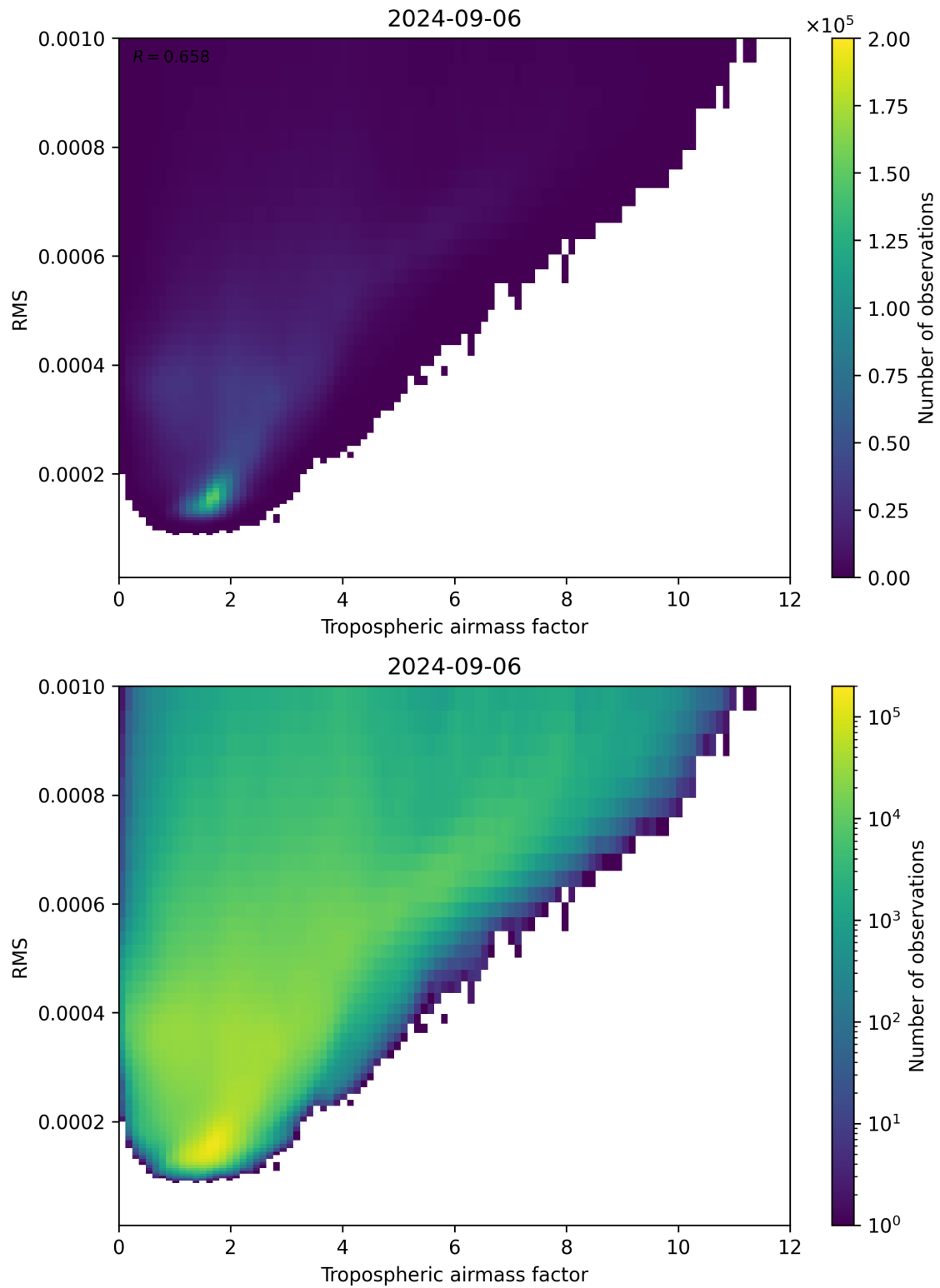
Figure 79: Scatter density plot of “Tropospheric airmass factor” against “RMS” for 2024-09-06 to 2024-09-07.
