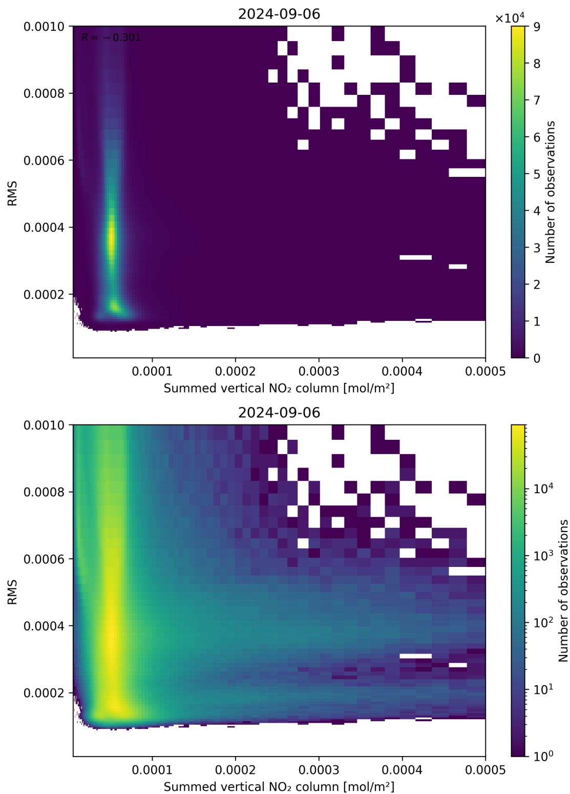
Figure 109: Scatter density plot of “Summed vertical NO 2 column” against “RMS” for 2024-09-06 to 2024-09-07.
