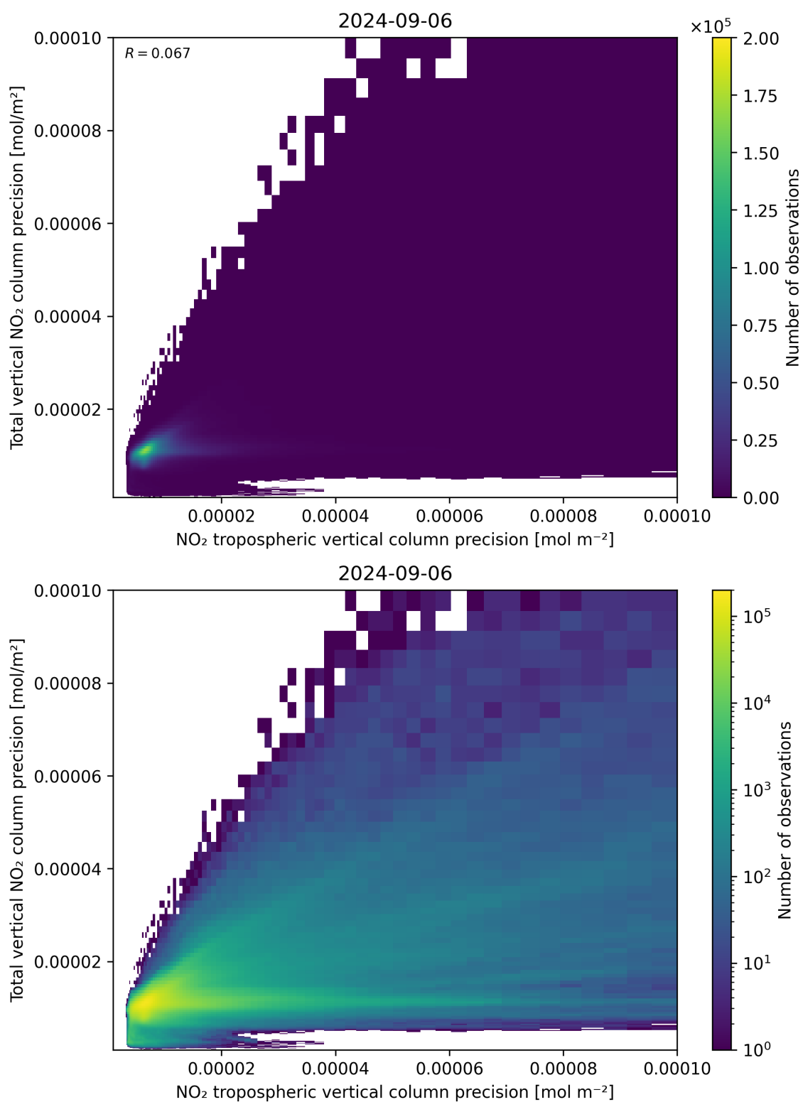
Figure 139: Scatter density plot of “NO 2 tropospheric vertical column precision” against “Total vertical NO 2 column precision” for 2024-09-06 to 2024-09-07.
