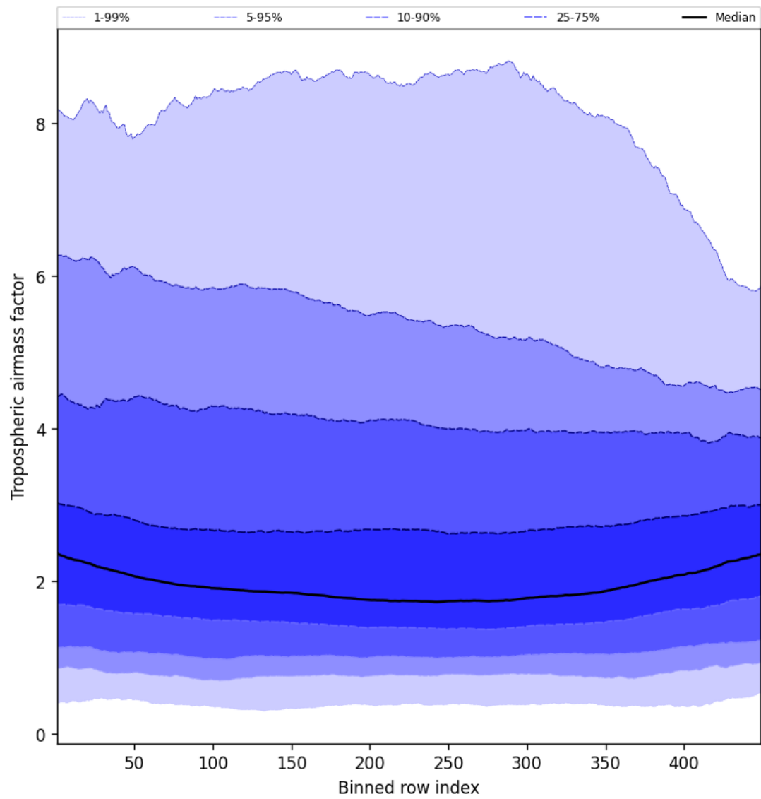
Figure 48: Along track statistics of “Tropospheric air mass factor” for 2024-09-06 to 2024-09-07
