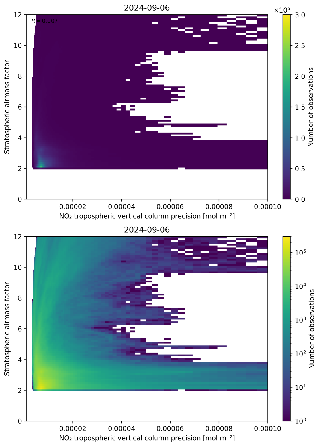
Figure 131: Scatter density plot of “NO 2 tropospheric vertical column precision” against “Stratospheric airmass factor” for 2024-09-06 to 2024-09-07.
