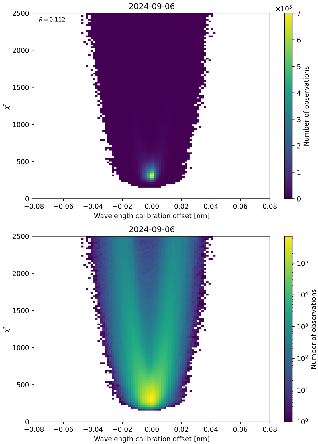
Figure 175: Scatter density plot of “Wavelength calibration offset” against “ \chi^2 ” for 2024-09-06 to 2024-09-07.
