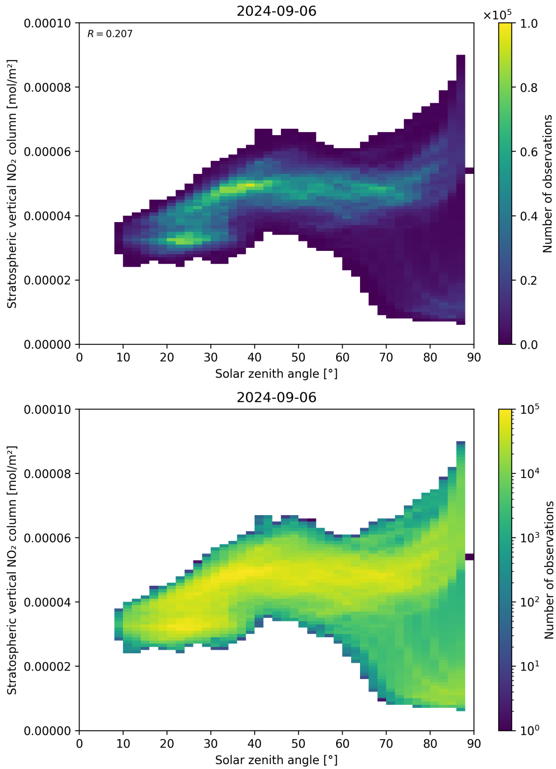
Figure 150: Scatter density plot of “Solar zenith angle” against “Stratospheric vertical \text{NO}_2 column” for 2024-09-06 to 2024-09-07.
