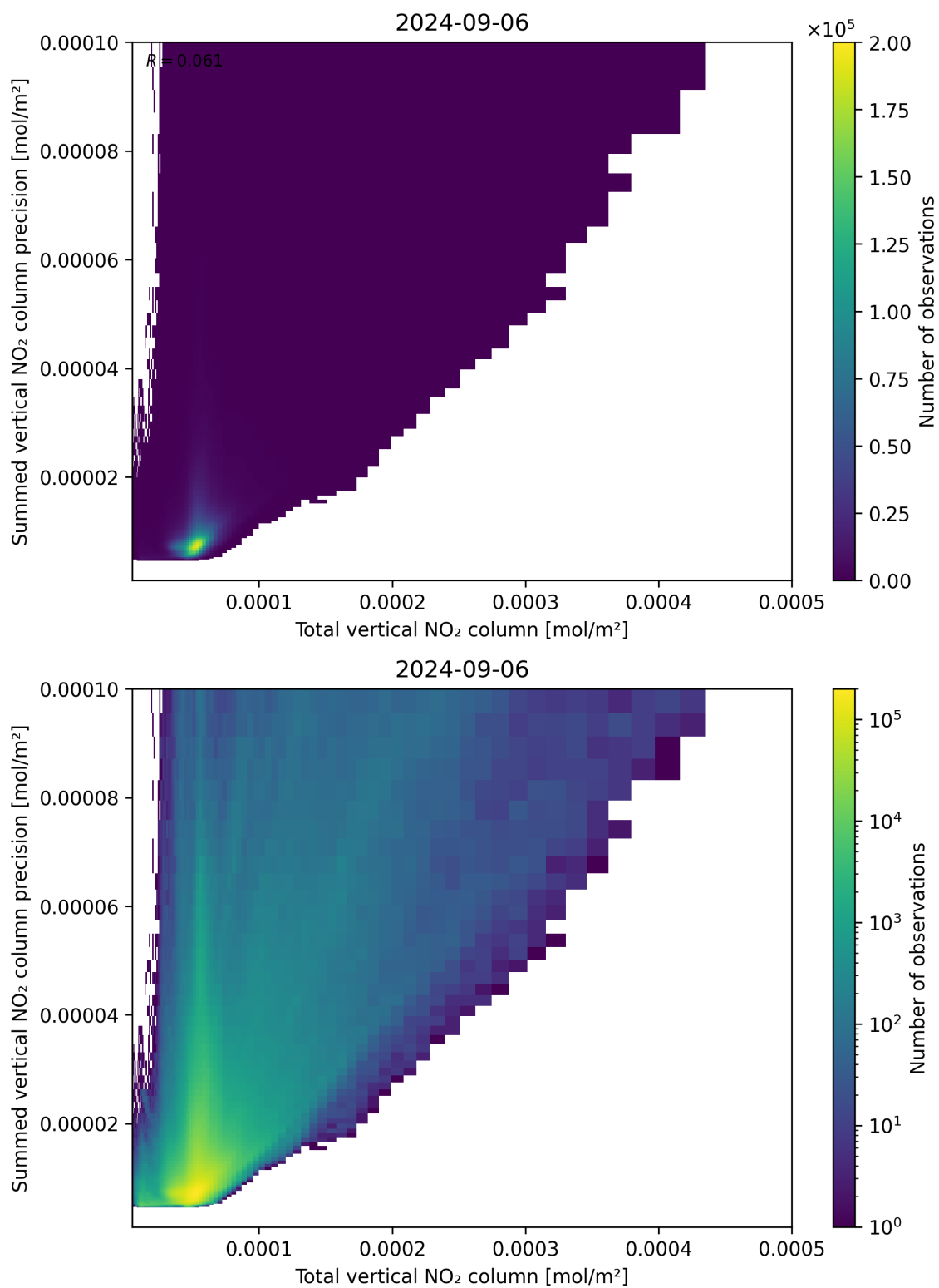
Figure 113: Scatter density plot of “Total vertical NO 2 column” against “Summed vertical NO 2 column precision” for 2024-09-06 to 2024-09-07.
