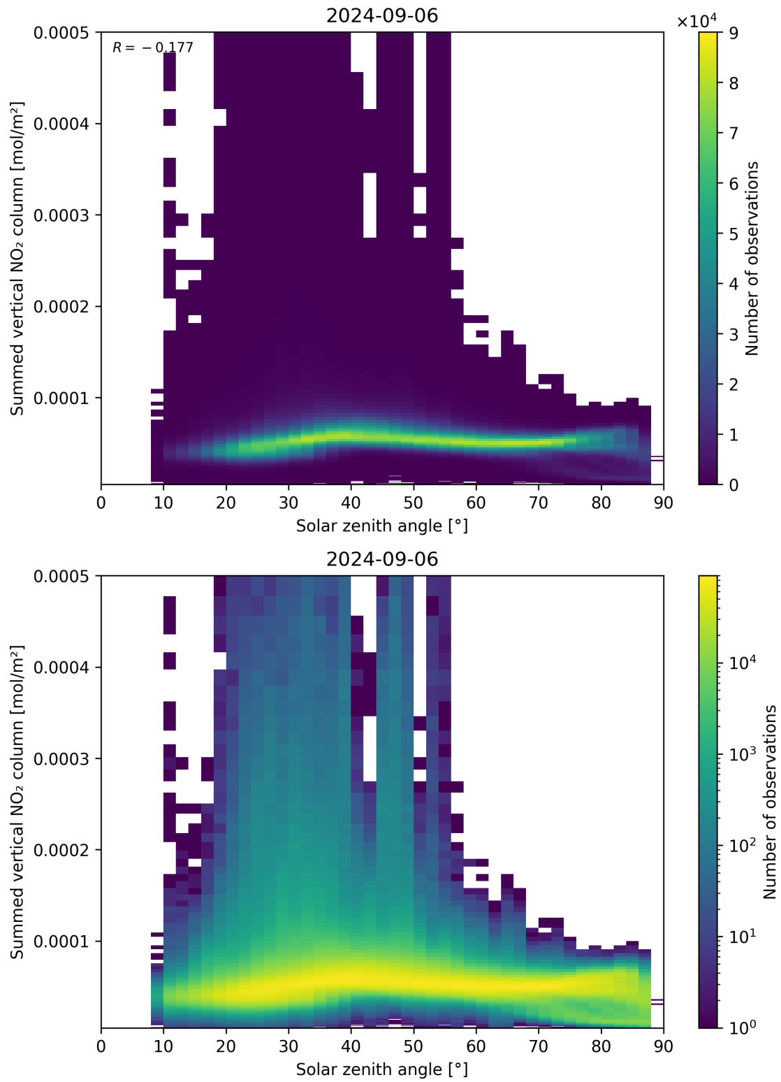
Figure 151: Scatter density plot of “Solar zenith angle” against “Summed vertical NO 2 column” for 2024-09-06 to 2024-09-07.
