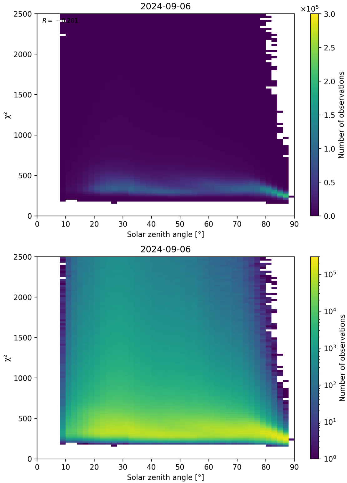
Figure 148: Scatter density plot of “Solar zenith angle” against “ \chi^2 ” for 2024-09-06 to 2024-09-07.
