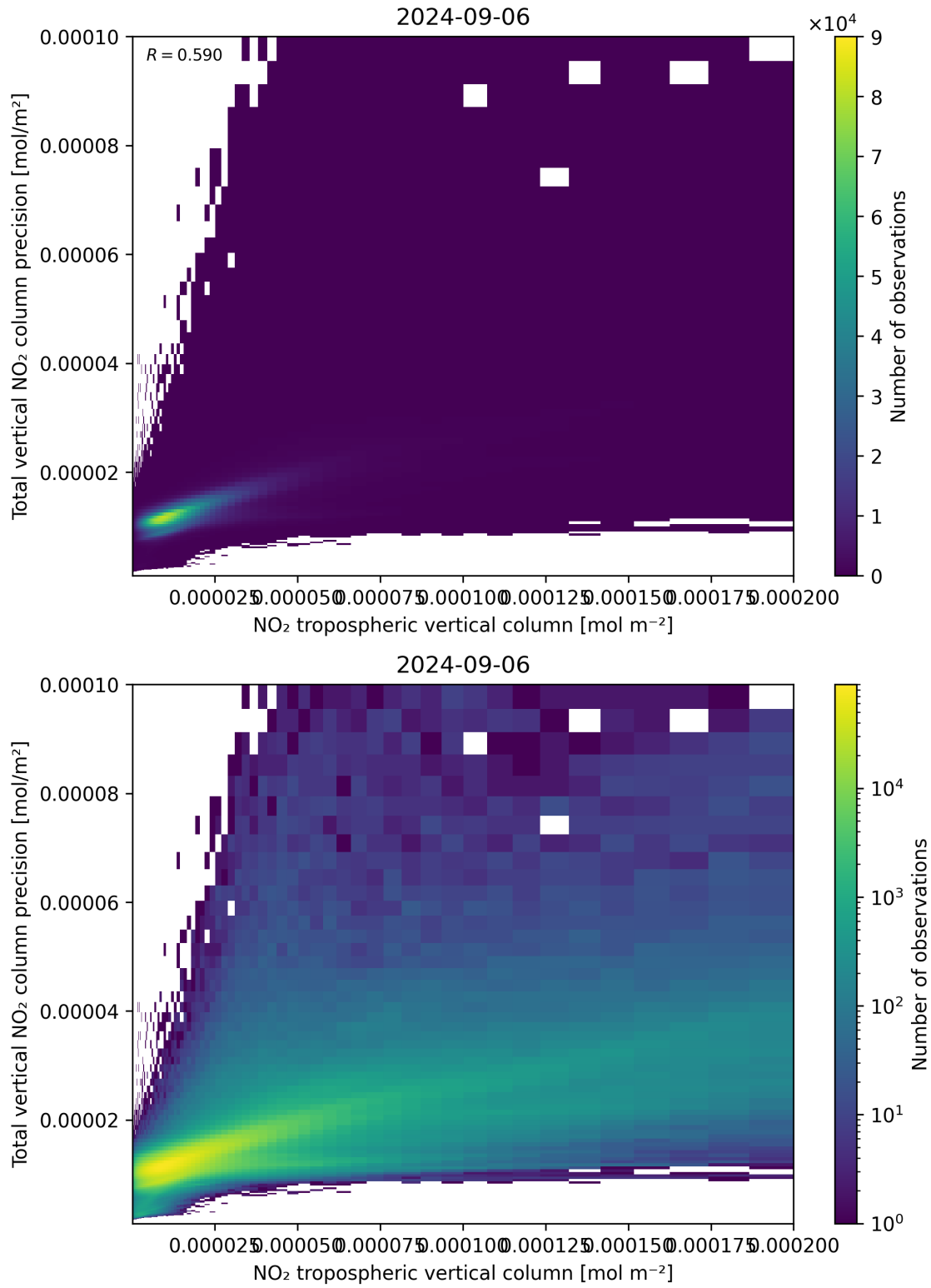
Figure 129: Scatter density plot of “NO 2 tropospheric vertical column” against “Total vertical NO 2 column precision” for 2024-09-06 to 2024-09-07.
