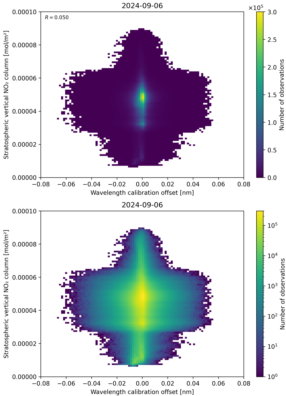
Figure 176: Scatter density plot of “Wavelength calibration offset” against “Stratospheric vertical NO 2 column” for 2024-09-06 to 2024-09-07.
