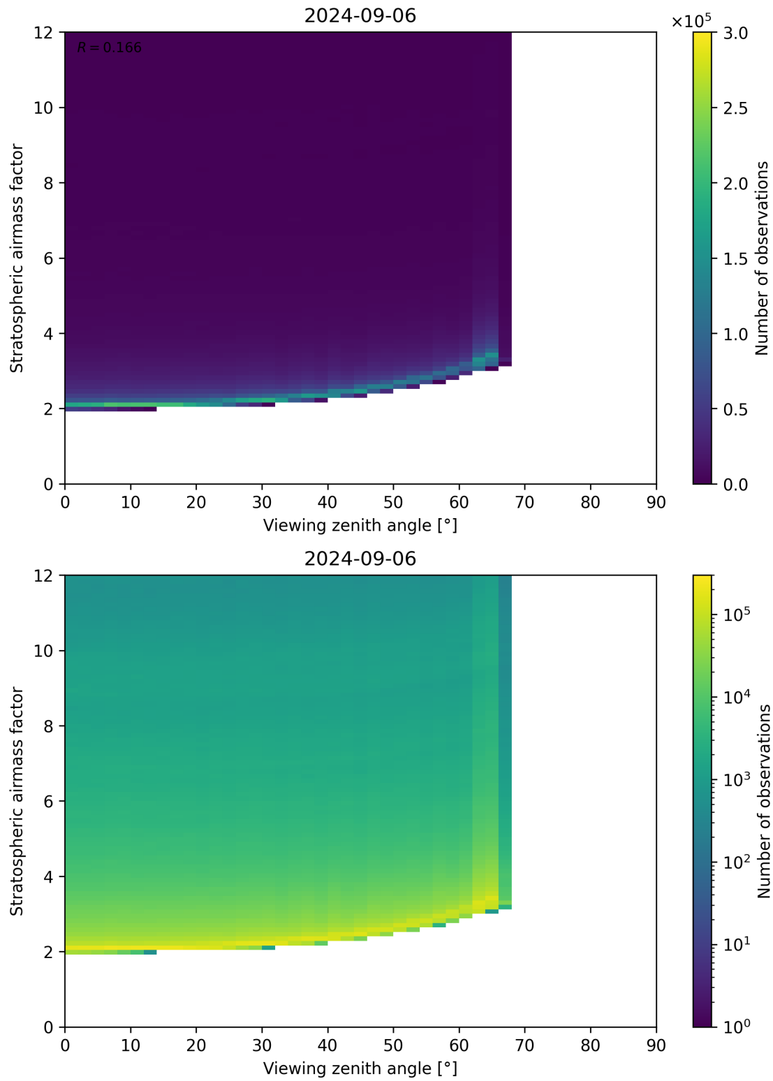
Figure 159: Scatter density plot of “Viewing zenith angle” against “Stratospheric airmass factor” for 2024-09-06 to 2024-09-07.
