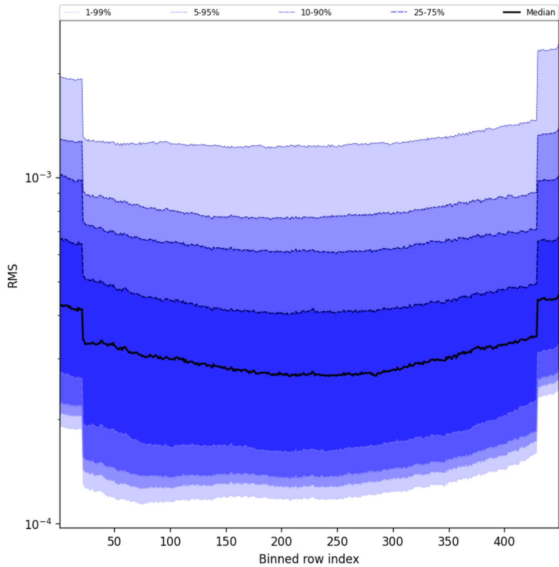
Figure 60: Along track statistics of “RMS” for 2024-09-06 to 2024-09-07
