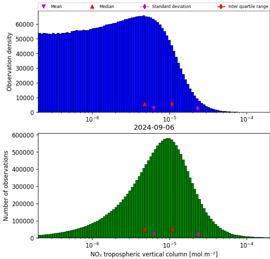
Figure 29: Histogram of “NO 2 tropospheric vertical column” for 2024-09-06 to 2024-09-07
