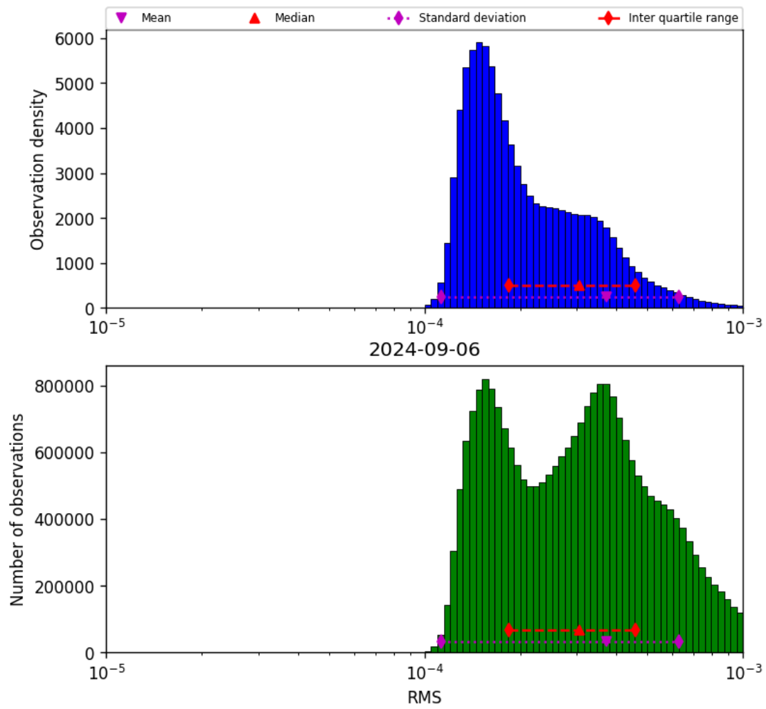
Figure 43: Histogram of “RMS” for 2024-09-06 to 2024-09-07
