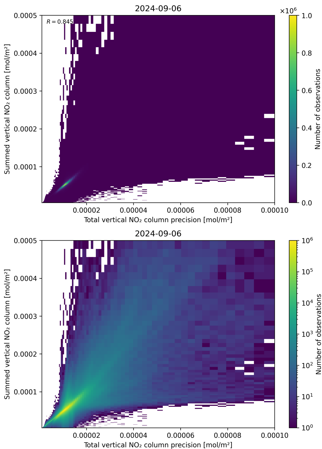
Figure 117: Scatter density plot of “Total vertical NO 2 column precision” against “Summed vertical NO 2 column” for 2024-09-06 to 2024-09-07.
