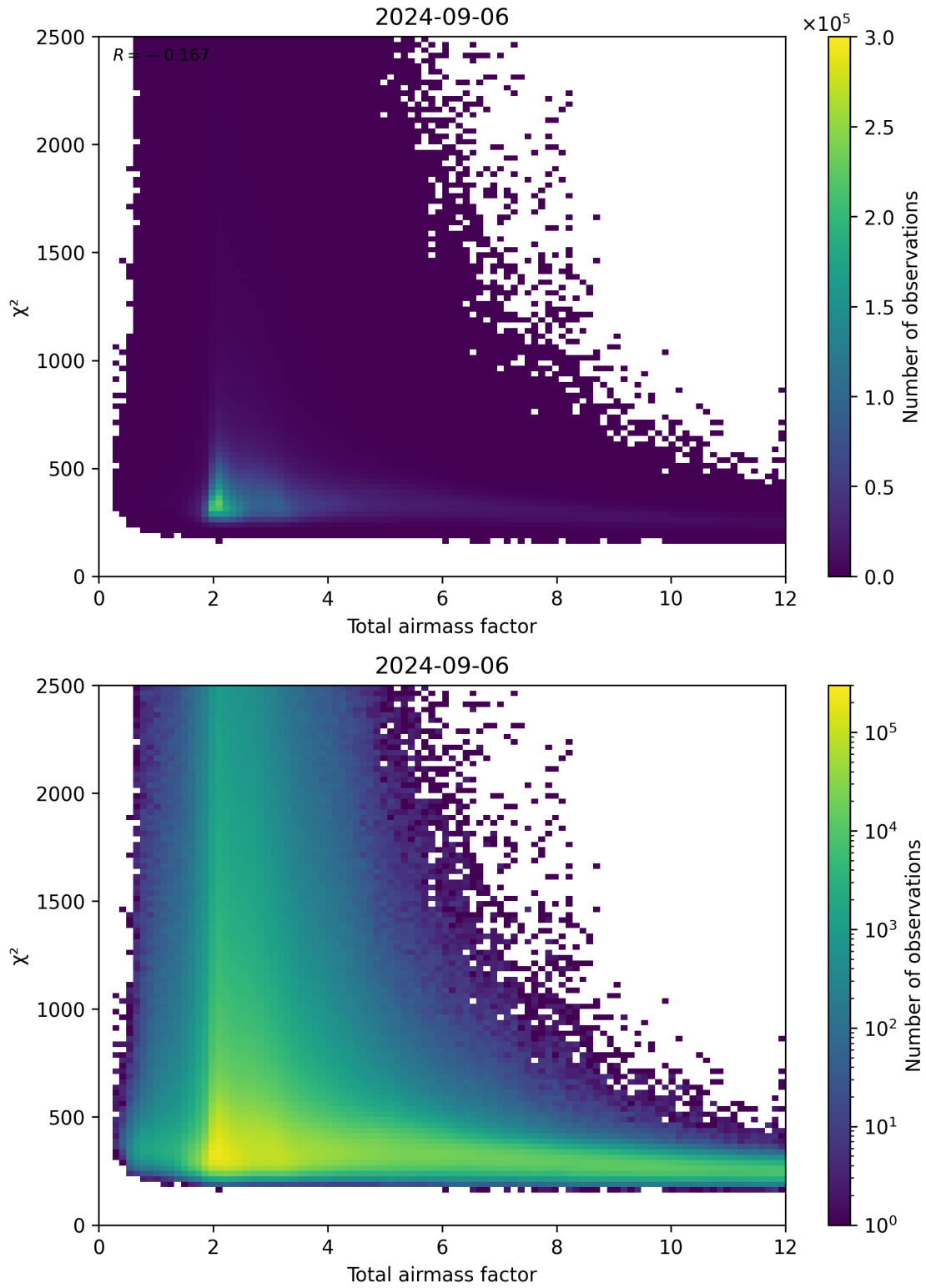
Figure 63: Scatter density plot of “Total airmass factor” against “ \chi^2 ” for 2024-09-06 to 2024-09-07.
