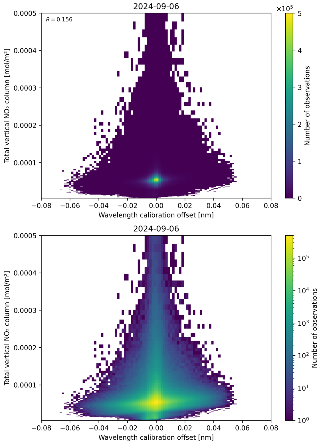
Figure 179: Scatter density plot of “Wavelength calibration offset” against “Total vertical NO 2 column” for 2024-09-06 to 2024-09-07.
