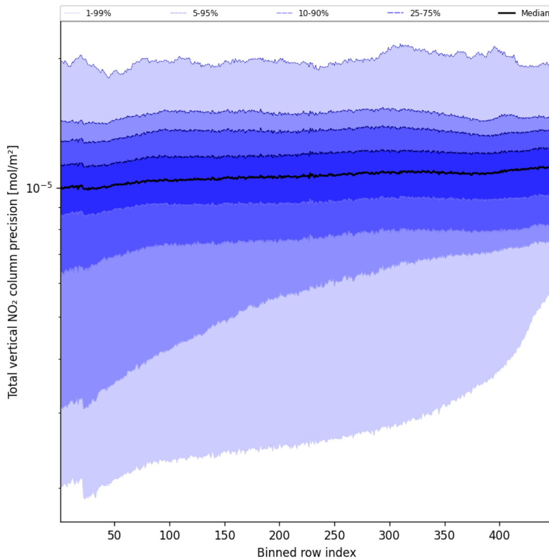
Figure 56: Along track statistics of “Total vertical NO 2 column precision” for 2024-09-06 to 2024-09-07
