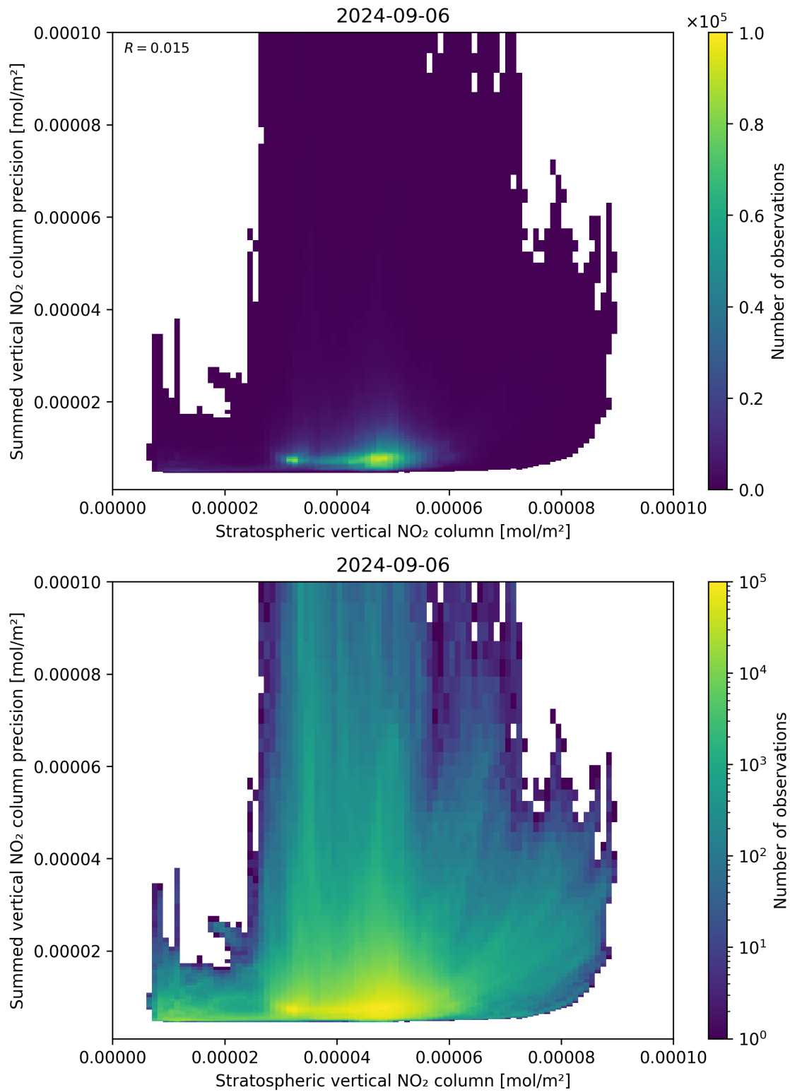
Figure 99: Scatter density plot of “Stratospheric vertical NO 2 column” against “Summed vertical NO 2 column precision” for 2024-09-06 to 2024-09-07.
