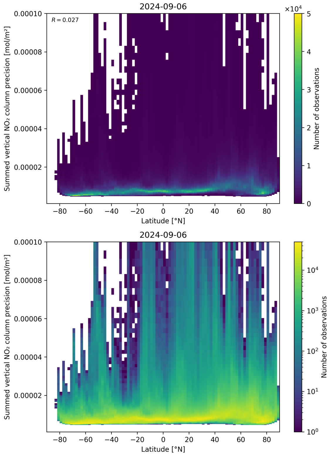
Figure 89: Scatter density plot of “Latitude” against “Summed vertical NO 2 column precision” for 2024-09-06 to 2024-09-07.
