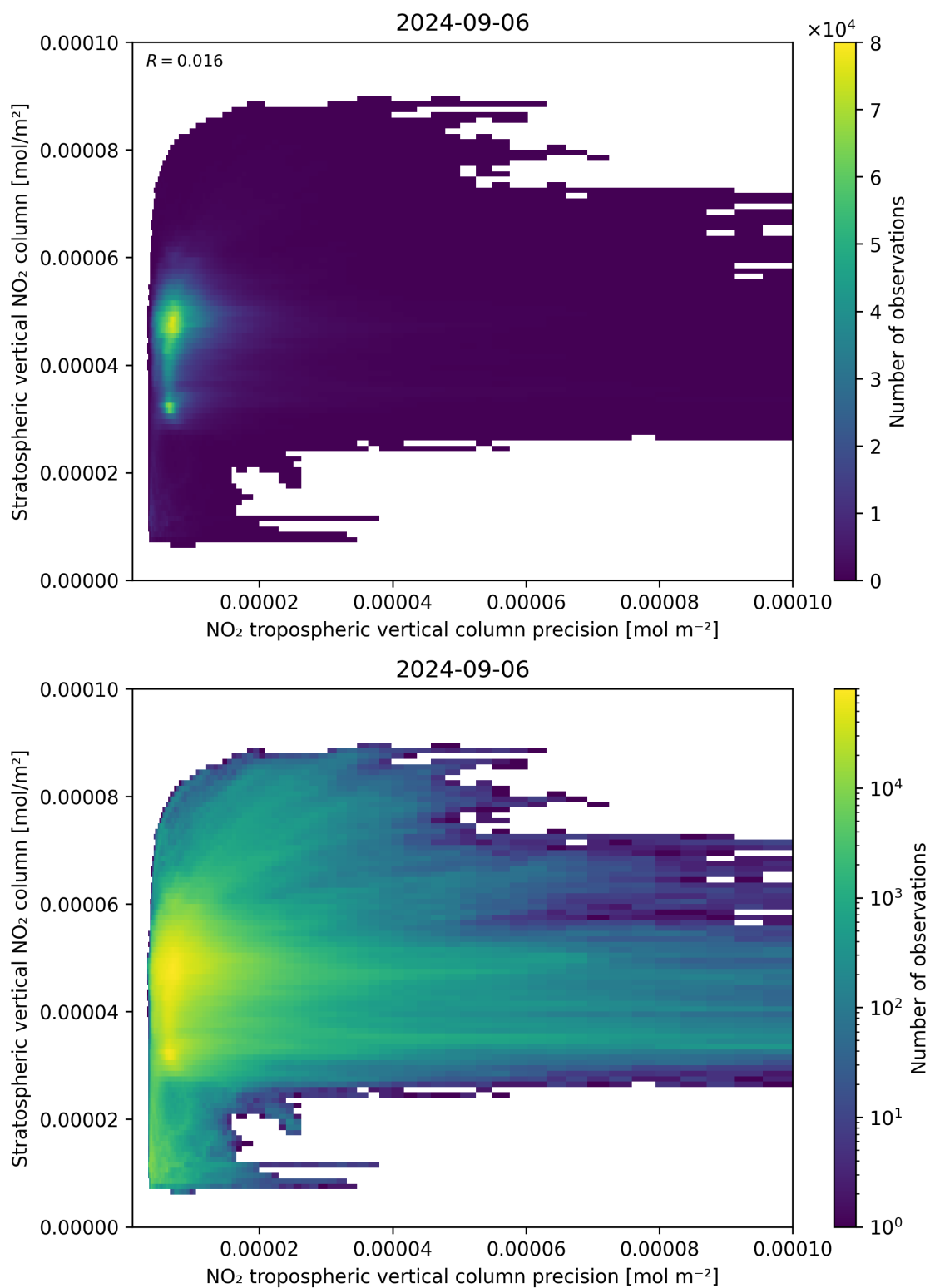
Figure 135: Scatter density plot of “NO 2 tropospheric vertical column precision” against “Stratospheric vertical NO 2 column” for 2024-09-06 to 2024-09-07.
