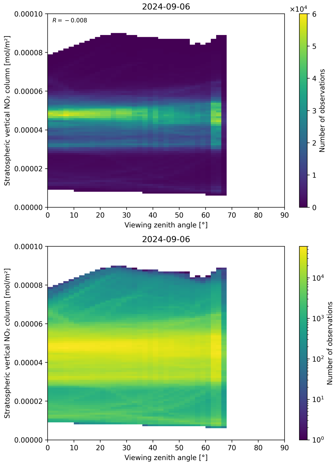
Figure 164: Scatter density plot of “Viewing zenith angle” against “Stratospheric vertical NO 2 column” for 2024-09-06 to 2024-09-07.
