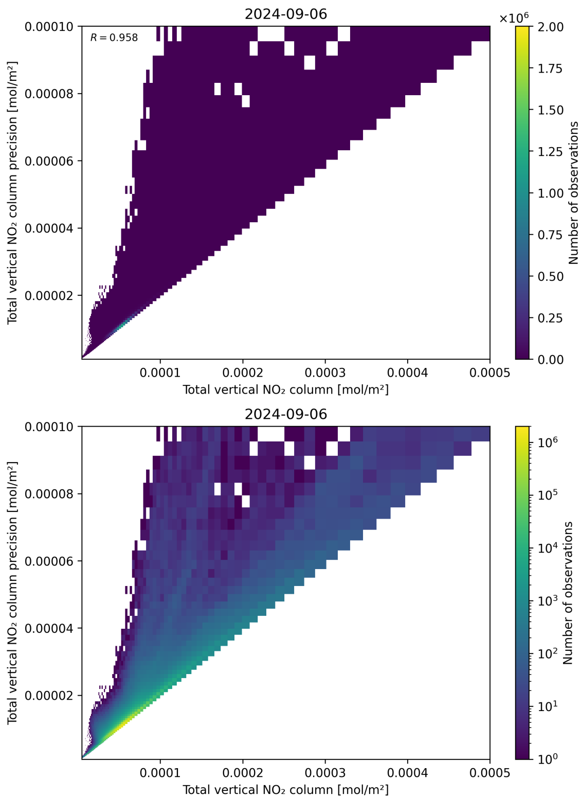
Figure 114: Scatter density plot of “Total vertical NO 2 column” against “Total vertical NO 2 column precision” for 2024-09-06 to 2024-09-07.
