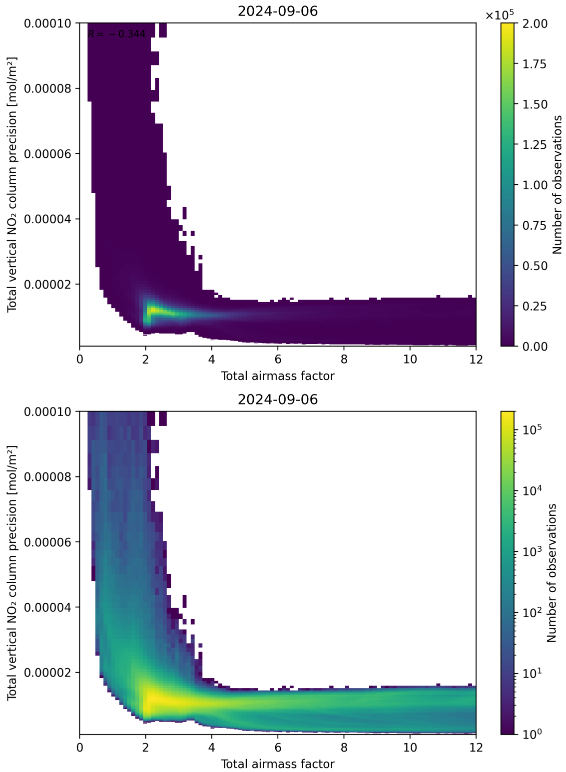
Figure 68: Scatter density plot of “Total airmass factor” against “Total vertical NO 2 column precision” for 2024-09-06 to 2024-09-07.
