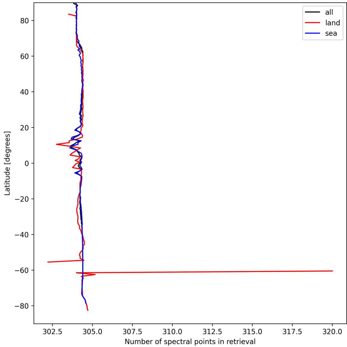
Figure 16: Zonal average of “Number of spectral points in retrieval” for 2024-09-06 to 2024-09-07.
