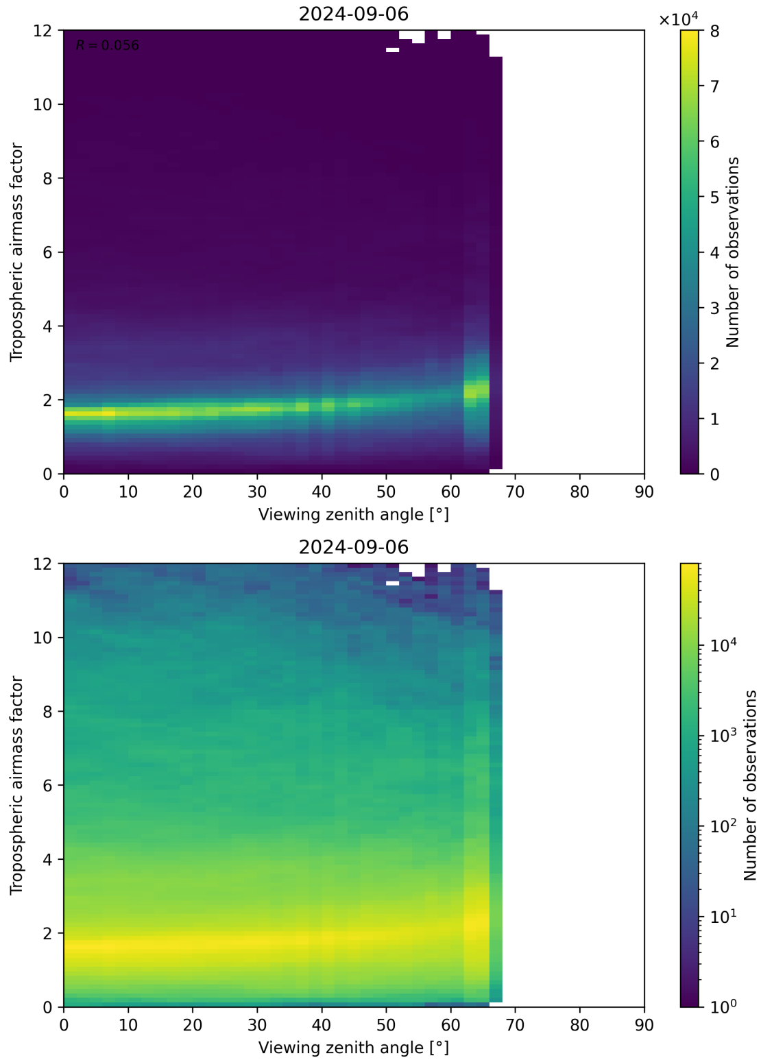
Figure 161: Scatter density plot of “Viewing zenith angle” against “Tropospheric airmass factor” for 2024-09-06 to 2024-09-07.
