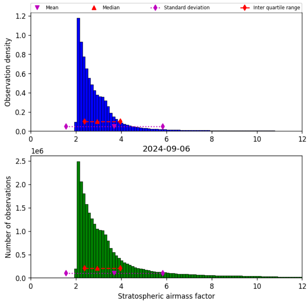
Figure 44: Histogram of “Stratospheric airmass factor” for 2024-09-06 to 2024-09-07
