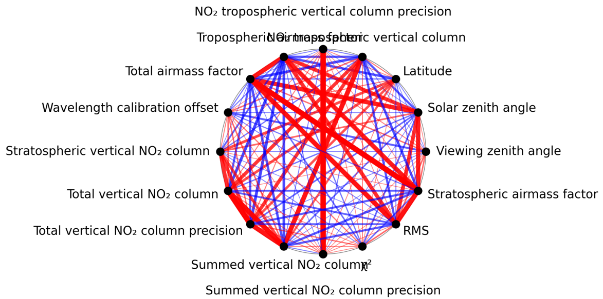
Figure 1: Map of correlation graph for 2024-09-06 to 2024-09-07.
