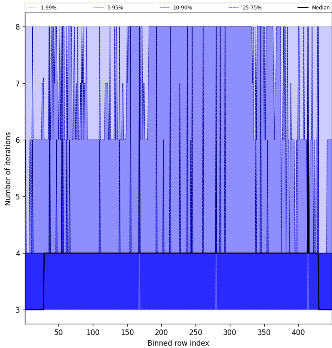
Figure 51: Along track statistics of "Number of iterations" for 2024-09-06 to 2024-09-07
