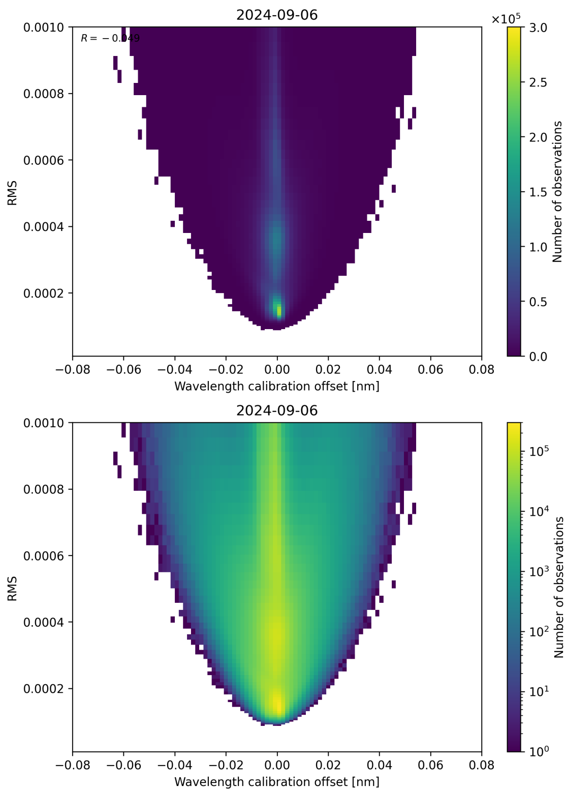
Figure 181: Scatter density plot of “Wavelength calibration offset” against “RMS” for 2024-09-06 to 2024-09-07.
