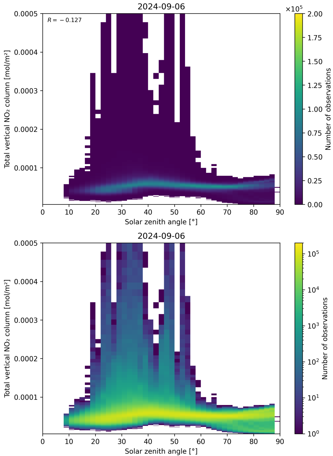
Figure 153: Scatter density plot of “Solar zenith angle” against “Total vertical NO 2 column” for 2024-09-06 to 2024-09-07.
