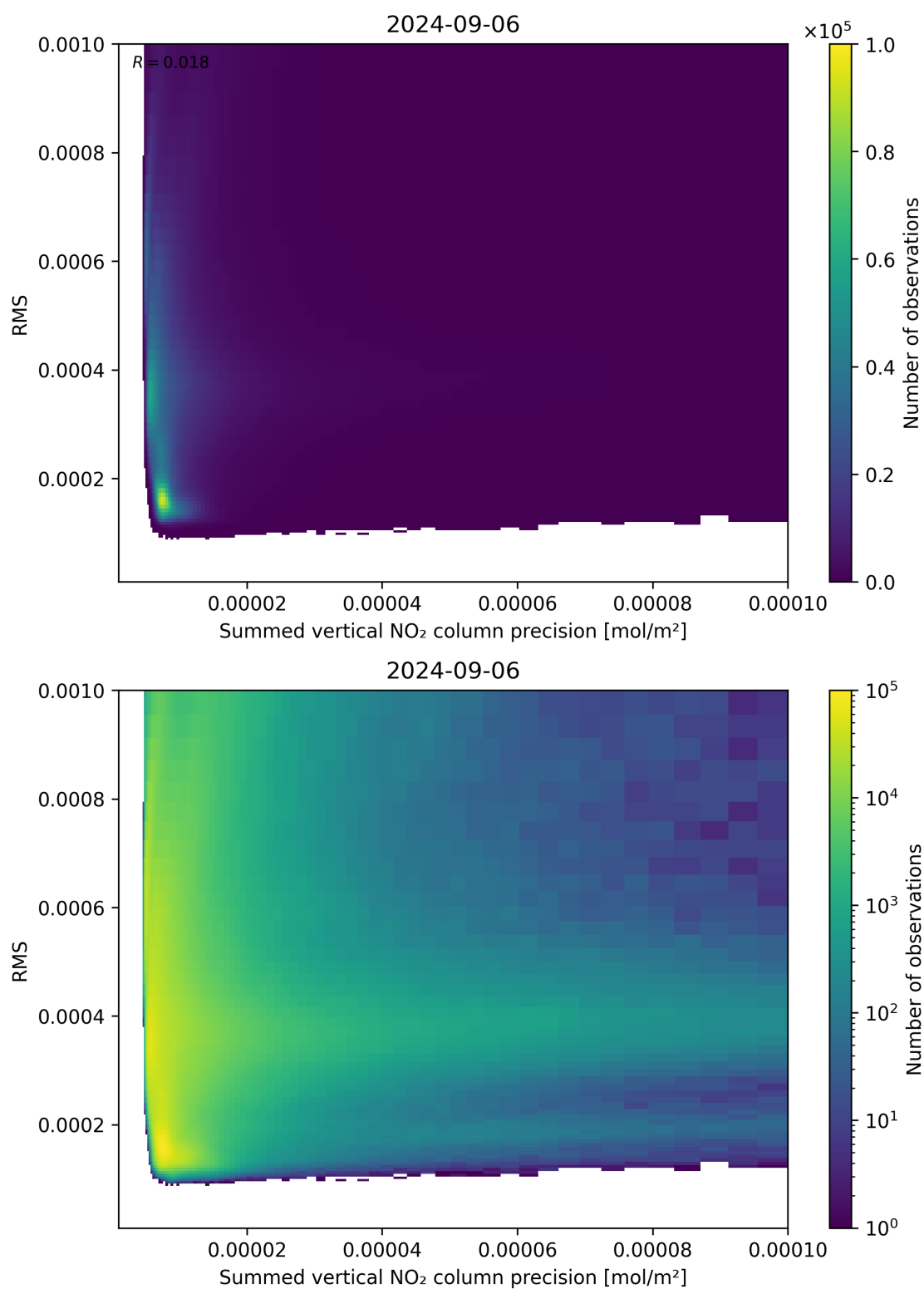
Figure 108: Scatter density plot of “Summed vertical NO 2 column precision” against “RMS” for 2024-09-06 to 2024-09-07.
