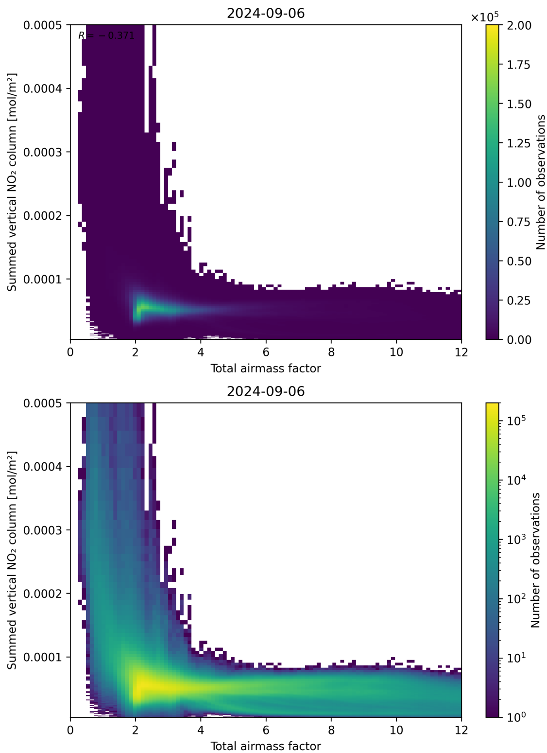
Figure 65: Scatter density plot of “Total airmass factor” against “Summed vertical NO 2 column” for 2024-09-06 to 2024-09-07.
