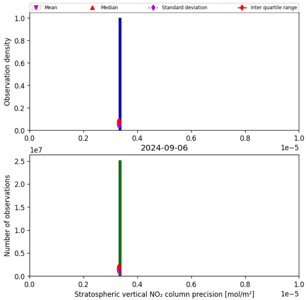
Figure 37: Histogram of “Stratospheric vertical NO 2 column precision” for 2024-09-06 to 2024-09-07
