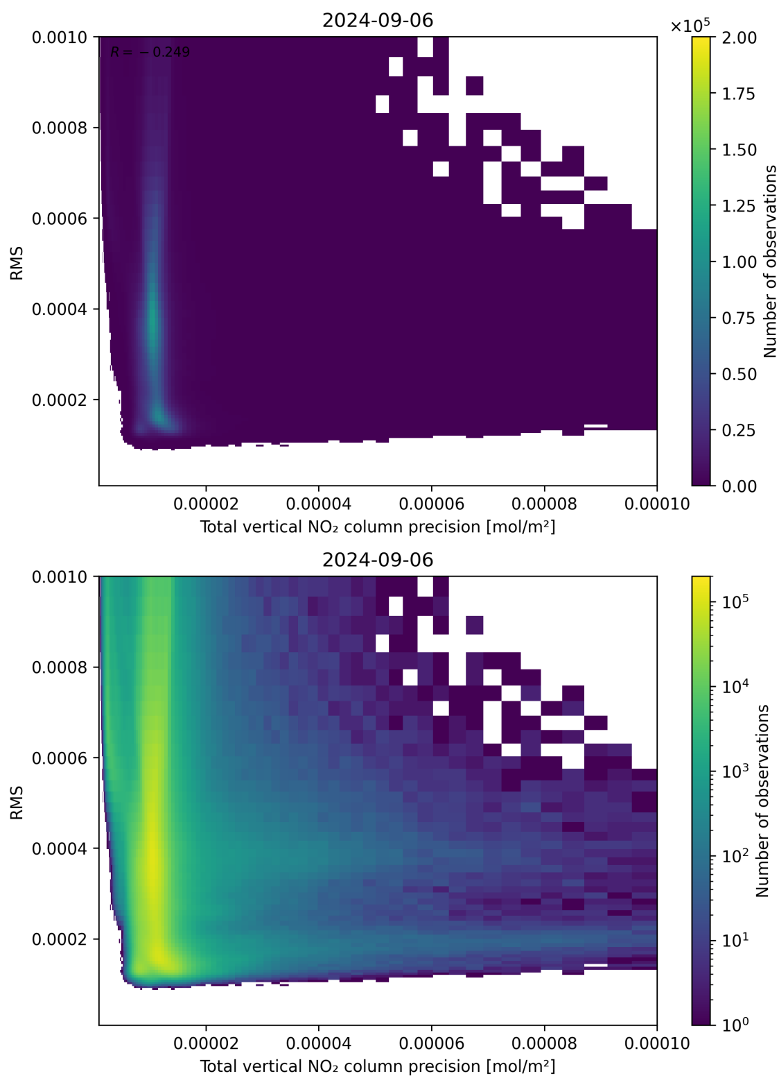
Figure 119: Scatter density plot of “Total vertical NO 2 column precision” against “RMS” for 2024-09-06 to 2024-09-07.
