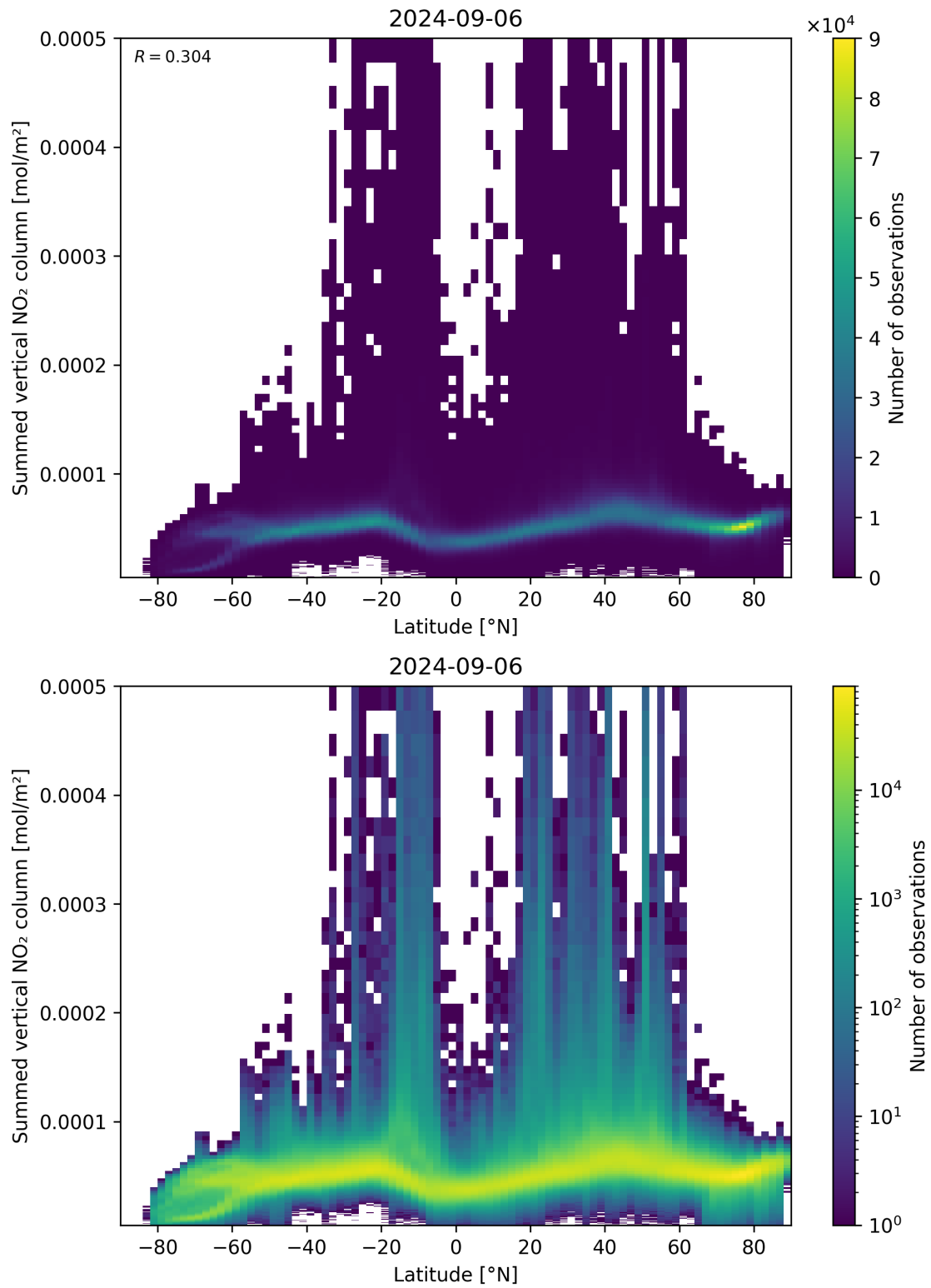
Figure 88: Scatter density plot of “Latitude” against “Summed vertical NO 2 column” for 2024-09-06 to 2024-09-07.
