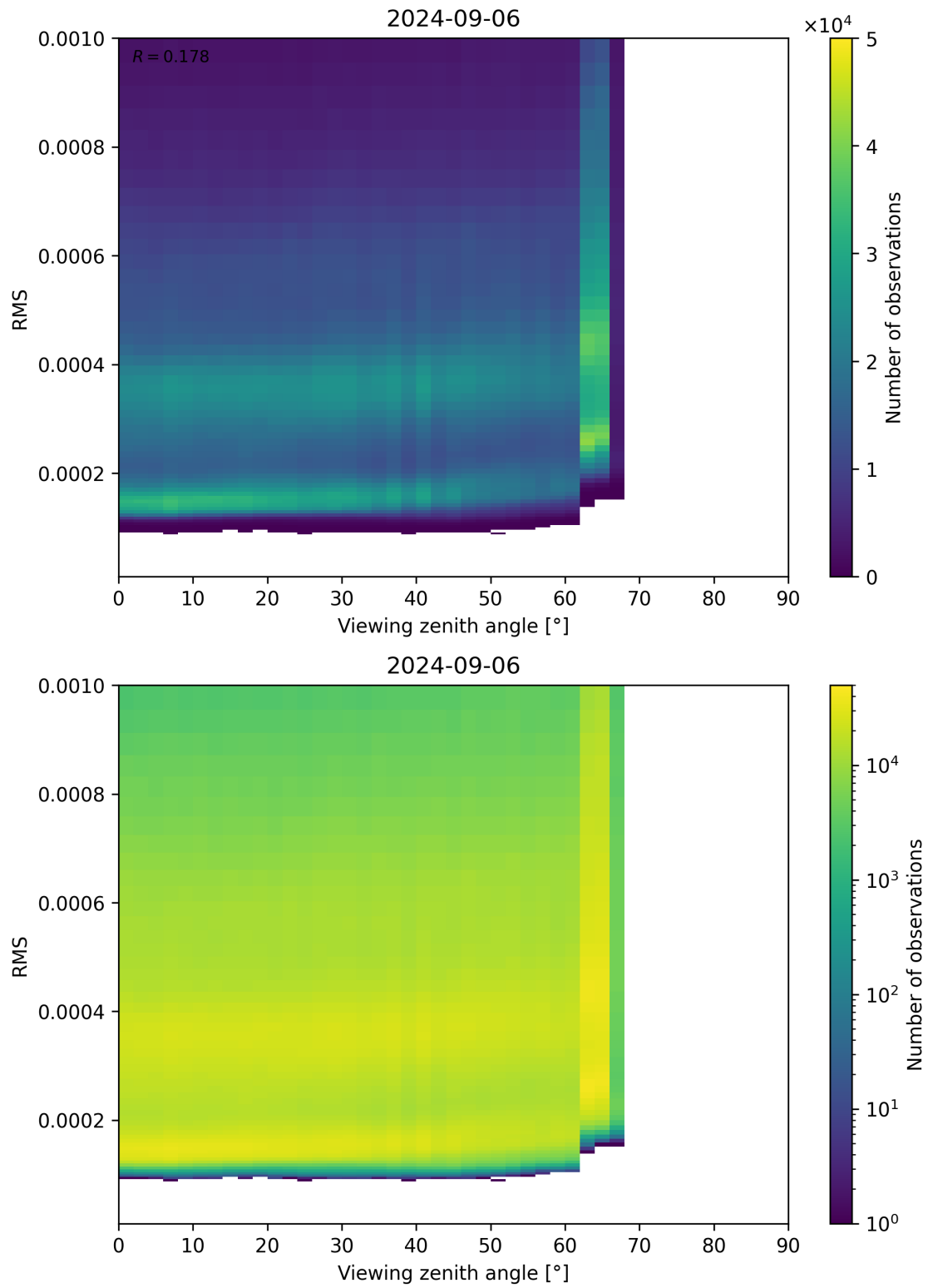
Figure 171: Scatter density plot of “Viewing zenith angle” against “RMS” for 2024-09-06 to 2024-09-07.
