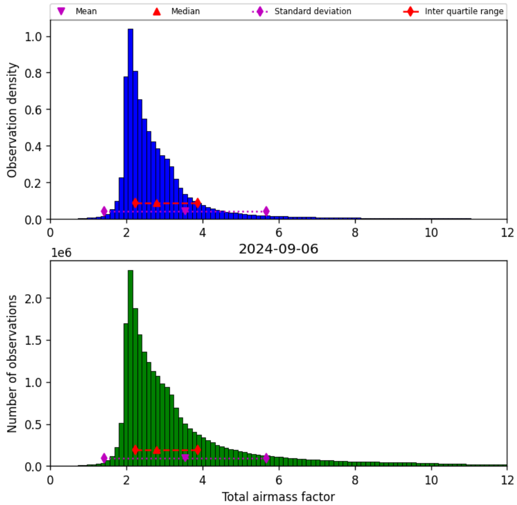
Figure 32: Histogram of “Total airmass factor” for 2024-09-06 to 2024-09-07
