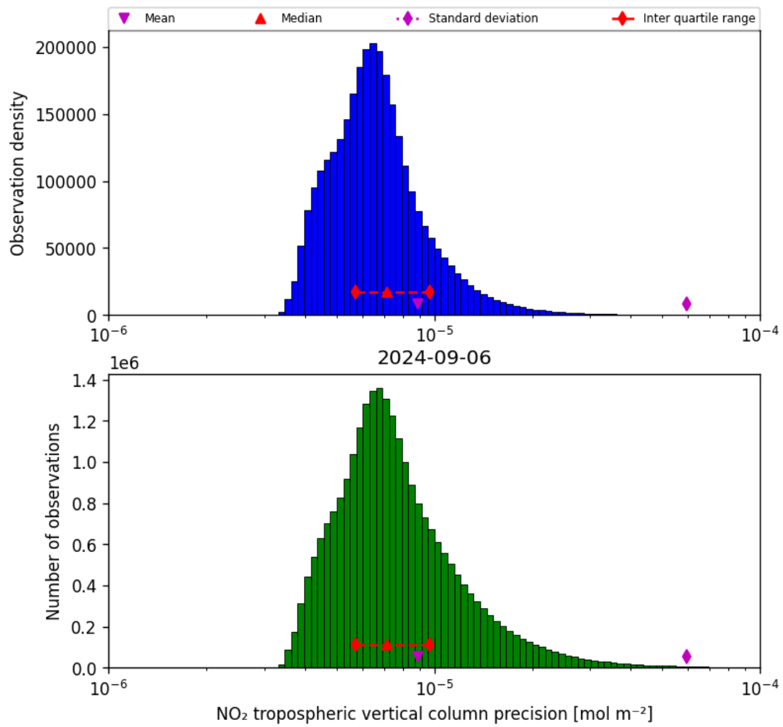
Figure 30: Histogram of “NO 2 tropospheric vertical column precision” for 2024-09-06 to 2024-09-07
