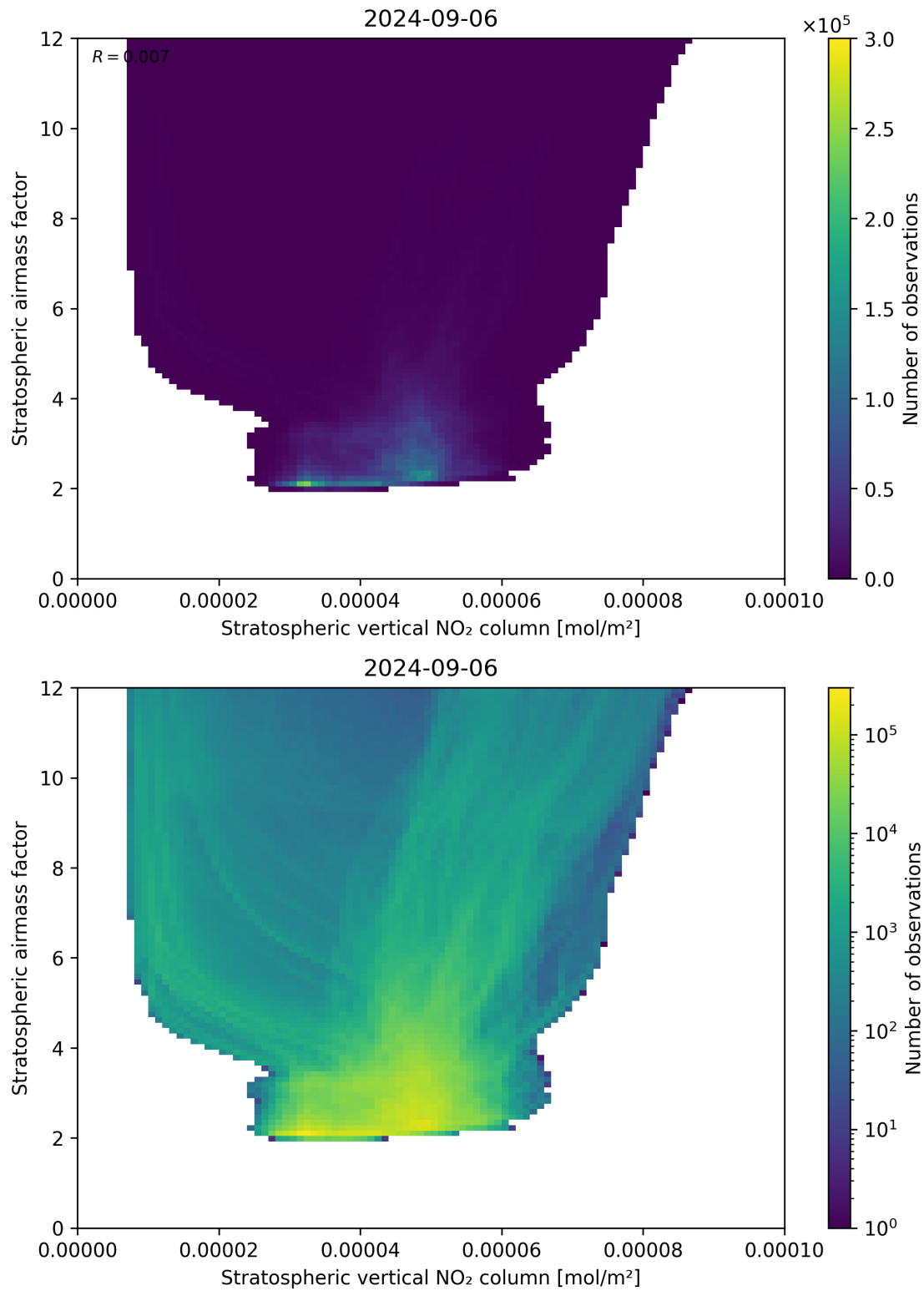
Figure 96: Scatter density plot of “Stratospheric vertical NO 2 column” against “Stratospheric airmass factor” for 2024-09-06 to 2024-09-07.
