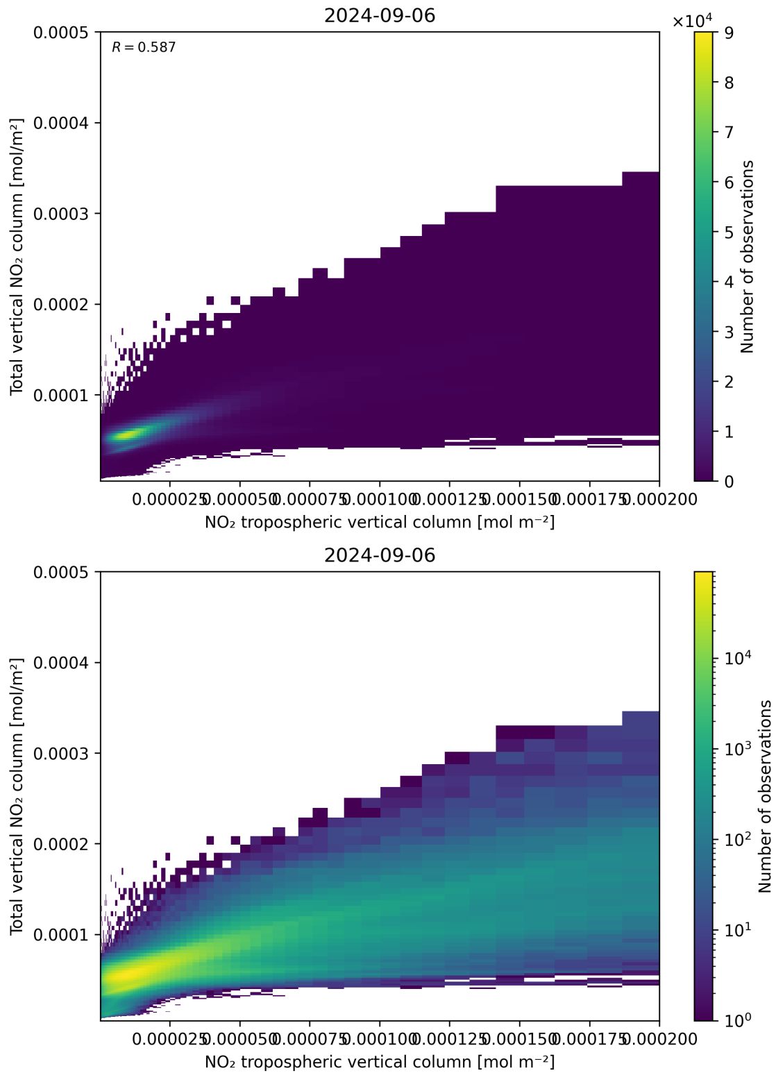
Figure 128: Scatter density plot of “NO 2 tropospheric vertical column” against “Total vertical NO 2 column” for 2024-09-06 to 2024-09-07.
