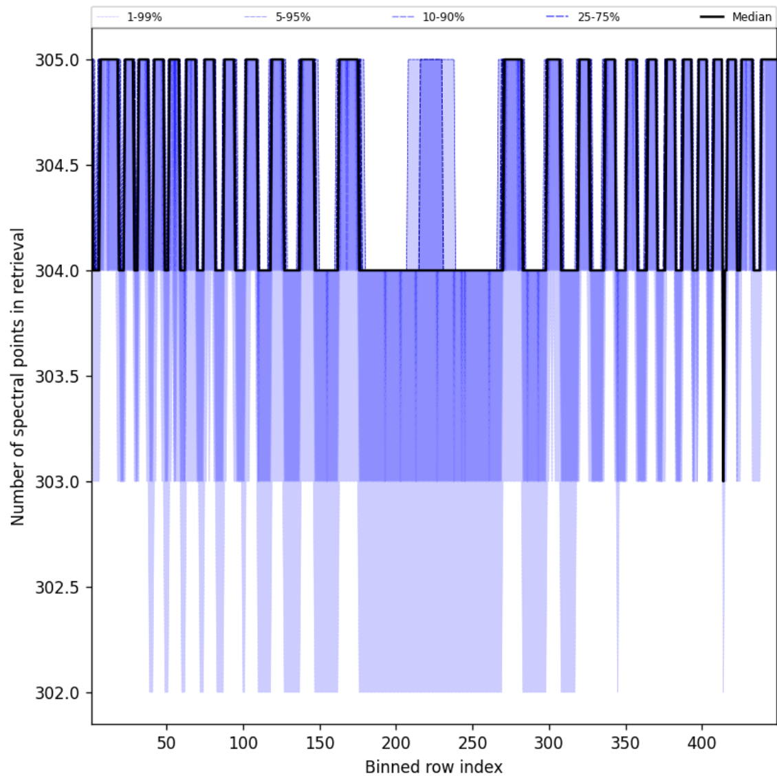
Figure 50: Along track statistics of “Number of spectral points in retrieval” for 2024-09-06 to 2024-09-07
