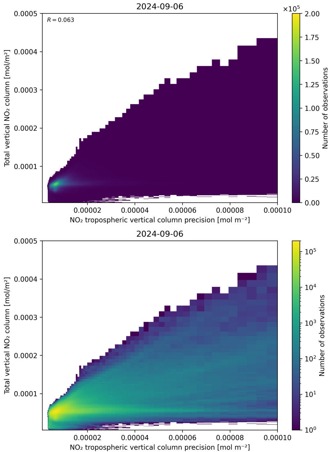
Figure 138: Scatter density plot of “ \text{NO}_2 tropospheric vertical column precision” against “Total vertical \text{NO}_2 column” for 2024-09-06 to 2024-09-07.
