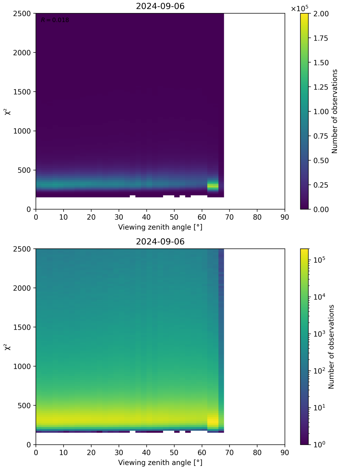
Figure 162: Scatter density plot of “Viewing zenith angle” against “ \chi^2 ” for 2024-09-06 to 2024-09-07.
