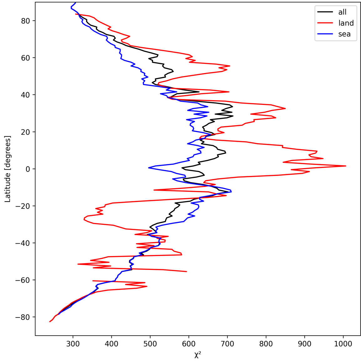
Figure 25: Zonal average of “ \chi^2 ” for 2024-09-06 to 2024-09-07.
