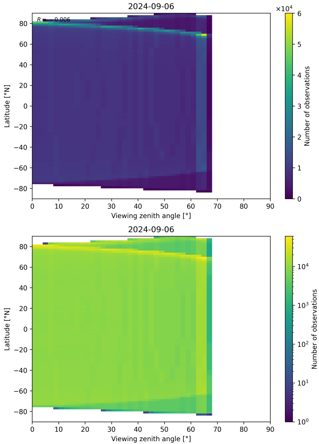
Figure 163: Scatter density plot of “Viewing zenith angle” against “Latitude” for 2024-09-06 to 2024-09-07.
