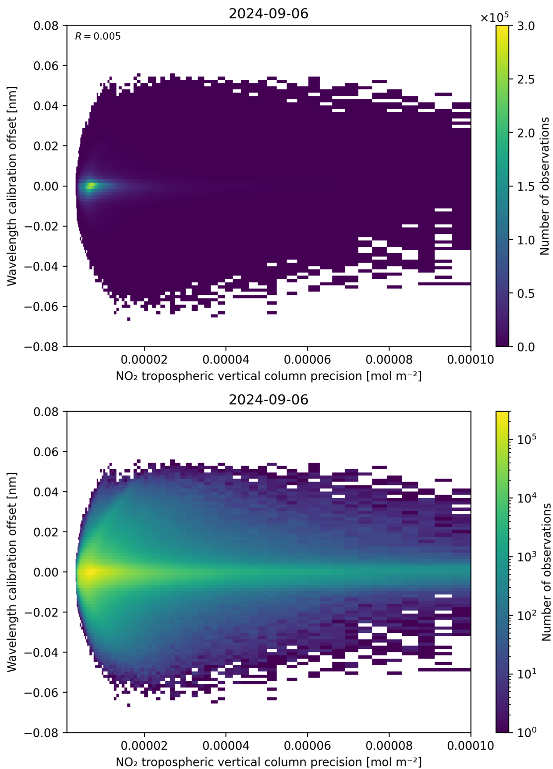
Figure 141: Scatter density plot of “NO 2 tropospheric vertical column precision” against “Wavelength calibration offset” for 2024-09-06 to 2024-09-07.
