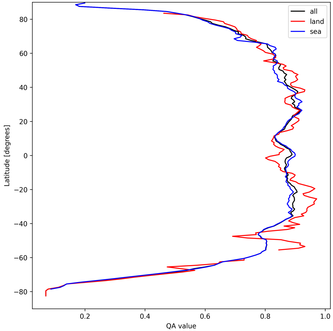
Figure 11: Zonal average of “QA value” for 2024-09-06 to 2024-09-07.
