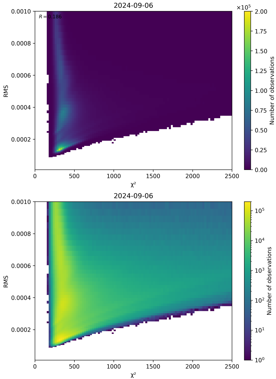
Figure 82: Scatter density plot of “ \chi^2 ” against “RMS” for 2024-09-06 to 2024-09-07.
