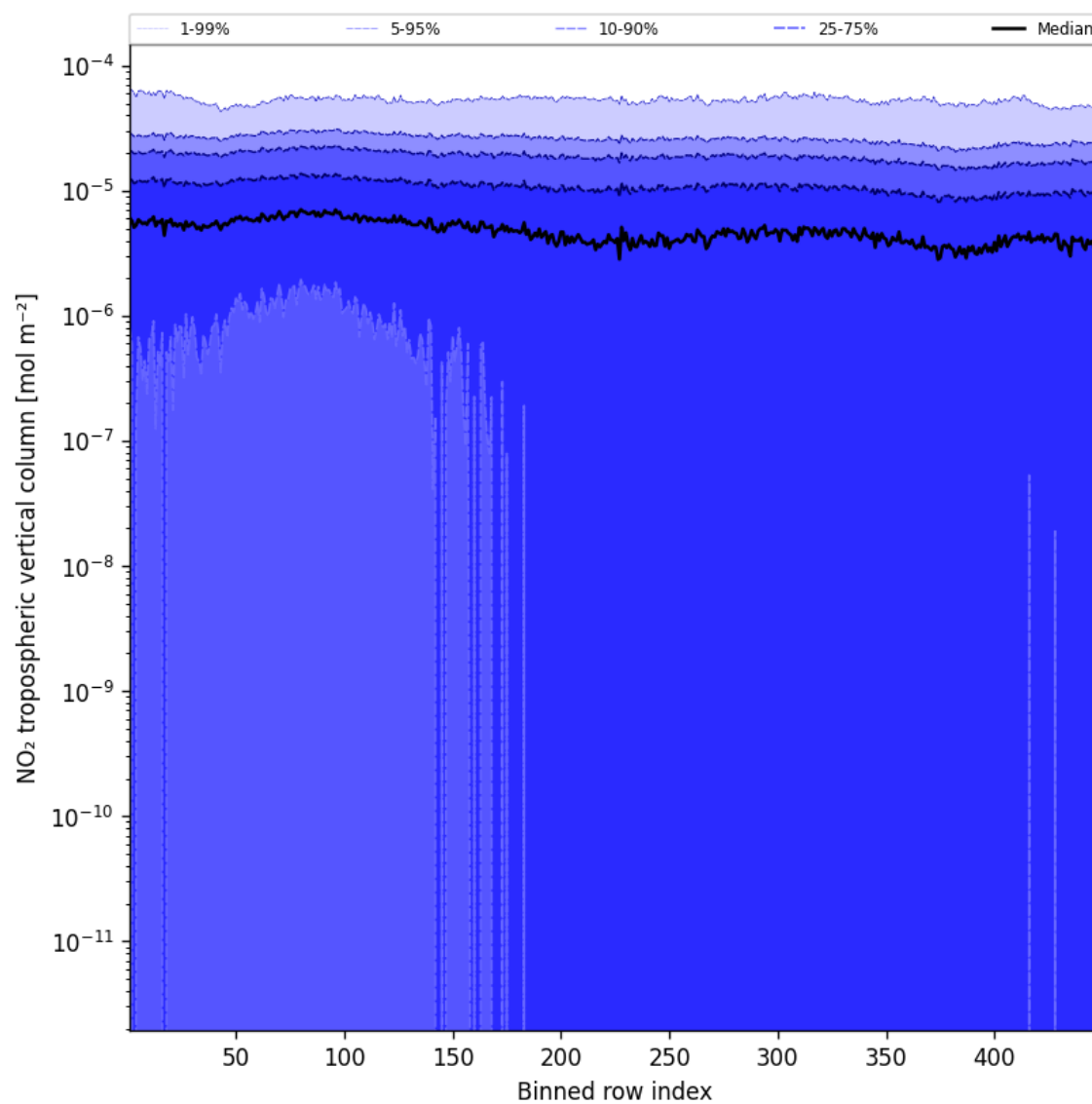
Figure 46: Along track statistics of “NO 2 tropospheric vertical column” for 2024-09-06 to 2024-09-07
