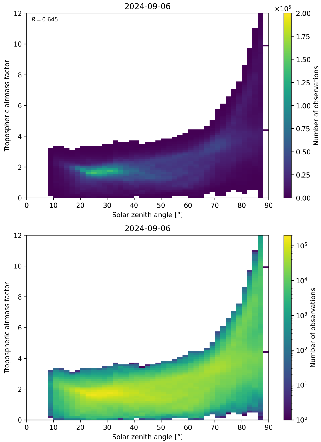
Figure 147: Scatter density plot of “Solar zenith angle” against “Tropospheric airmass factor” for 2024-09-06 to 2024-09-07.
