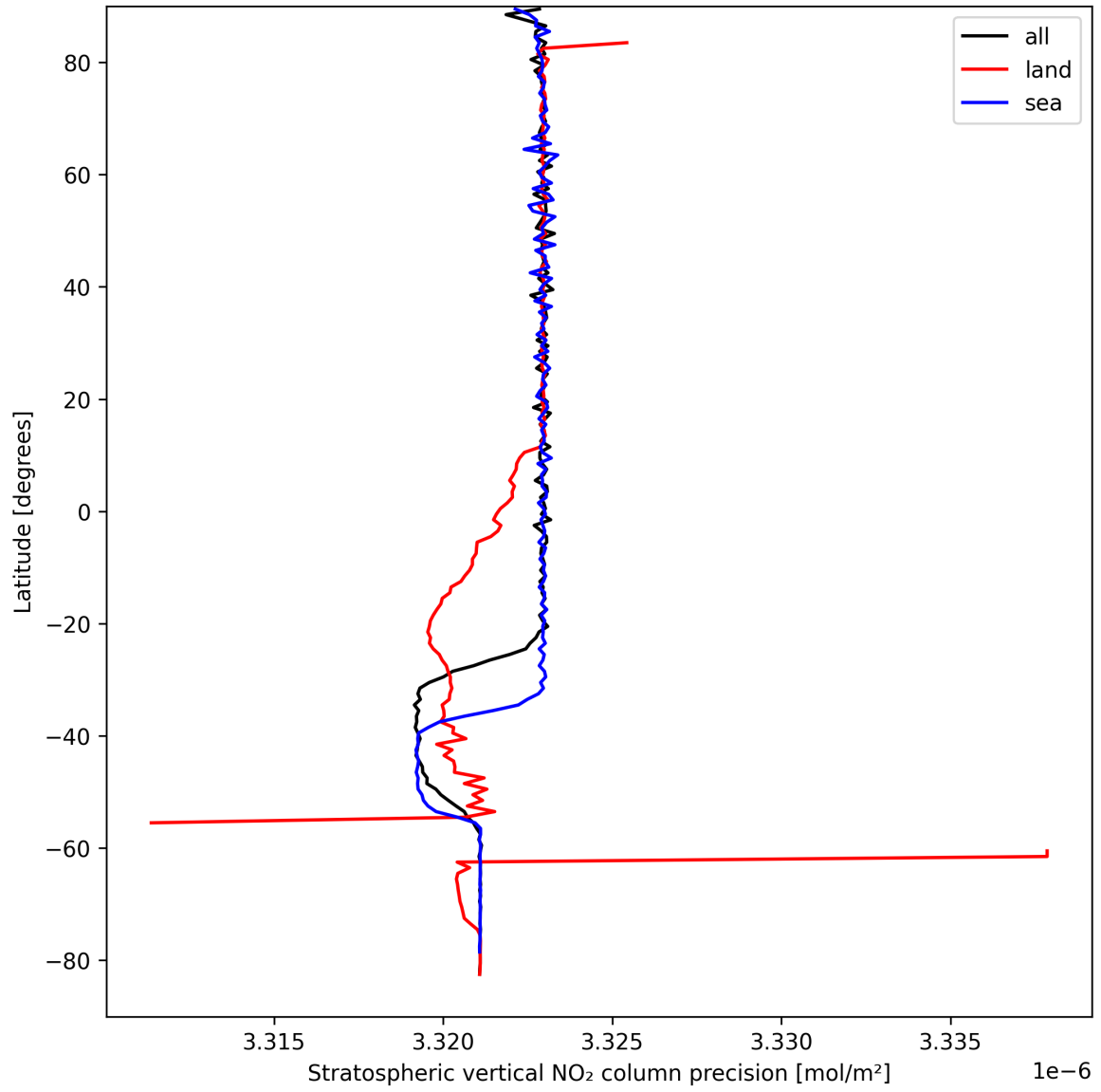
Figure 20: Zonal average of “Stratospheric vertical NO 2 column precision” for 2024-09-06 to 2024-09-07.
