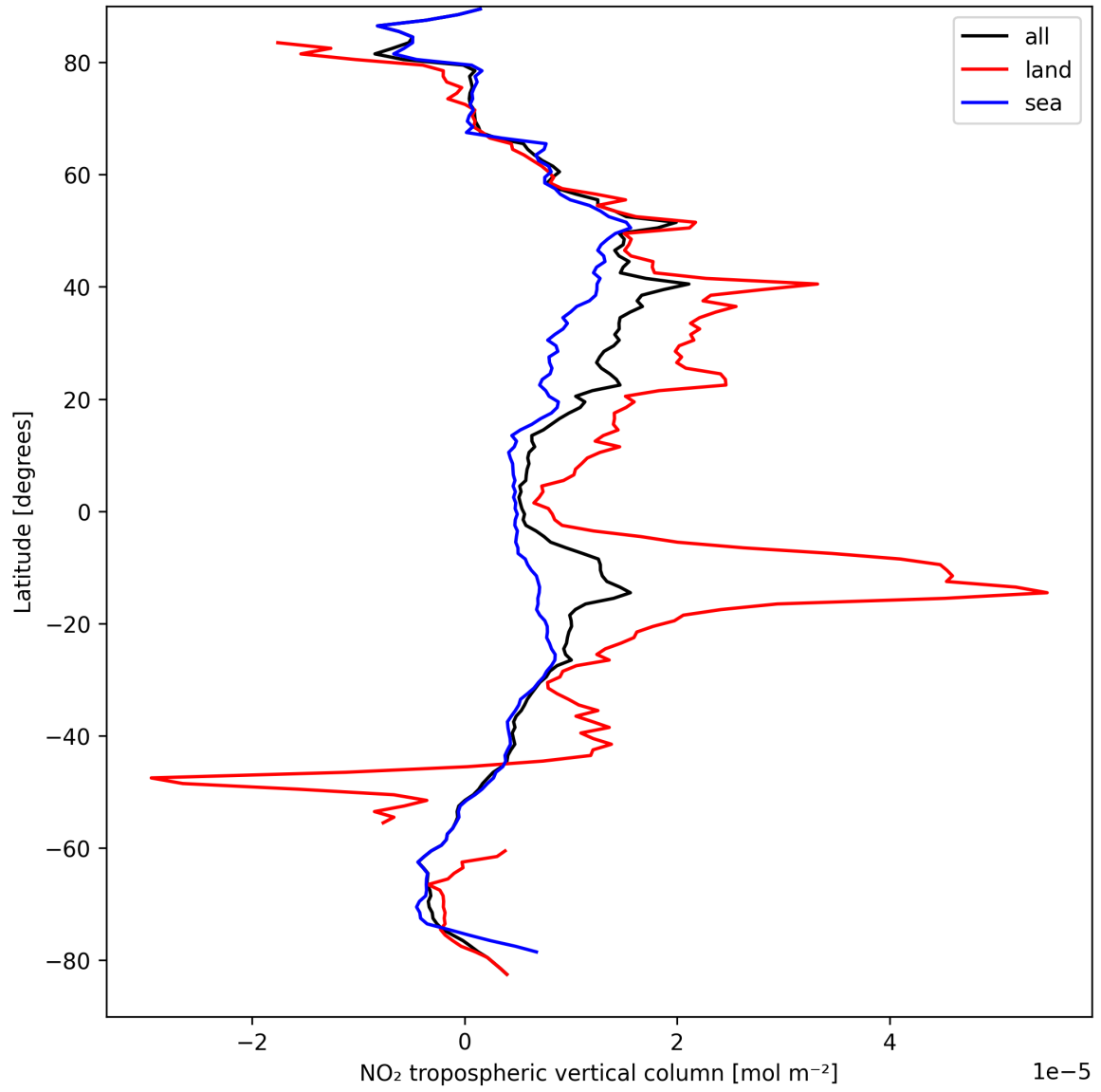
Figure 12: Zonal average of “NO 2 tropospheric vertical column” for 2024-09-06 to 2024-09-07.
