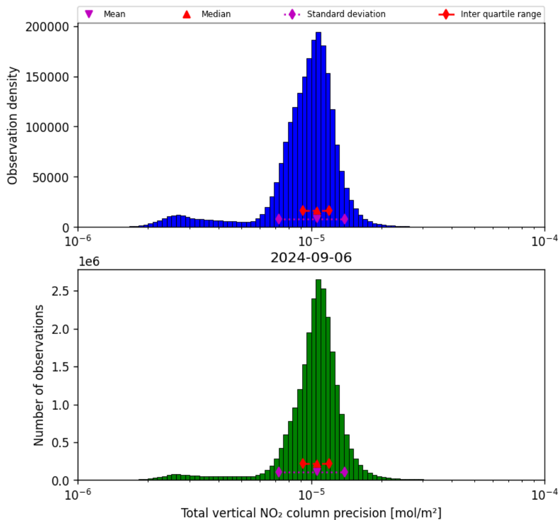
Figure 39: Histogram of “Total vertical NO 2 column precision” for 2024-09-06 to 2024-09-07
