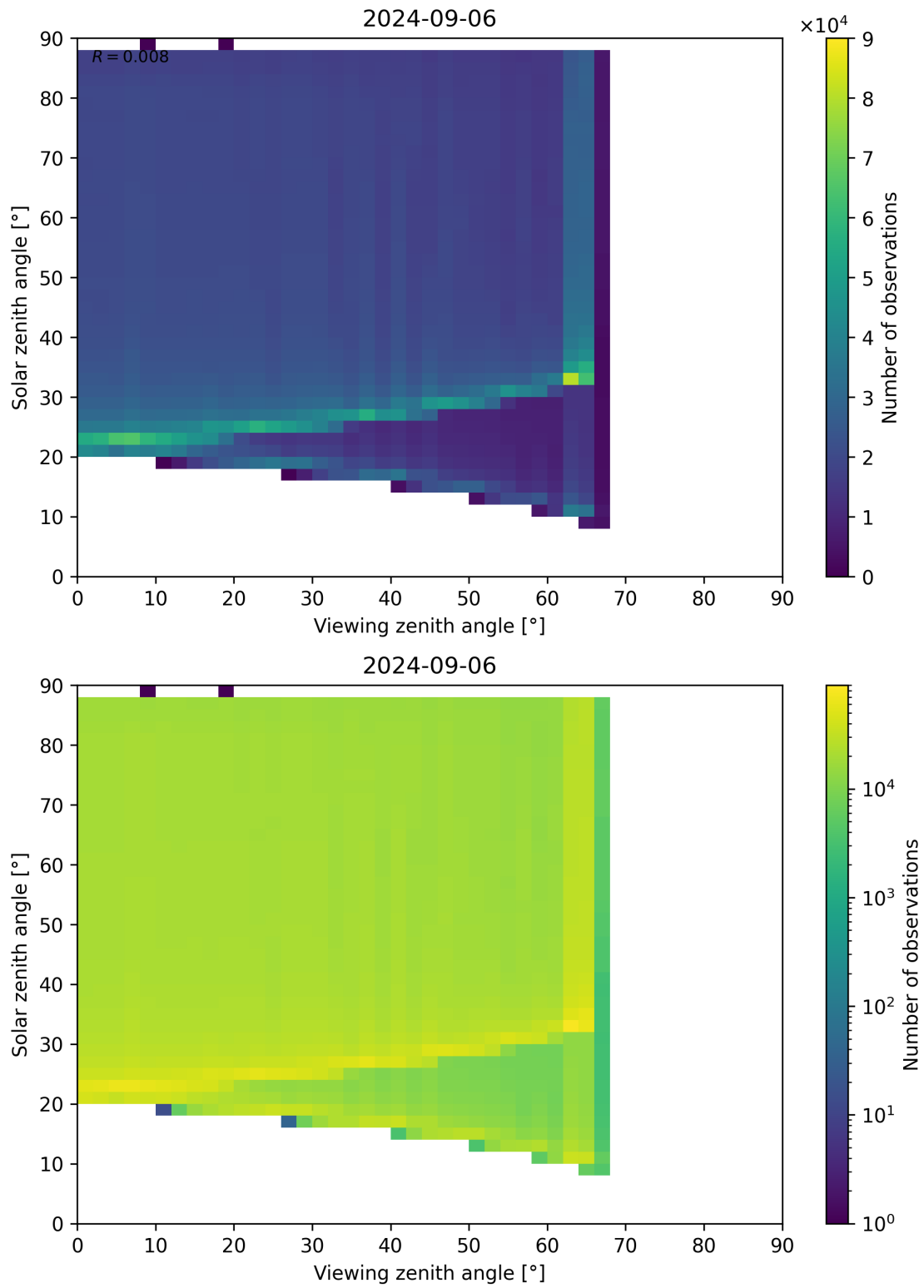
Figure 172: Scatter density plot of “Viewing zenith angle” against “Solar zenith angle” for 2024-09-06 to 2024-09-07.
