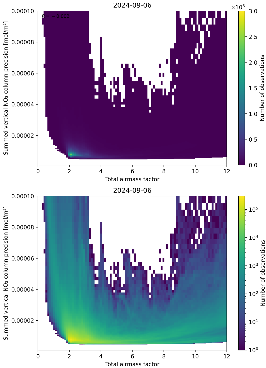
Figure 66: Scatter density plot of “Total airmass factor” against “Summed vertical NO 2 column precision” for 2024-09-06 to 2024-09-07.
