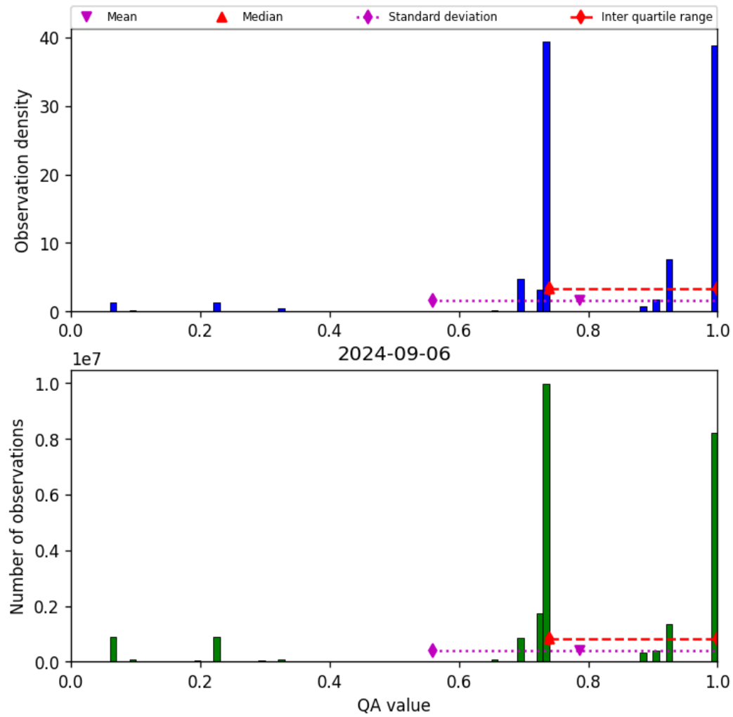
Figure 28: Histogram of “QA value” for 2024-09-06 to 2024-09-07
