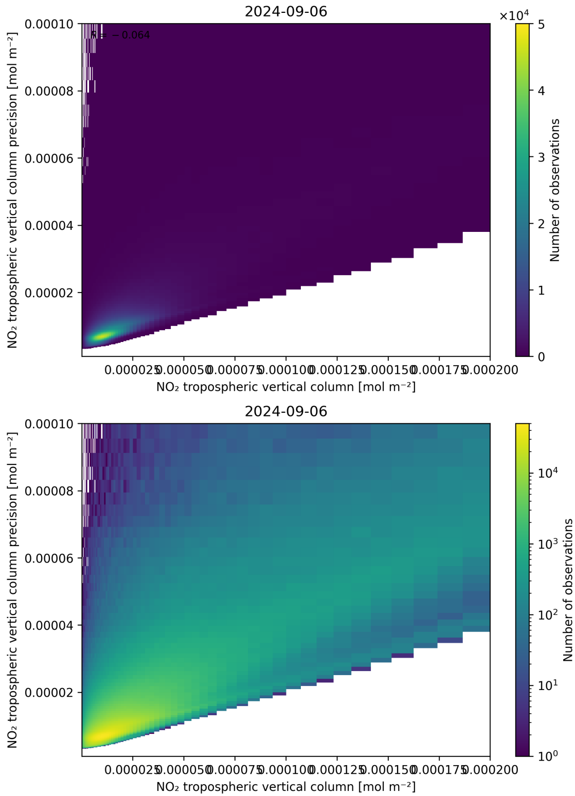
Figure 130: Scatter density plot of “NO 2 tropospheric vertical column” against “NO 2 tropospheric vertical column precision” for 2024-09-06 to 2024-09-07.
