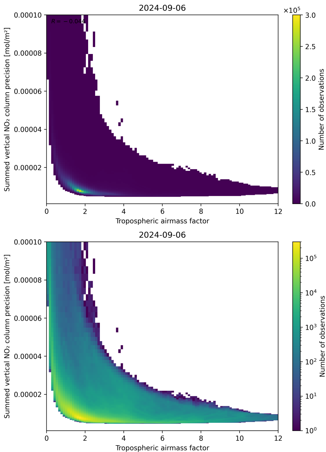
Figure 76: Scatter density plot of “Tropospheric air mass factor” against “Summed vertical NO 2 column precision” for 2024-09-06 to 2024-09-07.
