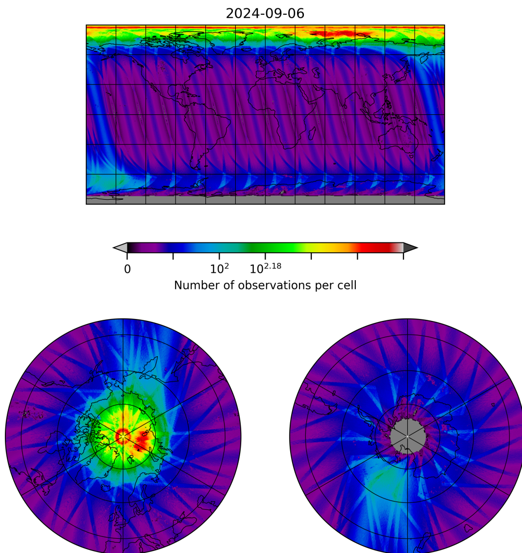
Figure 10: Map of the number of observations for 2024-09-06 to 2024-09-07
