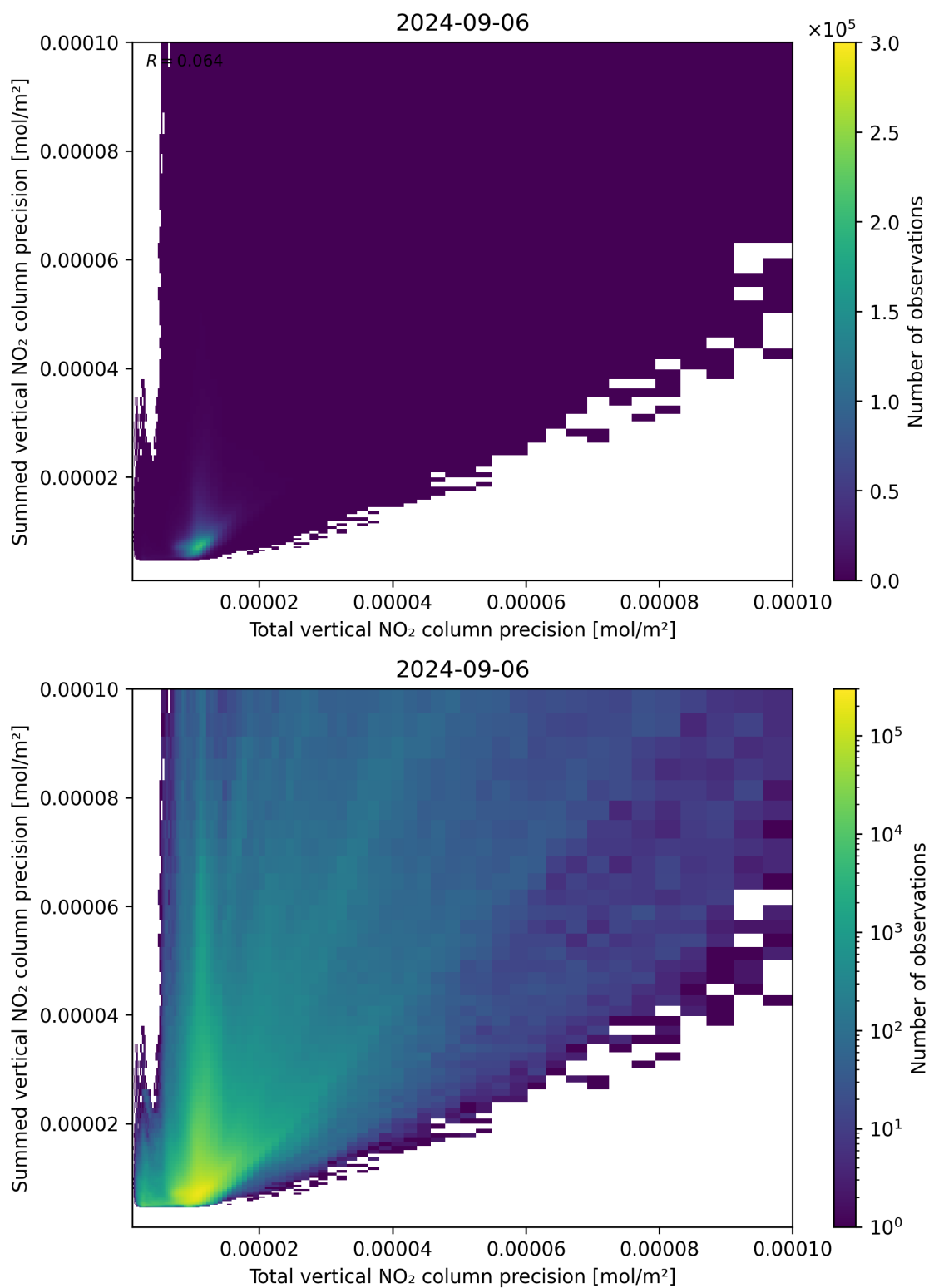
Figure 118: Scatter density plot of “Total vertical NO 2 column precision” against “Summed vertical NO 2 column precision” for 2024-09-06 to 2024-09-07.
