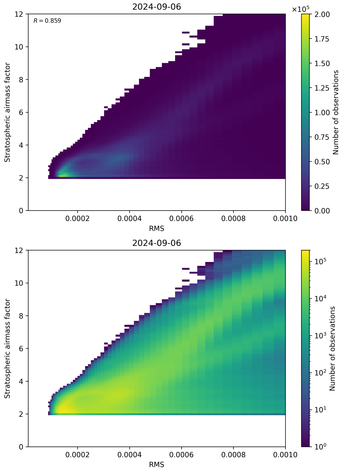
Figure 144: Scatter density plot of “RMS” against “Stratospheric airmass factor” for 2024-09-06 to 2024-09-07.
