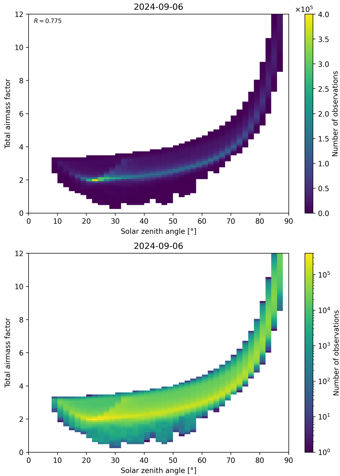
Figure 146: Scatter density plot of “Solar zenith angle” against “Total airmass factor” for 2024-09-06 to 2024-09-07.
