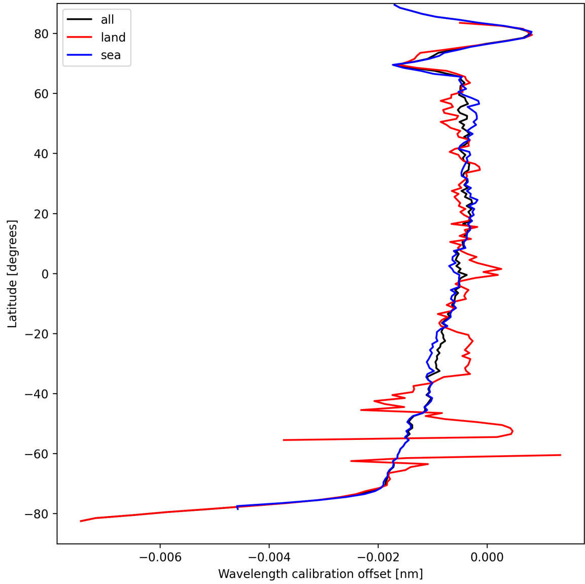
Figure 18: Zonal average of “Wavelength calibration offset” for 2024-09-06 to 2024-09-07.
