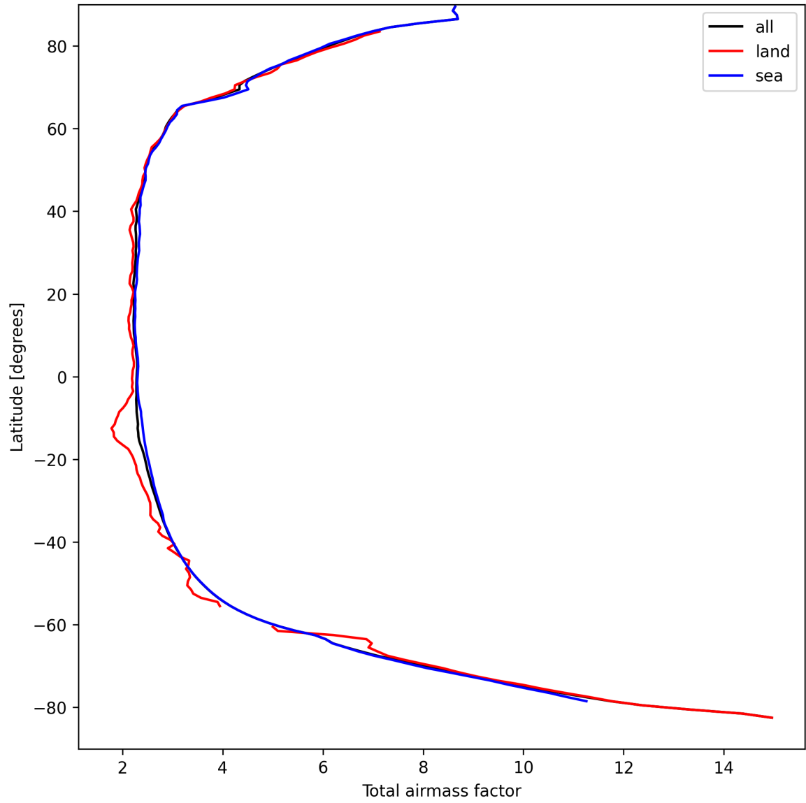
Figure 15: Zonal average of “Total airmass factor” for 2024-09-06 to 2024-09-07.
