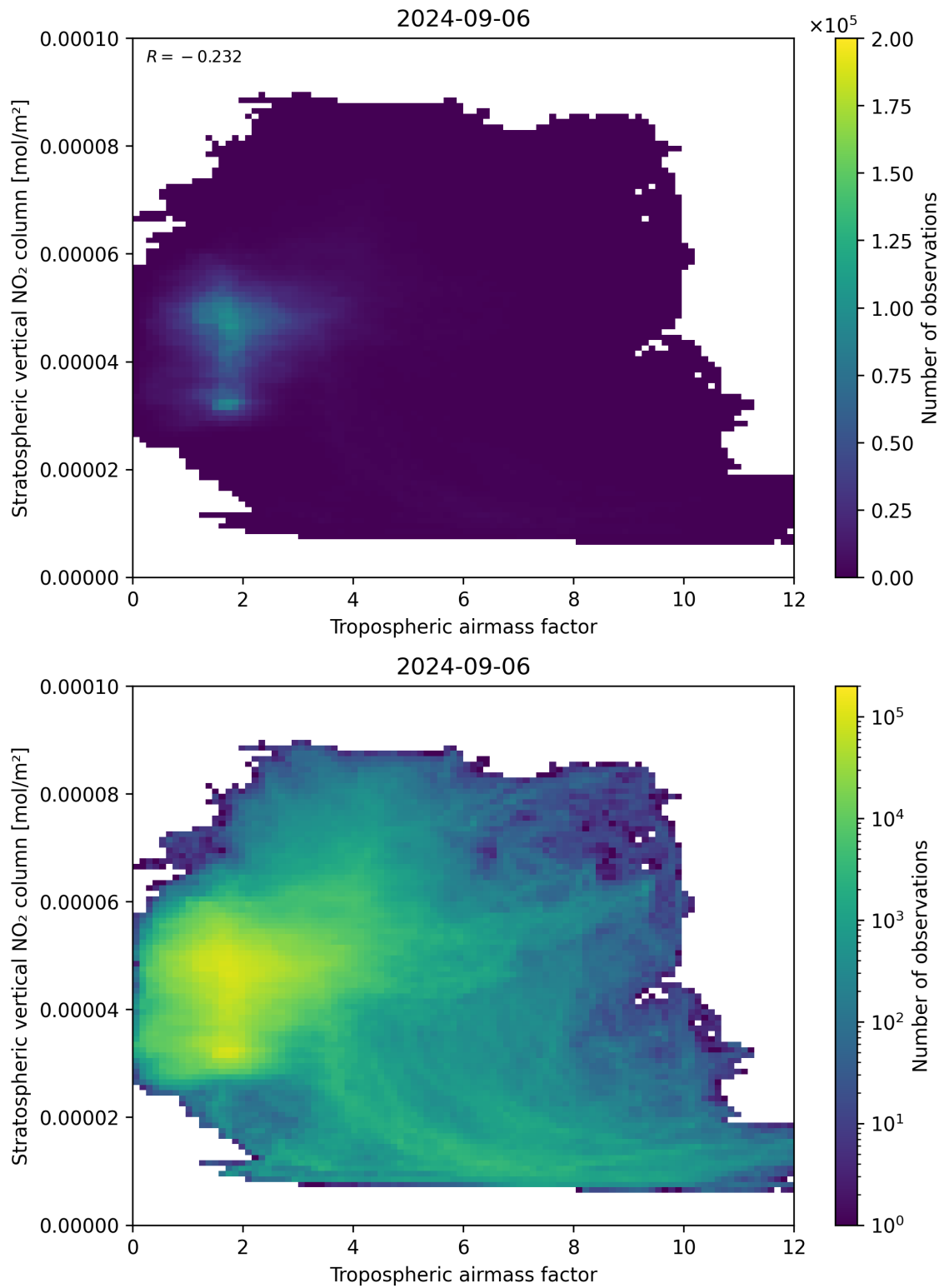
Figure 74: Scatter density plot of “Tropospheric air mass factor” against “Stratospheric vertical NO 2 column” for 2024-09-06 to 2024-09-07.
