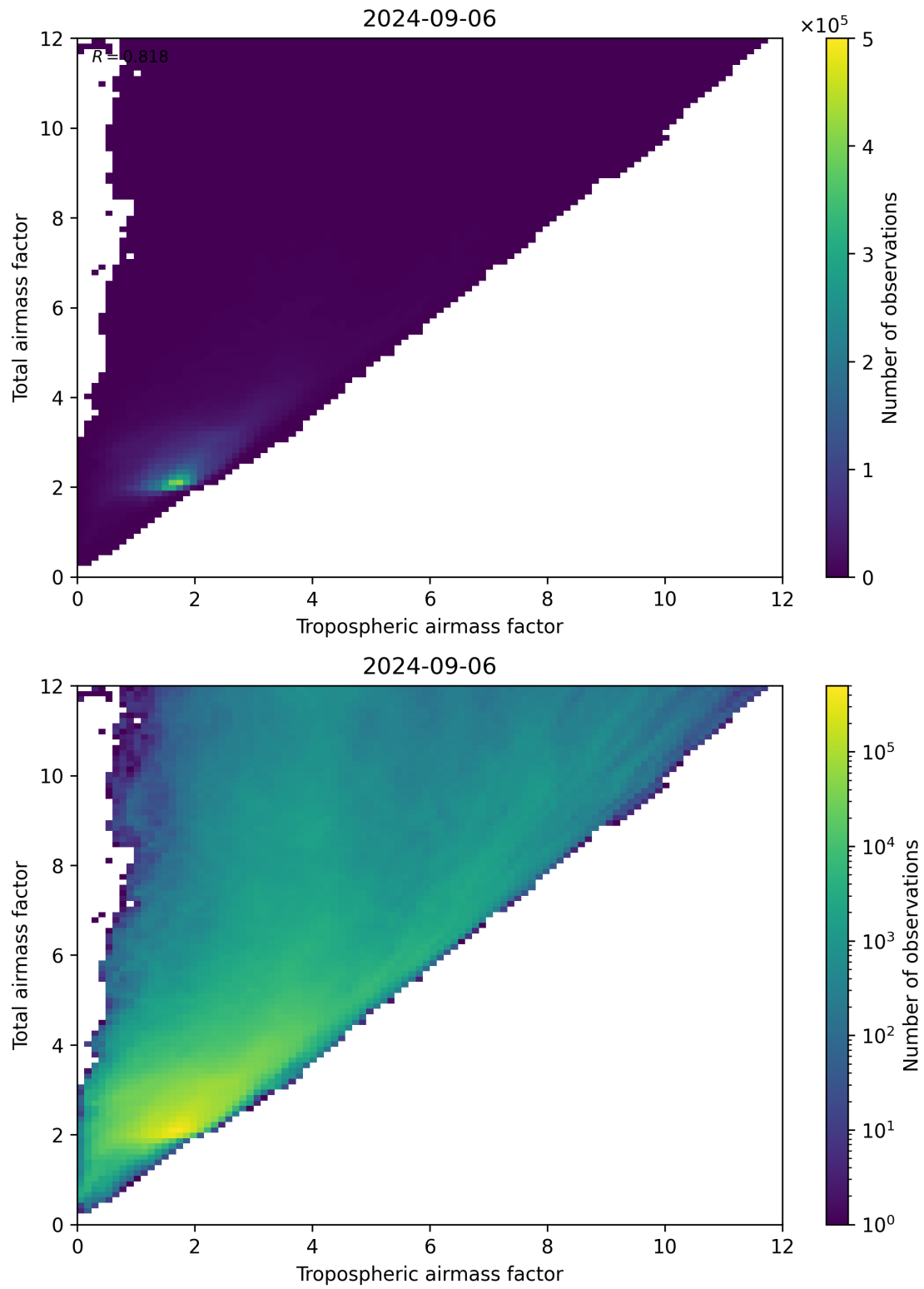
Figure 72: Scatter density plot of “Tropospheric airmass factor” against “Total airmass factor” for 2024-09-06 to 2024-09-07.
