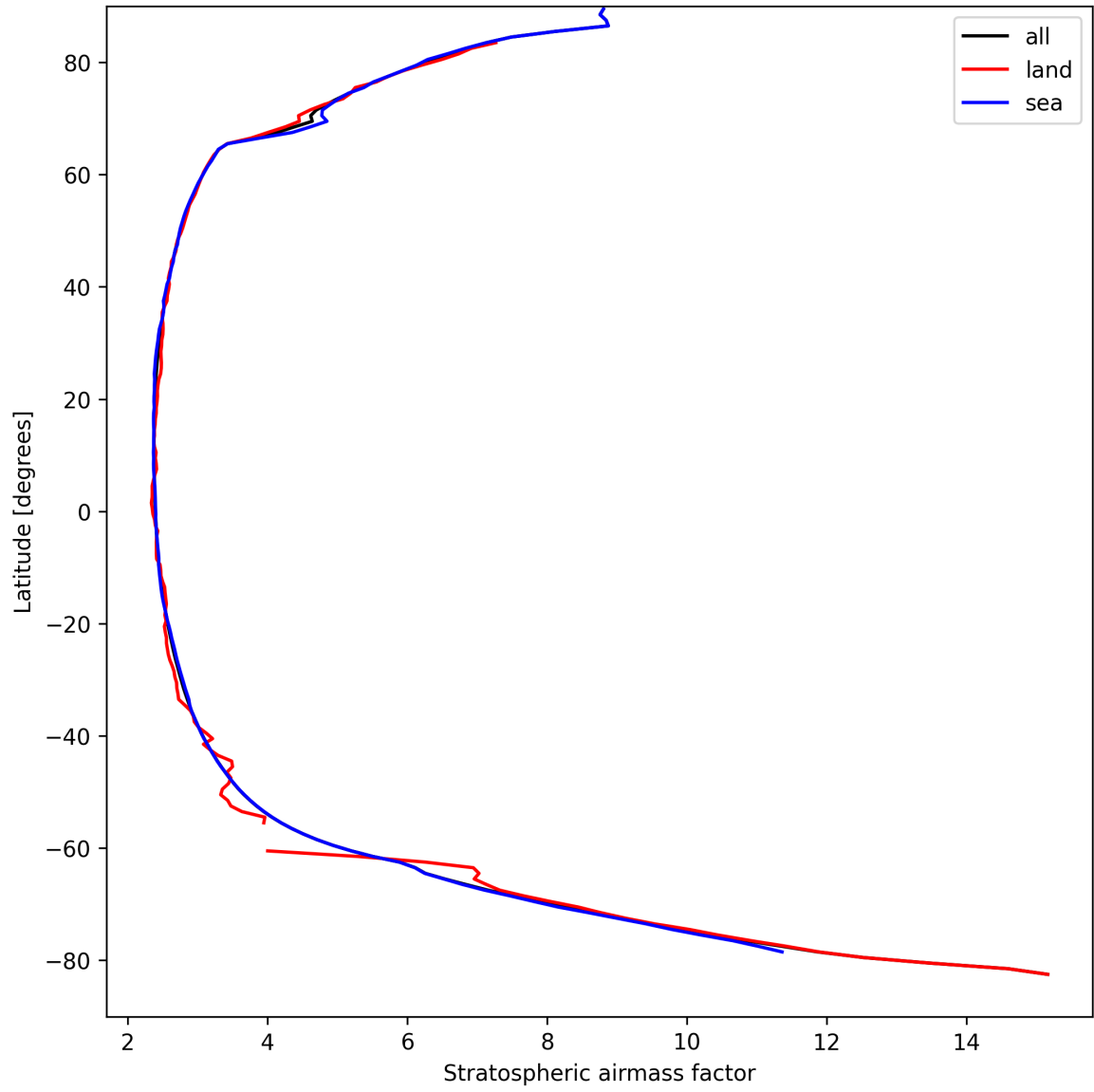
Figure 27: Zonal average of “Stratospheric airmass factor” for 2024-09-06 to 2024-09-07.
