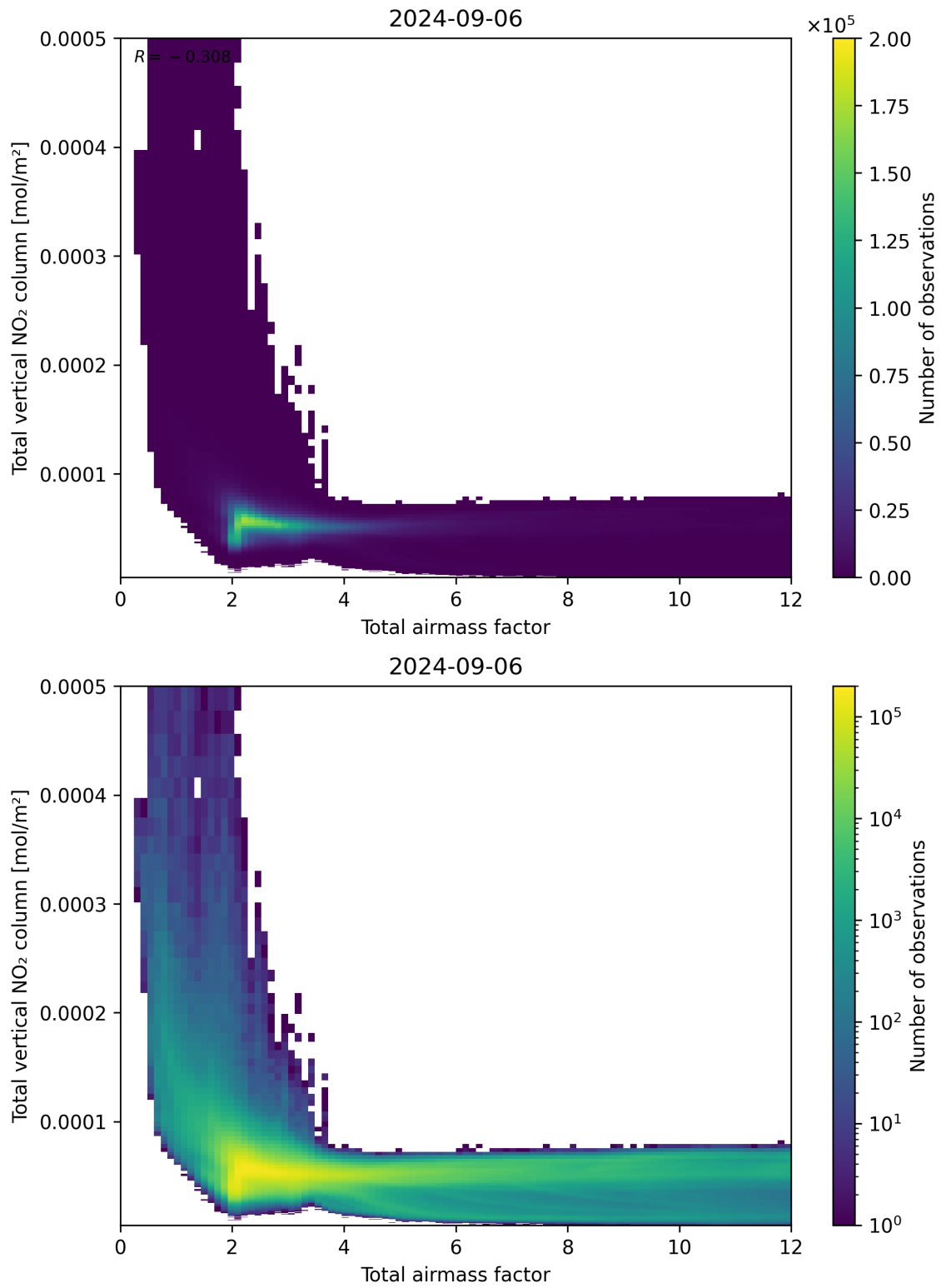
Figure 67: Scatter density plot of “Total airmass factor” against “Total vertical NO 2 column” for 2024-09-06 to 2024-09-07.
