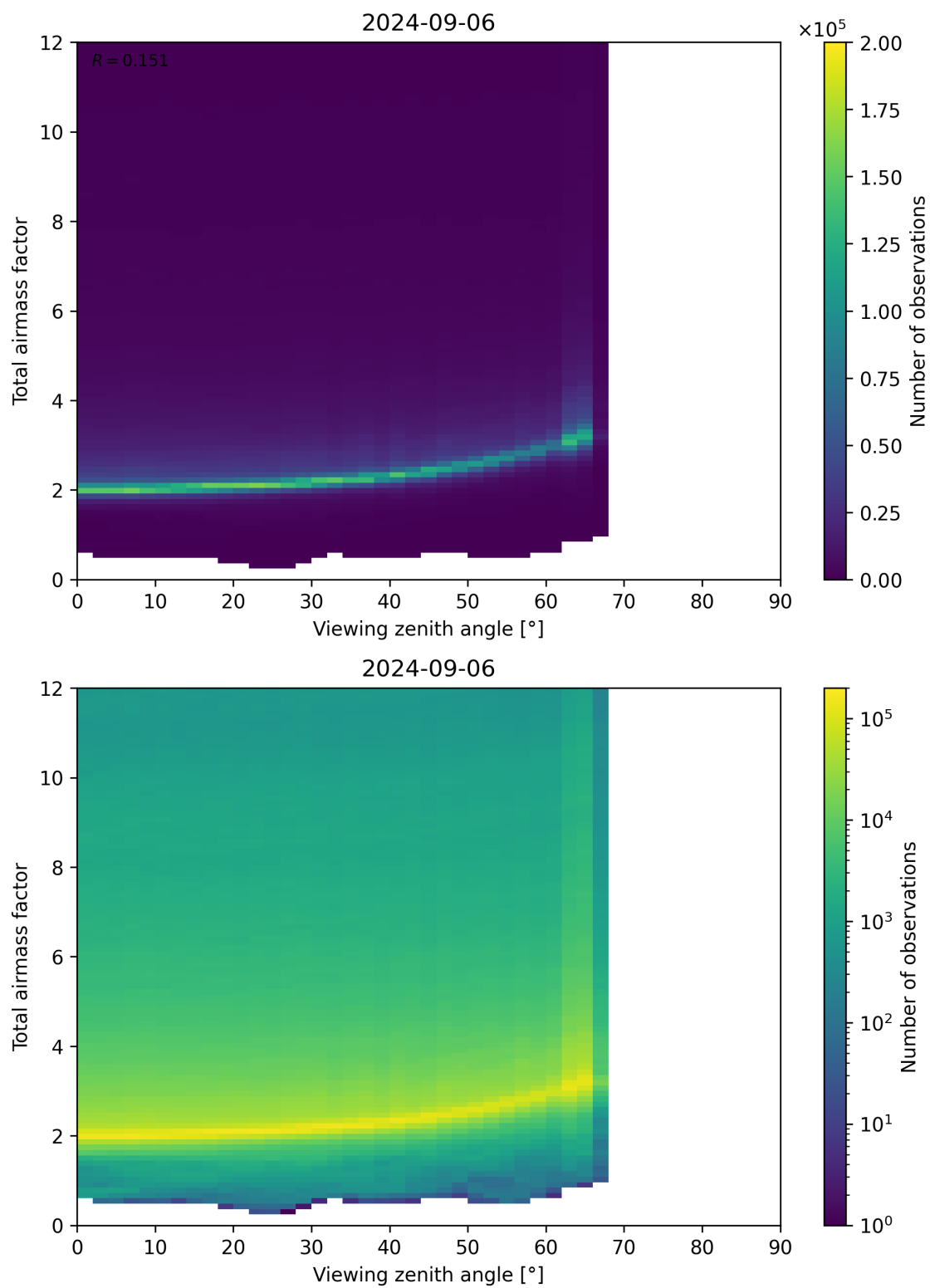
Figure 160: Scatter density plot of “Viewing zenith angle” against “Total airmass factor” for 2024-09-06 to 2024-09-07.
