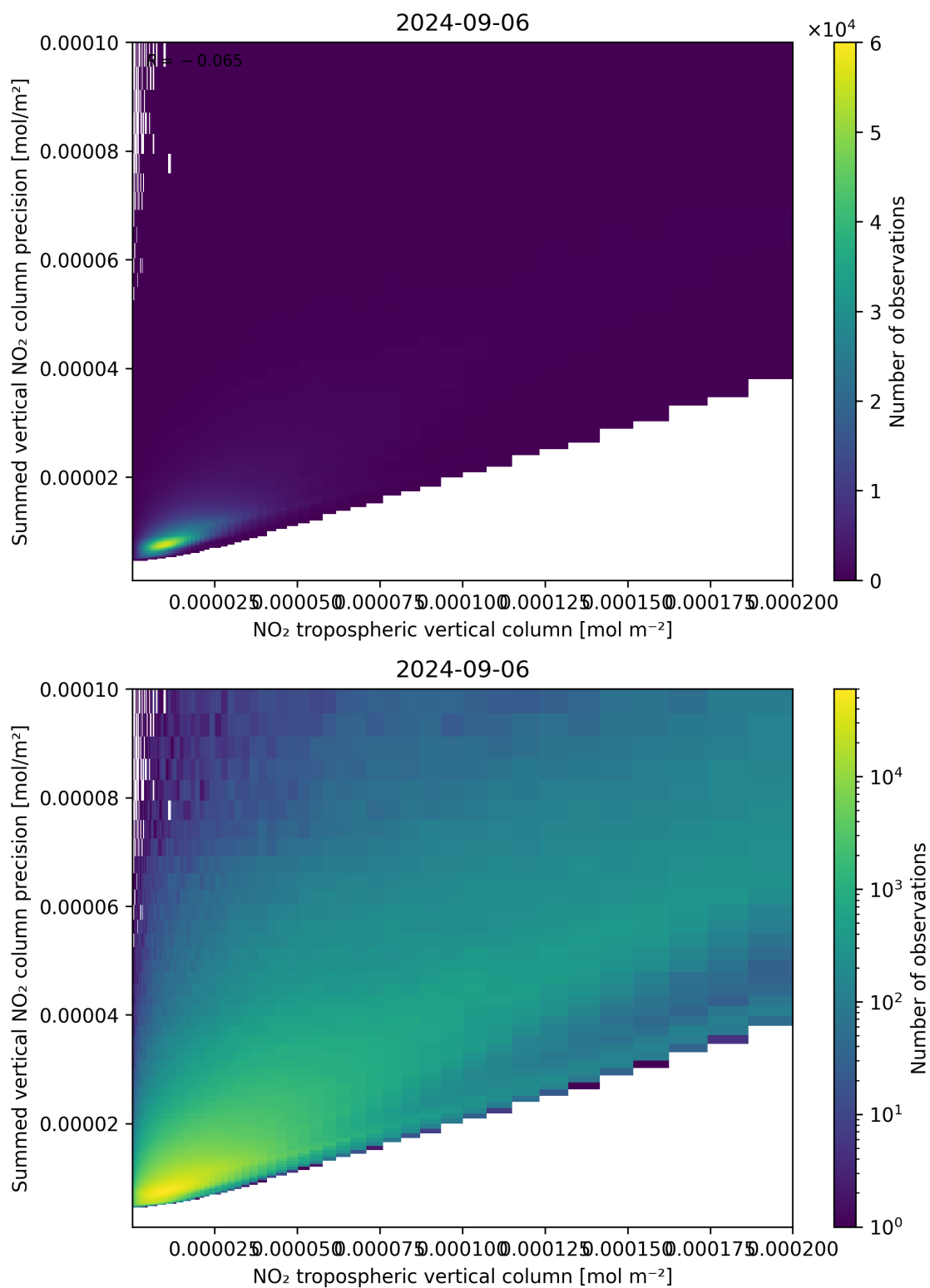
Figure 127: Scatter density plot of “NO 2 tropospheric vertical column” against “Summed vertical NO 2 column precision” for 2024-09-06 to 2024-09-07.
