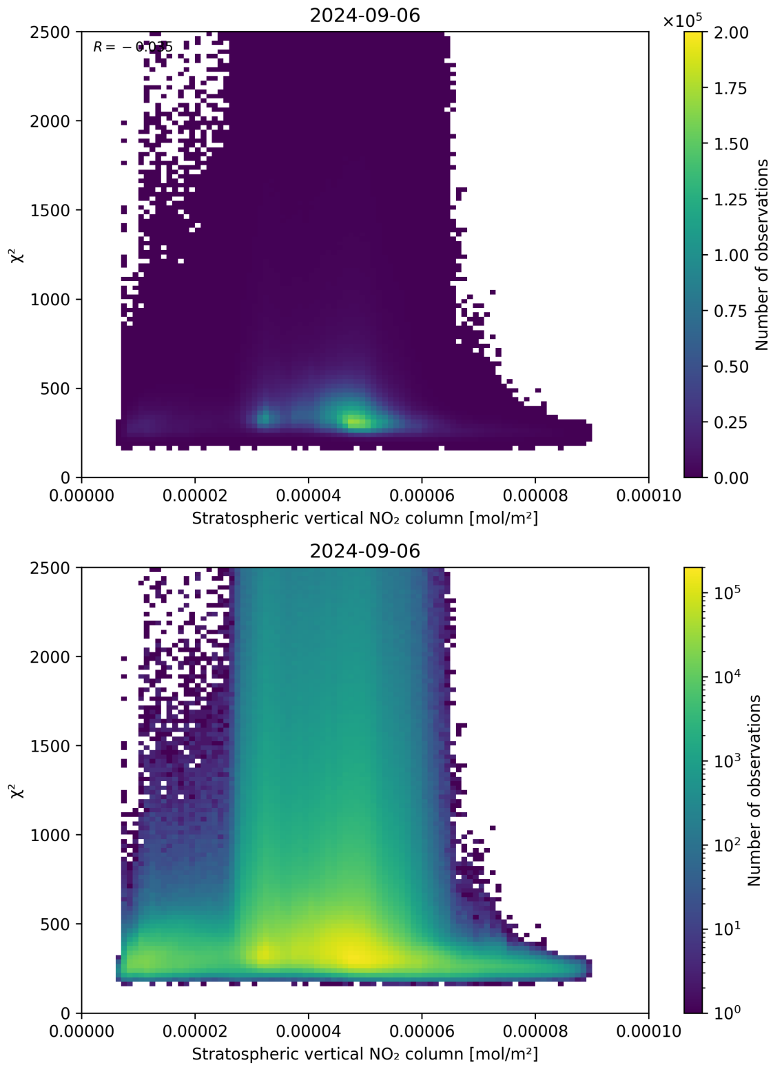
Figure 97: Scatter density plot of “Stratospheric vertical NO 2 column” against “ \chi^2 ” for 2024-09-06 to 2024-09-07.
