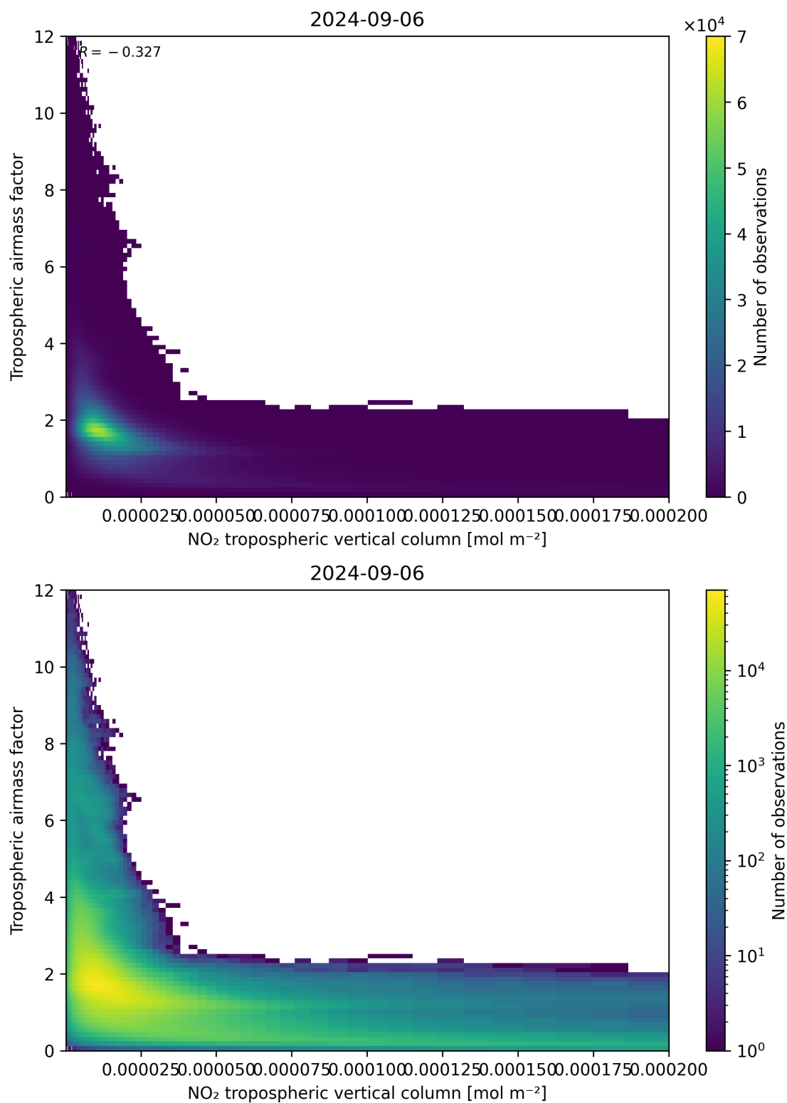
Figure 123: Scatter density plot of “NO 2 tropospheric vertical column” against “Tropospheric air mass factor” for 2024-09-06 to 2024-09-07.
