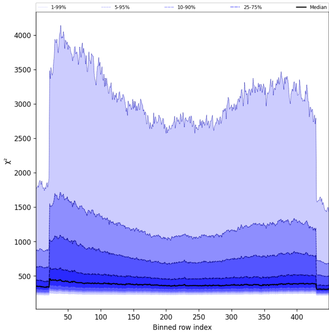
Figure 59: Along track statistics of “ \chi^2 ” for 2024-09-06 to 2024-09-07
