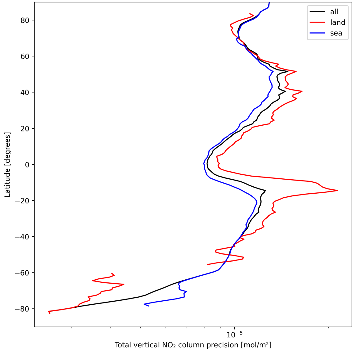
Figure 22: Zonal average of “Total vertical NO 2 column precision” for 2024-09-06 to 2024-09-07.
