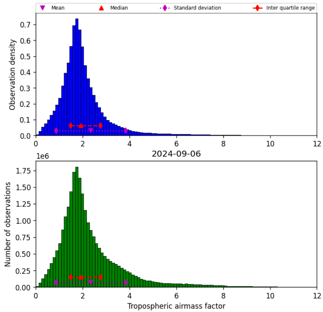
Figure 31: Histogram of “Tropospheric airmass factor” for 2024-09-06 to 2024-09-07
