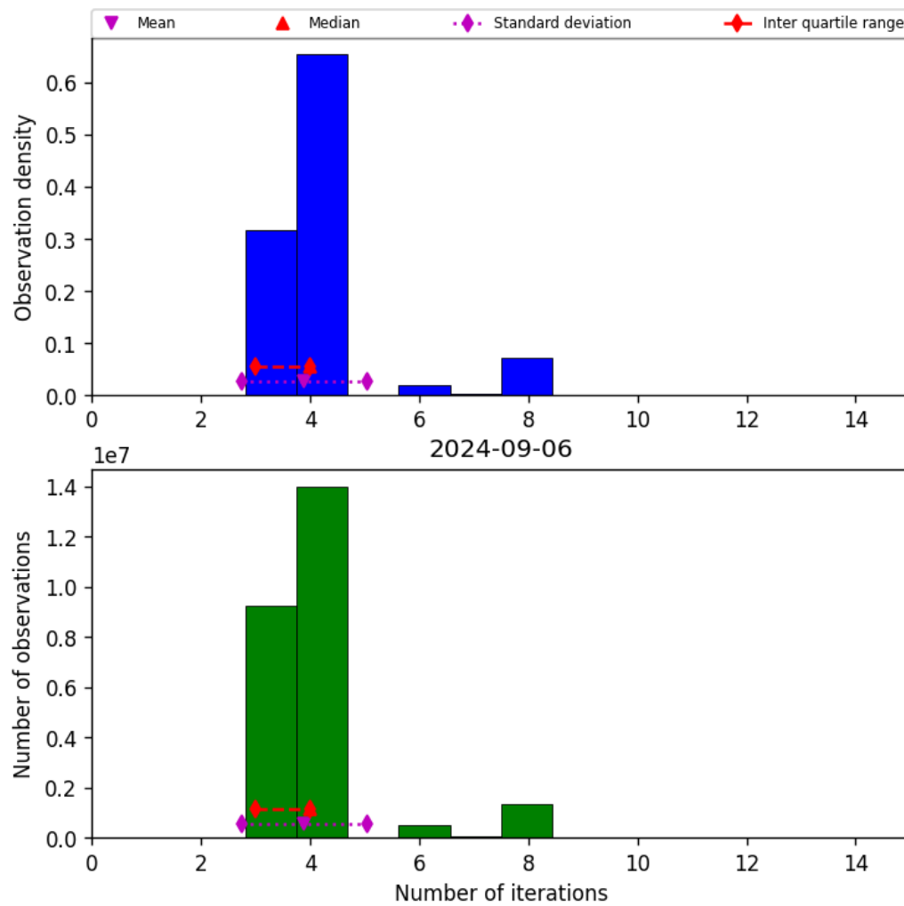
Figure 34: Histogram of “Number of iterations” for 2024-09-06 to 2024-09-07
