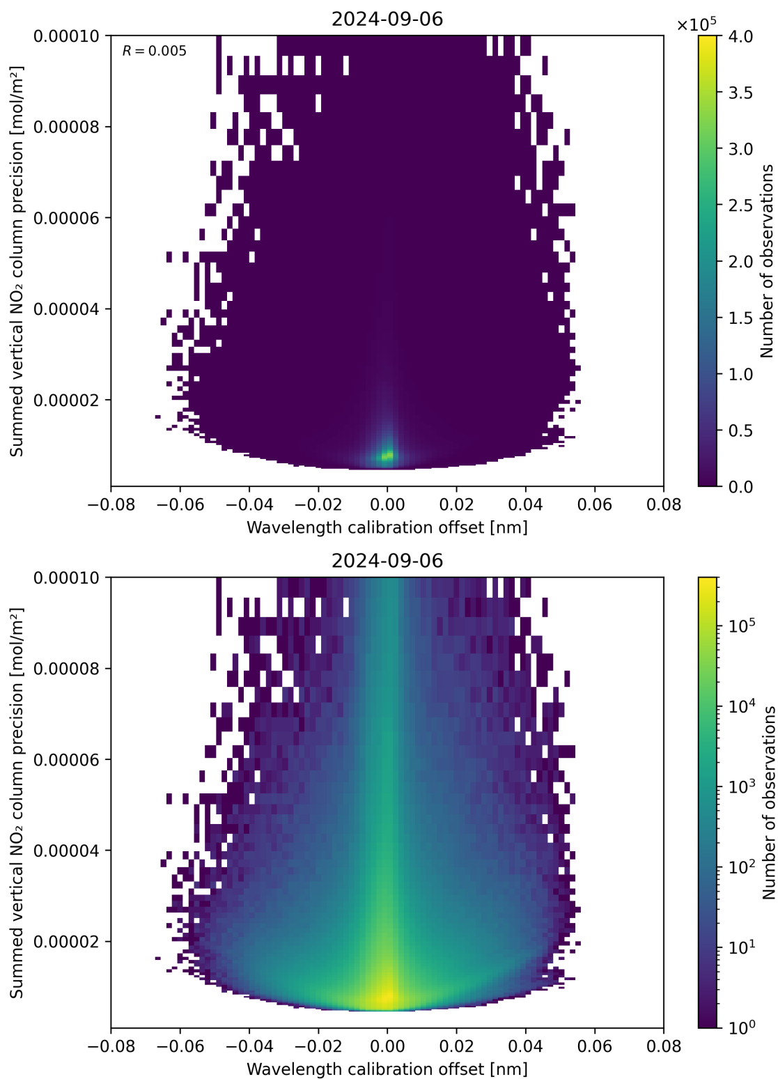
Figure 178: Scatter density plot of “Wavelength calibration offset” against “Summed vertical NO 2 column precision” for 2024-09-06 to 2024-09-07.
