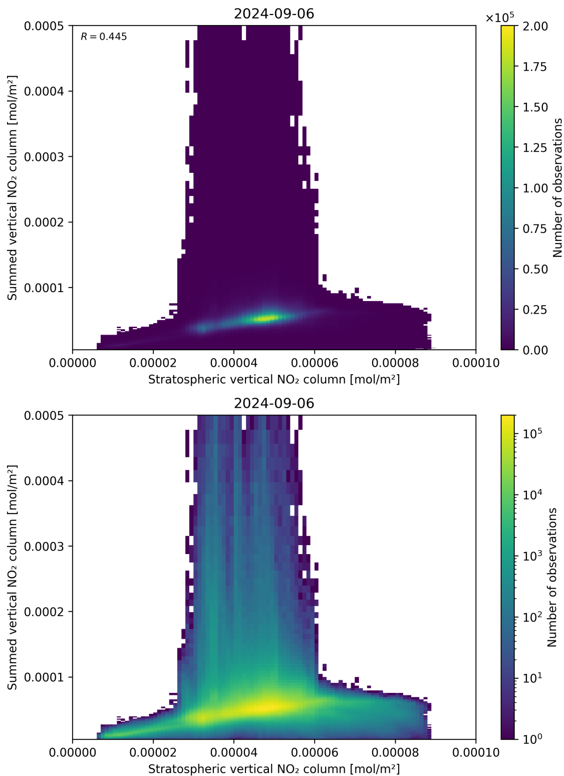
Figure 98: Scatter density plot of “Stratospheric vertical NO 2 column” against “Summed vertical NO 2 column” for 2024-09-06 to 2024-09-07.
