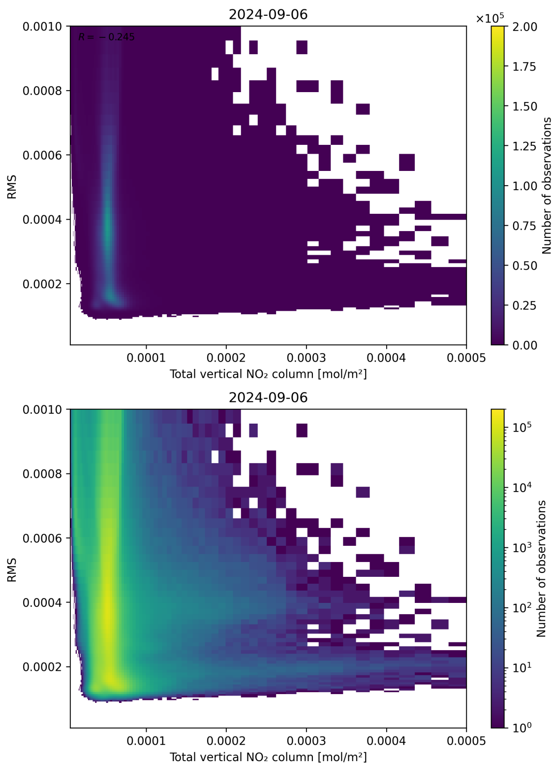
Figure 120: Scatter density plot of “Total vertical NO 2 column” against “RMS” for 2024-09-06 to 2024-09-07.
