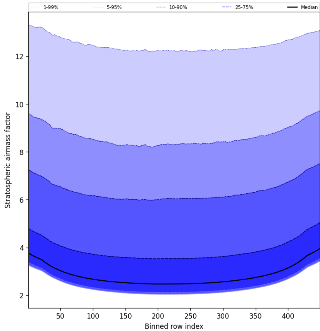
Figure 61: Along track statistics of “Stratospheric airmass factor” for 2024-09-06 to 2024-09-07
