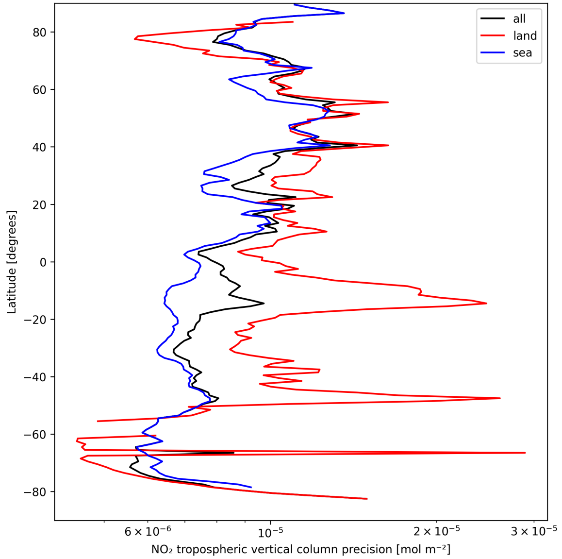
Figure 13: Zonal average of “NO 2 tropospheric vertical column precision” for 2024-09-06 to 2024-09-07.
