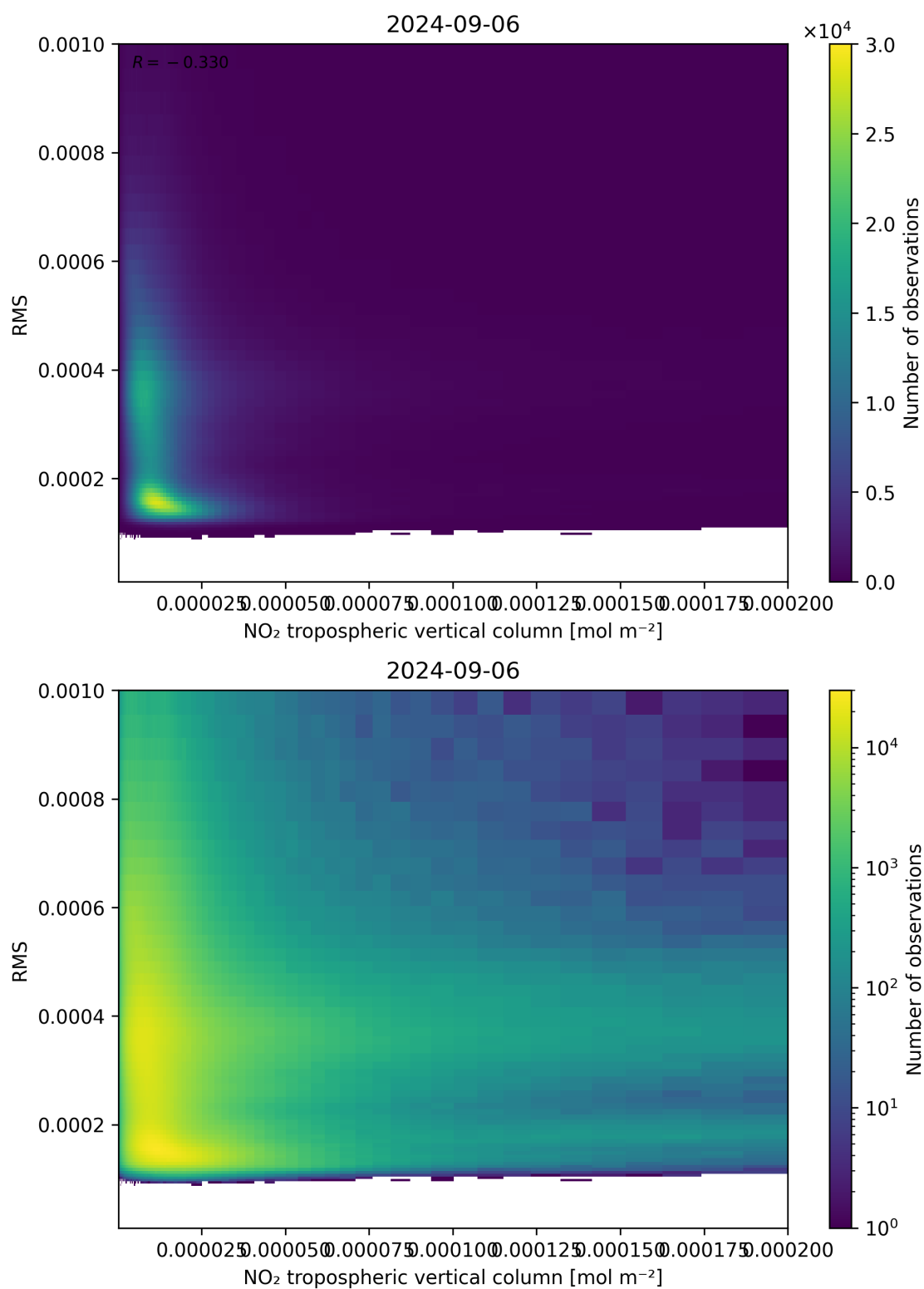
Figure 142: Scatter density plot of “NO 2 tropospheric vertical column” against “RMS” for 2024-09-06 to 2024-09-07.
