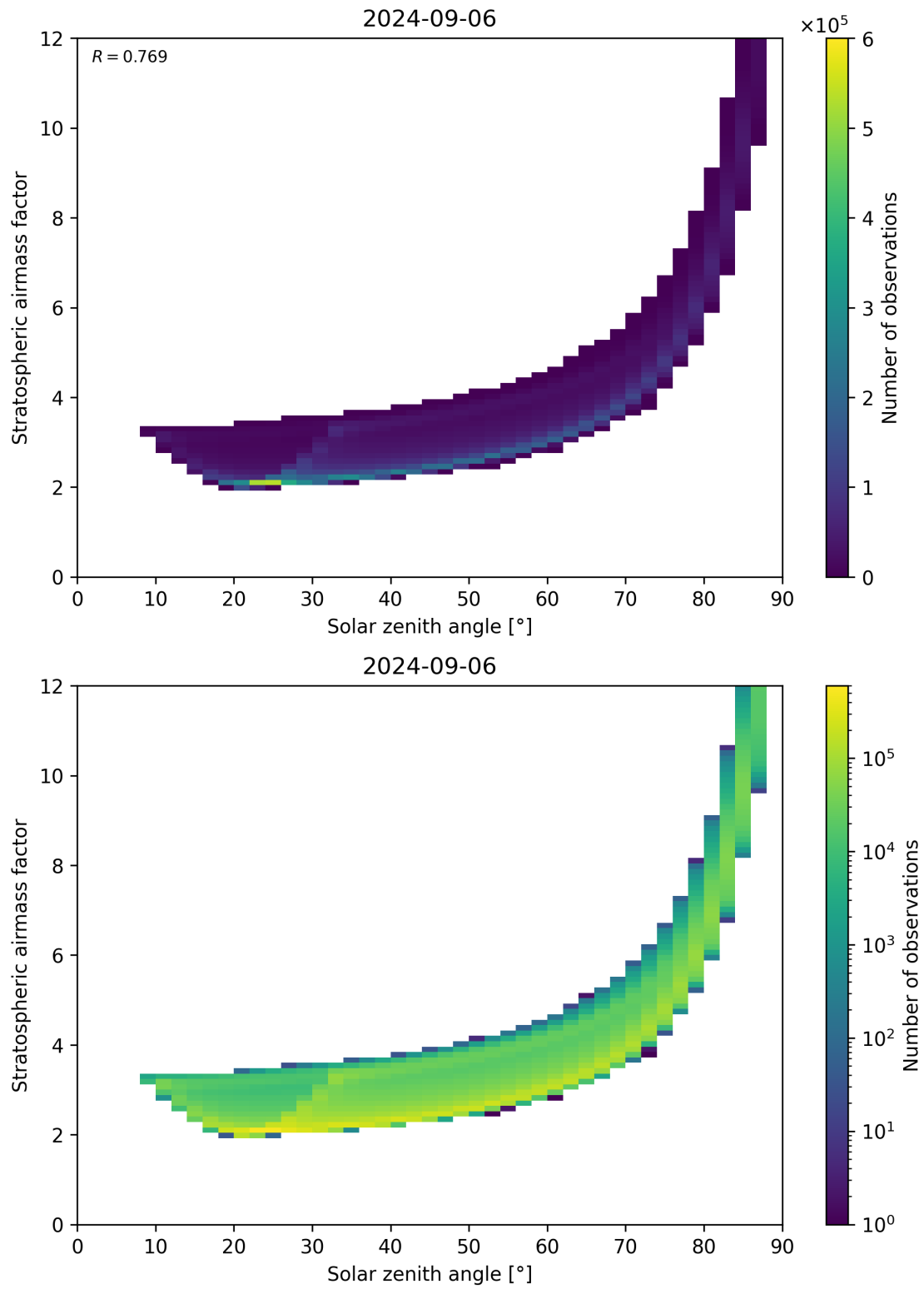
Figure 145: Scatter density plot of “Solar zenith angle” against “Stratospheric airmass factor” for 2024-09-06 to 2024-09-07.
