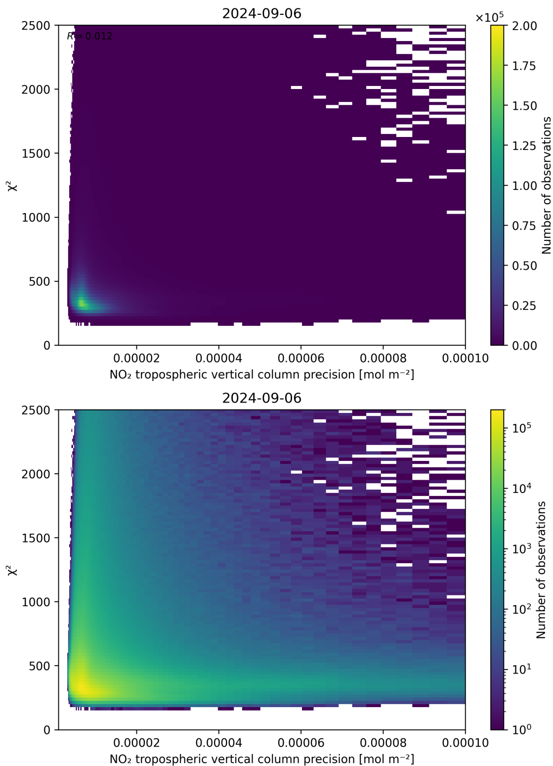
Figure 134: Scatter density plot of “NO 2 tropospheric vertical column precision” against “ \chi^2 ” for 2024-09-06 to 2024-09-07.
