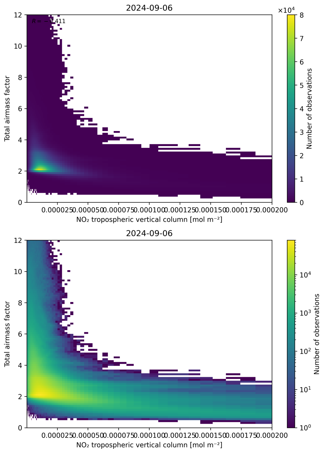
Figure 122: Scatter density plot of “NO 2 tropospheric vertical column” against “Total air mass factor” for 2024-09-06 to 2024-09-07.
