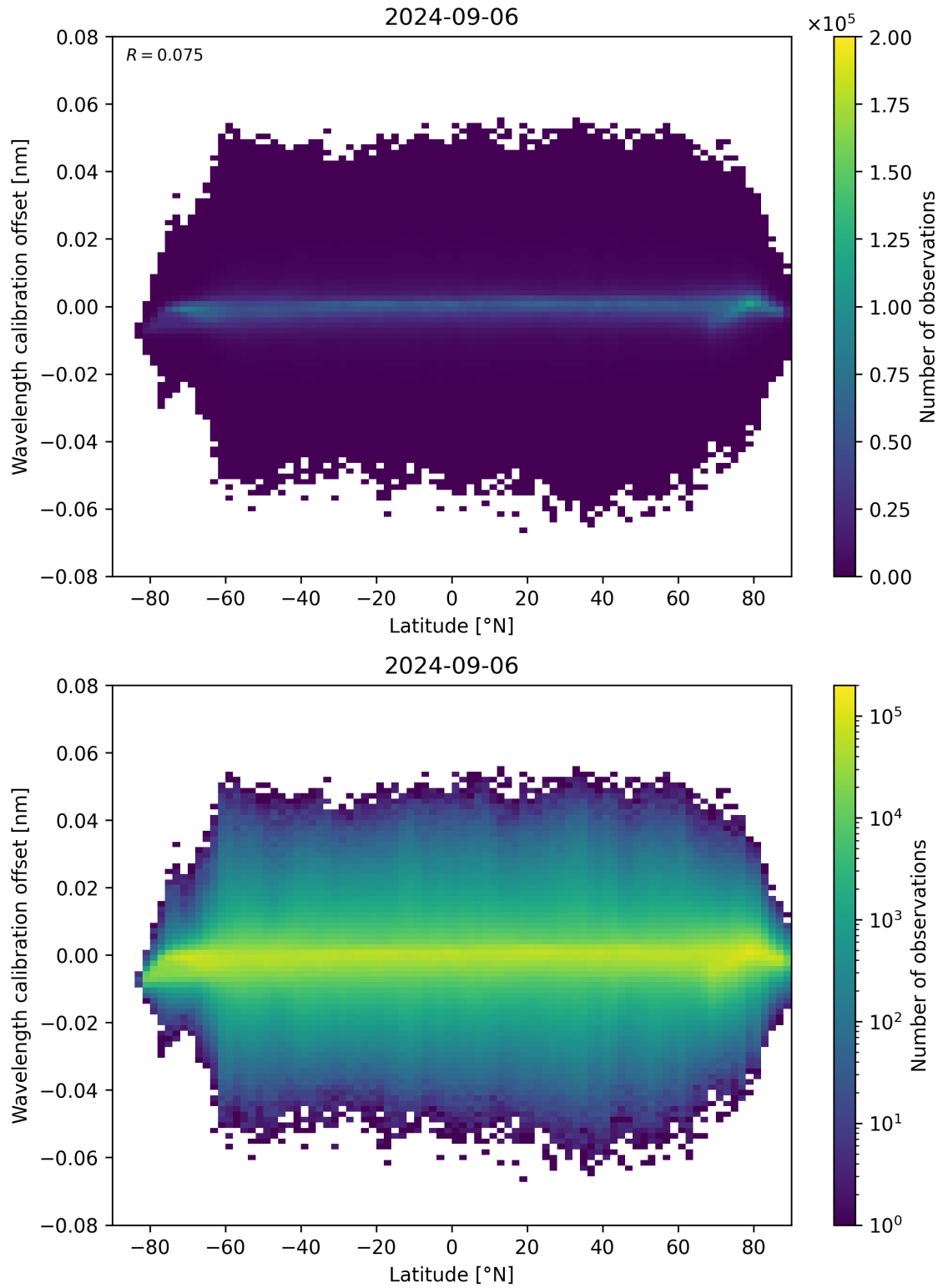
Figure 95: Scatter density plot of “Latitude” against “Wavelength calibration offset” for 2024-09-06 to 2024-09-07.
