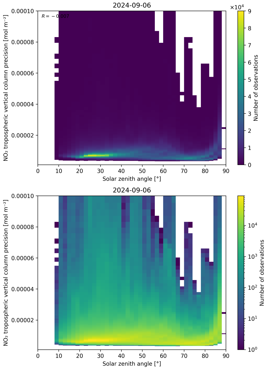
Figure 156: Scatter density plot of “Solar zenith angle” against “NO 2 tropospheric vertical column precision” for 2024-09-06 to 2024-09-07.
