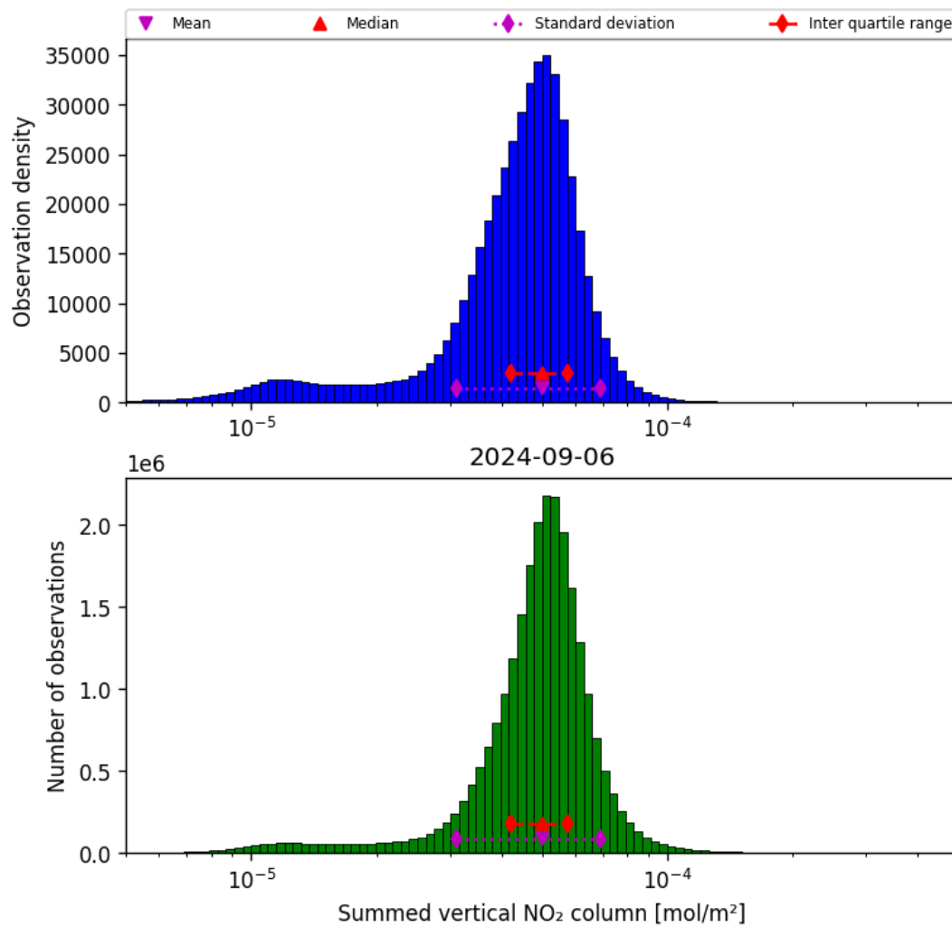
Figure 40: Histogram of “Summed vertical NO 2 column” for 2024-09-06 to 2024-09-07
