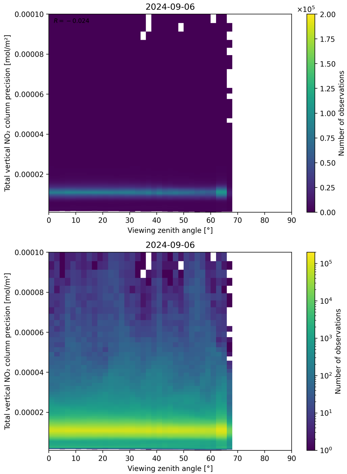
Figure 168: Scatter density plot of “Viewing zenith angle” against “Total vertical NO 2 column precision” for 2024-09-06 to 2024-09-07.
