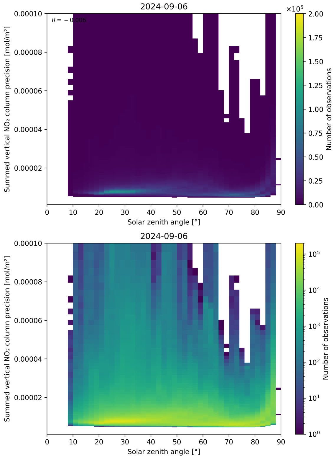
Figure 152: Scatter density plot of “Solar zenith angle” against “Summed vertical NO 2 column precision” for 2024-09-06 to 2024-09-07.
