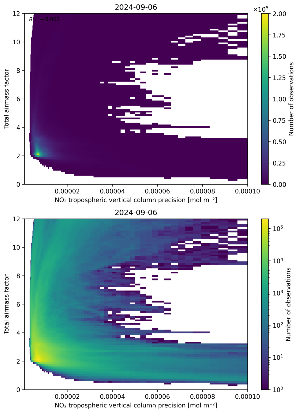
Figure 132: Scatter density plot of “NO 2 tropospheric vertical column precision” against “Total airmass factor” for 2024-09-06 to 2024-09-07.
