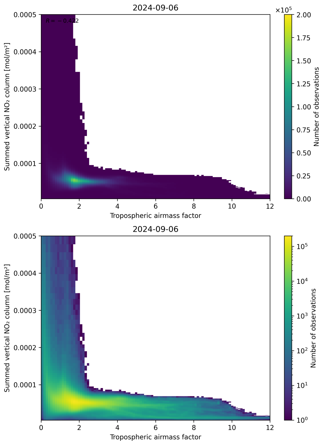
Figure 75: Scatter density plot of “Tropospheric airmass factor” against “Summed vertical NO 2 column” for 2024-09-06 to 2024-09-07.
