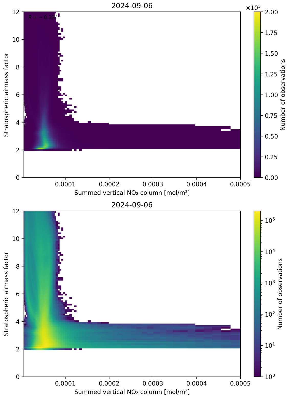
Figure 103: Scatter density plot of “Summed vertical NO 2 column” against “Stratospheric air mass factor” for 2024-09-06 to 2024-09-07.
