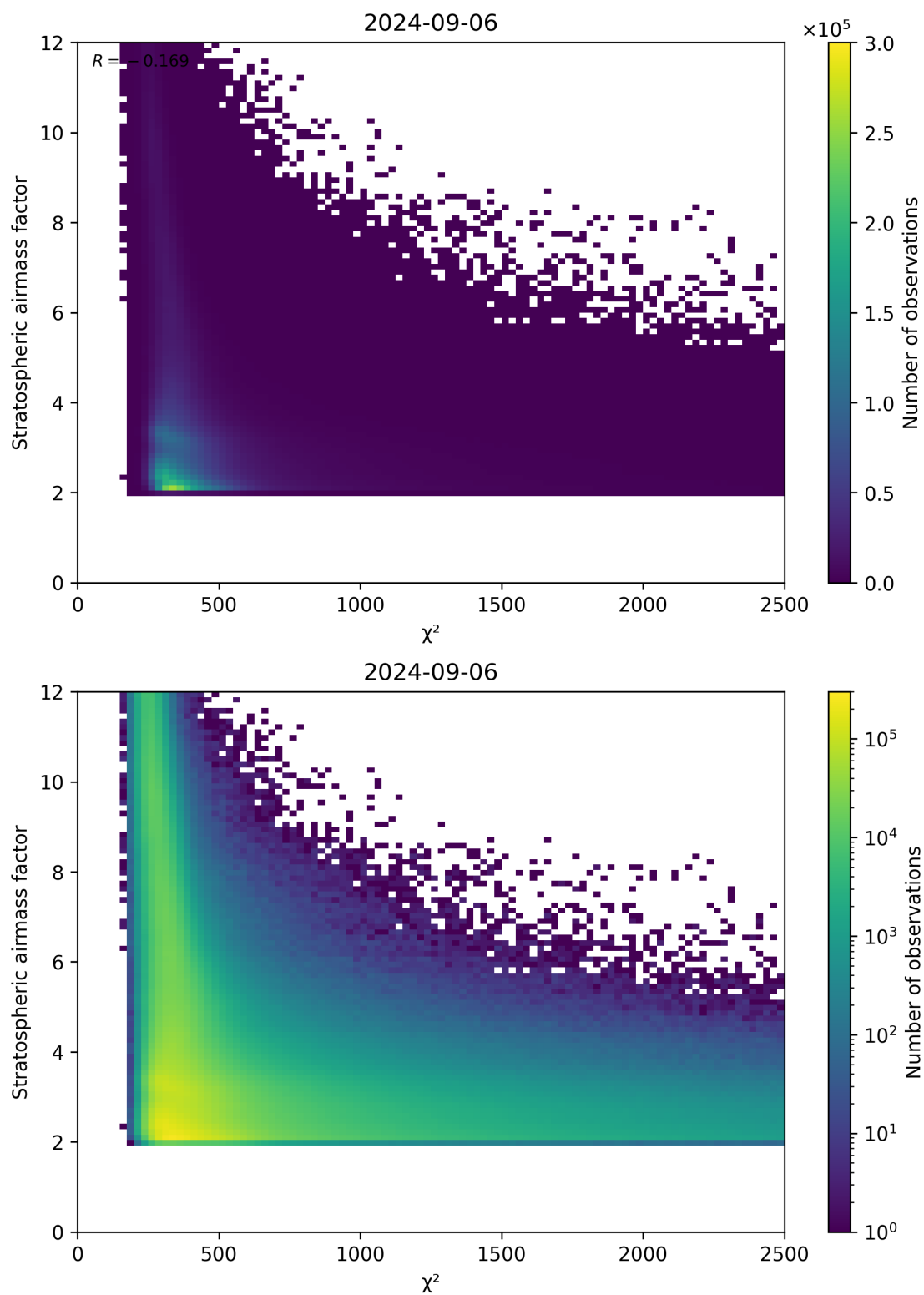
Figure 81: Scatter density plot of “ \chi^2 ” against “Stratospheric airmass factor” for 2024-09-06 to 2024-09-07.
