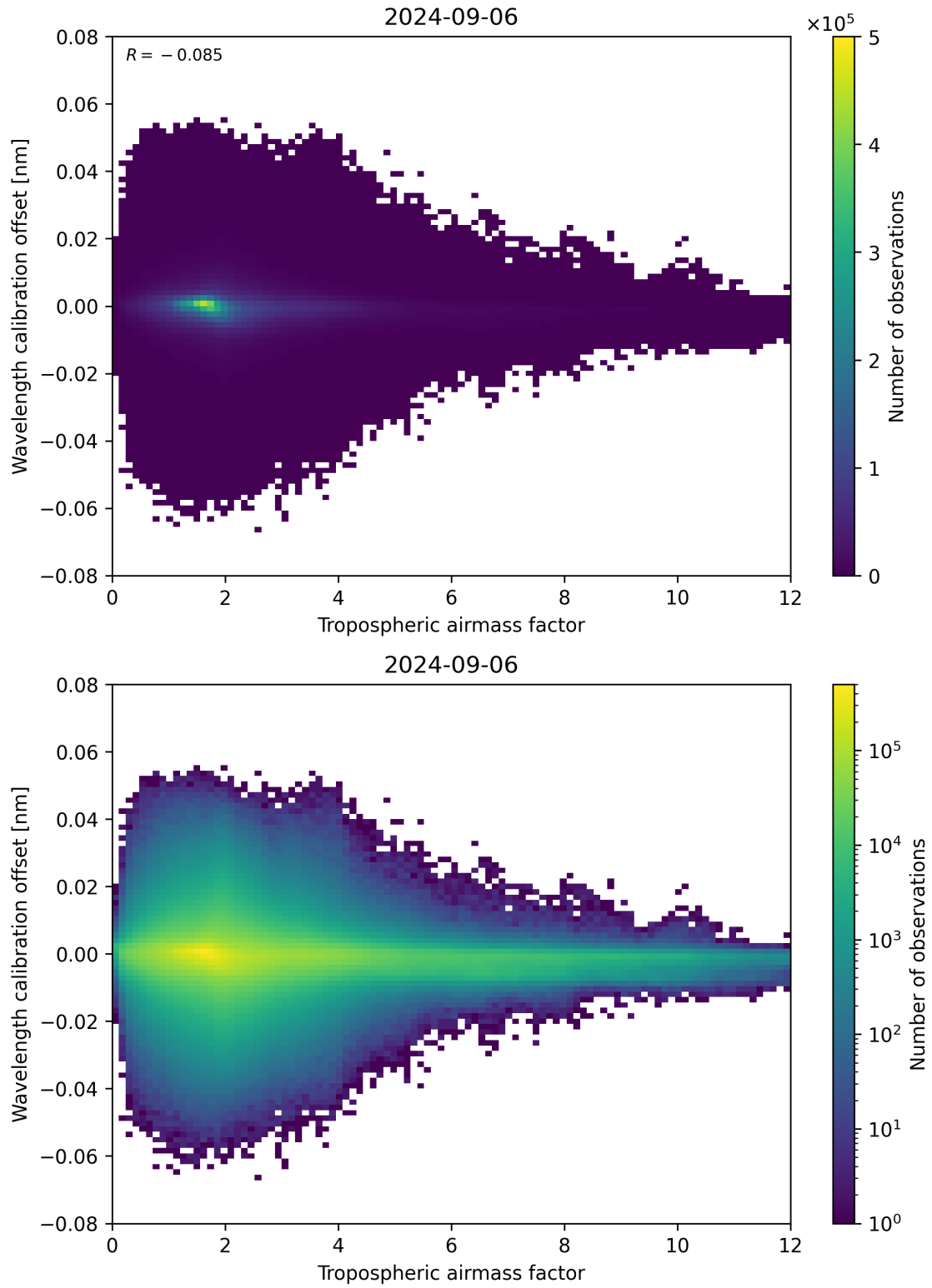
Figure 80: Scatter density plot of “Tropospheric airmass factor” against “Wavelength calibration offset” for 2024-09-06 to 2024-09-07.
