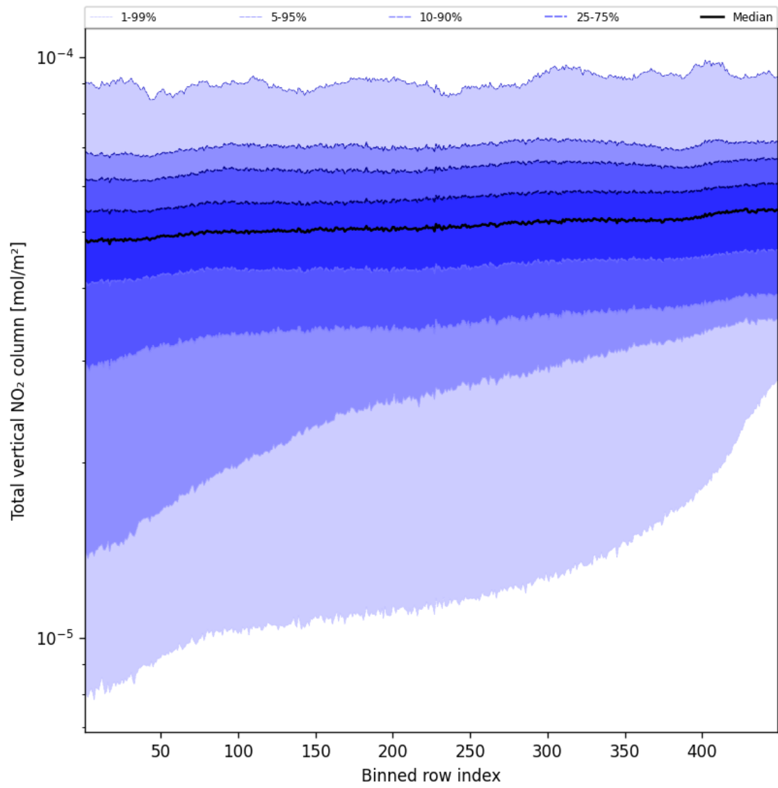
Figure 55: Along track statistics of “Total vertical NO 2 column” for 2024-09-06 to 2024-09-07
