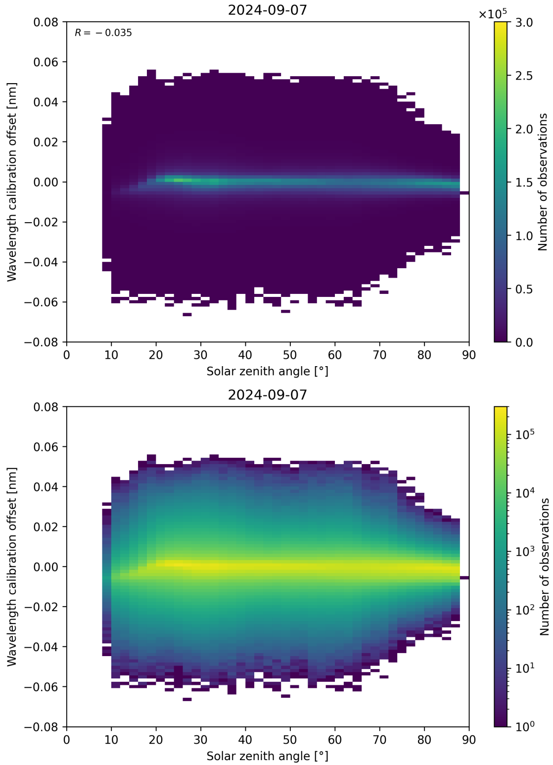
Figure 158: Scatter density plot of “Solar zenith angle” against “Wavelength calibration offset” for 2024-09-06 to 2024-09-08.
