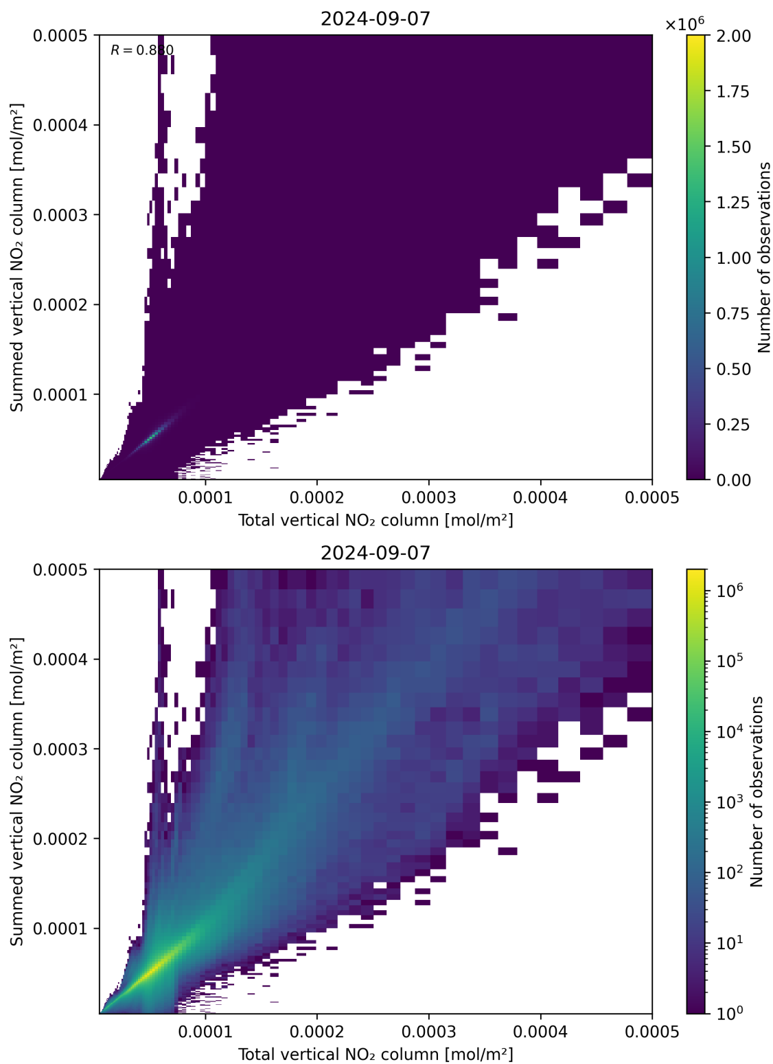
Figure 112: Scatter density plot of “Total vertical NO 2 column” against “Summed vertical NO 2 column” for 2024-09-06 to 2024-09-08.
