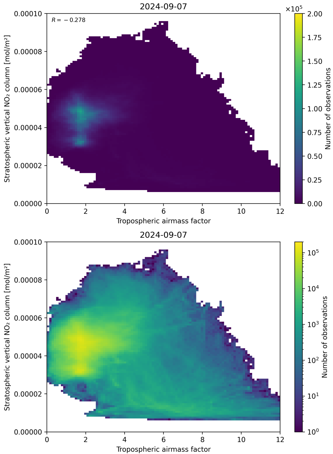
Figure 74: Scatter density plot of “Tropospheric airmass factor” against “Stratospheric vertical NO 2 column” for 2024-09-06 to 2024-09-08.
