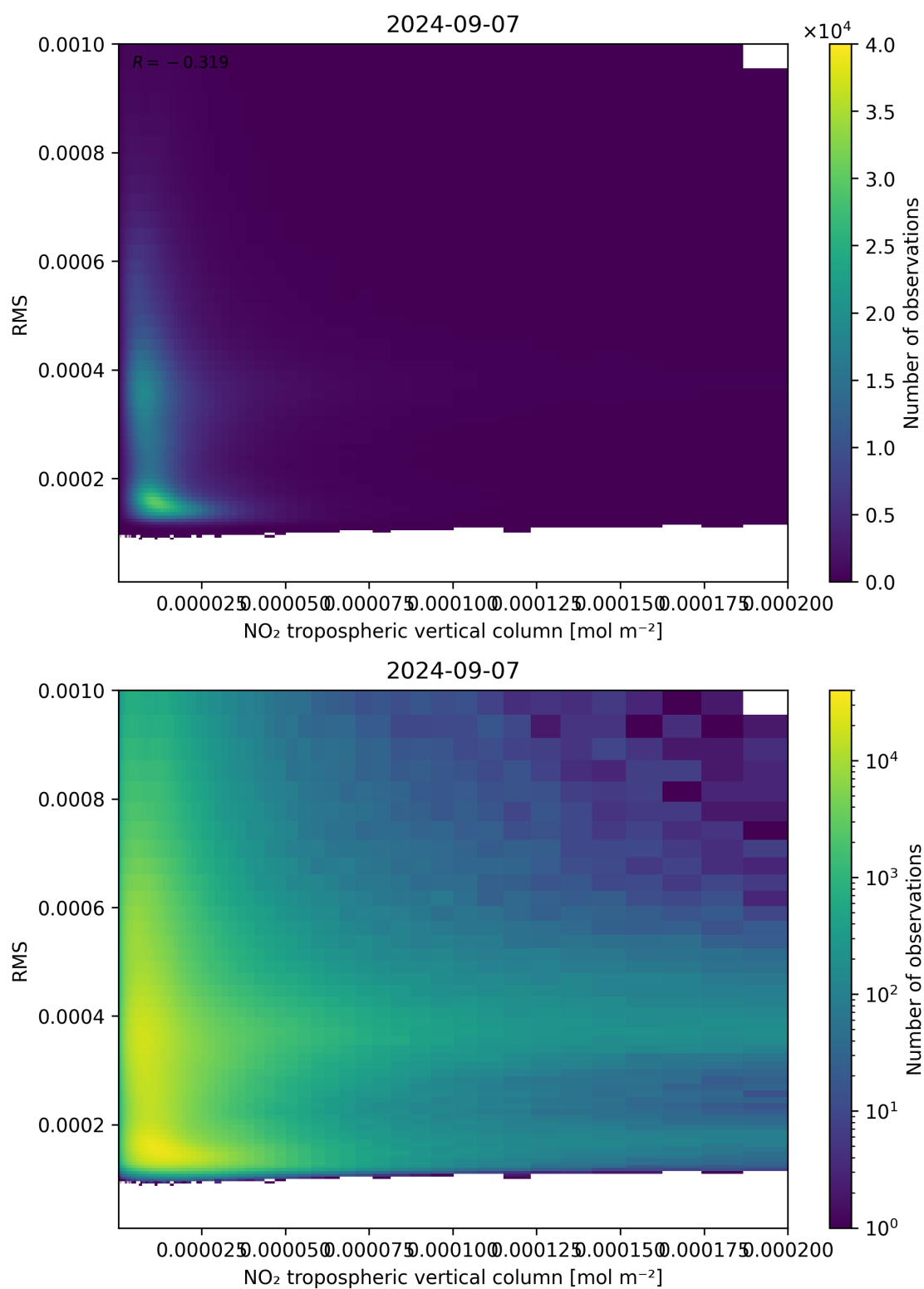
Figure 142: Scatter density plot of “NO 2 tropospheric vertical column” against “RMS” for 2024-09-06 to 2024-09-08.
