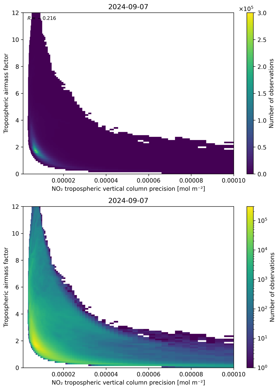
Figure 133: Scatter density plot of “NO 2 tropospheric vertical column precision” against “Tropospheric airmass factor” for 2024-09-06 to 2024-09-08.
