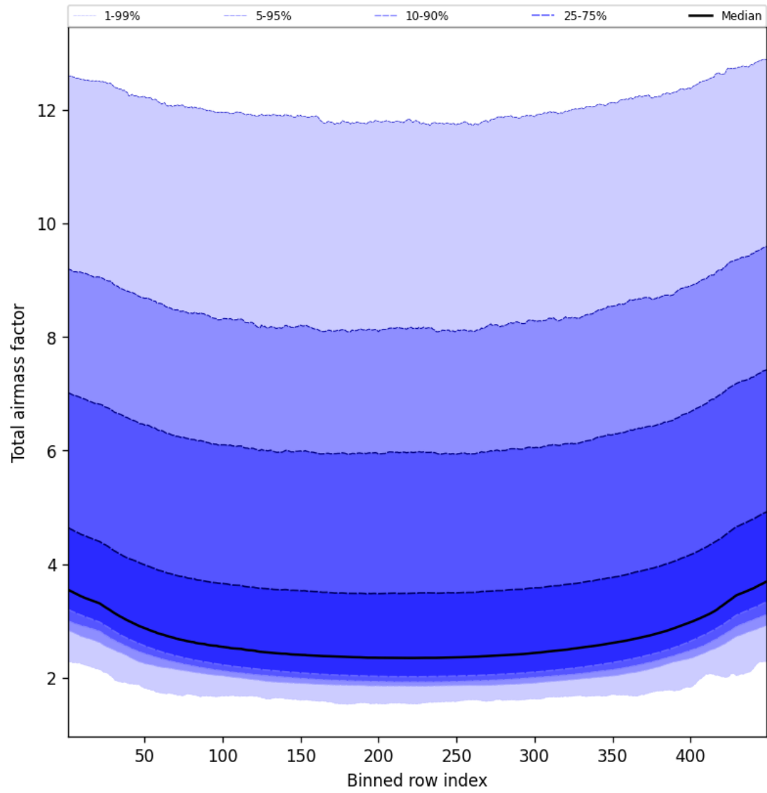
Figure 49: Along track statistics of “Total airmass factor” for 2024-09-06 to 2024-09-08
