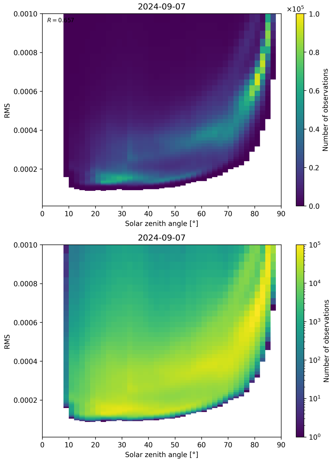
Figure 157: Scatter density plot of “Solar zenith angle” against “RMS” for 2024-09-06 to 2024-09-08.
