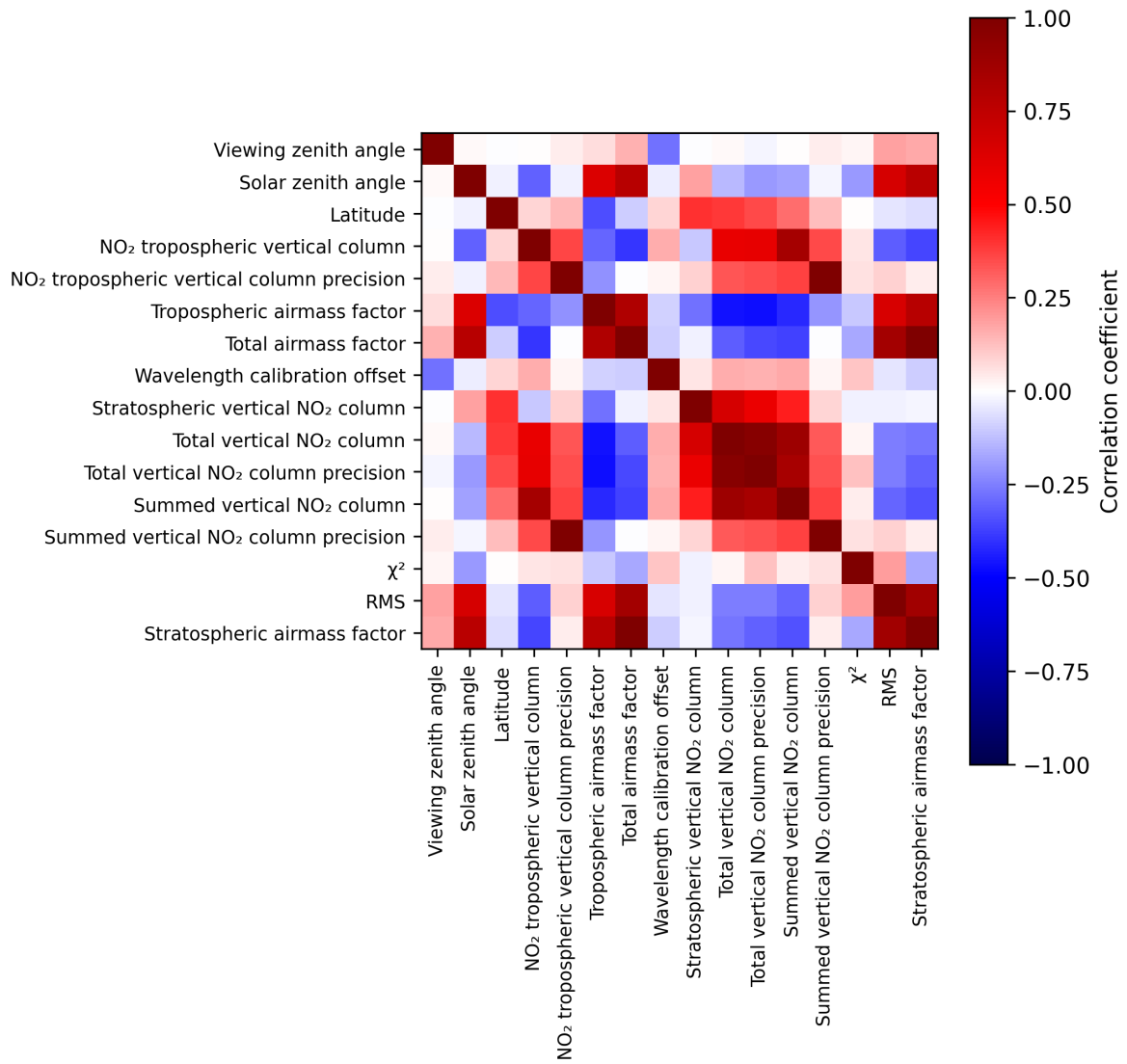
Figure 2: Map of correlation matrix for 2024-09-06 to 2024-09-08.
