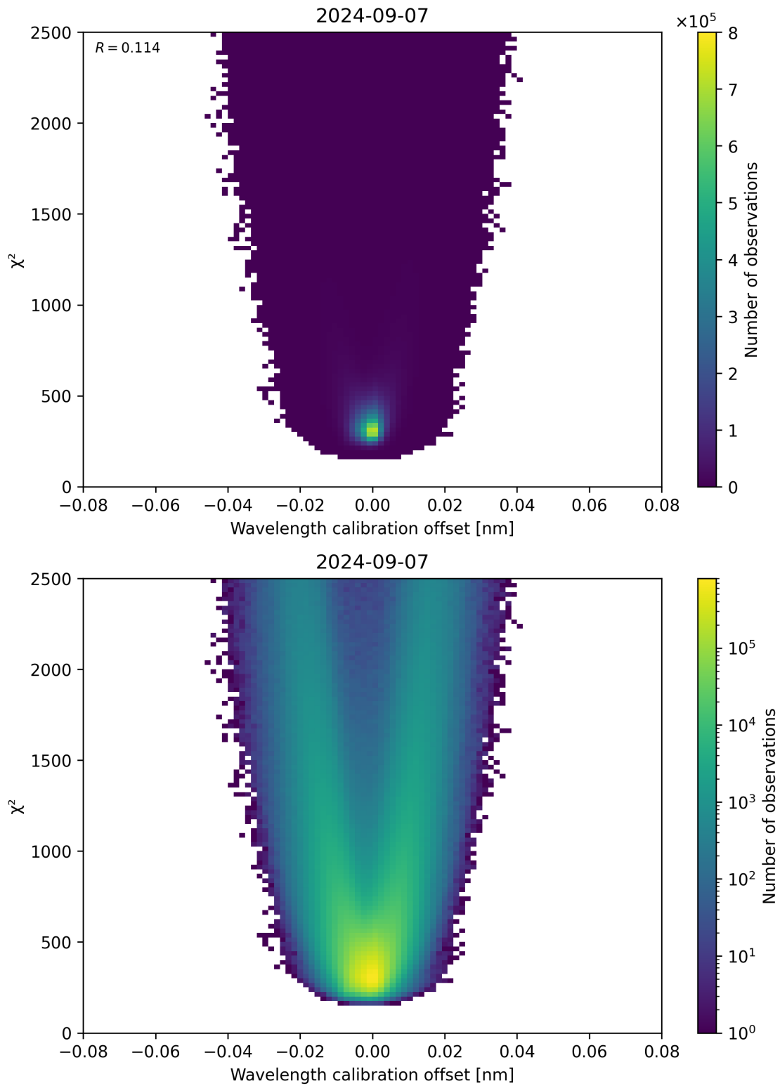
Figure 175: Scatter density plot of “Wavelength calibration offset” against “ \chi^2 ” for 2024-09-06 to 2024-09-08.
