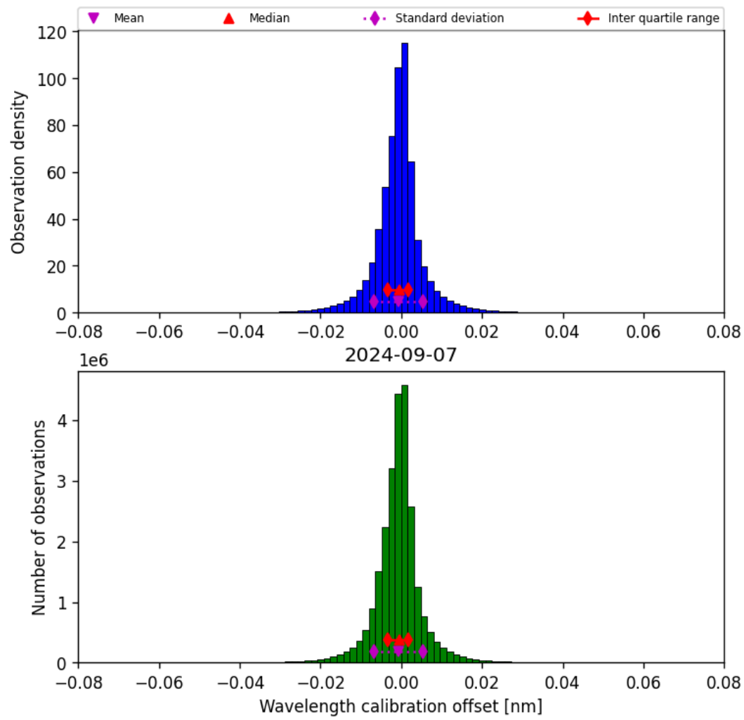
Figure 35: Histogram of “Wavelength calibration offset” for 2024-09-06 to 2024-09-08
