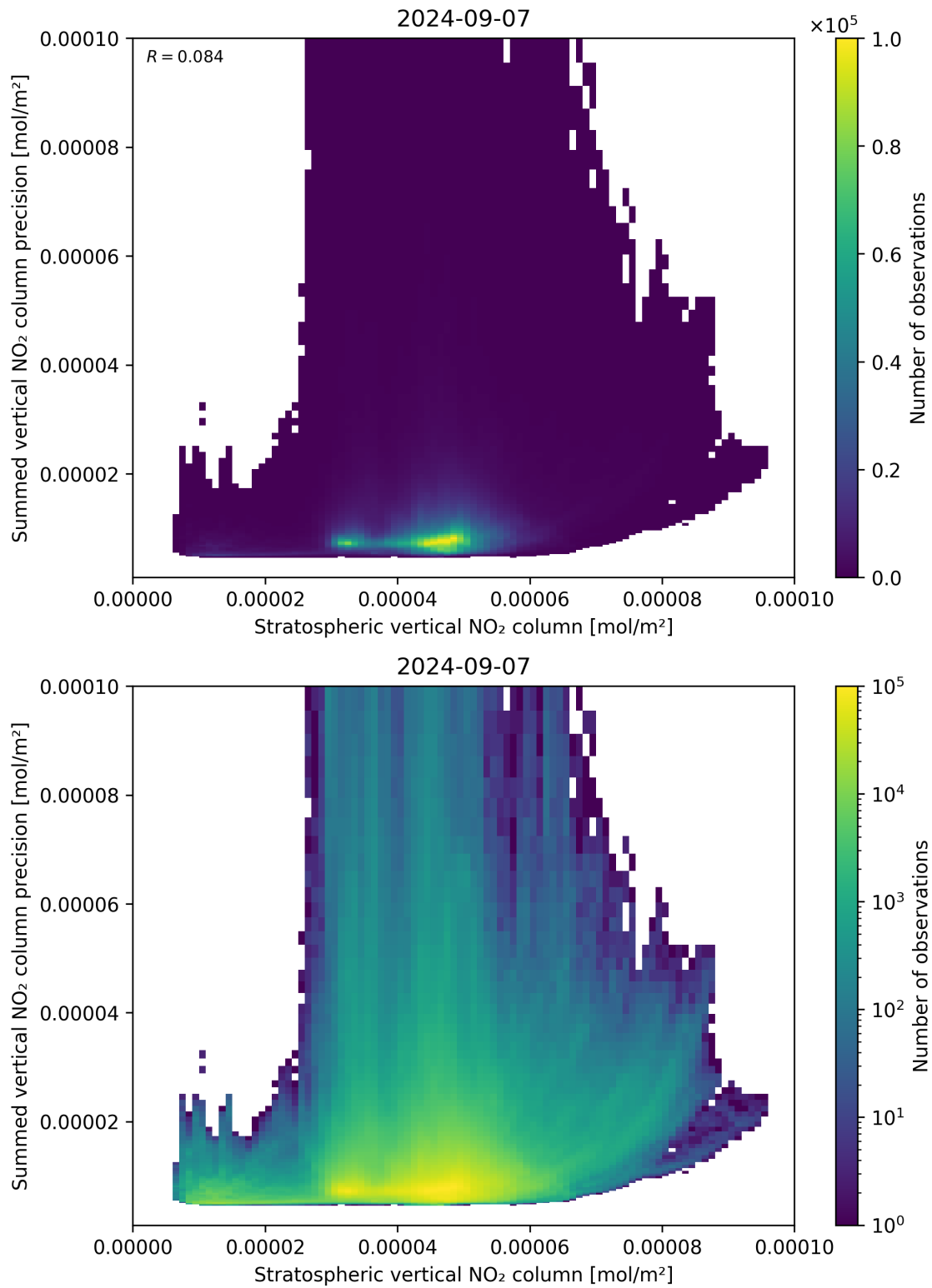
Figure 99: Scatter density plot of “Stratospheric vertical NO 2 column” against “Summed vertical NO 2 column precision” for 2024-09-06 to 2024-09-08.
