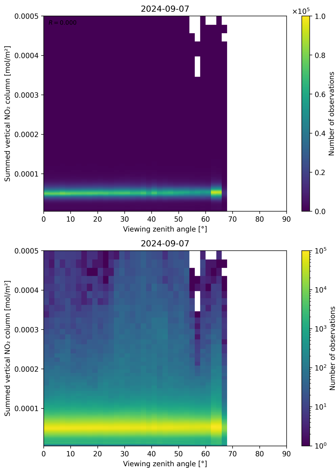
Figure 165: Scatter density plot of “Viewing zenith angle” against “Summed vertical NO 2 column” for 2024-09-06 to 2024-09-08.
