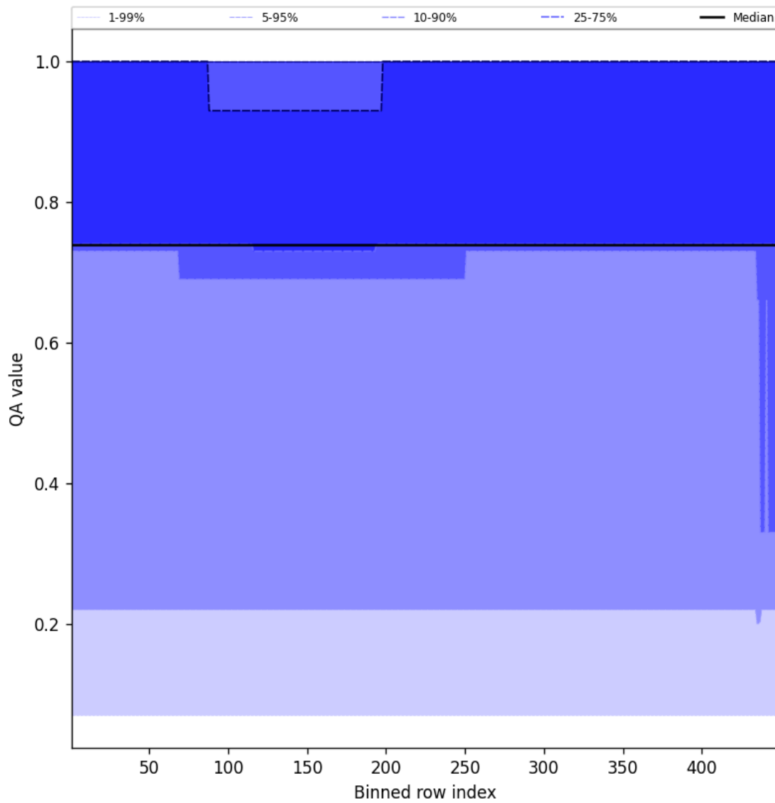
Figure 45: Along track statistics of “QA value” for 2024-09-06 to 2024-09-08
