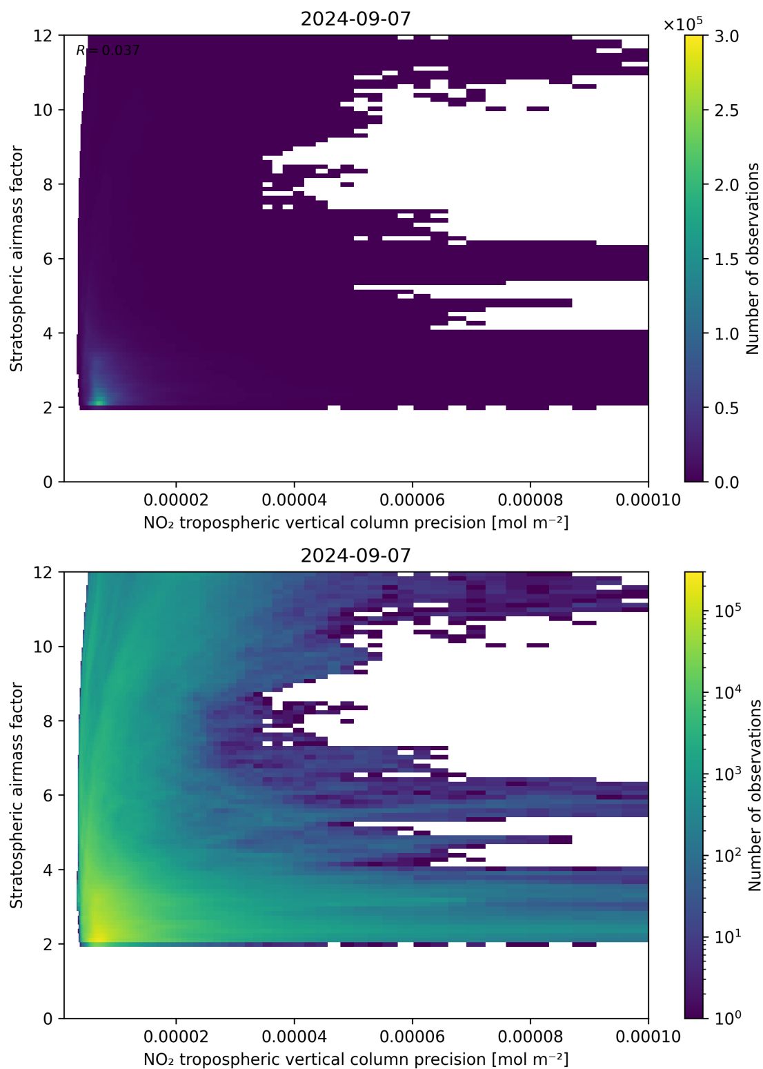
Figure 131: Scatter density plot of “NO 2 tropospheric vertical column precision” against “Stratospheric airmass factor” for 2024-09-06 to 2024-09-08.
