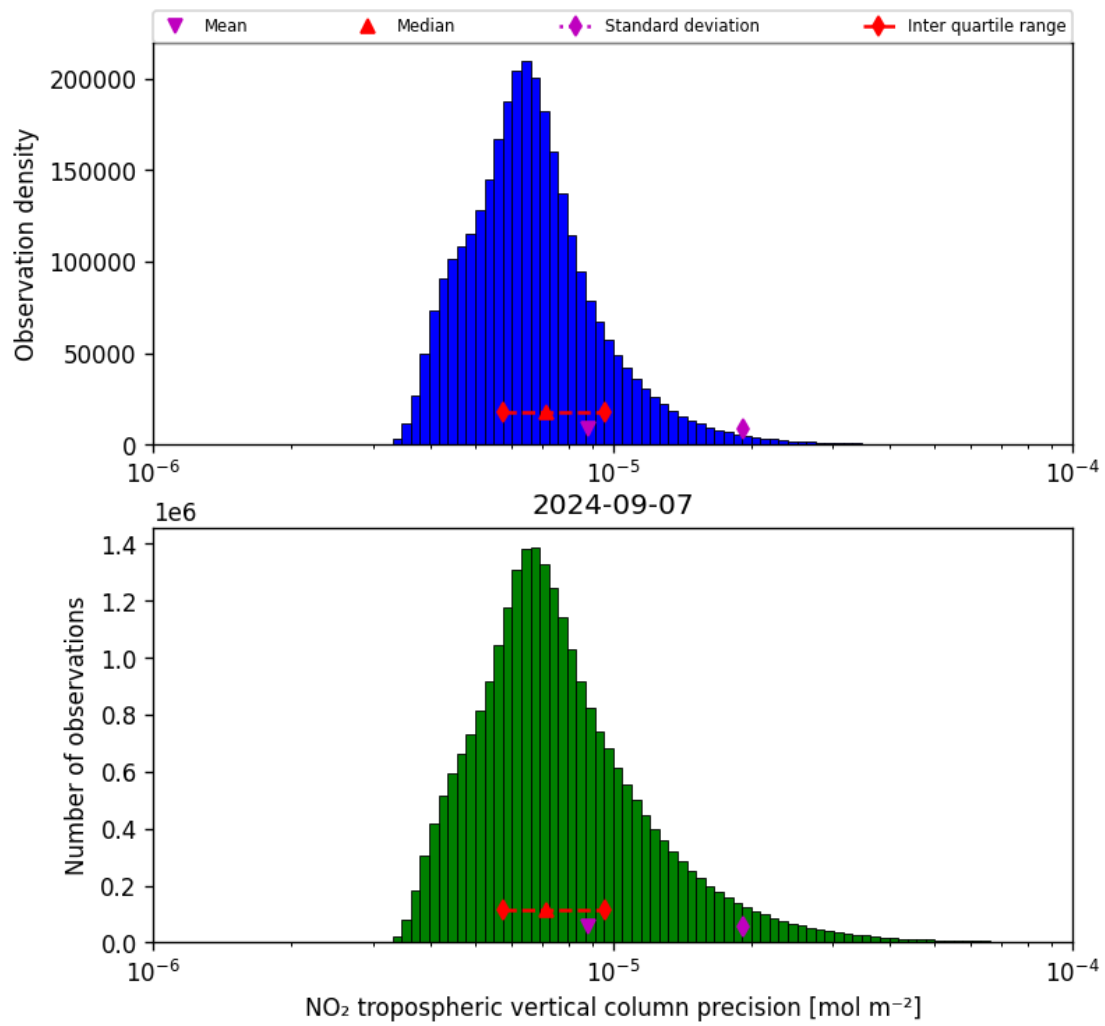
Figure 30: Histogram of “NO 2 tropospheric vertical column precision” for 2024-09-06 to 2024-09-08
