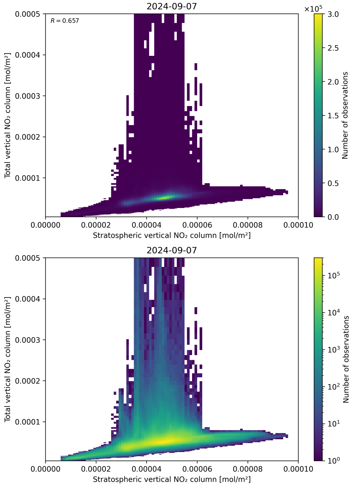
Figure 100: Scatter density plot of “Stratospheric vertical NO 2 column” against “Total vertical NO 2 column” for 2024-09-06 to 2024-09-08.
