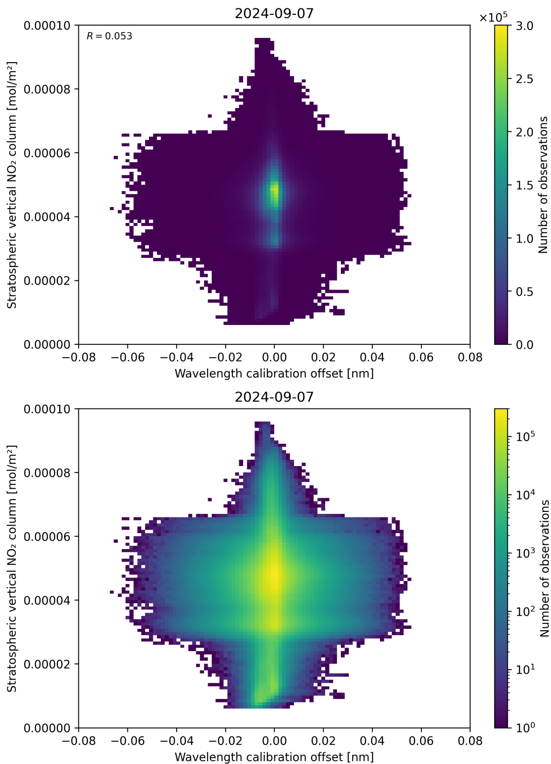
Figure 176: Scatter density plot of “Wavelength calibration offset” against “Stratospheric vertical NO 2 column” for 2024-09-06 to 2024-09-08.
