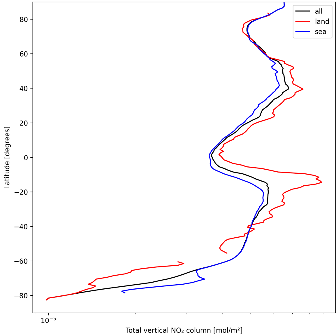
Figure 21: Zonal average of “Total vertical NO 2 column” for 2024-09-06 to 2024-09-08.
