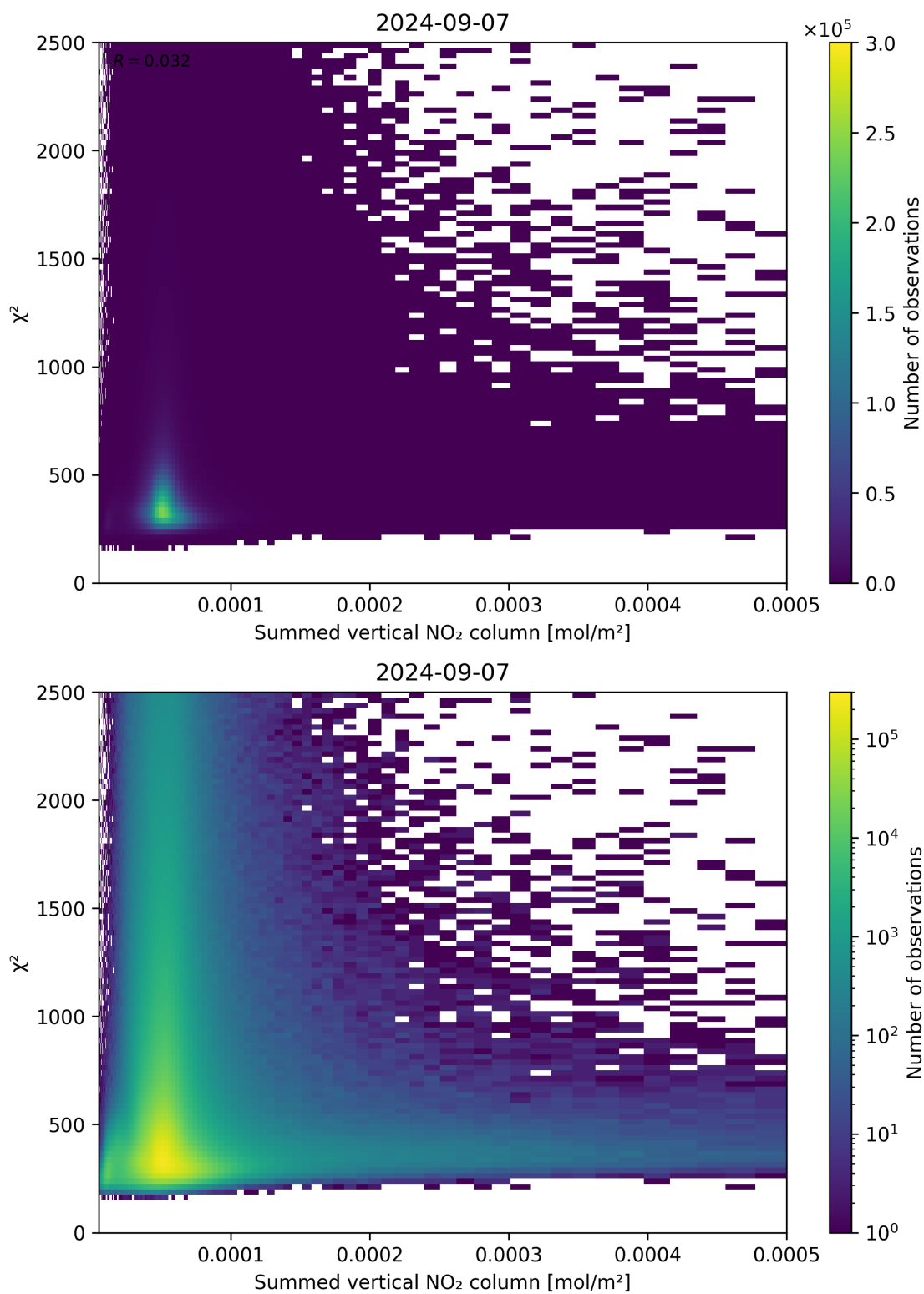
Figure 104: Scatter density plot of “Summed vertical NO 2 column” against “ \chi^2 ” for 2024-09-06 to 2024-09-08.
