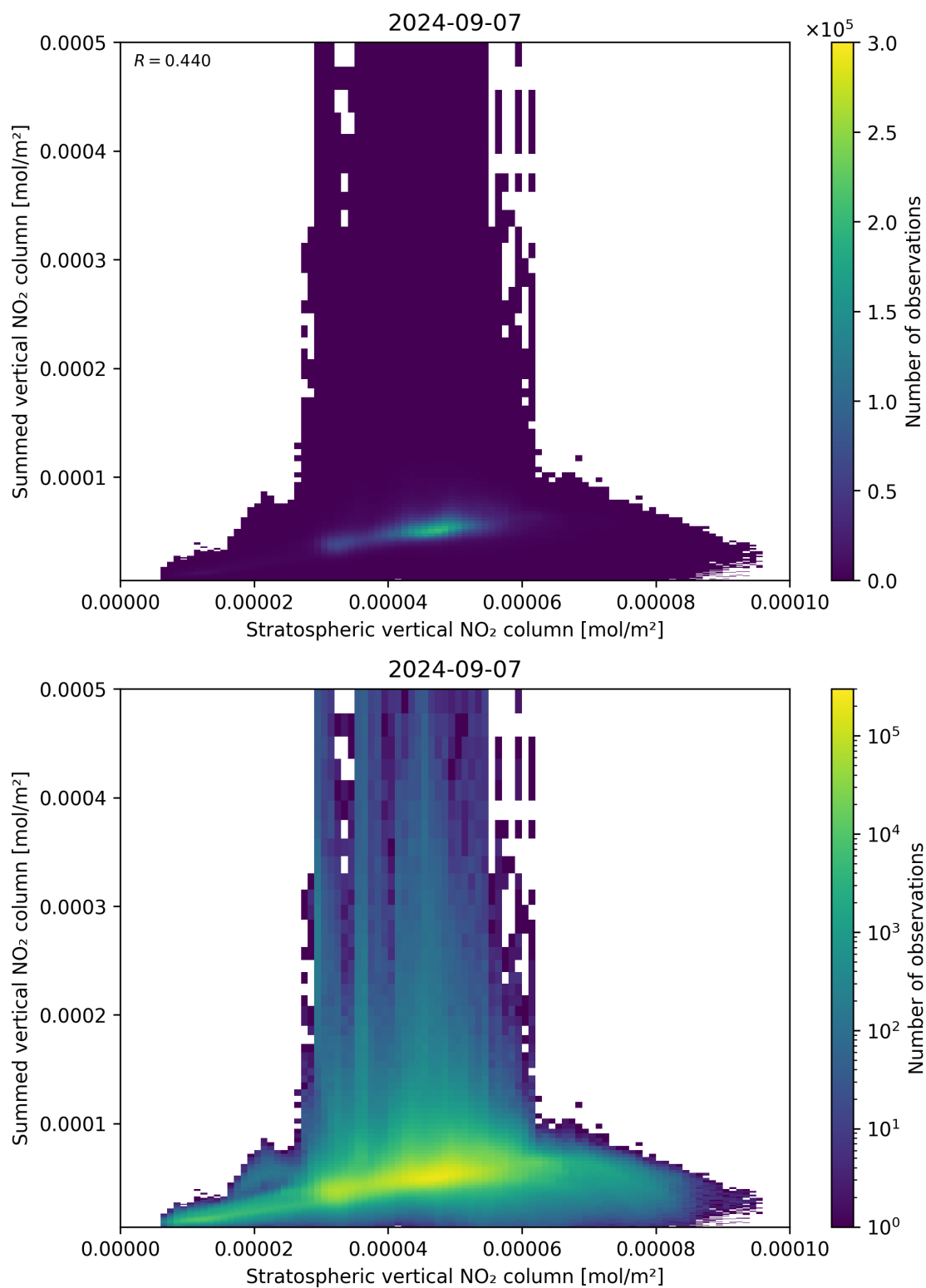
Figure 98: Scatter density plot of “Stratospheric vertical NO 2 column” against “Summed vertical NO 2 column” for 2024-09-06 to 2024-09-08.
