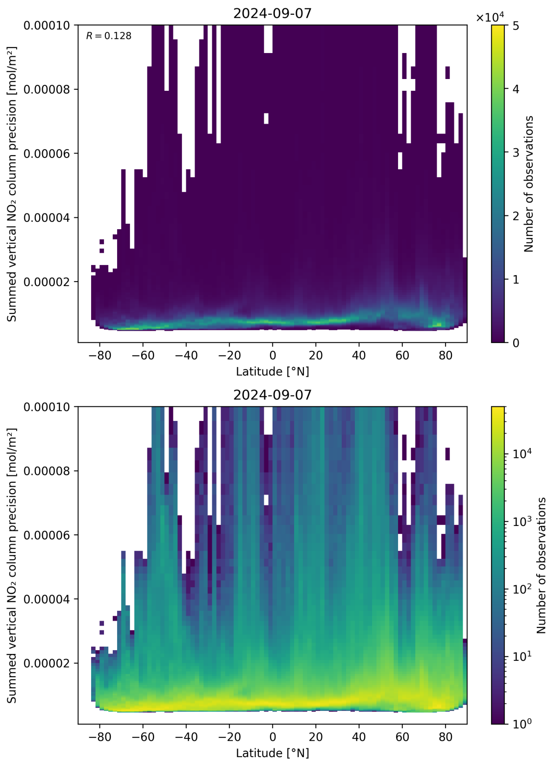
Figure 89: Scatter density plot of “Latitude” against “Summed vertical NO 2 column precision” for 2024-09-06 to 2024-09-08.
