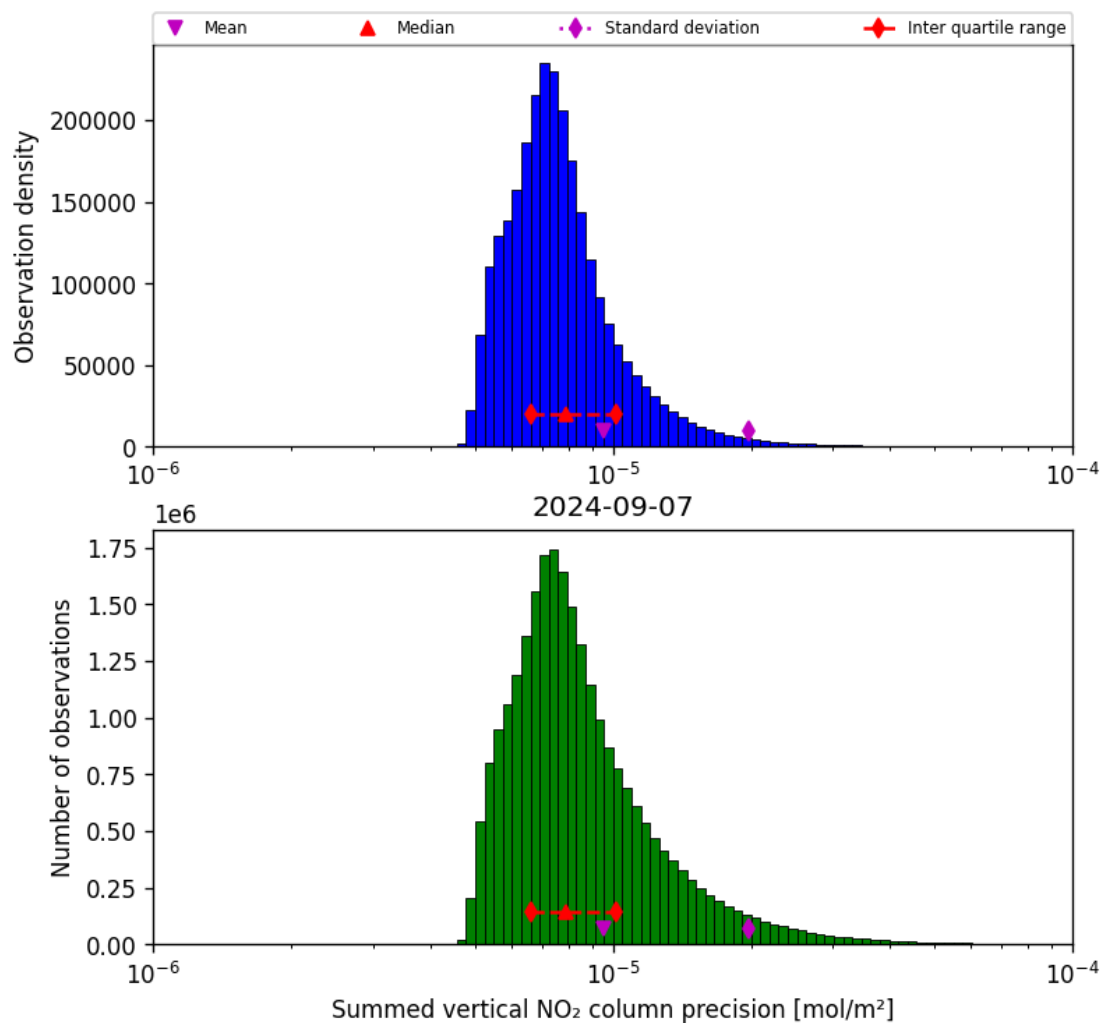
Figure 41: Histogram of “Summed vertical NO 2 column precision” for 2024-09-06 to 2024-09-08
