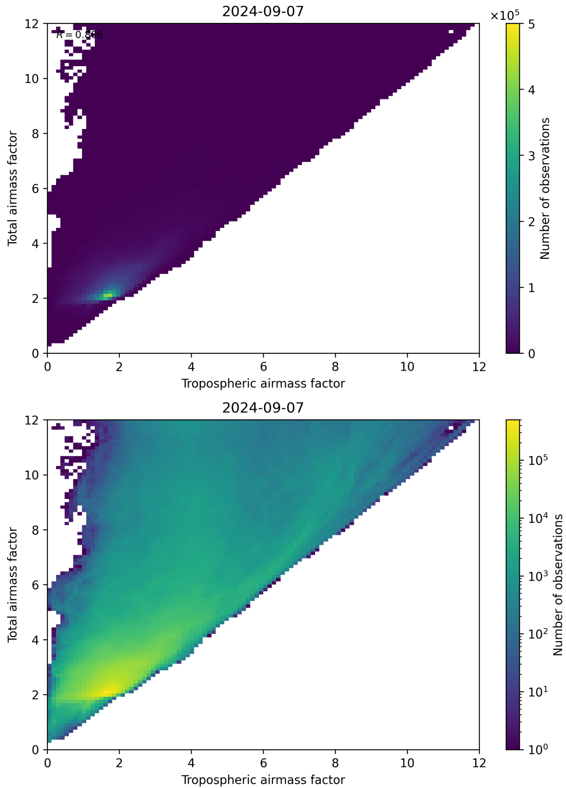
Figure 72: Scatter density plot of “Tropospheric airmass factor” against “Total airmass factor” for 2024-09-06 to 2024-09-08.
