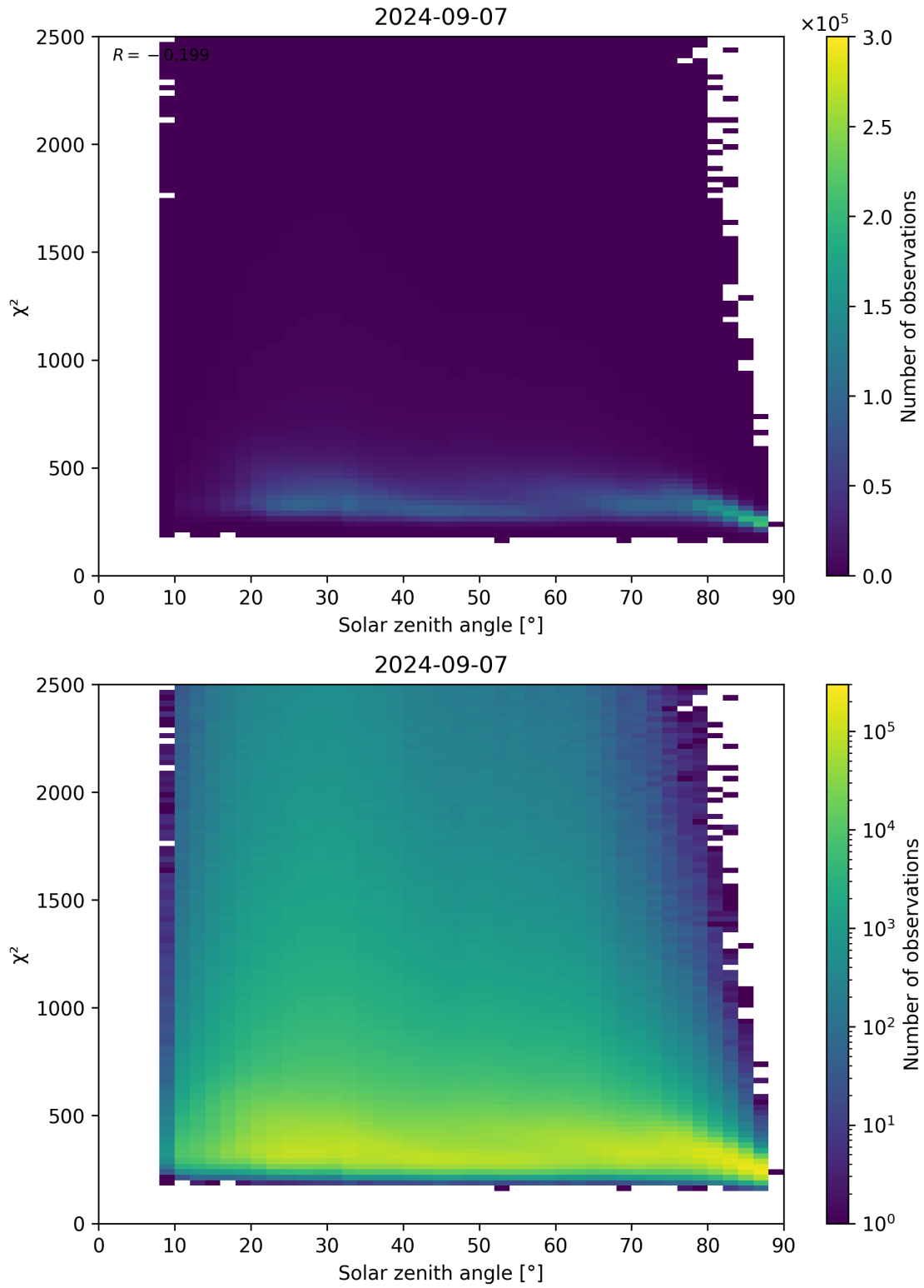
Figure 148: Scatter density plot of “Solar zenith angle” against “ \chi^2 ” for 2024-09-06 to 2024-09-08.
