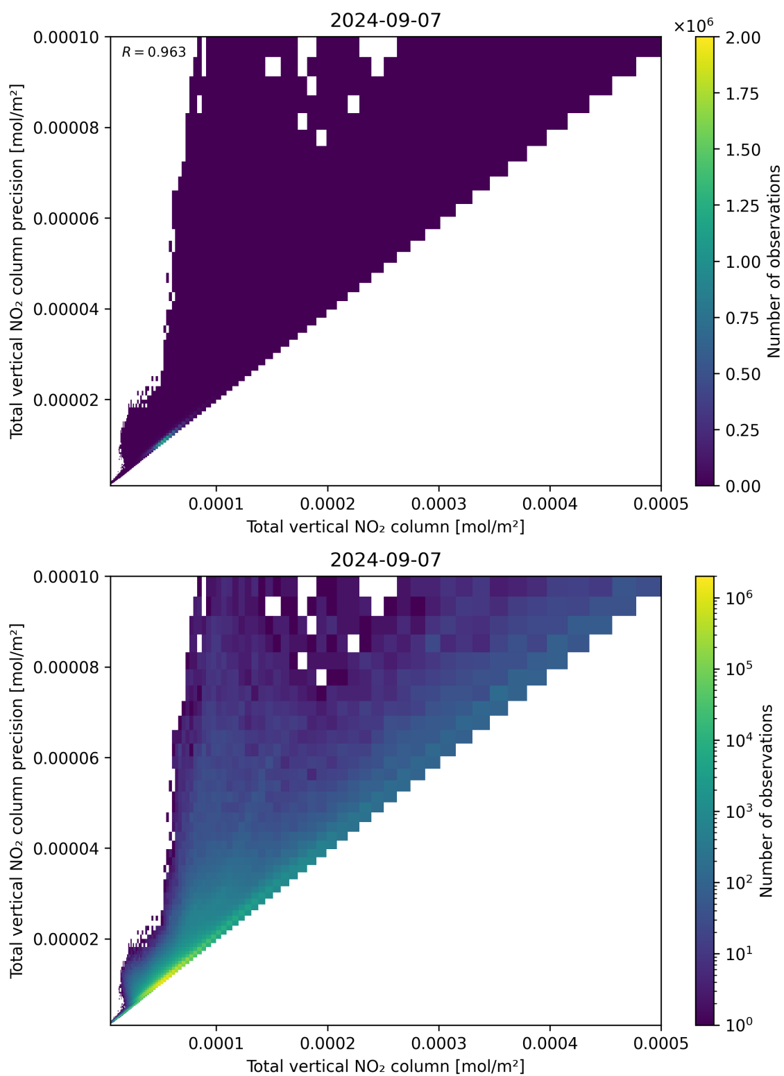
Figure 114: Scatter density plot of “Total vertical NO 2 column” against “Total vertical NO 2 column precision” for 2024-09-06 to 2024-09-08.
