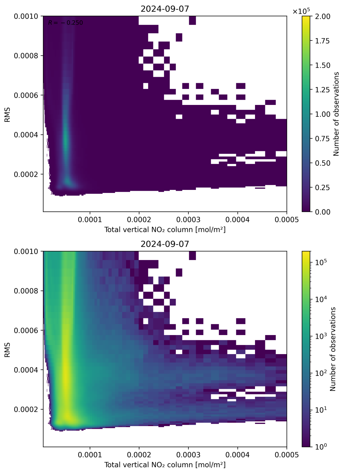
Figure 120: Scatter density plot of “Total vertical NO 2 column” against “RMS” for 2024-09-06 to 2024-09-08.
