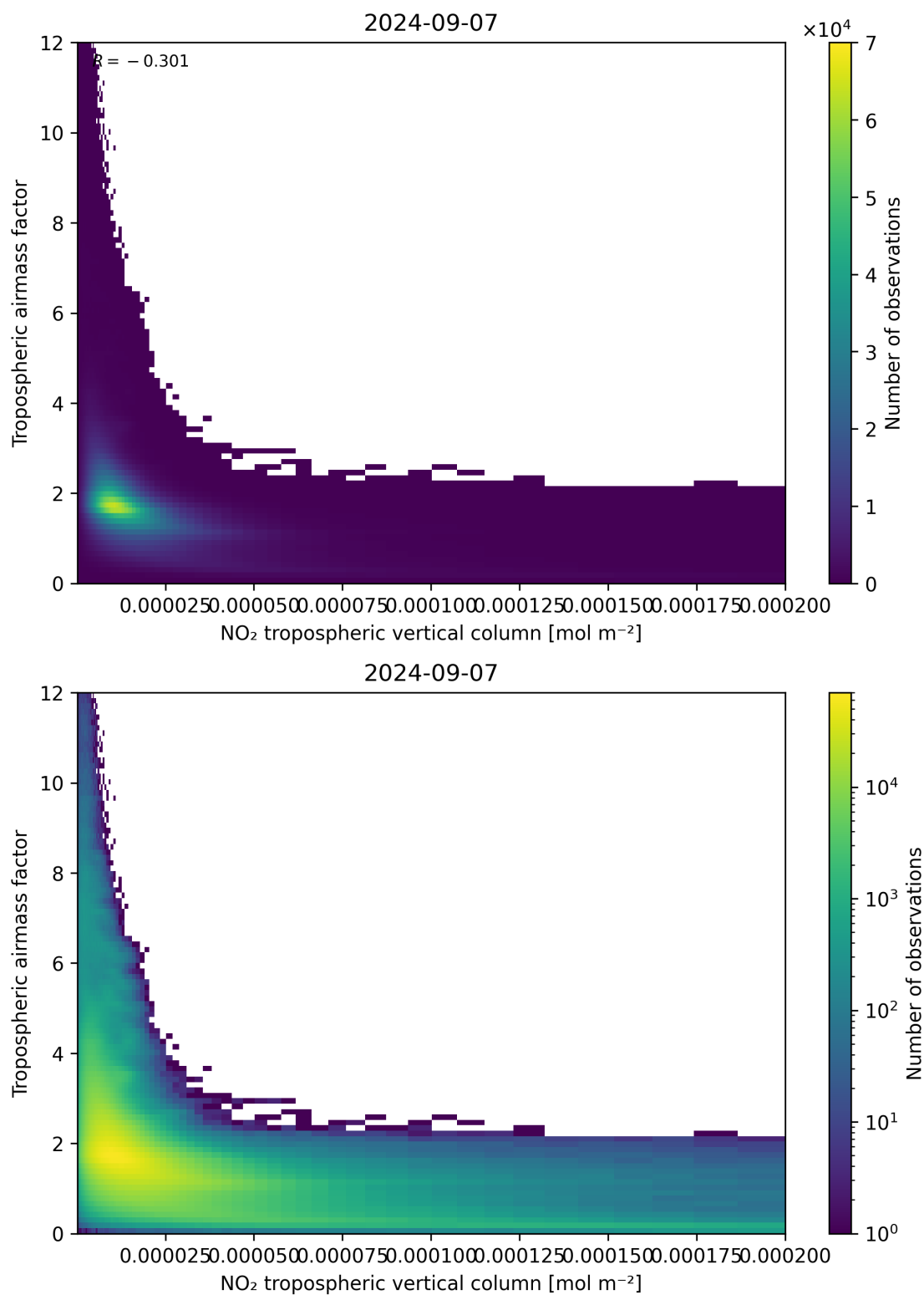
Figure 123: Scatter density plot of “NO 2 tropospheric vertical column” against “Tropospheric air mass factor” for 2024-09-06 to 2024-09-08.
