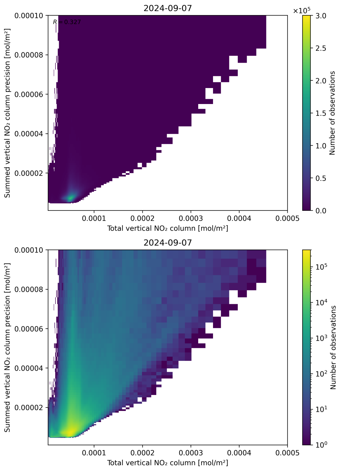
Figure 113: Scatter density plot of “Total vertical NO 2 column” against “Summed vertical NO 2 column precision” for 2024-09-06 to 2024-09-08.
