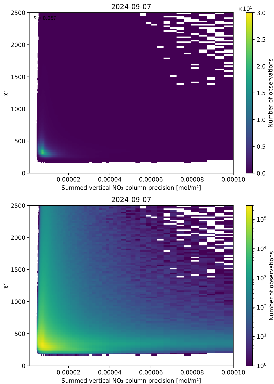
Figure 107: Scatter density plot of “Summed vertical NO 2 column precision” against “ \chi^2 ” for 2024-09-06 to 2024-09-08.
