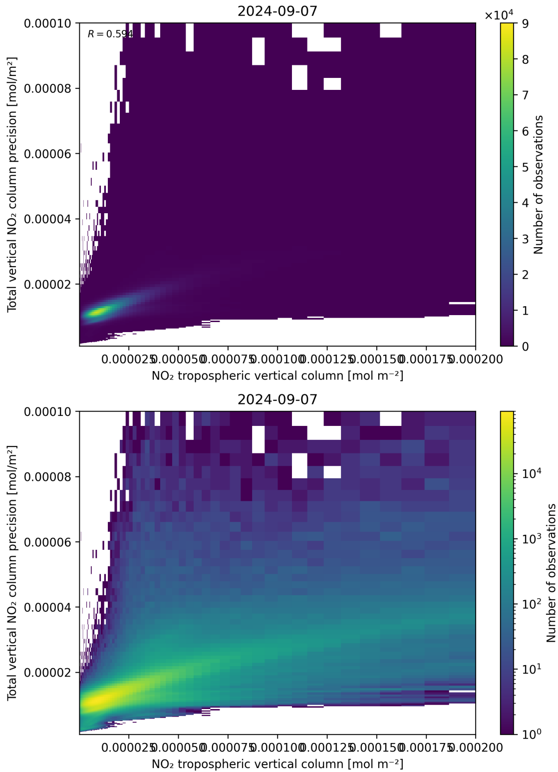
Figure 129: Scatter density plot of “NO 2 tropospheric vertical column” against “Total vertical NO 2 column precision” for 2024-09-06 to 2024-09-08.
