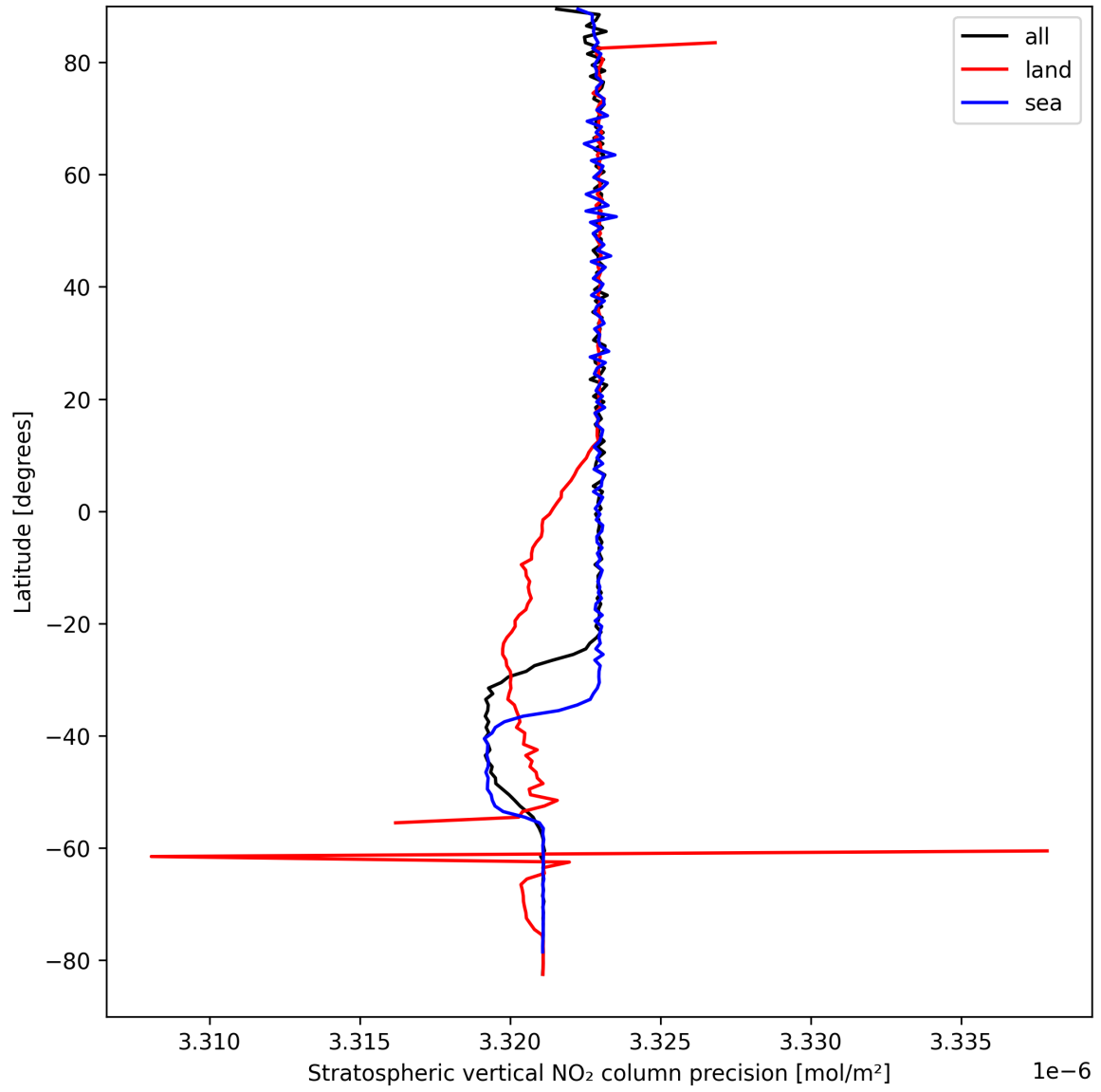
Figure 20: Zonal average of “Stratospheric vertical NO 2 column precision” for 2024-09-06 to 2024-09-08.
