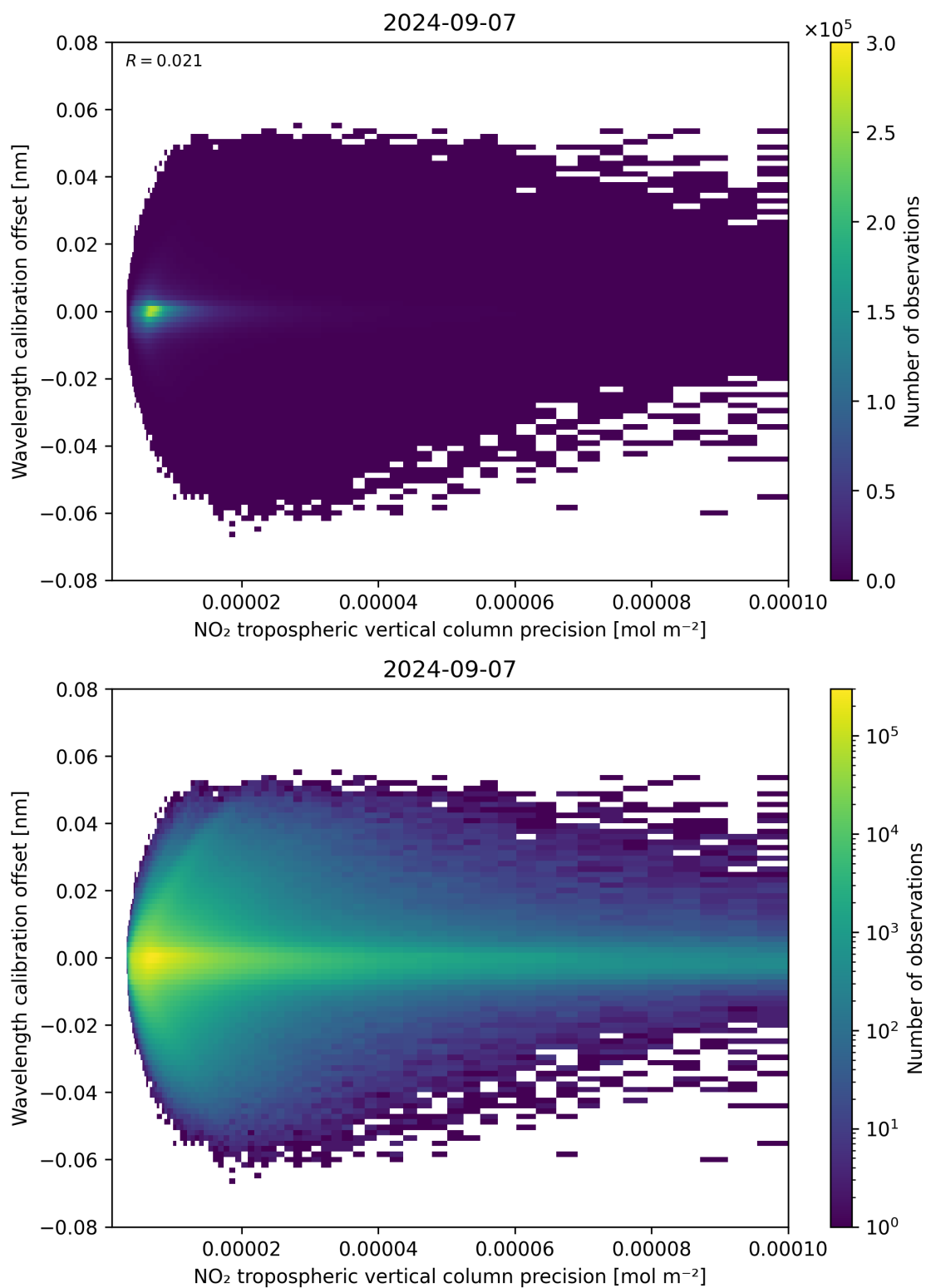
Figure 141: Scatter density plot of “NO 2 tropospheric vertical column precision” against “Wavelength calibration offset” for 2024-09-06 to 2024-09-08.
