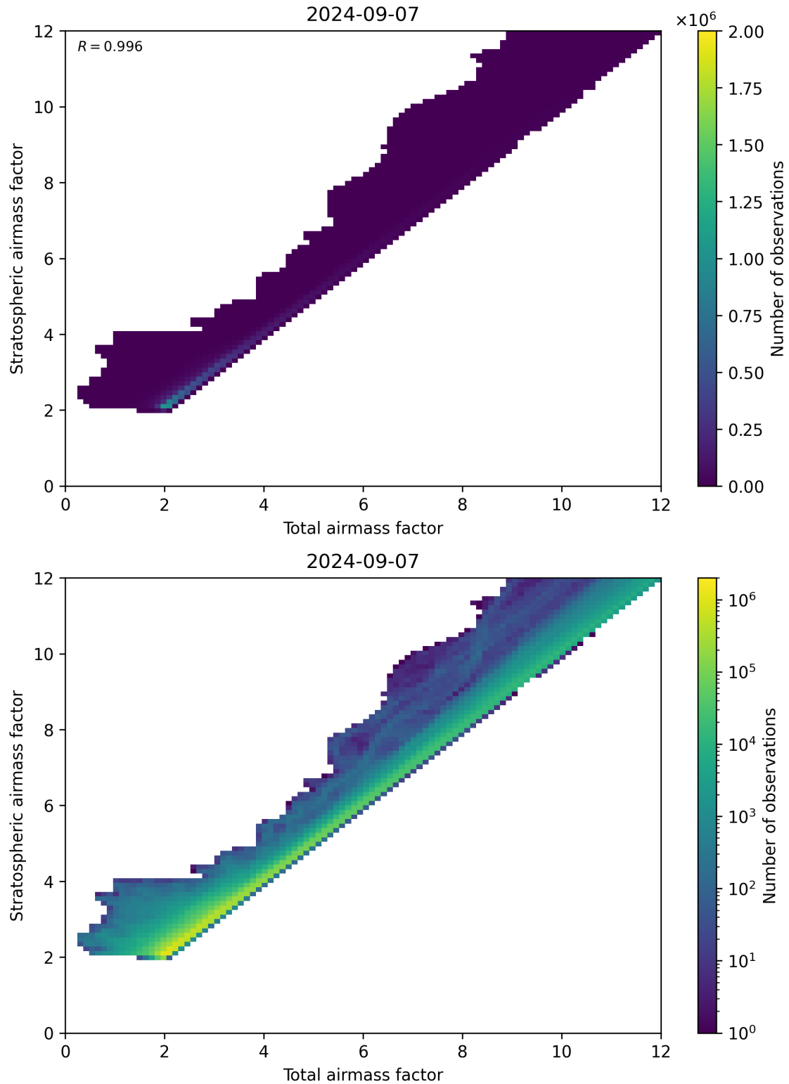
Figure 62: Scatter density plot of “Total airmass factor” against “Stratospheric airmass factor” for 2024-09-06 to 2024-09-08.
