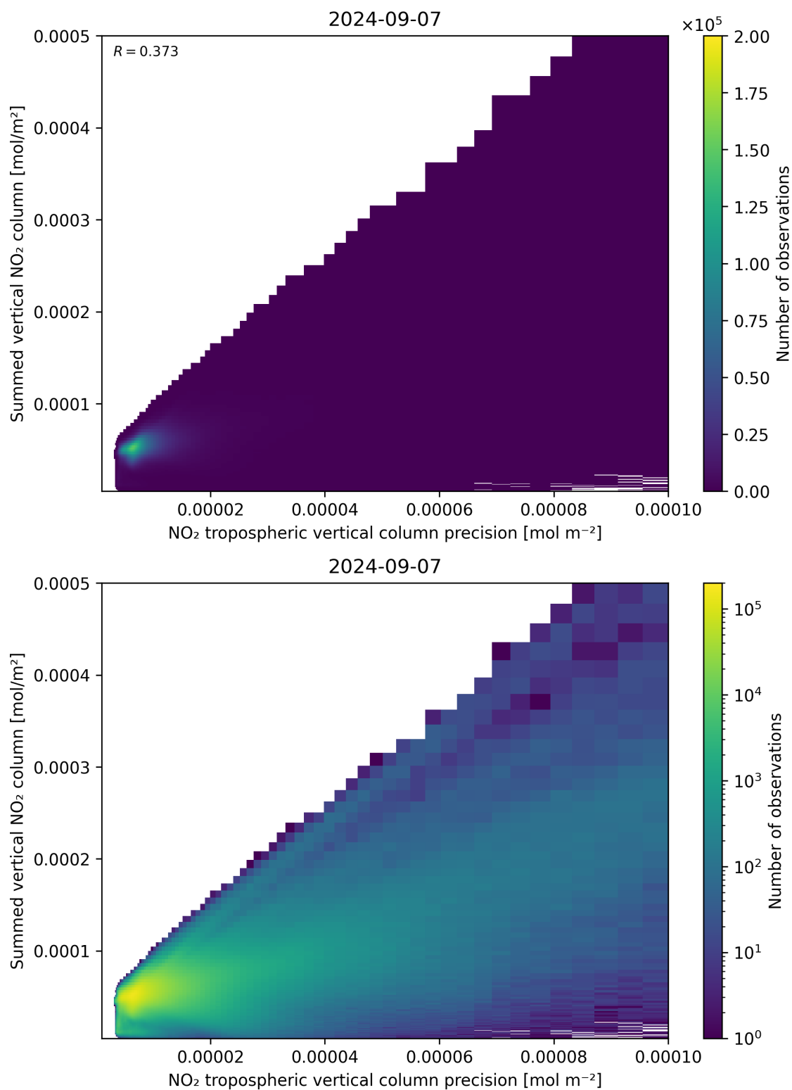
Figure 136: Scatter density plot of “NO 2 tropospheric vertical column precision” against “Summed vertical NO 2 column” for 2024-09-06 to 2024-09-08.
