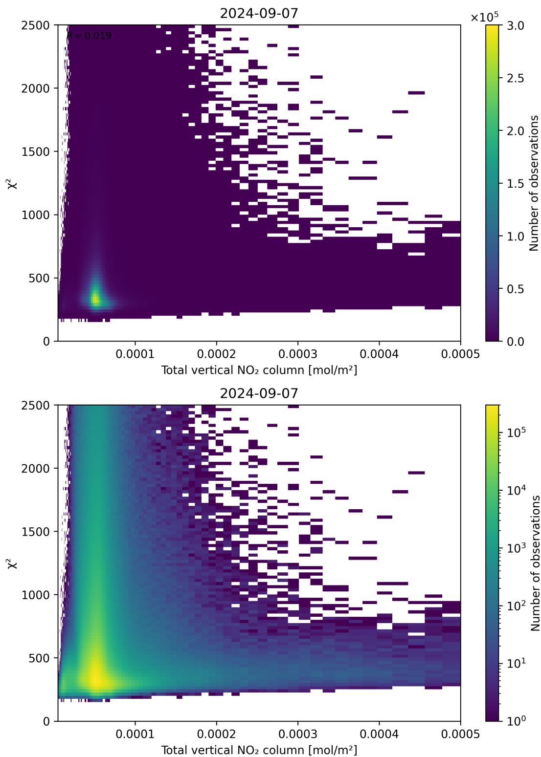
Figure 111: Scatter density plot of “Total vertical NO 2 column” against “ \chi^2 ” for 2024-09-06 to 2024-09-08.
