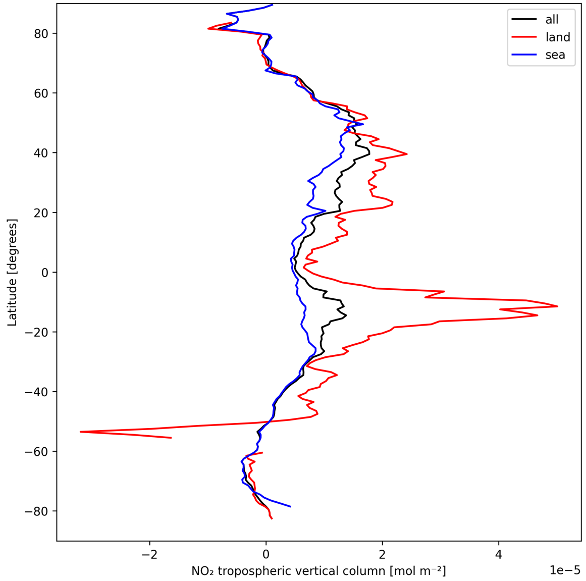
Figure 12: Zonal average of “NO 2 tropospheric vertical column” for 2024-09-06 to 2024-09-08.
