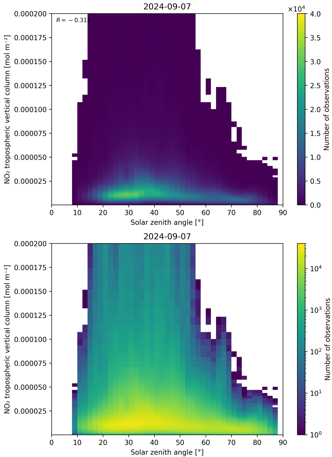
Figure 155: Scatter density plot of “Solar zenith angle” against “NO 2 tropospheric vertical column” for 2024-09-06 to 2024-09-08.
