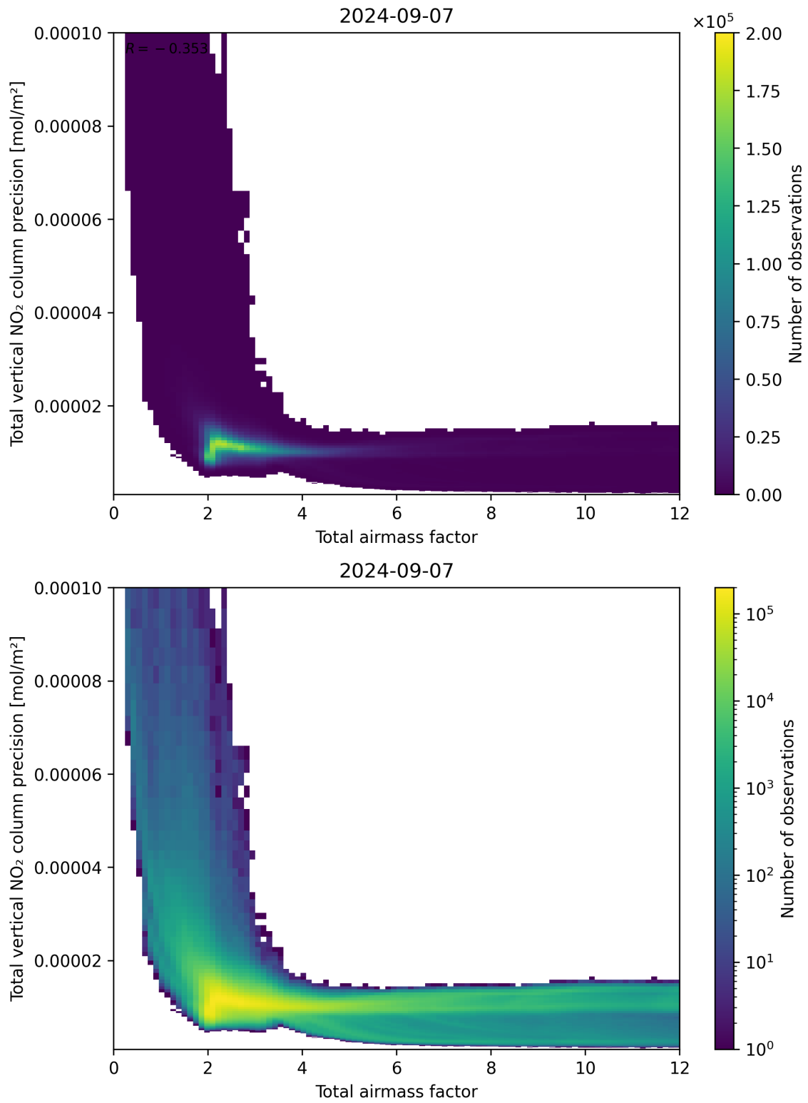
Figure 68: Scatter density plot of “Total airmass factor” against “Total vertical NO 2 column precision” for 2024-09-06 to 2024-09-08.
