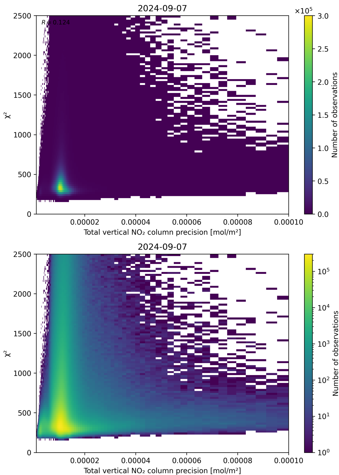
Figure 116: Scatter density plot of “Total vertical NO 2 column precision” against “ \chi^2 ” for 2024-09-06 to 2024-09-08.
