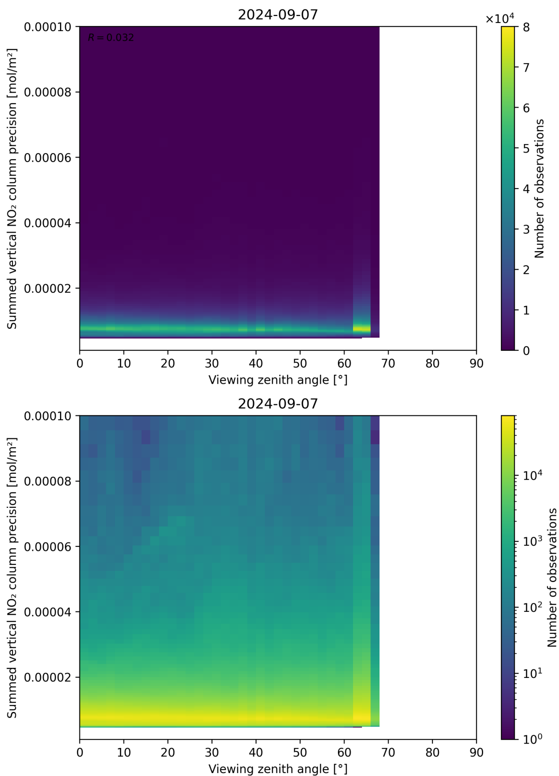
Figure 166: Scatter density plot of “Viewing zenith angle” against “Summed vertical NO 2 column precision” for 2024-09-06 to 2024-09-08.
