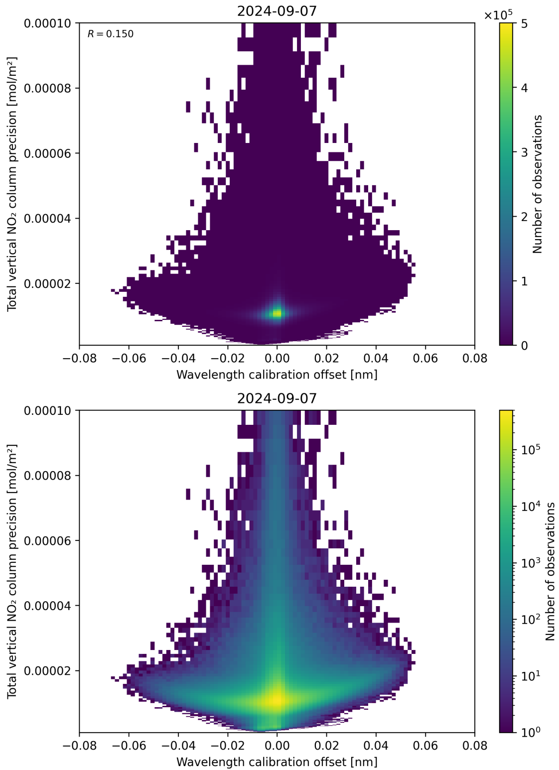
Figure 180: Scatter density plot of “Wavelength calibration offset” against “Total vertical NO 2 column precision” for 2024-09-06 to 2024-09-08.
