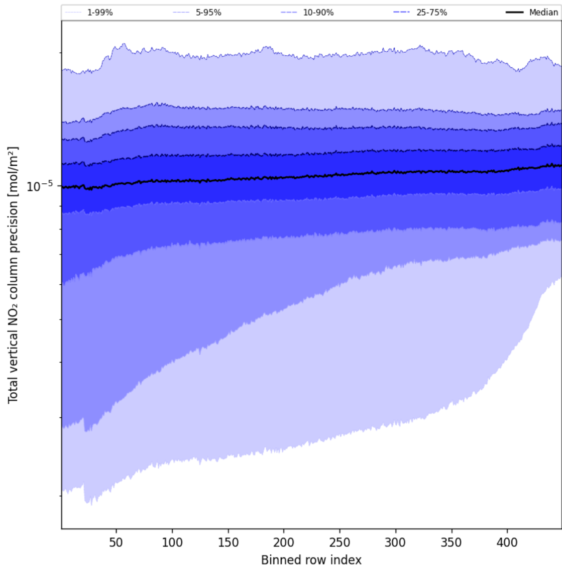
Figure 56: Along track statistics of “Total vertical NO 2 column precision” for 2024-09-06 to 2024-09-08
