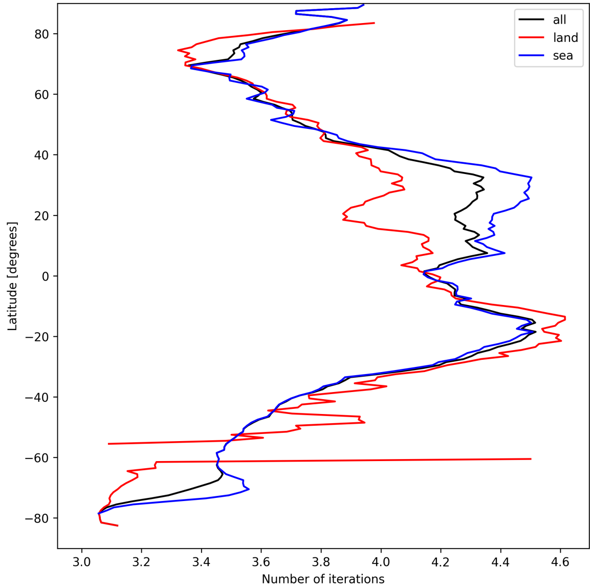
Figure 17: Zonal average of “Number of iterations” for 2024-09-06 to 2024-09-08.
