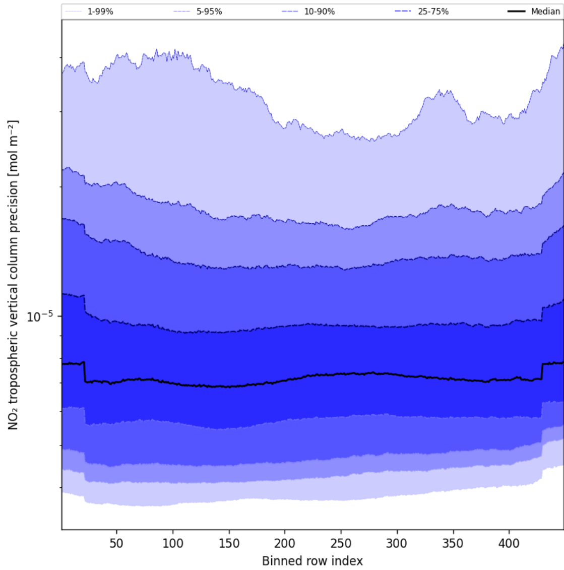
Figure 47: Along track statistics of “NO 2 tropospheric vertical column precision” for 2024-09-06 to 2024-09-08
