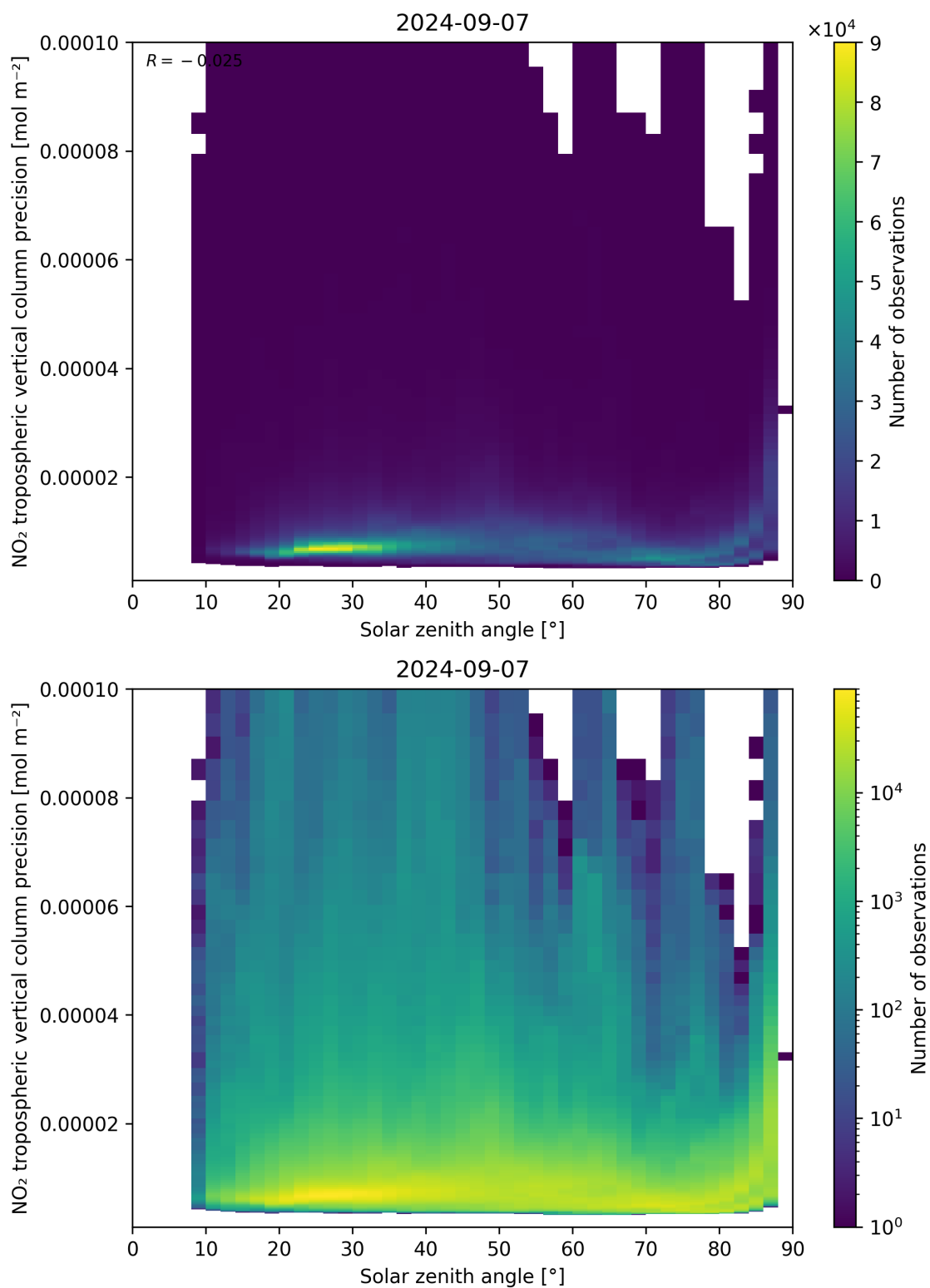
Figure 156: Scatter density plot of “Solar zenith angle” against “NO 2 tropospheric vertical column precision” for 2024-09-06 to 2024-09-08.
