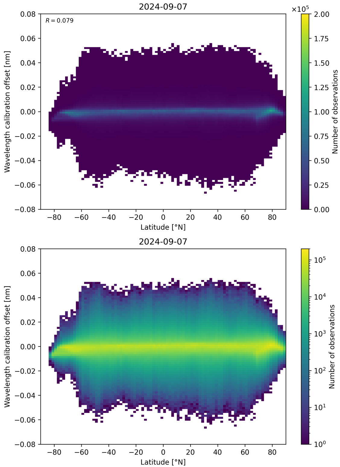
Figure 95: Scatter density plot of “Latitude” against “Wavelength calibration offset” for 2024-09-06 to 2024-09-08.
