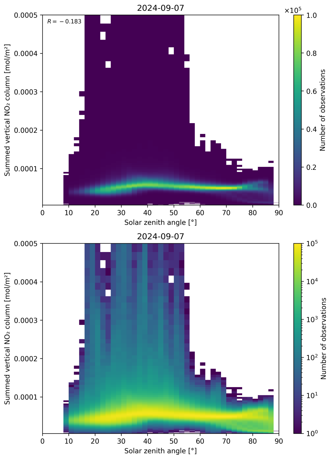
Figure 151: Scatter density plot of “Solar zenith angle” against “Summed vertical NO 2 column” for 2024-09-06 to 2024-09-08.
