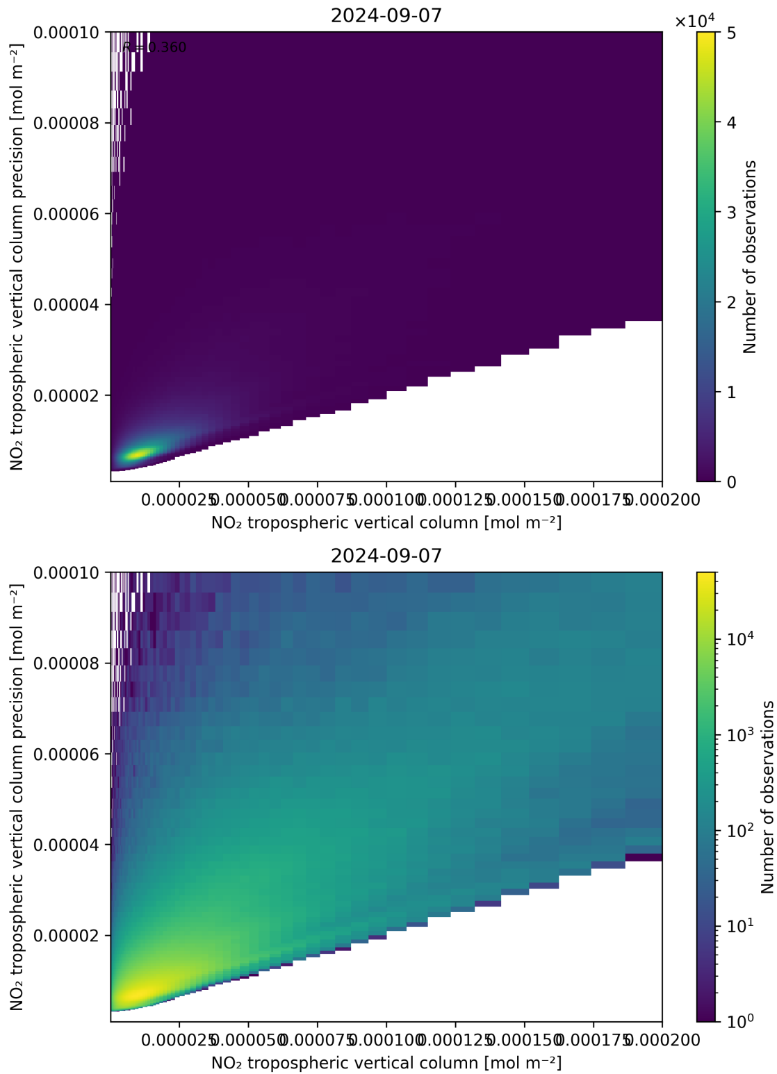
Figure 130: Scatter density plot of “NO 2 tropospheric vertical column” against “NO 2 tropospheric vertical column precision” for 2024-09-06 to 2024-09-08.
