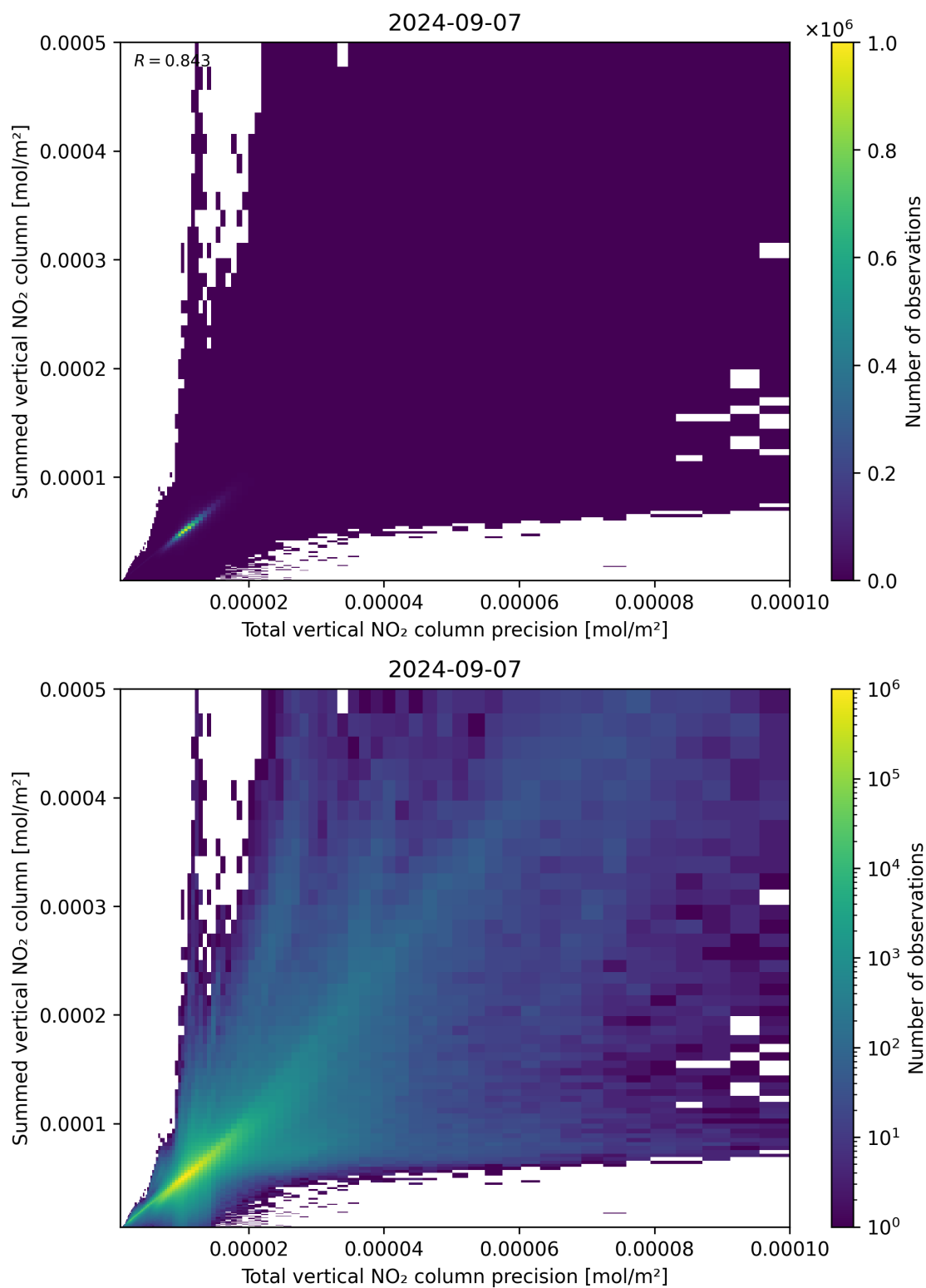
Figure 117: Scatter density plot of “Total vertical NO 2 column precision” against “Summed vertical NO 2 column” for 2024-09-06 to 2024-09-08.
