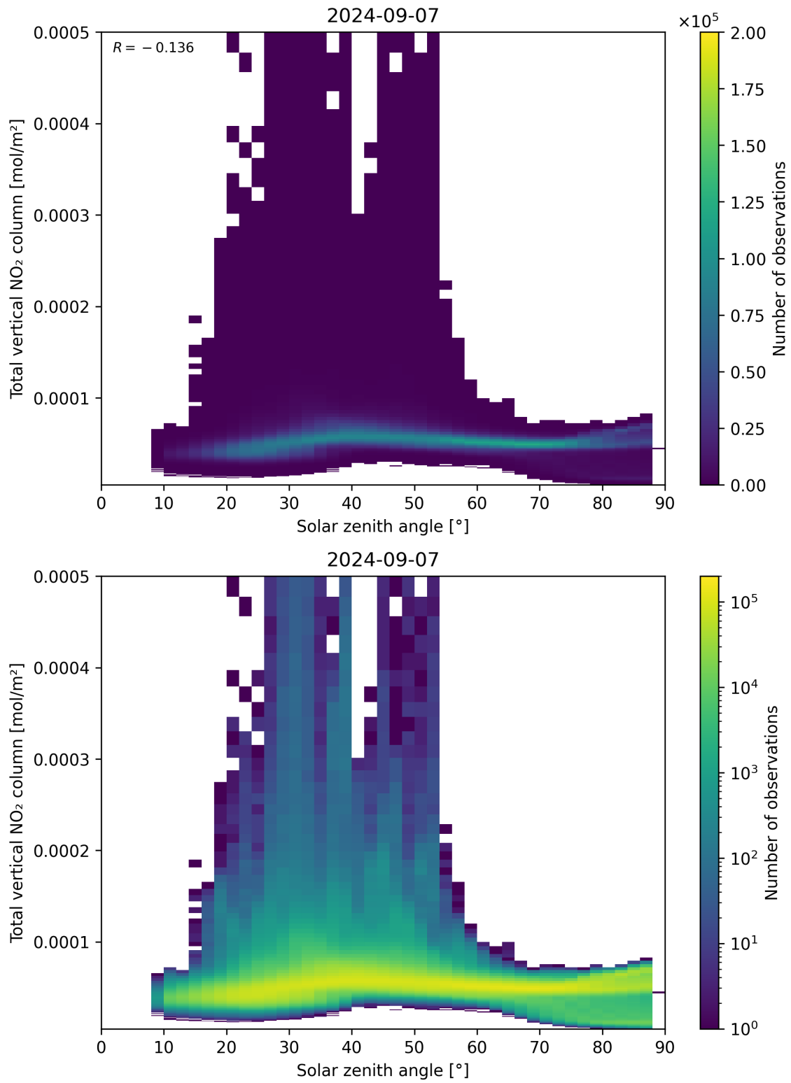
Figure 153: Scatter density plot of “Solar zenith angle” against “Total vertical NO 2 column” for 2024-09-06 to 2024-09-08.
