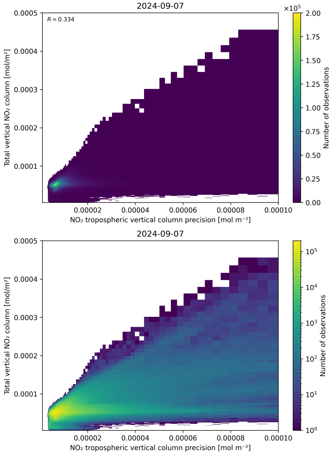
Figure 138: Scatter density plot of “NO 2 tropospheric vertical column precision” against “Total vertical NO 2 column” for 2024-09-06 to 2024-09-08.
