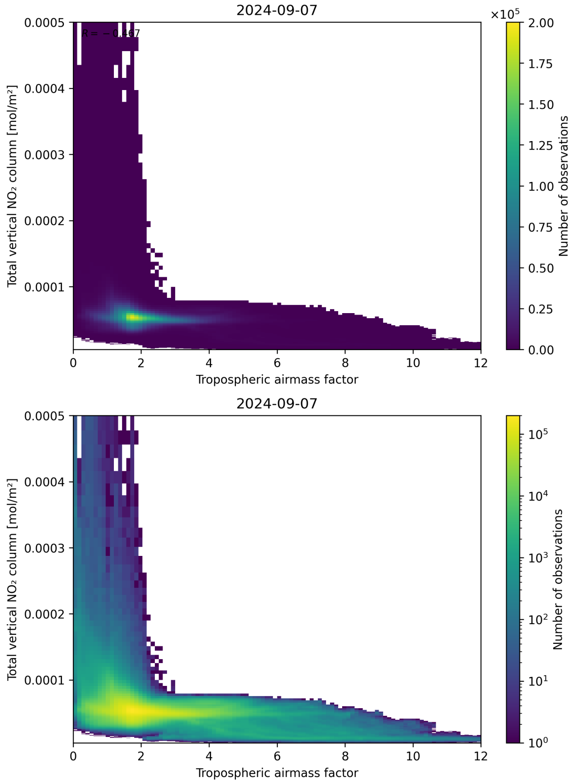
Figure 77: Scatter density plot of “Tropospheric airmass factor” against “Total vertical NO 2 column” for 2024-09-06 to 2024-09-08.
