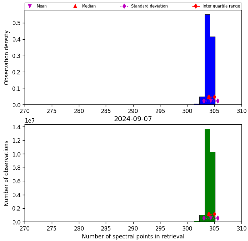
Figure 33: Histogram of “Number of spectral points in retrieval” for 2024-09-06 to 2024-09-08
