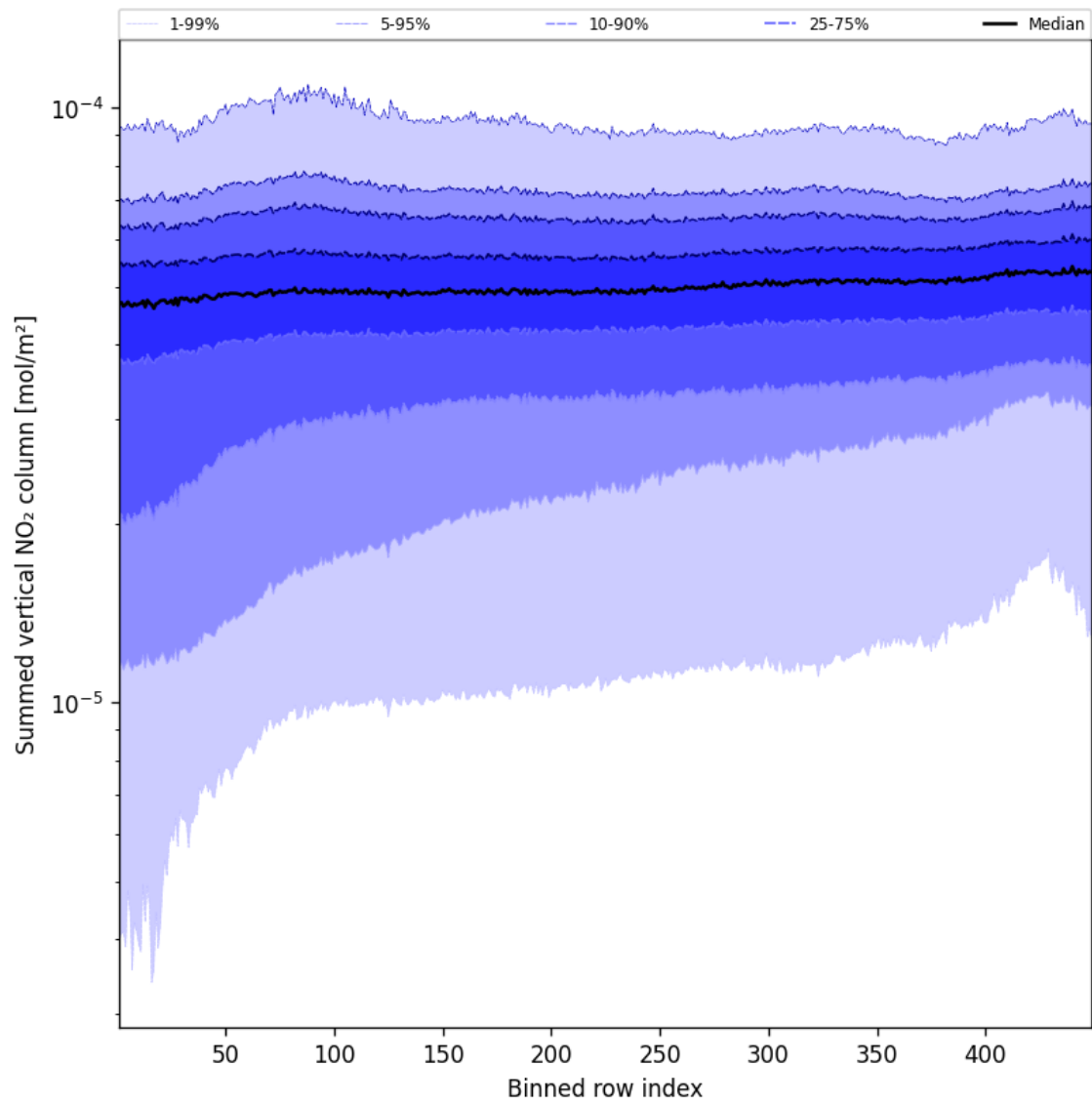
Figure 57: Along track statistics of “Summed vertical NO 2 column” for 2024-09-06 to 2024-09-08
