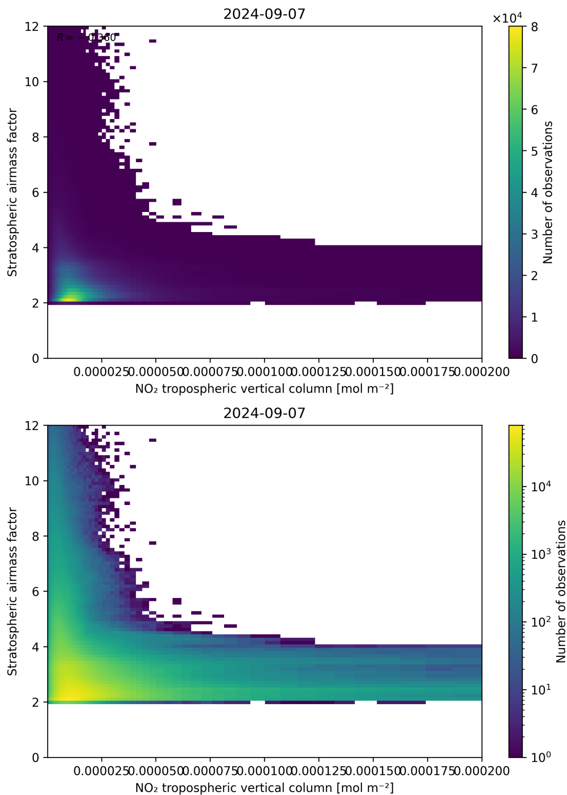
Figure 121: Scatter density plot of “NO 2 tropospheric vertical column” against “Stratospheric airmass factor” for 2024-09-06 to 2024-09-08.
