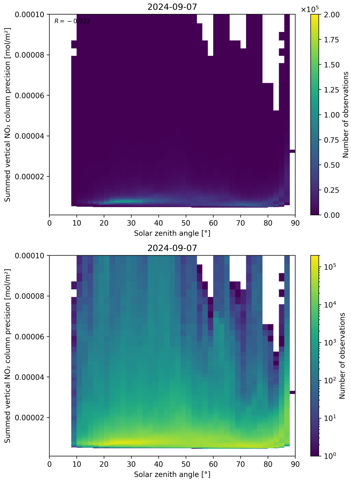
Figure 152: Scatter density plot of “Solar zenith angle” against “Summed vertical NO 2 column precision” for 2024-09-06 to 2024-09-08.
