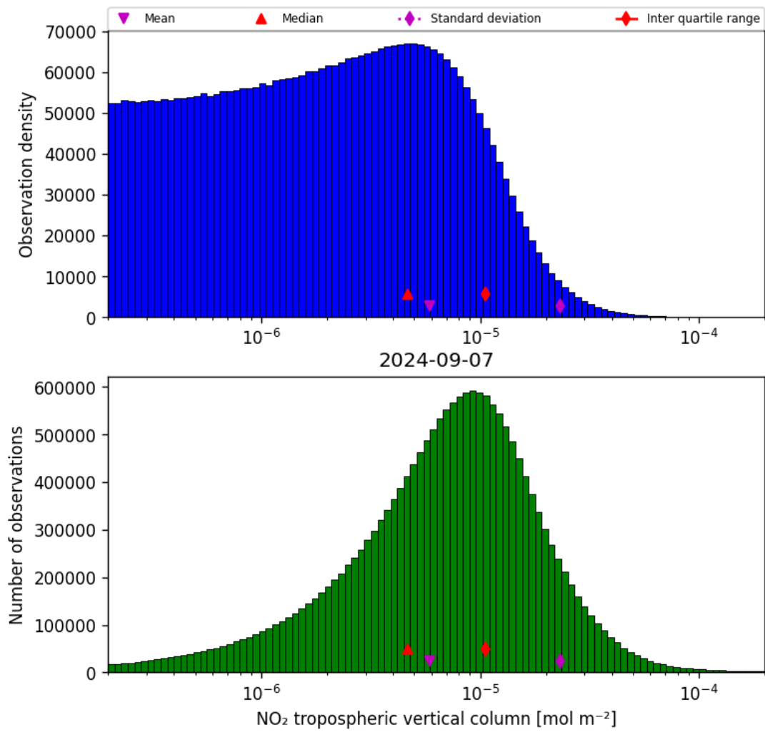
Figure 29: Histogram of “NO 2 tropospheric vertical column” for 2024-09-06 to 2024-09-08
