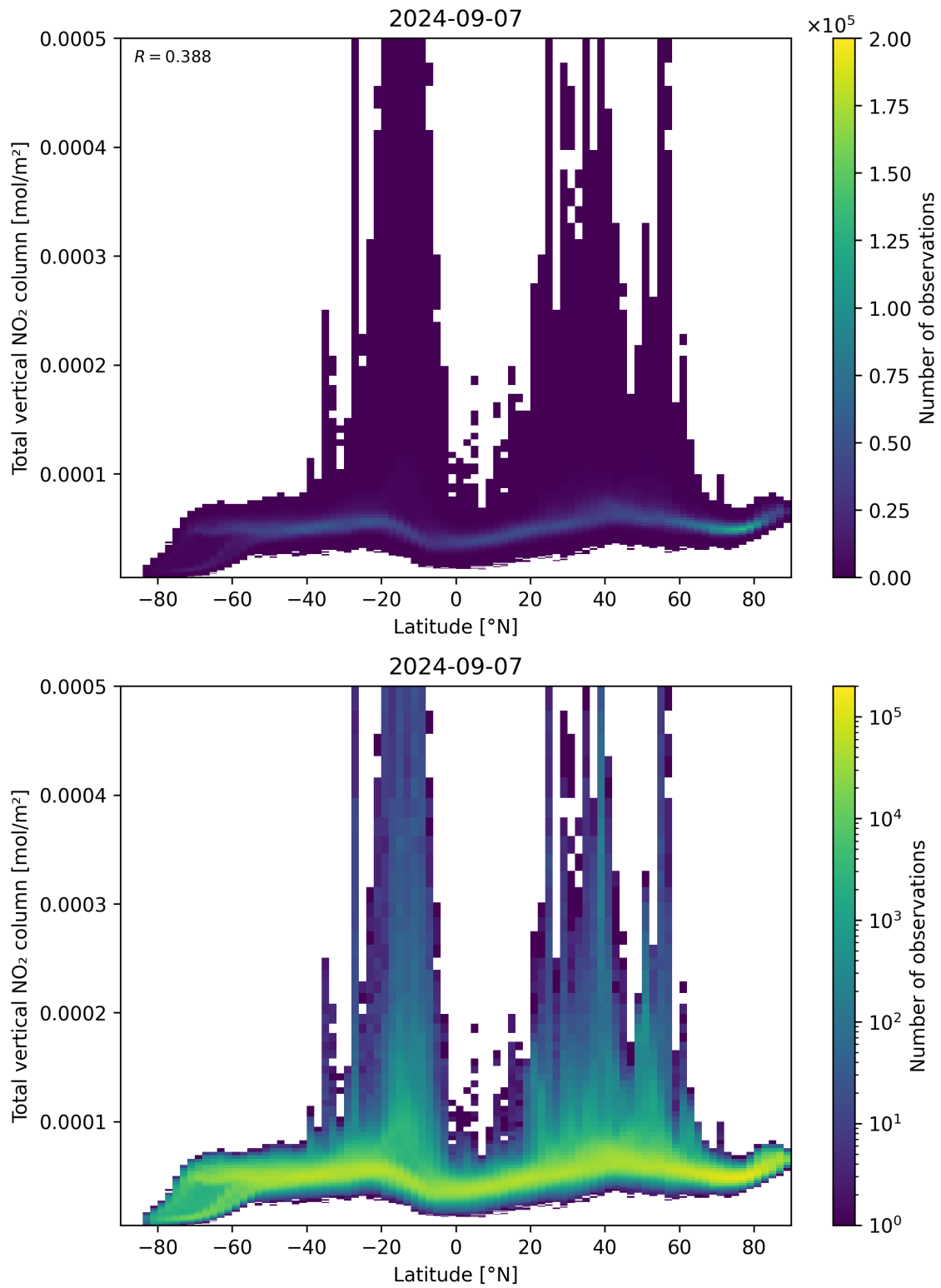
Figure 90: Scatter density plot of “Latitude” against “Total vertical NO 2 column” for 2024-09-06 to 2024-09-08.
