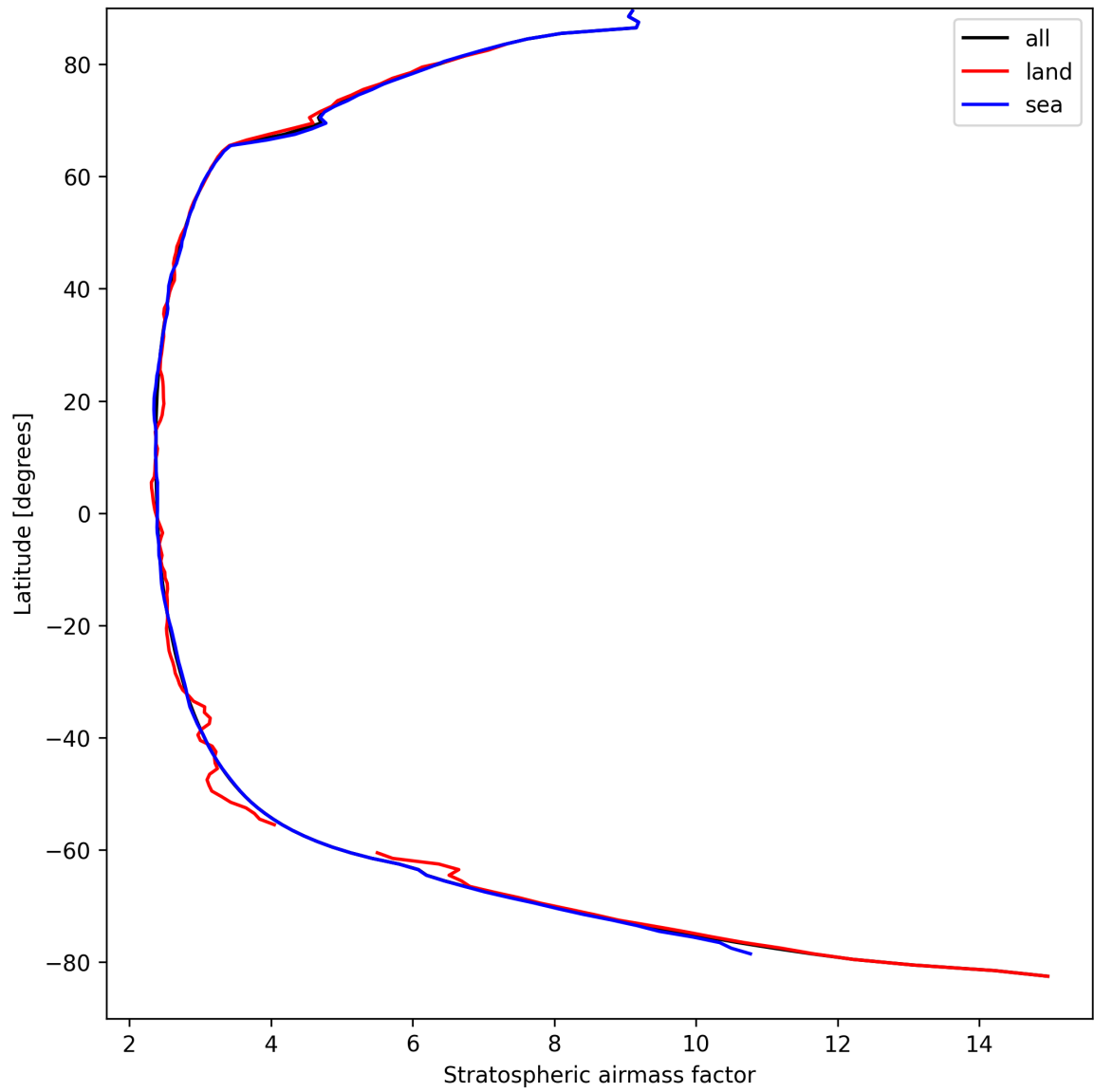
Figure 27: Zonal average of “Stratospheric airmass factor” for 2024-09-06 to 2024-09-08.
