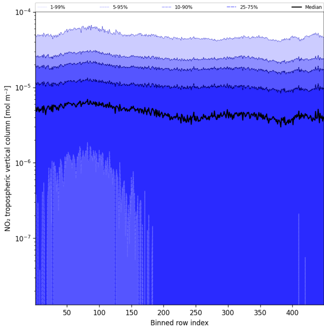
Figure 46: Along track statistics of “NO 2 tropospheric vertical column” for 2024-09-06 to 2024-09-08
