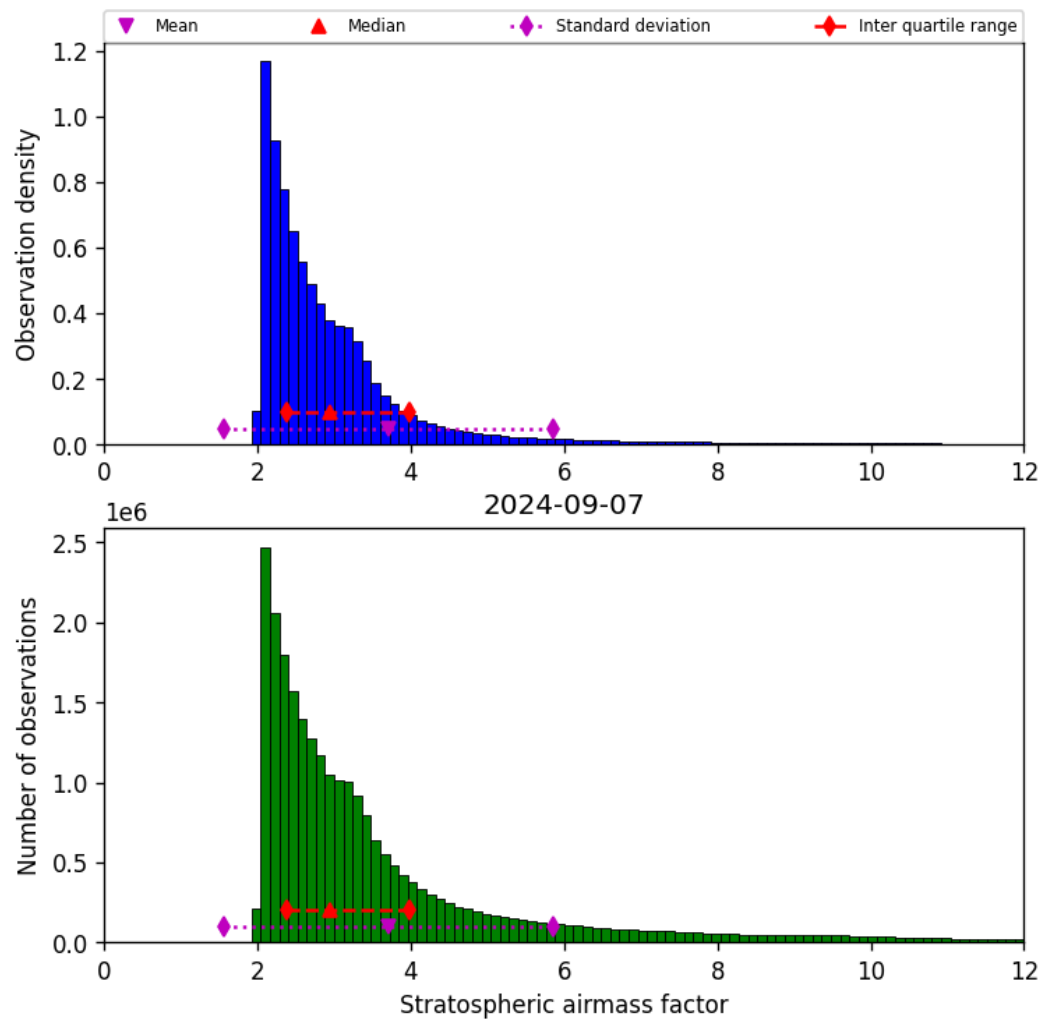
Figure 44: Histogram of “Stratospheric airmass factor” for 2024-09-06 to 2024-09-08
