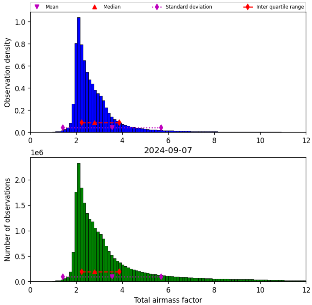
Figure 32: Histogram of “Total airmass factor” for 2024-09-06 to 2024-09-08
