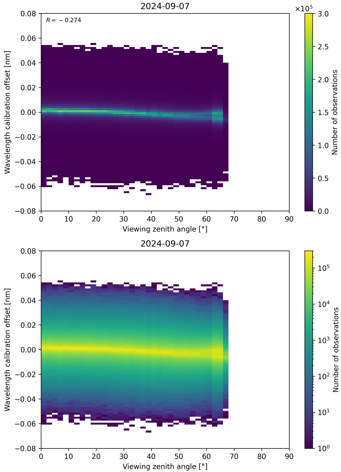
Figure 173: Scatter density plot of “Viewing zenith angle” against “Wavelength calibration offset” for 2024-09-06 to 2024-09-08.
