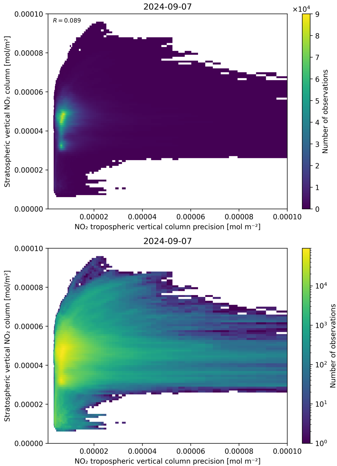
Figure 135: Scatter density plot of “NO 2 tropospheric vertical column precision” against “Stratospheric vertical NO 2 column” for 2024-09-06 to 2024-09-08.
