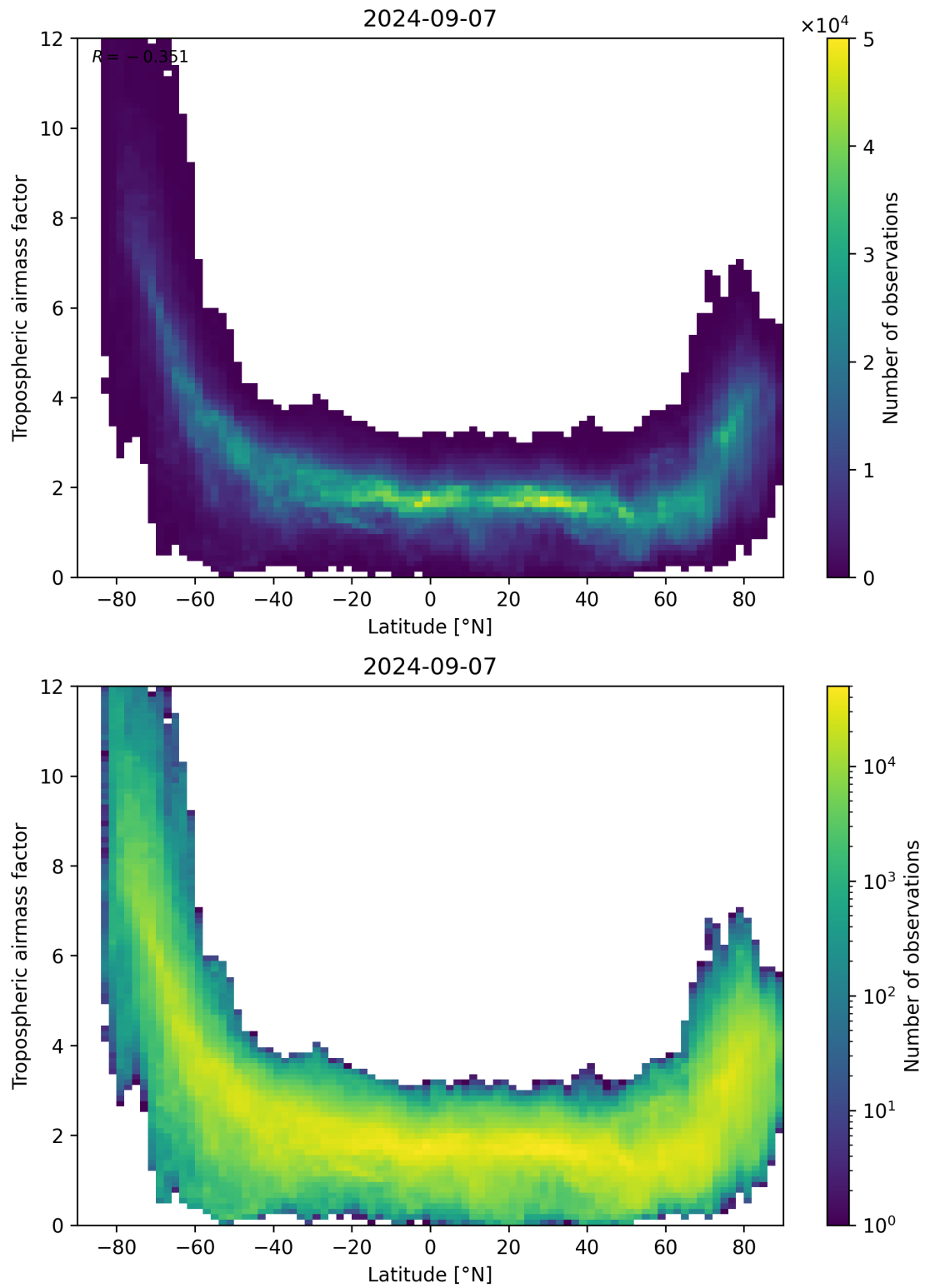
Figure 85: Scatter density plot of “Latitude” against “Tropospheric airmass factor” for 2024-09-06 to 2024-09-08.
