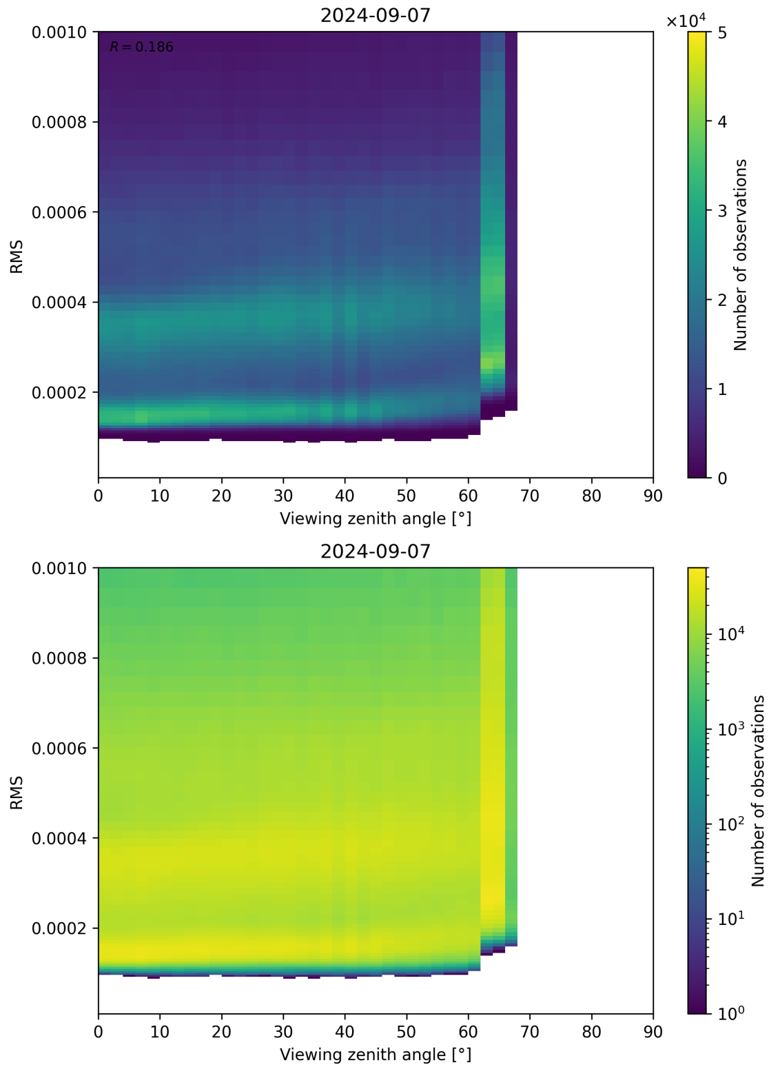
Figure 171: Scatter density plot of “Viewing zenith angle” against “RMS” for 2024-09-06 to 2024-09-08.
