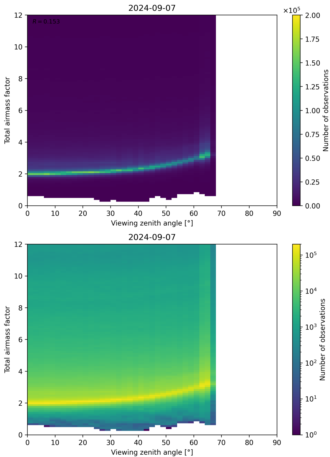
Figure 160: Scatter density plot of “Viewing zenith angle” against “Total airmass factor” for 2024-09-06 to 2024-09-08.
