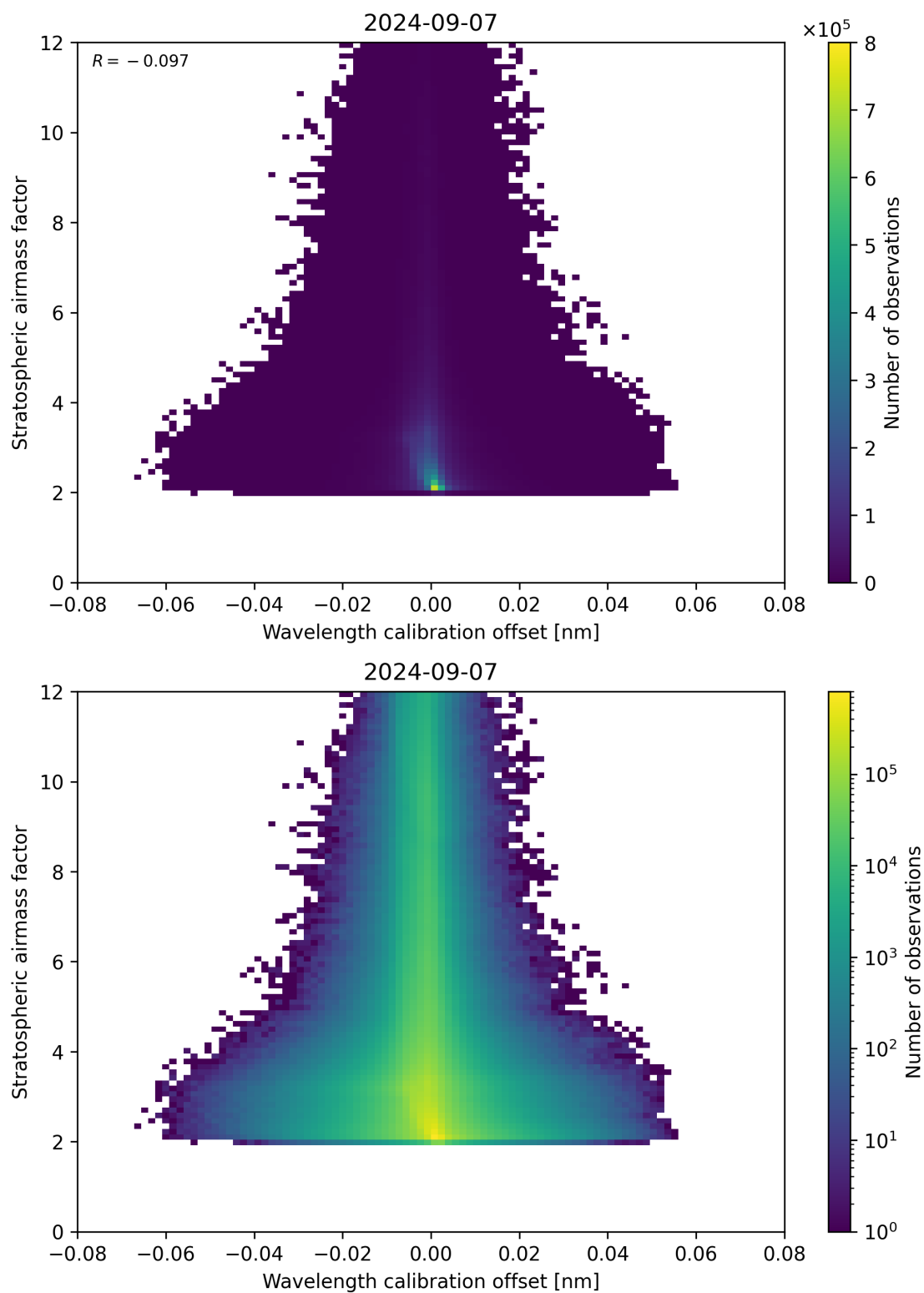
Figure 174: Scatter density plot of “Wavelength calibration offset” against “Stratospheric airmass factor” for 2024-09-06 to 2024-09-08.
