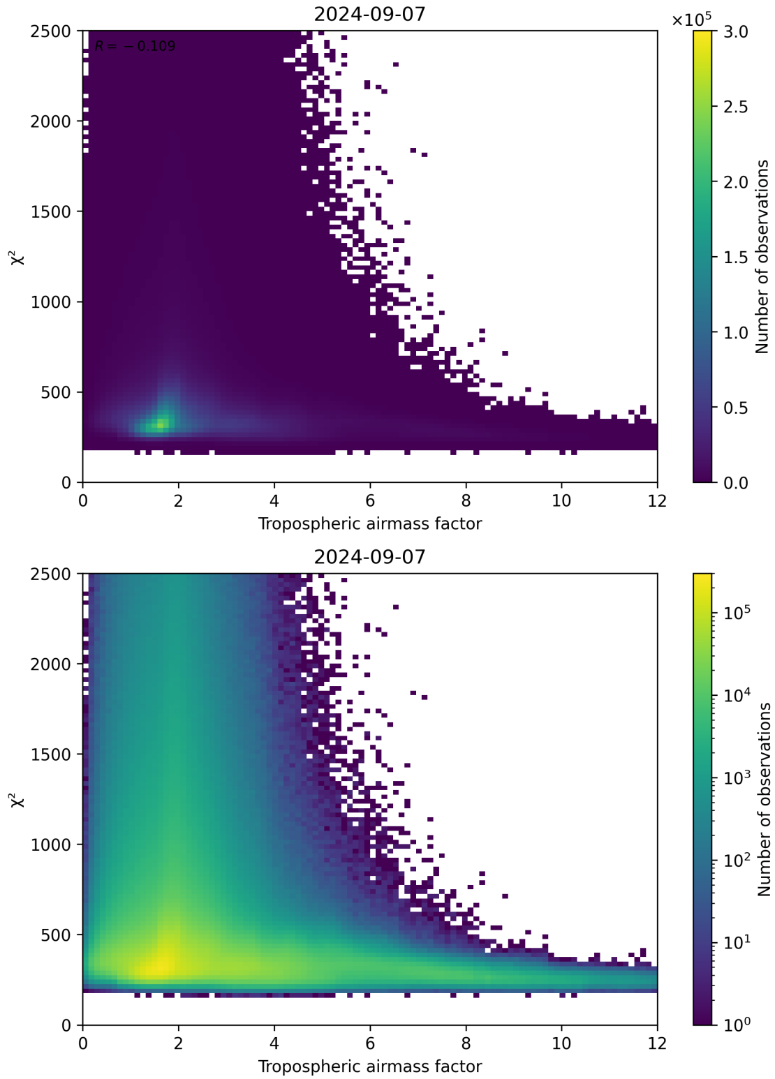
Figure 73: Scatter density plot of “Tropospheric airmass factor” against “ \chi^2 ” for 2024-09-06 to 2024-09-08.
