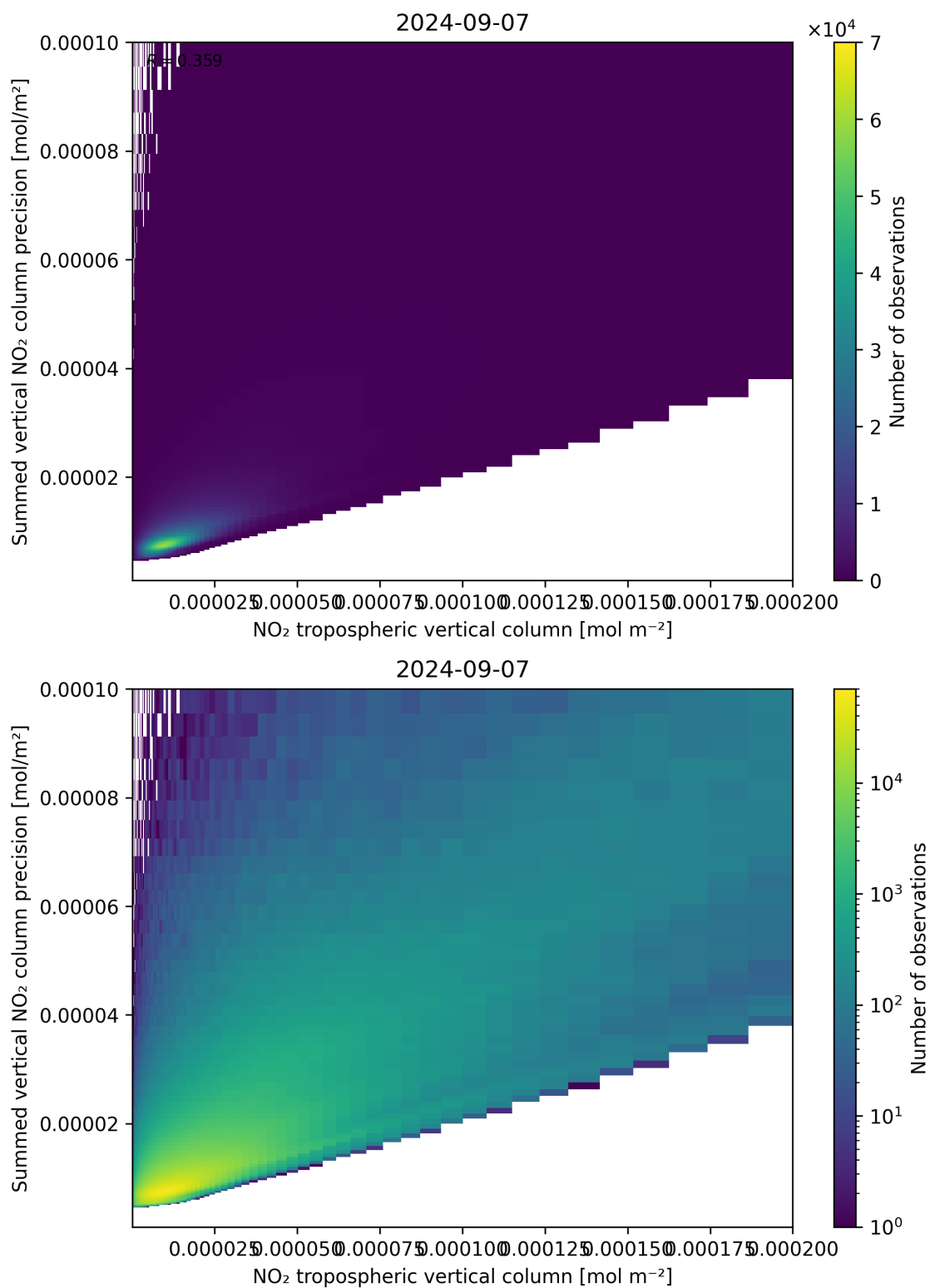
Figure 127: Scatter density plot of “NO 2 tropospheric vertical column” against “Summed vertical NO 2 column precision” for 2024-09-06 to 2024-09-08.
