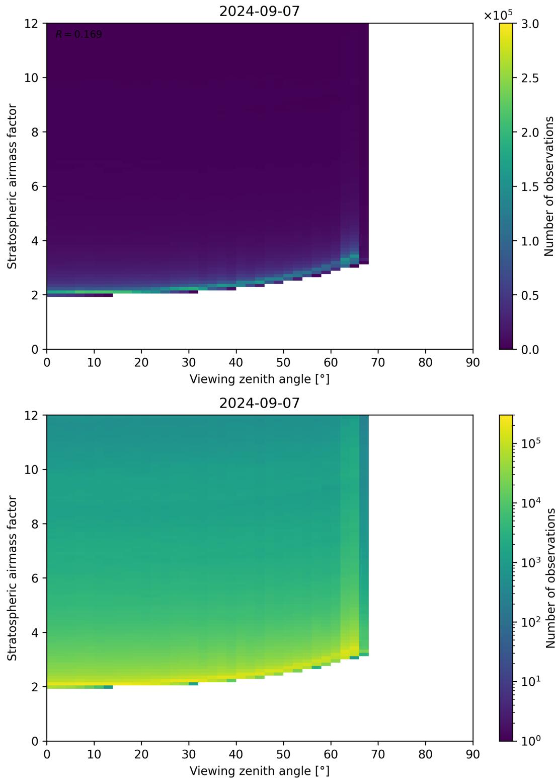
Figure 159: Scatter density plot of “Viewing zenith angle” against “Stratospheric airmass factor” for 2024-09-06 to 2024-09-08.
