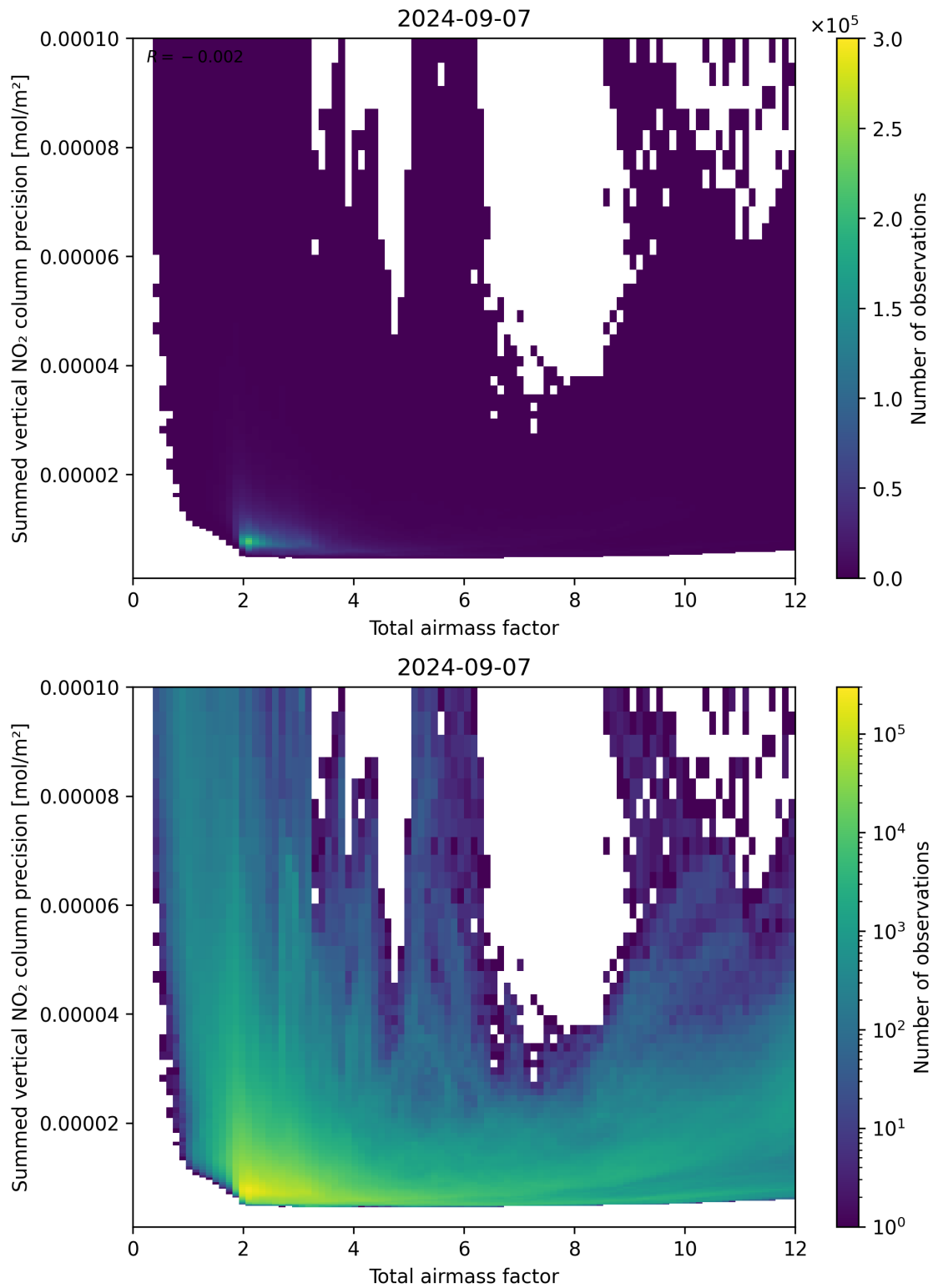
Figure 66: Scatter density plot of “Total airmass factor” against “Summed vertical NO 2 column precision” for 2024-09-06 to 2024-09-08.
