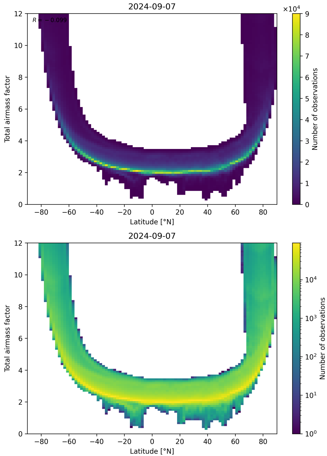
Figure 84: Scatter density plot of “Latitude” against “Total airmass factor” for 2024-09-06 to 2024-09-08.
