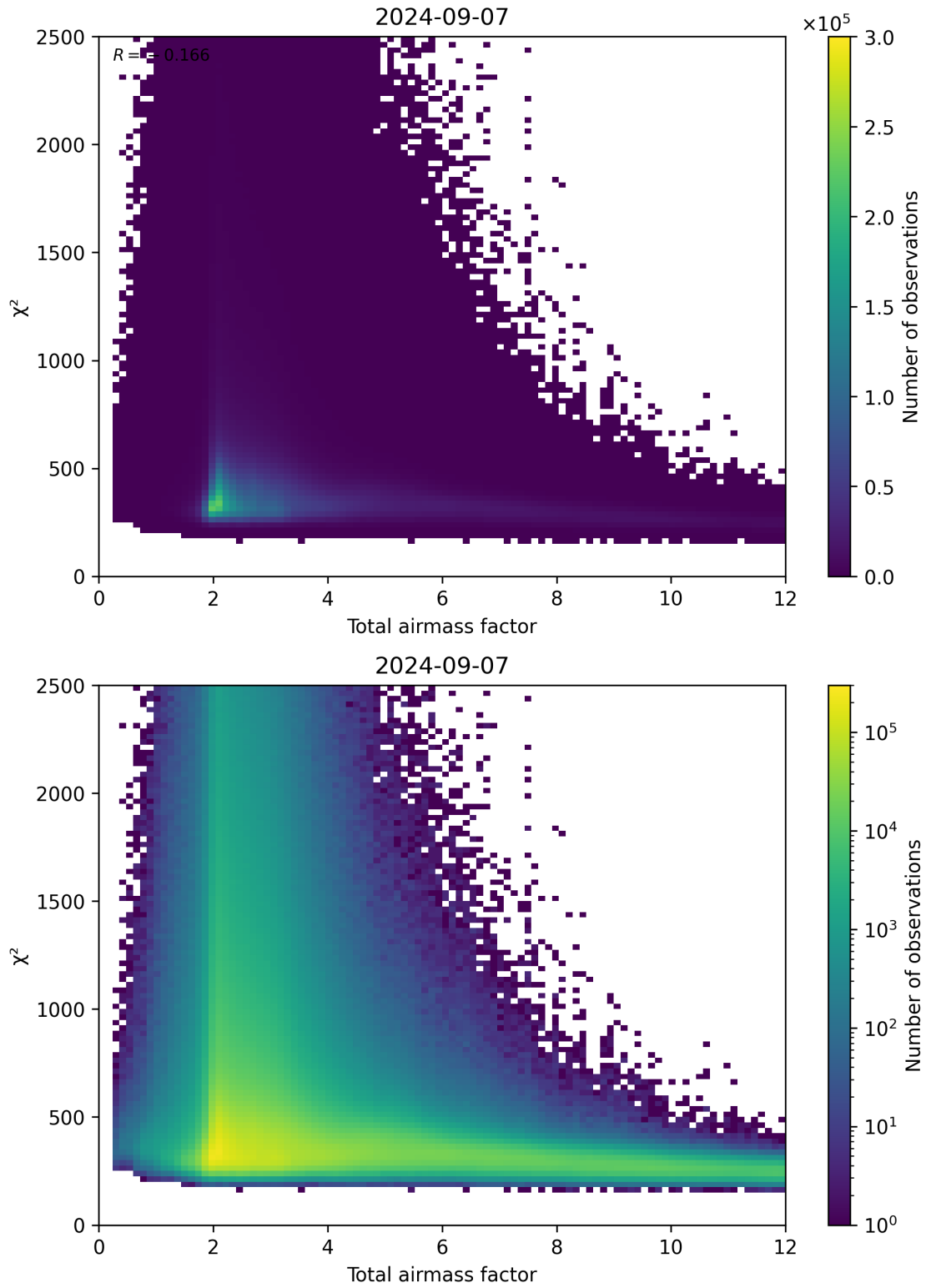
Figure 63: Scatter density plot of “Total airmass factor” against “ \chi^2 ” for 2024-09-06 to 2024-09-08.
