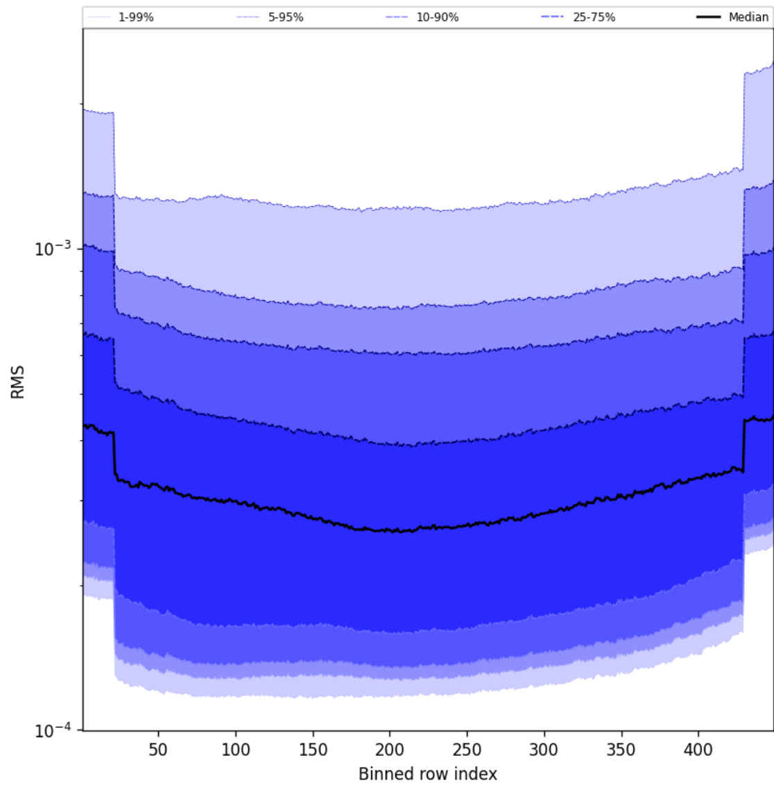
Figure 60: Along track statistics of “RMS” for 2024-09-06 to 2024-09-08
