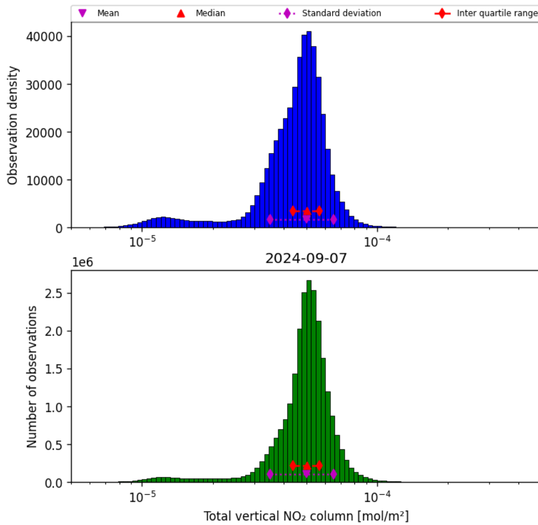
Figure 38: Histogram of "Total vertical NO 2 column" for 2024-09-06 to 2024-09-08
