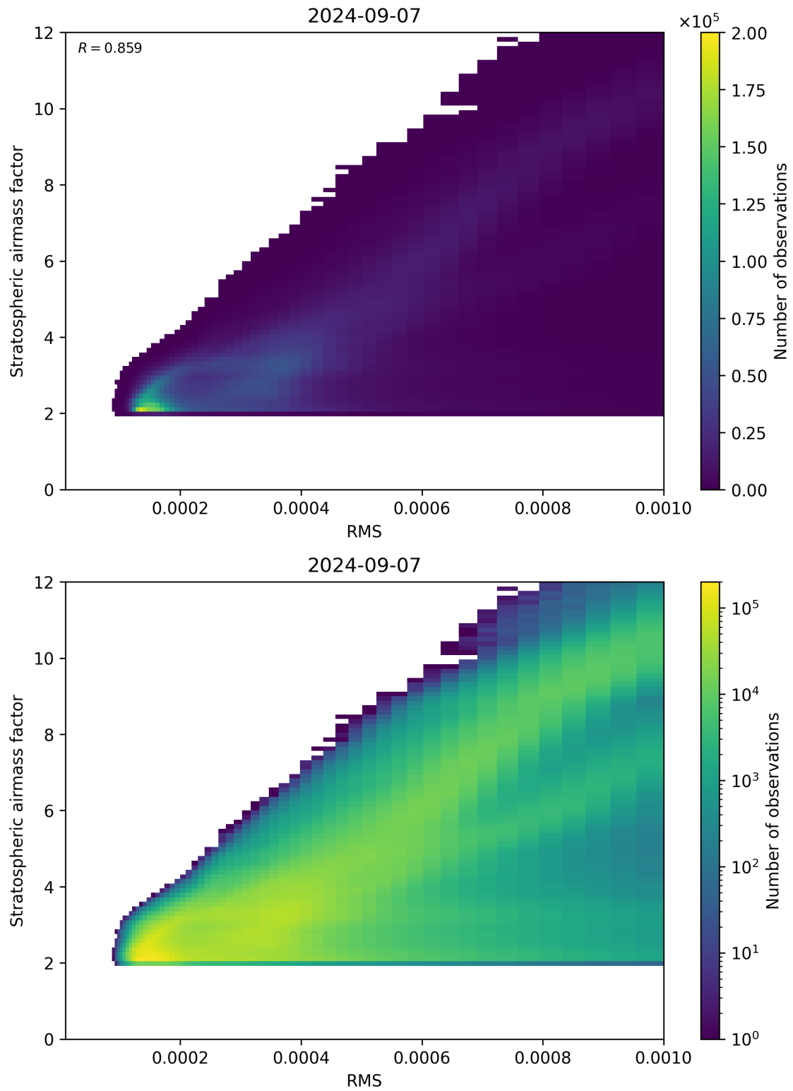
Figure 144: Scatter density plot of “RMS” against “Stratospheric airmass factor” for 2024-09-06 to 2024-09-08.
