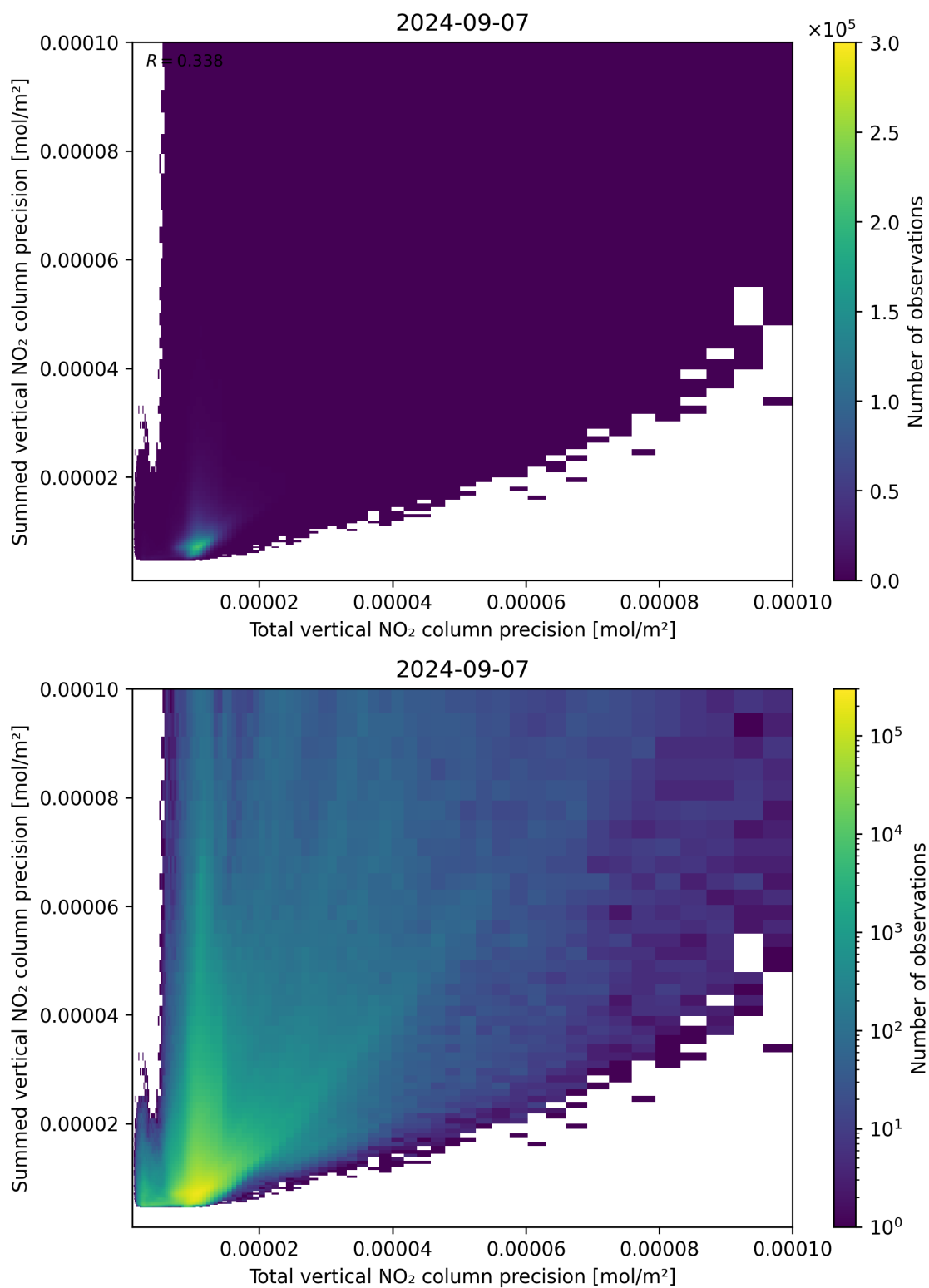
Figure 118: Scatter density plot of “Total vertical NO 2 column precision” against “Summed vertical NO 2 column precision” for 2024-09-06 to 2024-09-08.
