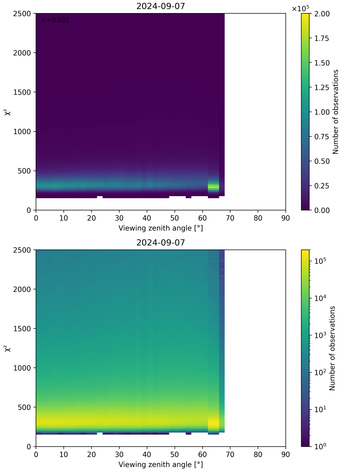
Figure 162: Scatter density plot of “Viewing zenith angle” against “ \chi^2 ” for 2024-09-06 to 2024-09-08.
