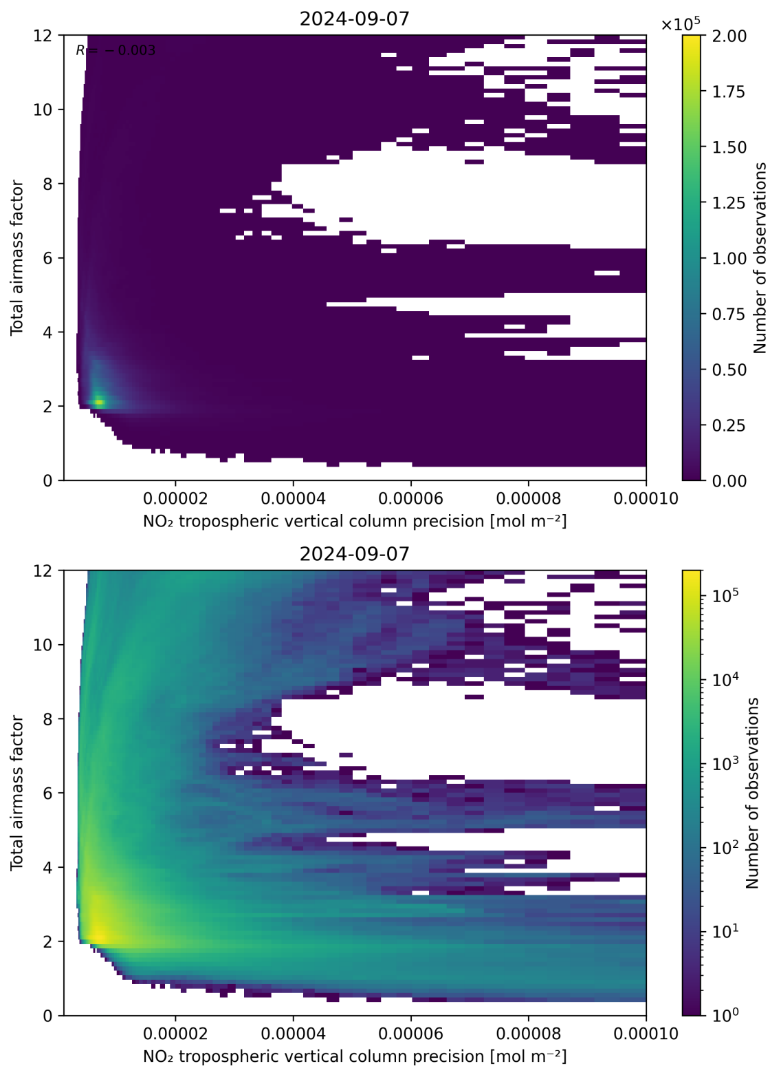
Figure 132: Scatter density plot of “NO 2 tropospheric vertical column precision” against “Total air mass factor” for 2024-09-06 to 2024-09-08.
