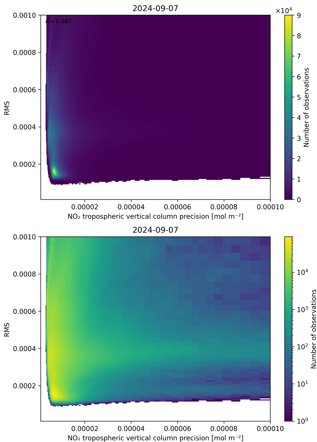
Figure 140: Scatter density plot of “NO 2 tropospheric vertical column precision” against “RMS” for 2024-09-06 to 2024-09-08.
