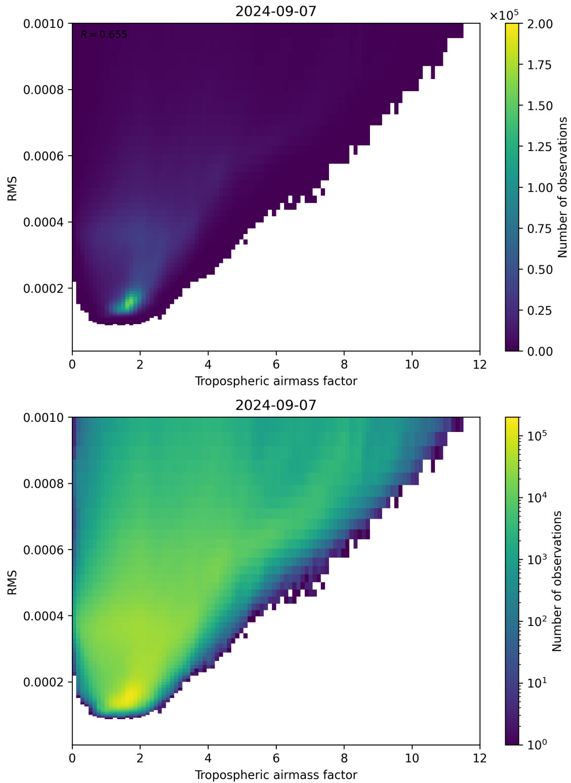
Figure 79: Scatter density plot of “Tropospheric airmass factor” against “RMS” for 2024-09-06 to 2024-09-08.
