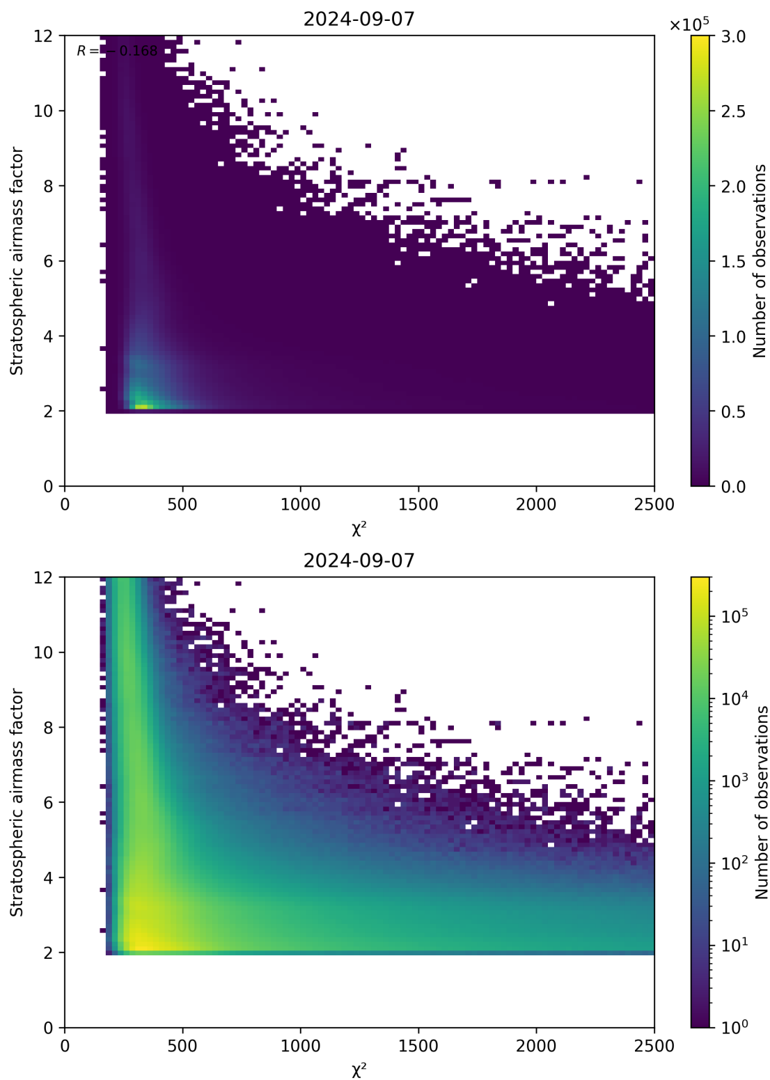
Figure 81: Scatter density plot of “ \chi^2 ” against “Stratospheric airmass factor” for 2024-09-06 to 2024-09-08.
