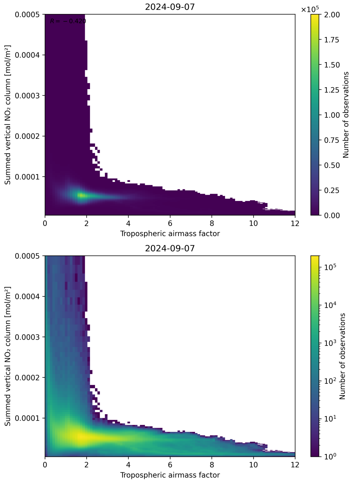
Figure 75: Scatter density plot of “Tropospheric air mass factor” against “Summed vertical NO 2 column” for 2024-09-06 to 2024-09-08.
