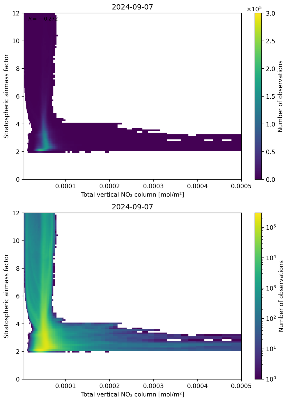
Figure 110: Scatter density plot of “Total vertical NO 2 column” against “Stratospheric airmass factor” for 2024-09-06 to 2024-09-08.
