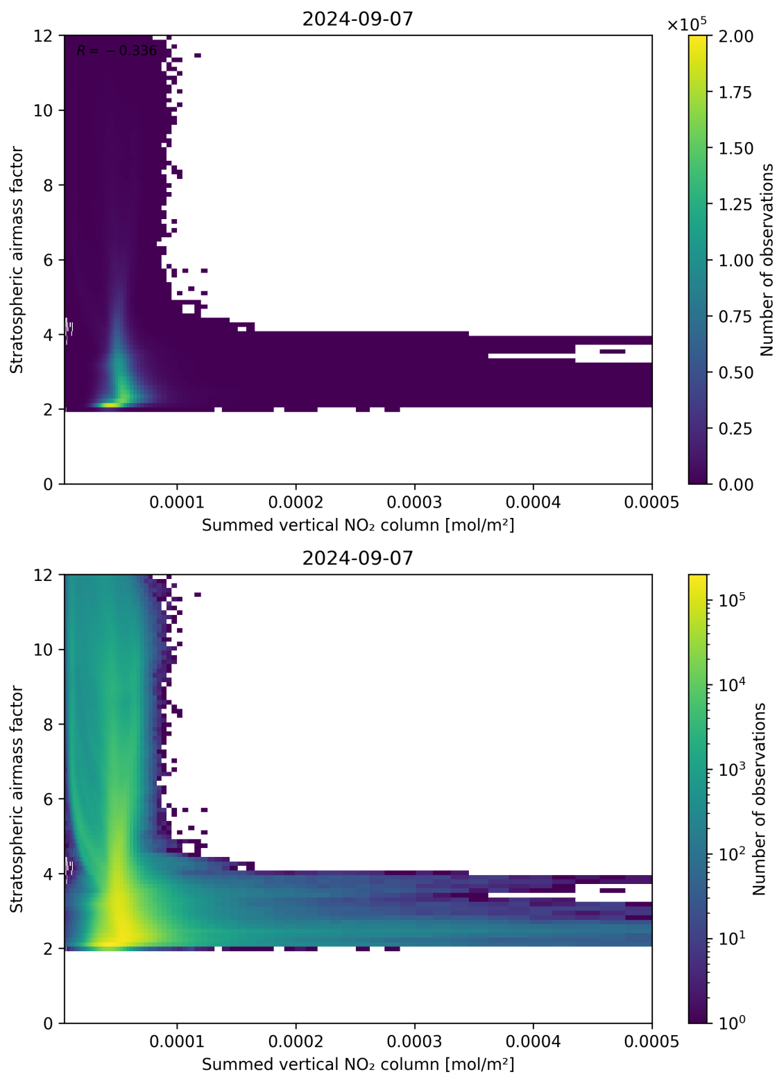
Figure 103: Scatter density plot of “Summed vertical NO 2 column” against “Stratospheric airmass factor” for 2024-09-06 to 2024-09-08.
