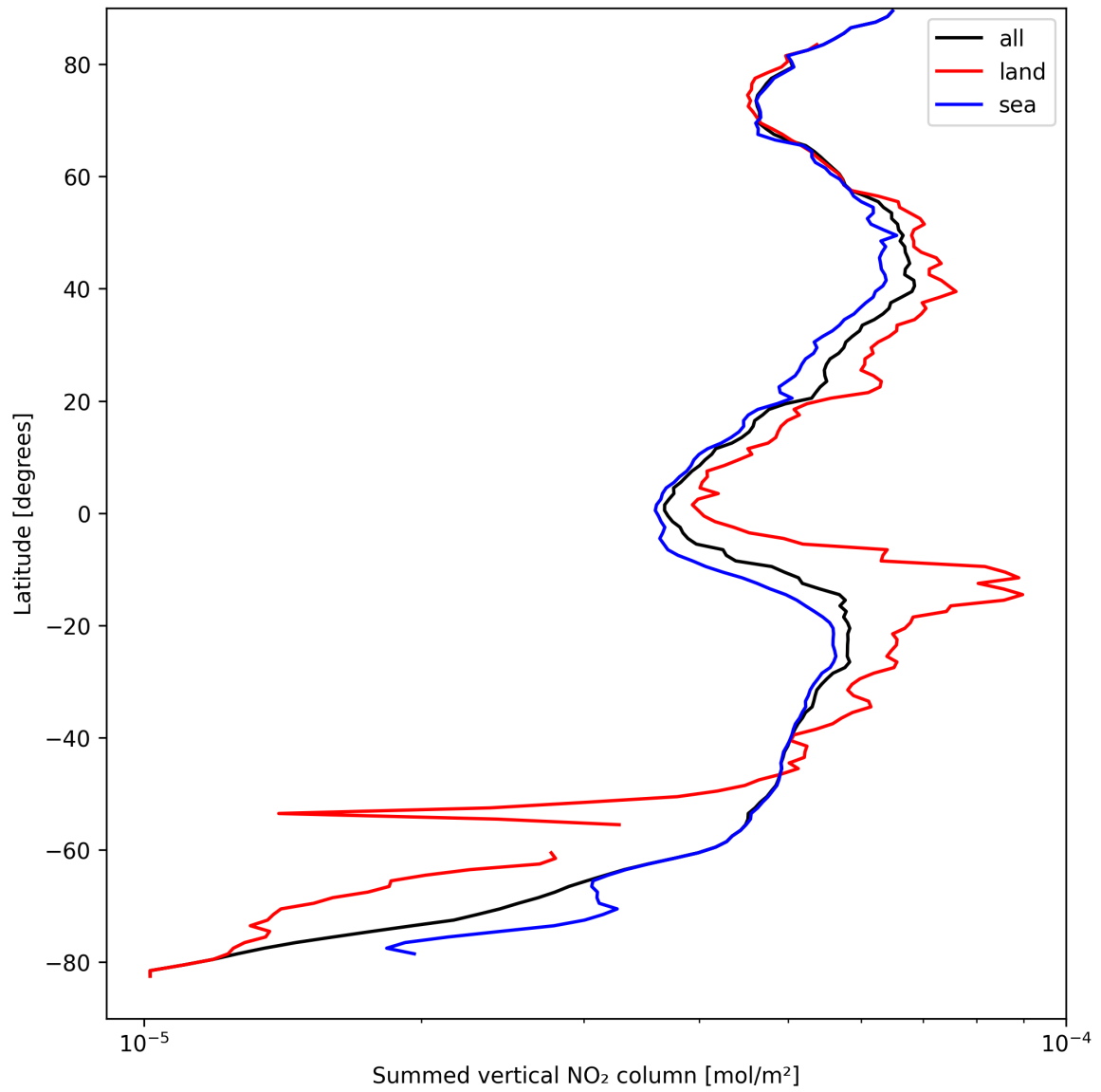
Figure 23: Zonal average of “Summed vertical NO 2 column” for 2024-09-06 to 2024-09-08.
