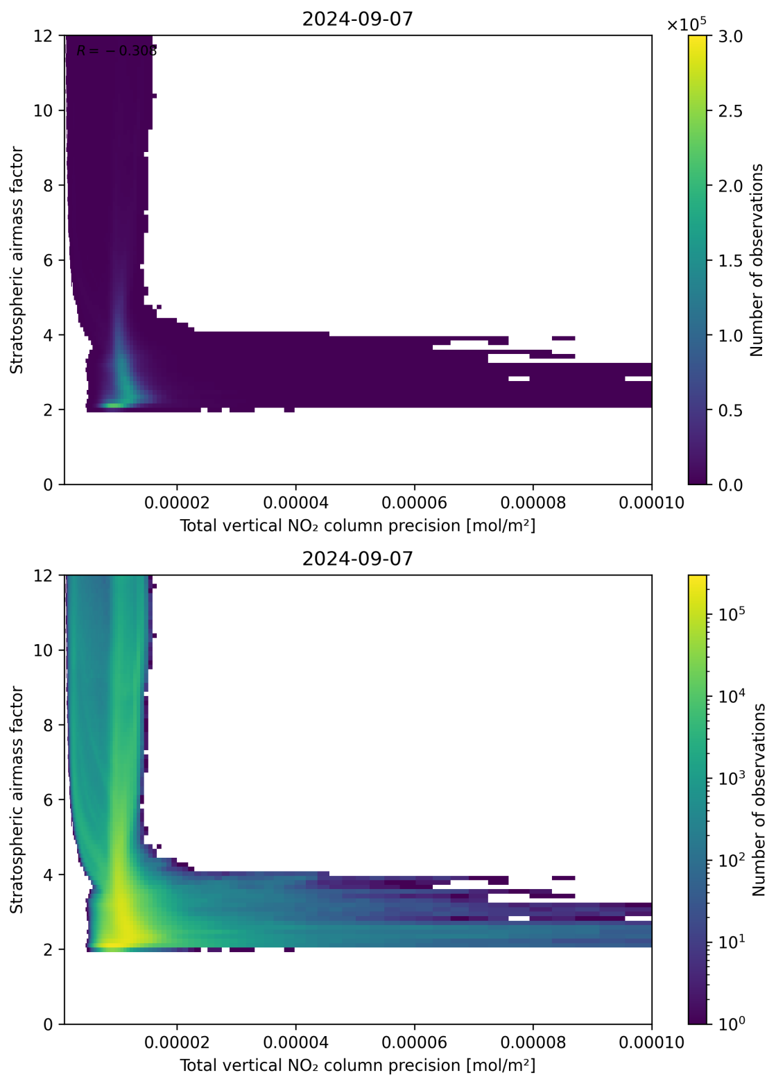
Figure 115: Scatter density plot of “Total vertical NO 2 column precision” against “Stratospheric air mass factor” for 2024-09-06 to 2024-09-08.
