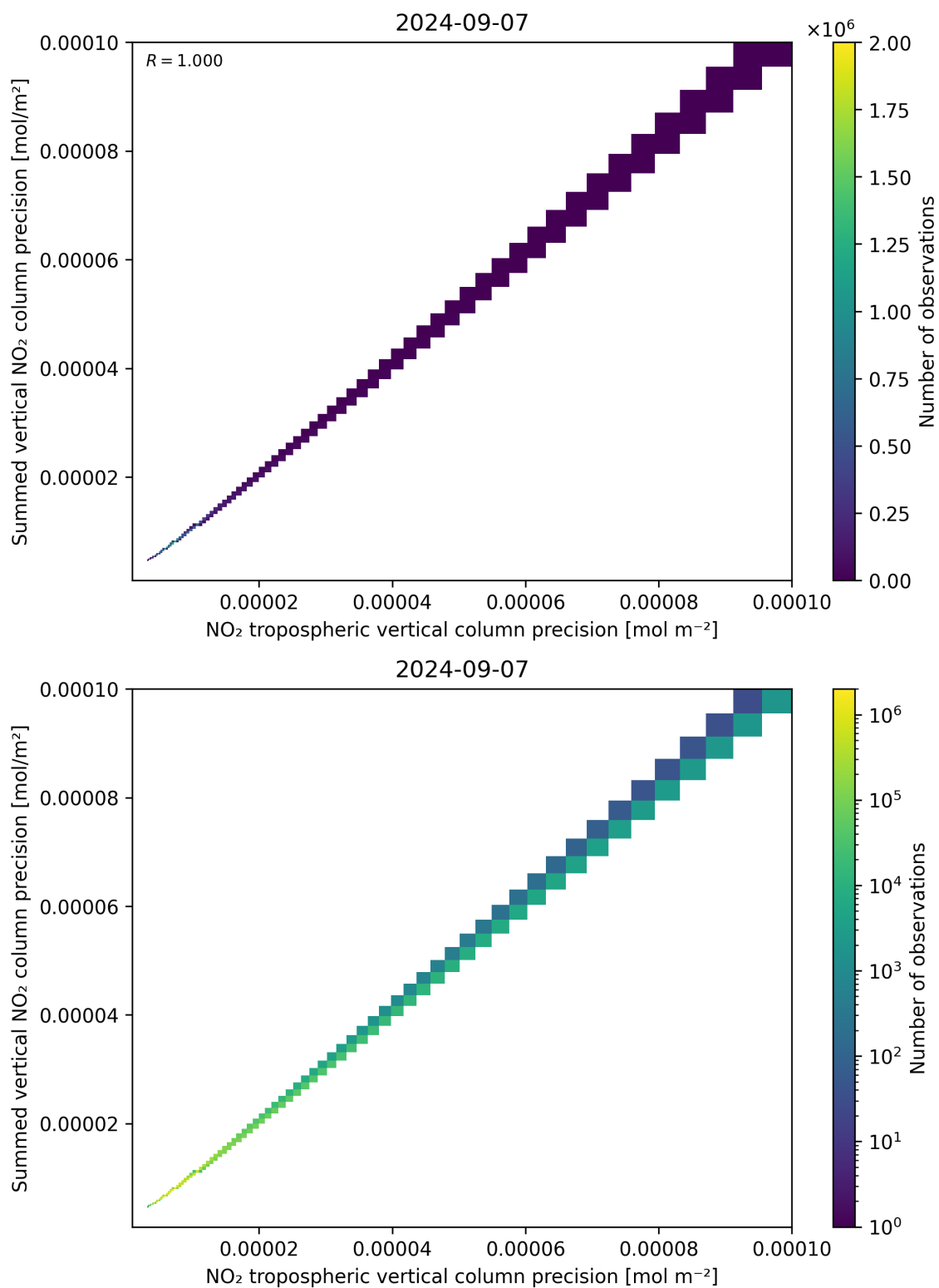
Figure 137: Scatter density plot of “NO 2 tropospheric vertical column precision” against “Summed vertical NO 2 column precision” for 2024-09-06 to 2024-09-08.
