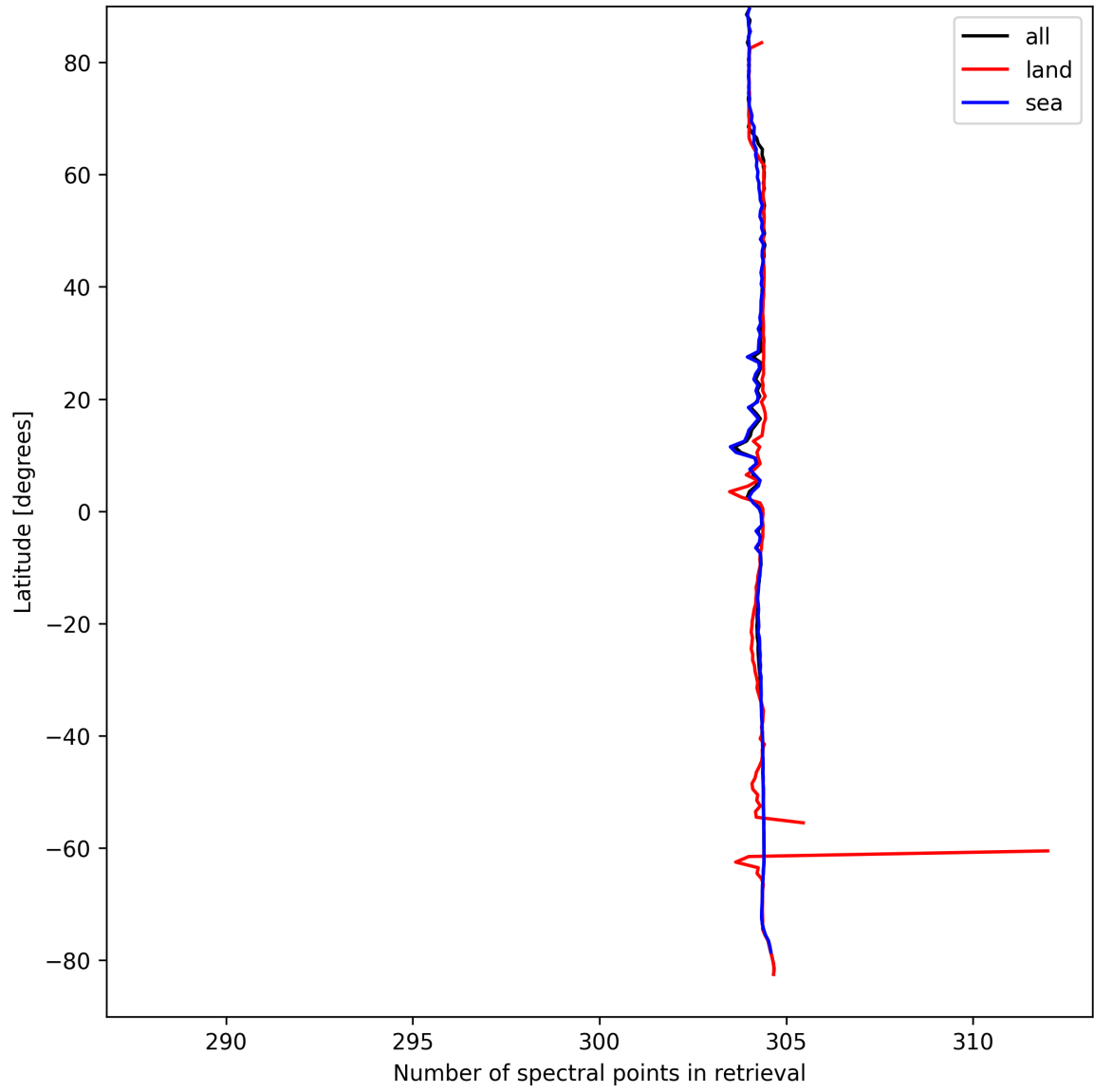
Figure 16: Zonal average of “Number of spectral points in retrieval” for 2024-09-06 to 2024-09-08.
