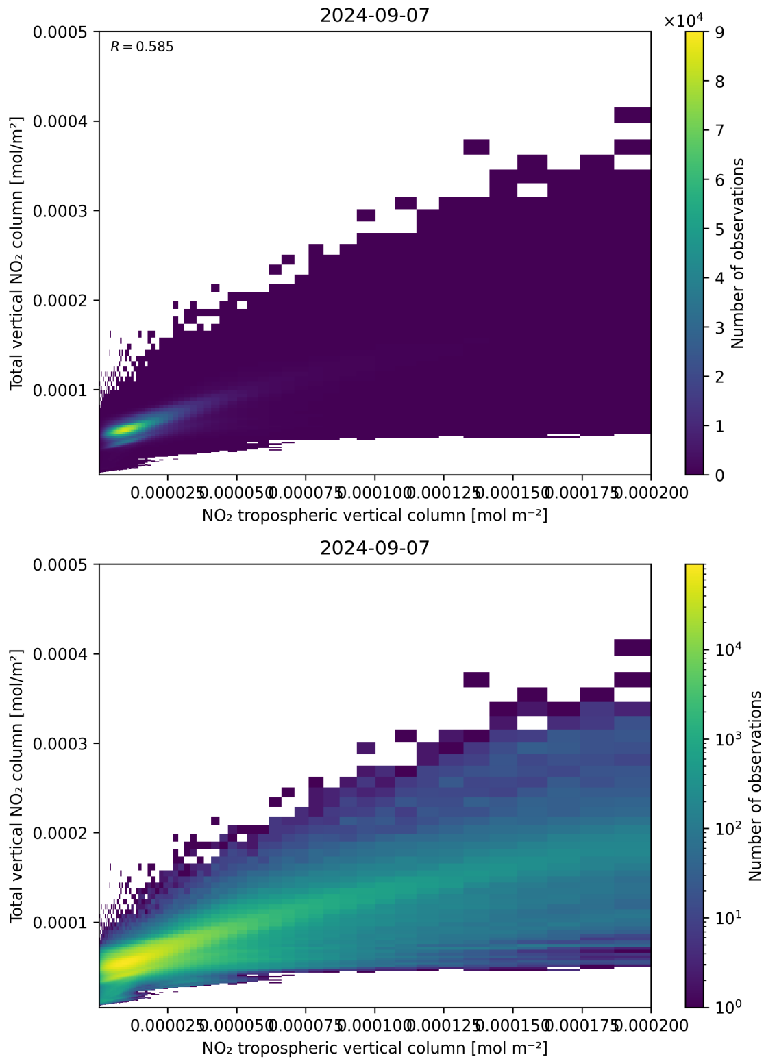
Figure 128: Scatter density plot of “NO 2 tropospheric vertical column” against “Total vertical NO 2 column” for 2024-09-06 to 2024-09-08.
