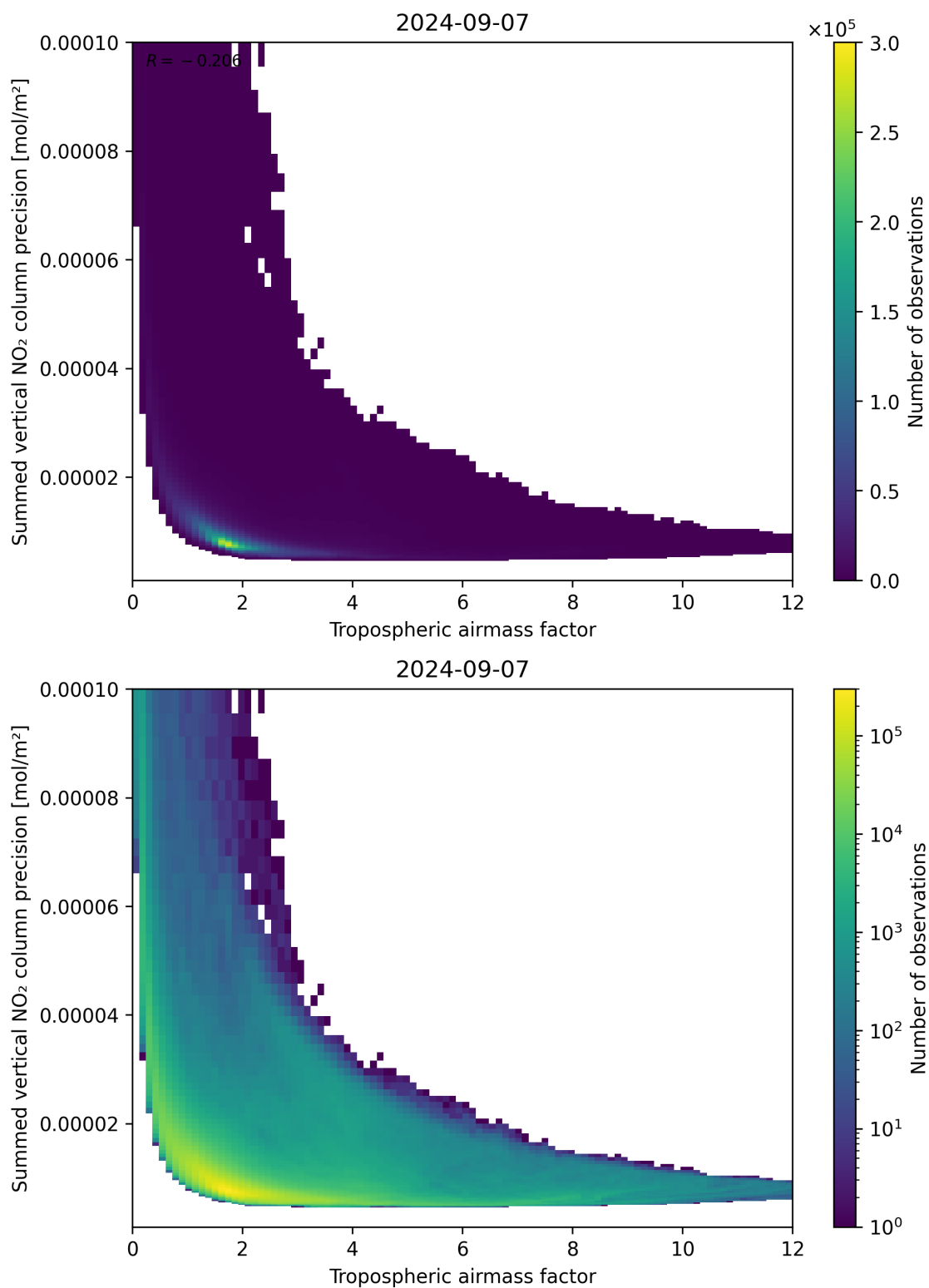
Figure 76: Scatter density plot of “Tropospheric air mass factor” against “Summed vertical NO 2 column precision” for 2024-09-06 to 2024-09-08.
