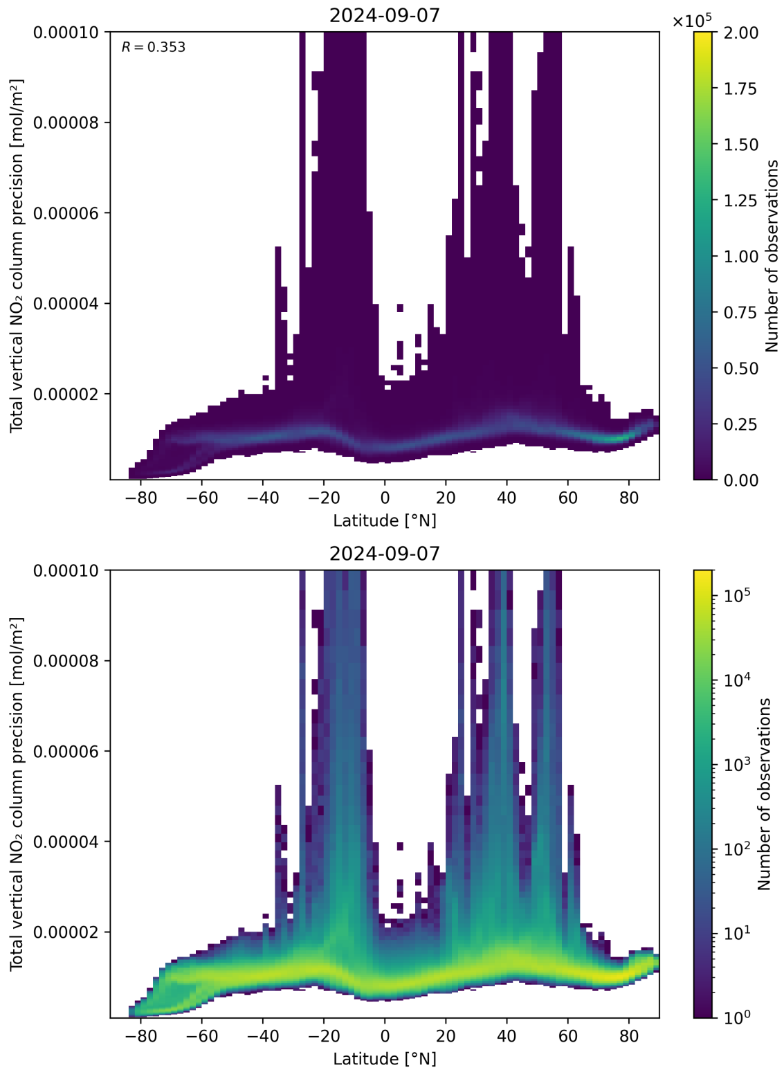
Figure 91: Scatter density plot of “Latitude” against “Total vertical NO 2 column precision” for 2024-09-06 to 2024-09-08.
