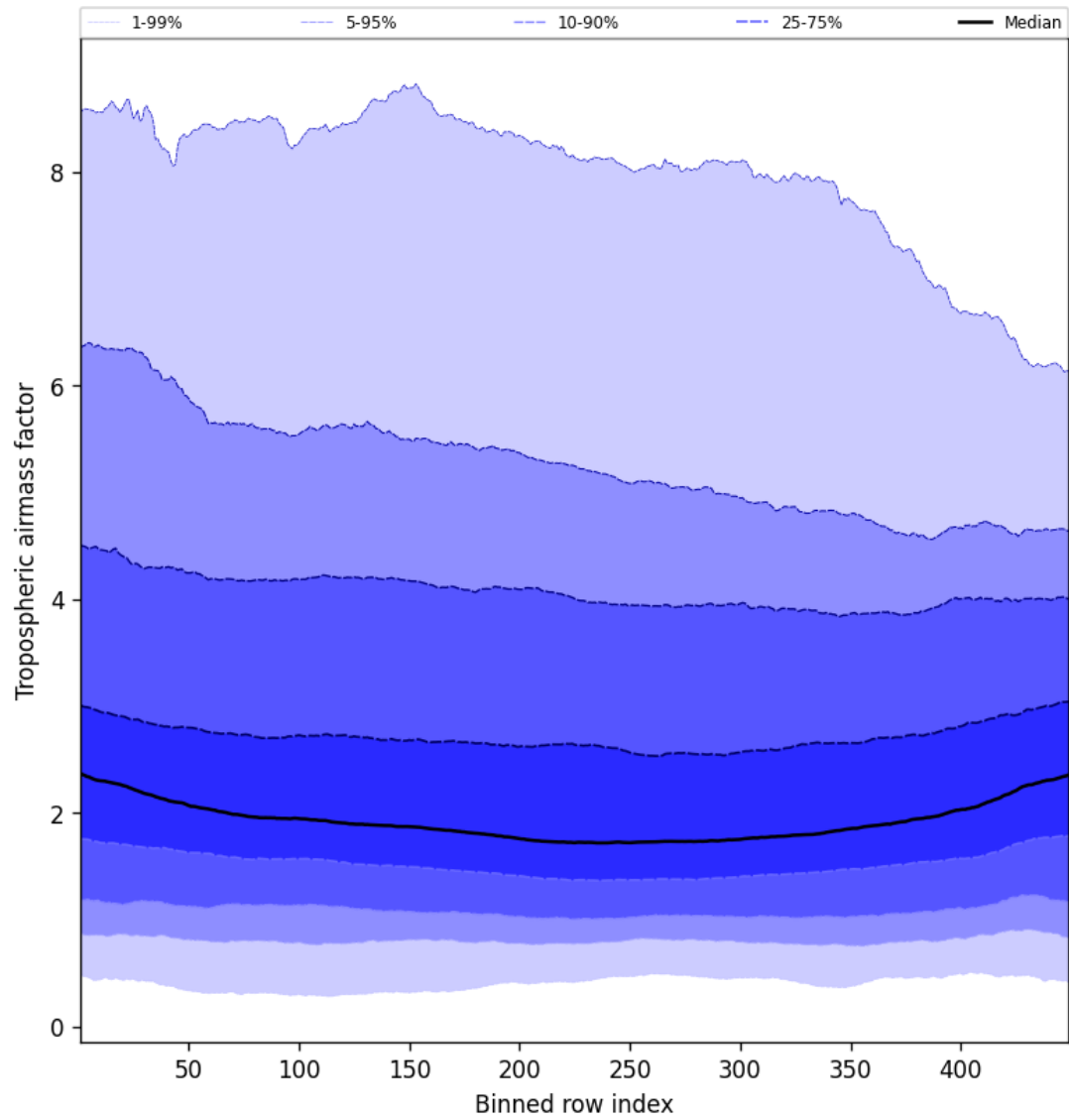
Figure 48: Along track statistics of “Tropospheric airmass factor” for 2024-09-06 to 2024-09-08
