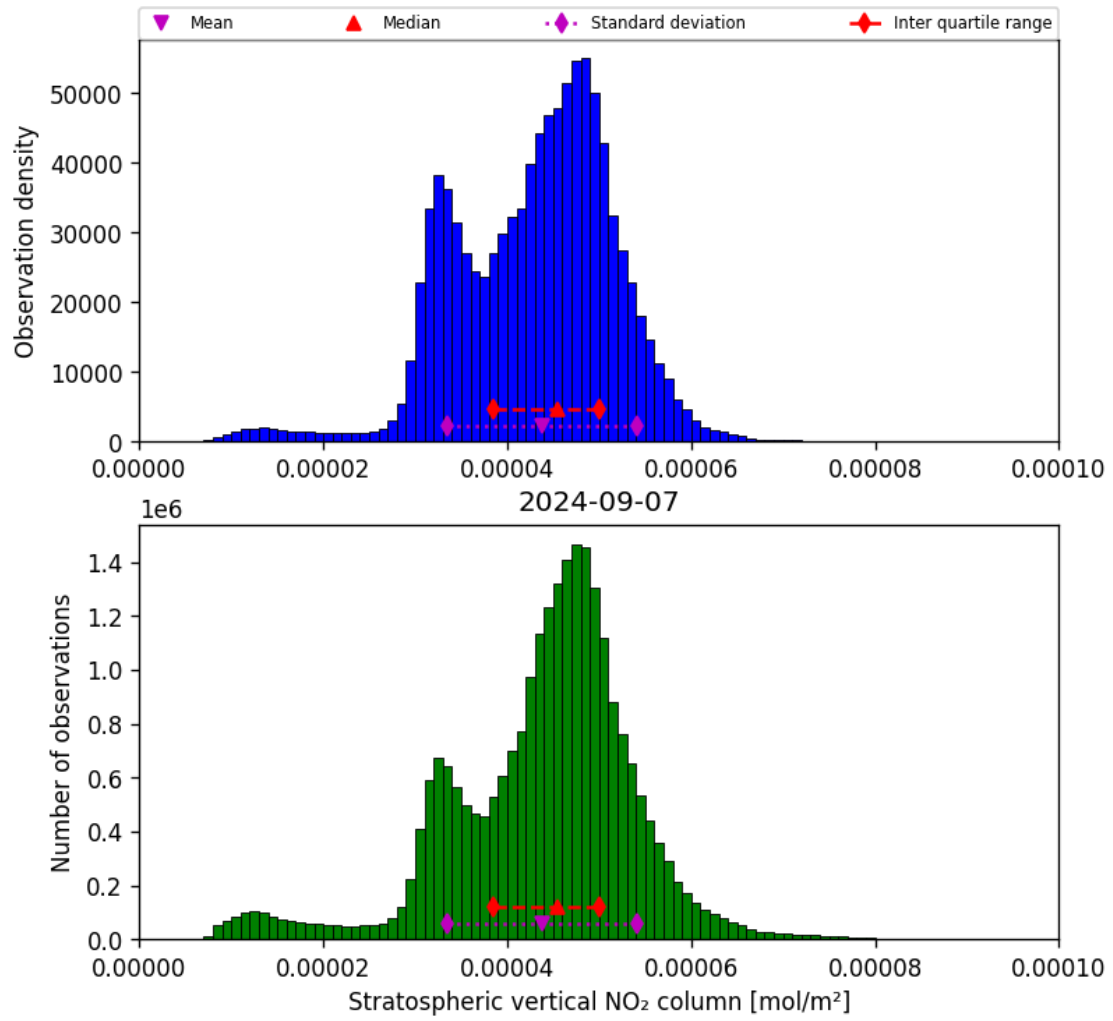
Figure 36: Histogram of “Stratospheric vertical NO 2 column” for 2024-09-06 to 2024-09-08
