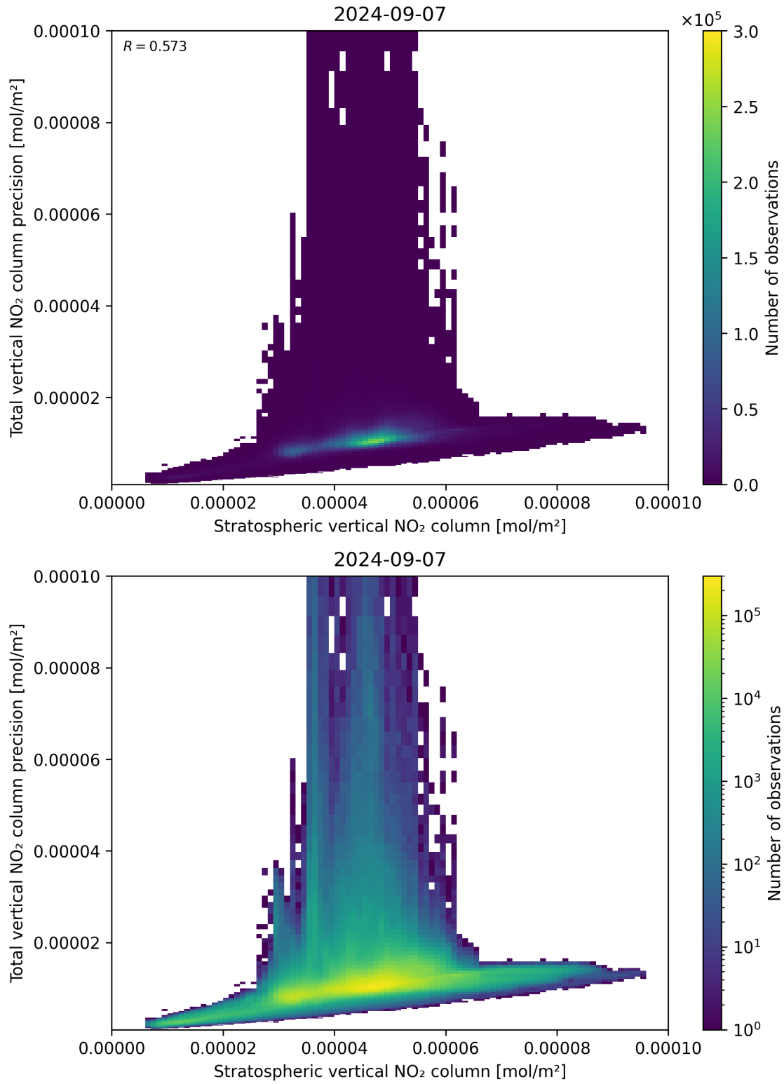
Figure 101: Scatter density plot of “Stratospheric vertical NO 2 column” against “Total vertical NO 2 column precision” for 2024-09-06 to 2024-09-08.
