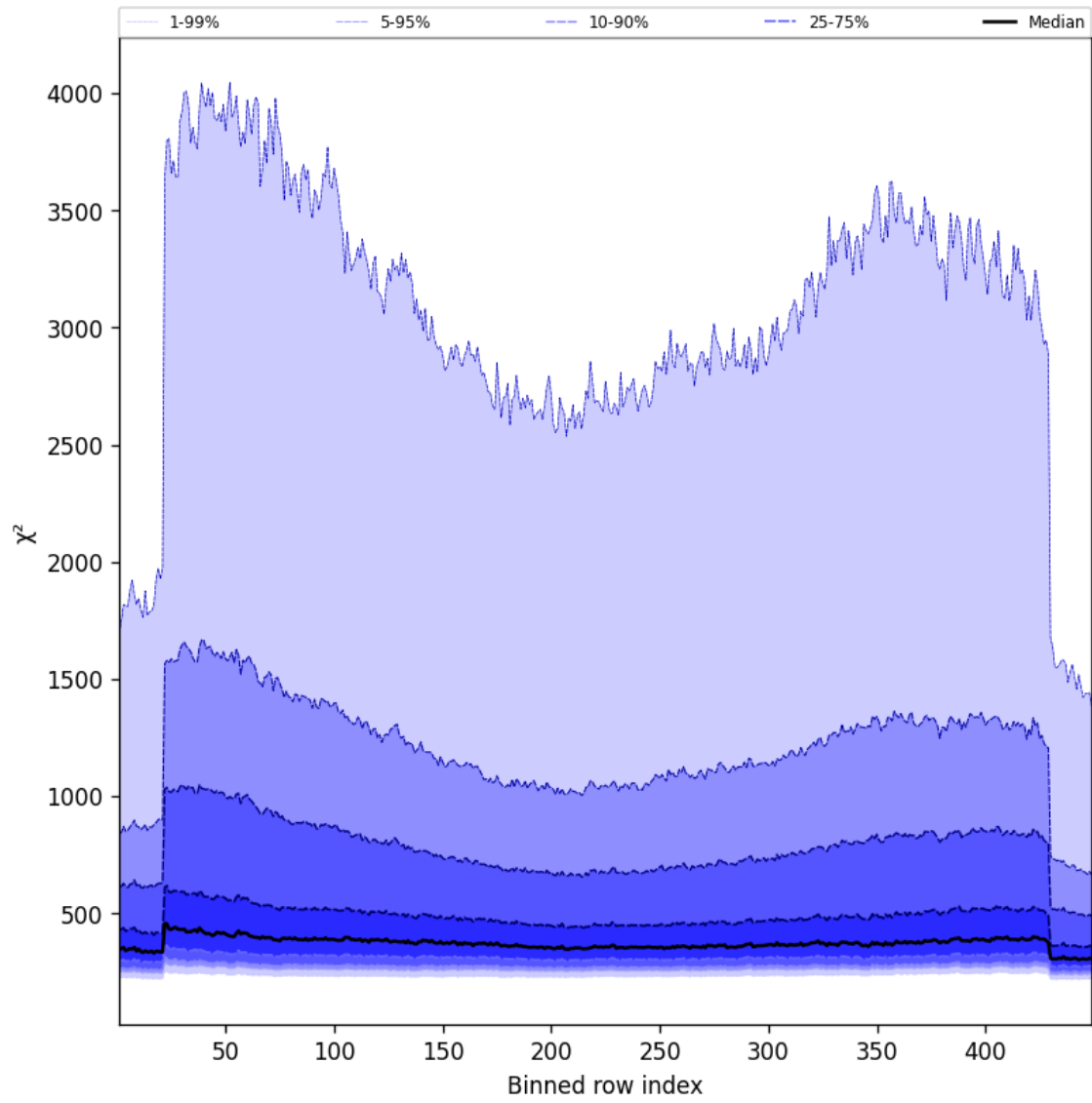
Figure 59: Along track statistics of “ \chi^2 ” for 2024-09-06 to 2024-09-08
