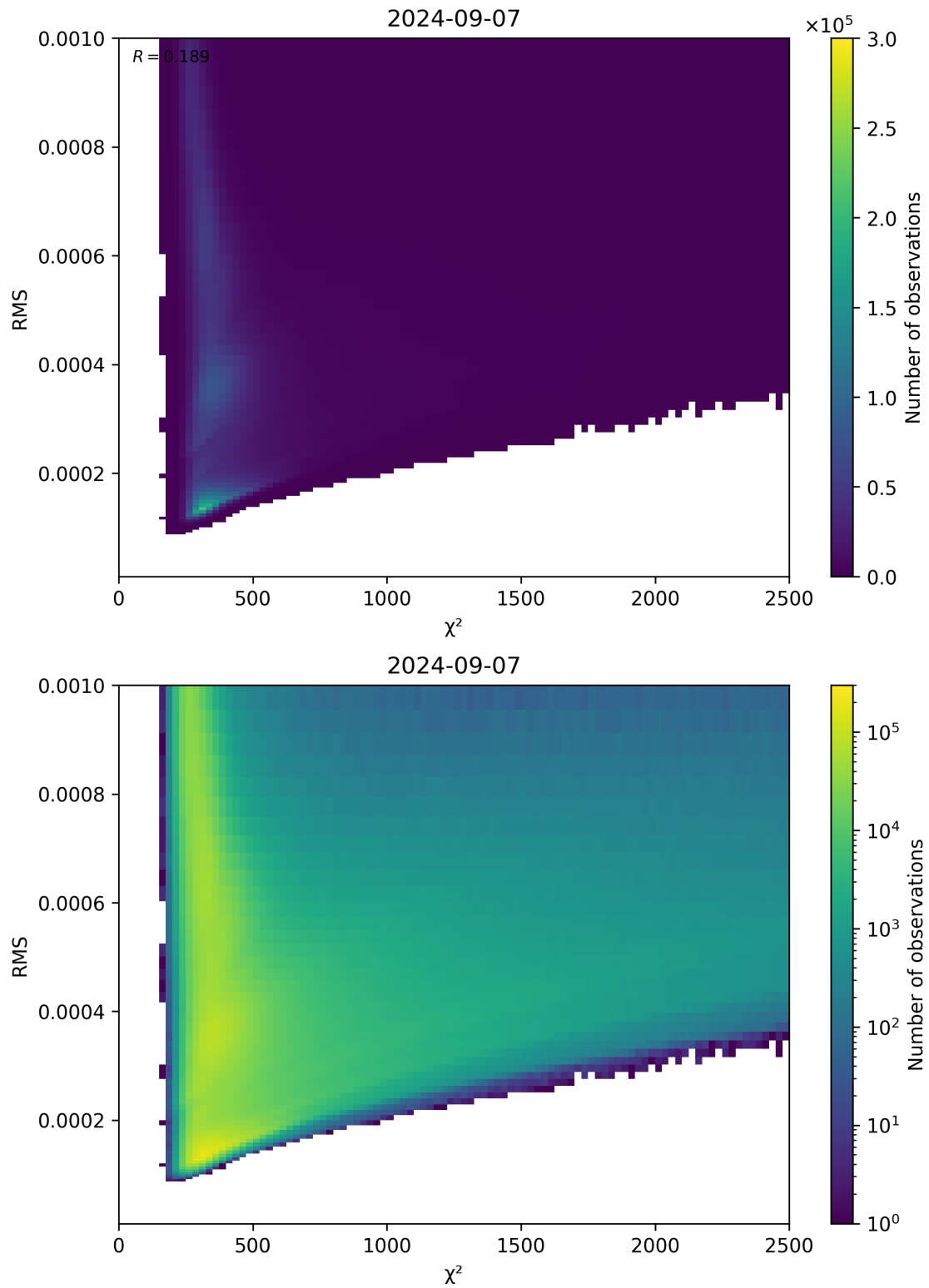
Figure 82: Scatter density plot of “ \chi^2 ” against “RMS” for 2024-09-06 to 2024-09-08.
