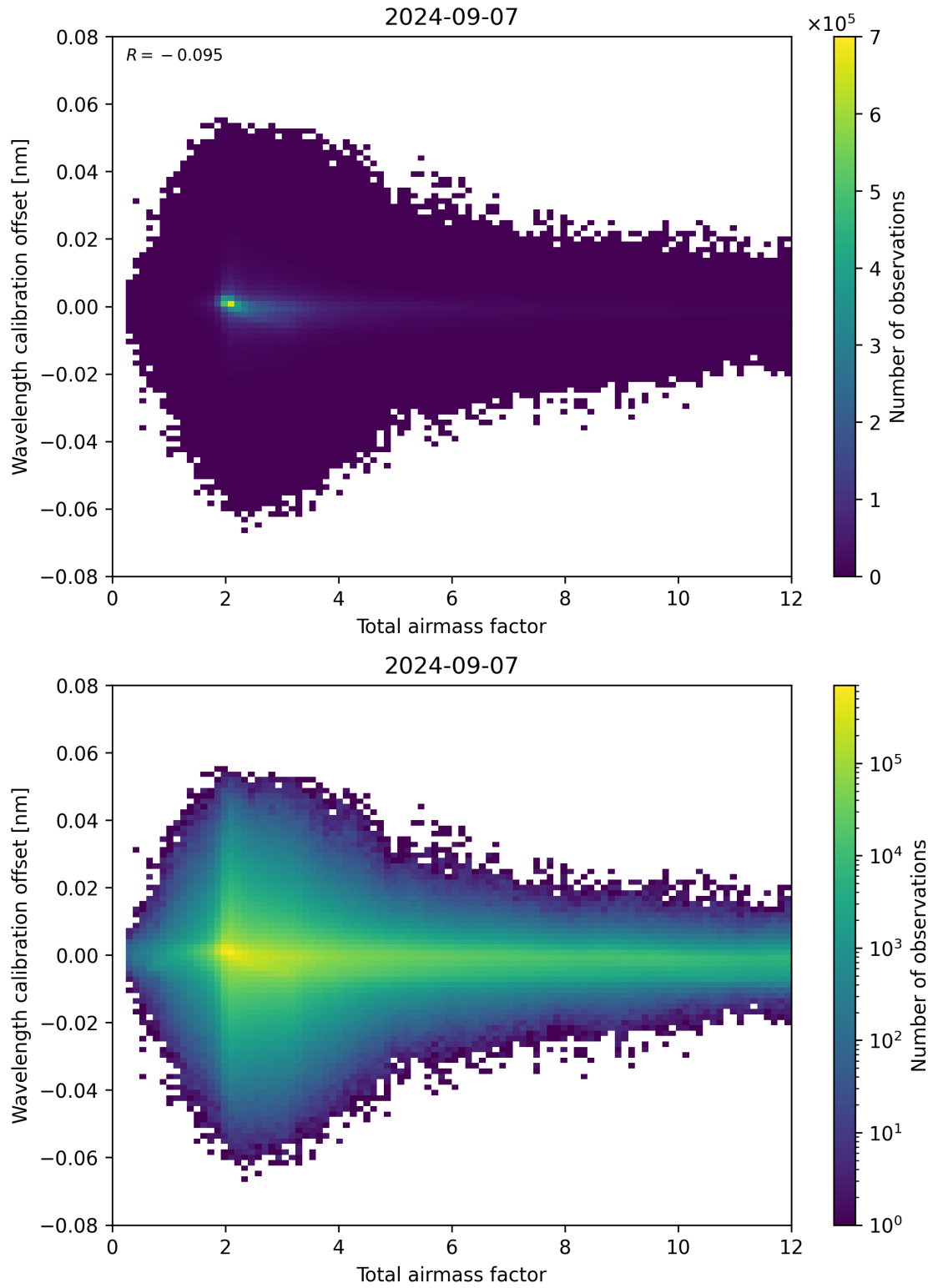
Figure 70: Scatter density plot of “Total airmass factor” against “Wavelength calibration offset” for 2024-09-06 to 2024-09-08.
