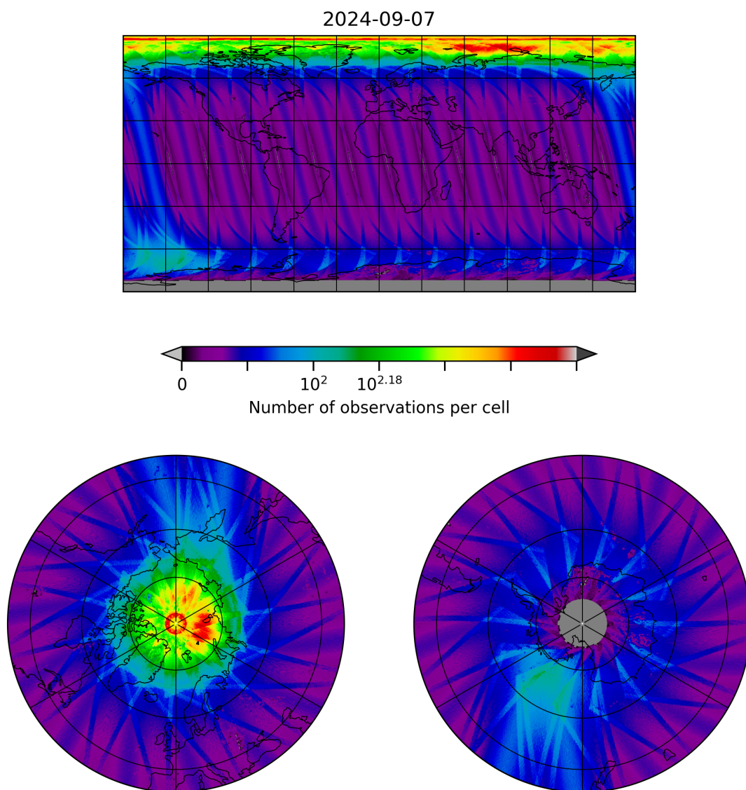
Figure 10: Map of the number of observations for 2024-09-06 to 2024-09-08
