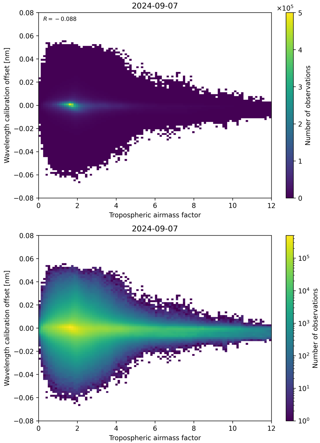
Figure 80: Scatter density plot of “Tropospheric airmass factor” against “Wavelength calibration offset” for 2024-09-06 to 2024-09-08.
