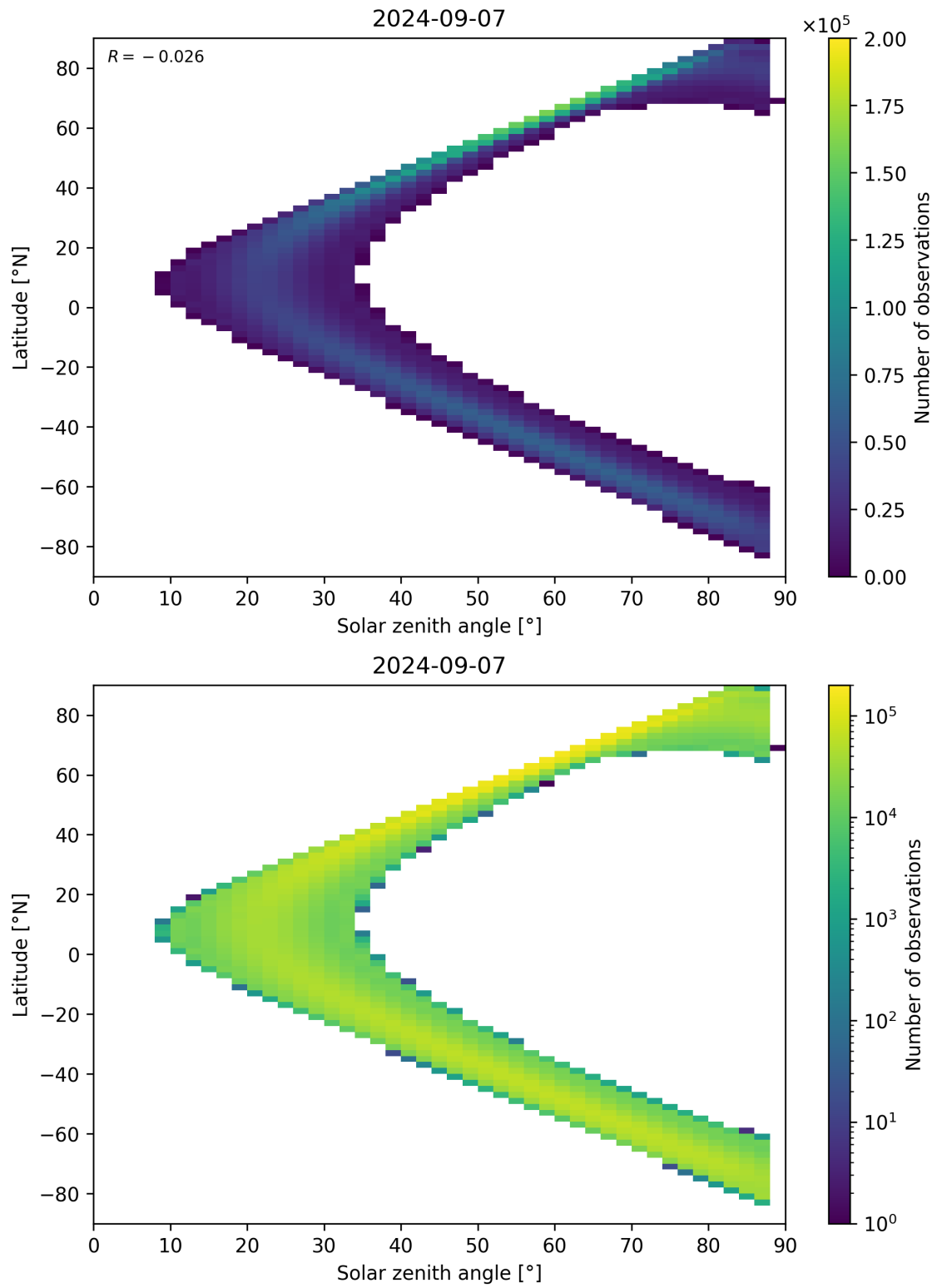
Figure 149: Scatter density plot of “Solar zenith angle” against “Latitude” for 2024-09-06 to 2024-09-08.
