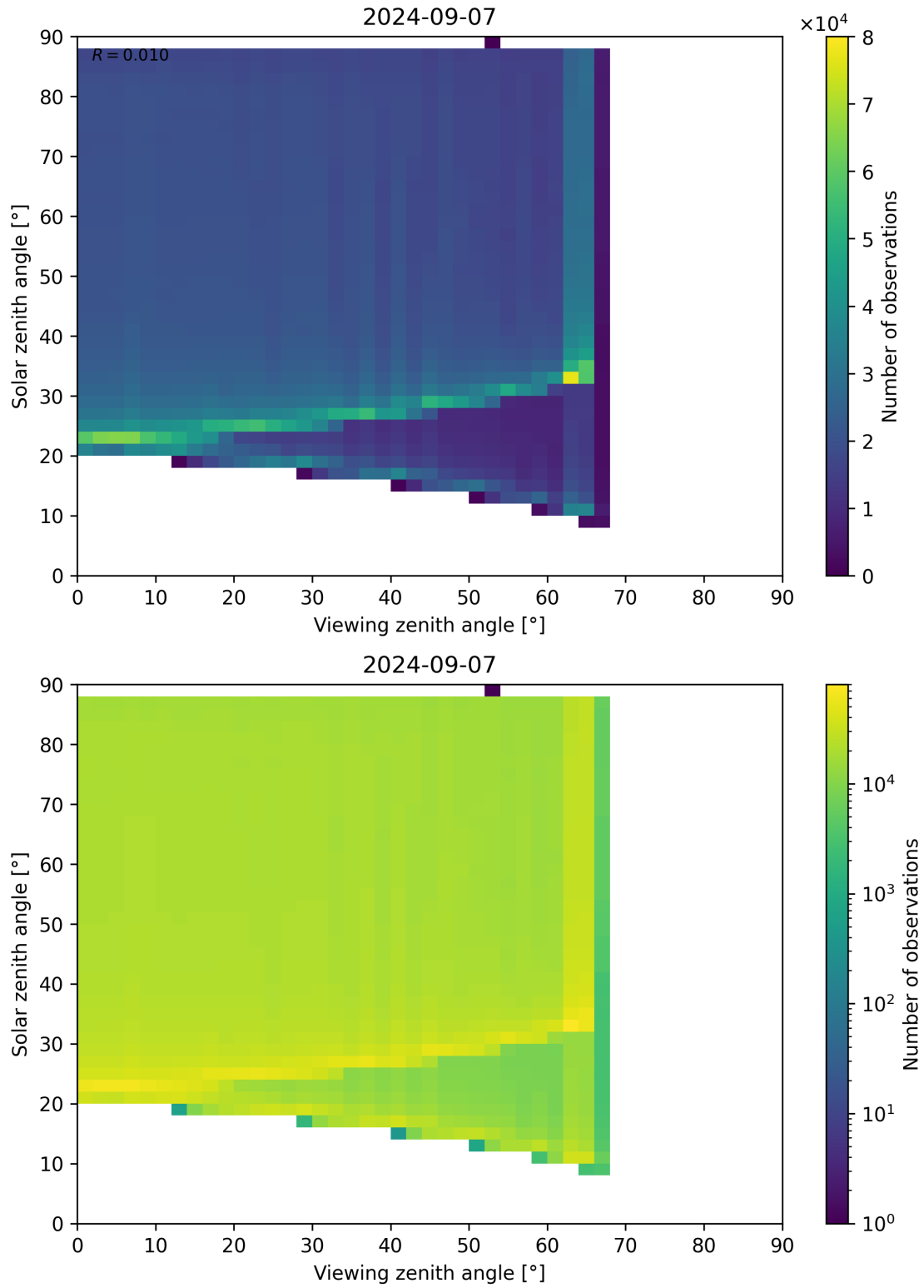
Figure 172: Scatter density plot of “Viewing zenith angle” against “Solar zenith angle” for 2024-09-06 to 2024-09-08.
