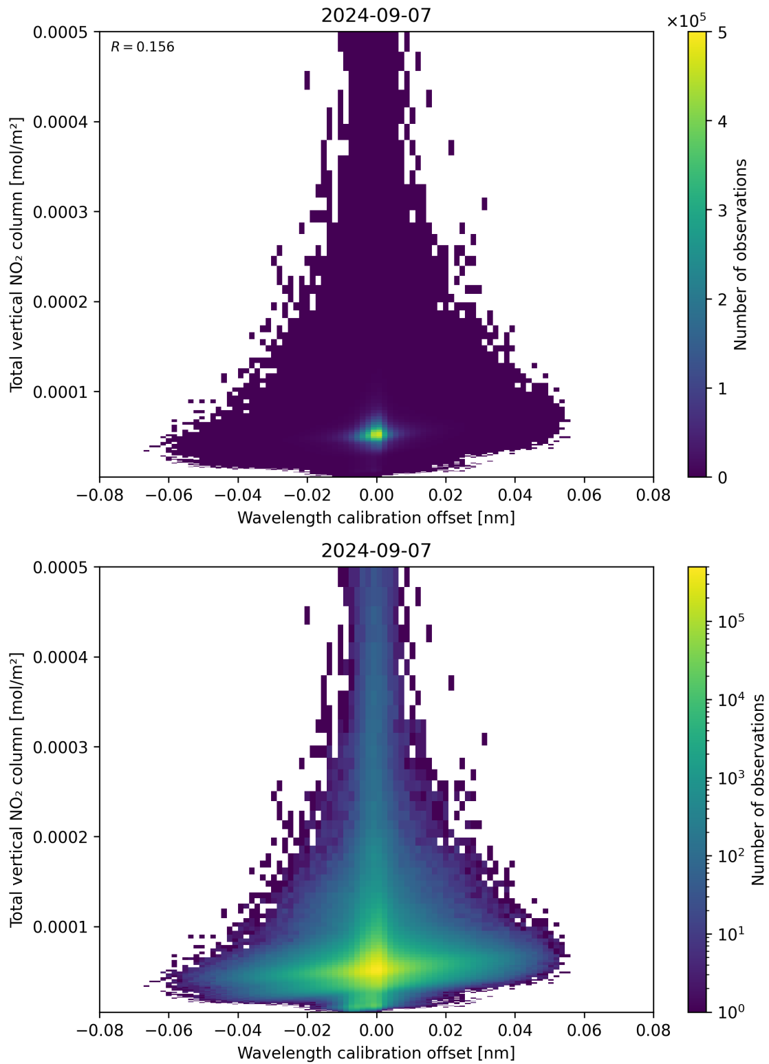
Figure 179: Scatter density plot of “Wavelength calibration offset” against “Total vertical NO 2 column” for 2024-09-06 to 2024-09-08.
