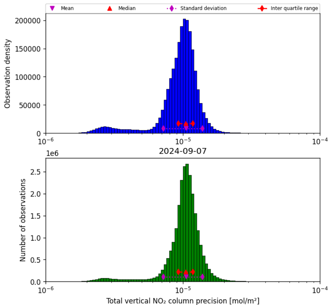
Figure 39: Histogram of “Total vertical NO 2 column precision” for 2024-09-06 to 2024-09-08
