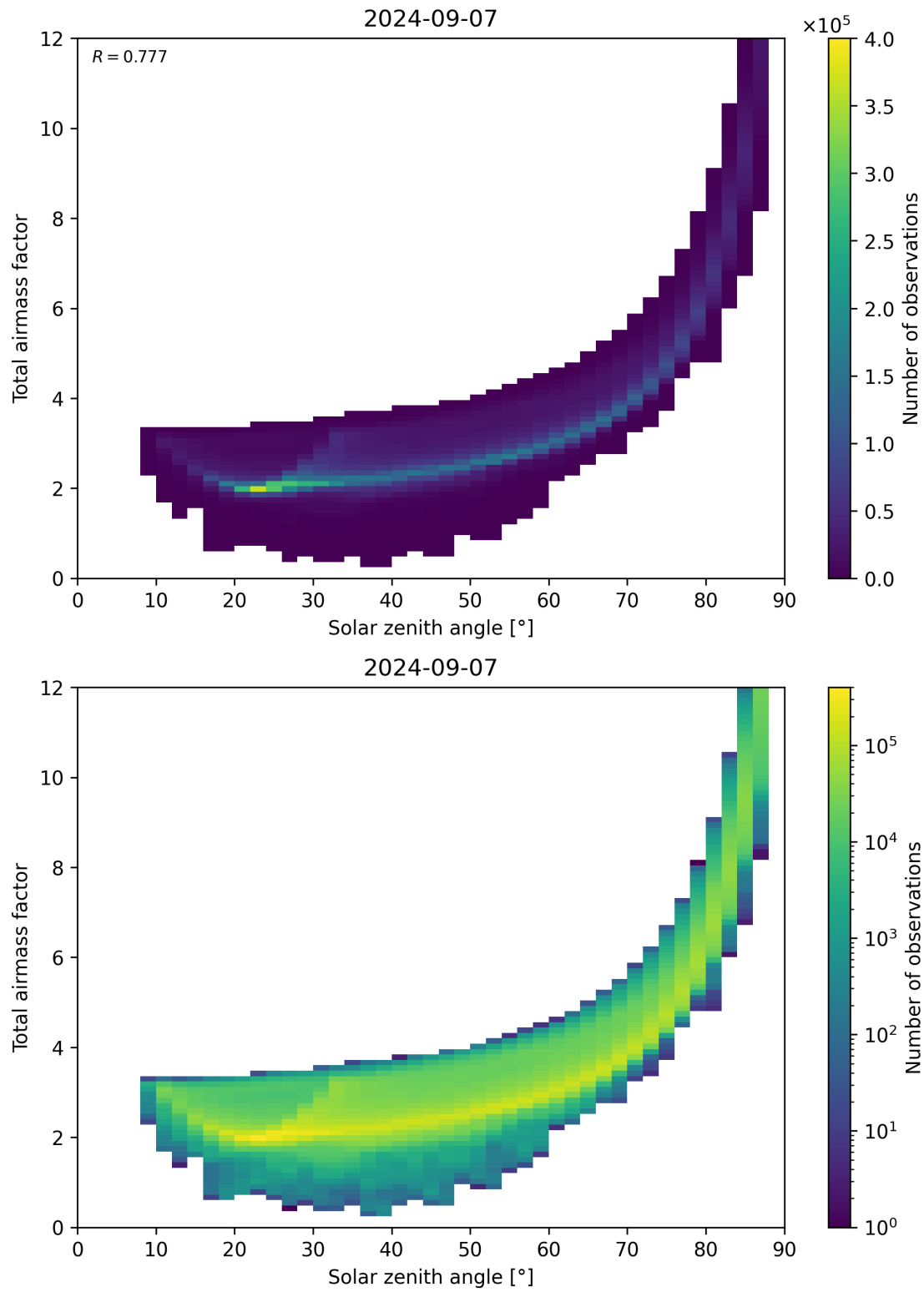
Figure 146: Scatter density plot of “Solar zenith angle” against “Total airmass factor” for 2024-09-06 to 2024-09-08.
