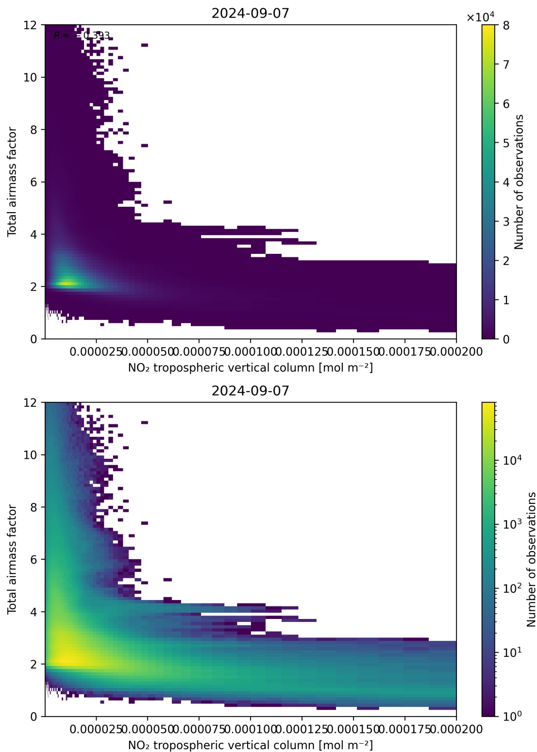
Figure 122: Scatter density plot of “NO 2 tropospheric vertical column” against “Total air mass factor” for 2024-09-06 to 2024-09-08.
