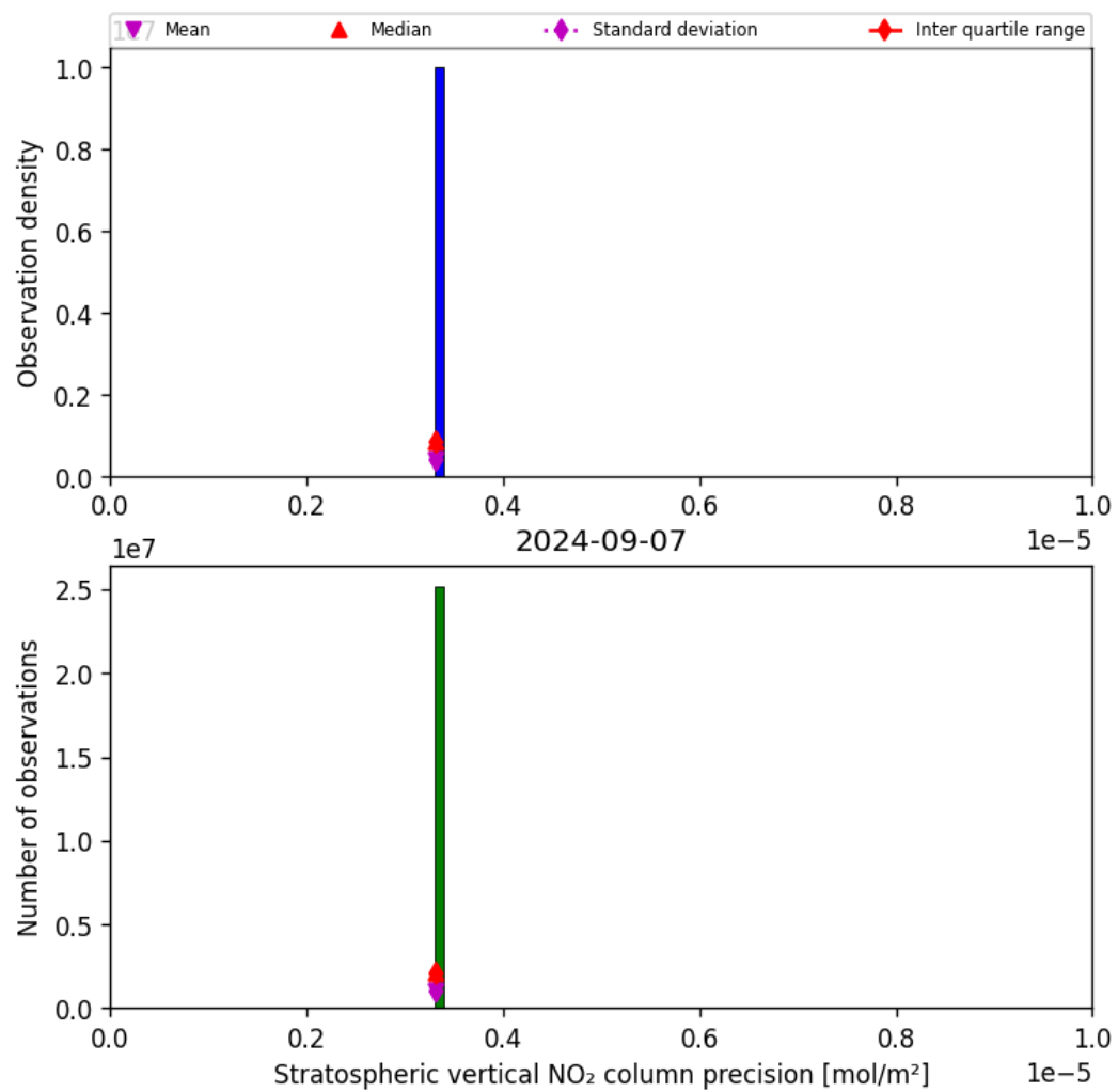
Figure 37: Histogram of “Stratospheric vertical NO 2 column precision” for 2024-09-06 to 2024-09-08
