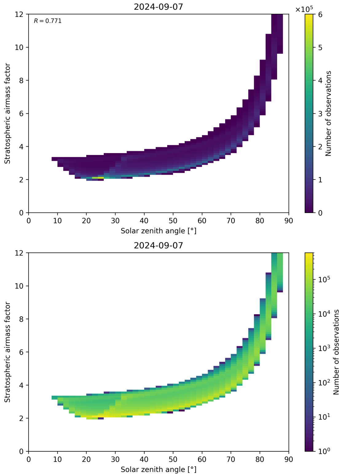
Figure 145: Scatter density plot of “Solar zenith angle” against “Stratospheric airmass factor” for 2024-09-06 to 2024-09-08.
