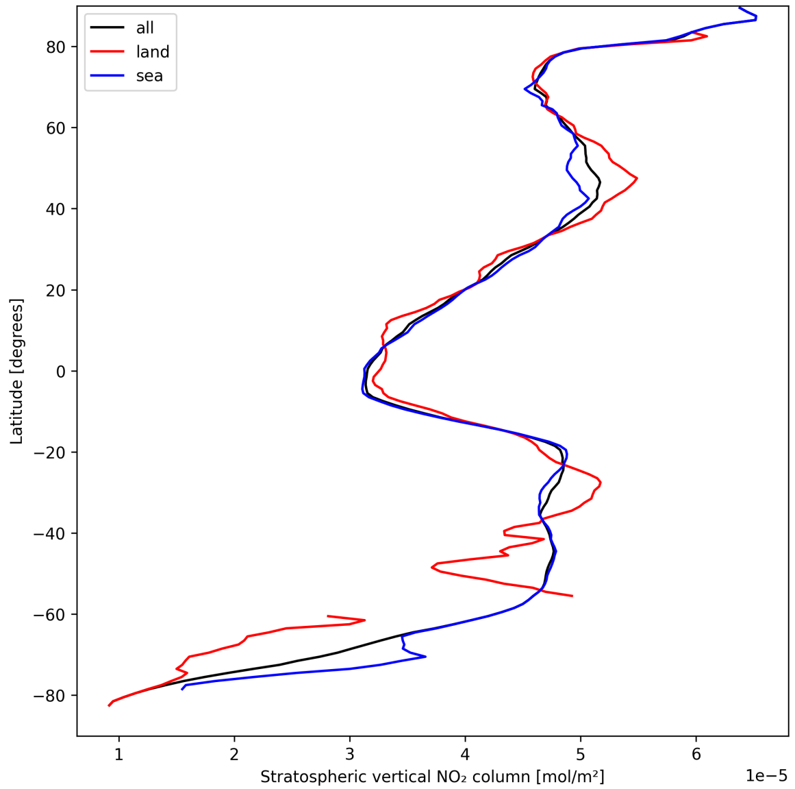
Figure 19: Zonal average of “Stratospheric vertical NO 2 column” for 2024-09-06 to 2024-09-08.
