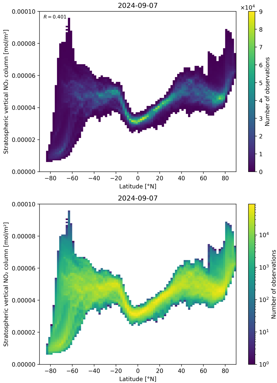
Figure 87: Scatter density plot of “Latitude” against “Stratospheric vertical NO 2 column” for 2024-09-06 to 2024-09-08.
