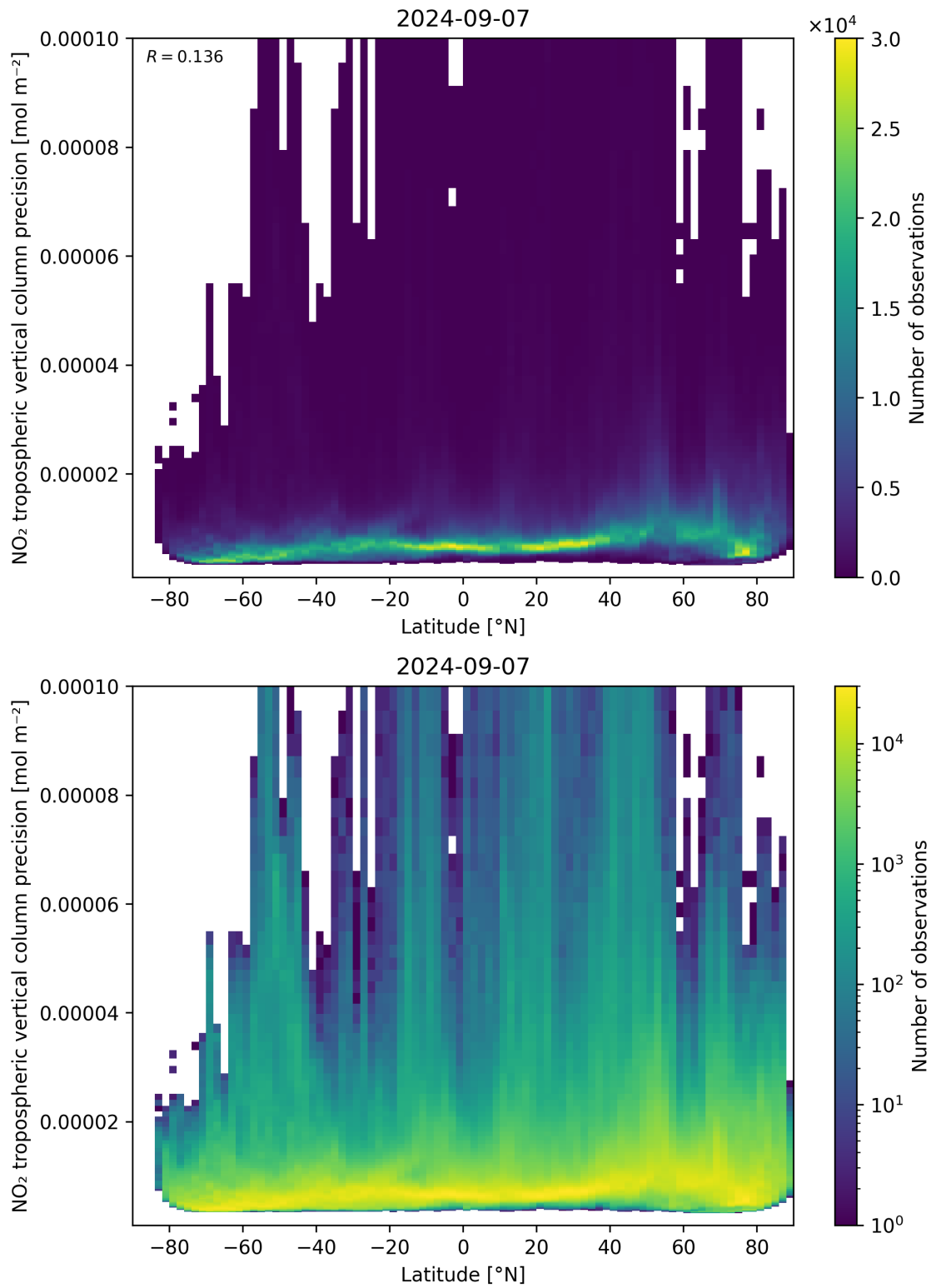
Figure 93: Scatter density plot of “Latitude” against “NO 2 tropospheric vertical column precision” for 2024-09-06 to 2024-09-08.
