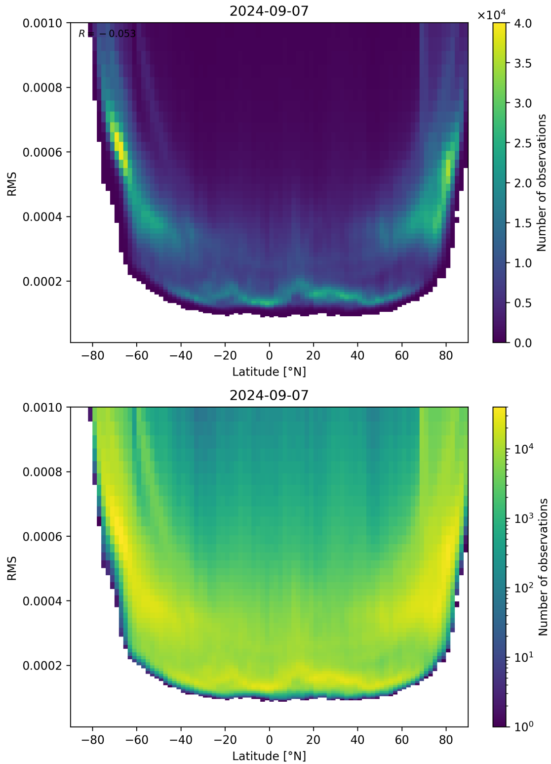
Figure 94: Scatter density plot of “Latitude” against “RMS” for 2024-09-06 to 2024-09-08.
