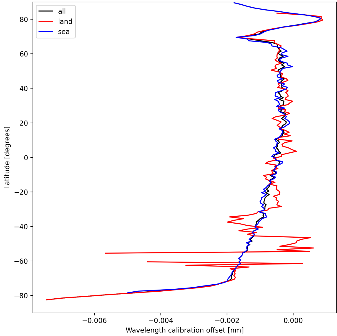
Figure 18: Zonal average of “Wavelength calibration offset” for 2024-09-06 to 2024-09-08.
