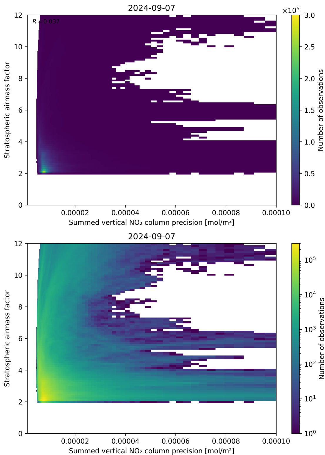
Figure 106: Scatter density plot of “Summed vertical NO 2 column precision” against “Stratospheric airmass factor” for 2024-09-06 to 2024-09-08.
