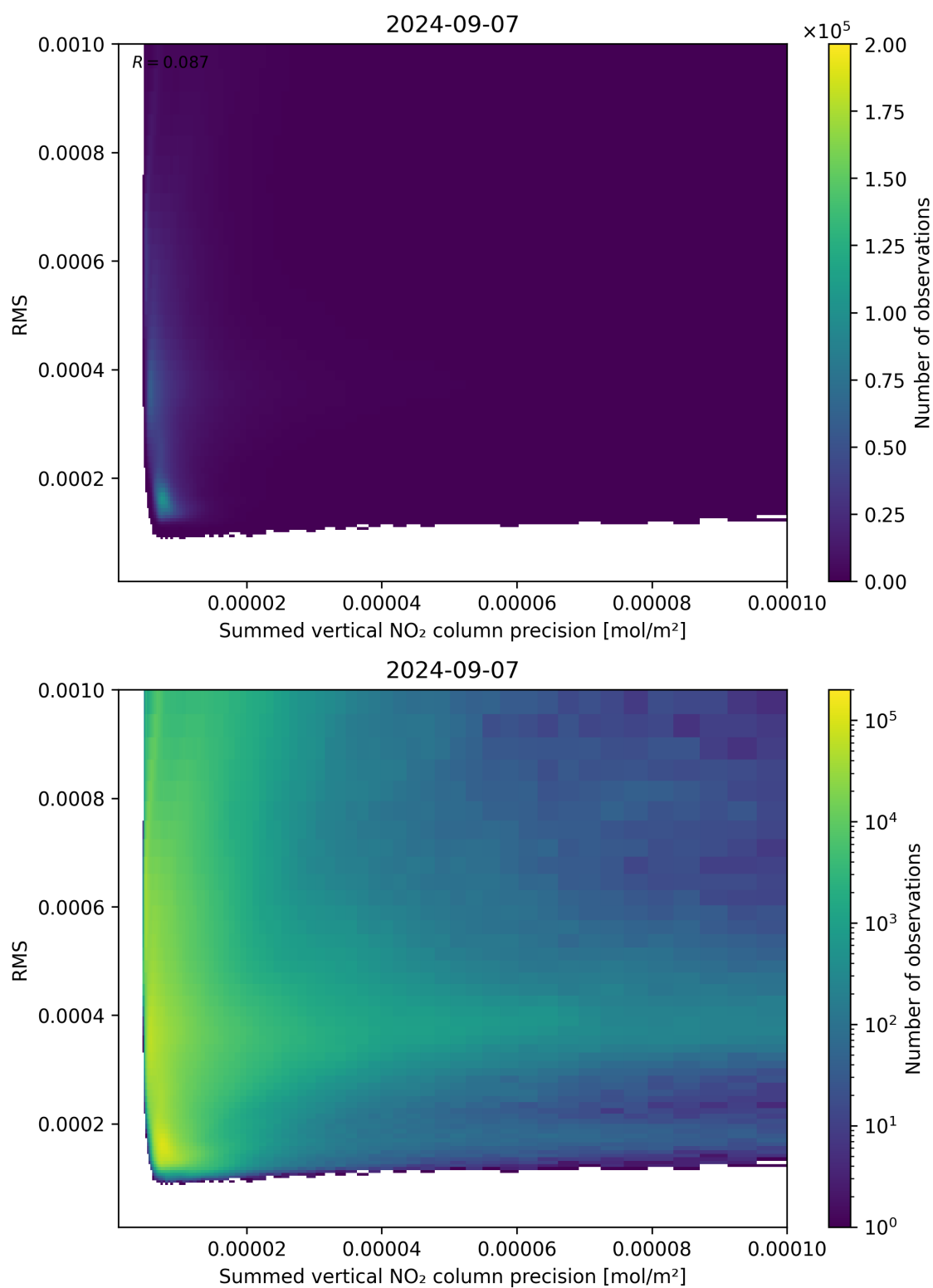
Figure 108: Scatter density plot of “Summed vertical NO 2 column precision” against “RMS” for 2024-09-06 to 2024-09-08.
