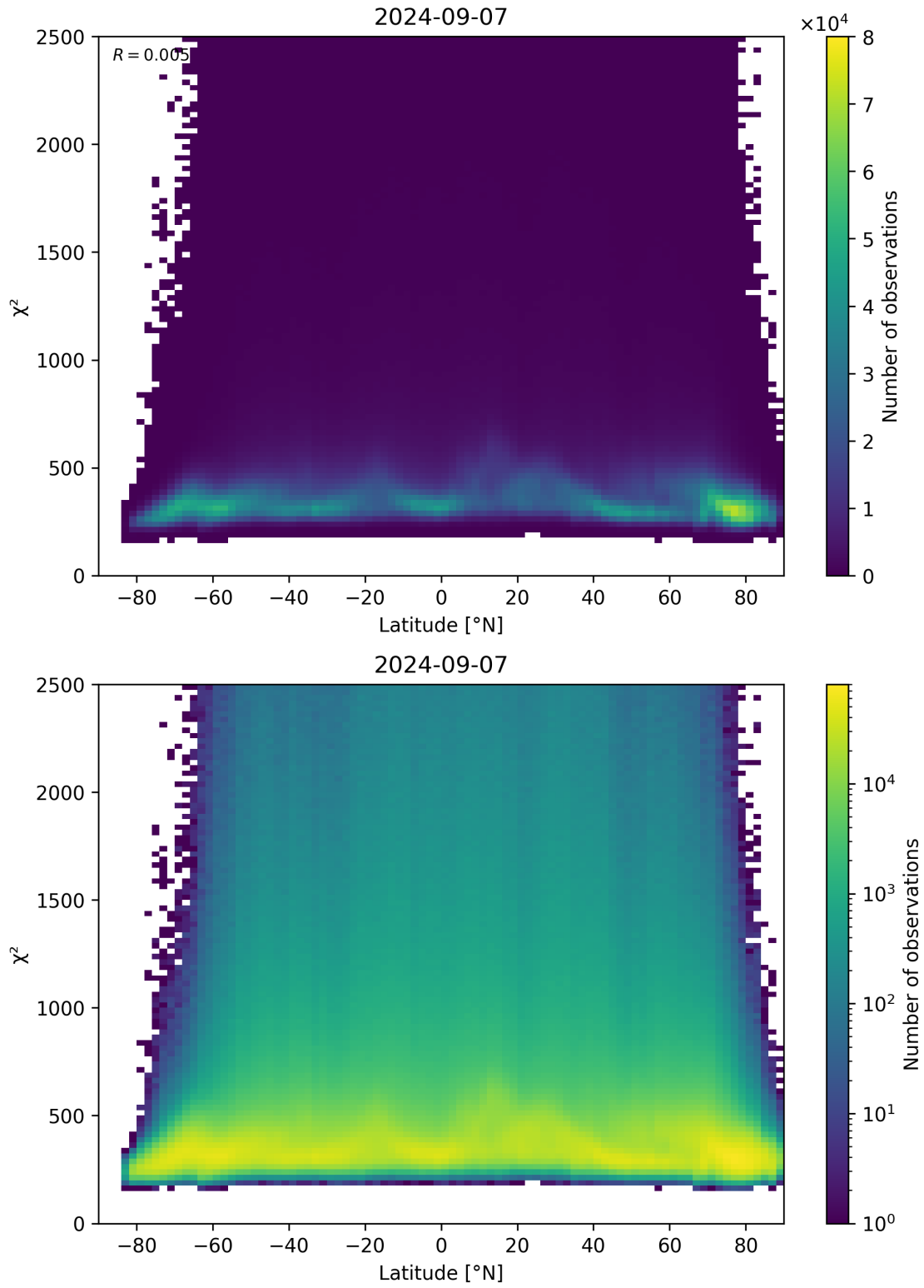
Figure 86: Scatter density plot of “Latitude” against “ \chi^2 ” for 2024-09-06 to 2024-09-08.
