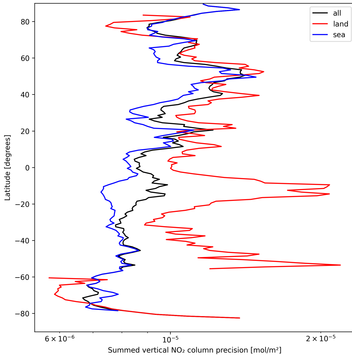
Figure 24: Zonal average of “Summed vertical NO 2 column precision” for 2024-09-06 to 2024-09-08.
