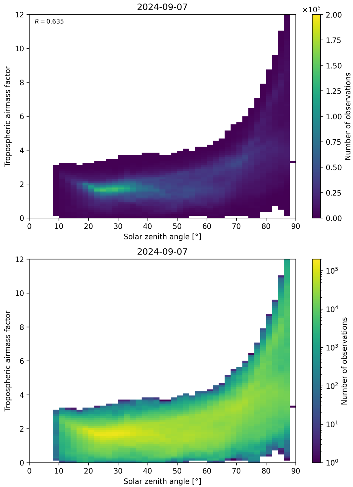
Figure 147: Scatter density plot of “Solar zenith angle” against “Tropospheric airmass factor” for 2024-09-06 to 2024-09-08.
