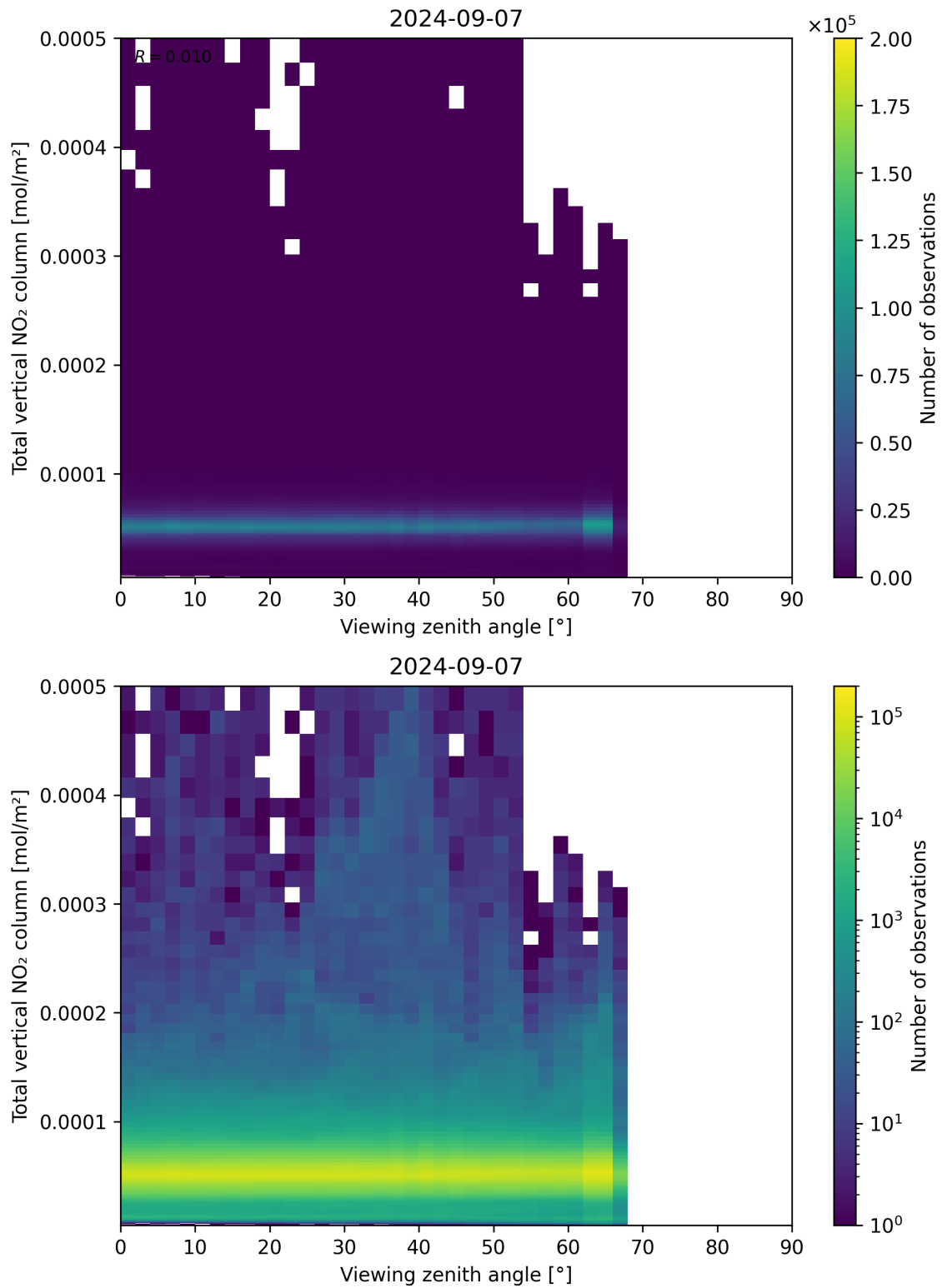
Figure 167: Scatter density plot of “Viewing zenith angle” against “Total vertical NO 2 column” for 2024-09-06 to 2024-09-08.
