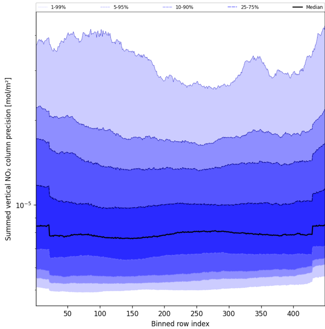
Figure 58: Along track statistics of “Summed vertical NO 2 column precision” for 2024-09-06 to 2024-09-08
