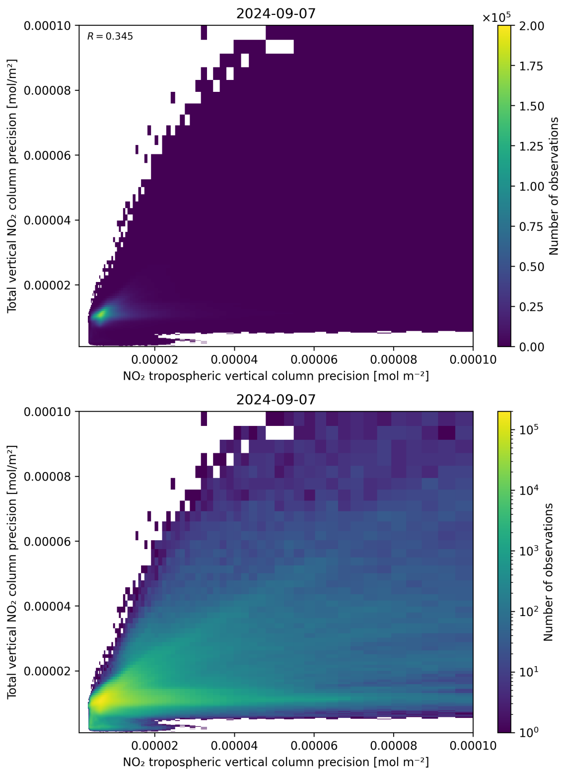
Figure 139: Scatter density plot of “NO 2 tropospheric vertical column precision” against “Total vertical NO 2 column precision” for 2024-09-06 to 2024-09-08.
