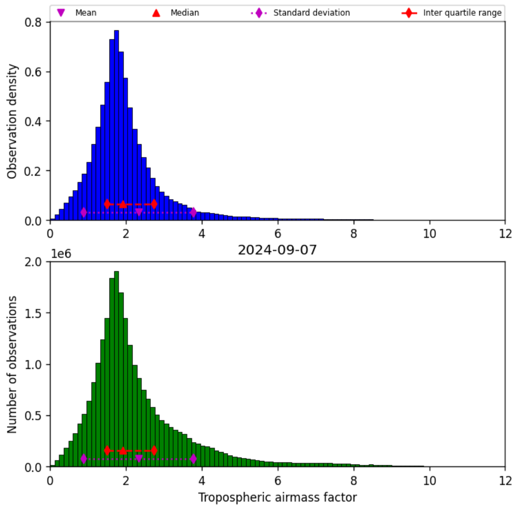
Figure 31: Histogram of “Tropospheric airmass factor” for 2024-09-06 to 2024-09-08
