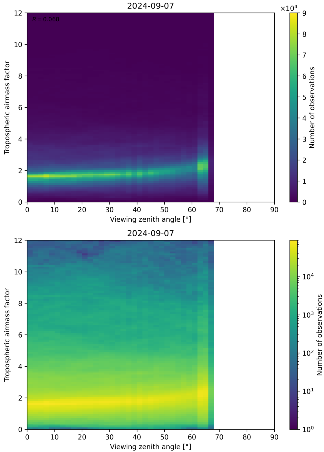
Figure 161: Scatter density plot of “Viewing zenith angle” against “Tropospheric airmass factor” for 2024-09-06 to 2024-09-08.
