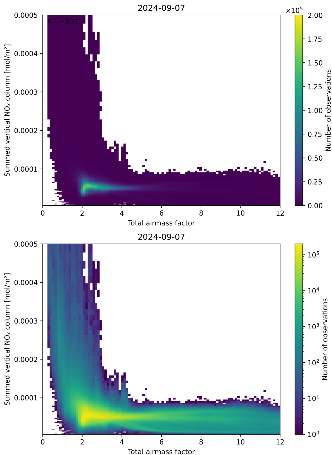
Figure 65: Scatter density plot of “Total airmass factor” against “Summed vertical NO 2 column” for 2024-09-06 to 2024-09-08.
