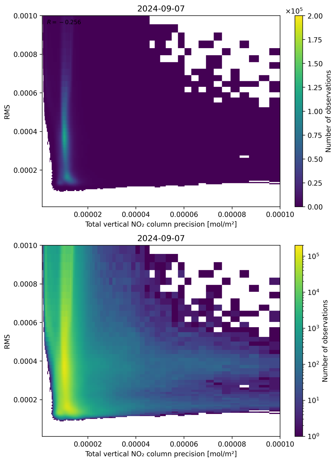
Figure 119: Scatter density plot of “Total vertical NO 2 column precision” against “RMS” for 2024-09-06 to 2024-09-08.
