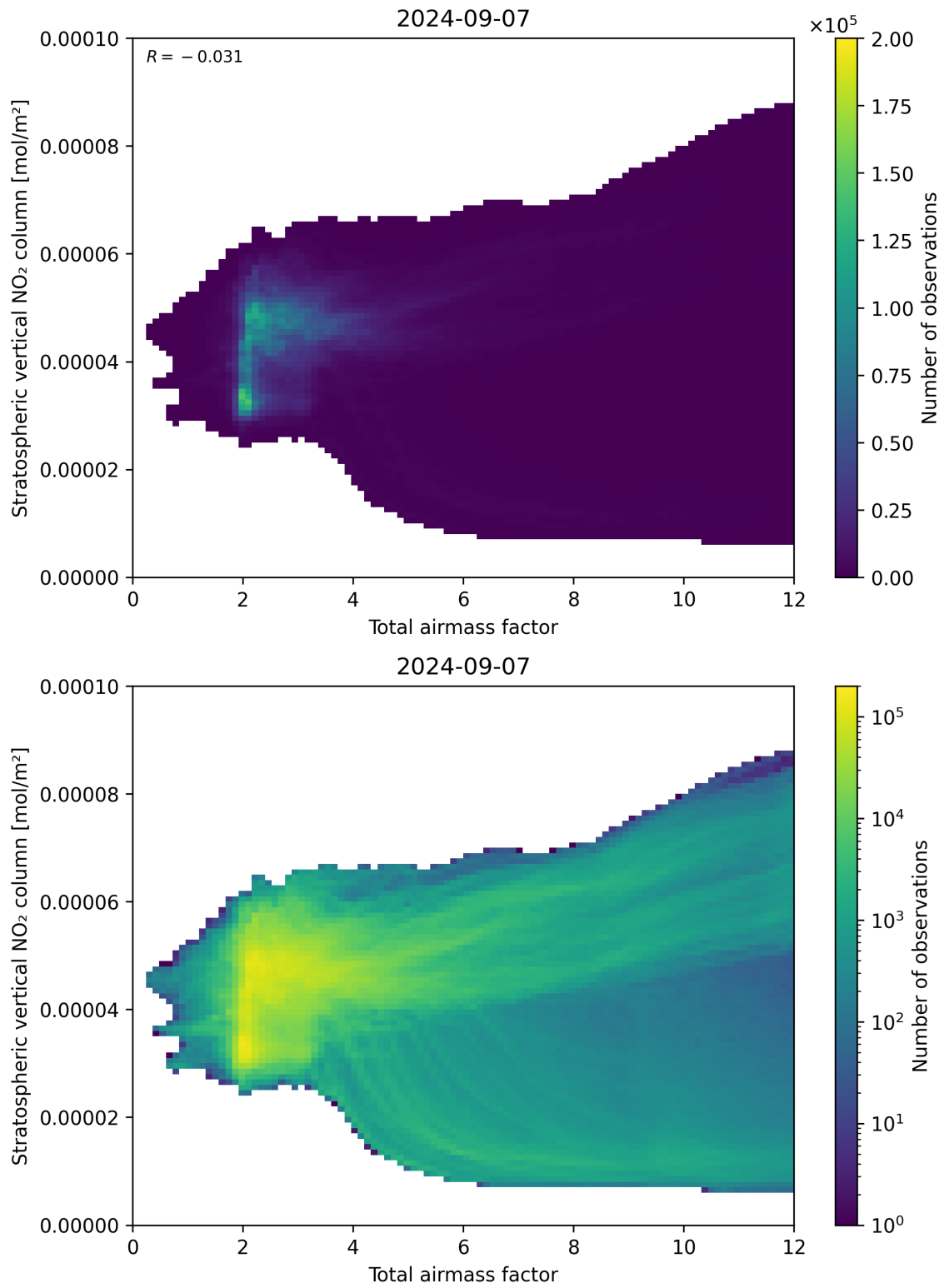
Figure 64: Scatter density plot of “Total airmass factor” against “Stratospheric vertical NO 2 column” for 2024-09-06 to 2024-09-08.
