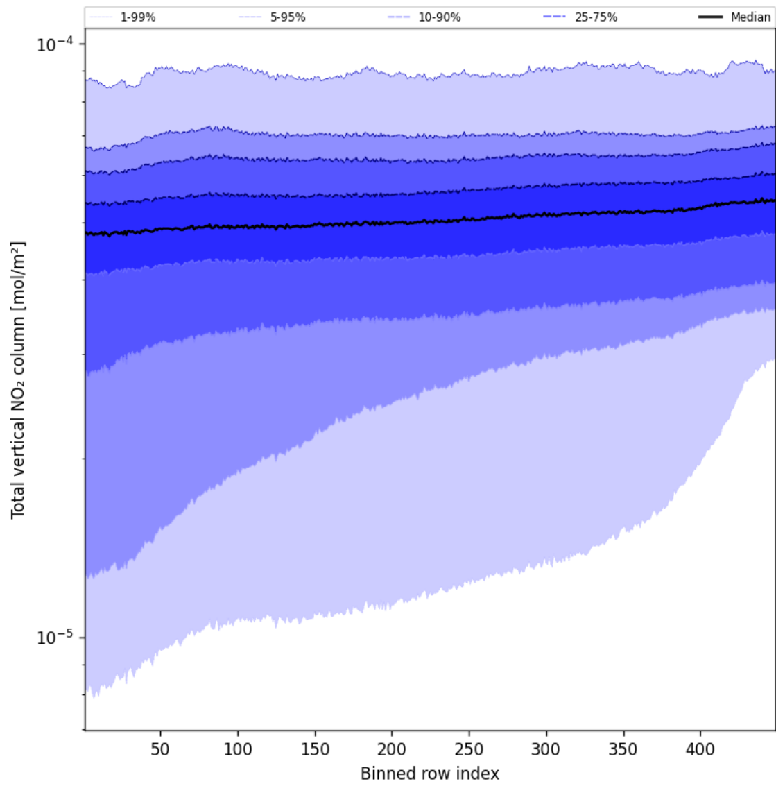
Figure 55: Along track statistics of “Total vertical NO 2 column” for 2024-09-06 to 2024-09-08
