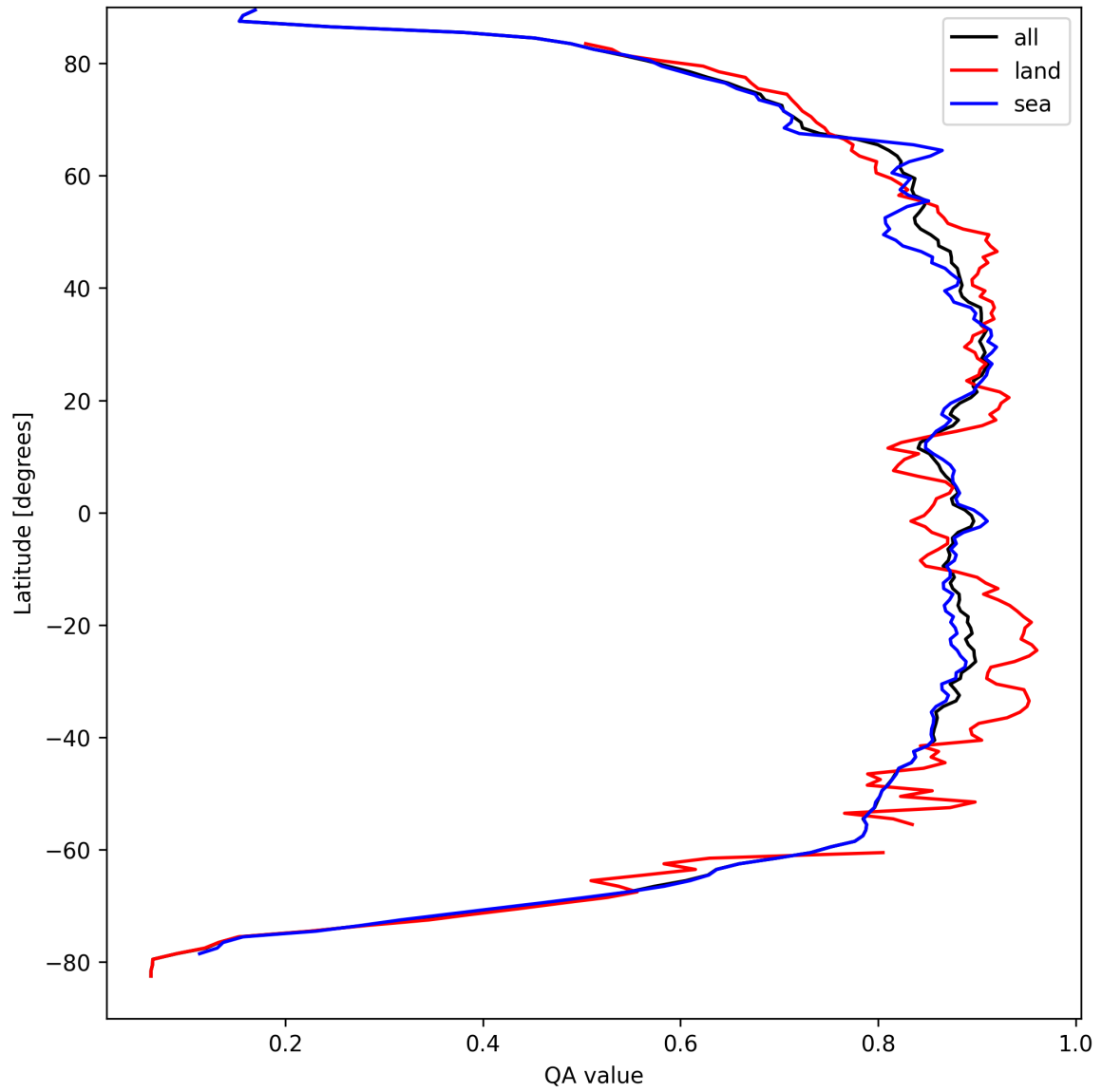
Figure 11: Zonal average of “QA value” for 2024-09-06 to 2024-09-08.
