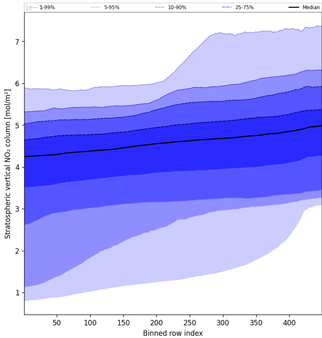
Figure 53: Along track statistics of “Stratospheric vertical NO 2 column” for 2024-09-06 to 2024-09-08
