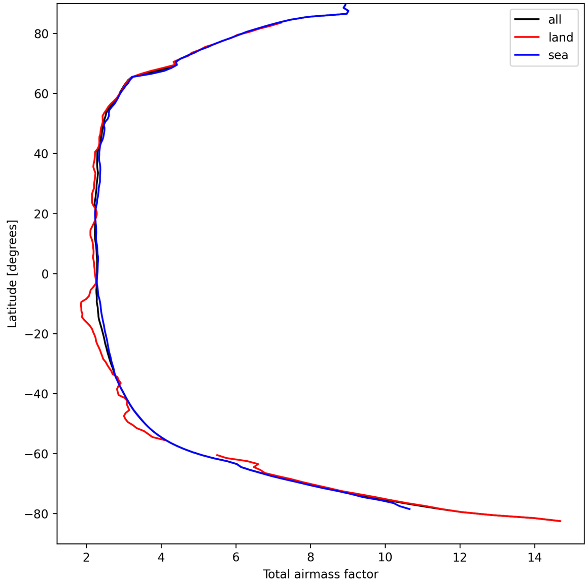
Figure 15: Zonal average of “Total airmass factor” for 2024-09-06 to 2024-09-08.
