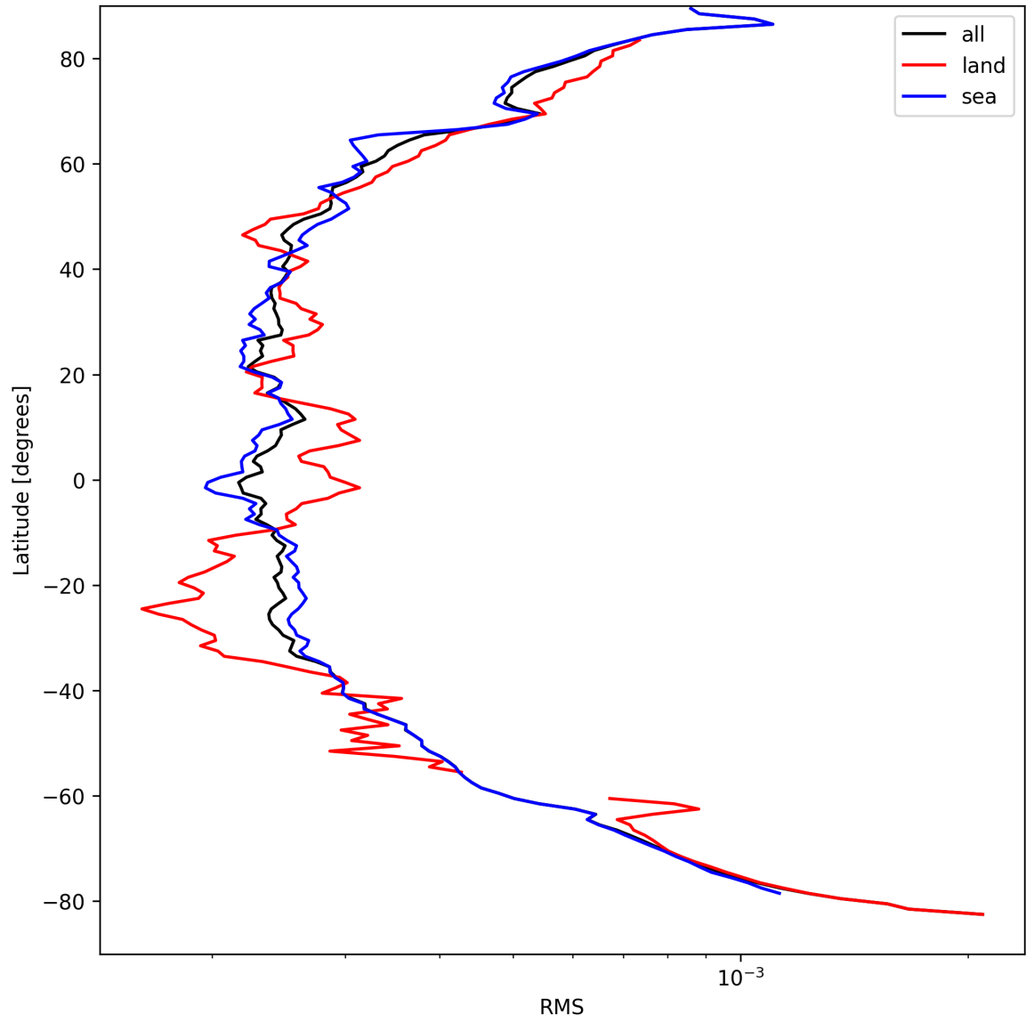
Figure 26: Zonal average of “RMS” for 2024-09-06 to 2024-09-08.
