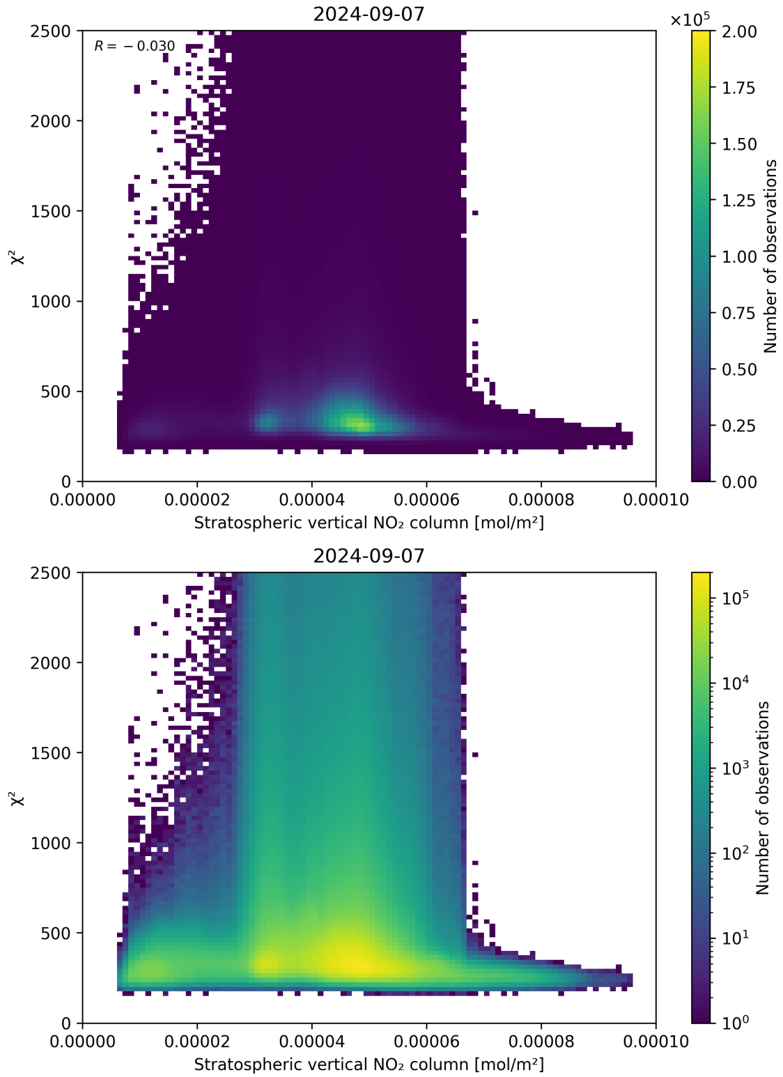
Figure 97: Scatter density plot of “Stratospheric vertical NO 2 column” against “ \chi^2 ” for 2024-09-06 to 2024-09-08.
