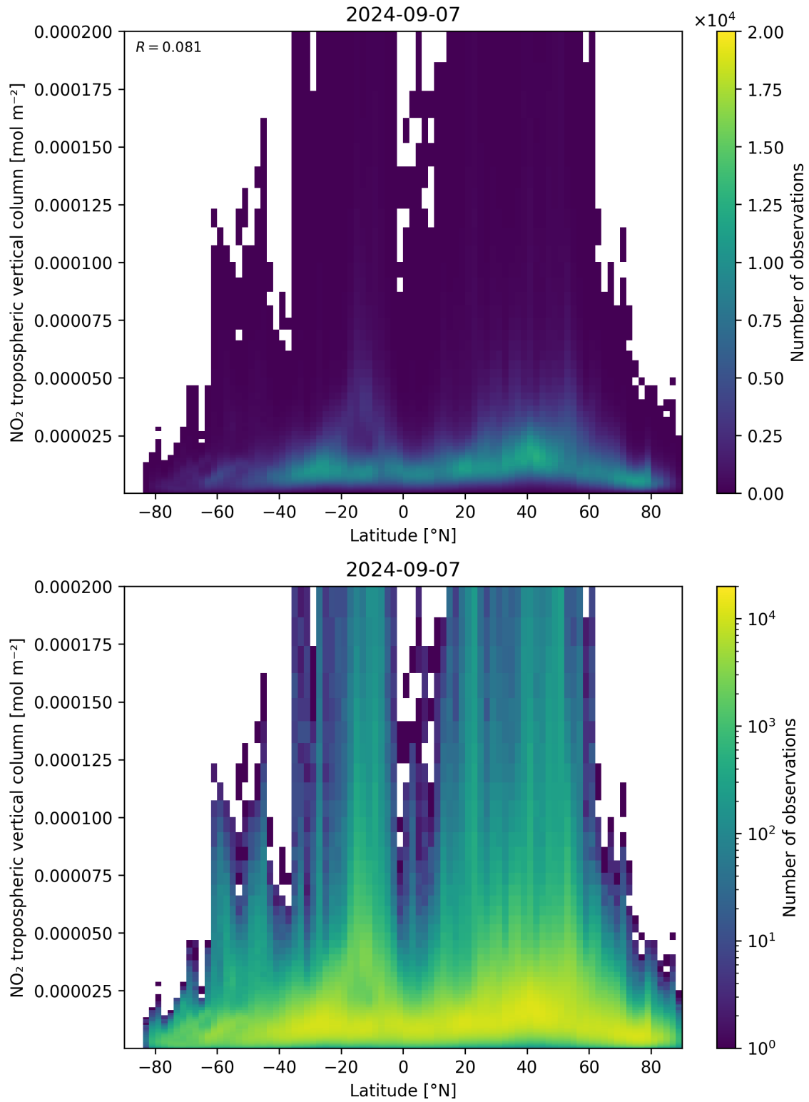
Figure 92: Scatter density plot of “Latitude” against “NO 2 tropospheric vertical column” for 2024-09-06 to 2024-09-08.
