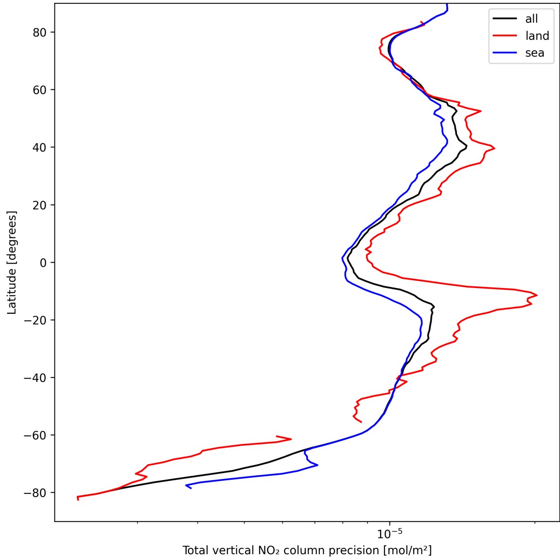
Figure 22: Zonal average of “Total vertical NO 2 column precision” for 2024-09-06 to 2024-09-08.
