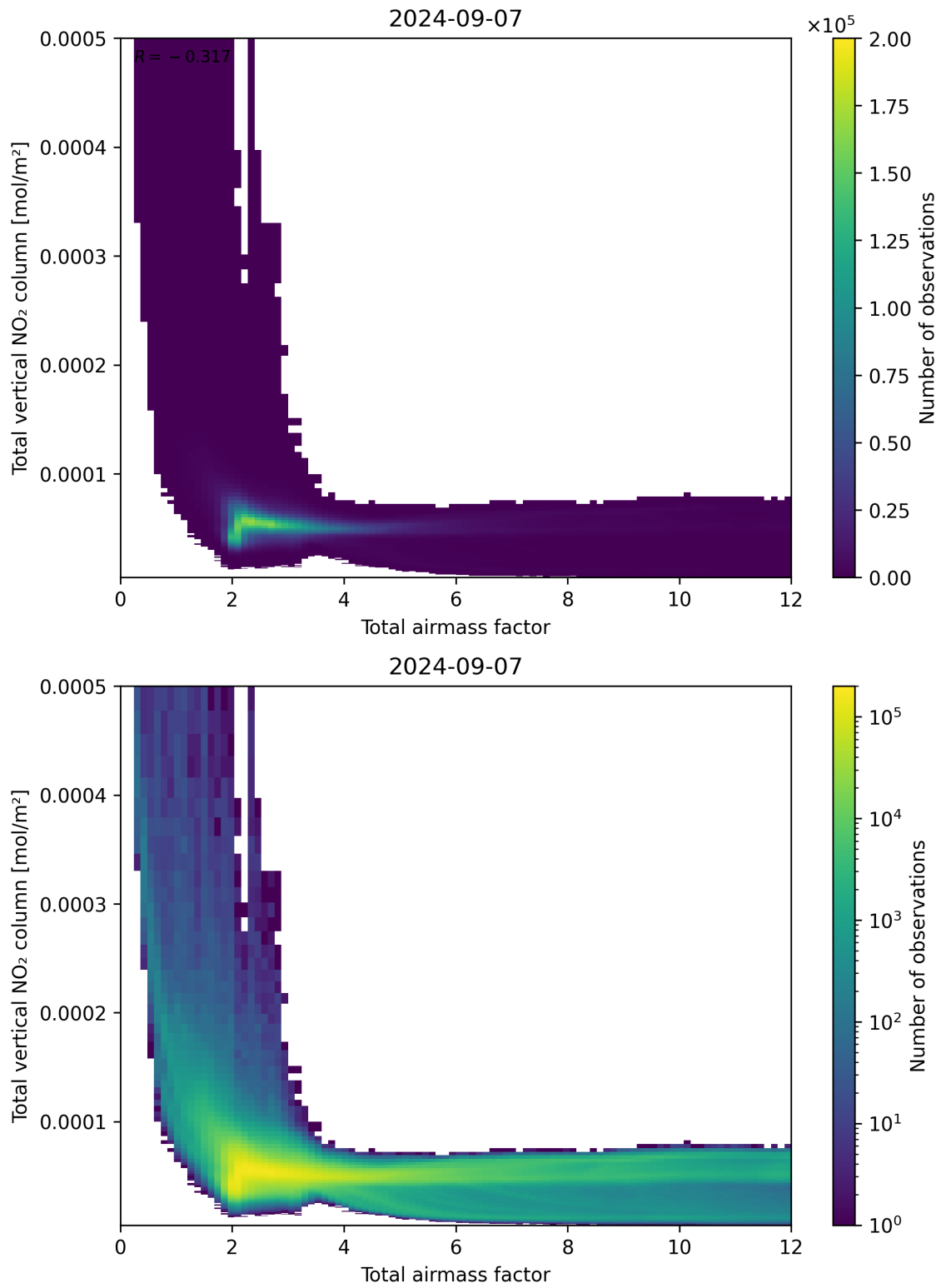
Figure 67: Scatter density plot of “Total airmass factor” against “Total vertical NO 2 column” for 2024-09-06 to 2024-09-08.
