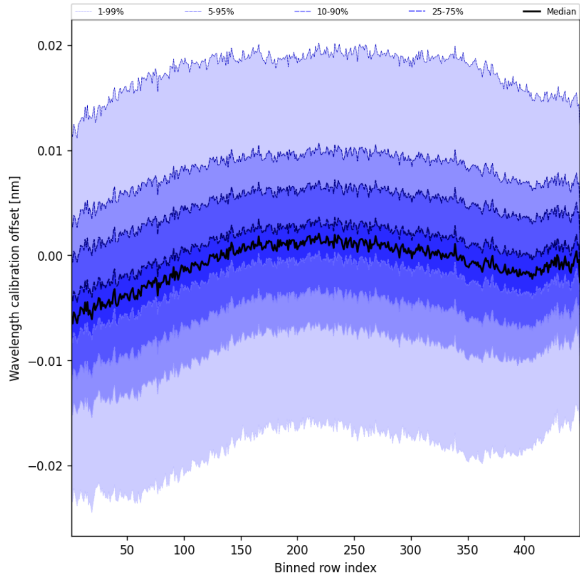
Figure 52: Along track statistics of “Wavelength calibration offset” for 2024-09-06 to 2024-09-08
