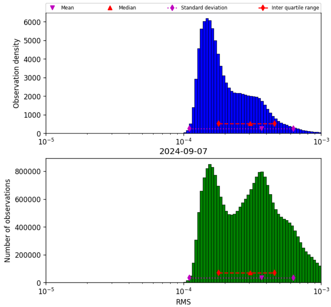
Figure 43: Histogram of “RMS” for 2024-09-06 to 2024-09-08
