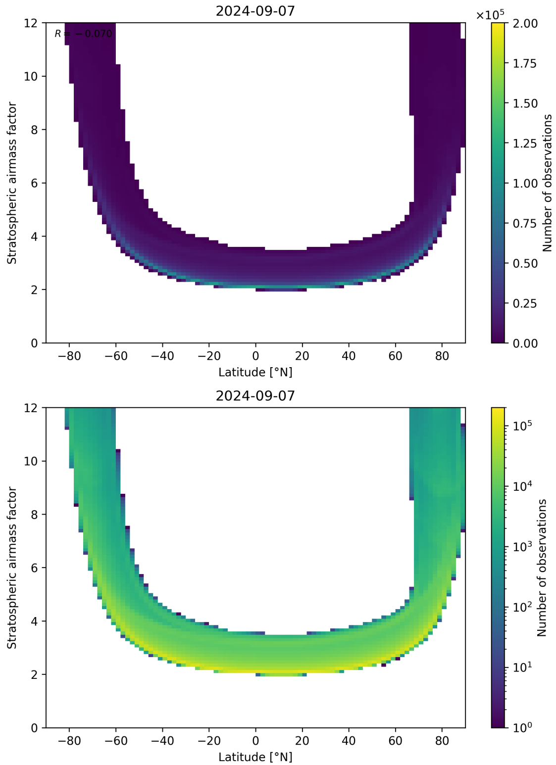
Figure 83: Scatter density plot of “Latitude” against “Stratospheric airmass factor” for 2024-09-06 to 2024-09-08.
