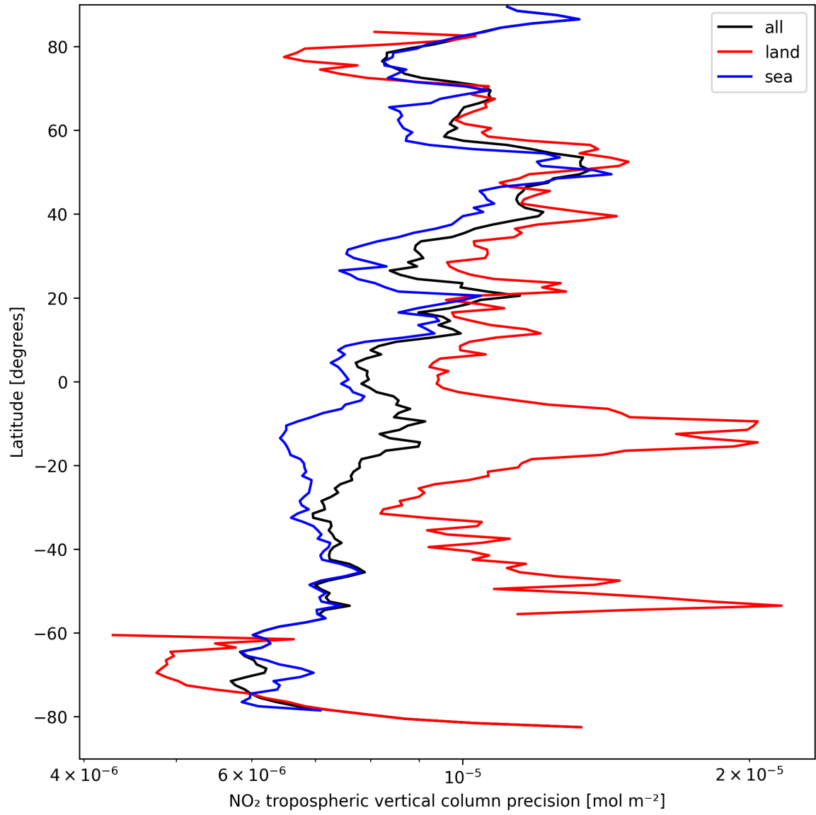
Figure 13: Zonal average of “NO 2 tropospheric vertical column precision” for 2024-09-06 to 2024-09-08.
