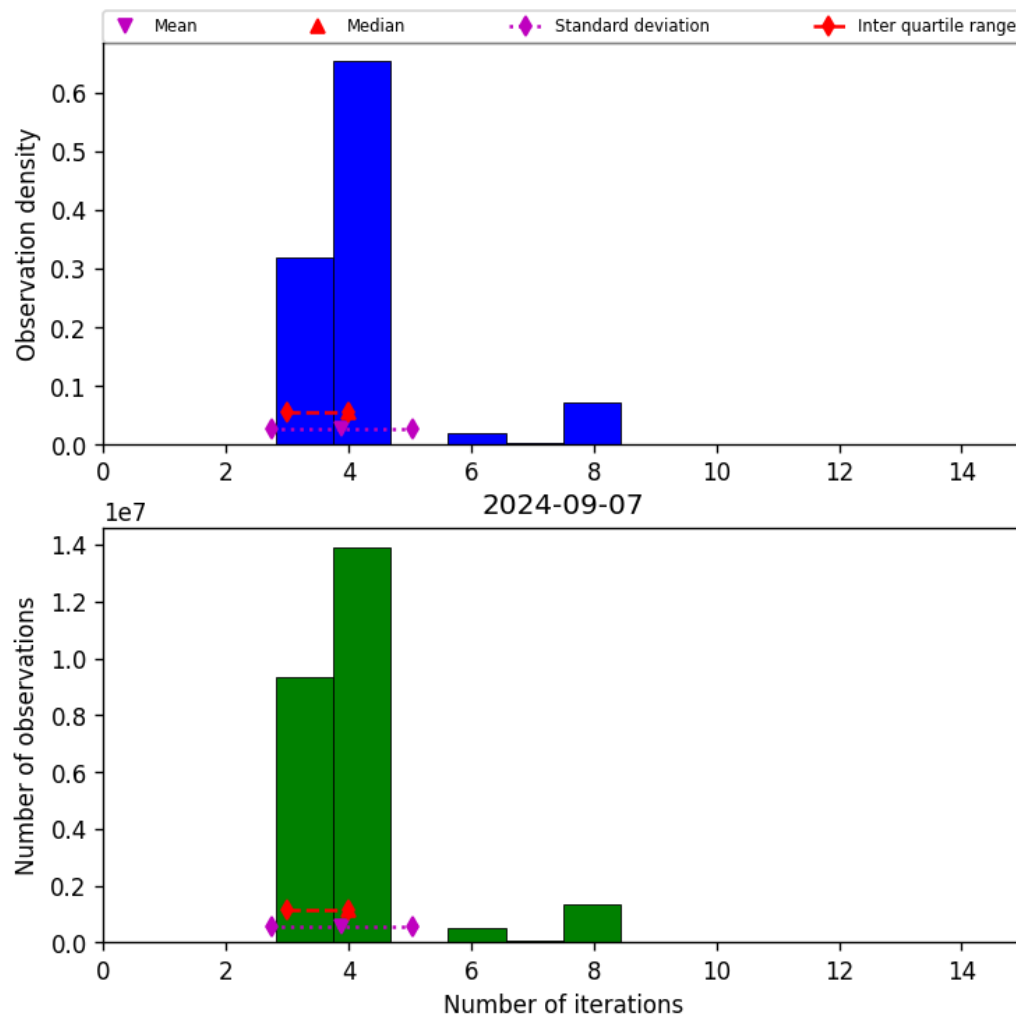
Figure 34: Histogram of “Number of iterations” for 2024-09-06 to 2024-09-08
