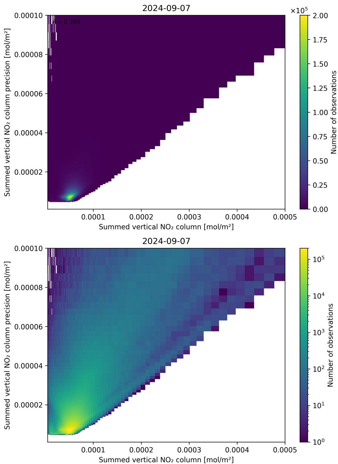
Figure 105: Scatter density plot of “Summed vertical NO 2 column” against “Summed vertical NO 2 column precision” for 2024-09-06 to 2024-09-08.
