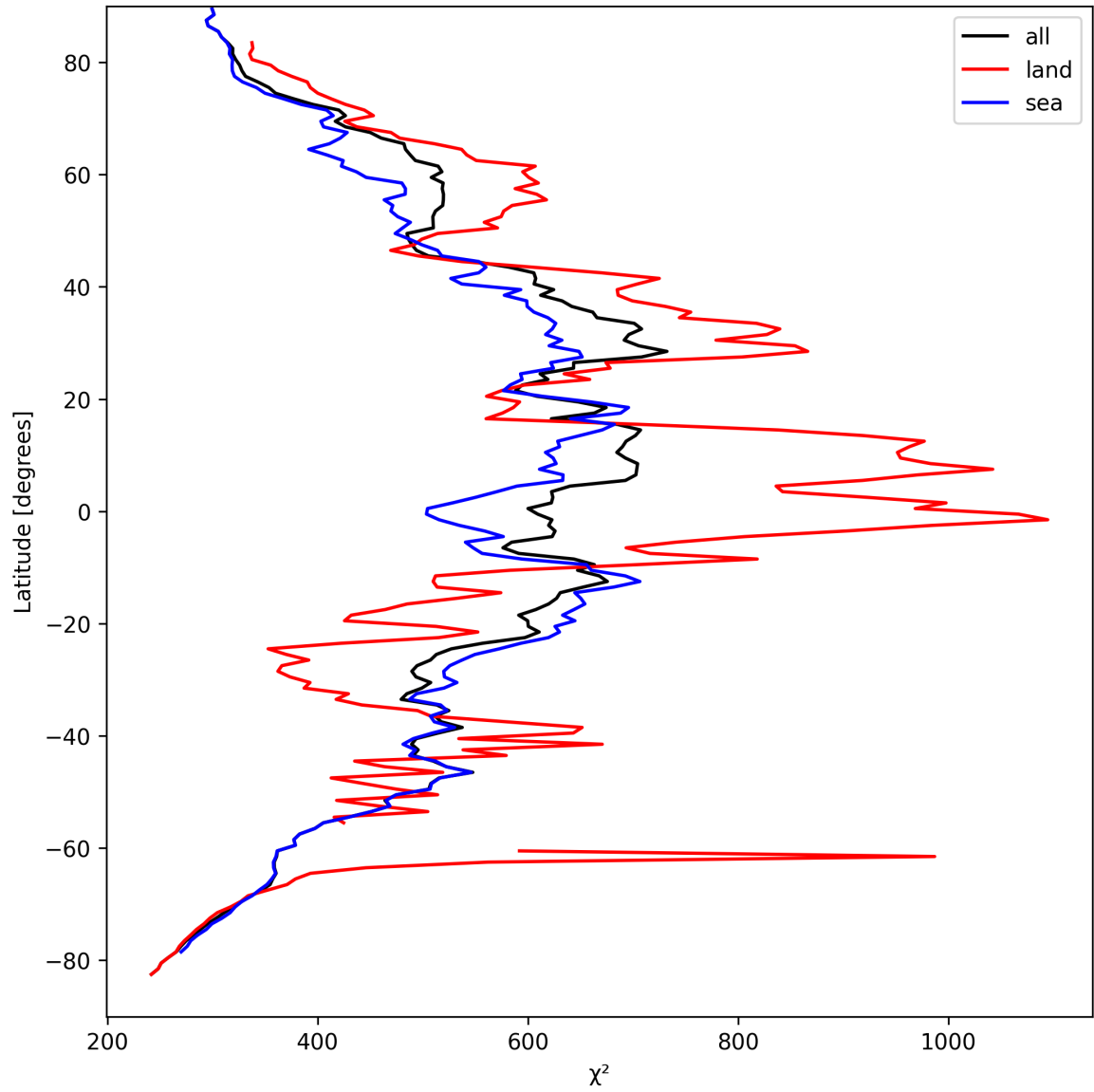
Figure 25: Zonal average of “ \chi^2 ” for 2024-09-06 to 2024-09-08.
