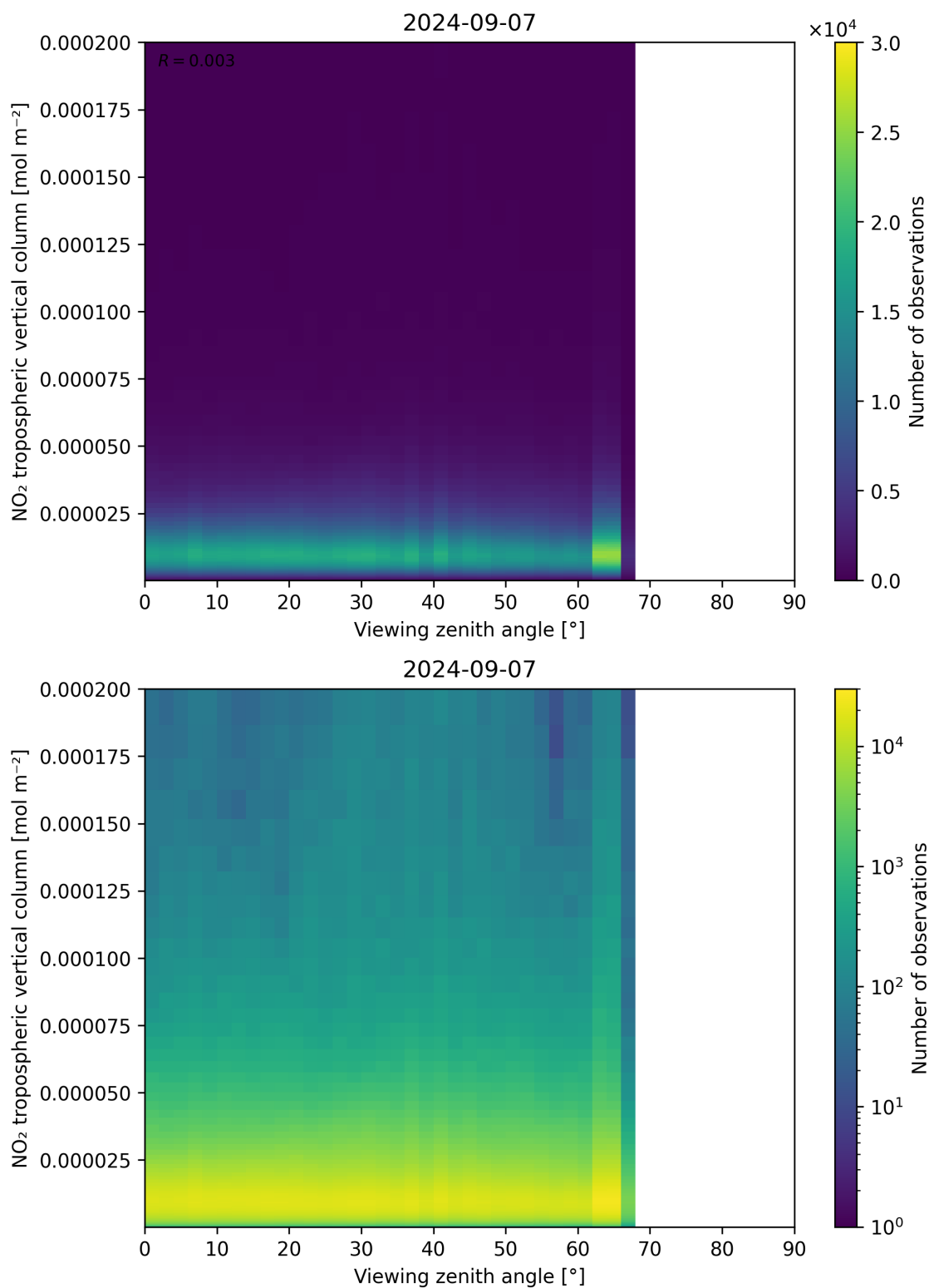
Figure 169: Scatter density plot of “Viewing zenith angle” against “NO 2 tropospheric vertical column” for 2024-09-06 to 2024-09-08.
