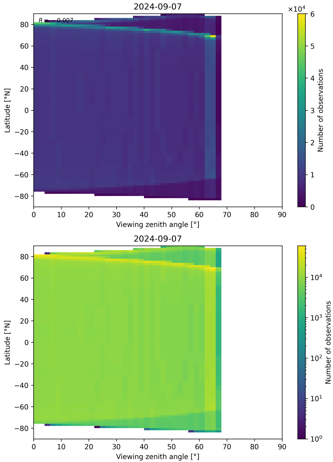
Figure 163: Scatter density plot of “Viewing zenith angle” against “Latitude” for 2024-09-06 to 2024-09-08.
