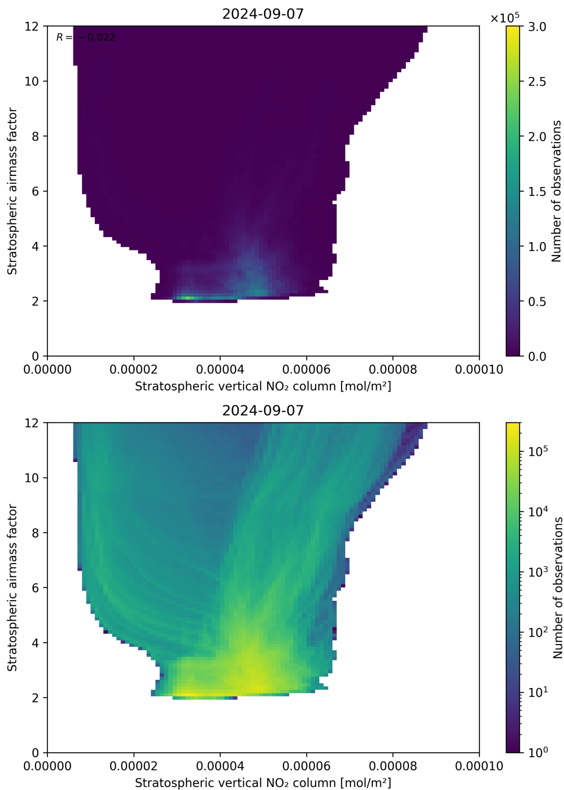
Figure 96: Scatter density plot of “Stratospheric vertical NO 2 column” against “Stratospheric airmass factor” for 2024-09-06 to 2024-09-08.
