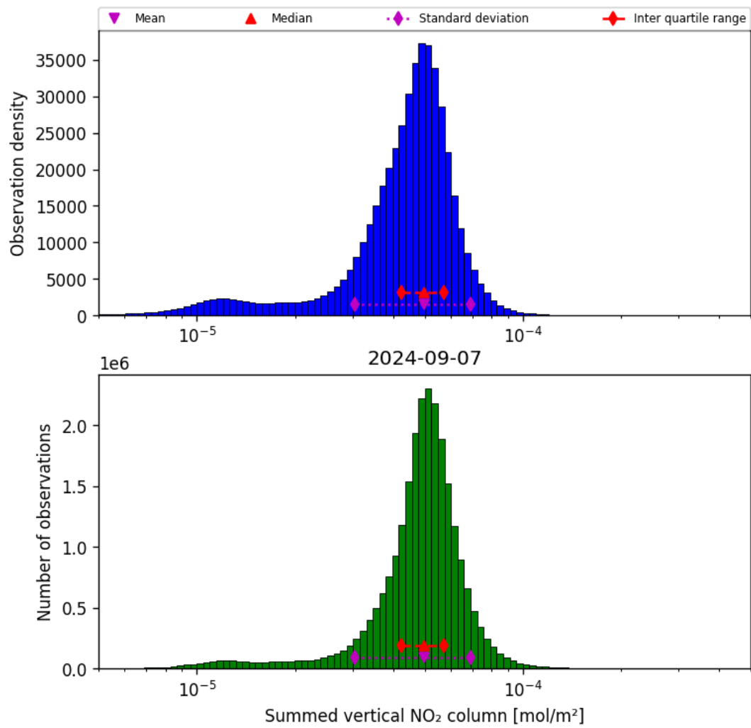
Figure 40: Histogram of “Summed vertical NO 2 column” for 2024-09-06 to 2024-09-08
