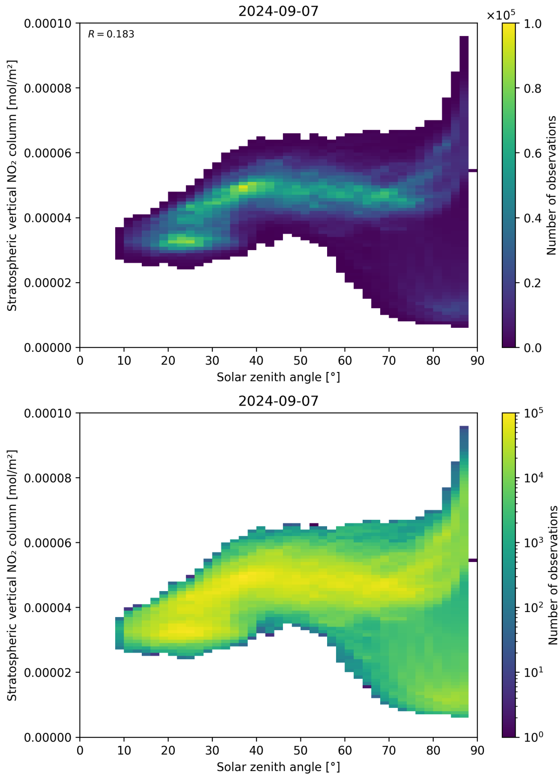
Figure 150: Scatter density plot of “Solar zenith angle” against “Stratospheric vertical NO 2 column” for 2024-09-06 to 2024-09-08.
