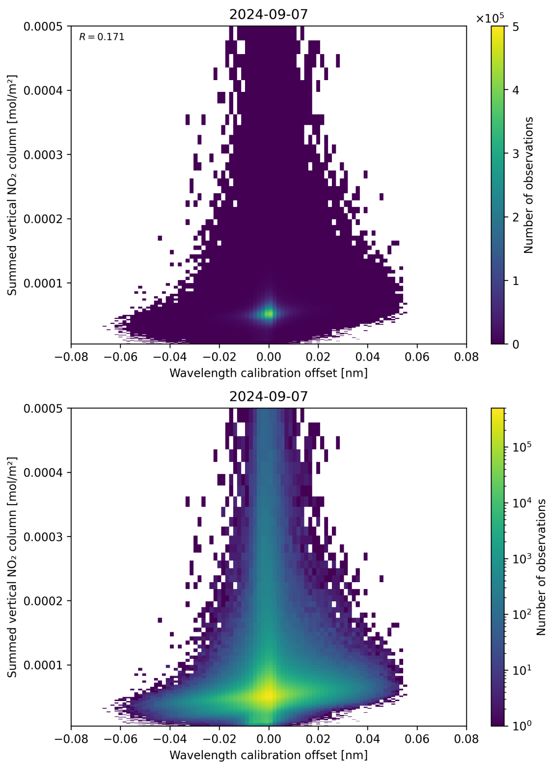
Figure 177: Scatter density plot of “Wavelength calibration offset” against “Summed vertical NO 2 column” for 2024-09-06 to 2024-09-08.
