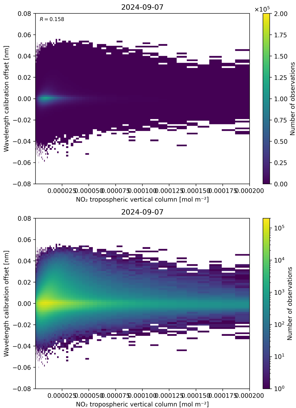
Figure 143: Scatter density plot of “NO 2 tropospheric vertical column” against “Wavelength calibration offset” for 2024-09-06 to 2024-09-08.
