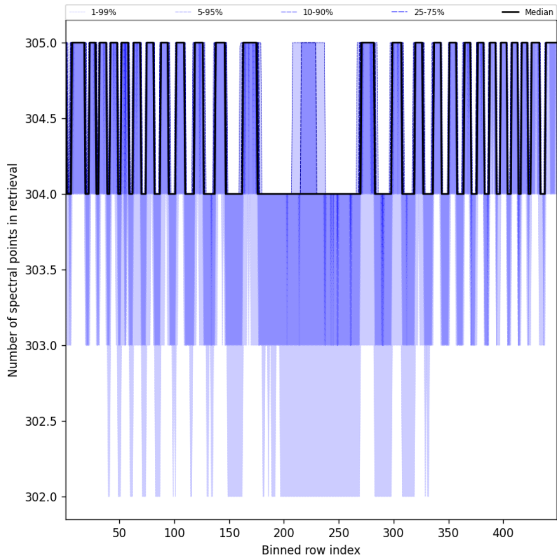
Figure 50: Along track statistics of “Number of spectral points in retrieval” for 2024-09-06 to 2024-09-08
