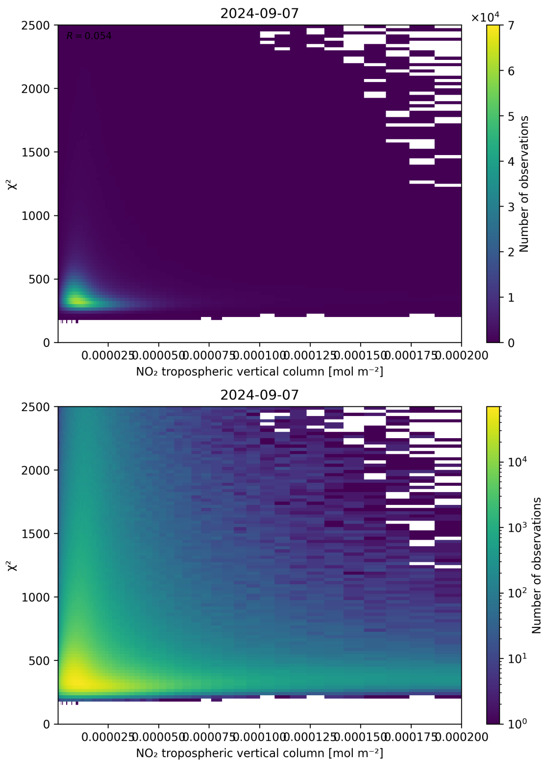
Figure 124: Scatter density plot of “NO 2 tropospheric vertical column” against “ \chi^2 ” for 2024-09-06 to 2024-09-08.
