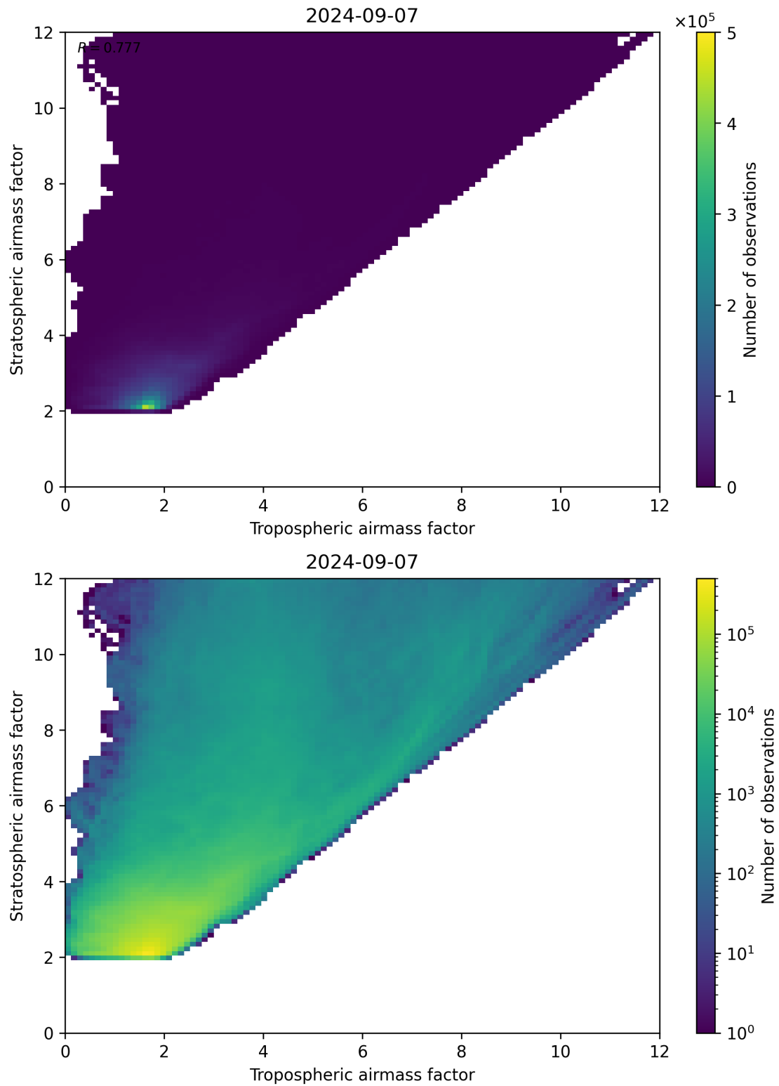
Figure 71: Scatter density plot of “Tropospheric airmass factor” against “Stratospheric airmass factor” for 2024-09-06 to 2024-09-08.
