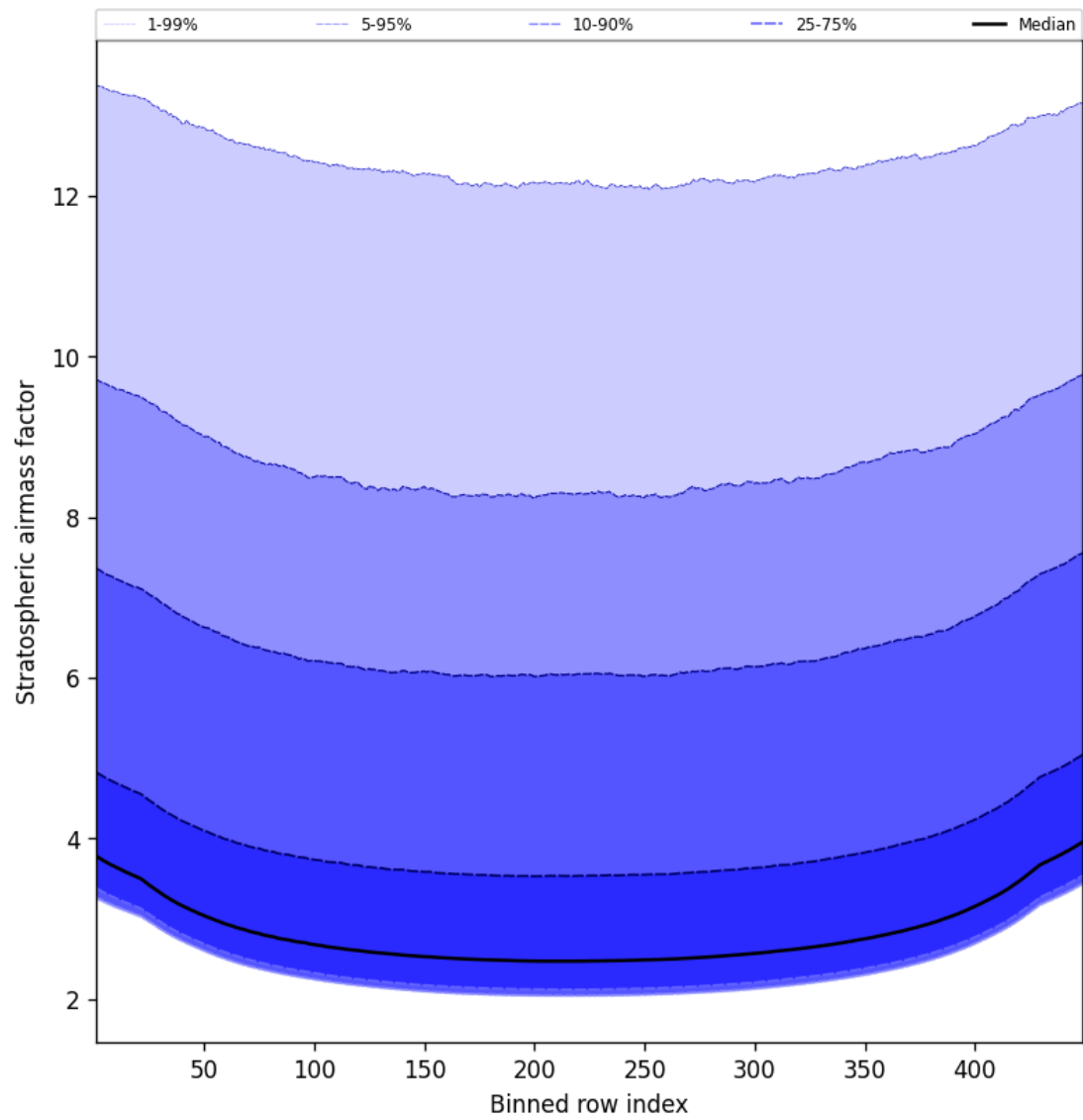
Figure 61: Along track statistics of “Stratospheric airmass factor” for 2024-09-06 to 2024-09-08
