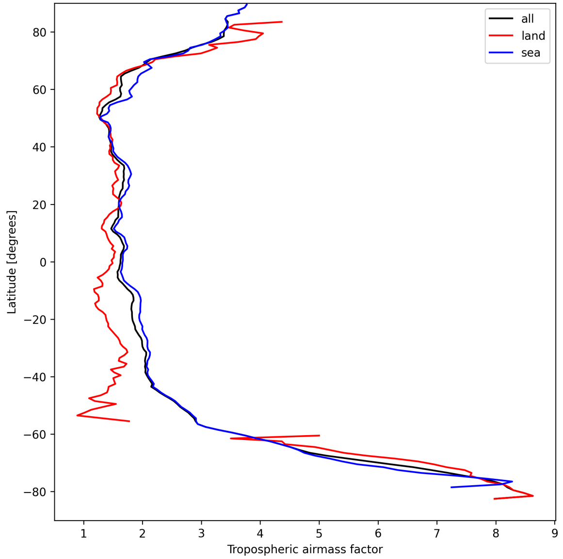
Figure 14: Zonal average of “Tropospheric airmass factor” for 2024-09-06 to 2024-09-08.
