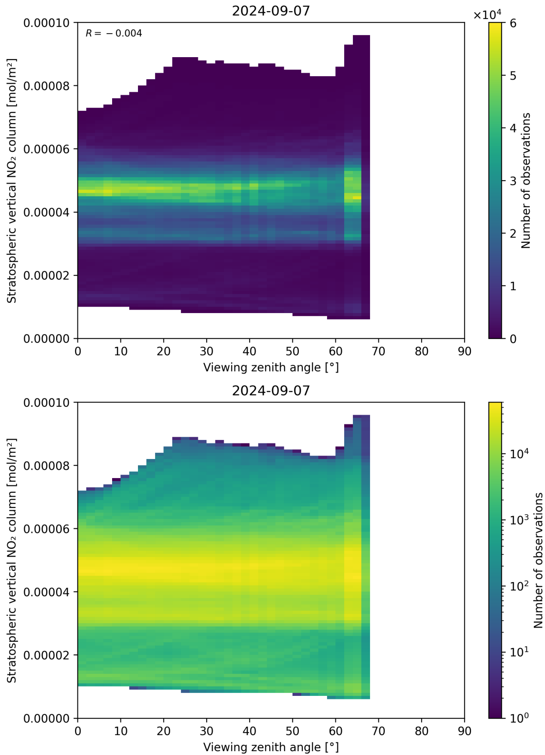
Figure 164: Scatter density plot of “Viewing zenith angle” against “Stratospheric vertical NO 2 column” for 2024-09-06 to 2024-09-08.
