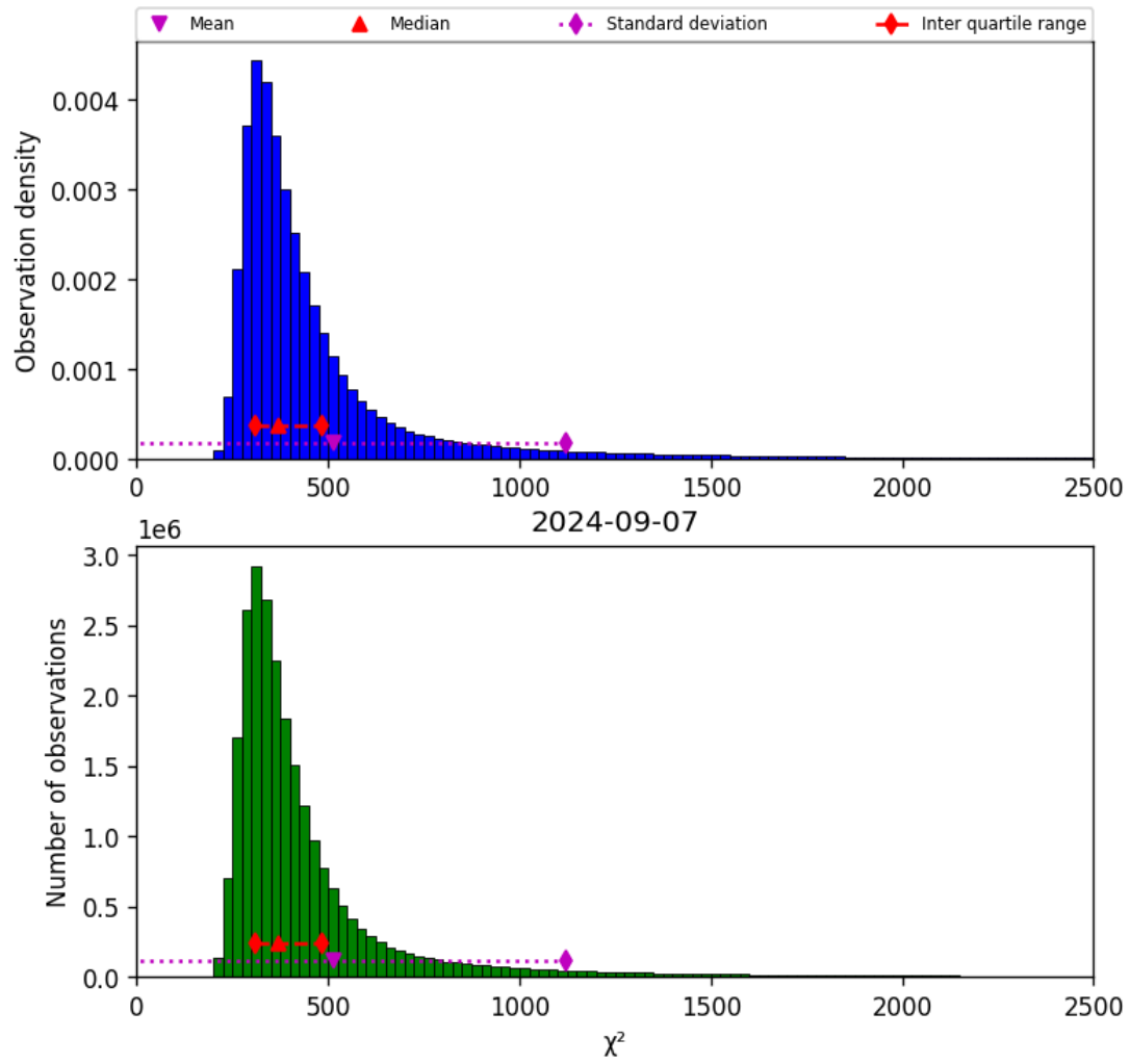
Figure 42: Histogram of “ \chi^2 ” for 2024-09-06 to 2024-09-08
