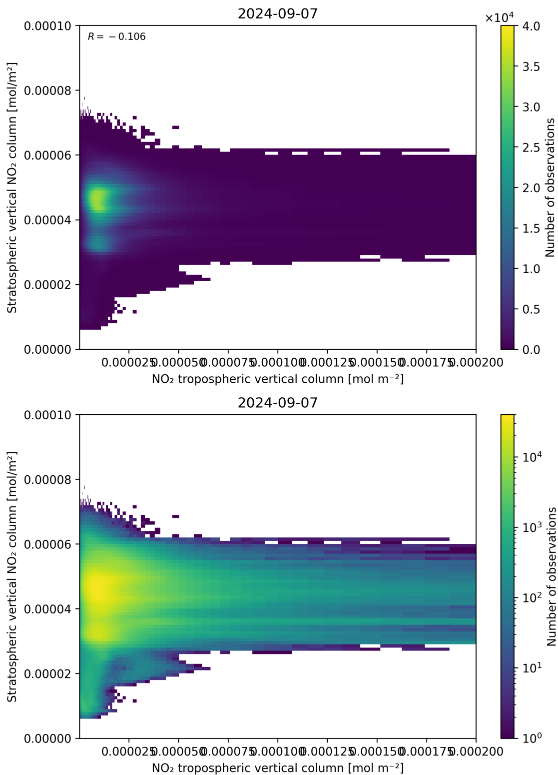
Figure 125: Scatter density plot of “NO 2 tropospheric vertical column” against “Stratospheric vertical NO 2 column” for 2024-09-06 to 2024-09-08.
