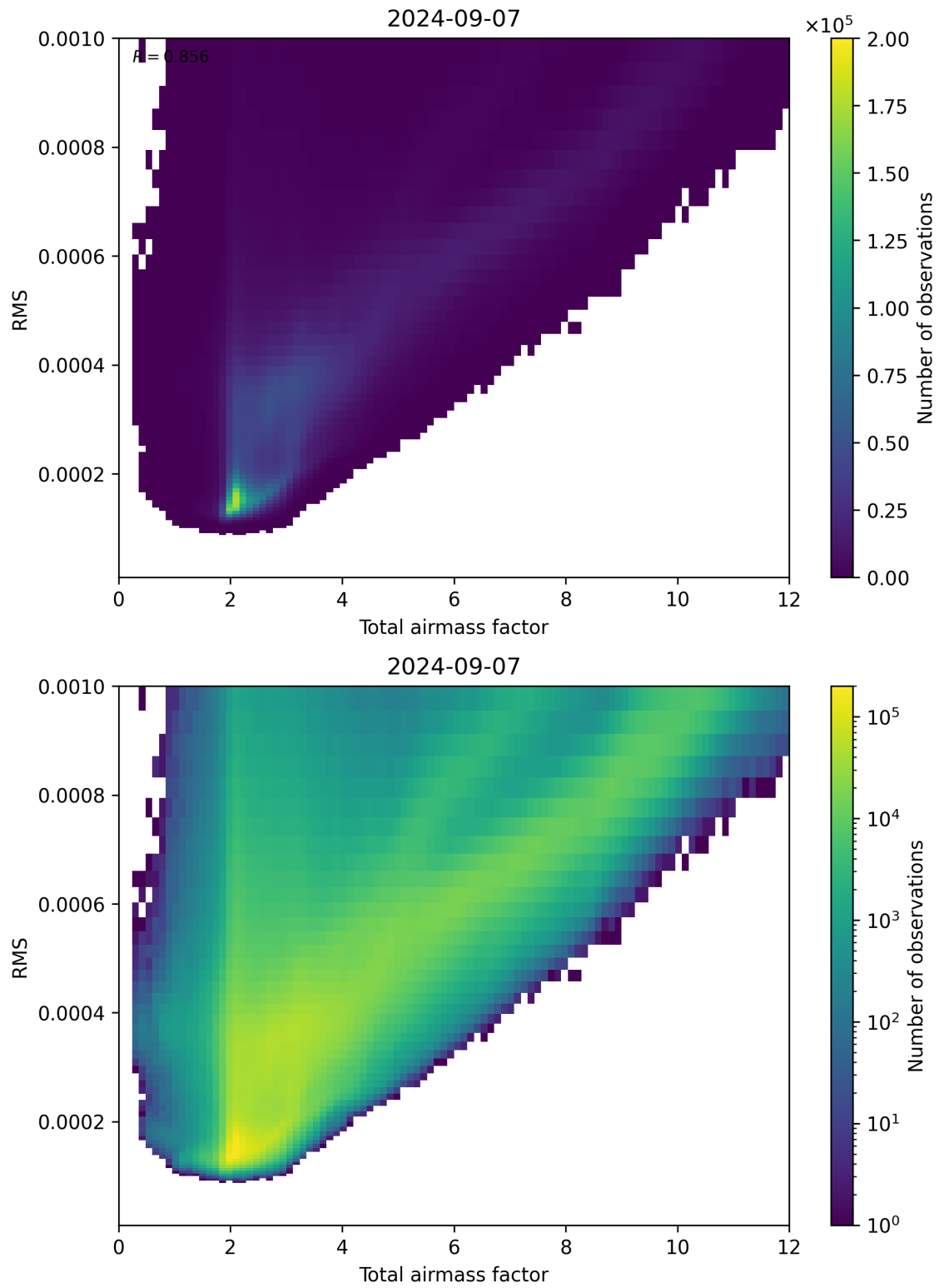
Figure 69: Scatter density plot of “Total airmass factor” against “RMS” for 2024-09-06 to 2024-09-08.
