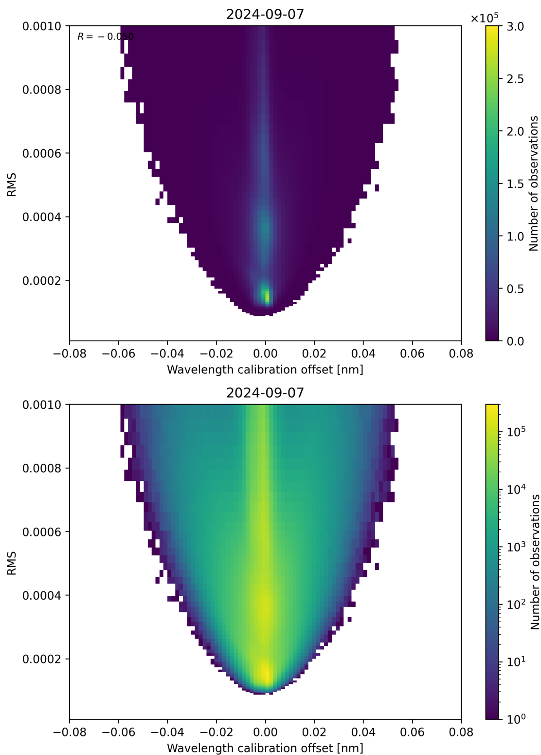
Figure 181: Scatter density plot of “Wavelength calibration offset” against “RMS” for 2024-09-06 to 2024-09-08.
