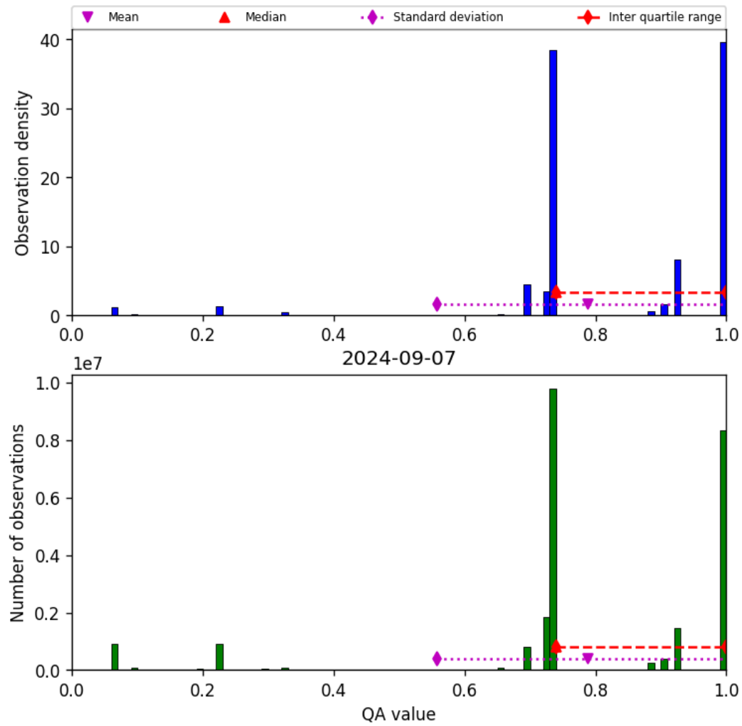
Figure 28: Histogram of “QA value” for 2024-09-06 to 2024-09-08
