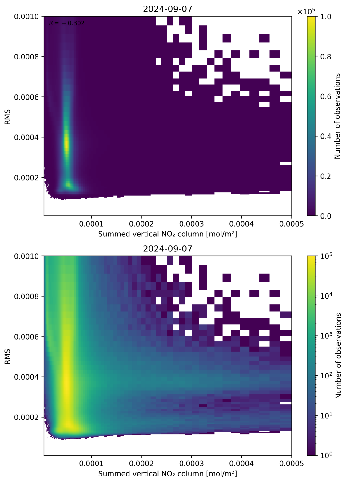
Figure 109: Scatter density plot of “Summed vertical NO 2 column” against “RMS” for 2024-09-06 to 2024-09-08.
