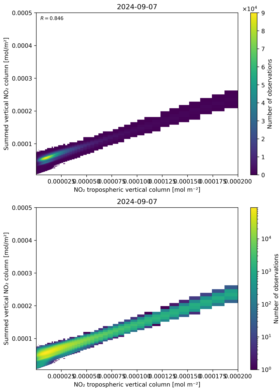
Figure 126: Scatter density plot of “NO 2 tropospheric vertical column” against “Summed vertical NO 2 column” for 2024-09-06 to 2024-09-08.
