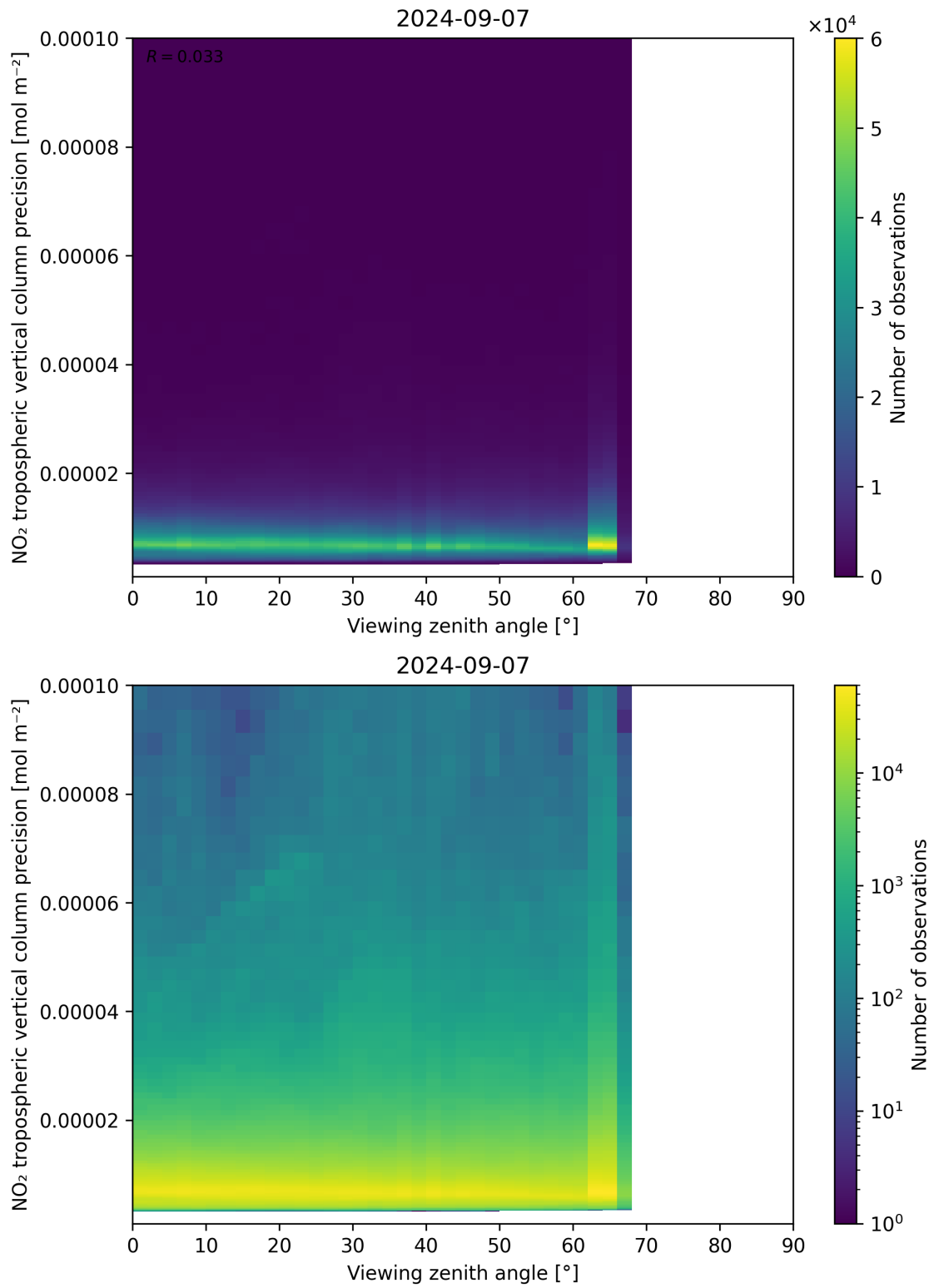
Figure 170: Scatter density plot of “Viewing zenith angle” against “NO 2 tropospheric vertical column precision” for 2024-09-06 to 2024-09-08.
