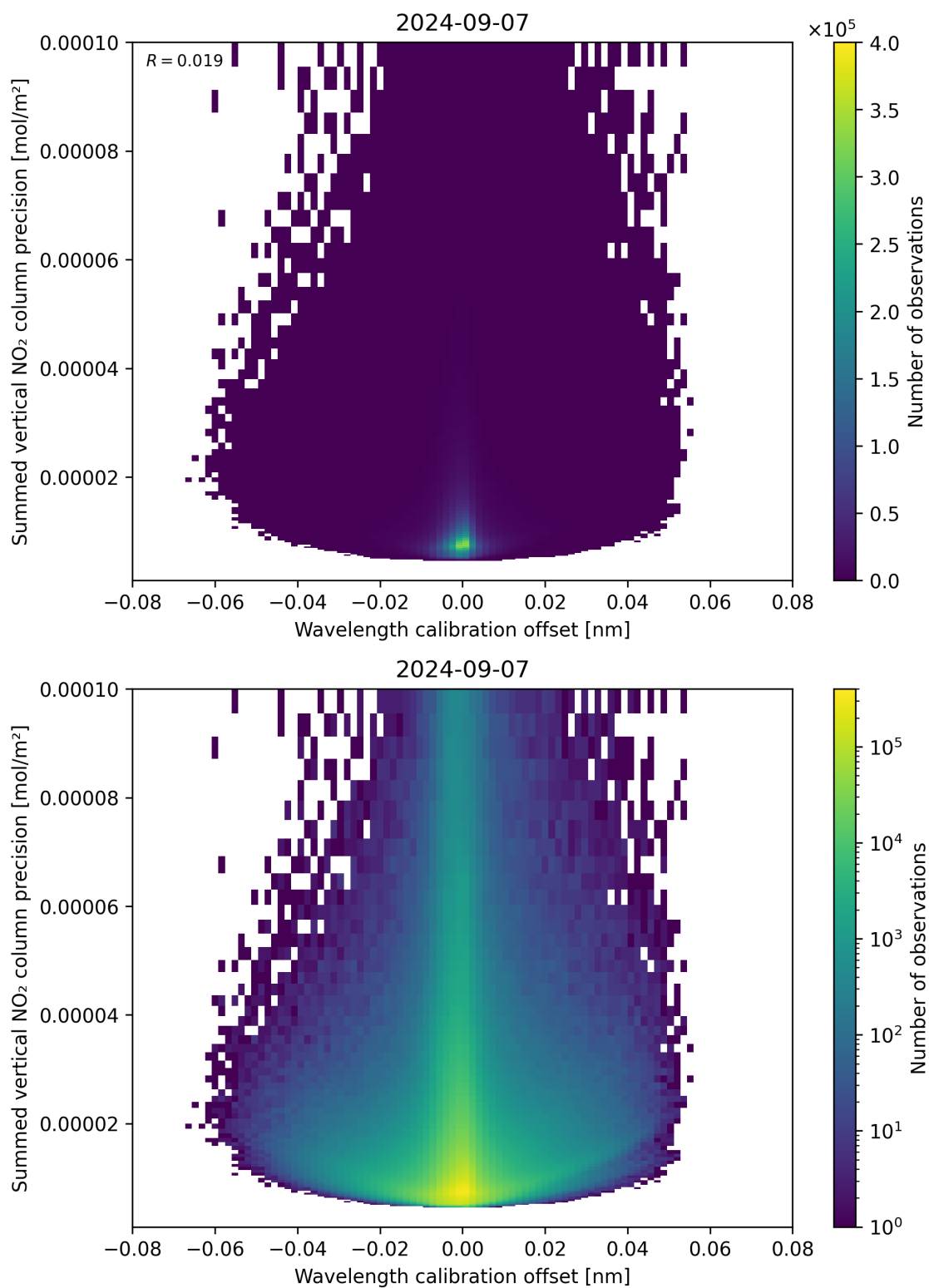
Figure 178: Scatter density plot of “Wavelength calibration offset” against “Summed vertical NO 2 column precision” for 2024-09-06 to 2024-09-08.
