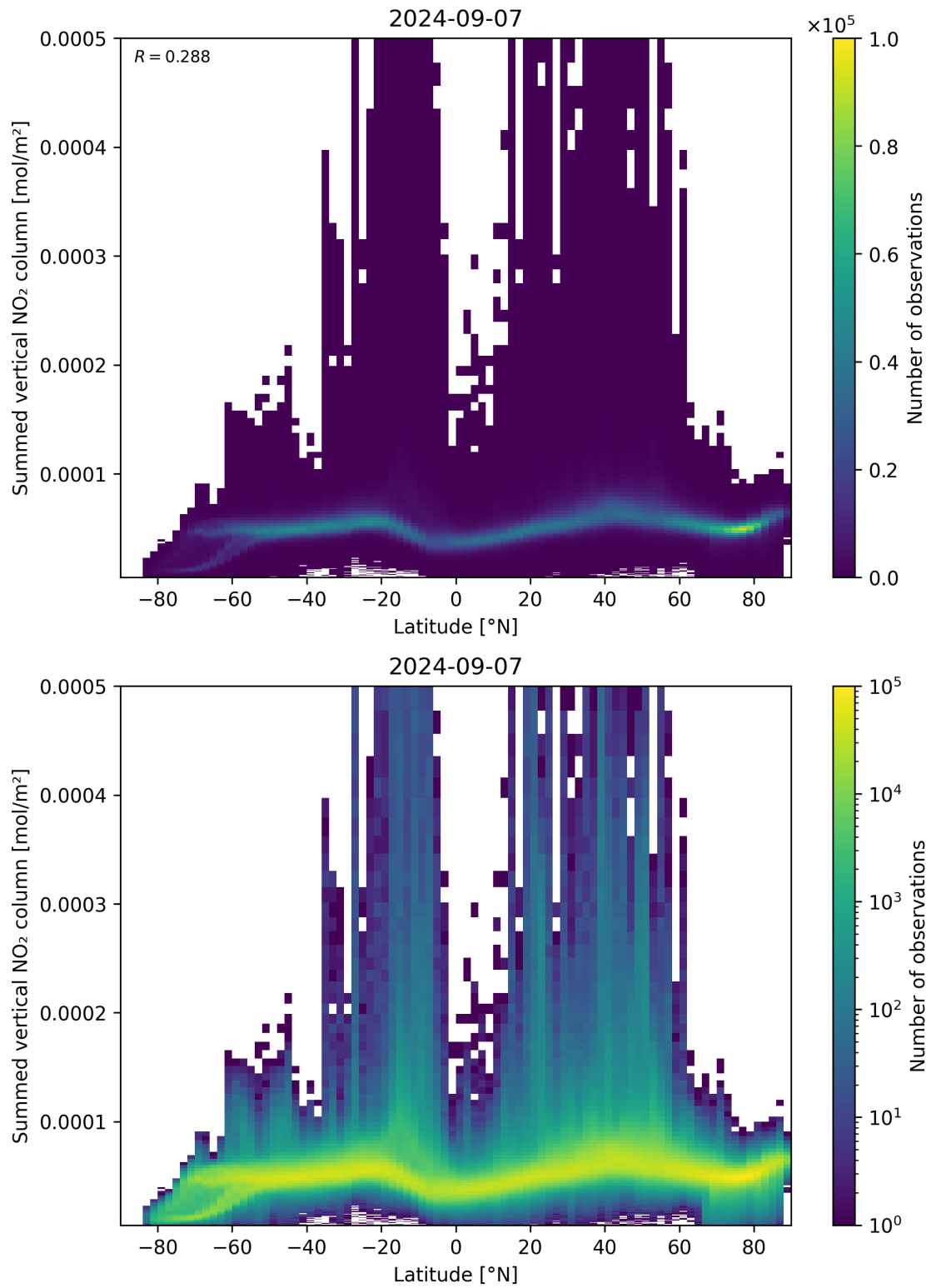
Figure 88: Scatter density plot of “Latitude” against “Summed vertical NO 2 column” for 2024-09-06 to 2024-09-08.
