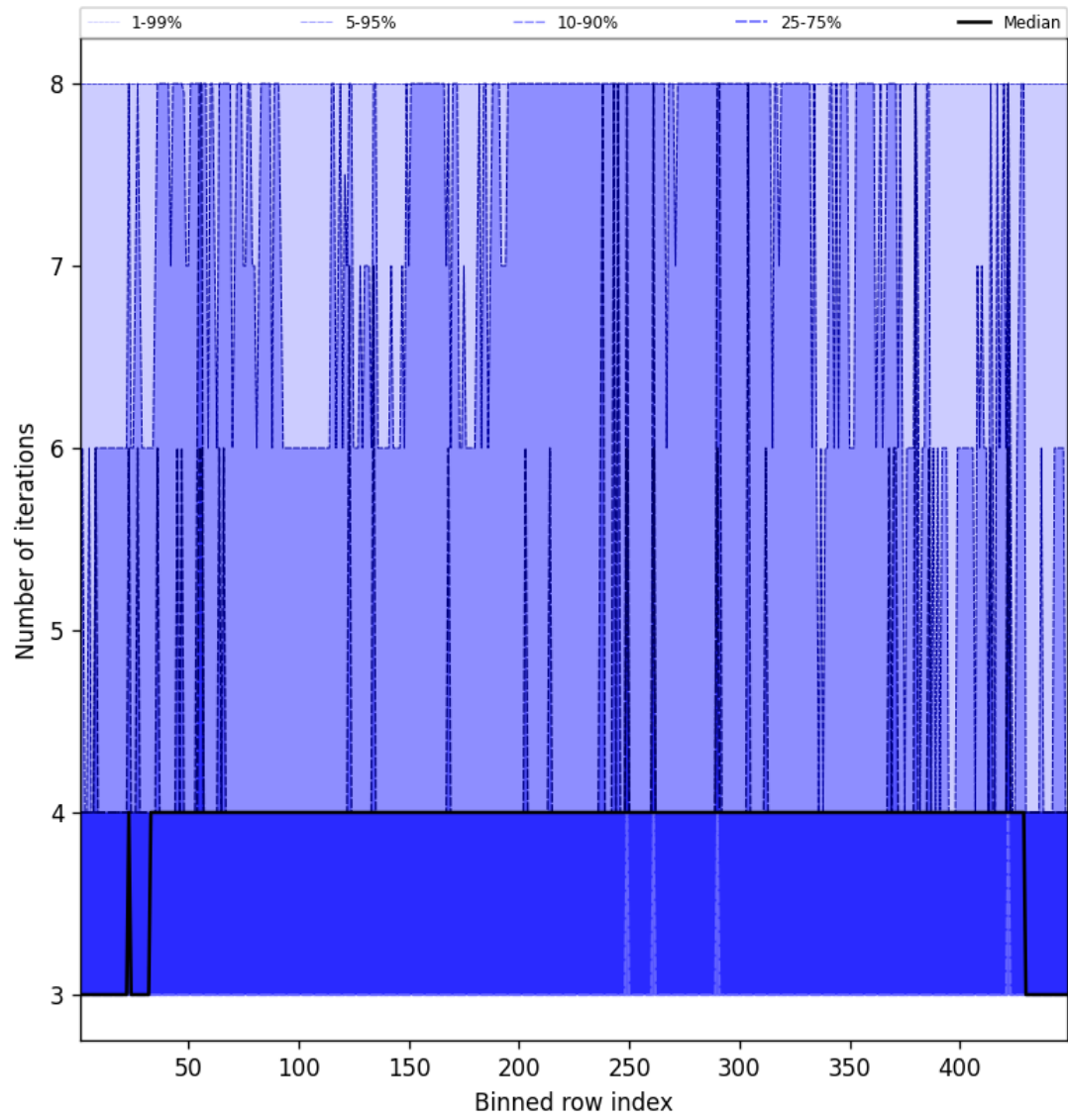
Figure 51: Along track statistics of “Number of iterations” for 2024-09-06 to 2024-09-08
