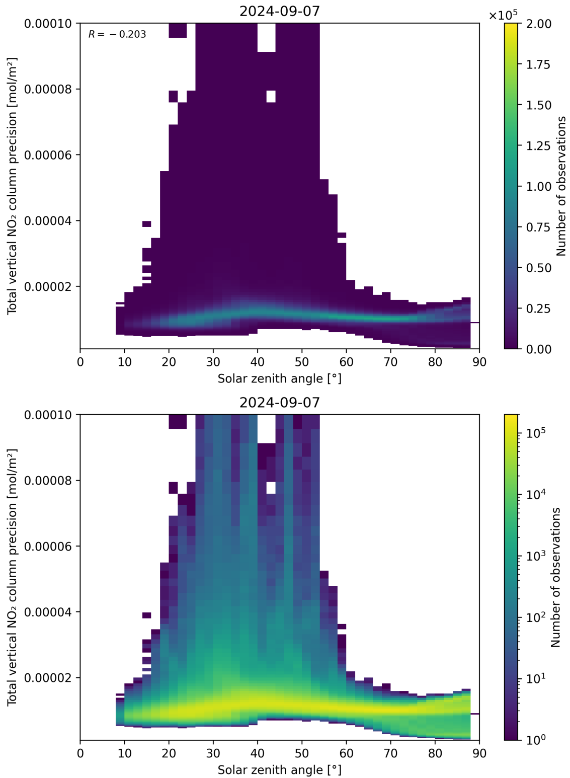
Figure 154: Scatter density plot of “Solar zenith angle” against “Total vertical NO 2 column precision” for 2024-09-06 to 2024-09-08.
