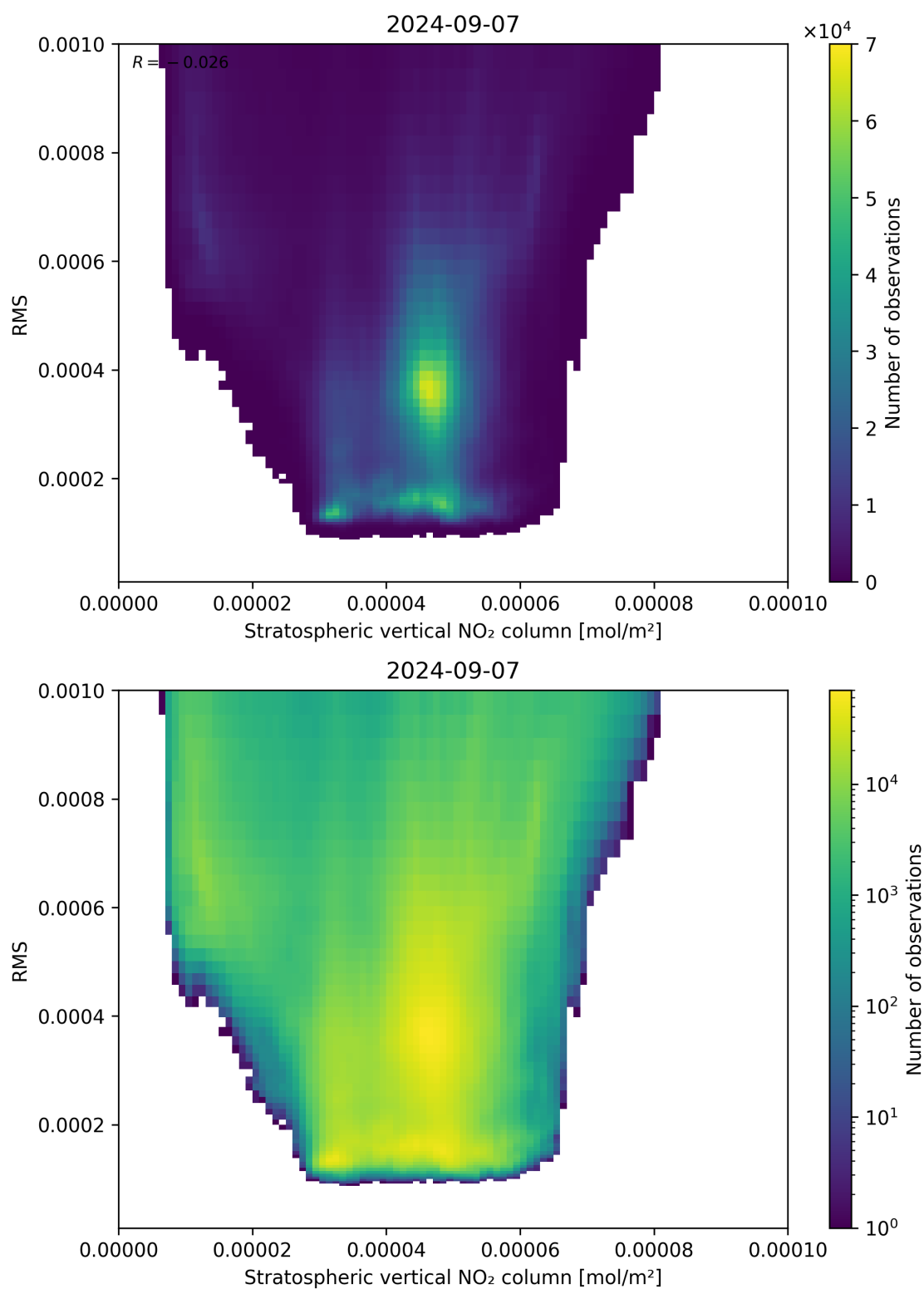
Figure 102: Scatter density plot of “Stratospheric vertical NO 2 column” against “RMS” for 2024-09-06 to 2024-09-08.
