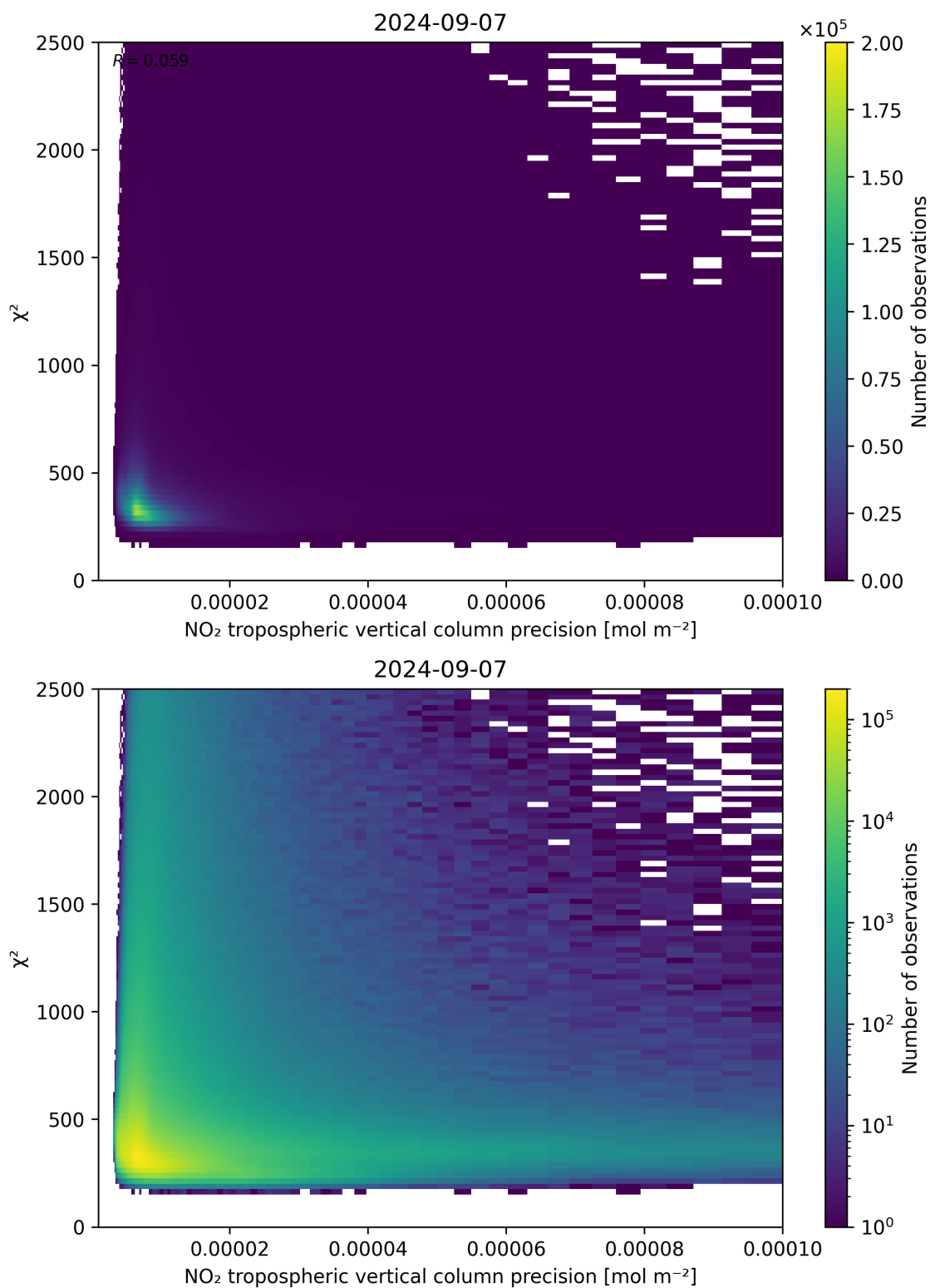
Figure 134: Scatter density plot of “NO 2 tropospheric vertical column precision” against “ \chi^2 ” for 2024-09-06 to 2024-09-08.
