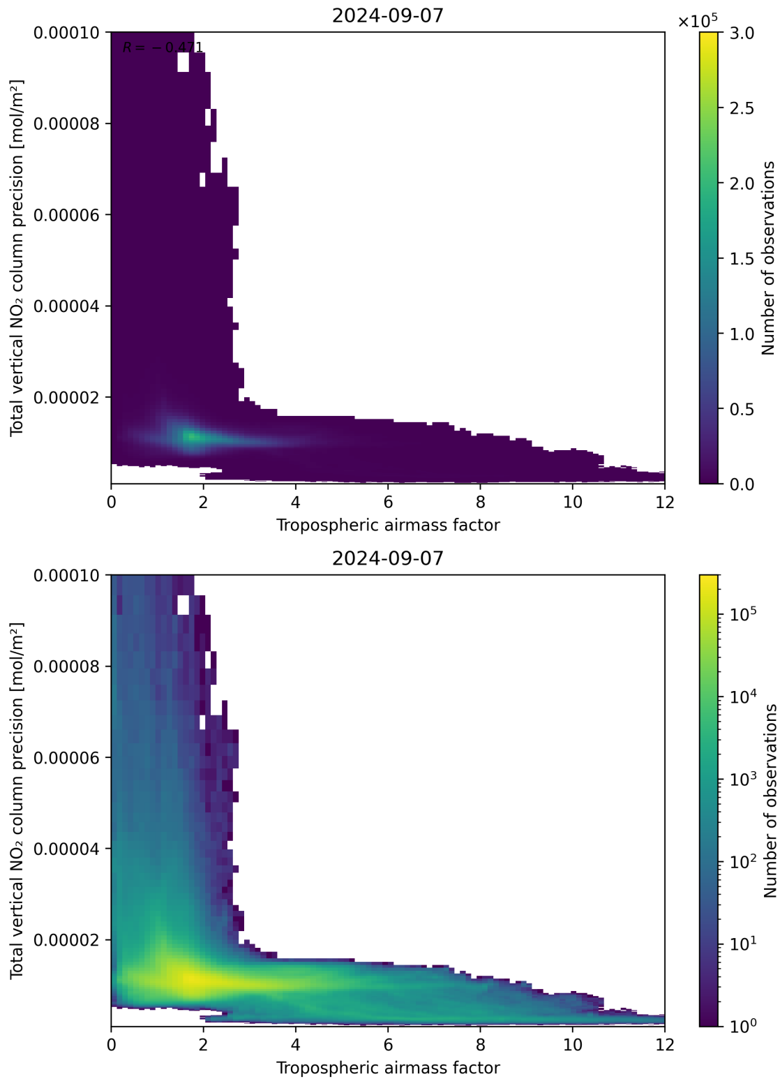
Figure 78: Scatter density plot of “Tropospheric air mass factor” against “Total vertical NO 2 column precision” for 2024-09-06 to 2024-09-08.
