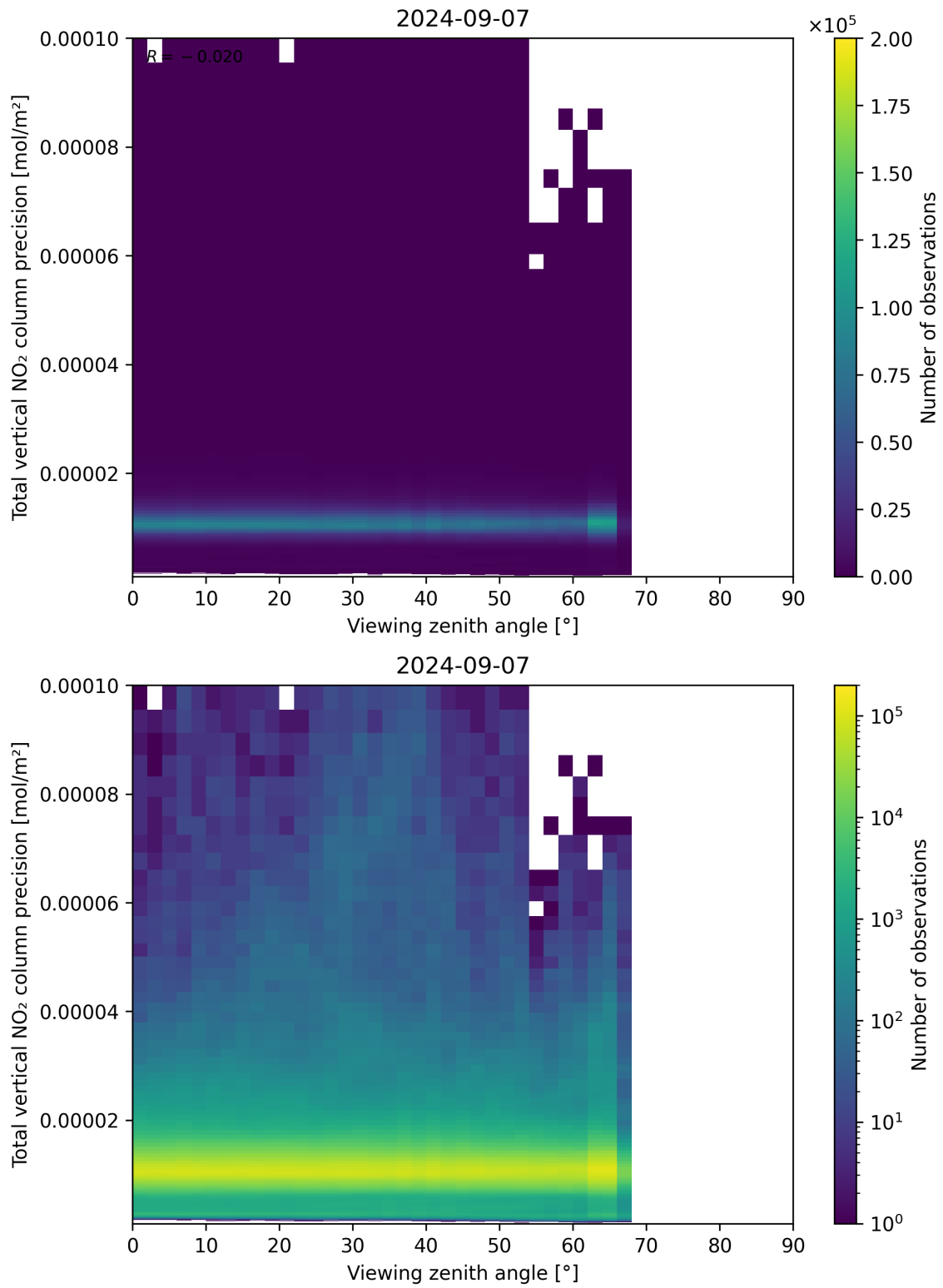
Figure 168: Scatter density plot of “Viewing zenith angle” against “Total vertical NO 2 column precision” for 2024-09-06 to 2024-09-08.
