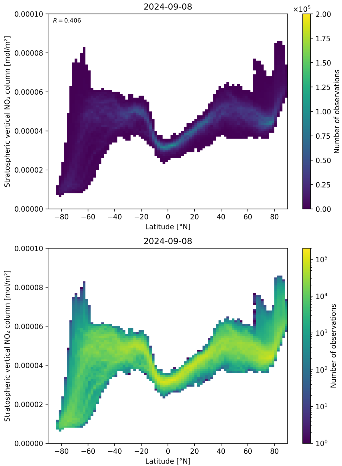
Figure 87: Scatter density plot of “Latitude” against “Stratospheric vertical \text{NO}_2 column” for 2024-09-07 to 2024-09-09.
