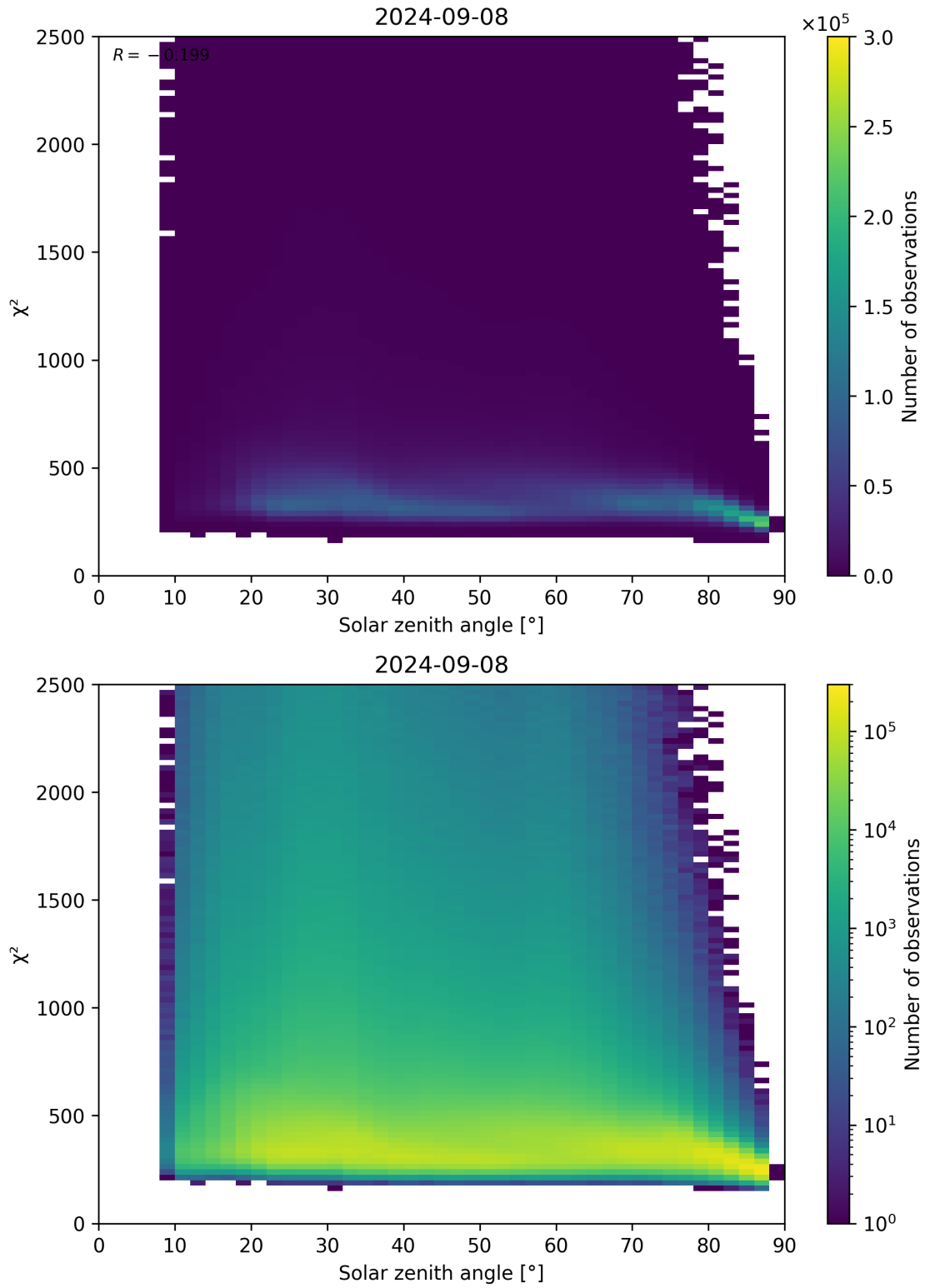
Figure 148: Scatter density plot of “Solar zenith angle” against “ \chi^2 ” for 2024-09-07 to 2024-09-09.
