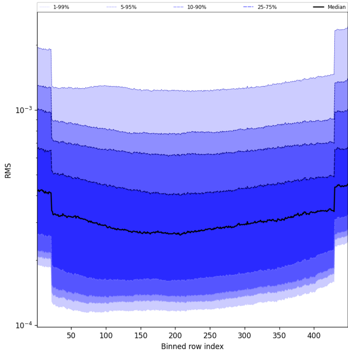
Figure 60: Along track statistics of “RMS” for 2024-09-07 to 2024-09-09
