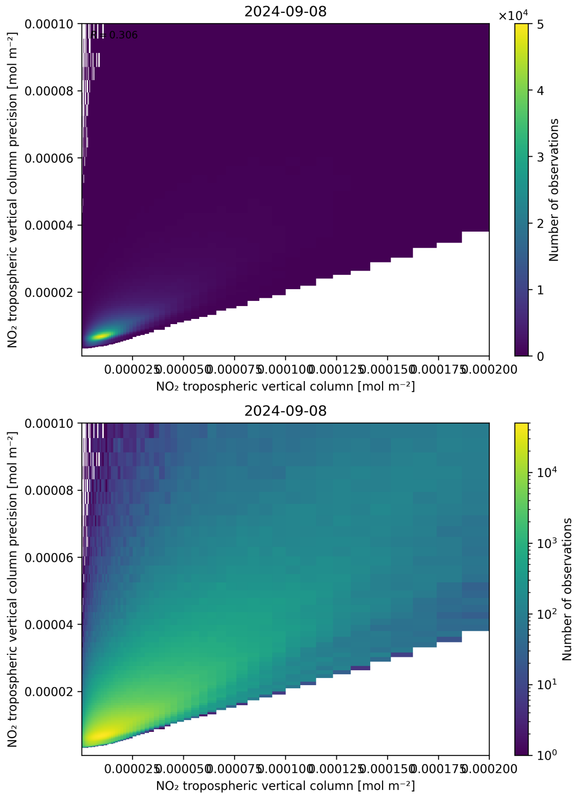
Figure 130: Scatter density plot of “NO 2 tropospheric vertical column” against “NO 2 tropospheric vertical column precision” for 2024-09-07 to 2024-09-09.
