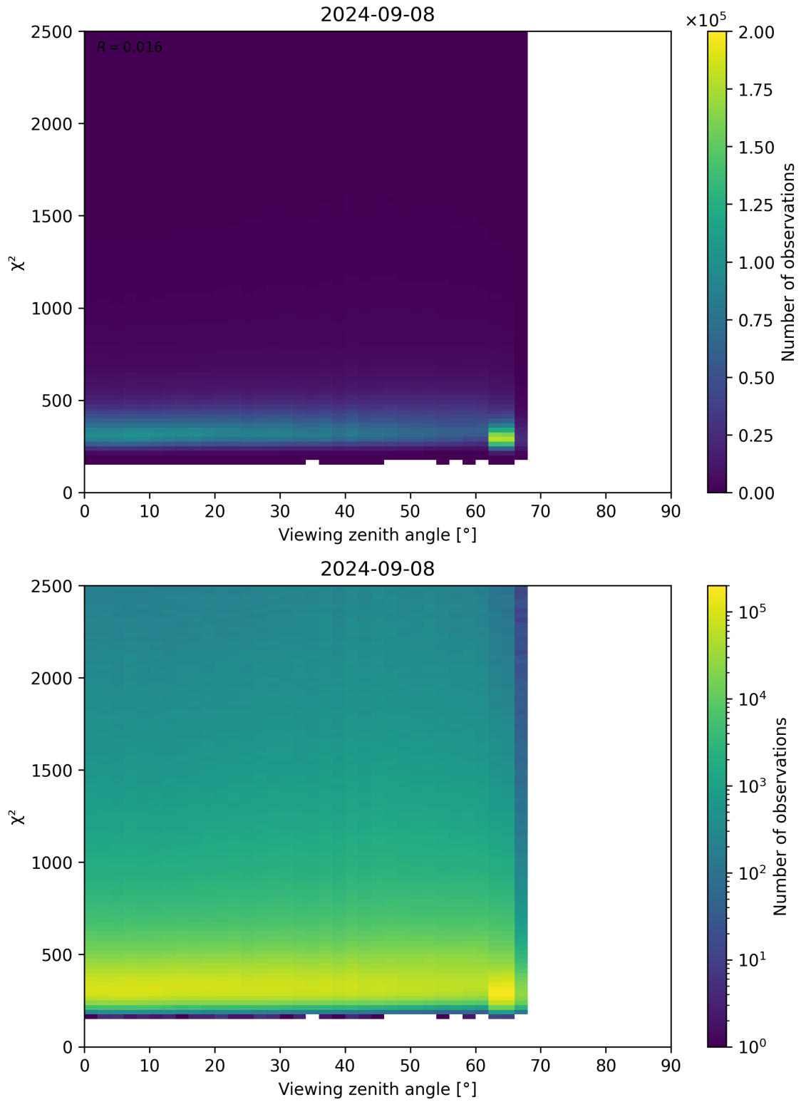
Figure 162: Scatter density plot of “Viewing zenith angle” against “ \chi^2 ” for 2024-09-07 to 2024-09-09.
