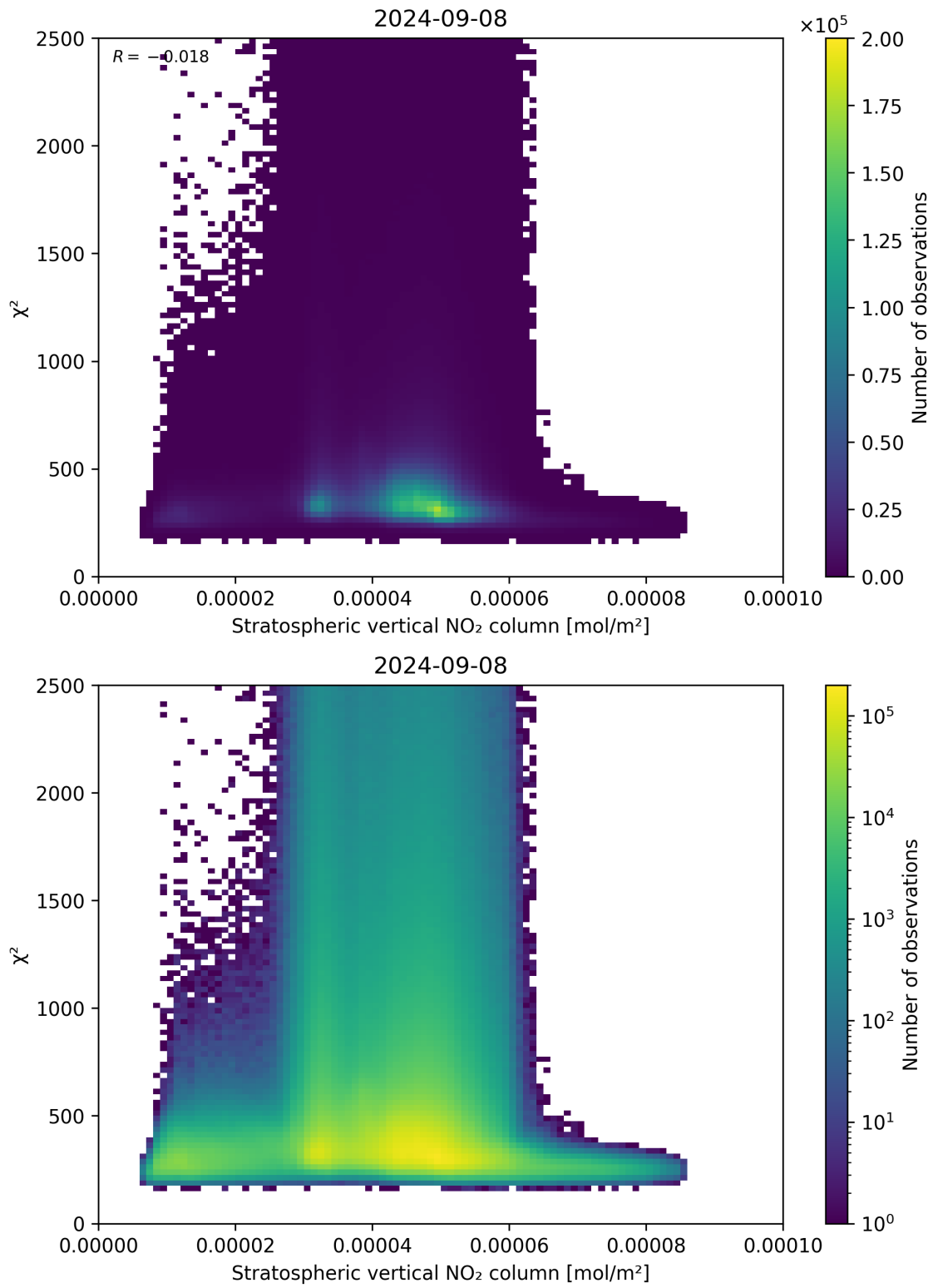
Figure 97: Scatter density plot of “Stratospheric vertical NO 2 column” against “ \chi^2 ” for 2024-09-07 to 2024-09-09.
