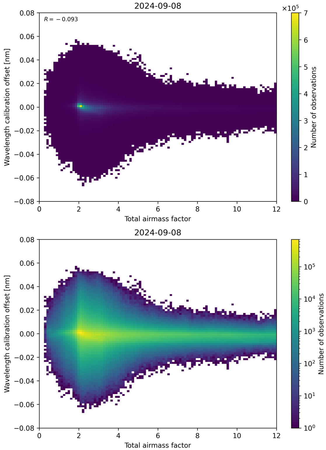
Figure 70: Scatter density plot of “Total airmass factor” against “Wavelength calibration offset” for 2024-09-07 to 2024-09-09.
