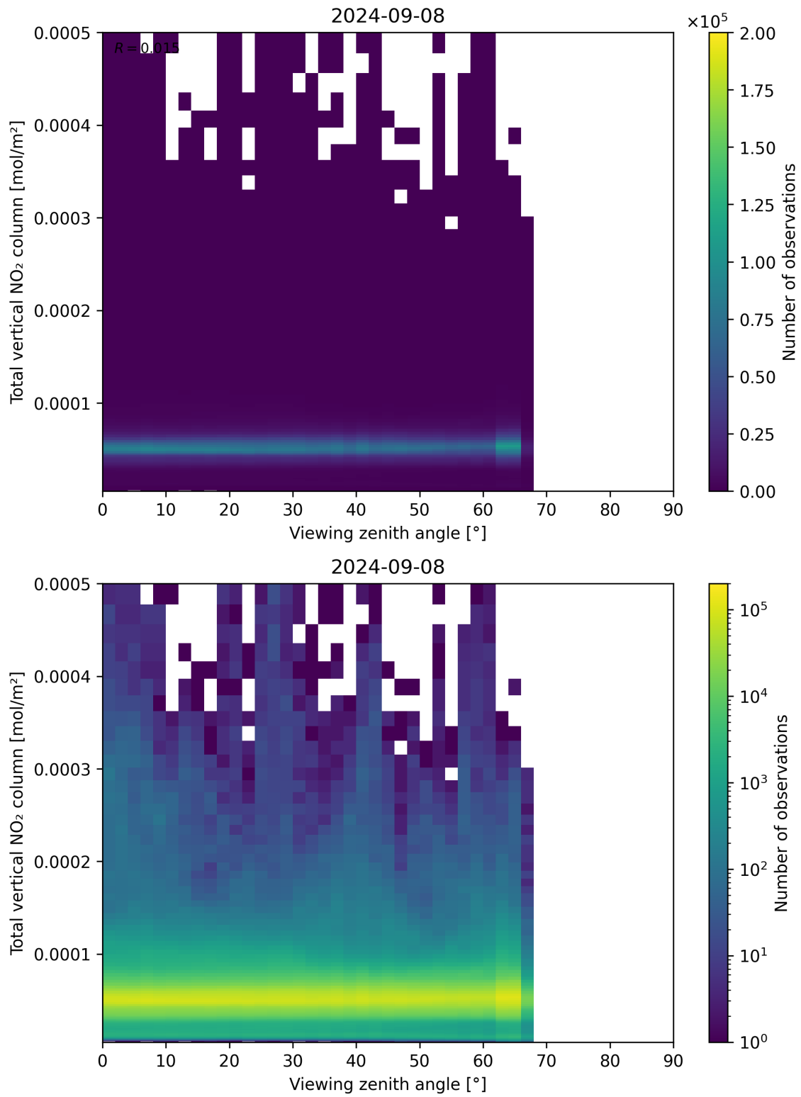
Figure 167: Scatter density plot of “Viewing zenith angle” against “Total vertical NO 2 column” for 2024-09-07 to 2024-09-09.
