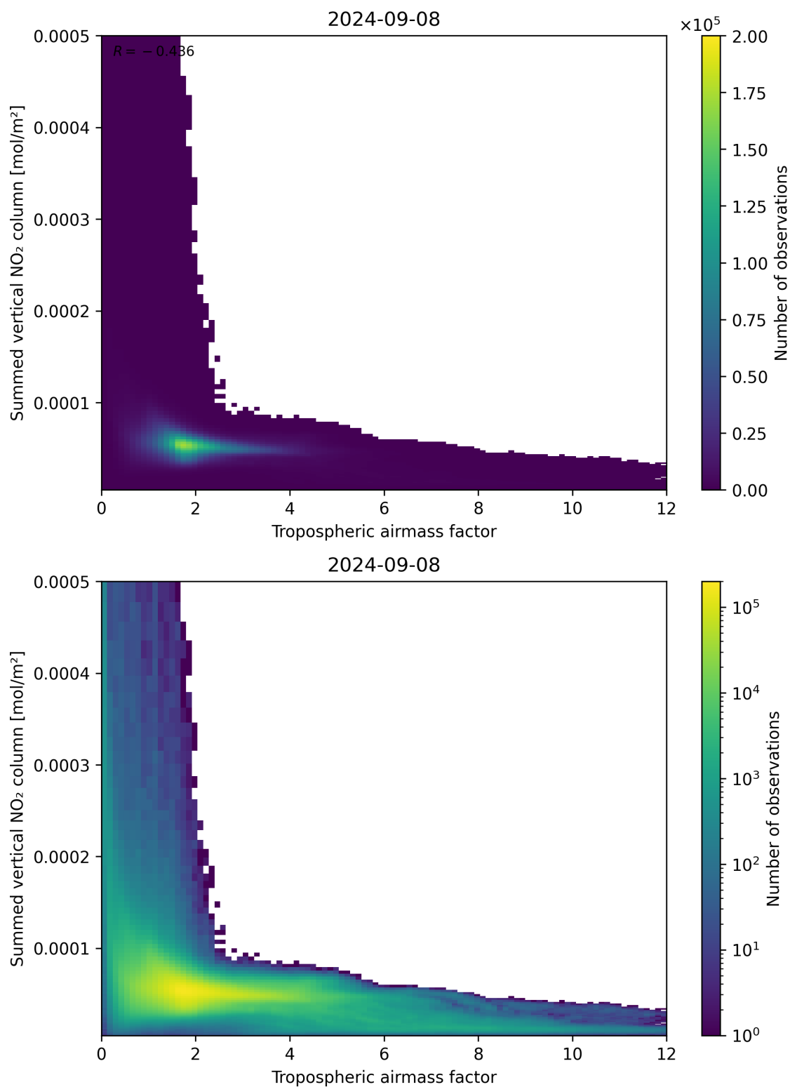
Figure 75: Scatter density plot of “Tropospheric airmass factor” against “Summed vertical NO 2 column” for 2024-09-07 to 2024-09-09.
