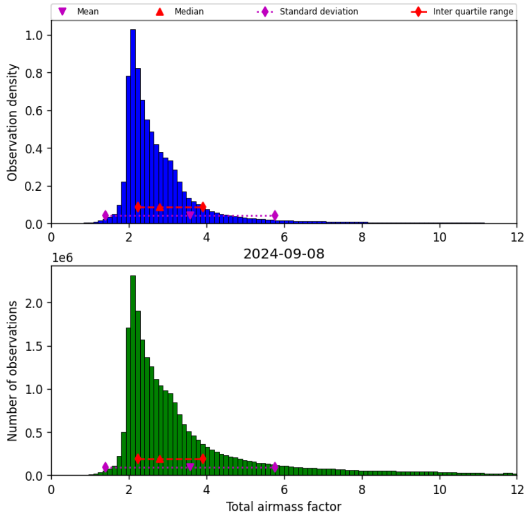
Figure 32: Histogram of “Total airmass factor” for 2024-09-07 to 2024-09-09
