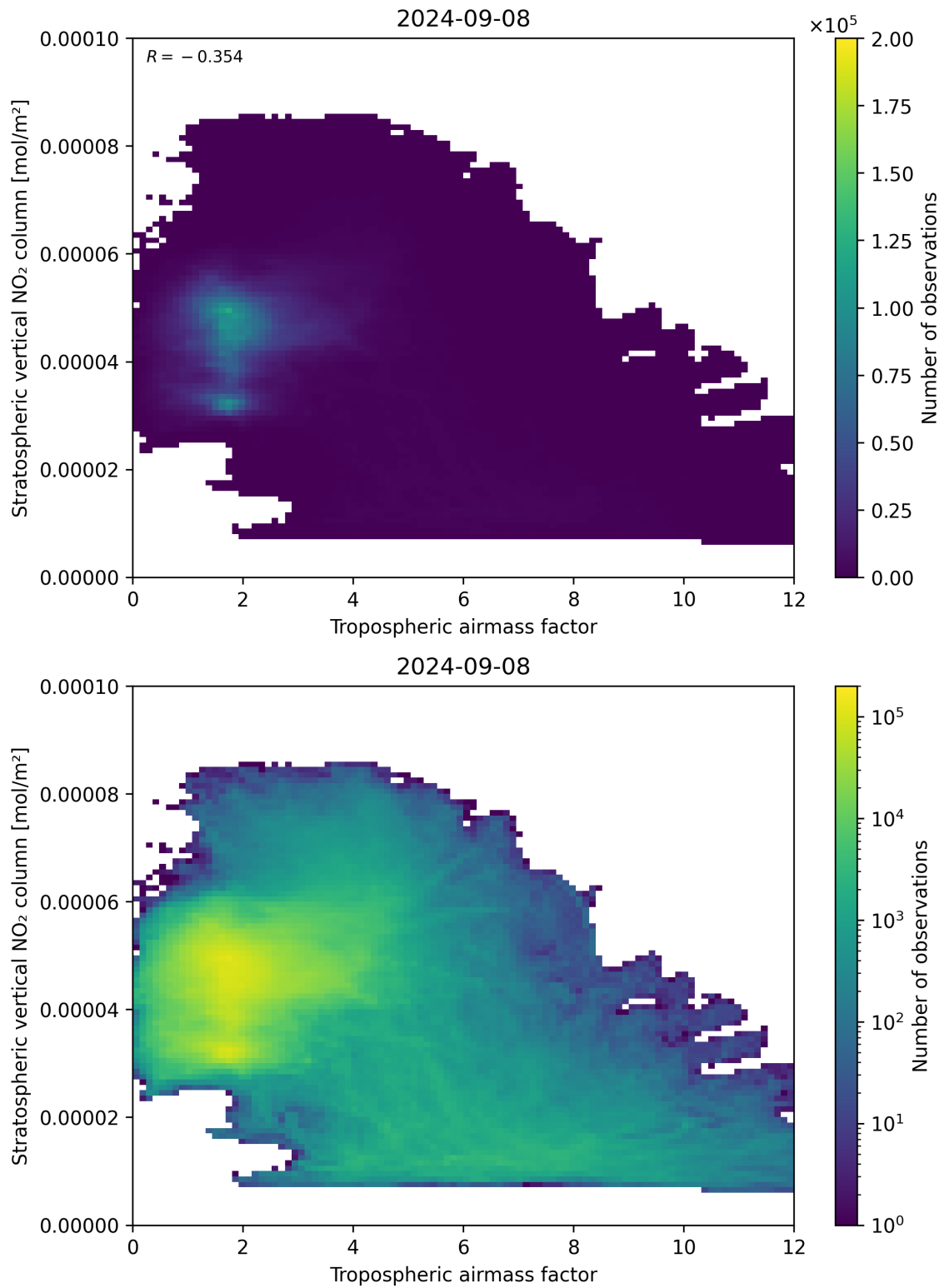
Figure 74: Scatter density plot of “Tropospheric air mass factor” against “Stratospheric vertical NO 2 column” for 2024-09-07 to 2024-09-09.
