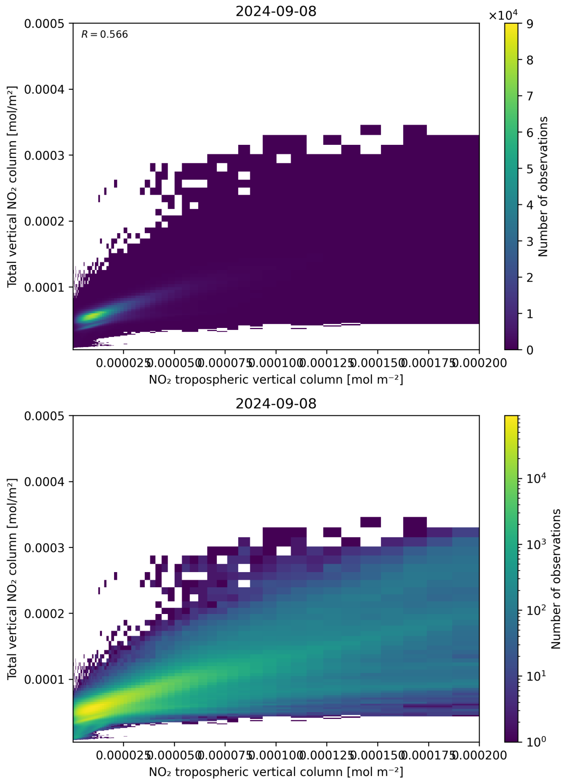
Figure 128: Scatter density plot of “NO 2 tropospheric vertical column” against “Total vertical NO 2 column” for 2024-09-07 to 2024-09-09.
