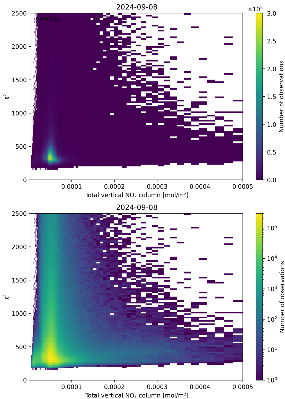
Figure 111: Scatter density plot of “Total vertical NO 2 column” against “ \chi^2 ” for 2024-09-07 to 2024-09-09.
