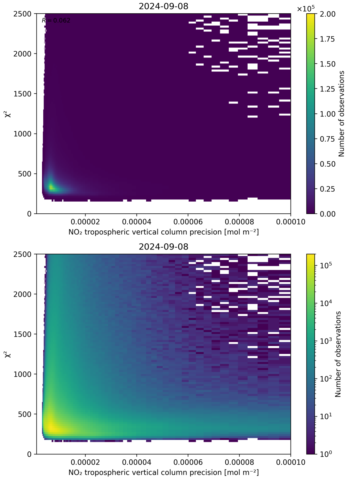
Figure 134: Scatter density plot of “NO 2 tropospheric vertical column precision” against “ \chi^2 ” for 2024-09-07 to 2024-09-09.
