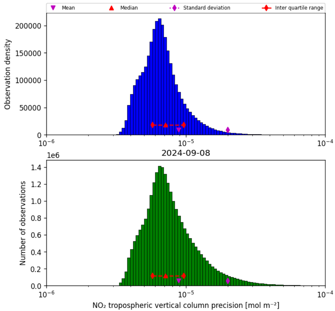
Figure 30: Histogram of “NO 2 tropospheric vertical column precision” for 2024-09-07 to 2024-09-09
