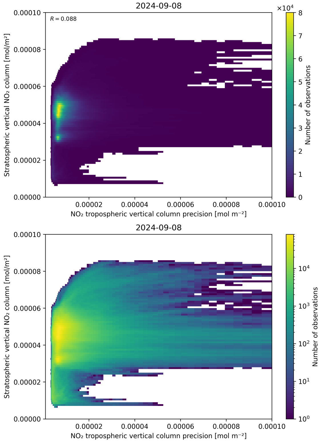
Figure 135: Scatter density plot of “NO 2 tropospheric vertical column precision” against “Stratospheric vertical NO 2 column” for 2024-09-07 to 2024-09-09.
