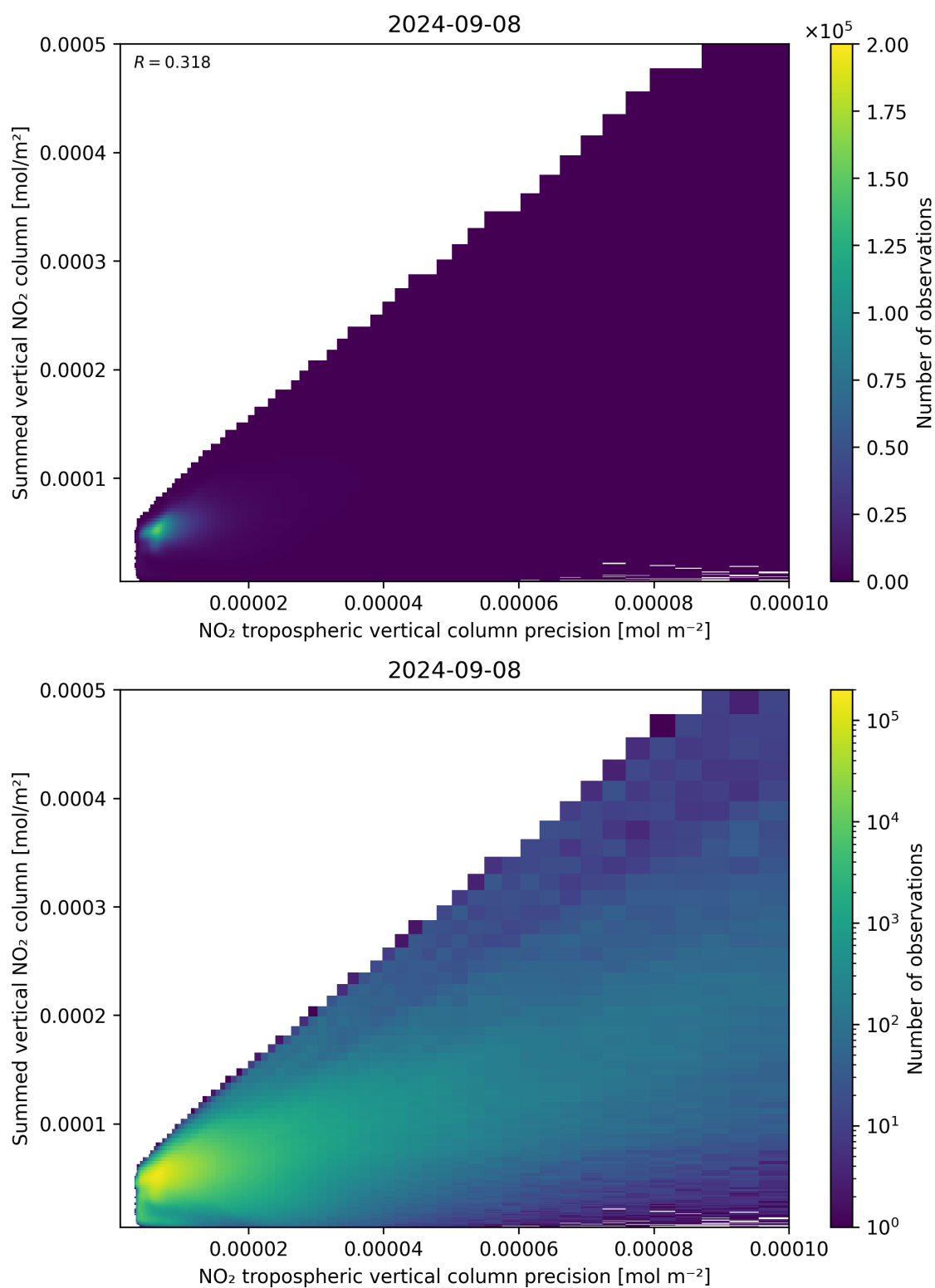
Figure 136: Scatter density plot of “NO 2 tropospheric vertical column precision” against “Summed vertical NO 2 column” for 2024-09-07 to 2024-09-09.
