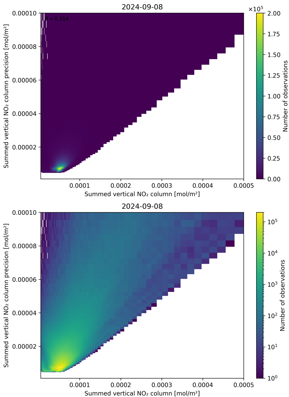
Figure 105: Scatter density plot of “Summed vertical NO 2 column” against “Summed vertical NO 2 column precision” for 2024-09-07 to 2024-09-09.
