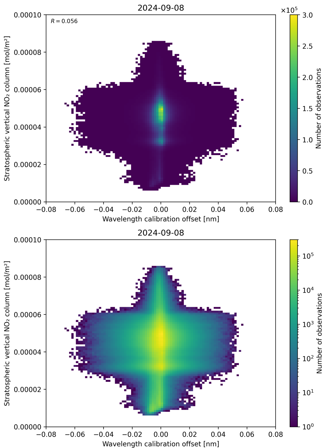
Figure 176: Scatter density plot of “Wavelength calibration offset” against “Stratospheric vertical NO 2 column” for 2024-09-07 to 2024-09-09.
