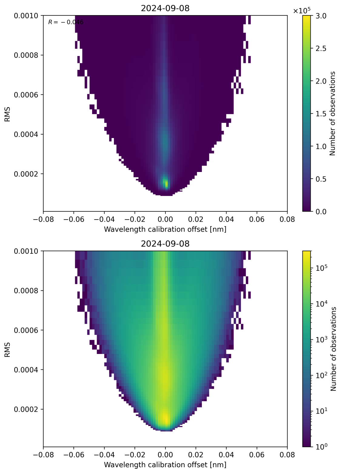
Figure 181: Scatter density plot of “Wavelength calibration offset” against “RMS” for 2024-09-07 to 2024-09-09.
