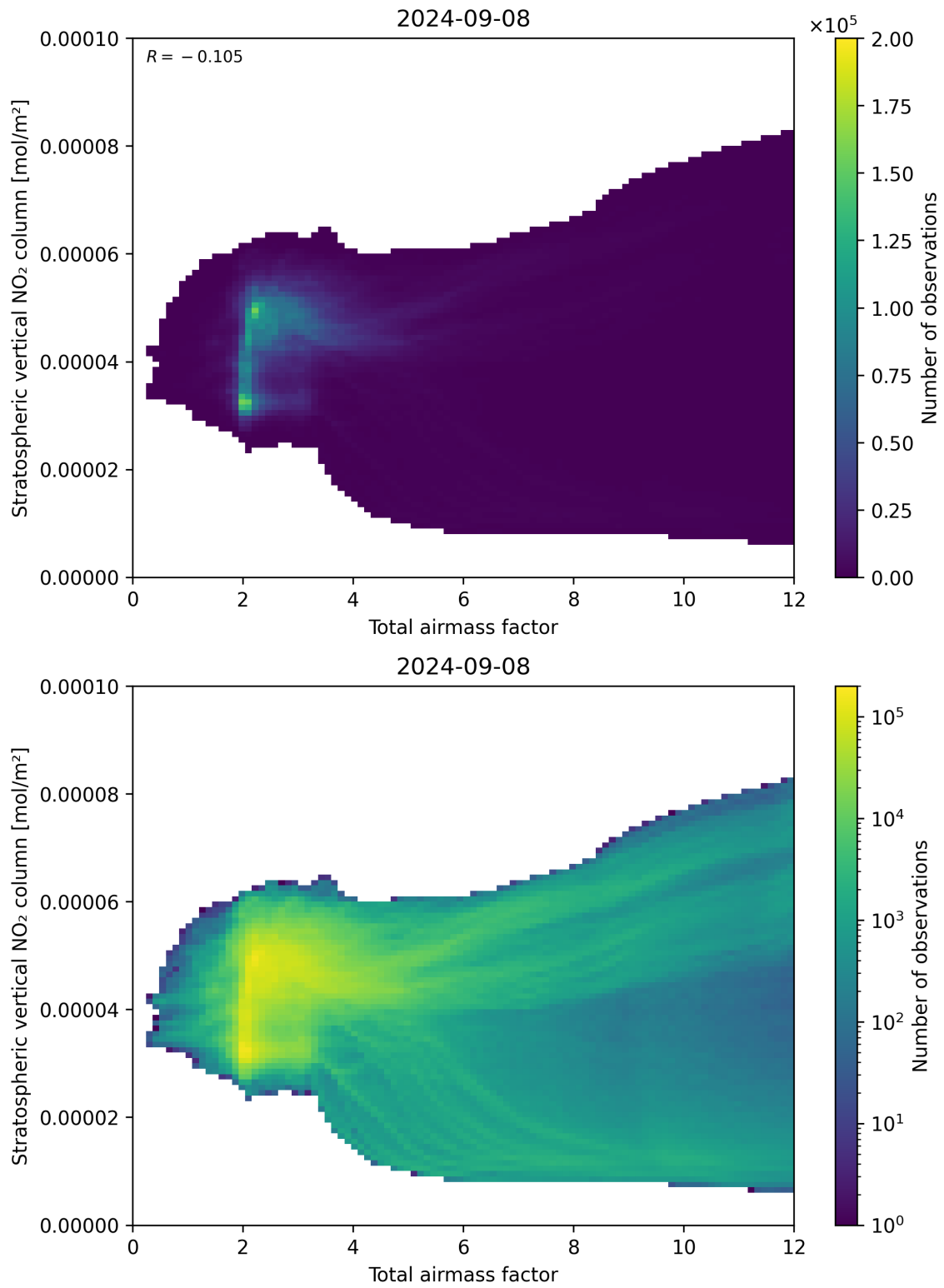
Figure 64: Scatter density plot of “Total airmass factor” against “Stratospheric vertical NO 2 column” for 2024-09-07 to 2024-09-09.
