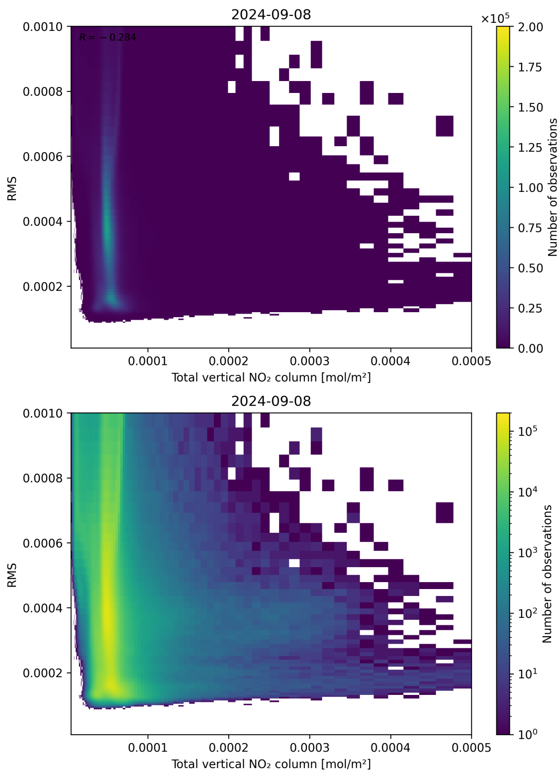
Figure 120: Scatter density plot of “Total vertical NO 2 column” against “RMS” for 2024-09-07 to 2024-09-09.
