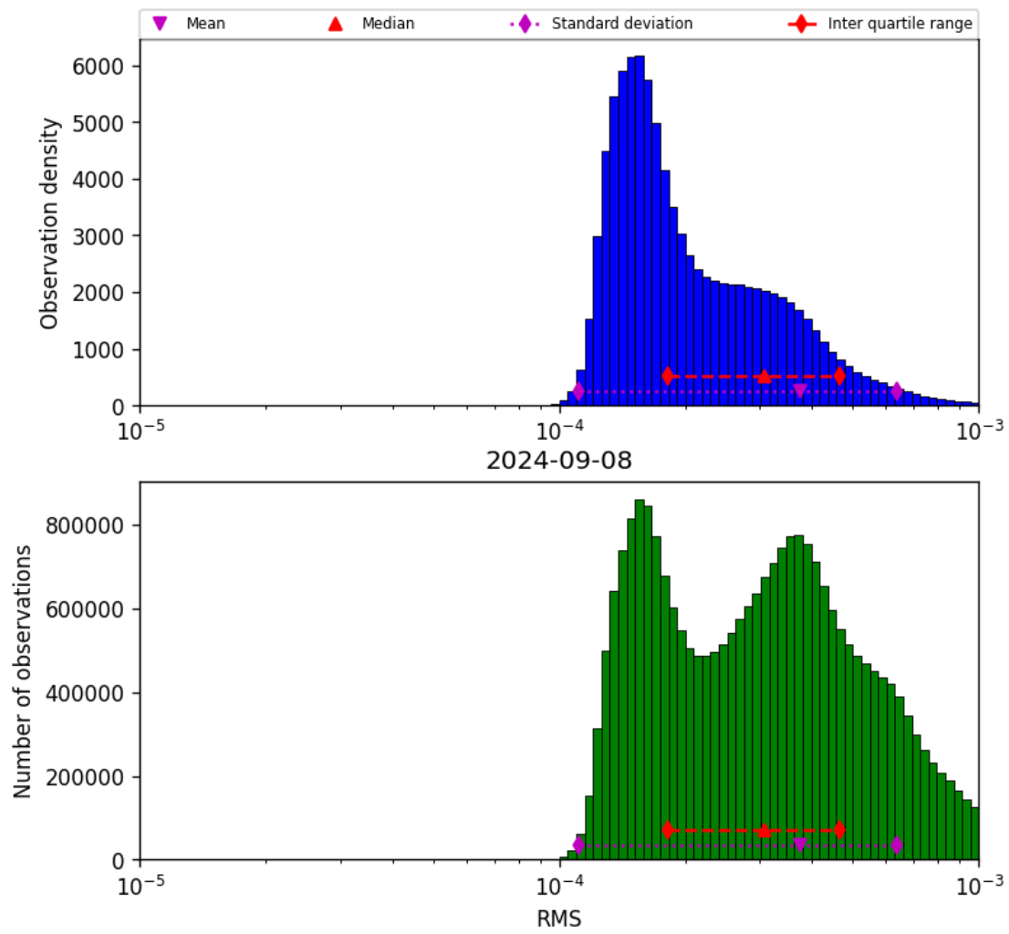
Figure 43: Histogram of “RMS” for 2024-09-07 to 2024-09-09
