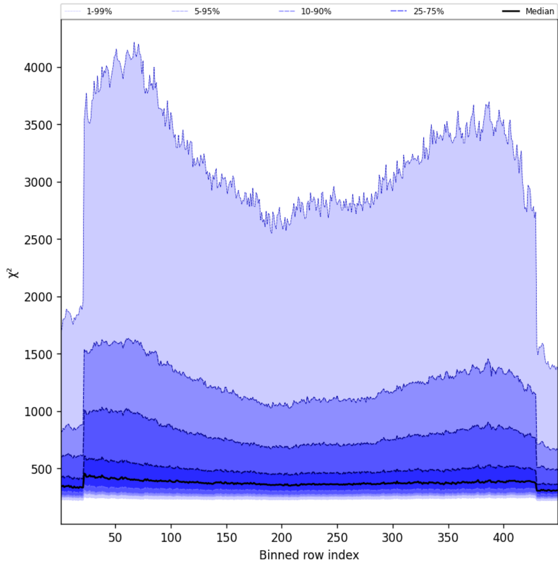
Figure 59: Along track statistics of “ \chi^2 ” for 2024-09-07 to 2024-09-09
