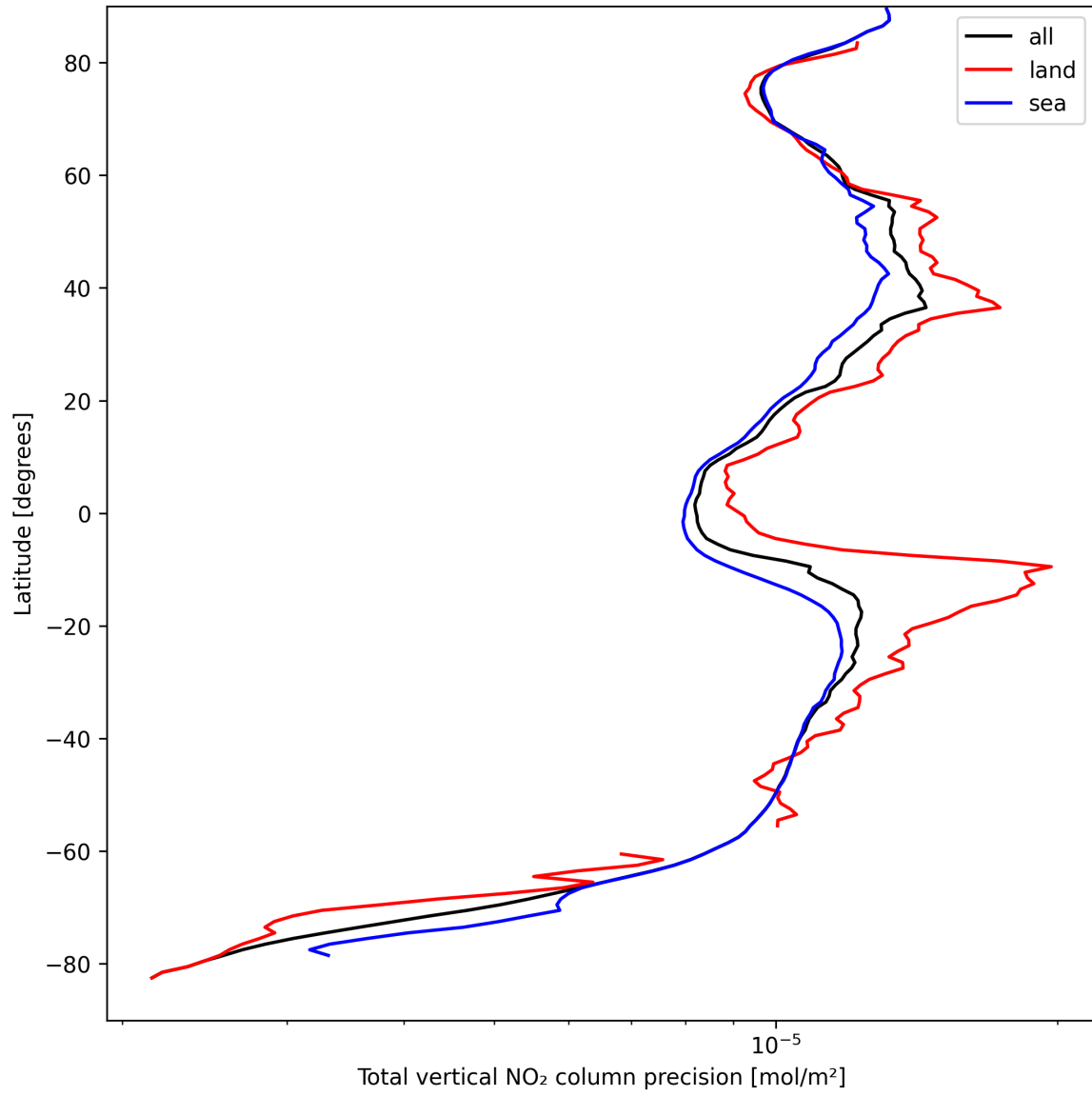
Figure 22: Zonal average of “Total vertical NO 2 column precision” for 2024-09-07 to 2024-09-09.
