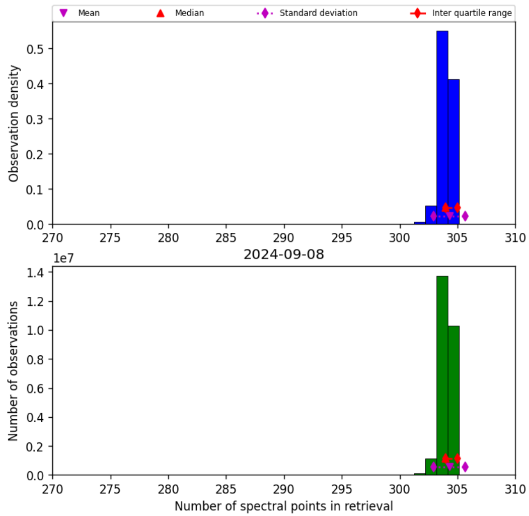
Figure 33: Histogram of “Number of spectral points in retrieval” for 2024-09-07 to 2024-09-09
