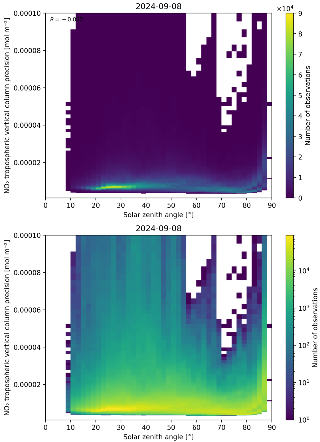
Figure 156: Scatter density plot of “Solar zenith angle” against “NO 2 tropospheric vertical column precision” for 2024-09-07 to 2024-09-09.
