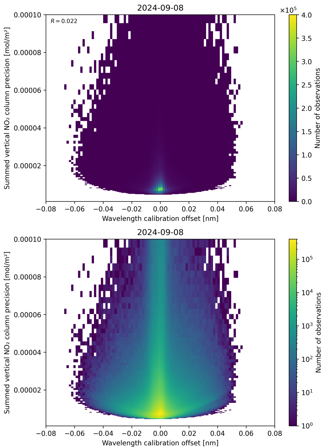
Figure 178: Scatter density plot of “Wavelength calibration offset” against “Summed vertical NO 2 column precision” for 2024-09-07 to 2024-09-09.
