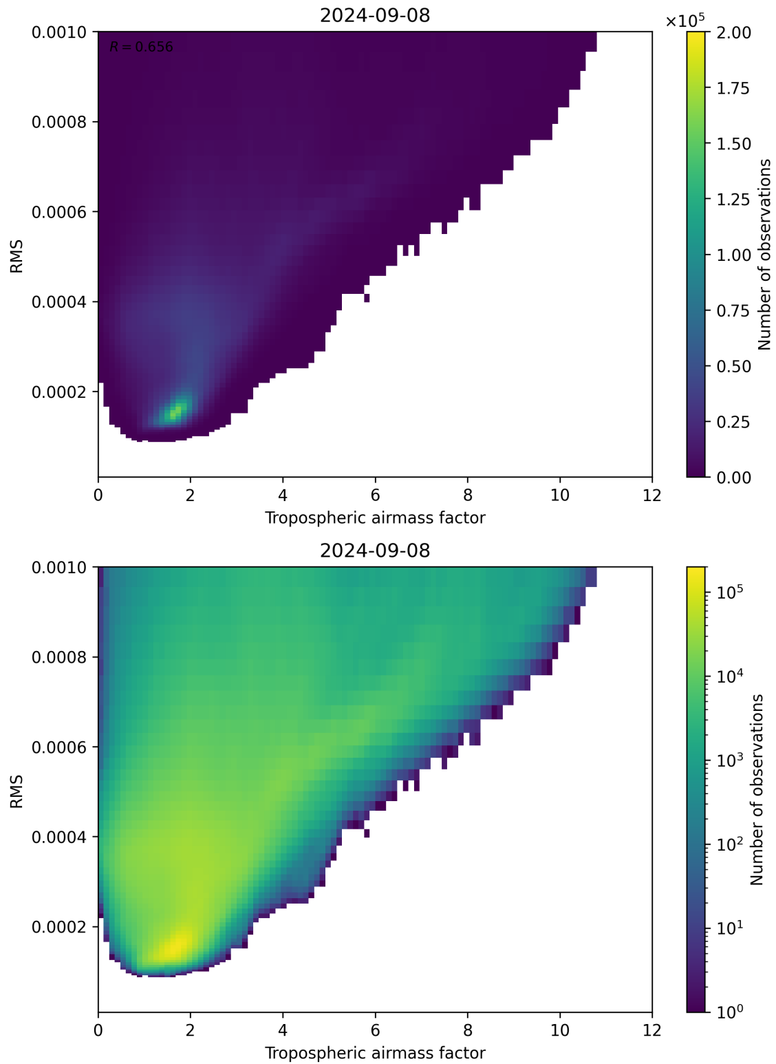
Figure 79: Scatter density plot of “Tropospheric airmass factor” against “RMS” for 2024-09-07 to 2024-09-09.
