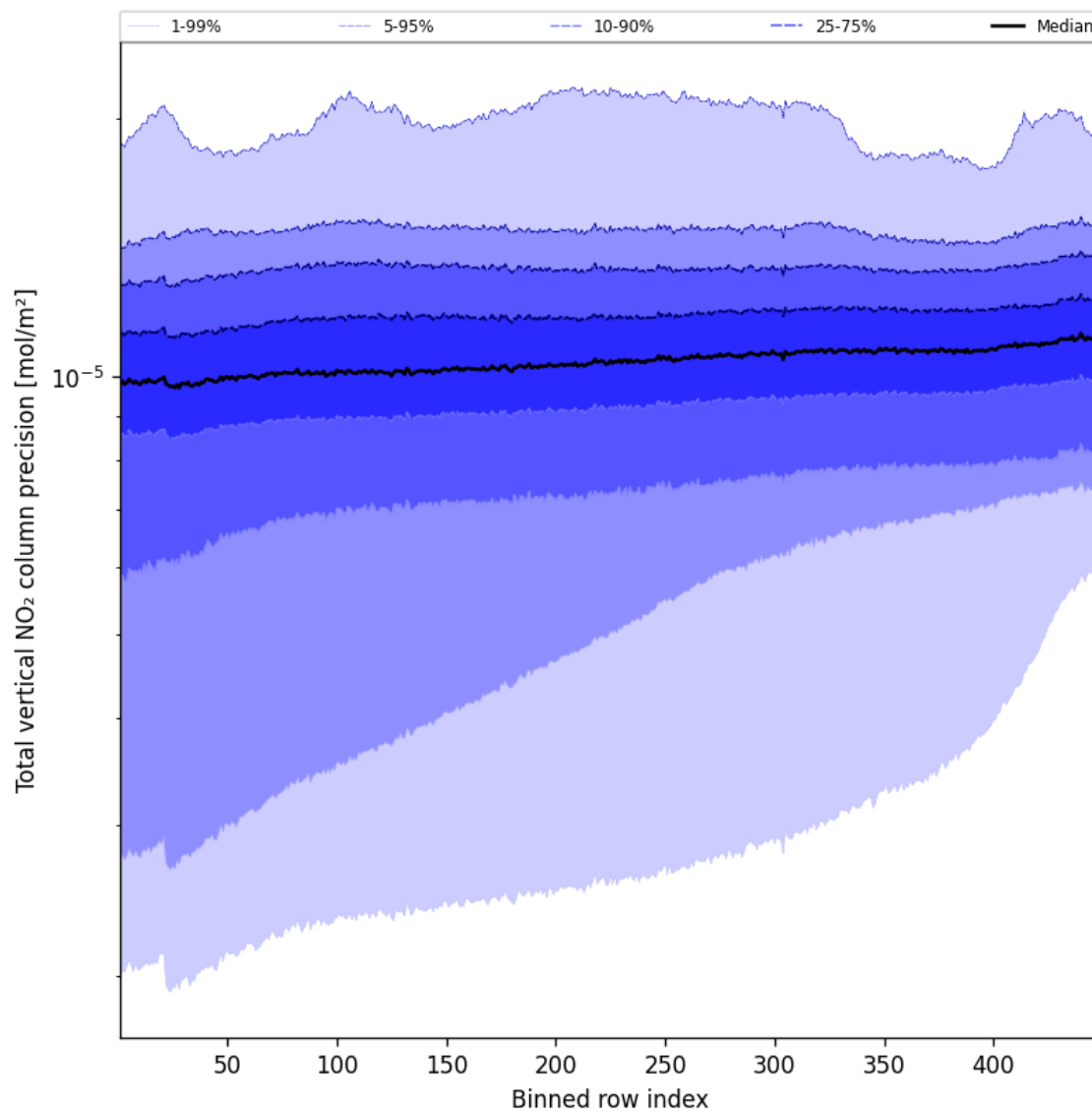
Figure 56: Along track statistics of “Total vertical NO 2 column precision” for 2024-09-07 to 2024-09-09
