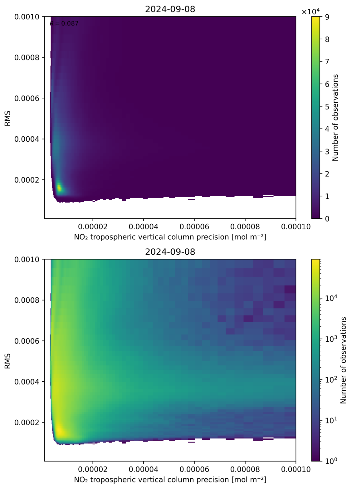
Figure 140: Scatter density plot of “NO 2 tropospheric vertical column precision” against “RMS” for 2024-09-07 to 2024-09-09.
