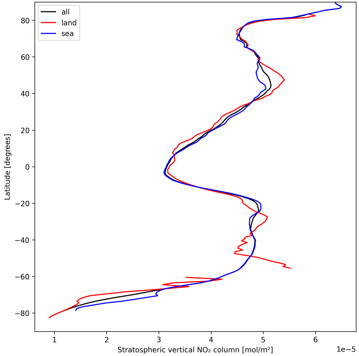
Figure 19: Zonal average of “Stratospheric vertical NO 2 column” for 2024-09-07 to 2024-09-09.
