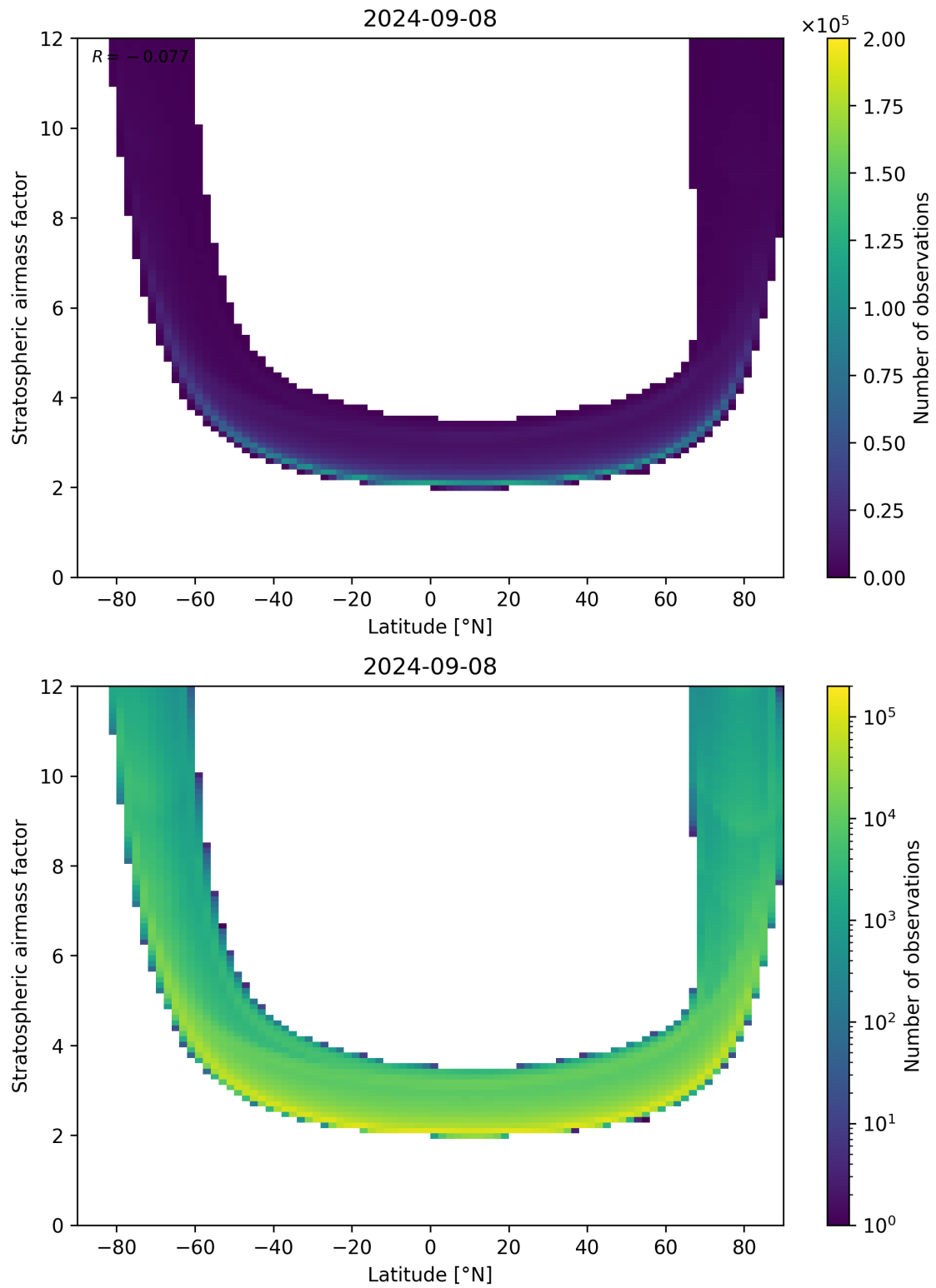
Figure 83: Scatter density plot of “Latitude” against “Stratospheric airmass factor” for 2024-09-07 to 2024-09-09.
