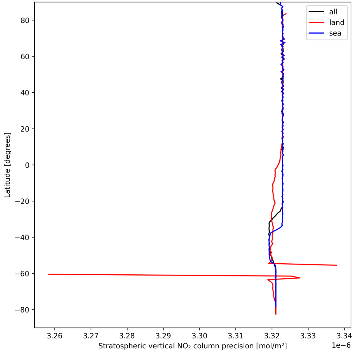
Figure 20: Zonal average of “Stratospheric vertical NO 2 column precision” for 2024-09-07 to 2024-09-09.
