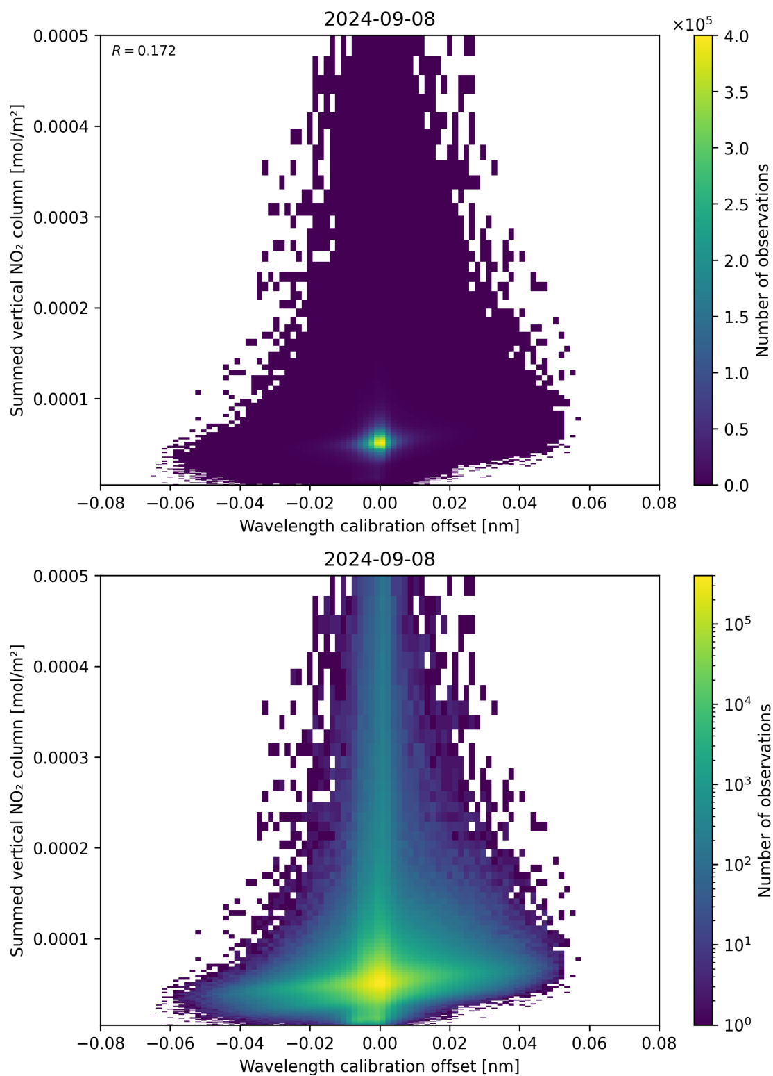
Figure 177: Scatter density plot of “Wavelength calibration offset” against “Summed vertical NO 2 column” for 2024-09-07 to 2024-09-09.
