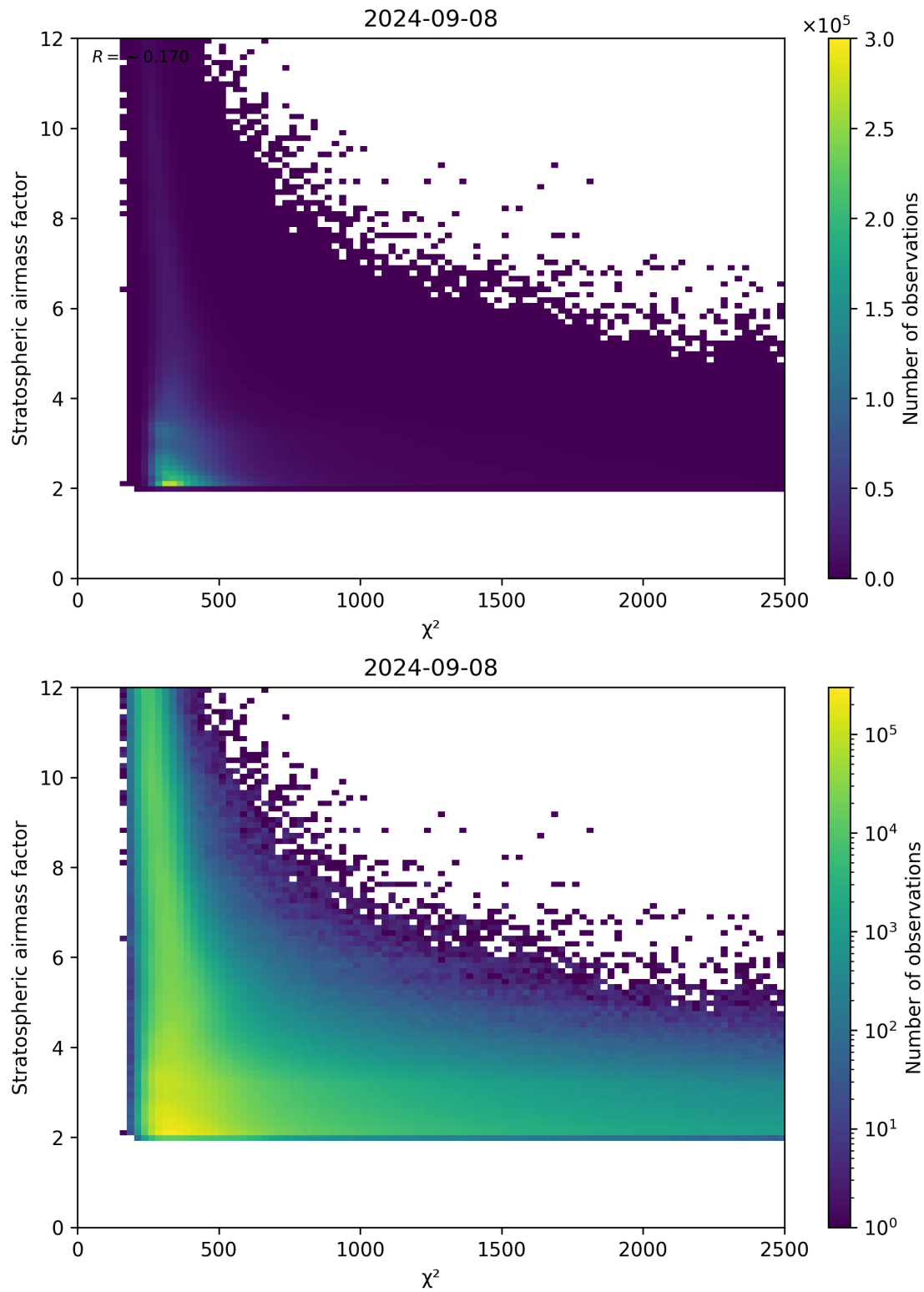
Figure 81: Scatter density plot of “ \chi^2 ” against “Stratospheric airmass factor” for 2024-09-07 to 2024-09-09.
