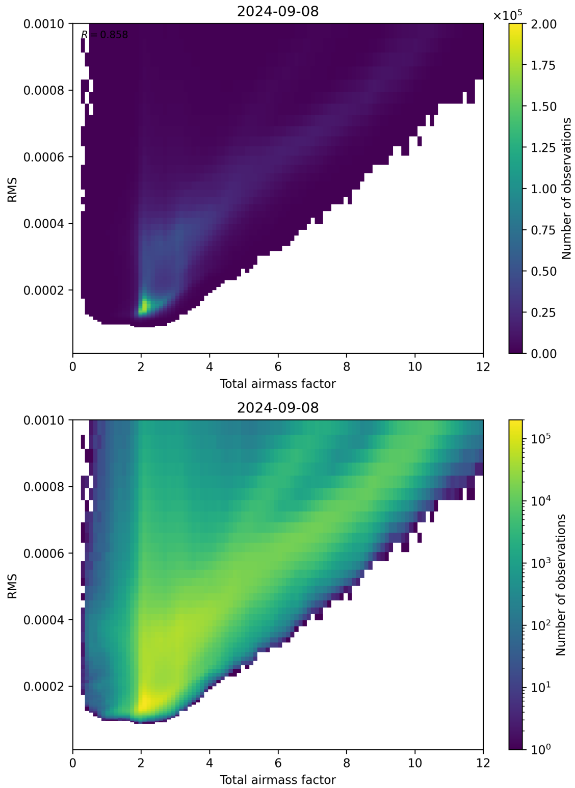
Figure 69: Scatter density plot of “Total airmass factor” against “RMS” for 2024-09-07 to 2024-09-09.
