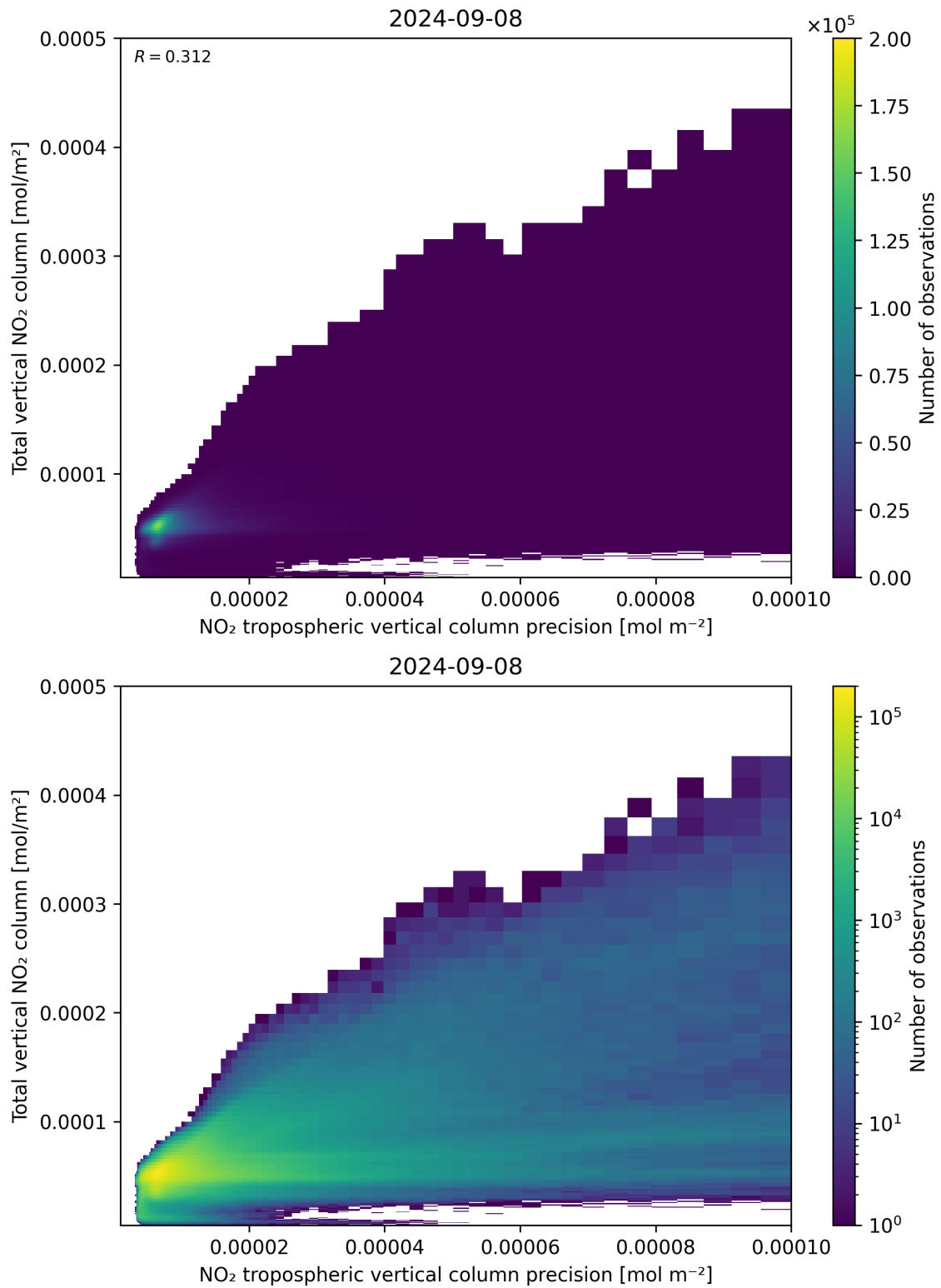
Figure 138: Scatter density plot of “NO 2 tropospheric vertical column precision” against “Total vertical NO 2 column” for 2024-09-07 to 2024-09-09.
