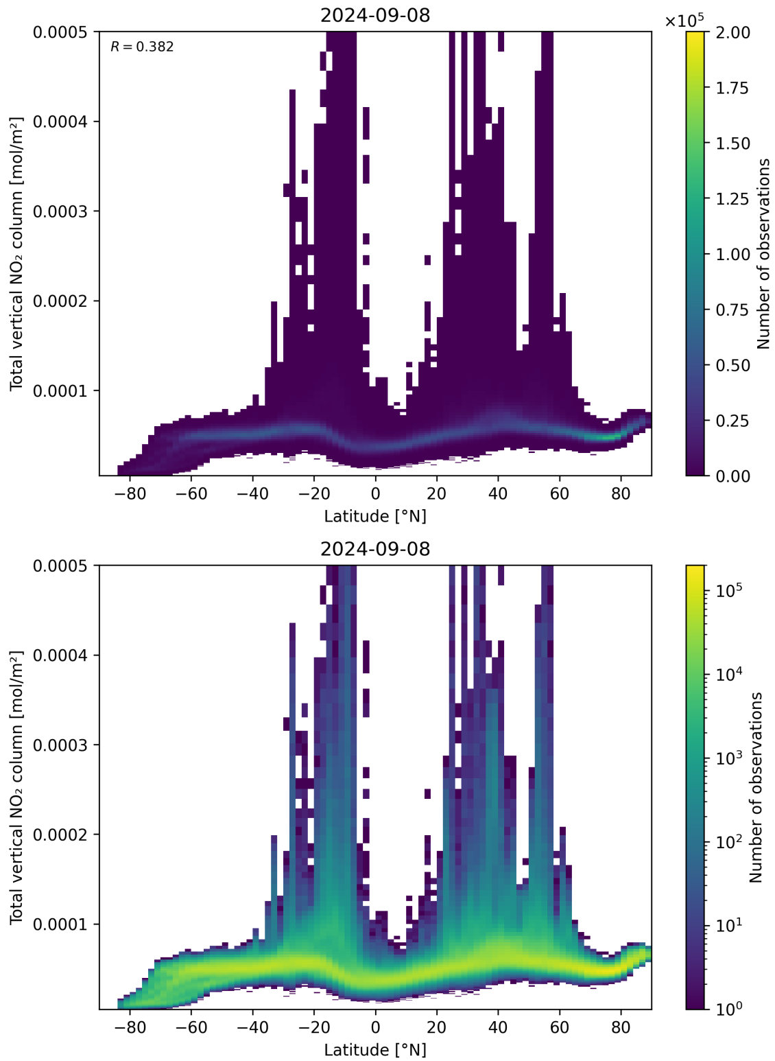
Figure 90: Scatter density plot of “Latitude” against “Total vertical NO 2 column” for 2024-09-07 to 2024-09-09.
