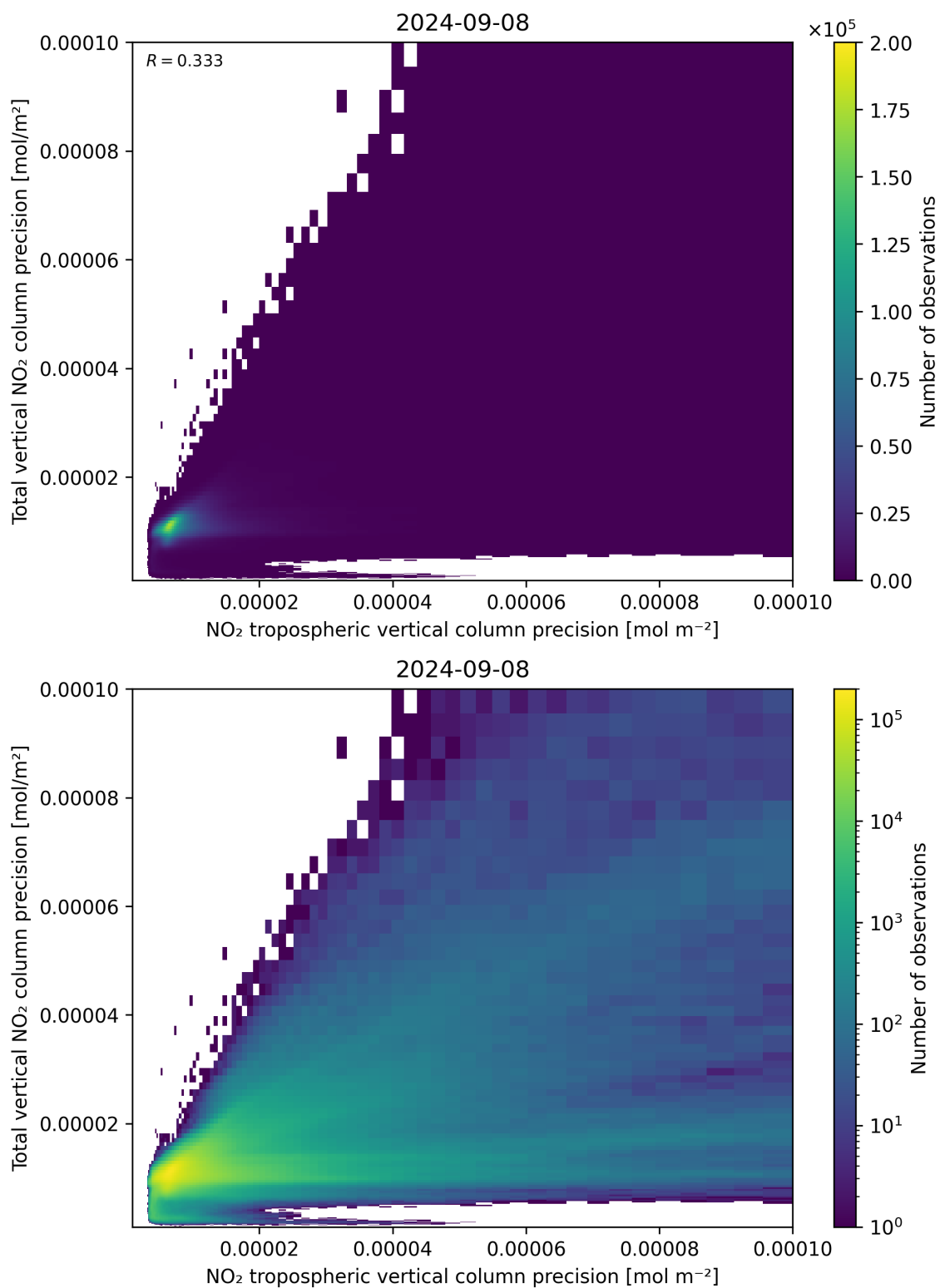
Figure 139: Scatter density plot of “NO 2 tropospheric vertical column precision” against “Total vertical NO 2 column precision” for 2024-09-07 to 2024-09-09.
