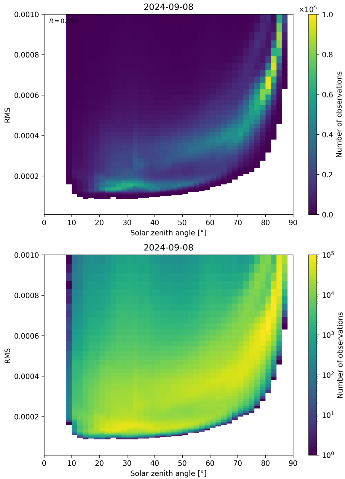
Figure 157: Scatter density plot of “Solar zenith angle” against “RMS” for 2024-09-07 to 2024-09-09.
