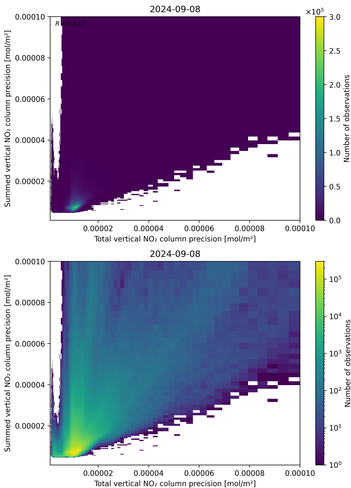
Figure 118: Scatter density plot of “Total vertical NO 2 column precision” against “Summed vertical NO 2 column precision” for 2024-09-07 to 2024-09-09.
