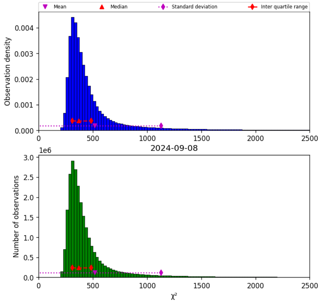
Figure 42: Histogram of “ \chi^2 ” for 2024-09-07 to 2024-09-09
