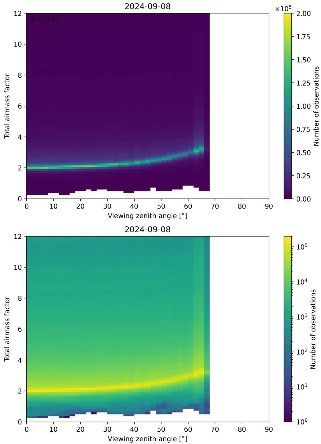
Figure 160: Scatter density plot of “Viewing zenith angle” against “Total airmass factor” for 2024-09-07 to 2024-09-09.
