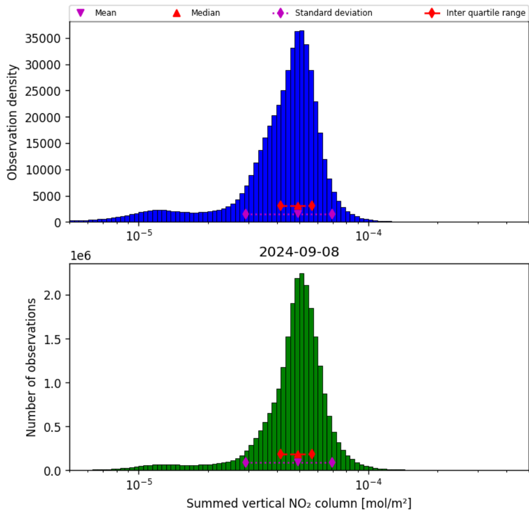
Figure 40: Histogram of “Summed vertical NO 2 column” for 2024-09-07 to 2024-09-09
