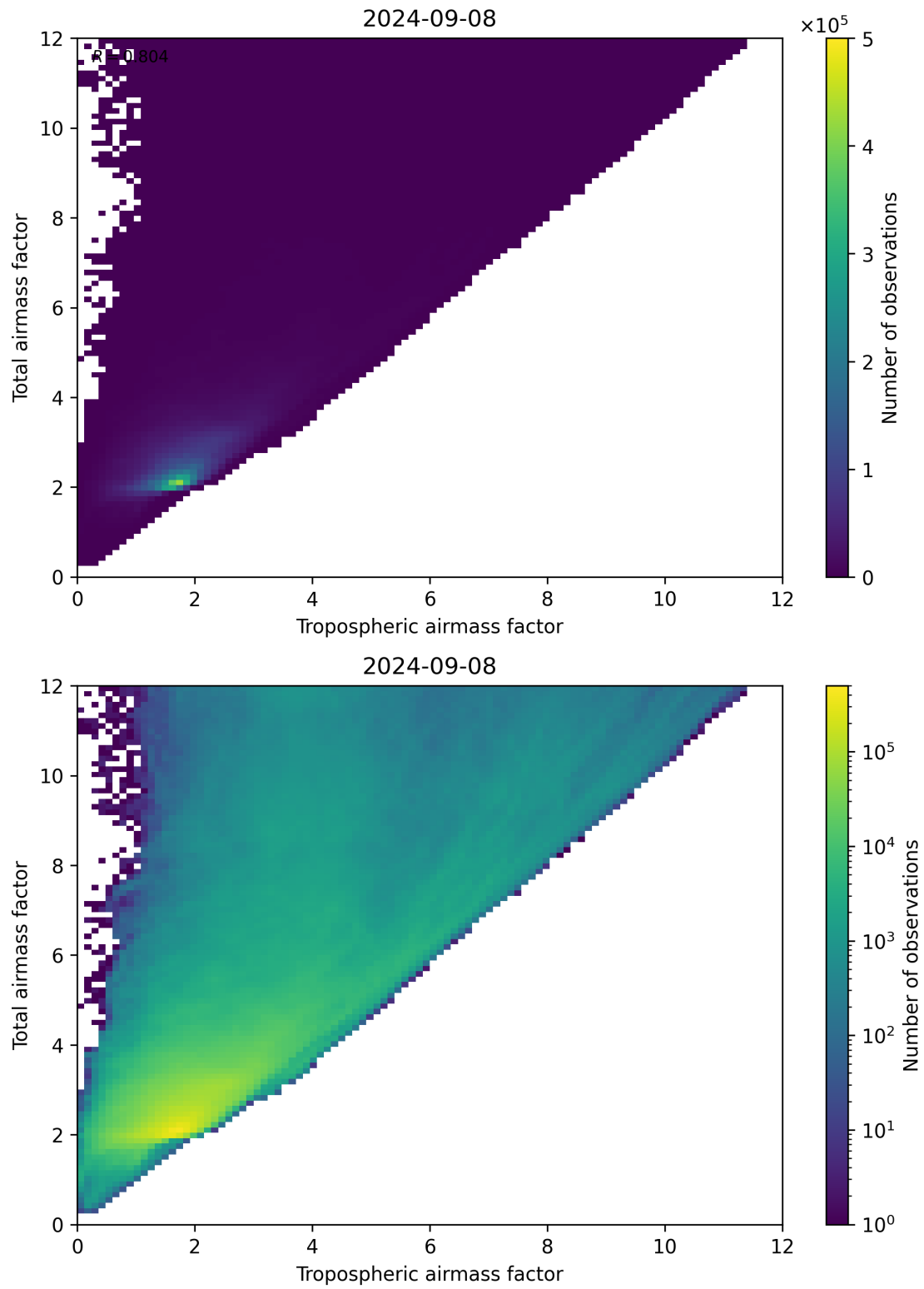
Figure 72: Scatter density plot of “Tropospheric airmass factor” against “Total airmass factor” for 2024-09-07 to 2024-09-09.
