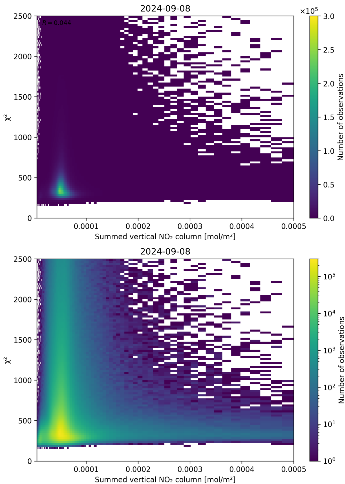
Figure 104: Scatter density plot of “Summed vertical NO 2 column” against “ \chi^2 ” for 2024-09-07 to 2024-09-09.
