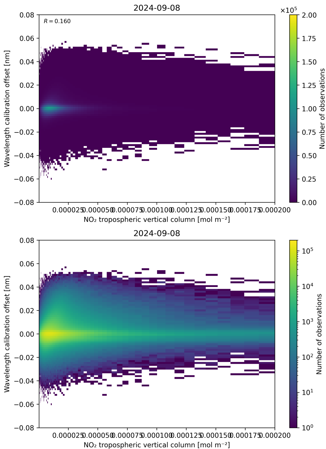
Figure 143: Scatter density plot of “NO 2 tropospheric vertical column” against “Wavelength calibration offset” for 2024-09-07 to 2024-09-09.
