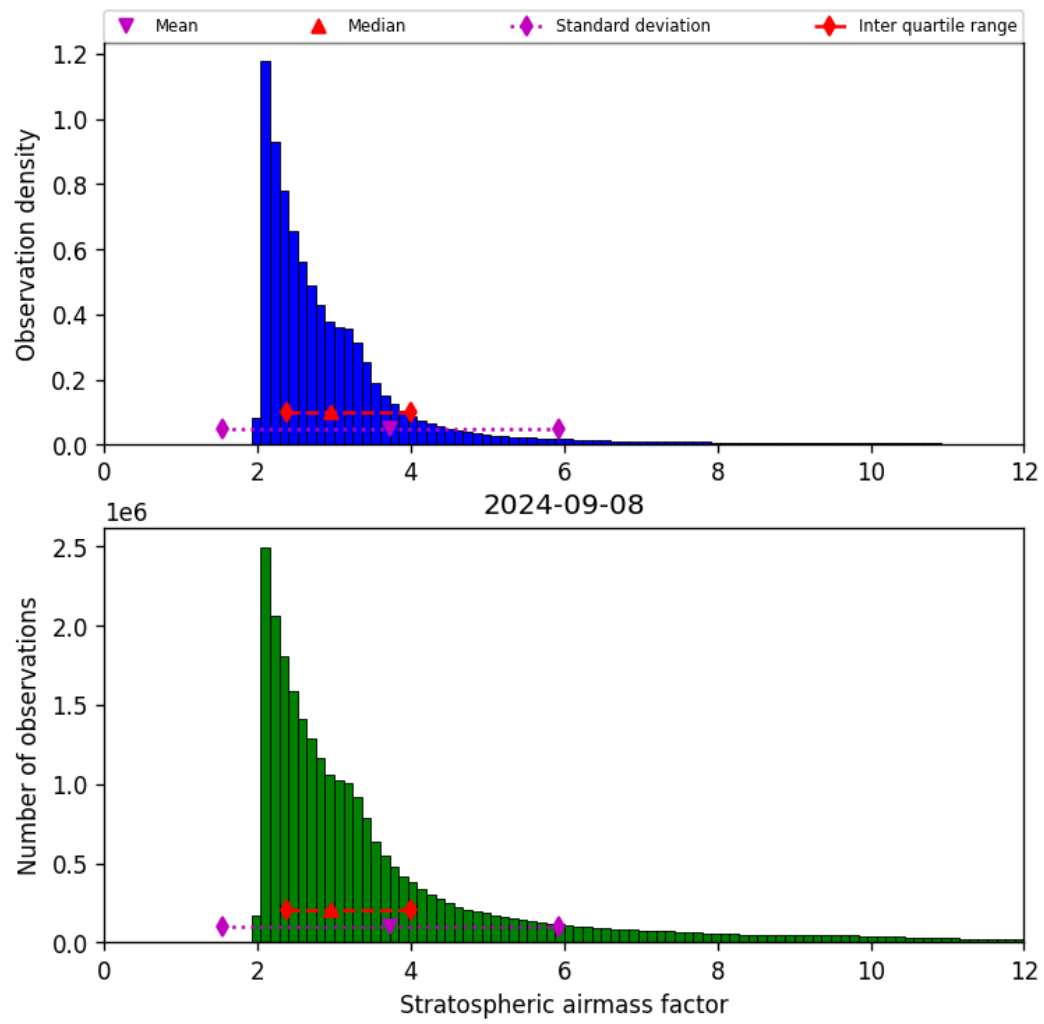
Figure 44: Histogram of “Stratospheric airmass factor” for 2024-09-07 to 2024-09-09
