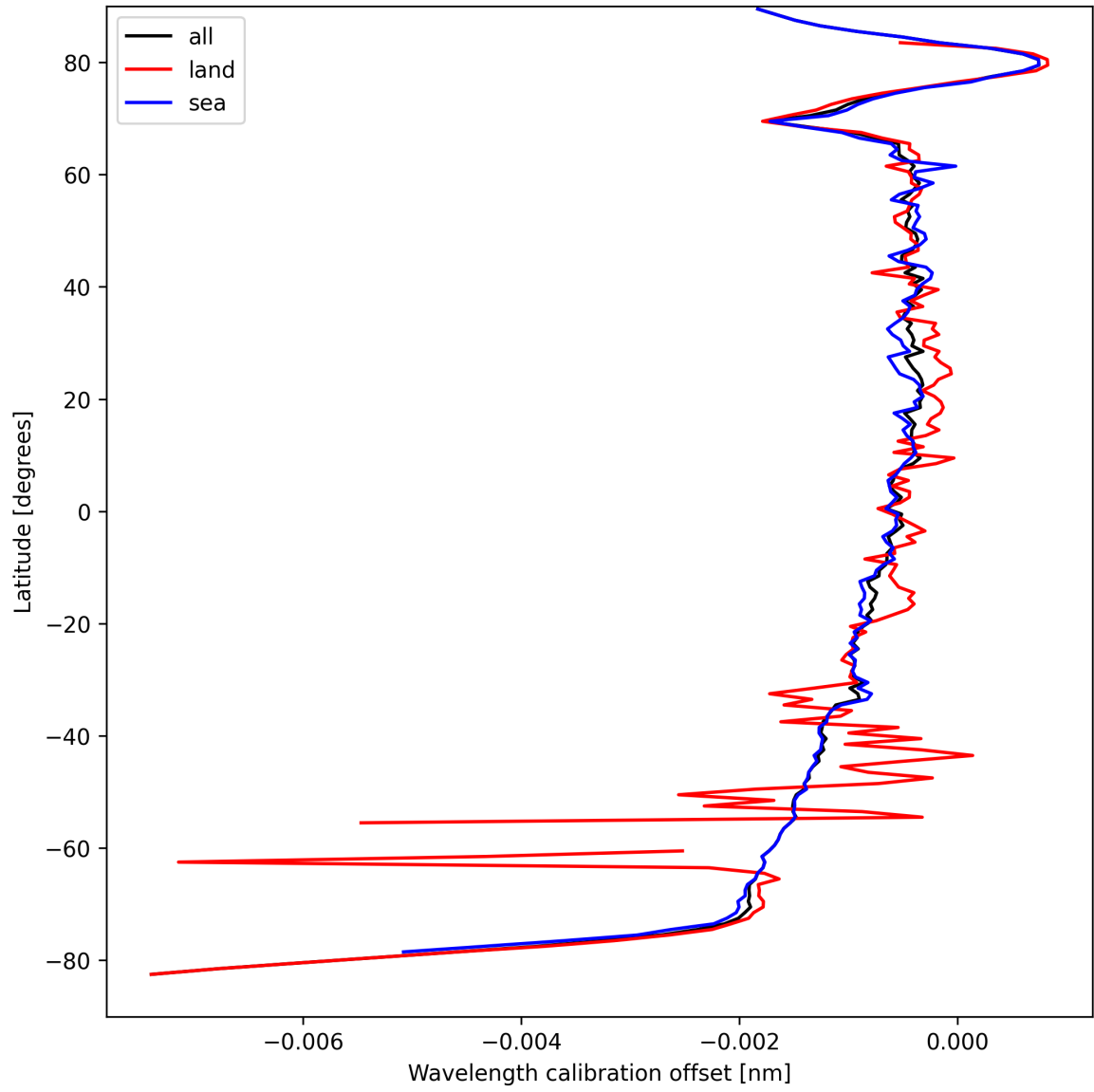
Figure 18: Zonal average of “Wavelength calibration offset” for 2024-09-07 to 2024-09-09.
