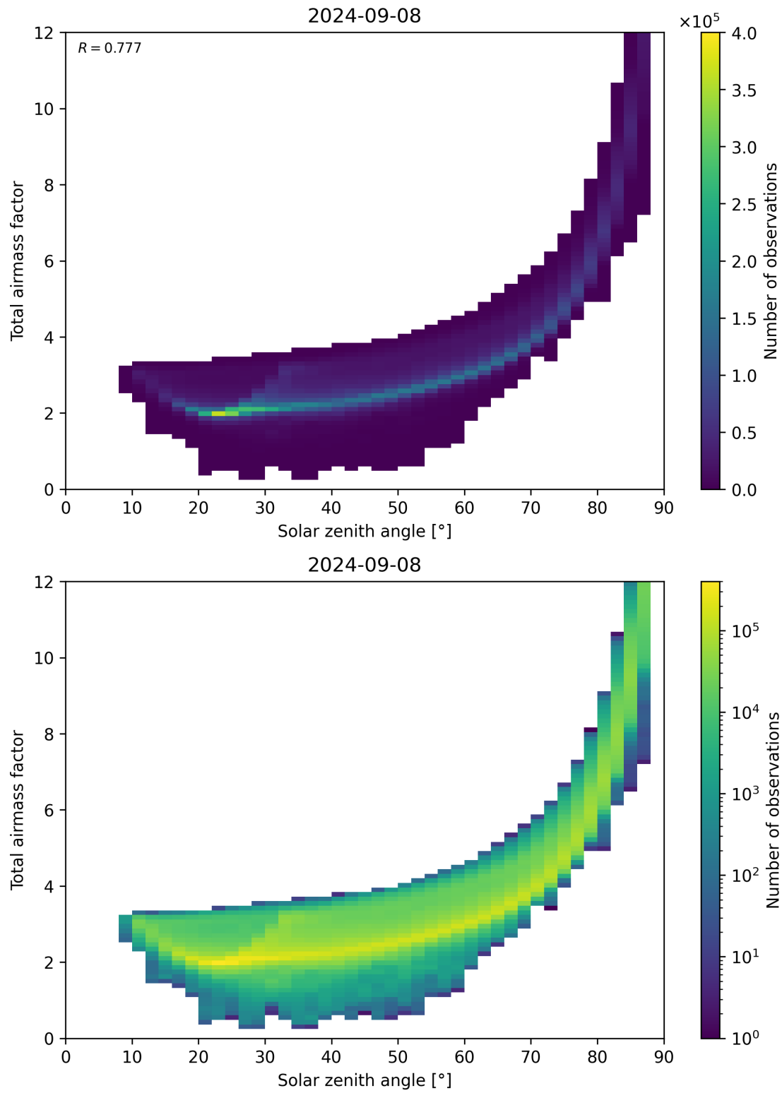
Figure 146: Scatter density plot of “Solar zenith angle” against “Total air mass factor” for 2024-09-07 to 2024-09-09.
