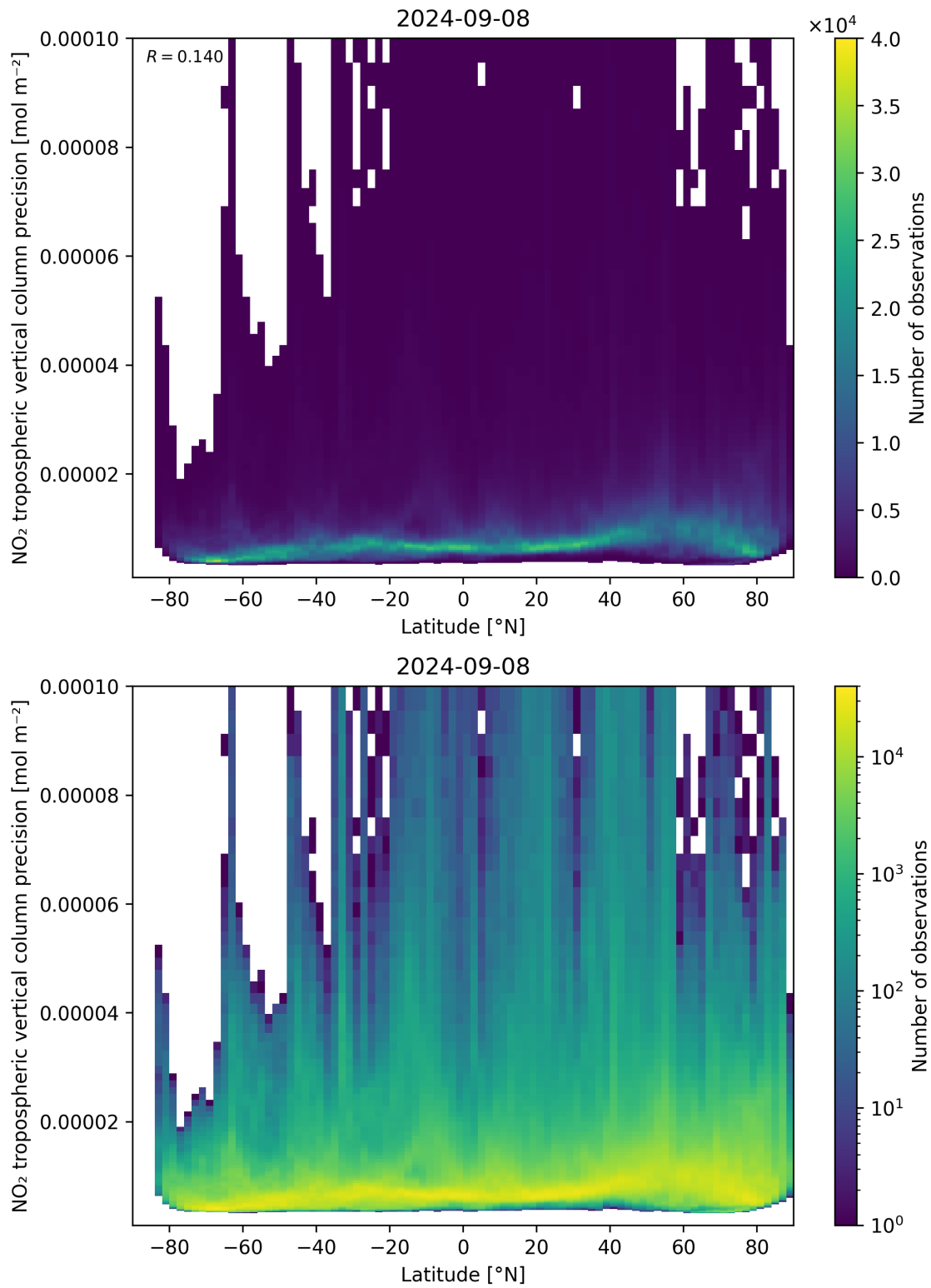
Figure 93: Scatter density plot of “Latitude” against “NO 2 tropospheric vertical column precision” for 2024-09-07 to 2024-09-09.
