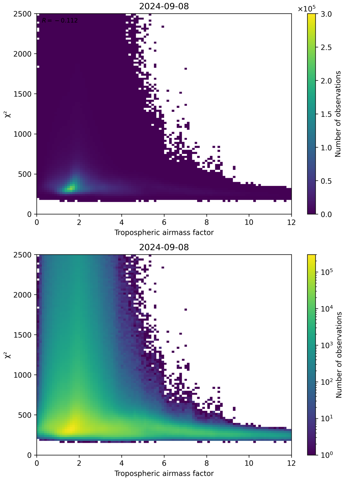
Figure 73: Scatter density plot of “Tropospheric airmass factor” against “ \chi^2 ” for 2024-09-07 to 2024-09-09.
