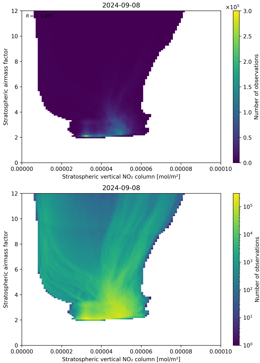
Figure 96: Scatter density plot of “Stratospheric vertical NO 2 column” against “Stratospheric airmass factor” for 2024-09-07 to 2024-09-09.
