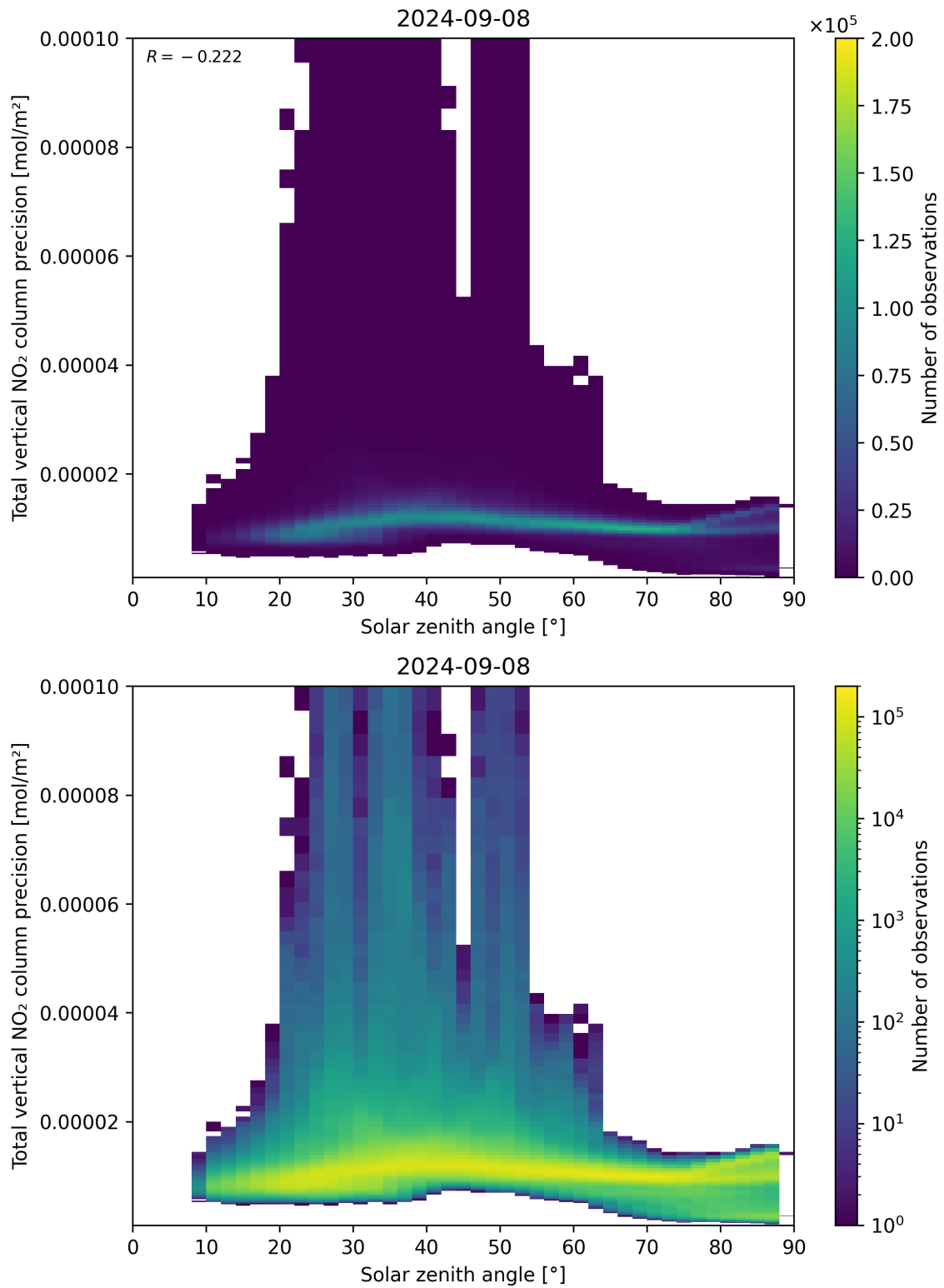
Figure 154: Scatter density plot of “Solar zenith angle” against “Total vertical NO 2 column precision” for 2024-09-07 to 2024-09-09.
