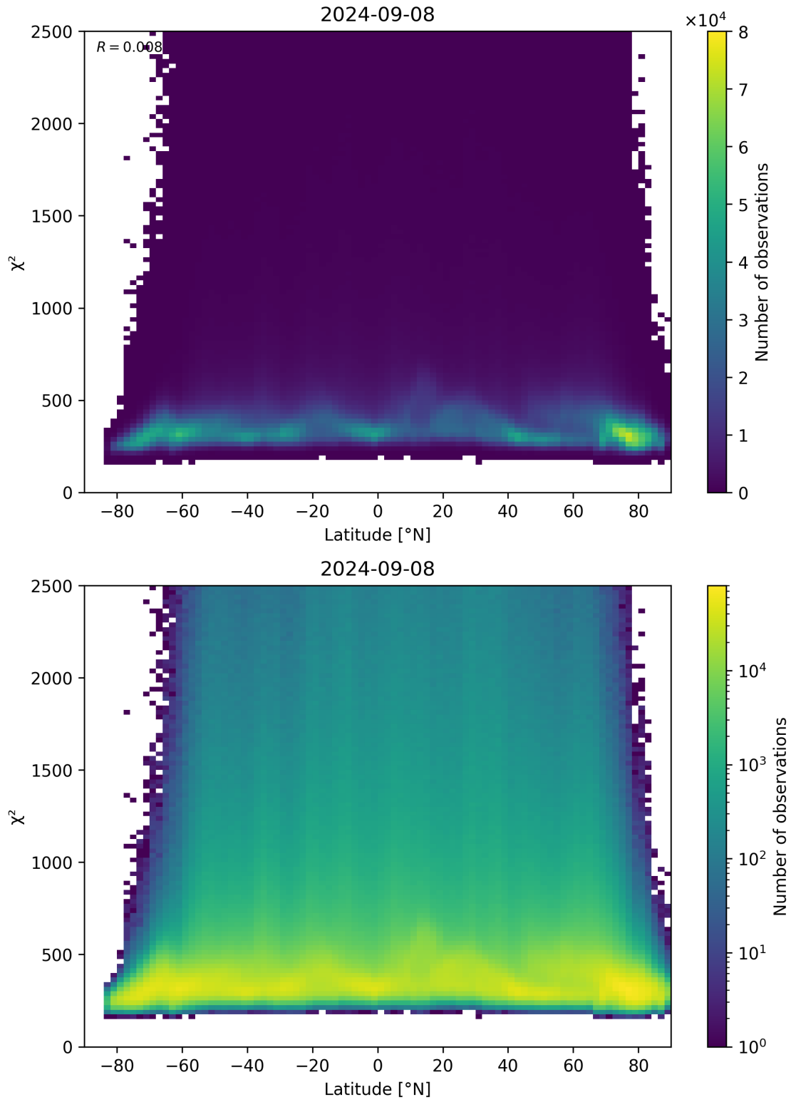
Figure 86: Scatter density plot of “Latitude” against “ \chi^2 ” for 2024-09-07 to 2024-09-09.
