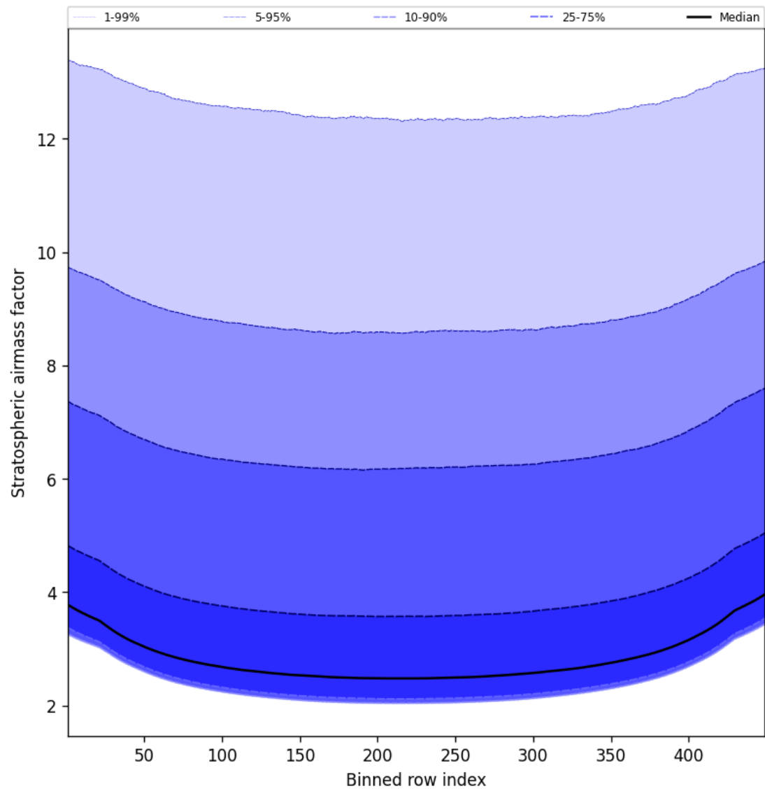
Figure 61: Along track statistics of “Stratospheric air mass factor” for 2024-09-07 to 2024-09-09
