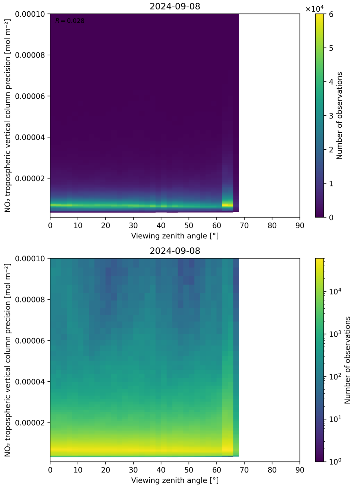
Figure 170: Scatter density plot of “Viewing zenith angle” against “NO 2 tropospheric vertical column precision” for 2024-09-07 to 2024-09-09.
