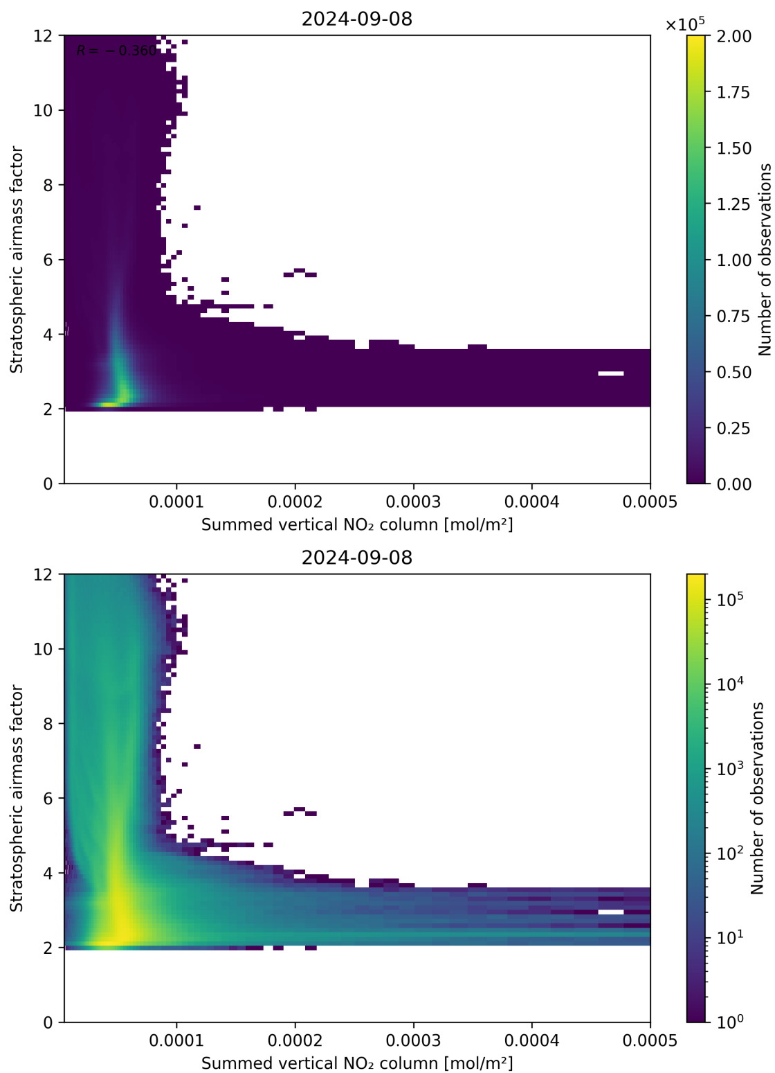
Figure 103: Scatter density plot of “Summed vertical NO 2 column” against “Stratospheric air mass factor” for 2024-09-07 to 2024-09-09.
