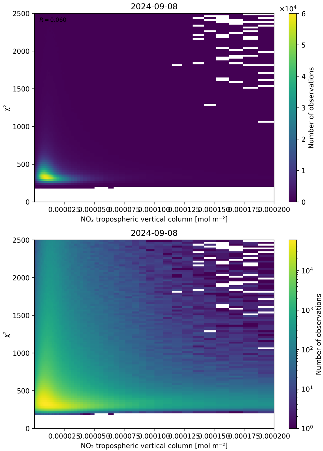
Figure 124: Scatter density plot of “NO 2 tropospheric vertical column” against “ \chi^2 ” for 2024-09-07 to 2024-09-09.
