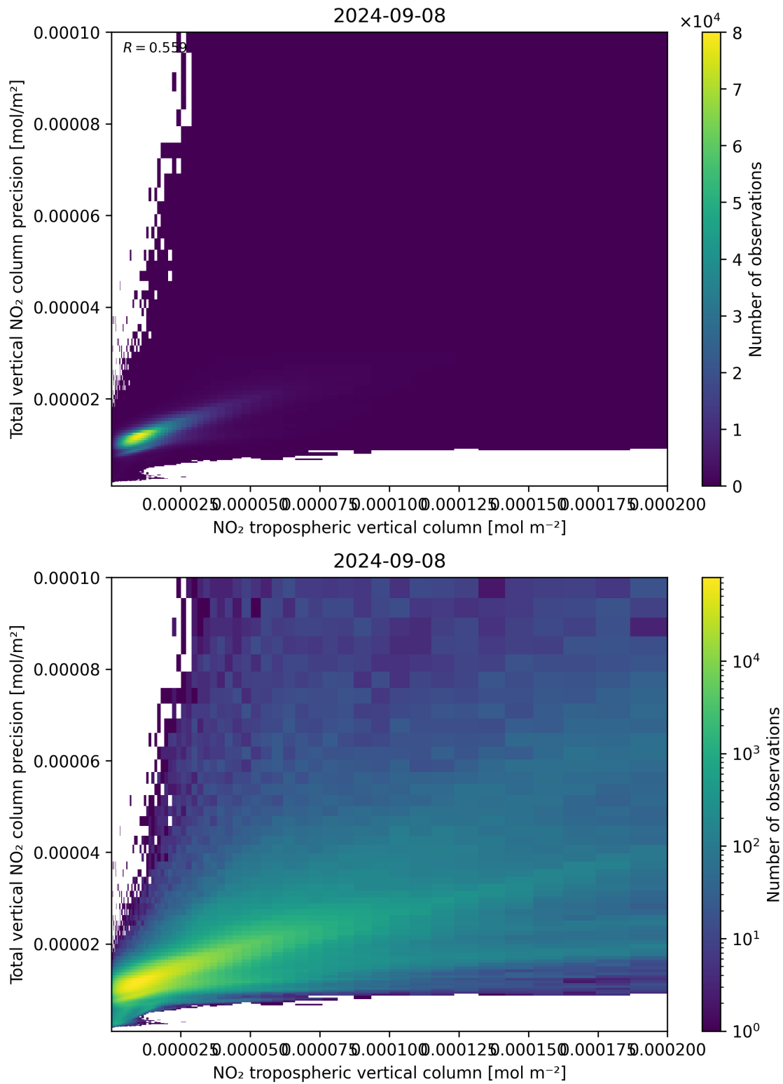
Figure 129: Scatter density plot of “NO 2 tropospheric vertical column” against “Total vertical NO 2 column precision” for 2024-09-07 to 2024-09-09.
