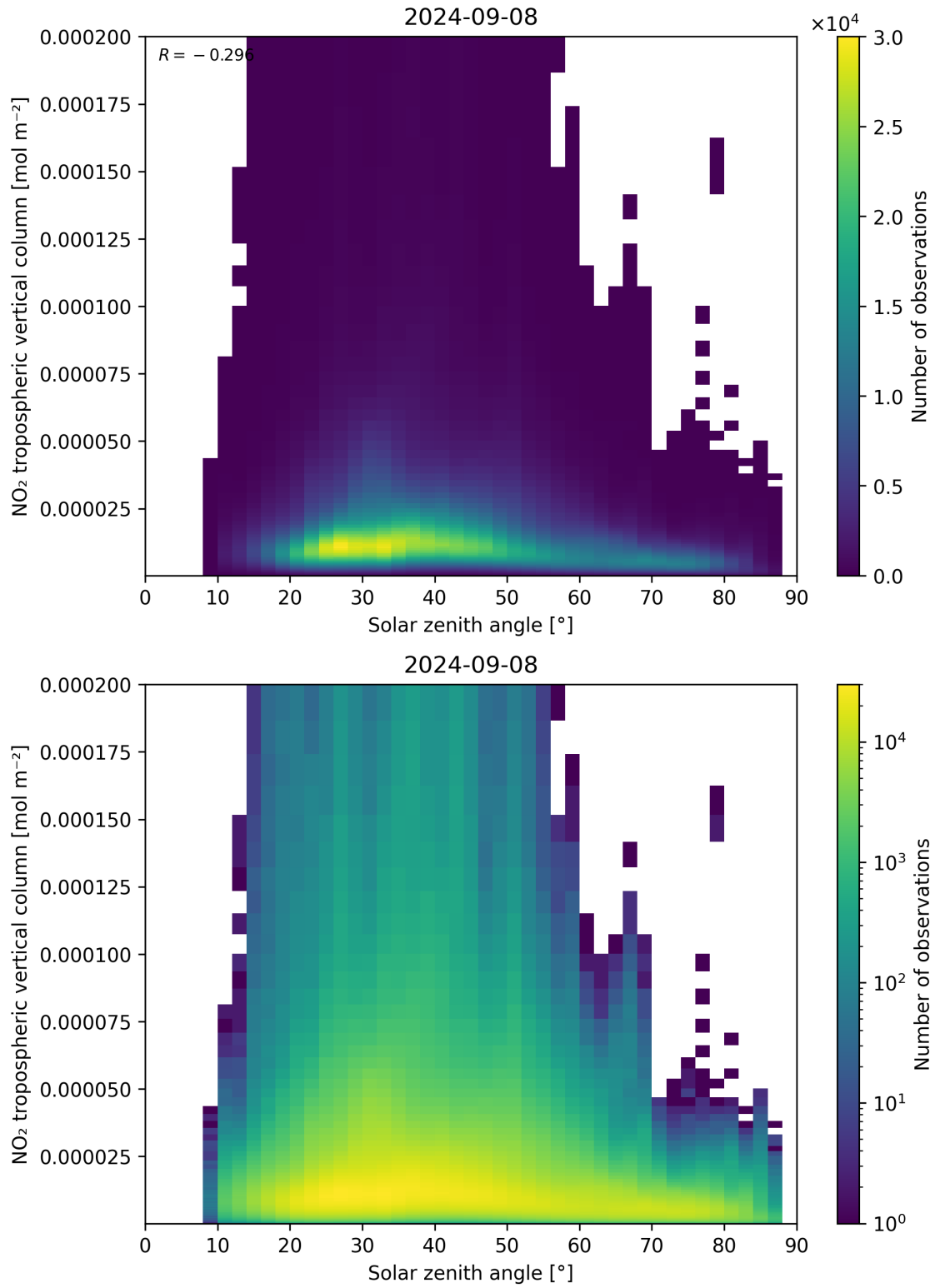
Figure 155: Scatter density plot of “Solar zenith angle” against “NO 2 tropospheric vertical column” for 2024-09-07 to 2024-09-09.
