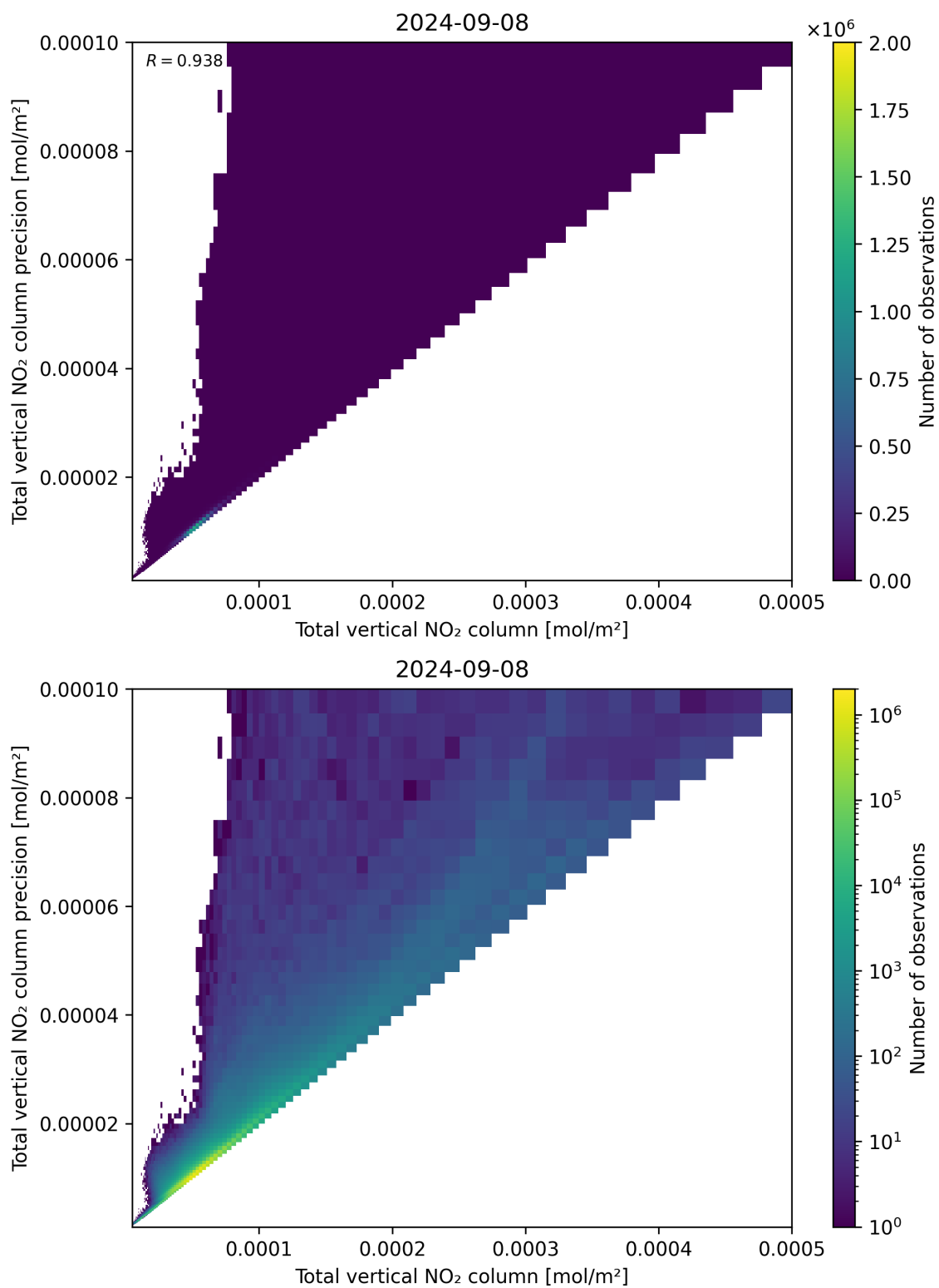
Figure 114: Scatter density plot of “Total vertical NO 2 column” against “Total vertical NO 2 column precision” for 2024-09-07 to 2024-09-09.
