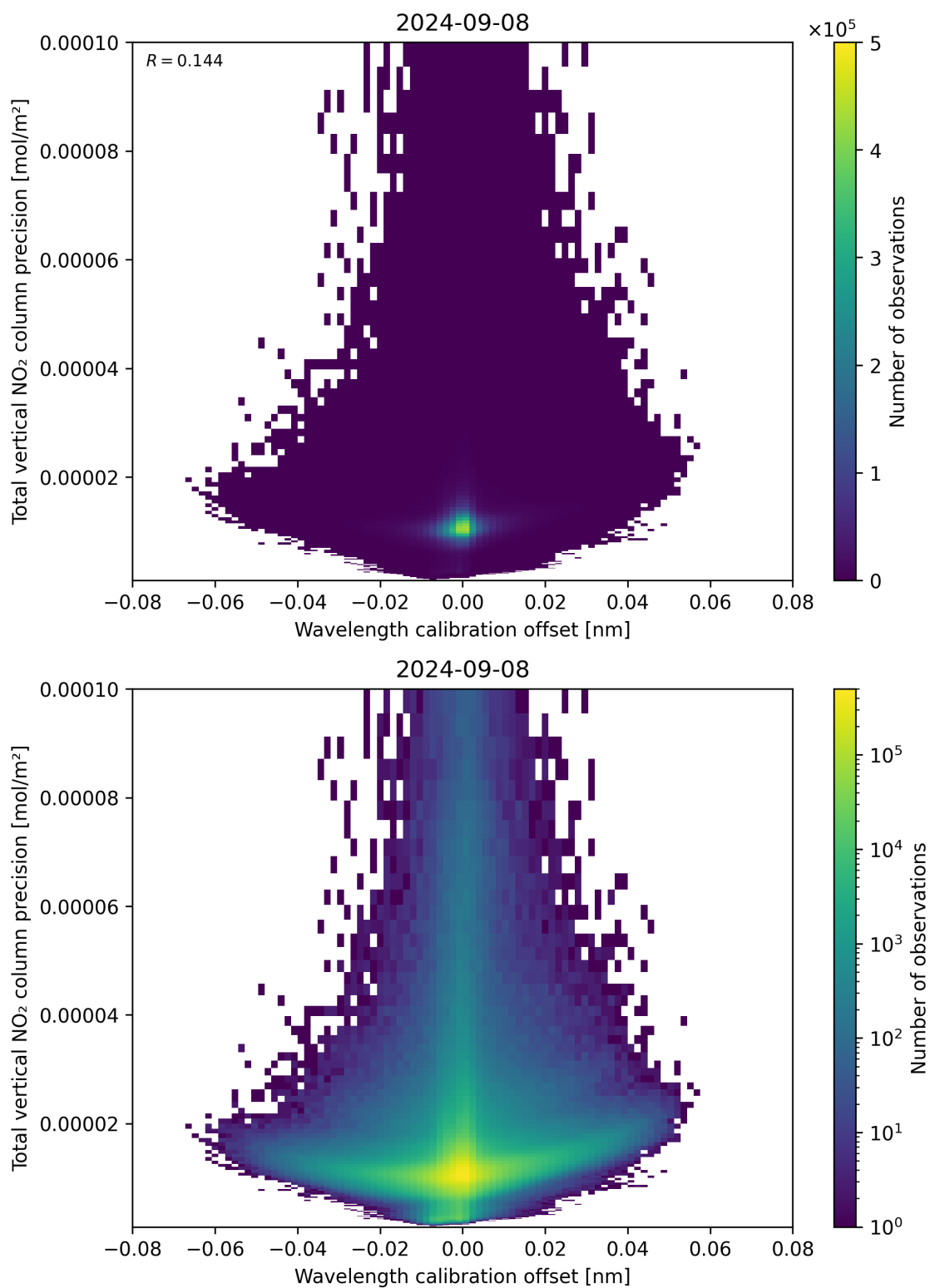
Figure 180: Scatter density plot of “Wavelength calibration offset” against “Total vertical NO 2 column precision” for 2024-09-07 to 2024-09-09.
