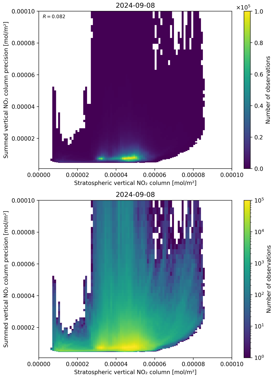
Figure 99: Scatter density plot of “Stratospheric vertical NO 2 column” against “Summed vertical NO 2 column precision” for 2024-09-07 to 2024-09-09.
