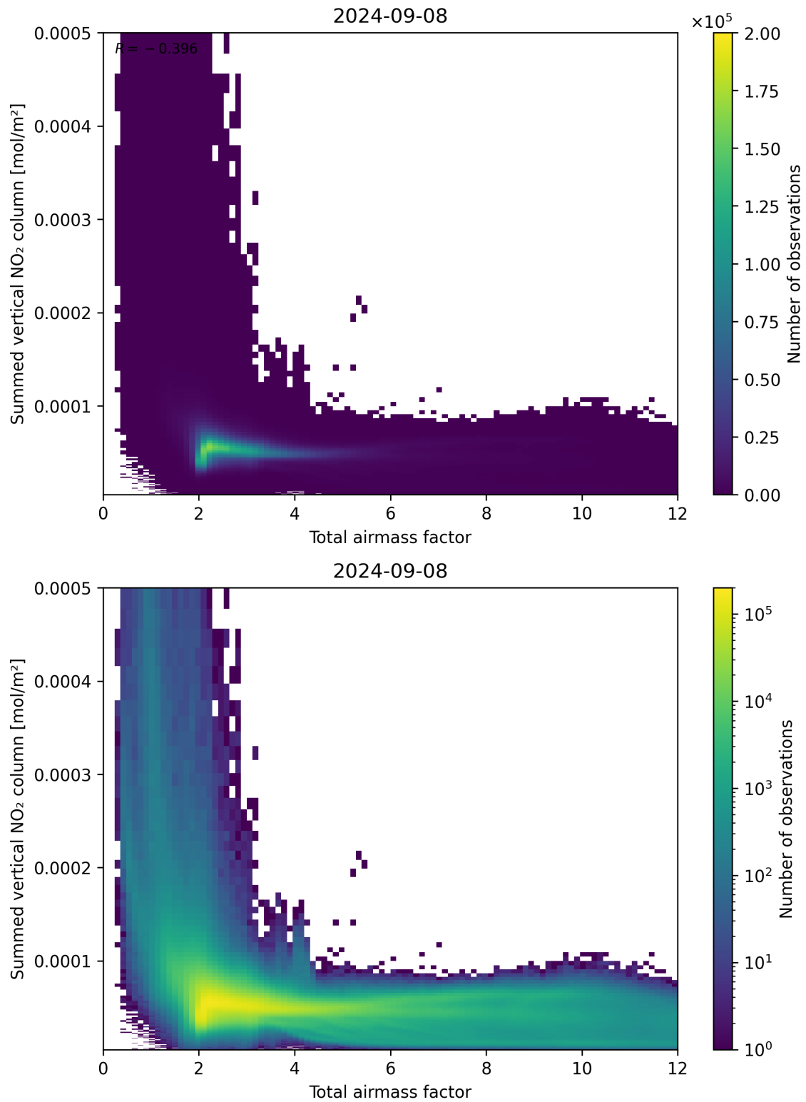
Figure 65: Scatter density plot of “Total airmass factor” against “Summed vertical NO 2 column” for 2024-09-07 to 2024-09-09.
