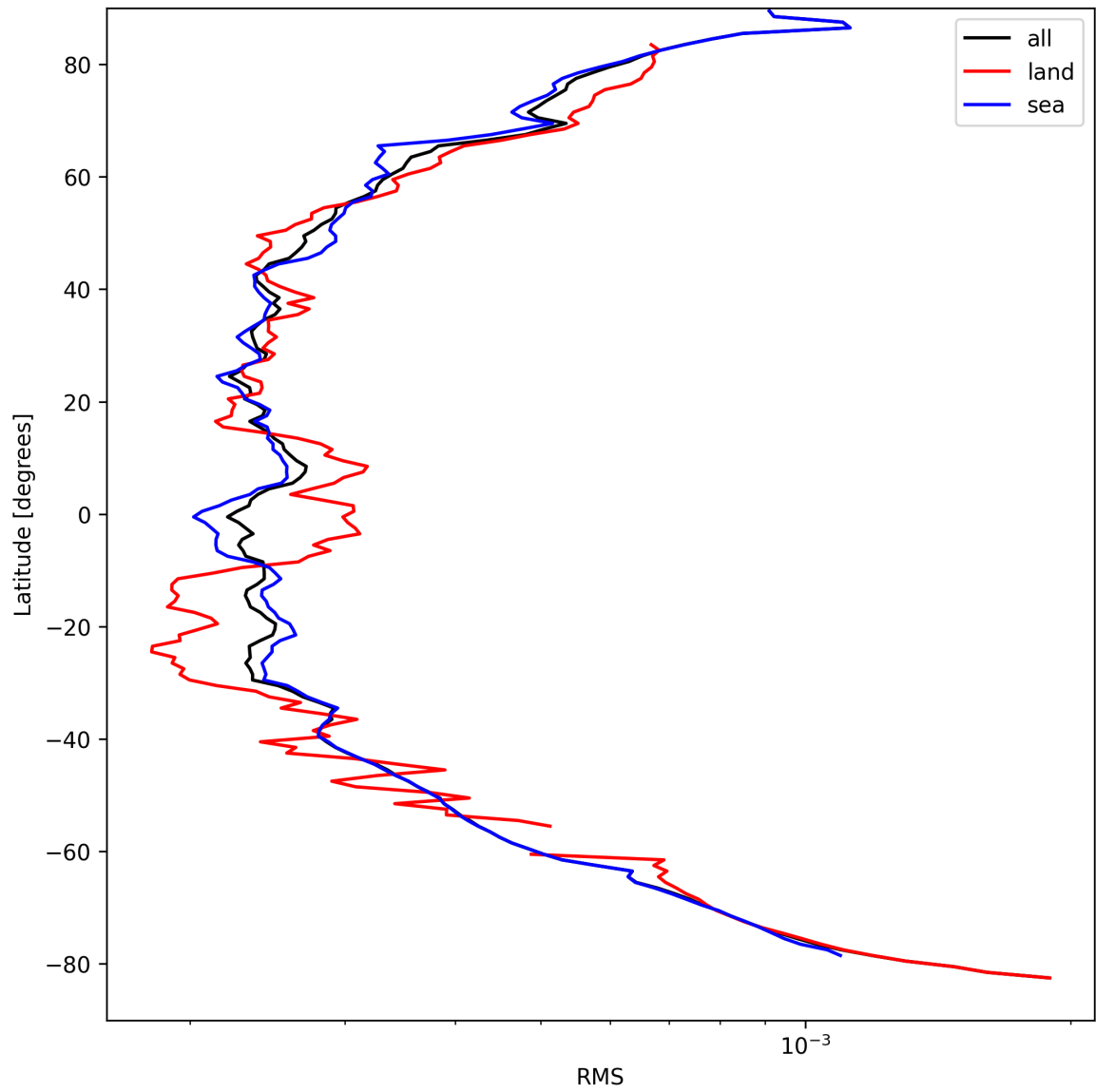
Figure 26: Zonal average of “RMS” for 2024-09-07 to 2024-09-09.
