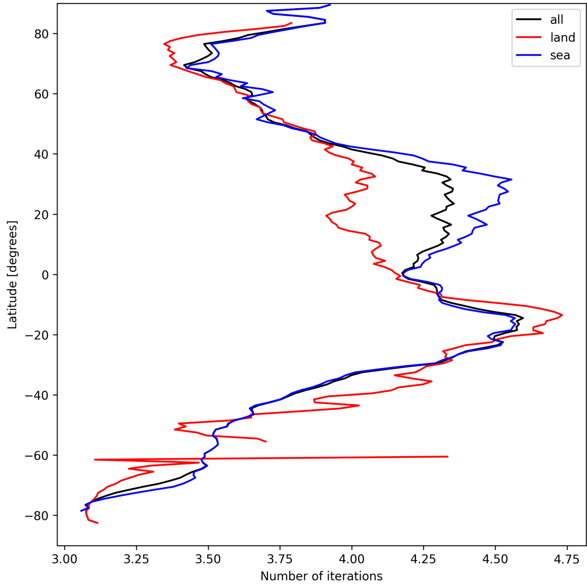
Figure 17: Zonal average of “Number of iterations” for 2024-09-07 to 2024-09-09.
