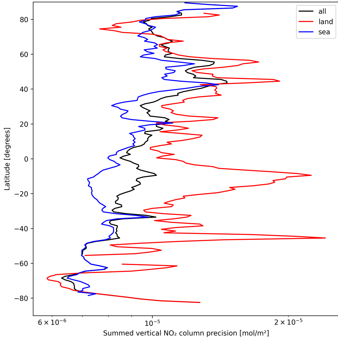
Figure 24: Zonal average of “Summed vertical NO 2 column precision” for 2024-09-07 to 2024-09-09.
