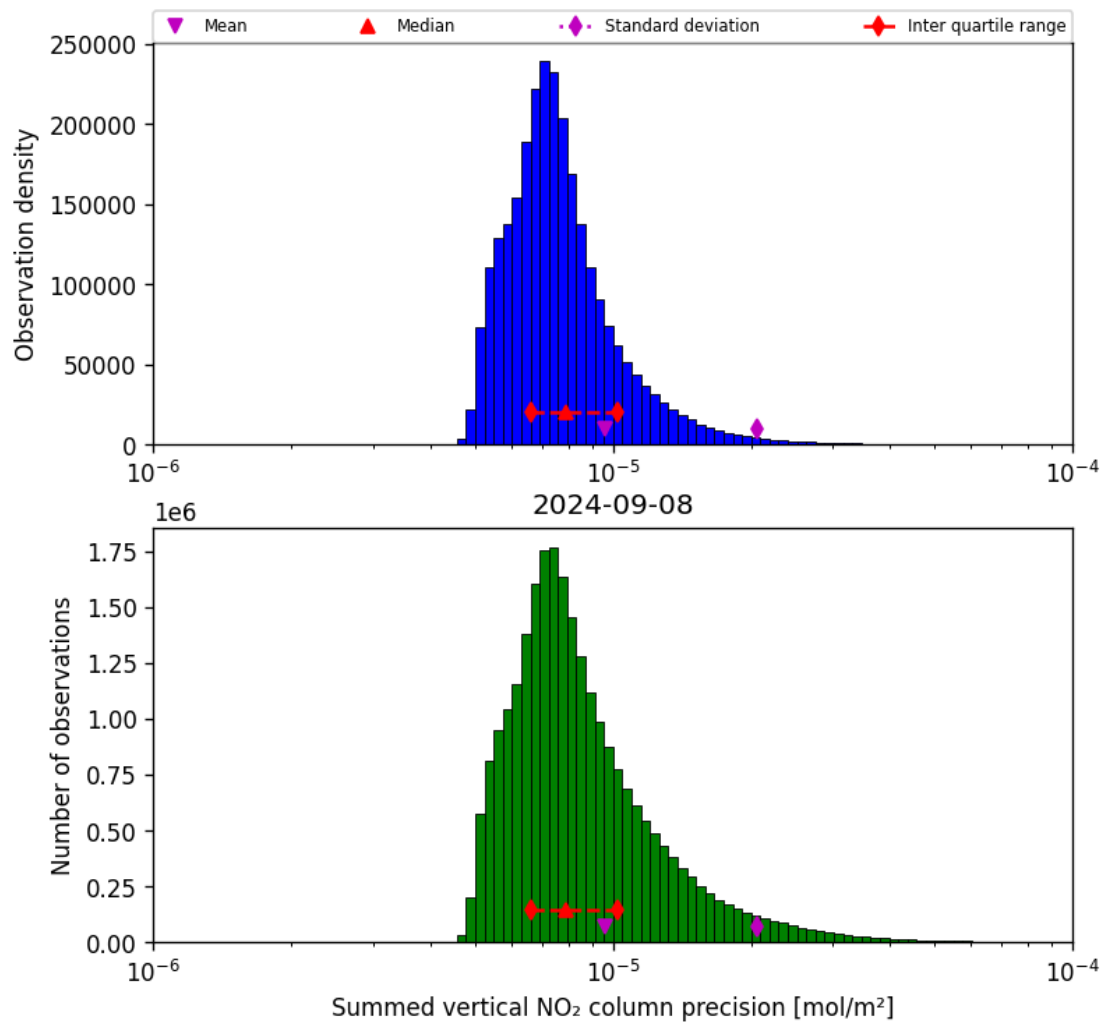
Figure 41: Histogram of "Summed vertical NO 2 column precision" for 2024-09-07 to 2024-09-09
