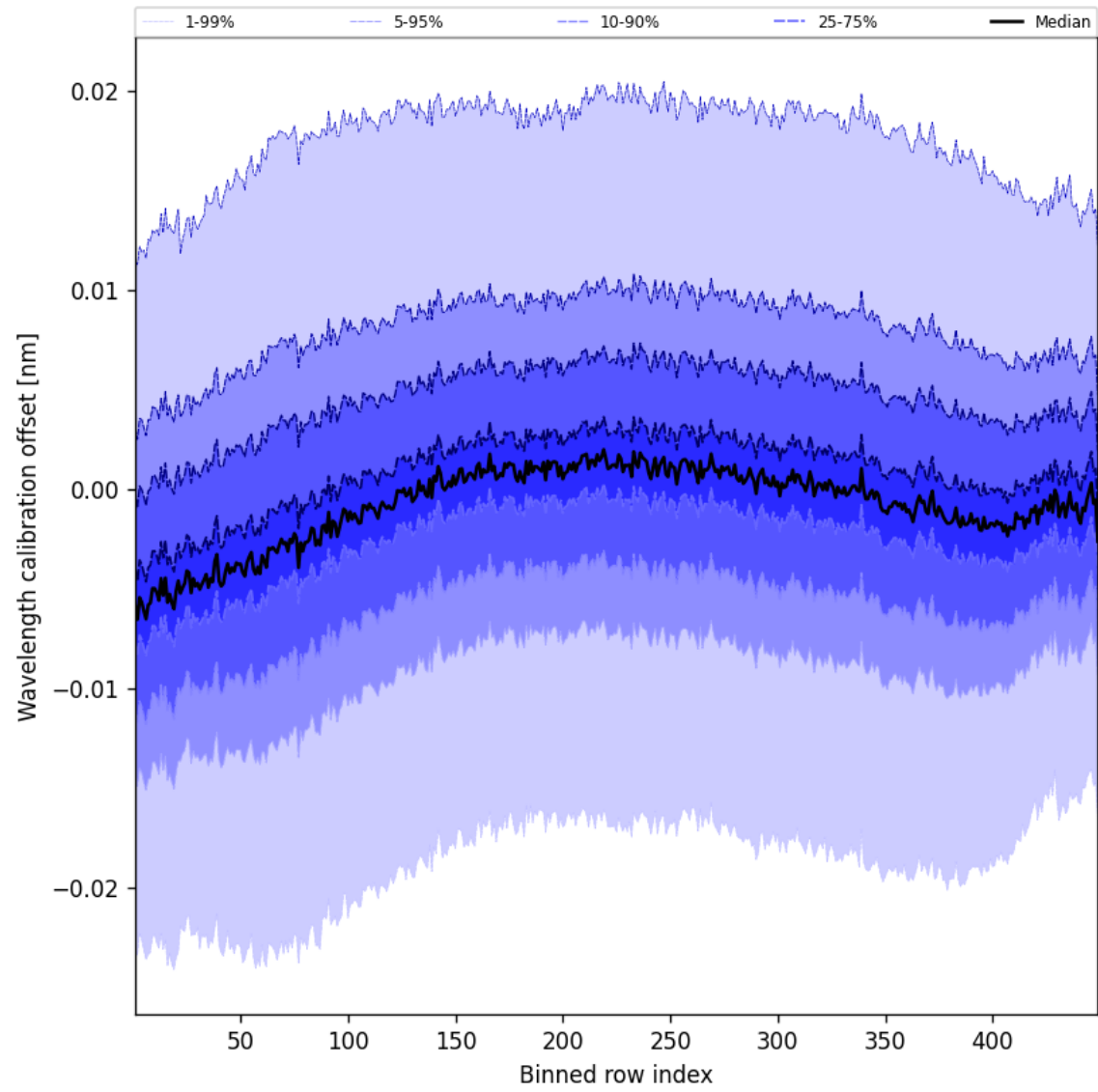
Figure 52: Along track statistics of “Wavelength calibration offset” for 2024-09-07 to 2024-09-09
