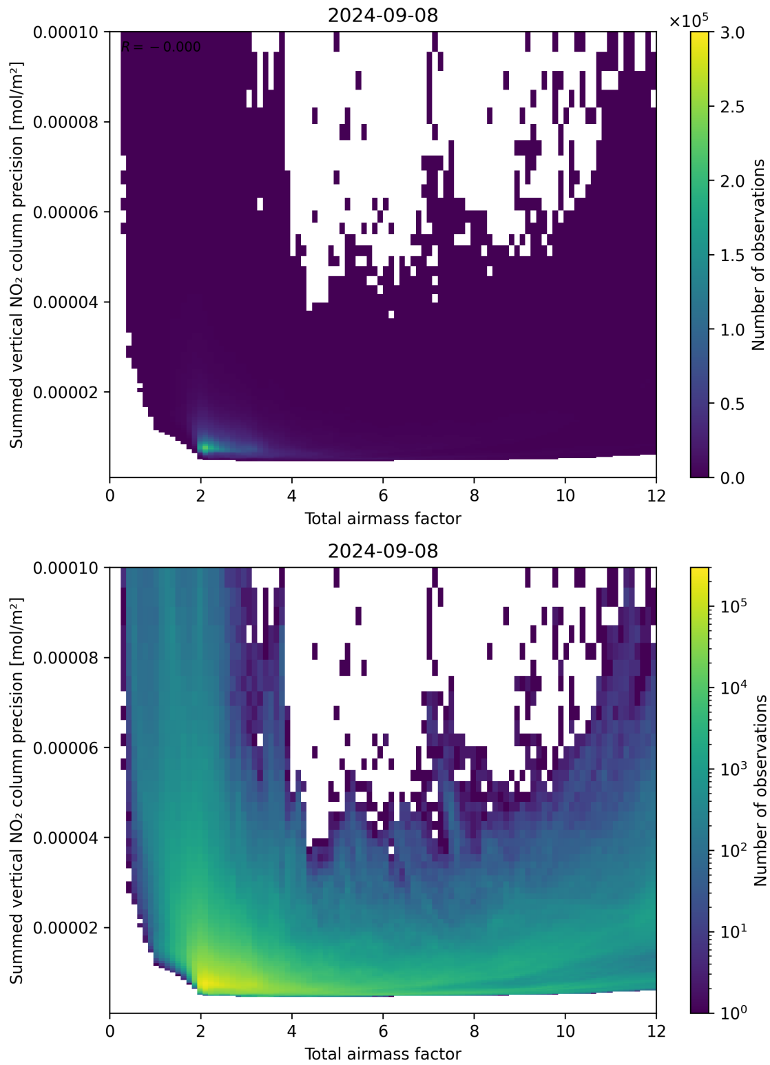
Figure 66: Scatter density plot of “Total airmass factor” against “Summed vertical NO 2 column precision” for 2024-09-07 to 2024-09-09.
