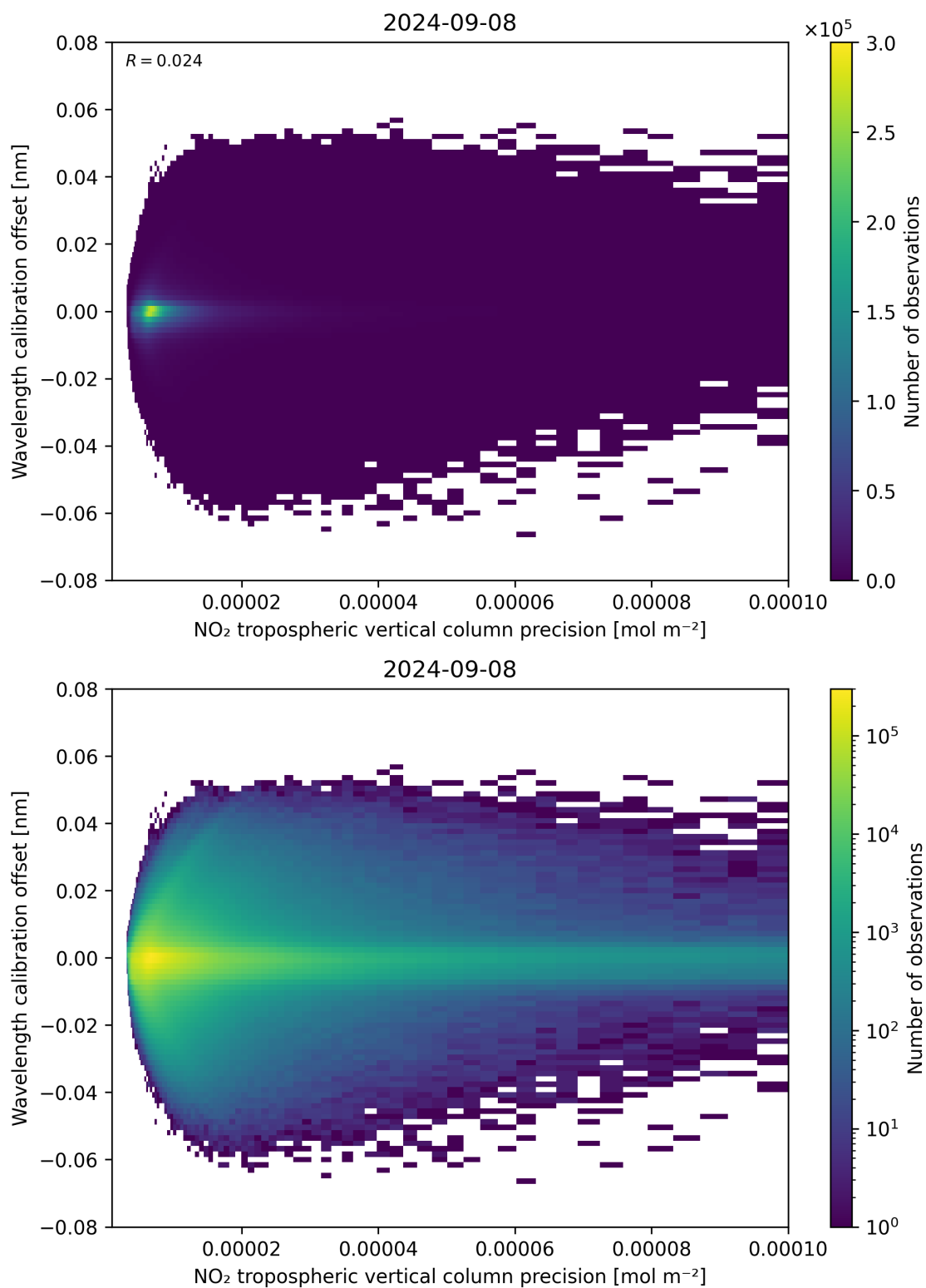
Figure 141: Scatter density plot of “NO 2 tropospheric vertical column precision” against “Wavelength calibration offset” for 2024-09-07 to 2024-09-09.
