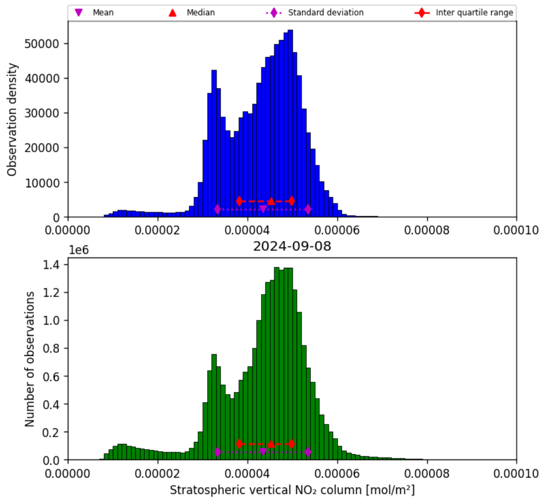
Figure 36: Histogram of “Stratospheric vertical NO 2 column” for 2024-09-07 to 2024-09-09
