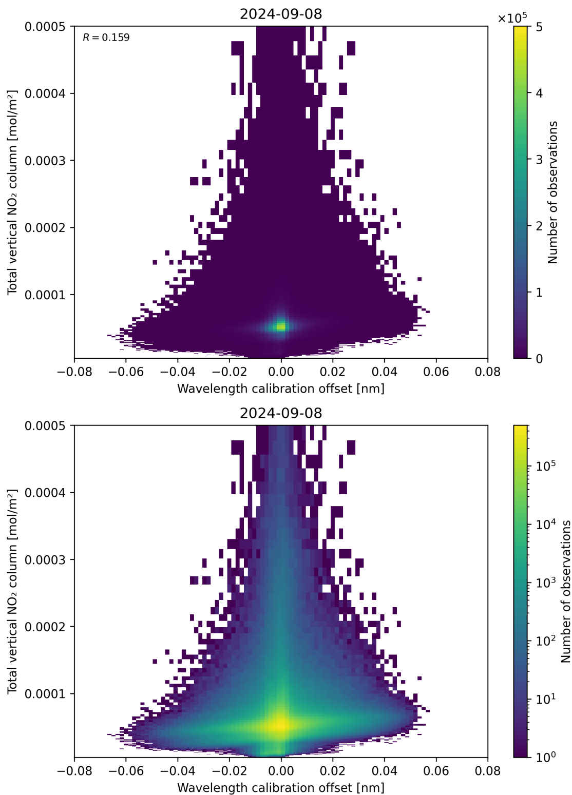
Figure 179: Scatter density plot of “Wavelength calibration offset” against “Total vertical NO 2 column” for 2024-09-07 to 2024-09-09.
