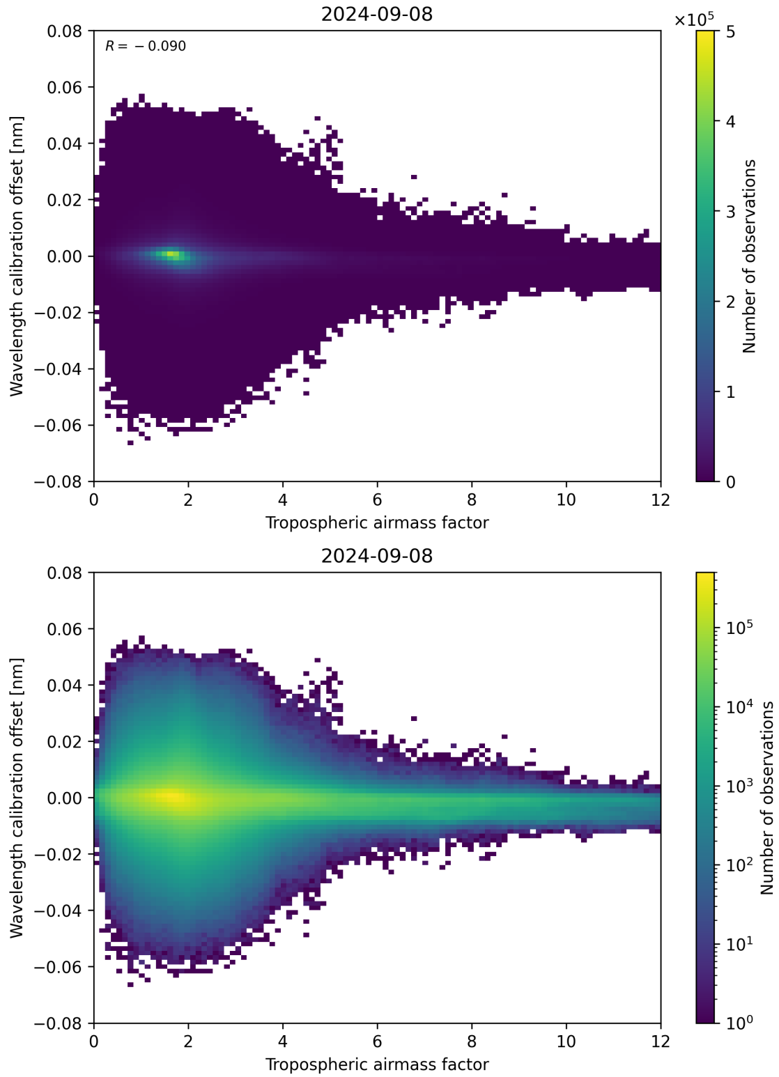
Figure 80: Scatter density plot of “Tropospheric airmass factor” against “Wavelength calibration offset” for 2024-09-07 to 2024-09-09.
