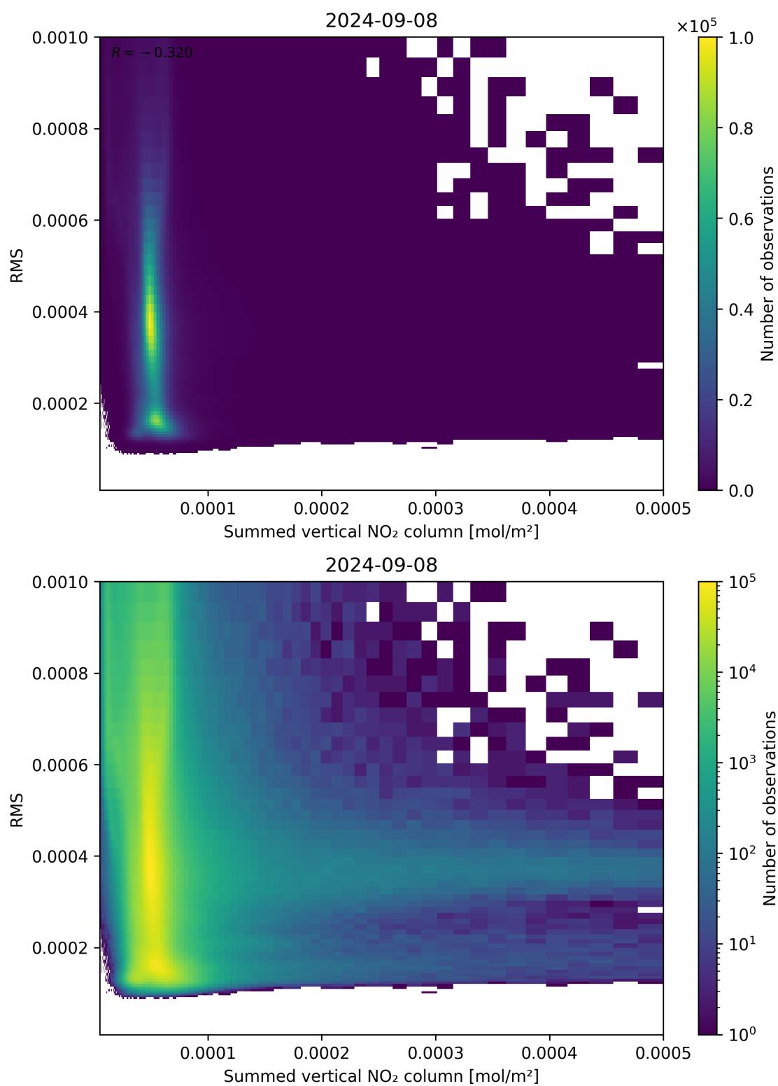
Figure 109: Scatter density plot of “Summed vertical NO 2 column” against “RMS” for 2024-09-07 to 2024-09-09.
