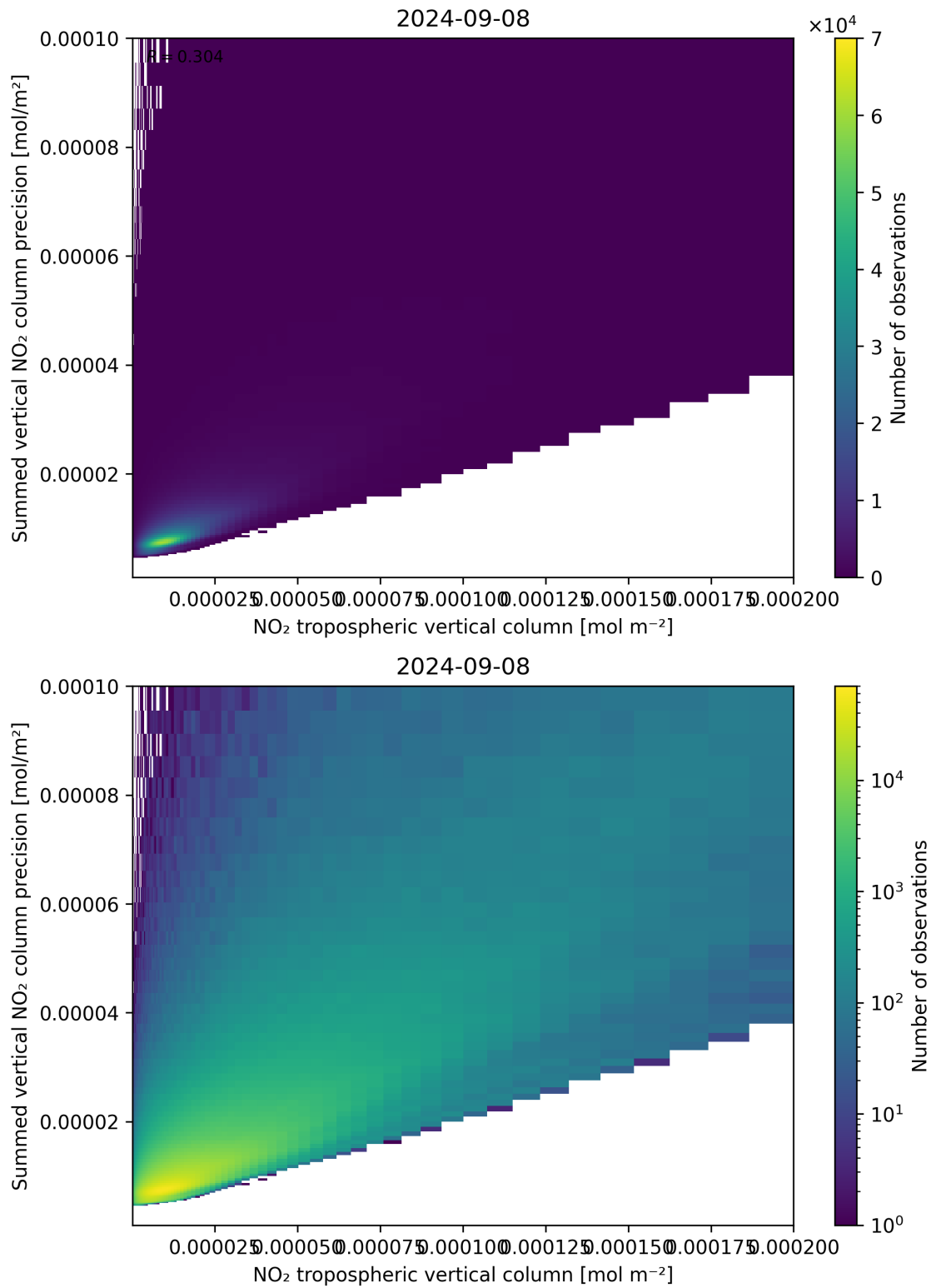
Figure 127: Scatter density plot of “NO 2 tropospheric vertical column” against “Summed vertical NO 2 column precision” for 2024-09-07 to 2024-09-09.
