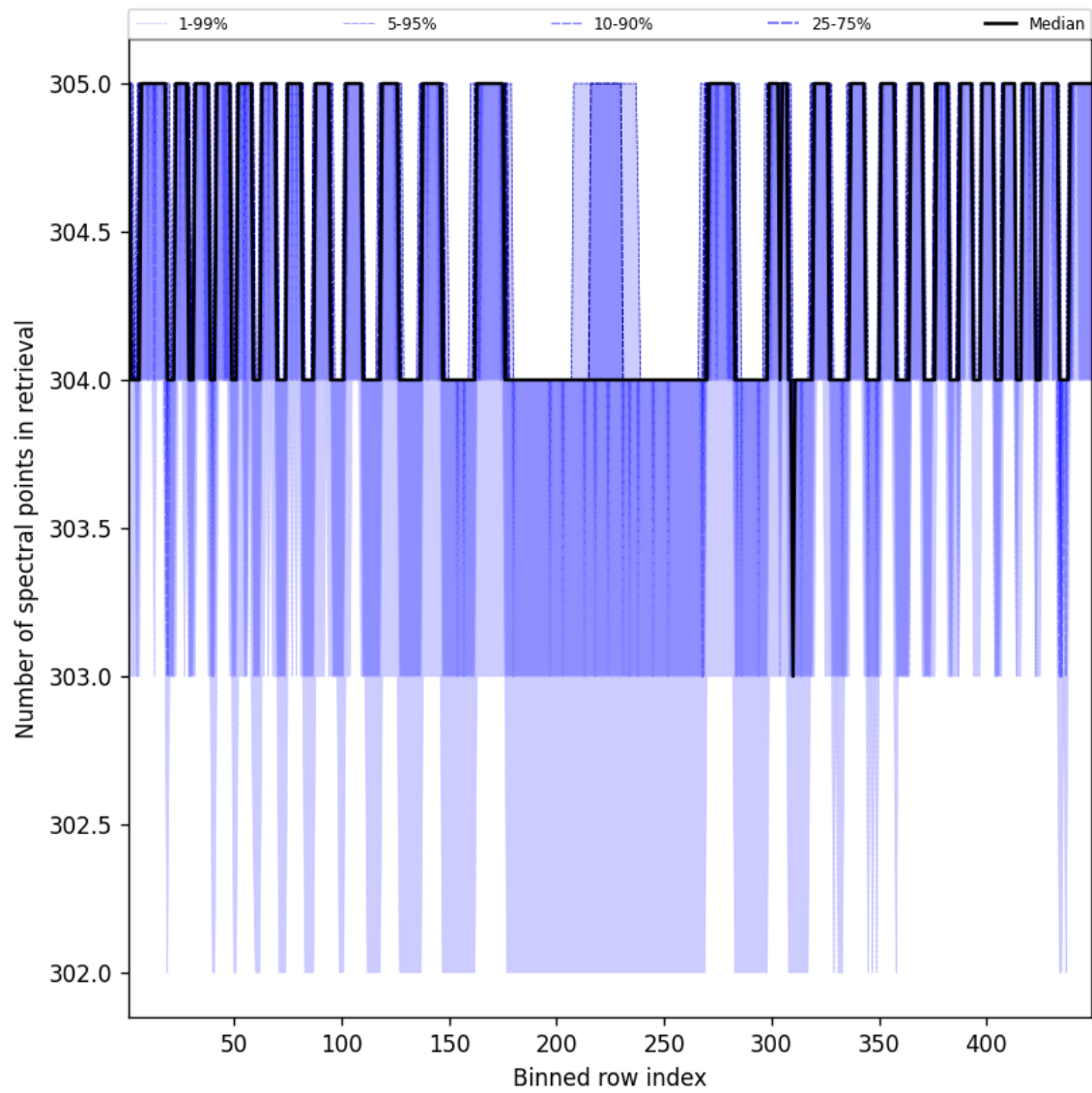
Figure 50: Along track statistics of “Number of spectral points in retrieval” for 2024-09-07 to 2024-09-09
