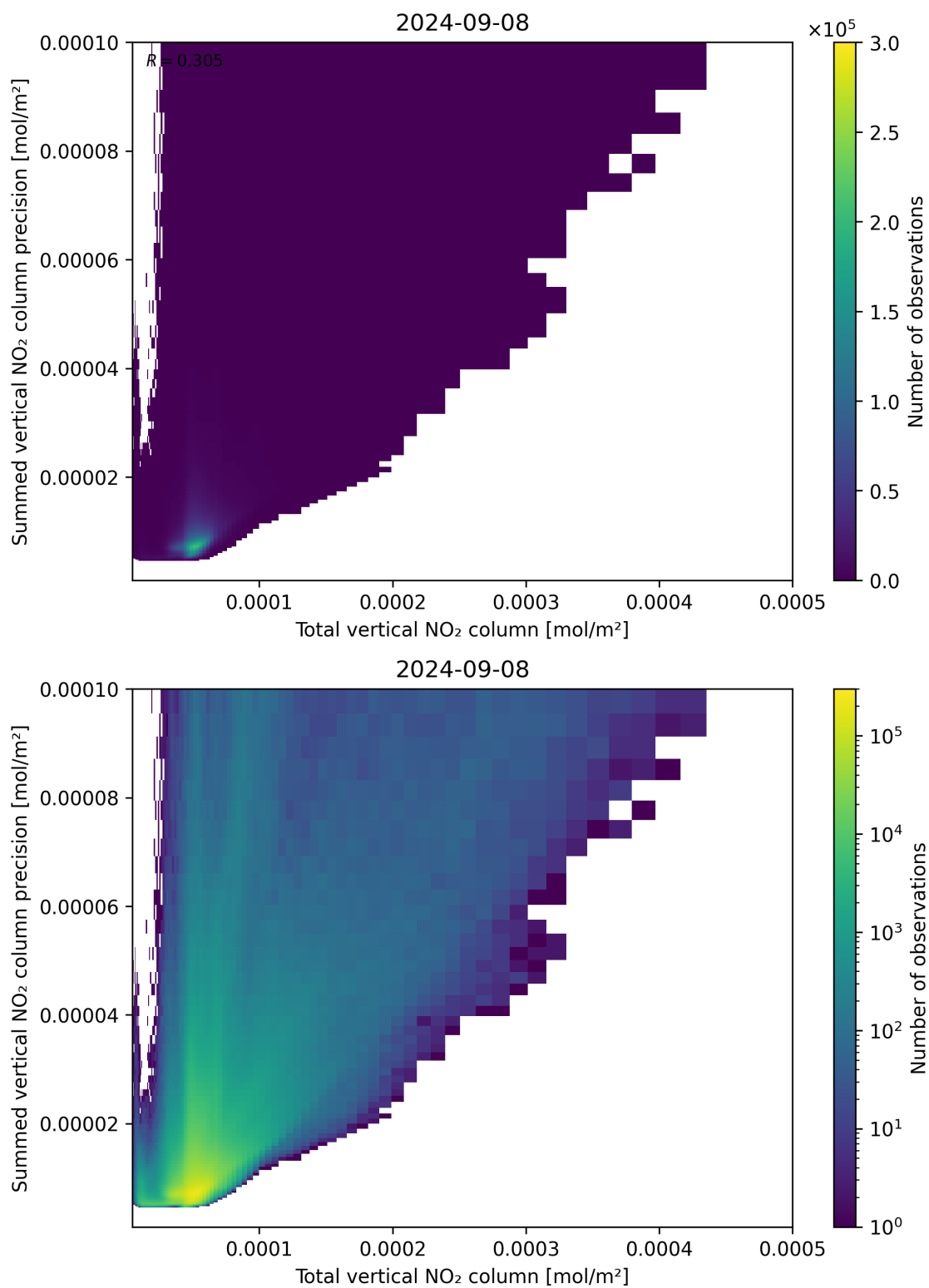
Figure 113: Scatter density plot of “Total vertical NO 2 column” against “Summed vertical NO 2 column precision” for 2024-09-07 to 2024-09-09.
