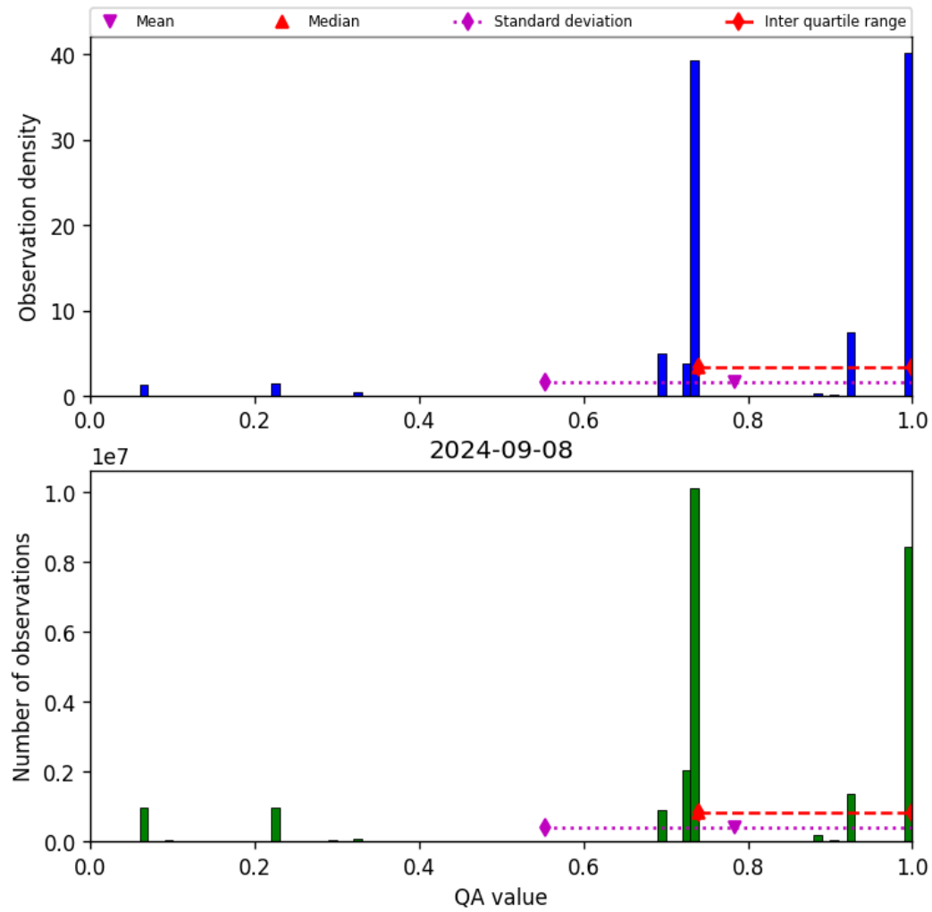
Figure 28: Histogram of “QA value” for 2024-09-07 to 2024-09-09
