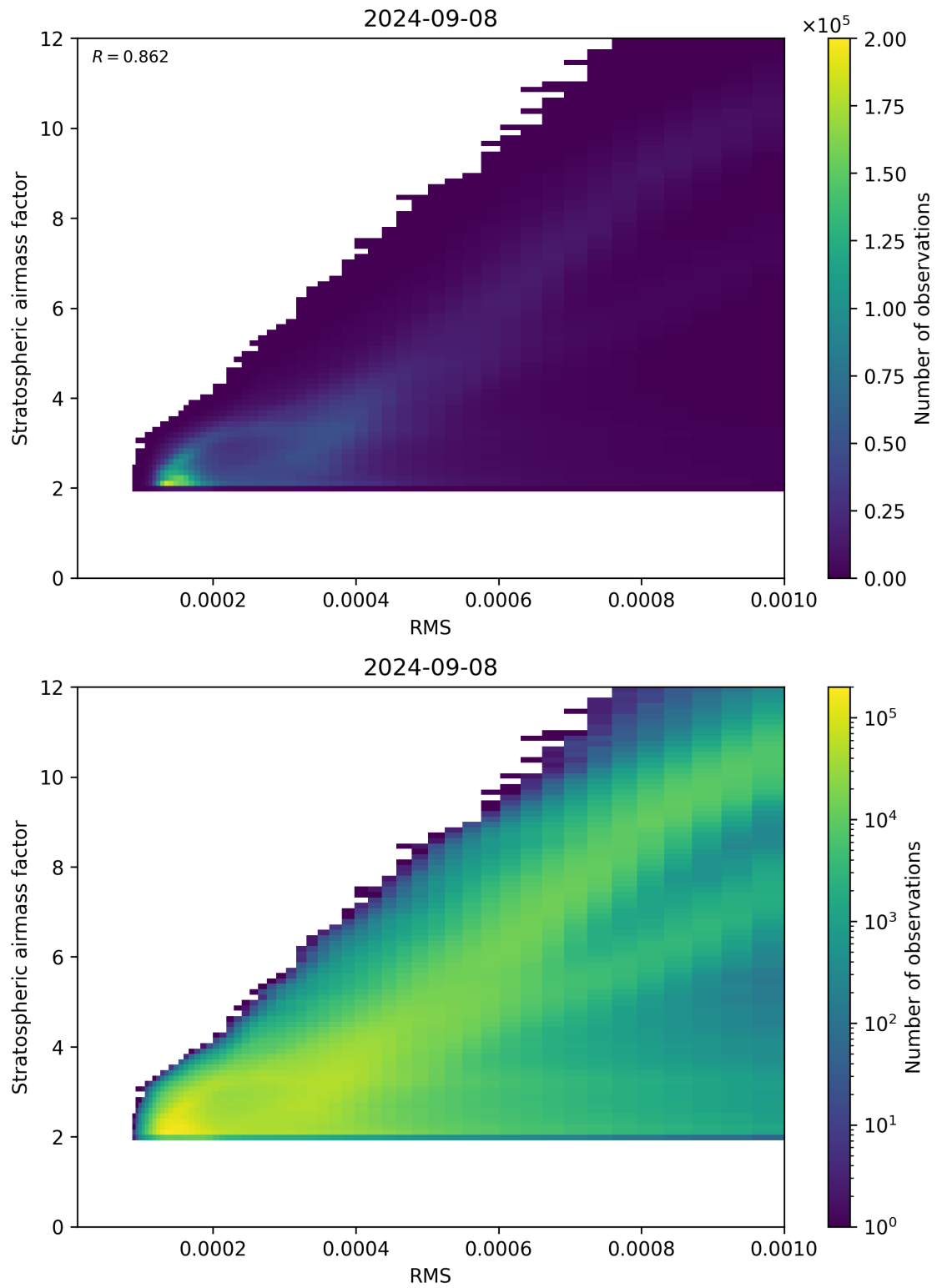
Figure 144: Scatter density plot of “RMS” against “Stratospheric airmass factor” for 2024-09-07 to 2024-09-09.
