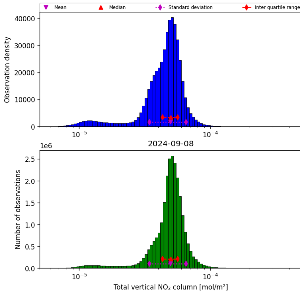
Figure 38: Histogram of “Total vertical NO 2 column” for 2024-09-07 to 2024-09-09
