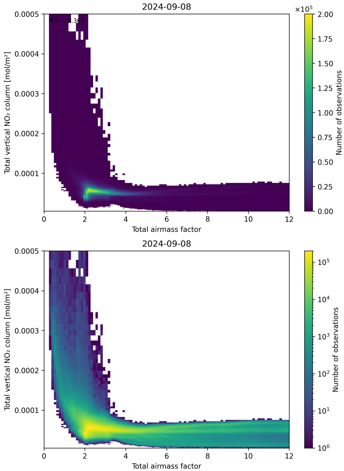
Figure 67: Scatter density plot of “Total airmass factor” against “Total vertical NO 2 column” for 2024-09-07 to 2024-09-09.
