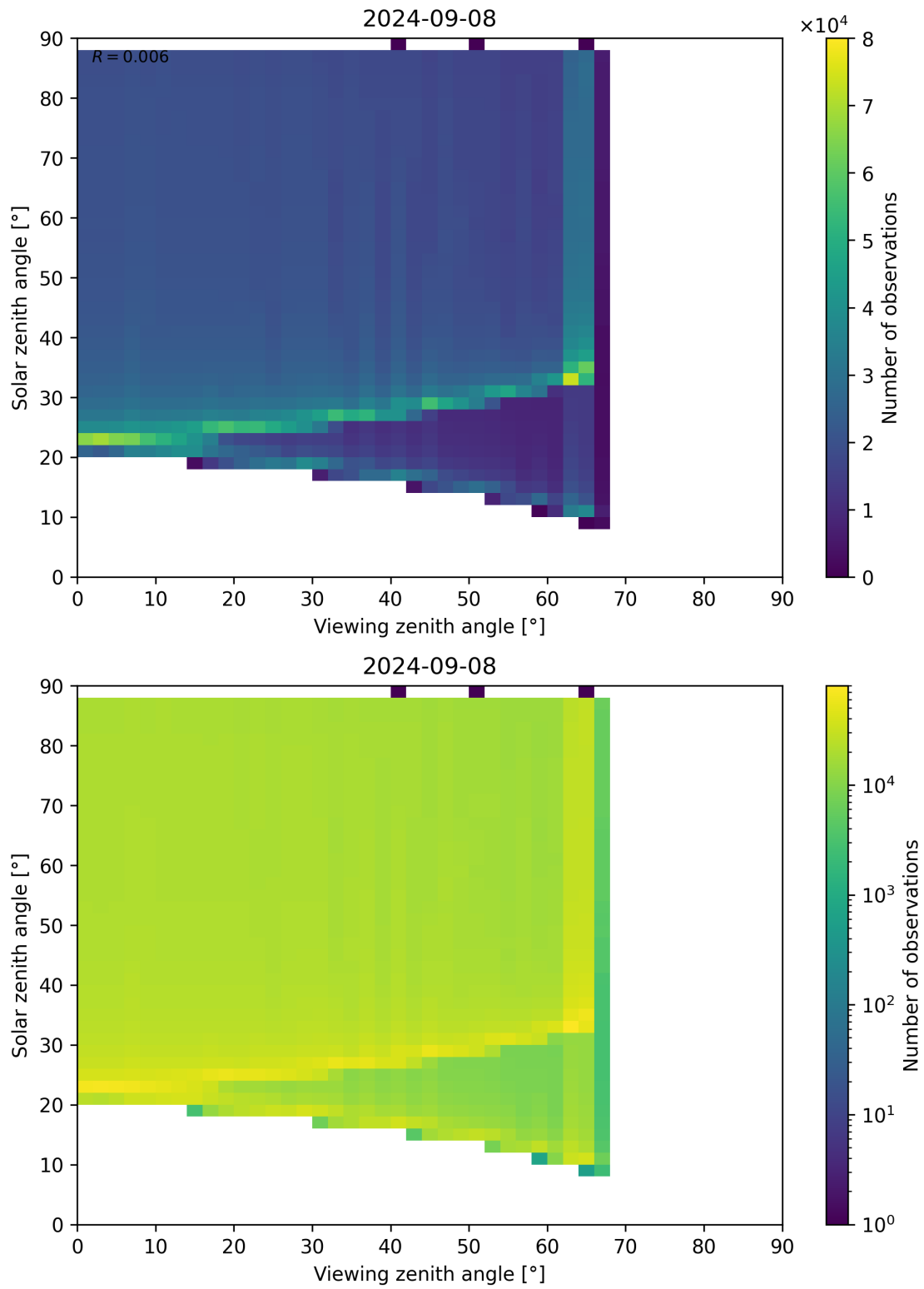
Figure 172: Scatter density plot of “Viewing zenith angle” against “Solar zenith angle” for 2024-09-07 to 2024-09-09.
