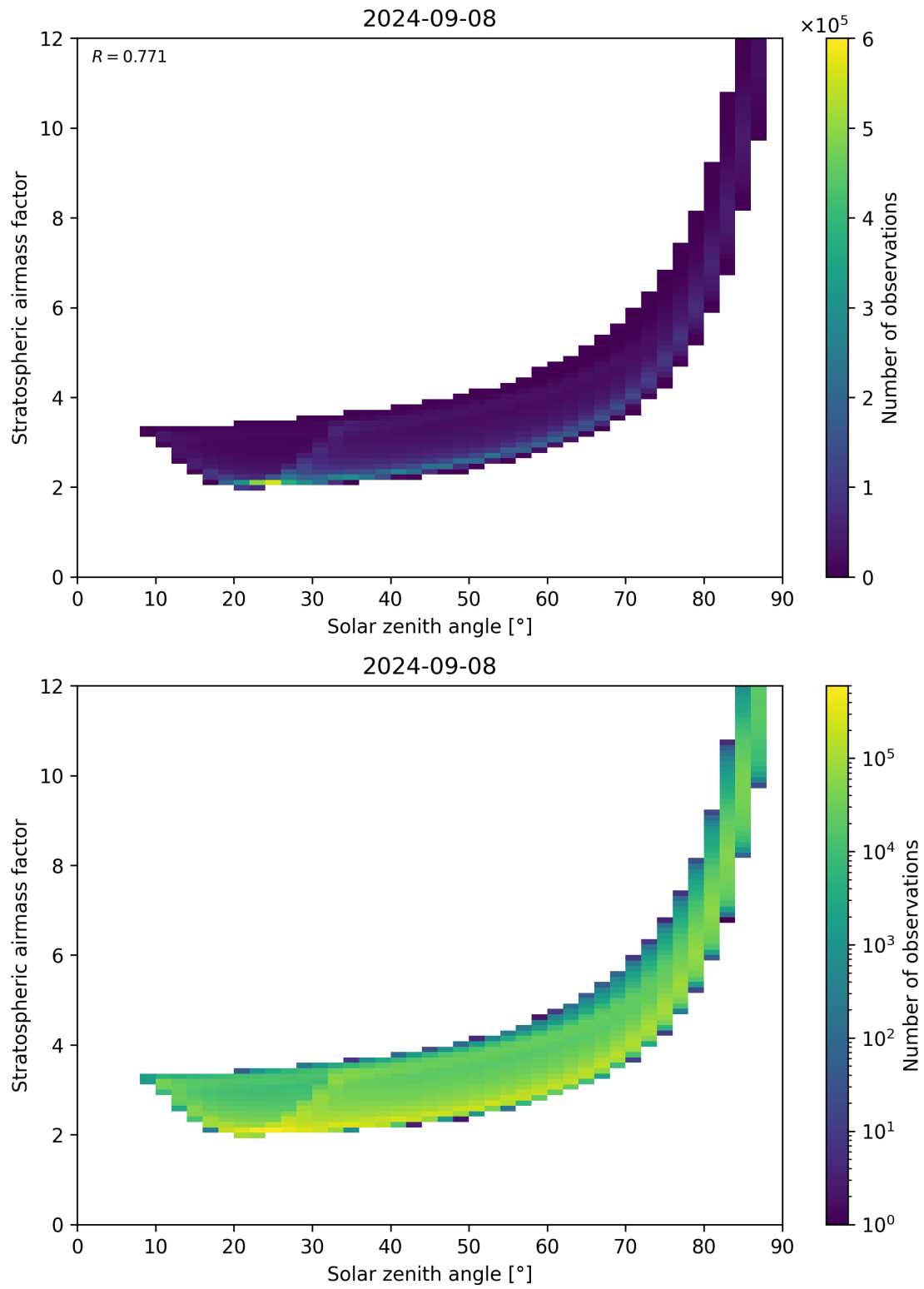
Figure 145: Scatter density plot of “Solar zenith angle” against “Stratospheric airmass factor” for 2024-09-07 to 2024-09-09.
