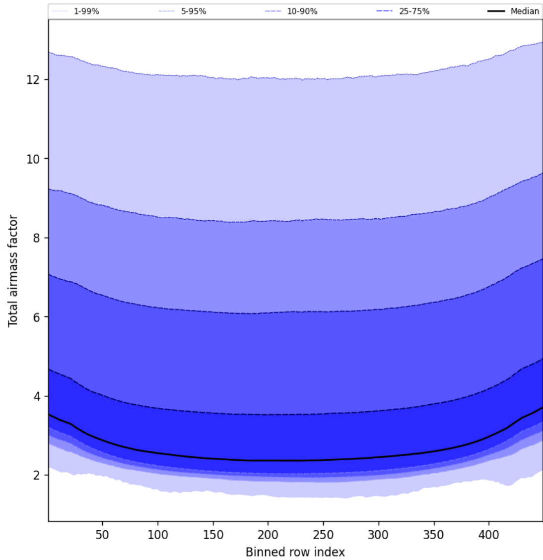
Figure 49: Along track statistics of “Total airmass factor” for 2024-09-07 to 2024-09-09
