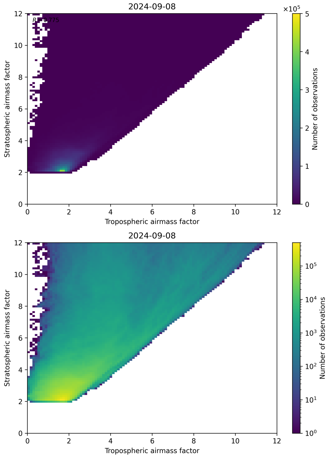
Figure 71: Scatter density plot of “Tropospheric airmass factor” against “Stratospheric airmass factor” for 2024-09-07 to 2024-09-09.
