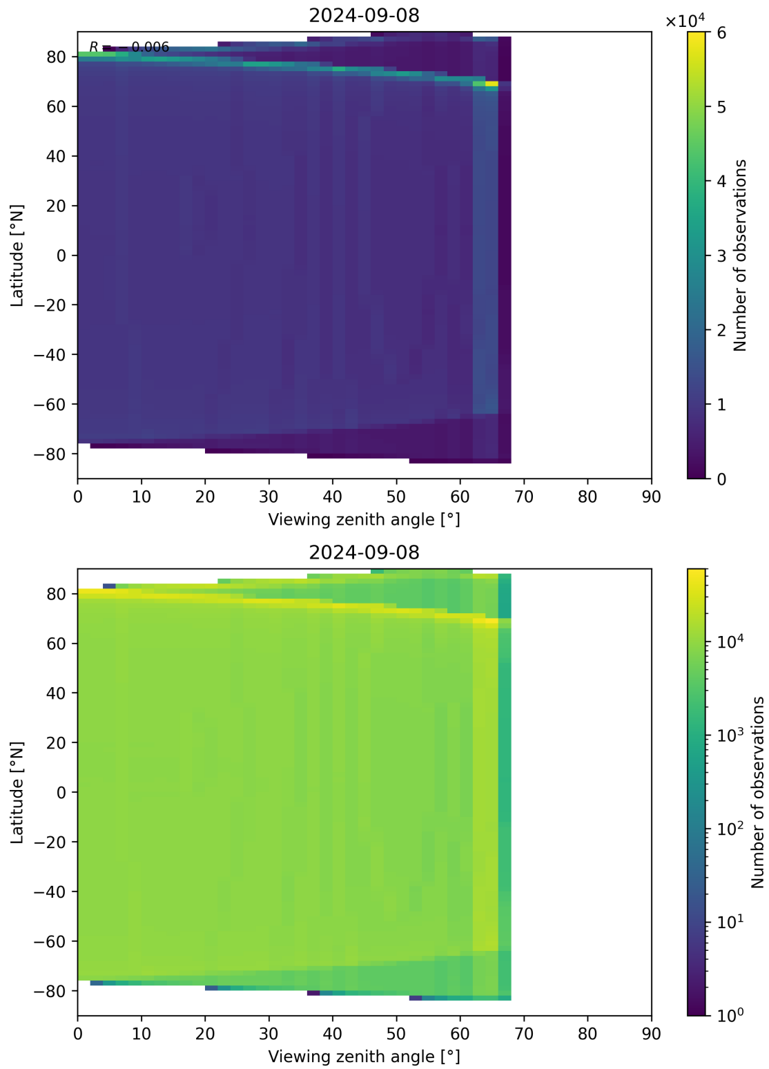
Figure 163: Scatter density plot of “Viewing zenith angle” against “Latitude” for 2024-09-07 to 2024-09-09.
