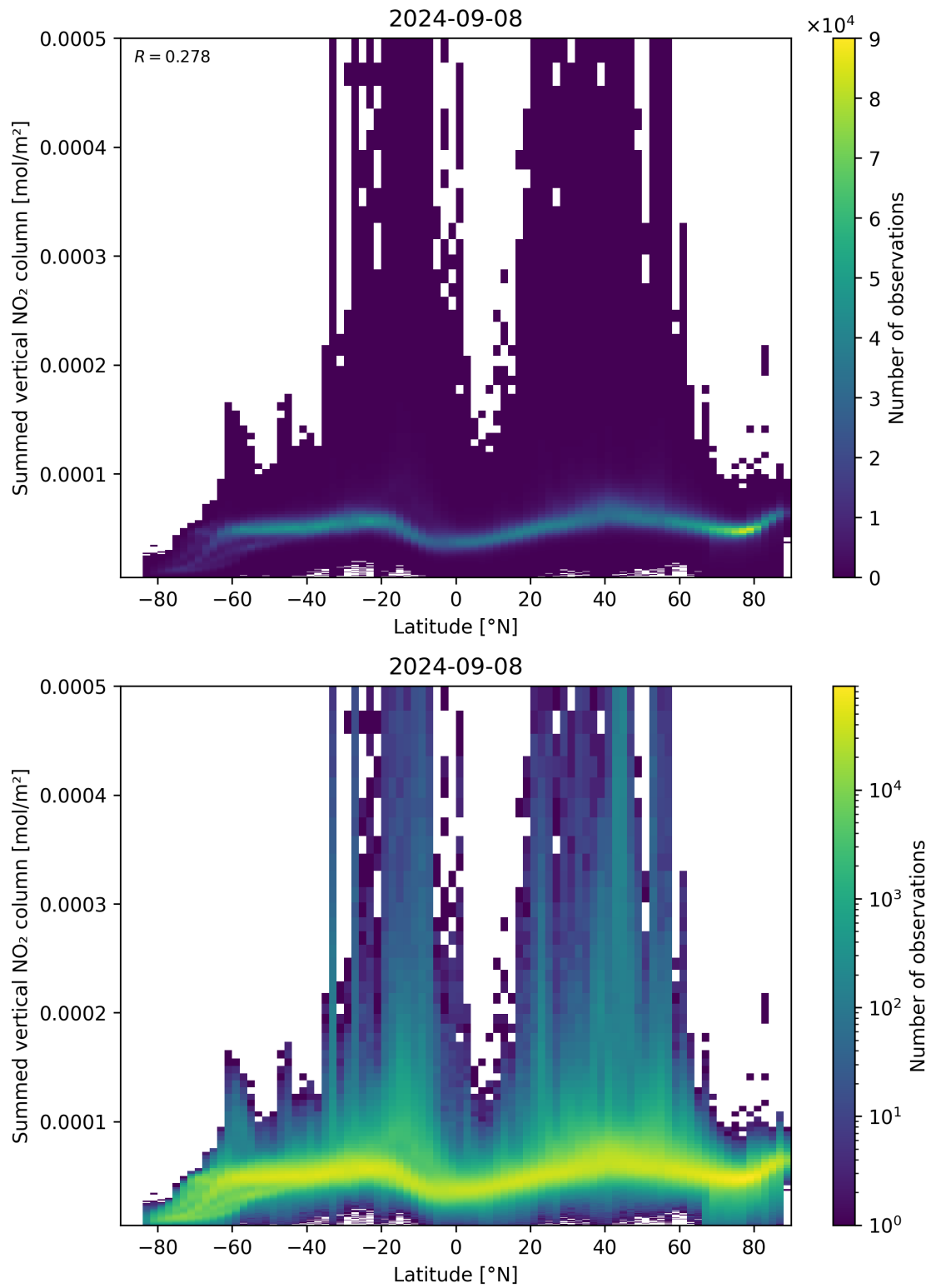
Figure 88: Scatter density plot of “Latitude” against “Summed vertical NO 2 column” for 2024-09-07 to 2024-09-09.
