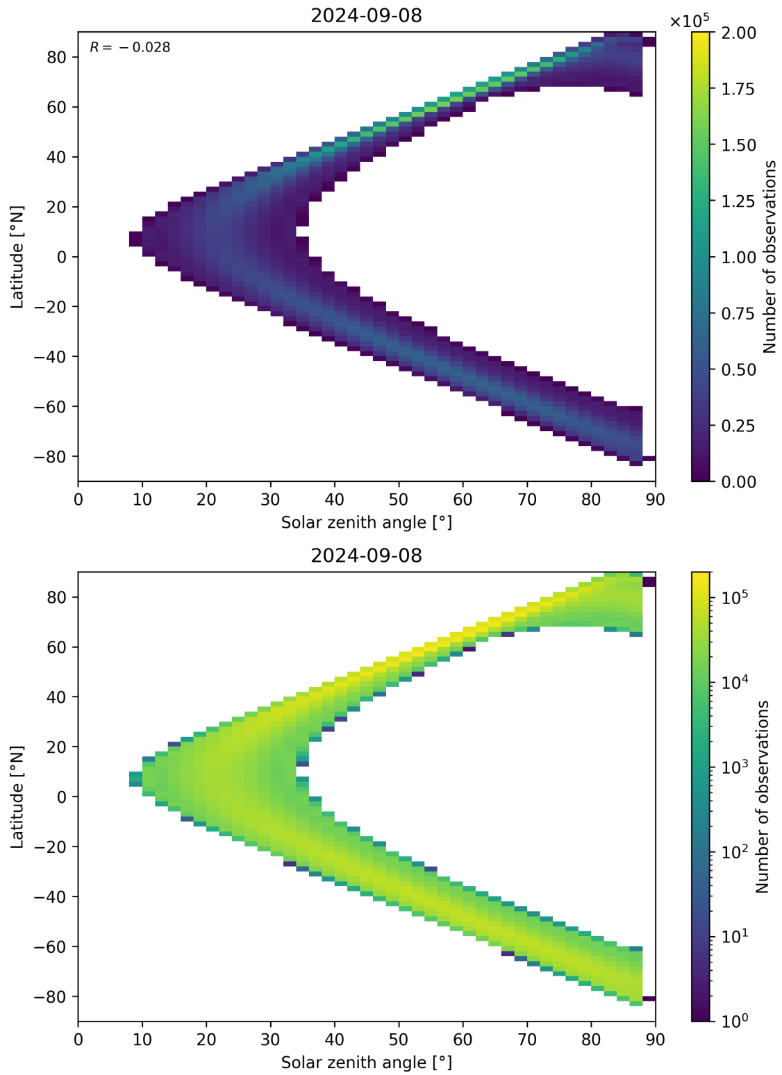
Figure 149: Scatter density plot of “Solar zenith angle” against “Latitude” for 2024-09-07 to 2024-09-09.
