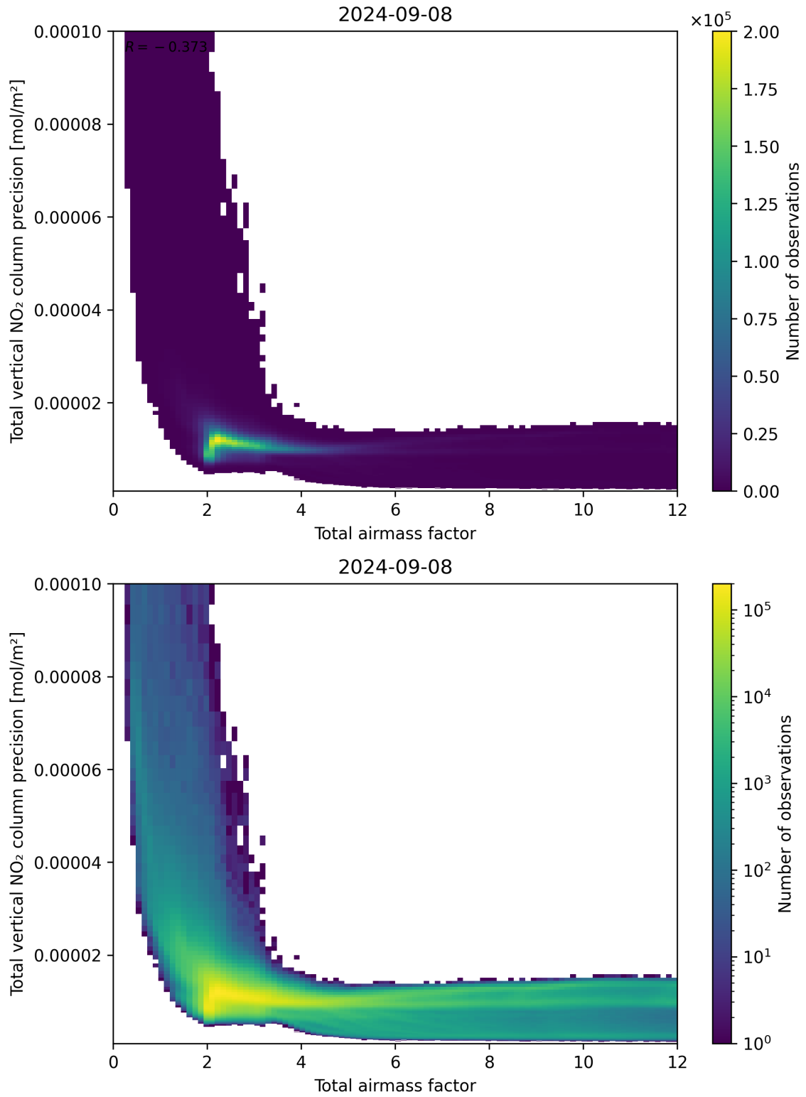
Figure 68: Scatter density plot of “Total airmass factor” against “Total vertical NO 2 column precision” for 2024-09-07 to 2024-09-09.
