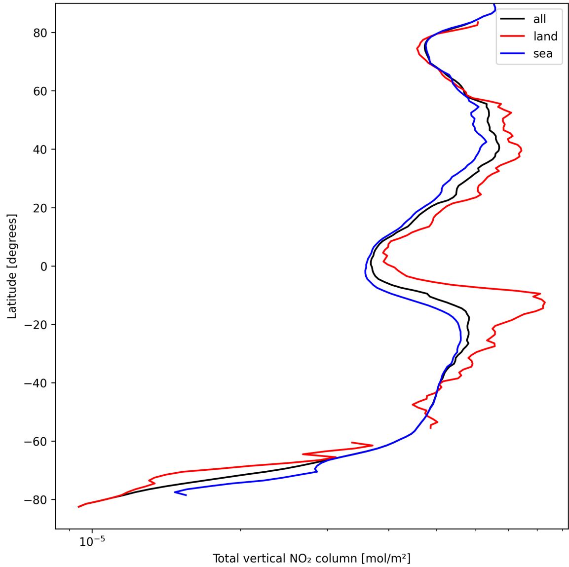
Figure 21: Zonal average of “Total vertical NO 2 column” for 2024-09-07 to 2024-09-09.
