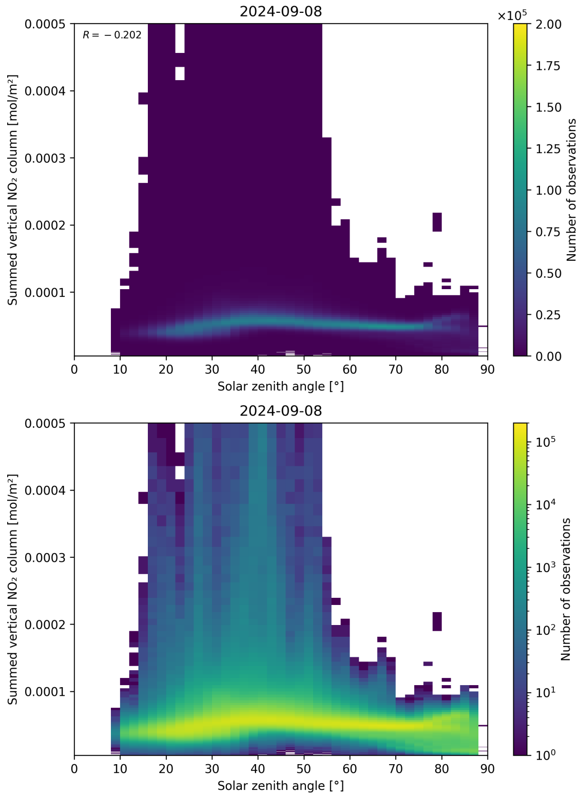
Figure 151: Scatter density plot of “Solar zenith angle” against “Summed vertical NO 2 column” for 2024-09-07 to 2024-09-09.
