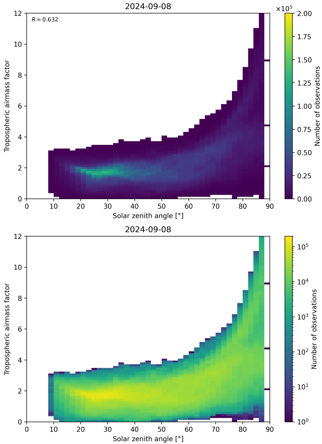
Figure 147: Scatter density plot of “Solar zenith angle” against “Tropospheric airmass factor” for 2024-09-07 to 2024-09-09.
