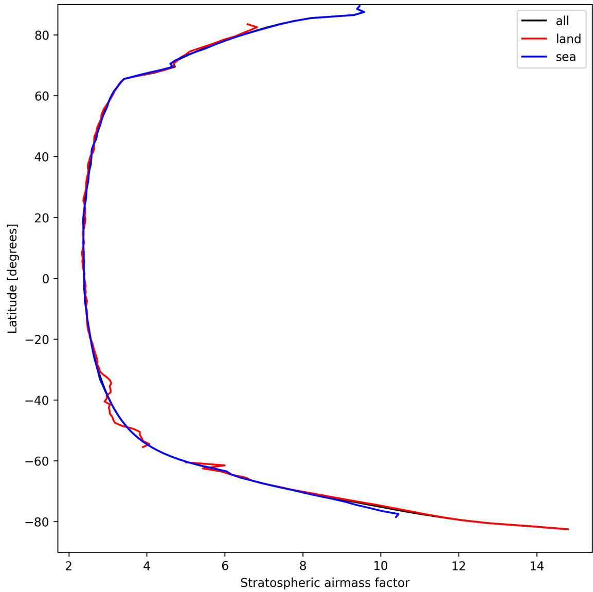
Figure 27: Zonal average of “Stratospheric air mass factor” for 2024-09-07 to 2024-09-09.
