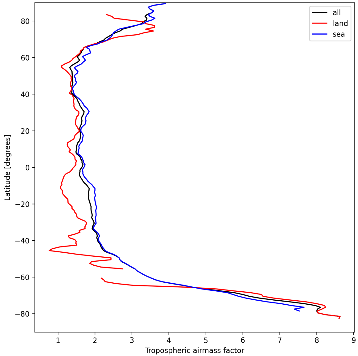
Figure 14: Zonal average of “Tropospheric airmass factor” for 2024-09-07 to 2024-09-09.
