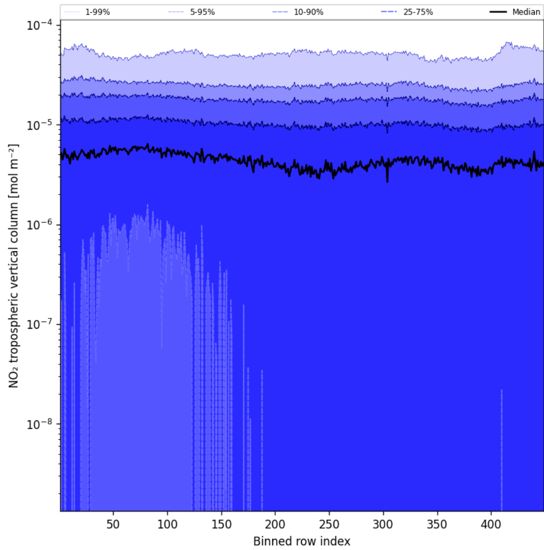
Figure 46: Along track statistics of “NO 2 tropospheric vertical column” for 2024-09-07 to 2024-09-09
