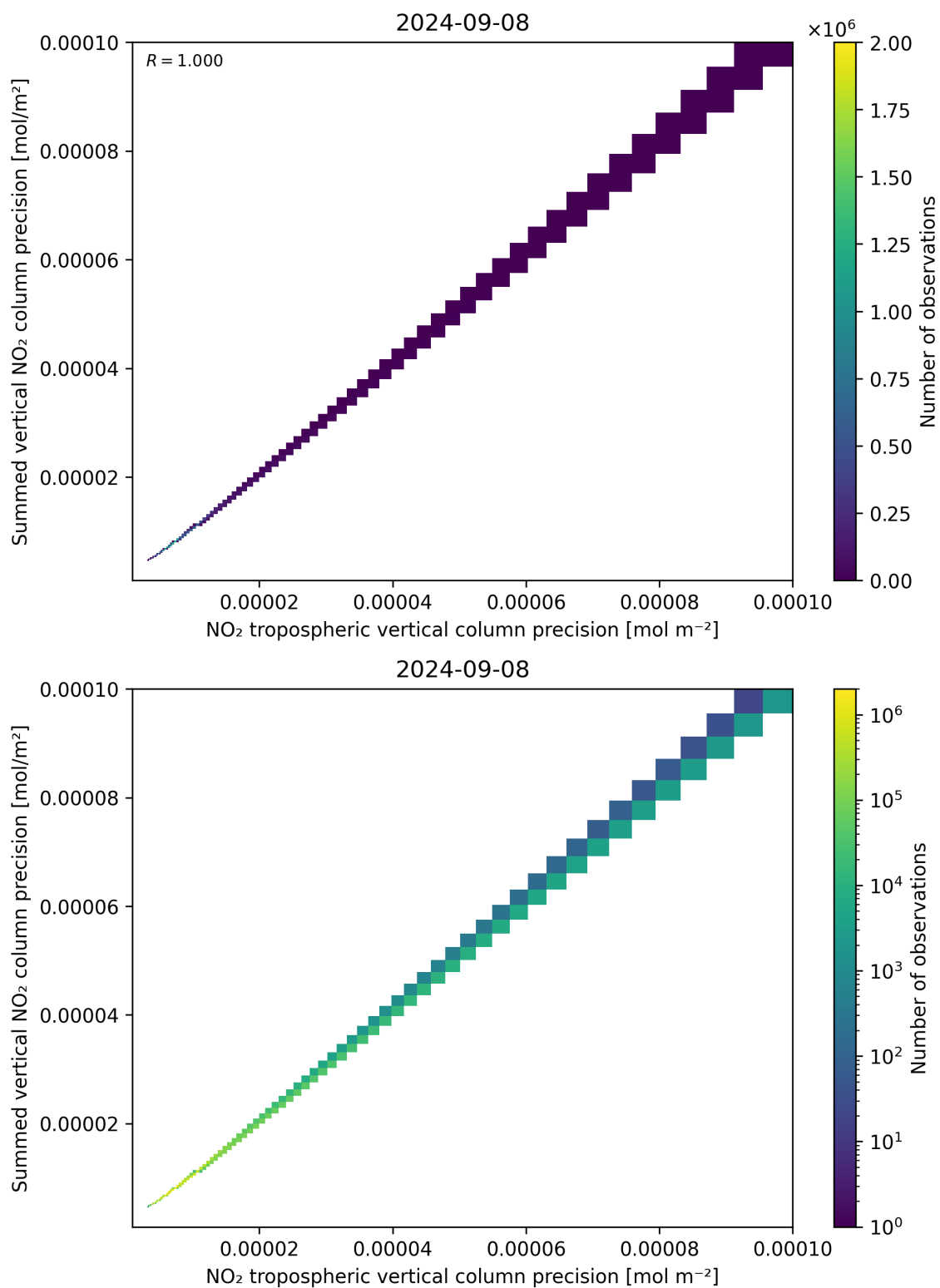
Figure 137: Scatter density plot of “NO 2 tropospheric vertical column precision” against “Summed vertical NO 2 column precision” for 2024-09-07 to 2024-09-09.
