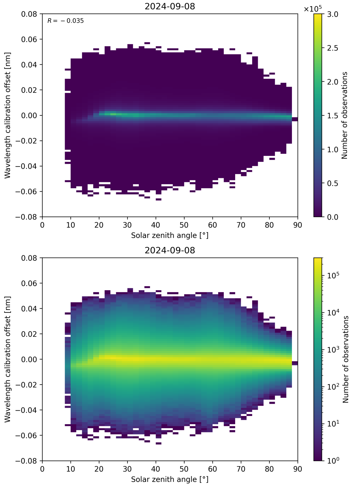
Figure 158: Scatter density plot of “Solar zenith angle” against “Wavelength calibration offset” for 2024-09-07 to 2024-09-09.
