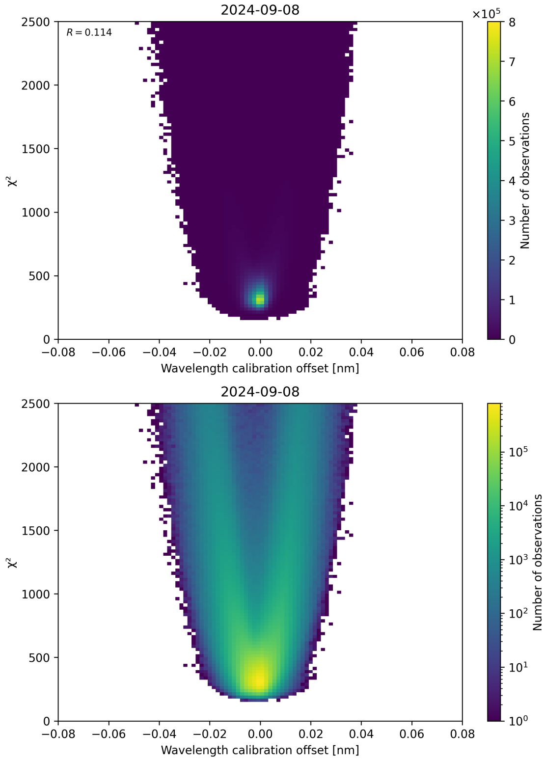
Figure 175: Scatter density plot of “Wavelength calibration offset” against “ \chi^2 ” for 2024-09-07 to 2024-09-09.
