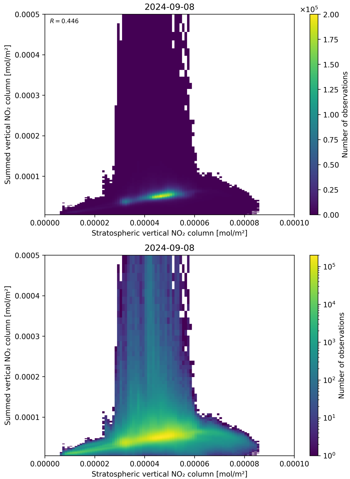
Figure 98: Scatter density plot of “Stratospheric vertical NO 2 column” against “Summed vertical NO 2 column” for 2024-09-07 to 2024-09-09.
