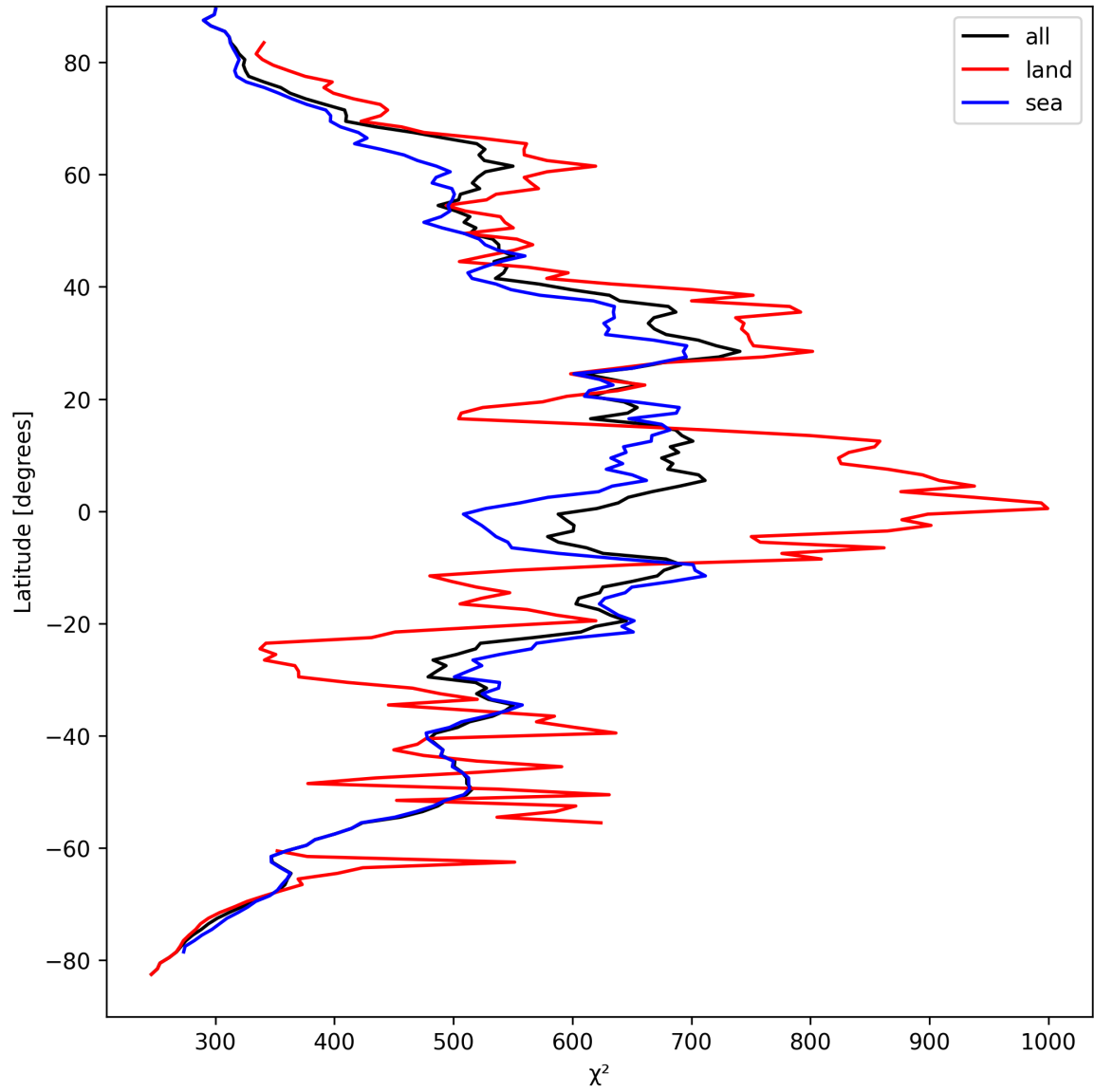
Figure 25: Zonal average of “ \chi^2 ” for 2024-09-07 to 2024-09-09.
