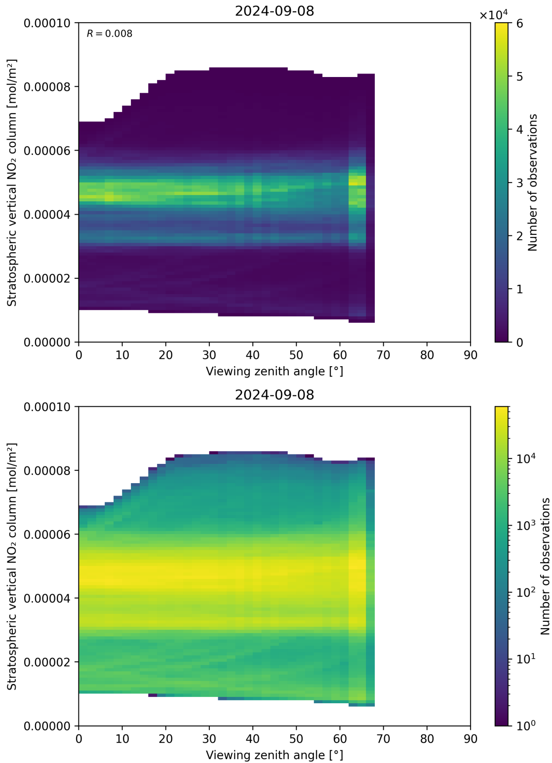
Figure 164: Scatter density plot of “Viewing zenith angle” against “Stratospheric vertical NO 2 column” for 2024-09-07 to 2024-09-09.
