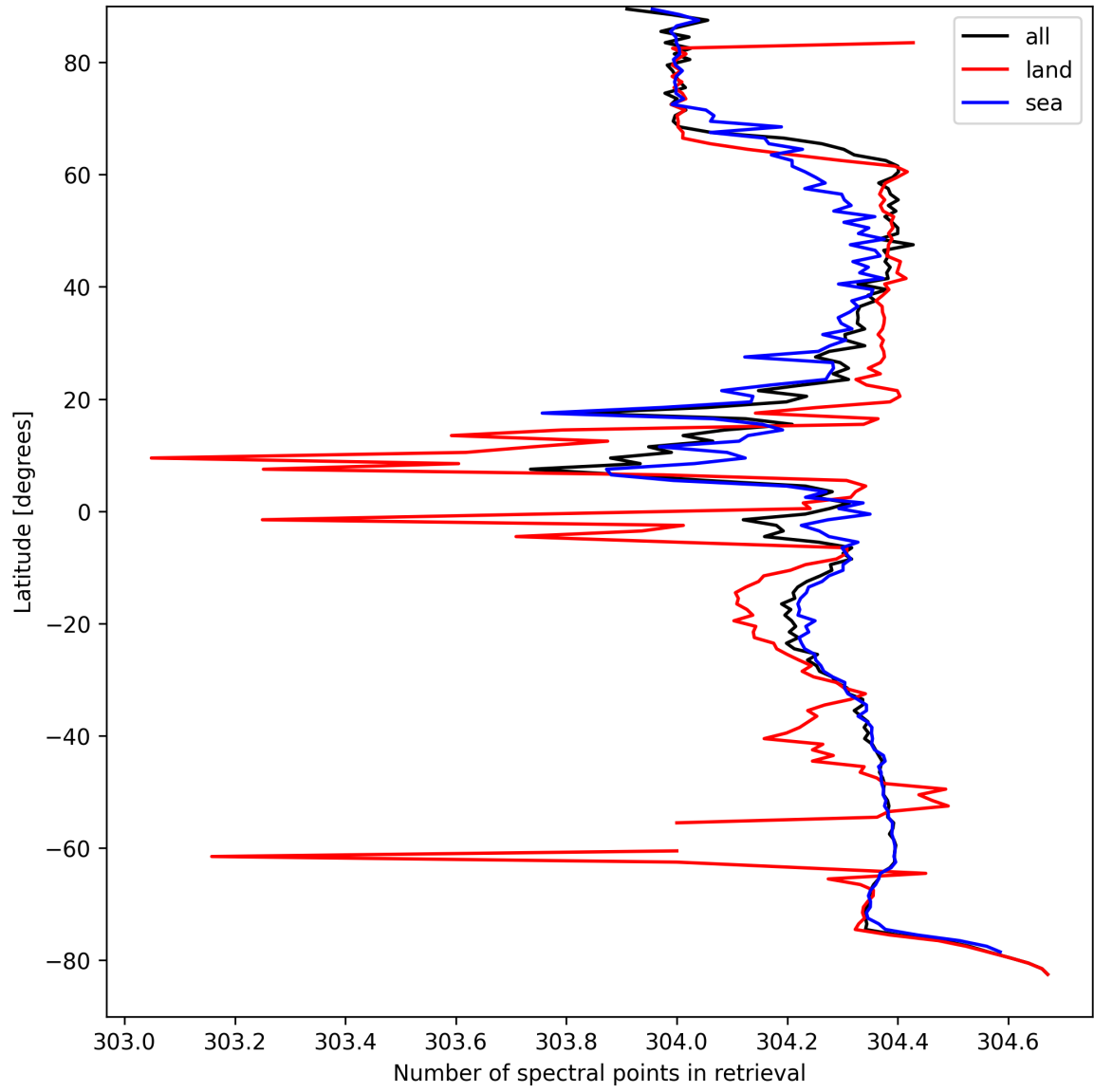
Figure 16: Zonal average of “Number of spectral points in retrieval” for 2024-09-07 to 2024-09-09.
