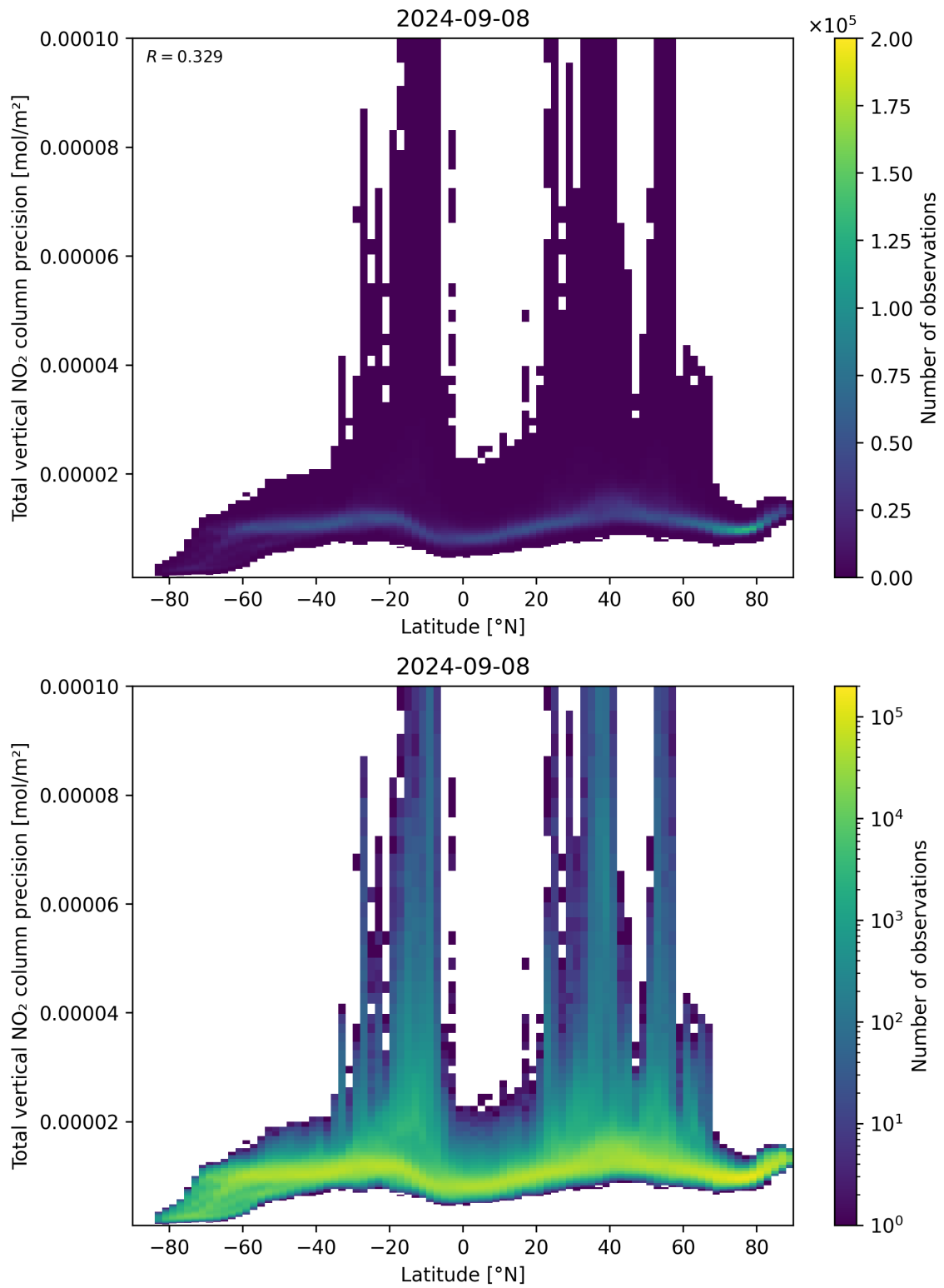
Figure 91: Scatter density plot of “Latitude” against “Total vertical NO 2 column precision” for 2024-09-07 to 2024-09-09.
