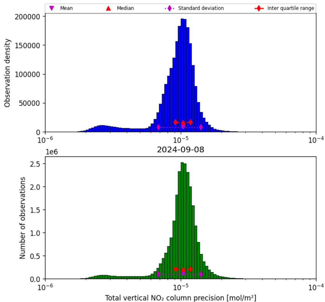
Figure 39: Histogram of “Total vertical NO 2 column precision” for 2024-09-07 to 2024-09-09
