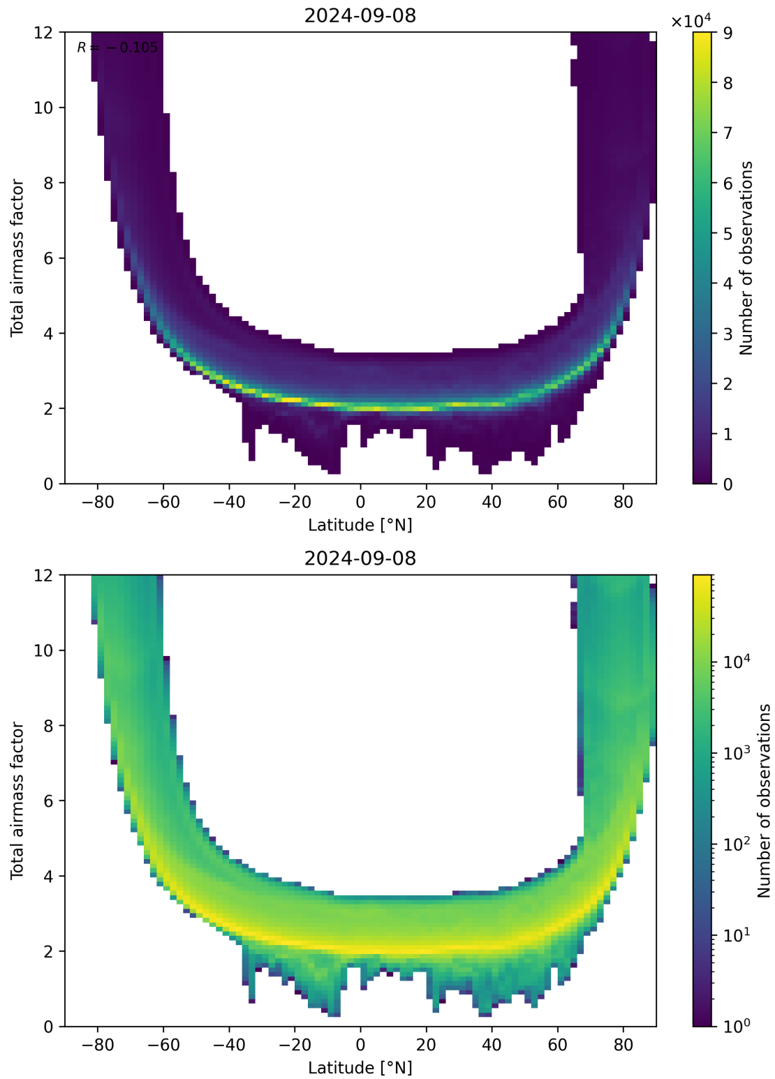
Figure 84: Scatter density plot of “Latitude” against “Total airmass factor” for 2024-09-07 to 2024-09-09.
