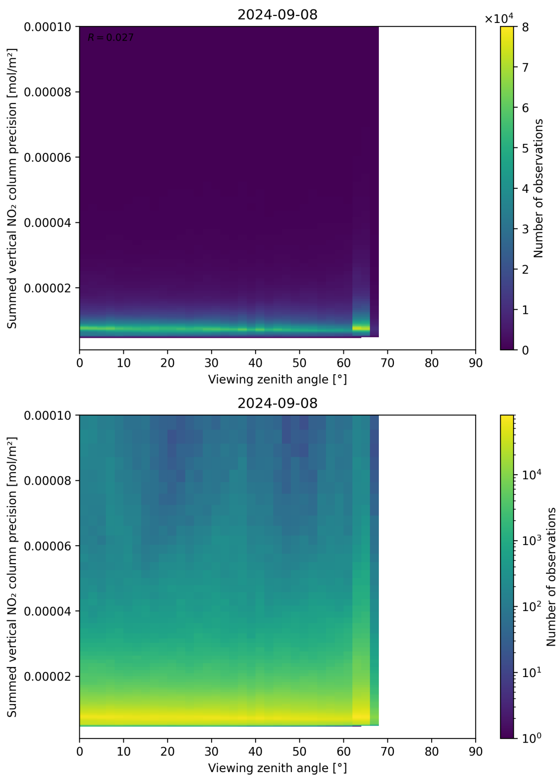
Figure 166: Scatter density plot of “Viewing zenith angle” against “Summed vertical NO 2 column precision” for 2024-09-07 to 2024-09-09.
