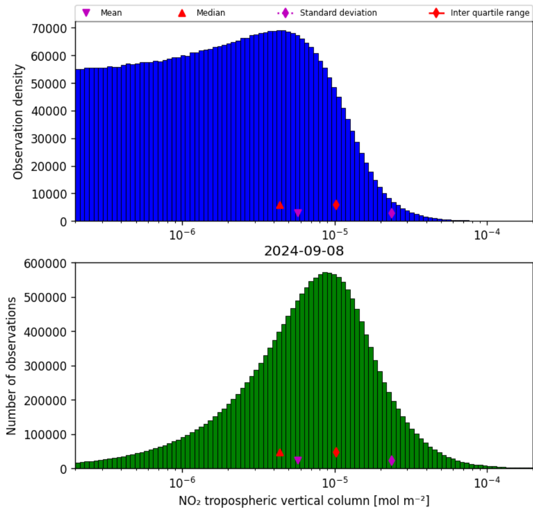
Figure 29: Histogram of “NO 2 tropospheric vertical column” for 2024-09-07 to 2024-09-09
