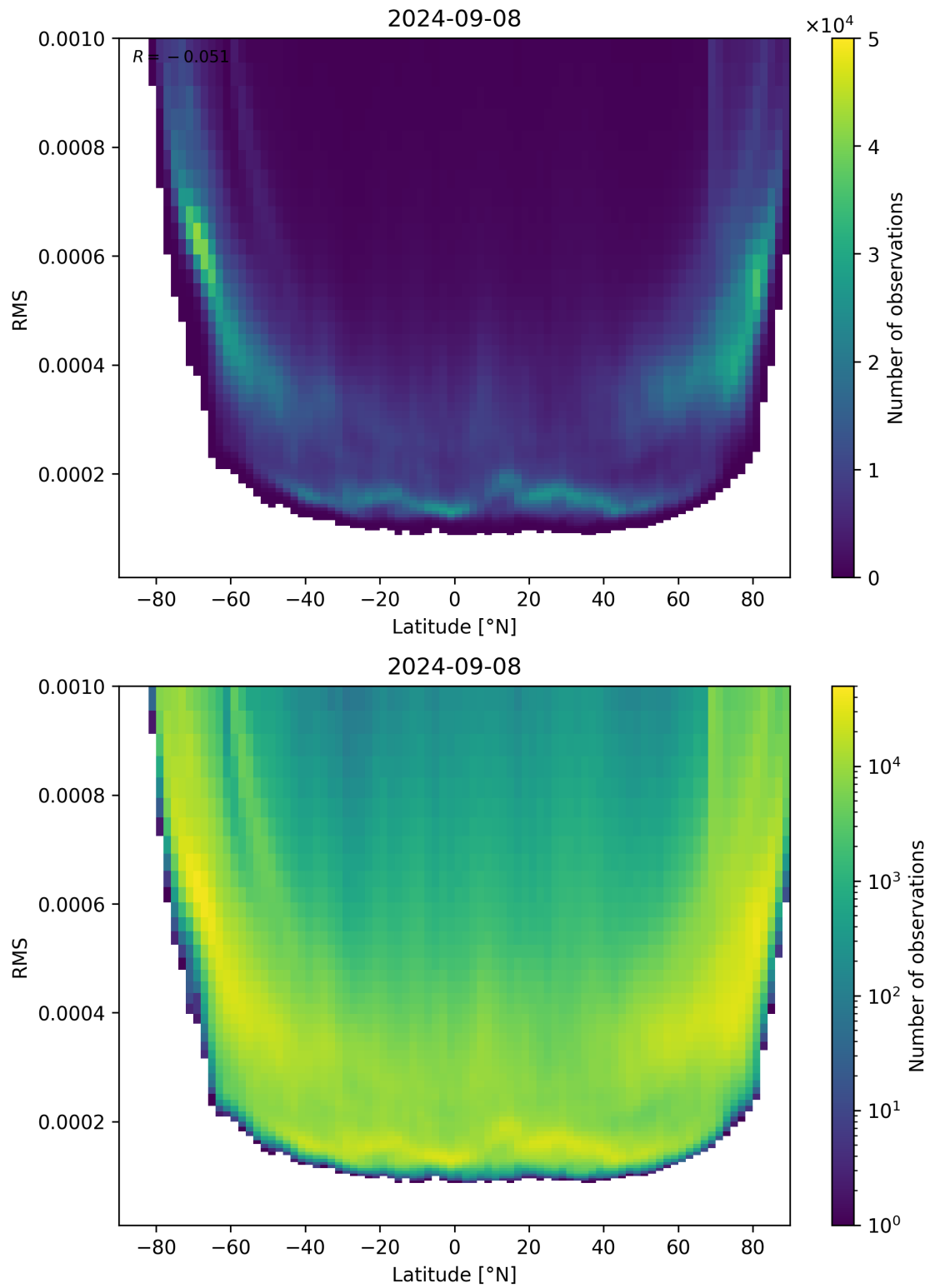
Figure 94: Scatter density plot of “Latitude” against “RMS” for 2024-09-07 to 2024-09-09.
