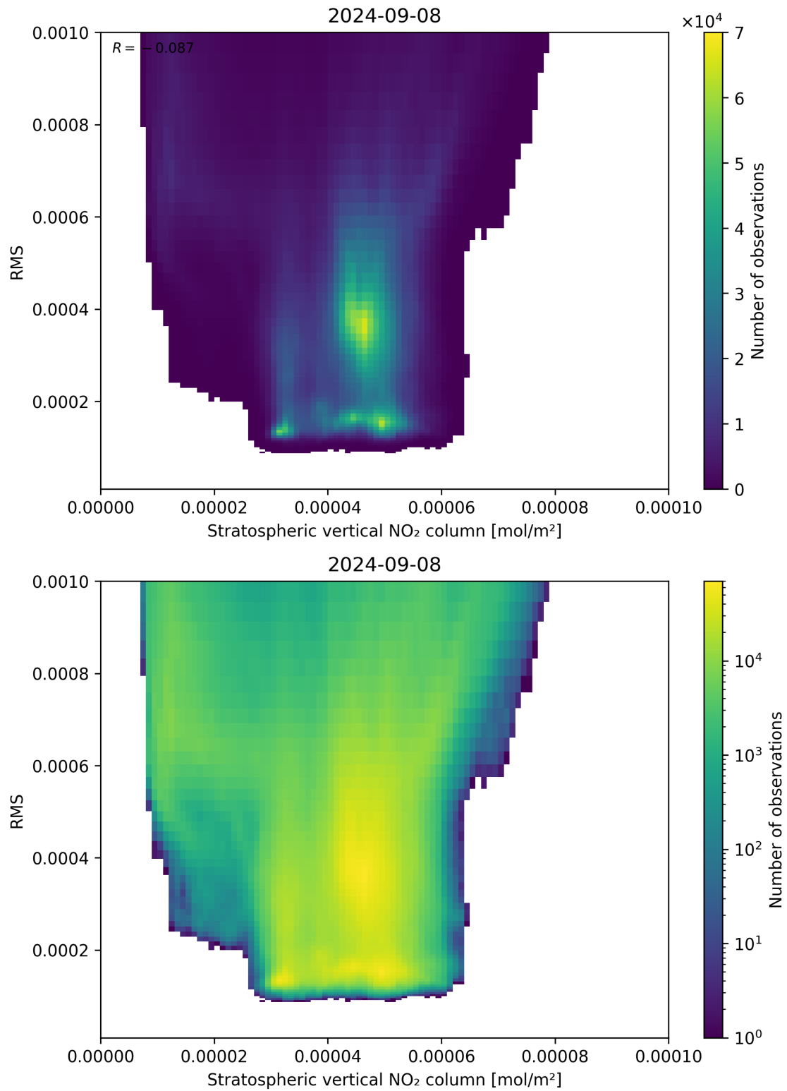
Figure 102: Scatter density plot of “Stratospheric vertical NO 2 column” against “RMS” for 2024-09-07 to 2024-09-09.
