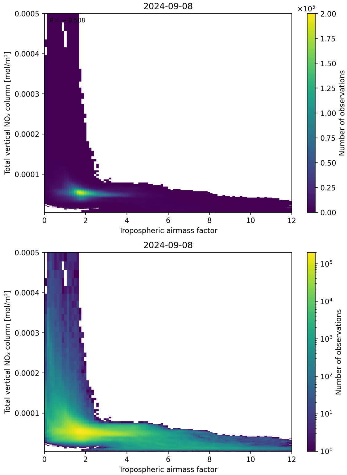
Figure 77: Scatter density plot of “Tropospheric airmass factor” against “Total vertical NO 2 column” for 2024-09-07 to 2024-09-09.
