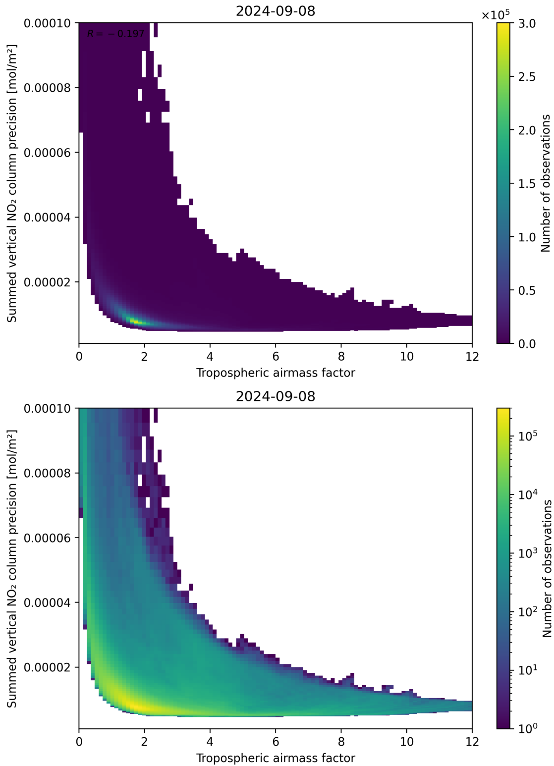
Figure 76: Scatter density plot of “Tropospheric air mass factor” against “Summed vertical NO 2 column precision” for 2024-09-07 to 2024-09-09.
