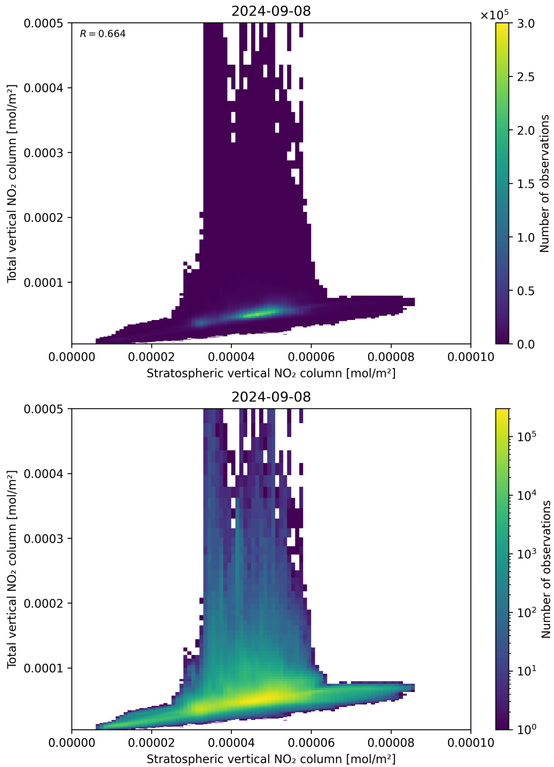
Figure 100: Scatter density plot of “Stratospheric vertical NO 2 column” against “Total vertical NO 2 column” for 2024-09-07 to 2024-09-09.
