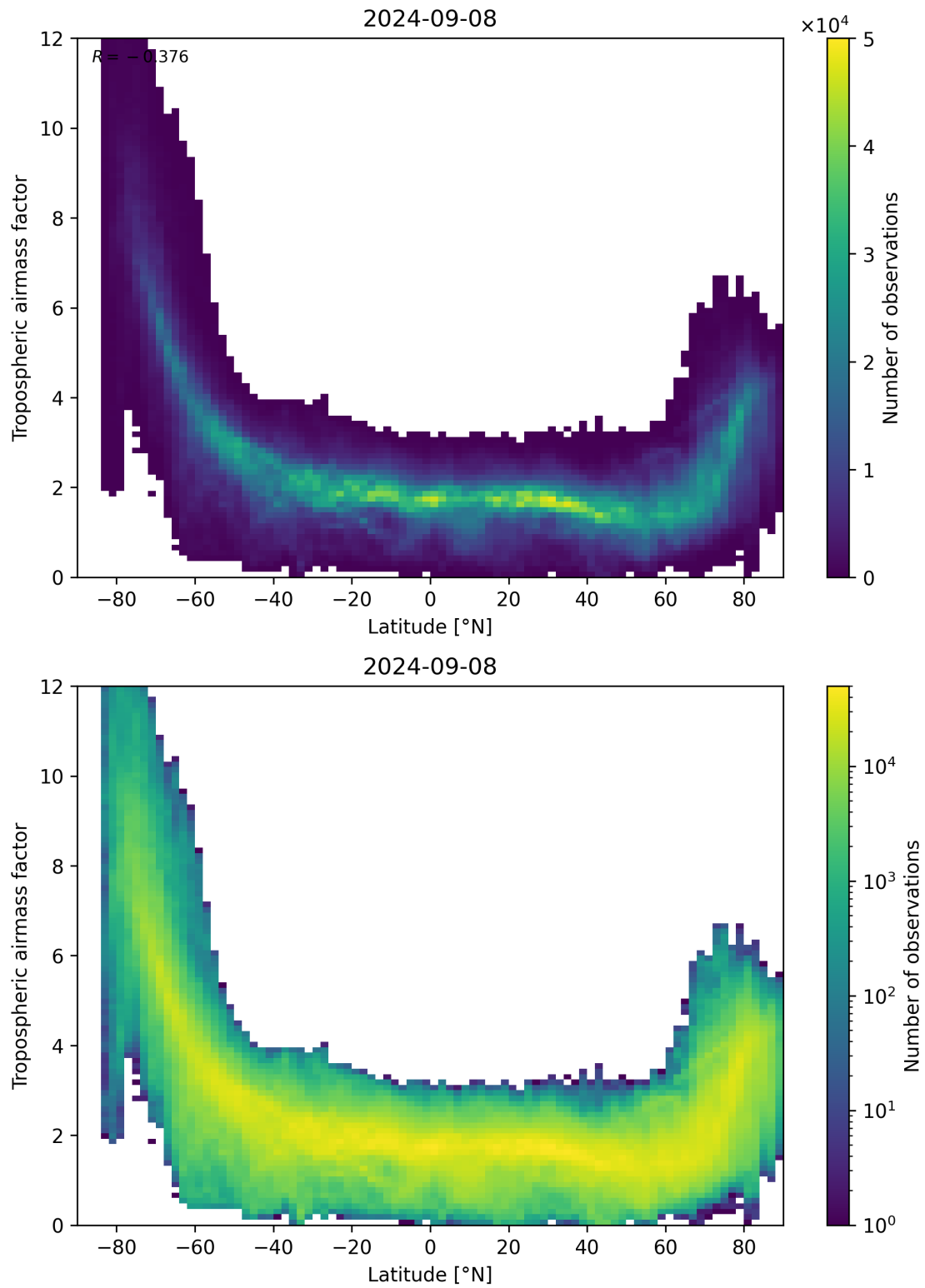
Figure 85: Scatter density plot of “Latitude” against “Tropospheric air mass factor” for 2024-09-07 to 2024-09-09.
