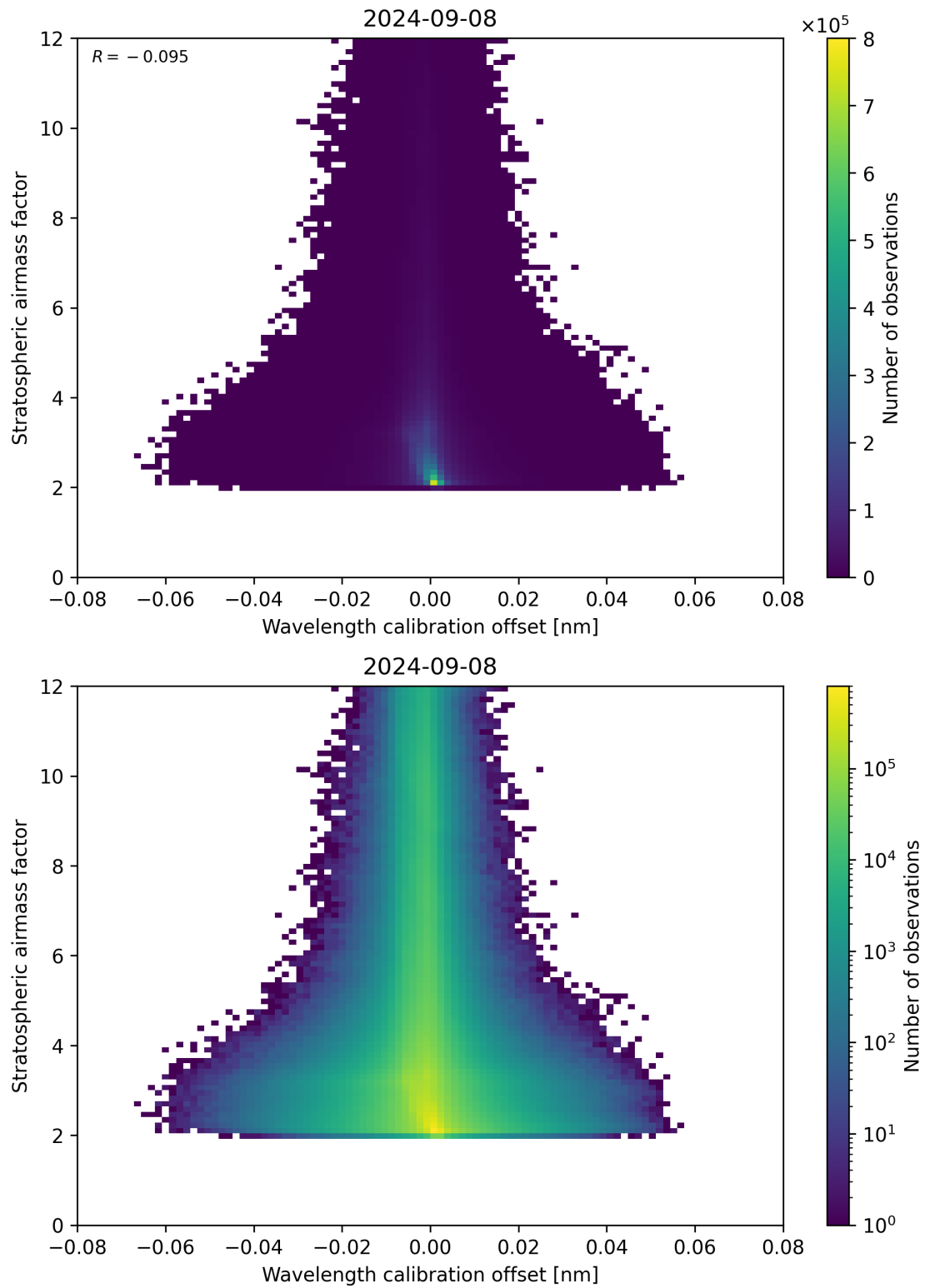
Figure 174: Scatter density plot of “Wavelength calibration offset” against “Stratospheric airmass factor” for 2024-09-07 to 2024-09-09.
