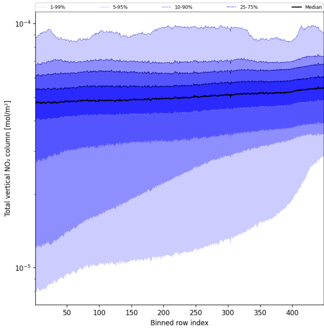
Figure 55: Along track statistics of “Total vertical NO 2 column” for 2024-09-07 to 2024-09-09
