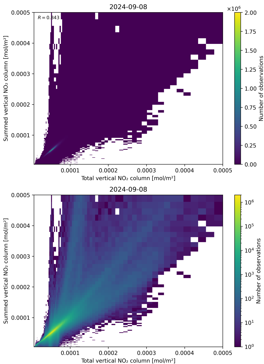
Figure 112: Scatter density plot of “Total vertical NO 2 column” against “Summed vertical NO 2 column” for 2024-09-07 to 2024-09-09.
