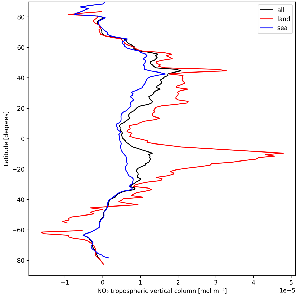
Figure 12: Zonal average of “NO 2 tropospheric vertical column” for 2024-09-07 to 2024-09-09.
