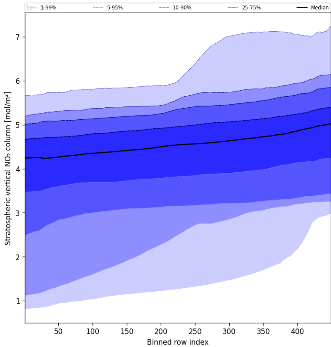
Figure 53: Along track statistics of “Stratospheric vertical NO 2 column” for 2024-09-07 to 2024-09-09
