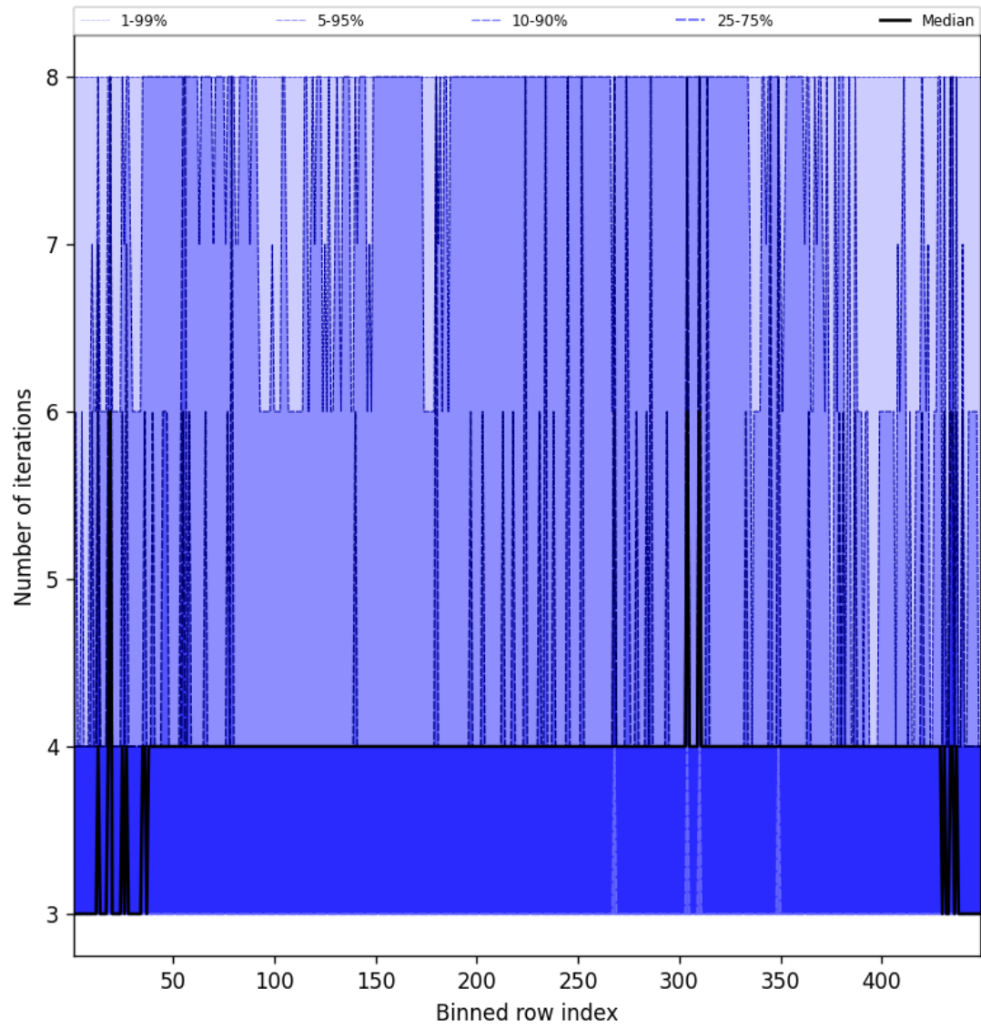
Figure 51: Along track statistics of “Number of iterations” for 2024-09-07 to 2024-09-09
