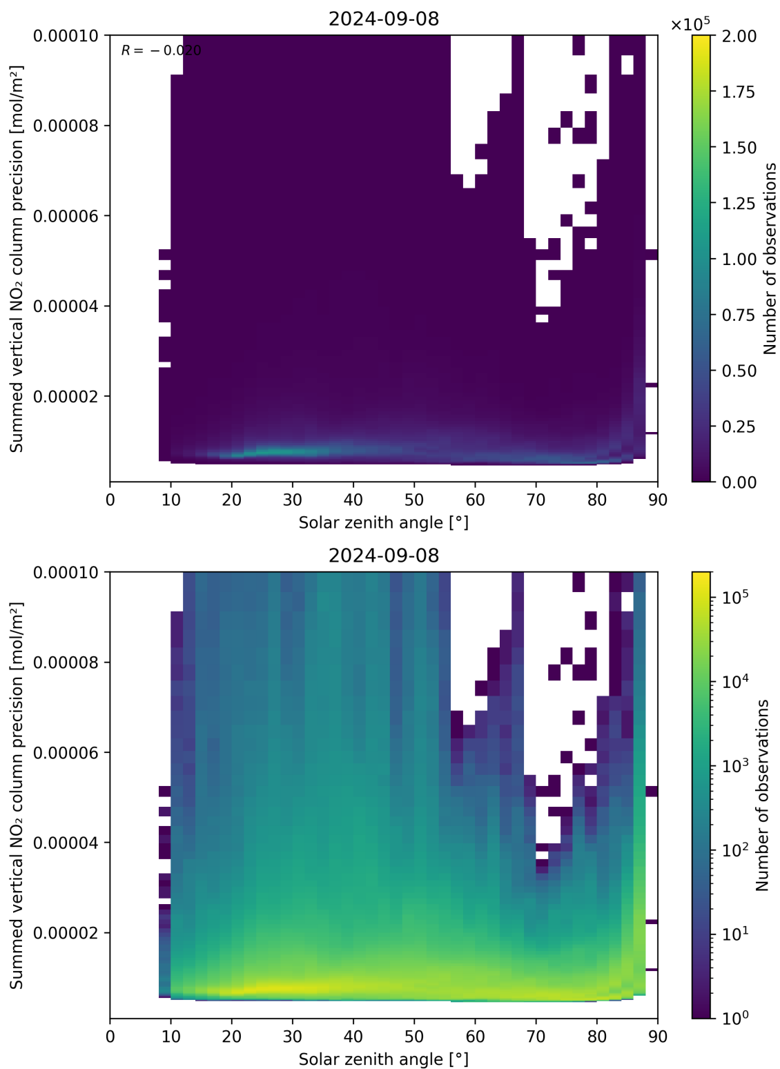
Figure 152: Scatter density plot of “Solar zenith angle” against “Summed vertical NO 2 column precision” for 2024-09-07 to 2024-09-09.
