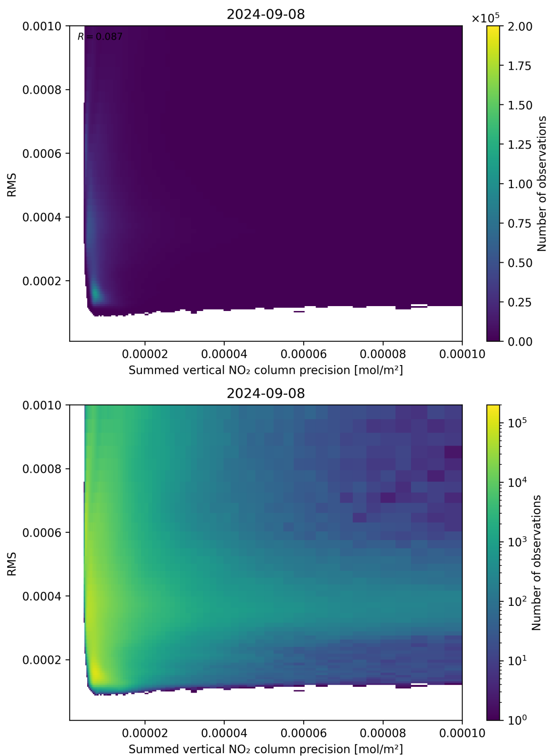
Figure 108: Scatter density plot of “Summed vertical NO 2 column precision” against “RMS” for 2024-09-07 to 2024-09-09.
