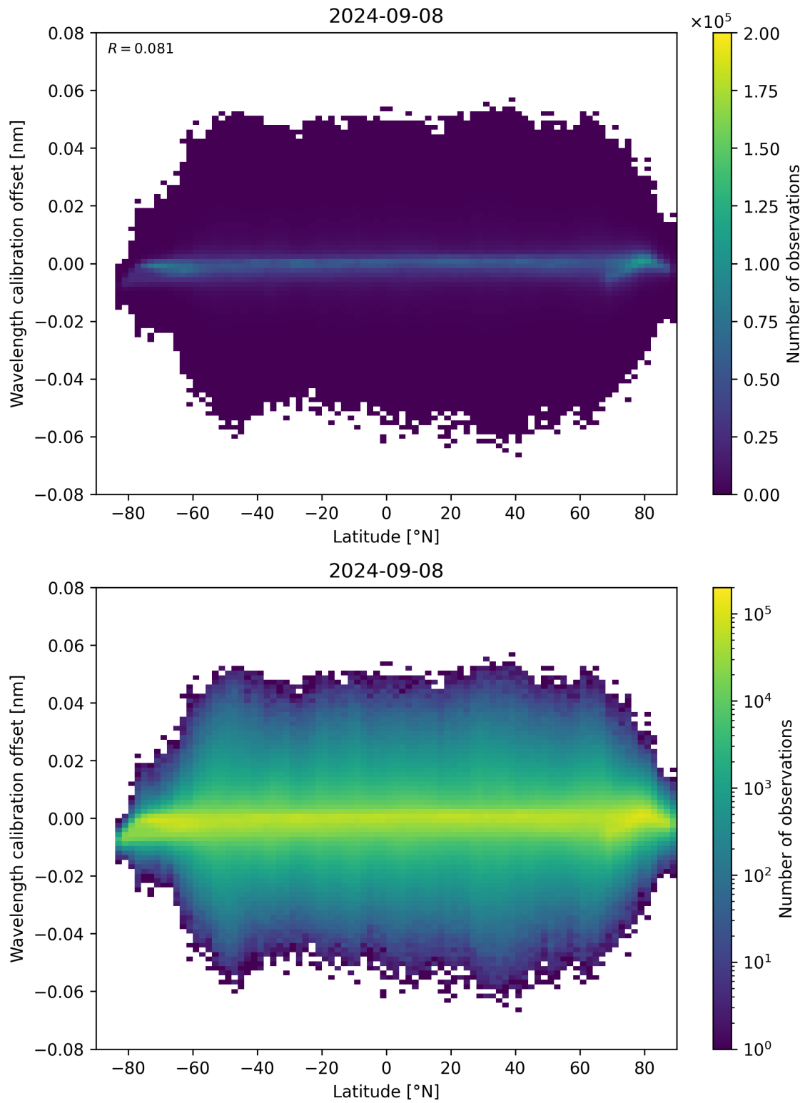
Figure 95: Scatter density plot of “Latitude” against “Wavelength calibration offset” for 2024-09-07 to 2024-09-09.
