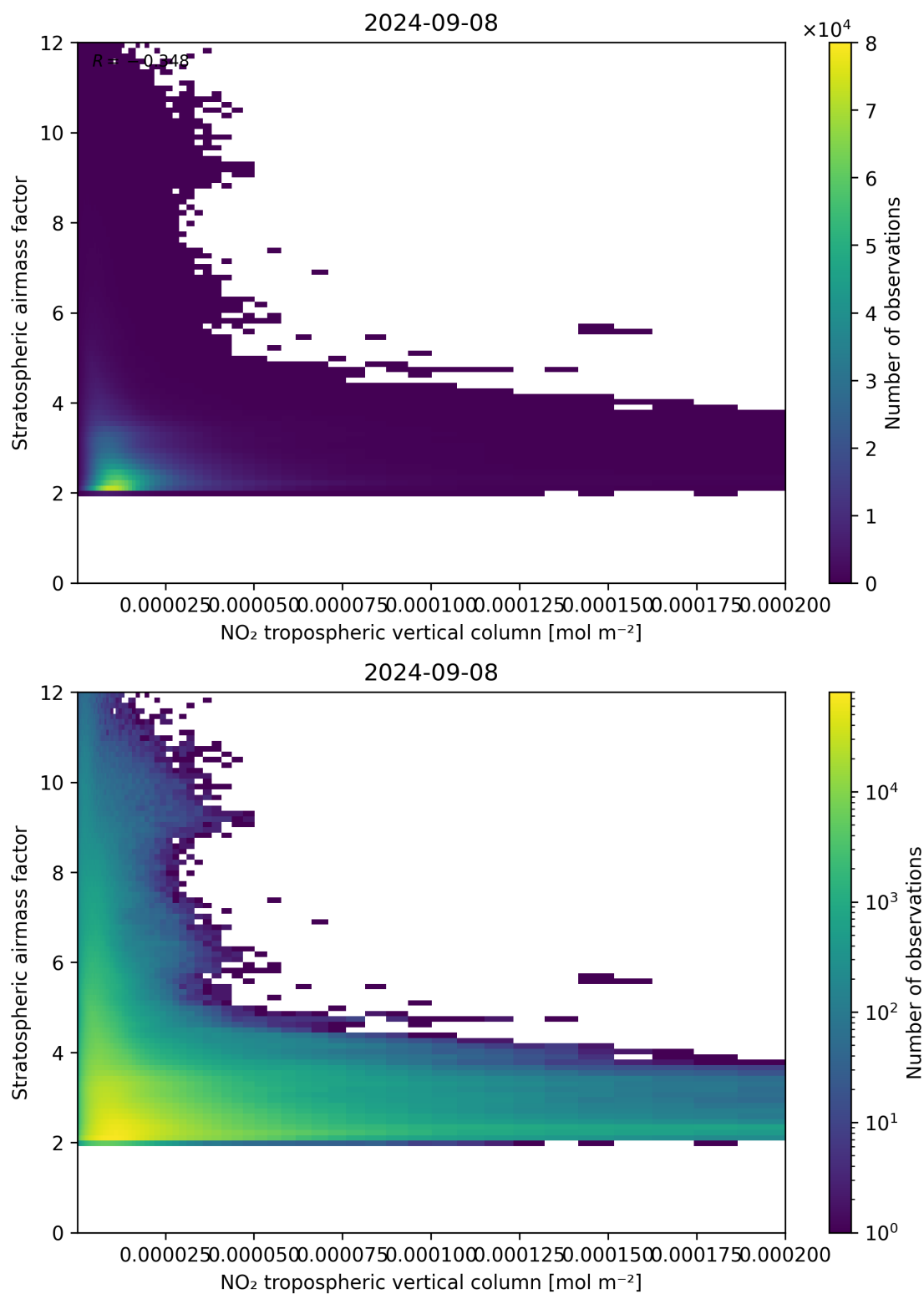
Figure 121: Scatter density plot of “NO 2 tropospheric vertical column” against “Stratospheric air mass factor” for 2024-09-07 to 2024-09-09.
