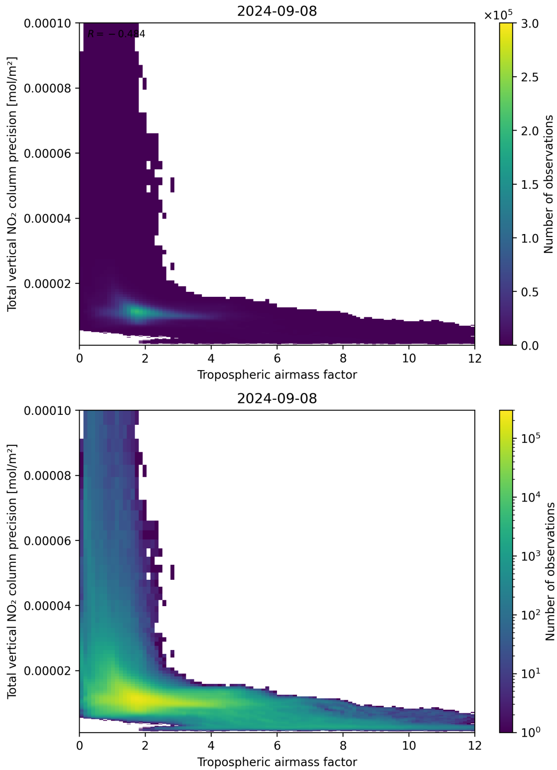
Figure 78: Scatter density plot of “Tropospheric air mass factor” against “Total vertical NO 2 column precision” for 2024-09-07 to 2024-09-09.
