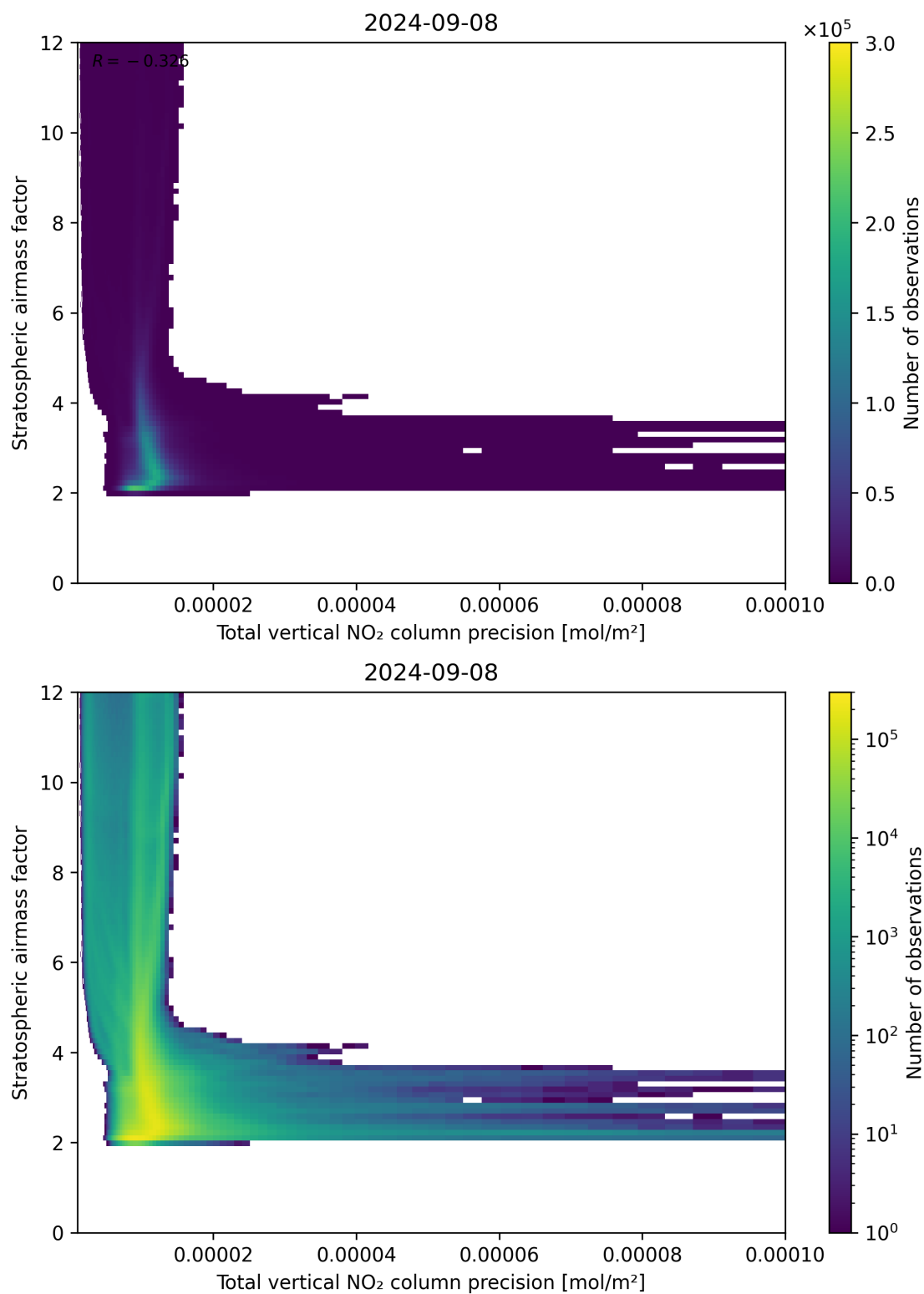
Figure 115: Scatter density plot of “Total vertical NO 2 column precision” against “Stratospheric air mass factor” for 2024-09-07 to 2024-09-09.
