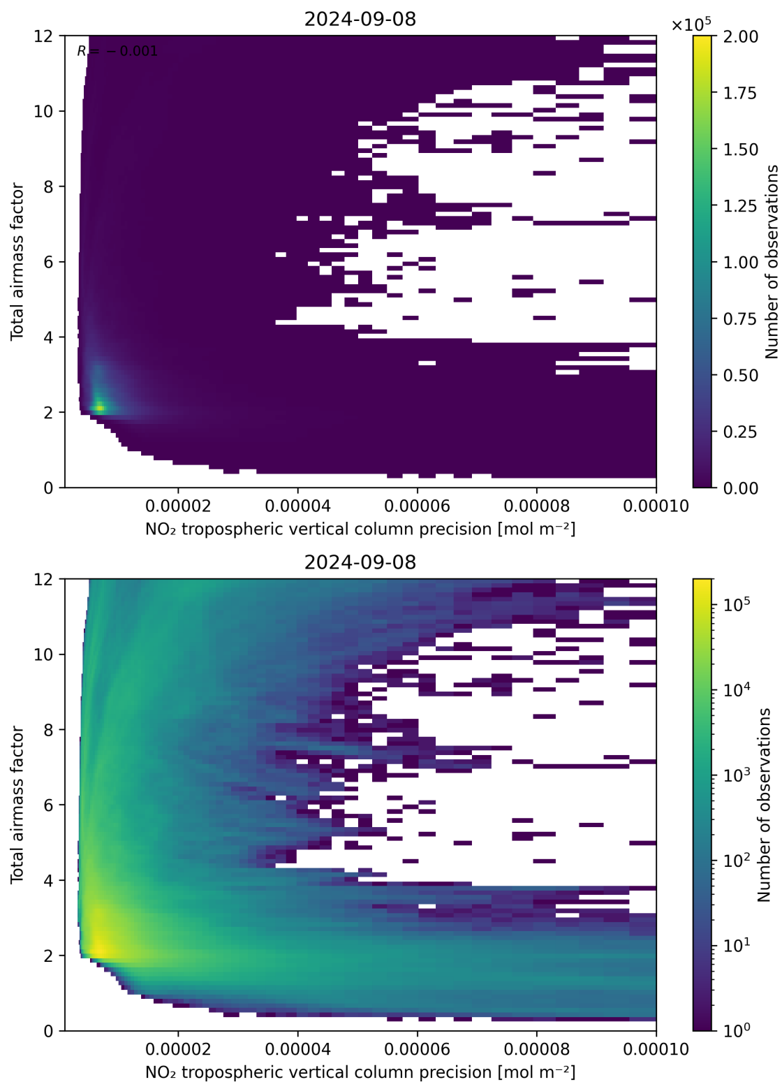
Figure 132: Scatter density plot of “NO 2 tropospheric vertical column precision” against “Total air mass factor” for 2024-09-07 to 2024-09-09.
