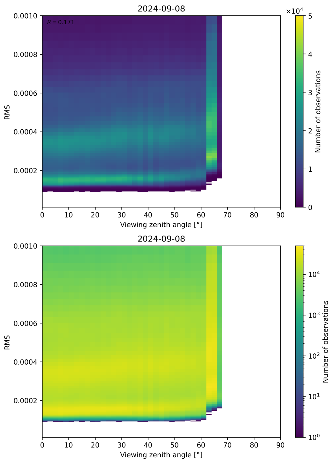
Figure 171: Scatter density plot of “Viewing zenith angle” against “RMS” for 2024-09-07 to 2024-09-09.
