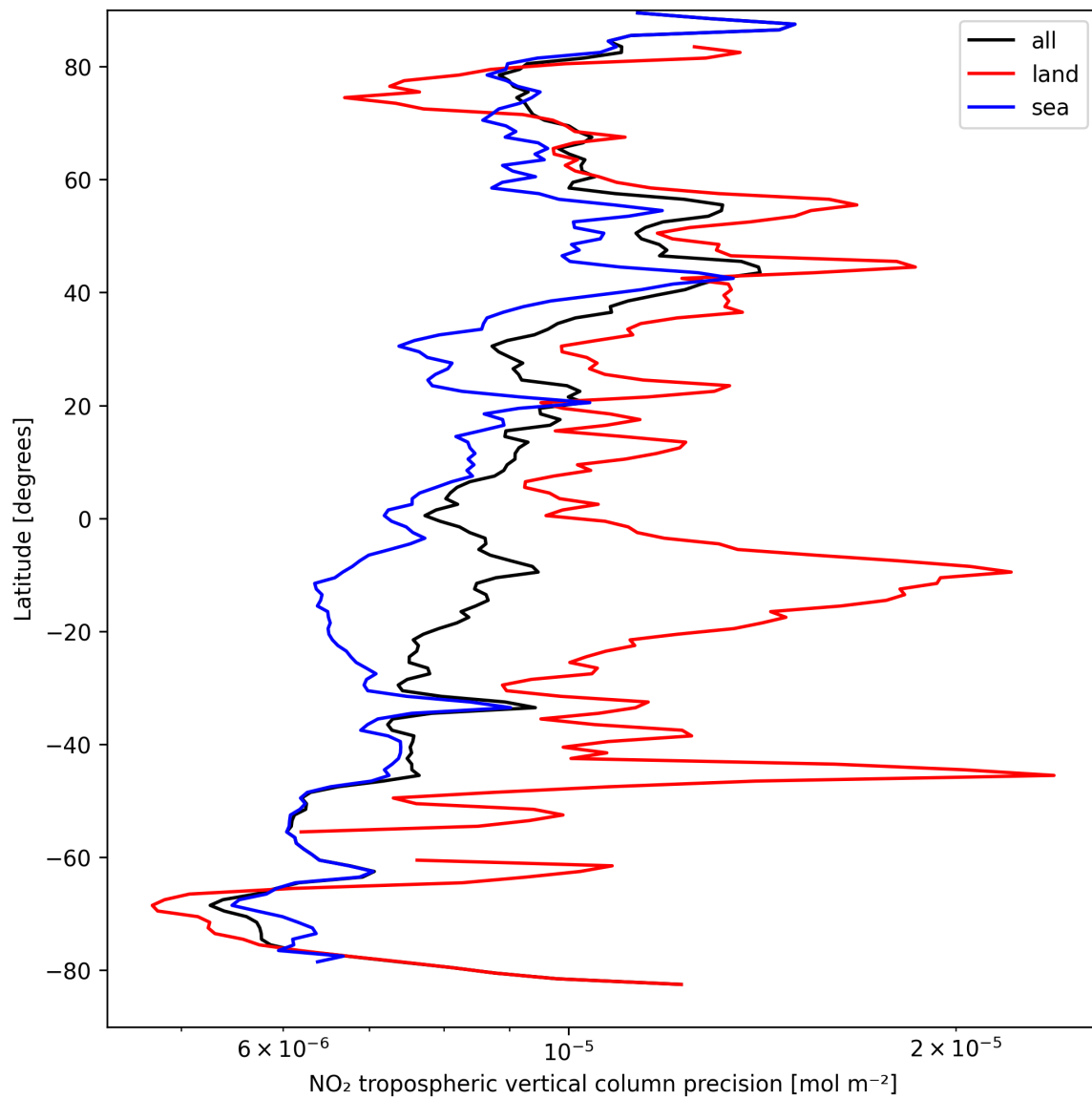
Figure 13: Zonal average of “NO 2 tropospheric vertical column precision” for 2024-09-07 to 2024-09-09.
