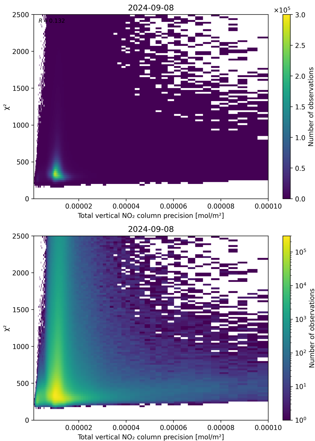
Figure 116: Scatter density plot of “Total vertical NO 2 column precision” against “ \chi^2 ” for 2024-09-07 to 2024-09-09.
