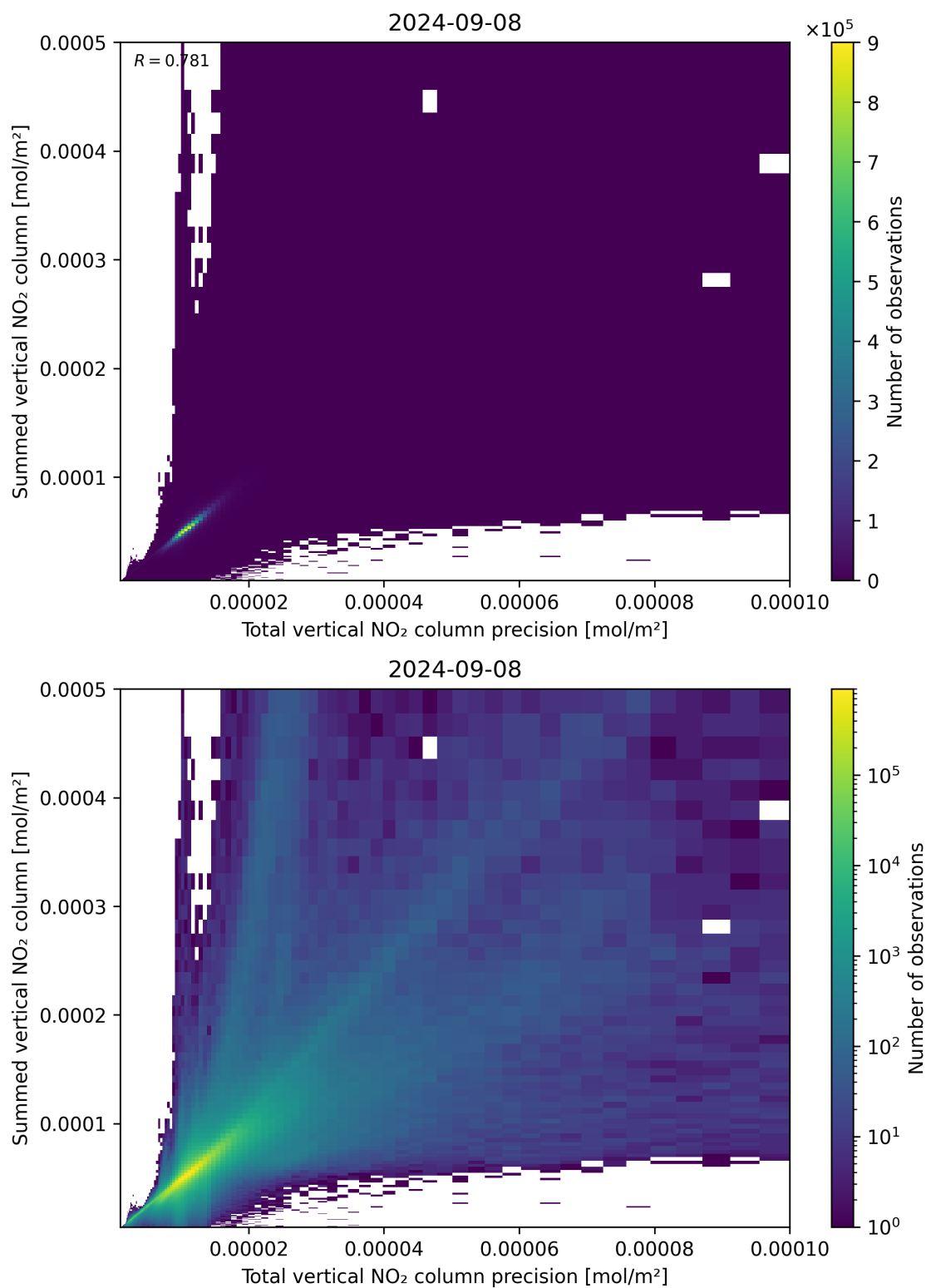
Figure 117: Scatter density plot of “Total vertical NO 2 column precision” against “Summed vertical NO 2 column” for 2024-09-07 to 2024-09-09.
