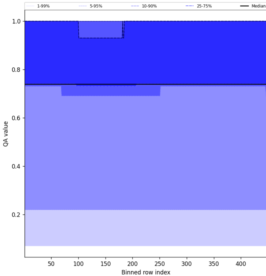
Figure 45: Along track statistics of “QA value” for 2024-09-07 to 2024-09-09
