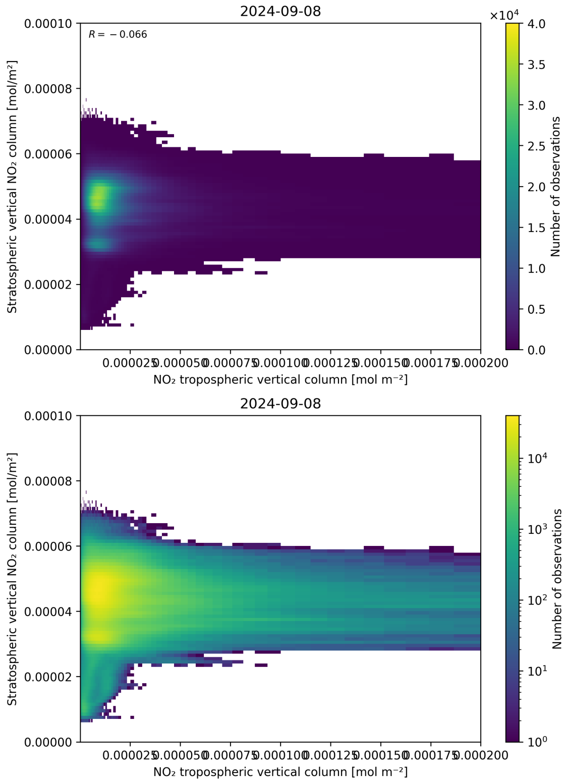
Figure 125: Scatter density plot of “NO 2 tropospheric vertical column” against “Stratospheric vertical NO 2 column” for 2024-09-07 to 2024-09-09.
