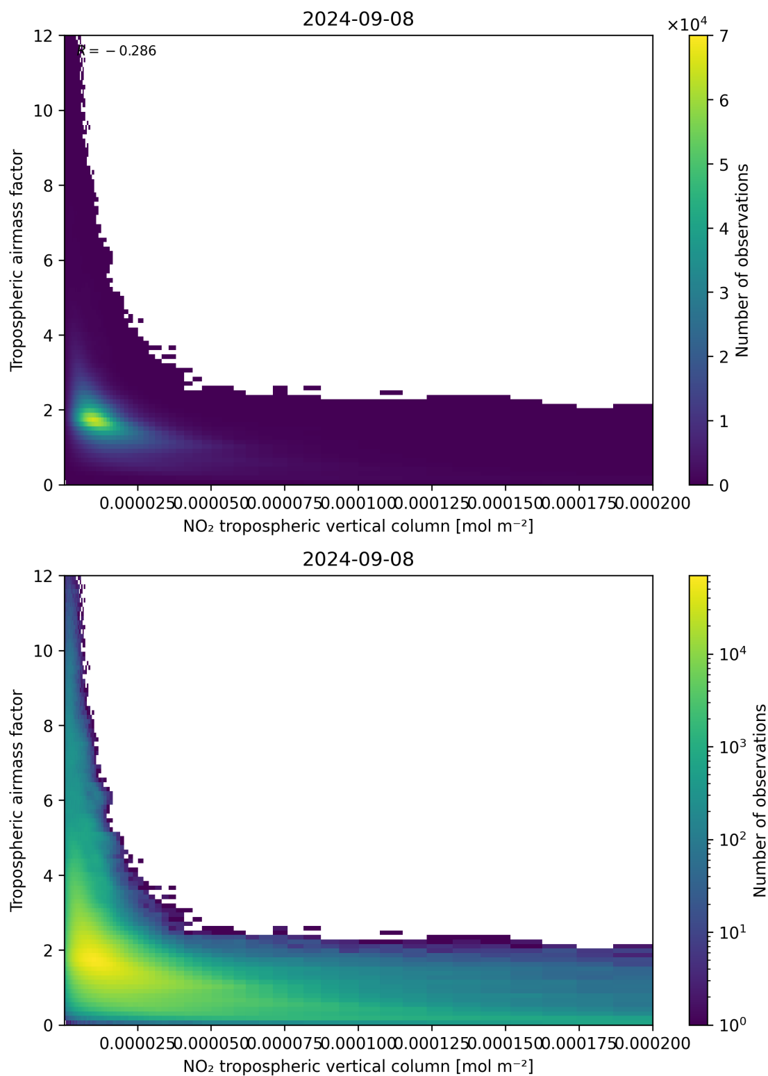
Figure 123: Scatter density plot of “NO 2 tropospheric vertical column” against “Tropospheric air mass factor” for 2024-09-07 to 2024-09-09.
