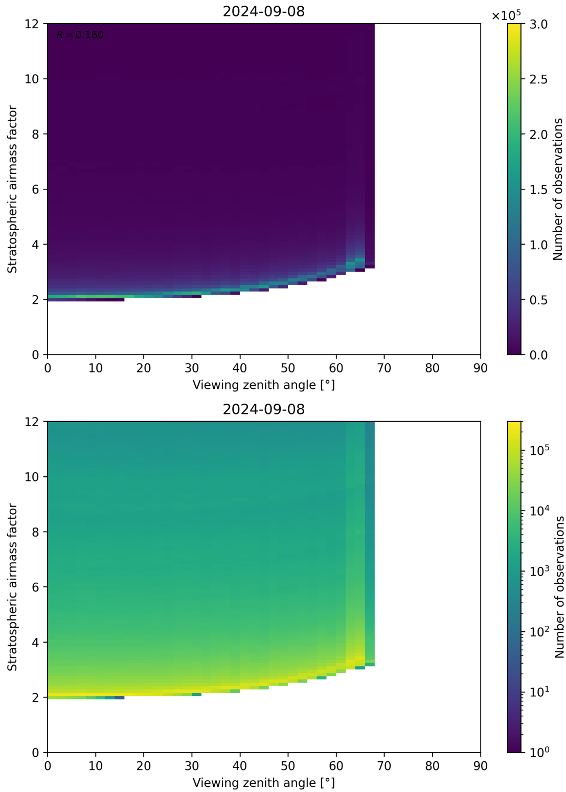
Figure 159: Scatter density plot of “Viewing zenith angle” against “Stratospheric airmass factor” for 2024-09-07 to 2024-09-09.
