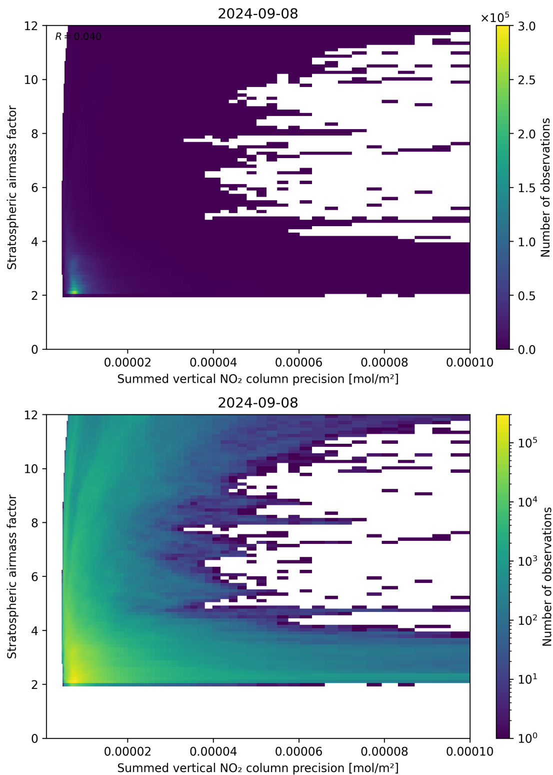
Figure 106: Scatter density plot of “Summed vertical NO 2 column precision” against “Stratospheric airmass factor” for 2024-09-07 to 2024-09-09.
