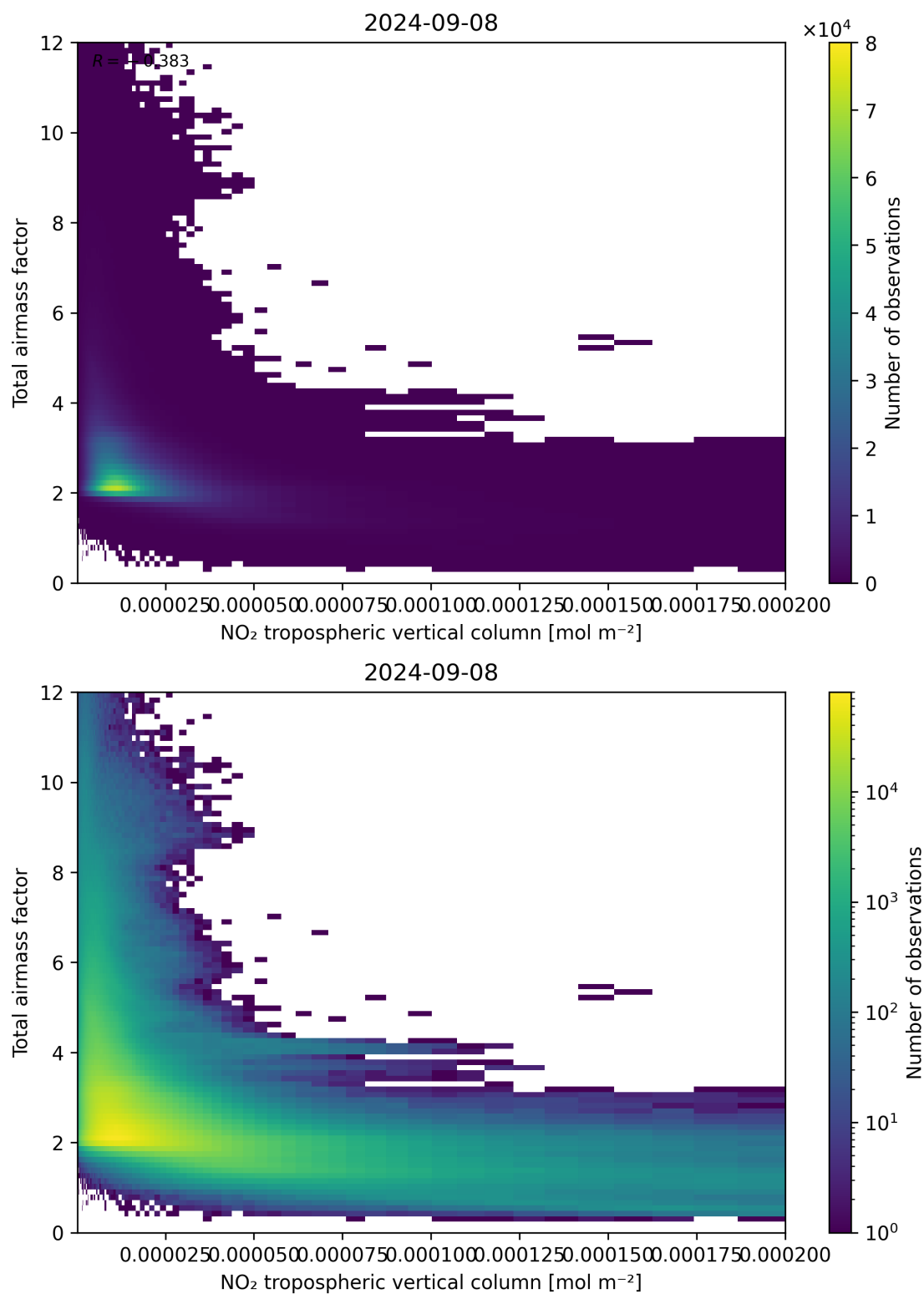
Figure 122: Scatter density plot of “NO 2 tropospheric vertical column” against “Total air mass factor” for 2024-09-07 to 2024-09-09.
