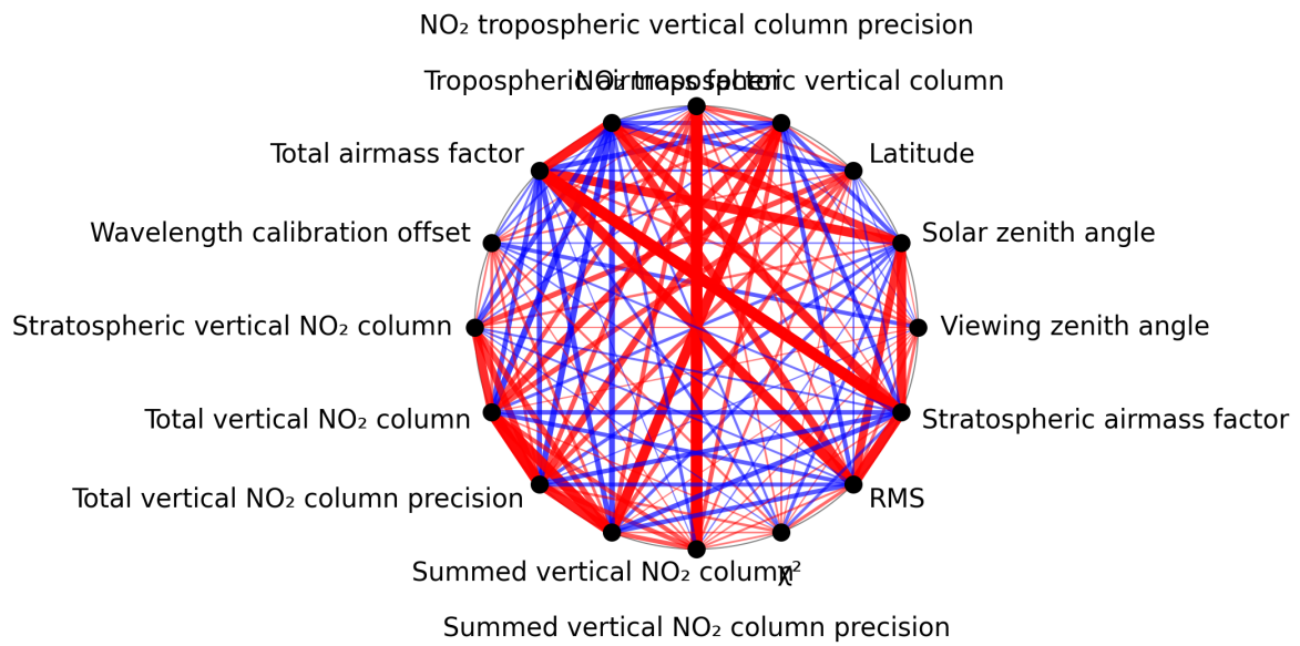
Figure 1: Map of correlation graph for 2024-09-07 to 2024-09-09.
