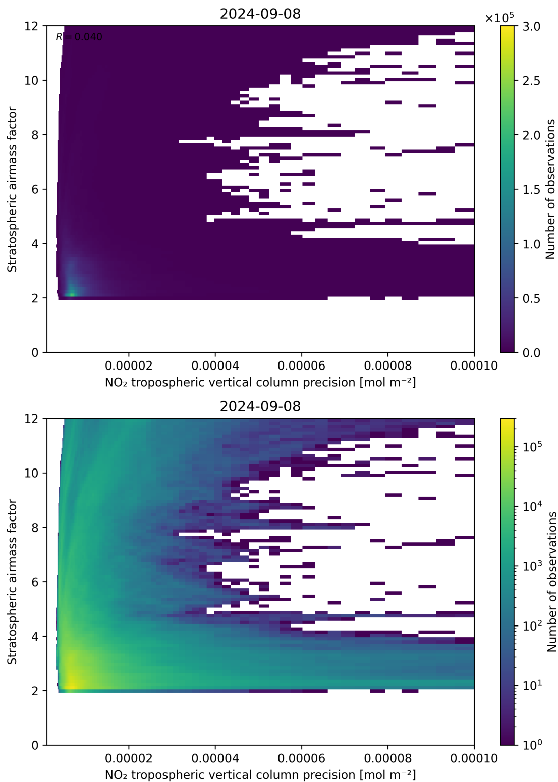
Figure 131: Scatter density plot of “NO 2 tropospheric vertical column precision” against “Stratospheric airmass factor” for 2024-09-07 to 2024-09-09.
