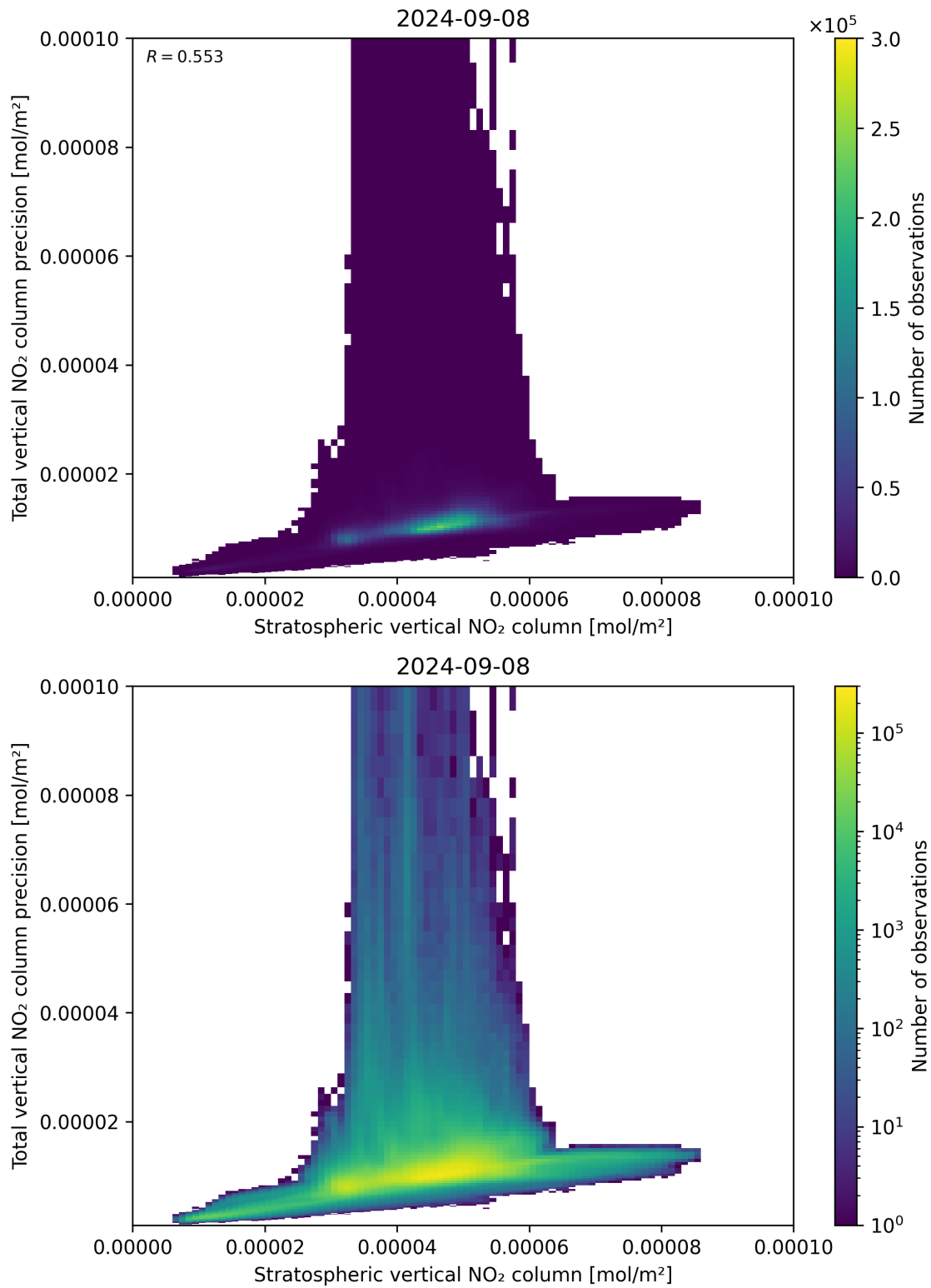
Figure 101: Scatter density plot of “Stratospheric vertical NO 2 column” against “Total vertical NO 2 column precision” for 2024-09-07 to 2024-09-09.
