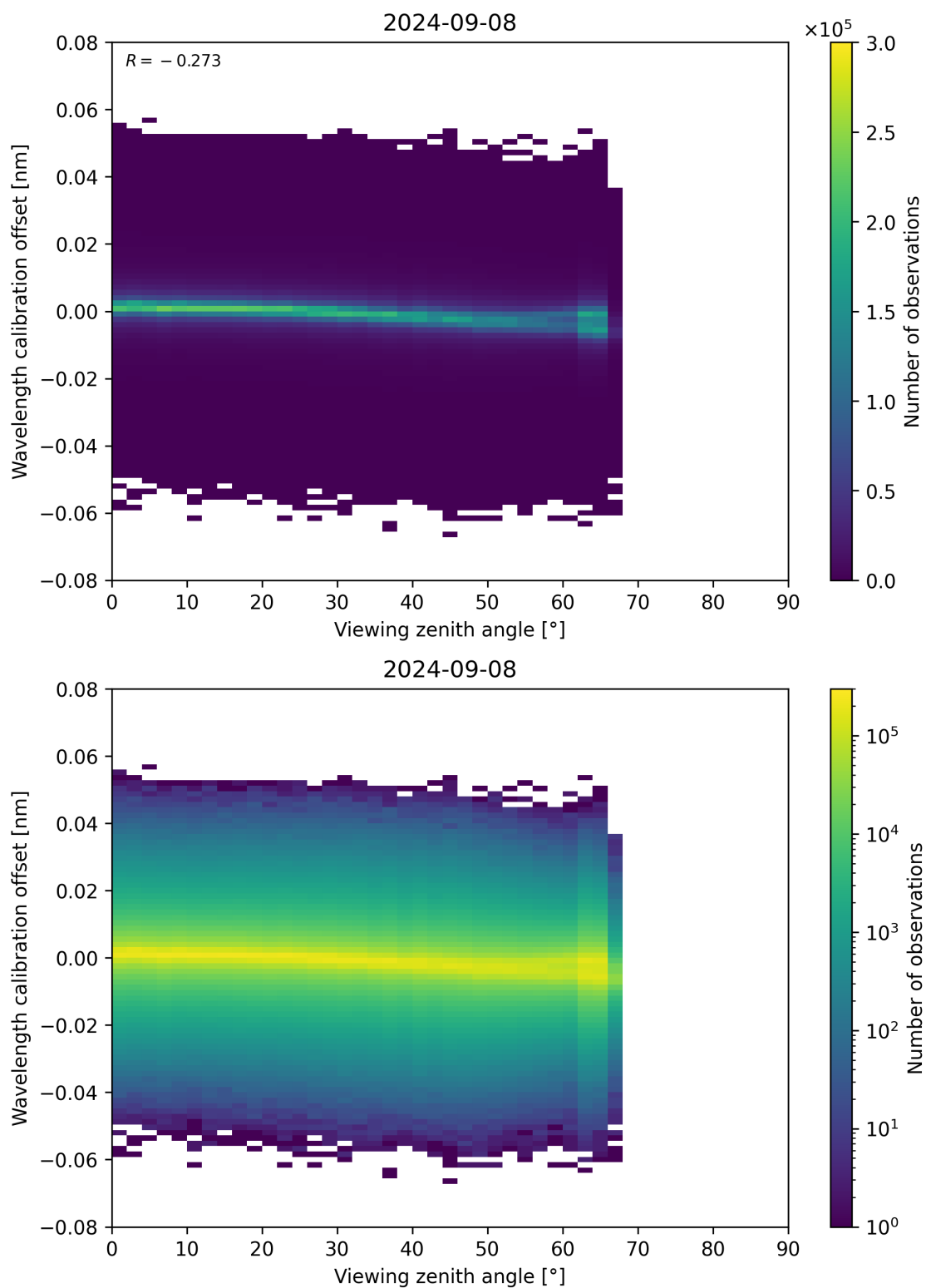
Figure 173: Scatter density plot of “Viewing zenith angle” against “Wavelength calibration offset” for 2024-09-07 to 2024-09-09.
