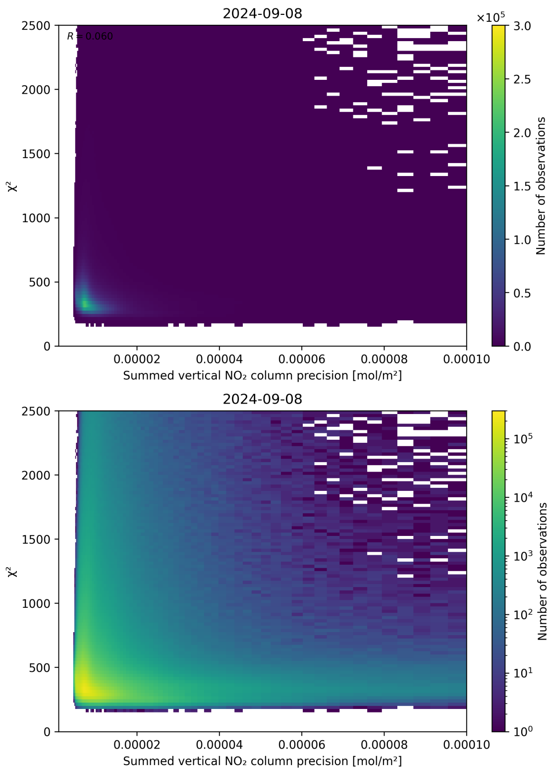
Figure 107: Scatter density plot of “Summed vertical NO 2 column precision” against “ \chi^2 ” for 2024-09-07 to 2024-09-09.
