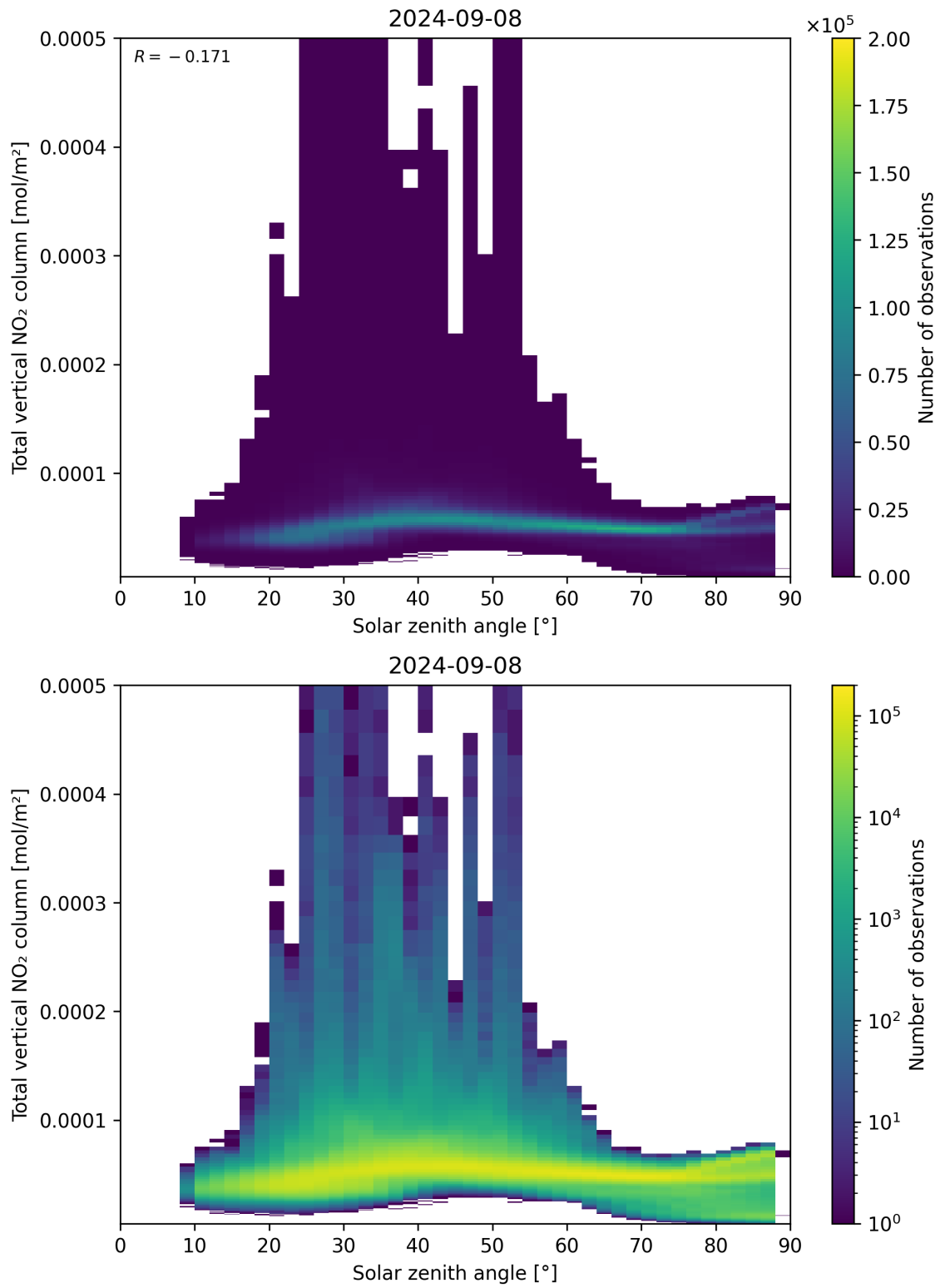
Figure 153: Scatter density plot of “Solar zenith angle” against “Total vertical NO 2 column” for 2024-09-07 to 2024-09-09.
