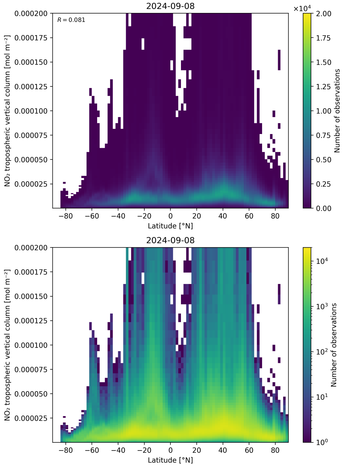
Figure 92: Scatter density plot of “Latitude” against “NO 2 tropospheric vertical column” for 2024-09-07 to 2024-09-09.
