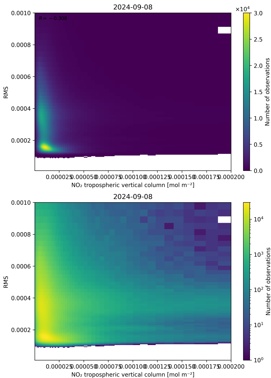
Figure 142: Scatter density plot of “NO 2 tropospheric vertical column” against “RMS” for 2024-09-07 to 2024-09-09.
