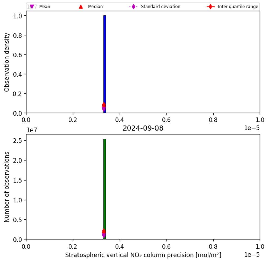
Figure 37: Histogram of “Stratospheric vertical NO 2 column precision” for 2024-09-07 to 2024-09-09
