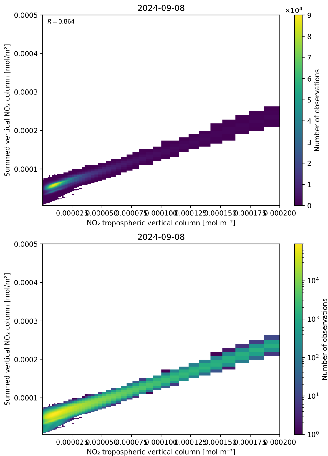
Figure 126: Scatter density plot of “NO 2 tropospheric vertical column” against “Summed vertical NO 2 column” for 2024-09-07 to 2024-09-09.
