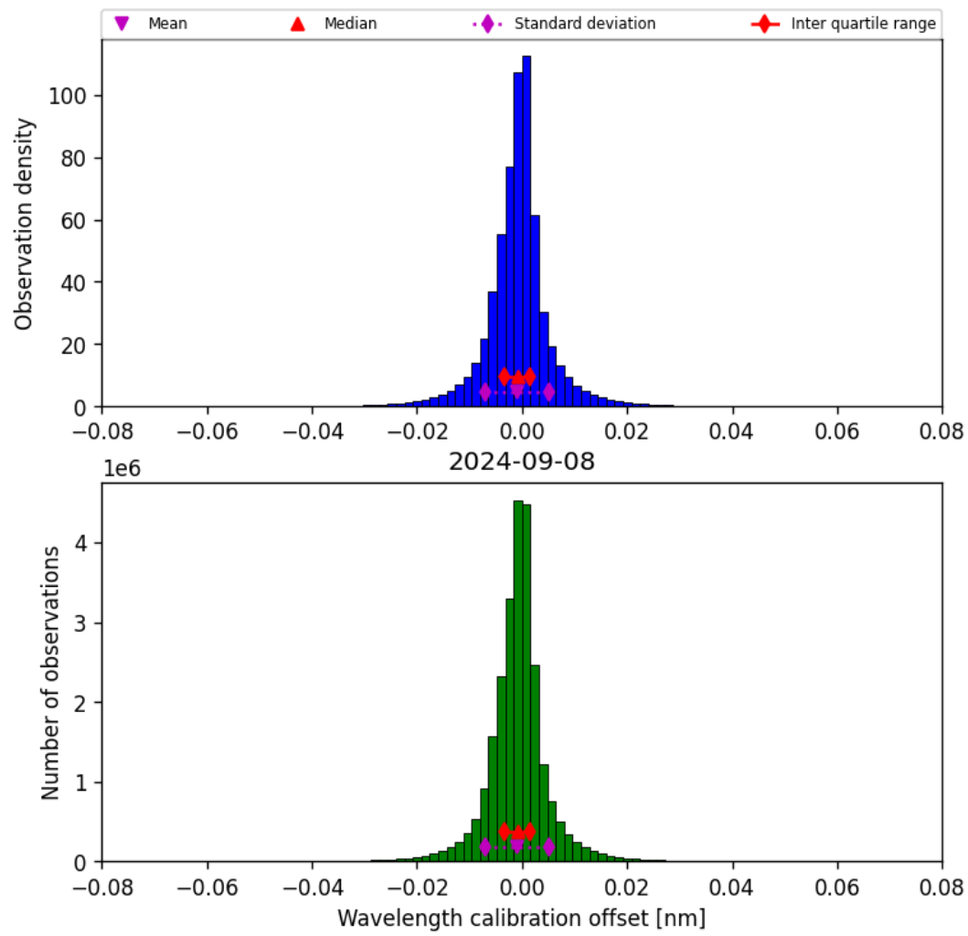
Figure 35: Histogram of “Wavelength calibration offset” for 2024-09-07 to 2024-09-09
