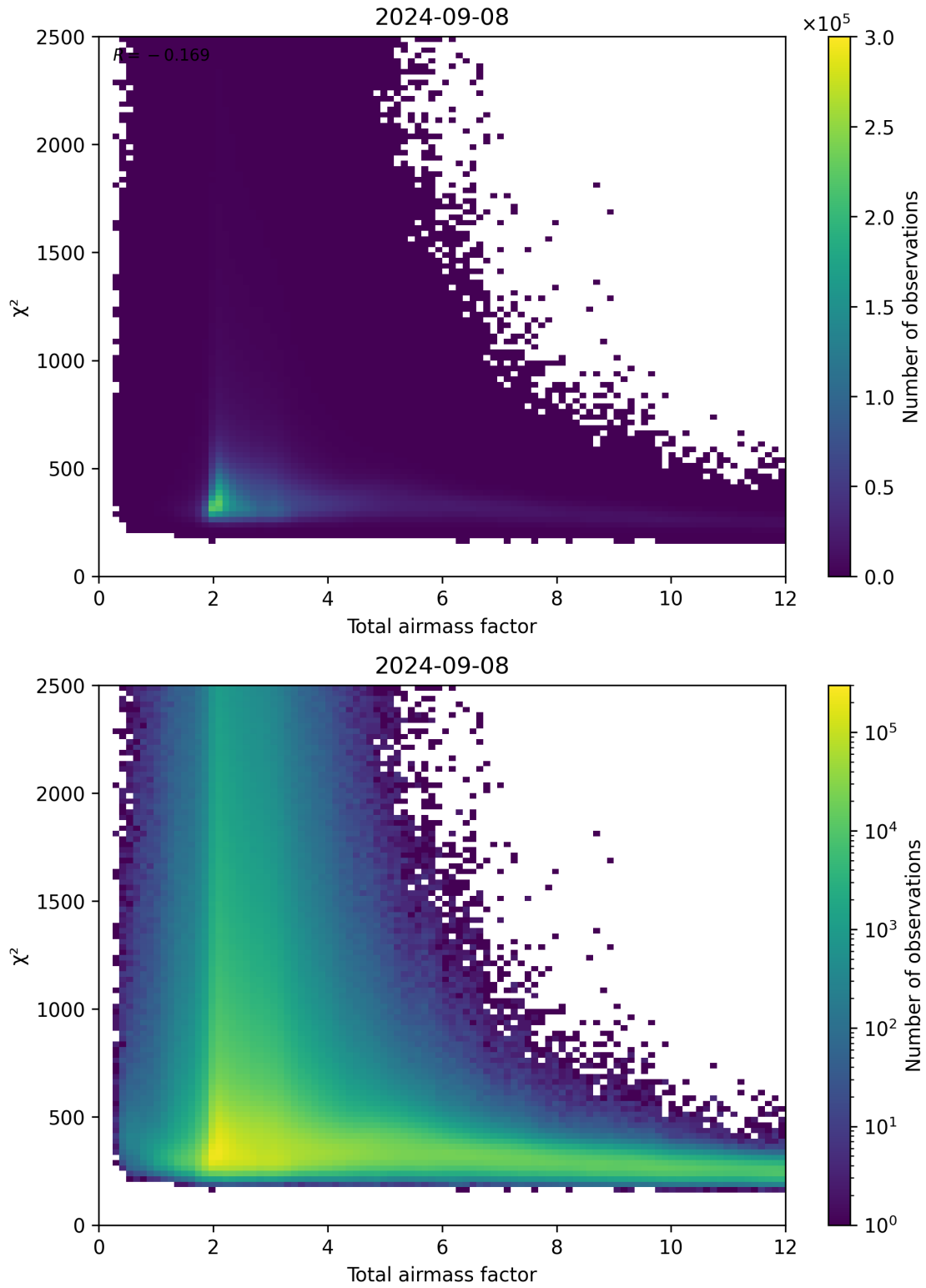
Figure 63: Scatter density plot of “Total airmass factor” against “ \chi^2 ” for 2024-09-07 to 2024-09-09.
