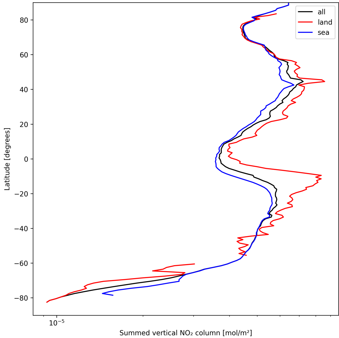
Figure 23: Zonal average of “Summed vertical NO 2 column” for 2024-09-07 to 2024-09-09.
