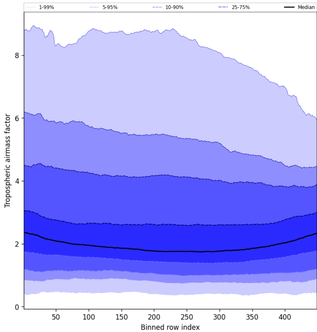
Figure 48: Along track statistics of “Tropospheric air mass factor” for 2024-09-07 to 2024-09-09
