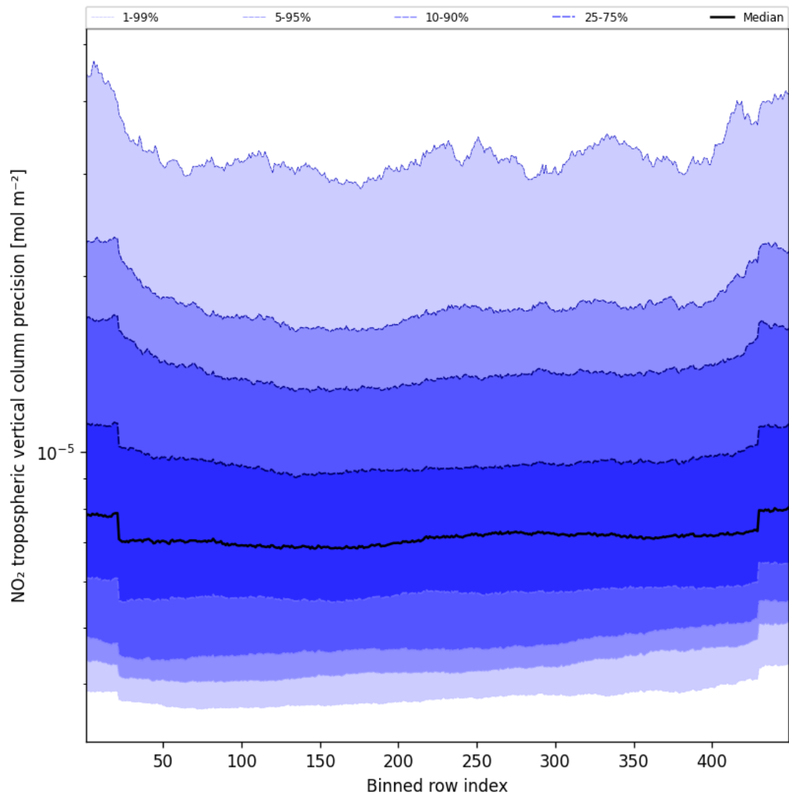
Figure 47: Along track statistics of “NO 2 tropospheric vertical column precision” for 2024-09-07 to 2024-09-09
