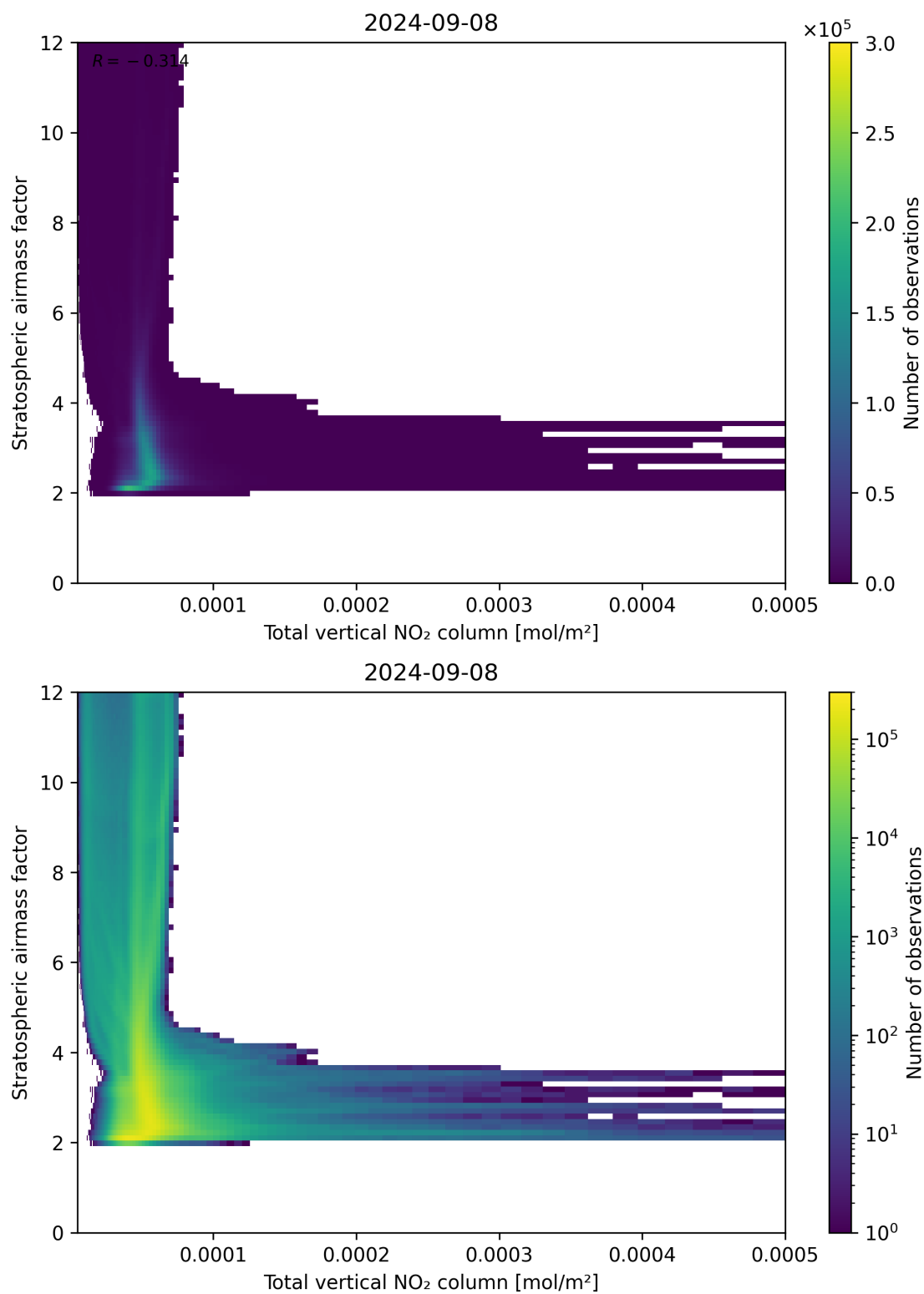
Figure 110: Scatter density plot of “Total vertical NO 2 column” against “Stratospheric airmass factor” for 2024-09-07 to 2024-09-09.
