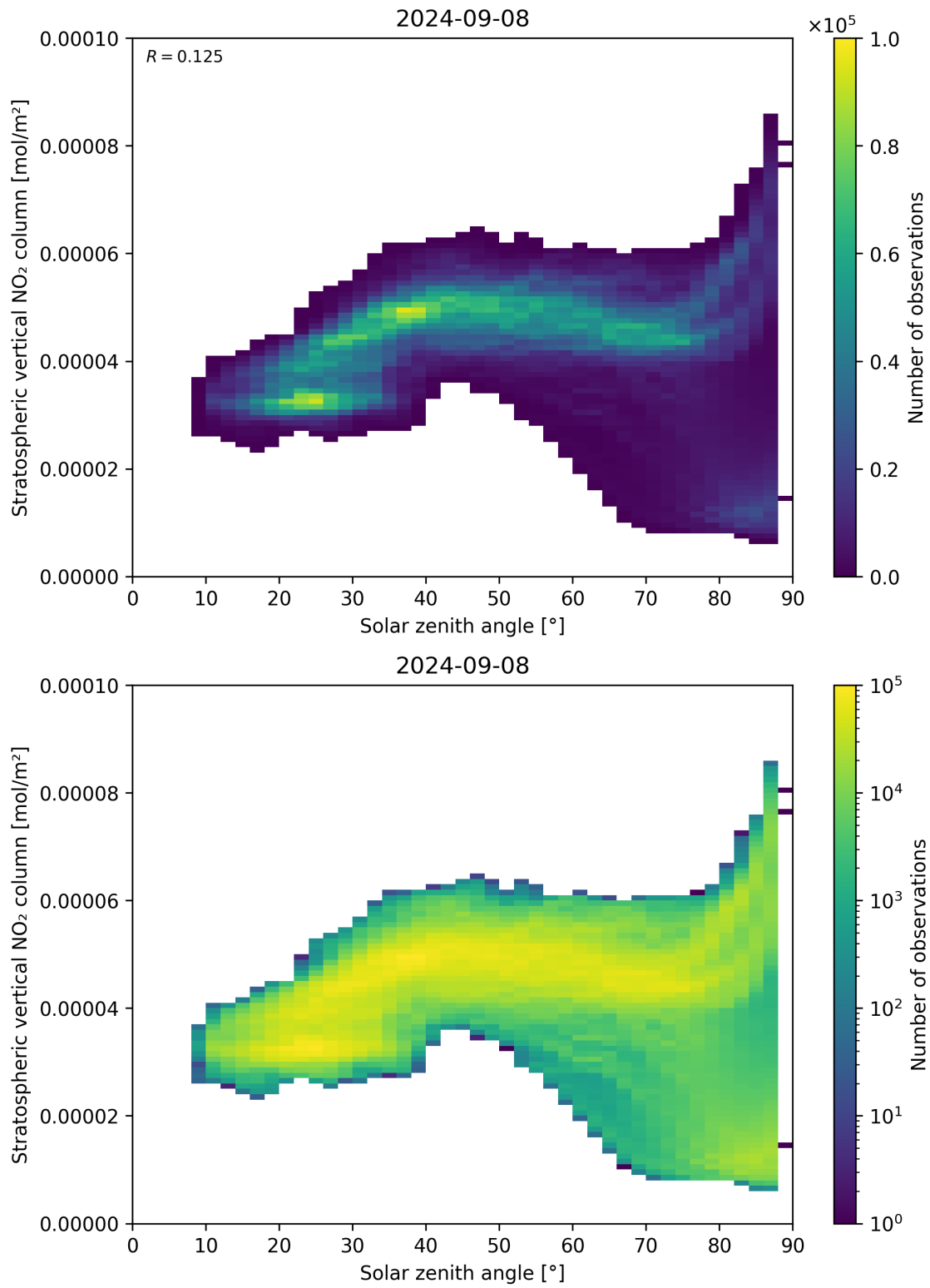
Figure 150: Scatter density plot of “Solar zenith angle” against “Stratospheric vertical NO 2 column” for 2024-09-07 to 2024-09-09.
