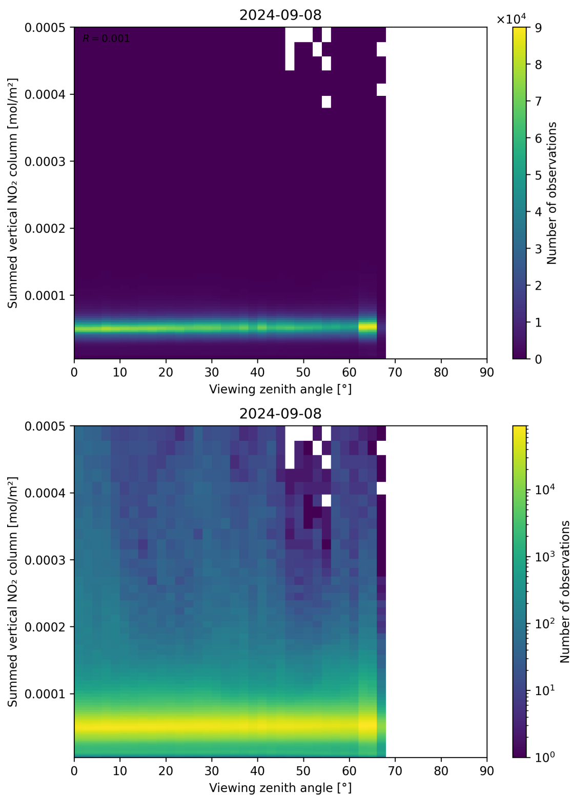
Figure 165: Scatter density plot of “Viewing zenith angle” against “Summed vertical NO 2 column” for 2024-09-07 to 2024-09-09.
