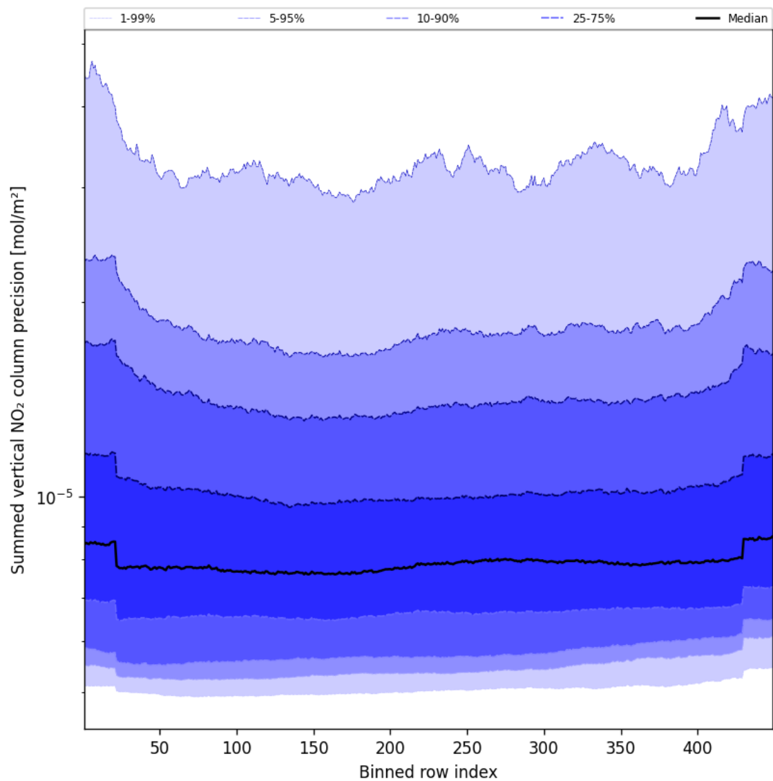
Figure 58: Along track statistics of “Summed vertical NO 2 column precision” for 2024-09-07 to 2024-09-09
