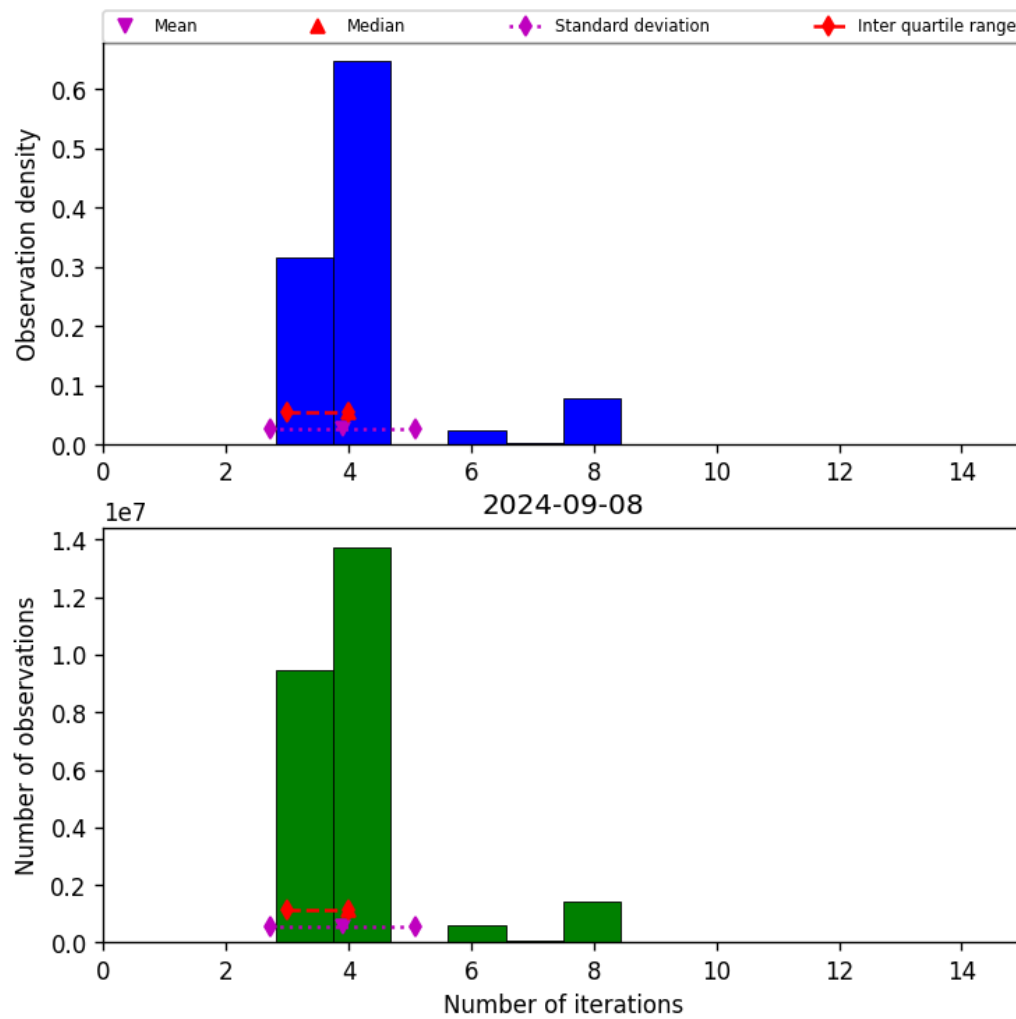
Figure 34: Histogram of “Number of iterations” for 2024-09-07 to 2024-09-09
