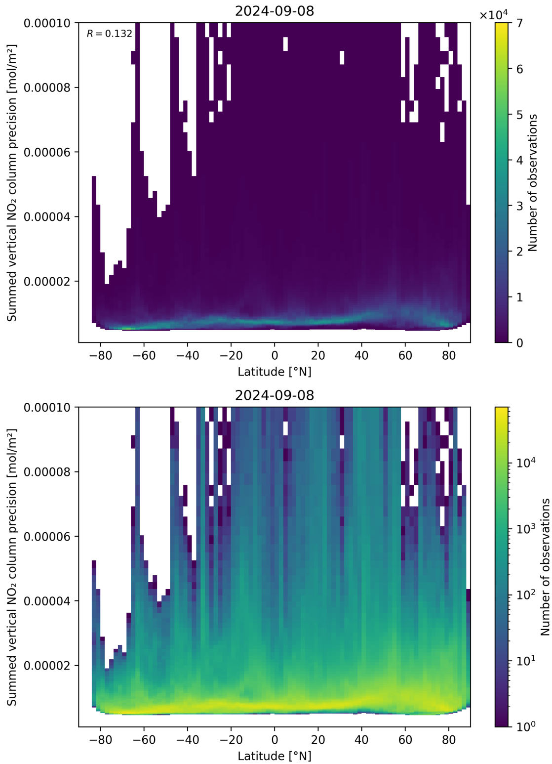
Figure 89: Scatter density plot of “Latitude” against “Summed vertical NO 2 column precision” for 2024-09-07 to 2024-09-09.
