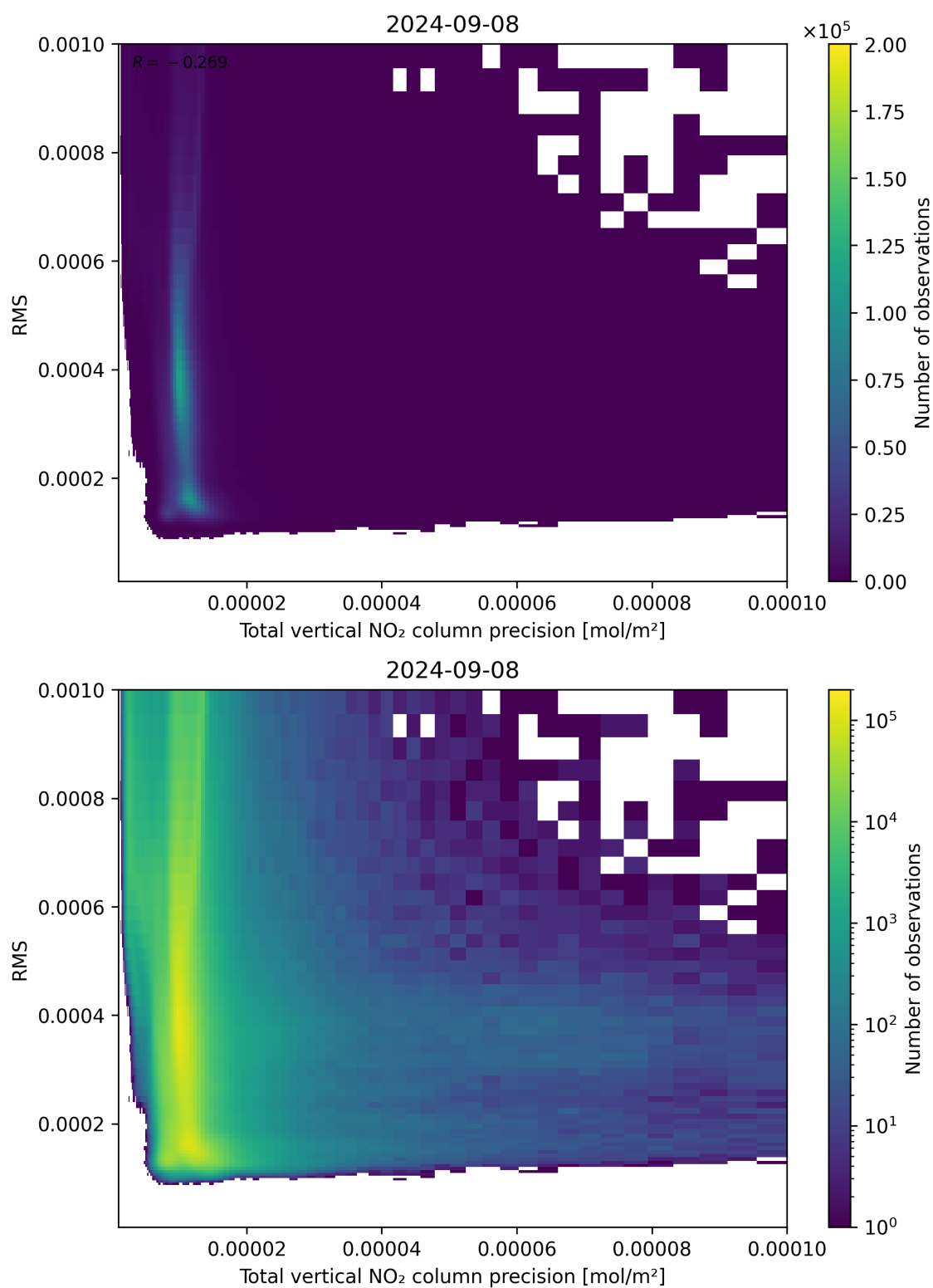
Figure 119: Scatter density plot of “Total vertical NO 2 column precision” against “RMS” for 2024-09-07 to 2024-09-09.
