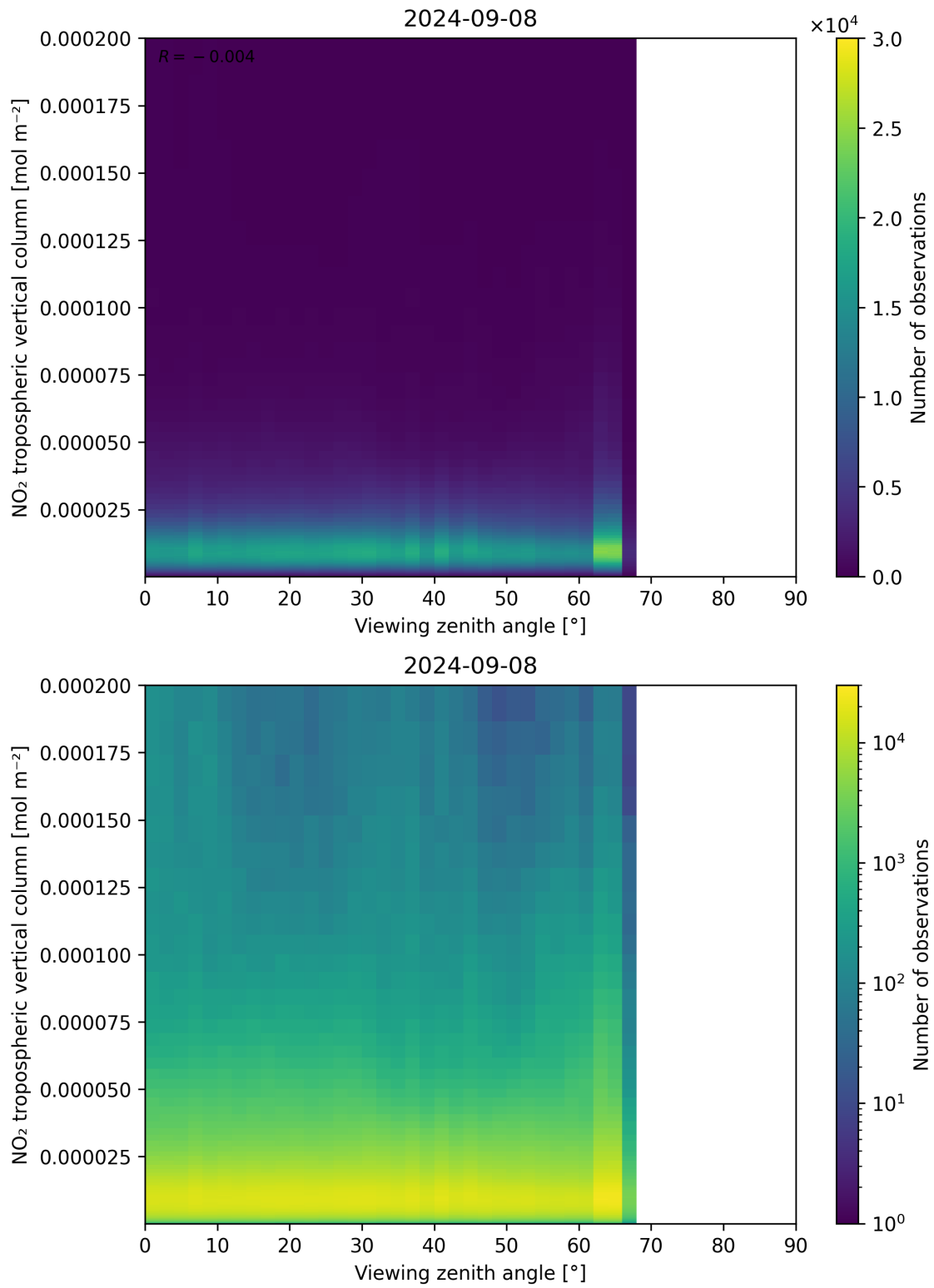
Figure 169: Scatter density plot of “Viewing zenith angle” against “NO 2 tropospheric vertical column” for 2024-09-07 to 2024-09-09.
