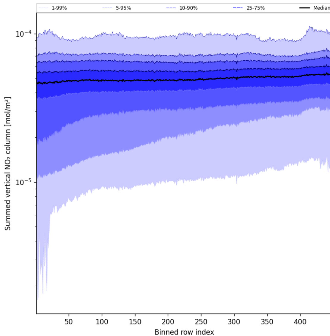
Figure 57: Along track statistics of “Summed vertical NO 2 column” for 2024-09-07 to 2024-09-09
