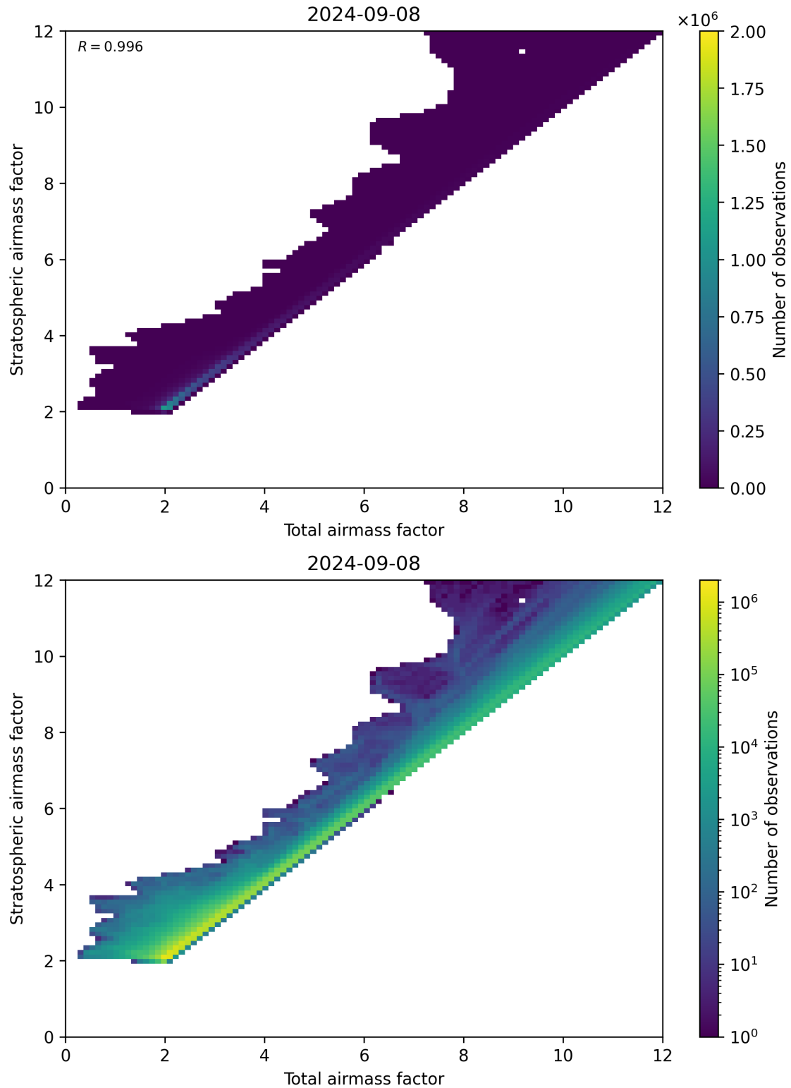
Figure 62: Scatter density plot of “Total air mass factor” against “Stratospheric air mass factor” for 2024-09-07 to 2024-09-09.
