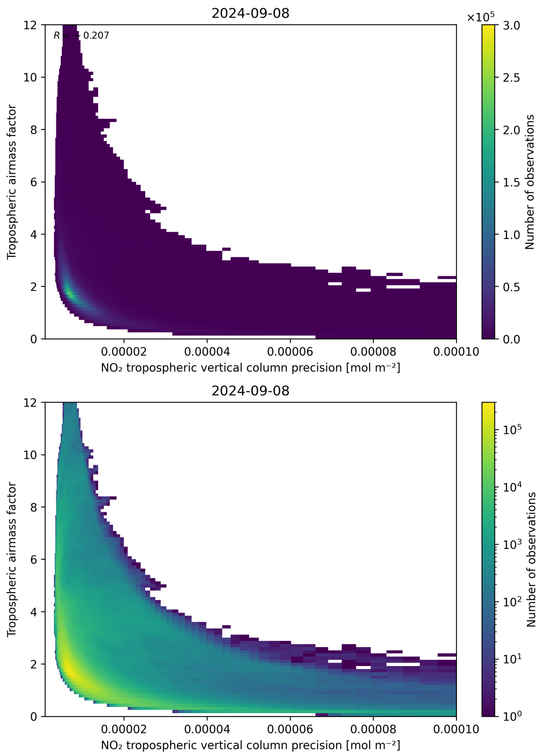
Figure 133: Scatter density plot of “NO 2 tropospheric vertical column precision” against “Tropospheric airmass factor” for 2024-09-07 to 2024-09-09.
