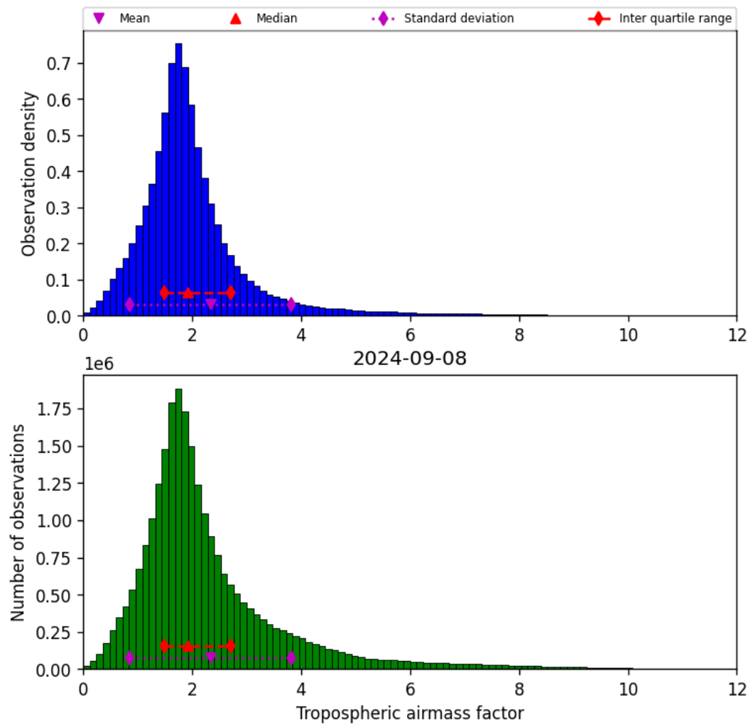
Figure 31: Histogram of “Tropospheric airmass factor” for 2024-09-07 to 2024-09-09
