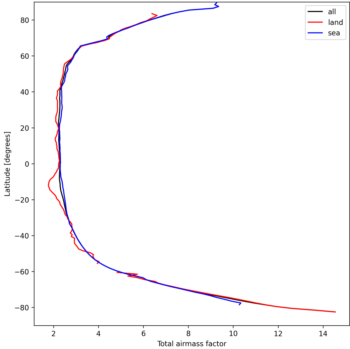
Figure 15: Zonal average of “Total airmass factor” for 2024-09-07 to 2024-09-09.
