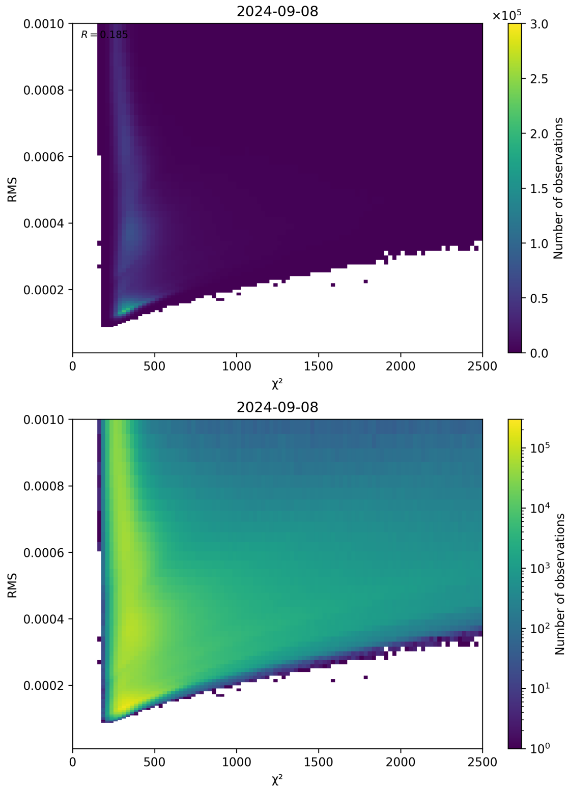
Figure 82: Scatter density plot of “ \chi^2 ” against “RMS” for 2024-09-07 to 2024-09-09.
