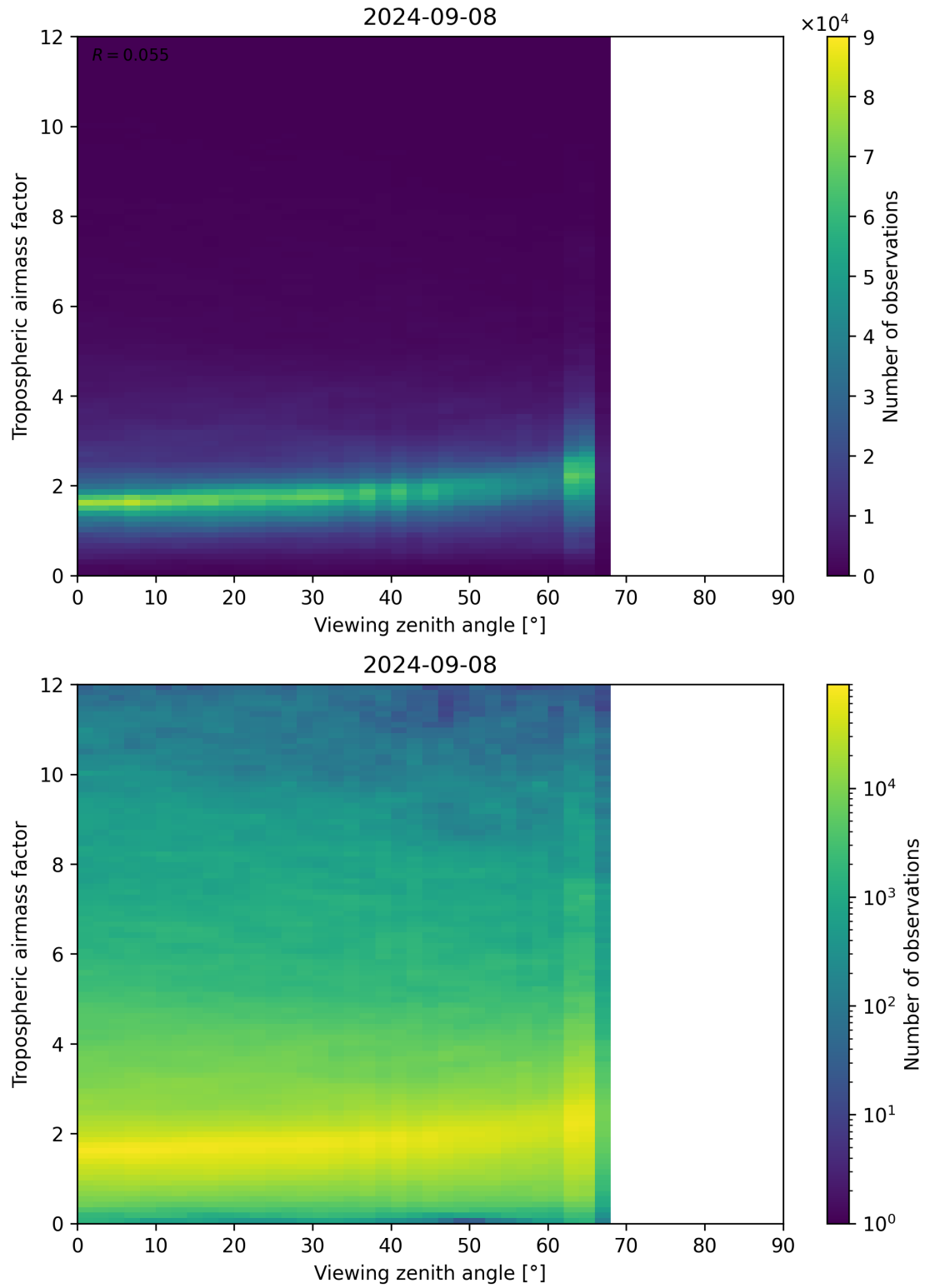
Figure 161: Scatter density plot of “Viewing zenith angle” against “Tropospheric airmass factor” for 2024-09-07 to 2024-09-09.
