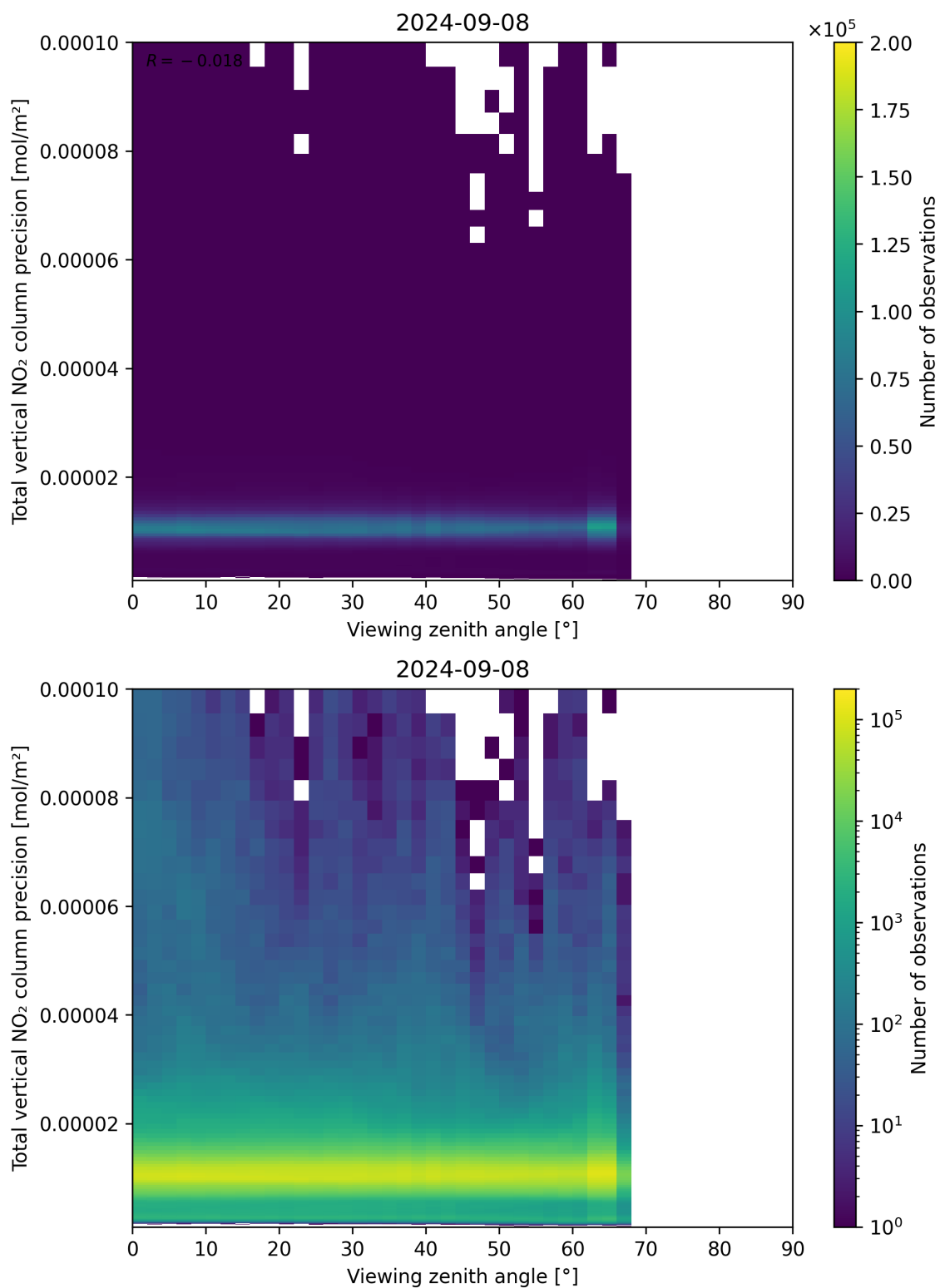
Figure 168: Scatter density plot of “Viewing zenith angle” against “Total vertical NO 2 column precision” for 2024-09-07 to 2024-09-09.
