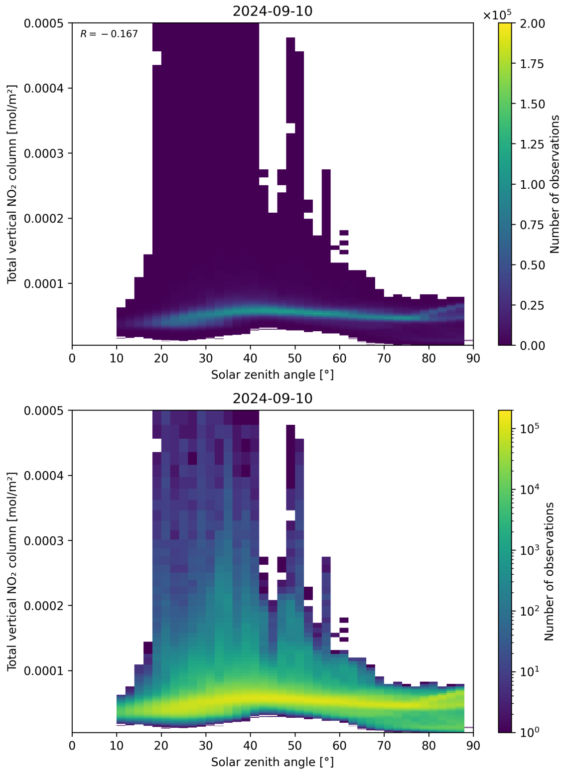
Figure 153: Scatter density plot of “Solar zenith angle” against “Total vertical NO 2 column” for 2024-09-09 to 2024-09-11.
