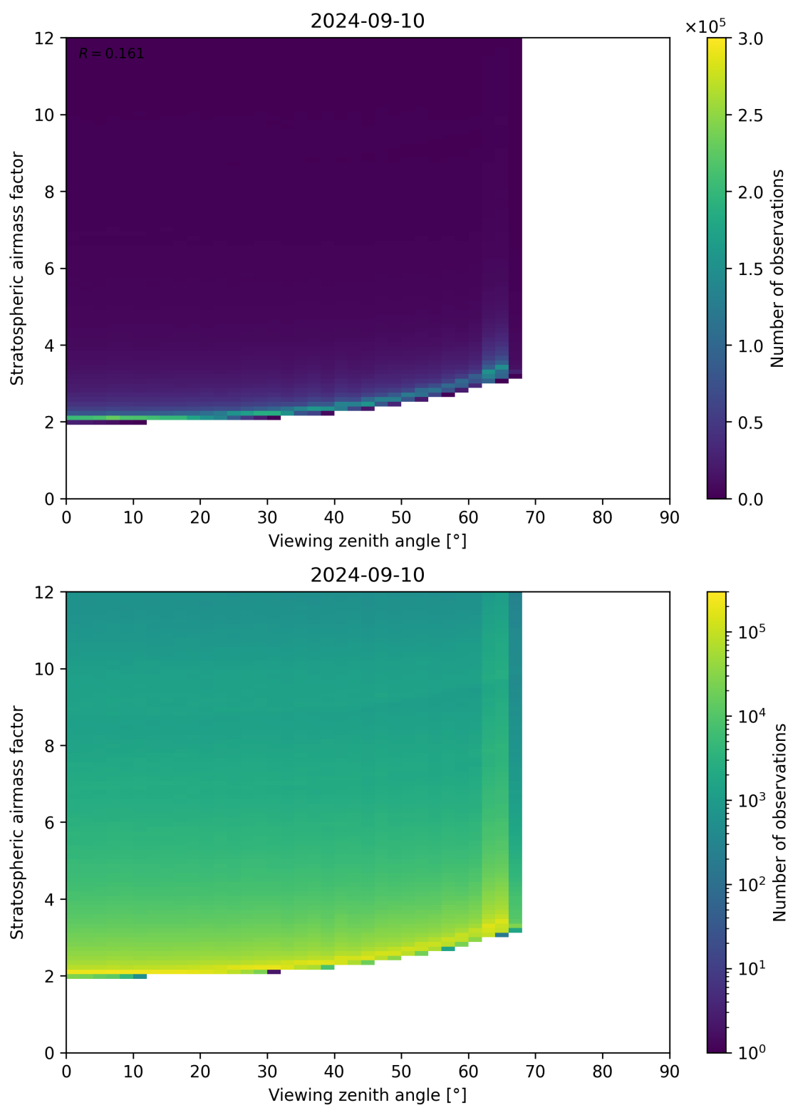
Figure 159: Scatter density plot of “Viewing zenith angle” against “Stratospheric airmass factor” for 2024-09-09 to 2024-09-11.
