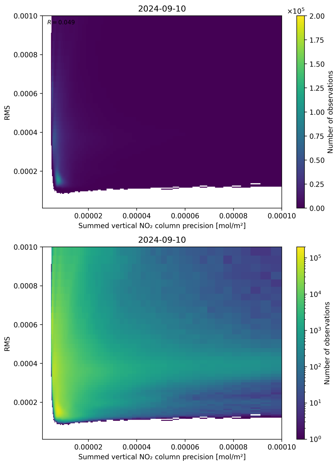
Figure 108: Scatter density plot of “Summed vertical NO 2 column precision” against “RMS” for 2024-09-09 to 2024-09-11.
