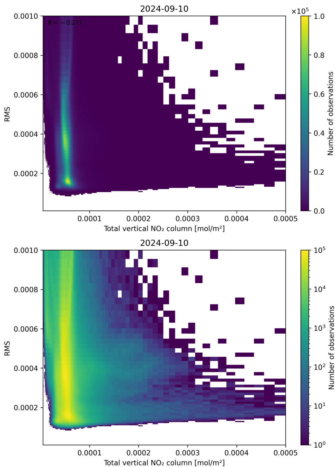
Figure 120: Scatter density plot of “Total vertical NO 2 column” against “RMS” for 2024-09-09 to 2024-09-11.
