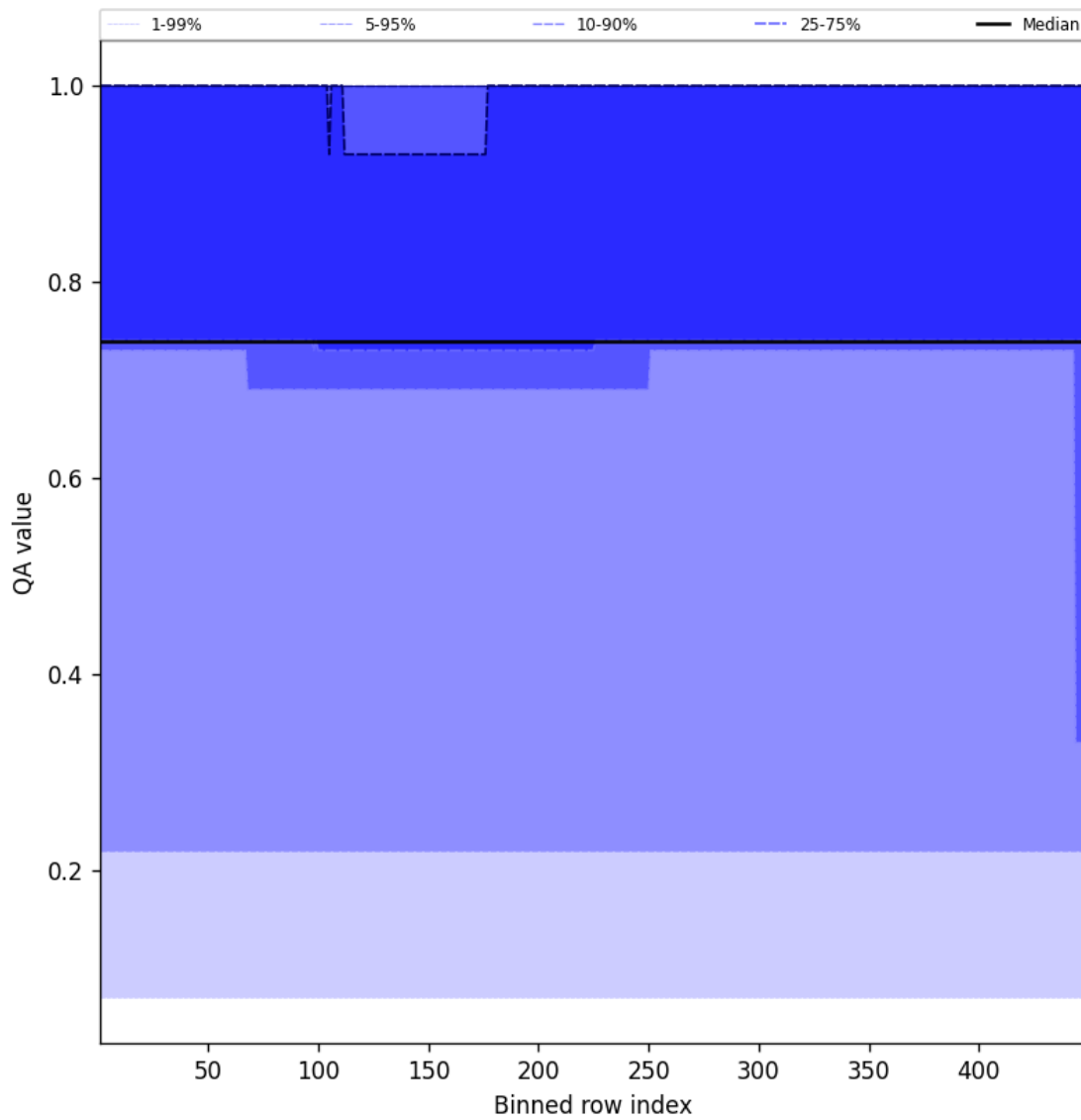
Figure 45: Along track statistics of “QA value” for 2024-09-09 to 2024-09-11
