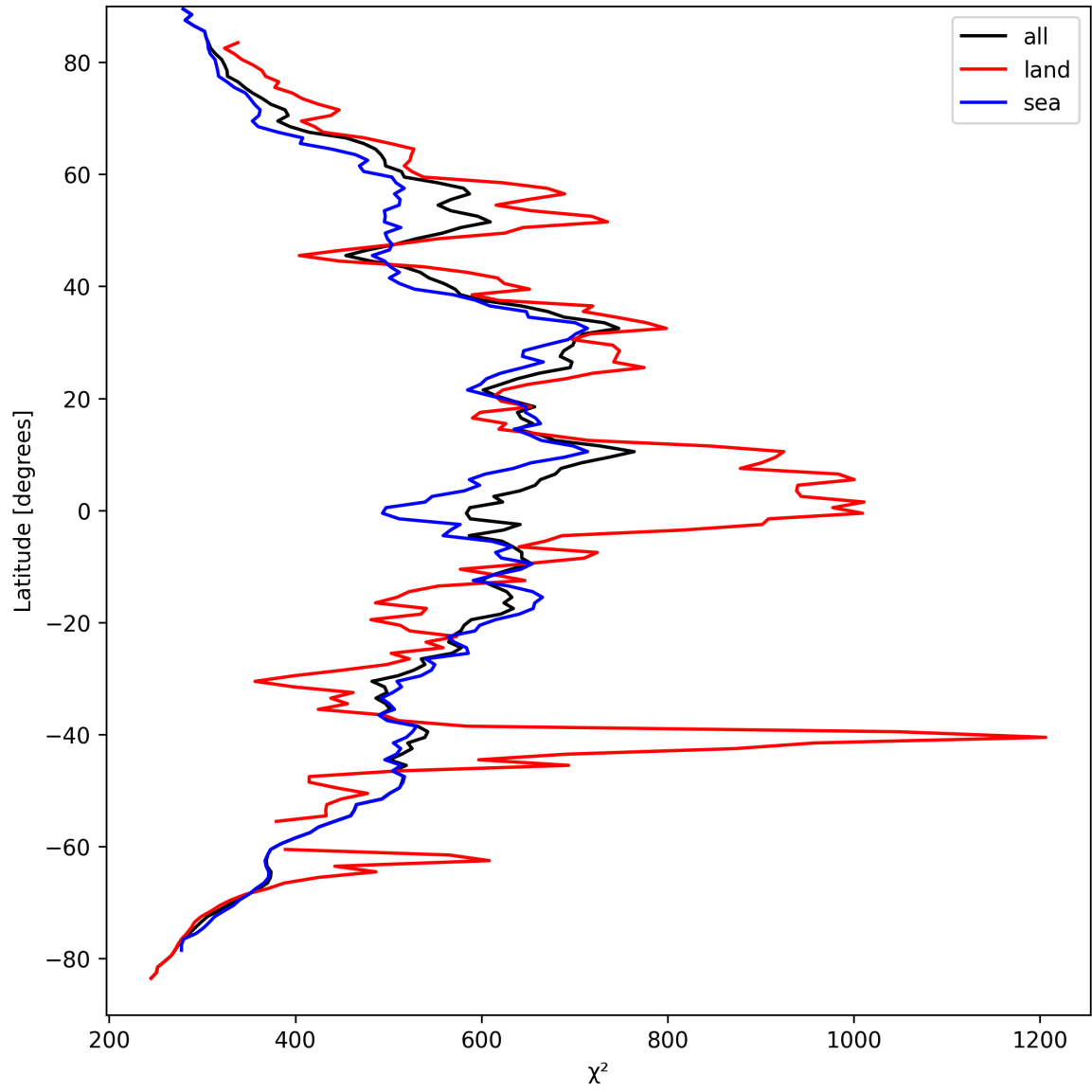
Figure 25: Zonal average of “ \chi^2 ” for 2024-09-09 to 2024-09-11.
