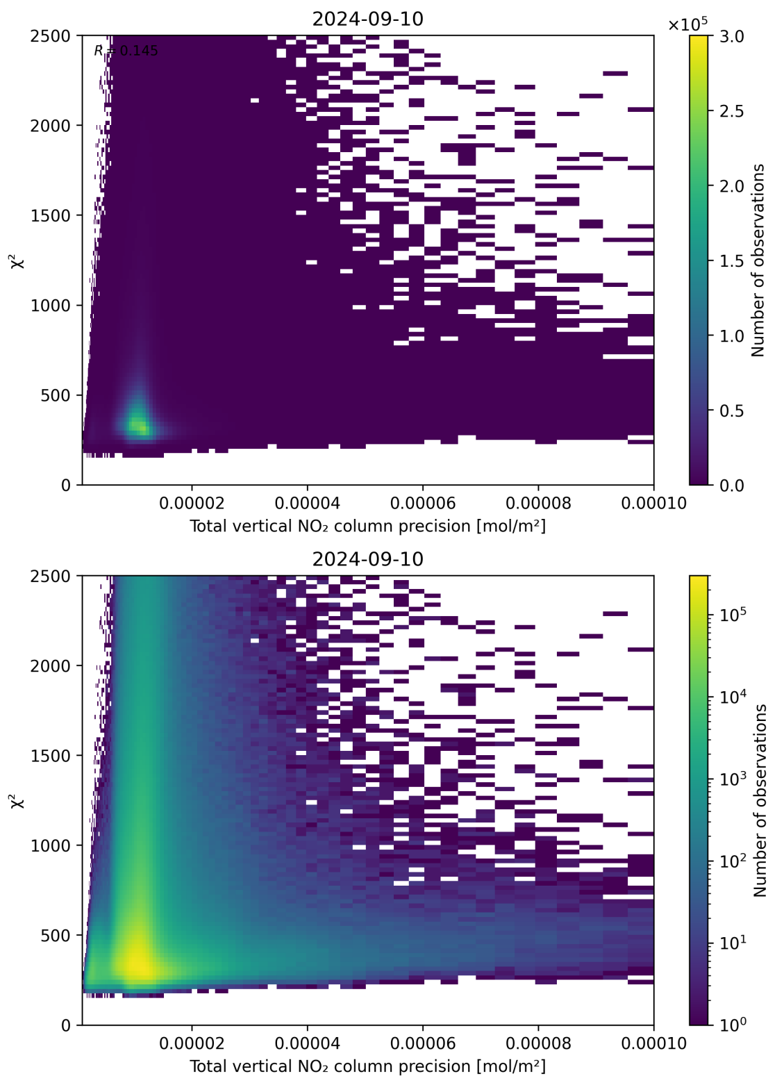
Figure 116: Scatter density plot of “Total vertical NO 2 column precision” against “ \chi^2 ” for 2024-09-09 to 2024-09-11.
