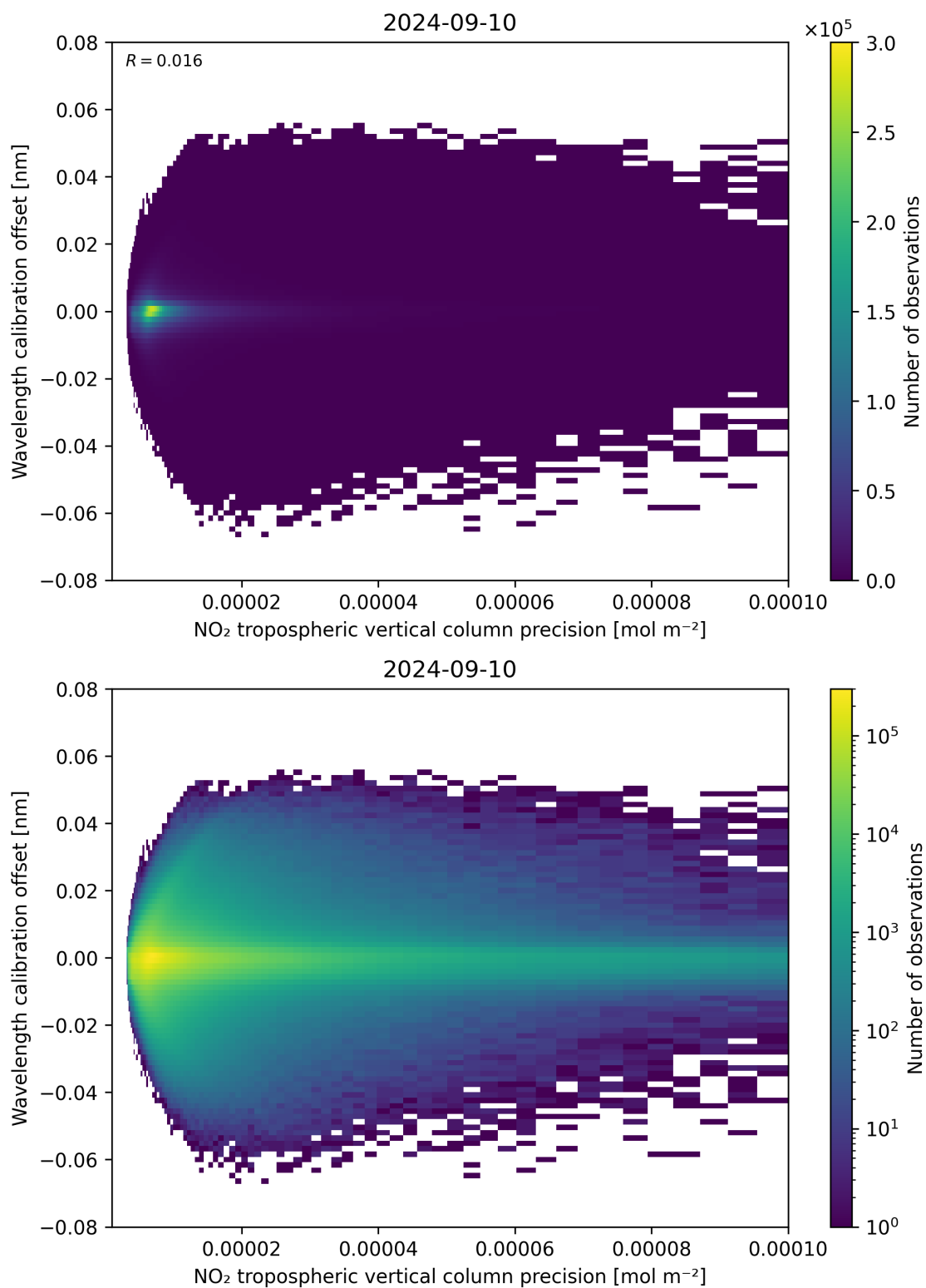
Figure 141: Scatter density plot of “NO 2 tropospheric vertical column precision” against “Wavelength calibration offset” for 2024-09-09 to 2024-09-11.
