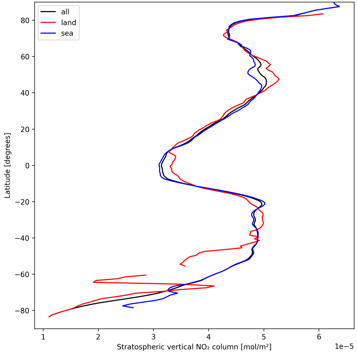
Figure 19: Zonal average of “Stratospheric vertical NO 2 column” for 2024-09-09 to 2024-09-11.
