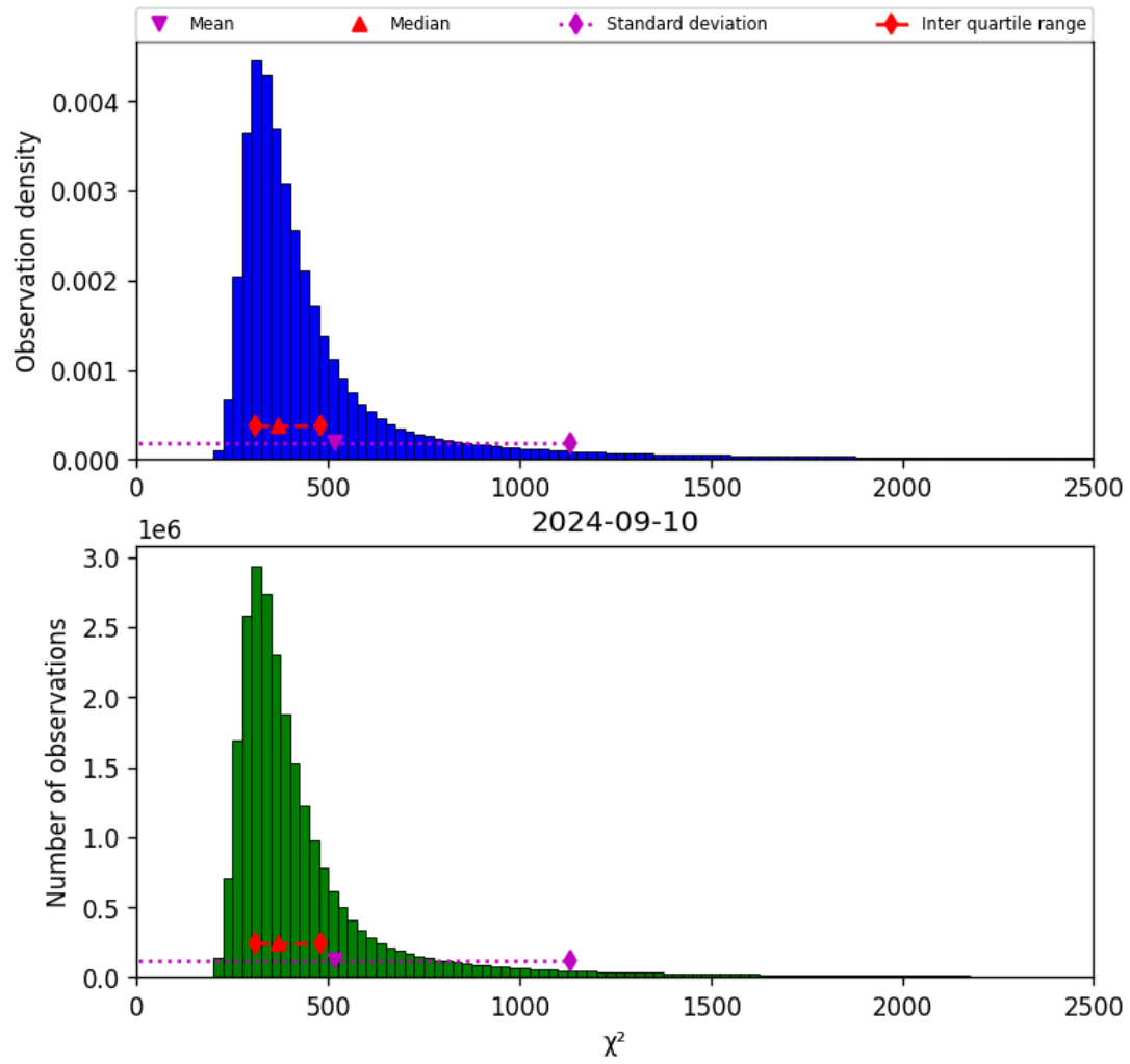
Figure 42: Histogram of “ \chi^2 ” for 2024-09-09 to 2024-09-11
