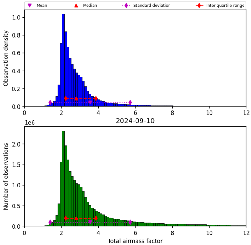
Figure 32: Histogram of “Total airmass factor” for 2024-09-09 to 2024-09-11
