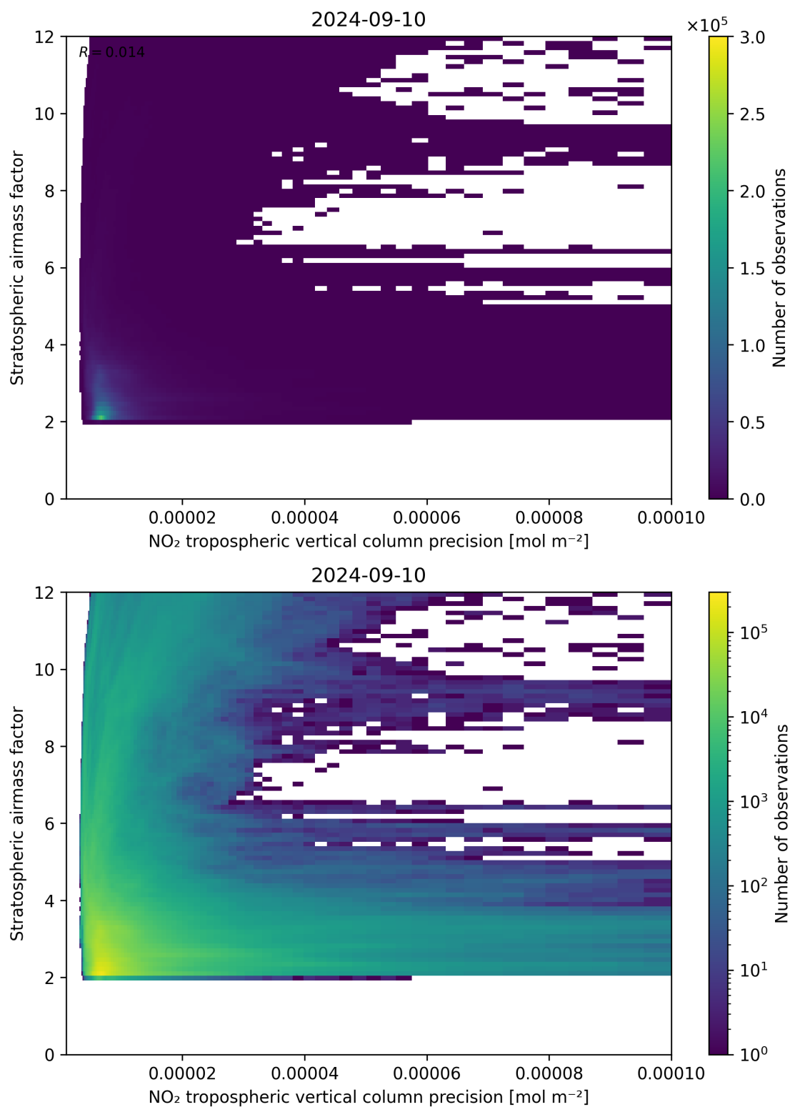
Figure 131: Scatter density plot of “NO 2 tropospheric vertical column precision” against “Stratospheric airmass factor” for 2024-09-09 to 2024-09-11.
