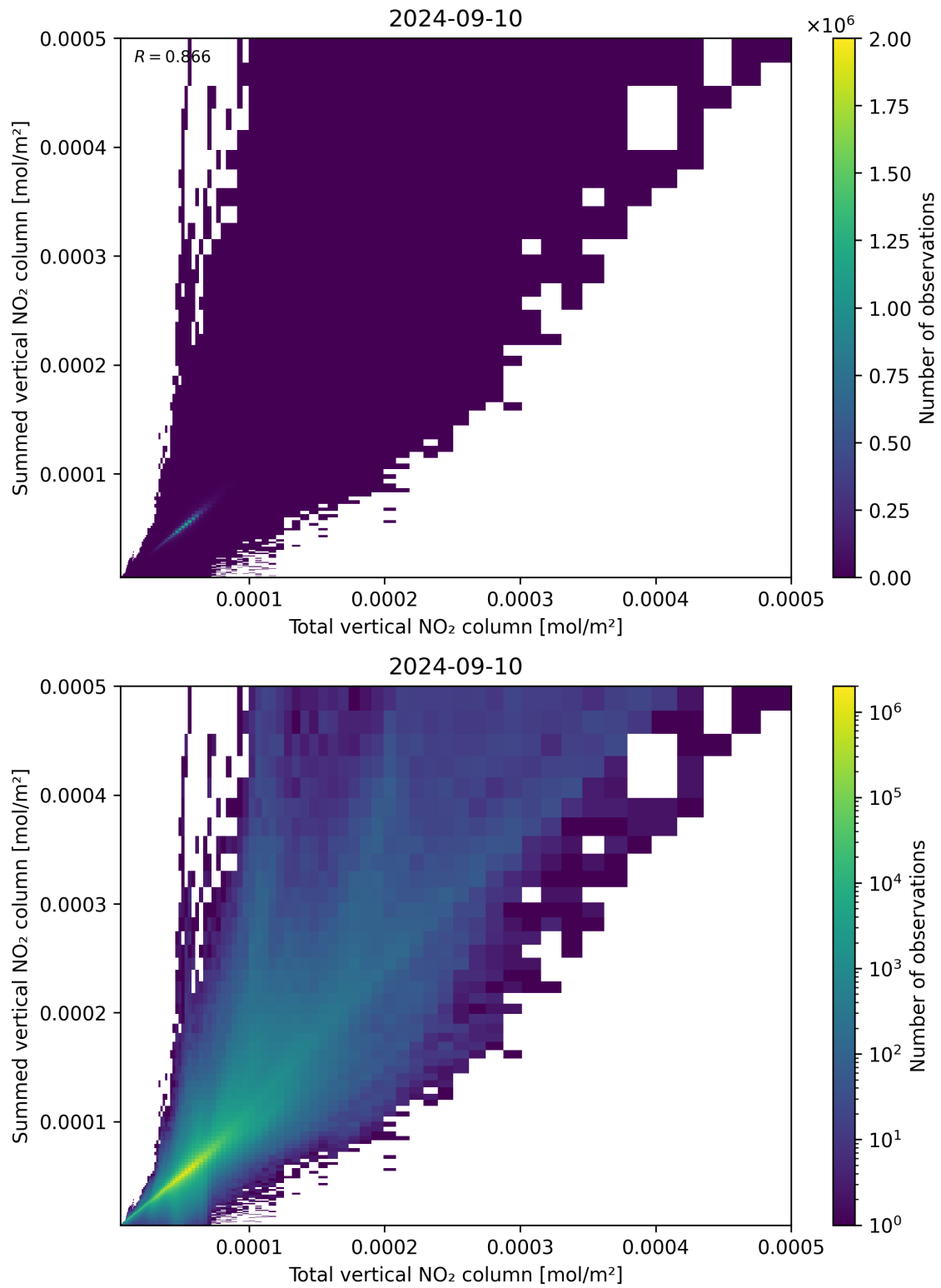
Figure 112: Scatter density plot of “Total vertical NO 2 column” against “Summed vertical NO 2 column” for 2024-09-09 to 2024-09-11.
