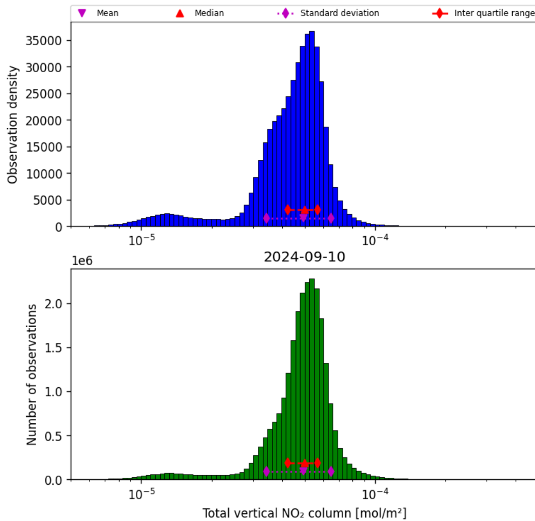
Figure 38: Histogram of “Total vertical NO 2 column” for 2024-09-09 to 2024-09-11
