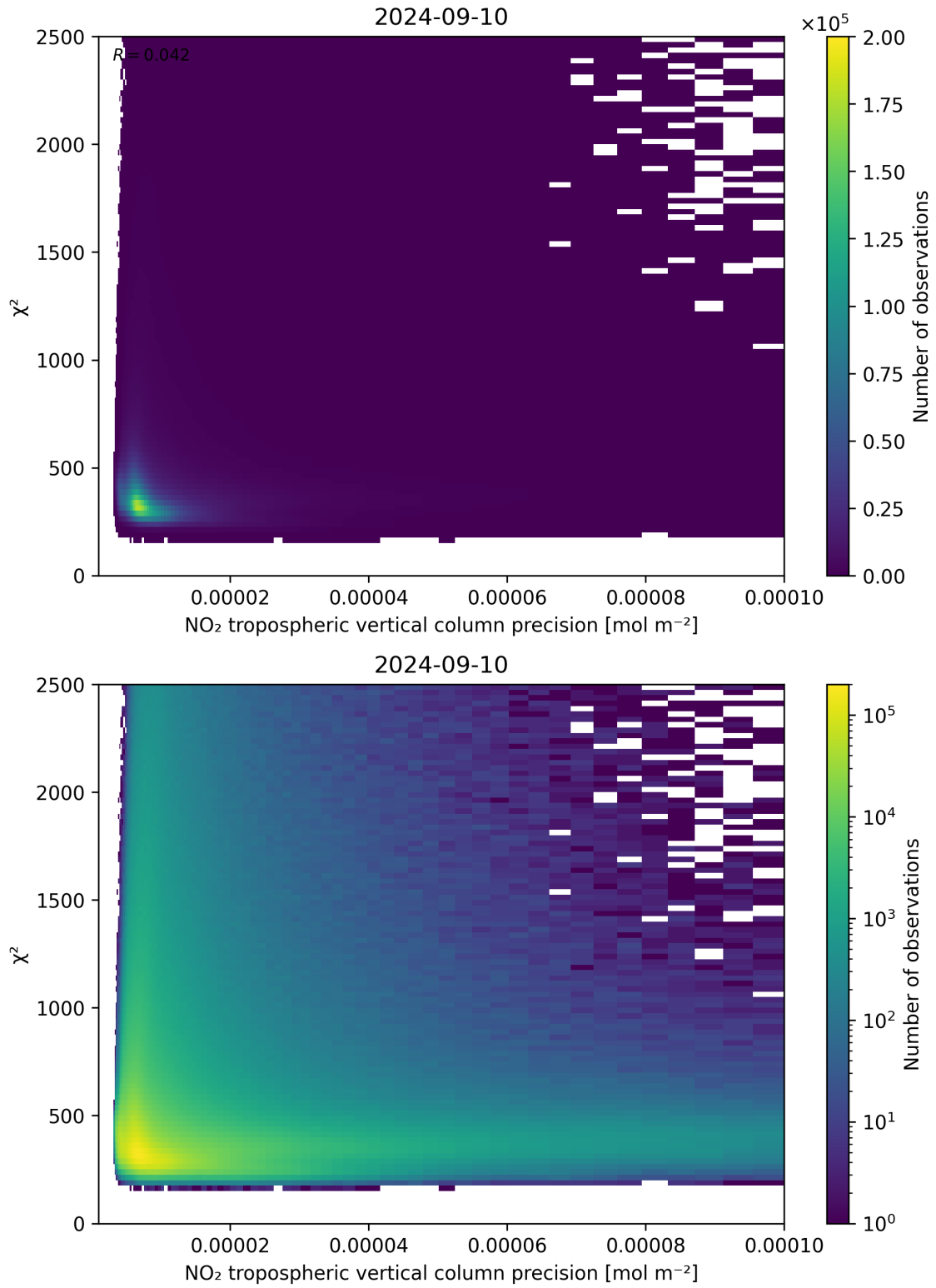
Figure 134: Scatter density plot of “NO 2 tropospheric vertical column precision” against “ \chi^2 ” for 2024-09-09 to 2024-09-11.
