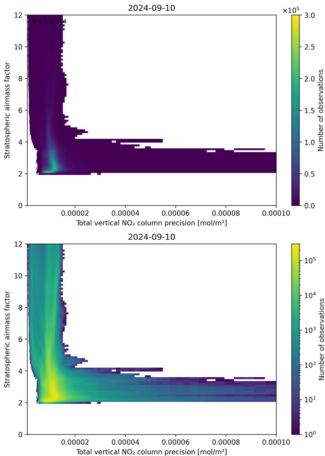
Figure 115: Scatter density plot of “Total vertical NO 2 column precision” against “Stratospheric air mass factor” for 2024-09-09 to 2024-09-11.
