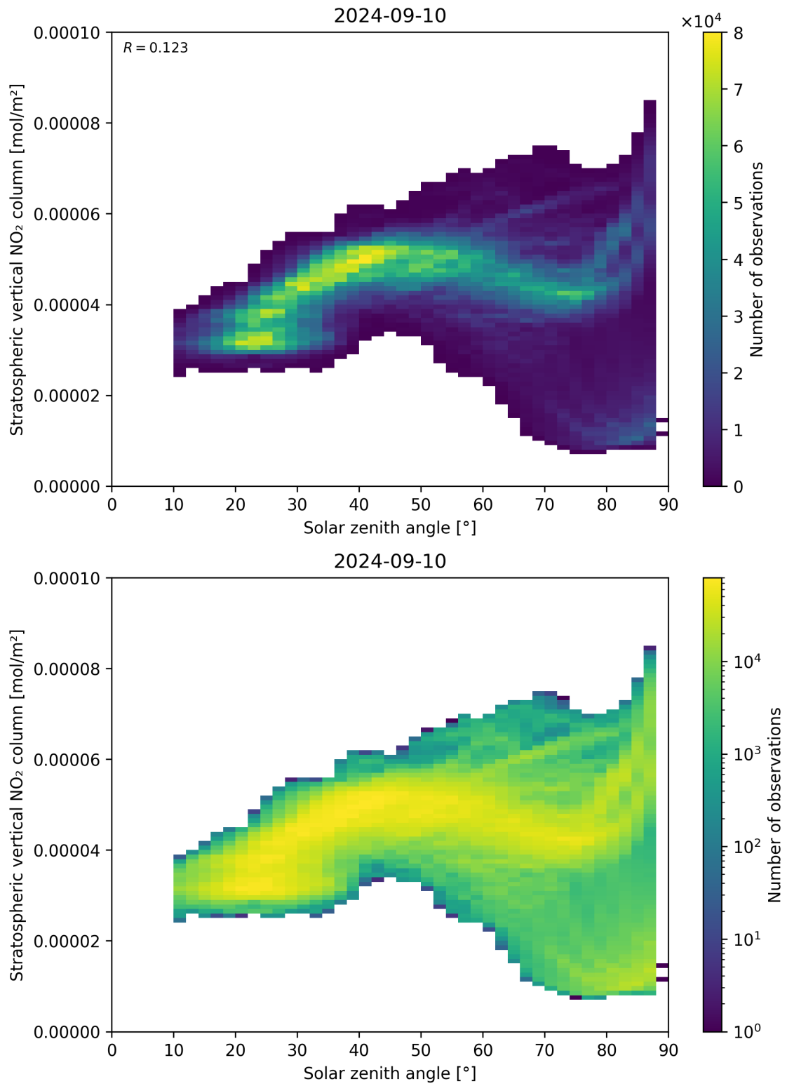
Figure 150: Scatter density plot of “Solar zenith angle” against “Stratospheric vertical NO 2 column” for 2024-09-09 to 2024-09-11.
