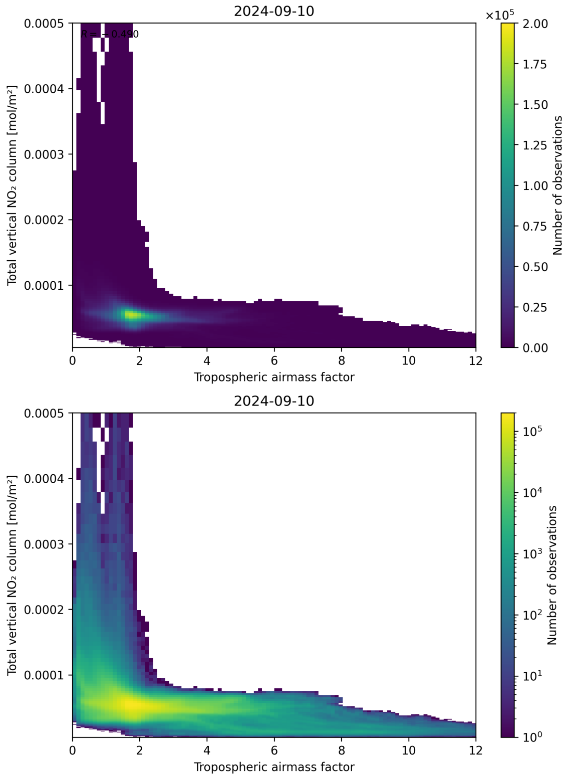
Figure 77: Scatter density plot of “Tropospheric airmass factor” against “Total vertical NO 2 column” for 2024-09-09 to 2024-09-11.
