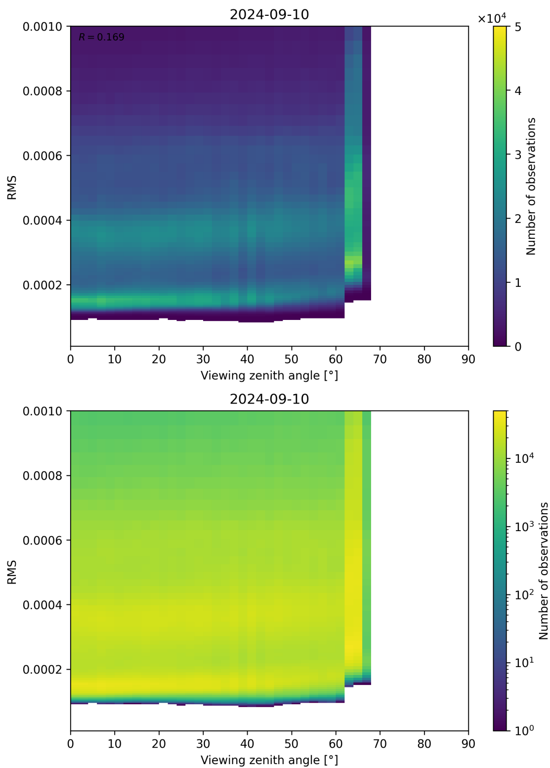
Figure 171: Scatter density plot of “Viewing zenith angle” against “RMS” for 2024-09-09 to 2024-09-11.
