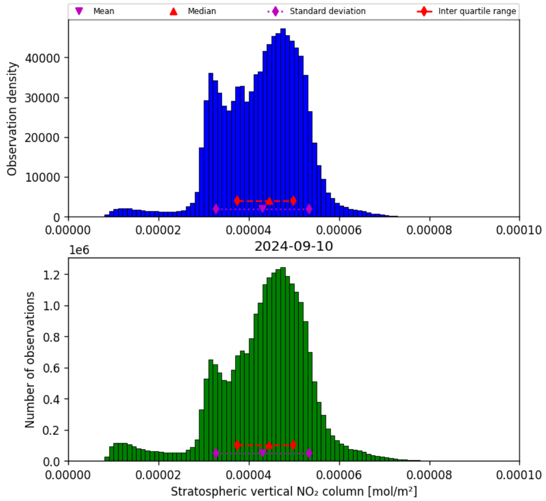
Figure 36: Histogram of “Stratospheric vertical NO 2 column” for 2024-09-09 to 2024-09-11
