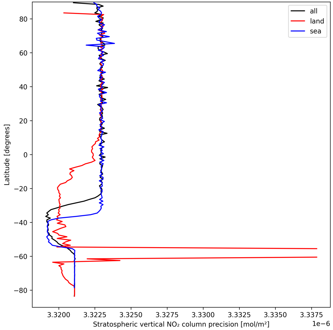
Figure 20: Zonal average of “Stratospheric vertical NO 2 column precision” for 2024-09-09 to 2024-09-11.
