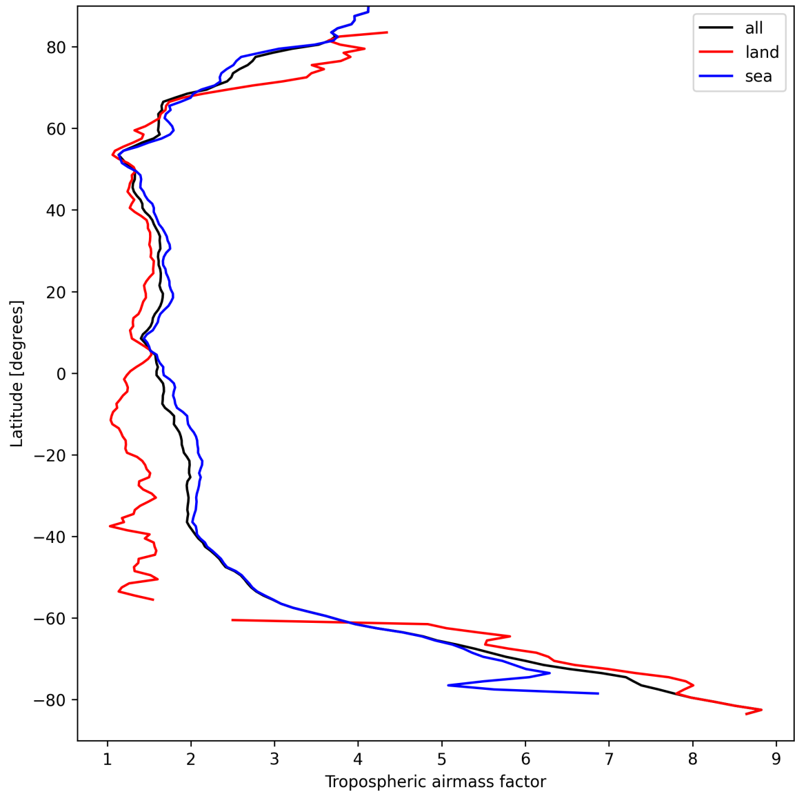
Figure 14: Zonal average of “Tropospheric airmass factor” for 2024-09-09 to 2024-09-11.
