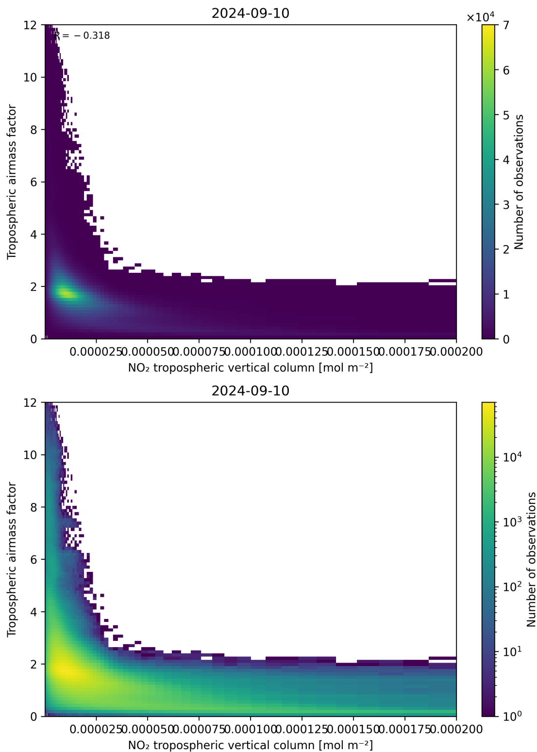
Figure 123: Scatter density plot of “NO 2 tropospheric vertical column” against “Tropospheric air mass factor” for 2024-09-09 to 2024-09-11.
