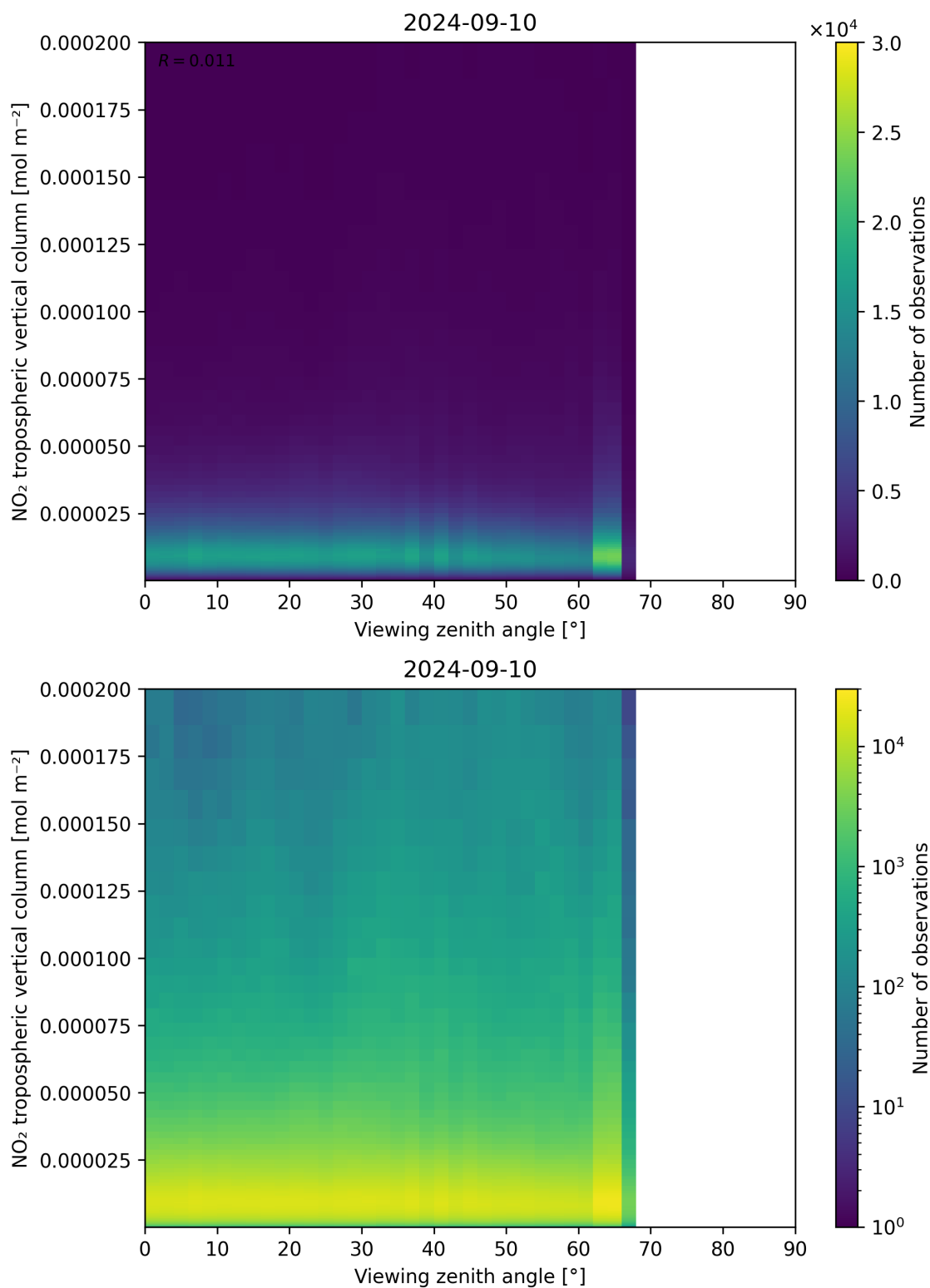
Figure 169: Scatter density plot of “Viewing zenith angle” against “NO 2 tropospheric vertical column” for 2024-09-09 to 2024-09-11.
