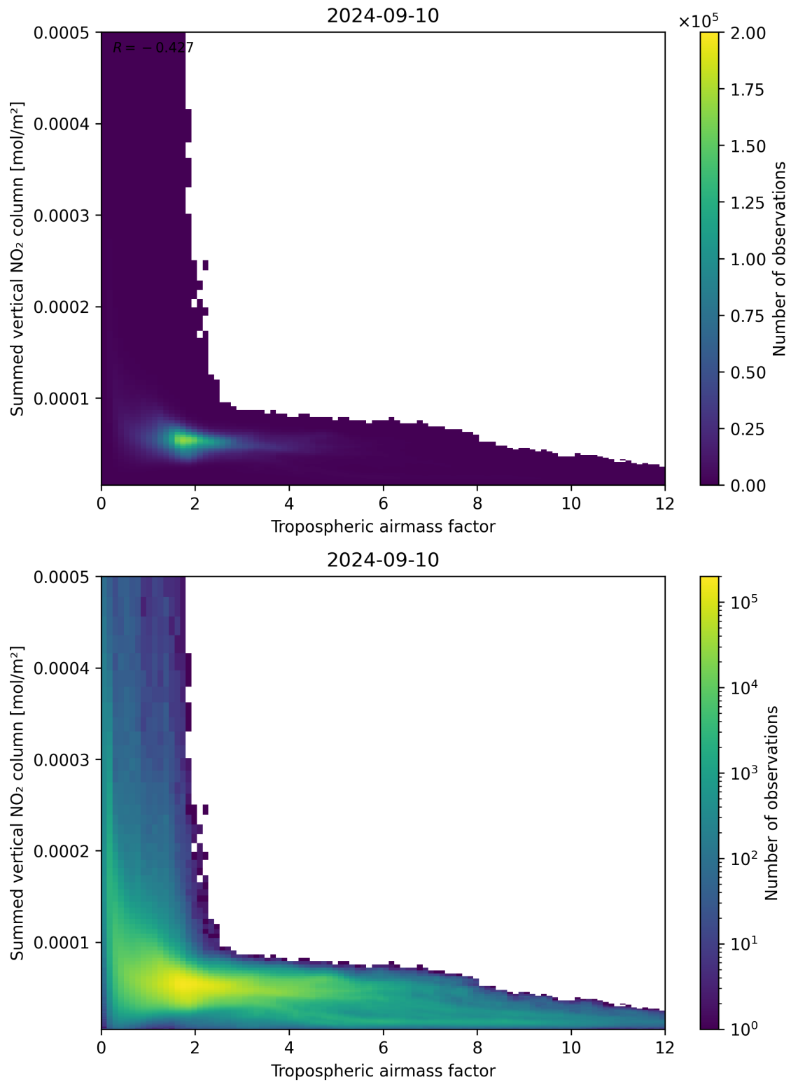
Figure 75: Scatter density plot of “Tropospheric air mass factor” against “Summed vertical NO 2 column” for 2024-09-09 to 2024-09-11.
