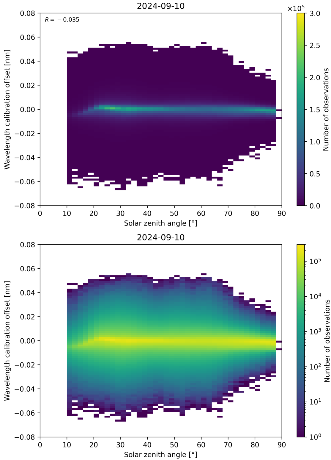
Figure 158: Scatter density plot of “Solar zenith angle” against “Wavelength calibration offset” for 2024-09-09 to 2024-09-11.
