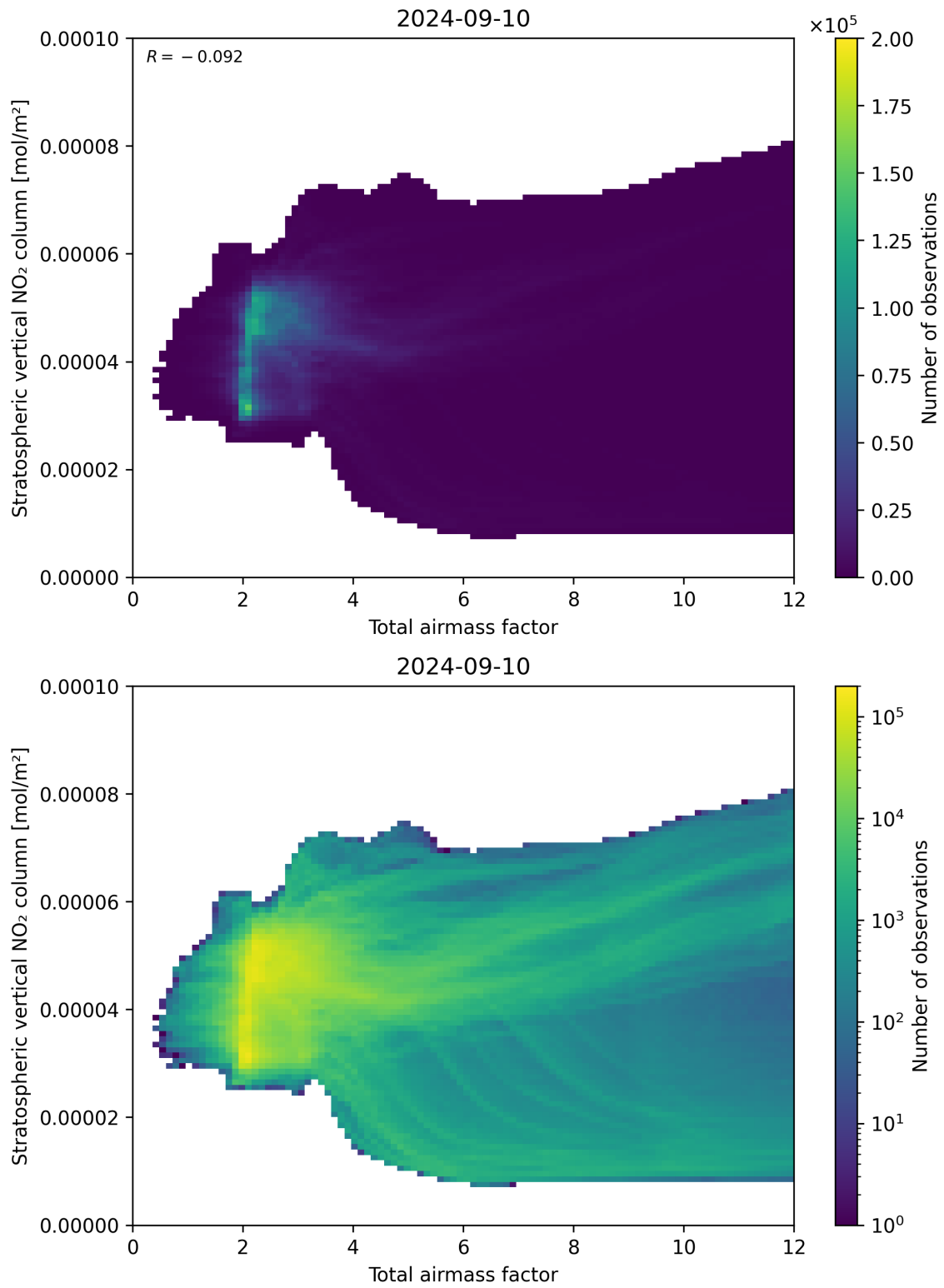
Figure 64: Scatter density plot of “Total airmass factor” against “Stratospheric vertical NO 2 column” for 2024-09-09 to 2024-09-11.
