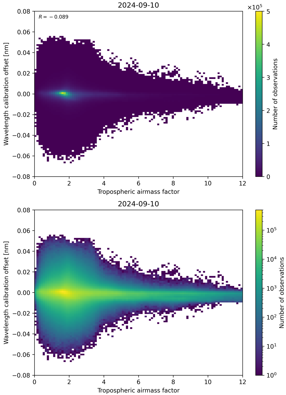
Figure 80: Scatter density plot of “Tropospheric airmass factor” against “Wavelength calibration offset” for 2024-09-09 to 2024-09-11.
