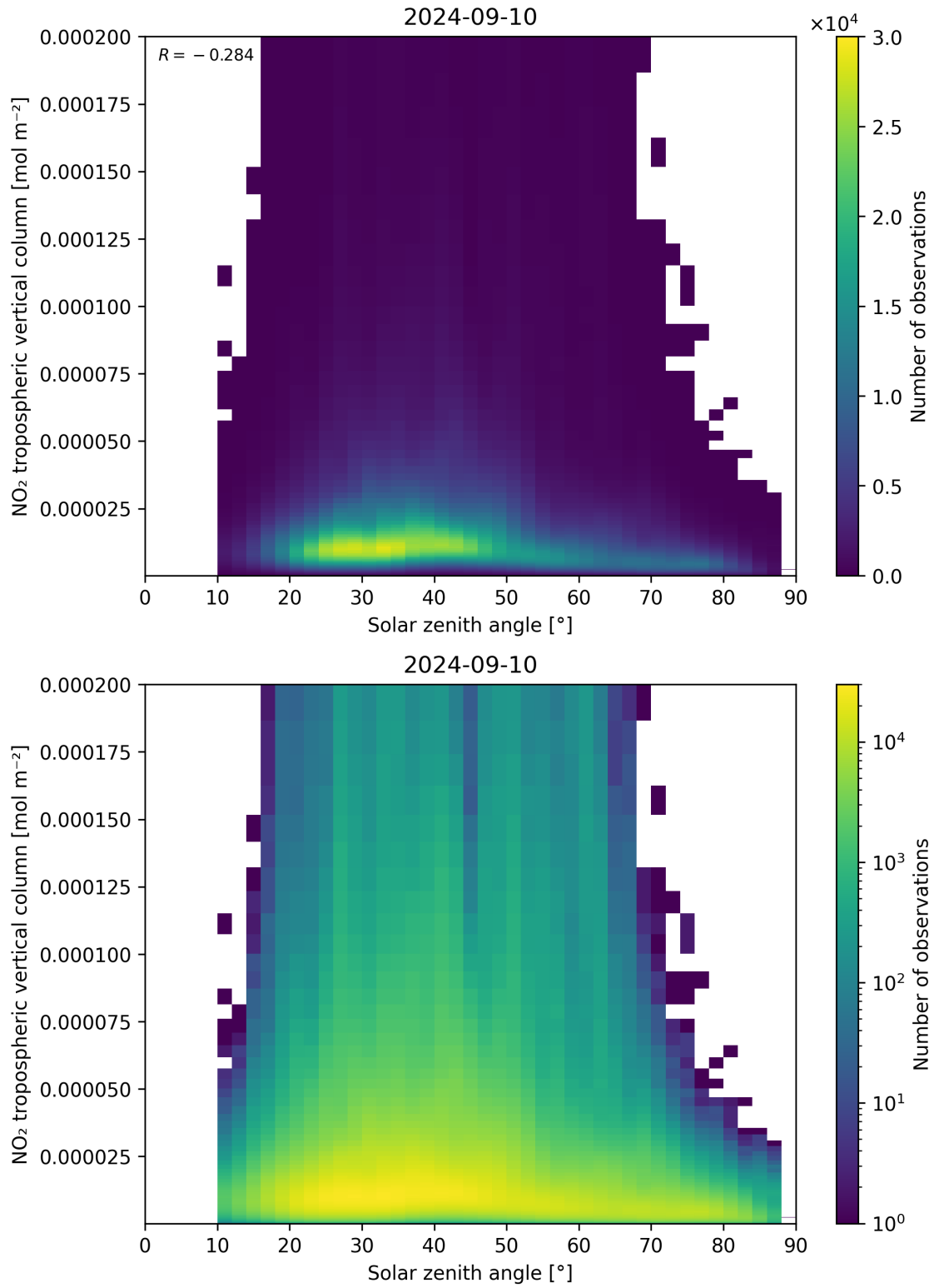
Figure 155: Scatter density plot of “Solar zenith angle” against “NO 2 tropospheric vertical column” for 2024-09-09 to 2024-09-11.
