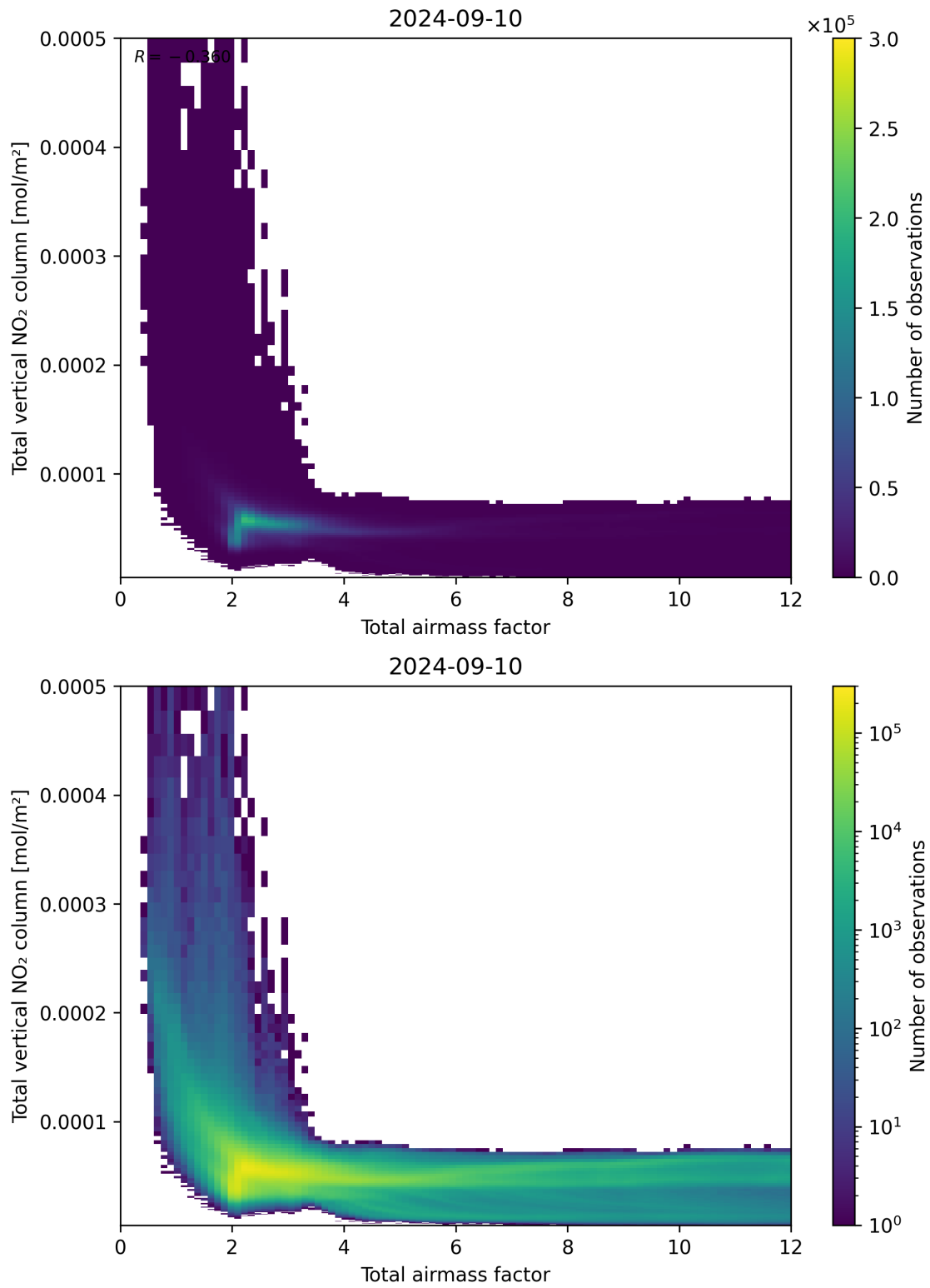
Figure 67: Scatter density plot of “Total airmass factor” against “Total vertical NO 2 column” for 2024-09-09 to 2024-09-11.
