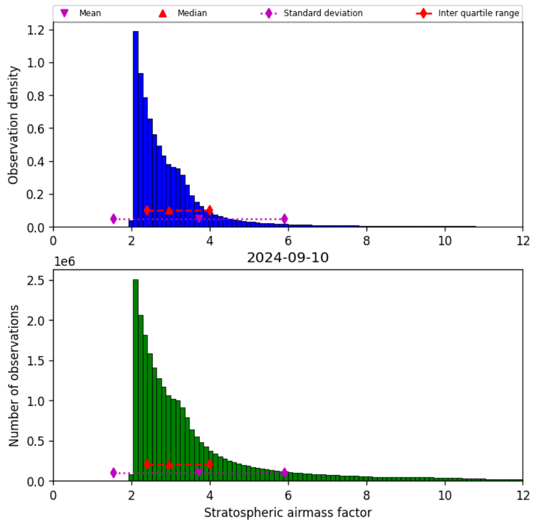
Figure 44: Histogram of “Stratospheric airmass factor” for 2024-09-09 to 2024-09-11
