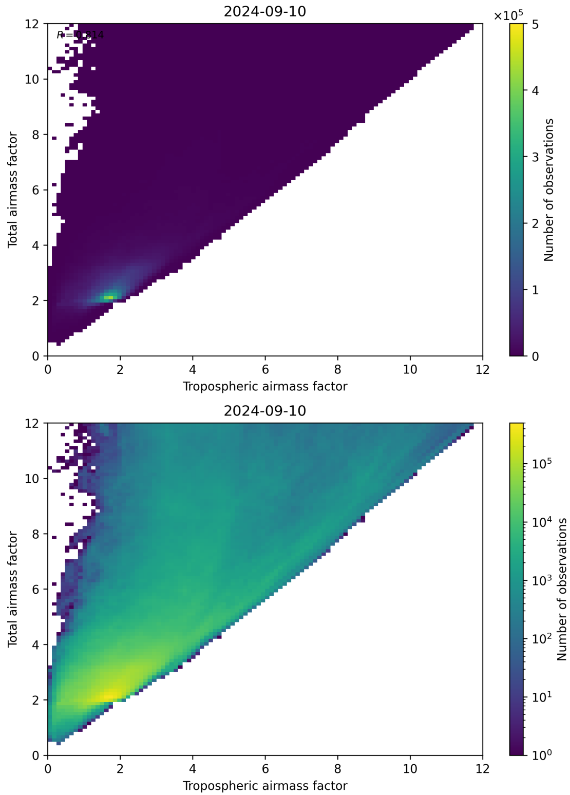
Figure 72: Scatter density plot of “Tropospheric airmass factor” against “Total airmass factor” for 2024-09-09 to 2024-09-11.
