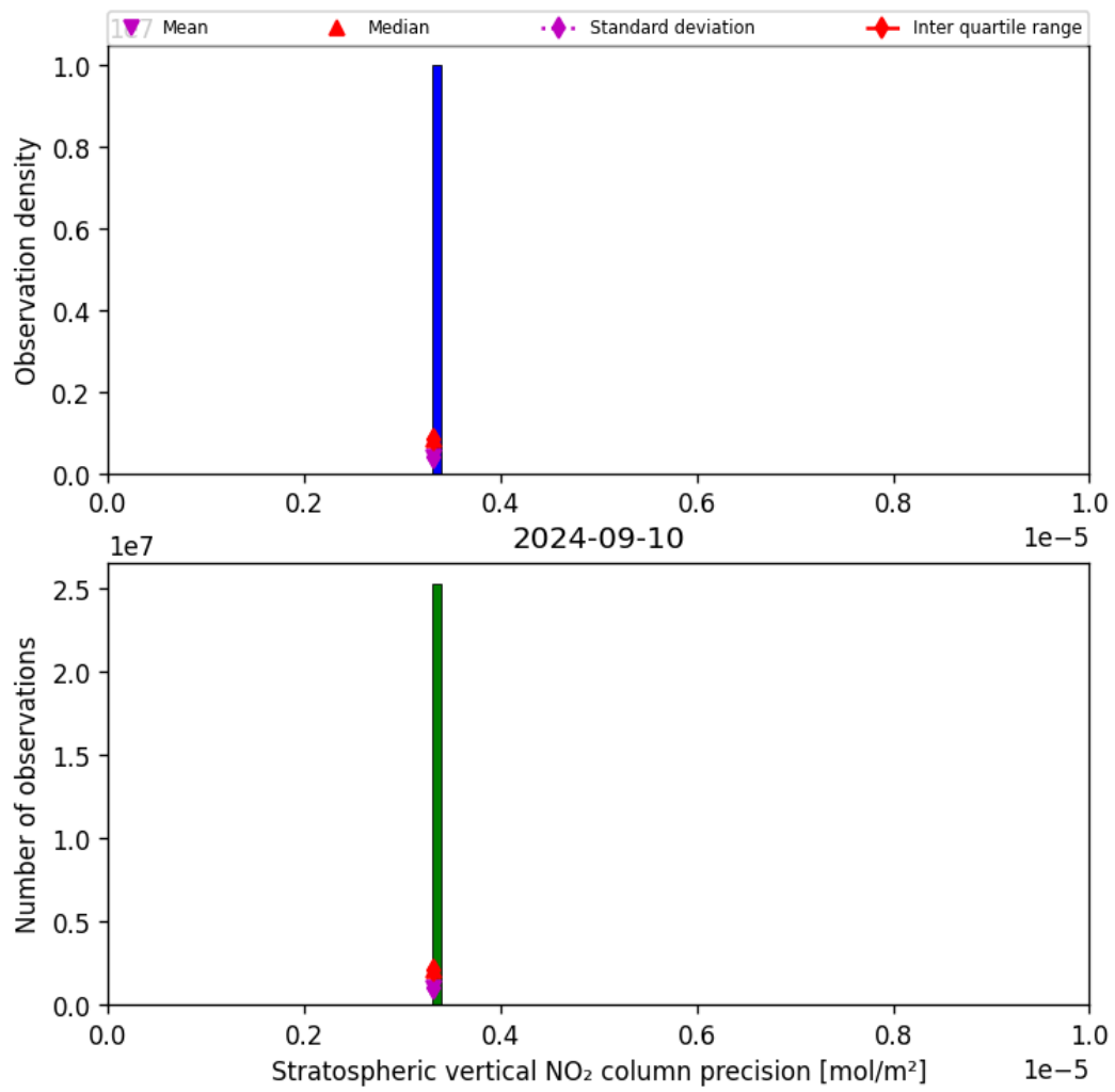
Figure 37: Histogram of “Stratospheric vertical NO 2 column precision” for 2024-09-09 to 2024-09-11
