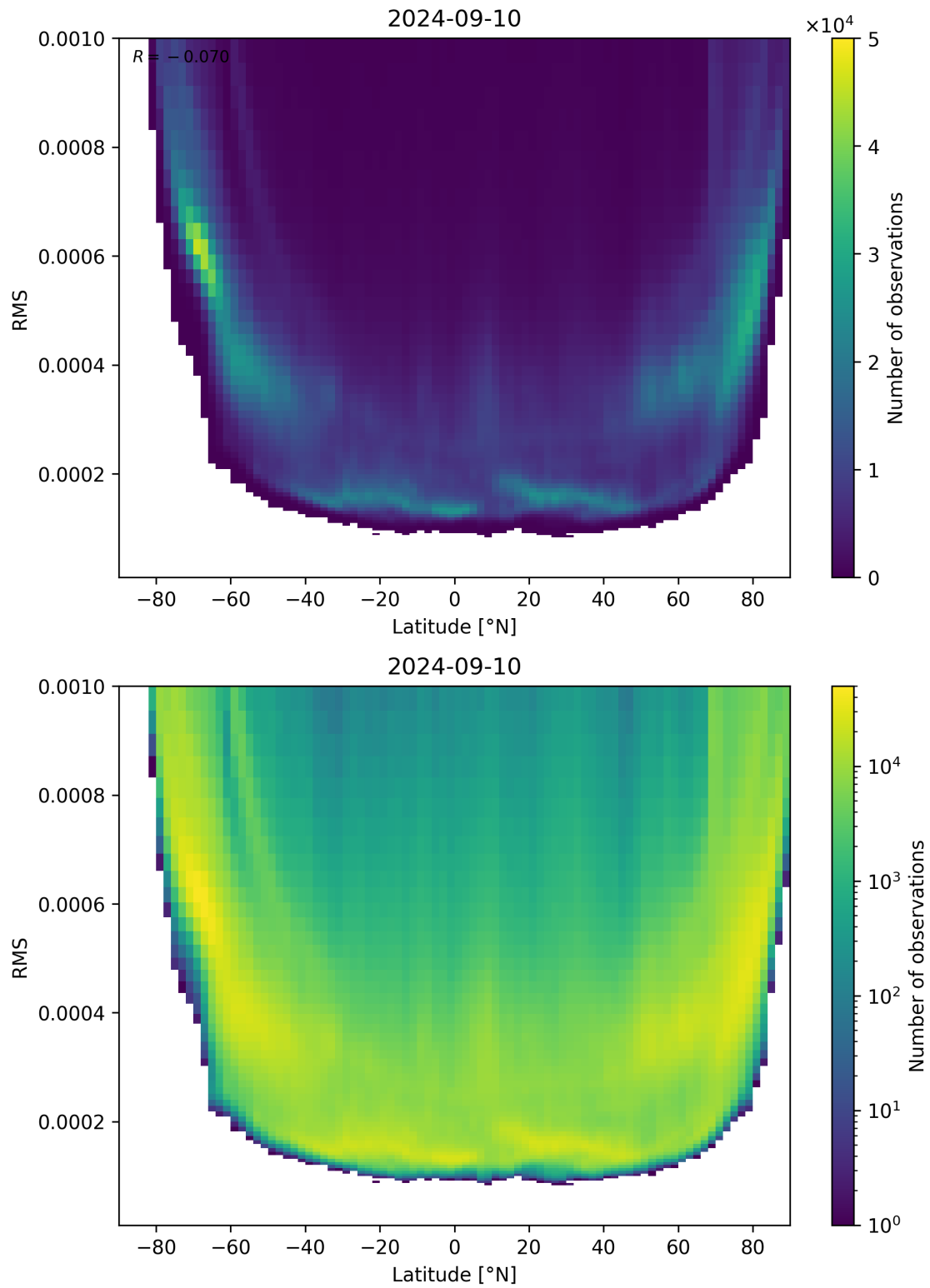
Figure 94: Scatter density plot of “Latitude” against “RMS” for 2024-09-09 to 2024-09-11.
