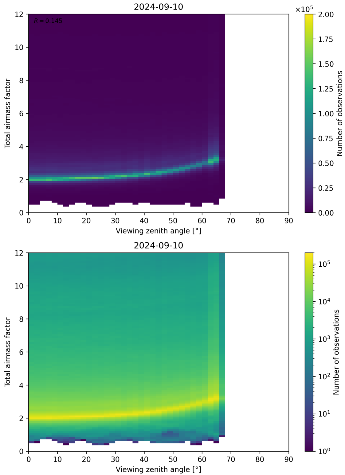
Figure 160: Scatter density plot of “Viewing zenith angle” against “Total airmass factor” for 2024-09-09 to 2024-09-11.
