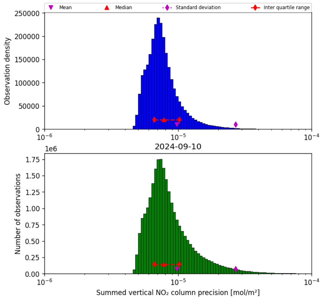
Figure 41: Histogram of "Summed vertical NO 2 column precision" for 2024-09-09 to 2024-09-11
