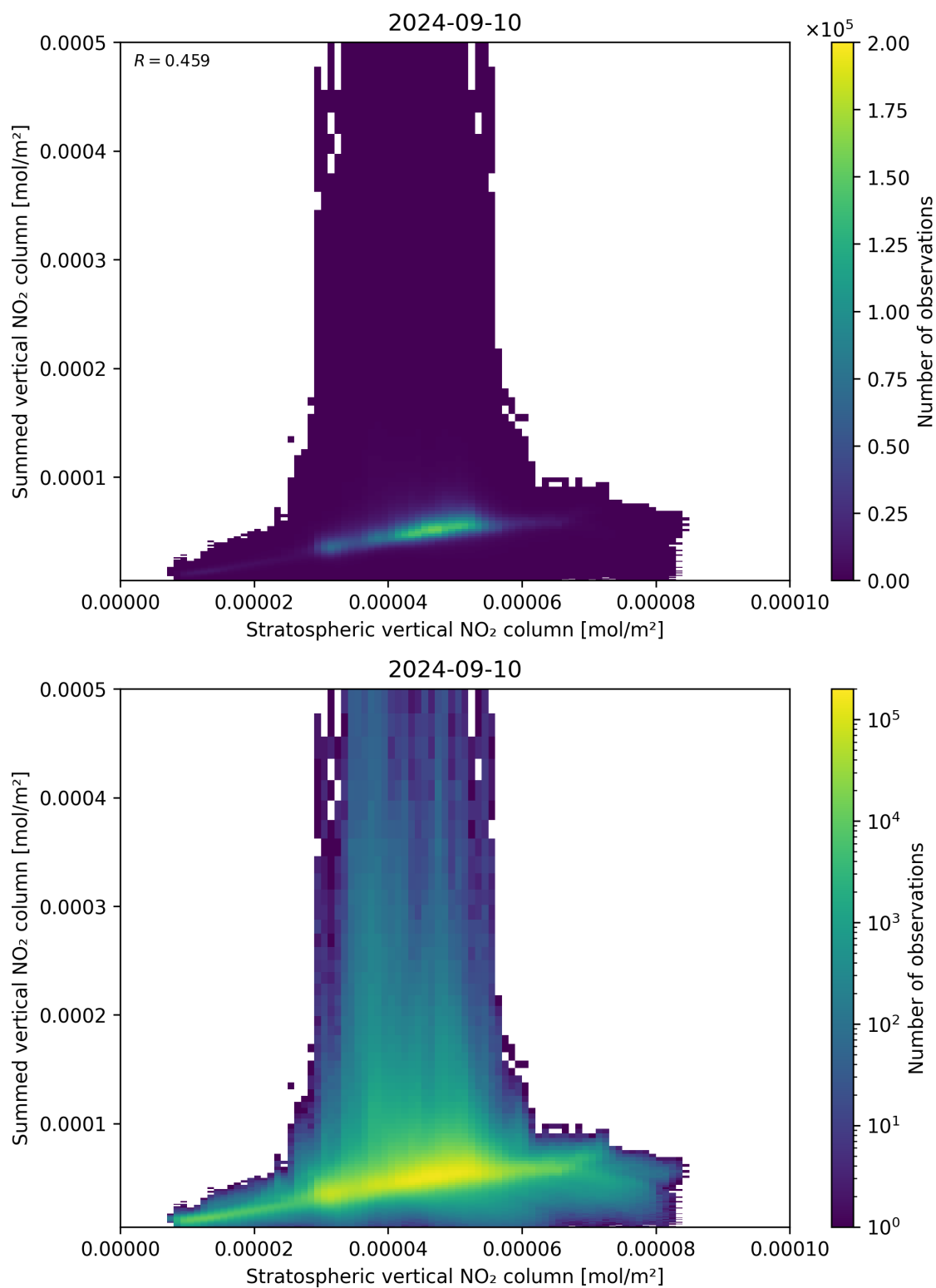
Figure 98: Scatter density plot of “Stratospheric vertical NO 2 column” against “Summed vertical NO 2 column” for 2024-09-09 to 2024-09-11.
