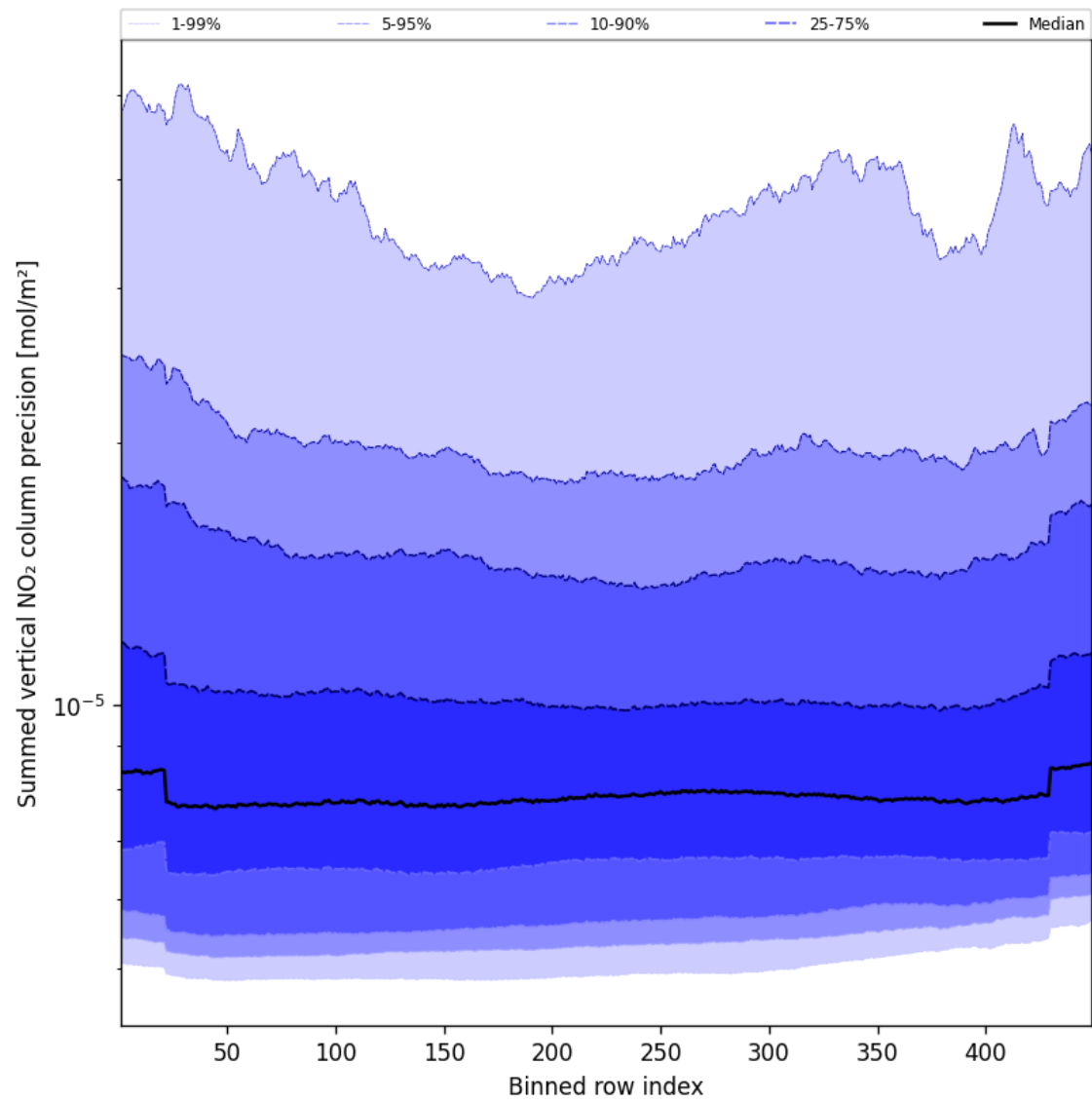
Figure 58: Along track statistics of “Summed vertical NO 2 column precision” for 2024-09-09 to 2024-09-11
