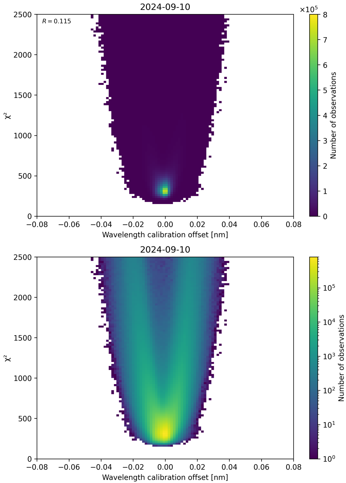
Figure 175: Scatter density plot of “Wavelength calibration offset” against “ \chi^2 ” for 2024-09-09 to 2024-09-11.
