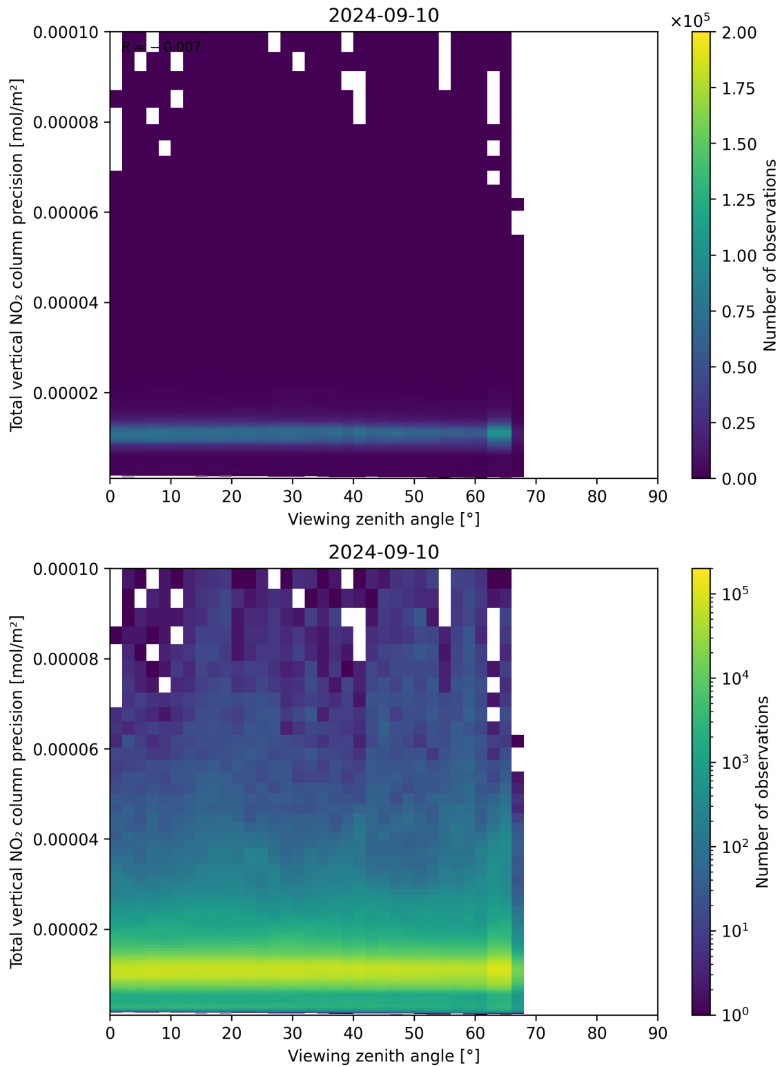
Figure 168: Scatter density plot of “Viewing zenith angle” against “Total vertical NO 2 column precision” for 2024-09-09 to 2024-09-11.
