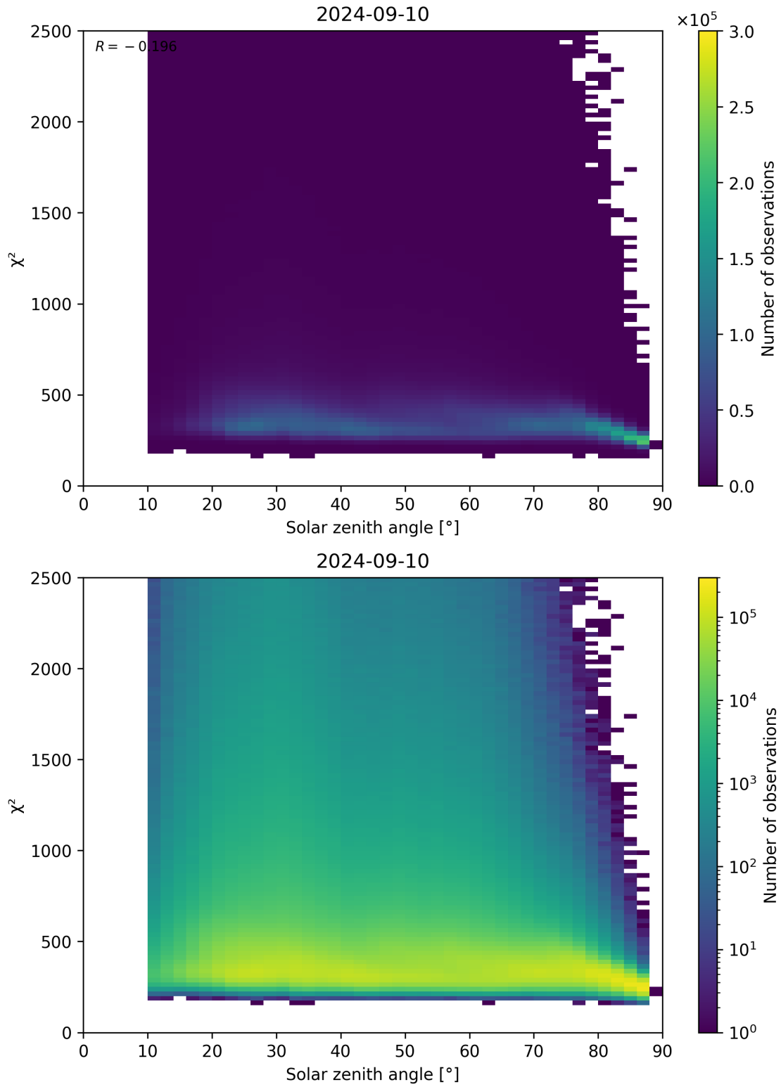
Figure 148: Scatter density plot of “Solar zenith angle” against “ \chi^2 ” for 2024-09-09 to 2024-09-11.
