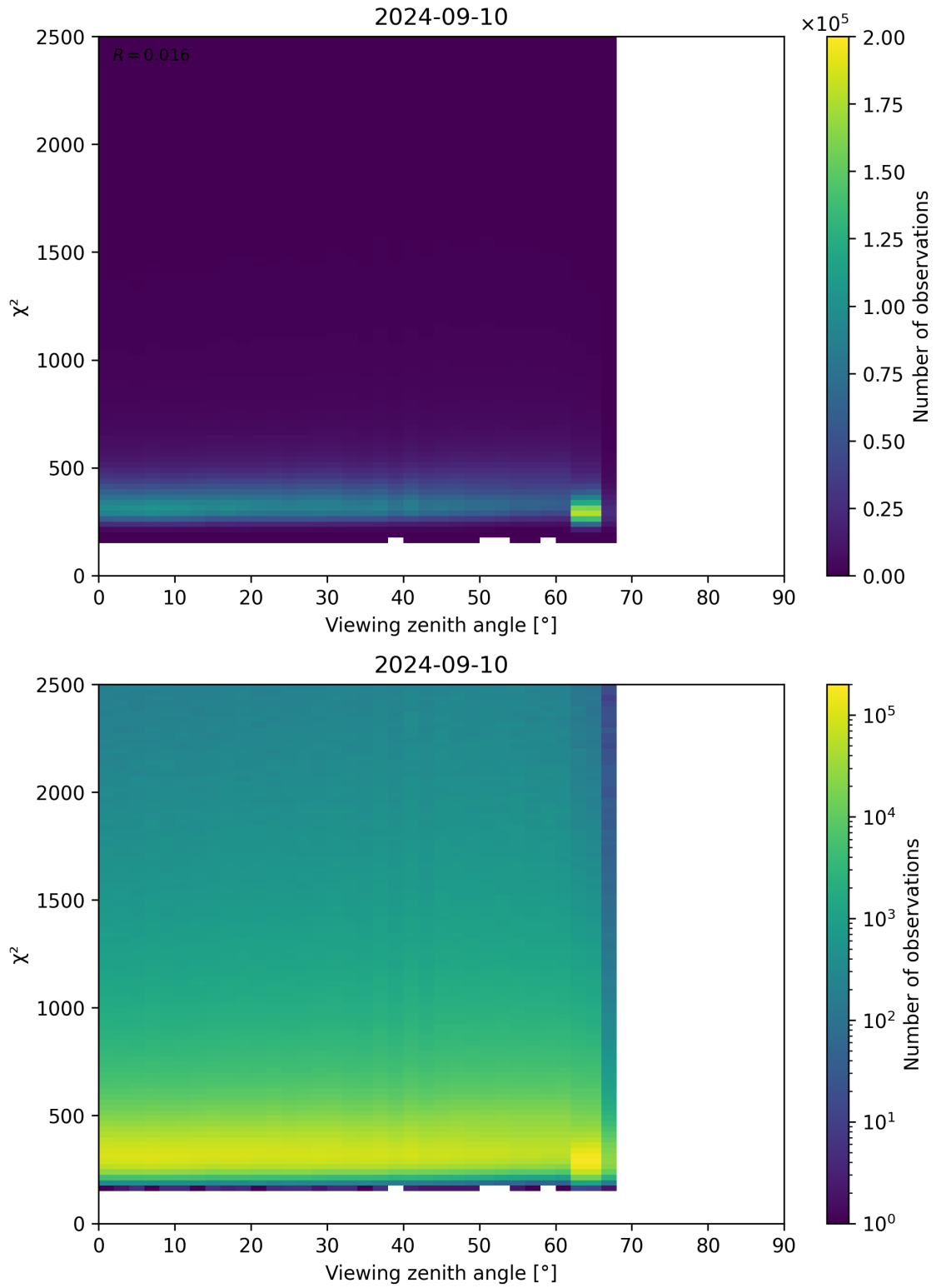
Figure 162: Scatter density plot of “Viewing zenith angle” against “ \chi^2 ” for 2024-09-09 to 2024-09-11.
