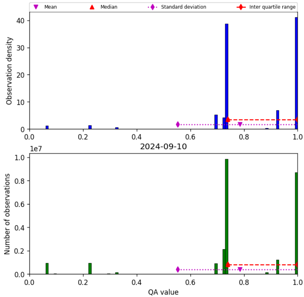
Figure 28: Histogram of “QA value” for 2024-09-09 to 2024-09-11
