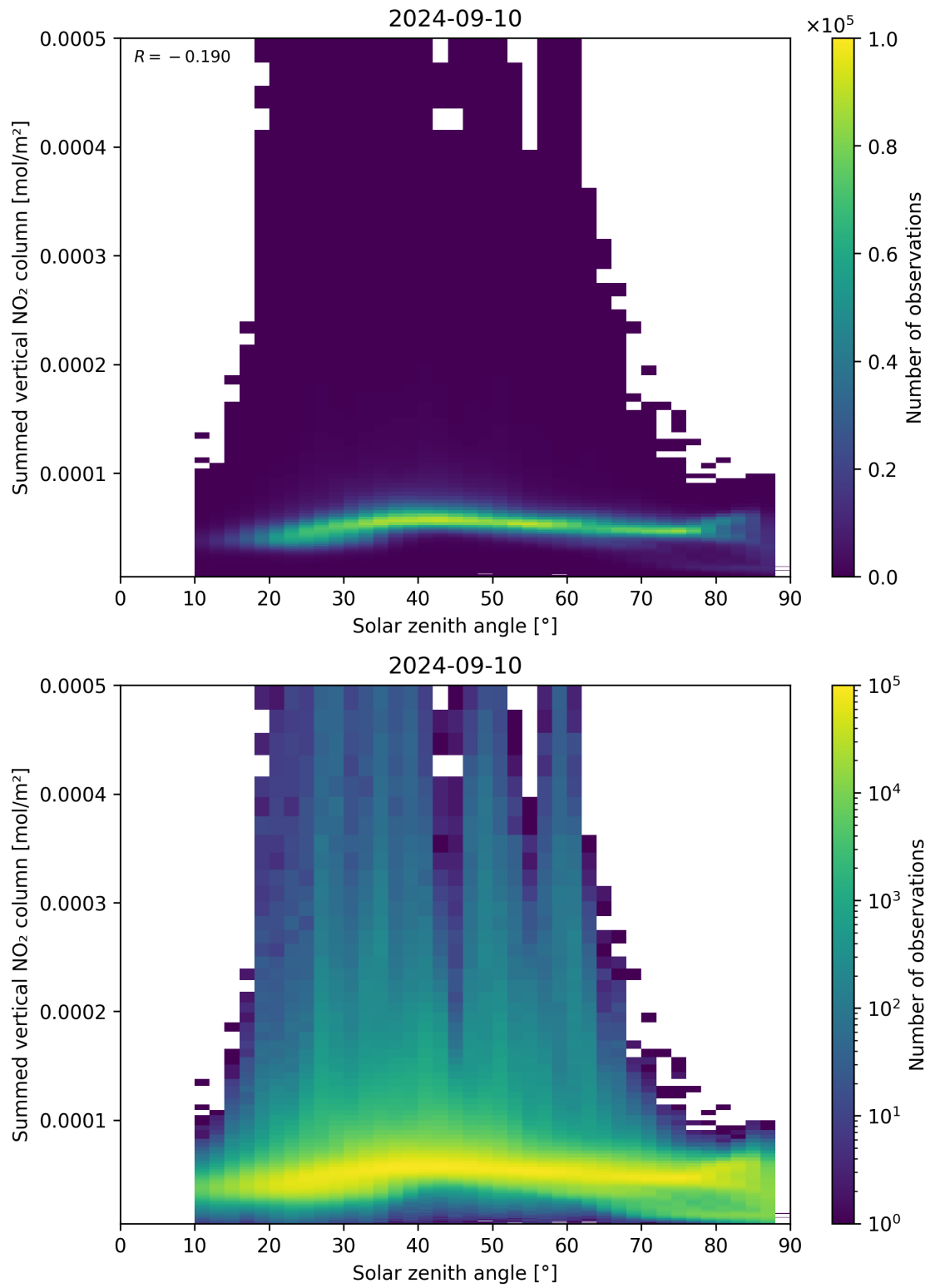
Figure 151: Scatter density plot of “Solar zenith angle” against “Summed vertical NO 2 column” for 2024-09-09 to 2024-09-11.
