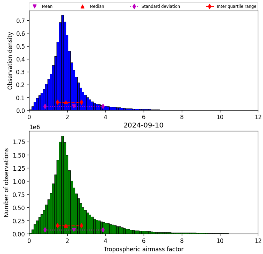
Figure 31: Histogram of “Tropospheric airmass factor” for 2024-09-09 to 2024-09-11
