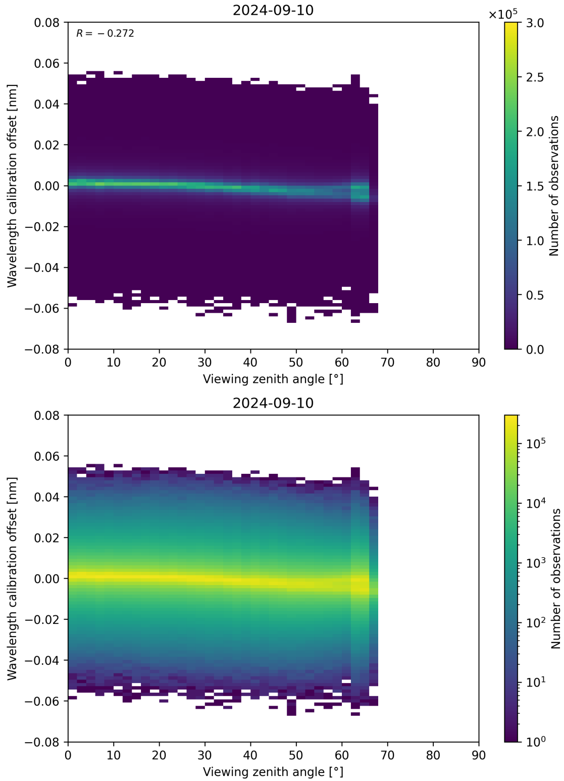
Figure 173: Scatter density plot of “Viewing zenith angle” against “Wavelength calibration offset” for 2024-09-09 to 2024-09-11.
