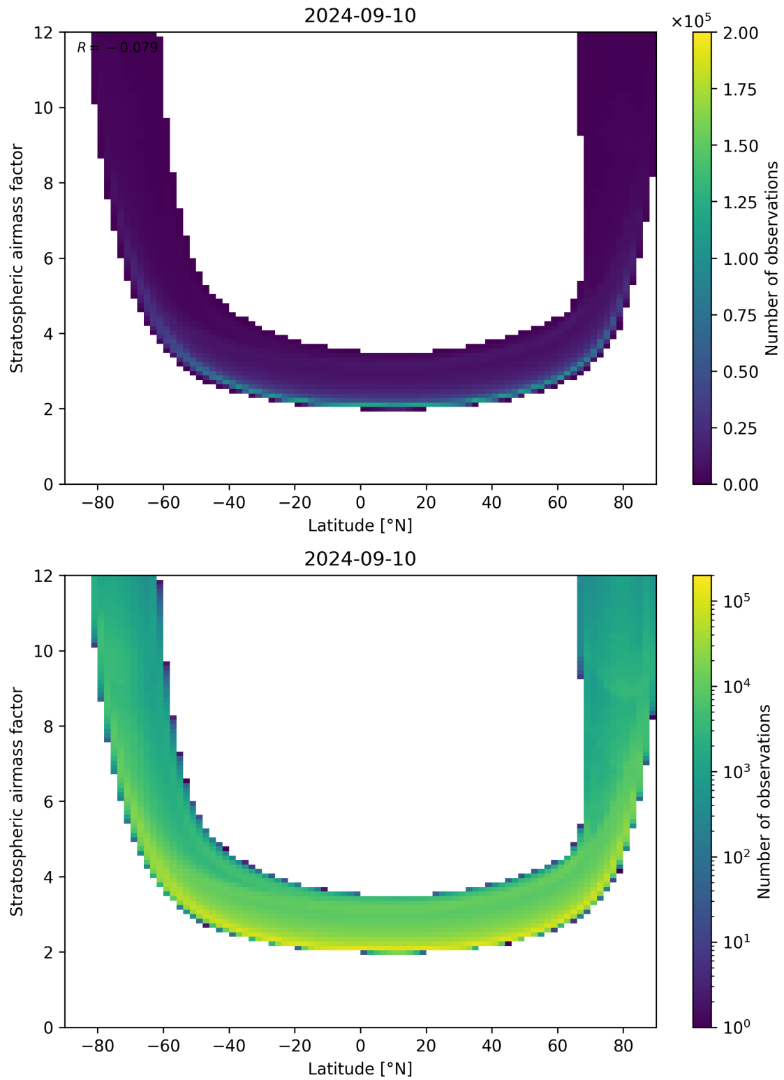
Figure 83: Scatter density plot of “Latitude” against “Stratospheric airmass factor” for 2024-09-09 to 2024-09-11.
