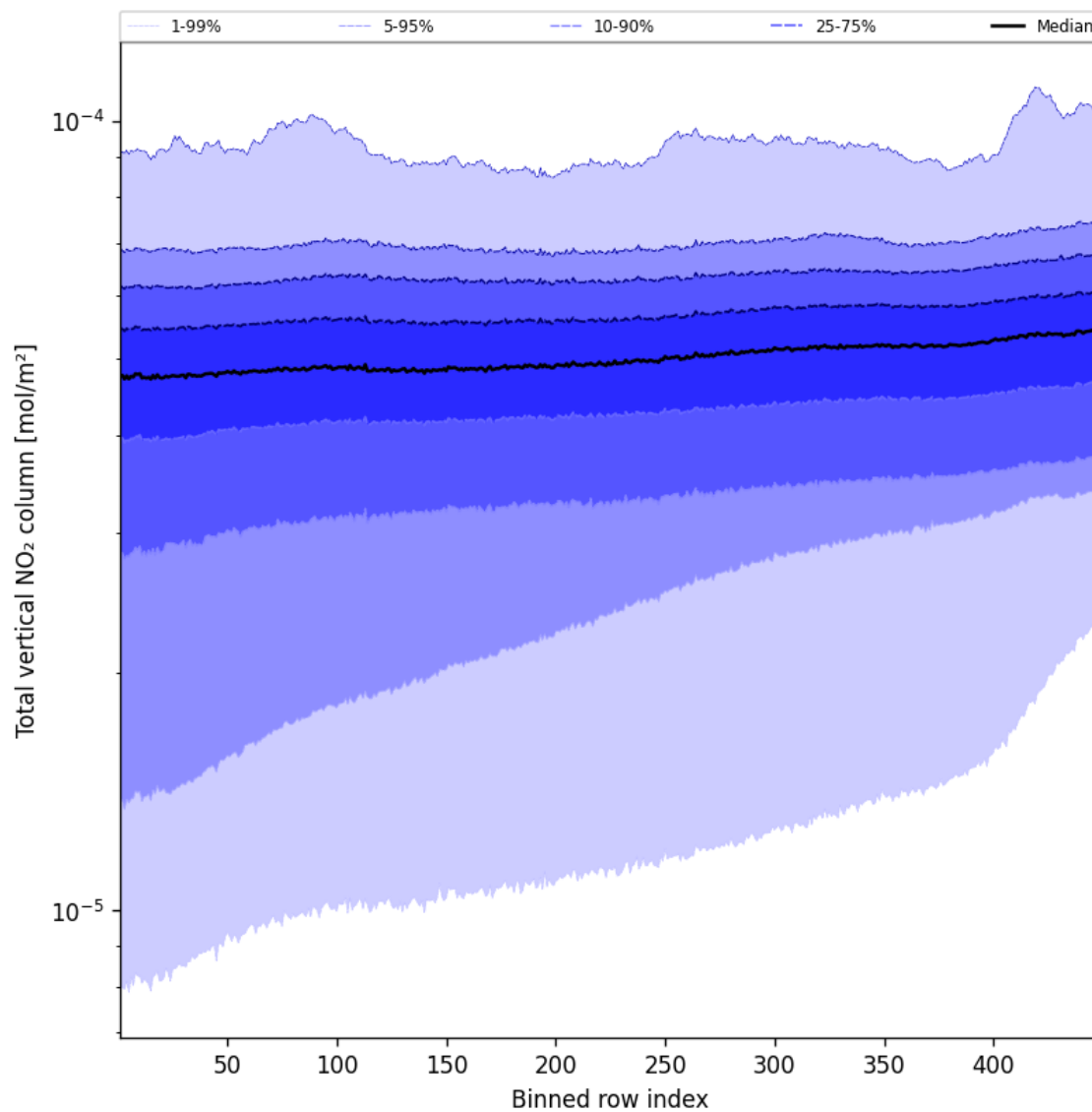
Figure 55: Along track statistics of “Total vertical NO 2 column” for 2024-09-09 to 2024-09-11
