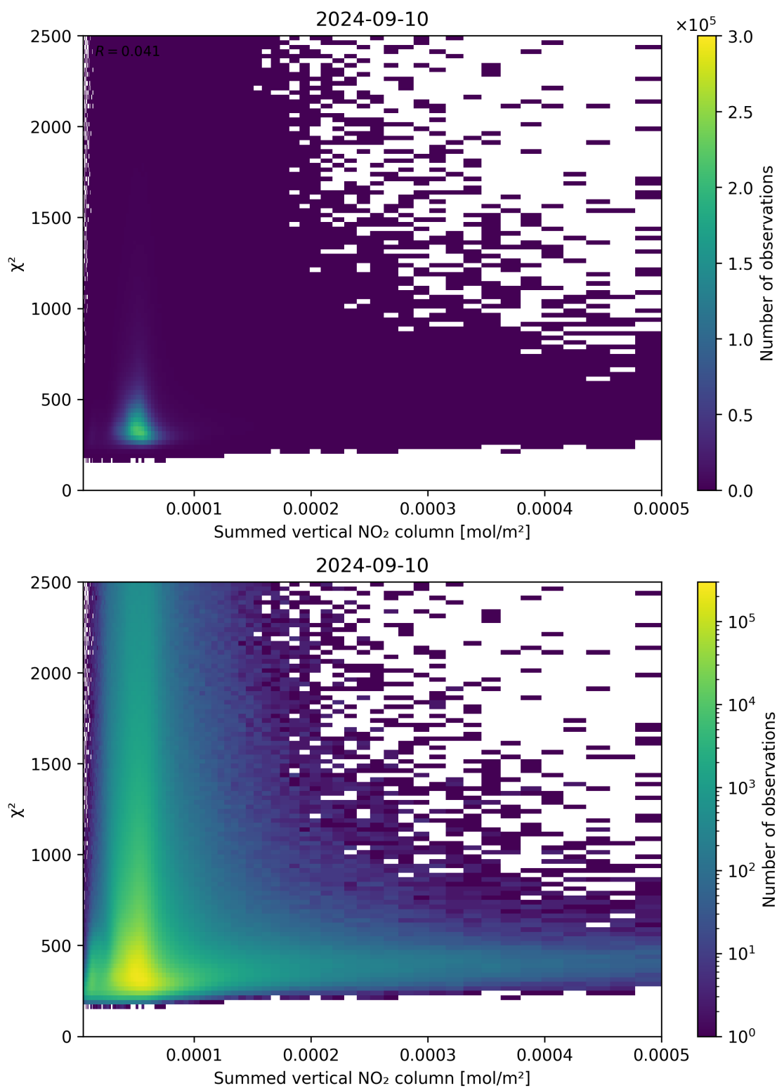
Figure 104: Scatter density plot of “Summed vertical NO 2 column” against “ \chi^2 ” for 2024-09-09 to 2024-09-11.
