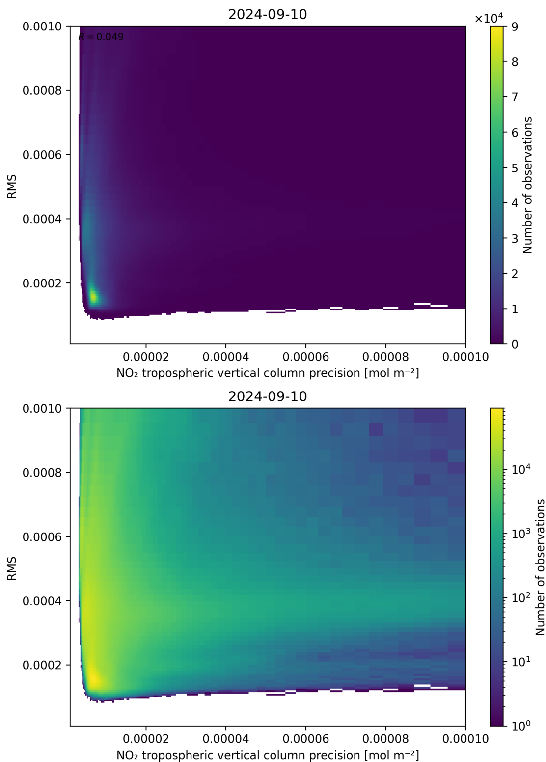
Figure 140: Scatter density plot of “NO 2 tropospheric vertical column precision” against “RMS” for 2024-09-09 to 2024-09-11.
