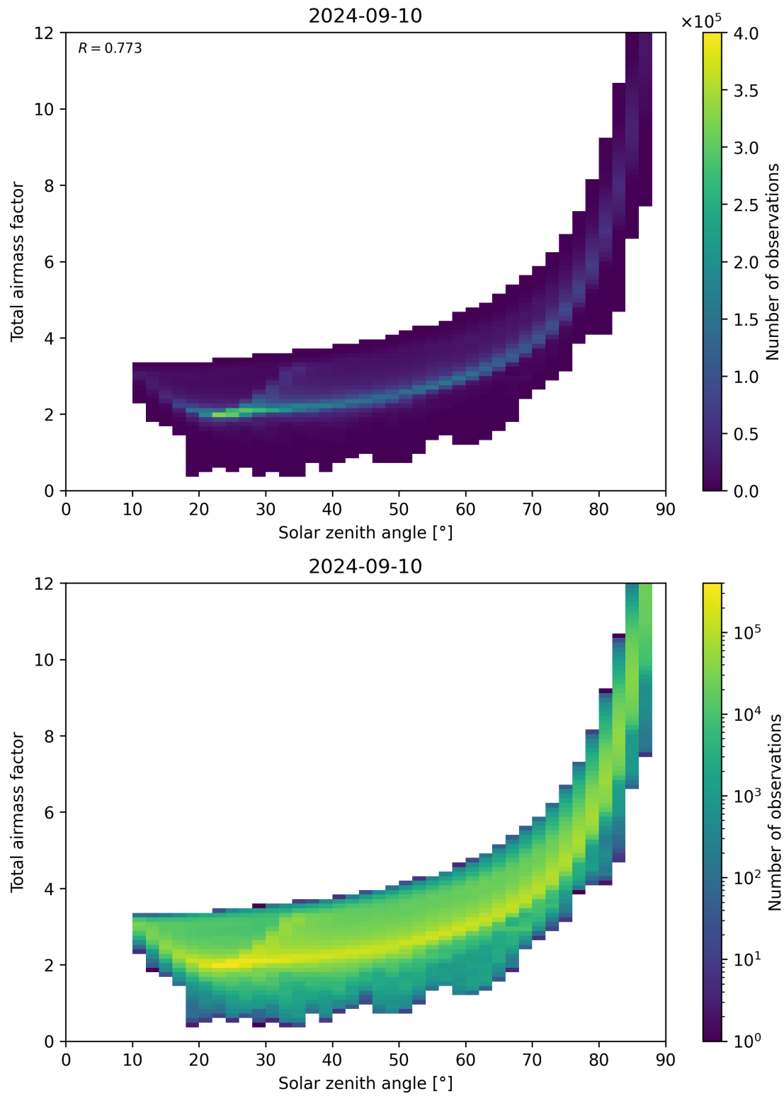
Figure 146: Scatter density plot of “Solar zenith angle” against “Total air mass factor” for 2024-09-09 to 2024-09-11.
