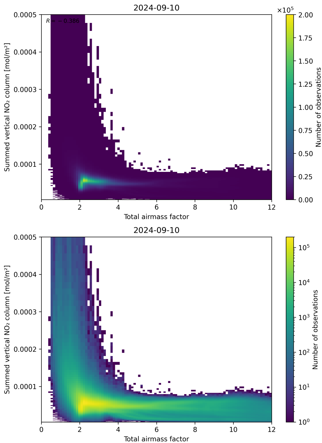
Figure 65: Scatter density plot of “Total airmass factor” against “Summed vertical NO 2 column” for 2024-09-09 to 2024-09-11.
