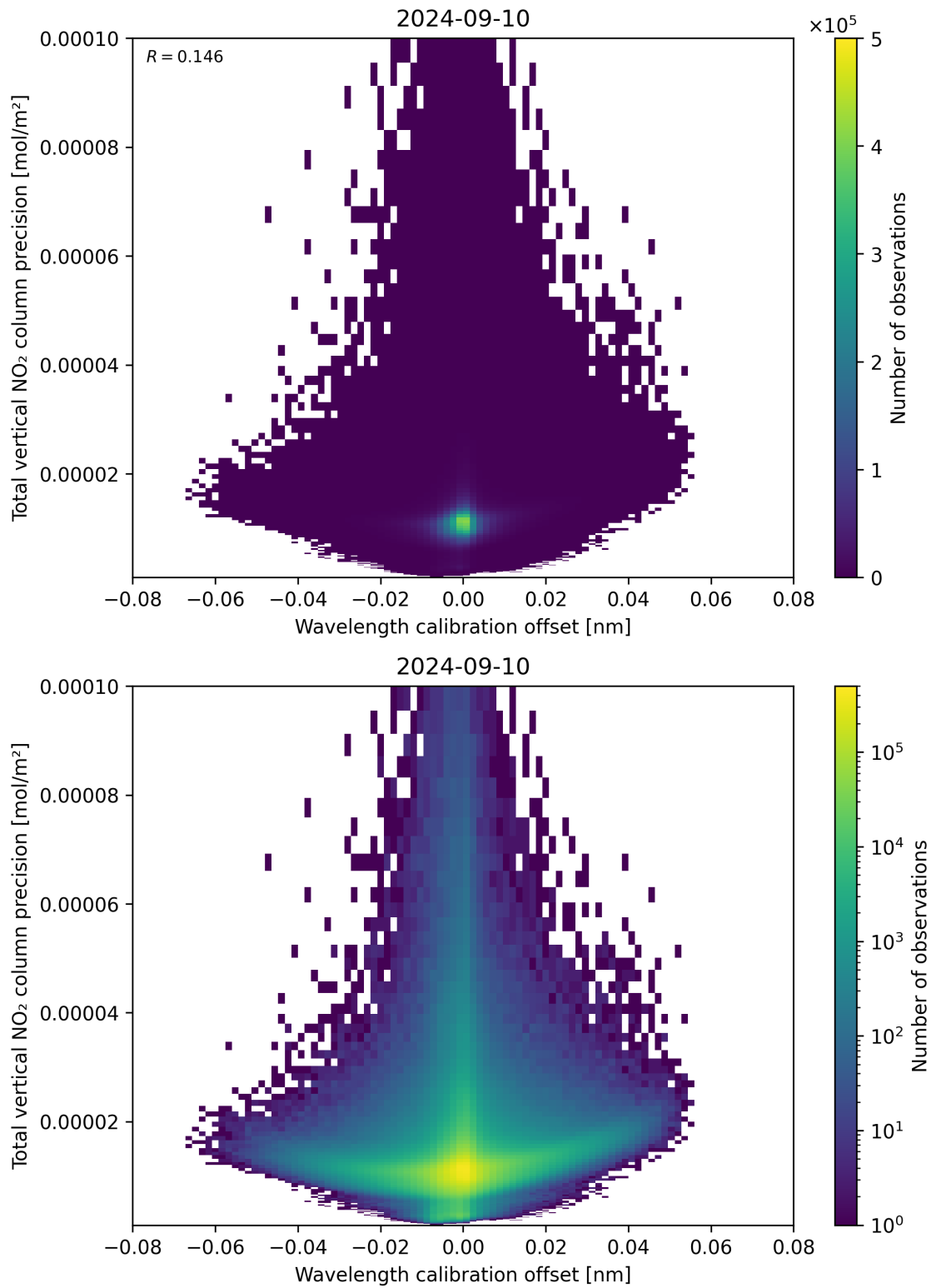
Figure 180: Scatter density plot of “Wavelength calibration offset” against “Total vertical NO 2 column precision” for 2024-09-09 to 2024-09-11.
