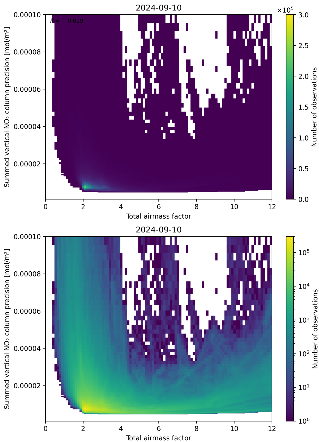
Figure 66: Scatter density plot of “Total airmass factor” against “Summed vertical NO 2 column precision” for 2024-09-09 to 2024-09-11.
