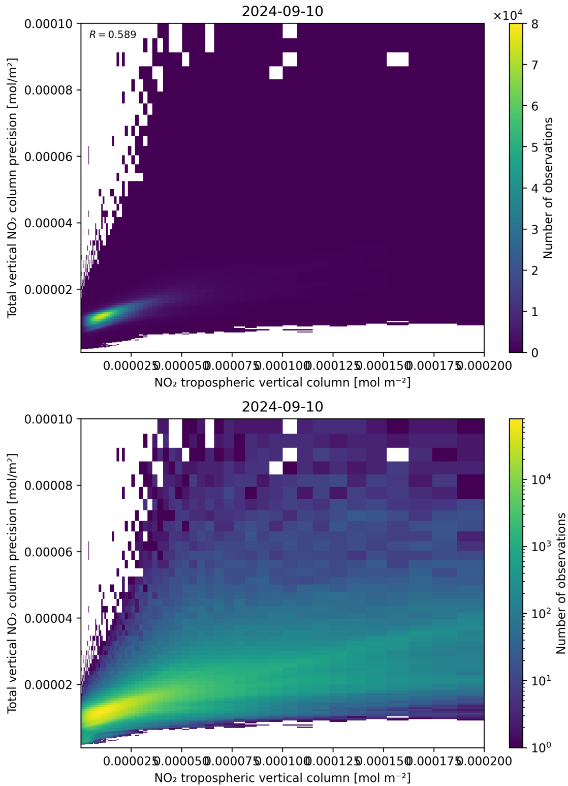
Figure 129: Scatter density plot of “NO 2 tropospheric vertical column” against “Total vertical NO 2 column precision” for 2024-09-09 to 2024-09-11.
