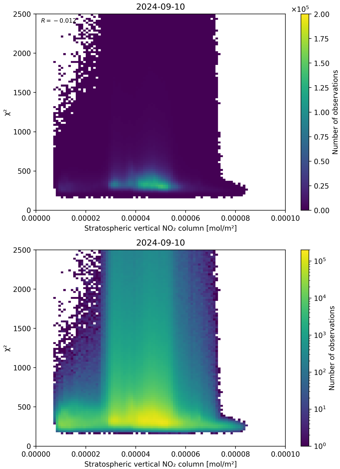
Figure 97: Scatter density plot of “Stratospheric vertical NO 2 column” against “ \chi^2 ” for 2024-09-09 to 2024-09-11.
