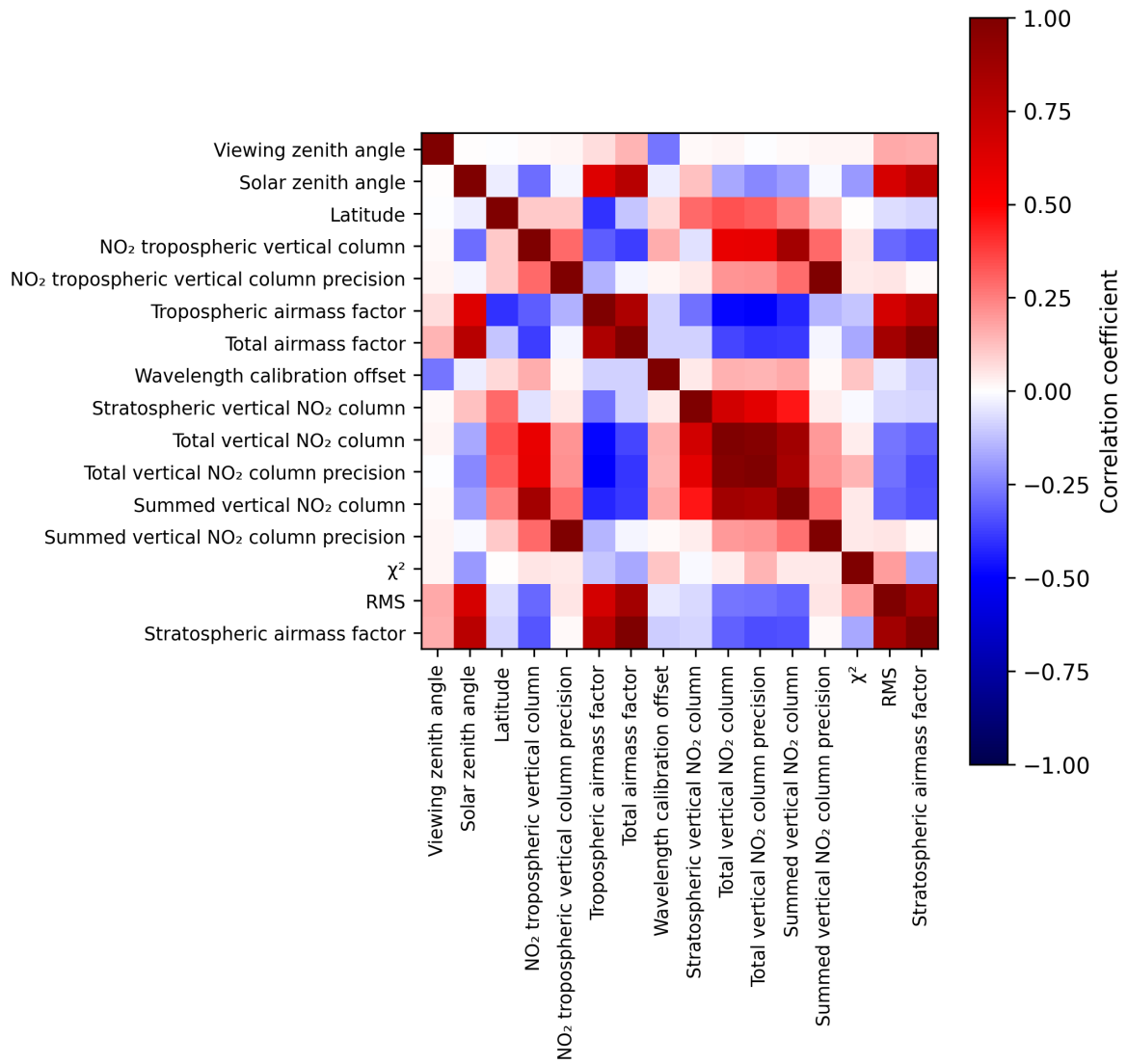
Figure 2: Map of correlation matrix for 2024-09-09 to 2024-09-11.
