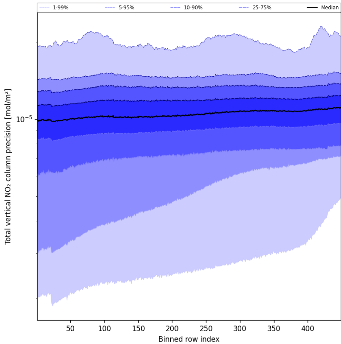
Figure 56: Along track statistics of “Total vertical NO 2 column precision” for 2024-09-09 to 2024-09-11
