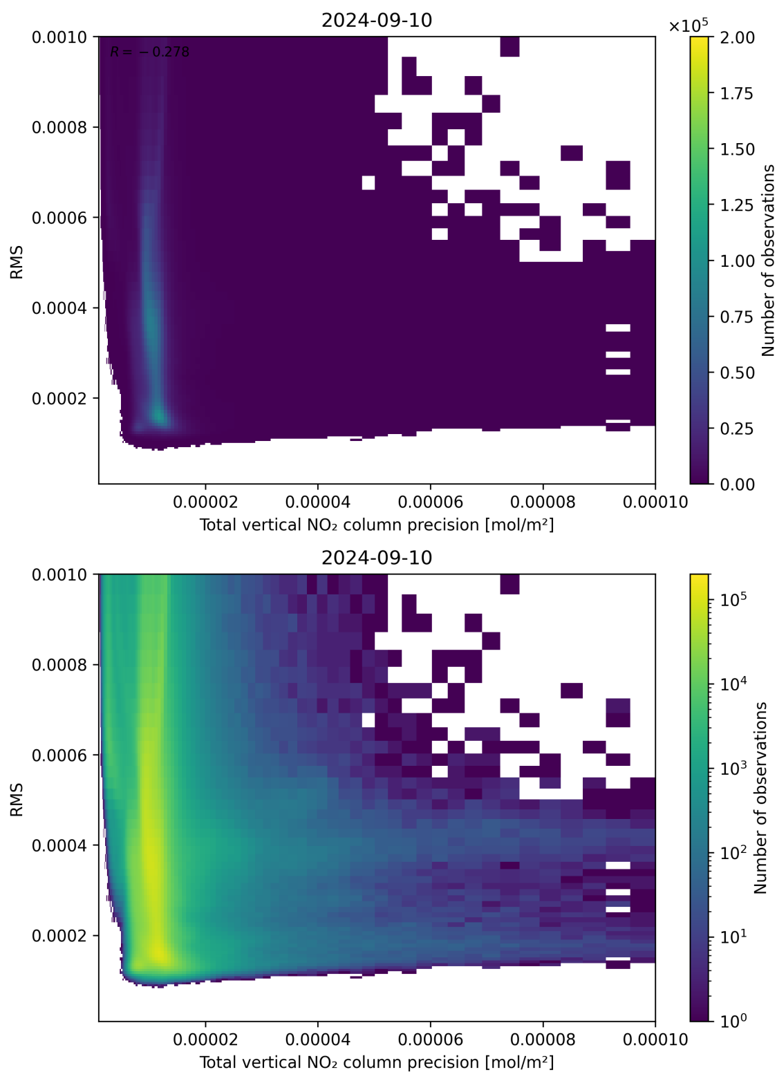
Figure 119: Scatter density plot of “Total vertical NO 2 column precision” against “RMS” for 2024-09-09 to 2024-09-11.
