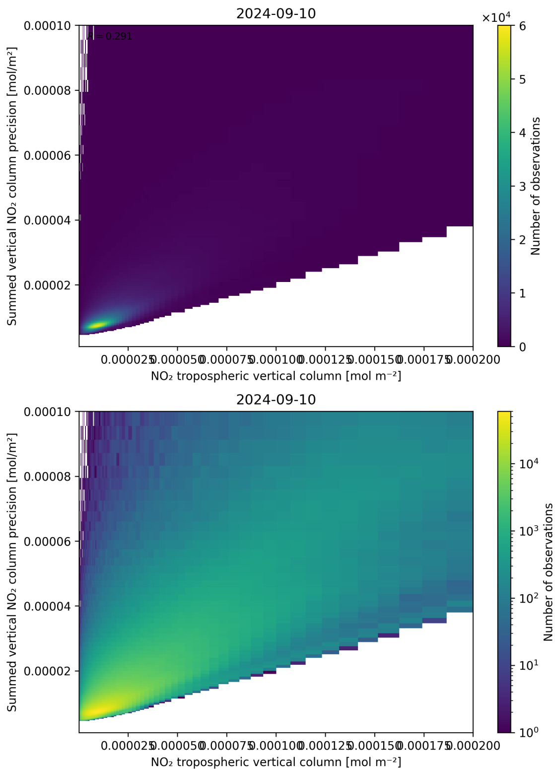
Figure 127: Scatter density plot of “NO 2 tropospheric vertical column” against “Summed vertical NO 2 column precision” for 2024-09-09 to 2024-09-11.
