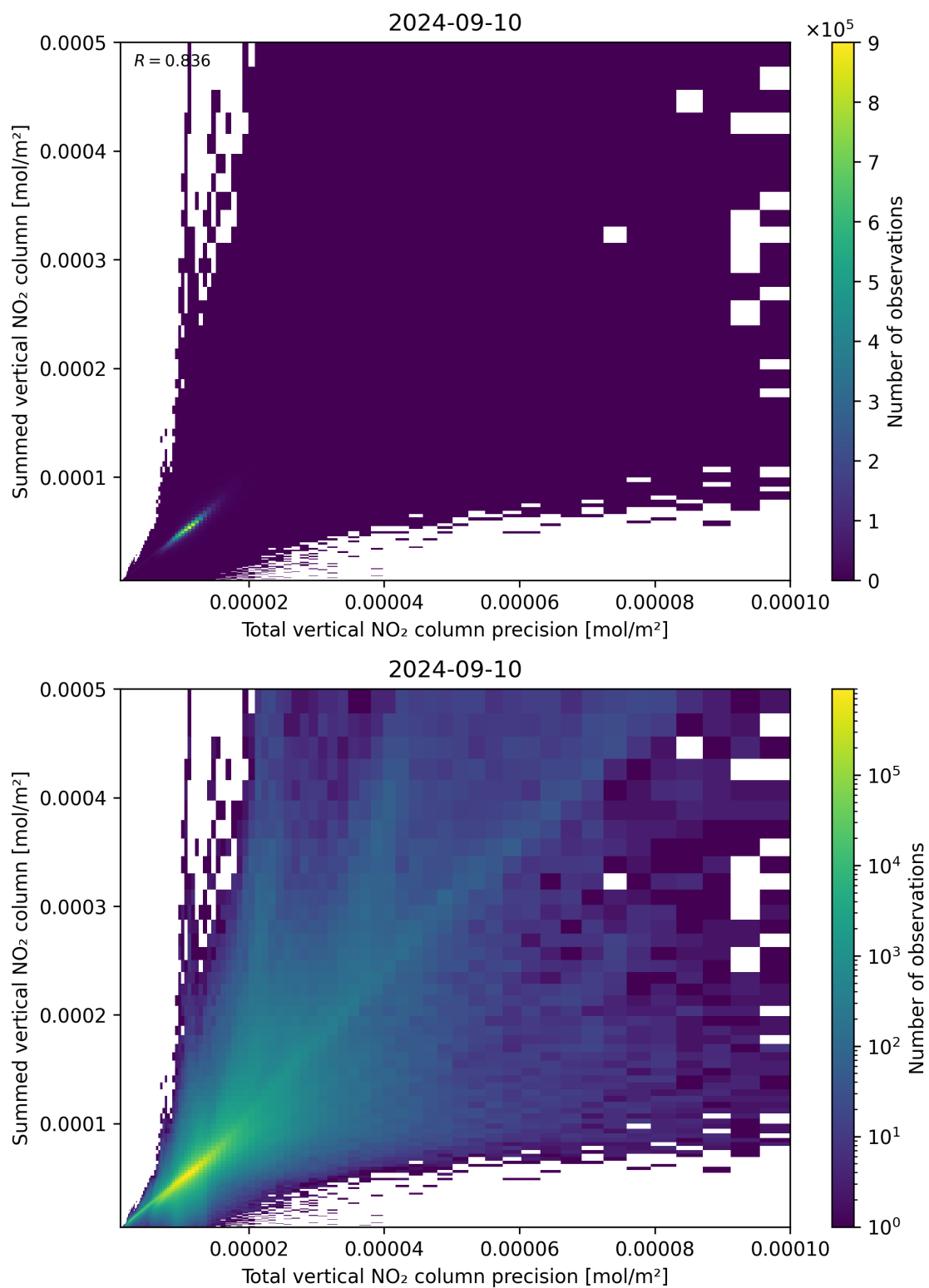
Figure 117: Scatter density plot of “Total vertical NO 2 column precision” against “Summed vertical NO 2 column” for 2024-09-09 to 2024-09-11.
