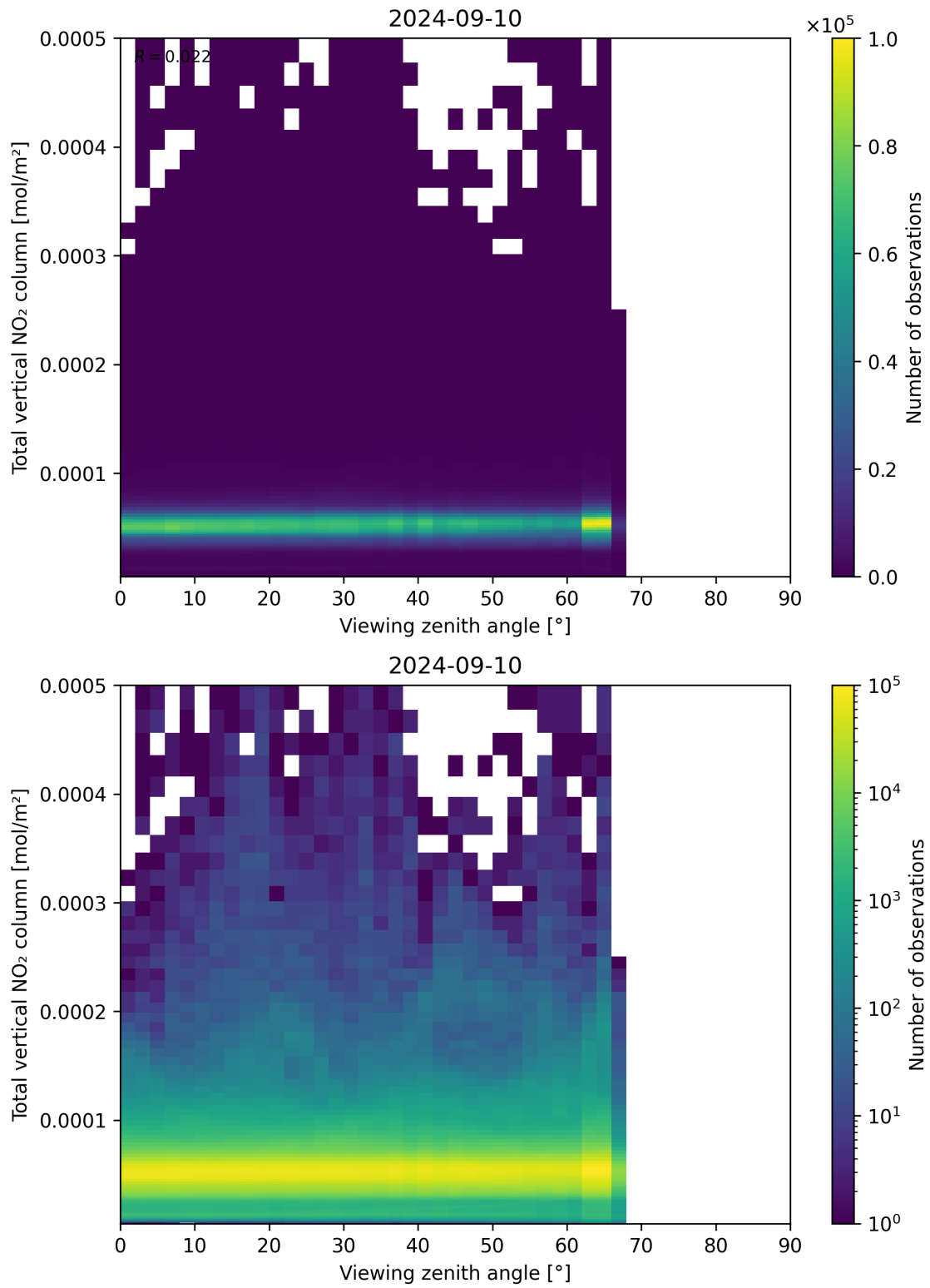
Figure 167: Scatter density plot of “Viewing zenith angle” against “Total vertical NO 2 column” for 2024-09-09 to 2024-09-11.
