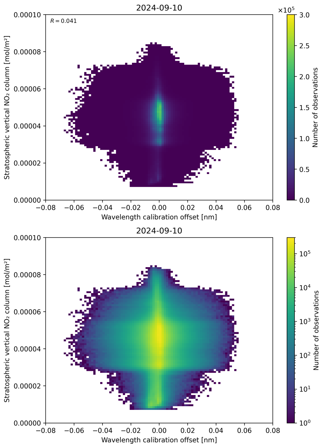
Figure 176: Scatter density plot of “Wavelength calibration offset” against “Stratospheric vertical NO 2 column” for 2024-09-09 to 2024-09-11.
