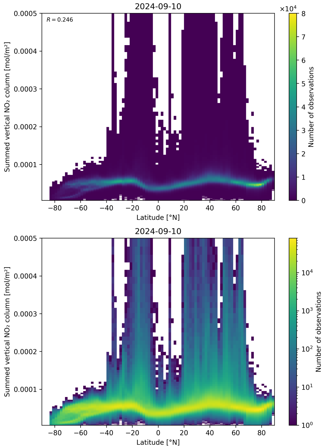
Figure 88: Scatter density plot of “Latitude” against “Summed vertical NO 2 column” for 2024-09-09 to 2024-09-11.
