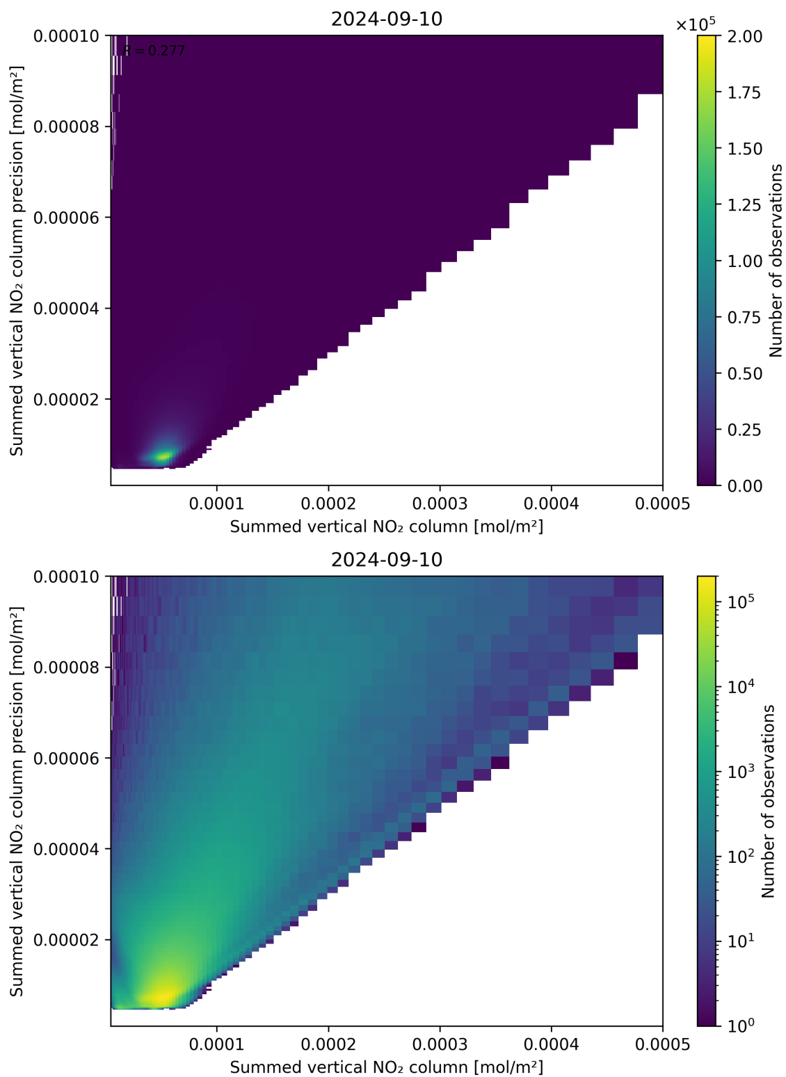
Figure 105: Scatter density plot of “Summed vertical NO 2 column” against “Summed vertical NO 2 column precision” for 2024-09-09 to 2024-09-11.
