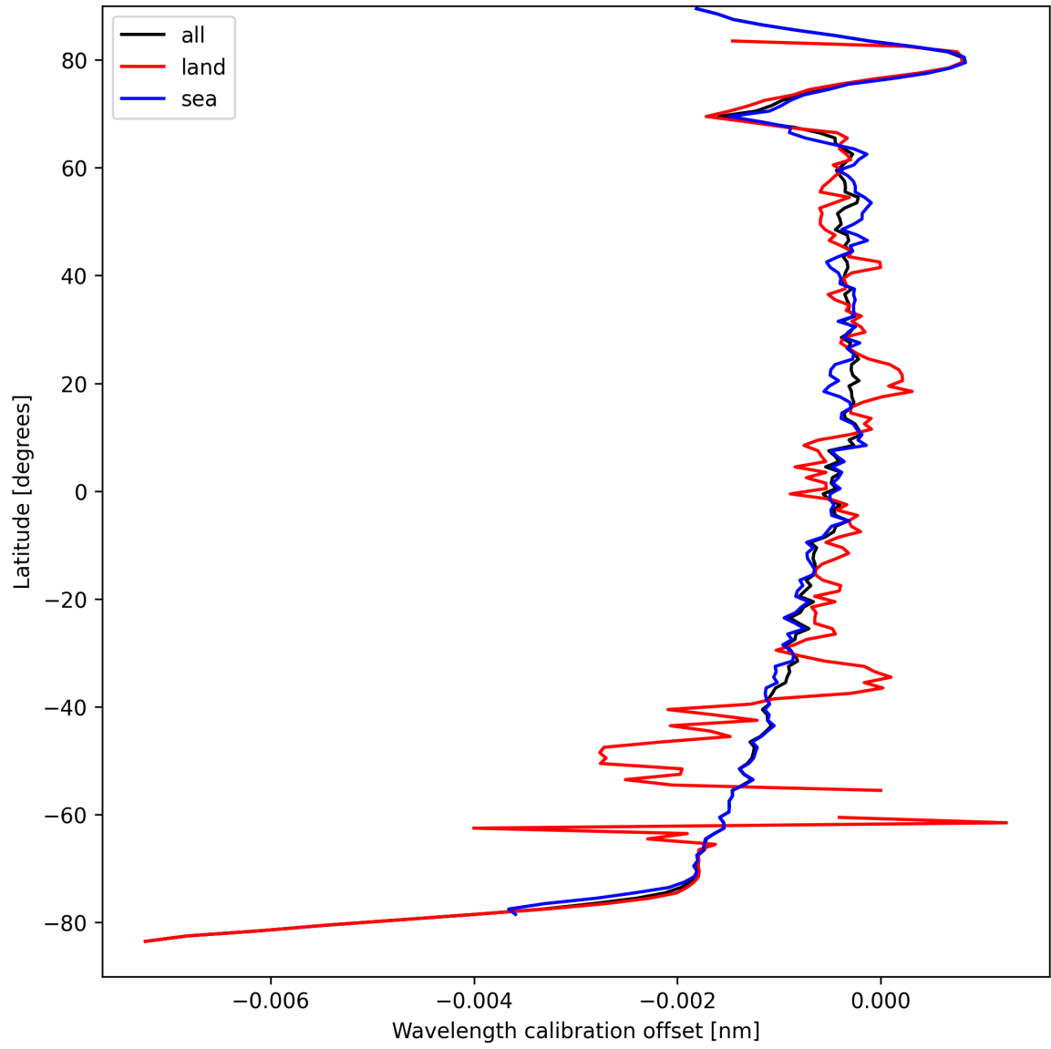
Figure 18: Zonal average of “Wavelength calibration offset” for 2024-09-09 to 2024-09-11.
