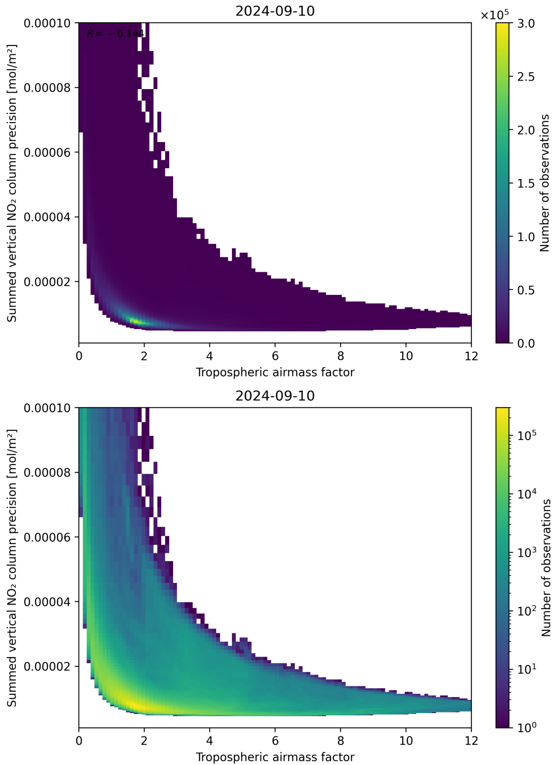
Figure 76: Scatter density plot of “Tropospheric air mass factor” against “Summed vertical NO 2 column precision” for 2024-09-09 to 2024-09-11.
