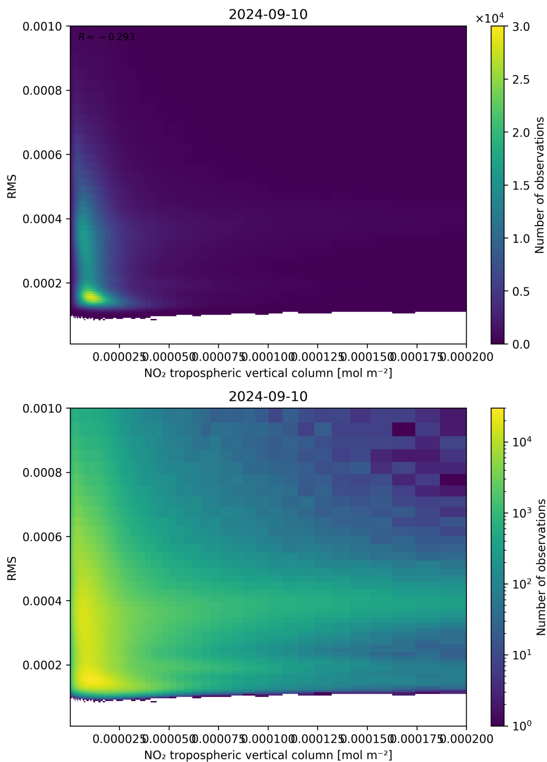
Figure 142: Scatter density plot of “NO 2 tropospheric vertical column” against “RMS” for 2024-09-09 to 2024-09-11.
