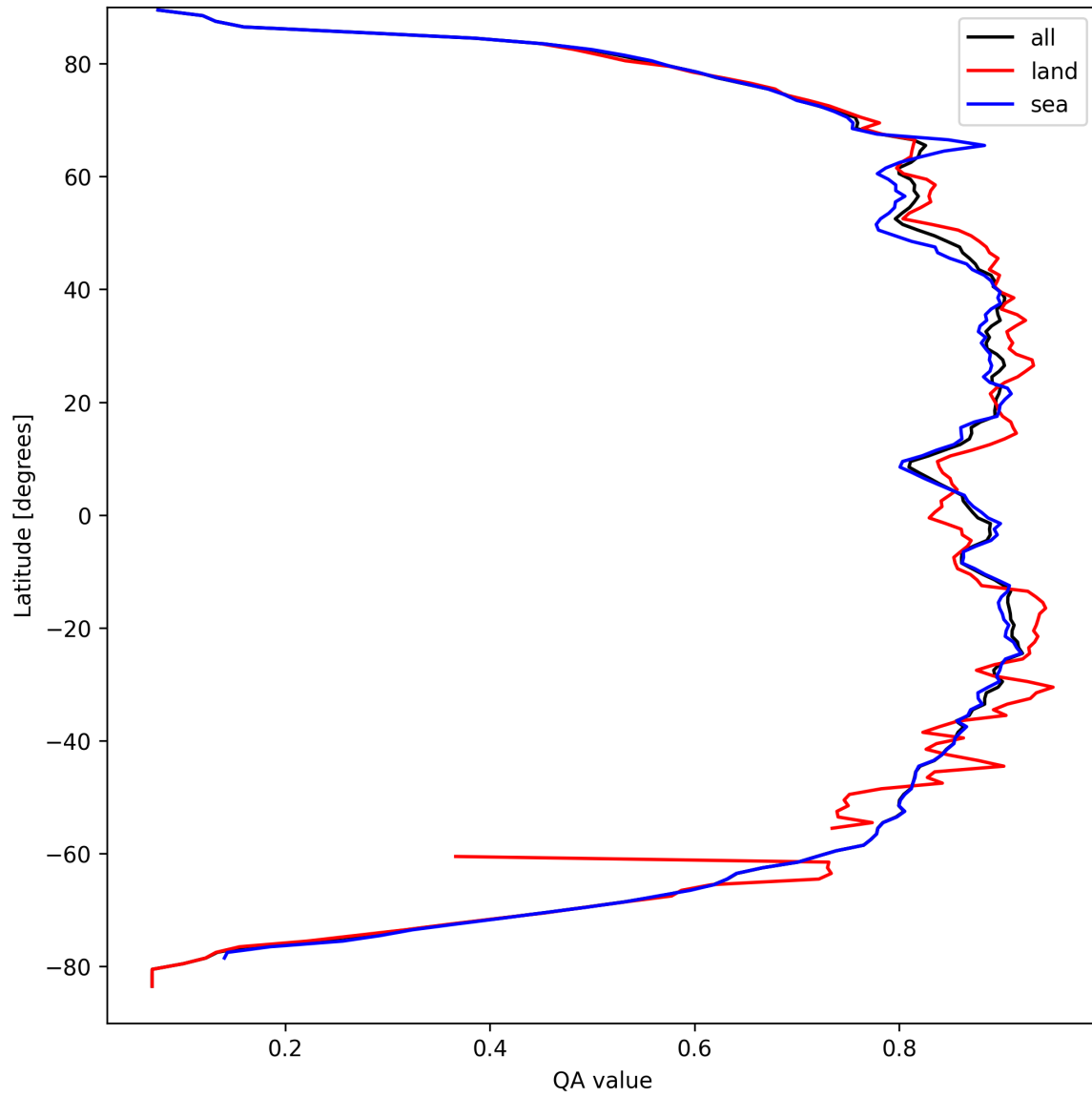
Figure 11: Zonal average of “QA value” for 2024-09-09 to 2024-09-11.
