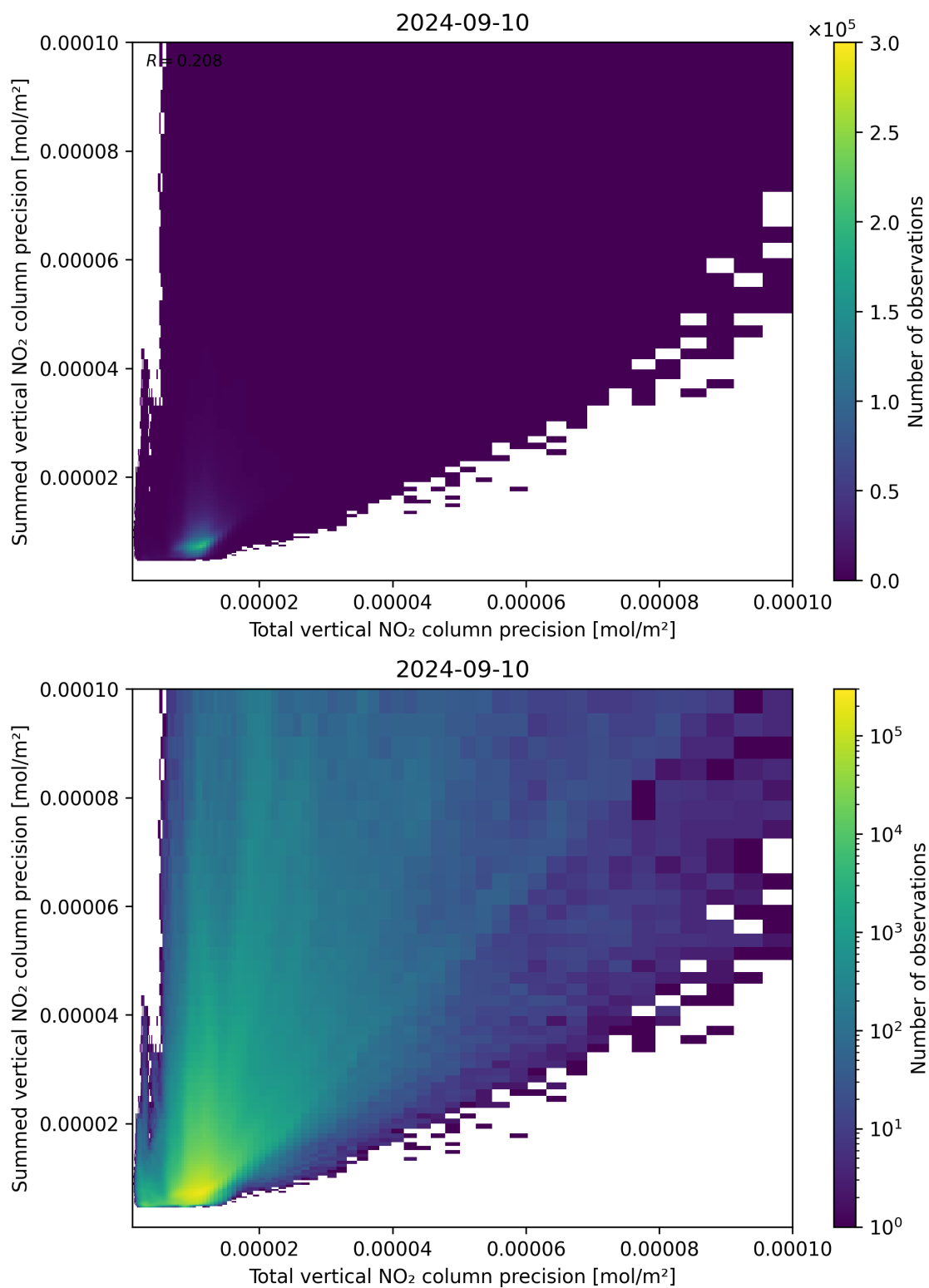
Figure 118: Scatter density plot of “Total vertical NO 2 column precision” against “Summed vertical NO 2 column precision” for 2024-09-09 to 2024-09-11.
