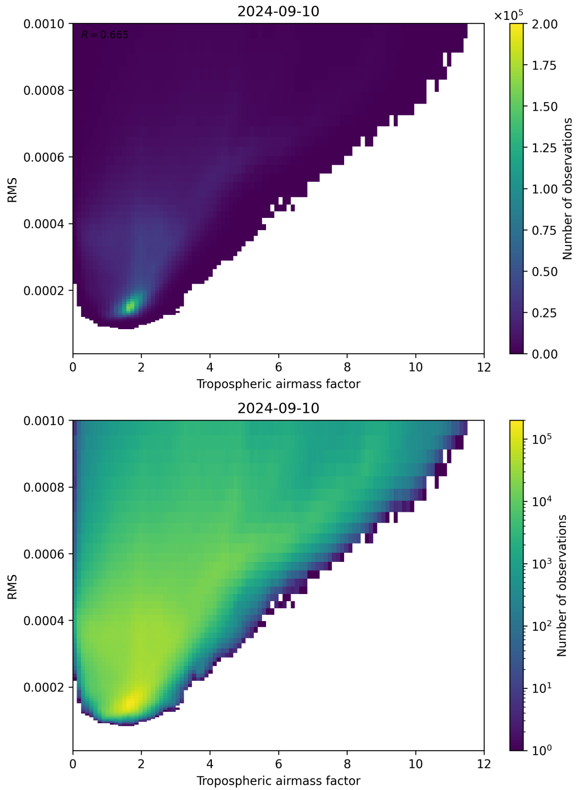
Figure 79: Scatter density plot of “Tropospheric airmass factor” against “RMS” for 2024-09-09 to 2024-09-11.
