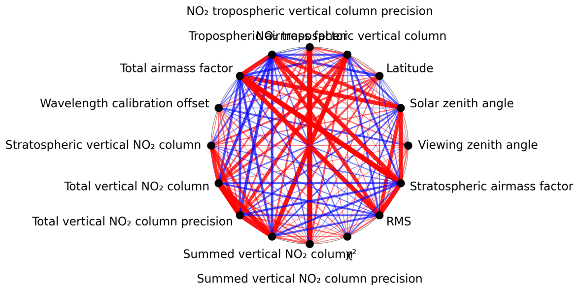
Figure 1: Map of correlation graph for 2024-09-09 to 2024-09-11.
