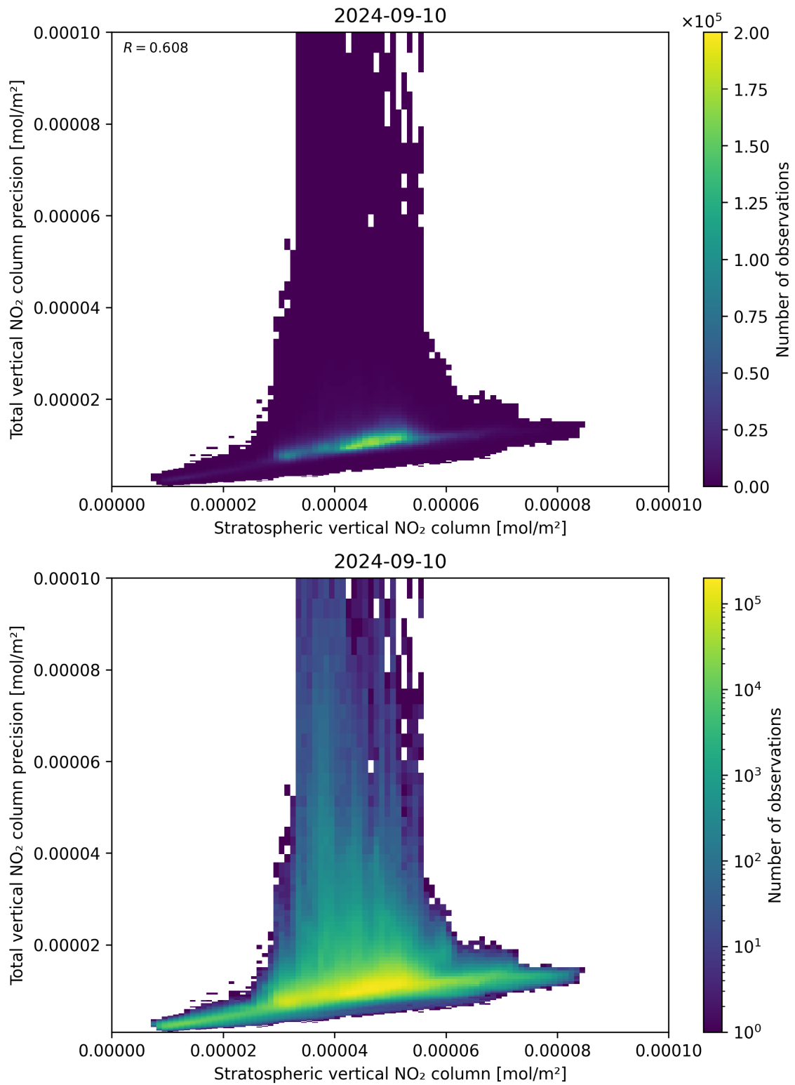
Figure 101: Scatter density plot of “Stratospheric vertical NO 2 column” against “Total vertical NO 2 column precision” for 2024-09-09 to 2024-09-11.
