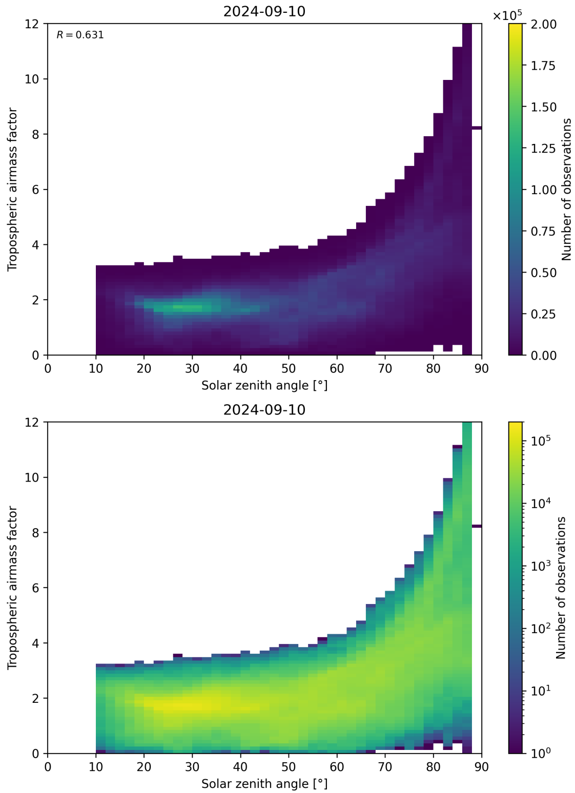
Figure 147: Scatter density plot of “Solar zenith angle” against “Tropospheric airmass factor” for 2024-09-09 to 2024-09-11.
