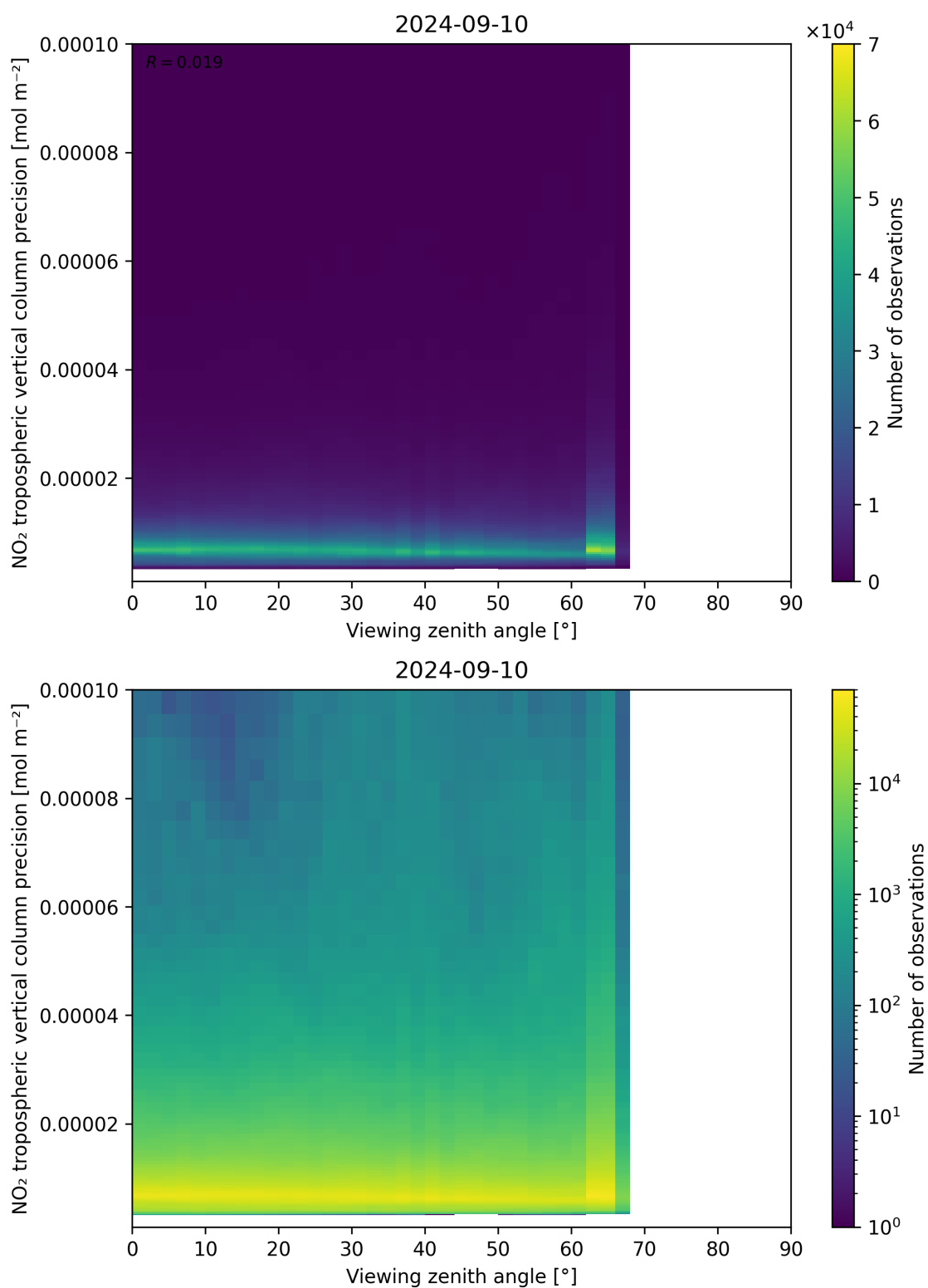
Figure 170: Scatter density plot of “Viewing zenith angle” against “NO 2 tropospheric vertical column precision” for 2024-09-09 to 2024-09-11.
