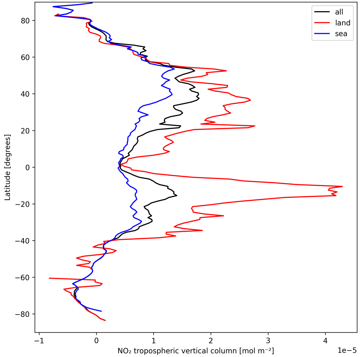
Figure 12: Zonal average of “NO 2 tropospheric vertical column” for 2024-09-09 to 2024-09-11.
