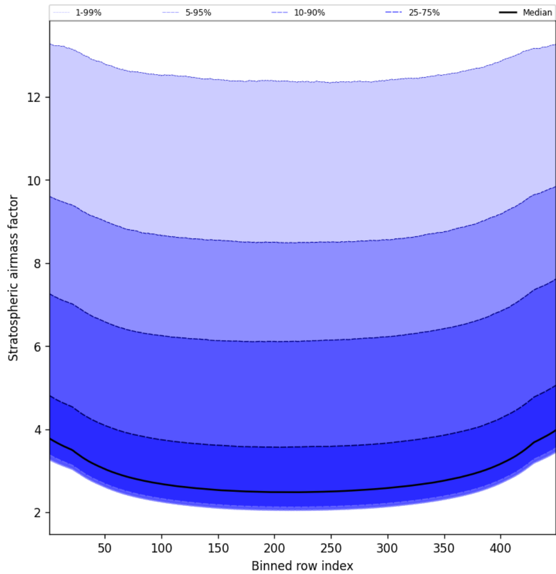
Figure 61: Along track statistics of “Stratospheric airmass factor” for 2024-09-09 to 2024-09-11
