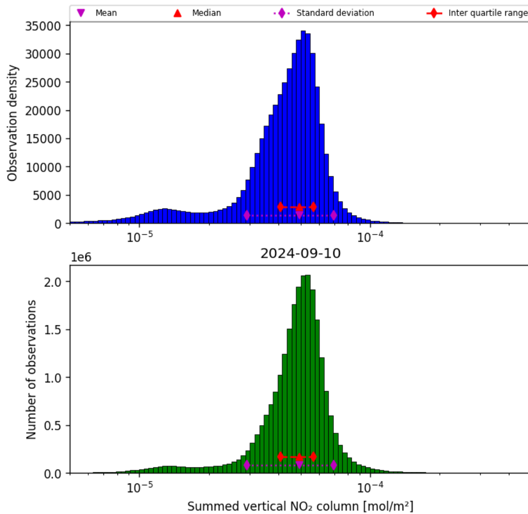
Figure 40: Histogram of “Summed vertical NO 2 column” for 2024-09-09 to 2024-09-11
