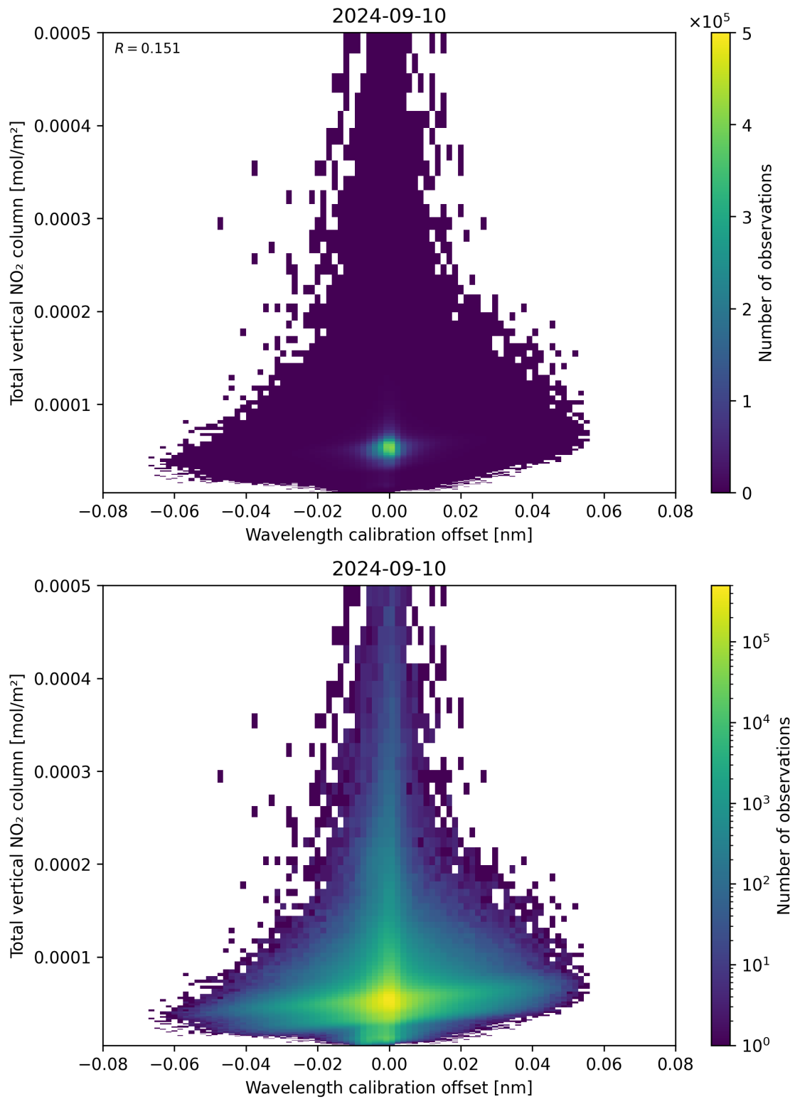
Figure 179: Scatter density plot of “Wavelength calibration offset” against “Total vertical NO 2 column” for 2024-09-09 to 2024-09-11.
