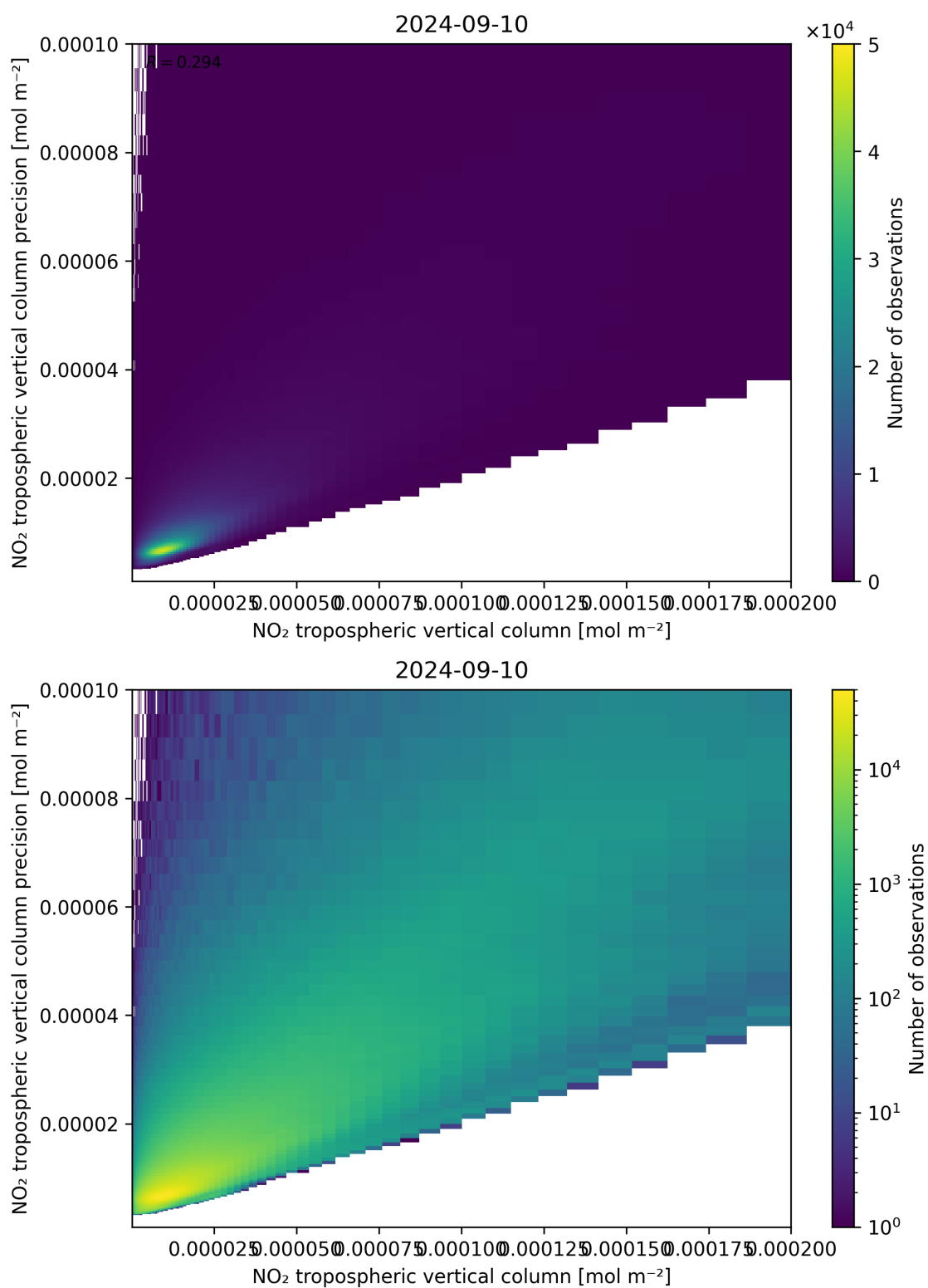
Figure 130: Scatter density plot of “NO 2 tropospheric vertical column” against “NO 2 tropospheric vertical column precision” for 2024-09-09 to 2024-09-11.
