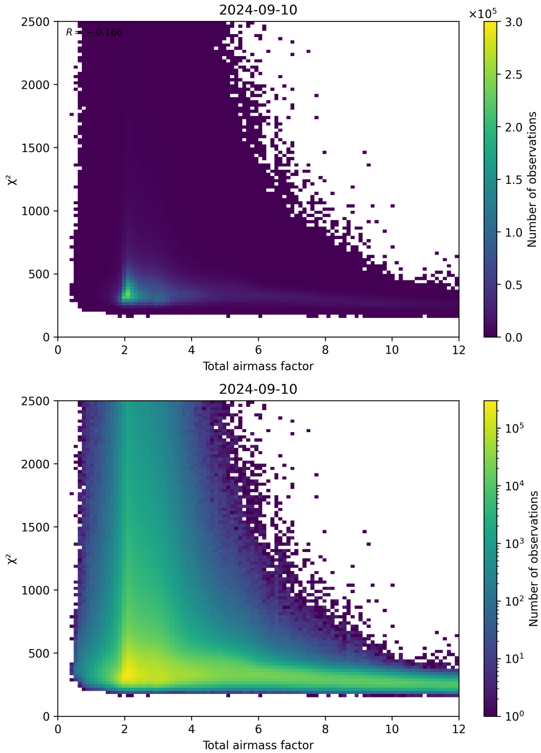
Figure 63: Scatter density plot of “Total airmass factor” against “ \chi^2 ” for 2024-09-09 to 2024-09-11.
