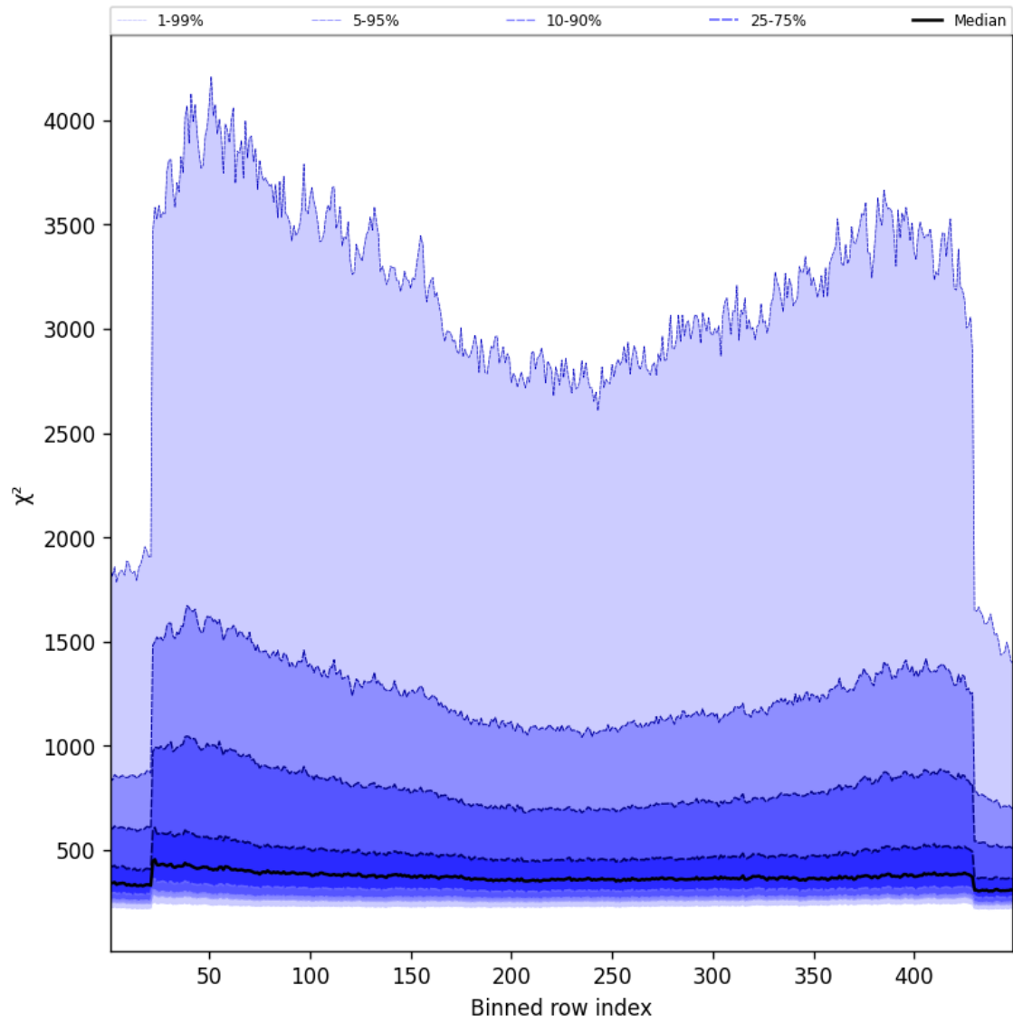
Figure 59: Along track statistics of “ \chi^2 ” for 2024-09-09 to 2024-09-11
