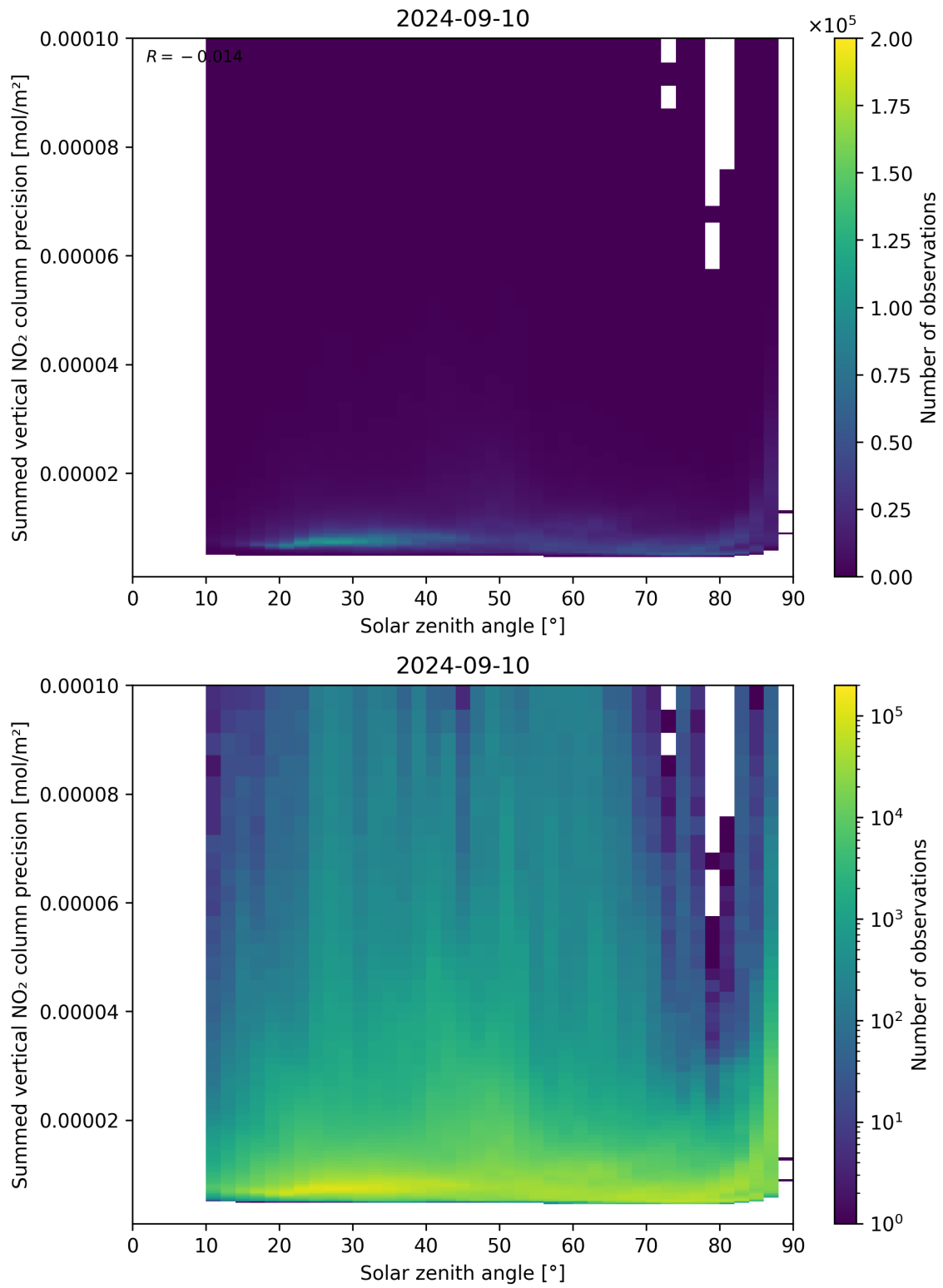
Figure 152: Scatter density plot of “Solar zenith angle” against “Summed vertical NO 2 column precision” for 2024-09-09 to 2024-09-11.
