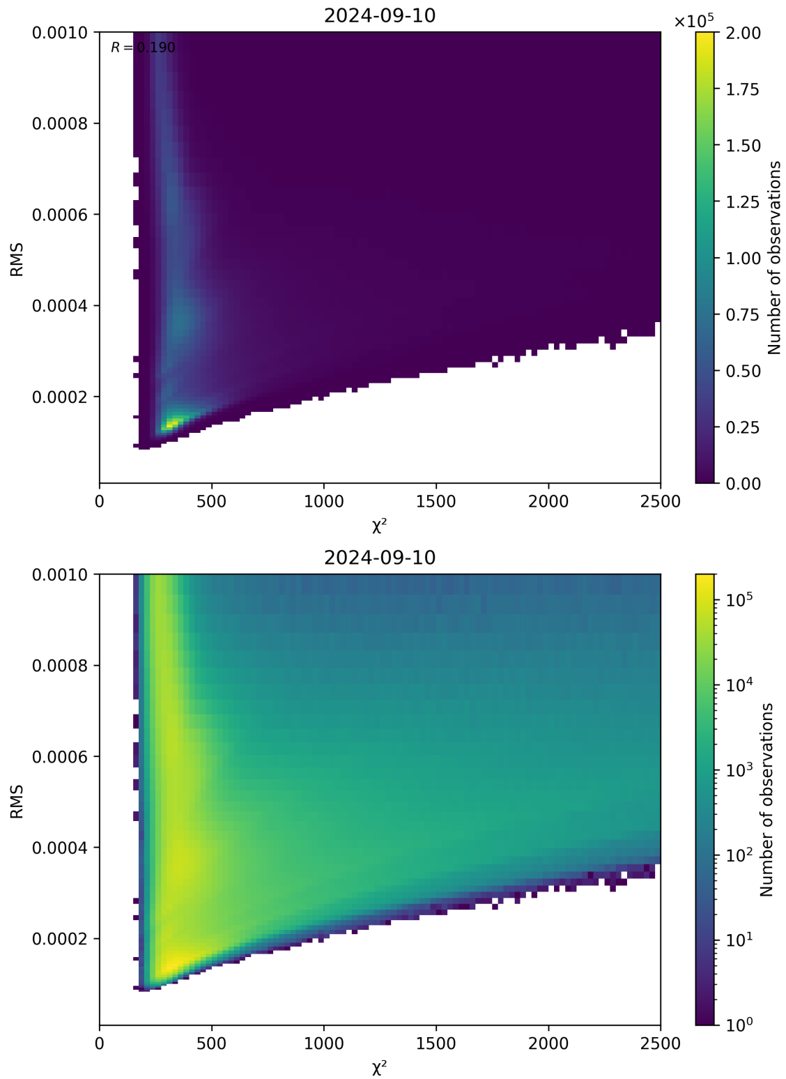
Figure 82: Scatter density plot of “ \chi^2 ” against “RMS” for 2024-09-09 to 2024-09-11.
