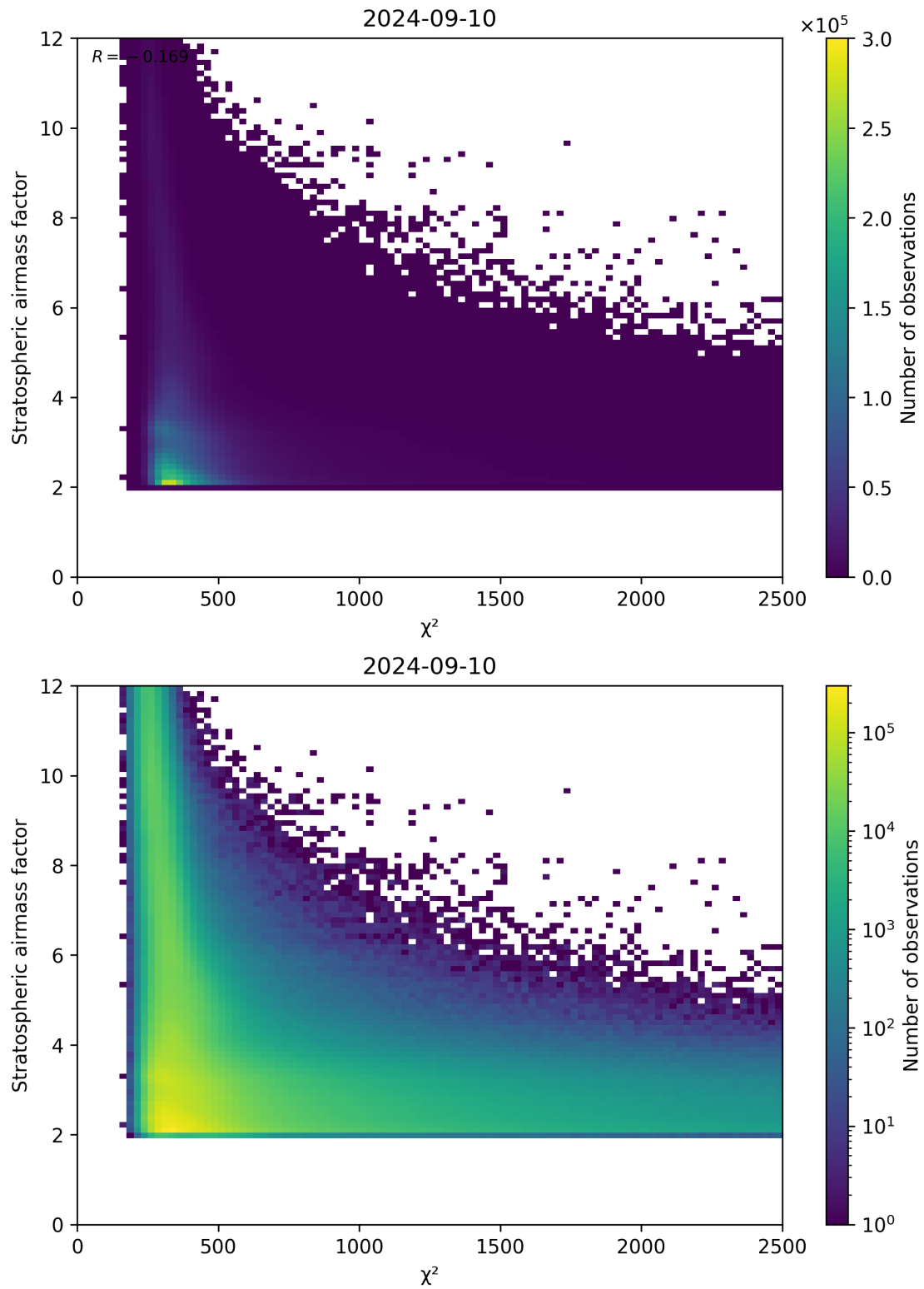
Figure 81: Scatter density plot of “ \chi^2 ” against “Stratospheric airmass factor” for 2024-09-09 to 2024-09-11.
