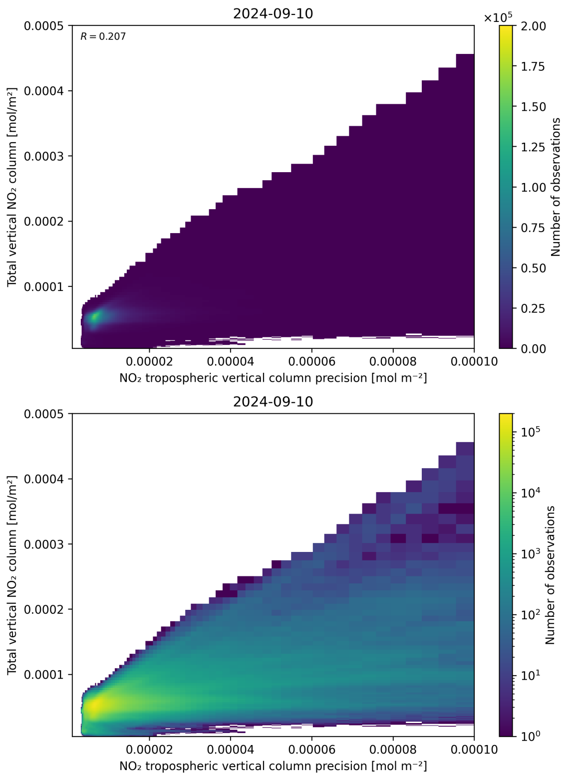
Figure 138: Scatter density plot of “NO 2 tropospheric vertical column precision” against “Total vertical NO 2 column” for 2024-09-09 to 2024-09-11.
