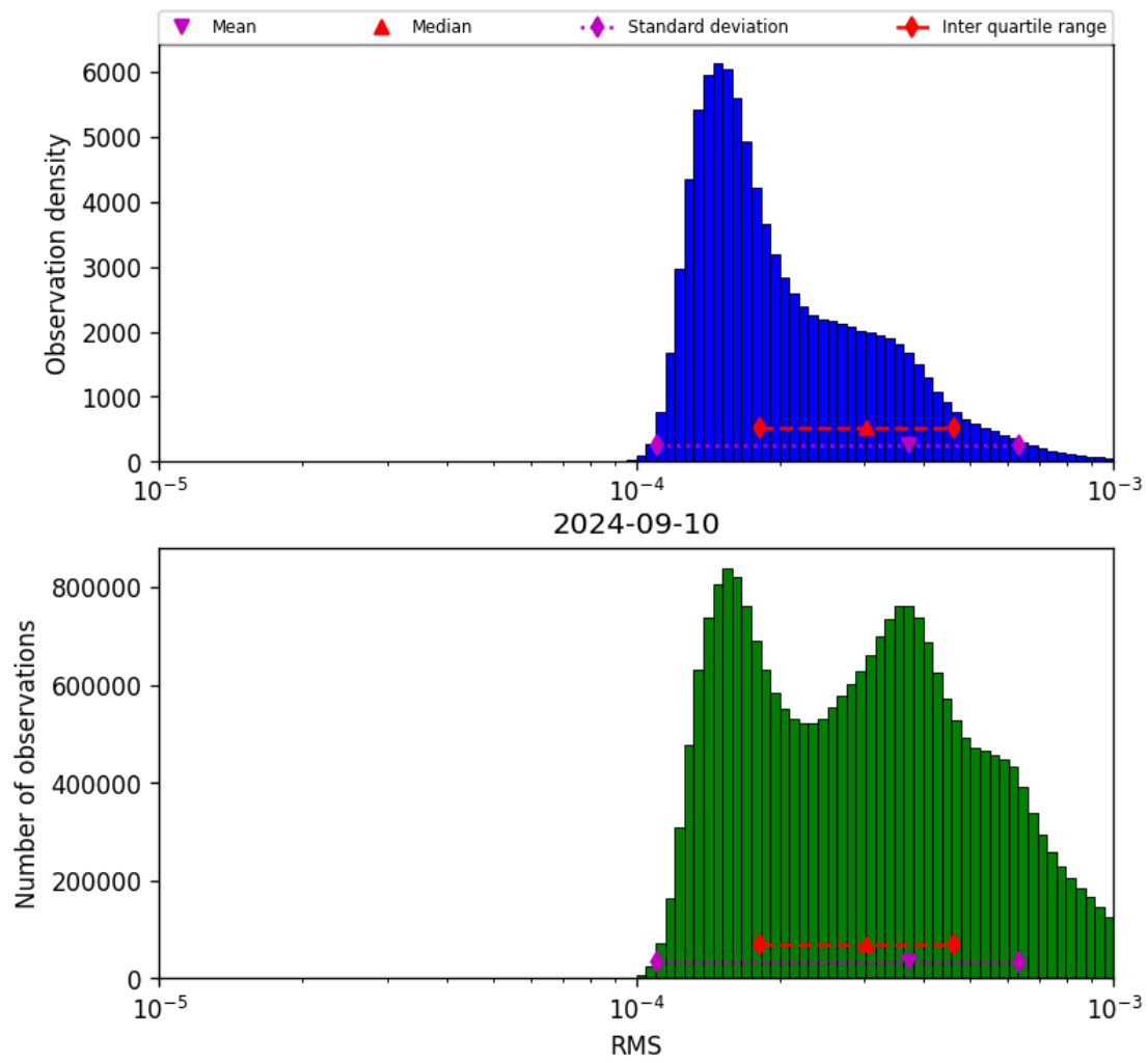
Figure 43: Histogram of “RMS” for 2024-09-09 to 2024-09-11
