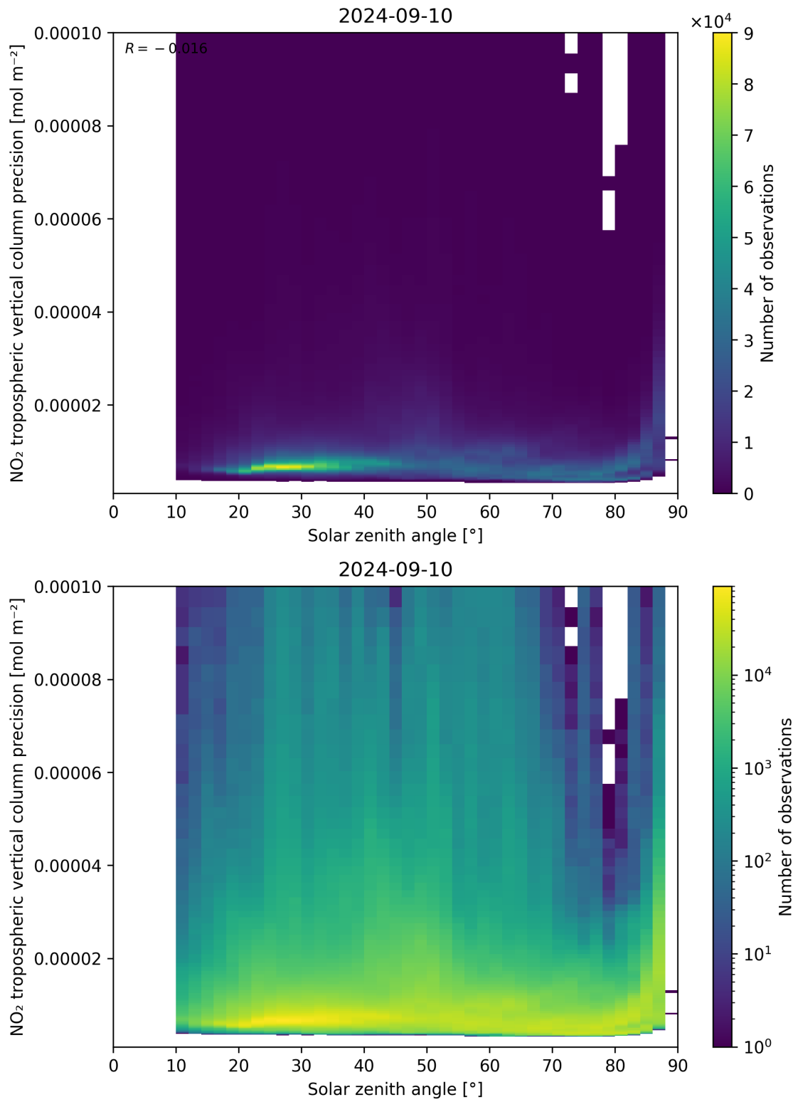
Figure 156: Scatter density plot of “Solar zenith angle” against “NO 2 tropospheric vertical column precision” for 2024-09-09 to 2024-09-11.
