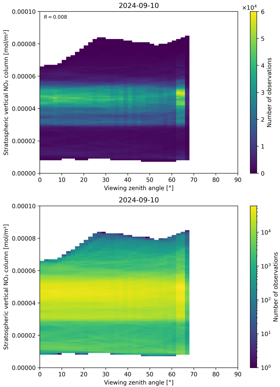
Figure 164: Scatter density plot of “Viewing zenith angle” against “Stratospheric vertical NO 2 column” for 2024-09-09 to 2024-09-11.
