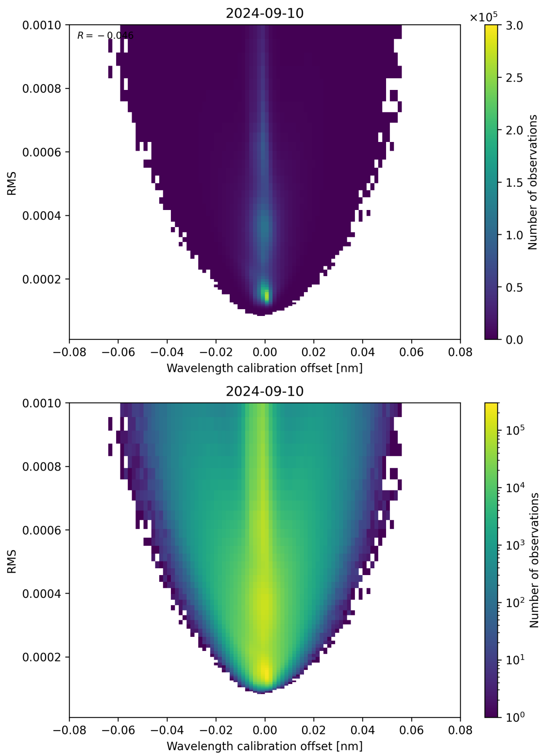
Figure 181: Scatter density plot of “Wavelength calibration offset” against “RMS” for 2024-09-09 to 2024-09-11.
