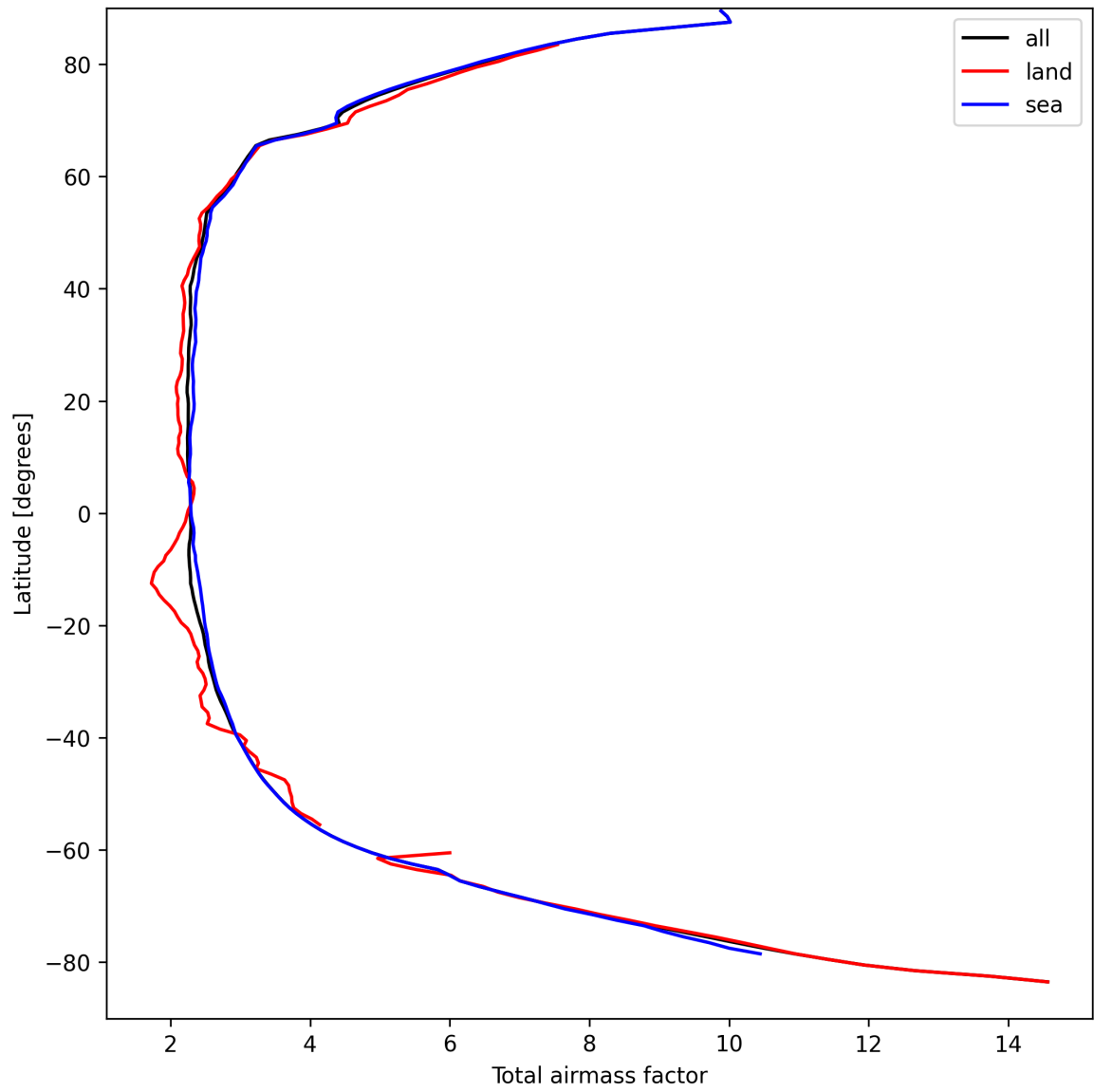
Figure 15: Zonal average of “Total airmass factor” for 2024-09-09 to 2024-09-11.
