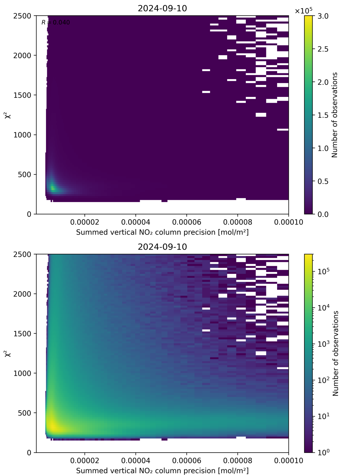
Figure 107: Scatter density plot of “Summed vertical NO 2 column precision” against “ \chi^2 ” for 2024-09-09 to 2024-09-11.
