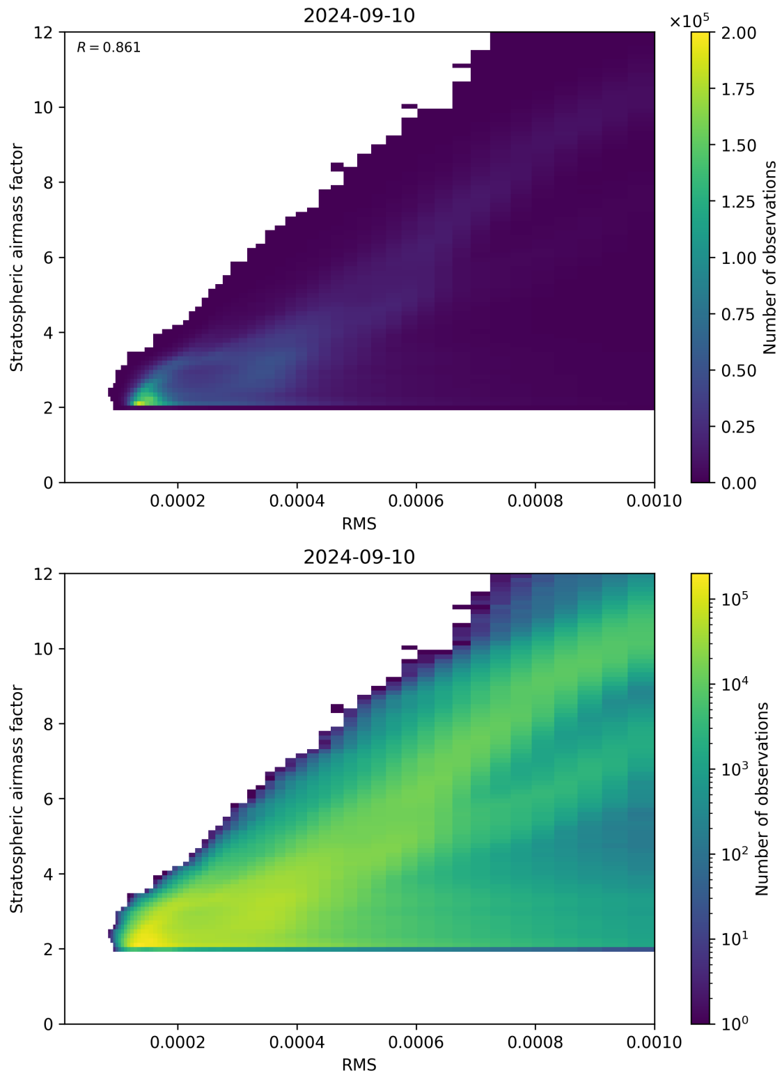
Figure 144: Scatter density plot of “RMS” against “Stratospheric airmass factor” for 2024-09-09 to 2024-09-11.
