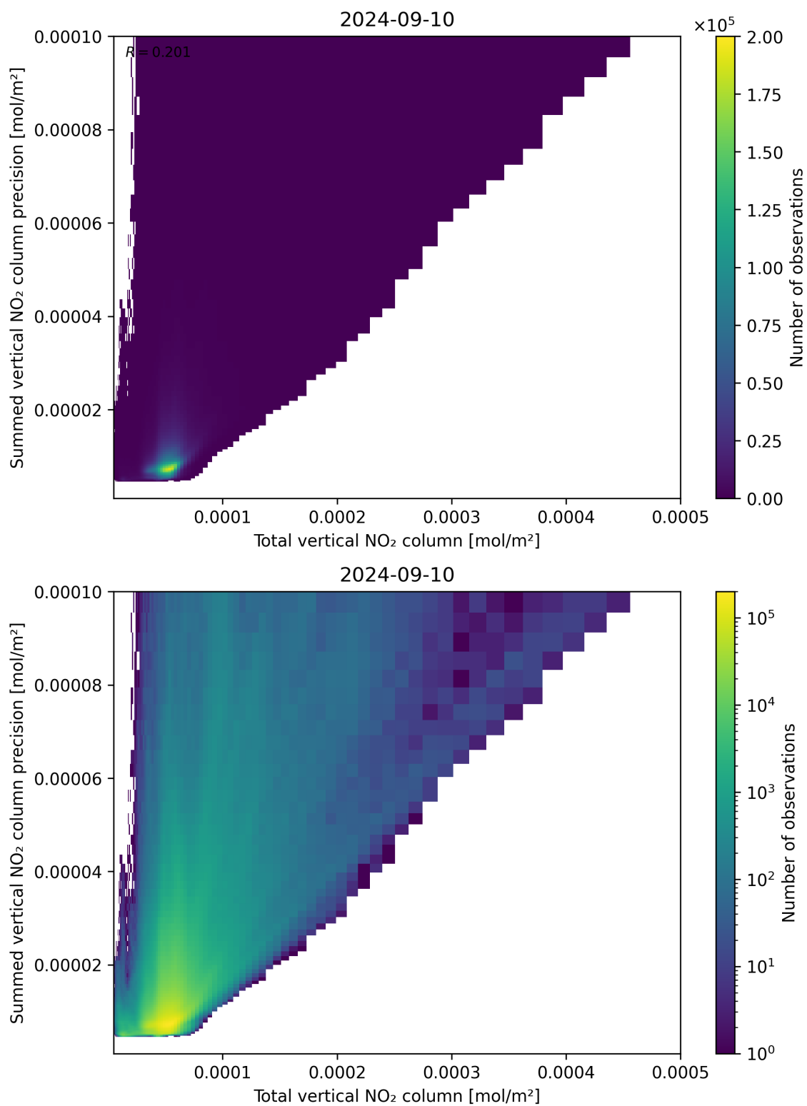
Figure 113: Scatter density plot of “Total vertical NO 2 column” against “Summed vertical NO 2 column precision” for 2024-09-09 to 2024-09-11.
