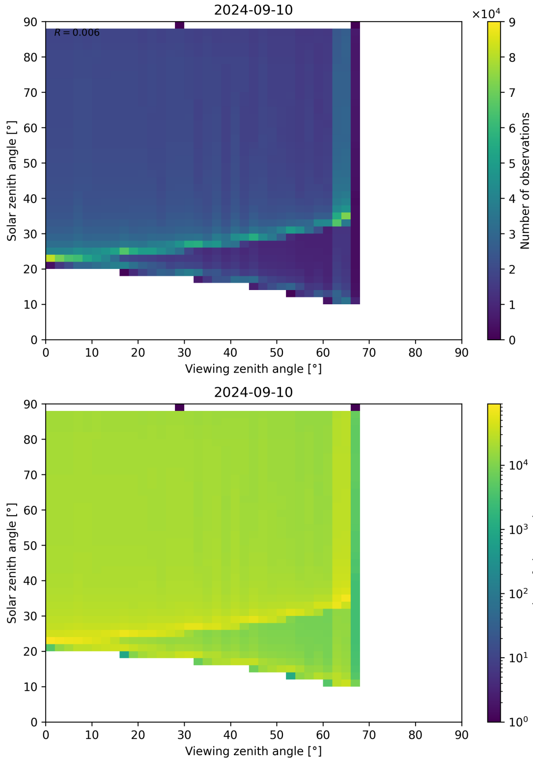
Figure 172: Scatter density plot of “Viewing zenith angle” against “Solar zenith angle” for 2024-09-09 to 2024-09-11.
