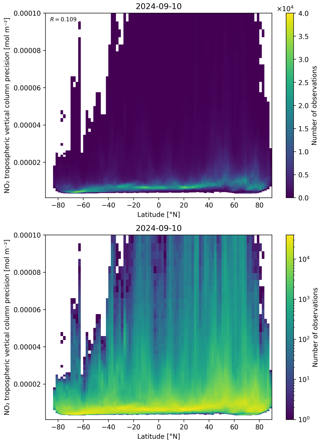
Figure 93: Scatter density plot of “Latitude” against “NO 2 tropospheric vertical column precision” for 2024-09-09 to 2024-09-11.
