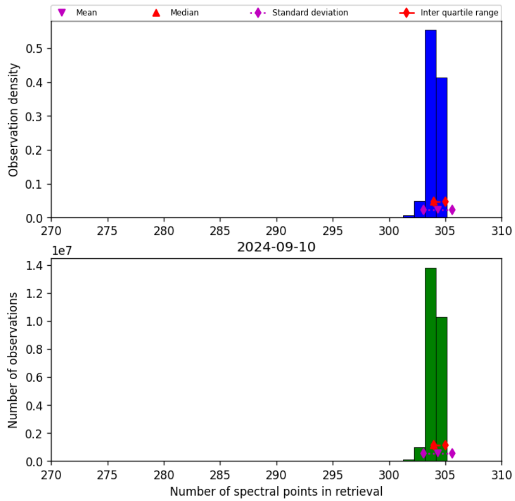
Figure 33: Histogram of “Number of spectral points in retrieval” for 2024-09-09 to 2024-09-11
