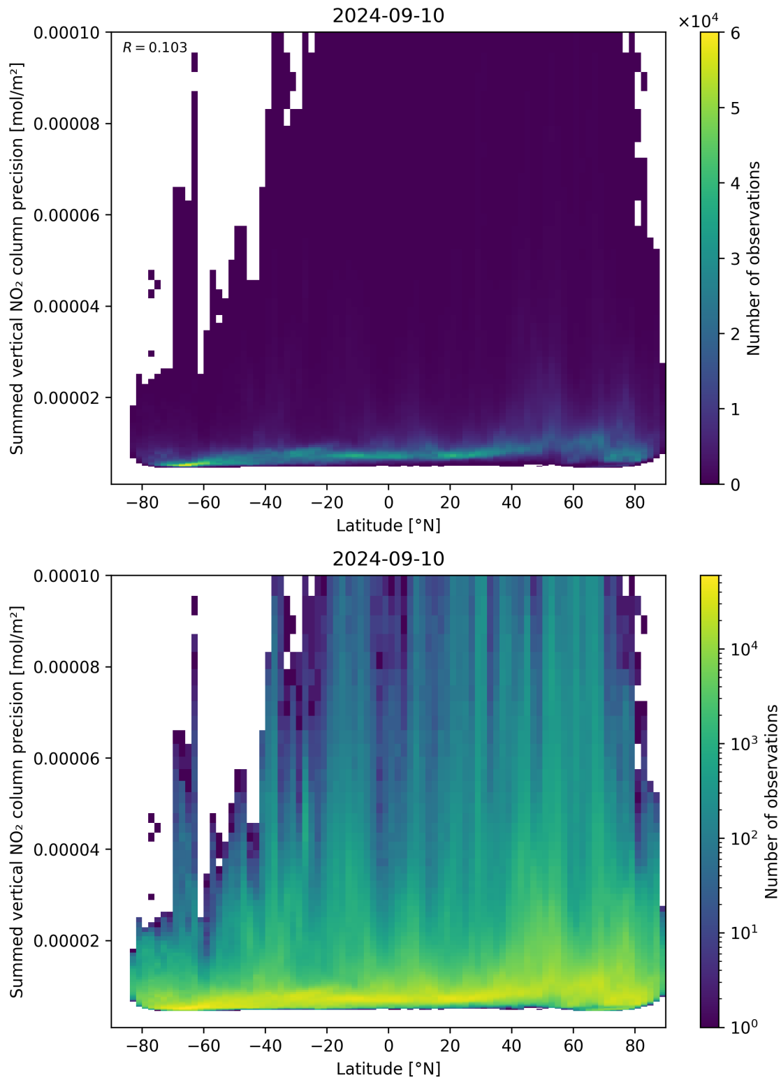
Figure 89: Scatter density plot of “Latitude” against “Summed vertical NO 2 column precision” for 2024-09-09 to 2024-09-11.
