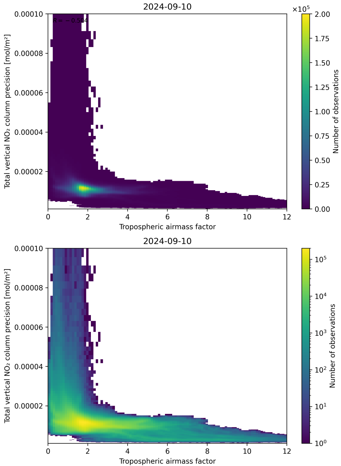
Figure 78: Scatter density plot of “Tropospheric air mass factor” against “Total vertical NO 2 column precision” for 2024-09-09 to 2024-09-11.
