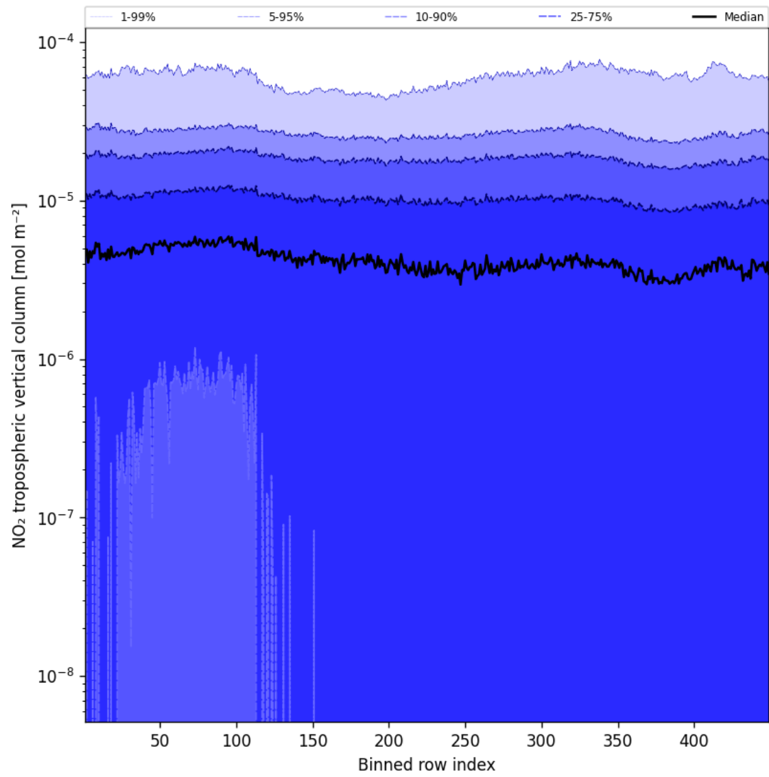
Figure 46: Along track statistics of “NO 2 tropospheric vertical column” for 2024-09-09 to 2024-09-11
