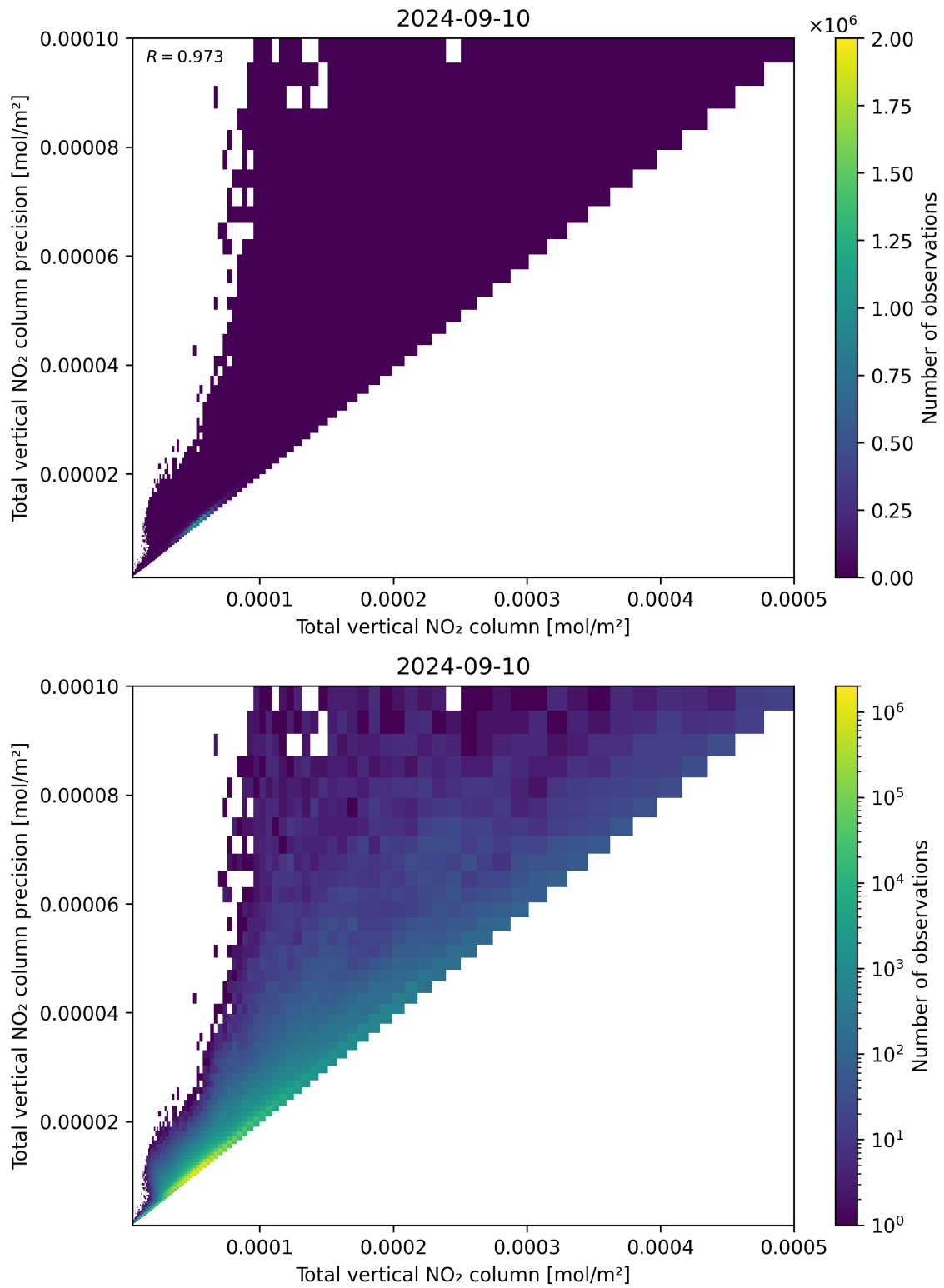
Figure 114: Scatter density plot of “Total vertical NO 2 column” against “Total vertical NO 2 column precision” for 2024-09-09 to 2024-09-11.
