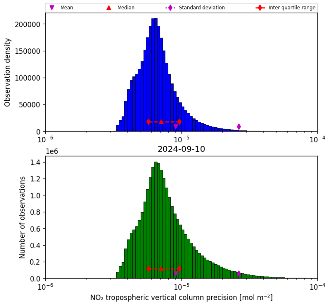
Figure 30: Histogram of “NO 2 tropospheric vertical column precision” for 2024-09-09 to 2024-09-11
