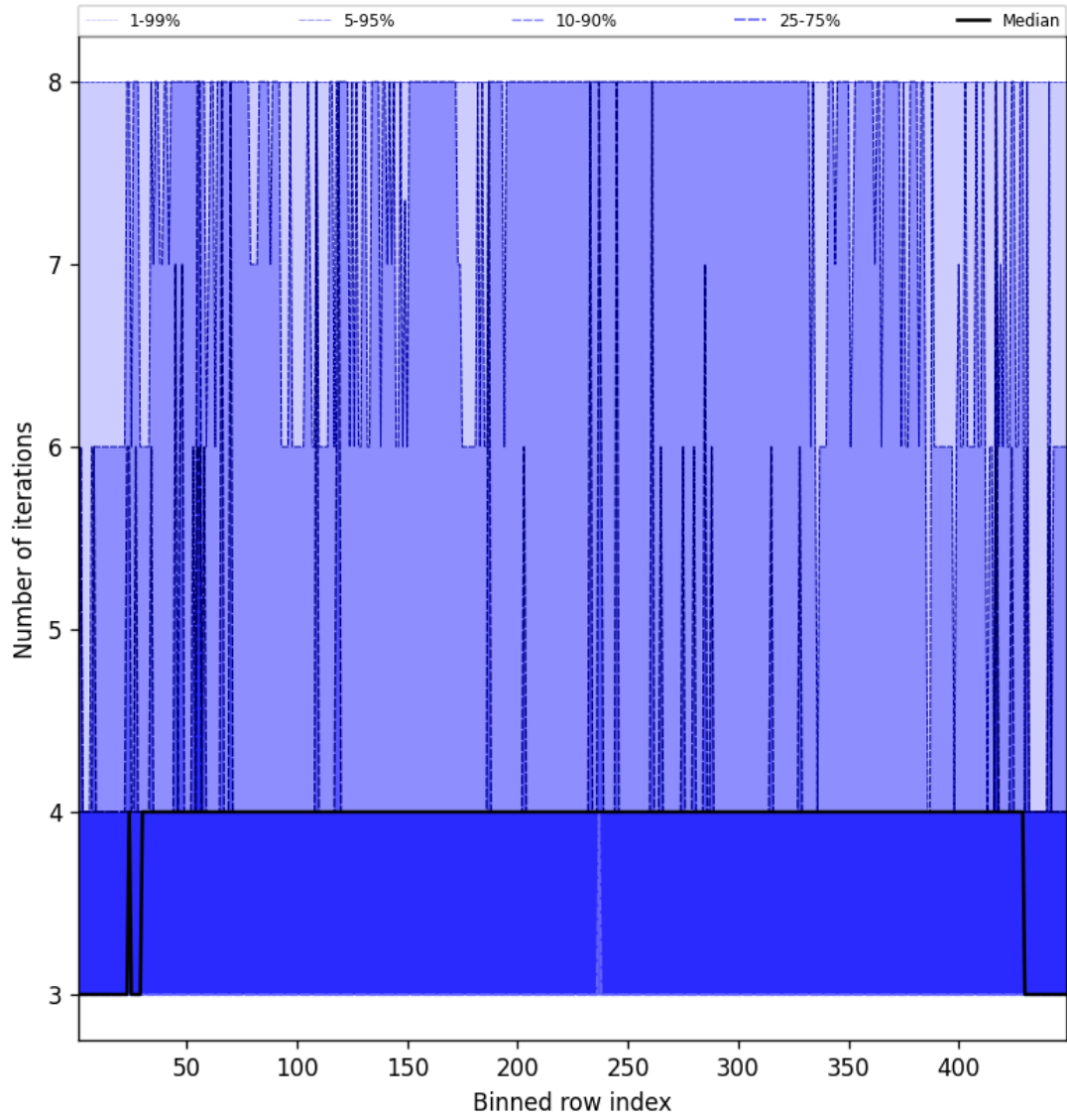
Figure 51: Along track statistics of “Number of iterations” for 2024-09-09 to 2024-09-11
