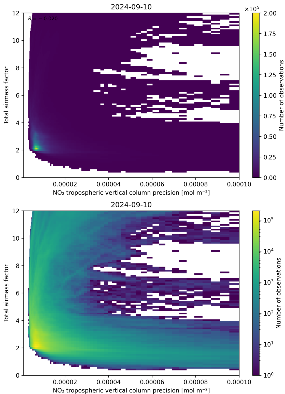
Figure 132: Scatter density plot of “NO 2 tropospheric vertical column precision” against “Total air mass factor” for 2024-09-09 to 2024-09-11.
