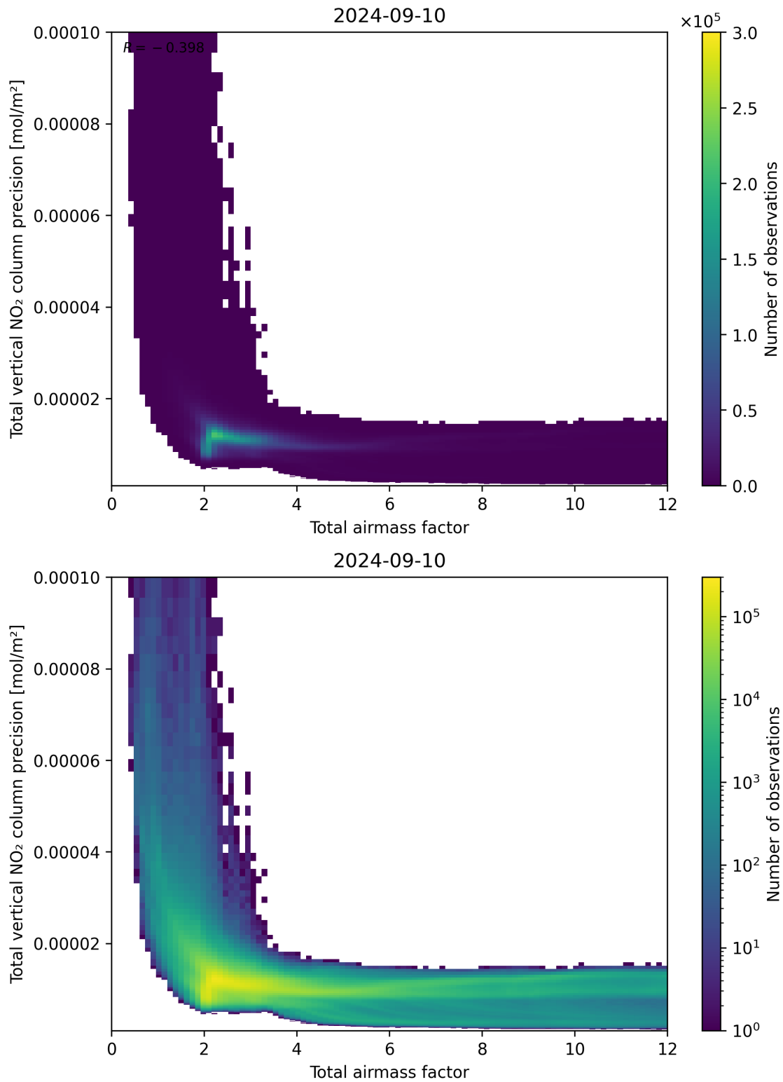
Figure 68: Scatter density plot of “Total airmass factor” against “Total vertical NO 2 column precision” for 2024-09-09 to 2024-09-11.
