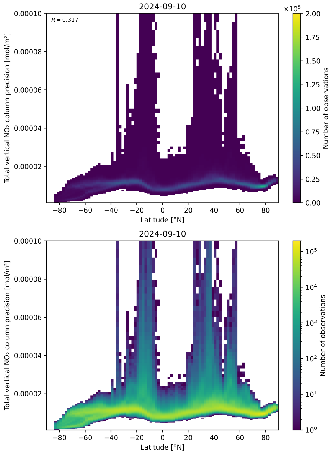
Figure 91: Scatter density plot of “Latitude” against “Total vertical NO 2 column precision” for 2024-09-09 to 2024-09-11.
