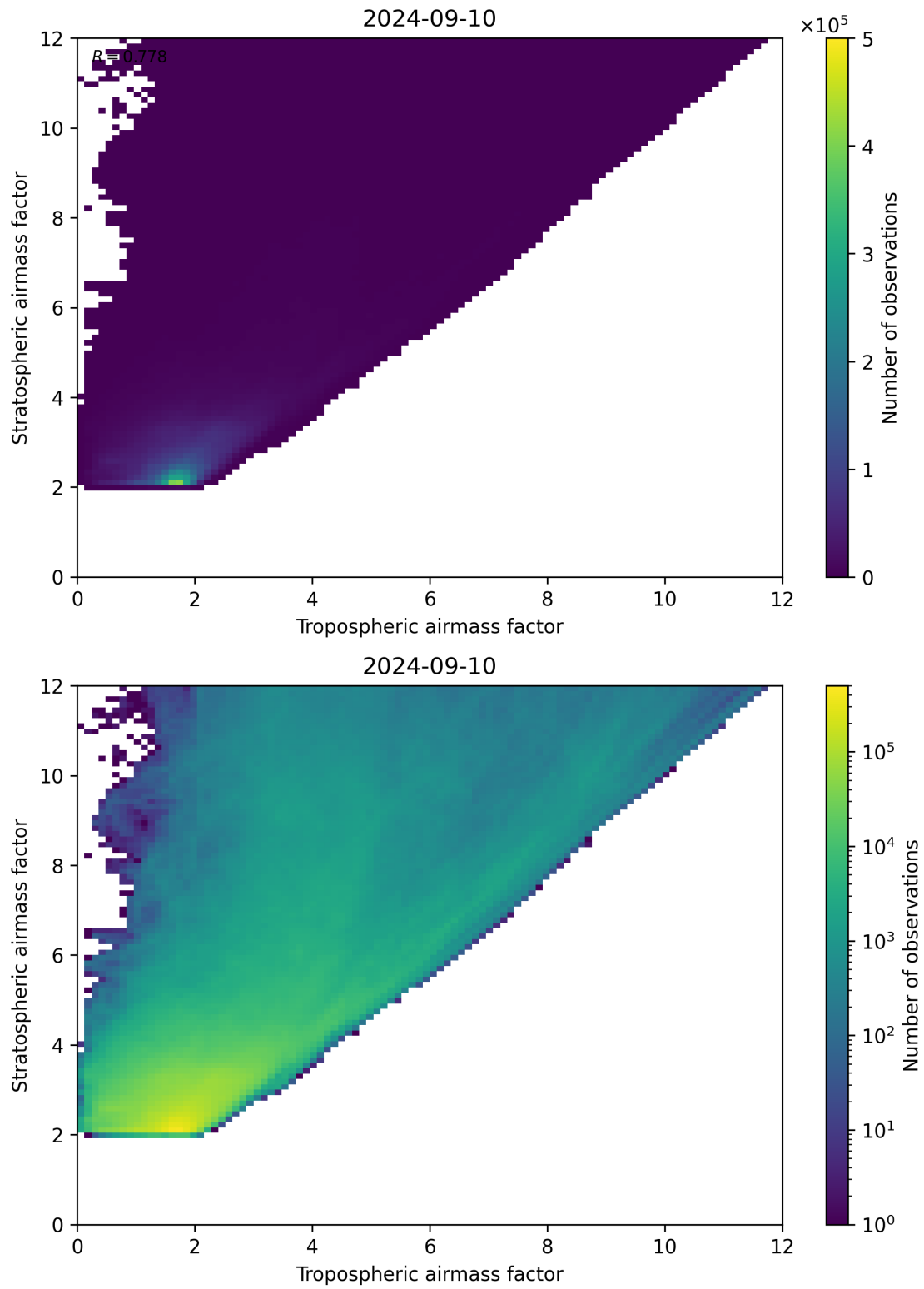
Figure 71: Scatter density plot of “Tropospheric airmass factor” against “Stratospheric airmass factor” for 2024-09-09 to 2024-09-11.
