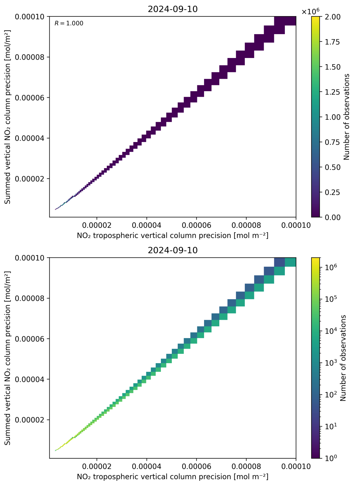
Figure 137: Scatter density plot of “NO 2 tropospheric vertical column precision” against “Summed vertical NO 2 column precision” for 2024-09-09 to 2024-09-11.
