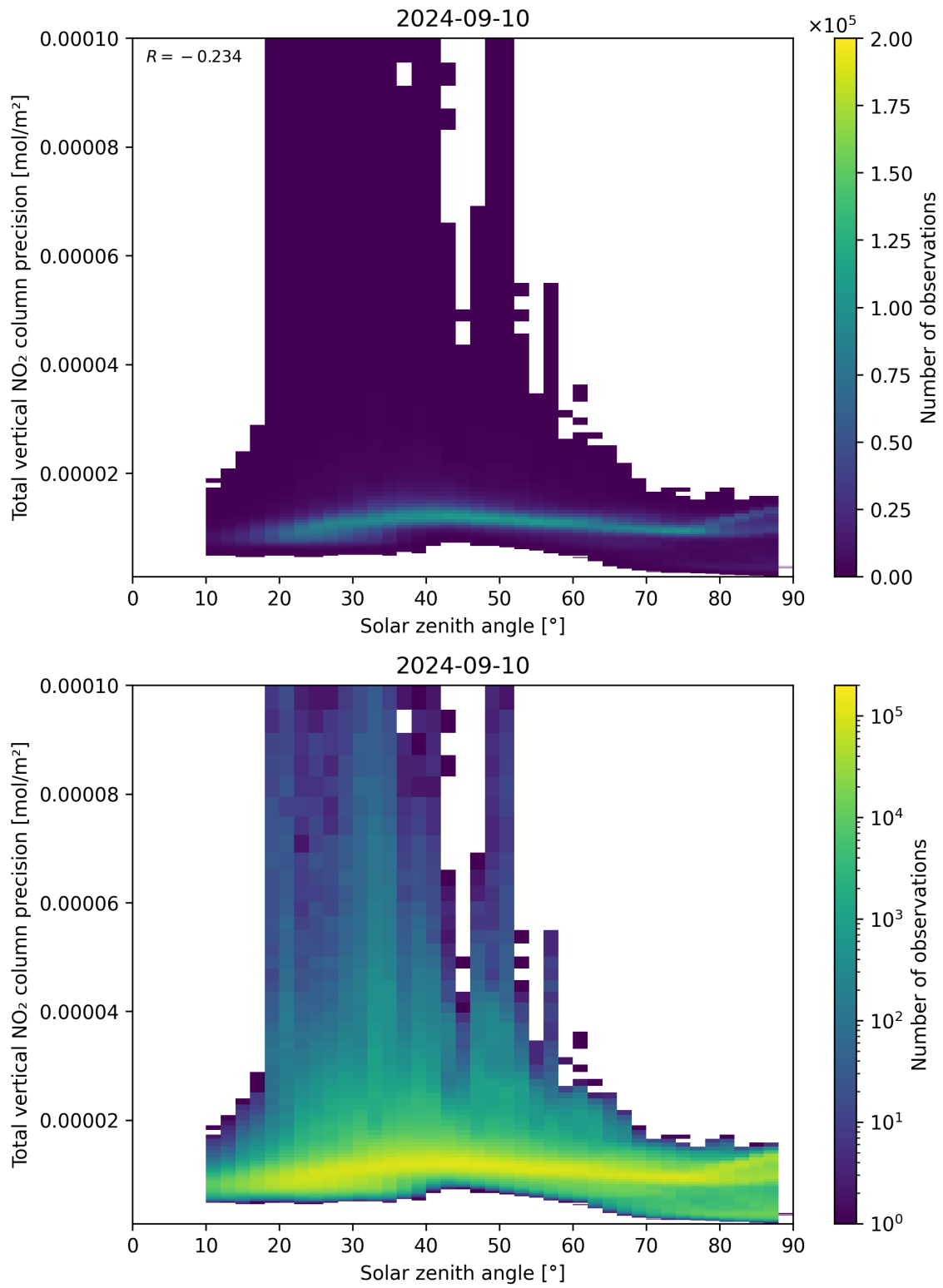
Figure 154: Scatter density plot of “Solar zenith angle” against “Total vertical NO 2 column precision” for 2024-09-09 to 2024-09-11.
