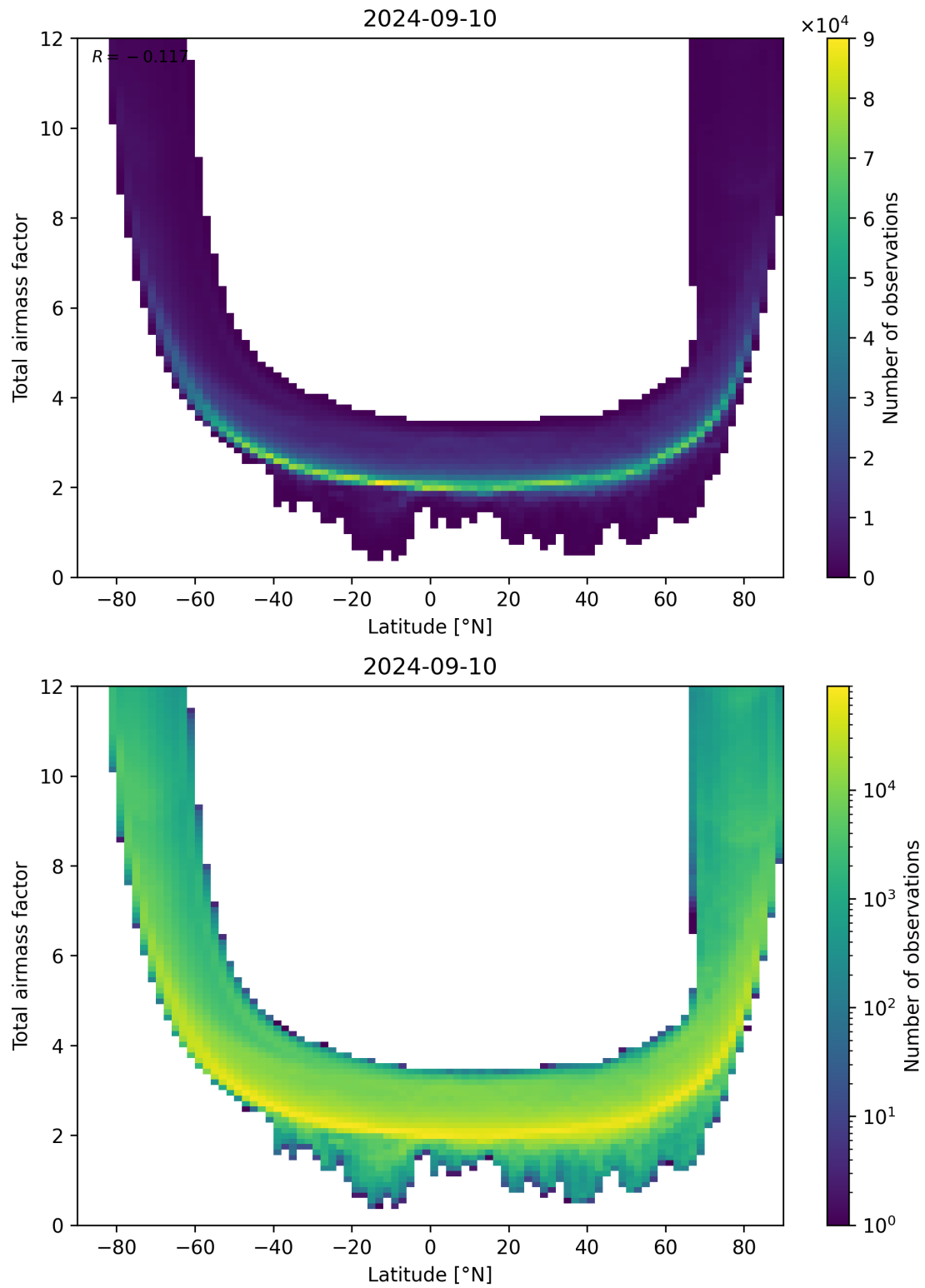
Figure 84: Scatter density plot of “Latitude” against “Total airmass factor” for 2024-09-09 to 2024-09-11.
