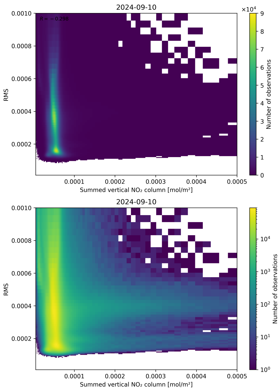
Figure 109: Scatter density plot of “Summed vertical NO 2 column” against “RMS” for 2024-09-09 to 2024-09-11.
