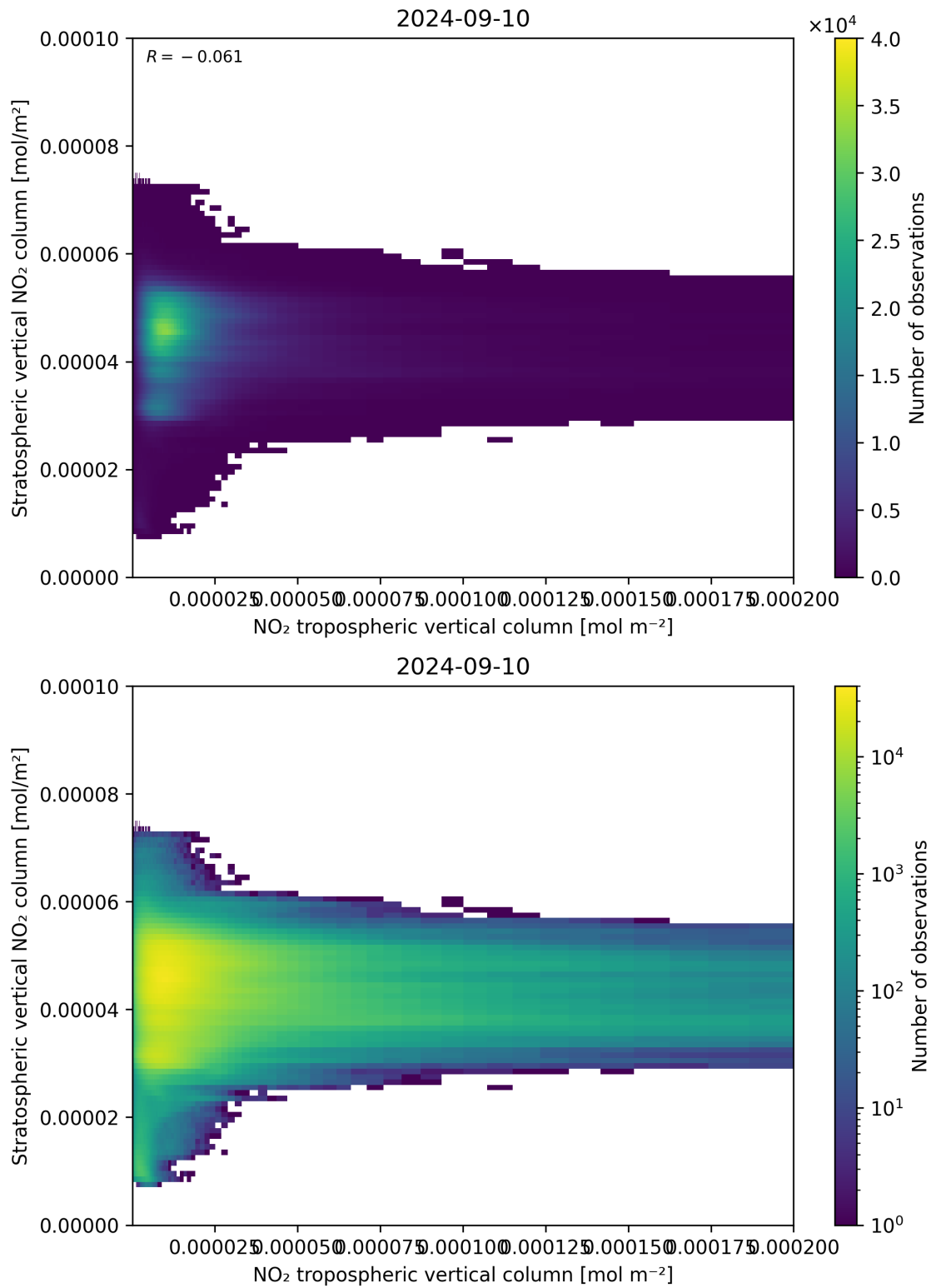
Figure 125: Scatter density plot of “NO 2 tropospheric vertical column” against “Stratospheric vertical NO 2 column” for 2024-09-09 to 2024-09-11.
