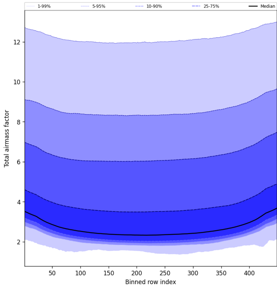
Figure 49: Along track statistics of “Total airmass factor” for 2024-09-09 to 2024-09-11
