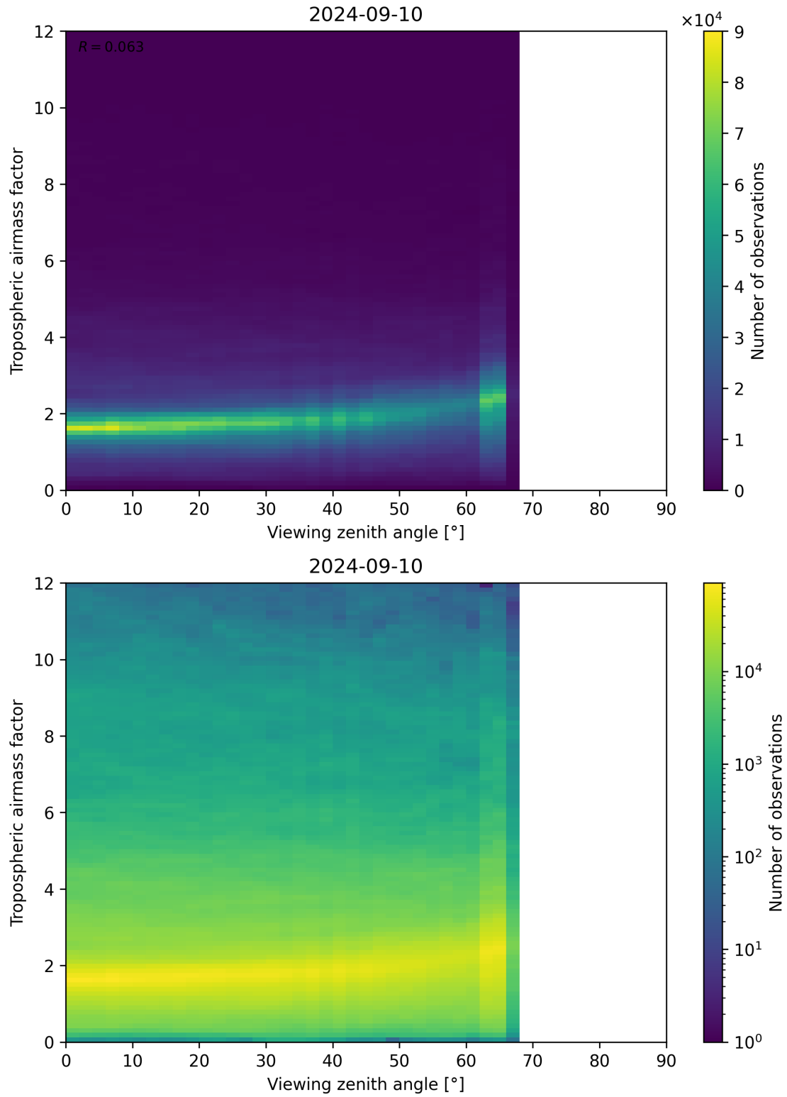
Figure 161: Scatter density plot of “Viewing zenith angle” against “Tropospheric airmass factor” for 2024-09-09 to 2024-09-11.
