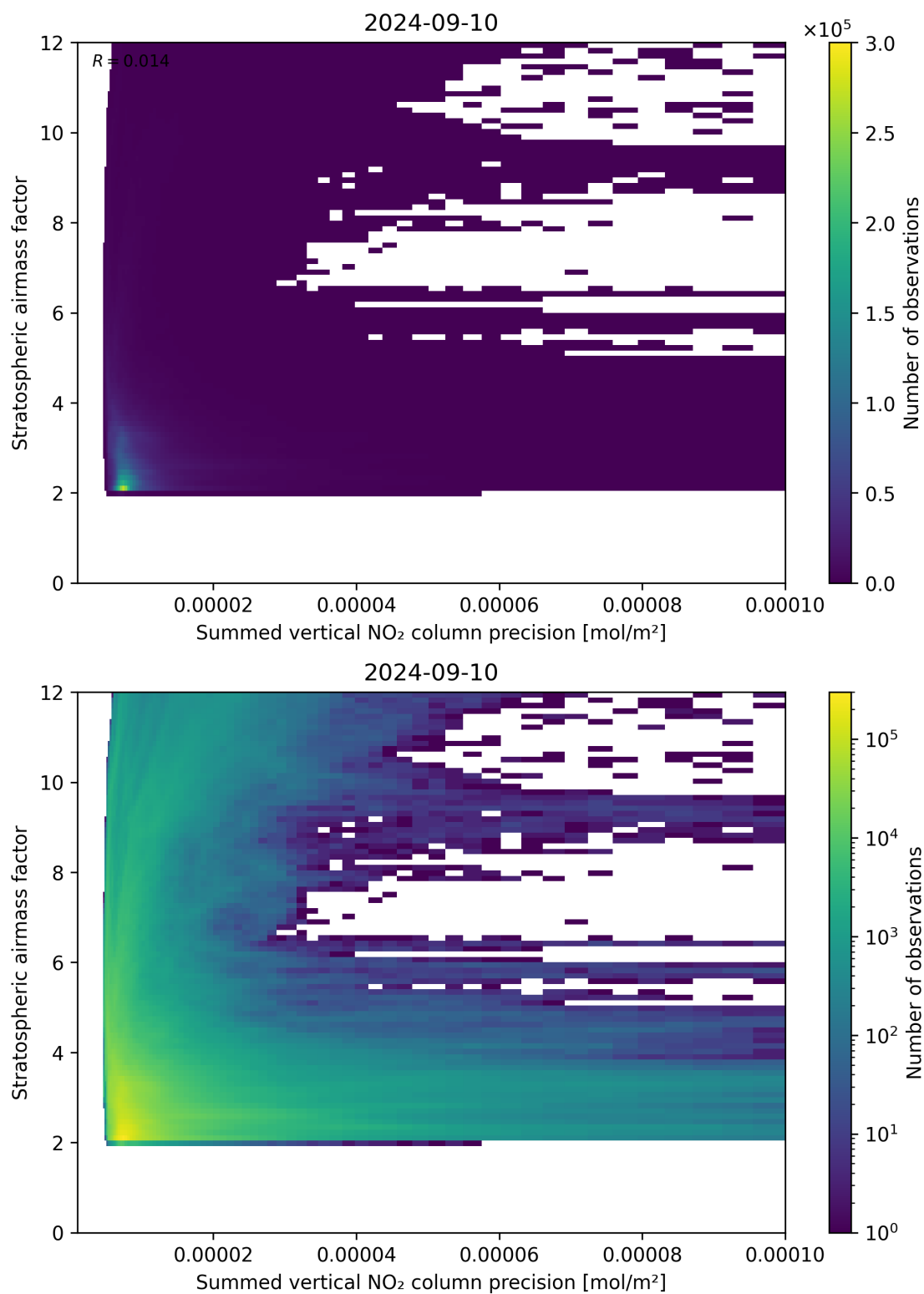
Figure 106: Scatter density plot of “Summed vertical NO 2 column precision” against “Stratospheric airmass factor” for 2024-09-09 to 2024-09-11.
