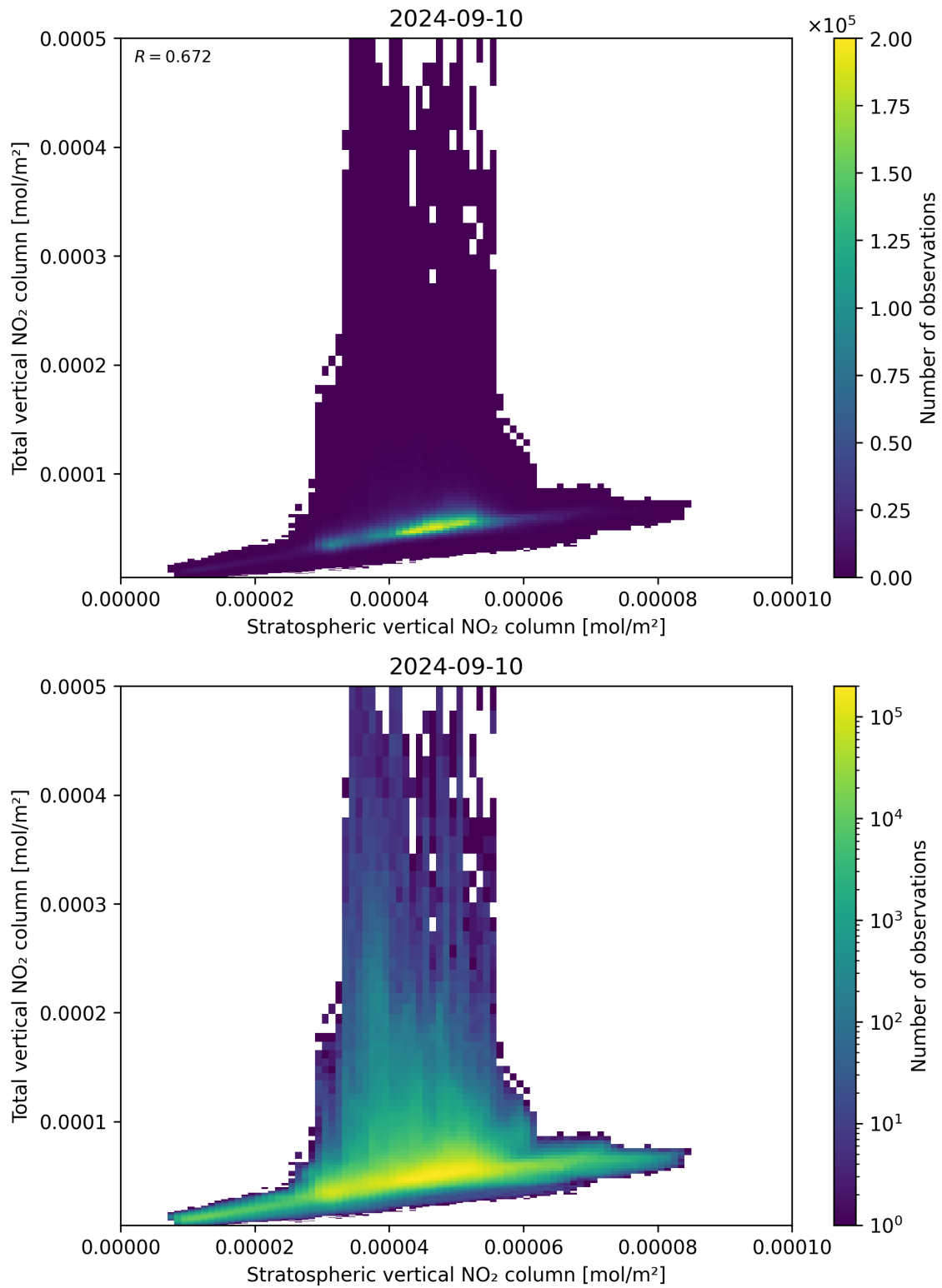
Figure 100: Scatter density plot of “Stratospheric vertical NO 2 column” against “Total vertical NO 2 column” for 2024-09-09 to 2024-09-11.
