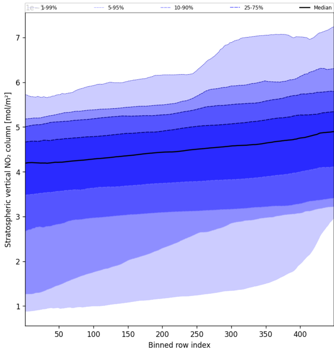
Figure 53: Along track statistics of “Stratospheric vertical NO 2 column” for 2024-09-09 to 2024-09-11
