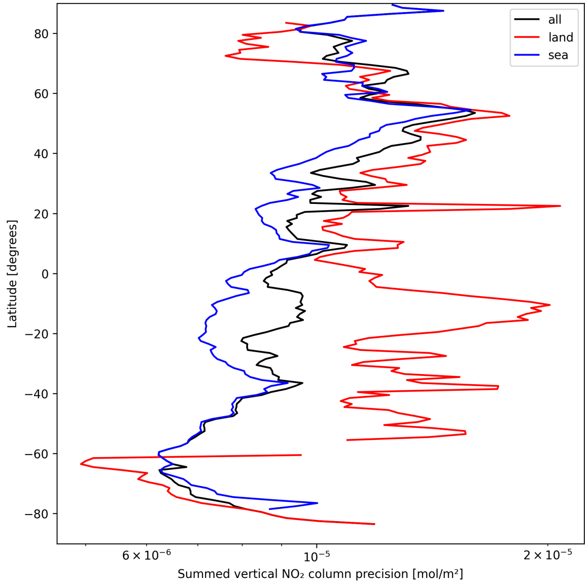
Figure 24: Zonal average of “Summed vertical NO 2 column precision” for 2024-09-09 to 2024-09-11.
