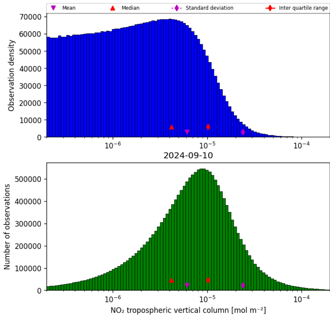
Figure 29: Histogram of “NO 2 tropospheric vertical column” for 2024-09-09 to 2024-09-11
