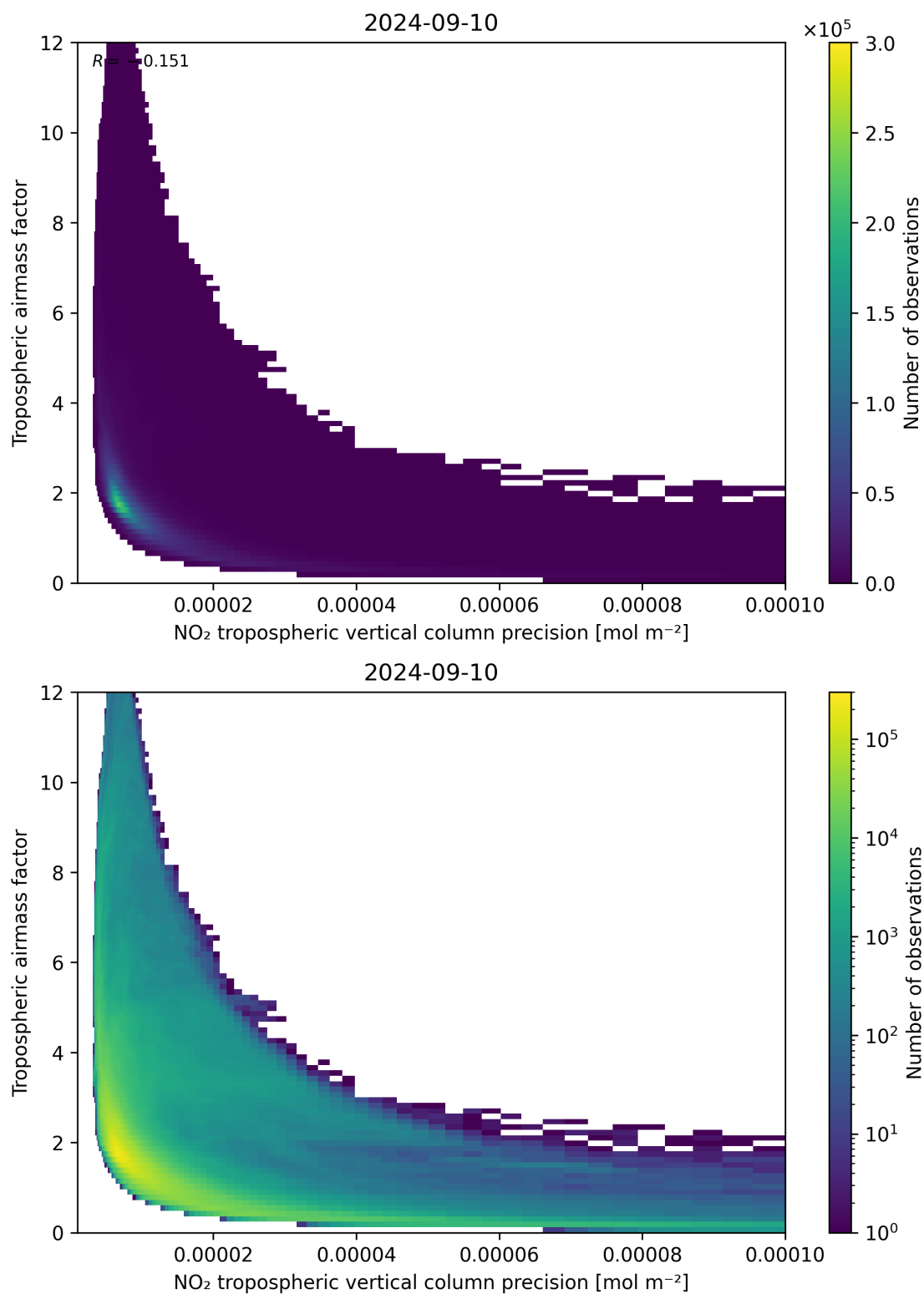
Figure 133: Scatter density plot of “NO 2 tropospheric vertical column precision” against “Tropospheric airmass factor” for 2024-09-09 to 2024-09-11.
