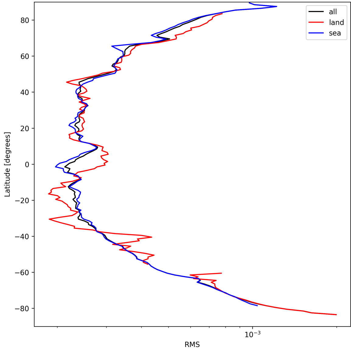
Figure 26: Zonal average of “RMS” for 2024-09-09 to 2024-09-11.
