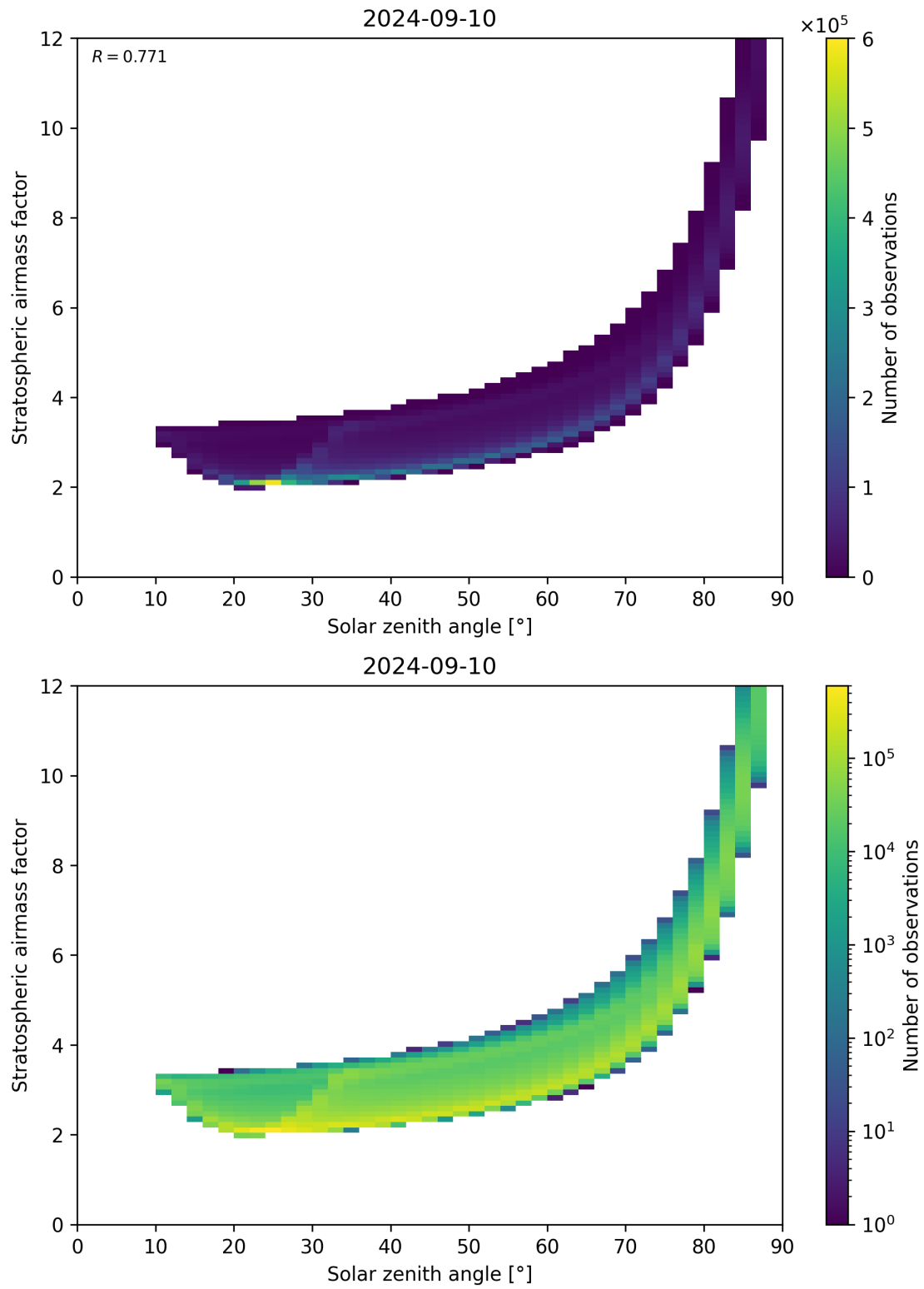
Figure 145: Scatter density plot of “Solar zenith angle” against “Stratospheric airmass factor” for 2024-09-09 to 2024-09-11.
