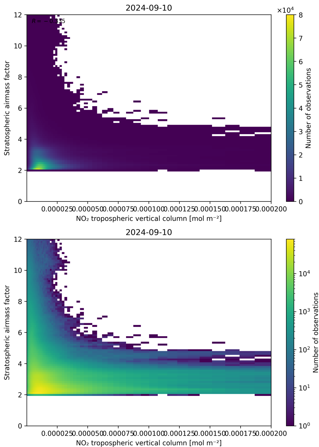
Figure 121: Scatter density plot of “NO 2 tropospheric vertical column” against “Stratospheric air mass factor” for 2024-09-09 to 2024-09-11.
