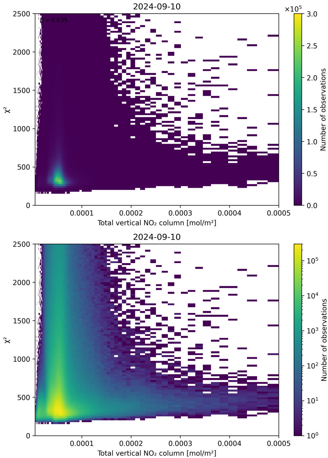
Figure 111: Scatter density plot of “Total vertical NO 2 column” against “ \chi^2 ” for 2024-09-09 to 2024-09-11.
