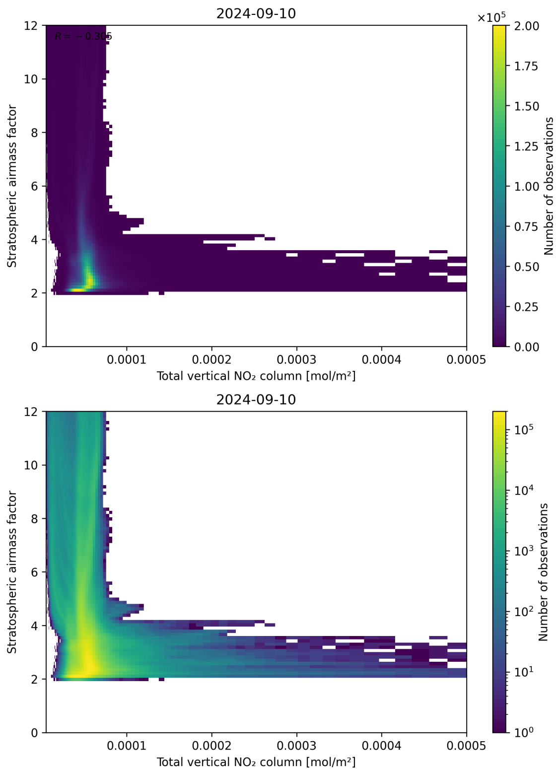
Figure 110: Scatter density plot of “Total vertical NO 2 column” against “Stratospheric airmass factor” for 2024-09-09 to 2024-09-11.
