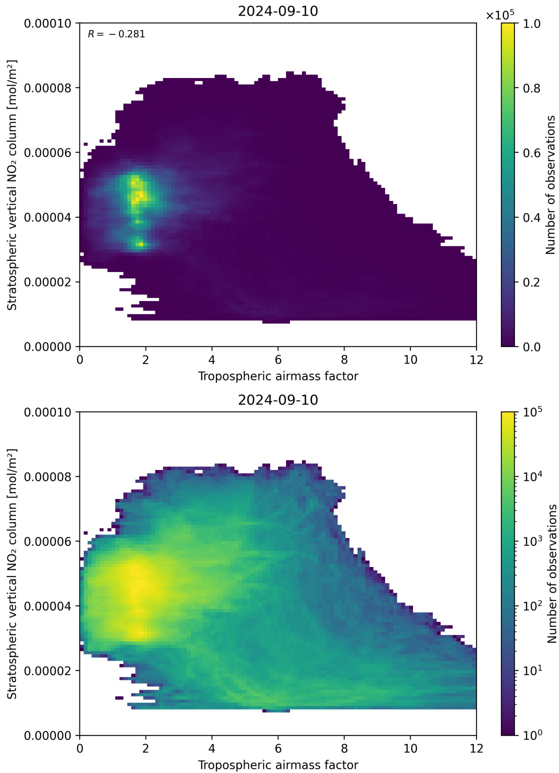
Figure 74: Scatter density plot of “Tropospheric air mass factor” against “Stratospheric vertical NO 2 column” for 2024-09-09 to 2024-09-11.
