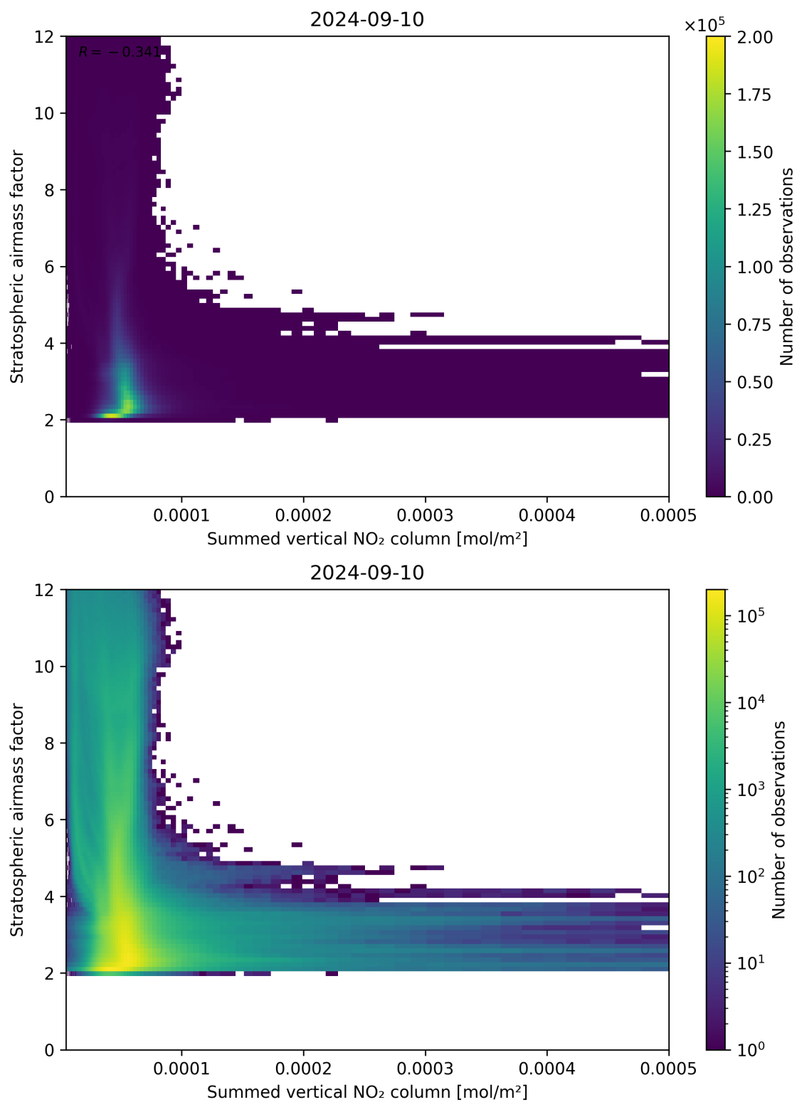
Figure 103: Scatter density plot of “Summed vertical NO 2 column” against “Stratospheric airmass factor” for 2024-09-09 to 2024-09-11.
