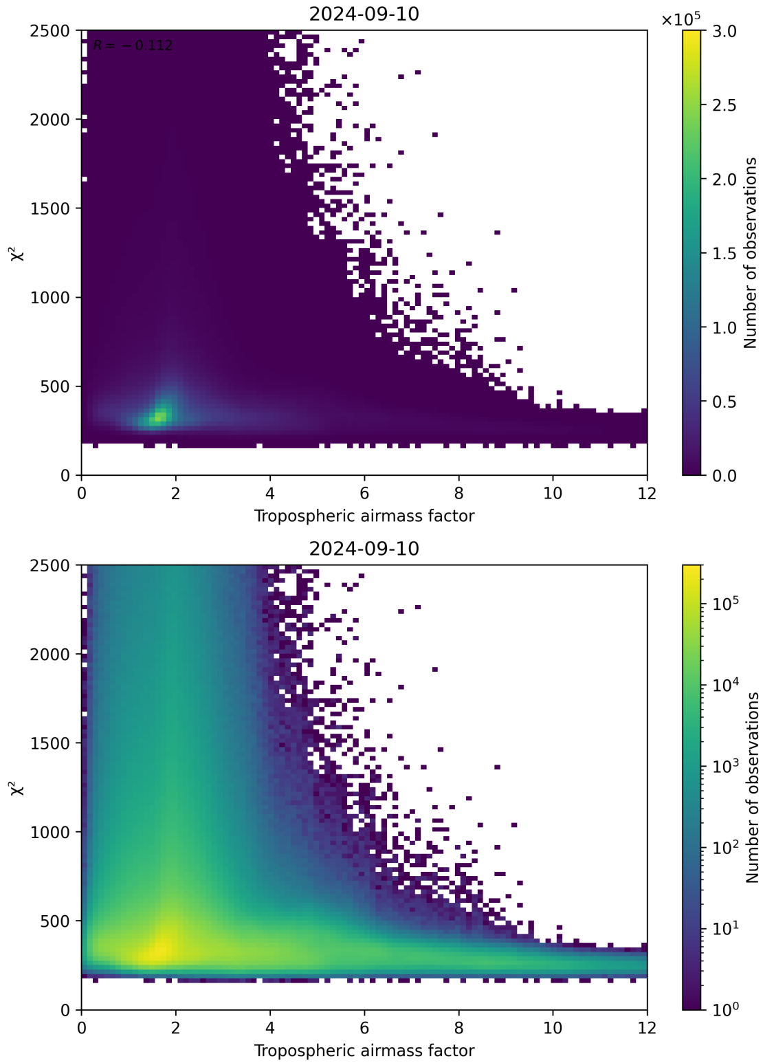
Figure 73: Scatter density plot of “Tropospheric airmass factor” against “ \chi^2 ” for 2024-09-09 to 2024-09-11.
