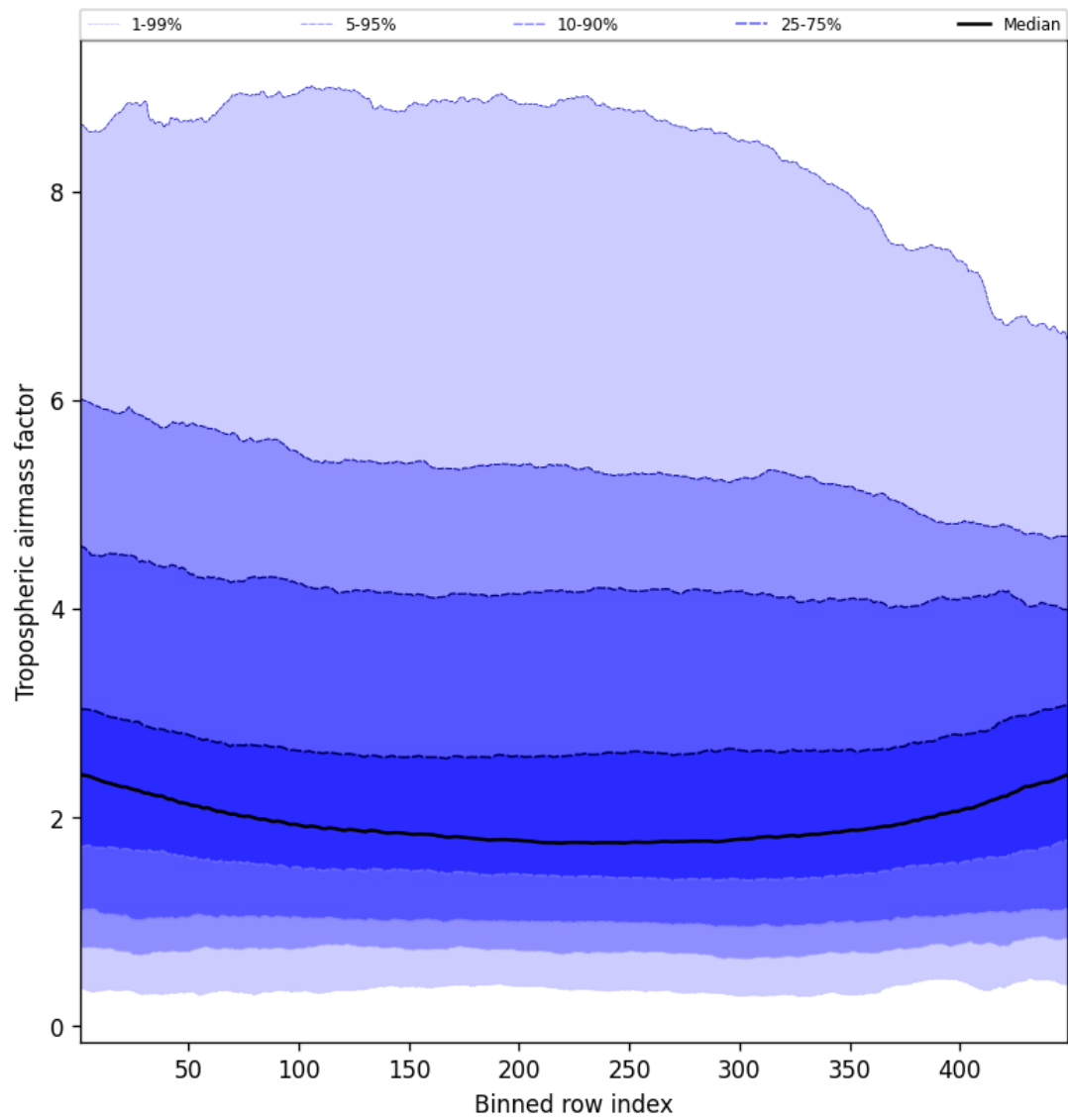
Figure 48: Along track statistics of “Tropospheric air mass factor” for 2024-09-09 to 2024-09-11
