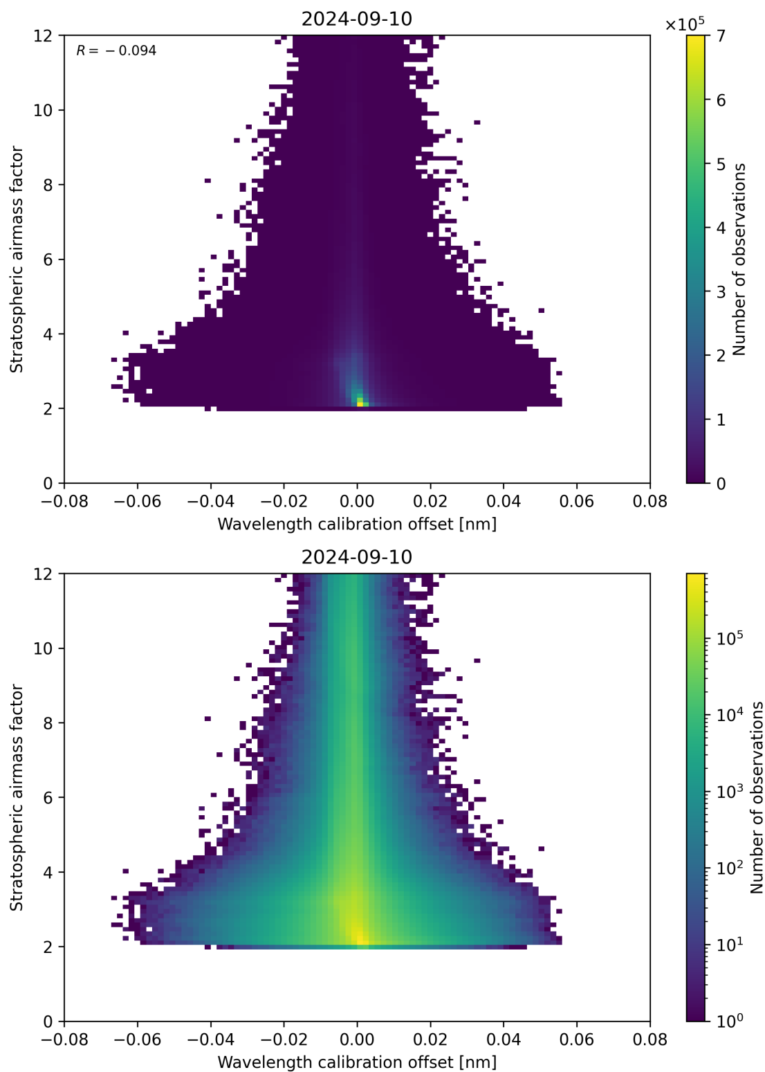
Figure 174: Scatter density plot of “Wavelength calibration offset” against “Stratospheric airmass factor” for 2024-09-09 to 2024-09-11.
