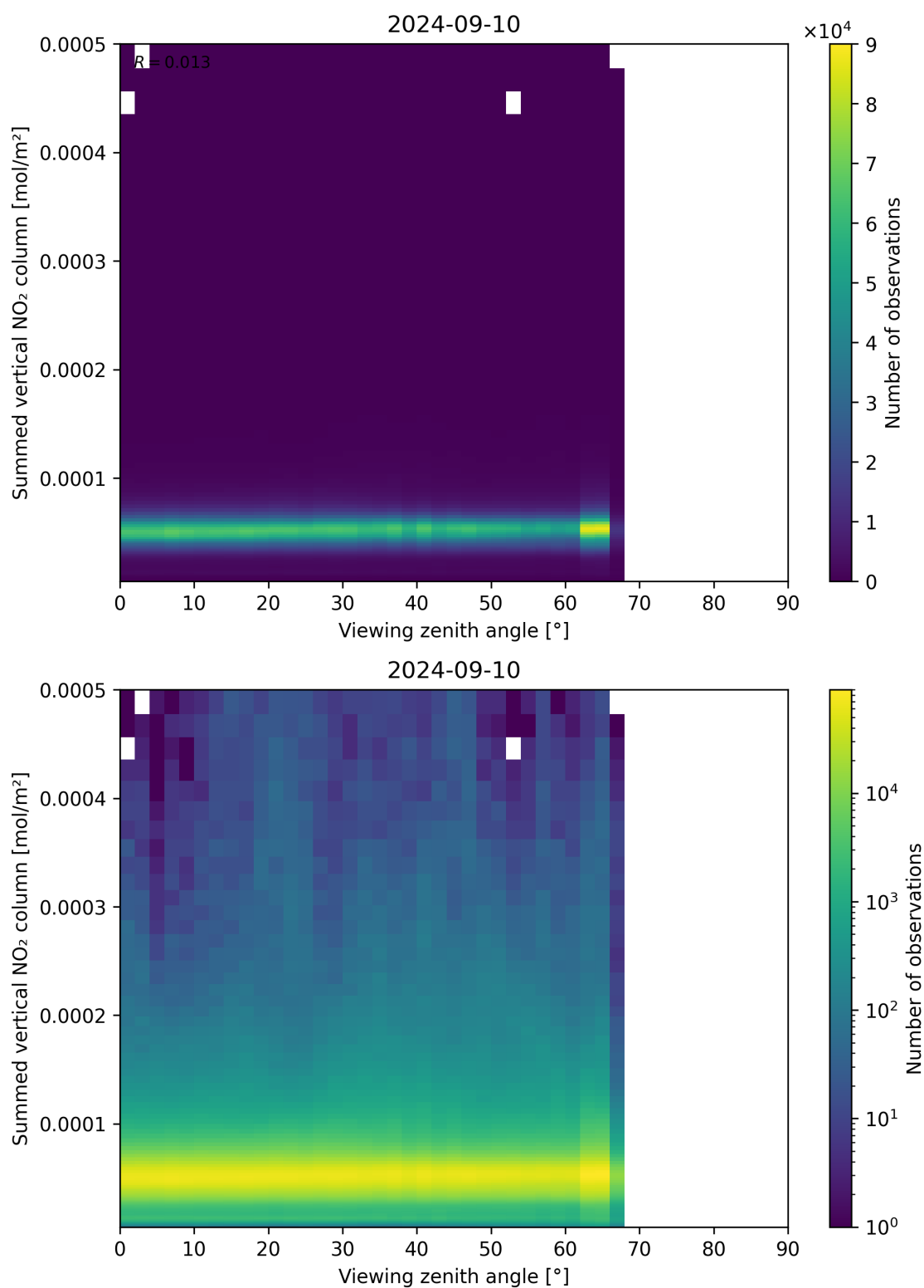
Figure 165: Scatter density plot of “Viewing zenith angle” against “Summed vertical NO 2 column” for 2024-09-09 to 2024-09-11.
