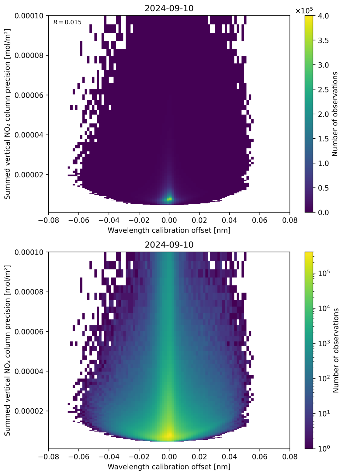
Figure 178: Scatter density plot of “Wavelength calibration offset” against “Summed vertical NO 2 column precision” for 2024-09-09 to 2024-09-11.
