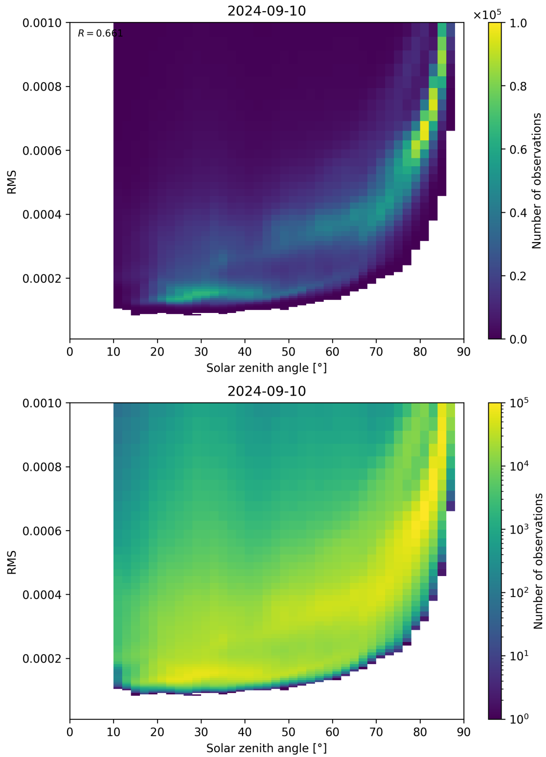
Figure 157: Scatter density plot of “Solar zenith angle” against “RMS” for 2024-09-09 to 2024-09-11.
