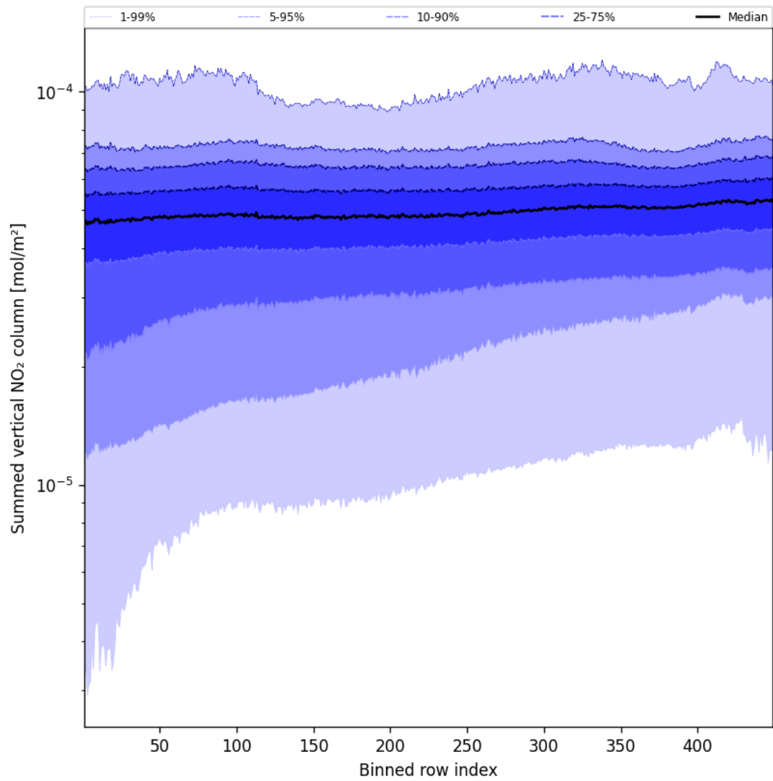
Figure 57: Along track statistics of “Summed vertical NO 2 column” for 2024-09-09 to 2024-09-11
