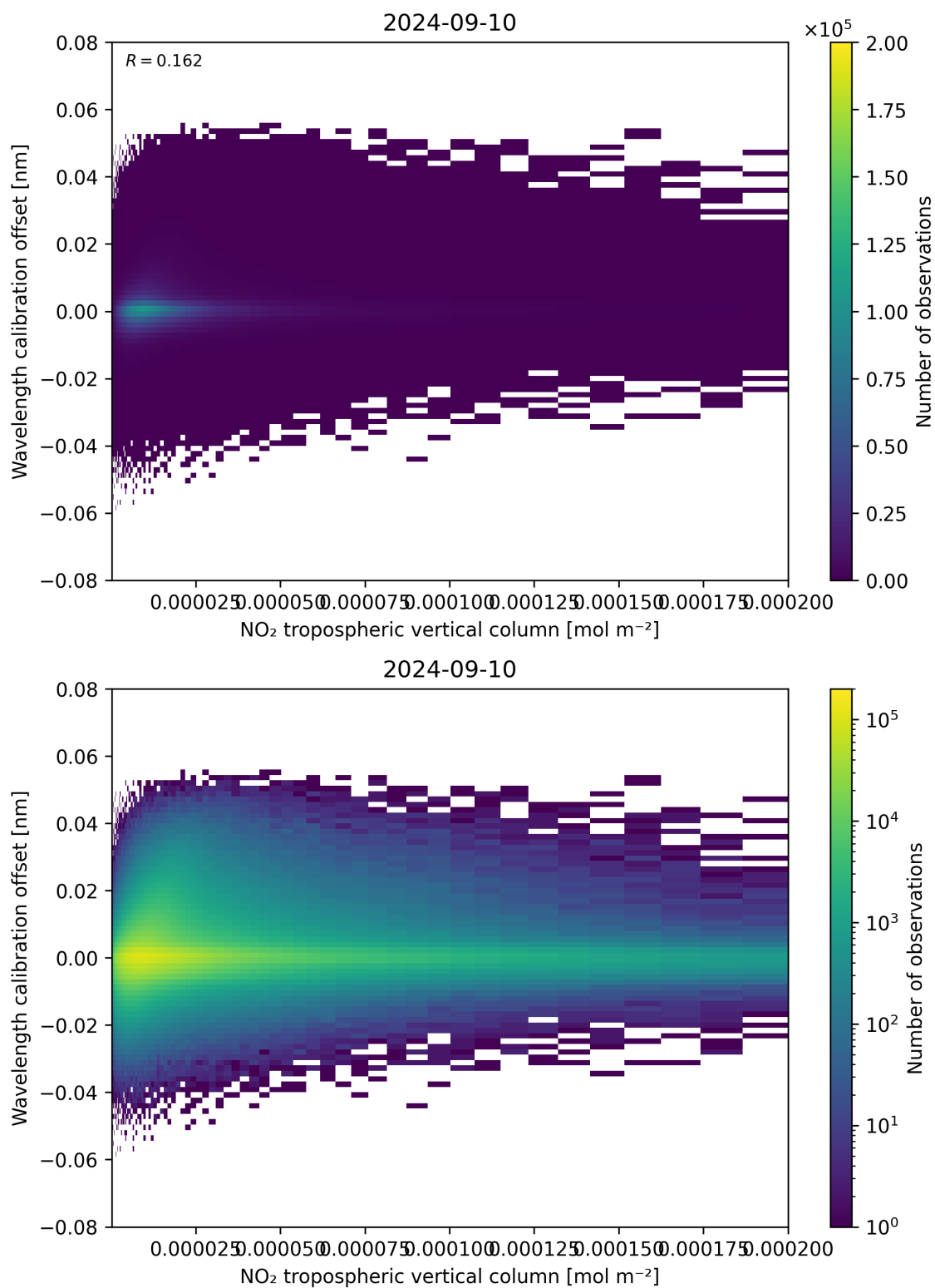
Figure 143: Scatter density plot of “NO 2 tropospheric vertical column” against “Wavelength calibration offset” for 2024-09-09 to 2024-09-11.
