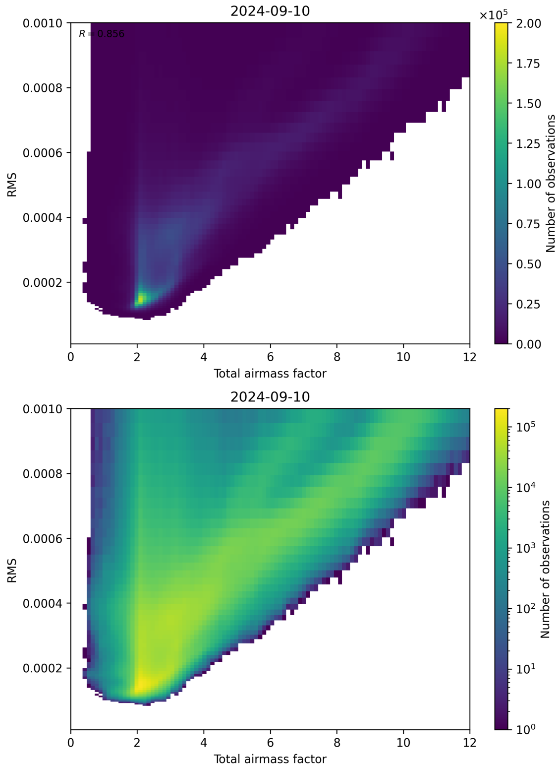
Figure 69: Scatter density plot of “Total airmass factor” against “RMS” for 2024-09-09 to 2024-09-11.
