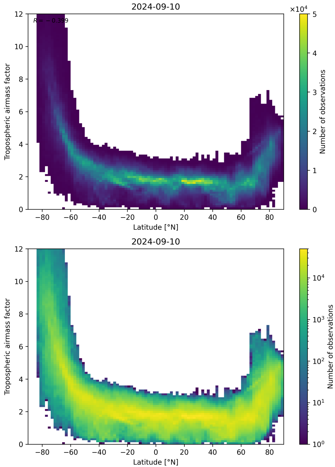
Figure 85: Scatter density plot of “Latitude” against “Tropospheric air mass factor” for 2024-09-09 to 2024-09-11.
