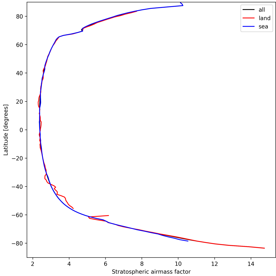
Figure 27: Zonal average of “Stratospheric airmass factor” for 2024-09-09 to 2024-09-11.
