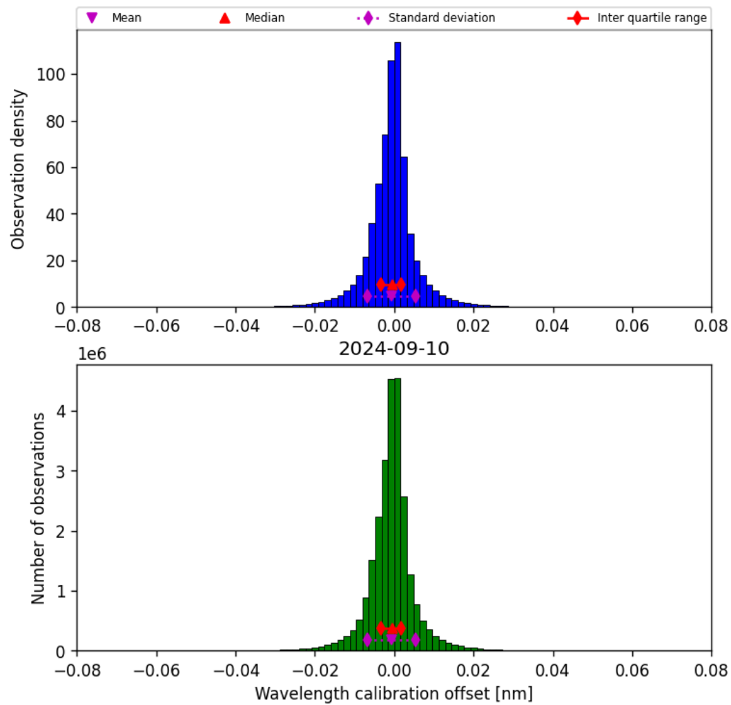
Figure 35: Histogram of “Wavelength calibration offset” for 2024-09-09 to 2024-09-11
