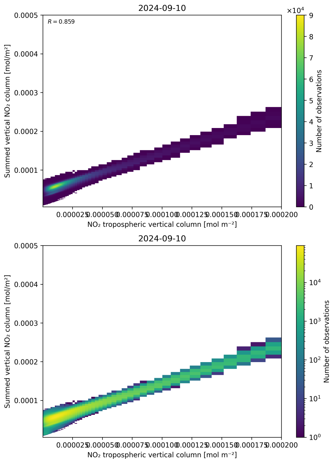
Figure 126: Scatter density plot of “NO 2 tropospheric vertical column” against “Summed vertical NO 2 column” for 2024-09-09 to 2024-09-11.
