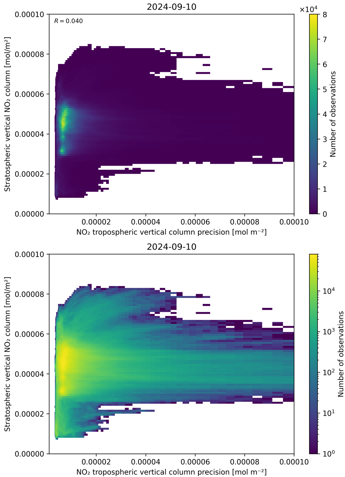
Figure 135: Scatter density plot of “NO 2 tropospheric vertical column precision” against “Stratospheric vertical NO 2 column” for 2024-09-09 to 2024-09-11.
