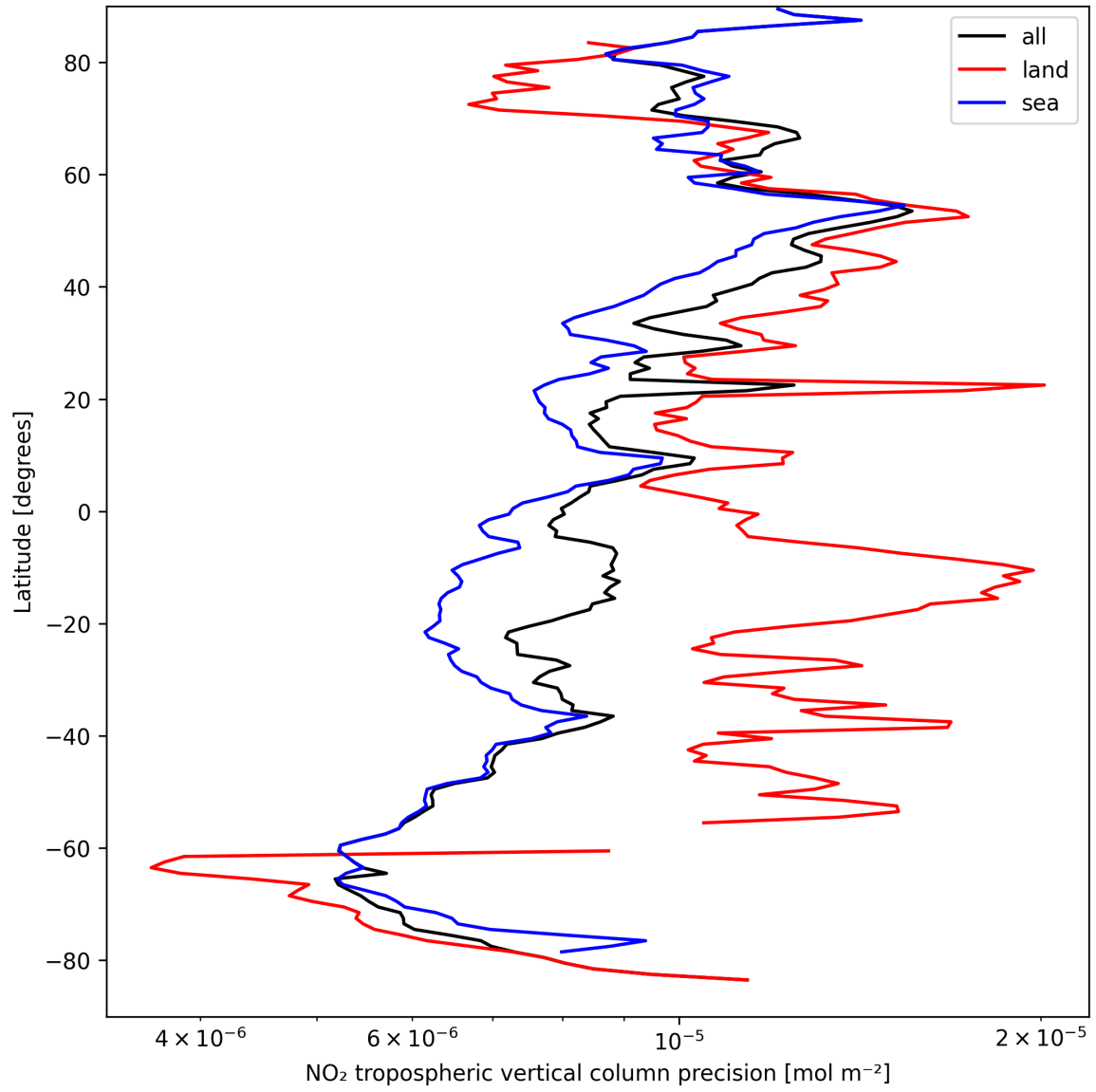
Figure 13: Zonal average of “NO 2 tropospheric vertical column precision” for 2024-09-09 to 2024-09-11.
