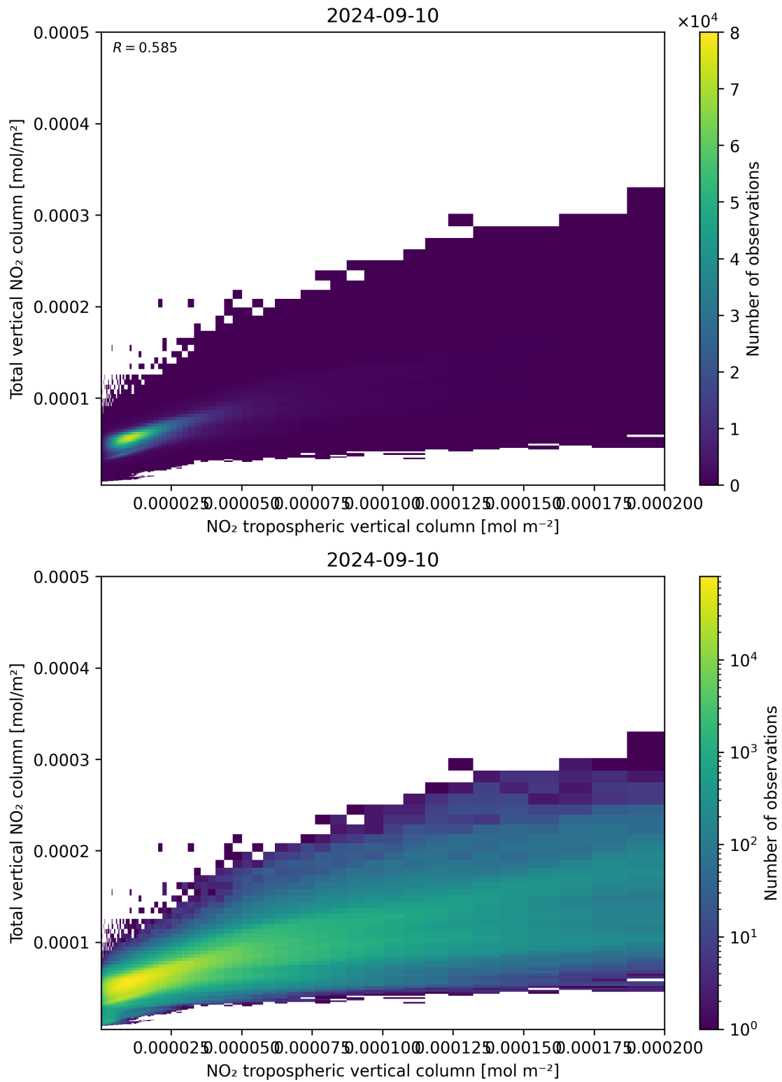
Figure 128: Scatter density plot of “NO 2 tropospheric vertical column” against “Total vertical NO 2 column” for 2024-09-09 to 2024-09-11.
