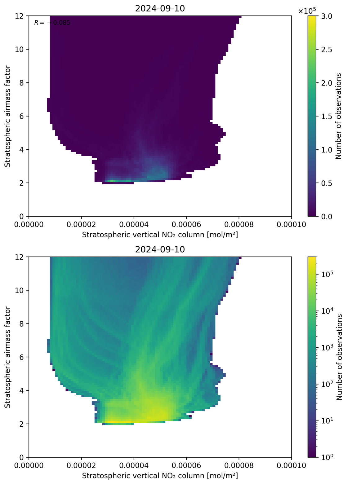
Figure 96: Scatter density plot of “Stratospheric vertical NO 2 column” against “Stratospheric airmass factor” for 2024-09-09 to 2024-09-11.
