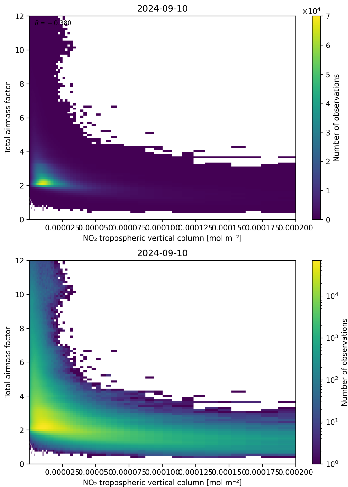
Figure 122: Scatter density plot of “NO 2 tropospheric vertical column” against “Total air mass factor” for 2024-09-09 to 2024-09-11.
