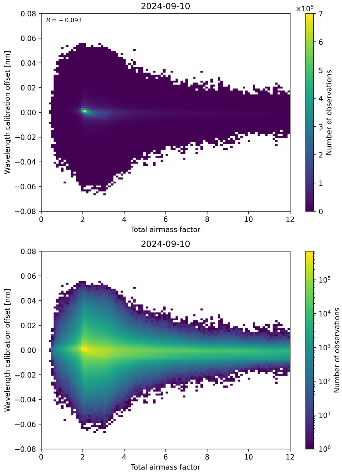
Figure 70: Scatter density plot of “Total airmass factor” against “Wavelength calibration offset” for 2024-09-09 to 2024-09-11.
