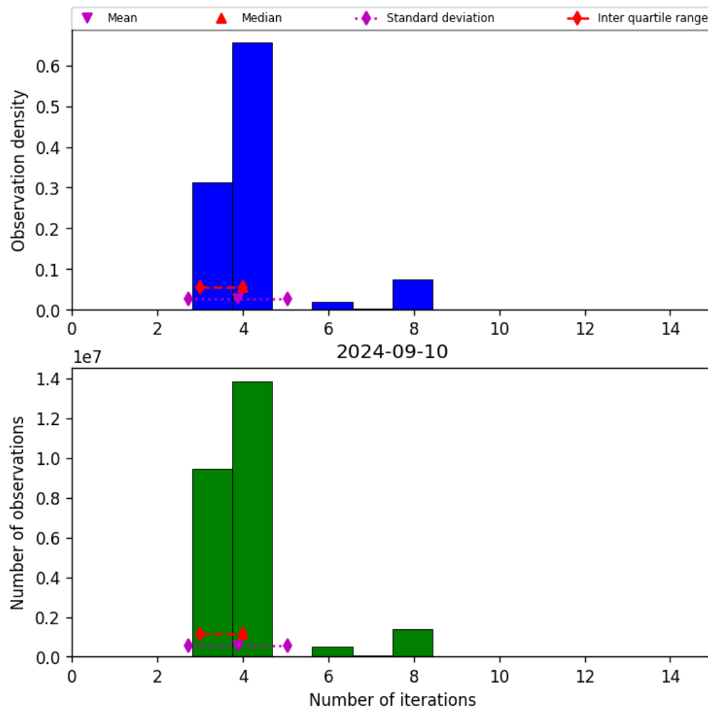
Figure 34: Histogram of “Number of iterations” for 2024-09-09 to 2024-09-11
