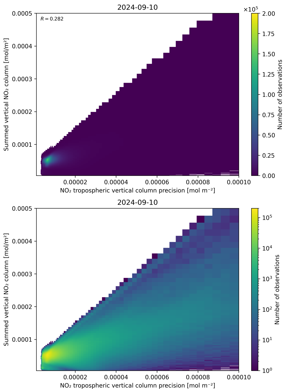
Figure 136: Scatter density plot of “NO 2 tropospheric vertical column precision” against “Summed vertical NO 2 column” for 2024-09-09 to 2024-09-11.
