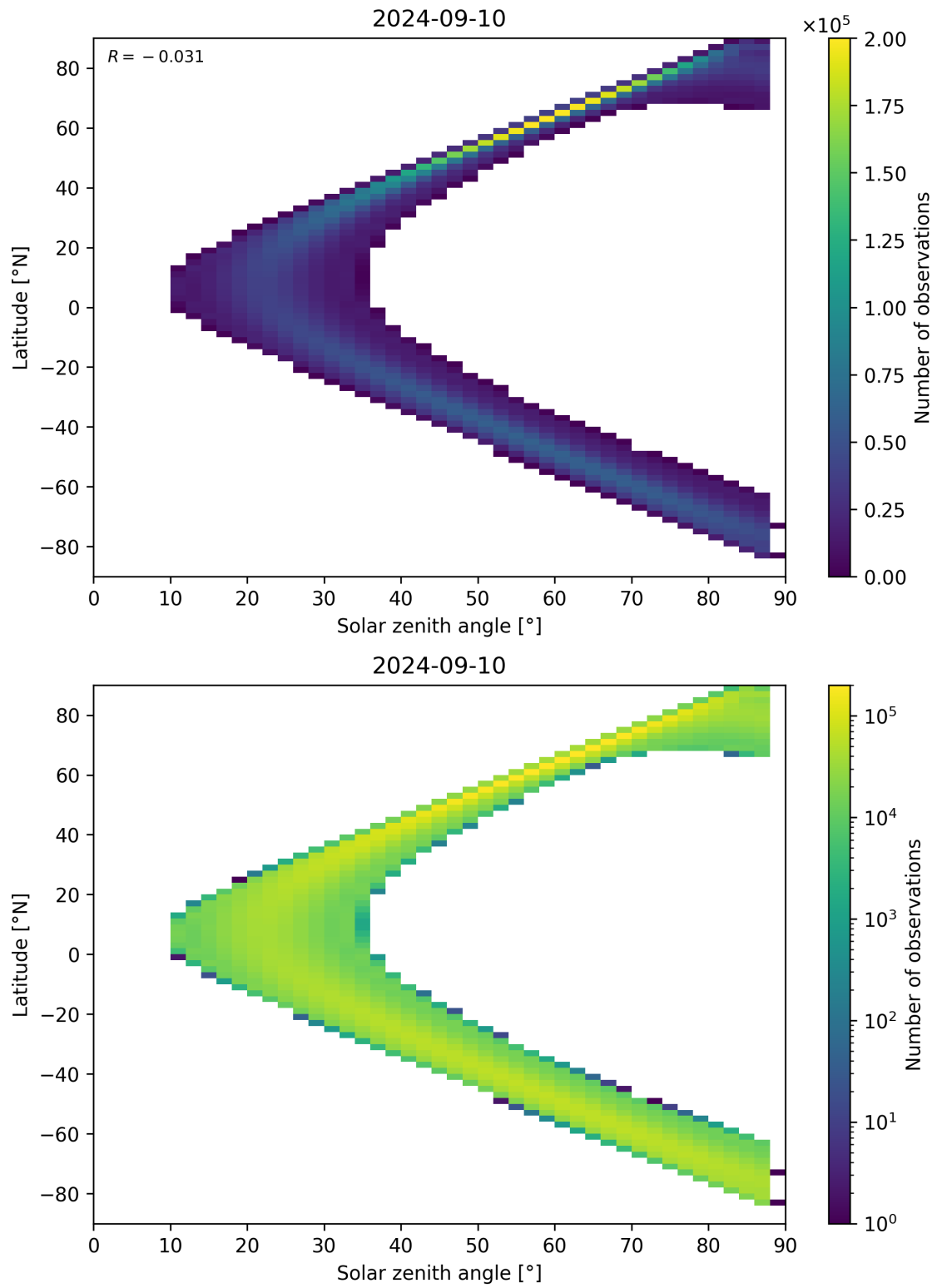
Figure 149: Scatter density plot of “Solar zenith angle” against “Latitude” for 2024-09-09 to 2024-09-11.
