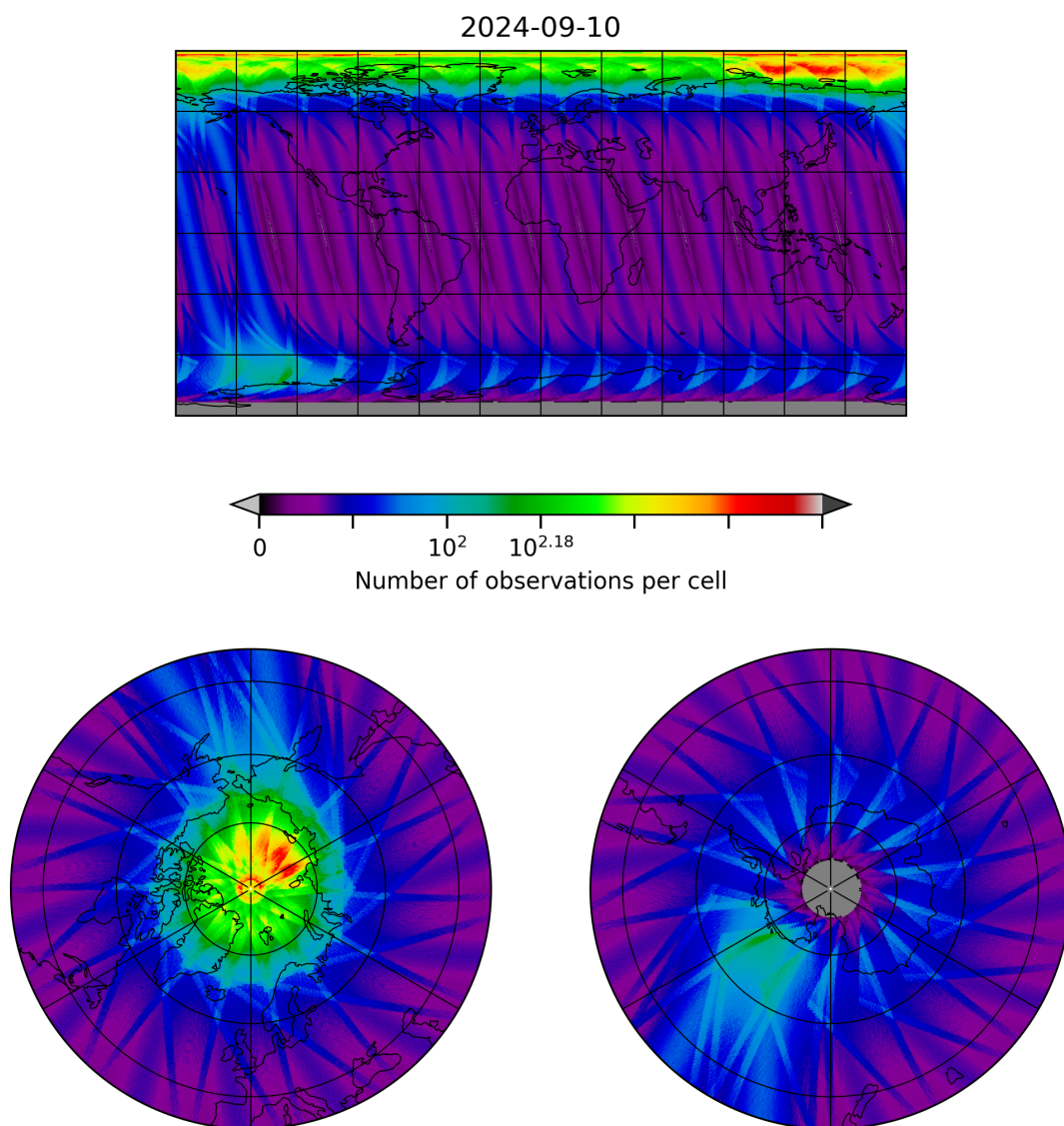
Figure 10: Map of the number of observations for 2024-09-09 to 2024-09-11
