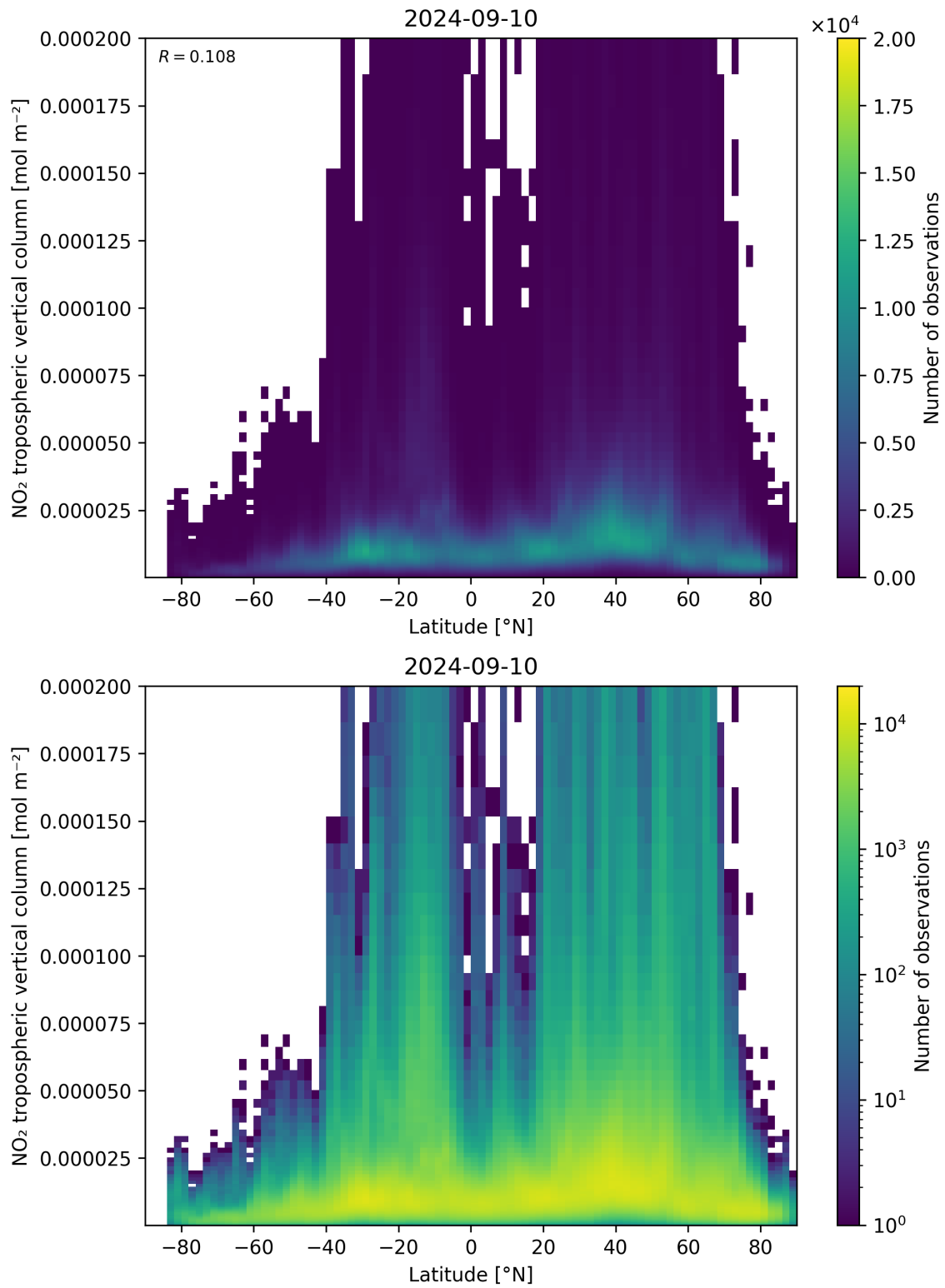
Figure 92: Scatter density plot of “Latitude” against “NO 2 tropospheric vertical column” for 2024-09-09 to 2024-09-11.
