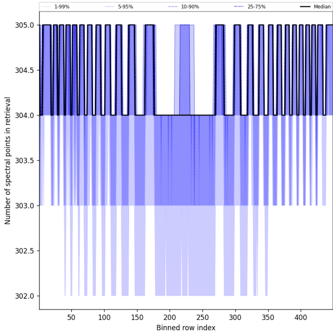
Figure 50: Along track statistics of “Number of spectral points in retrieval” for 2024-09-09 to 2024-09-11
