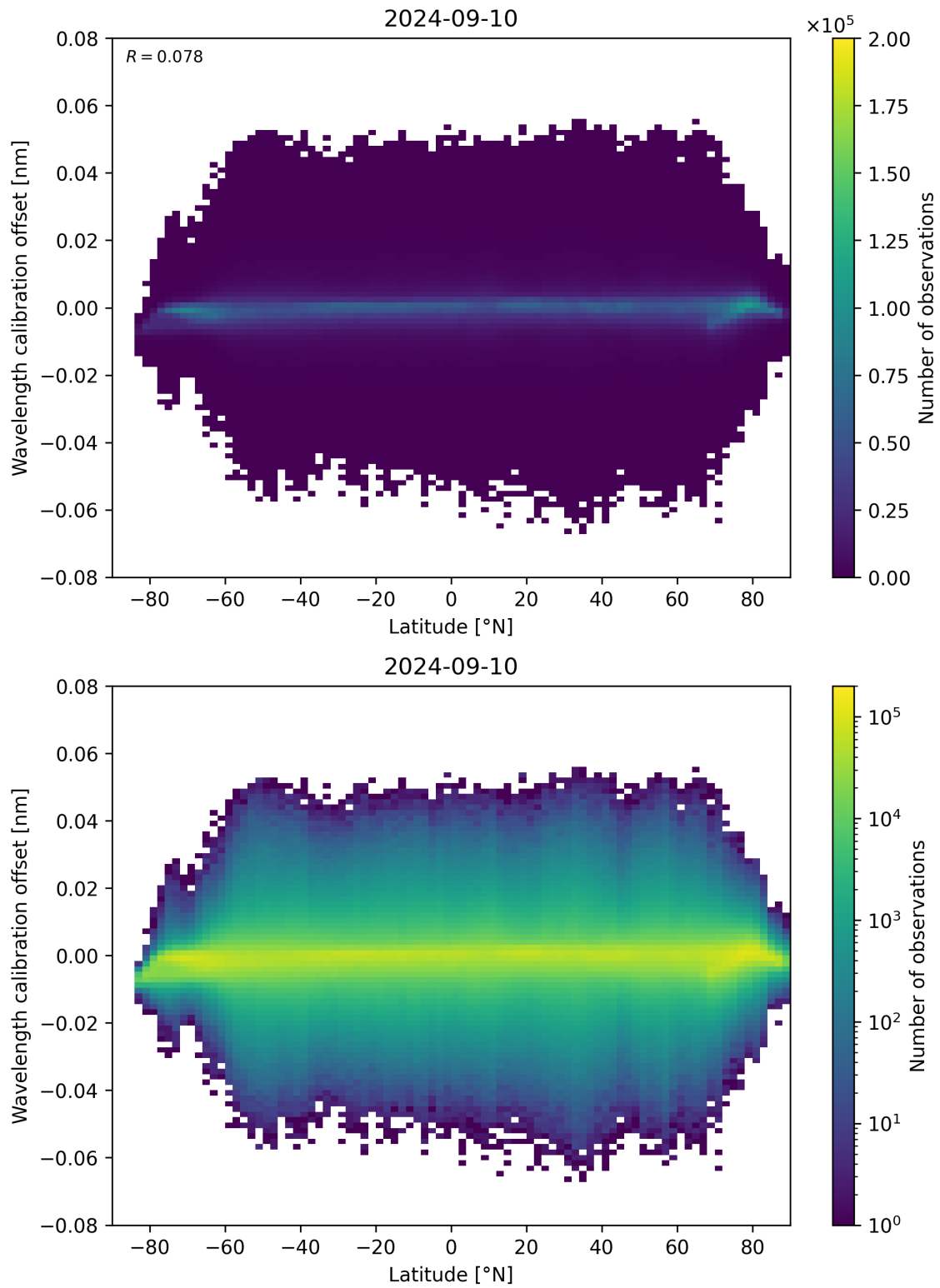
Figure 95: Scatter density plot of “Latitude” against “Wavelength calibration offset” for 2024-09-09 to 2024-09-11.
