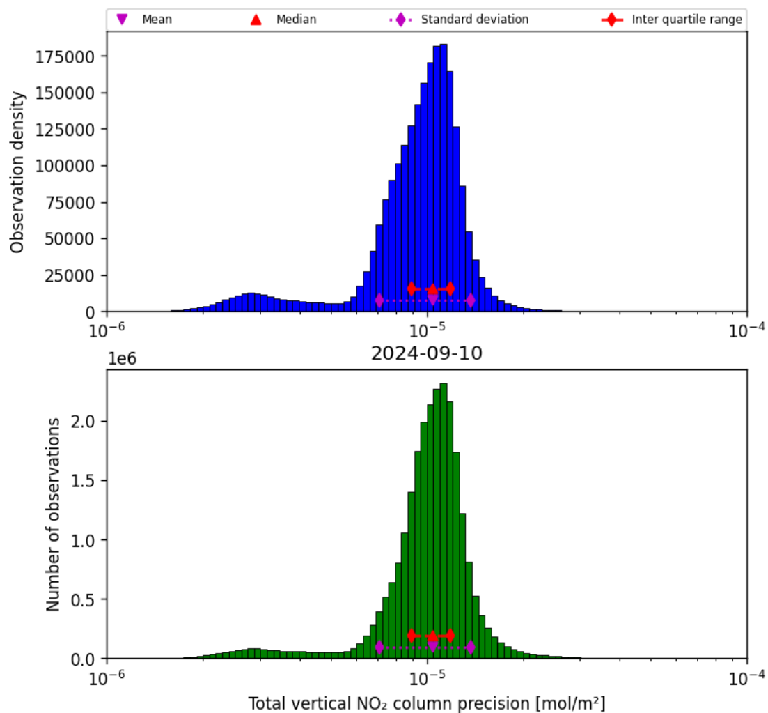
Figure 39: Histogram of “Total vertical NO 2 column precision” for 2024-09-09 to 2024-09-11
