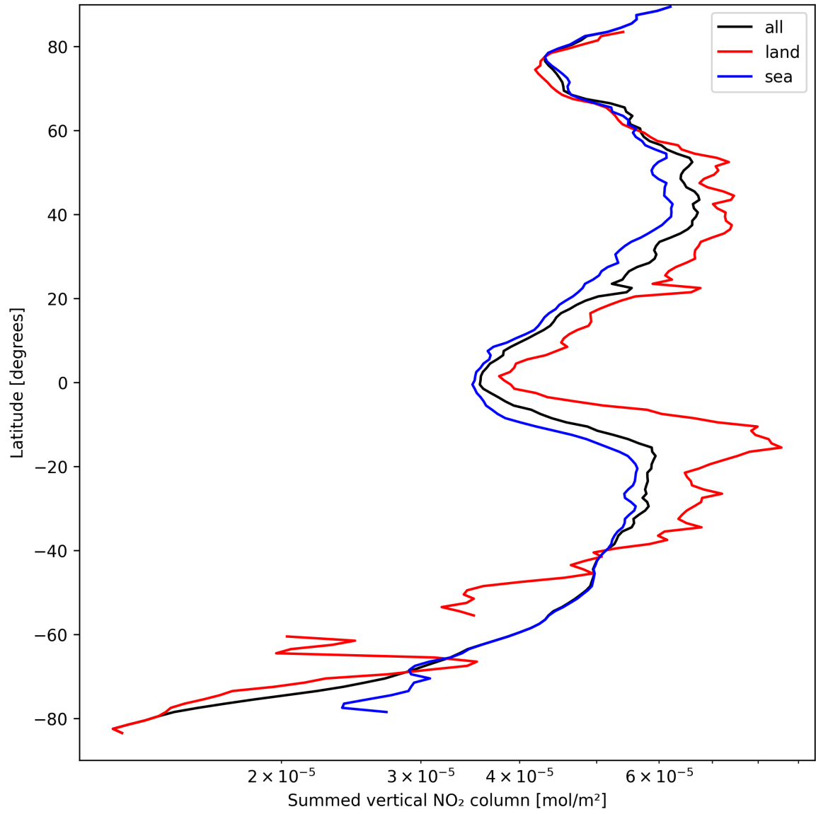
Figure 23: Zonal average of “Summed vertical NO 2 column” for 2024-09-09 to 2024-09-11.
