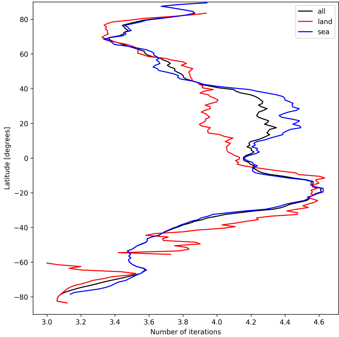
Figure 17: Zonal average of “Number of iterations” for 2024-09-09 to 2024-09-11.
