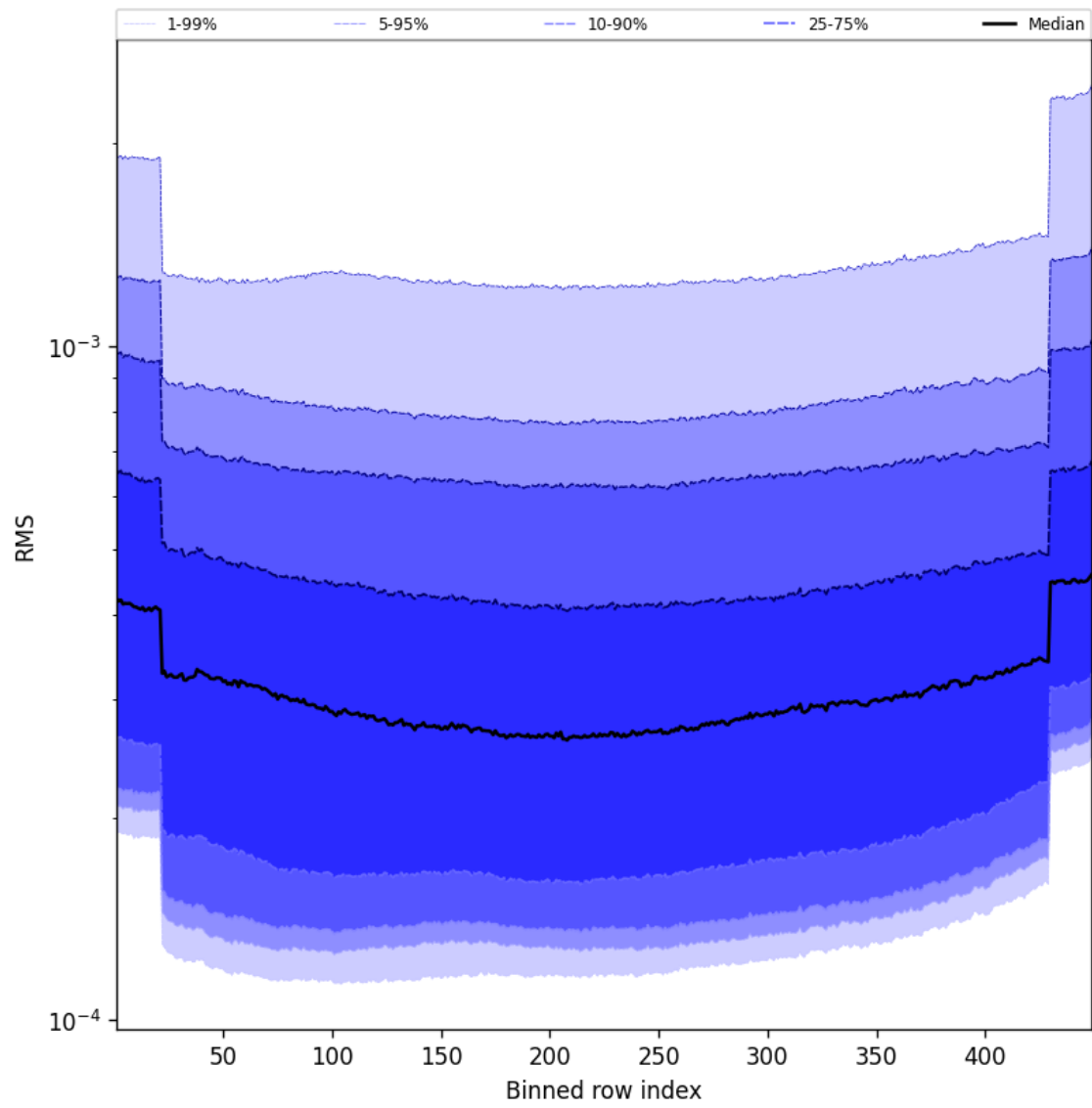
Figure 60: Along track statistics of “RMS” for 2024-09-09 to 2024-09-11
