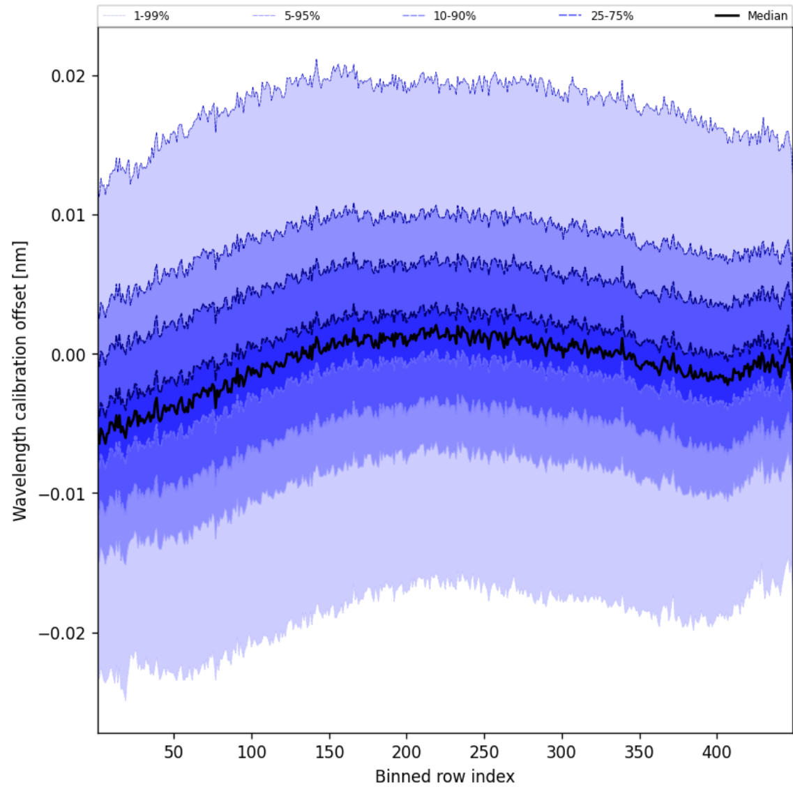
Figure 52: Along track statistics of “Wavelength calibration offset” for 2024-09-09 to 2024-09-11
