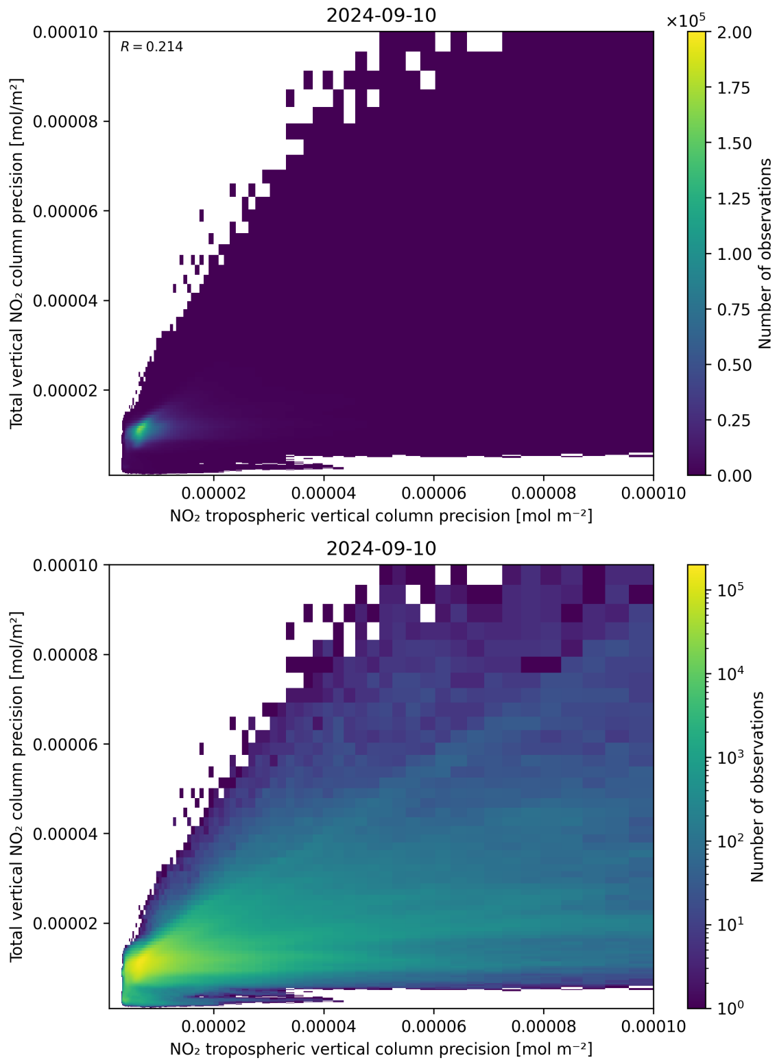
Figure 139: Scatter density plot of “NO 2 tropospheric vertical column precision” against “Total vertical NO 2 column precision” for 2024-09-09 to 2024-09-11.
