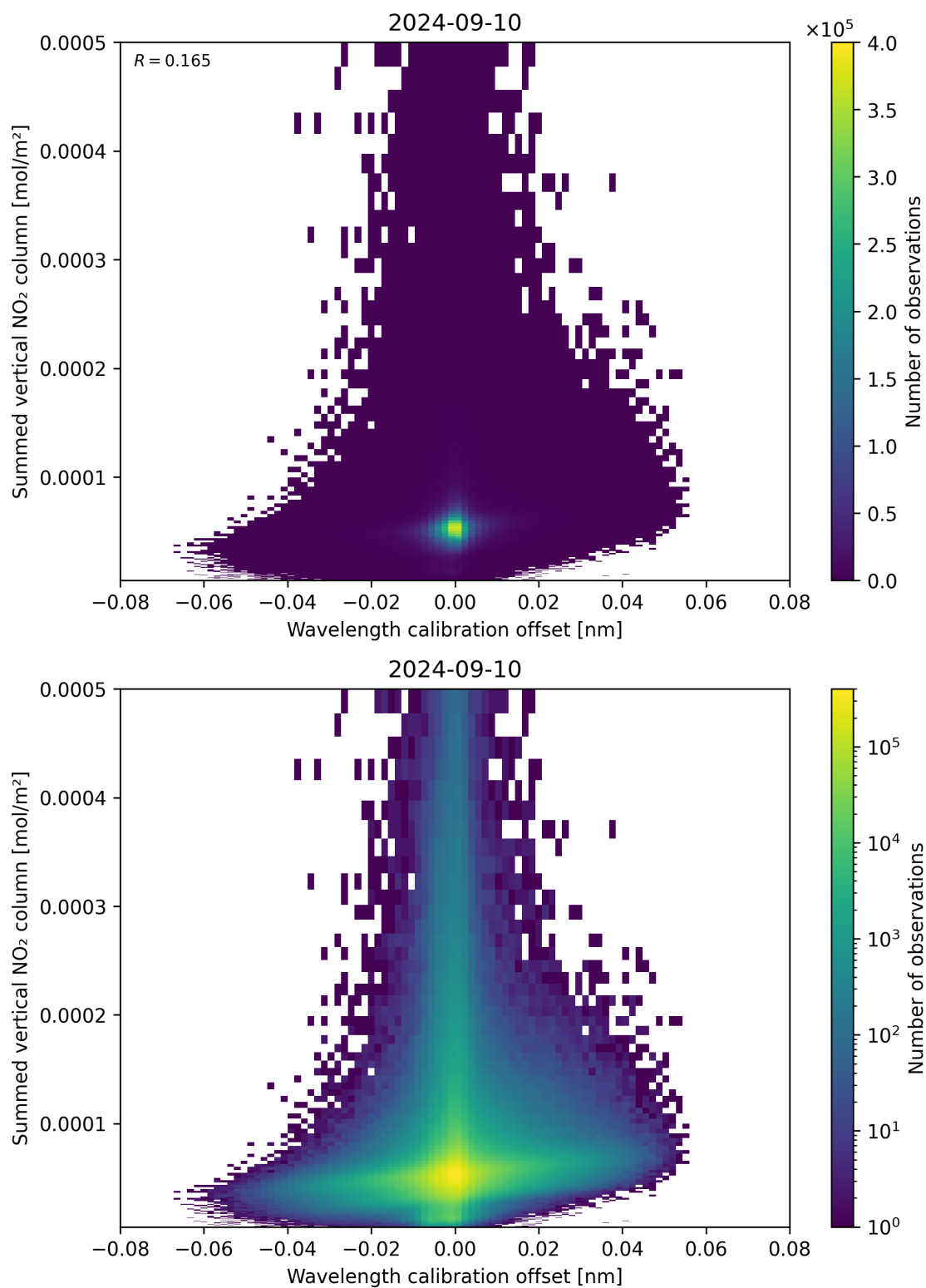
Figure 177: Scatter density plot of “Wavelength calibration offset” against “Summed vertical NO 2 column” for 2024-09-09 to 2024-09-11.
