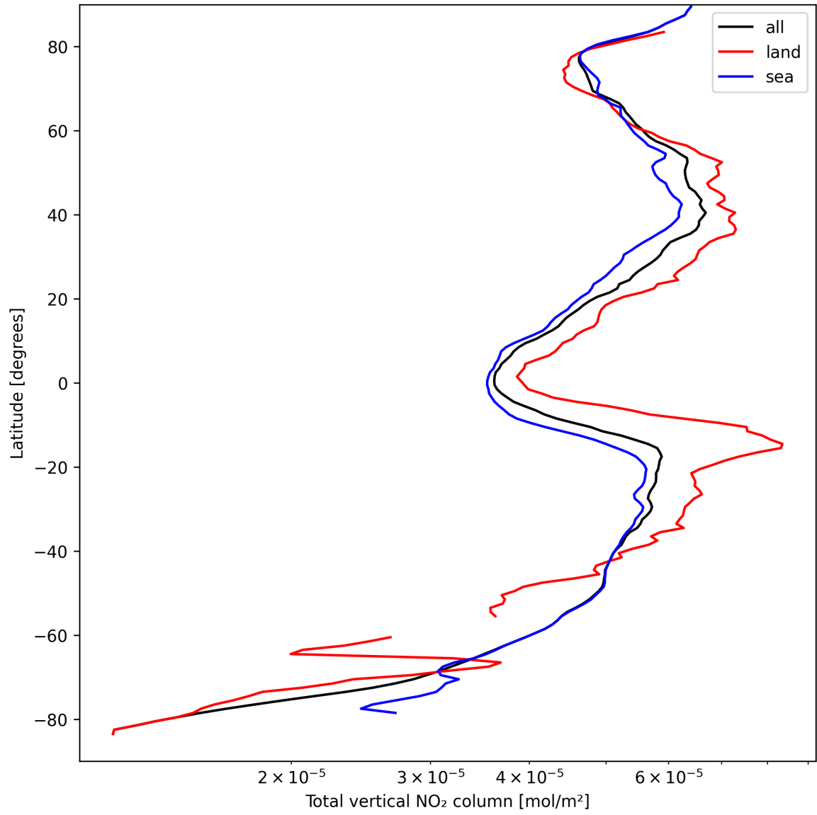
Figure 21: Zonal average of “Total vertical NO 2 column” for 2024-09-09 to 2024-09-11.
