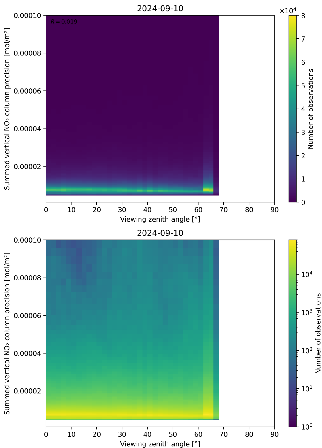
Figure 166: Scatter density plot of “Viewing zenith angle” against “Summed vertical NO 2 column precision” for 2024-09-09 to 2024-09-11.
