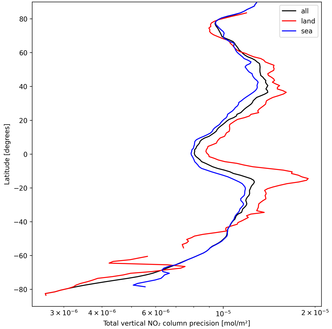
Figure 22: Zonal average of “Total vertical NO 2 column precision” for 2024-09-09 to 2024-09-11.
