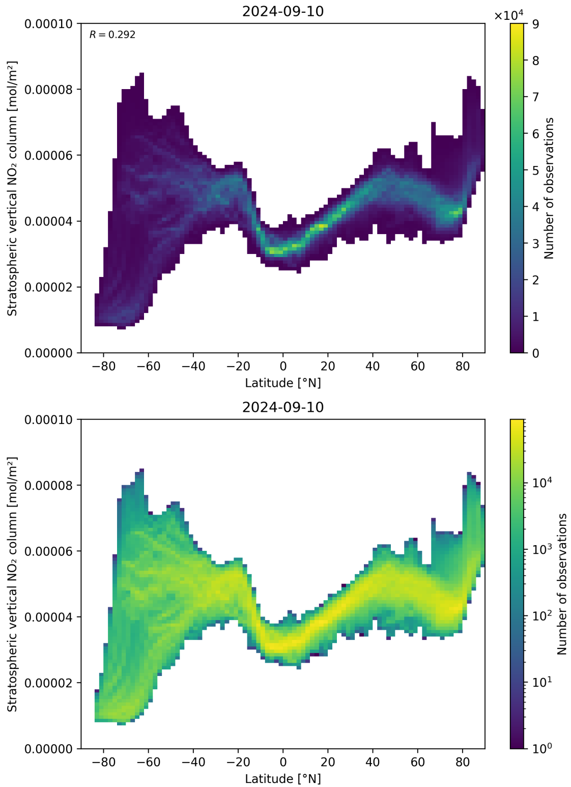
Figure 87: Scatter density plot of “Latitude” against “Stratospheric vertical \text{NO}_2 column” for 2024-09-09 to 2024-09-11.
