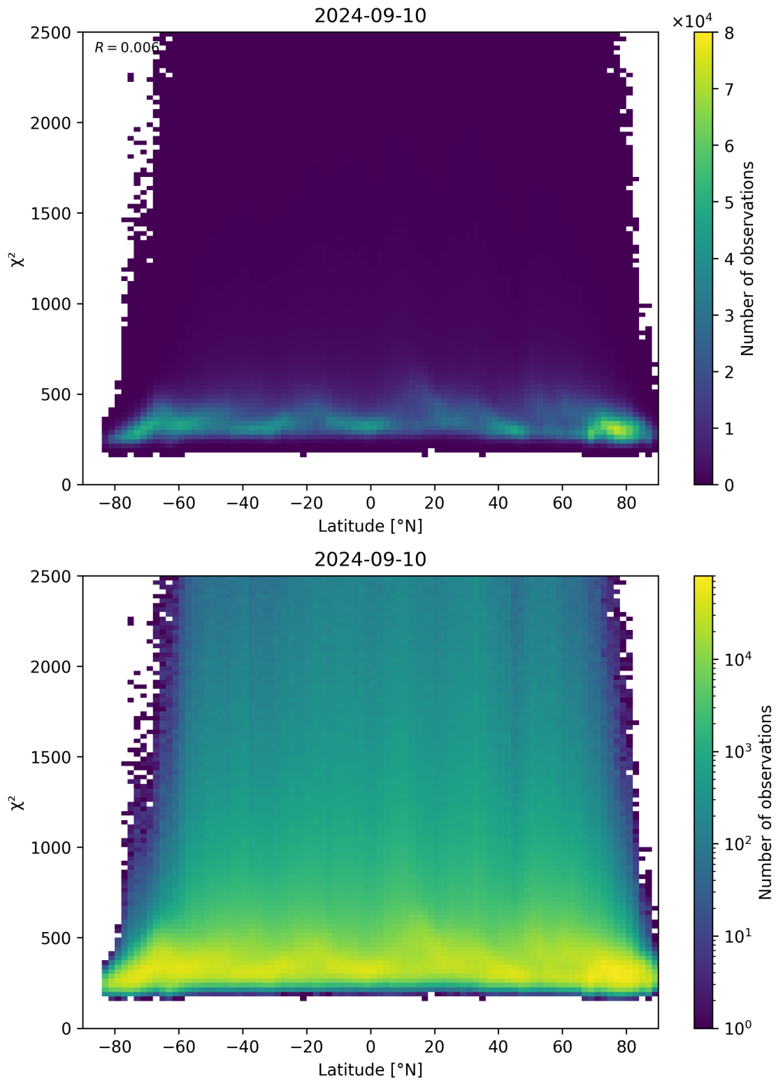
Figure 86: Scatter density plot of “Latitude” against “ \chi^2 ” for 2024-09-09 to 2024-09-11.
