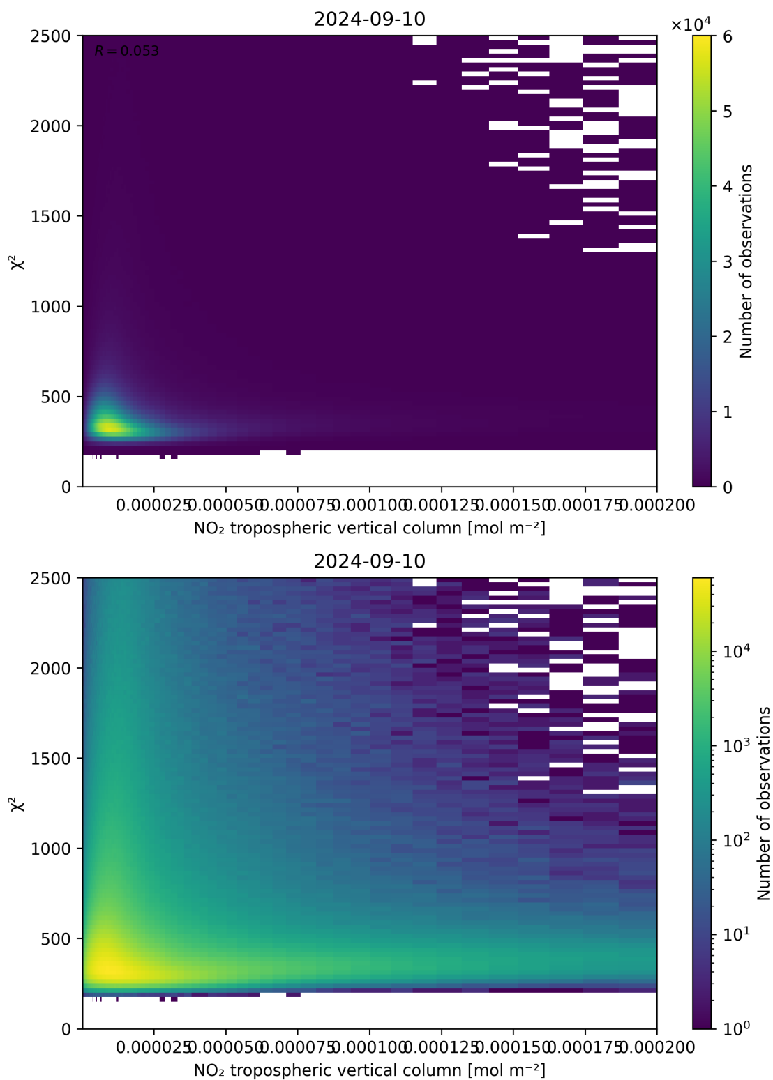
Figure 124: Scatter density plot of “NO 2 tropospheric vertical column” against “ \chi^2 ” for 2024-09-09 to 2024-09-11.
