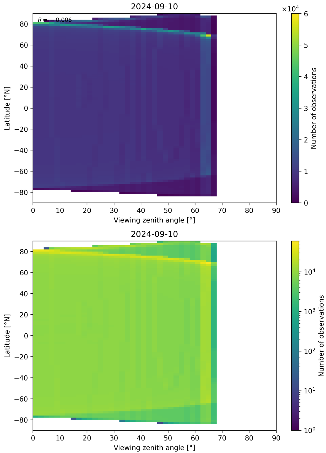
Figure 163: Scatter density plot of “Viewing zenith angle” against “Latitude” for 2024-09-09 to 2024-09-11.
