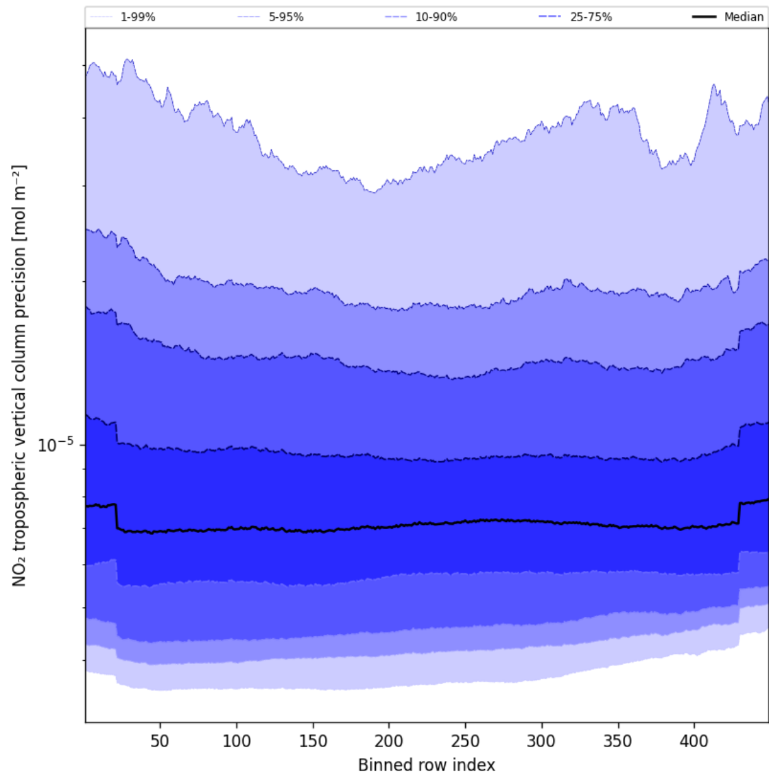
Figure 47: Along track statistics of “NO 2 tropospheric vertical column precision” for 2024-09-09 to 2024-09-11
