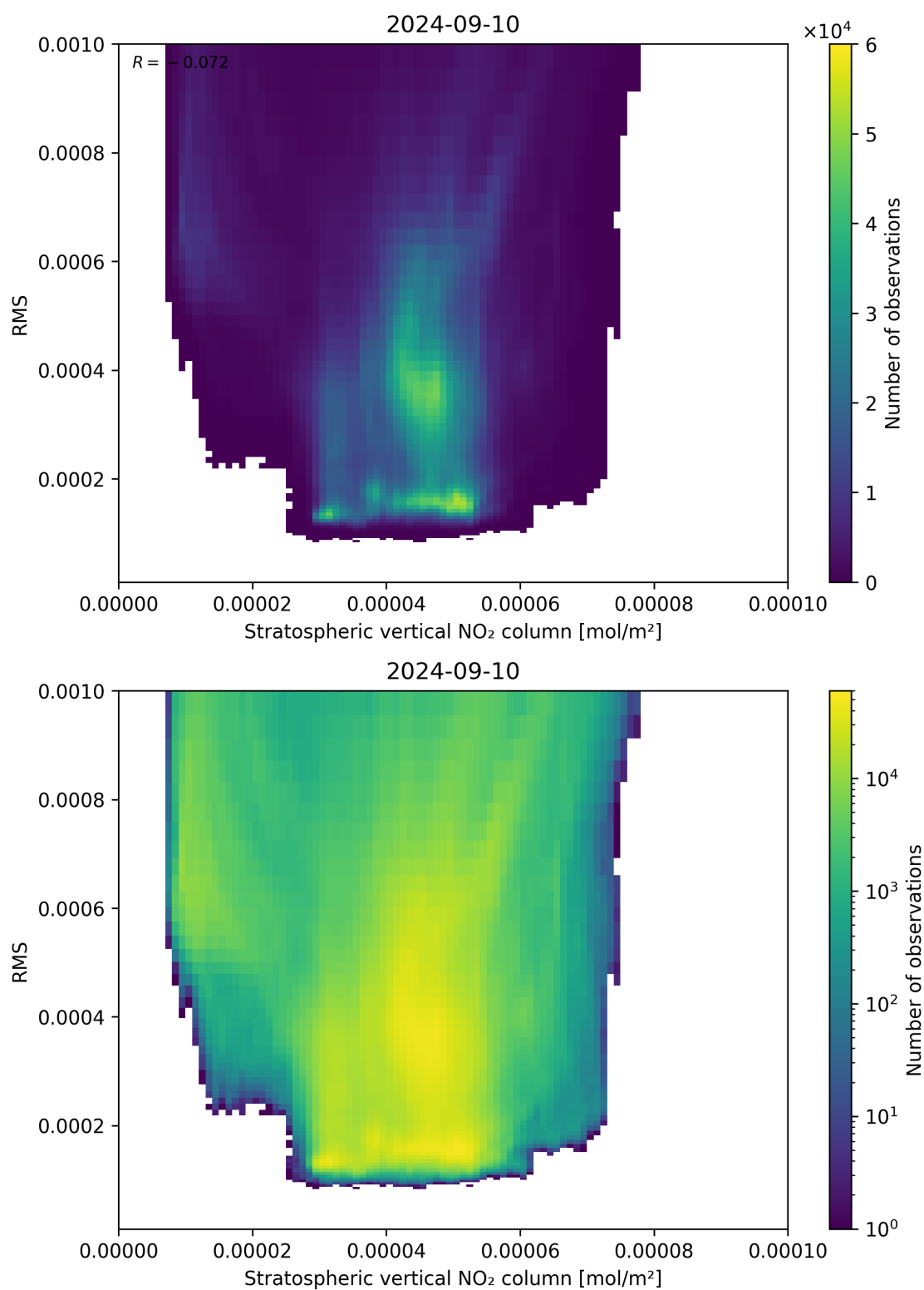
Figure 102: Scatter density plot of “Stratospheric vertical NO 2 column” against “RMS” for 2024-09-09 to 2024-09-11.
