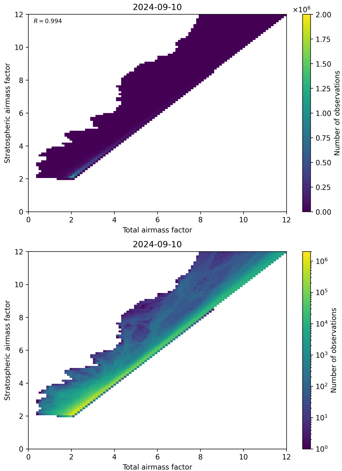
Figure 62: Scatter density plot of “Total airmass factor” against “Stratospheric airmass factor” for 2024-09-09 to 2024-09-11.
