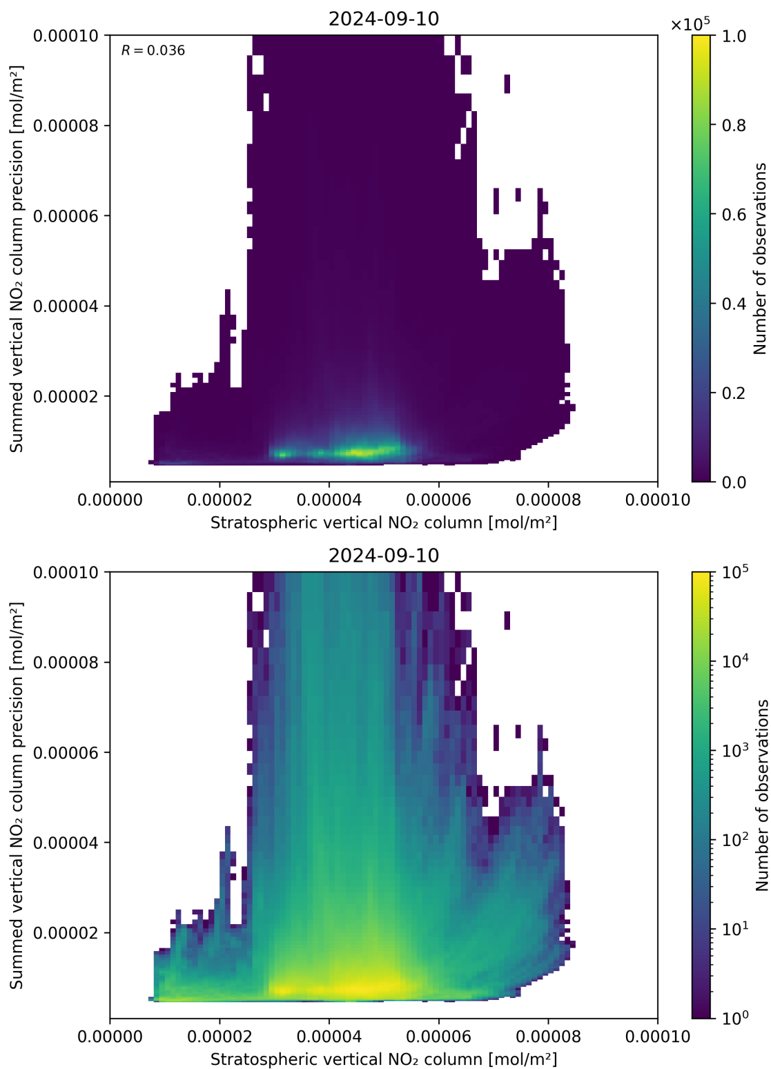
Figure 99: Scatter density plot of “Stratospheric vertical NO 2 column” against “Summed vertical NO 2 column precision” for 2024-09-09 to 2024-09-11.
