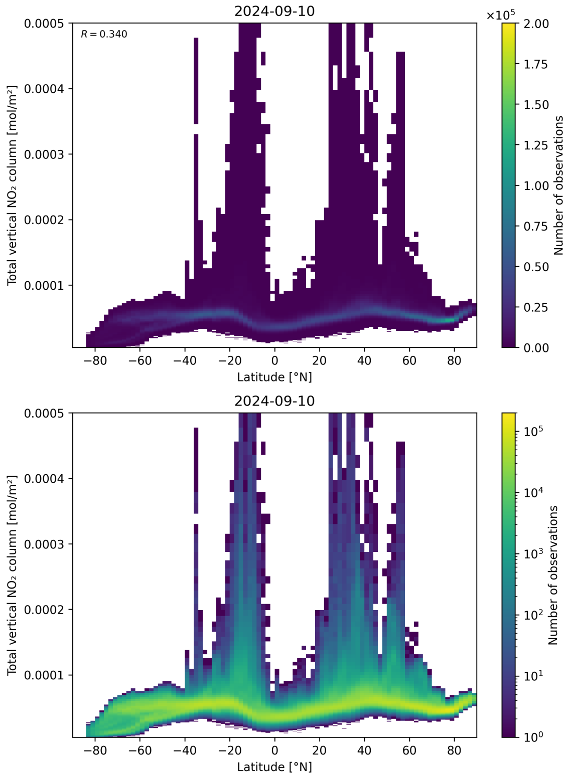
Figure 90: Scatter density plot of “Latitude” against “Total vertical NO 2 column” for 2024-09-09 to 2024-09-11.
