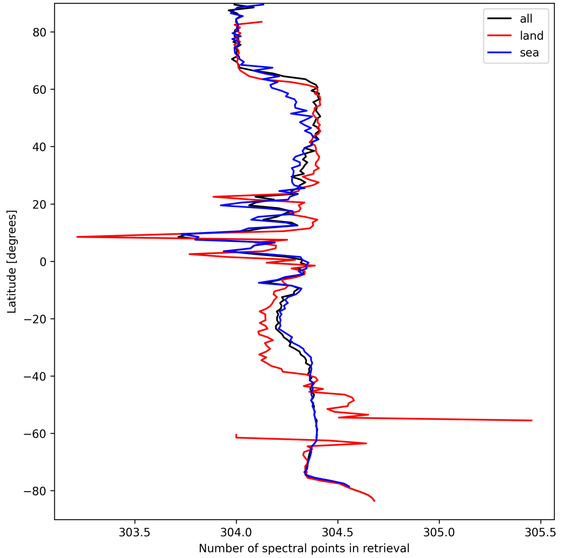
Figure 16: Zonal average of “Number of spectral points in retrieval” for 2024-09-09 to 2024-09-11.
