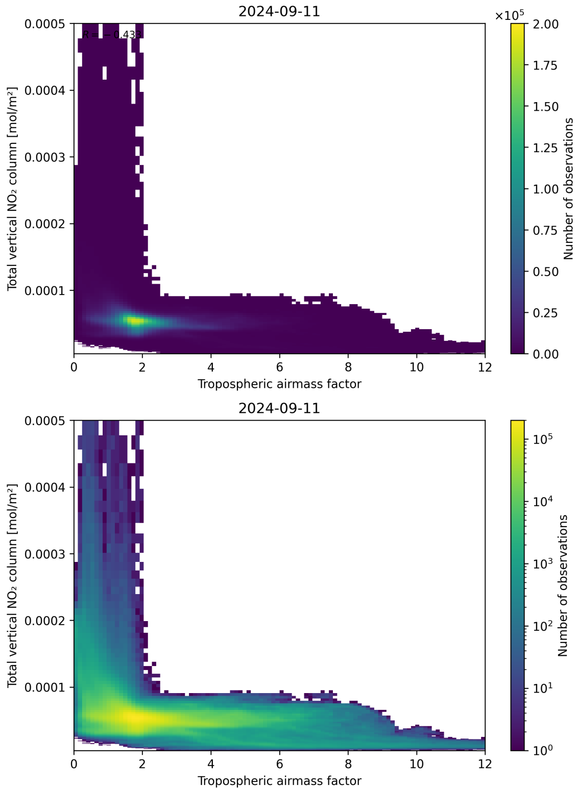
Figure 77: Scatter density plot of “Tropospheric airmass factor” against “Total vertical NO 2 column” for 2024-09-10 to 2024-09-12.
