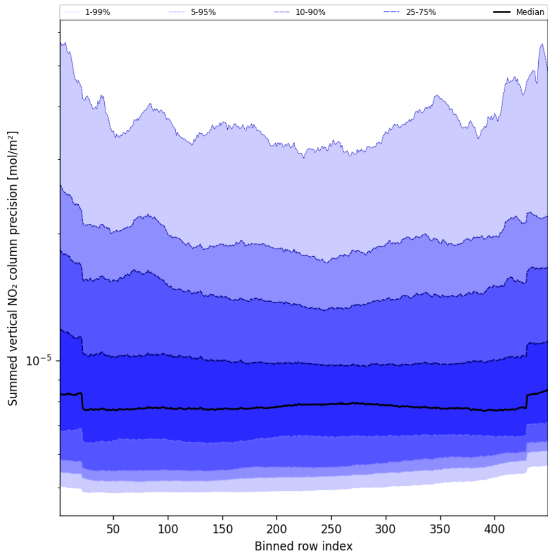
Figure 58: Along track statistics of “Summed vertical NO 2 column precision” for 2024-09-10 to 2024-09-12
