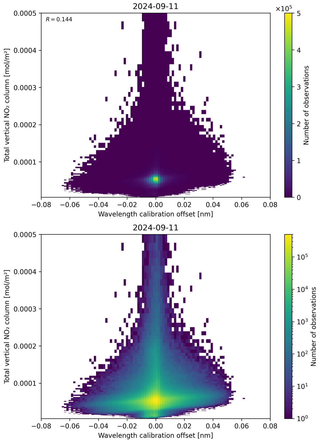
Figure 179: Scatter density plot of “Wavelength calibration offset” against “Total vertical NO 2 column” for 2024-09-10 to 2024-09-12.
