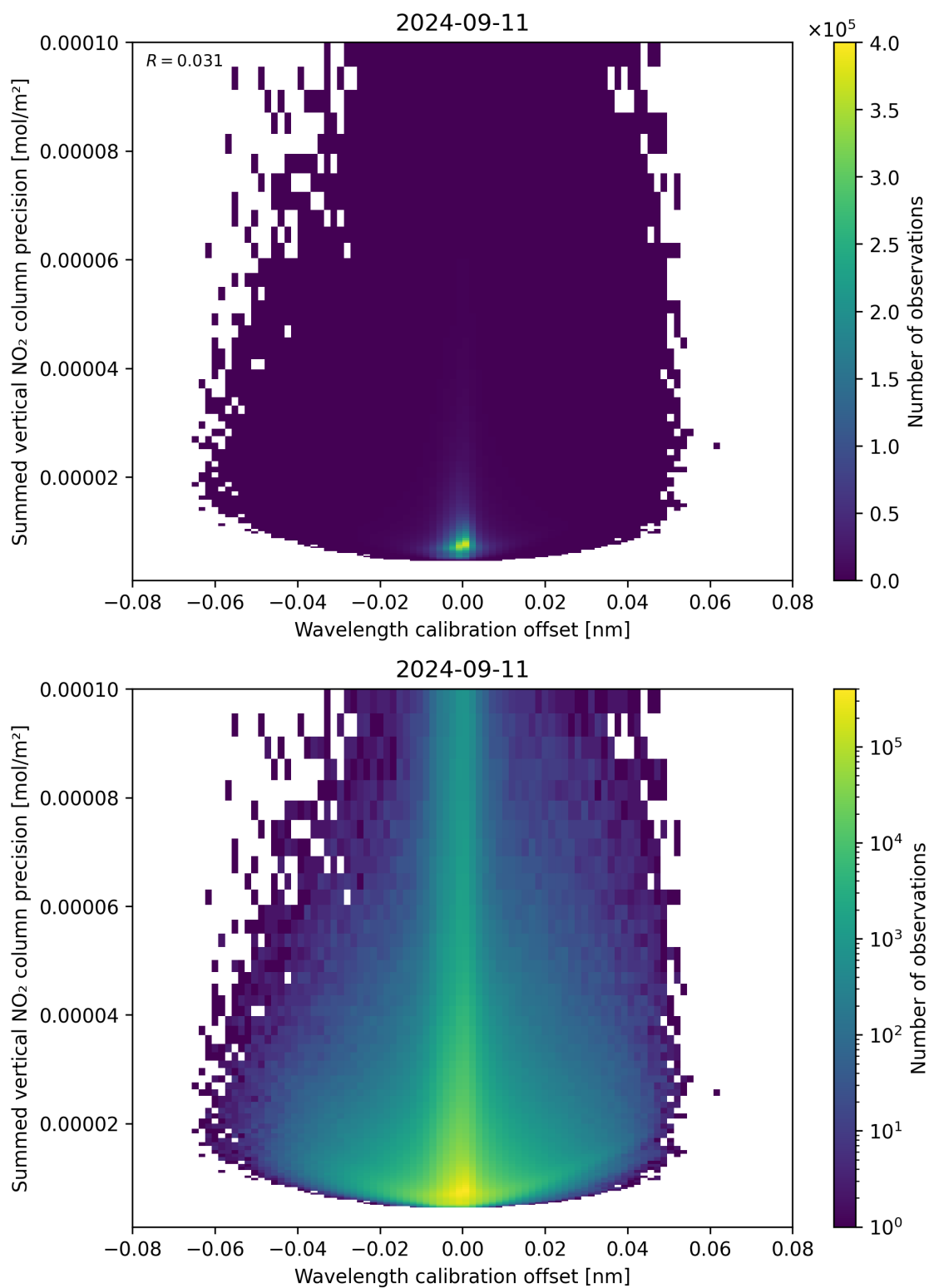
Figure 178: Scatter density plot of “Wavelength calibration offset” against “Summed vertical NO 2 column precision” for 2024-09-10 to 2024-09-12.
