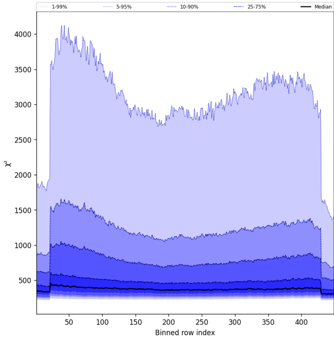
Figure 59: Along track statistics of “ \chi^2 ” for 2024-09-10 to 2024-09-12
