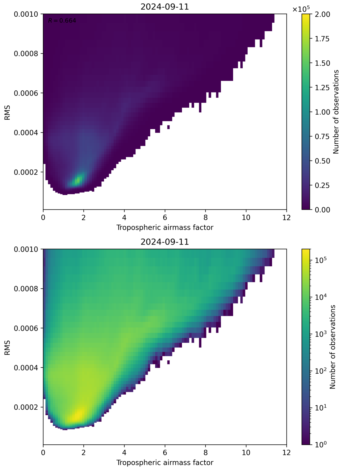
Figure 79: Scatter density plot of “Tropospheric airmass factor” against “RMS” for 2024-09-10 to 2024-09-12.
