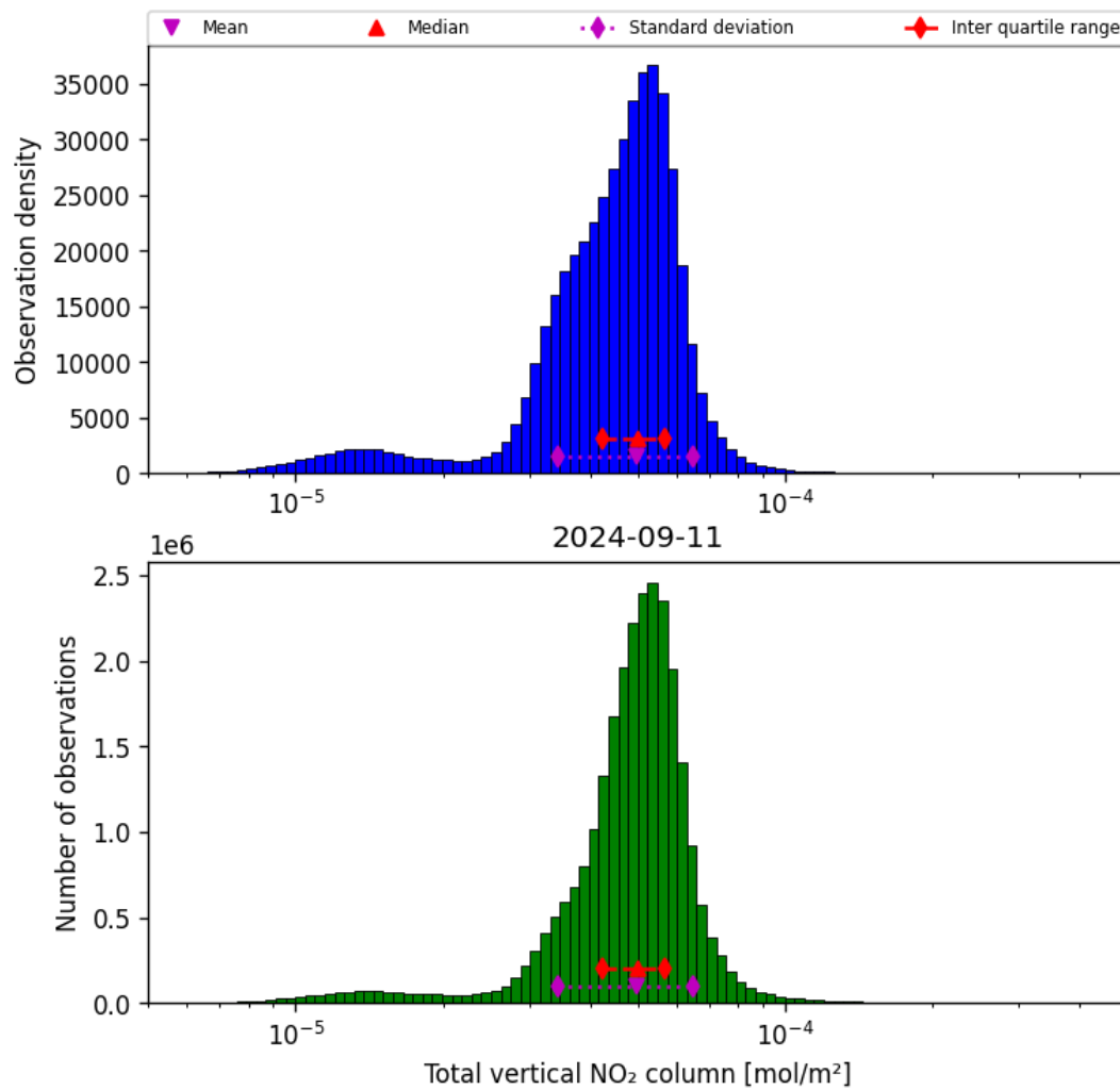
Figure 38: Histogram of “Total vertical NO 2 column” for 2024-09-10 to 2024-09-12
