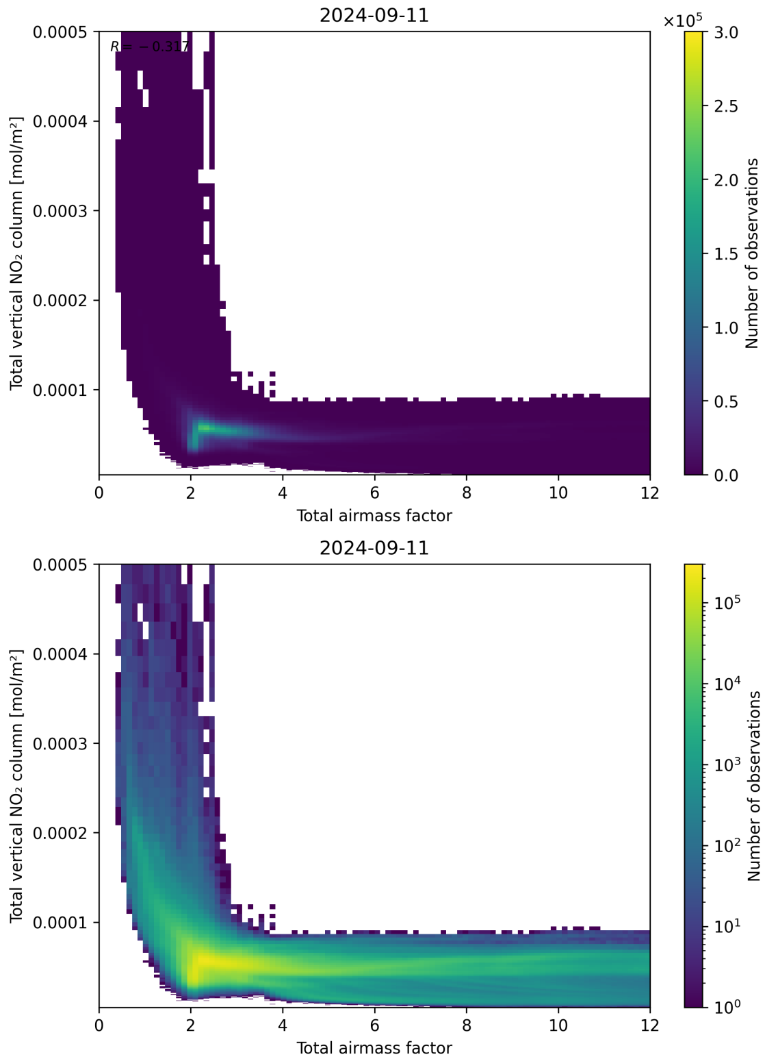
Figure 67: Scatter density plot of “Total airmass factor” against “Total vertical NO 2 column” for 2024-09-10 to 2024-09-12.
