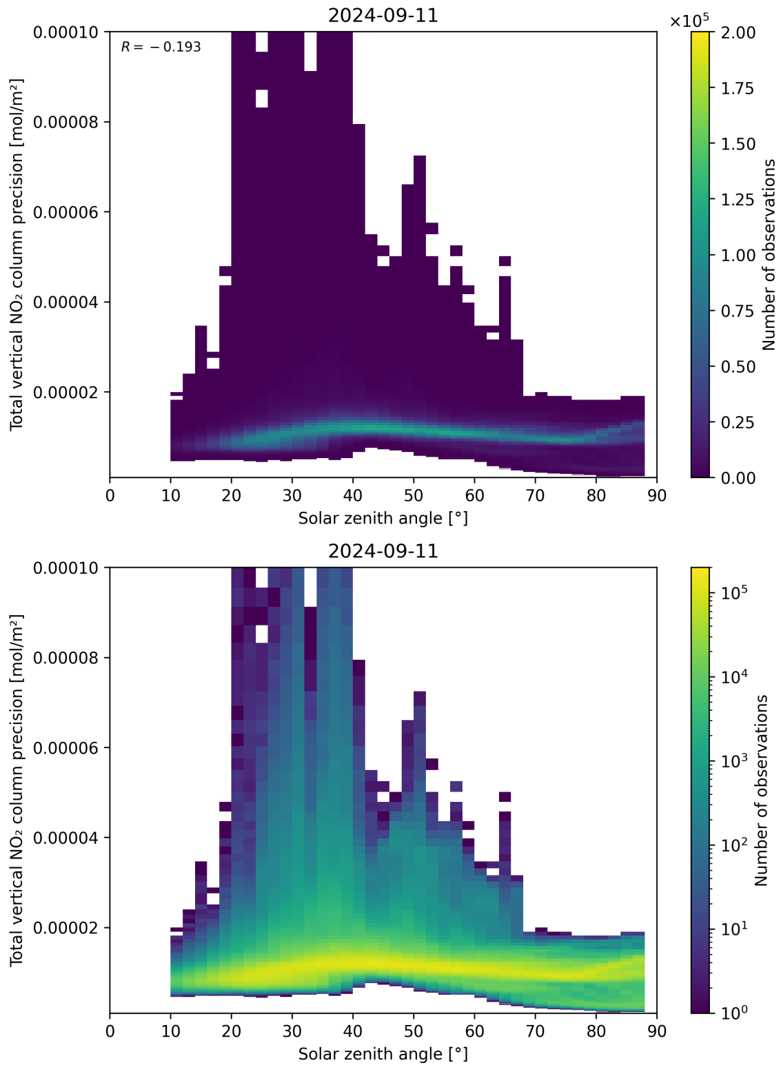
Figure 154: Scatter density plot of “Solar zenith angle” against “Total vertical NO 2 column precision” for 2024-09-10 to 2024-09-12.
