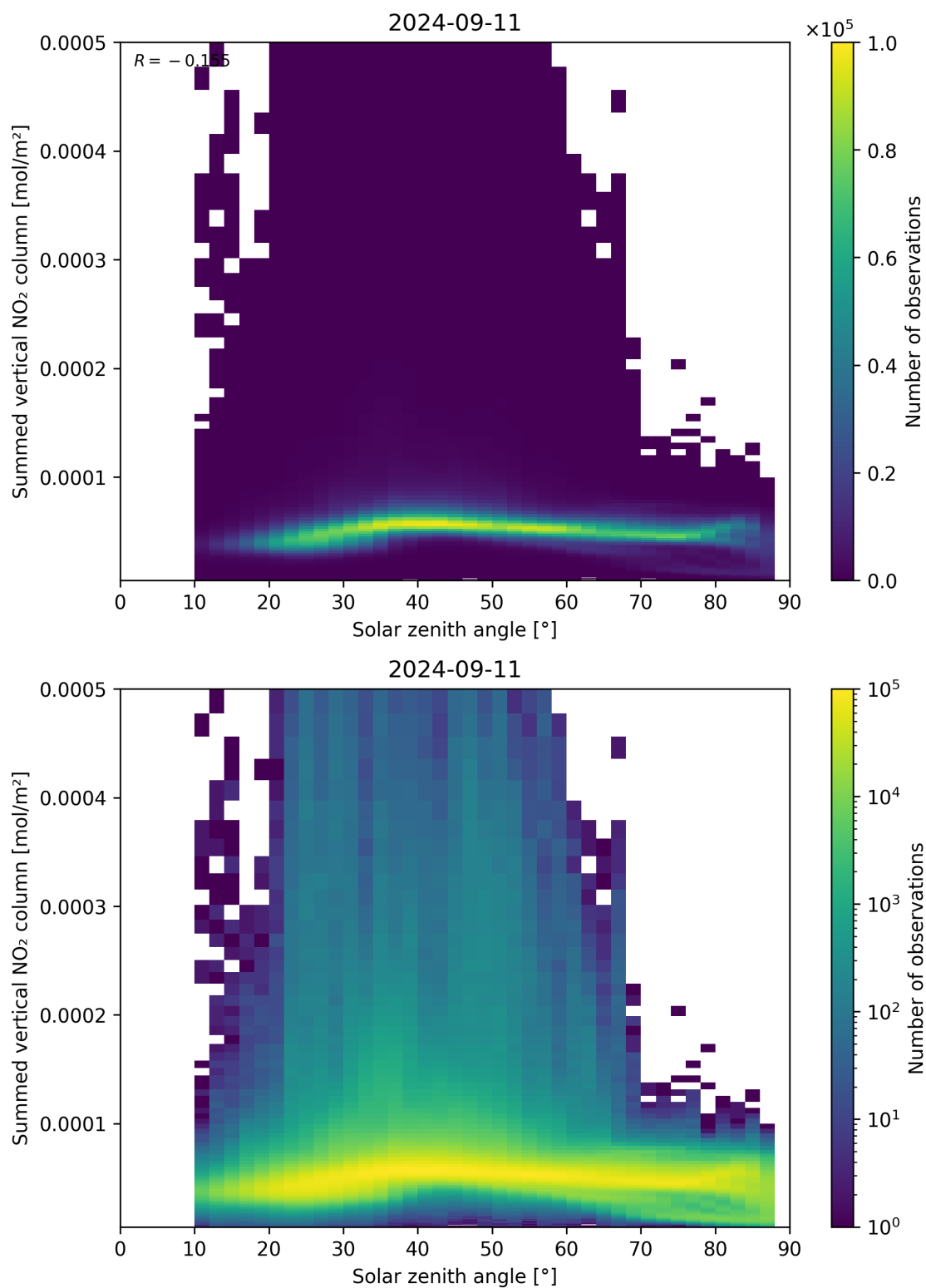
Figure 151: Scatter density plot of “Solar zenith angle” against “Summed vertical NO 2 column” for 2024-09-10 to 2024-09-12.
