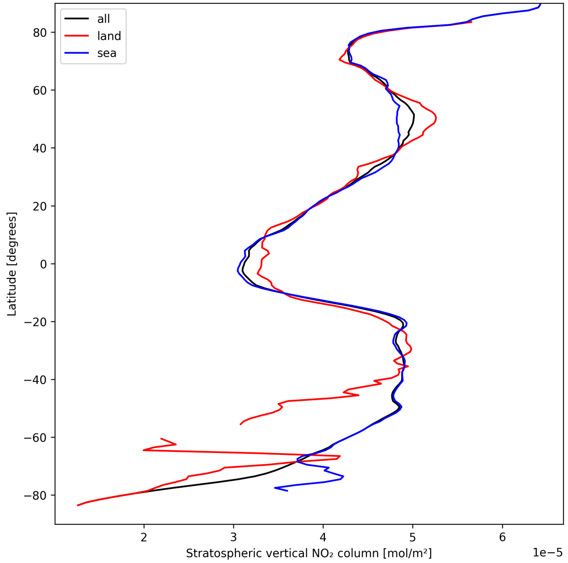
Figure 19: Zonal average of “Stratospheric vertical NO 2 column” for 2024-09-10 to 2024-09-12.
