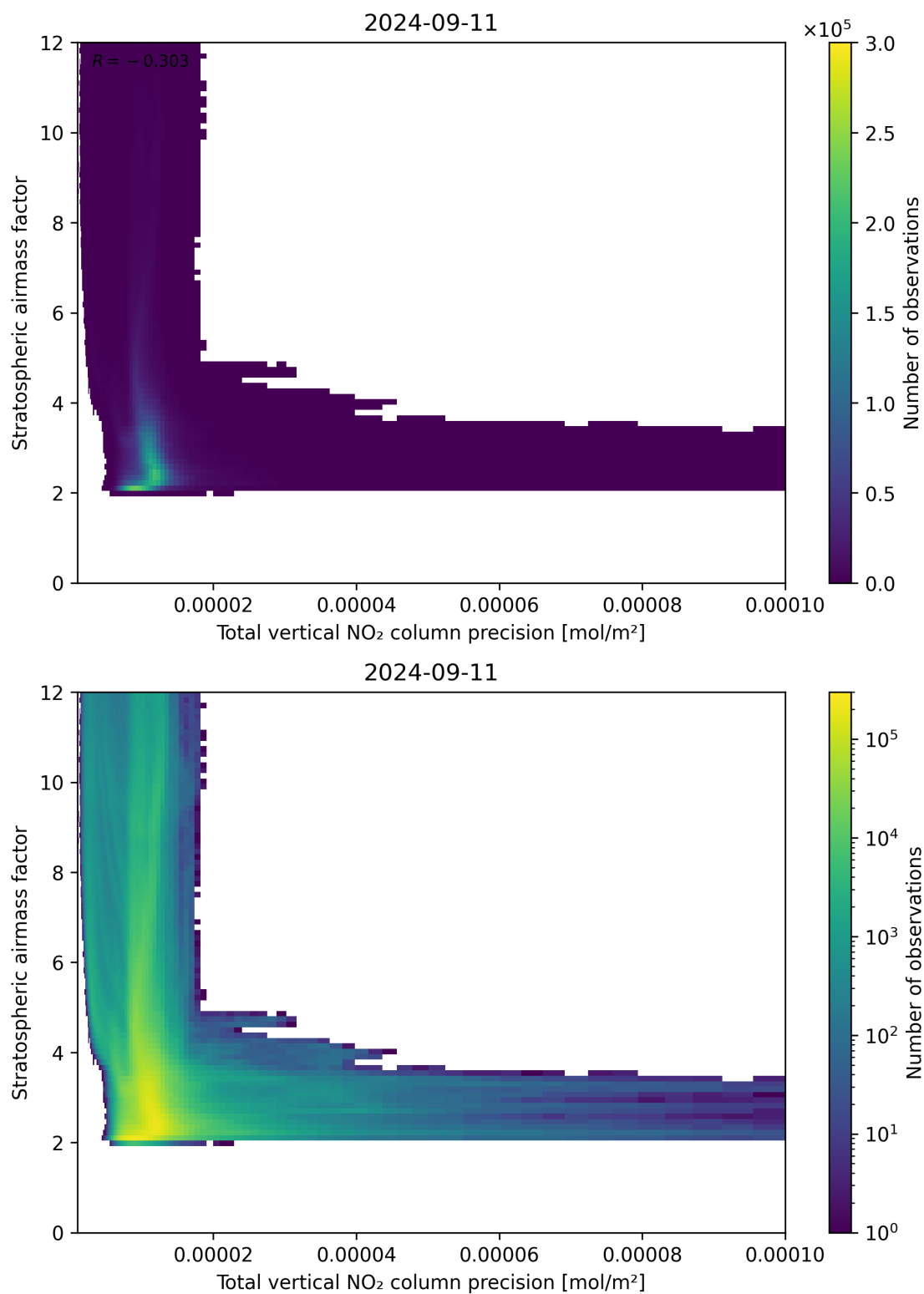
Figure 115: Scatter density plot of “Total vertical NO 2 column precision” against “Stratospheric air mass factor” for 2024-09-10 to 2024-09-12.
