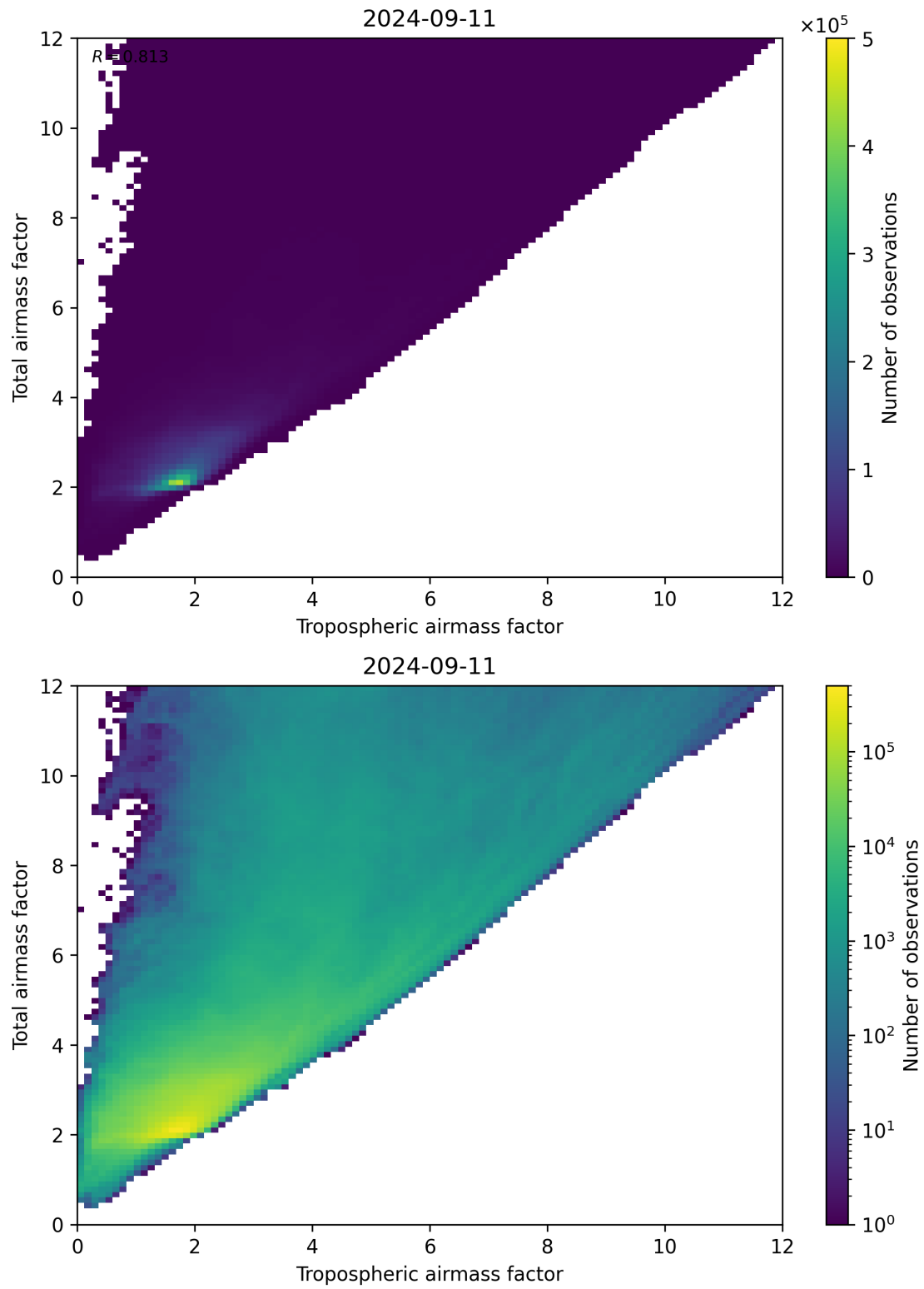
Figure 72: Scatter density plot of “Tropospheric airmass factor” against “Total airmass factor” for 2024-09-10 to 2024-09-12.
