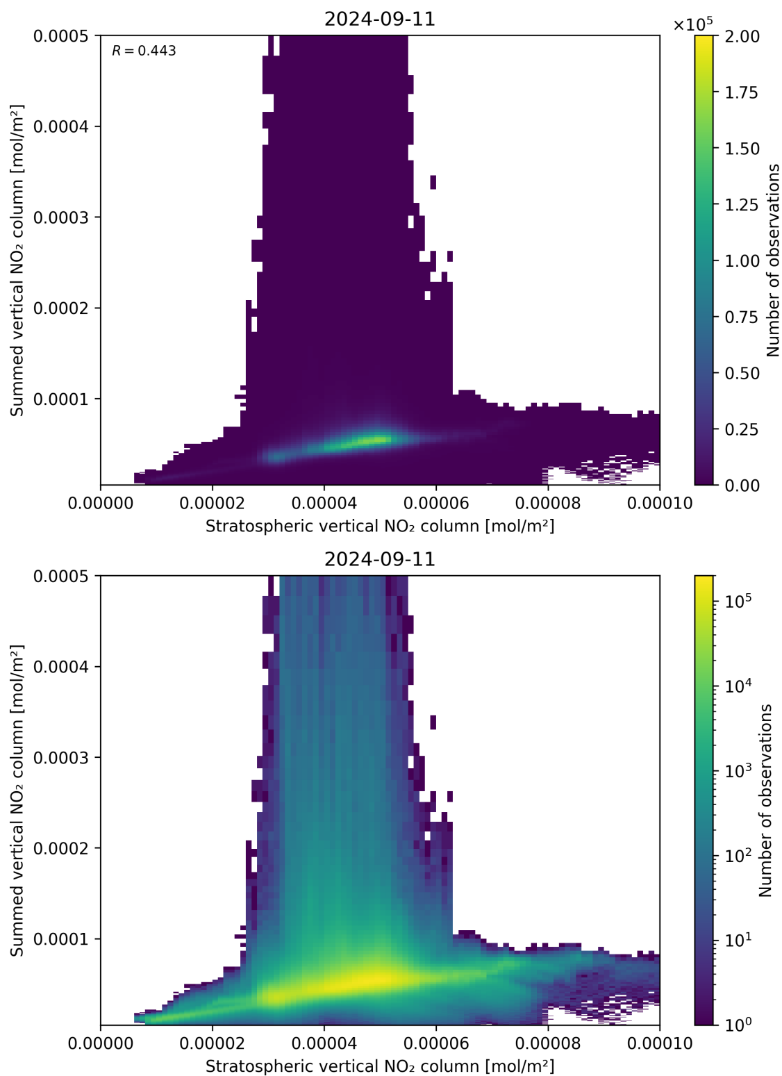
Figure 98: Scatter density plot of “Stratospheric vertical NO 2 column” against “Summed vertical NO 2 column” for 2024-09-10 to 2024-09-12.
