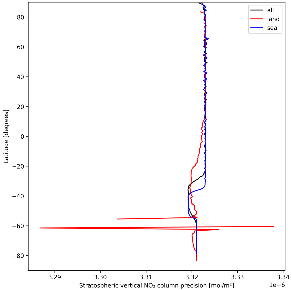
Figure 20: Zonal average of “Stratospheric vertical NO 2 column precision” for 2024-09-10 to 2024-09-12.
