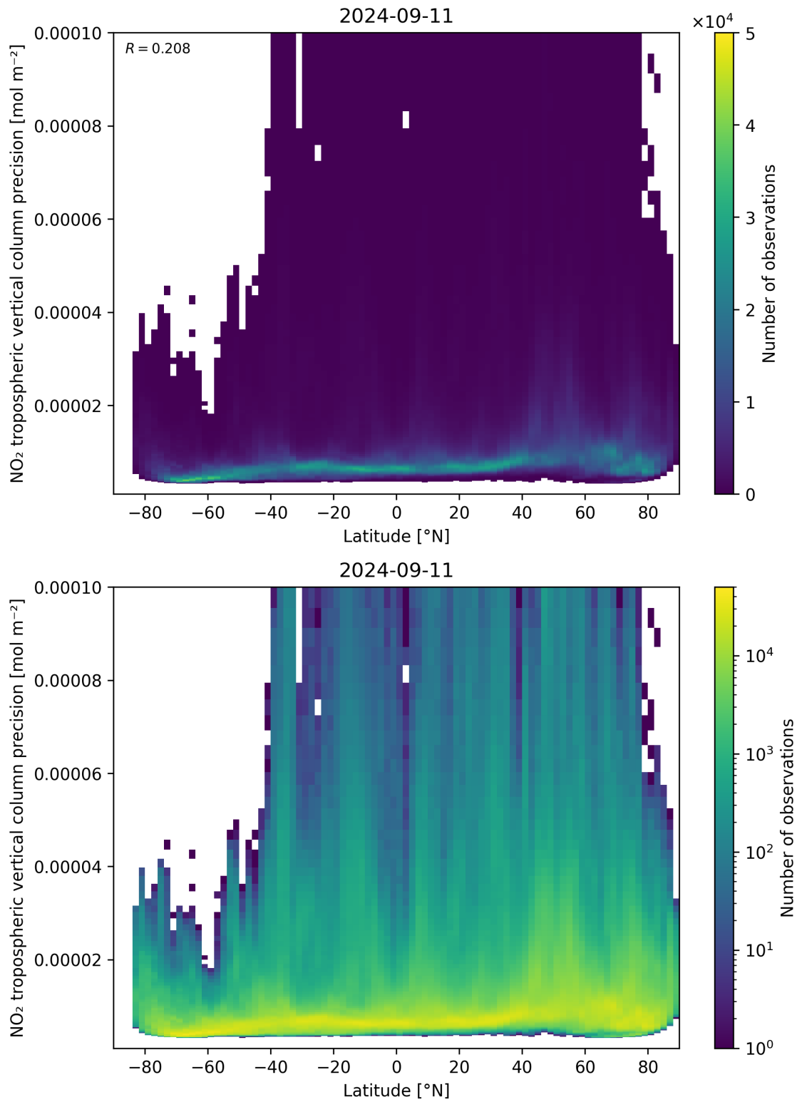
Figure 93: Scatter density plot of “Latitude” against “NO 2 tropospheric vertical column precision” for 2024-09-10 to 2024-09-12.
