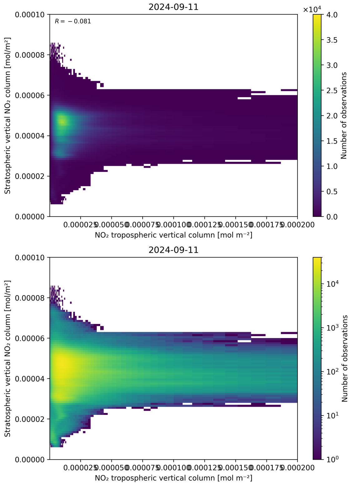
Figure 125: Scatter density plot of “NO 2 tropospheric vertical column” against “Stratospheric vertical NO 2 column” for 2024-09-10 to 2024-09-12.
