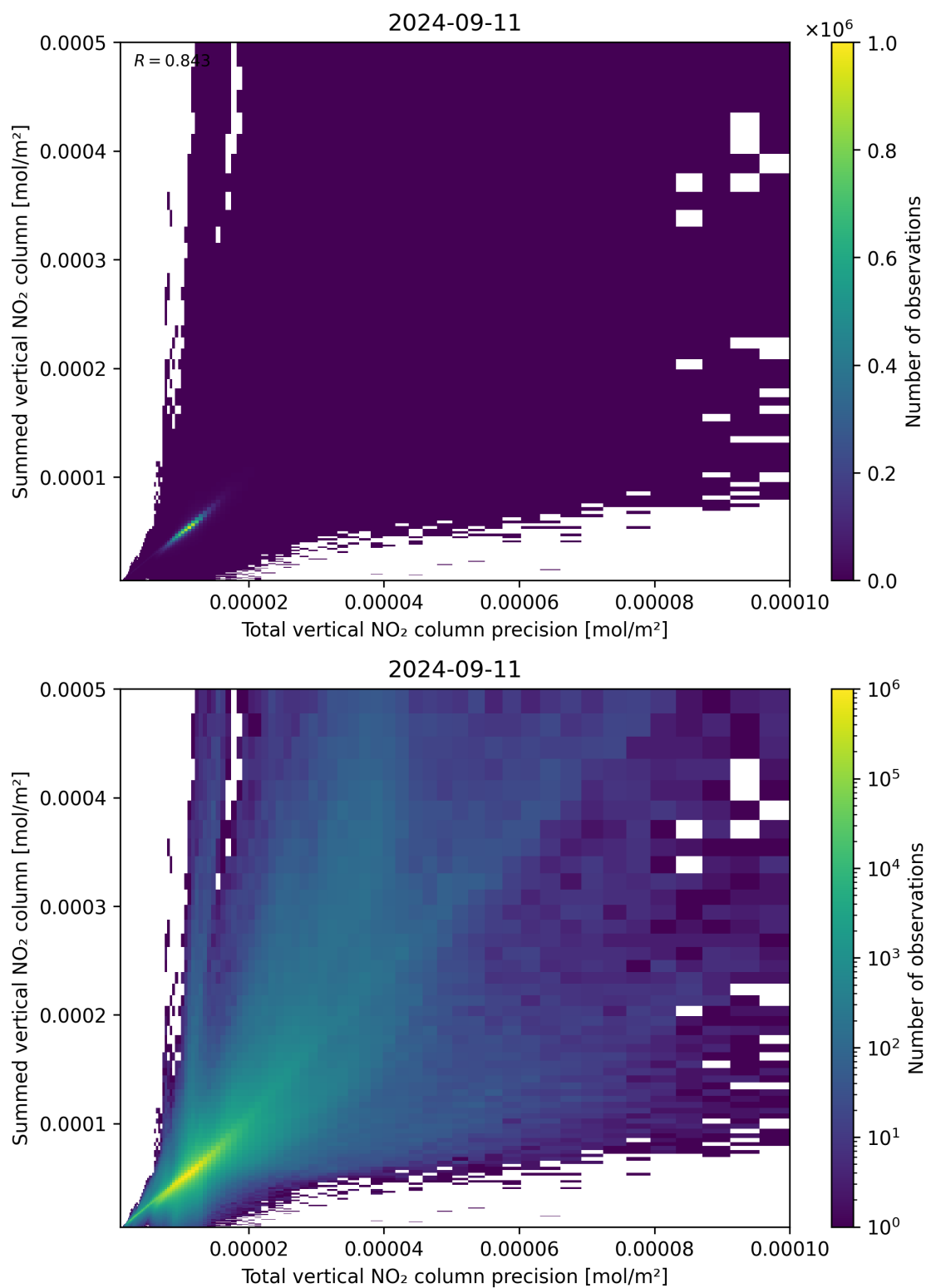
Figure 117: Scatter density plot of “Total vertical NO 2 column precision” against “Summed vertical NO 2 column” for 2024-09-10 to 2024-09-12.
