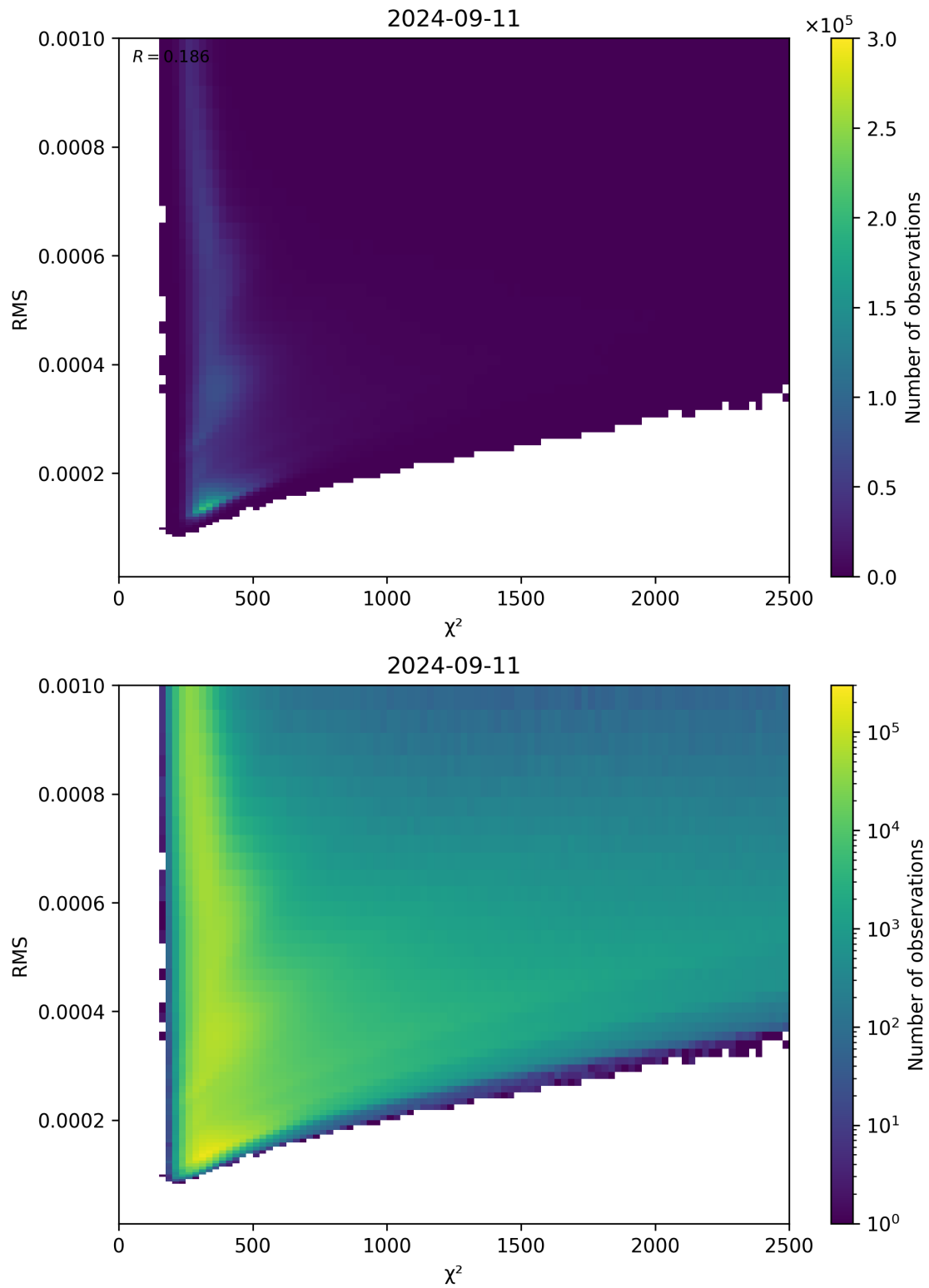
Figure 82: Scatter density plot of “ \chi^2 ” against “RMS” for 2024-09-10 to 2024-09-12.
