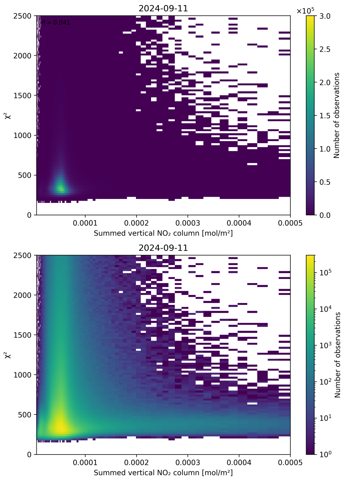
Figure 104: Scatter density plot of “Summed vertical NO 2 column” against “ \chi^2 ” for 2024-09-10 to 2024-09-12.
