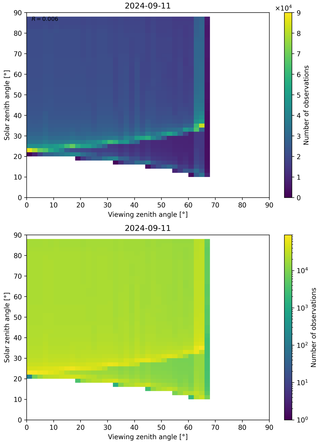
Figure 172: Scatter density plot of “Viewing zenith angle” against “Solar zenith angle” for 2024-09-10 to 2024-09-12.
