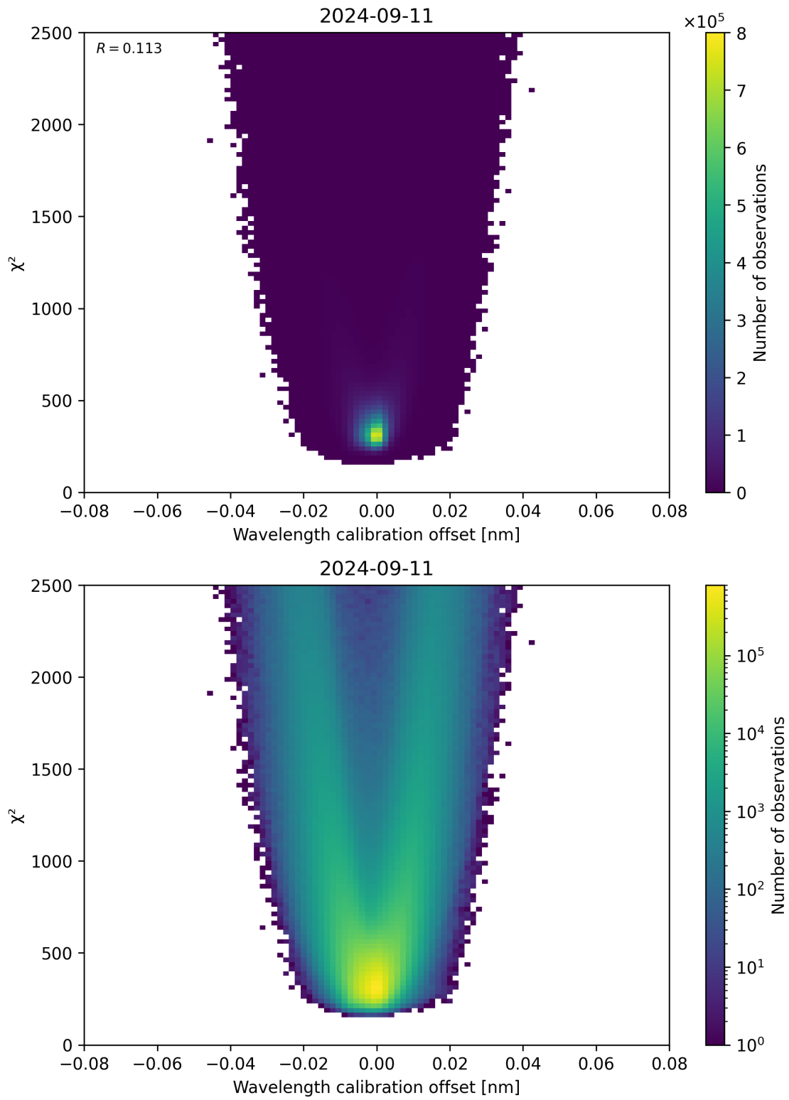
Figure 175: Scatter density plot of “Wavelength calibration offset” against “ \chi^2 ” for 2024-09-10 to 2024-09-12.
