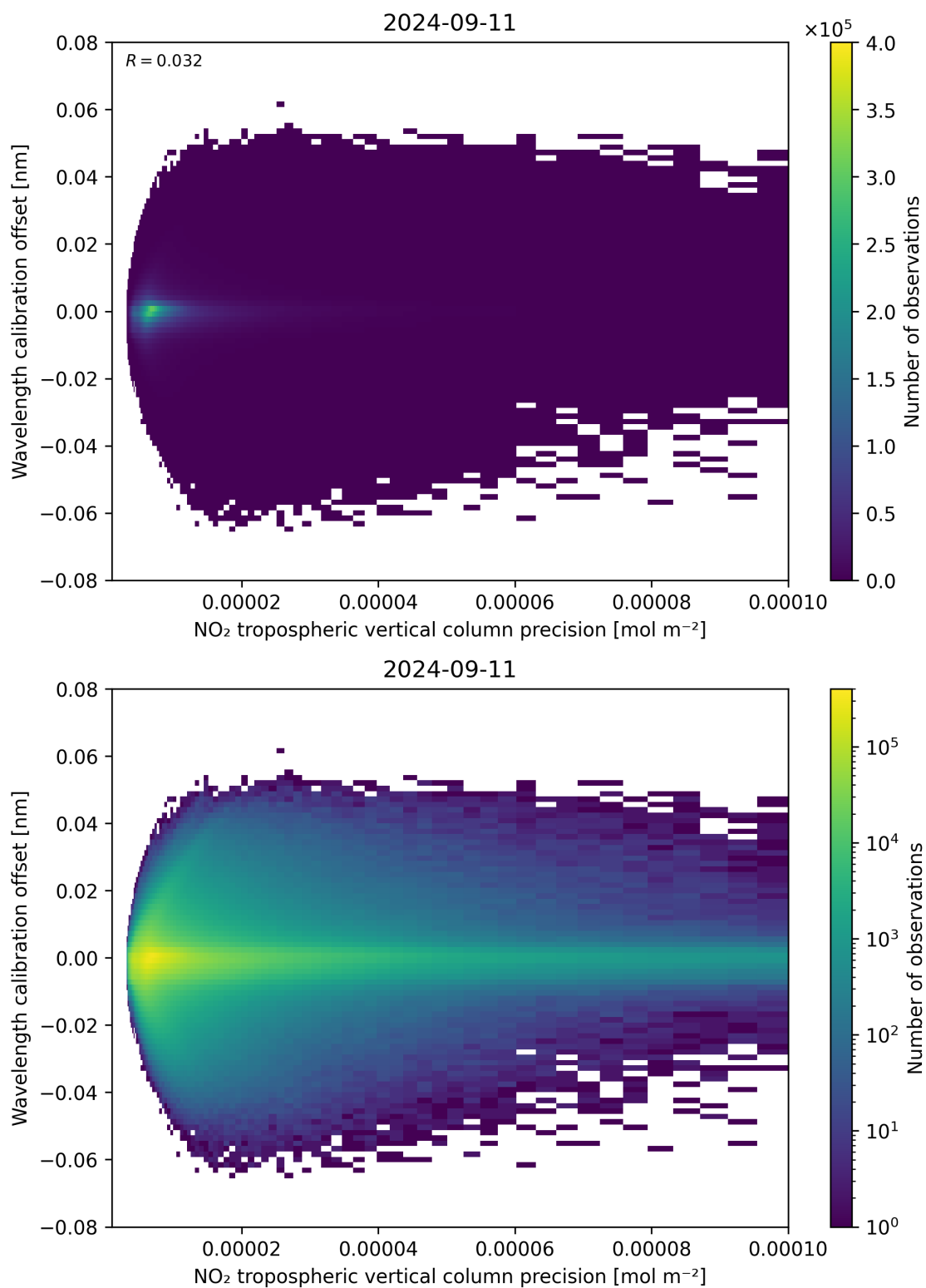
Figure 141: Scatter density plot of “NO 2 tropospheric vertical column precision” against “Wavelength calibration offset” for 2024-09-10 to 2024-09-12.
