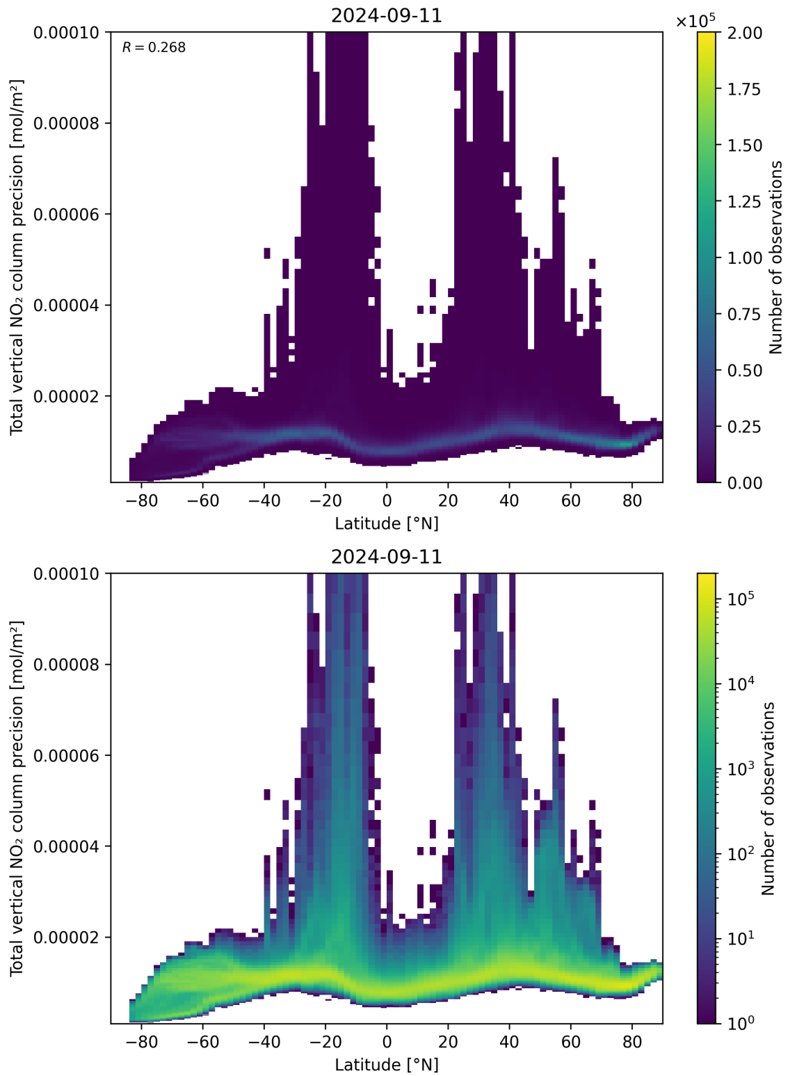
Figure 91: Scatter density plot of “Latitude” against “Total vertical NO 2 column precision” for 2024-09-10 to 2024-09-12.
