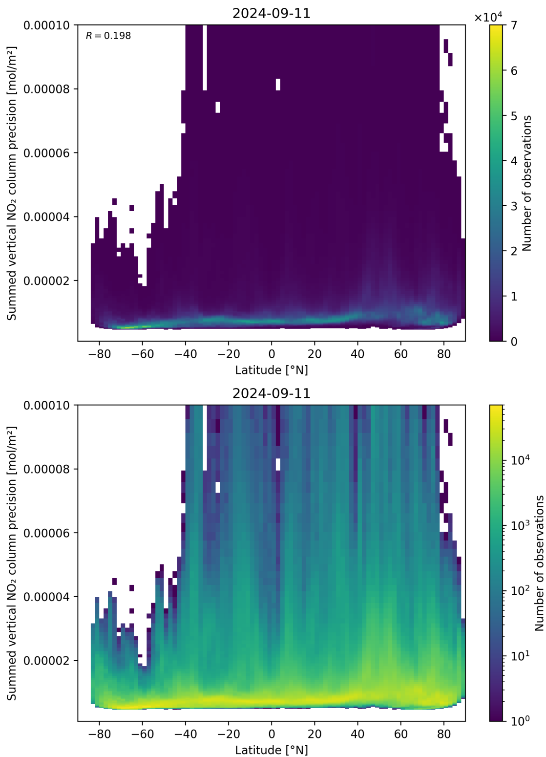
Figure 89: Scatter density plot of “Latitude” against “Summed vertical NO 2 column precision” for 2024-09-10 to 2024-09-12.
