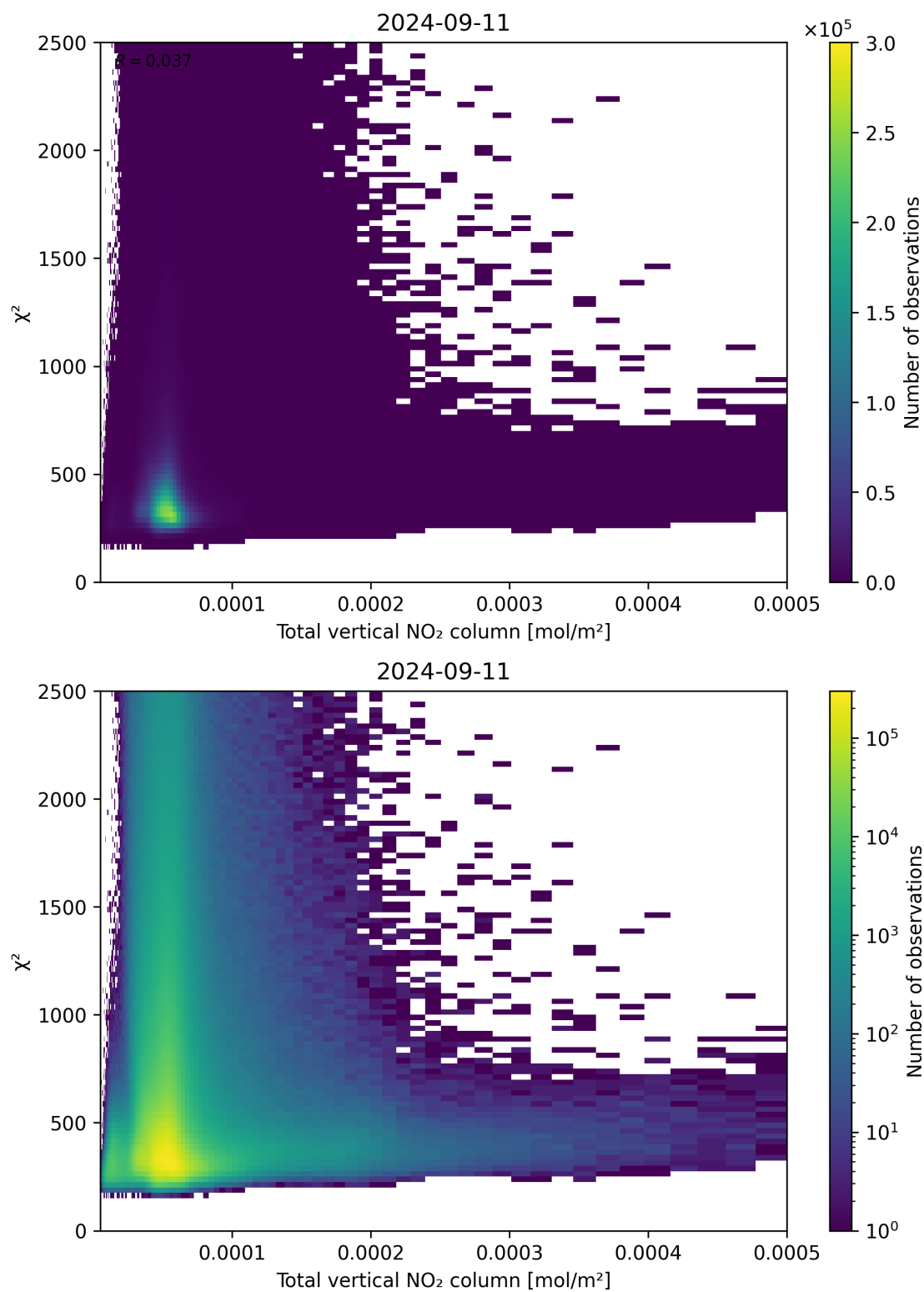
Figure 111: Scatter density plot of “Total vertical NO 2 column” against “ \chi^2 ” for 2024-09-10 to 2024-09-12.
