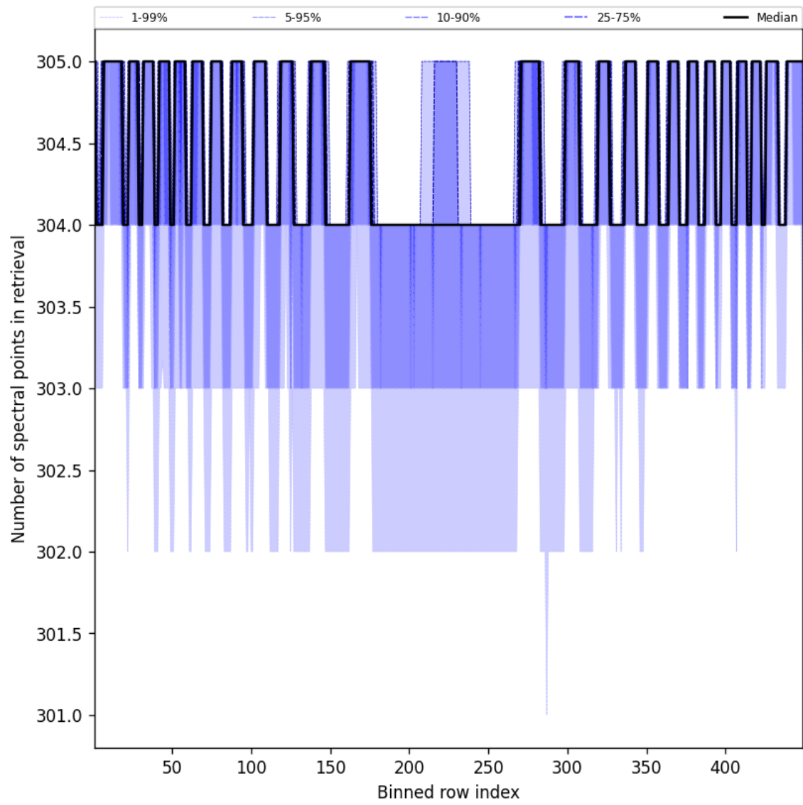
Figure 50: Along track statistics of “Number of spectral points in retrieval” for 2024-09-10 to 2024-09-12
