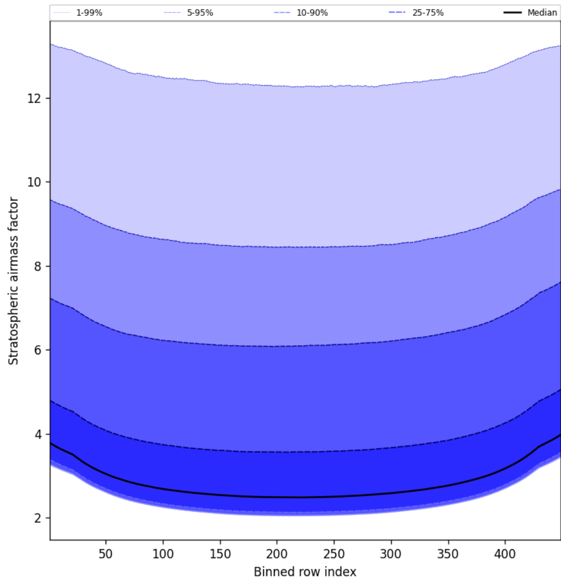
Figure 61: Along track statistics of “Stratospheric airmass factor” for 2024-09-10 to 2024-09-12
