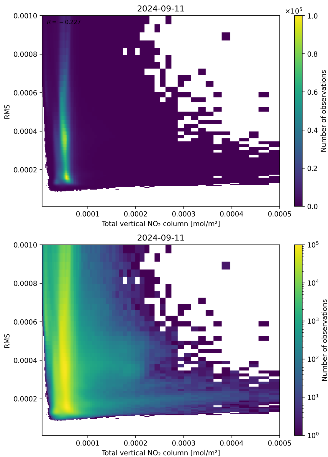
Figure 120: Scatter density plot of “Total vertical NO 2 column” against “RMS” for 2024-09-10 to 2024-09-12.
