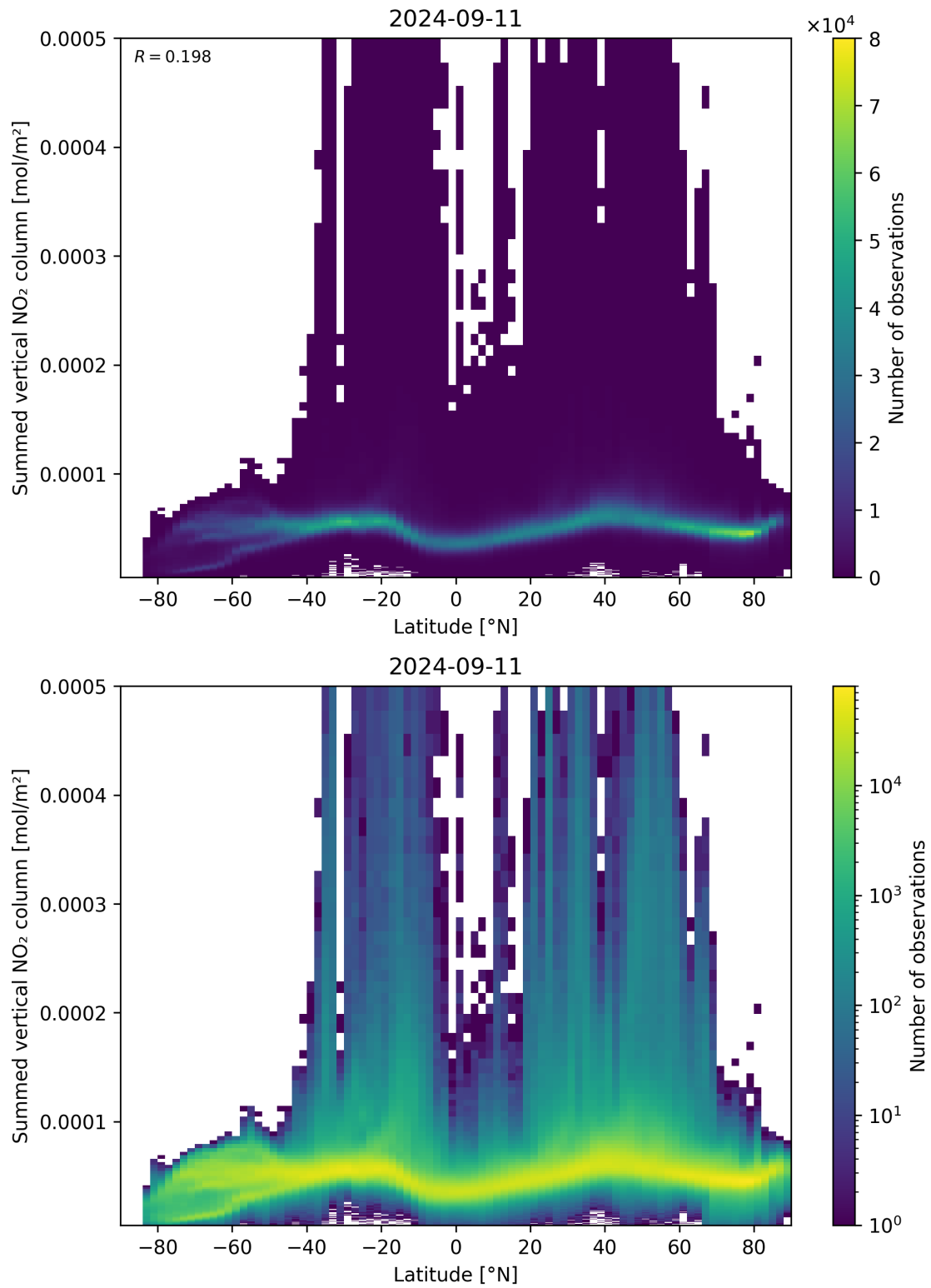
Figure 88: Scatter density plot of “Latitude” against “Summed vertical NO 2 column” for 2024-09-10 to 2024-09-12.
