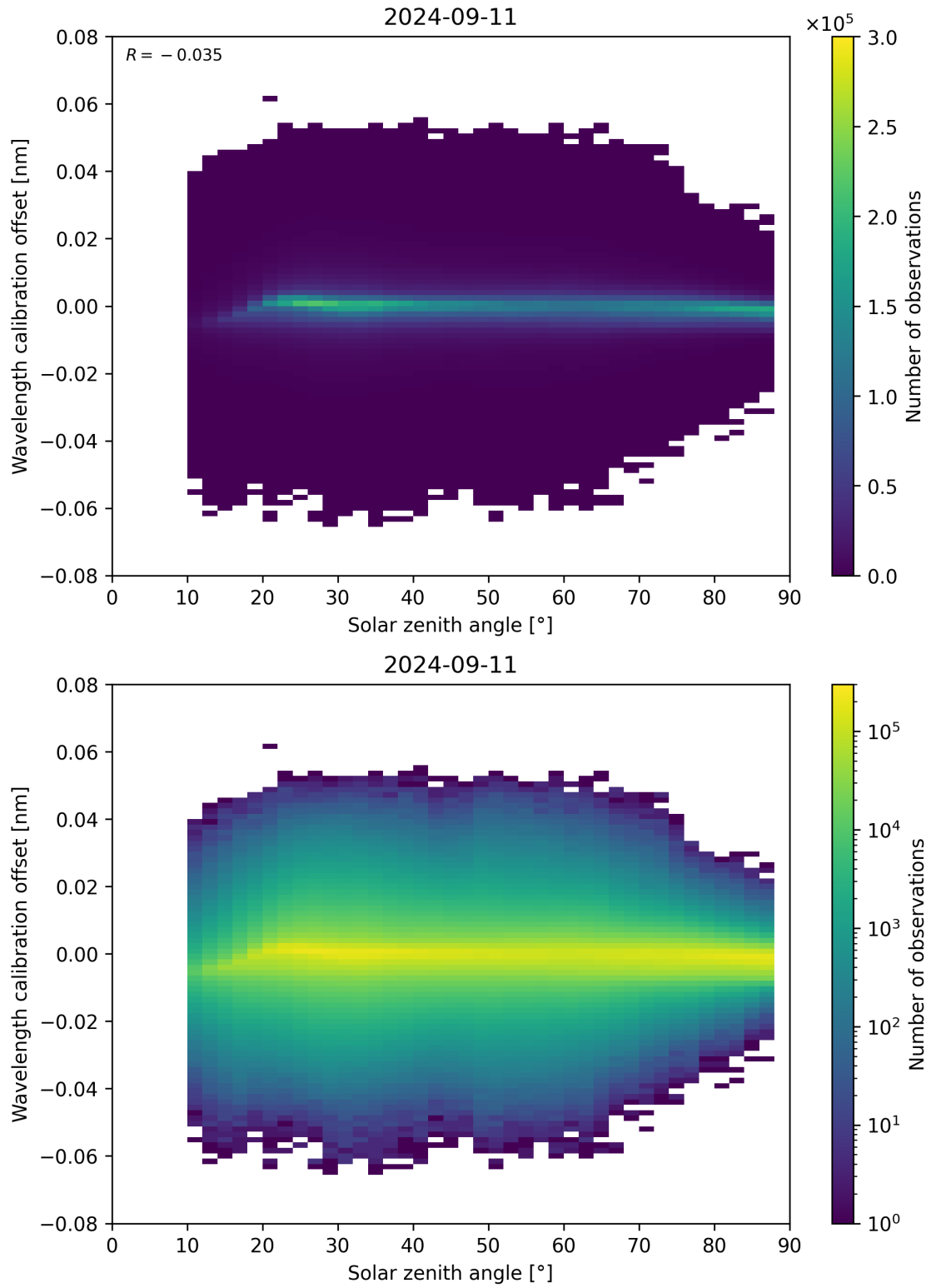
Figure 158: Scatter density plot of “Solar zenith angle” against “Wavelength calibration offset” for 2024-09-10 to 2024-09-12.
