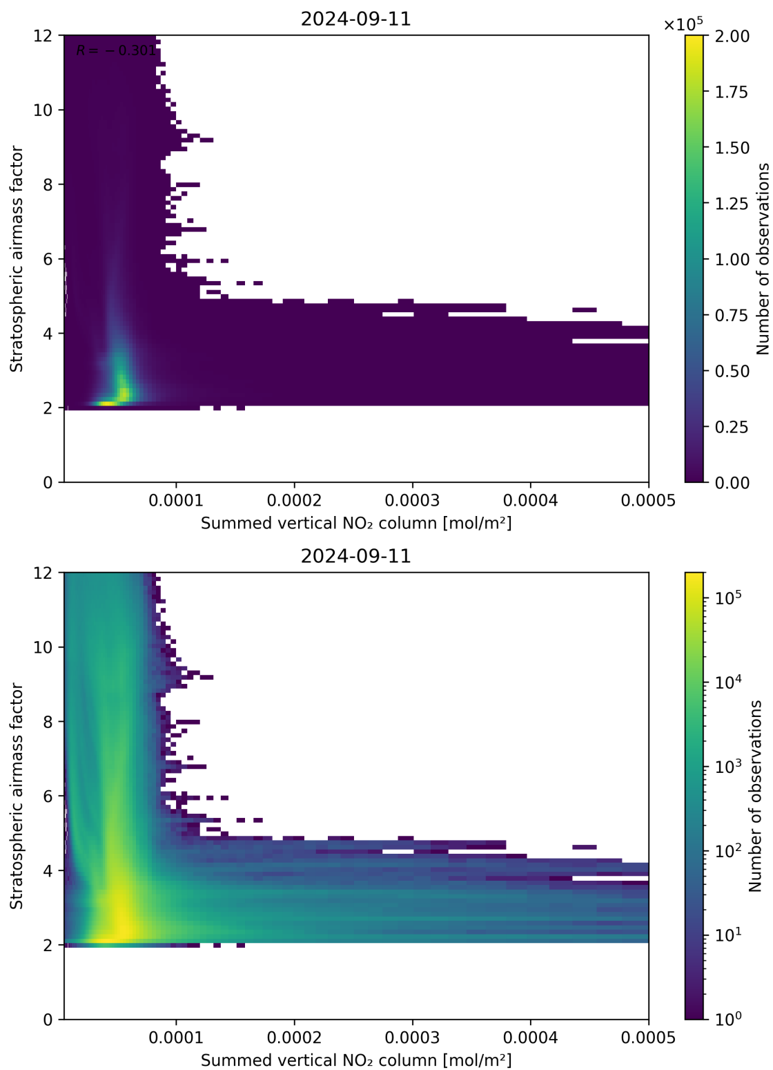
Figure 103: Scatter density plot of “Summed vertical NO 2 column” against “Stratospheric airmass factor” for 2024-09-10 to 2024-09-12.
