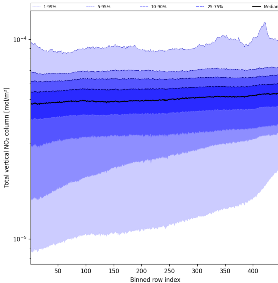
Figure 55: Along track statistics of “Total vertical NO 2 column” for 2024-09-10 to 2024-09-12
