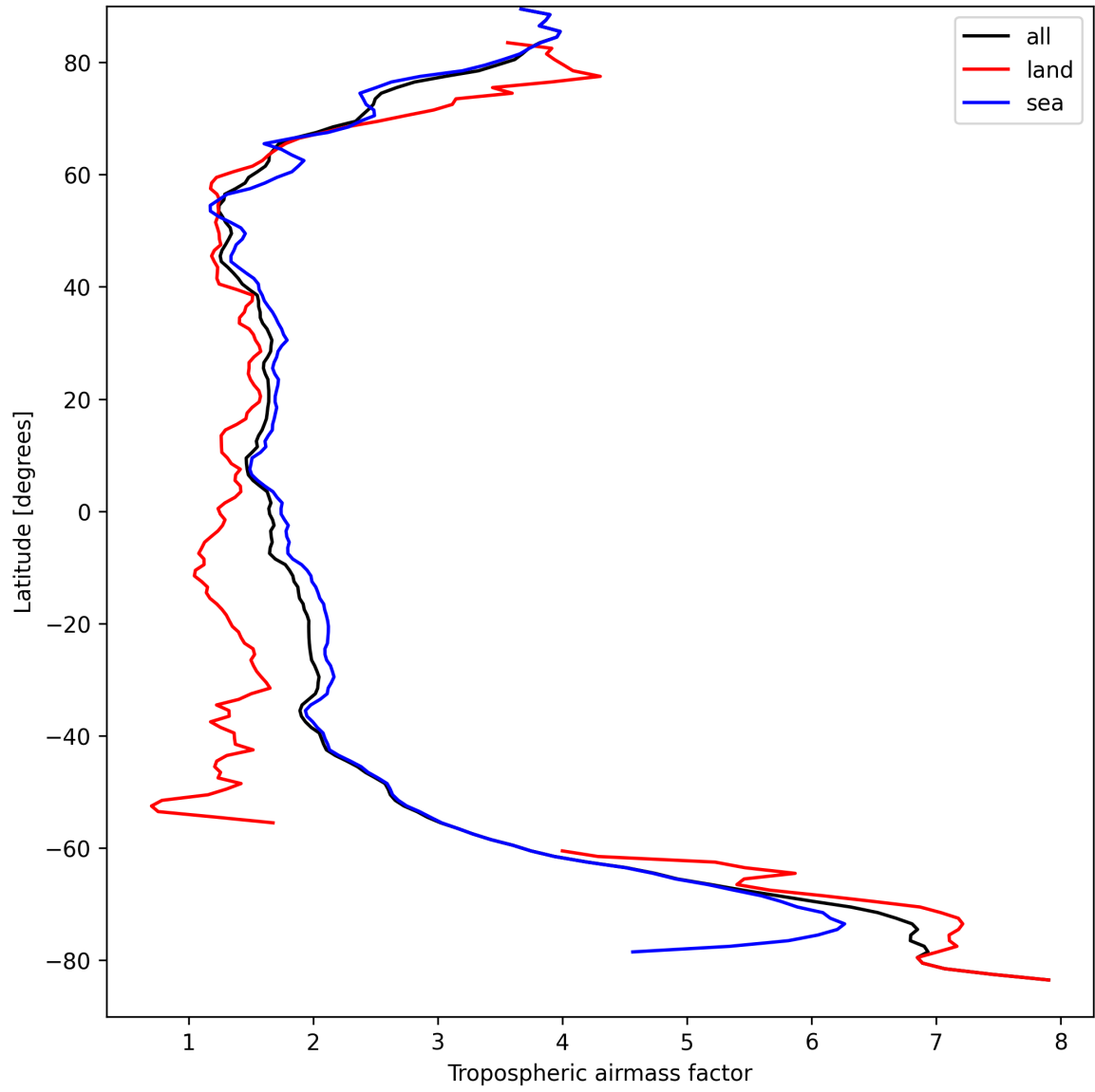
Figure 14: Zonal average of “Tropospheric air mass factor” for 2024-09-10 to 2024-09-12.
