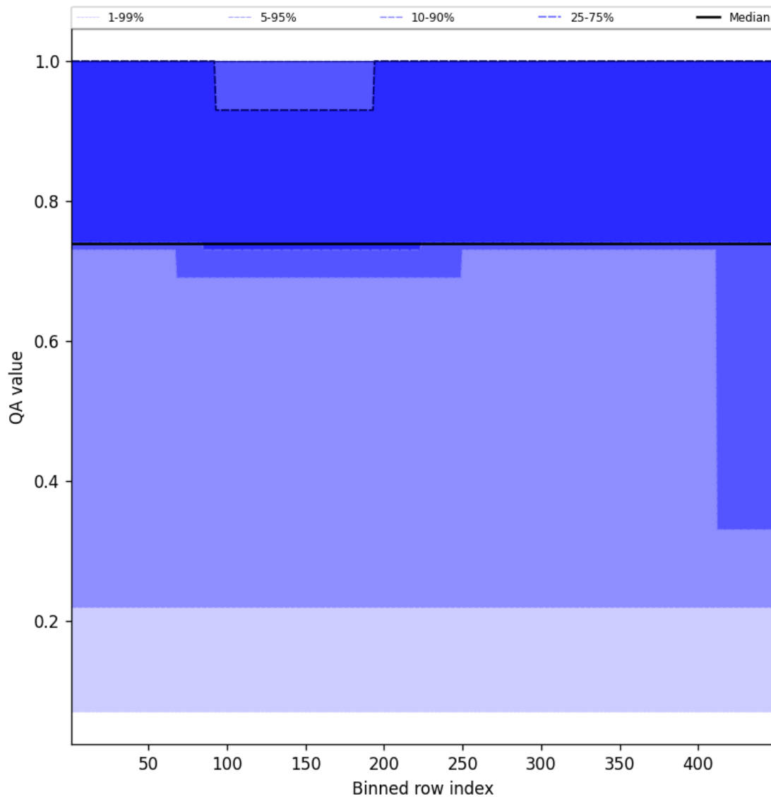
Figure 45: Along track statistics of “QA value” for 2024-09-10 to 2024-09-12
