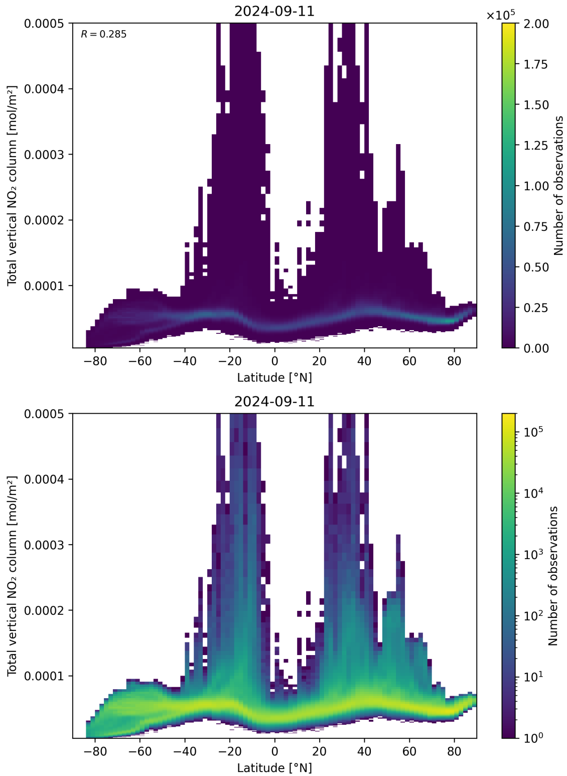
Figure 90: Scatter density plot of “Latitude” against “Total vertical NO 2 column” for 2024-09-10 to 2024-09-12.
