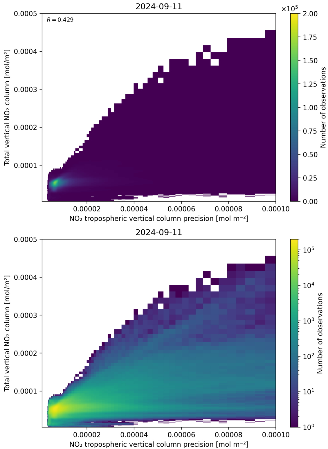
Figure 138: Scatter density plot of “NO 2 tropospheric vertical column precision” against “Total vertical NO 2 column” for 2024-09-10 to 2024-09-12.
