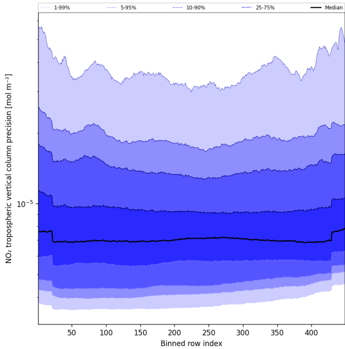
Figure 47: Along track statistics of “NO 2 tropospheric vertical column precision” for 2024-09-10 to 2024-09-12
