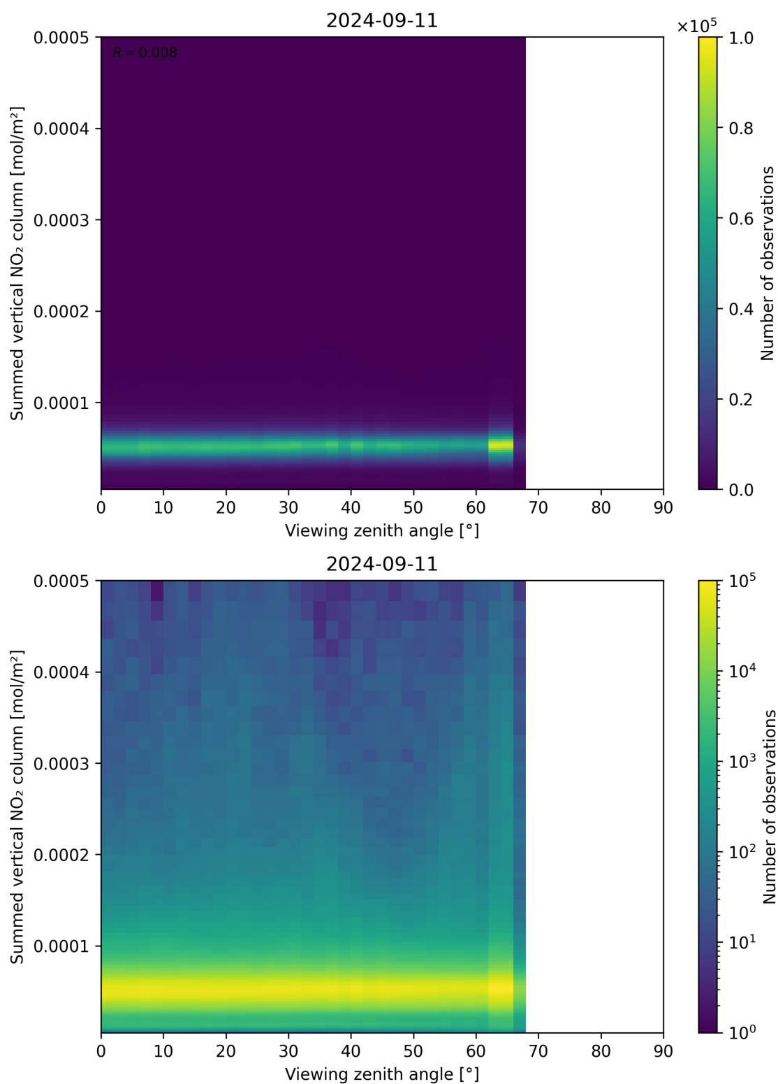
Figure 165: Scatter density plot of “Viewing zenith angle” against “Summed vertical NO 2 column” for 2024-09-10 to 2024-09-12.
