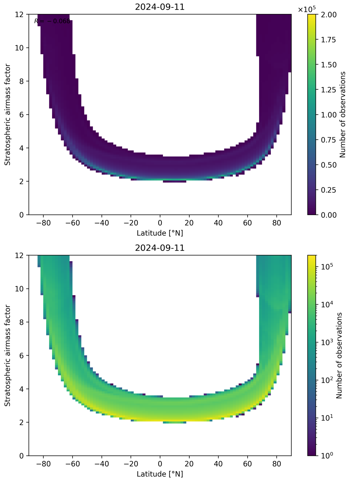
Figure 83: Scatter density plot of “Latitude” against “Stratospheric air mass factor” for 2024-09-10 to 2024-09-12.
