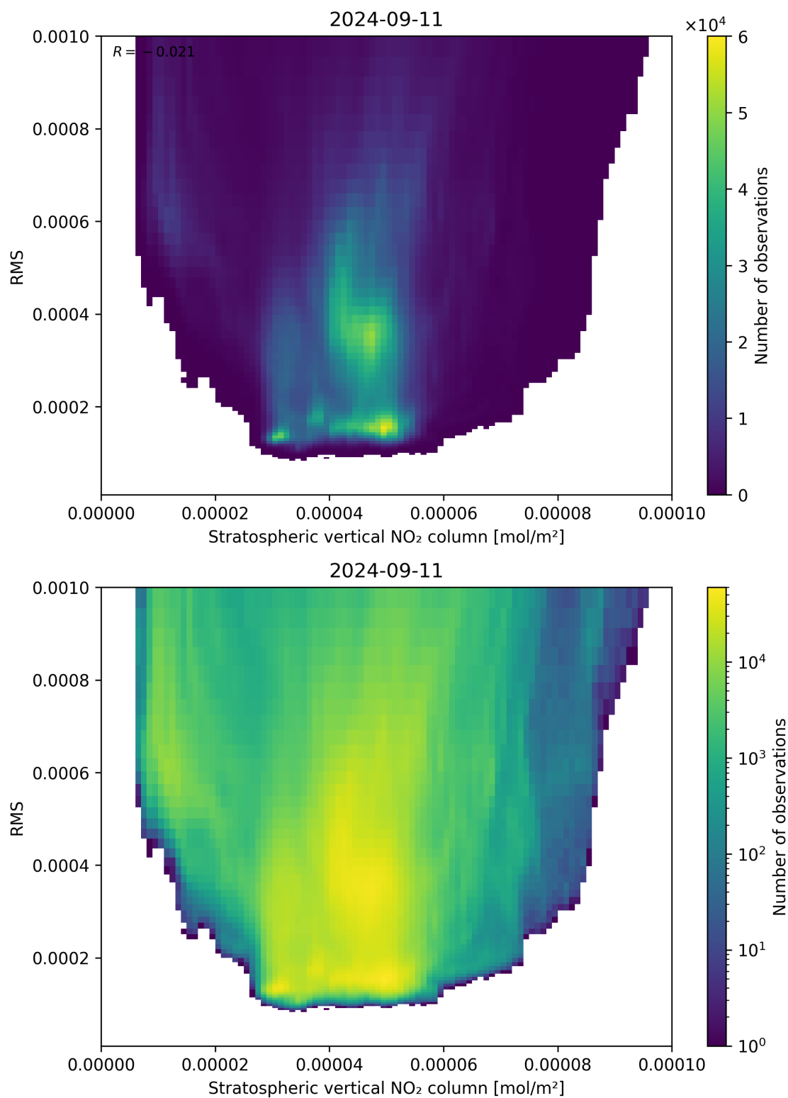
Figure 102: Scatter density plot of “Stratospheric vertical NO 2 column” against “RMS” for 2024-09-10 to 2024-09-12.
