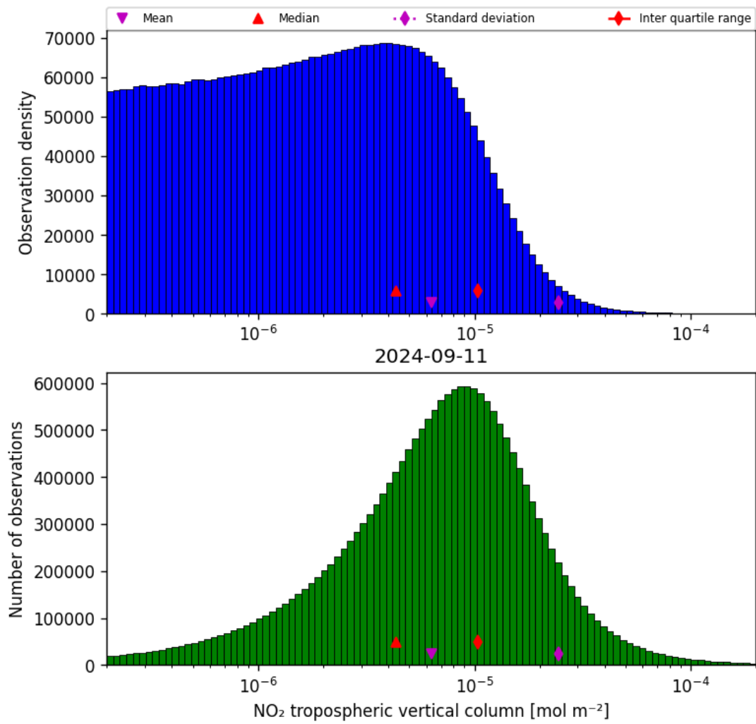
Figure 29: Histogram of “NO 2 tropospheric vertical column” for 2024-09-10 to 2024-09-12
