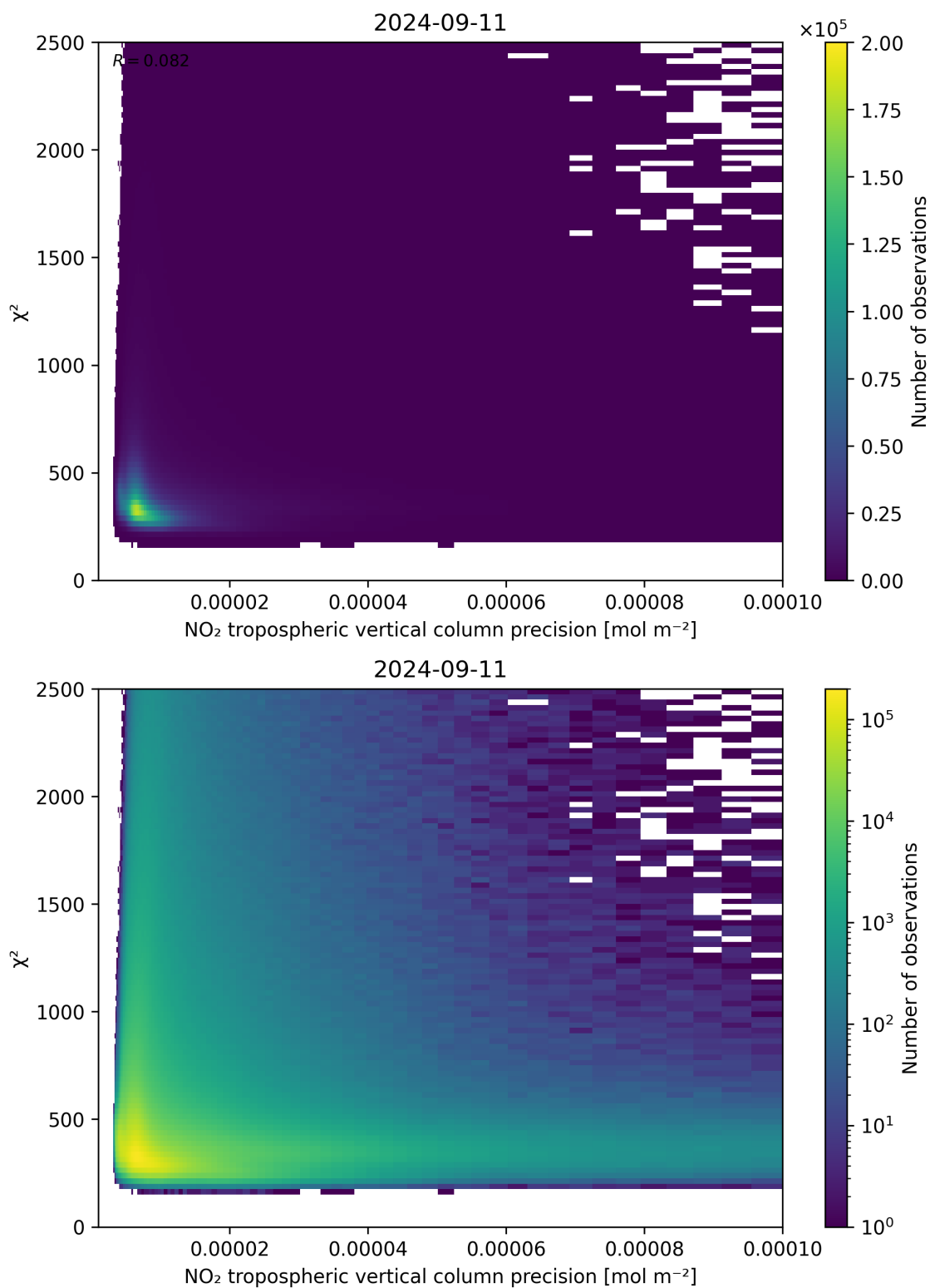
Figure 134: Scatter density plot of “NO 2 tropospheric vertical column precision” against “ \chi^2 ” for 2024-09-10 to 2024-09-12.
