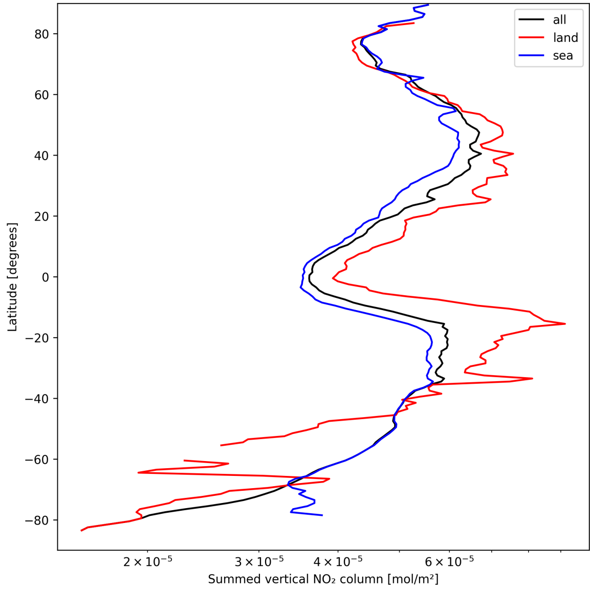
Figure 23: Zonal average of “Summed vertical NO 2 column” for 2024-09-10 to 2024-09-12.
