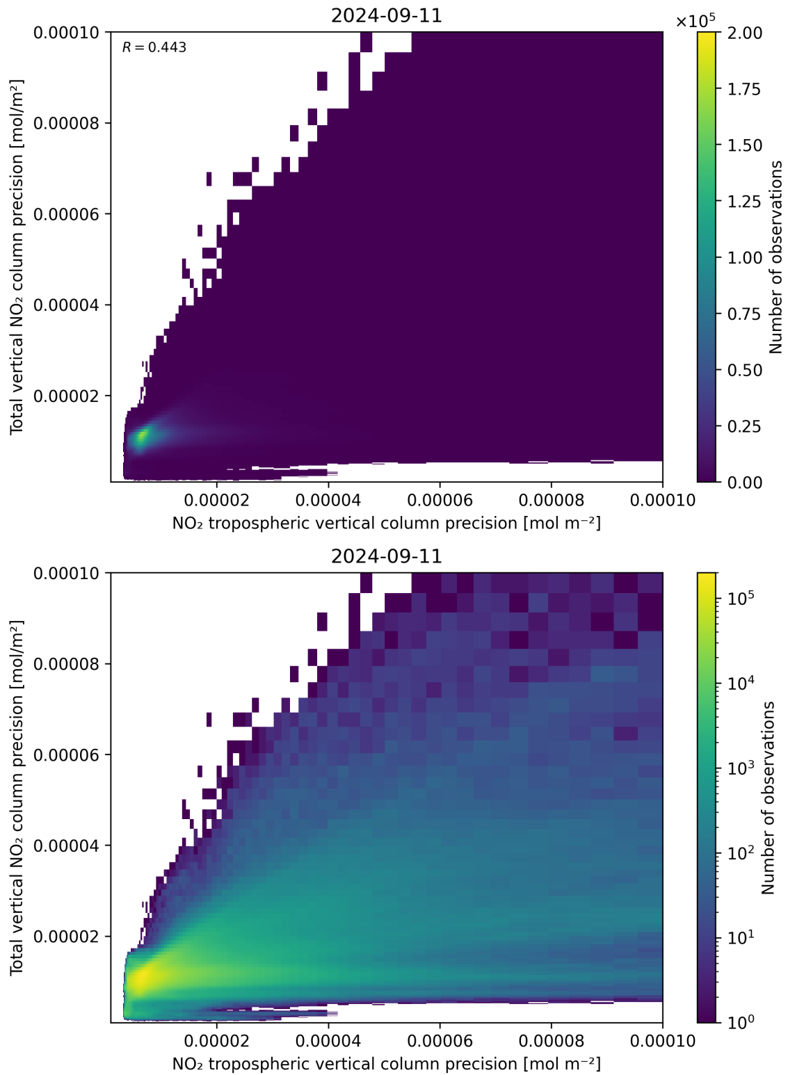
Figure 139: Scatter density plot of “NO 2 tropospheric vertical column precision” against “Total vertical NO 2 column precision” for 2024-09-10 to 2024-09-12.
