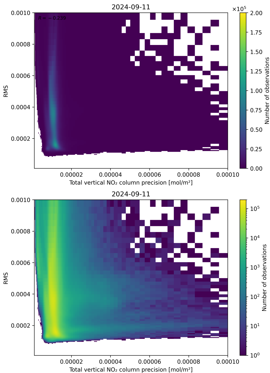
Figure 119: Scatter density plot of “Total vertical NO 2 column precision” against “RMS” for 2024-09-10 to 2024-09-12.
