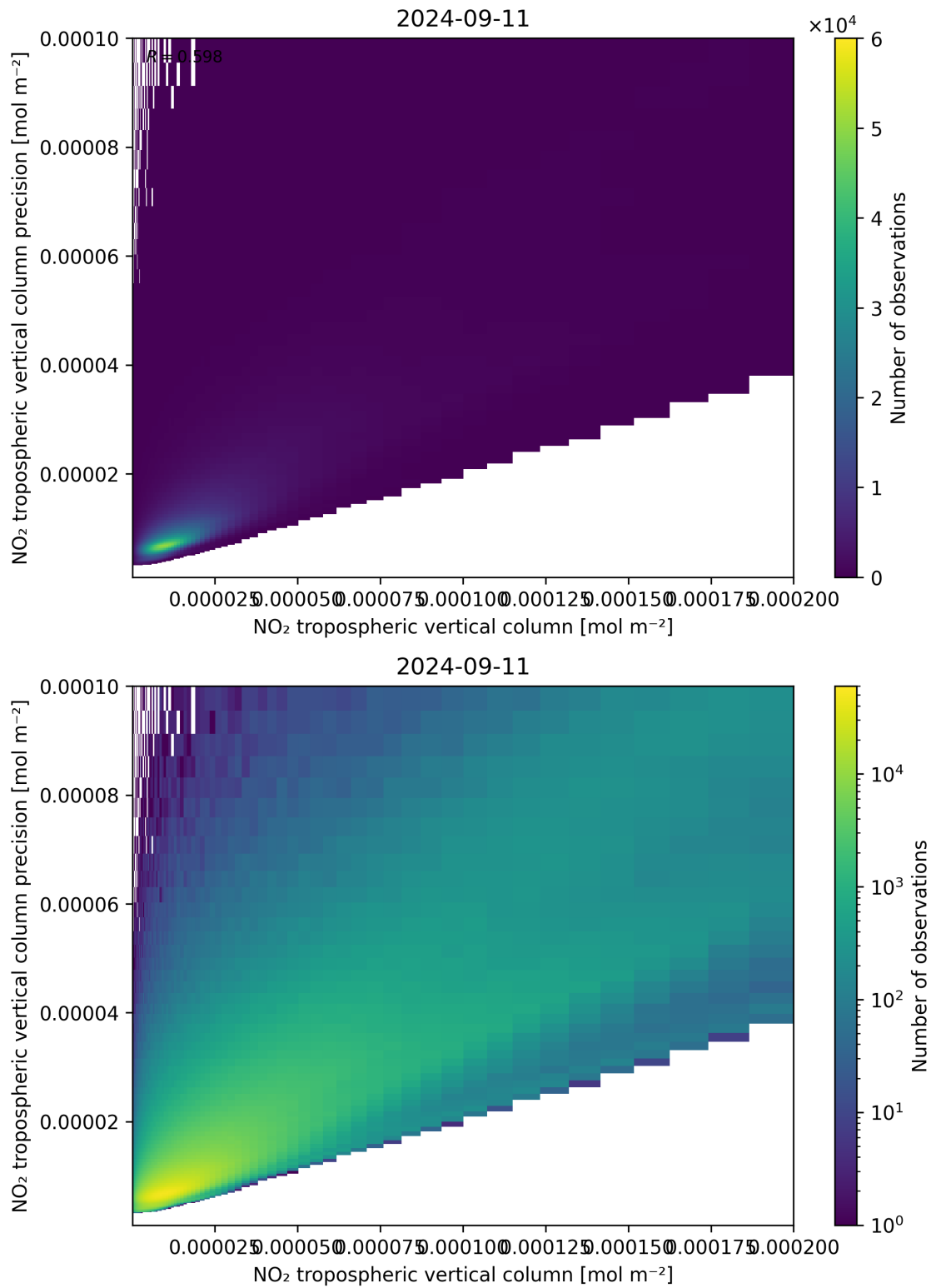
Figure 130: Scatter density plot of “NO 2 tropospheric vertical column” against “NO 2 tropospheric vertical column precision” for 2024-09-10 to 2024-09-12.
