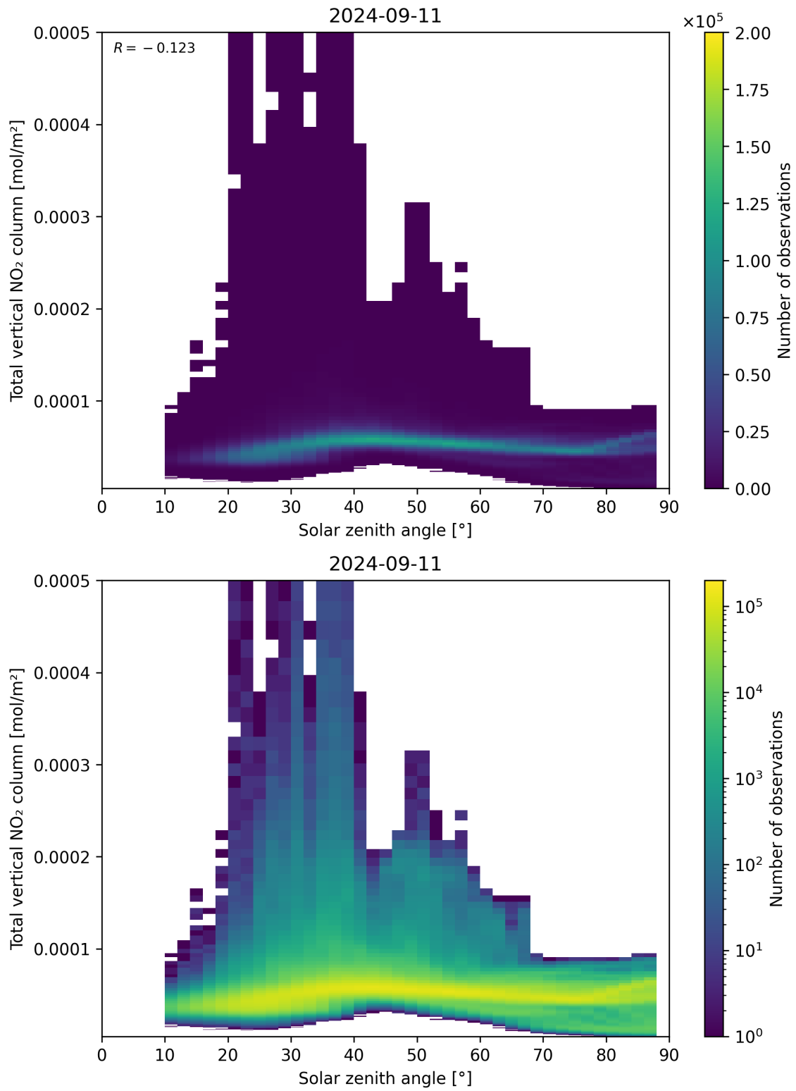
Figure 153: Scatter density plot of “Solar zenith angle” against “Total vertical NO 2 column” for 2024-09-10 to 2024-09-12.
