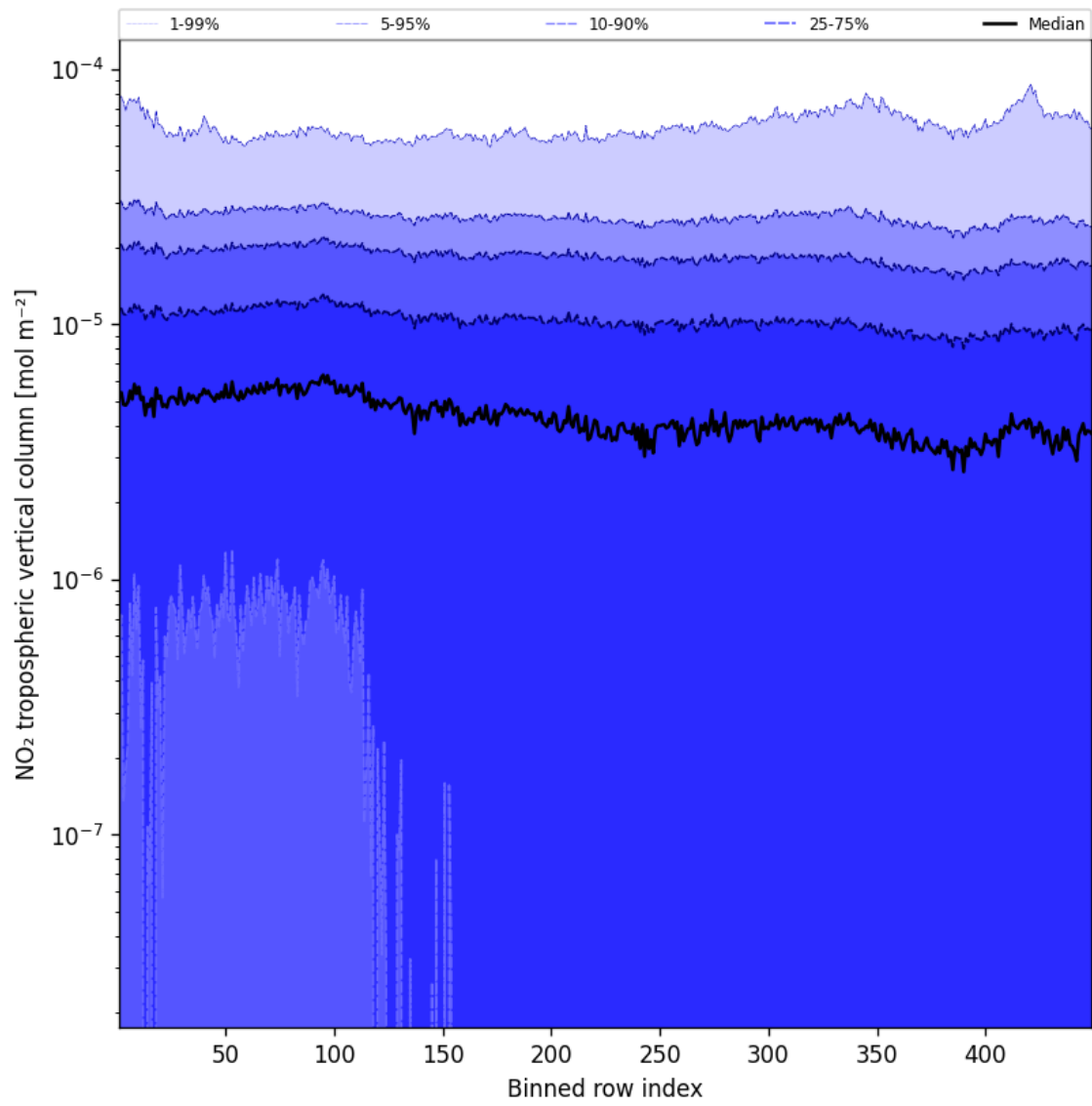
Figure 46: Along track statistics of “NO 2 tropospheric vertical column” for 2024-09-10 to 2024-09-12
