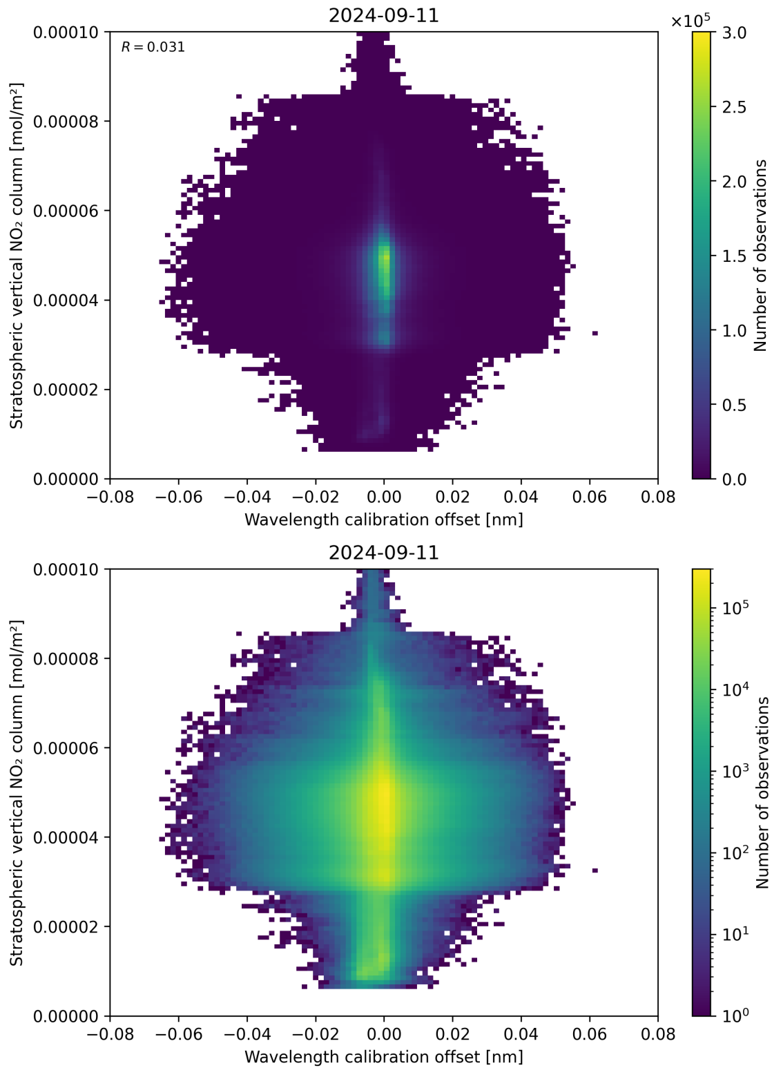
Figure 176: Scatter density plot of “Wavelength calibration offset” against “Stratospheric vertical NO 2 column” for 2024-09-10 to 2024-09-12.
