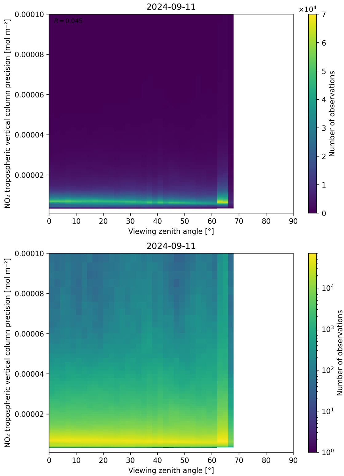
Figure 170: Scatter density plot of “Viewing zenith angle” against “NO 2 tropospheric vertical column precision” for 2024-09-10 to 2024-09-12.
