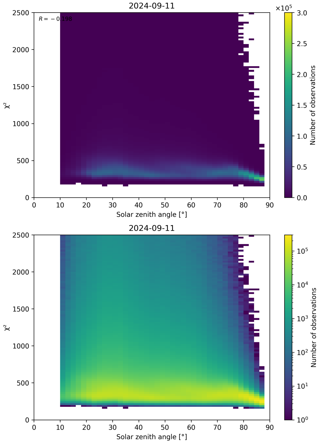
Figure 148: Scatter density plot of “Solar zenith angle” against “ \chi^2 ” for 2024-09-10 to 2024-09-12.
