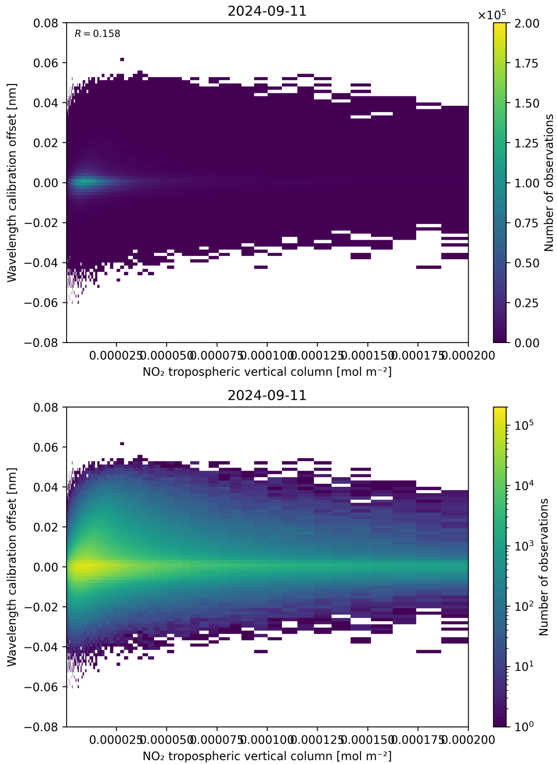
Figure 143: Scatter density plot of “NO 2 tropospheric vertical column” against “Wavelength calibration offset” for 2024-09-10 to 2024-09-12.
