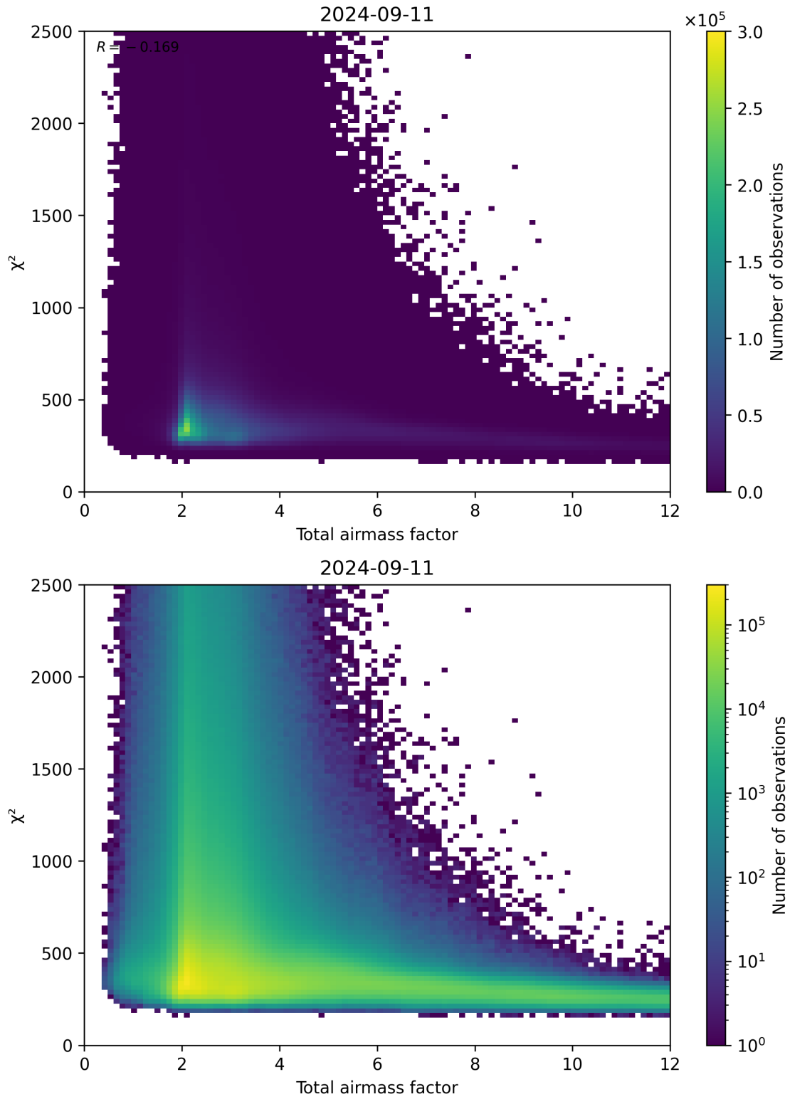
Figure 63: Scatter density plot of “Total airmass factor” against “ \chi^2 ” for 2024-09-10 to 2024-09-12.
