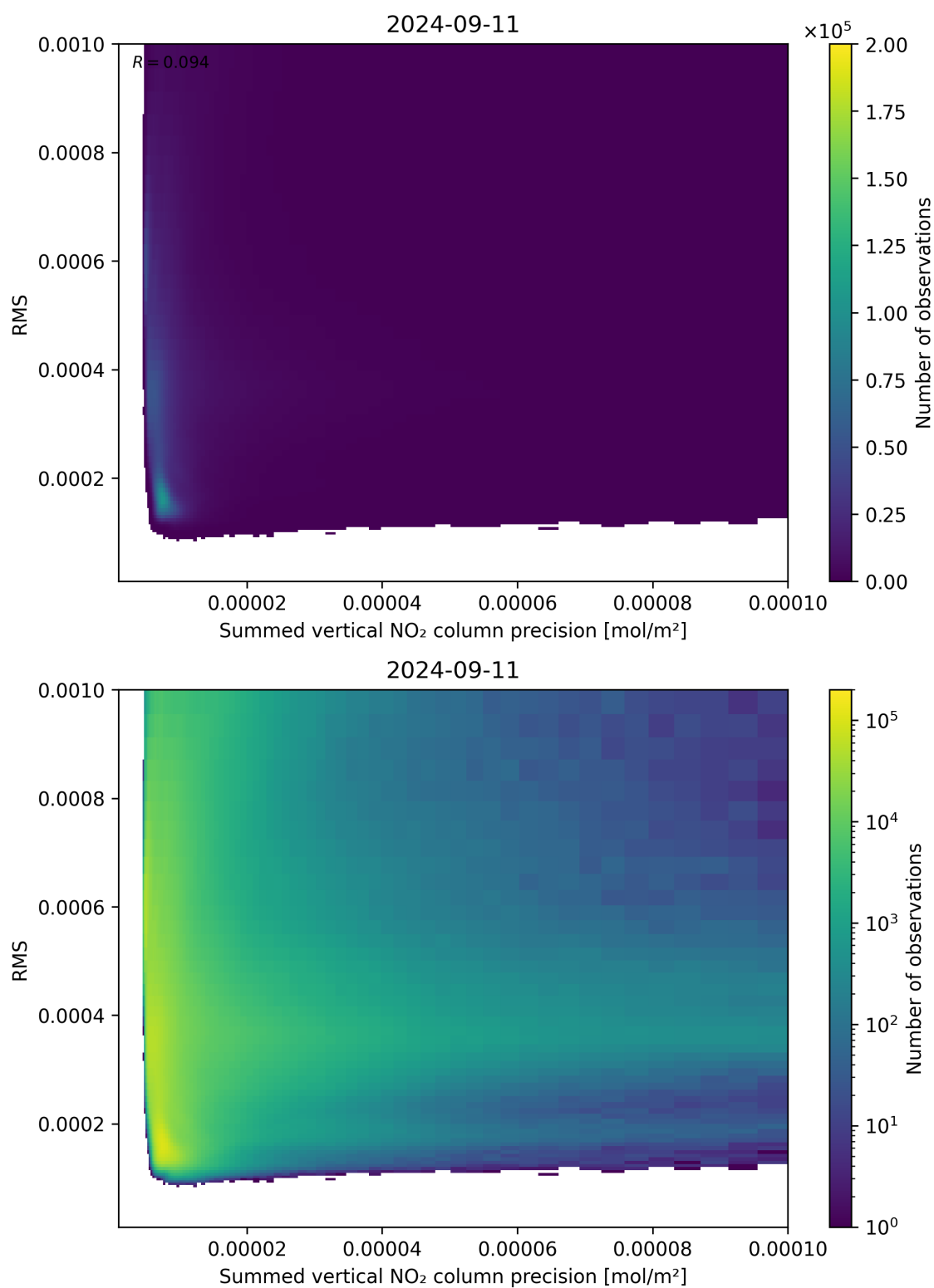
Figure 108: Scatter density plot of “Summed vertical NO 2 column precision” against “RMS” for 2024-09-10 to 2024-09-12.
