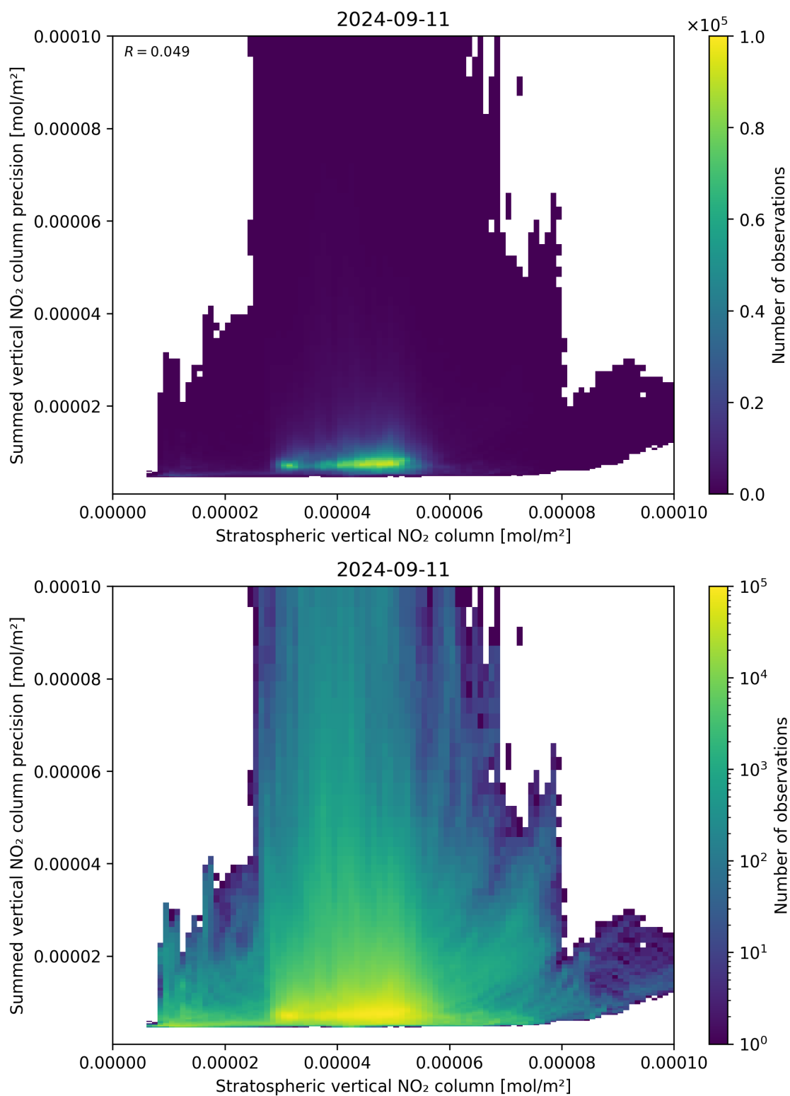
Figure 99: Scatter density plot of “Stratospheric vertical NO 2 column” against “Summed vertical NO 2 column precision” for 2024-09-10 to 2024-09-12.
