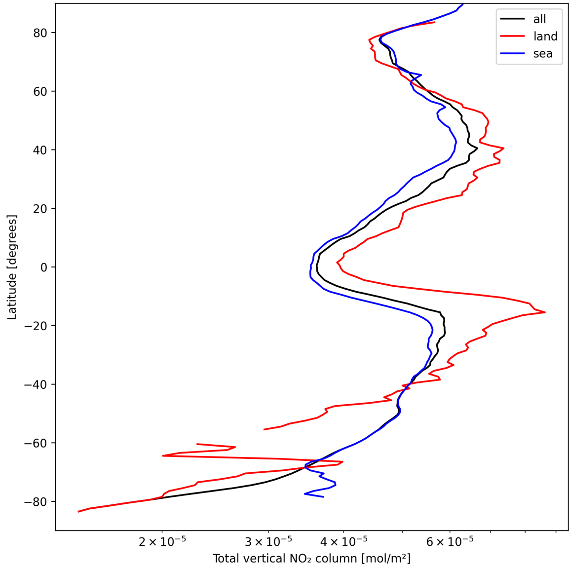
Figure 21: Zonal average of “Total vertical NO 2 column” for 2024-09-10 to 2024-09-12.
