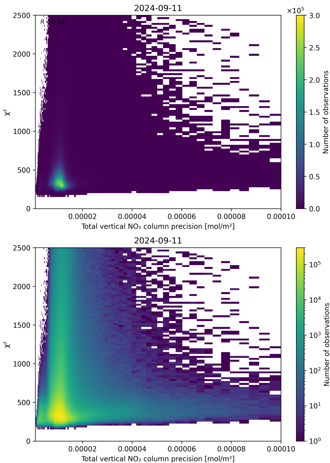
Figure 116: Scatter density plot of “Total vertical NO 2 column precision” against “ \chi^2 ” for 2024-09-10 to 2024-09-12.
