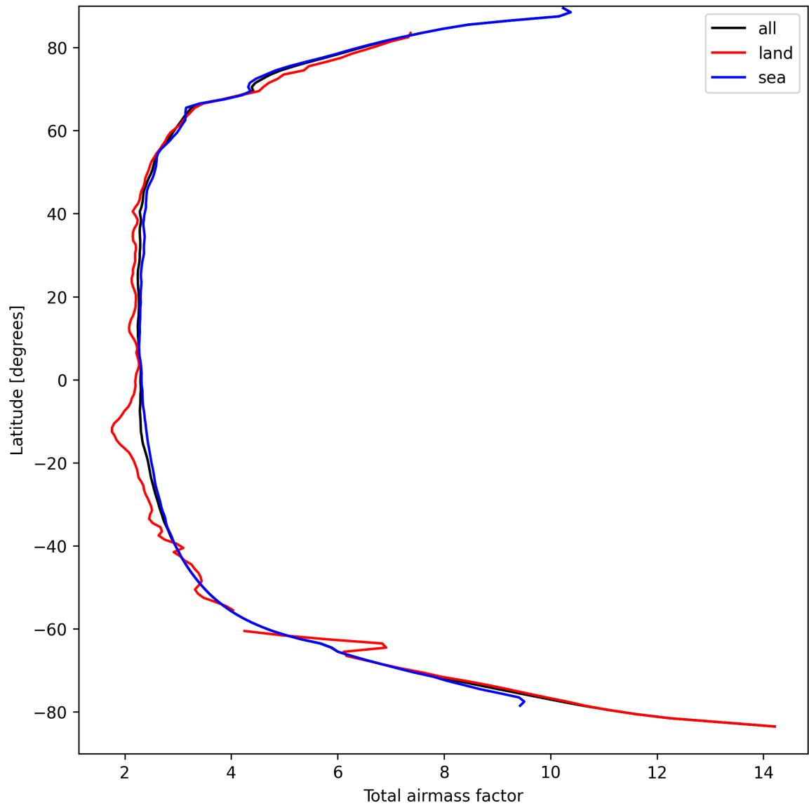
Figure 15: Zonal average of “Total airmass factor” for 2024-09-10 to 2024-09-12.
