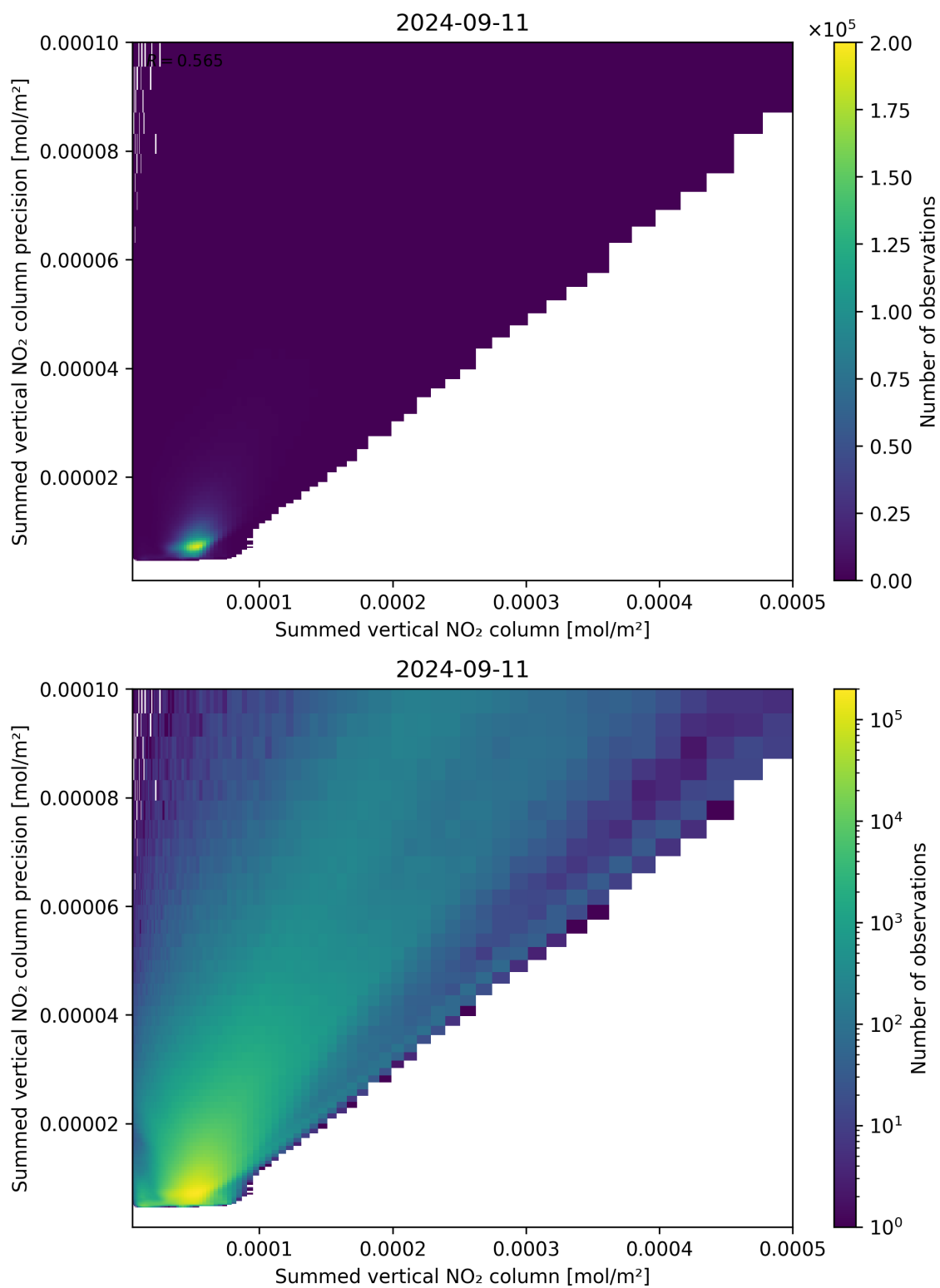
Figure 105: Scatter density plot of “Summed vertical NO 2 column” against “Summed vertical NO 2 column precision” for 2024-09-10 to 2024-09-12.
