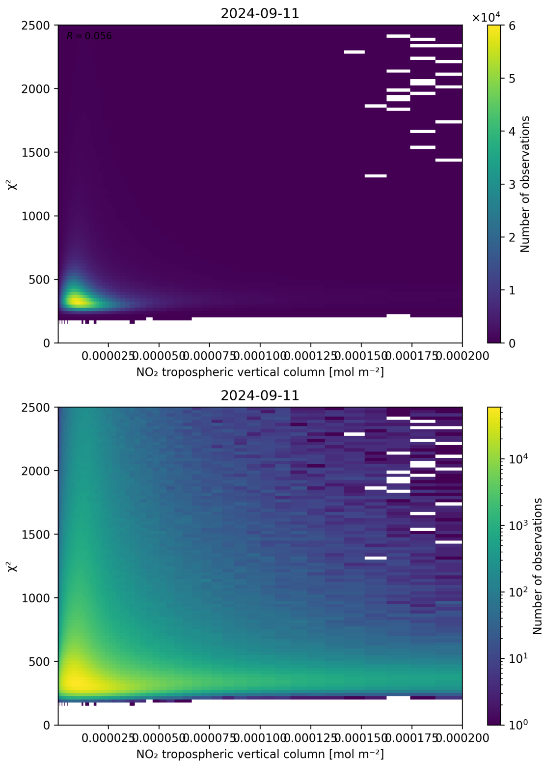
Figure 124: Scatter density plot of “NO 2 tropospheric vertical column” against “ \chi^2 ” for 2024-09-10 to 2024-09-12.
