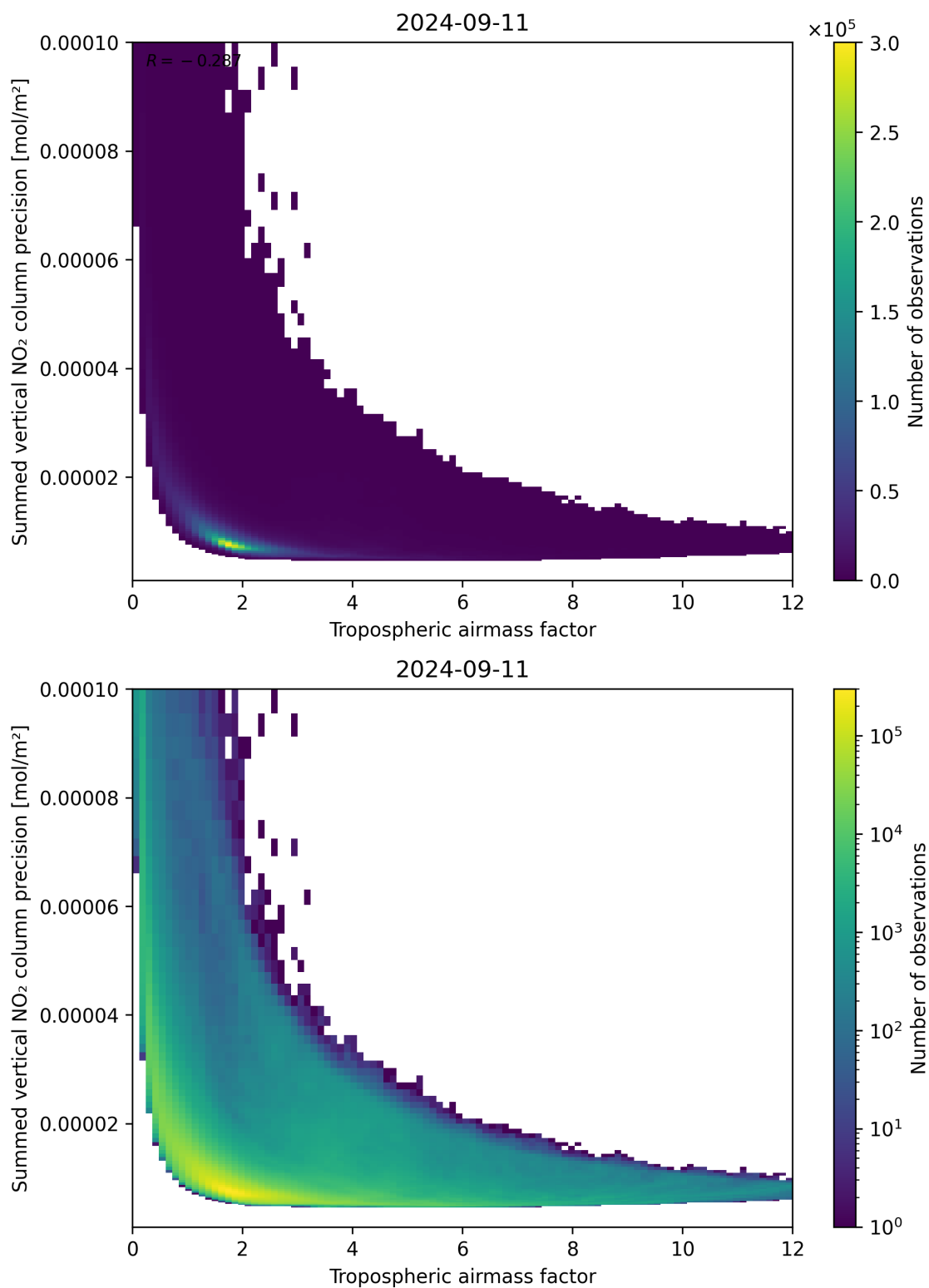
Figure 76: Scatter density plot of “Tropospheric air mass factor” against “Summed vertical NO 2 column precision” for 2024-09-10 to 2024-09-12.
