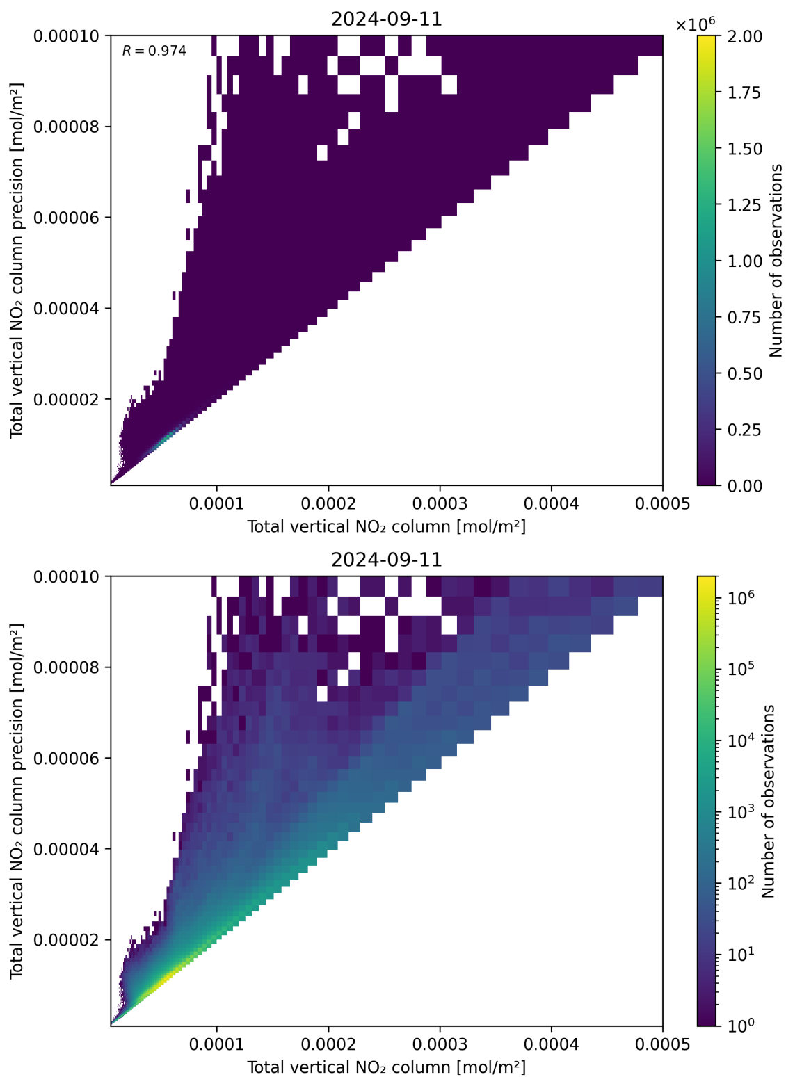
Figure 114: Scatter density plot of “Total vertical NO 2 column” against “Total vertical NO 2 column precision” for 2024-09-10 to 2024-09-12.
