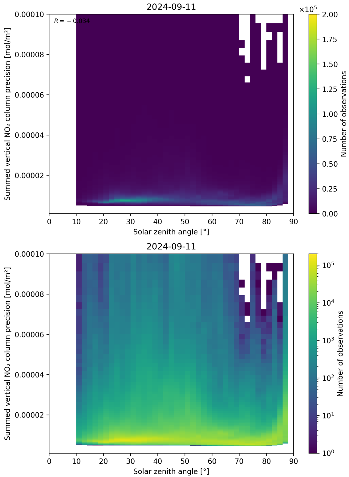
Figure 152: Scatter density plot of “Solar zenith angle” against “Summed vertical NO 2 column precision” for 2024-09-10 to 2024-09-12.
