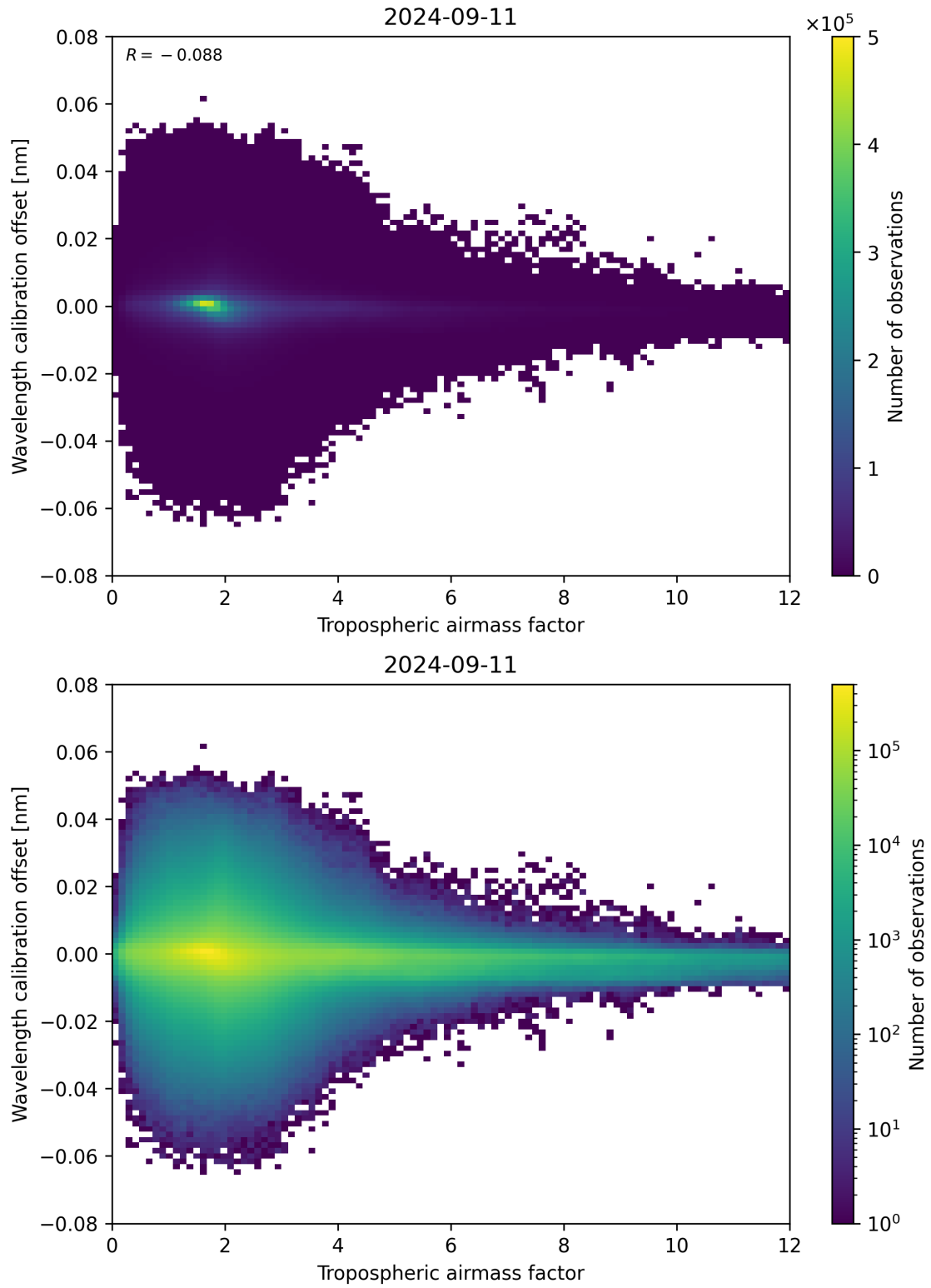
Figure 80: Scatter density plot of “Tropospheric airmass factor” against “Wavelength calibration offset” for 2024-09-10 to 2024-09-12.
