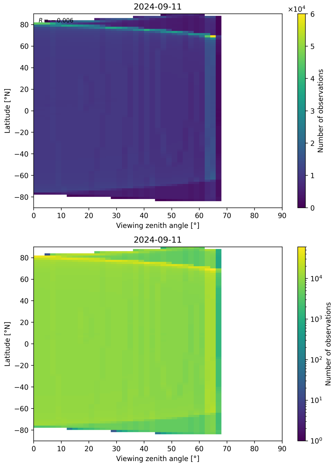
Figure 163: Scatter density plot of “Viewing zenith angle” against “Latitude” for 2024-09-10 to 2024-09-12.
