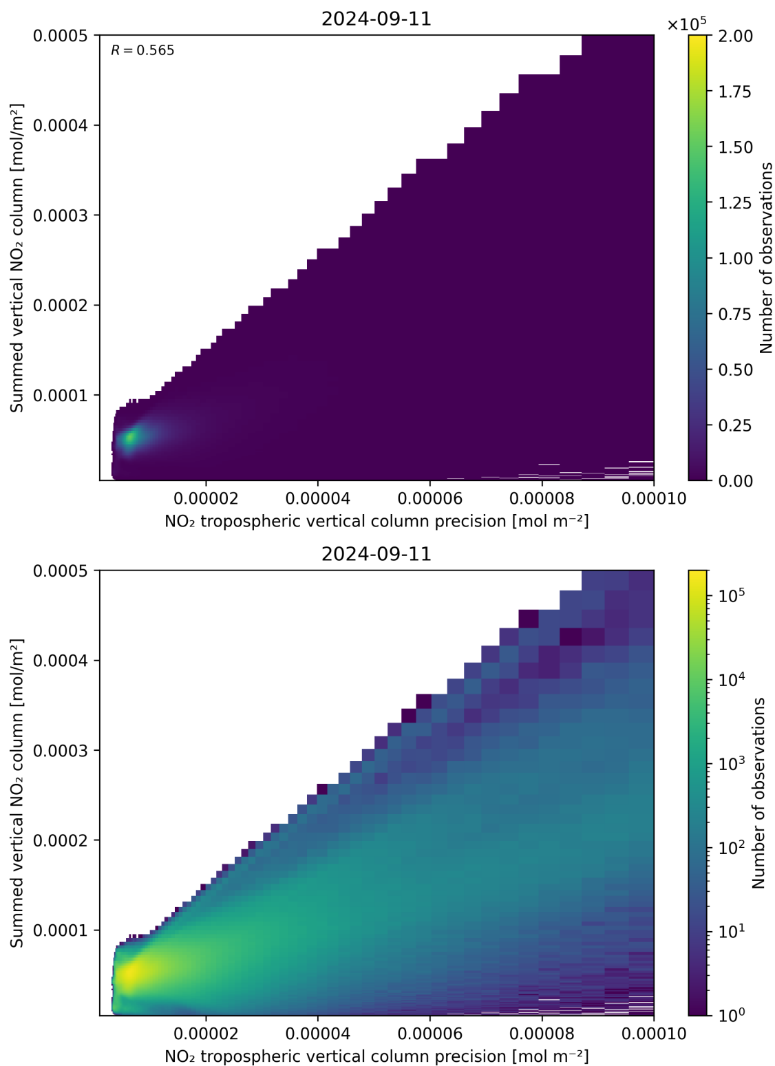
Figure 136: Scatter density plot of “NO 2 tropospheric vertical column precision” against “Summed vertical NO 2 column” for 2024-09-10 to 2024-09-12.
