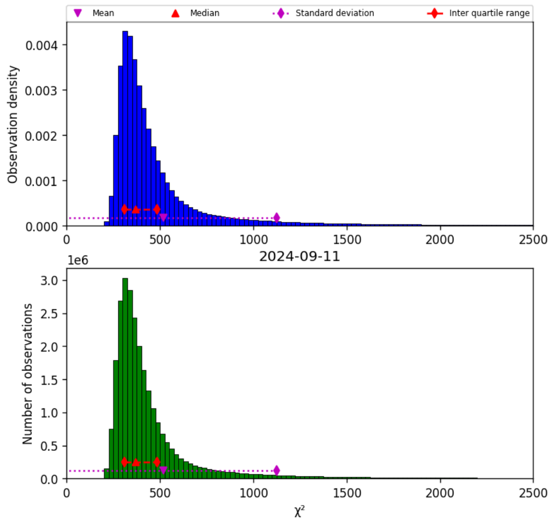
Figure 42: Histogram of “ \chi^2 ” for 2024-09-10 to 2024-09-12
