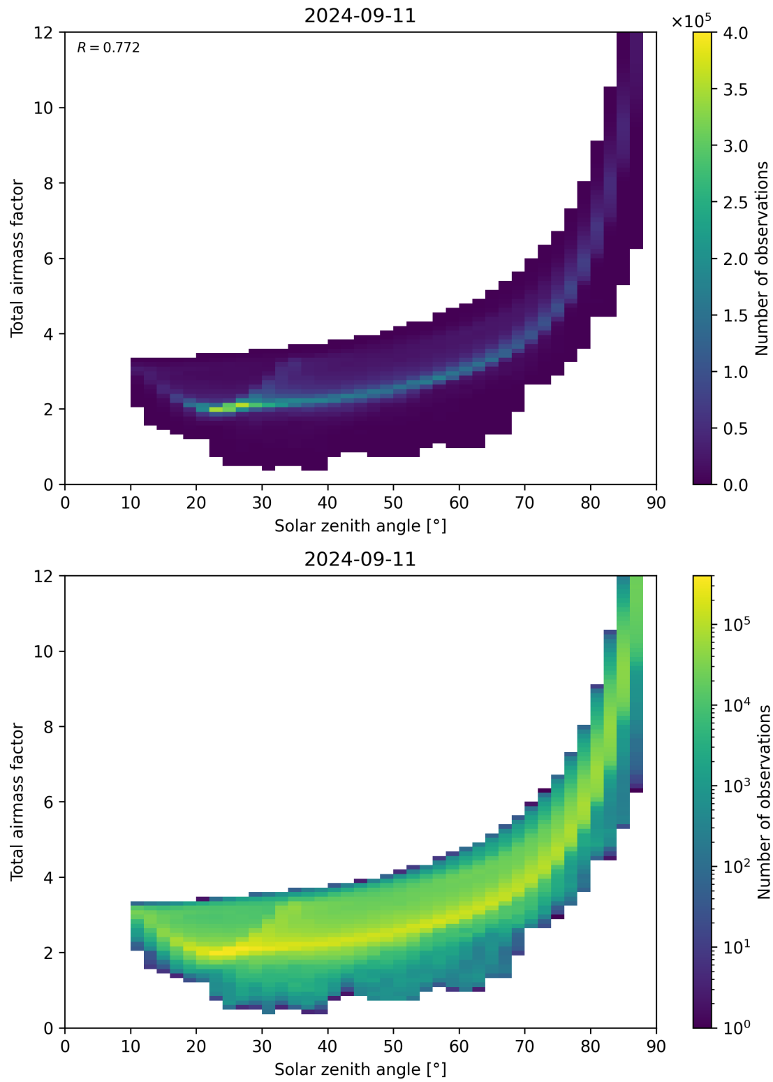
Figure 146: Scatter density plot of “Solar zenith angle” against “Total air mass factor” for 2024-09-10 to 2024-09-12.
