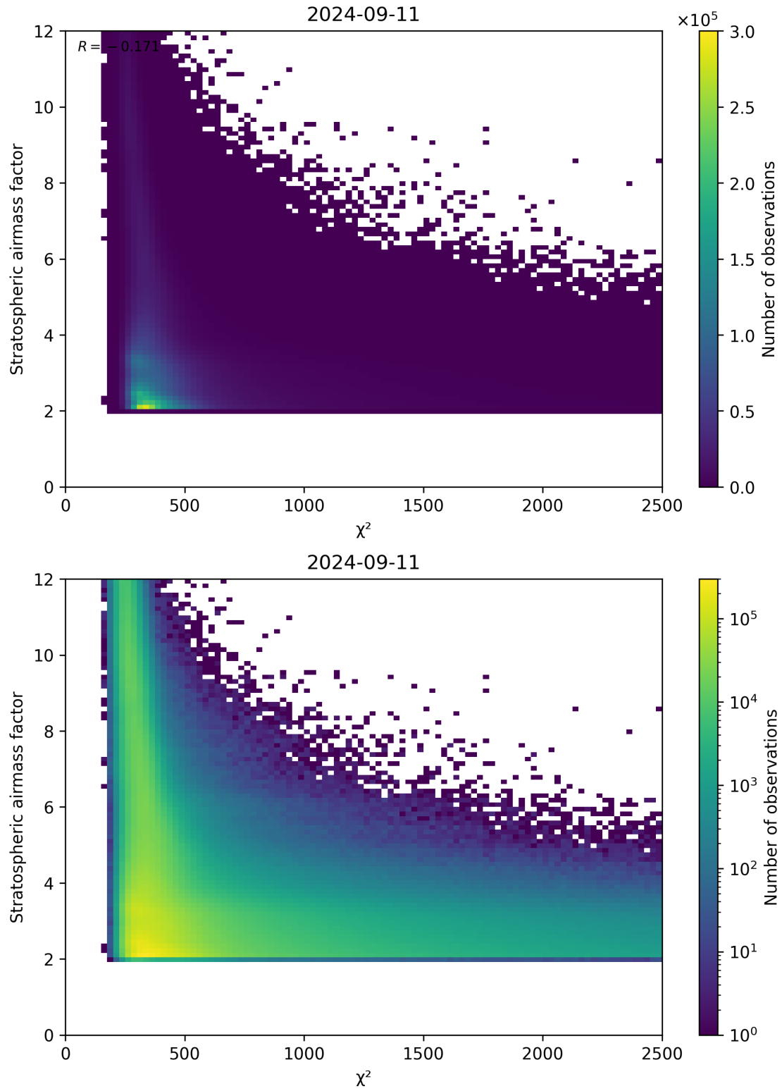
Figure 81: Scatter density plot of “ \chi^2 ” against “Stratospheric airmass factor” for 2024-09-10 to 2024-09-12.
