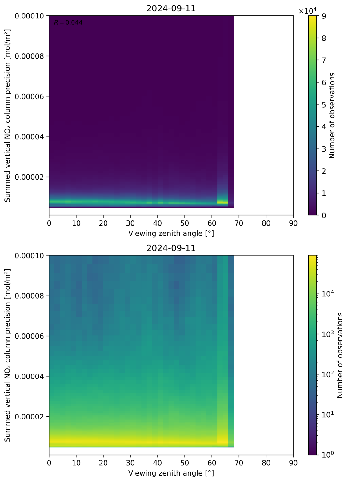
Figure 166: Scatter density plot of “Viewing zenith angle” against “Summed vertical NO 2 column precision” for 2024-09-10 to 2024-09-12.
