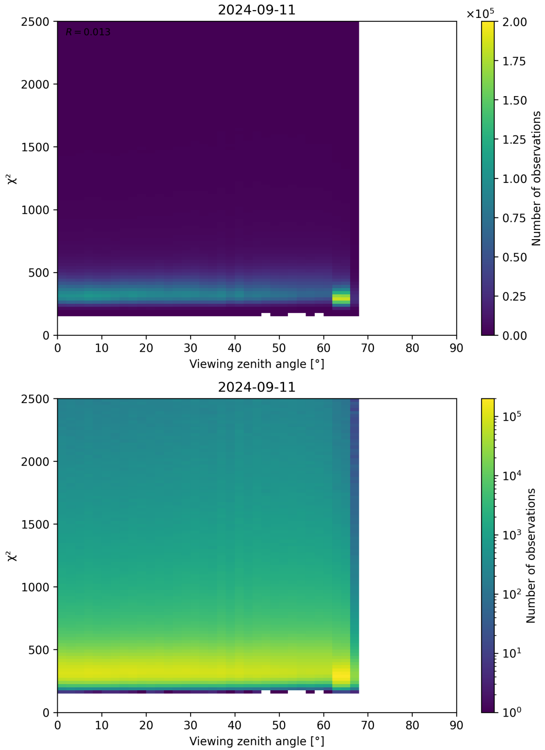
Figure 162: Scatter density plot of “Viewing zenith angle” against “ \chi^2 ” for 2024-09-10 to 2024-09-12.
