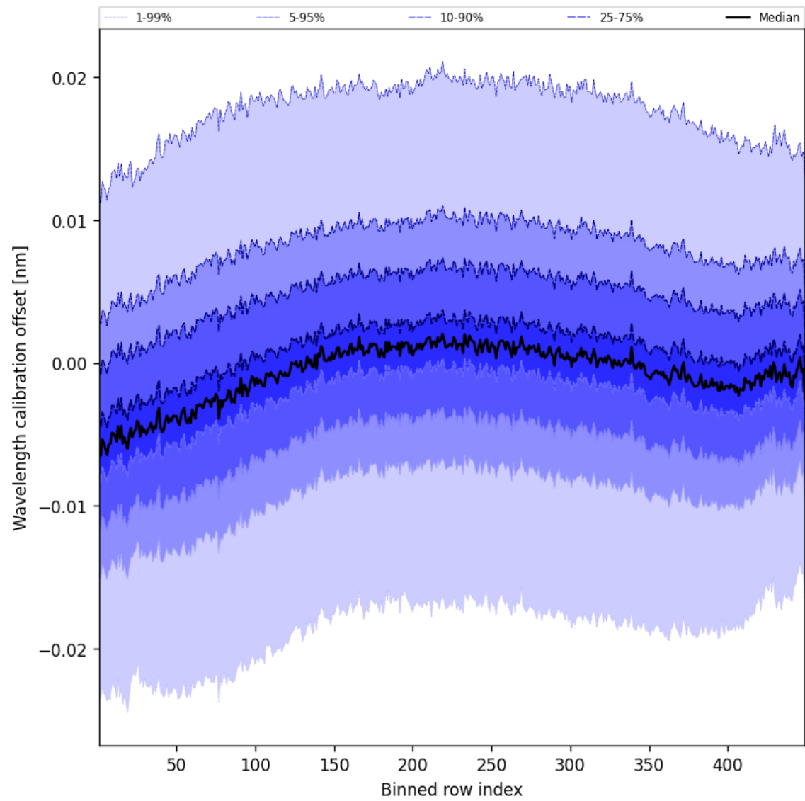
Figure 52: Along track statistics of “Wavelength calibration offset” for 2024-09-10 to 2024-09-12
