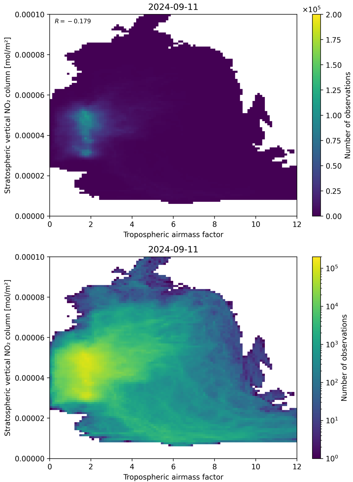
Figure 74: Scatter density plot of “Tropospheric air mass factor” against “Stratospheric vertical NO 2 column” for 2024-09-10 to 2024-09-12.
