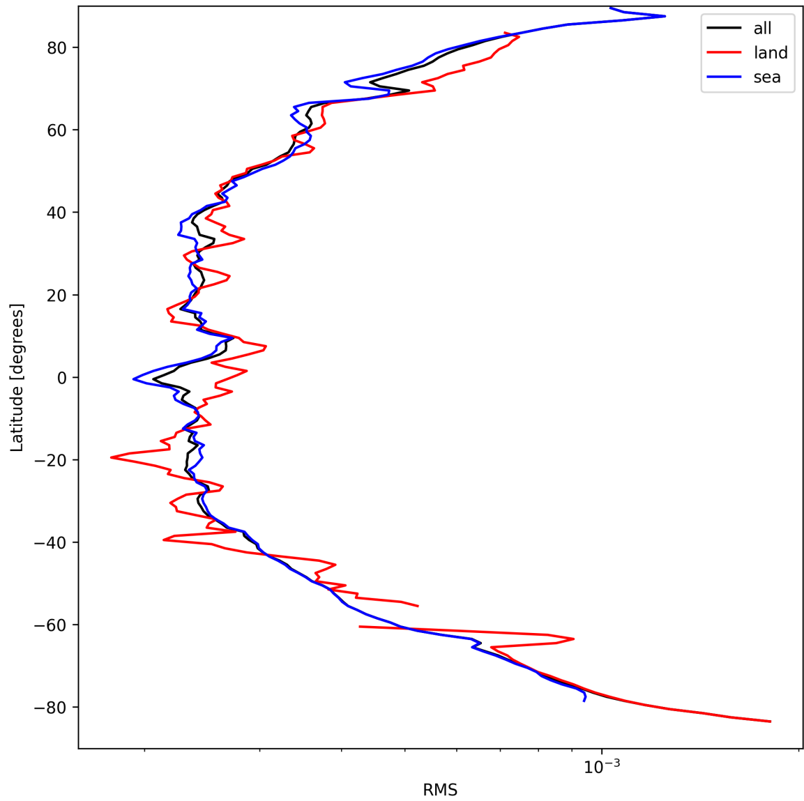
Figure 26: Zonal average of “RMS” for 2024-09-10 to 2024-09-12.
