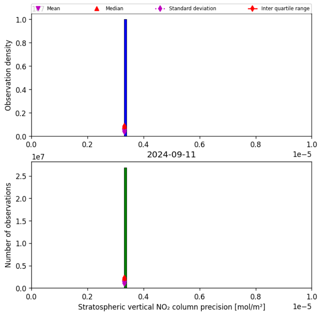
Figure 37: Histogram of “Stratospheric vertical NO 2 column precision” for 2024-09-10 to 2024-09-12
