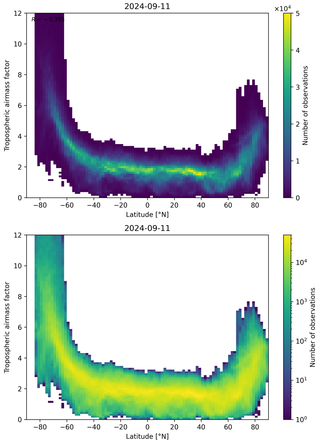
Figure 85: Scatter density plot of “Latitude” against “Tropospheric air mass factor” for 2024-09-10 to 2024-09-12.
