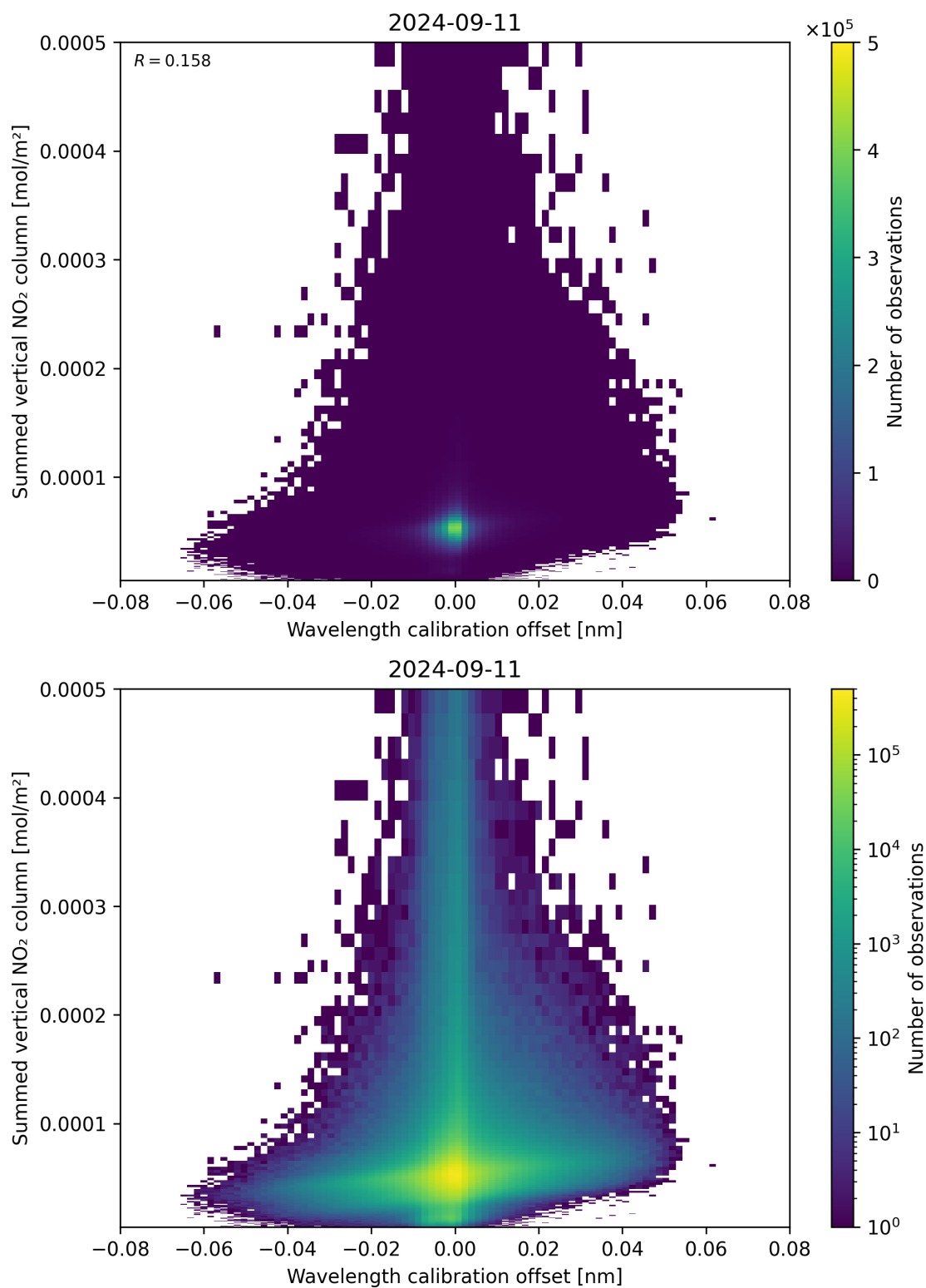
Figure 177: Scatter density plot of “Wavelength calibration offset” against “Summed vertical NO 2 column” for 2024-09-10 to 2024-09-12.
