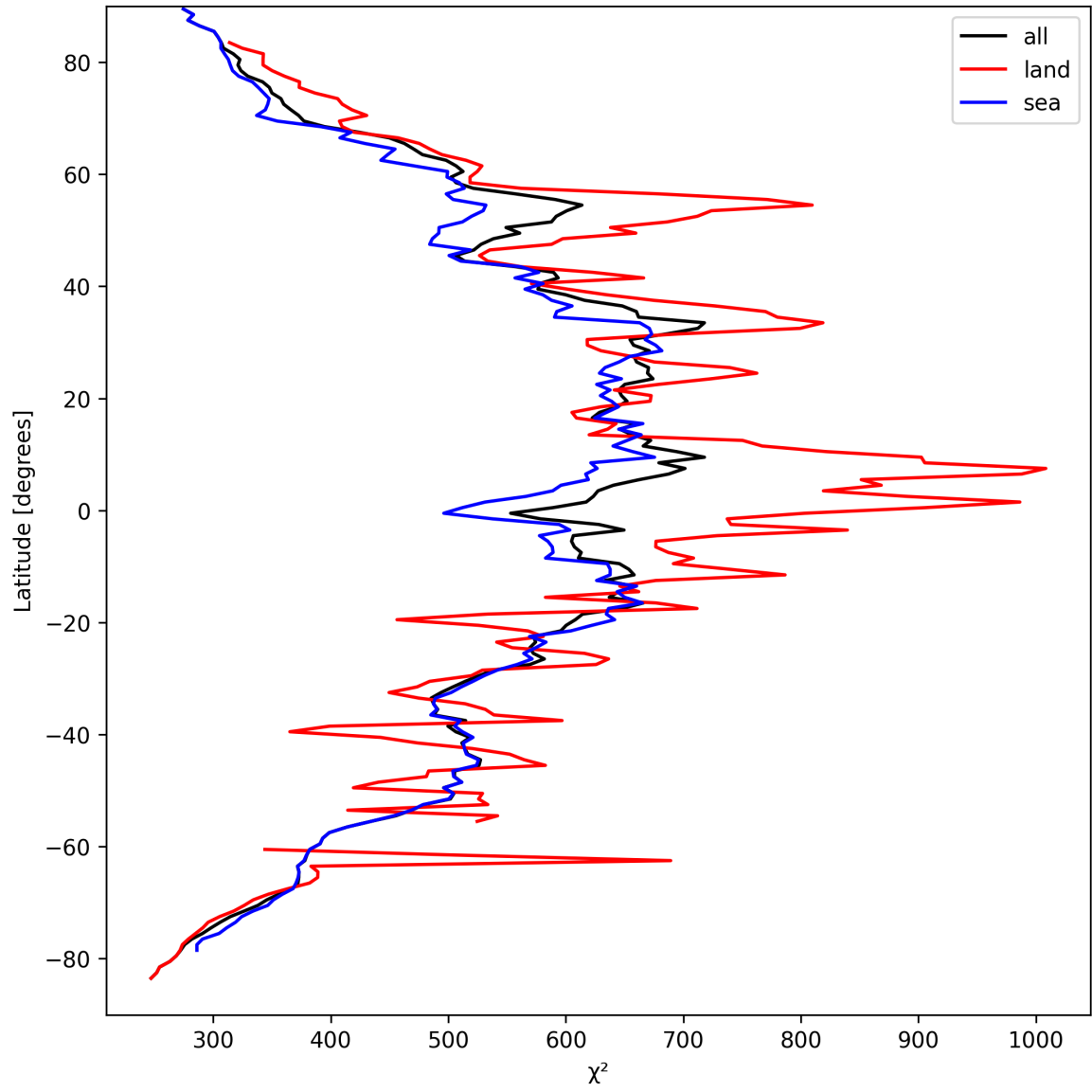
Figure 25: Zonal average of “ \chi^2 ” for 2024-09-10 to 2024-09-12.
