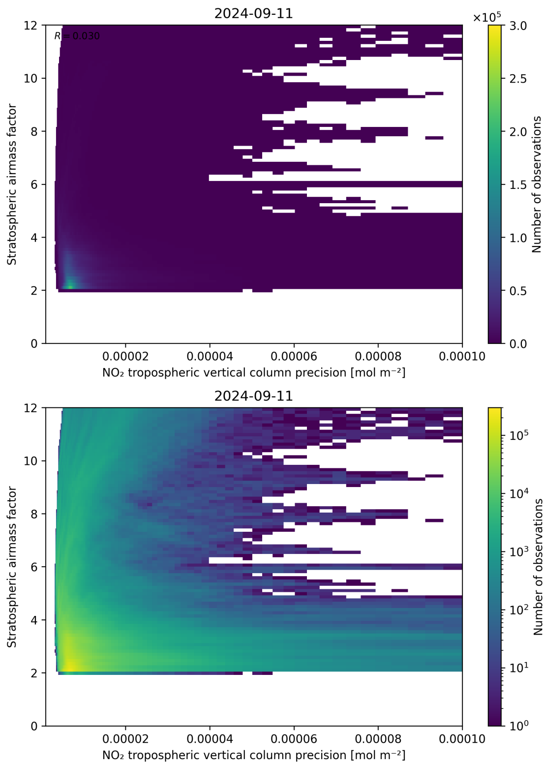
Figure 131: Scatter density plot of “NO 2 tropospheric vertical column precision” against “Stratospheric airmass factor” for 2024-09-10 to 2024-09-12.
