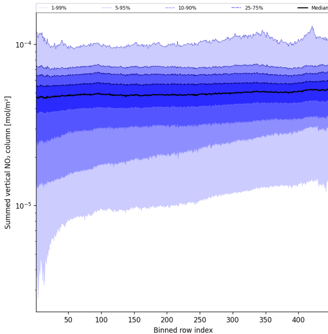
Figure 57: Along track statistics of “Summed vertical NO 2 column” for 2024-09-10 to 2024-09-12
