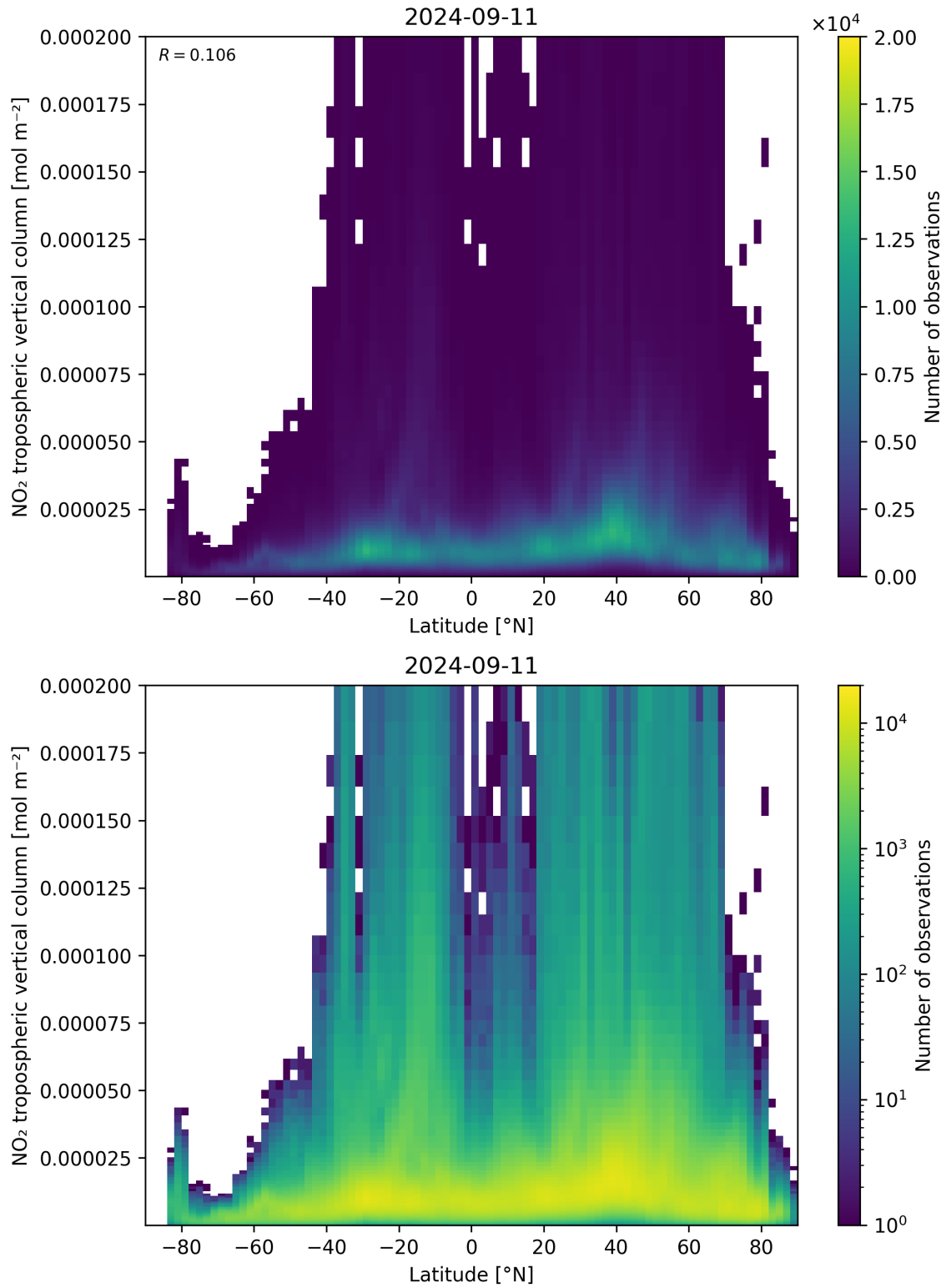
Figure 92: Scatter density plot of “Latitude” against “NO 2 tropospheric vertical column” for 2024-09-10 to 2024-09-12.
