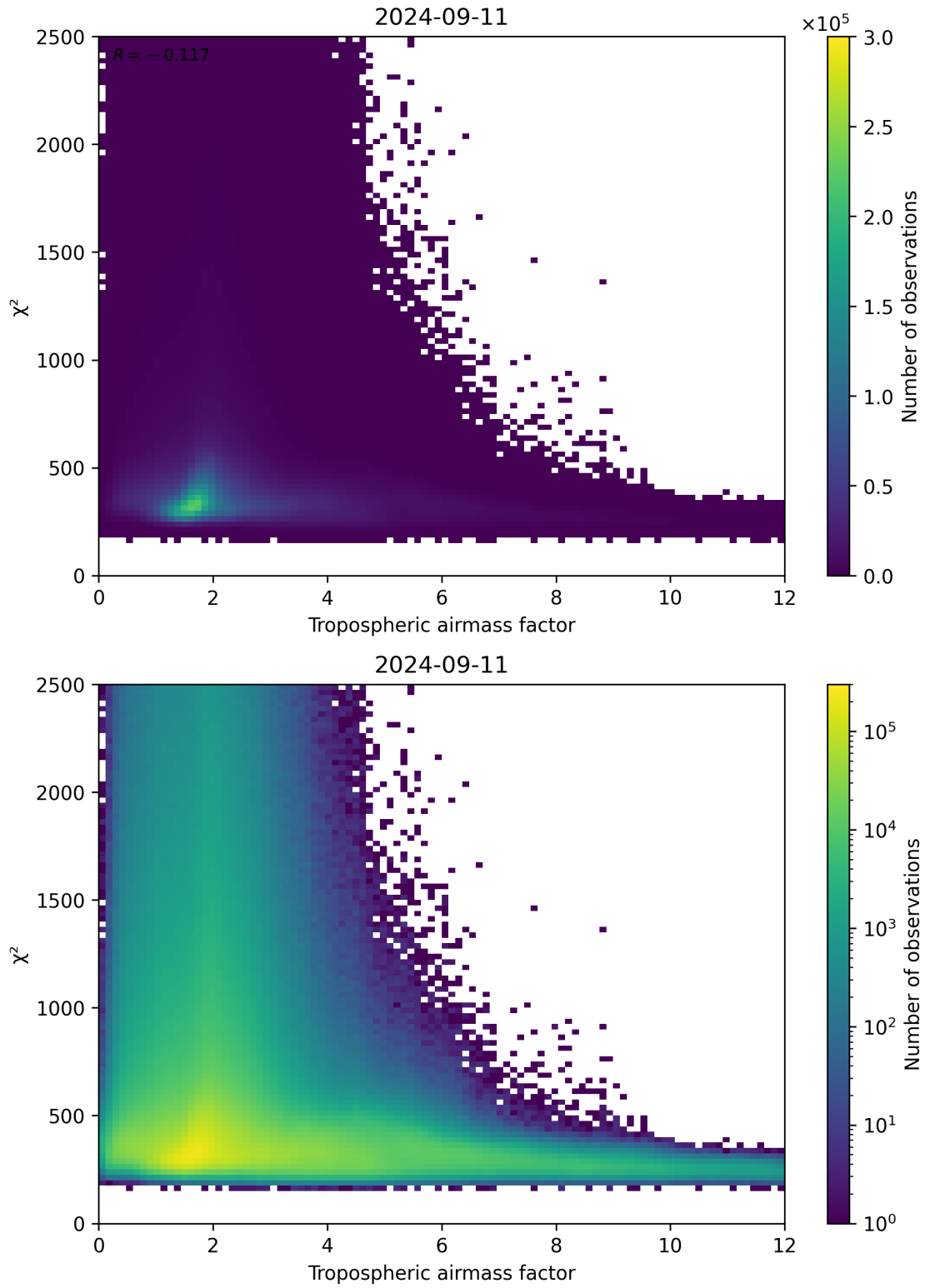
Figure 73: Scatter density plot of “Tropospheric airmass factor” against “ \chi^2 ” for 2024-09-10 to 2024-09-12.
