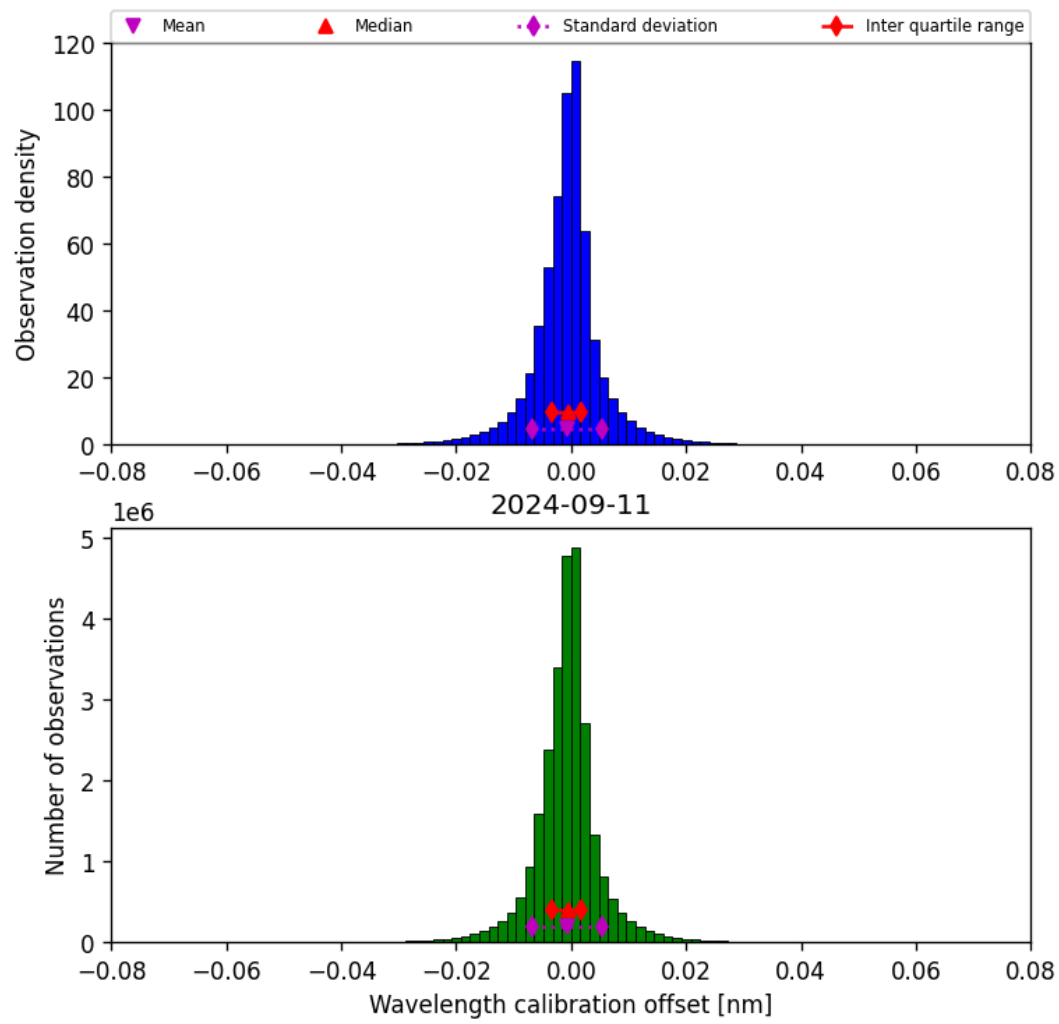
Figure 35: Histogram of “Wavelength calibration offset” for 2024-09-10 to 2024-09-12
