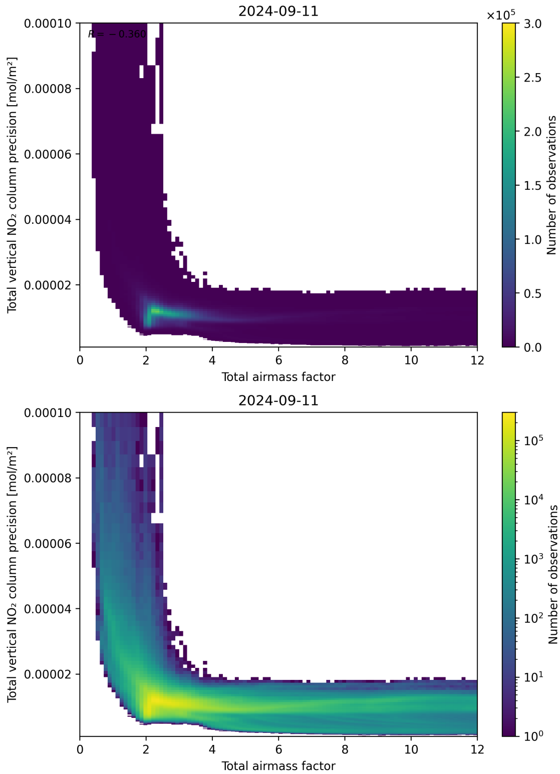
Figure 68: Scatter density plot of “Total airmass factor” against “Total vertical NO 2 column precision” for 2024-09-10 to 2024-09-12.
