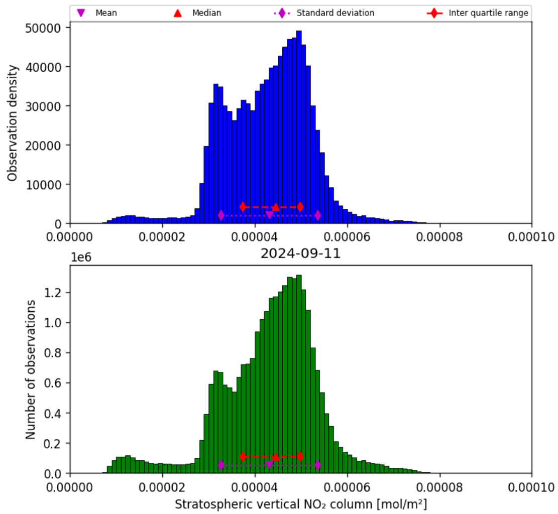
Figure 36: Histogram of “Stratospheric vertical NO 2 column” for 2024-09-10 to 2024-09-12
