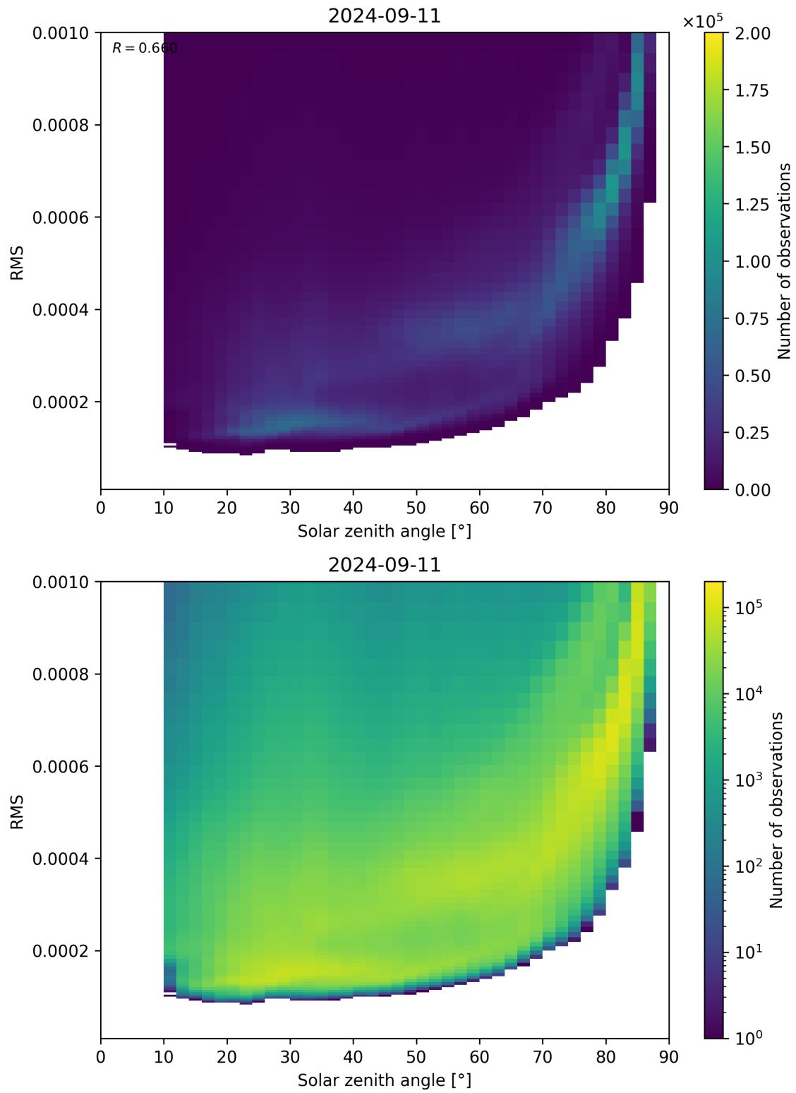
Figure 157: Scatter density plot of “Solar zenith angle” against “RMS” for 2024-09-10 to 2024-09-12.
