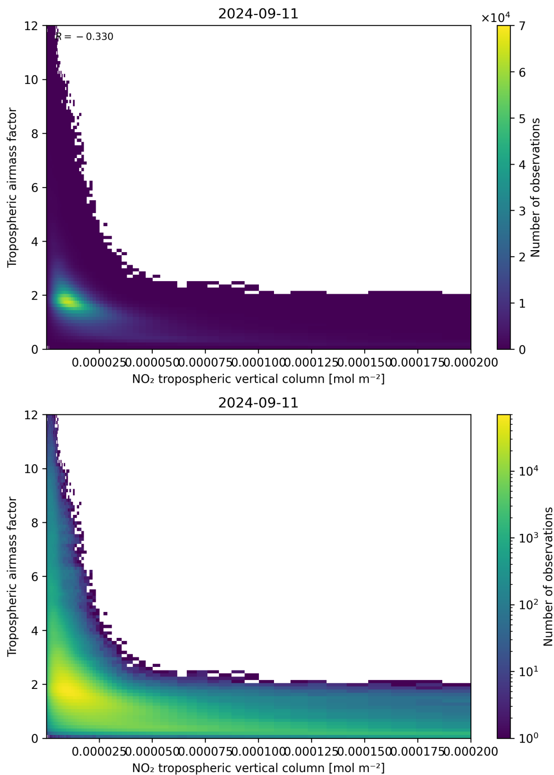
Figure 123: Scatter density plot of “NO 2 tropospheric vertical column” against “Tropospheric air mass factor” for 2024-09-10 to 2024-09-12.
