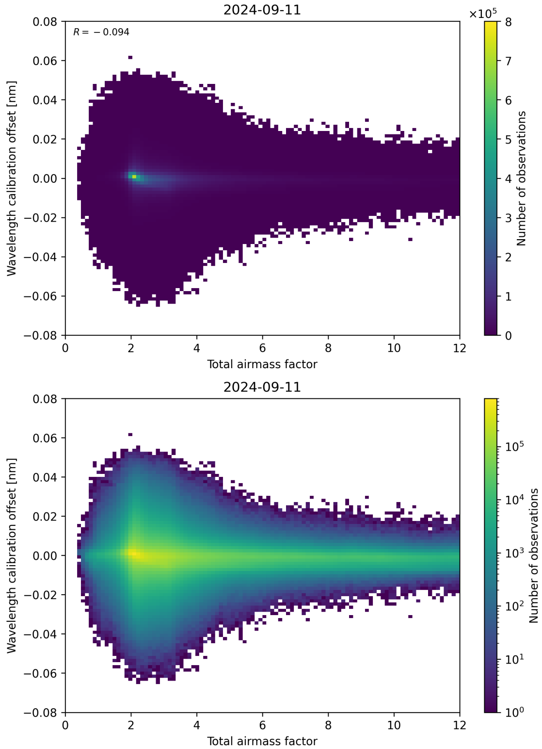
Figure 70: Scatter density plot of “Total airmass factor” against “Wavelength calibration offset” for 2024-09-10 to 2024-09-12.
