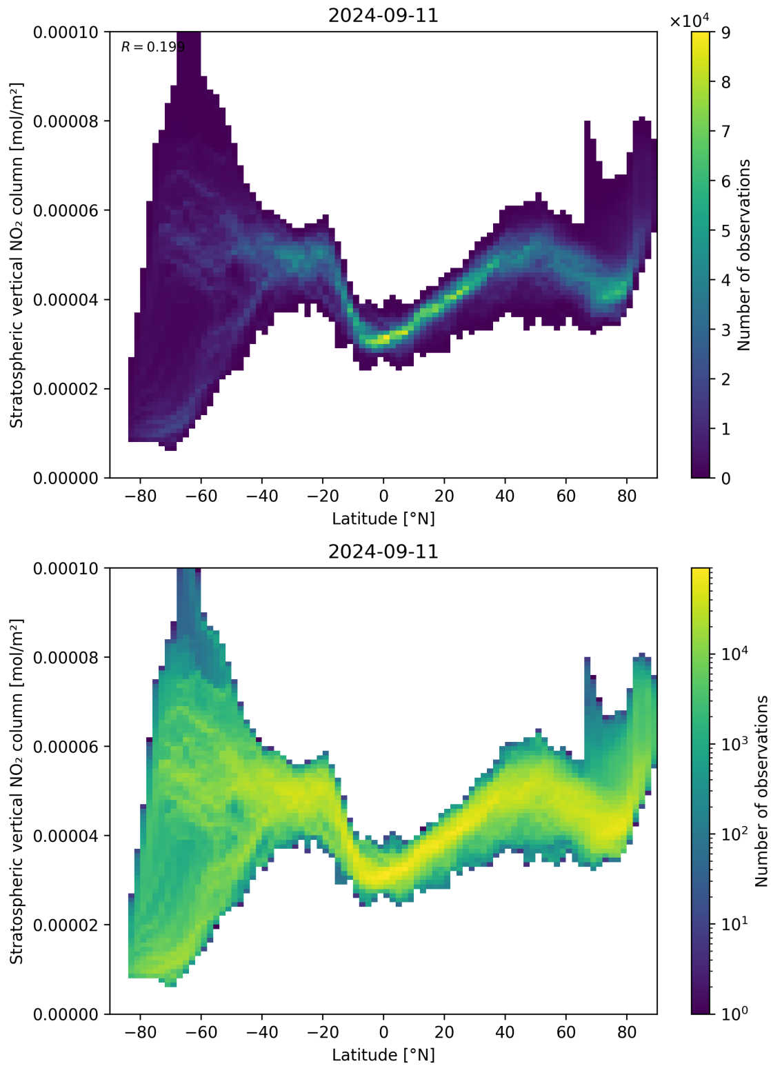
Figure 87: Scatter density plot of “Latitude” against “Stratospheric vertical NO 2 column” for 2024-09-10 to 2024-09-12.
