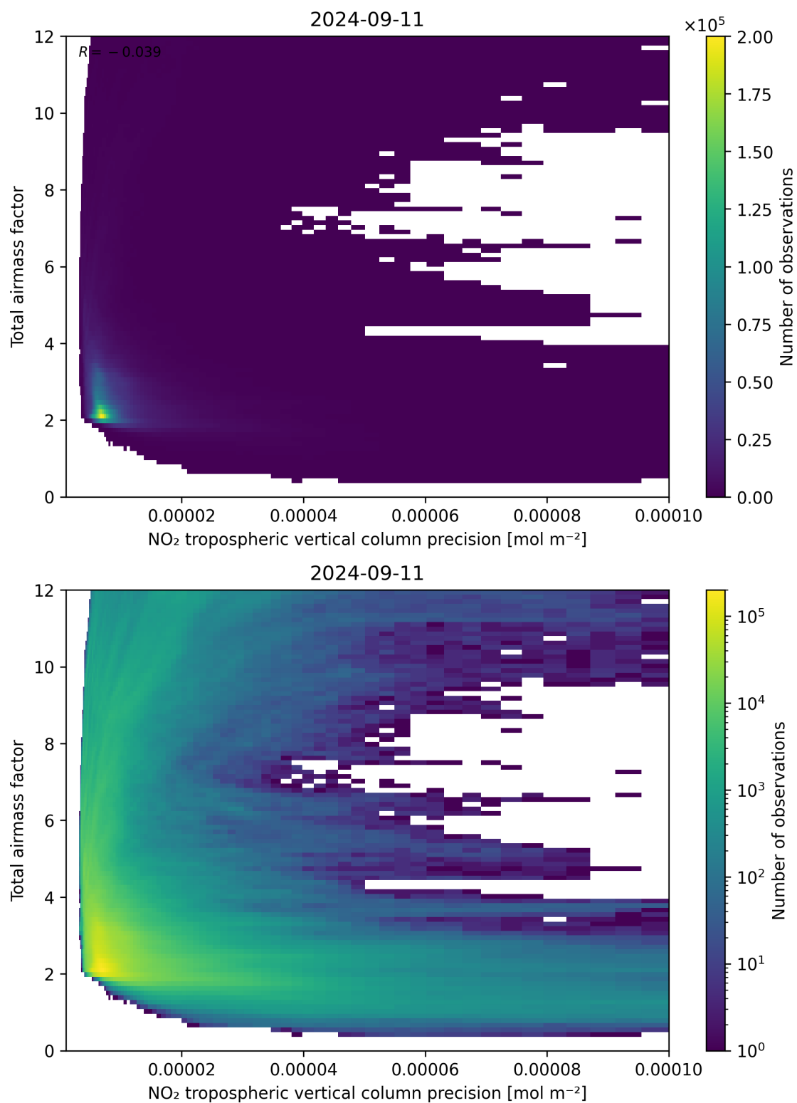
Figure 132: Scatter density plot of “NO 2 tropospheric vertical column precision” against “Total air mass factor” for 2024-09-10 to 2024-09-12.
