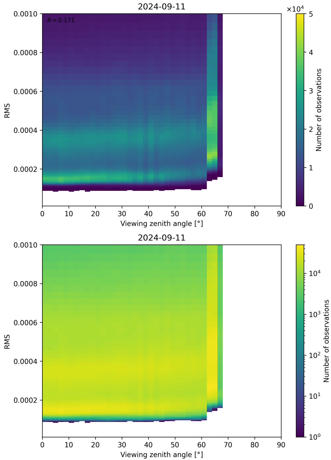
Figure 171: Scatter density plot of “Viewing zenith angle” against “RMS” for 2024-09-10 to 2024-09-12.
