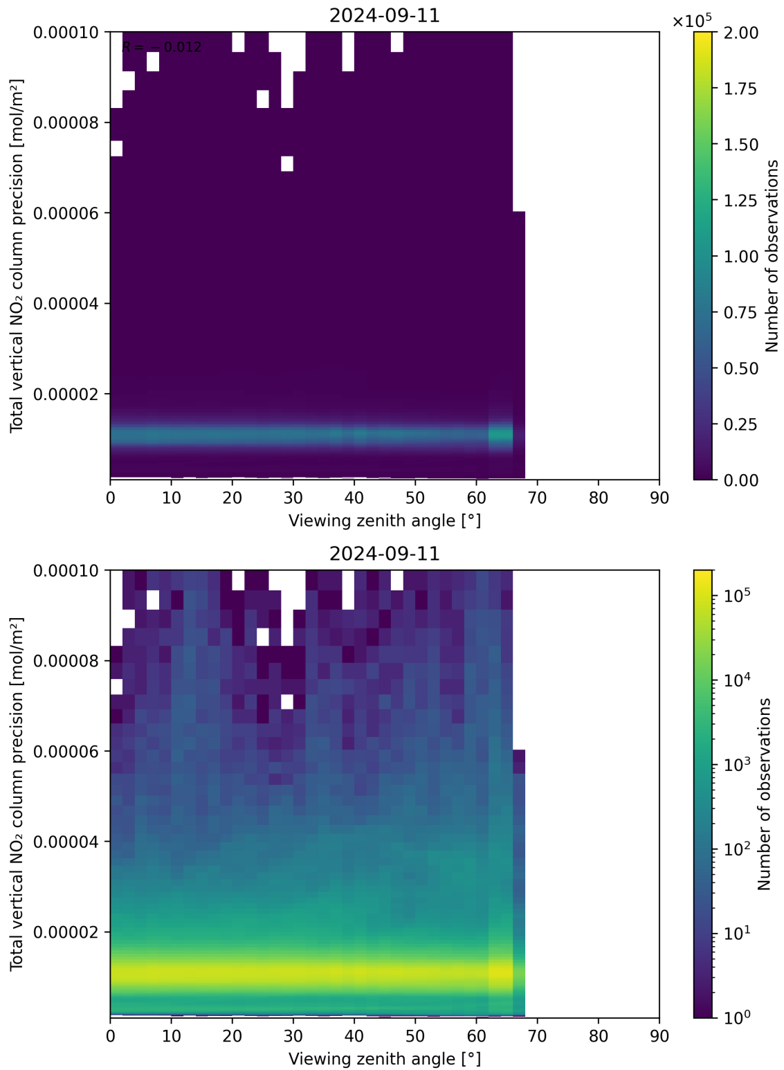
Figure 168: Scatter density plot of “Viewing zenith angle” against “Total vertical NO 2 column precision” for 2024-09-10 to 2024-09-12.
