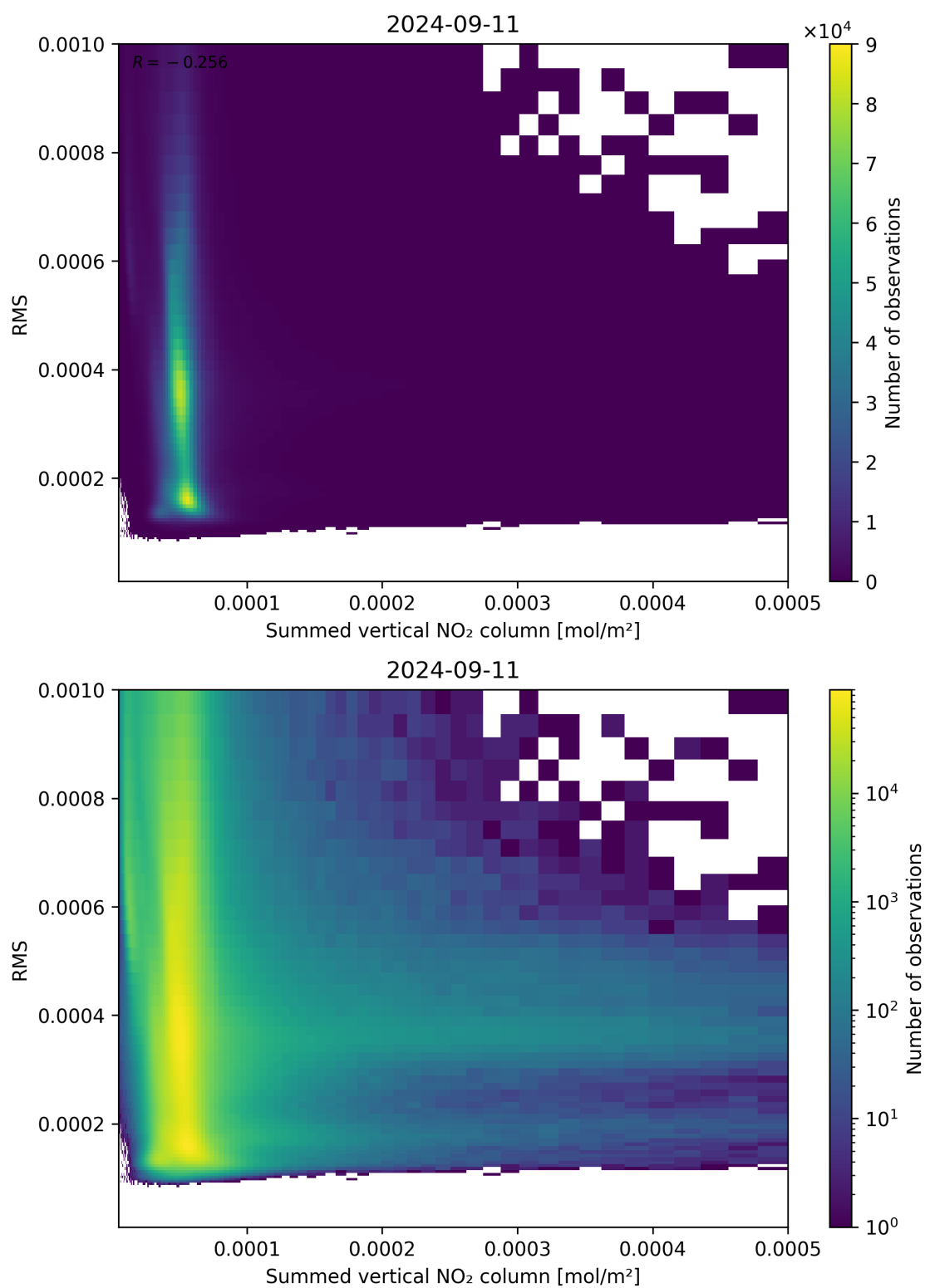
Figure 109: Scatter density plot of “Summed vertical NO 2 column” against “RMS” for 2024-09-10 to 2024-09-12.
