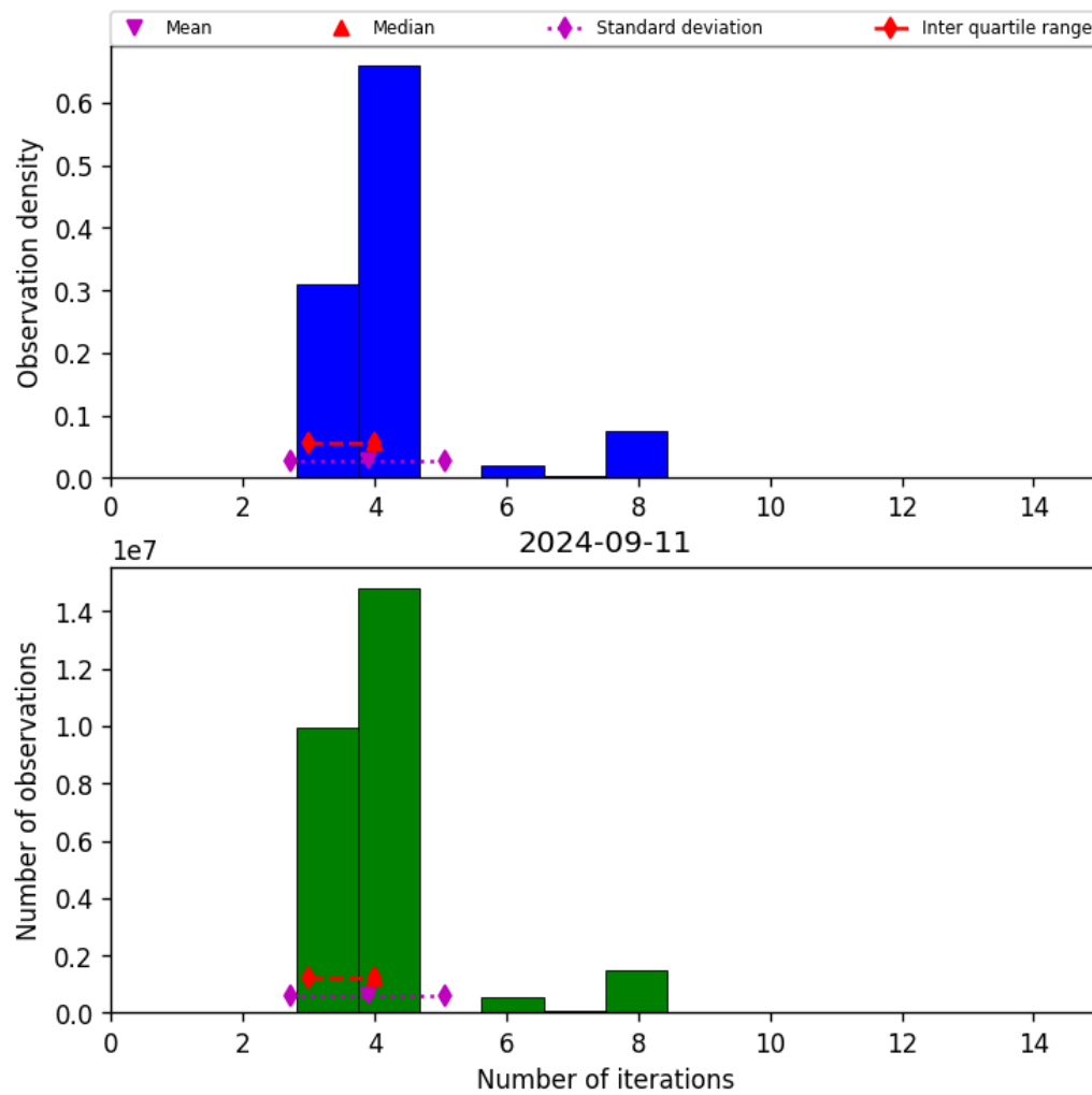
Figure 34: Histogram of “Number of iterations” for 2024-09-10 to 2024-09-12
