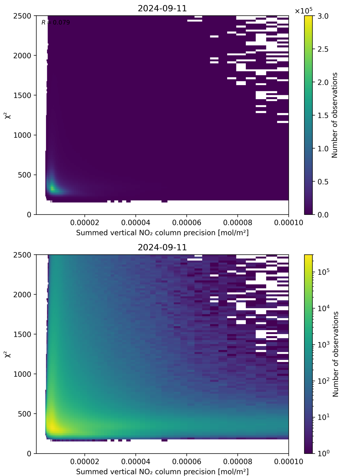
Figure 107: Scatter density plot of “Summed vertical NO 2 column precision” against “ \chi^2 ” for 2024-09-10 to 2024-09-12.
