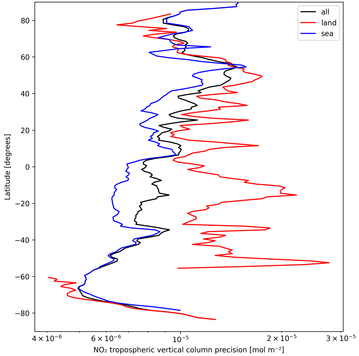
Figure 13: Zonal average of “NO 2 tropospheric vertical column precision” for 2024-09-10 to 2024-09-12.
