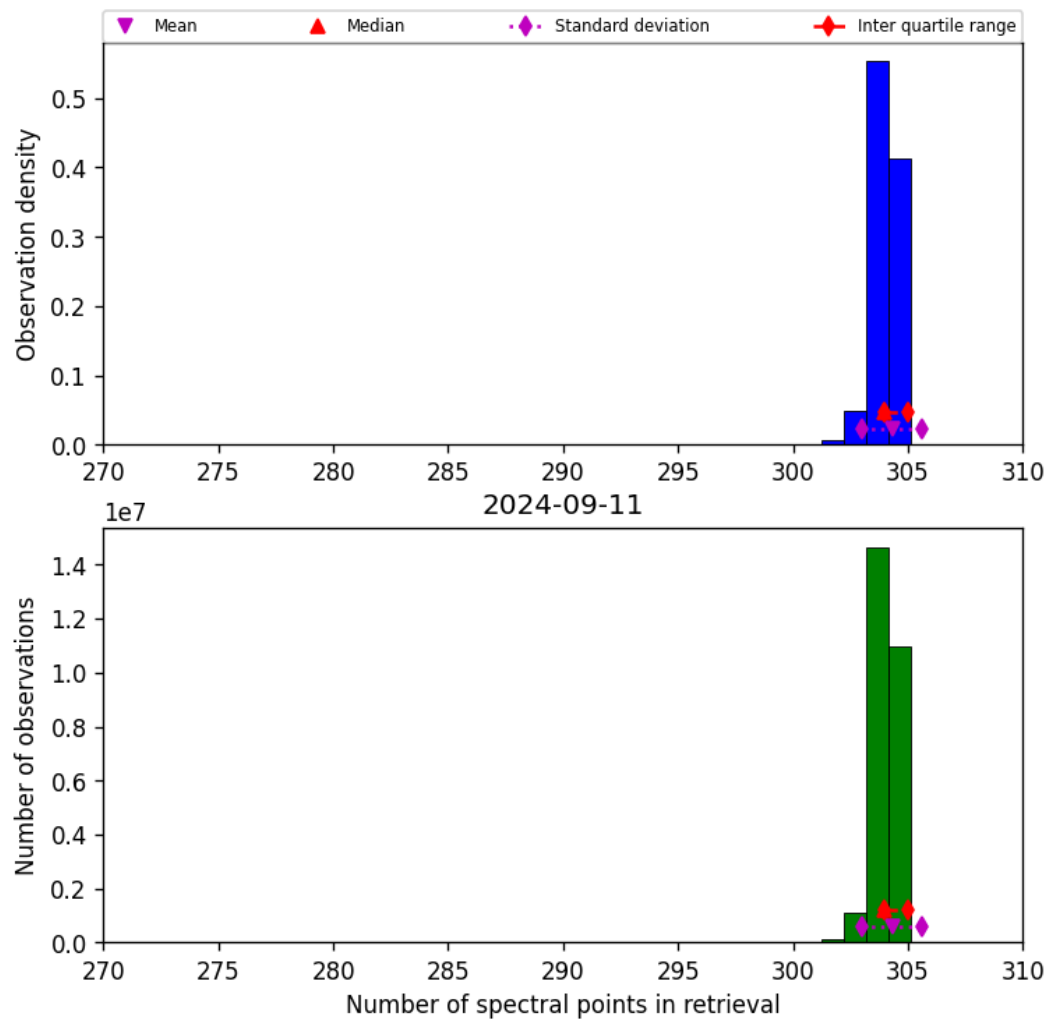
Figure 33: Histogram of "Number of spectral points in retrieval" for 2024-09-10 to 2024-09-12
