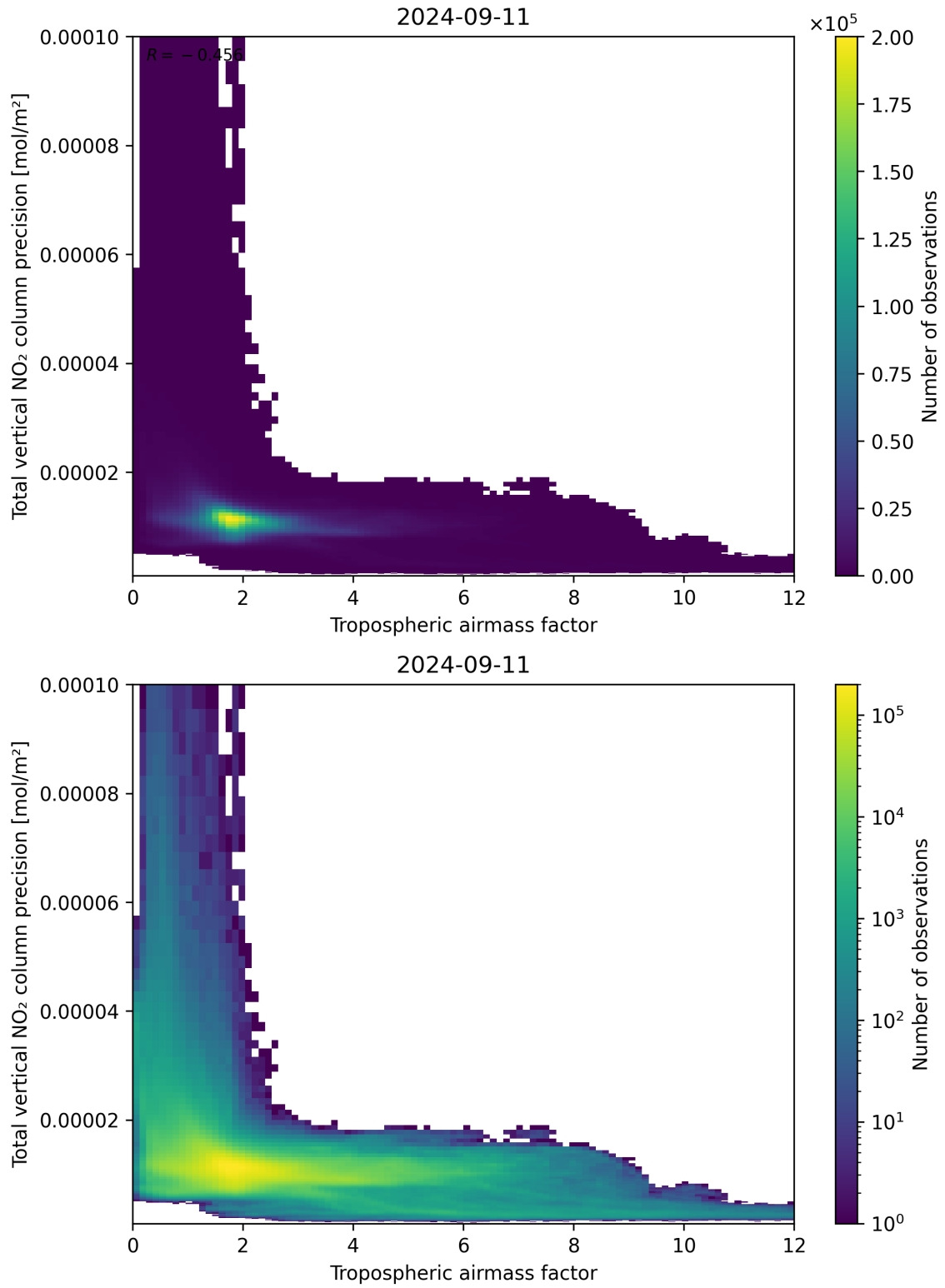
Figure 78: Scatter density plot of “Tropospheric air mass factor” against “Total vertical NO 2 column precision” for 2024-09-10 to 2024-09-12.
