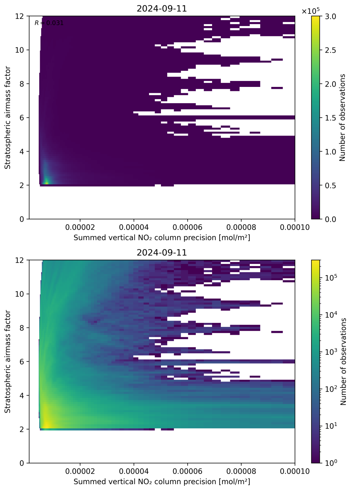
Figure 106: Scatter density plot of “Summed vertical NO 2 column precision” against “Stratospheric airmass factor” for 2024-09-10 to 2024-09-12.
