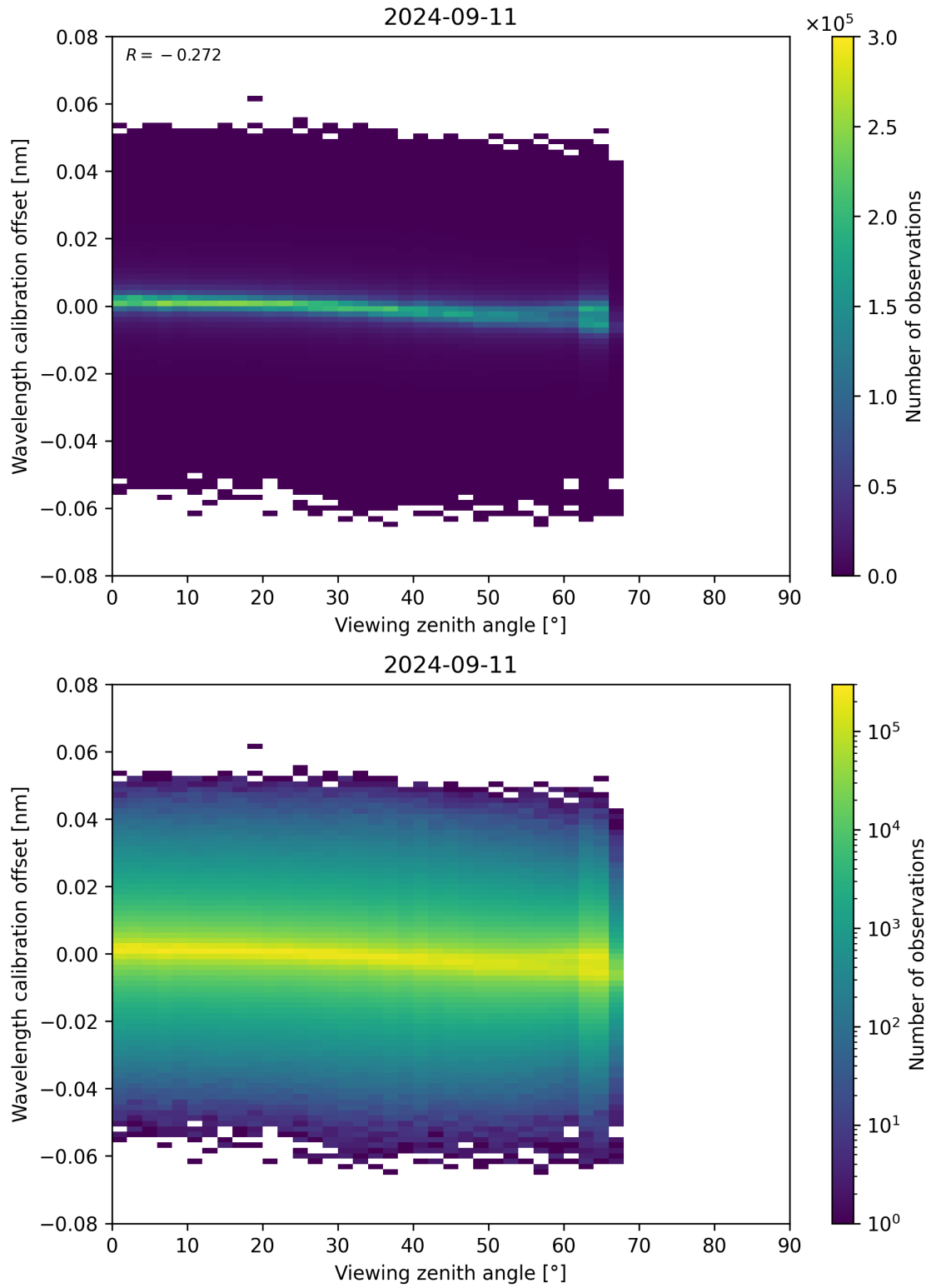
Figure 173: Scatter density plot of “Viewing zenith angle” against “Wavelength calibration offset” for 2024-09-10 to 2024-09-12.
