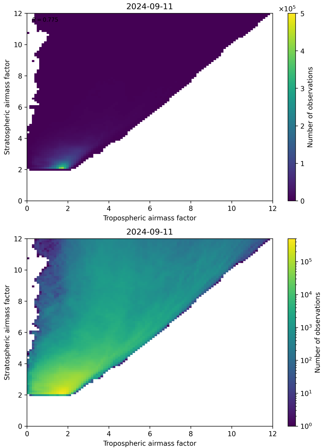
Figure 71: Scatter density plot of “Tropospheric airmass factor” against “Stratospheric airmass factor” for 2024-09-10 to 2024-09-12.
