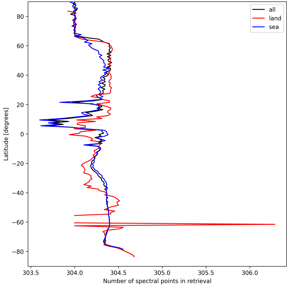
Figure 16: Zonal average of “Number of spectral points in retrieval” for 2024-09-10 to 2024-09-12.
