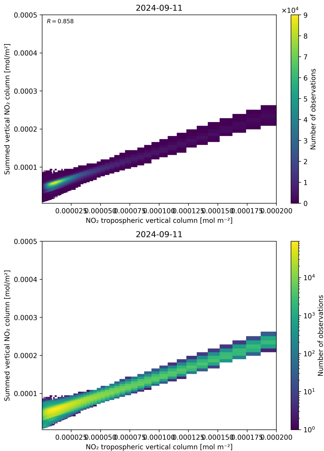
Figure 126: Scatter density plot of “NO 2 tropospheric vertical column” against “Summed vertical NO 2 column” for 2024-09-10 to 2024-09-12.
