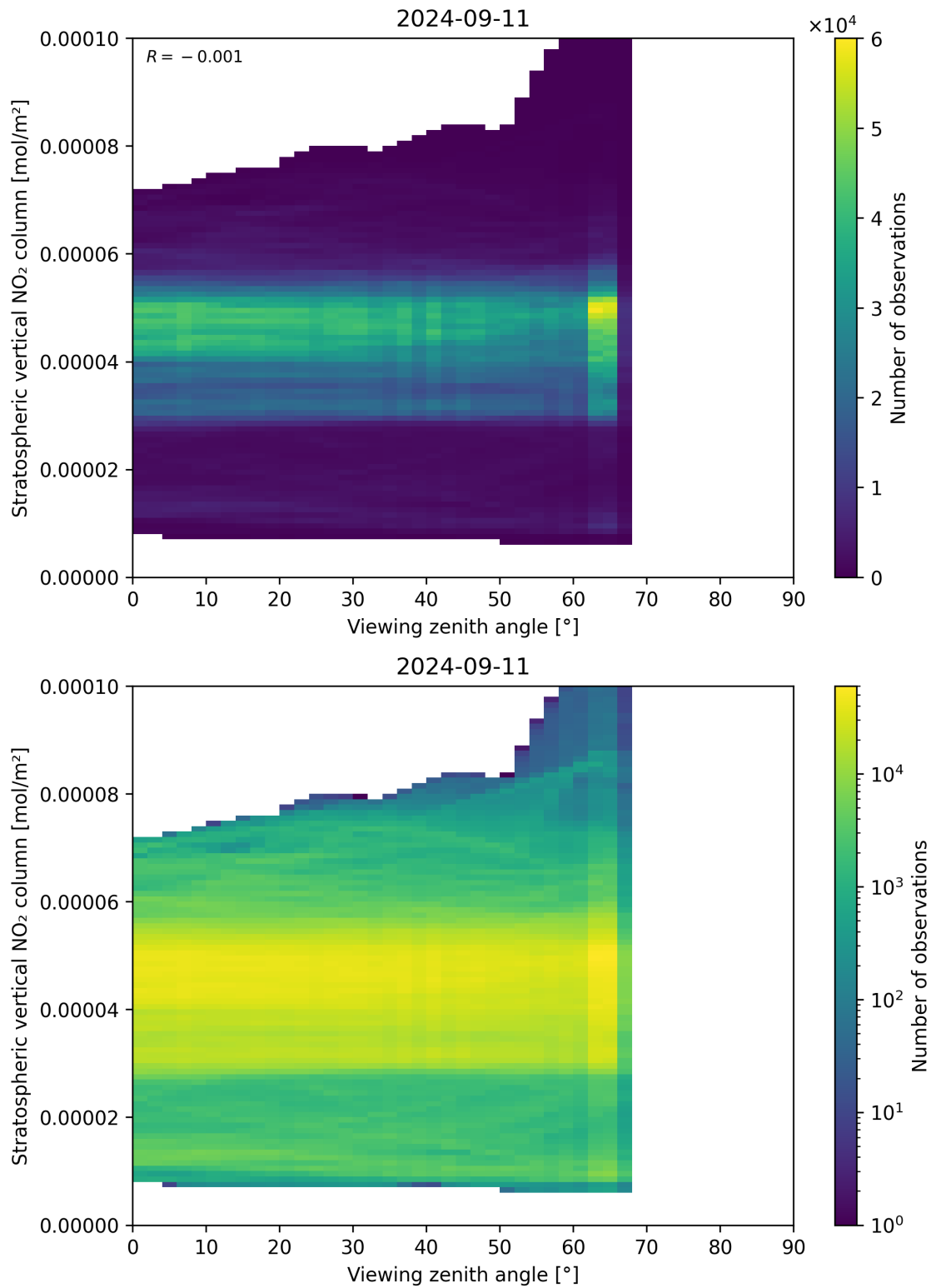
Figure 164: Scatter density plot of “Viewing zenith angle” against “Stratospheric vertical NO 2 column” for 2024-09-10 to 2024-09-12.
