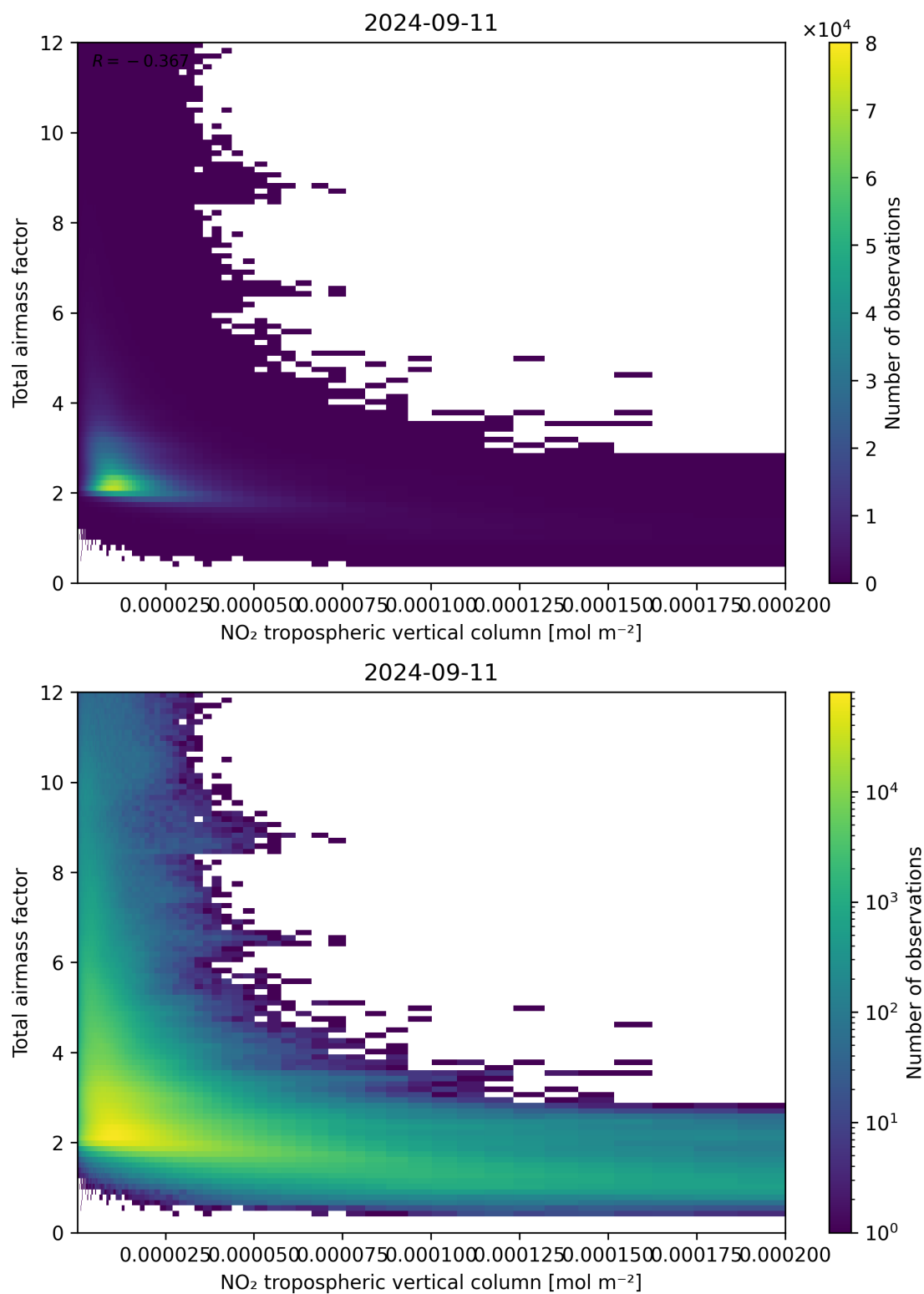
Figure 122: Scatter density plot of “NO 2 tropospheric vertical column” against “Total air mass factor” for 2024-09-10 to 2024-09-12.
