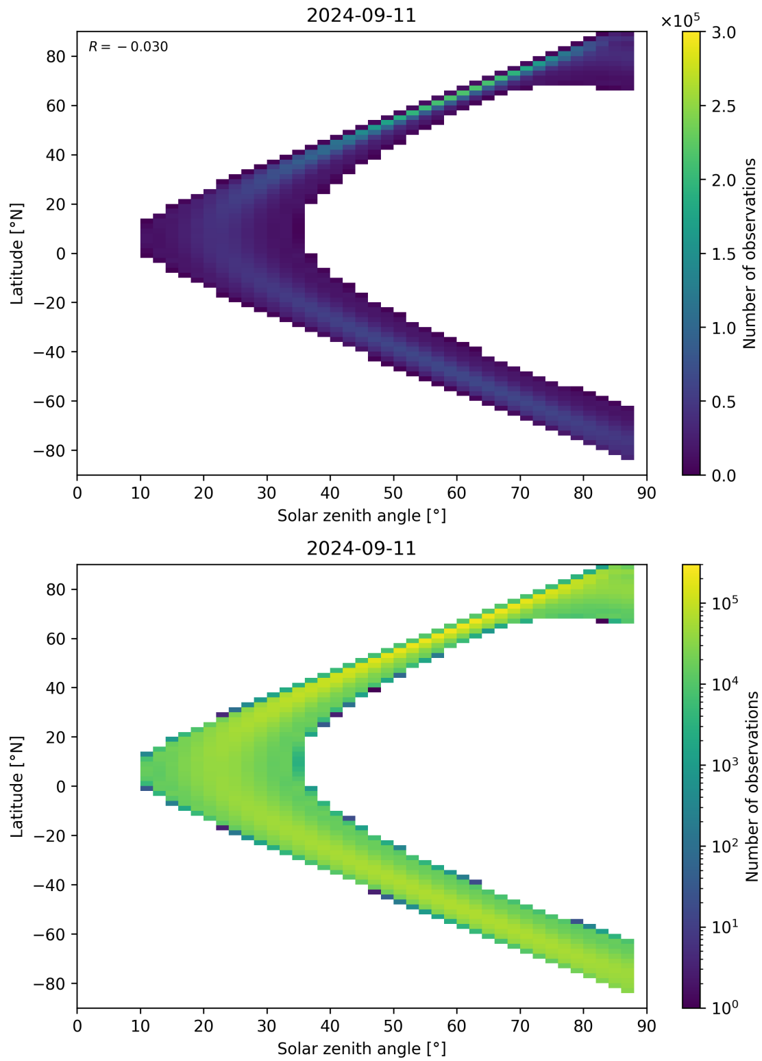
Figure 149: Scatter density plot of “Solar zenith angle” against “Latitude” for 2024-09-10 to 2024-09-12.
