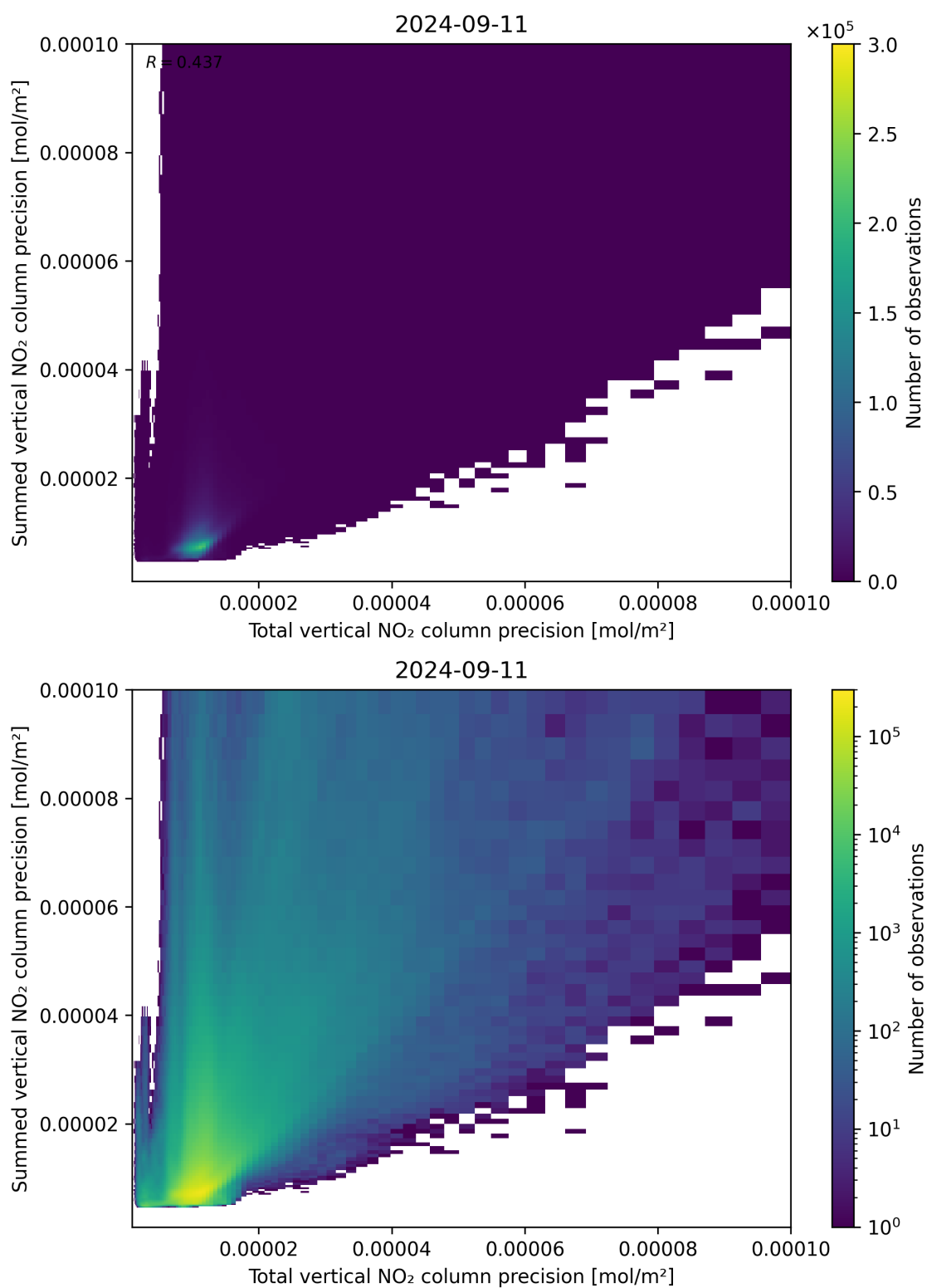
Figure 118: Scatter density plot of “Total vertical NO 2 column precision” against “Summed vertical NO 2 column precision” for 2024-09-10 to 2024-09-12.
