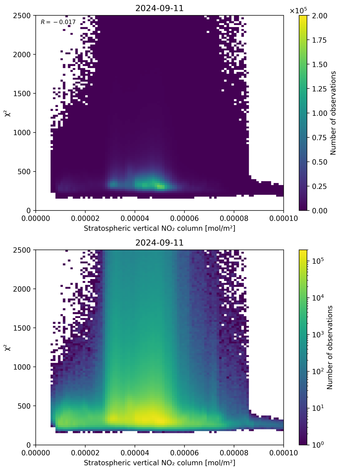
Figure 97: Scatter density plot of “Stratospheric vertical NO 2 column” against “ \chi^2 ” for 2024-09-10 to 2024-09-12.
