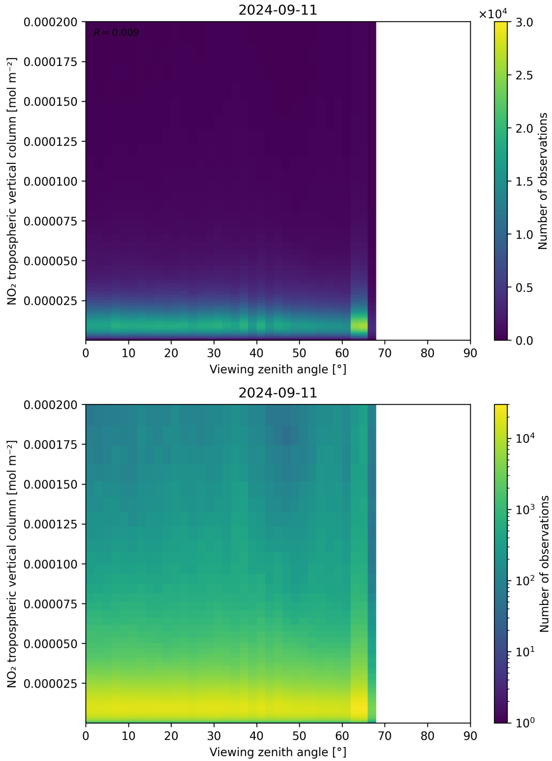
Figure 169: Scatter density plot of “Viewing zenith angle” against “NO 2 tropospheric vertical column” for 2024-09-10 to 2024-09-12.
