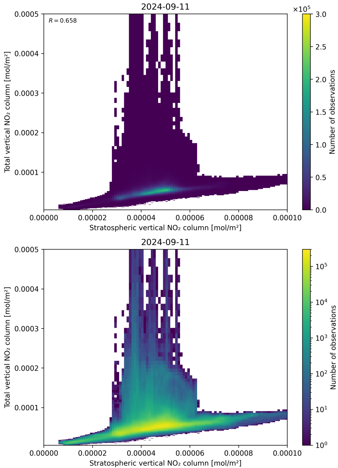
Figure 100: Scatter density plot of “Stratospheric vertical NO 2 column” against “Total vertical NO 2 column” for 2024-09-10 to 2024-09-12.
