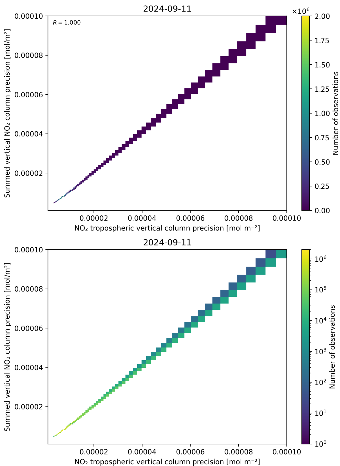
Figure 137: Scatter density plot of “NO 2 tropospheric vertical column precision” against “Summed vertical NO 2 column precision” for 2024-09-10 to 2024-09-12.
