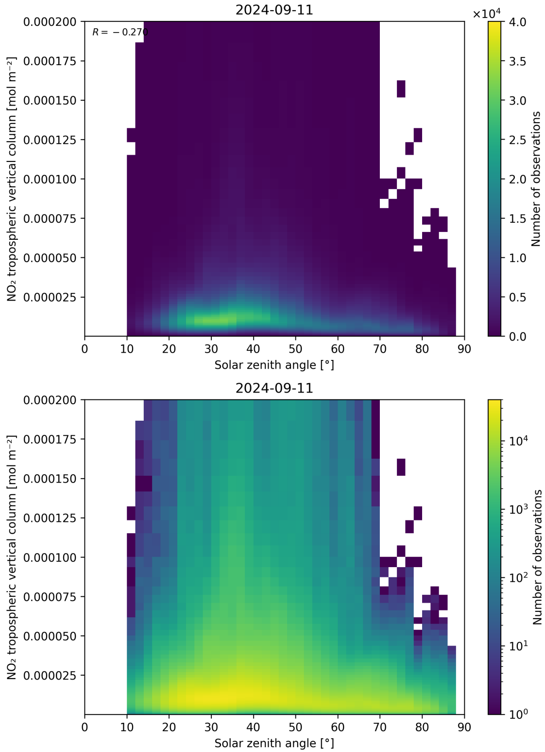
Figure 155: Scatter density plot of “Solar zenith angle” against “NO 2 tropospheric vertical column” for 2024-09-10 to 2024-09-12.
