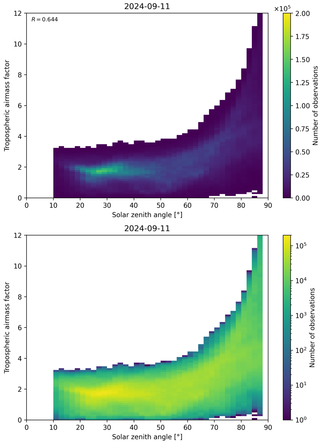
Figure 147: Scatter density plot of “Solar zenith angle” against “Tropospheric airmass factor” for 2024-09-10 to 2024-09-12.
