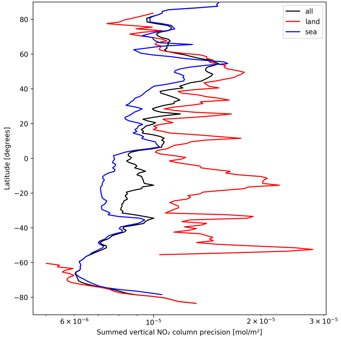
Figure 24: Zonal average of “Summed vertical NO 2 column precision” for 2024-09-10 to 2024-09-12.
