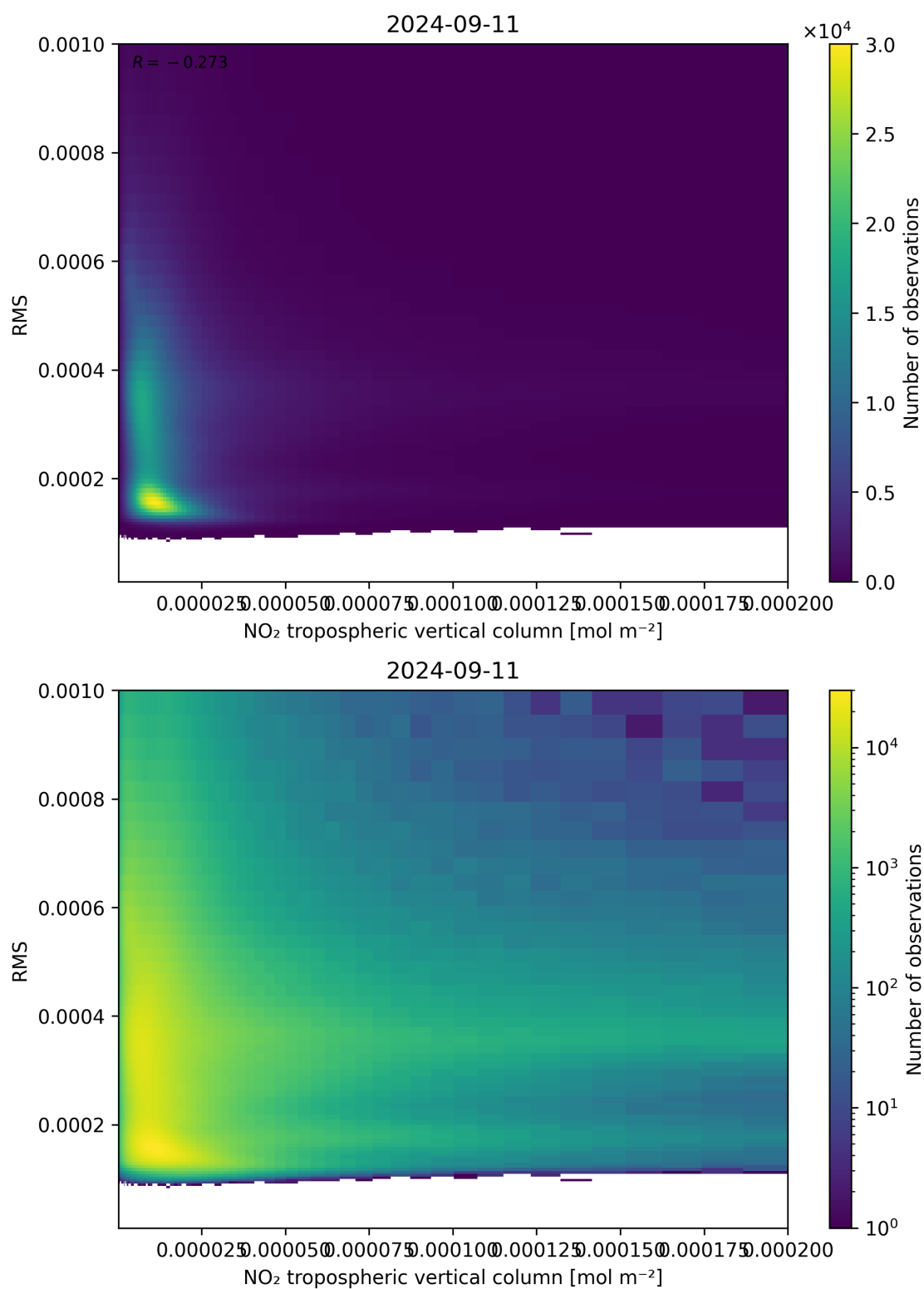
Figure 142: Scatter density plot of “NO 2 tropospheric vertical column” against “RMS” for 2024-09-10 to 2024-09-12.
