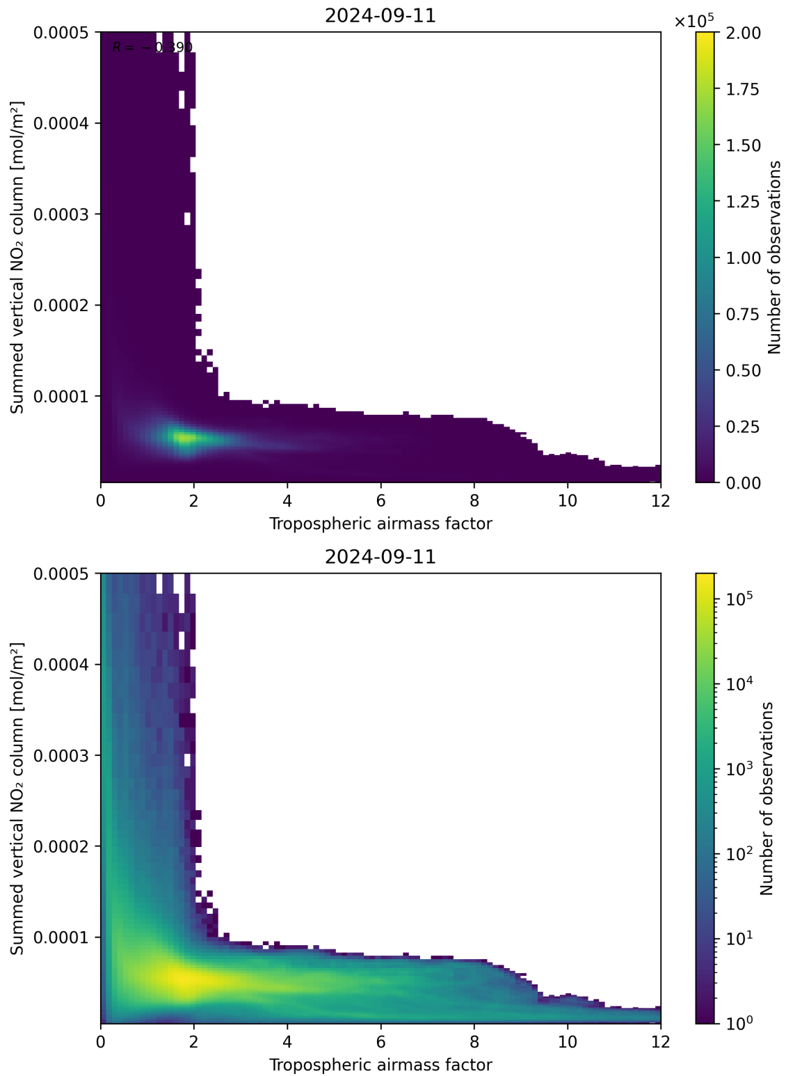
Figure 75: Scatter density plot of “Tropospheric air mass factor” against “Summed vertical NO 2 column” for 2024-09-10 to 2024-09-12.
