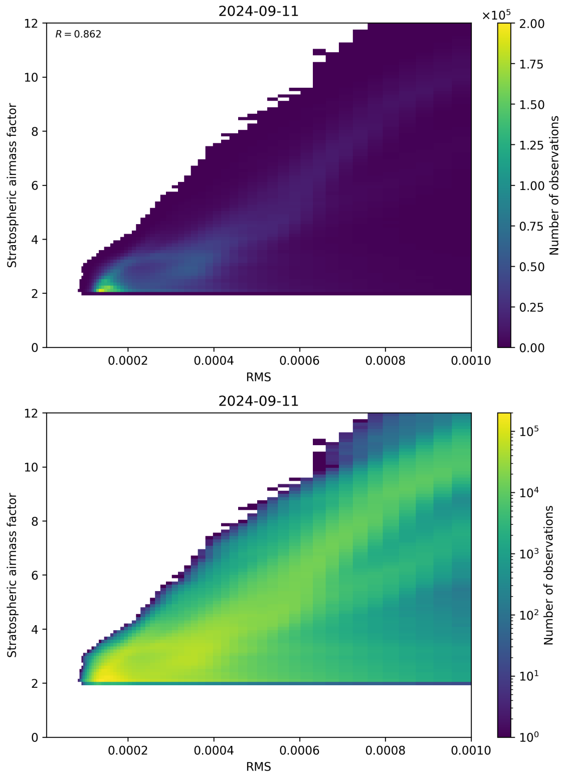
Figure 144: Scatter density plot of “RMS” against “Stratospheric airmass factor” for 2024-09-10 to 2024-09-12.
