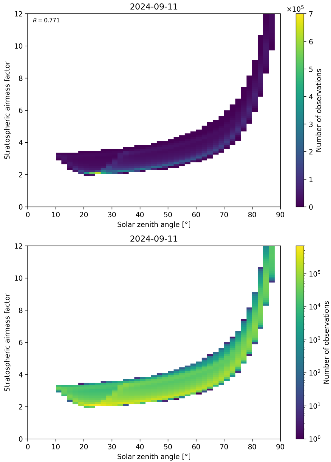
Figure 145: Scatter density plot of “Solar zenith angle” against “Stratospheric airmass factor” for 2024-09-10 to 2024-09-12.
