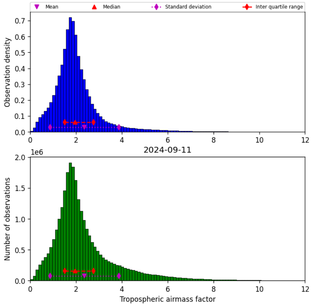
Figure 31: Histogram of “Tropospheric airmass factor” for 2024-09-10 to 2024-09-12
