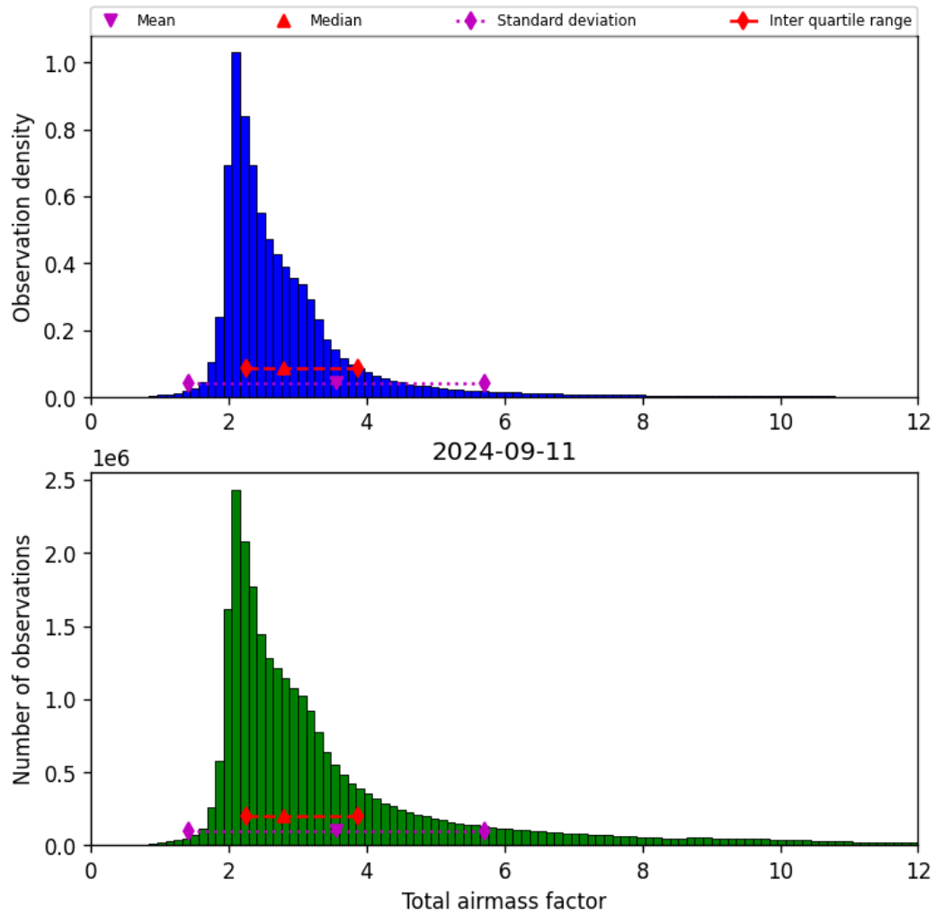
Figure 32: Histogram of “Total airmass factor” for 2024-09-10 to 2024-09-12
