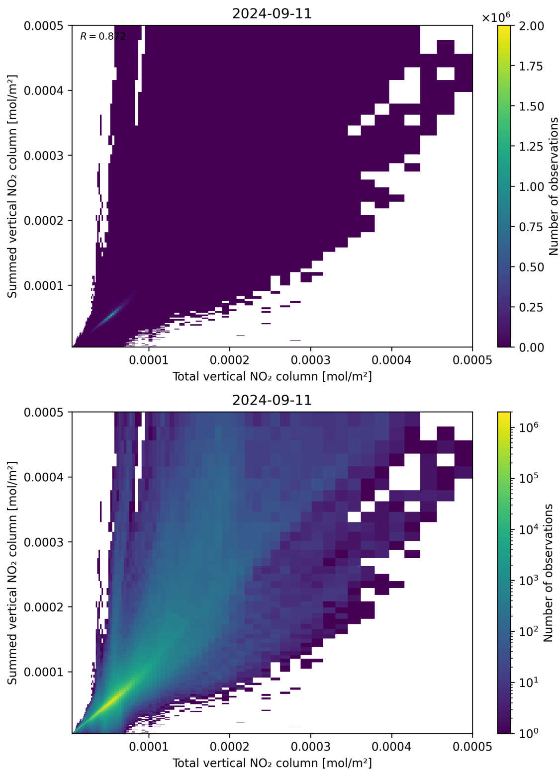
Figure 112: Scatter density plot of “Total vertical NO 2 column” against “Summed vertical NO 2 column” for 2024-09-10 to 2024-09-12.
