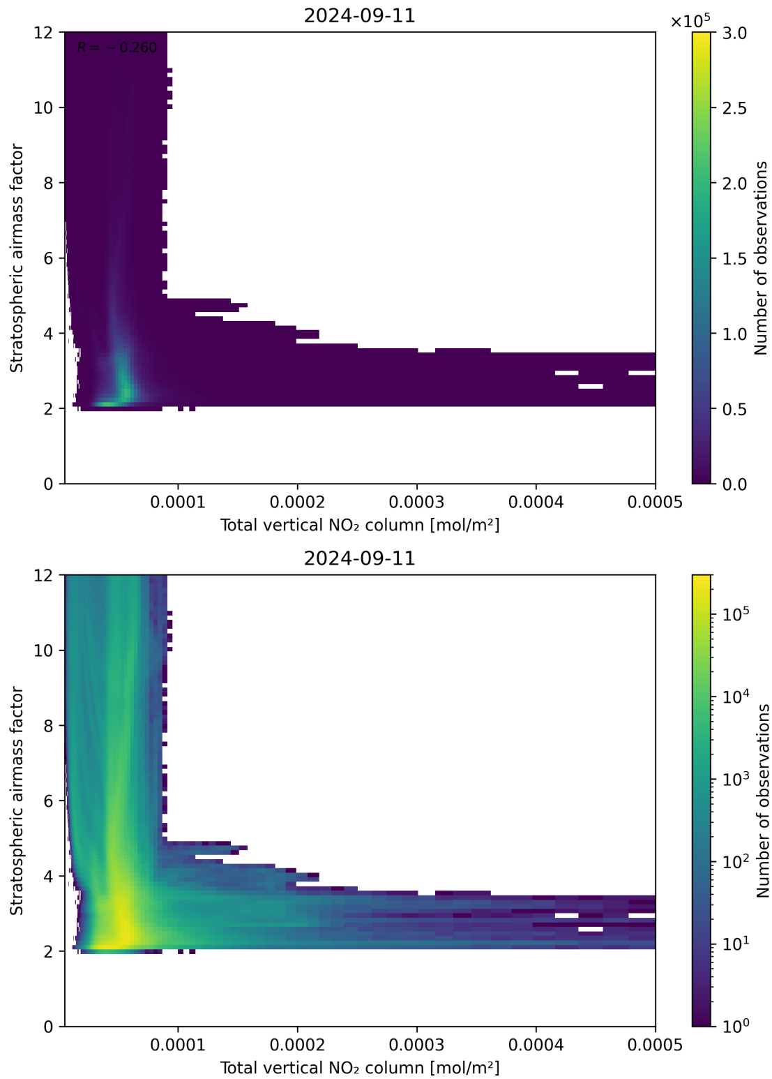
Figure 110: Scatter density plot of “Total vertical NO 2 column” against “Stratospheric airmass factor” for 2024-09-10 to 2024-09-12.
