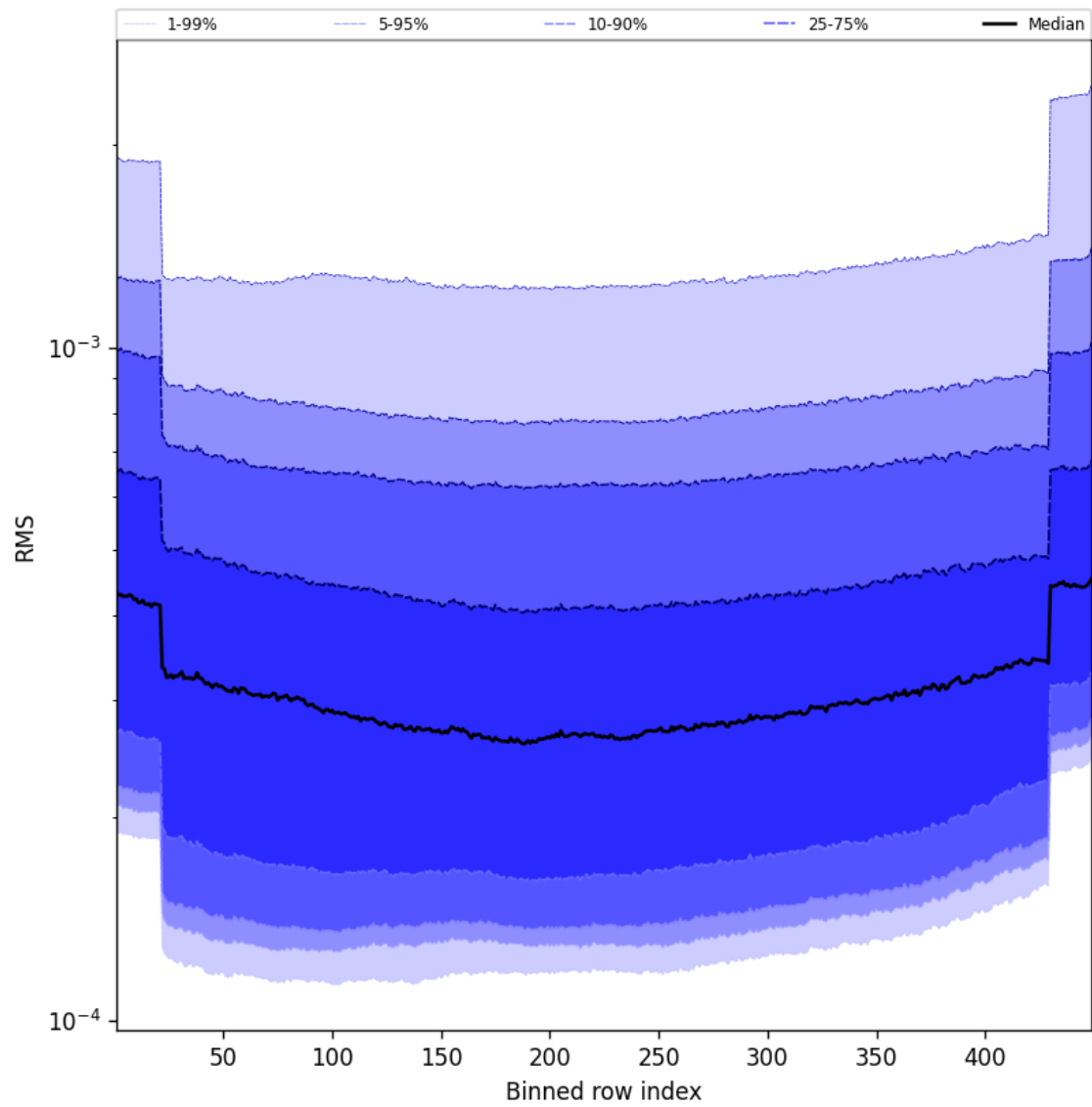
Figure 60: Along track statistics of “RMS” for 2024-09-10 to 2024-09-12
