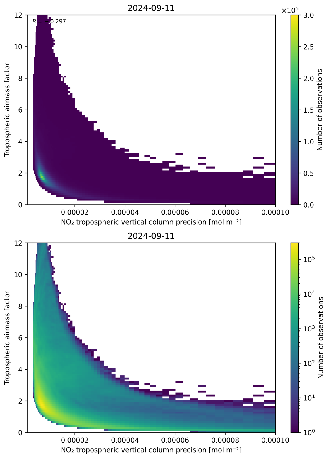
Figure 133: Scatter density plot of “NO 2 tropospheric vertical column precision” against “Tropospheric airmass factor” for 2024-09-10 to 2024-09-12.
