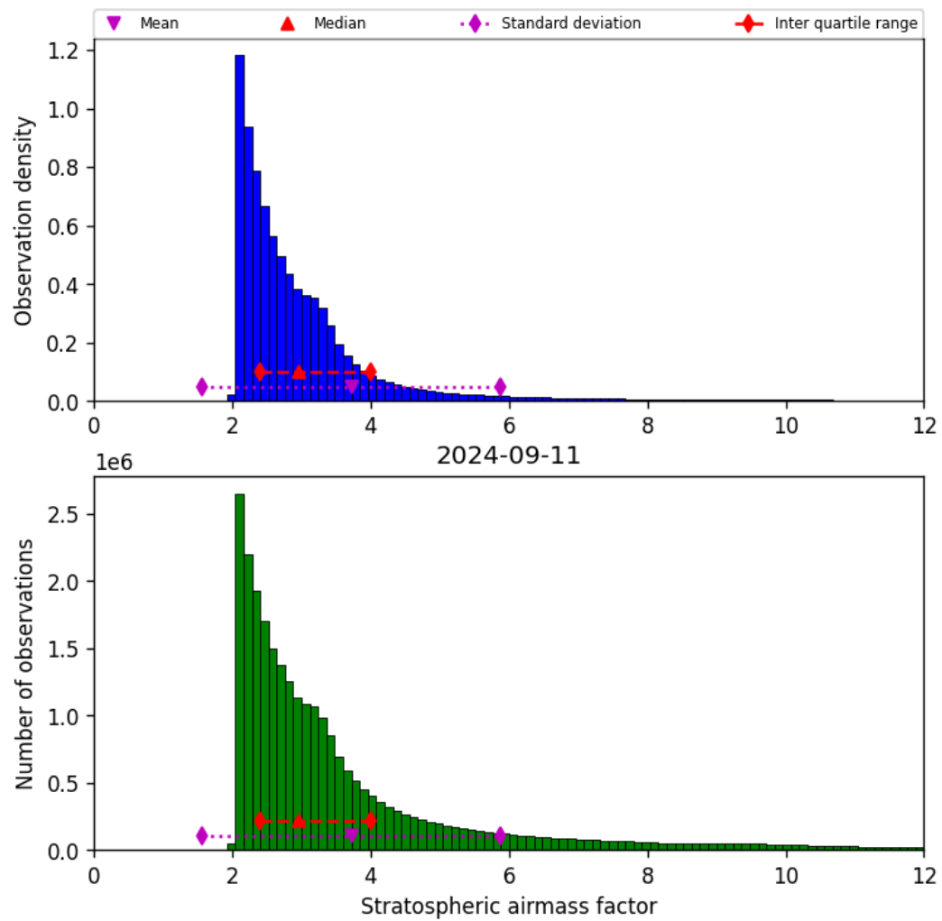
Figure 44: Histogram of “Stratospheric airmass factor” for 2024-09-10 to 2024-09-12
