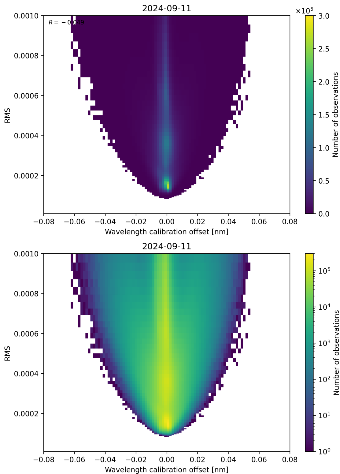
Figure 181: Scatter density plot of “Wavelength calibration offset” against “RMS” for 2024-09-10 to 2024-09-12.
