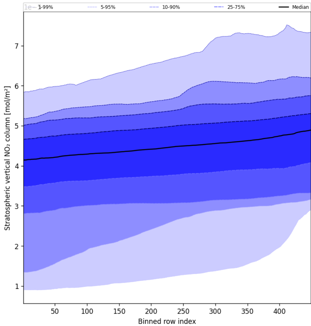
Figure 53: Along track statistics of “Stratospheric vertical NO 2 column” for 2024-09-10 to 2024-09-12
