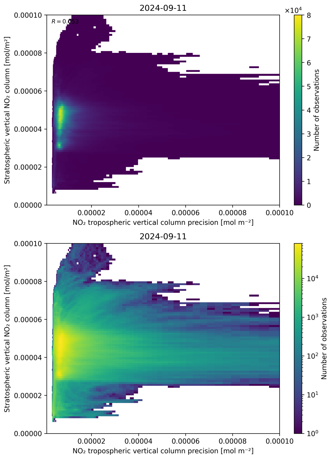
Figure 135: Scatter density plot of “NO 2 tropospheric vertical column precision” against “Stratospheric vertical NO 2 column” for 2024-09-10 to 2024-09-12.
