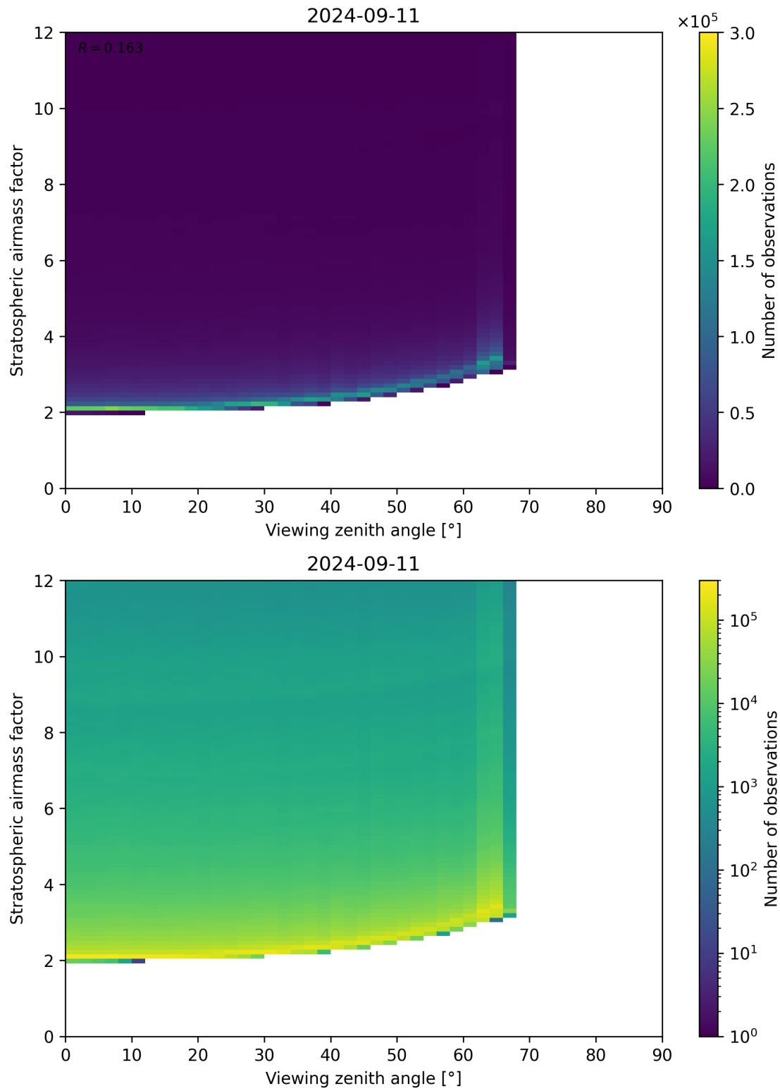
Figure 159: Scatter density plot of “Viewing zenith angle” against “Stratospheric airmass factor” for 2024-09-10 to 2024-09-12.
