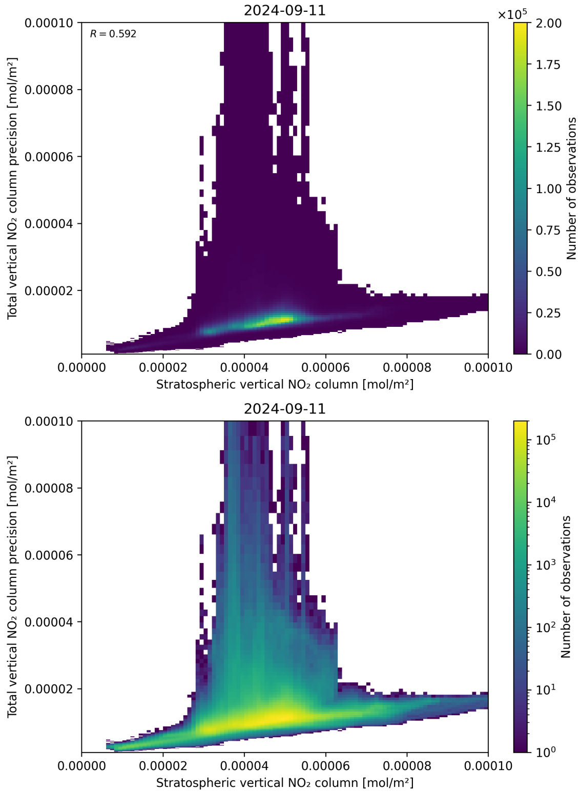
Figure 101: Scatter density plot of “Stratospheric vertical NO 2 column” against “Total vertical NO 2 column precision” for 2024-09-10 to 2024-09-12.
