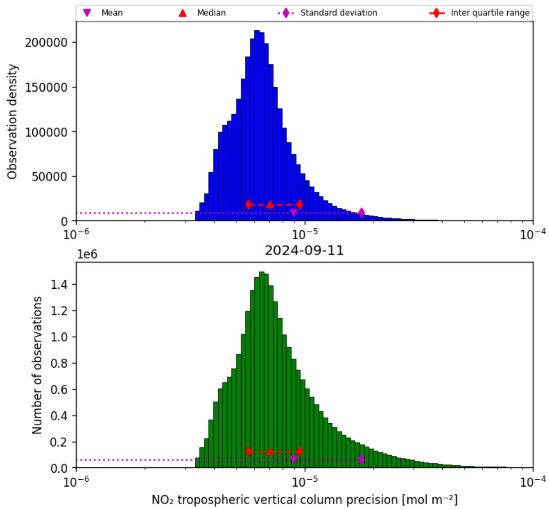
Figure 30: Histogram of “NO 2 tropospheric vertical column precision” for 2024-09-10 to 2024-09-12
