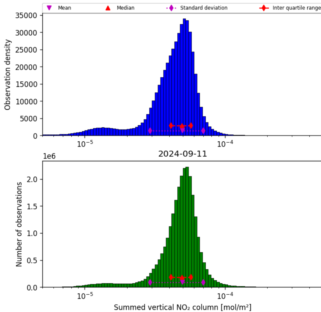
Figure 40: Histogram of “Summed vertical NO 2 column” for 2024-09-10 to 2024-09-12
