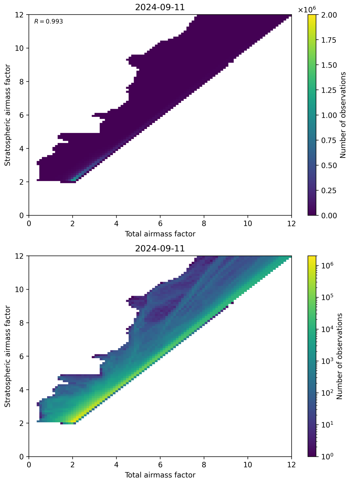
Figure 62: Scatter density plot of “Total air mass factor” against “Stratospheric air mass factor” for 2024-09-10 to 2024-09-12.
