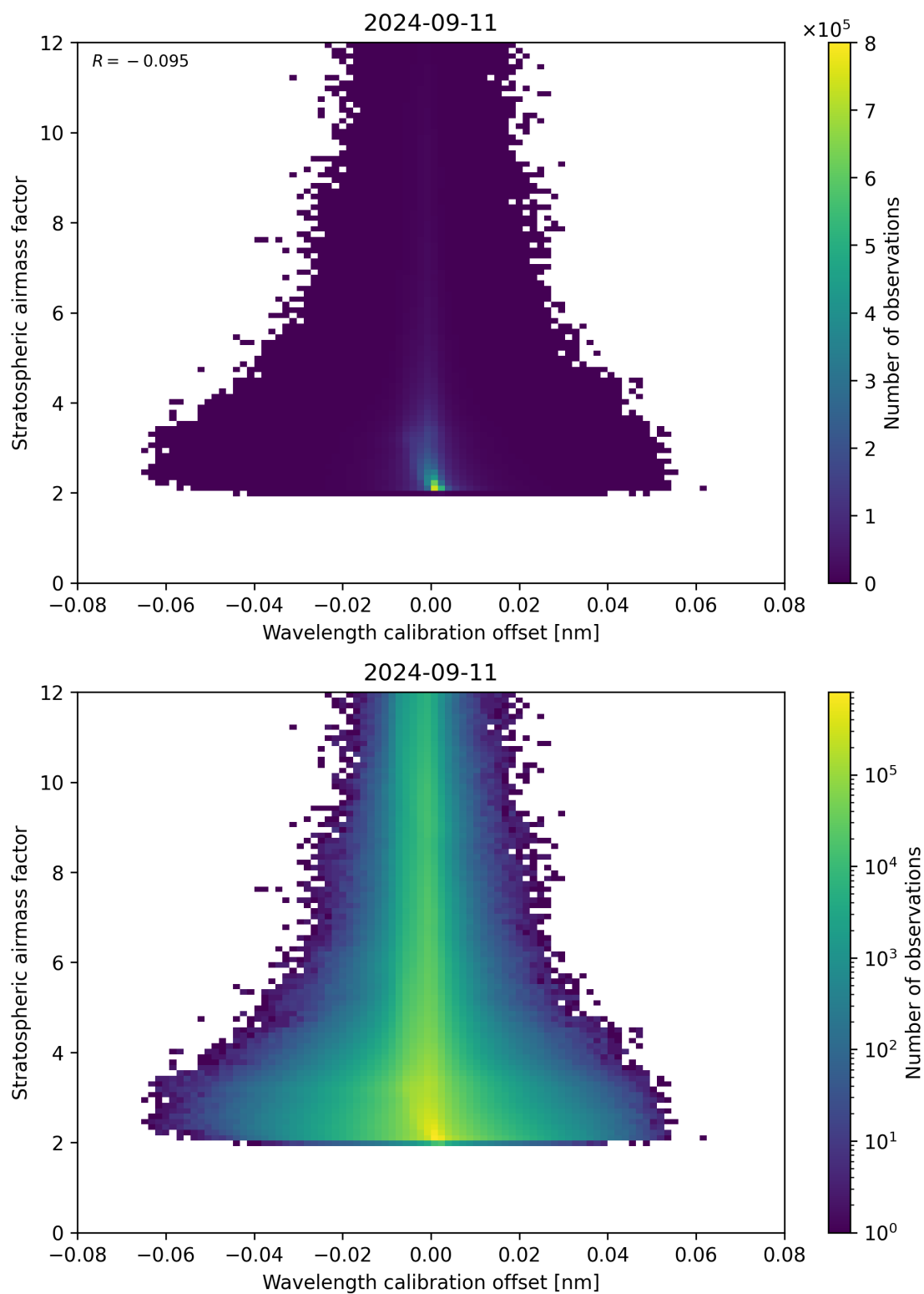
Figure 174: Scatter density plot of “Wavelength calibration offset” against “Stratospheric airmass factor” for 2024-09-10 to 2024-09-12.
