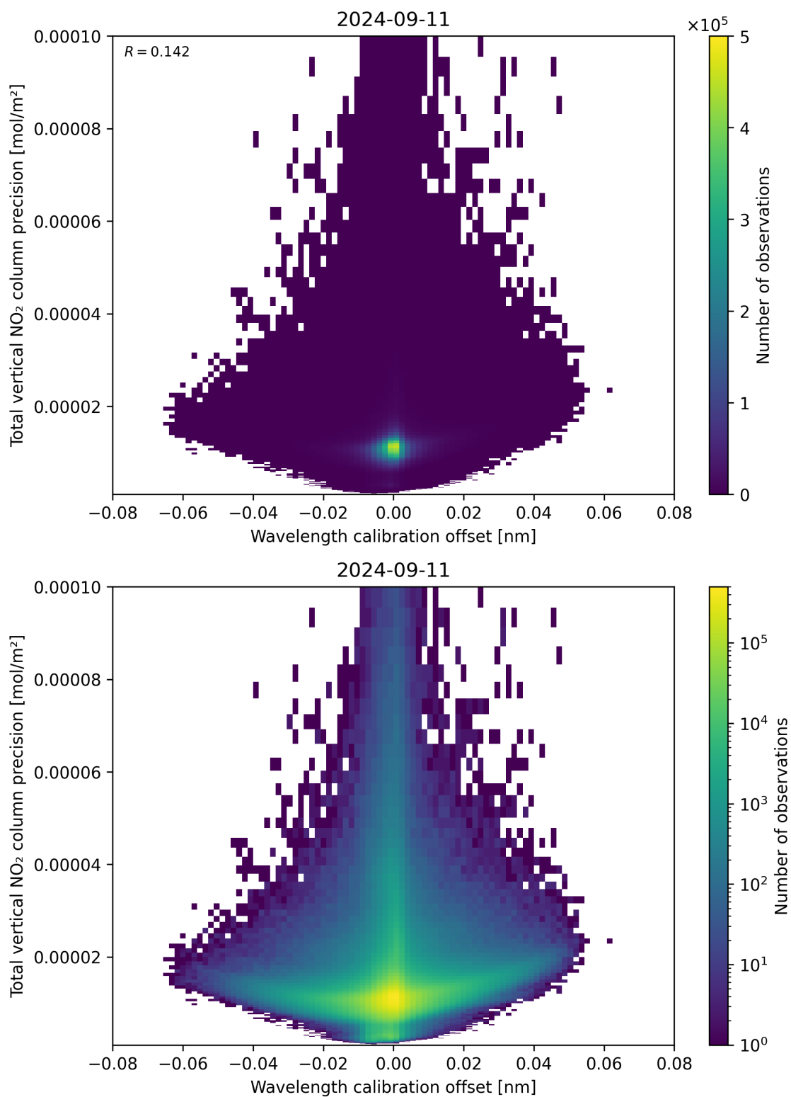
Figure 180: Scatter density plot of “Wavelength calibration offset” against “Total vertical NO 2 column precision” for 2024-09-10 to 2024-09-12.
