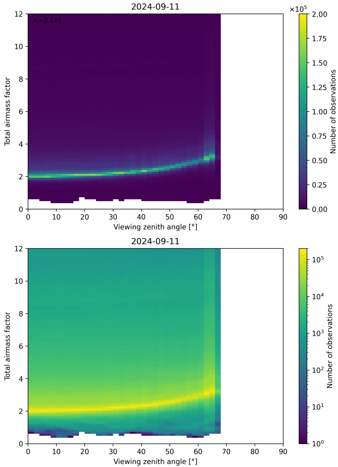
Figure 160: Scatter density plot of “Viewing zenith angle” against “Total airmass factor” for 2024-09-10 to 2024-09-12.
