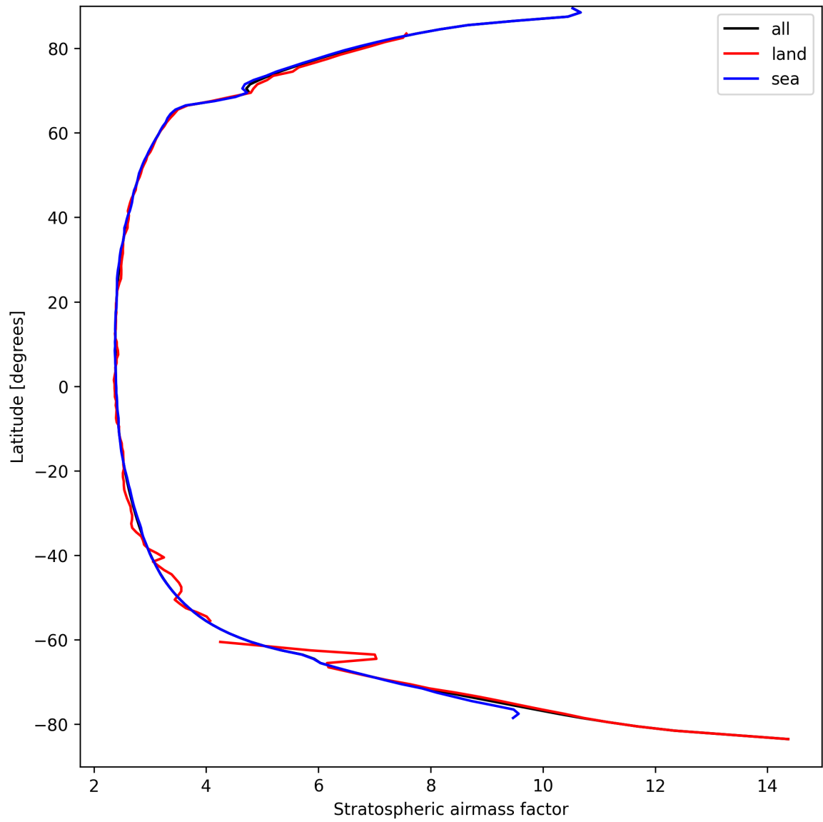
Figure 27: Zonal average of “Stratospheric airmass factor” for 2024-09-10 to 2024-09-12.
