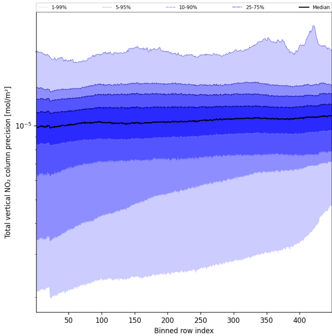
Figure 56: Along track statistics of “Total vertical NO 2 column precision” for 2024-09-10 to 2024-09-12
