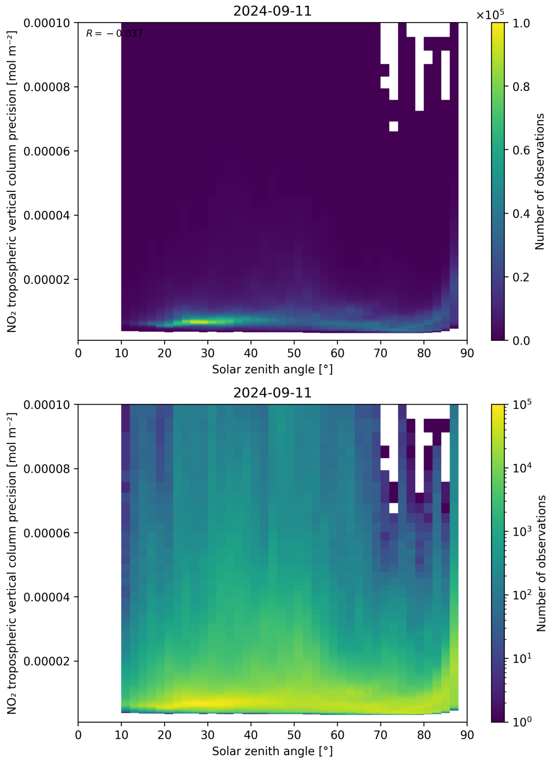
Figure 156: Scatter density plot of “Solar zenith angle” against “NO 2 tropospheric vertical column precision” for 2024-09-10 to 2024-09-12.
