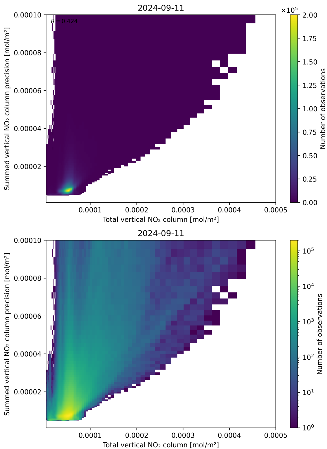
Figure 113: Scatter density plot of “Total vertical NO 2 column” against “Summed vertical NO 2 column precision” for 2024-09-10 to 2024-09-12.
