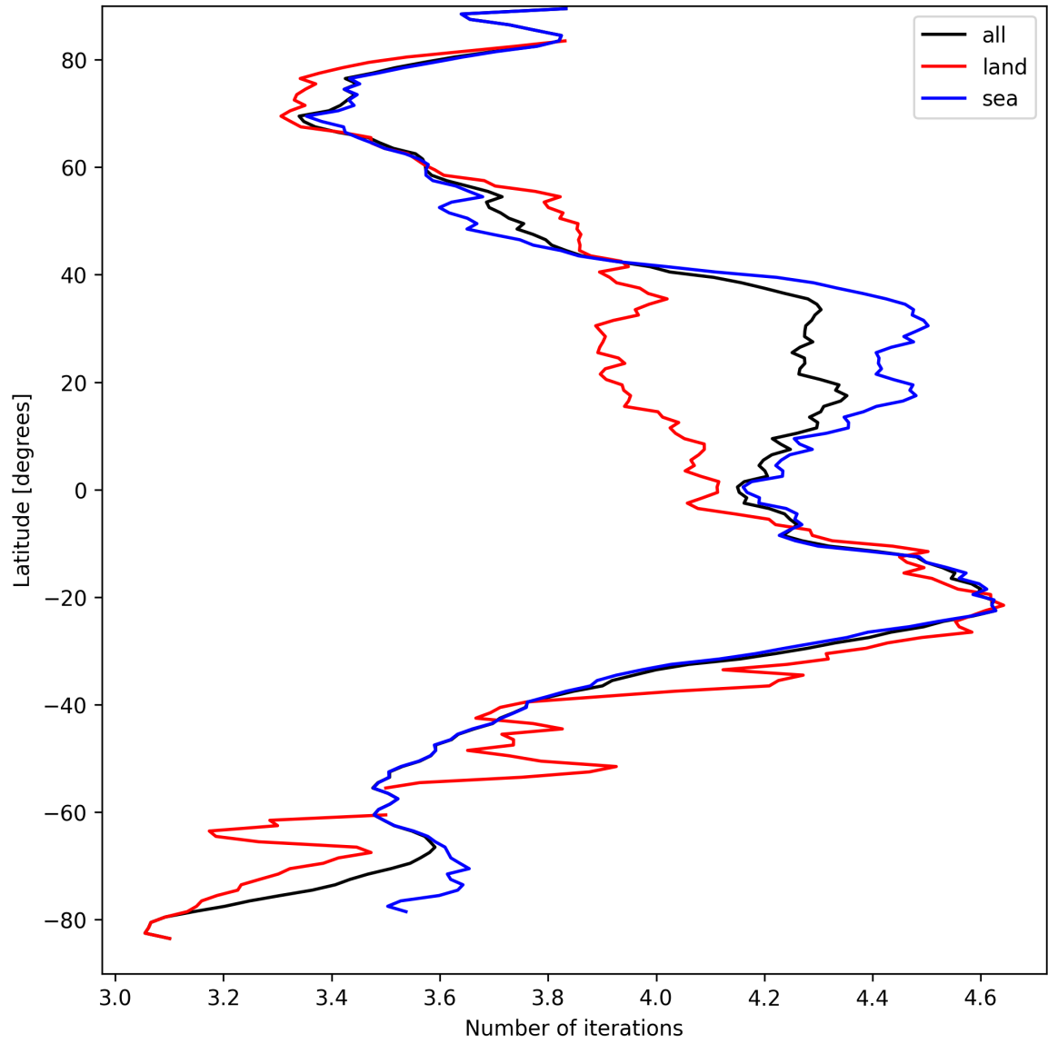
Figure 17: Zonal average of “Number of iterations” for 2024-09-10 to 2024-09-12.
