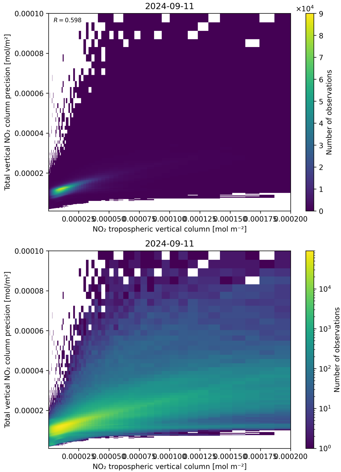
Figure 129: Scatter density plot of “NO 2 tropospheric vertical column” against “Total vertical NO 2 column precision” for 2024-09-10 to 2024-09-12.
