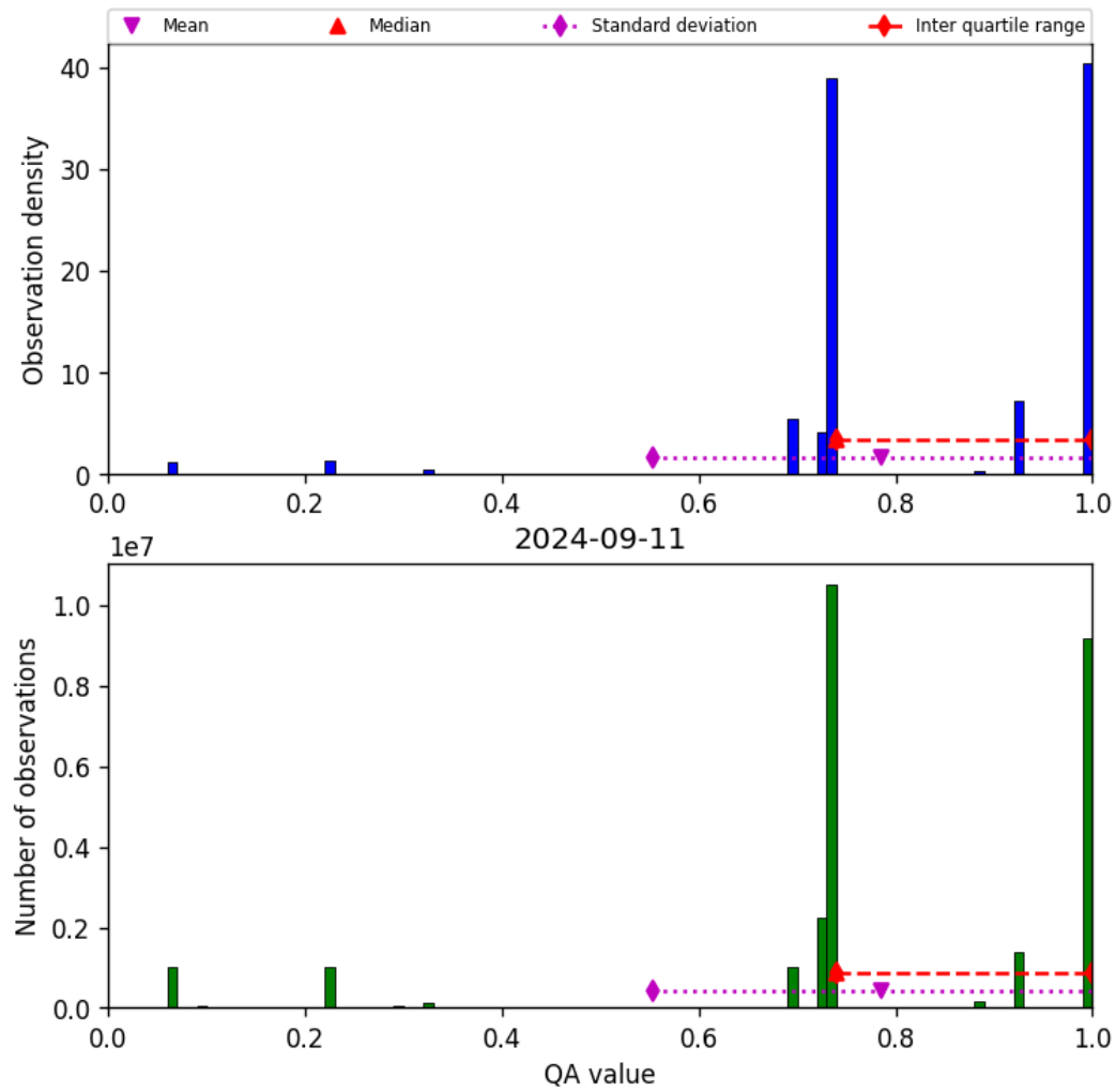
Figure 28: Histogram of “QA value” for 2024-09-10 to 2024-09-12
