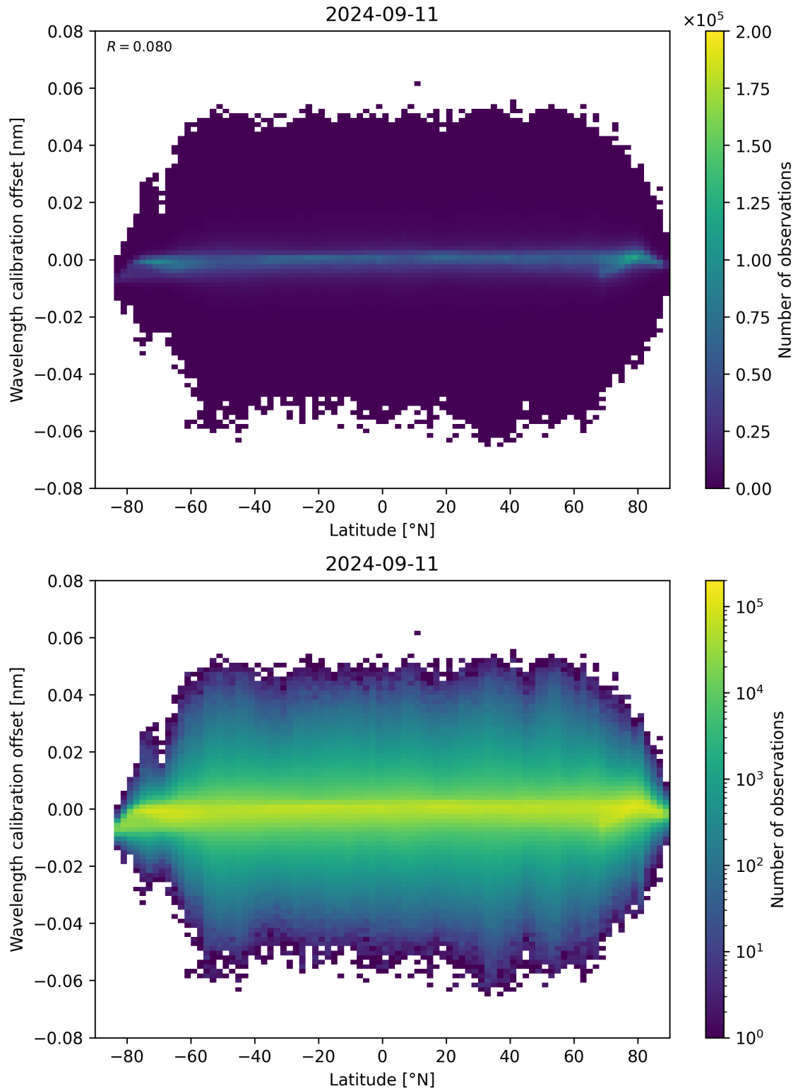
Figure 95: Scatter density plot of “Latitude” against “Wavelength calibration offset” for 2024-09-10 to 2024-09-12.
