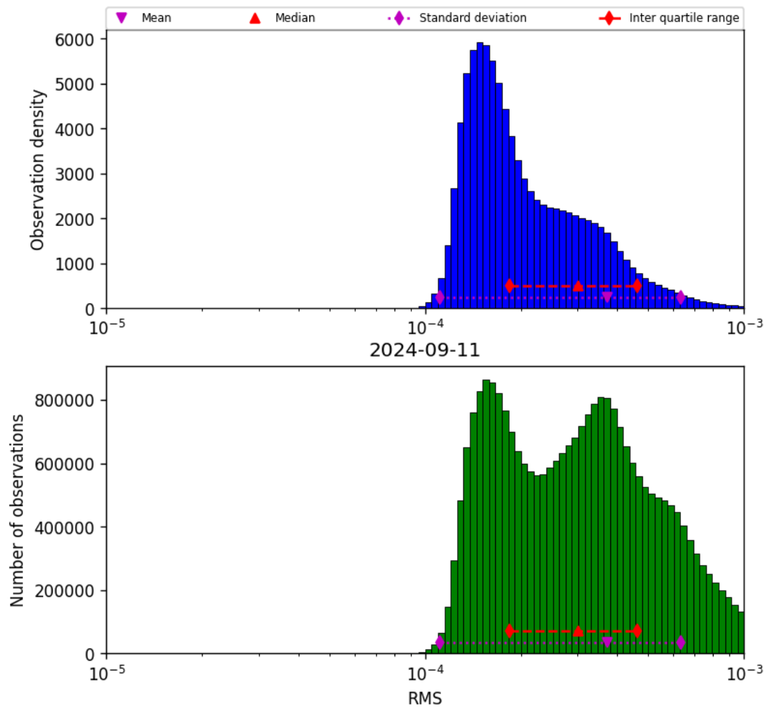
Figure 43: Histogram of “RMS” for 2024-09-10 to 2024-09-12
