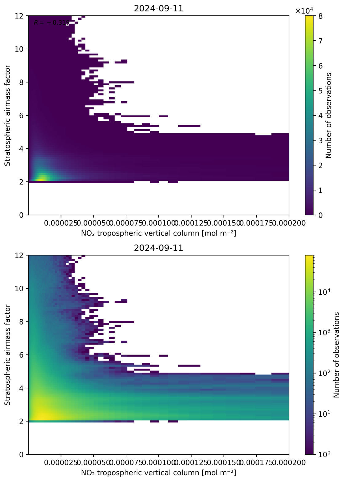
Figure 121: Scatter density plot of “NO 2 tropospheric vertical column” against “Stratospheric air mass factor” for 2024-09-10 to 2024-09-12.
