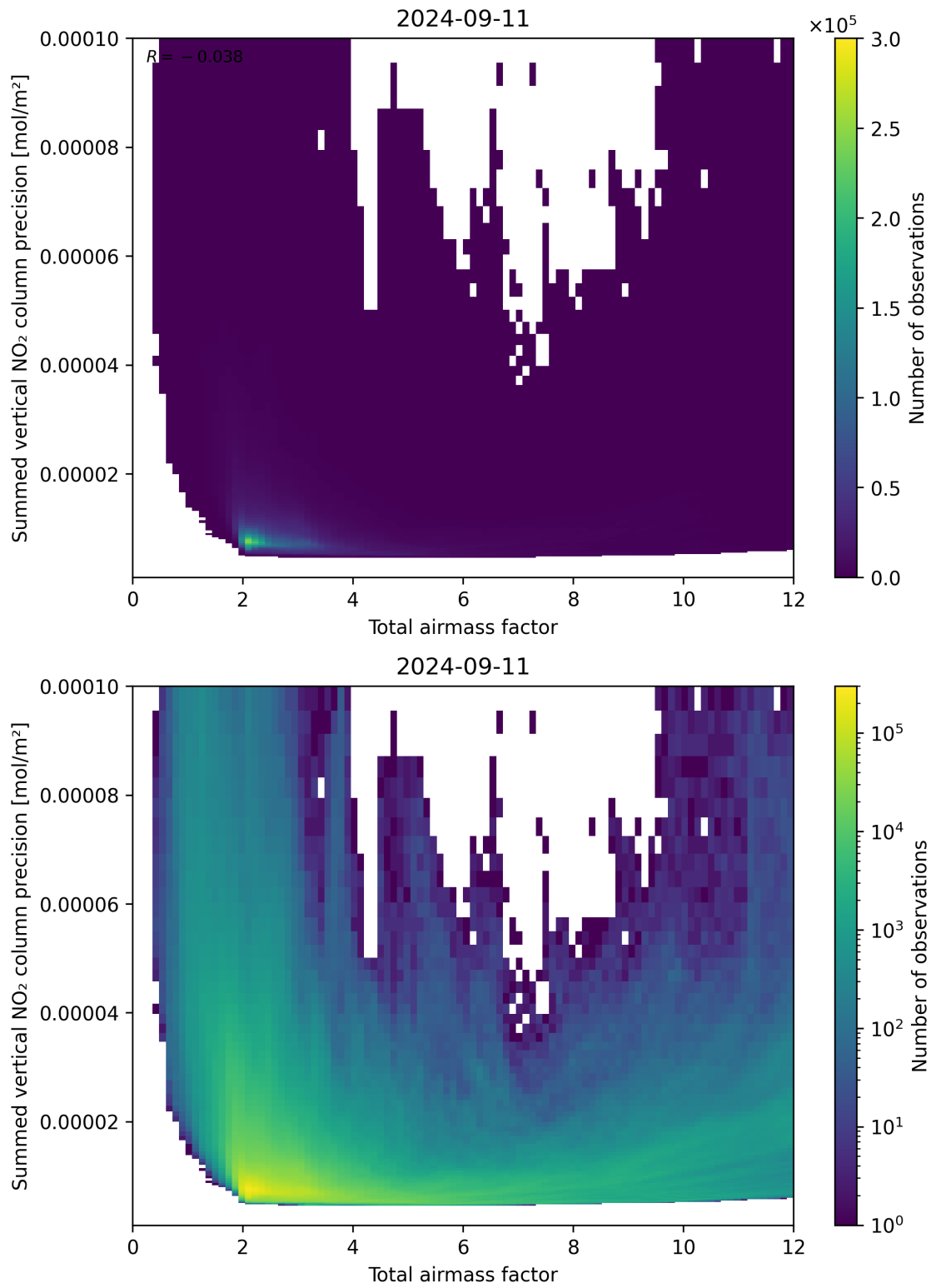
Figure 66: Scatter density plot of “Total airmass factor” against “Summed vertical NO 2 column precision” for 2024-09-10 to 2024-09-12.
