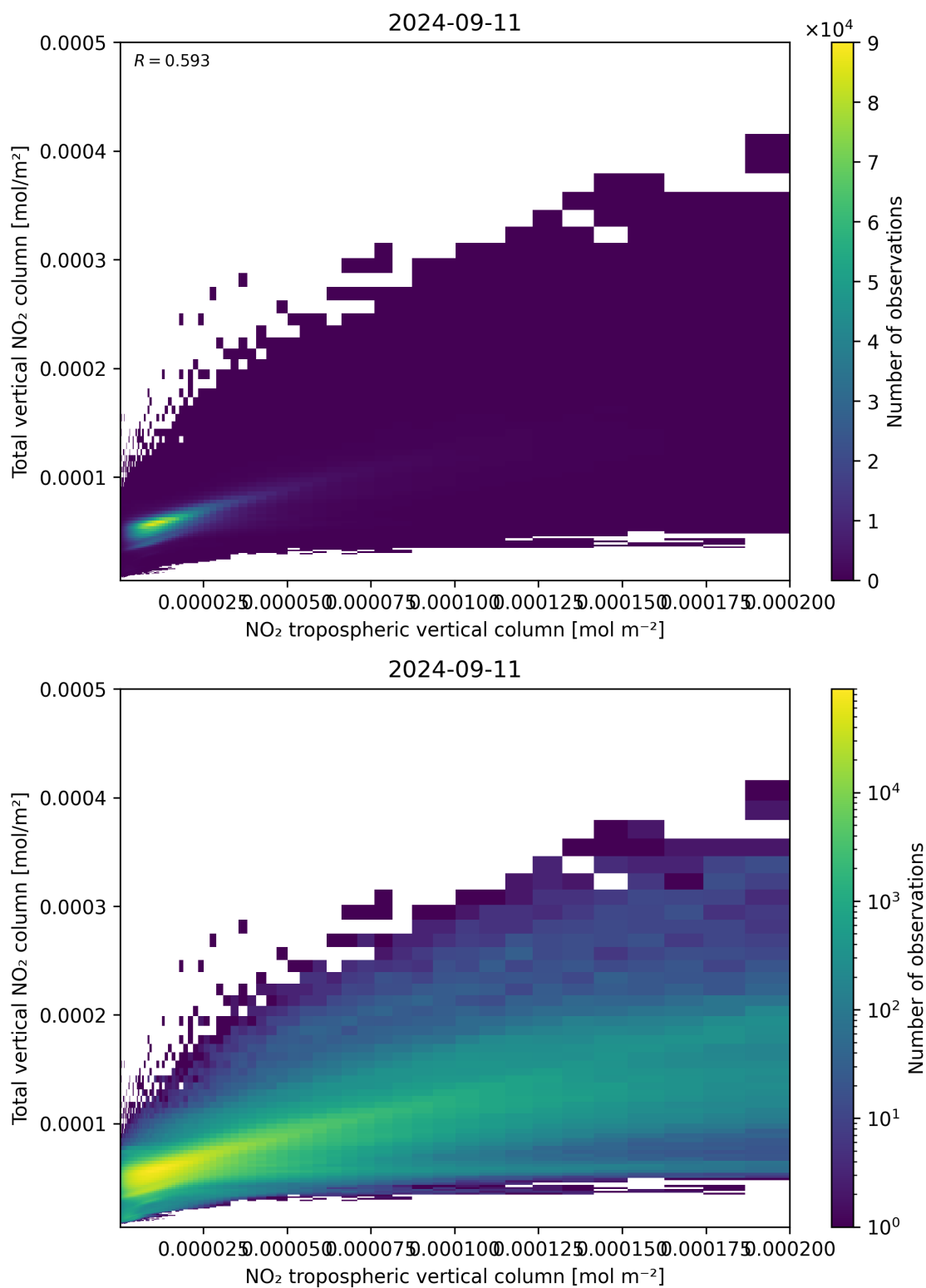
Figure 128: Scatter density plot of “NO 2 tropospheric vertical column” against “Total vertical NO 2 column” for 2024-09-10 to 2024-09-12.
