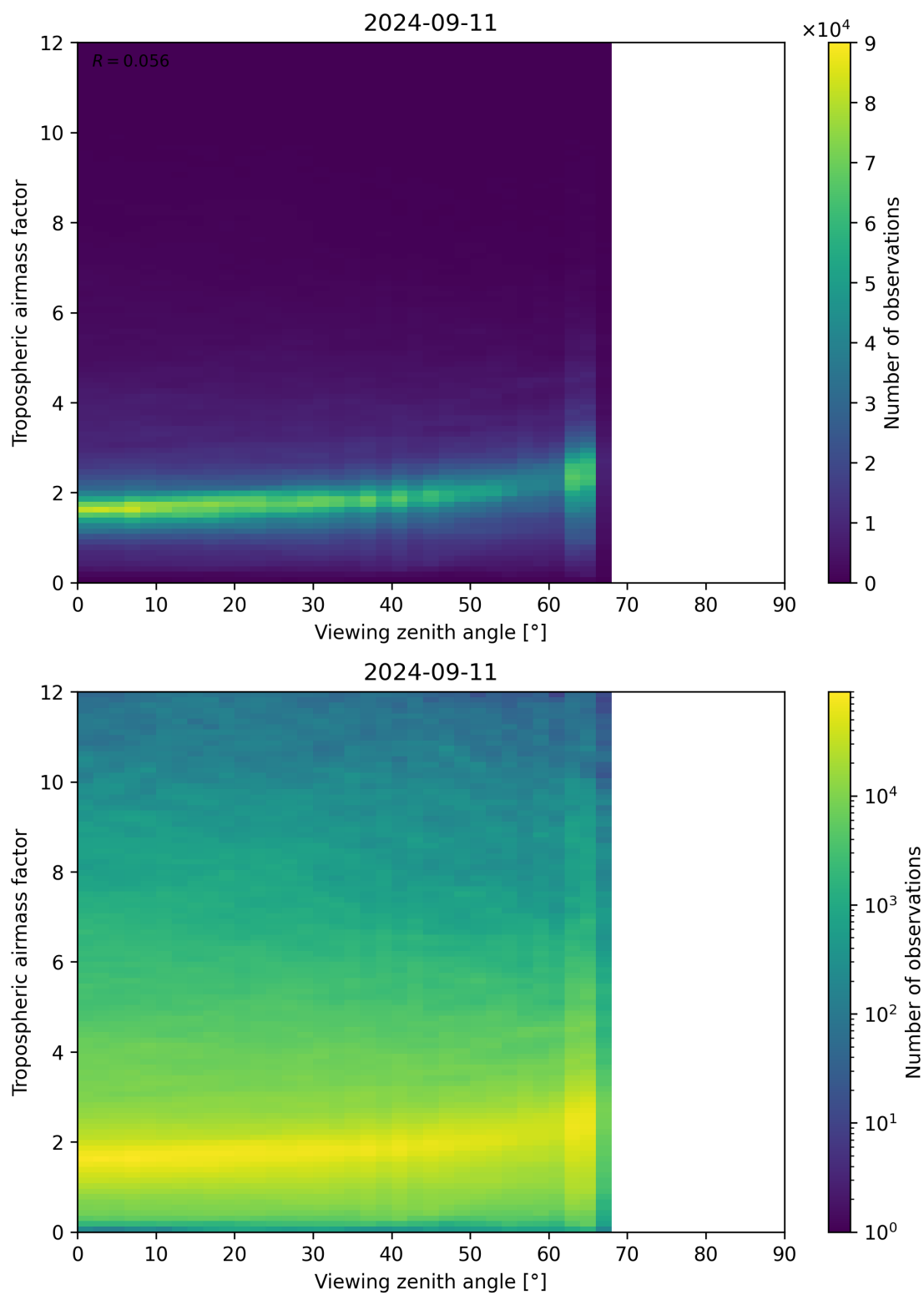
Figure 161: Scatter density plot of “Viewing zenith angle” against “Tropospheric airmass factor” for 2024-09-10 to 2024-09-12.
