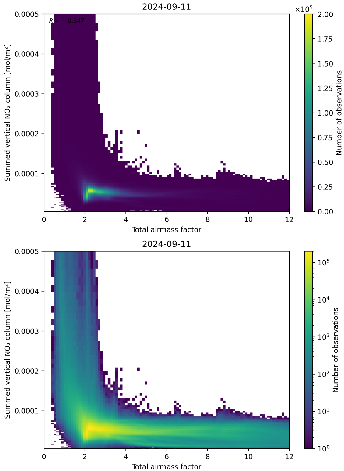
Figure 65: Scatter density plot of “Total airmass factor” against “Summed vertical NO 2 column” for 2024-09-10 to 2024-09-12.
