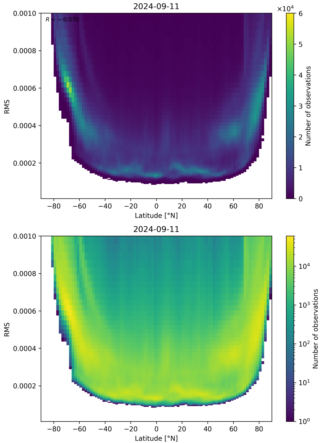
Figure 94: Scatter density plot of “Latitude” against “RMS” for 2024-09-10 to 2024-09-12.
