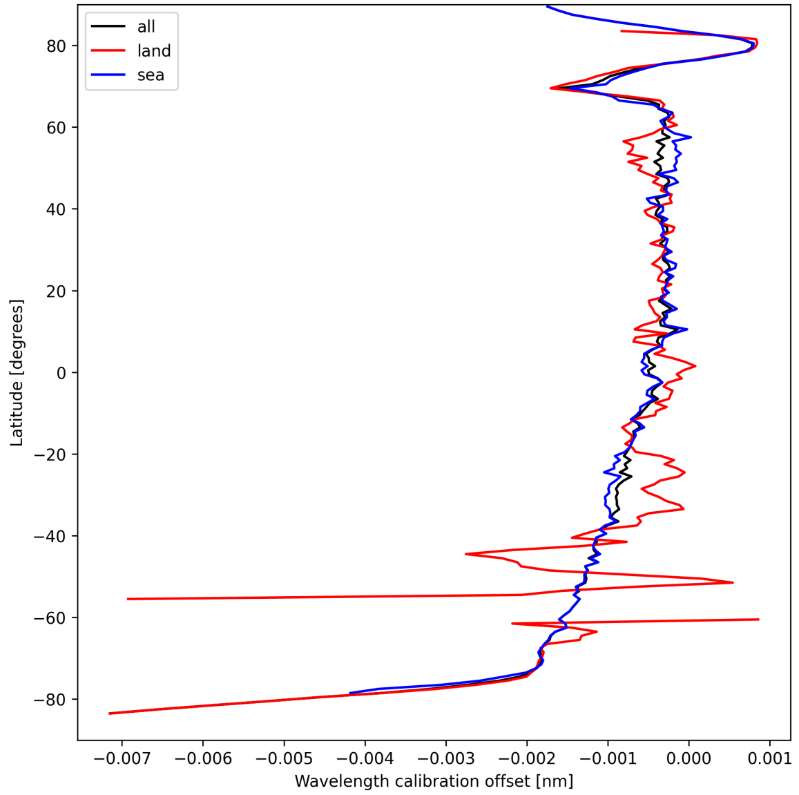
Figure 18: Zonal average of “Wavelength calibration offset” for 2024-09-10 to 2024-09-12.
