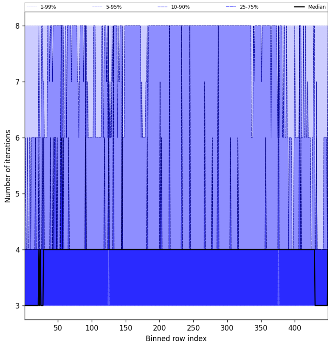
Figure 51: Along track statistics of “Number of iterations” for 2024-09-10 to 2024-09-12
