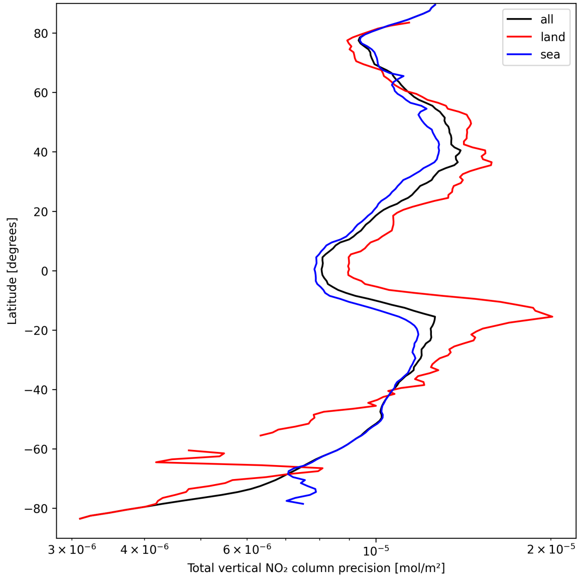
Figure 22: Zonal average of “Total vertical NO 2 column precision” for 2024-09-10 to 2024-09-12.
