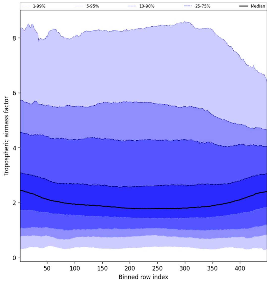
Figure 48: Along track statistics of “Tropospheric air mass factor” for 2024-09-10 to 2024-09-12
