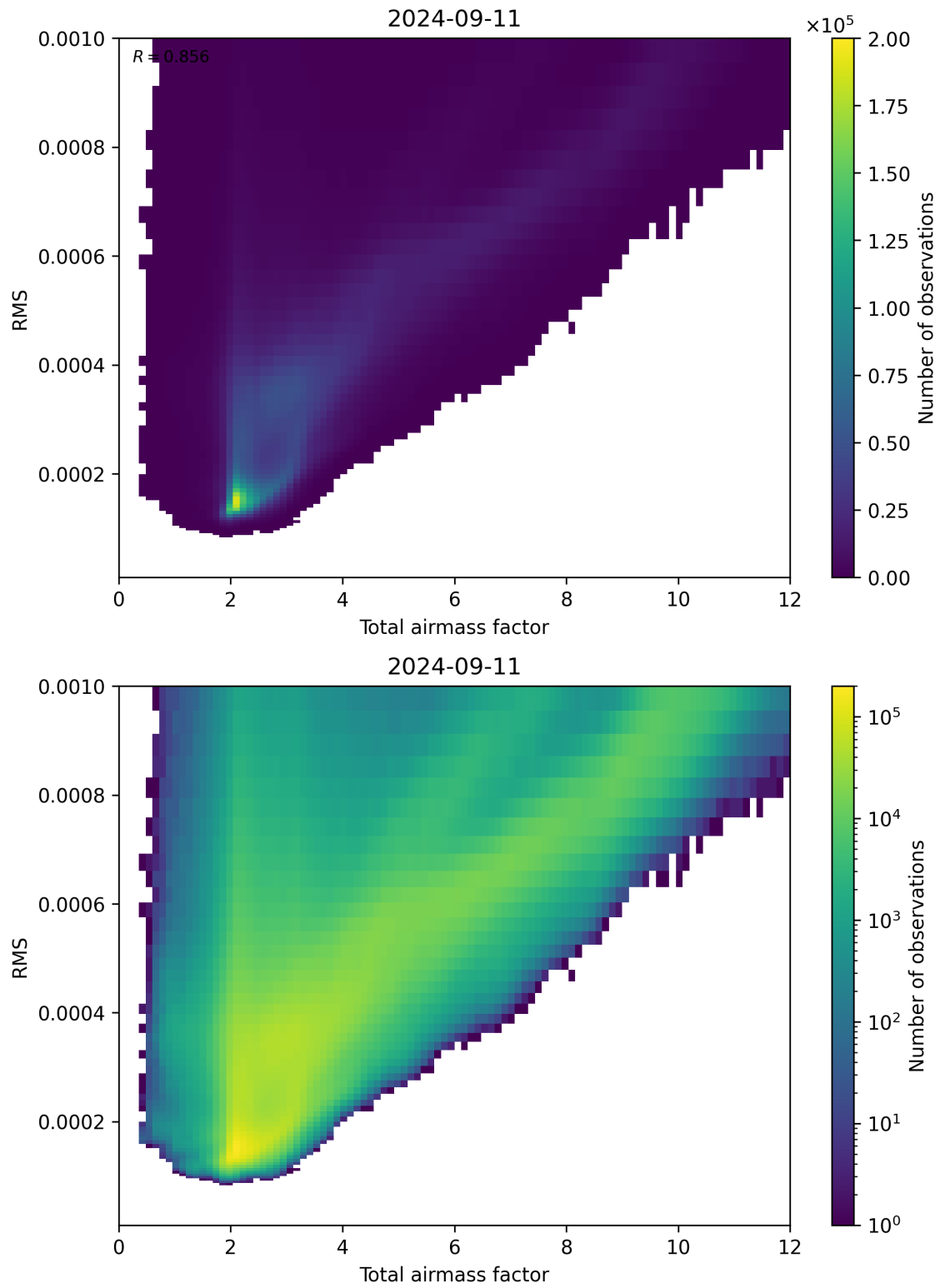
Figure 69: Scatter density plot of “Total airmass factor” against “RMS” for 2024-09-10 to 2024-09-12.
