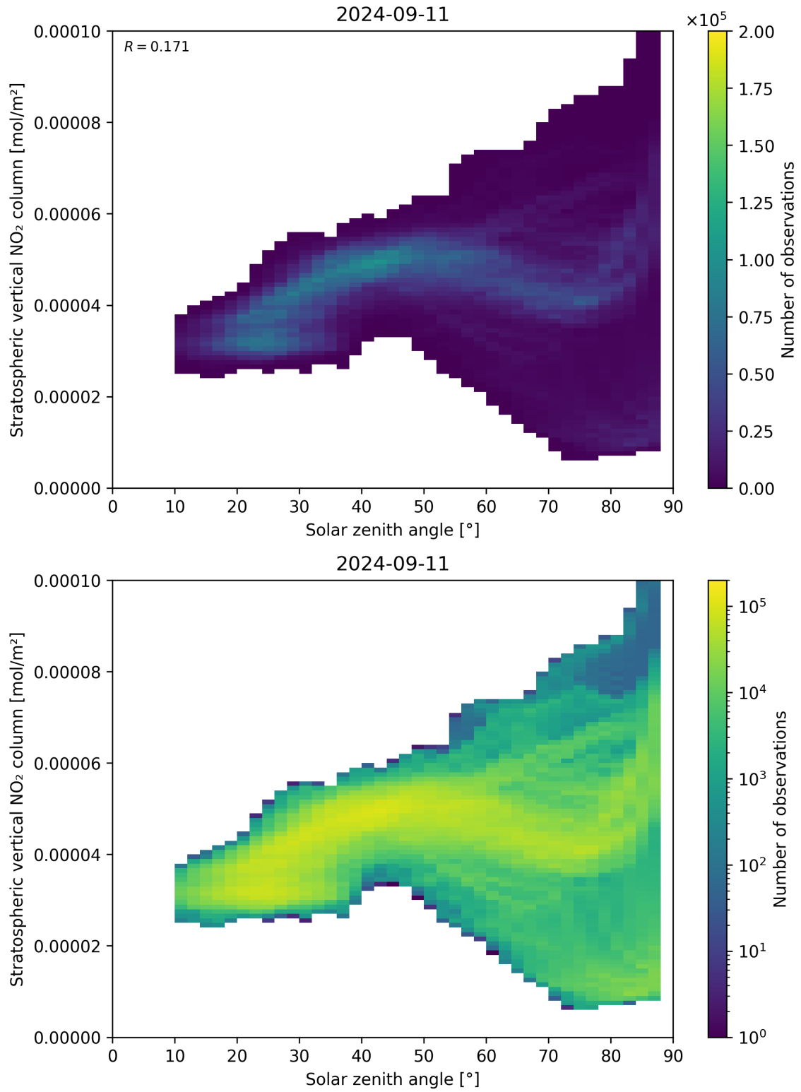
Figure 150: Scatter density plot of “Solar zenith angle” against “Stratospheric vertical NO 2 column” for 2024-09-10 to 2024-09-12.
