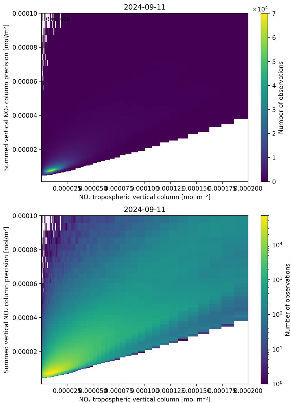
Figure 127: Scatter density plot of “NO 2 tropospheric vertical column” against “Summed vertical NO 2 column precision” for 2024-09-10 to 2024-09-12.
