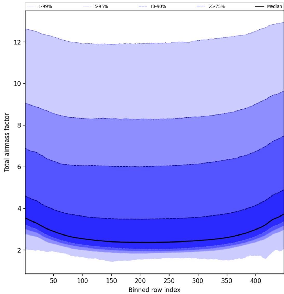
Figure 49: Along track statistics of “Total airmass factor” for 2024-09-10 to 2024-09-12
