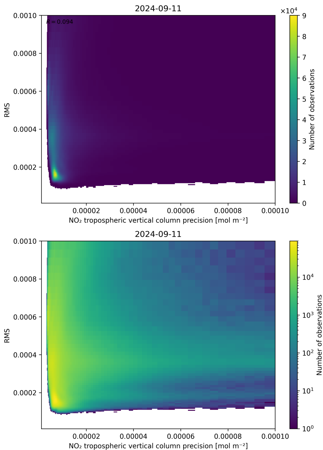
Figure 140: Scatter density plot of “NO 2 tropospheric vertical column precision” against “RMS” for 2024-09-10 to 2024-09-12.
