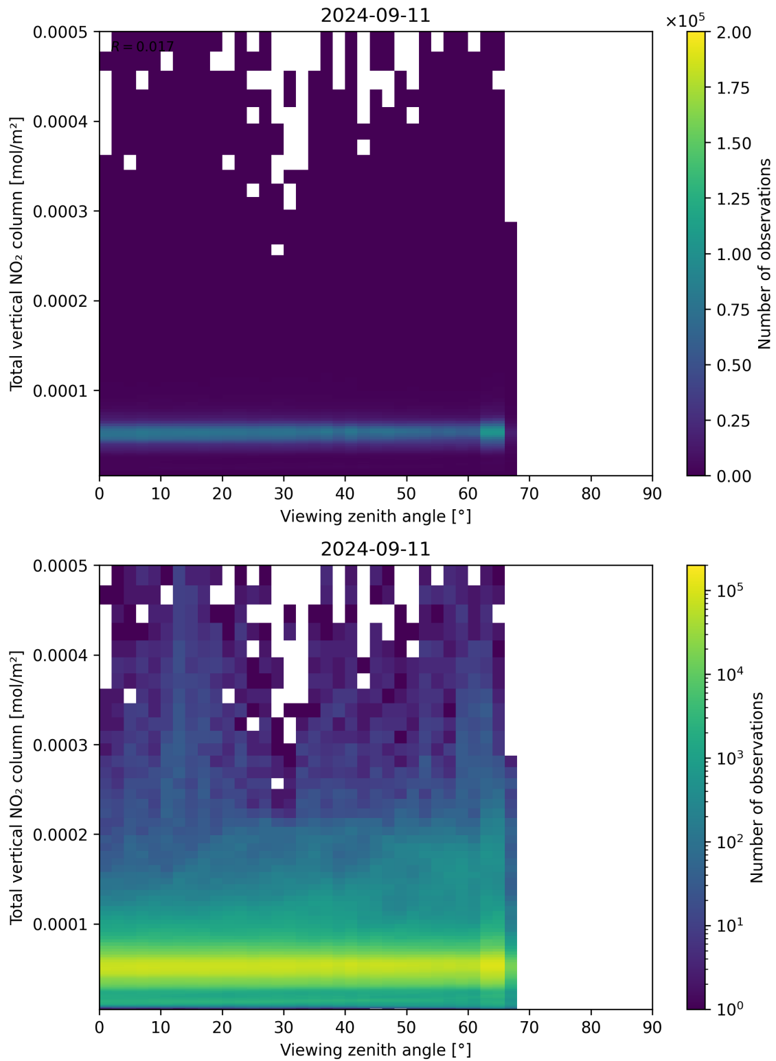
Figure 167: Scatter density plot of “Viewing zenith angle” against “Total vertical NO 2 column” for 2024-09-10 to 2024-09-12.
