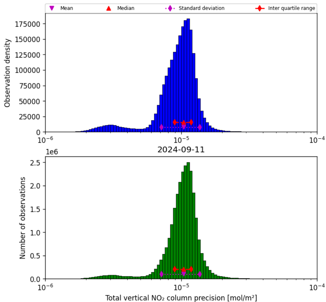
Figure 39: Histogram of “Total vertical NO 2 column precision” for 2024-09-10 to 2024-09-12
