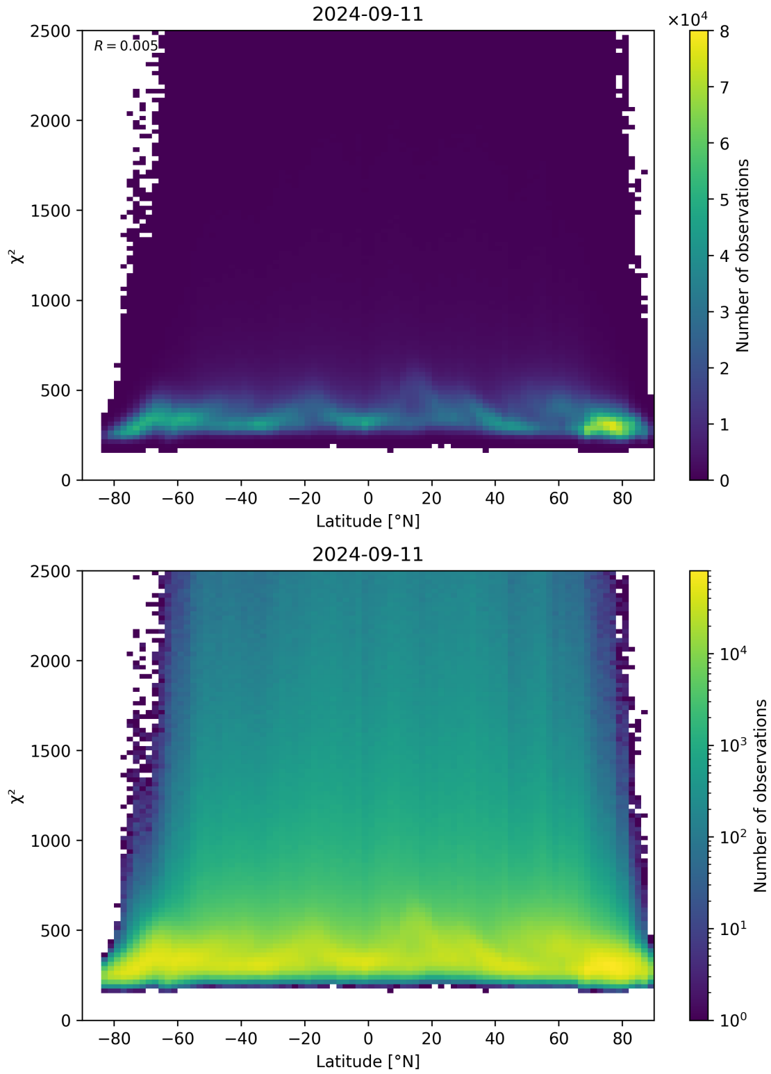
Figure 86: Scatter density plot of “Latitude” against “ \chi^2 ” for 2024-09-10 to 2024-09-12.
