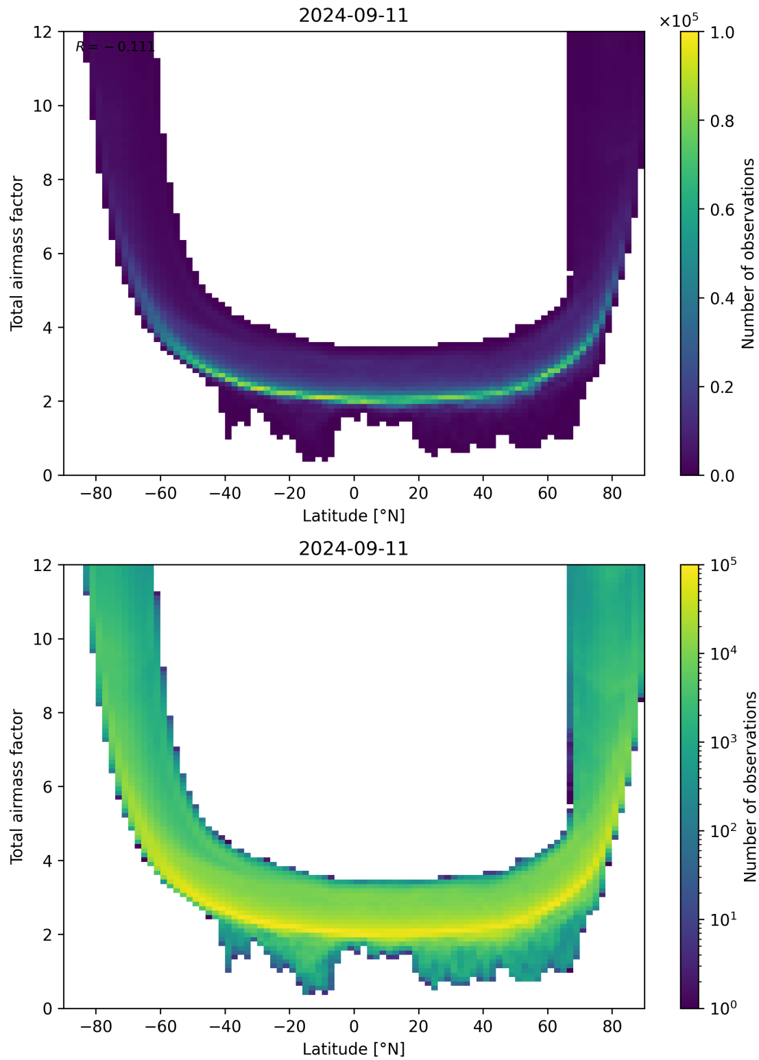
Figure 84: Scatter density plot of “Latitude” against “Total airmass factor” for 2024-09-10 to 2024-09-12.
