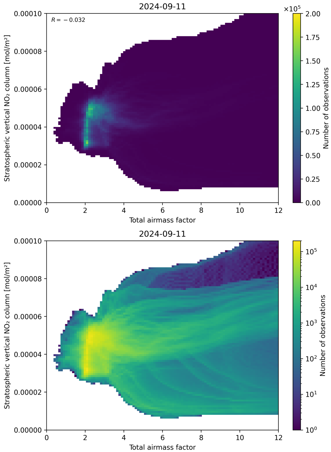
Figure 64: Scatter density plot of “Total airmass factor” against “Stratospheric vertical NO 2 column” for 2024-09-10 to 2024-09-12.
