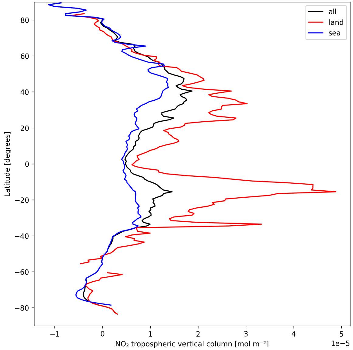
Figure 12: Zonal average of “NO 2 tropospheric vertical column” for 2024-09-10 to 2024-09-12.
