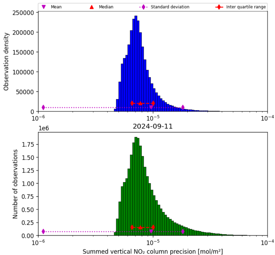
Figure 41: Histogram of “Summed vertical NO 2 column precision” for 2024-09-10 to 2024-09-12
