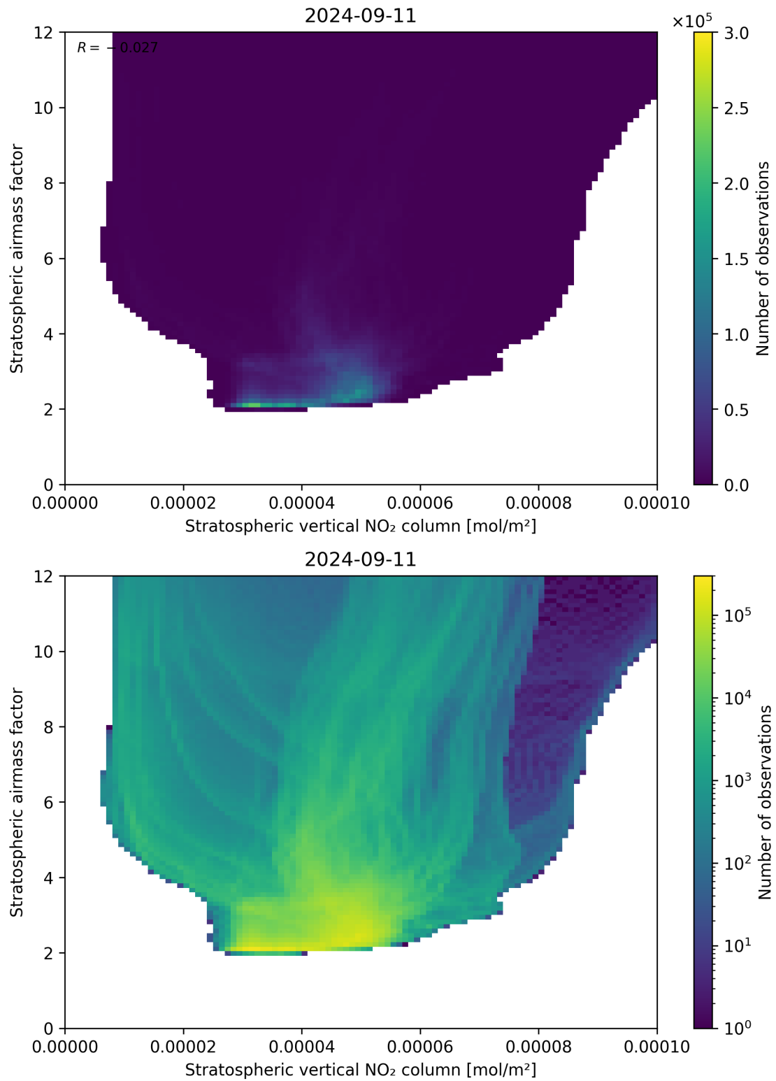
Figure 96: Scatter density plot of “Stratospheric vertical NO 2 column” against “Stratospheric airmass factor” for 2024-09-10 to 2024-09-12.
