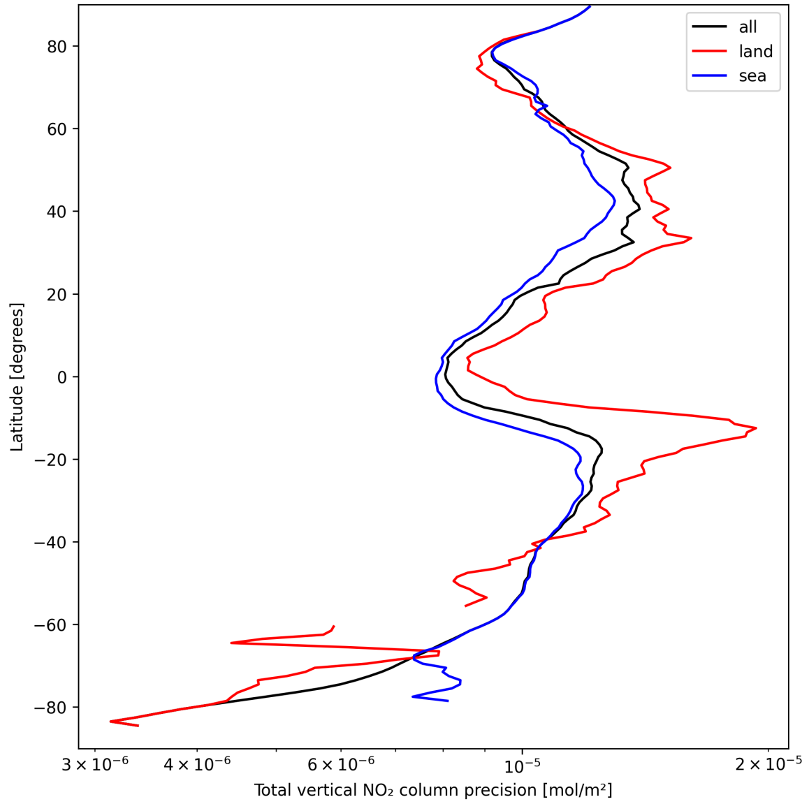
Figure 22: Zonal average of “Total vertical NO 2 column precision” for 2024-09-12 to 2024-09-13.
