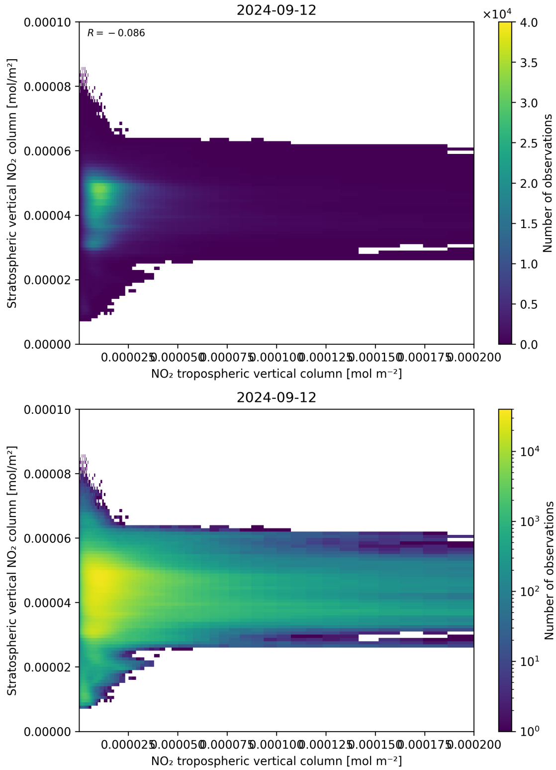
Figure 125: Scatter density plot of “NO 2 tropospheric vertical column” against “Stratospheric vertical NO 2 column” for 2024-09-12 to 2024-09-13.
