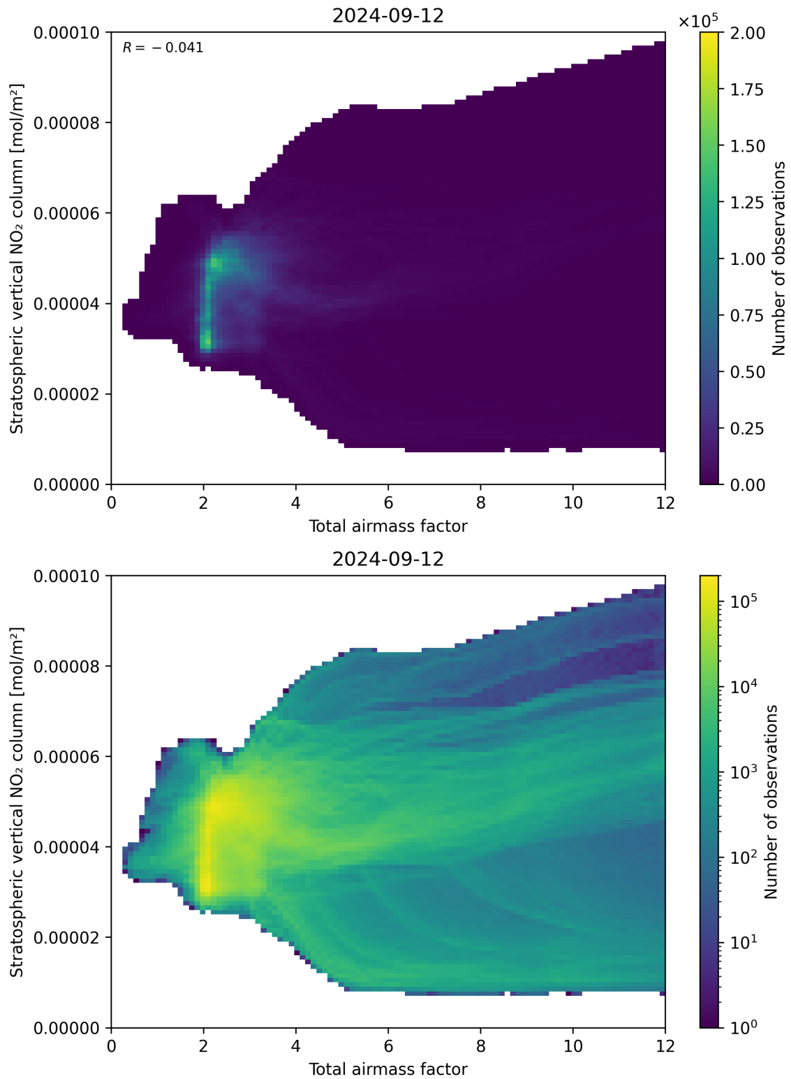
Figure 64: Scatter density plot of “Total airmass factor” against “Stratospheric vertical NO 2 column” for 2024-09-12 to 2024-09-13.
