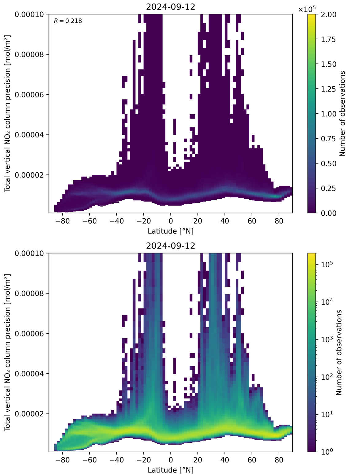
Figure 91: Scatter density plot of “Latitude” against “Total vertical NO 2 column precision” for 2024-09-12 to 2024-09-13.
