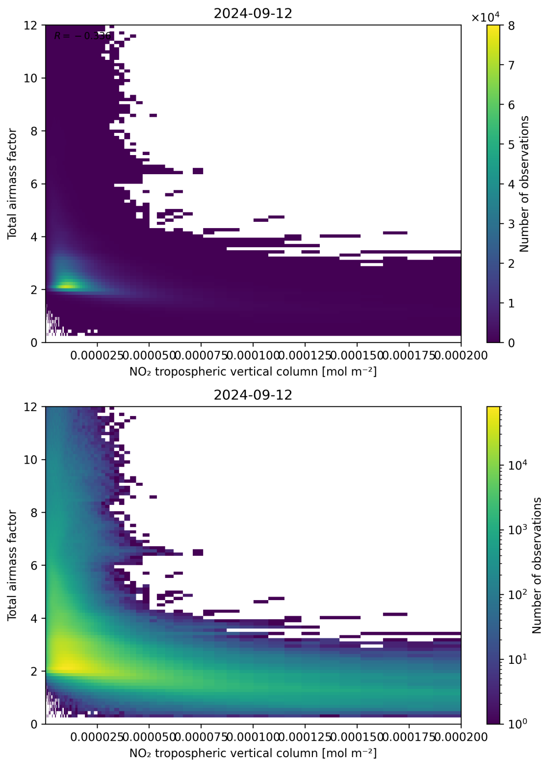
Figure 122: Scatter density plot of “NO 2 tropospheric vertical column” against “Total air mass factor” for 2024-09-12 to 2024-09-13.
