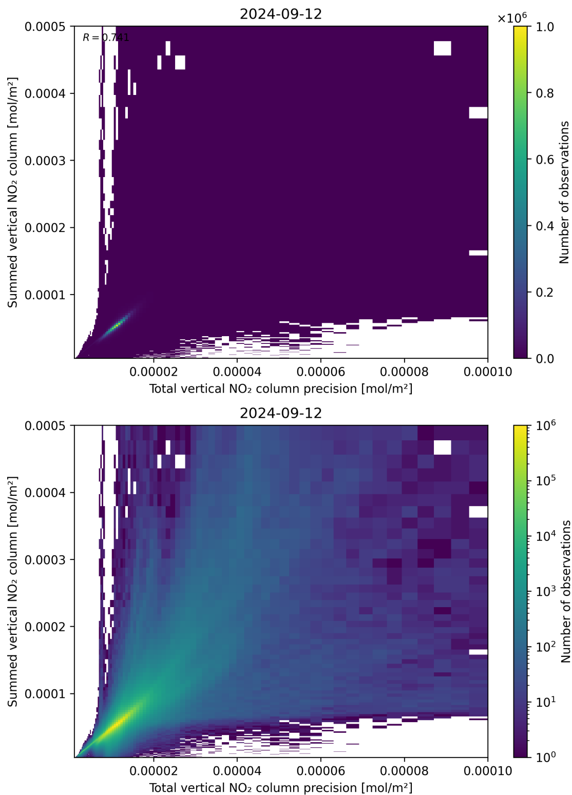
Figure 117: Scatter density plot of “Total vertical NO 2 column precision” against “Summed vertical NO 2 column” for 2024-09-12 to 2024-09-13.
