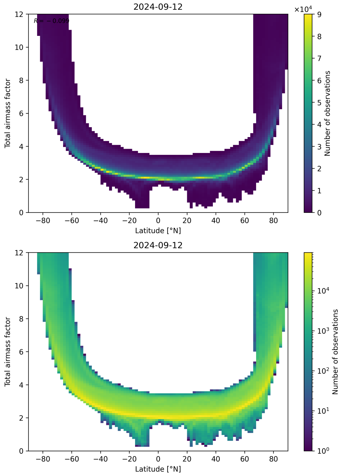
Figure 84: Scatter density plot of “Latitude” against “Total airmass factor” for 2024-09-12 to 2024-09-13.
