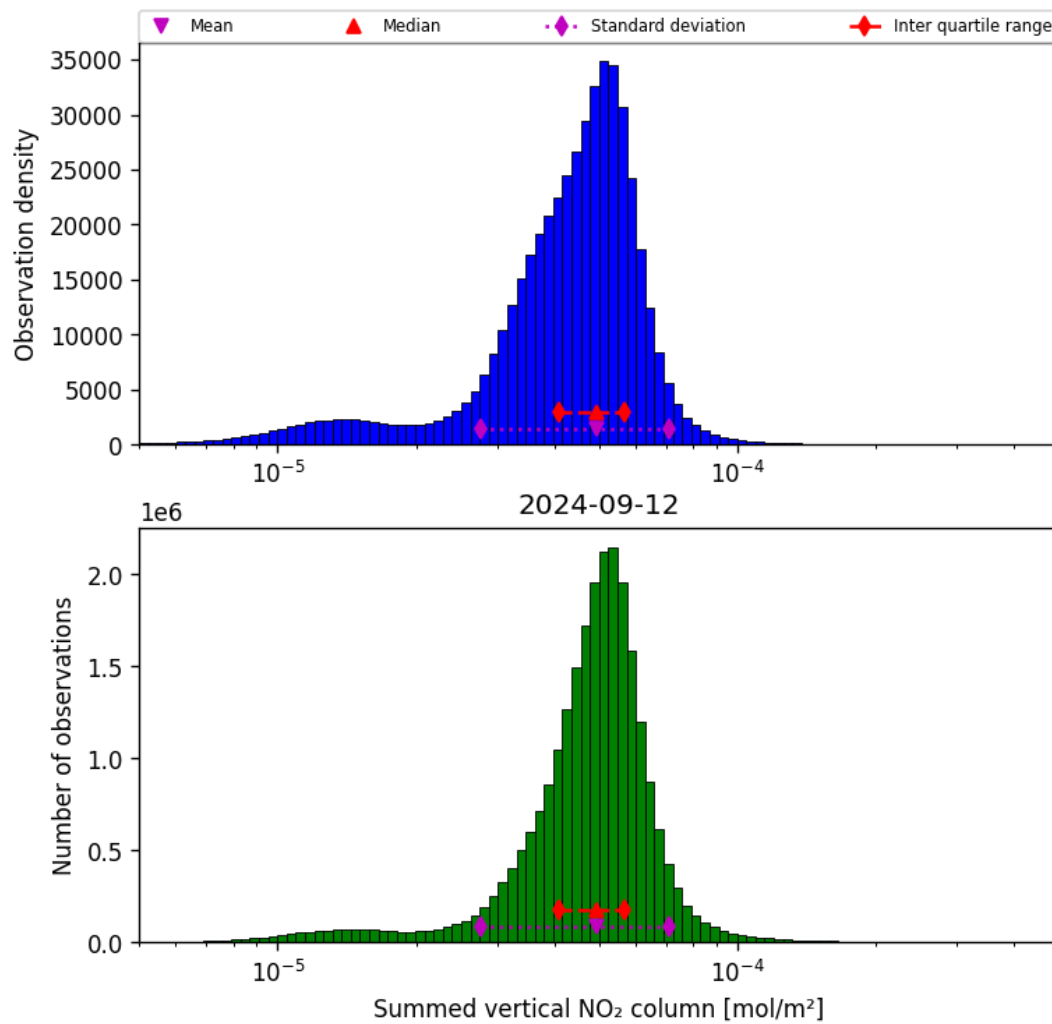
Figure 40: Histogram of “Summed vertical NO 2 column” for 2024-09-12 to 2024-09-13
