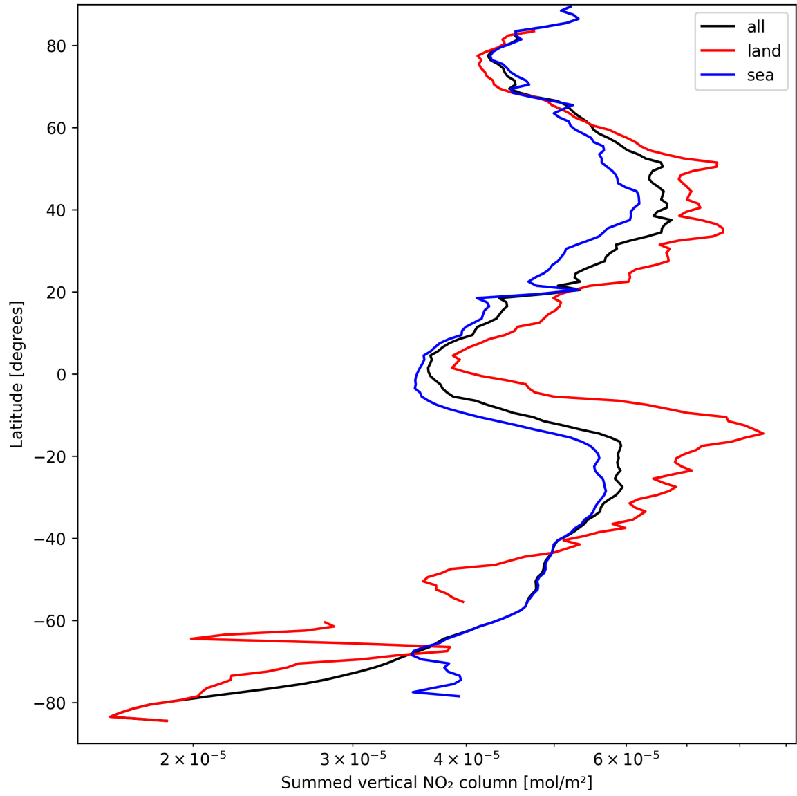
Figure 23: Zonal average of “Summed vertical NO 2 column” for 2024-09-12 to 2024-09-13.
