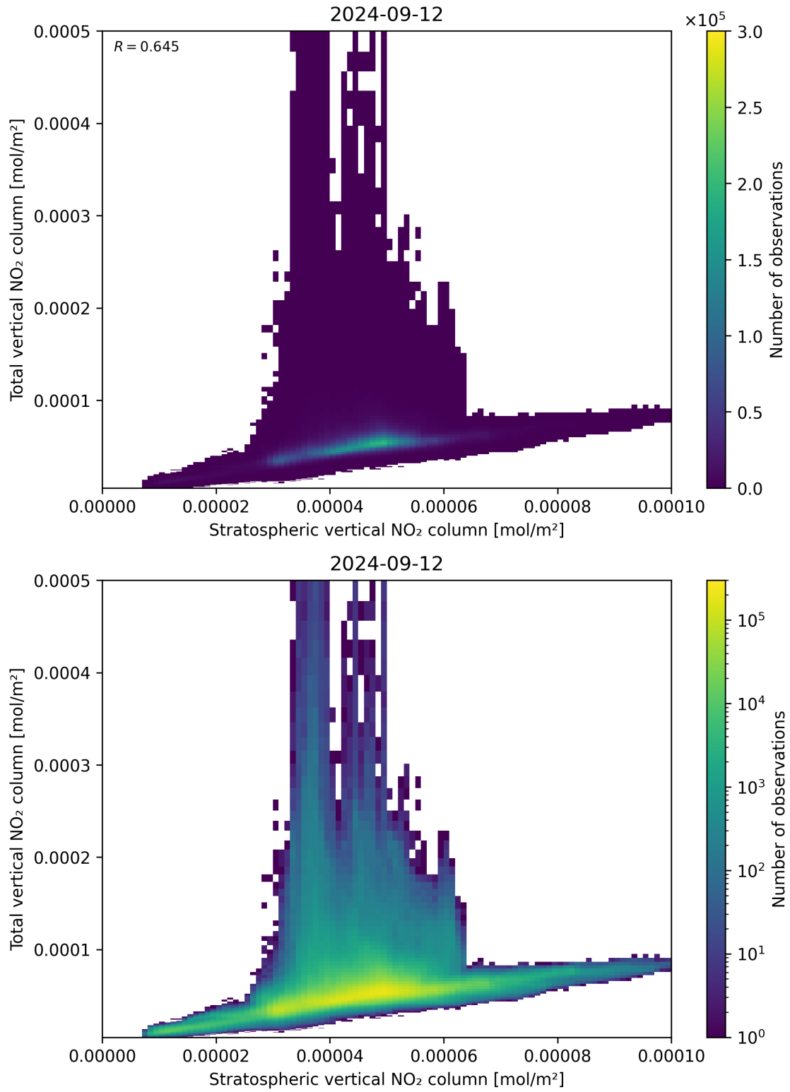
Figure 100: Scatter density plot of “Stratospheric vertical NO 2 column” against “Total vertical NO 2 column” for 2024-09-12 to 2024-09-13.
