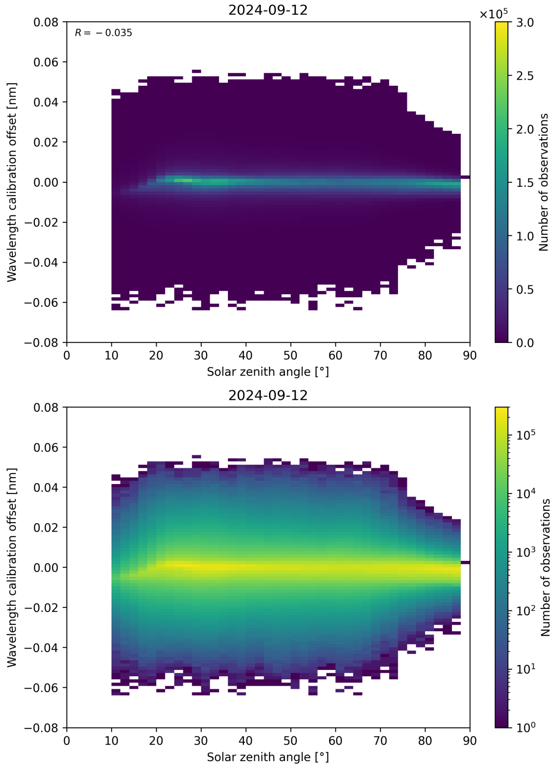
Figure 158: Scatter density plot of “Solar zenith angle” against “Wavelength calibration offset” for 2024-09-12 to 2024-09-13.
