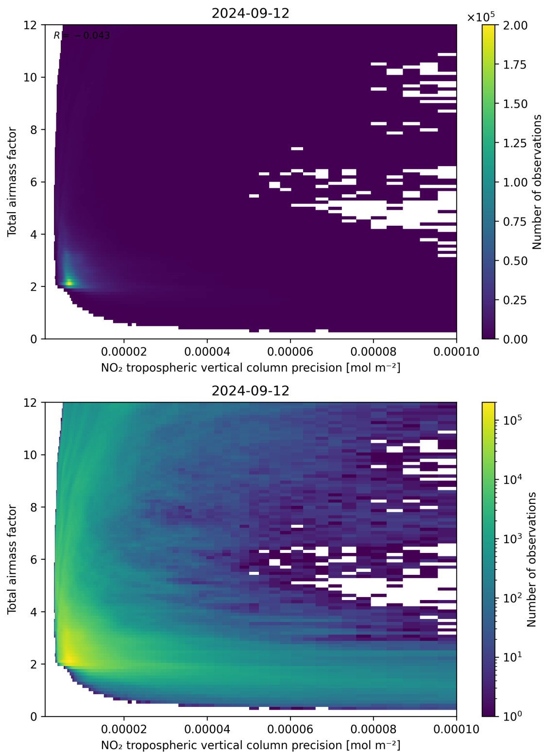
Figure 132: Scatter density plot of “NO 2 tropospheric vertical column precision” against “Total air mass factor” for 2024-09-12 to 2024-09-13.
