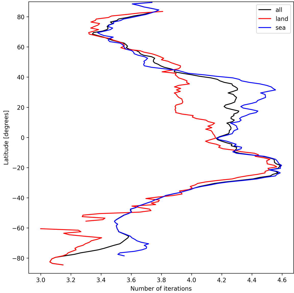
Figure 17: Zonal average of “Number of iterations” for 2024-09-12 to 2024-09-13.
