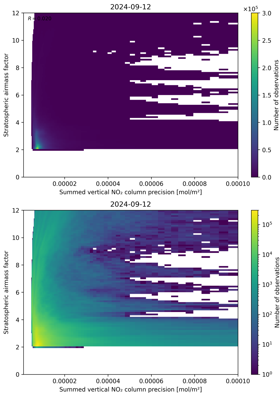
Figure 106: Scatter density plot of “Summed vertical NO 2 column precision” against “Stratospheric airmass factor” for 2024-09-12 to 2024-09-13.
