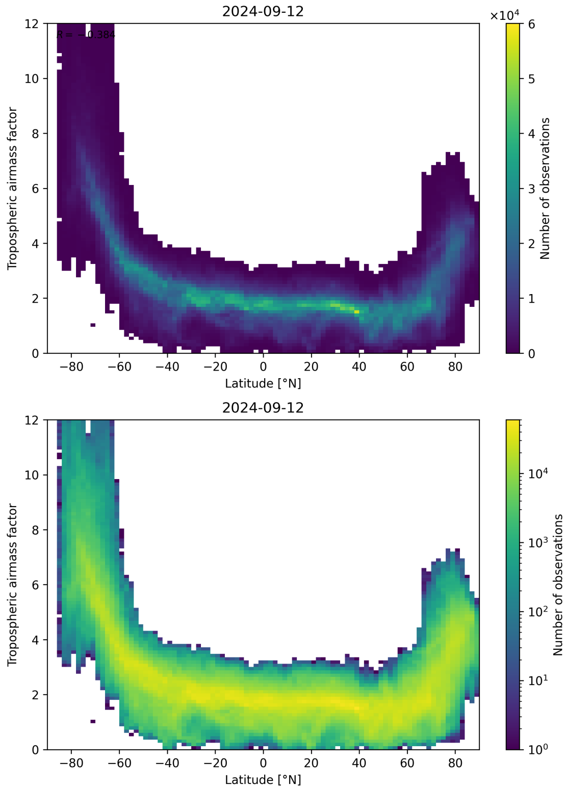
Figure 85: Scatter density plot of “Latitude” against “Tropospheric airmass factor” for 2024-09-12 to 2024-09-13.
