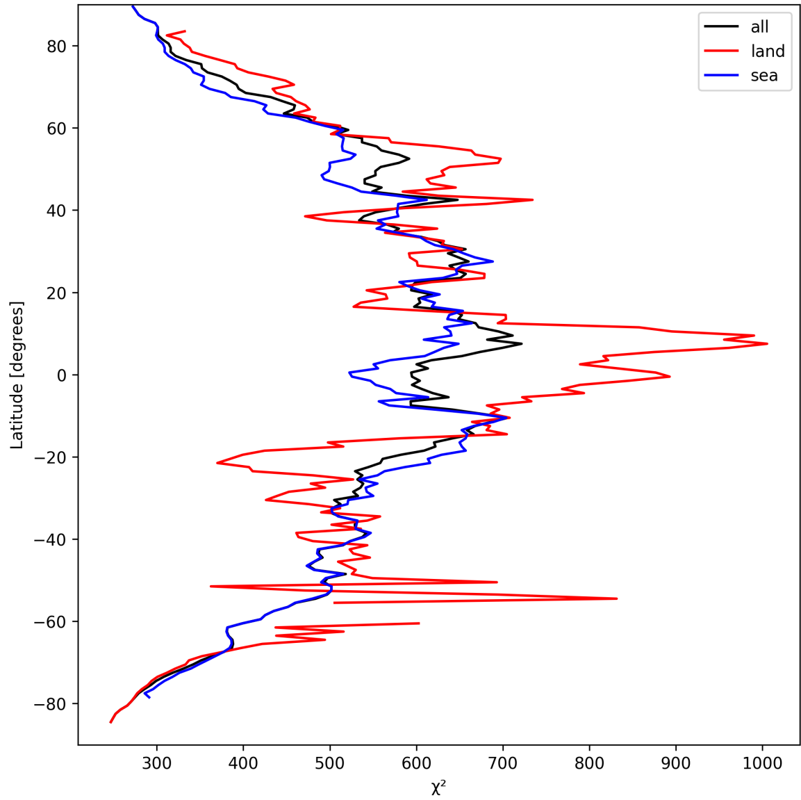
Figure 25: Zonal average of “ \chi^2 ” for 2024-09-12 to 2024-09-13.
