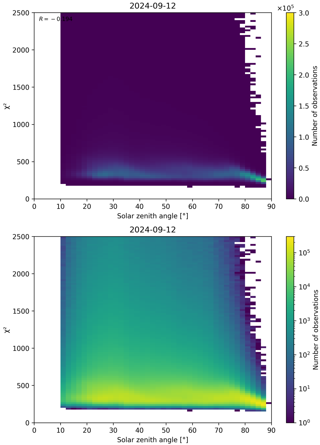
Figure 148: Scatter density plot of “Solar zenith angle” against “ \chi^2 ” for 2024-09-12 to 2024-09-13.
