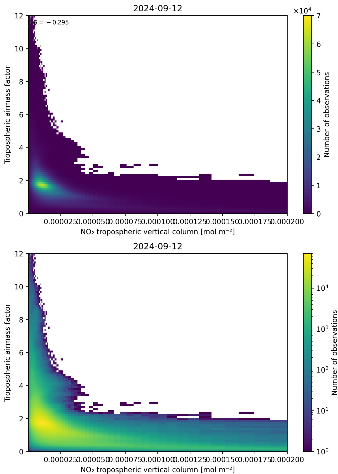
Figure 123: Scatter density plot of “NO 2 tropospheric vertical column” against “Tropospheric air mass factor” for 2024-09-12 to 2024-09-13.
