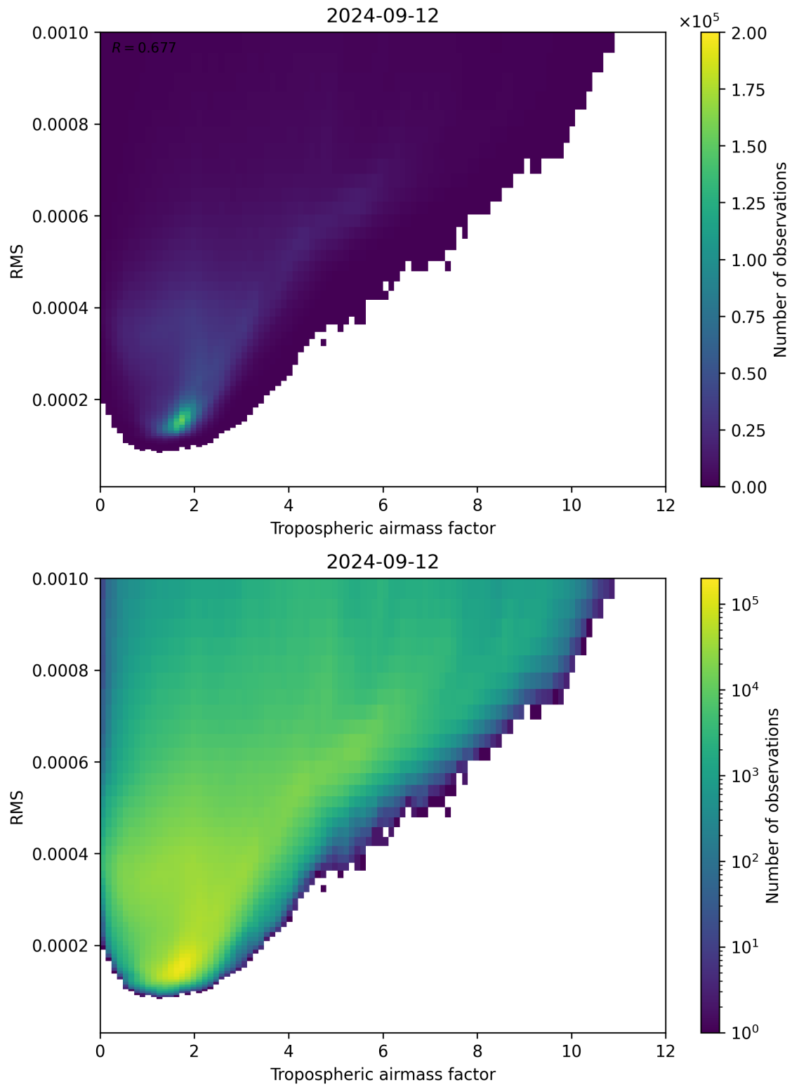
Figure 79: Scatter density plot of “Tropospheric airmass factor” against “RMS” for 2024-09-12 to 2024-09-13.
