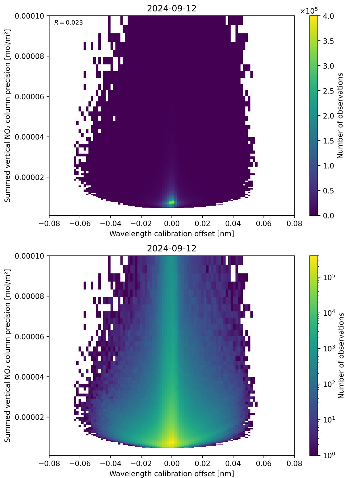
Figure 178: Scatter density plot of “Wavelength calibration offset” against “Summed vertical NO 2 column precision” for 2024-09-12 to 2024-09-13.
