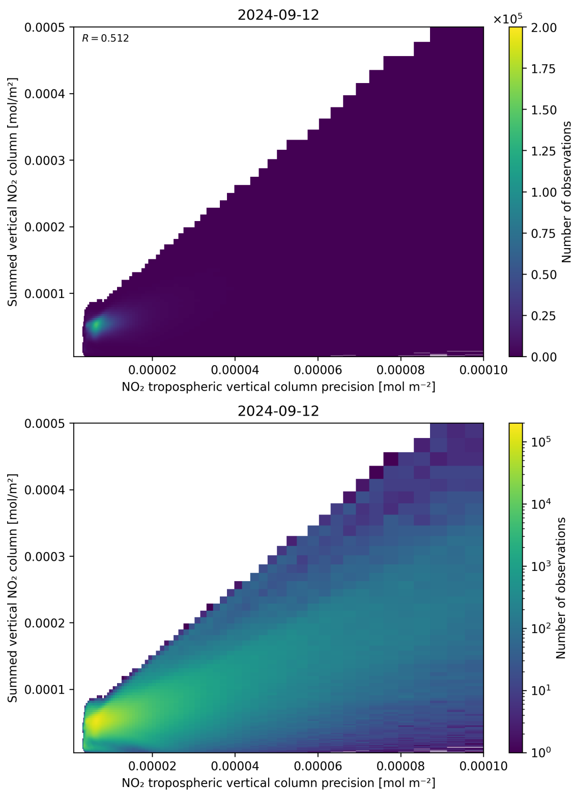
Figure 136: Scatter density plot of “NO 2 tropospheric vertical column precision” against “Summed vertical NO 2 column” for 2024-09-12 to 2024-09-13.
