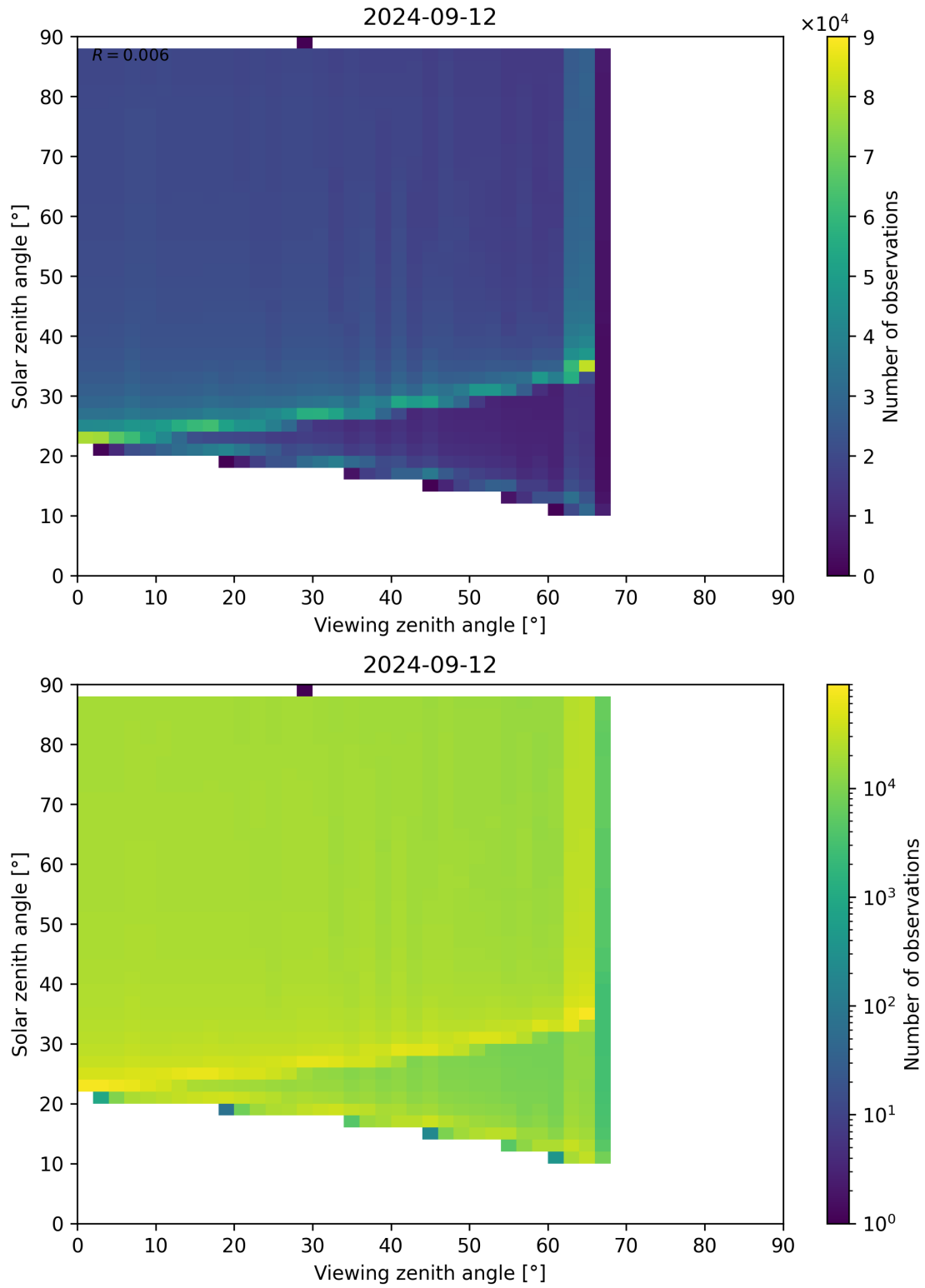
Figure 172: Scatter density plot of “Viewing zenith angle” against “Solar zenith angle” for 2024-09-12 to 2024-09-13.
