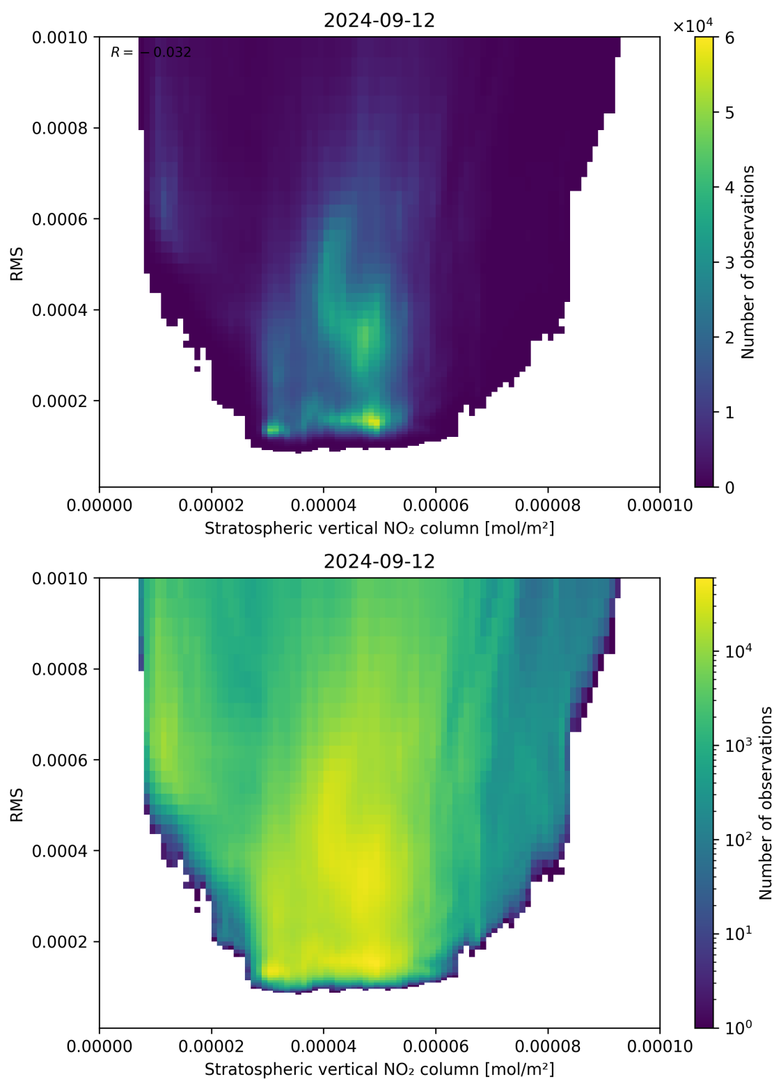
Figure 102: Scatter density plot of “Stratospheric vertical NO 2 column” against “RMS” for 2024-09-12 to 2024-09-13.
