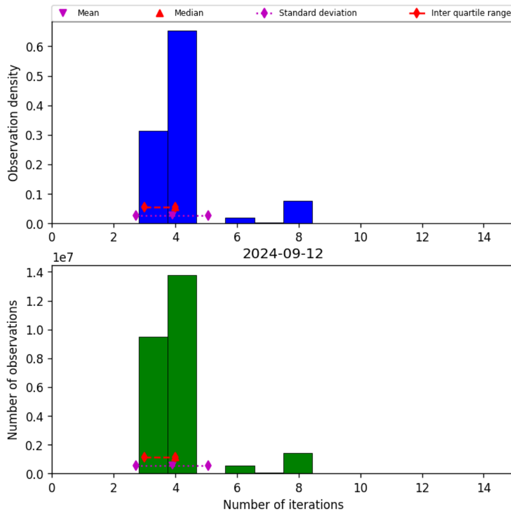
Figure 34: Histogram of “Number of iterations” for 2024-09-12 to 2024-09-13
