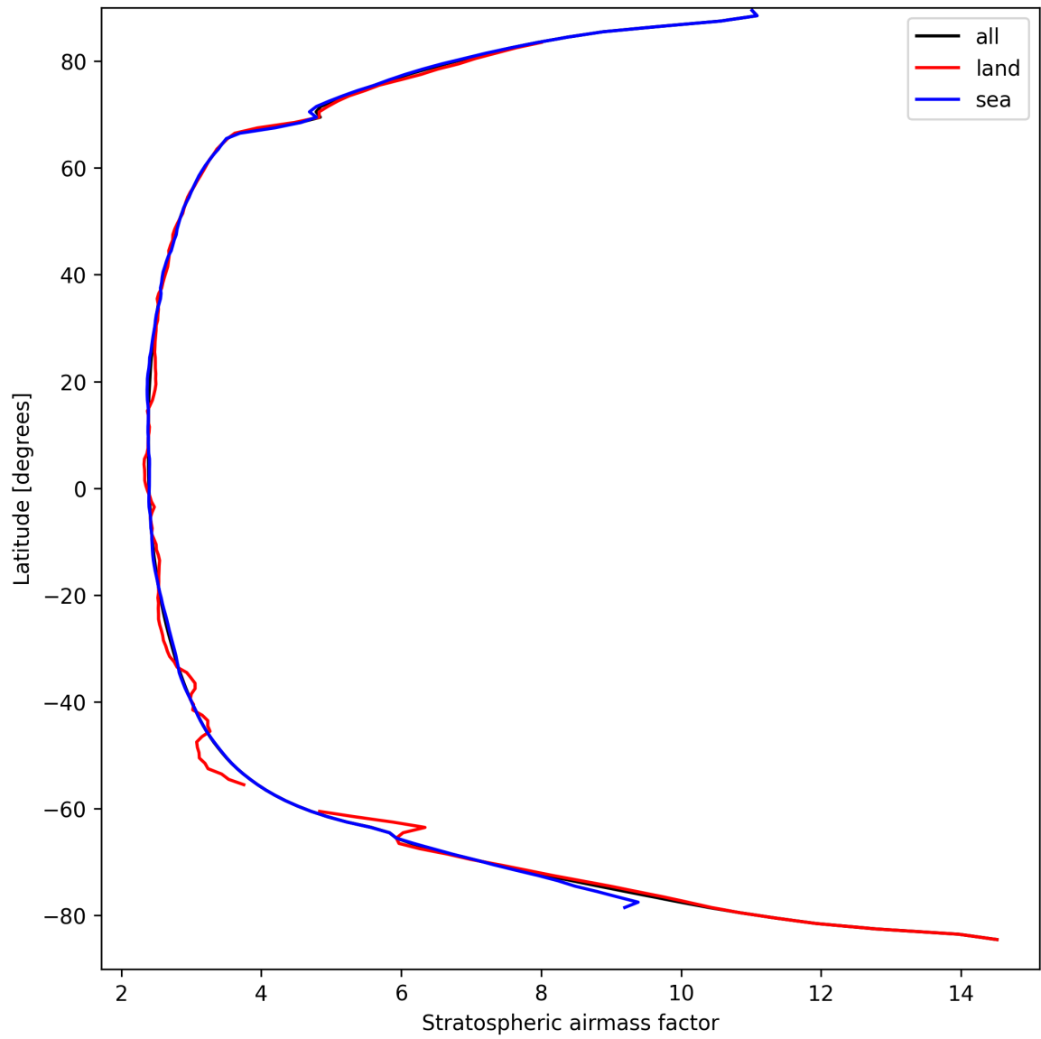
Figure 27: Zonal average of “Stratospheric airmass factor” for 2024-09-12 to 2024-09-13.
