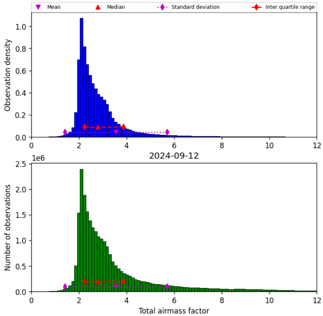
Figure 32: Histogram of “Total airmass factor” for 2024-09-12 to 2024-09-13
