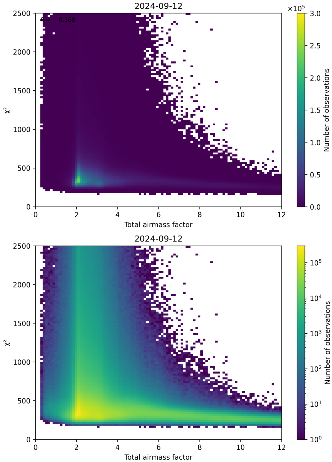
Figure 63: Scatter density plot of “Total airmass factor” against “ \chi^2 ” for 2024-09-12 to 2024-09-13.
