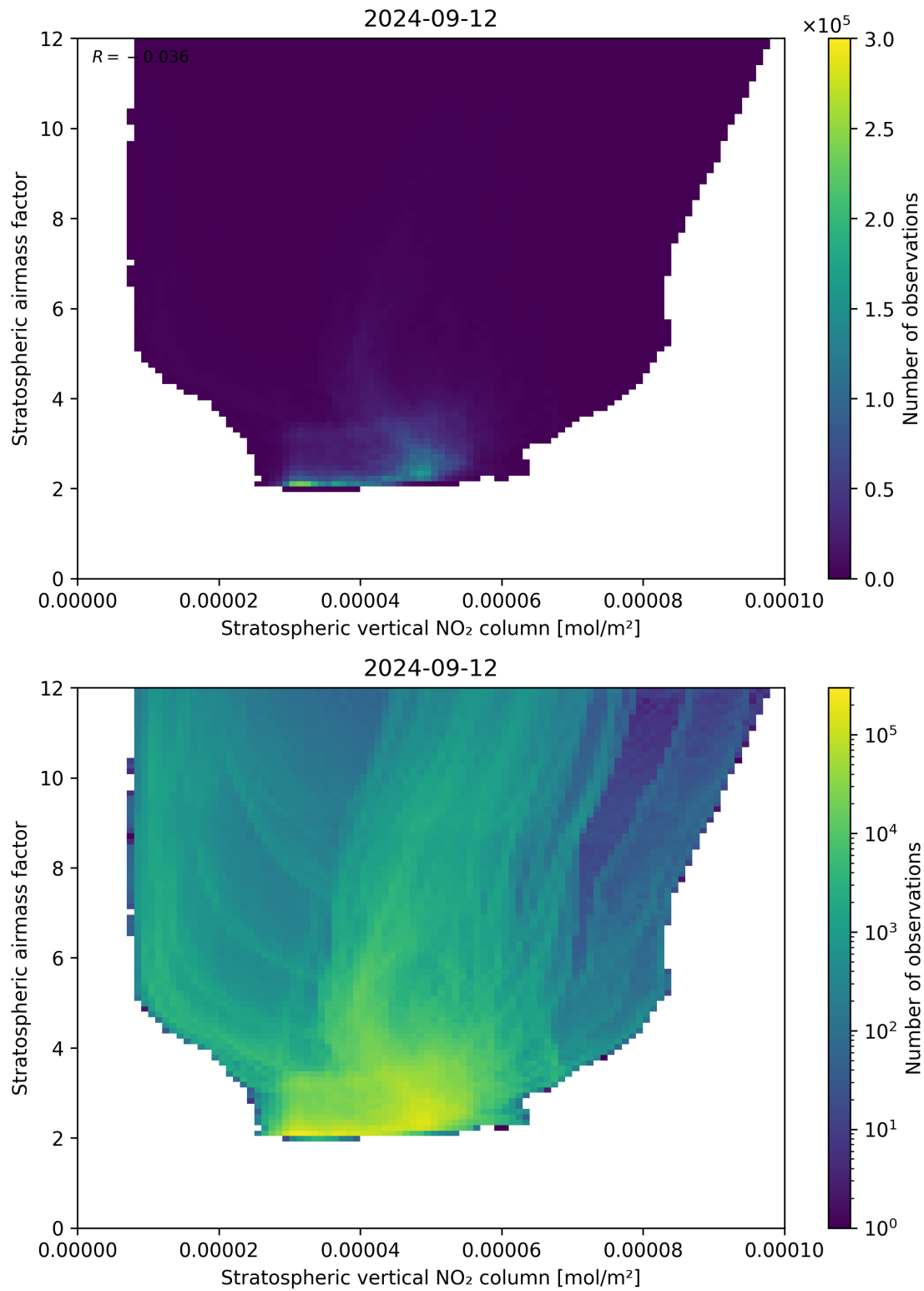
Figure 96: Scatter density plot of “Stratospheric vertical NO 2 column” against “Stratospheric airmass factor” for 2024-09-12 to 2024-09-13.
