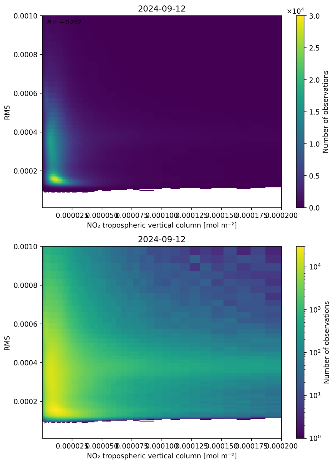
Figure 142: Scatter density plot of “NO 2 tropospheric vertical column” against “RMS” for 2024-09-12 to 2024-09-13.
