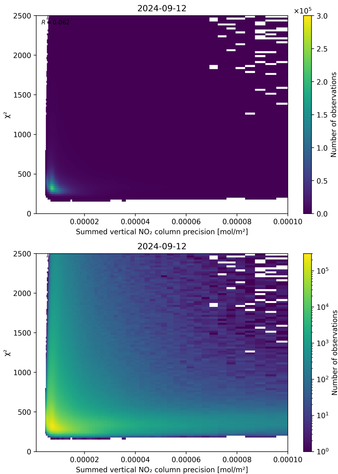
Figure 107: Scatter density plot of “Summed vertical NO 2 column precision” against “ \chi^2 ” for 2024-09-12 to 2024-09-13.
