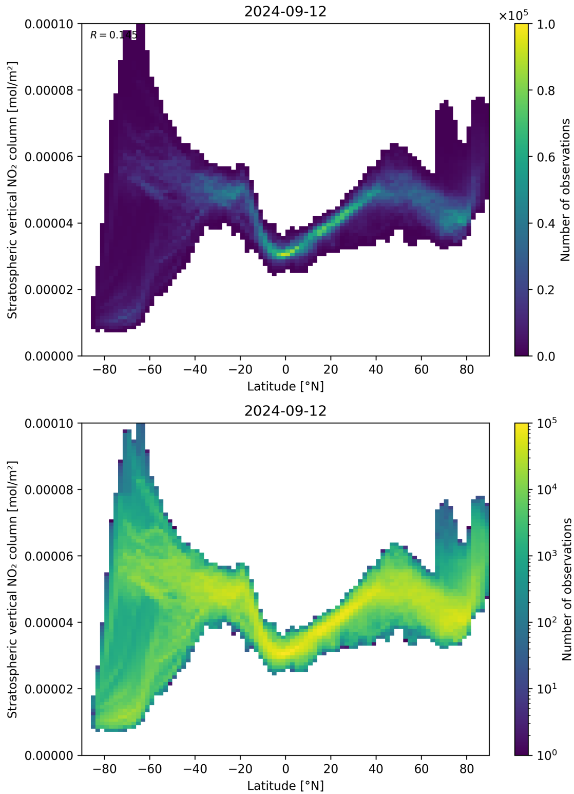
Figure 87: Scatter density plot of “Latitude” against “Stratospheric vertical NO 2 column” for 2024-09-12 to 2024-09-13.
