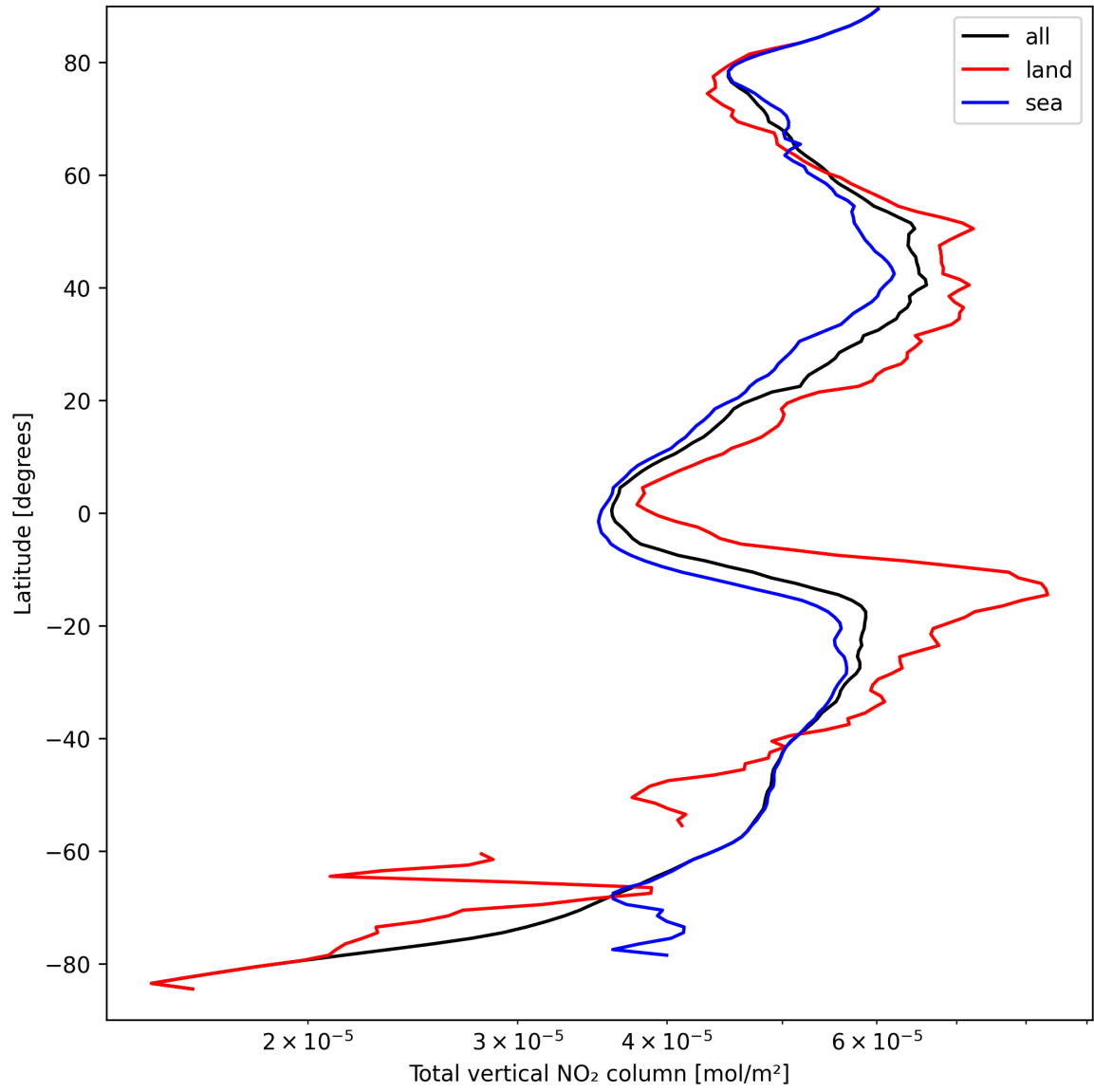
Figure 21: Zonal average of “Total vertical NO 2 column” for 2024-09-12 to 2024-09-13.
