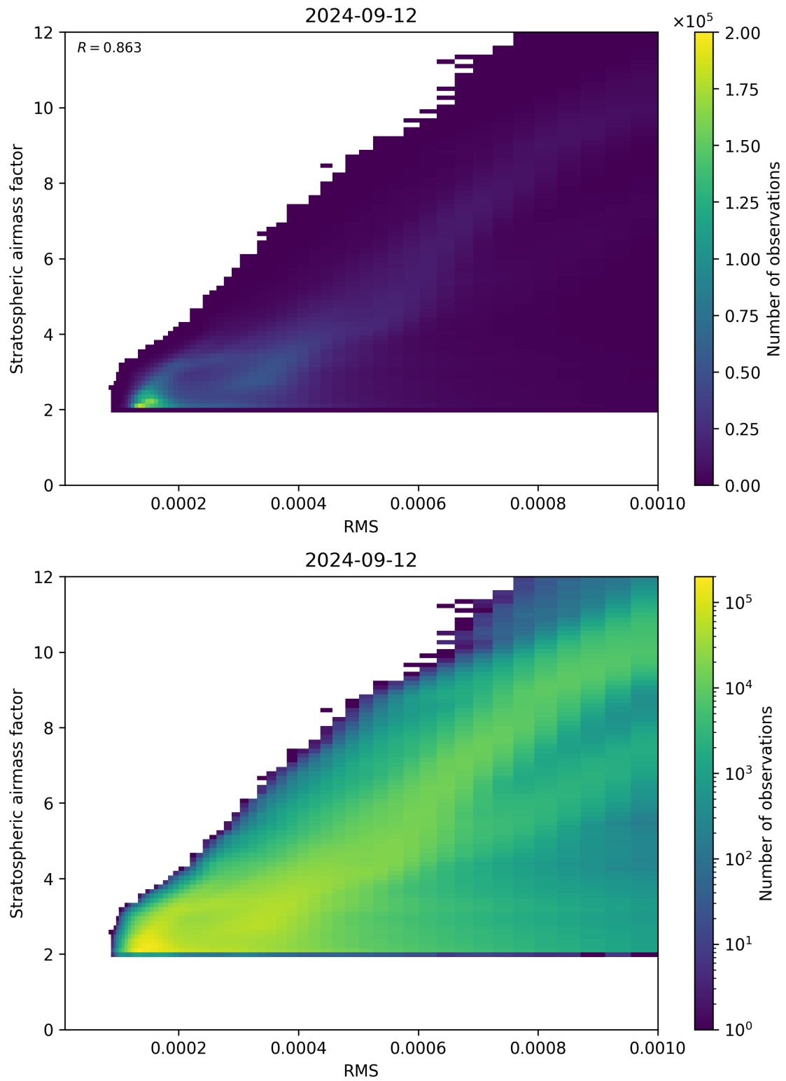
Figure 144: Scatter density plot of “RMS” against “Stratospheric airmass factor” for 2024-09-12 to 2024-09-13.
