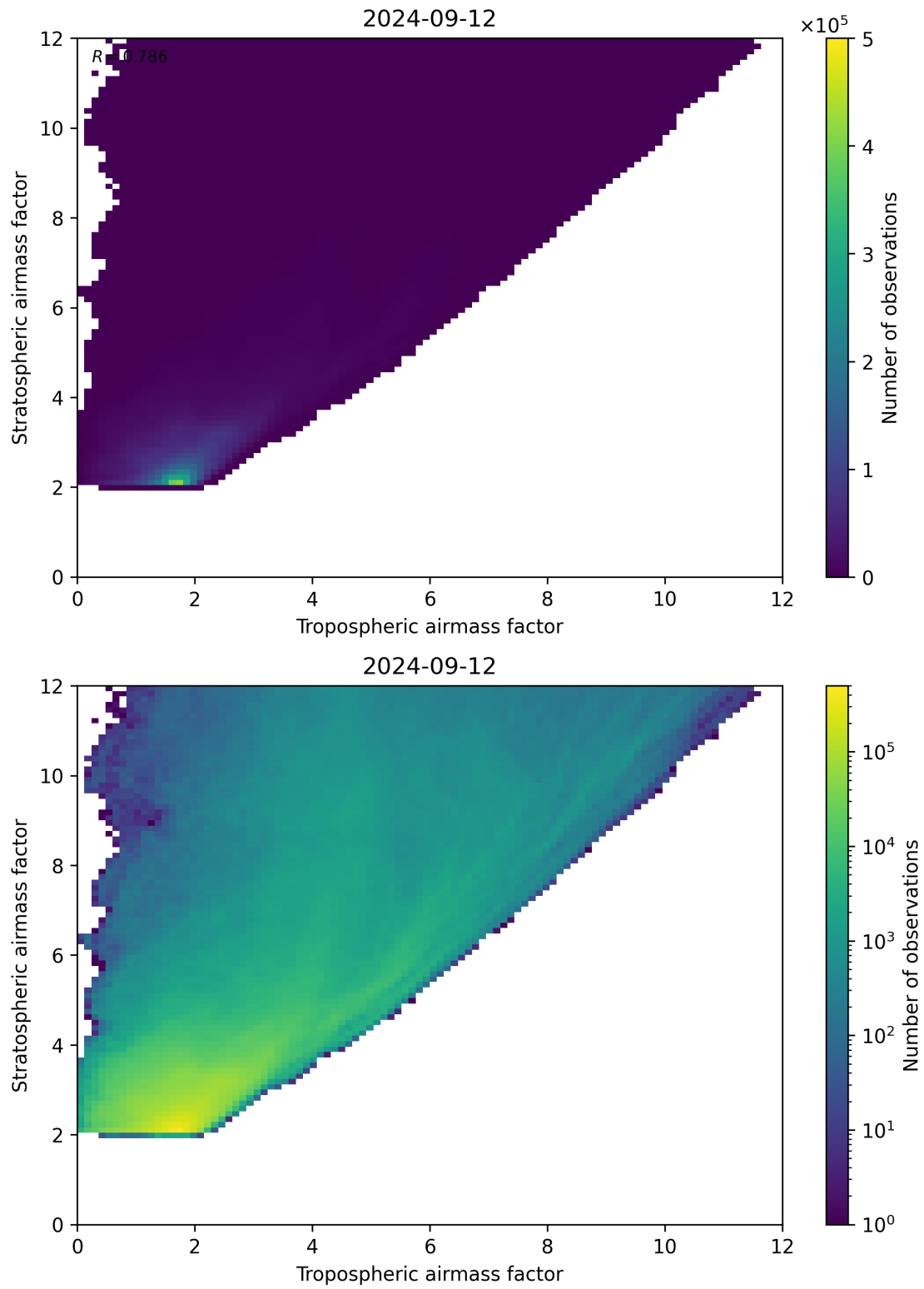
Figure 71: Scatter density plot of “Tropospheric airmass factor” against “Stratospheric airmass factor” for 2024-09-12 to 2024-09-13.
