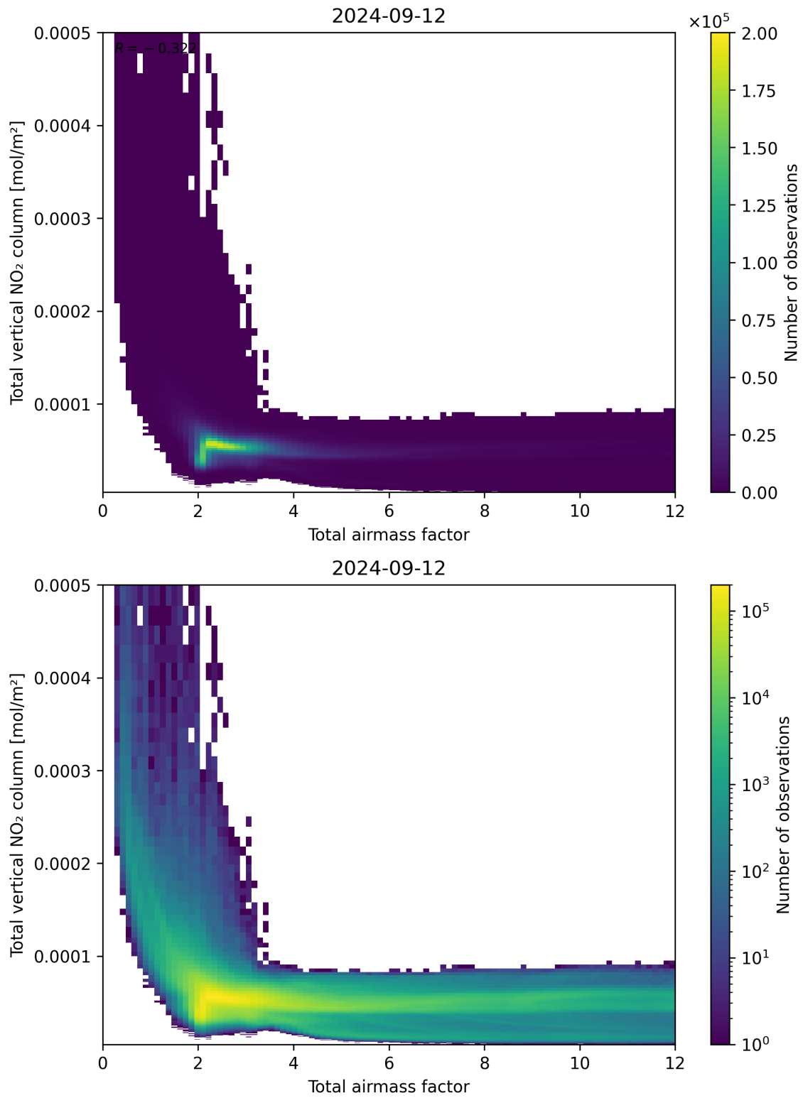
Figure 67: Scatter density plot of “Total airmass factor” against “Total vertical NO 2 column” for 2024-09-12 to 2024-09-13.
