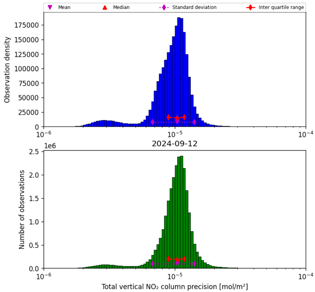
Figure 39: Histogram of “Total vertical NO 2 column precision” for 2024-09-12 to 2024-09-13
