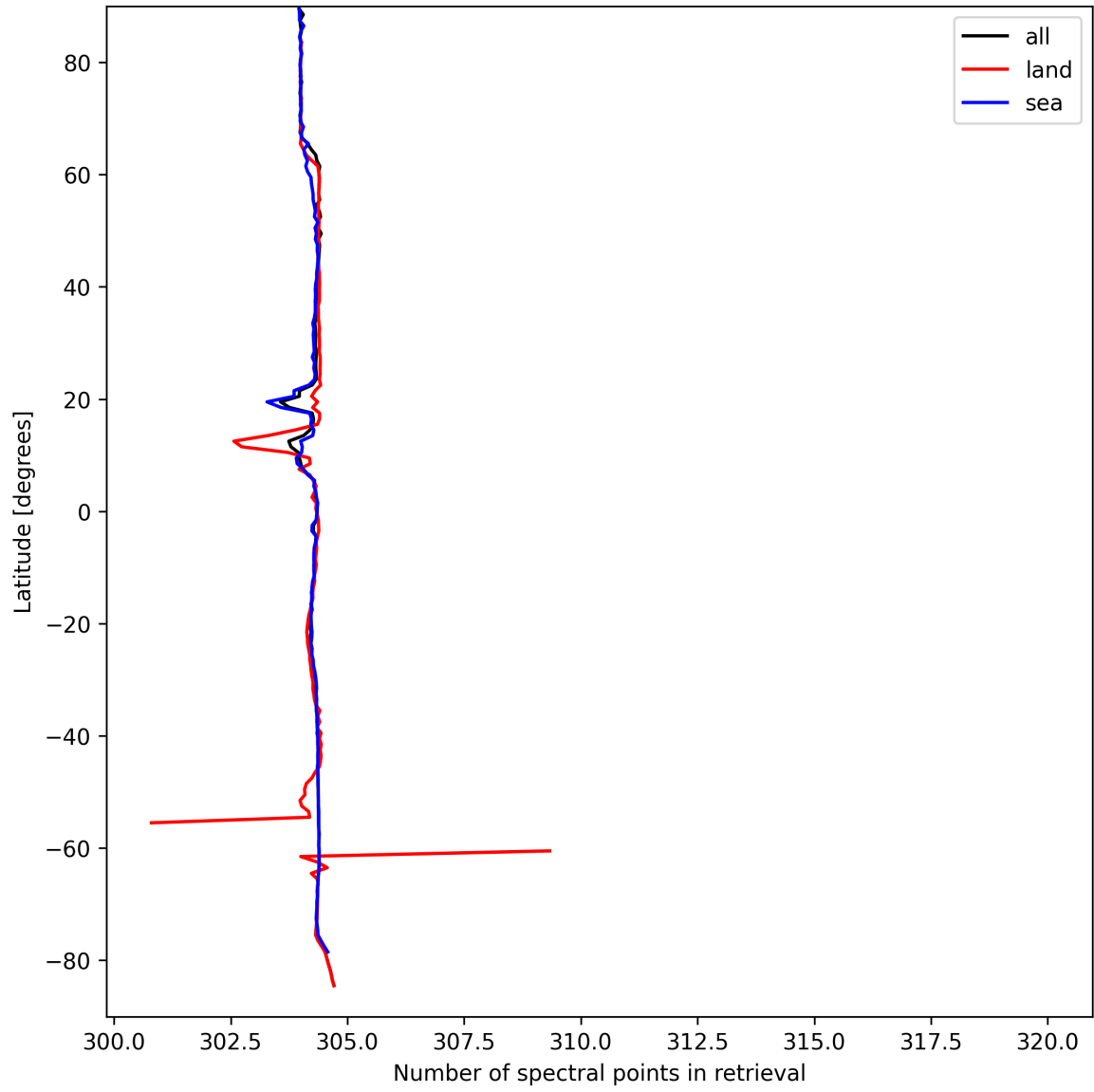
Figure 16: Zonal average of “Number of spectral points in retrieval” for 2024-09-12 to 2024-09-13.
