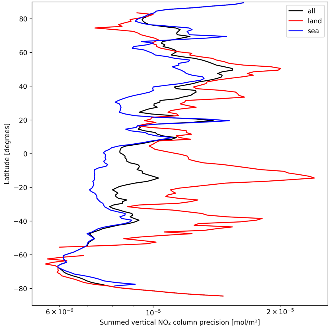
Figure 24: Zonal average of “Summed vertical NO 2 column precision” for 2024-09-12 to 2024-09-13.
