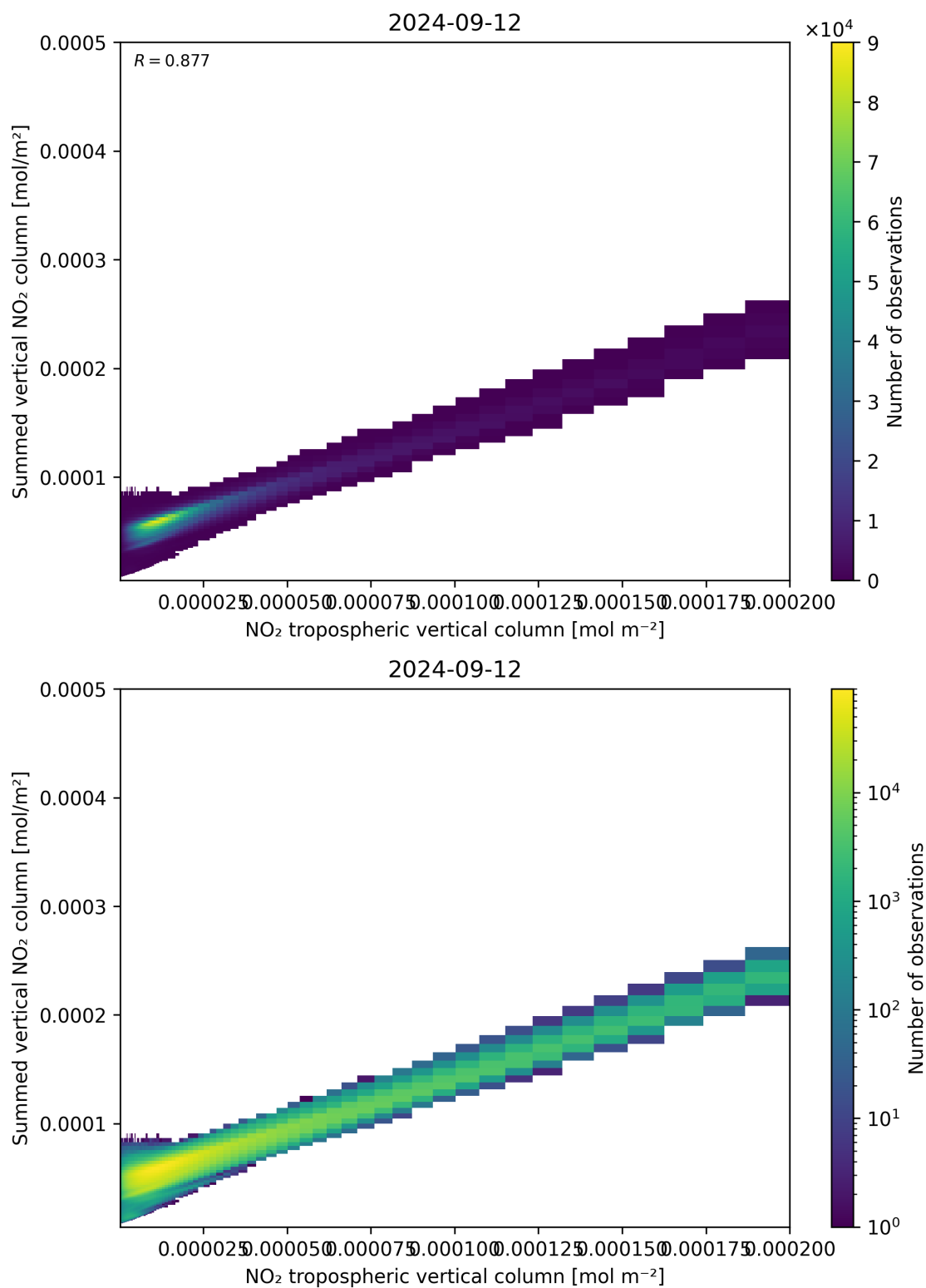
Figure 126: Scatter density plot of “NO 2 tropospheric vertical column” against “Summed vertical NO 2 column” for 2024-09-12 to 2024-09-13.
