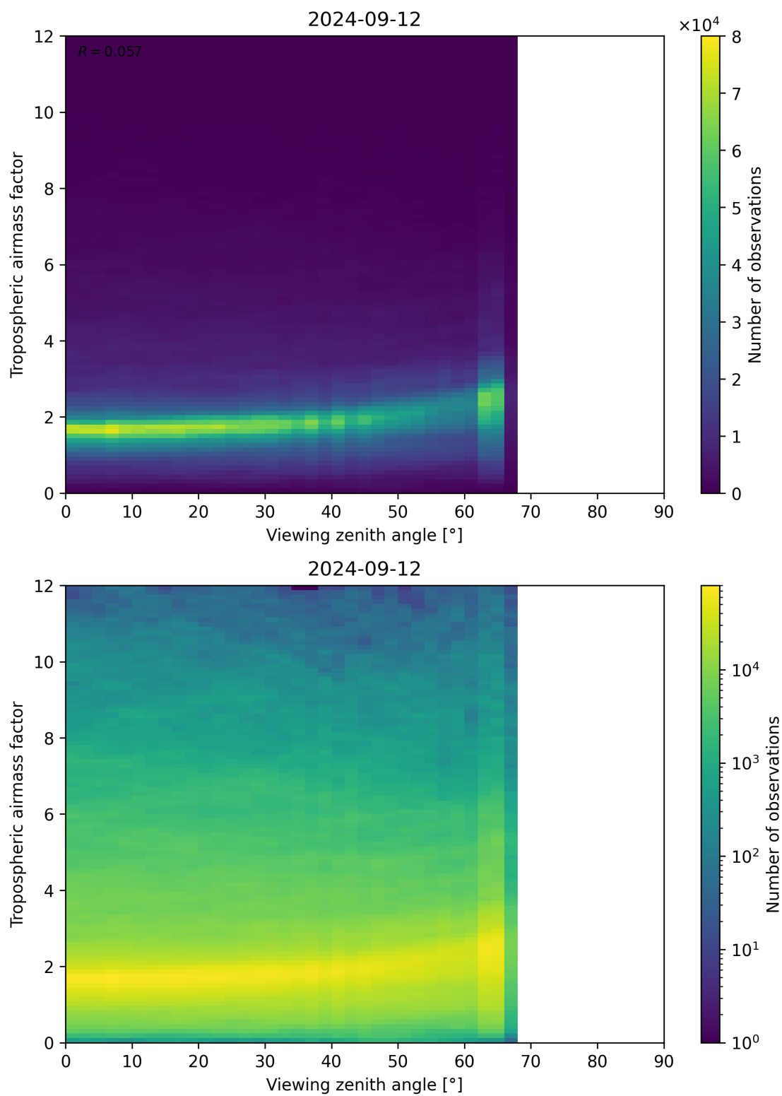
Figure 161: Scatter density plot of “Viewing zenith angle” against “Tropospheric airmass factor” for 2024-09-12 to 2024-09-13.
