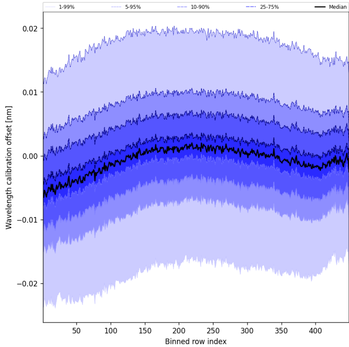
Figure 52: Along track statistics of “Wavelength calibration offset” for 2024-09-12 to 2024-09-13
