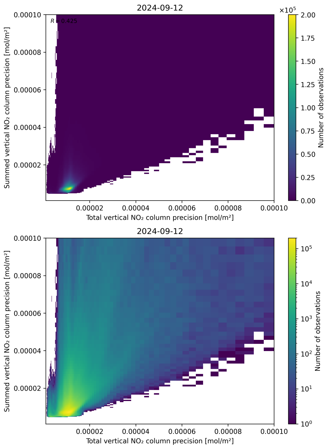
Figure 118: Scatter density plot of “Total vertical NO 2 column precision” against “Summed vertical NO 2 column precision” for 2024-09-12 to 2024-09-13.
