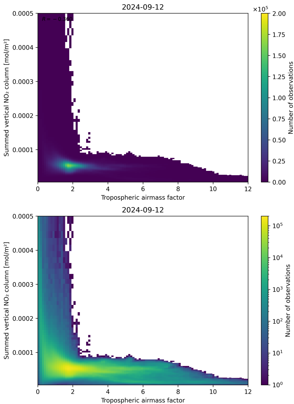
Figure 75: Scatter density plot of “Tropospheric air mass factor” against “Summed vertical NO 2 column” for 2024-09-12 to 2024-09-13.
