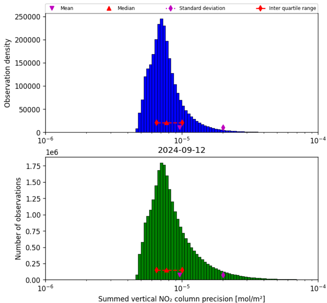
Figure 41: Histogram of “Summed vertical NO 2 column precision” for 2024-09-12 to 2024-09-13
