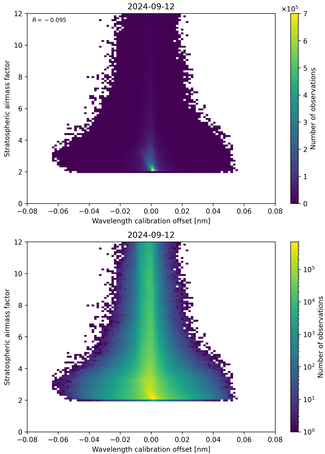
Figure 174: Scatter density plot of “Wavelength calibration offset” against “Stratospheric air mass factor” for 2024-09-12 to 2024-09-13.
