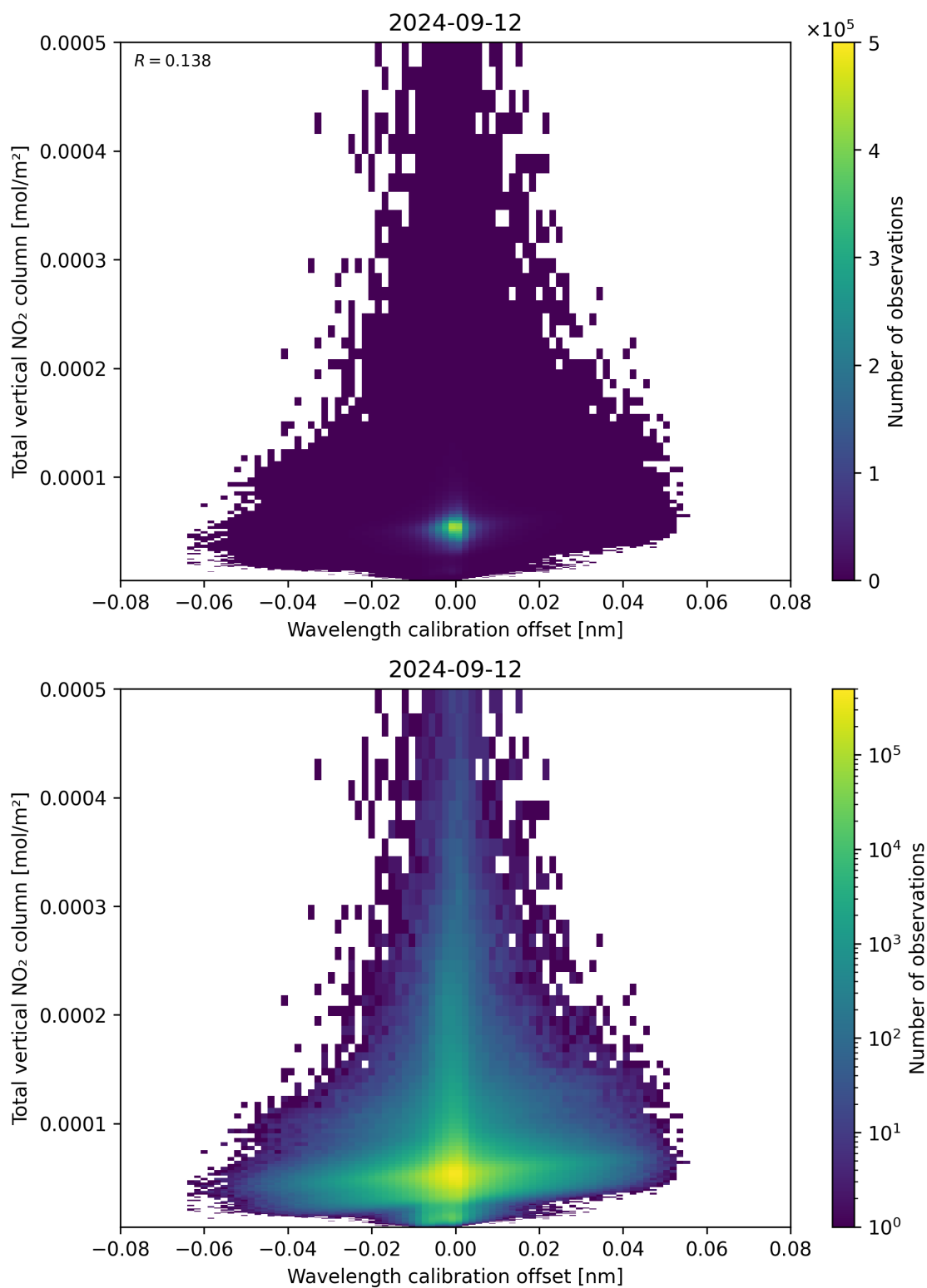
Figure 179: Scatter density plot of “Wavelength calibration offset” against “Total vertical NO 2 column” for 2024-09-12 to 2024-09-13.
