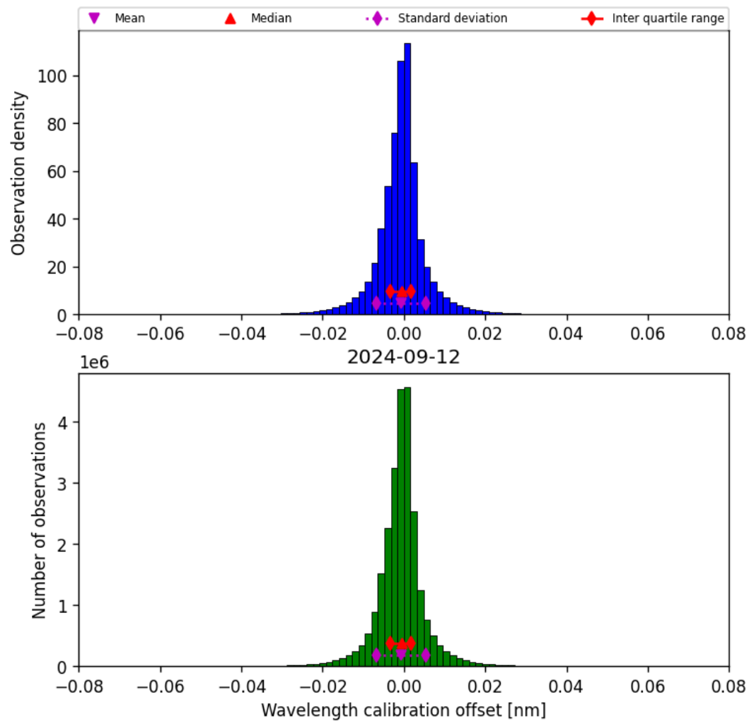
Figure 35: Histogram of “Wavelength calibration offset” for 2024-09-12 to 2024-09-13
