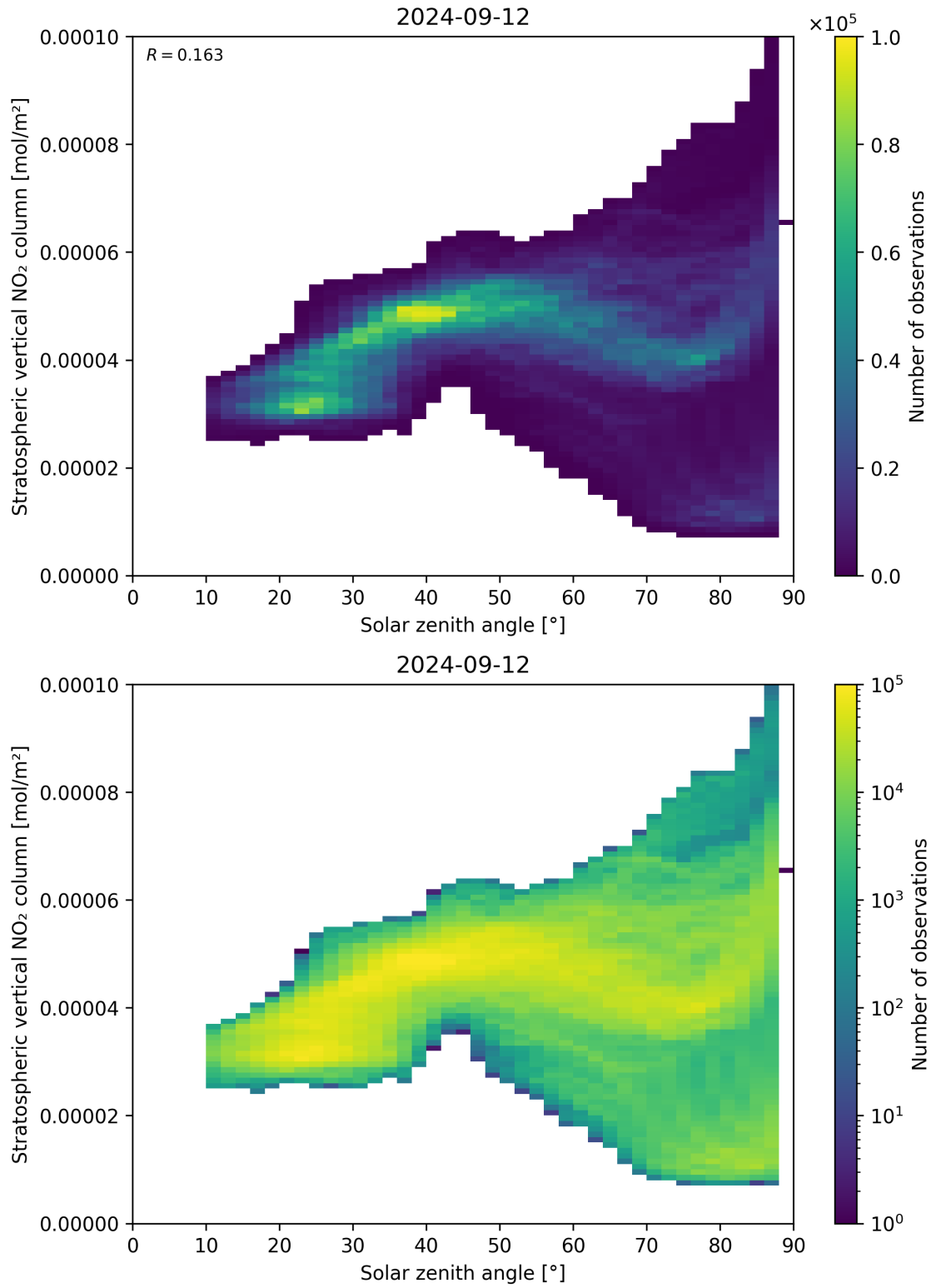
Figure 150: Scatter density plot of “Solar zenith angle” against “Stratospheric vertical NO 2 column” for 2024-09-12 to 2024-09-13.
