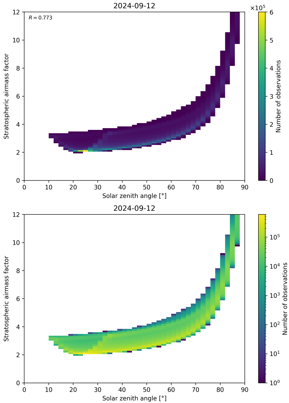
Figure 145: Scatter density plot of “Solar zenith angle” against “Stratospheric airmass factor” for 2024-09-12 to 2024-09-13.
