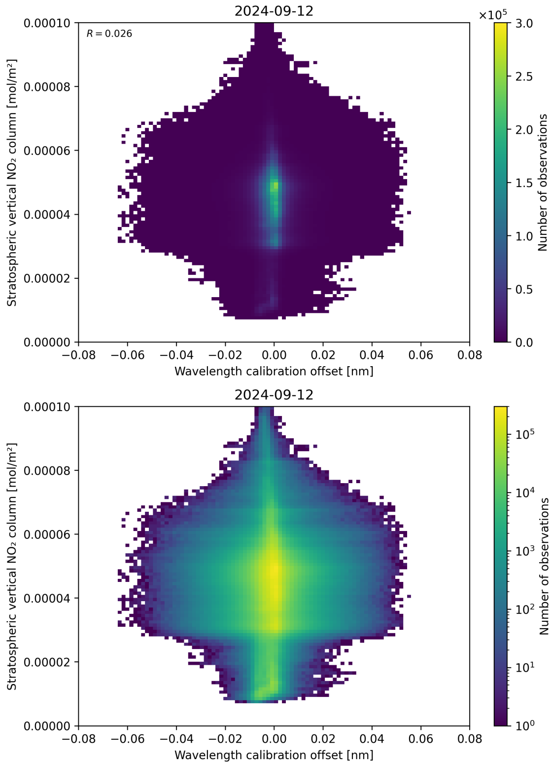
Figure 176: Scatter density plot of “Wavelength calibration offset” against “Stratospheric vertical NO 2 column” for 2024-09-12 to 2024-09-13.
