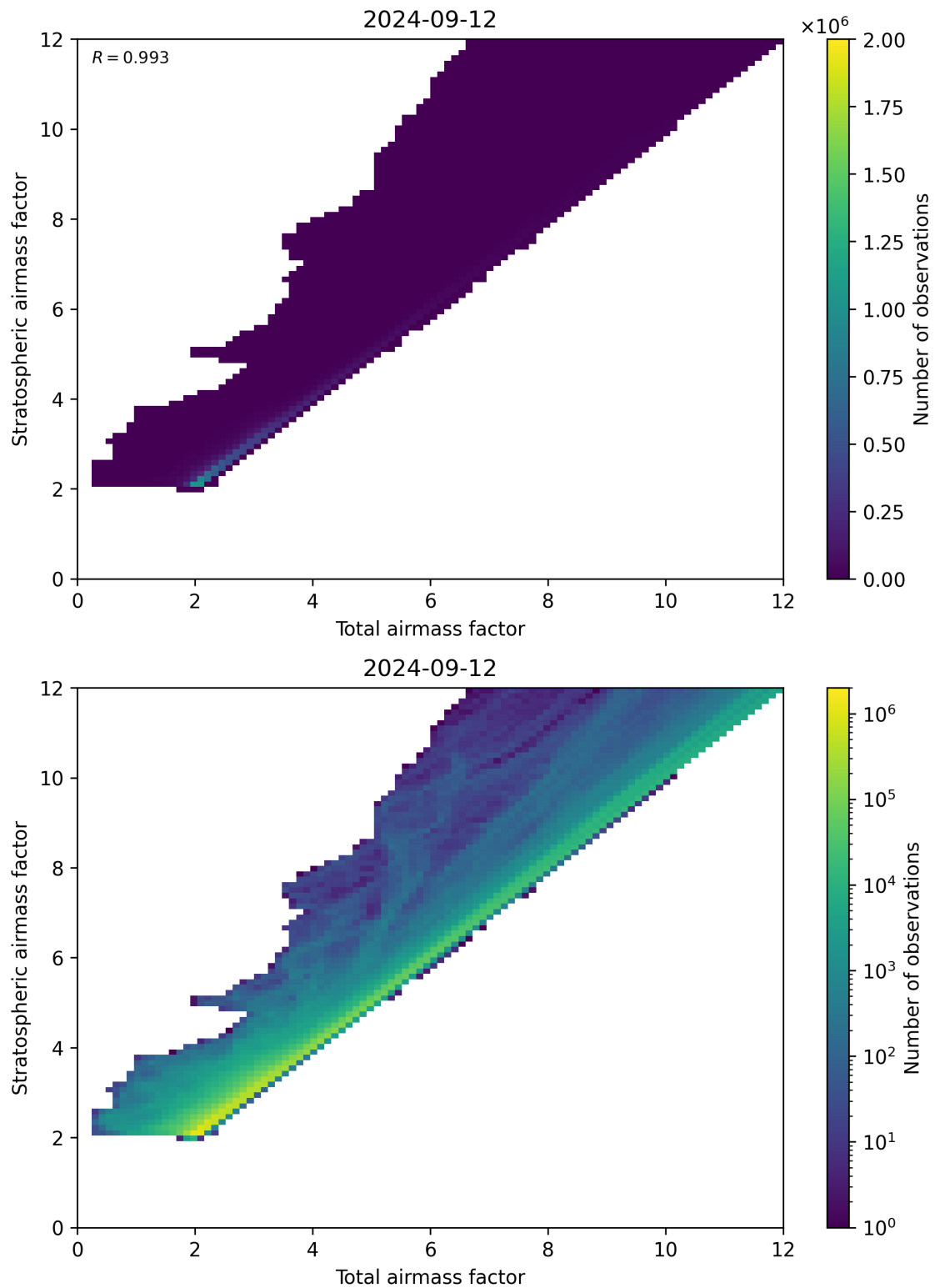
Figure 62: Scatter density plot of “Total airmass factor” against “Stratospheric airmass factor” for 2024-09-12 to 2024-09-13.
