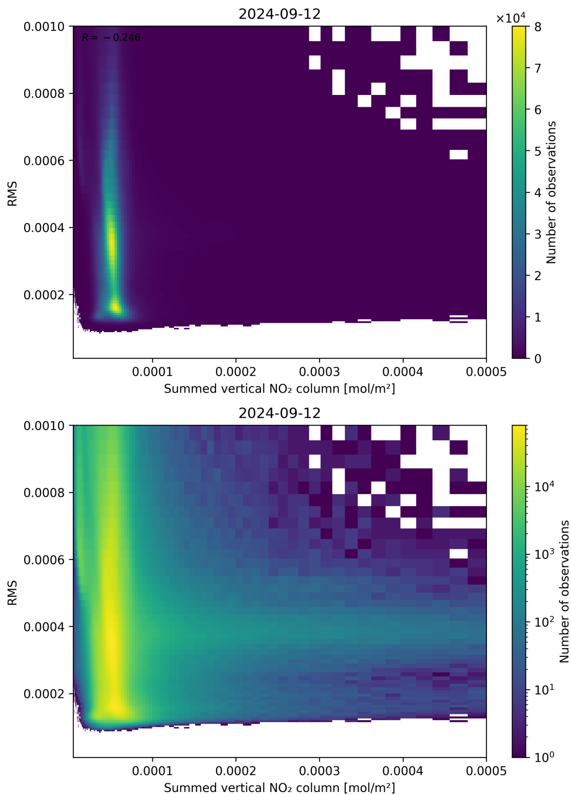
Figure 109: Scatter density plot of “Summed vertical NO 2 column” against “RMS” for 2024-09-12 to 2024-09-13.
