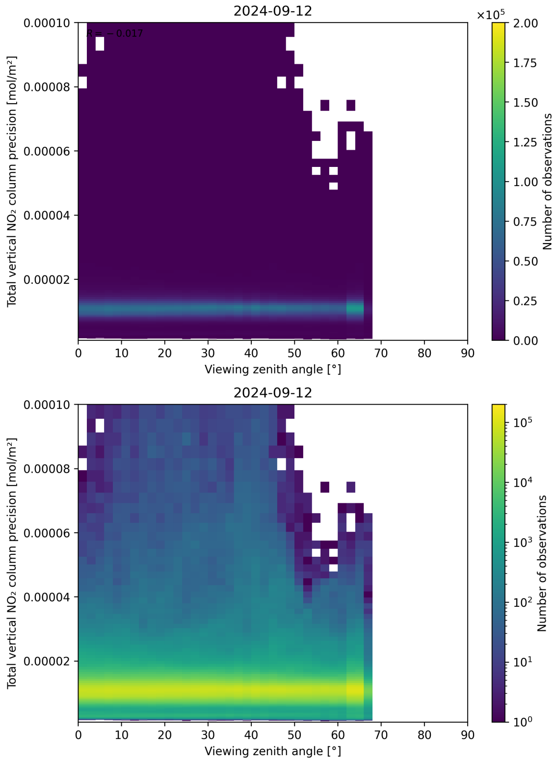
Figure 168: Scatter density plot of “Viewing zenith angle” against “Total vertical NO 2 column precision” for 2024-09-12 to 2024-09-13.
