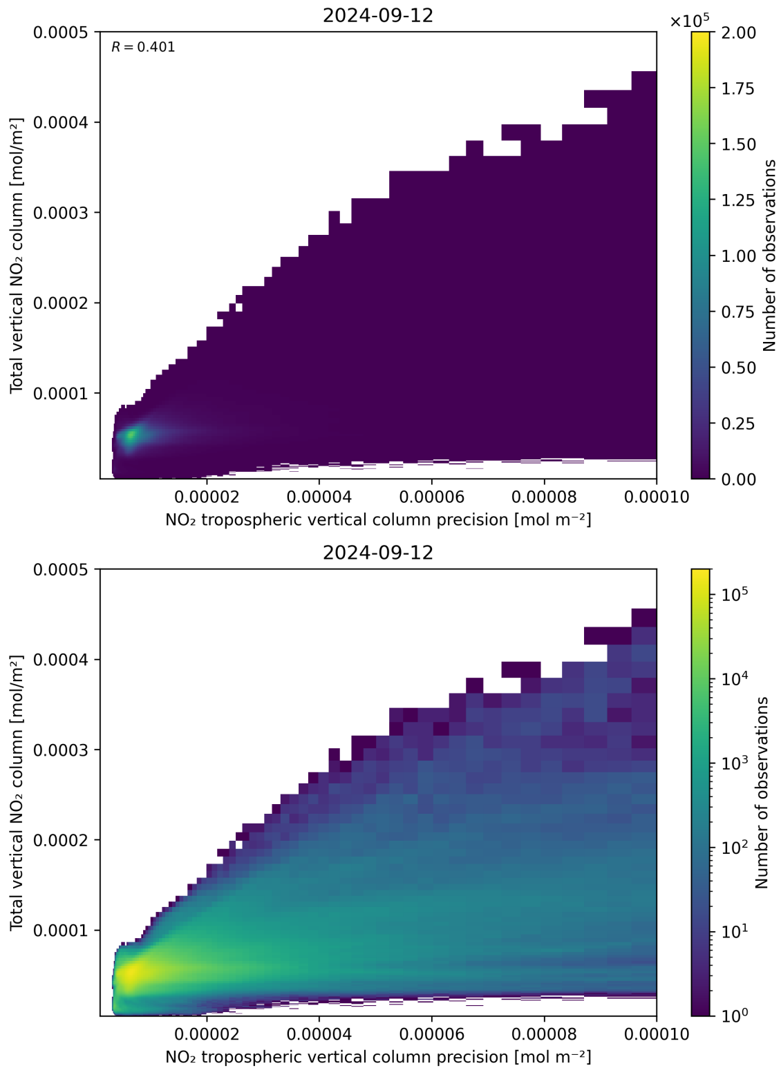
Figure 138: Scatter density plot of “NO 2 tropospheric vertical column precision” against “Total vertical NO 2 column” for 2024-09-12 to 2024-09-13.
