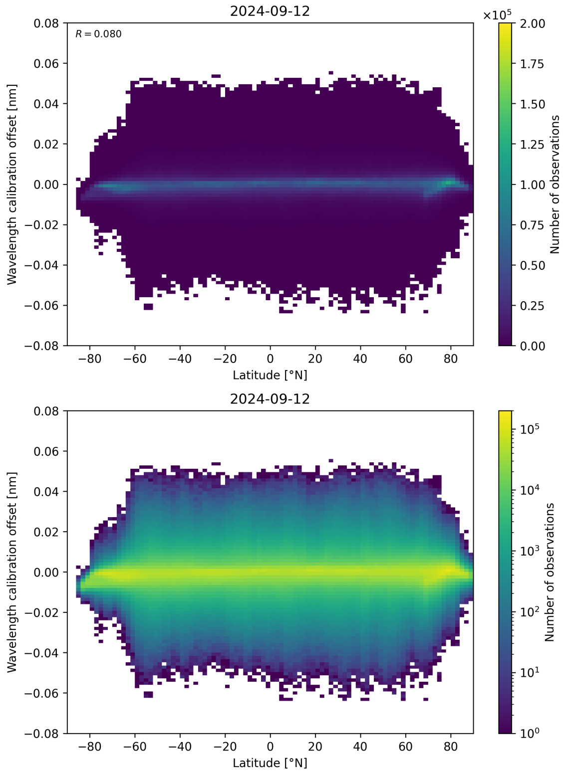
Figure 95: Scatter density plot of “Latitude” against “Wavelength calibration offset” for 2024-09-12 to 2024-09-13.
