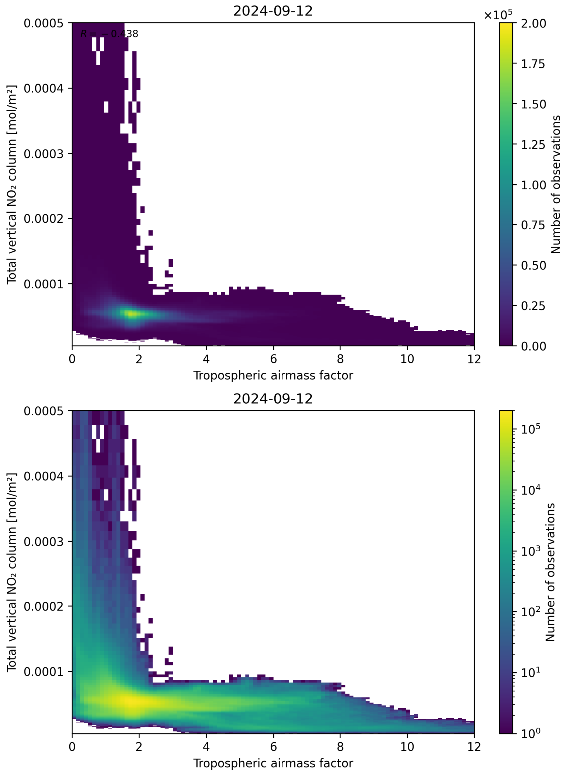
Figure 77: Scatter density plot of “Tropospheric airmass factor” against “Total vertical NO 2 column” for 2024-09-12 to 2024-09-13.
