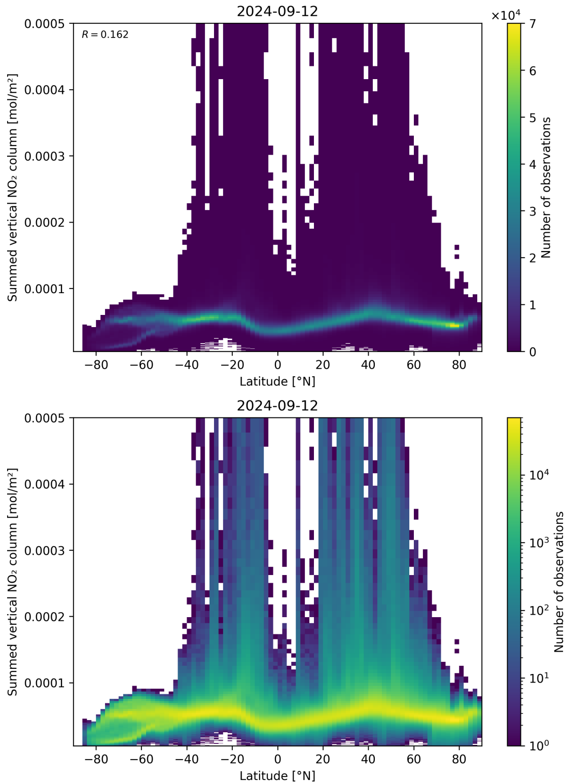
Figure 88: Scatter density plot of “Latitude” against “Summed vertical NO 2 column” for 2024-09-12 to 2024-09-13.
