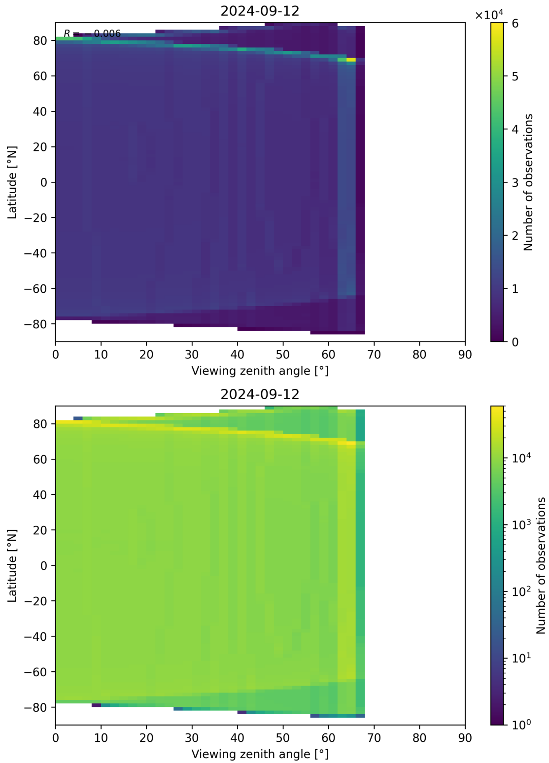
Figure 163: Scatter density plot of “Viewing zenith angle” against “Latitude” for 2024-09-12 to 2024-09-13.
