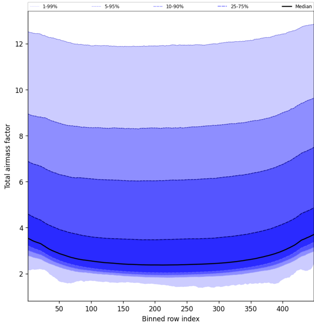
Figure 49: Along track statistics of “Total airmass factor” for 2024-09-12 to 2024-09-13
