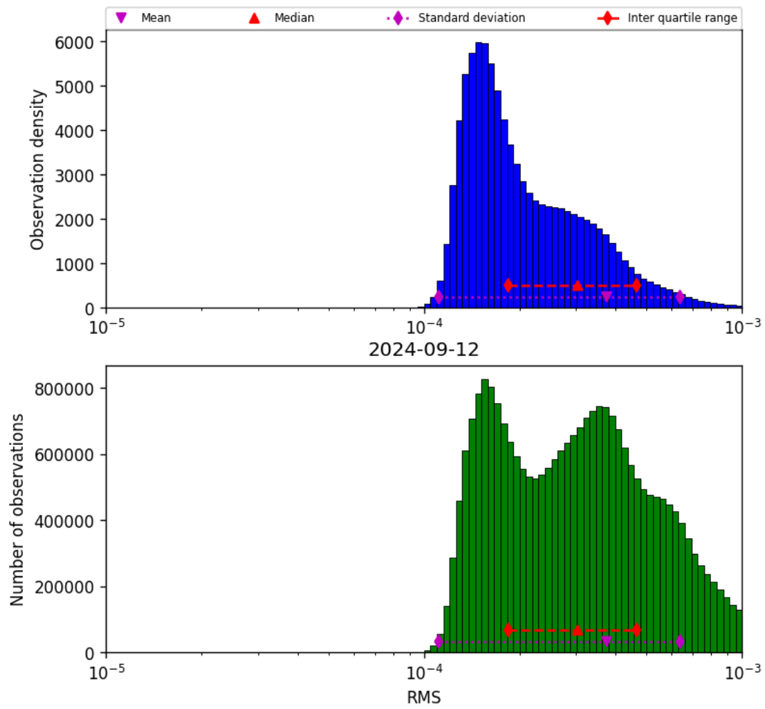
Figure 43: Histogram of “RMS” for 2024-09-12 to 2024-09-13
