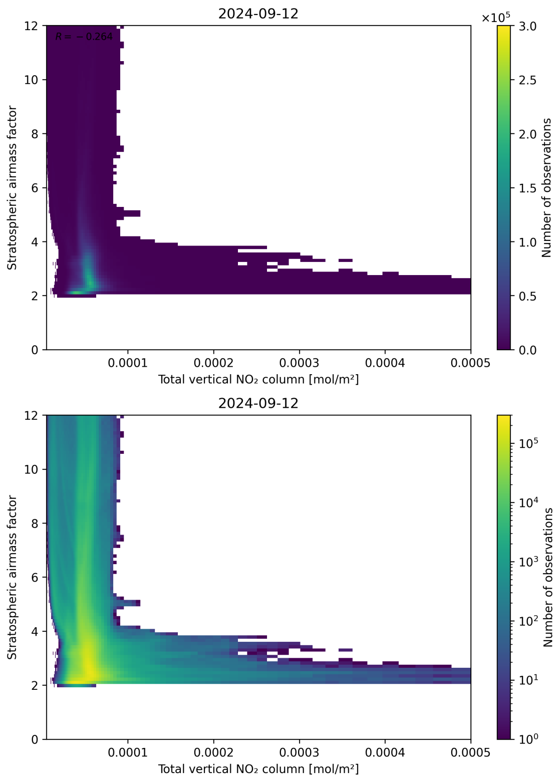
Figure 110: Scatter density plot of “Total vertical NO 2 column” against “Stratospheric air mass factor” for 2024-09-12 to 2024-09-13.
