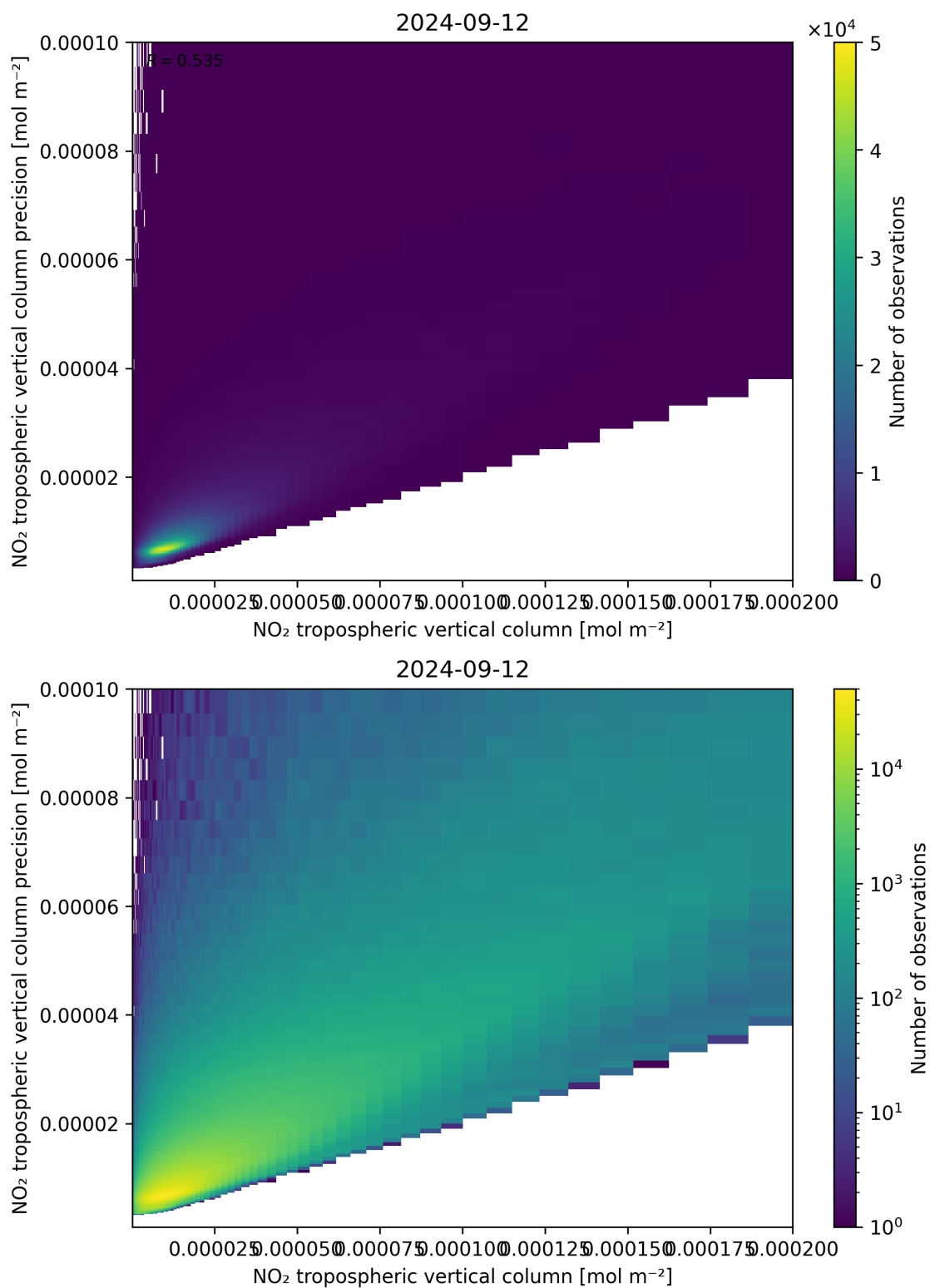
Figure 130: Scatter density plot of “NO 2 tropospheric vertical column” against “NO 2 tropospheric vertical column precision” for 2024-09-12 to 2024-09-13.
