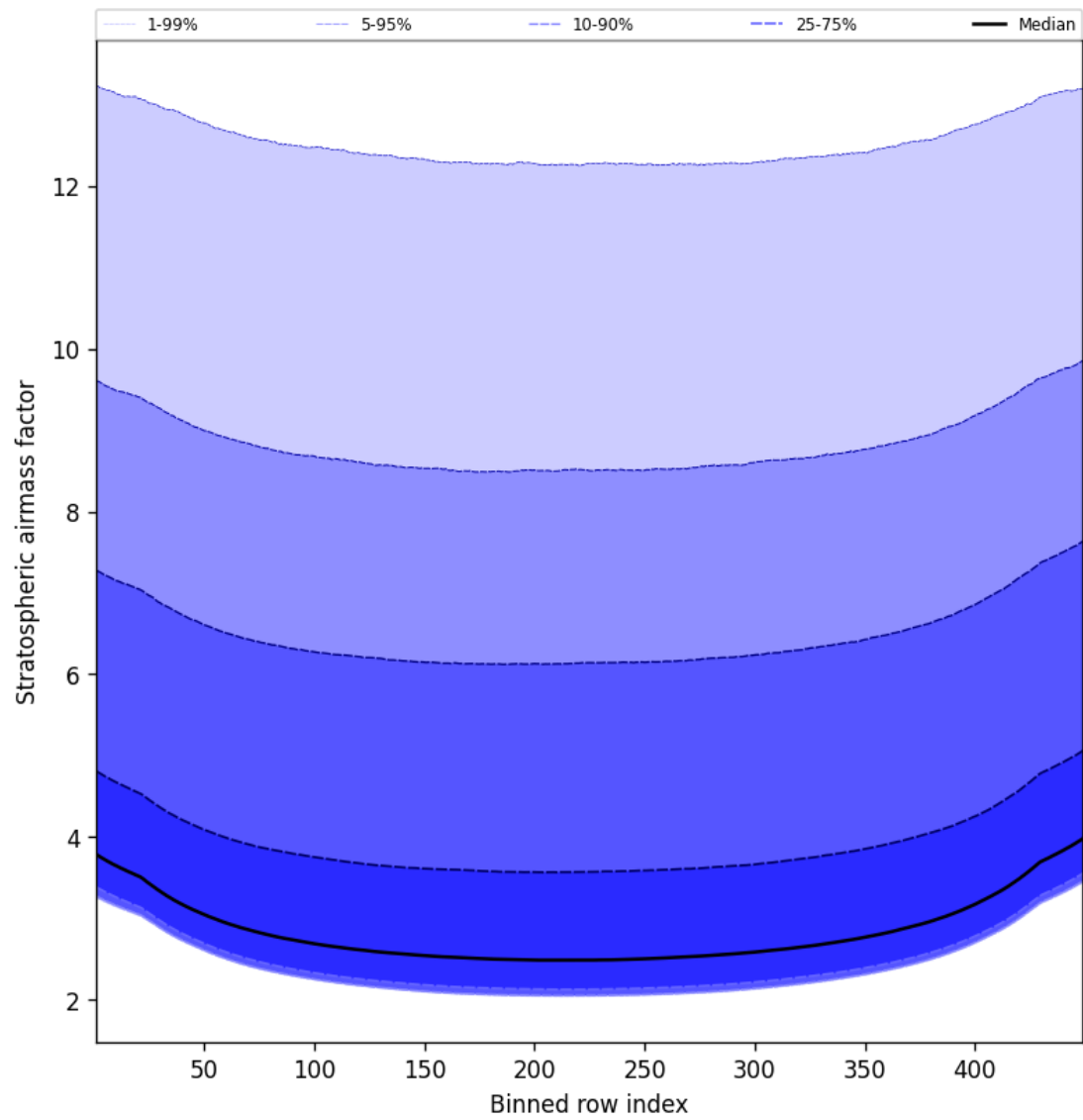
Figure 61: Along track statistics of “Stratospheric airmass factor” for 2024-09-12 to 2024-09-13
