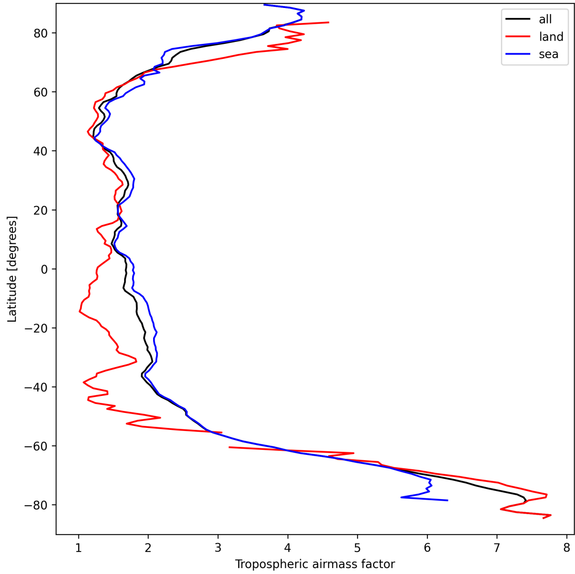
Figure 14: Zonal average of “Tropospheric airmass factor” for 2024-09-12 to 2024-09-13.
