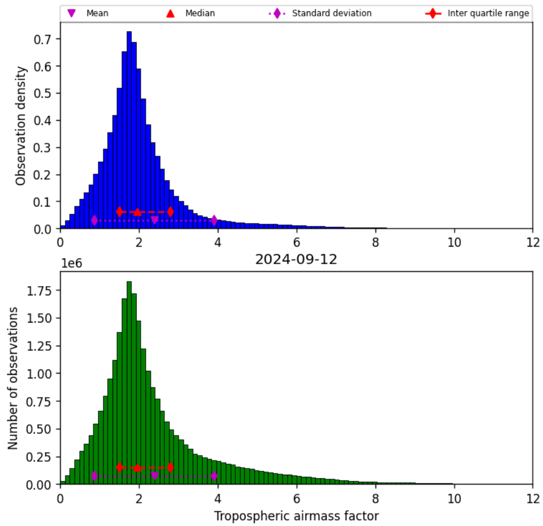
Figure 31: Histogram of “Tropospheric air mass factor” for 2024-09-12 to 2024-09-13
