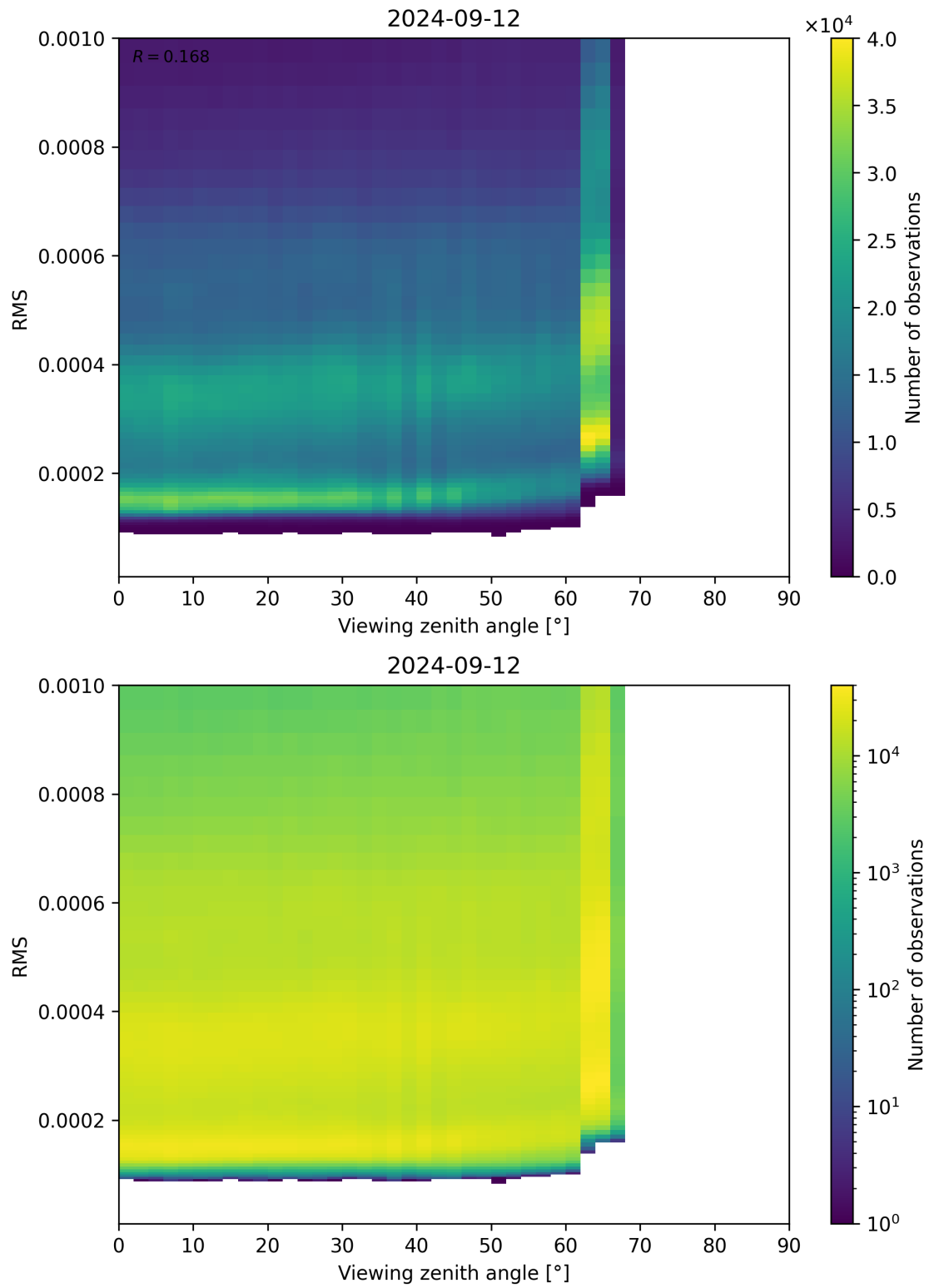
Figure 171: Scatter density plot of “Viewing zenith angle” against “RMS” for 2024-09-12 to 2024-09-13.
