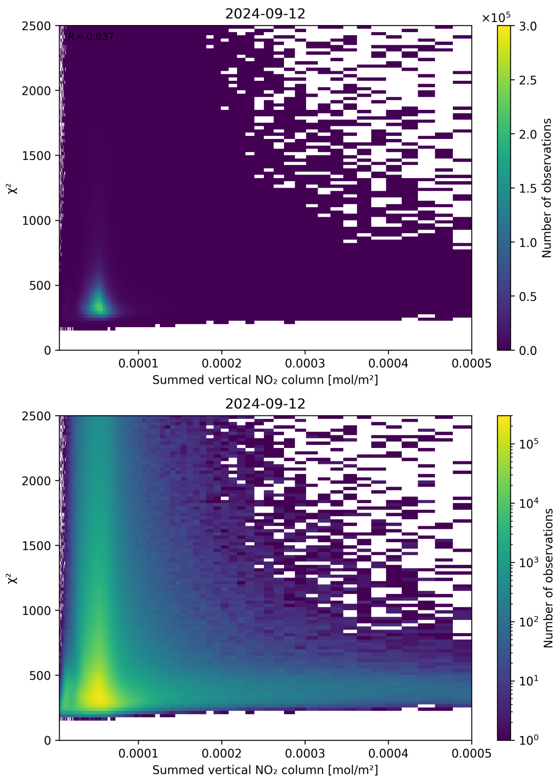
Figure 104: Scatter density plot of “Summed vertical NO 2 column” against “ \chi^2 ” for 2024-09-12 to 2024-09-13.
