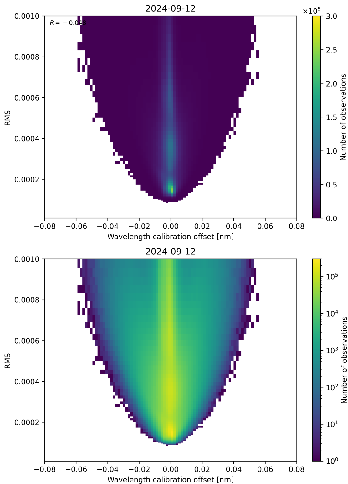
Figure 181: Scatter density plot of “Wavelength calibration offset” against “RMS” for 2024-09-12 to 2024-09-13.
