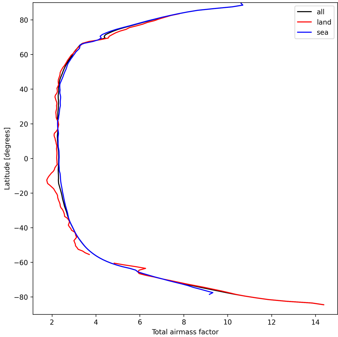
Figure 15: Zonal average of “Total airmass factor” for 2024-09-12 to 2024-09-13.
