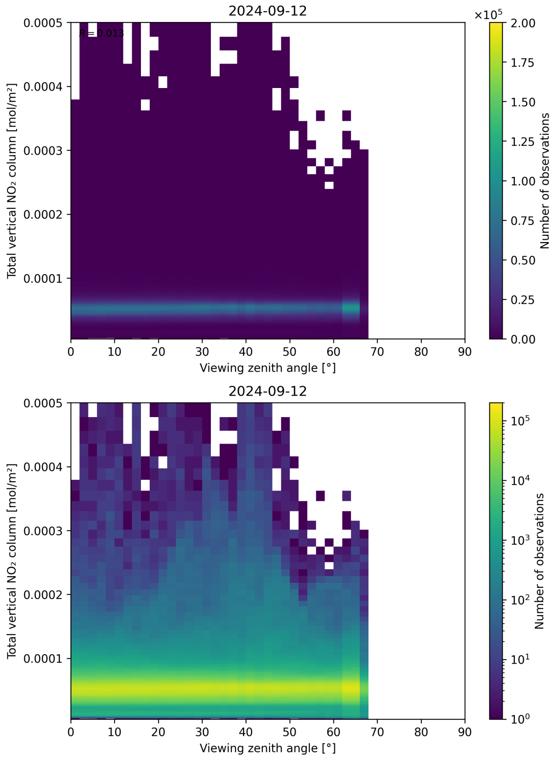
Figure 167: Scatter density plot of “Viewing zenith angle” against “Total vertical NO 2 column” for 2024-09-12 to 2024-09-13.
