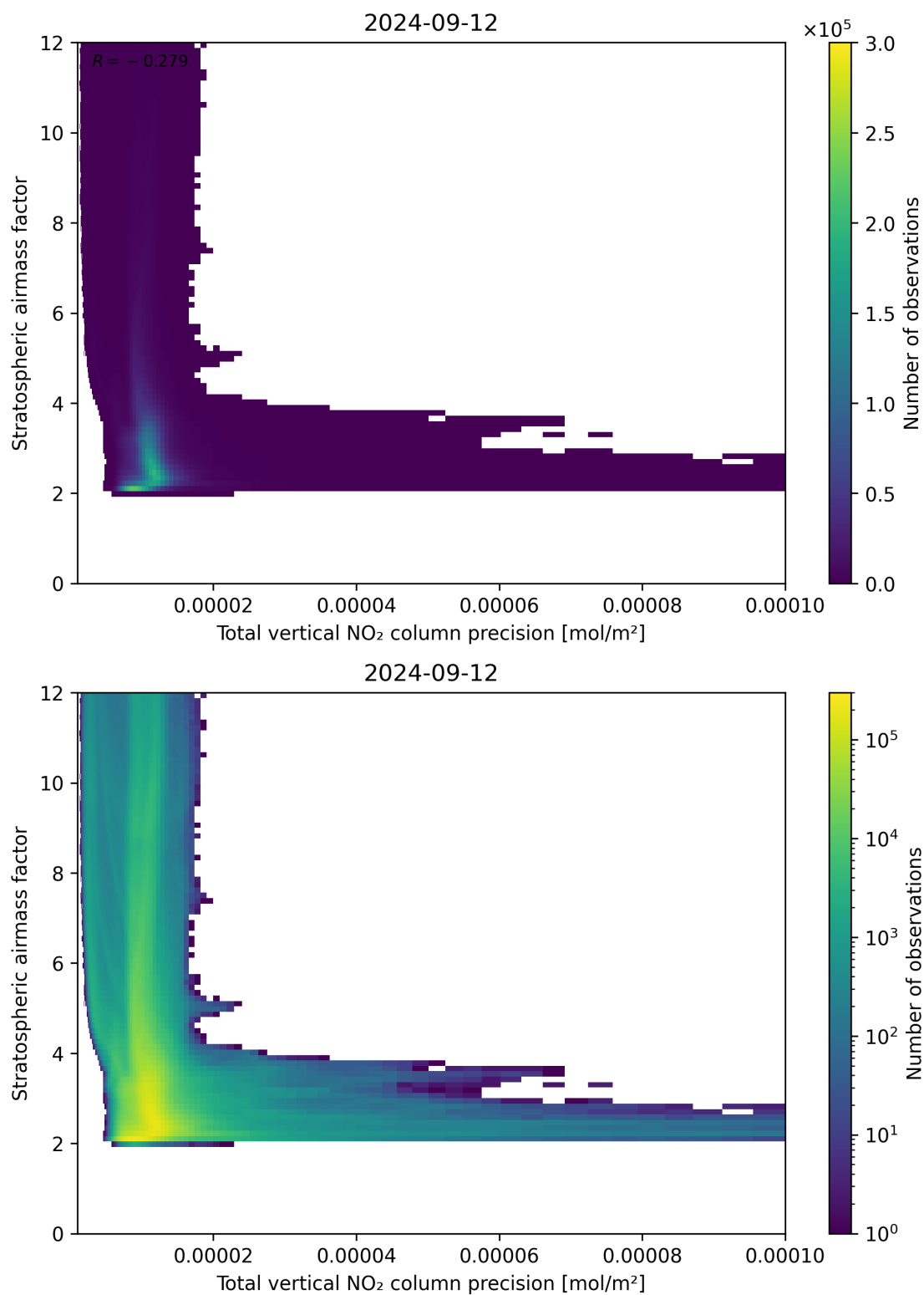
Figure 115: Scatter density plot of “Total vertical NO 2 column precision” against “Stratospheric airmass factor” for 2024-09-12 to 2024-09-13.
