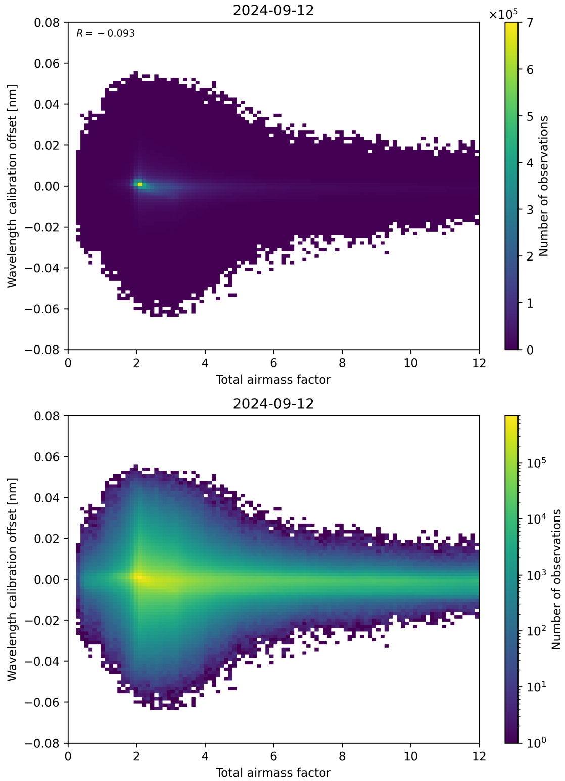
Figure 70: Scatter density plot of “Total airmass factor” against “Wavelength calibration offset” for 2024-09-12 to 2024-09-13.
