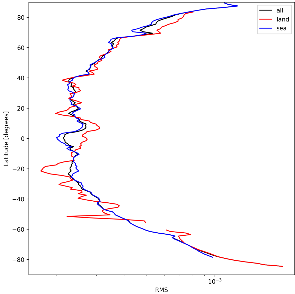
Figure 26: Zonal average of “RMS” for 2024-09-12 to 2024-09-13.
