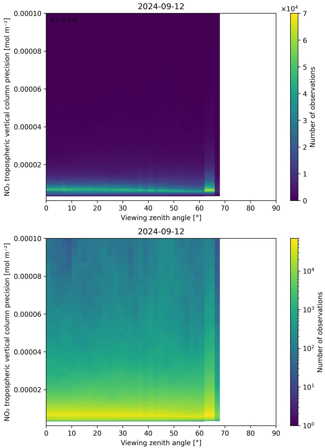
Figure 170: Scatter density plot of “Viewing zenith angle” against “NO 2 tropospheric vertical column precision” for 2024-09-12 to 2024-09-13.
