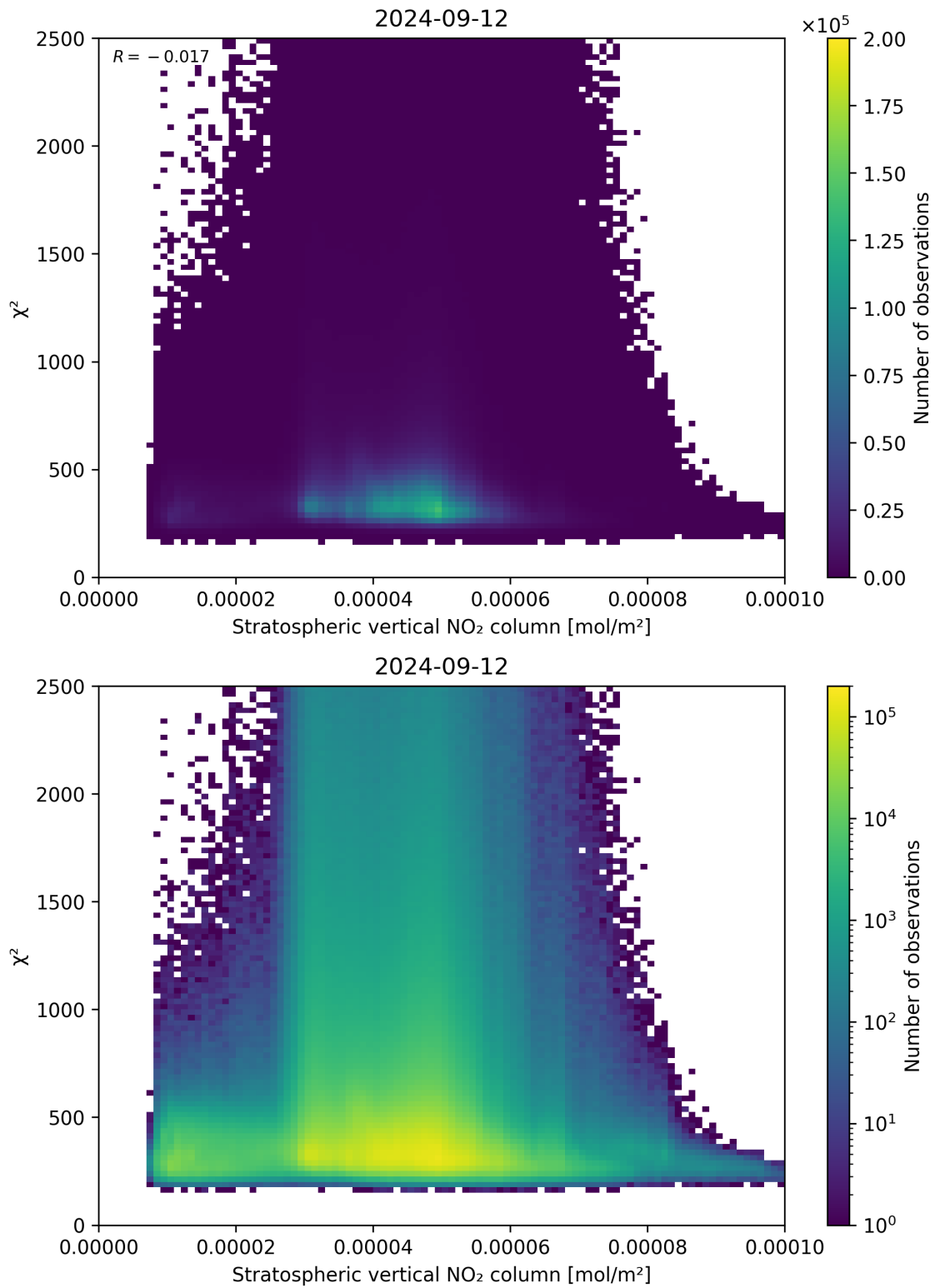
Figure 97: Scatter density plot of “Stratospheric vertical NO 2 column” against “ \chi^2 ” for 2024-09-12 to 2024-09-13.
