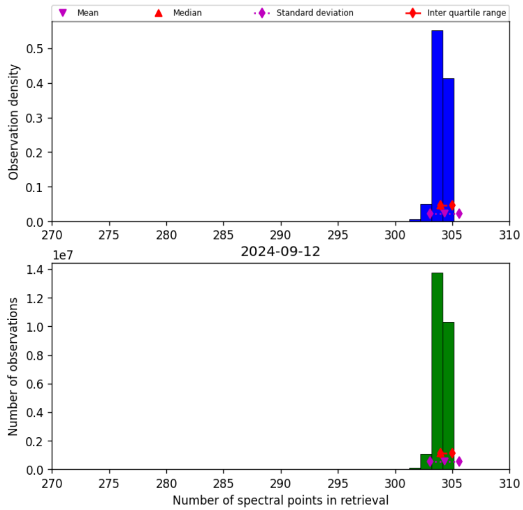
Figure 33: Histogram of “Number of spectral points in retrieval” for 2024-09-12 to 2024-09-13
