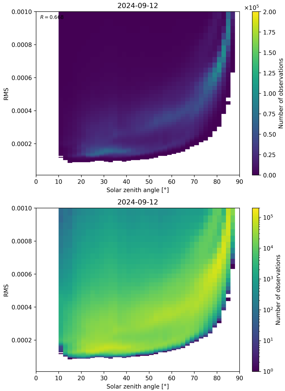
Figure 157: Scatter density plot of “Solar zenith angle” against “RMS” for 2024-09-12 to 2024-09-13.
