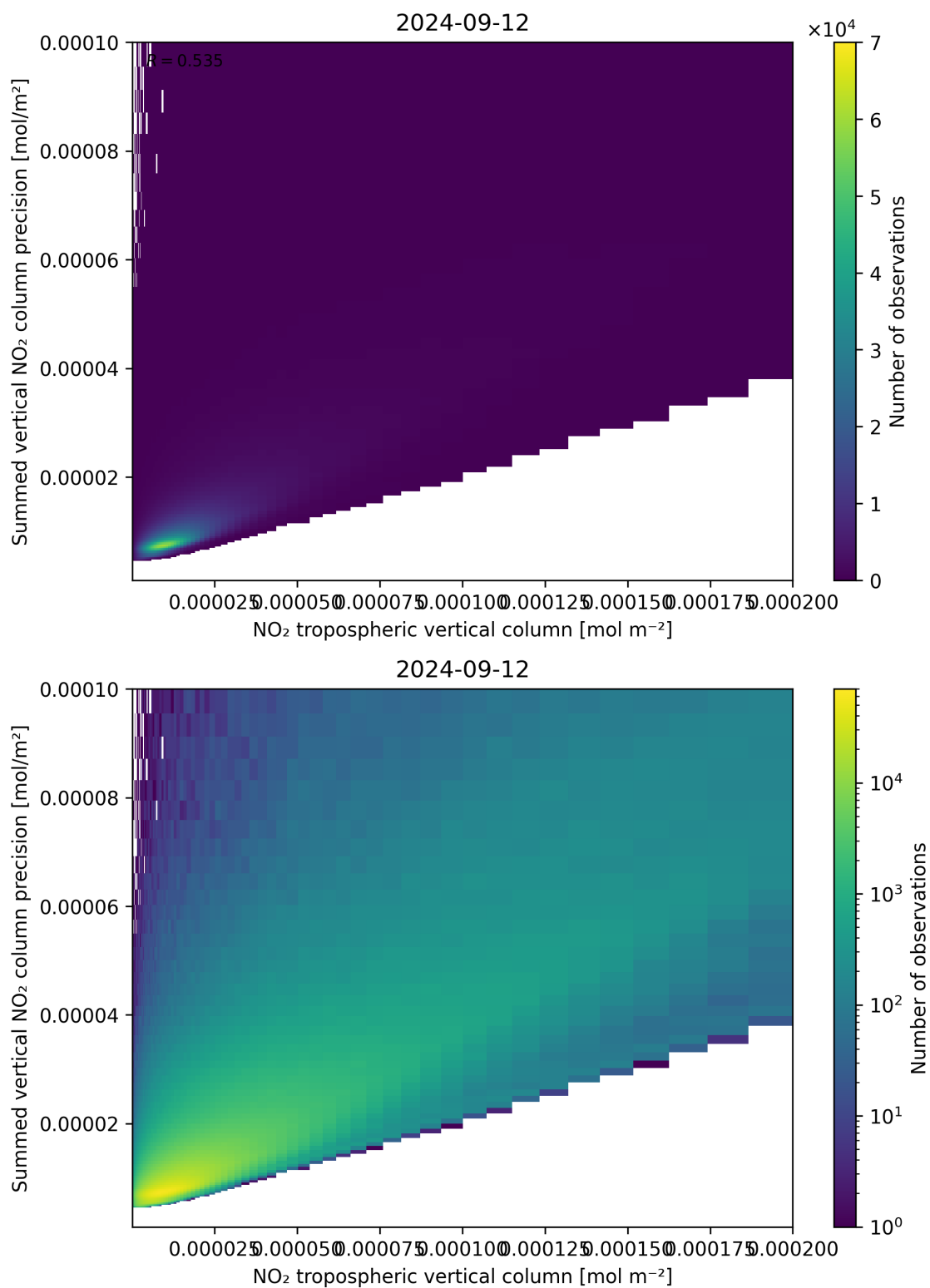
Figure 127: Scatter density plot of “NO 2 tropospheric vertical column” against “Summed vertical NO 2 column precision” for 2024-09-12 to 2024-09-13.
