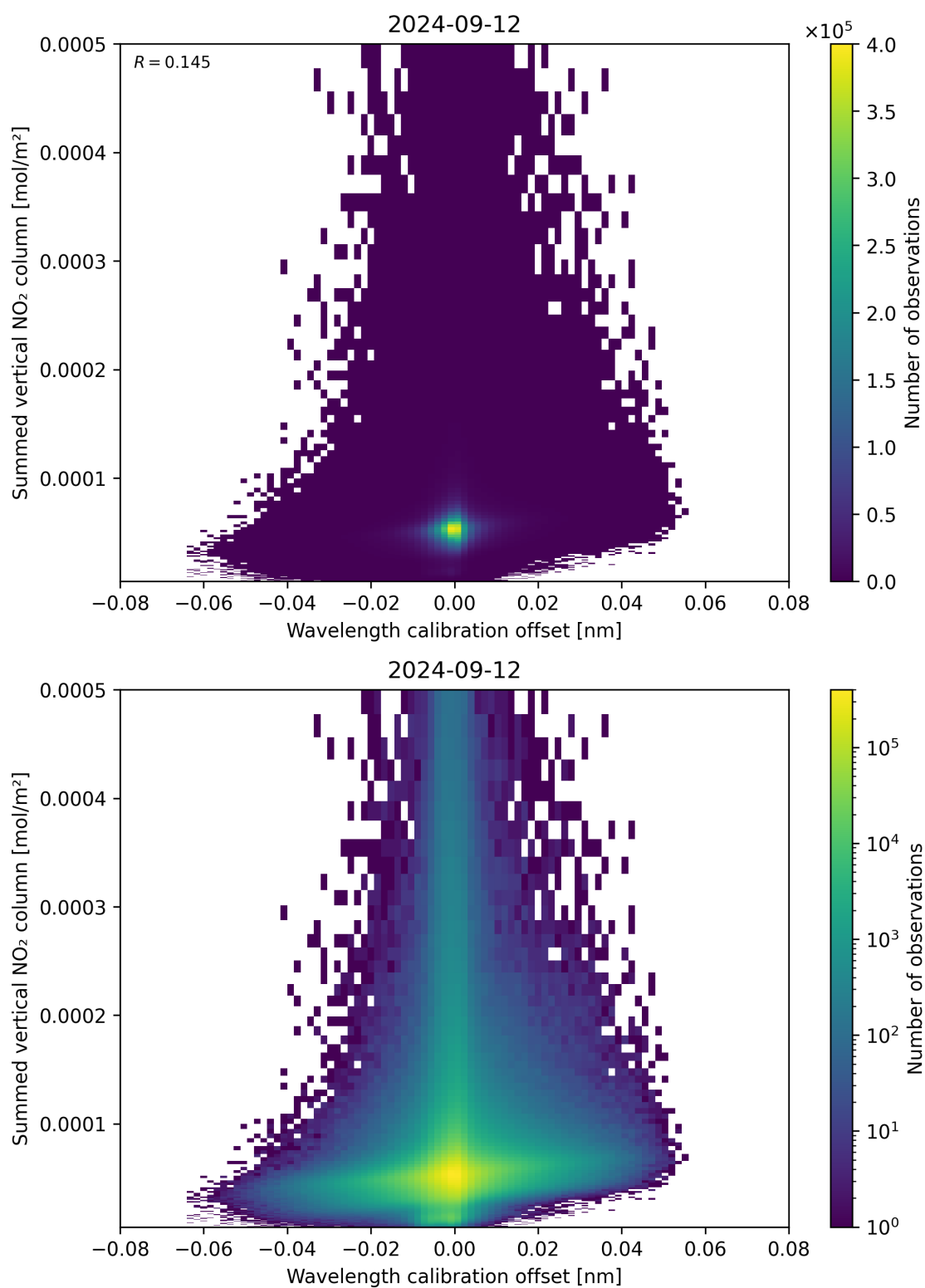
Figure 177: Scatter density plot of “Wavelength calibration offset” against “Summed vertical NO 2 column” for 2024-09-12 to 2024-09-13.
