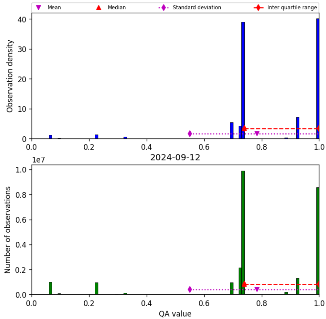
Figure 28: Histogram of “QA value” for 2024-09-12 to 2024-09-13
