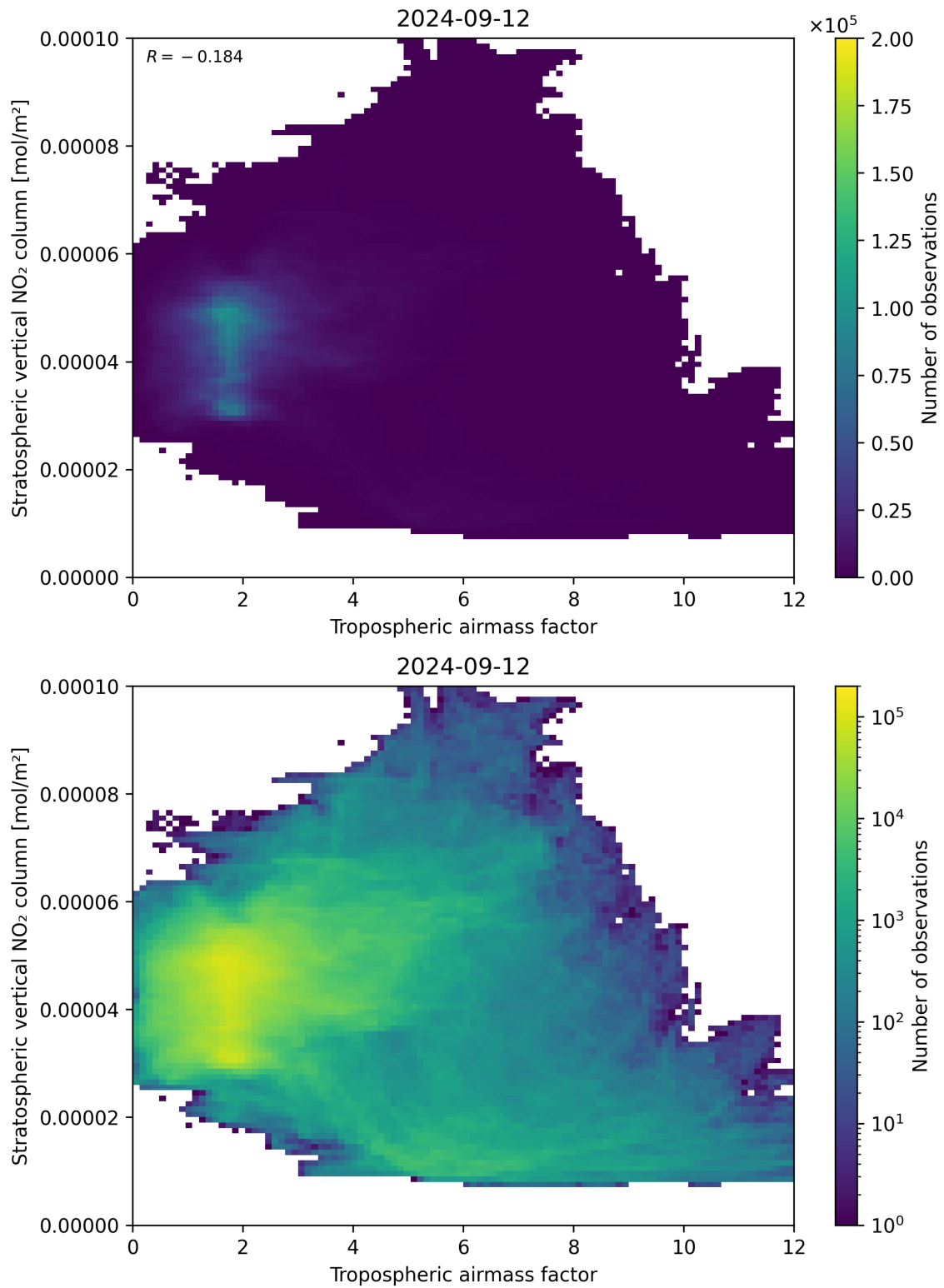
Figure 74: Scatter density plot of “Tropospheric air mass factor” against “Stratospheric vertical NO 2 column” for 2024-09-12 to 2024-09-13.
