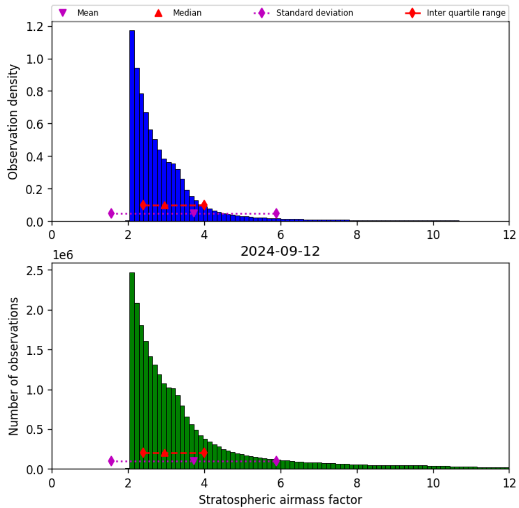
Figure 44: Histogram of “Stratospheric airmass factor” for 2024-09-12 to 2024-09-13
