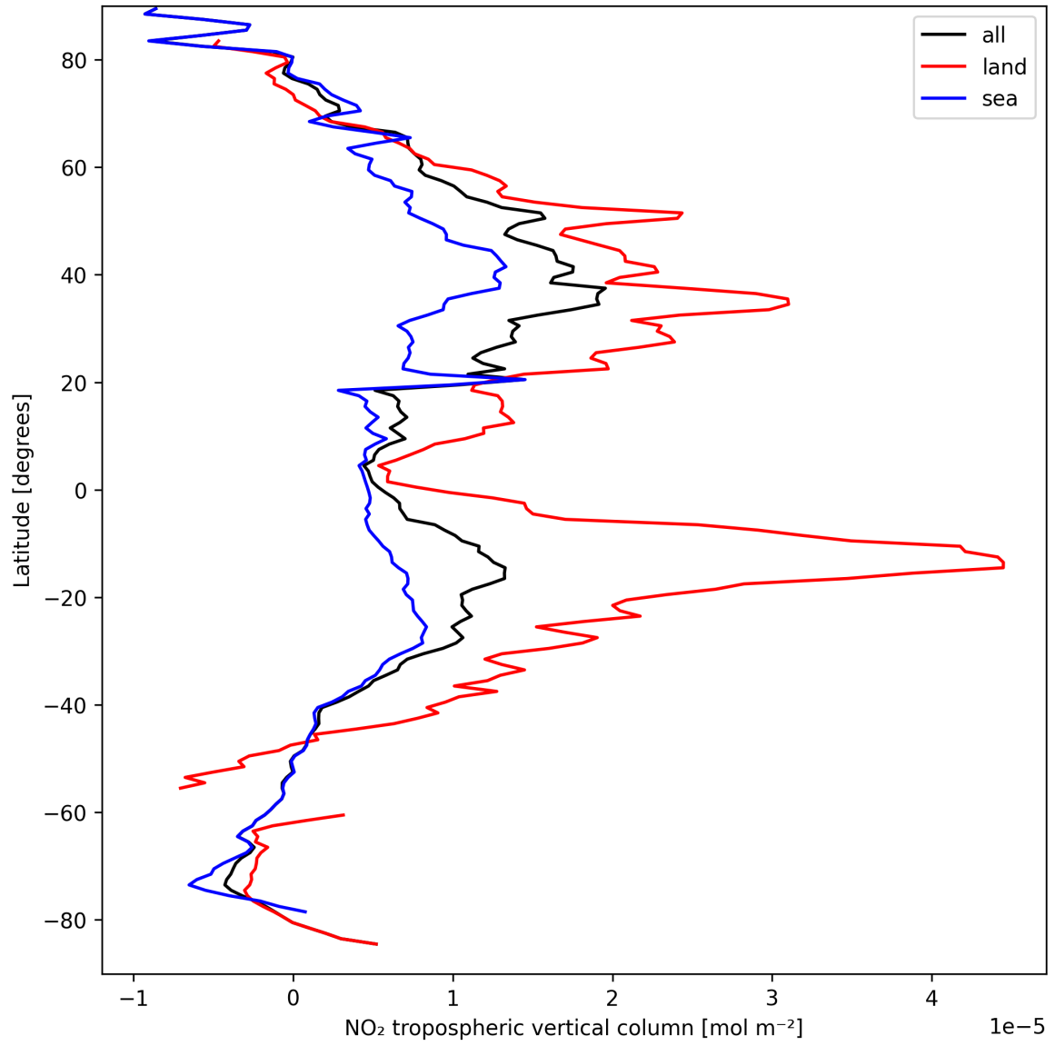
Figure 12: Zonal average of “NO 2 tropospheric vertical column” for 2024-09-12 to 2024-09-13.
