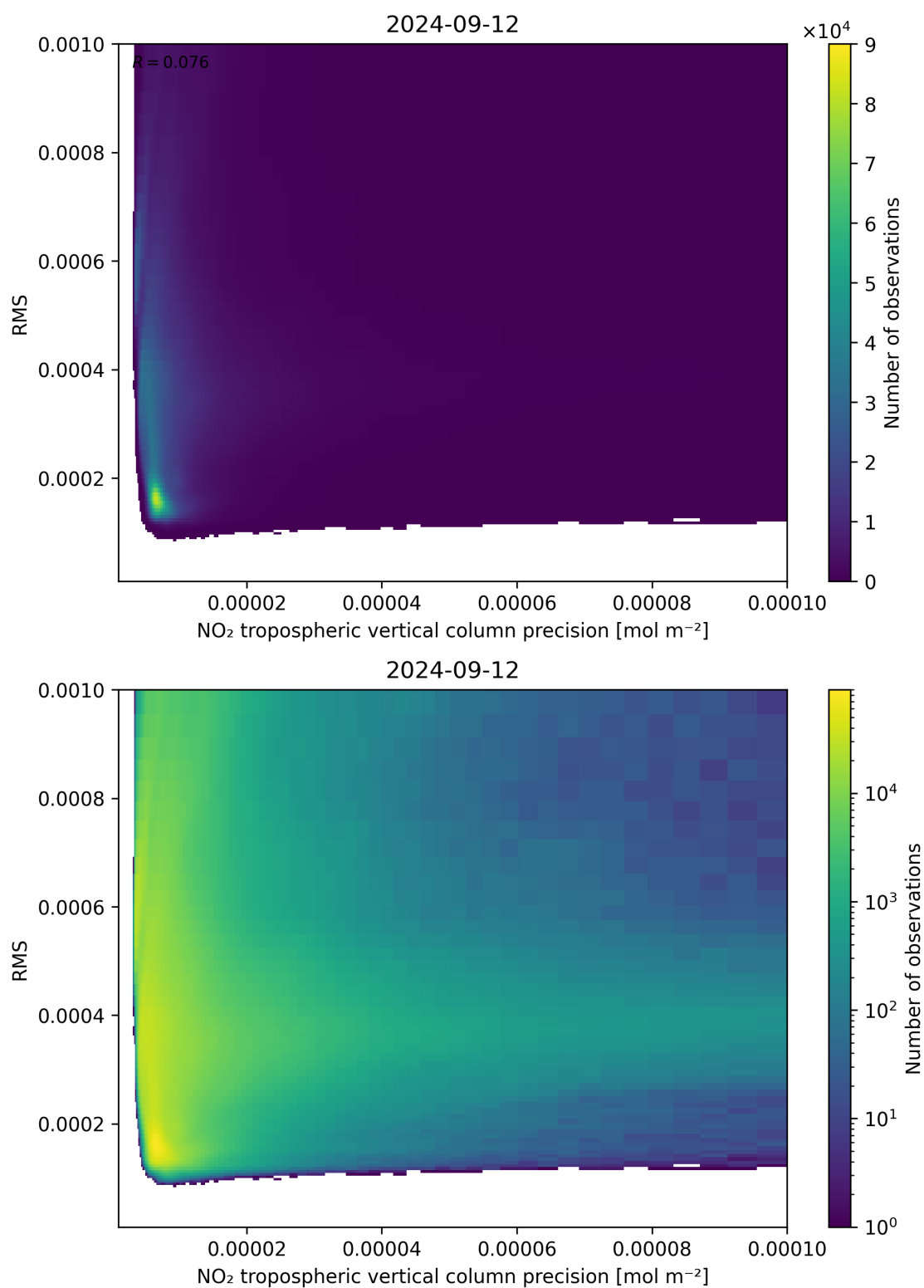
Figure 140: Scatter density plot of “NO 2 tropospheric vertical column precision” against “RMS” for 2024-09-12 to 2024-09-13.
