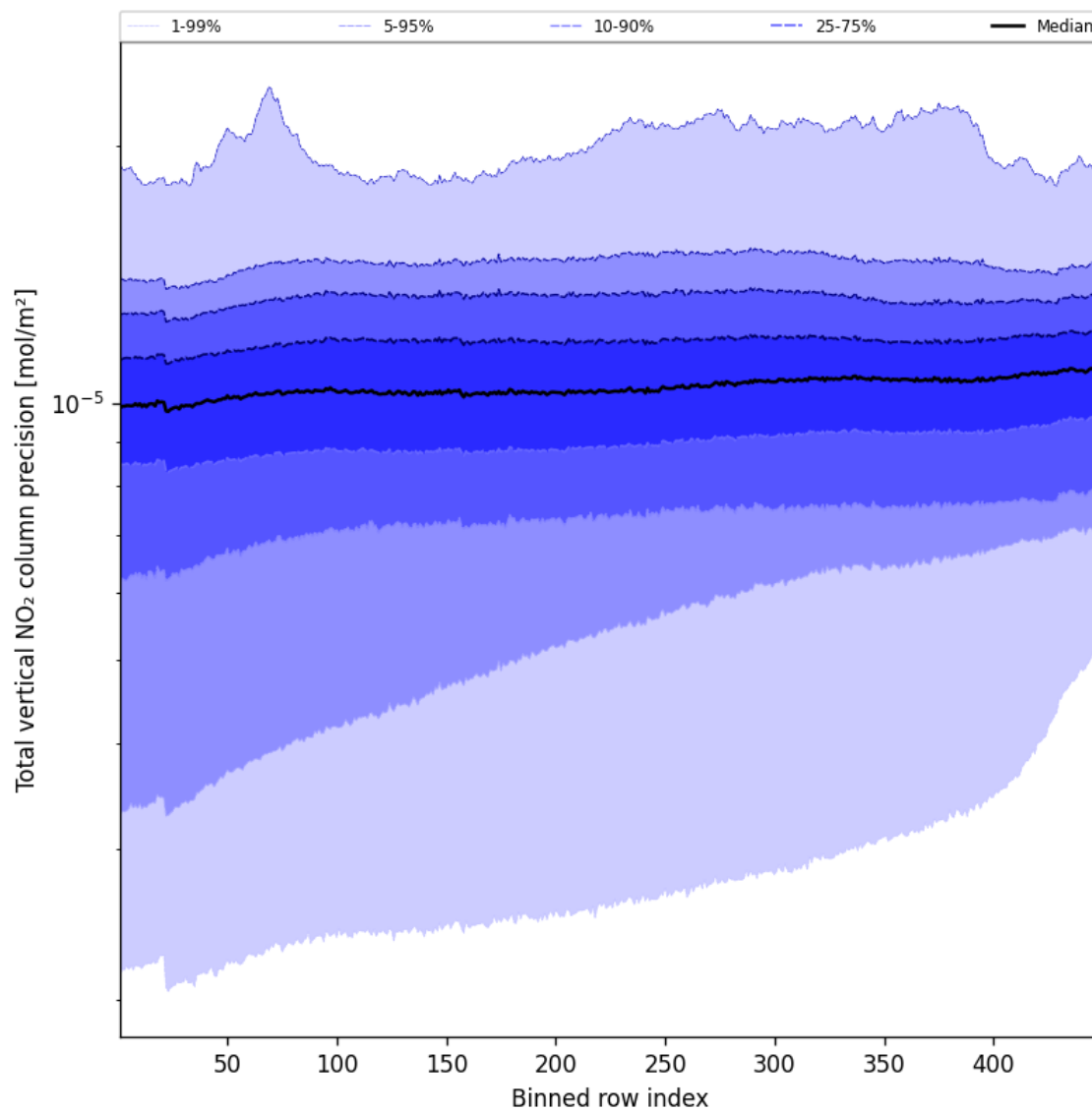
Figure 56: Along track statistics of “Total vertical NO 2 column precision” for 2024-09-12 to 2024-09-13
