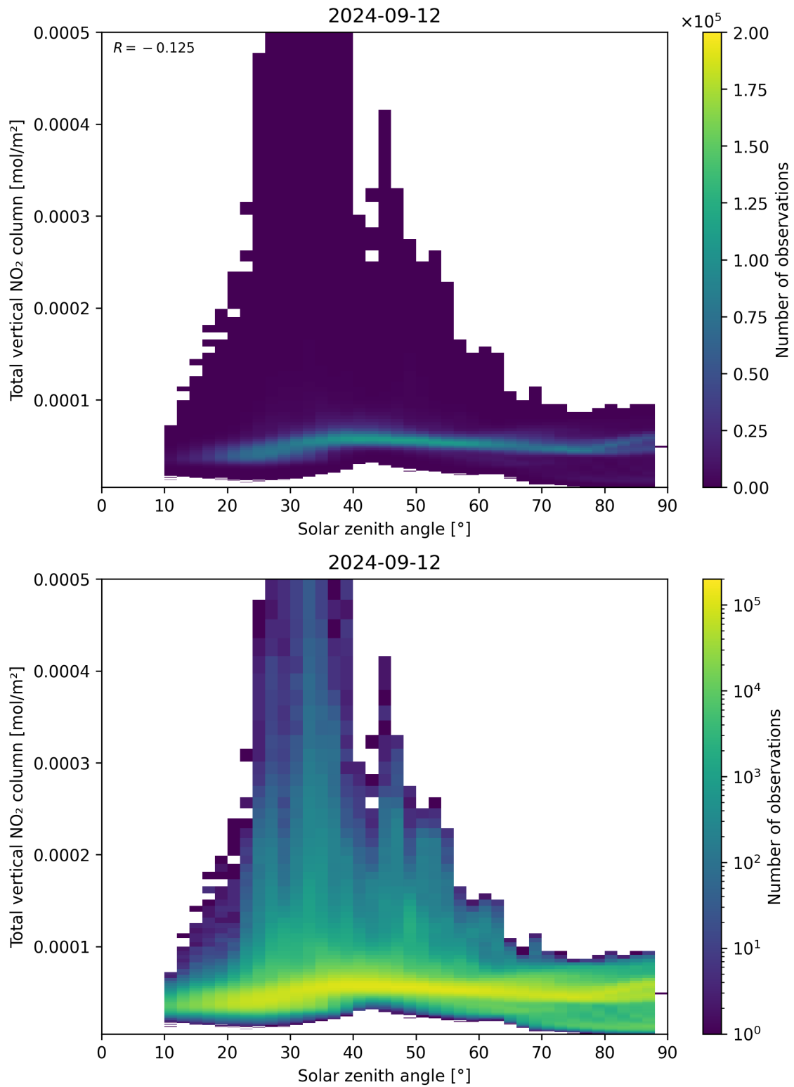
Figure 153: Scatter density plot of “Solar zenith angle” against “Total vertical NO 2 column” for 2024-09-12 to 2024-09-13.
