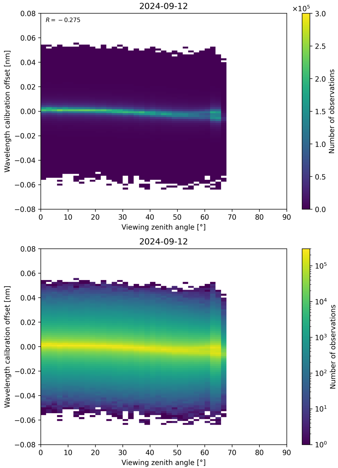
Figure 173: Scatter density plot of “Viewing zenith angle” against “Wavelength calibration offset” for 2024-09-12 to 2024-09-13.
