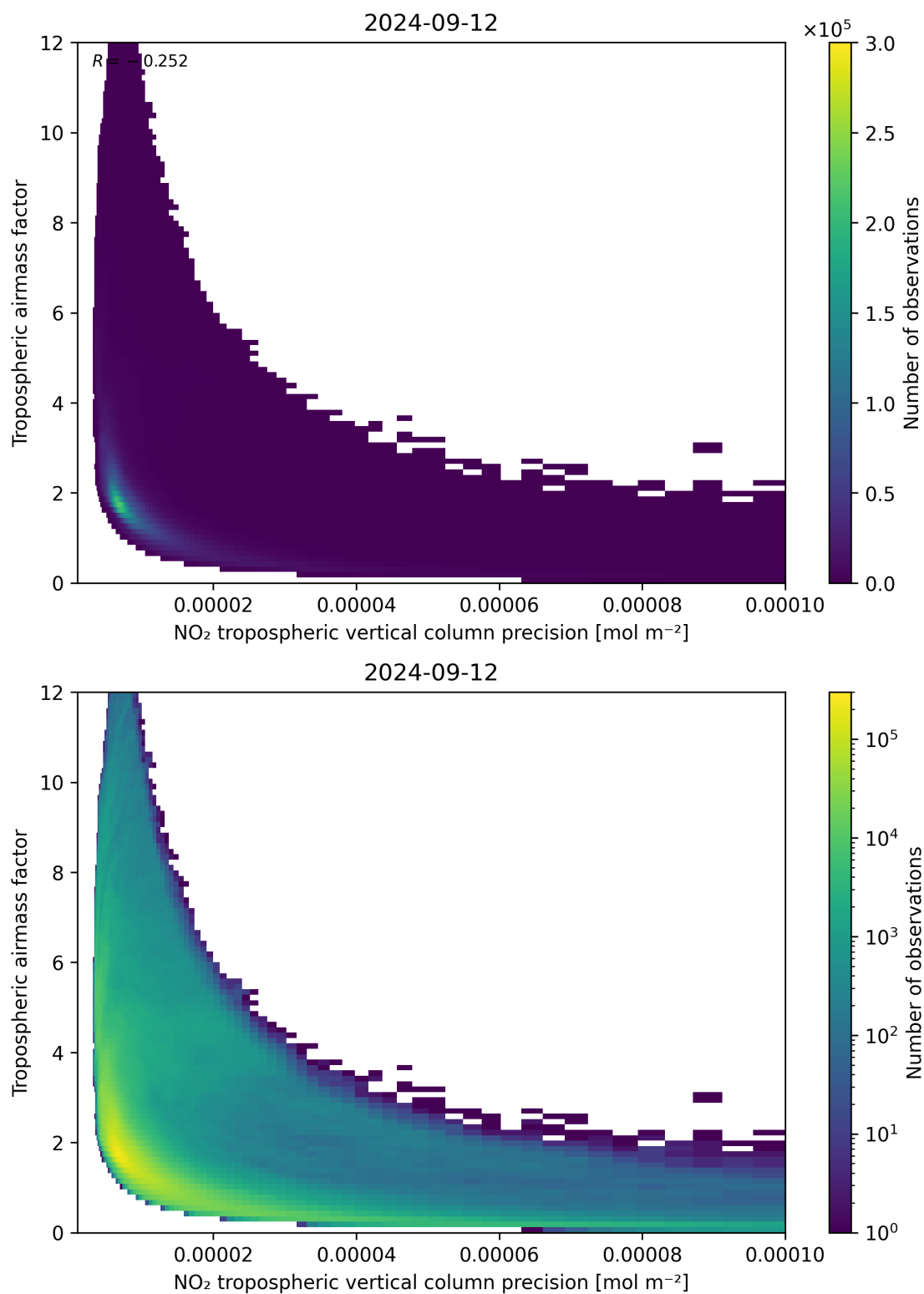
Figure 133: Scatter density plot of “NO 2 tropospheric vertical column precision” against “Tropospheric air mass factor” for 2024-09-12 to 2024-09-13.
