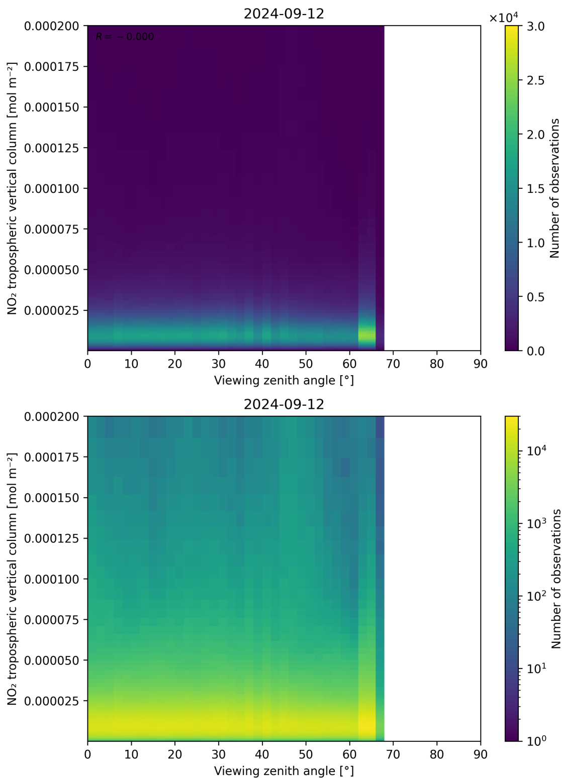
Figure 169: Scatter density plot of “Viewing zenith angle” against “NO 2 tropospheric vertical column” for 2024-09-12 to 2024-09-13.
