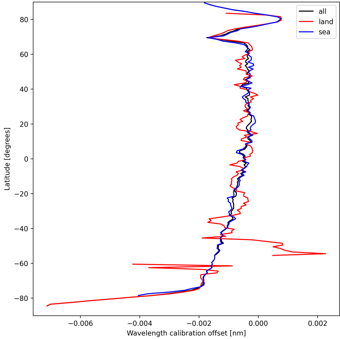
Figure 18: Zonal average of “Wavelength calibration offset” for 2024-09-12 to 2024-09-13.
