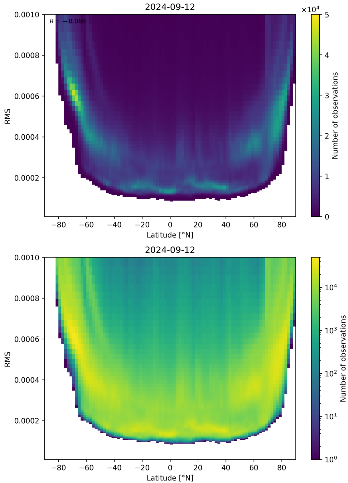
Figure 94: Scatter density plot of “Latitude” against “RMS” for 2024-09-12 to 2024-09-13.
