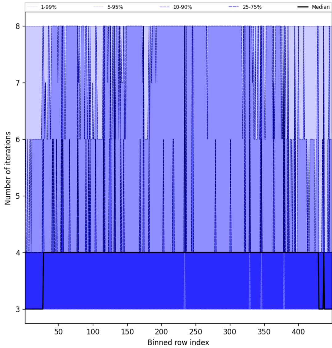
Figure 51: Along track statistics of “Number of iterations” for 2024-09-12 to 2024-09-13
