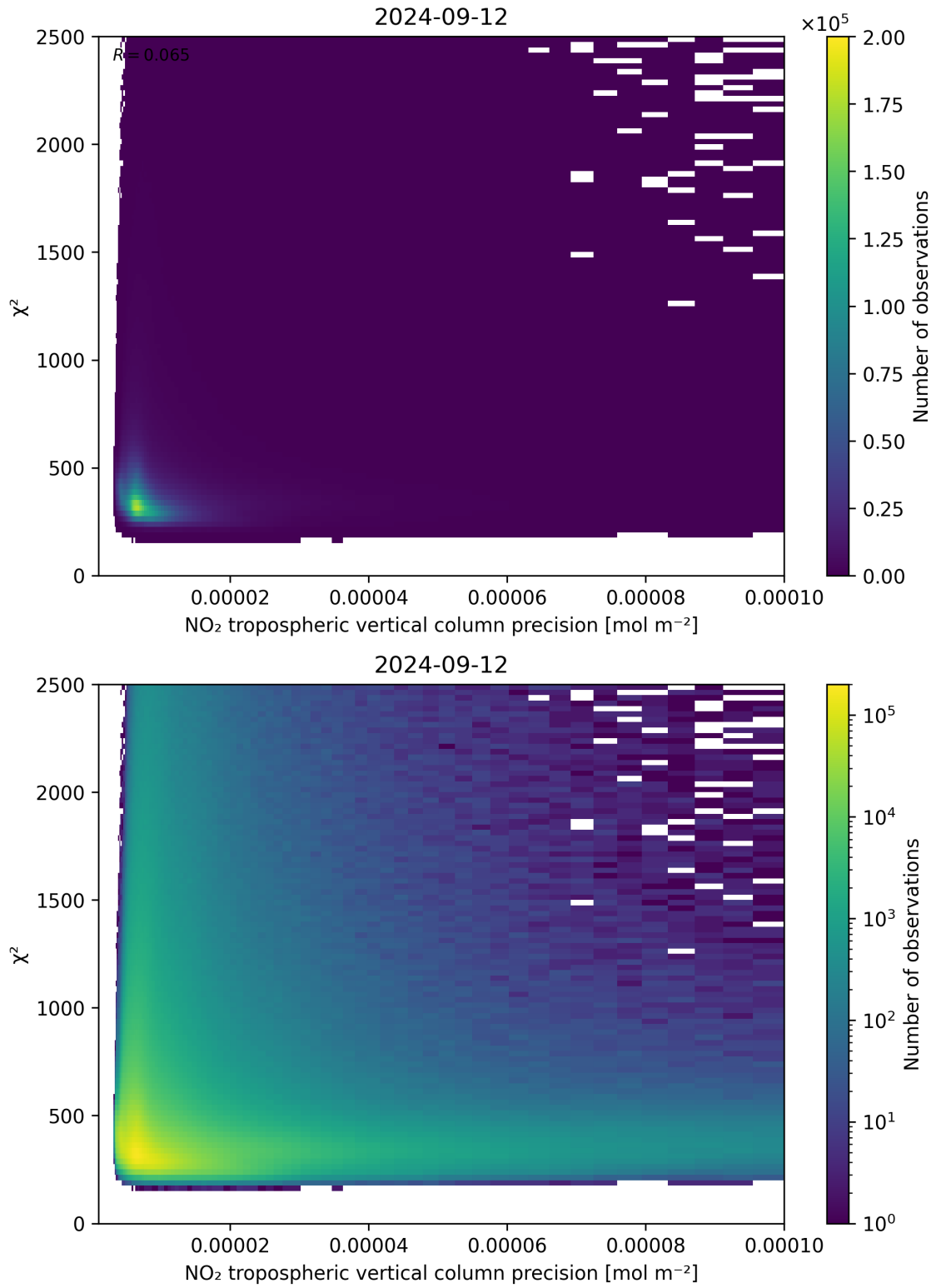
Figure 134: Scatter density plot of “NO 2 tropospheric vertical column precision” against “ \chi^2 ” for 2024-09-12 to 2024-09-13.
