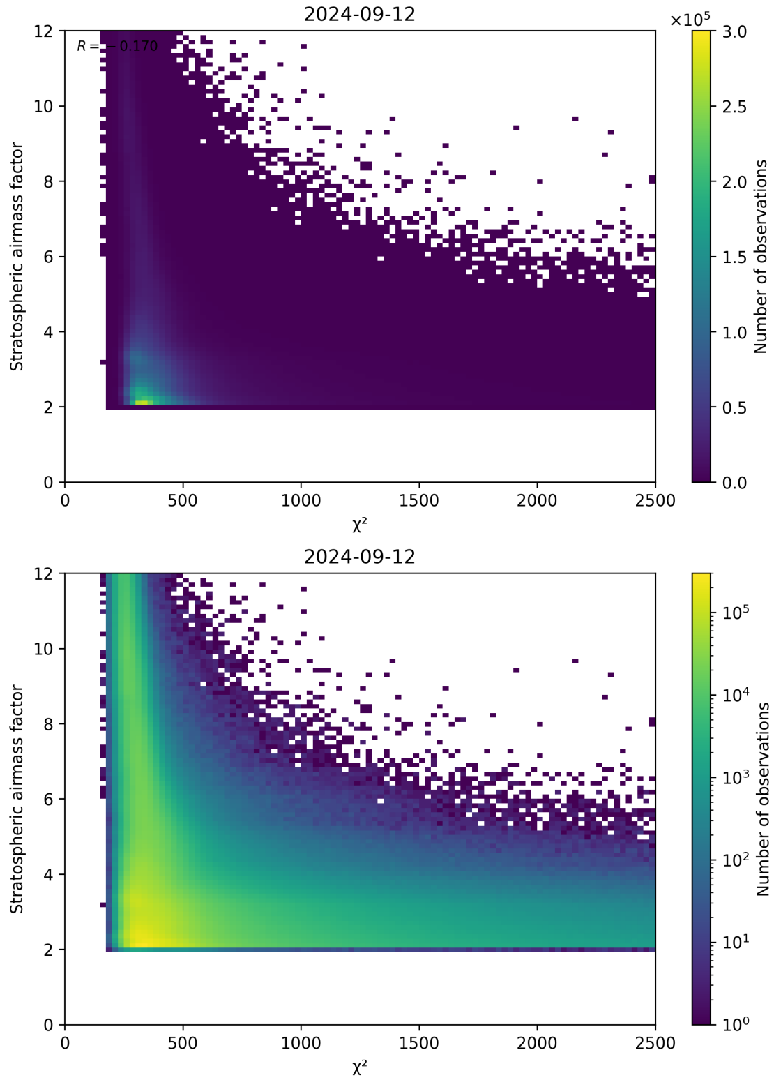
Figure 81: Scatter density plot of “ \chi^2 ” against “Stratospheric airmass factor” for 2024-09-12 to 2024-09-13.
