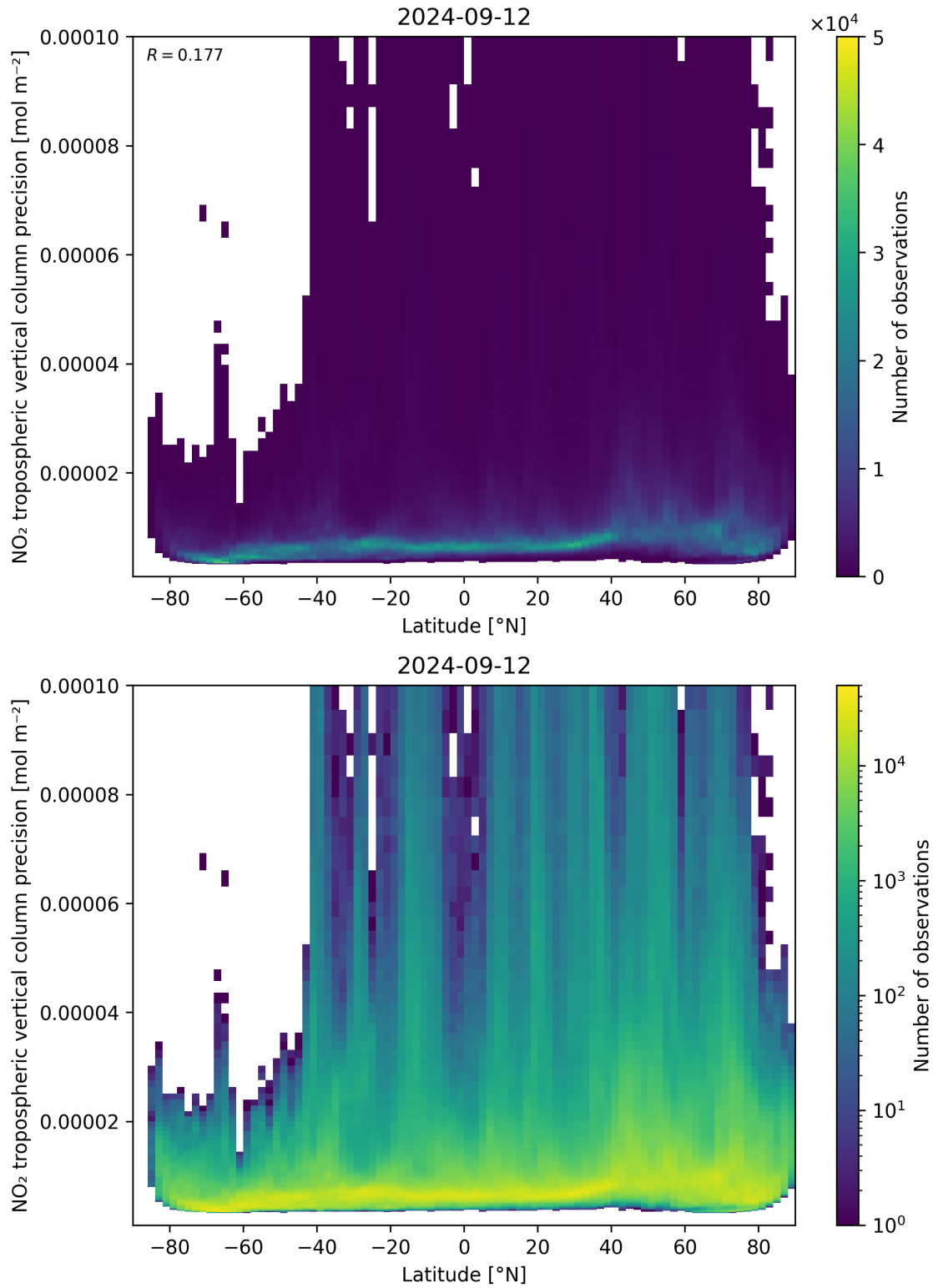
Figure 93: Scatter density plot of “Latitude” against “NO 2 tropospheric vertical column precision” for 2024-09-12 to 2024-09-13.
