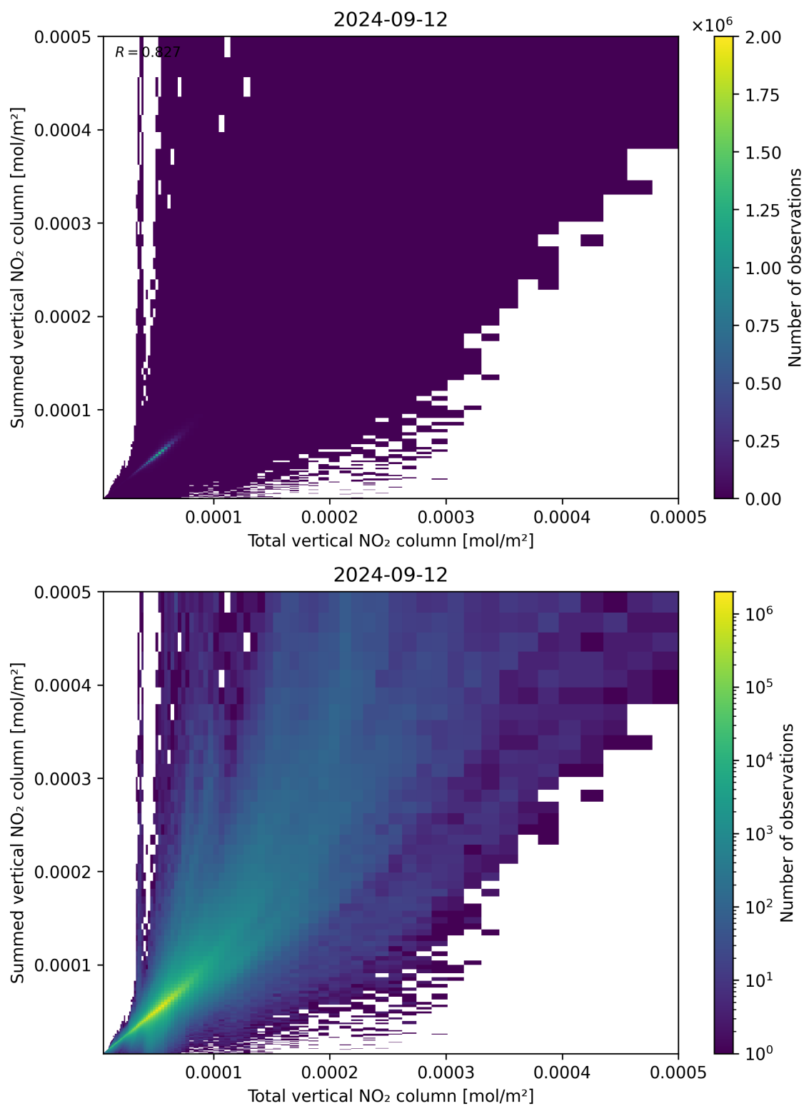
Figure 112: Scatter density plot of “Total vertical NO 2 column” against “Summed vertical NO 2 column” for 2024-09-12 to 2024-09-13.
