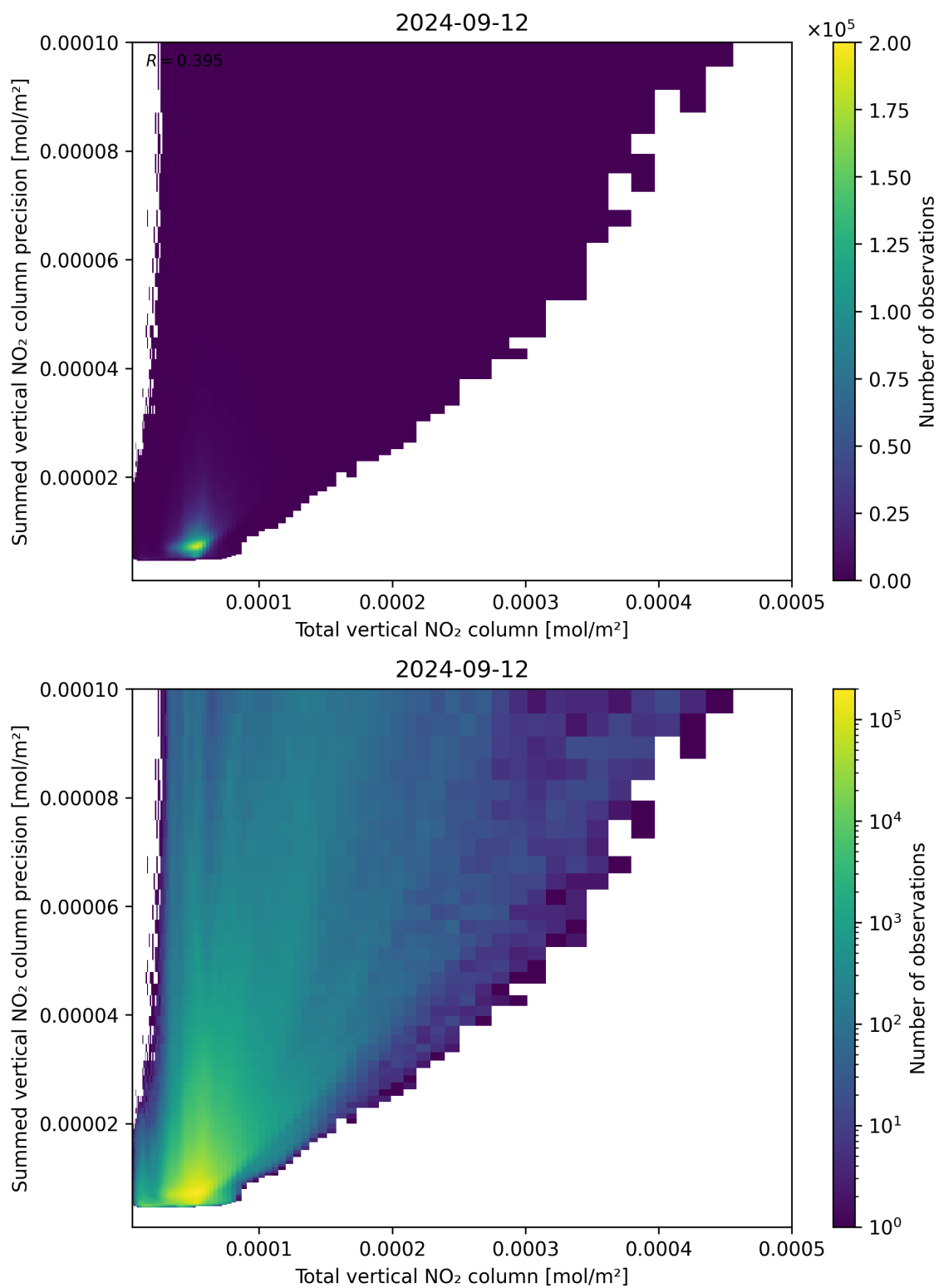
Figure 113: Scatter density plot of “Total vertical NO 2 column” against “Summed vertical NO 2 column precision” for 2024-09-12 to 2024-09-13.
