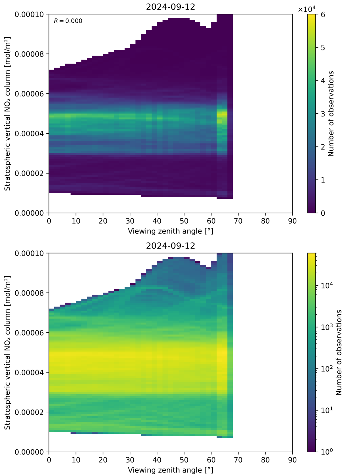
Figure 164: Scatter density plot of “Viewing zenith angle” against “Stratospheric vertical NO 2 column” for 2024-09-12 to 2024-09-13.
