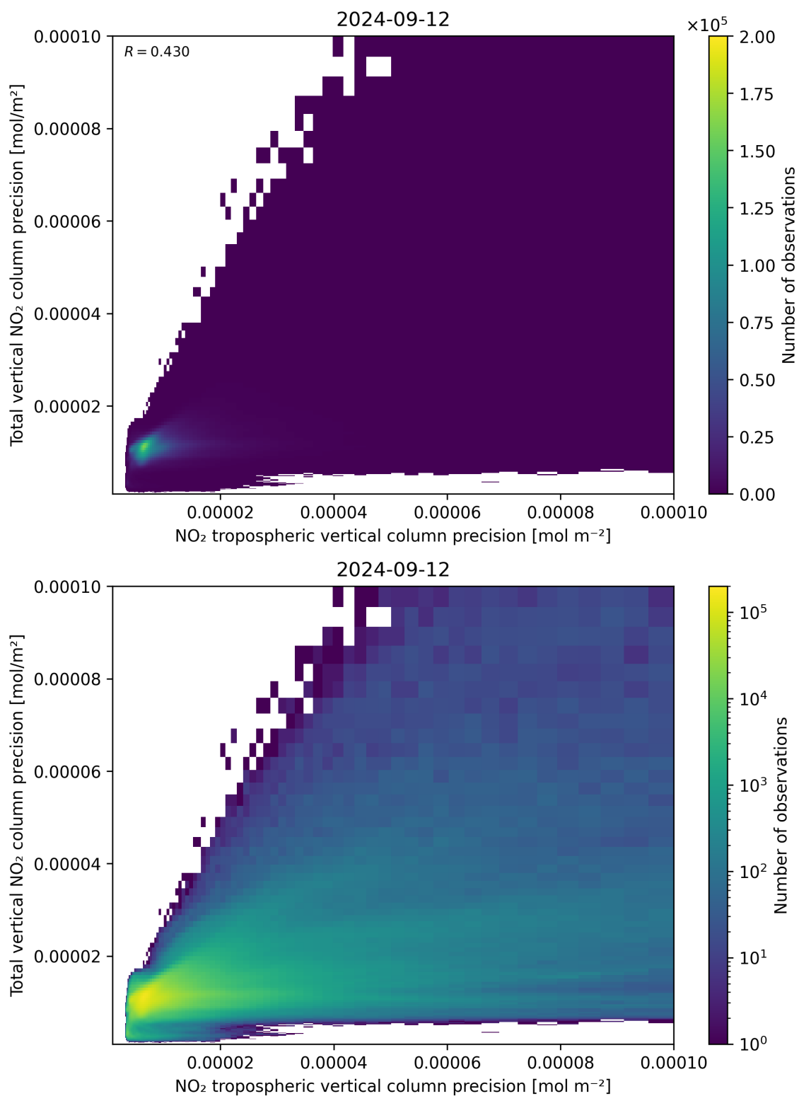
Figure 139: Scatter density plot of “NO 2 tropospheric vertical column precision” against “Total vertical NO 2 column precision” for 2024-09-12 to 2024-09-13.
