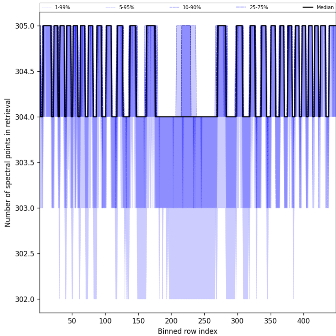
Figure 50: Along track statistics of “Number of spectral points in retrieval” for 2024-09-12 to 2024-09-13
