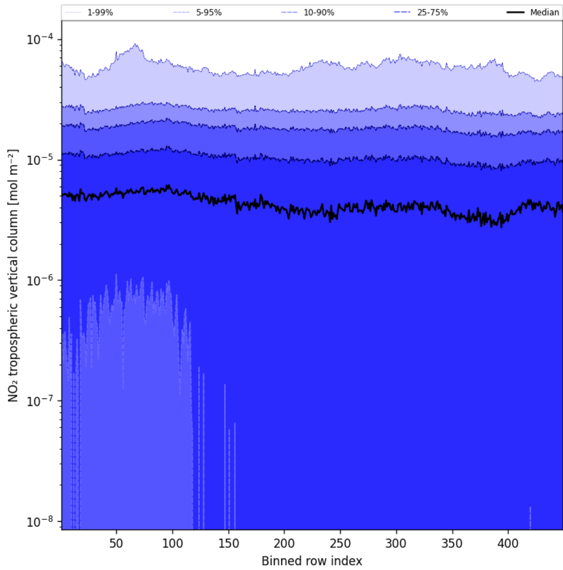
Figure 46: Along track statistics of “NO 2 tropospheric vertical column” for 2024-09-12 to 2024-09-13
