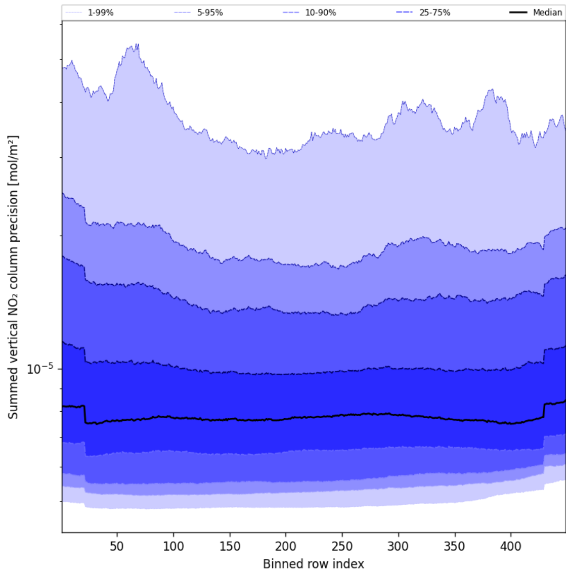
Figure 58: Along track statistics of “Summed vertical NO 2 column precision” for 2024-09-12 to 2024-09-13
