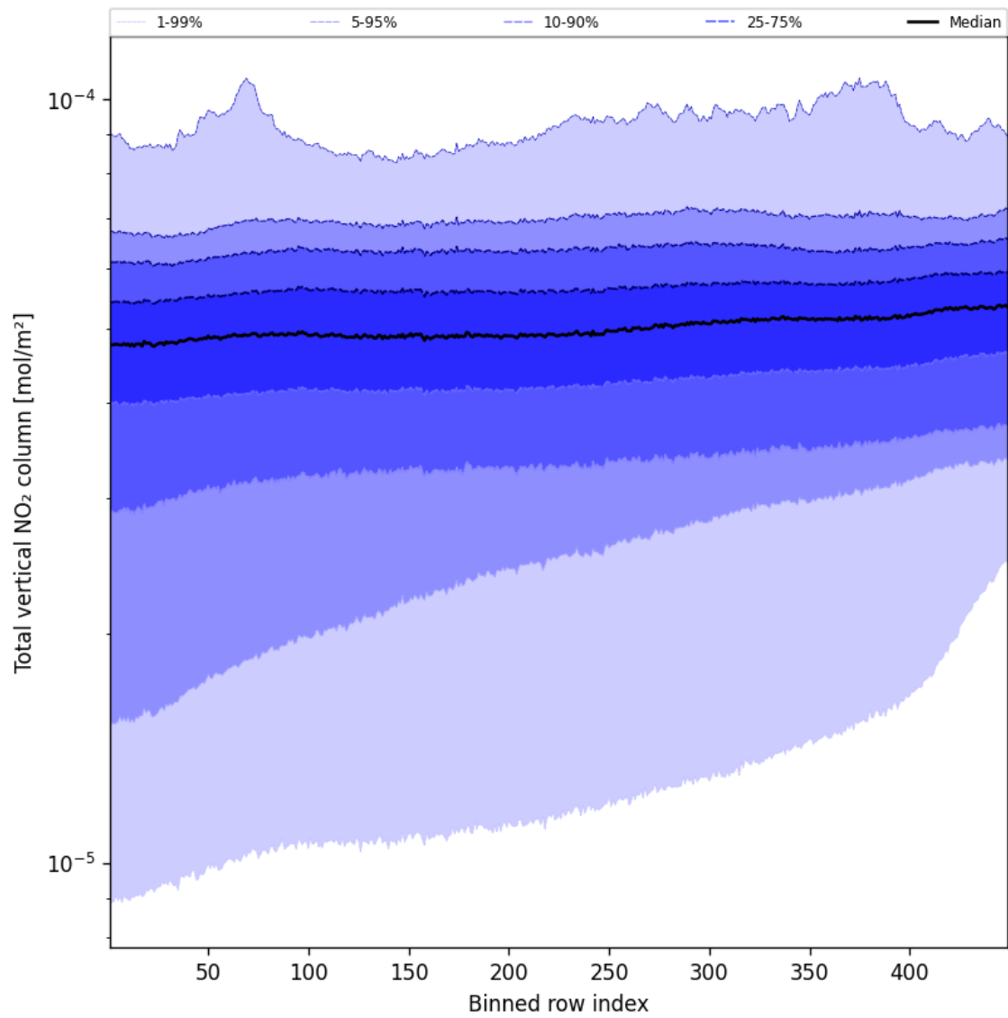
Figure 55: Along track statistics of “Total vertical NO 2 column” for 2024-09-12 to 2024-09-13
