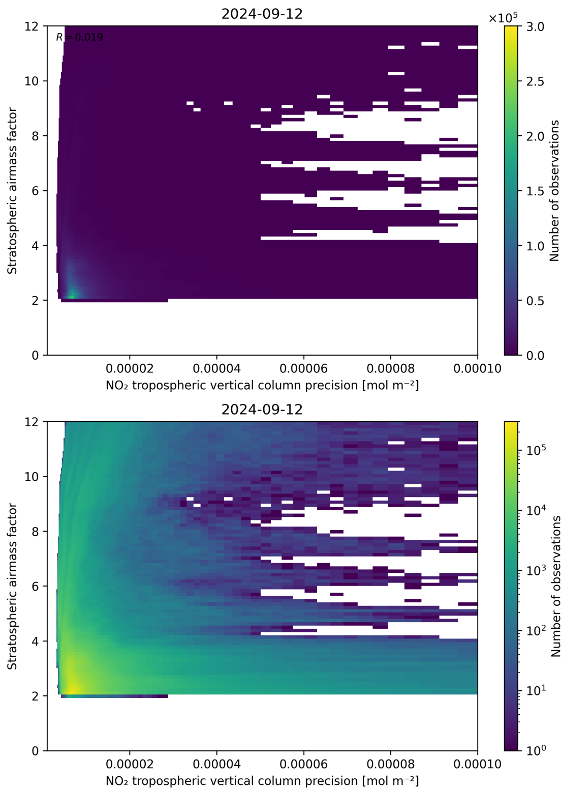
Figure 131: Scatter density plot of “NO 2 tropospheric vertical column precision” against “Stratospheric airmass factor” for 2024-09-12 to 2024-09-13.
