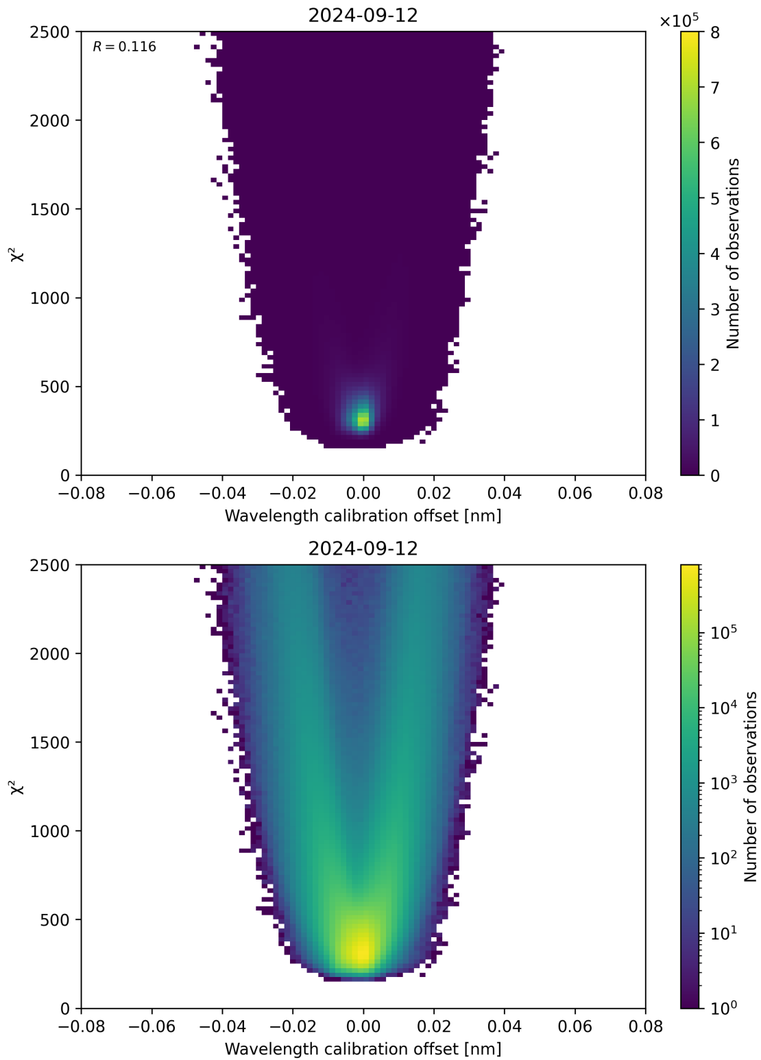
Figure 175: Scatter density plot of “Wavelength calibration offset” against “ \chi^2 ” for 2024-09-12 to 2024-09-13.
