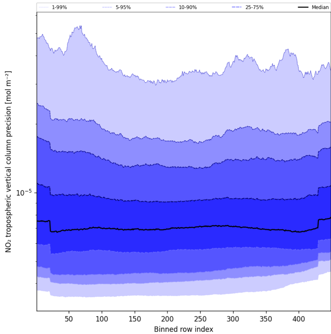
Figure 47: Along track statistics of “NO 2 tropospheric vertical column precision” for 2024-09-12 to 2024-09-13
