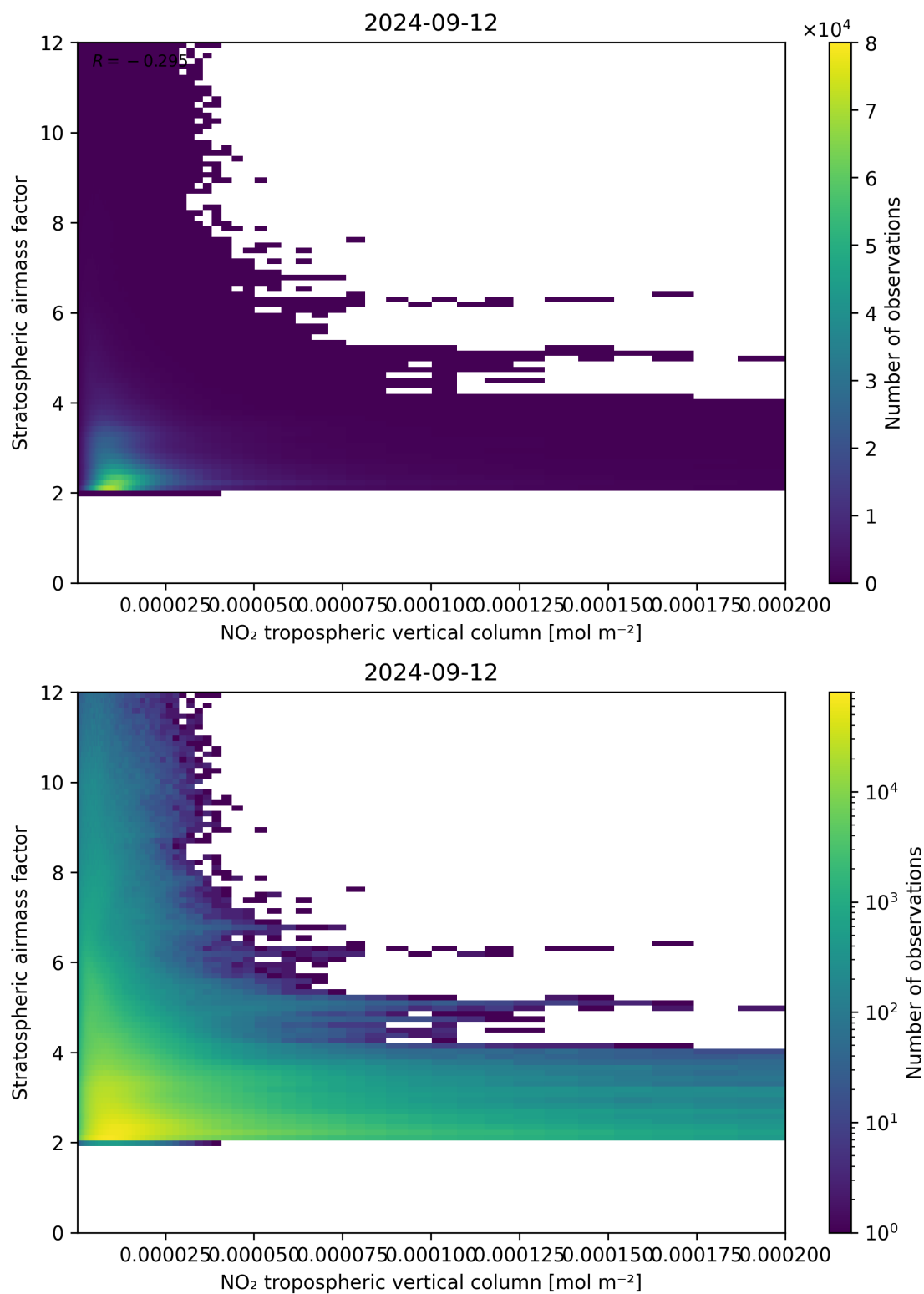
Figure 121: Scatter density plot of “NO 2 tropospheric vertical column” against “Stratospheric air mass factor” for 2024-09-12 to 2024-09-13.
