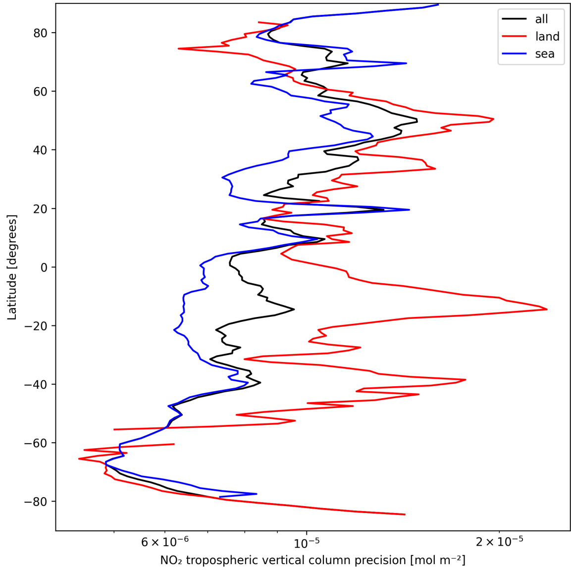
Figure 13: Zonal average of “NO 2 tropospheric vertical column precision” for 2024-09-12 to 2024-09-13.
