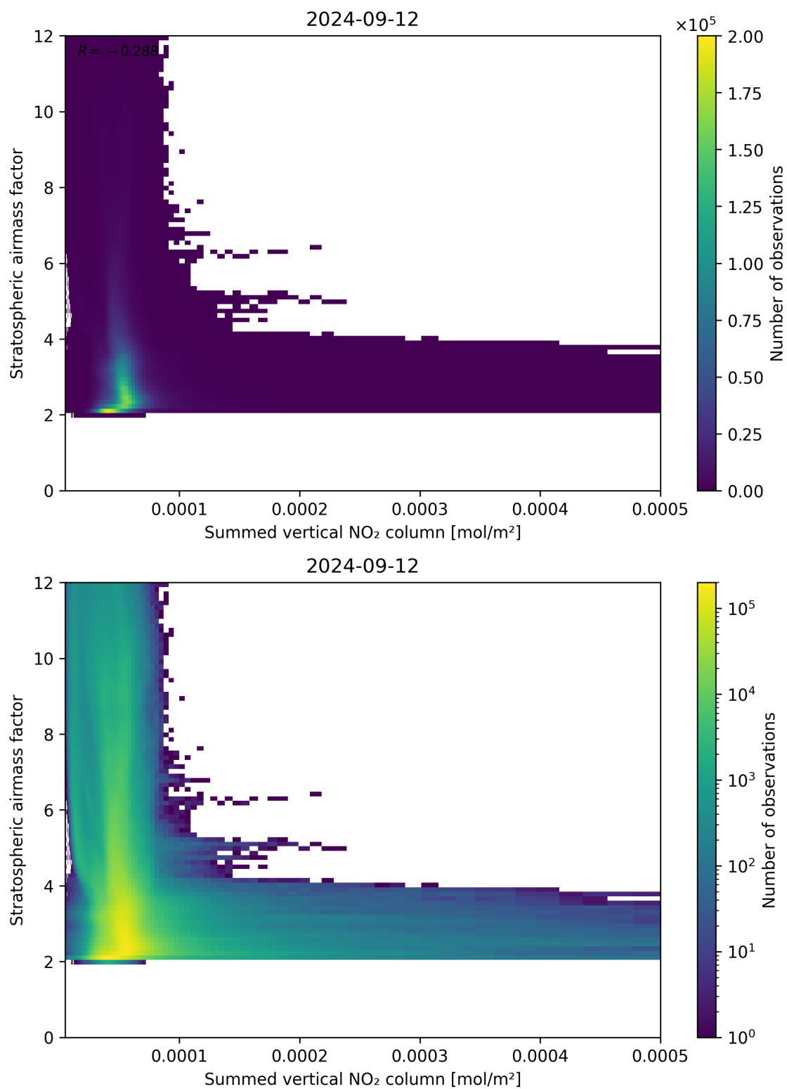
Figure 103: Scatter density plot of “Summed vertical NO 2 column” against “Stratospheric airmass factor” for 2024-09-12 to 2024-09-13.
