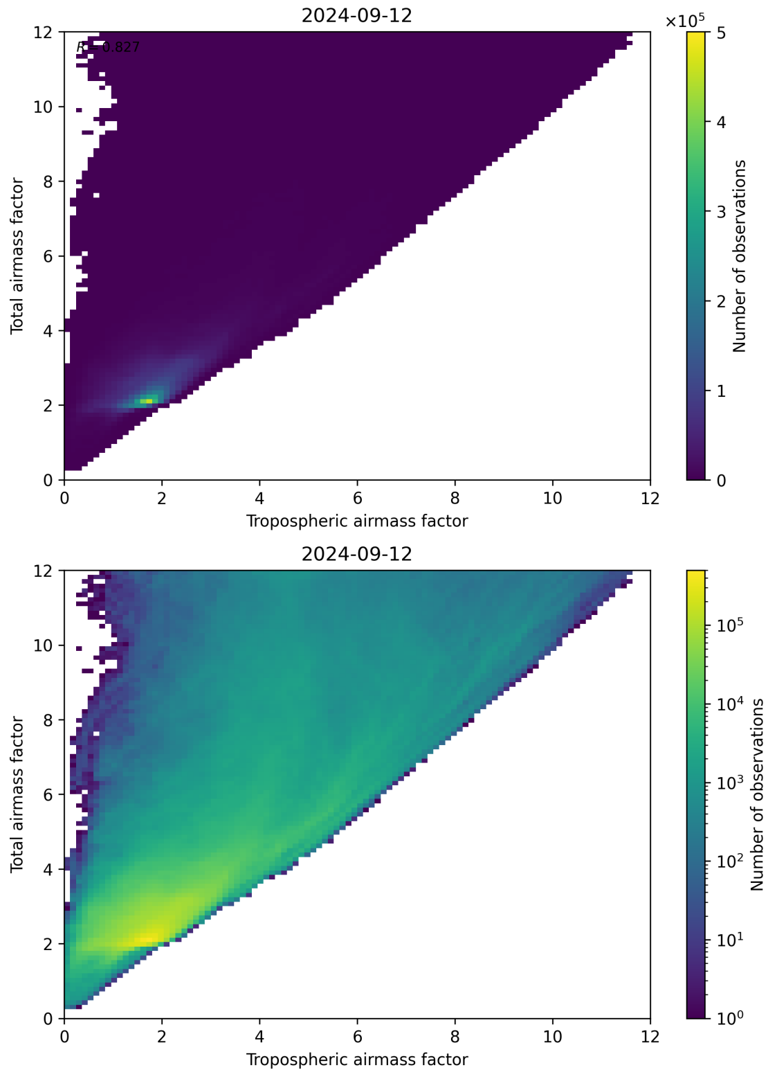
Figure 72: Scatter density plot of “Tropospheric airmass factor” against “Total airmass factor” for 2024-09-12 to 2024-09-13.
