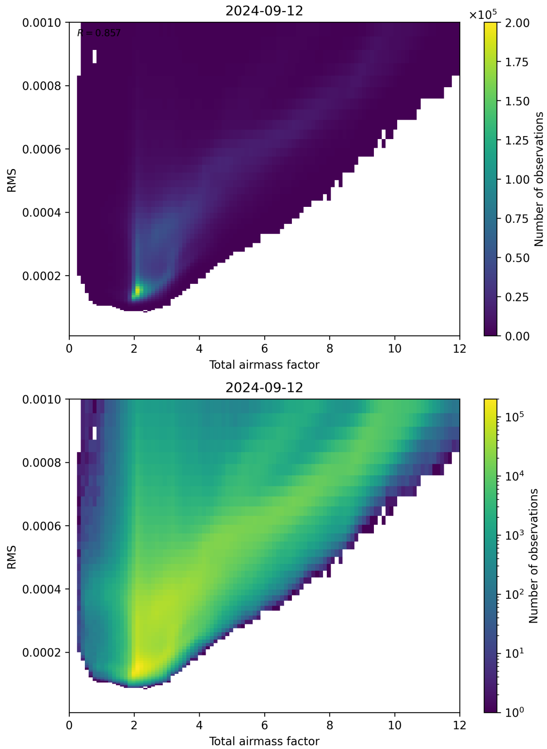
Figure 69: Scatter density plot of “Total airmass factor” against “RMS” for 2024-09-12 to 2024-09-13.
