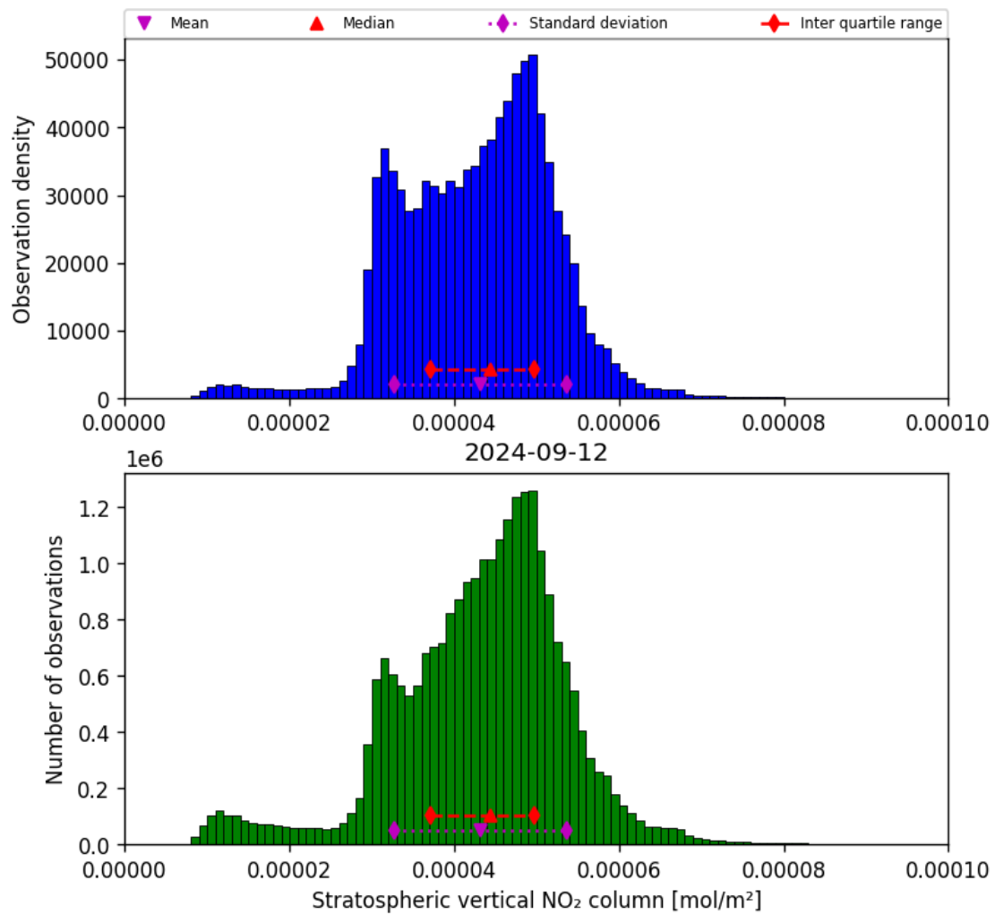
Figure 36: Histogram of “Stratospheric vertical NO 2 column” for 2024-09-12 to 2024-09-13
