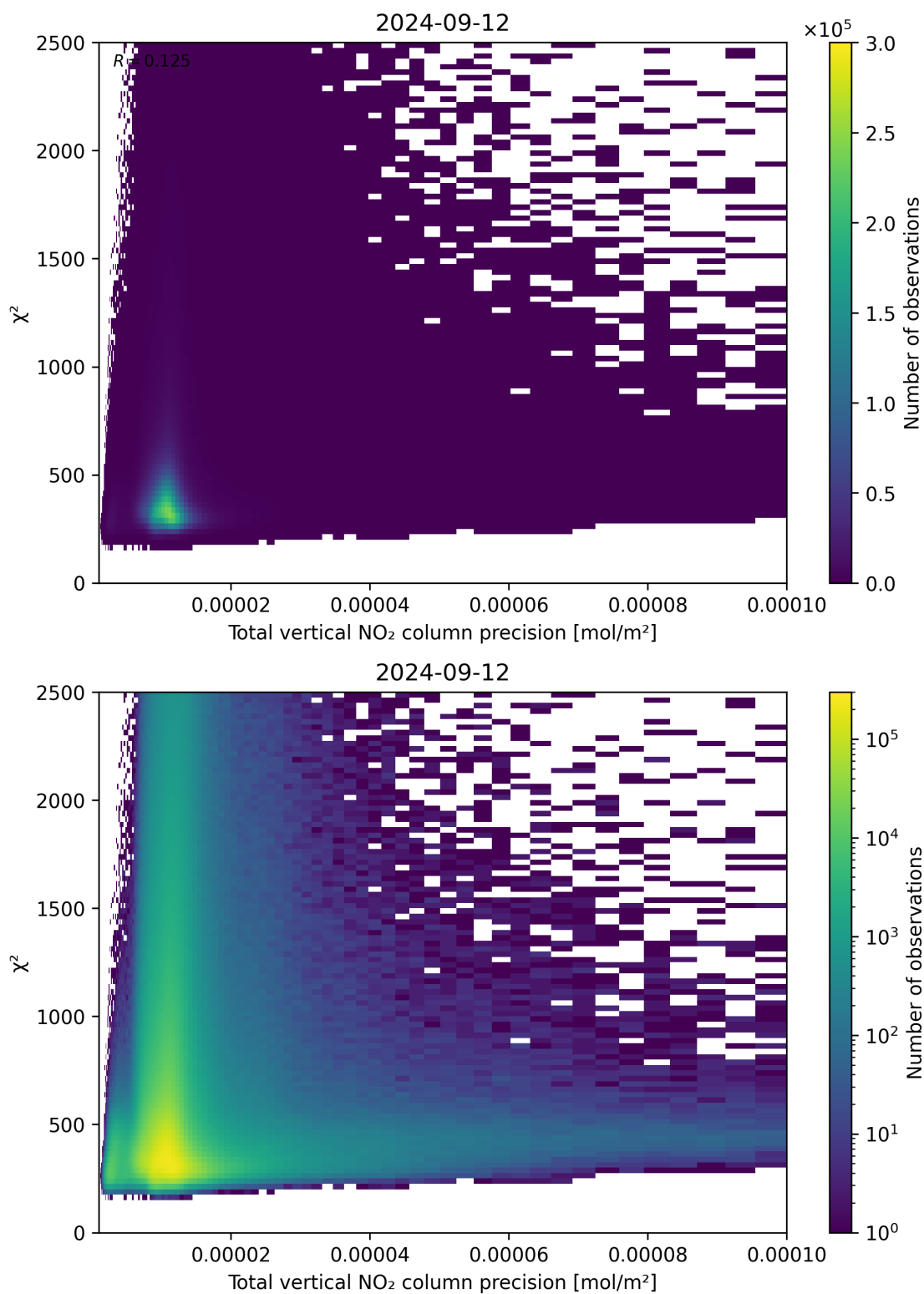
Figure 116: Scatter density plot of “Total vertical NO 2 column precision” against “ \chi^2 ” for 2024-09-12 to 2024-09-13.
