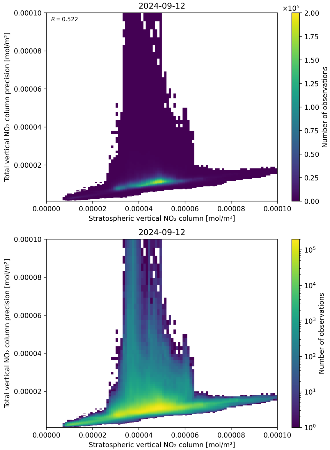
Figure 101: Scatter density plot of “Stratospheric vertical NO 2 column” against “Total vertical NO 2 column precision” for 2024-09-12 to 2024-09-13.
