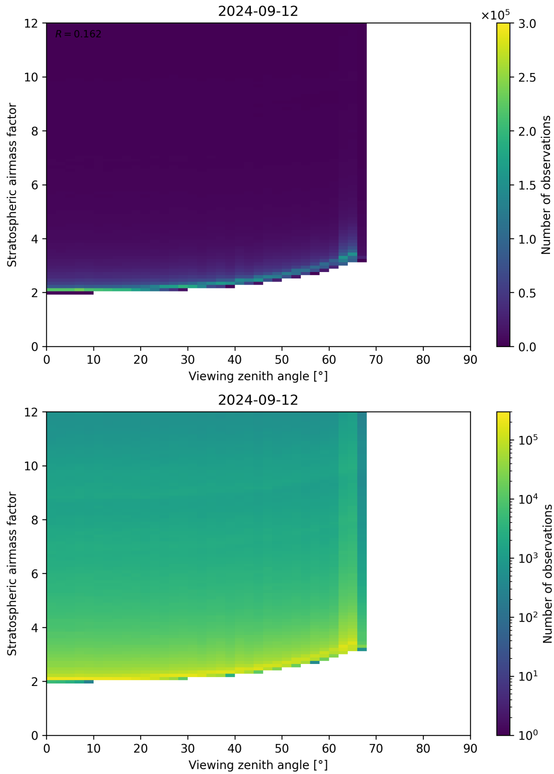
Figure 159: Scatter density plot of “Viewing zenith angle” against “Stratospheric airmass factor” for 2024-09-12 to 2024-09-13.
