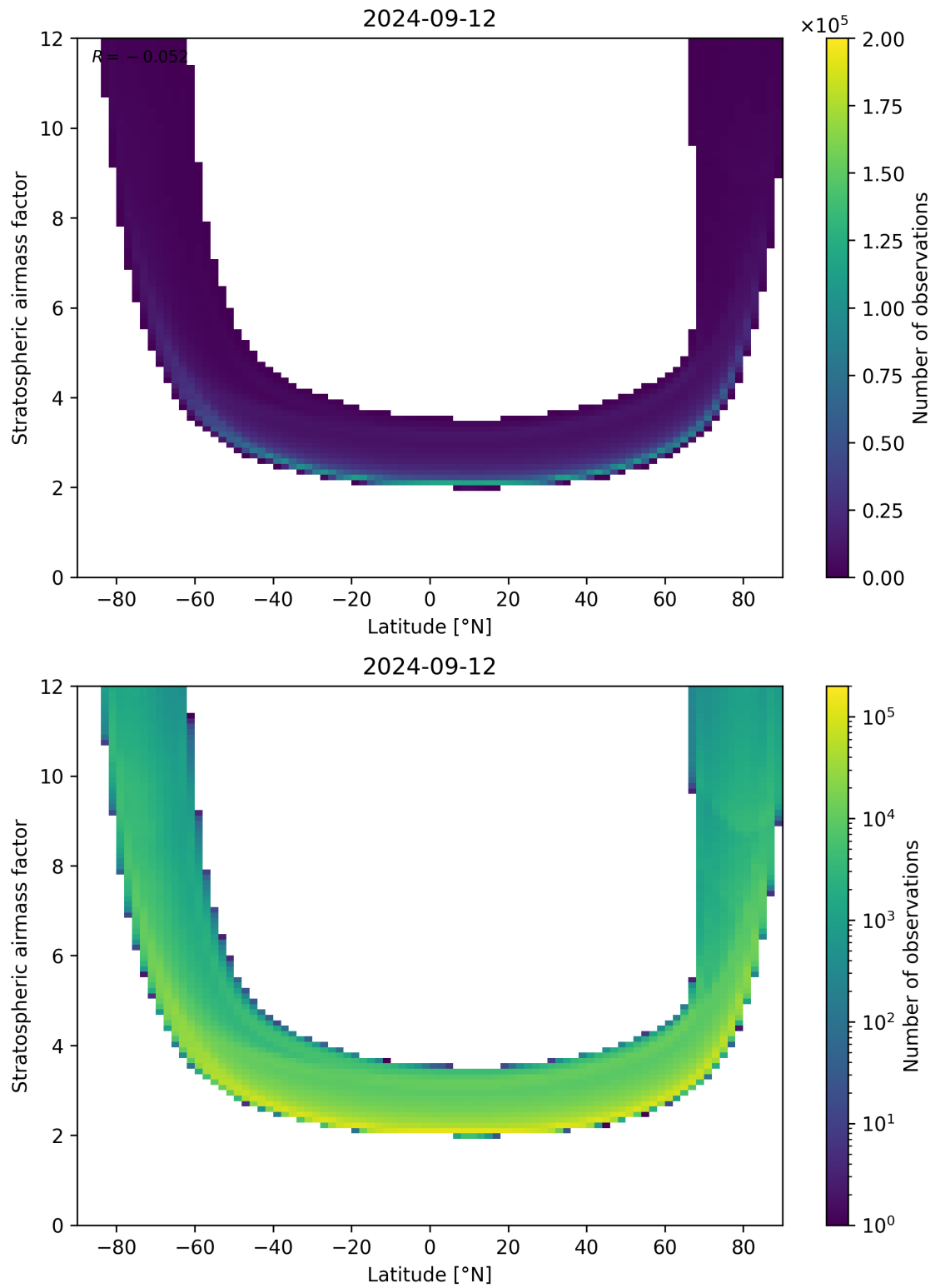
Figure 83: Scatter density plot of “Latitude” against “Stratospheric airmass factor” for 2024-09-12 to 2024-09-13.
