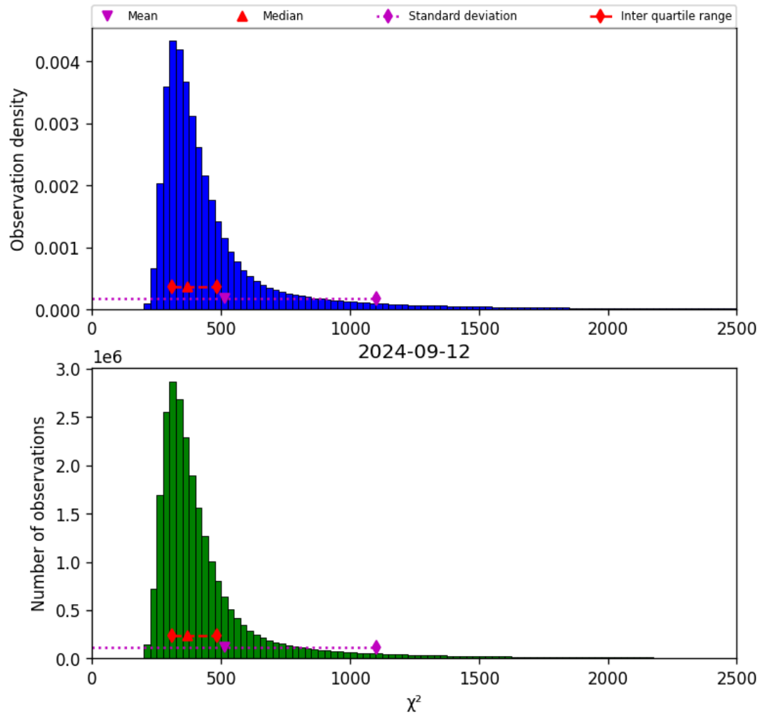
Figure 42: Histogram of “ \chi^2 ” for 2024-09-12 to 2024-09-13
