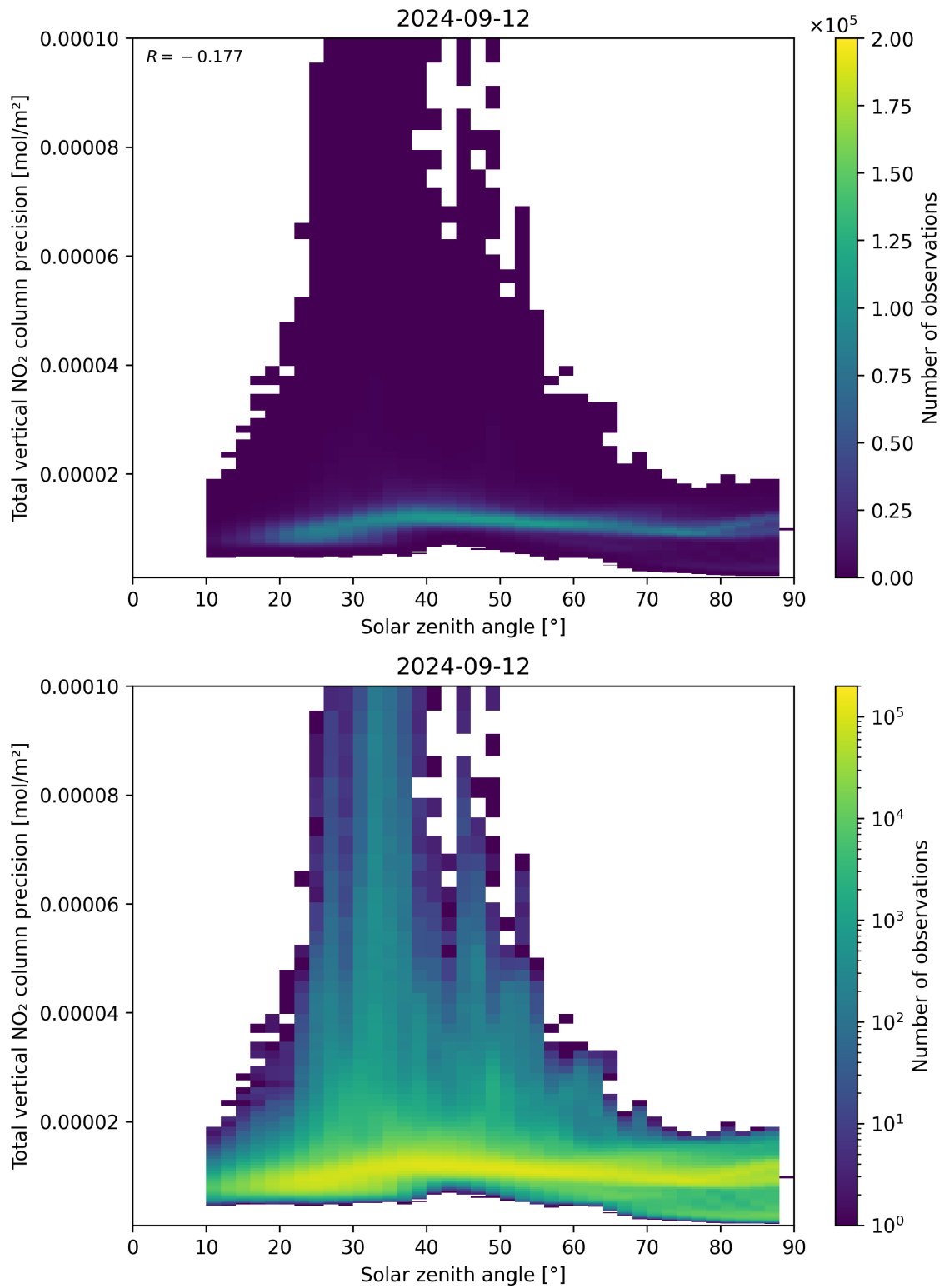
Figure 154: Scatter density plot of “Solar zenith angle” against “Total vertical NO 2 column precision” for 2024-09-12 to 2024-09-13.
