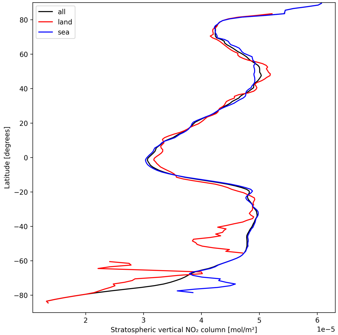
Figure 19: Zonal average of “Stratospheric vertical NO 2 column” for 2024-09-12 to 2024-09-13.
