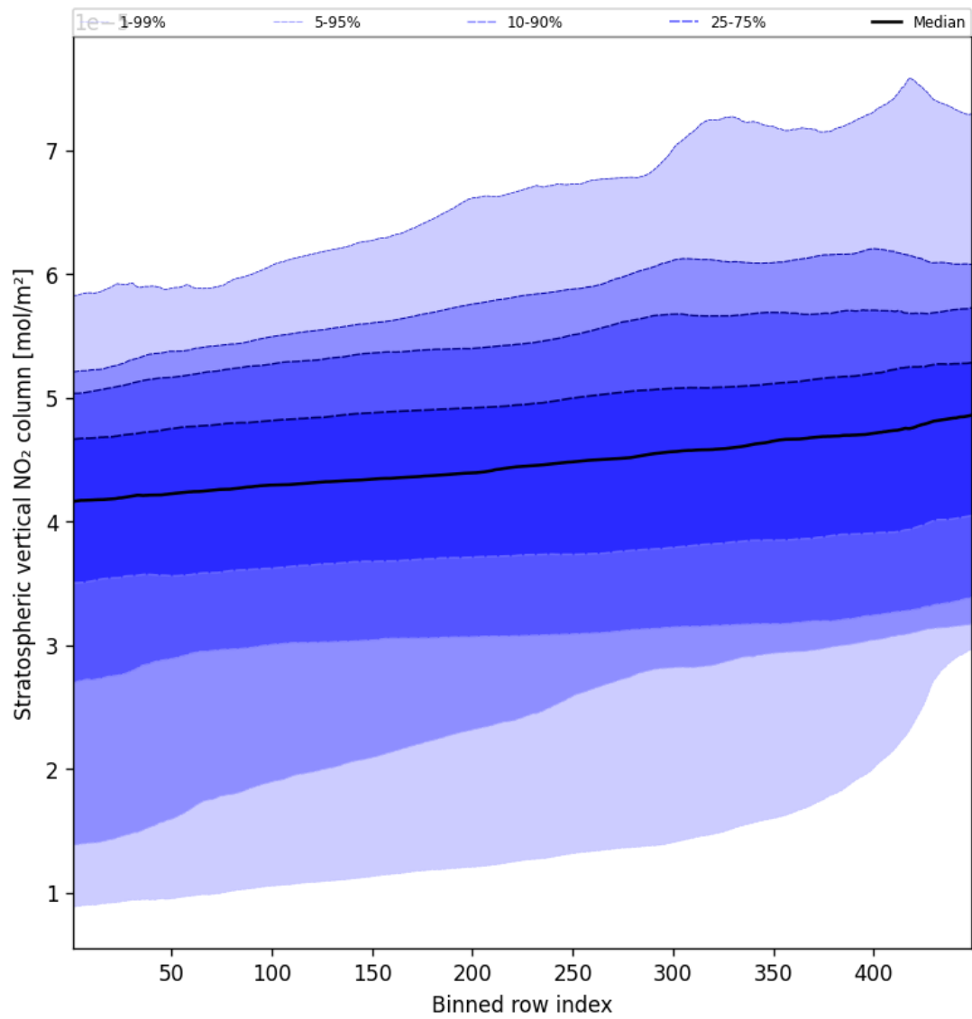
Figure 53: Along track statistics of “Stratospheric vertical NO 2 column” for 2024-09-12 to 2024-09-13
