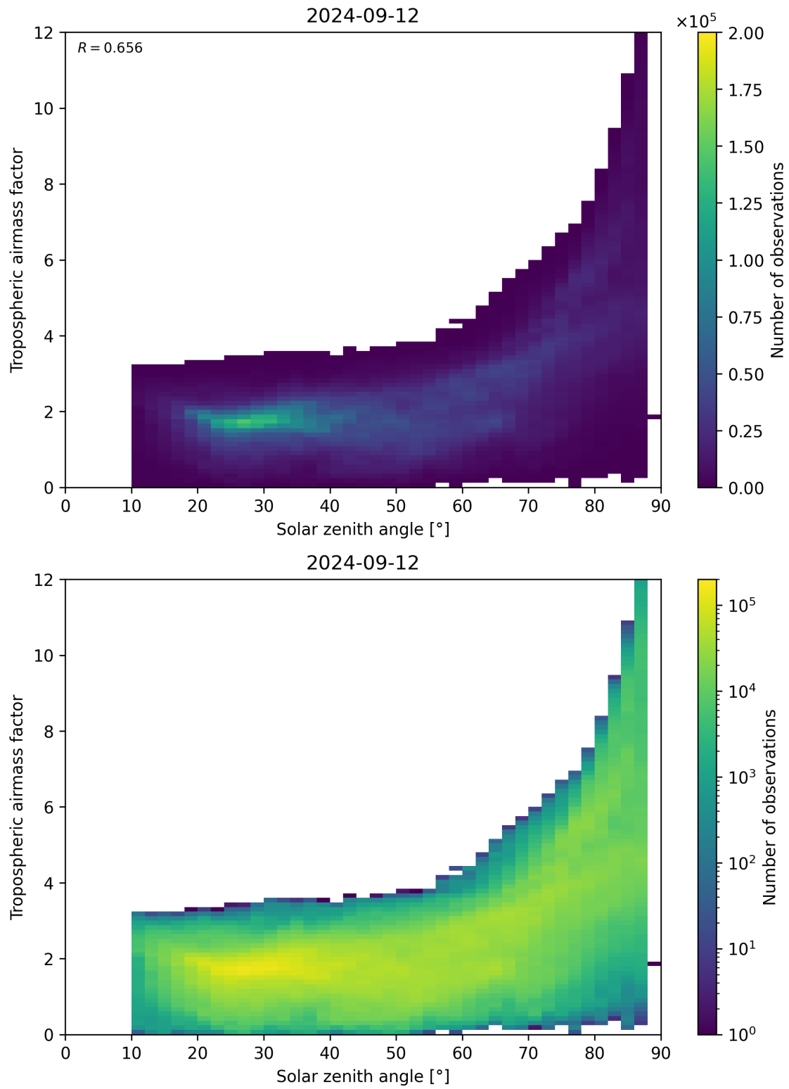
Figure 147: Scatter density plot of “Solar zenith angle” against “Tropospheric airmass factor” for 2024-09-12 to 2024-09-13.
