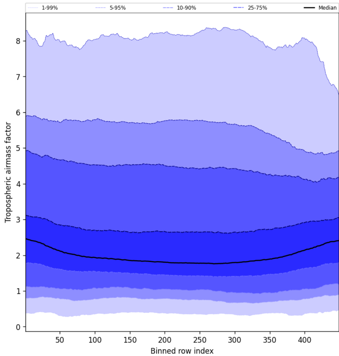
Figure 48: Along track statistics of “Tropospheric air mass factor” for 2024-09-12 to 2024-09-13
