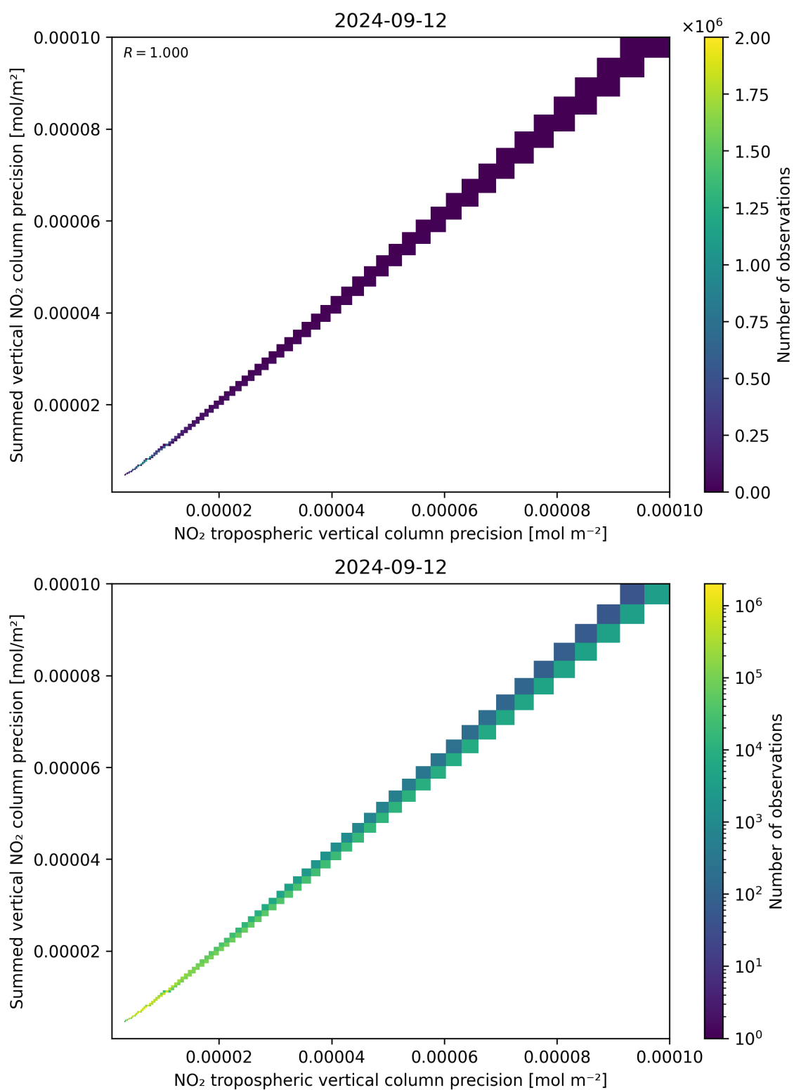
Figure 137: Scatter density plot of “NO 2 tropospheric vertical column precision” against “Summed vertical NO 2 column precision” for 2024-09-12 to 2024-09-13.
