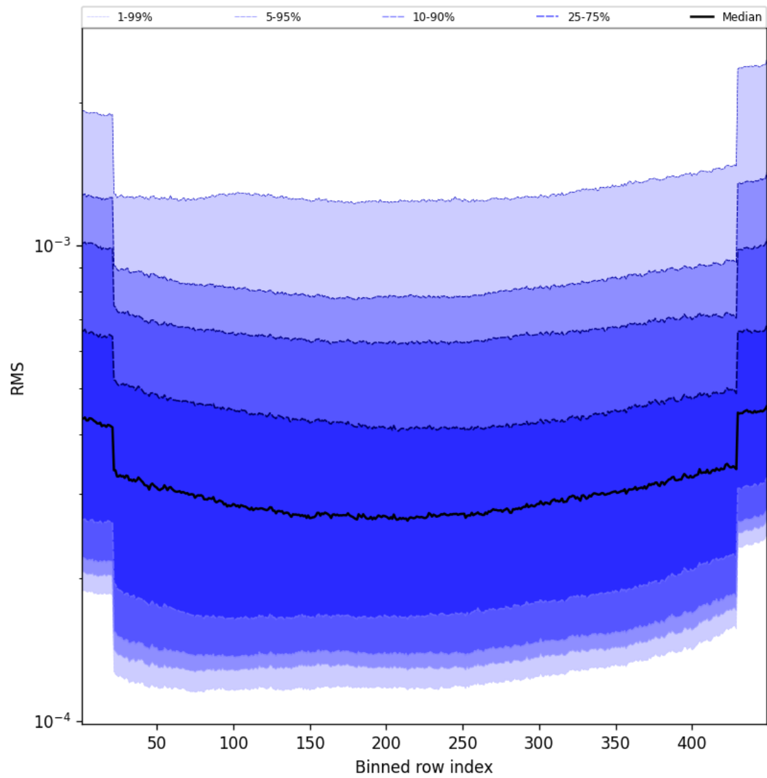
Figure 60: Along track statistics of “RMS” for 2024-09-12 to 2024-09-13
