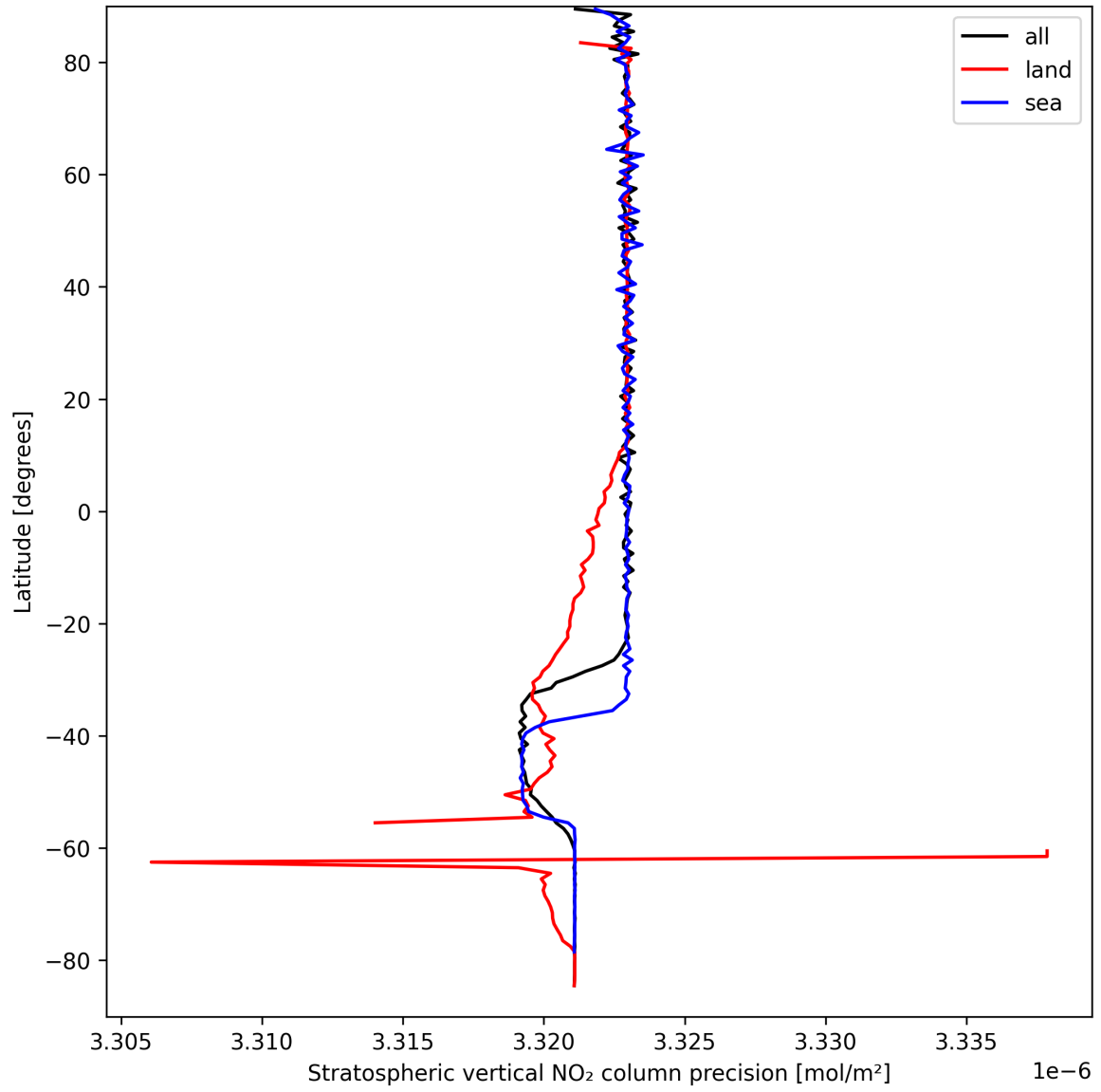
Figure 20: Zonal average of “Stratospheric vertical NO 2 column precision” for 2024-09-12 to 2024-09-13.
