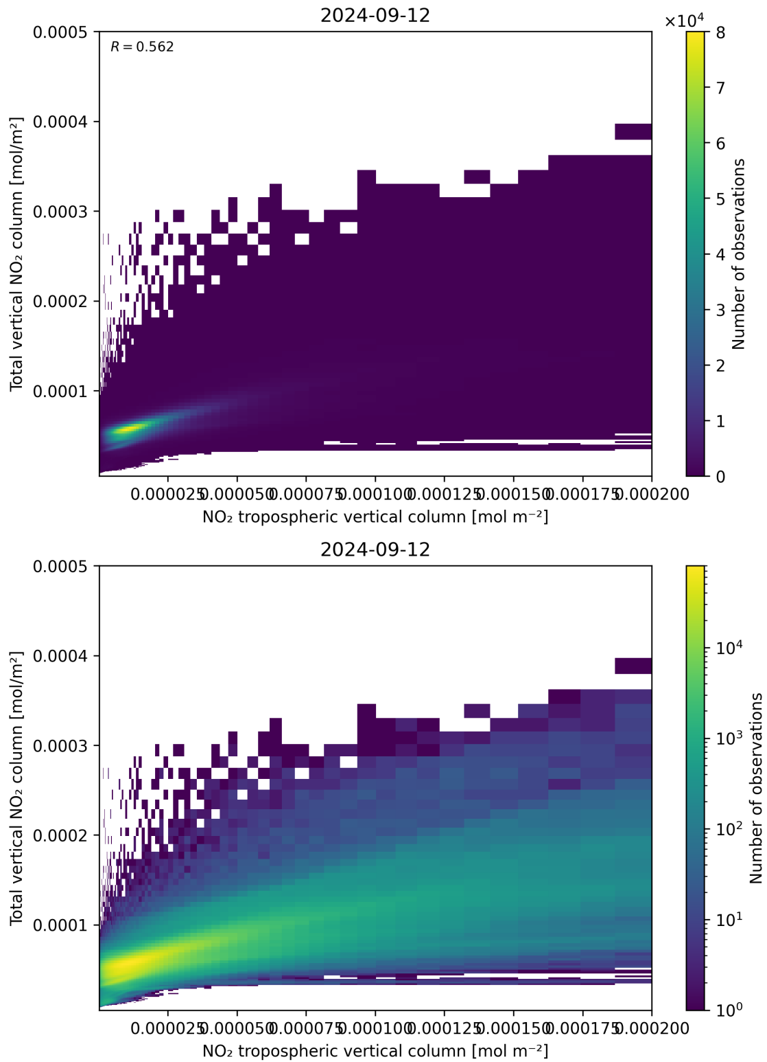
Figure 128: Scatter density plot of “NO 2 tropospheric vertical column” against “Total vertical NO 2 column” for 2024-09-12 to 2024-09-13.
