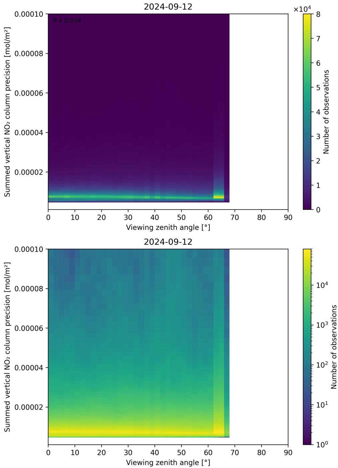
Figure 166: Scatter density plot of “Viewing zenith angle” against “Summed vertical NO 2 column precision” for 2024-09-12 to 2024-09-13.
