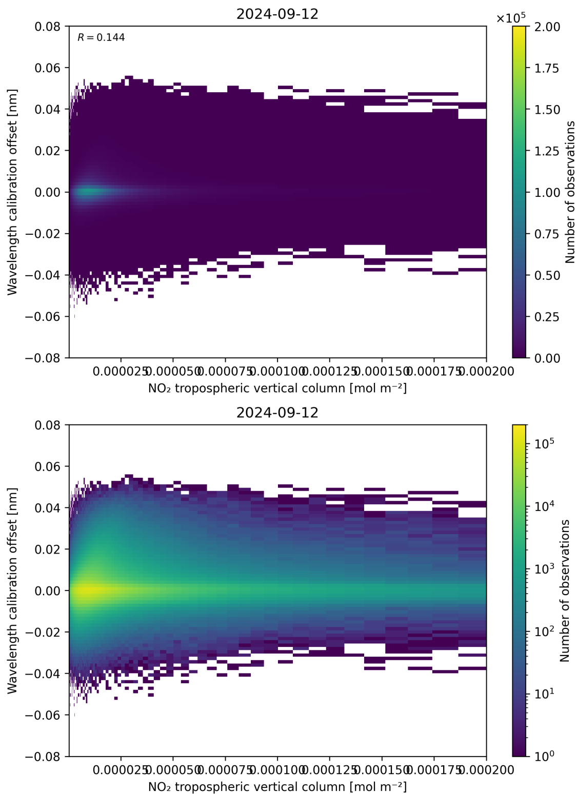
Figure 143: Scatter density plot of “NO 2 tropospheric vertical column” against “Wavelength calibration offset” for 2024-09-12 to 2024-09-13.
