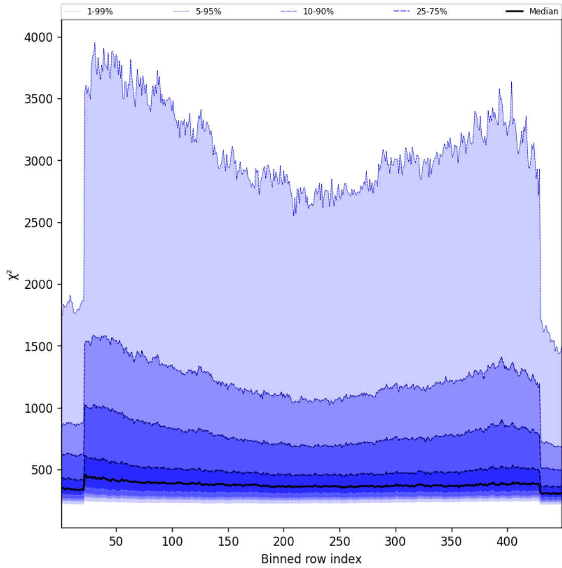
Figure 59: Along track statistics of “ \chi^2 ” for 2024-09-12 to 2024-09-13
