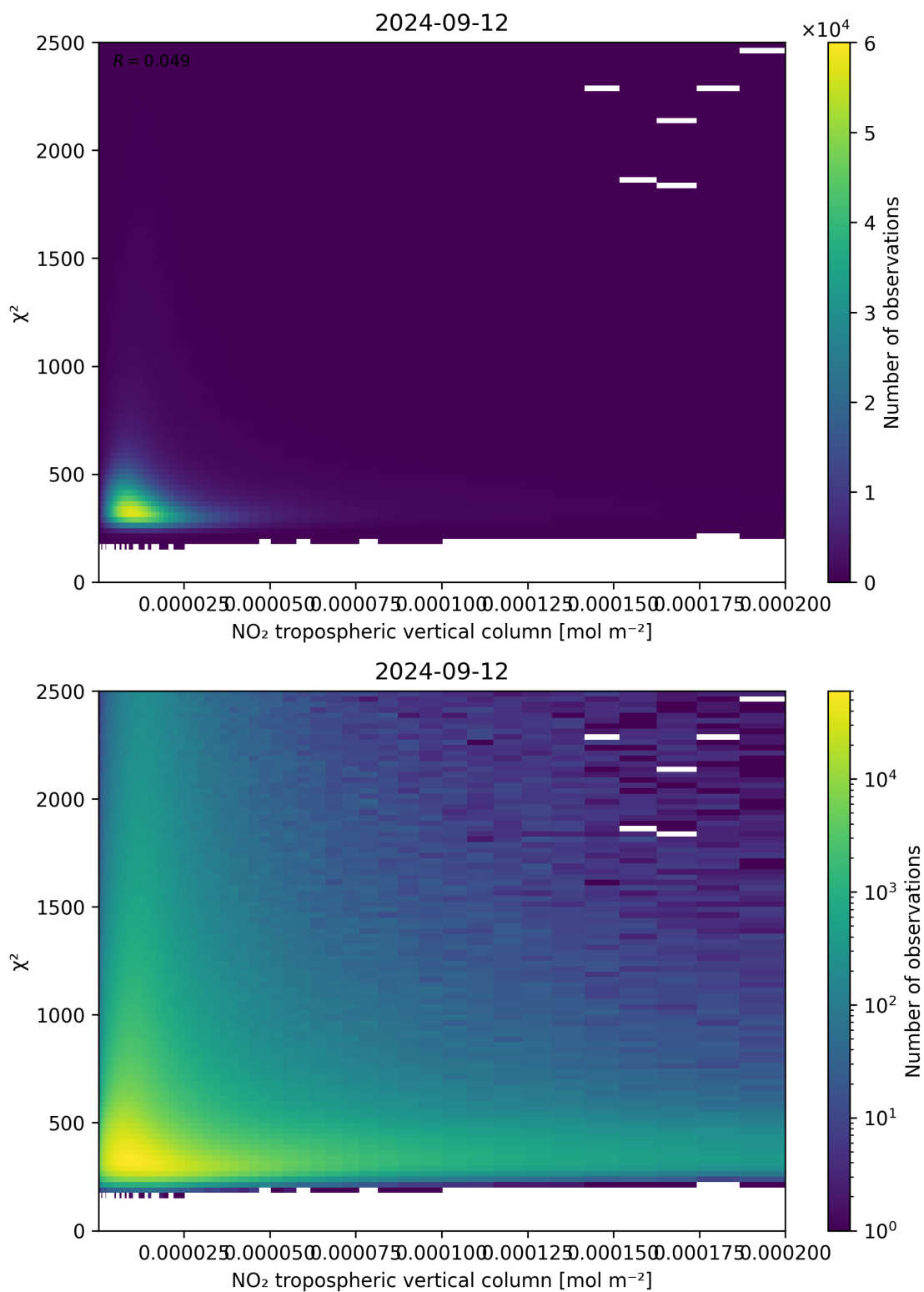
Figure 124: Scatter density plot of “NO 2 tropospheric vertical column” against “ \chi^2 ” for 2024-09-12 to 2024-09-13.
