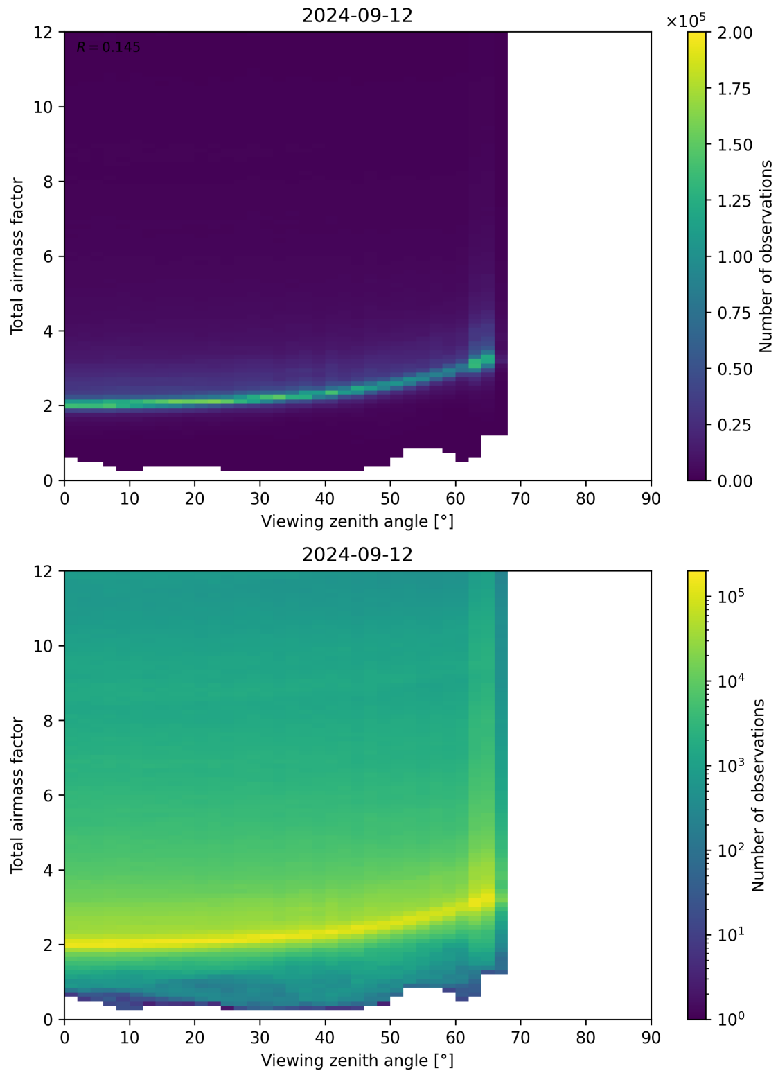
Figure 160: Scatter density plot of “Viewing zenith angle” against “Total airmass factor” for 2024-09-12 to 2024-09-13.
