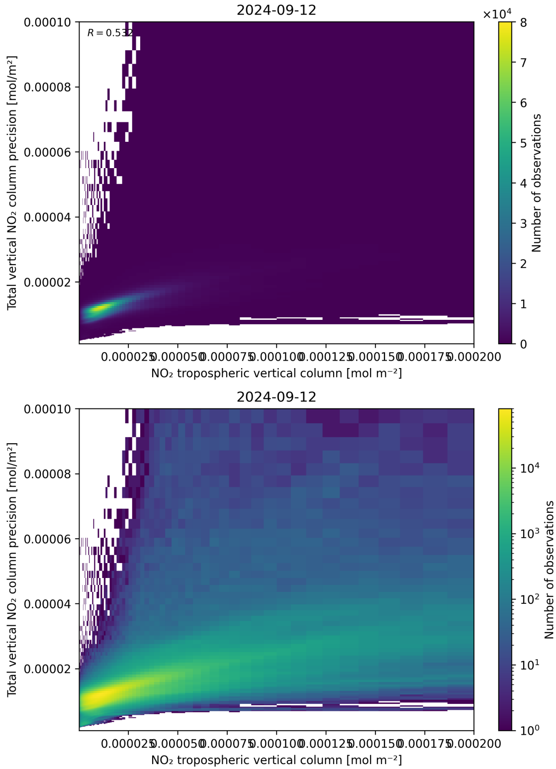
Figure 129: Scatter density plot of “NO 2 tropospheric vertical column” against “Total vertical NO 2 column precision” for 2024-09-12 to 2024-09-13.
