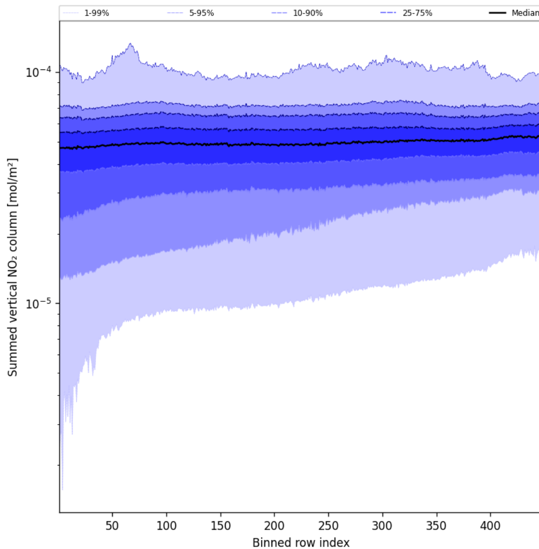
Figure 57: Along track statistics of “Summed vertical NO 2 column” for 2024-09-12 to 2024-09-13
