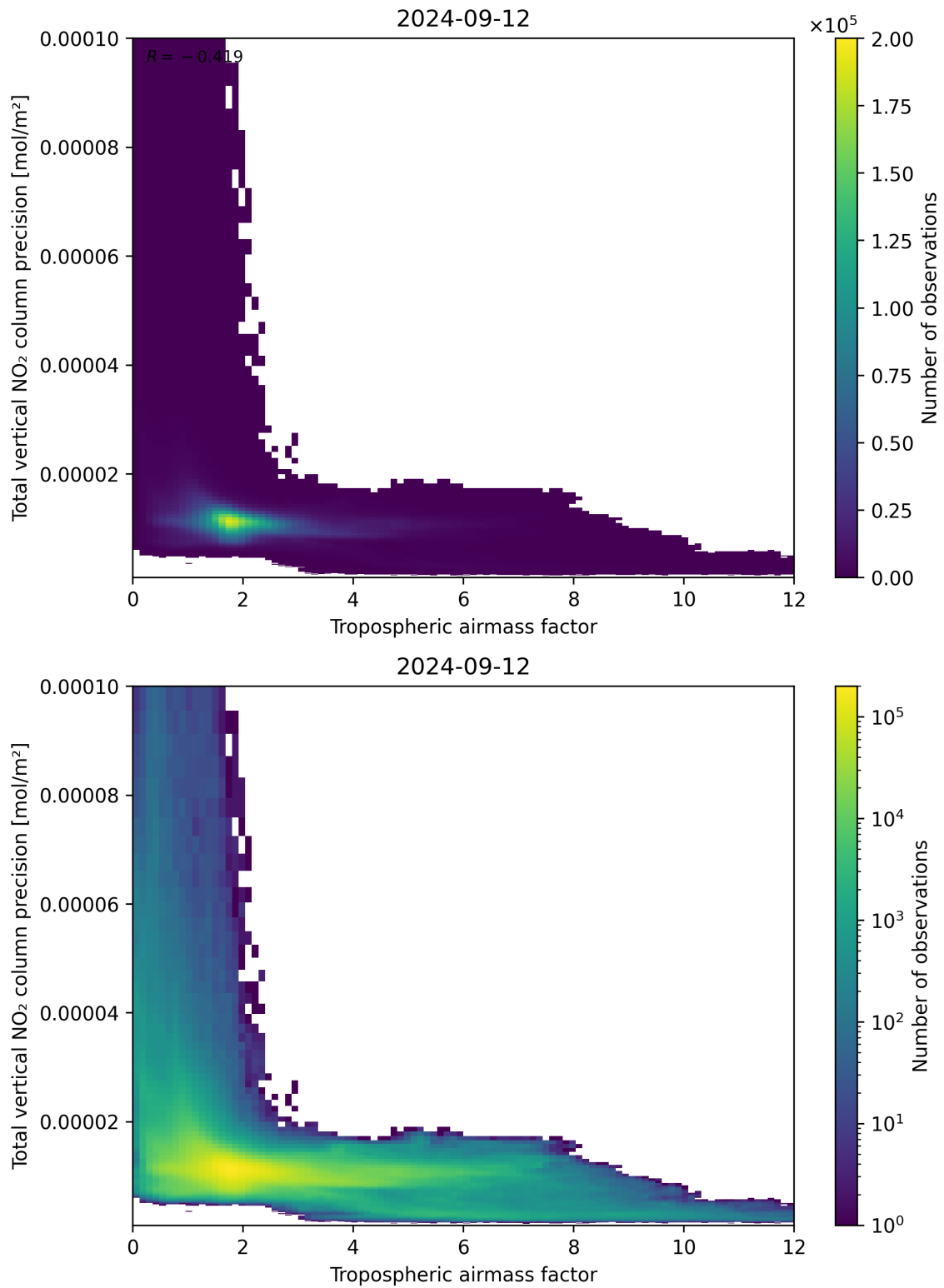
Figure 78: Scatter density plot of “Tropospheric airmass factor” against “Total vertical NO 2 column precision” for 2024-09-12 to 2024-09-13.
