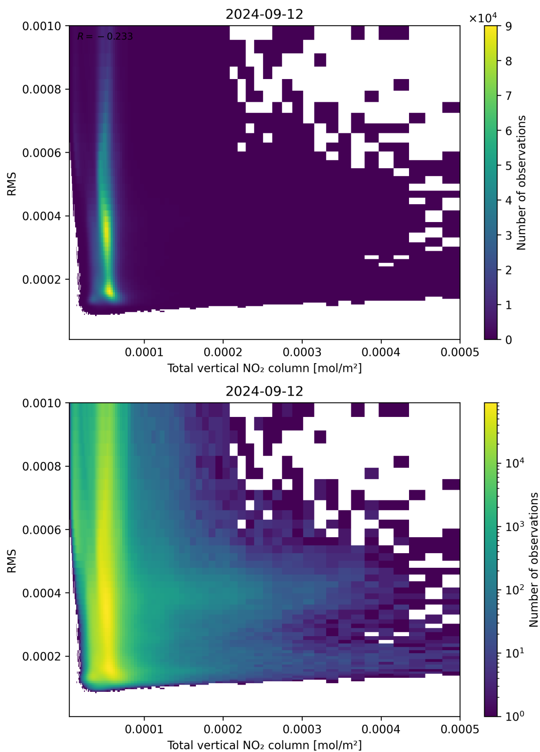
Figure 120: Scatter density plot of “Total vertical NO 2 column” against “RMS” for 2024-09-12 to 2024-09-13.
