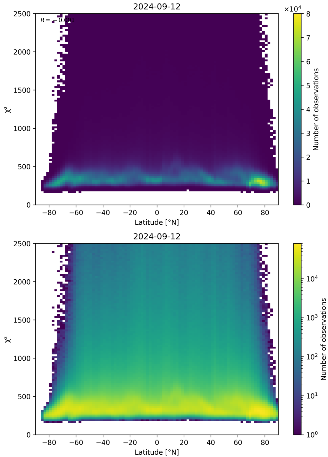
Figure 86: Scatter density plot of “Latitude” against “ \chi^2 ” for 2024-09-12 to 2024-09-13.
