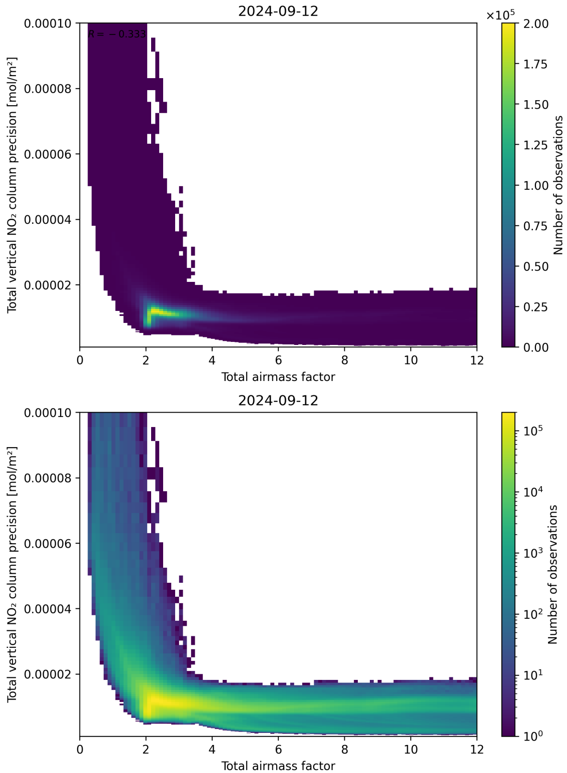
Figure 68: Scatter density plot of “Total airmass factor” against “Total vertical NO 2 column precision” for 2024-09-12 to 2024-09-13.
