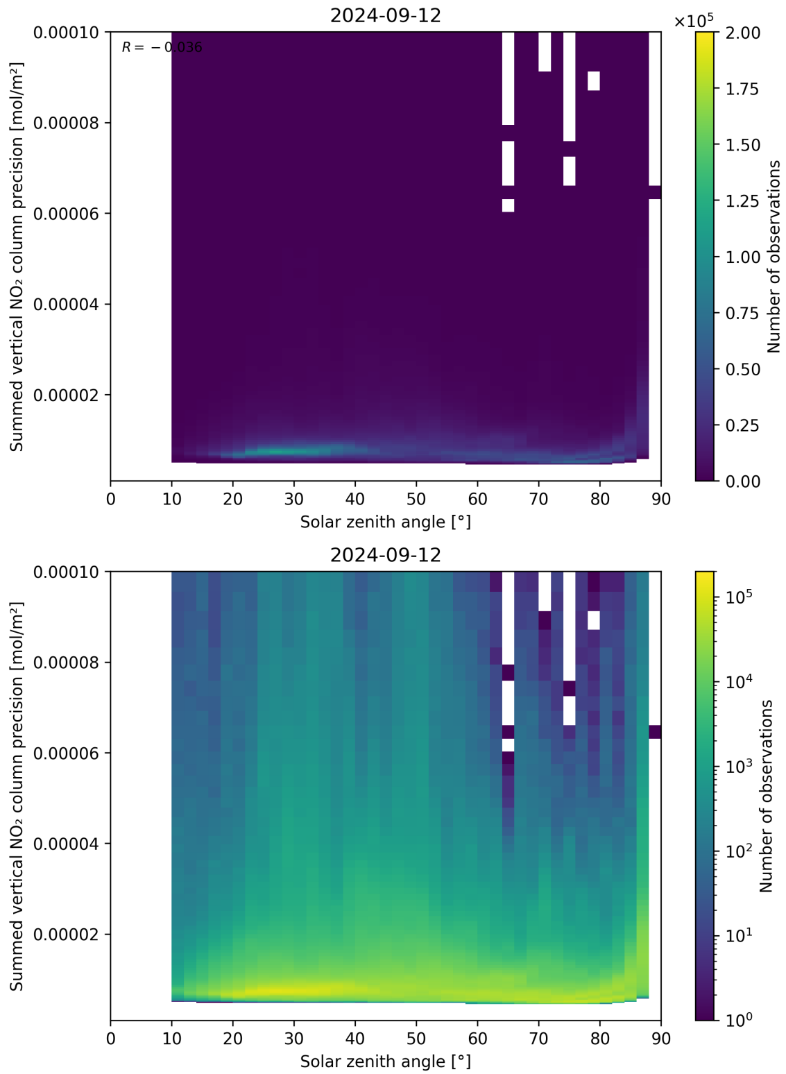
Figure 152: Scatter density plot of “Solar zenith angle” against “Summed vertical NO 2 column precision” for 2024-09-12 to 2024-09-13.
