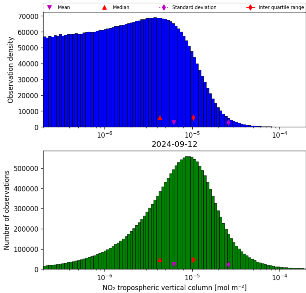
Figure 29: Histogram of “NO 2 tropospheric vertical column” for 2024-09-12 to 2024-09-13
