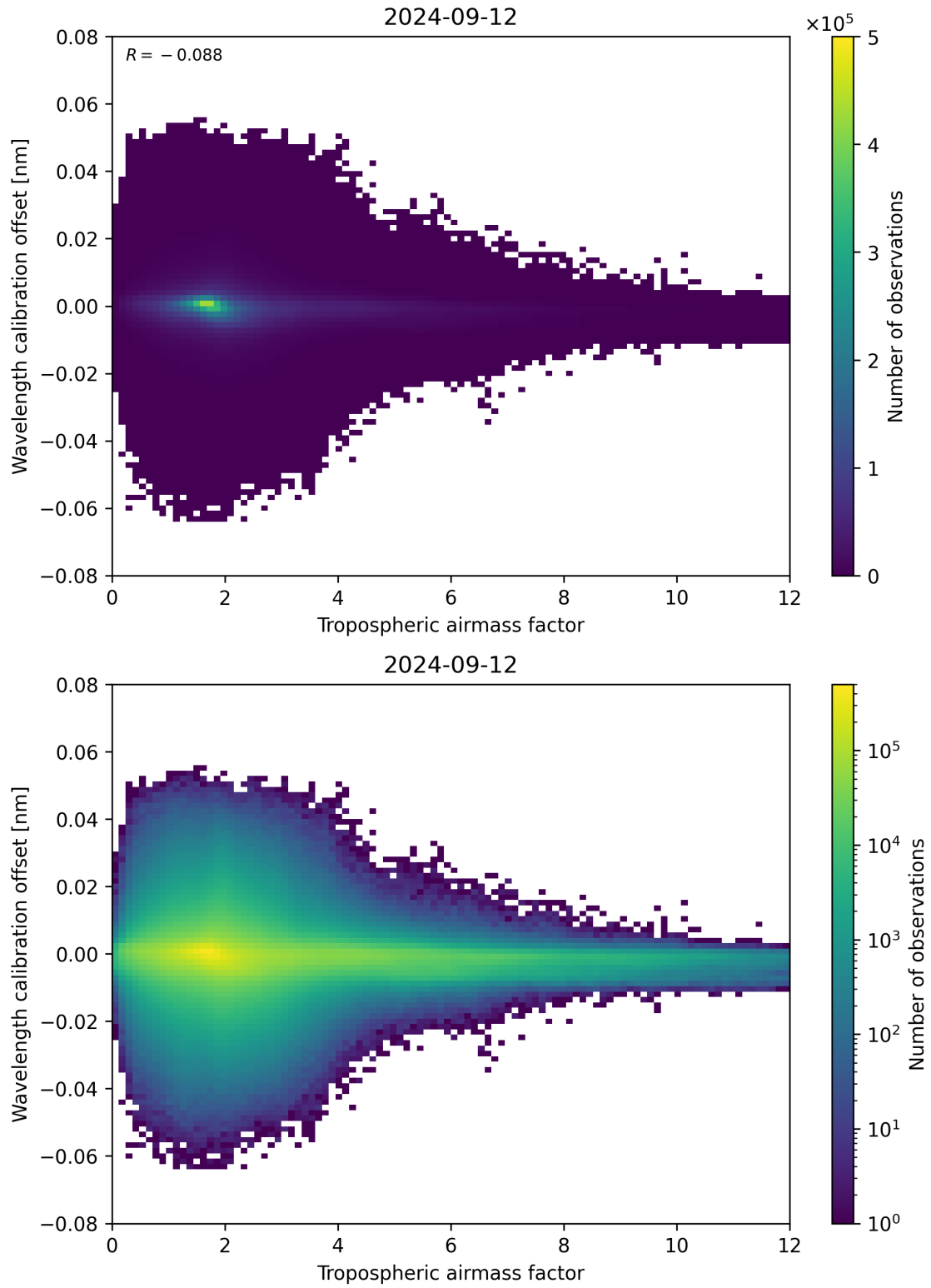
Figure 80: Scatter density plot of “Tropospheric airmass factor” against “Wavelength calibration offset” for 2024-09-12 to 2024-09-13.
