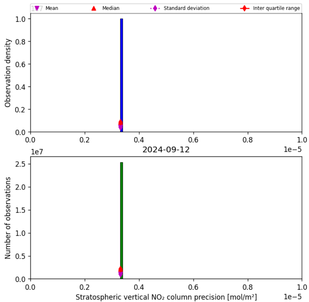
Figure 37: Histogram of “Stratospheric vertical NO 2 column precision” for 2024-09-12 to 2024-09-13
