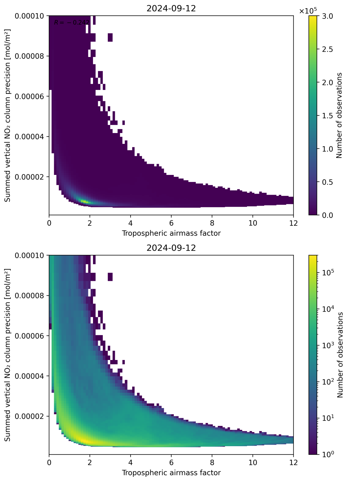
Figure 76: Scatter density plot of “Tropospheric air mass factor” against “Summed vertical NO 2 column precision” for 2024-09-12 to 2024-09-13.
