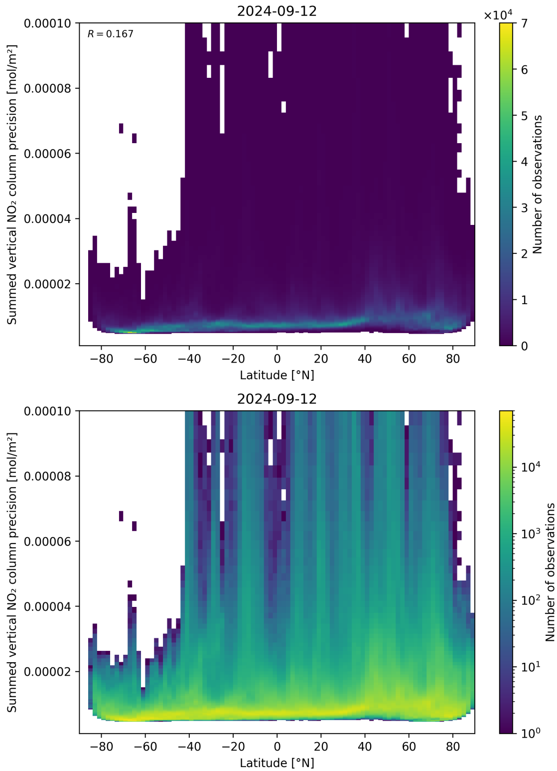
Figure 89: Scatter density plot of “Latitude” against “Summed vertical NO 2 column precision” for 2024-09-12 to 2024-09-13.
