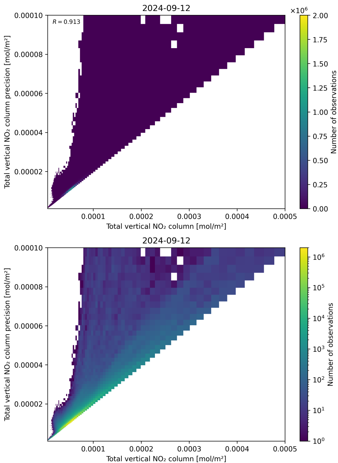
Figure 114: Scatter density plot of “Total vertical NO 2 column” against “Total vertical NO 2 column precision” for 2024-09-12 to 2024-09-13.
