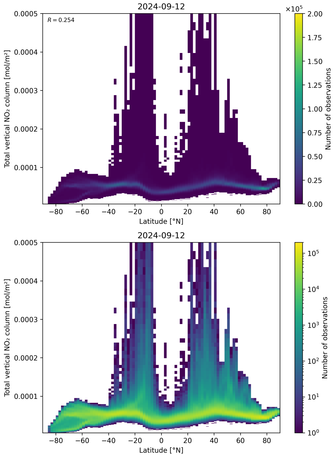
Figure 90: Scatter density plot of “Latitude” against “Total vertical NO 2 column” for 2024-09-12 to 2024-09-13.
