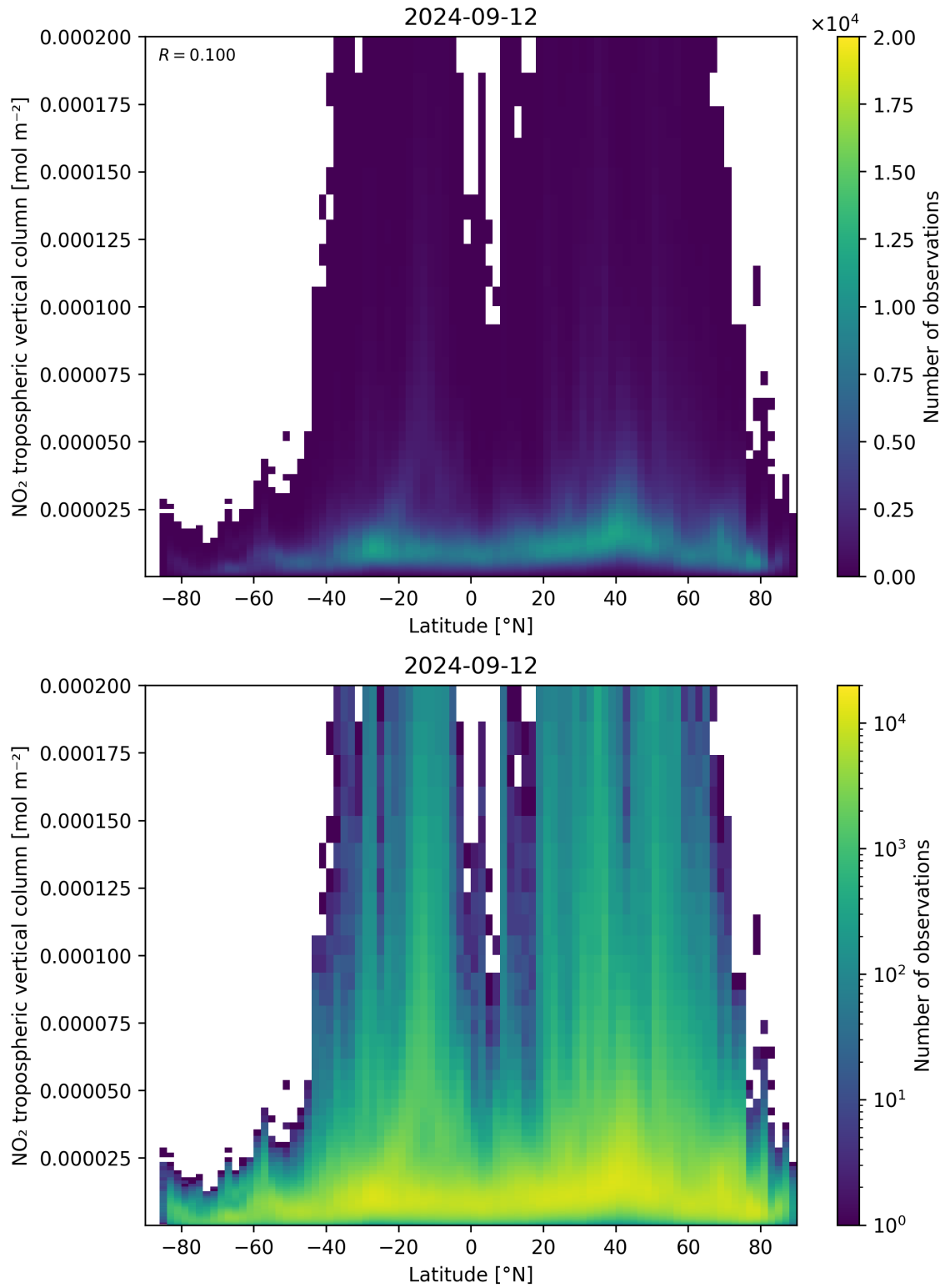
Figure 92: Scatter density plot of “Latitude” against “NO 2 tropospheric vertical column” for 2024-09-12 to 2024-09-13.
