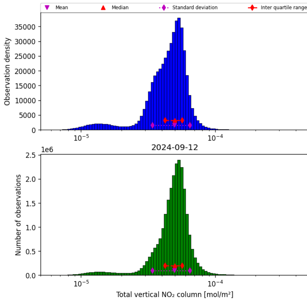
Figure 38: Histogram of “Total vertical NO 2 column” for 2024-09-12 to 2024-09-13
