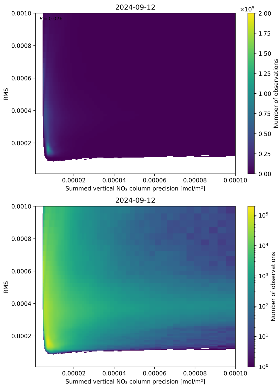
Figure 108: Scatter density plot of “Summed vertical NO 2 column precision” against “RMS” for 2024-09-12 to 2024-09-13.
