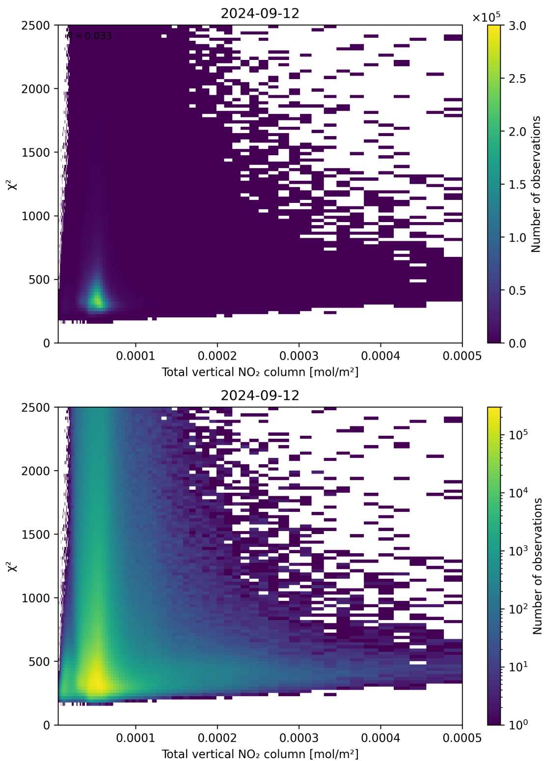
Figure 111: Scatter density plot of “Total vertical NO 2 column” against “ \chi^2 ” for 2024-09-12 to 2024-09-13.
