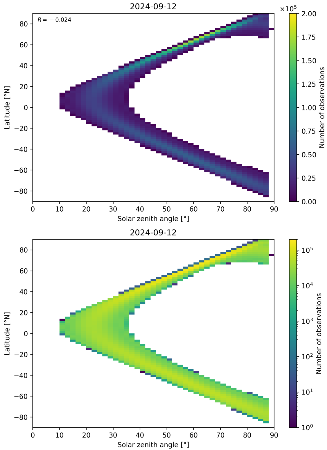
Figure 149: Scatter density plot of “Solar zenith angle” against “Latitude” for 2024-09-12 to 2024-09-13.
