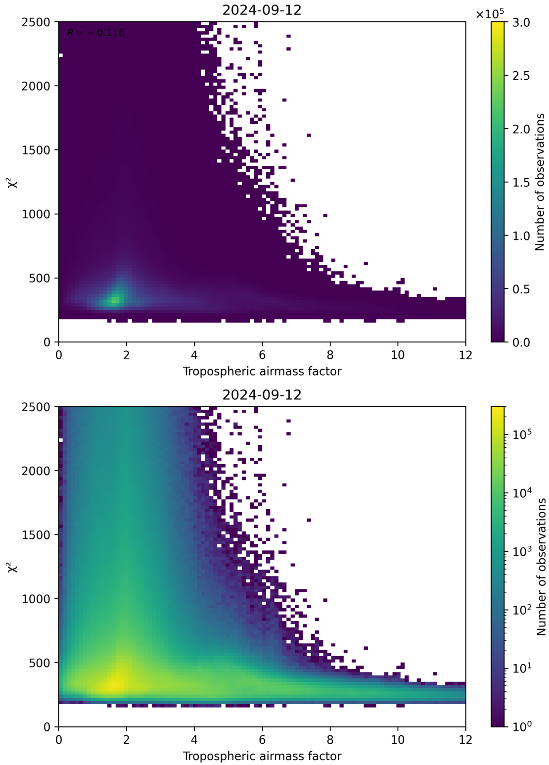
Figure 73: Scatter density plot of “Tropospheric airmass factor” against “ \chi^2 ” for 2024-09-12 to 2024-09-13.
