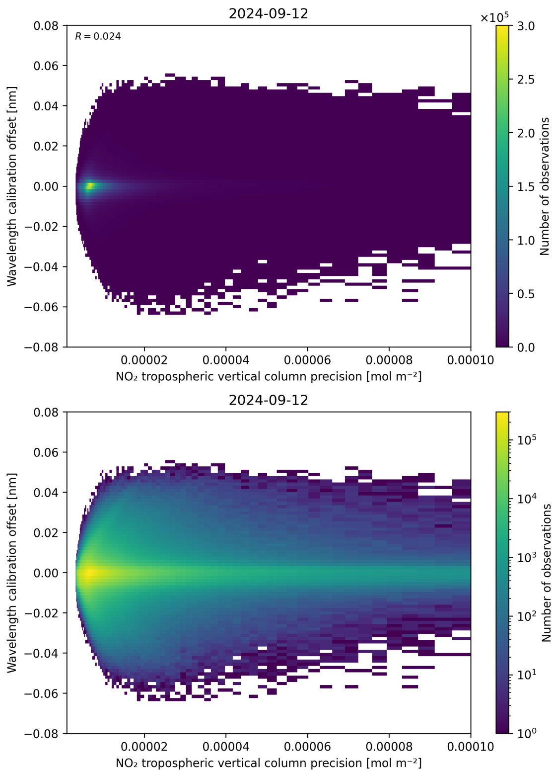
Figure 141: Scatter density plot of “NO 2 tropospheric vertical column precision” against “Wavelength calibration offset” for 2024-09-12 to 2024-09-13.
