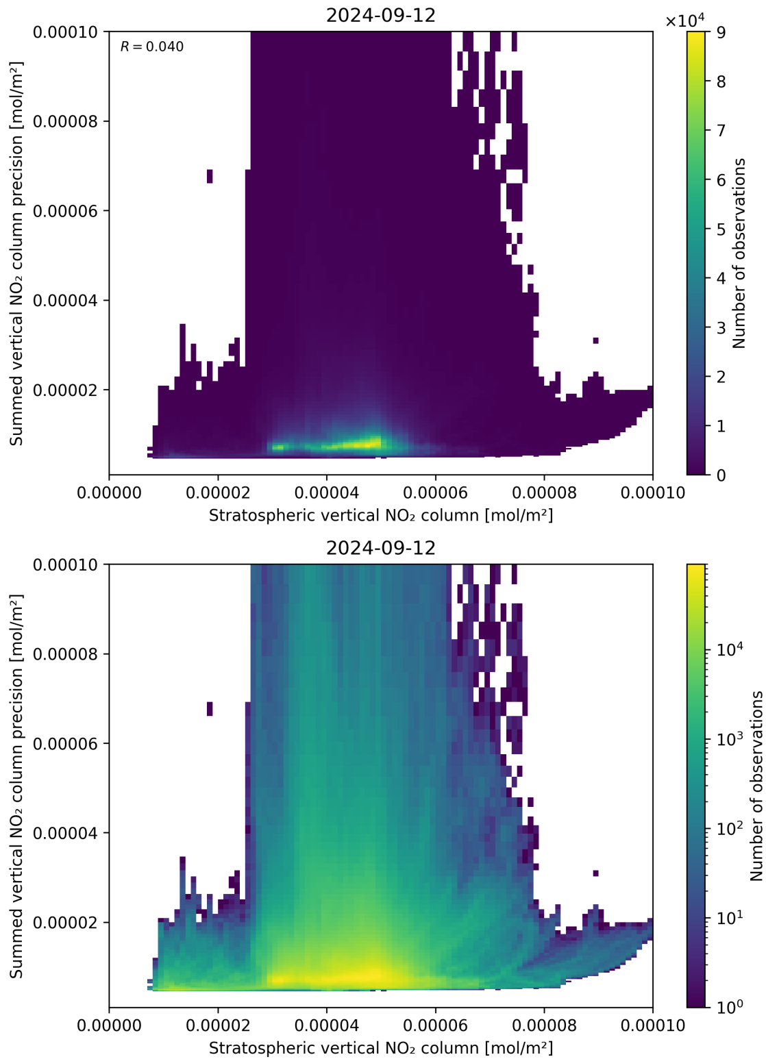
Figure 99: Scatter density plot of “Stratospheric vertical NO 2 column” against “Summed vertical NO 2 column precision” for 2024-09-12 to 2024-09-13.
