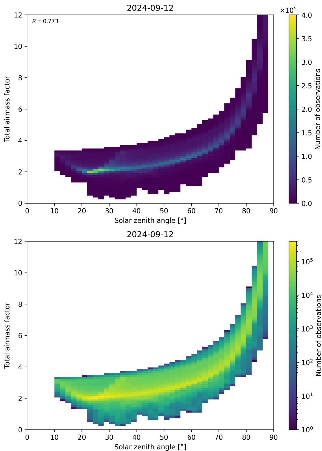
Figure 146: Scatter density plot of “Solar zenith angle” against “Total airmass factor” for 2024-09-12 to 2024-09-13.
