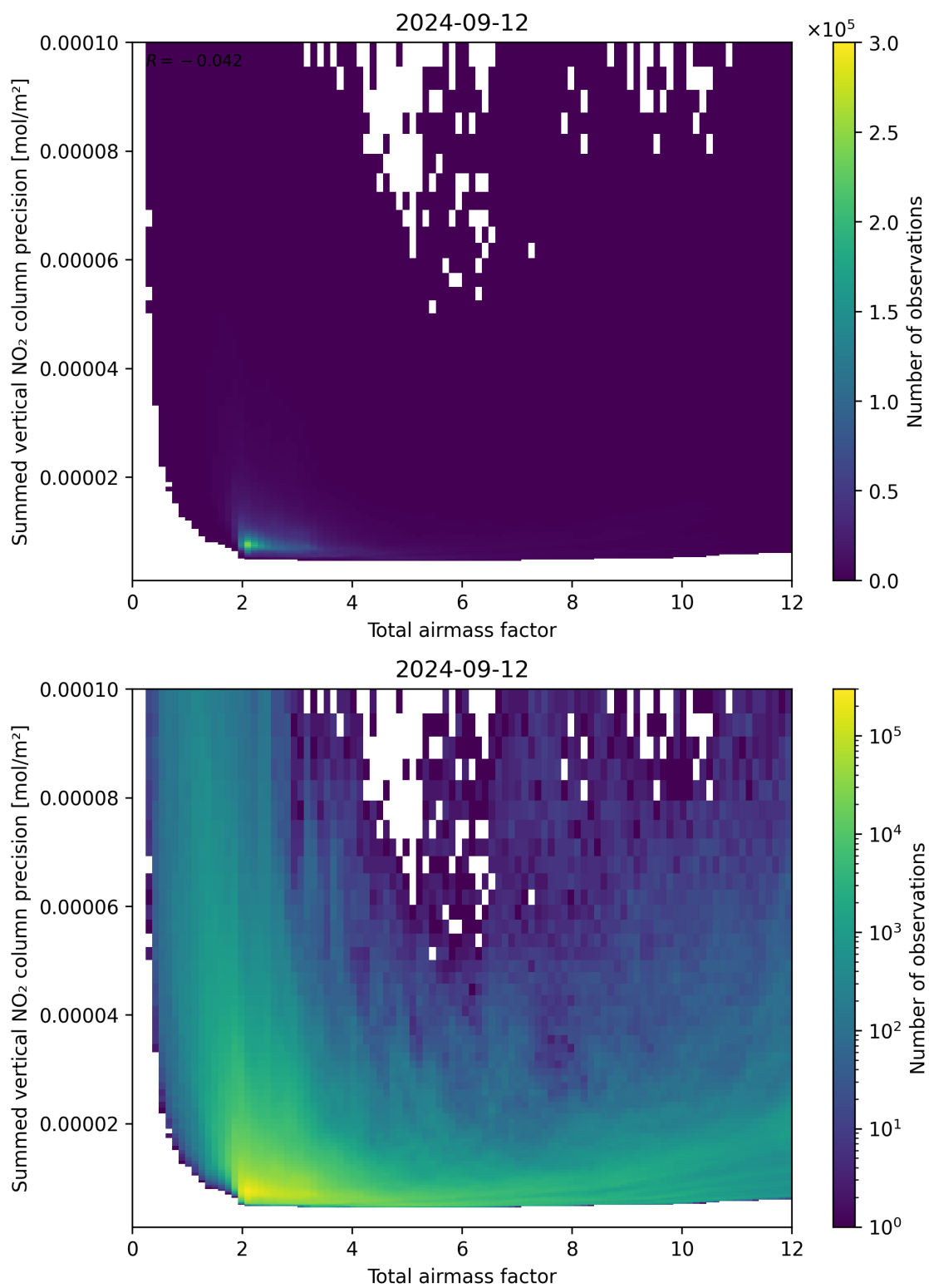
Figure 66: Scatter density plot of “Total airmass factor” against “Summed vertical NO 2 column precision” for 2024-09-12 to 2024-09-13.
