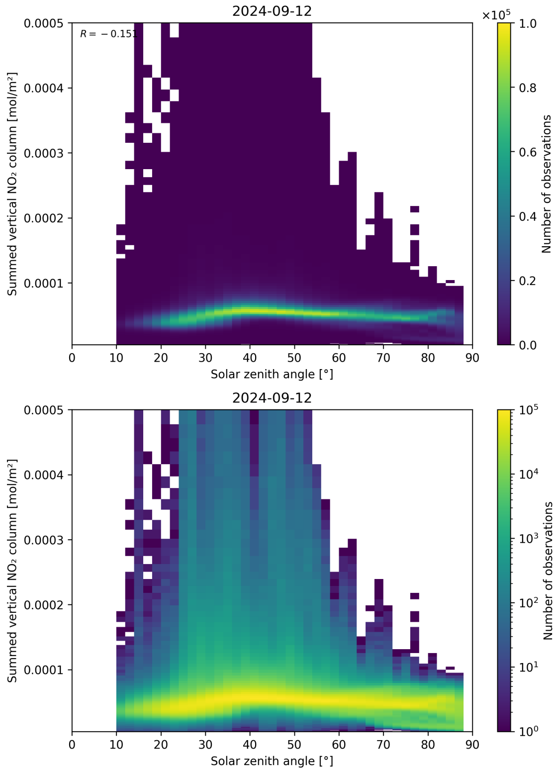
Figure 151: Scatter density plot of “Solar zenith angle” against “Summed vertical NO 2 column” for 2024-09-12 to 2024-09-13.
