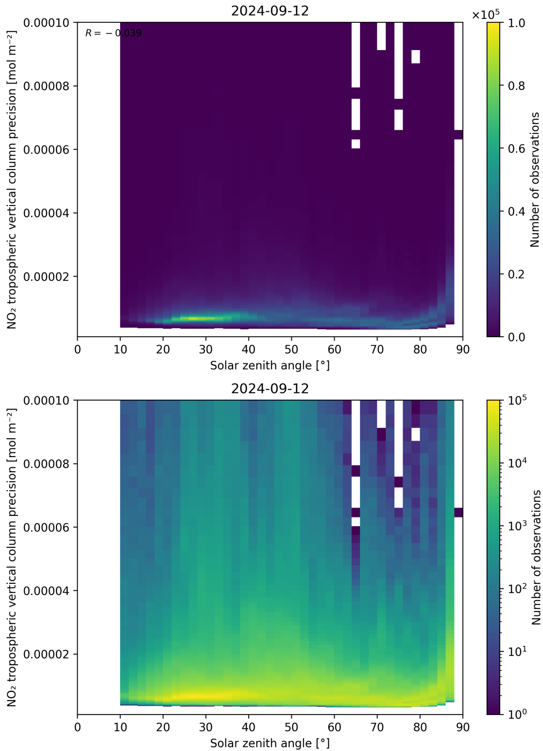
Figure 156: Scatter density plot of “Solar zenith angle” against “NO 2 tropospheric vertical column precision” for 2024-09-12 to 2024-09-13.
