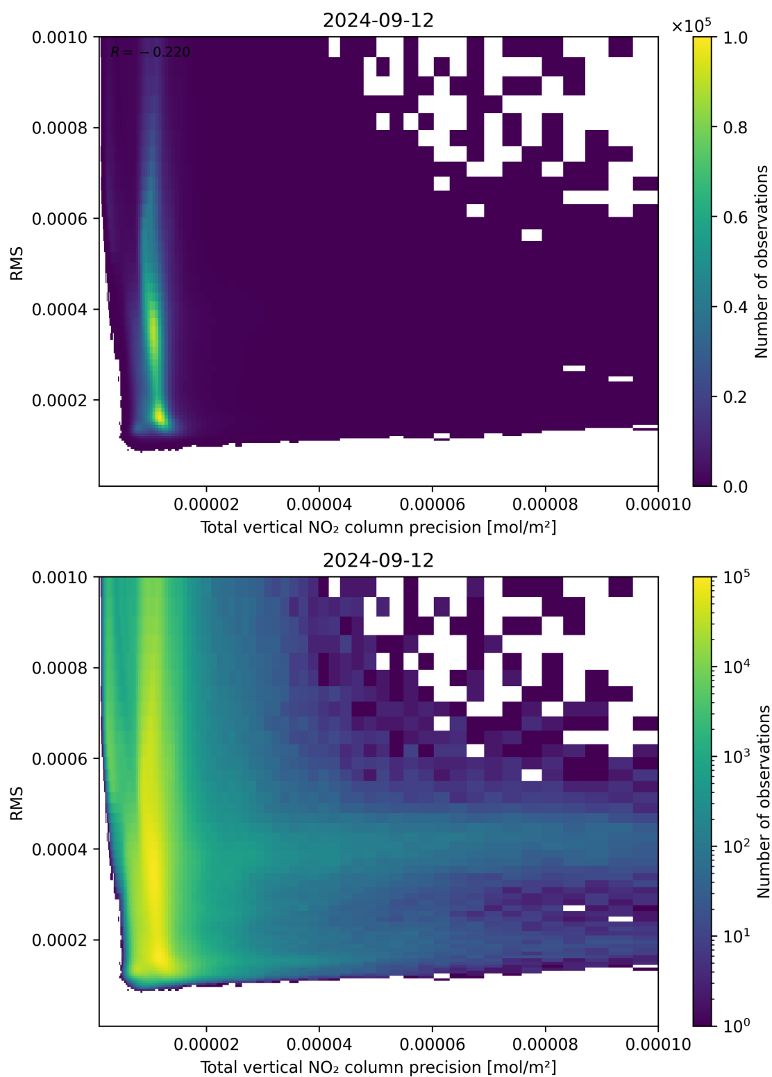
Figure 119: Scatter density plot of “Total vertical NO 2 column precision” against “RMS” for 2024-09-12 to 2024-09-13.
