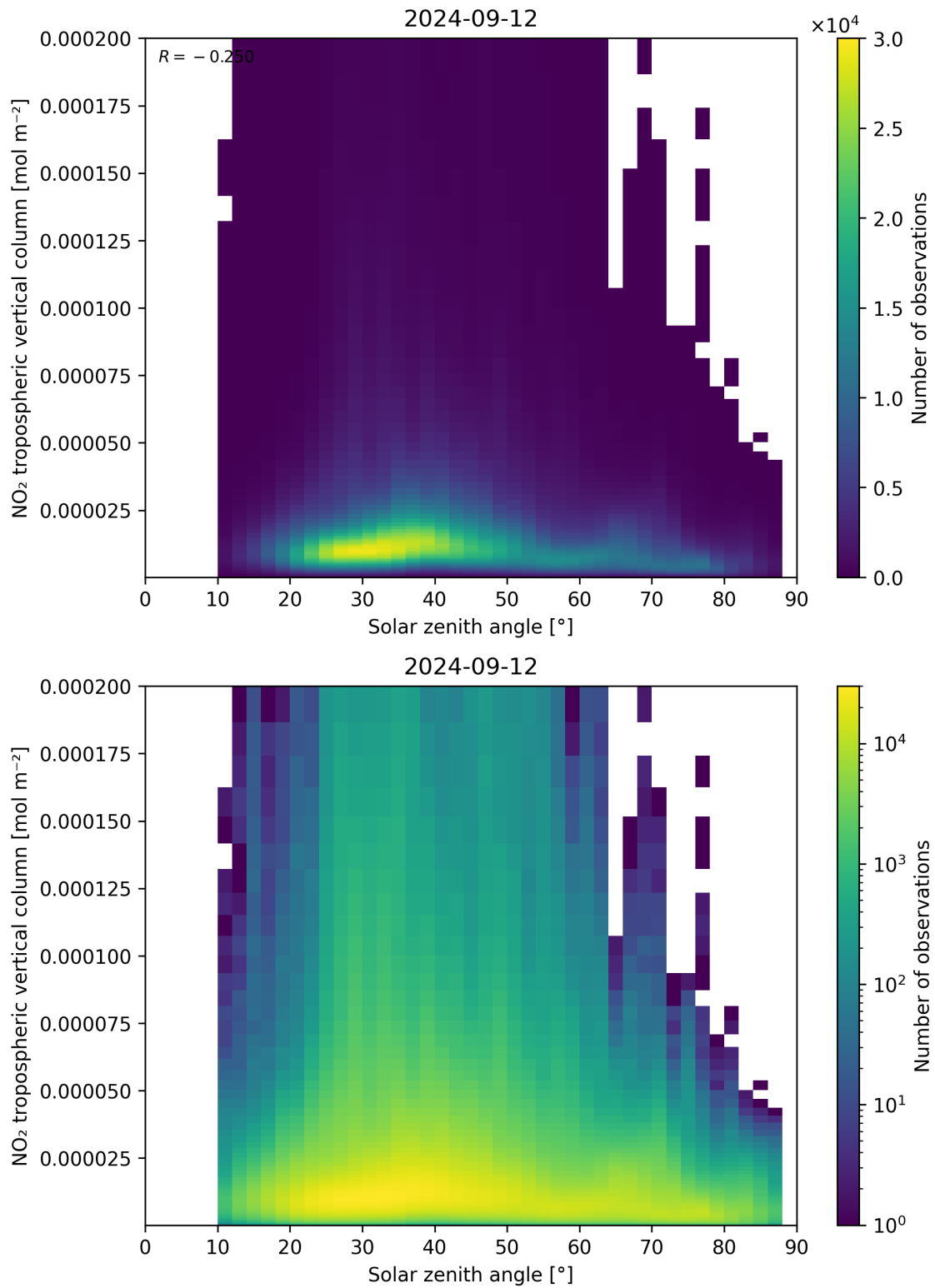
Figure 155: Scatter density plot of “Solar zenith angle” against “NO 2 tropospheric vertical column” for 2024-09-12 to 2024-09-13.
