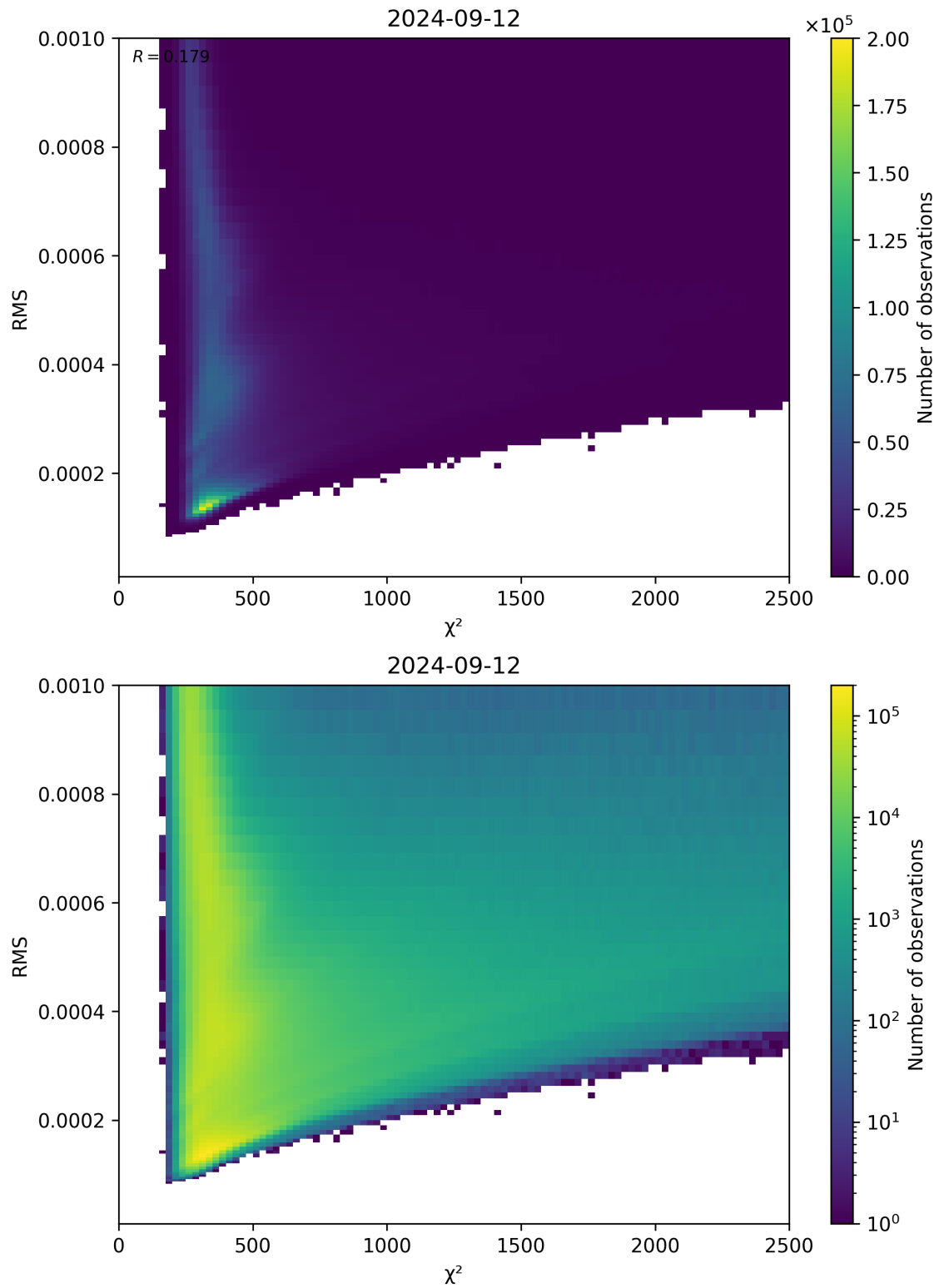
Figure 82: Scatter density plot of “ \chi^2 ” against “RMS” for 2024-09-12 to 2024-09-13.
