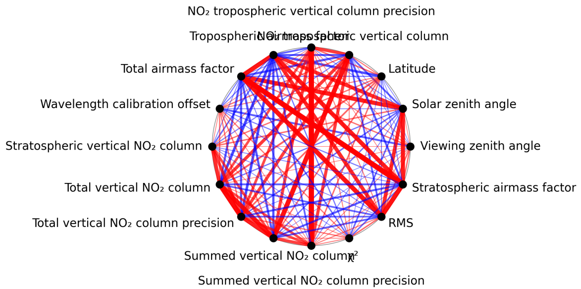
Figure 1: Map of correlation graph for 2024-09-12 to 2024-09-13.
