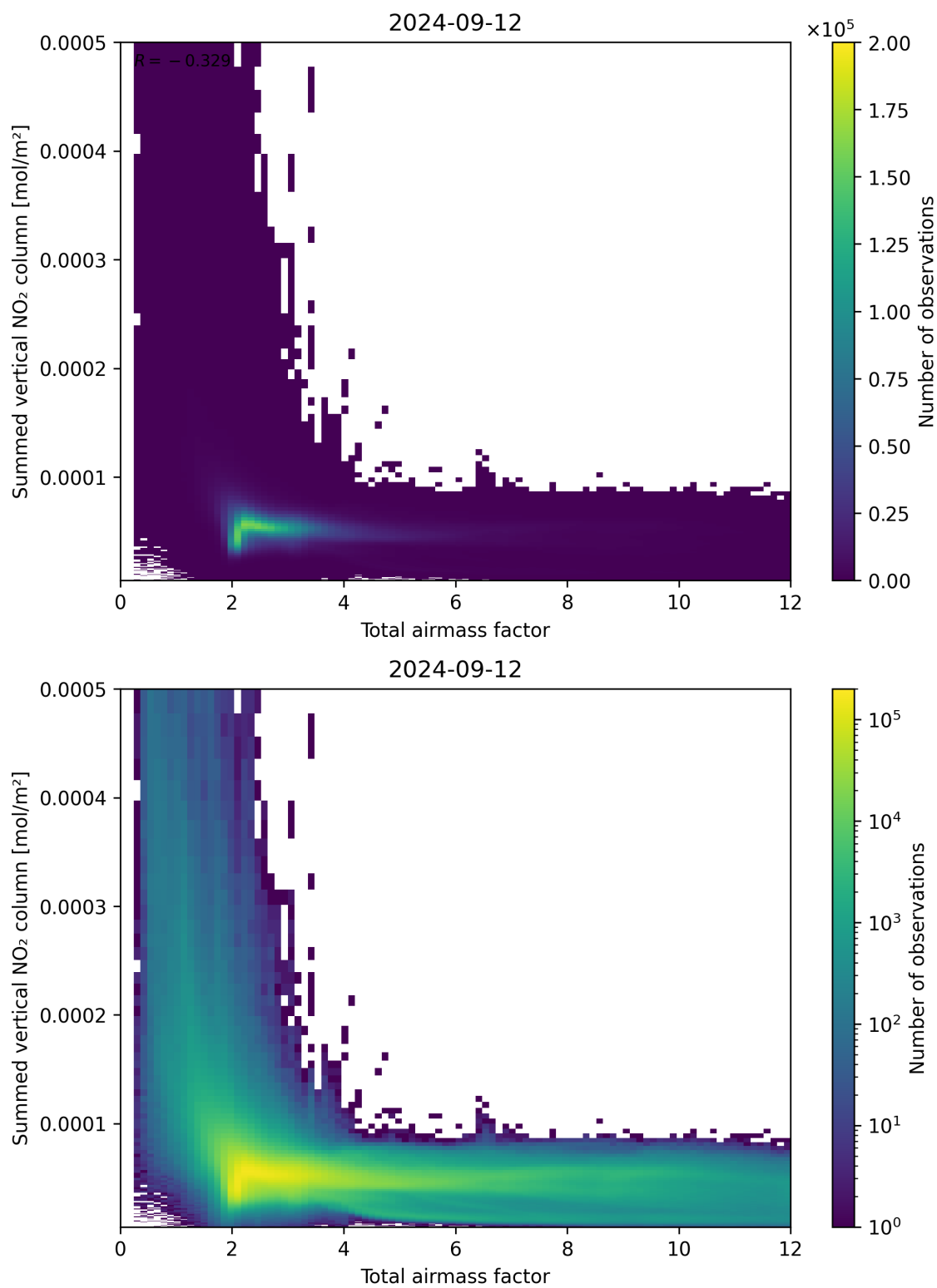
Figure 65: Scatter density plot of “Total airmass factor” against “Summed vertical NO 2 column” for 2024-09-12 to 2024-09-13.
