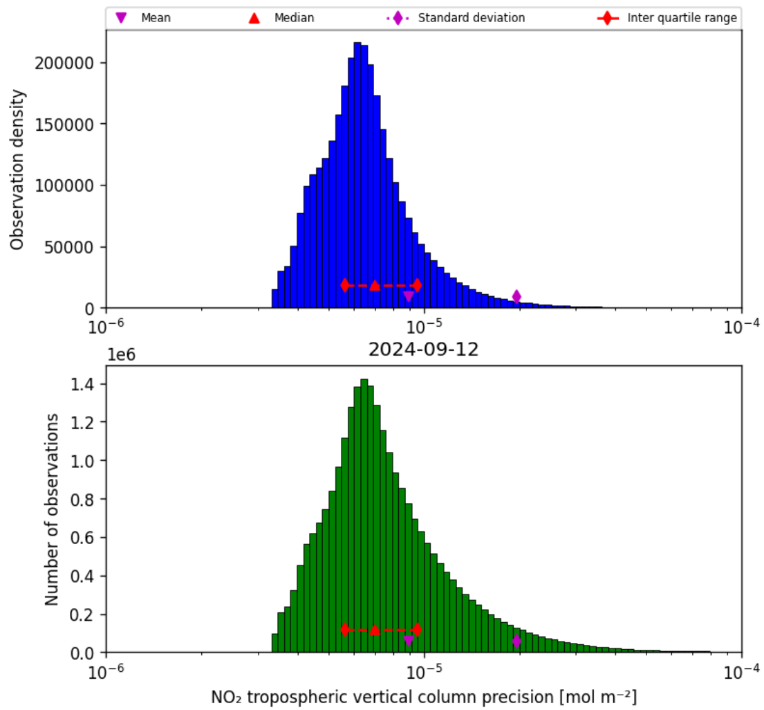
Figure 30: Histogram of “NO 2 tropospheric vertical column precision” for 2024-09-12 to 2024-09-13
