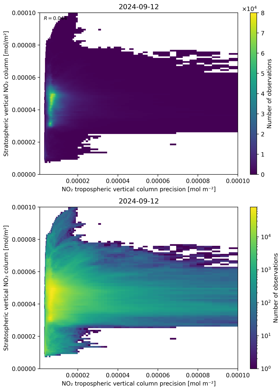
Figure 135: Scatter density plot of “NO 2 tropospheric vertical column precision” against “Stratospheric vertical NO 2 column” for 2024-09-12 to 2024-09-13.
