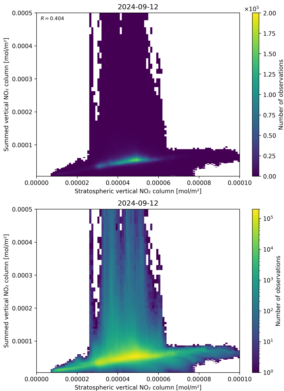
Figure 98: Scatter density plot of “Stratospheric vertical NO 2 column” against “Summed vertical NO 2 column” for 2024-09-12 to 2024-09-13.
