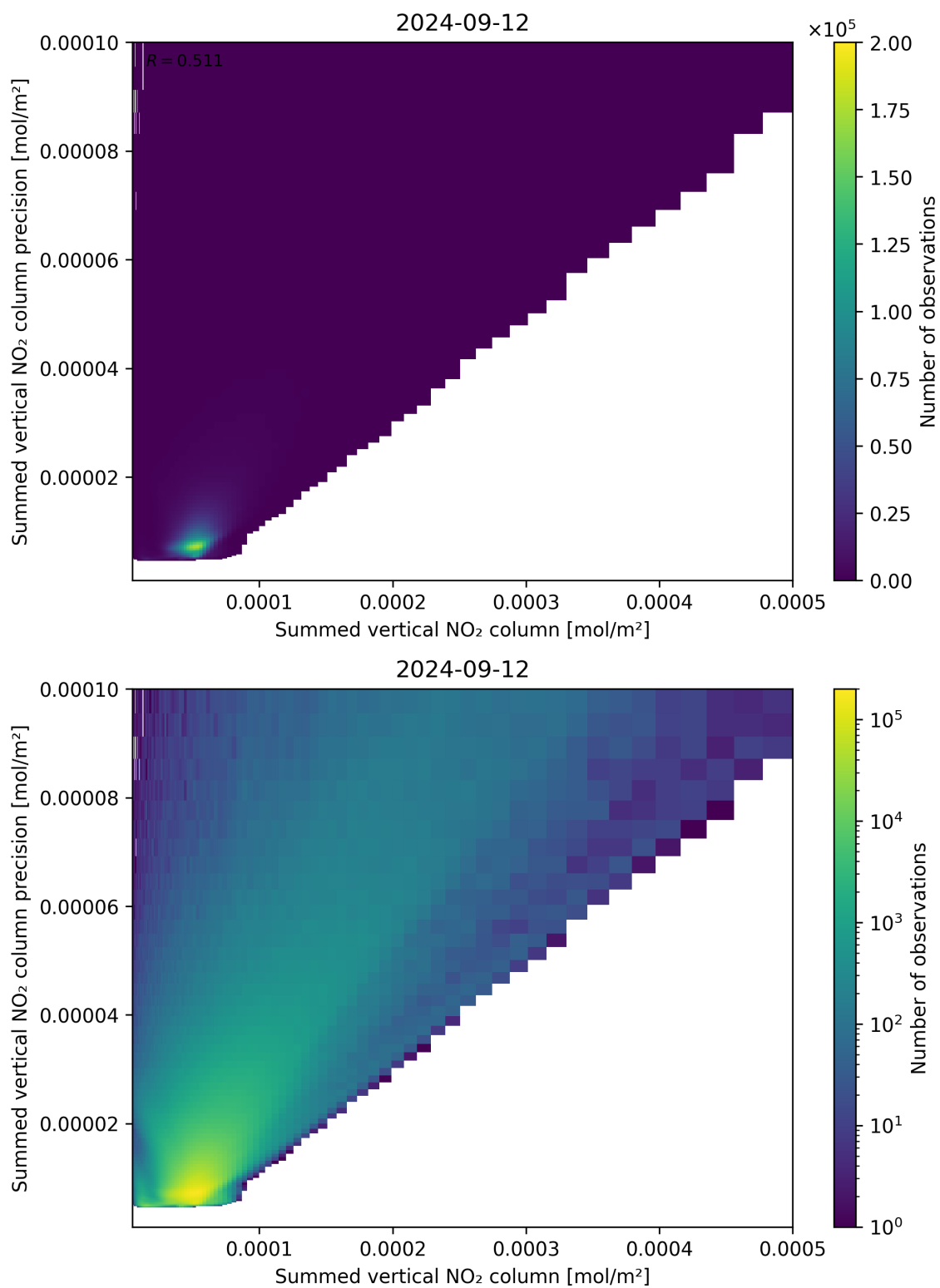
Figure 105: Scatter density plot of “Summed vertical NO 2 column” against “Summed vertical NO 2 column precision” for 2024-09-12 to 2024-09-13.
