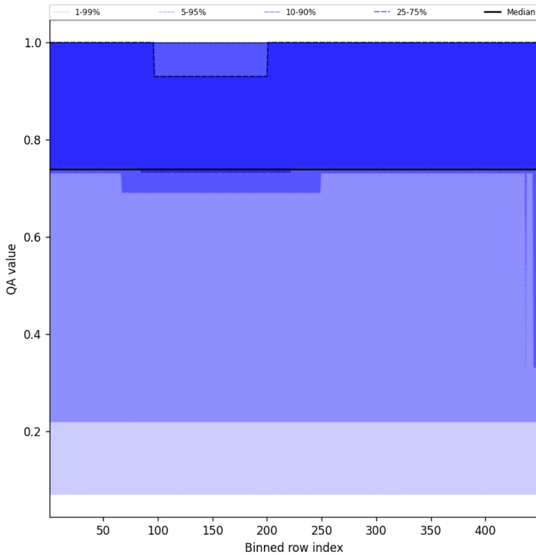
Figure 45: Along track statistics of “QA value” for 2024-09-12 to 2024-09-13
