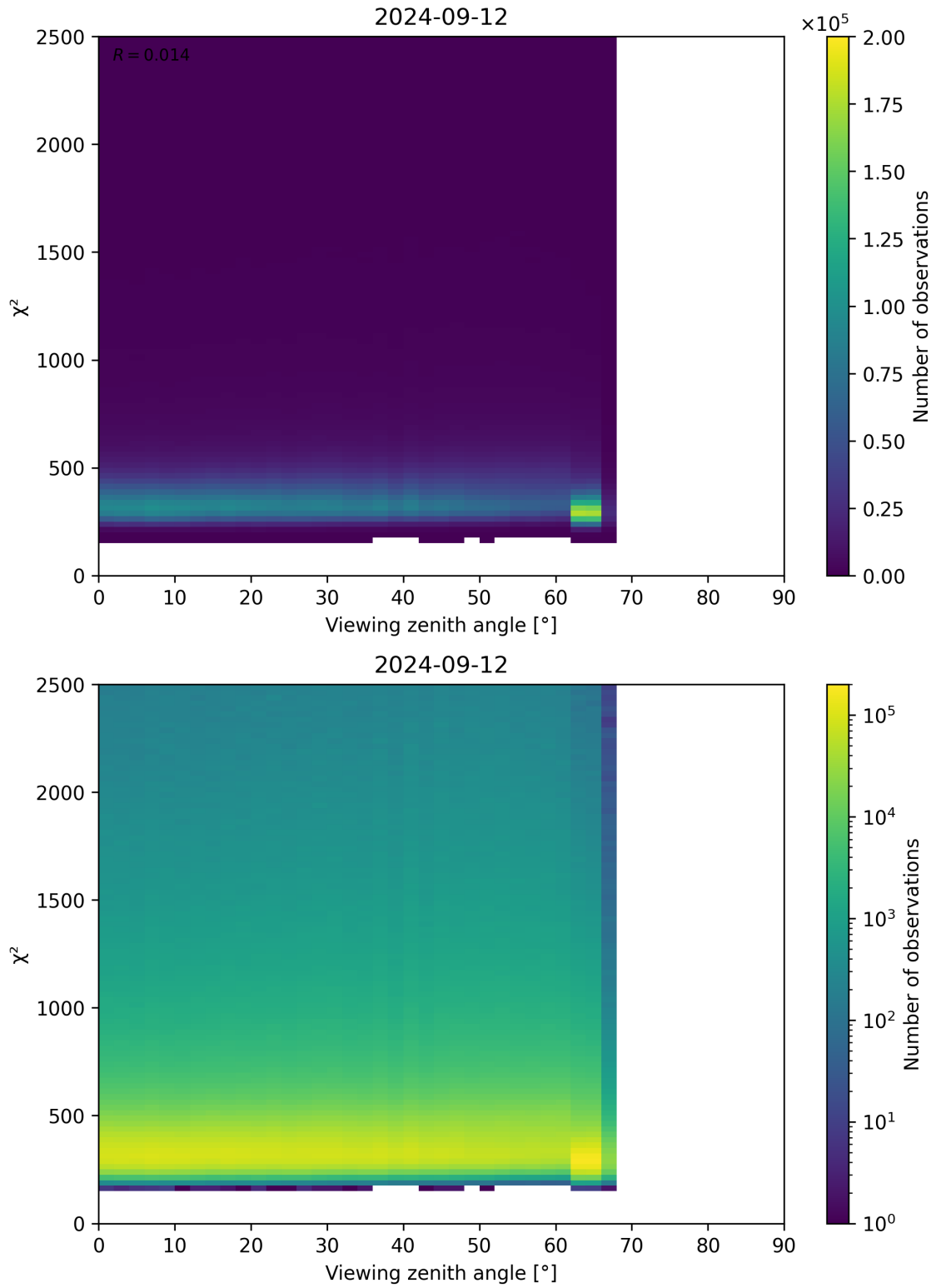
Figure 162: Scatter density plot of “Viewing zenith angle” against “ \chi^2 ” for 2024-09-12 to 2024-09-13.
