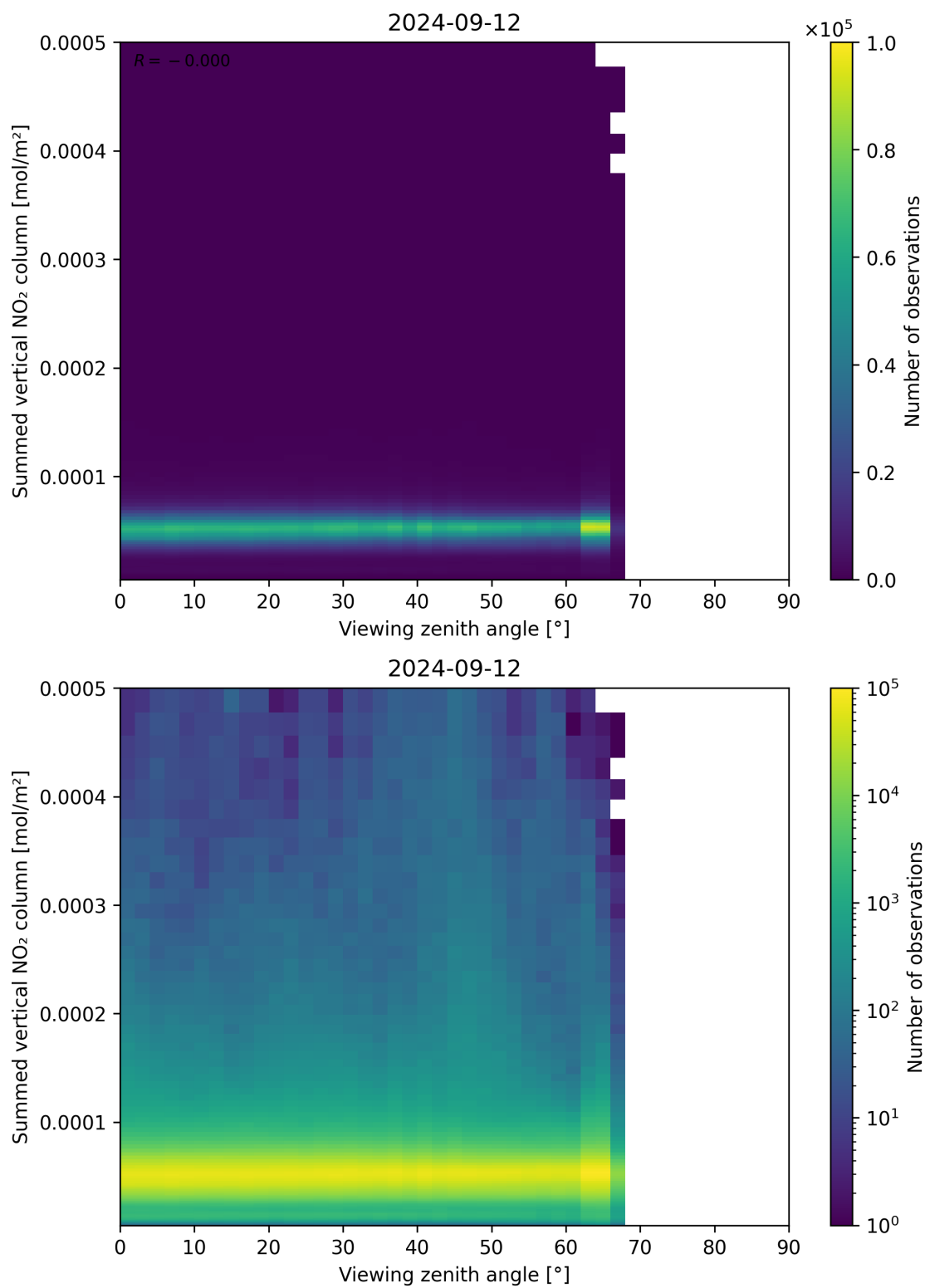
Figure 165: Scatter density plot of “Viewing zenith angle” against “Summed vertical NO 2 column” for 2024-09-12 to 2024-09-13.
