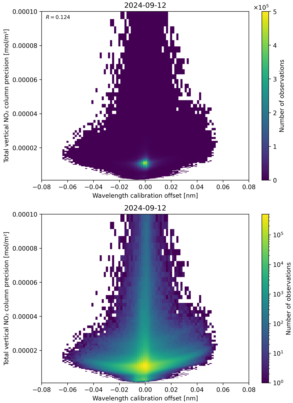
Figure 180: Scatter density plot of “Wavelength calibration offset” against “Total vertical NO 2 column precision” for 2024-09-12 to 2024-09-13.
