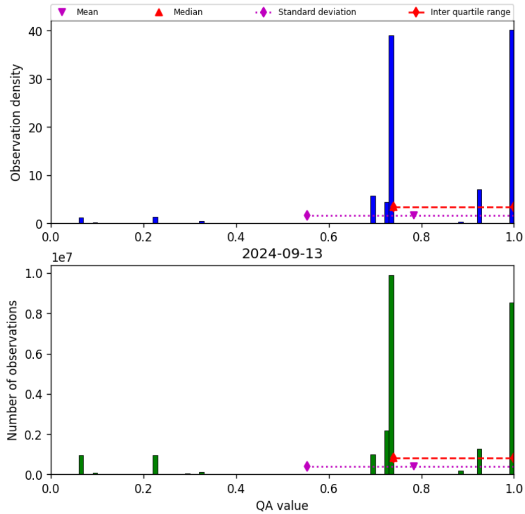
Figure 28: Histogram of “QA value” for 2024-09-12 to 2024-09-14
