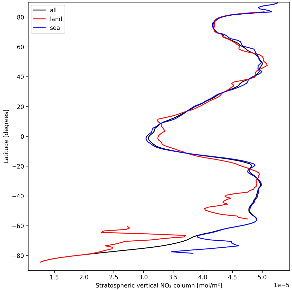
Figure 19: Zonal average of “Stratospheric vertical NO 2 column” for 2024-09-12 to 2024-09-14.
