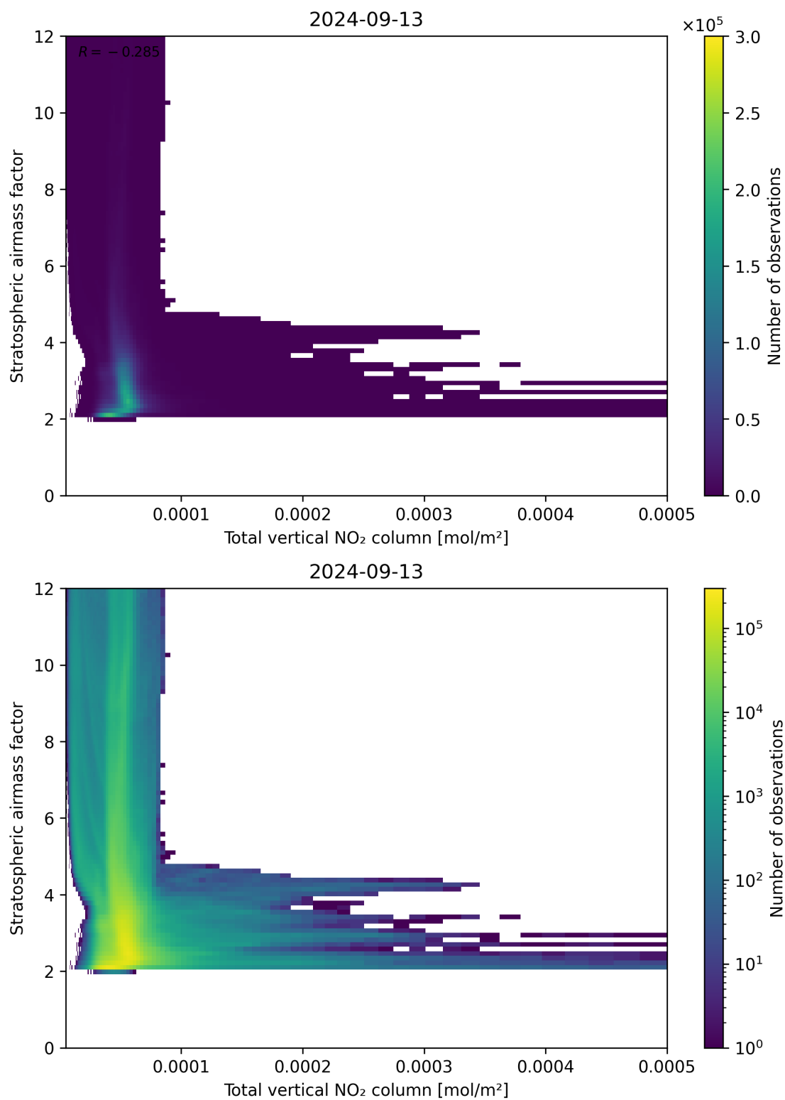
Figure 110: Scatter density plot of “Total vertical NO 2 column” against “Stratospheric airmass factor” for 2024-09-12 to 2024-09-14.
