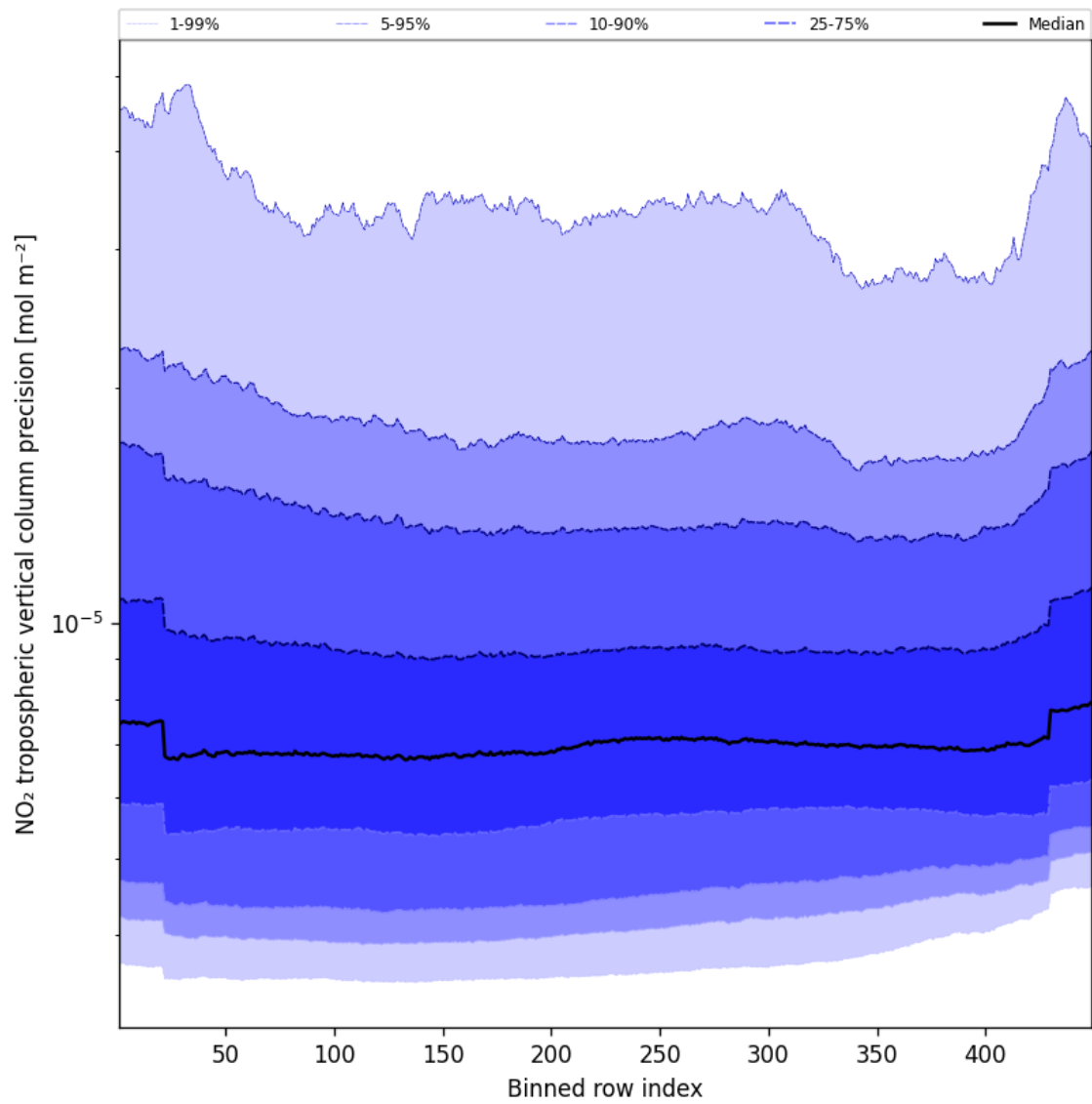
Figure 47: Along track statistics of “NO 2 tropospheric vertical column precision” for 2024-09-12 to 2024-09-14
