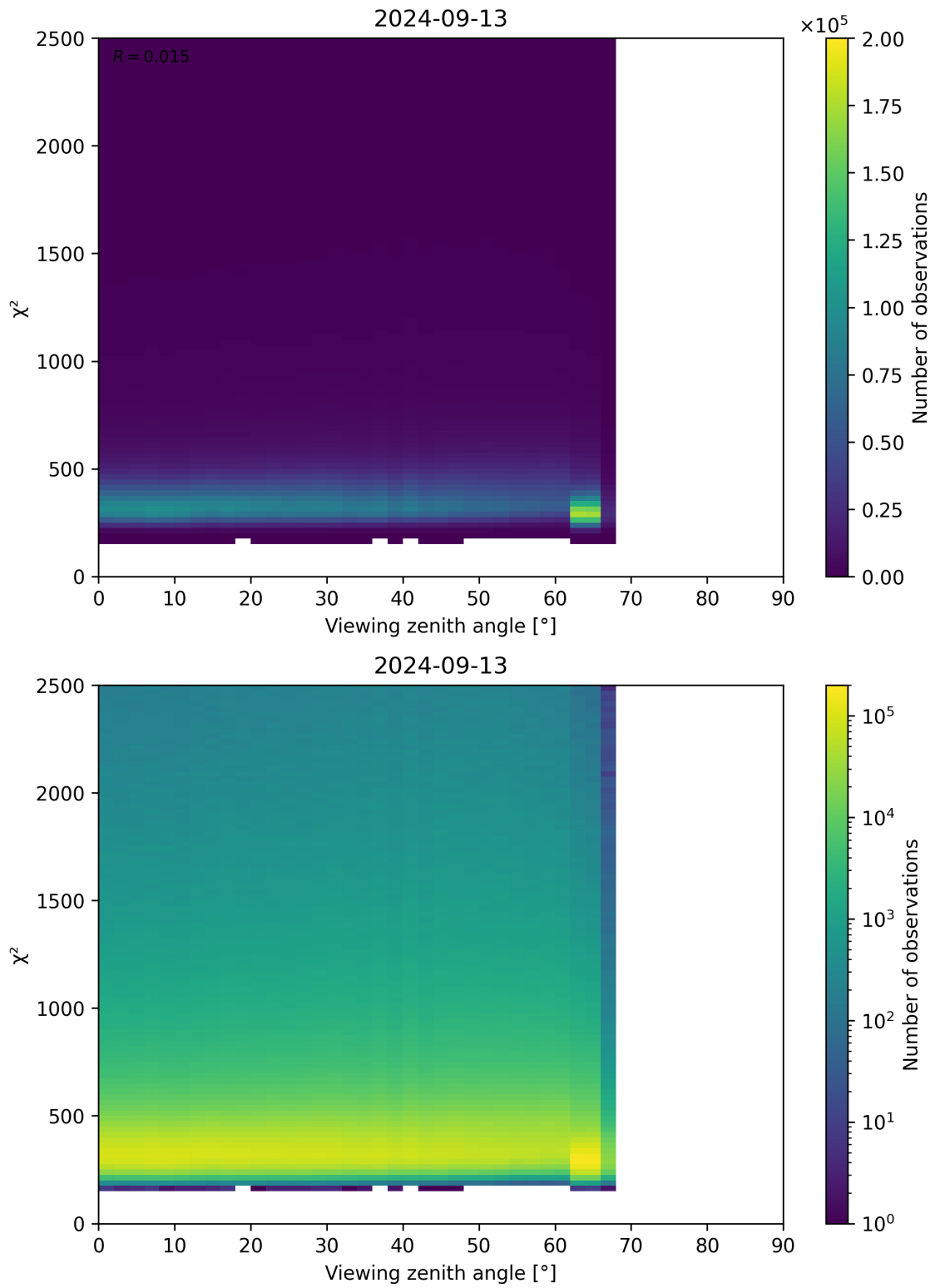
Figure 162: Scatter density plot of “Viewing zenith angle” against “ \chi^2 ” for 2024-09-12 to 2024-09-14.
