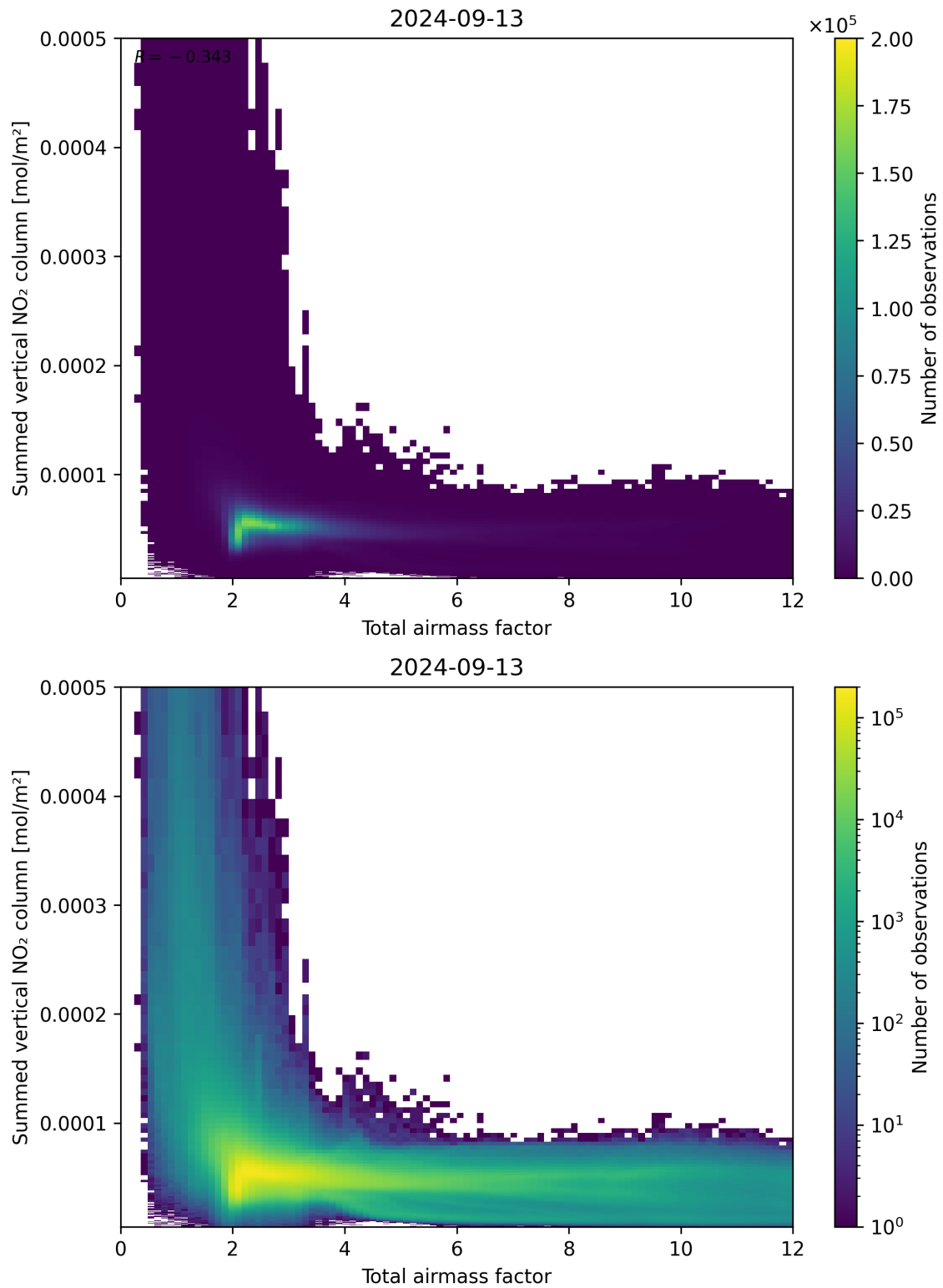
Figure 65: Scatter density plot of “Total airmass factor” against “Summed vertical NO 2 column” for 2024-09-12 to 2024-09-14.
