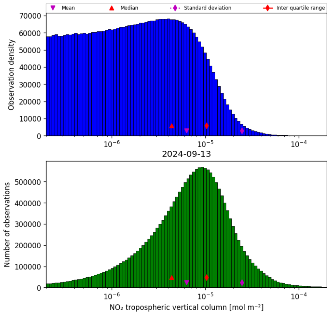
Figure 29: Histogram of “NO 2 tropospheric vertical column” for 2024-09-12 to 2024-09-14
