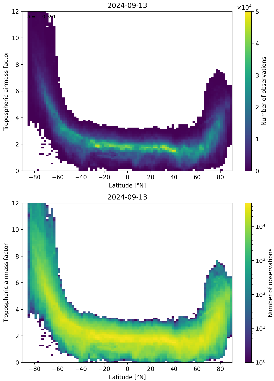
Figure 85: Scatter density plot of “Latitude” against “Tropospheric air mass factor” for 2024-09-12 to 2024-09-14.
