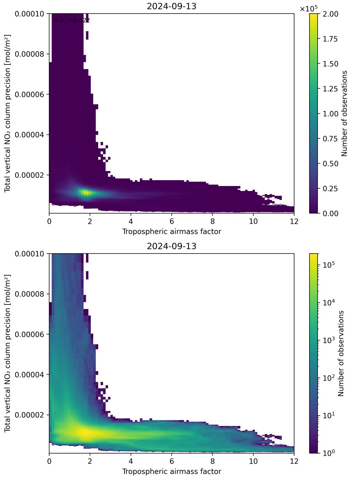
Figure 78: Scatter density plot of “Tropospheric air mass factor” against “Total vertical NO 2 column precision” for 2024-09-12 to 2024-09-14.
