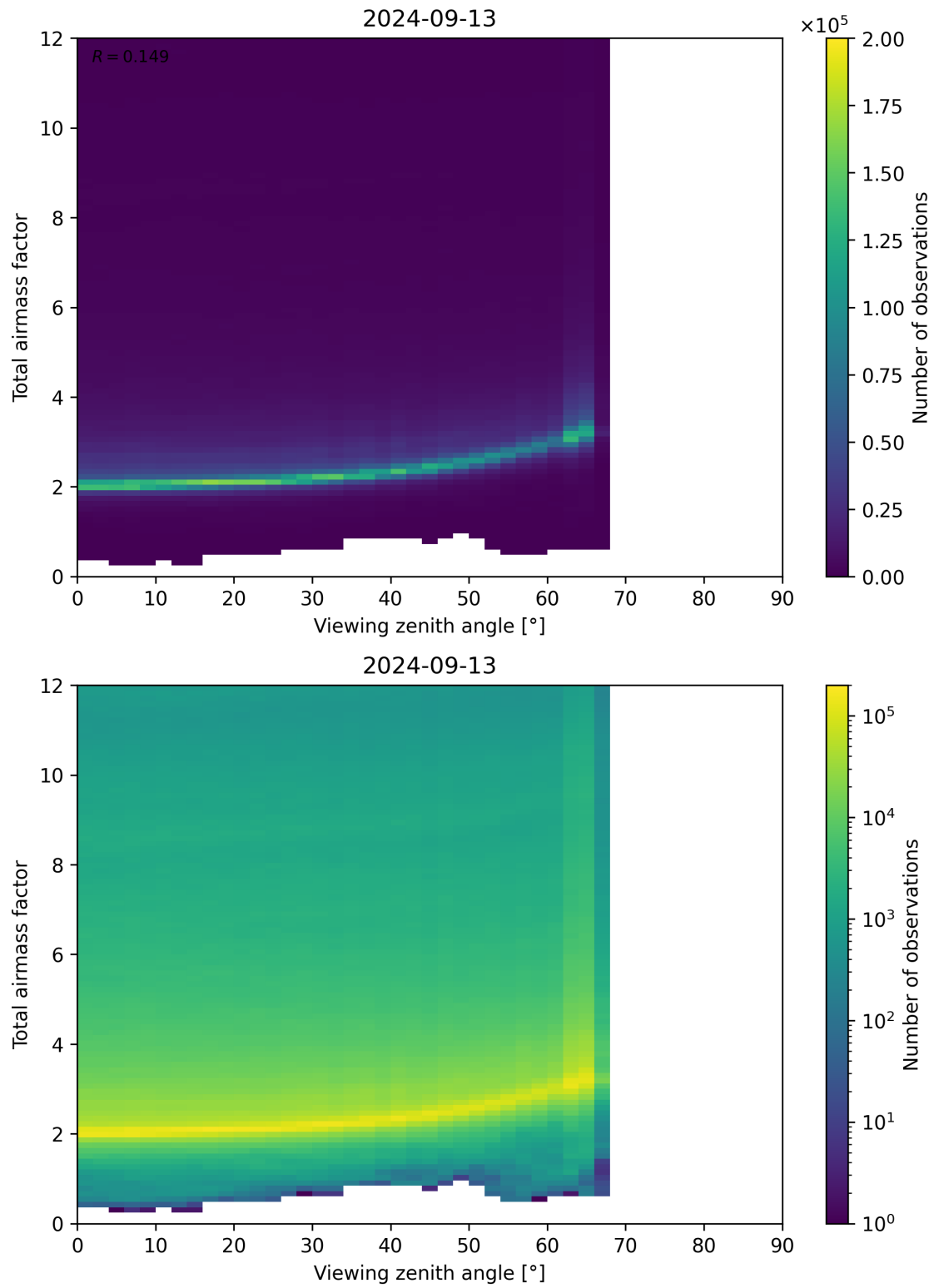
Figure 160: Scatter density plot of “Viewing zenith angle” against “Total airmass factor” for 2024-09-12 to 2024-09-14.
