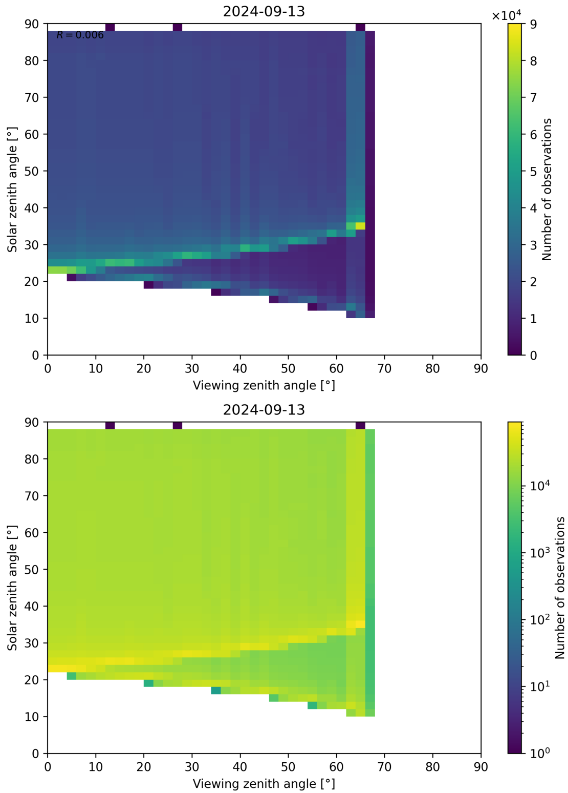
Figure 172: Scatter density plot of “Viewing zenith angle” against “Solar zenith angle” for 2024-09-12 to 2024-09-14.
