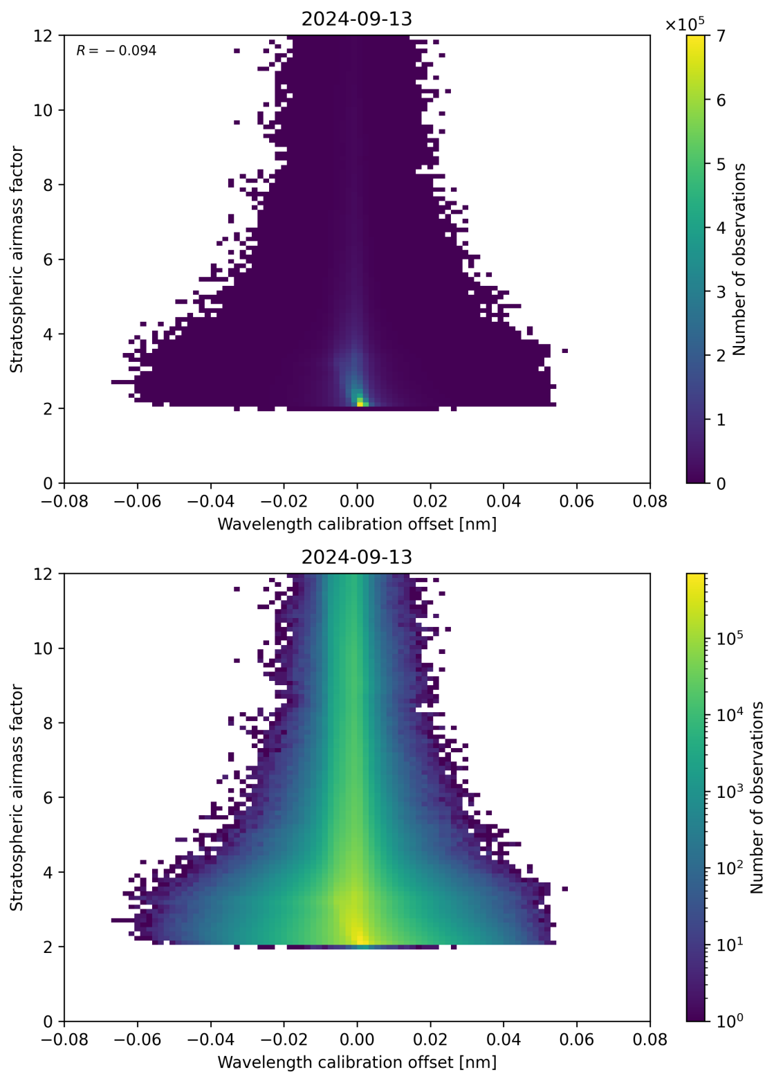
Figure 174: Scatter density plot of “Wavelength calibration offset” against “Stratospheric air mass factor” for 2024-09-12 to 2024-09-14.
