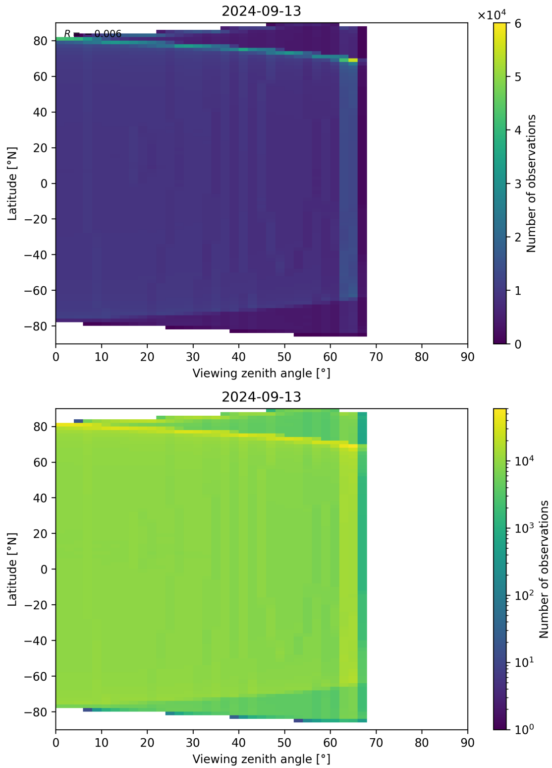
Figure 163: Scatter density plot of “Viewing zenith angle” against “Latitude” for 2024-09-12 to 2024-09-14.
