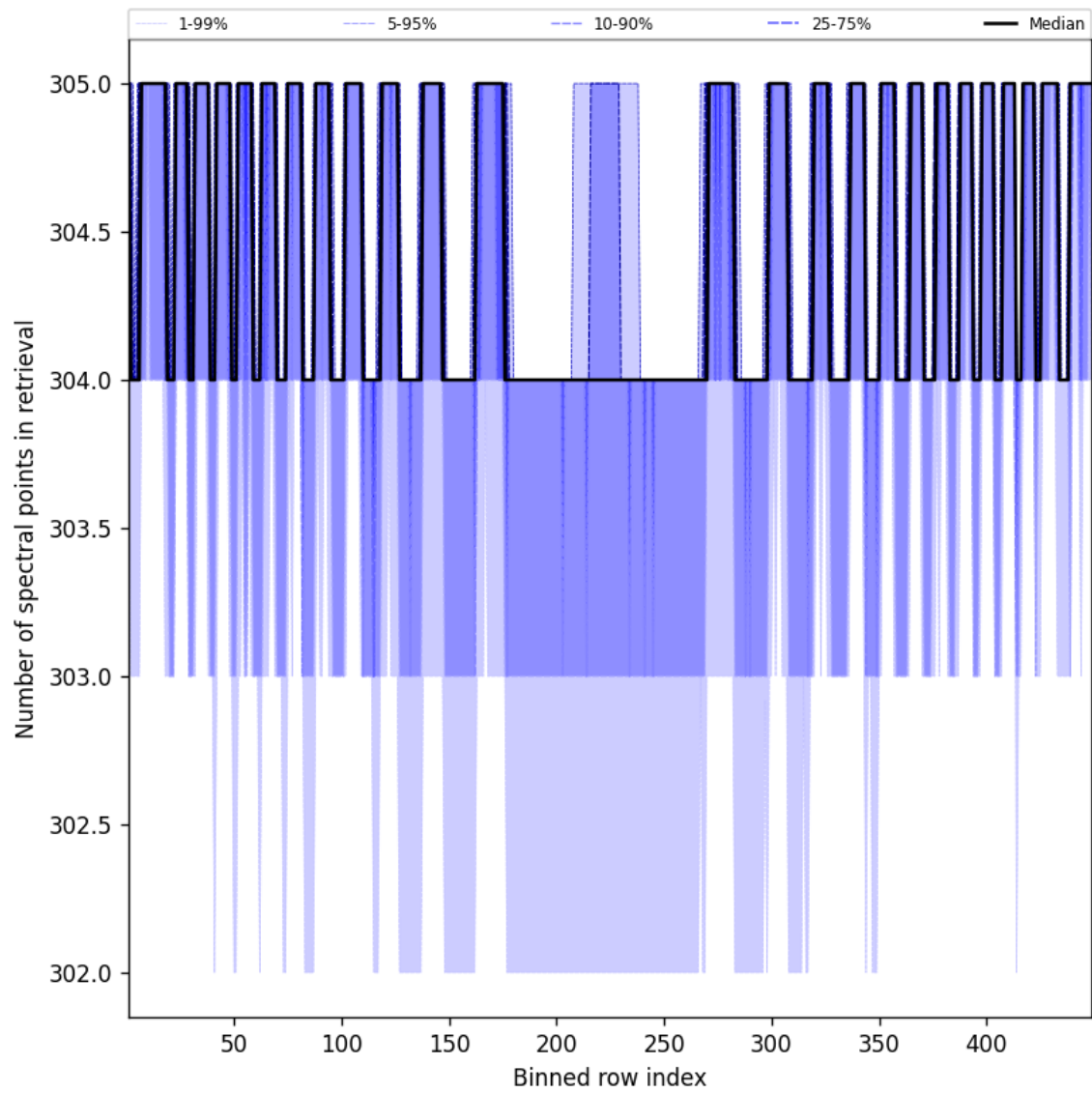
Figure 50: Along track statistics of “Number of spectral points in retrieval” for 2024-09-12 to 2024-09-14
