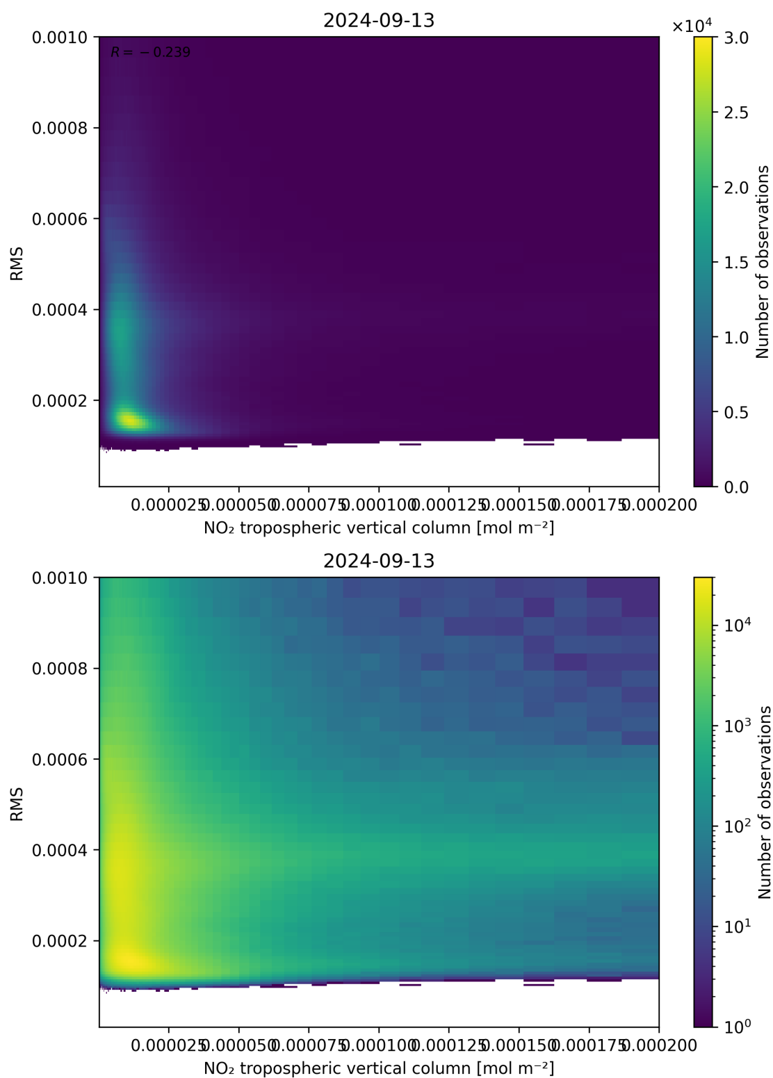
Figure 142: Scatter density plot of “NO 2 tropospheric vertical column” against “RMS” for 2024-09-12 to 2024-09-14.
