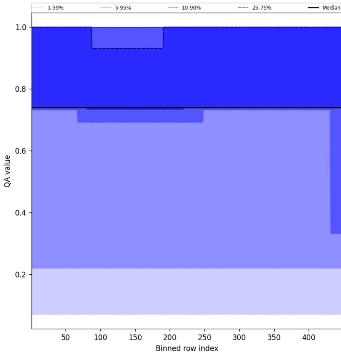
Figure 45: Along track statistics of “QA value” for 2024-09-12 to 2024-09-14
