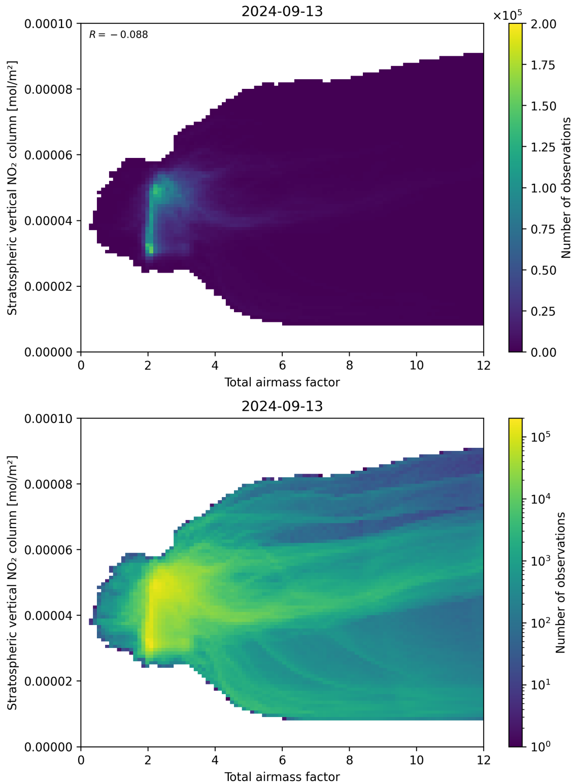
Figure 64: Scatter density plot of “Total airmass factor” against “Stratospheric vertical NO 2 column” for 2024-09-12 to 2024-09-14.
