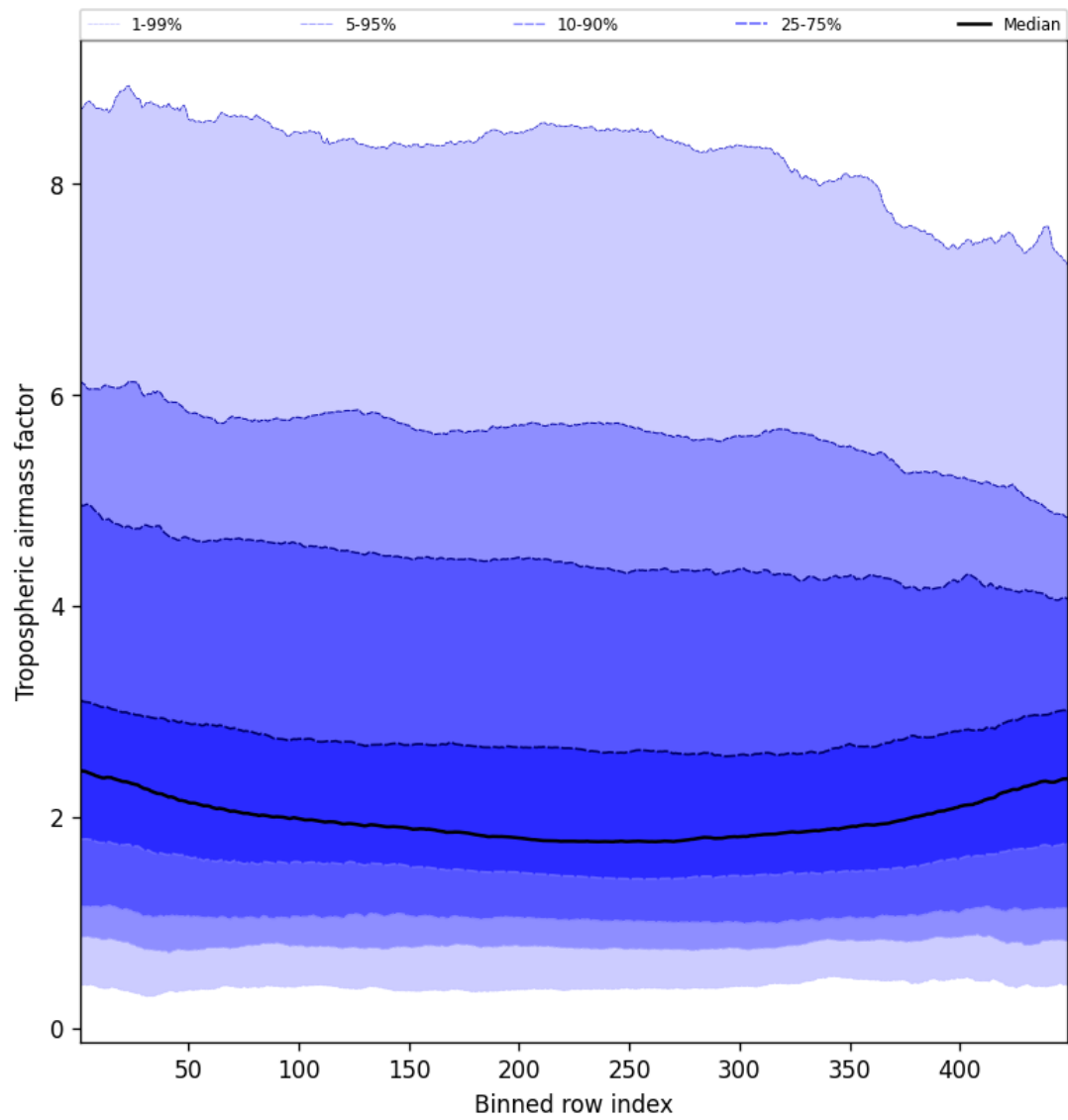
Figure 48: Along track statistics of “Tropospheric air mass factor” for 2024-09-12 to 2024-09-14
