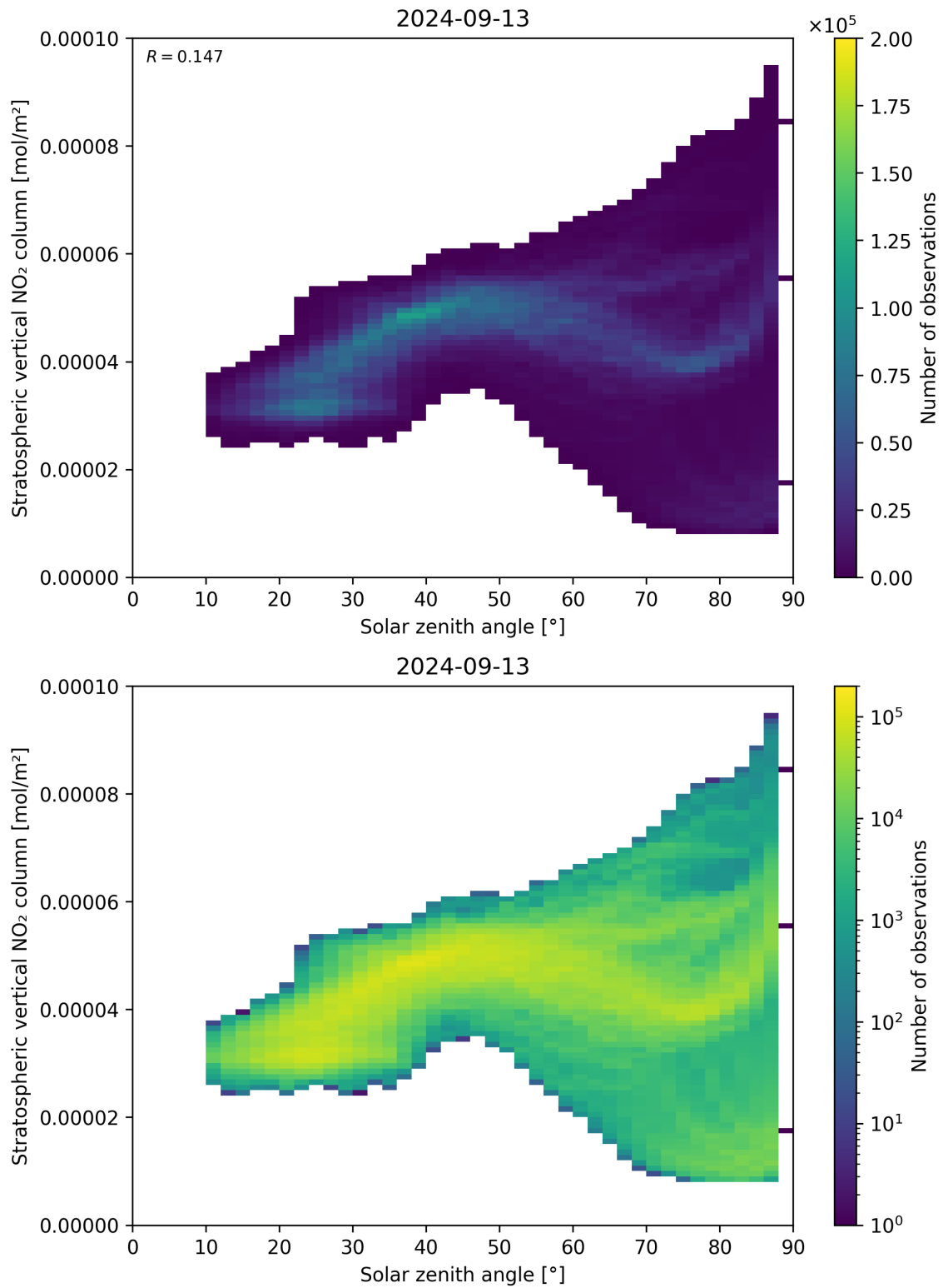
Figure 150: Scatter density plot of “Solar zenith angle” against “Stratospheric vertical NO 2 column” for 2024-09-12 to 2024-09-14.
