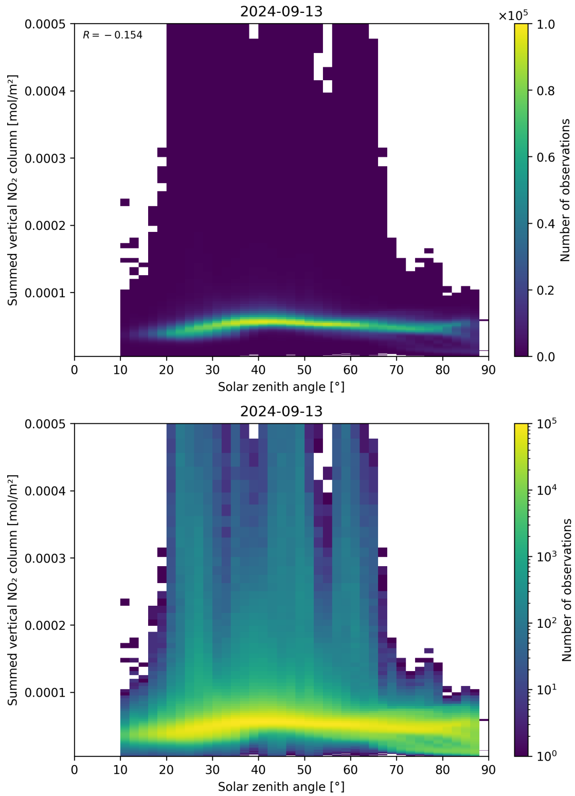
Figure 151: Scatter density plot of “Solar zenith angle” against “Summed vertical NO 2 column” for 2024-09-12 to 2024-09-14.
