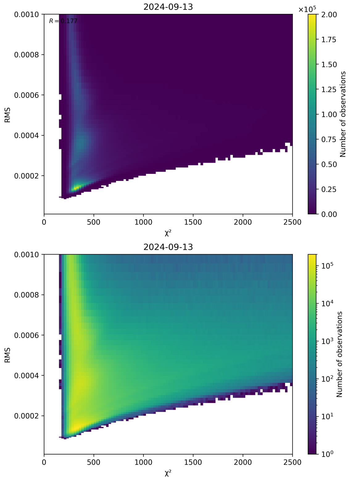
Figure 82: Scatter density plot of “ \chi^2 ” against “RMS” for 2024-09-12 to 2024-09-14.
