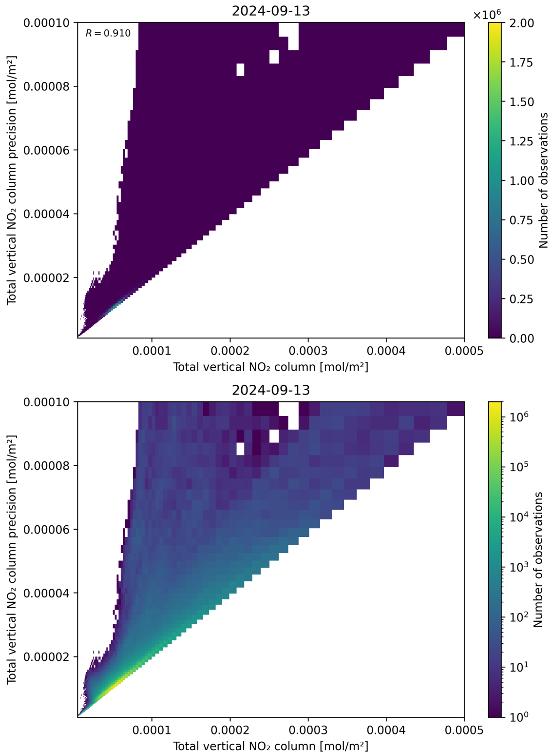
Figure 114: Scatter density plot of “Total vertical NO 2 column” against “Total vertical NO 2 column precision” for 2024-09-12 to 2024-09-14.
