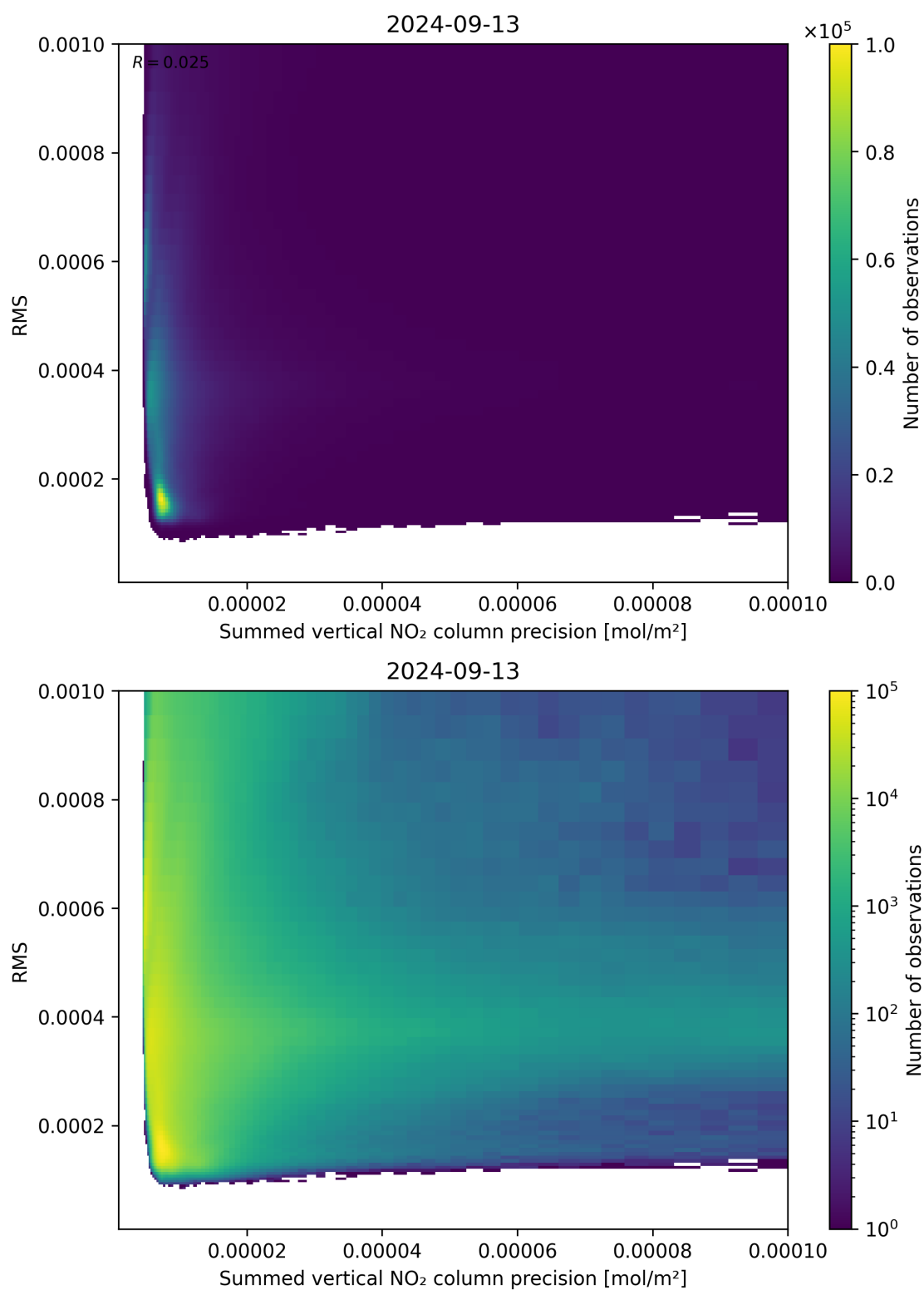
Figure 108: Scatter density plot of “Summed vertical NO 2 column precision” against “RMS” for 2024-09-12 to 2024-09-14.
