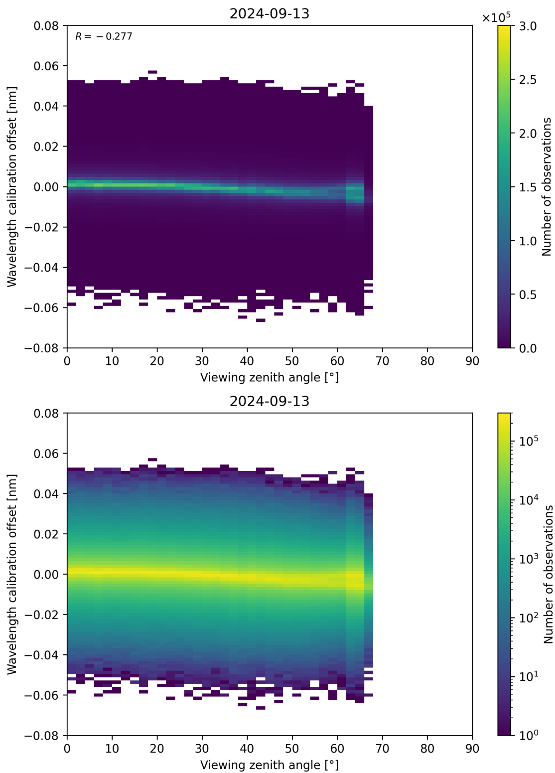
Figure 173: Scatter density plot of “Viewing zenith angle” against “Wavelength calibration offset” for 2024-09-12 to 2024-09-14.
