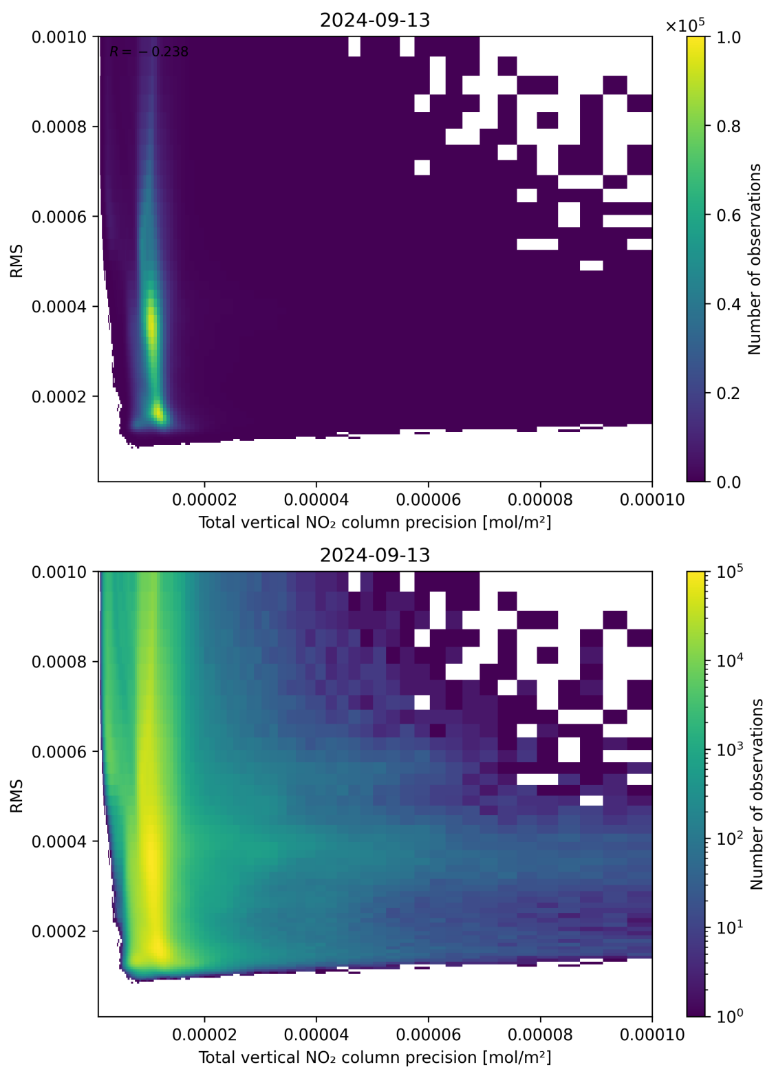
Figure 119: Scatter density plot of “Total vertical NO 2 column precision” against “RMS” for 2024-09-12 to 2024-09-14.
