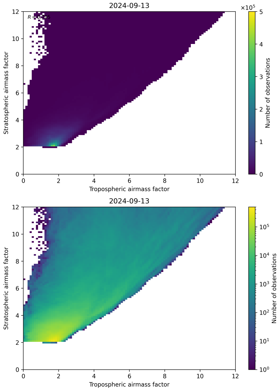
Figure 71: Scatter density plot of “Tropospheric airmass factor” against “Stratospheric airmass factor” for 2024-09-12 to 2024-09-14.
