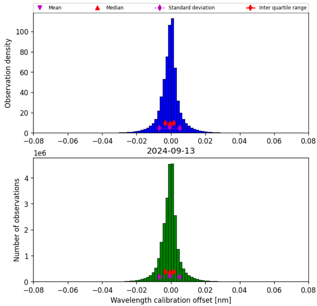
Figure 35: Histogram of “Wavelength calibration offset” for 2024-09-12 to 2024-09-14
