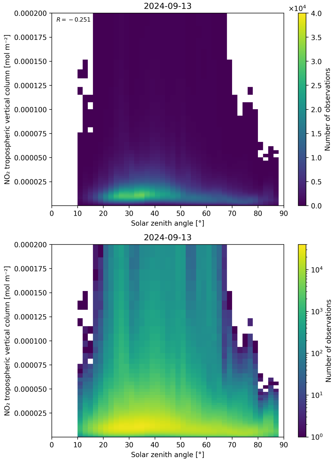
Figure 155: Scatter density plot of “Solar zenith angle” against “NO 2 tropospheric vertical column” for 2024-09-12 to 2024-09-14.
