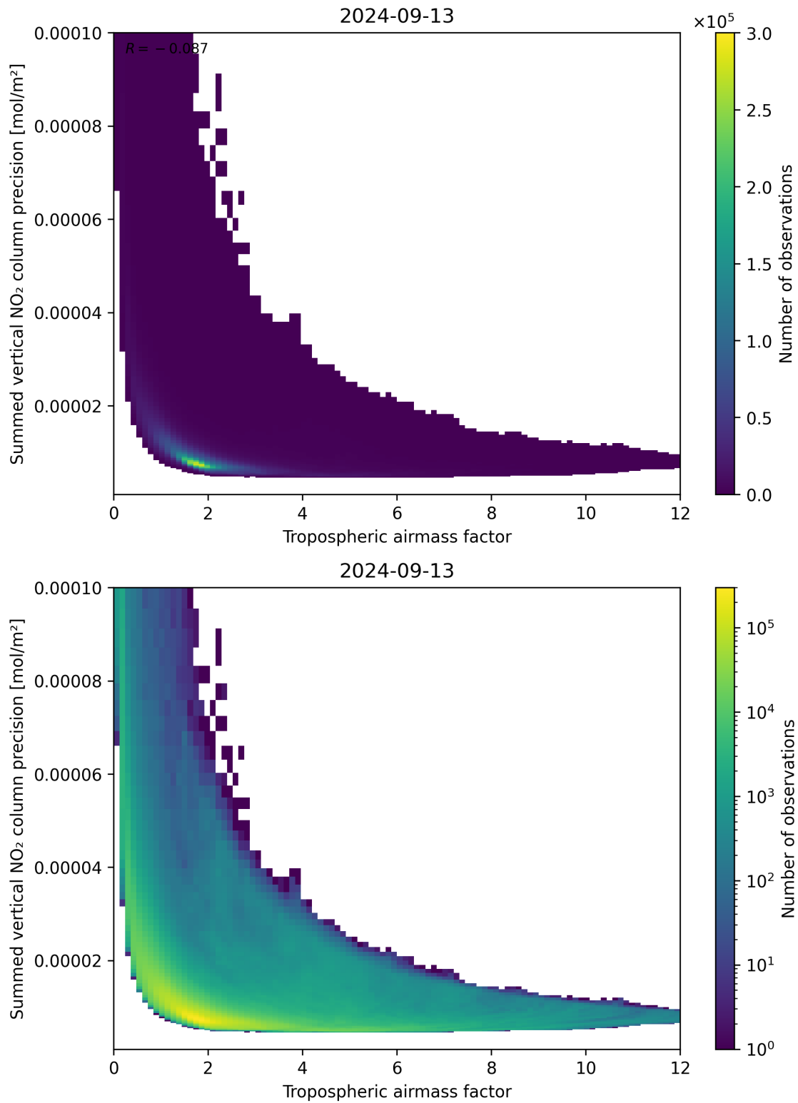
Figure 76: Scatter density plot of “Tropospheric airmass factor” against “Summed vertical NO 2 column precision” for 2024-09-12 to 2024-09-14.
