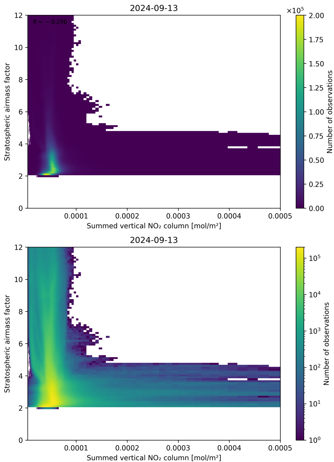
Figure 103: Scatter density plot of “Summed vertical NO 2 column” against “Stratospheric airmass factor” for 2024-09-12 to 2024-09-14.
