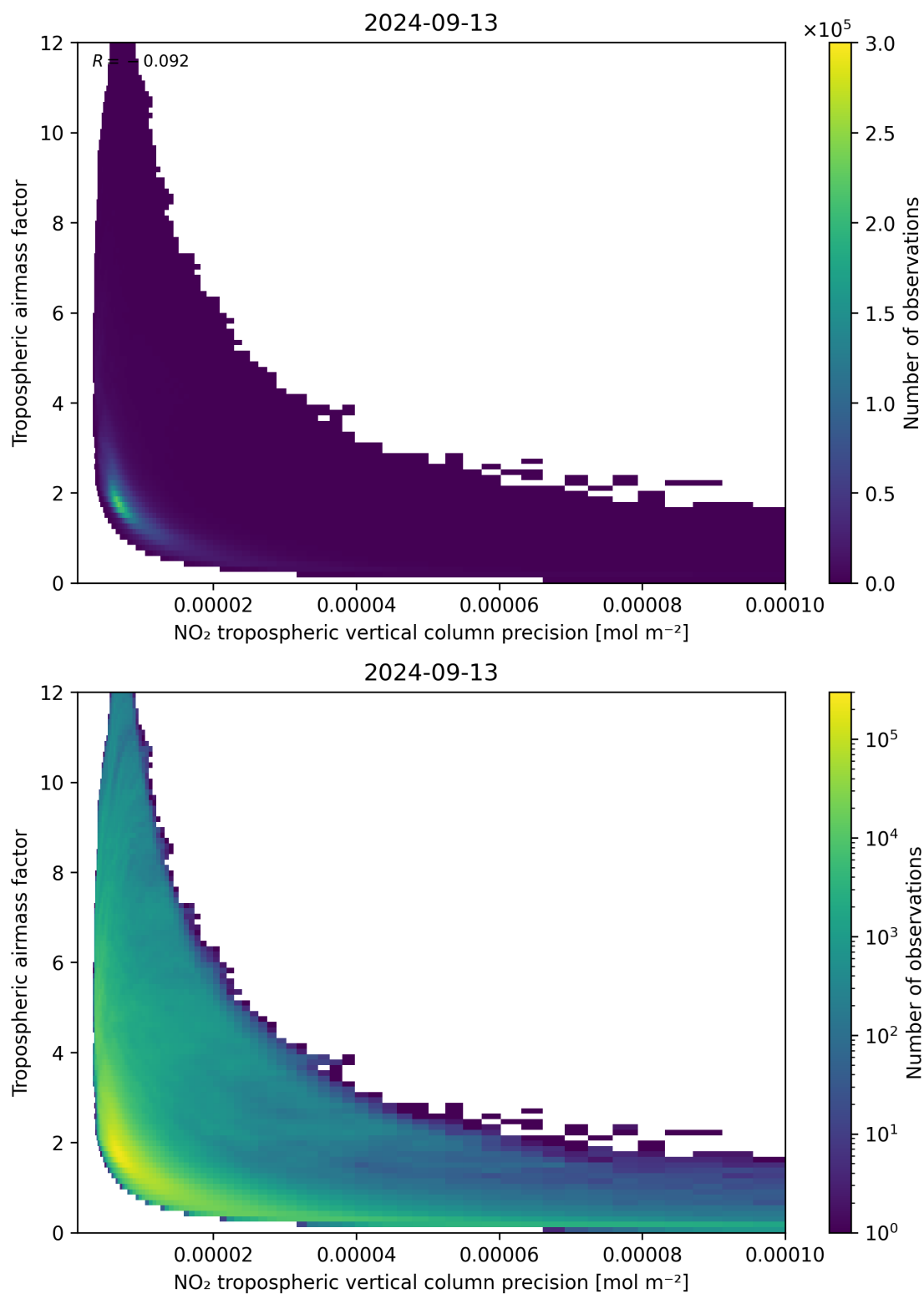
Figure 133: Scatter density plot of “NO 2 tropospheric vertical column precision” against “Tropospheric air mass factor” for 2024-09-12 to 2024-09-14.
