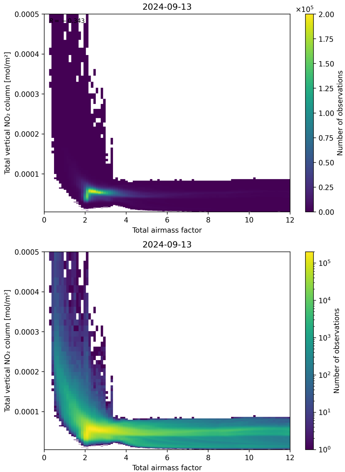
Figure 67: Scatter density plot of “Total airmass factor” against “Total vertical NO 2 column” for 2024-09-12 to 2024-09-14.
