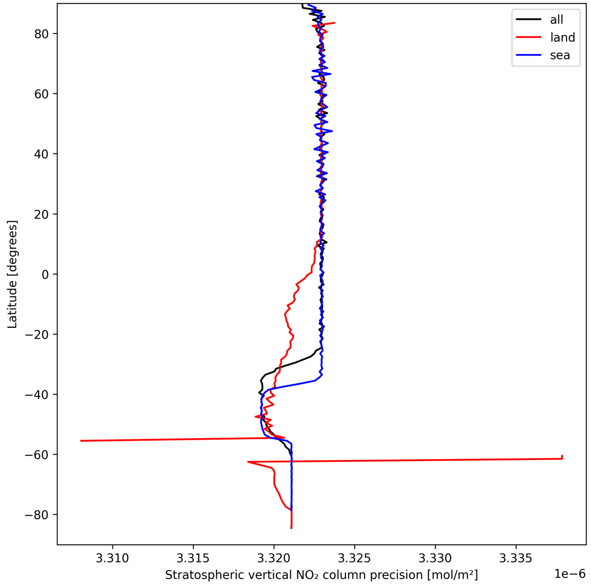
Figure 20: Zonal average of “Stratospheric vertical NO 2 column precision” for 2024-09-12 to 2024-09-14.
