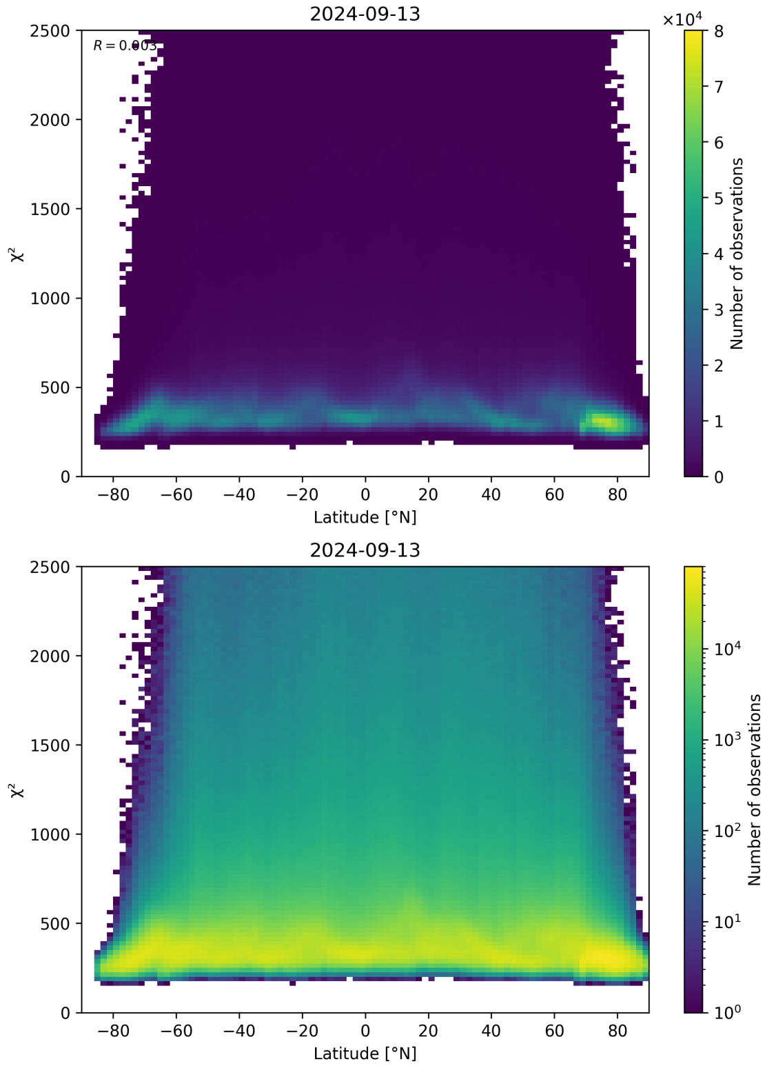
Figure 86: Scatter density plot of “Latitude” against “ \chi^2 ” for 2024-09-12 to 2024-09-14.
