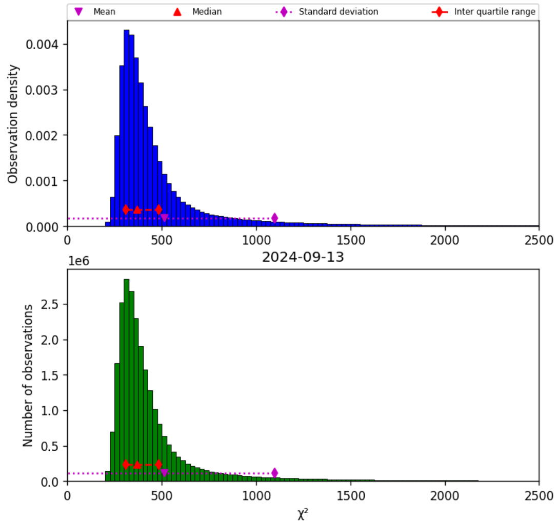
Figure 42: Histogram of “ \chi^2 ” for 2024-09-12 to 2024-09-14
