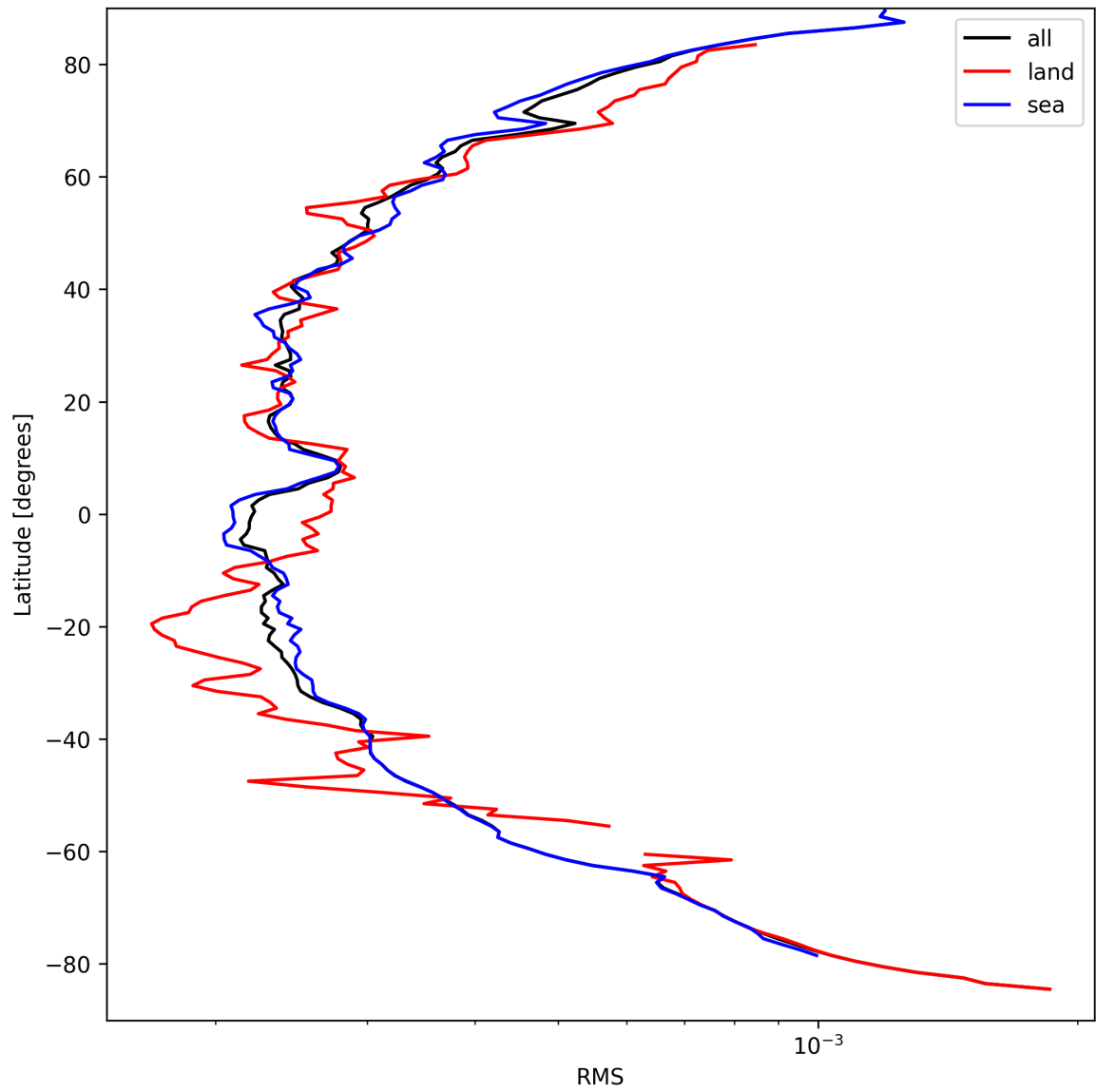
Figure 26: Zonal average of “RMS” for 2024-09-12 to 2024-09-14.
