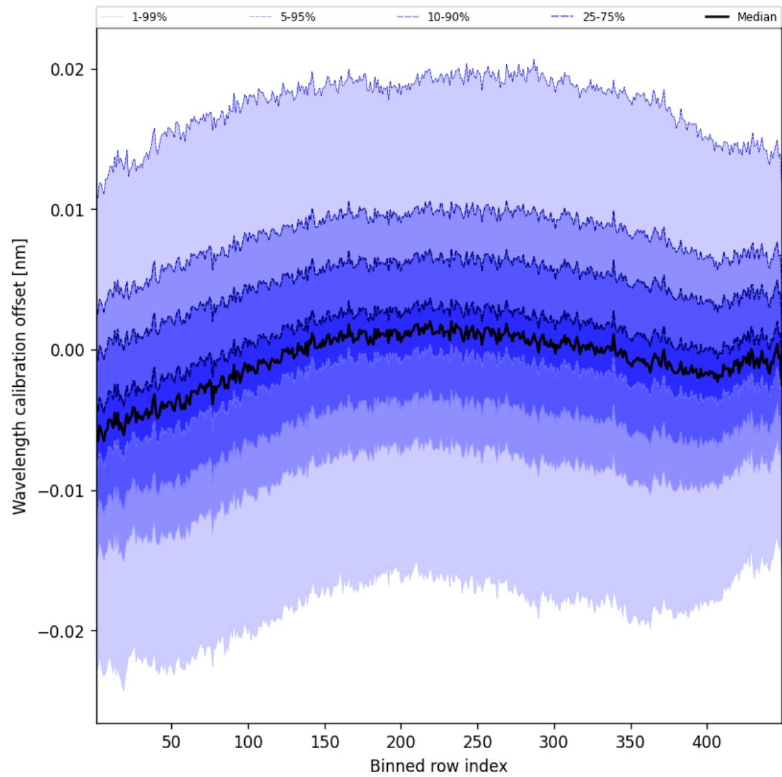
Figure 52: Along track statistics of “Wavelength calibration offset” for 2024-09-12 to 2024-09-14
