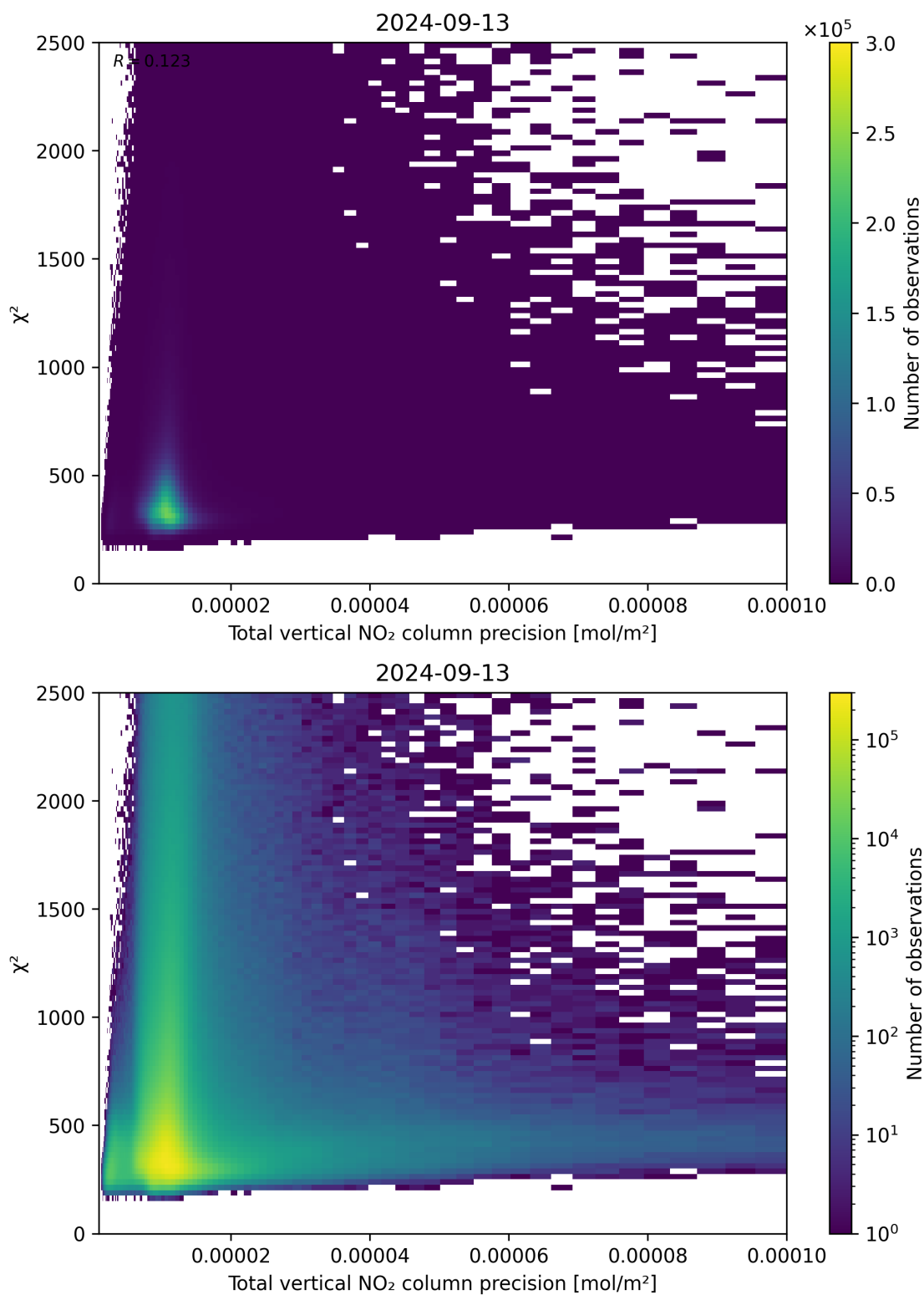
Figure 116: Scatter density plot of “Total vertical NO 2 column precision” against “ \chi^2 ” for 2024-09-12 to 2024-09-14.
