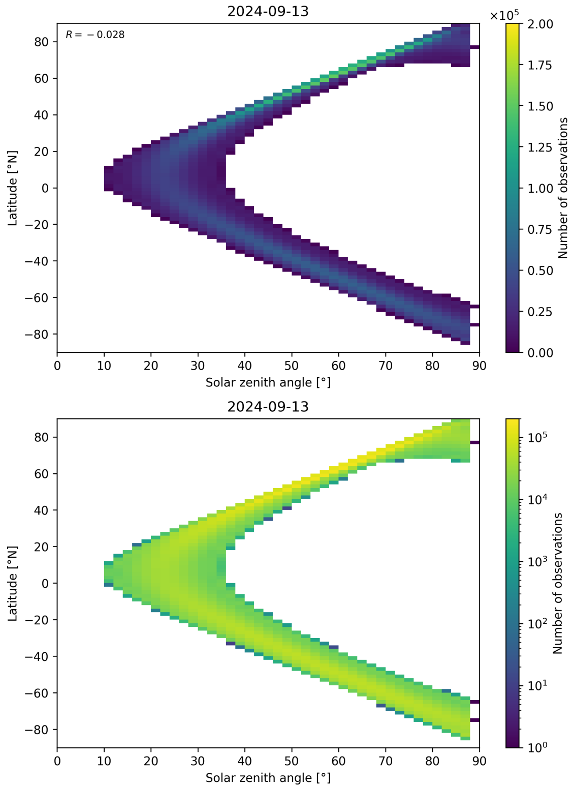
Figure 149: Scatter density plot of “Solar zenith angle” against “Latitude” for 2024-09-12 to 2024-09-14.
