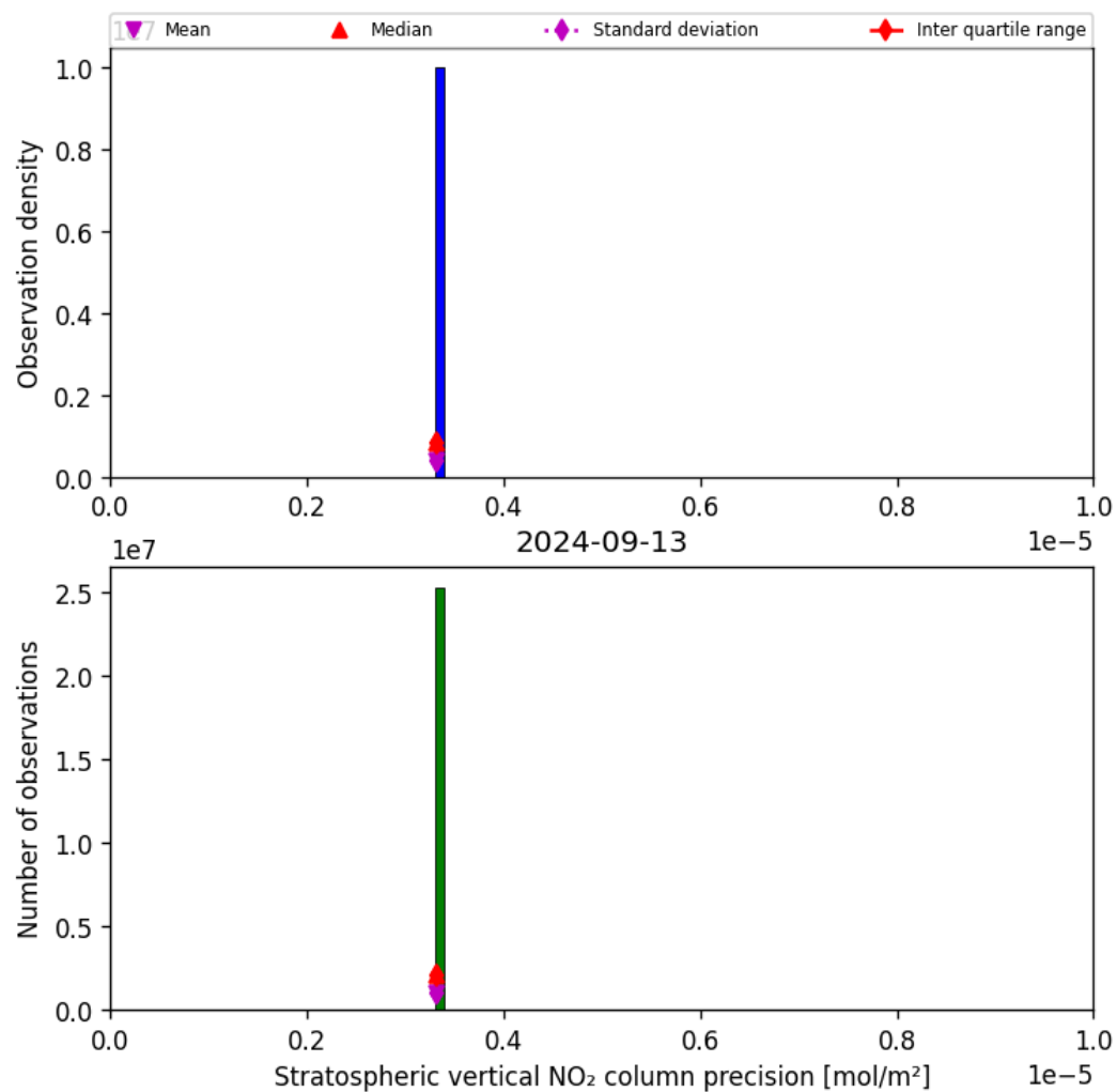
Figure 37: Histogram of “Stratospheric vertical NO 2 column precision” for 2024-09-12 to 2024-09-14
