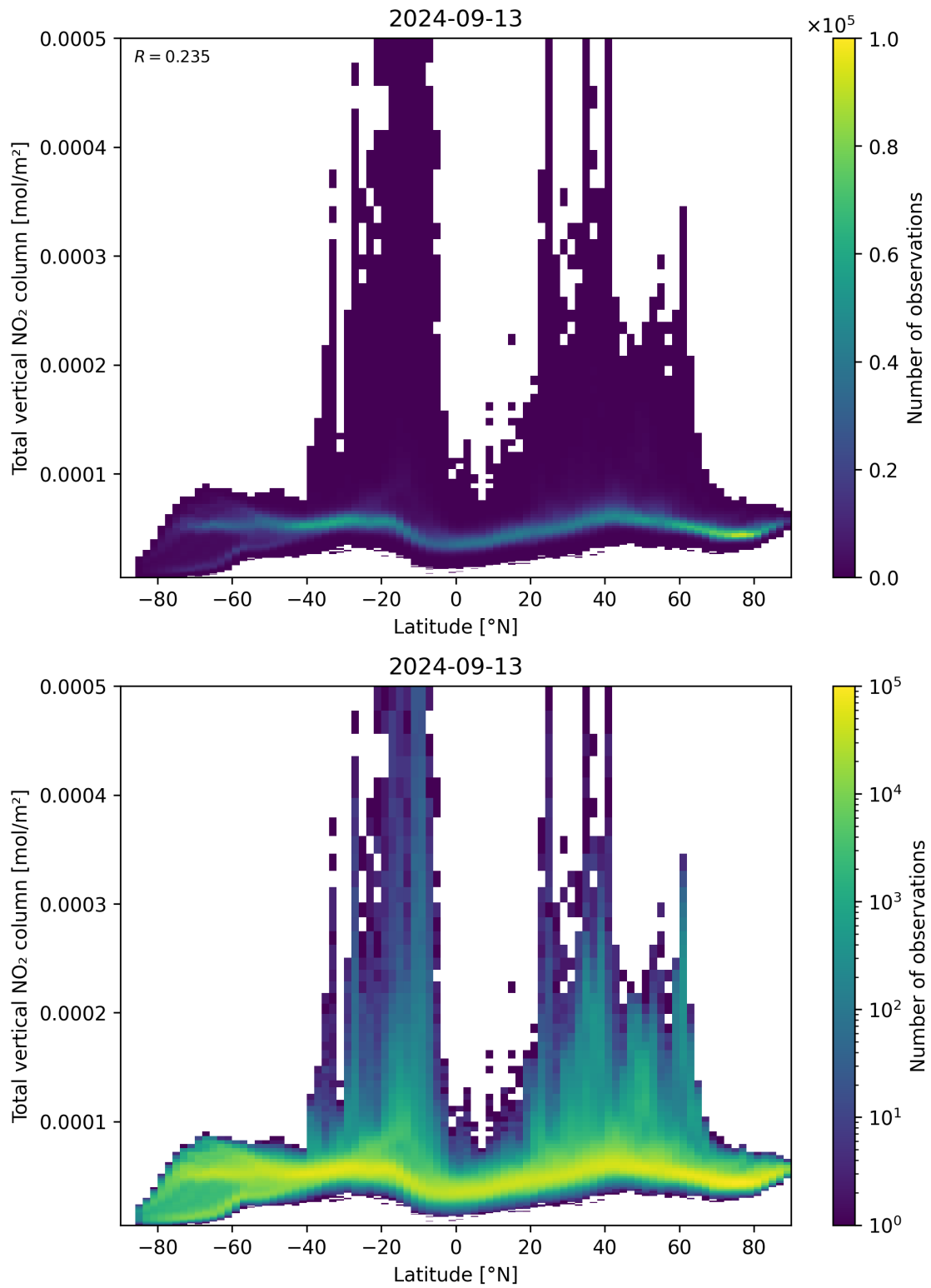
Figure 90: Scatter density plot of “Latitude” against “Total vertical \text{NO}_2 column” for 2024-09-12 to 2024-09-14.
