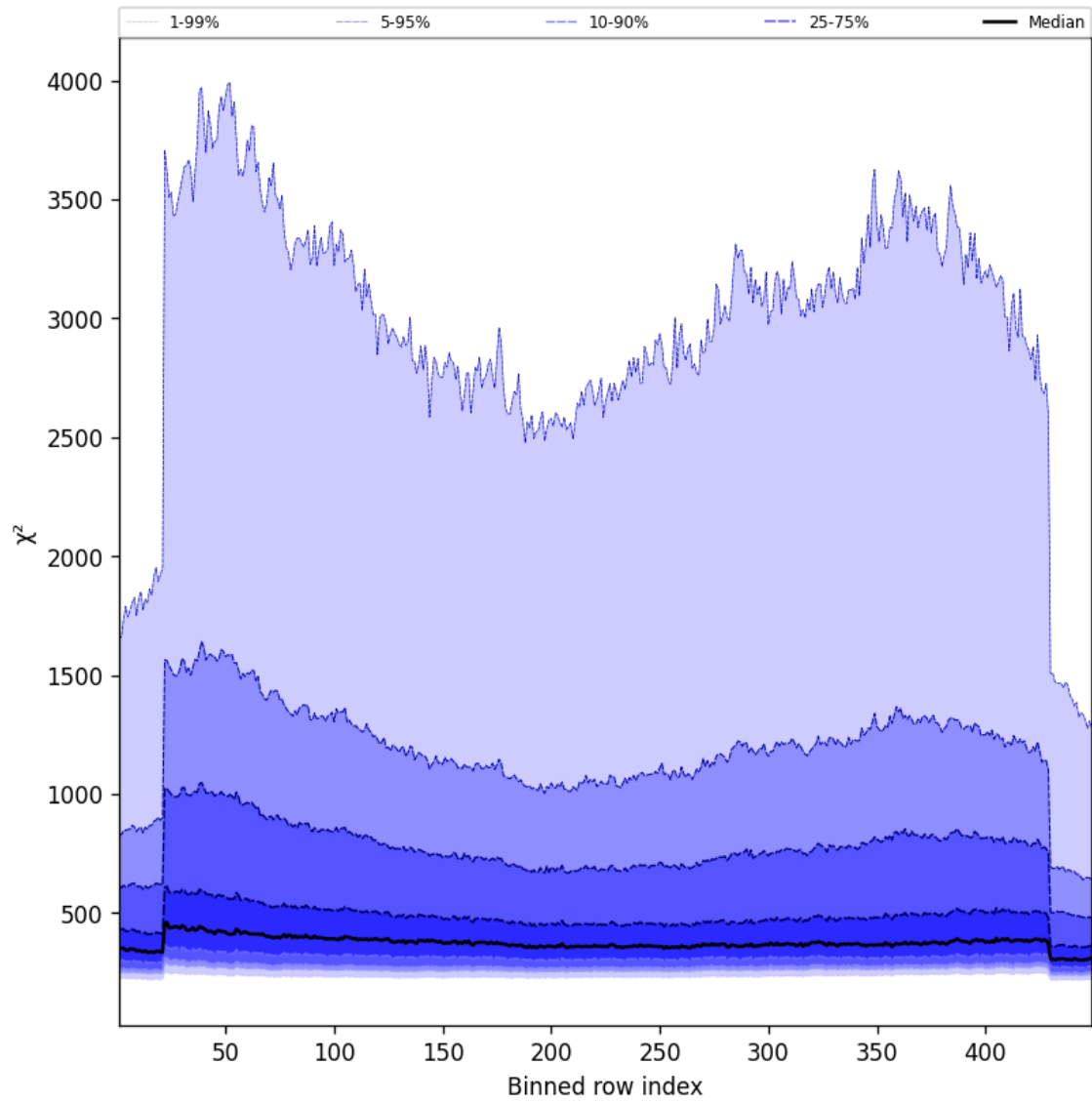
Figure 59: Along track statistics of “ \chi^2 ” for 2024-09-12 to 2024-09-14
