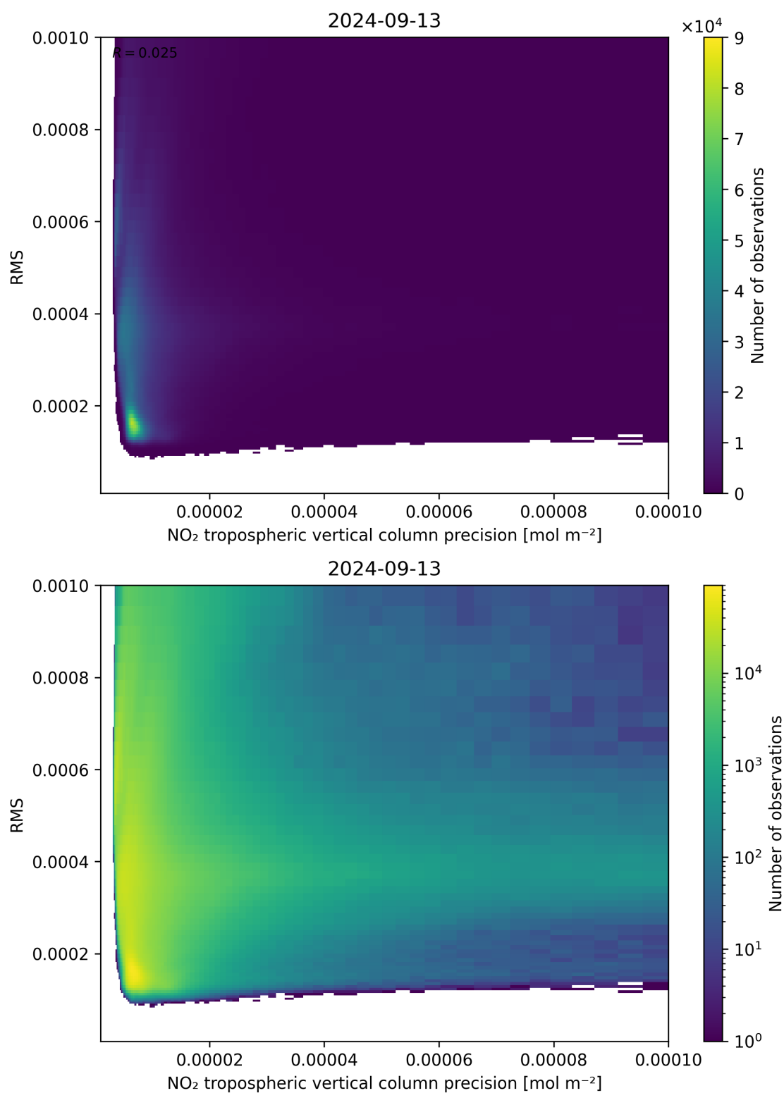
Figure 140: Scatter density plot of “NO 2 tropospheric vertical column precision” against “RMS” for 2024-09-12 to 2024-09-14.
