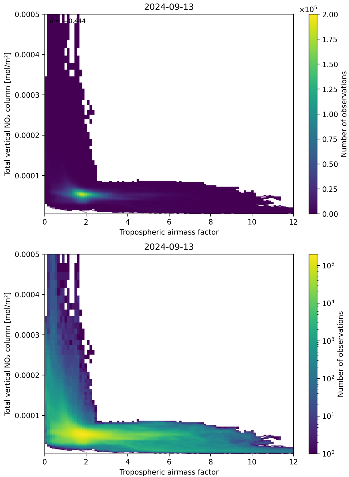
Figure 77: Scatter density plot of “Tropospheric airmass factor” against “Total vertical NO 2 column” for 2024-09-12 to 2024-09-14.
