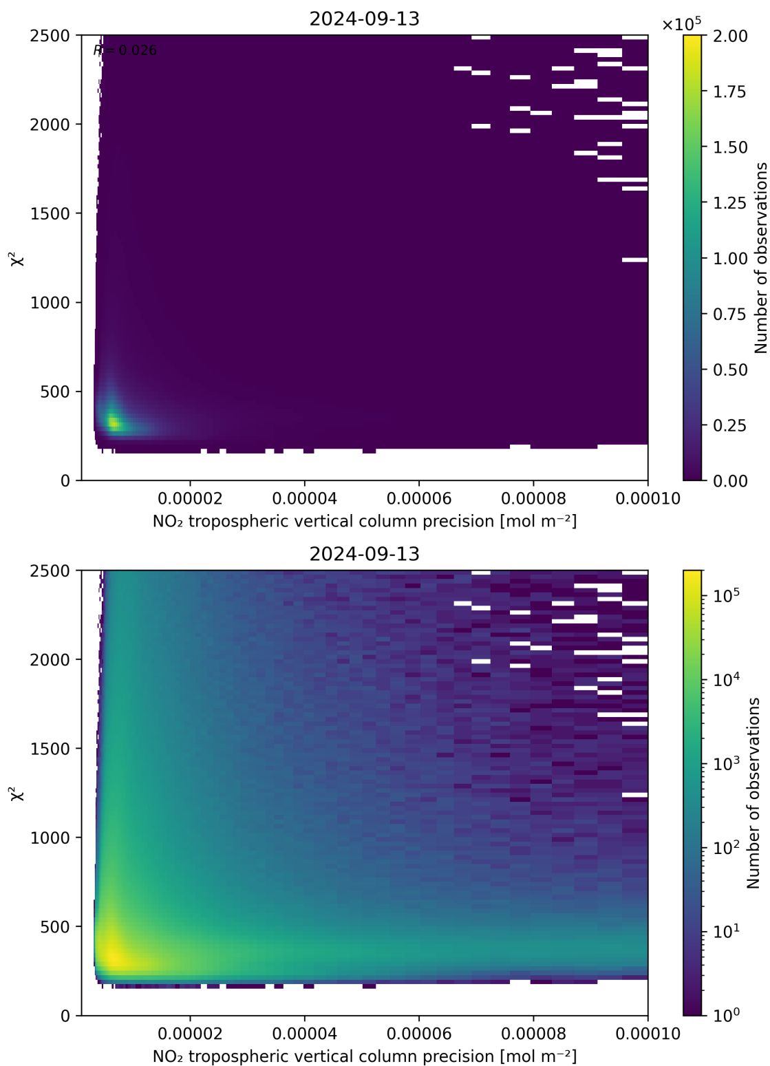
Figure 134: Scatter density plot of “NO 2 tropospheric vertical column precision” against “ \chi^2 ” for 2024-09-12 to 2024-09-14.
