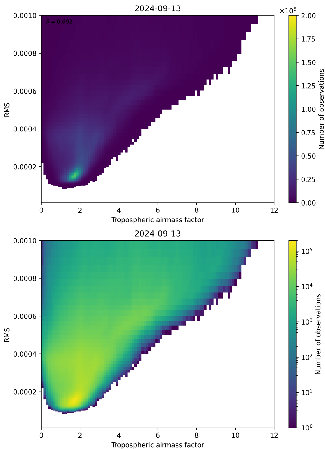
Figure 79: Scatter density plot of “Tropospheric airmass factor” against “RMS” for 2024-09-12 to 2024-09-14.
