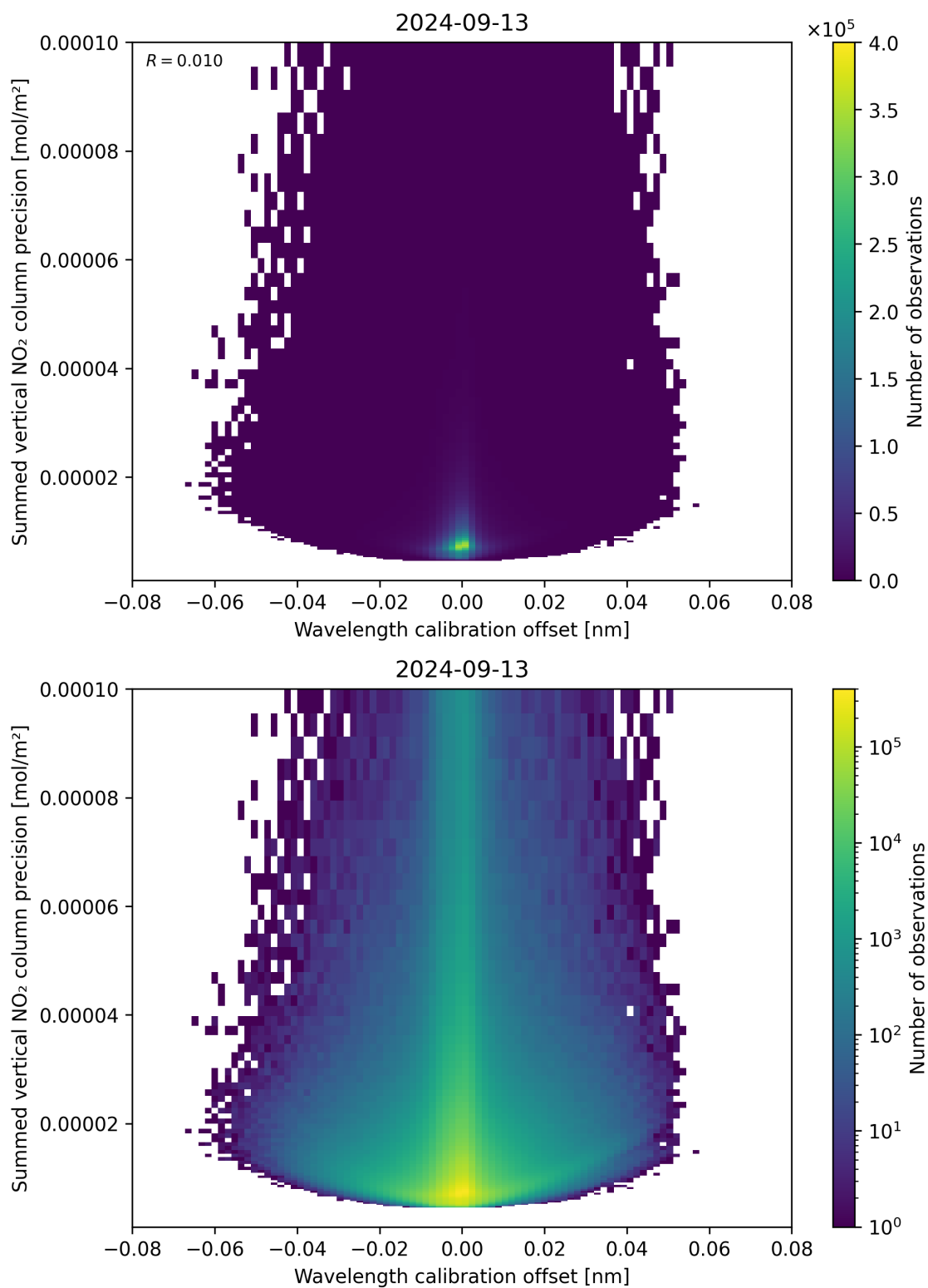
Figure 178: Scatter density plot of “Wavelength calibration offset” against “Summed vertical NO 2 column precision” for 2024-09-12 to 2024-09-14.
