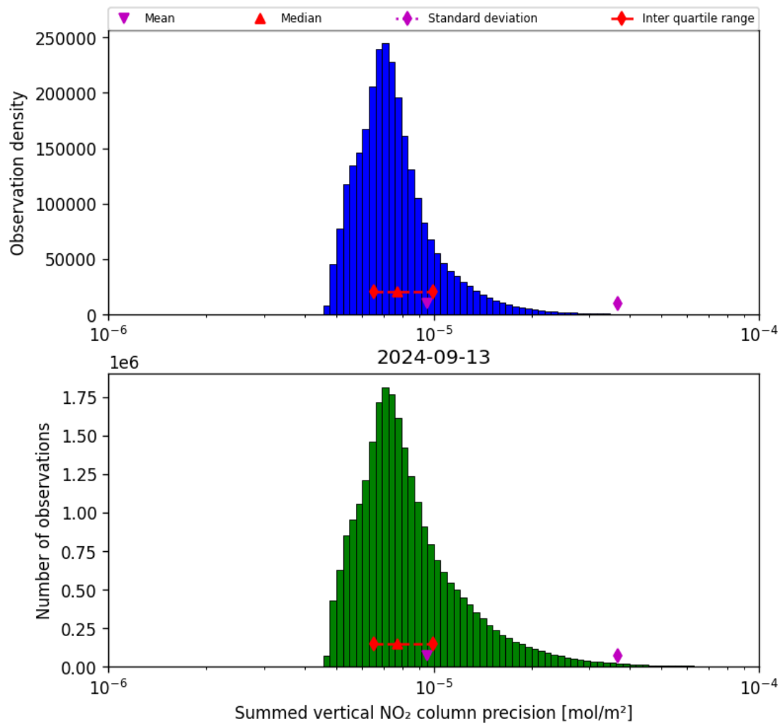
Figure 41: Histogram of "Summed vertical NO 2 column precision" for 2024-09-12 to 2024-09-14
