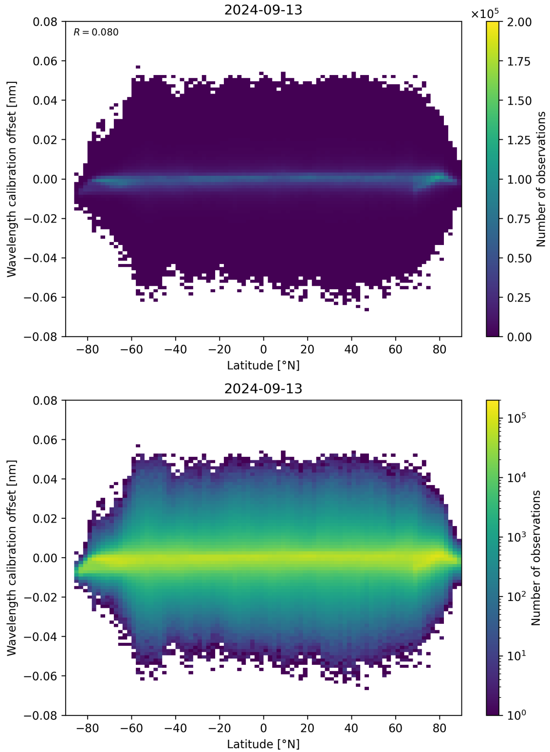
Figure 95: Scatter density plot of “Latitude” against “Wavelength calibration offset” for 2024-09-12 to 2024-09-14.
