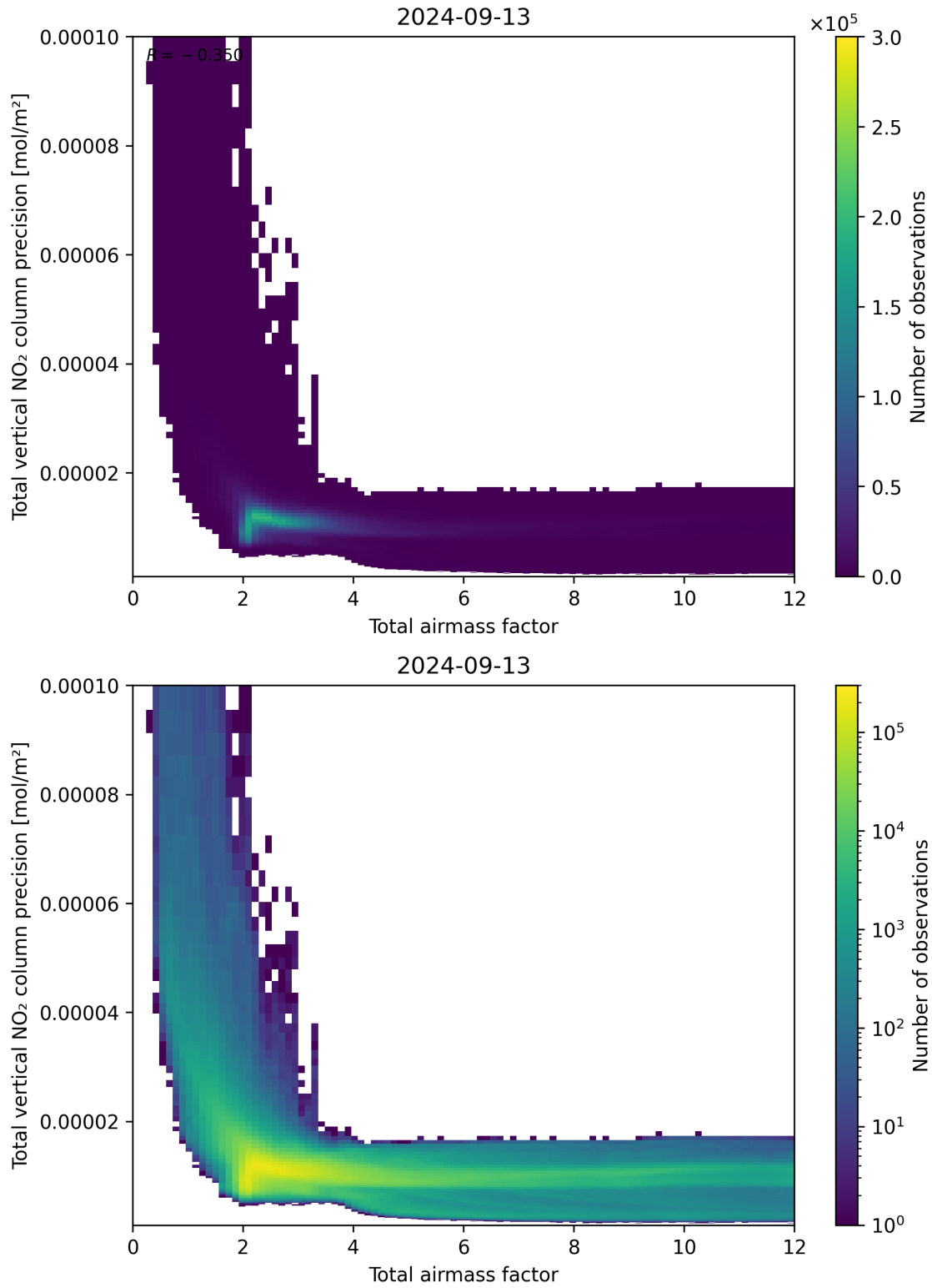
Figure 68: Scatter density plot of “Total airmass factor” against “Total vertical NO 2 column precision” for 2024-09-12 to 2024-09-14.
