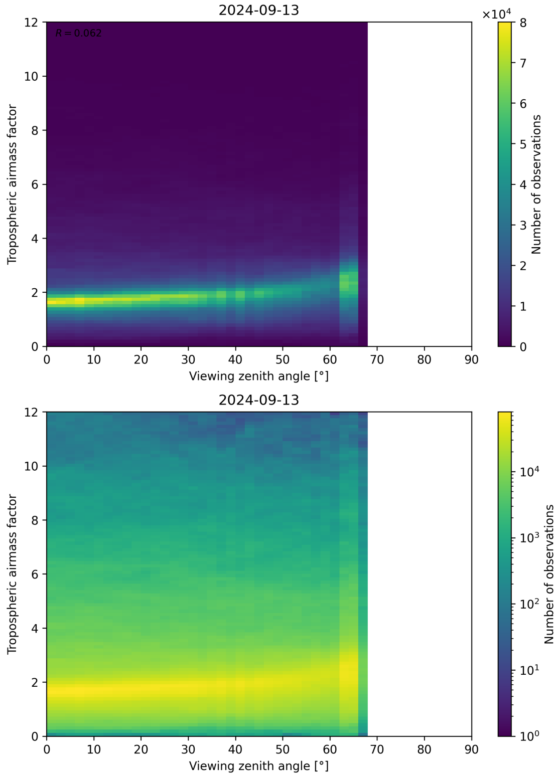
Figure 161: Scatter density plot of “Viewing zenith angle” against “Tropospheric airmass factor” for 2024-09-12 to 2024-09-14.
