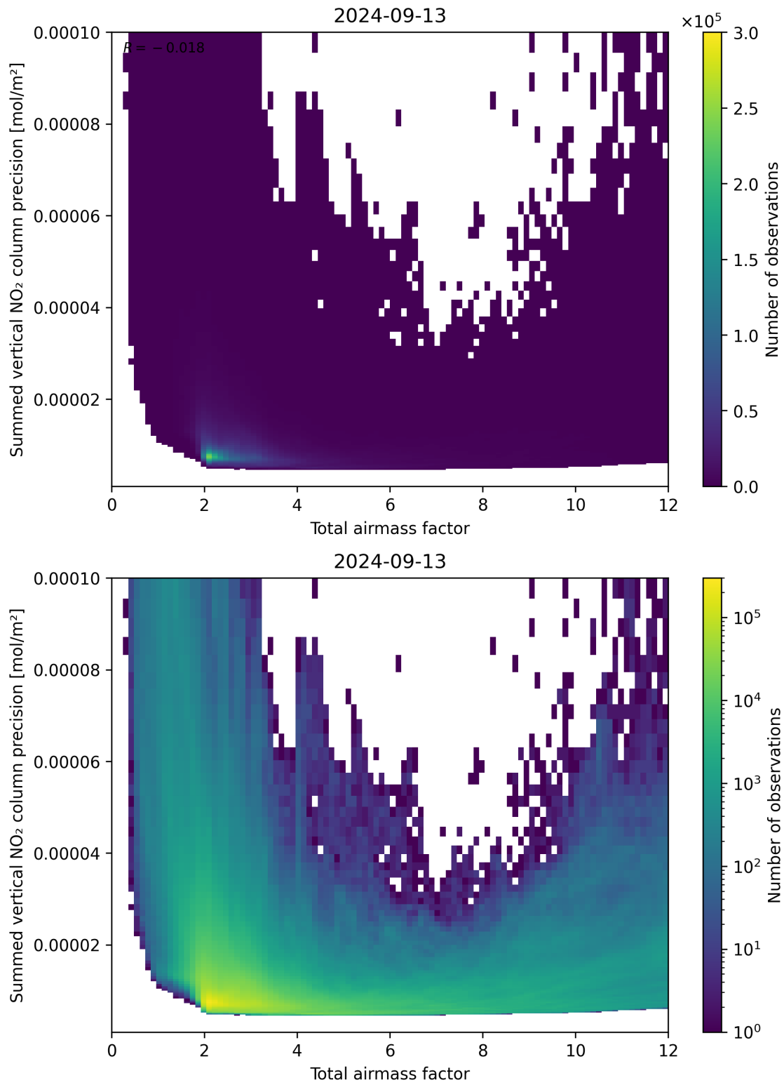
Figure 66: Scatter density plot of “Total airmass factor” against “Summed vertical NO 2 column precision” for 2024-09-12 to 2024-09-14.
