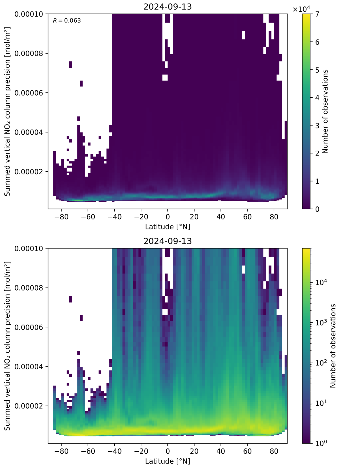
Figure 89: Scatter density plot of “Latitude” against “Summed vertical NO 2 column precision” for 2024-09-12 to 2024-09-14.
