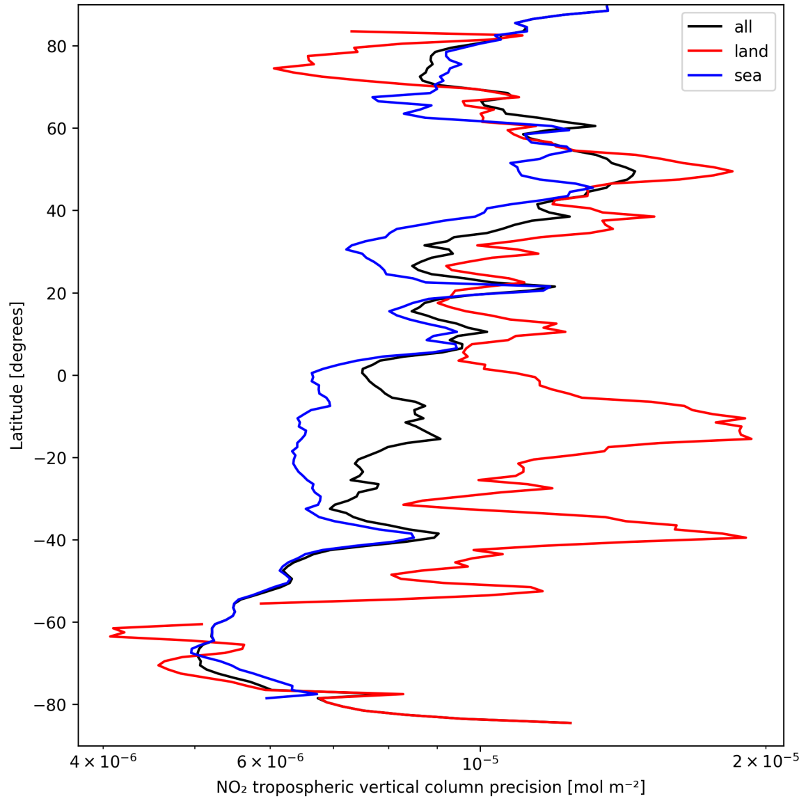
Figure 13: Zonal average of “NO 2 tropospheric vertical column precision” for 2024-09-12 to 2024-09-14.
