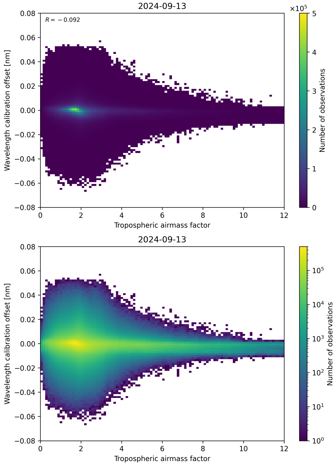
Figure 80: Scatter density plot of “Tropospheric airmass factor” against “Wavelength calibration offset” for 2024-09-12 to 2024-09-14.
