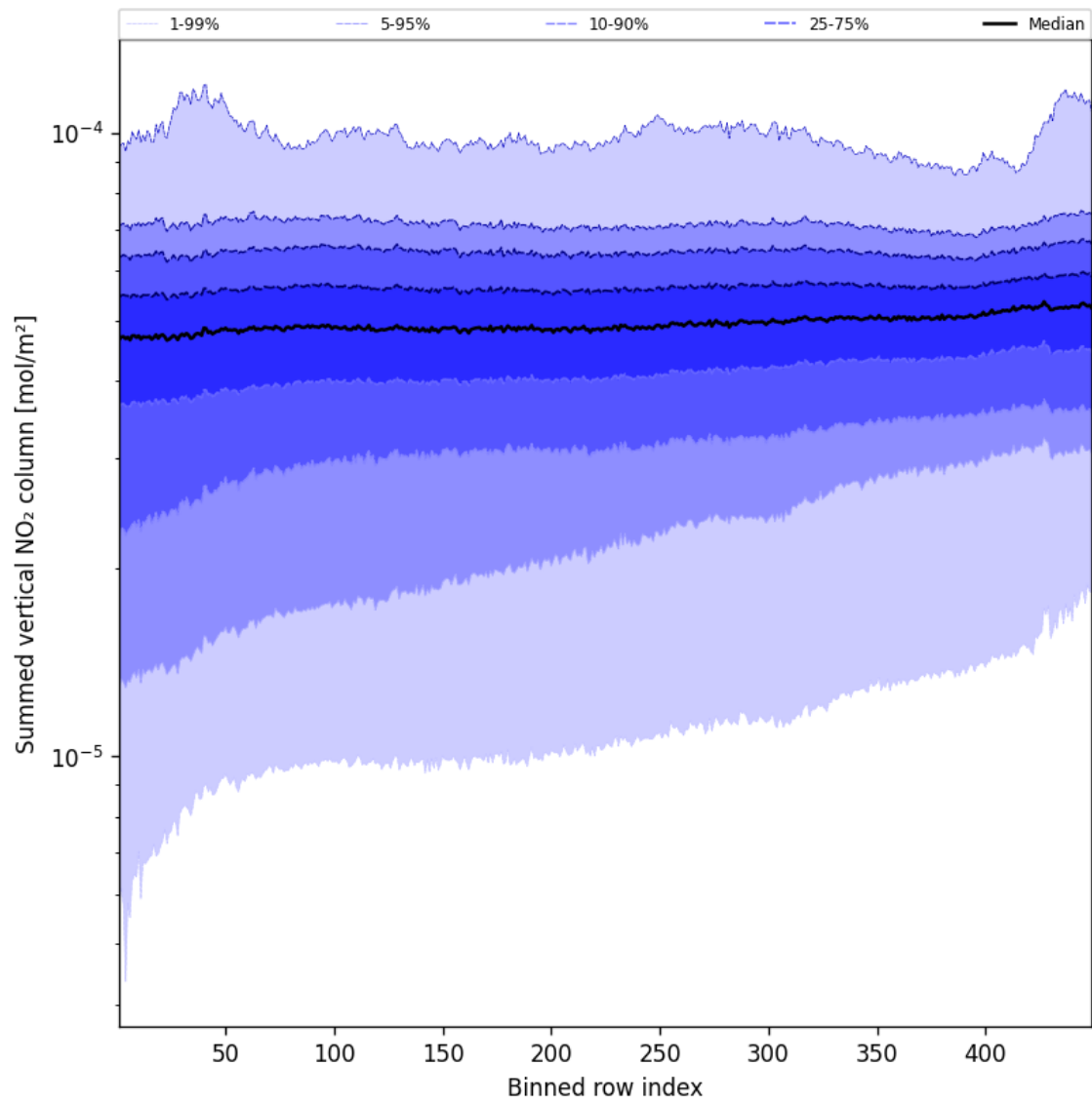
Figure 57: Along track statistics of “Summed vertical NO 2 column” for 2024-09-12 to 2024-09-14
