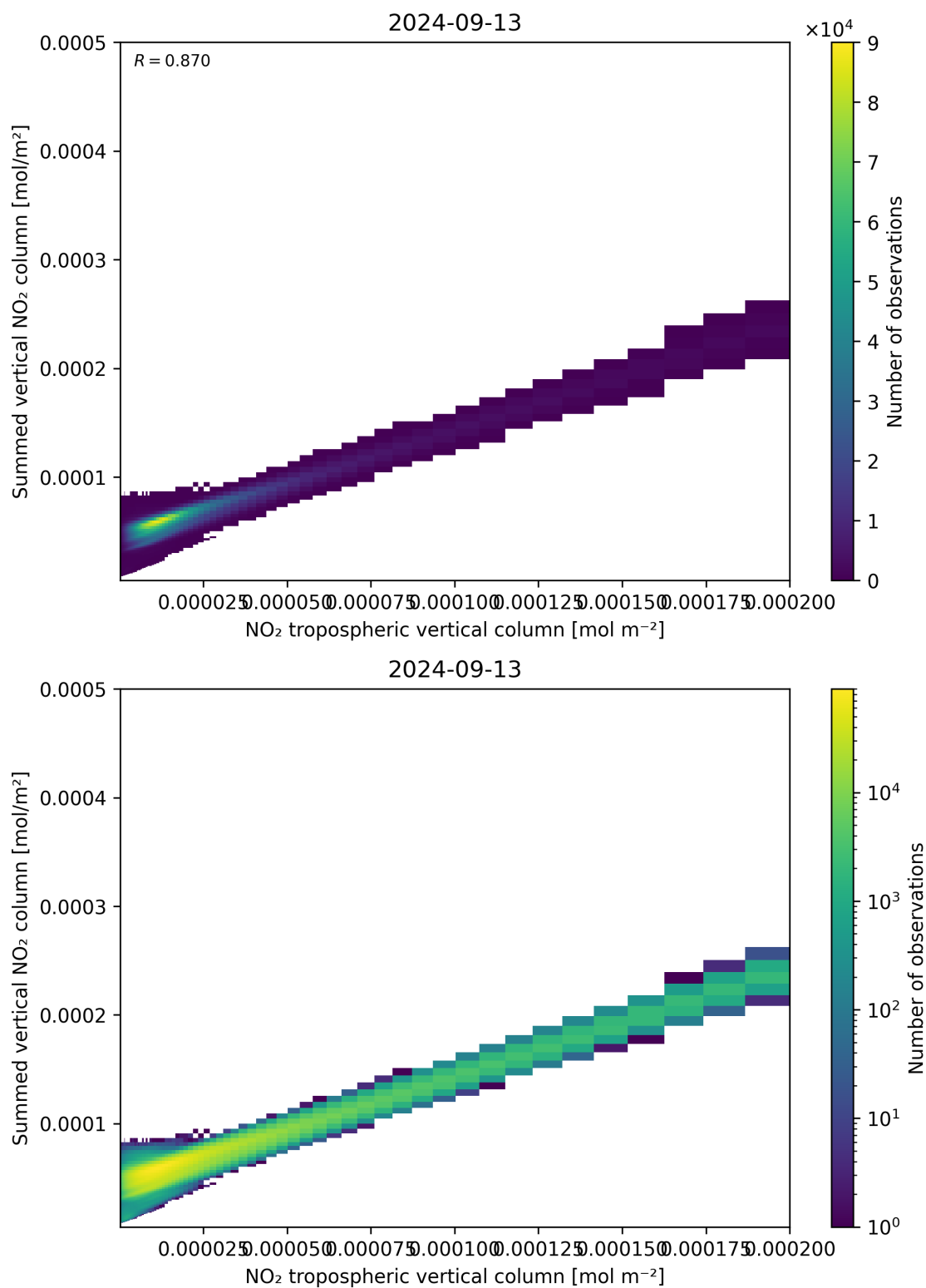
Figure 126: Scatter density plot of “NO 2 tropospheric vertical column” against “Summed vertical NO 2 column” for 2024-09-12 to 2024-09-14.
