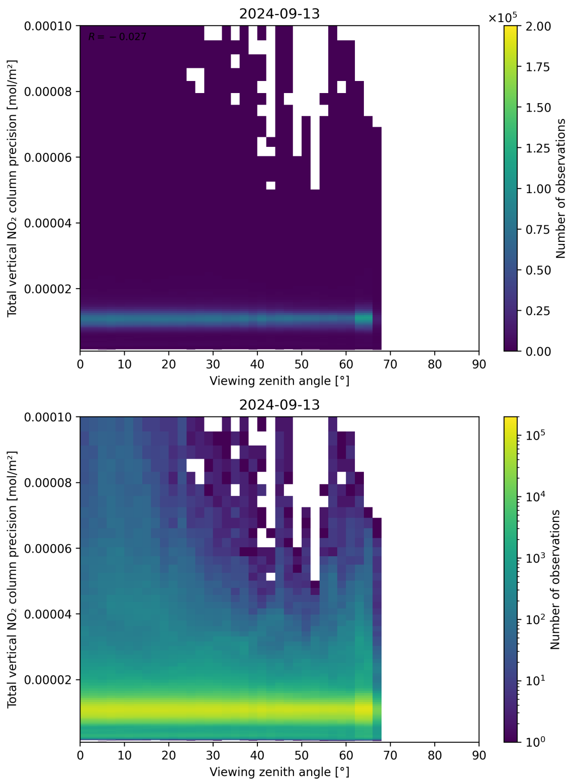
Figure 168: Scatter density plot of “Viewing zenith angle” against “Total vertical NO 2 column precision” for 2024-09-12 to 2024-09-14.
