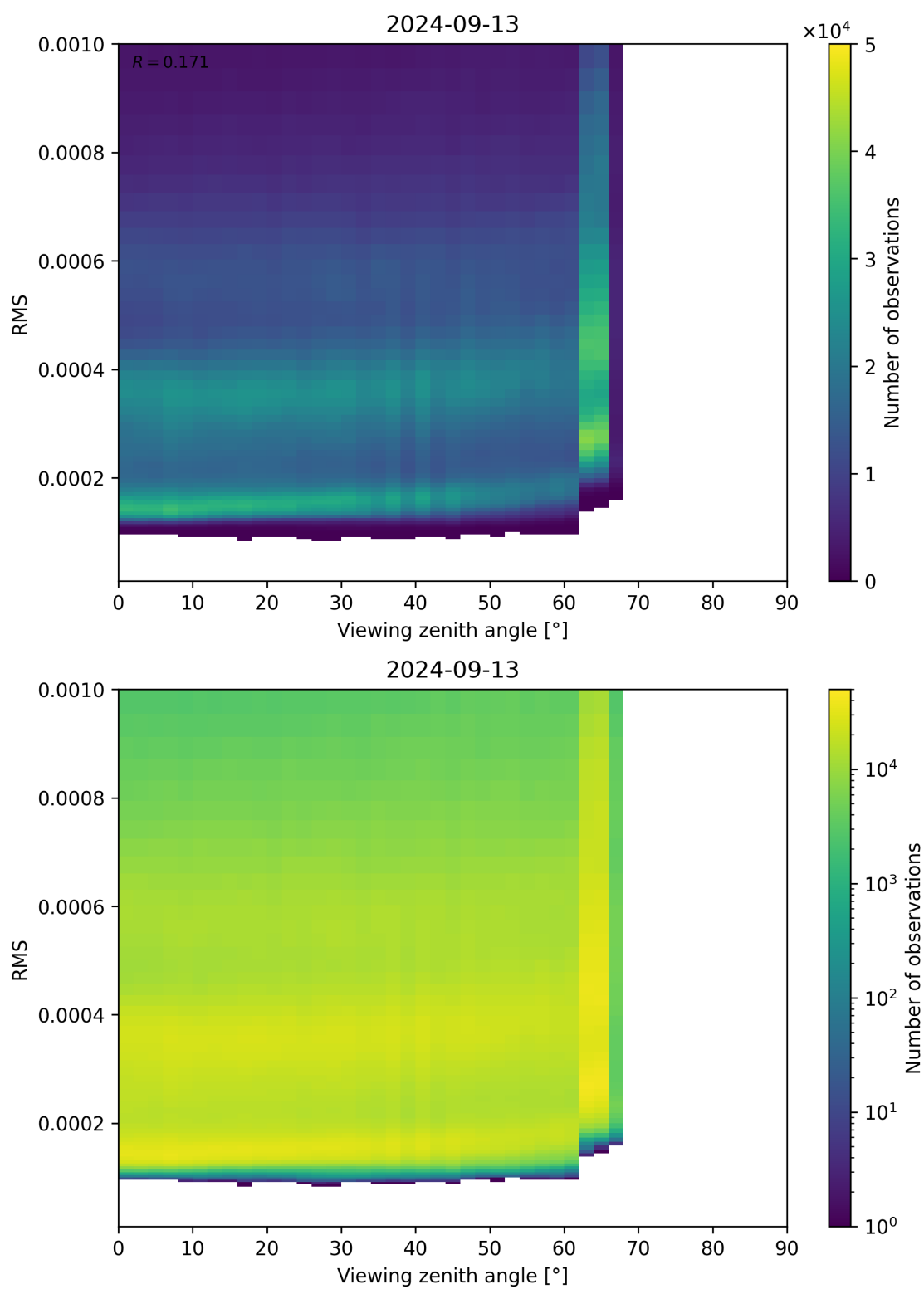
Figure 171: Scatter density plot of “Viewing zenith angle” against “RMS” for 2024-09-12 to 2024-09-14.
