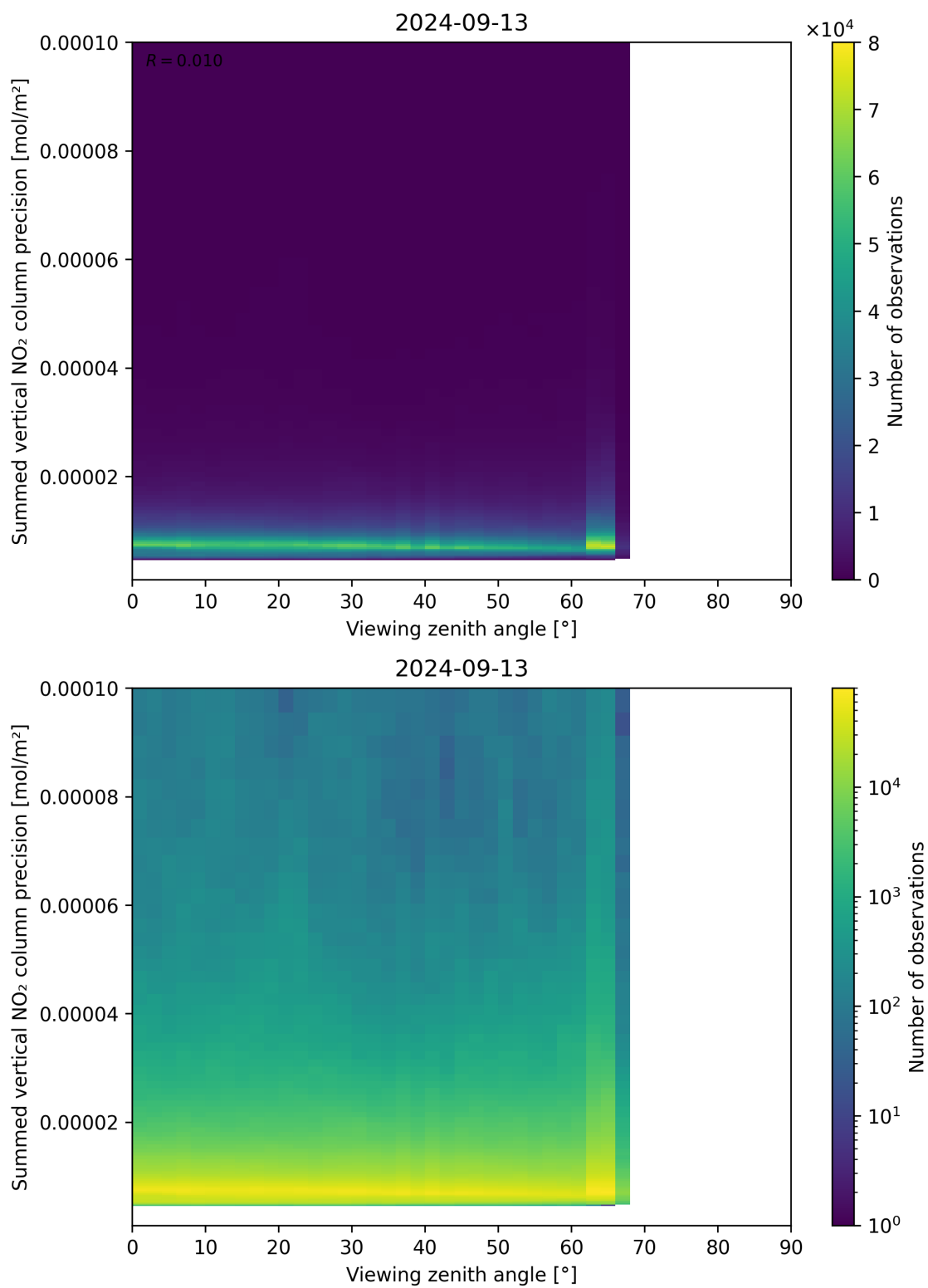
Figure 166: Scatter density plot of “Viewing zenith angle” against “Summed vertical NO 2 column precision” for 2024-09-12 to 2024-09-14.
