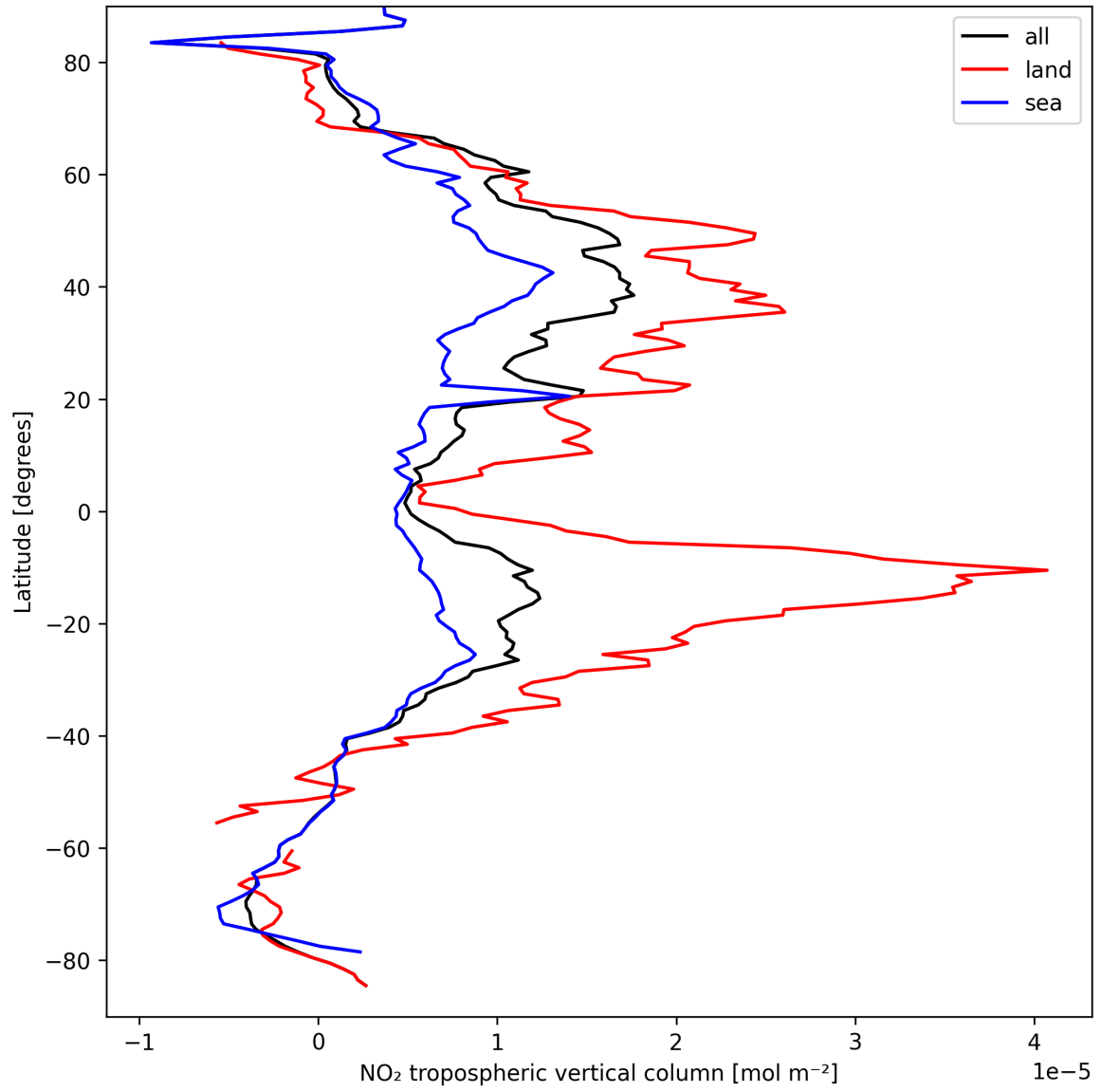
Figure 12: Zonal average of “NO 2 tropospheric vertical column” for 2024-09-12 to 2024-09-14.
