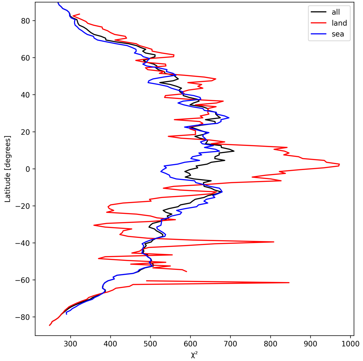
Figure 25: Zonal average of “ \chi^2 ” for 2024-09-12 to 2024-09-14.
