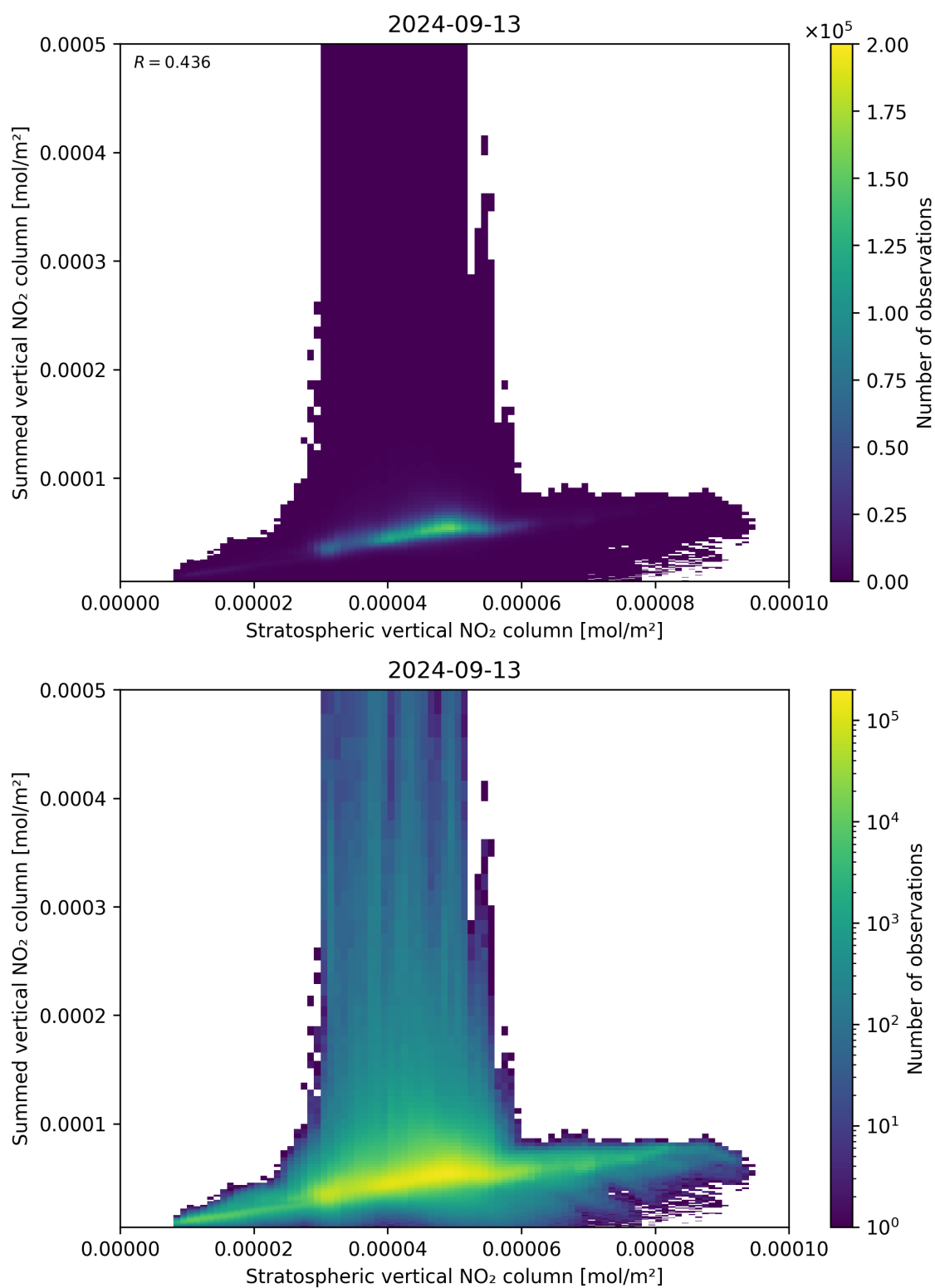
Figure 98: Scatter density plot of “Stratospheric vertical NO 2 column” against “Summed vertical NO 2 column” for 2024-09-12 to 2024-09-14.
