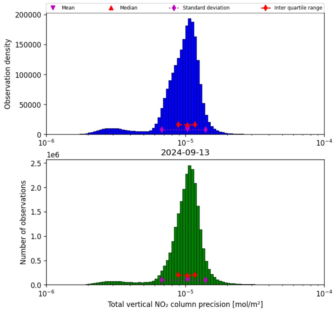
Figure 39: Histogram of "Total vertical NO 2 column precision" for 2024-09-12 to 2024-09-14
