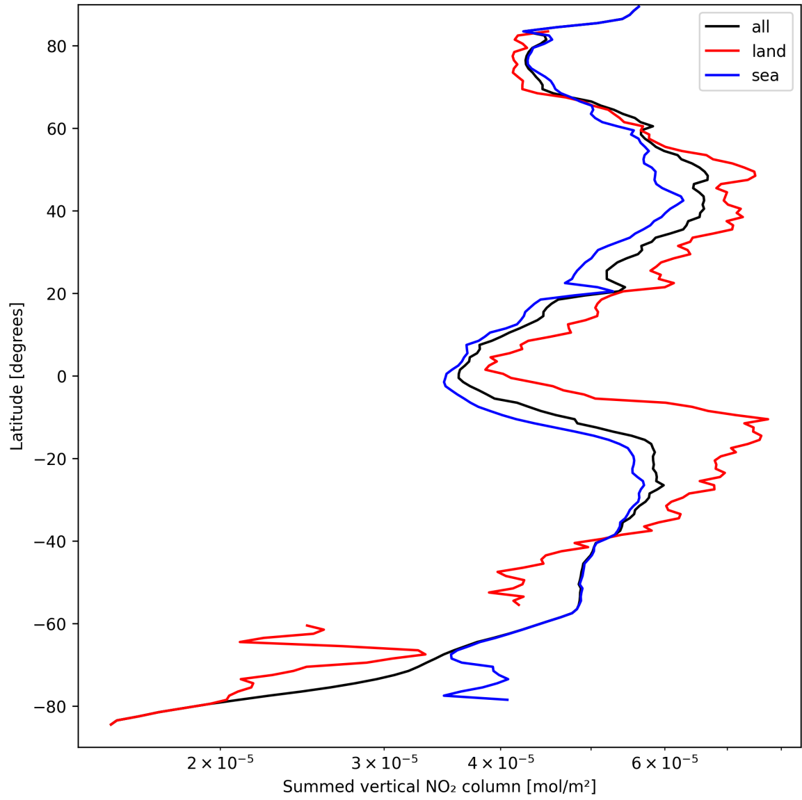
Figure 23: Zonal average of “Summed vertical NO 2 column” for 2024-09-12 to 2024-09-14.
