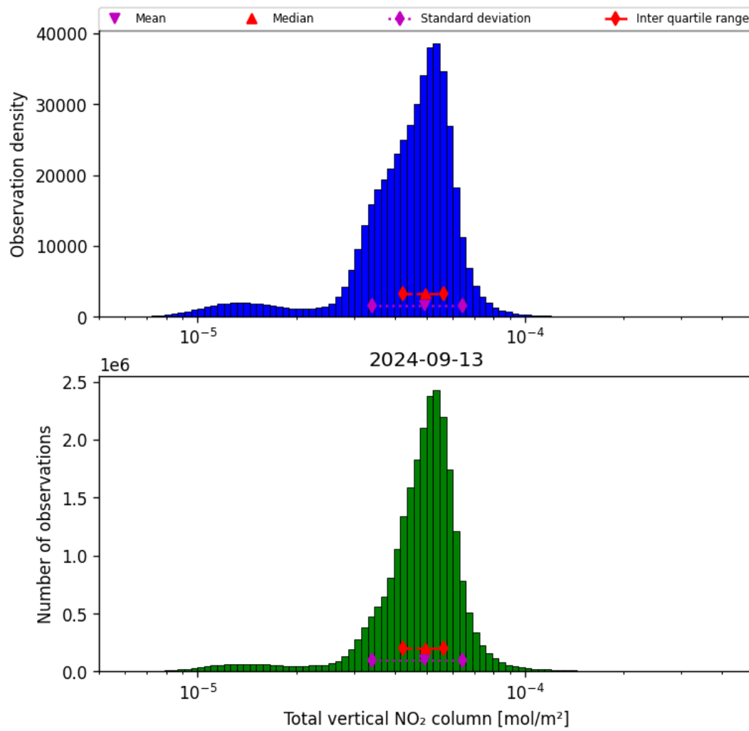
Figure 38: Histogram of “Total vertical NO 2 column” for 2024-09-12 to 2024-09-14
