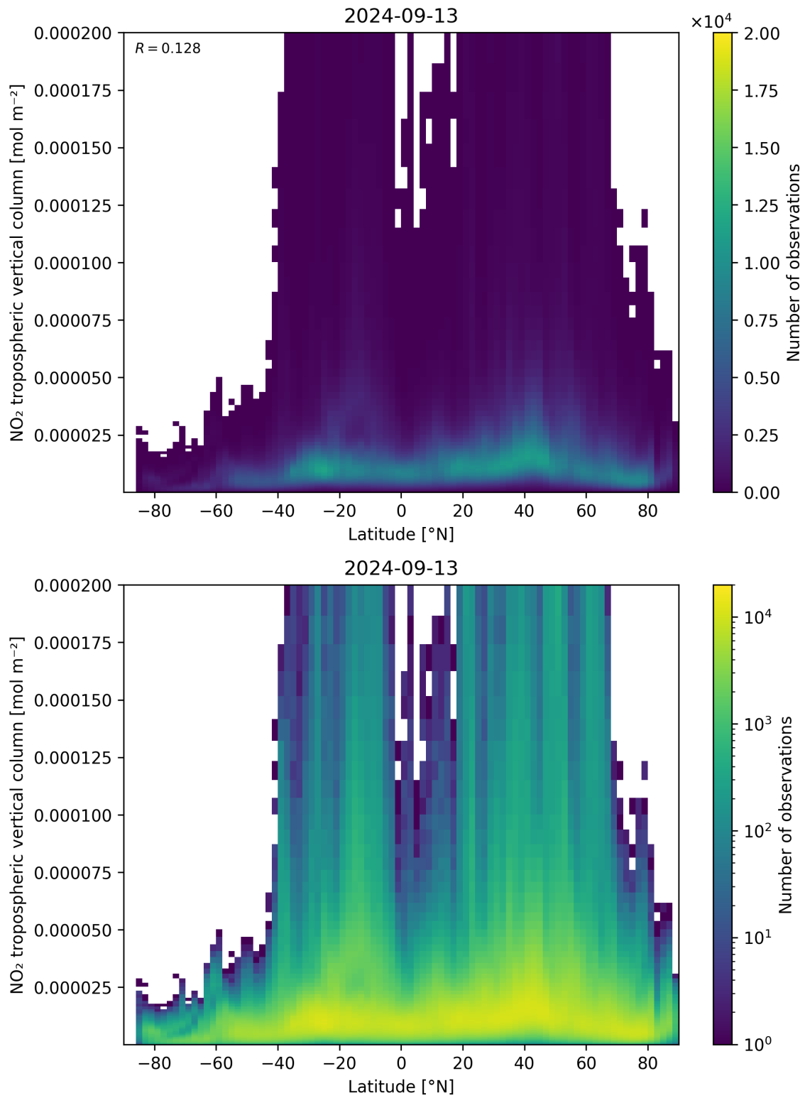
Figure 92: Scatter density plot of “Latitude” against “NO 2 tropospheric vertical column” for 2024-09-12 to 2024-09-14.
