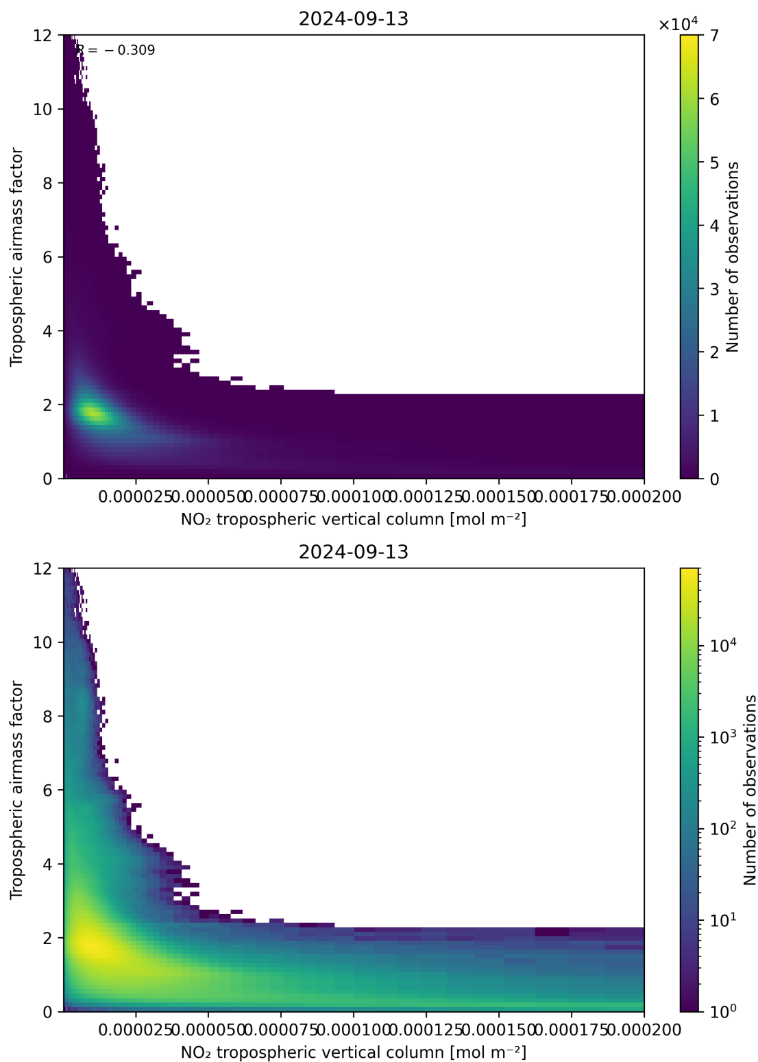
Figure 123: Scatter density plot of “NO 2 tropospheric vertical column” against “Tropospheric air mass factor” for 2024-09-12 to 2024-09-14.
