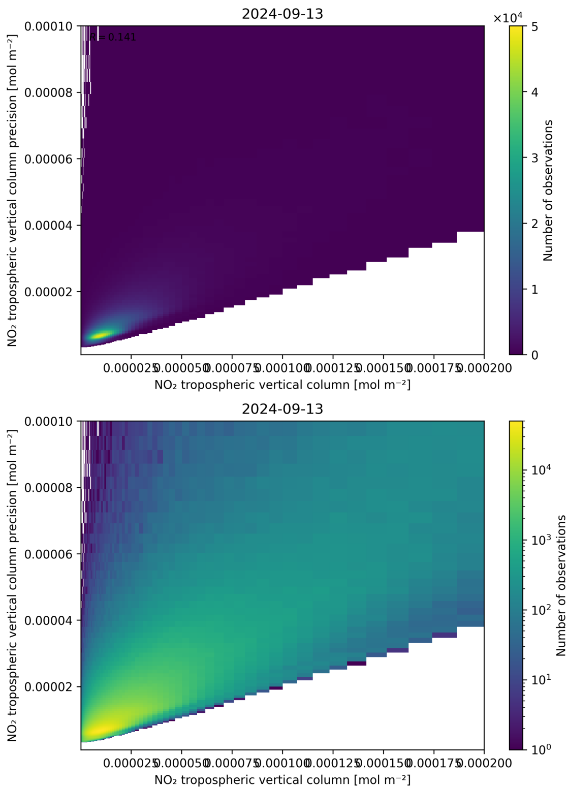
Figure 130: Scatter density plot of “NO 2 tropospheric vertical column” against “NO 2 tropospheric vertical column precision” for 2024-09-12 to 2024-09-14.
