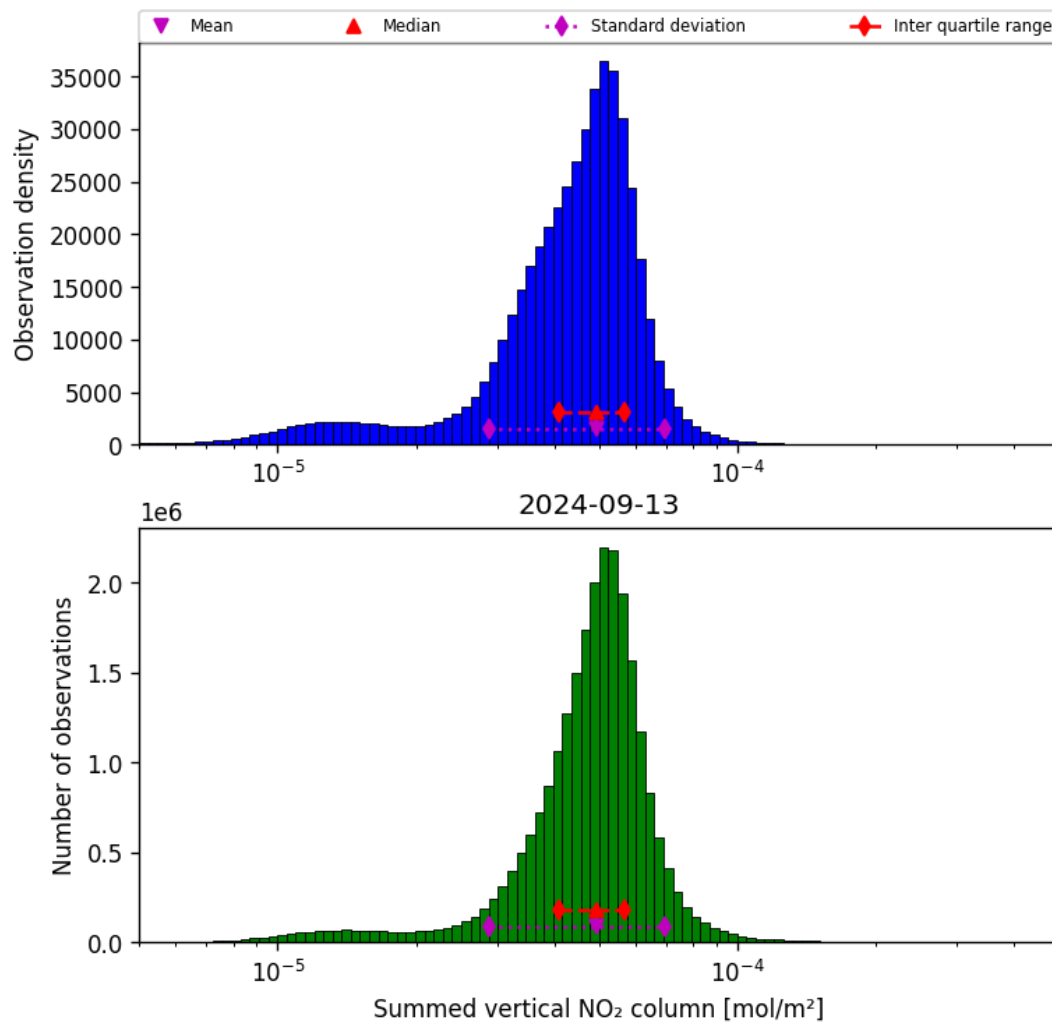
Figure 40: Histogram of “Summed vertical NO 2 column” for 2024-09-12 to 2024-09-14
