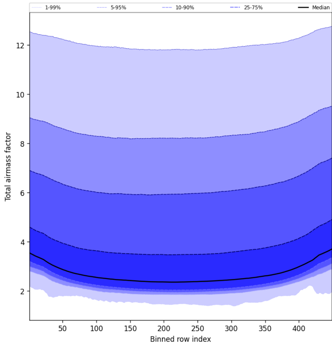
Figure 49: Along track statistics of “Total airmass factor” for 2024-09-12 to 2024-09-14
