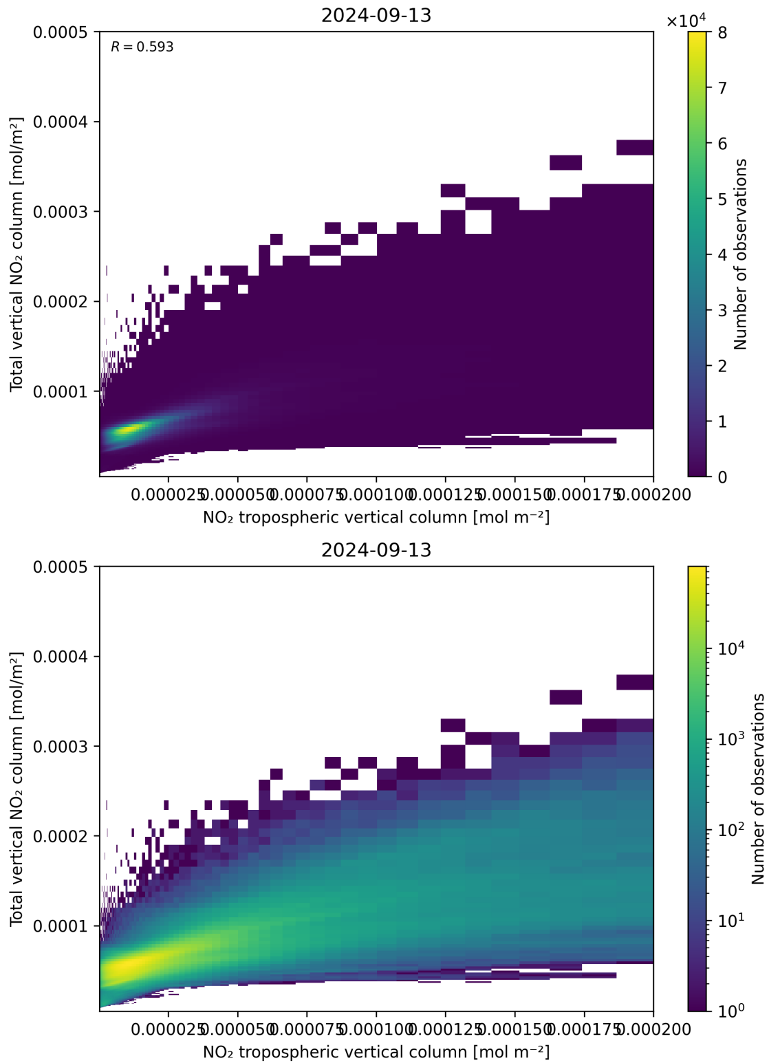
Figure 128: Scatter density plot of “NO 2 tropospheric vertical column” against “Total vertical NO 2 column” for 2024-09-12 to 2024-09-14.
