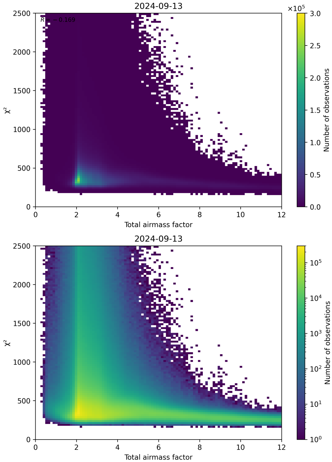
Figure 63: Scatter density plot of “Total airmass factor” against “ \chi^2 ” for 2024-09-12 to 2024-09-14.
