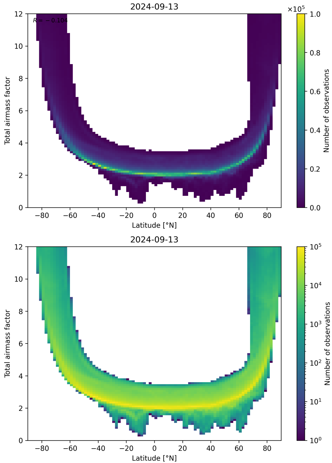
Figure 84: Scatter density plot of “Latitude” against “Total airmass factor” for 2024-09-12 to 2024-09-14.
