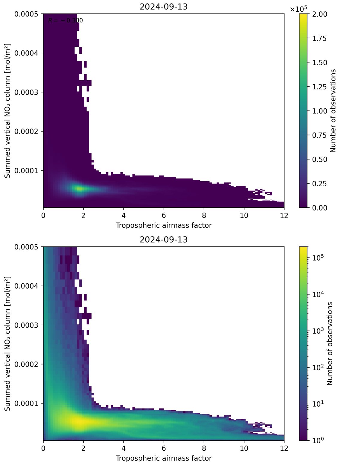
Figure 75: Scatter density plot of “Tropospheric air mass factor” against “Summed vertical NO 2 column” for 2024-09-12 to 2024-09-14.
