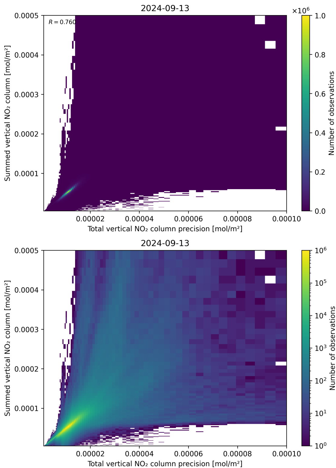
Figure 117: Scatter density plot of “Total vertical NO 2 column precision” against “Summed vertical NO 2 column” for 2024-09-12 to 2024-09-14.
