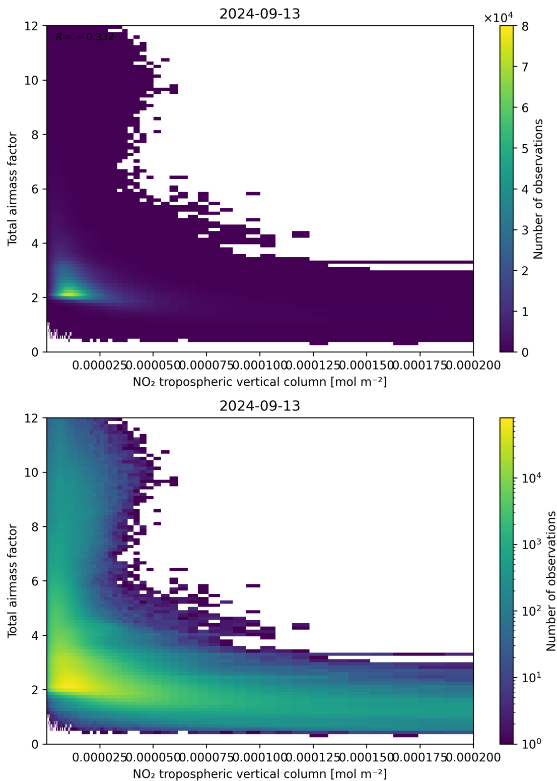
Figure 122: Scatter density plot of “NO 2 tropospheric vertical column” against “Total air mass factor” for 2024-09-12 to 2024-09-14.
