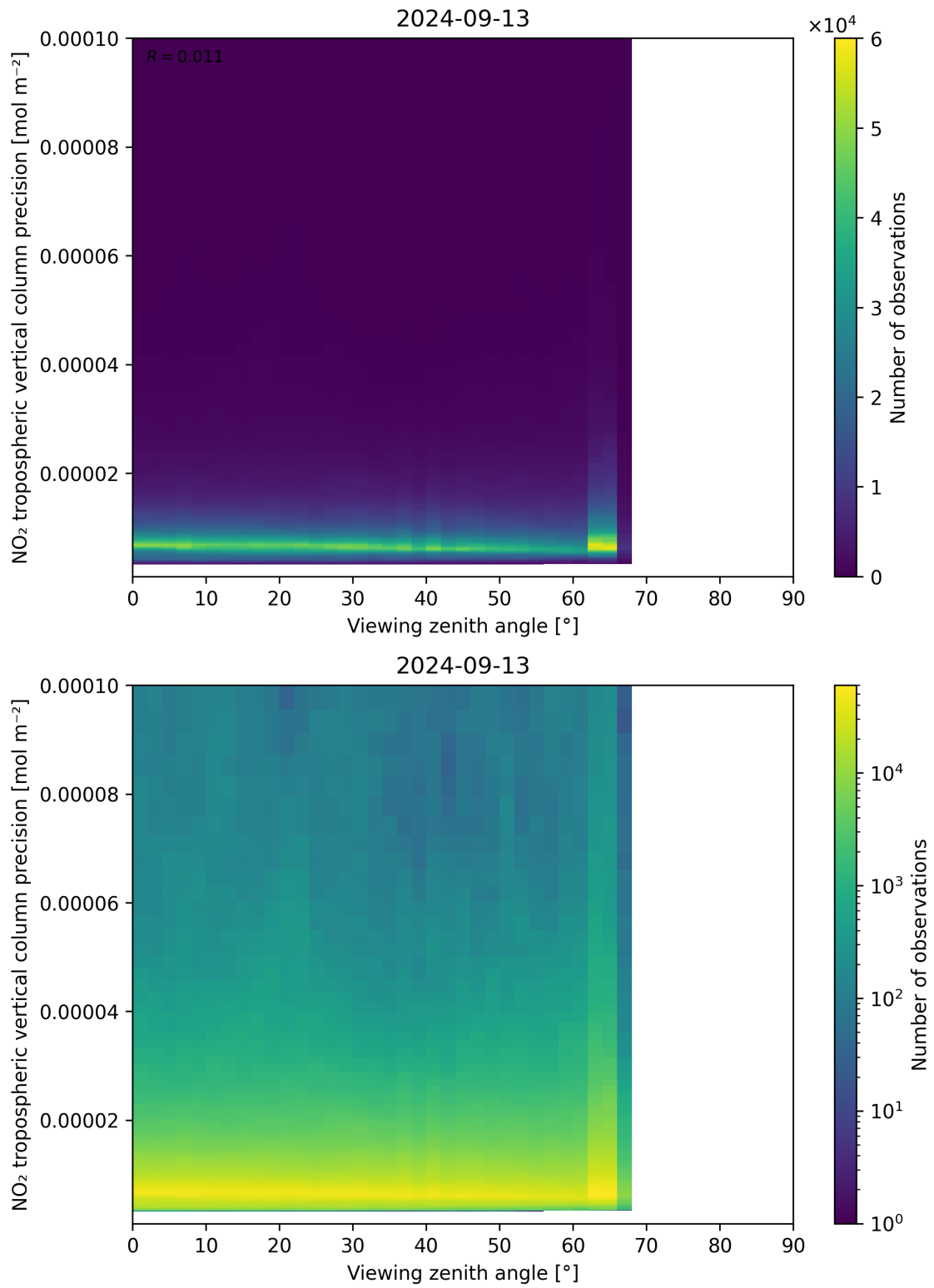
Figure 170: Scatter density plot of “Viewing zenith angle” against “NO 2 tropospheric vertical column precision” for 2024-09-12 to 2024-09-14.
