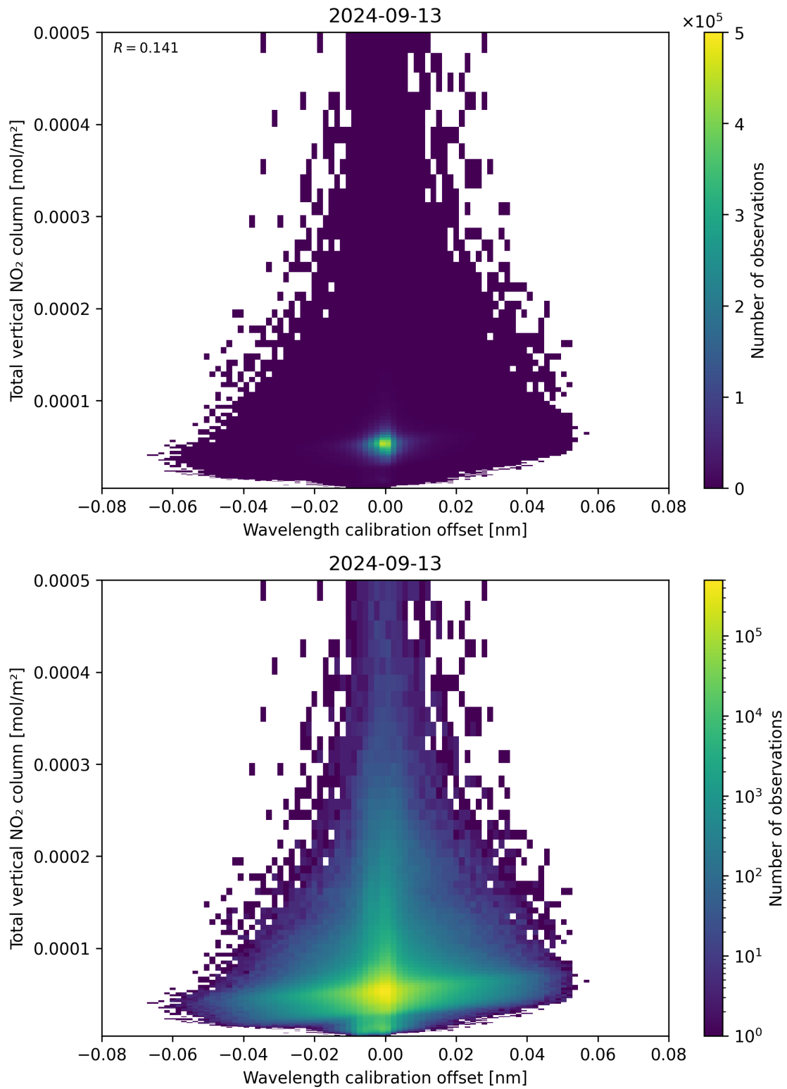
Figure 179: Scatter density plot of “Wavelength calibration offset” against “Total vertical NO 2 column” for 2024-09-12 to 2024-09-14.
