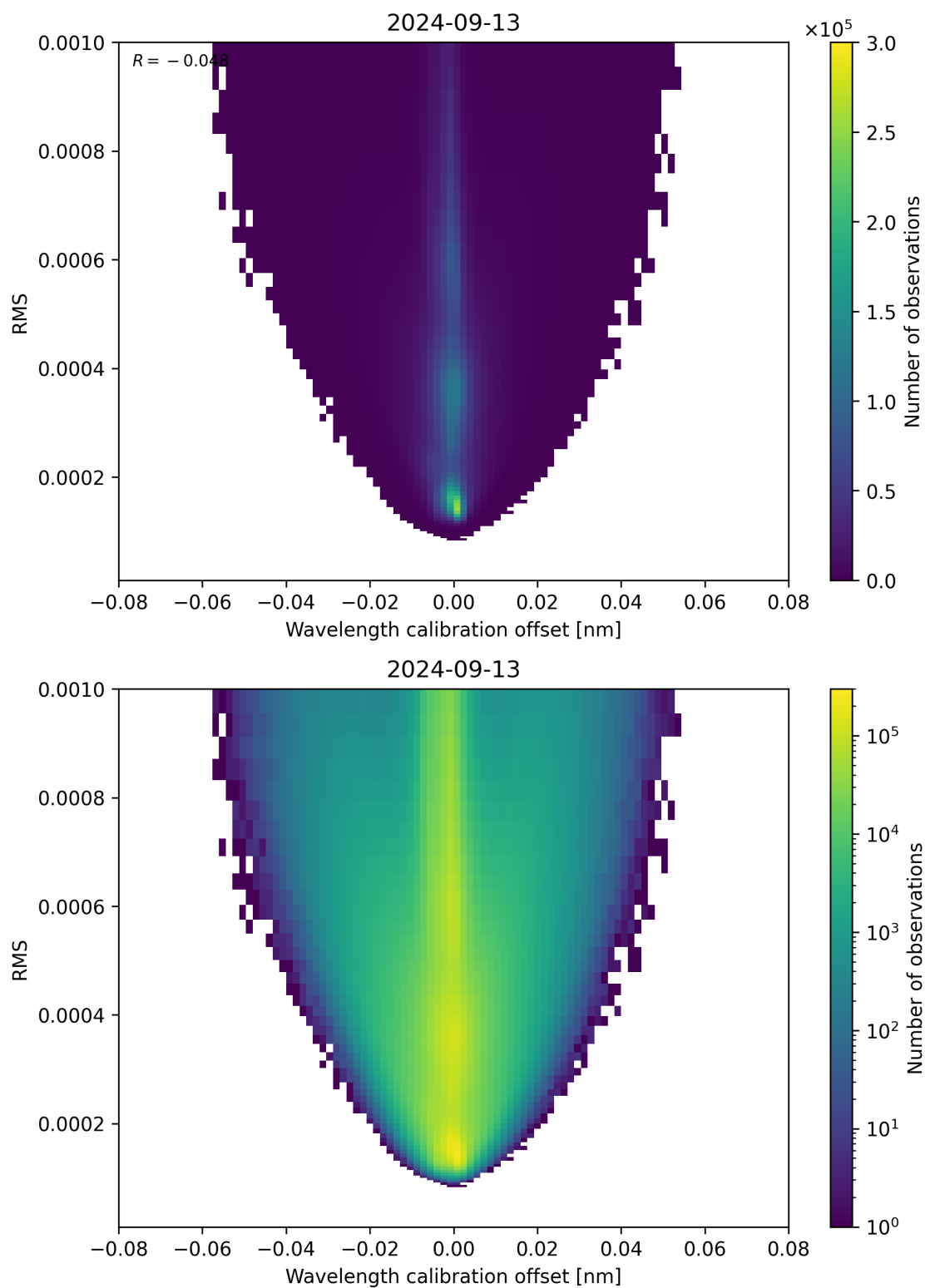
Figure 181: Scatter density plot of “Wavelength calibration offset” against “RMS” for 2024-09-12 to 2024-09-14.
