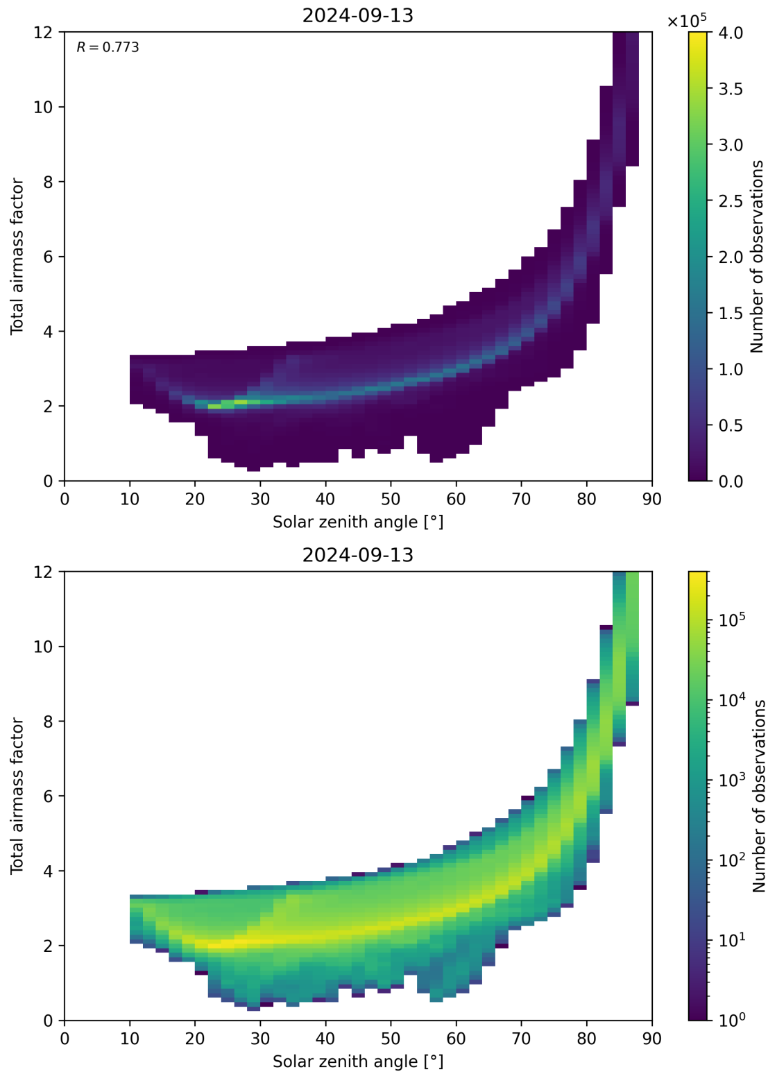
Figure 146: Scatter density plot of “Solar zenith angle” against “Total airmass factor” for 2024-09-12 to 2024-09-14.
