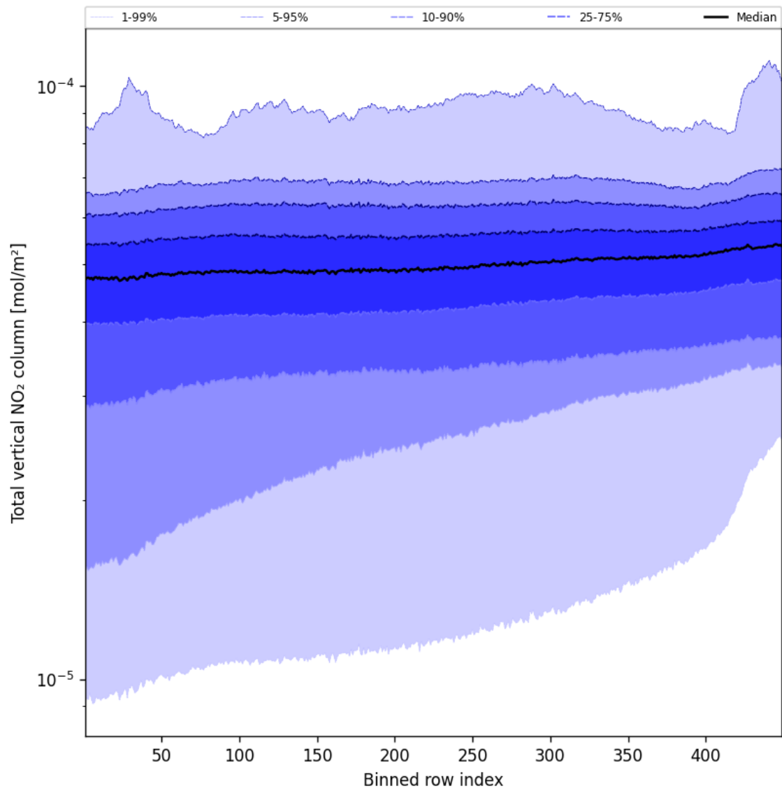
Figure 55: Along track statistics of “Total vertical NO 2 column” for 2024-09-12 to 2024-09-14
