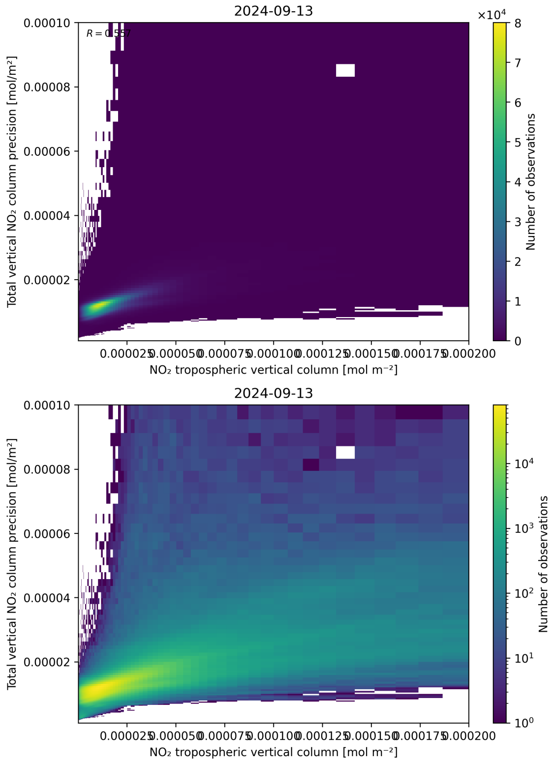
Figure 129: Scatter density plot of “NO 2 tropospheric vertical column” against “Total vertical NO 2 column precision” for 2024-09-12 to 2024-09-14.
