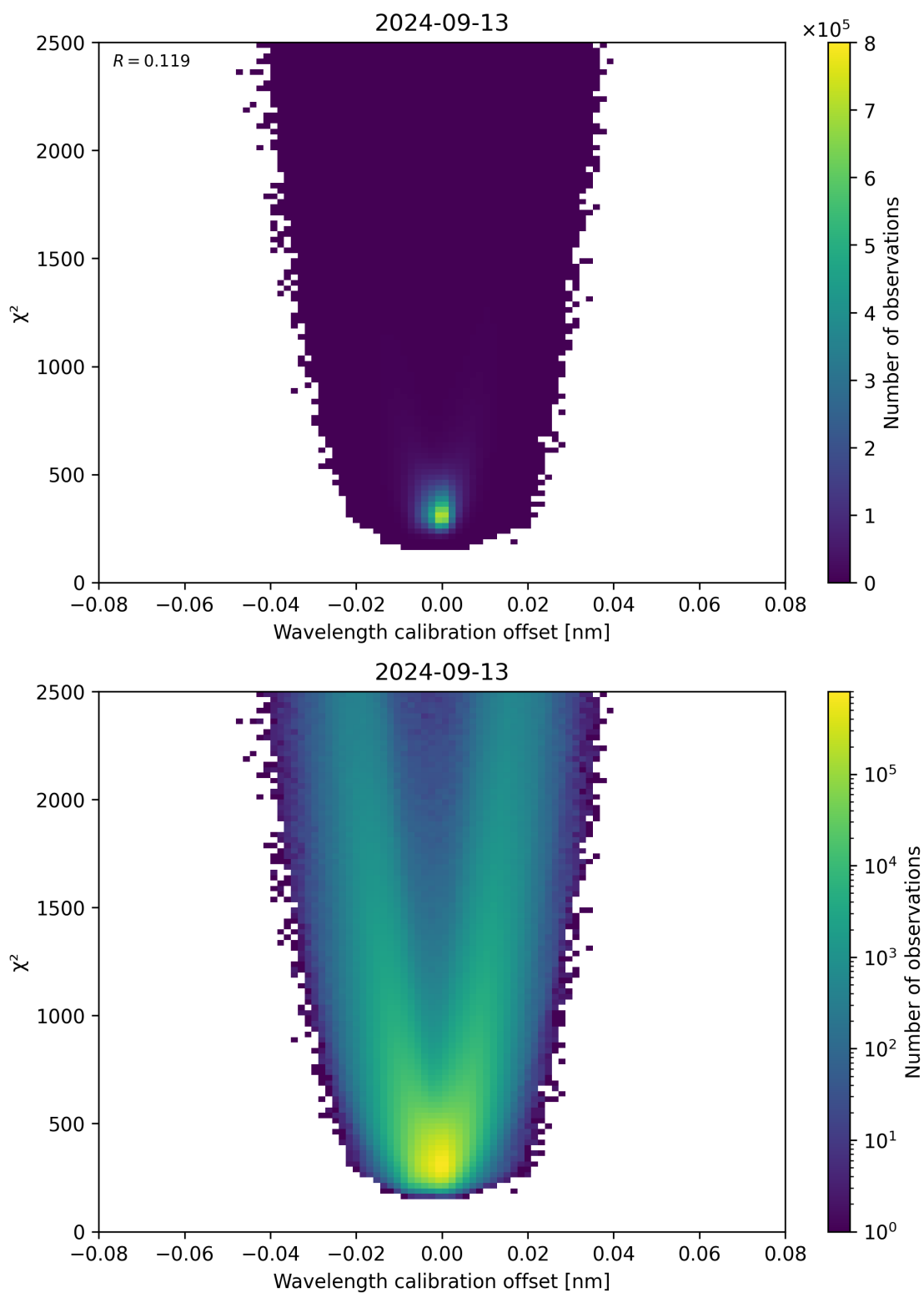
Figure 175: Scatter density plot of “Wavelength calibration offset” against “ \chi^2 ” for 2024-09-12 to 2024-09-14.
