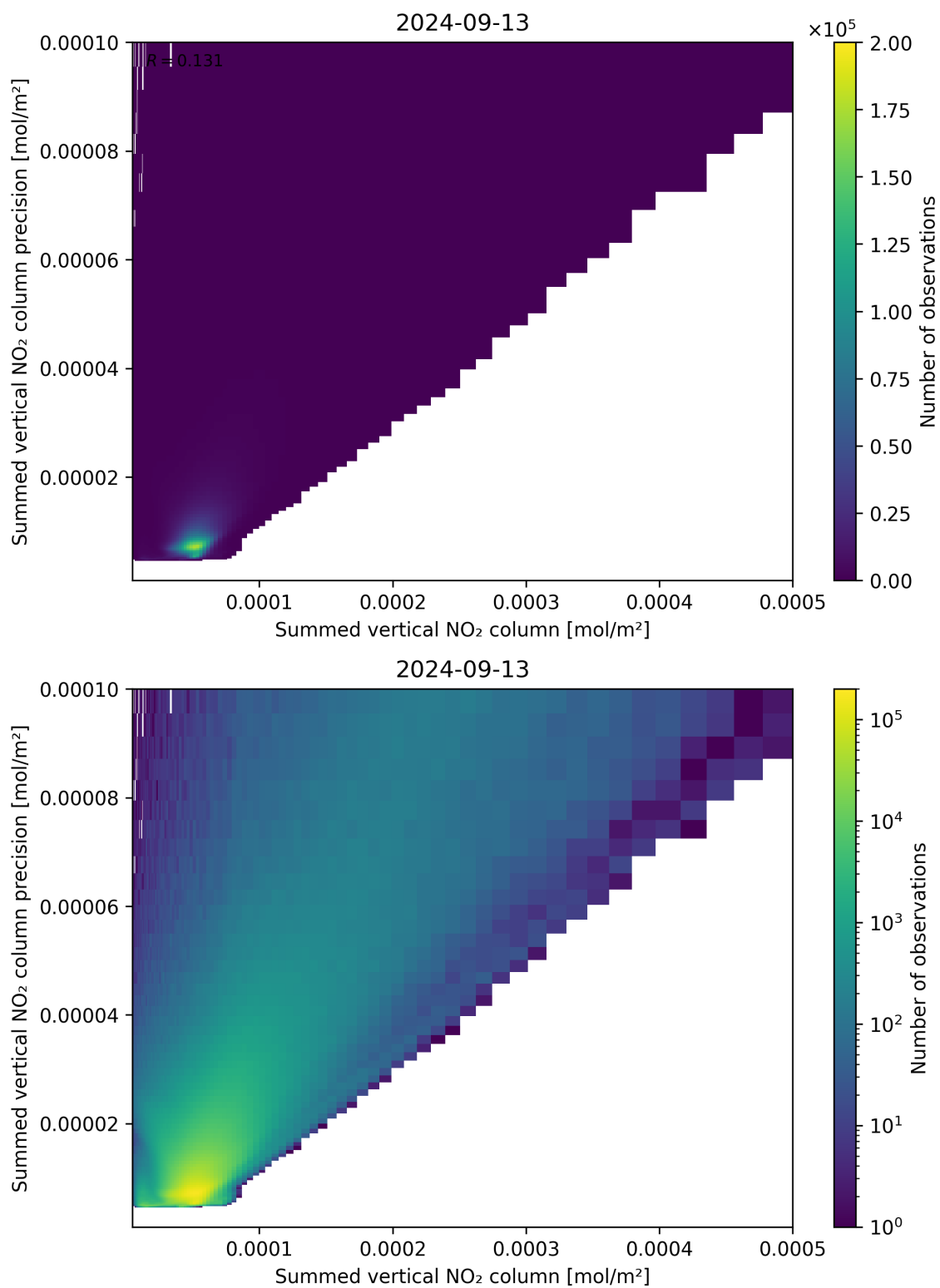
Figure 105: Scatter density plot of “Summed vertical NO 2 column” against “Summed vertical NO 2 column precision” for 2024-09-12 to 2024-09-14.
