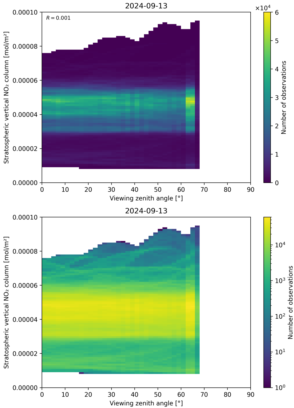
Figure 164: Scatter density plot of “Viewing zenith angle” against “Stratospheric vertical NO 2 column” for 2024-09-12 to 2024-09-14.
