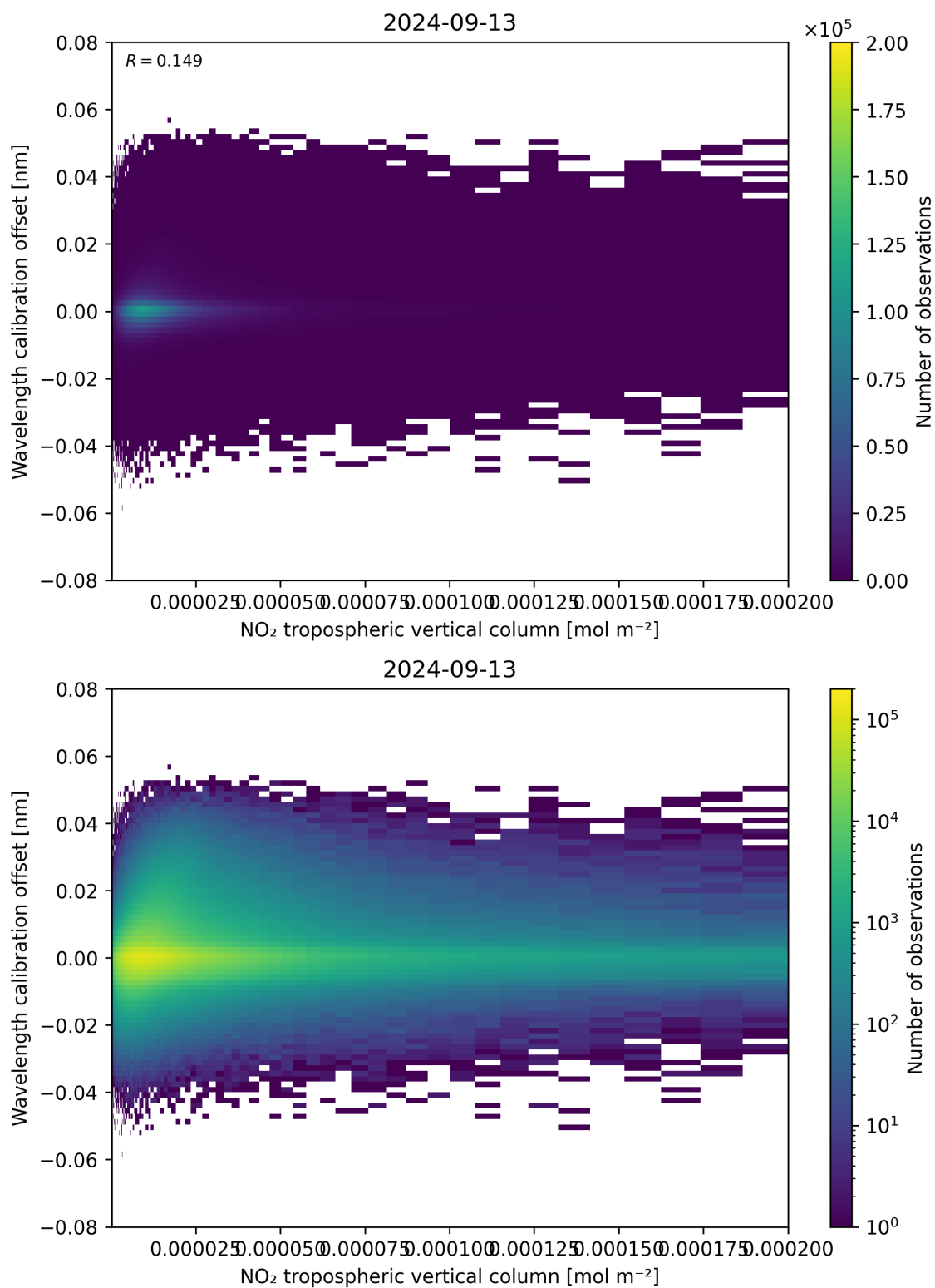
Figure 143: Scatter density plot of “NO 2 tropospheric vertical column” against “Wavelength calibration offset” for 2024-09-12 to 2024-09-14.
