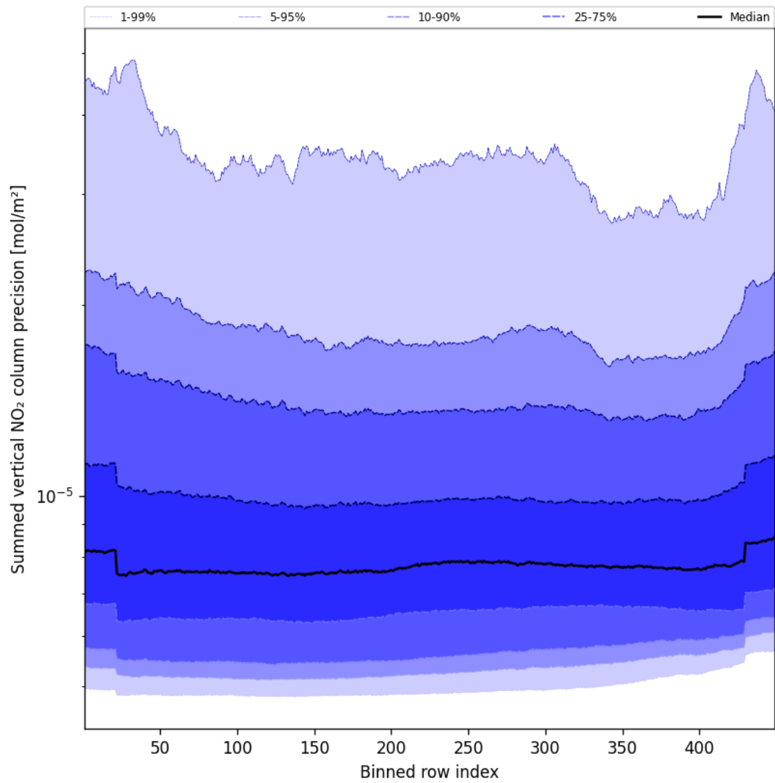
Figure 58: Along track statistics of “Summed vertical NO 2 column precision” for 2024-09-12 to 2024-09-14
