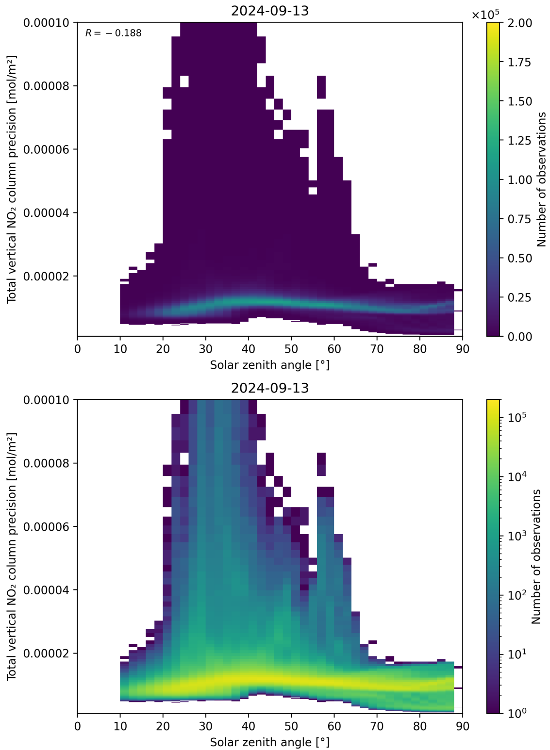
Figure 154: Scatter density plot of “Solar zenith angle” against “Total vertical NO 2 column precision” for 2024-09-12 to 2024-09-14.
