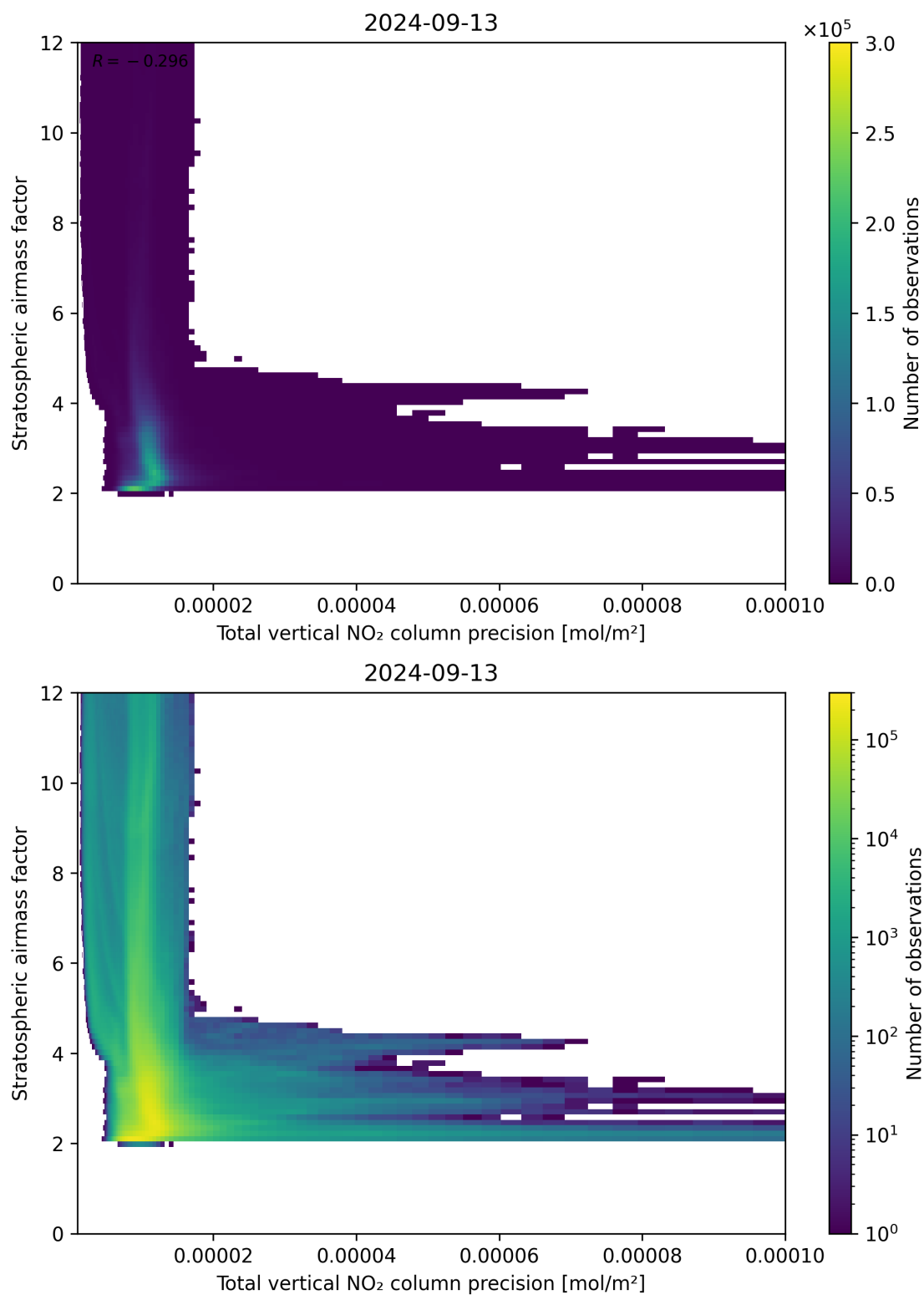
Figure 115: Scatter density plot of “Total vertical NO 2 column precision” against “Stratospheric airmass factor” for 2024-09-12 to 2024-09-14.
