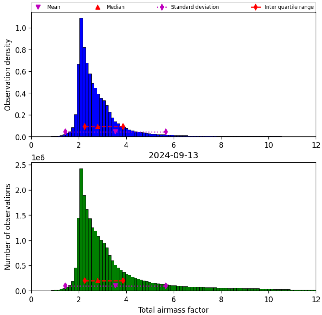
Figure 32: Histogram of “Total airmass factor” for 2024-09-12 to 2024-09-14
