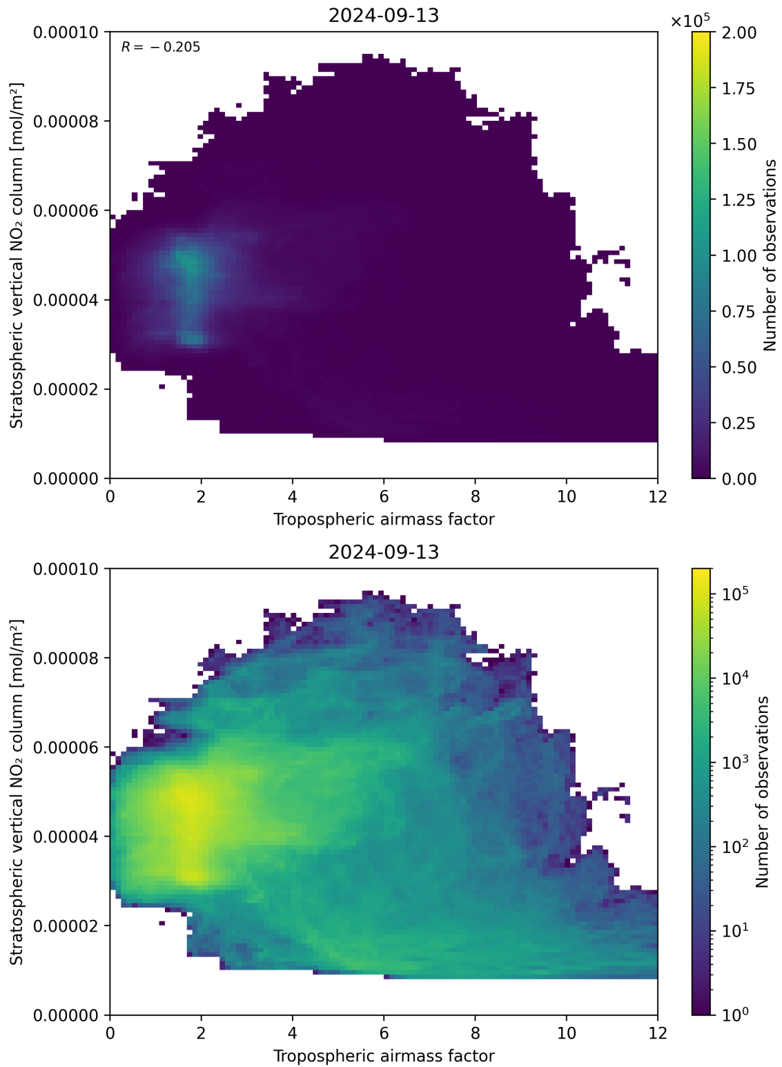
Figure 74: Scatter density plot of “Tropospheric air mass factor” against “Stratospheric vertical NO 2 column” for 2024-09-12 to 2024-09-14.
