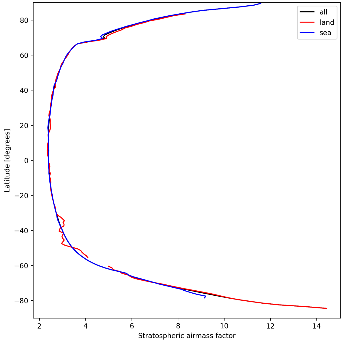
Figure 27: Zonal average of “Stratospheric airmass factor” for 2024-09-12 to 2024-09-14.
