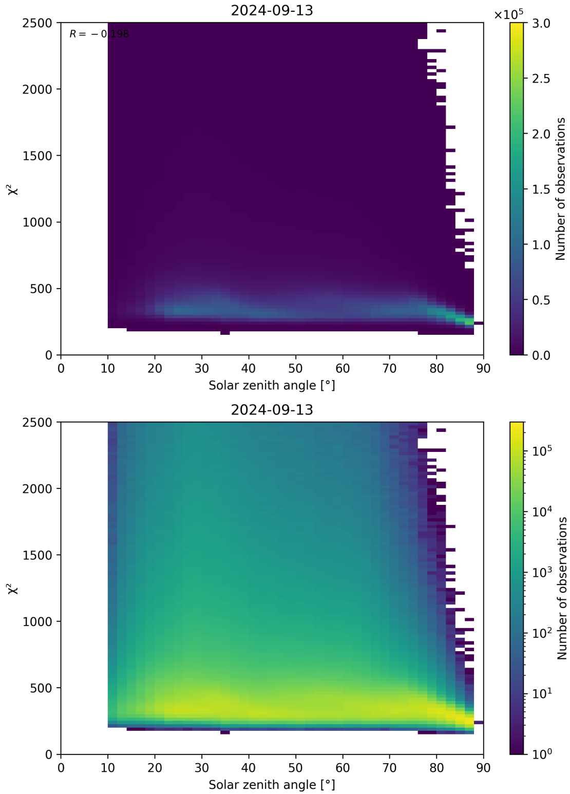
Figure 148: Scatter density plot of “Solar zenith angle” against “ \chi^2 ” for 2024-09-12 to 2024-09-14.
