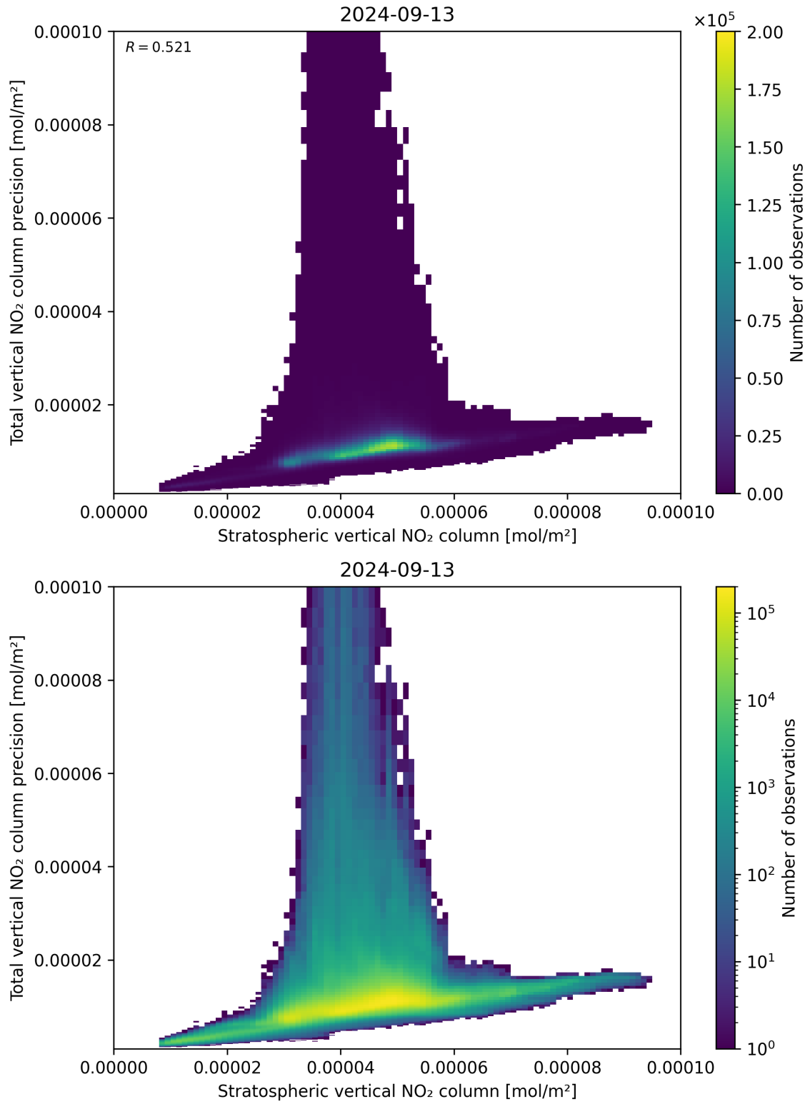
Figure 101: Scatter density plot of “Stratospheric vertical NO 2 column” against “Total vertical NO 2 column precision” for 2024-09-12 to 2024-09-14.
