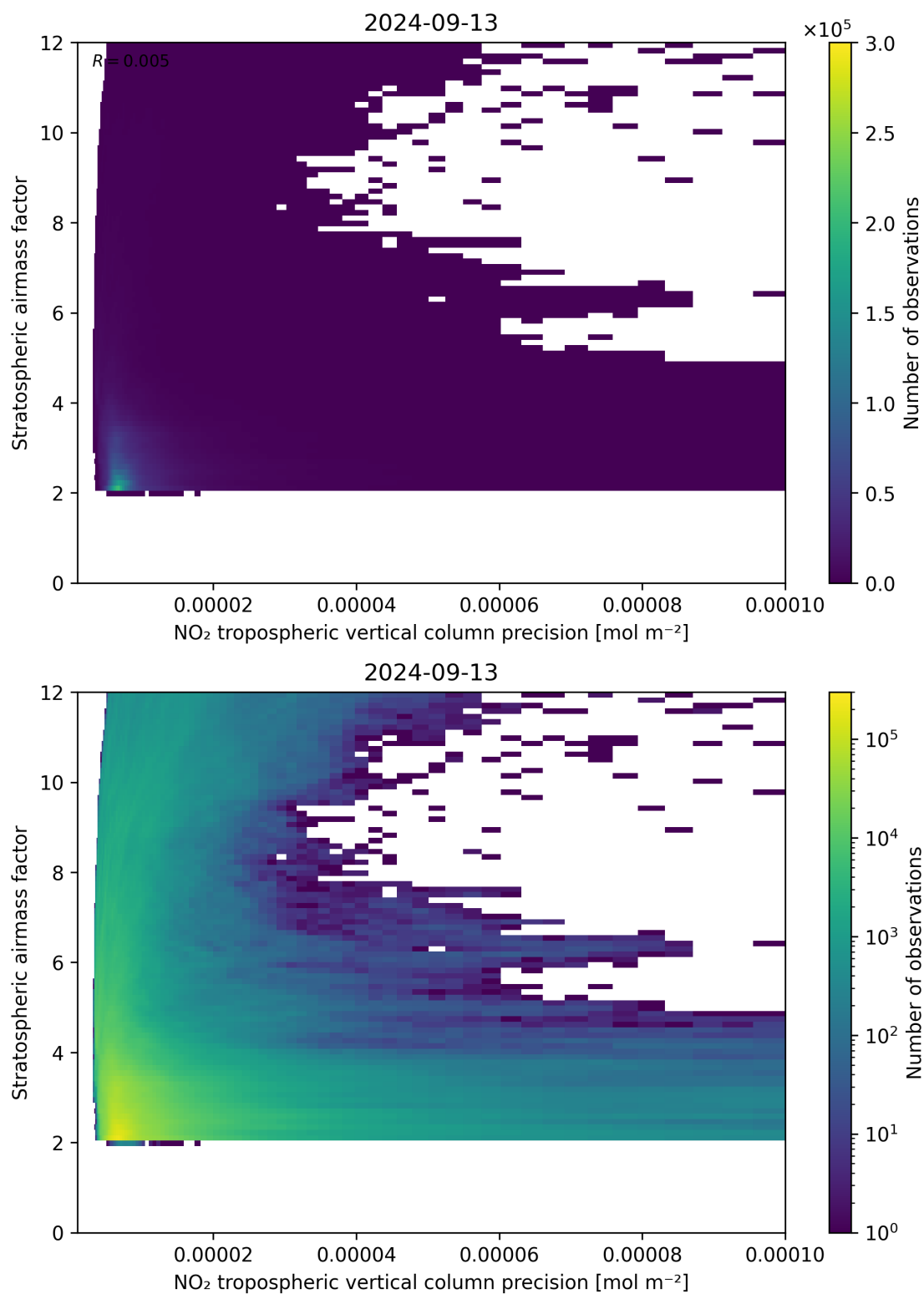
Figure 131: Scatter density plot of “NO 2 tropospheric vertical column precision” against “Stratospheric airmass factor” for 2024-09-12 to 2024-09-14.
