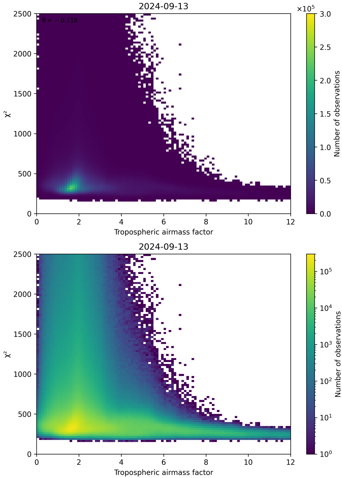
Figure 73: Scatter density plot of “Tropospheric airmass factor” against “ \chi^2 ” for 2024-09-12 to 2024-09-14.
