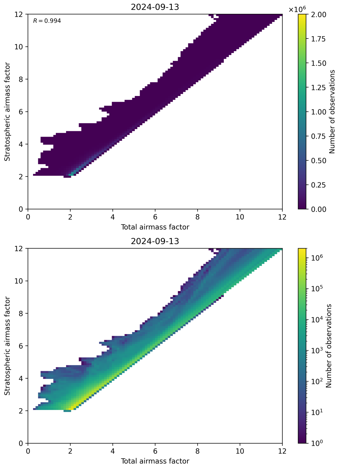
Figure 62: Scatter density plot of “Total airmass factor” against “Stratospheric airmass factor” for 2024-09-12 to 2024-09-14.
