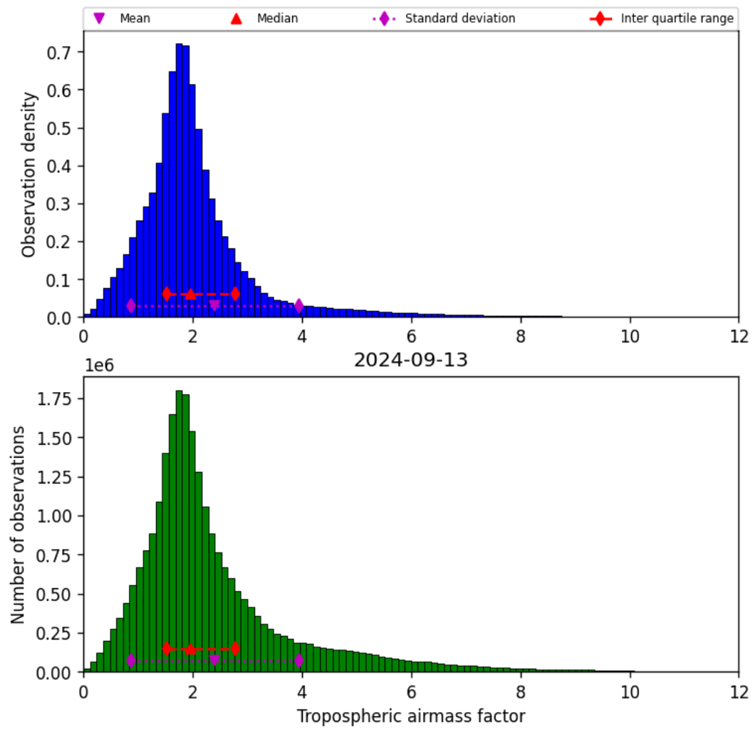
Figure 31: Histogram of “Tropospheric airmass factor” for 2024-09-12 to 2024-09-14
