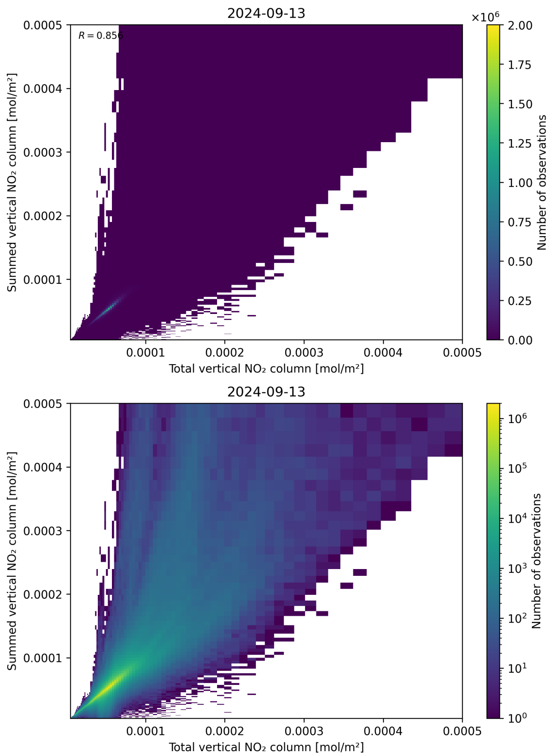
Figure 112: Scatter density plot of “Total vertical NO 2 column” against “Summed vertical NO 2 column” for 2024-09-12 to 2024-09-14.
