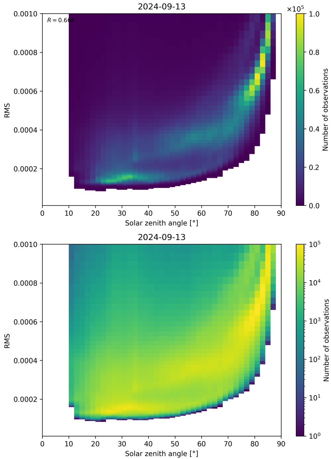
Figure 157: Scatter density plot of “Solar zenith angle” against “RMS” for 2024-09-12 to 2024-09-14.
