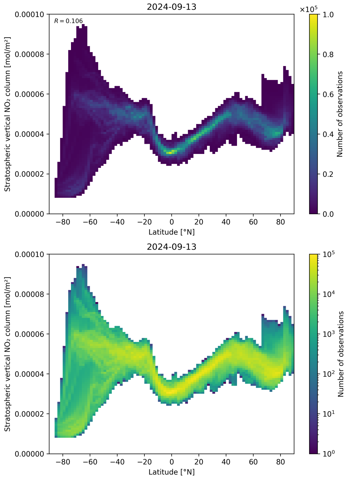
Figure 87: Scatter density plot of “Latitude” against “Stratospheric vertical NO 2 column” for 2024-09-12 to 2024-09-14.
