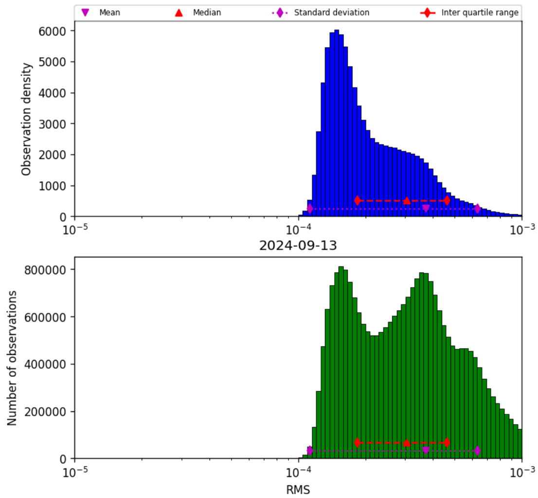
Figure 43: Histogram of “RMS” for 2024-09-12 to 2024-09-14
