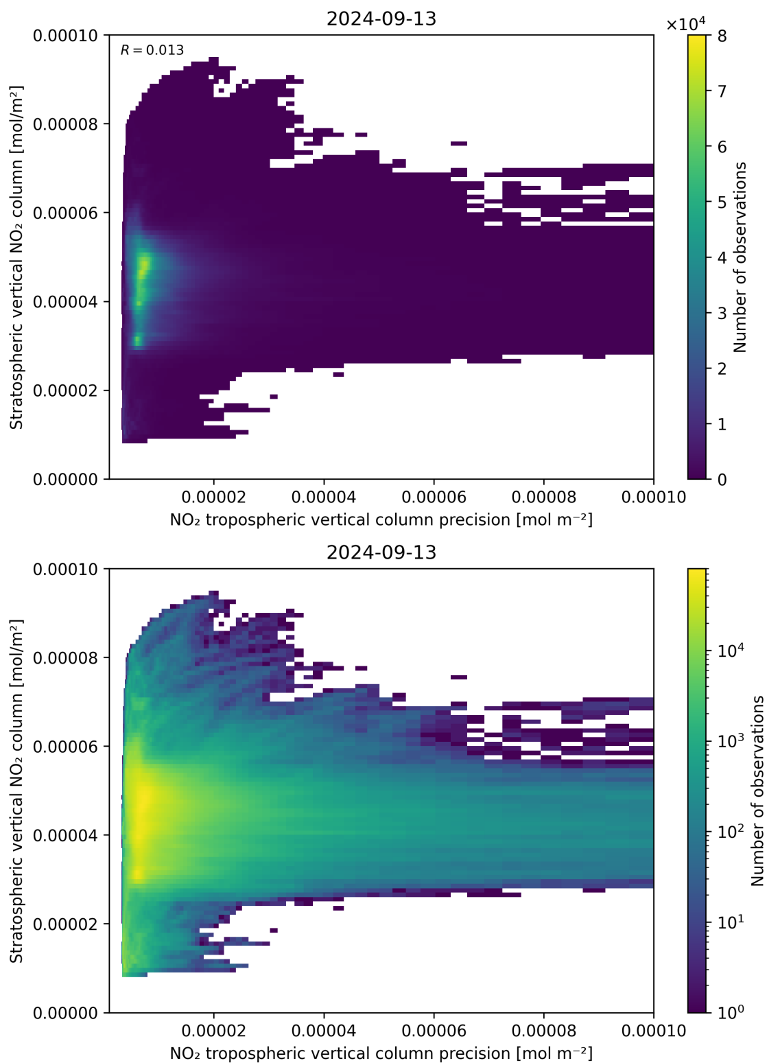
Figure 135: Scatter density plot of “NO 2 tropospheric vertical column precision” against “Stratospheric vertical NO 2 column” for 2024-09-12 to 2024-09-14.
