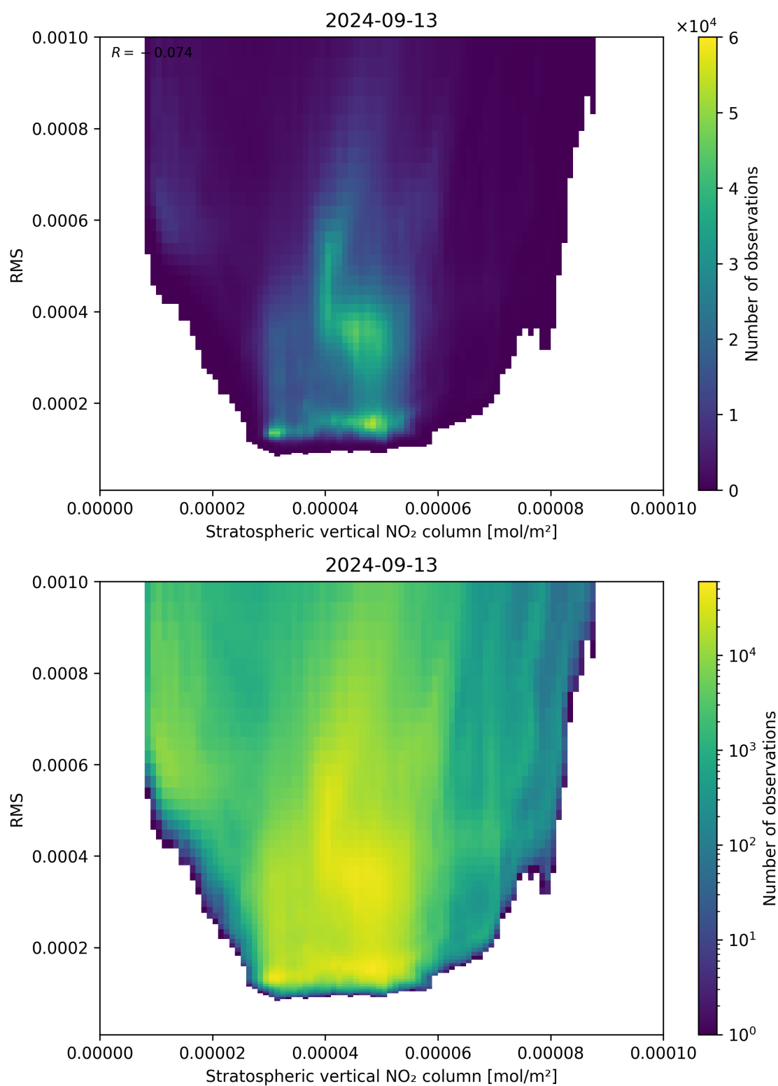
Figure 102: Scatter density plot of “Stratospheric vertical NO 2 column” against “RMS” for 2024-09-12 to 2024-09-14.
