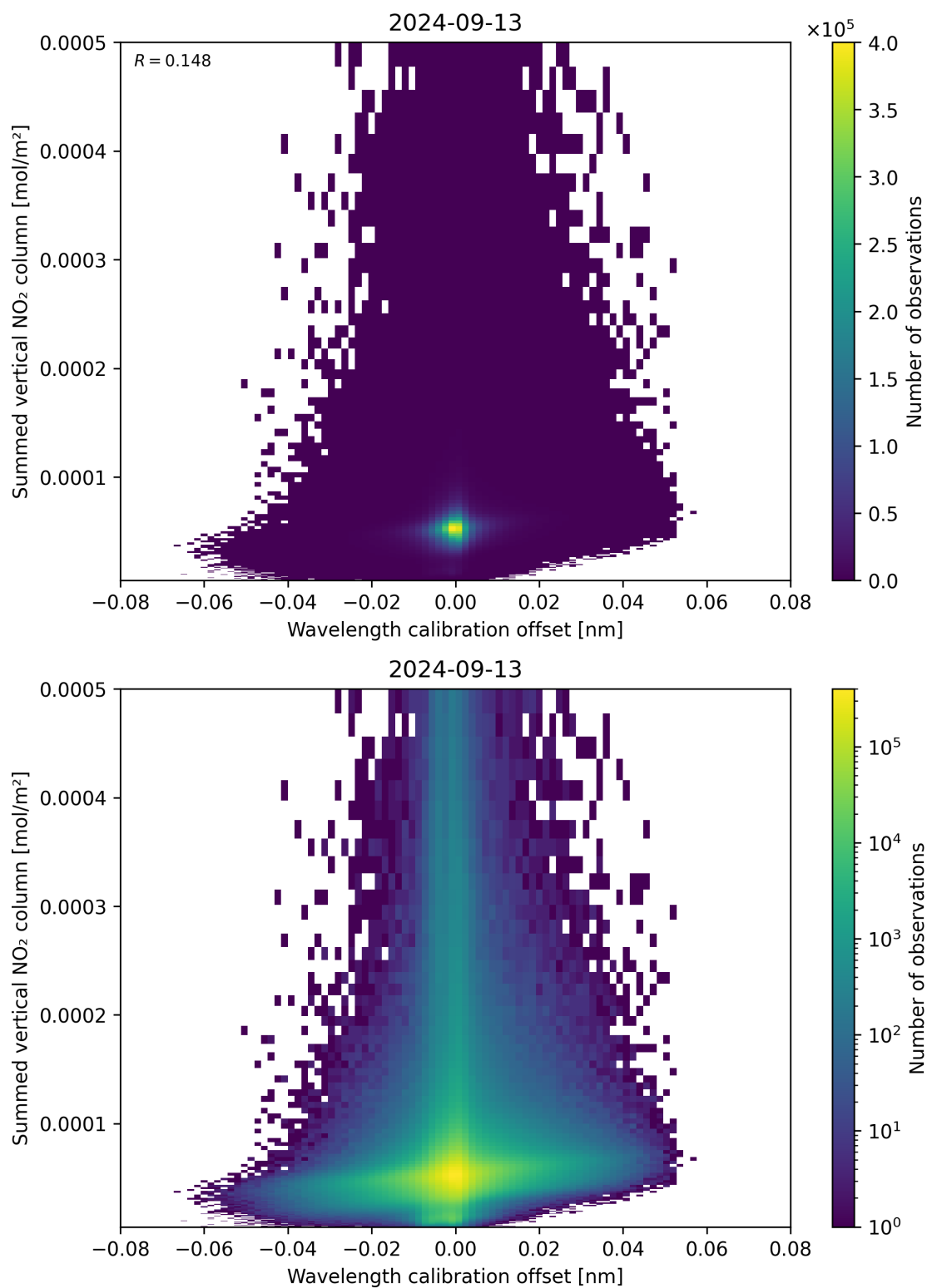
Figure 177: Scatter density plot of “Wavelength calibration offset” against “Summed vertical NO 2 column” for 2024-09-12 to 2024-09-14.
