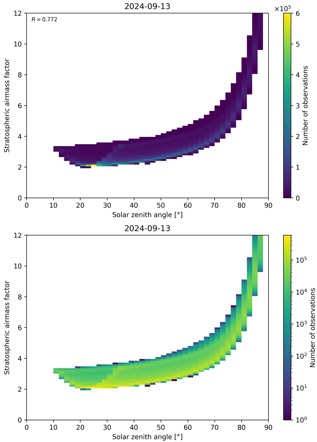
Figure 145: Scatter density plot of “Solar zenith angle” against “Stratospheric airmass factor” for 2024-09-12 to 2024-09-14.
