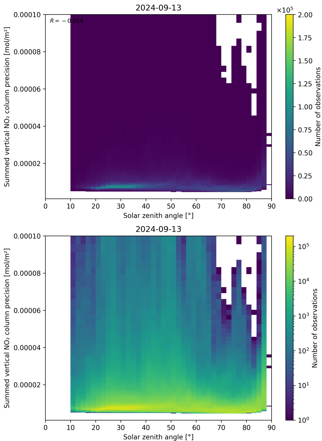
Figure 152: Scatter density plot of “Solar zenith angle” against “Summed vertical NO 2 column precision” for 2024-09-12 to 2024-09-14.
