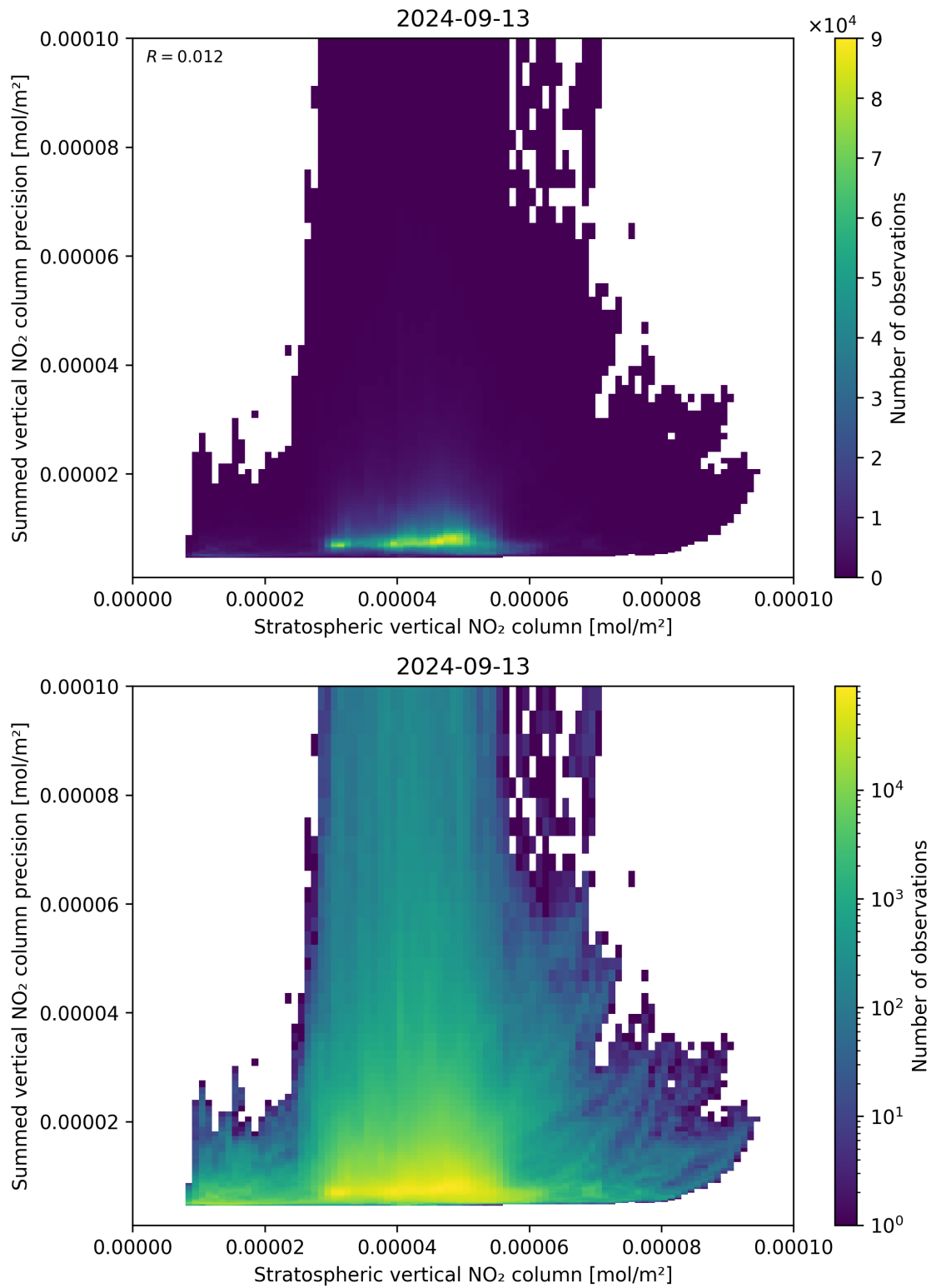
Figure 99: Scatter density plot of “Stratospheric vertical NO 2 column” against “Summed vertical NO 2 column precision” for 2024-09-12 to 2024-09-14.
