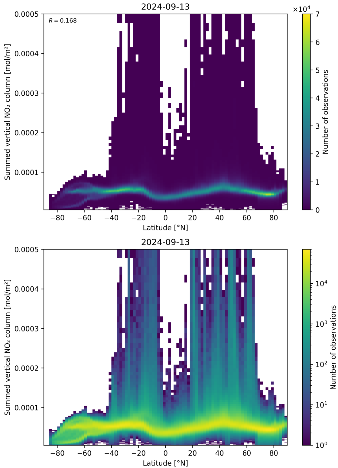
Figure 88: Scatter density plot of “Latitude” against “Summed vertical NO 2 column” for 2024-09-12 to 2024-09-14.
