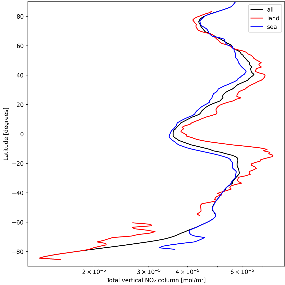
Figure 21: Zonal average of “Total vertical NO 2 column” for 2024-09-13 to 2024-09-15.
