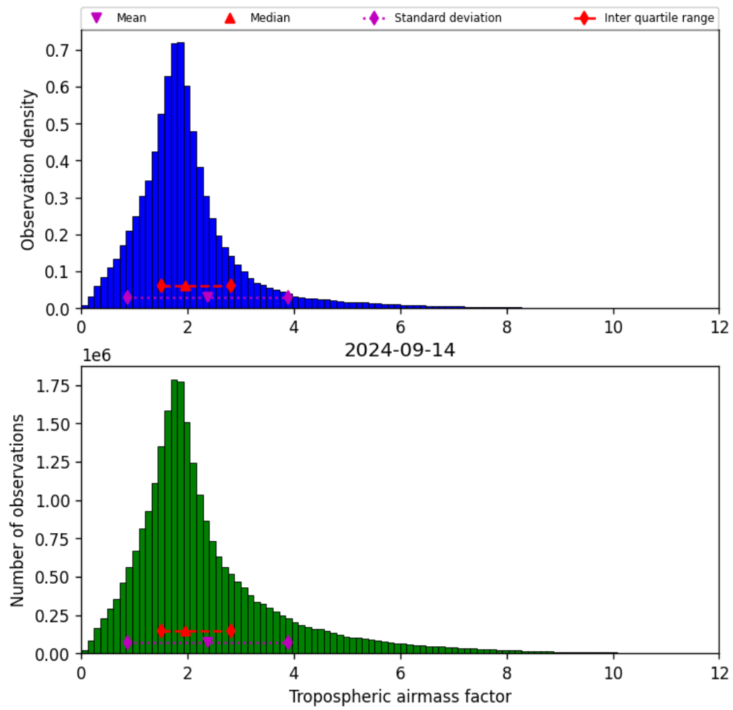
Figure 31: Histogram of “Tropospheric airmass factor” for 2024-09-13 to 2024-09-15
