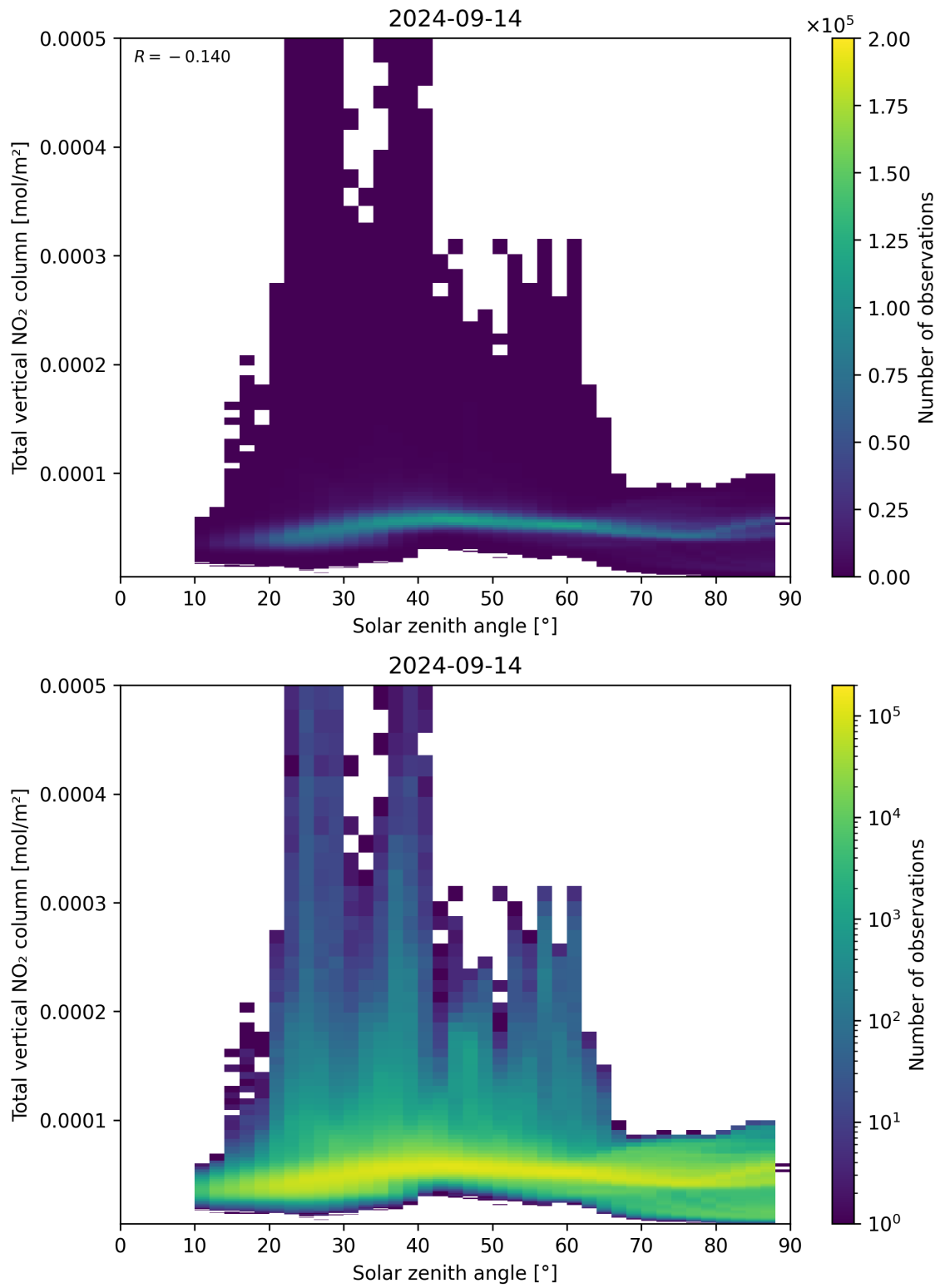
Figure 153: Scatter density plot of “Solar zenith angle” against “Total vertical NO 2 column” for 2024-09-13 to 2024-09-15.
