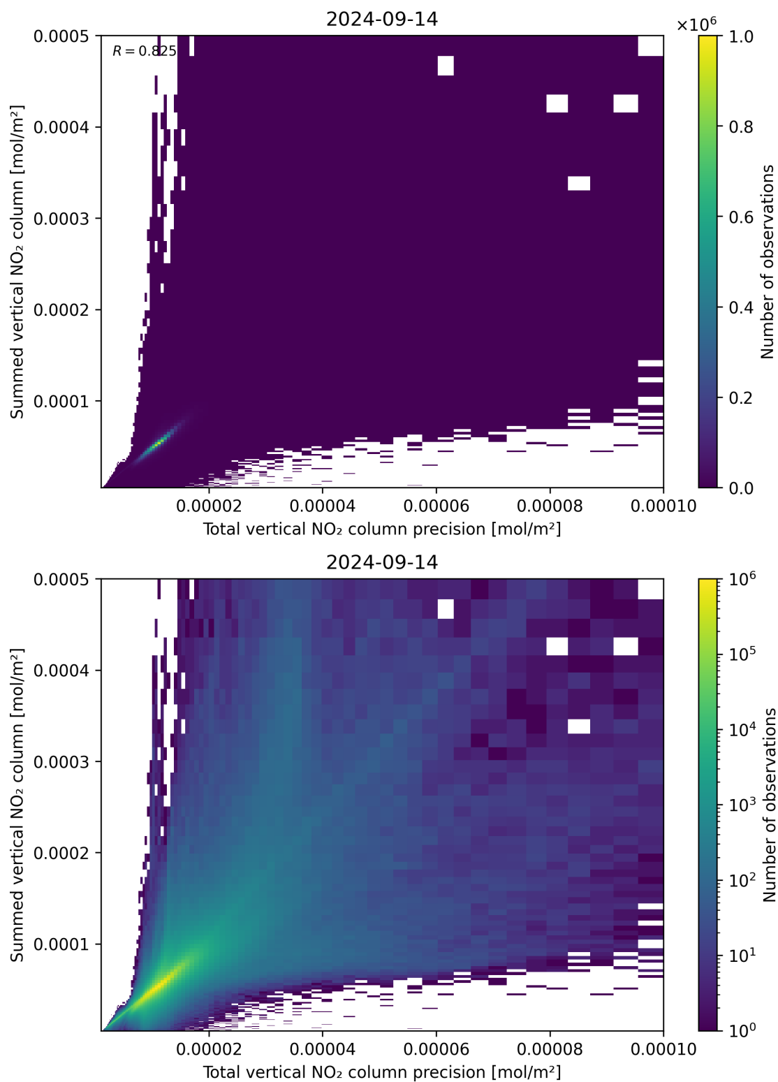
Figure 117: Scatter density plot of “Total vertical NO 2 column precision” against “Summed vertical NO 2 column” for 2024-09-13 to 2024-09-15.
