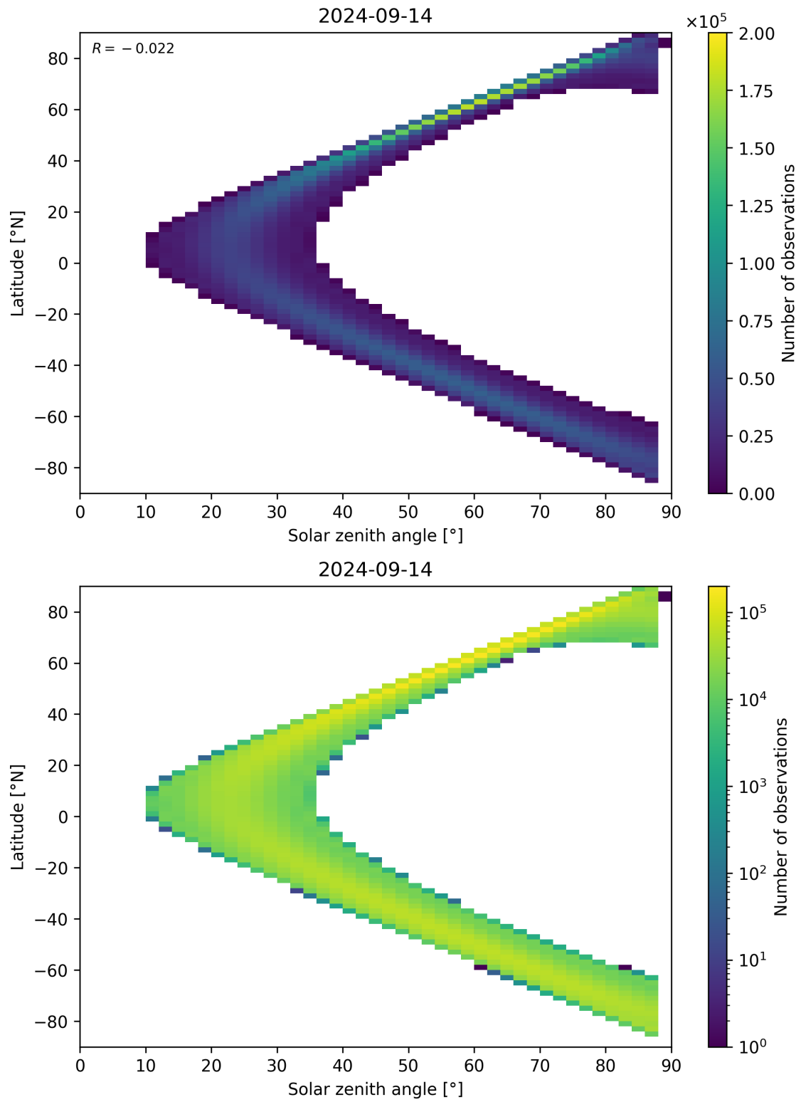
Figure 149: Scatter density plot of “Solar zenith angle” against “Latitude” for 2024-09-13 to 2024-09-15.
