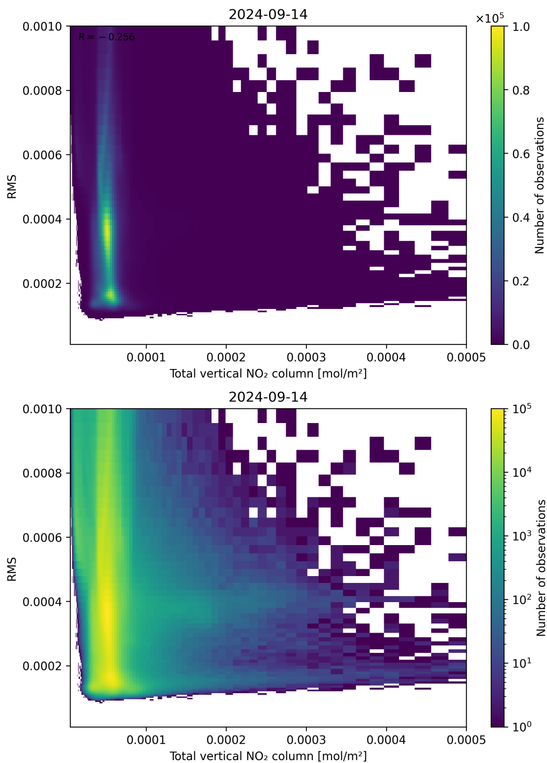
Figure 120: Scatter density plot of “Total vertical NO 2 column” against “RMS” for 2024-09-13 to 2024-09-15.
