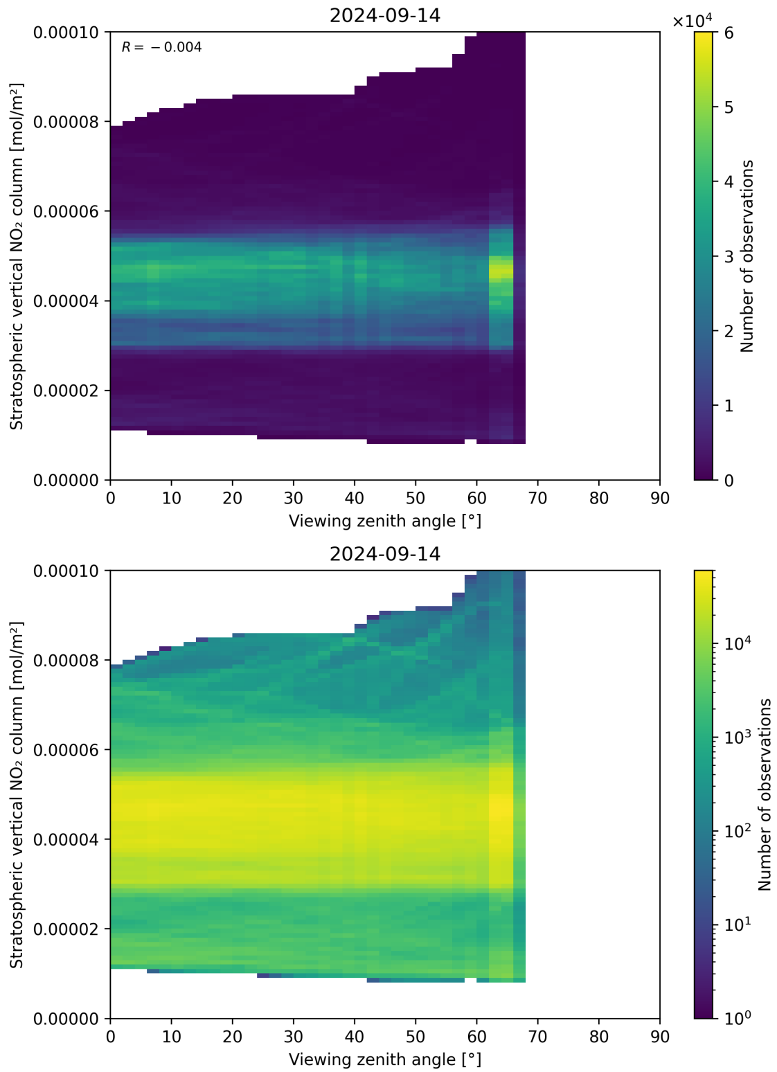
Figure 164: Scatter density plot of “Viewing zenith angle” against “Stratospheric vertical NO 2 column” for 2024-09-13 to 2024-09-15.
