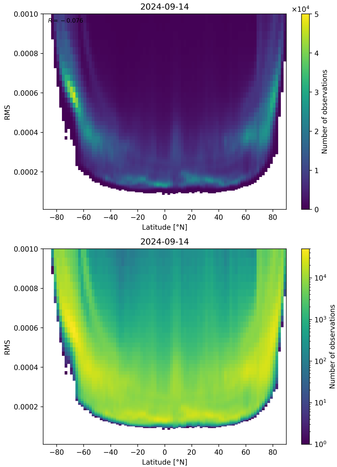
Figure 94: Scatter density plot of “Latitude” against “RMS” for 2024-09-13 to 2024-09-15.
