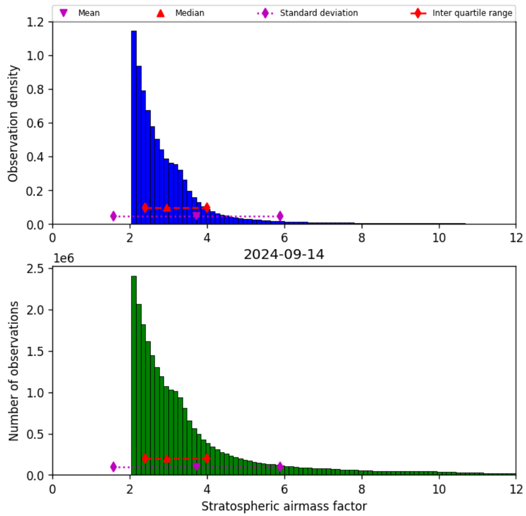
Figure 44: Histogram of “Stratospheric airmass factor” for 2024-09-13 to 2024-09-15
