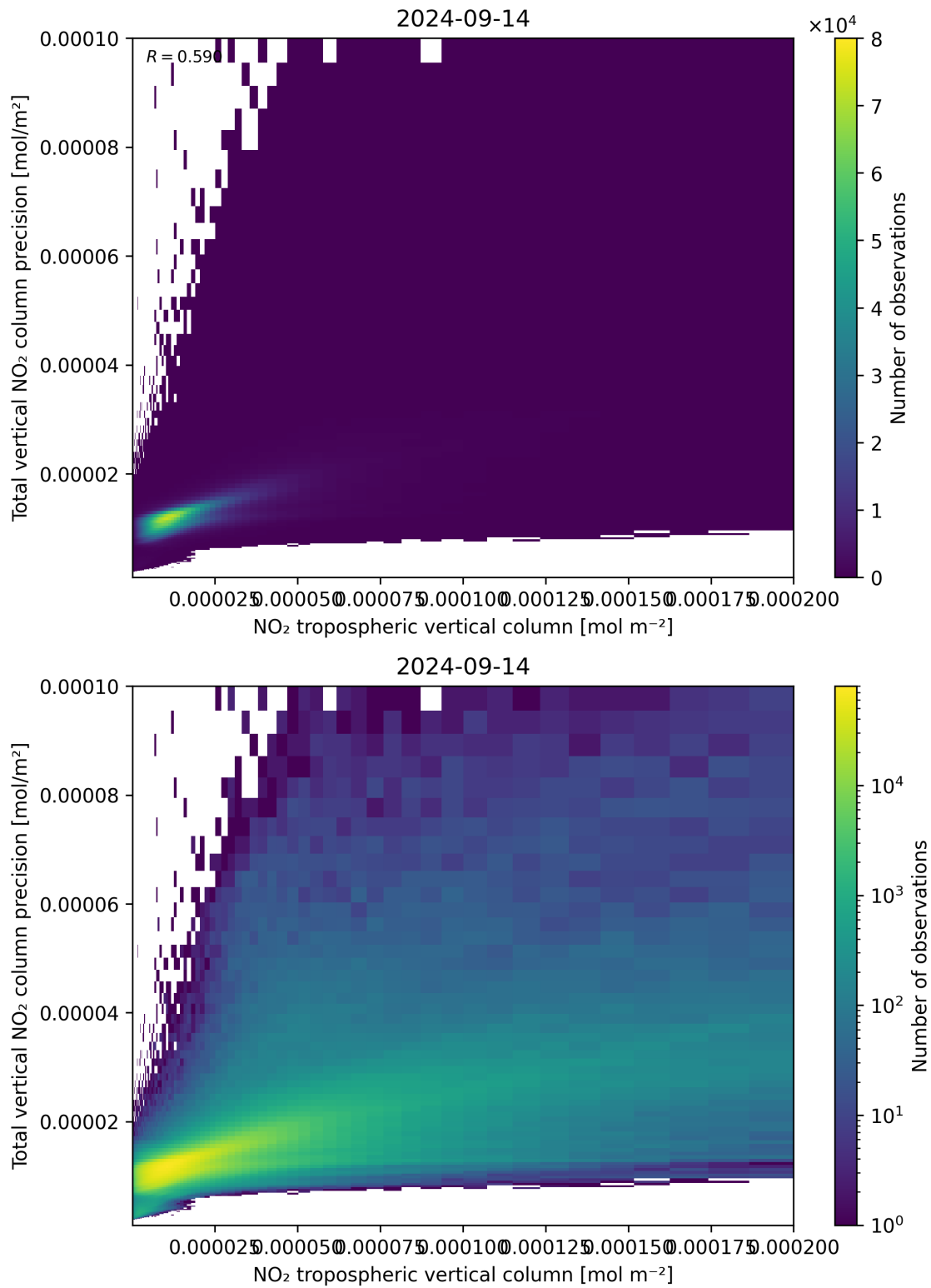
Figure 129: Scatter density plot of “NO 2 tropospheric vertical column” against “Total vertical NO 2 column precision” for 2024-09-13 to 2024-09-15.
