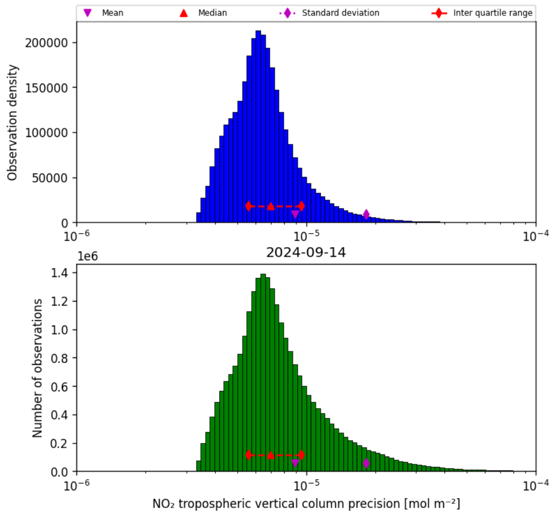
Figure 30: Histogram of “NO 2 tropospheric vertical column precision” for 2024-09-13 to 2024-09-15
