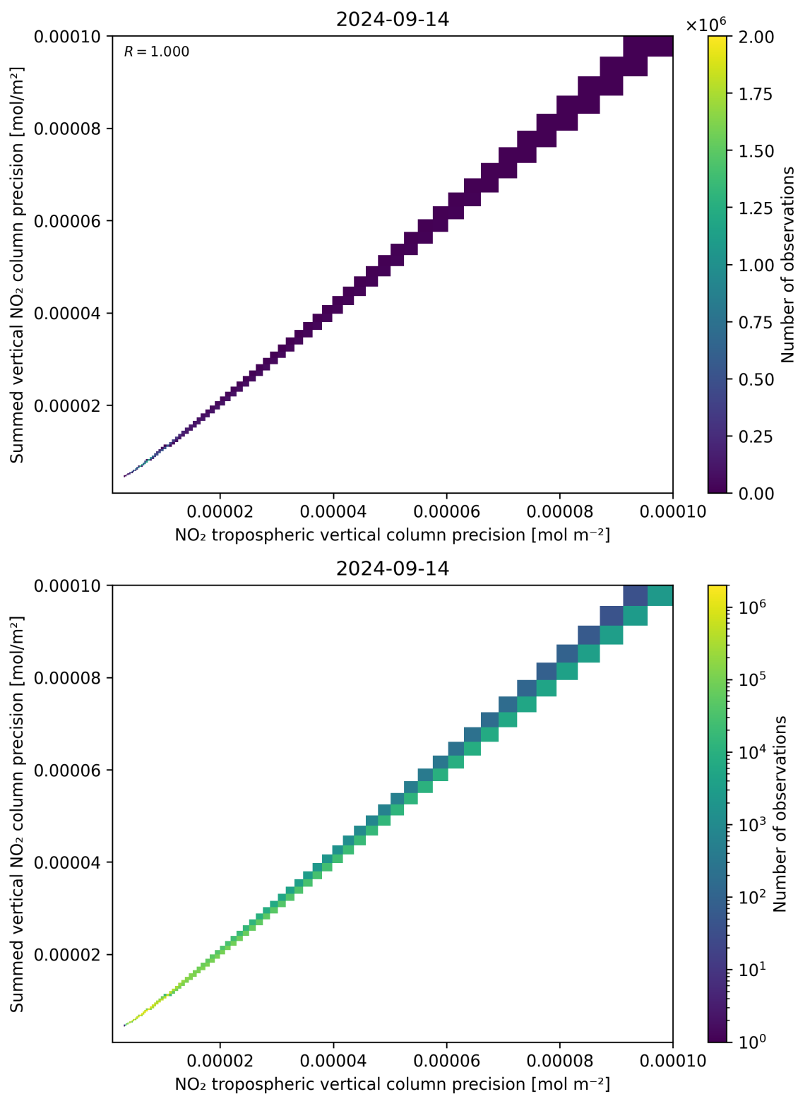
Figure 137: Scatter density plot of “NO 2 tropospheric vertical column precision” against “Summed vertical NO 2 column precision” for 2024-09-13 to 2024-09-15.
