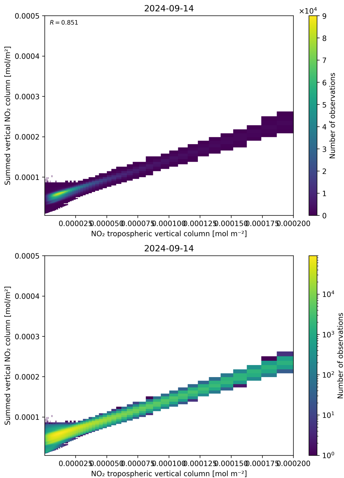
Figure 126: Scatter density plot of “NO 2 tropospheric vertical column” against “Summed vertical NO 2 column” for 2024-09-13 to 2024-09-15.
