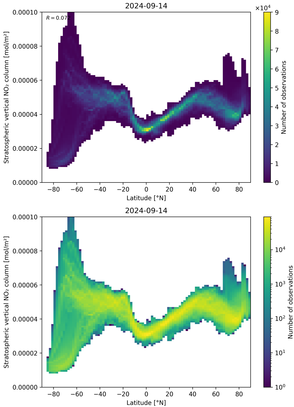
Figure 87: Scatter density plot of “Latitude” against “Stratospheric vertical NO 2 column” for 2024-09-13 to 2024-09-15.
