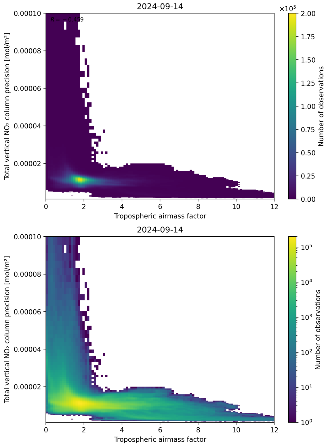
Figure 78: Scatter density plot of “Tropospheric air mass factor” against “Total vertical NO 2 column precision” for 2024-09-13 to 2024-09-15.
