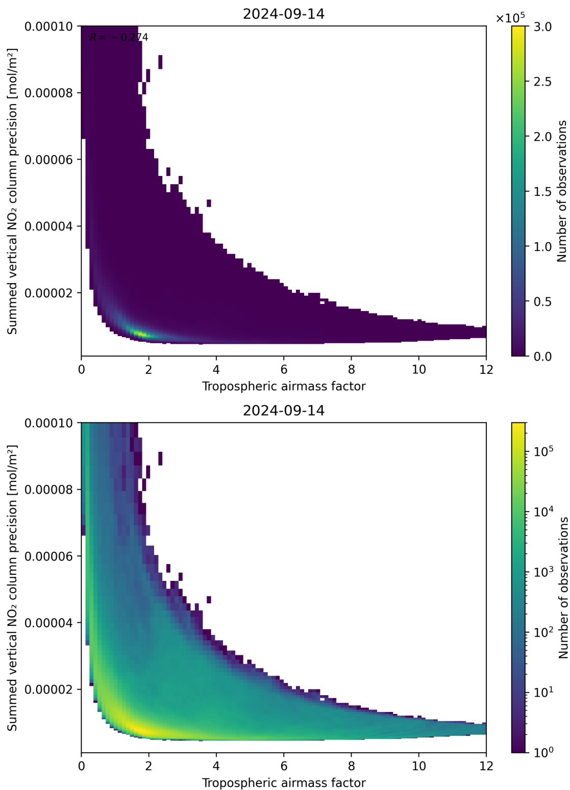
Figure 76: Scatter density plot of “Tropospheric air mass factor” against “Summed vertical NO 2 column precision” for 2024-09-13 to 2024-09-15.
