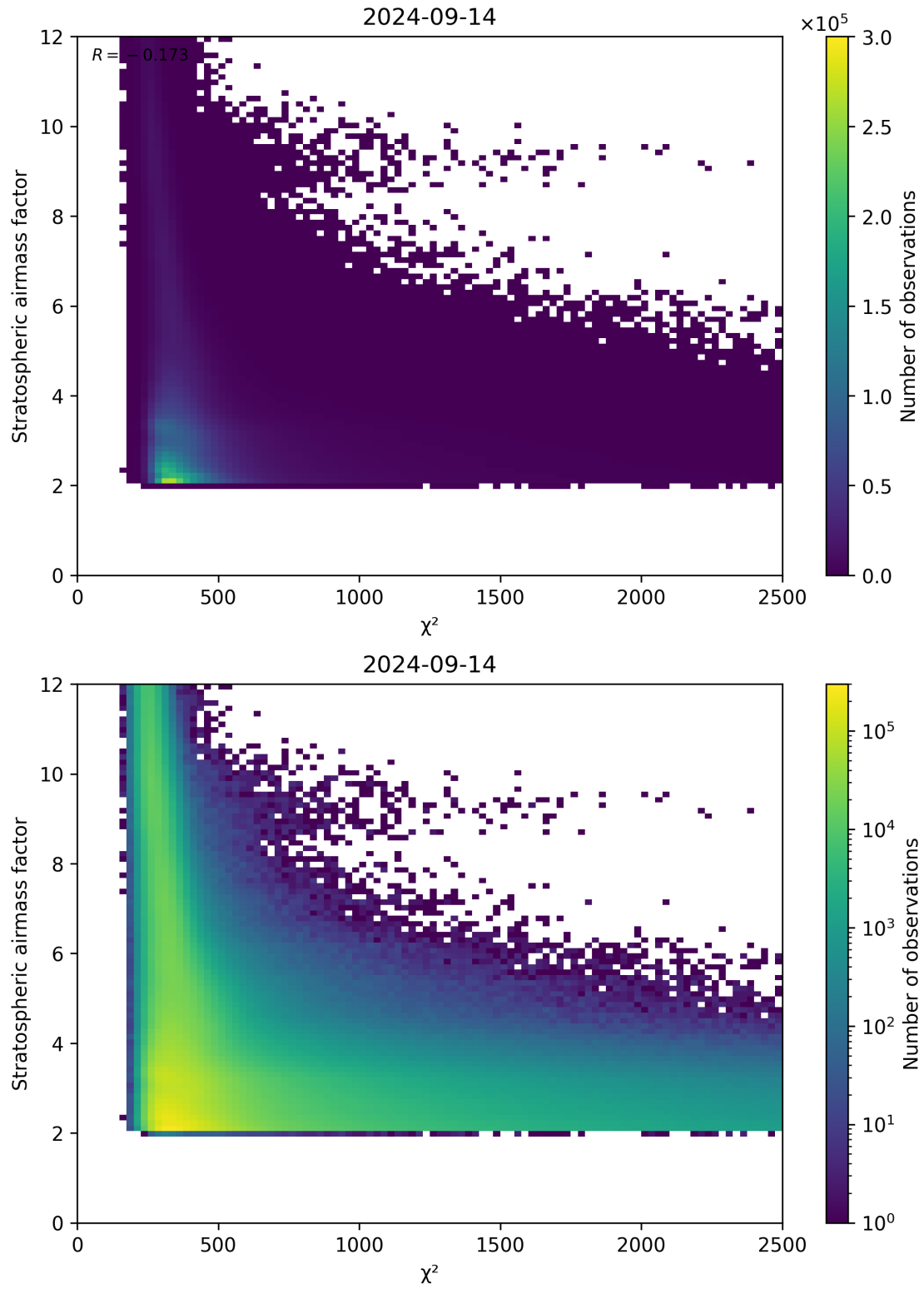
Figure 81: Scatter density plot of “ \chi^2 ” against “Stratospheric airmass factor” for 2024-09-13 to 2024-09-15.
