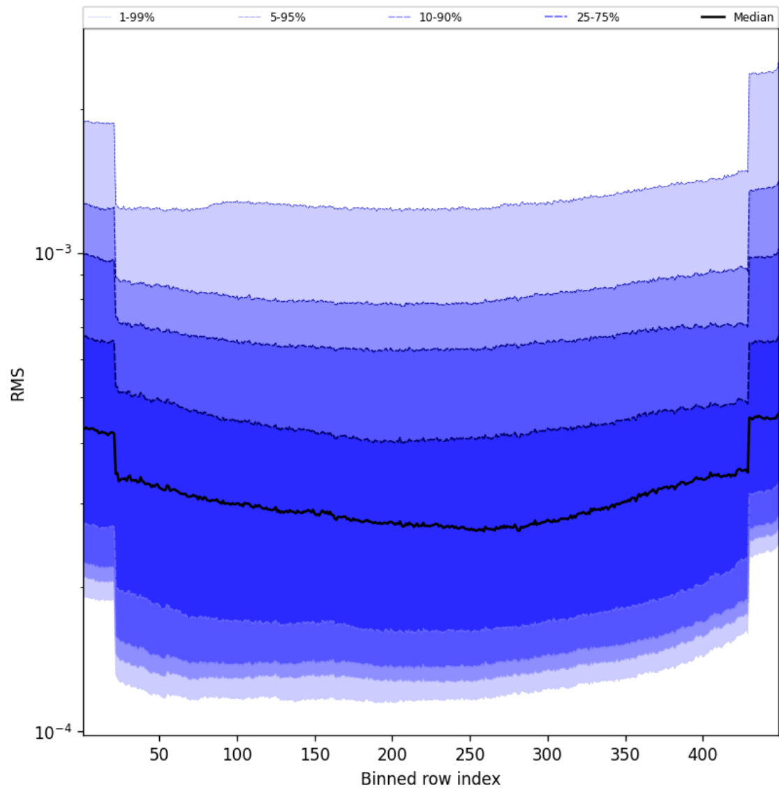
Figure 60: Along track statistics of “RMS” for 2024-09-13 to 2024-09-15
