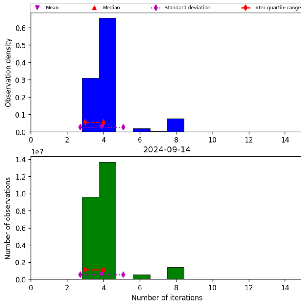
Figure 34: Histogram of “Number of iterations” for 2024-09-13 to 2024-09-15
