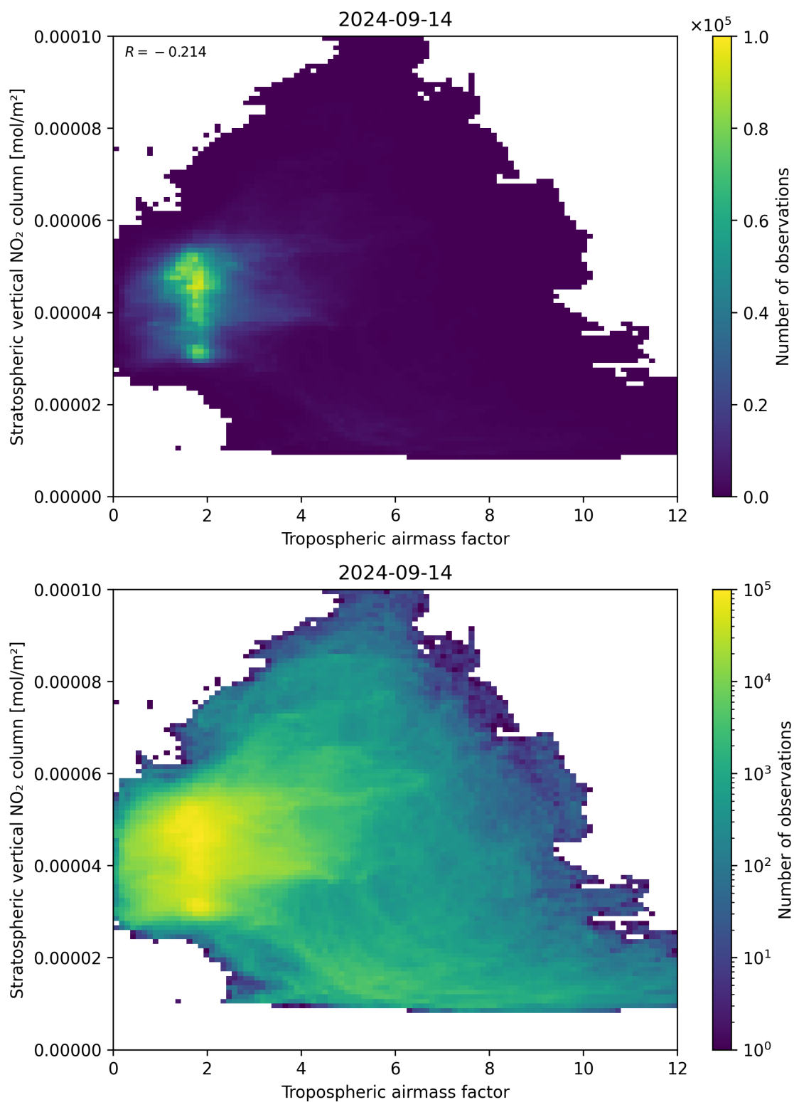
Figure 74: Scatter density plot of “Tropospheric air mass factor” against “Stratospheric vertical NO 2 column” for 2024-09-13 to 2024-09-15.
