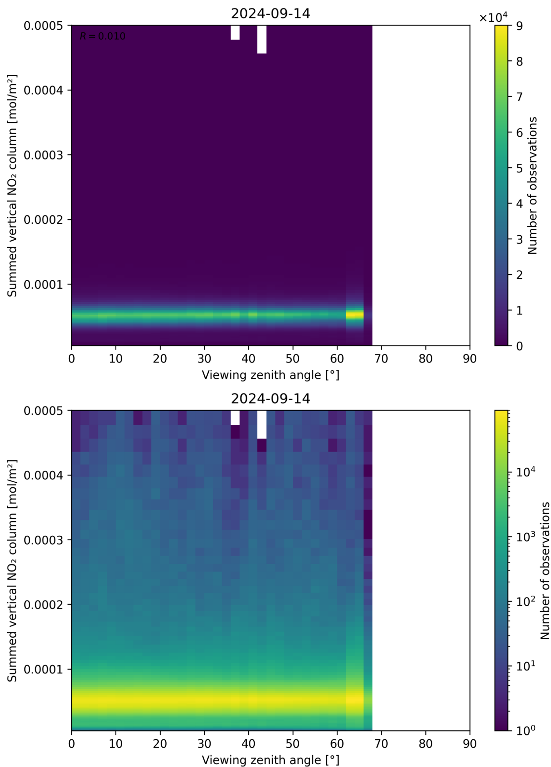
Figure 165: Scatter density plot of “Viewing zenith angle” against “Summed vertical NO 2 column” for 2024-09-13 to 2024-09-15.
