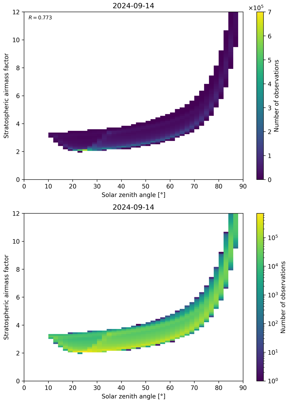
Figure 145: Scatter density plot of “Solar zenith angle” against “Stratospheric airmass factor” for 2024-09-13 to 2024-09-15.
