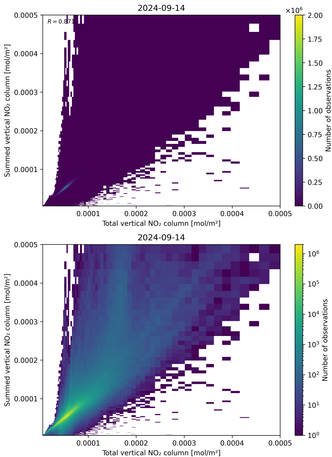
Figure 112: Scatter density plot of “Total vertical NO 2 column” against “Summed vertical NO 2 column” for 2024-09-13 to 2024-09-15.
