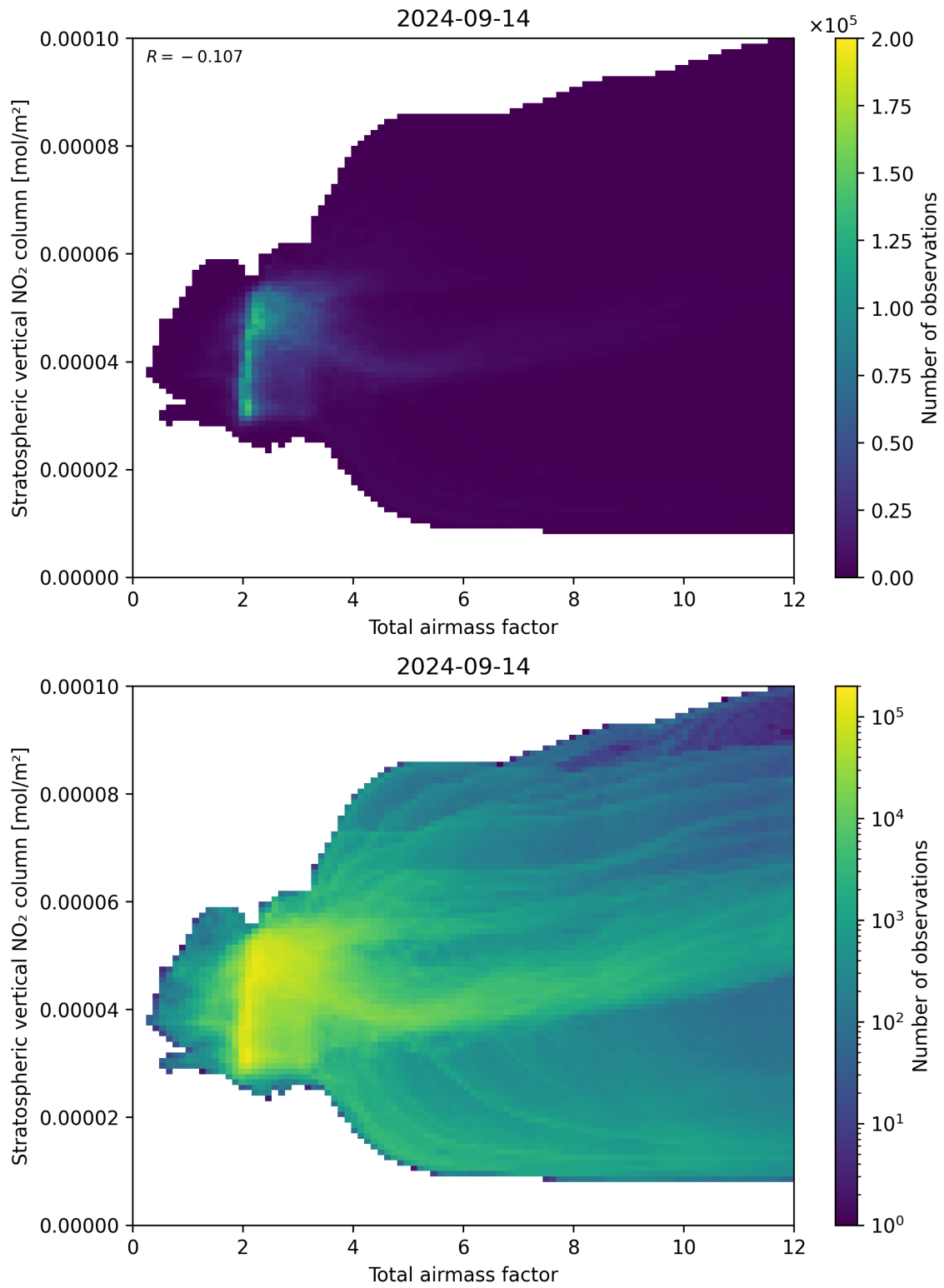
Figure 64: Scatter density plot of “Total airmass factor” against “Stratospheric vertical NO 2 column” for 2024-09-13 to 2024-09-15.
