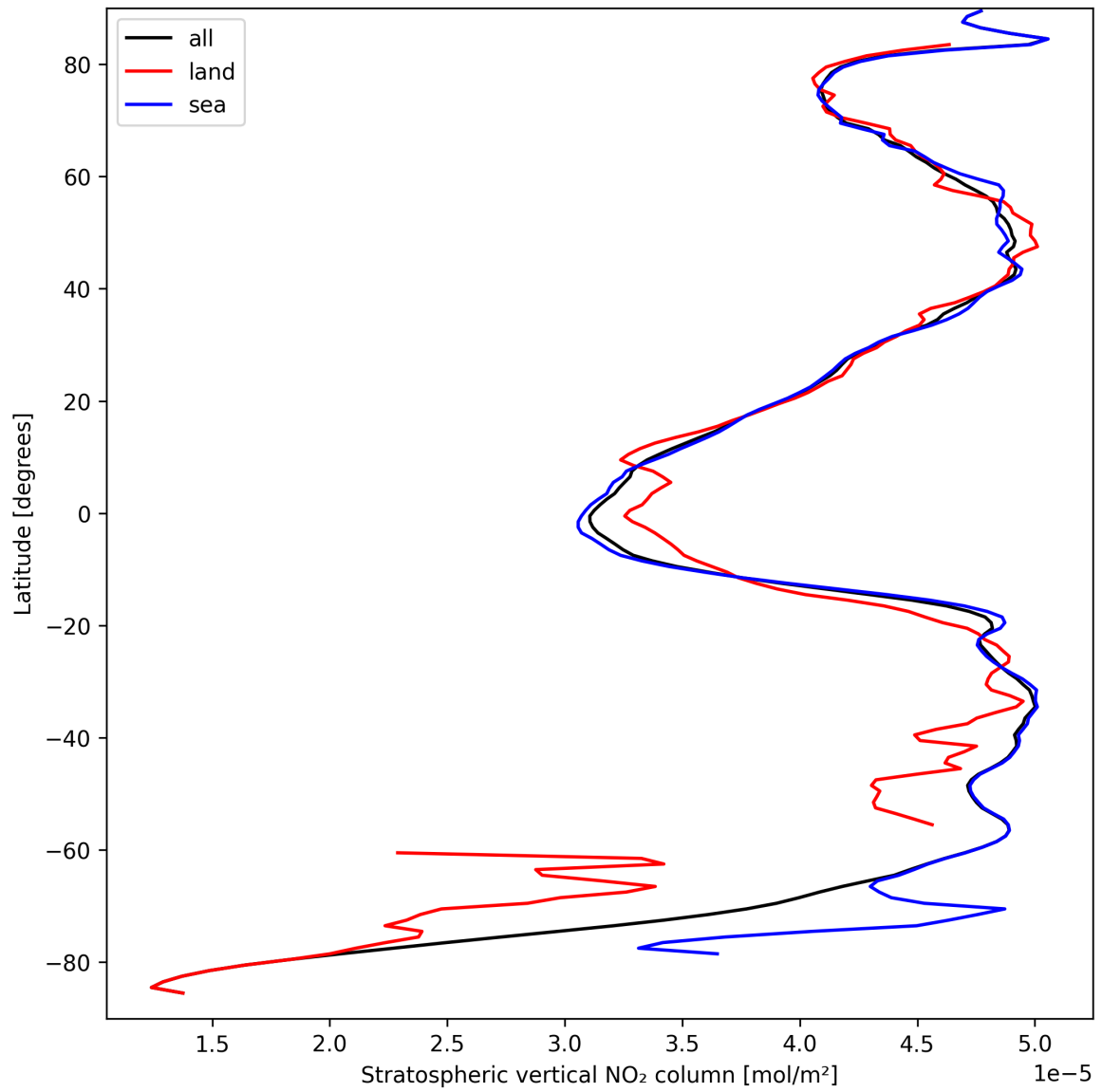
Figure 19: Zonal average of “Stratospheric vertical NO 2 column” for 2024-09-13 to 2024-09-15.
