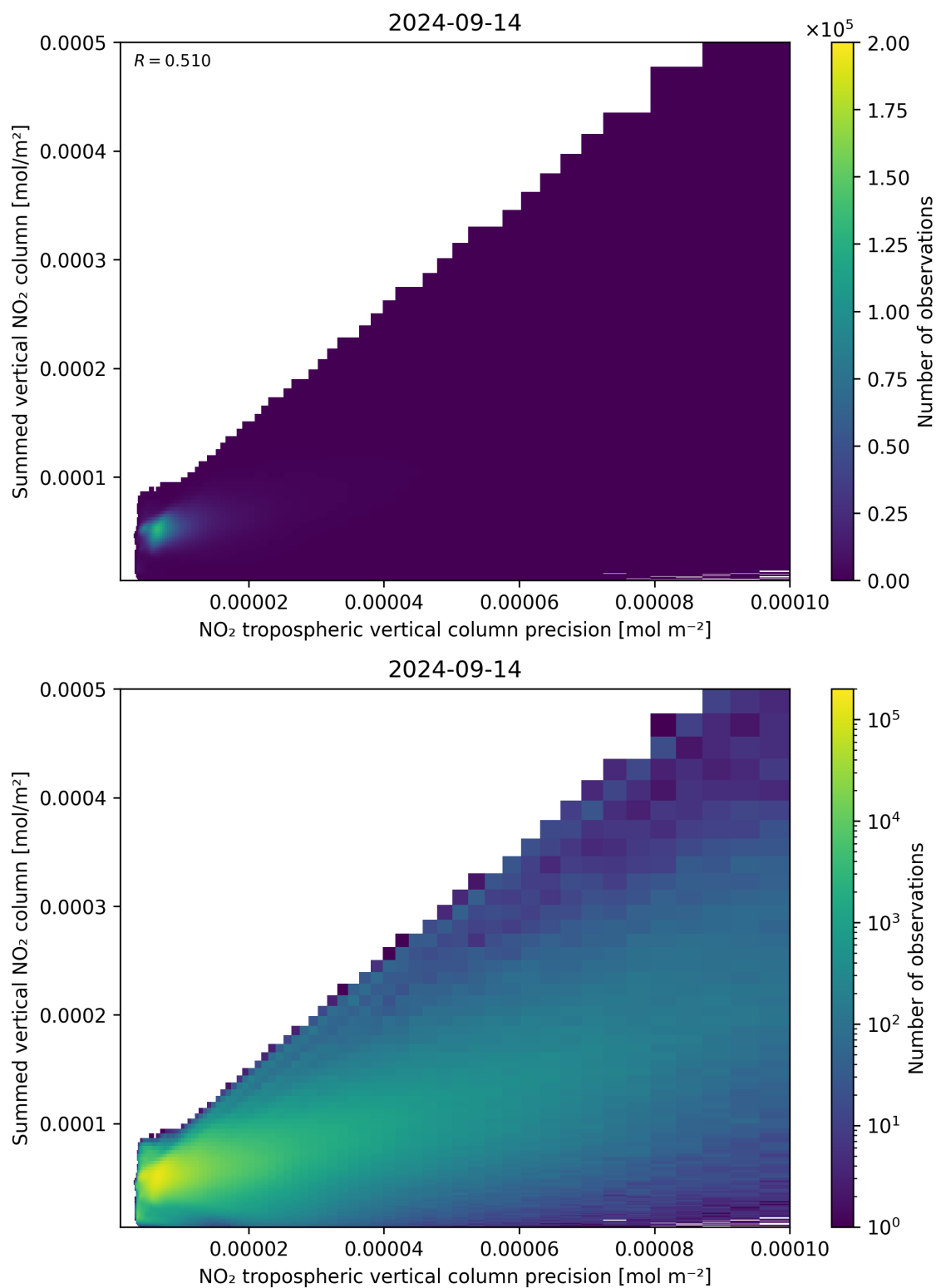
Figure 136: Scatter density plot of “NO 2 tropospheric vertical column precision” against “Summed vertical NO 2 column” for 2024-09-13 to 2024-09-15.
