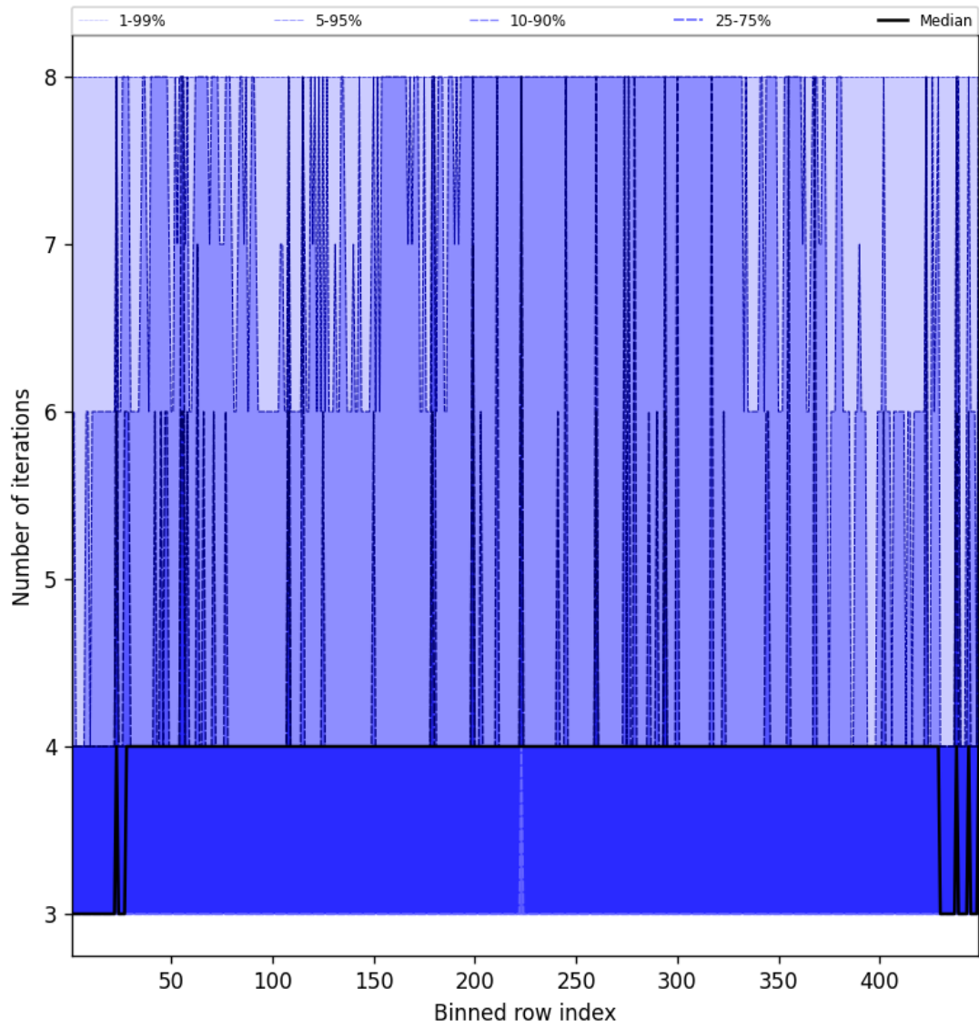
Figure 51: Along track statistics of “Number of iterations” for 2024-09-13 to 2024-09-15
