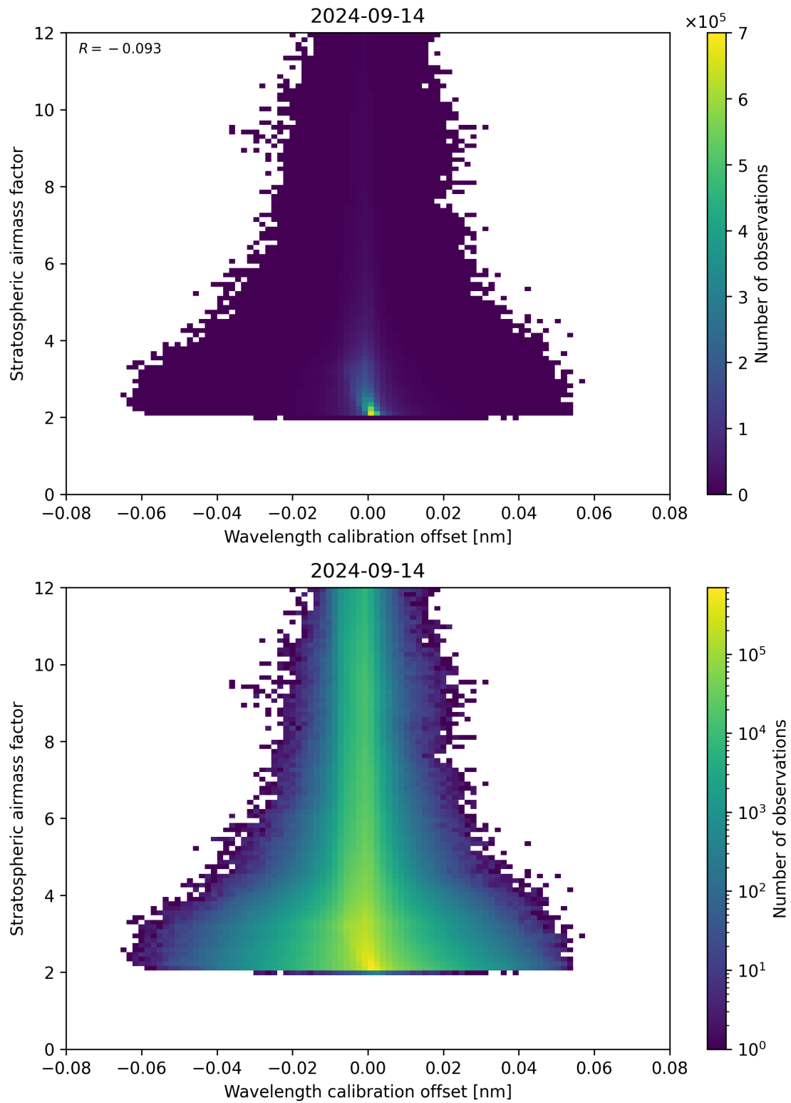
Figure 174: Scatter density plot of “Wavelength calibration offset” against “Stratospheric airmass factor” for 2024-09-13 to 2024-09-15.
