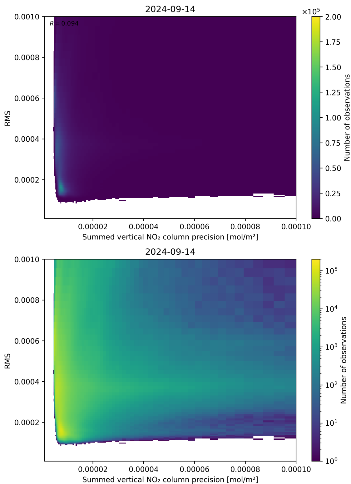
Figure 108: Scatter density plot of “Summed vertical NO 2 column precision” against “RMS” for 2024-09-13 to 2024-09-15.
