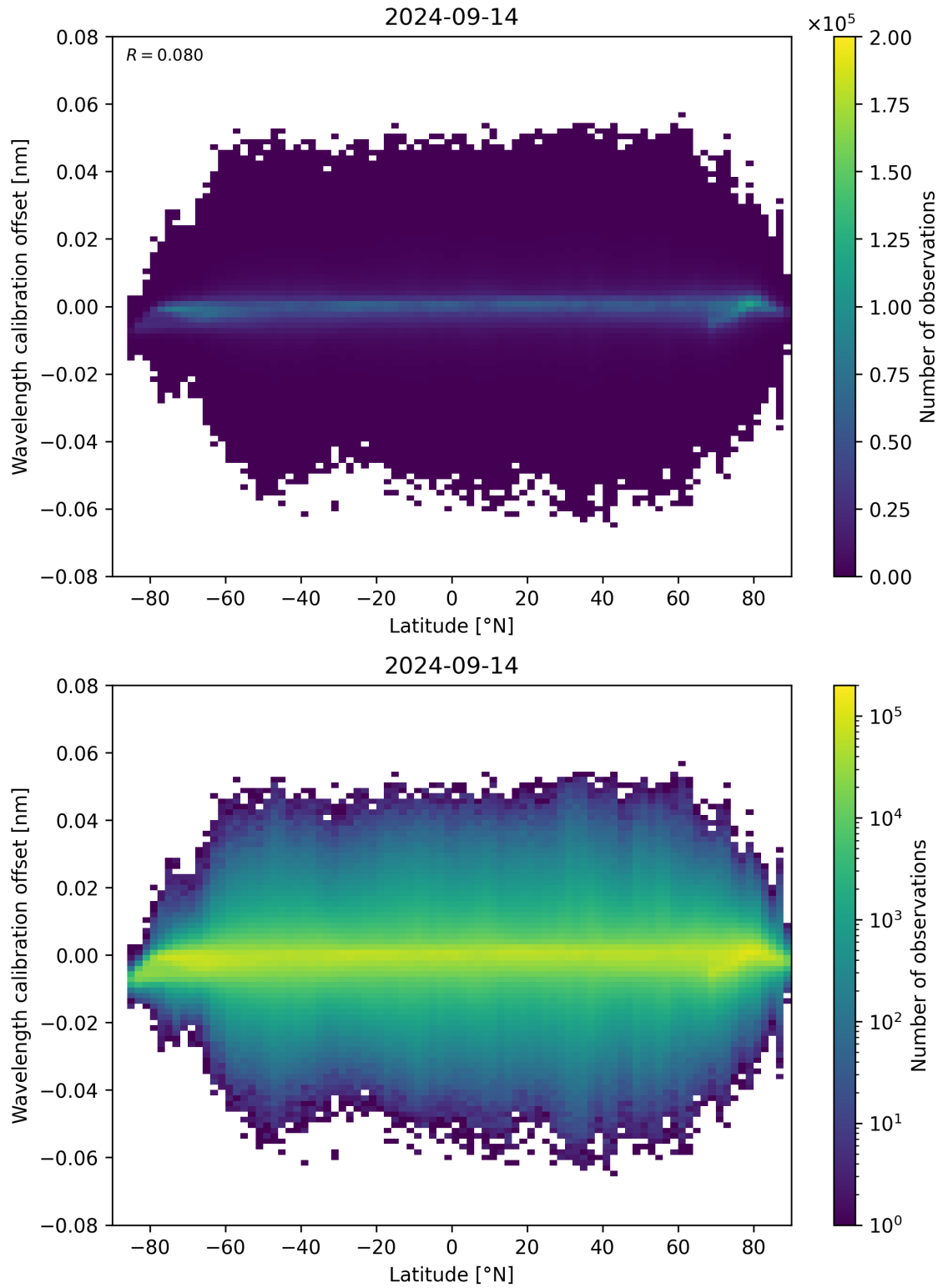
Figure 95: Scatter density plot of “Latitude” against “Wavelength calibration offset” for 2024-09-13 to 2024-09-15.
