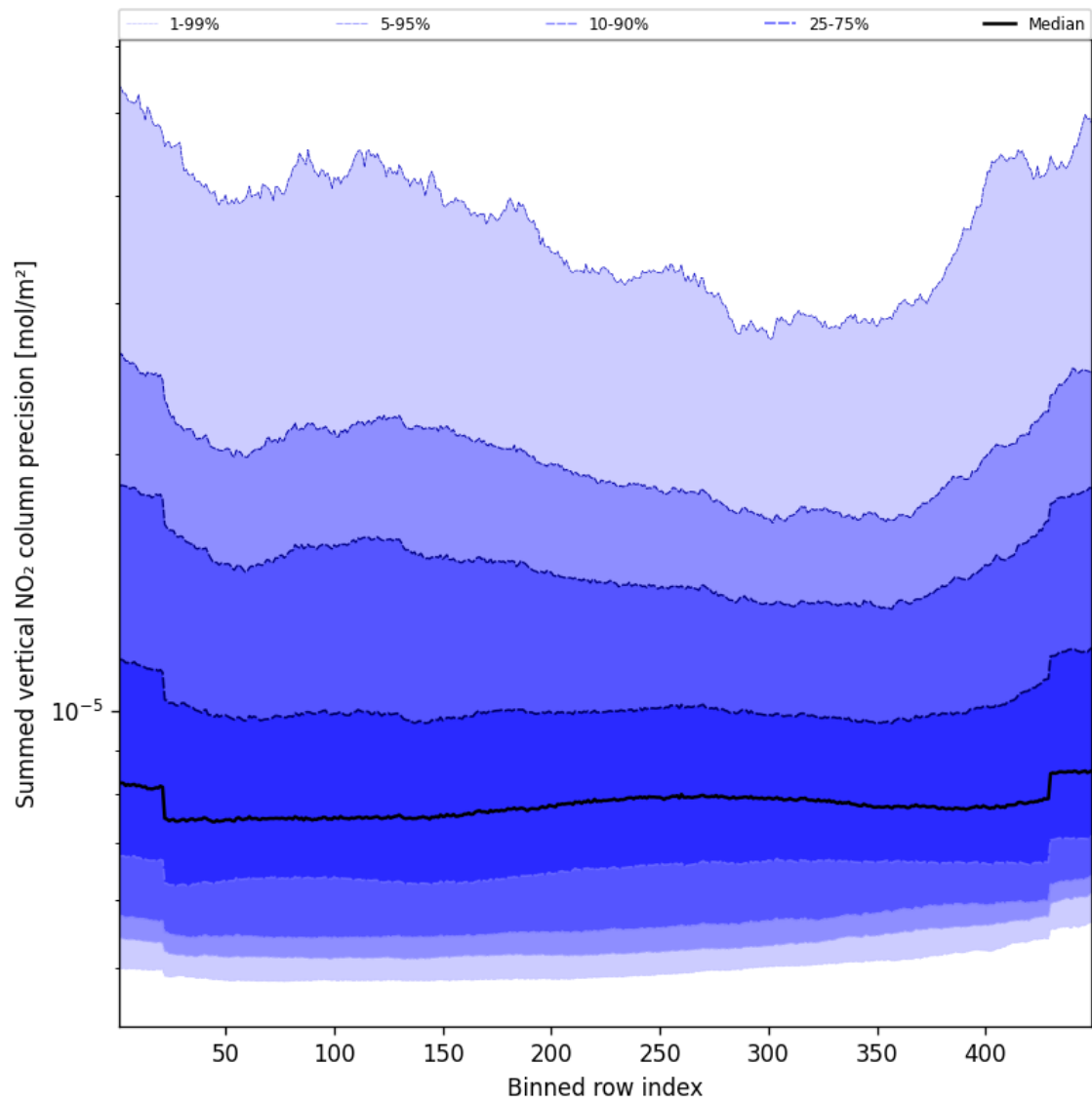
Figure 58: Along track statistics of “Summed vertical NO 2 column precision” for 2024-09-13 to 2024-09-15
