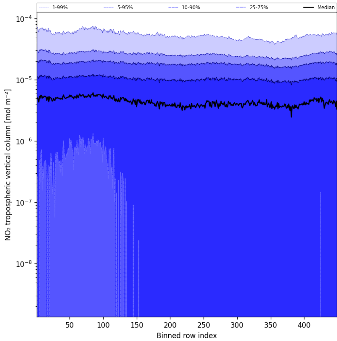
Figure 46: Along track statistics of “NO 2 tropospheric vertical column” for 2024-09-13 to 2024-09-15
