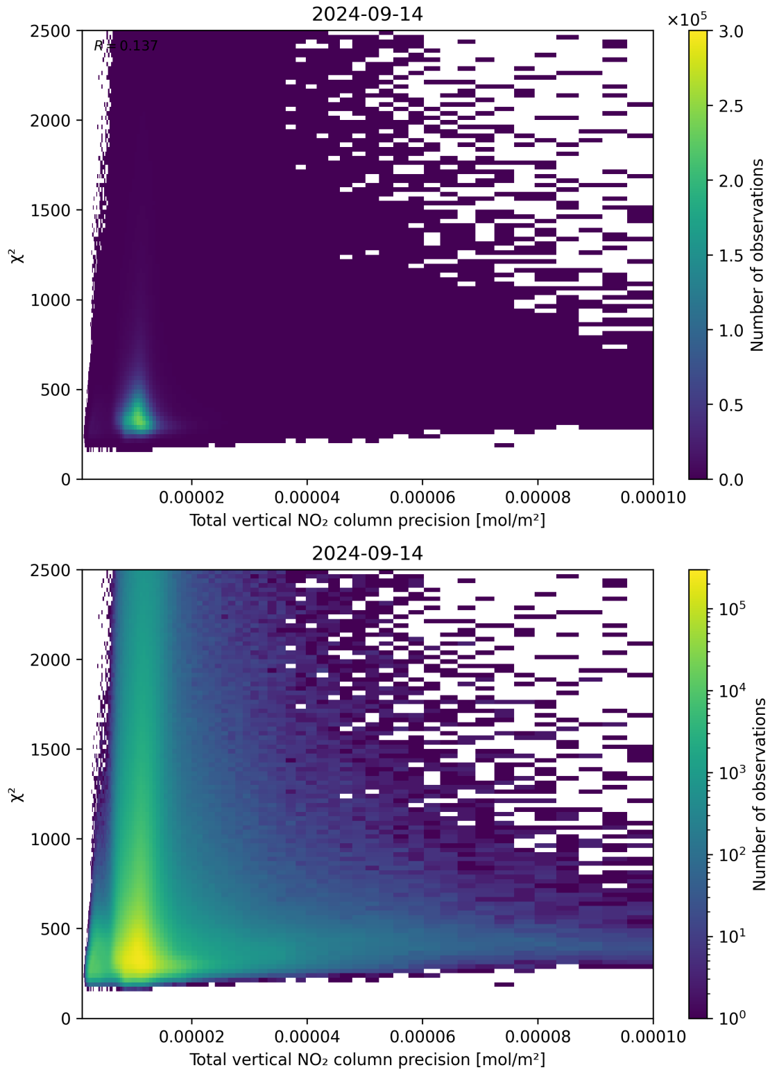
Figure 116: Scatter density plot of “Total vertical NO 2 column precision” against “ \chi^2 ” for 2024-09-13 to 2024-09-15.
