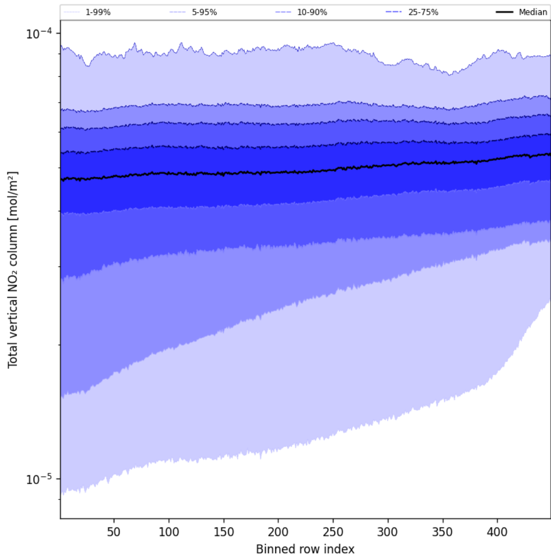
Figure 55: Along track statistics of “Total vertical NO 2 column” for 2024-09-13 to 2024-09-15
