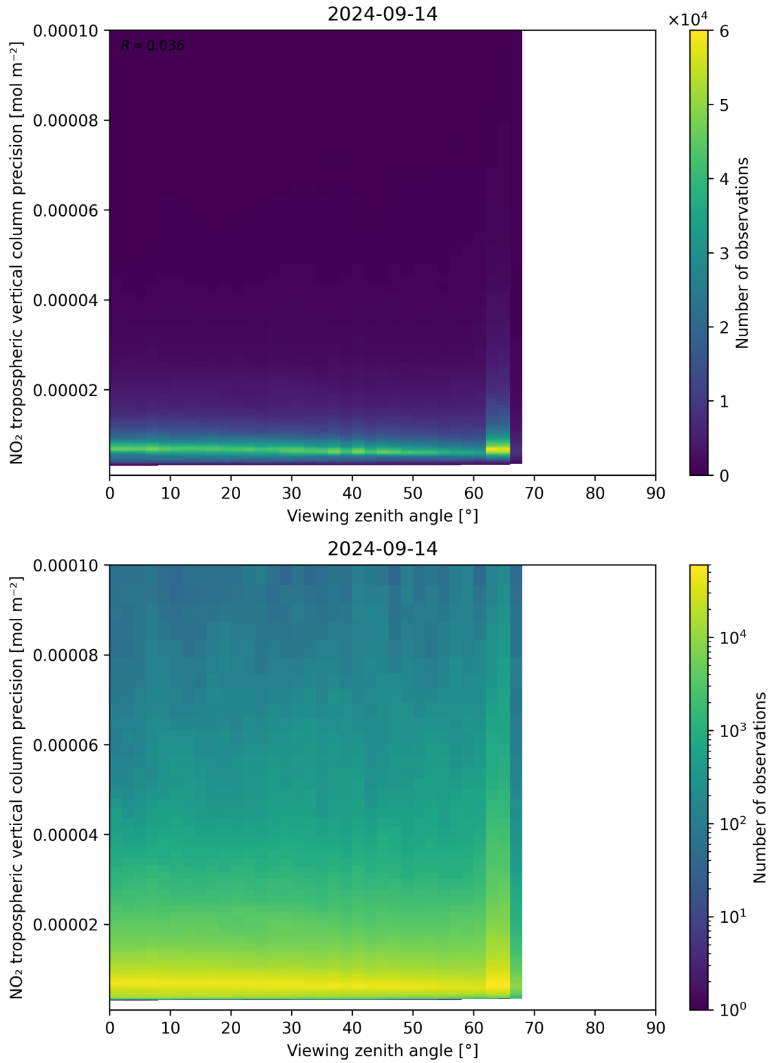
Figure 170: Scatter density plot of “Viewing zenith angle” against “NO 2 tropospheric vertical column precision” for 2024-09-13 to 2024-09-15.
