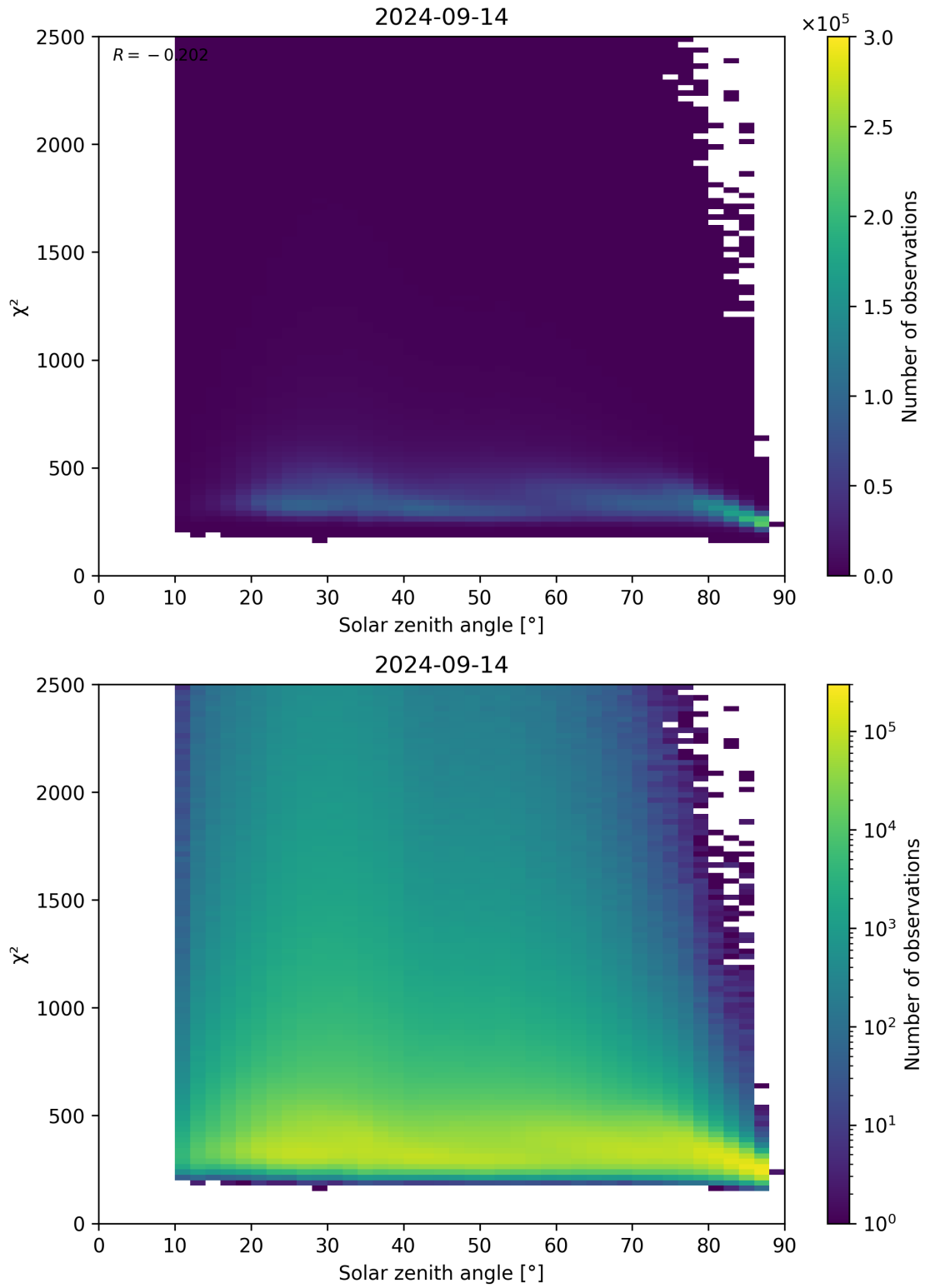
Figure 148: Scatter density plot of “Solar zenith angle” against “ \chi^2 ” for 2024-09-13 to 2024-09-15.
