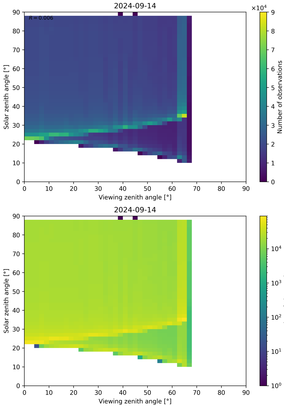
Figure 172: Scatter density plot of “Viewing zenith angle” against “Solar zenith angle” for 2024-09-13 to 2024-09-15.
