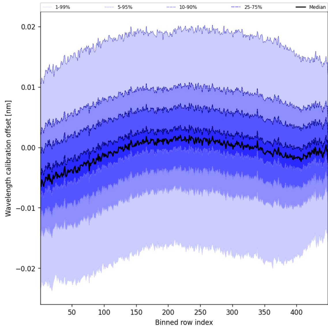
Figure 52: Along track statistics of “Wavelength calibration offset” for 2024-09-13 to 2024-09-15
