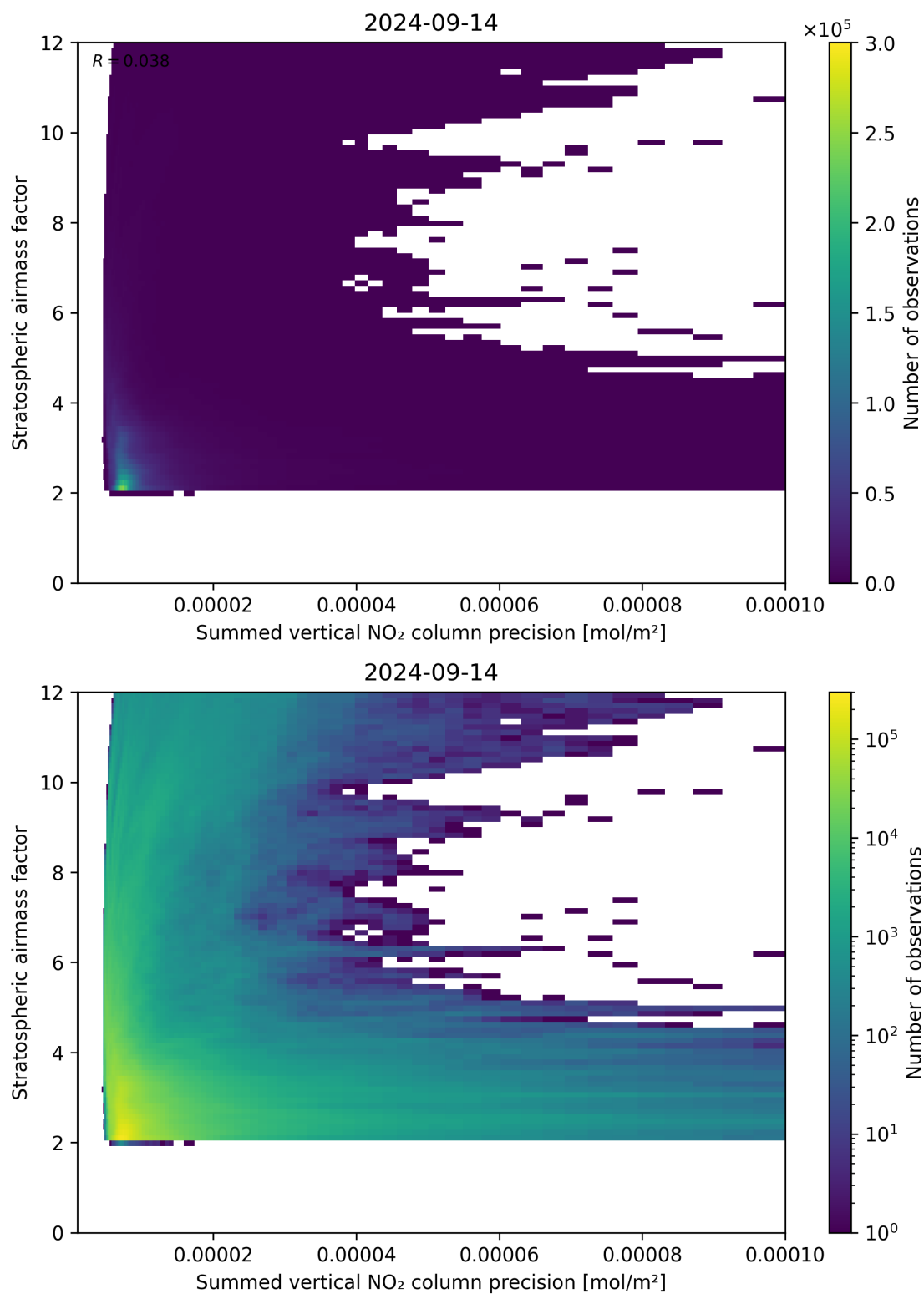
Figure 106: Scatter density plot of “Summed vertical NO 2 column precision” against “Stratospheric airmass factor” for 2024-09-13 to 2024-09-15.
