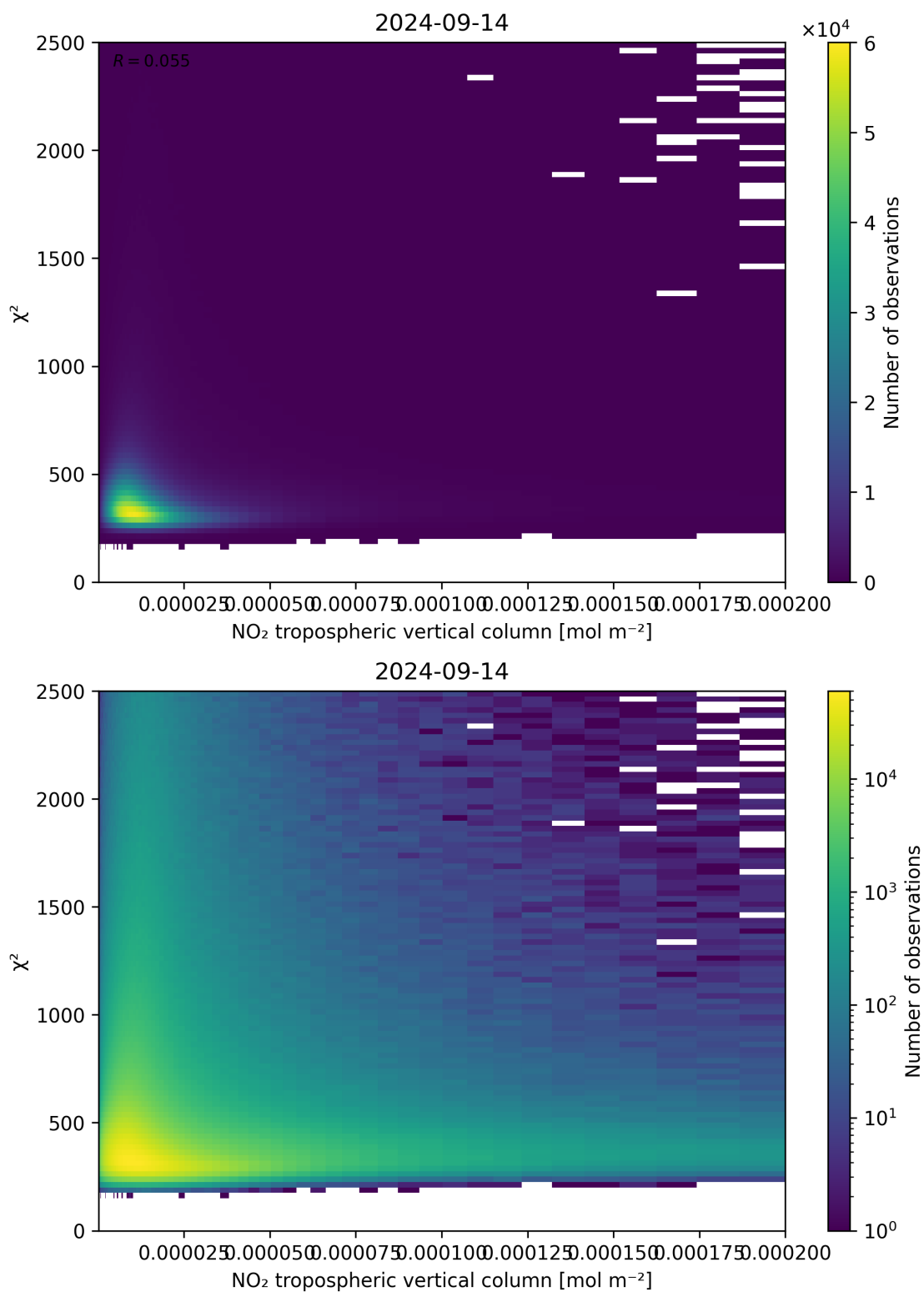
Figure 124: Scatter density plot of “NO 2 tropospheric vertical column” against “ \chi^2 ” for 2024-09-13 to 2024-09-15.
