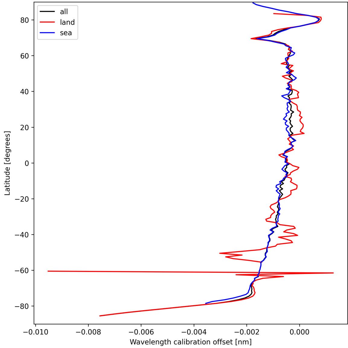
Figure 18: Zonal average of “Wavelength calibration offset” for 2024-09-13 to 2024-09-15.
