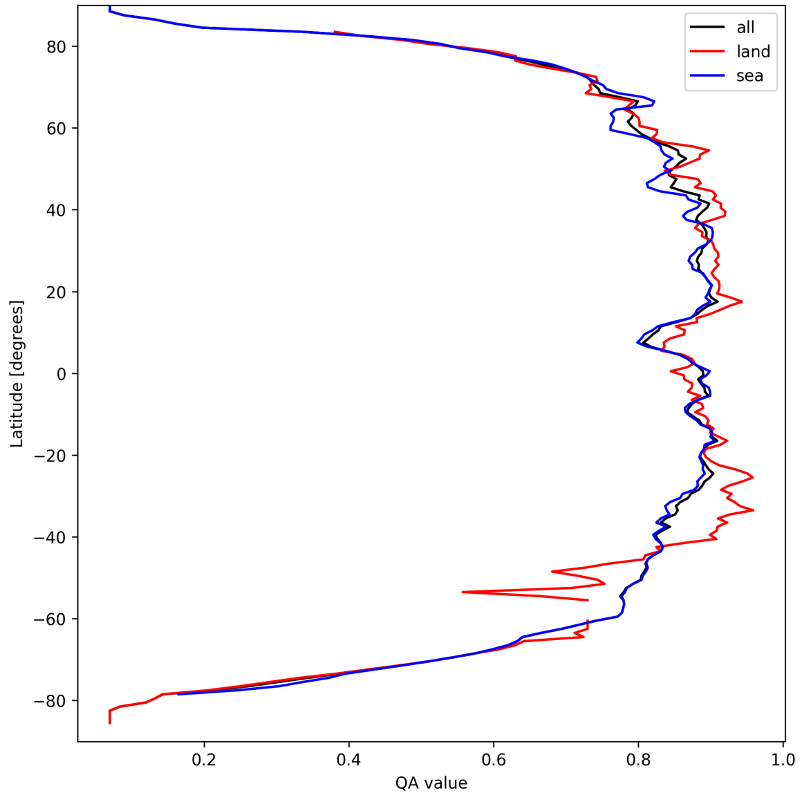
Figure 11: Zonal average of “QA value” for 2024-09-13 to 2024-09-15.
