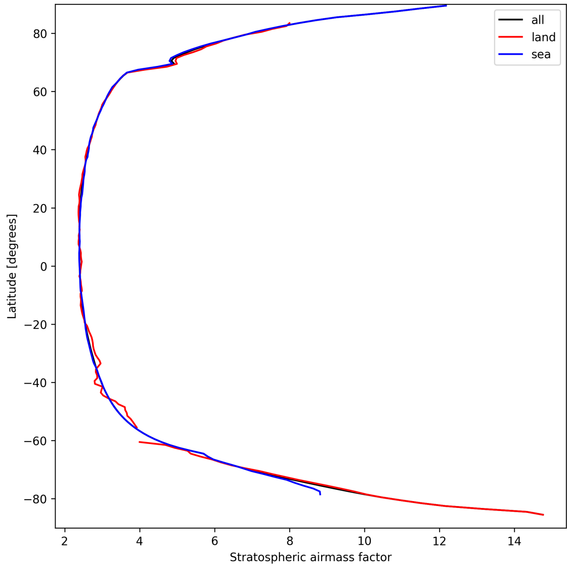
Figure 27: Zonal average of “Stratospheric airmass factor” for 2024-09-13 to 2024-09-15.
