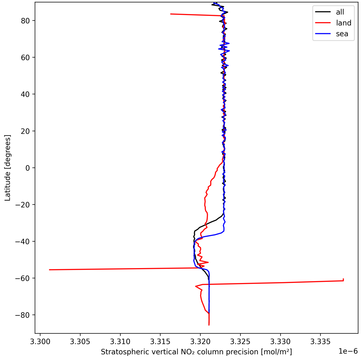
Figure 20: Zonal average of “Stratospheric vertical NO 2 column precision” for 2024-09-13 to 2024-09-15.
