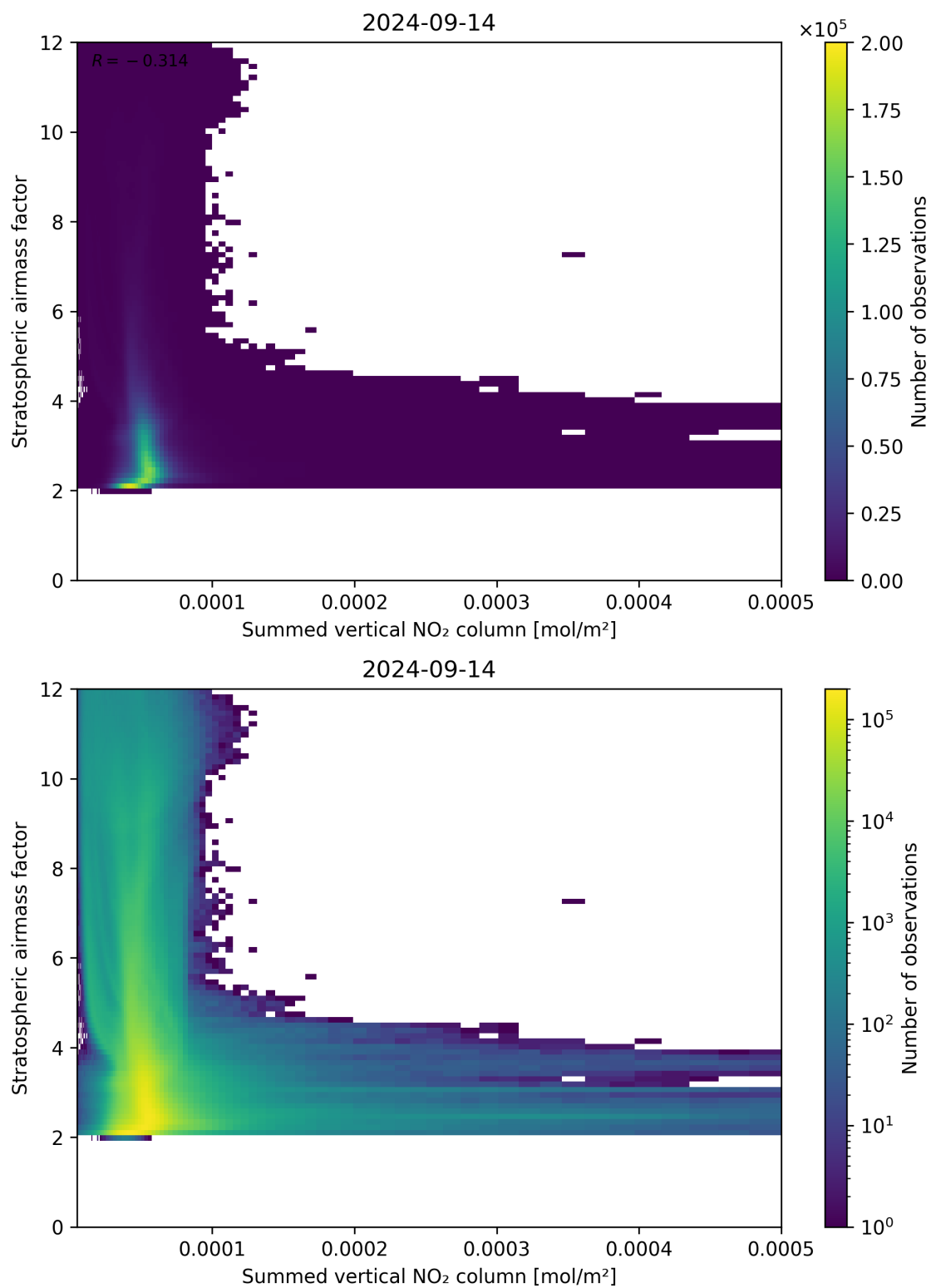
Figure 103: Scatter density plot of “Summed vertical NO 2 column” against “Stratospheric air mass factor” for 2024-09-13 to 2024-09-15.
