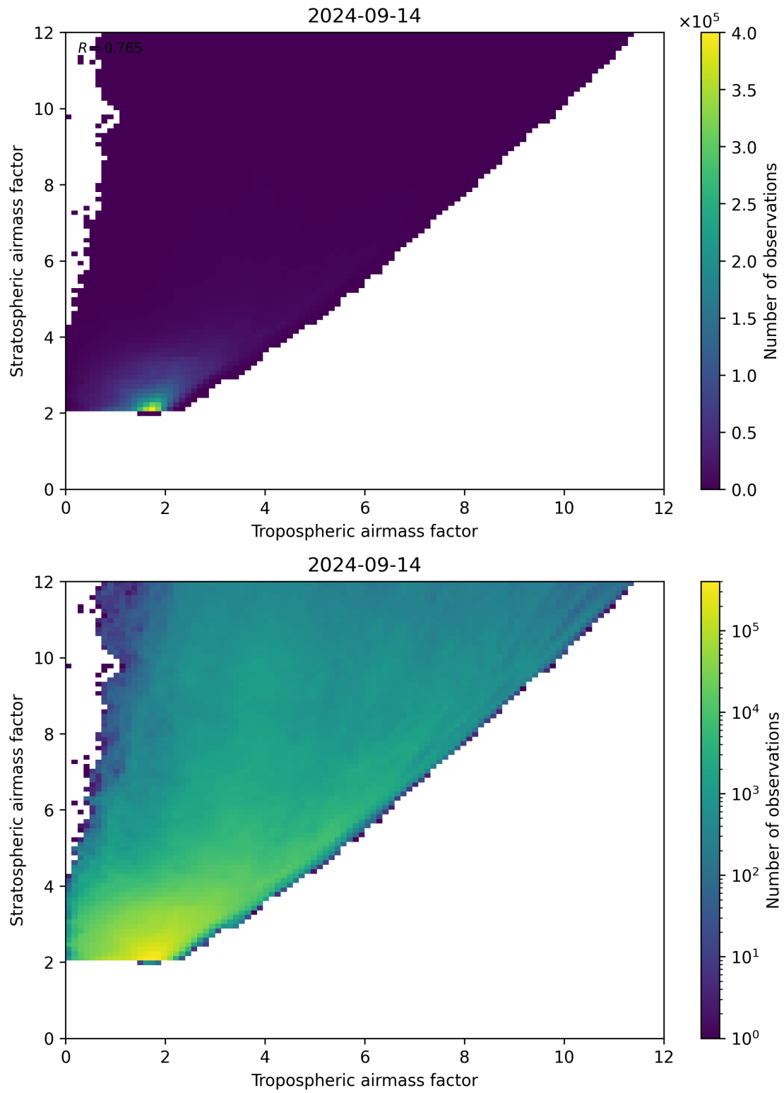
Figure 71: Scatter density plot of “Tropospheric airmass factor” against “Stratospheric airmass factor” for 2024-09-13 to 2024-09-15.
