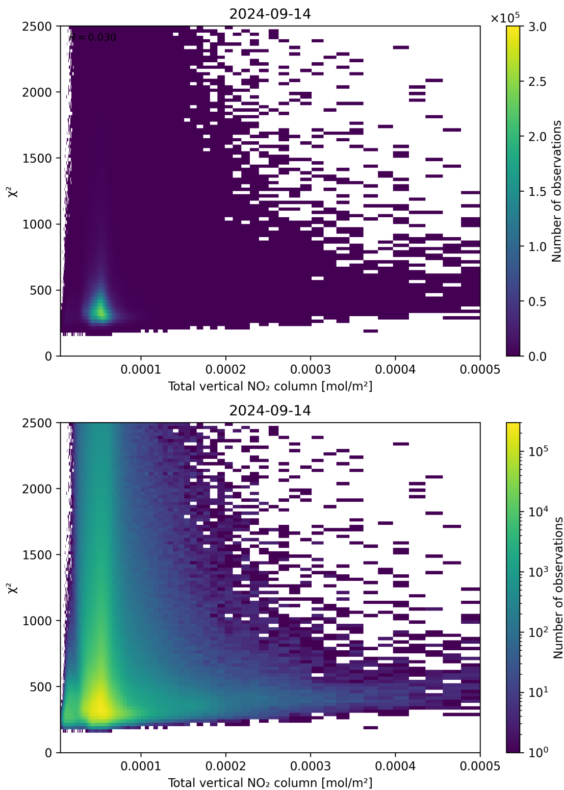
Figure 111: Scatter density plot of “Total vertical NO 2 column” against “ \chi^2 ” for 2024-09-13 to 2024-09-15.
