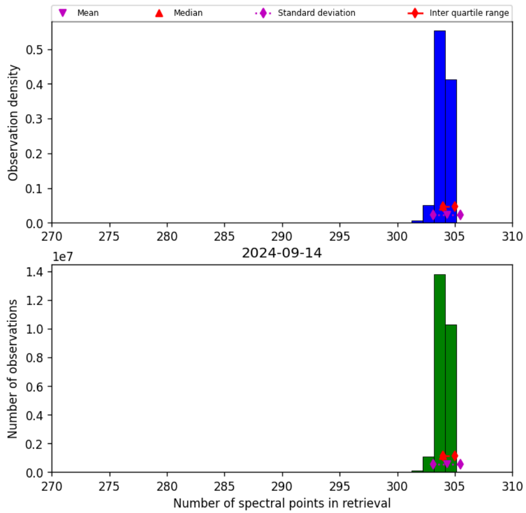
Figure 33: Histogram of “Number of spectral points in retrieval” for 2024-09-13 to 2024-09-15
