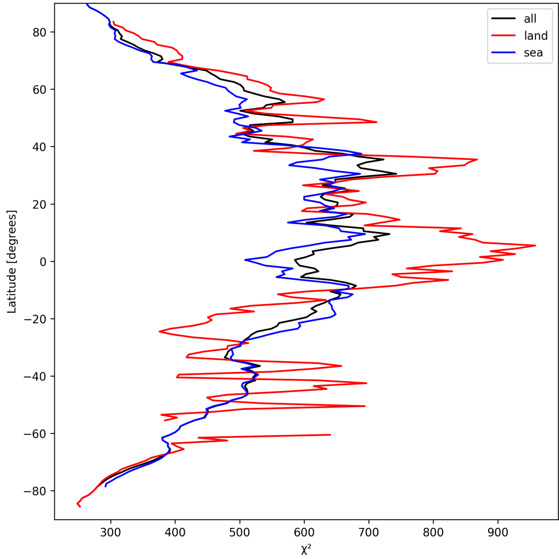
Figure 25: Zonal average of “ \chi^2 ” for 2024-09-13 to 2024-09-15.
