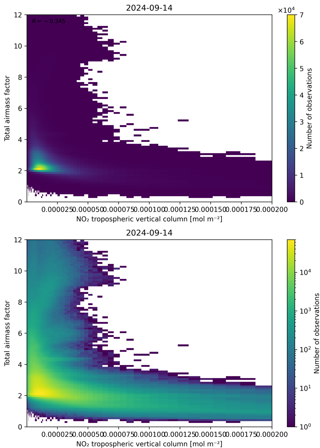
Figure 122: Scatter density plot of “NO 2 tropospheric vertical column” against “Total airmass factor” for 2024-09-13 to 2024-09-15.
