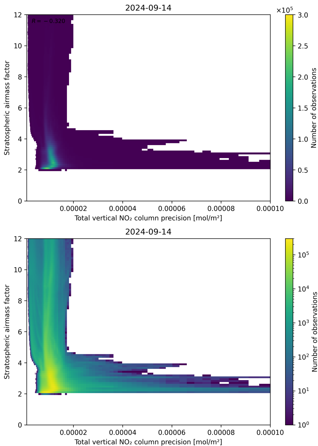
Figure 115: Scatter density plot of “Total vertical NO 2 column precision” against “Stratospheric air mass factor” for 2024-09-13 to 2024-09-15.
