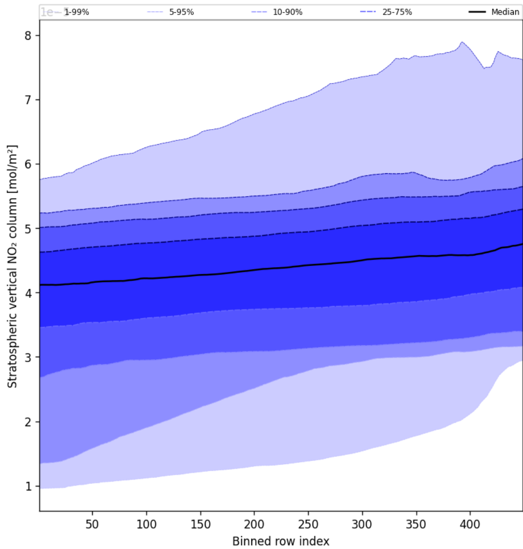
Figure 53: Along track statistics of “Stratospheric vertical NO 2 column” for 2024-09-13 to 2024-09-15
