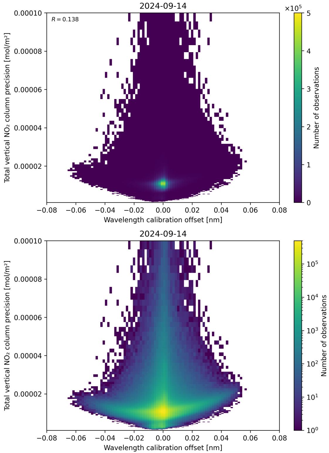
Figure 180: Scatter density plot of “Wavelength calibration offset” against “Total vertical NO 2 column precision” for 2024-09-13 to 2024-09-15.
