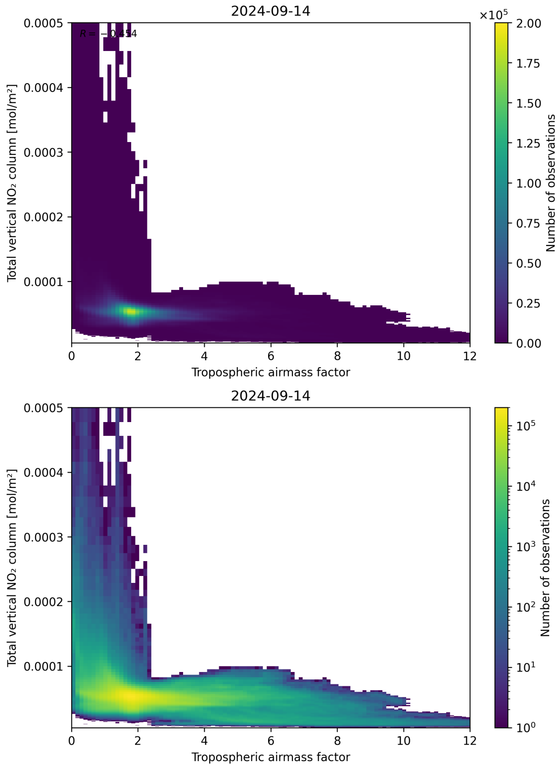
Figure 77: Scatter density plot of “Tropospheric airmass factor” against “Total vertical NO 2 column” for 2024-09-13 to 2024-09-15.
