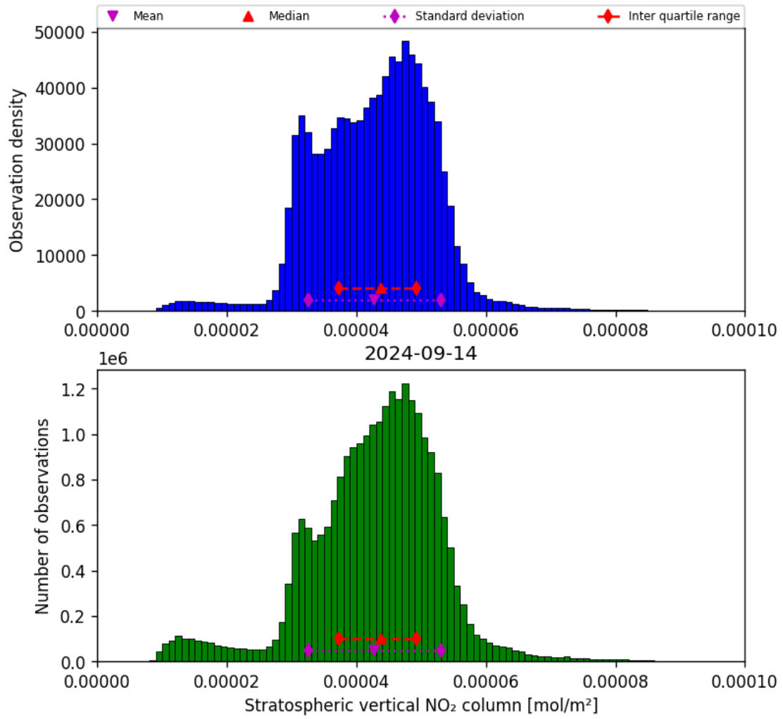
Figure 36: Histogram of “Stratospheric vertical NO 2 column” for 2024-09-13 to 2024-09-15
