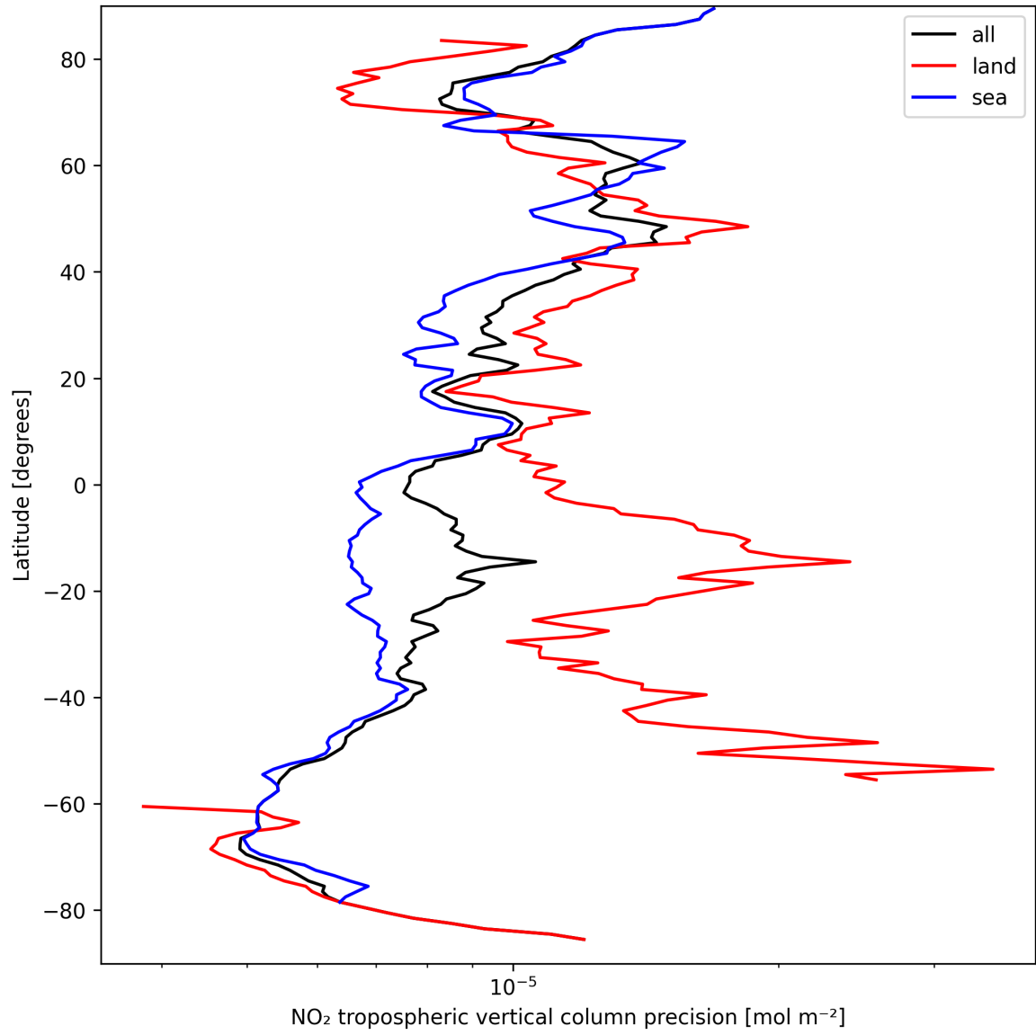
Figure 13: Zonal average of “NO 2 tropospheric vertical column precision” for 2024-09-13 to 2024-09-15.
