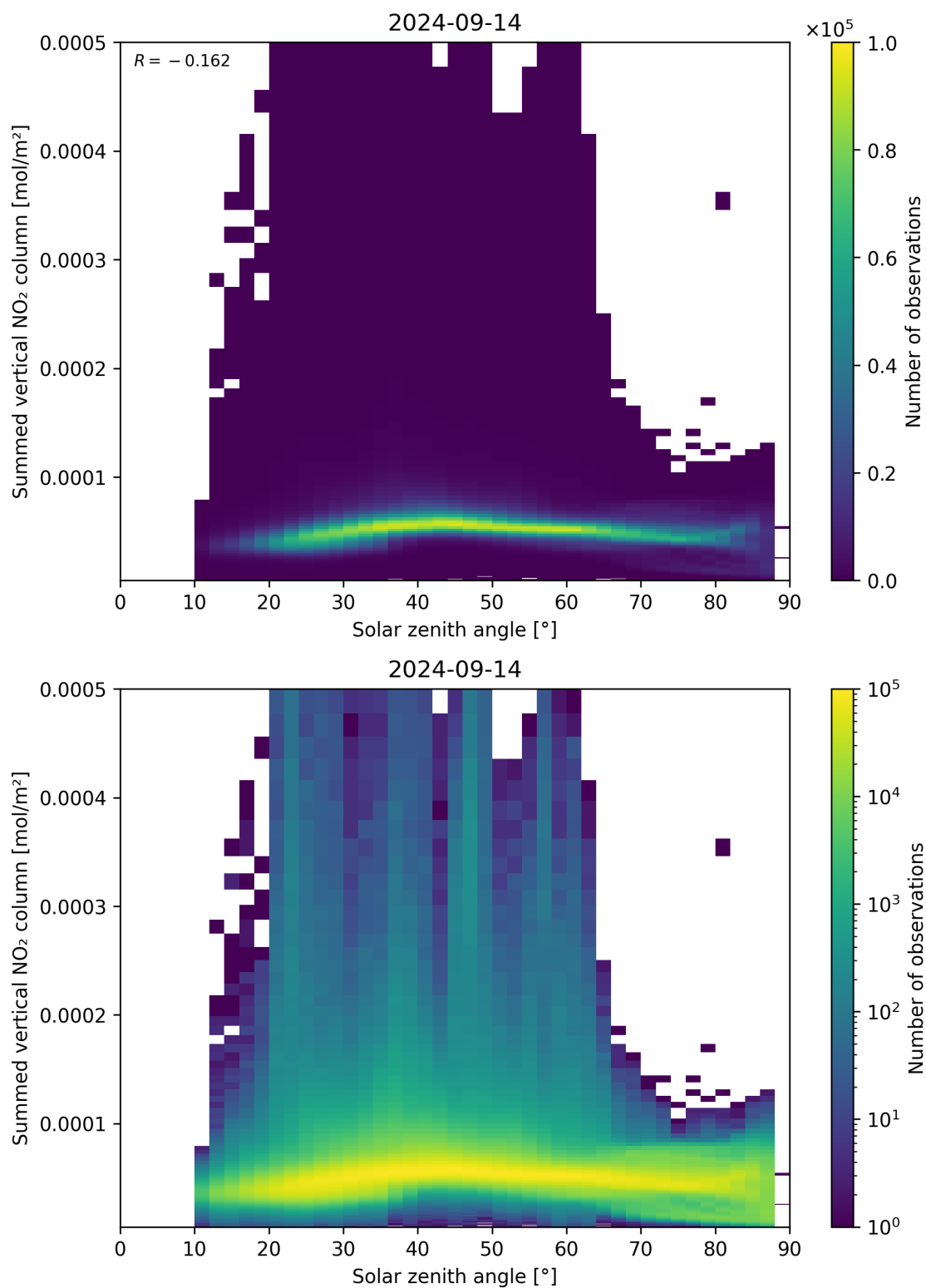
Figure 151: Scatter density plot of “Solar zenith angle” against “Summed vertical NO 2 column” for 2024-09-13 to 2024-09-15.
