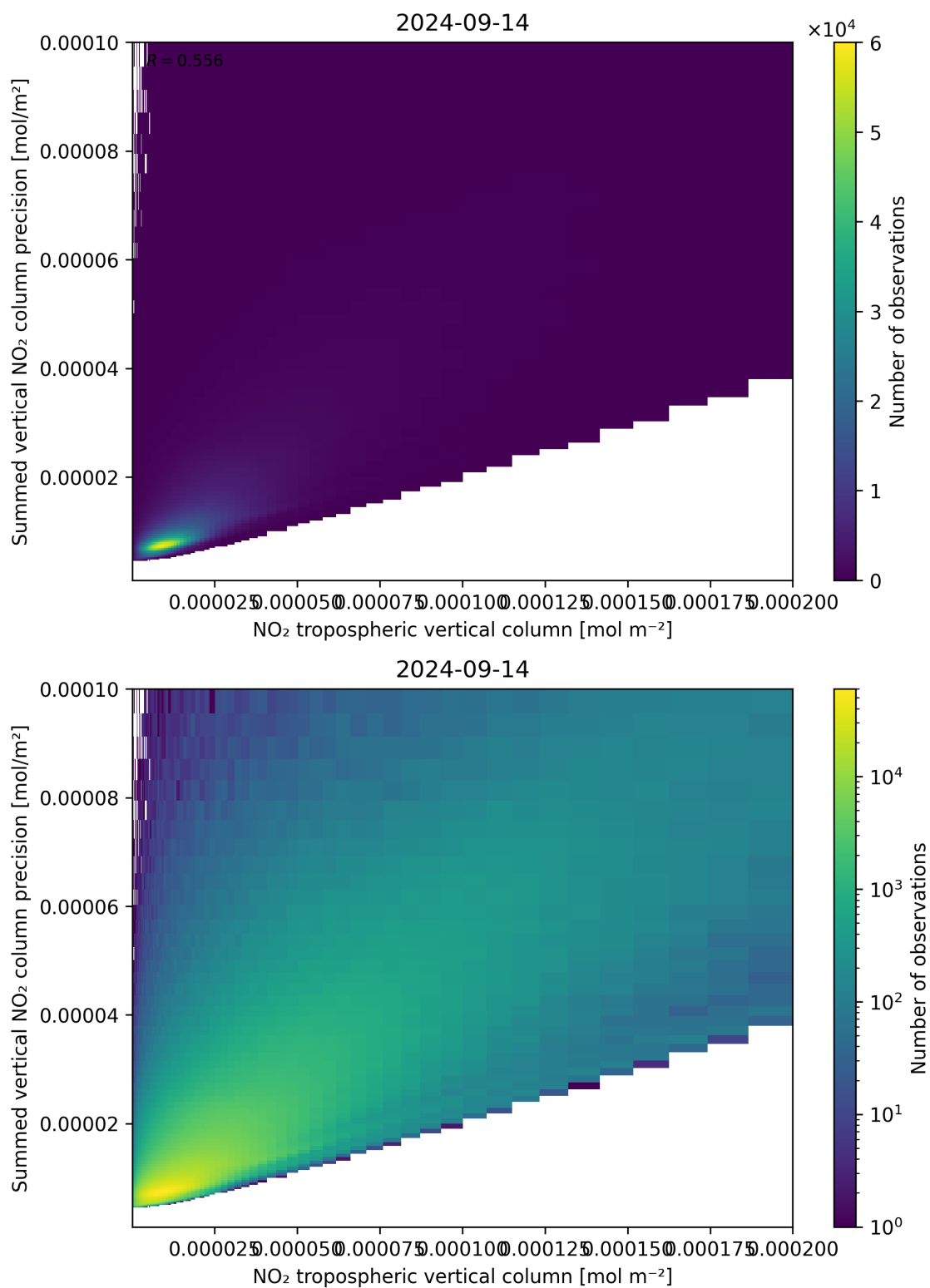
Figure 127: Scatter density plot of “NO 2 tropospheric vertical column” against “Summed vertical NO 2 column precision” for 2024-09-13 to 2024-09-15.
