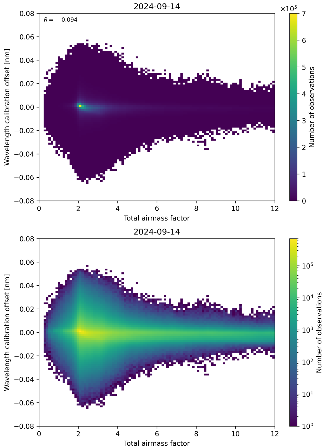
Figure 70: Scatter density plot of “Total airmass factor” against “Wavelength calibration offset” for 2024-09-13 to 2024-09-15.
