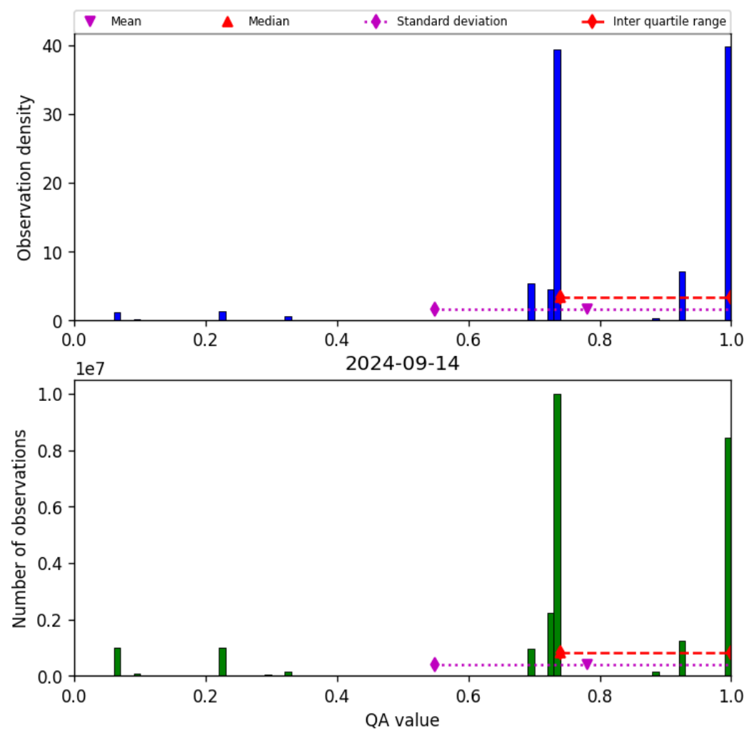
Figure 28: Histogram of “QA value” for 2024-09-13 to 2024-09-15
