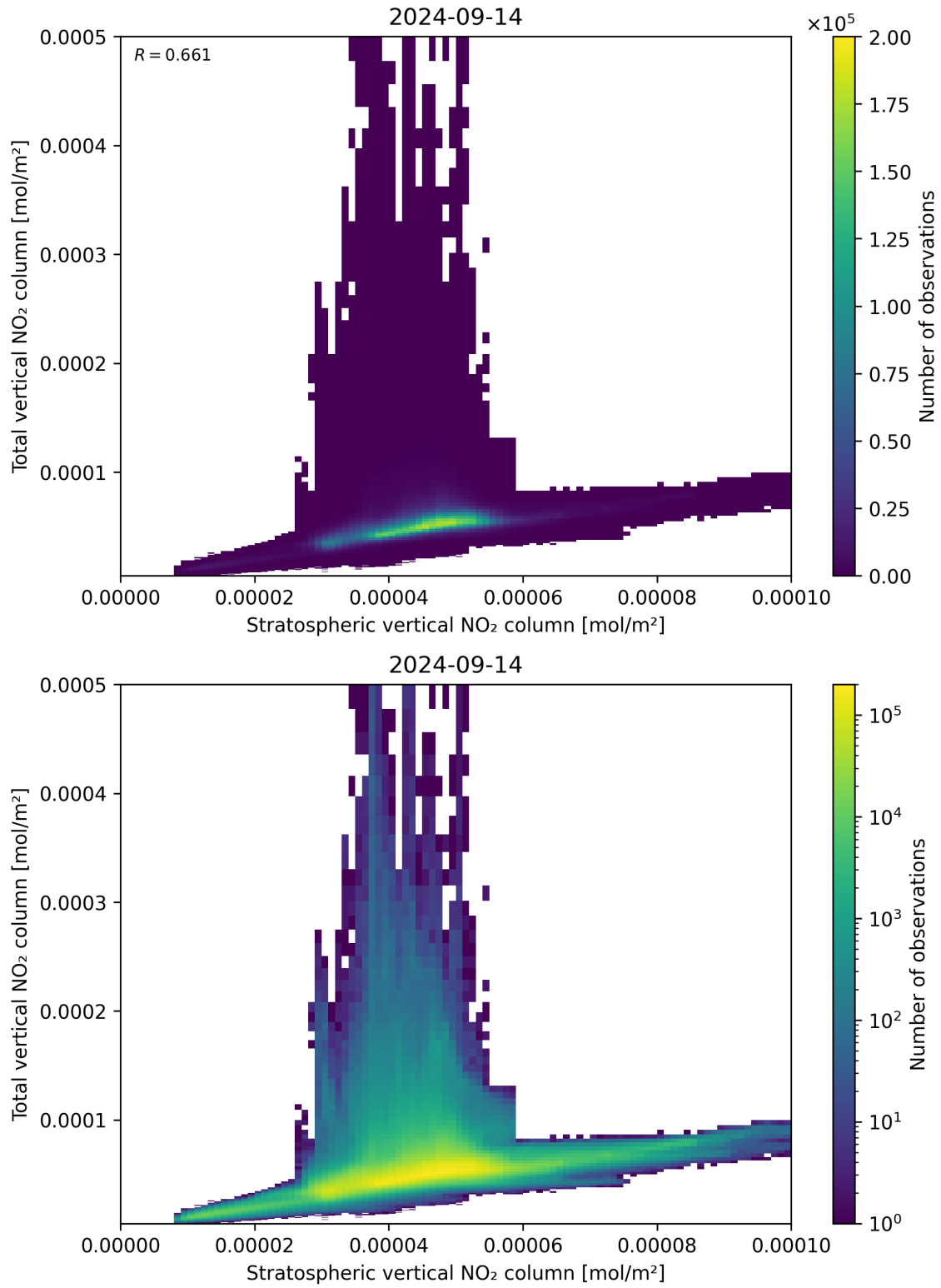
Figure 100: Scatter density plot of “Stratospheric vertical NO 2 column” against “Total vertical NO 2 column” for 2024-09-13 to 2024-09-15.
