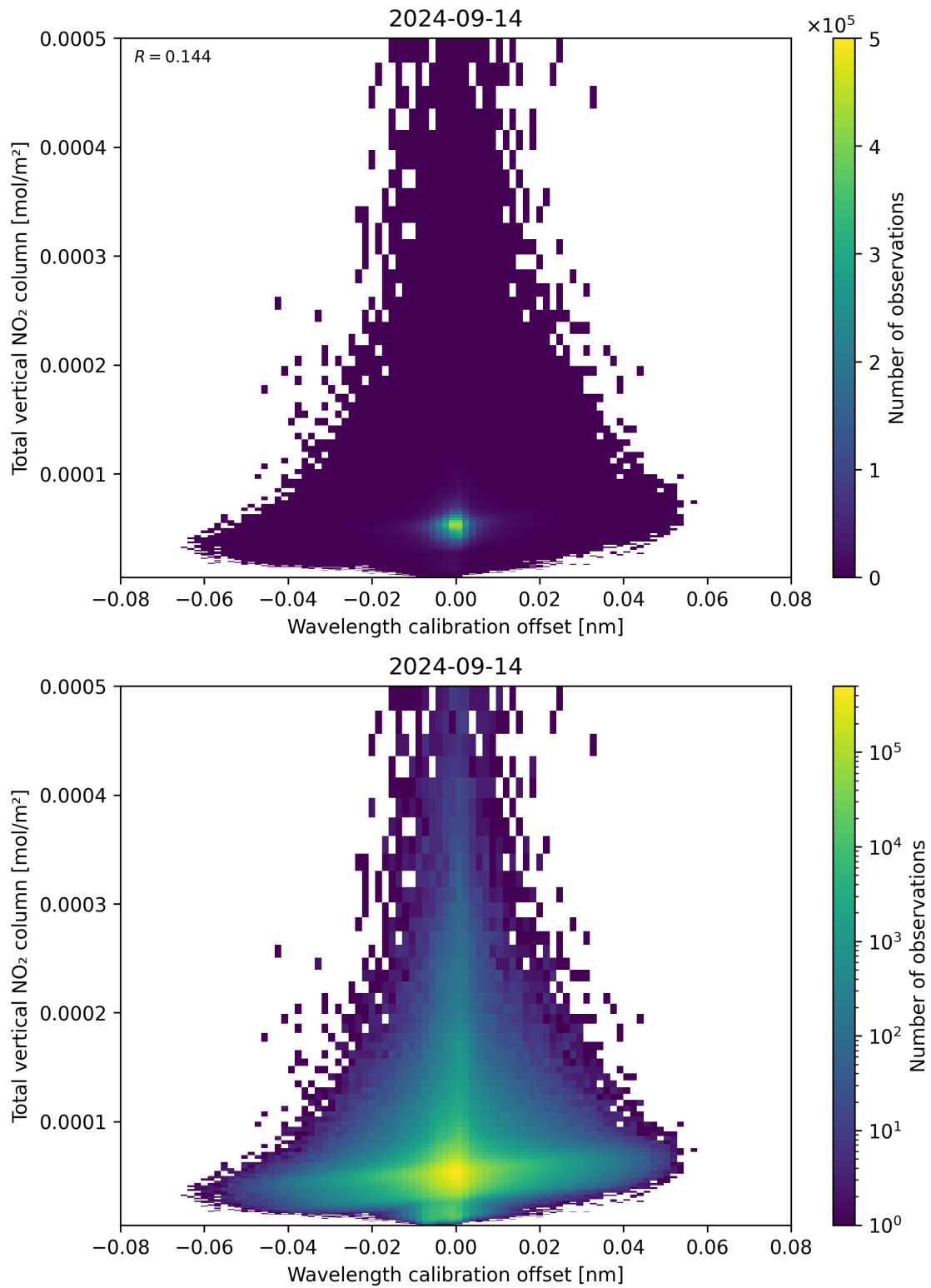
Figure 179: Scatter density plot of “Wavelength calibration offset” against “Total vertical NO 2 column” for 2024-09-13 to 2024-09-15.
