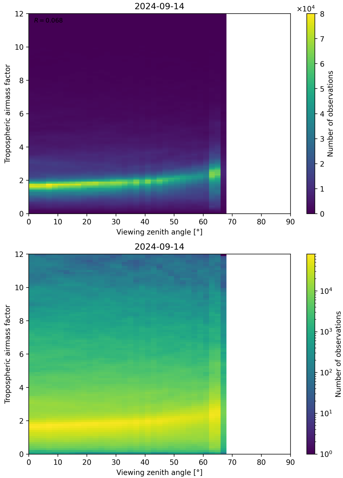
Figure 161: Scatter density plot of “Viewing zenith angle” against “Tropospheric airmass factor” for 2024-09-13 to 2024-09-15.
