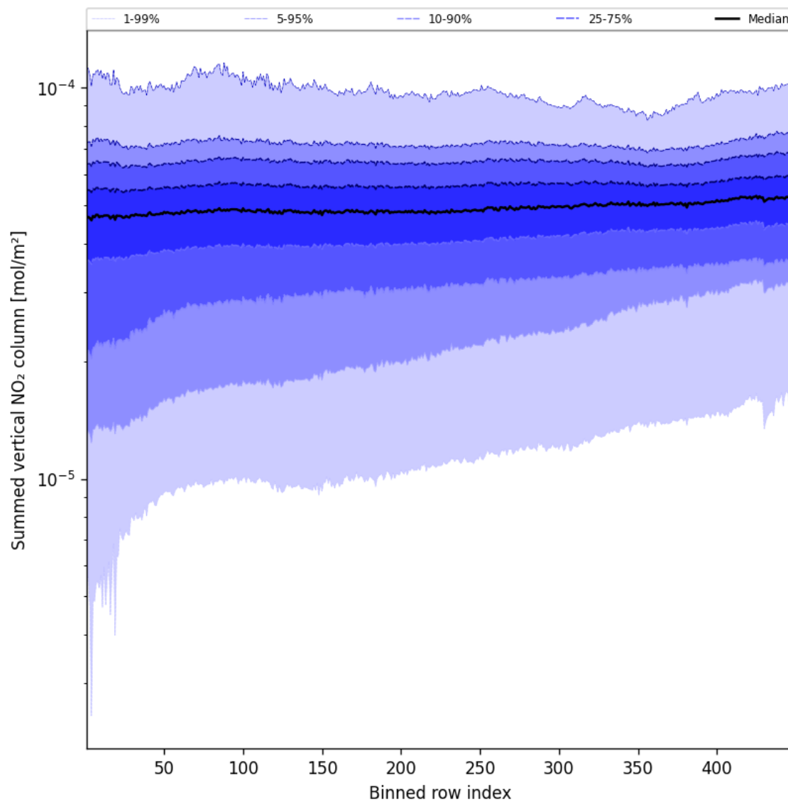
Figure 57: Along track statistics of “Summed vertical NO 2 column” for 2024-09-13 to 2024-09-15
