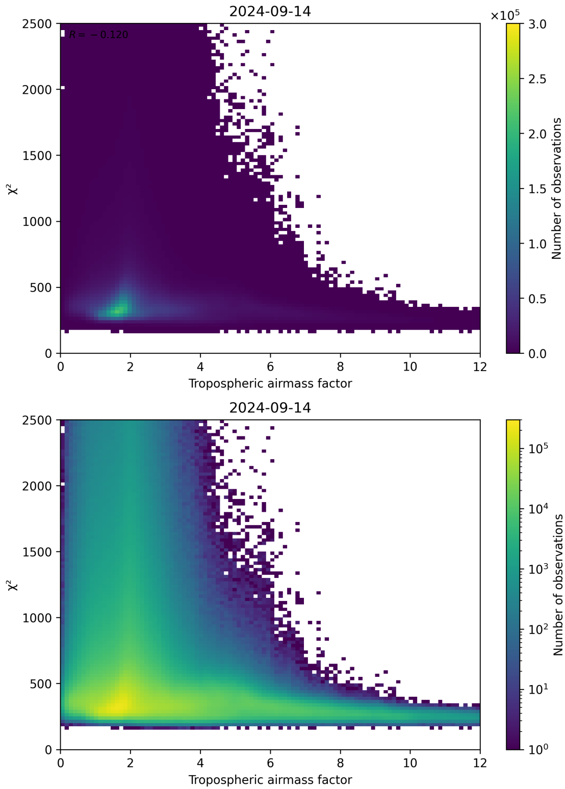
Figure 73: Scatter density plot of “Tropospheric airmass factor” against “ \chi^2 ” for 2024-09-13 to 2024-09-15.
