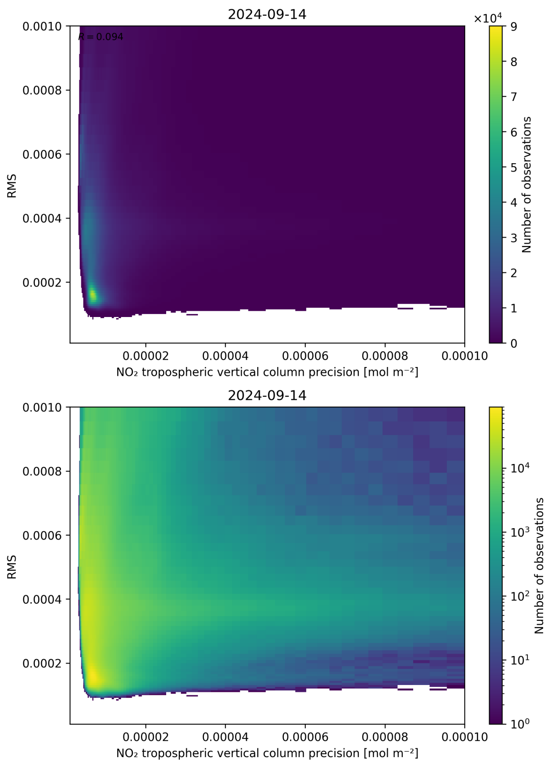
Figure 140: Scatter density plot of “NO 2 tropospheric vertical column precision” against “RMS” for 2024-09-13 to 2024-09-15.
