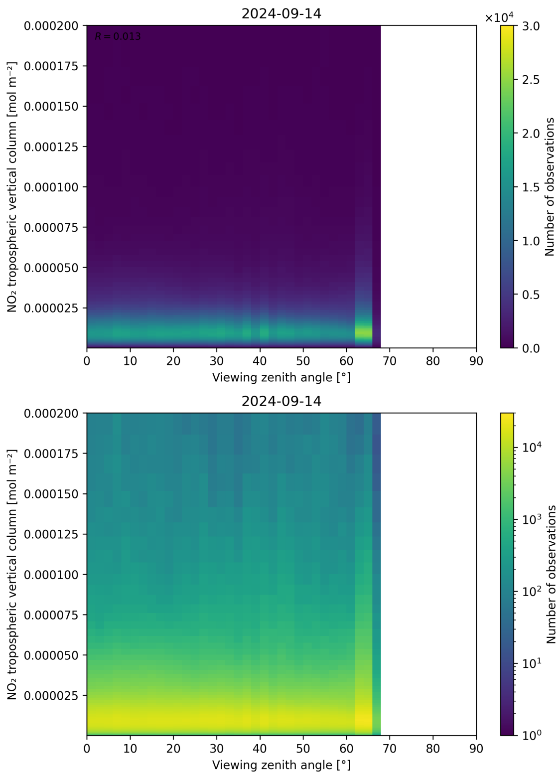
Figure 169: Scatter density plot of “Viewing zenith angle” against “NO 2 tropospheric vertical column” for 2024-09-13 to 2024-09-15.
