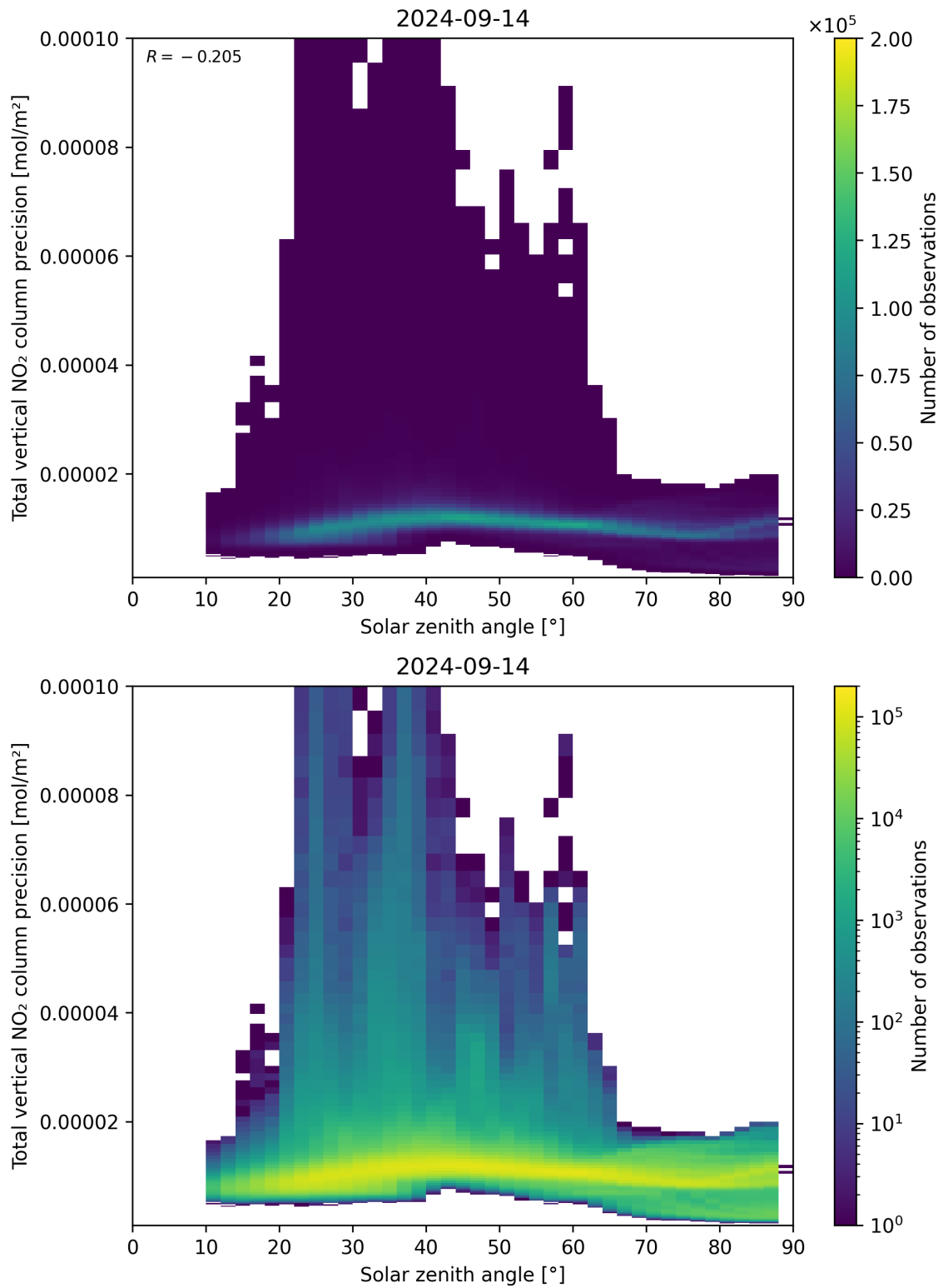
Figure 154: Scatter density plot of “Solar zenith angle” against “Total vertical NO 2 column precision” for 2024-09-13 to 2024-09-15.
