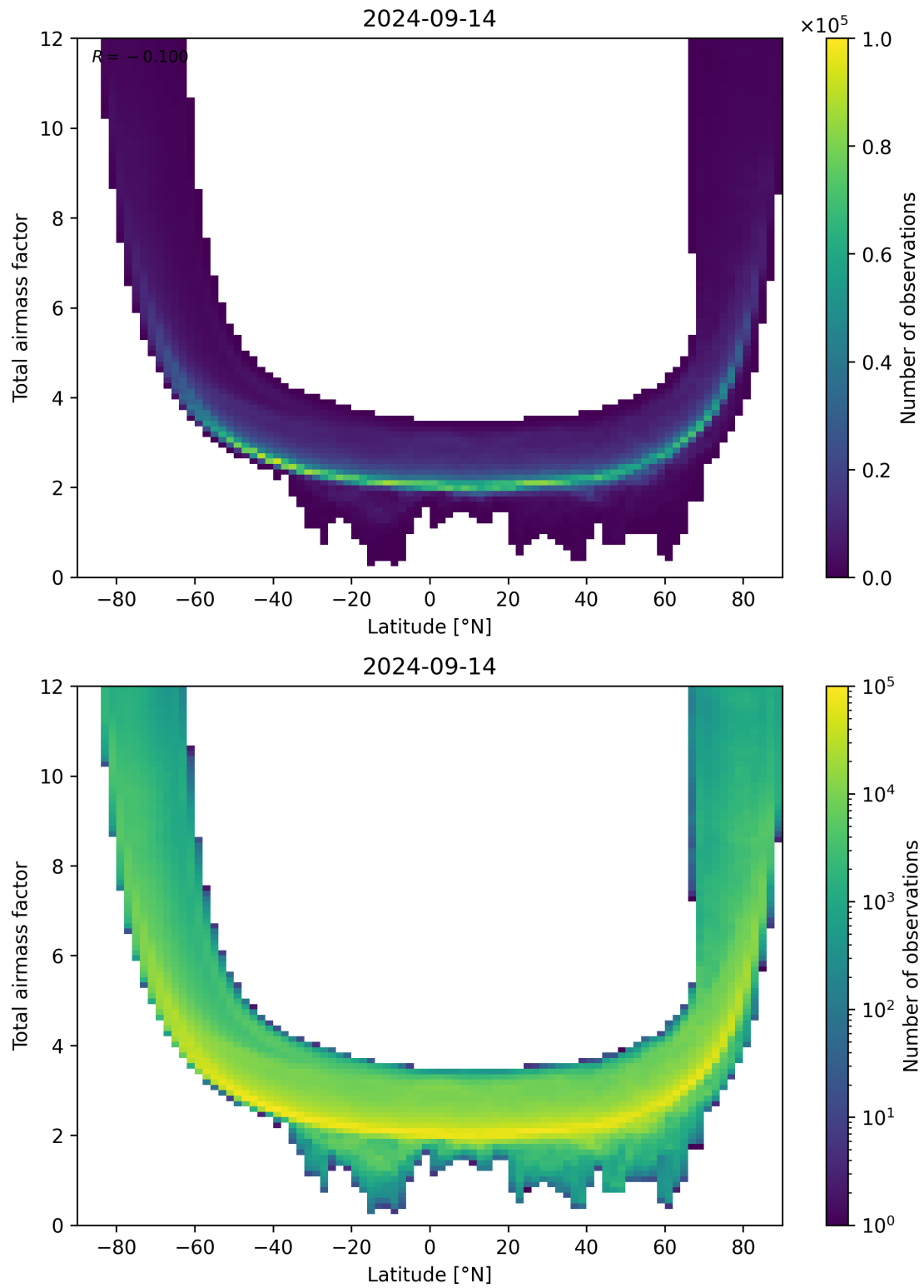
Figure 84: Scatter density plot of “Latitude” against “Total airmass factor” for 2024-09-13 to 2024-09-15.
