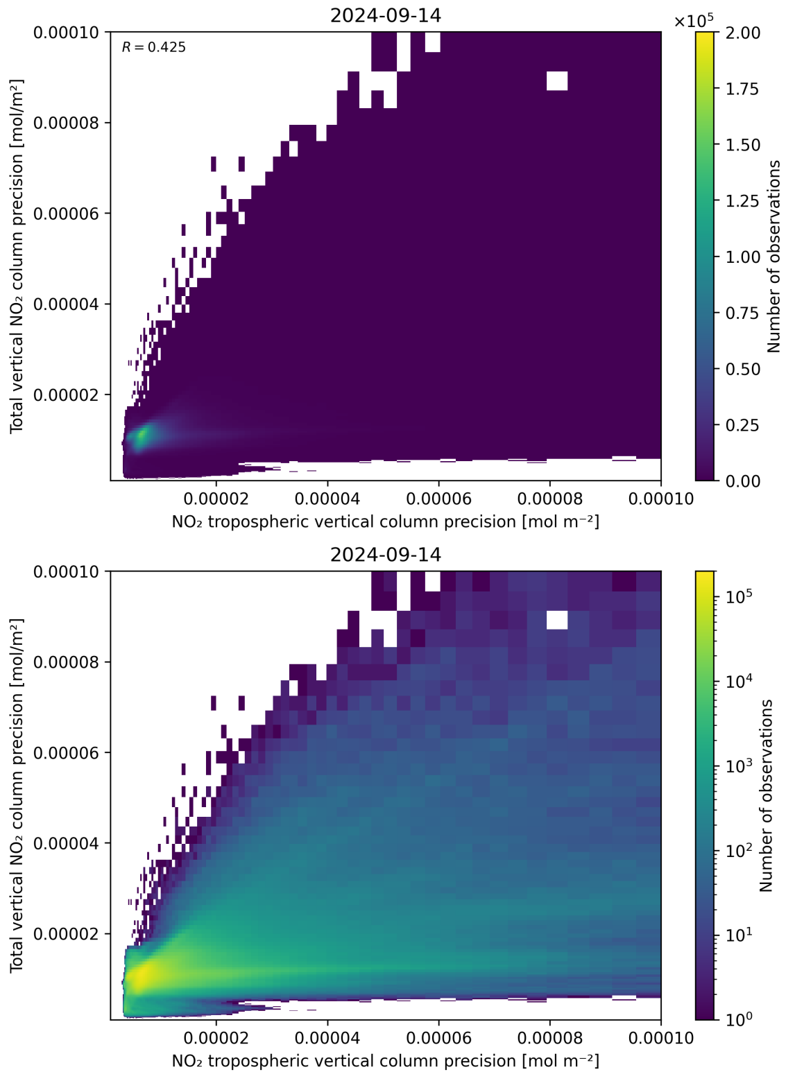
Figure 139: Scatter density plot of “NO 2 tropospheric vertical column precision” against “Total vertical NO 2 column precision” for 2024-09-13 to 2024-09-15.
