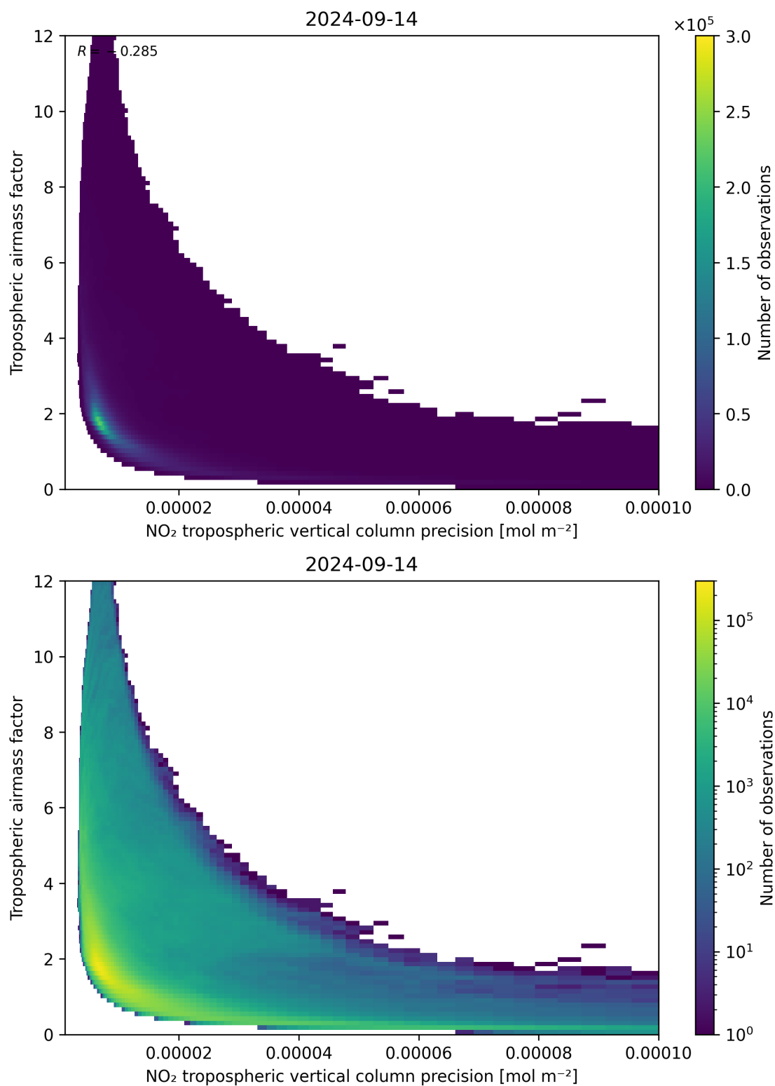
Figure 133: Scatter density plot of “NO 2 tropospheric vertical column precision” against “Tropospheric air mass factor” for 2024-09-13 to 2024-09-15.
