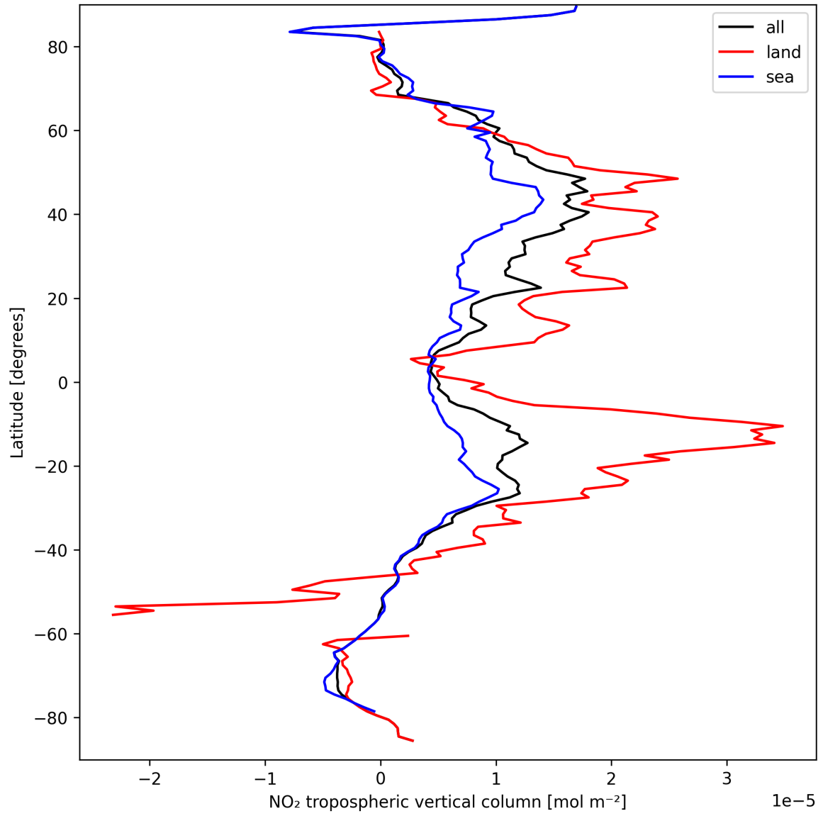
Figure 12: Zonal average of “NO 2 tropospheric vertical column” for 2024-09-13 to 2024-09-15.
