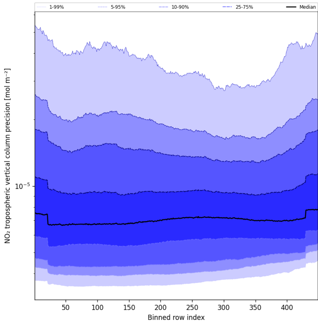
Figure 47: Along track statistics of “NO 2 tropospheric vertical column precision” for 2024-09-13 to 2024-09-15
