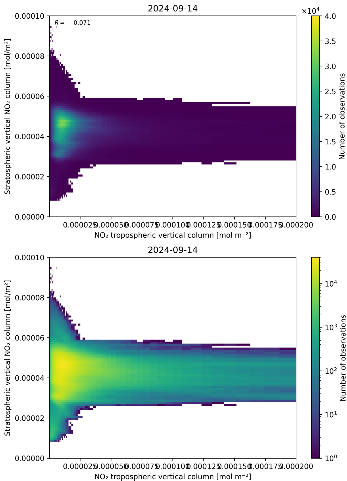
Figure 125: Scatter density plot of “NO 2 tropospheric vertical column” against “Stratospheric vertical NO 2 column” for 2024-09-13 to 2024-09-15.
