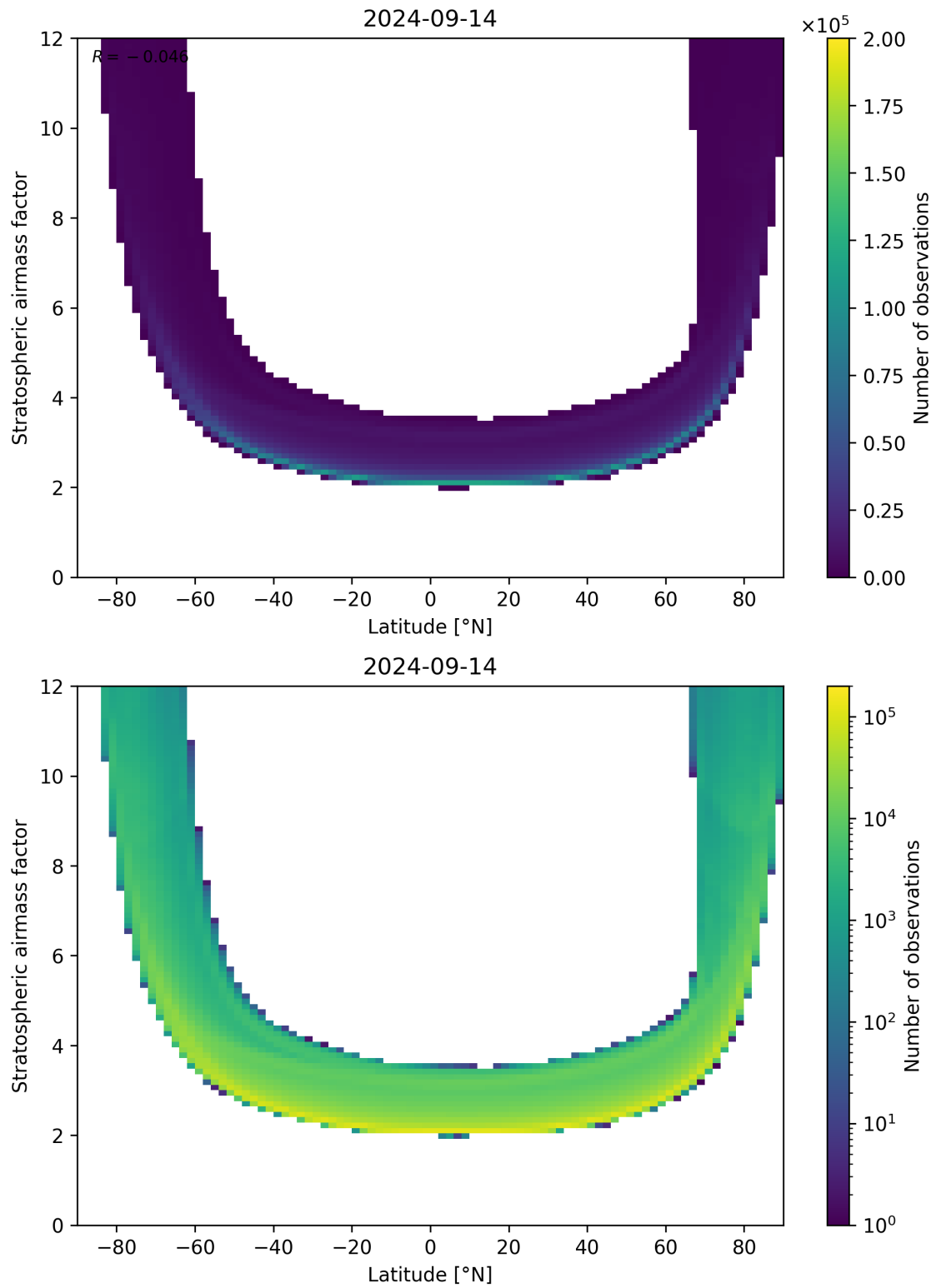
Figure 83: Scatter density plot of “Latitude” against “Stratospheric airmass factor” for 2024-09-13 to 2024-09-15.
