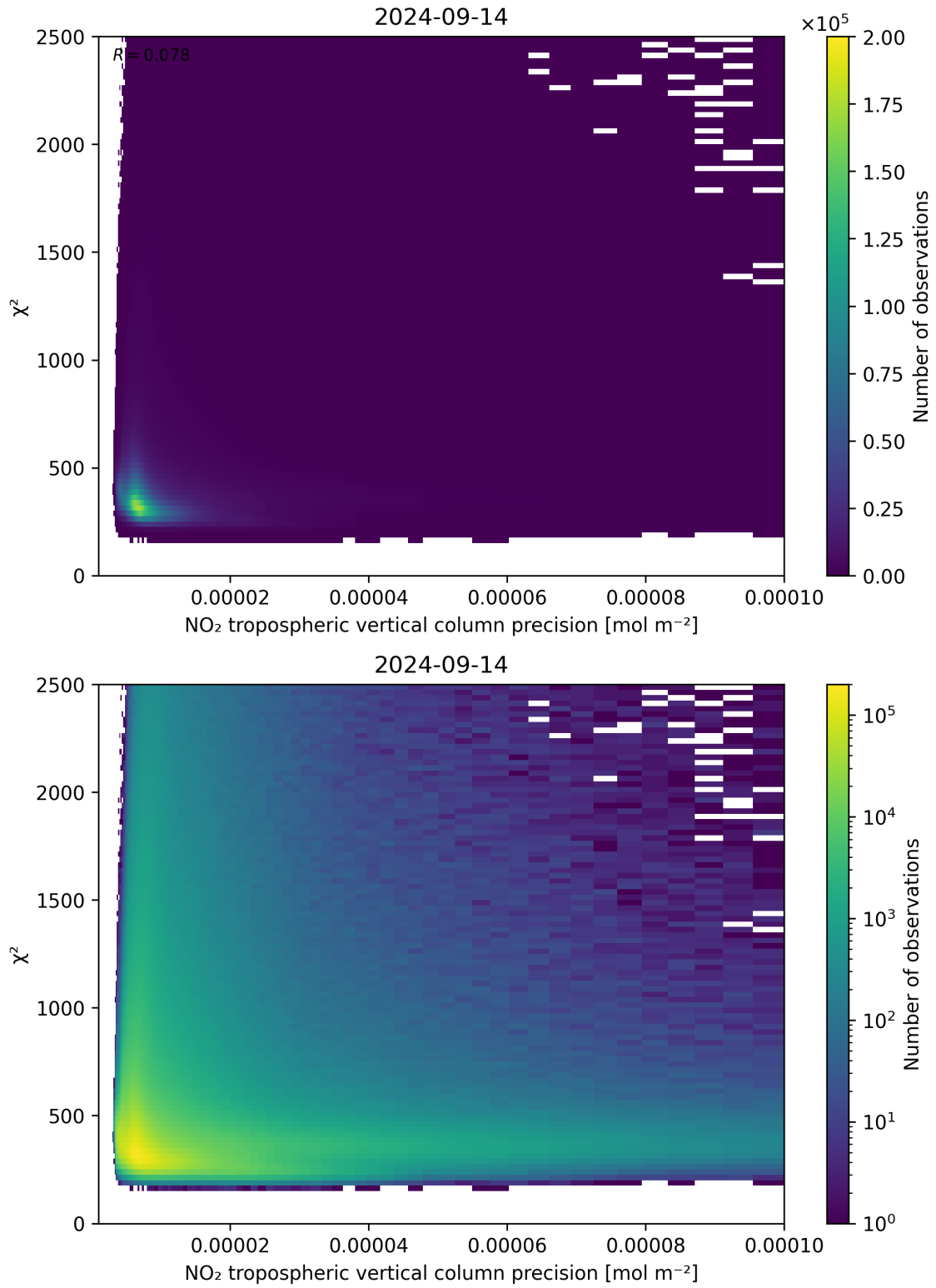
Figure 134: Scatter density plot of “NO 2 tropospheric vertical column precision” against “ \chi^2 ” for 2024-09-13 to 2024-09-15.
