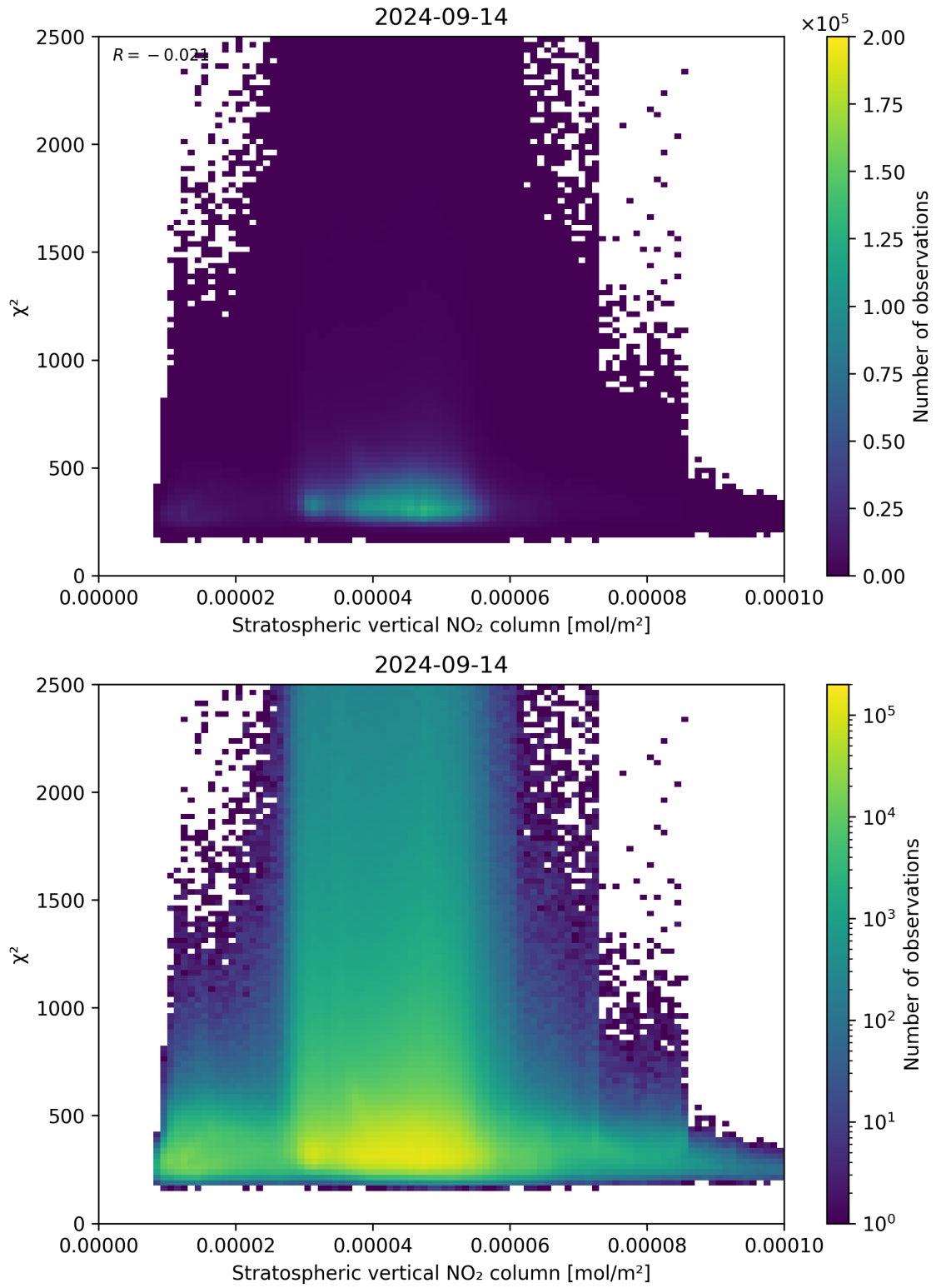
Figure 97: Scatter density plot of “Stratospheric vertical NO 2 column” against “ \chi^2 ” for 2024-09-13 to 2024-09-15.
