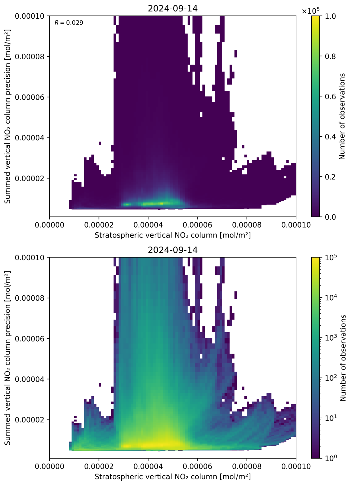
Figure 99: Scatter density plot of “Stratospheric vertical NO 2 column” against “Summed vertical NO 2 column precision” for 2024-09-13 to 2024-09-15.
