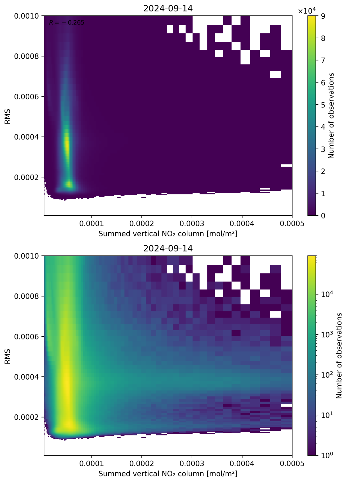
Figure 109: Scatter density plot of “Summed vertical NO 2 column” against “RMS” for 2024-09-13 to 2024-09-15.
