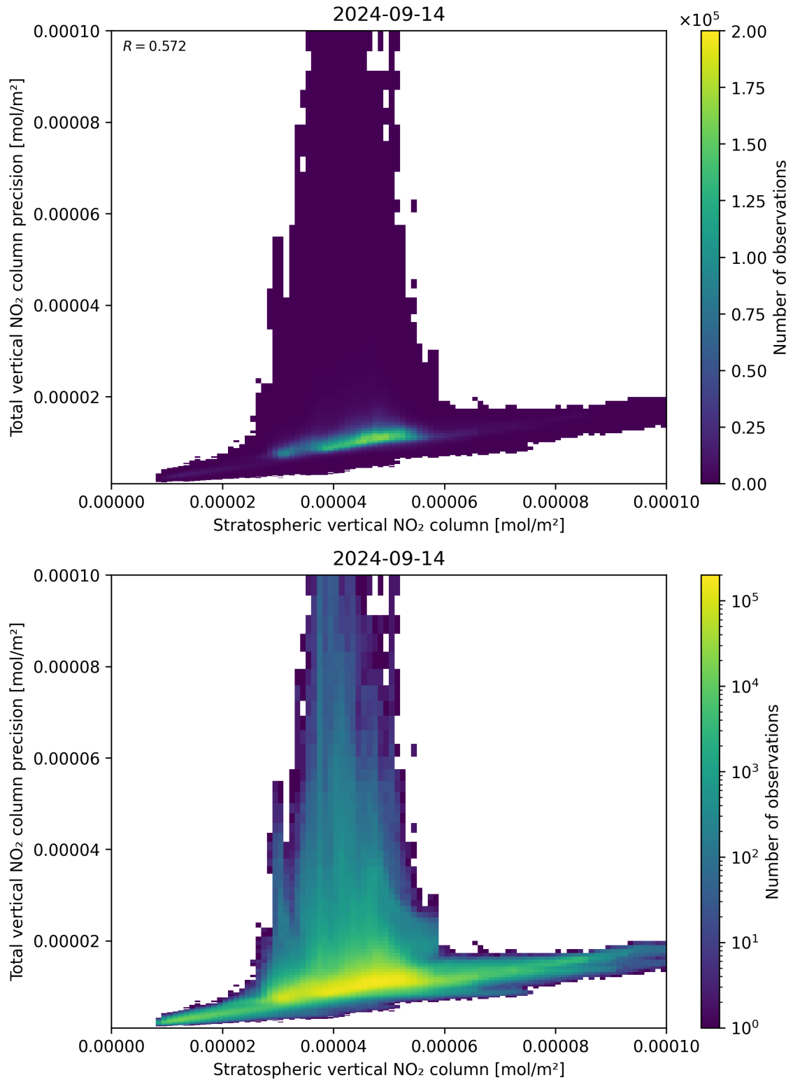
Figure 101: Scatter density plot of “Stratospheric vertical NO 2 column” against “Total vertical NO 2 column precision” for 2024-09-13 to 2024-09-15.
