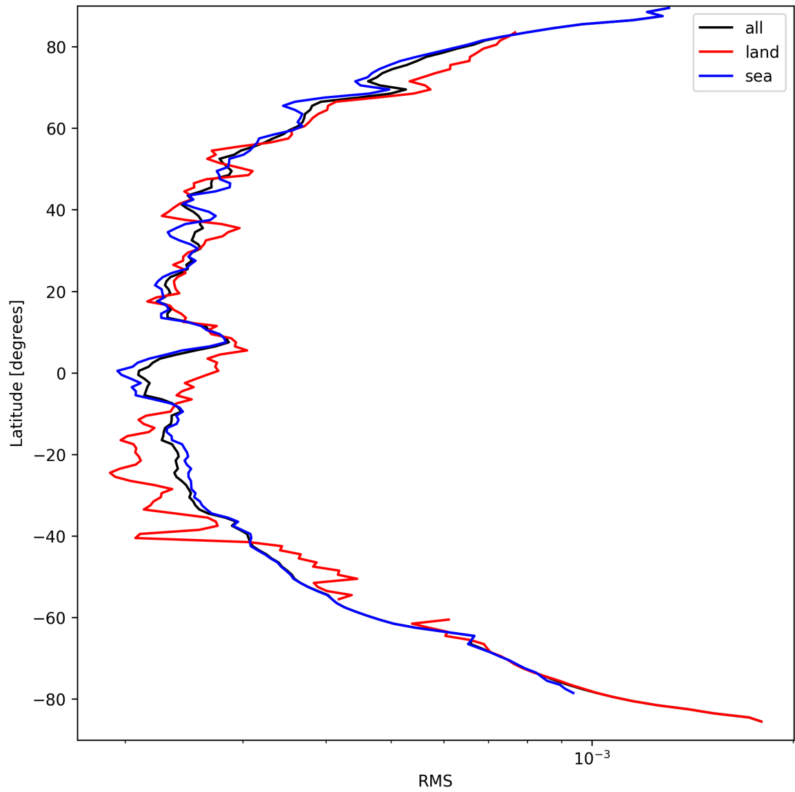
Figure 26: Zonal average of “RMS” for 2024-09-13 to 2024-09-15.
