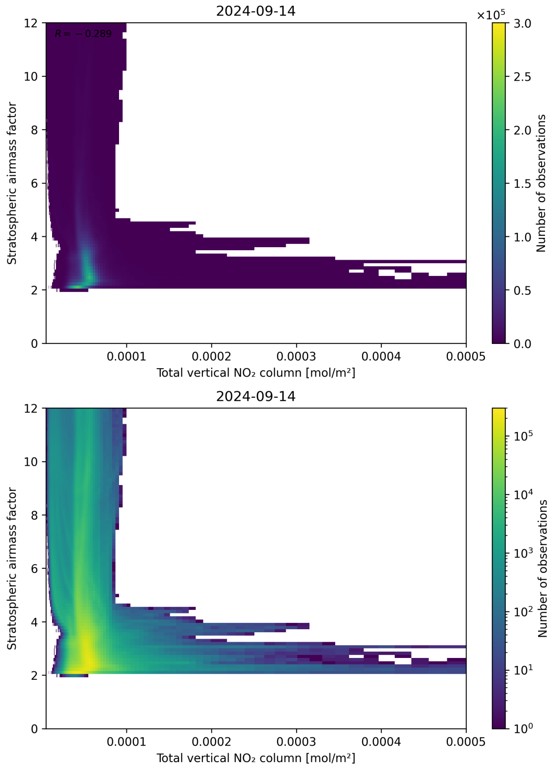
Figure 110: Scatter density plot of “Total vertical NO 2 column” against “Stratospheric airmass factor” for 2024-09-13 to 2024-09-15.
