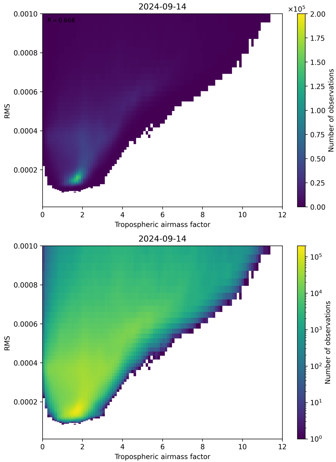
Figure 79: Scatter density plot of “Tropospheric airmass factor” against “RMS” for 2024-09-13 to 2024-09-15.
