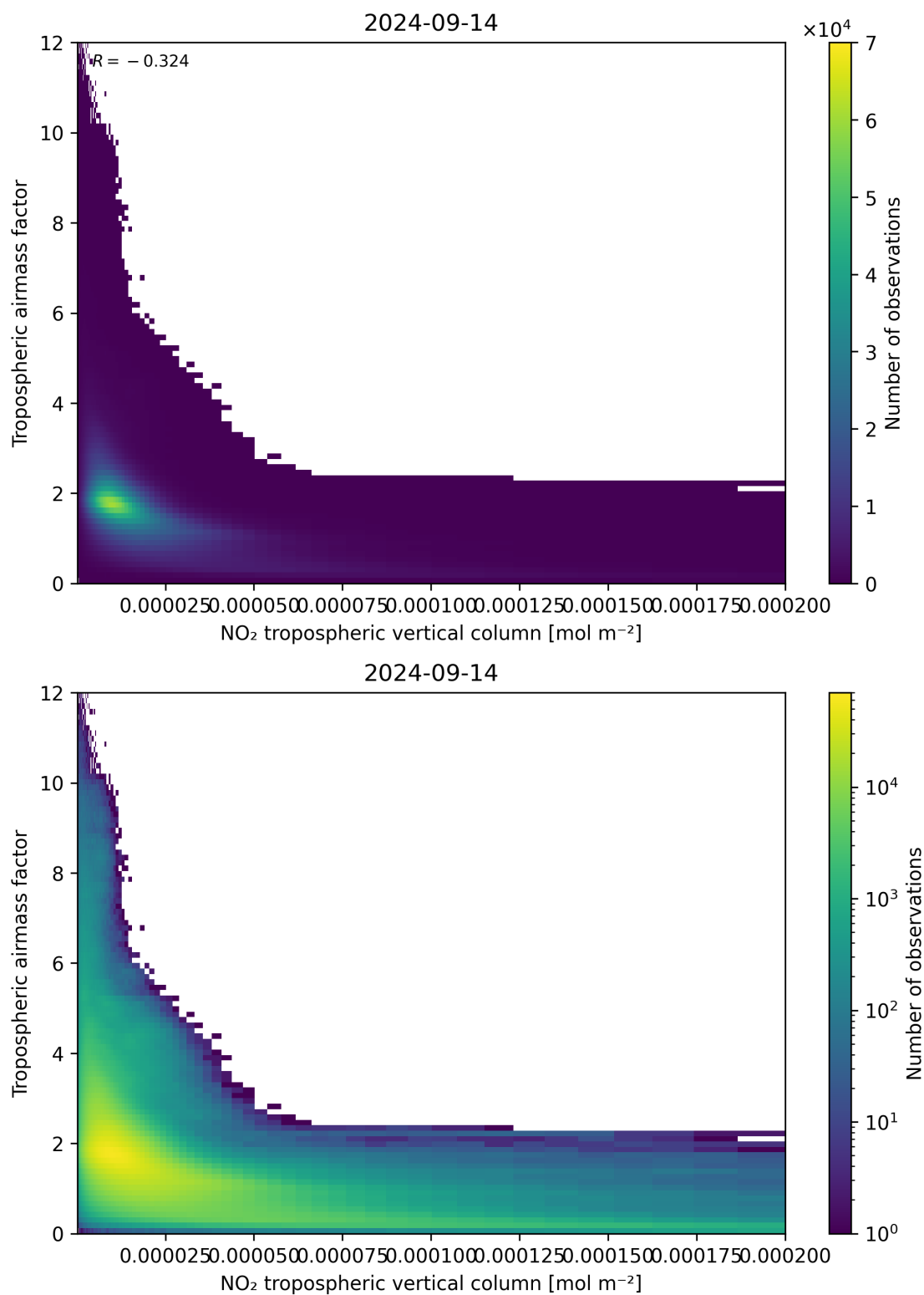
Figure 123: Scatter density plot of “NO 2 tropospheric vertical column” against “Tropospheric air mass factor” for 2024-09-13 to 2024-09-15.
