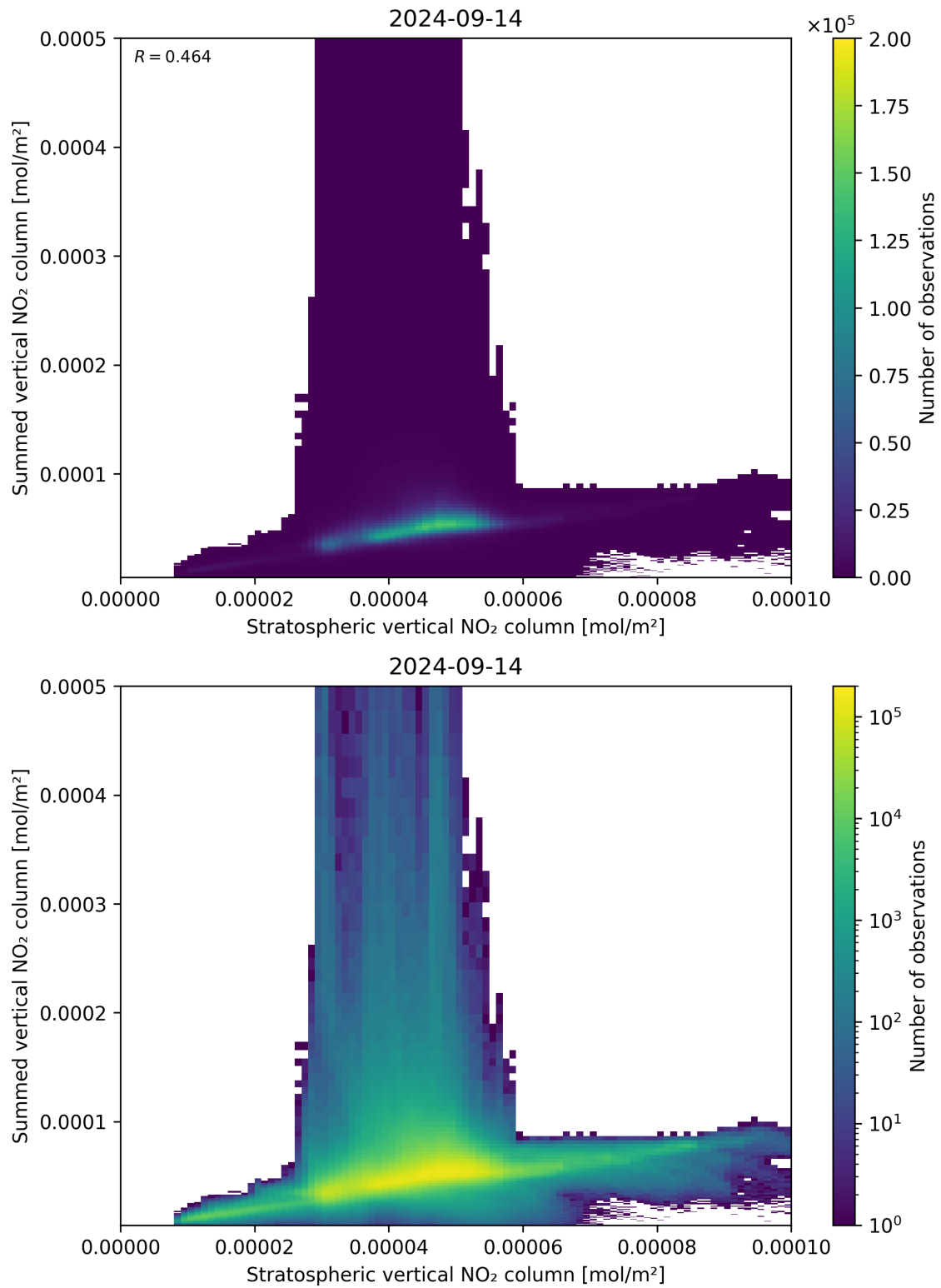
Figure 98: Scatter density plot of “Stratospheric vertical NO 2 column” against “Summed vertical NO 2 column” for 2024-09-13 to 2024-09-15.
