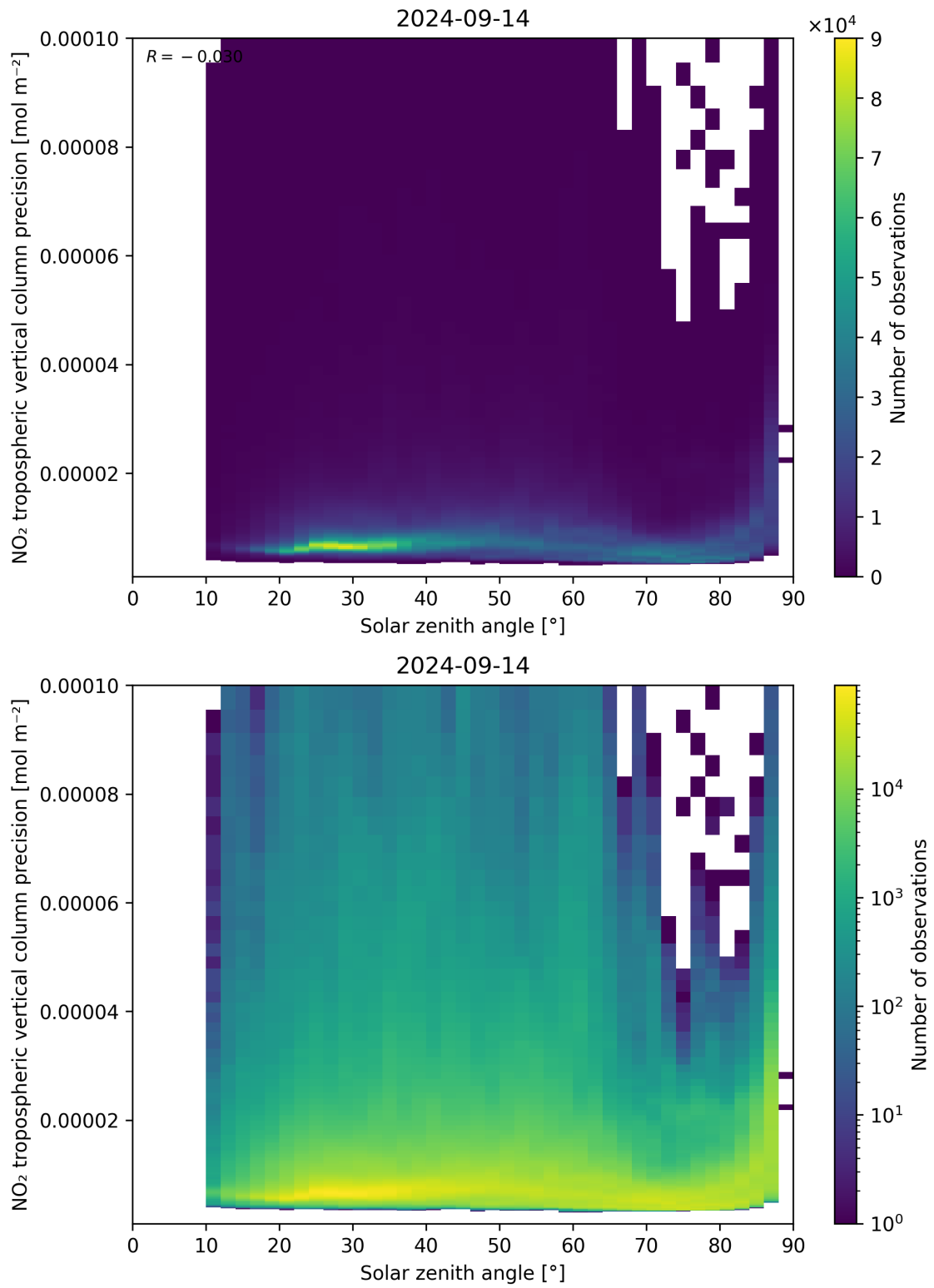
Figure 156: Scatter density plot of “Solar zenith angle” against “NO 2 tropospheric vertical column precision” for 2024-09-13 to 2024-09-15.
