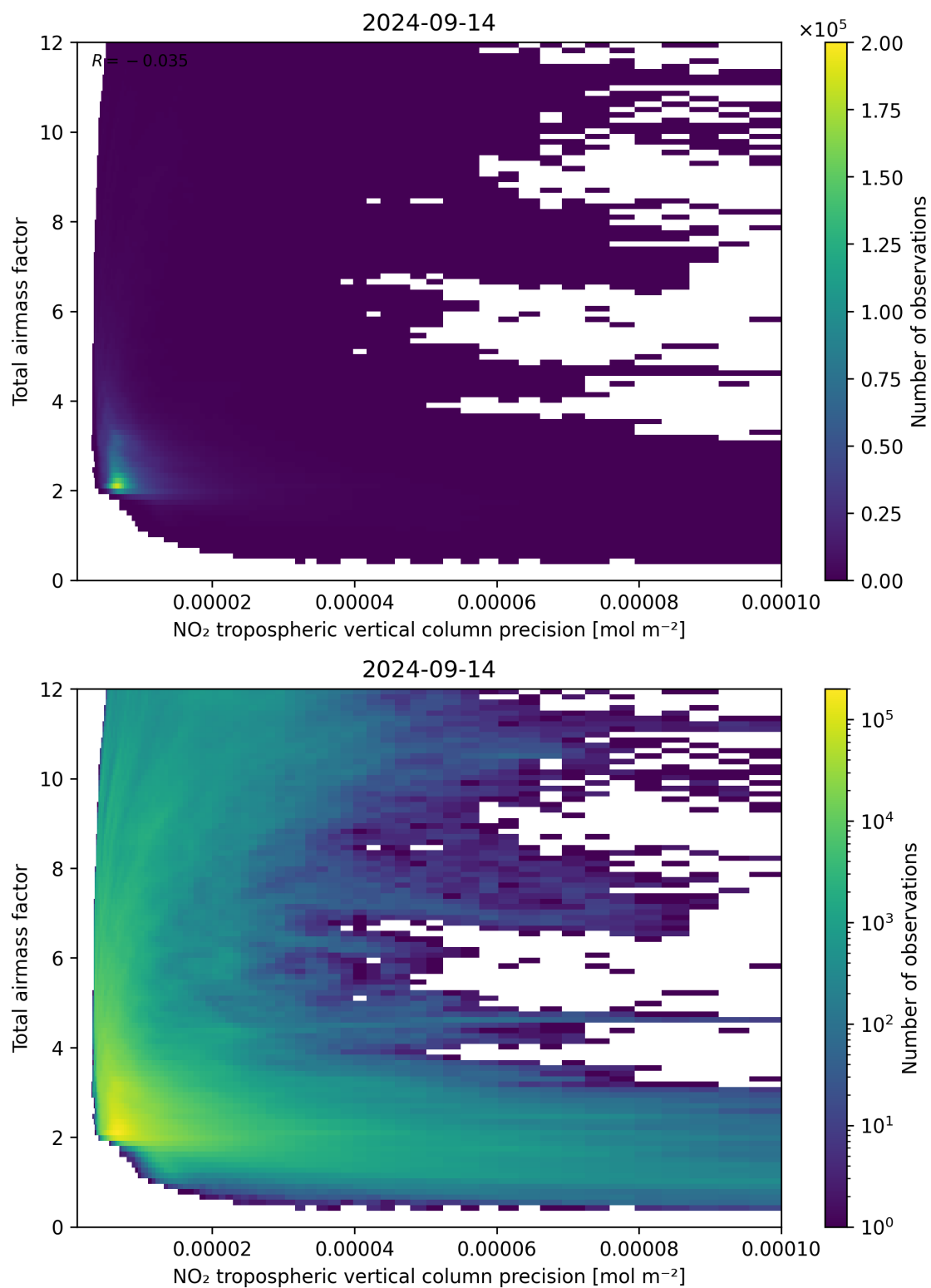
Figure 132: Scatter density plot of “NO 2 tropospheric vertical column precision” against “Total air mass factor” for 2024-09-13 to 2024-09-15.
