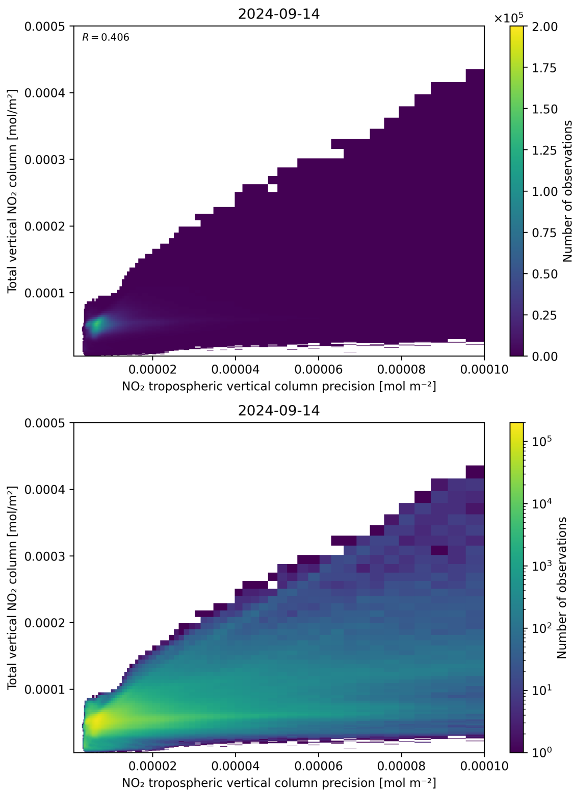
Figure 138: Scatter density plot of “NO 2 tropospheric vertical column precision” against “Total vertical NO 2 column” for 2024-09-13 to 2024-09-15.
