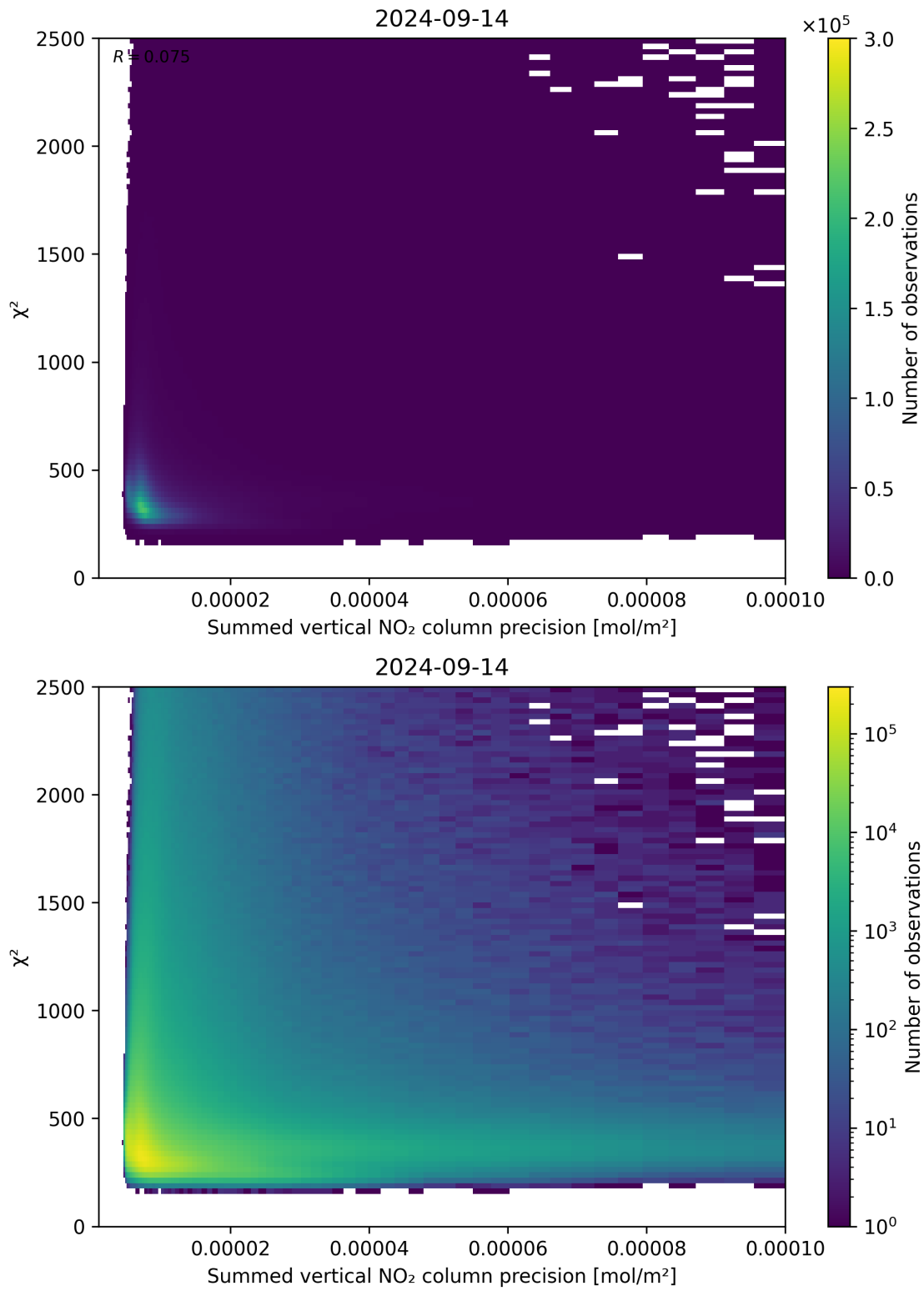
Figure 107: Scatter density plot of “Summed vertical NO 2 column precision” against “ \chi^2 ” for 2024-09-13 to 2024-09-15.
