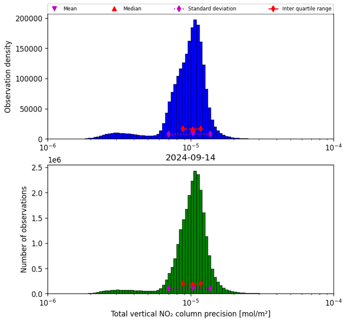
Figure 39: Histogram of “Total vertical NO 2 column precision” for 2024-09-13 to 2024-09-15
