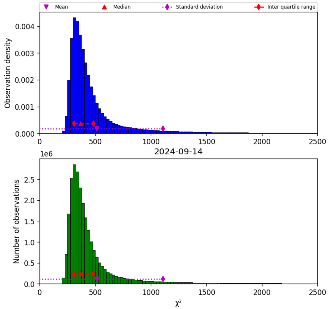
Figure 42: Histogram of “ \chi^2 ” for 2024-09-13 to 2024-09-15
