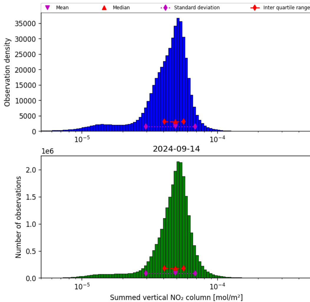
Figure 40: Histogram of “Summed vertical NO 2 column” for 2024-09-13 to 2024-09-15
