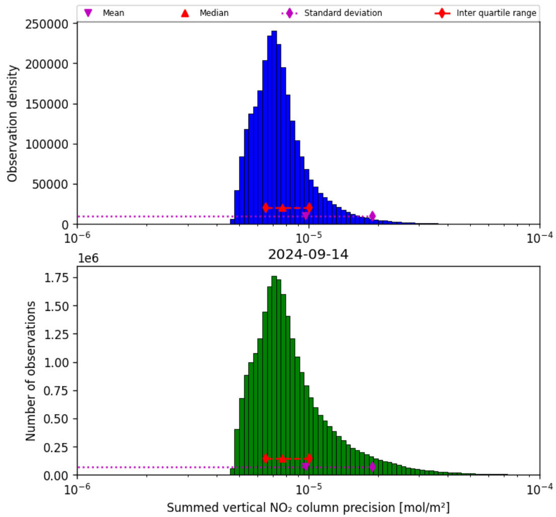
Figure 41: Histogram of "Summed vertical NO 2 column precision" for 2024-09-13 to 2024-09-15
