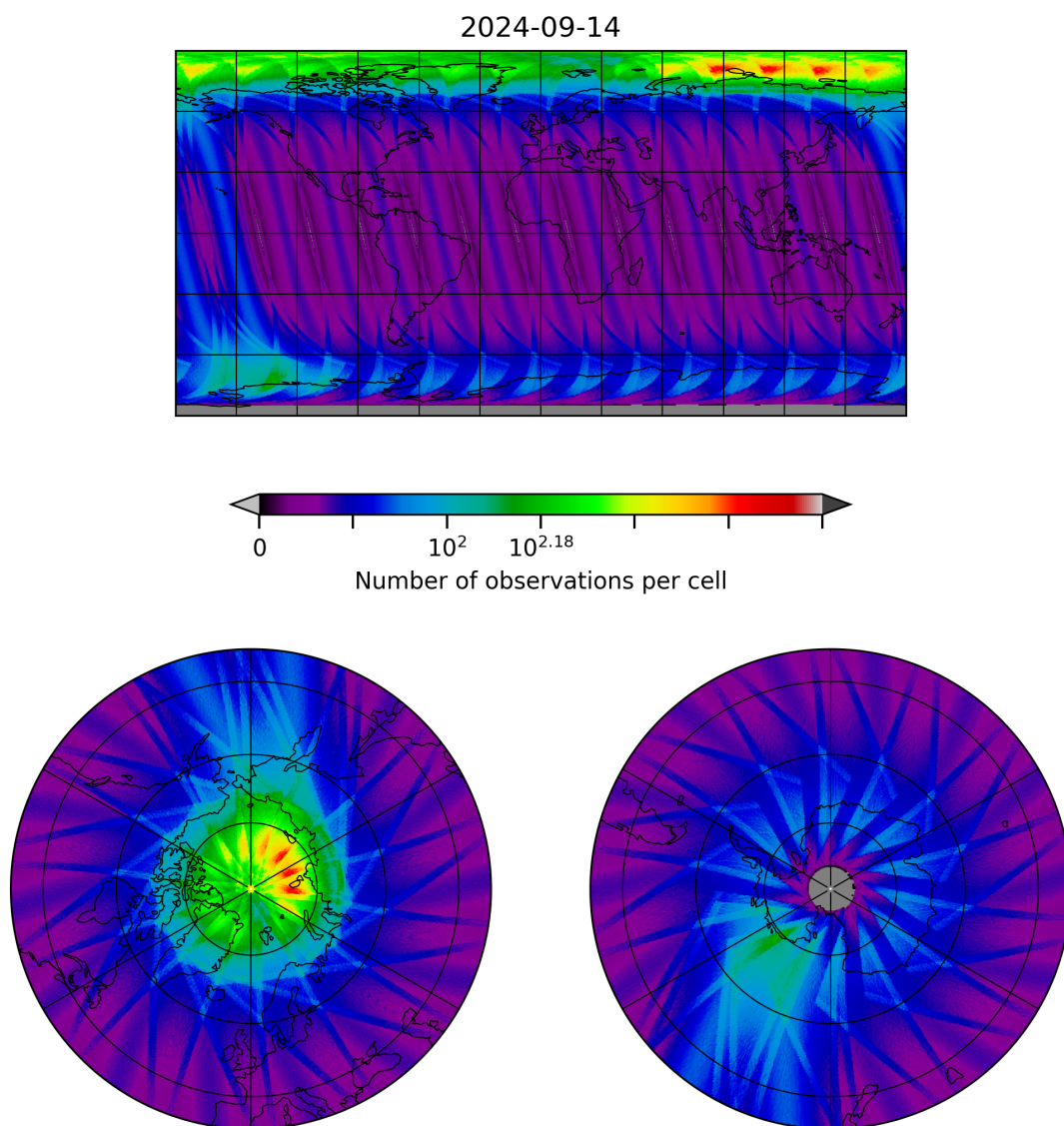
Figure 10: Map of the number of observations for 2024-09-13 to 2024-09-15
