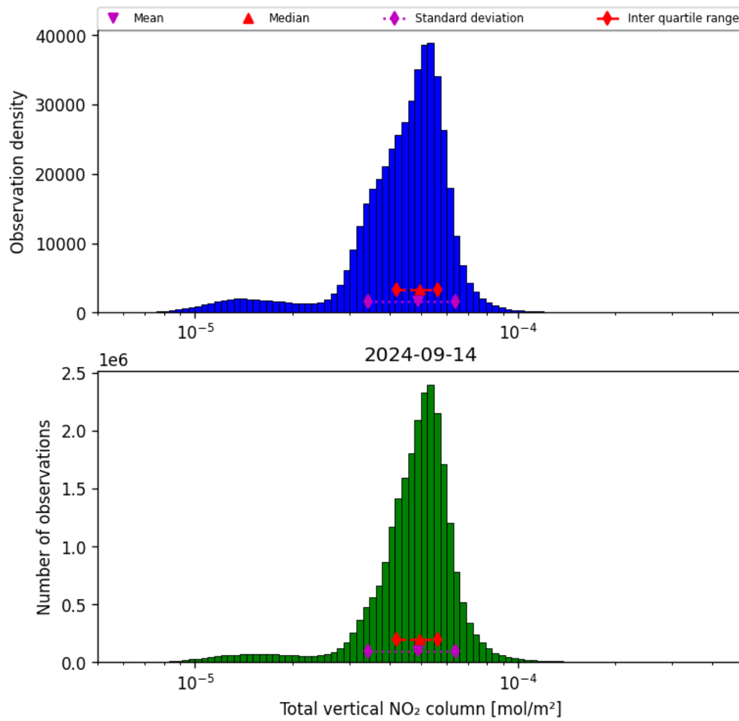
Figure 38: Histogram of "Total vertical NO 2 column" for 2024-09-13 to 2024-09-15
