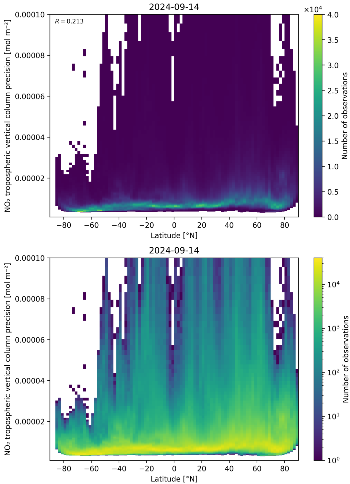
Figure 93: Scatter density plot of “Latitude” against “NO 2 tropospheric vertical column precision” for 2024-09-13 to 2024-09-15.
