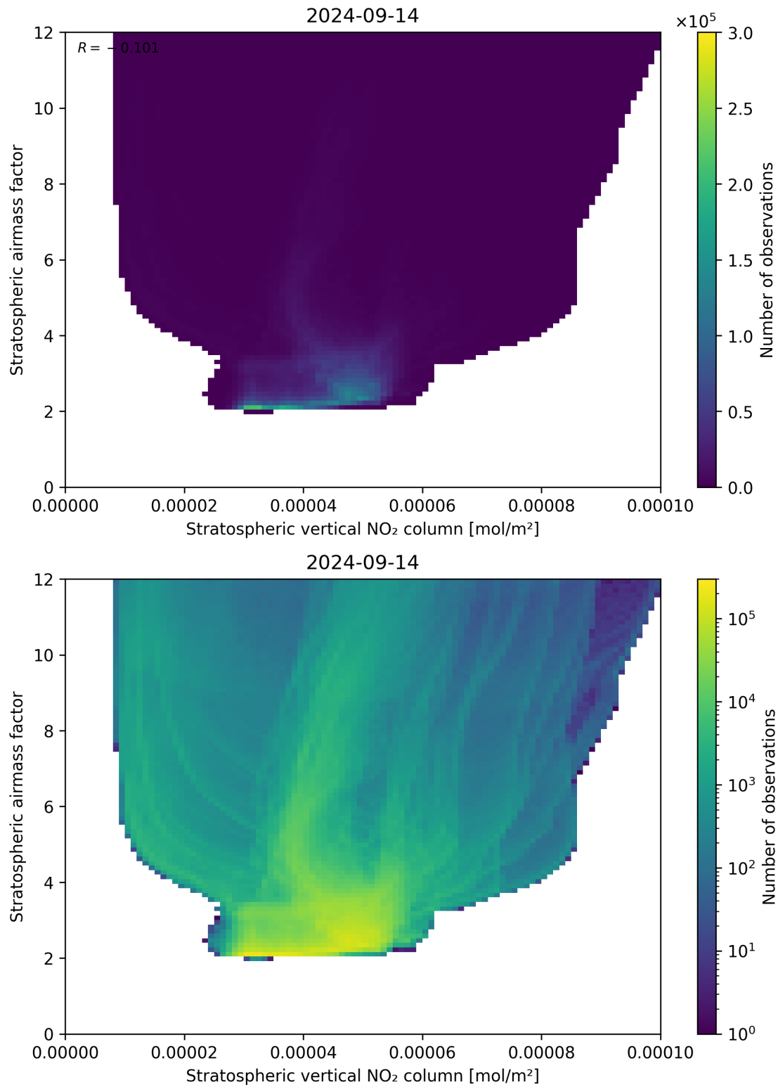
Figure 96: Scatter density plot of “Stratospheric vertical NO 2 column” against “Stratospheric airmass factor” for 2024-09-13 to 2024-09-15.
