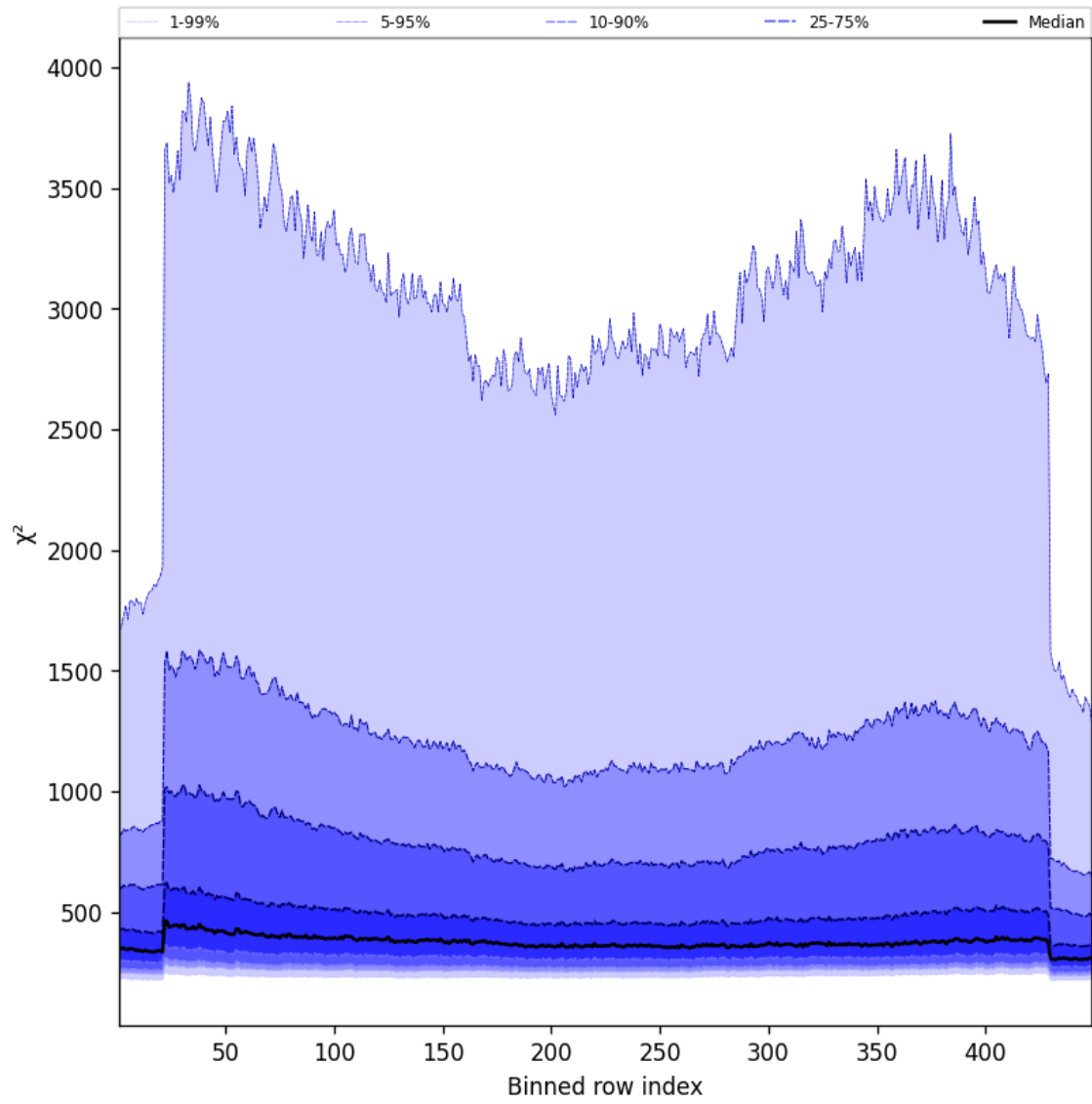
Figure 59: Along track statistics of “ \chi^2 ” for 2024-09-13 to 2024-09-15
