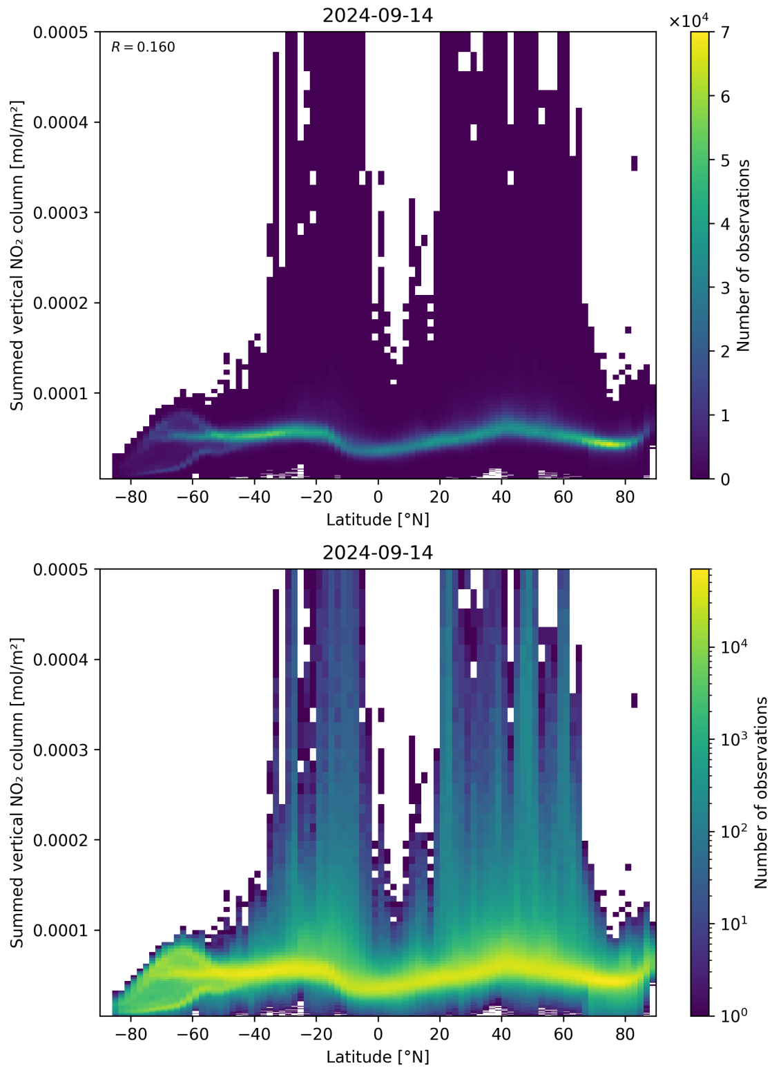
Figure 88: Scatter density plot of “Latitude” against “Summed vertical NO 2 column” for 2024-09-13 to 2024-09-15.
