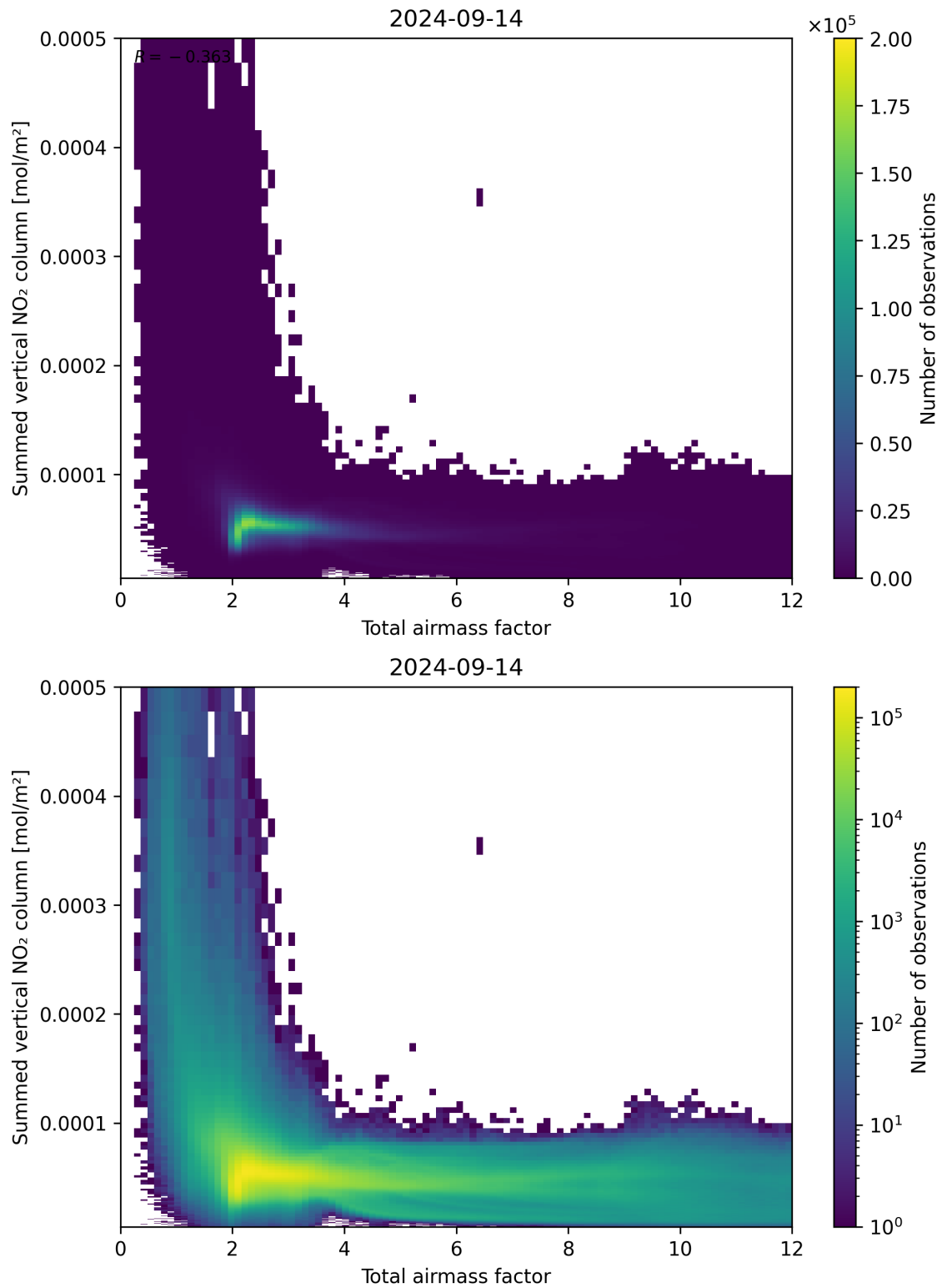
Figure 65: Scatter density plot of “Total airmass factor” against “Summed vertical NO 2 column” for 2024-09-13 to 2024-09-15.
