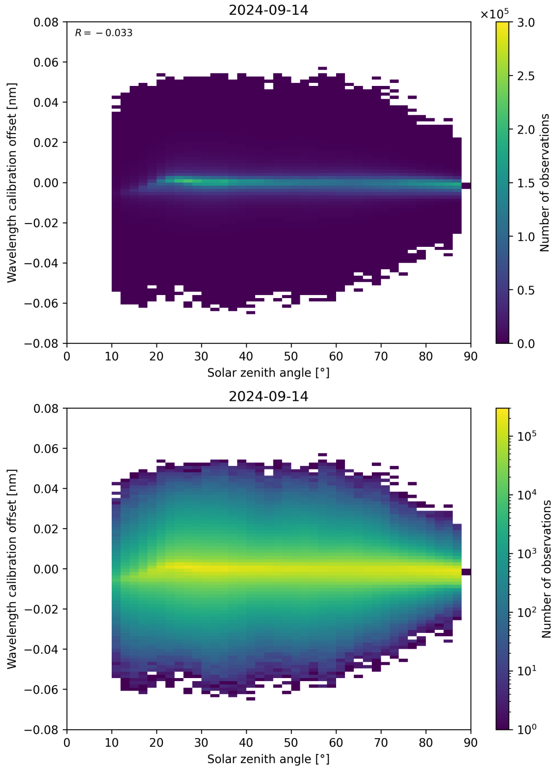
Figure 158: Scatter density plot of “Solar zenith angle” against “Wavelength calibration offset” for 2024-09-13 to 2024-09-15.
