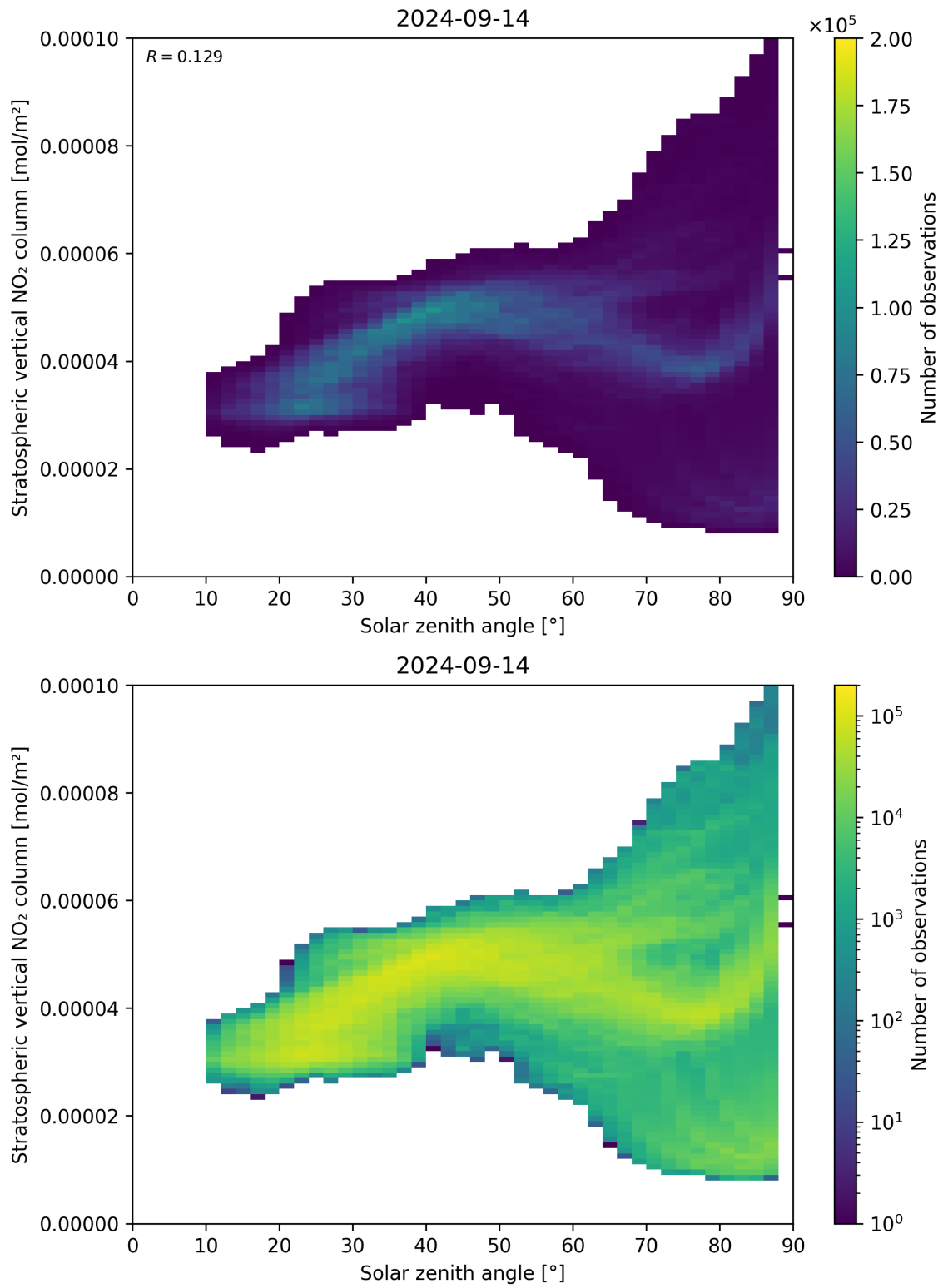
Figure 150: Scatter density plot of “Solar zenith angle” against “Stratospheric vertical NO 2 column” for 2024-09-13 to 2024-09-15.
