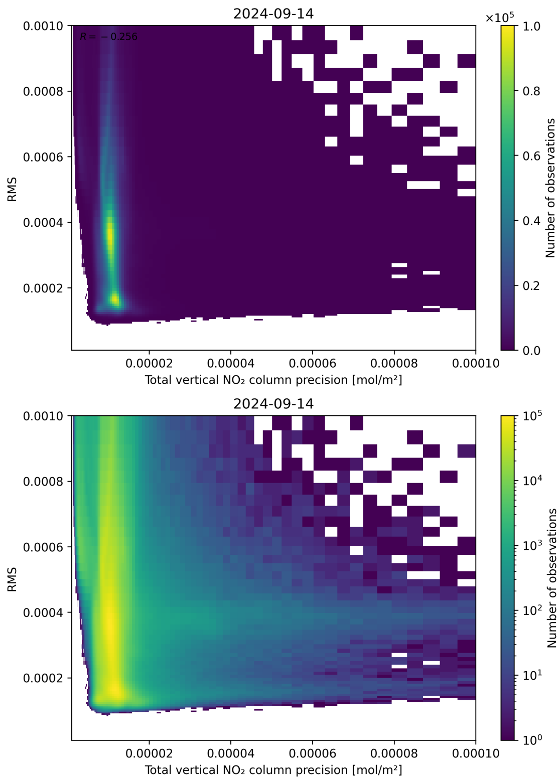
Figure 119: Scatter density plot of “Total vertical NO 2 column precision” against “RMS” for 2024-09-13 to 2024-09-15.
