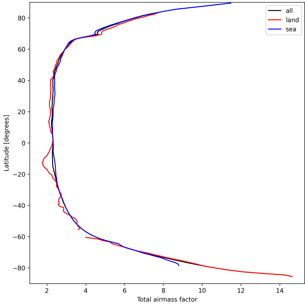
Figure 15: Zonal average of “Total airmass factor” for 2024-09-13 to 2024-09-15.
