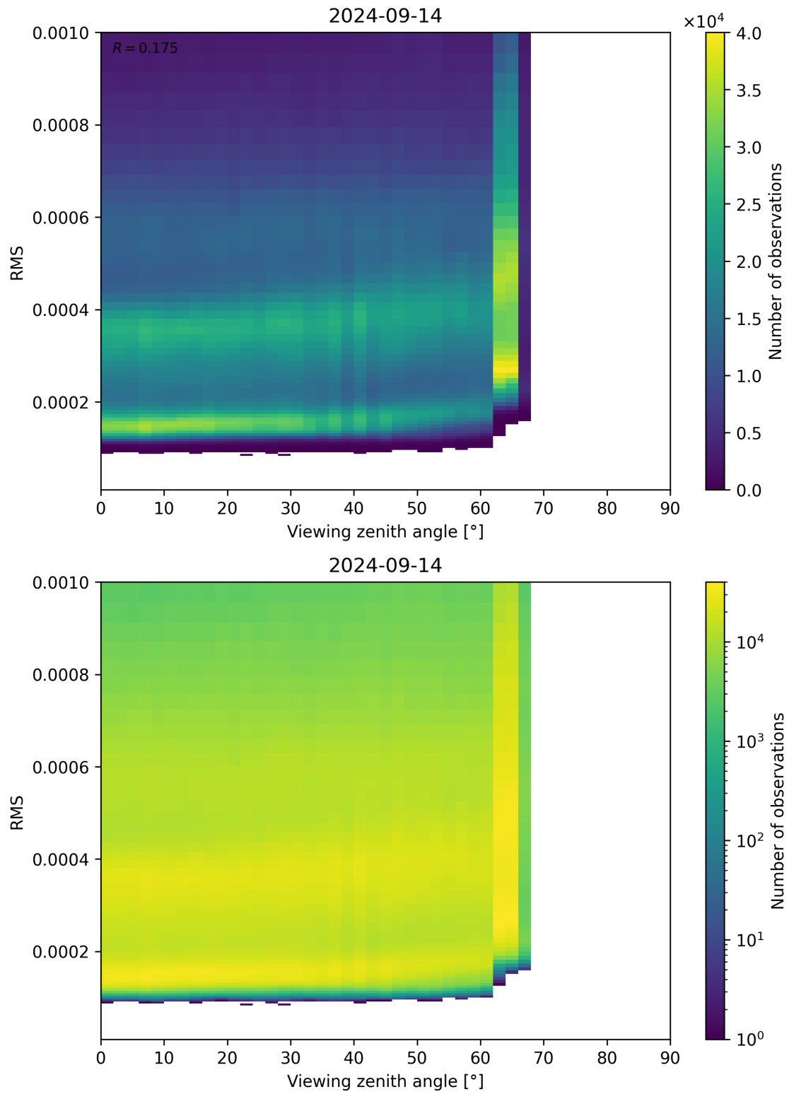
Figure 171: Scatter density plot of “Viewing zenith angle” against “RMS” for 2024-09-13 to 2024-09-15.
