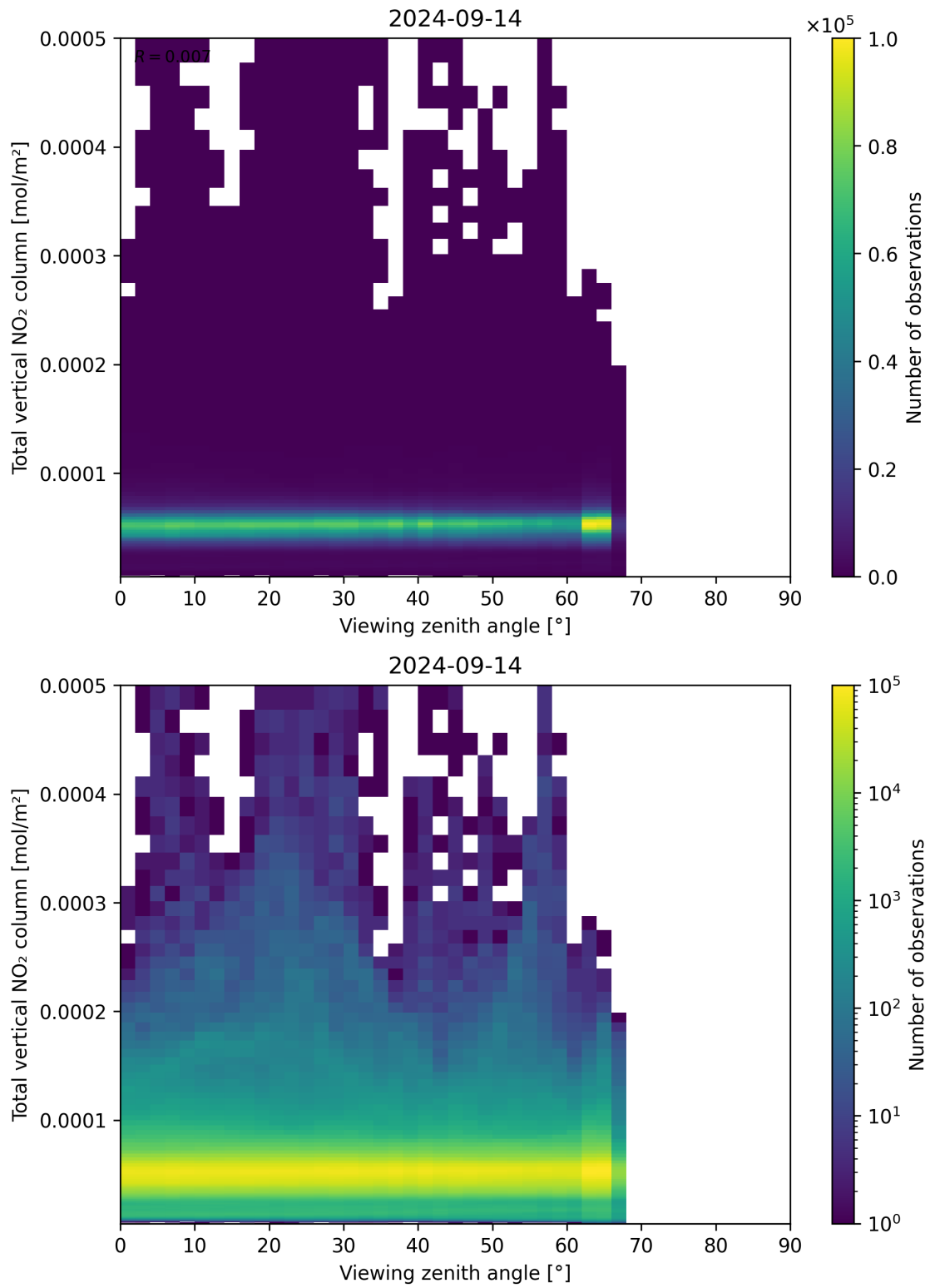
Figure 167: Scatter density plot of “Viewing zenith angle” against “Total vertical NO 2 column” for 2024-09-13 to 2024-09-15.
