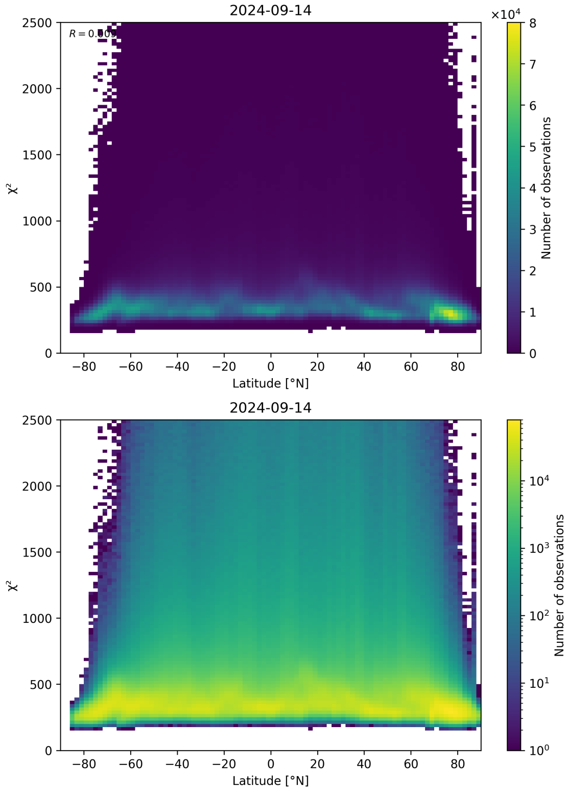
Figure 86: Scatter density plot of “Latitude” against “ \chi^2 ” for 2024-09-13 to 2024-09-15.
