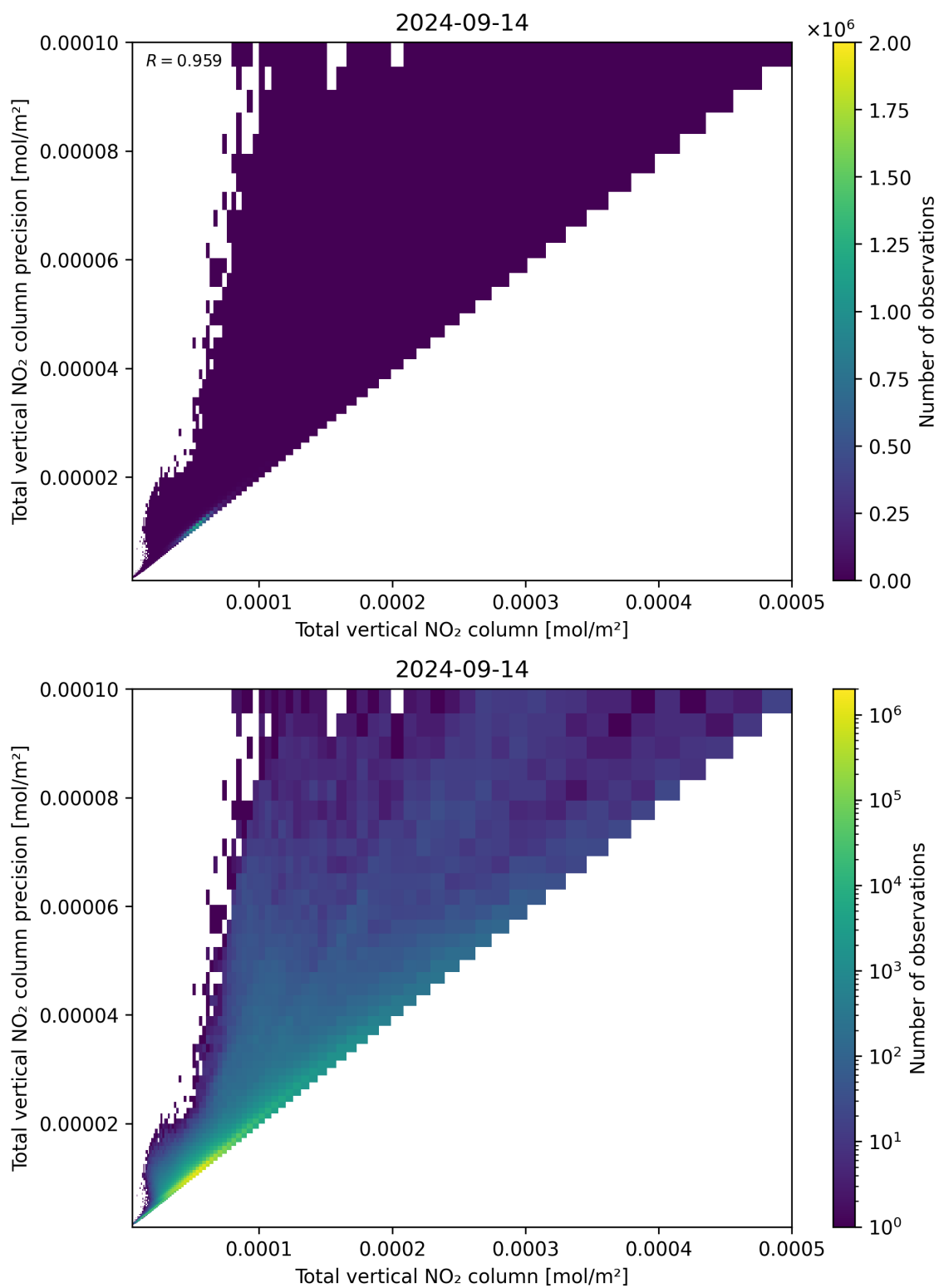
Figure 114: Scatter density plot of “Total vertical NO 2 column” against “Total vertical NO 2 column precision” for 2024-09-13 to 2024-09-15.
