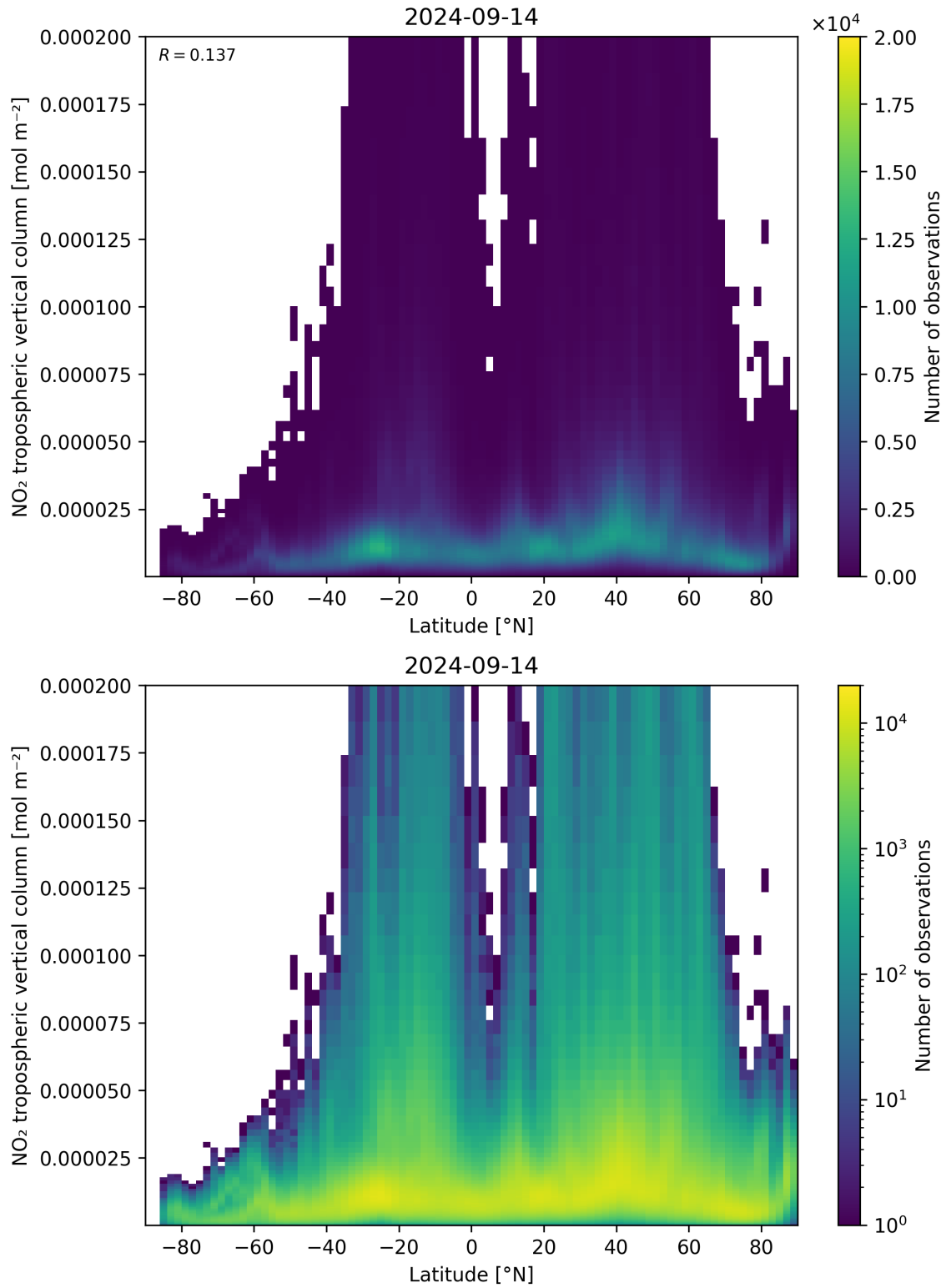
Figure 92: Scatter density plot of “Latitude” against “NO 2 tropospheric vertical column” for 2024-09-13 to 2024-09-15.
