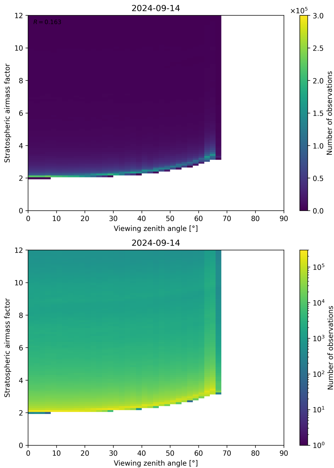
Figure 159: Scatter density plot of “Viewing zenith angle” against “Stratospheric airmass factor” for 2024-09-13 to 2024-09-15.
