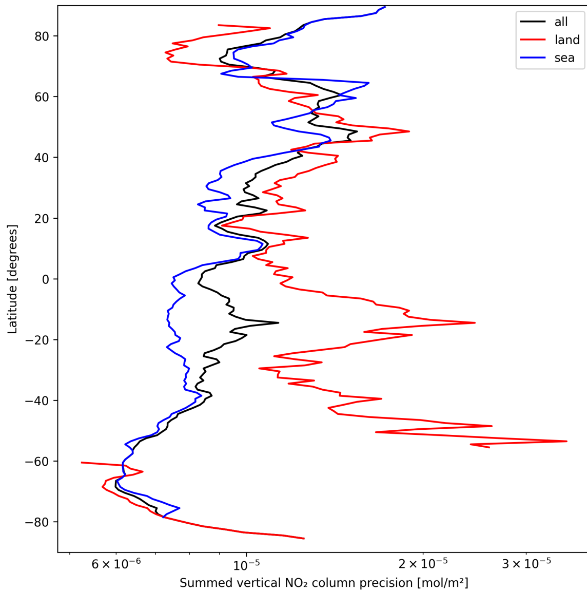
Figure 24: Zonal average of “Summed vertical NO 2 column precision” for 2024-09-13 to 2024-09-15.
