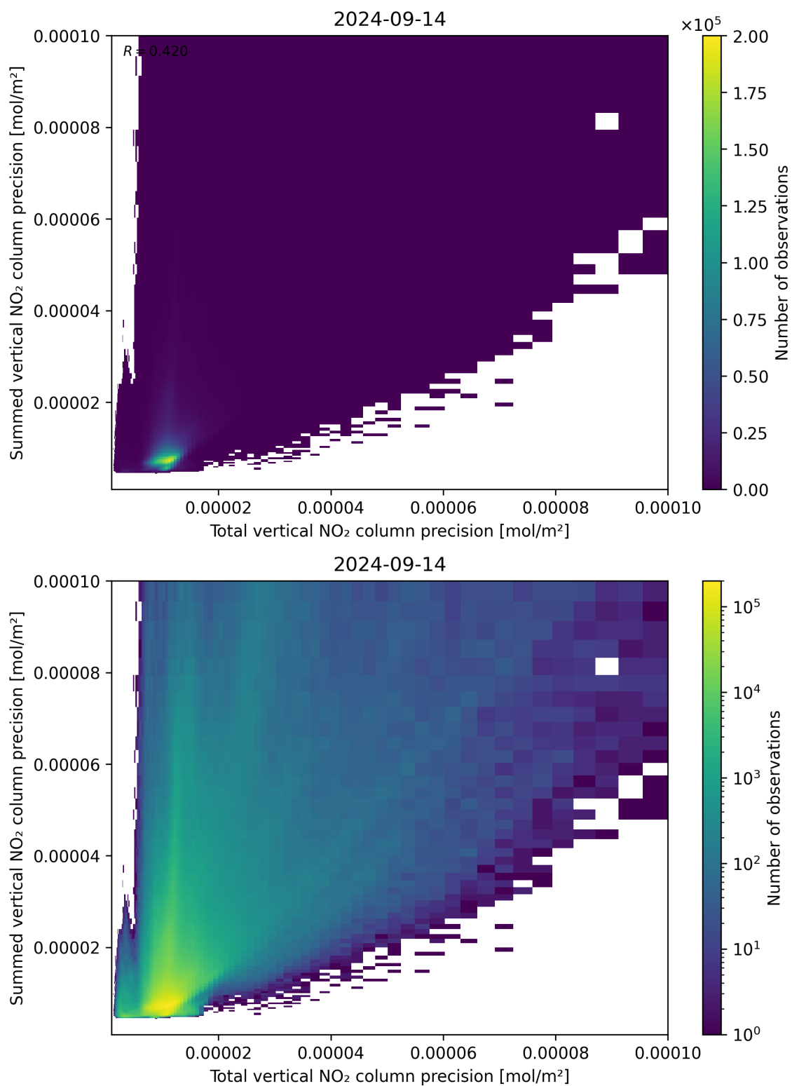
Figure 118: Scatter density plot of “Total vertical NO 2 column precision” against “Summed vertical NO 2 column precision” for 2024-09-13 to 2024-09-15.
