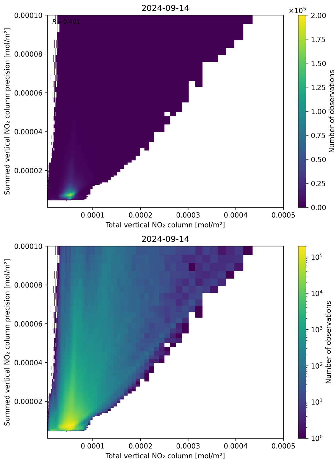
Figure 113: Scatter density plot of “Total vertical NO 2 column” against “Summed vertical NO 2 column precision” for 2024-09-13 to 2024-09-15.
