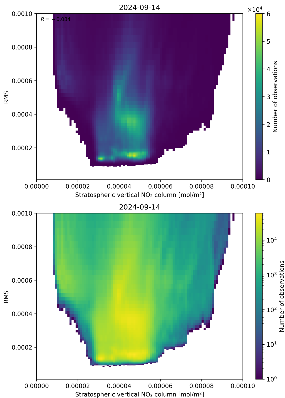
Figure 102: Scatter density plot of “Stratospheric vertical NO 2 column” against “RMS” for 2024-09-13 to 2024-09-15.
