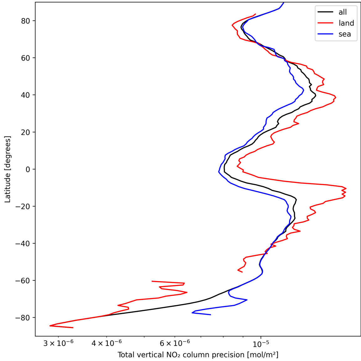
Figure 22: Zonal average of “Total vertical NO 2 column precision” for 2024-09-13 to 2024-09-15.
