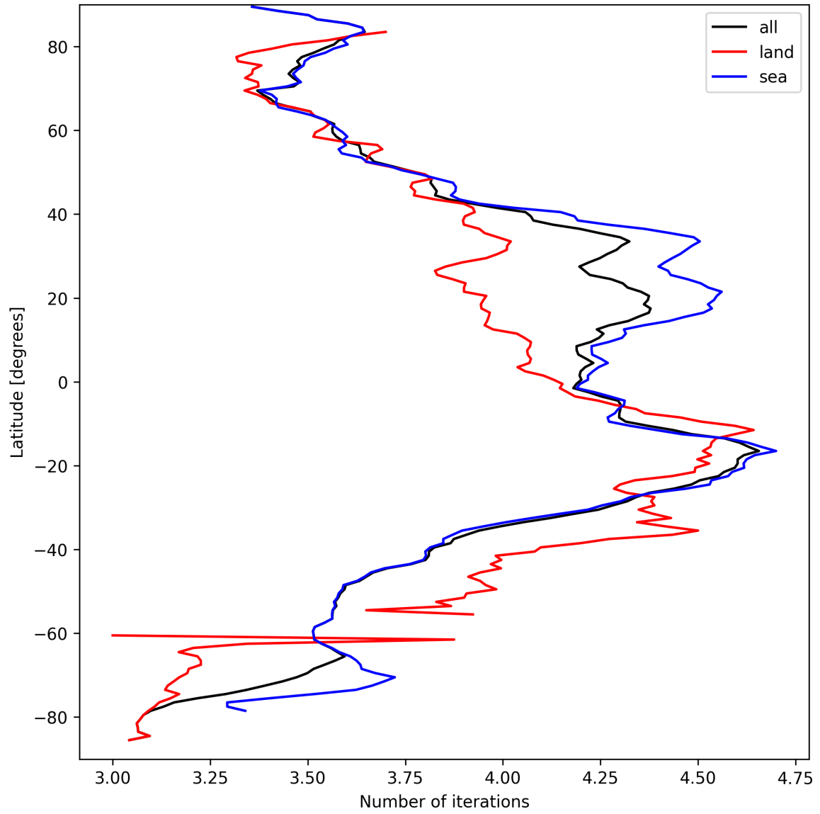
Figure 17: Zonal average of “Number of iterations” for 2024-09-13 to 2024-09-15.
