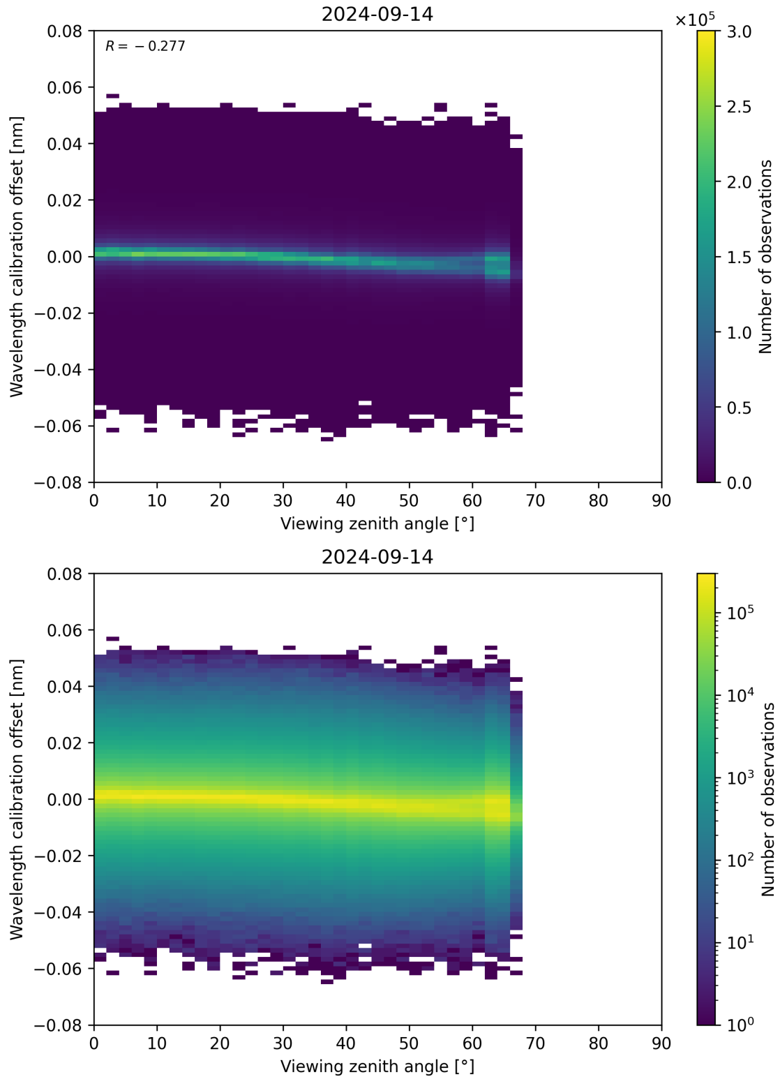
Figure 173: Scatter density plot of “Viewing zenith angle” against “Wavelength calibration offset” for 2024-09-13 to 2024-09-15.
