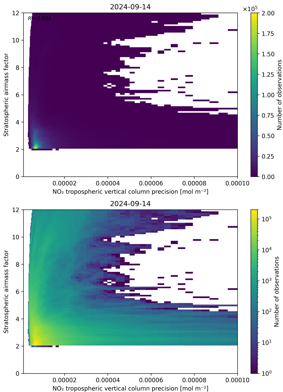
Figure 131: Scatter density plot of “NO 2 tropospheric vertical column precision” against “Stratospheric airmass factor” for 2024-09-13 to 2024-09-15.
