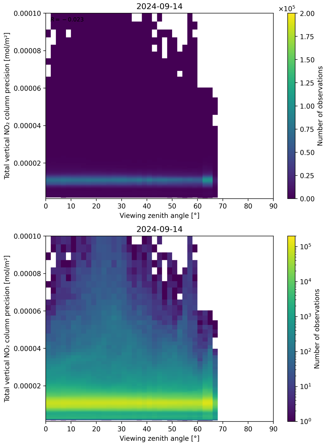
Figure 168: Scatter density plot of “Viewing zenith angle” against “Total vertical NO 2 column precision” for 2024-09-13 to 2024-09-15.
