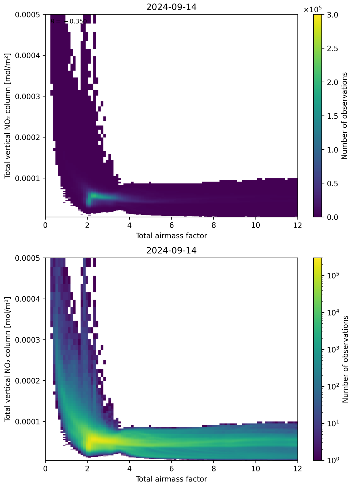
Figure 67: Scatter density plot of “Total airmass factor” against “Total vertical NO 2 column” for 2024-09-13 to 2024-09-15.
