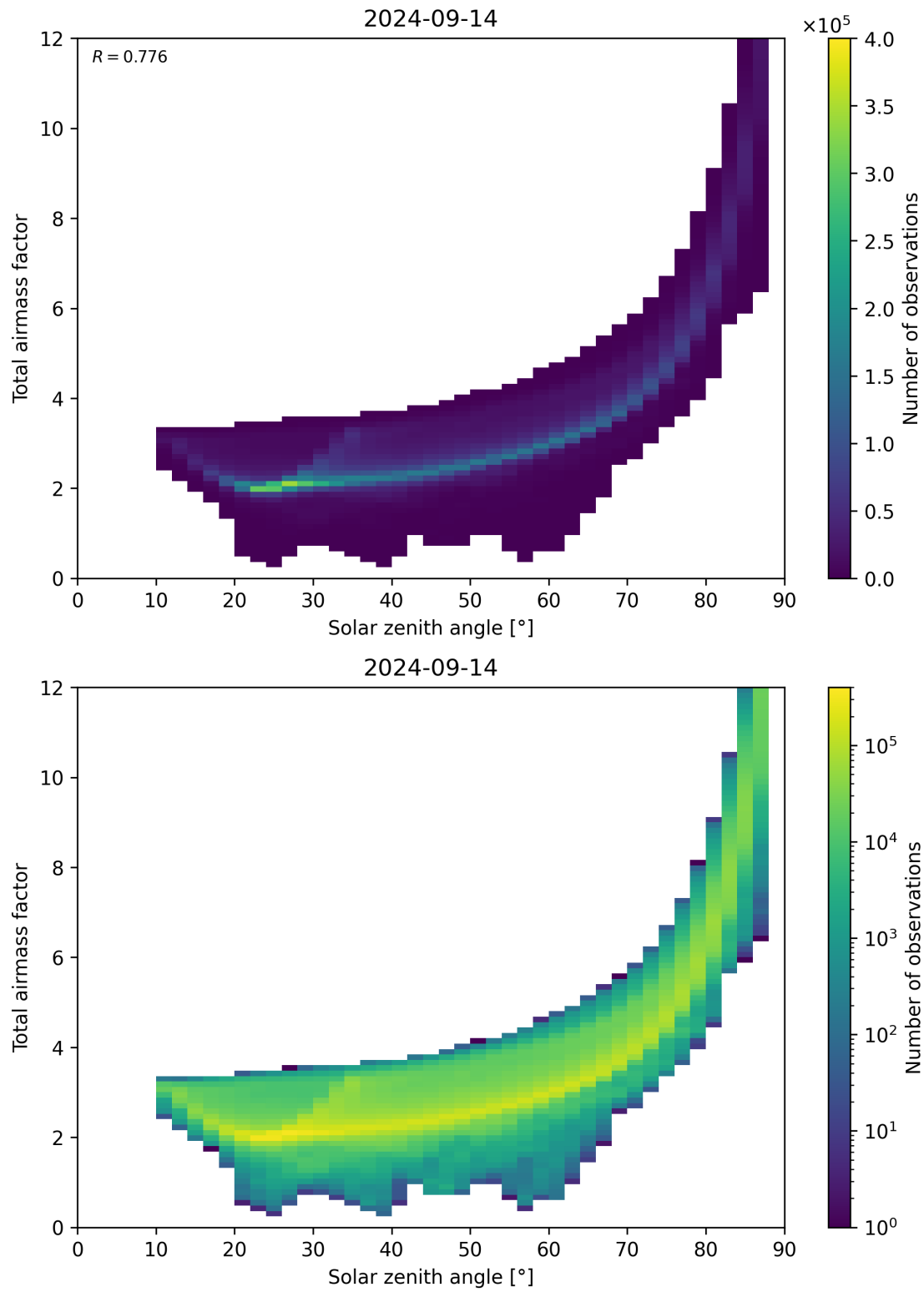
Figure 146: Scatter density plot of “Solar zenith angle” against “Total air mass factor” for 2024-09-13 to 2024-09-15.
