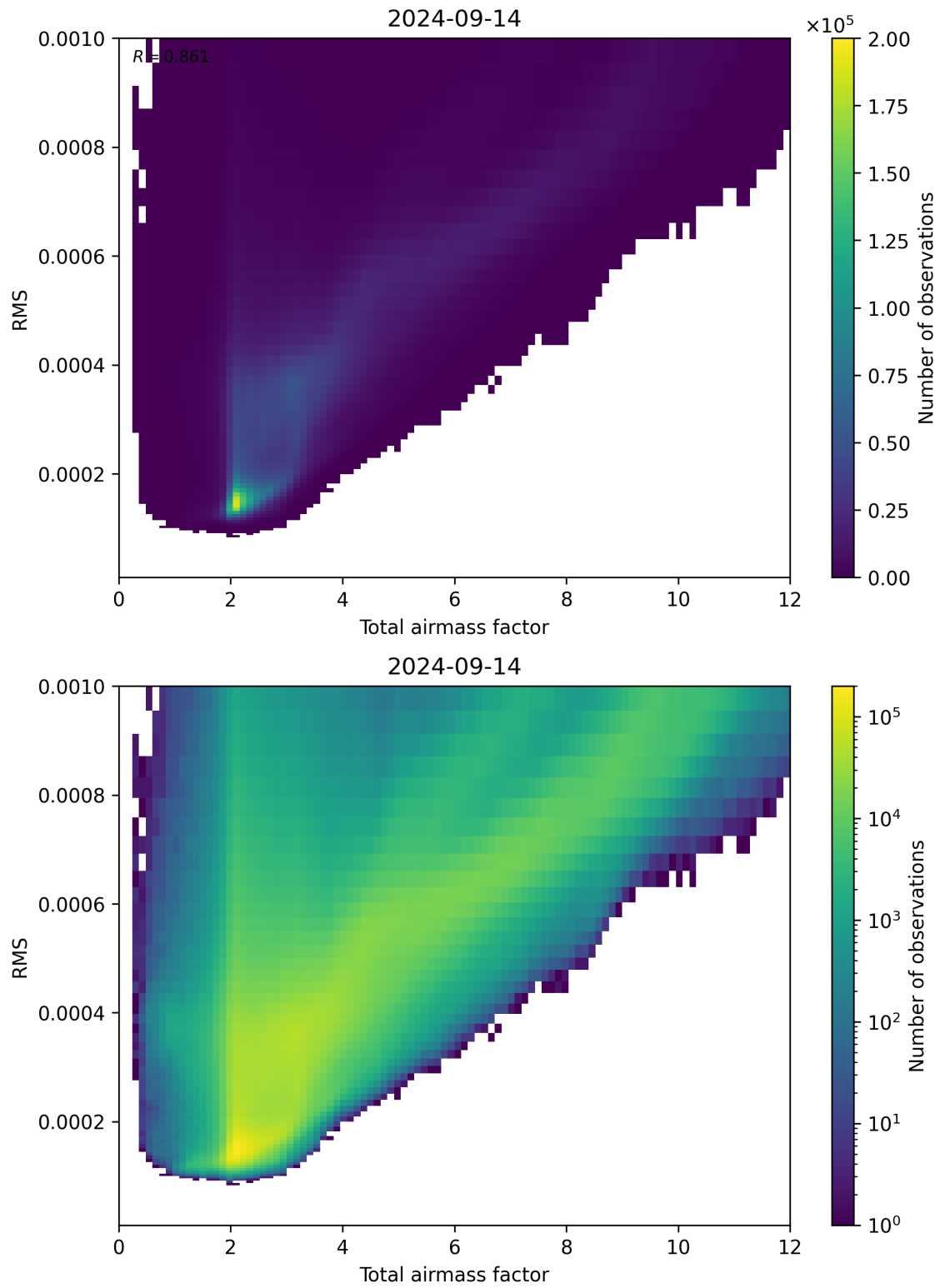
Figure 69: Scatter density plot of “Total airmass factor” against “RMS” for 2024-09-13 to 2024-09-15.
