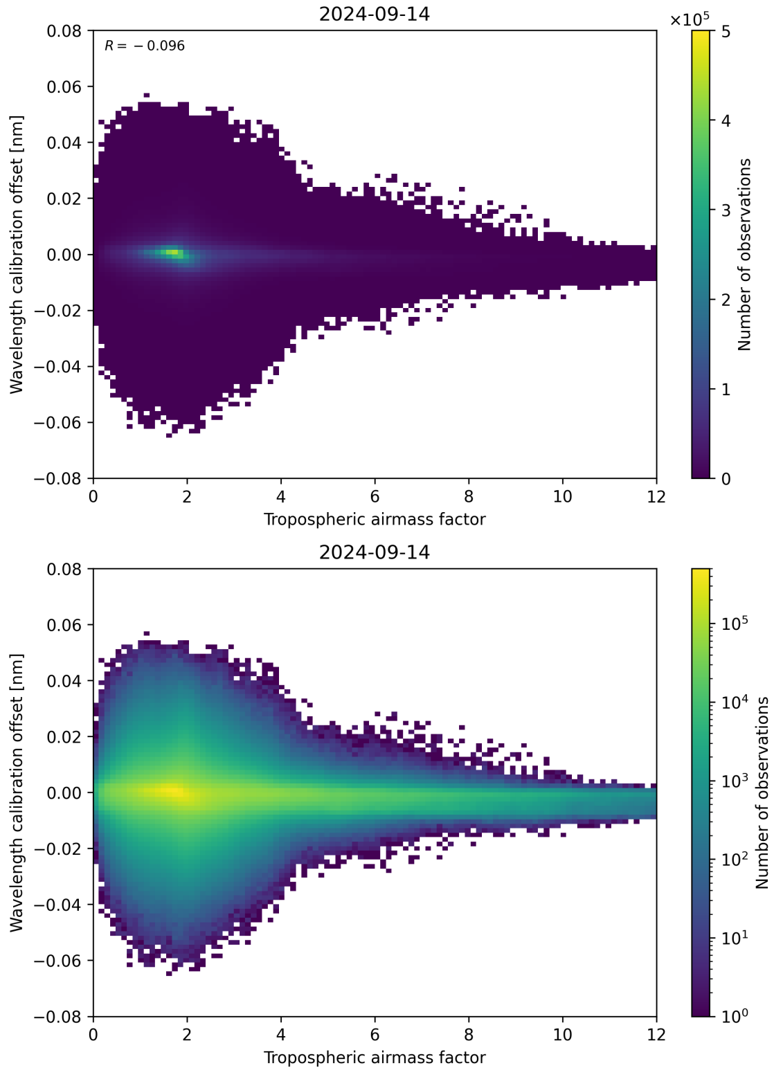
Figure 80: Scatter density plot of “Tropospheric airmass factor” against “Wavelength calibration offset” for 2024-09-13 to 2024-09-15.
