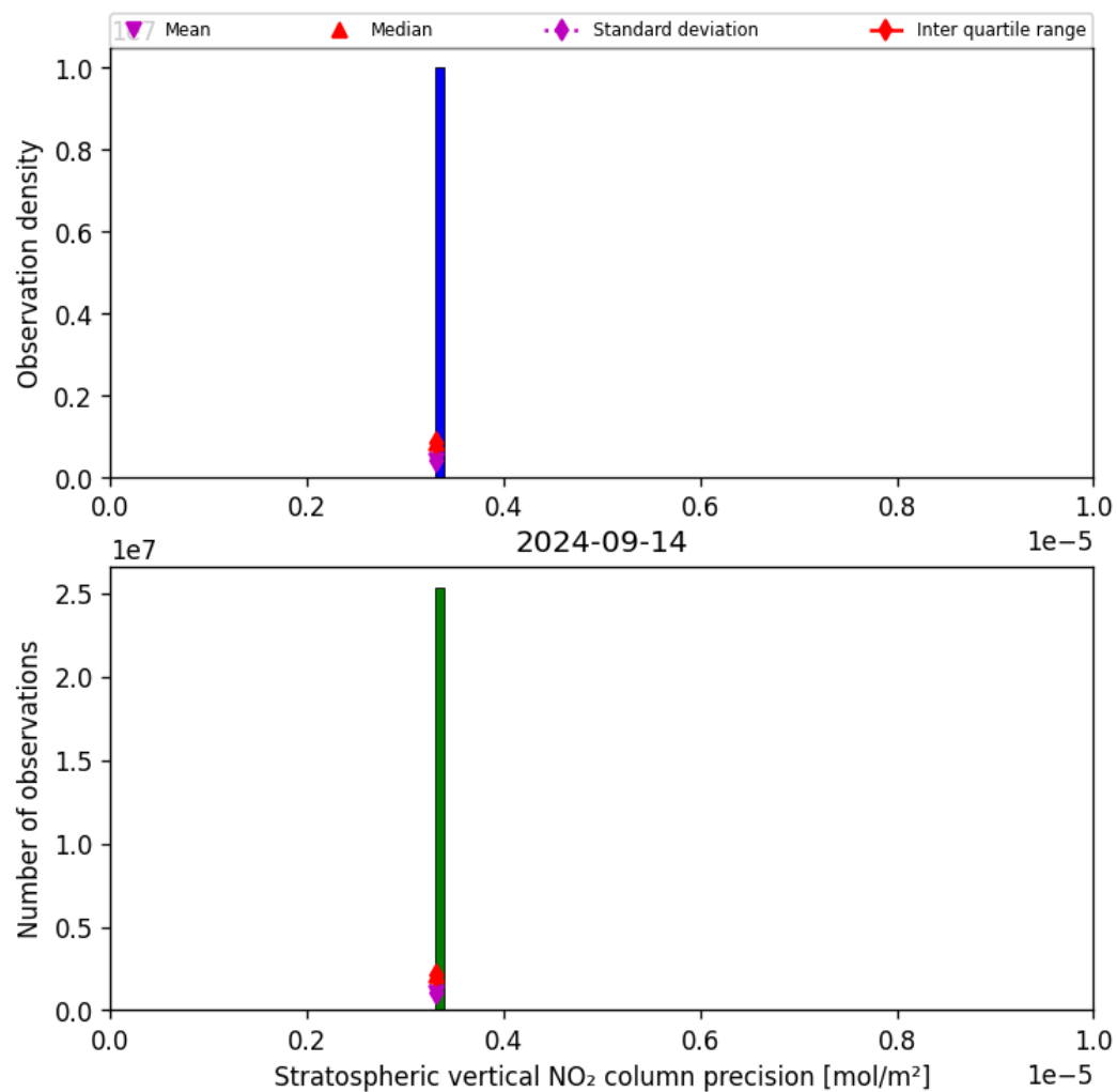
Figure 37: Histogram of “Stratospheric vertical NO 2 column precision” for 2024-09-13 to 2024-09-15
