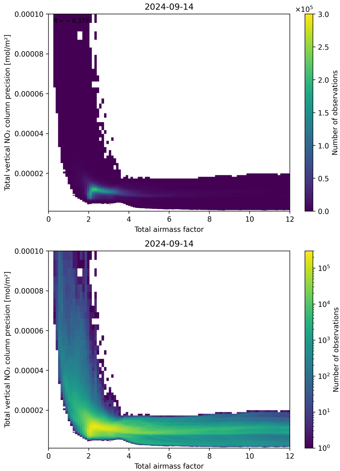
Figure 68: Scatter density plot of “Total airmass factor” against “Total vertical NO 2 column precision” for 2024-09-13 to 2024-09-15.
