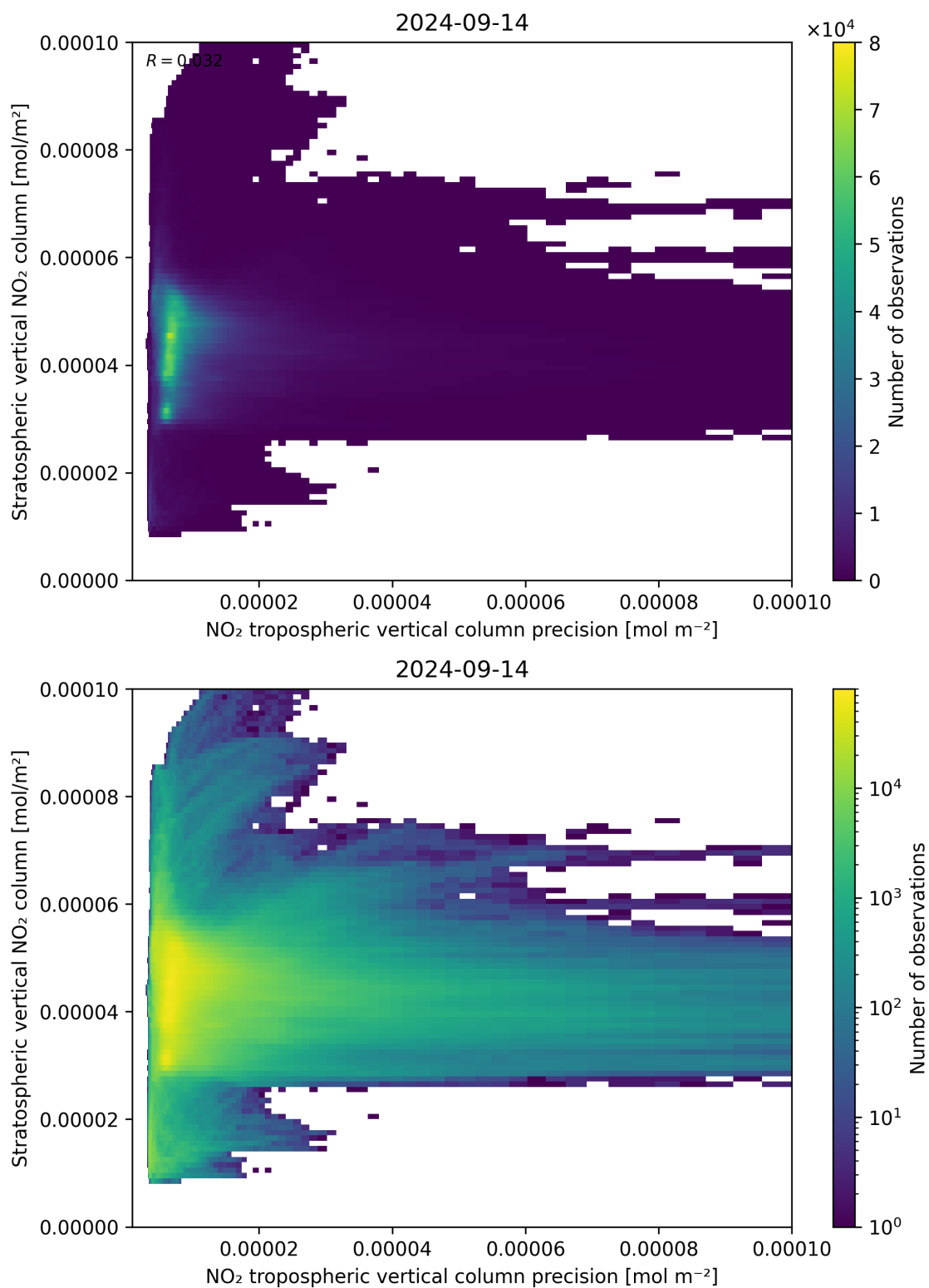
Figure 135: Scatter density plot of “NO 2 tropospheric vertical column precision” against “Stratospheric vertical NO 2 column” for 2024-09-13 to 2024-09-15.
