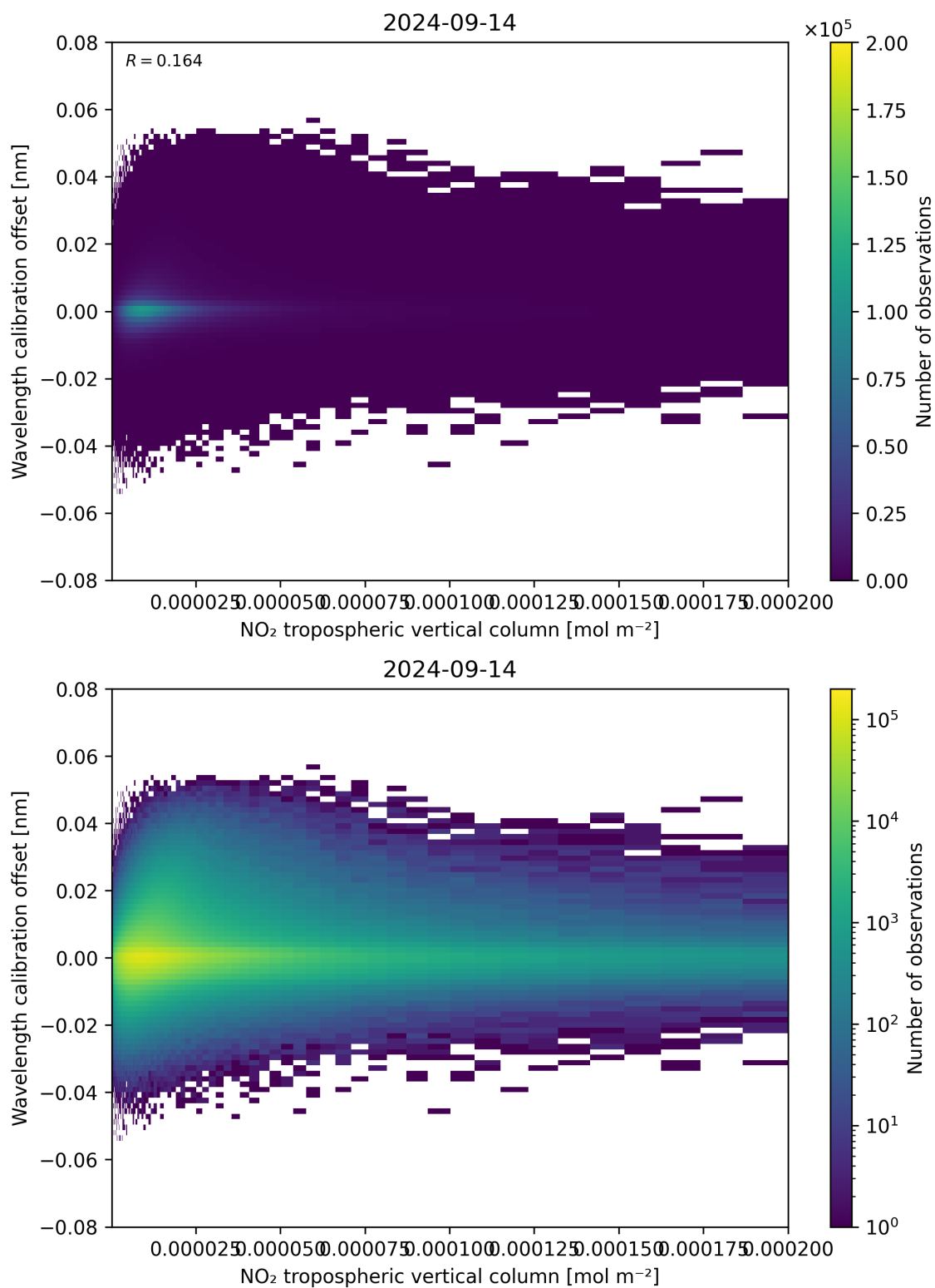
Figure 143: Scatter density plot of “NO 2 tropospheric vertical column” against “Wavelength calibration offset” for 2024-09-13 to 2024-09-15.
