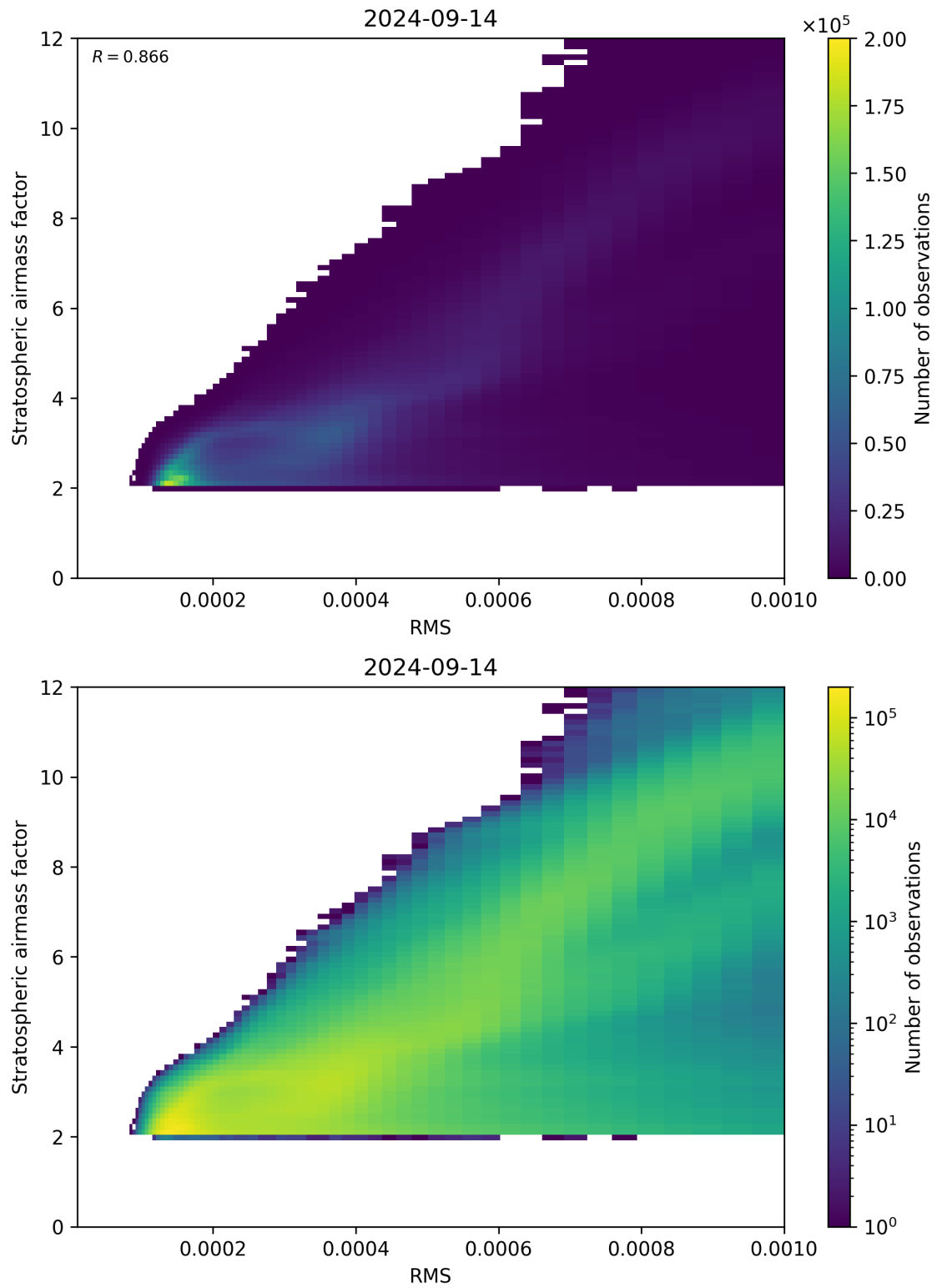
Figure 144: Scatter density plot of “RMS” against “Stratospheric airmass factor” for 2024-09-13 to 2024-09-15.
