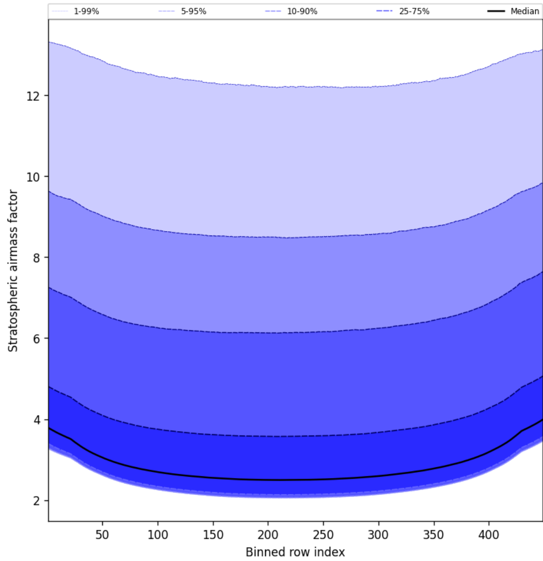
Figure 61: Along track statistics of “Stratospheric airmass factor” for 2024-09-13 to 2024-09-15
