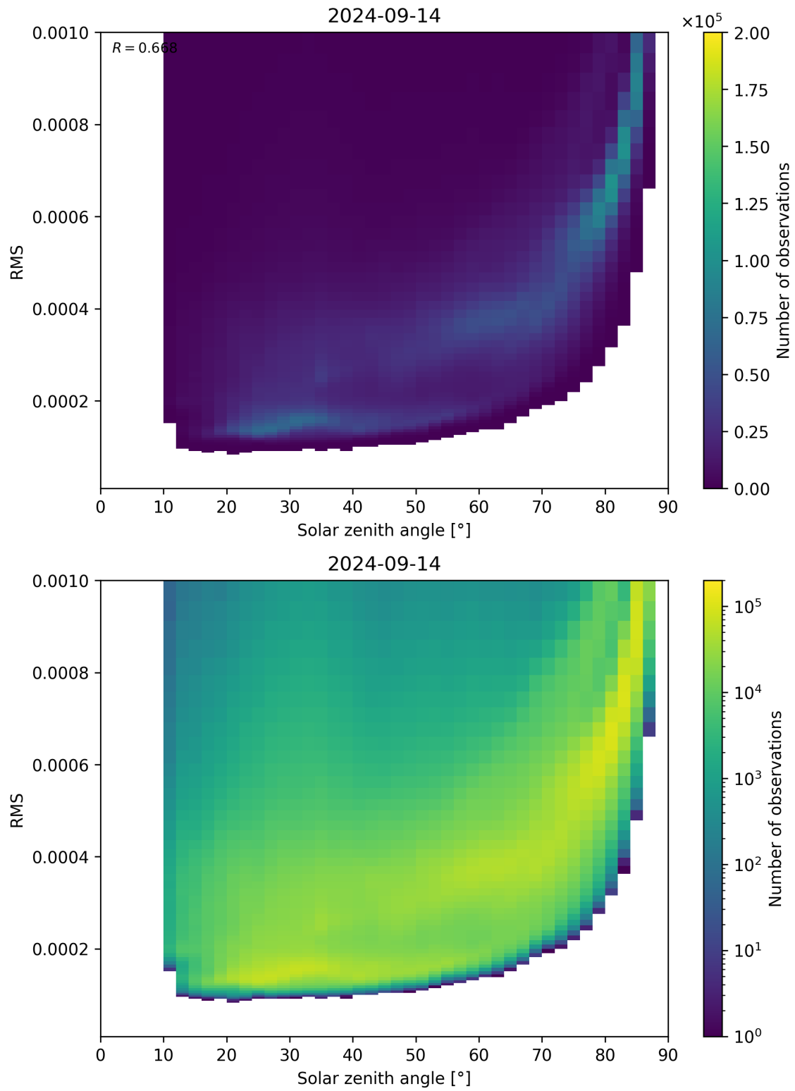
Figure 157: Scatter density plot of “Solar zenith angle” against “RMS” for 2024-09-13 to 2024-09-15.
