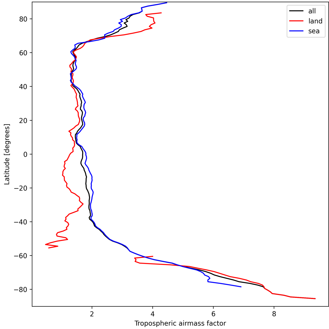
Figure 14: Zonal average of “Tropospheric airmass factor” for 2024-09-13 to 2024-09-15.
