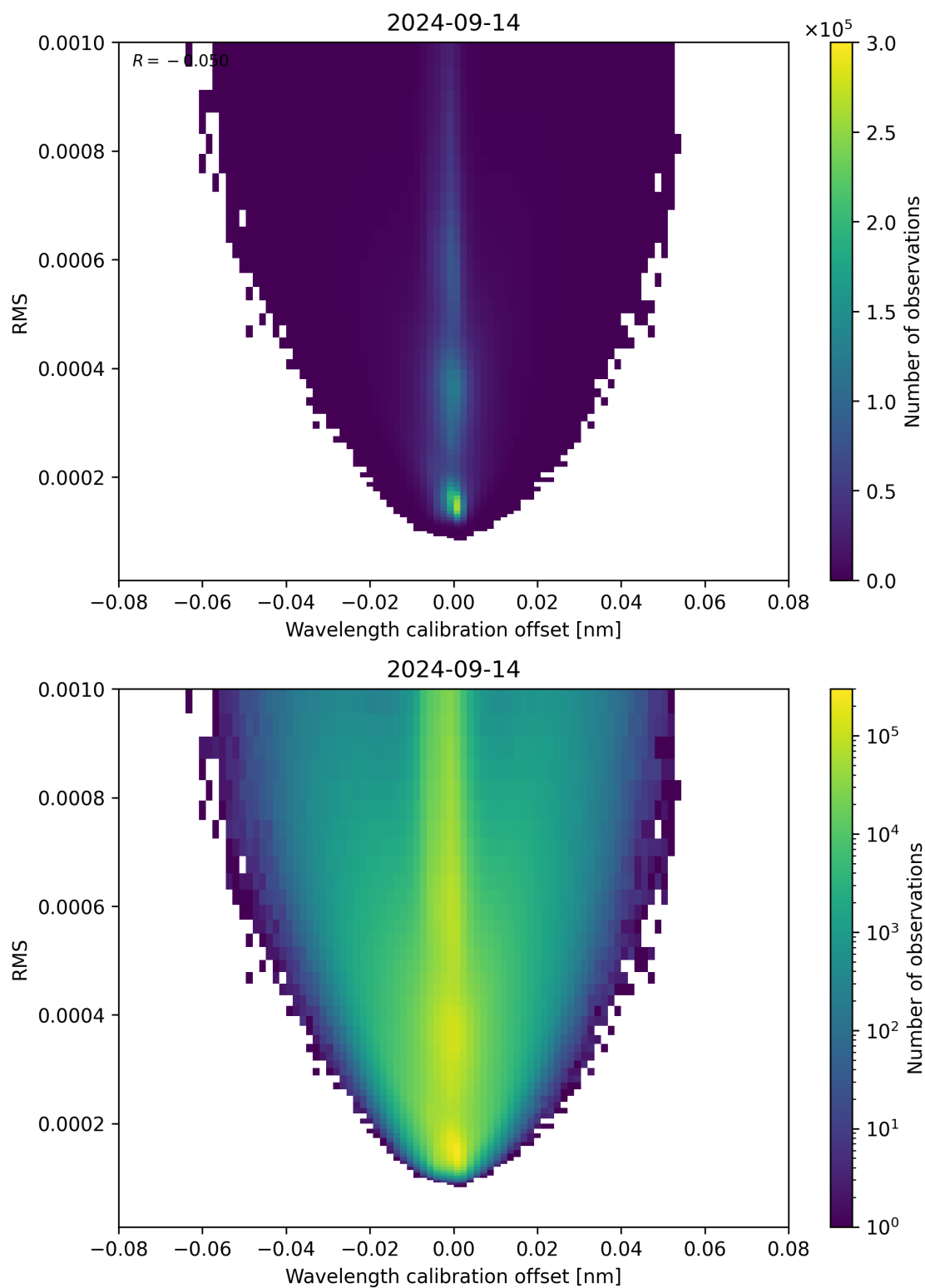
Figure 181: Scatter density plot of “Wavelength calibration offset” against “RMS” for 2024-09-13 to 2024-09-15.
