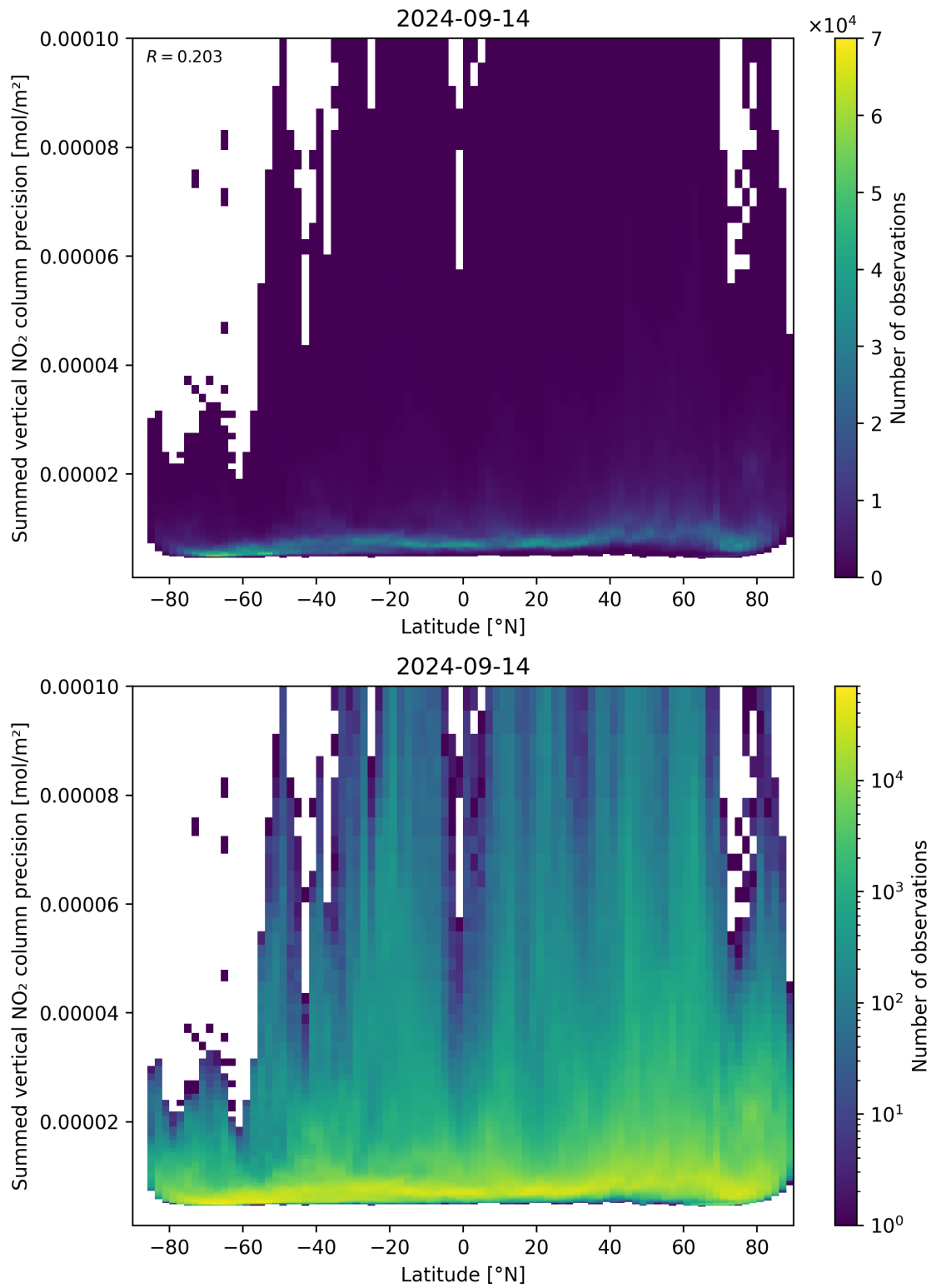
Figure 89: Scatter density plot of “Latitude” against “Summed vertical NO 2 column precision” for 2024-09-13 to 2024-09-15.
