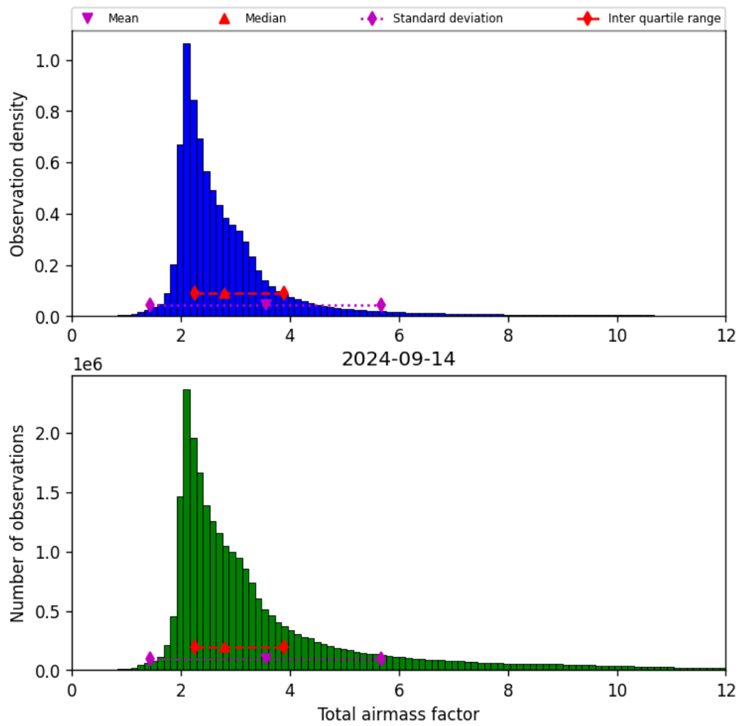
Figure 32: Histogram of “Total airmass factor” for 2024-09-13 to 2024-09-15
