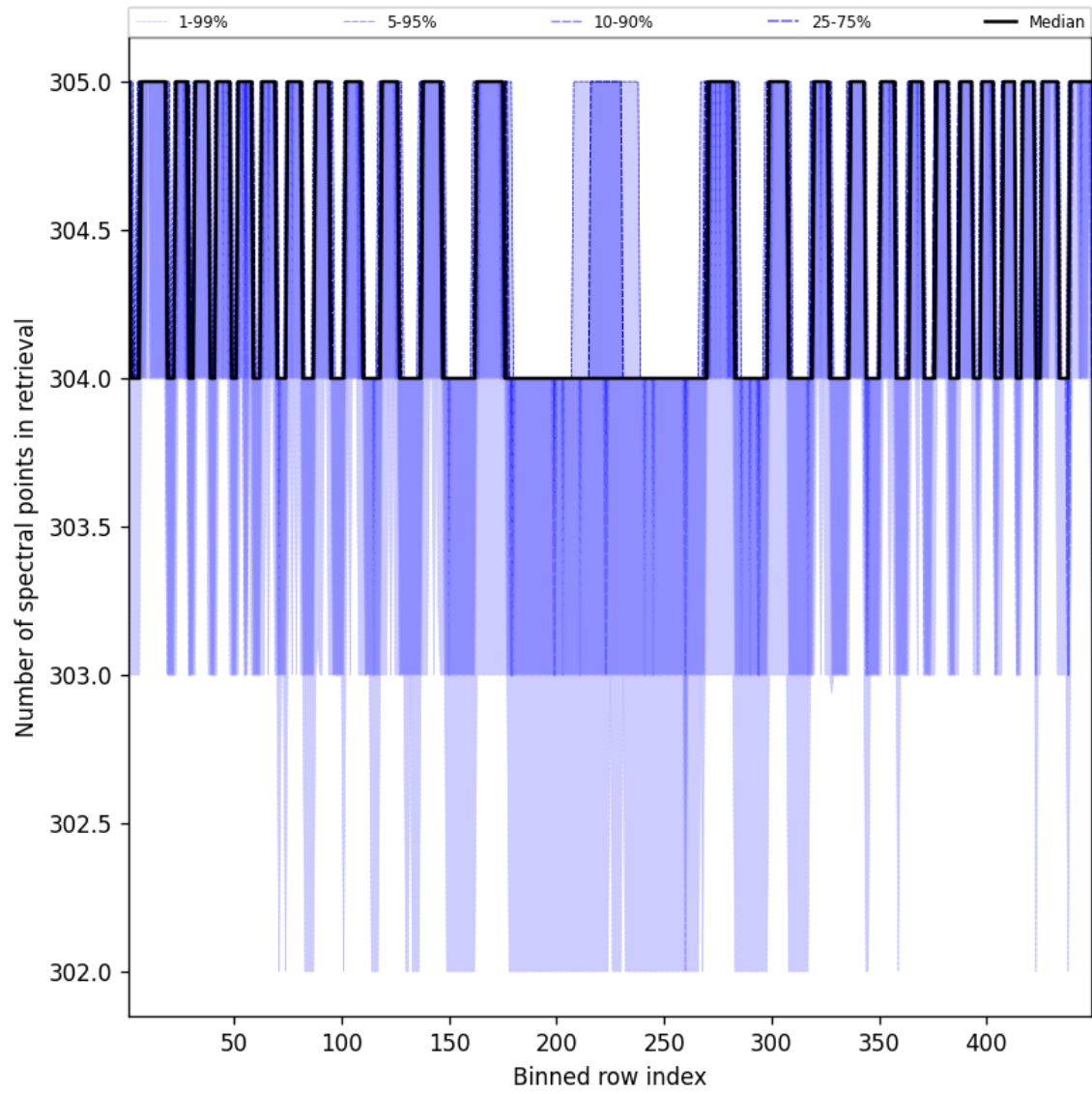
Figure 50: Along track statistics of “Number of spectral points in retrieval” for 2024-09-13 to 2024-09-15
