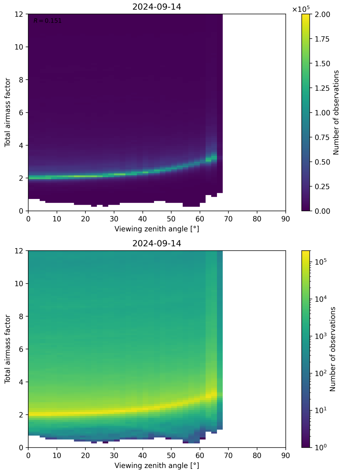
Figure 160: Scatter density plot of “Viewing zenith angle” against “Total airmass factor” for 2024-09-13 to 2024-09-15.
