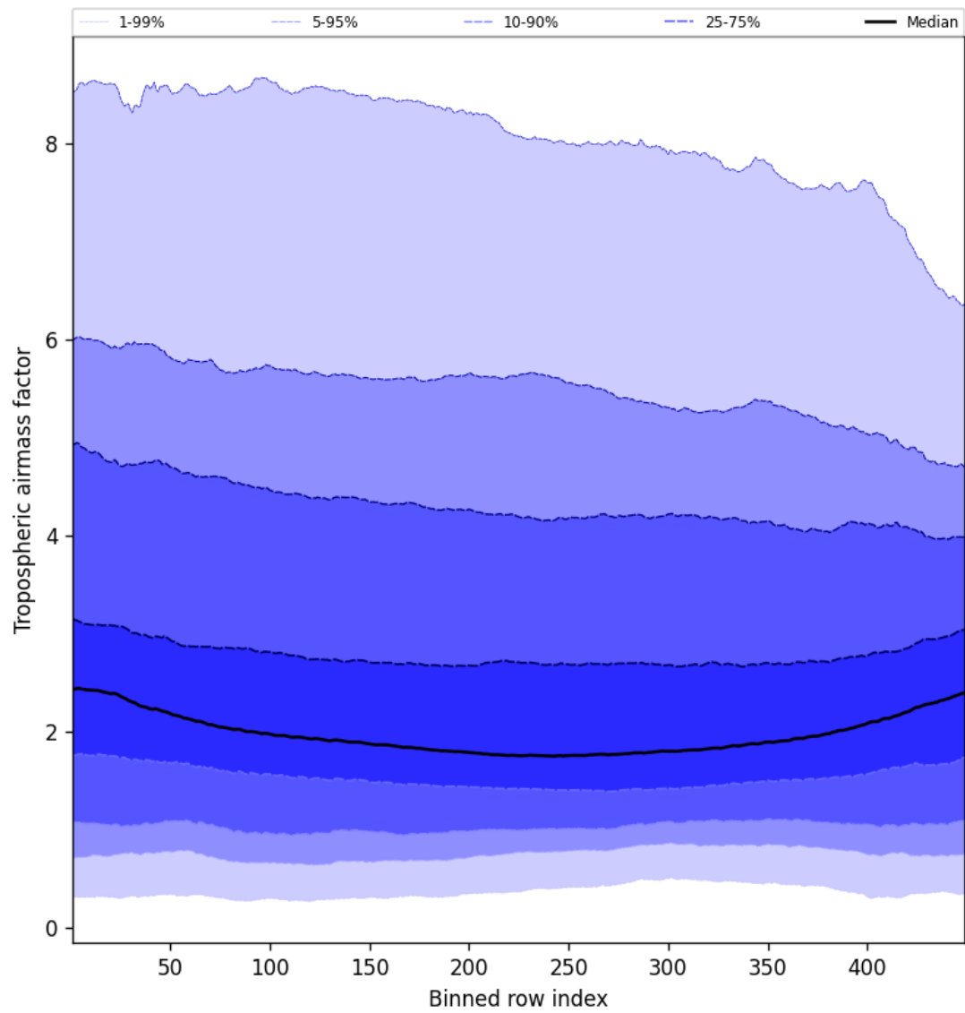
Figure 48: Along track statistics of “Tropospheric air mass factor” for 2024-09-13 to 2024-09-15
