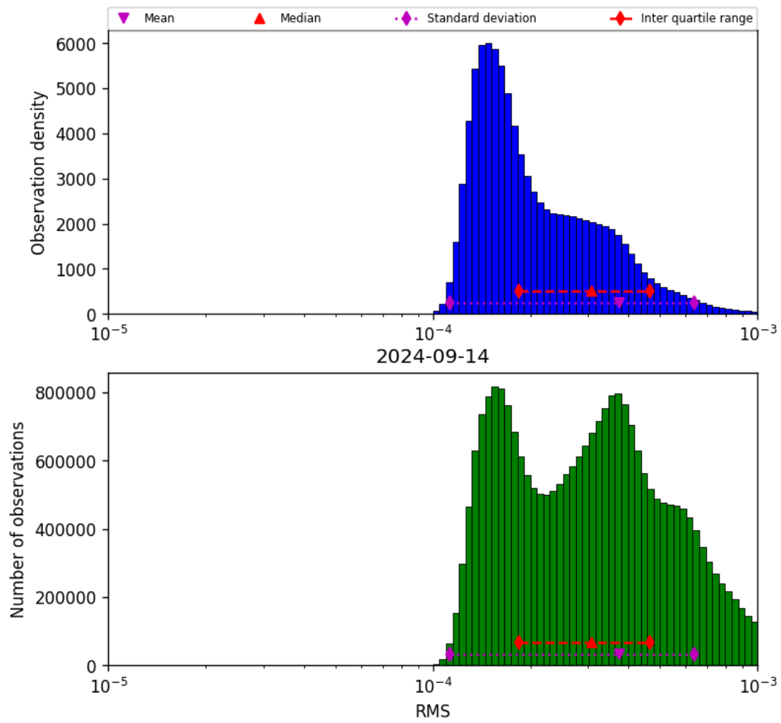
Figure 43: Histogram of “RMS” for 2024-09-13 to 2024-09-15
