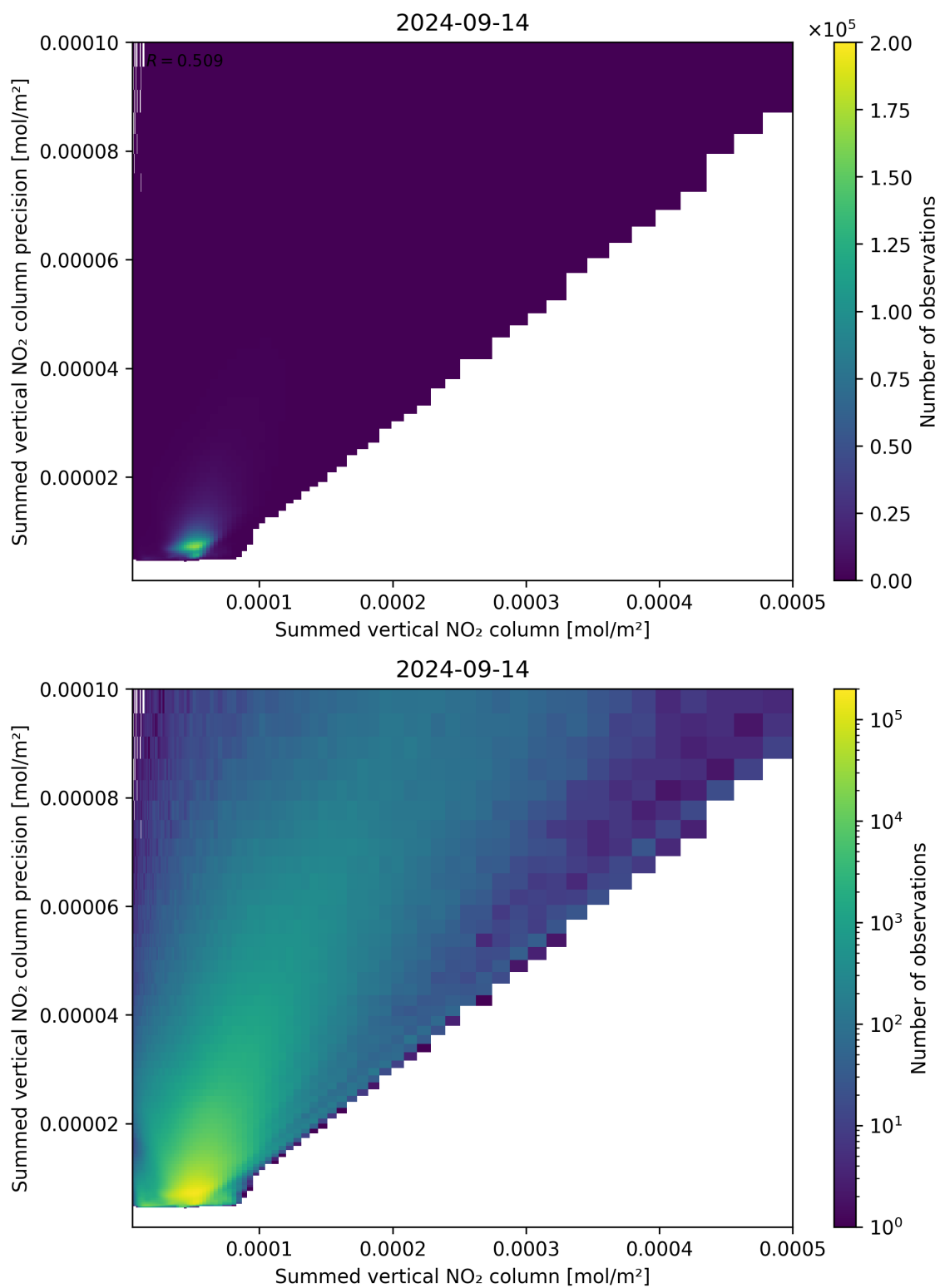
Figure 105: Scatter density plot of “Summed vertical NO 2 column” against “Summed vertical NO 2 column precision” for 2024-09-13 to 2024-09-15.
