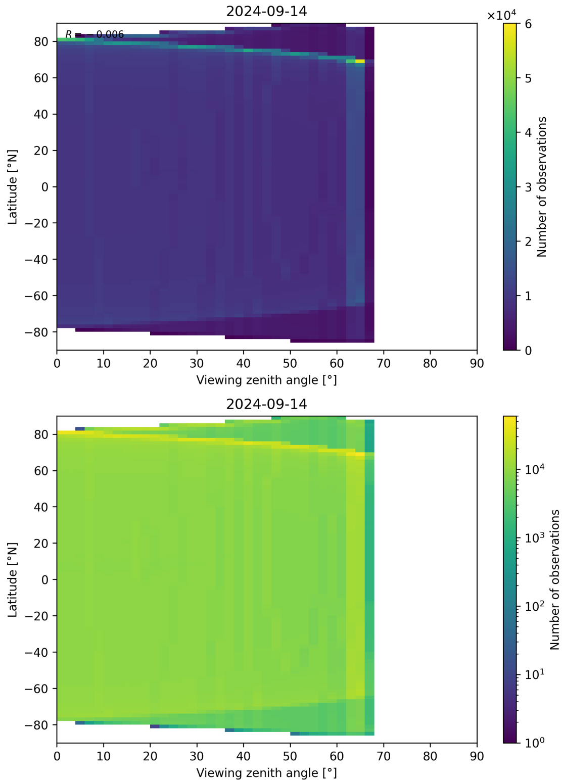
Figure 163: Scatter density plot of “Viewing zenith angle” against “Latitude” for 2024-09-13 to 2024-09-15.
