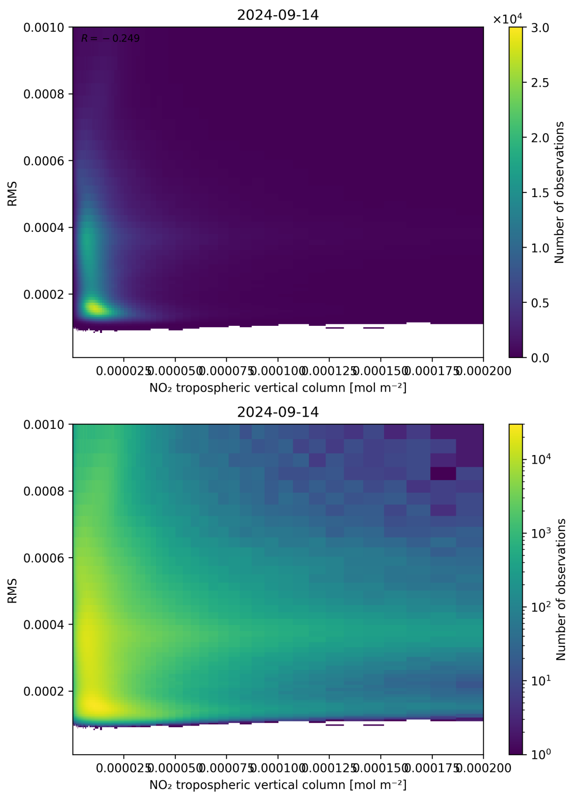
Figure 142: Scatter density plot of “NO 2 tropospheric vertical column” against “RMS” for 2024-09-13 to 2024-09-15.
