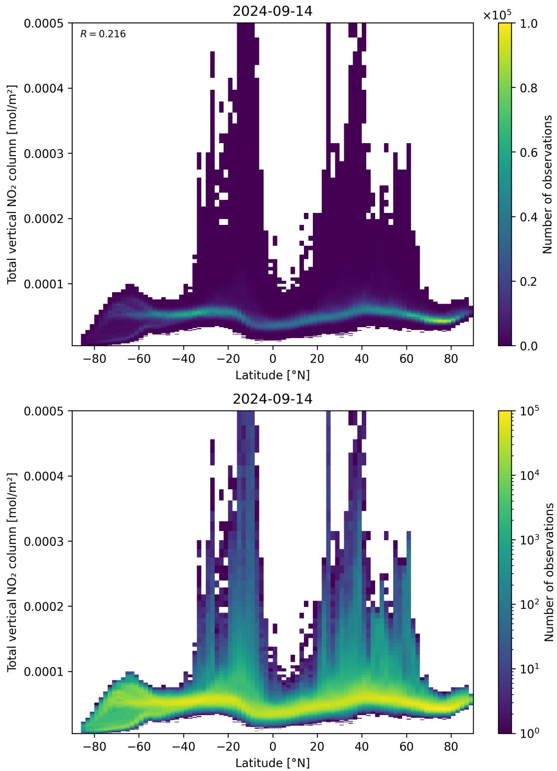
Figure 90: Scatter density plot of “Latitude” against “Total vertical NO 2 column” for 2024-09-13 to 2024-09-15.
