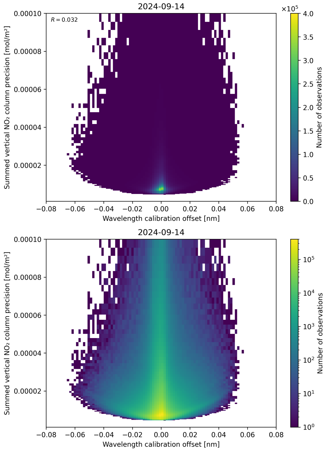
Figure 178: Scatter density plot of “Wavelength calibration offset” against “Summed vertical NO 2 column precision” for 2024-09-13 to 2024-09-15.
