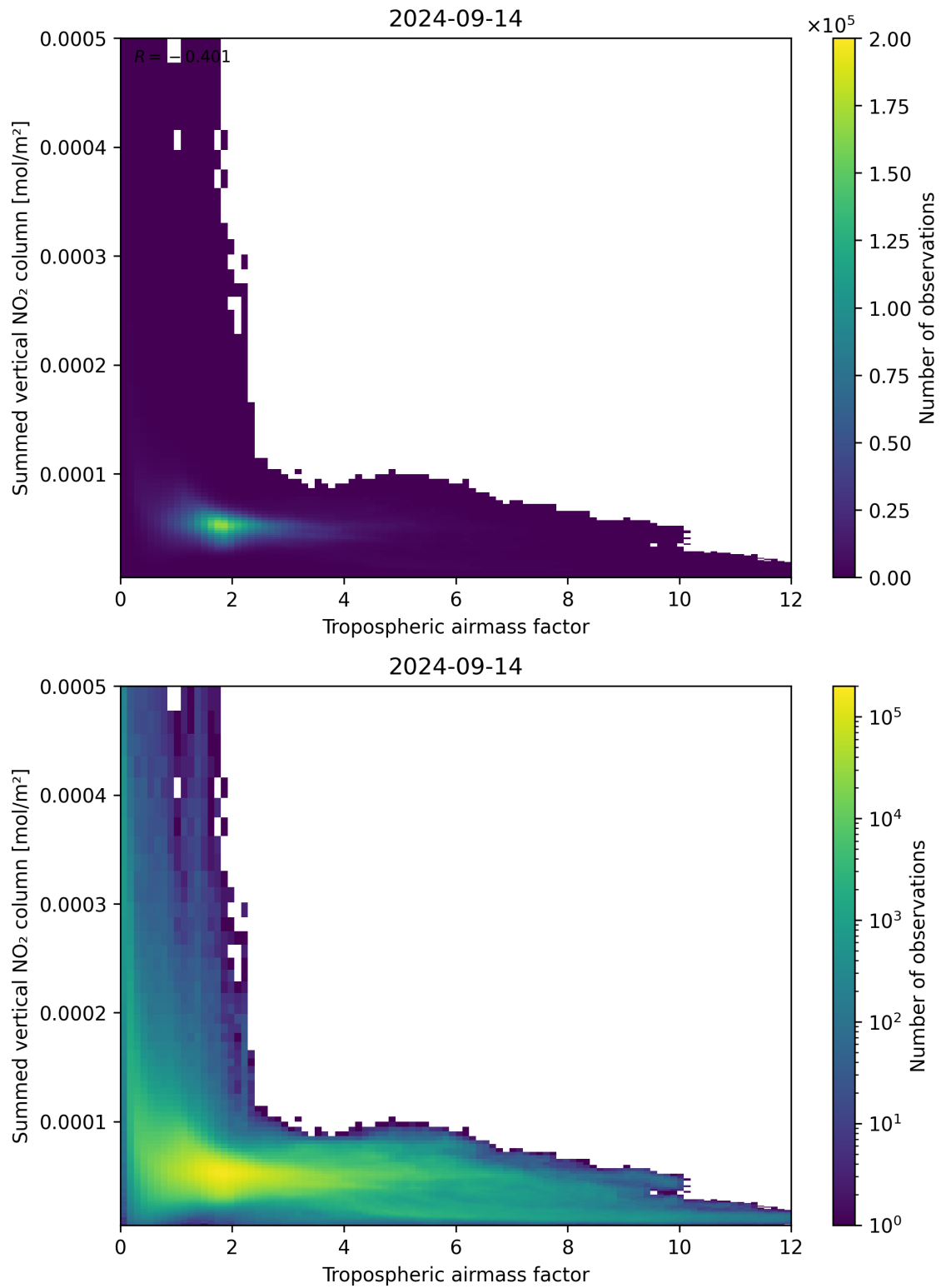
Figure 75: Scatter density plot of “Tropospheric airmass factor” against “Summed vertical NO 2 column” for 2024-09-13 to 2024-09-15.
