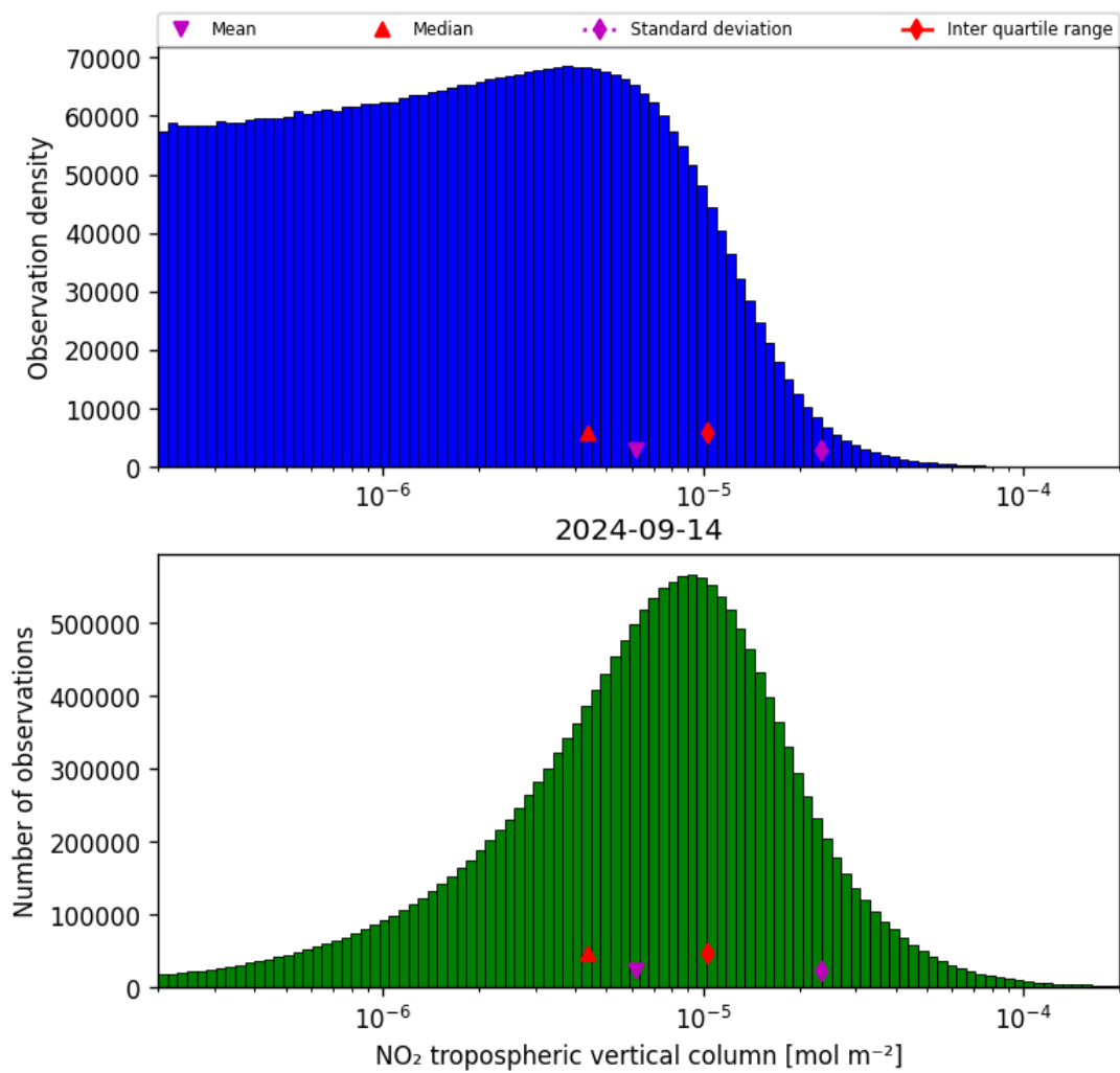
Figure 29: Histogram of “NO 2 tropospheric vertical column” for 2024-09-13 to 2024-09-15
