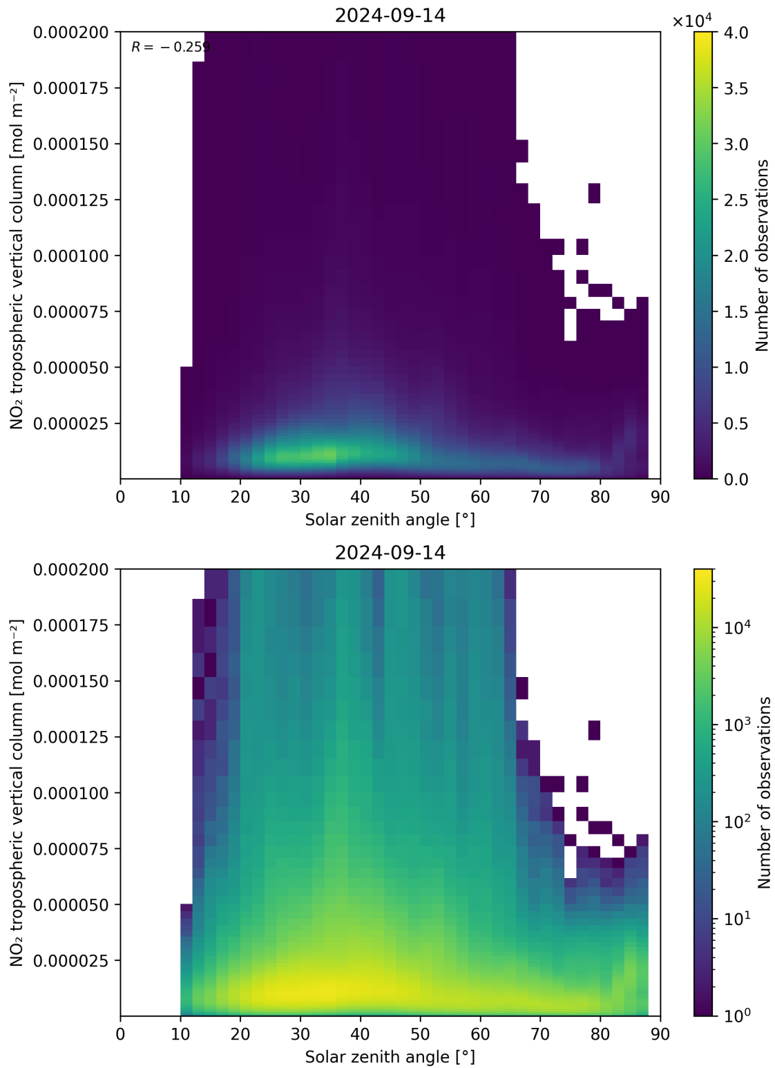
Figure 155: Scatter density plot of “Solar zenith angle” against “NO 2 tropospheric vertical column” for 2024-09-13 to 2024-09-15.
