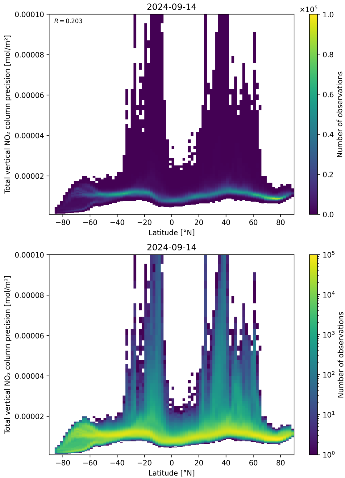
Figure 91: Scatter density plot of “Latitude” against “Total vertical NO 2 column precision” for 2024-09-13 to 2024-09-15.
