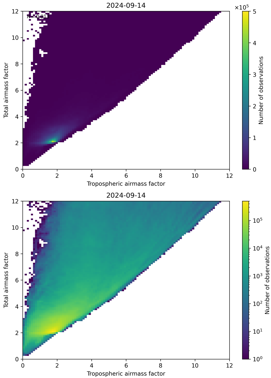
Figure 72: Scatter density plot of “Tropospheric airmass factor” against “Total airmass factor” for 2024-09-13 to 2024-09-15.
