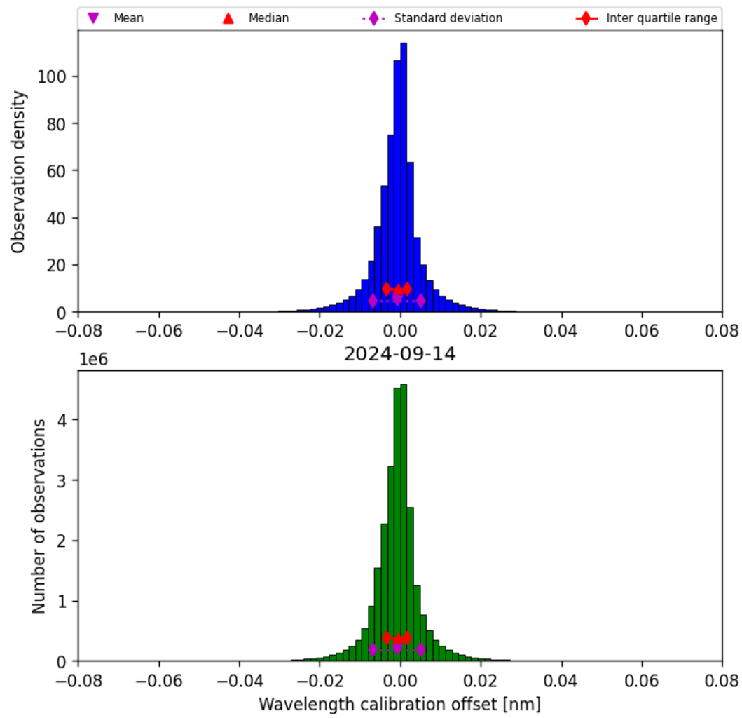
Figure 35: Histogram of “Wavelength calibration offset” for 2024-09-13 to 2024-09-15
