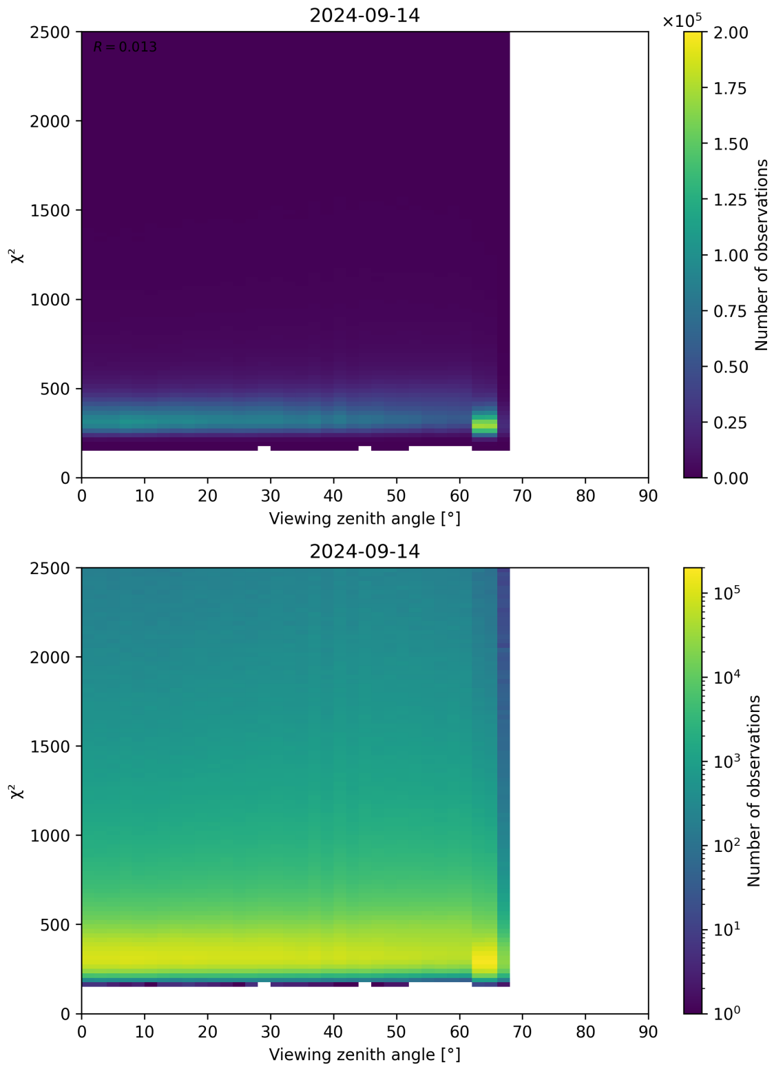
Figure 162: Scatter density plot of “Viewing zenith angle” against “ \chi^2 ” for 2024-09-13 to 2024-09-15.
