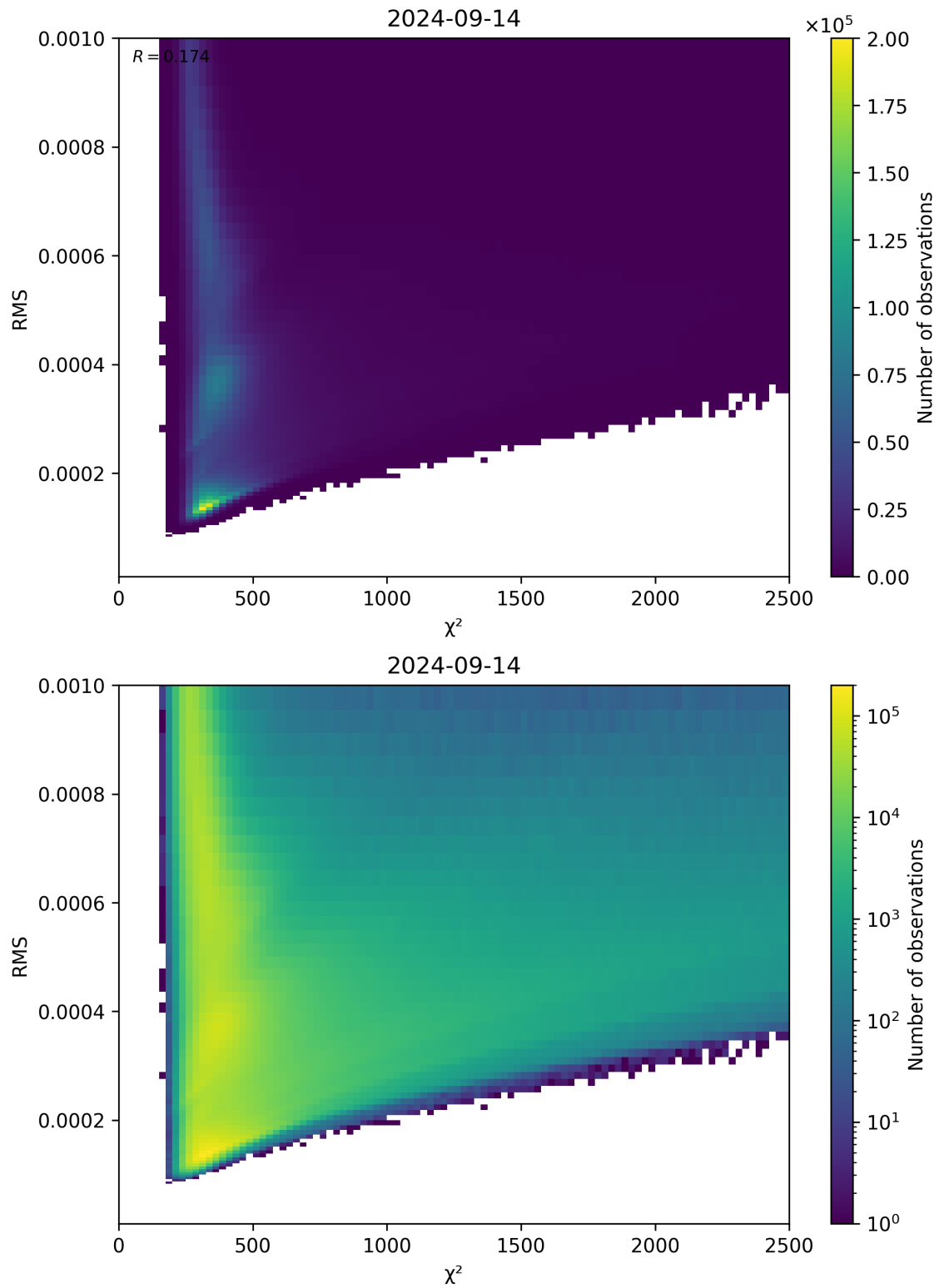
Figure 82: Scatter density plot of “ \chi^2 ” against “RMS” for 2024-09-13 to 2024-09-15.
