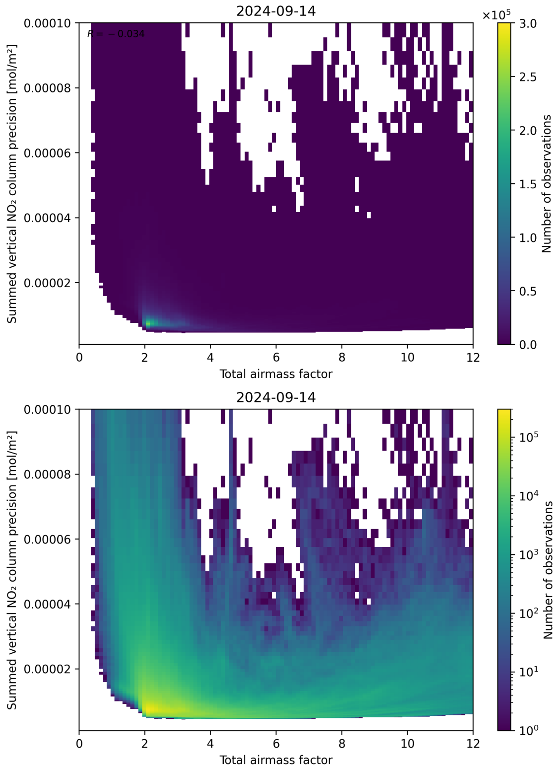
Figure 66: Scatter density plot of “Total airmass factor” against “Summed vertical NO 2 column precision” for 2024-09-13 to 2024-09-15.
