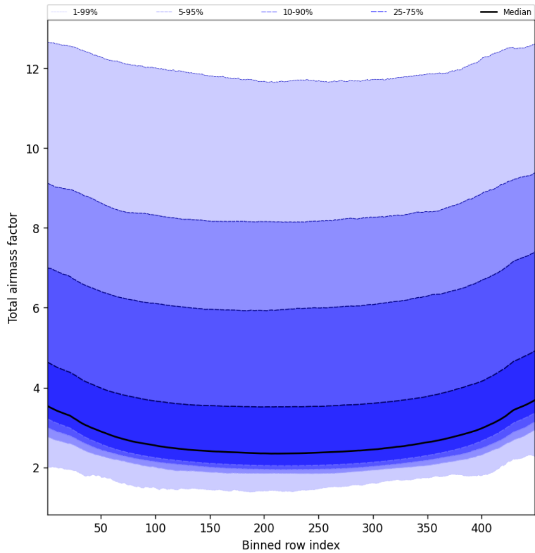
Figure 49: Along track statistics of “Total airmass factor” for 2024-09-13 to 2024-09-15
