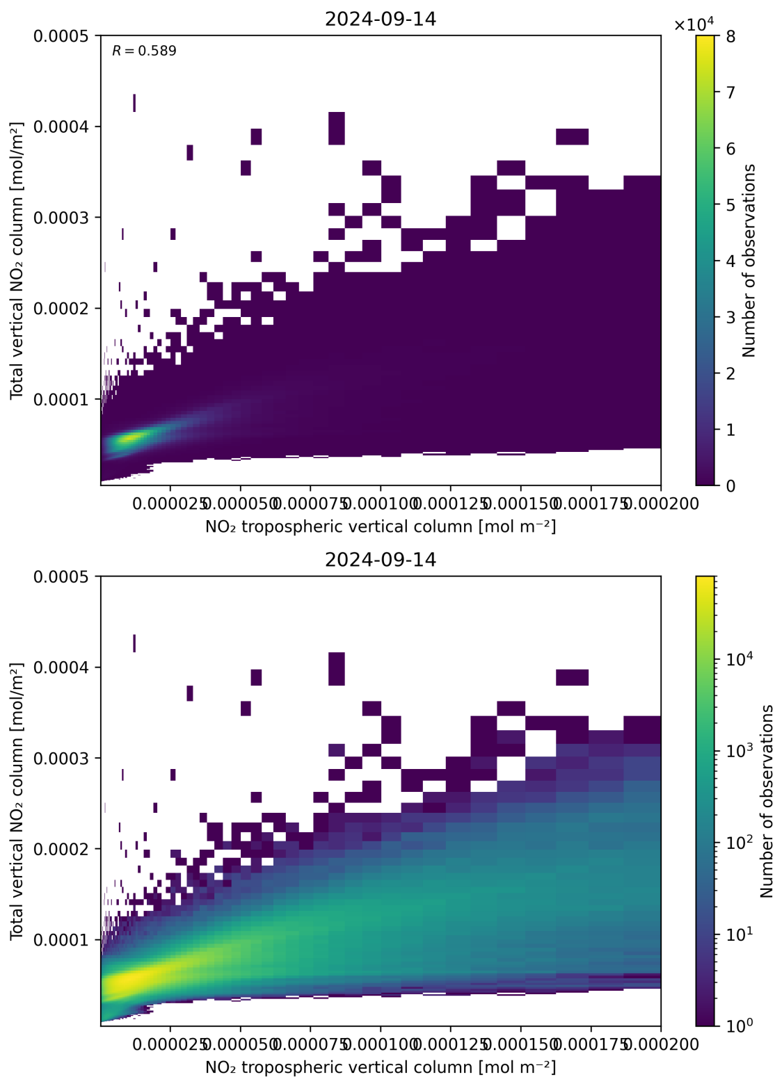
Figure 128: Scatter density plot of “NO 2 tropospheric vertical column” against “Total vertical NO 2 column” for 2024-09-13 to 2024-09-15.
