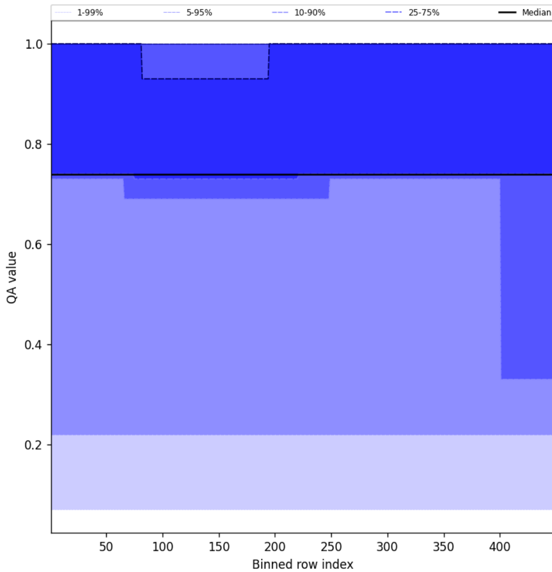
Figure 45: Along track statistics of “QA value” for 2024-09-13 to 2024-09-15
