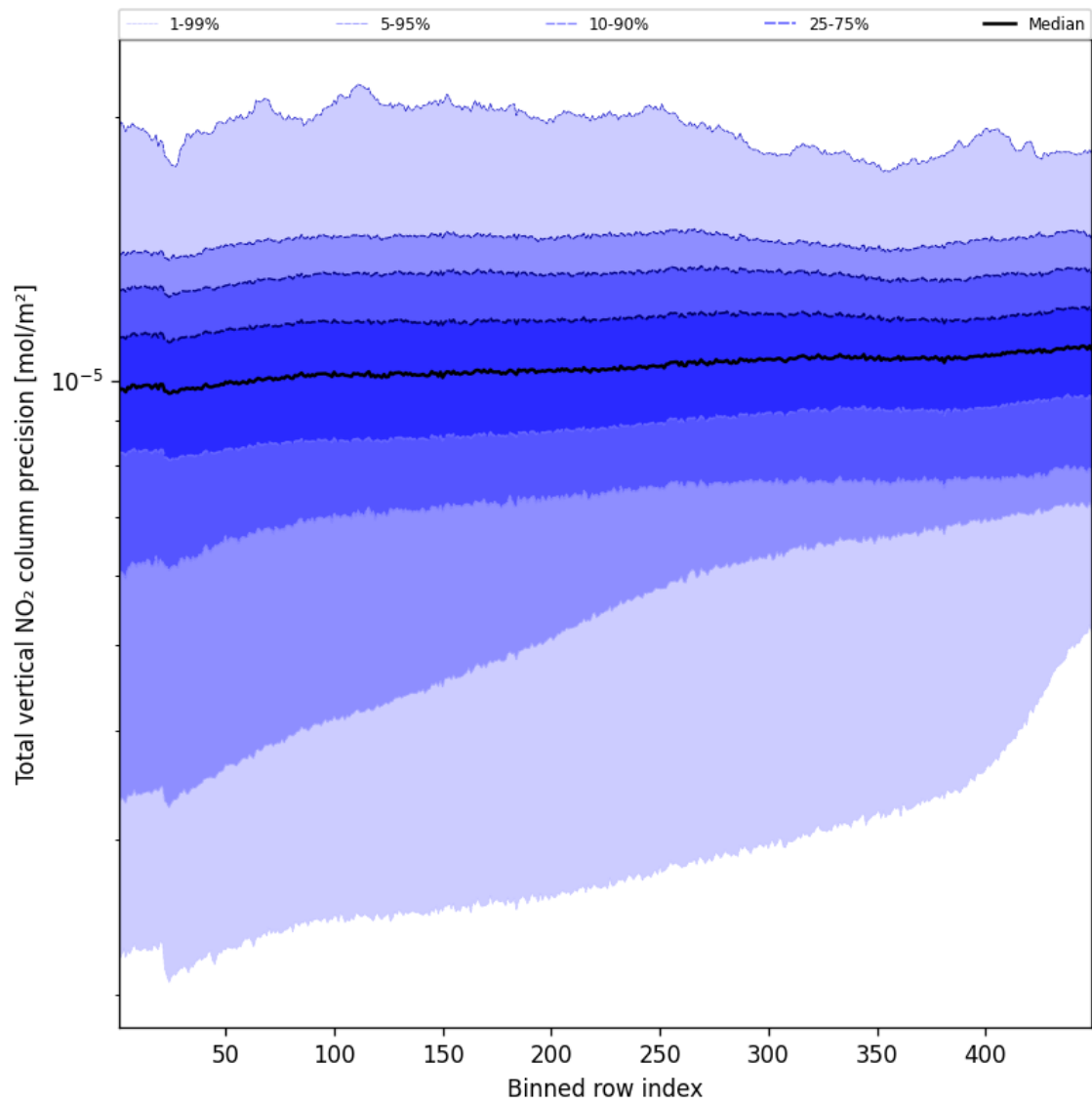
Figure 56: Along track statistics of “Total vertical NO 2 column precision” for 2024-09-13 to 2024-09-15
