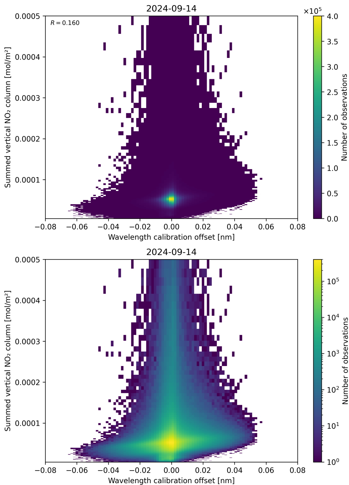
Figure 177: Scatter density plot of “Wavelength calibration offset” against “Summed vertical NO 2 column” for 2024-09-13 to 2024-09-15.
