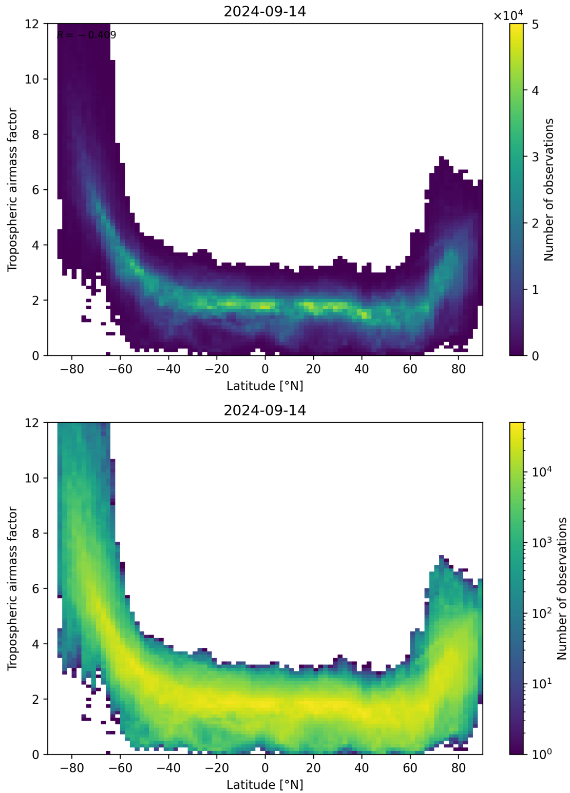
Figure 85: Scatter density plot of “Latitude” against “Tropospheric air mass factor” for 2024-09-13 to 2024-09-15.
