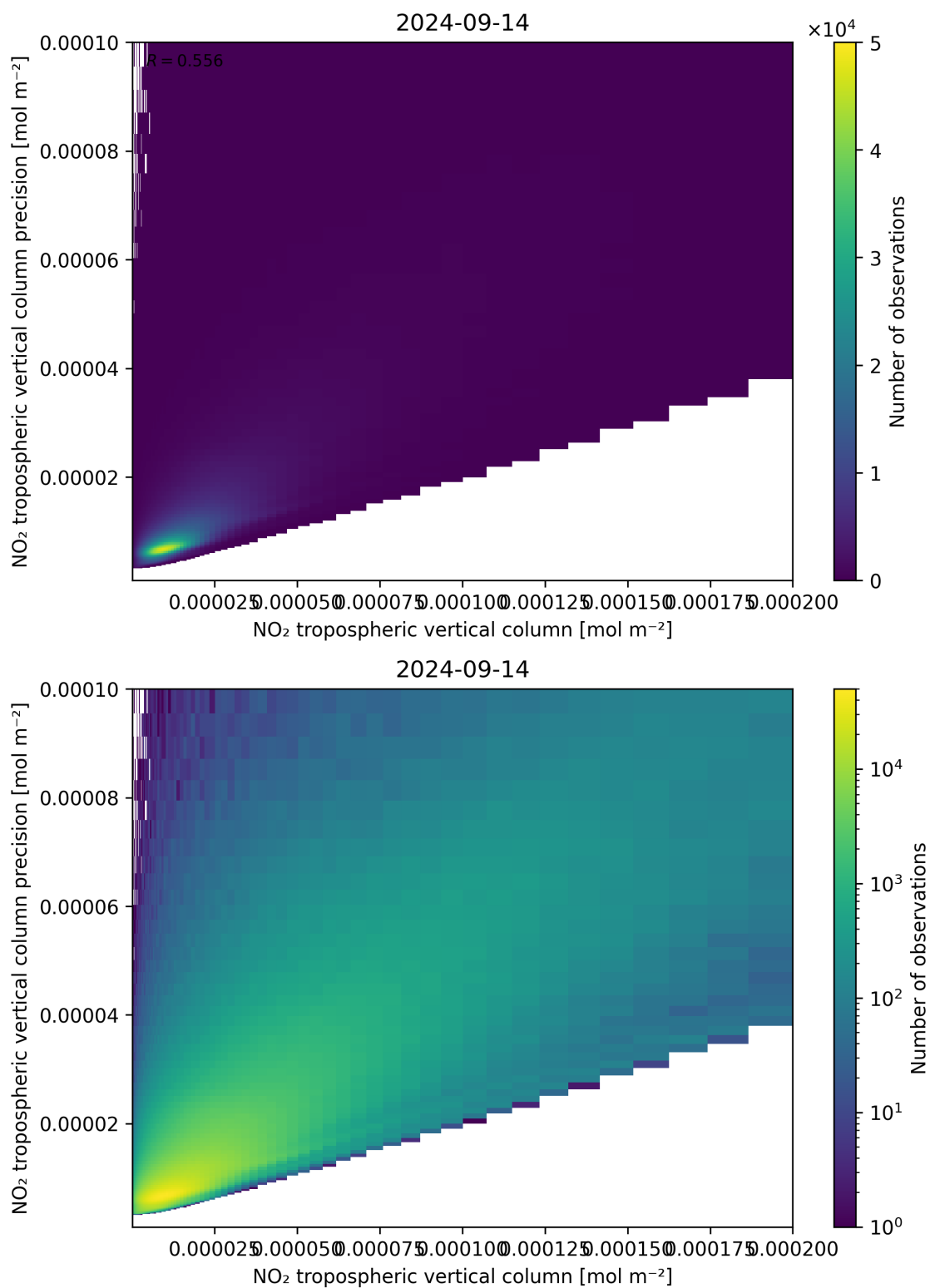
Figure 130: Scatter density plot of “NO 2 tropospheric vertical column” against “NO 2 tropospheric vertical column precision” for 2024-09-13 to 2024-09-15.
