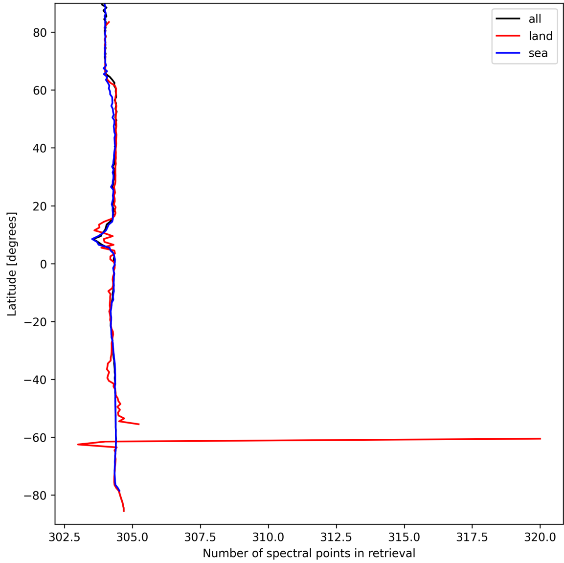
Figure 16: Zonal average of “Number of spectral points in retrieval” for 2024-09-13 to 2024-09-15.
