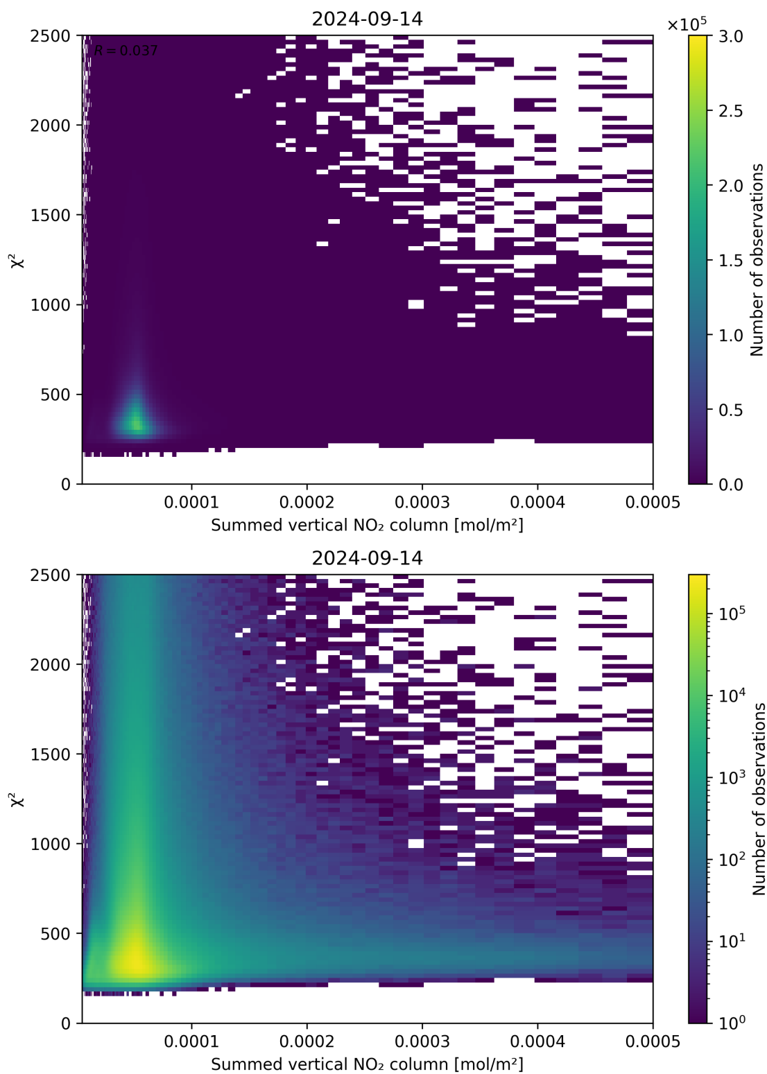
Figure 104: Scatter density plot of “Summed vertical NO 2 column” against “ \chi^2 ” for 2024-09-13 to 2024-09-15.
