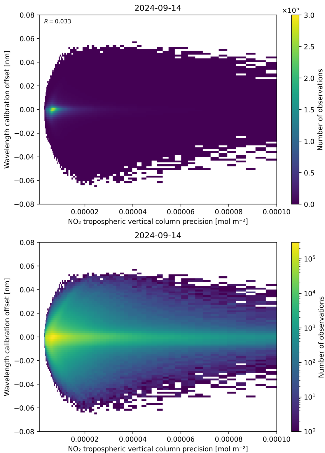
Figure 141: Scatter density plot of “NO 2 tropospheric vertical column precision” against “Wavelength calibration offset” for 2024-09-13 to 2024-09-15.
