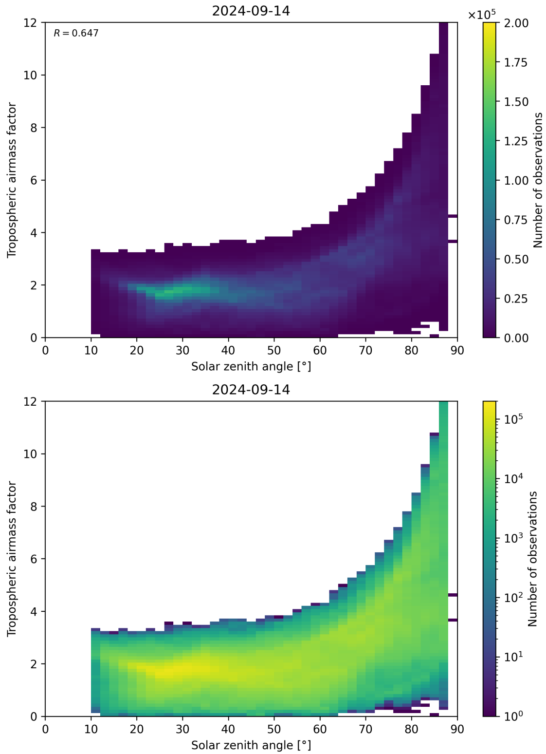
Figure 147: Scatter density plot of “Solar zenith angle” against “Tropospheric airmass factor” for 2024-09-13 to 2024-09-15.
