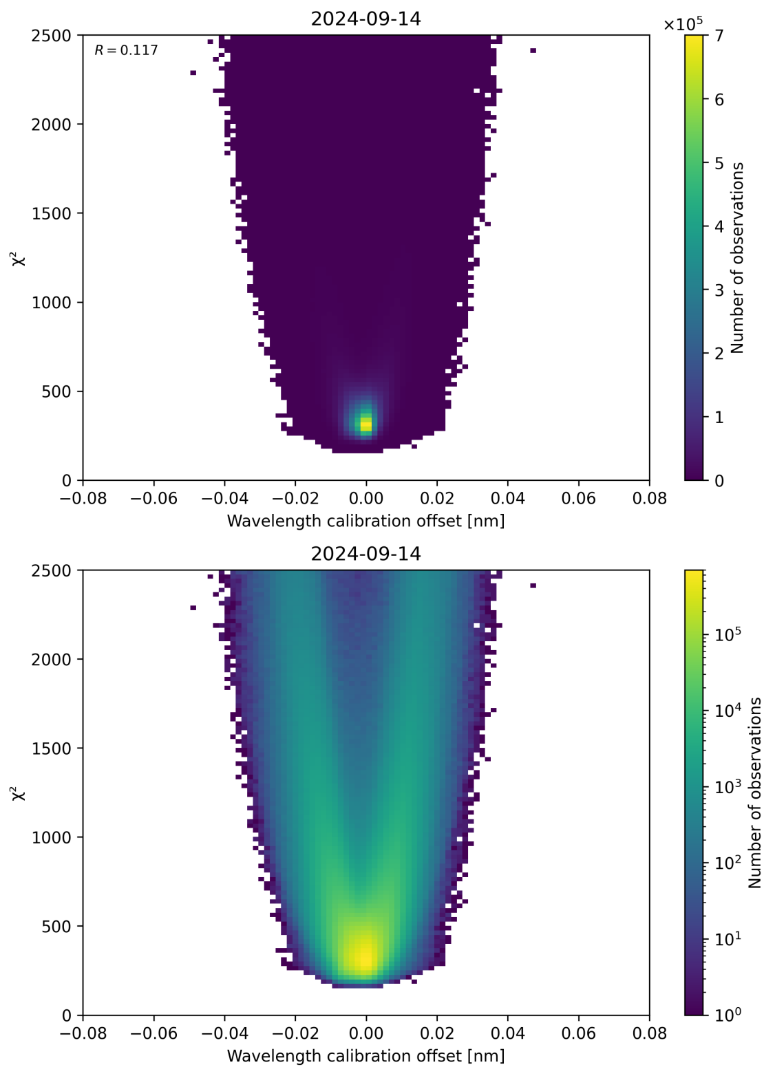
Figure 175: Scatter density plot of “Wavelength calibration offset” against “ \chi^2 ” for 2024-09-13 to 2024-09-15.
