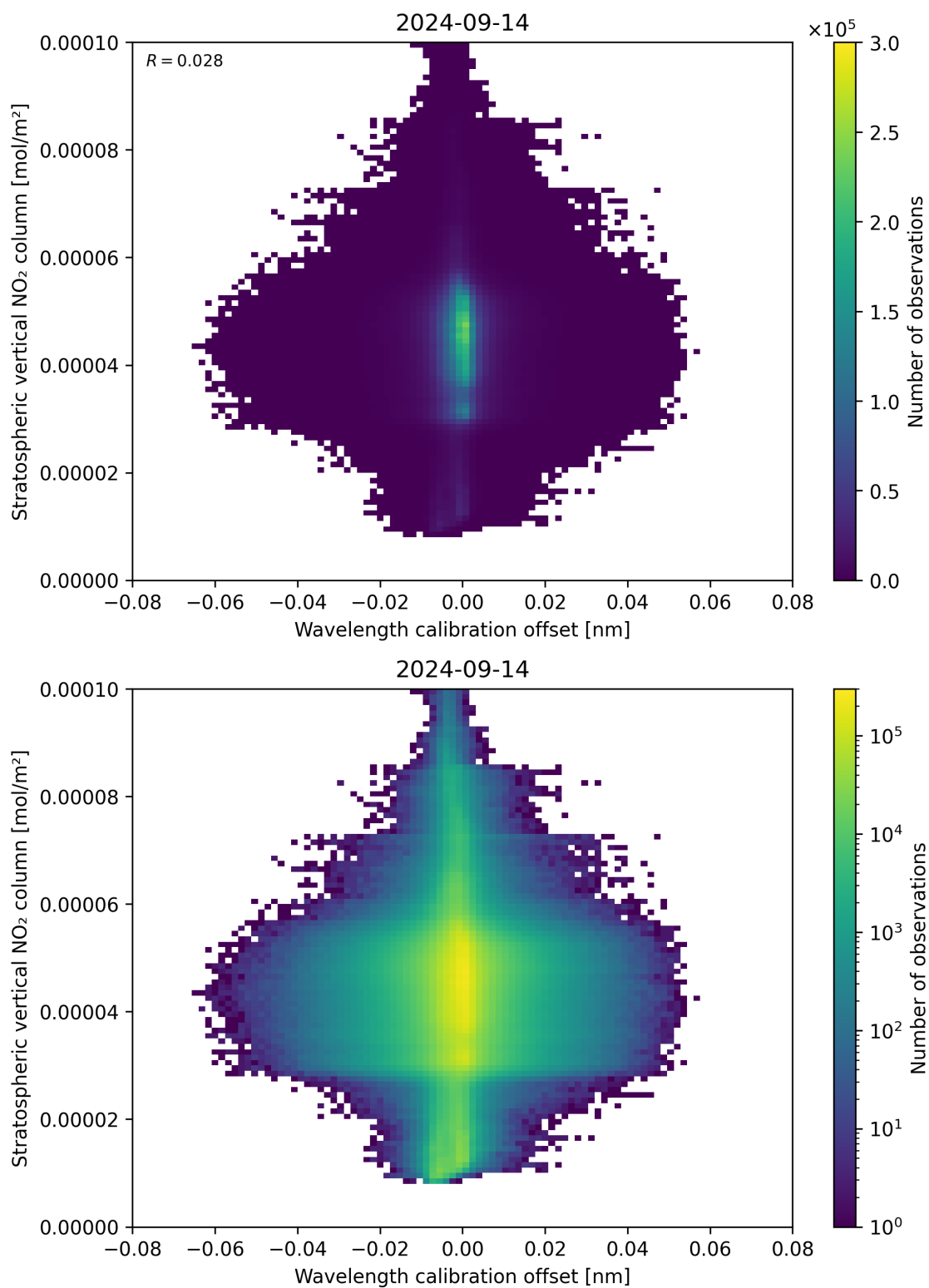
Figure 176: Scatter density plot of “Wavelength calibration offset” against “Stratospheric vertical NO 2 column” for 2024-09-13 to 2024-09-15.
