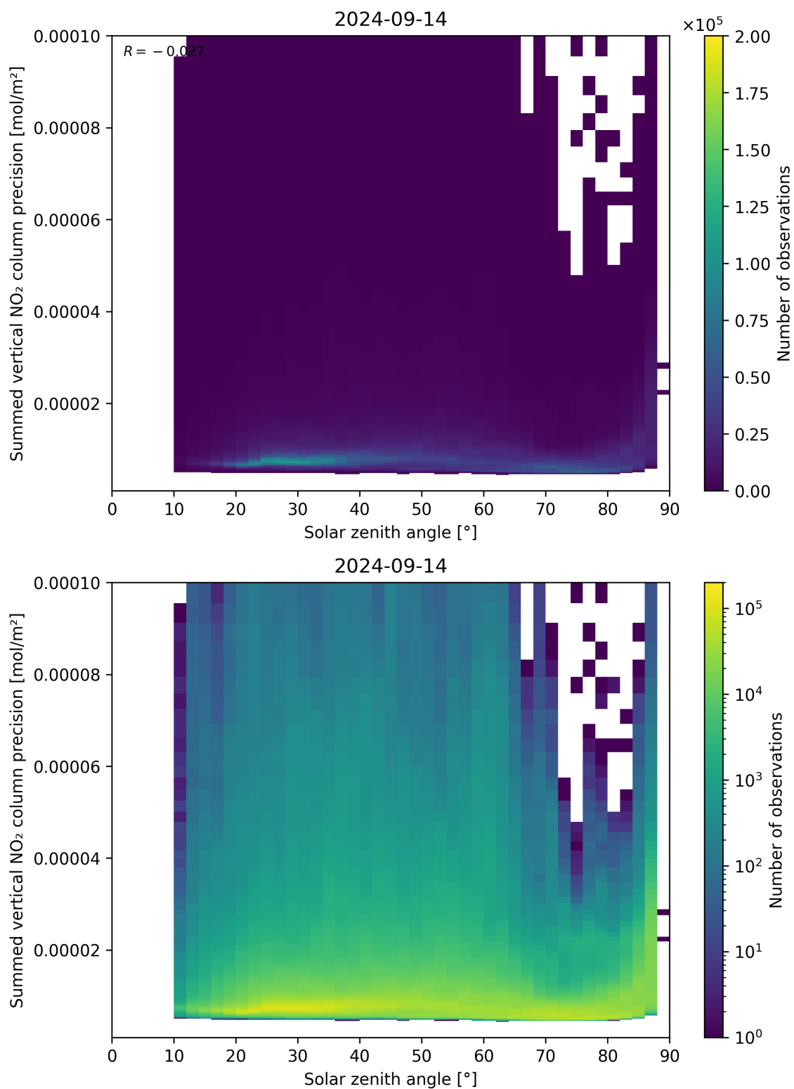
Figure 152: Scatter density plot of “Solar zenith angle” against “Summed vertical NO 2 column precision” for 2024-09-13 to 2024-09-15.
