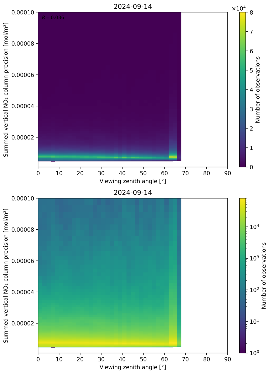
Figure 166: Scatter density plot of “Viewing zenith angle” against “Summed vertical NO 2 column precision” for 2024-09-13 to 2024-09-15.
