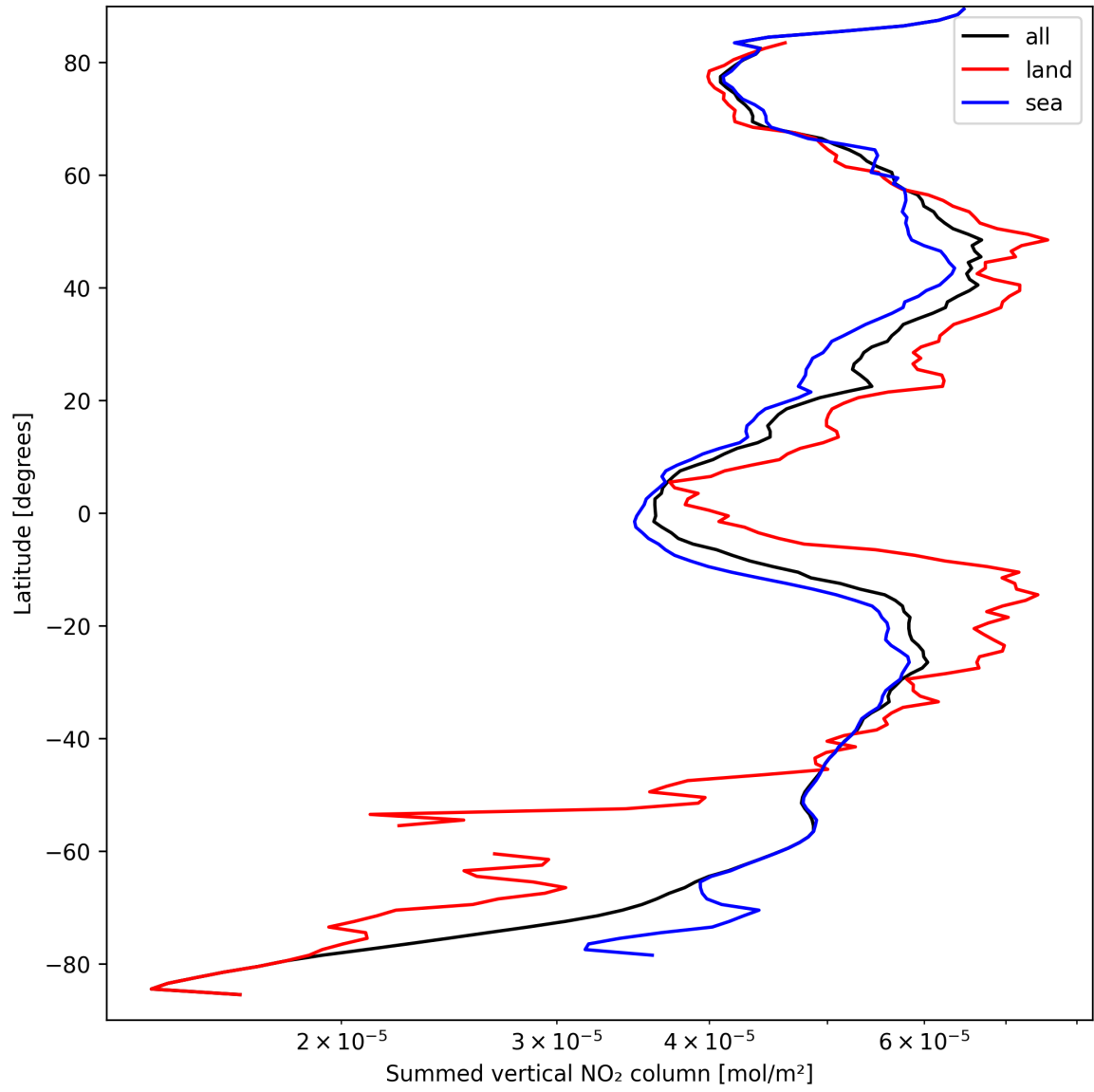
Figure 23: Zonal average of “Summed vertical NO 2 column” for 2024-09-13 to 2024-09-15.
