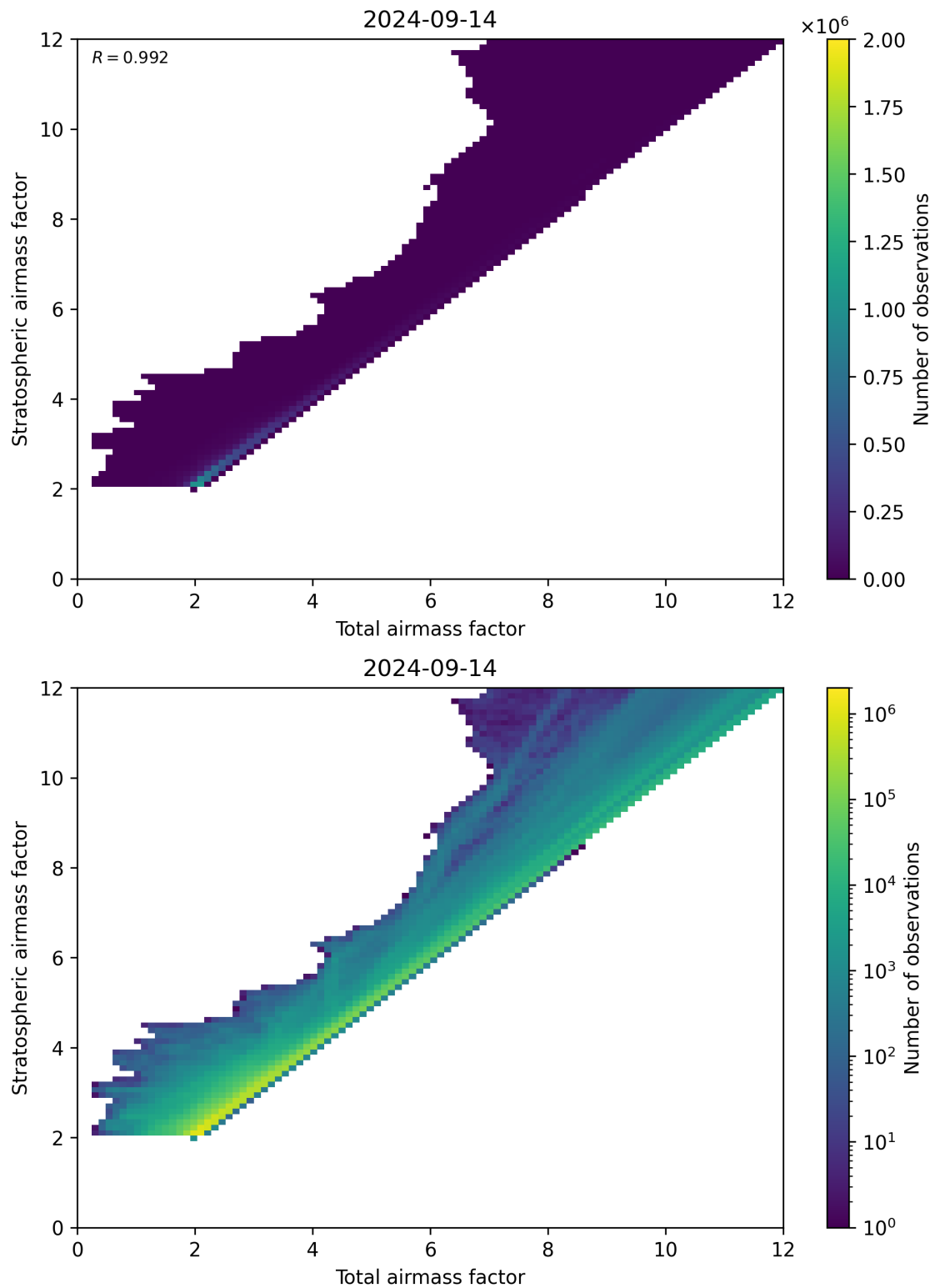
Figure 62: Scatter density plot of “Total airmass factor” against “Stratospheric airmass factor” for 2024-09-13 to 2024-09-15.
