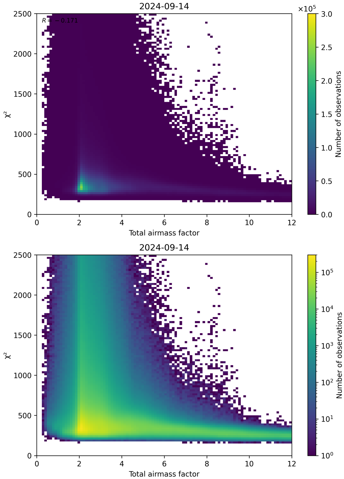
Figure 63: Scatter density plot of “Total airmass factor” against “ \chi^2 ” for 2024-09-13 to 2024-09-15.
