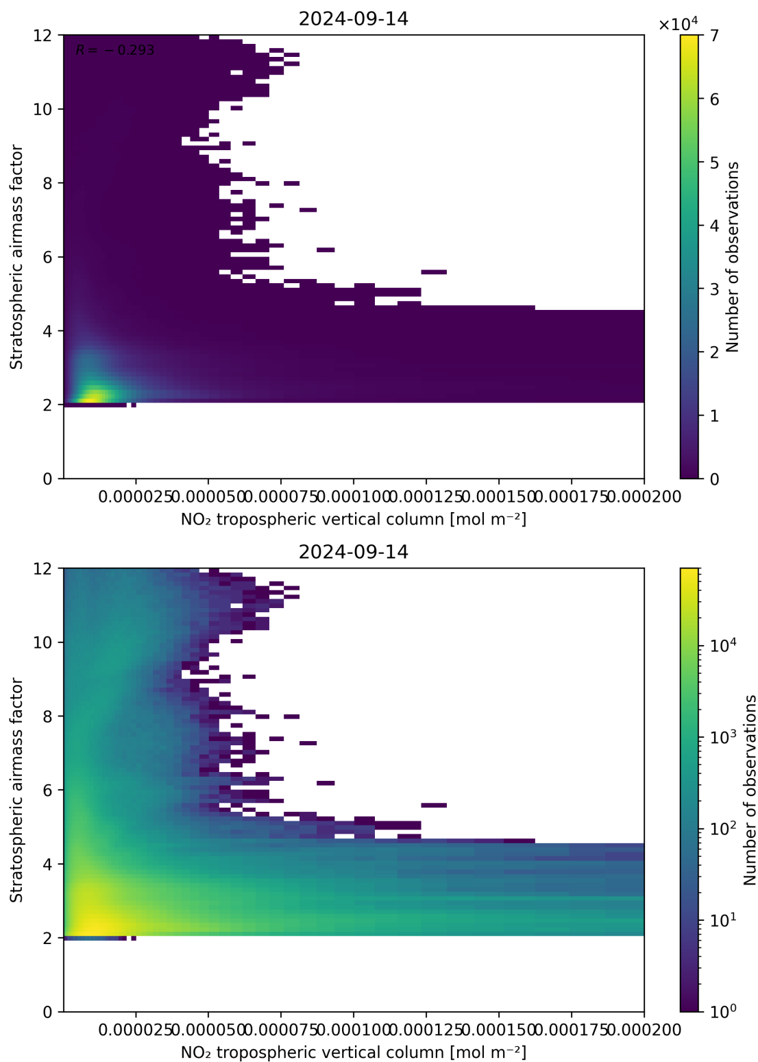
Figure 121: Scatter density plot of “NO 2 tropospheric vertical column” against “Stratospheric air mass factor” for 2024-09-13 to 2024-09-15.
