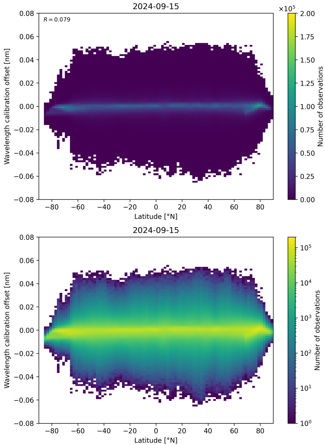
Figure 95: Scatter density plot of “Latitude” against “Wavelength calibration offset” for 2024-09-14 to 2024-09-16.
