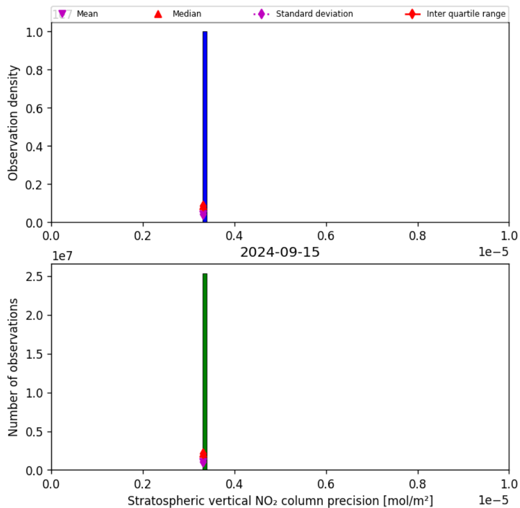
Figure 37: Histogram of “Stratospheric vertical NO 2 column precision” for 2024-09-14 to 2024-09-16
