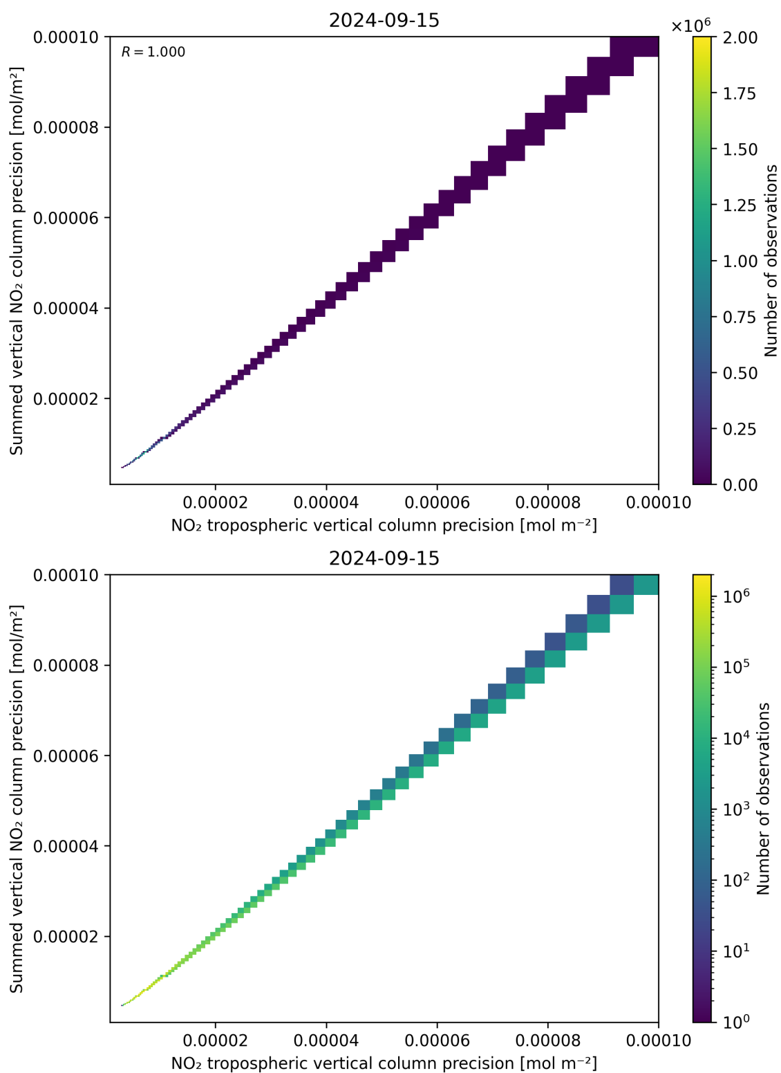
Figure 137: Scatter density plot of “NO 2 tropospheric vertical column precision” against “Summed vertical NO 2 column precision” for 2024-09-14 to 2024-09-16.
