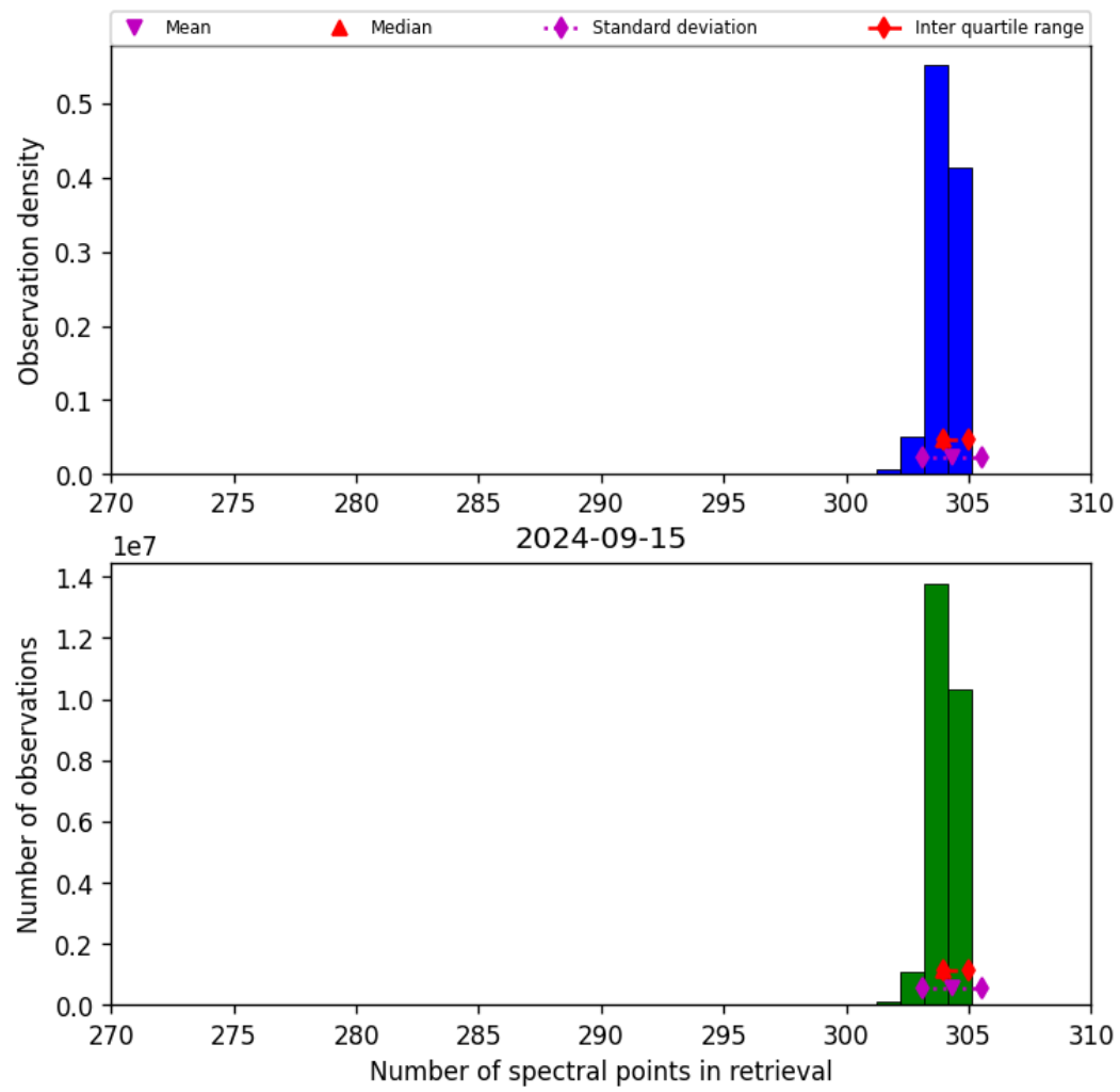
Figure 33: Histogram of “Number of spectral points in retrieval” for 2024-09-14 to 2024-09-16
