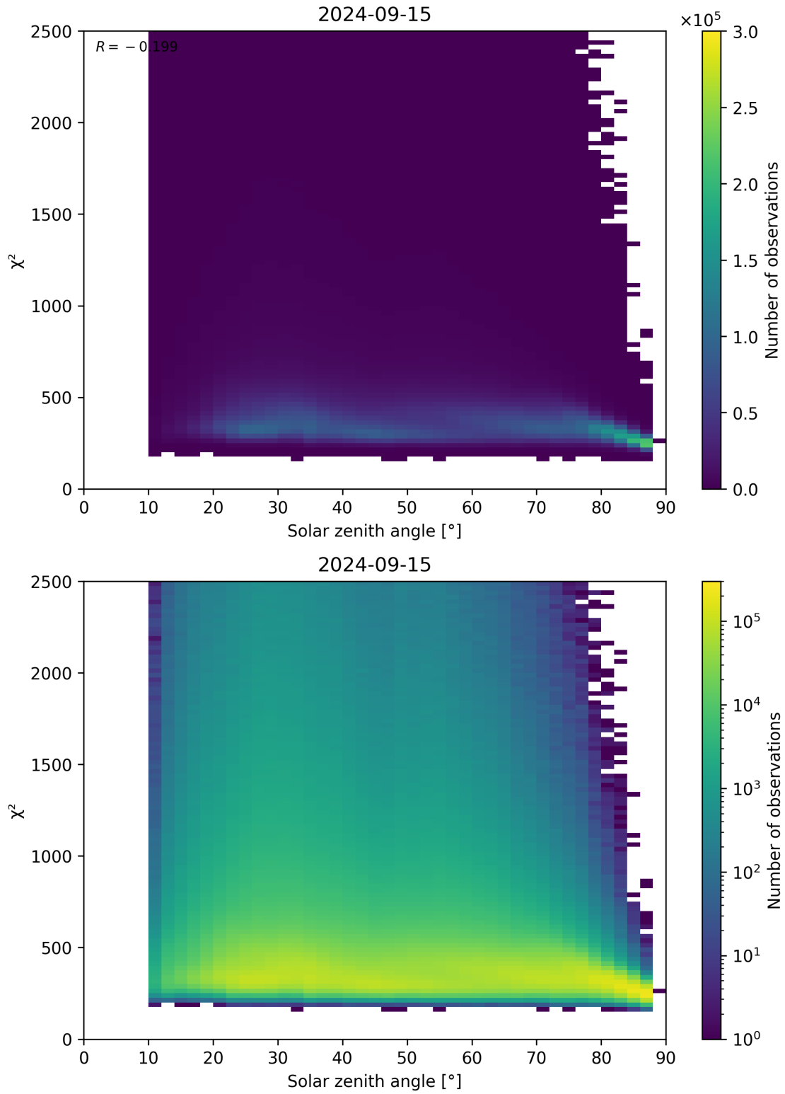
Figure 148: Scatter density plot of “Solar zenith angle” against “ \chi^2 ” for 2024-09-14 to 2024-09-16.
