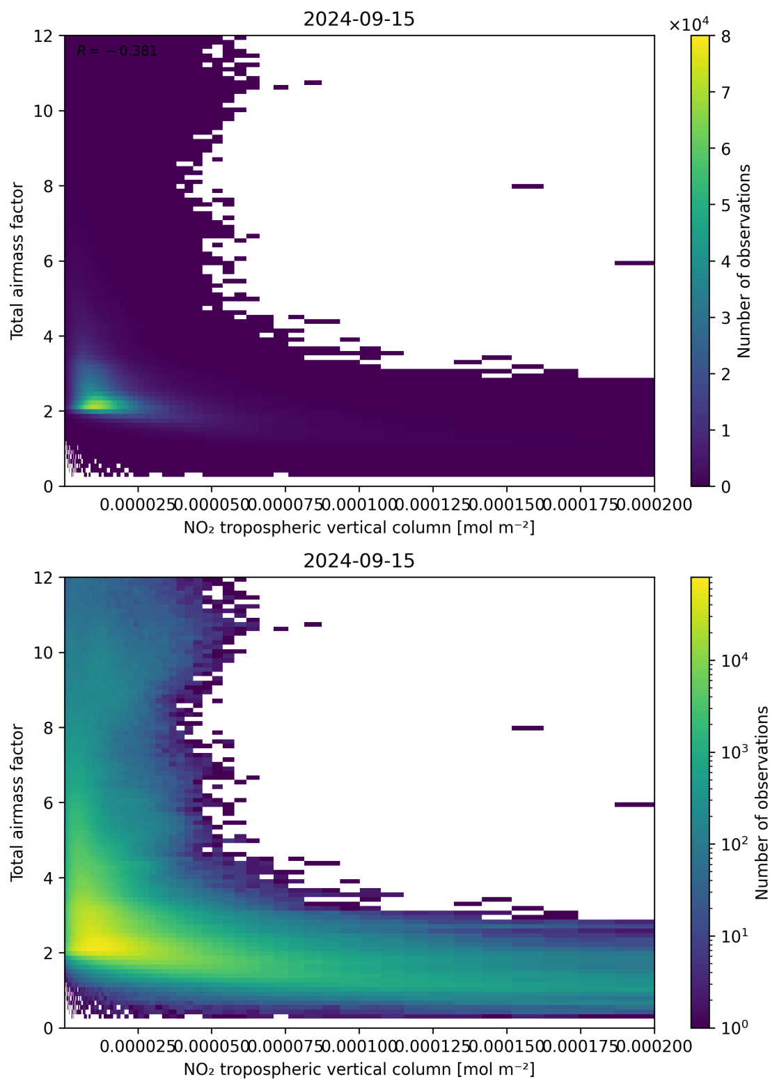
Figure 122: Scatter density plot of “NO 2 tropospheric vertical column” against “Total air mass factor” for 2024-09-14 to 2024-09-16.
