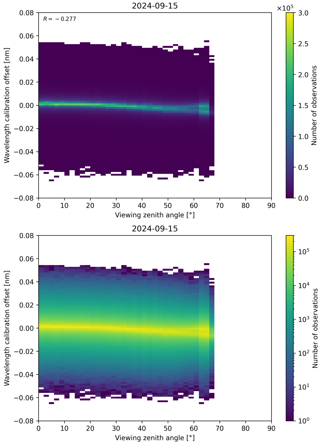
Figure 173: Scatter density plot of “Viewing zenith angle” against “Wavelength calibration offset” for 2024-09-14 to 2024-09-16.
