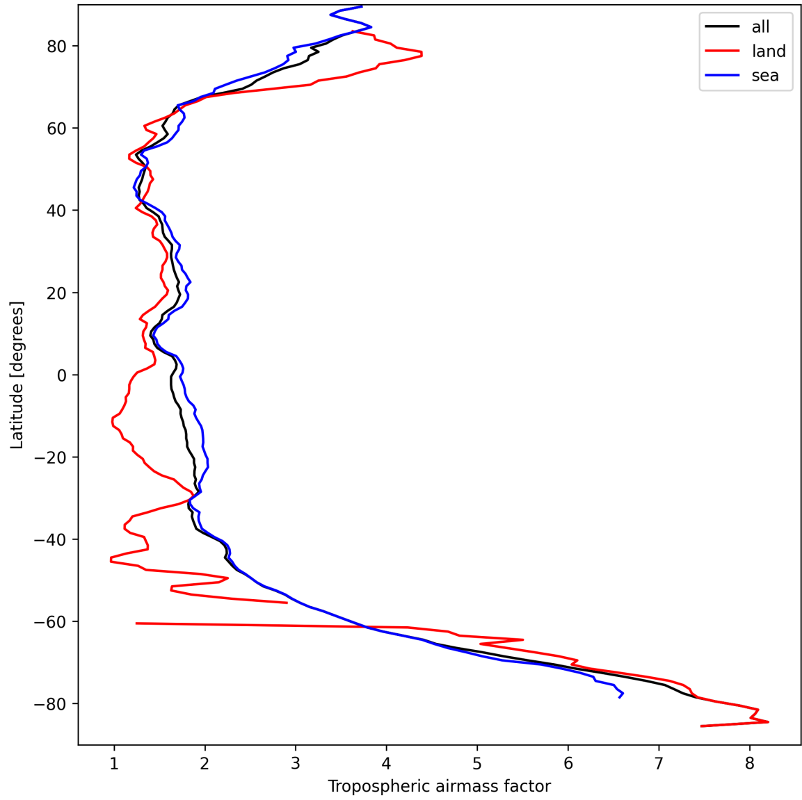
Figure 14: Zonal average of “Tropospheric airmass factor” for 2024-09-14 to 2024-09-16.
