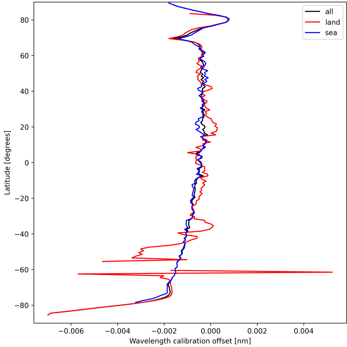
Figure 18: Zonal average of “Wavelength calibration offset” for 2024-09-14 to 2024-09-16.
