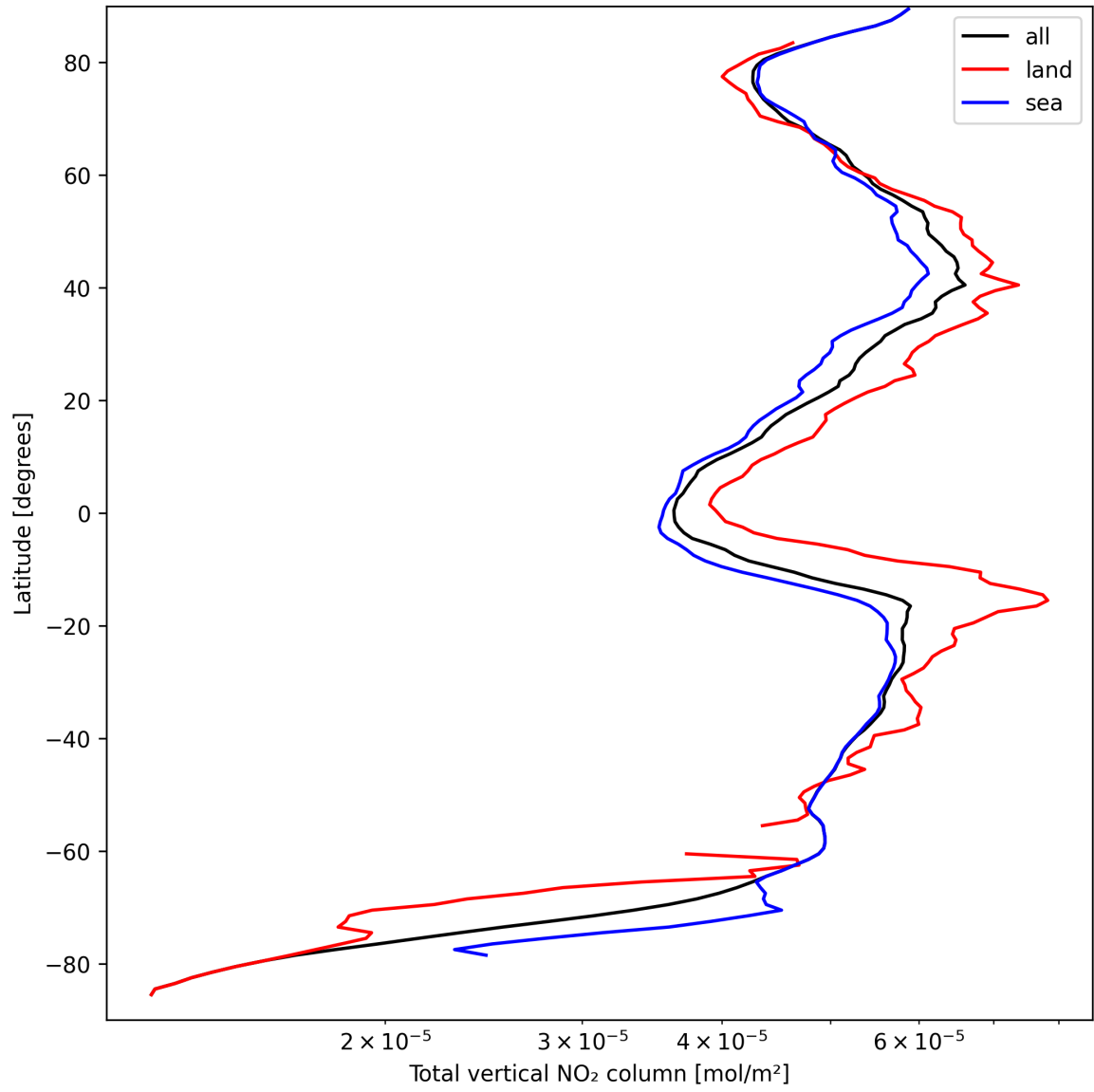
Figure 21: Zonal average of “Total vertical NO 2 column” for 2024-09-14 to 2024-09-16.
