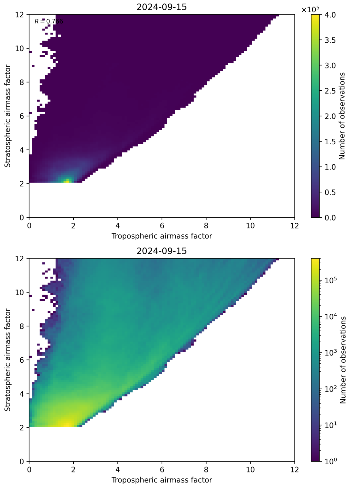
Figure 71: Scatter density plot of “Tropospheric airmass factor” against “Stratospheric airmass factor” for 2024-09-14 to 2024-09-16.
