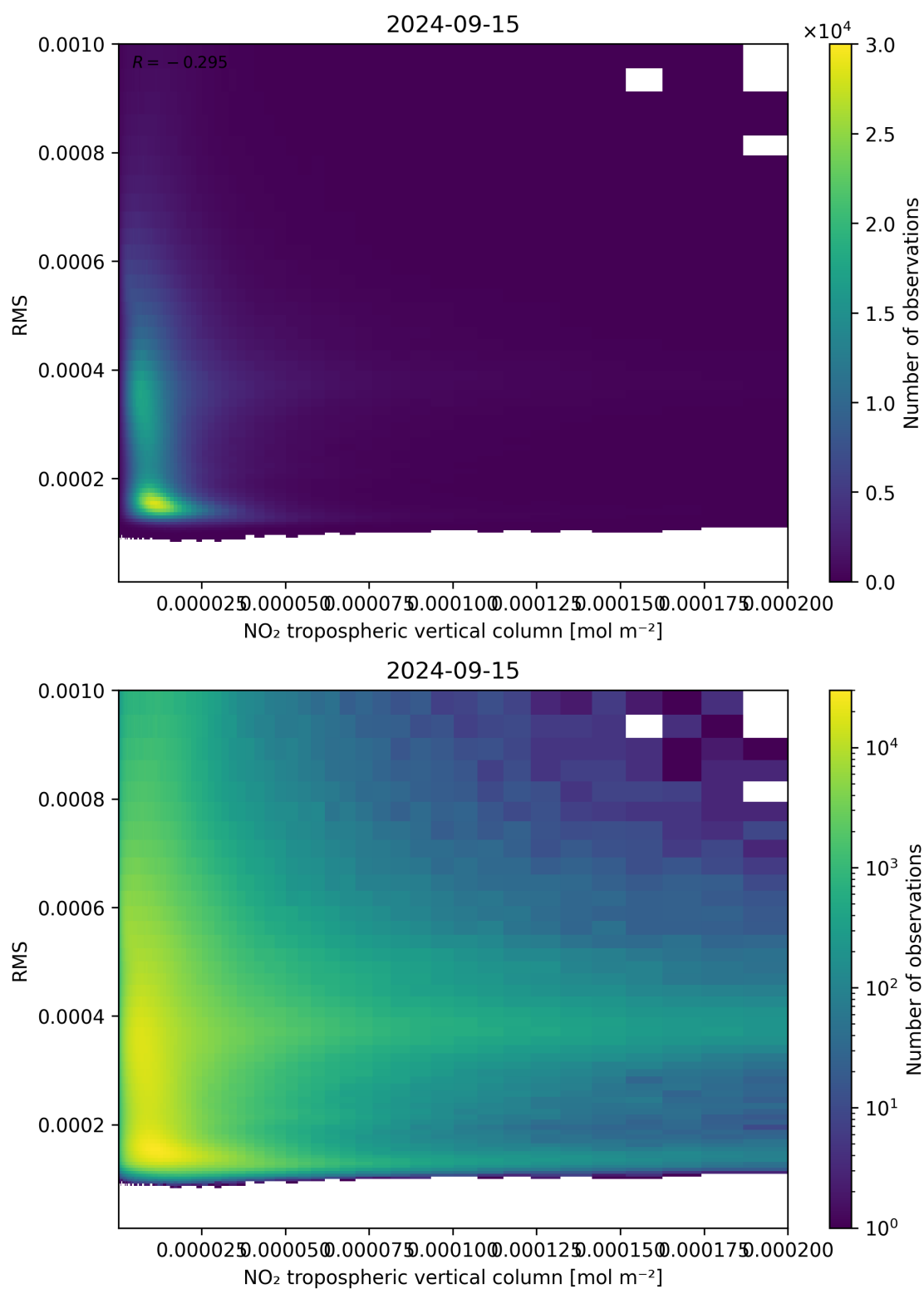
Figure 142: Scatter density plot of “NO 2 tropospheric vertical column” against “RMS” for 2024-09-14 to 2024-09-16.
