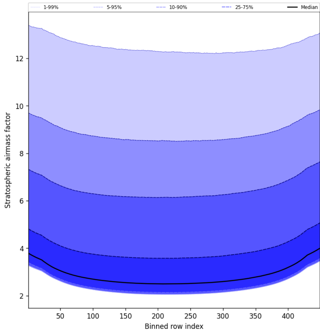
Figure 61: Along track statistics of “Stratospheric airmass factor” for 2024-09-14 to 2024-09-16
