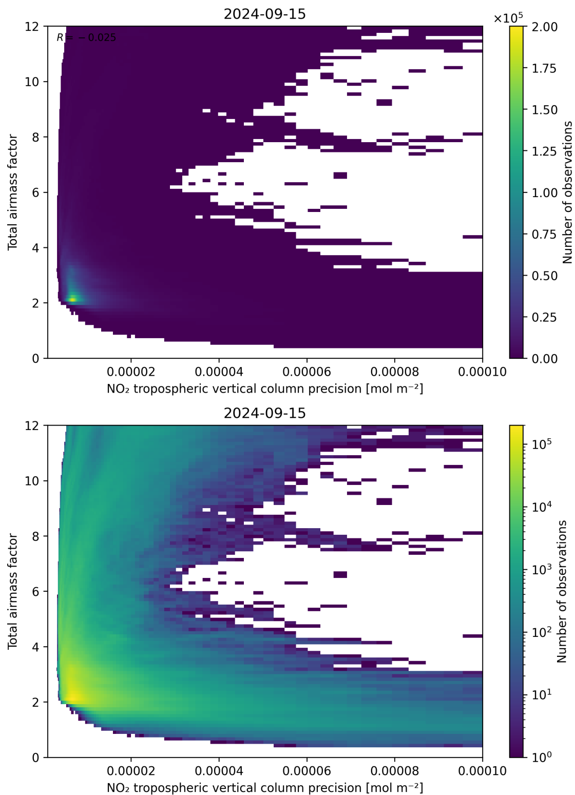
Figure 132: Scatter density plot of “NO 2 tropospheric vertical column precision” against “Total airmass factor” for 2024-09-14 to 2024-09-16.
