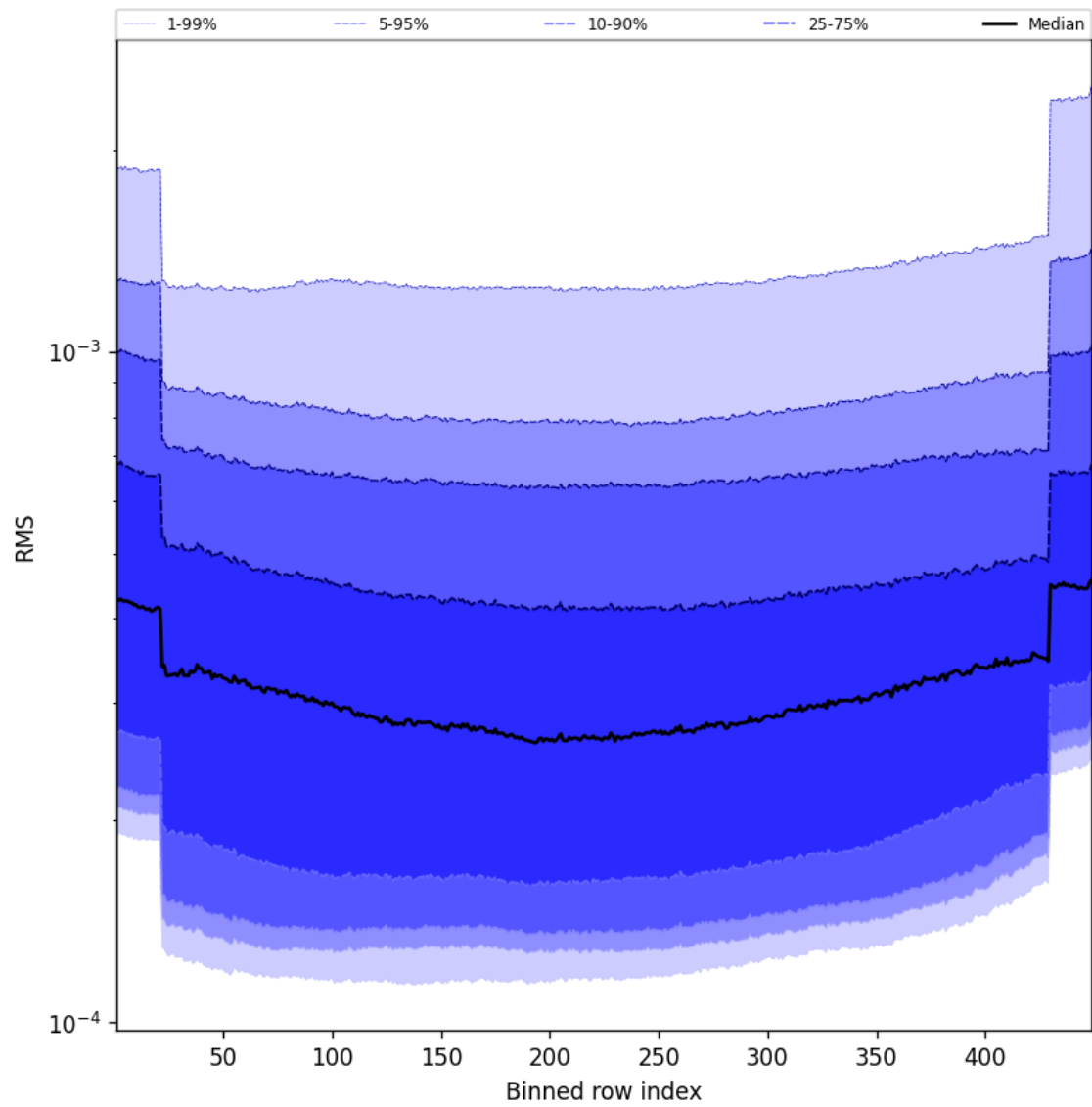
Figure 60: Along track statistics of “RMS” for 2024-09-14 to 2024-09-16
