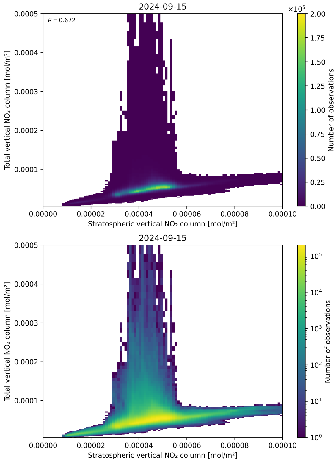
Figure 100: Scatter density plot of “Stratospheric vertical NO 2 column” against “Total vertical NO 2 column” for 2024-09-14 to 2024-09-16.
