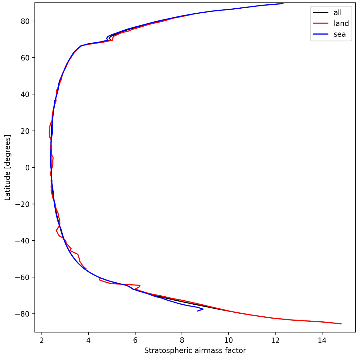
Figure 27: Zonal average of “Stratospheric airmass factor” for 2024-09-14 to 2024-09-16.
