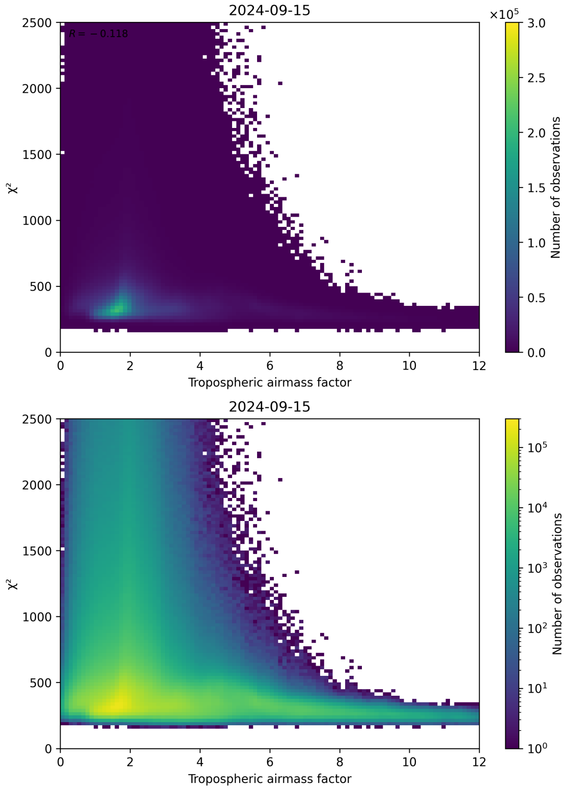
Figure 73: Scatter density plot of “Tropospheric airmass factor” against “ \chi^2 ” for 2024-09-14 to 2024-09-16.
