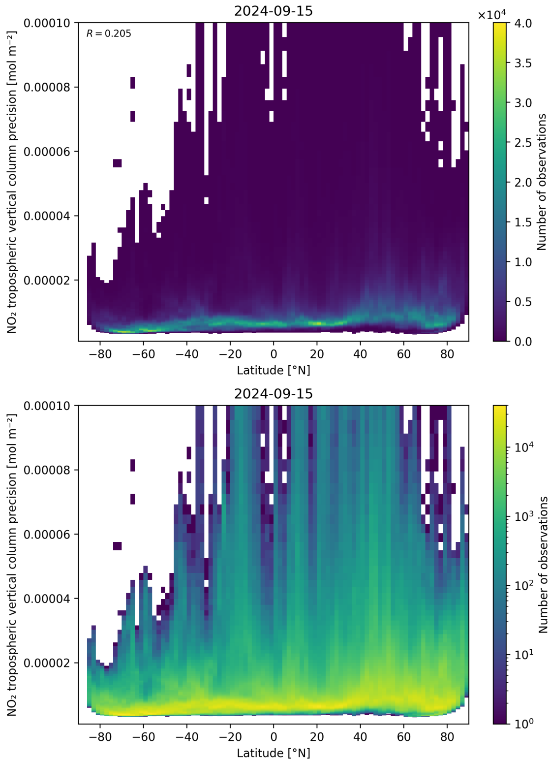
Figure 93: Scatter density plot of “Latitude” against “NO 2 tropospheric vertical column precision” for 2024-09-14 to 2024-09-16.
