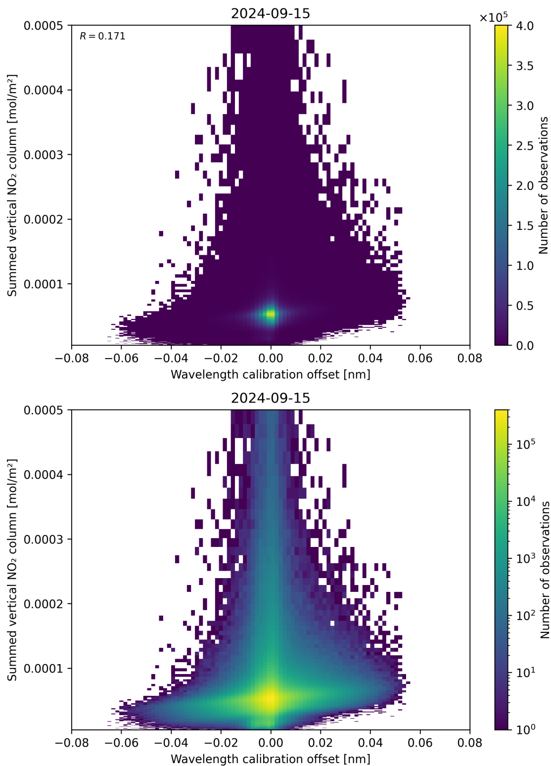
Figure 177: Scatter density plot of “Wavelength calibration offset” against “Summed vertical NO 2 column” for 2024-09-14 to 2024-09-16.
