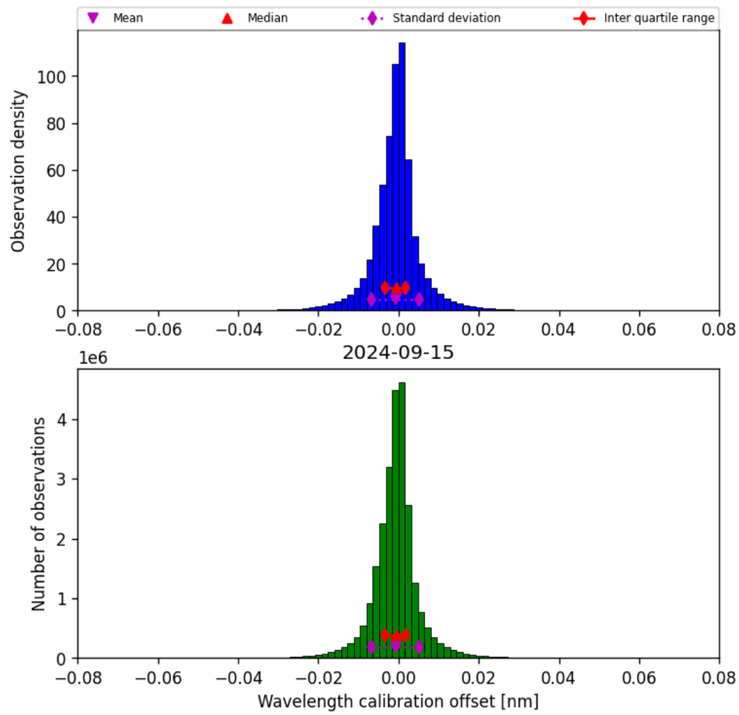
Figure 35: Histogram of “Wavelength calibration offset” for 2024-09-14 to 2024-09-16
