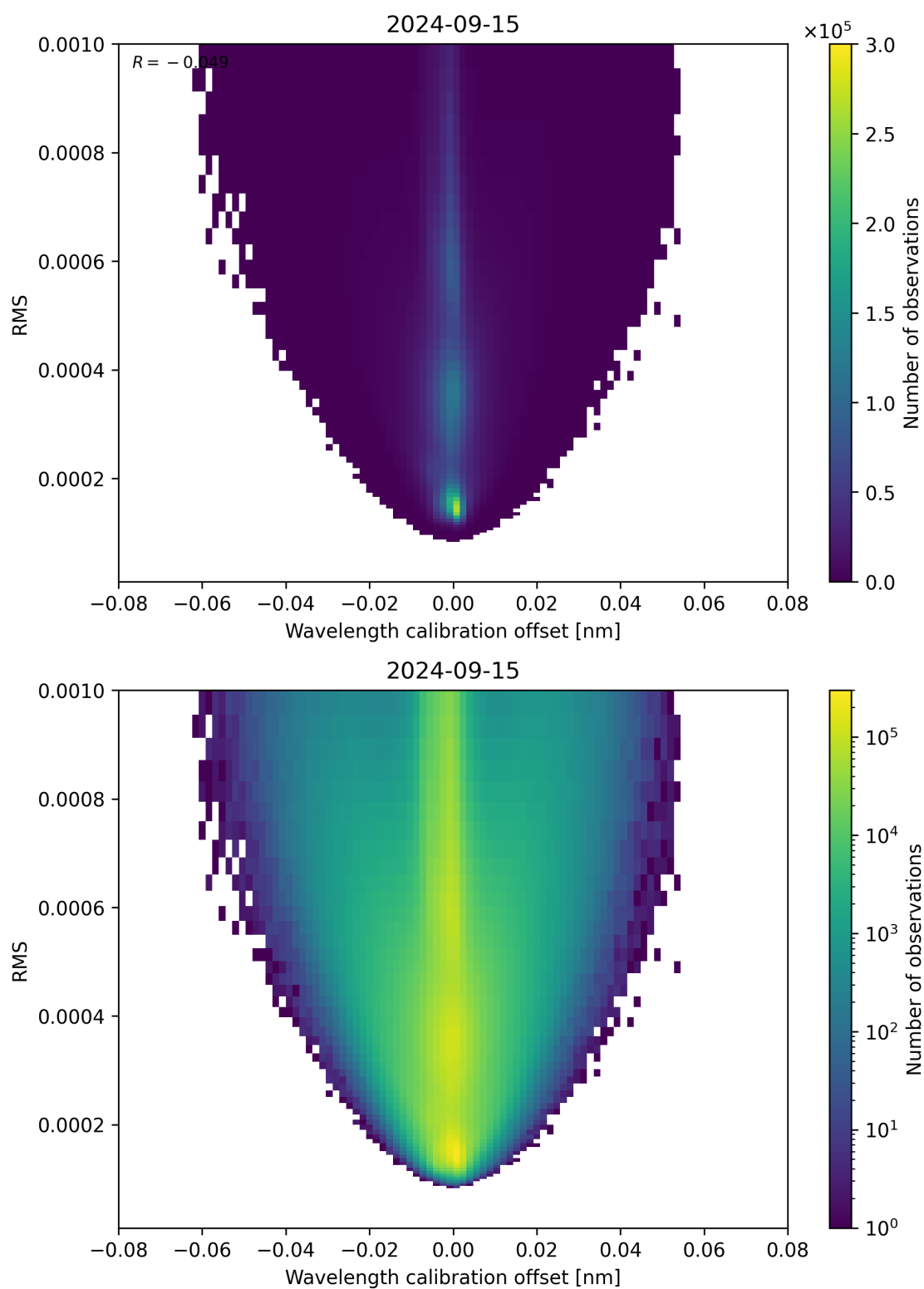
Figure 181: Scatter density plot of “Wavelength calibration offset” against “RMS” for 2024-09-14 to 2024-09-16.
