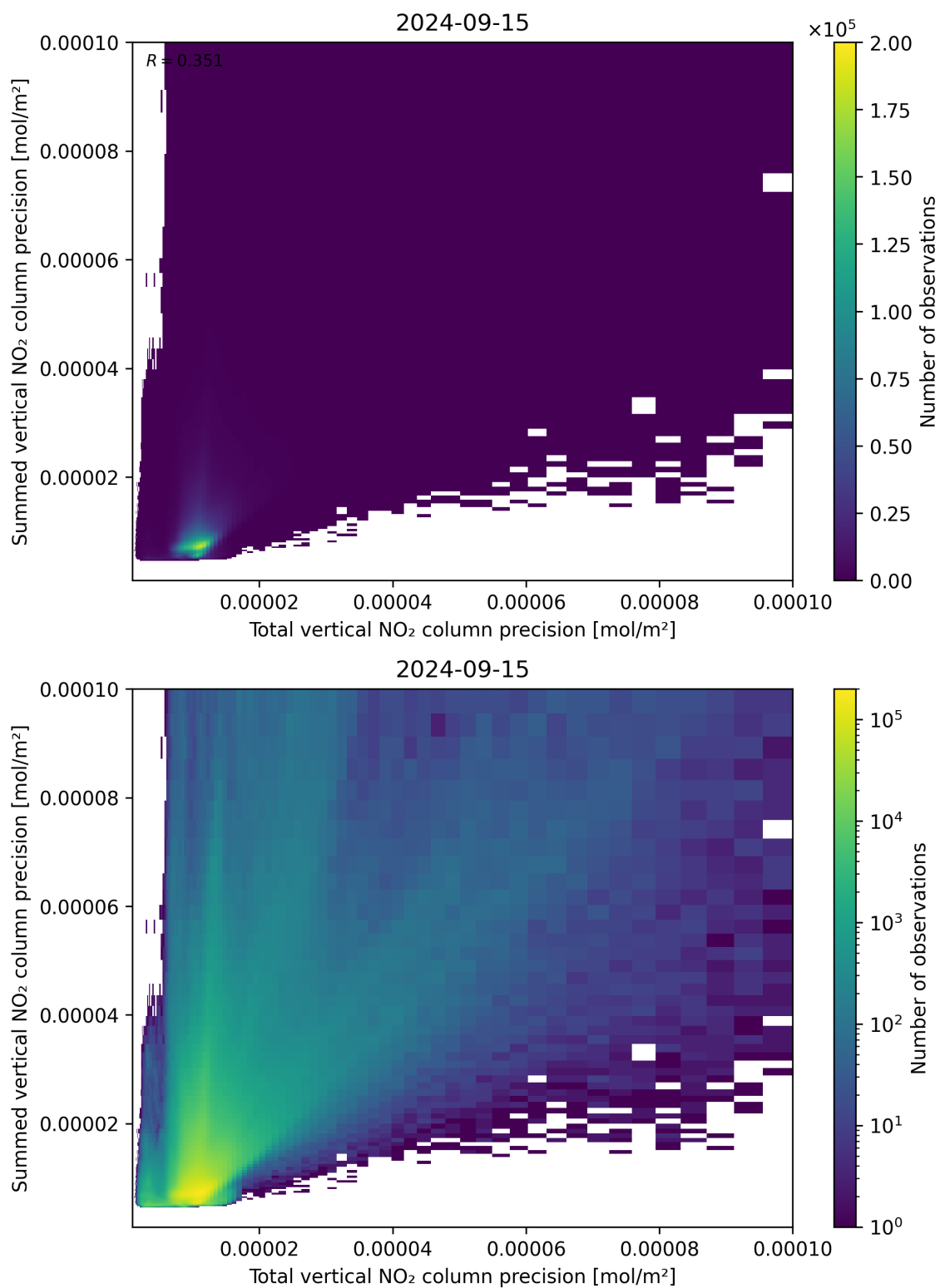
Figure 118: Scatter density plot of “Total vertical NO 2 column precision” against “Summed vertical NO 2 column precision” for 2024-09-14 to 2024-09-16.
