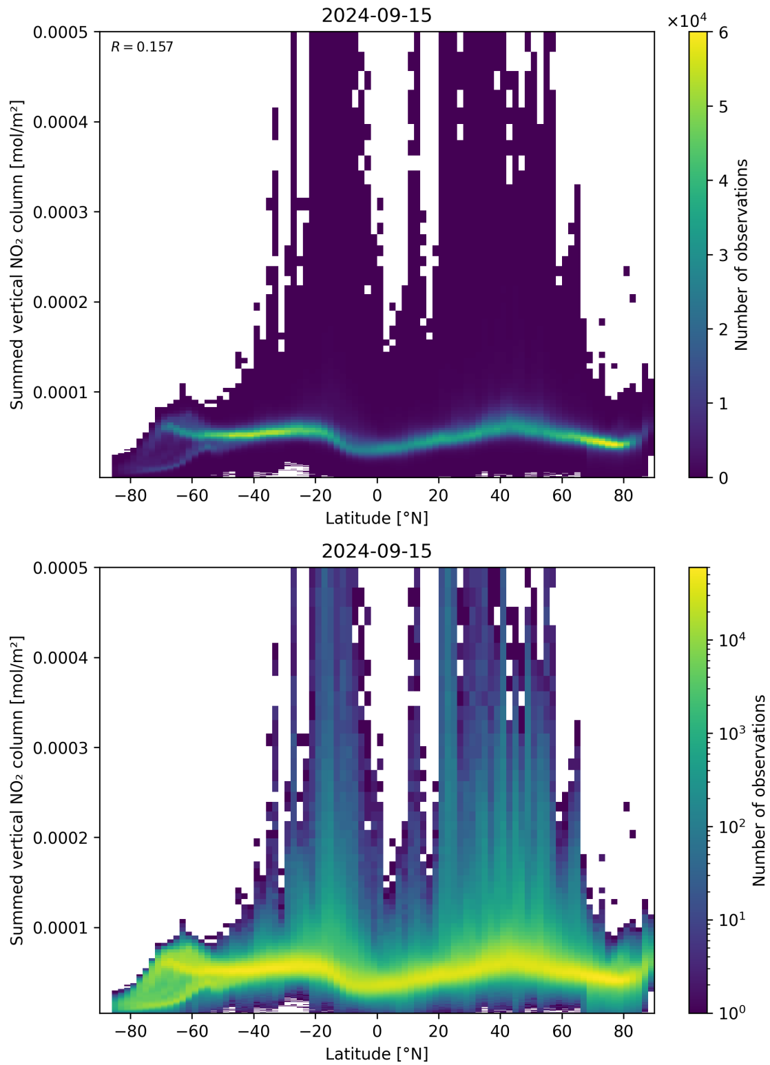
Figure 88: Scatter density plot of “Latitude” against “Summed vertical NO 2 column” for 2024-09-14 to 2024-09-16.
