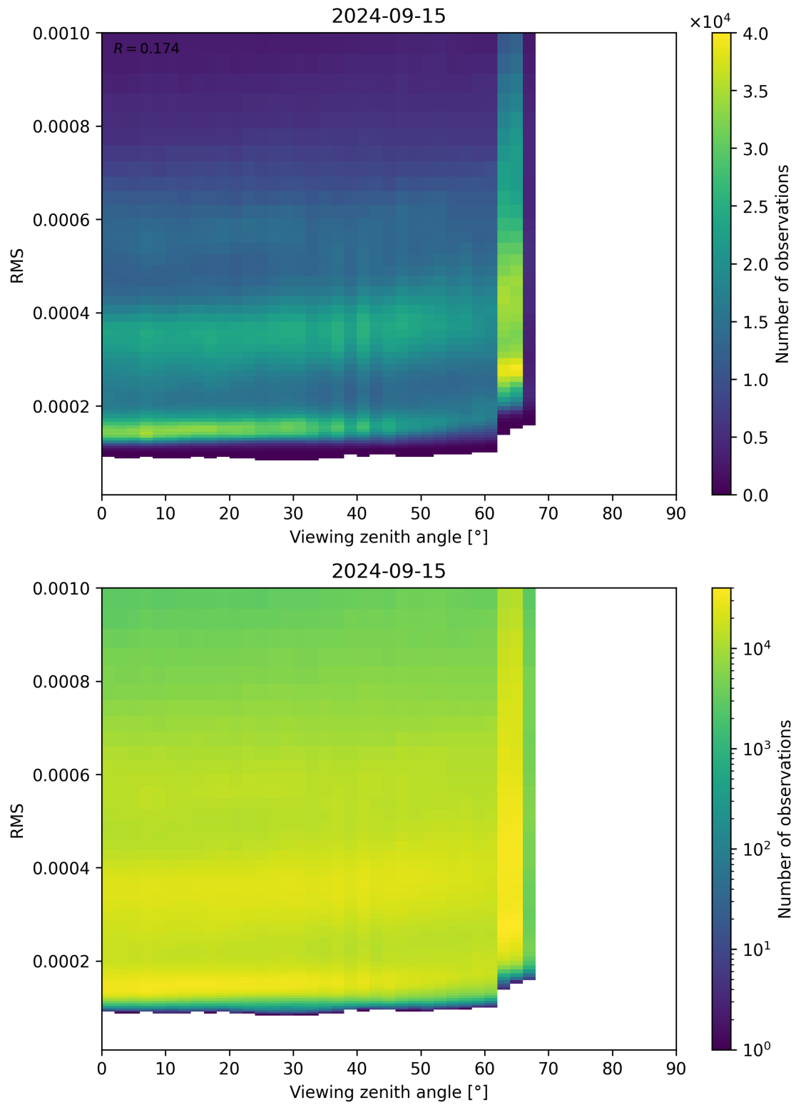
Figure 171: Scatter density plot of “Viewing zenith angle” against “RMS” for 2024-09-14 to 2024-09-16.
