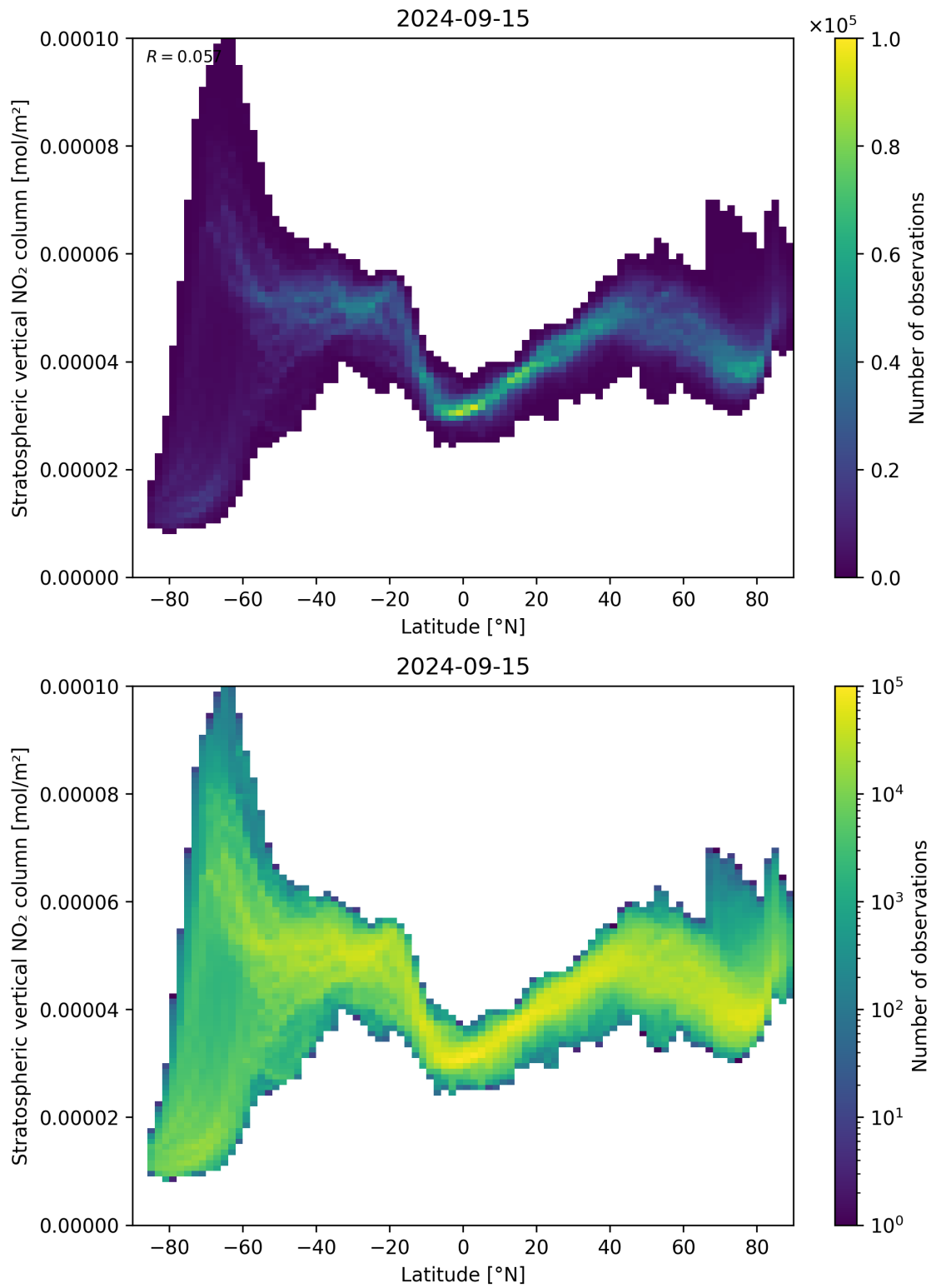
Figure 87: Scatter density plot of “Latitude” against “Stratospheric vertical NO 2 column” for 2024-09-14 to 2024-09-16.
