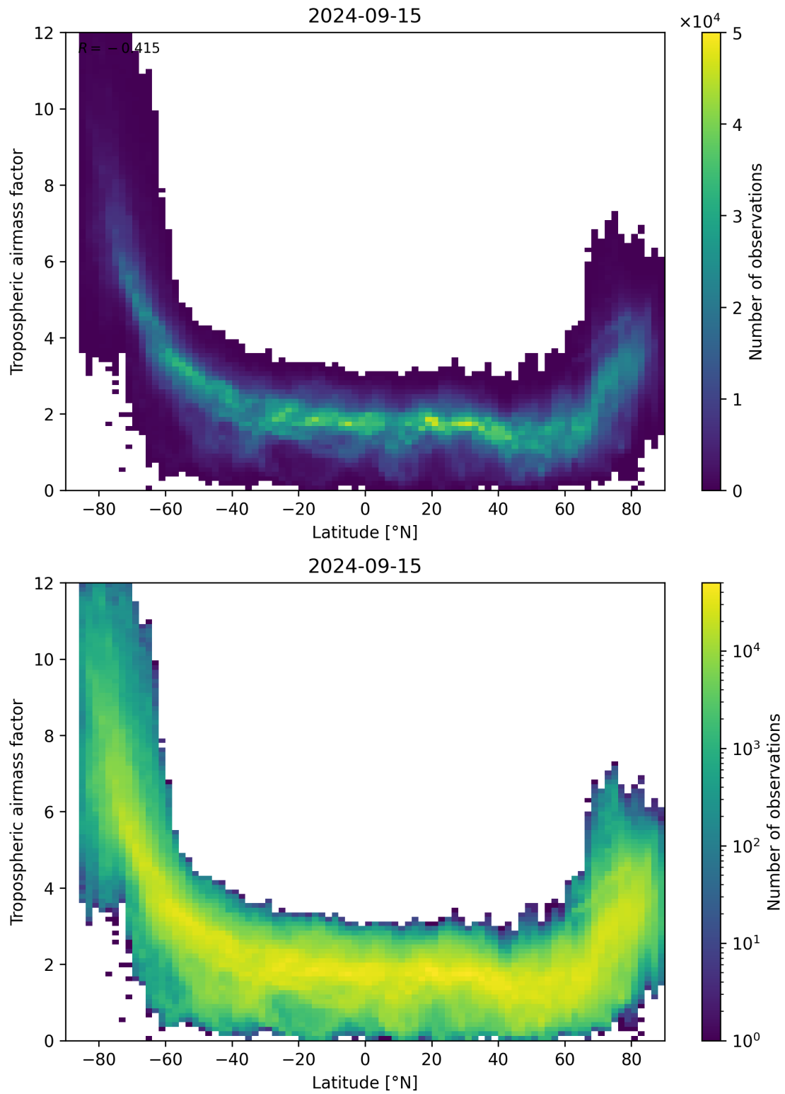
Figure 85: Scatter density plot of “Latitude” against “Tropospheric airmass factor” for 2024-09-14 to 2024-09-16.
