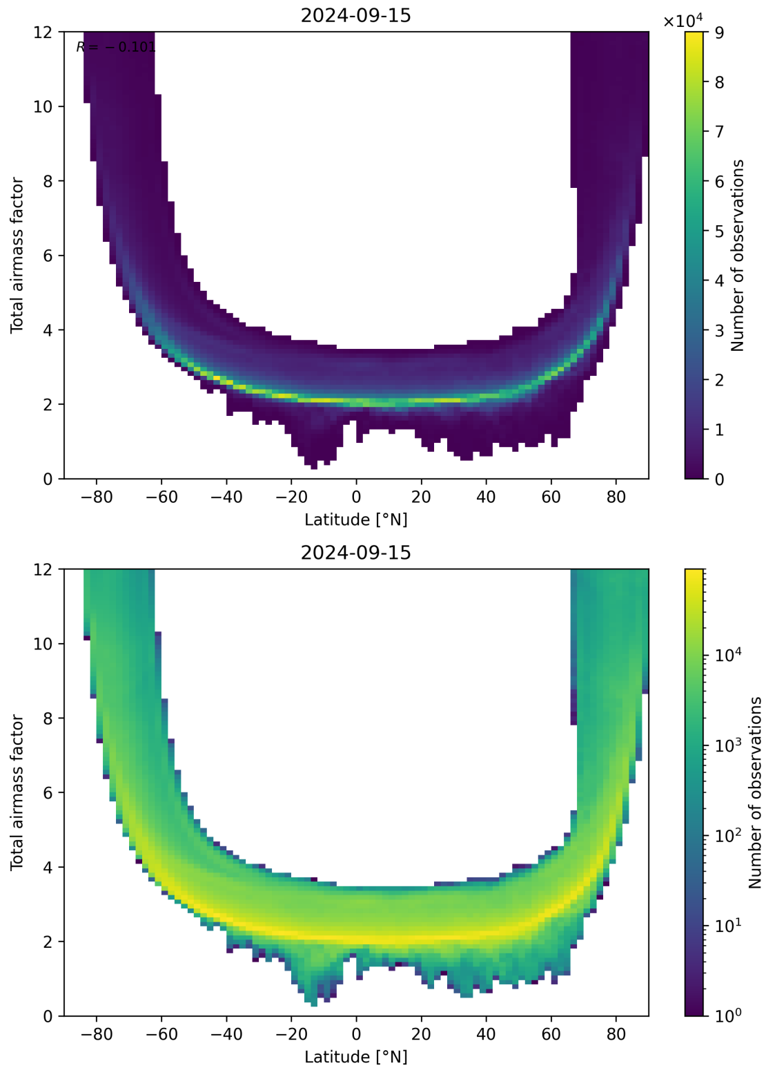
Figure 84: Scatter density plot of “Latitude” against “Total airmass factor” for 2024-09-14 to 2024-09-16.
