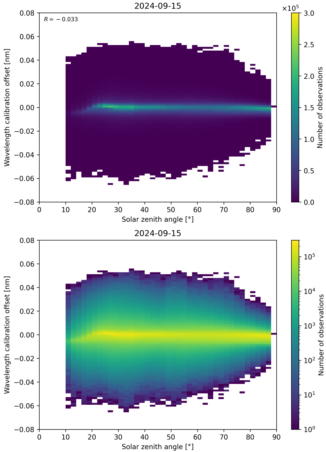
Figure 158: Scatter density plot of “Solar zenith angle” against “Wavelength calibration offset” for 2024-09-14 to 2024-09-16.
