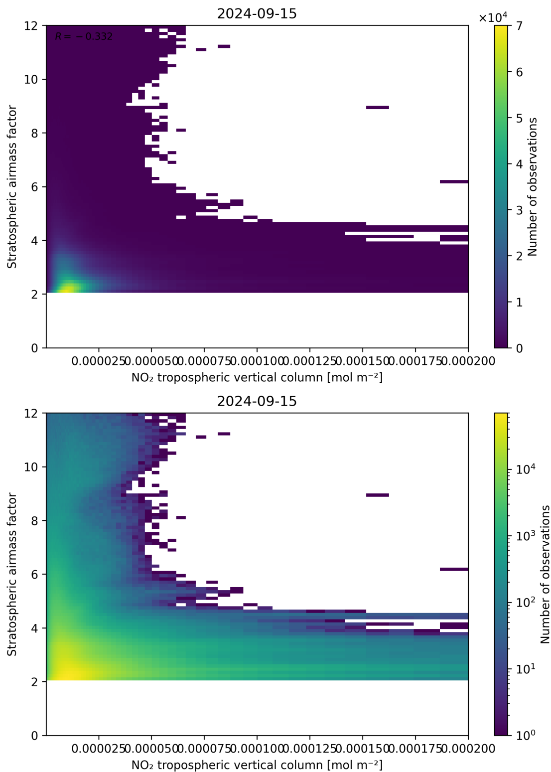
Figure 121: Scatter density plot of “NO 2 tropospheric vertical column” against “Stratospheric air mass factor” for 2024-09-14 to 2024-09-16.
