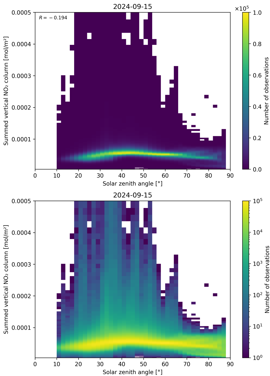
Figure 151: Scatter density plot of “Solar zenith angle” against “Summed vertical NO 2 column” for 2024-09-14 to 2024-09-16.
