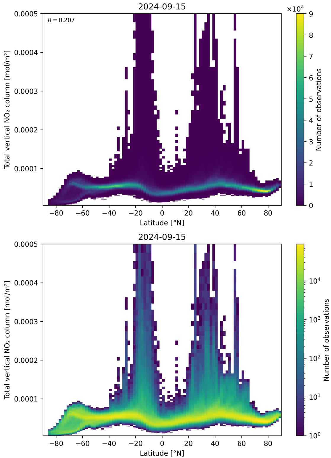
Figure 90: Scatter density plot of “Latitude” against “Total vertical NO 2 column” for 2024-09-14 to 2024-09-16.
