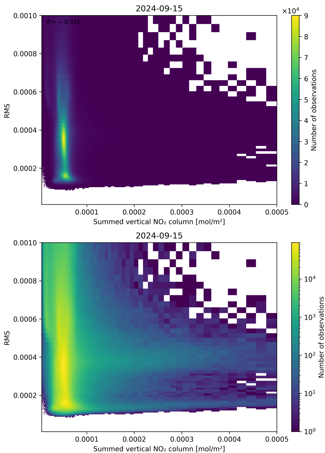
Figure 109: Scatter density plot of “Summed vertical NO 2 column” against “RMS” for 2024-09-14 to 2024-09-16.
