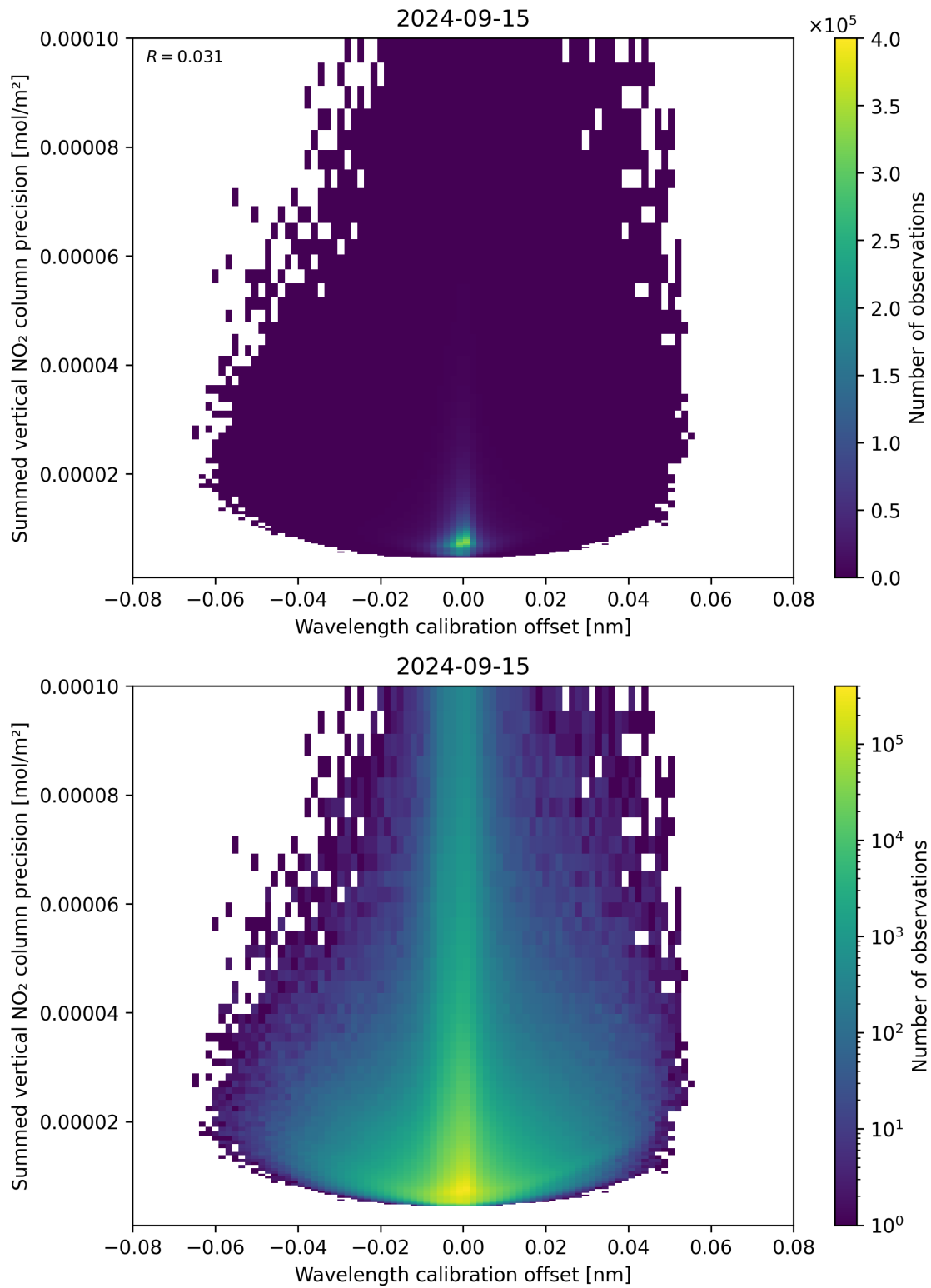
Figure 178: Scatter density plot of “Wavelength calibration offset” against “Summed vertical NO 2 column precision” for 2024-09-14 to 2024-09-16.
