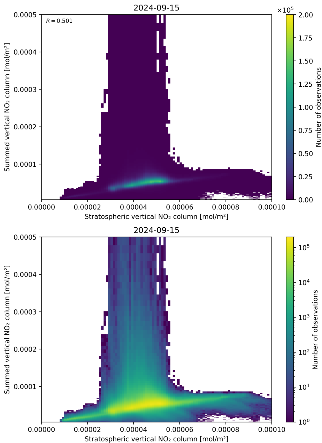
Figure 98: Scatter density plot of “Stratospheric vertical NO 2 column” against “Summed vertical NO 2 column” for 2024-09-14 to 2024-09-16.
