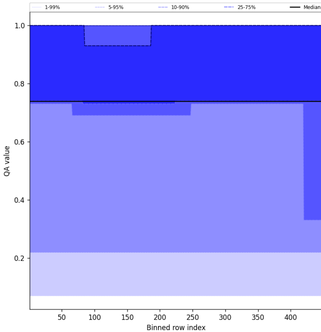
Figure 45: Along track statistics of “QA value” for 2024-09-14 to 2024-09-16
