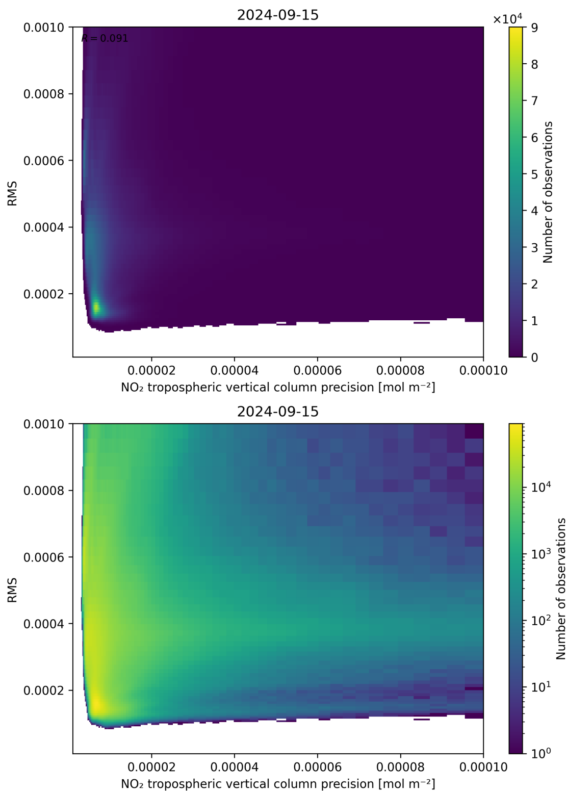
Figure 140: Scatter density plot of “NO 2 tropospheric vertical column precision” against “RMS” for 2024-09-14 to 2024-09-16.
