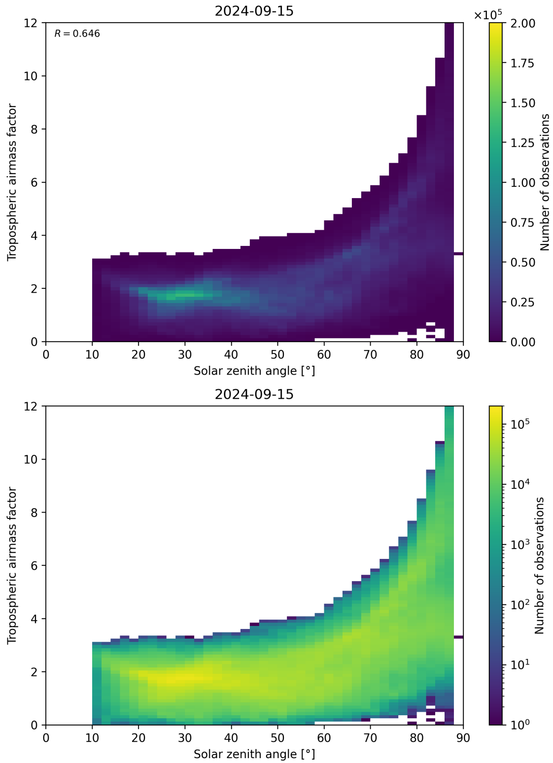
Figure 147: Scatter density plot of “Solar zenith angle” against “Tropospheric airmass factor” for 2024-09-14 to 2024-09-16.
