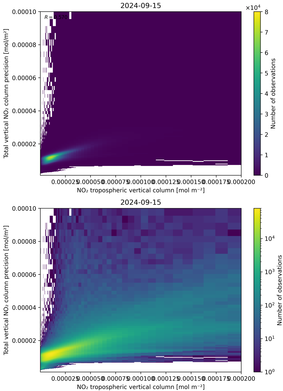
Figure 129: Scatter density plot of “NO 2 tropospheric vertical column” against “Total vertical NO 2 column precision” for 2024-09-14 to 2024-09-16.
