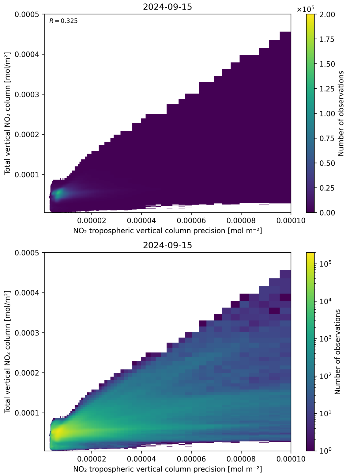
Figure 138: Scatter density plot of “NO 2 tropospheric vertical column precision” against “Total vertical NO 2 column” for 2024-09-14 to 2024-09-16.
