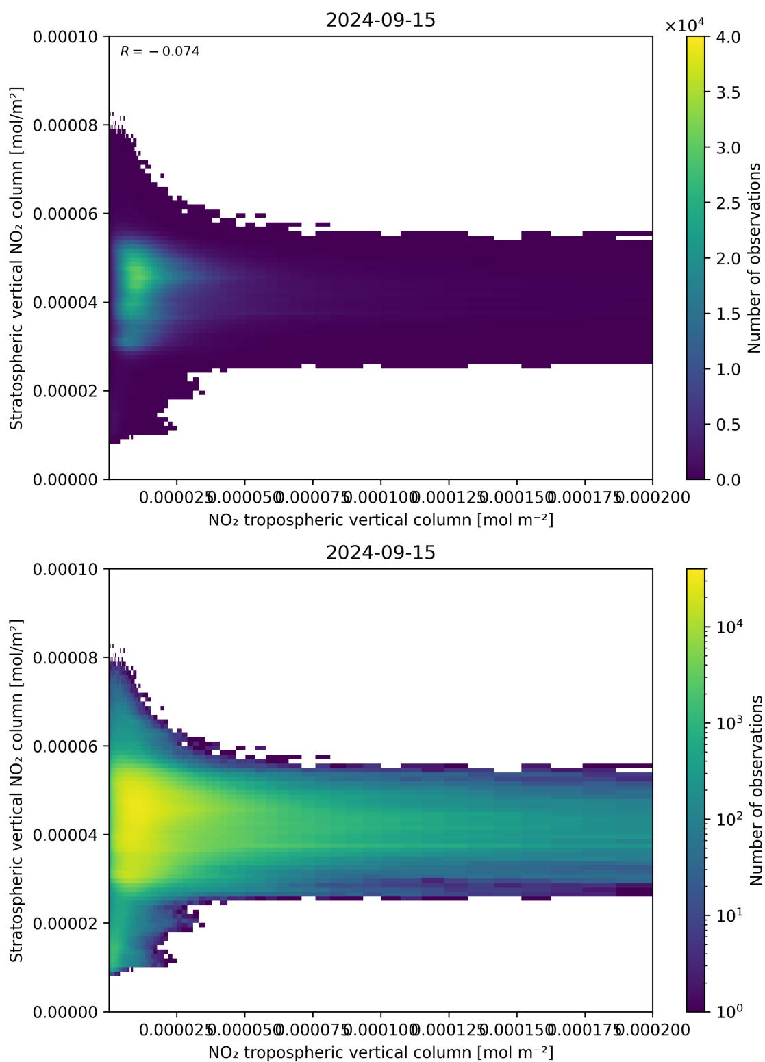
Figure 125: Scatter density plot of “NO 2 tropospheric vertical column” against “Stratospheric vertical NO 2 column” for 2024-09-14 to 2024-09-16.
