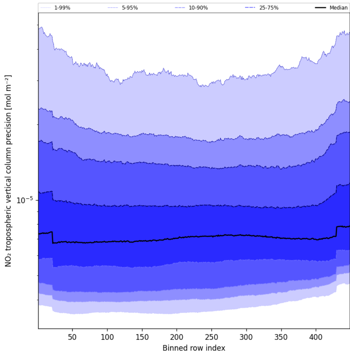
Figure 47: Along track statistics of “NO 2 tropospheric vertical column precision” for 2024-09-14 to 2024-09-16
