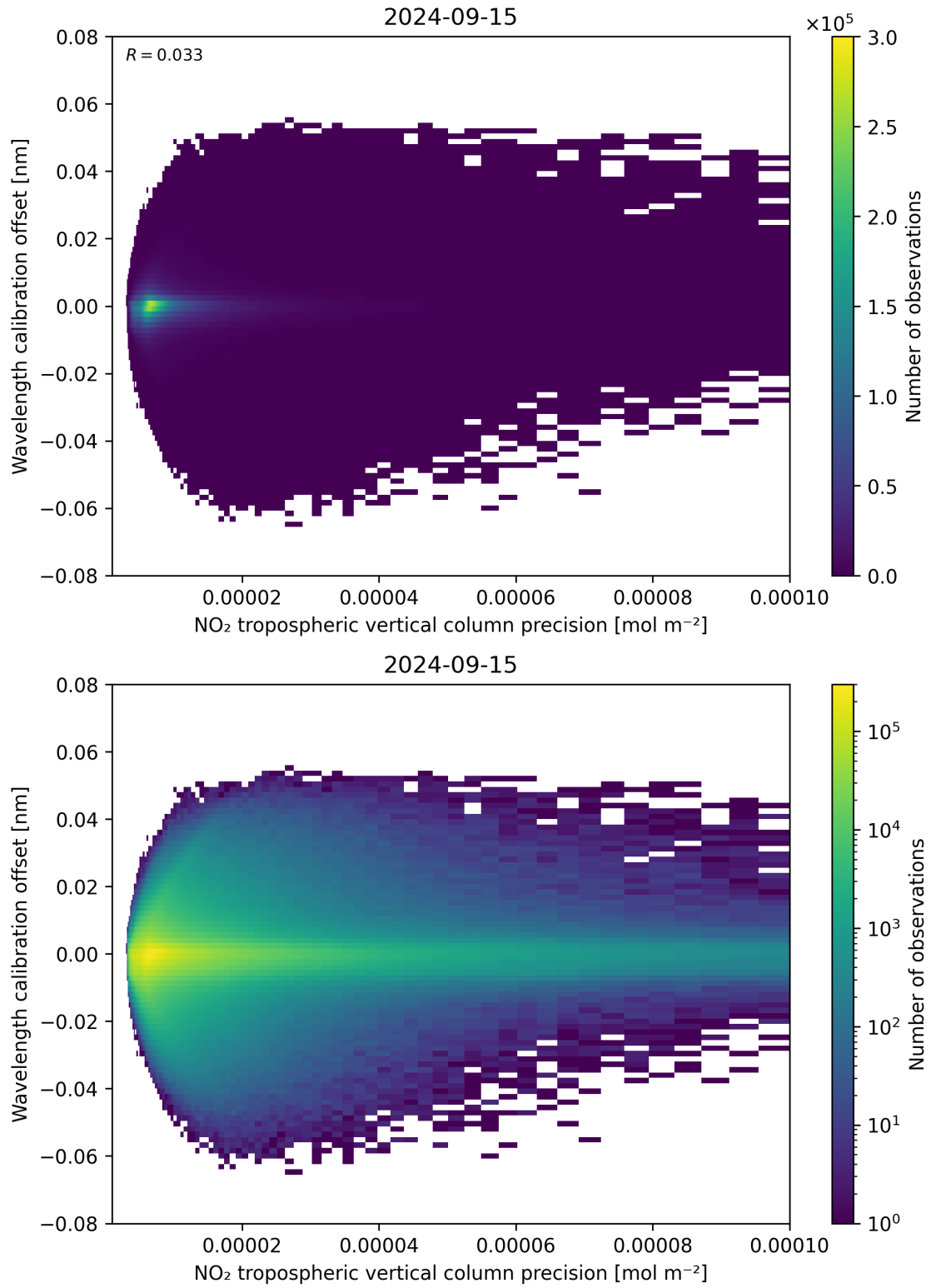
Figure 141: Scatter density plot of “NO 2 tropospheric vertical column precision” against “Wavelength calibration offset” for 2024-09-14 to 2024-09-16.
