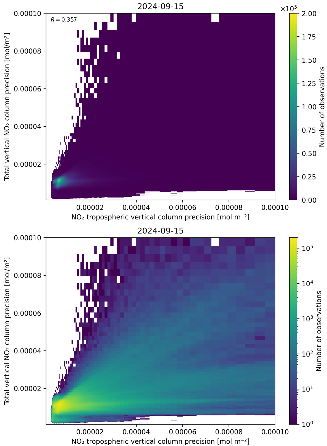
Figure 139: Scatter density plot of “NO 2 tropospheric vertical column precision” against “Total vertical NO 2 column precision” for 2024-09-14 to 2024-09-16.
