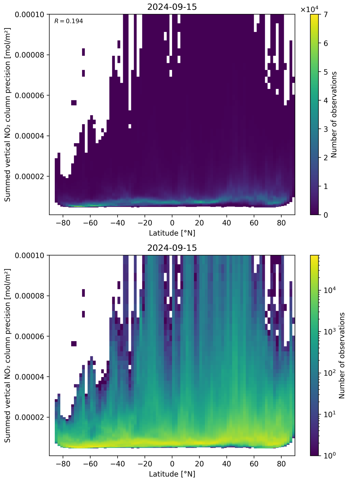
Figure 89: Scatter density plot of “Latitude” against “Summed vertical NO 2 column precision” for 2024-09-14 to 2024-09-16.
