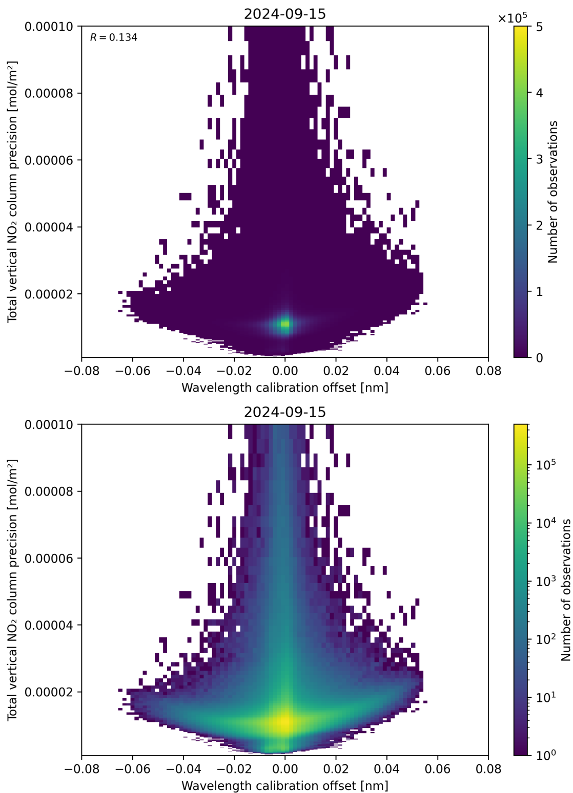
Figure 180: Scatter density plot of “Wavelength calibration offset” against “Total vertical NO 2 column precision” for 2024-09-14 to 2024-09-16.
