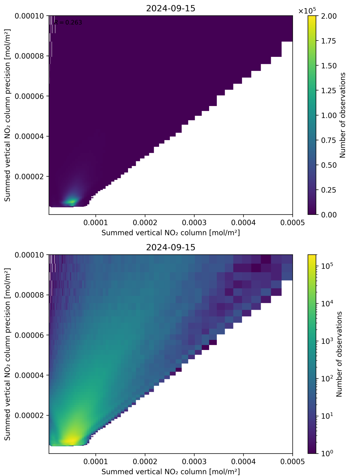
Figure 105: Scatter density plot of “Summed vertical NO 2 column” against “Summed vertical NO 2 column precision” for 2024-09-14 to 2024-09-16.
