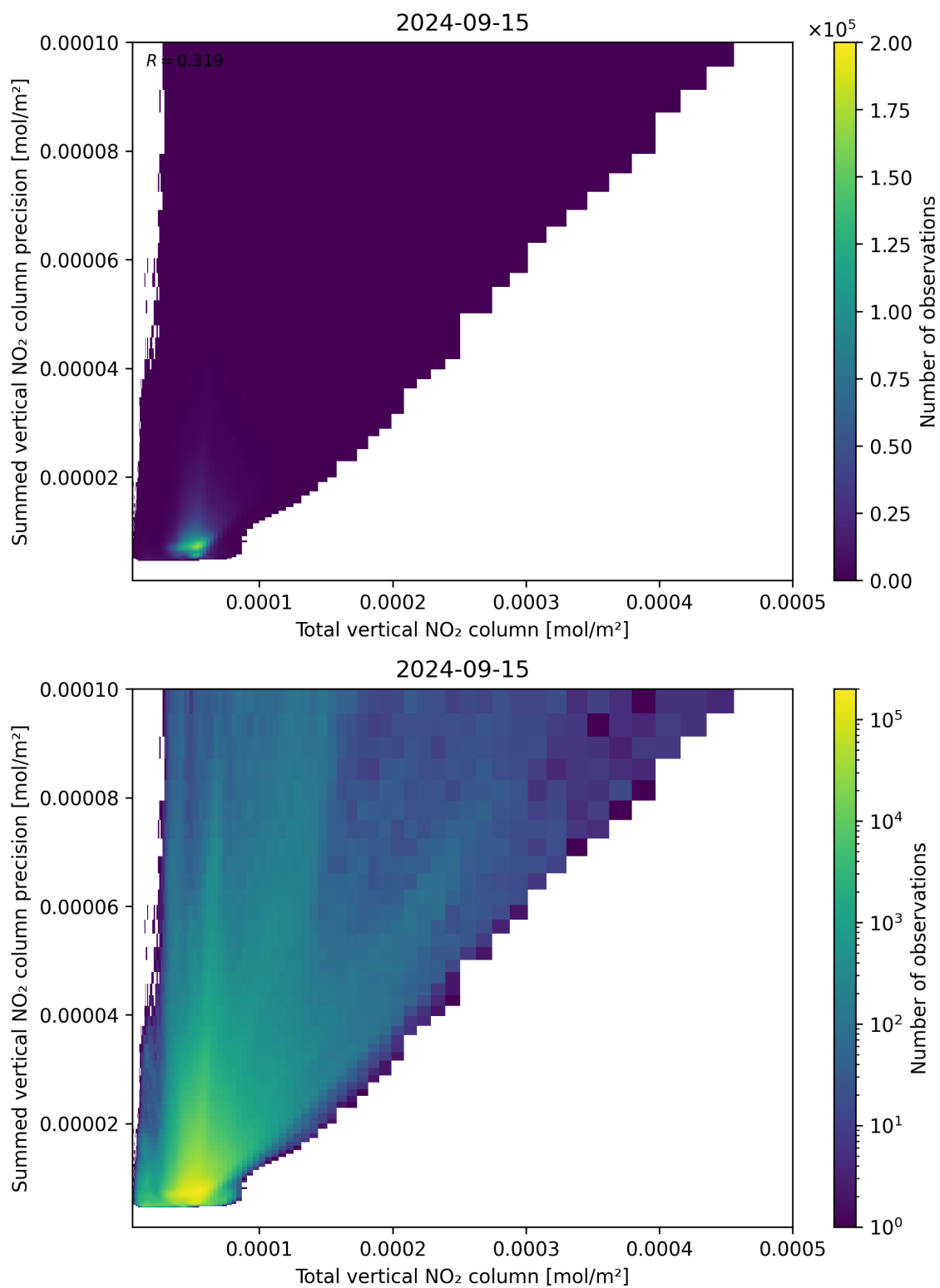
Figure 113: Scatter density plot of “Total vertical NO 2 column” against “Summed vertical NO 2 column precision” for 2024-09-14 to 2024-09-16.
