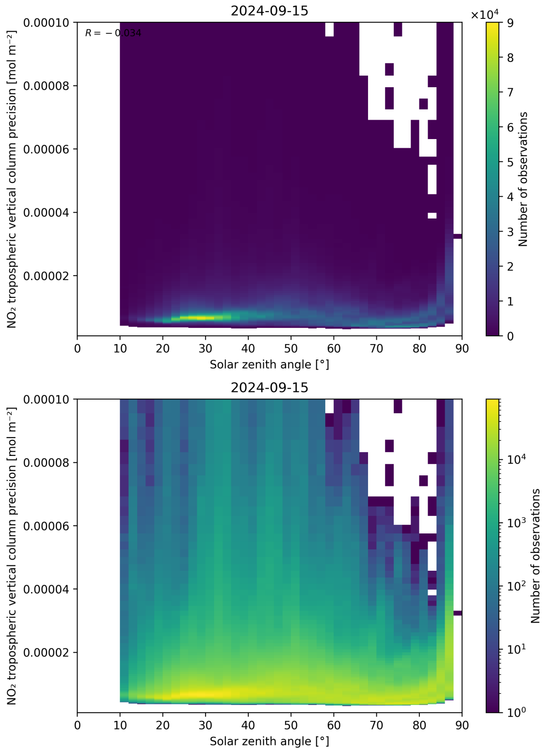
Figure 156: Scatter density plot of “Solar zenith angle” against “NO 2 tropospheric vertical column precision” for 2024-09-14 to 2024-09-16.
