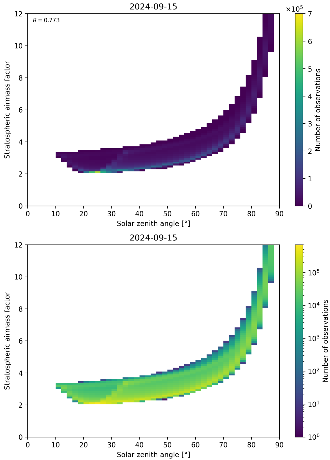
Figure 145: Scatter density plot of “Solar zenith angle” against “Stratospheric airmass factor” for 2024-09-14 to 2024-09-16.
