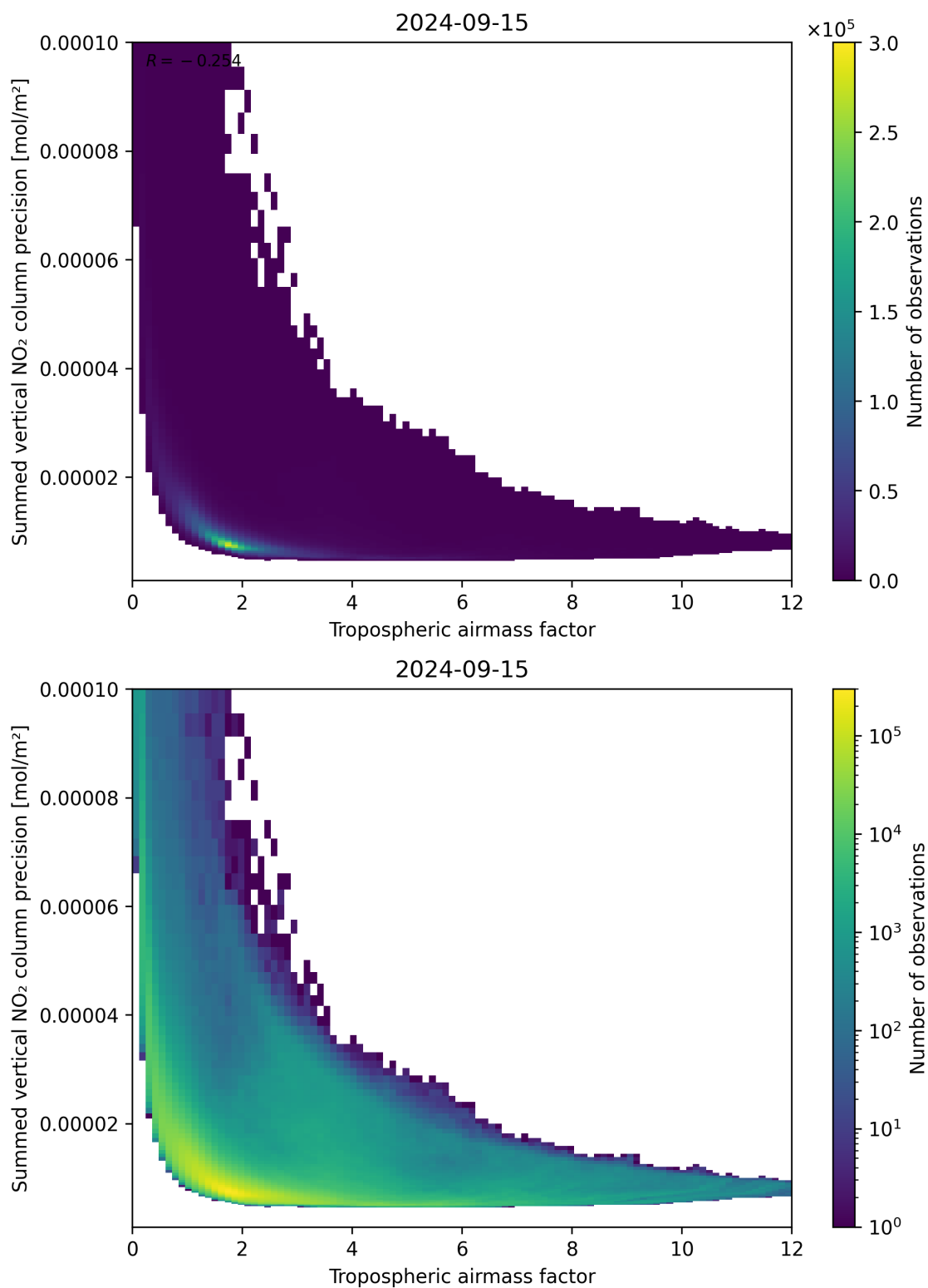
Figure 76: Scatter density plot of “Tropospheric air mass factor” against “Summed vertical NO 2 column precision” for 2024-09-14 to 2024-09-16.
