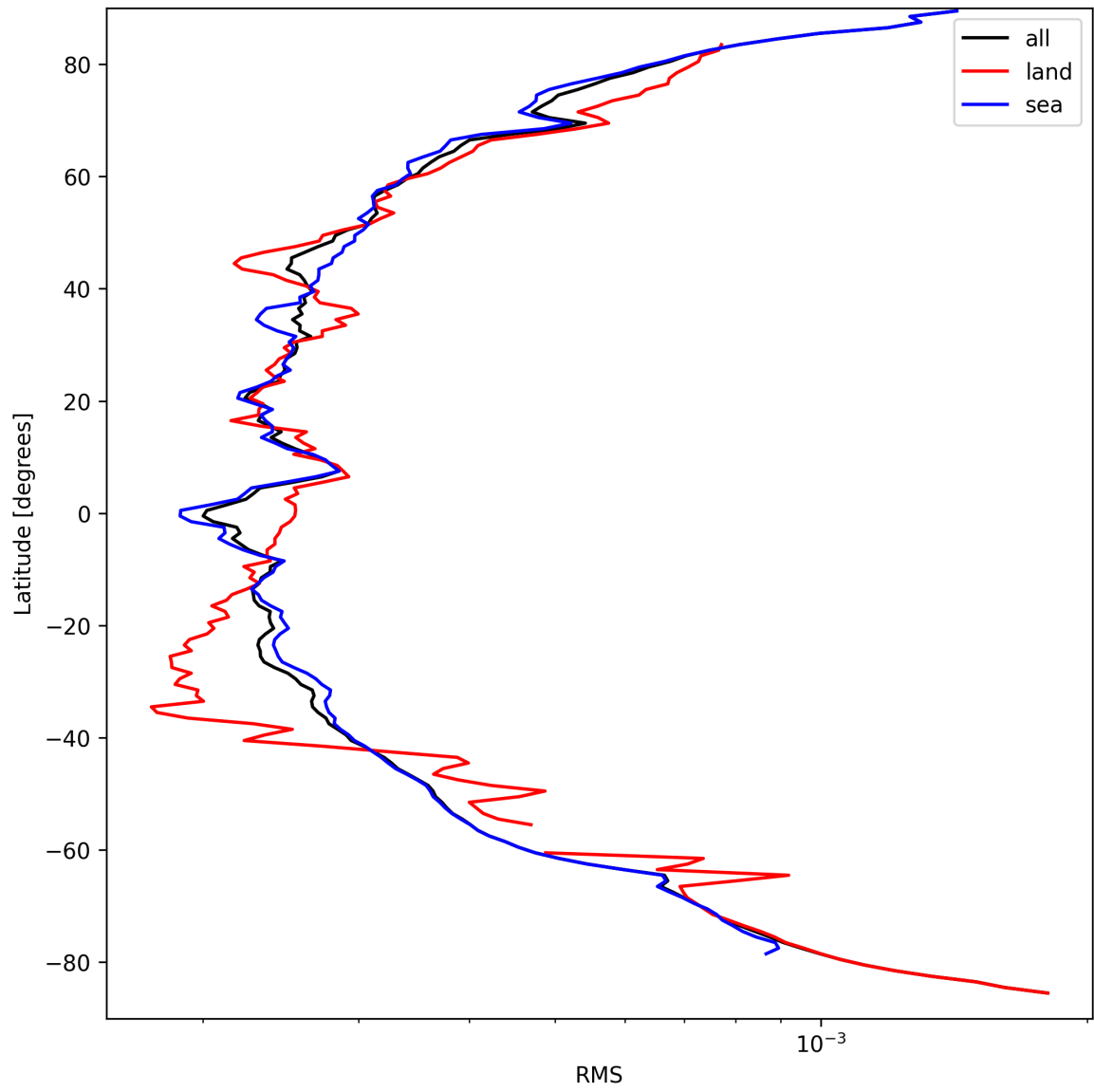
Figure 26: Zonal average of “RMS” for 2024-09-14 to 2024-09-16.
