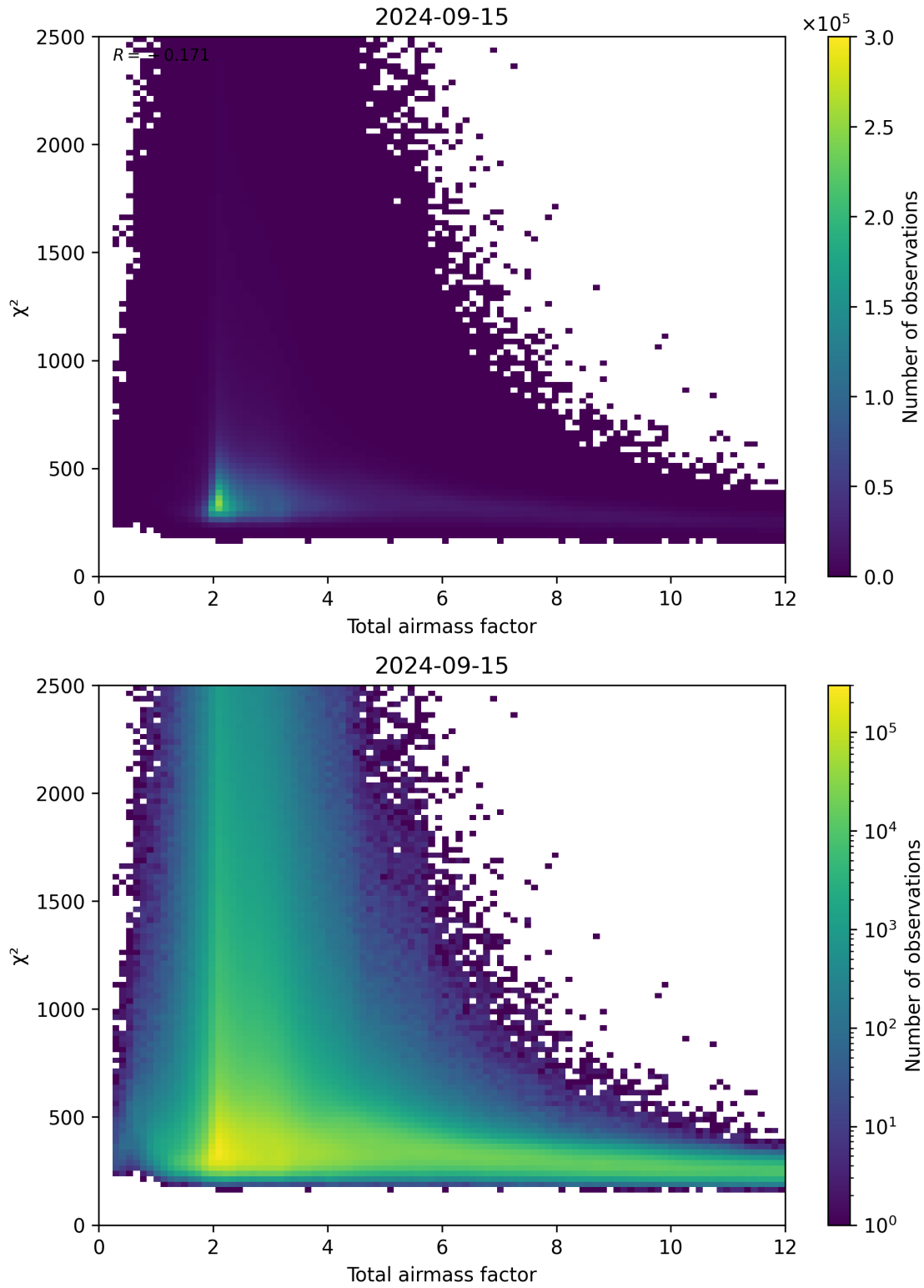
Figure 63: Scatter density plot of “Total airmass factor” against “ \chi^2 ” for 2024-09-14 to 2024-09-16.
