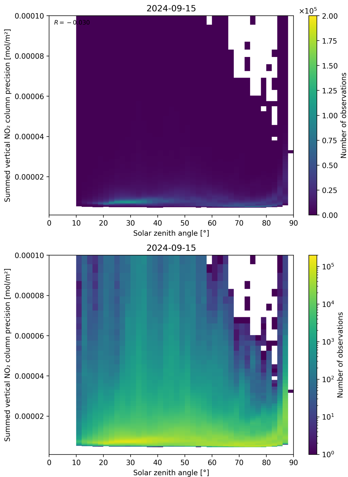
Figure 152: Scatter density plot of “Solar zenith angle” against “Summed vertical NO 2 column precision” for 2024-09-14 to 2024-09-16.
