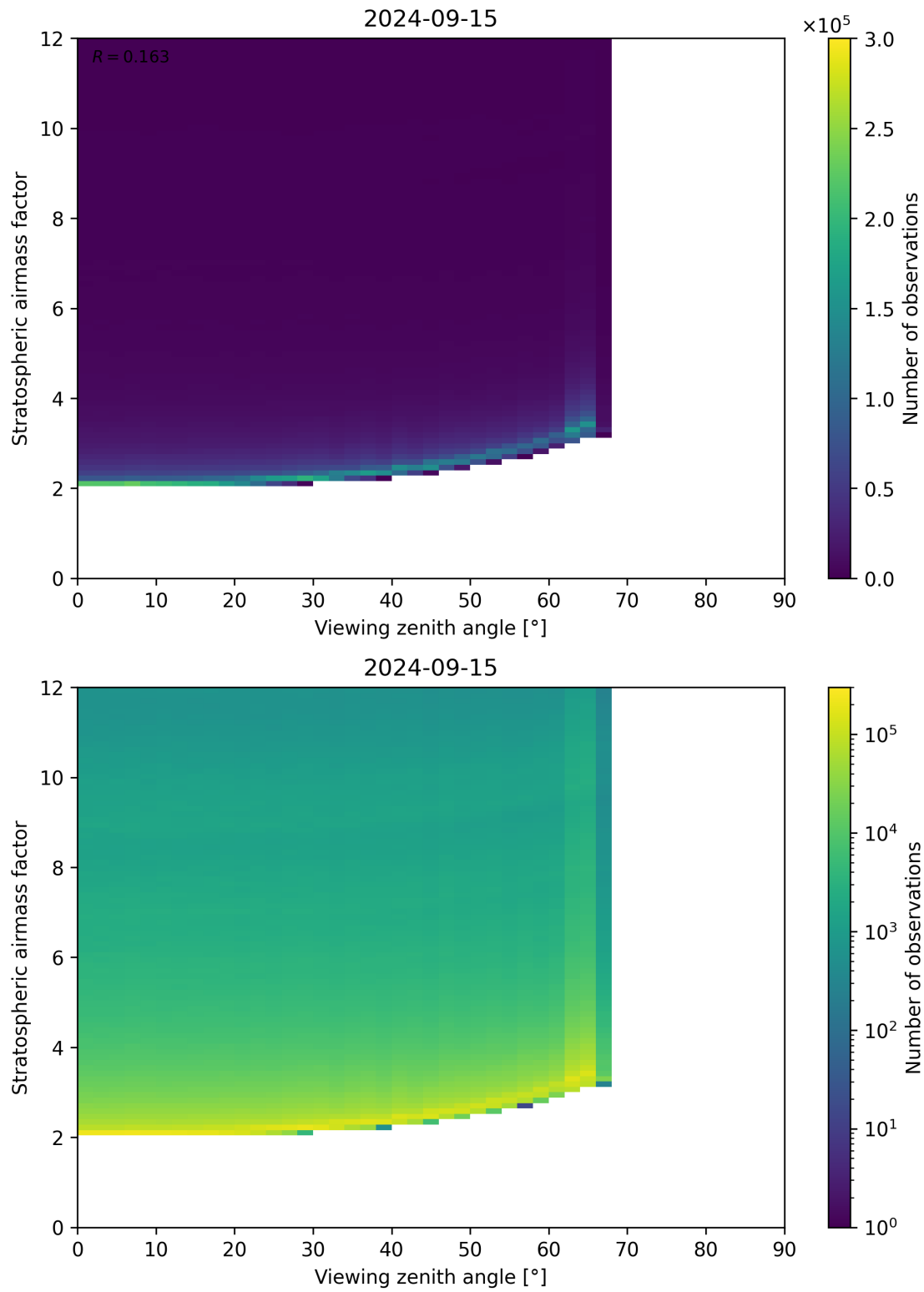
Figure 159: Scatter density plot of “Viewing zenith angle” against “Stratospheric airmass factor” for 2024-09-14 to 2024-09-16.
