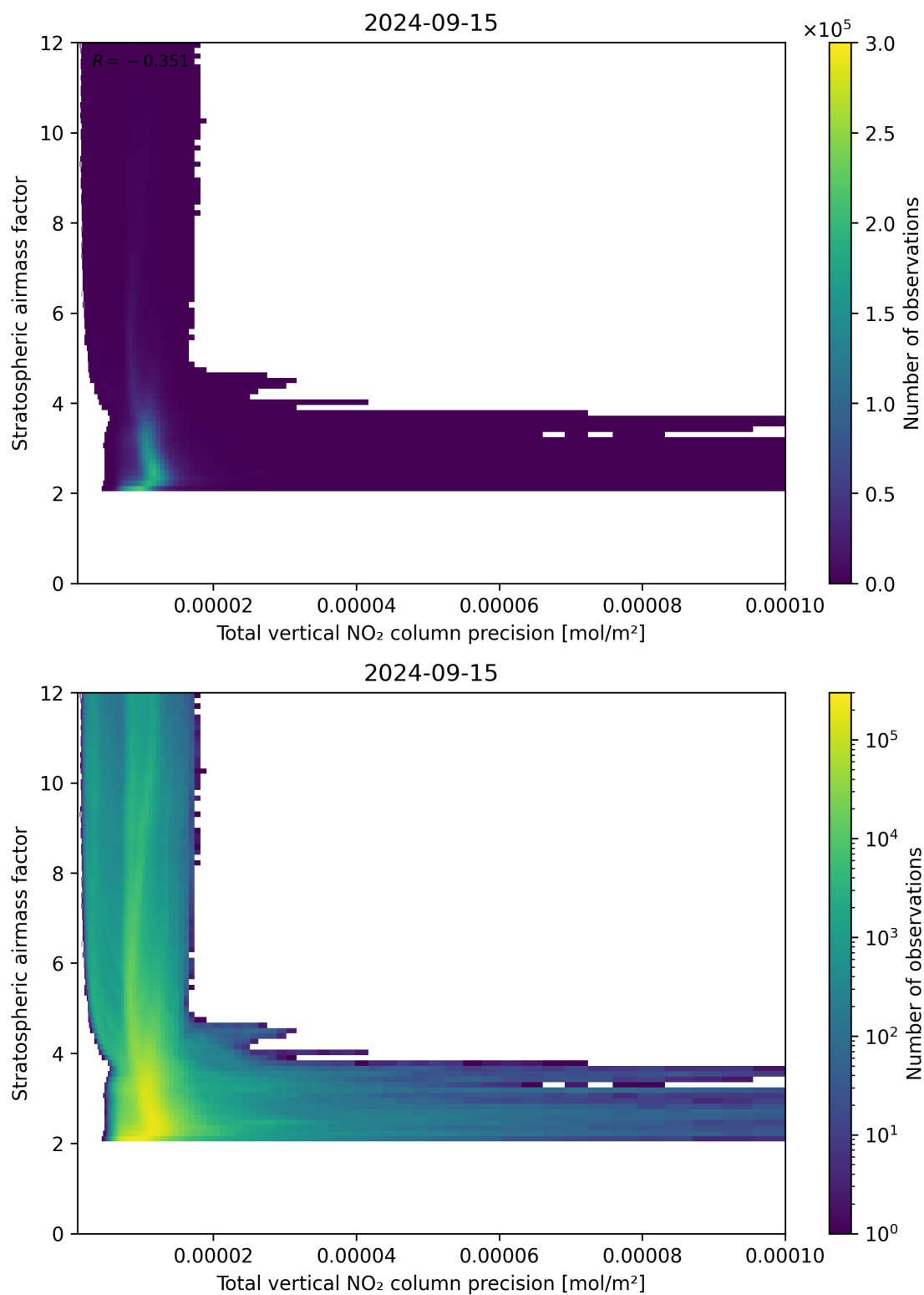
Figure 115: Scatter density plot of “Total vertical NO 2 column precision” against “Stratospheric air mass factor” for 2024-09-14 to 2024-09-16.
