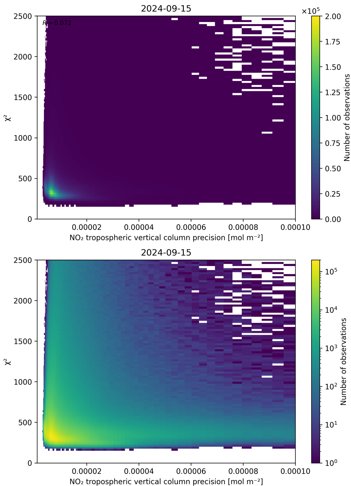
Figure 134: Scatter density plot of “NO 2 tropospheric vertical column precision” against “ \chi^2 ” for 2024-09-14 to 2024-09-16.
