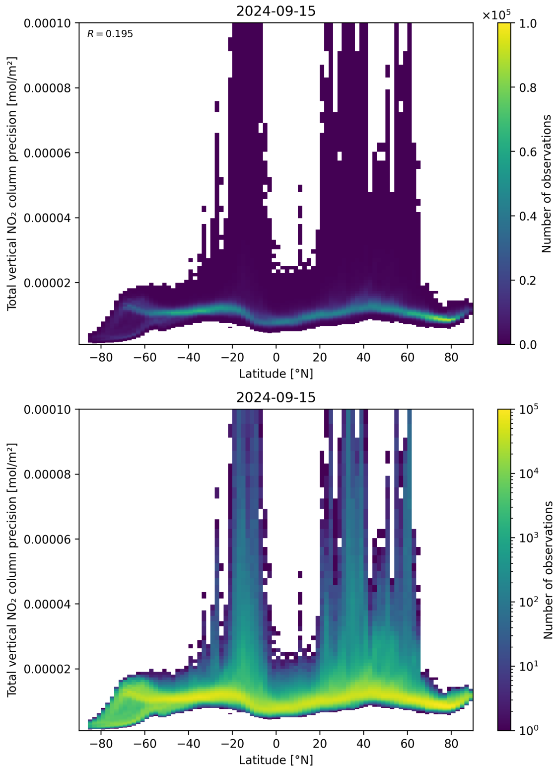
Figure 91: Scatter density plot of “Latitude” against “Total vertical NO 2 column precision” for 2024-09-14 to 2024-09-16.
