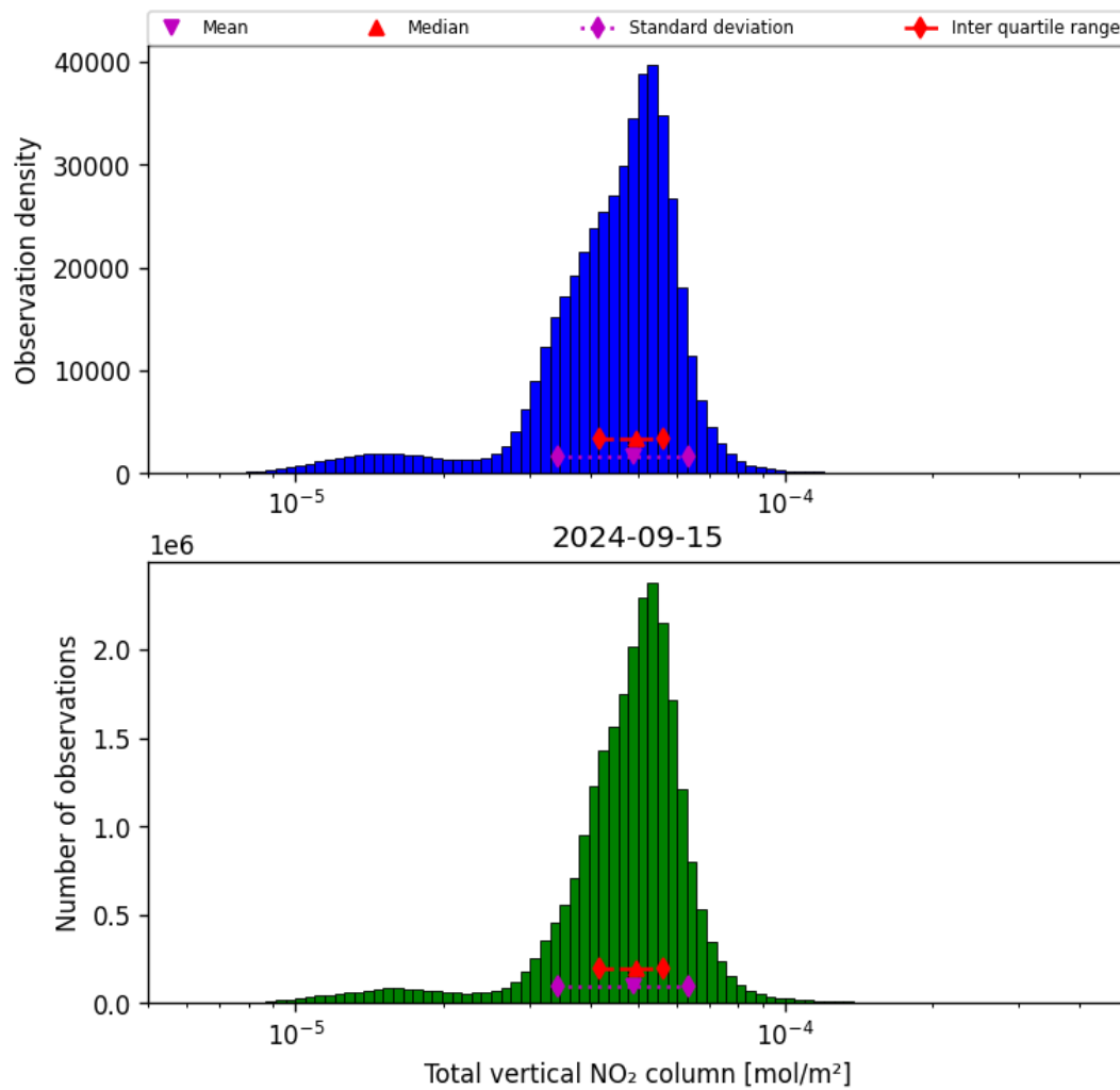
Figure 38: Histogram of “Total vertical NO 2 column” for 2024-09-14 to 2024-09-16
