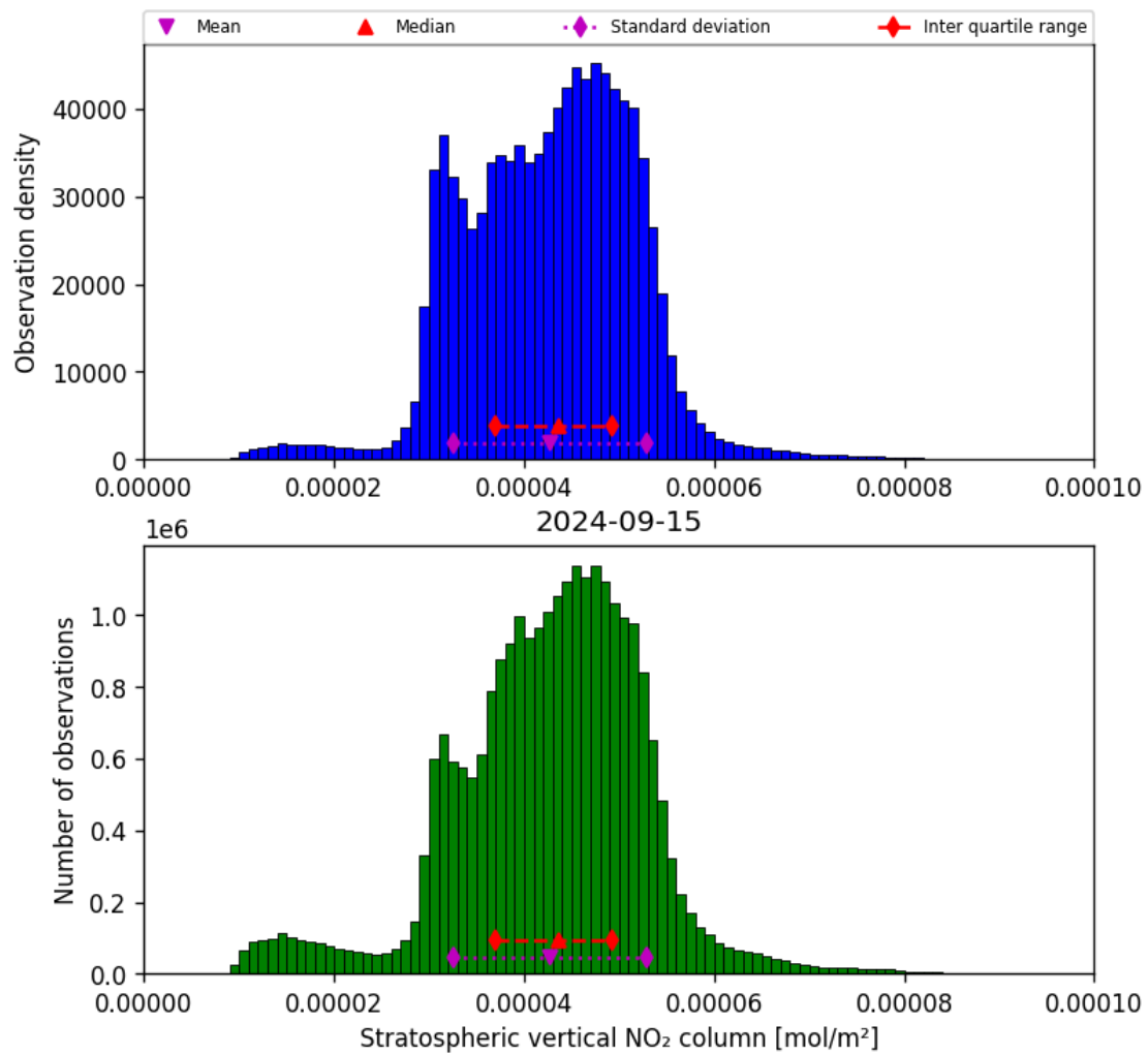
Figure 36: Histogram of “Stratospheric vertical NO 2 column” for 2024-09-14 to 2024-09-16
