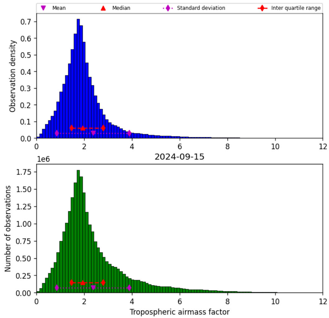
Figure 31: Histogram of “Tropospheric airmass factor” for 2024-09-14 to 2024-09-16
