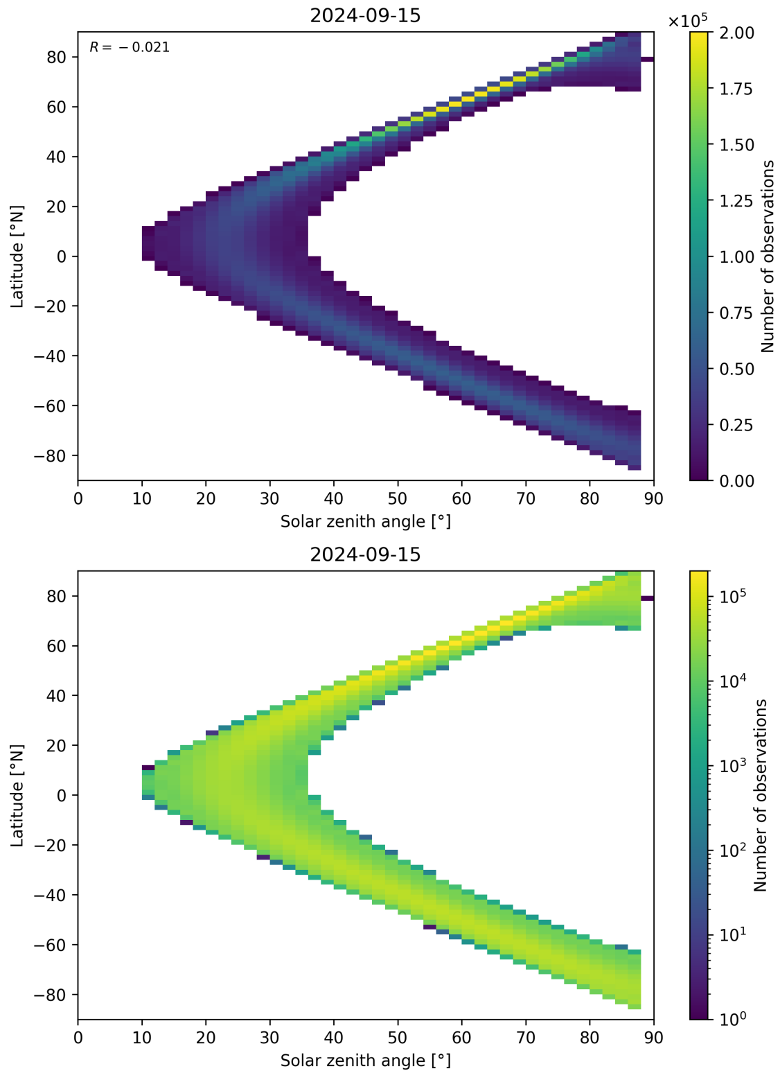
Figure 149: Scatter density plot of “Solar zenith angle” against “Latitude” for 2024-09-14 to 2024-09-16.
