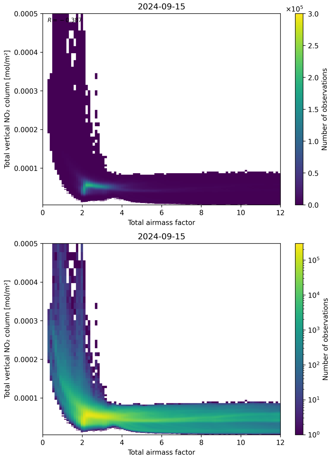
Figure 67: Scatter density plot of “Total airmass factor” against “Total vertical NO 2 column” for 2024-09-14 to 2024-09-16.
