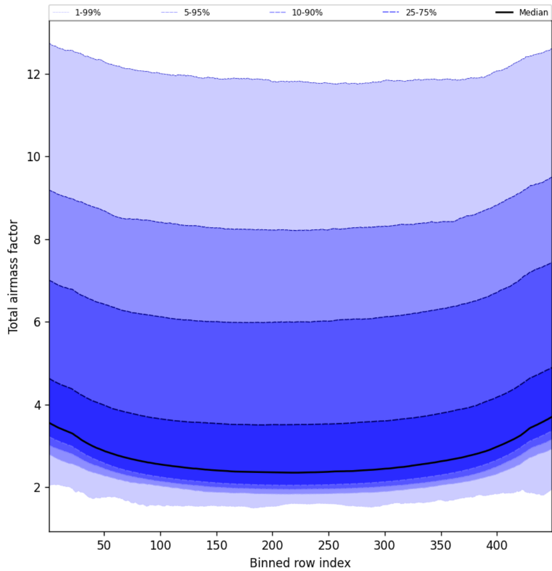
Figure 49: Along track statistics of “Total airmass factor” for 2024-09-14 to 2024-09-16
