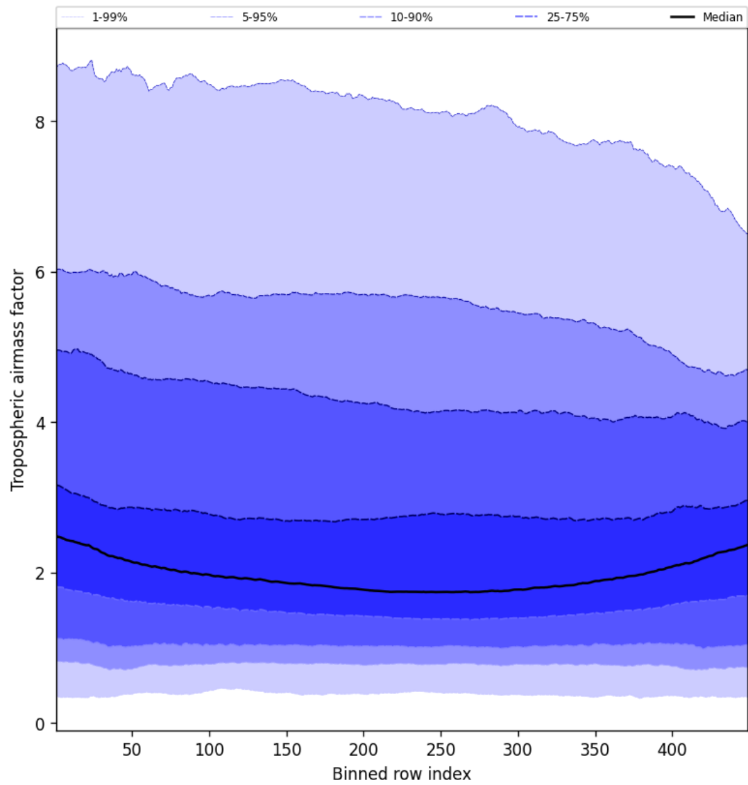
Figure 48: Along track statistics of “Tropospheric air mass factor” for 2024-09-14 to 2024-09-16
