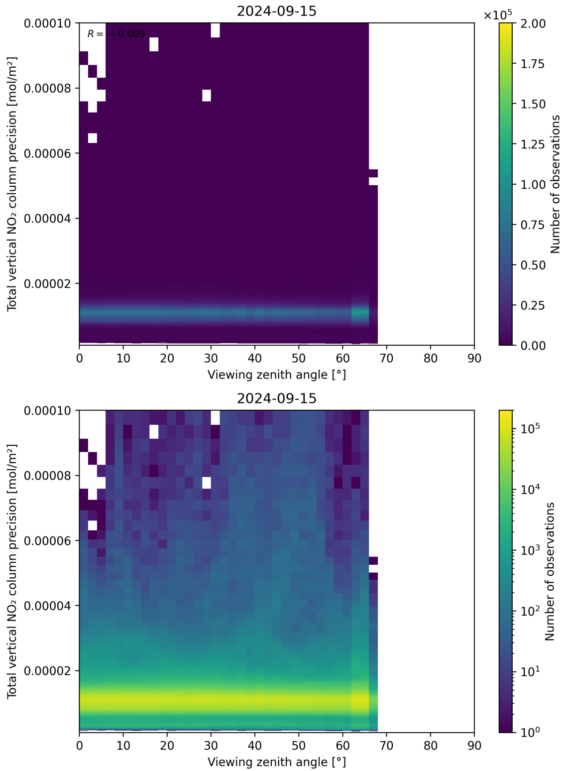
Figure 168: Scatter density plot of “Viewing zenith angle” against “Total vertical NO 2 column precision” for 2024-09-14 to 2024-09-16.
