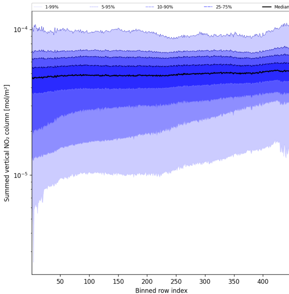
Figure 57: Along track statistics of “Summed vertical NO 2 column” for 2024-09-14 to 2024-09-16
