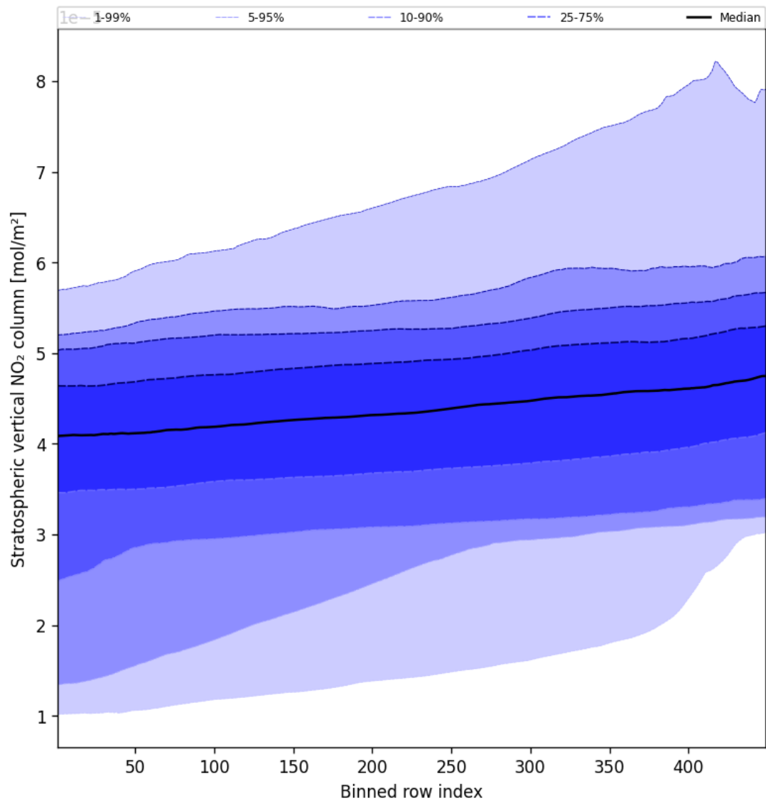
Figure 53: Along track statistics of “Stratospheric vertical NO 2 column” for 2024-09-14 to 2024-09-16
