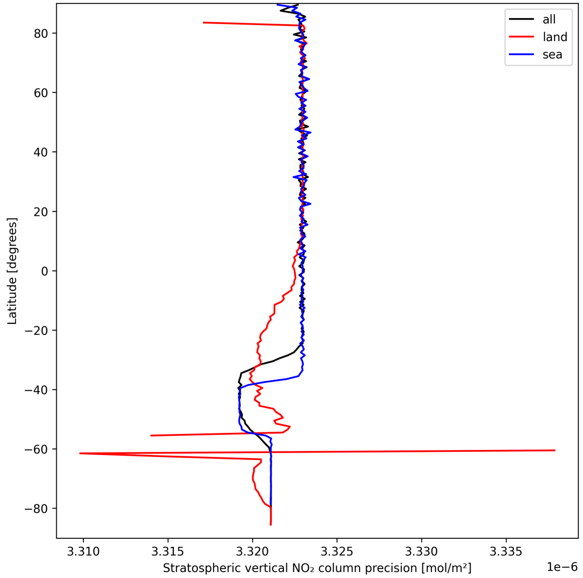
Figure 20: Zonal average of “Stratospheric vertical NO 2 column precision” for 2024-09-14 to 2024-09-16.
