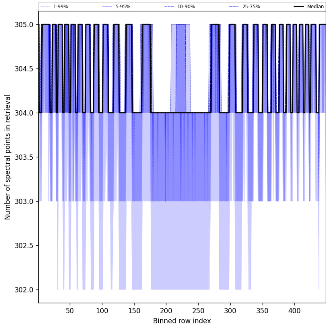
Figure 50: Along track statistics of “Number of spectral points in retrieval” for 2024-09-14 to 2024-09-16
