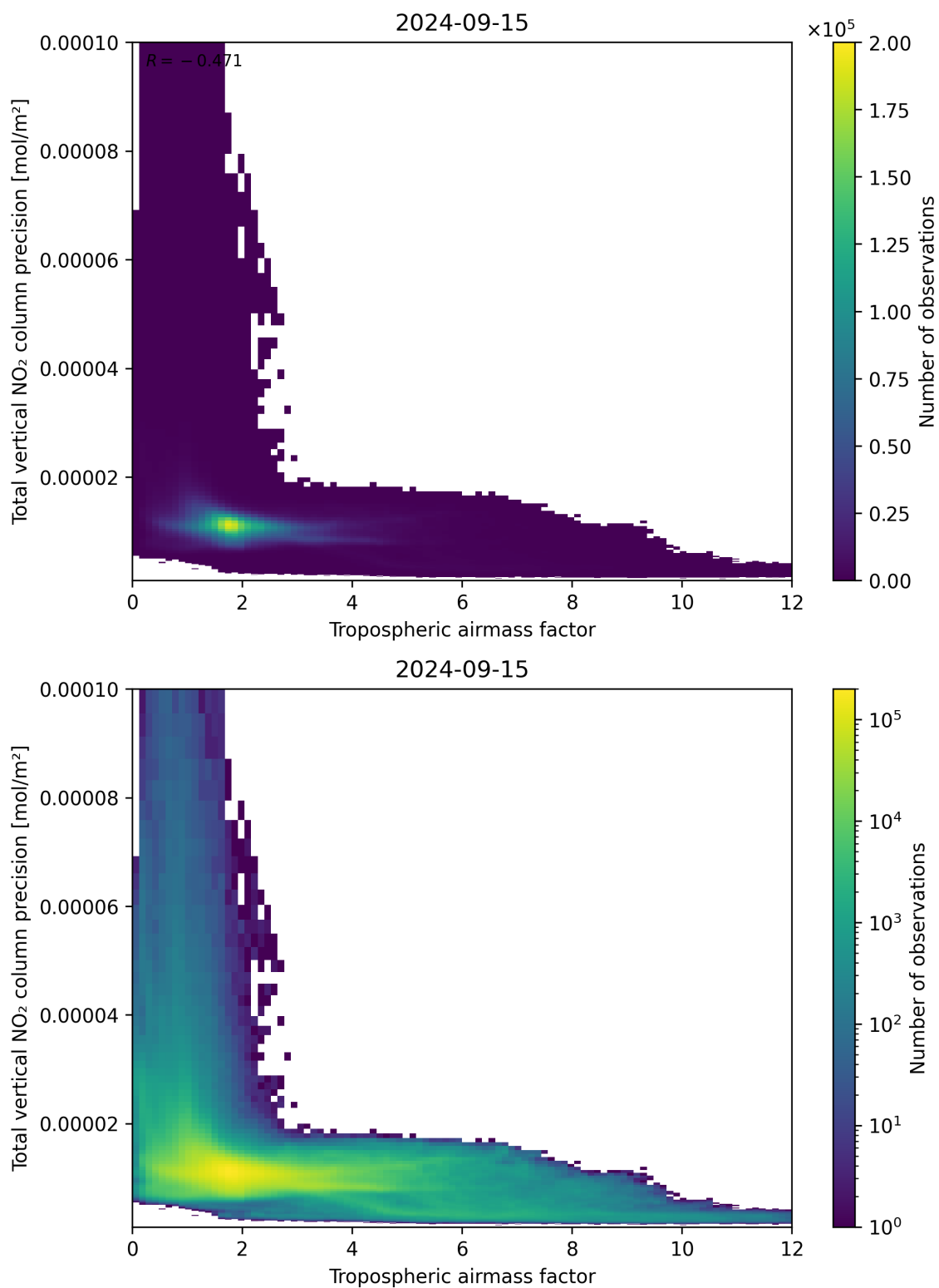
Figure 78: Scatter density plot of “Tropospheric air mass factor” against “Total vertical NO 2 column precision” for 2024-09-14 to 2024-09-16.
