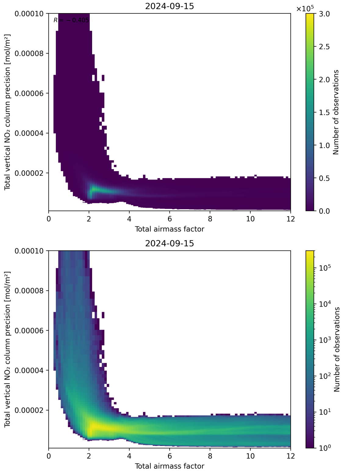
Figure 68: Scatter density plot of “Total airmass factor” against “Total vertical NO 2 column precision” for 2024-09-14 to 2024-09-16.
