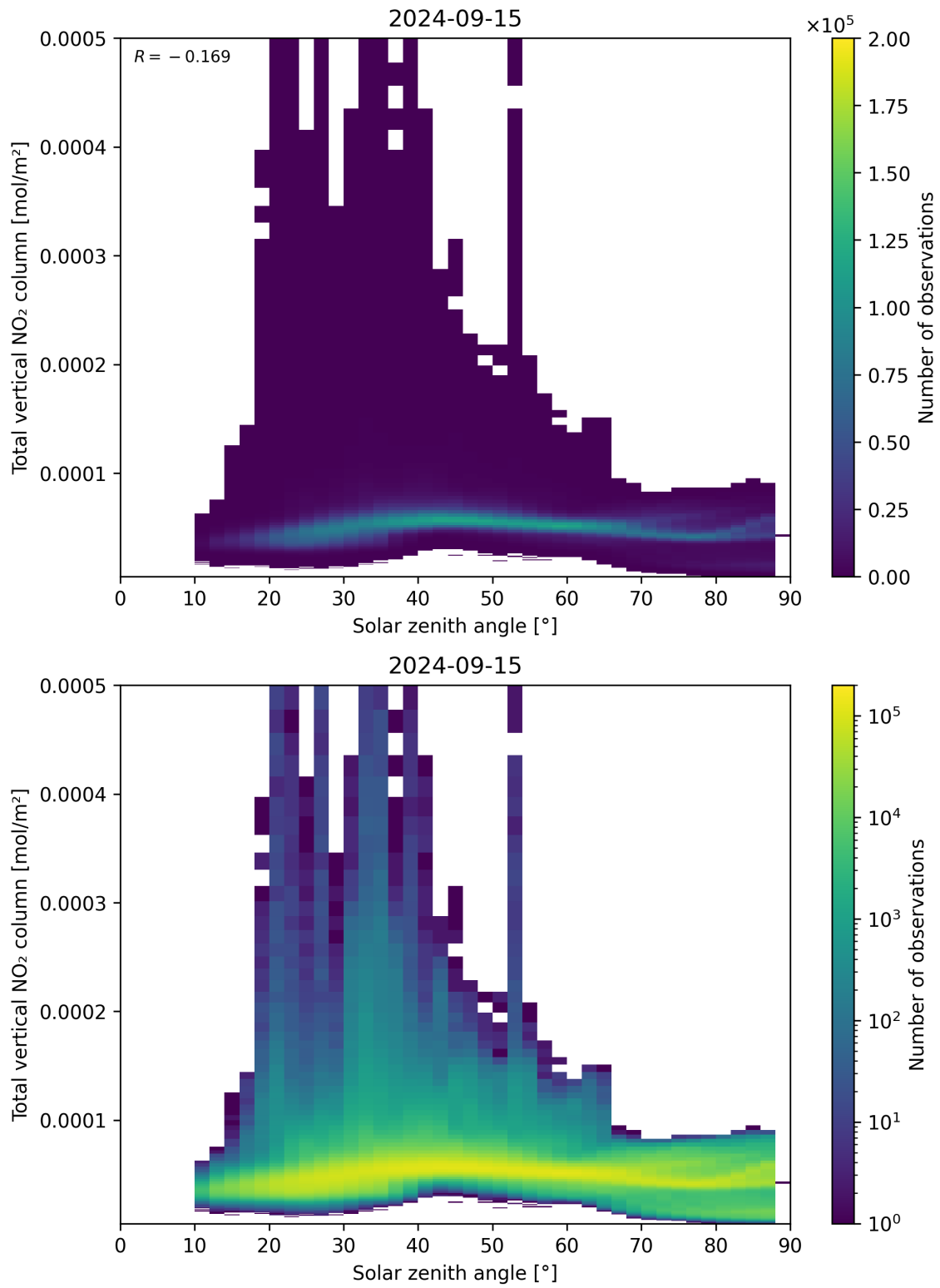
Figure 153: Scatter density plot of “Solar zenith angle” against “Total vertical NO 2 column” for 2024-09-14 to 2024-09-16.
