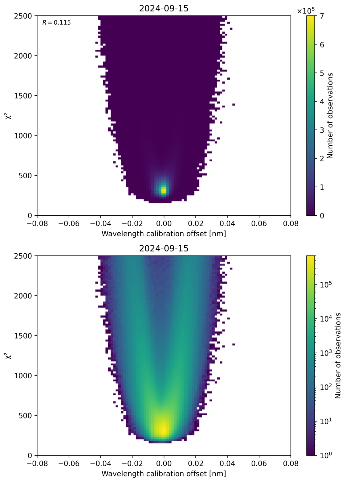
Figure 175: Scatter density plot of “Wavelength calibration offset” against “ \chi^2 ” for 2024-09-14 to 2024-09-16.
