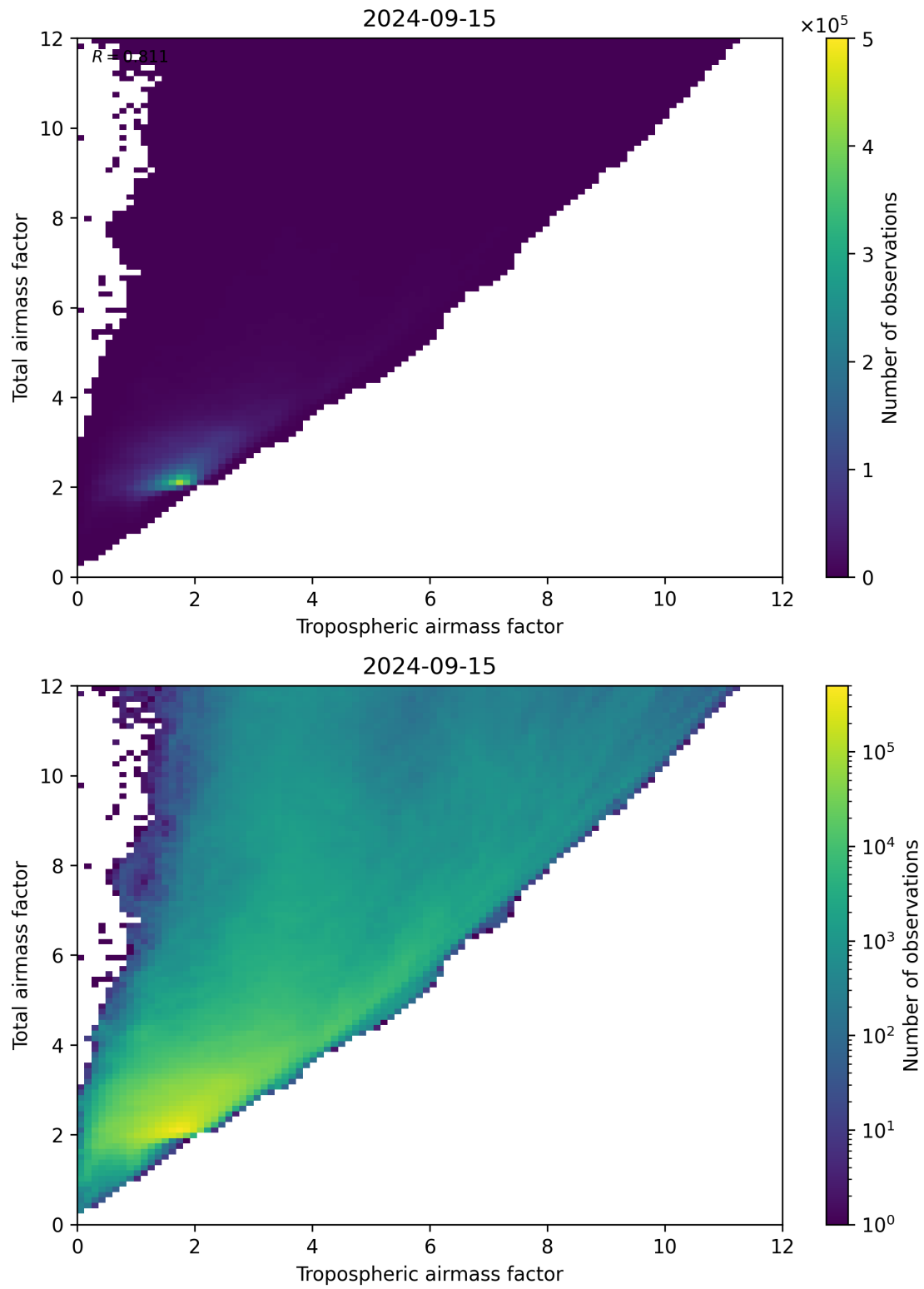
Figure 72: Scatter density plot of “Tropospheric airmass factor” against “Total airmass factor” for 2024-09-14 to 2024-09-16.
