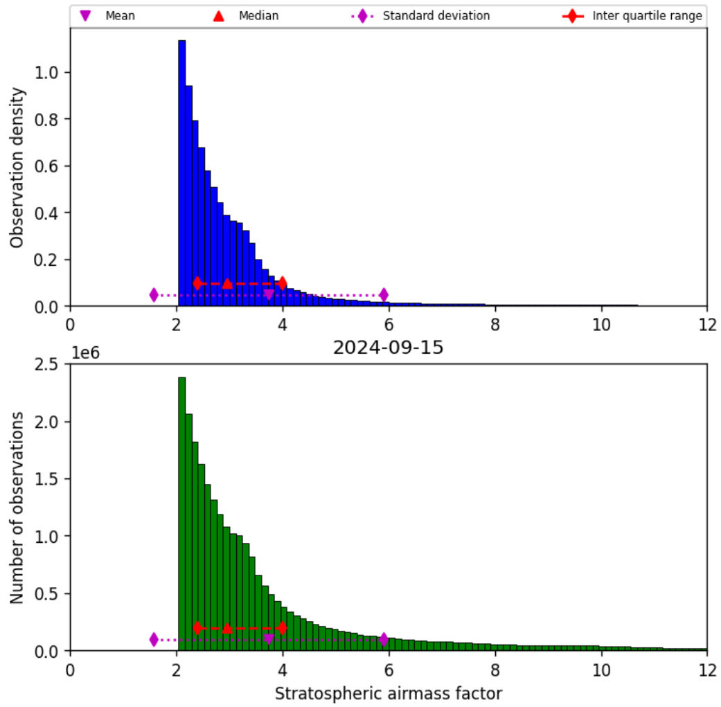
Figure 44: Histogram of “Stratospheric airmass factor” for 2024-09-14 to 2024-09-16
