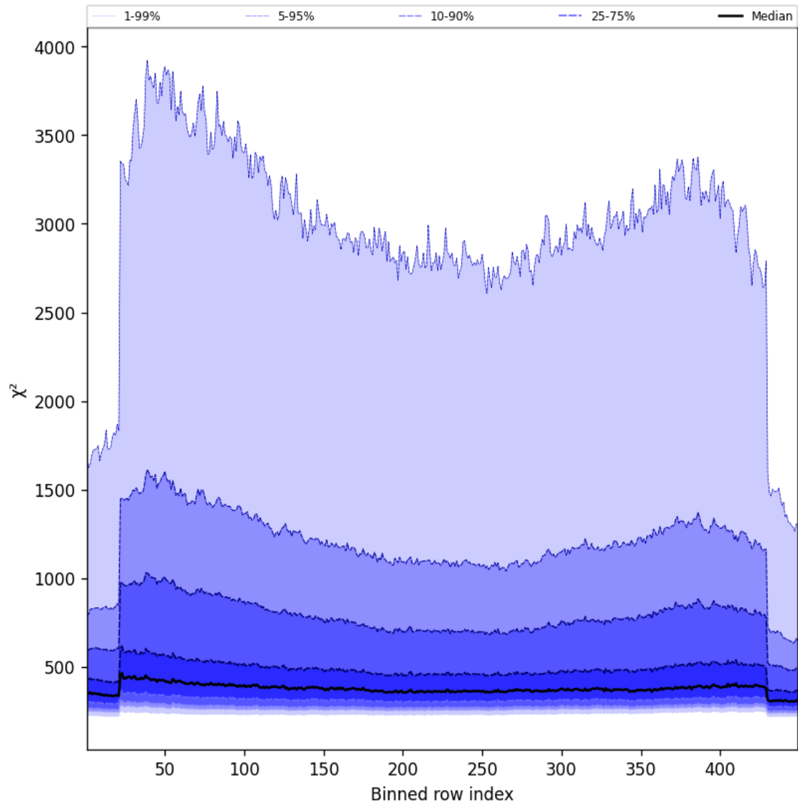
Figure 59: Along track statistics of “ \chi^2 ” for 2024-09-14 to 2024-09-16
