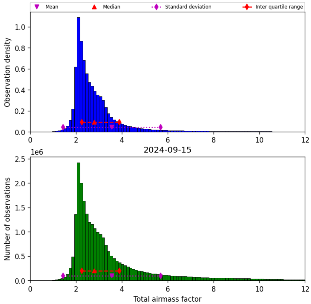
Figure 32: Histogram of “Total airmass factor” for 2024-09-14 to 2024-09-16
