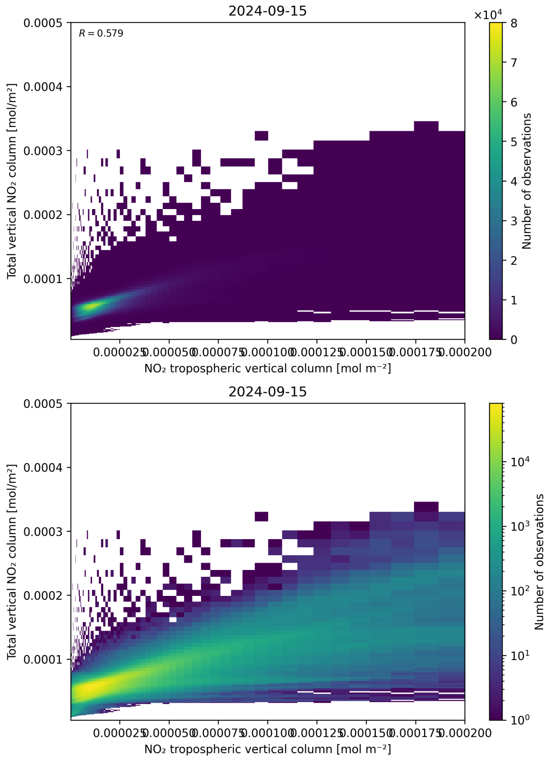
Figure 128: Scatter density plot of “NO 2 tropospheric vertical column” against “Total vertical NO 2 column” for 2024-09-14 to 2024-09-16.
