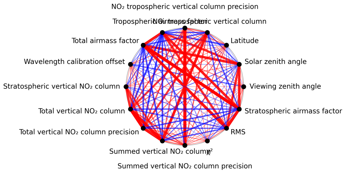
Figure 1: Map of correlation graph for 2024-09-14 to 2024-09-16.
