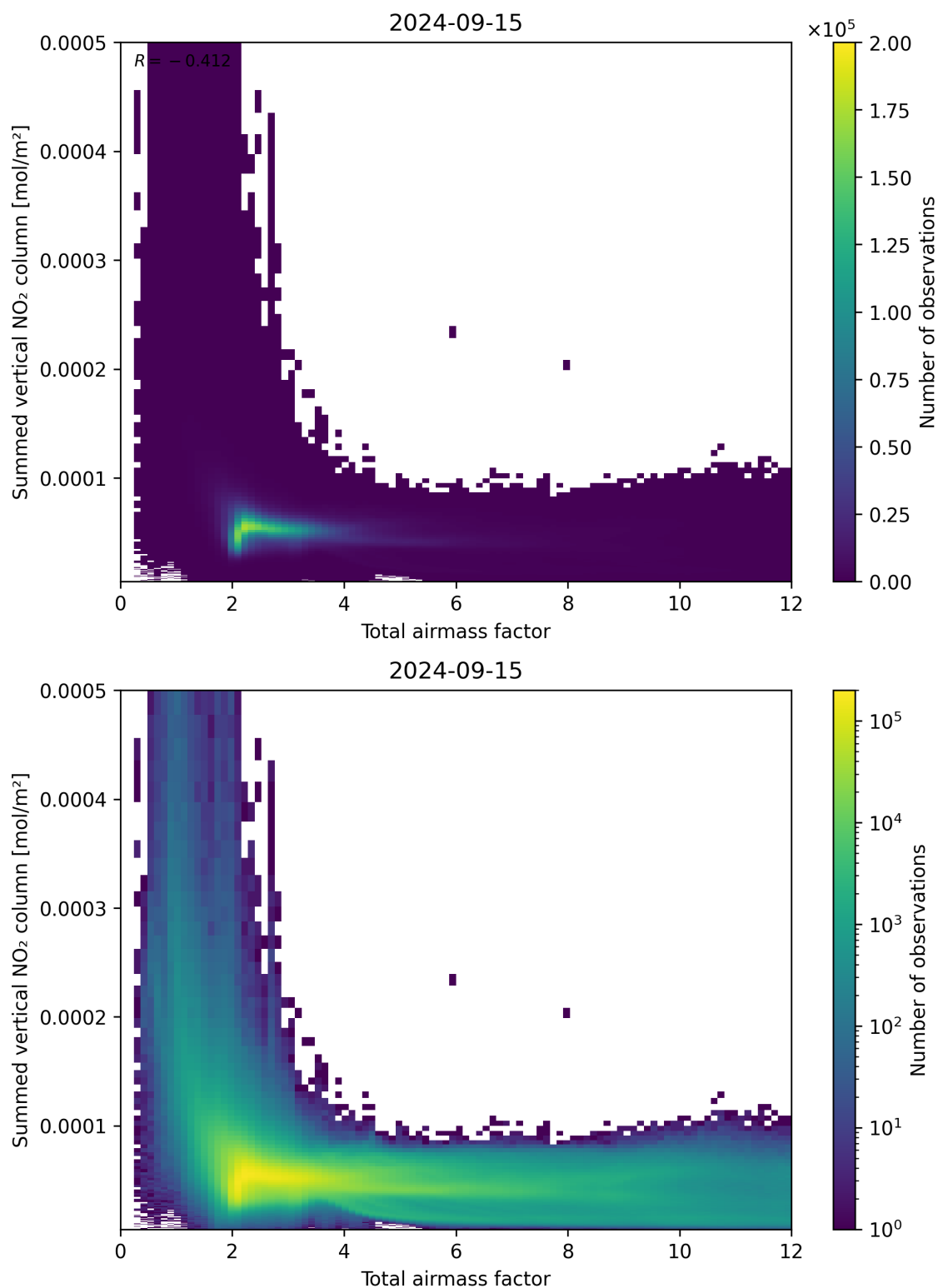
Figure 65: Scatter density plot of “Total airmass factor” against “Summed vertical NO 2 column” for 2024-09-14 to 2024-09-16.
