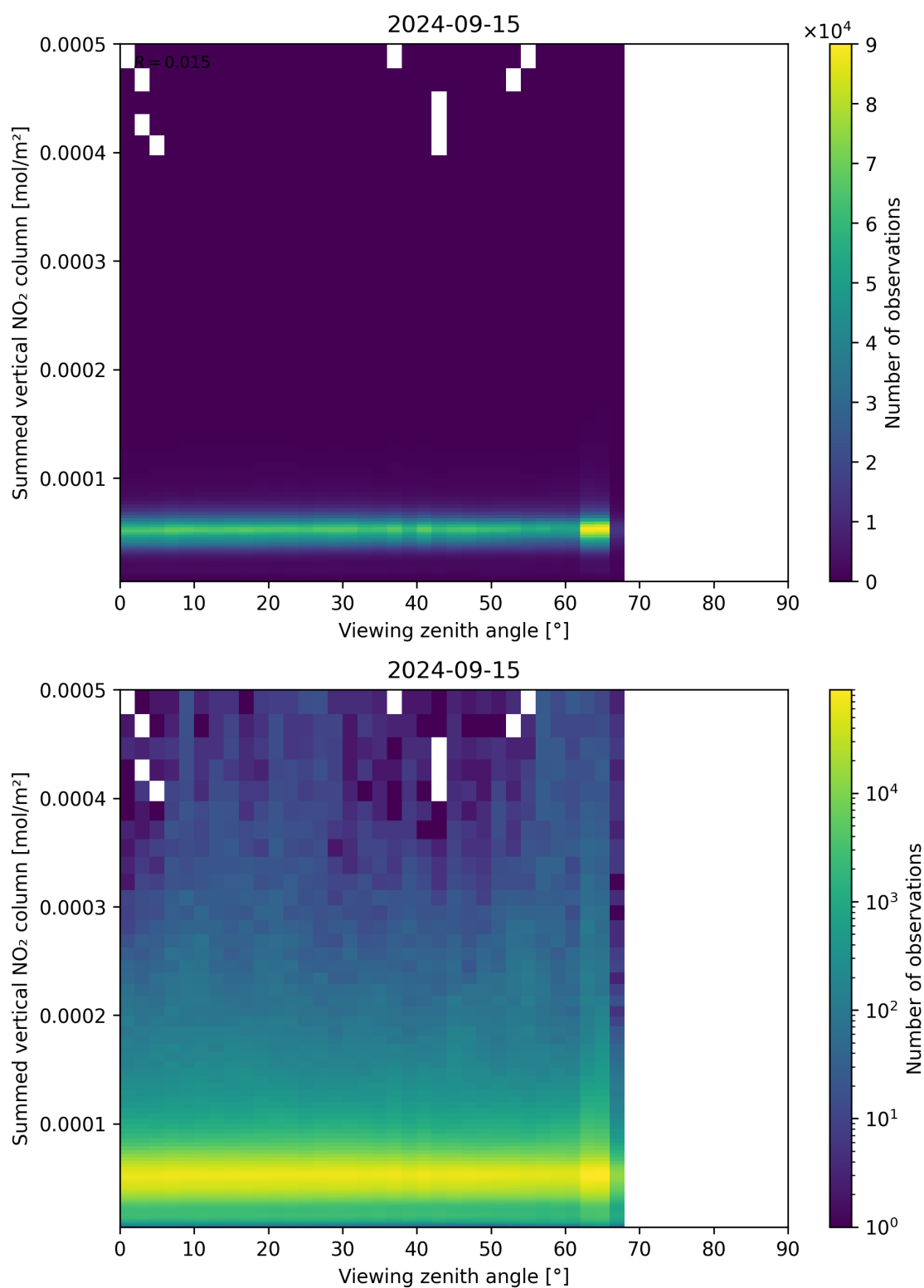
Figure 165: Scatter density plot of “Viewing zenith angle” against “Summed vertical NO 2 column” for 2024-09-14 to 2024-09-16.
