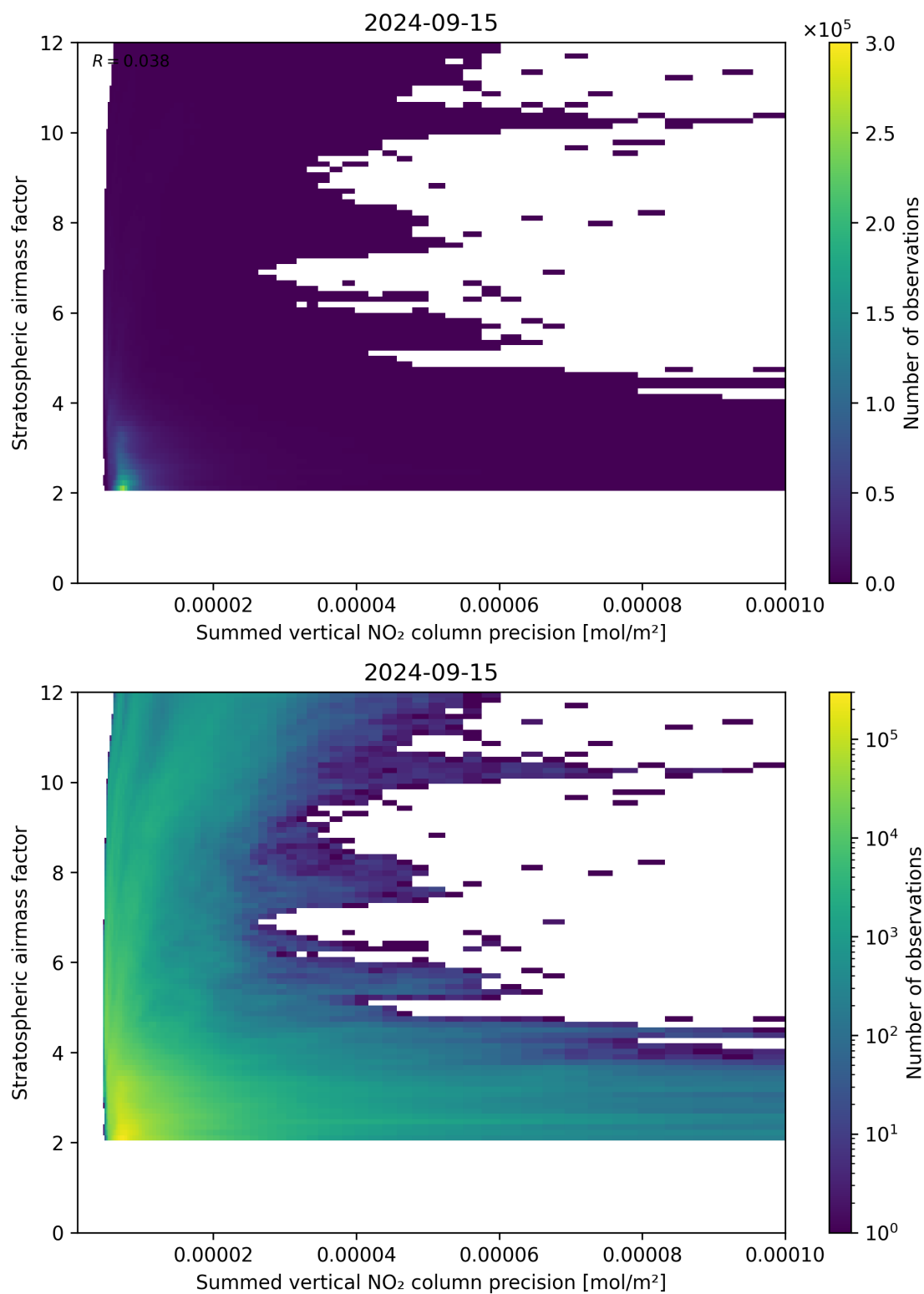
Figure 106: Scatter density plot of “Summed vertical NO 2 column precision” against “Stratospheric airmass factor” for 2024-09-14 to 2024-09-16.
