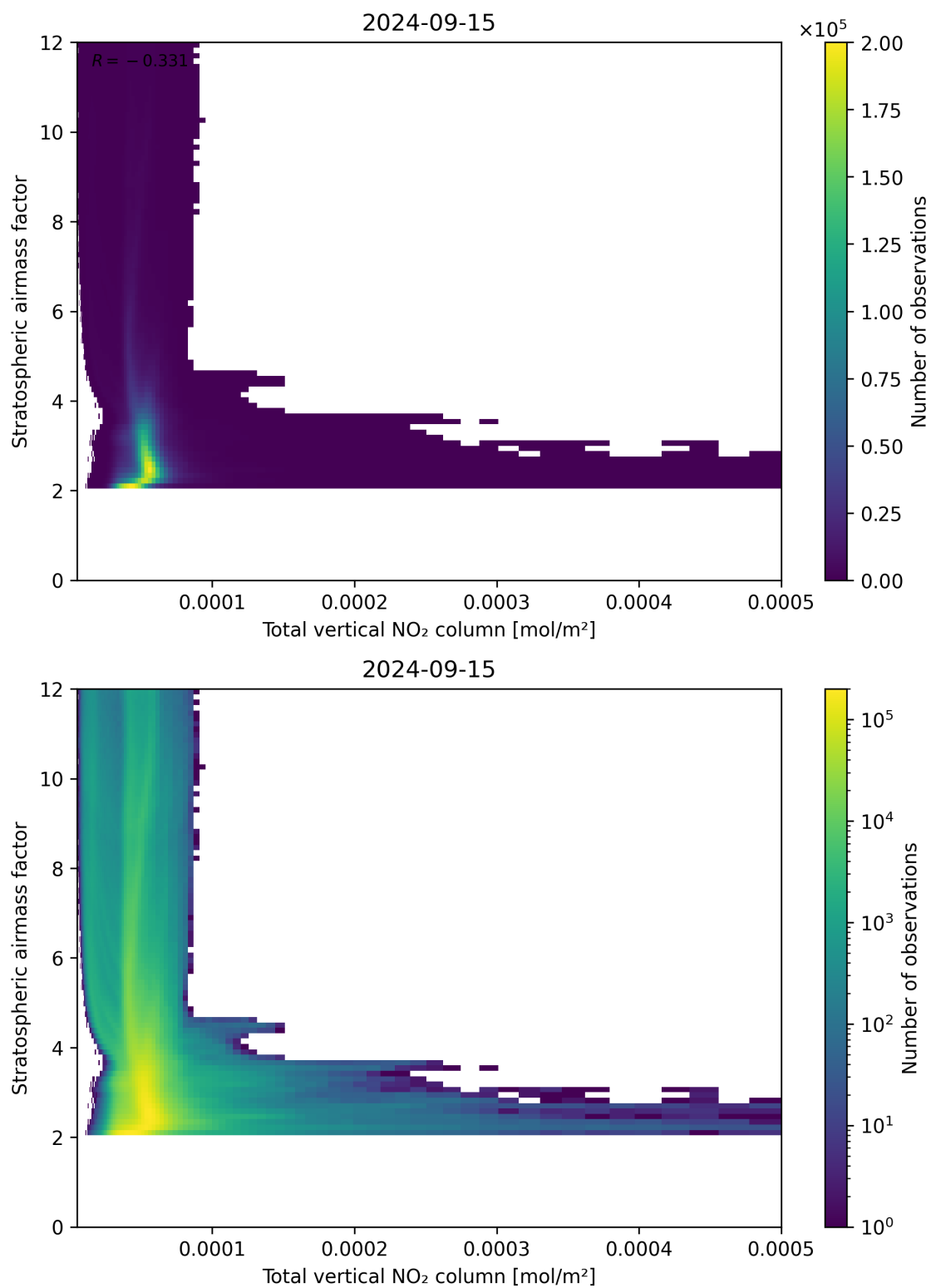
Figure 110: Scatter density plot of “Total vertical NO 2 column” against “Stratospheric airmass factor” for 2024-09-14 to 2024-09-16.
