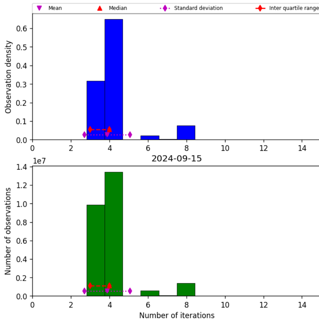
Figure 34: Histogram of “Number of iterations” for 2024-09-14 to 2024-09-16
