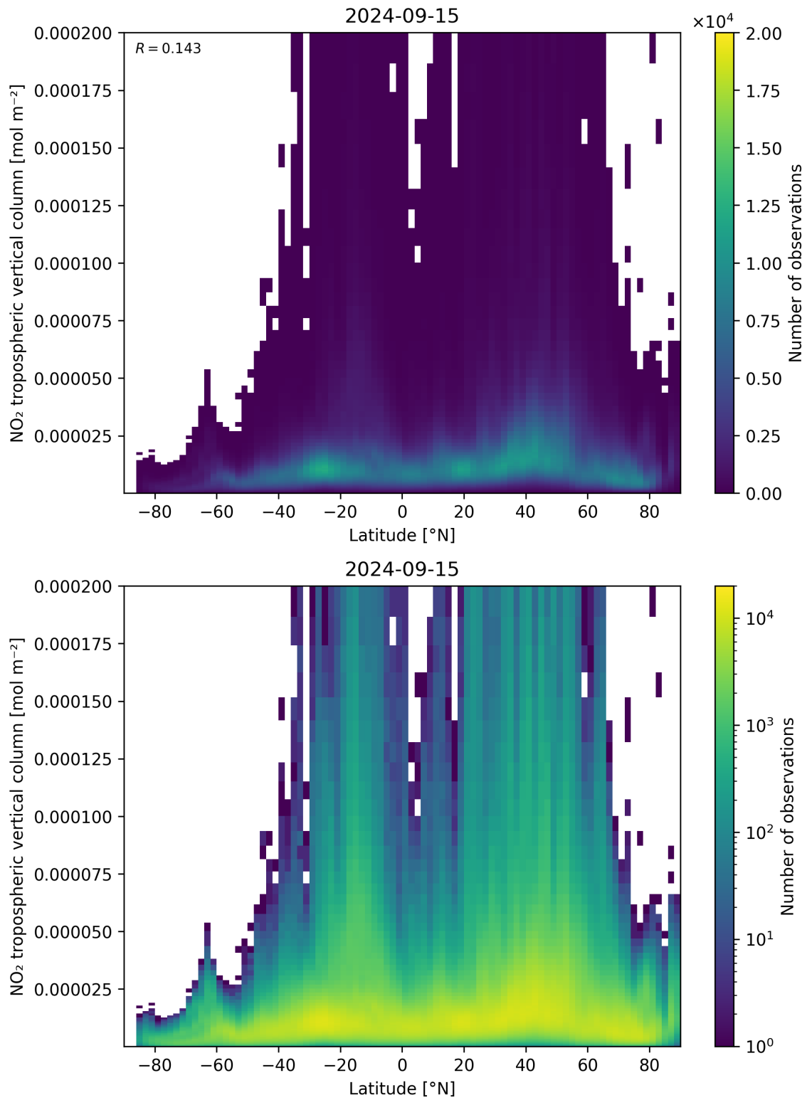
Figure 92: Scatter density plot of “Latitude” against “NO 2 tropospheric vertical column” for 2024-09-14 to 2024-09-16.
