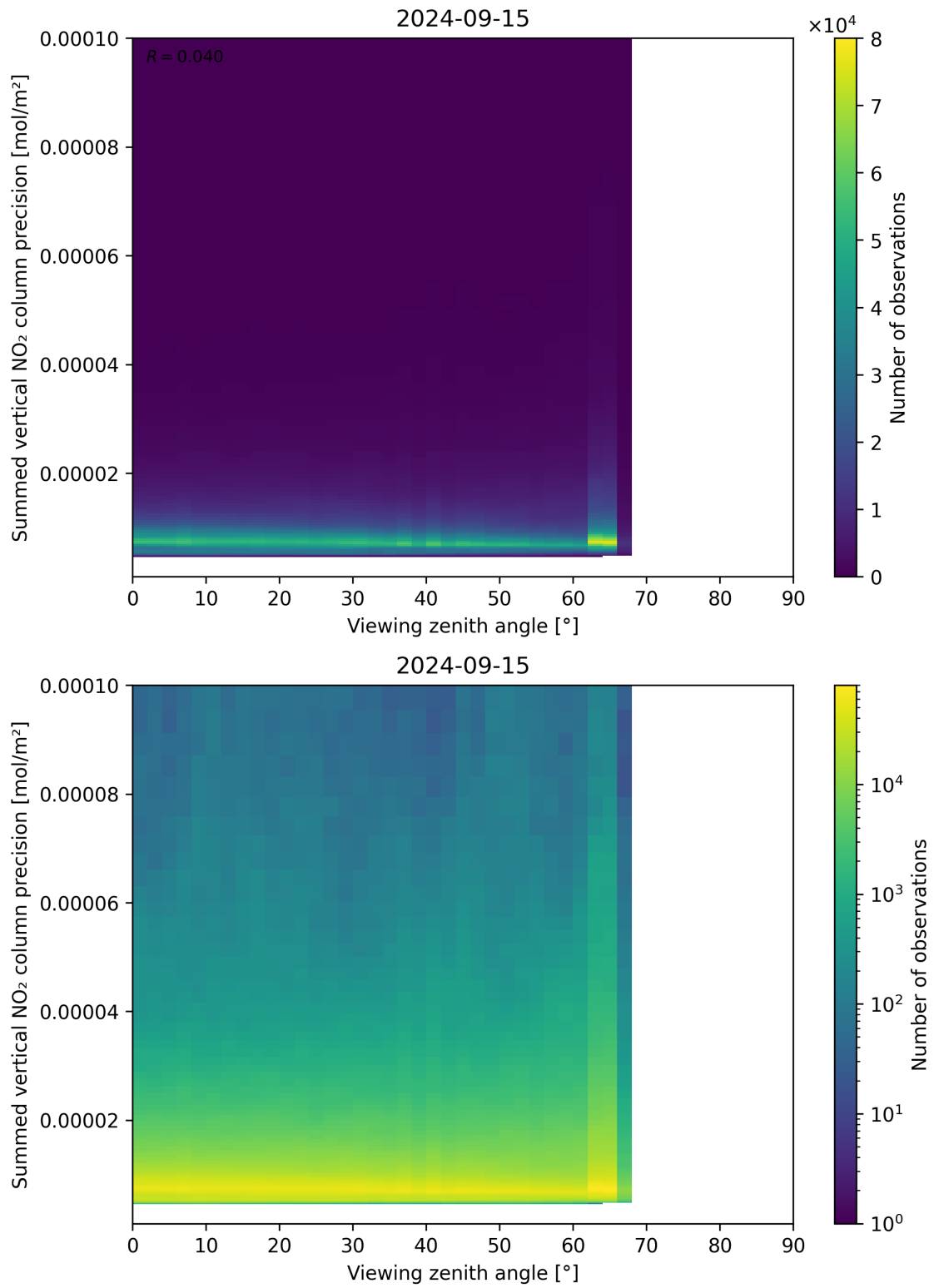
Figure 166: Scatter density plot of “Viewing zenith angle” against “Summed vertical NO 2 column precision” for 2024-09-14 to 2024-09-16.
