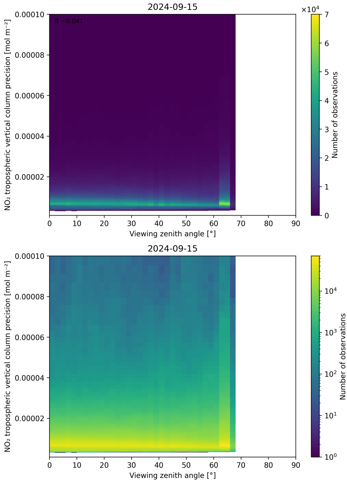
Figure 170: Scatter density plot of “Viewing zenith angle” against “NO 2 tropospheric vertical column precision” for 2024-09-14 to 2024-09-16.
