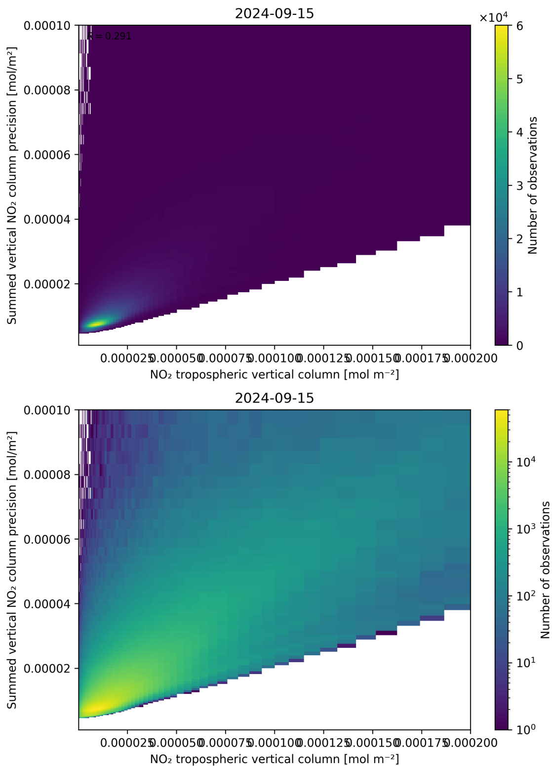
Figure 127: Scatter density plot of “NO 2 tropospheric vertical column” against “Summed vertical NO 2 column precision” for 2024-09-14 to 2024-09-16.
