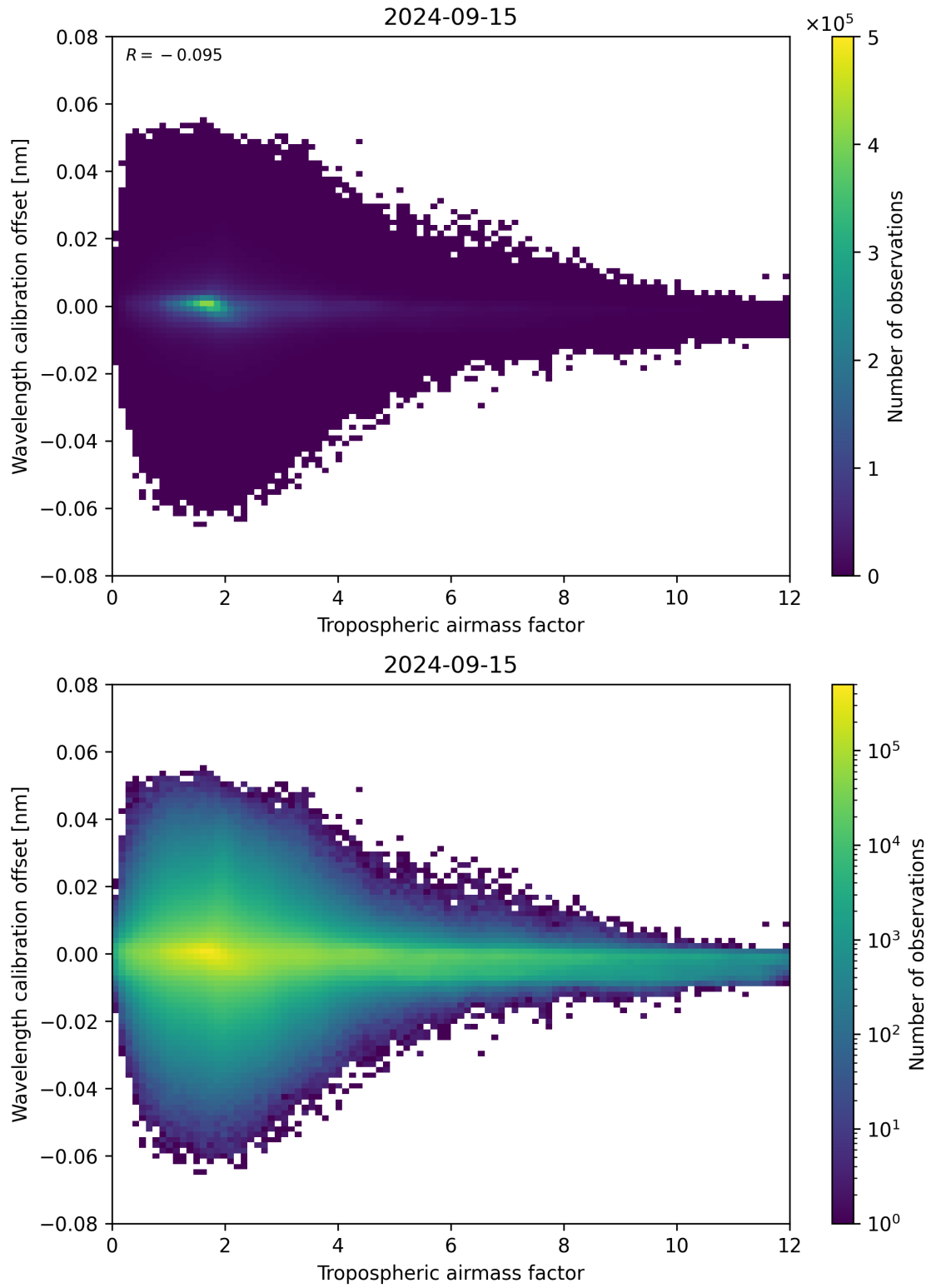
Figure 80: Scatter density plot of “Tropospheric airmass factor” against “Wavelength calibration offset” for 2024-09-14 to 2024-09-16.
