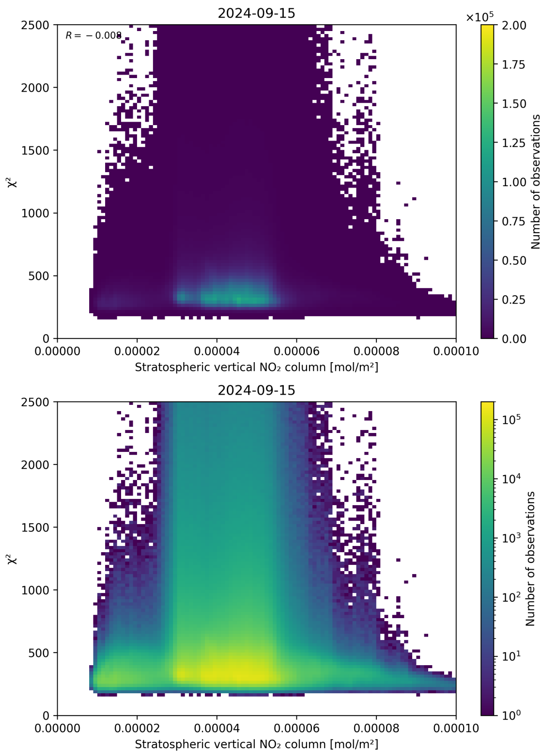
Figure 97: Scatter density plot of “Stratospheric vertical NO 2 column” against “ \chi^2 ” for 2024-09-14 to 2024-09-16.
