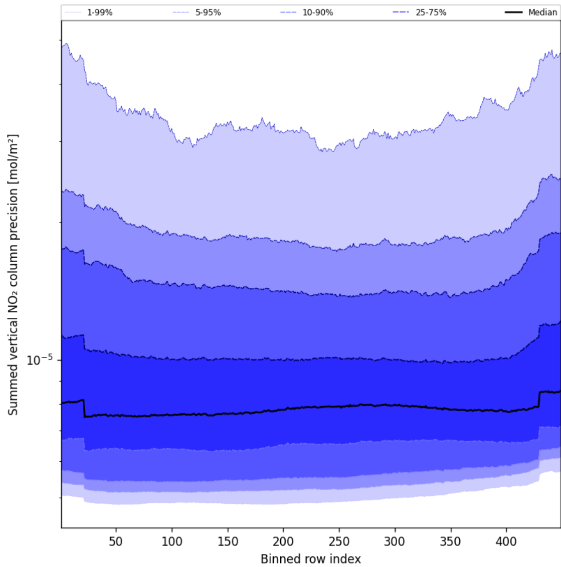
Figure 58: Along track statistics of “Summed vertical NO 2 column precision” for 2024-09-14 to 2024-09-16
