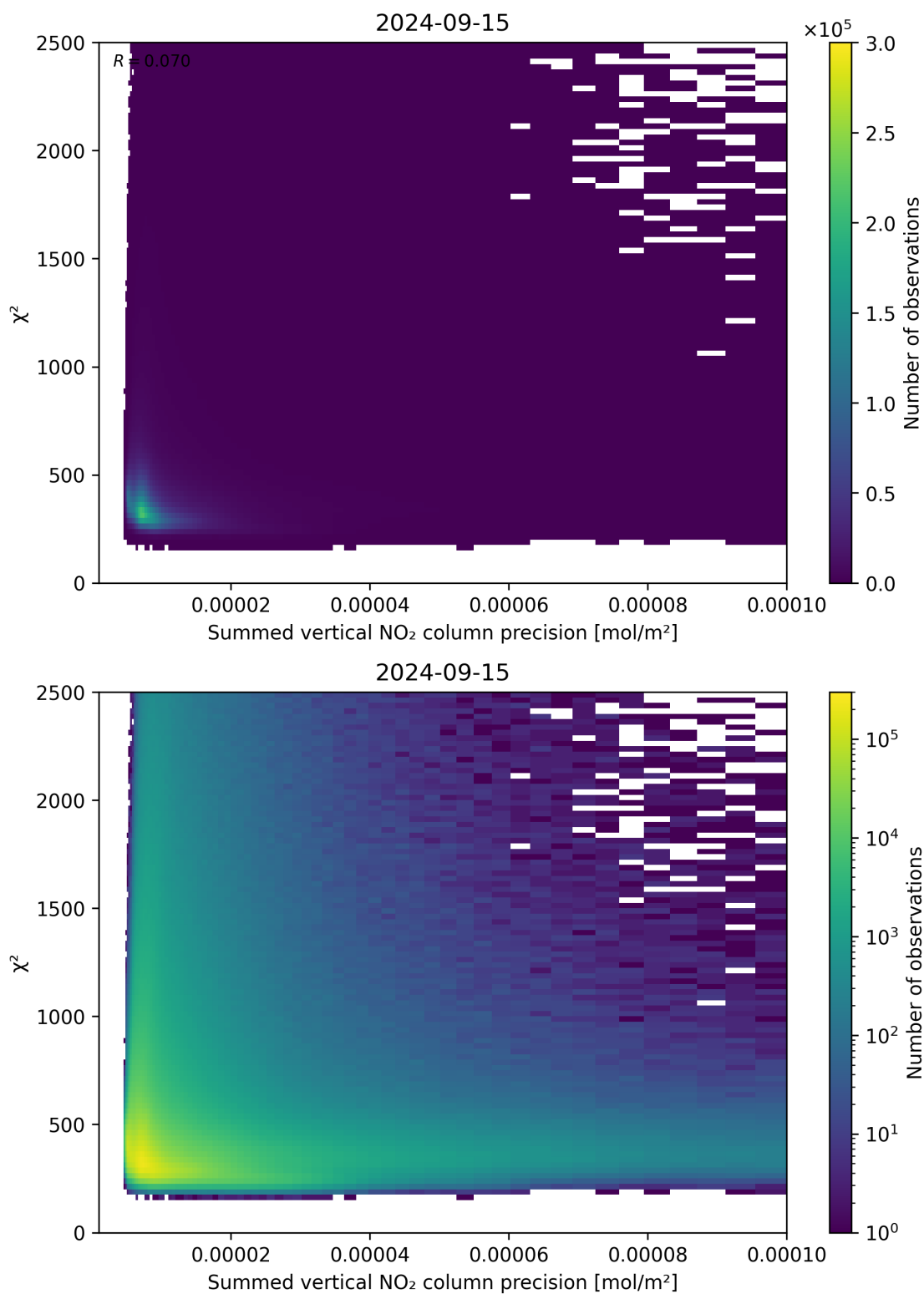
Figure 107: Scatter density plot of “Summed vertical NO 2 column precision” against “ \chi^2 ” for 2024-09-14 to 2024-09-16.
