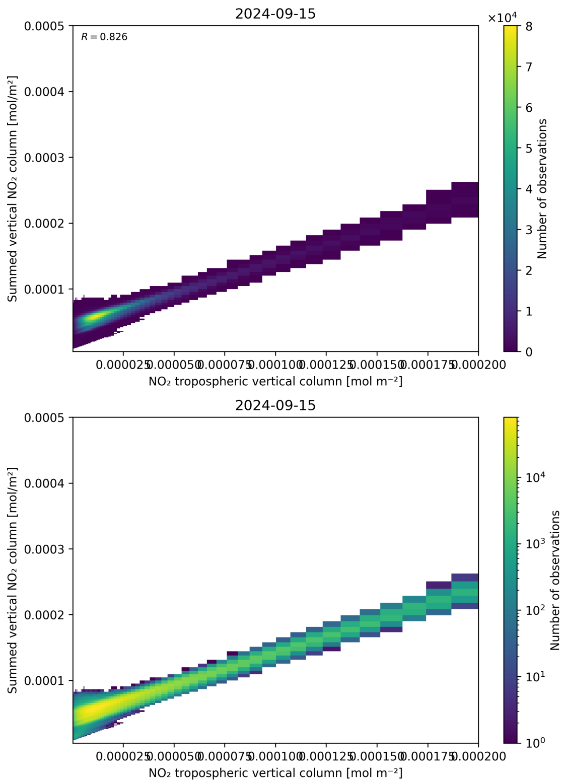
Figure 126: Scatter density plot of “NO 2 tropospheric vertical column” against “Summed vertical NO 2 column” for 2024-09-14 to 2024-09-16.
