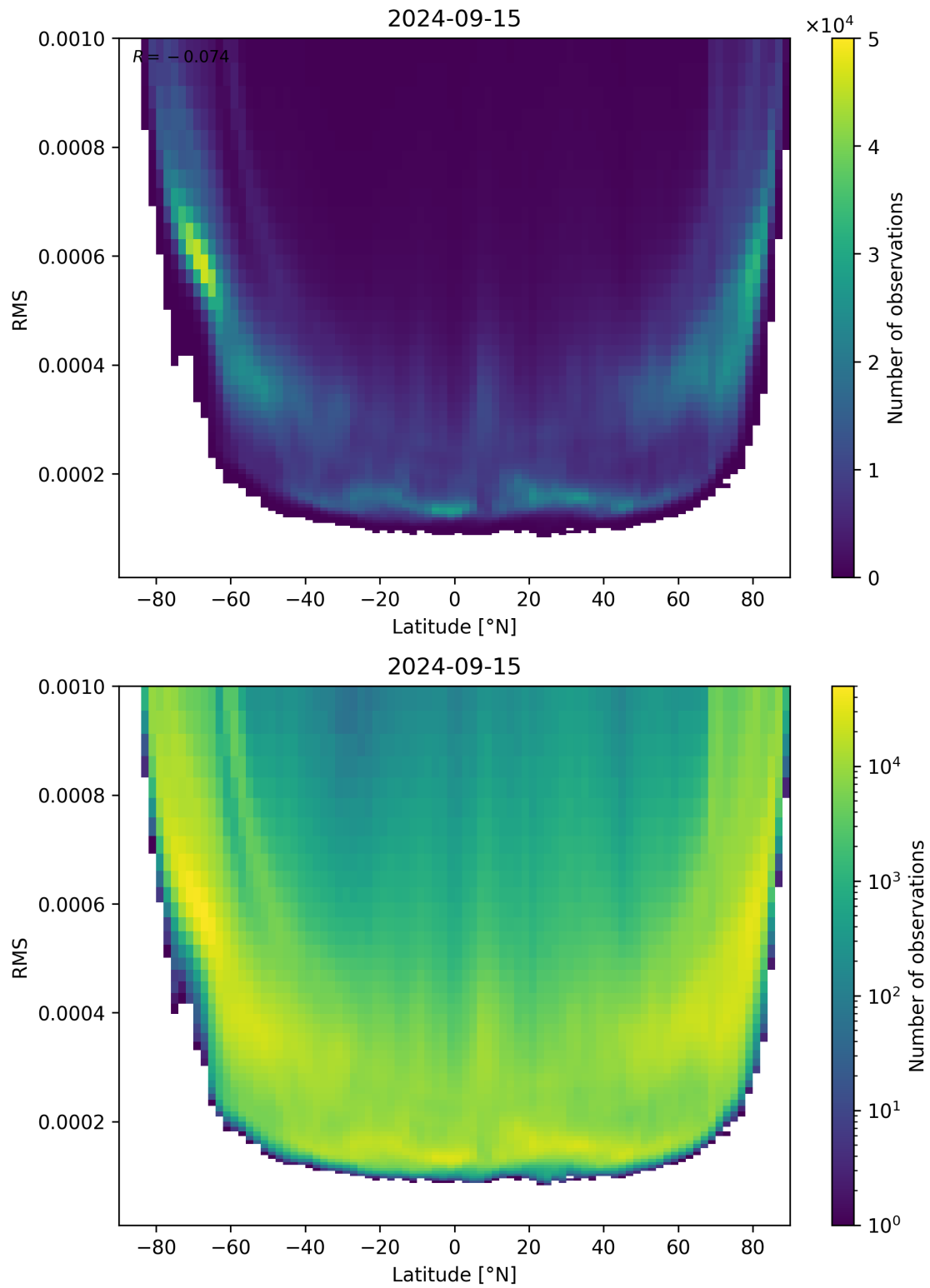
Figure 94: Scatter density plot of “Latitude” against “RMS” for 2024-09-14 to 2024-09-16.
