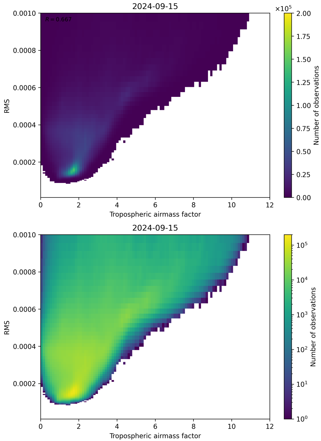
Figure 79: Scatter density plot of “Tropospheric airmass factor” against “RMS” for 2024-09-14 to 2024-09-16.
