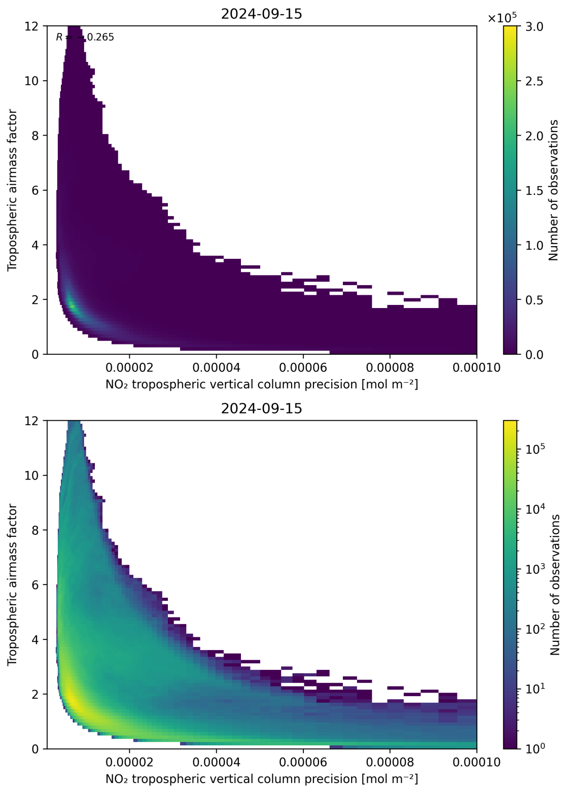
Figure 133: Scatter density plot of “NO 2 tropospheric vertical column precision” against “Tropospheric air mass factor” for 2024-09-14 to 2024-09-16.
