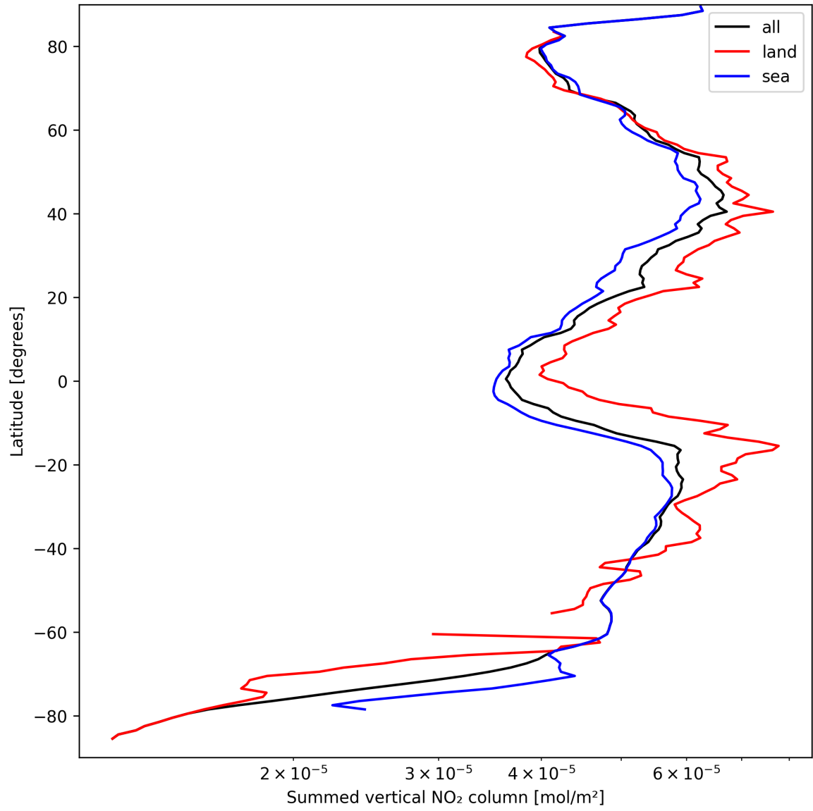
Figure 23: Zonal average of “Summed vertical NO 2 column” for 2024-09-14 to 2024-09-16.
