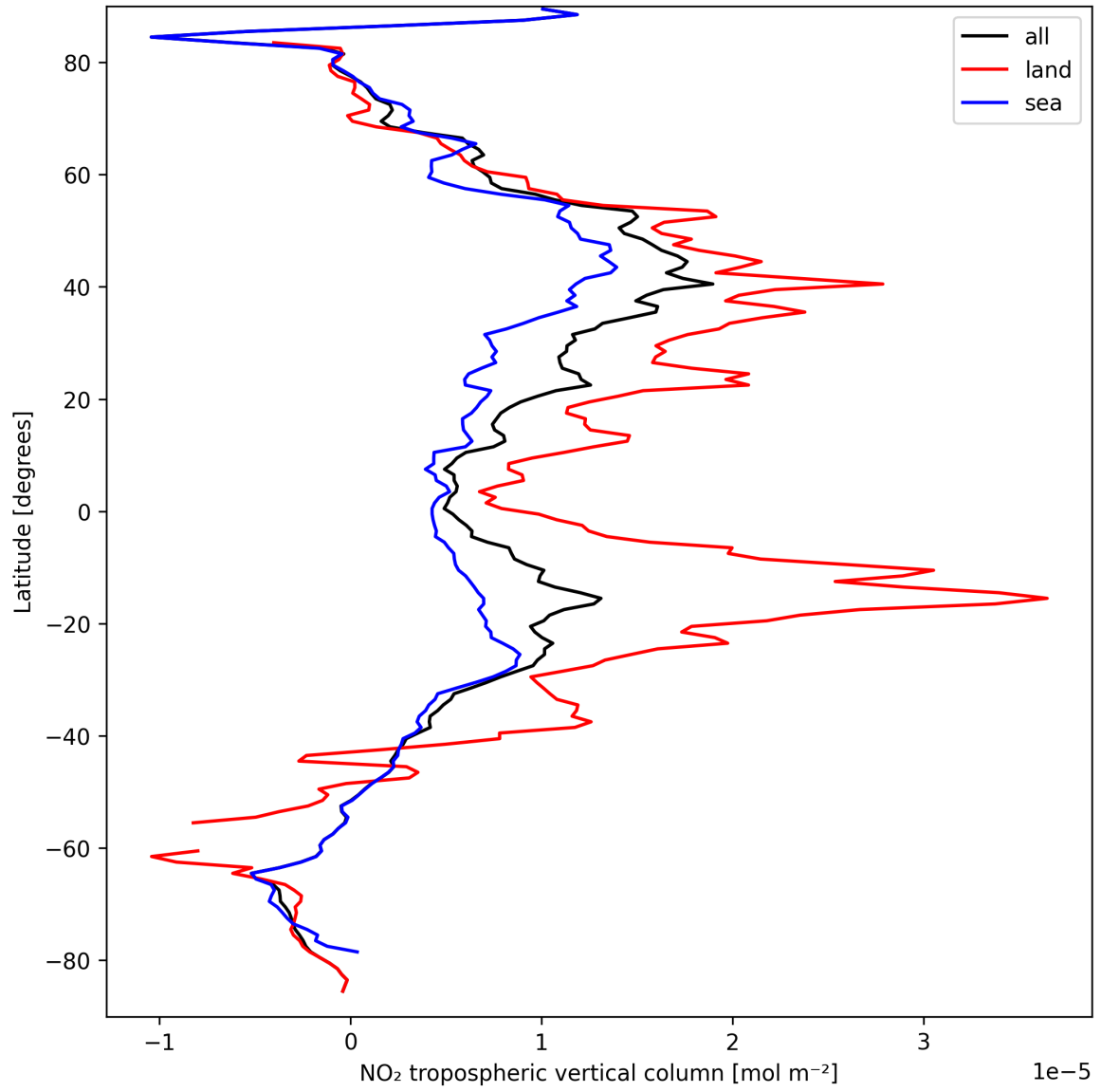
Figure 12: Zonal average of “NO 2 tropospheric vertical column” for 2024-09-14 to 2024-09-16.
