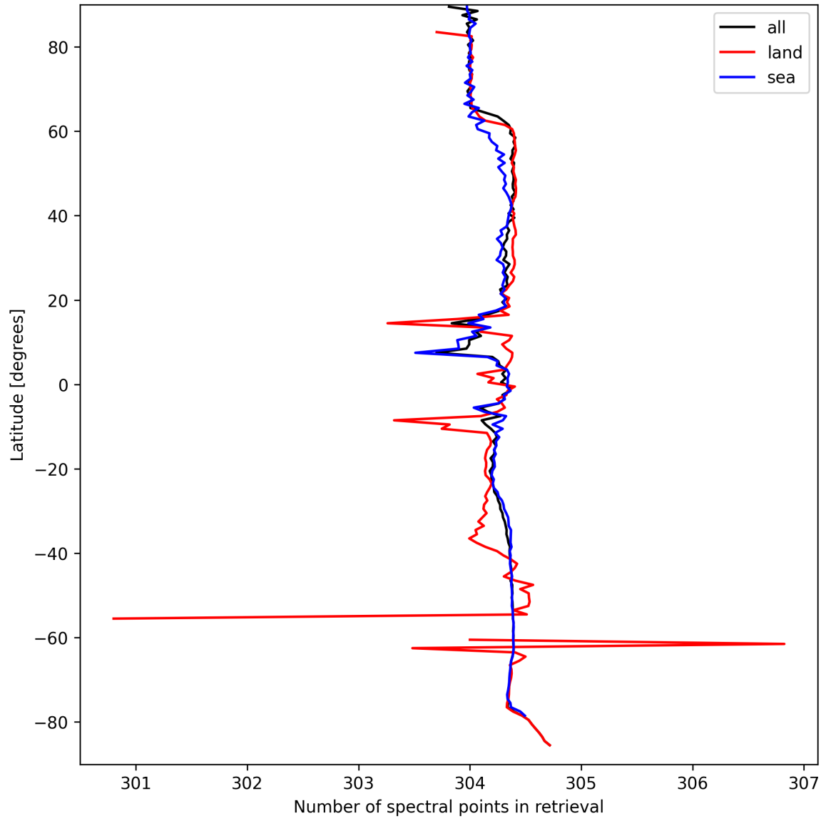
Figure 16: Zonal average of “Number of spectral points in retrieval” for 2024-09-14 to 2024-09-16.
