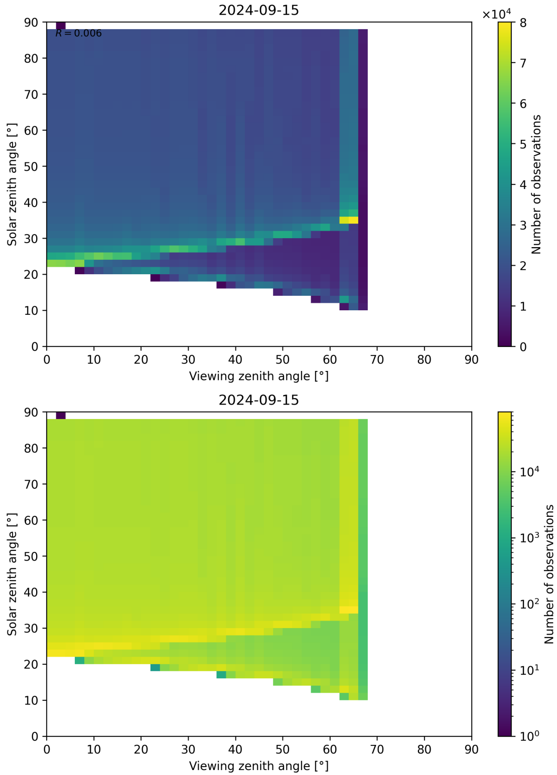
Figure 172: Scatter density plot of “Viewing zenith angle” against “Solar zenith angle” for 2024-09-14 to 2024-09-16.
