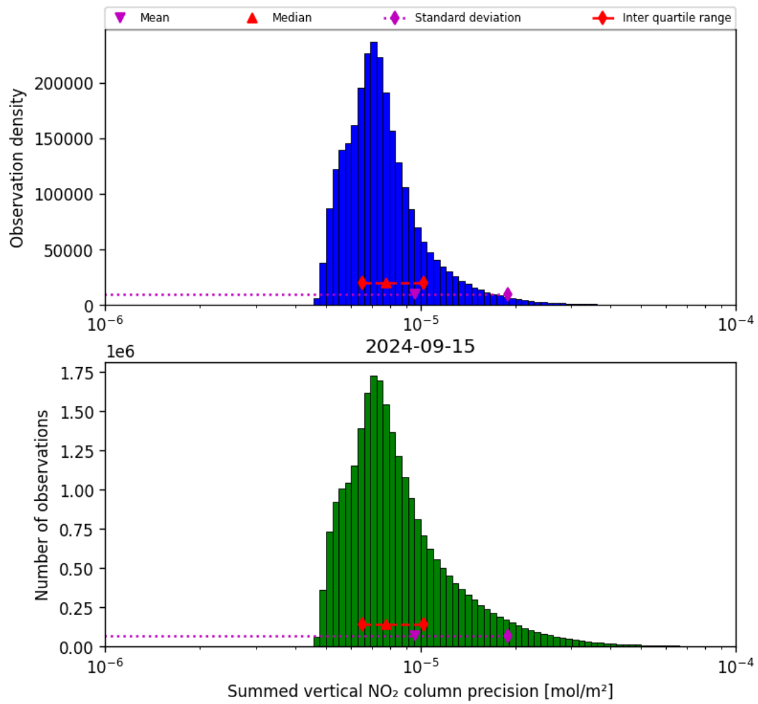
Figure 41: Histogram of “Summed vertical NO 2 column precision” for 2024-09-14 to 2024-09-16
