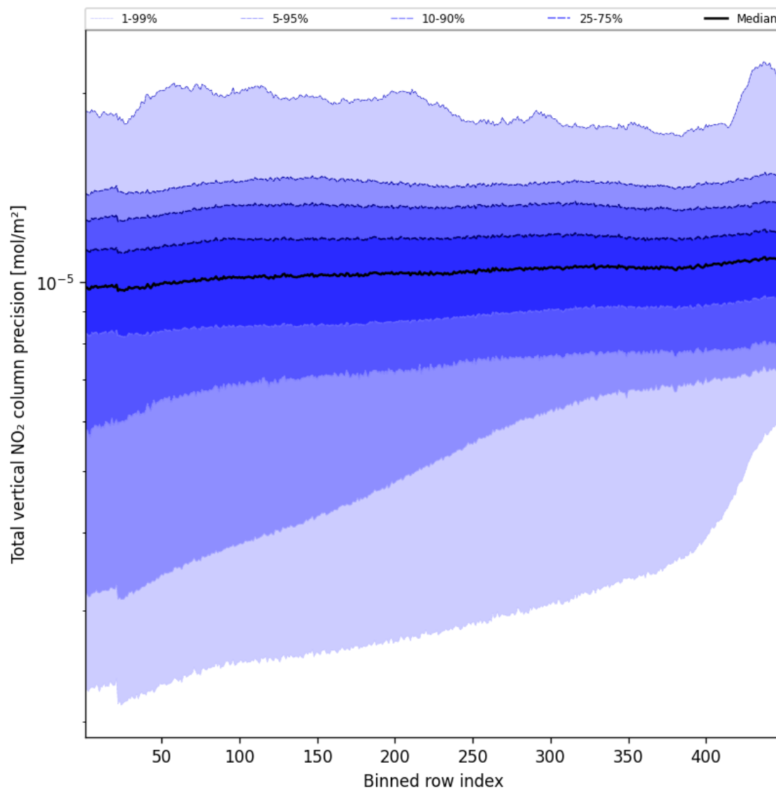
Figure 56: Along track statistics of “Total vertical NO 2 column precision” for 2024-09-14 to 2024-09-16
