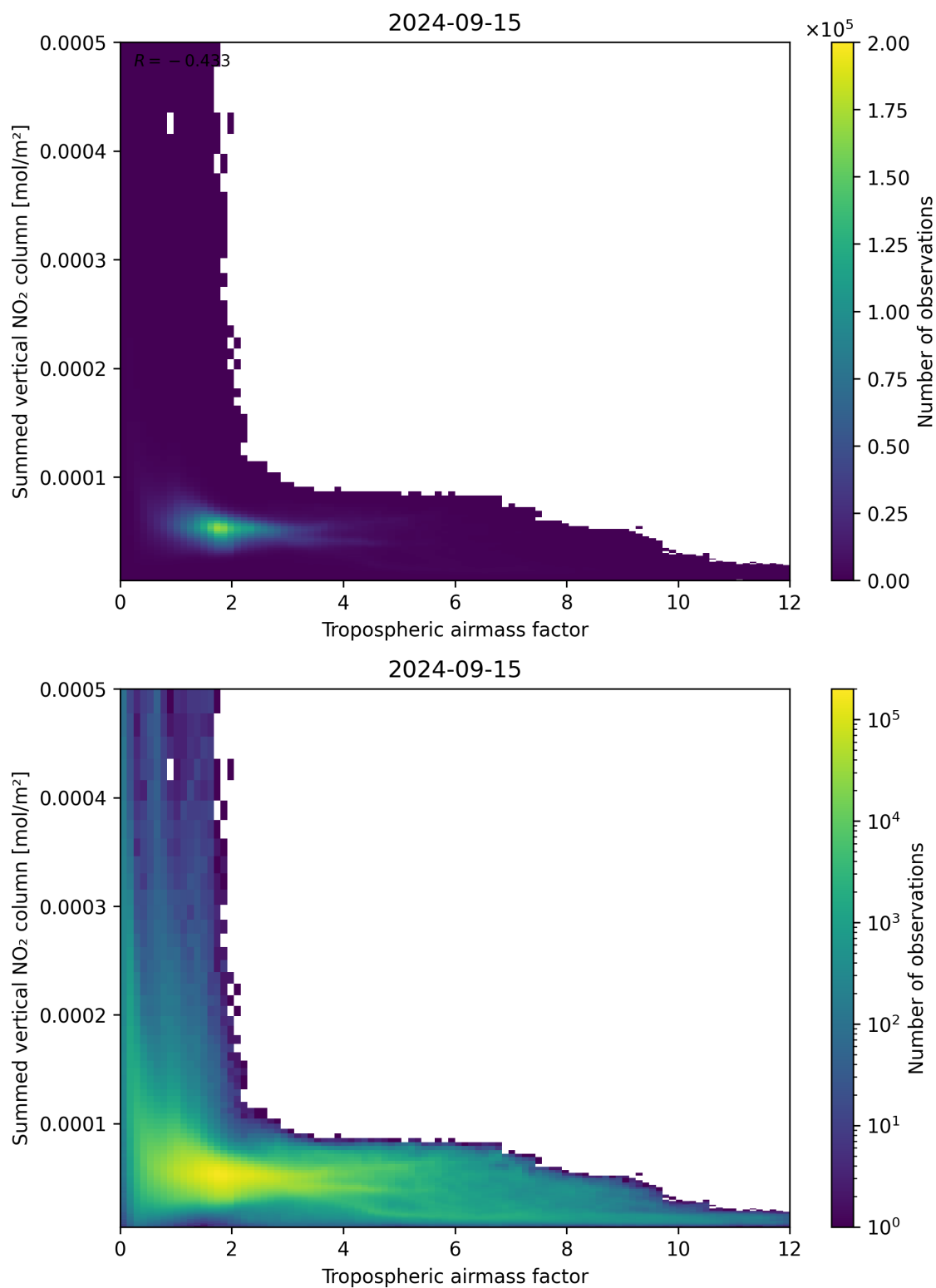
Figure 75: Scatter density plot of “Tropospheric air mass factor” against “Summed vertical NO 2 column” for 2024-09-14 to 2024-09-16.
