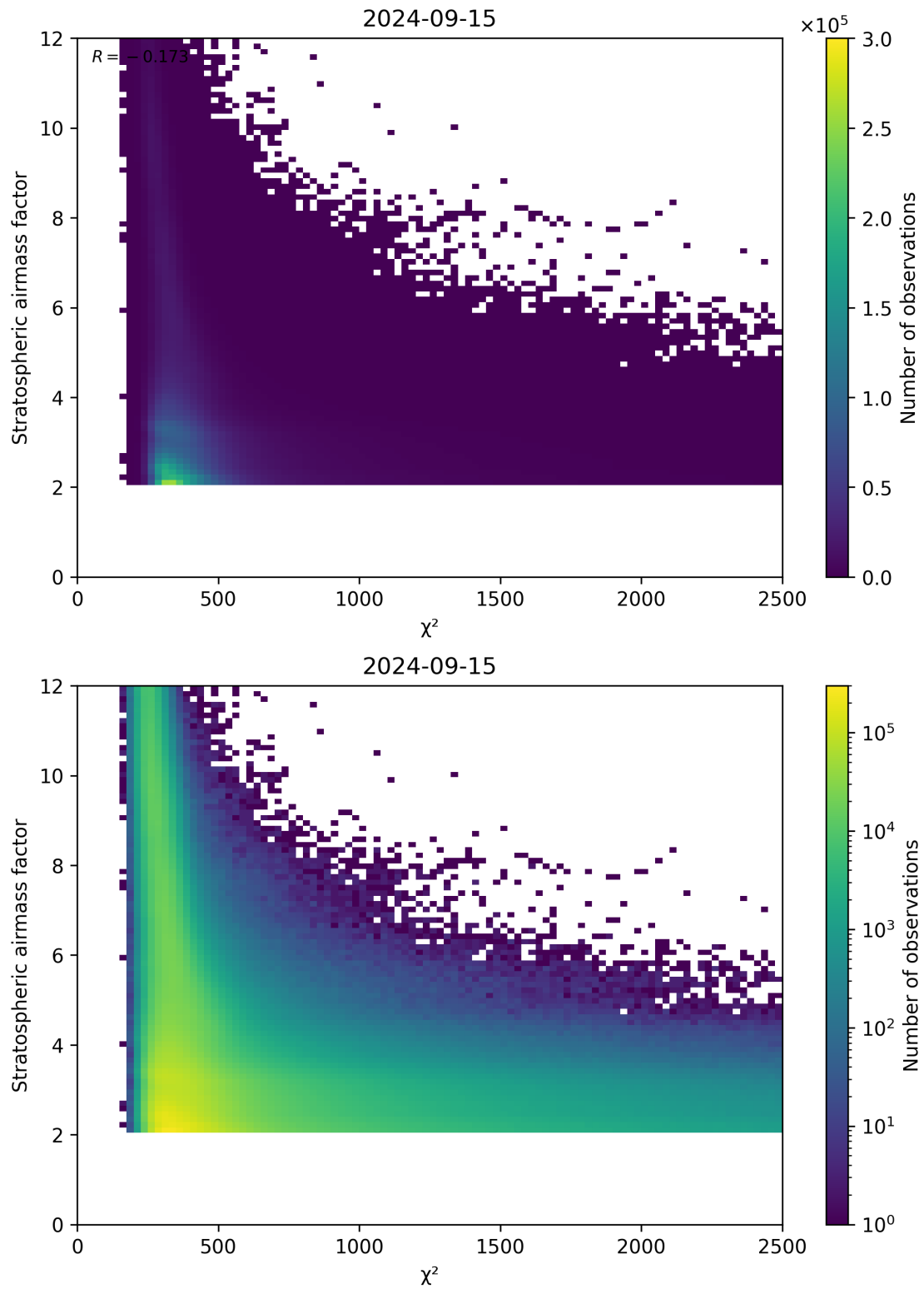
Figure 81: Scatter density plot of “ \chi^2 ” against “Stratospheric airmass factor” for 2024-09-14 to 2024-09-16.
