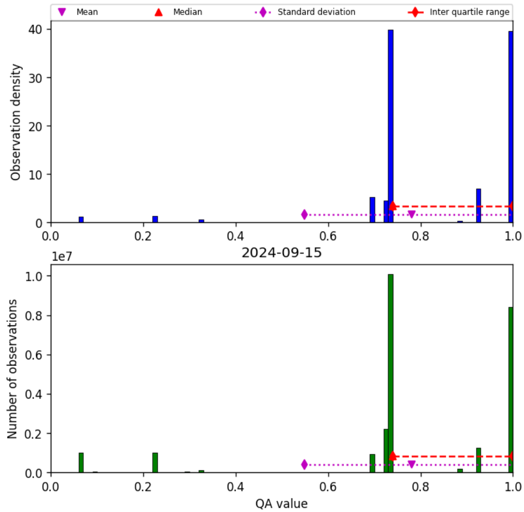
Figure 28: Histogram of “QA value” for 2024-09-14 to 2024-09-16
