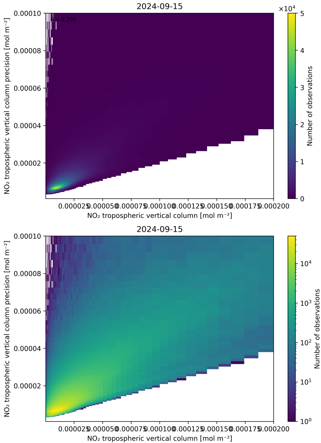
Figure 130: Scatter density plot of “NO 2 tropospheric vertical column” against “NO 2 tropospheric vertical column precision” for 2024-09-14 to 2024-09-16.
