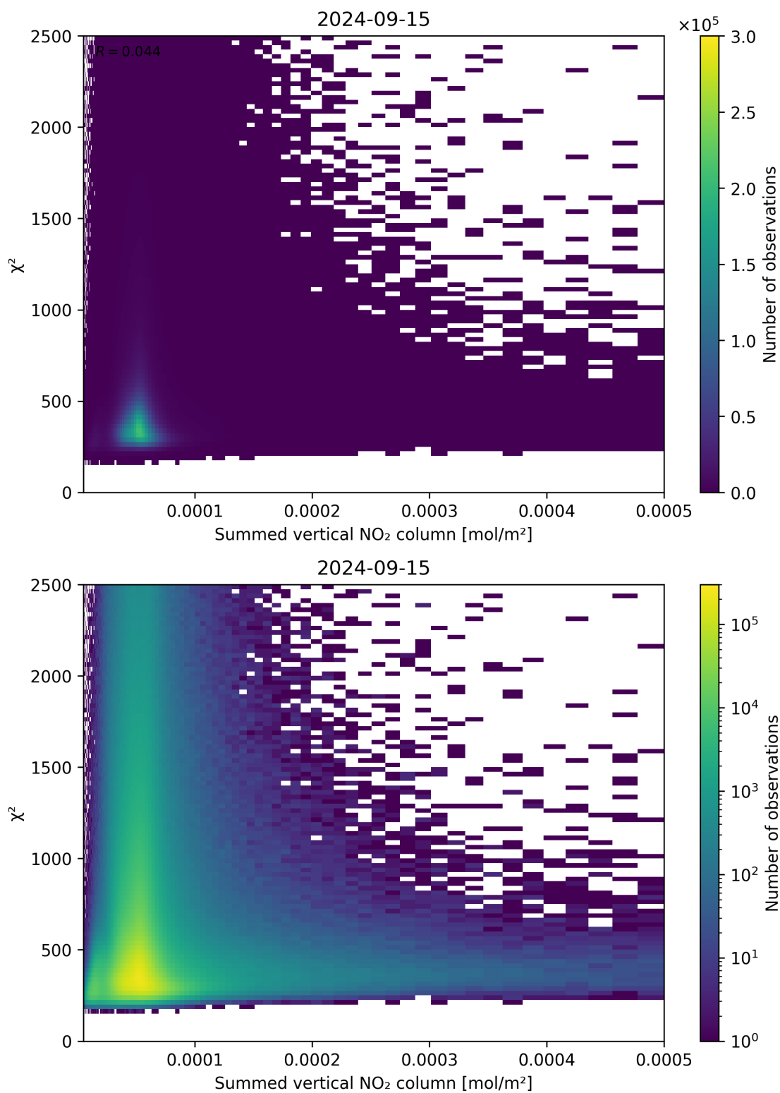
Figure 104: Scatter density plot of “Summed vertical NO 2 column” against “ \chi^2 ” for 2024-09-14 to 2024-09-16.
