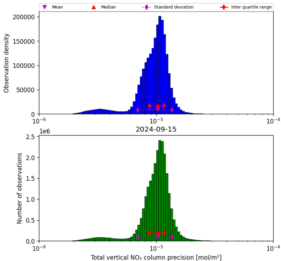
Figure 39: Histogram of “Total vertical NO 2 column precision” for 2024-09-14 to 2024-09-16
