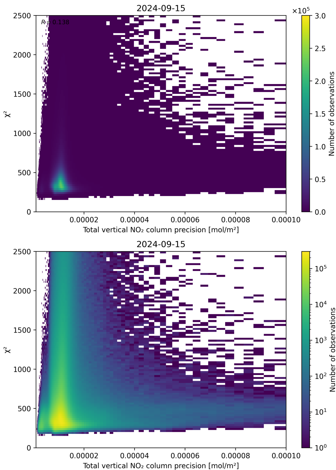
Figure 116: Scatter density plot of “Total vertical NO 2 column precision” against “ \chi^2 ” for 2024-09-14 to 2024-09-16.
