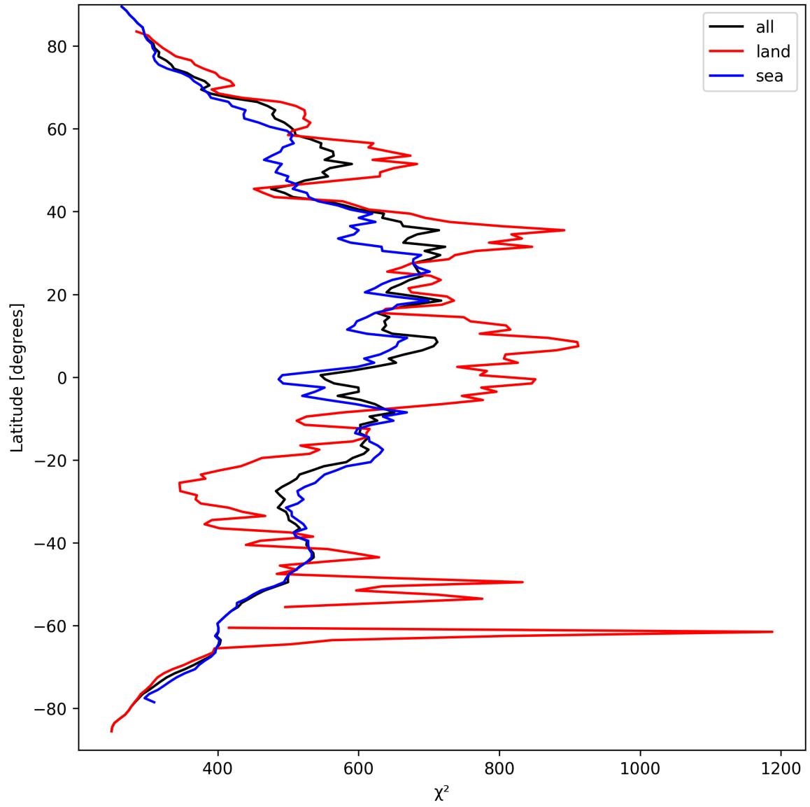
Figure 25: Zonal average of “ \chi^2 ” for 2024-09-14 to 2024-09-16.
