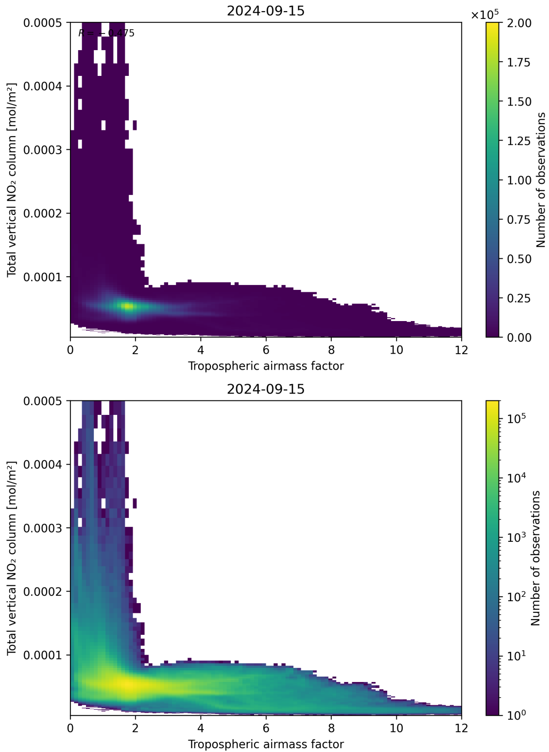
Figure 77: Scatter density plot of “Tropospheric airmass factor” against “Total vertical NO 2 column” for 2024-09-14 to 2024-09-16.
