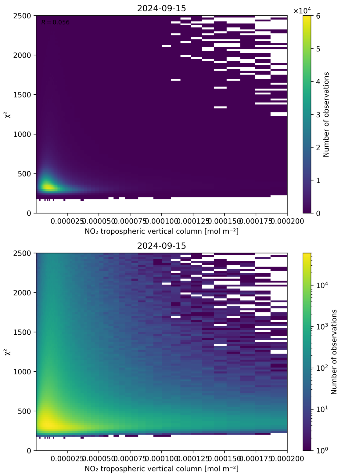
Figure 124: Scatter density plot of “NO 2 tropospheric vertical column” against “ \chi^2 ” for 2024-09-14 to 2024-09-16.
