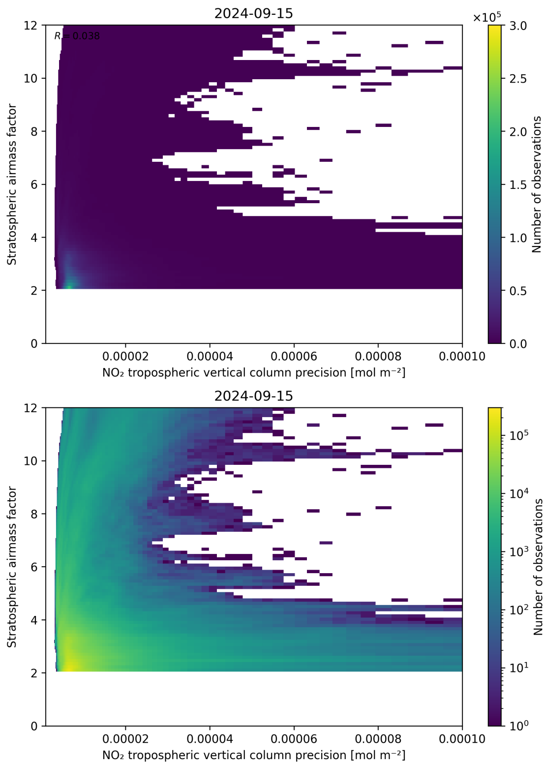
Figure 131: Scatter density plot of “NO 2 tropospheric vertical column precision” against “Stratospheric airmass factor” for 2024-09-14 to 2024-09-16.
