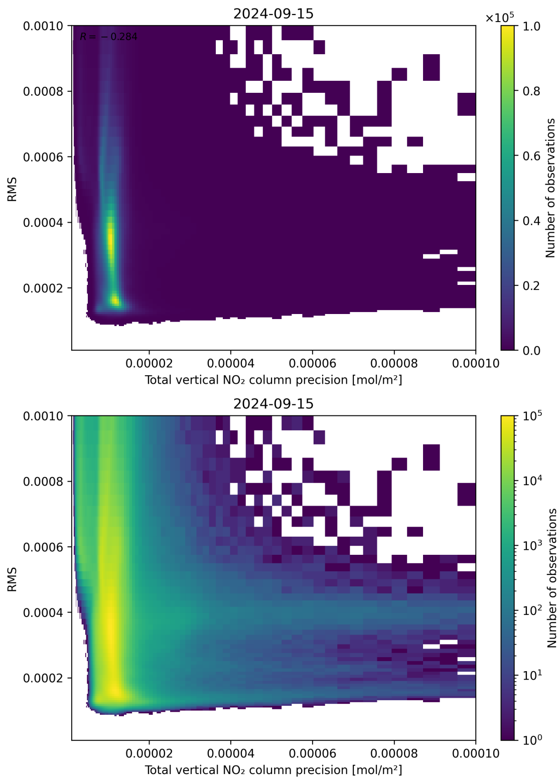
Figure 119: Scatter density plot of “Total vertical NO 2 column precision” against “RMS” for 2024-09-14 to 2024-09-16.
