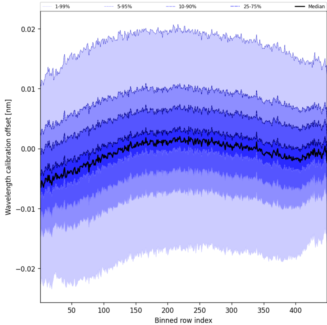
Figure 52: Along track statistics of “Wavelength calibration offset” for 2024-09-14 to 2024-09-16
