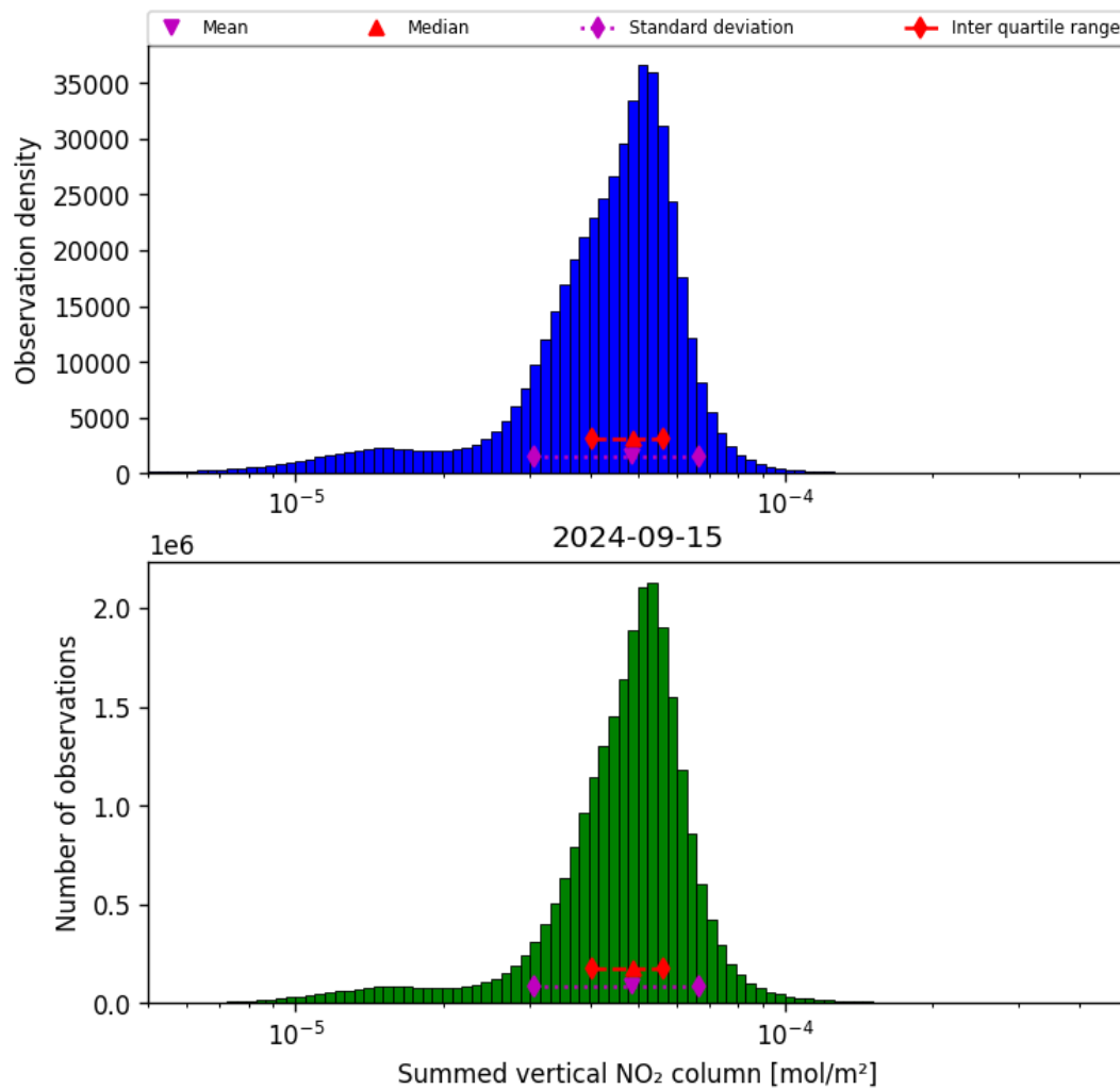
Figure 40: Histogram of “Summed vertical NO 2 column” for 2024-09-14 to 2024-09-16
