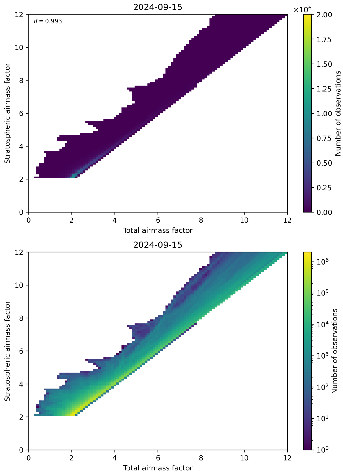
Figure 62: Scatter density plot of “Total airmass factor” against “Stratospheric airmass factor” for 2024-09-14 to 2024-09-16.
