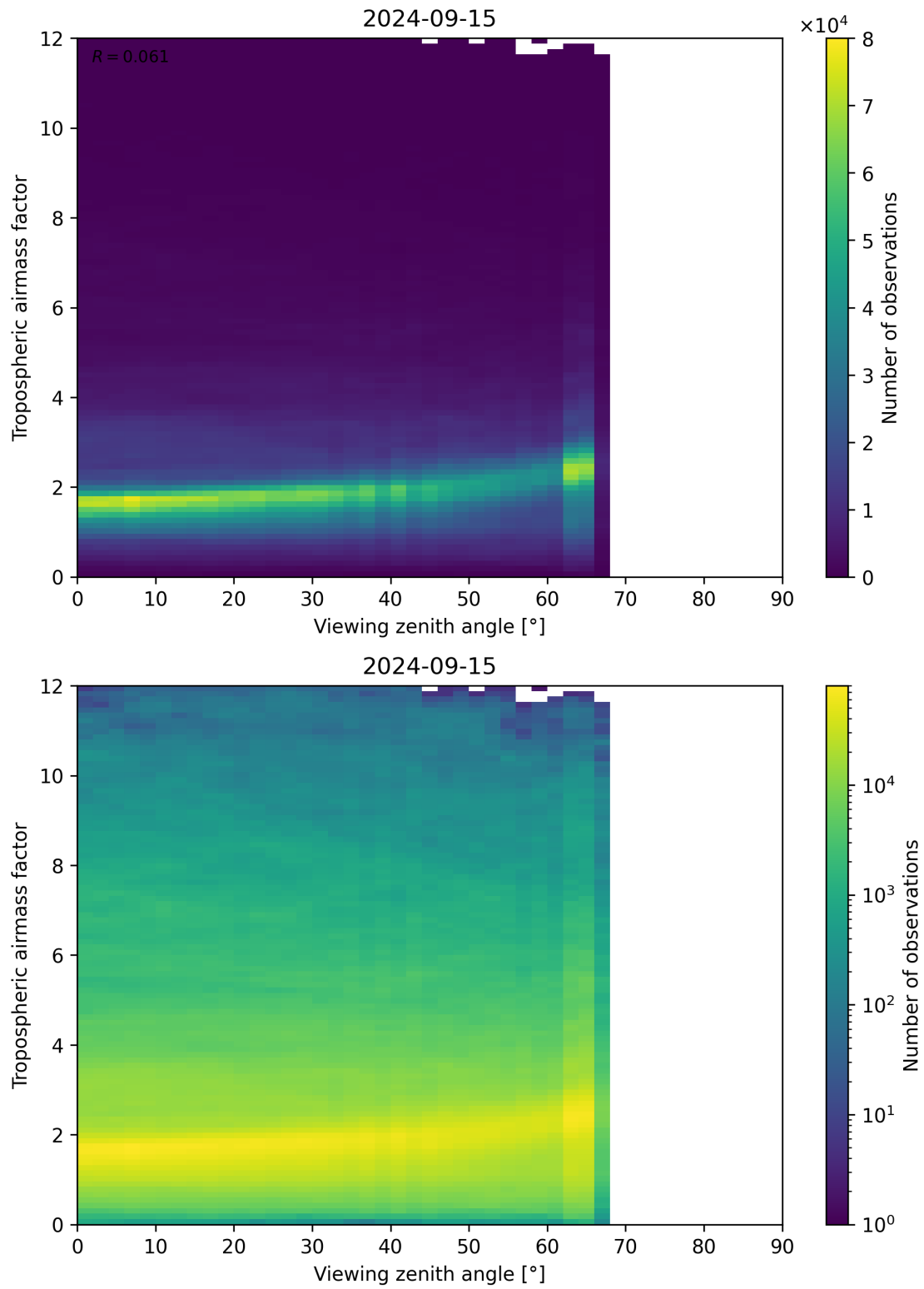
Figure 161: Scatter density plot of “Viewing zenith angle” against “Tropospheric airmass factor” for 2024-09-14 to 2024-09-16.
