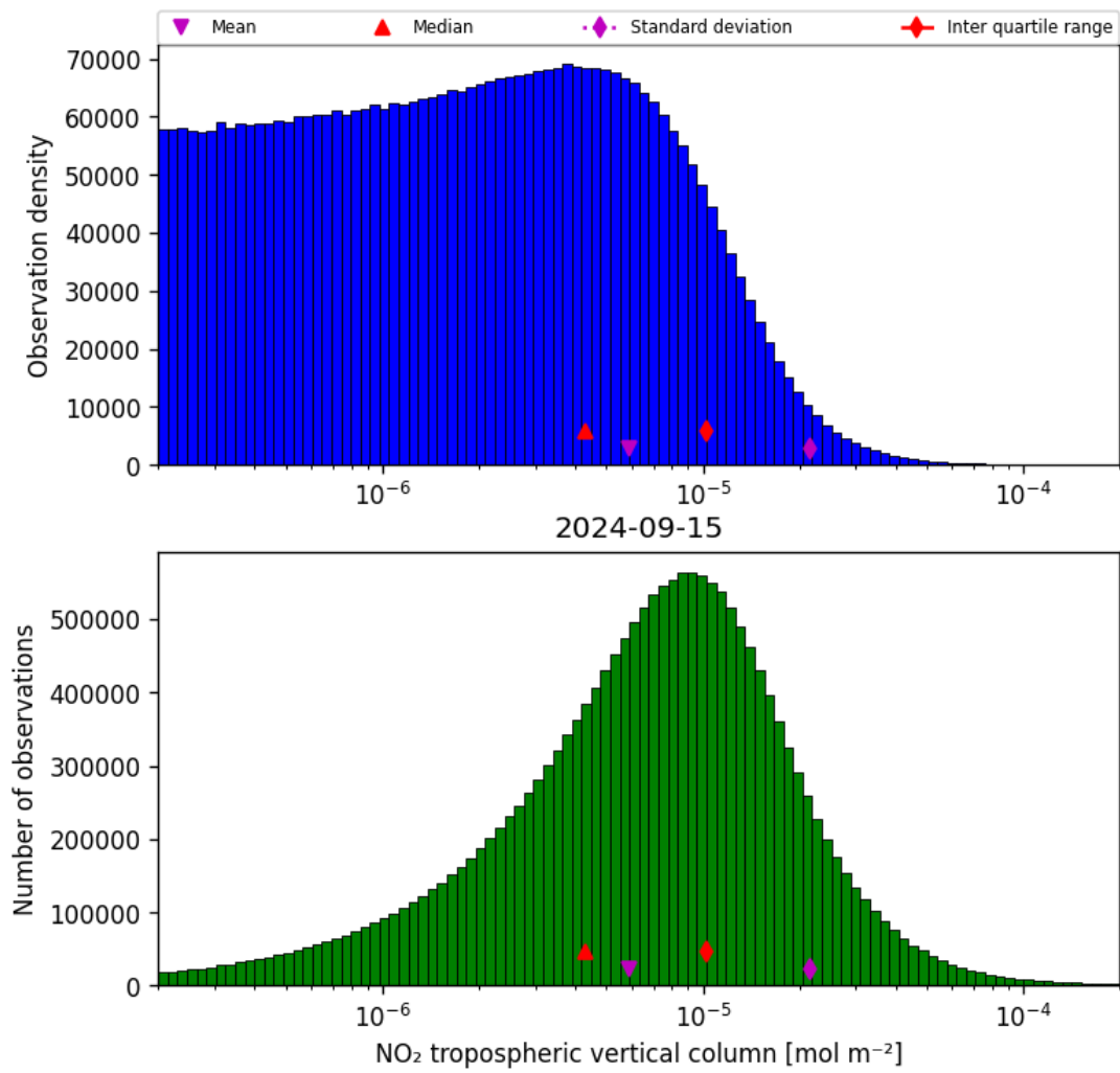
Figure 29: Histogram of “NO 2 tropospheric vertical column” for 2024-09-14 to 2024-09-16
