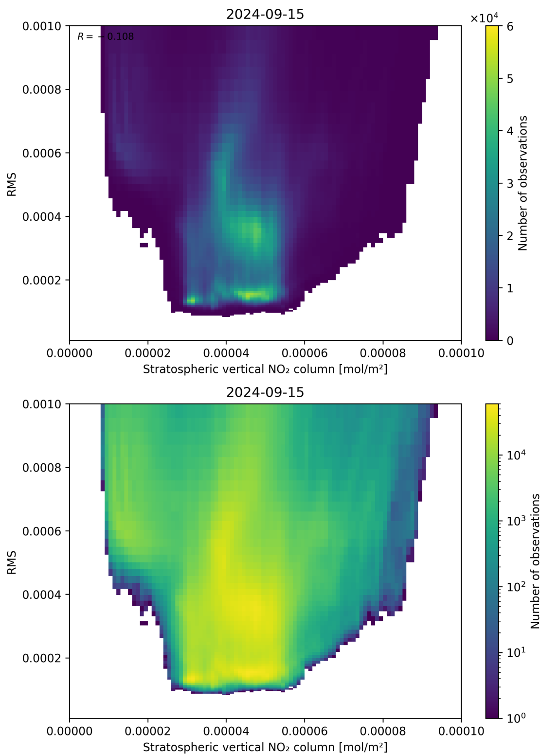
Figure 102: Scatter density plot of “Stratospheric vertical NO 2 column” against “RMS” for 2024-09-14 to 2024-09-16.
