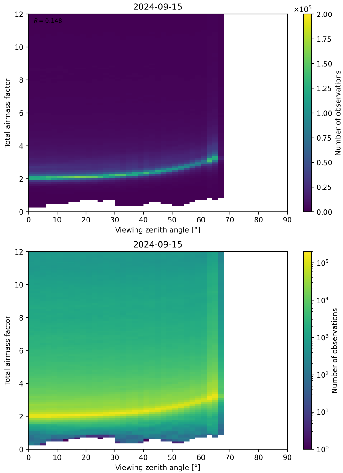
Figure 160: Scatter density plot of “Viewing zenith angle” against “Total airmass factor” for 2024-09-14 to 2024-09-16.
