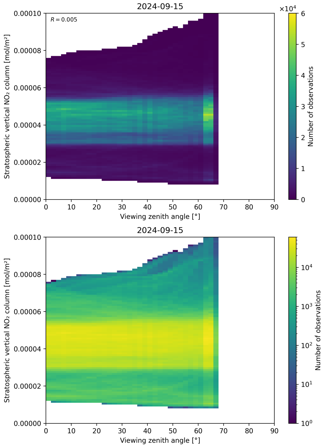
Figure 164: Scatter density plot of “Viewing zenith angle” against “Stratospheric vertical NO 2 column” for 2024-09-14 to 2024-09-16.
