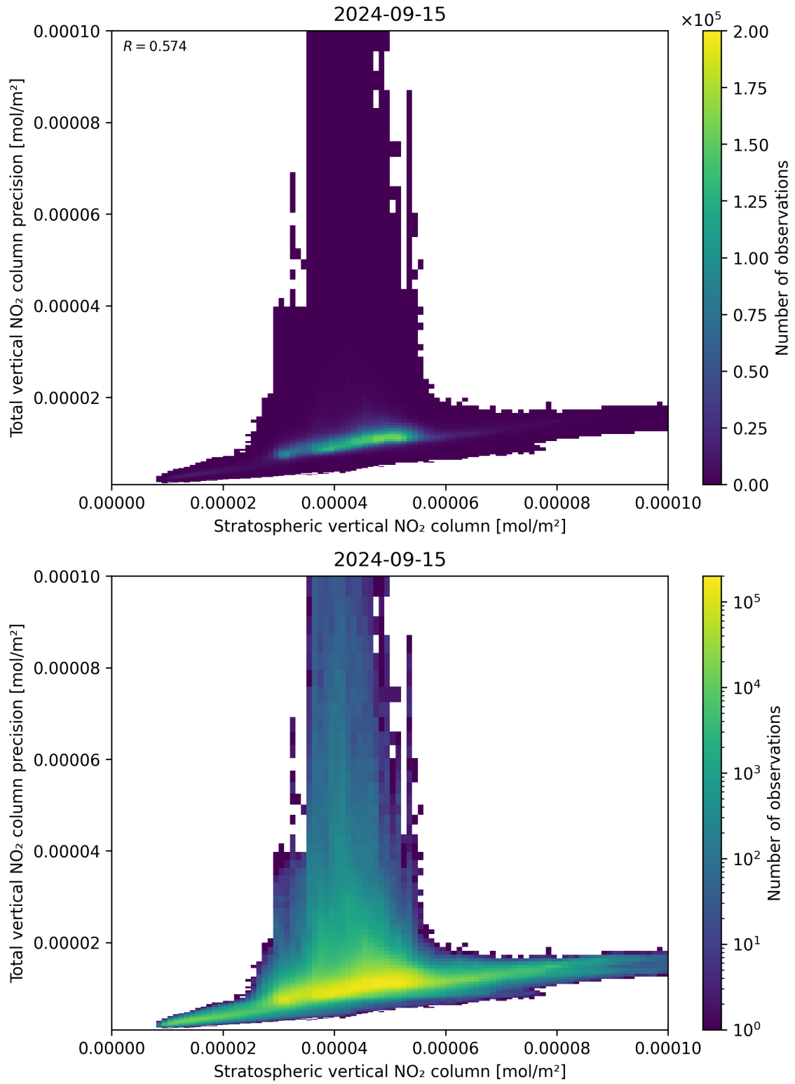
Figure 101: Scatter density plot of “Stratospheric vertical NO 2 column” against “Total vertical NO 2 column precision” for 2024-09-14 to 2024-09-16.
