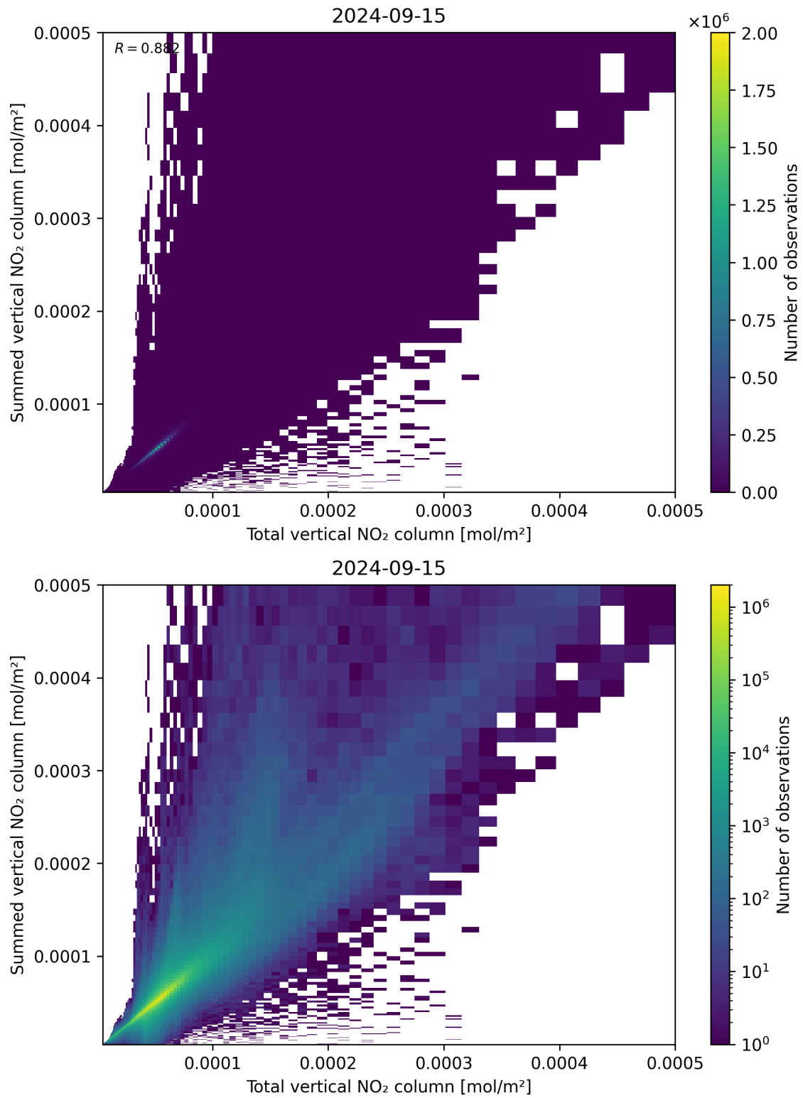
Figure 112: Scatter density plot of “Total vertical NO 2 column” against “Summed vertical NO 2 column” for 2024-09-14 to 2024-09-16.
