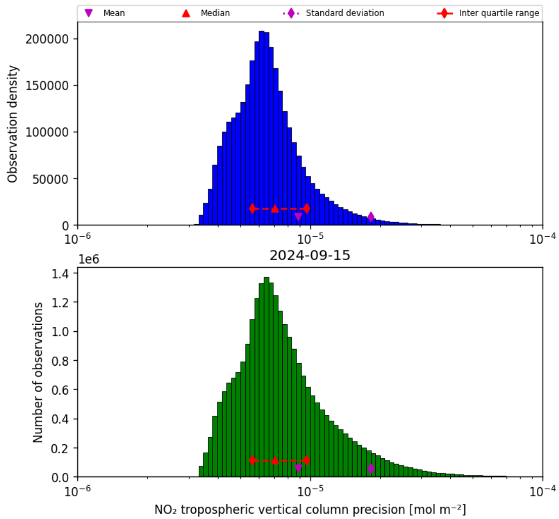
Figure 30: Histogram of “NO 2 tropospheric vertical column precision” for 2024-09-14 to 2024-09-16
