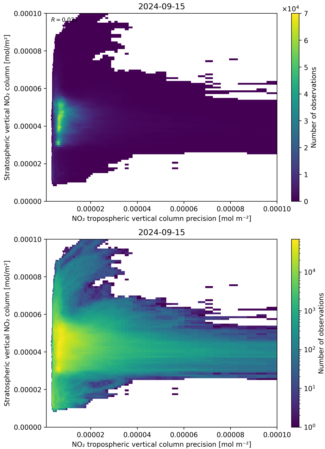
Figure 135: Scatter density plot of “NO 2 tropospheric vertical column precision” against “Stratospheric vertical NO 2 column” for 2024-09-14 to 2024-09-16.
