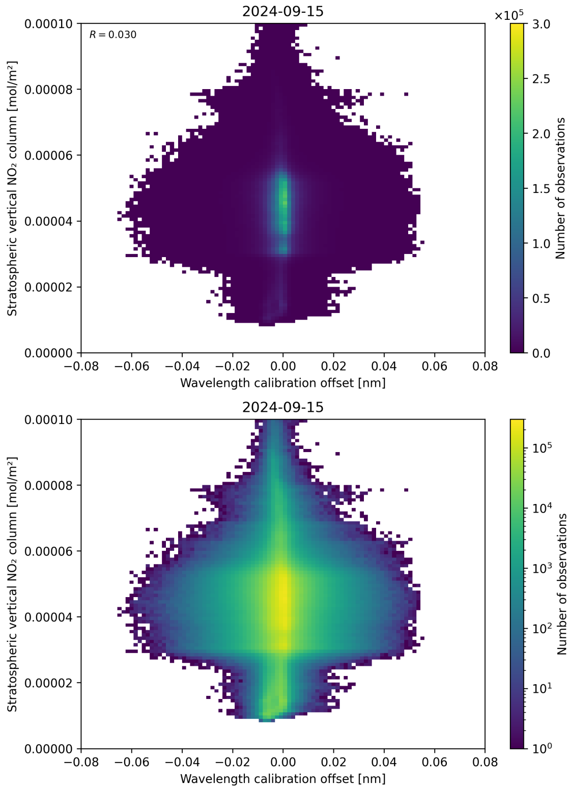
Figure 176: Scatter density plot of “Wavelength calibration offset” against “Stratospheric vertical NO 2 column” for 2024-09-14 to 2024-09-16.
