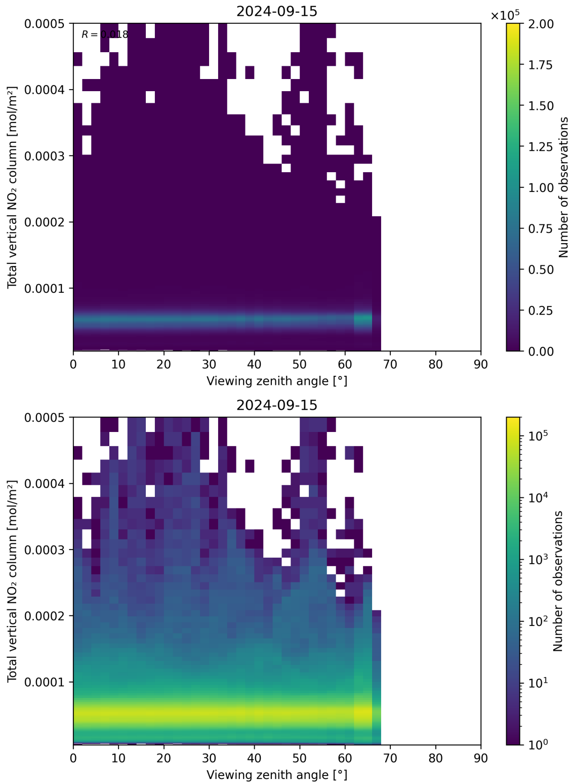
Figure 167: Scatter density plot of “Viewing zenith angle” against “Total vertical NO 2 column” for 2024-09-14 to 2024-09-16.
