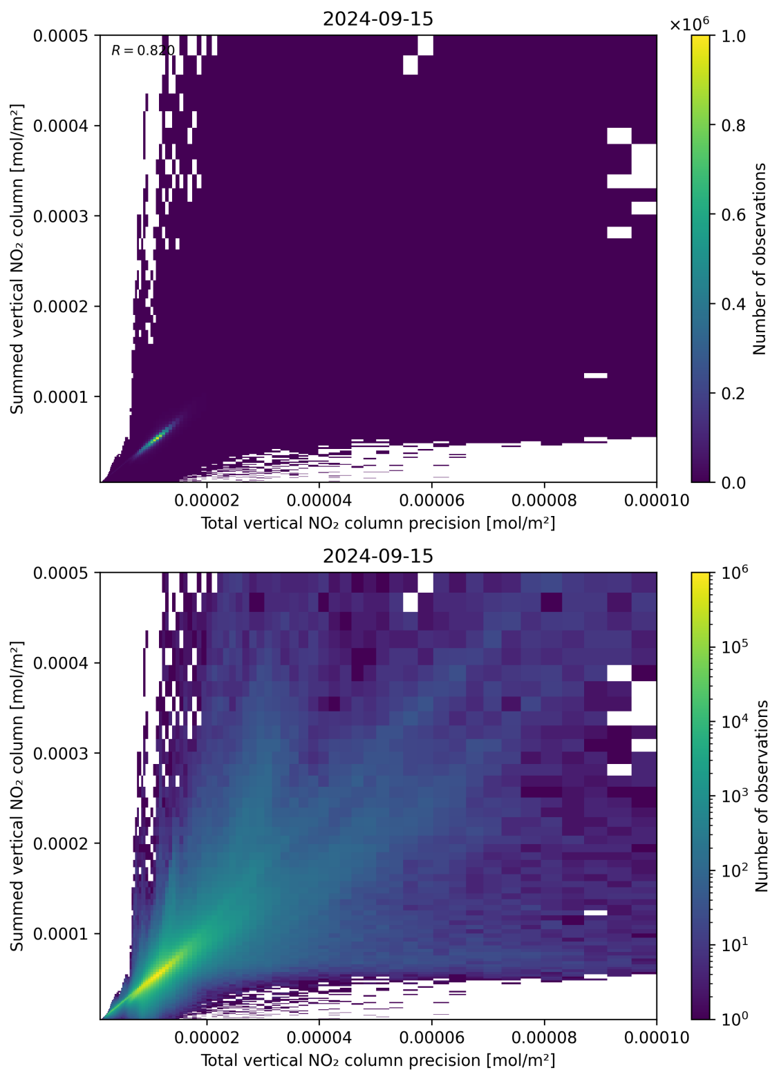
Figure 117: Scatter density plot of “Total vertical NO 2 column precision” against “Summed vertical NO 2 column” for 2024-09-14 to 2024-09-16.
