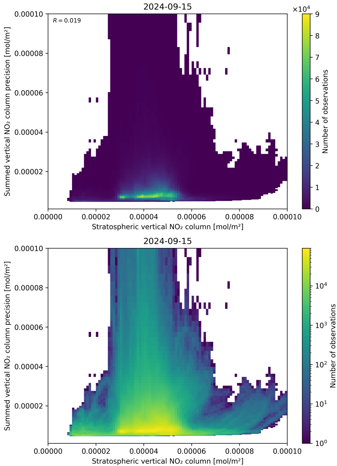
Figure 99: Scatter density plot of “Stratospheric vertical NO 2 column” against “Summed vertical NO 2 column precision” for 2024-09-14 to 2024-09-16.
