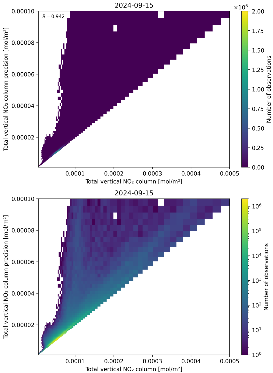
Figure 114: Scatter density plot of “Total vertical NO 2 column” against “Total vertical NO 2 column precision” for 2024-09-14 to 2024-09-16.
