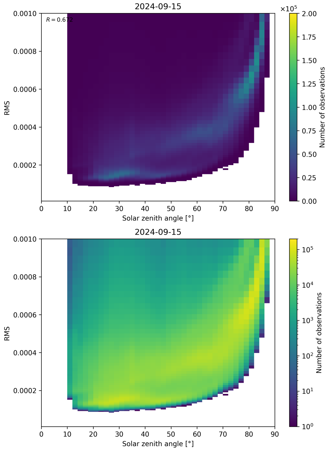
Figure 157: Scatter density plot of “Solar zenith angle” against “RMS” for 2024-09-14 to 2024-09-16.
