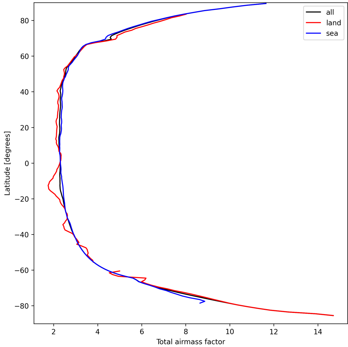
Figure 15: Zonal average of “Total airmass factor” for 2024-09-14 to 2024-09-16.
