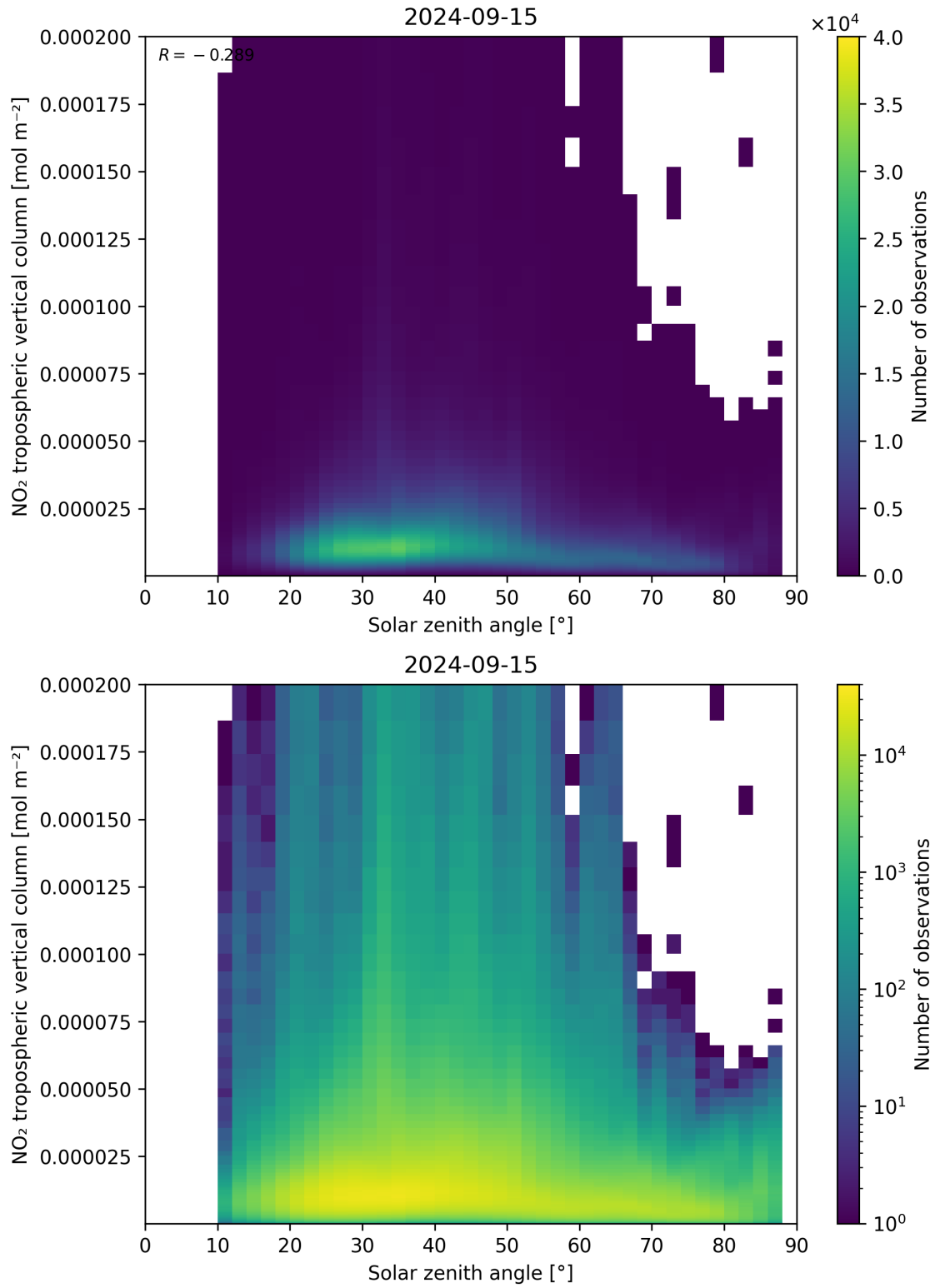
Figure 155: Scatter density plot of “Solar zenith angle” against “NO 2 tropospheric vertical column” for 2024-09-14 to 2024-09-16.
