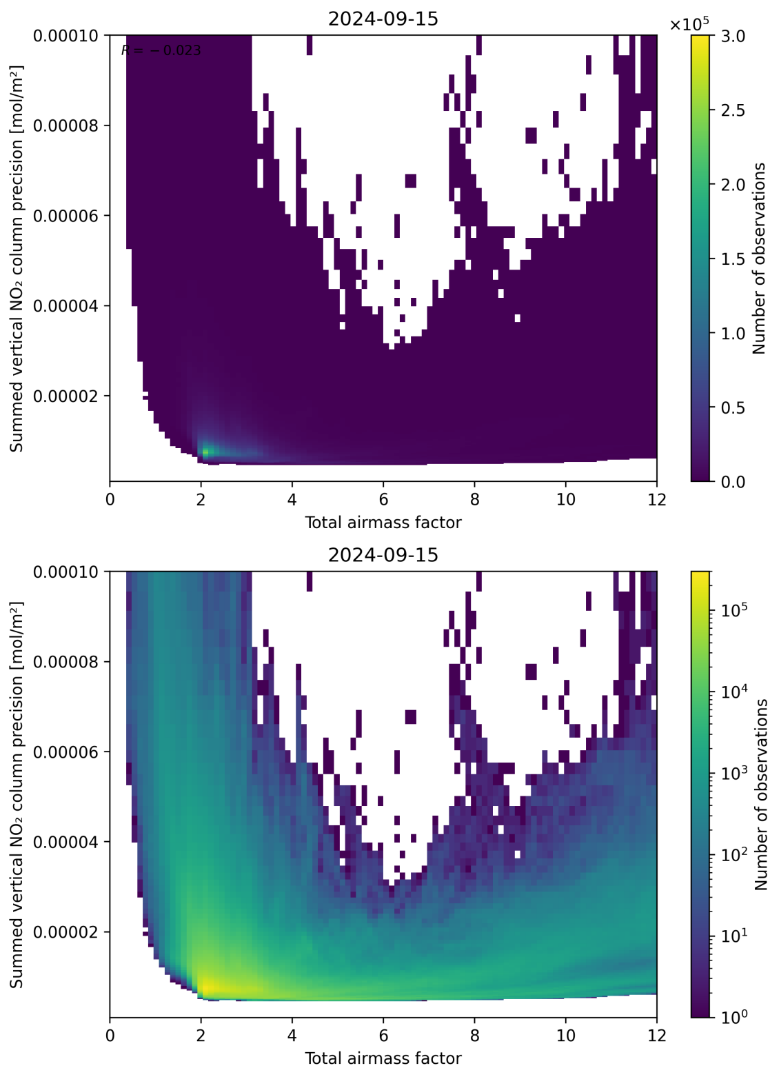
Figure 66: Scatter density plot of “Total airmass factor” against “Summed vertical NO 2 column precision” for 2024-09-14 to 2024-09-16.
