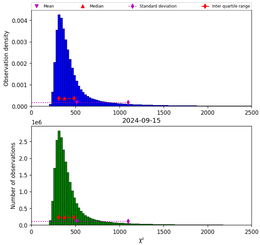
Figure 42: Histogram of “ \chi^2 ” for 2024-09-14 to 2024-09-16
