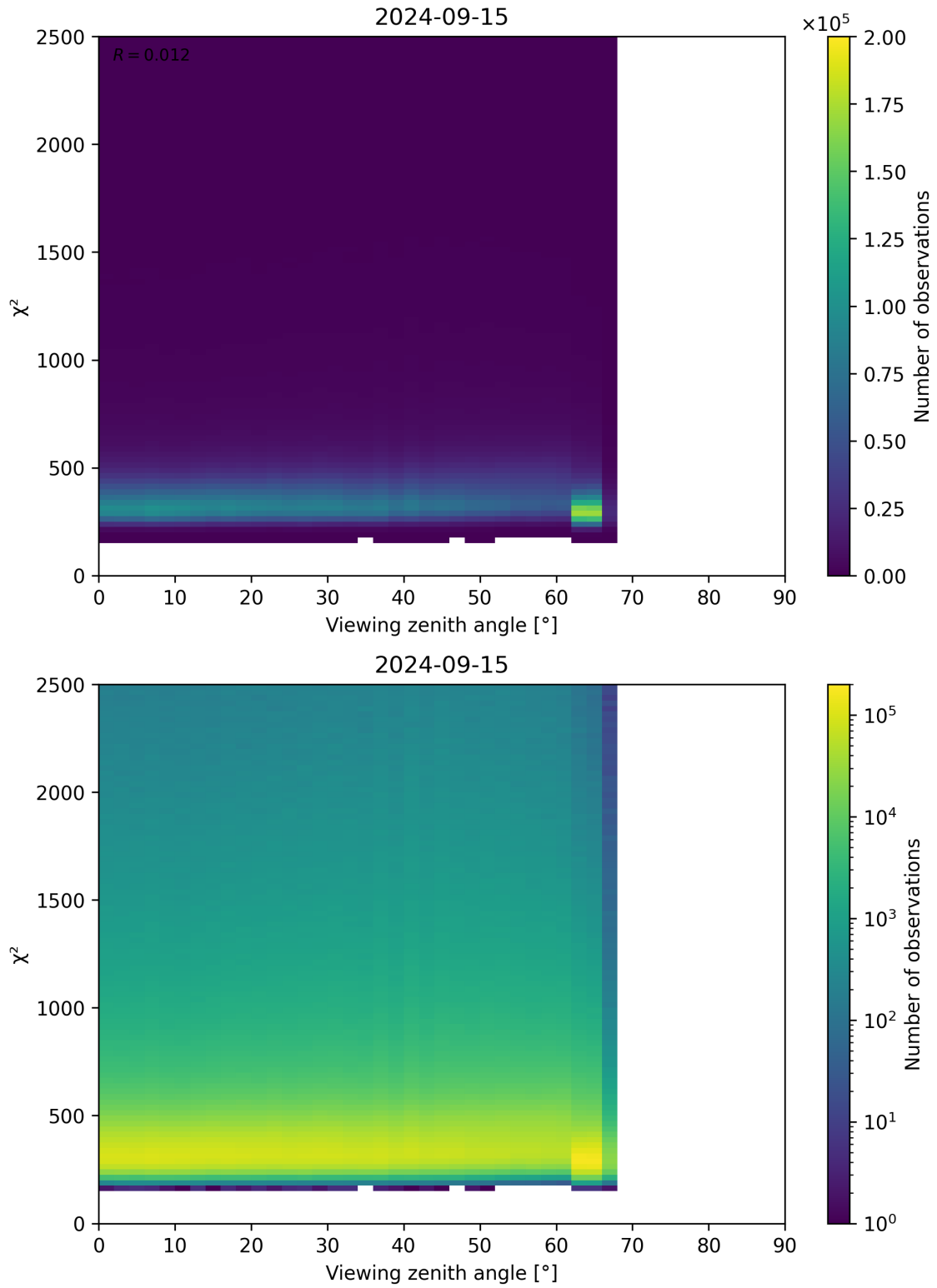
Figure 162: Scatter density plot of “Viewing zenith angle” against “ \chi^2 ” for 2024-09-14 to 2024-09-16.
