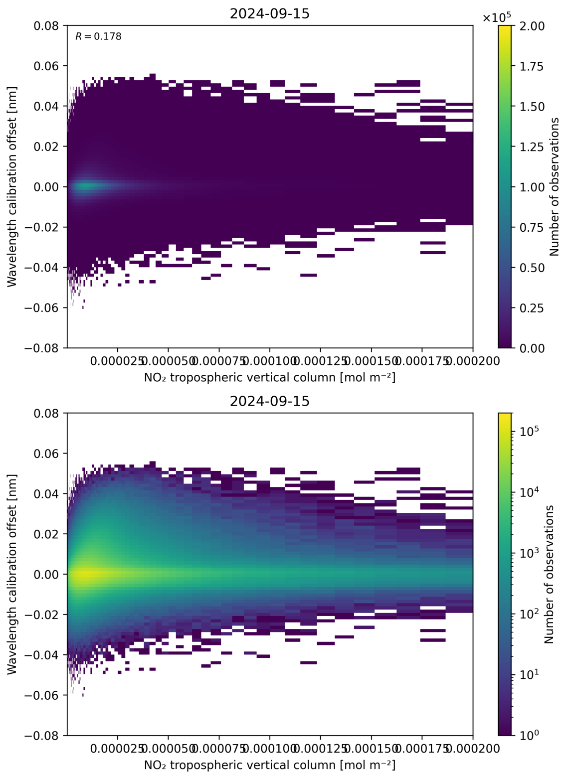
Figure 143: Scatter density plot of “NO 2 tropospheric vertical column” against “Wavelength calibration offset” for 2024-09-14 to 2024-09-16.
