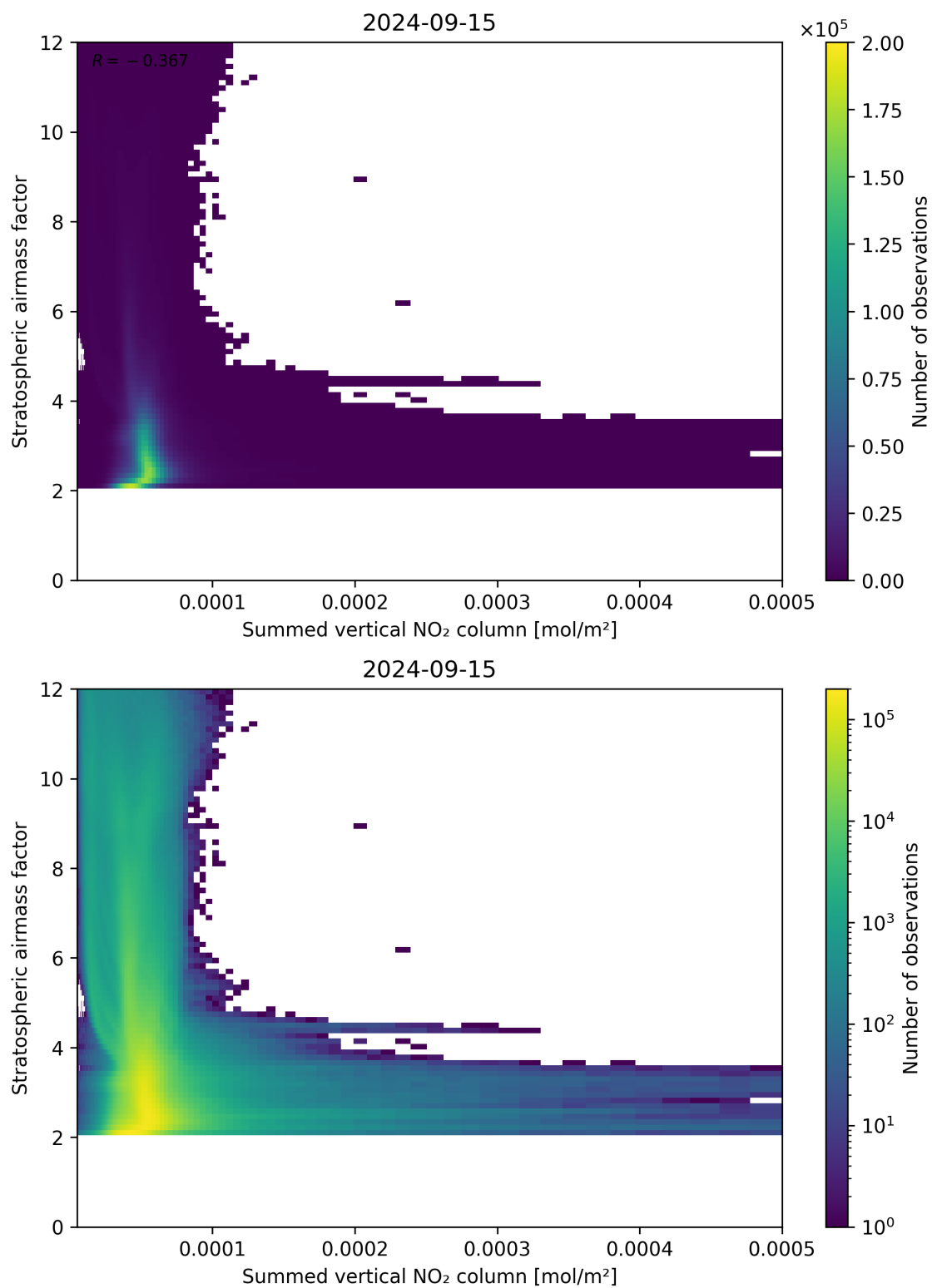
Figure 103: Scatter density plot of “Summed vertical NO 2 column” against “Stratospheric airmass factor” for 2024-09-14 to 2024-09-16.
