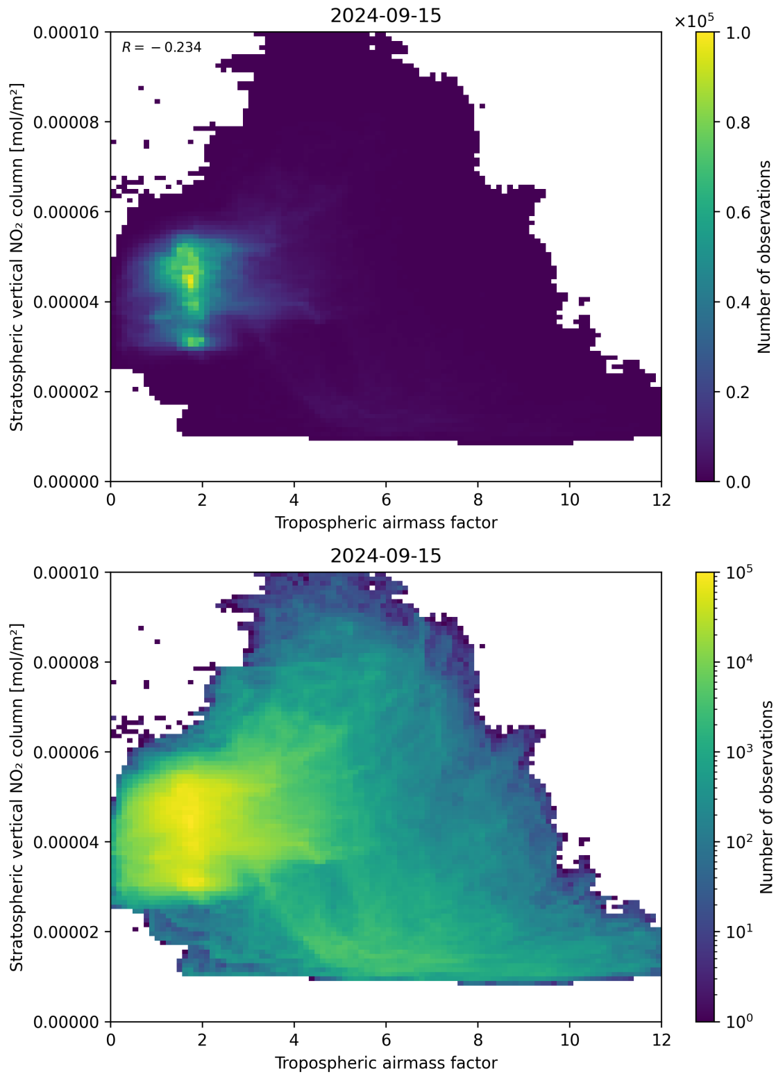
Figure 74: Scatter density plot of “Tropospheric air mass factor” against “Stratospheric vertical NO 2 column” for 2024-09-14 to 2024-09-16.
