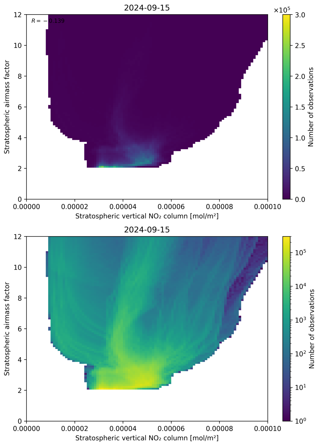
Figure 96: Scatter density plot of “Stratospheric vertical NO 2 column” against “Stratospheric airmass factor” for 2024-09-14 to 2024-09-16.
