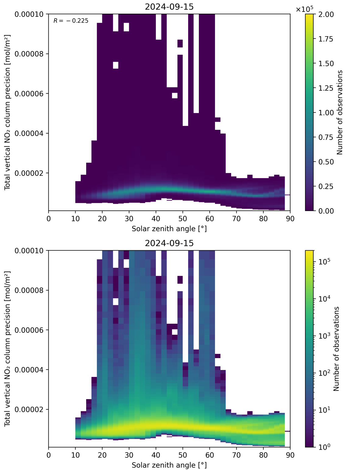
Figure 154: Scatter density plot of “Solar zenith angle” against “Total vertical NO 2 column precision” for 2024-09-14 to 2024-09-16.
