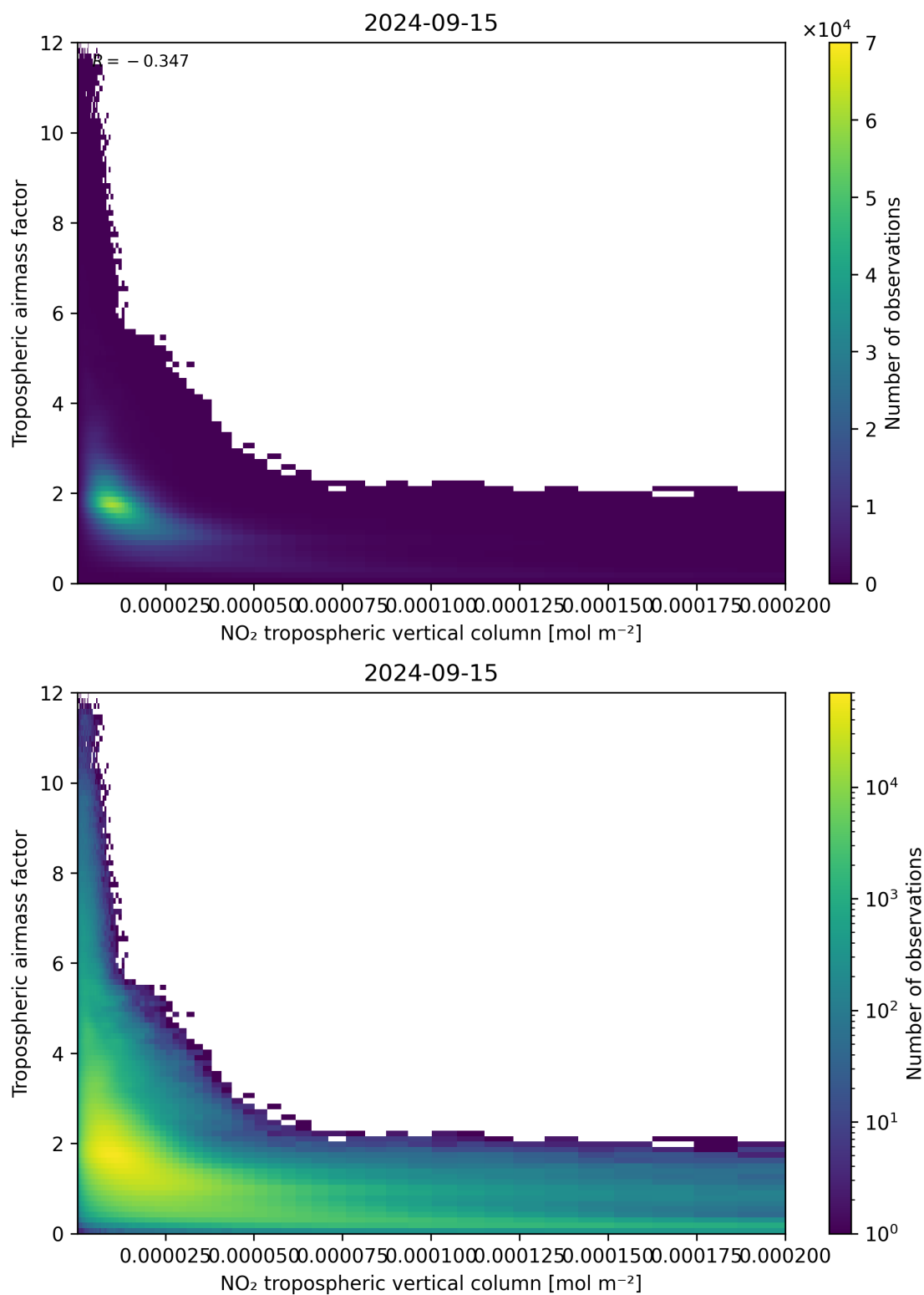
Figure 123: Scatter density plot of “NO 2 tropospheric vertical column” against “Tropospheric air mass factor” for 2024-09-14 to 2024-09-16.
