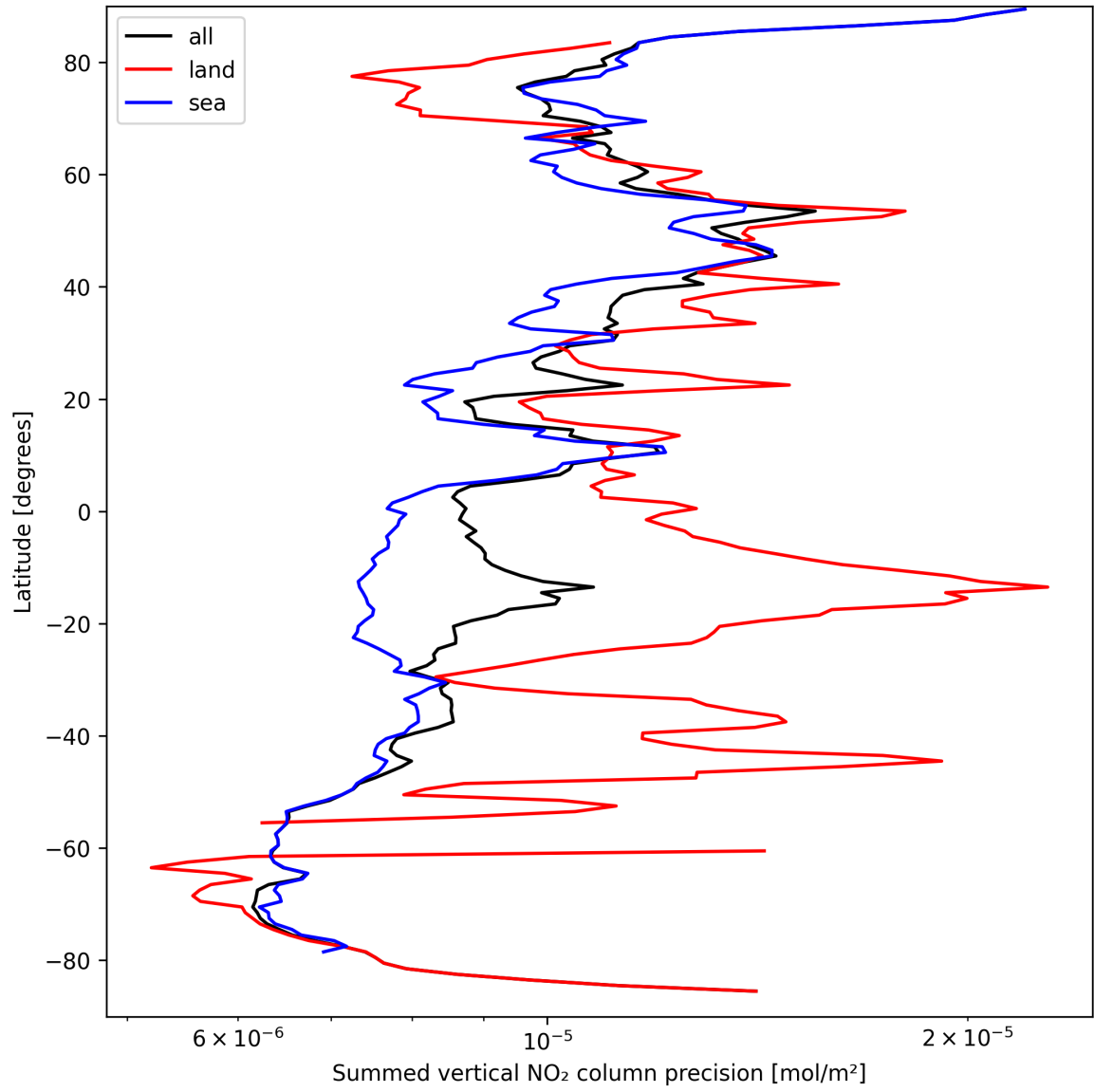
Figure 24: Zonal average of “Summed vertical NO 2 column precision” for 2024-09-14 to 2024-09-16.
