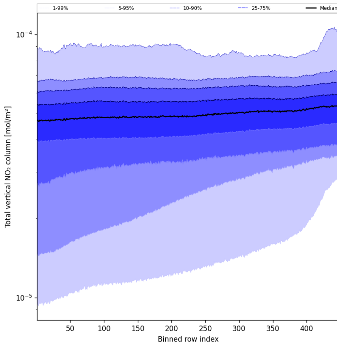
Figure 55: Along track statistics of “Total vertical NO 2 column” for 2024-09-14 to 2024-09-16
