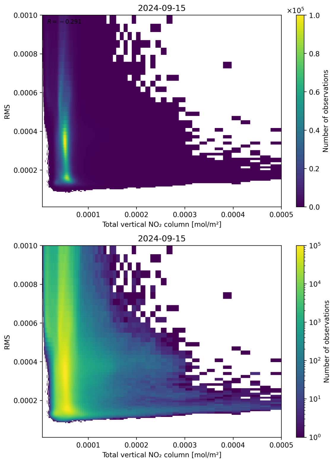
Figure 120: Scatter density plot of “Total vertical NO 2 column” against “RMS” for 2024-09-14 to 2024-09-16.
