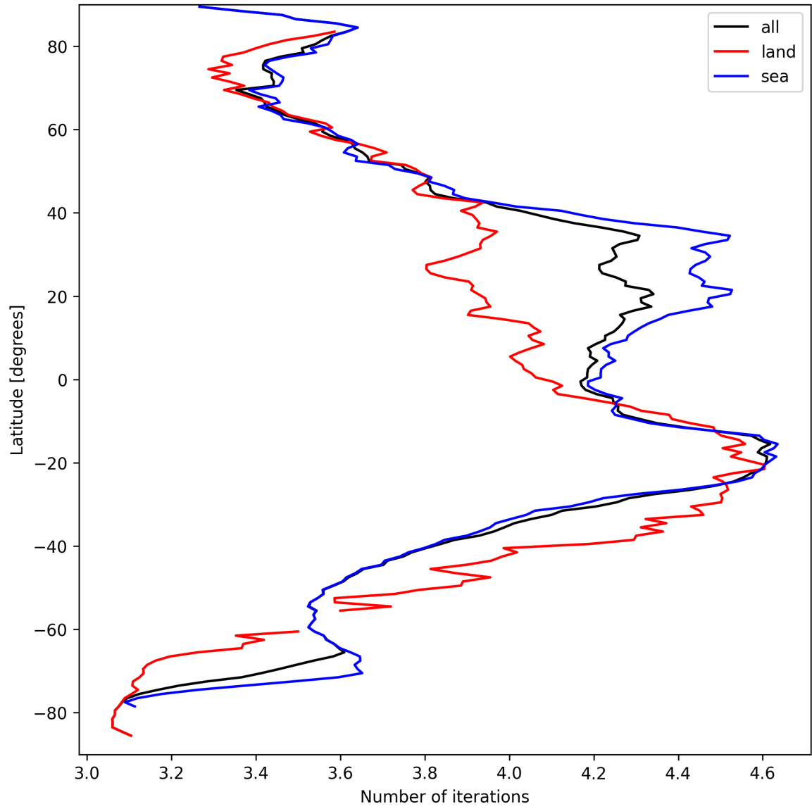
Figure 17: Zonal average of “Number of iterations” for 2024-09-14 to 2024-09-16.
