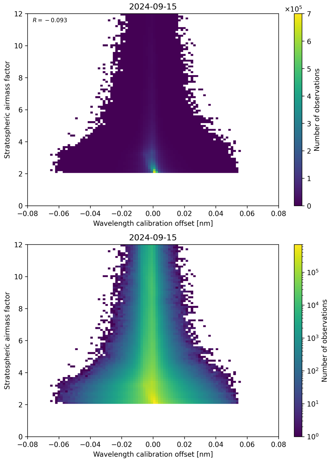
Figure 174: Scatter density plot of “Wavelength calibration offset” against “Stratospheric air mass factor” for 2024-09-14 to 2024-09-16.
