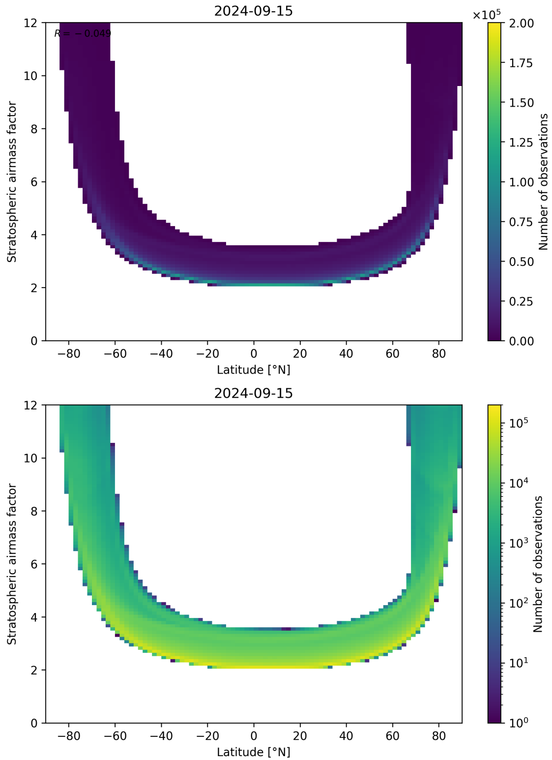
Figure 83: Scatter density plot of “Latitude” against “Stratospheric air mass factor” for 2024-09-14 to 2024-09-16.
