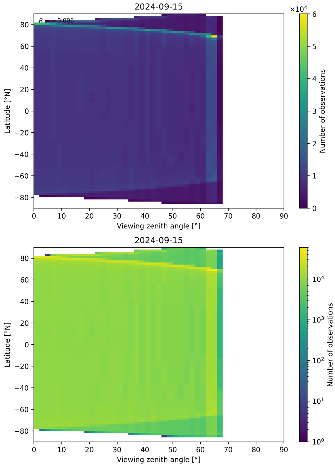
Figure 163: Scatter density plot of “Viewing zenith angle” against “Latitude” for 2024-09-14 to 2024-09-16.
