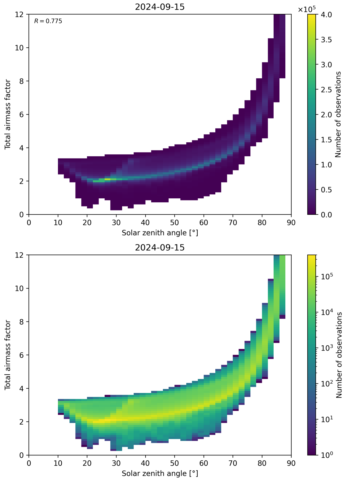
Figure 146: Scatter density plot of “Solar zenith angle” against “Total air mass factor” for 2024-09-14 to 2024-09-16.
