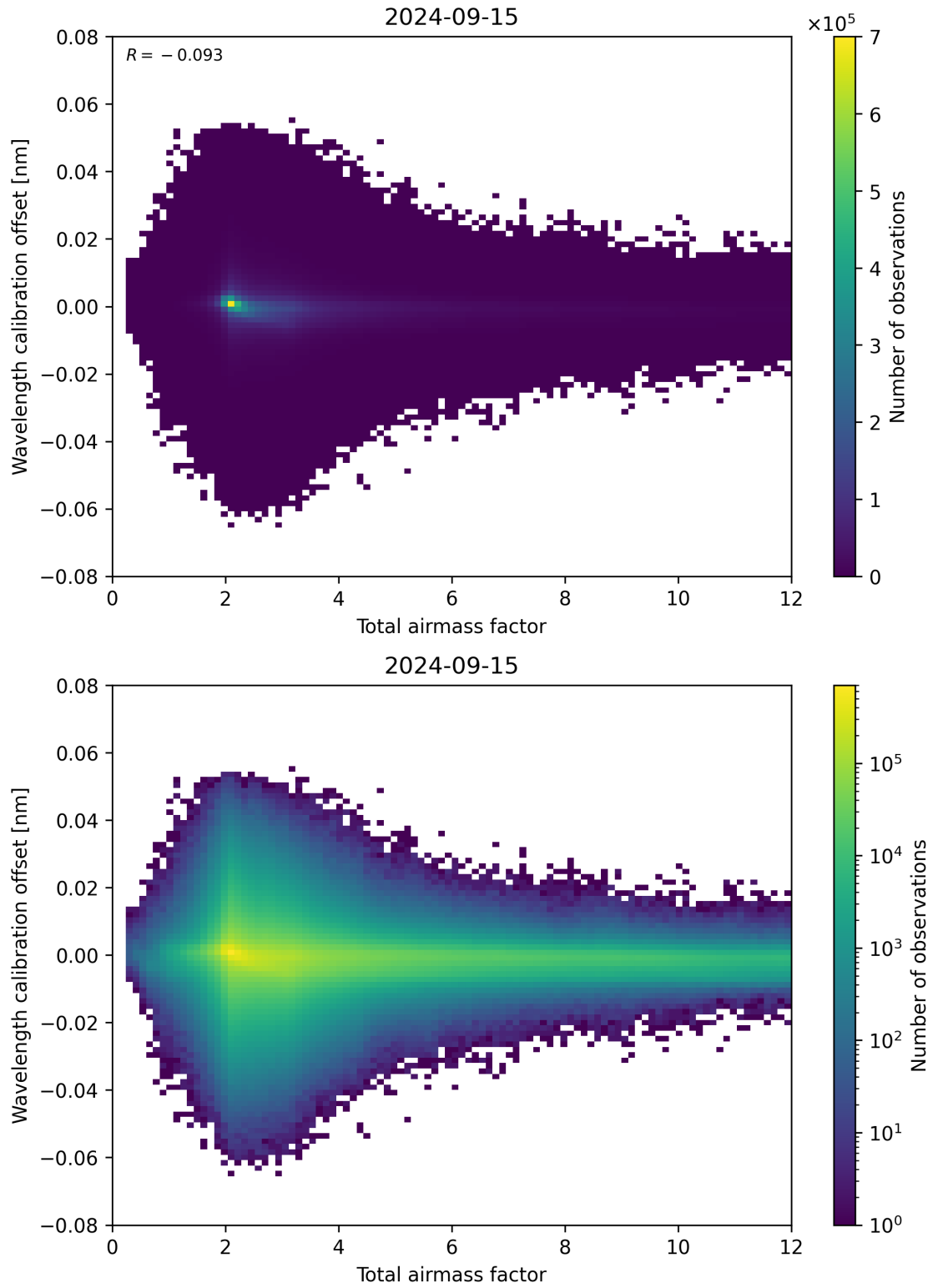
Figure 70: Scatter density plot of “Total airmass factor” against “Wavelength calibration offset” for 2024-09-14 to 2024-09-16.
