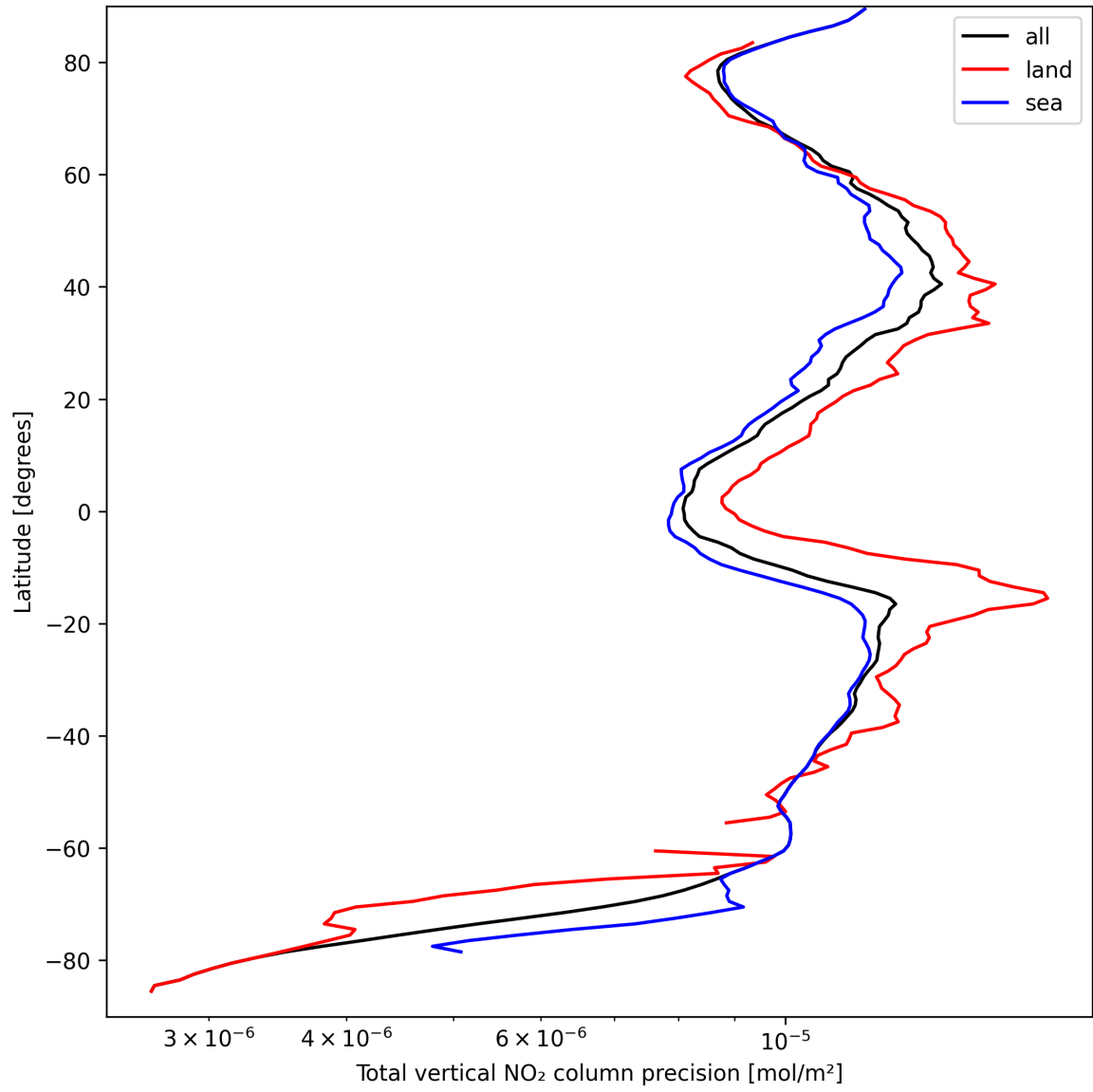
Figure 22: Zonal average of “Total vertical NO 2 column precision” for 2024-09-14 to 2024-09-16.
