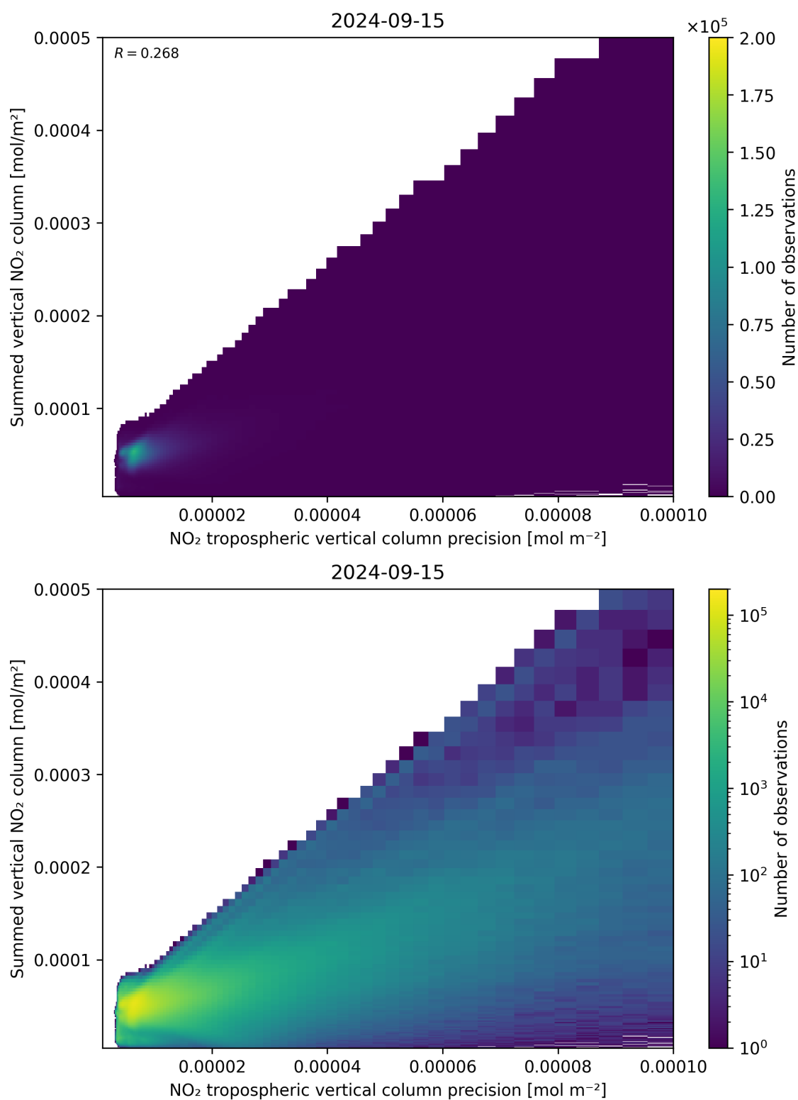
Figure 136: Scatter density plot of “NO 2 tropospheric vertical column precision” against “Summed vertical NO 2 column” for 2024-09-14 to 2024-09-16.
