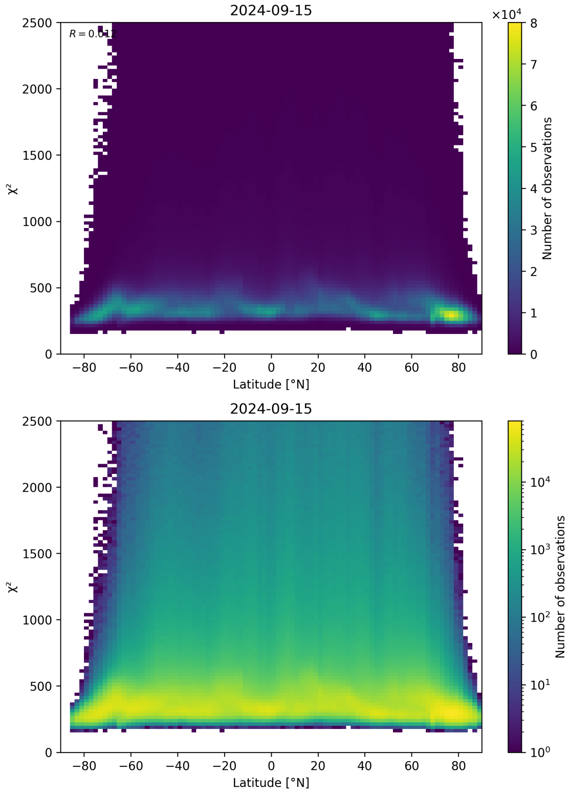
Figure 86: Scatter density plot of “Latitude” against “ \chi^2 ” for 2024-09-14 to 2024-09-16.
