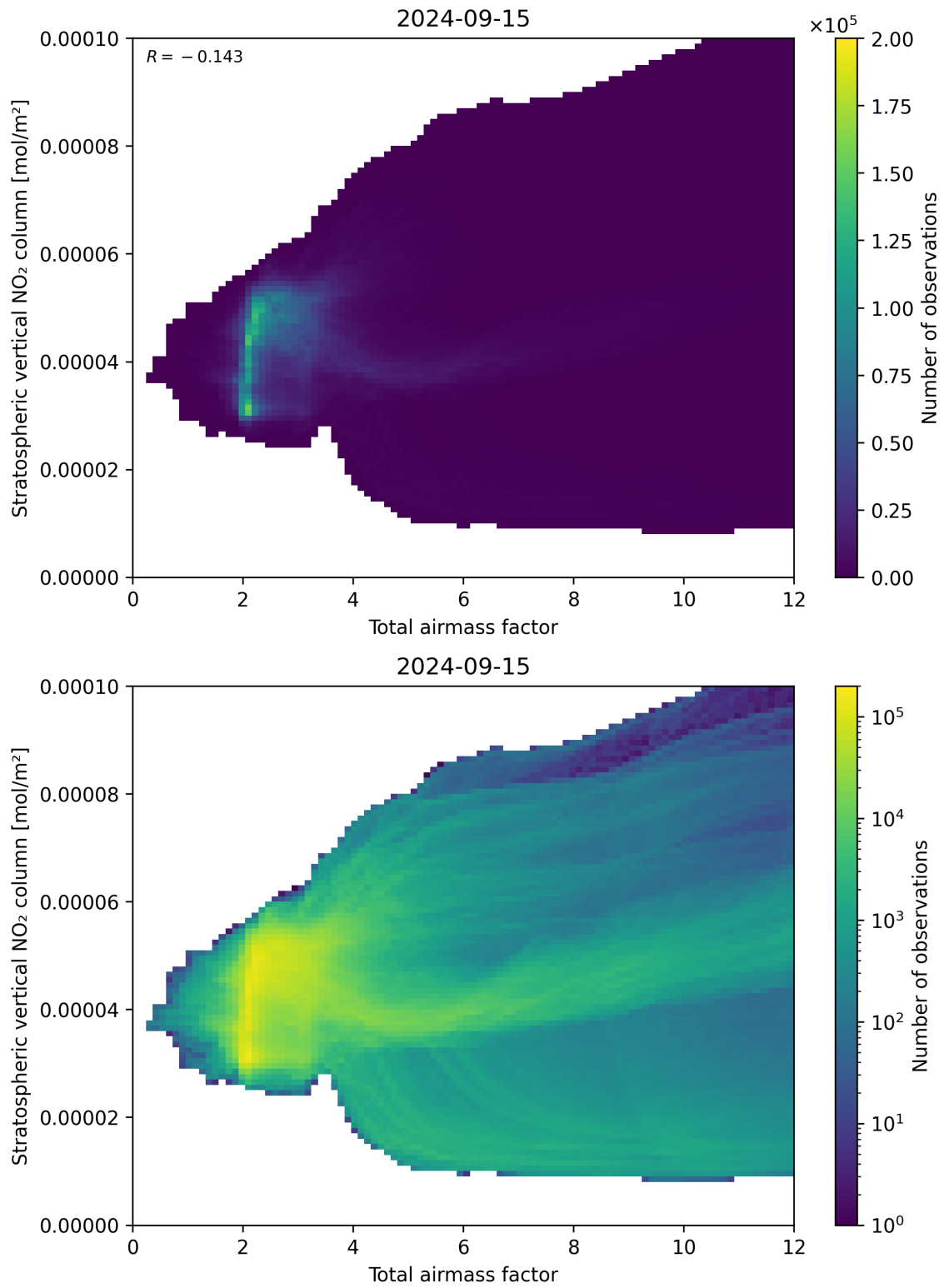
Figure 64: Scatter density plot of “Total airmass factor” against “Stratospheric vertical NO 2 column” for 2024-09-14 to 2024-09-16.
