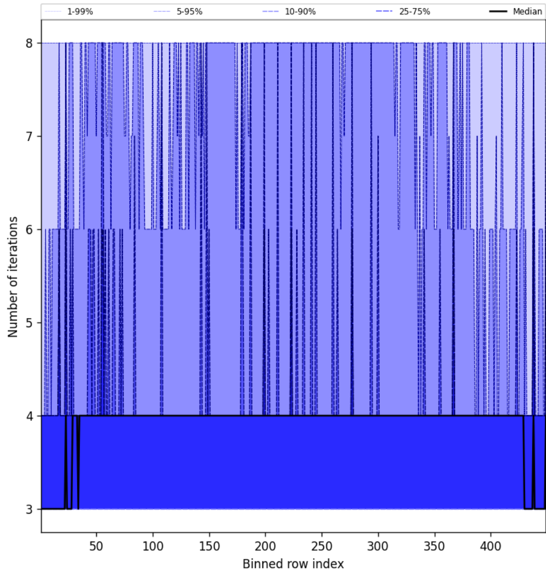
Figure 51: Along track statistics of “Number of iterations” for 2024-09-14 to 2024-09-16
