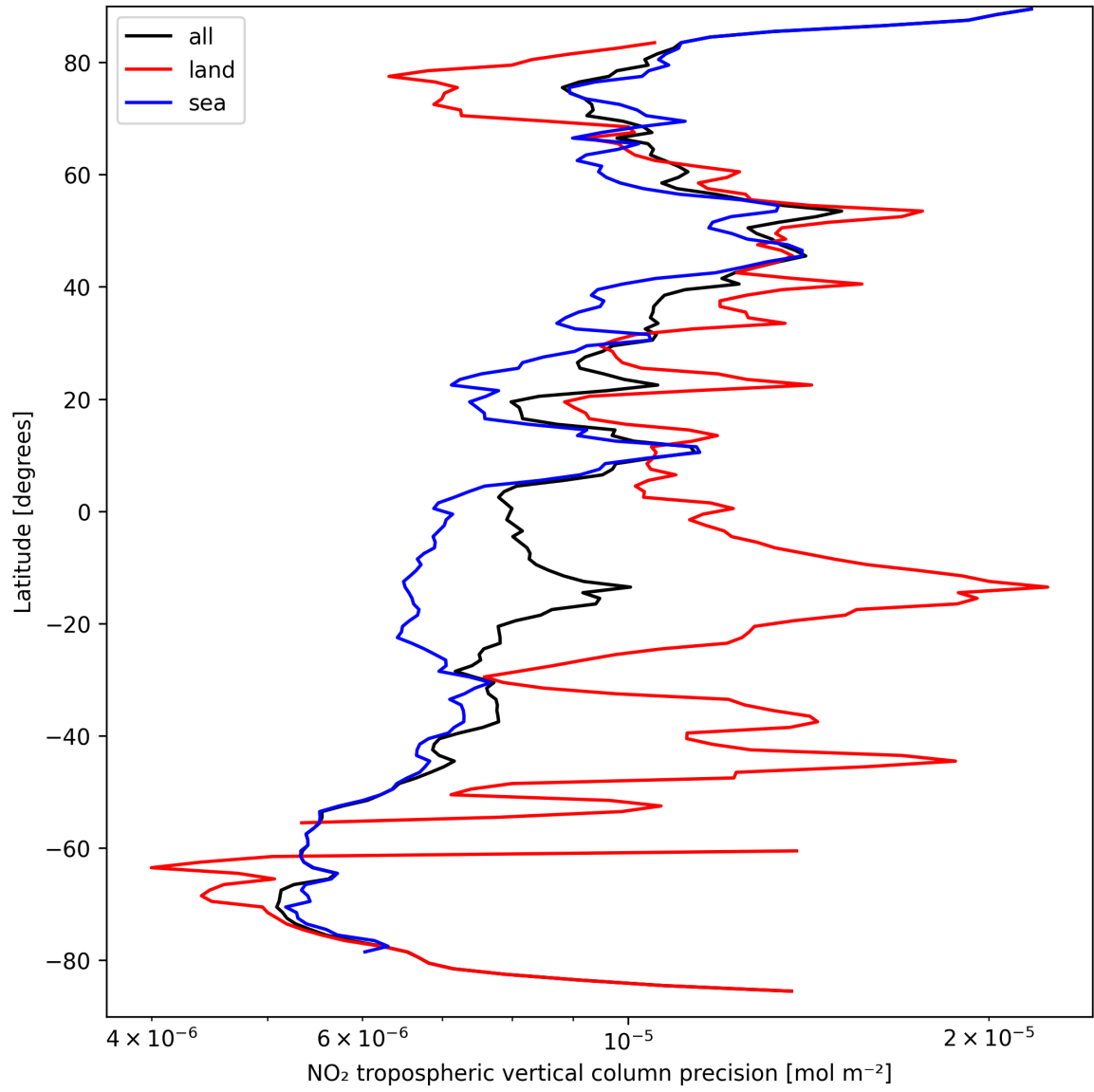
Figure 13: Zonal average of “NO 2 tropospheric vertical column precision” for 2024-09-14 to 2024-09-16.
