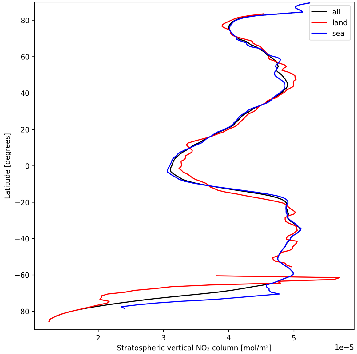
Figure 19: Zonal average of “Stratospheric vertical NO 2 column” for 2024-09-14 to 2024-09-16.
