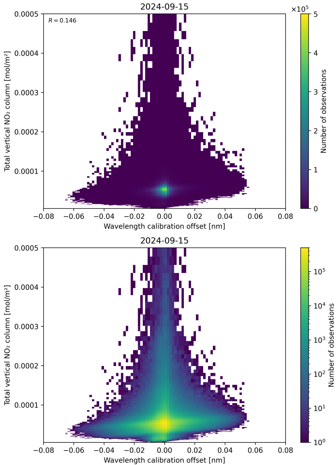
Figure 179: Scatter density plot of “Wavelength calibration offset” against “Total vertical NO 2 column” for 2024-09-14 to 2024-09-16.
