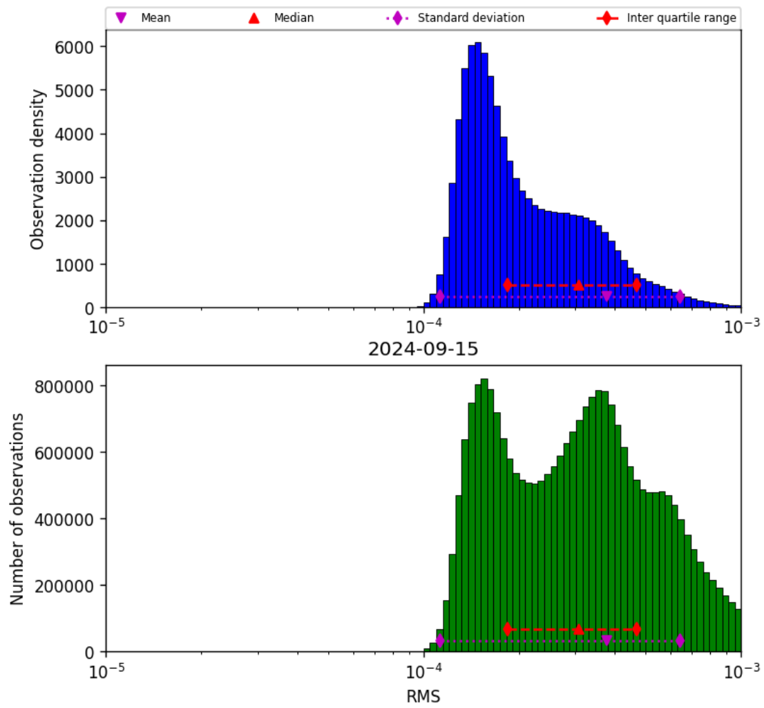
Figure 43: Histogram of “RMS” for 2024-09-14 to 2024-09-16
