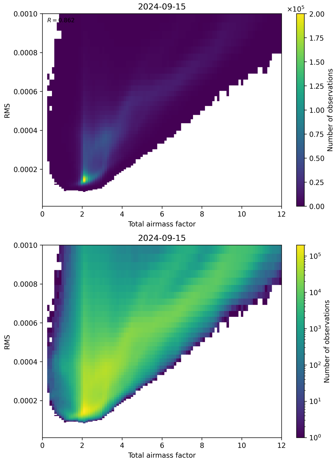
Figure 69: Scatter density plot of “Total airmass factor” against “RMS” for 2024-09-14 to 2024-09-16.
