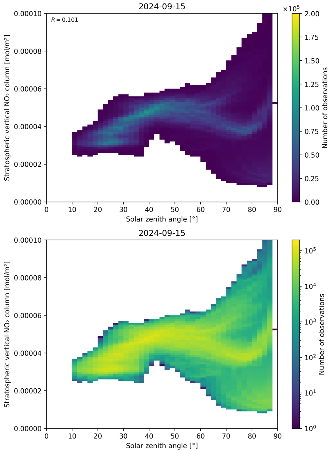
Figure 150: Scatter density plot of “Solar zenith angle” against “Stratospheric vertical NO 2 column” for 2024-09-14 to 2024-09-16.
