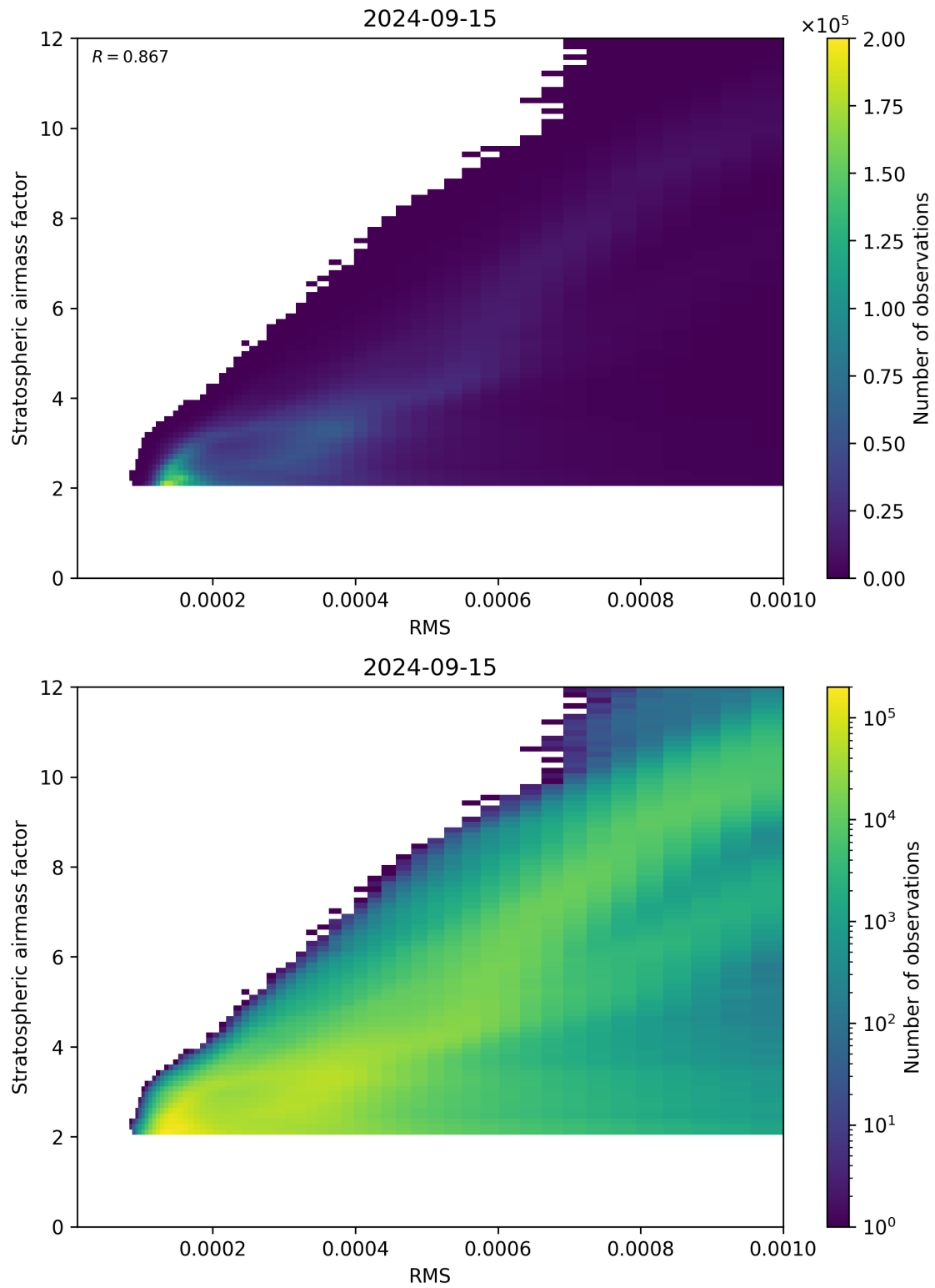
Figure 144: Scatter density plot of “RMS” against “Stratospheric airmass factor” for 2024-09-14 to 2024-09-16.
