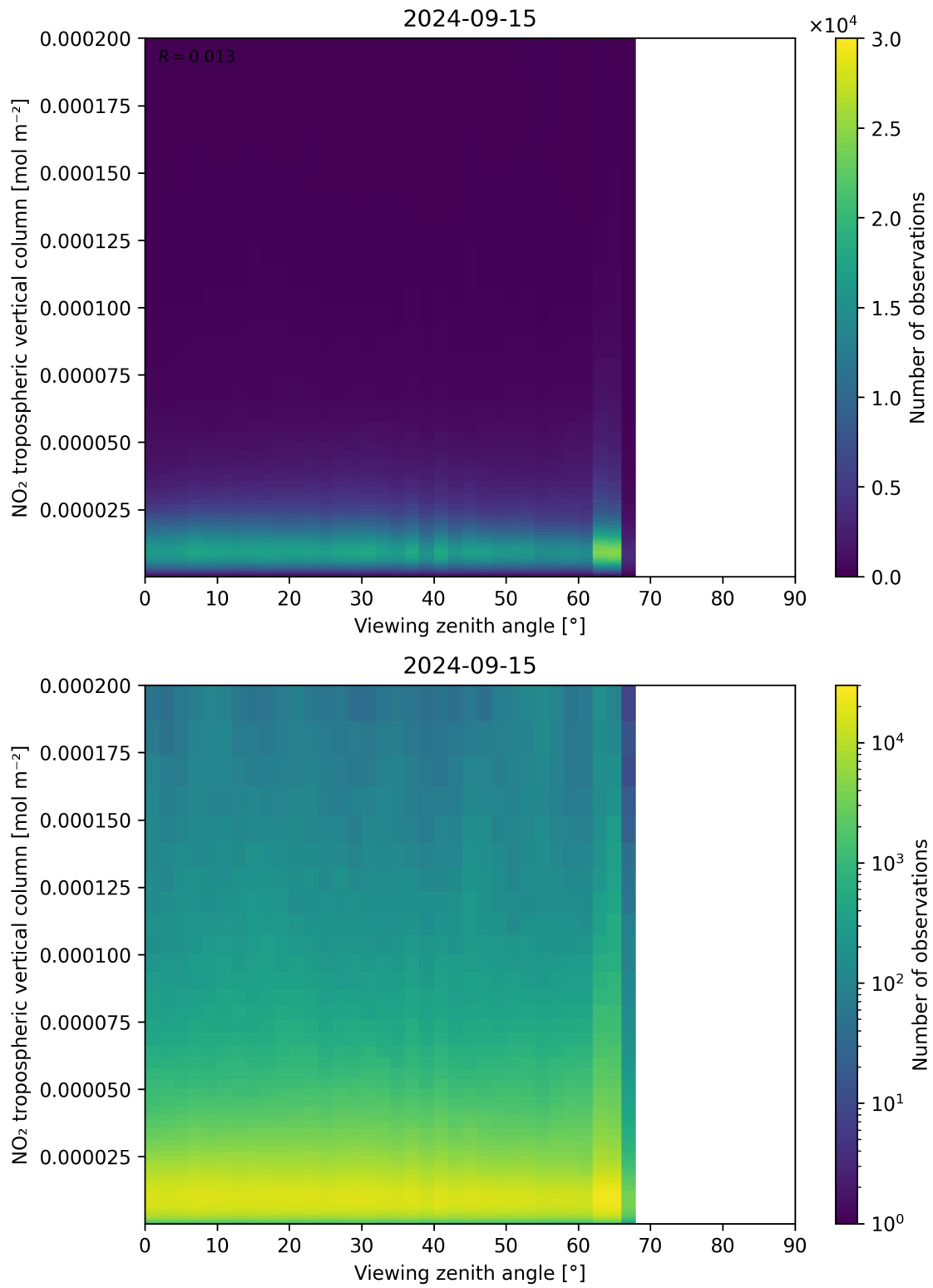
Figure 169: Scatter density plot of “Viewing zenith angle” against “NO 2 tropospheric vertical column” for 2024-09-14 to 2024-09-16.
