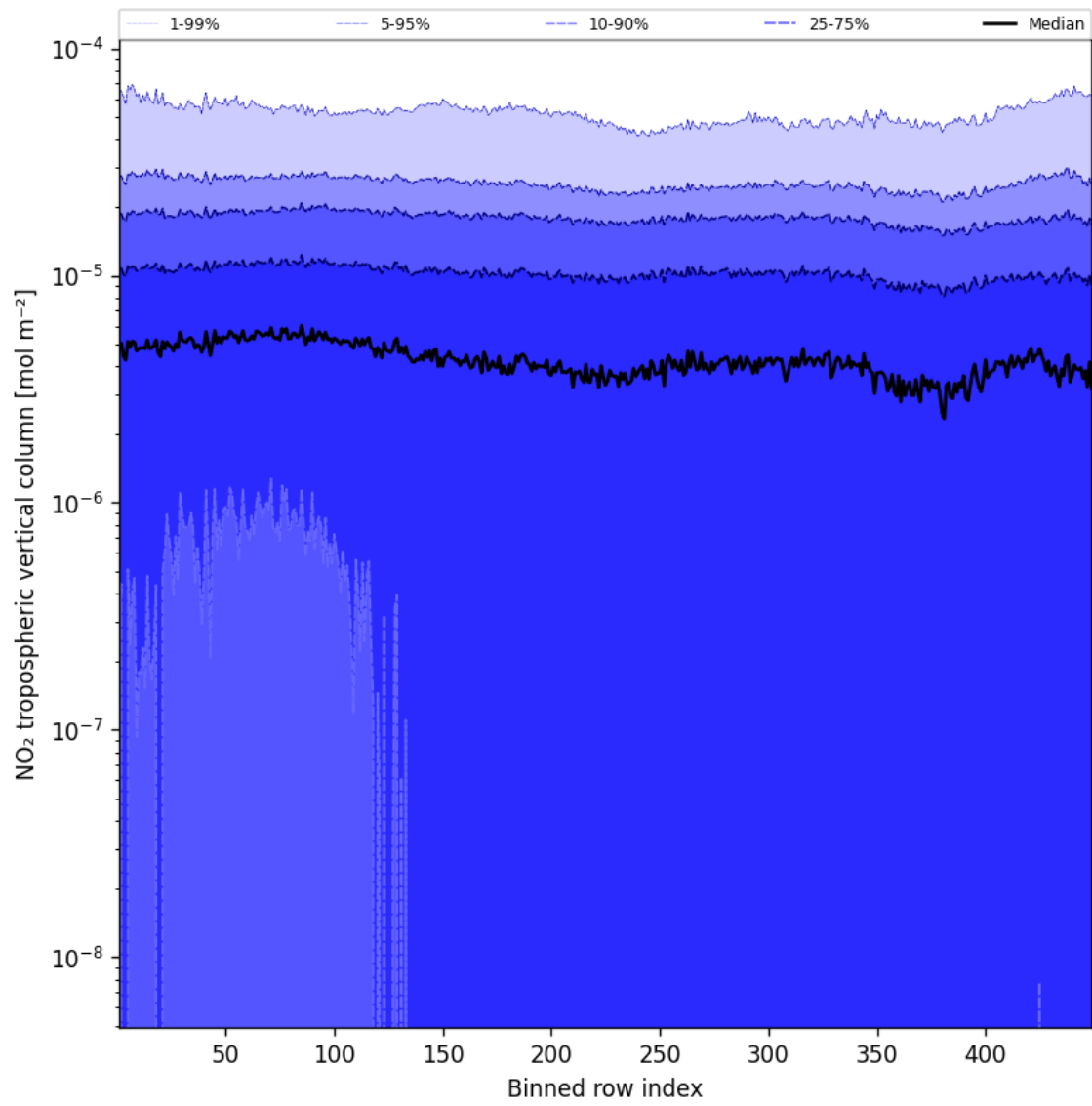
Figure 46: Along track statistics of “NO 2 tropospheric vertical column” for 2024-09-14 to 2024-09-16
