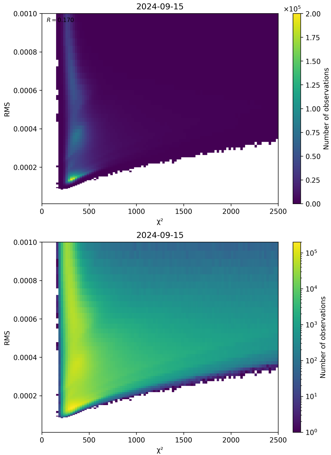
Figure 82: Scatter density plot of “ \chi^2 ” against “RMS” for 2024-09-14 to 2024-09-16.
