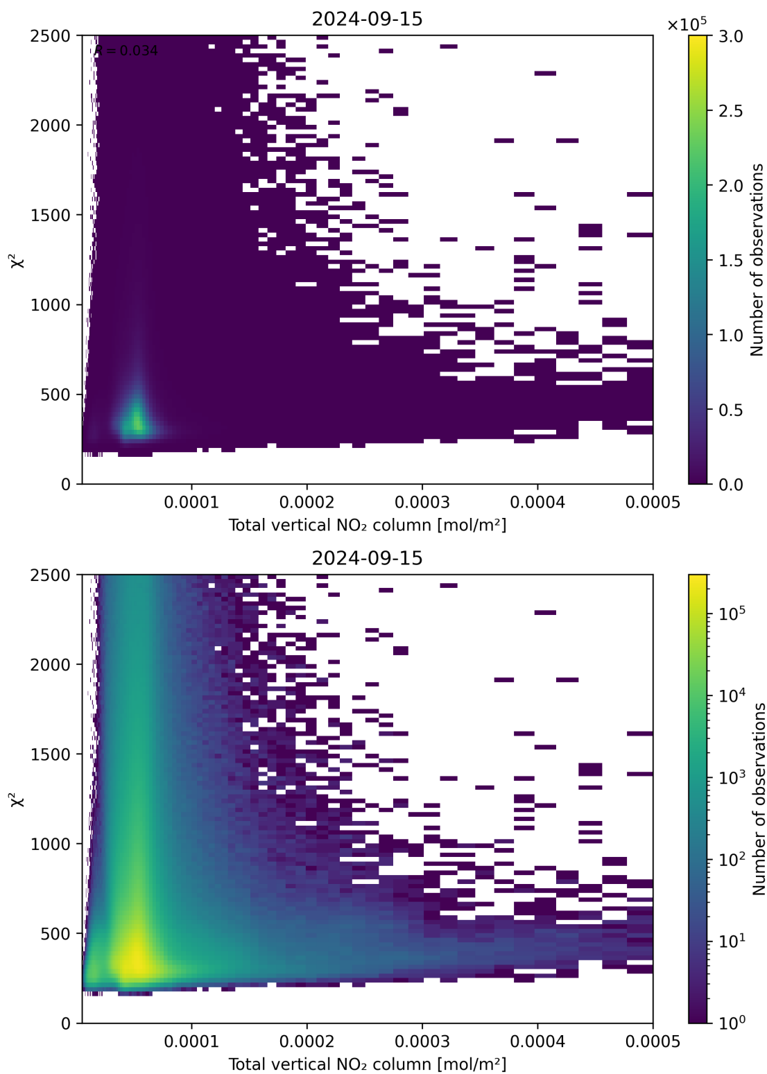
Figure 111: Scatter density plot of “Total vertical NO 2 column” against “ \chi^2 ” for 2024-09-14 to 2024-09-16.
