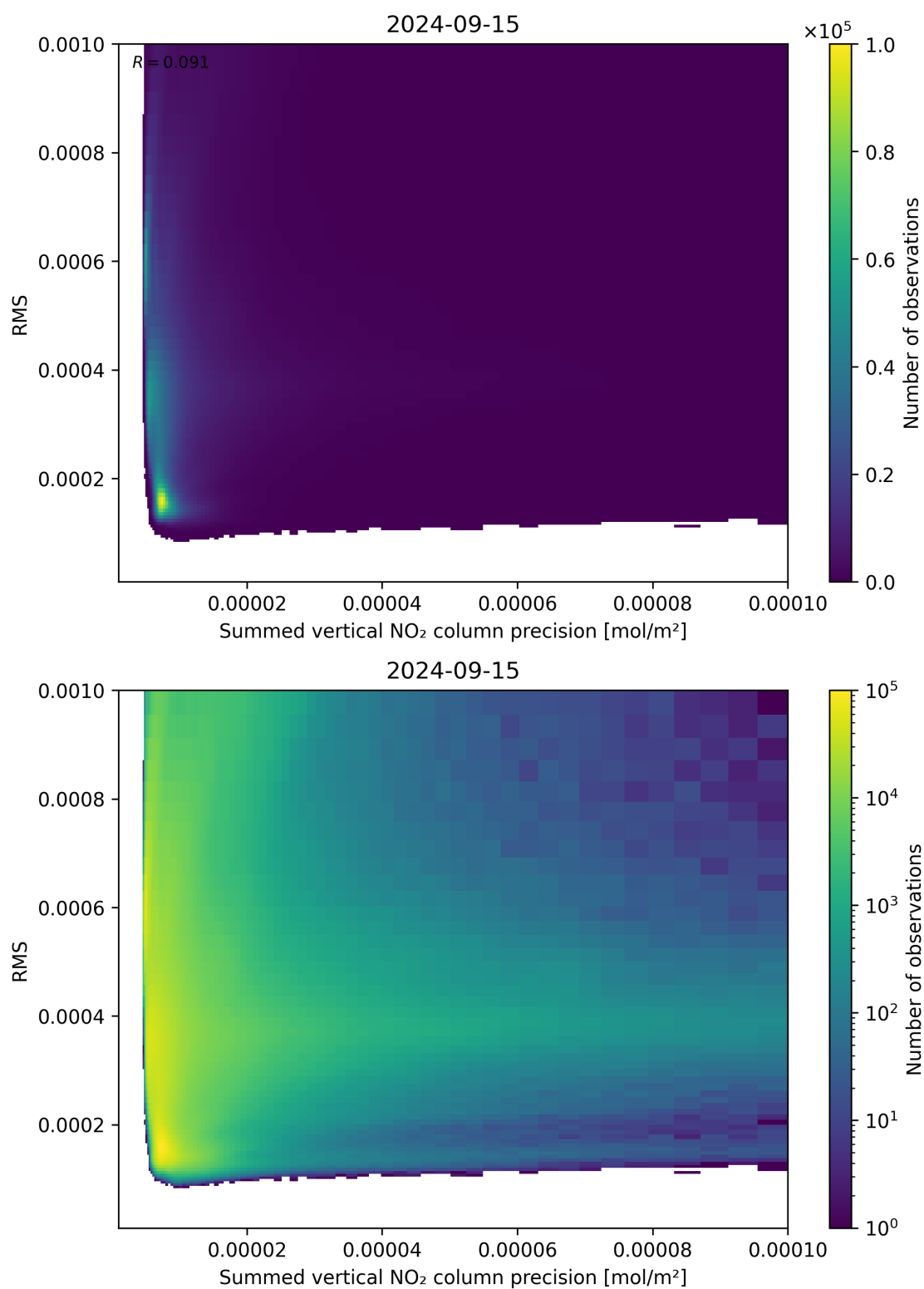
Figure 108: Scatter density plot of “Summed vertical NO 2 column precision” against “RMS” for 2024-09-14 to 2024-09-16.
