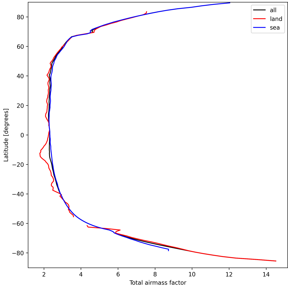
Figure 15: Zonal average of “Total airmass factor” for 2024-09-15 to 2024-09-17.
