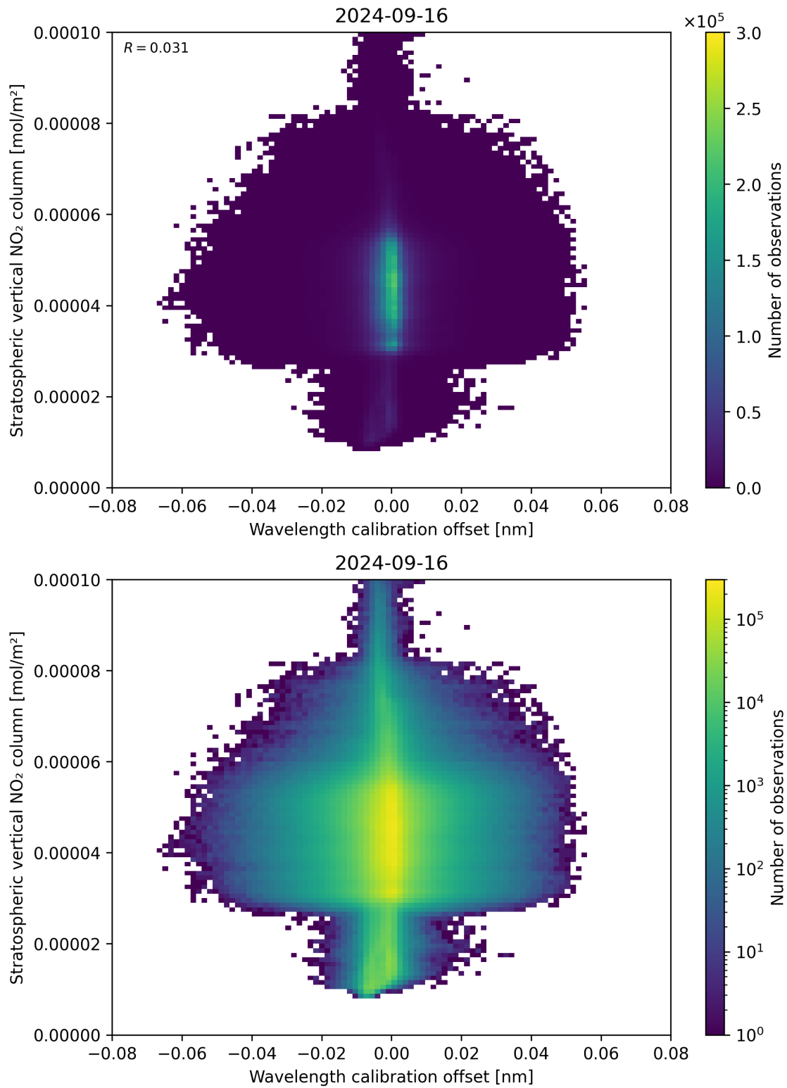
Figure 176: Scatter density plot of “Wavelength calibration offset” against “Stratospheric vertical NO 2 column” for 2024-09-15 to 2024-09-17.
