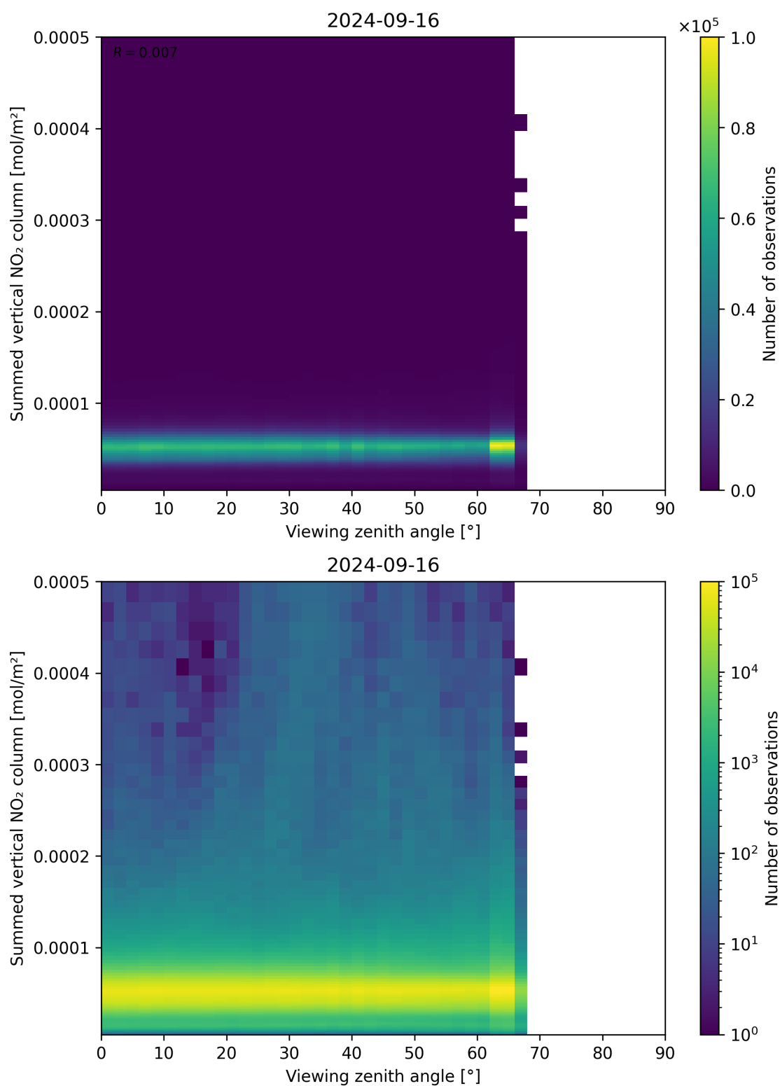
Figure 165: Scatter density plot of “Viewing zenith angle” against “Summed vertical NO 2 column” for 2024-09-15 to 2024-09-17.
