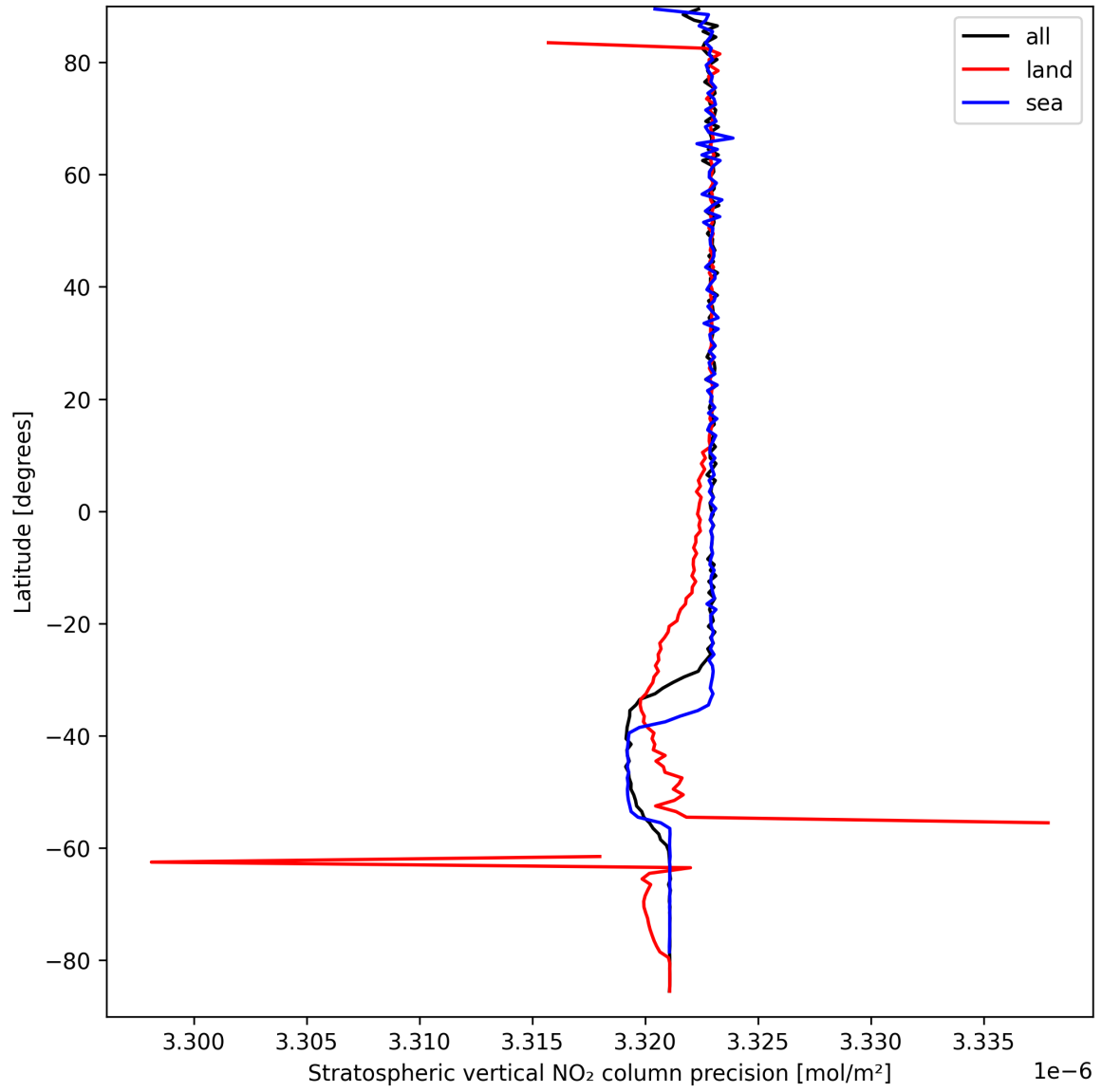
Figure 20: Zonal average of “Stratospheric vertical NO 2 column precision” for 2024-09-15 to 2024-09-17.
