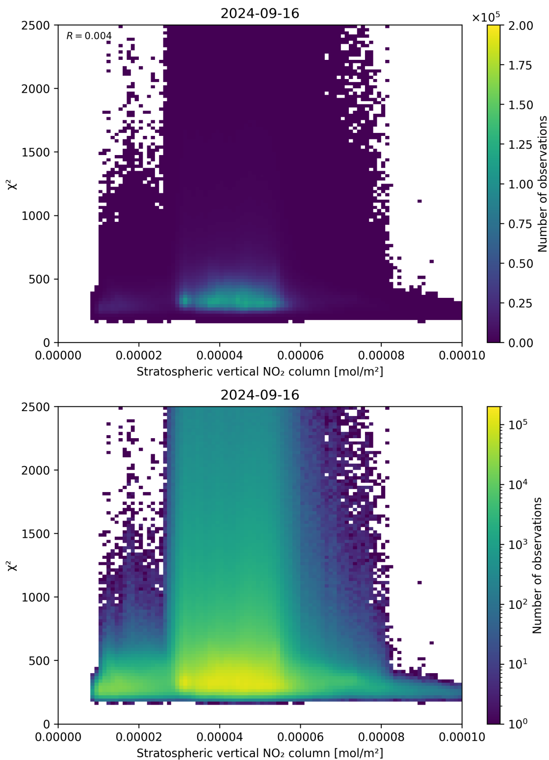
Figure 97: Scatter density plot of “Stratospheric vertical NO 2 column” against “ \chi^2 ” for 2024-09-15 to 2024-09-17.
