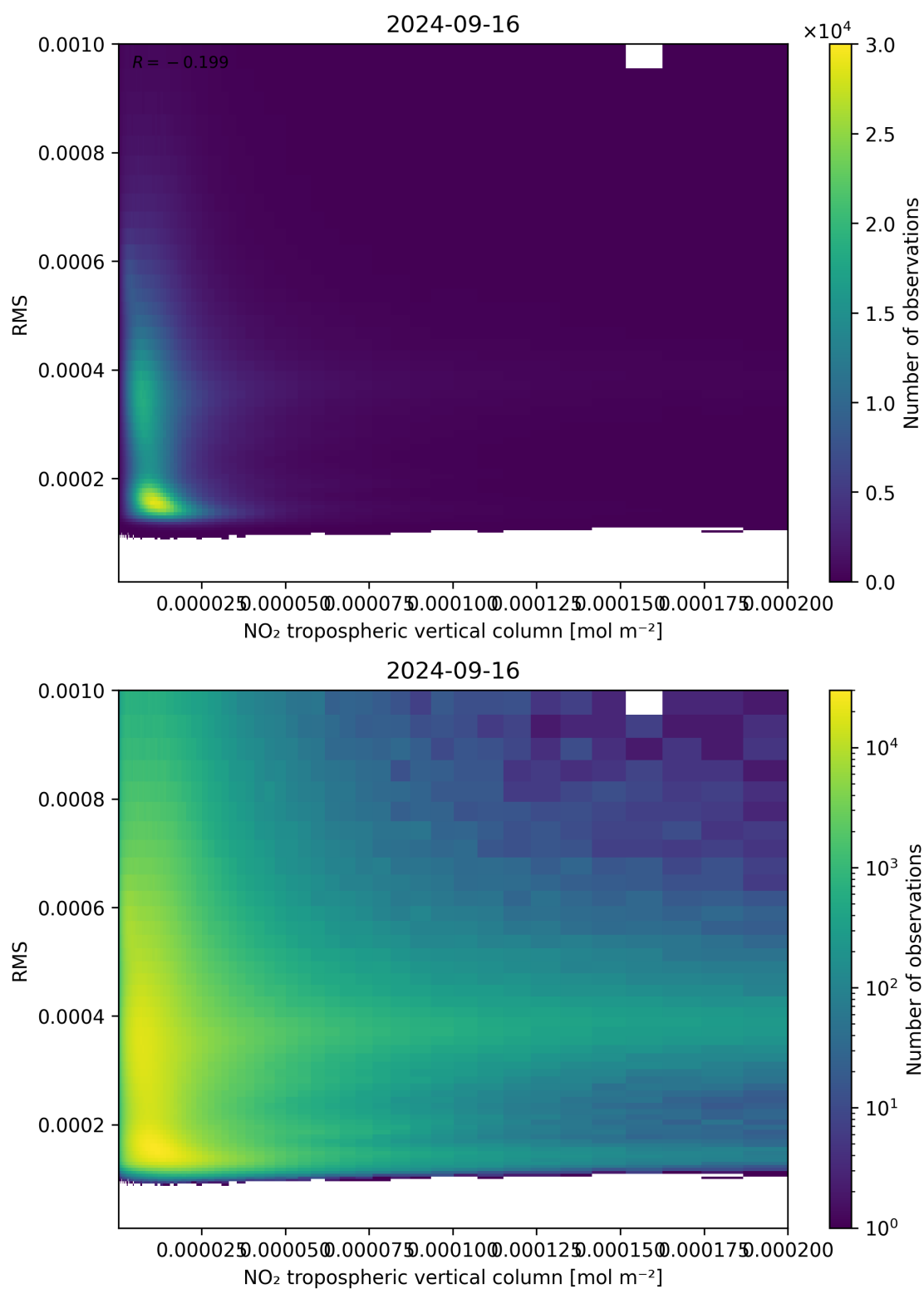
Figure 142: Scatter density plot of “NO 2 tropospheric vertical column” against “RMS” for 2024-09-15 to 2024-09-17.
