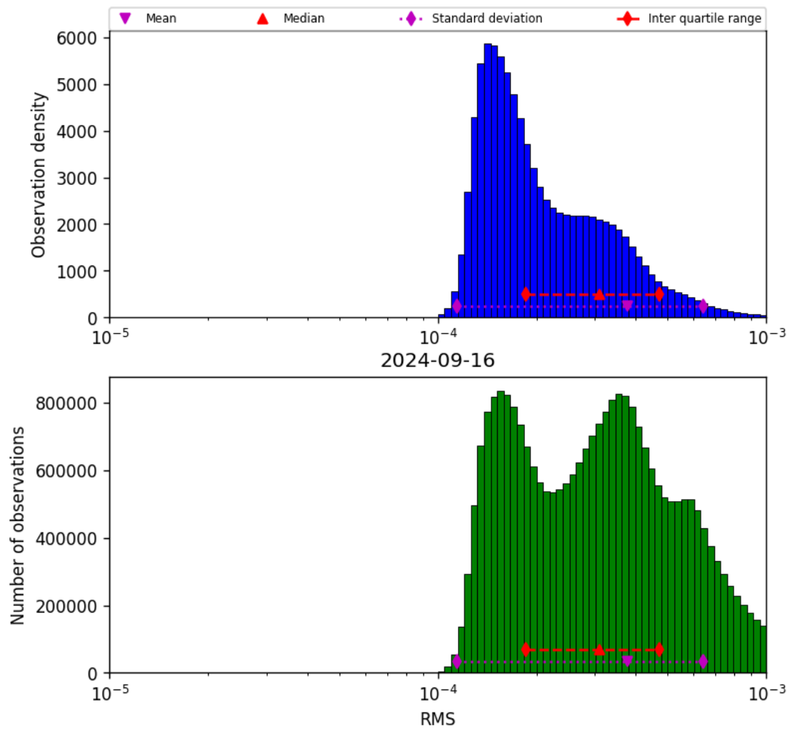
Figure 43: Histogram of “RMS” for 2024-09-15 to 2024-09-17
