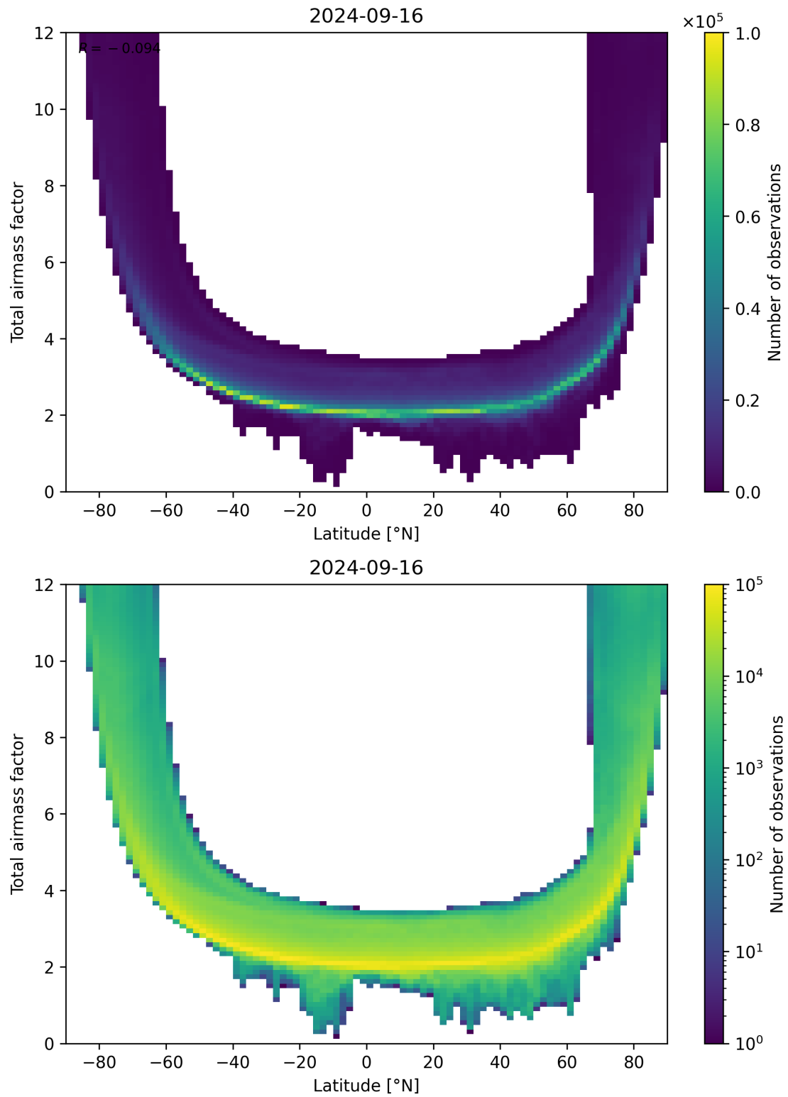
Figure 84: Scatter density plot of “Latitude” against “Total airmass factor” for 2024-09-15 to 2024-09-17.
