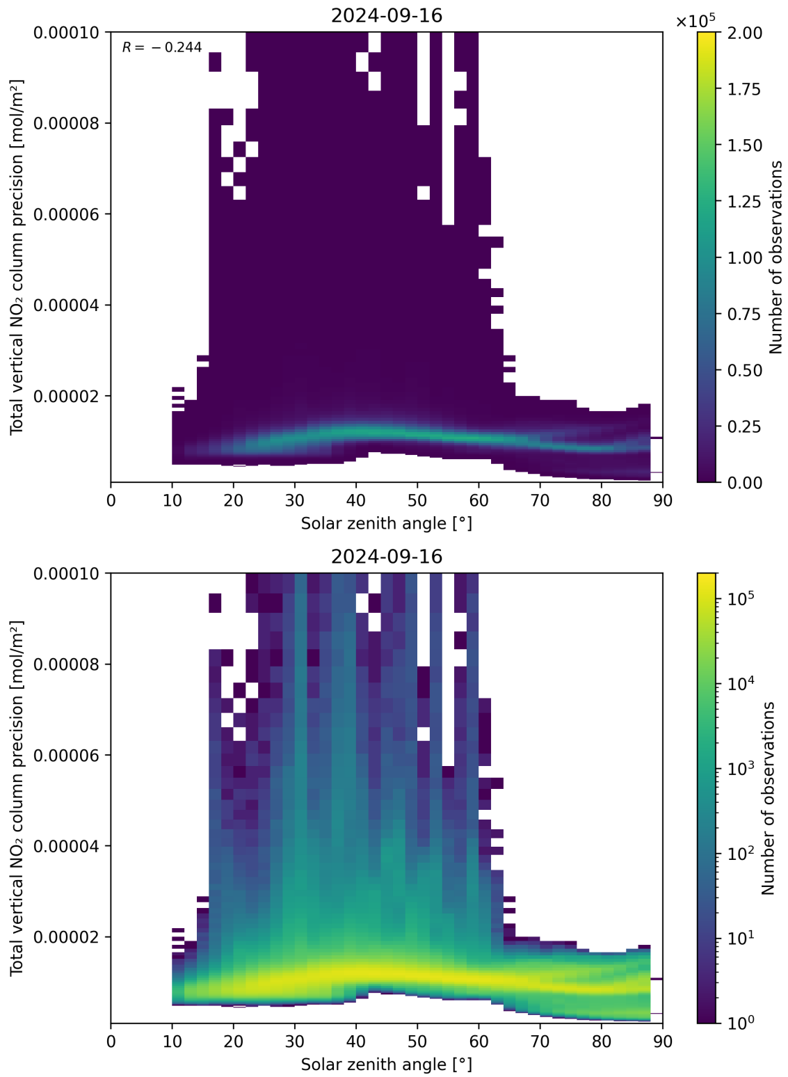
Figure 154: Scatter density plot of “Solar zenith angle” against “Total vertical NO 2 column precision” for 2024-09-15 to 2024-09-17.
