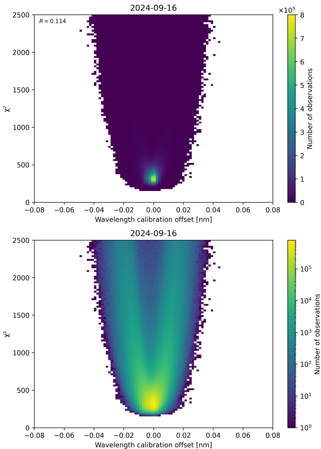
Figure 175: Scatter density plot of “Wavelength calibration offset” against “ \chi^2 ” for 2024-09-15 to 2024-09-17.
