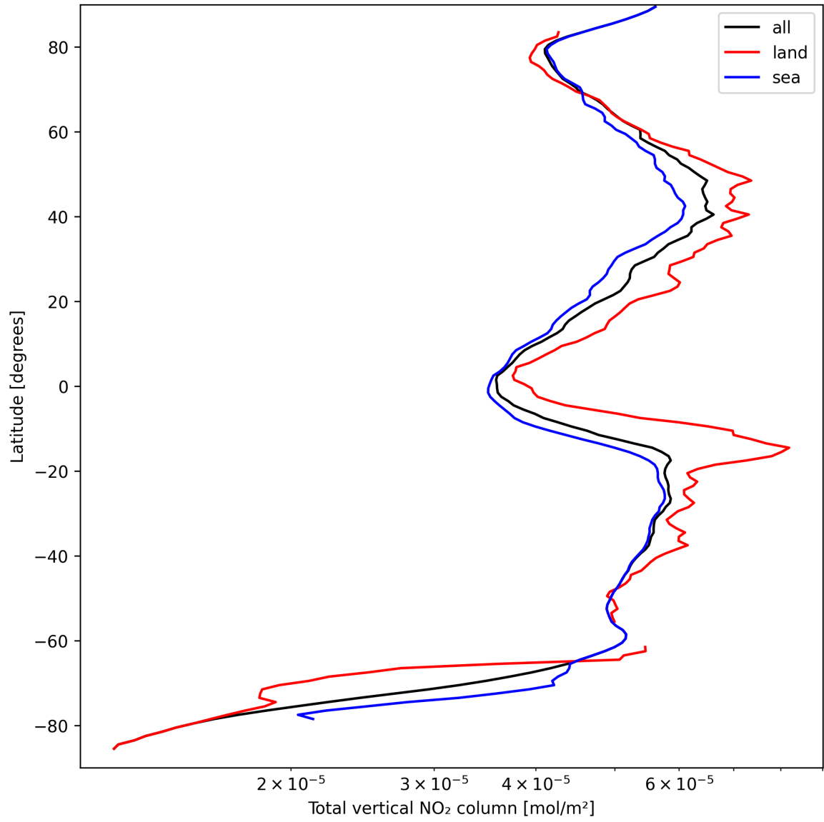
Figure 21: Zonal average of “Total vertical NO 2 column” for 2024-09-15 to 2024-09-17.
