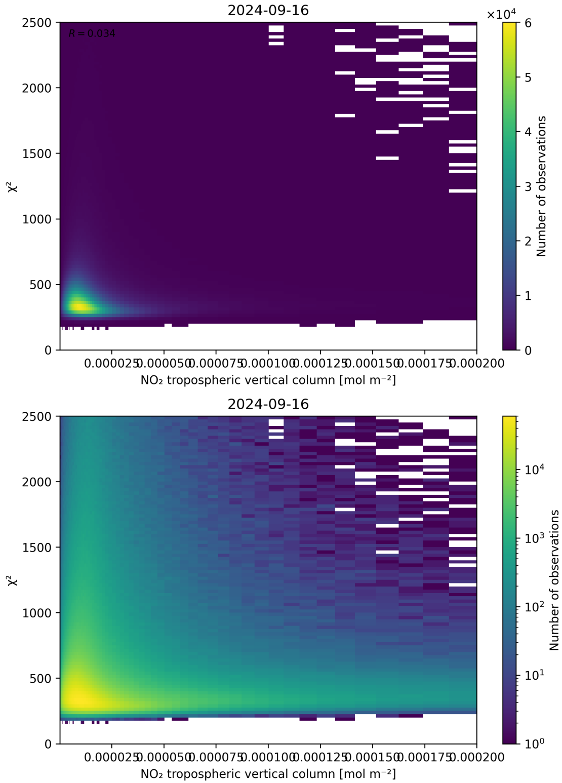
Figure 124: Scatter density plot of “NO 2 tropospheric vertical column” against “ \chi^2 ” for 2024-09-15 to 2024-09-17.
