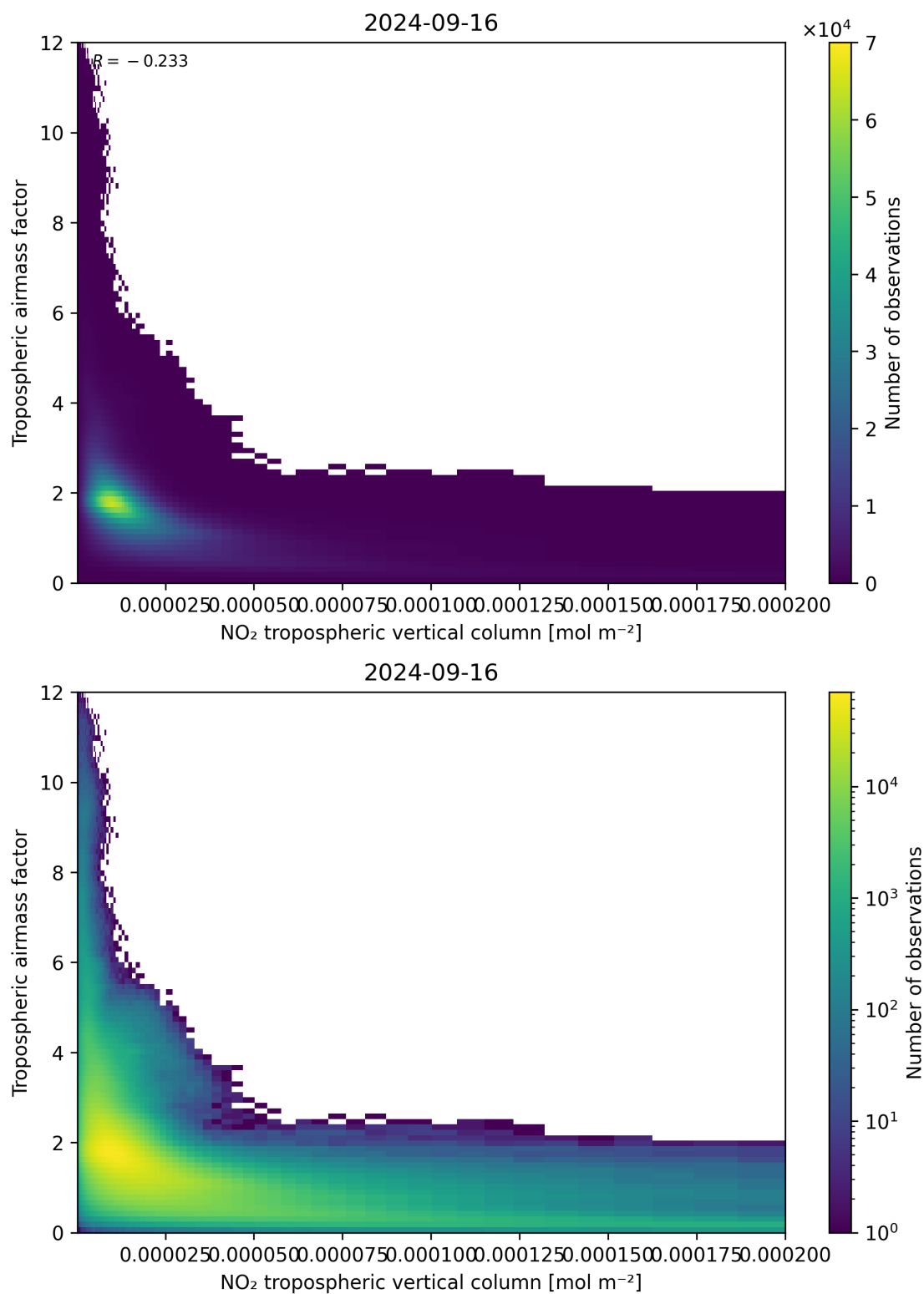
Figure 123: Scatter density plot of “NO 2 tropospheric vertical column” against “Tropospheric air mass factor” for 2024-09-15 to 2024-09-17.
