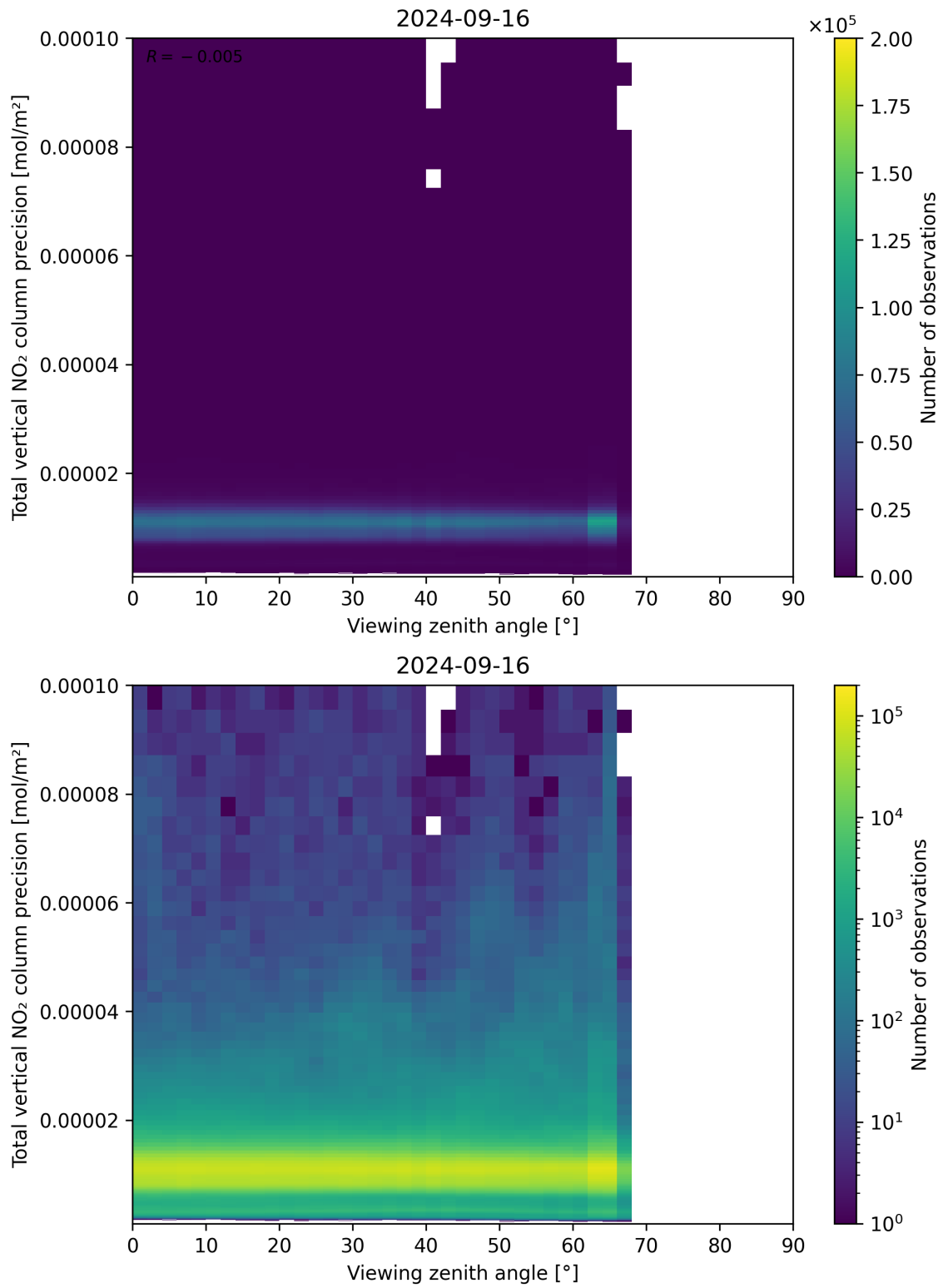
Figure 168: Scatter density plot of “Viewing zenith angle” against “Total vertical NO 2 column precision” for 2024-09-15 to 2024-09-17.
