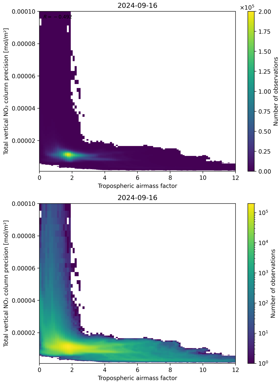
Figure 78: Scatter density plot of “Tropospheric air mass factor” against “Total vertical NO 2 column precision” for 2024-09-15 to 2024-09-17.
