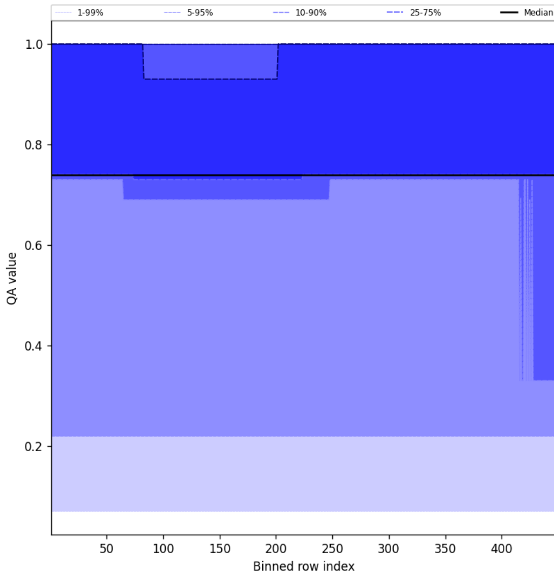
Figure 45: Along track statistics of “QA value” for 2024-09-15 to 2024-09-17
