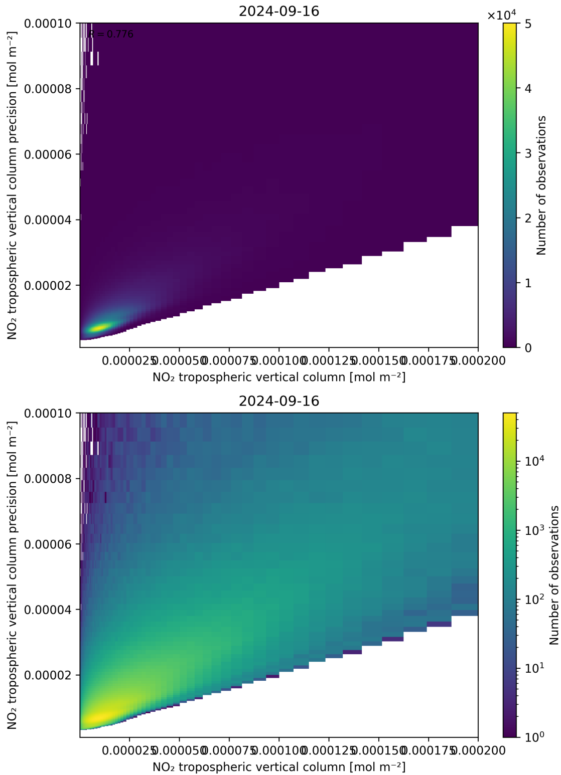
Figure 130: Scatter density plot of “NO 2 tropospheric vertical column” against “NO 2 tropospheric vertical column precision” for 2024-09-15 to 2024-09-17.
