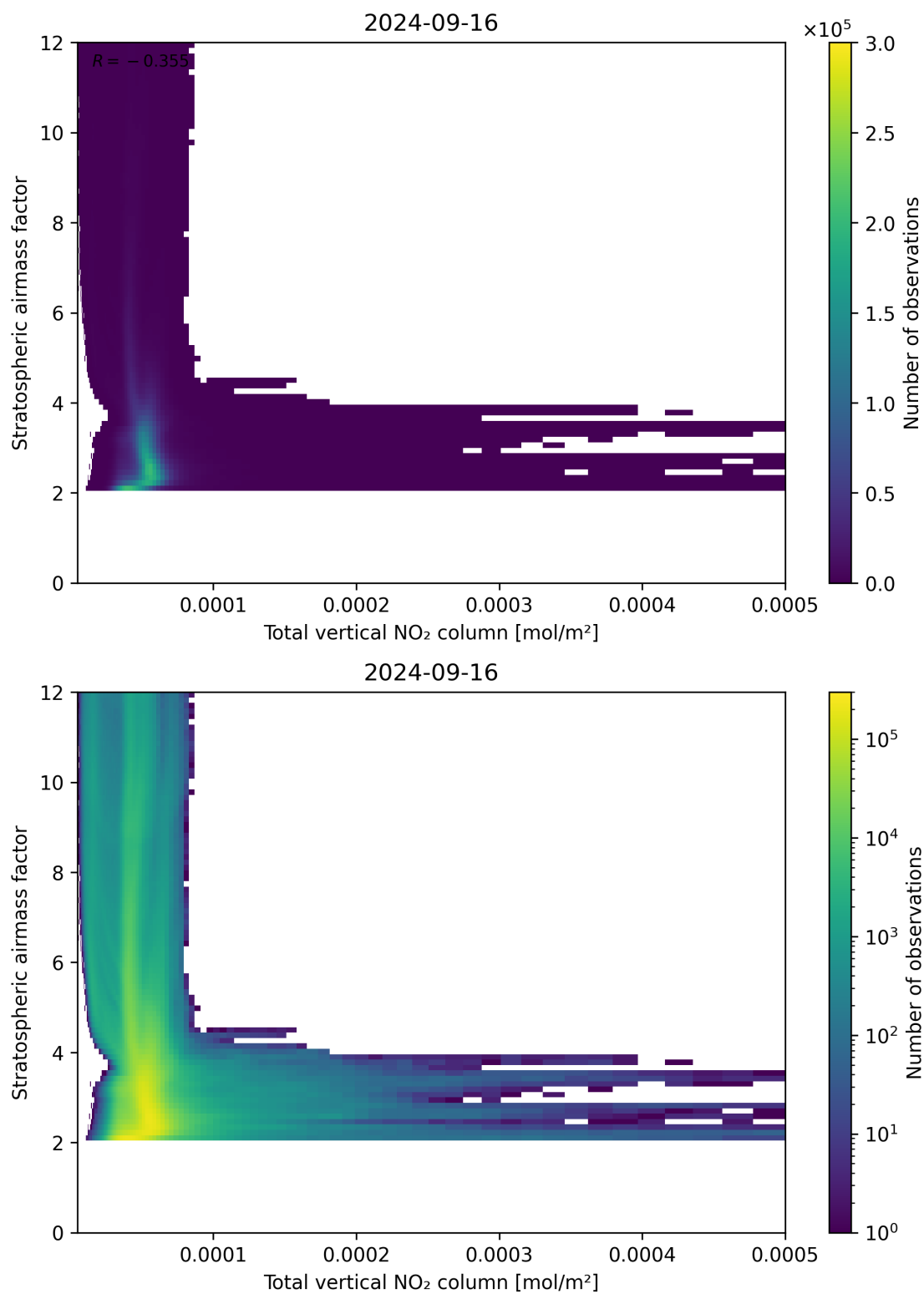
Figure 110: Scatter density plot of “Total vertical NO 2 column” against “Stratospheric airmass factor” for 2024-09-15 to 2024-09-17.
