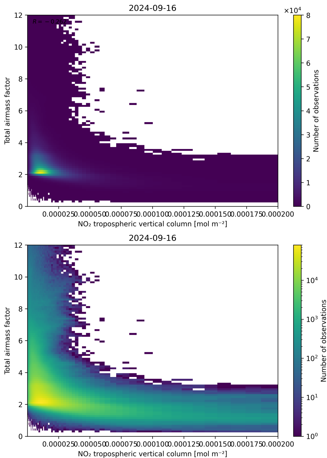
Figure 122: Scatter density plot of “NO 2 tropospheric vertical column” against “Total airmass factor” for 2024-09-15 to 2024-09-17.
