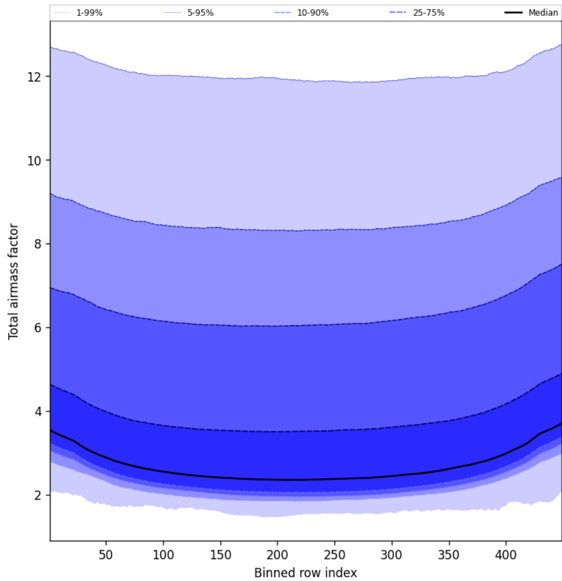
Figure 49: Along track statistics of “Total airmass factor” for 2024-09-15 to 2024-09-17
