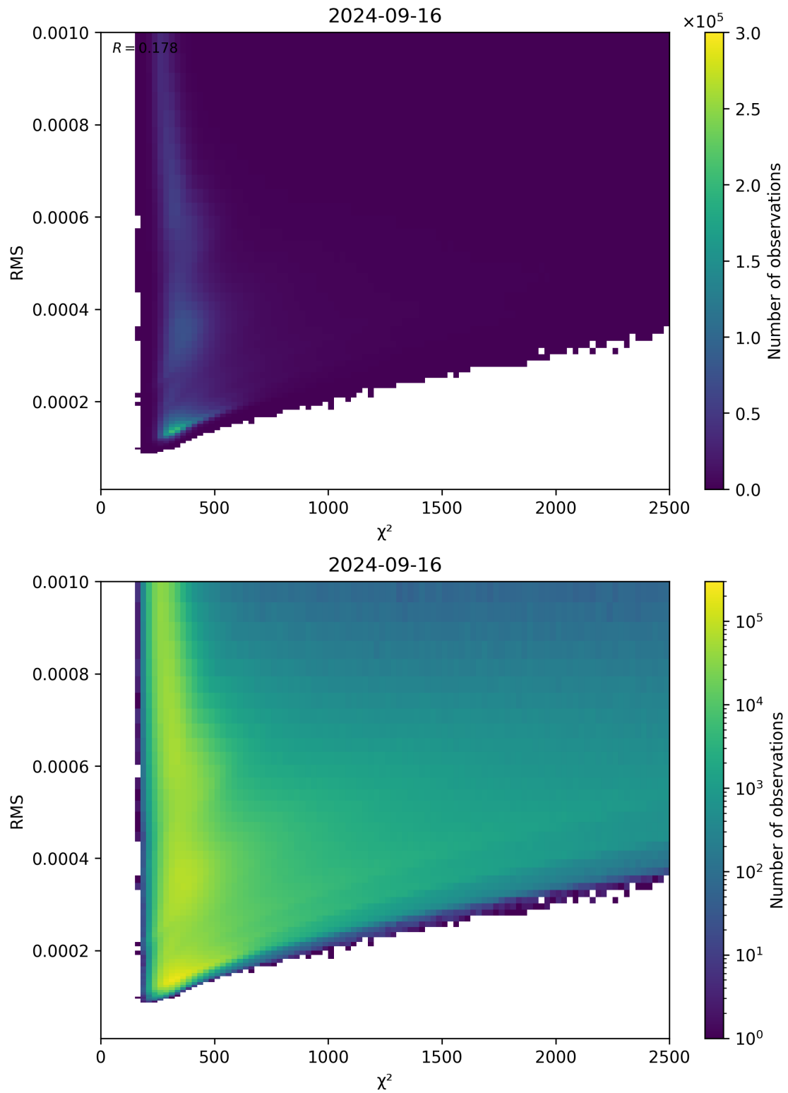
Figure 82: Scatter density plot of “ \chi^2 ” against “RMS” for 2024-09-15 to 2024-09-17.
