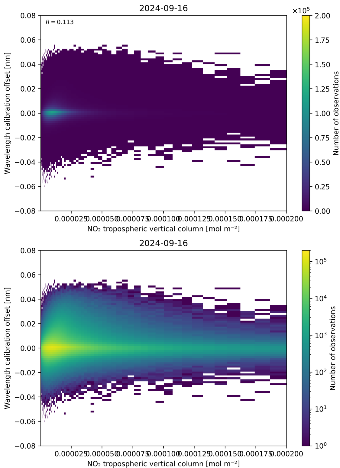
Figure 143: Scatter density plot of “NO 2 tropospheric vertical column” against “Wavelength calibration offset” for 2024-09-15 to 2024-09-17.
