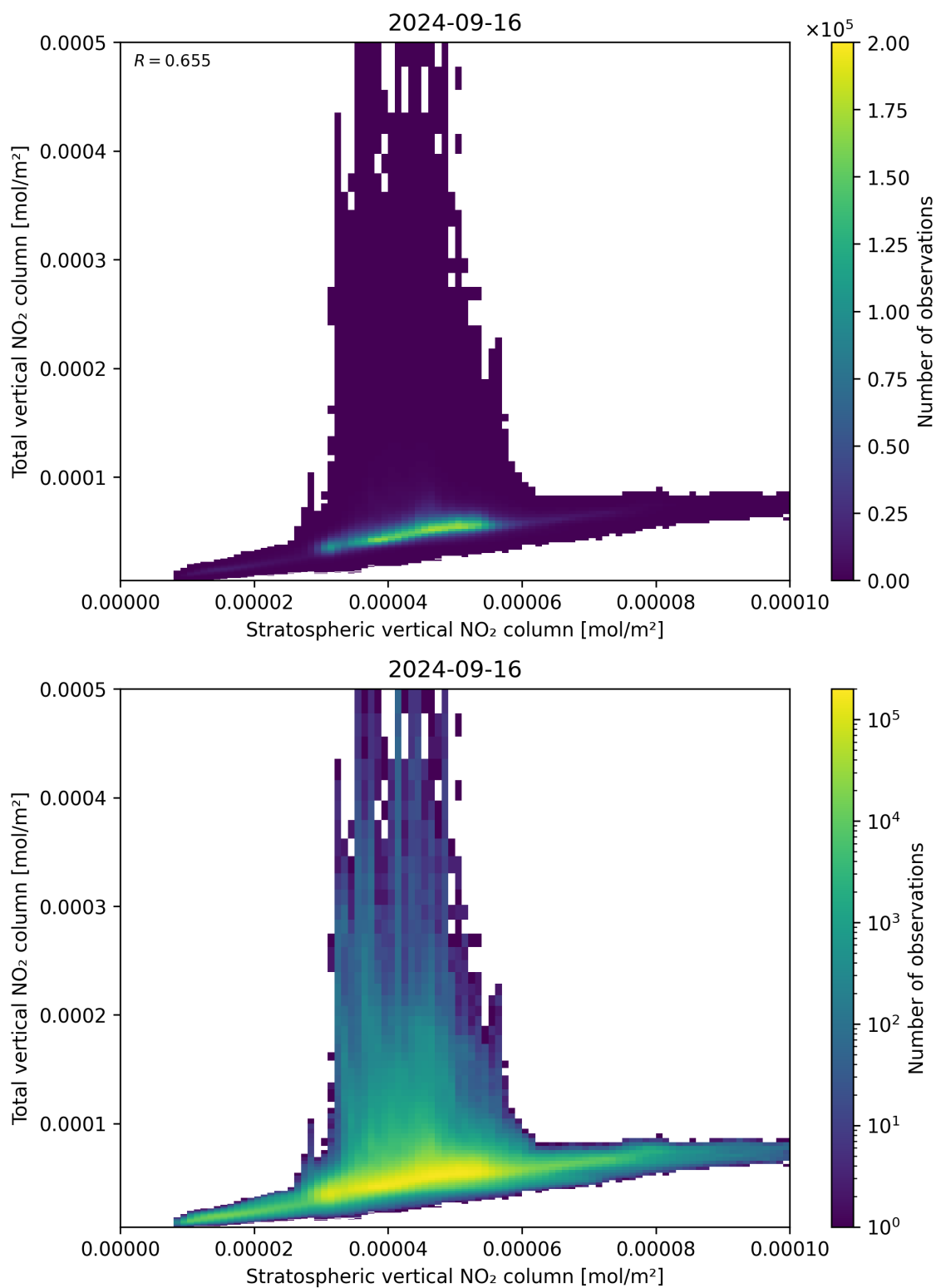
Figure 100: Scatter density plot of “Stratospheric vertical NO 2 column” against “Total vertical NO 2 column” for 2024-09-15 to 2024-09-17.
