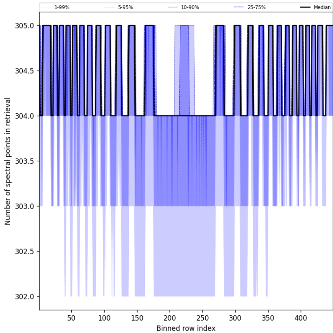
Figure 50: Along track statistics of “Number of spectral points in retrieval” for 2024-09-15 to 2024-09-17
