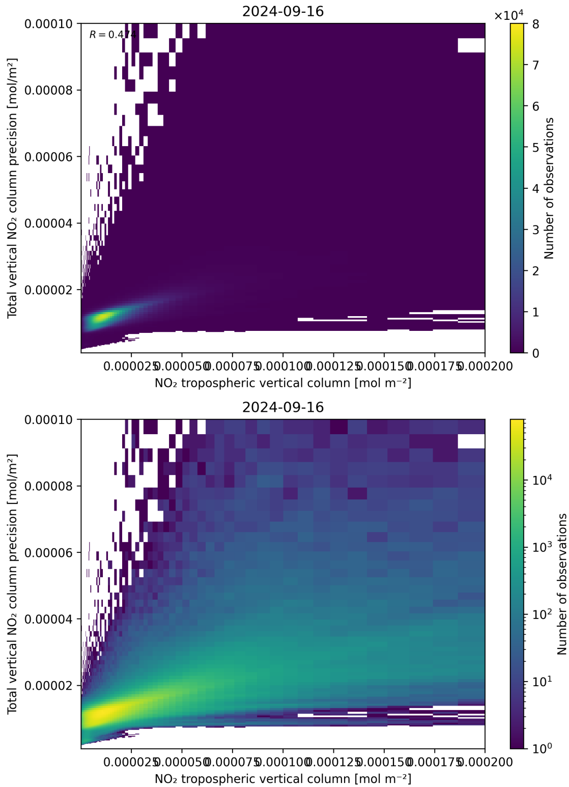
Figure 129: Scatter density plot of “NO 2 tropospheric vertical column” against “Total vertical NO 2 column precision” for 2024-09-15 to 2024-09-17.
