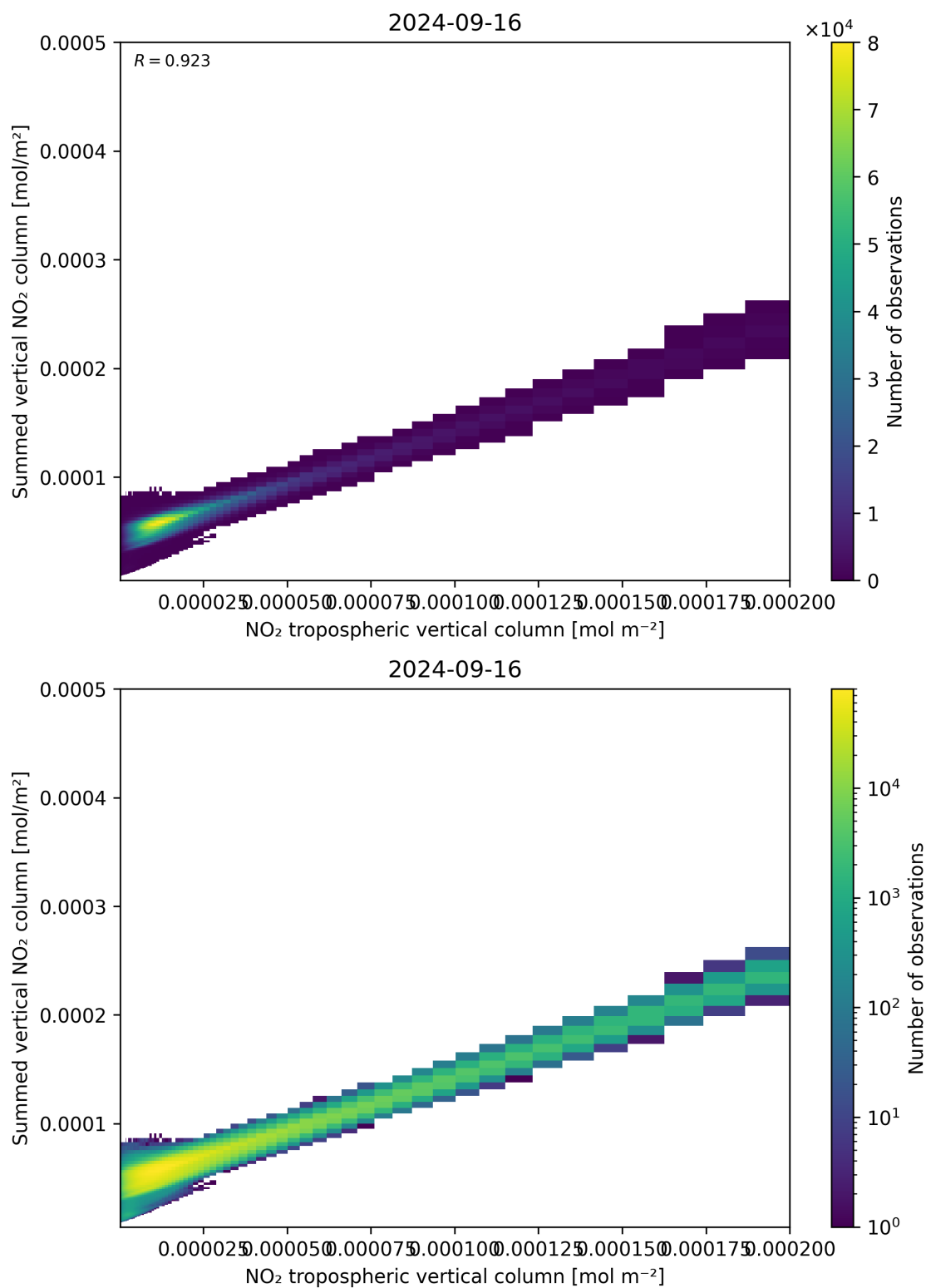
Figure 126: Scatter density plot of “NO 2 tropospheric vertical column” against “Summed vertical NO 2 column” for 2024-09-15 to 2024-09-17.
