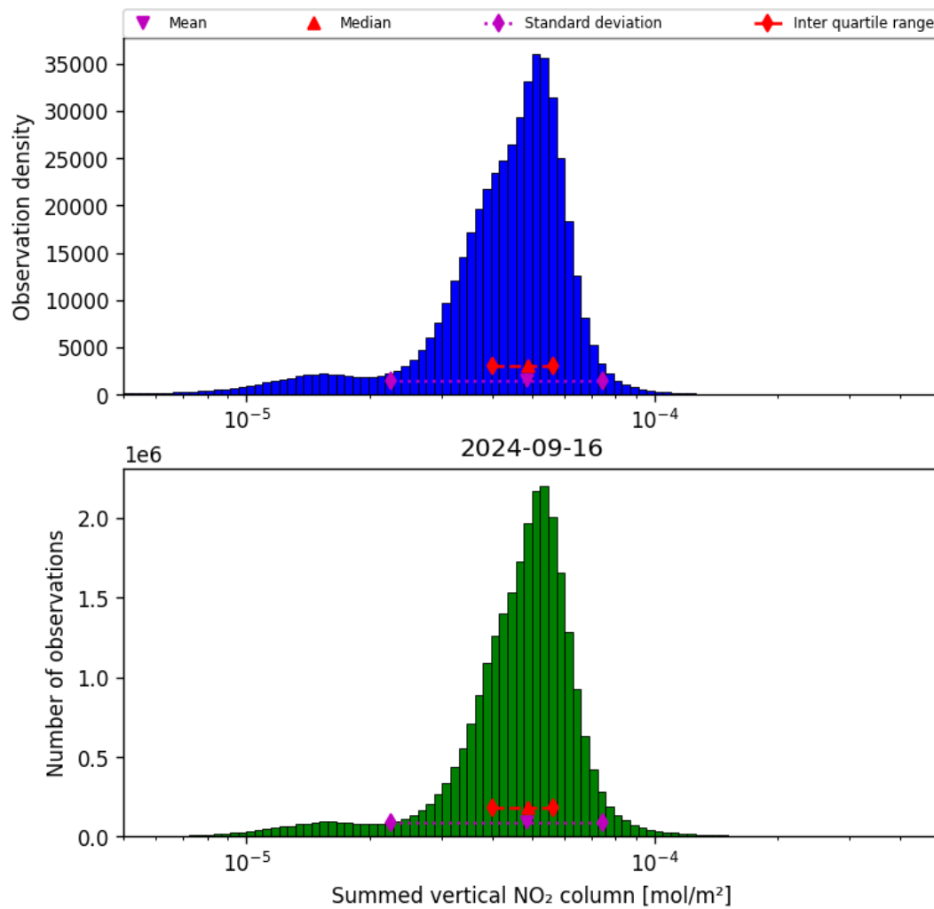
Figure 40: Histogram of “Summed vertical NO 2 column” for 2024-09-15 to 2024-09-17
