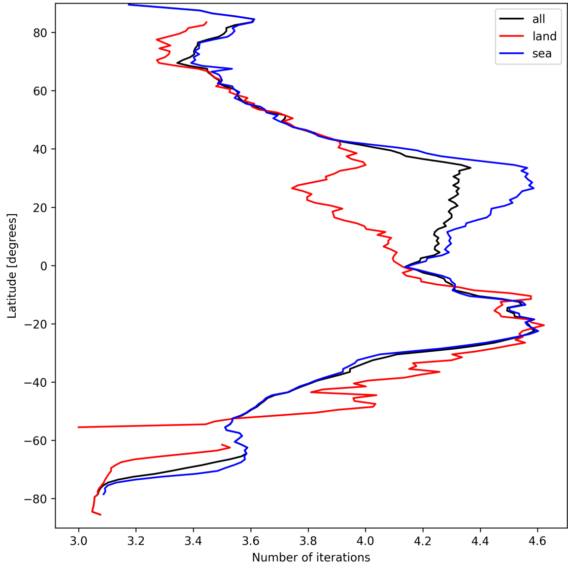
Figure 17: Zonal average of “Number of iterations” for 2024-09-15 to 2024-09-17.
