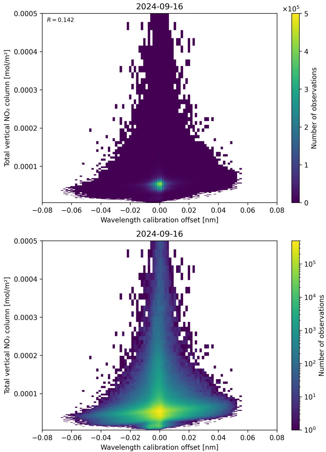
Figure 179: Scatter density plot of “Wavelength calibration offset” against “Total vertical NO 2 column” for 2024-09-15 to 2024-09-17.
