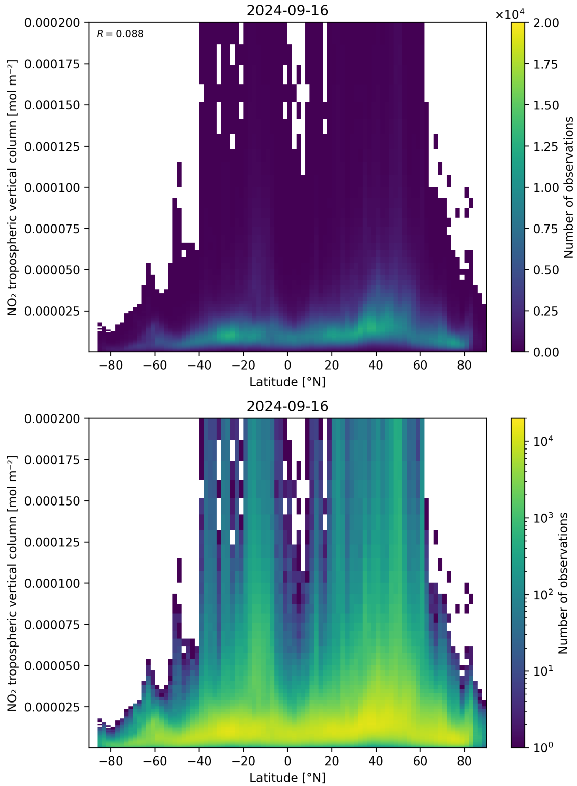
Figure 92: Scatter density plot of “Latitude” against “NO 2 tropospheric vertical column” for 2024-09-15 to 2024-09-17.
