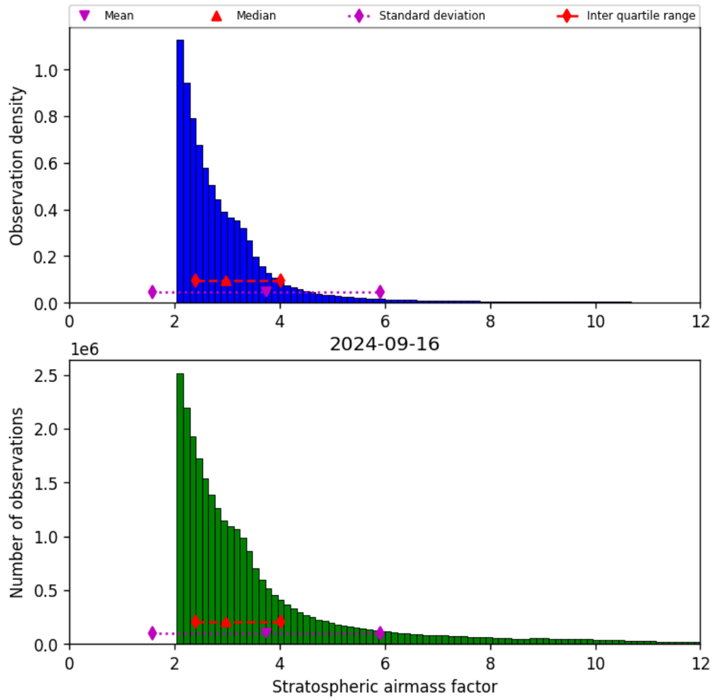
Figure 44: Histogram of “Stratospheric airmass factor” for 2024-09-15 to 2024-09-17
