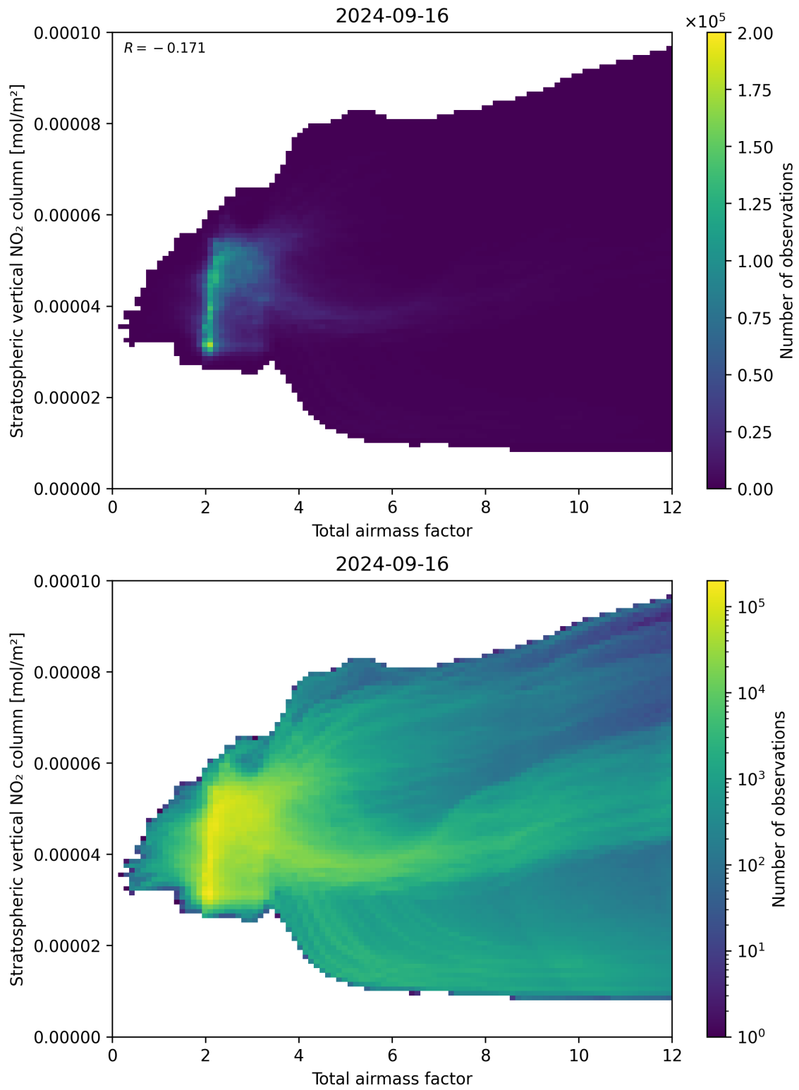
Figure 64: Scatter density plot of “Total airmass factor” against “Stratospheric vertical NO 2 column” for 2024-09-15 to 2024-09-17.
