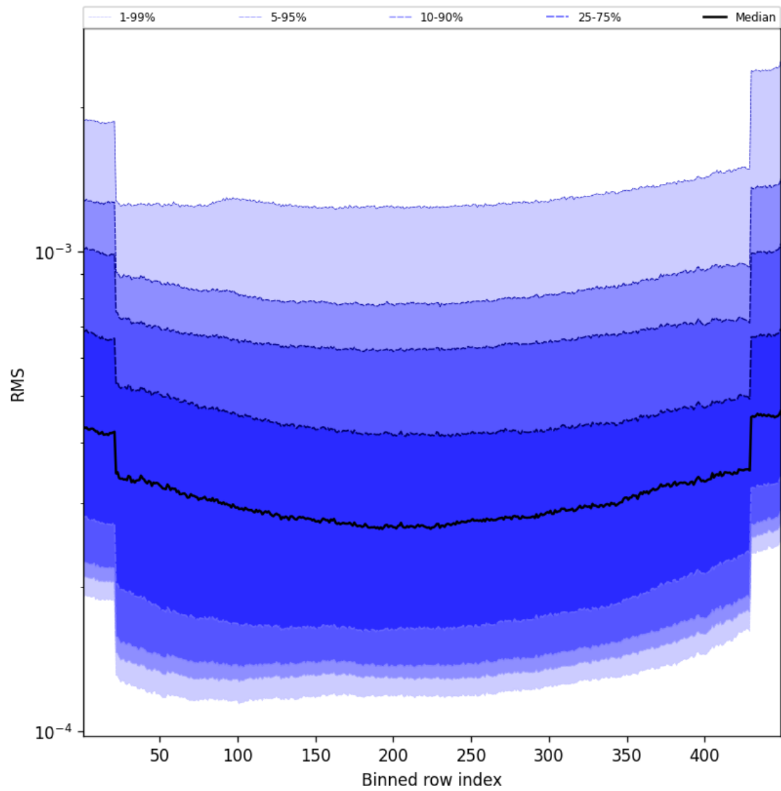
Figure 60: Along track statistics of “RMS” for 2024-09-15 to 2024-09-17
