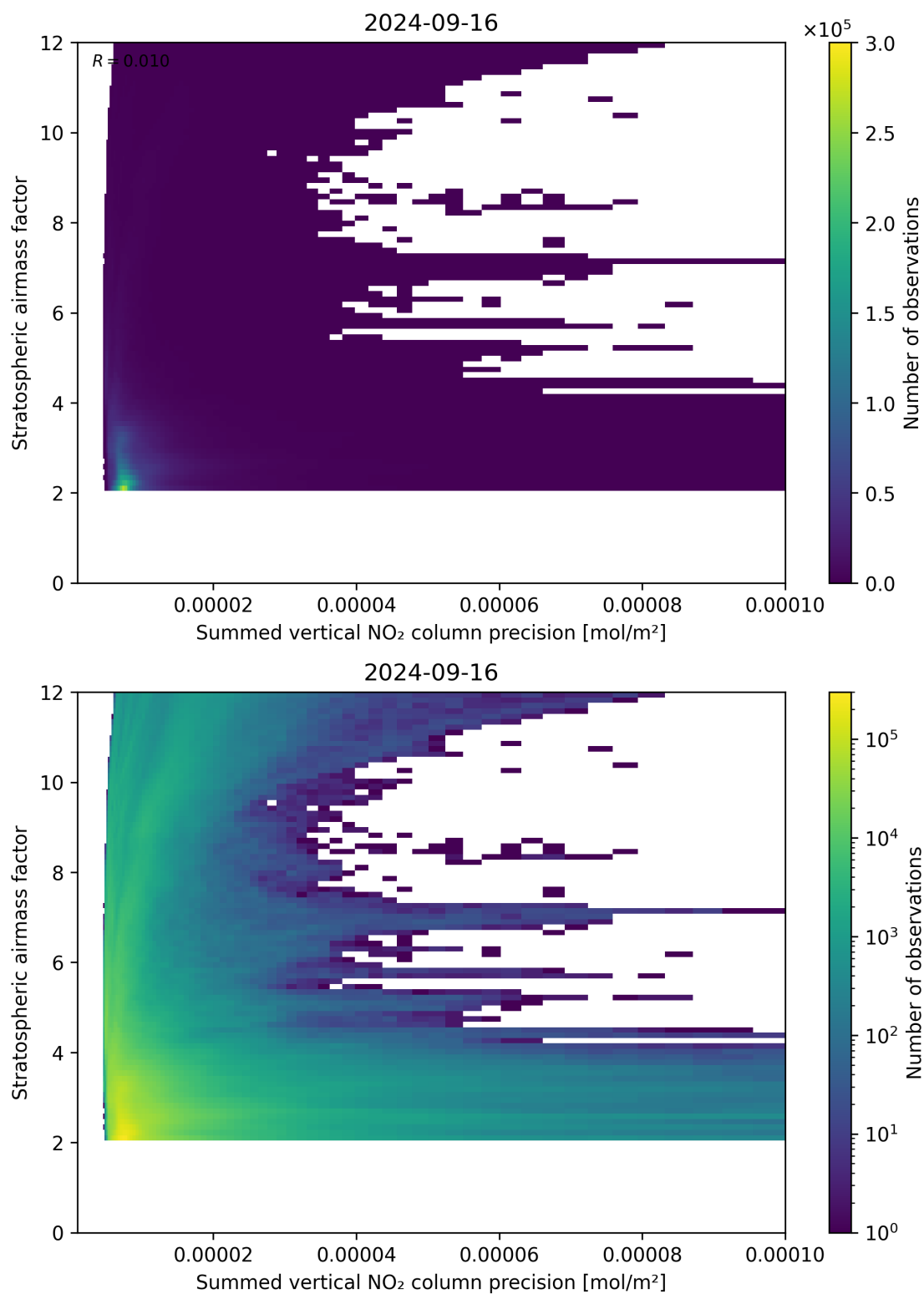
Figure 106: Scatter density plot of “Summed vertical NO 2 column precision” against “Stratospheric airmass factor” for 2024-09-15 to 2024-09-17.
