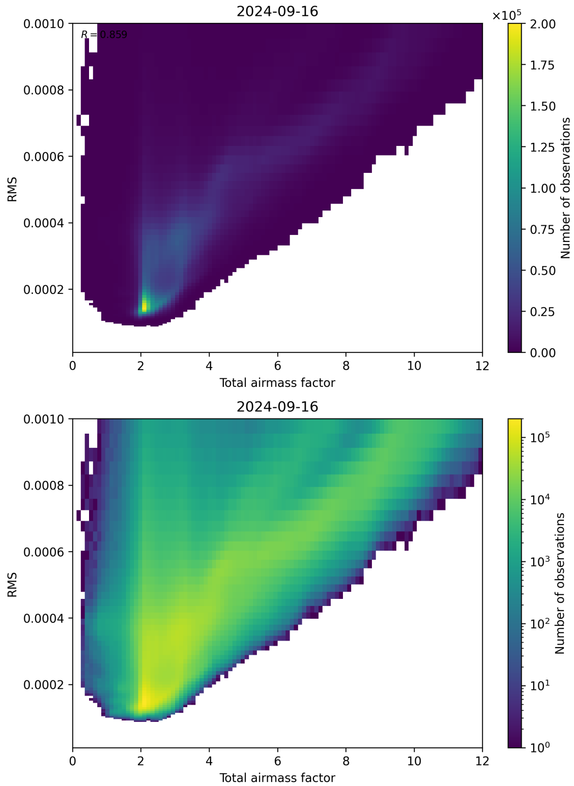
Figure 69: Scatter density plot of “Total airmass factor” against “RMS” for 2024-09-15 to 2024-09-17.
