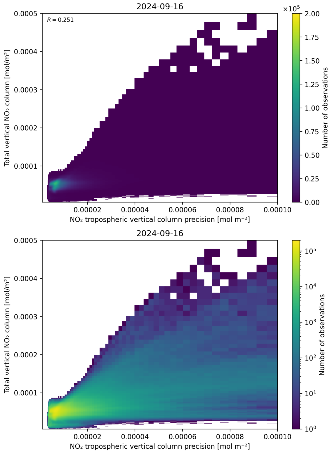
Figure 138: Scatter density plot of “NO 2 tropospheric vertical column precision” against “Total vertical NO 2 column” for 2024-09-15 to 2024-09-17.
