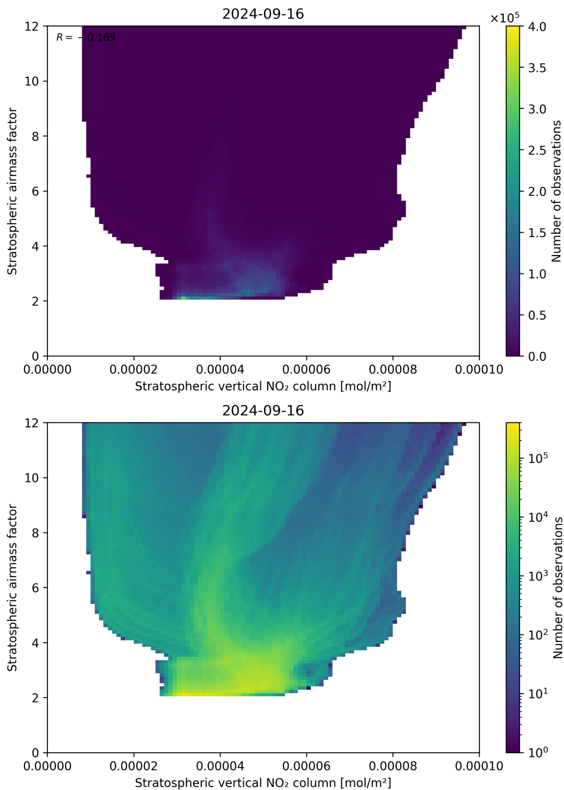
Figure 96: Scatter density plot of “Stratospheric vertical NO 2 column” against “Stratospheric airmass factor” for 2024-09-15 to 2024-09-17.
