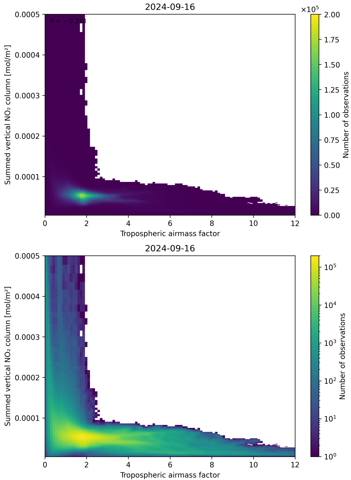
Figure 75: Scatter density plot of “Tropospheric air mass factor” against “Summed vertical NO 2 column” for 2024-09-15 to 2024-09-17.
