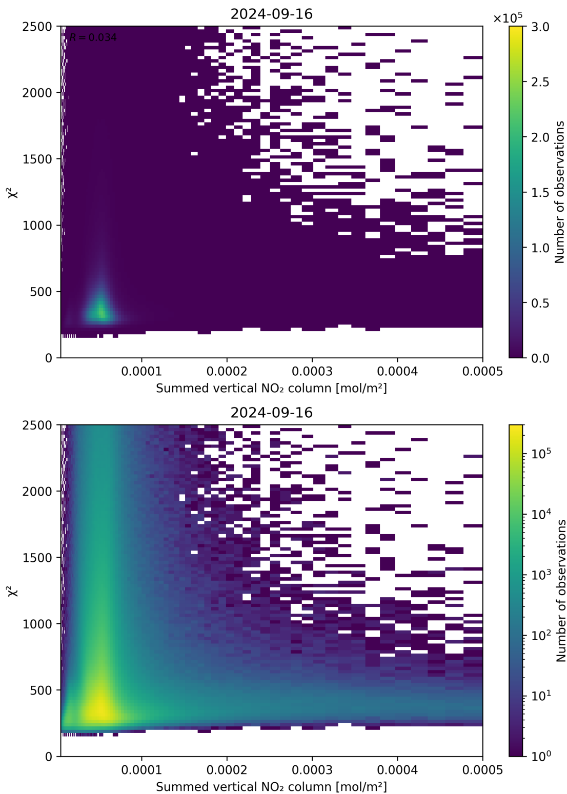
Figure 104: Scatter density plot of “Summed vertical NO 2 column” against “ \chi^2 ” for 2024-09-15 to 2024-09-17.
