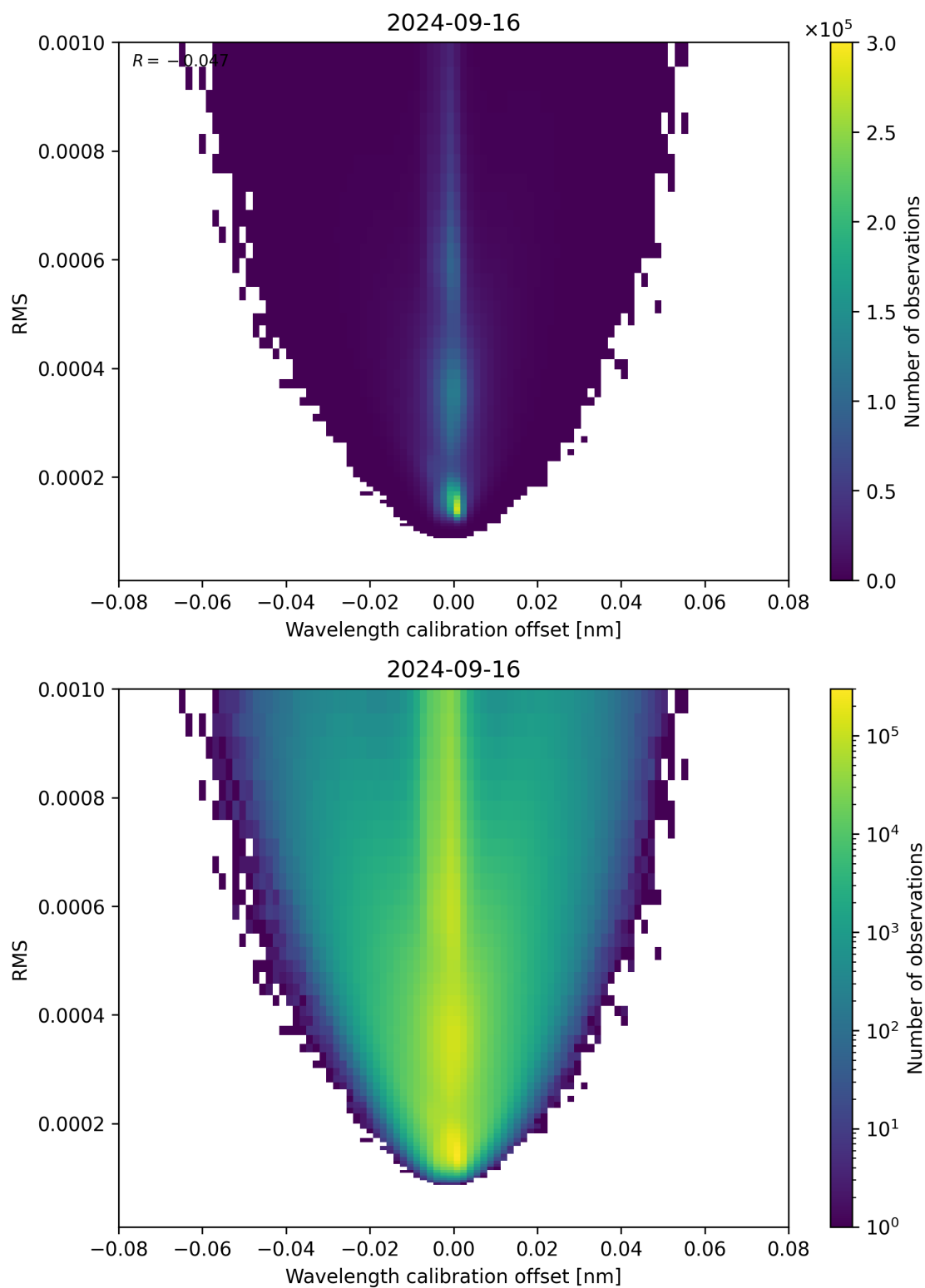
Figure 181: Scatter density plot of “Wavelength calibration offset” against “RMS” for 2024-09-15 to 2024-09-17.
