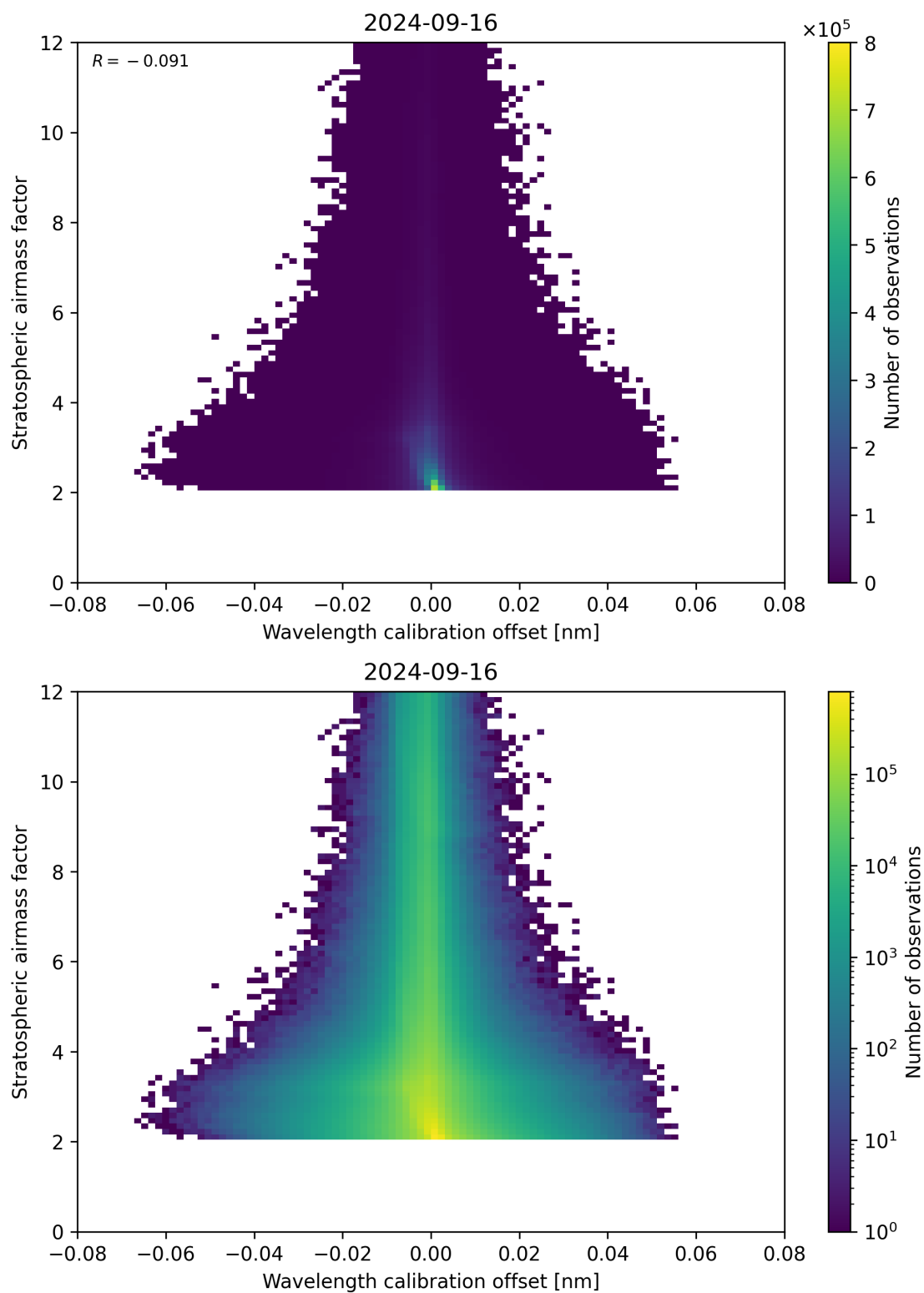
Figure 174: Scatter density plot of “Wavelength calibration offset” against “Stratospheric airmass factor” for 2024-09-15 to 2024-09-17.
