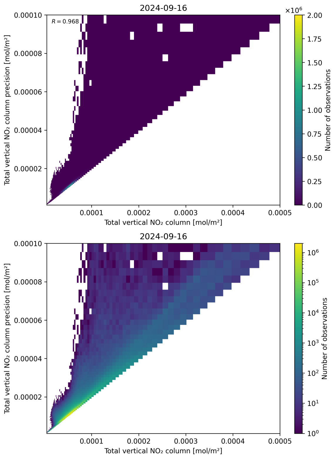
Figure 114: Scatter density plot of “Total vertical NO 2 column” against “Total vertical NO 2 column precision” for 2024-09-15 to 2024-09-17.
