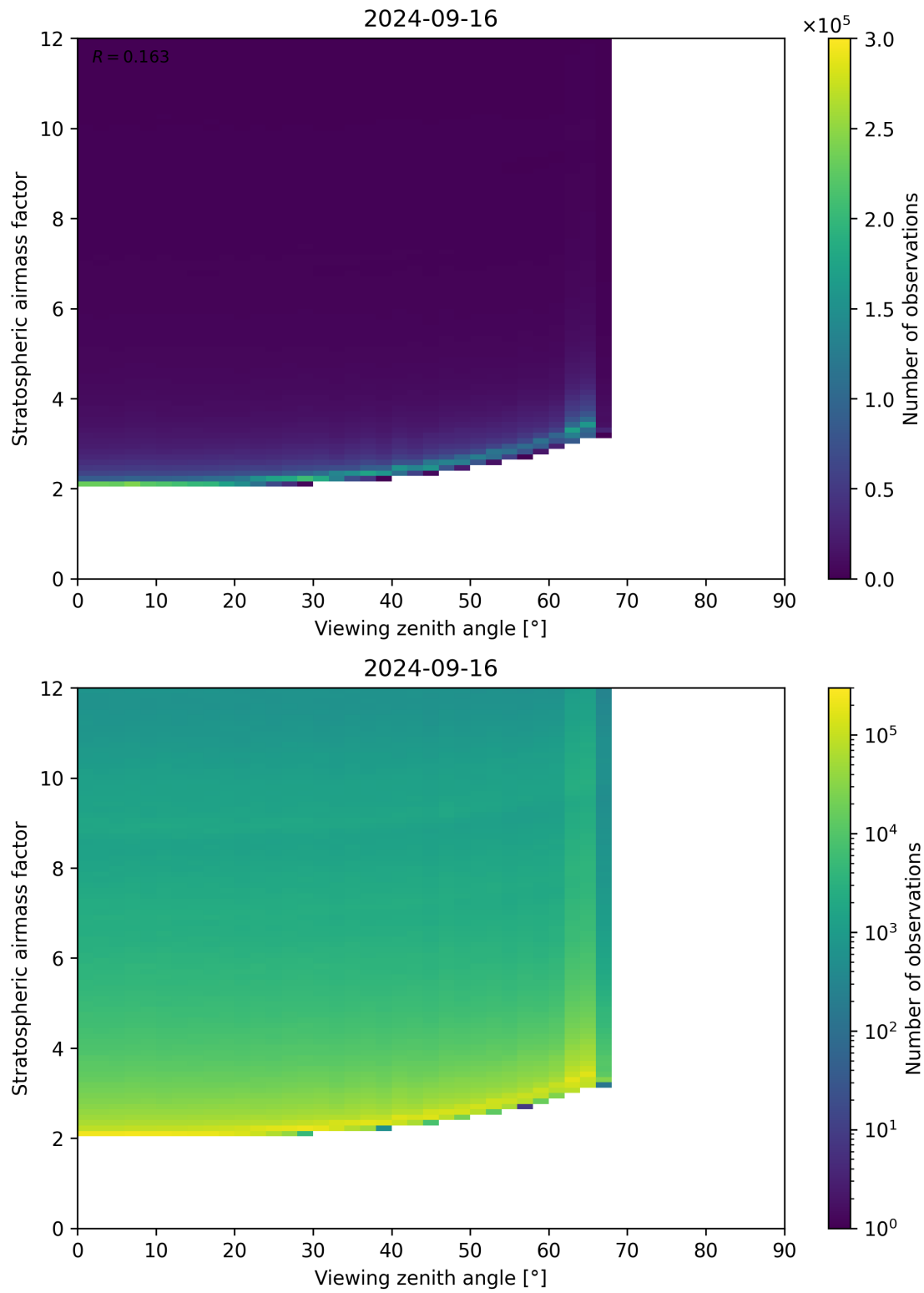
Figure 159: Scatter density plot of “Viewing zenith angle” against “Stratospheric airmass factor” for 2024-09-15 to 2024-09-17.
