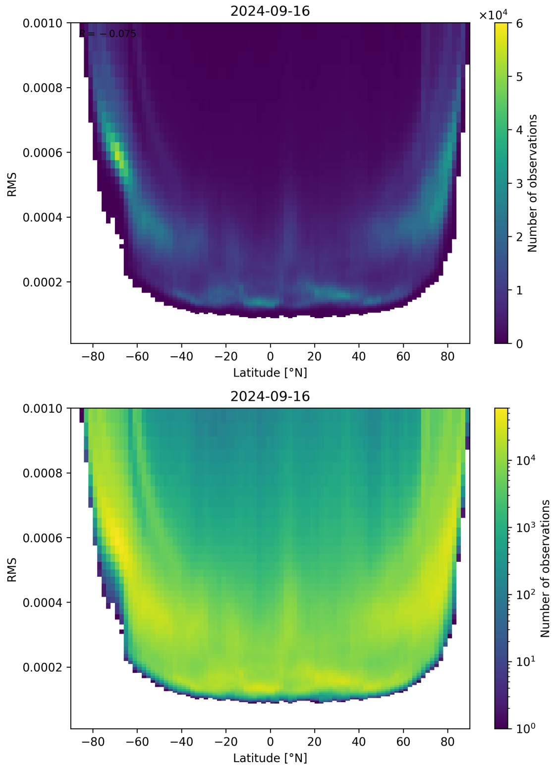
Figure 94: Scatter density plot of “Latitude” against “RMS” for 2024-09-15 to 2024-09-17.
