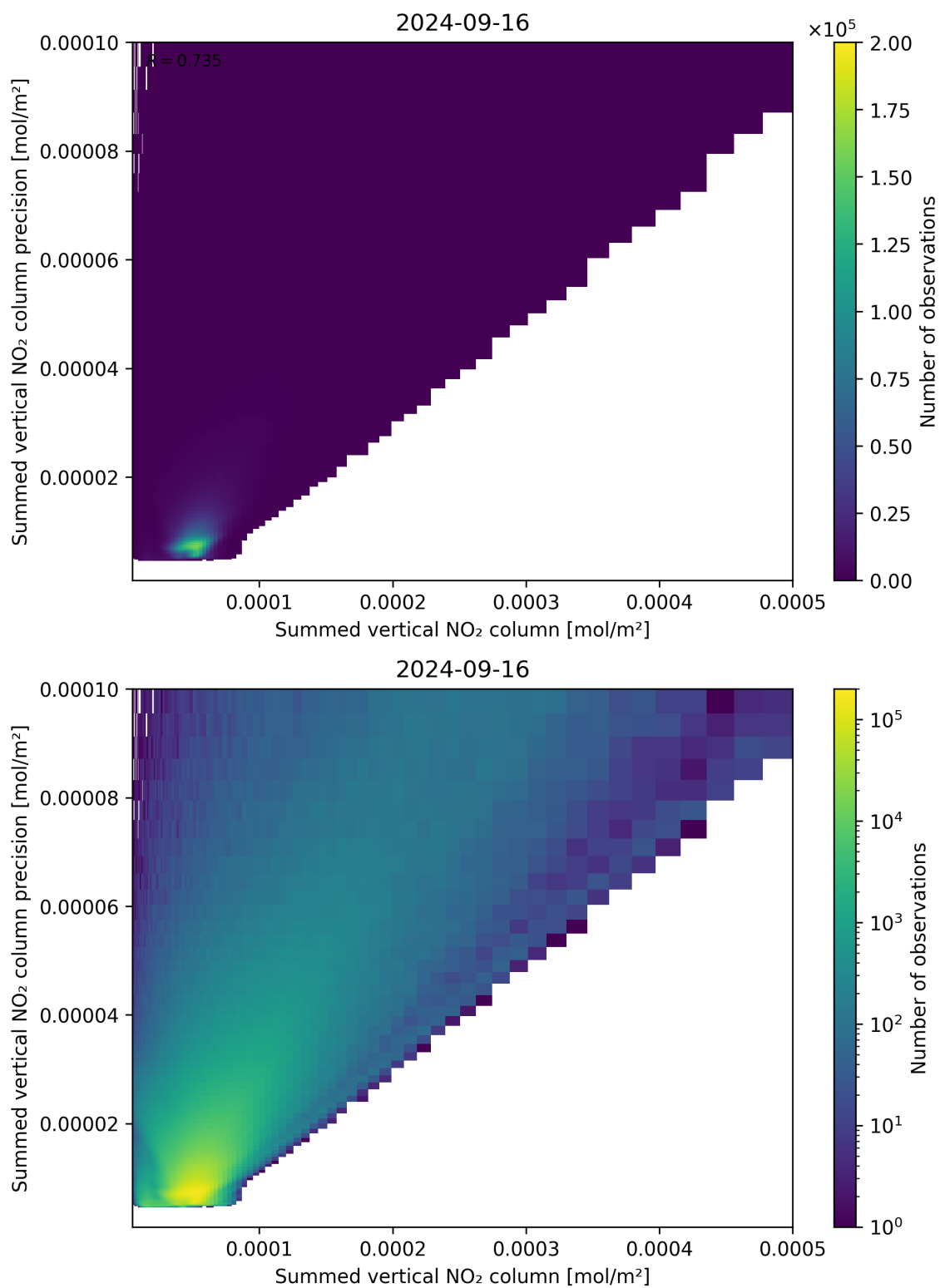
Figure 105: Scatter density plot of “Summed vertical NO 2 column” against “Summed vertical NO 2 column precision” for 2024-09-15 to 2024-09-17.
