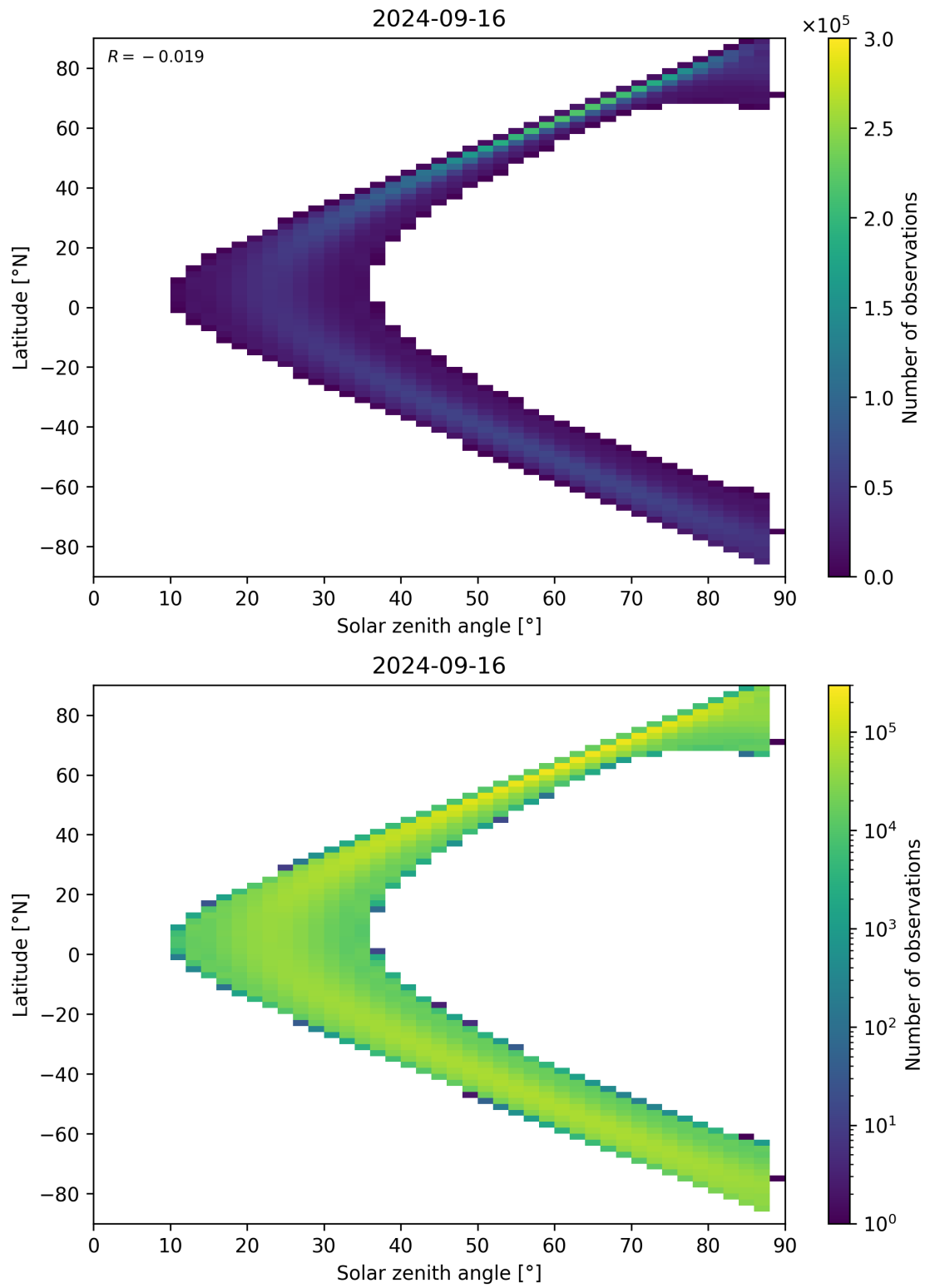
Figure 149: Scatter density plot of “Solar zenith angle” against “Latitude” for 2024-09-15 to 2024-09-17.
