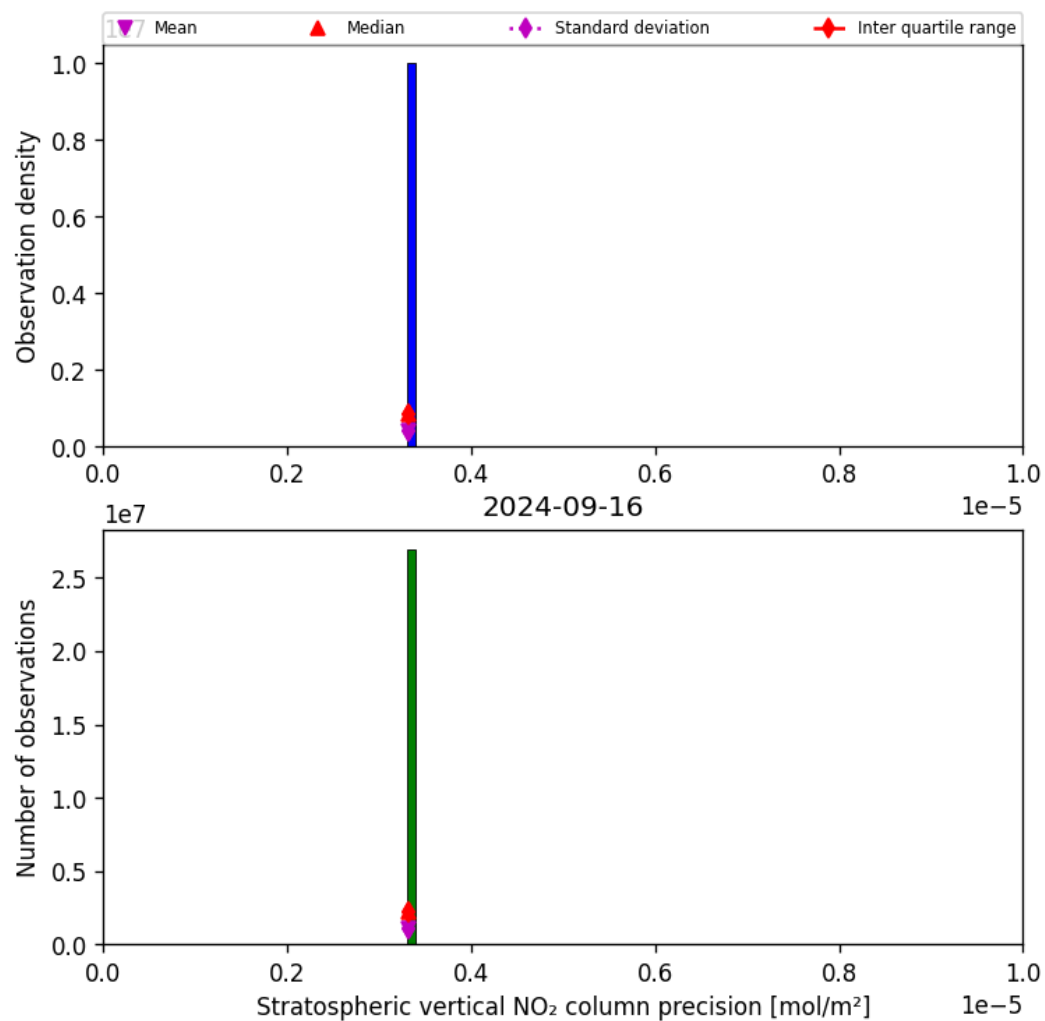
Figure 37: Histogram of “Stratospheric vertical NO 2 column precision” for 2024-09-15 to 2024-09-17
