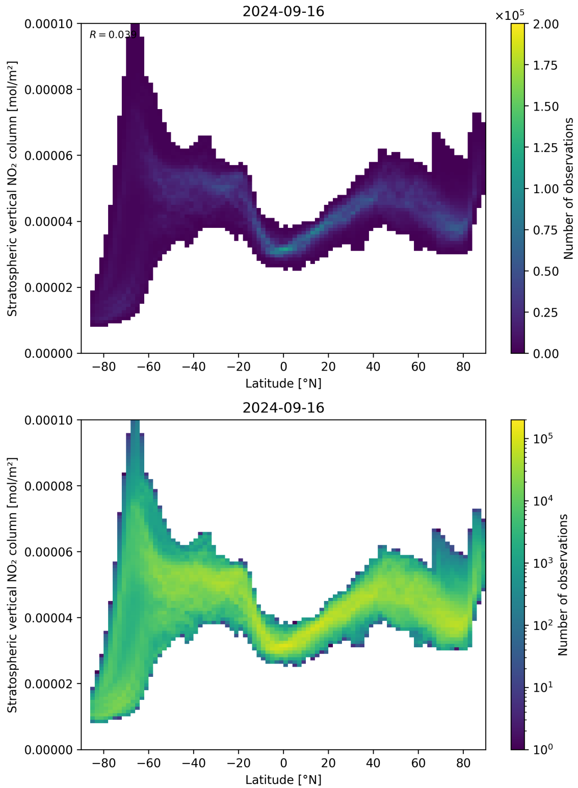
Figure 87: Scatter density plot of “Latitude” against “Stratospheric vertical NO 2 column” for 2024-09-15 to 2024-09-17.
