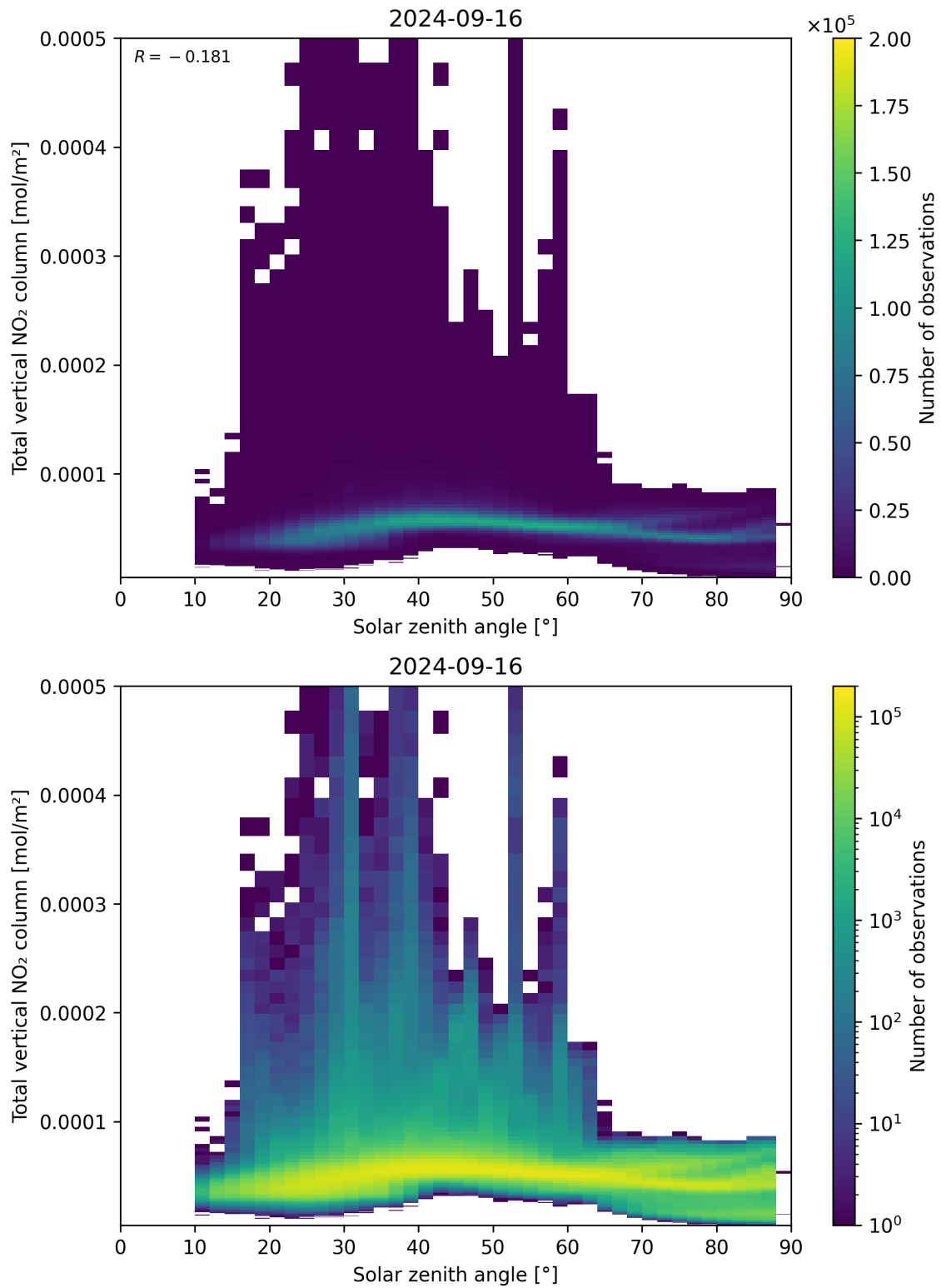
Figure 153: Scatter density plot of “Solar zenith angle” against “Total vertical NO 2 column” for 2024-09-15 to 2024-09-17.
