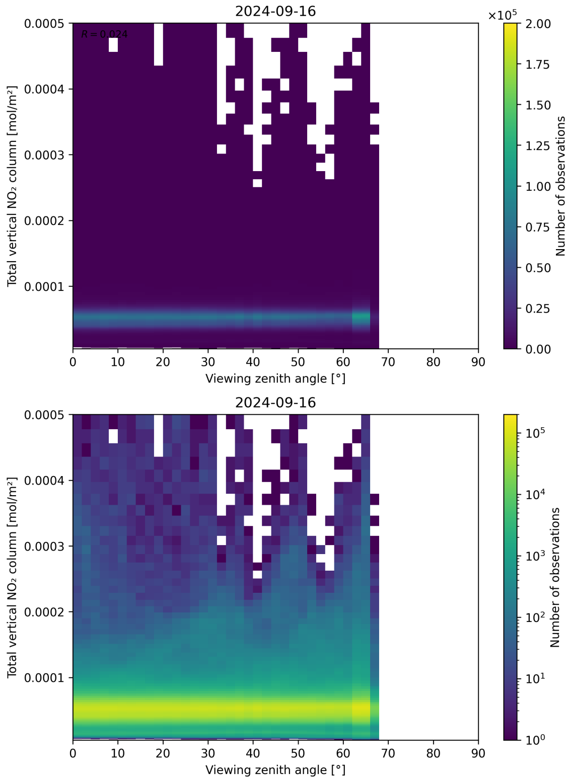
Figure 167: Scatter density plot of “Viewing zenith angle” against “Total vertical NO 2 column” for 2024-09-15 to 2024-09-17.
