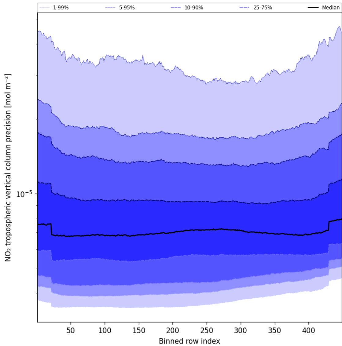
Figure 47: Along track statistics of “NO 2 tropospheric vertical column precision” for 2024-09-15 to 2024-09-17
