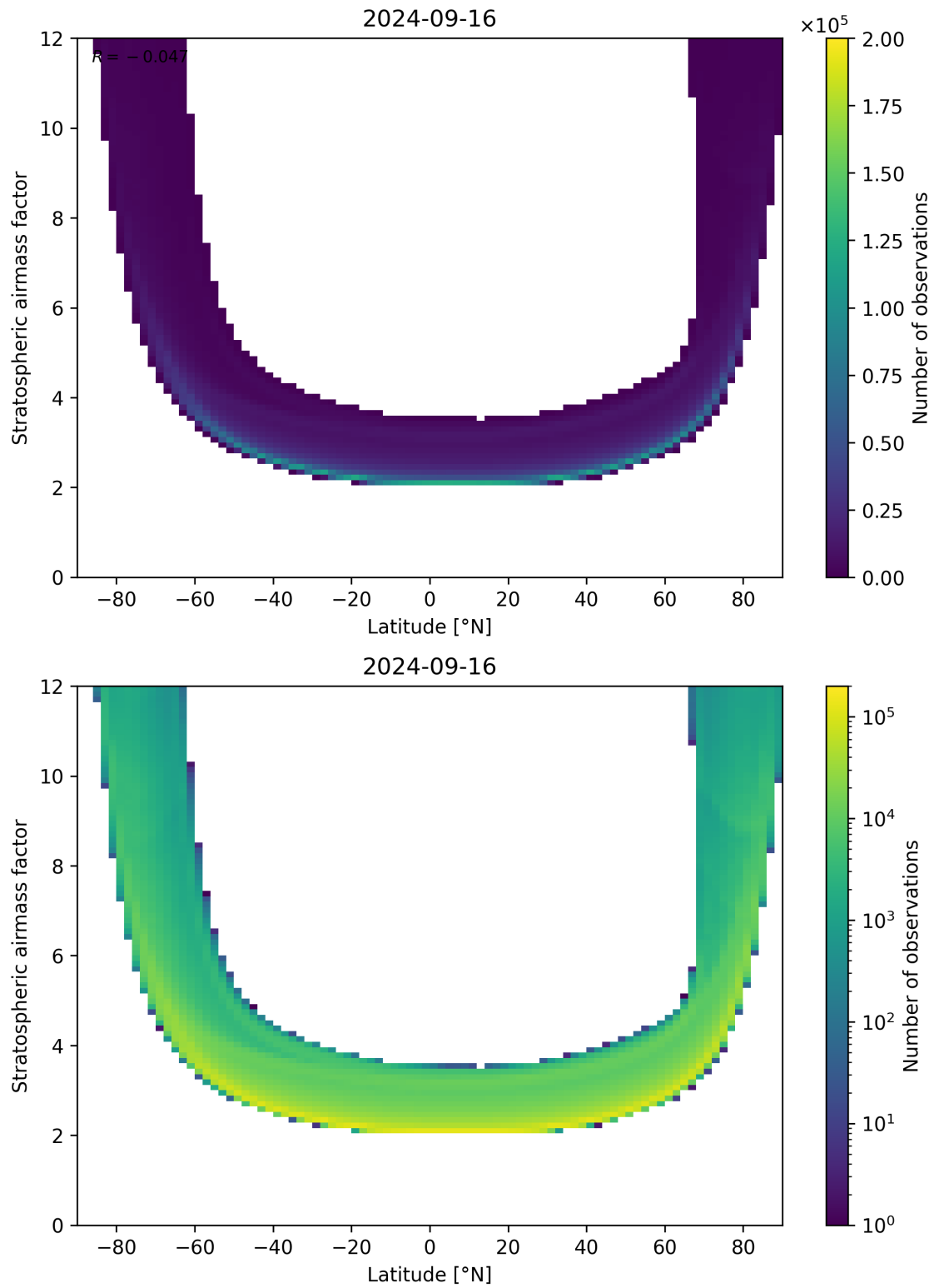
Figure 83: Scatter density plot of “Latitude” against “Stratospheric airmass factor” for 2024-09-15 to 2024-09-17.
