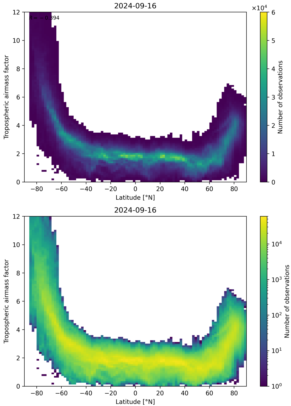
Figure 85: Scatter density plot of “Latitude” against “Tropospheric air mass factor” for 2024-09-15 to 2024-09-17.
