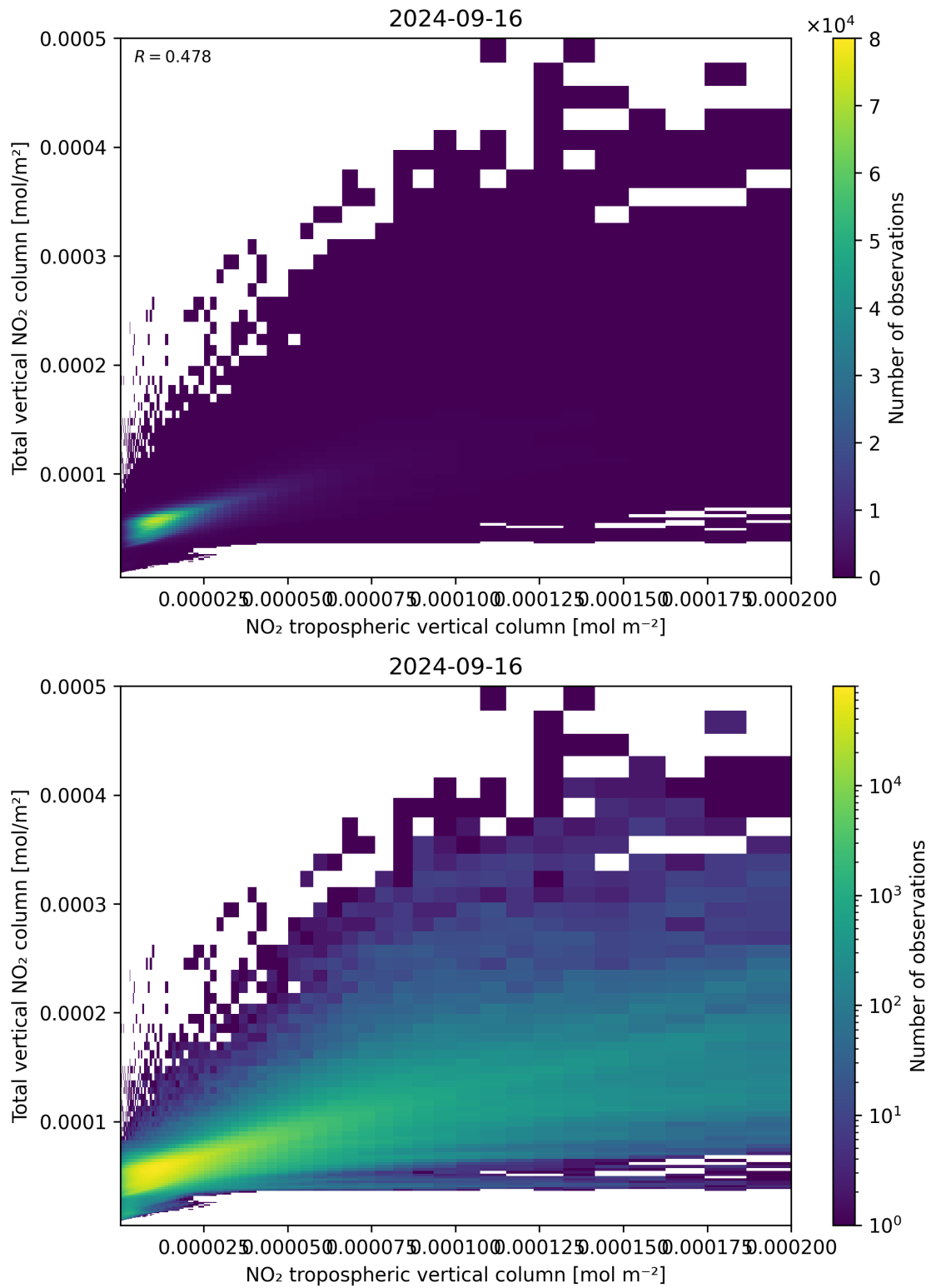
Figure 128: Scatter density plot of “NO 2 tropospheric vertical column” against “Total vertical NO 2 column” for 2024-09-15 to 2024-09-17.
