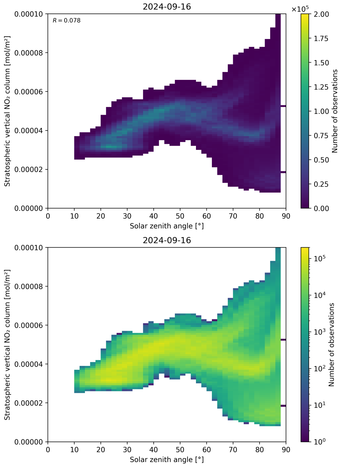
Figure 150: Scatter density plot of “Solar zenith angle” against “Stratospheric vertical NO 2 column” for 2024-09-15 to 2024-09-17.
