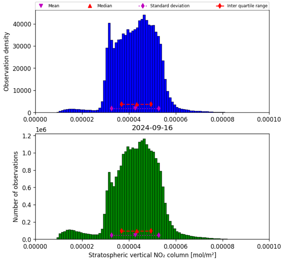
Figure 36: Histogram of “Stratospheric vertical NO 2 column” for 2024-09-15 to 2024-09-17
