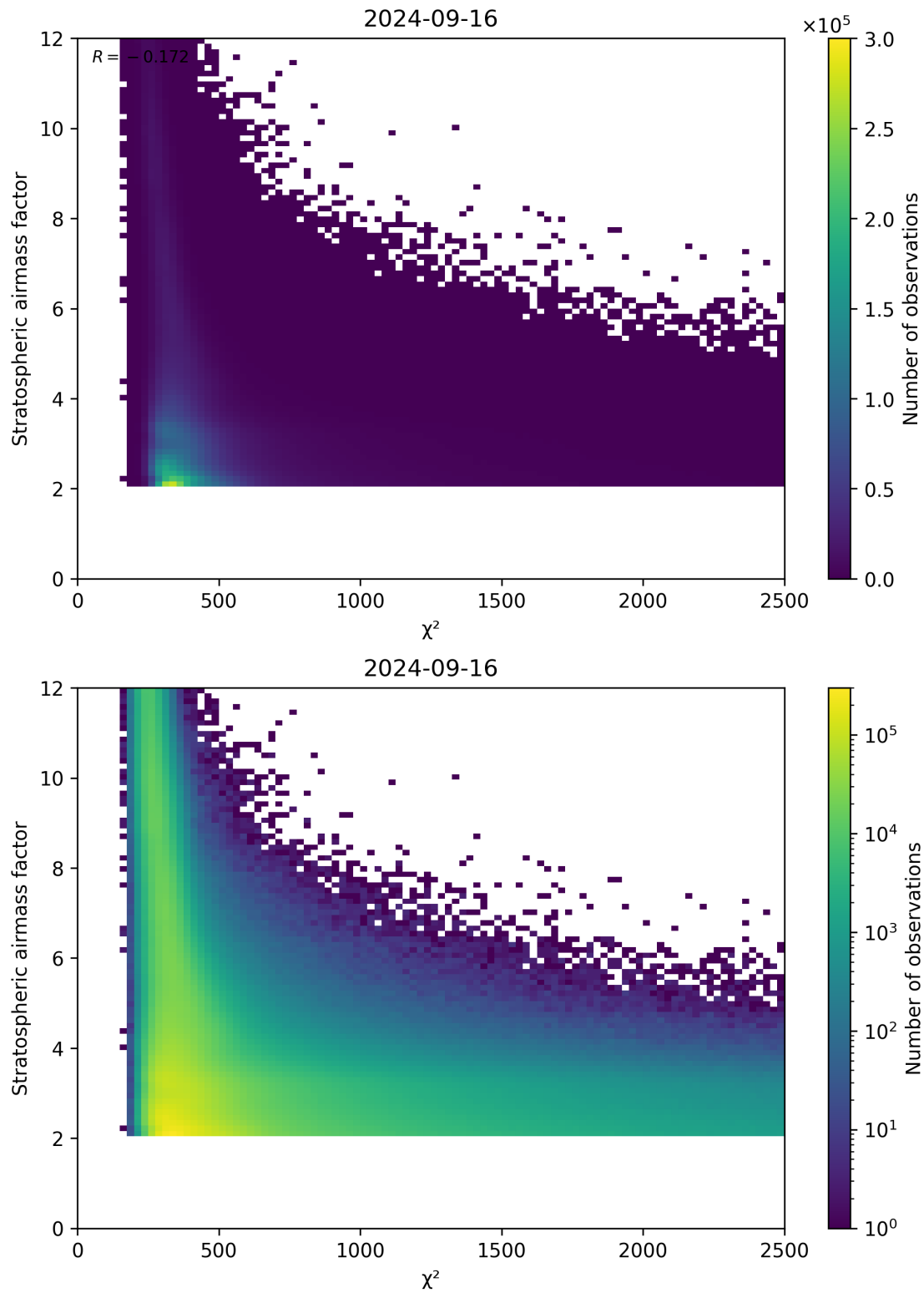
Figure 81: Scatter density plot of “ \chi^2 ” against “Stratospheric airmass factor” for 2024-09-15 to 2024-09-17.
