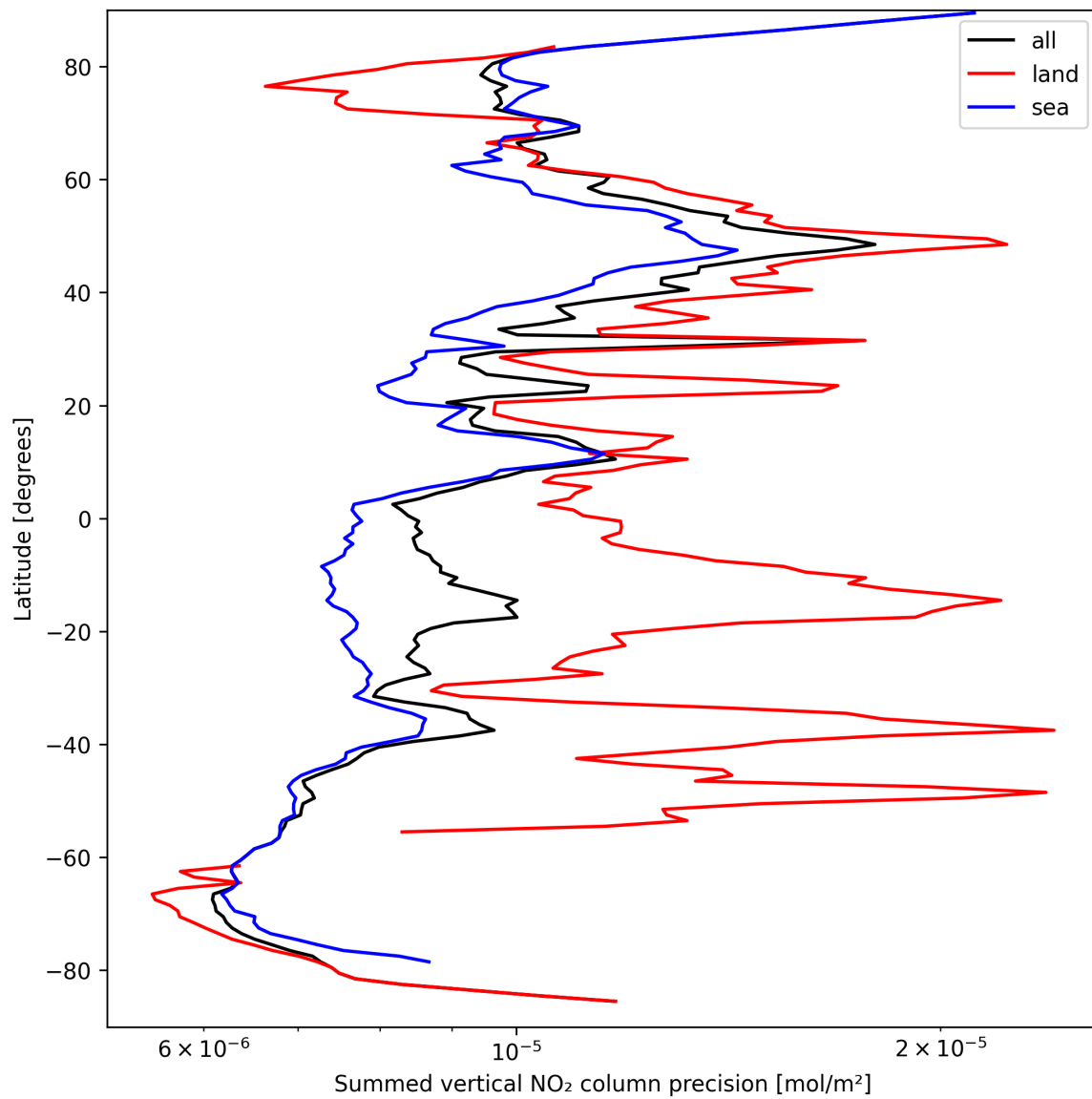
Figure 24: Zonal average of “Summed vertical NO 2 column precision” for 2024-09-15 to 2024-09-17.
