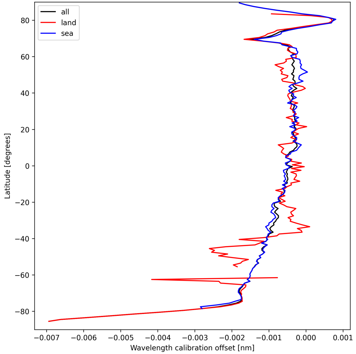
Figure 18: Zonal average of “Wavelength calibration offset” for 2024-09-15 to 2024-09-17.
