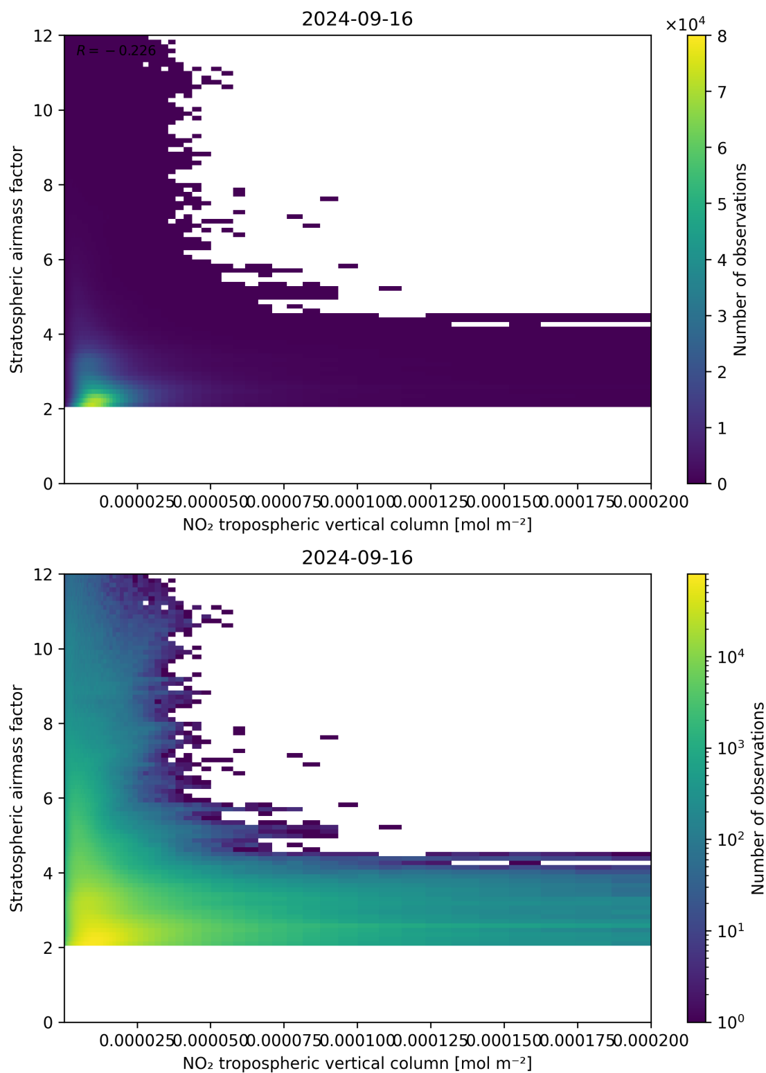
Figure 121: Scatter density plot of “NO 2 tropospheric vertical column” against “Stratospheric airmass factor” for 2024-09-15 to 2024-09-17.
