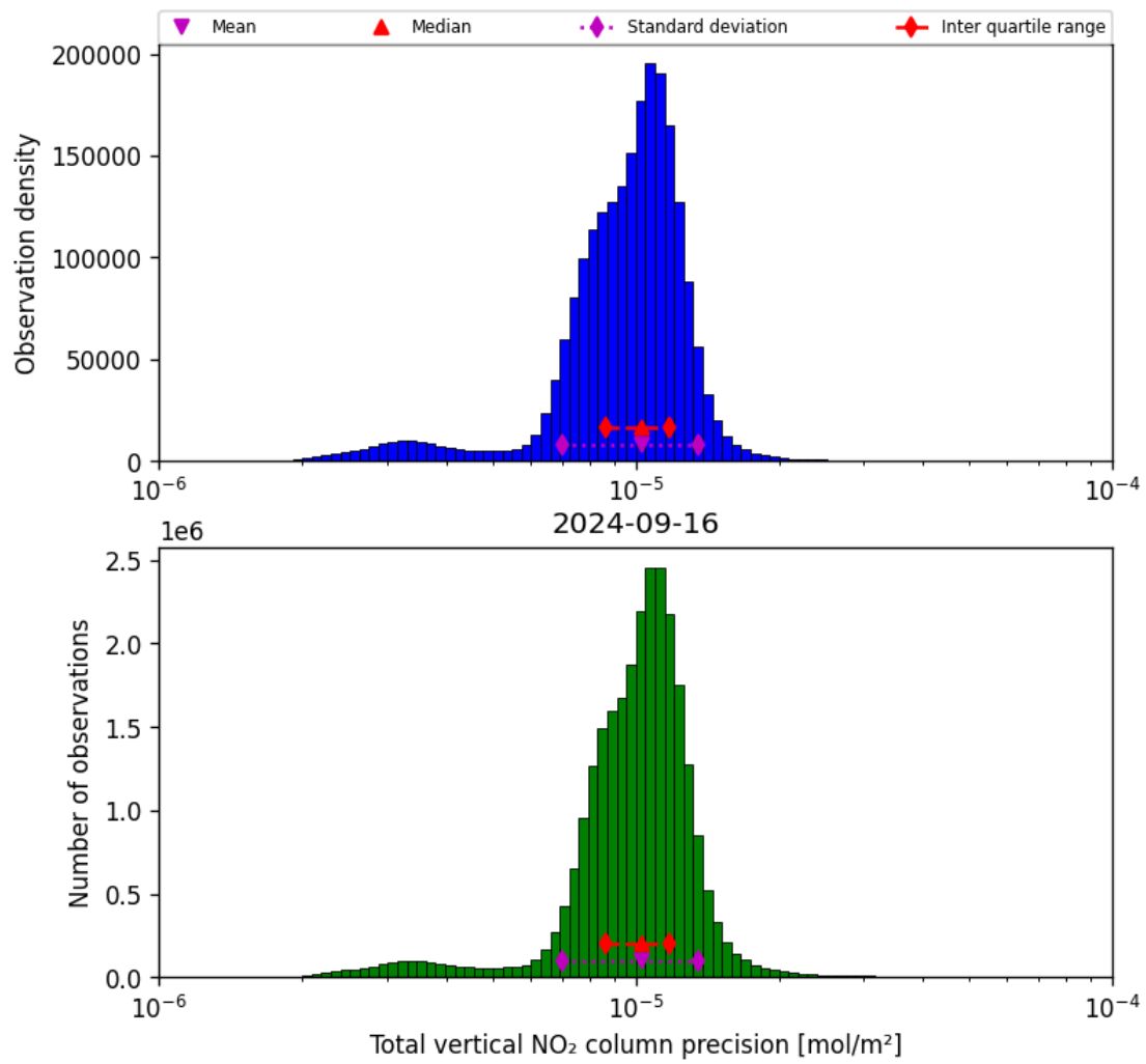
Figure 39: Histogram of "Total vertical NO 2 column precision" for 2024-09-15 to 2024-09-17
