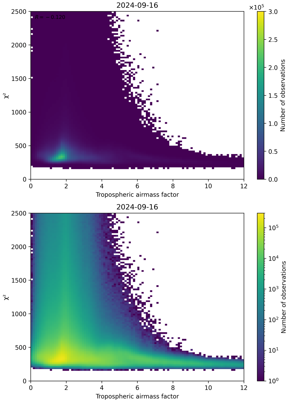
Figure 73: Scatter density plot of “Tropospheric airmass factor” against “ \chi^2 ” for 2024-09-15 to 2024-09-17.
