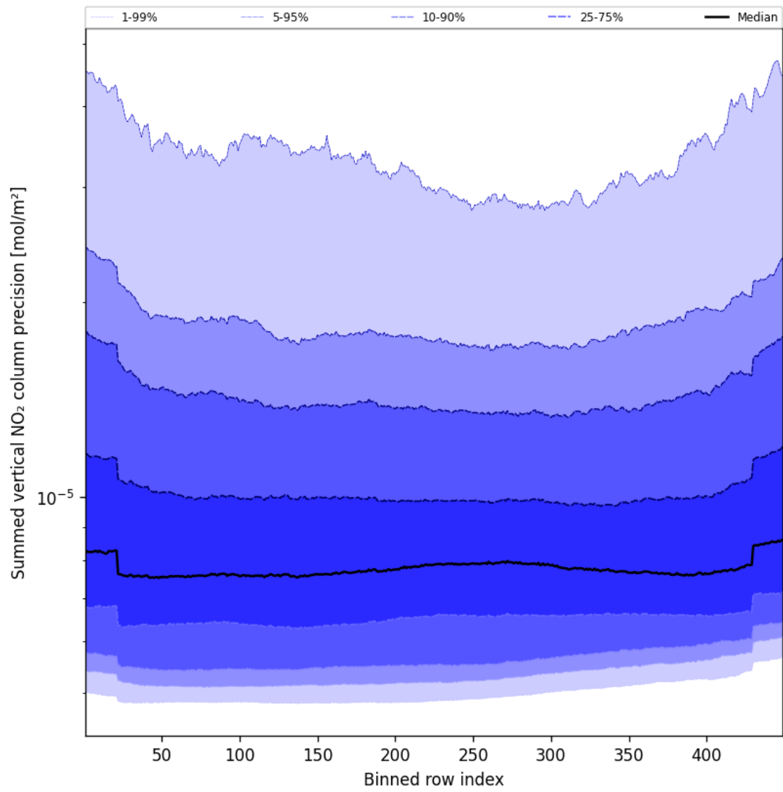
Figure 58: Along track statistics of “Summed vertical NO 2 column precision” for 2024-09-15 to 2024-09-17
