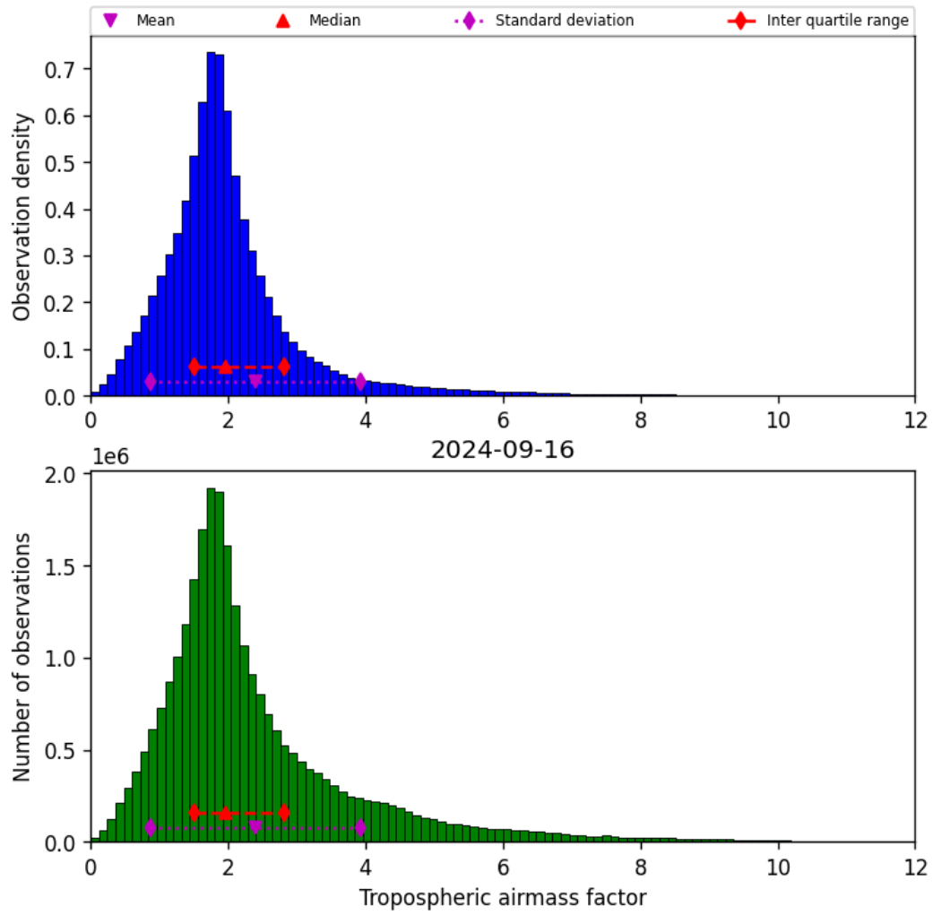
Figure 31: Histogram of “Tropospheric airmass factor” for 2024-09-15 to 2024-09-17
