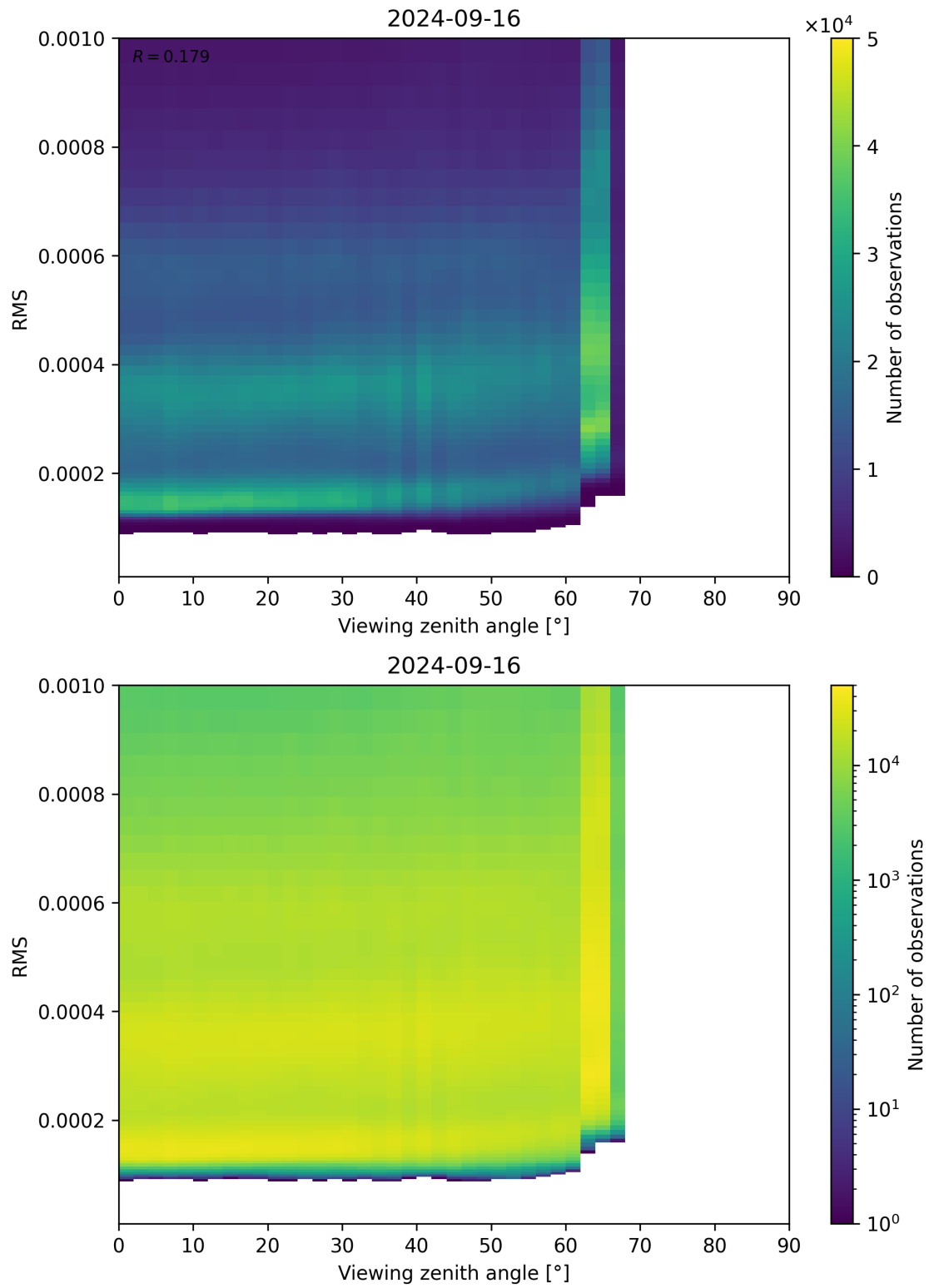
Figure 171: Scatter density plot of “Viewing zenith angle” against “RMS” for 2024-09-15 to 2024-09-17.
