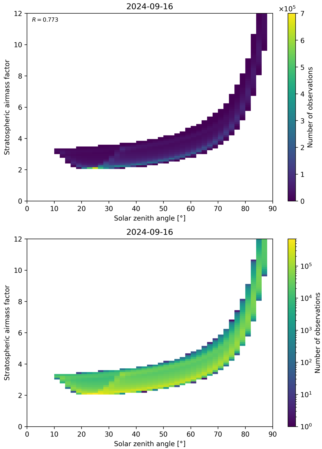
Figure 145: Scatter density plot of “Solar zenith angle” against “Stratospheric airmass factor” for 2024-09-15 to 2024-09-17.
