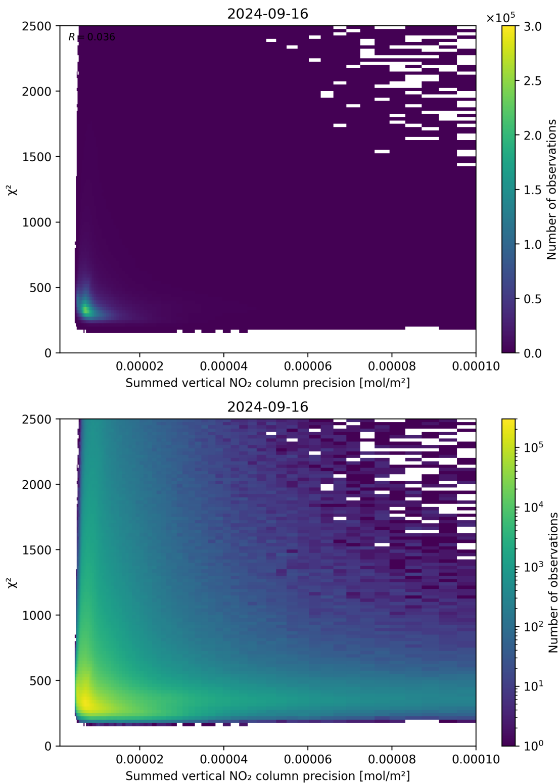
Figure 107: Scatter density plot of “Summed vertical NO 2 column precision” against “ \chi^2 ” for 2024-09-15 to 2024-09-17.
