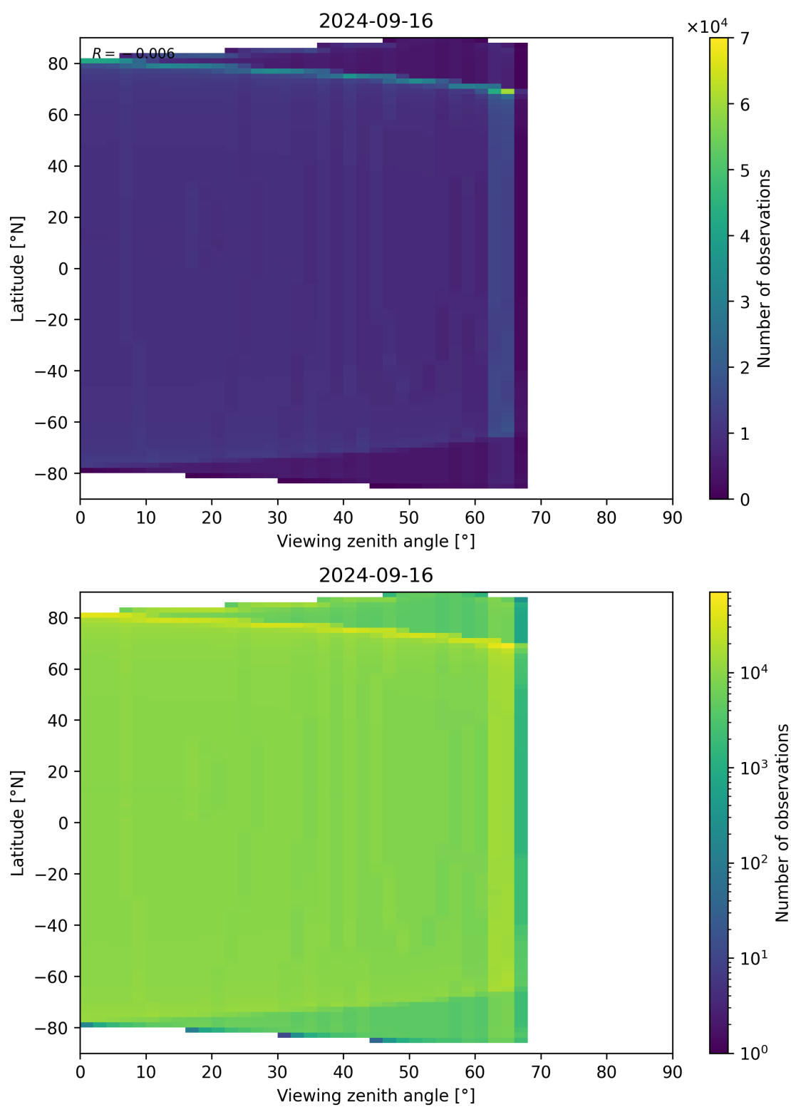
Figure 163: Scatter density plot of “Viewing zenith angle” against “Latitude” for 2024-09-15 to 2024-09-17.
