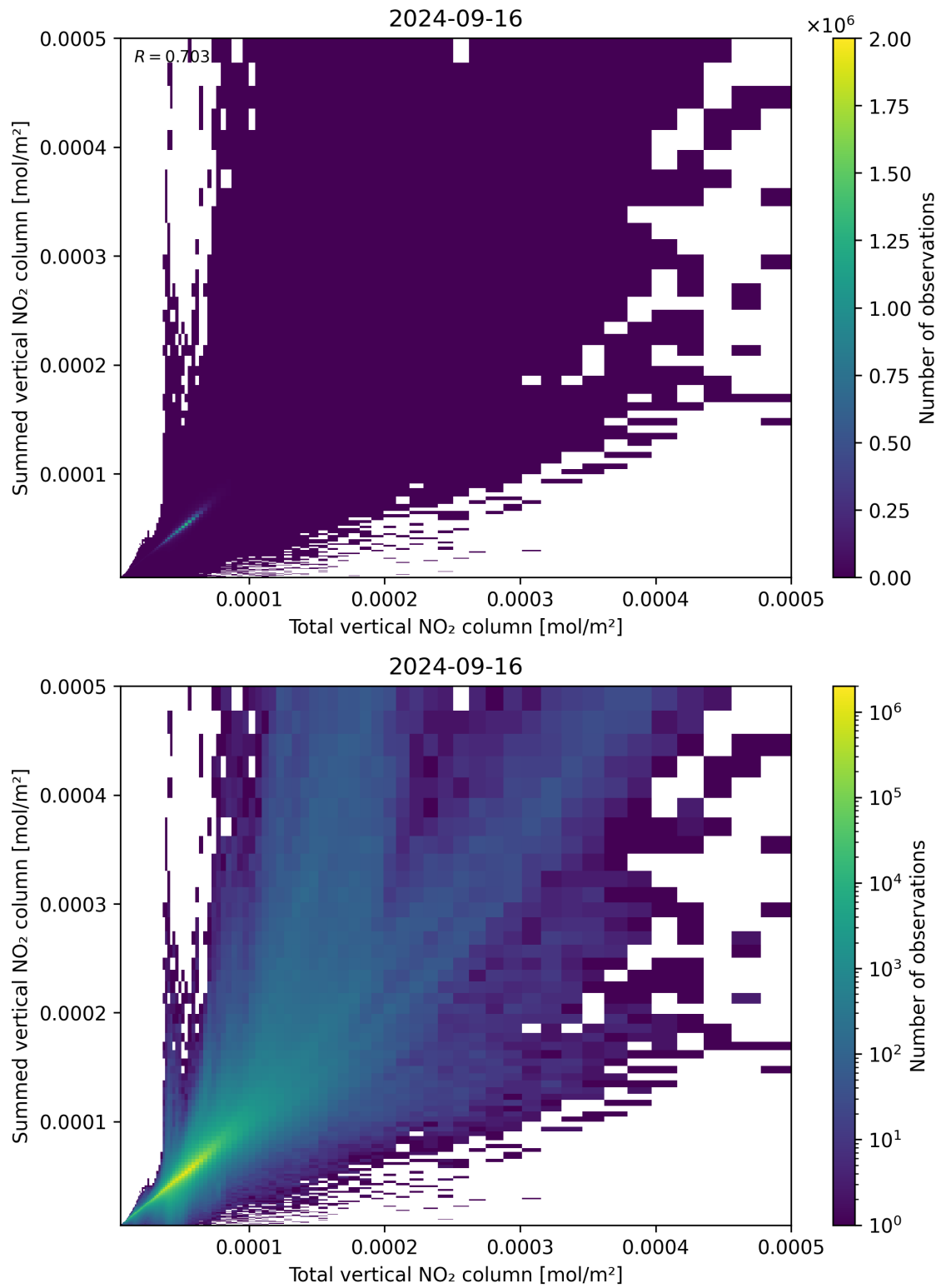
Figure 112: Scatter density plot of “Total vertical NO 2 column” against “Summed vertical NO 2 column” for 2024-09-15 to 2024-09-17.
