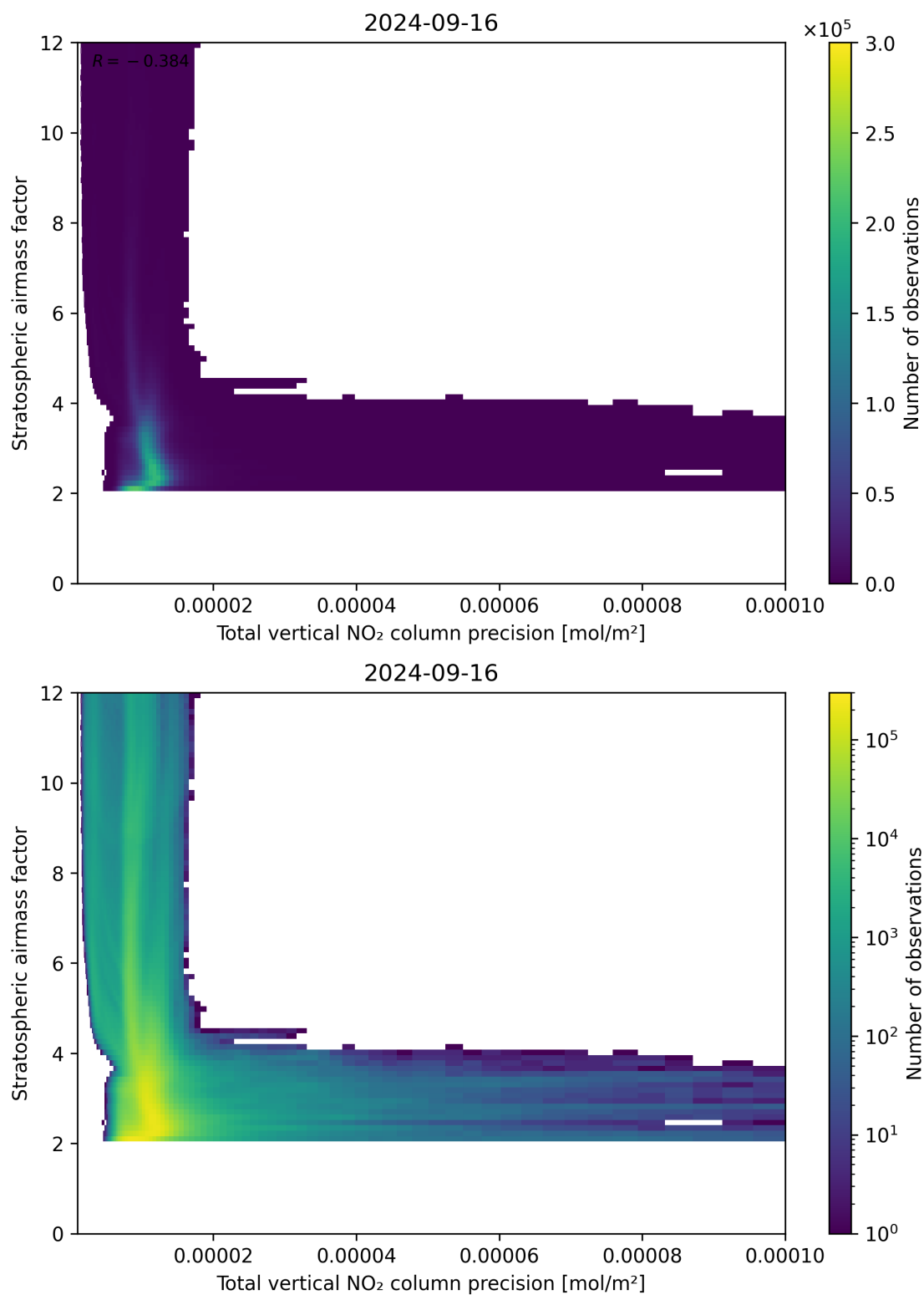
Figure 115: Scatter density plot of “Total vertical NO 2 column precision” against “Stratospheric air mass factor” for 2024-09-15 to 2024-09-17.
