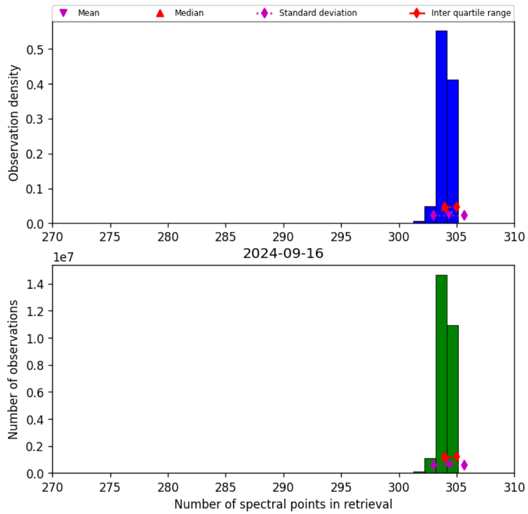
Figure 33: Histogram of “Number of spectral points in retrieval” for 2024-09-15 to 2024-09-17
