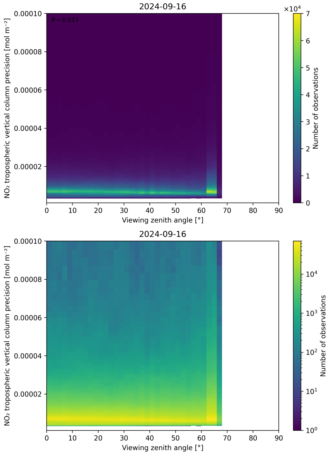
Figure 170: Scatter density plot of “Viewing zenith angle” against “NO 2 tropospheric vertical column precision” for 2024-09-15 to 2024-09-17.
