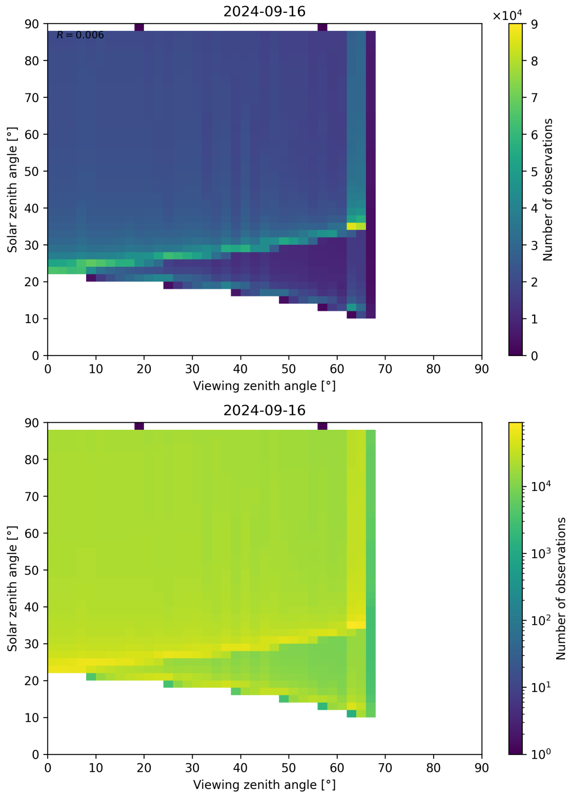
Figure 172: Scatter density plot of “Viewing zenith angle” against “Solar zenith angle” for 2024-09-15 to 2024-09-17.
