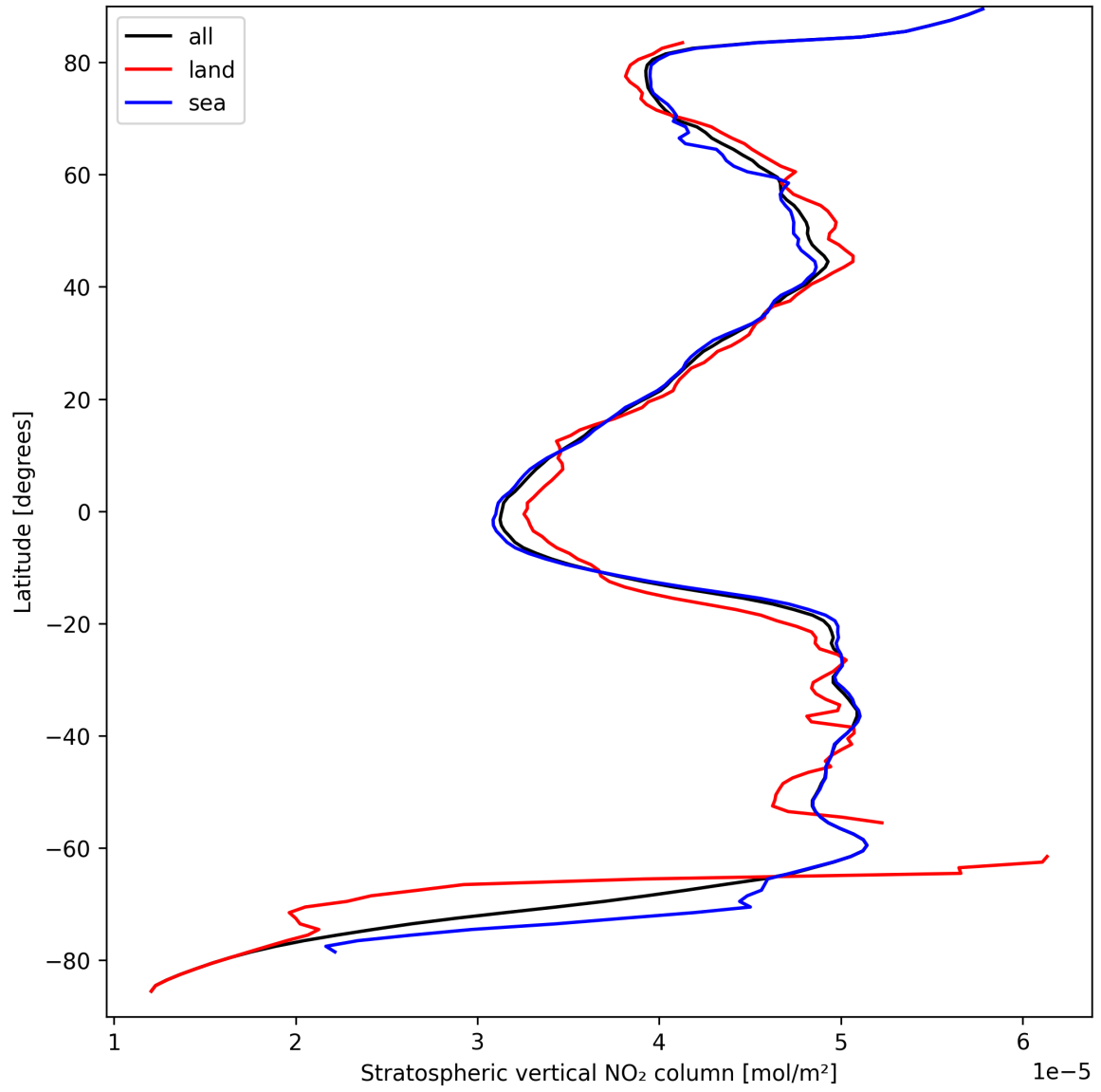
Figure 19: Zonal average of “Stratospheric vertical NO 2 column” for 2024-09-15 to 2024-09-17.
