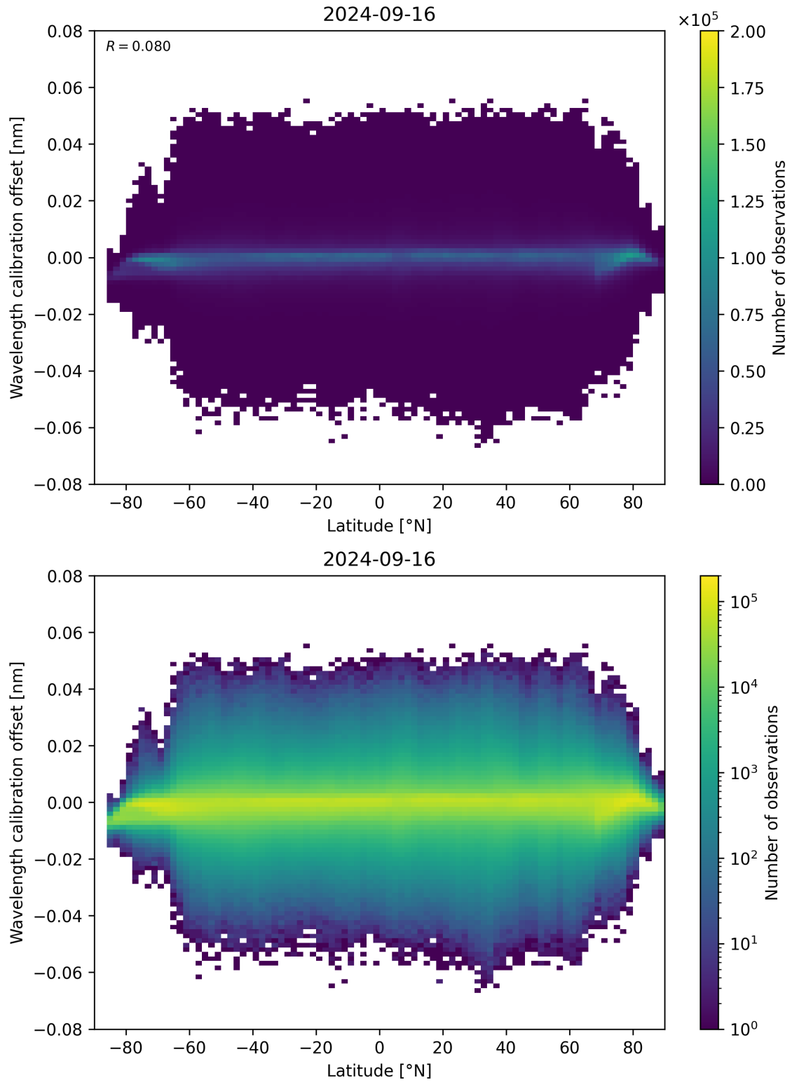
Figure 95: Scatter density plot of “Latitude” against “Wavelength calibration offset” for 2024-09-15 to 2024-09-17.
