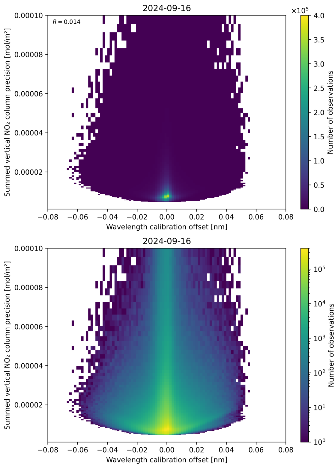
Figure 178: Scatter density plot of “Wavelength calibration offset” against “Summed vertical NO 2 column precision” for 2024-09-15 to 2024-09-17.
