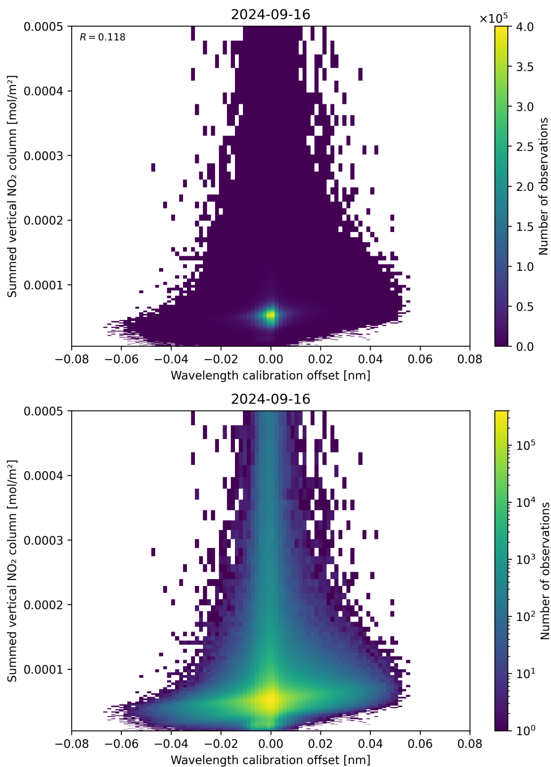
Figure 177: Scatter density plot of “Wavelength calibration offset” against “Summed vertical NO 2 column” for 2024-09-15 to 2024-09-17.
