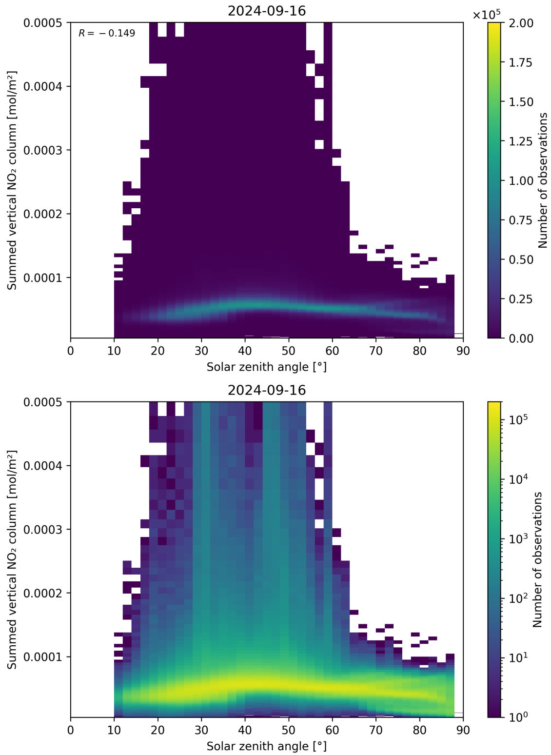
Figure 151: Scatter density plot of “Solar zenith angle” against “Summed vertical NO 2 column” for 2024-09-15 to 2024-09-17.
