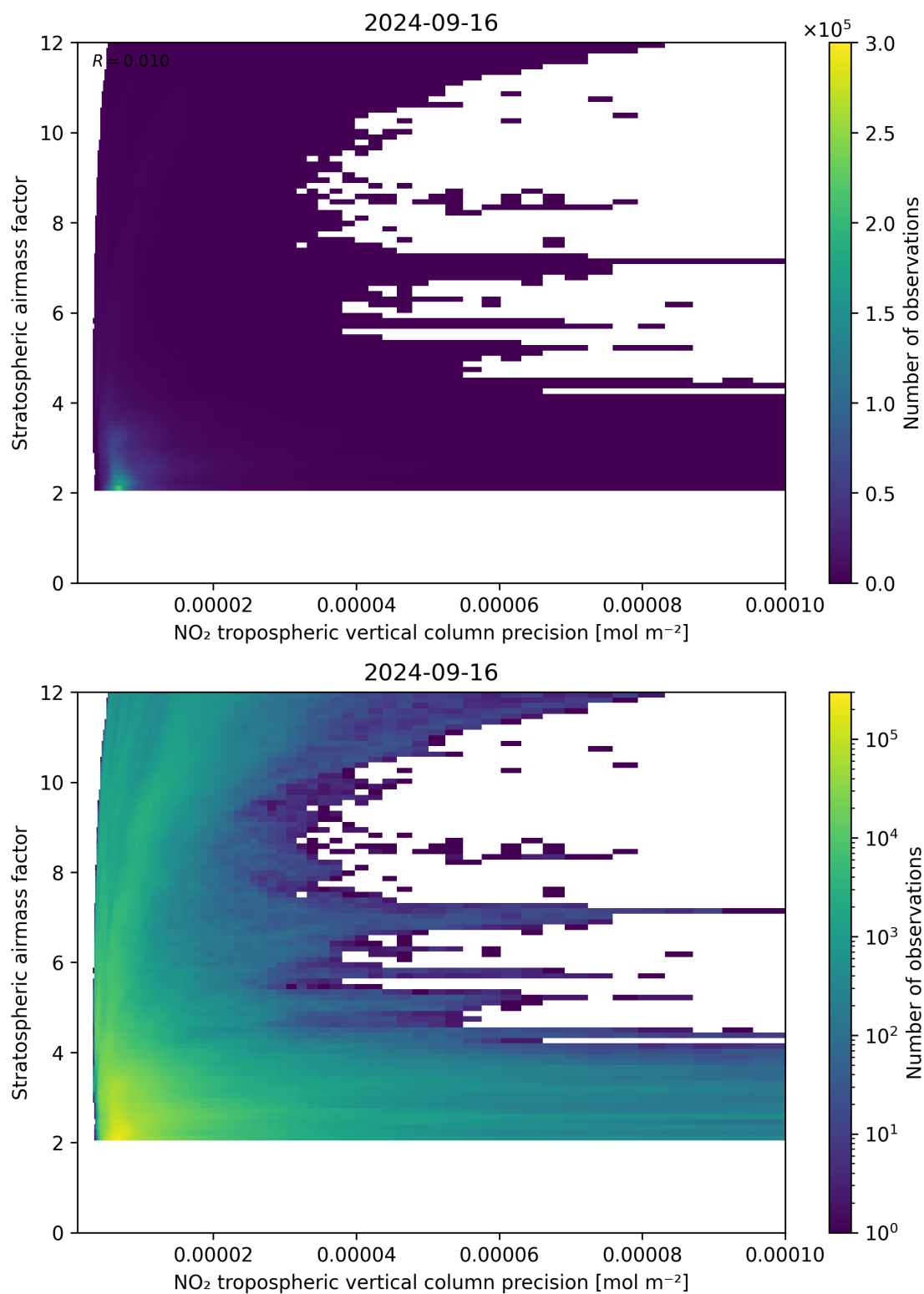
Figure 131: Scatter density plot of “NO 2 tropospheric vertical column precision” against “Stratospheric airmass factor” for 2024-09-15 to 2024-09-17.
