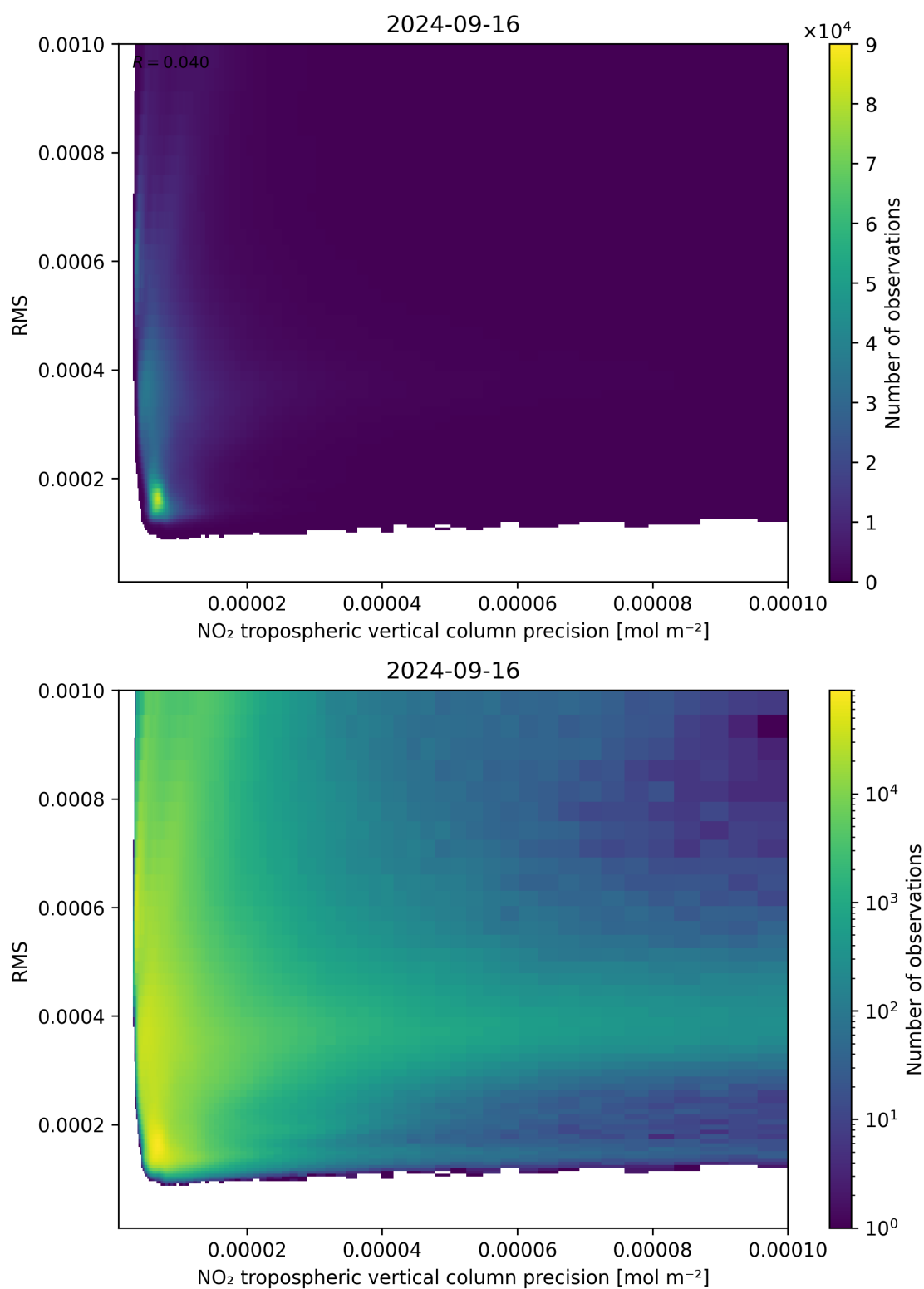
Figure 140: Scatter density plot of “NO 2 tropospheric vertical column precision” against “RMS” for 2024-09-15 to 2024-09-17.
