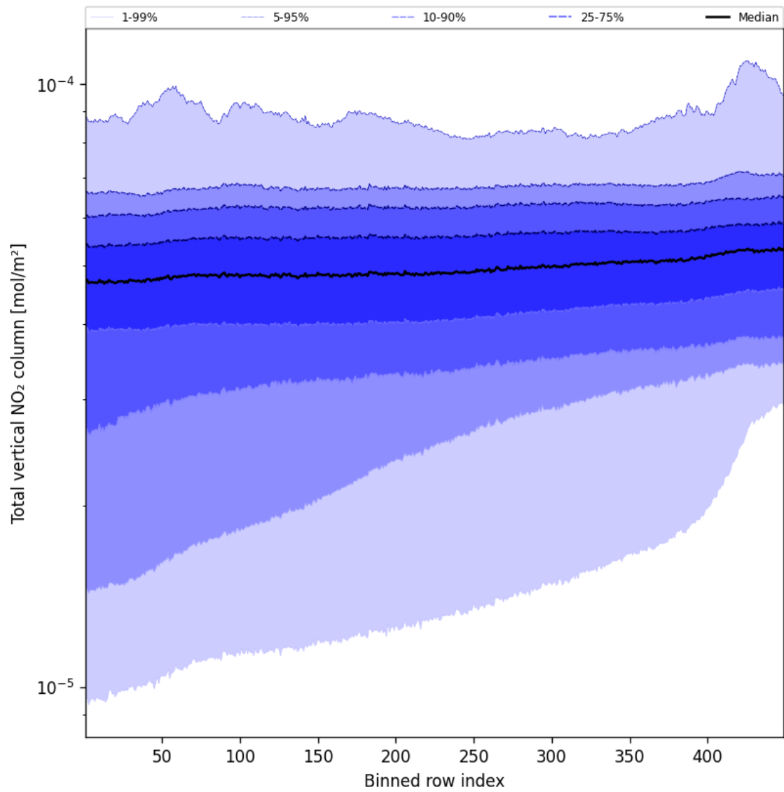
Figure 55: Along track statistics of “Total vertical NO 2 column” for 2024-09-15 to 2024-09-17
