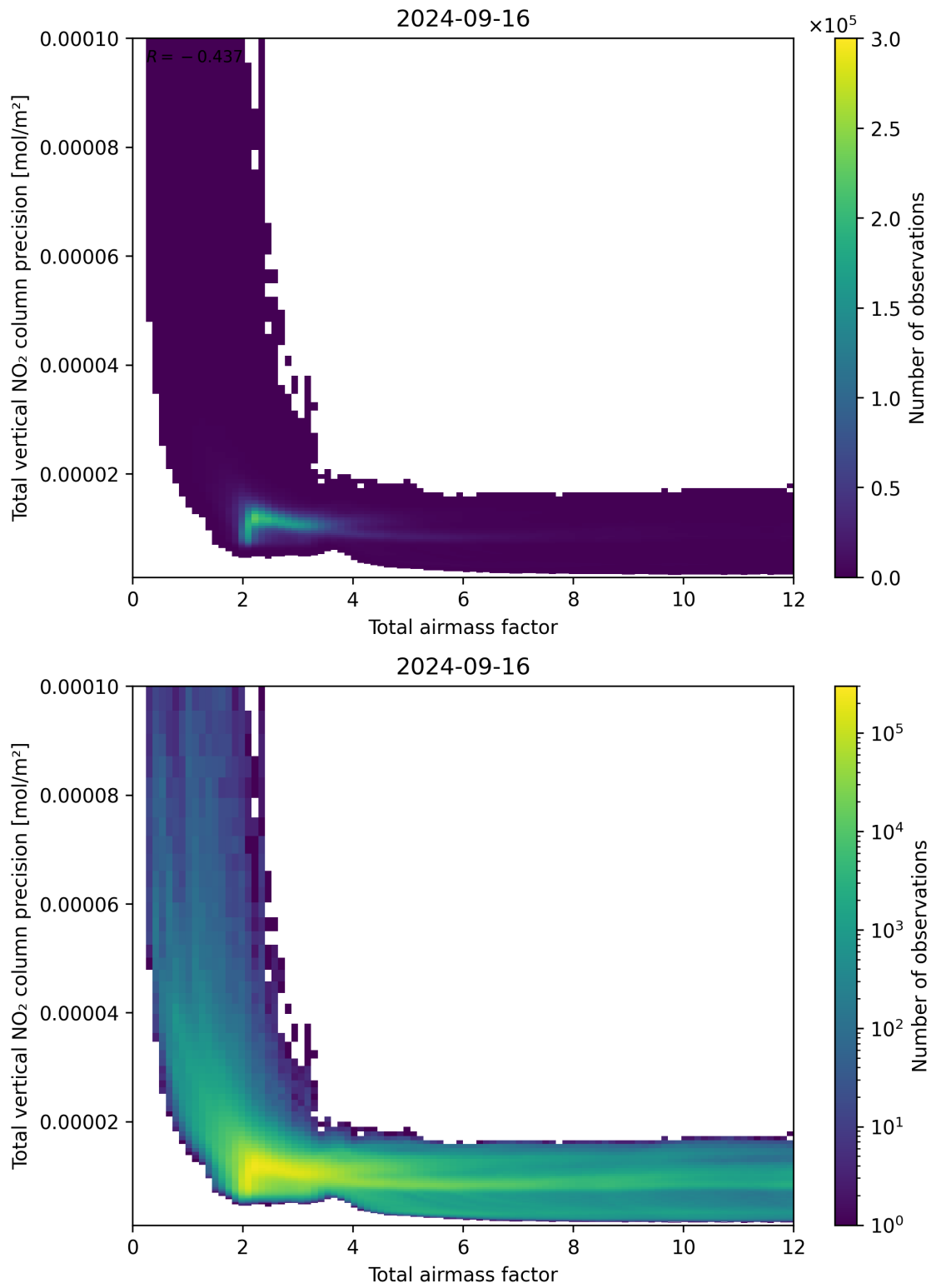
Figure 68: Scatter density plot of “Total airmass factor” against “Total vertical NO 2 column precision” for 2024-09-15 to 2024-09-17.
