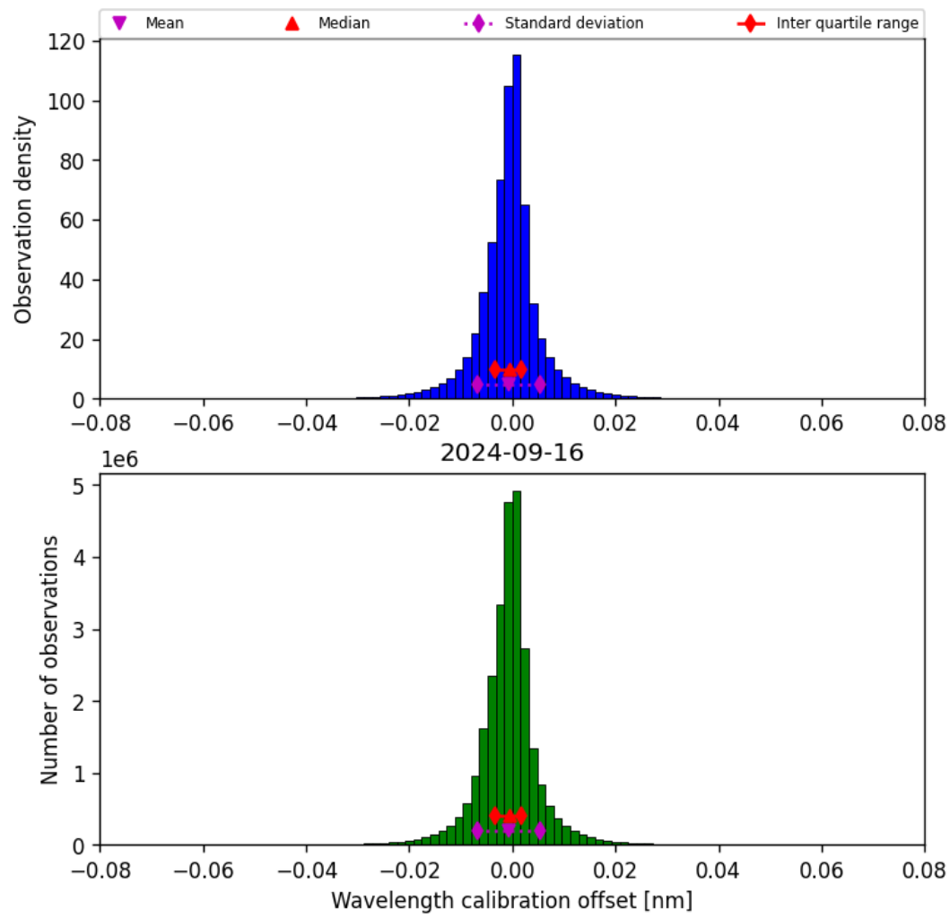
Figure 35: Histogram of “Wavelength calibration offset” for 2024-09-15 to 2024-09-17
