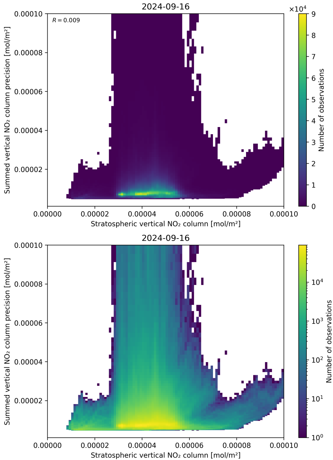
Figure 99: Scatter density plot of “Stratospheric vertical NO 2 column” against “Summed vertical NO 2 column precision” for 2024-09-15 to 2024-09-17.
