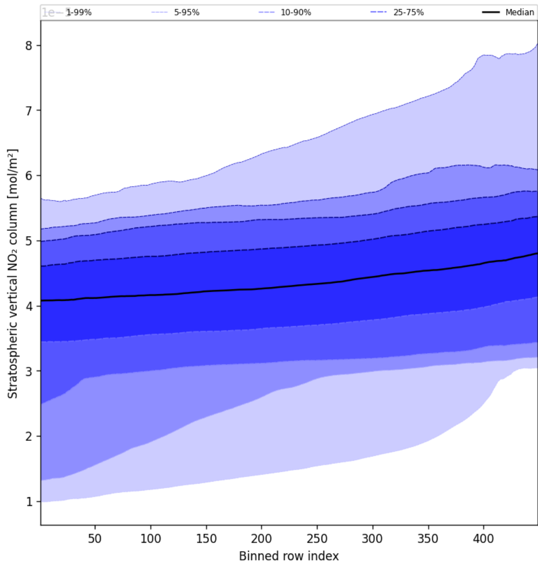
Figure 53: Along track statistics of “Stratospheric vertical NO 2 column” for 2024-09-15 to 2024-09-17
