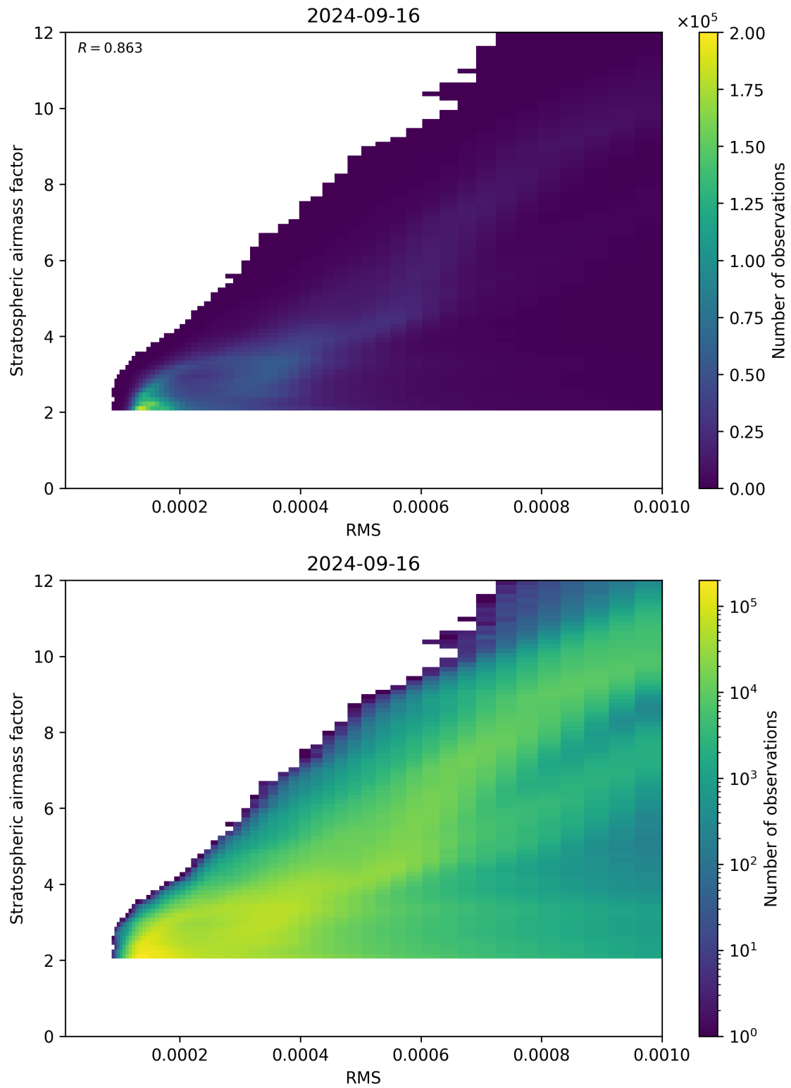
Figure 144: Scatter density plot of “RMS” against “Stratospheric airmass factor” for 2024-09-15 to 2024-09-17.
