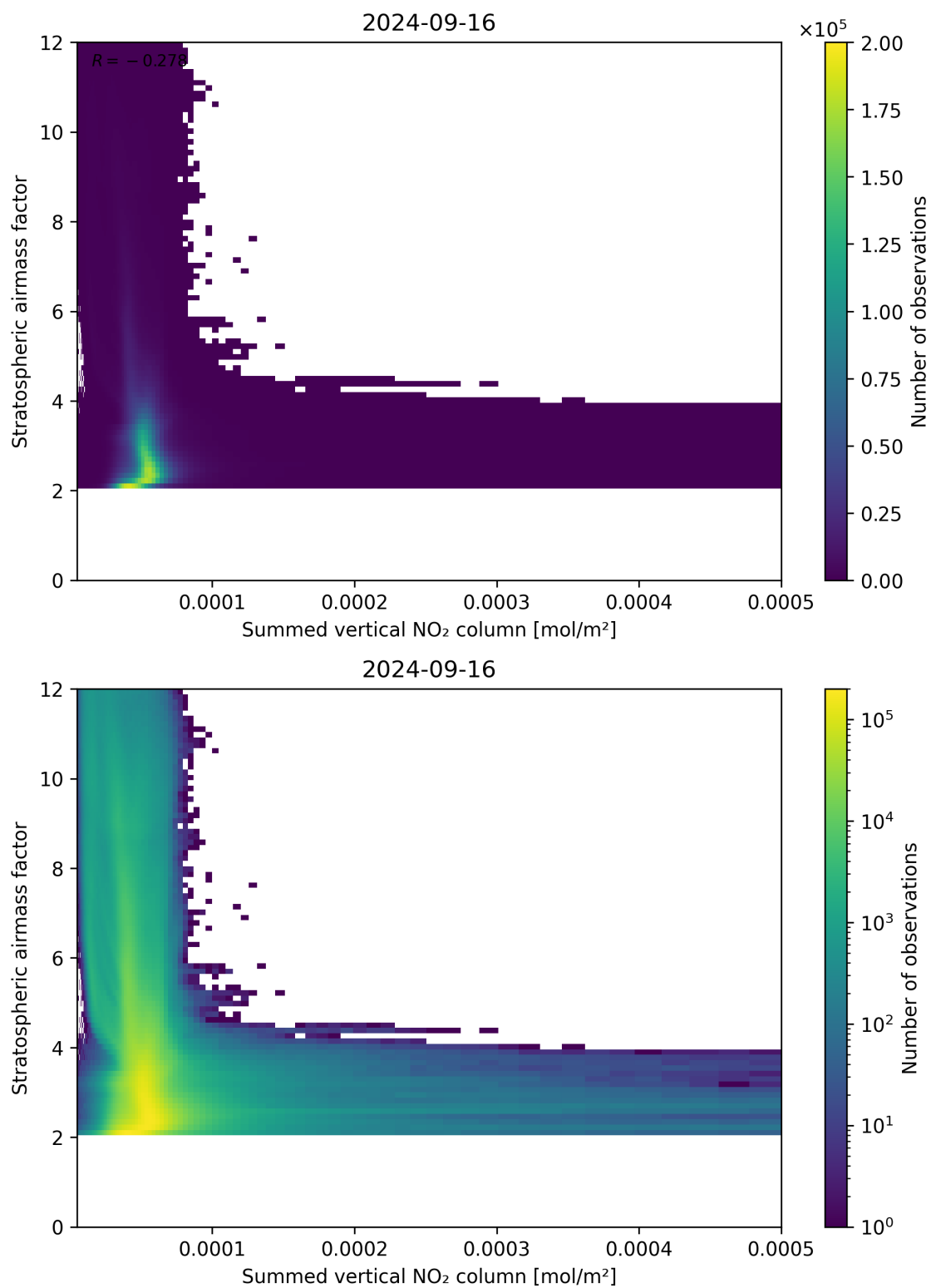
Figure 103: Scatter density plot of “Summed vertical NO 2 column” against “Stratospheric air mass factor” for 2024-09-15 to 2024-09-17.
