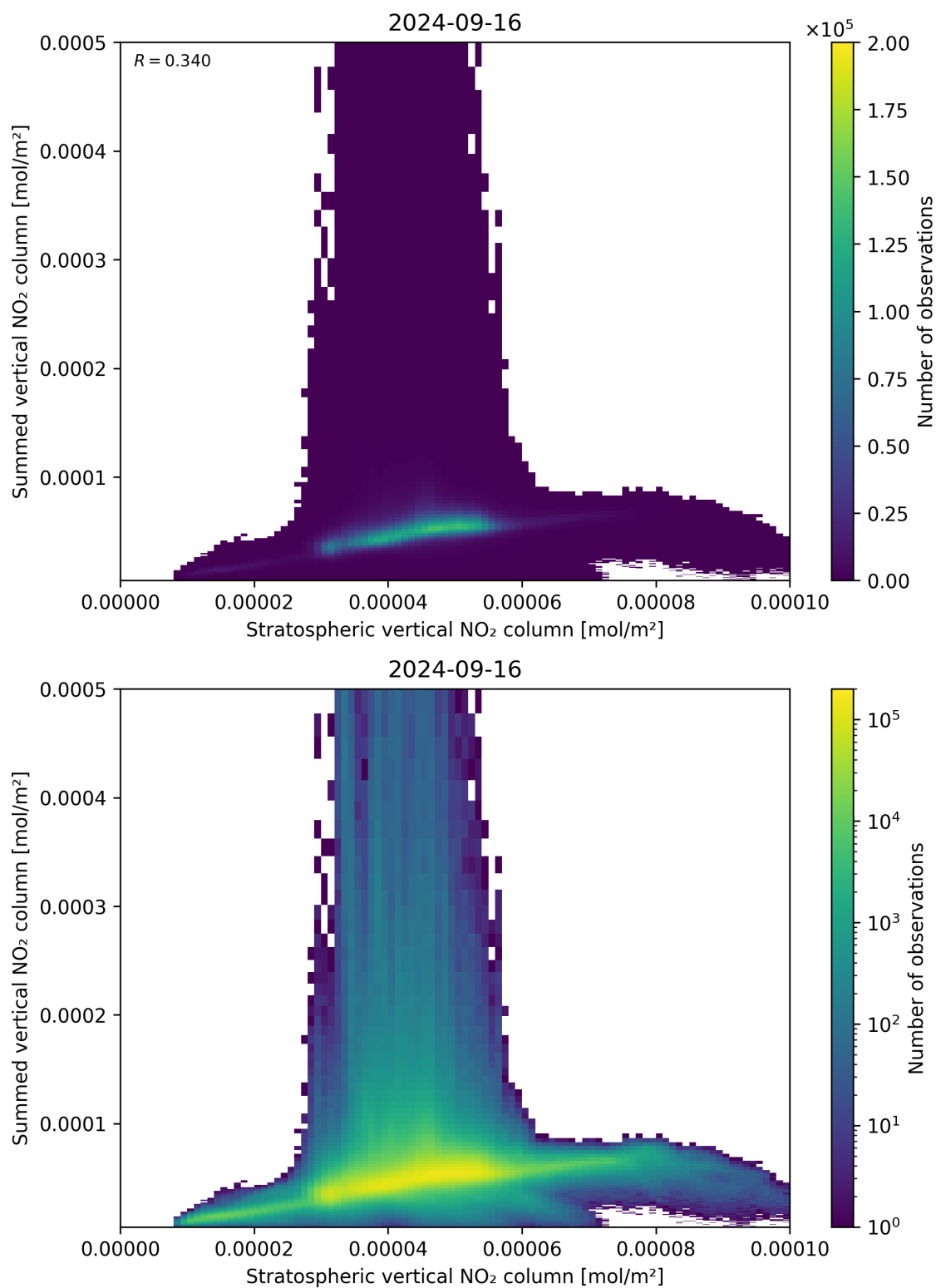
Figure 98: Scatter density plot of “Stratospheric vertical NO 2 column” against “Summed vertical NO 2 column” for 2024-09-15 to 2024-09-17.
