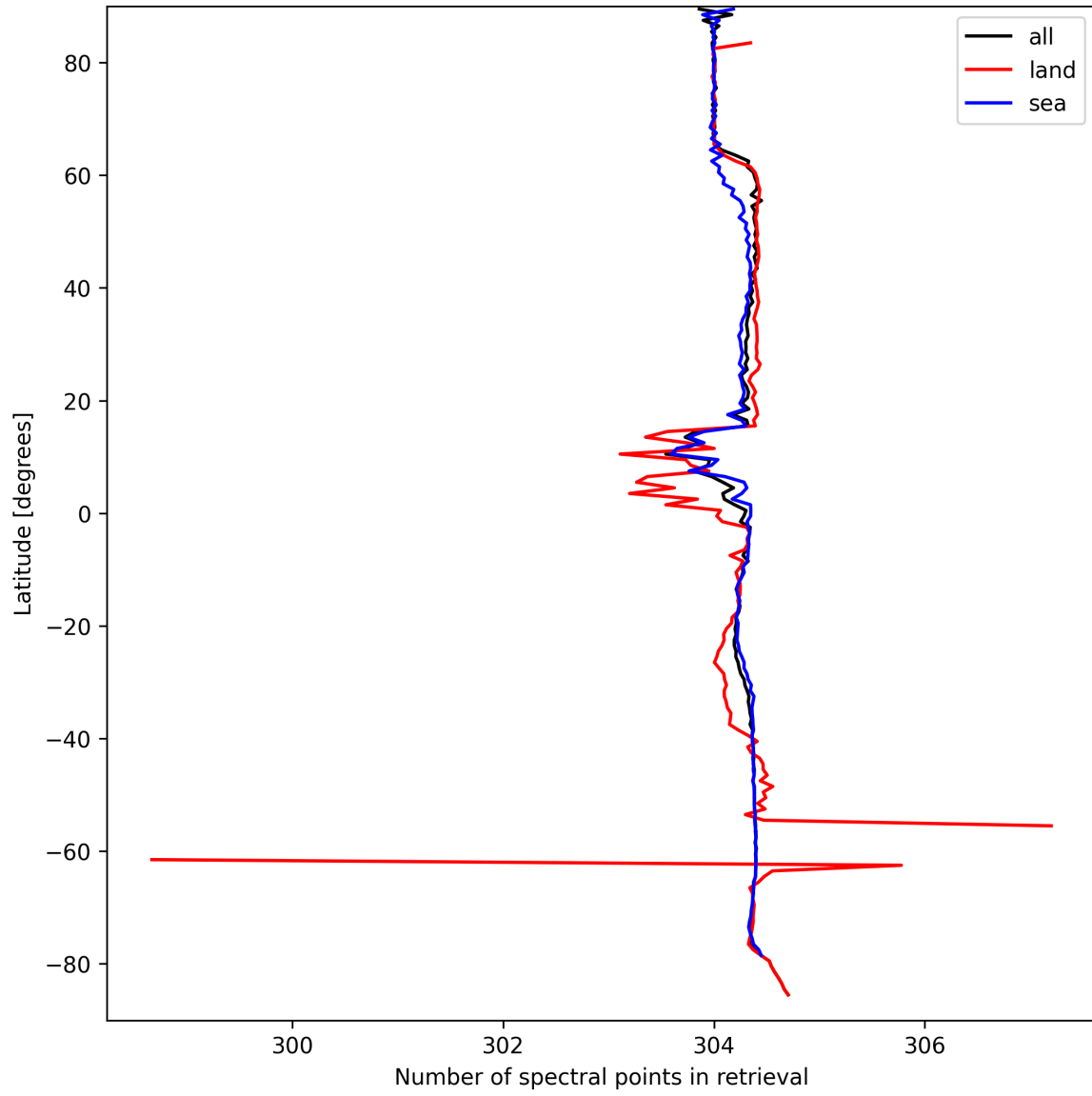
Figure 16: Zonal average of “Number of spectral points in retrieval” for 2024-09-15 to 2024-09-17.
