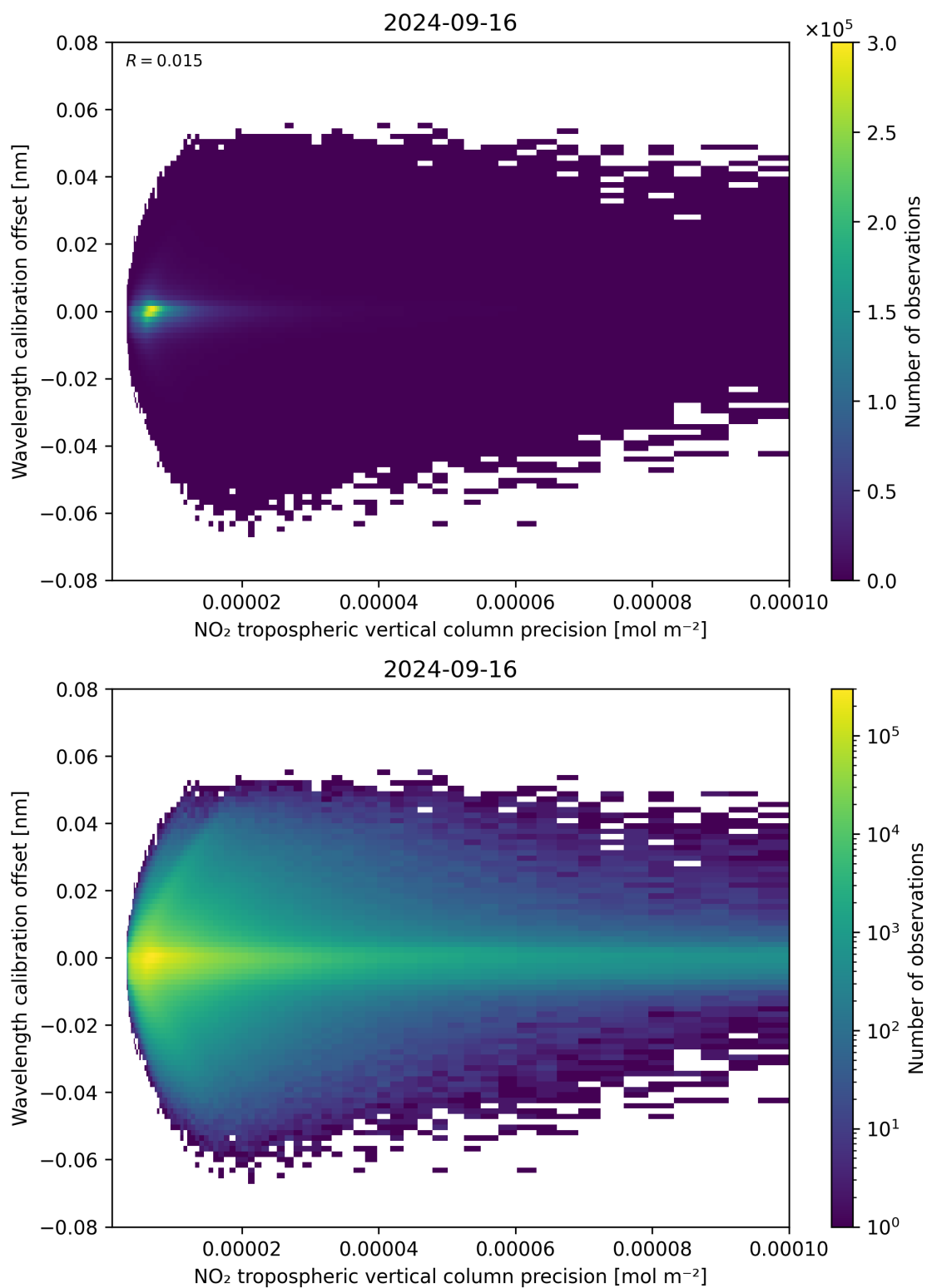
Figure 141: Scatter density plot of “NO 2 tropospheric vertical column precision” against “Wavelength calibration offset” for 2024-09-15 to 2024-09-17.
