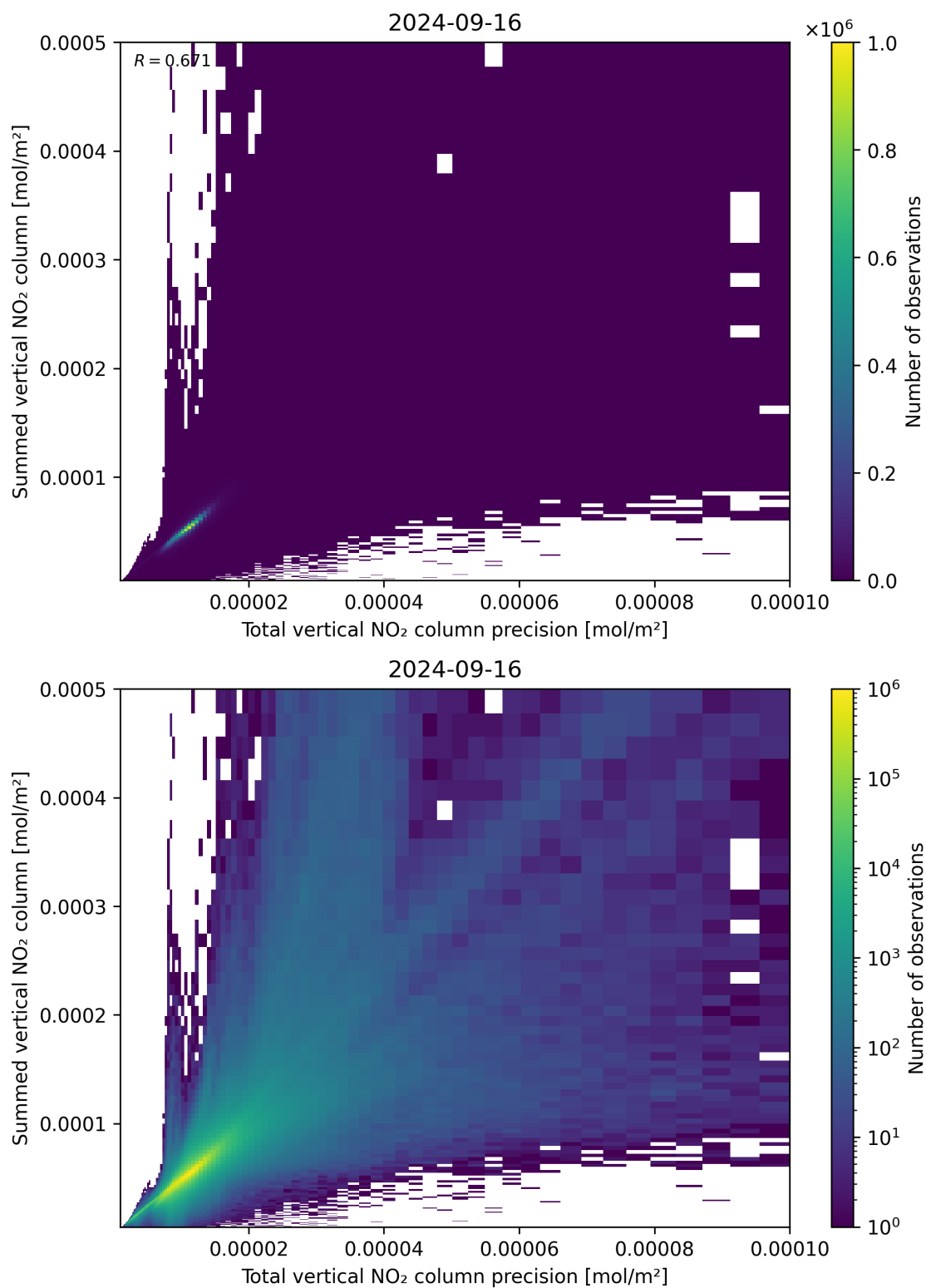
Figure 117: Scatter density plot of “Total vertical NO 2 column precision” against “Summed vertical NO 2 column” for 2024-09-15 to 2024-09-17.
