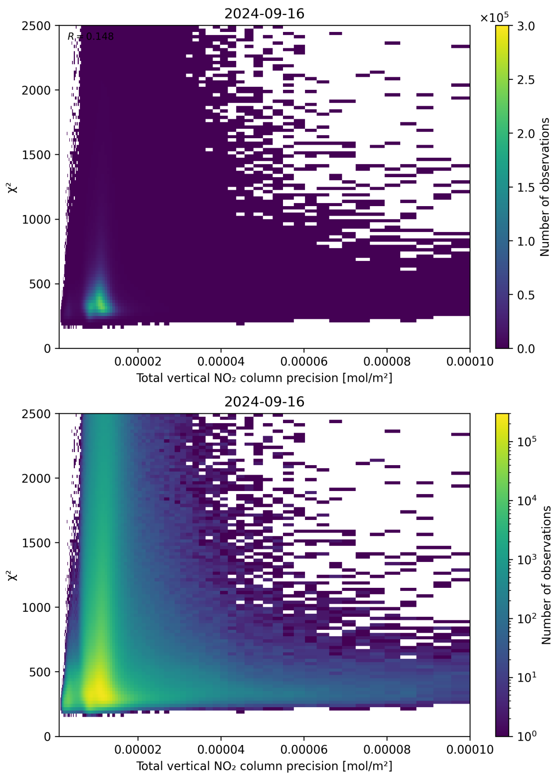
Figure 116: Scatter density plot of “Total vertical NO 2 column precision” against “ \chi^2 ” for 2024-09-15 to 2024-09-17.
