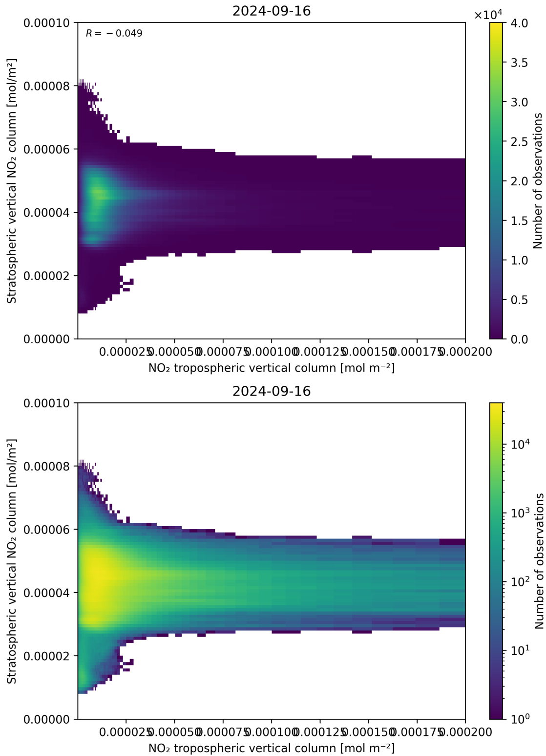
Figure 125: Scatter density plot of “NO 2 tropospheric vertical column” against “Stratospheric vertical NO 2 column” for 2024-09-15 to 2024-09-17.
