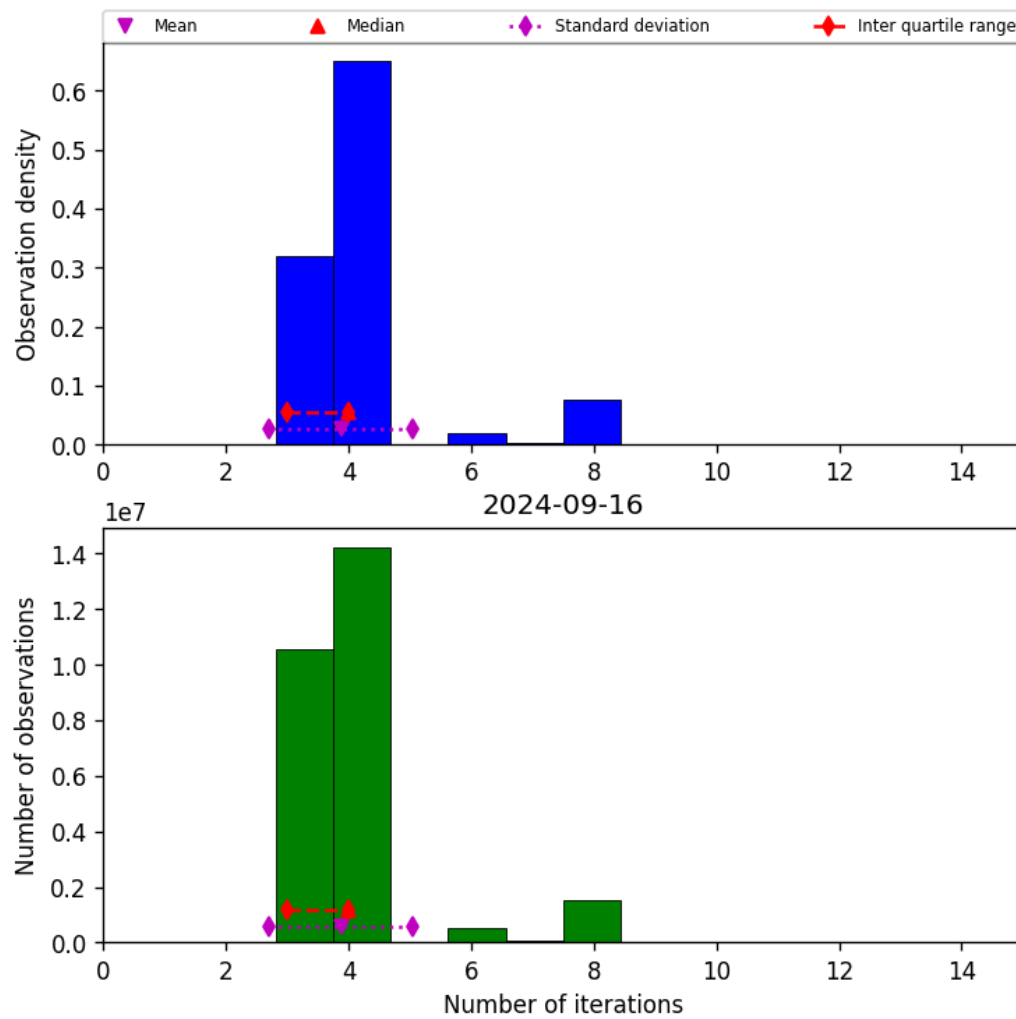
Figure 34: Histogram of “Number of iterations” for 2024-09-15 to 2024-09-17
