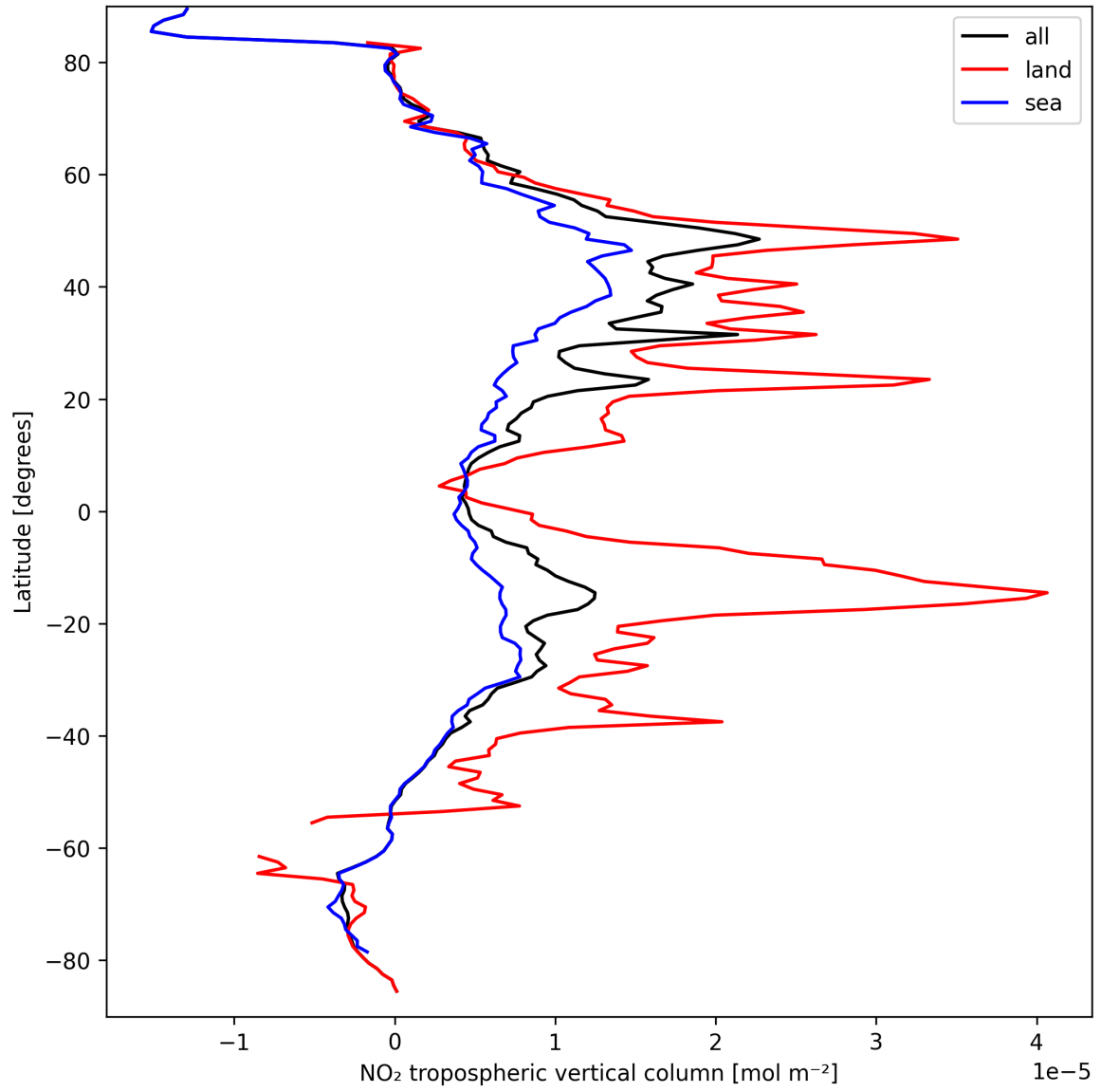
Figure 12: Zonal average of “NO 2 tropospheric vertical column” for 2024-09-15 to 2024-09-17.
