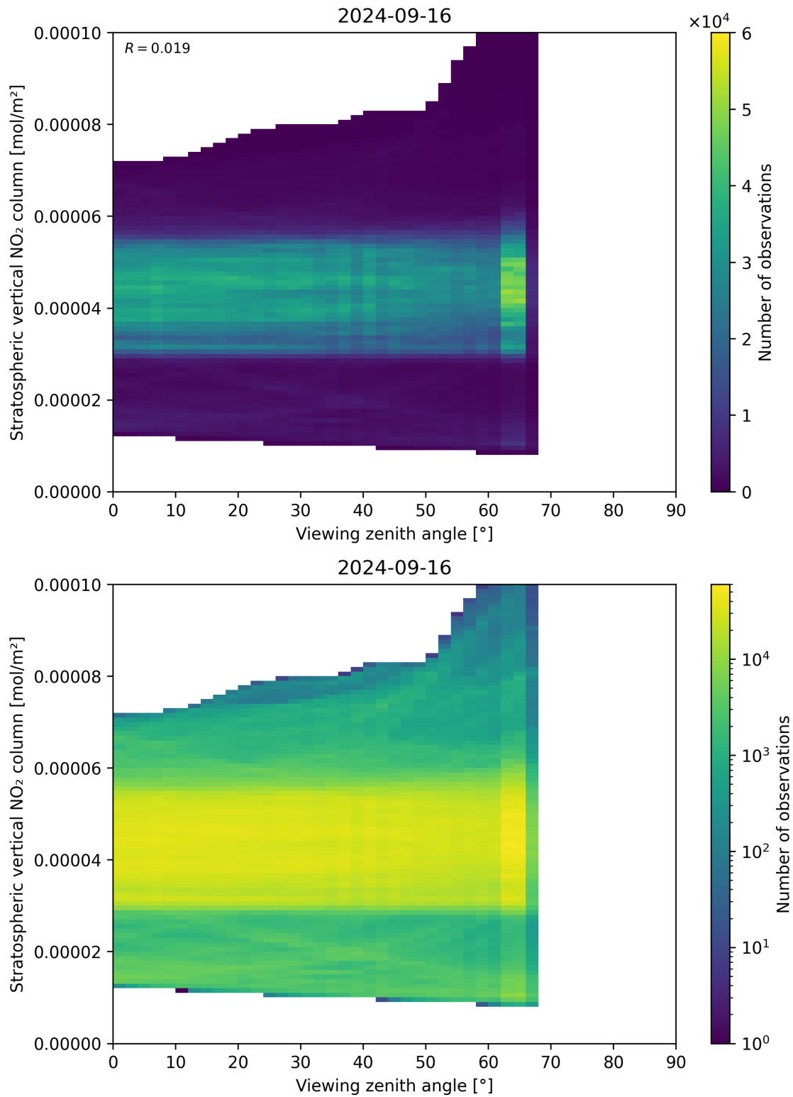
Figure 164: Scatter density plot of “Viewing zenith angle” against “Stratospheric vertical NO 2 column” for 2024-09-15 to 2024-09-17.
