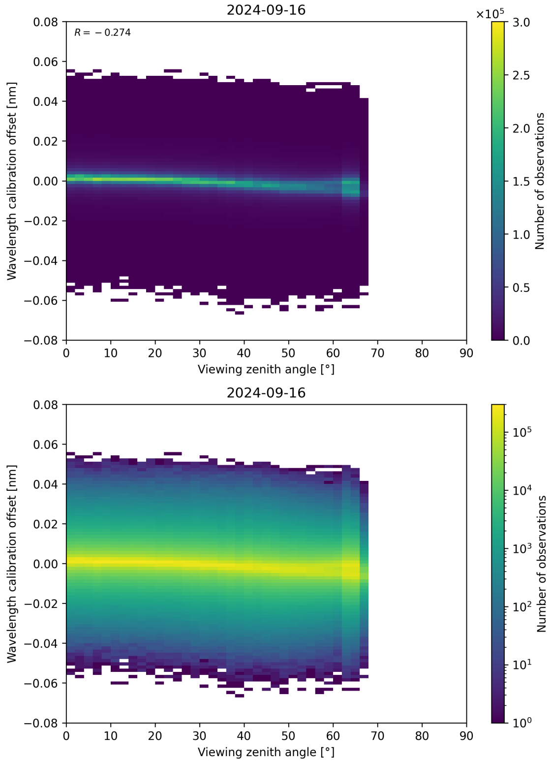
Figure 173: Scatter density plot of “Viewing zenith angle” against “Wavelength calibration offset” for 2024-09-15 to 2024-09-17.
