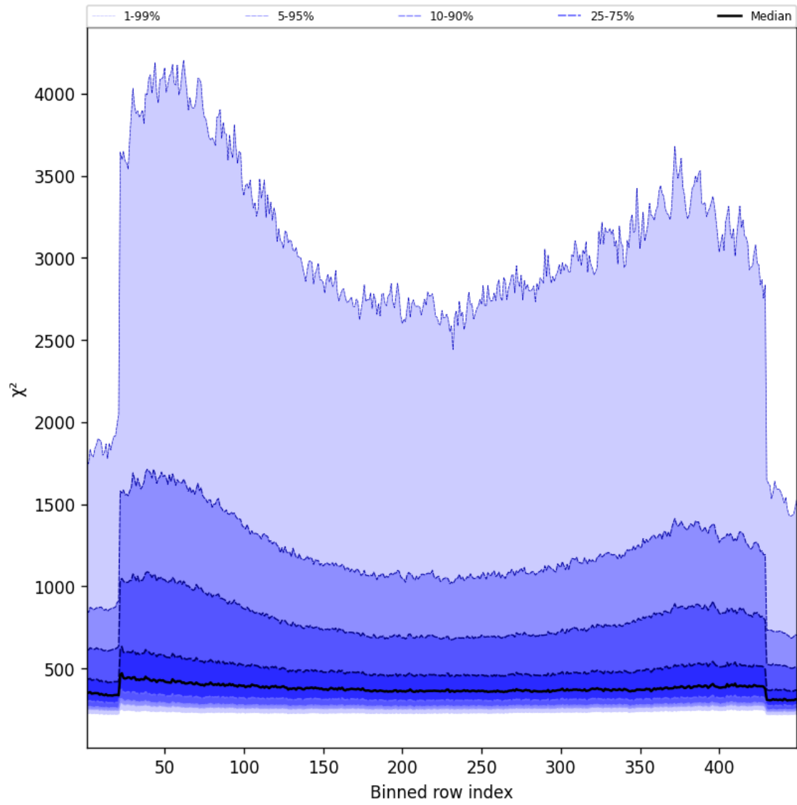
Figure 59: Along track statistics of “ \chi^2 ” for 2024-09-15 to 2024-09-17
