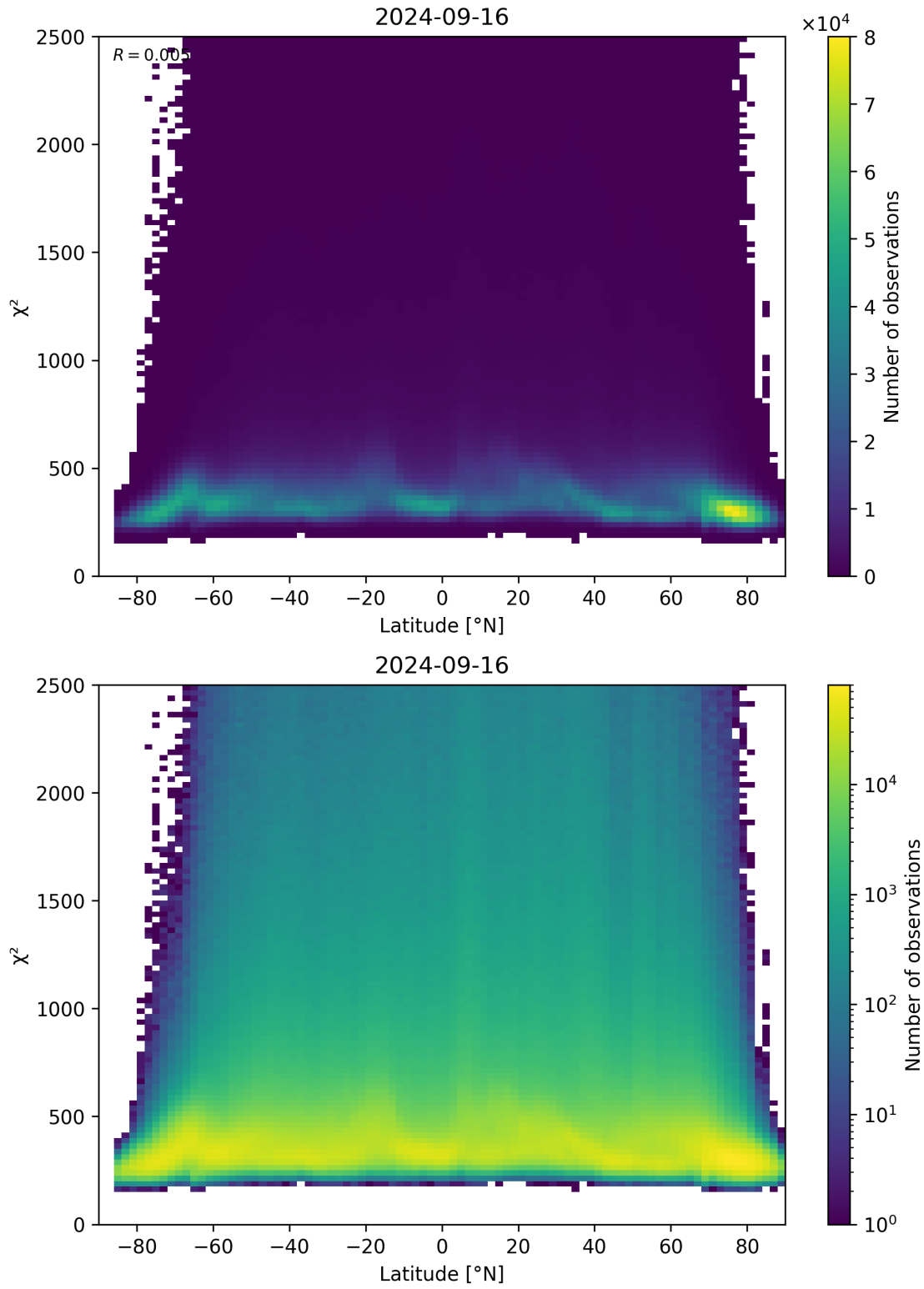
Figure 86: Scatter density plot of “Latitude” against “ \chi^2 ” for 2024-09-15 to 2024-09-17.
