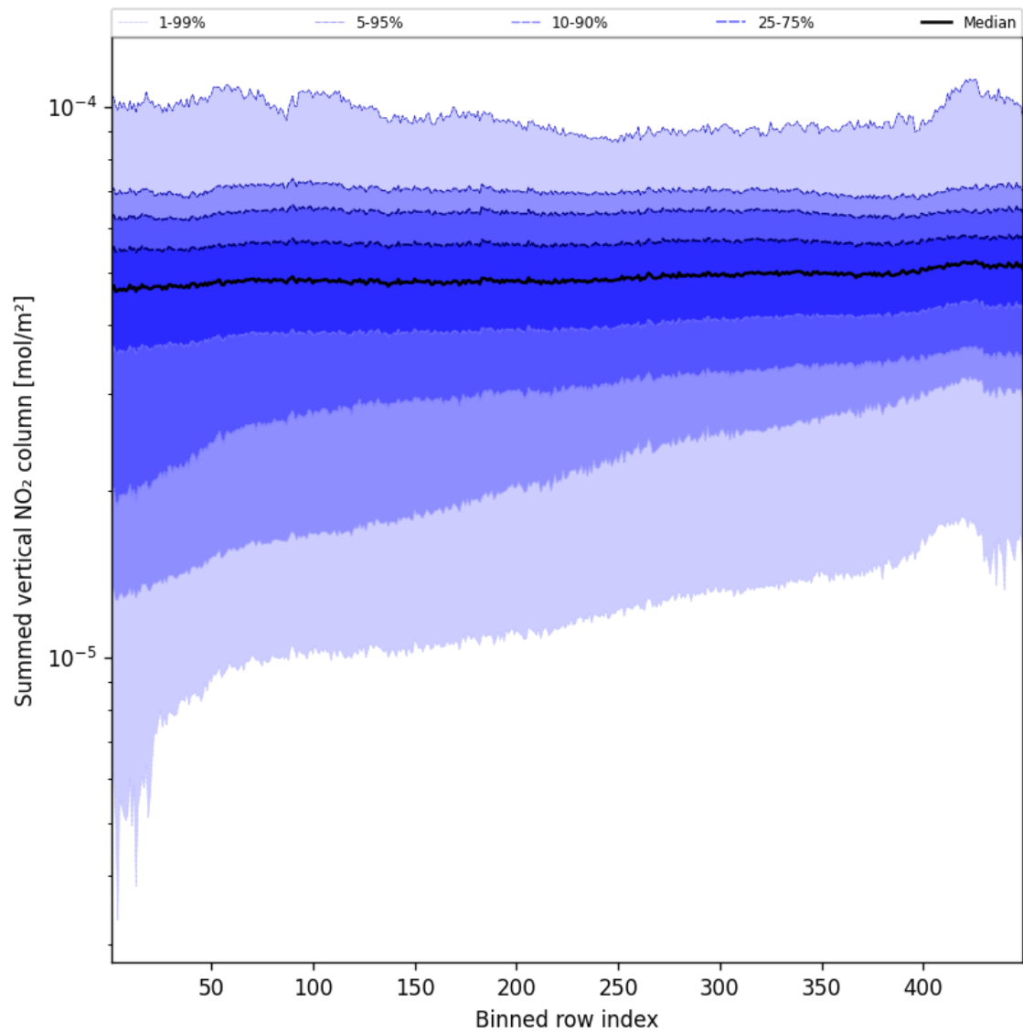
Figure 57: Along track statistics of “Summed vertical NO 2 column” for 2024-09-15 to 2024-09-17
