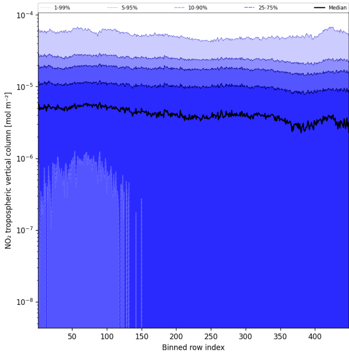
Figure 46: Along track statistics of “NO 2 tropospheric vertical column” for 2024-09-15 to 2024-09-17
