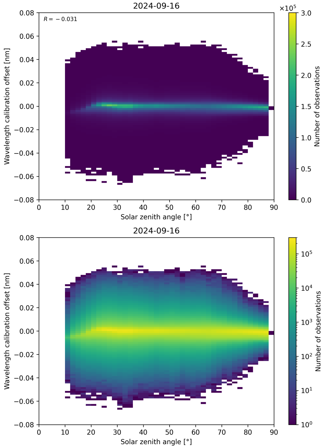
Figure 158: Scatter density plot of “Solar zenith angle” against “Wavelength calibration offset” for 2024-09-15 to 2024-09-17.
