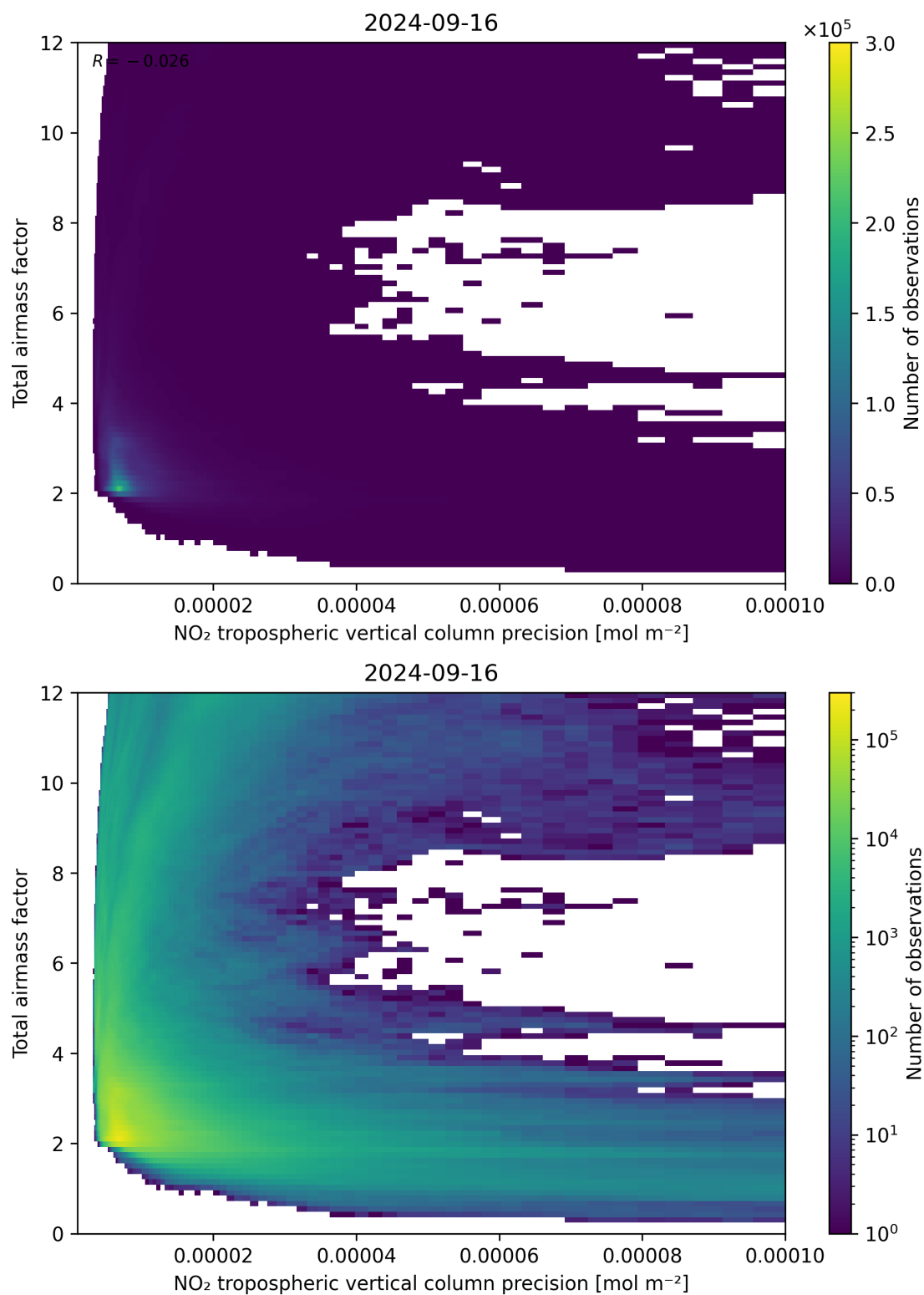
Figure 132: Scatter density plot of “NO 2 tropospheric vertical column precision” against “Total air mass factor” for 2024-09-15 to 2024-09-17.
