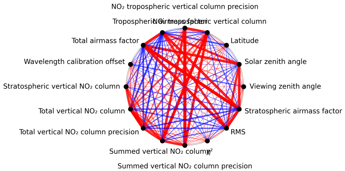
Figure 1: Map of correlation graph for 2024-09-15 to 2024-09-17.
