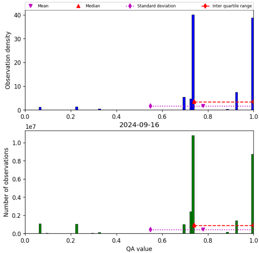
Figure 28: Histogram of “QA value” for 2024-09-15 to 2024-09-17
