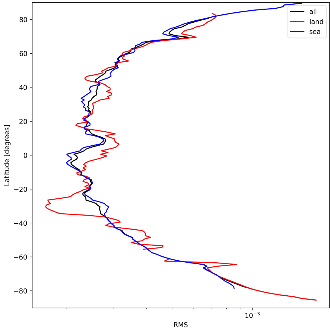
Figure 26: Zonal average of “RMS” for 2024-09-15 to 2024-09-17.
