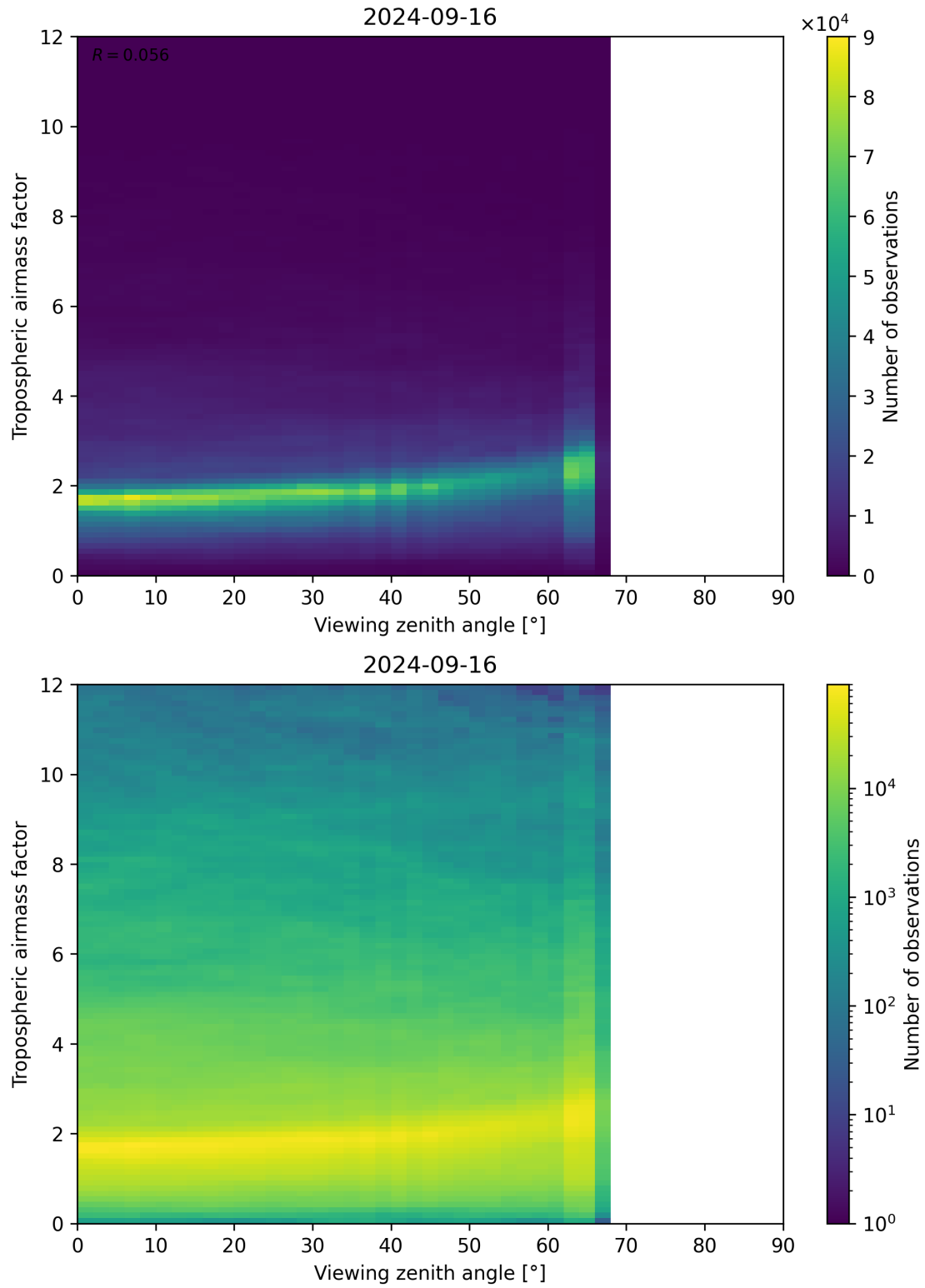
Figure 161: Scatter density plot of “Viewing zenith angle” against “Tropospheric airmass factor” for 2024-09-15 to 2024-09-17.
