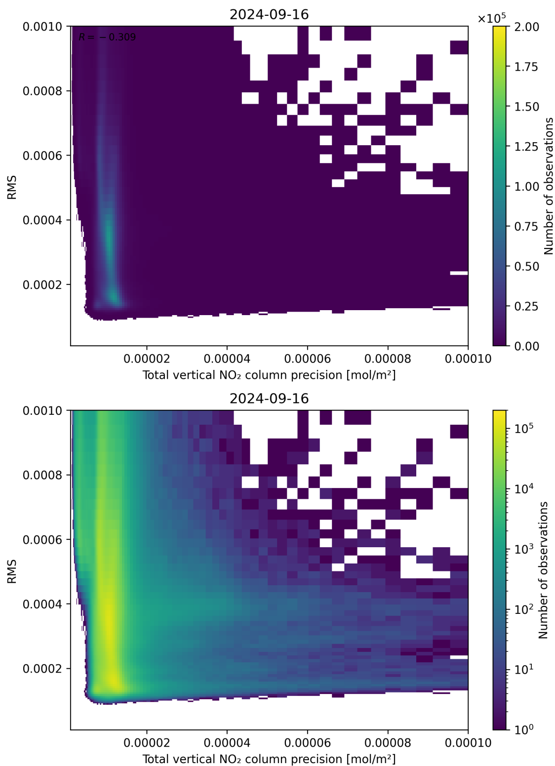
Figure 119: Scatter density plot of “Total vertical NO 2 column precision” against “RMS” for 2024-09-15 to 2024-09-17.
