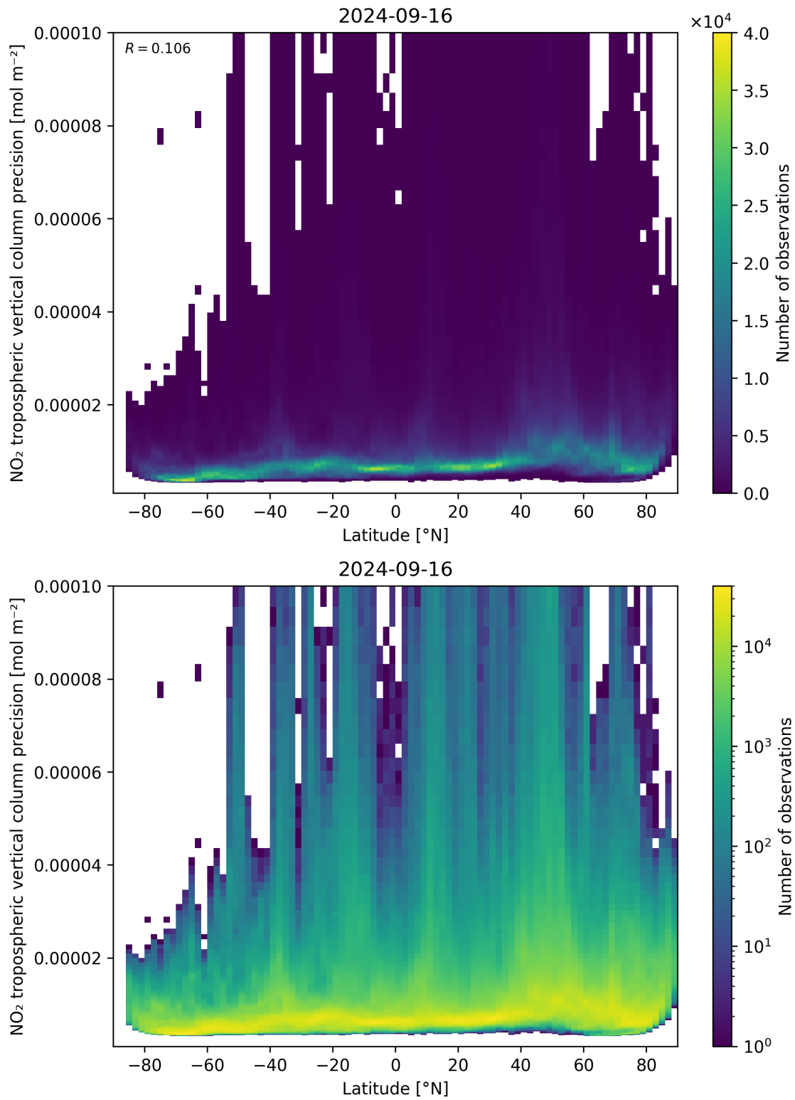
Figure 93: Scatter density plot of “Latitude” against “NO 2 tropospheric vertical column precision” for 2024-09-15 to 2024-09-17.
