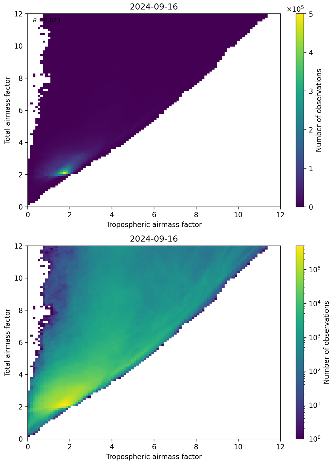
Figure 72: Scatter density plot of “Tropospheric airmass factor” against “Total airmass factor” for 2024-09-15 to 2024-09-17.
