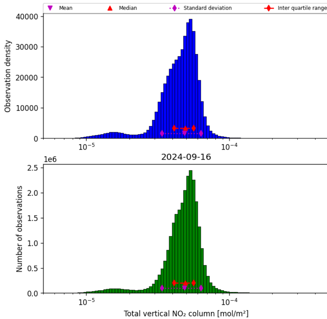
Figure 38: Histogram of “Total vertical NO 2 column” for 2024-09-15 to 2024-09-17
