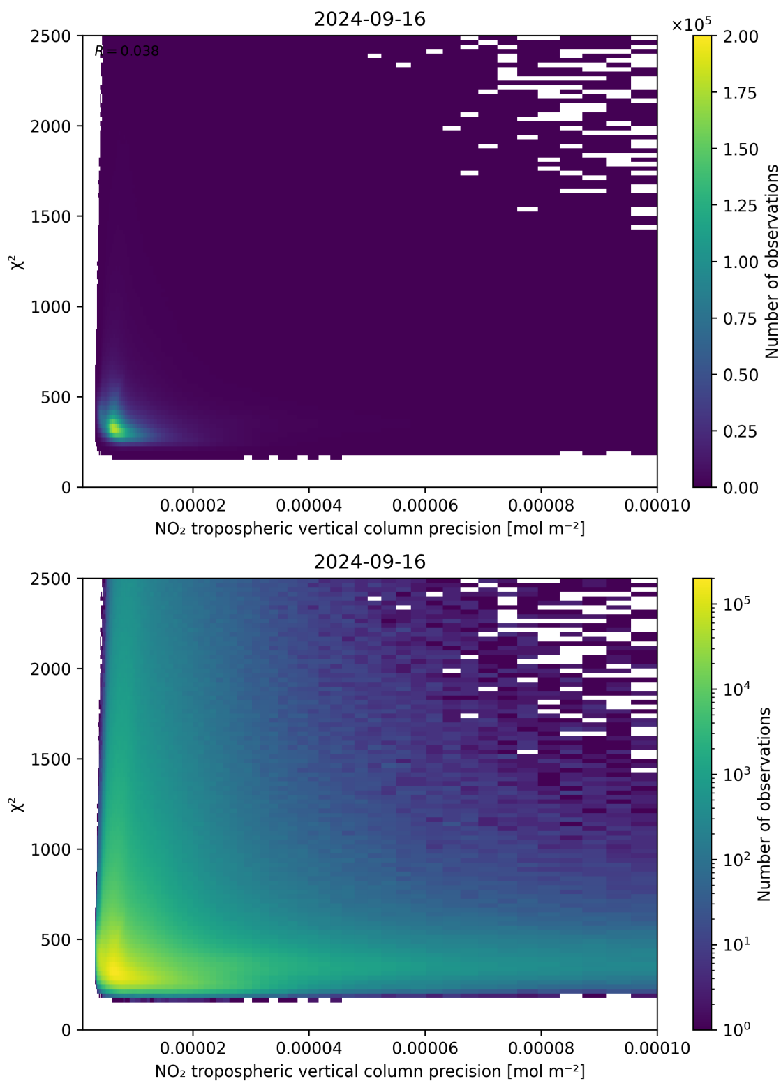
Figure 134: Scatter density plot of “NO 2 tropospheric vertical column precision” against “ \chi^2 ” for 2024-09-15 to 2024-09-17.
