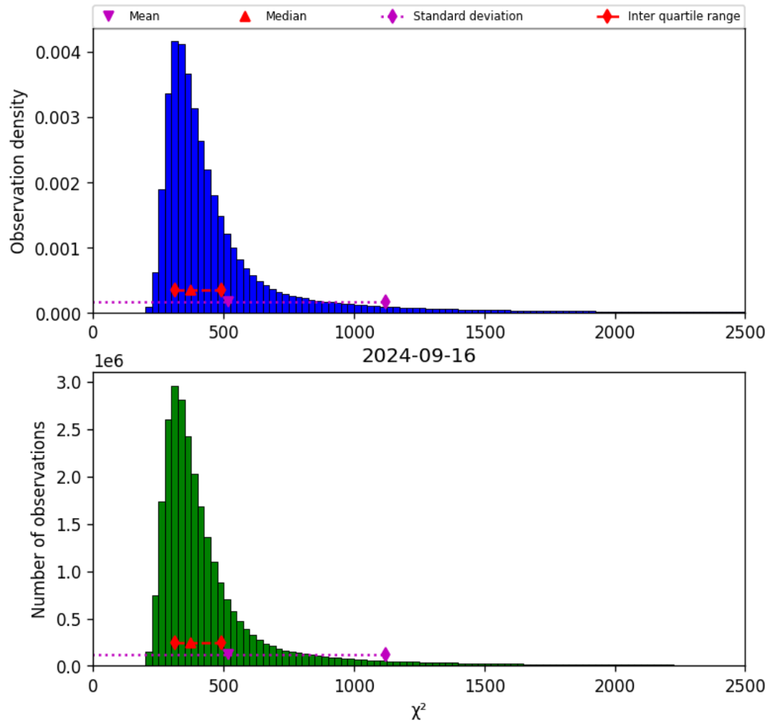
Figure 42: Histogram of “ \chi^2 ” for 2024-09-15 to 2024-09-17
