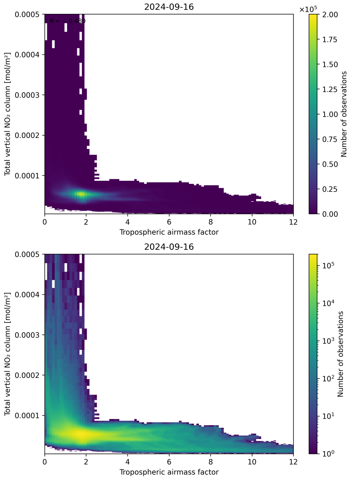
Figure 77: Scatter density plot of “Tropospheric airmass factor” against “Total vertical NO 2 column” for 2024-09-15 to 2024-09-17.
