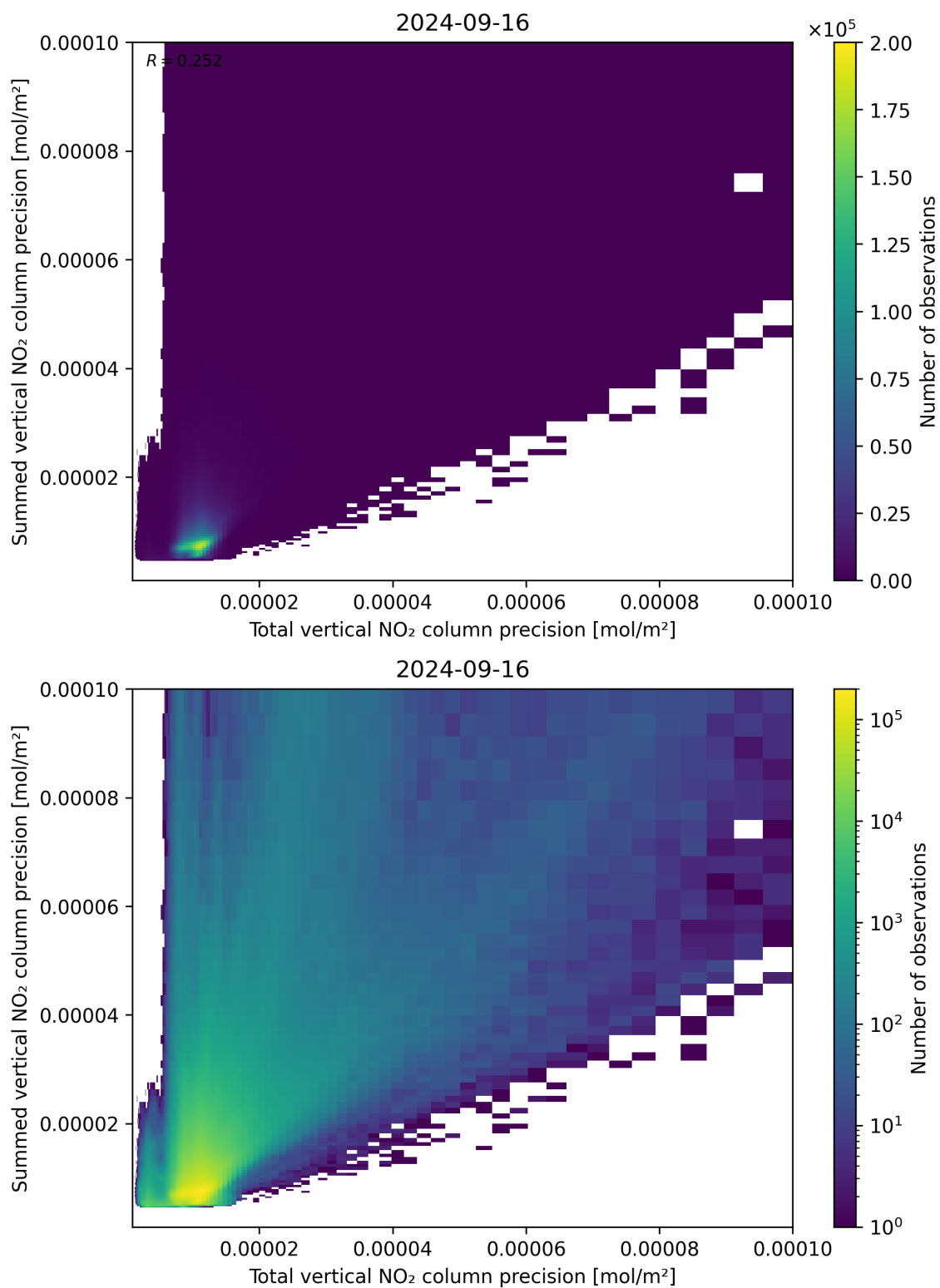
Figure 118: Scatter density plot of “Total vertical NO 2 column precision” against “Summed vertical NO 2 column precision” for 2024-09-15 to 2024-09-17.
