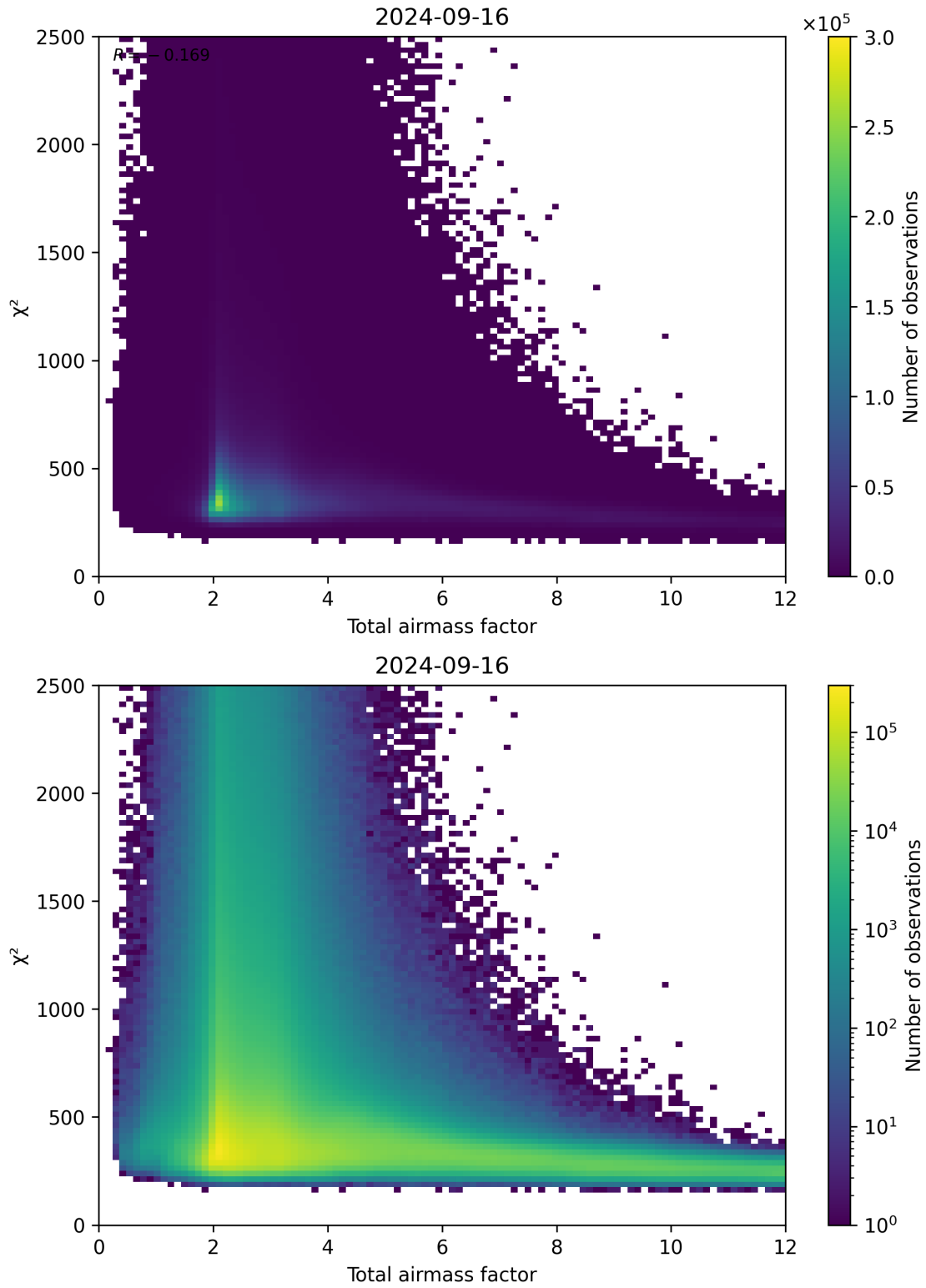
Figure 63: Scatter density plot of “Total airmass factor” against “ \chi^2 ” for 2024-09-15 to 2024-09-17.
