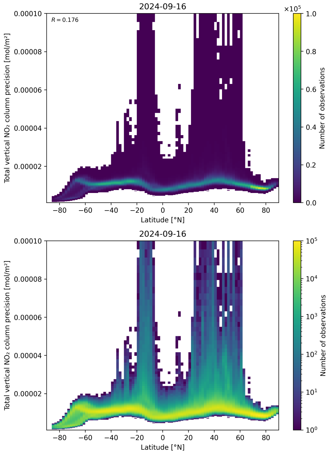
Figure 91: Scatter density plot of “Latitude” against “Total vertical NO 2 column precision” for 2024-09-15 to 2024-09-17.
