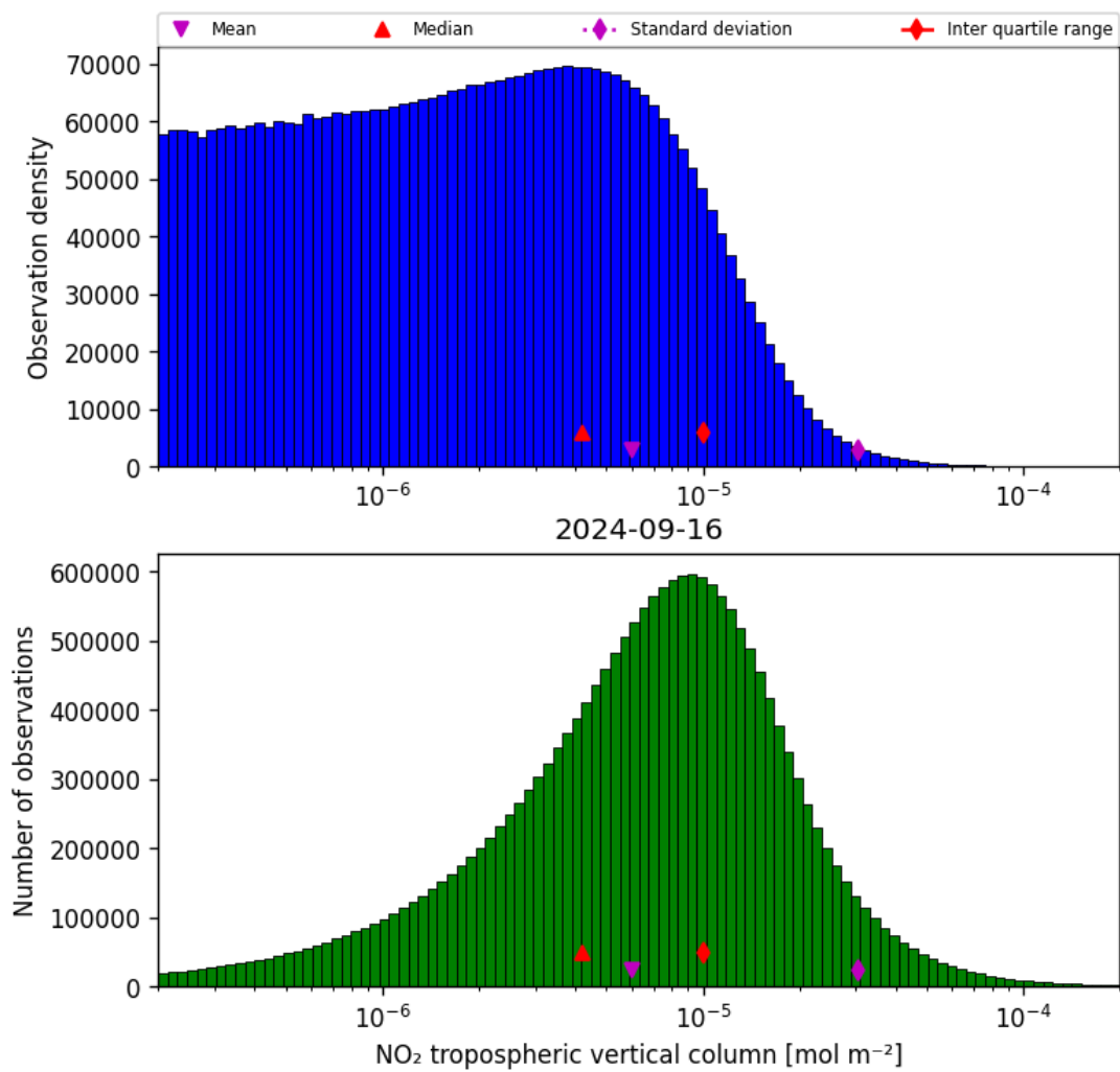
Figure 29: Histogram of “NO 2 tropospheric vertical column” for 2024-09-15 to 2024-09-17
