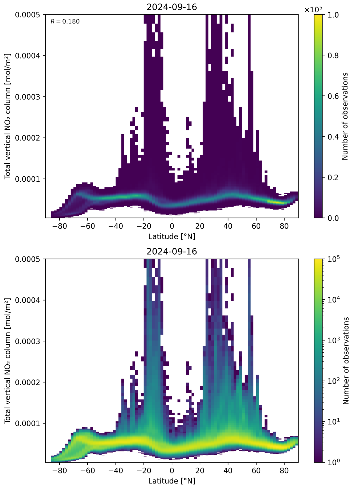
Figure 90: Scatter density plot of “Latitude” against “Total vertical NO 2 column” for 2024-09-15 to 2024-09-17.
