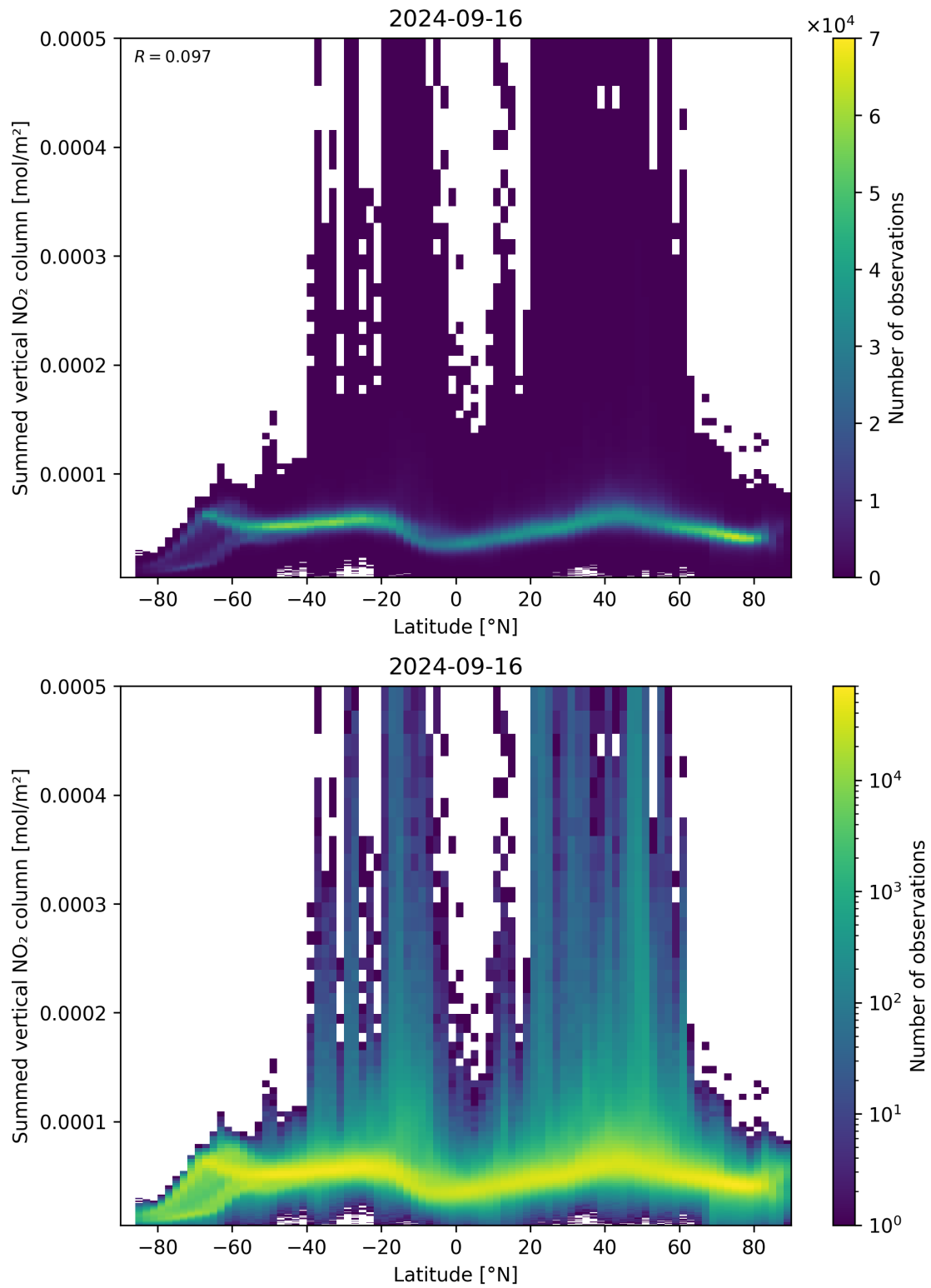
Figure 88: Scatter density plot of “Latitude” against “Summed vertical NO 2 column” for 2024-09-15 to 2024-09-17.
