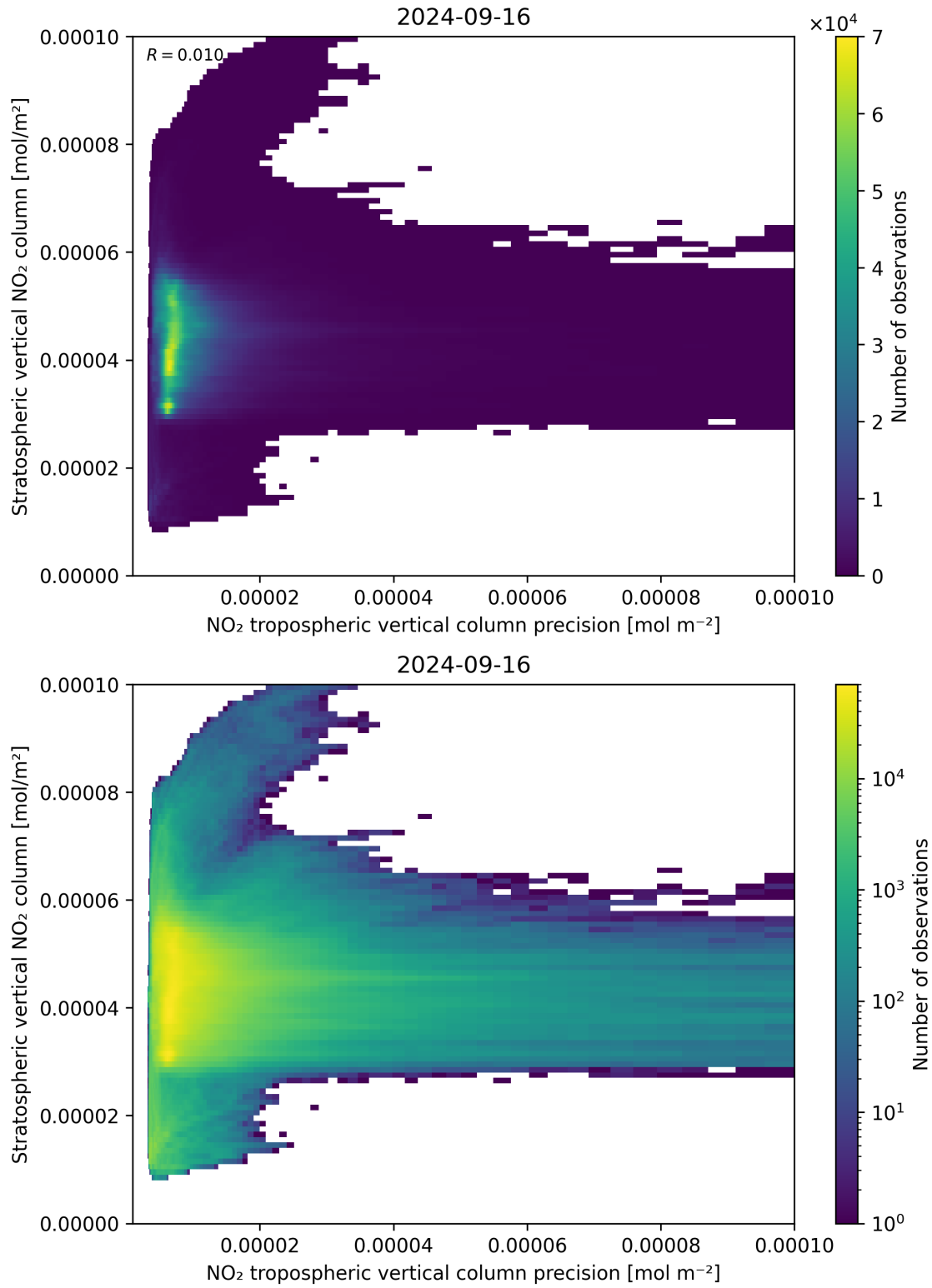
Figure 135: Scatter density plot of “NO 2 tropospheric vertical column precision” against “Stratospheric vertical NO 2 column” for 2024-09-15 to 2024-09-17.
