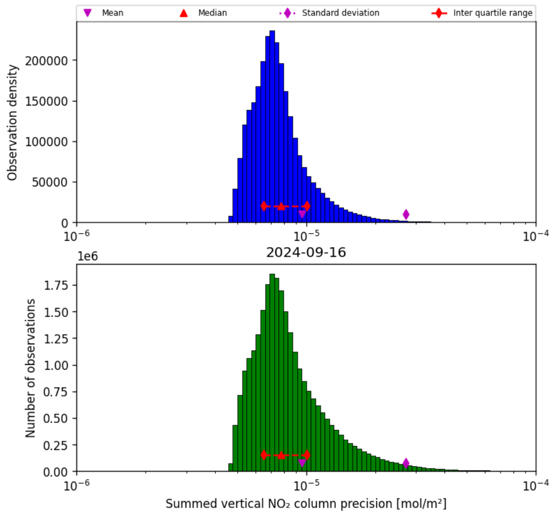
Figure 41: Histogram of "Summed vertical NO 2 column precision" for 2024-09-15 to 2024-09-17
