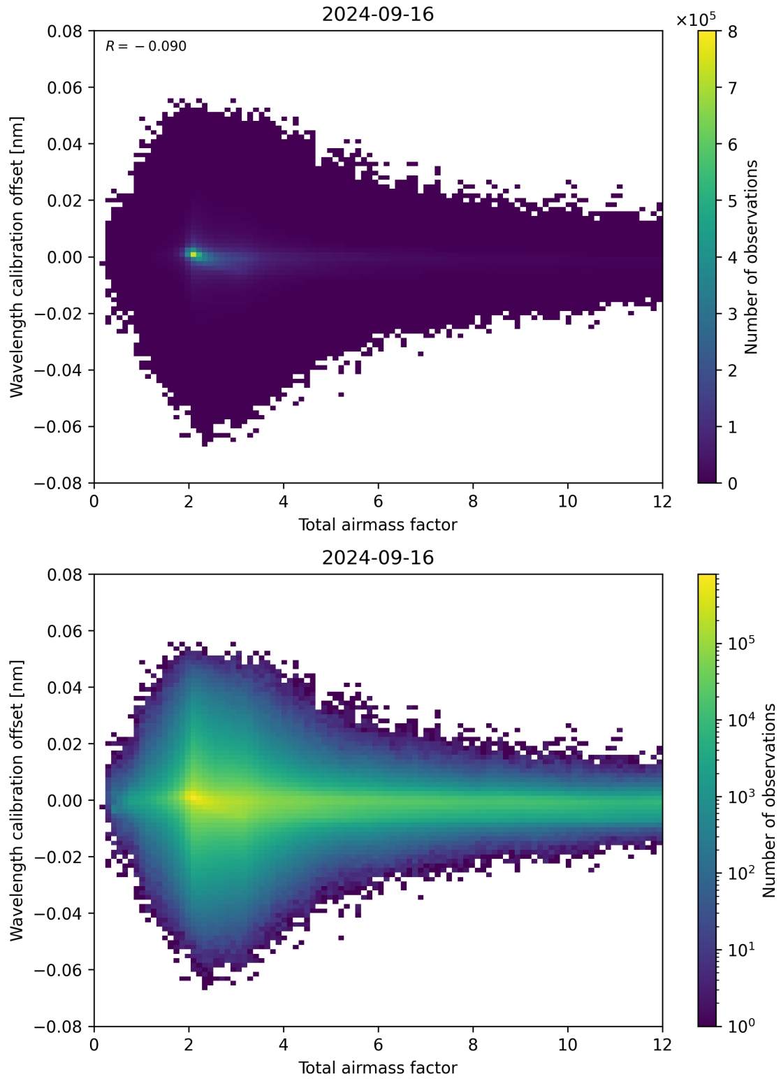
Figure 70: Scatter density plot of “Total airmass factor” against “Wavelength calibration offset” for 2024-09-15 to 2024-09-17.
