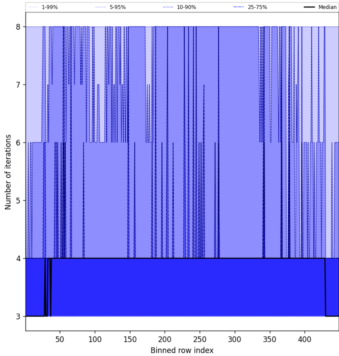
Figure 51: Along track statistics of “Number of iterations” for 2024-09-15 to 2024-09-17
