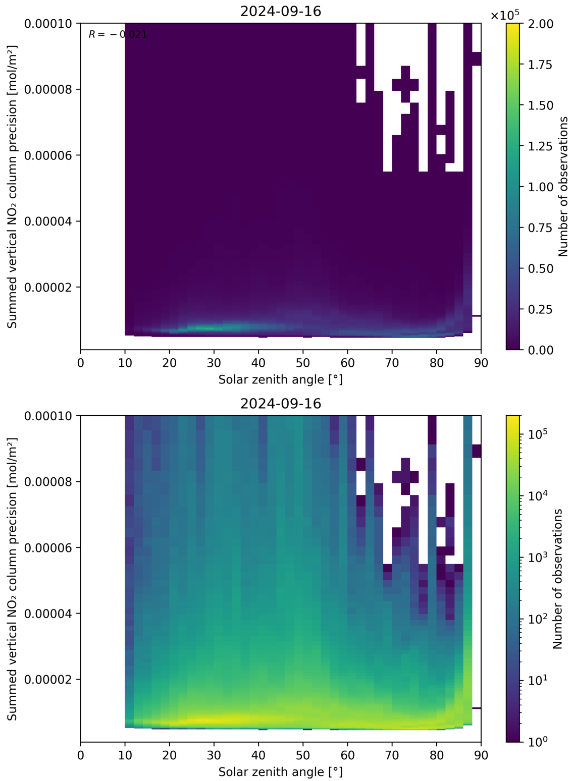
Figure 152: Scatter density plot of “Solar zenith angle” against “Summed vertical NO 2 column precision” for 2024-09-15 to 2024-09-17.
