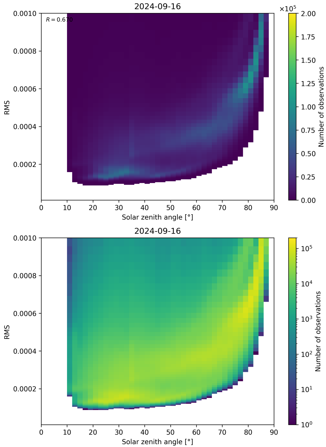
Figure 157: Scatter density plot of “Solar zenith angle” against “RMS” for 2024-09-15 to 2024-09-17.
