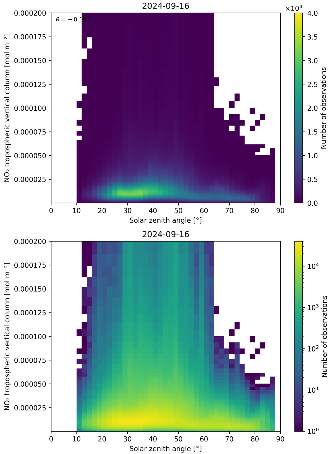
Figure 155: Scatter density plot of “Solar zenith angle” against “NO 2 tropospheric vertical column” for 2024-09-15 to 2024-09-17.
