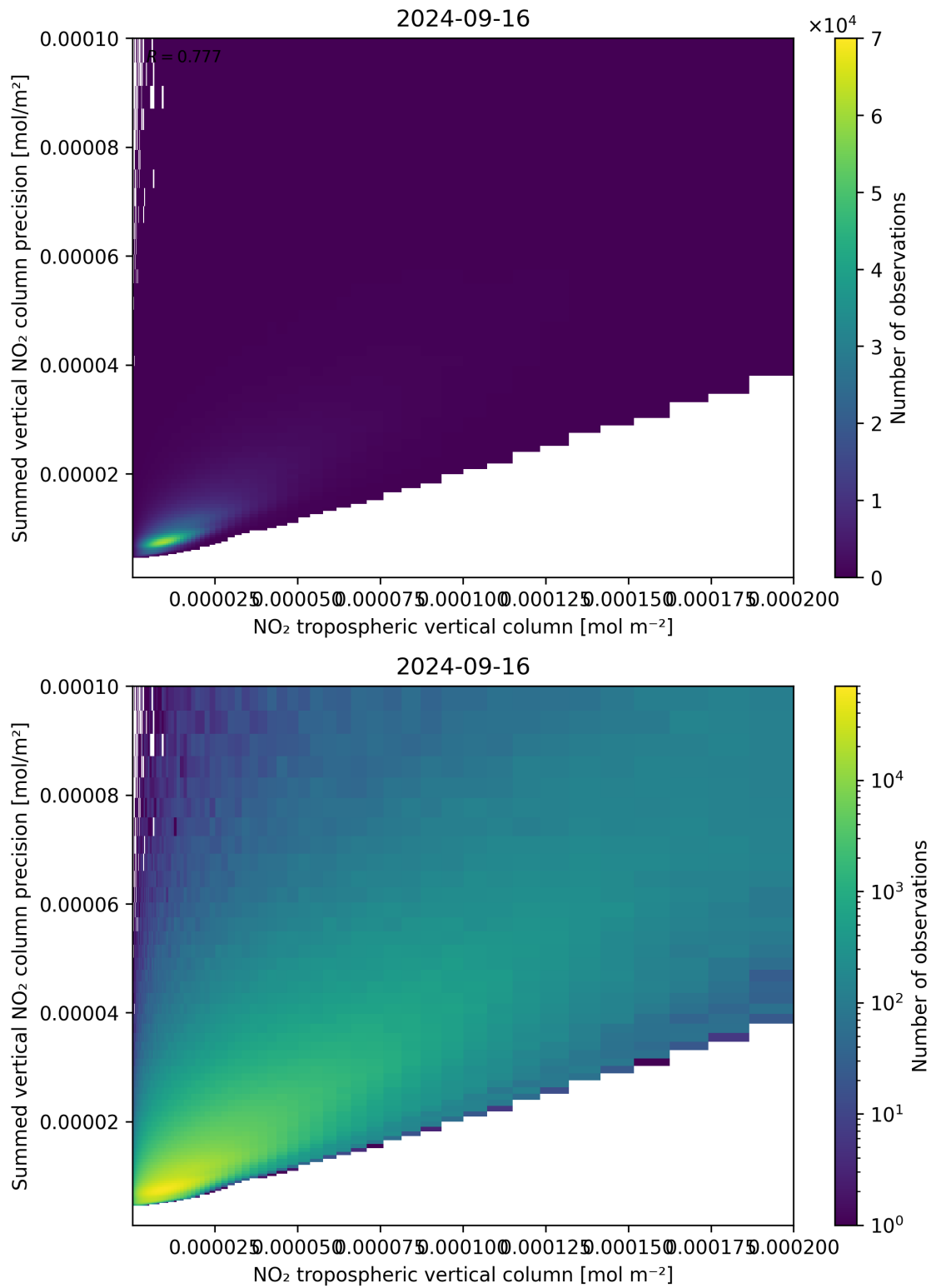
Figure 127: Scatter density plot of “NO 2 tropospheric vertical column” against “Summed vertical NO 2 column precision” for 2024-09-15 to 2024-09-17.
