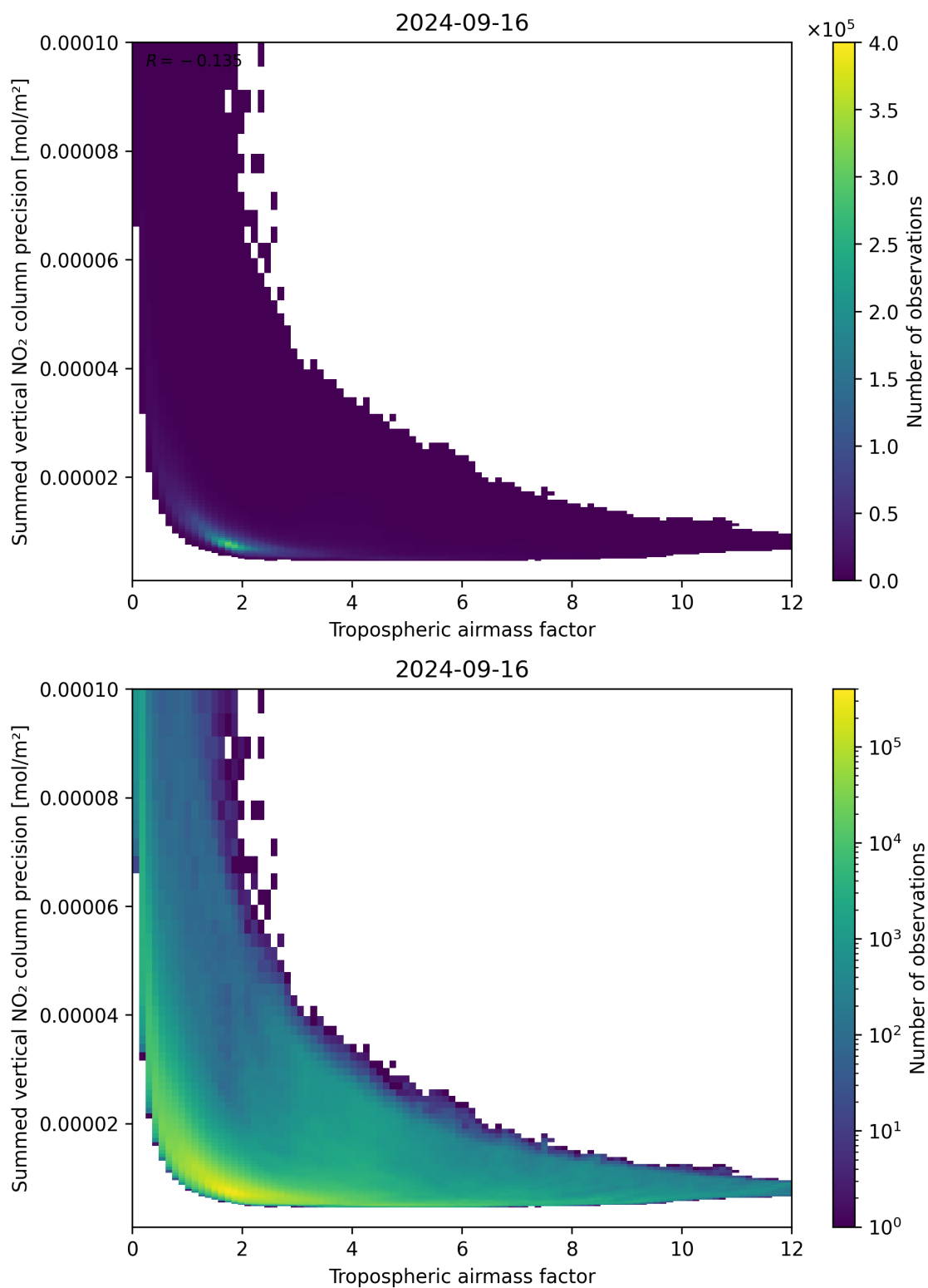
Figure 76: Scatter density plot of “Tropospheric air mass factor” against “Summed vertical NO 2 column precision” for 2024-09-15 to 2024-09-17.
