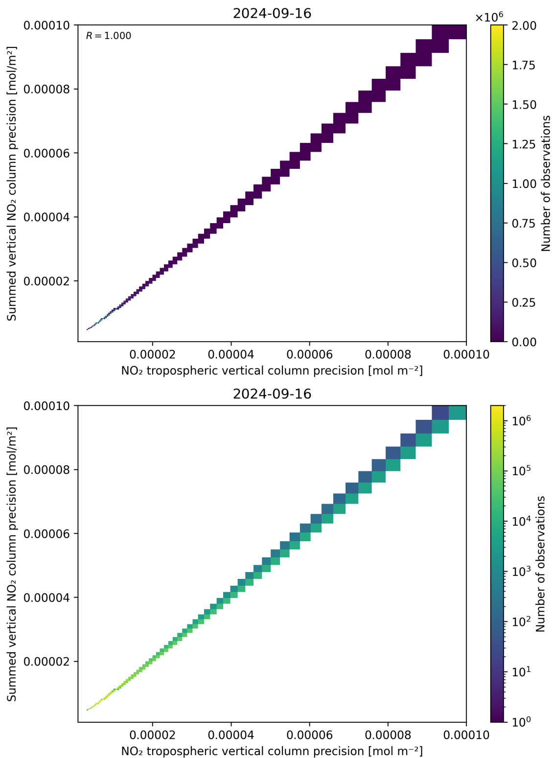
Figure 137: Scatter density plot of “NO 2 tropospheric vertical column precision” against “Summed vertical NO 2 column precision” for 2024-09-15 to 2024-09-17.
