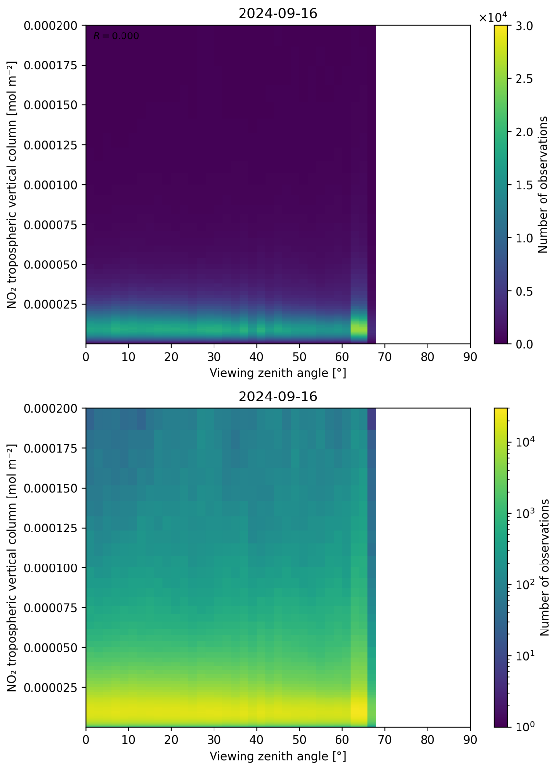
Figure 169: Scatter density plot of “Viewing zenith angle” against “NO 2 tropospheric vertical column” for 2024-09-15 to 2024-09-17.
