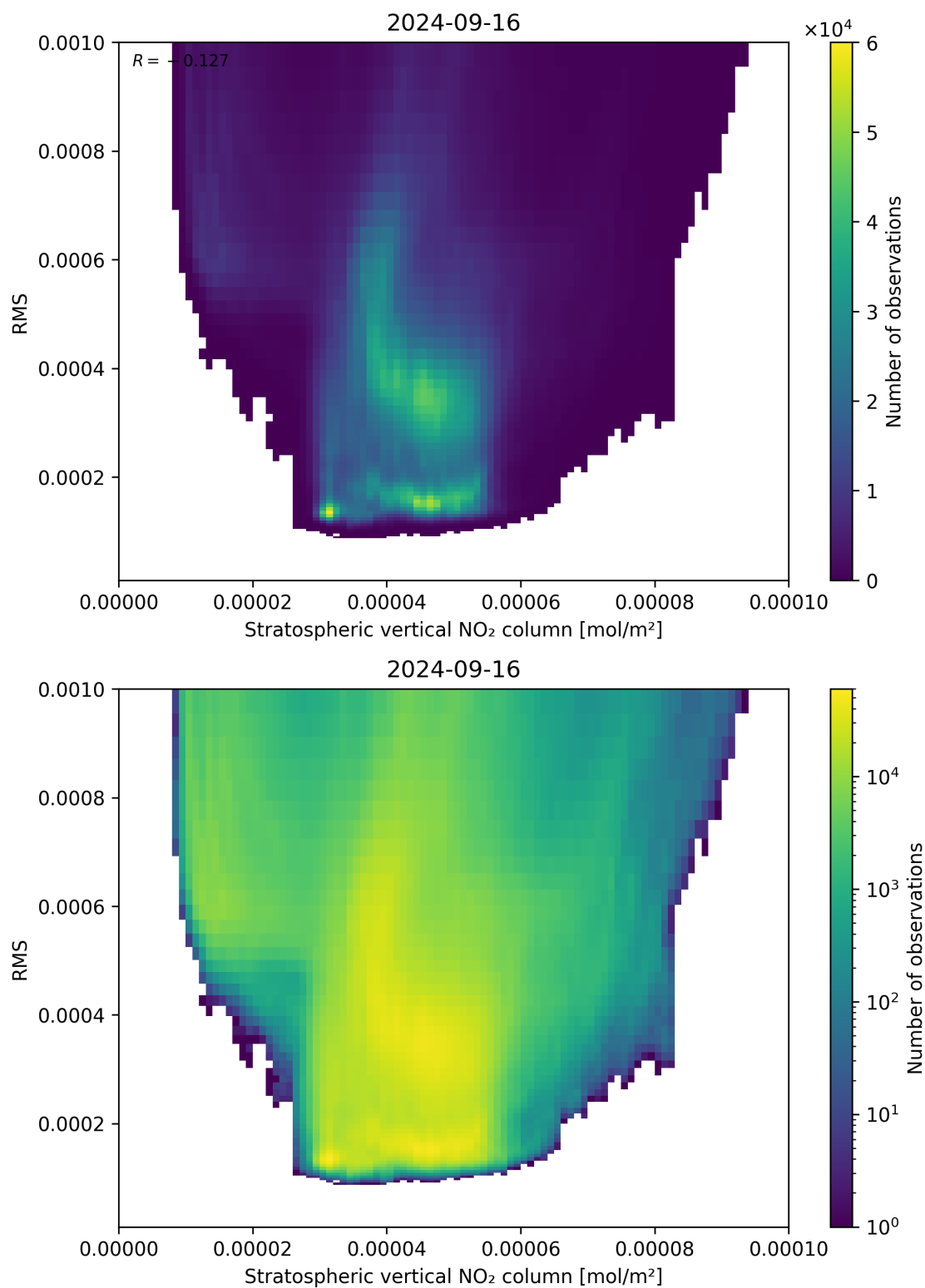
Figure 102: Scatter density plot of “Stratospheric vertical NO 2 column” against “RMS” for 2024-09-15 to 2024-09-17.
