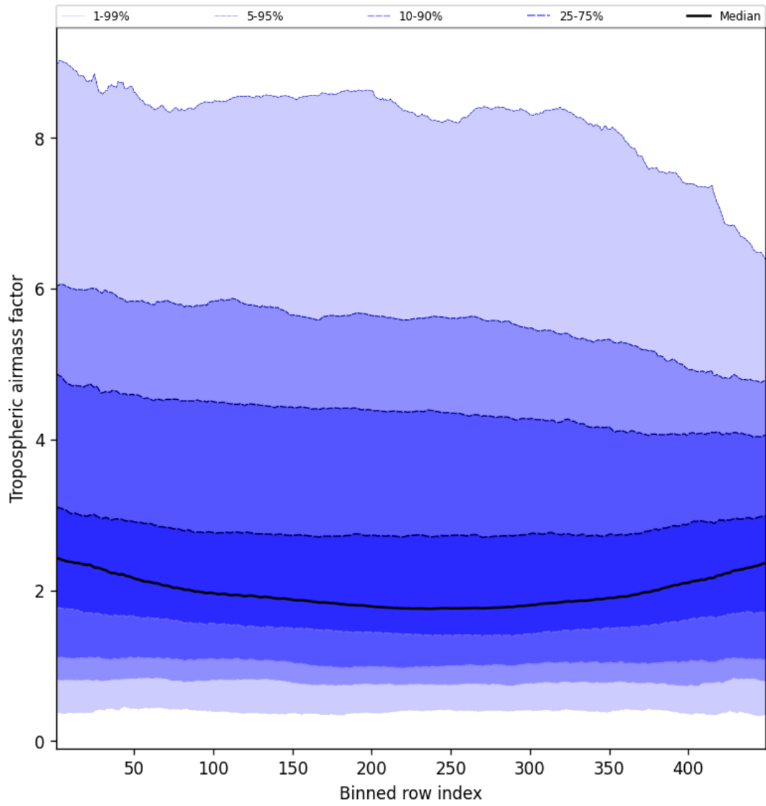
Figure 48: Along track statistics of “Tropospheric air mass factor” for 2024-09-15 to 2024-09-17
