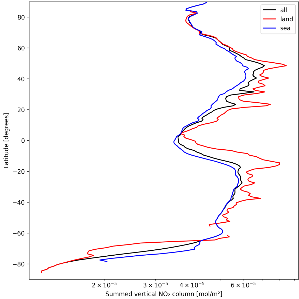
Figure 23: Zonal average of “Summed vertical NO 2 column” for 2024-09-15 to 2024-09-17.
