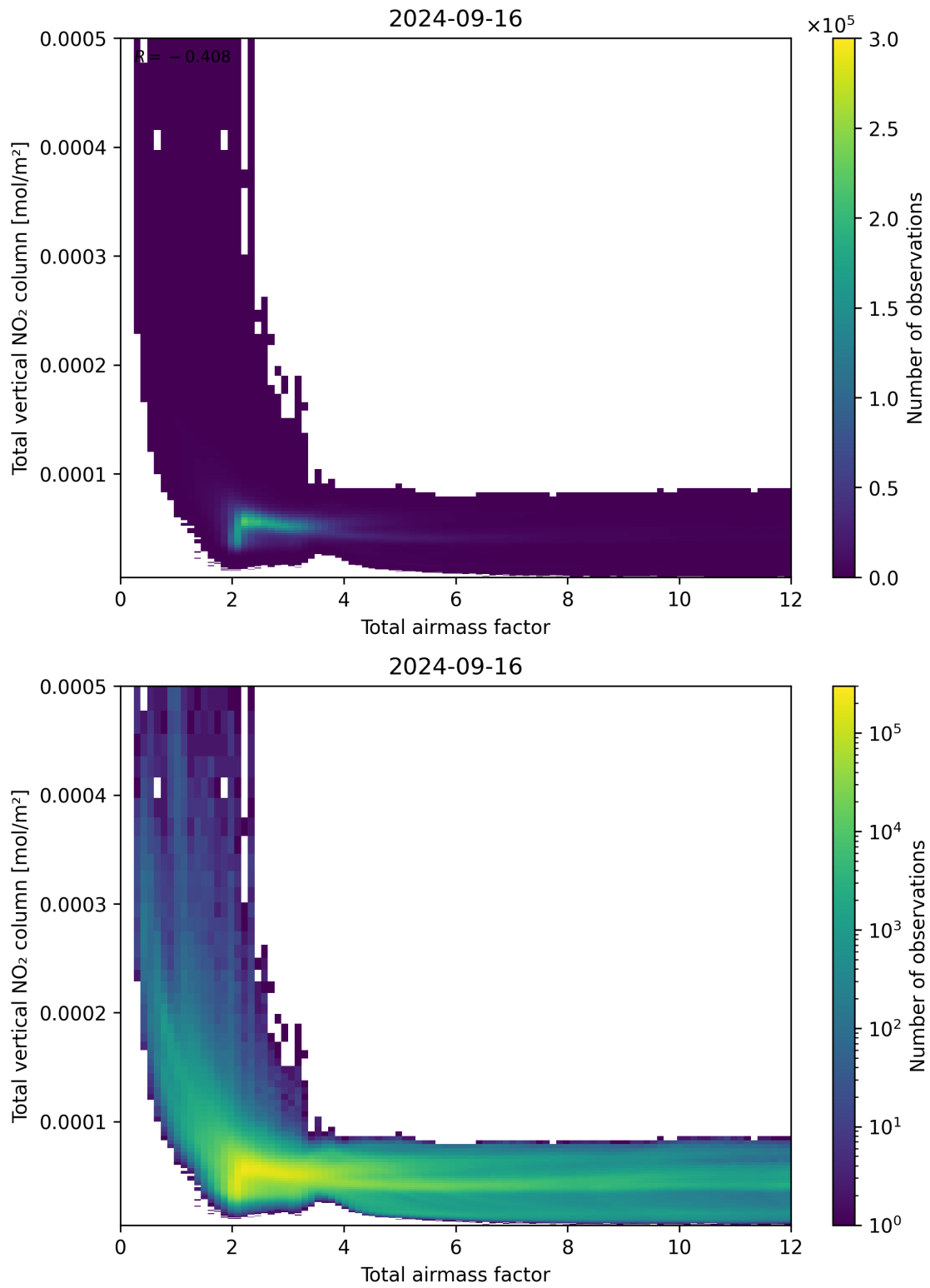
Figure 67: Scatter density plot of “Total airmass factor” against “Total vertical NO 2 column” for 2024-09-15 to 2024-09-17.
