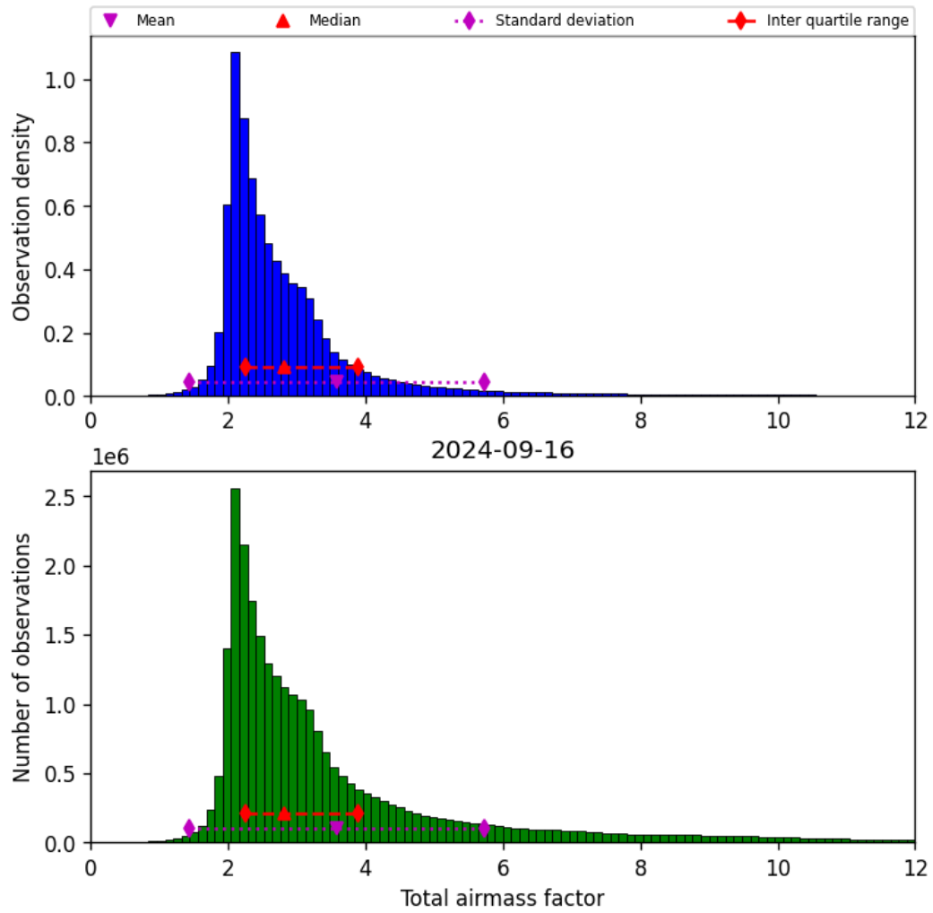
Figure 32: Histogram of “Total airmass factor” for 2024-09-15 to 2024-09-17
