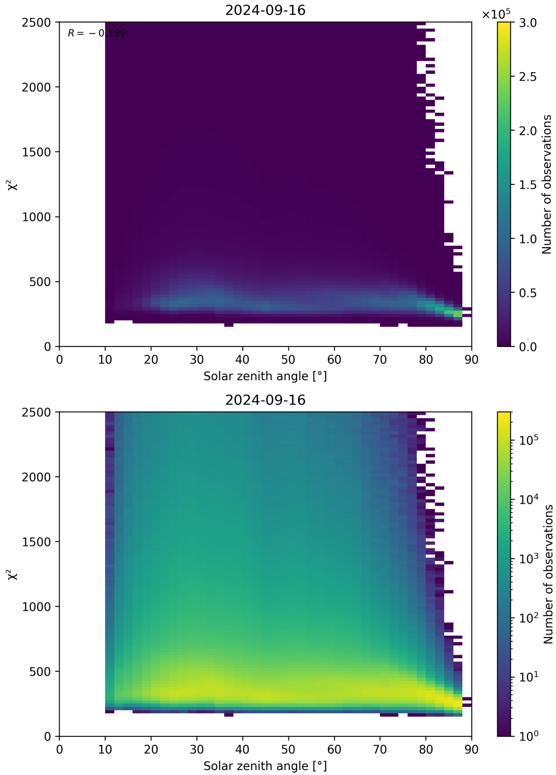
Figure 148: Scatter density plot of “Solar zenith angle” against “ \chi^2 ” for 2024-09-15 to 2024-09-17.
