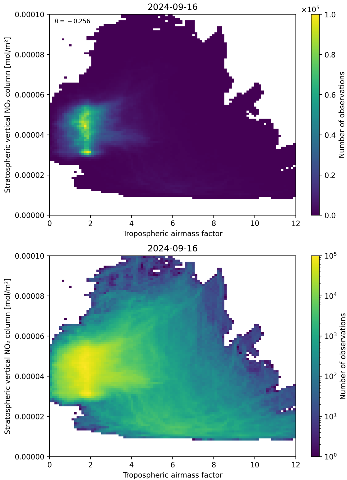
Figure 74: Scatter density plot of “Tropospheric air mass factor” against “Stratospheric vertical NO 2 column” for 2024-09-15 to 2024-09-17.
