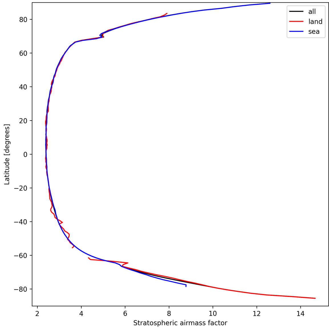
Figure 27: Zonal average of “Stratospheric airmass factor” for 2024-09-15 to 2024-09-17.
