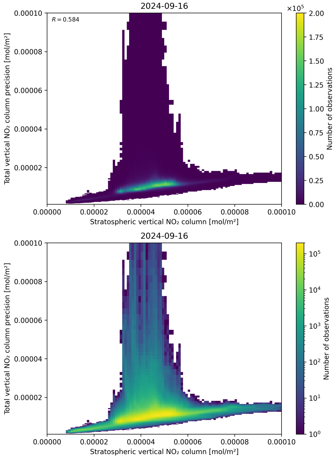
Figure 101: Scatter density plot of “Stratospheric vertical NO 2 column” against “Total vertical NO 2 column precision” for 2024-09-15 to 2024-09-17.
