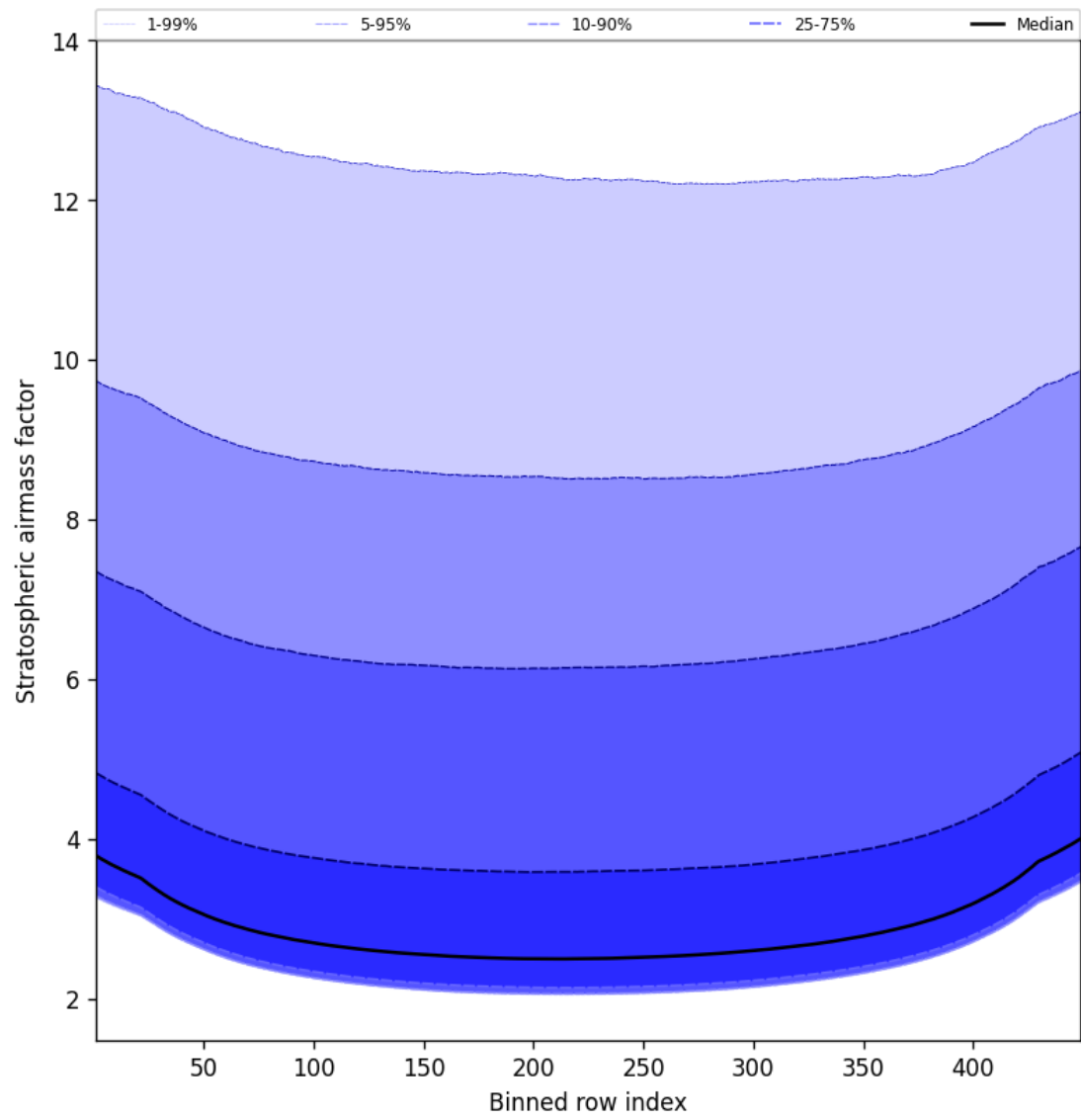
Figure 61: Along track statistics of “Stratospheric air mass factor” for 2024-09-15 to 2024-09-17
