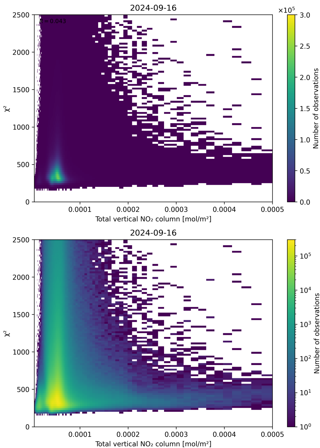
Figure 111: Scatter density plot of “Total vertical NO 2 column” against “ \chi^2 ” for 2024-09-15 to 2024-09-17.
