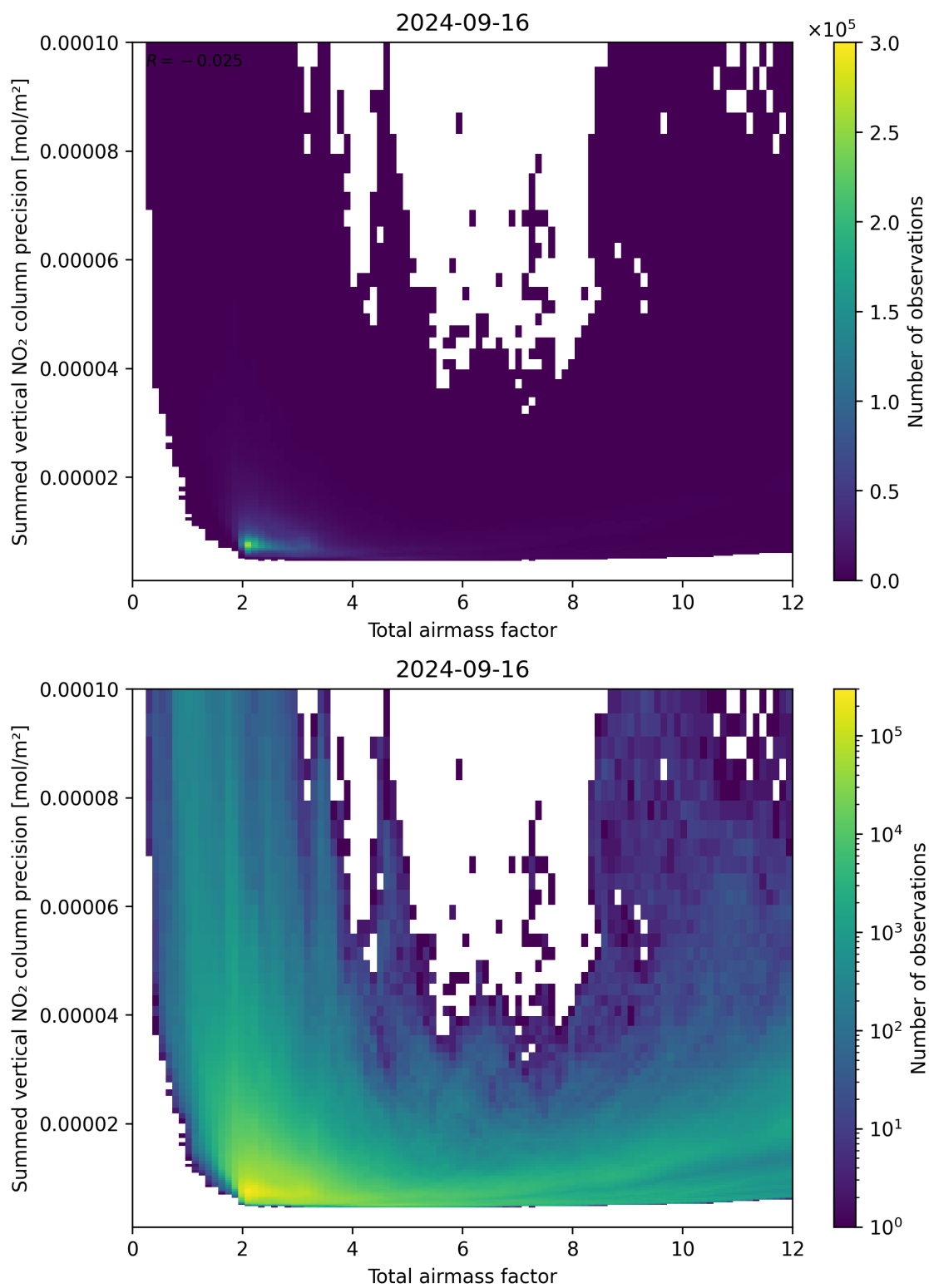
Figure 66: Scatter density plot of “Total airmass factor” against “Summed vertical NO 2 column precision” for 2024-09-15 to 2024-09-17.
