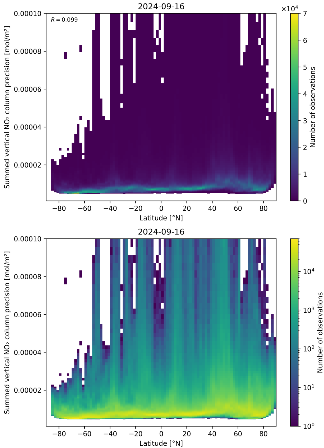
Figure 89: Scatter density plot of “Latitude” against “Summed vertical NO 2 column precision” for 2024-09-15 to 2024-09-17.
