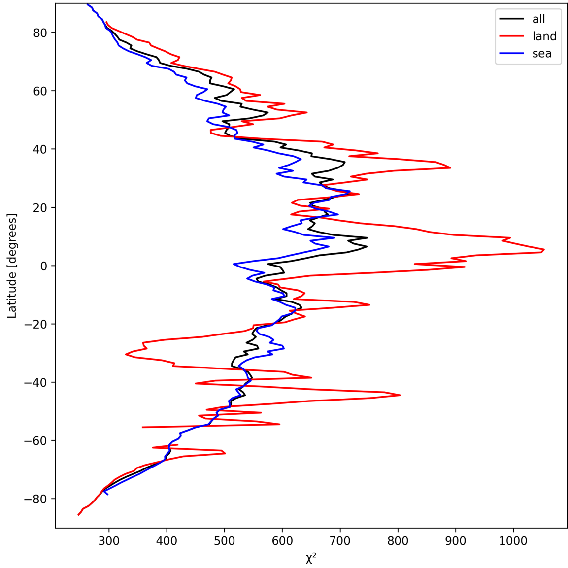
Figure 25: Zonal average of “ \chi^2 ” for 2024-09-15 to 2024-09-17.
