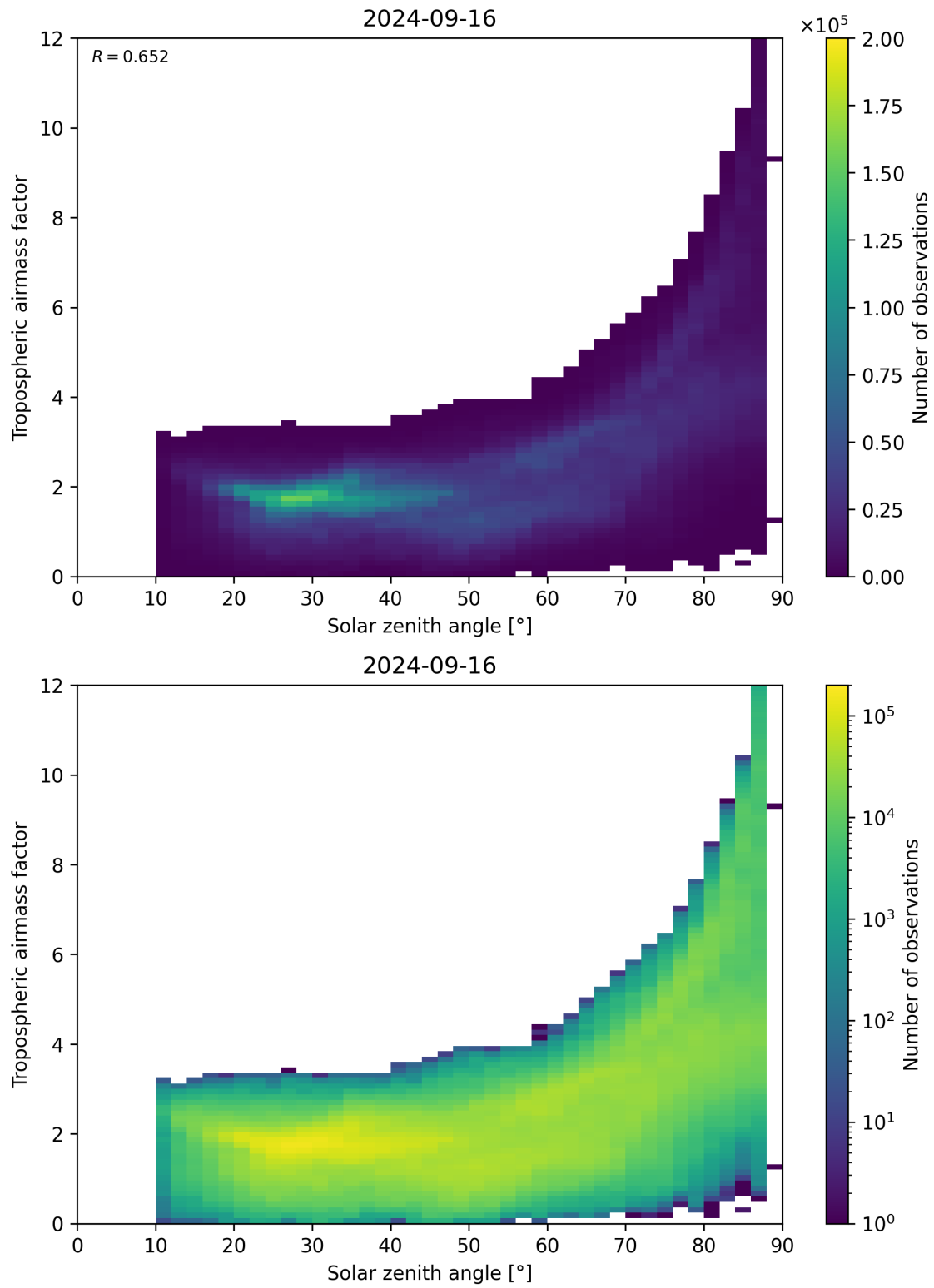
Figure 147: Scatter density plot of “Solar zenith angle” against “Tropospheric airmass factor” for 2024-09-15 to 2024-09-17.
