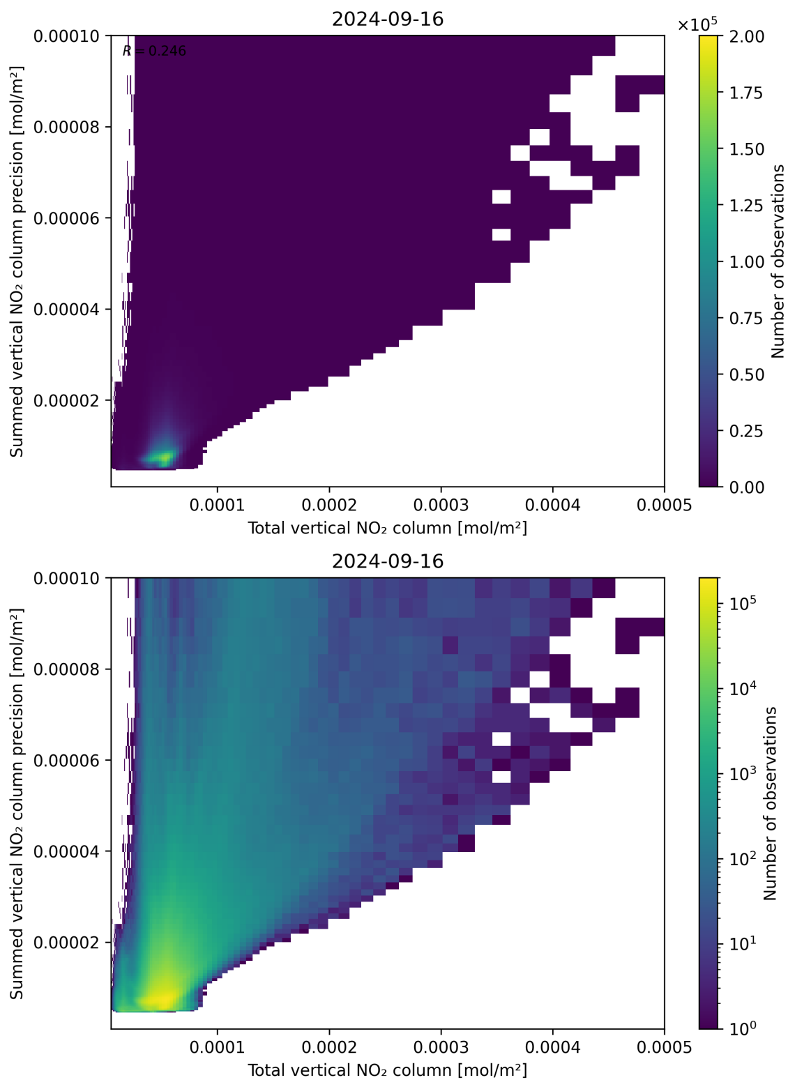
Figure 113: Scatter density plot of “Total vertical NO 2 column” against “Summed vertical NO 2 column precision” for 2024-09-15 to 2024-09-17.
