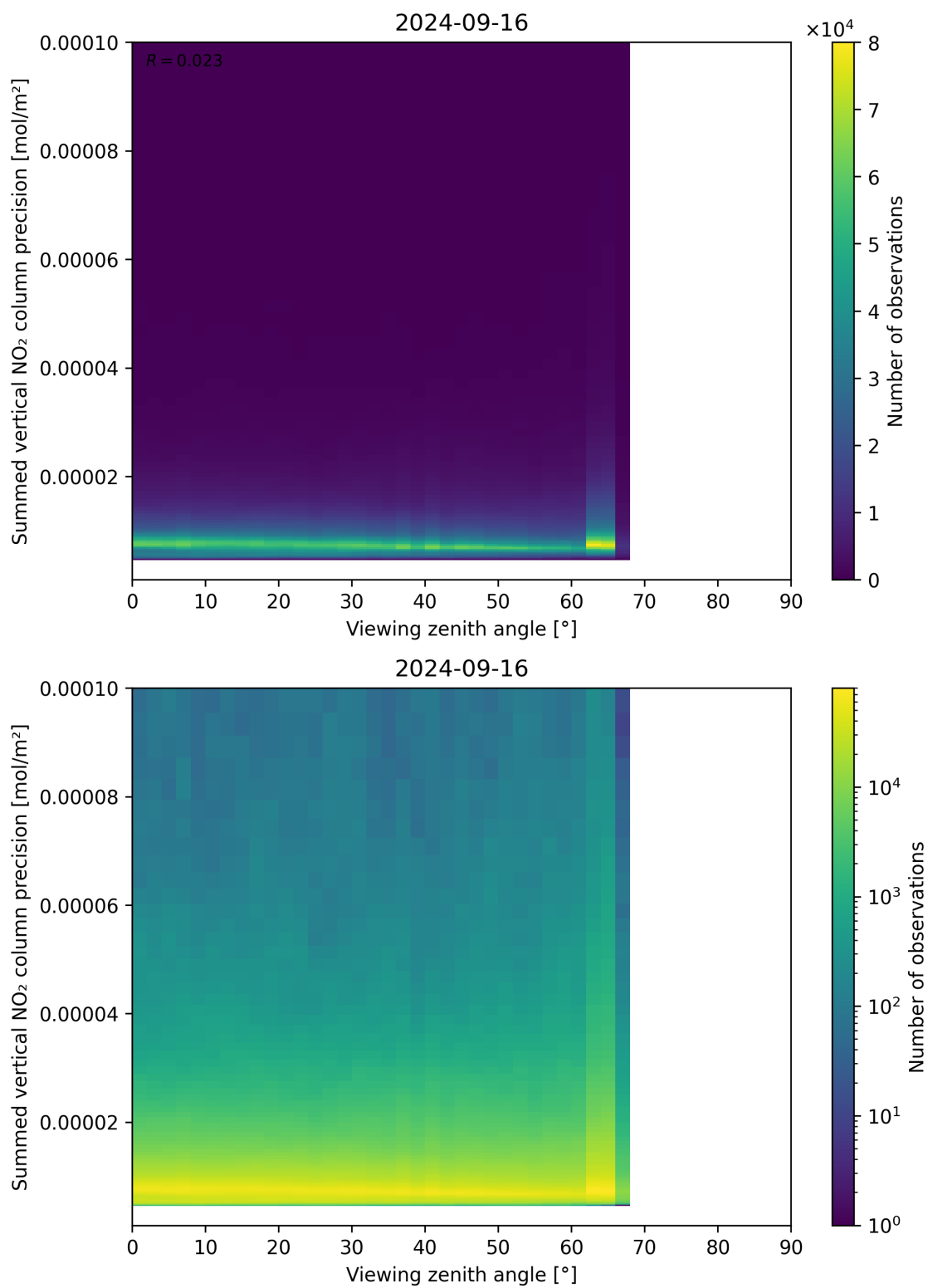
Figure 166: Scatter density plot of “Viewing zenith angle” against “Summed vertical NO 2 column precision” for 2024-09-15 to 2024-09-17.
