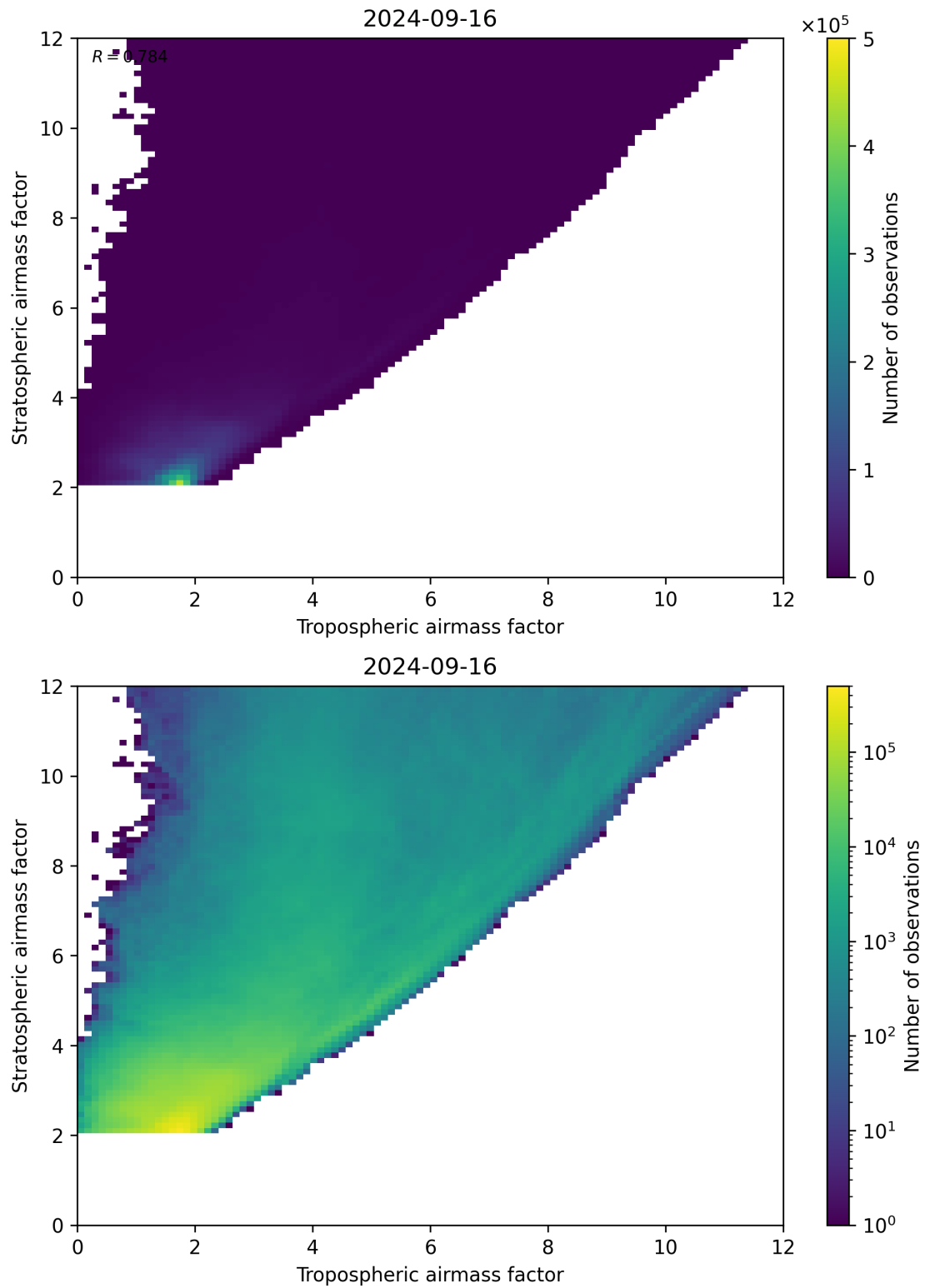
Figure 71: Scatter density plot of “Tropospheric airmass factor” against “Stratospheric airmass factor” for 2024-09-15 to 2024-09-17.
