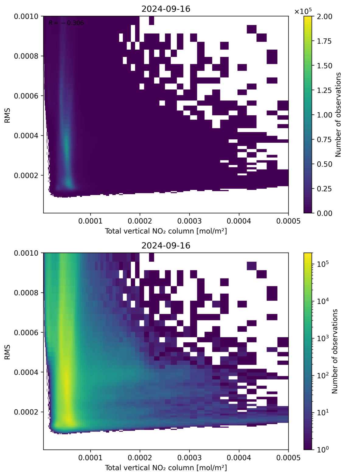
Figure 120: Scatter density plot of “Total vertical NO 2 column” against “RMS” for 2024-09-15 to 2024-09-17.
