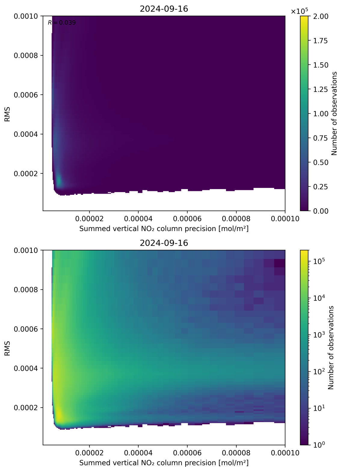
Figure 108: Scatter density plot of “Summed vertical NO 2 column precision” against “RMS” for 2024-09-15 to 2024-09-17.
