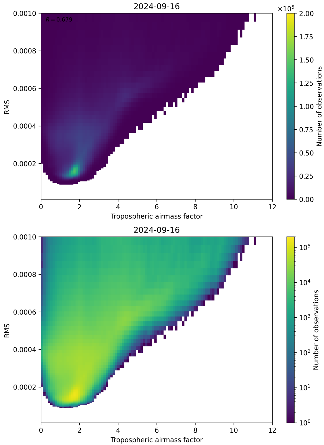
Figure 79: Scatter density plot of “Tropospheric airmass factor” against “RMS” for 2024-09-15 to 2024-09-17.
