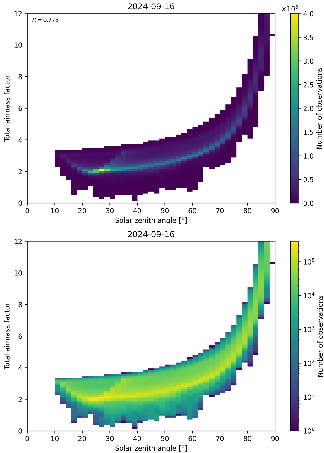
Figure 146: Scatter density plot of “Solar zenith angle” against “Total air mass factor” for 2024-09-15 to 2024-09-17.
