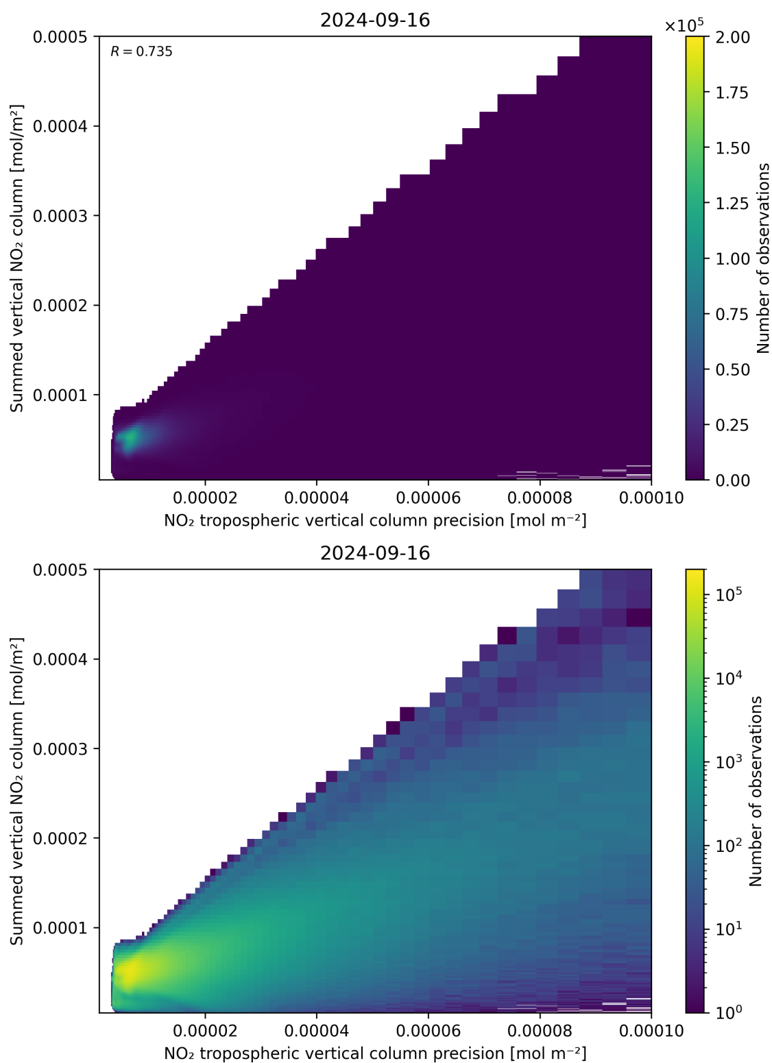
Figure 136: Scatter density plot of “NO 2 tropospheric vertical column precision” against “Summed vertical NO 2 column” for 2024-09-15 to 2024-09-17.
