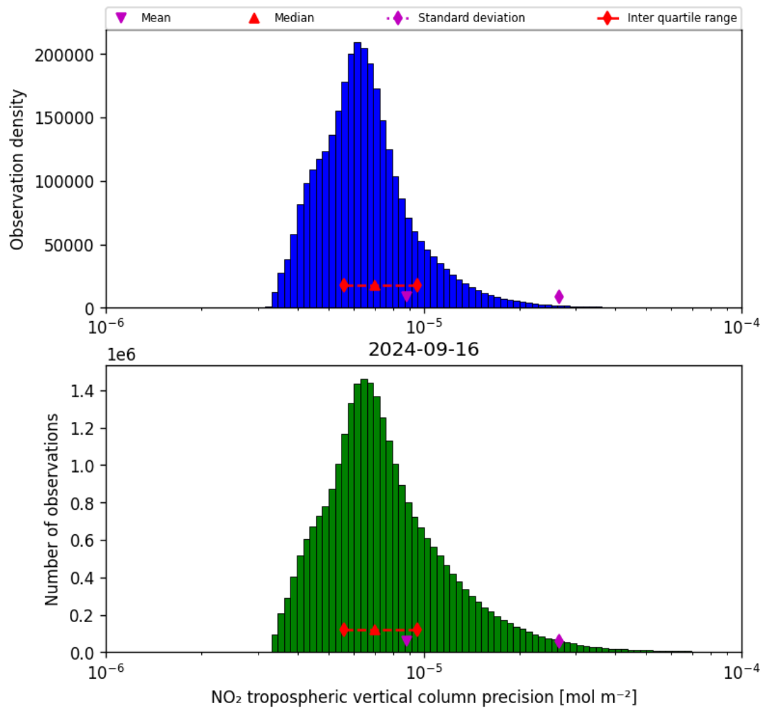
Figure 30: Histogram of “NO 2 tropospheric vertical column precision” for 2024-09-15 to 2024-09-17
