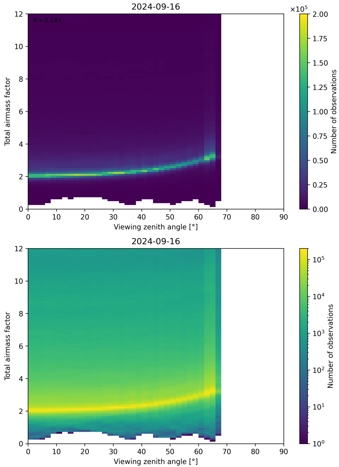
Figure 160: Scatter density plot of “Viewing zenith angle” against “Total airmass factor” for 2024-09-15 to 2024-09-17.
