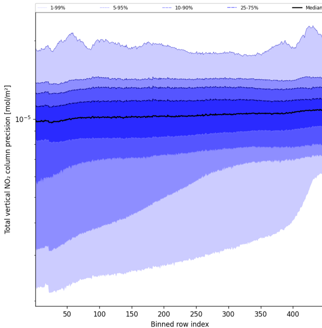
Figure 56: Along track statistics of “Total vertical NO 2 column precision” for 2024-09-15 to 2024-09-17
