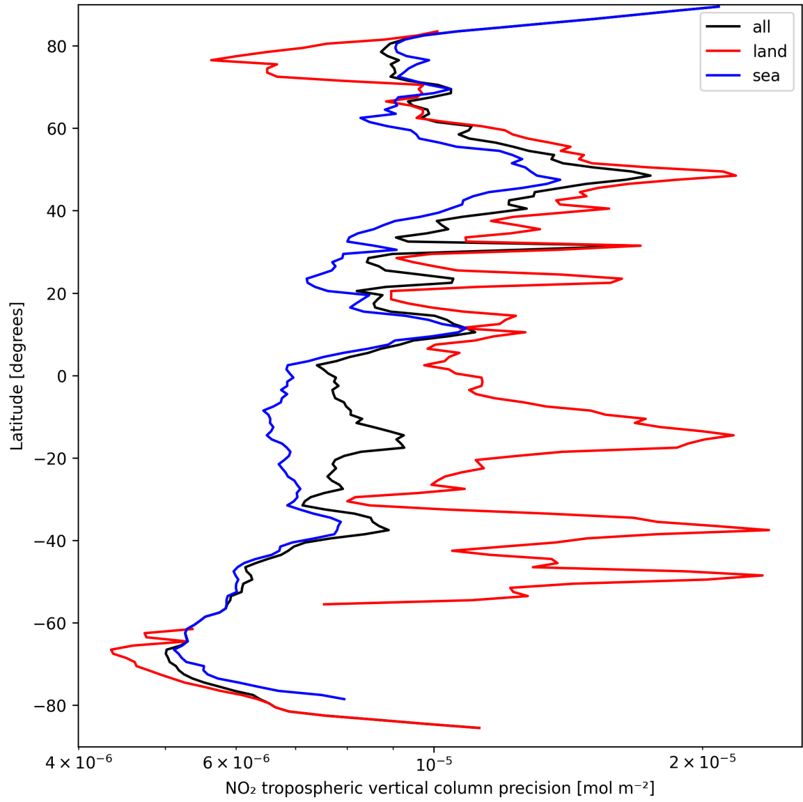
Figure 13: Zonal average of “NO 2 tropospheric vertical column precision” for 2024-09-15 to 2024-09-17.
