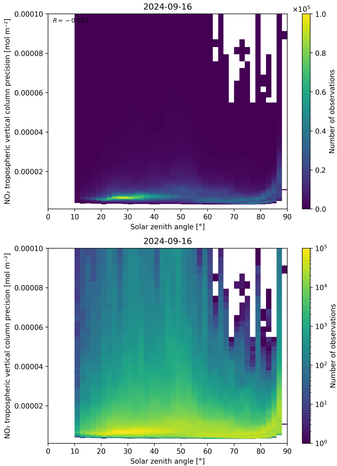
Figure 156: Scatter density plot of “Solar zenith angle” against “NO 2 tropospheric vertical column precision” for 2024-09-15 to 2024-09-17.
