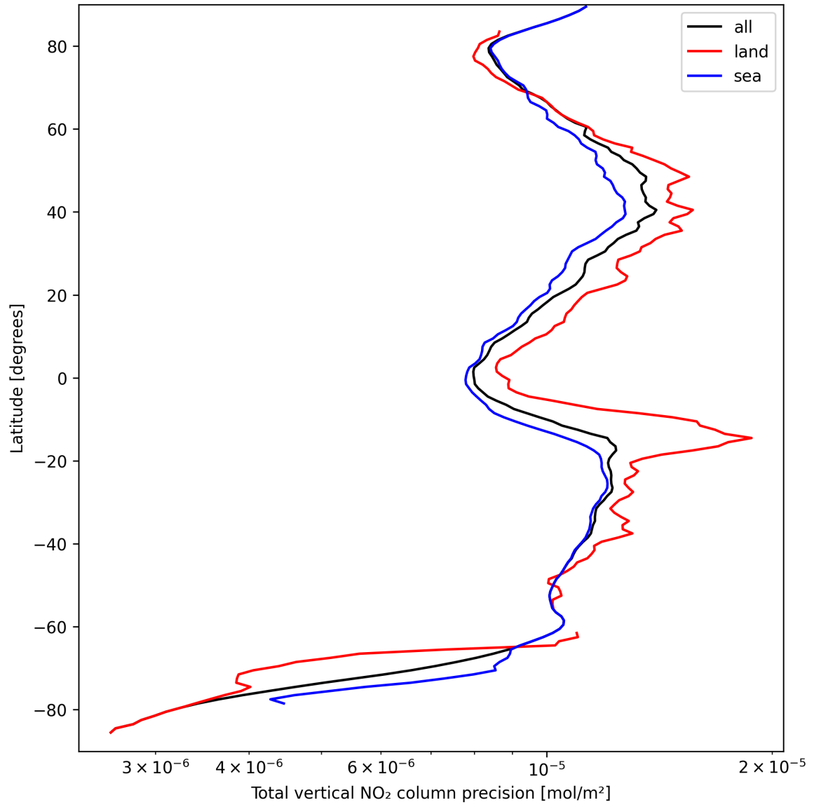
Figure 22: Zonal average of “Total vertical NO 2 column precision” for 2024-09-15 to 2024-09-17.
