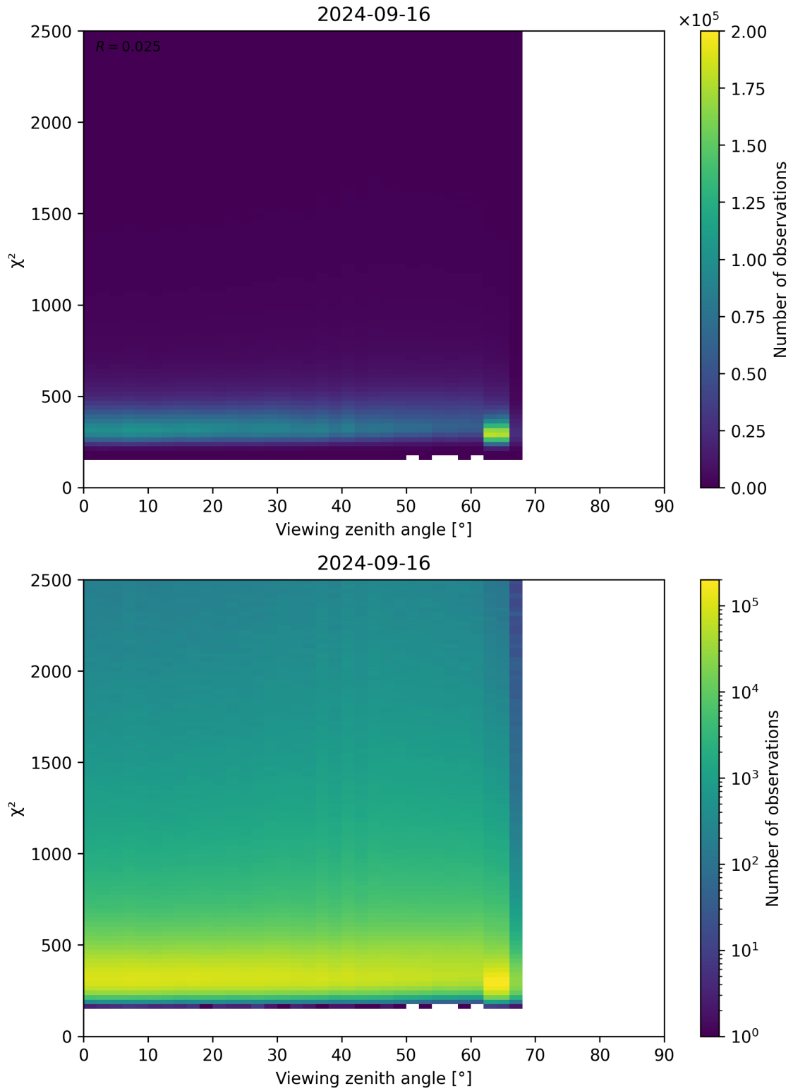
Figure 162: Scatter density plot of “Viewing zenith angle” against “ \chi^2 ” for 2024-09-15 to 2024-09-17.
