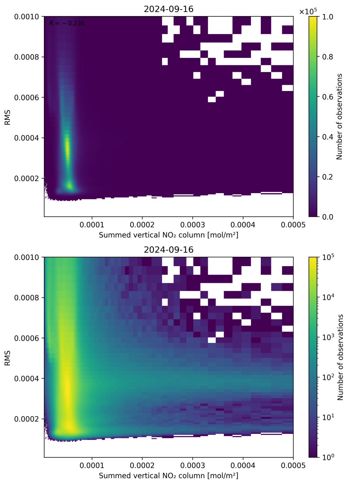
Figure 109: Scatter density plot of “Summed vertical NO 2 column” against “RMS” for 2024-09-15 to 2024-09-17.
