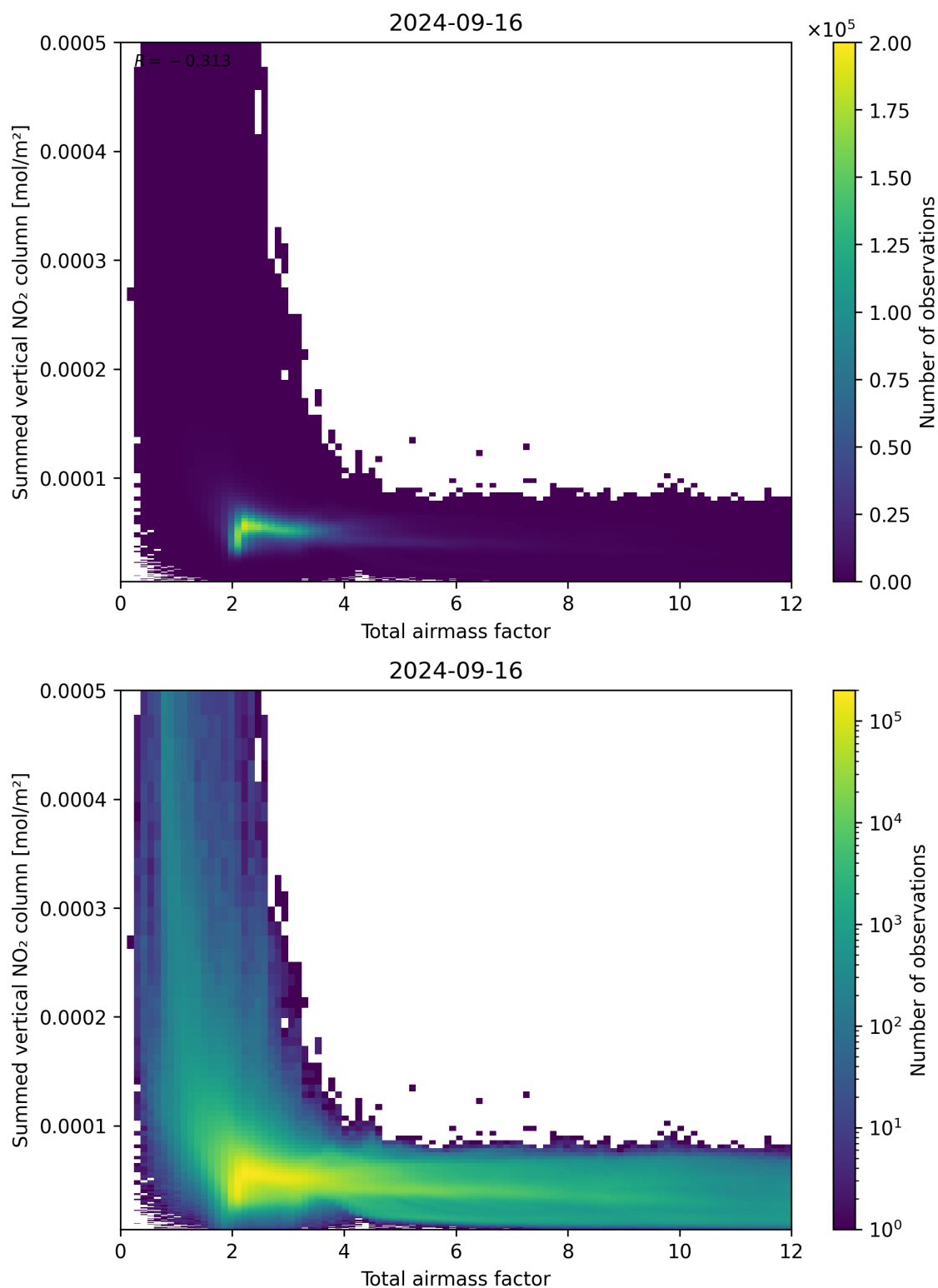
Figure 65: Scatter density plot of “Total airmass factor” against “Summed vertical NO 2 column” for 2024-09-15 to 2024-09-17.
