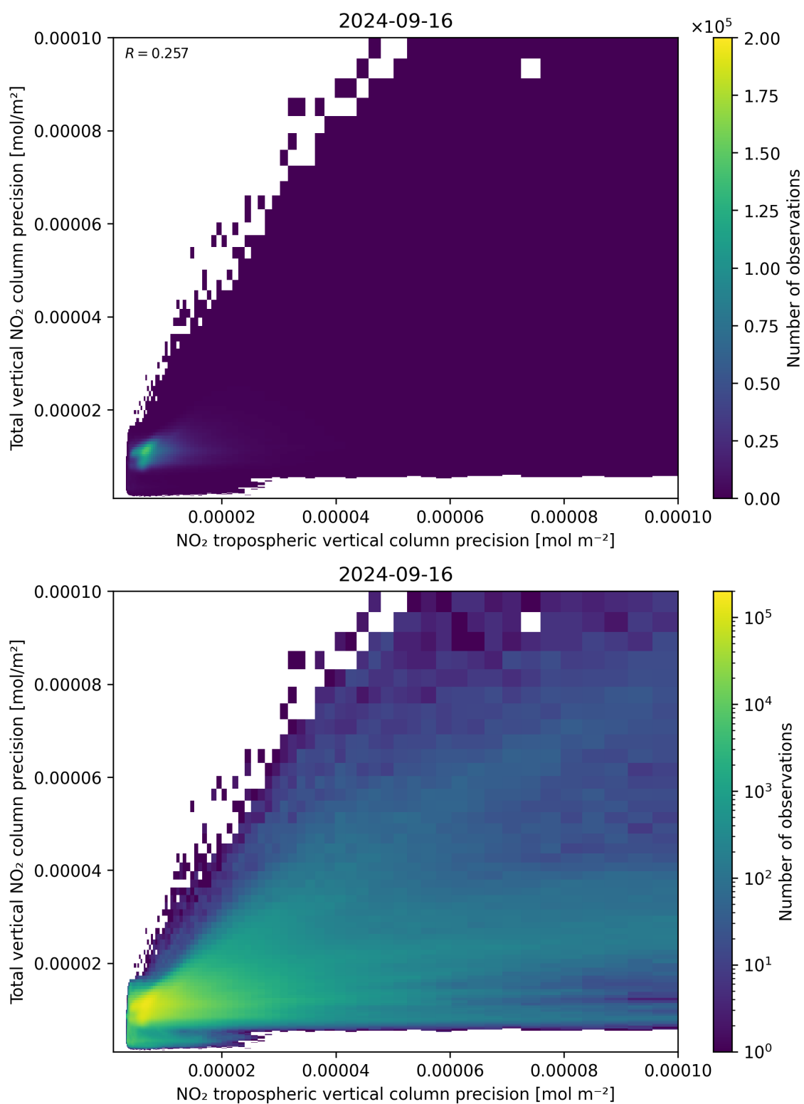
Figure 139: Scatter density plot of “NO 2 tropospheric vertical column precision” against “Total vertical NO 2 column precision” for 2024-09-15 to 2024-09-17.
