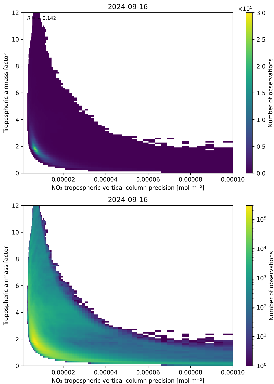
Figure 133: Scatter density plot of “NO 2 tropospheric vertical column precision” against “Tropospheric airmass factor” for 2024-09-15 to 2024-09-17.
