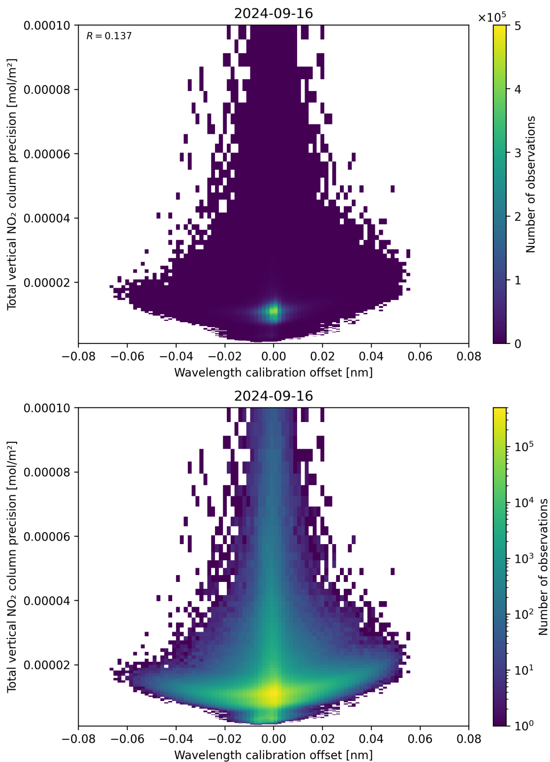
Figure 180: Scatter density plot of “Wavelength calibration offset” against “Total vertical NO 2 column precision” for 2024-09-15 to 2024-09-17.
