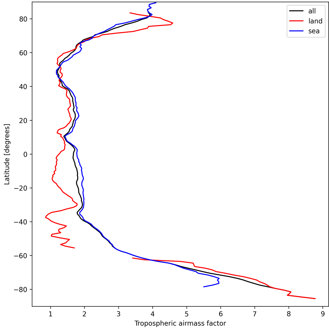
Figure 14: Zonal average of “Tropospheric airmass factor” for 2024-09-15 to 2024-09-17.
