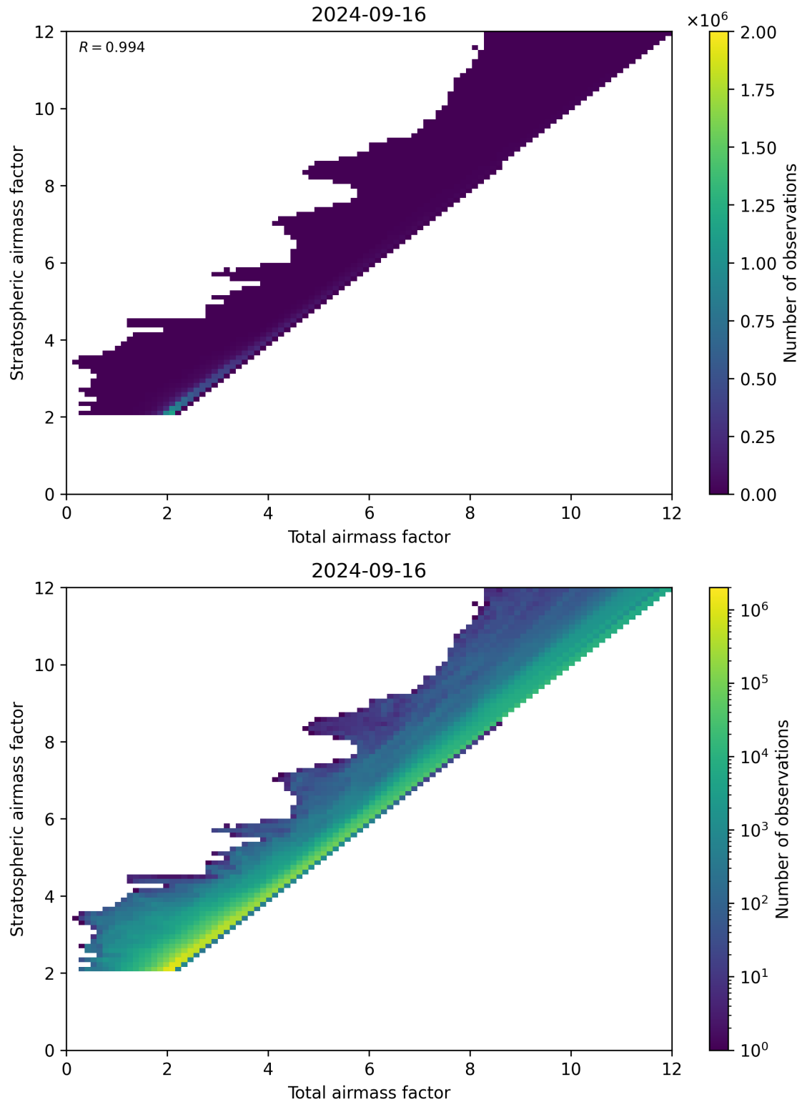
Figure 62: Scatter density plot of “Total airmass factor” against “Stratospheric airmass factor” for 2024-09-15 to 2024-09-17.
