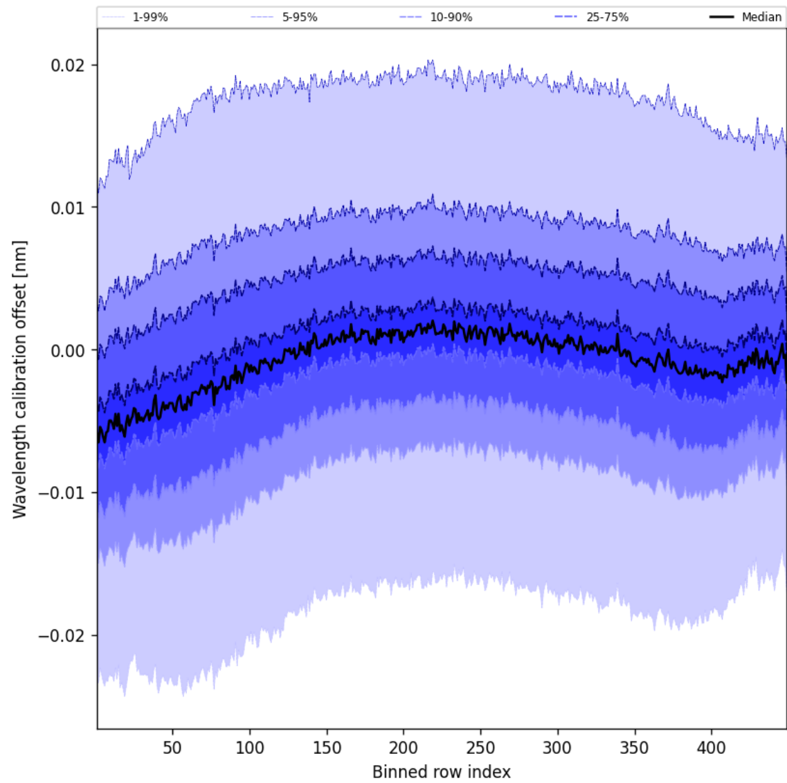
Figure 52: Along track statistics of “Wavelength calibration offset” for 2024-09-15 to 2024-09-17
