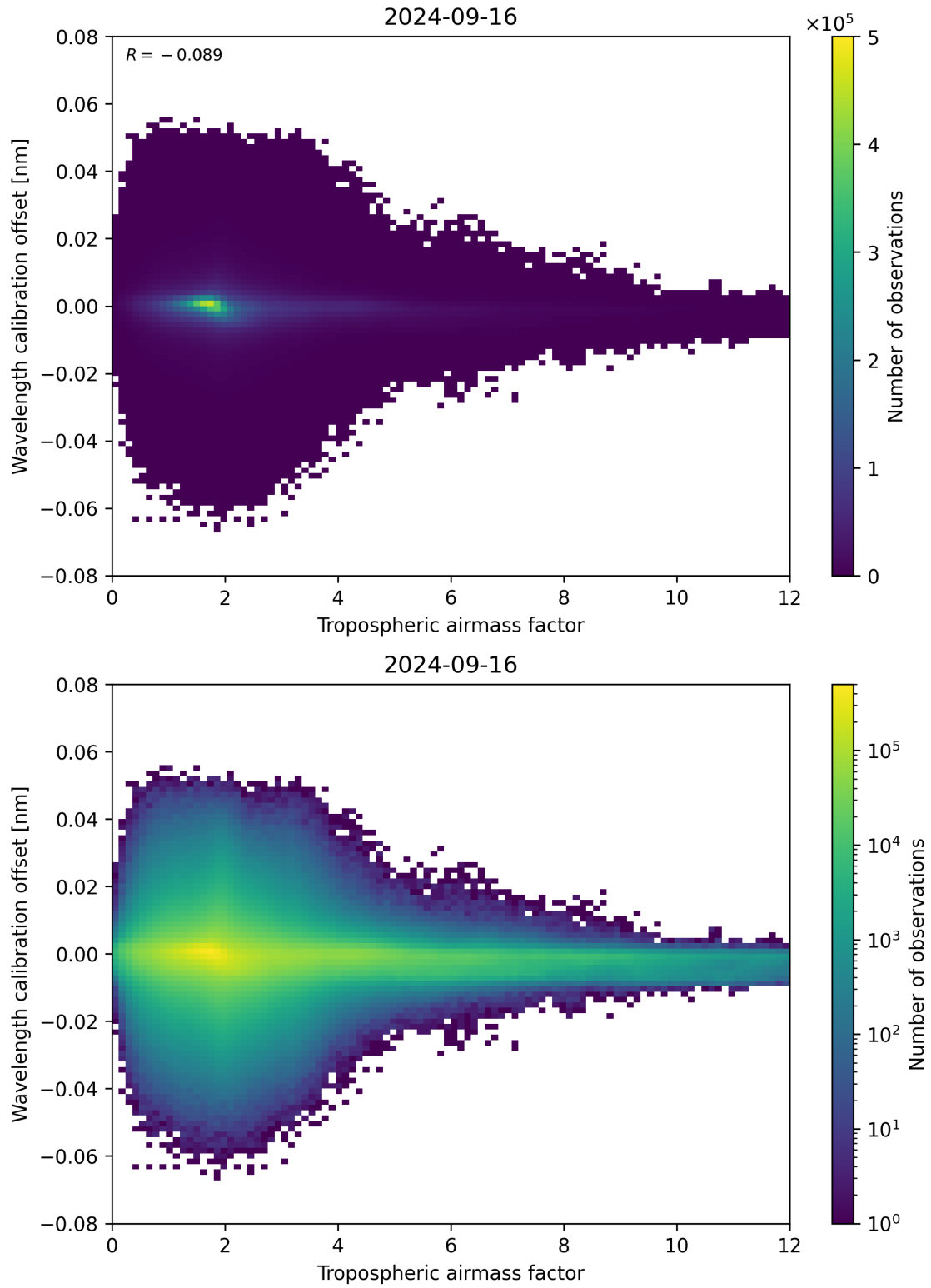
Figure 80: Scatter density plot of “Tropospheric airmass factor” against “Wavelength calibration offset” for 2024-09-15 to 2024-09-17.
