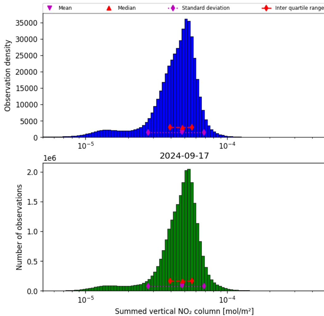
Figure 40: Histogram of “Summed vertical NO 2 column” for 2024-09-17 to 2024-09-18
