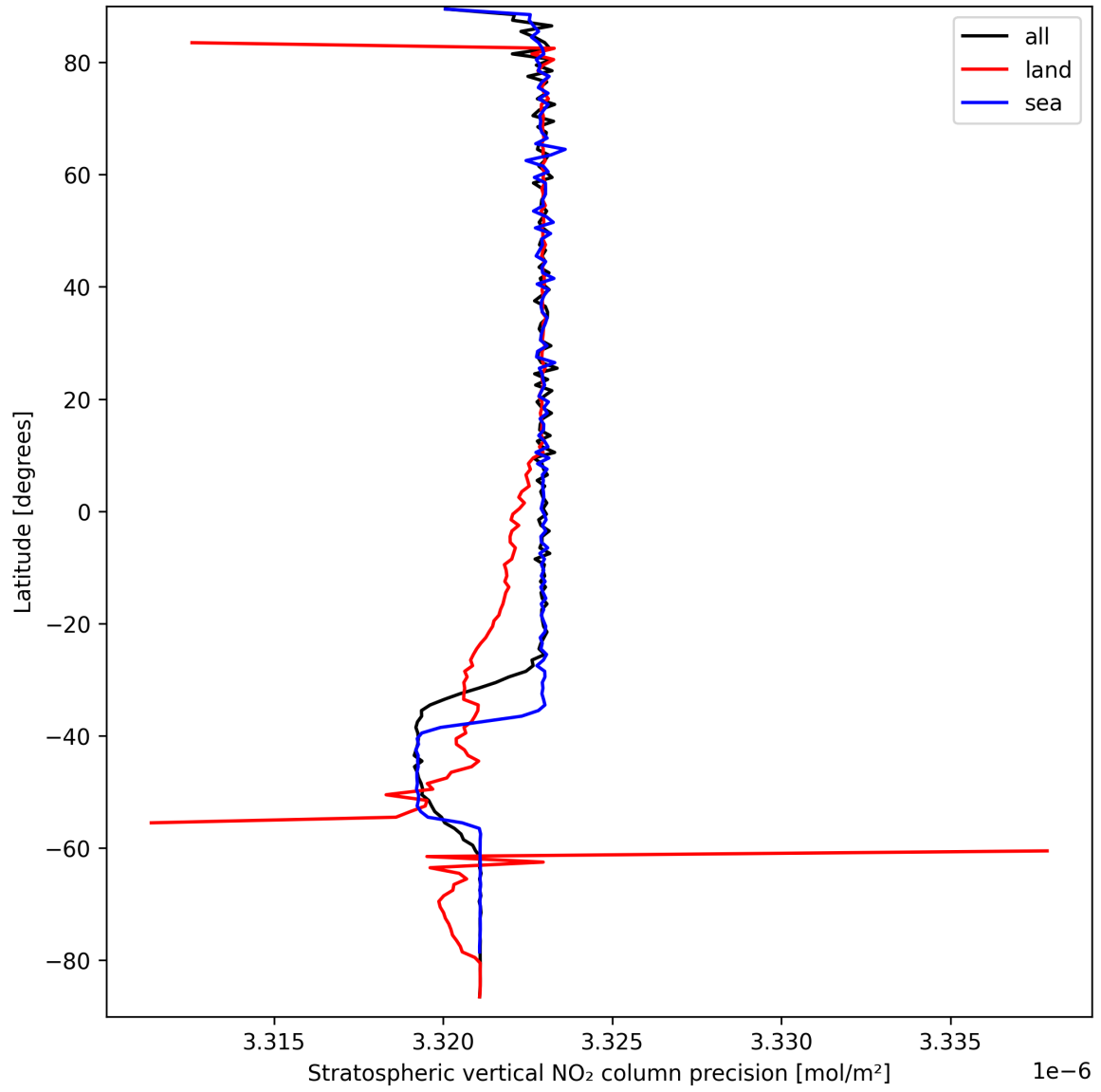
Figure 20: Zonal average of “Stratospheric vertical NO 2 column precision” for 2024-09-17 to 2024-09-18.
