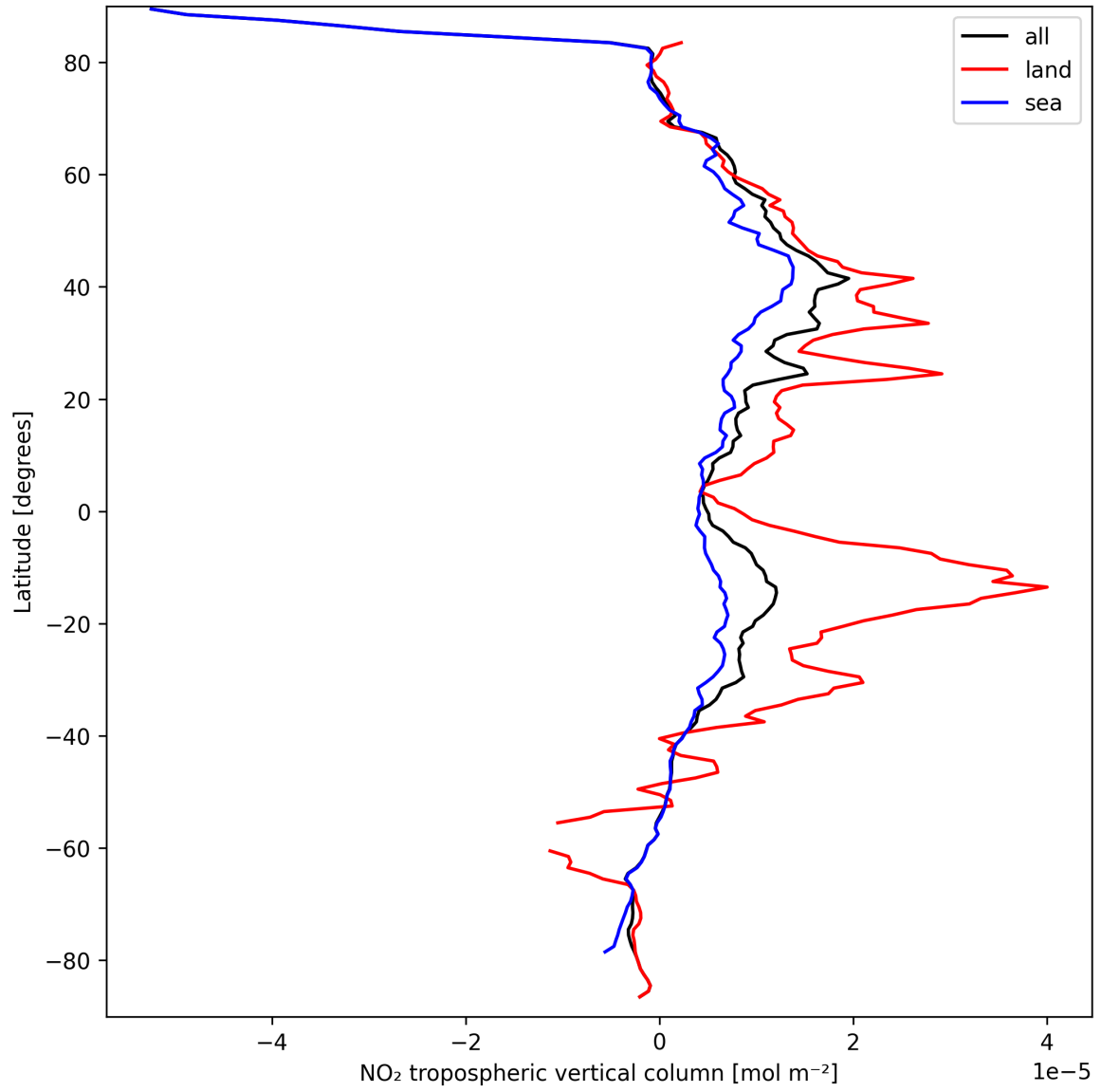
Figure 12: Zonal average of “NO 2 tropospheric vertical column” for 2024-09-17 to 2024-09-18.
