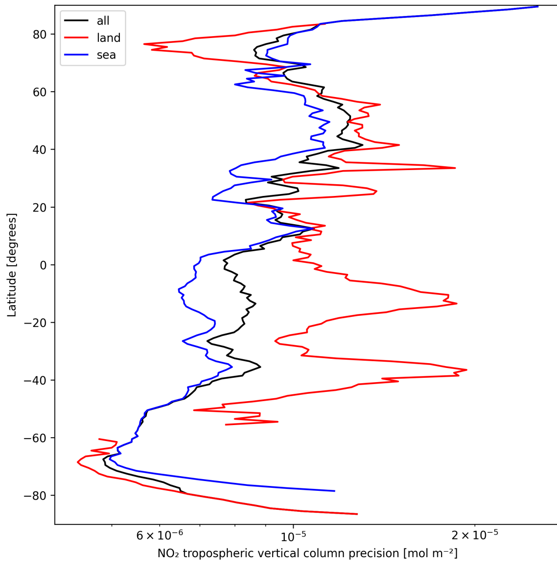
Figure 13: Zonal average of “NO 2 tropospheric vertical column precision” for 2024-09-17 to 2024-09-18.
