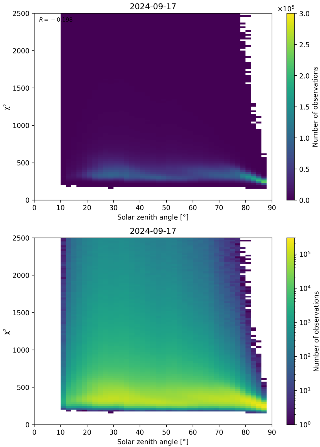
Figure 148: Scatter density plot of “Solar zenith angle” against “ \chi^2 ” for 2024-09-17 to 2024-09-18.
