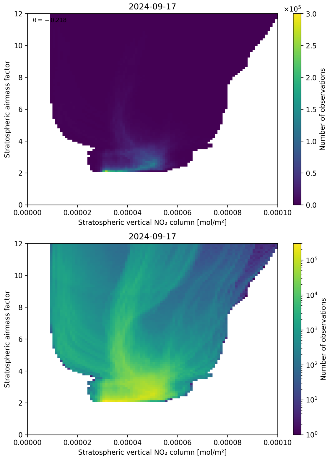
Figure 96: Scatter density plot of “Stratospheric vertical NO 2 column” against “Stratospheric airmass factor” for 2024-09-17 to 2024-09-18.
