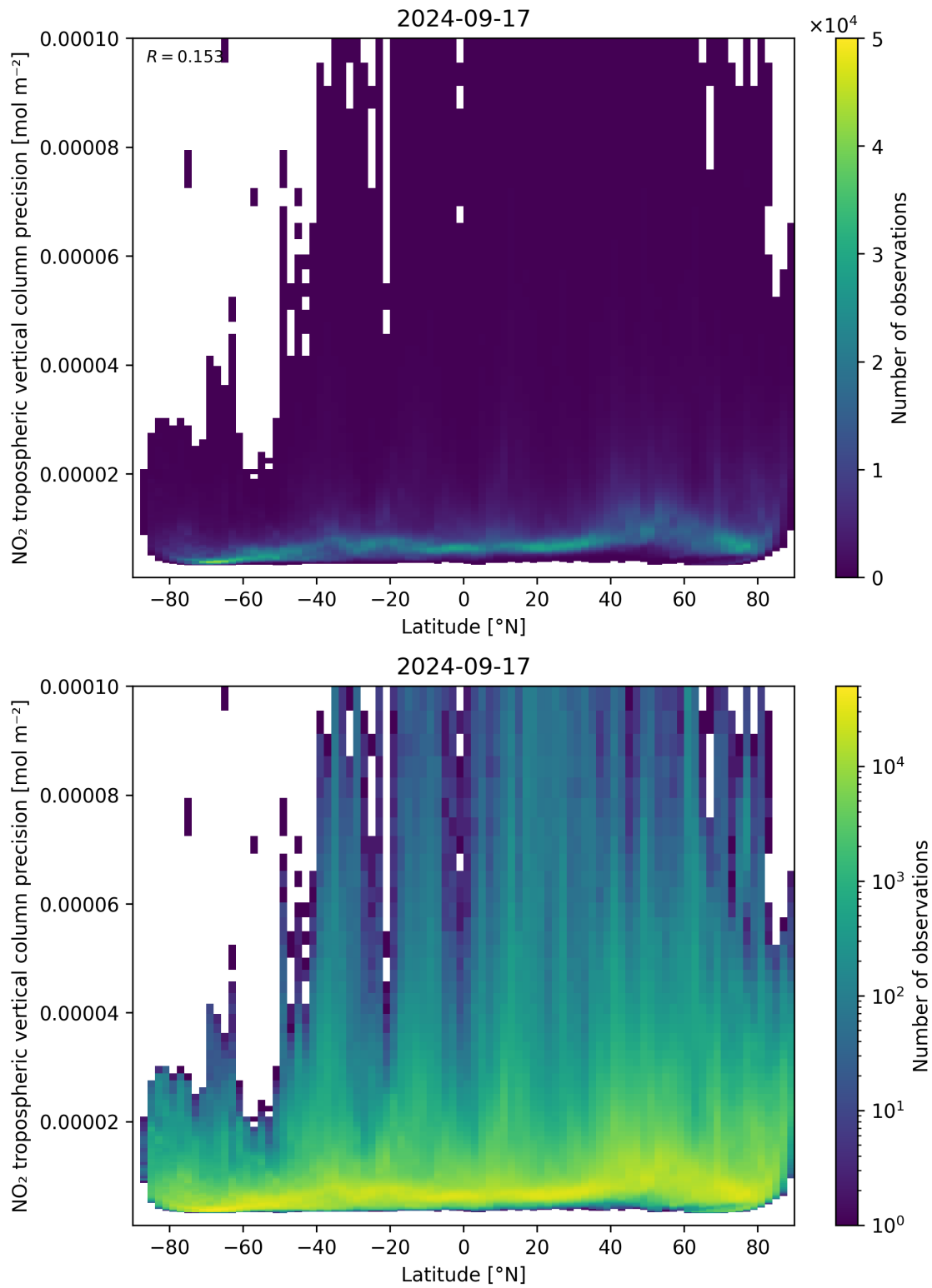
Figure 93: Scatter density plot of “Latitude” against “NO 2 tropospheric vertical column precision” for 2024-09-17 to 2024-09-18.
