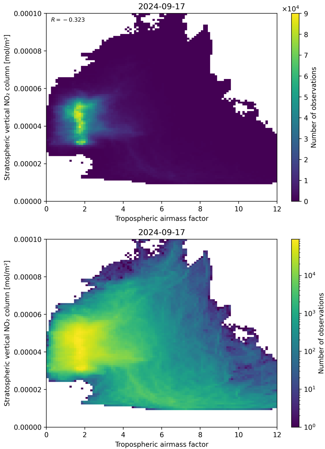
Figure 74: Scatter density plot of “Tropospheric air mass factor” against “Stratospheric vertical NO 2 column” for 2024-09-17 to 2024-09-18.
