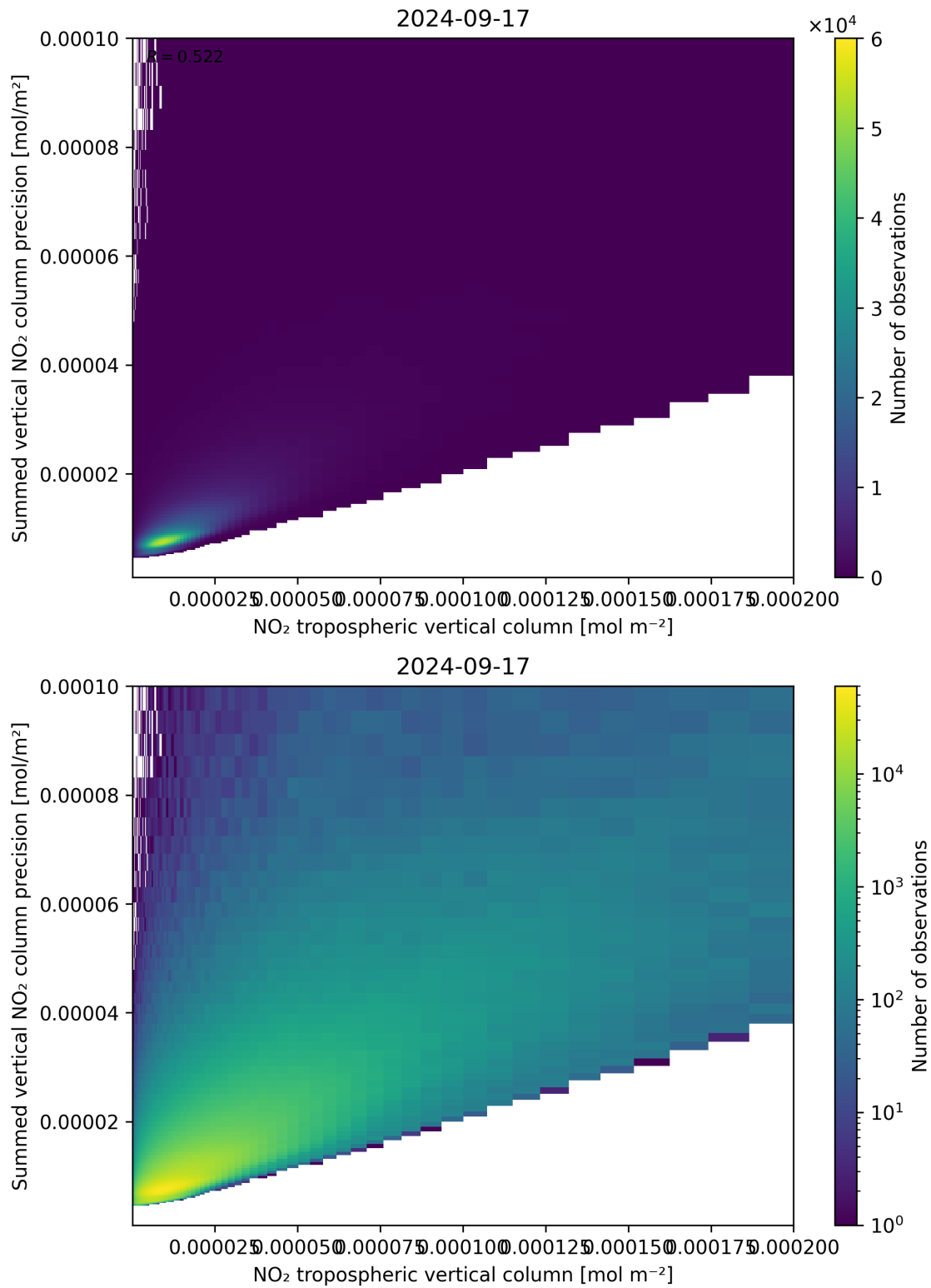
Figure 127: Scatter density plot of “NO 2 tropospheric vertical column” against “Summed vertical NO 2 column precision” for 2024-09-17 to 2024-09-18.
