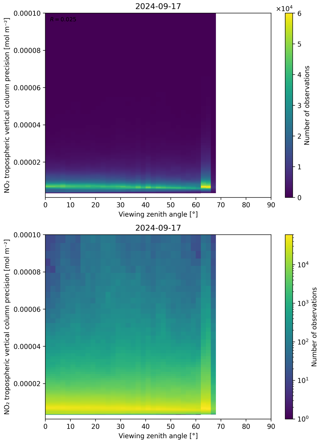
Figure 170: Scatter density plot of “Viewing zenith angle” against “NO 2 tropospheric vertical column precision” for 2024-09-17 to 2024-09-18.
