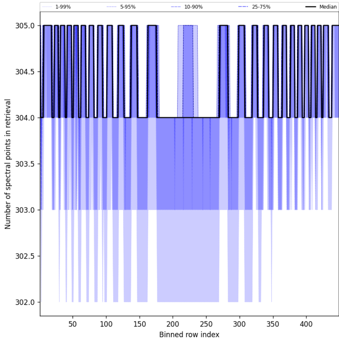
Figure 50: Along track statistics of “Number of spectral points in retrieval” for 2024-09-17 to 2024-09-18
