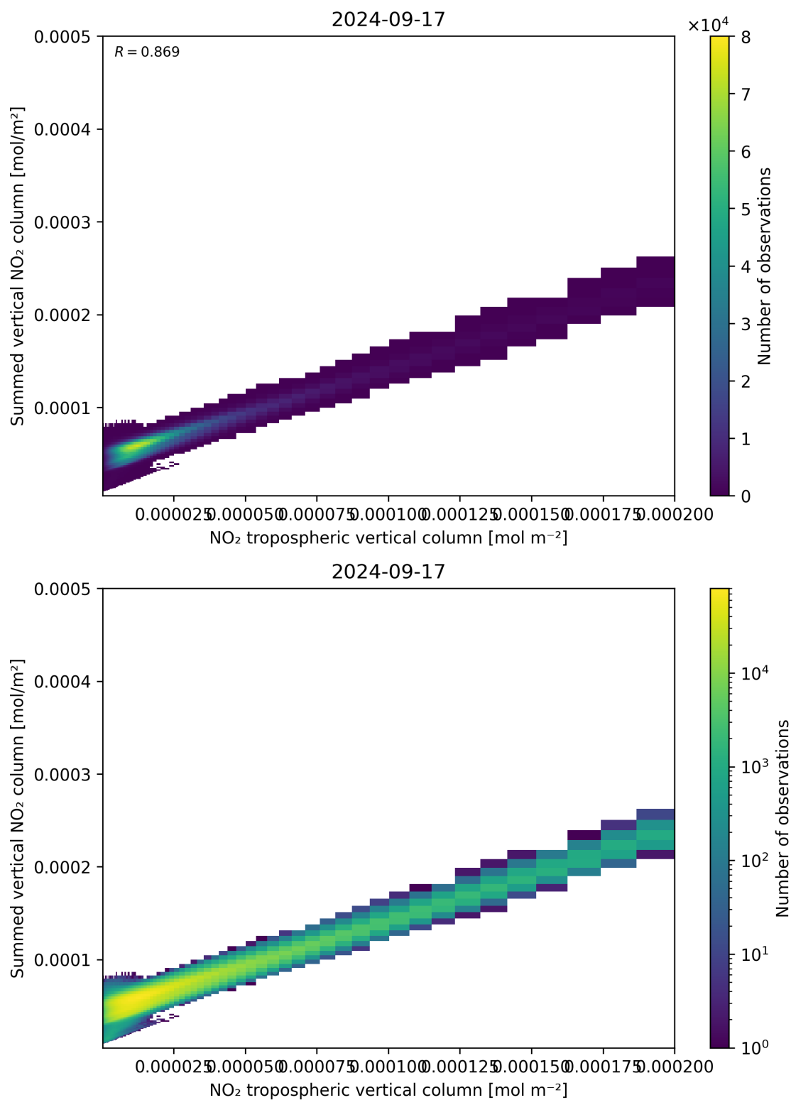
Figure 126: Scatter density plot of “NO 2 tropospheric vertical column” against “Summed vertical NO 2 column” for 2024-09-17 to 2024-09-18.
