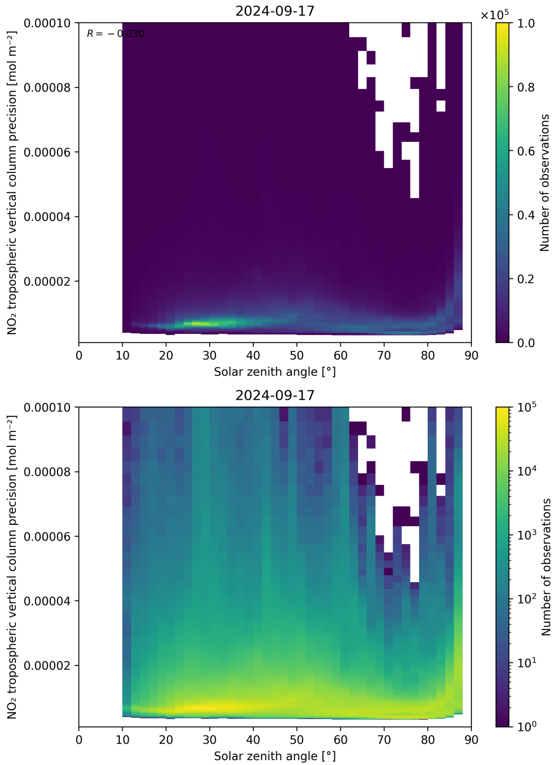
Figure 156: Scatter density plot of “Solar zenith angle” against “NO 2 tropospheric vertical column precision” for 2024-09-17 to 2024-09-18.
