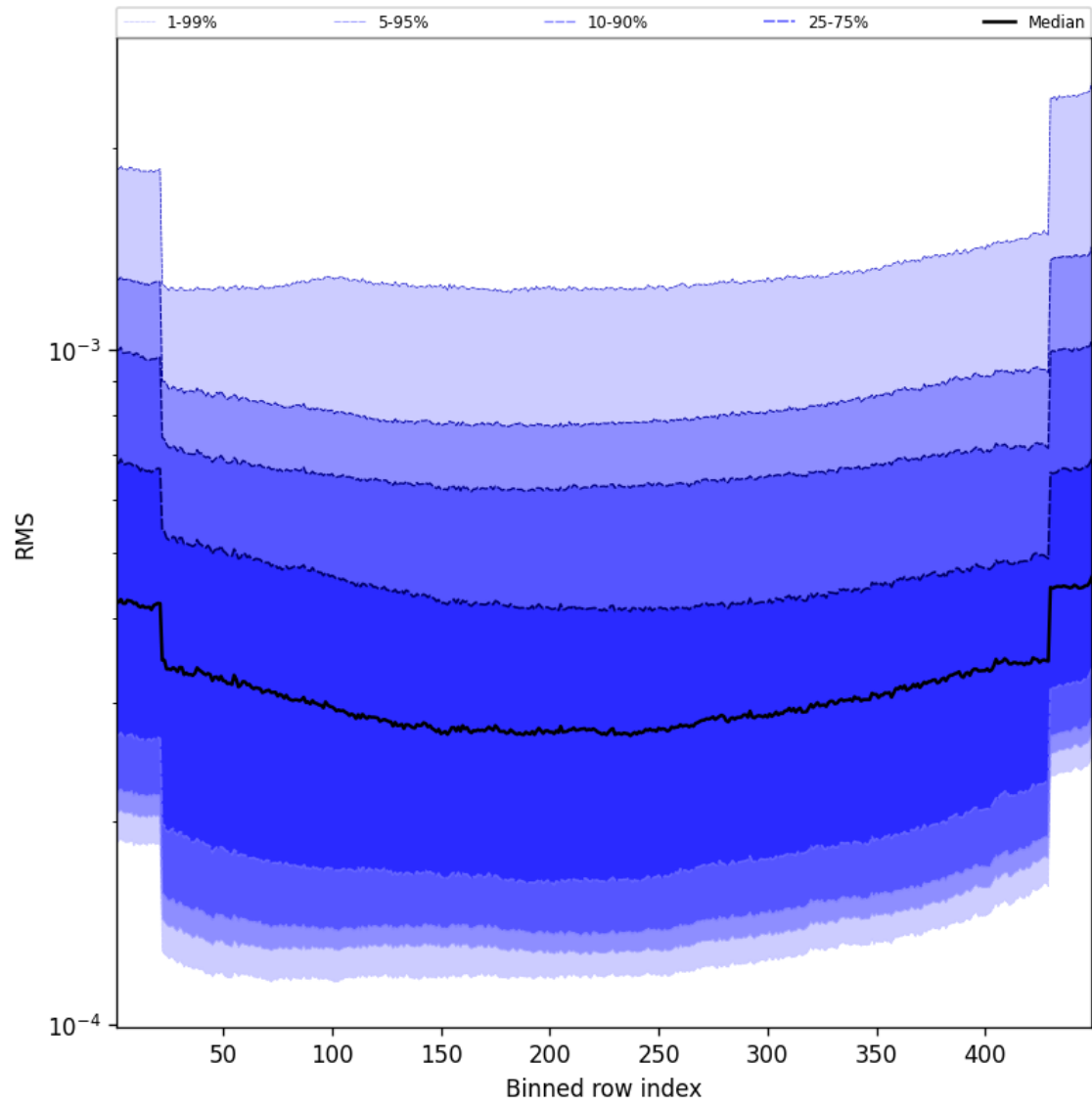
Figure 60: Along track statistics of “RMS” for 2024-09-17 to 2024-09-18
