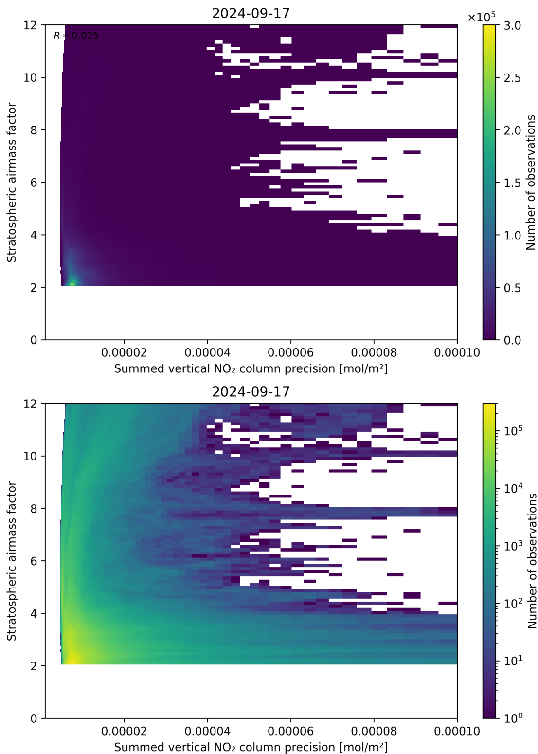
Figure 106: Scatter density plot of “Summed vertical NO 2 column precision” against “Stratospheric airmass factor” for 2024-09-17 to 2024-09-18.
