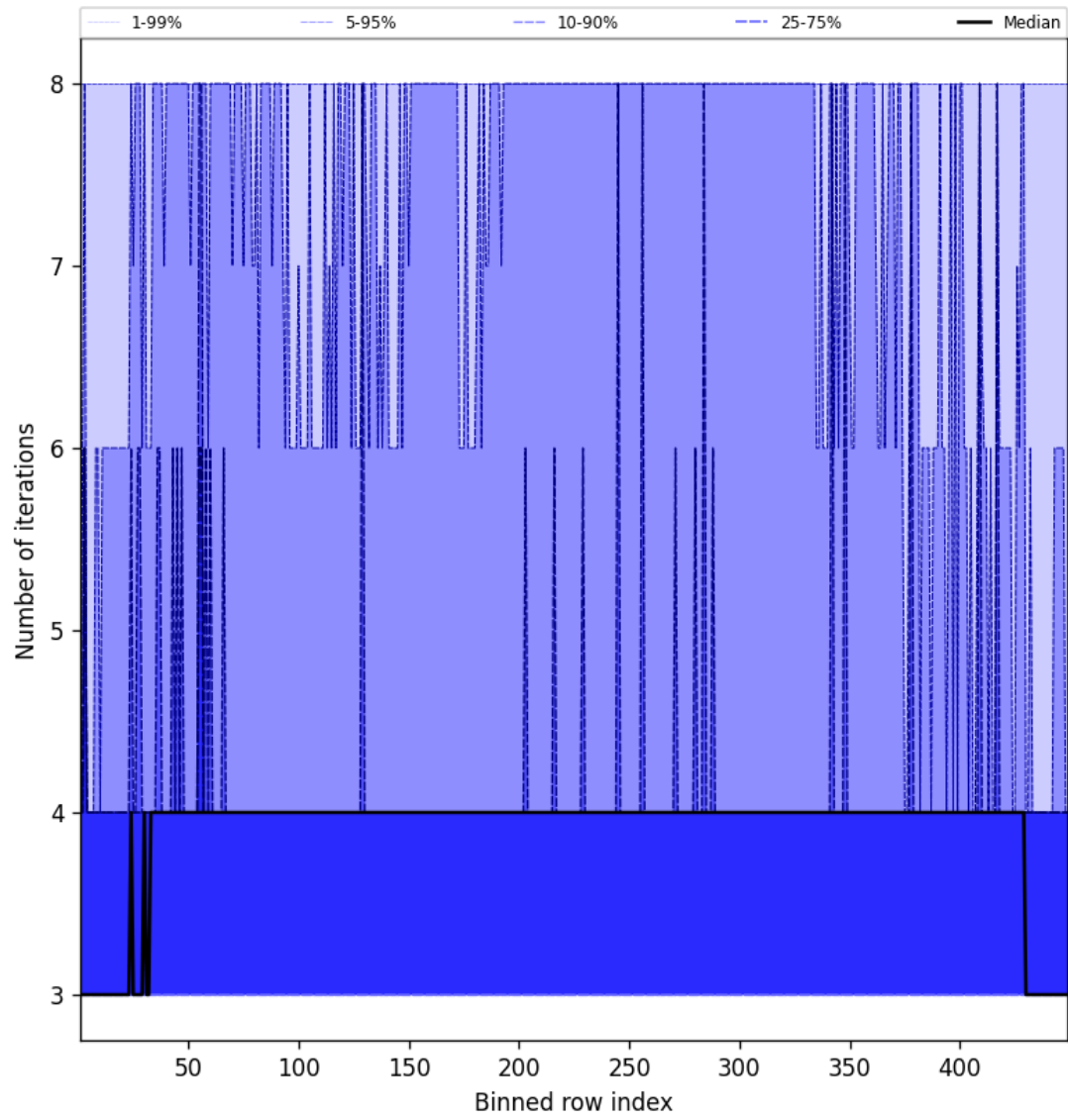
Figure 51: Along track statistics of “Number of iterations” for 2024-09-17 to 2024-09-18
