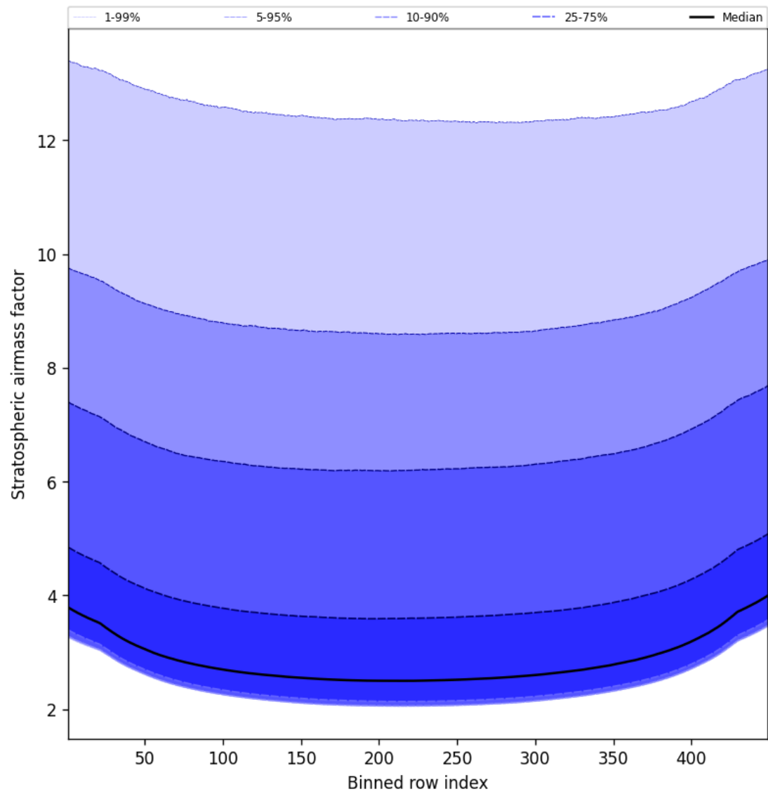
Figure 61: Along track statistics of “Stratospheric airmass factor” for 2024-09-17 to 2024-09-18
