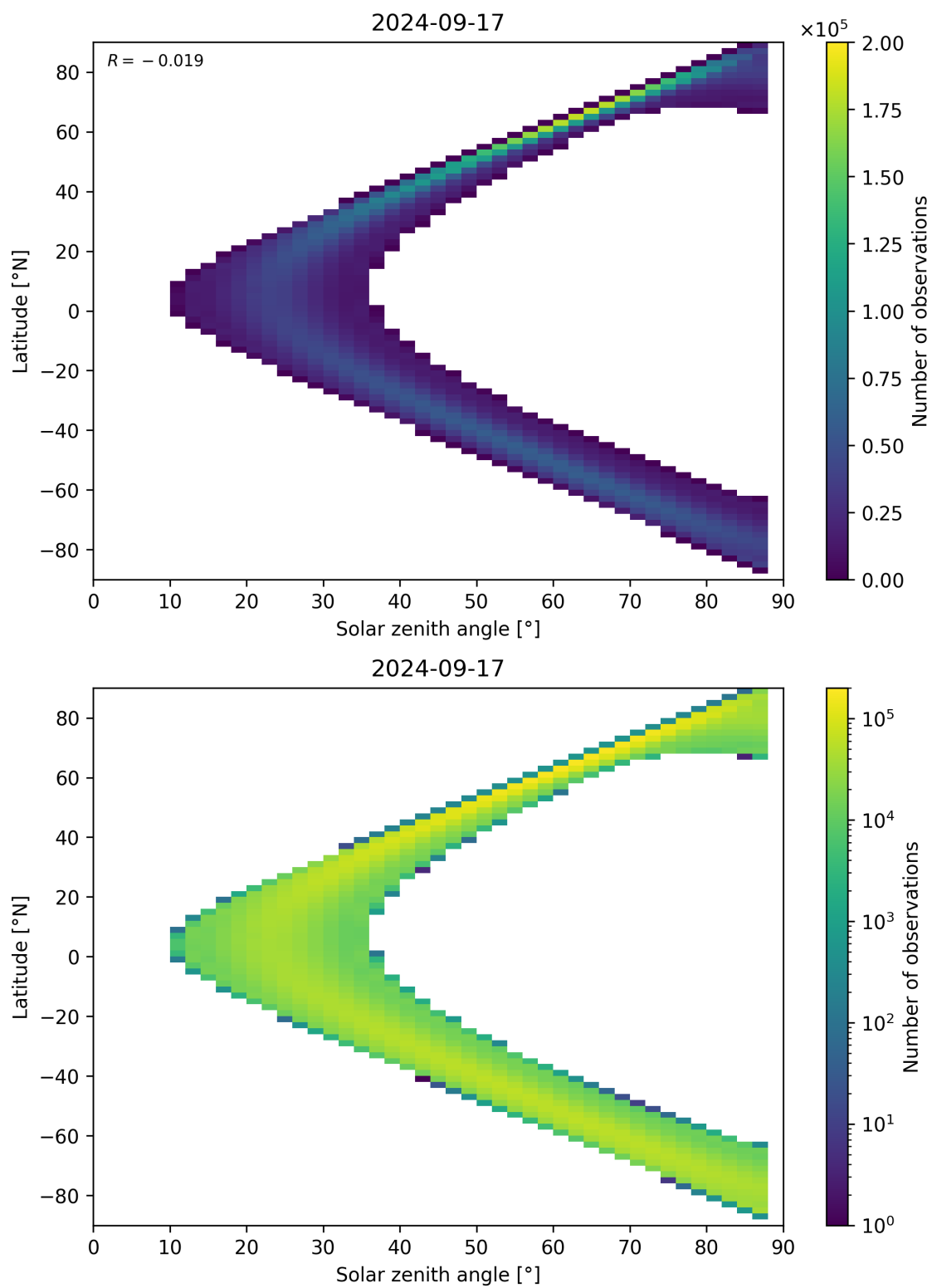
Figure 149: Scatter density plot of “Solar zenith angle” against “Latitude” for 2024-09-17 to 2024-09-18.
