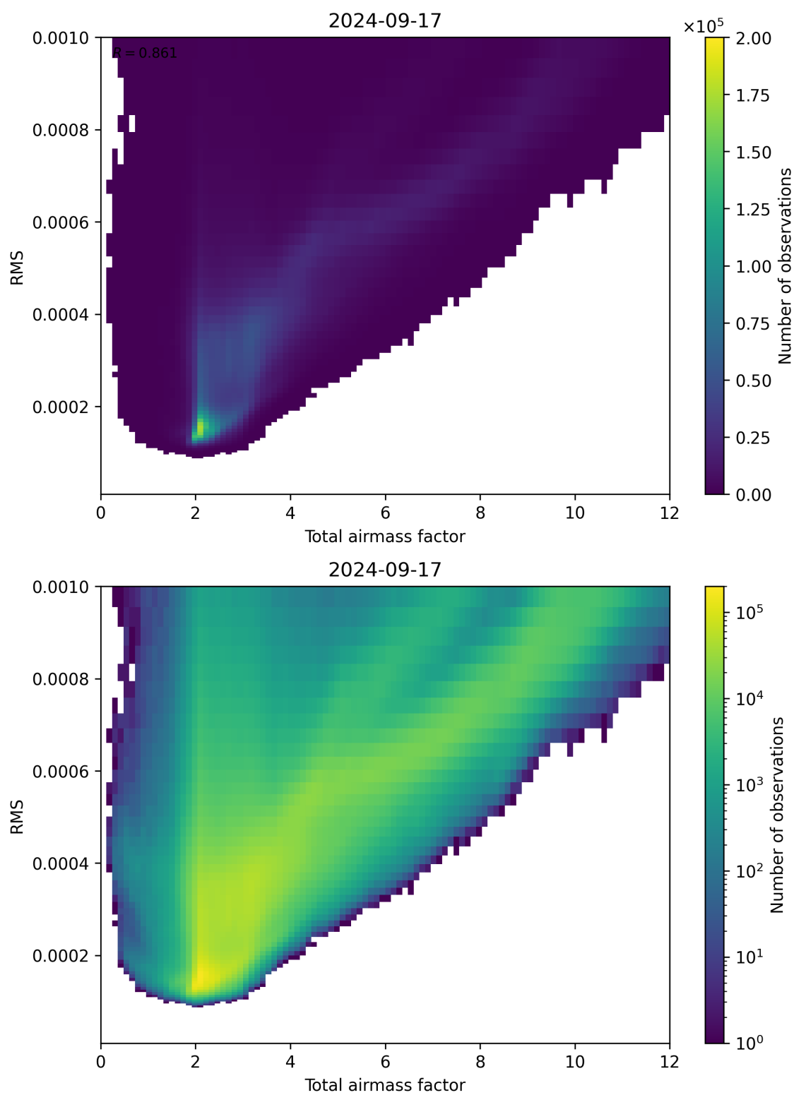
Figure 69: Scatter density plot of “Total airmass factor” against “RMS” for 2024-09-17 to 2024-09-18.
