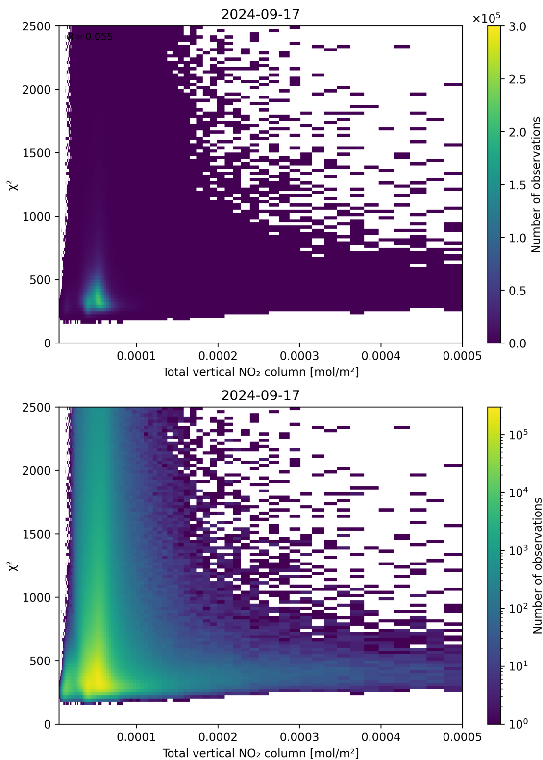
Figure 111: Scatter density plot of “Total vertical NO 2 column” against “ \chi^2 ” for 2024-09-17 to 2024-09-18.
