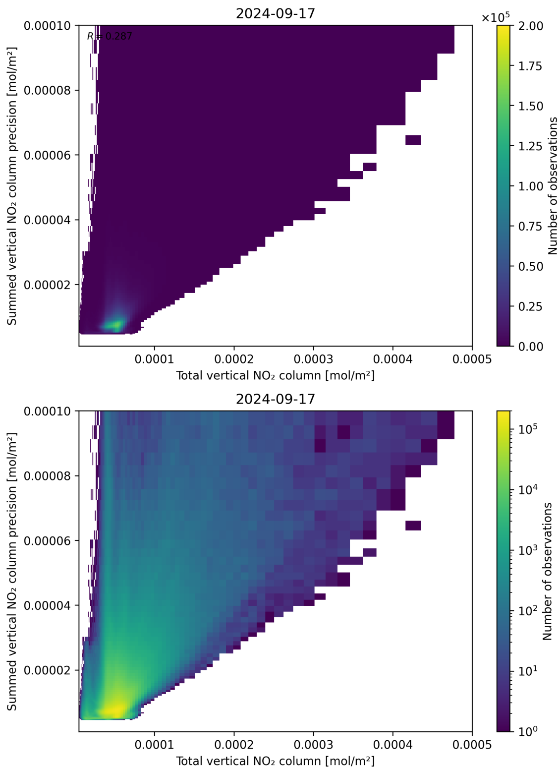
Figure 113: Scatter density plot of “Total vertical NO 2 column” against “Summed vertical NO 2 column precision” for 2024-09-17 to 2024-09-18.
