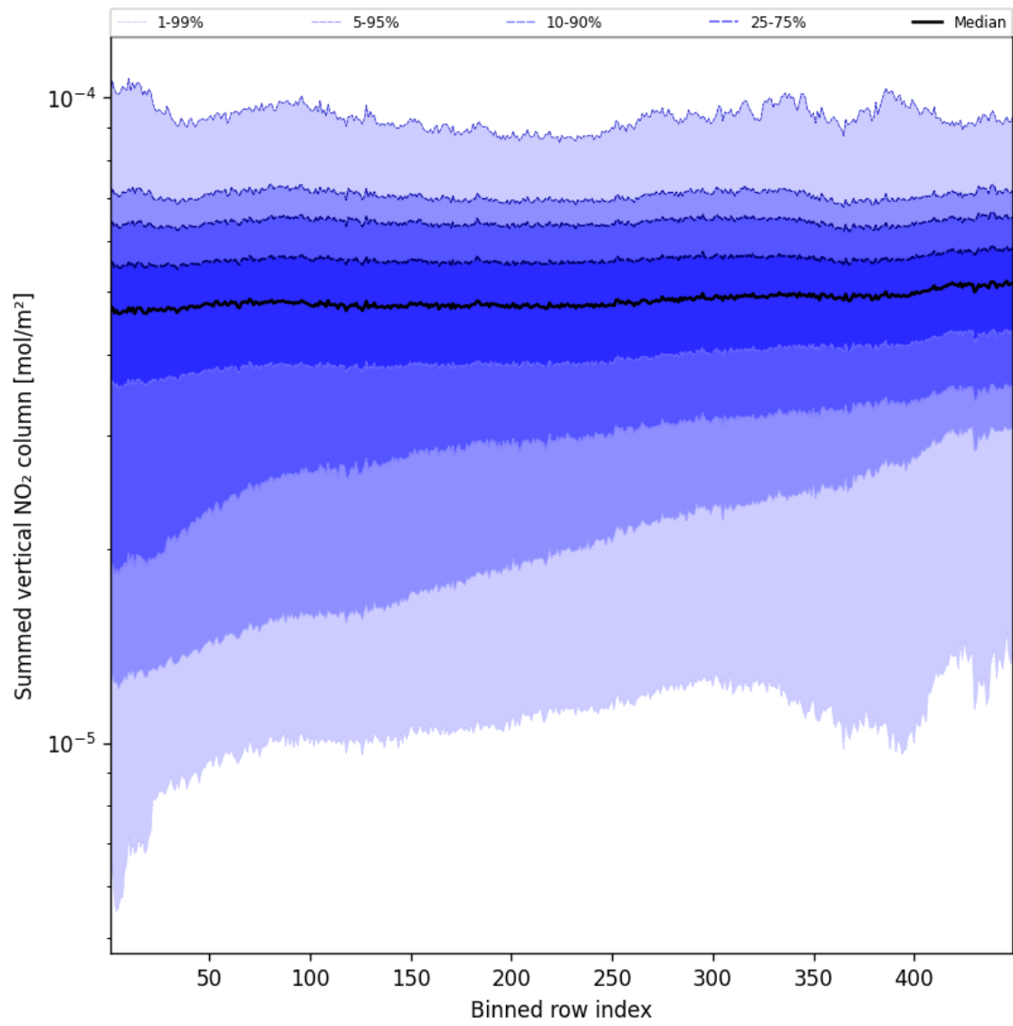
Figure 57: Along track statistics of “Summed vertical NO 2 column” for 2024-09-17 to 2024-09-18
