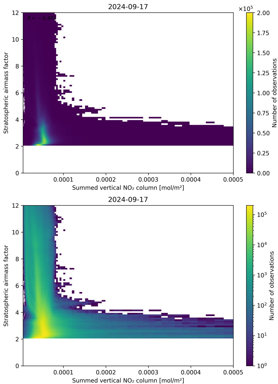
Figure 103: Scatter density plot of “Summed vertical NO 2 column” against “Stratospheric air mass factor” for 2024-09-17 to 2024-09-18.
