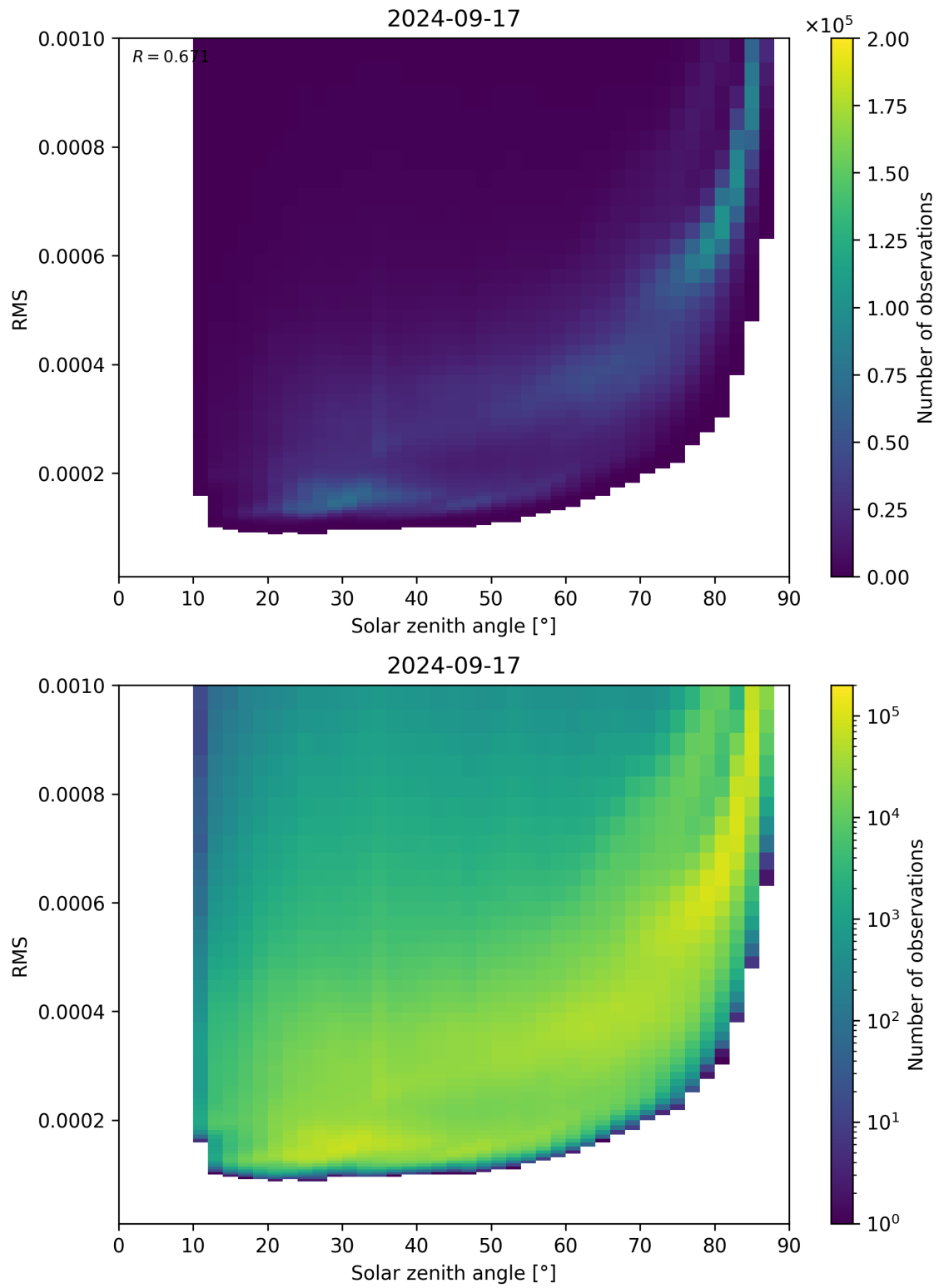
Figure 157: Scatter density plot of “Solar zenith angle” against “RMS” for 2024-09-17 to 2024-09-18.
