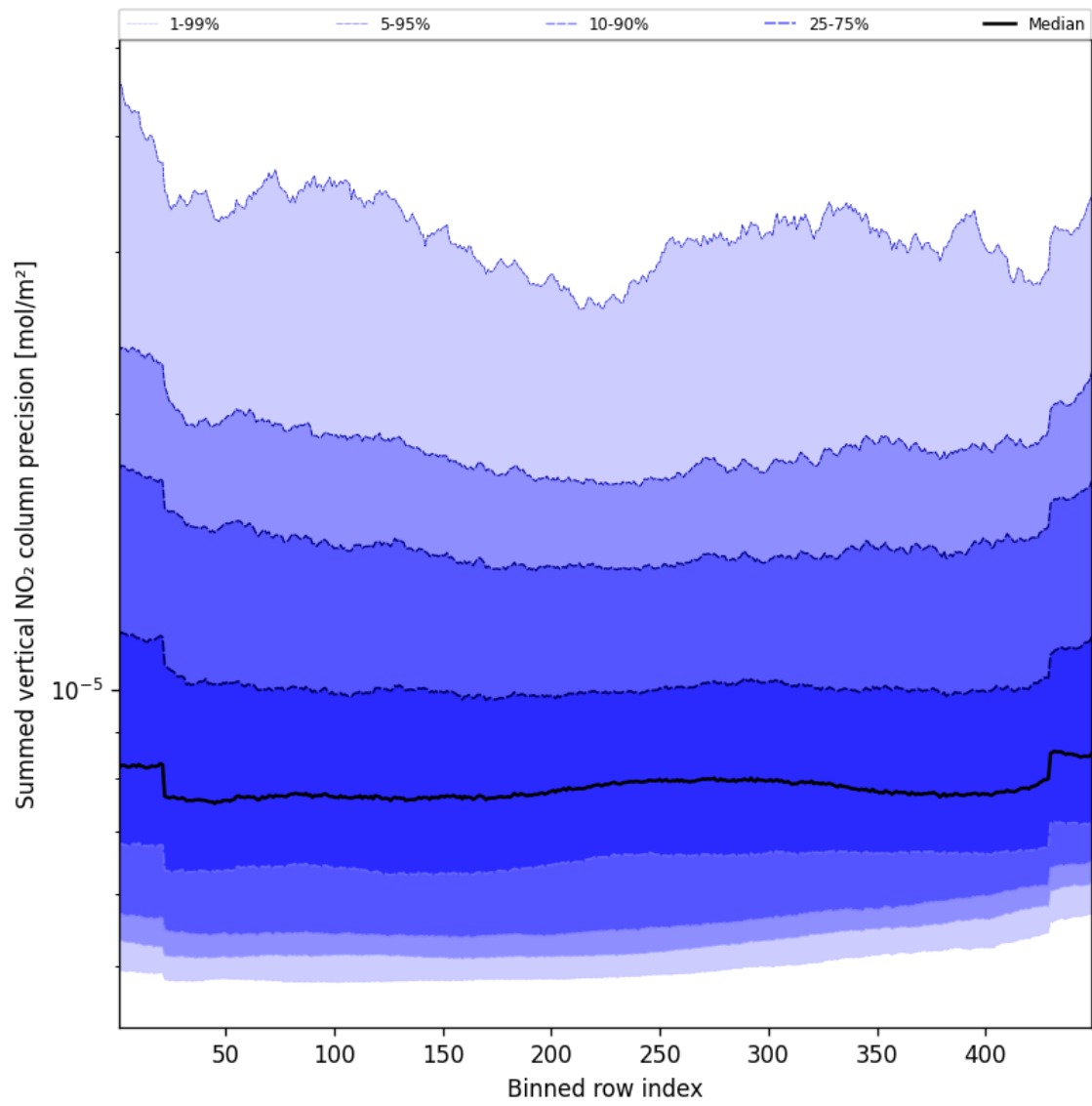
Figure 58: Along track statistics of “Summed vertical NO 2 column precision” for 2024-09-17 to 2024-09-18
