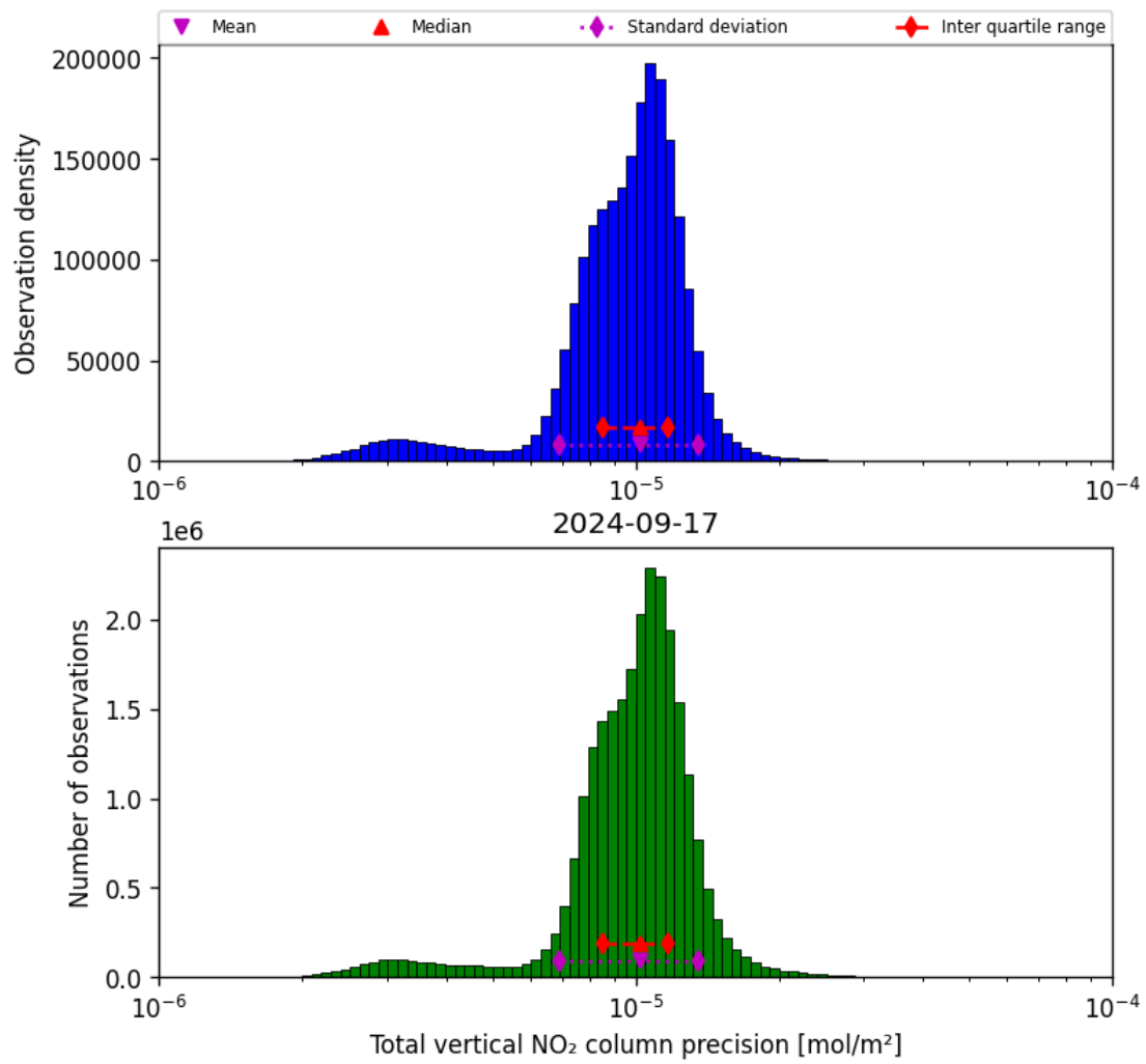
Figure 39: Histogram of “Total vertical NO 2 column precision” for 2024-09-17 to 2024-09-18
