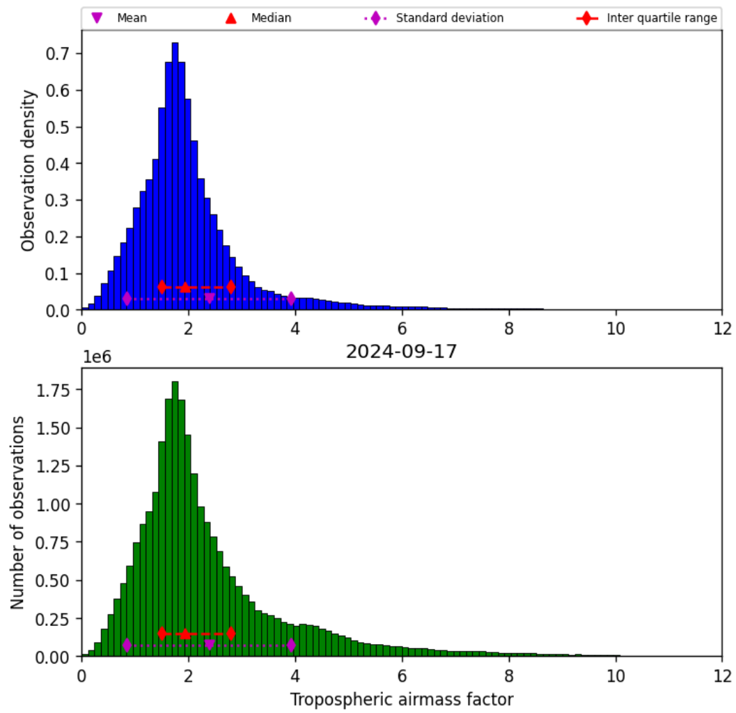
Figure 31: Histogram of “Tropospheric airmass factor” for 2024-09-17 to 2024-09-18
