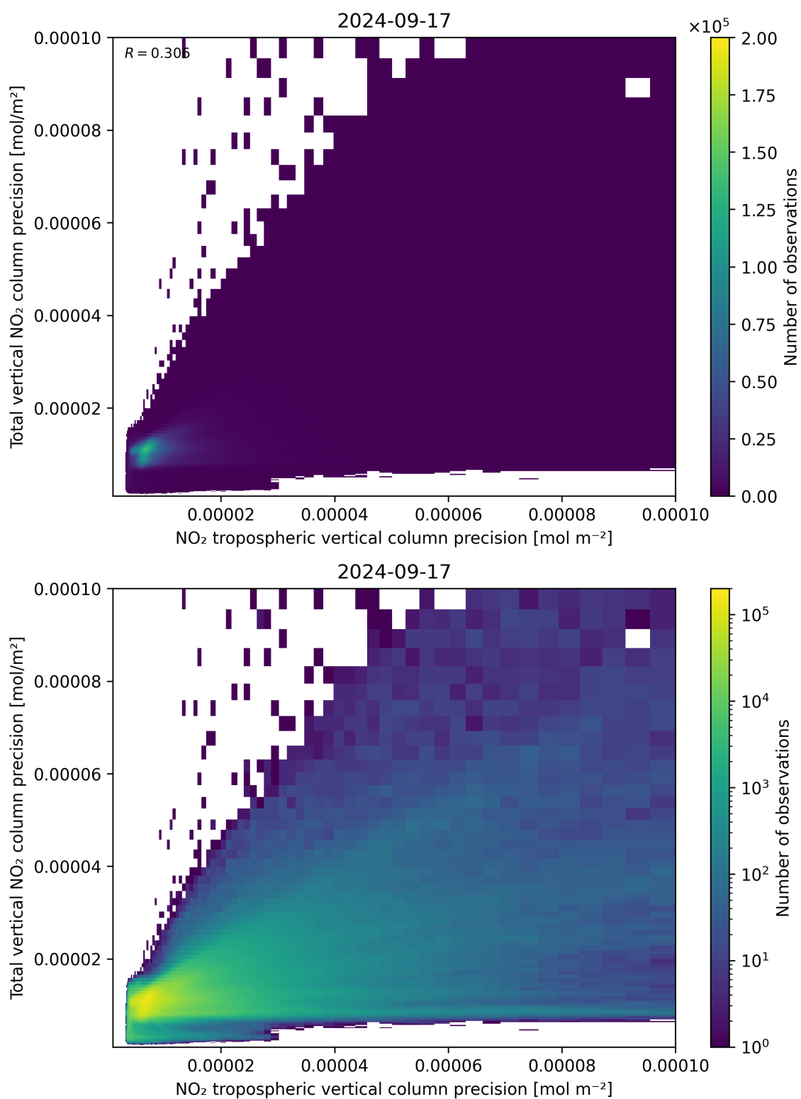
Figure 139: Scatter density plot of “NO 2 tropospheric vertical column precision” against “Total vertical NO 2 column precision” for 2024-09-17 to 2024-09-18.
