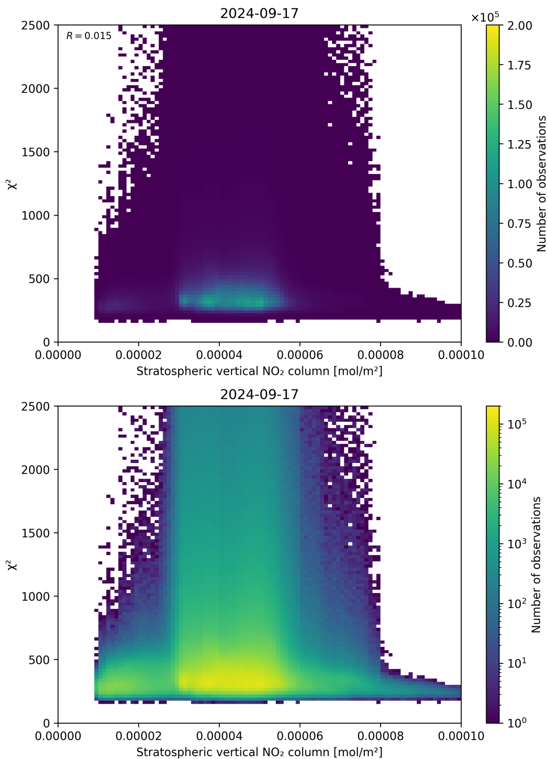
Figure 97: Scatter density plot of “Stratospheric vertical NO 2 column” against “ \chi^2 ” for 2024-09-17 to 2024-09-18.
