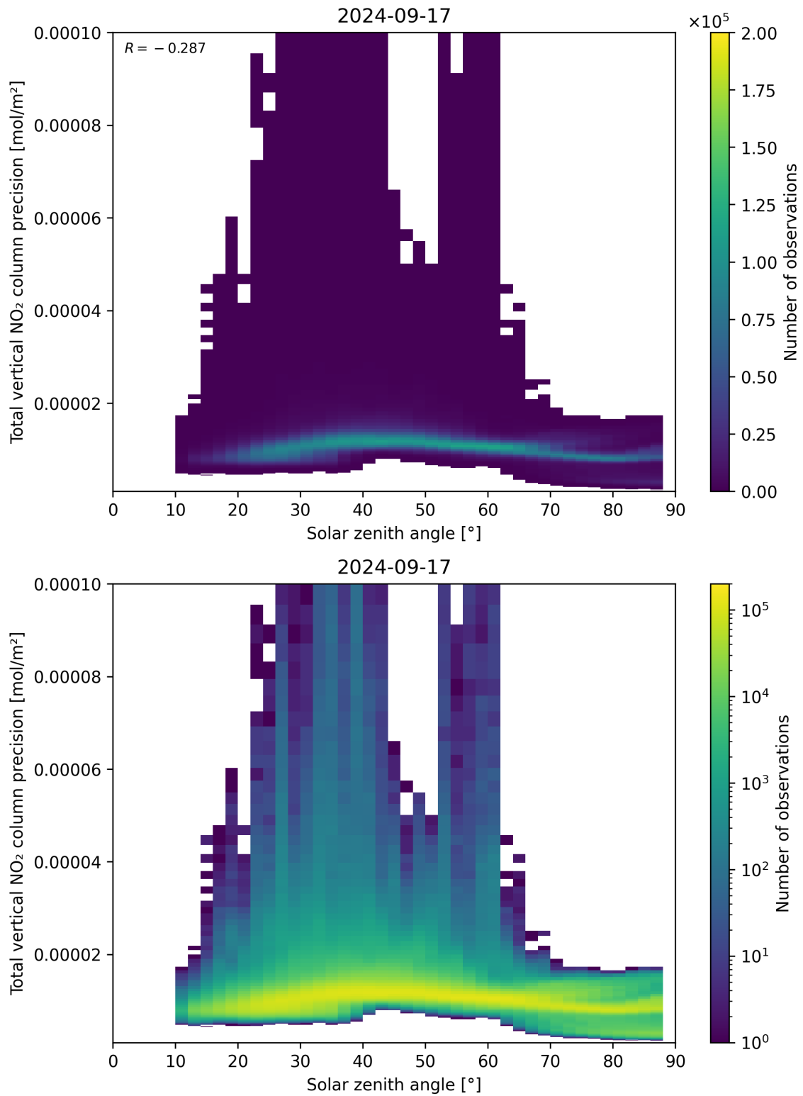
Figure 154: Scatter density plot of “Solar zenith angle” against “Total vertical NO 2 column precision” for 2024-09-17 to 2024-09-18.
