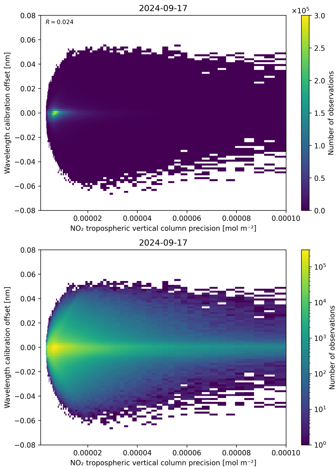
Figure 141: Scatter density plot of “NO 2 tropospheric vertical column precision” against “Wavelength calibration offset” for 2024-09-17 to 2024-09-18.
