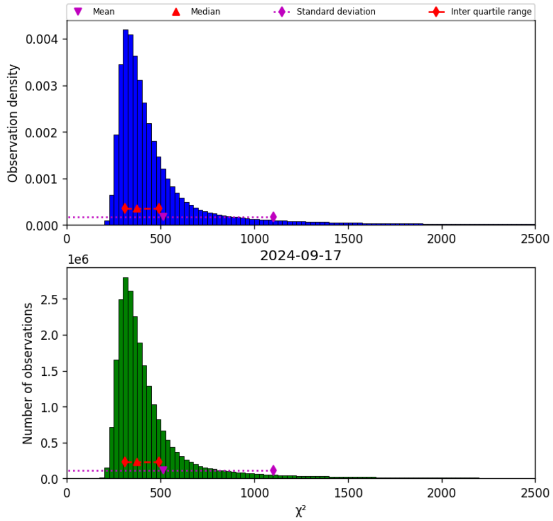
Figure 42: Histogram of “ \chi^2 ” for 2024-09-17 to 2024-09-18
