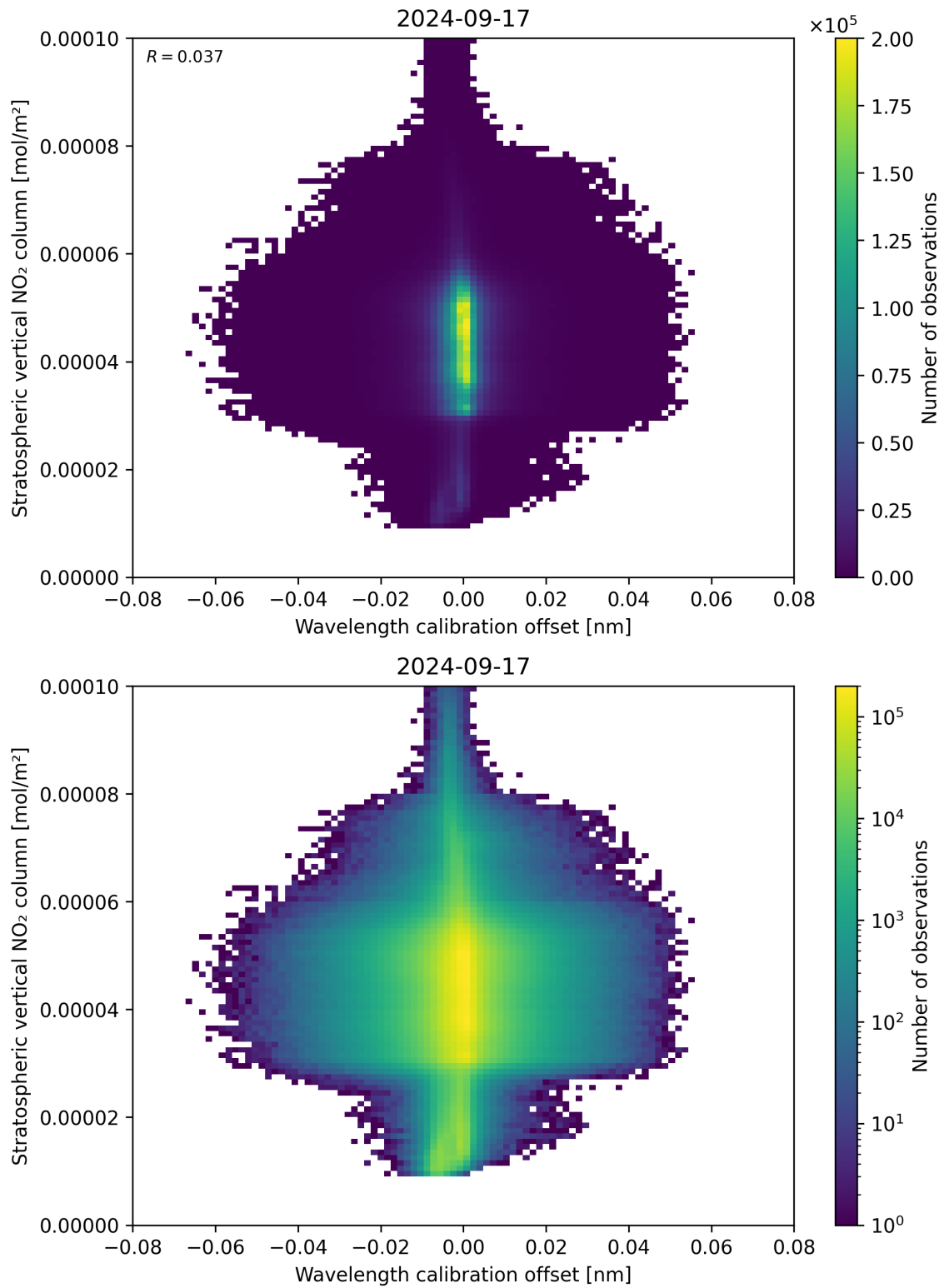
Figure 176: Scatter density plot of “Wavelength calibration offset” against “Stratospheric vertical NO 2 column” for 2024-09-17 to 2024-09-18.
