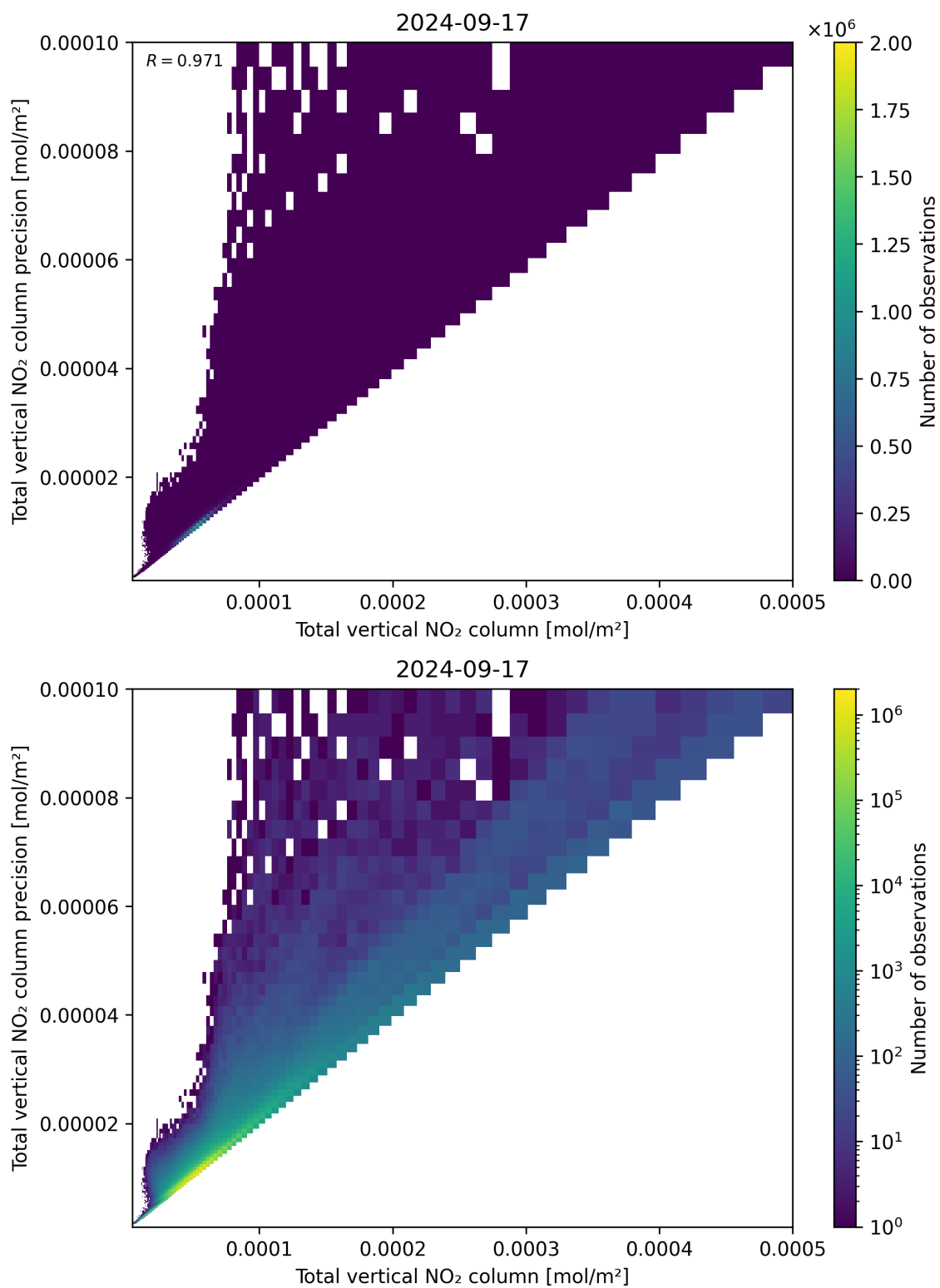
Figure 114: Scatter density plot of “Total vertical NO 2 column” against “Total vertical NO 2 column precision” for 2024-09-17 to 2024-09-18.
