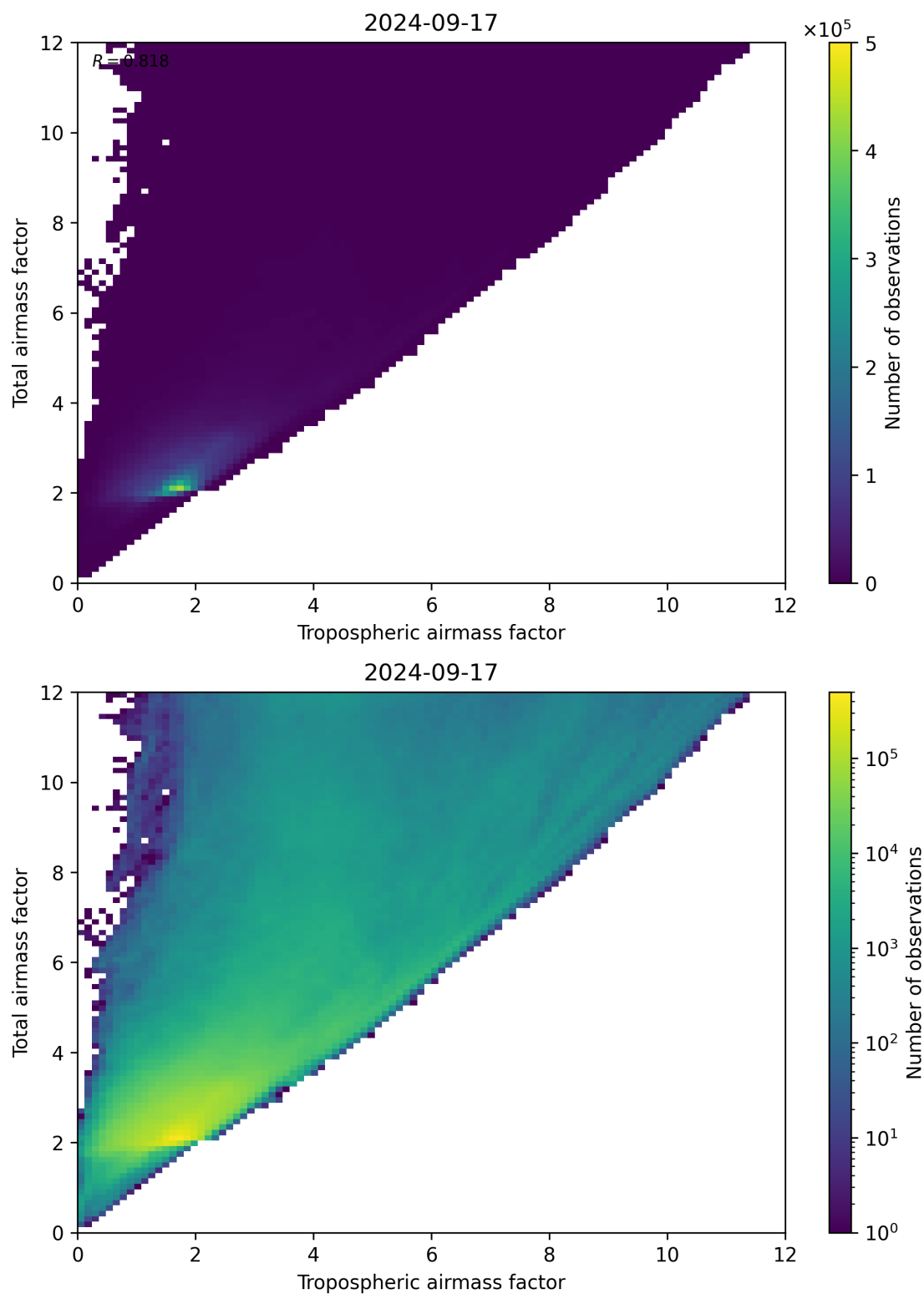
Figure 72: Scatter density plot of “Tropospheric airmass factor” against “Total airmass factor” for 2024-09-17 to 2024-09-18.
