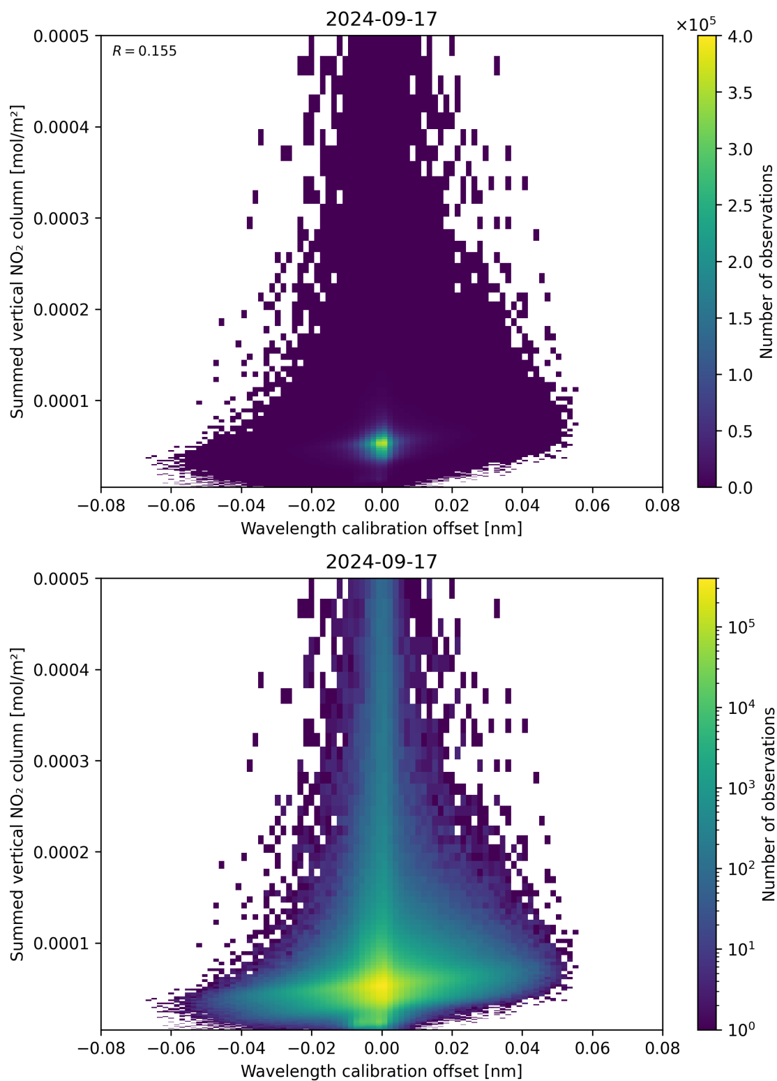
Figure 177: Scatter density plot of “Wavelength calibration offset” against “Summed vertical NO 2 column” for 2024-09-17 to 2024-09-18.
