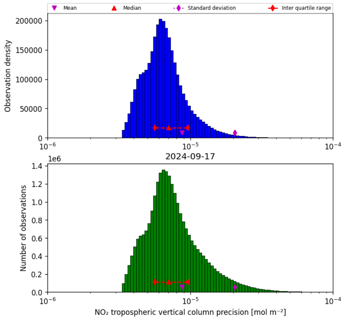
Figure 30: Histogram of “NO 2 tropospheric vertical column precision” for 2024-09-17 to 2024-09-18
