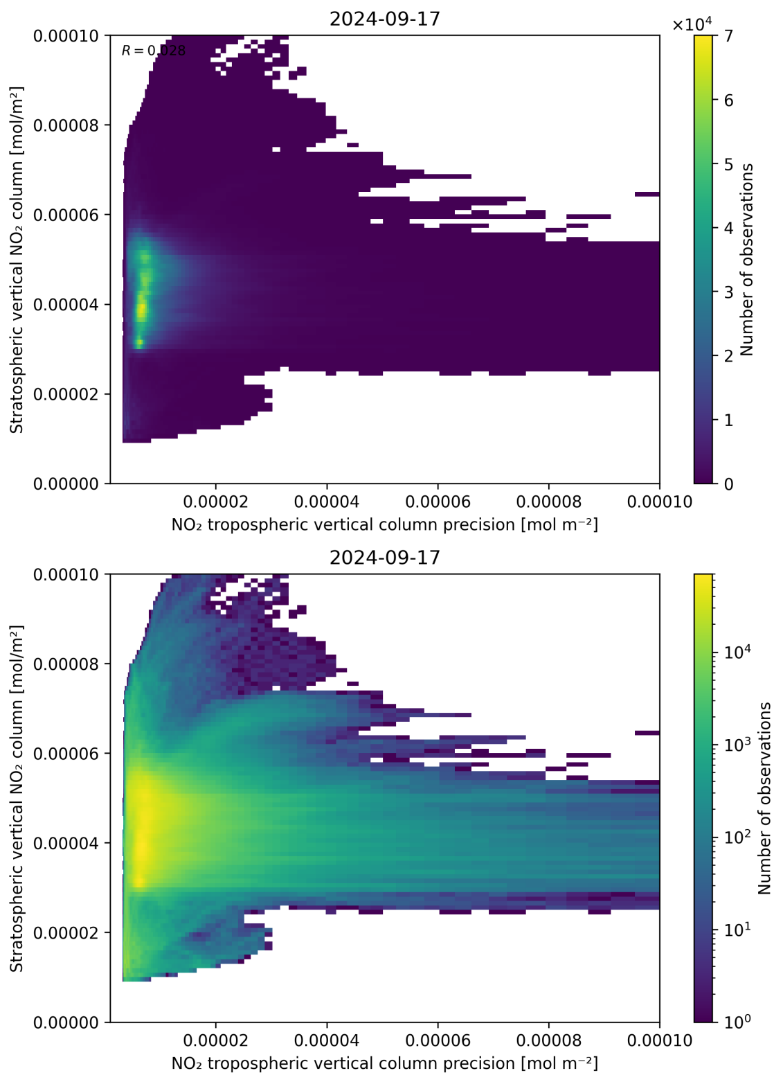
Figure 135: Scatter density plot of “NO 2 tropospheric vertical column precision” against “Stratospheric vertical NO 2 column” for 2024-09-17 to 2024-09-18.
