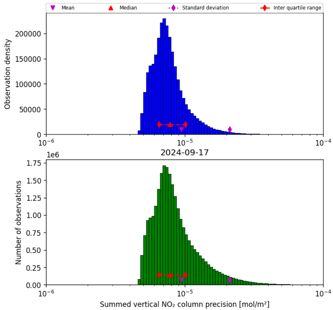
Figure 41: Histogram of "Summed vertical NO 2 column precision" for 2024-09-17 to 2024-09-18
