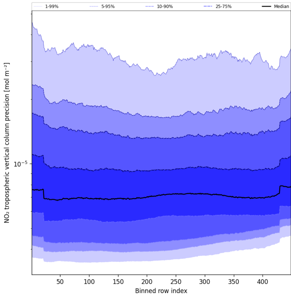
Figure 47: Along track statistics of “NO 2 tropospheric vertical column precision” for 2024-09-17 to 2024-09-18
