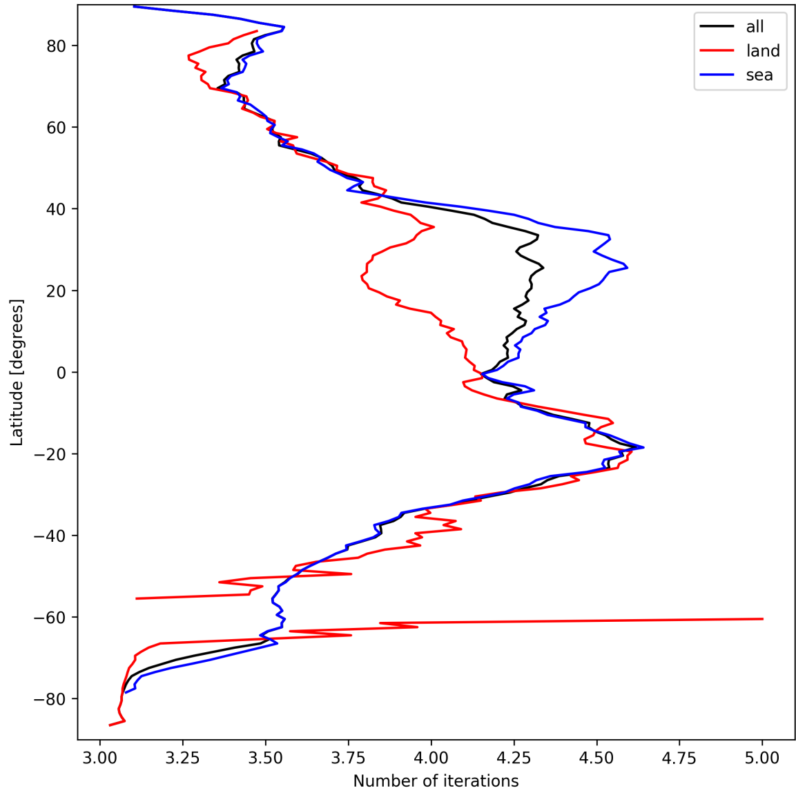
Figure 17: Zonal average of “Number of iterations” for 2024-09-17 to 2024-09-18.
