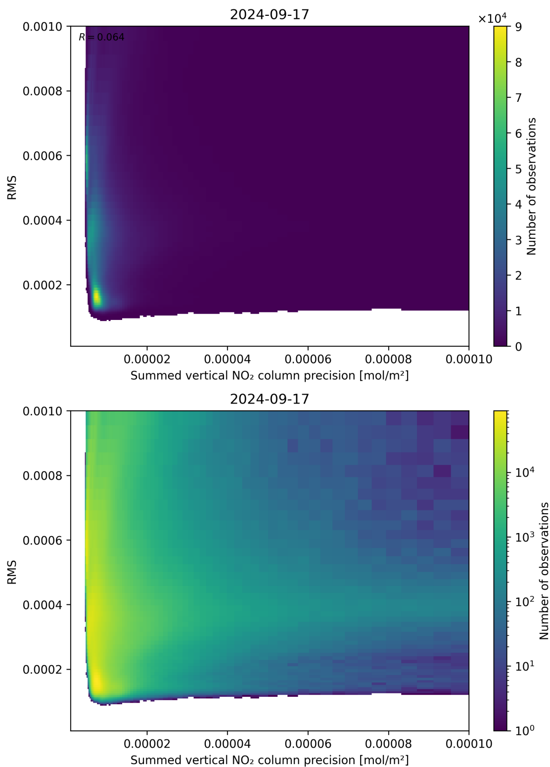
Figure 108: Scatter density plot of “Summed vertical NO 2 column precision” against “RMS” for 2024-09-17 to 2024-09-18.
