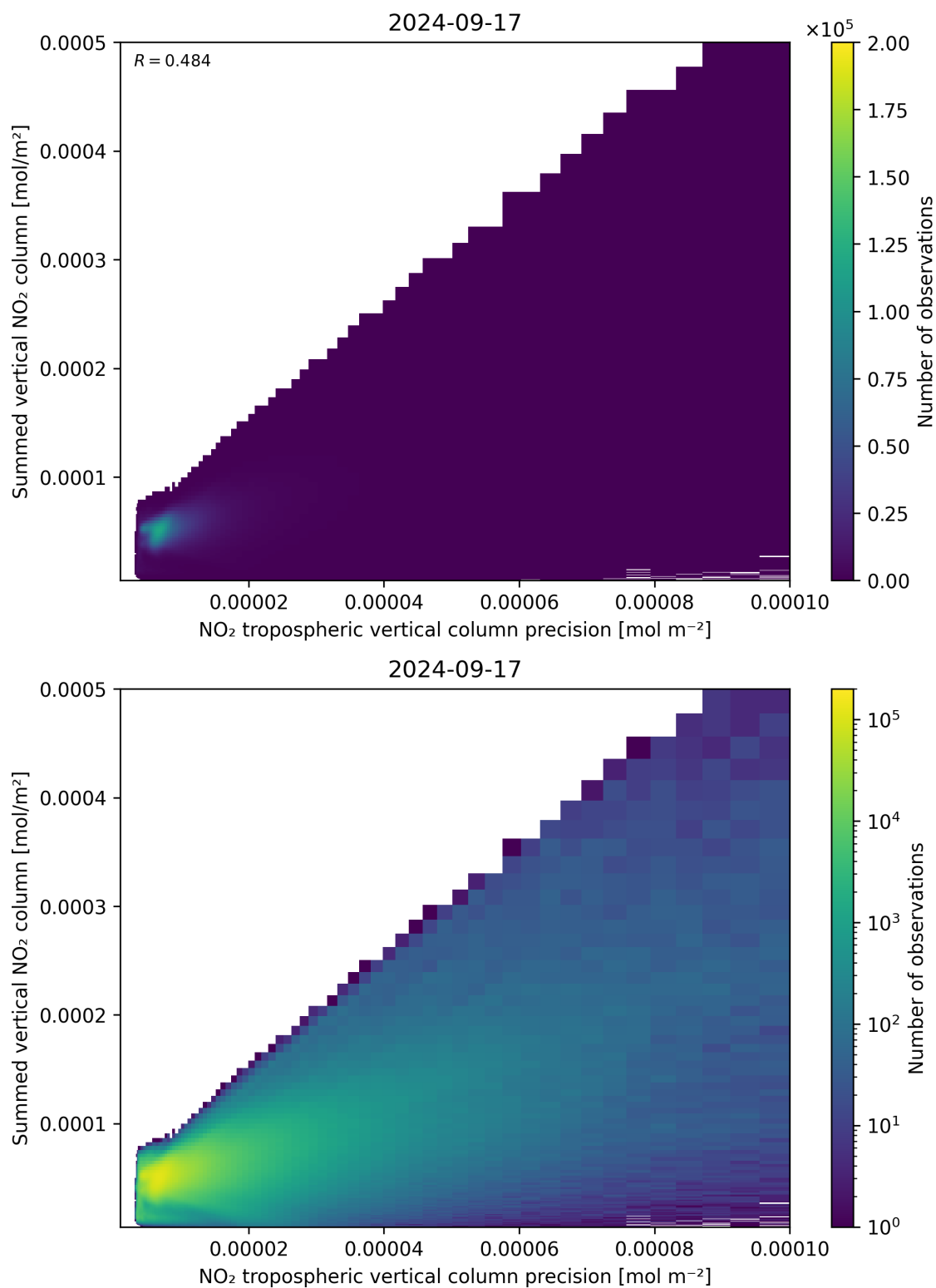
Figure 136: Scatter density plot of “NO 2 tropospheric vertical column precision” against “Summed vertical NO 2 column” for 2024-09-17 to 2024-09-18.
