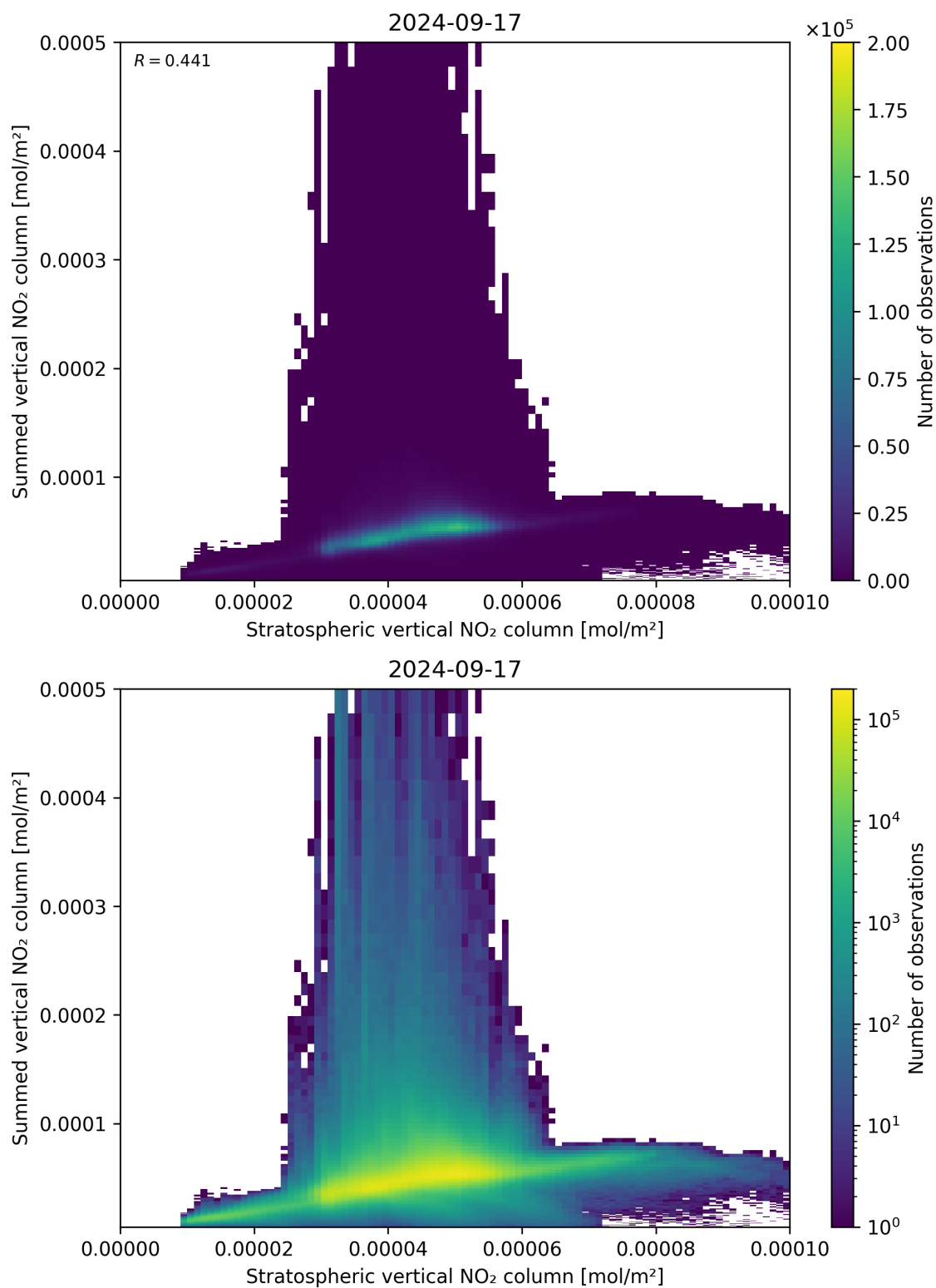
Figure 98: Scatter density plot of “Stratospheric vertical NO 2 column” against “Summed vertical NO 2 column” for 2024-09-17 to 2024-09-18.
