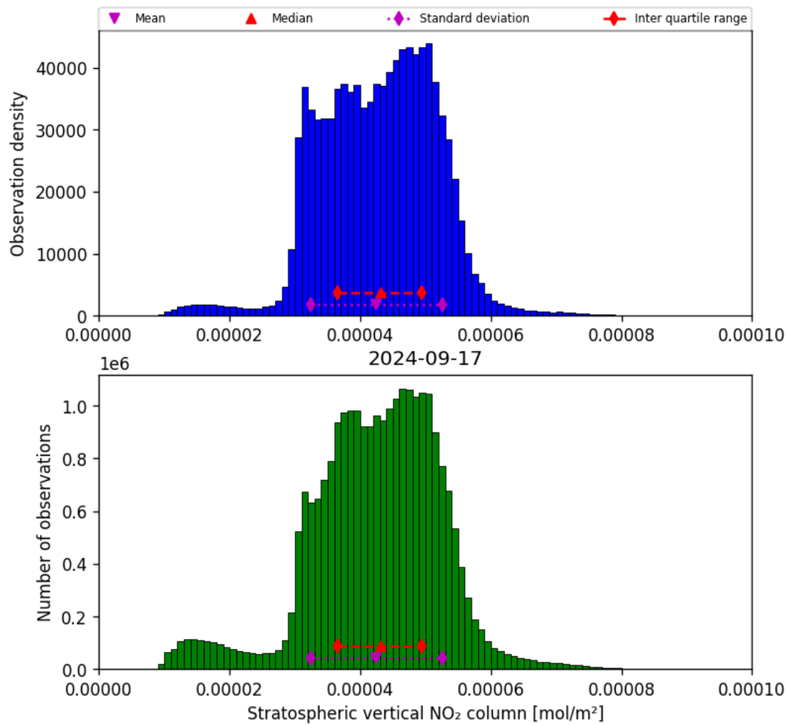
Figure 36: Histogram of “Stratospheric vertical NO 2 column” for 2024-09-17 to 2024-09-18
