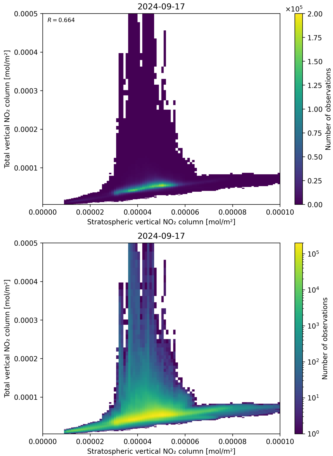
Figure 100: Scatter density plot of “Stratospheric vertical NO 2 column” against “Total vertical NO 2 column” for 2024-09-17 to 2024-09-18.
