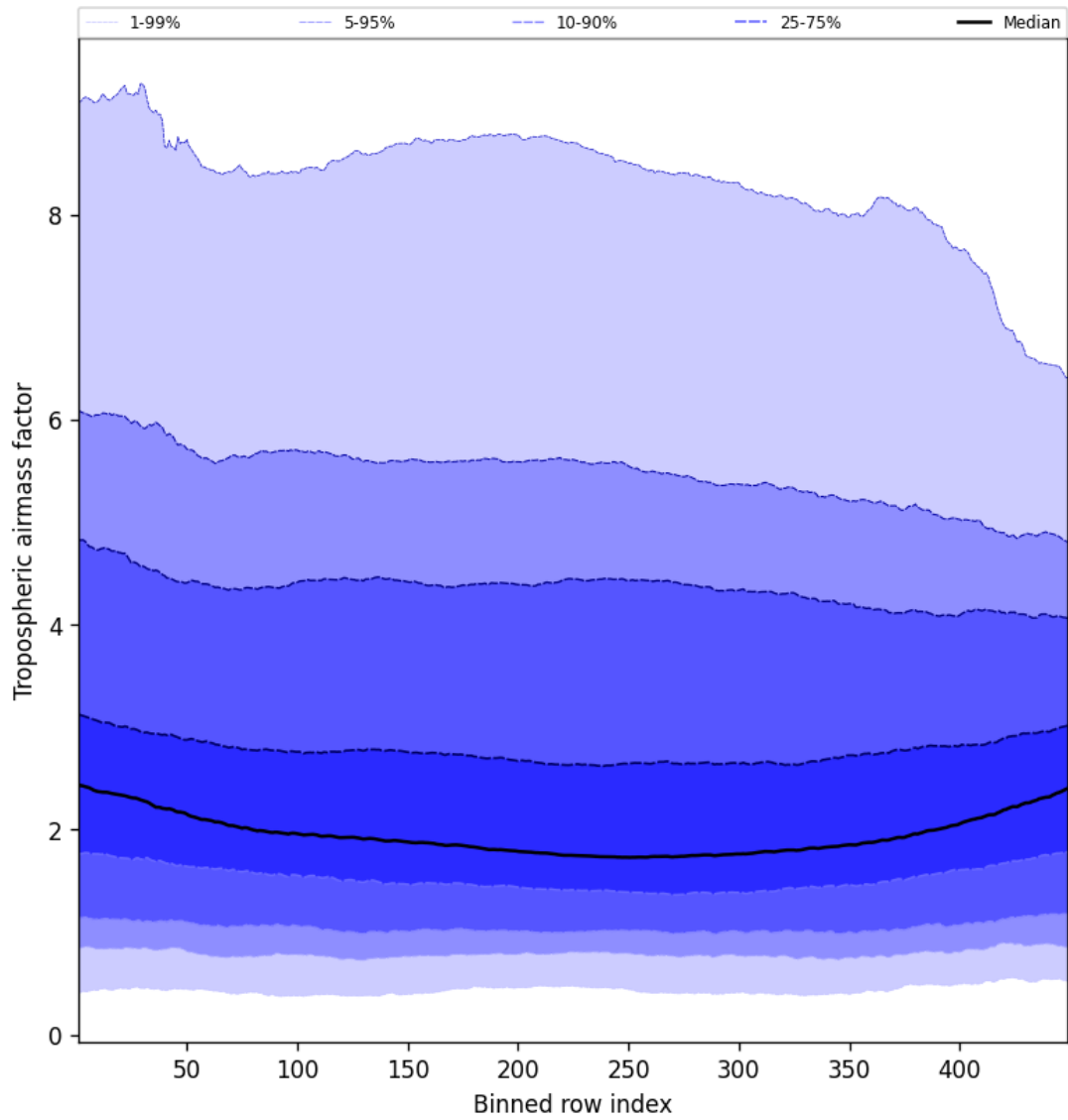
Figure 48: Along track statistics of “Tropospheric air mass factor” for 2024-09-17 to 2024-09-18
