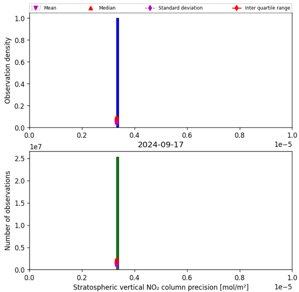
Figure 37: Histogram of “Stratospheric vertical NO 2 column precision” for 2024-09-17 to 2024-09-18
