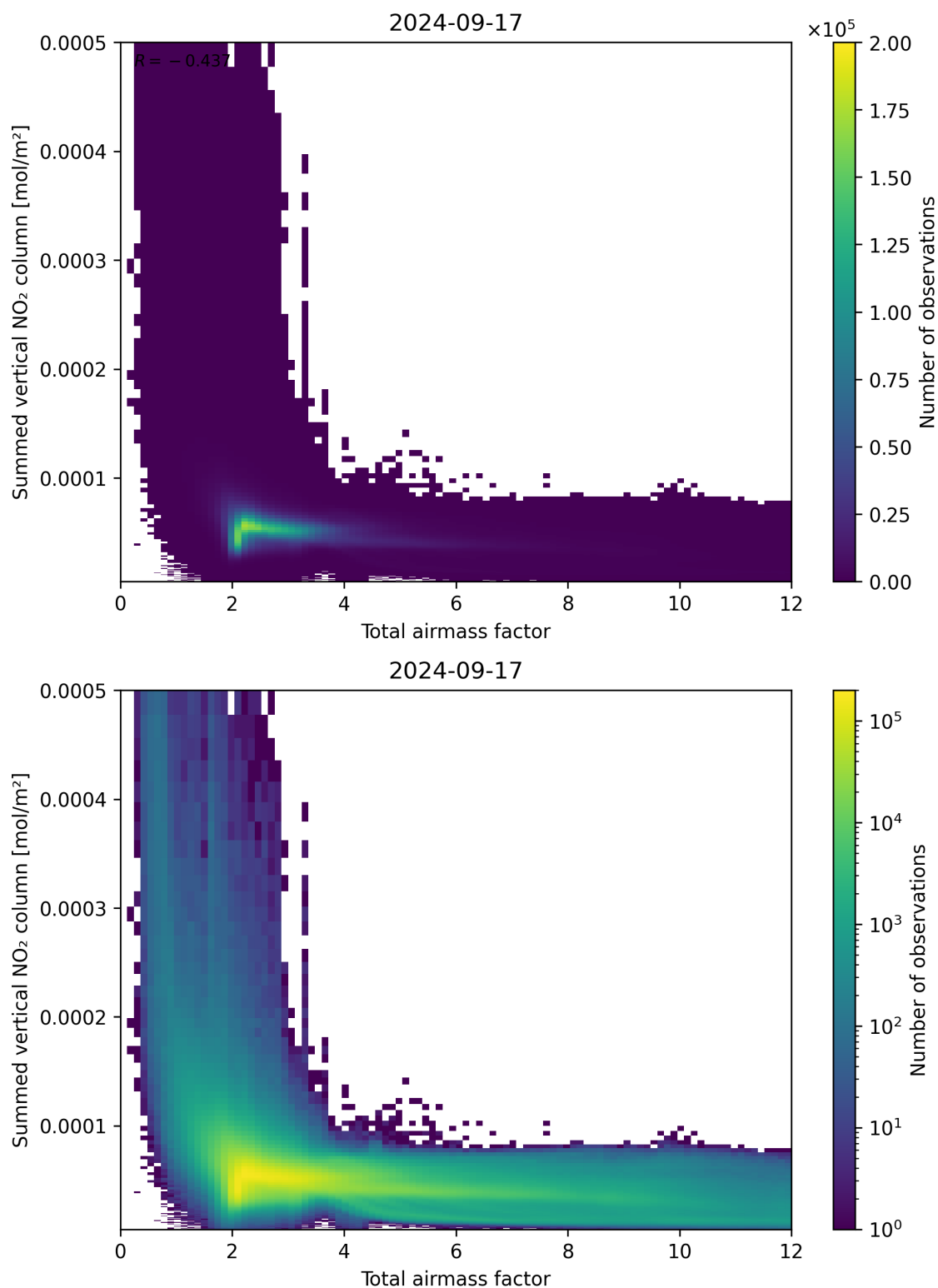
Figure 65: Scatter density plot of “Total airmass factor” against “Summed vertical NO 2 column” for 2024-09-17 to 2024-09-18.
