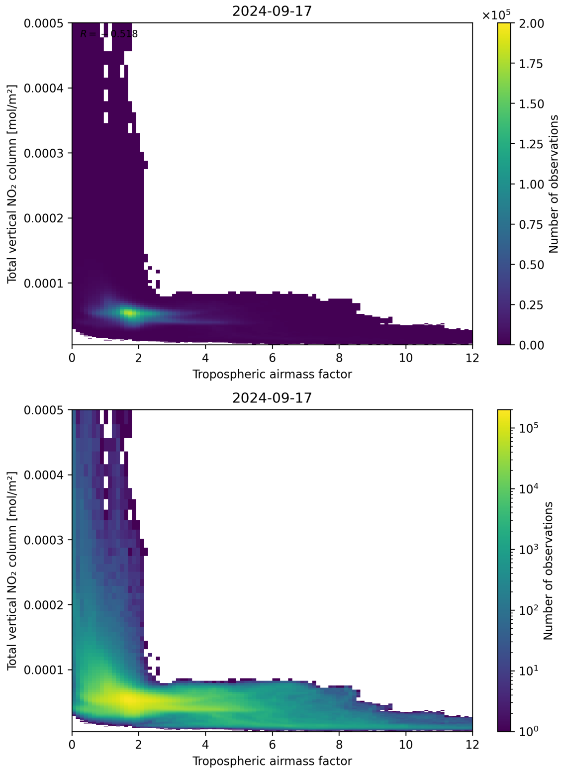
Figure 77: Scatter density plot of “Tropospheric airmass factor” against “Total vertical NO 2 column” for 2024-09-17 to 2024-09-18.
