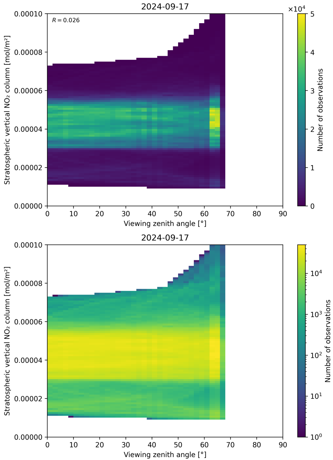
Figure 164: Scatter density plot of “Viewing zenith angle” against “Stratospheric vertical NO 2 column” for 2024-09-17 to 2024-09-18.
