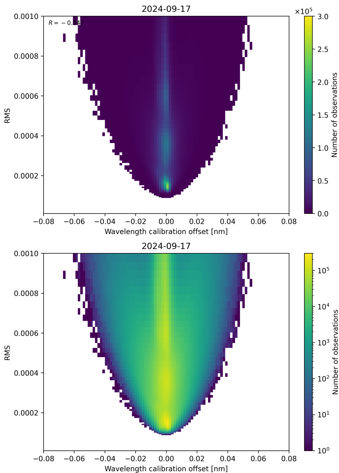
Figure 181: Scatter density plot of “Wavelength calibration offset” against “RMS” for 2024-09-17 to 2024-09-18.
