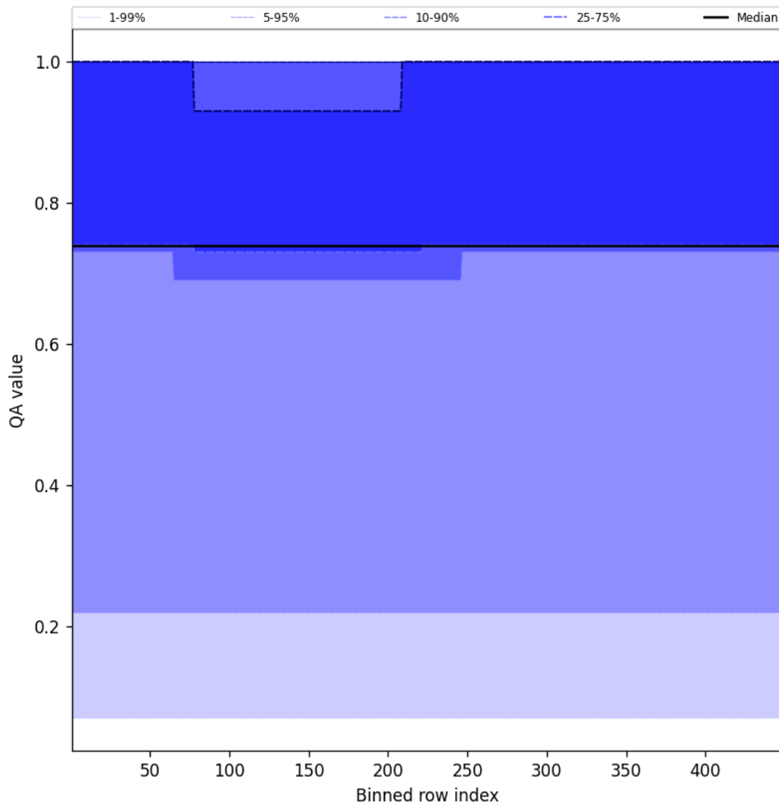
Figure 45: Along track statistics of “QA value” for 2024-09-17 to 2024-09-18
