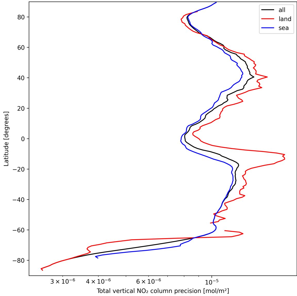
Figure 22: Zonal average of “Total vertical NO 2 column precision” for 2024-09-17 to 2024-09-18.
