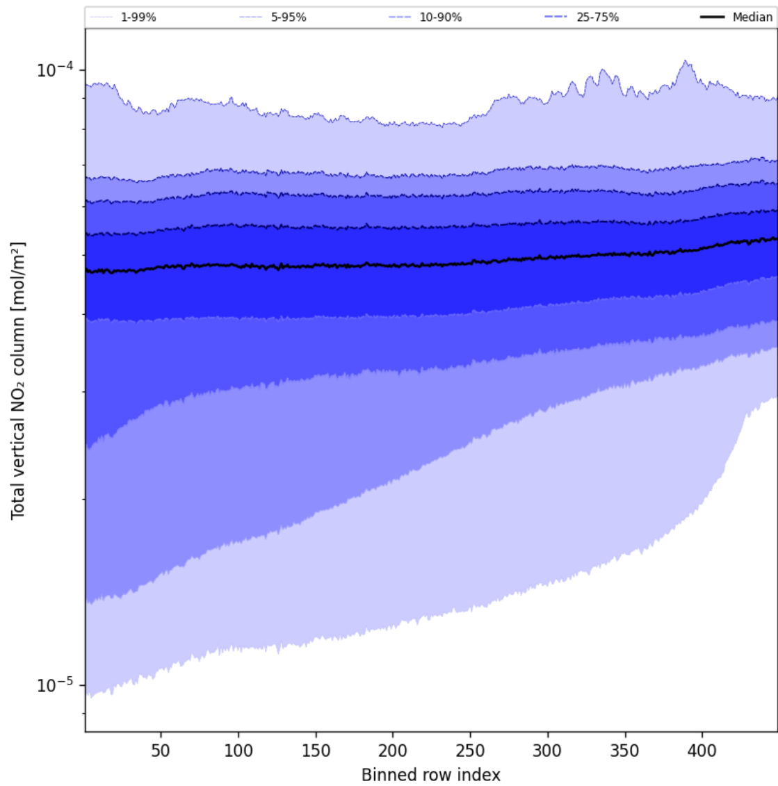
Figure 55: Along track statistics of “Total vertical NO 2 column” for 2024-09-17 to 2024-09-18
