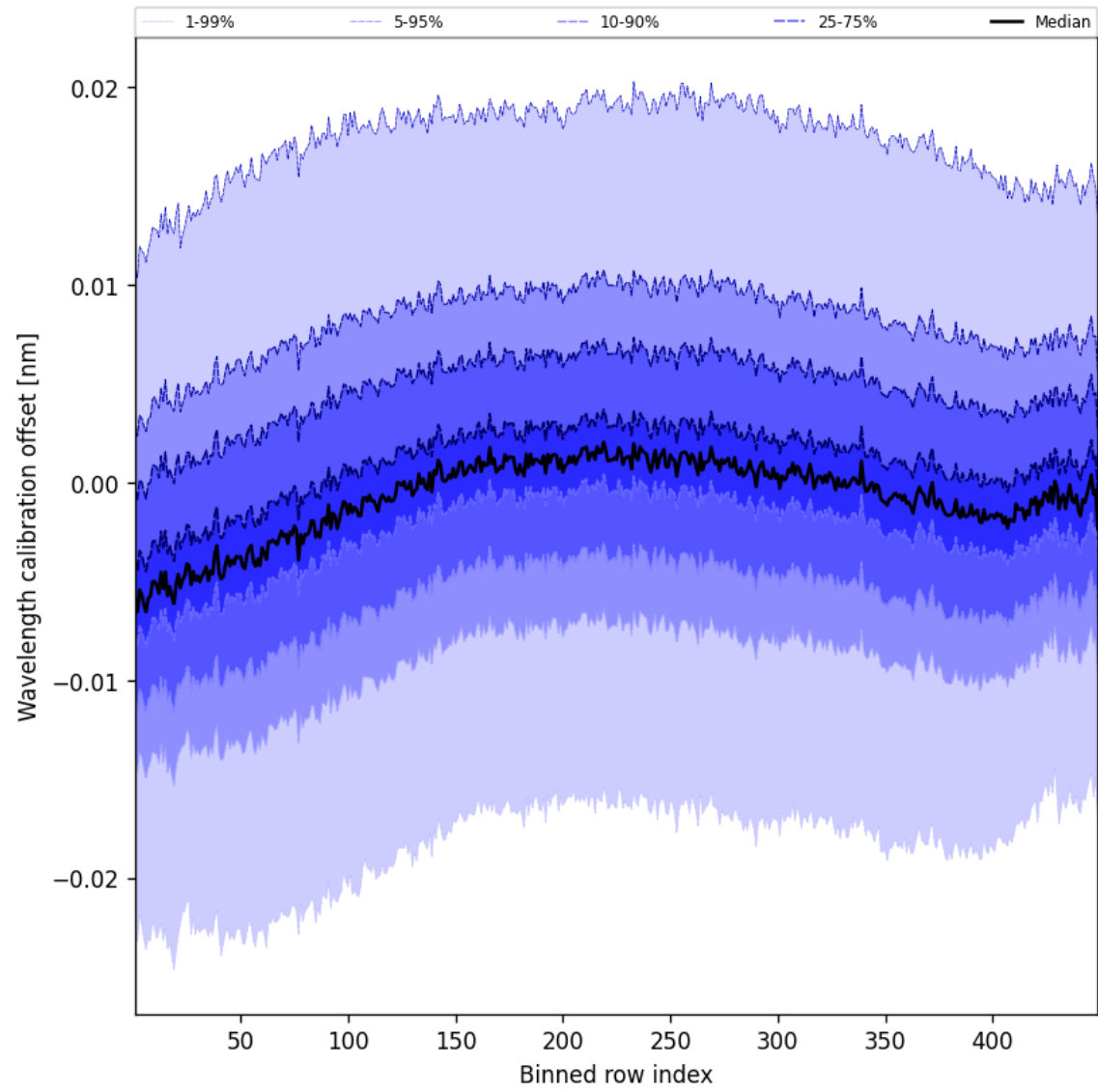
Figure 52: Along track statistics of “Wavelength calibration offset” for 2024-09-17 to 2024-09-18
