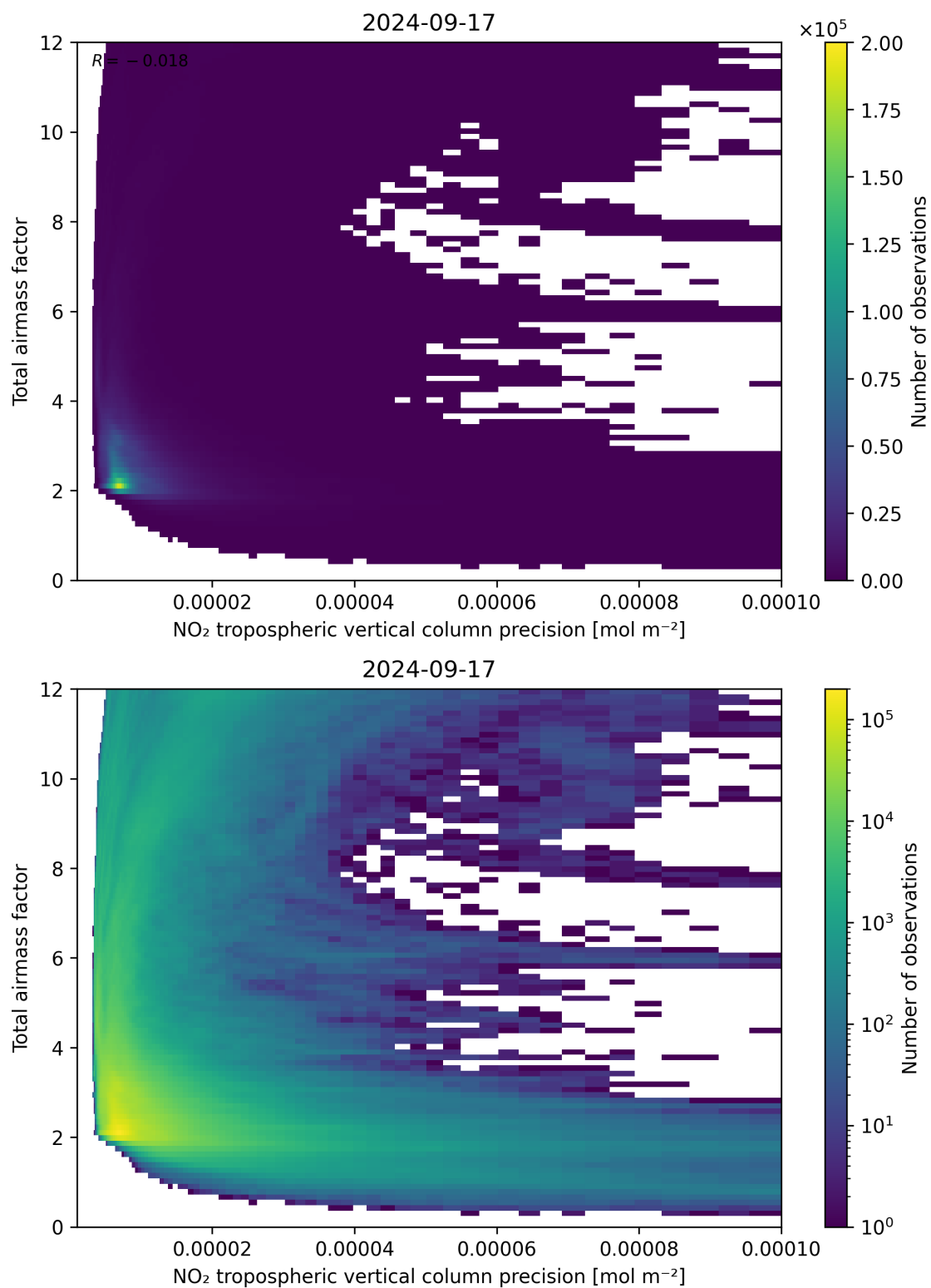
Figure 132: Scatter density plot of “NO 2 tropospheric vertical column precision” against “Total airmass factor” for 2024-09-17 to 2024-09-18.
