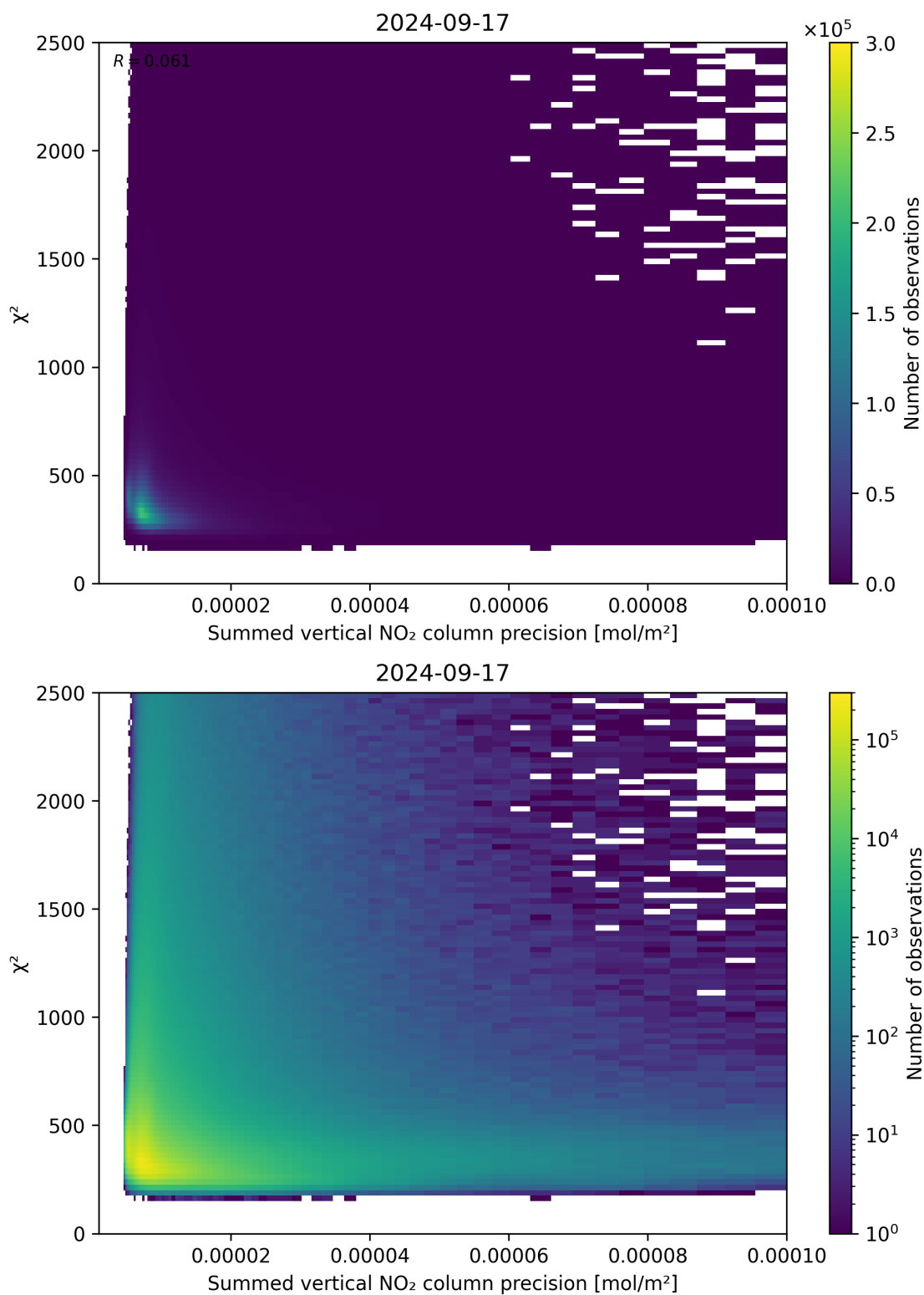
Figure 107: Scatter density plot of “Summed vertical NO 2 column precision” against “ \chi^2 ” for 2024-09-17 to 2024-09-18.
