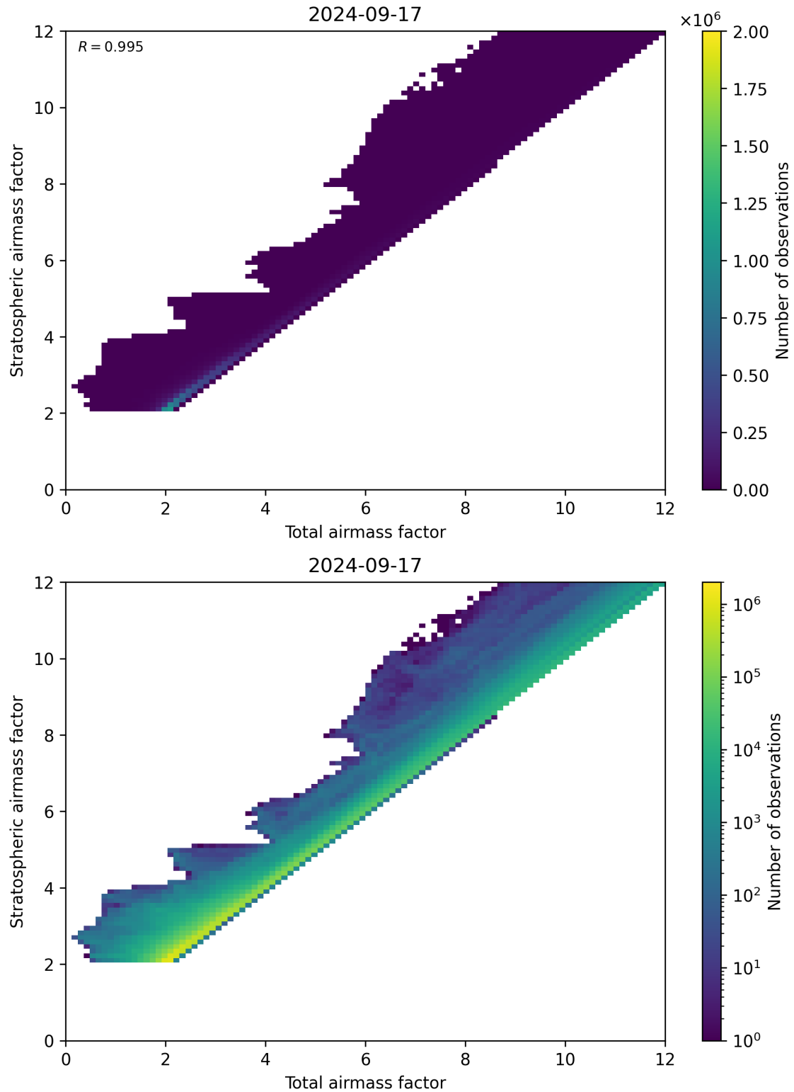
Figure 62: Scatter density plot of “Total airmass factor” against “Stratospheric airmass factor” for 2024-09-17 to 2024-09-18.
