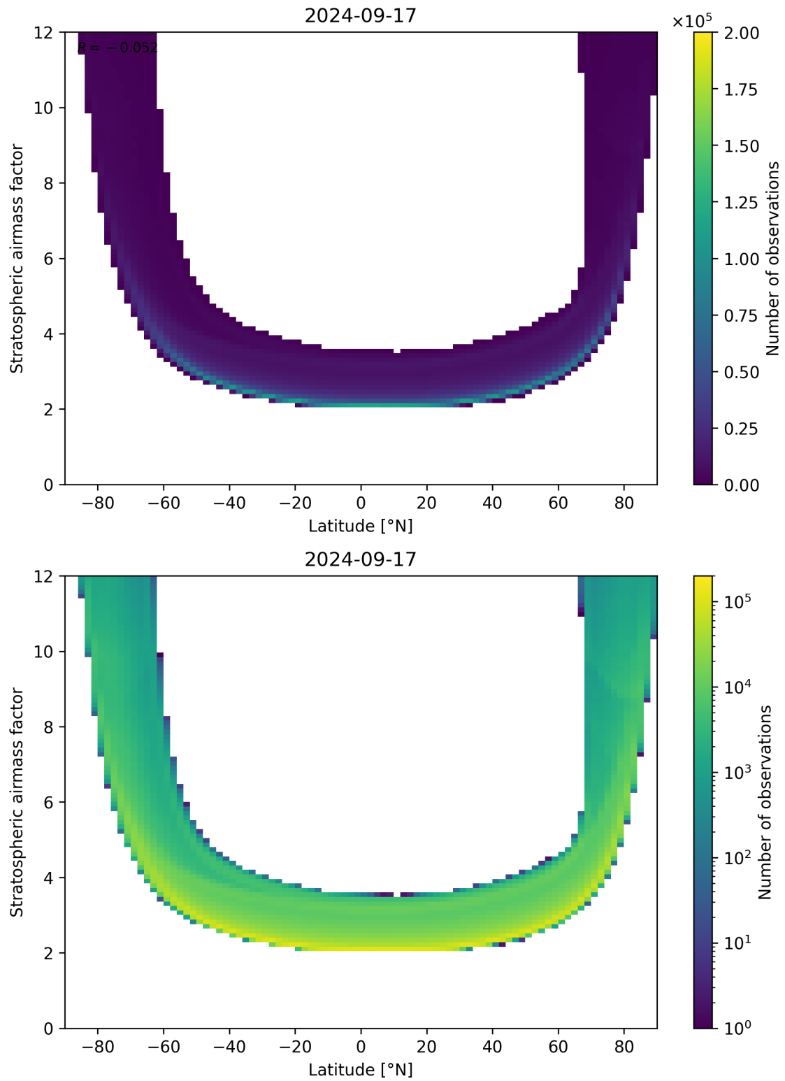
Figure 83: Scatter density plot of “Latitude” against “Stratospheric air mass factor” for 2024-09-17 to 2024-09-18.
