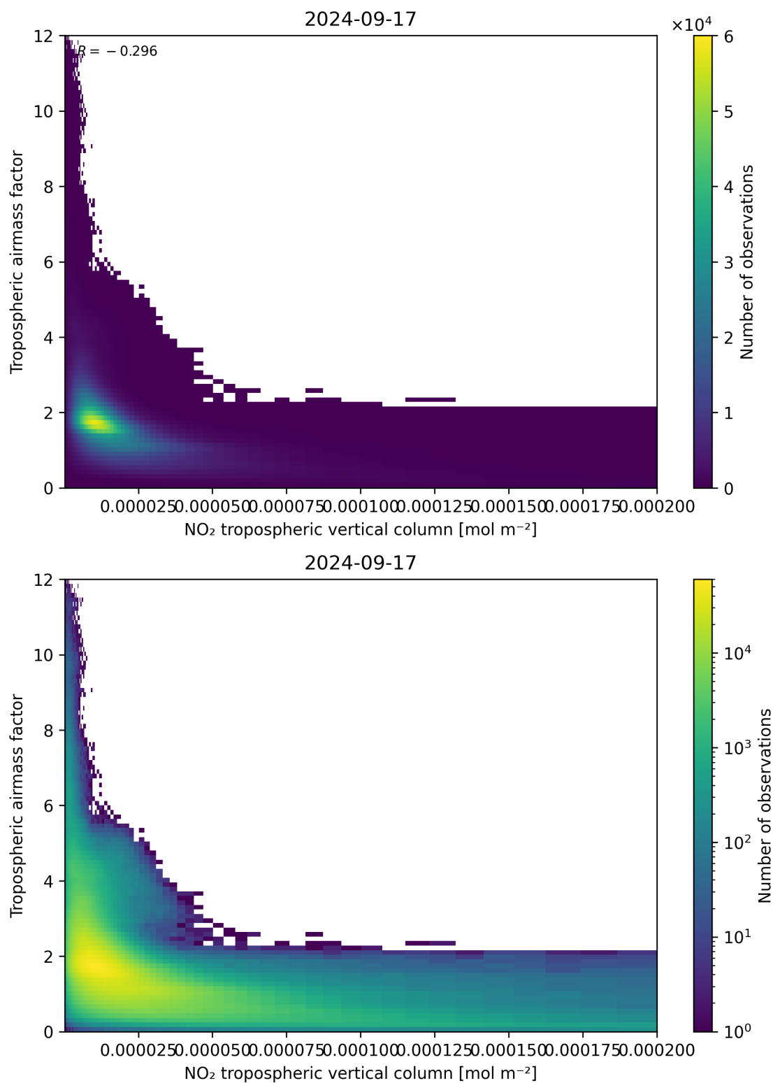
Figure 123: Scatter density plot of “NO 2 tropospheric vertical column” against “Tropospheric air mass factor” for 2024-09-17 to 2024-09-18.
