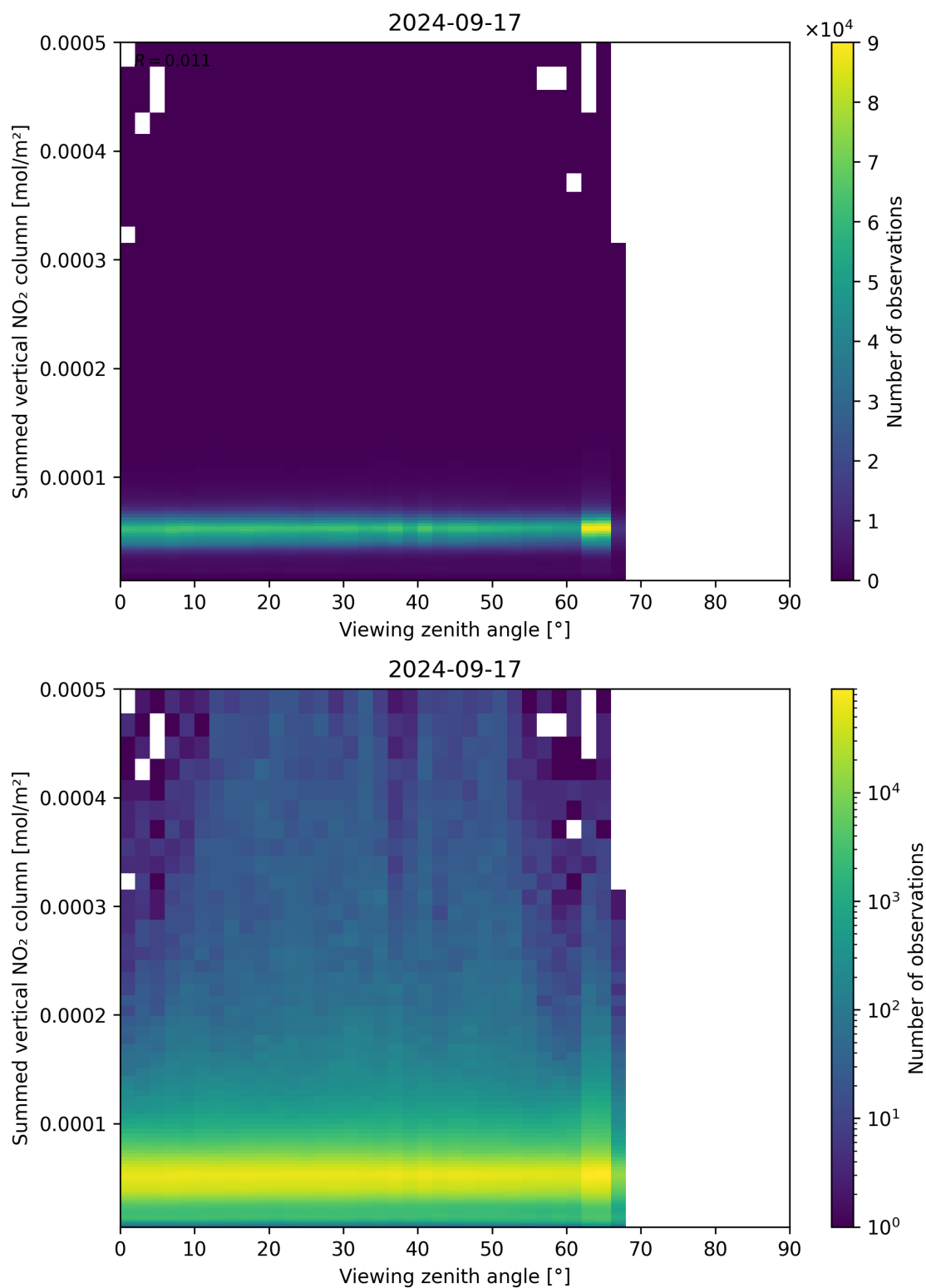
Figure 165: Scatter density plot of “Viewing zenith angle” against “Summed vertical NO 2 column” for 2024-09-17 to 2024-09-18.
