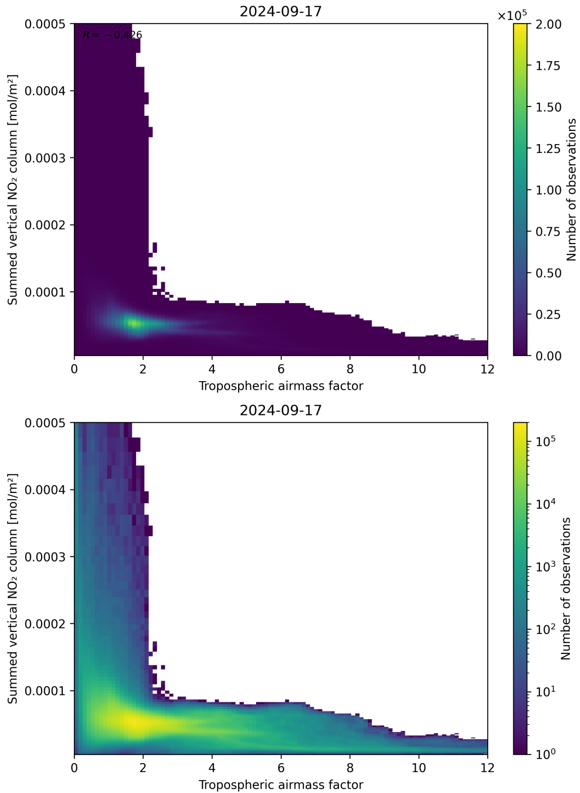
Figure 75: Scatter density plot of “Tropospheric air mass factor” against “Summed vertical NO 2 column” for 2024-09-17 to 2024-09-18.
