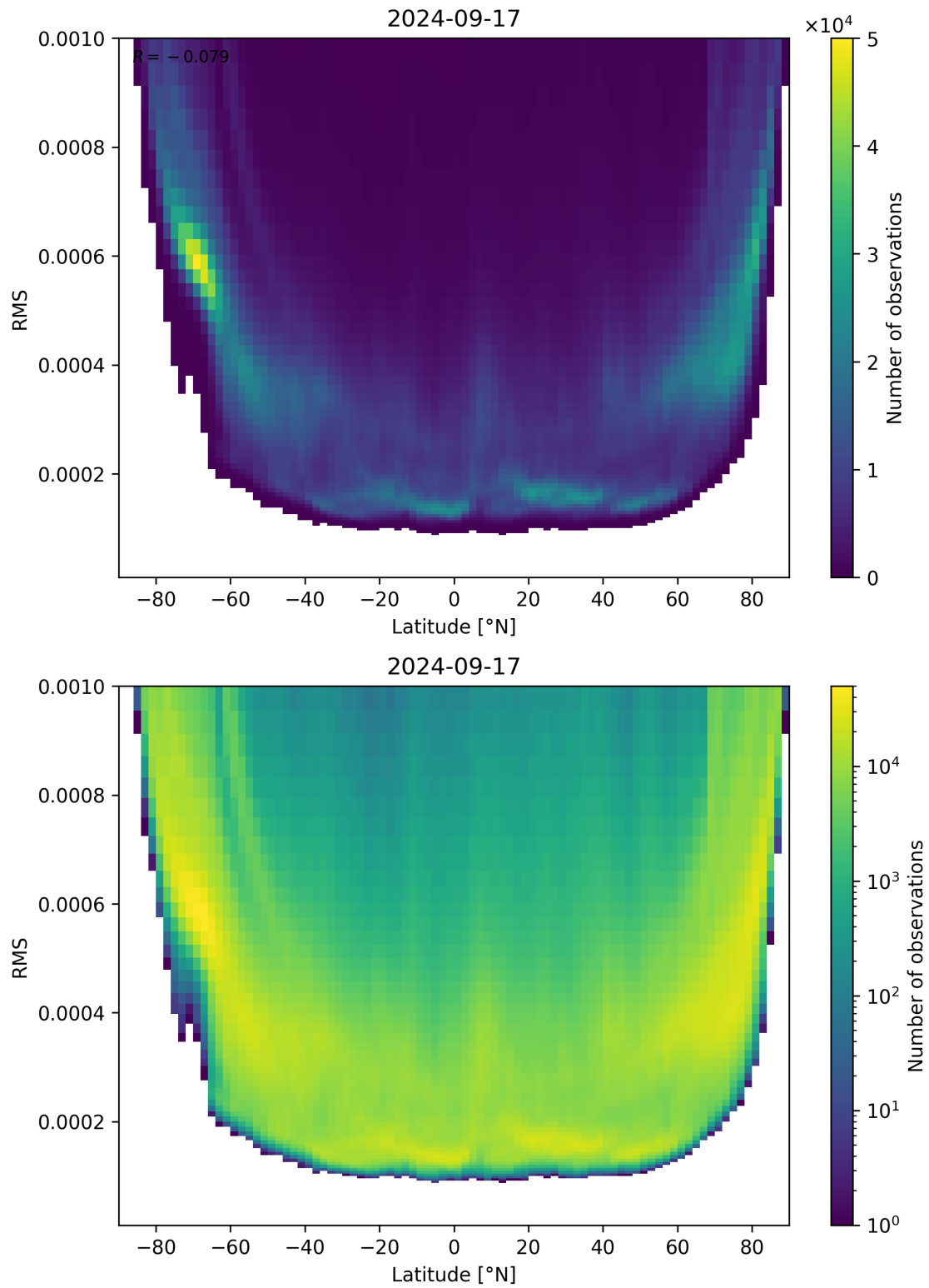
Figure 94: Scatter density plot of “Latitude” against “RMS” for 2024-09-17 to 2024-09-18.
