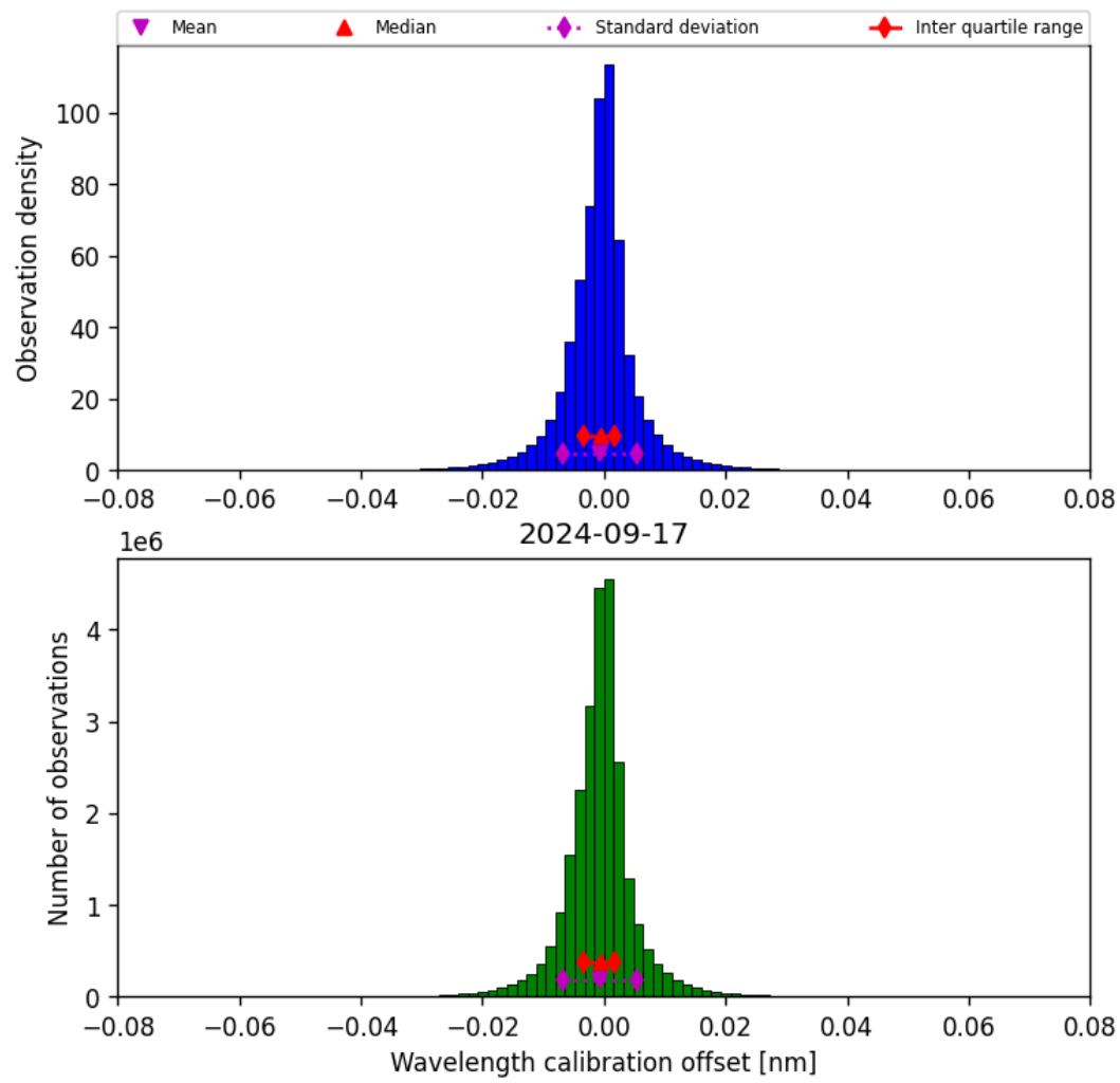
Figure 35: Histogram of “Wavelength calibration offset” for 2024-09-17 to 2024-09-18
