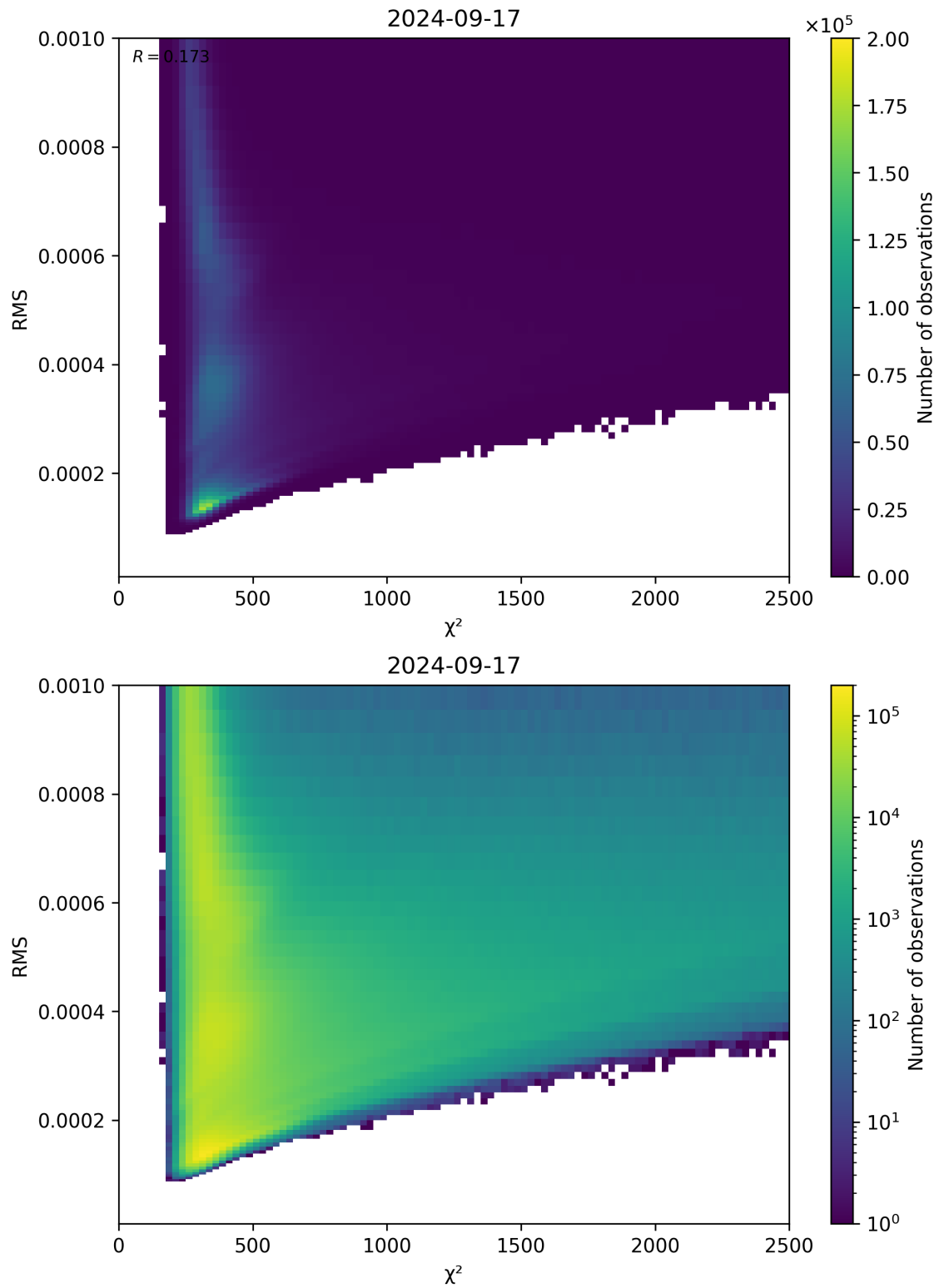
Figure 82: Scatter density plot of “ \chi^2 ” against “RMS” for 2024-09-17 to 2024-09-18.
