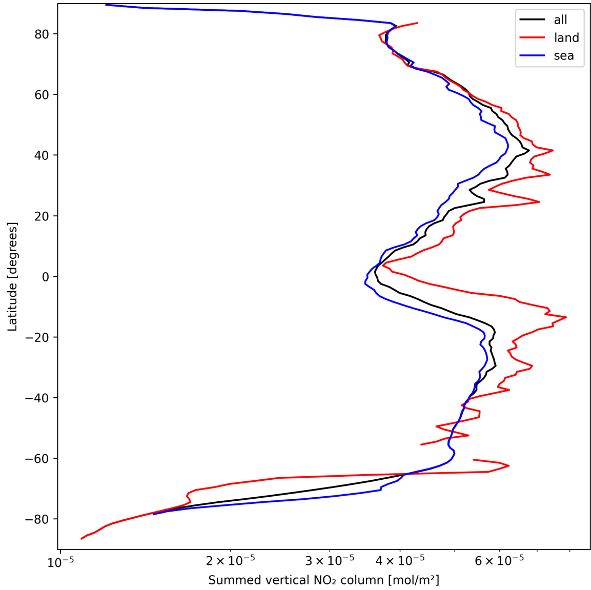
Figure 23: Zonal average of “Summed vertical NO 2 column” for 2024-09-17 to 2024-09-18.
