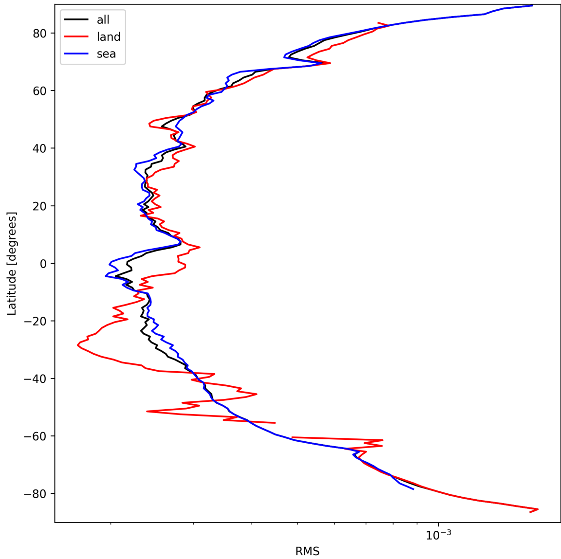
Figure 26: Zonal average of “RMS” for 2024-09-17 to 2024-09-18.
