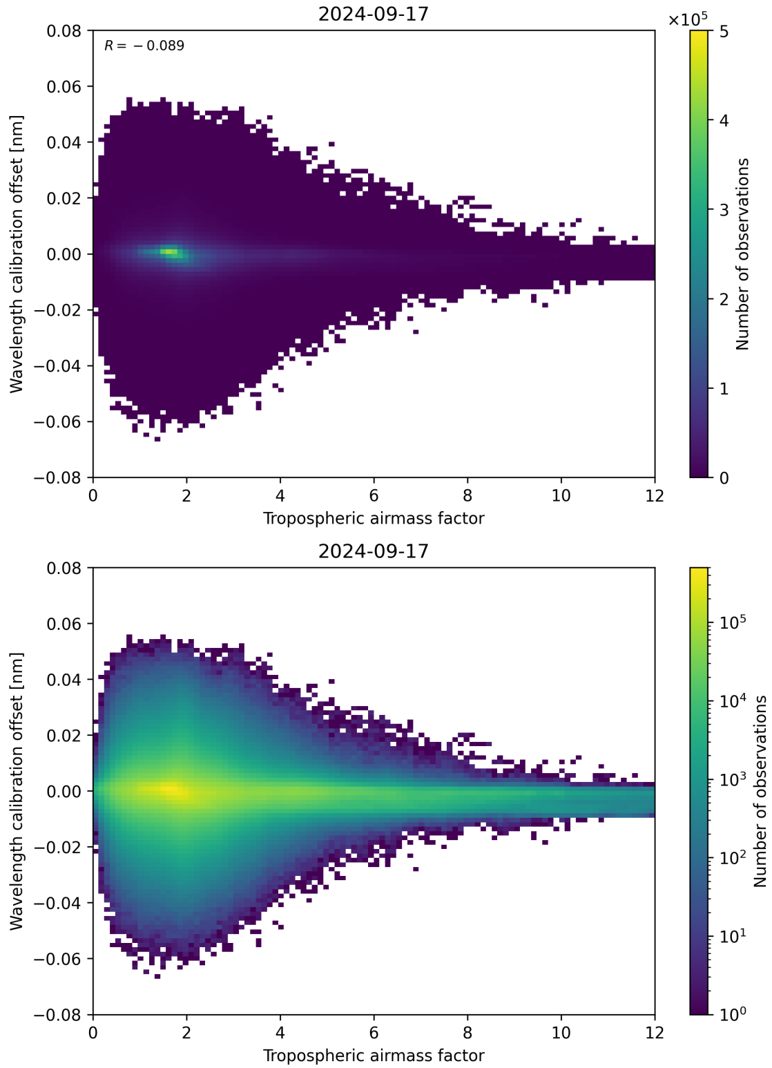
Figure 80: Scatter density plot of “Tropospheric airmass factor” against “Wavelength calibration offset” for 2024-09-17 to 2024-09-18.
