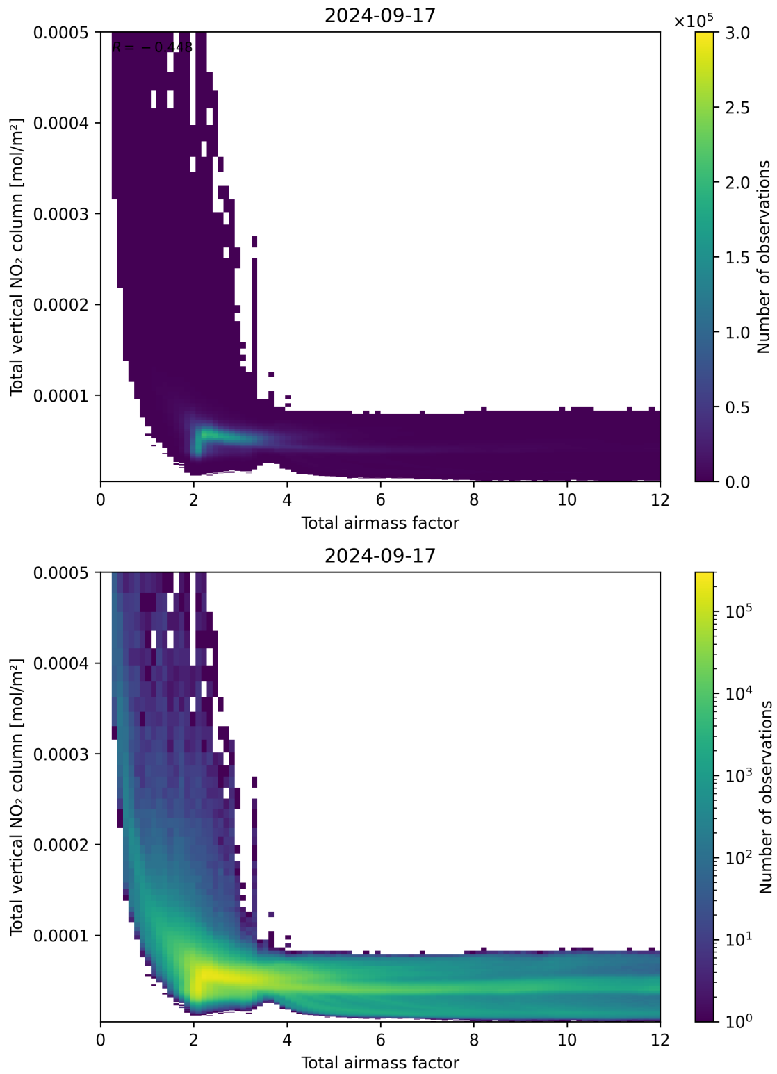
Figure 67: Scatter density plot of “Total airmass factor” against “Total vertical NO 2 column” for 2024-09-17 to 2024-09-18.
