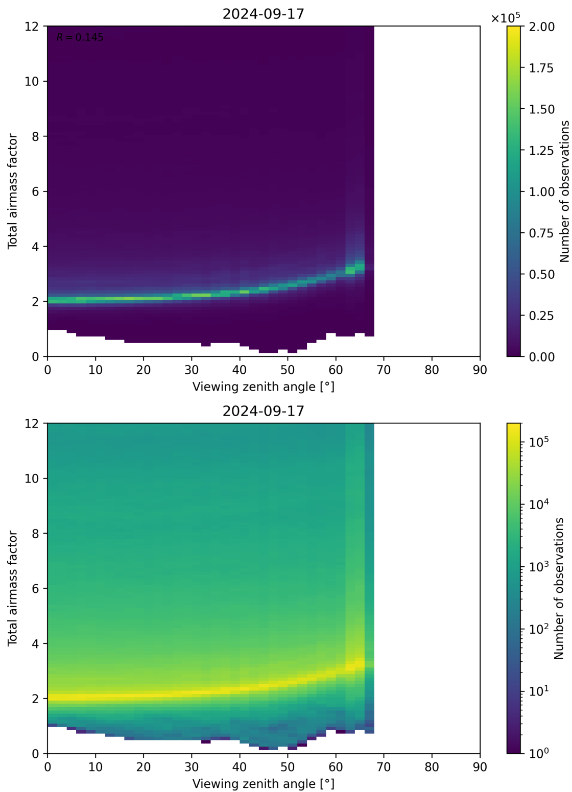
Figure 160: Scatter density plot of “Viewing zenith angle” against “Total airmass factor” for 2024-09-17 to 2024-09-18.
