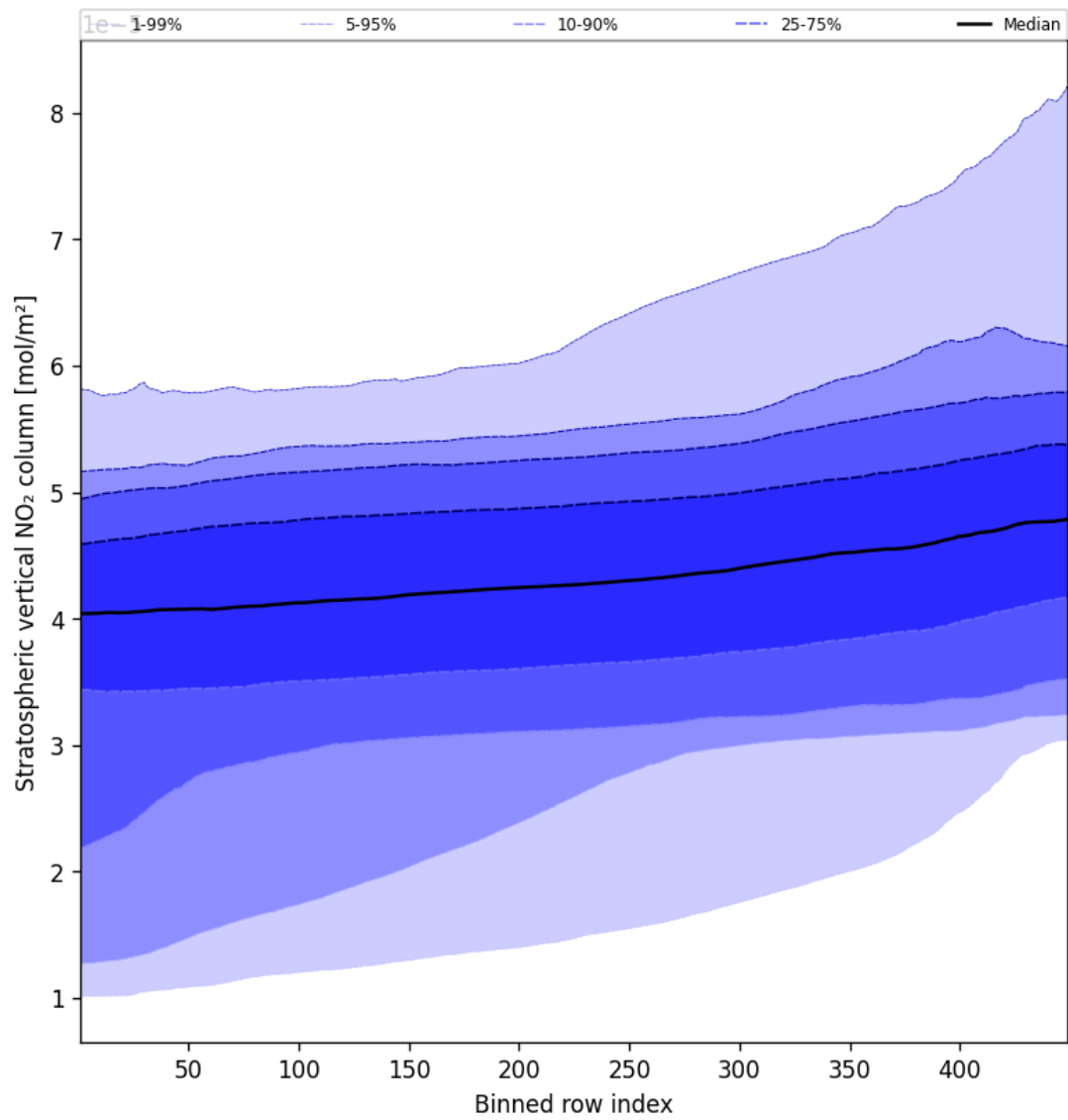
Figure 53: Along track statistics of “Stratospheric vertical NO 2 column” for 2024-09-17 to 2024-09-18
