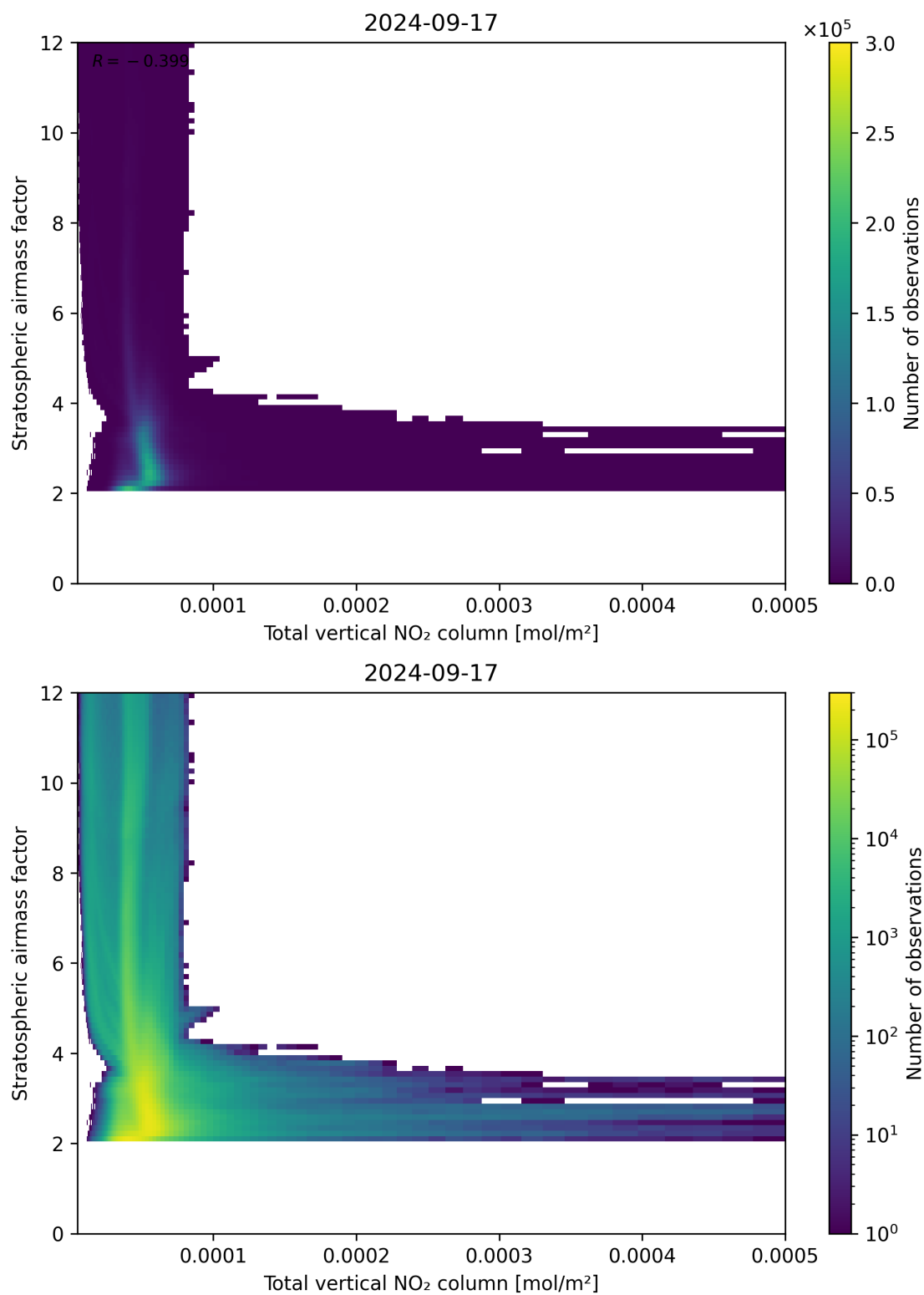
Figure 110: Scatter density plot of “Total vertical NO 2 column” against “Stratospheric airmass factor” for 2024-09-17 to 2024-09-18.
