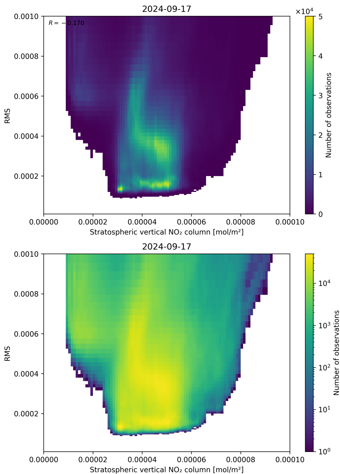
Figure 102: Scatter density plot of “Stratospheric vertical NO 2 column” against “RMS” for 2024-09-17 to 2024-09-18.
