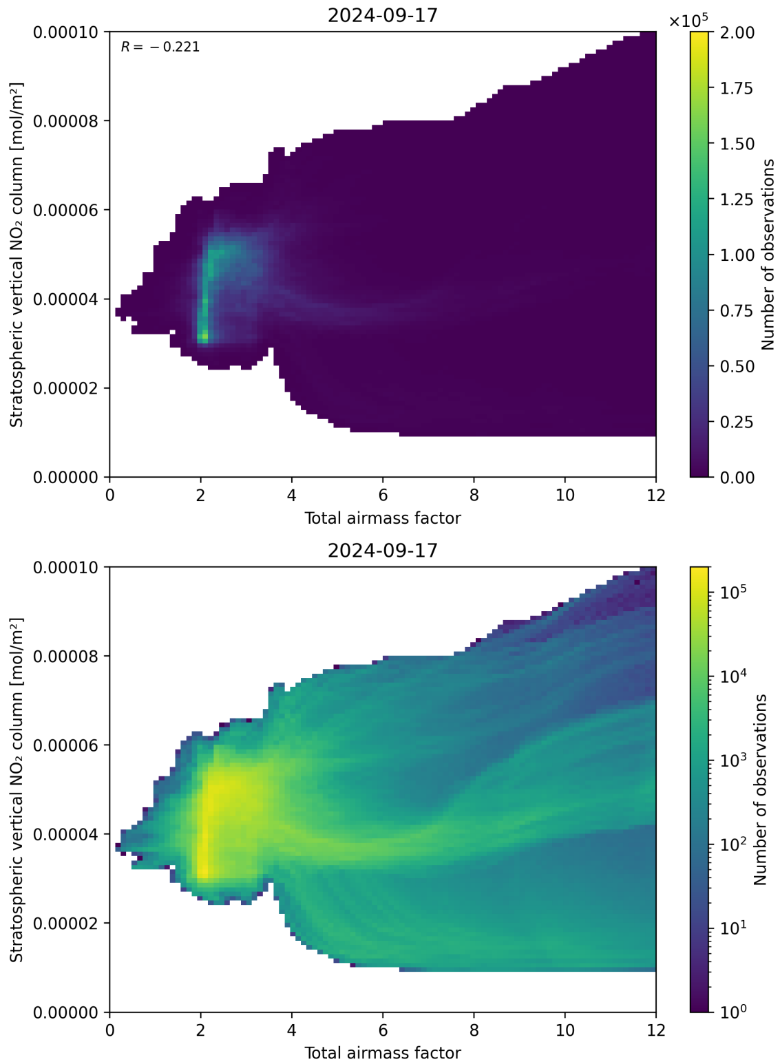
Figure 64: Scatter density plot of “Total airmass factor” against “Stratospheric vertical NO 2 column” for 2024-09-17 to 2024-09-18.
