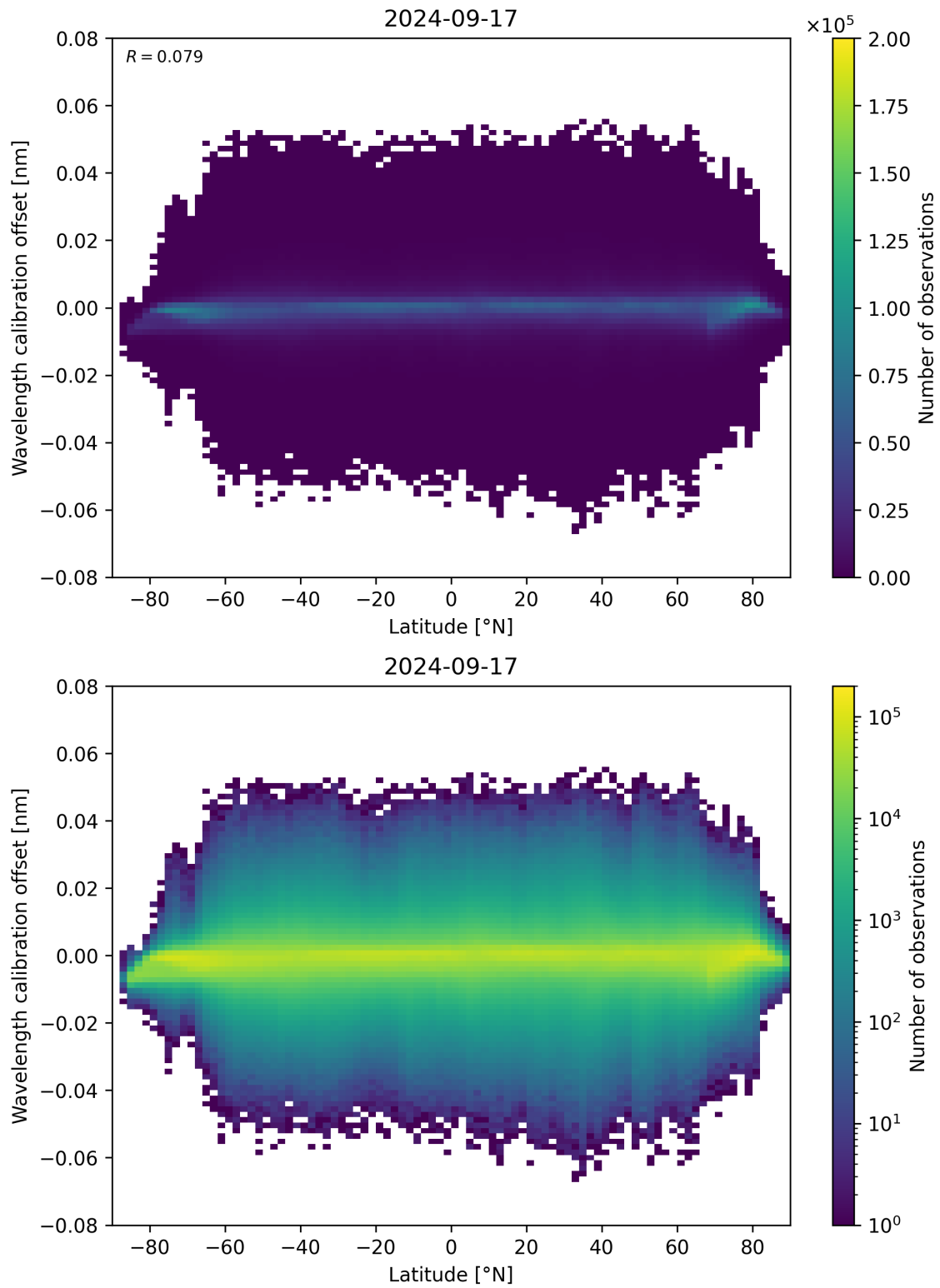
Figure 95: Scatter density plot of “Latitude” against “Wavelength calibration offset” for 2024-09-17 to 2024-09-18.
