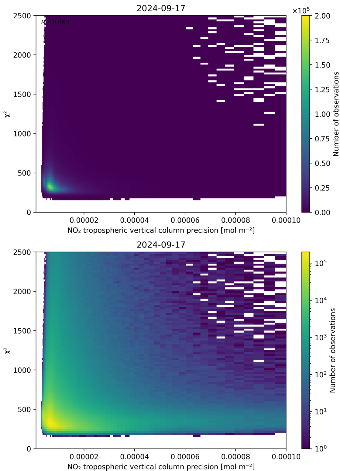
Figure 134: Scatter density plot of “NO 2 tropospheric vertical column precision” against “ \chi^2 ” for 2024-09-17 to 2024-09-18.
