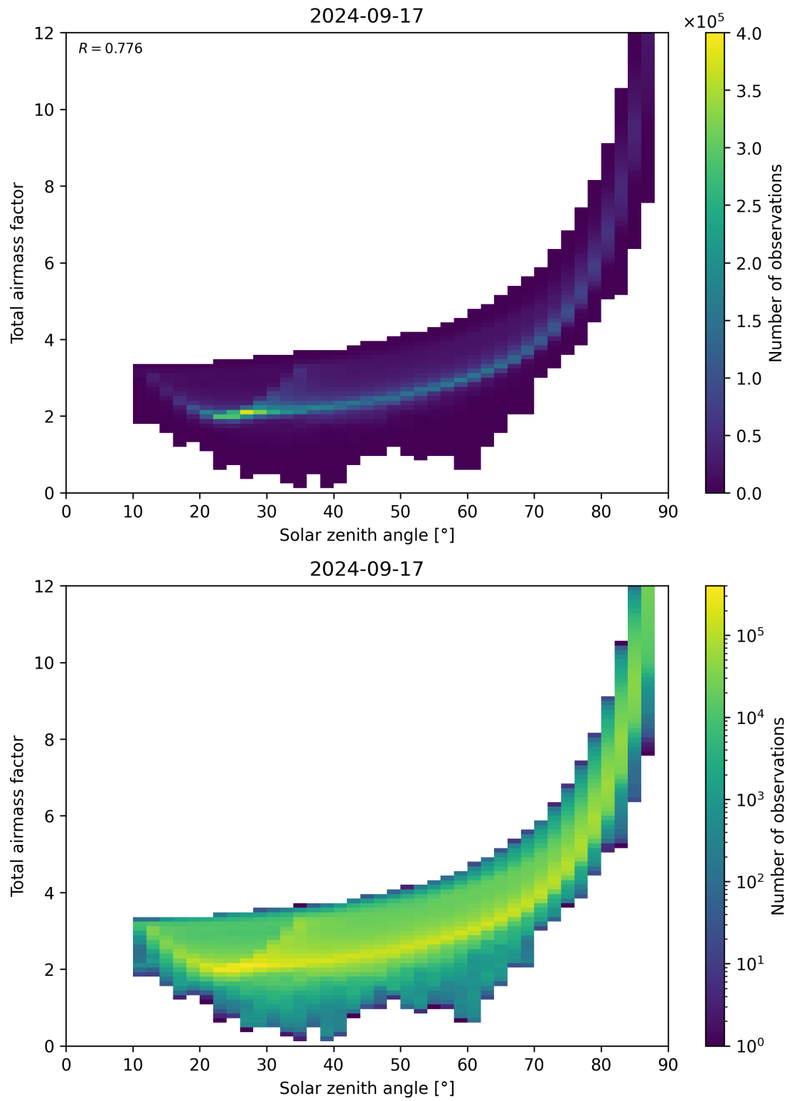
Figure 146: Scatter density plot of “Solar zenith angle” against “Total air mass factor” for 2024-09-17 to 2024-09-18.
