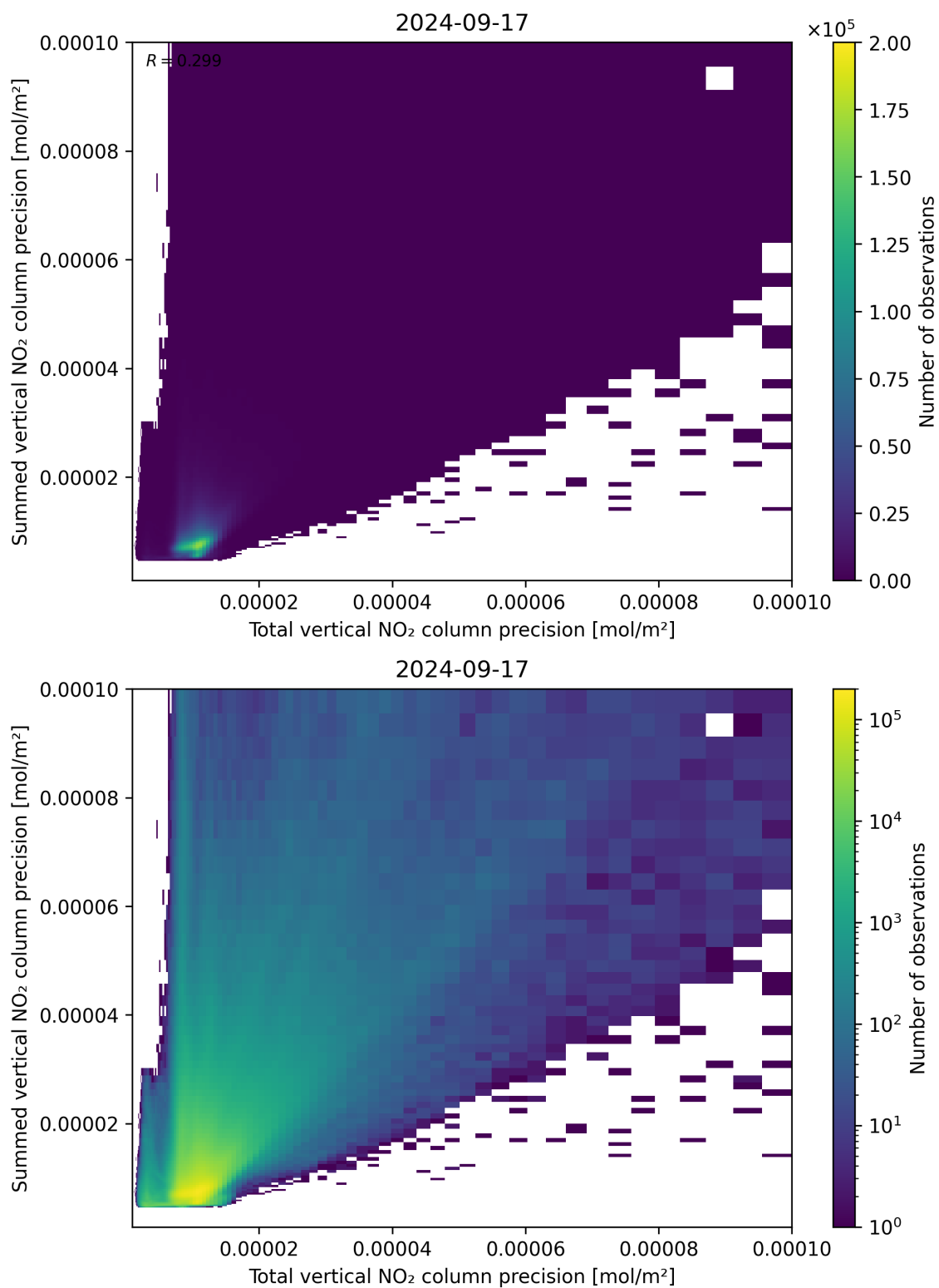
Figure 118: Scatter density plot of “Total vertical NO 2 column precision” against “Summed vertical NO 2 column precision” for 2024-09-17 to 2024-09-18.
