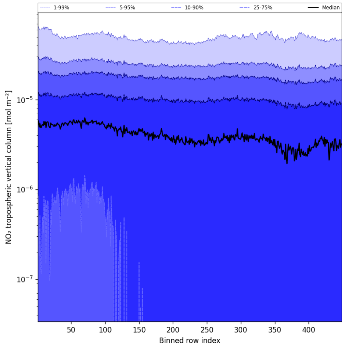
Figure 46: Along track statistics of “NO 2 tropospheric vertical column” for 2024-09-17 to 2024-09-18
