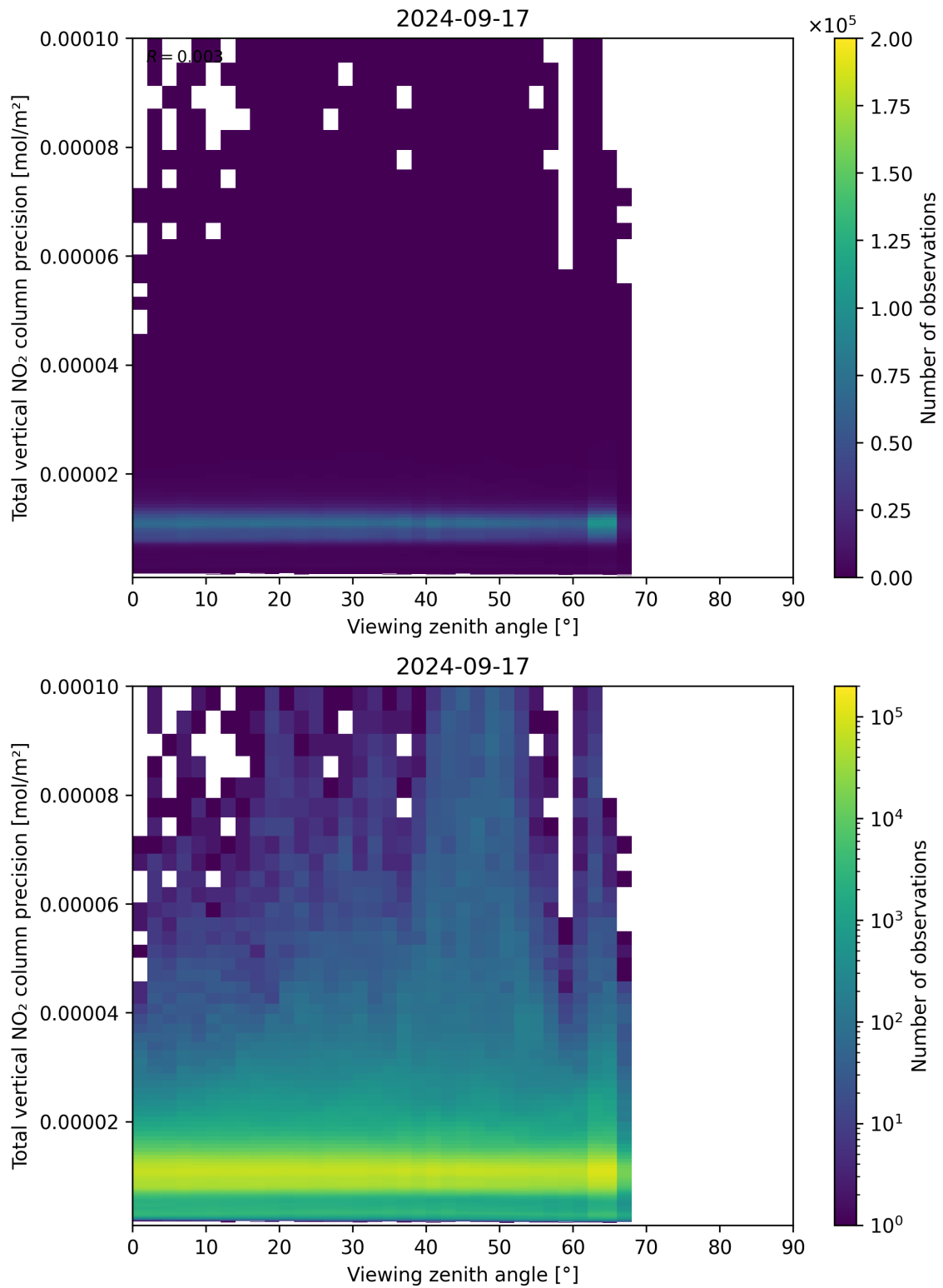
Figure 168: Scatter density plot of “Viewing zenith angle” against “Total vertical NO 2 column precision” for 2024-09-17 to 2024-09-18.
