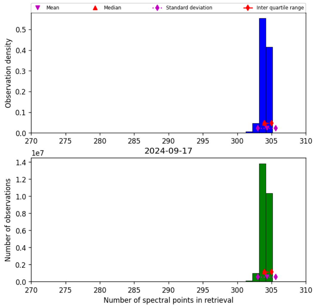
Figure 33: Histogram of “Number of spectral points in retrieval” for 2024-09-17 to 2024-09-18
