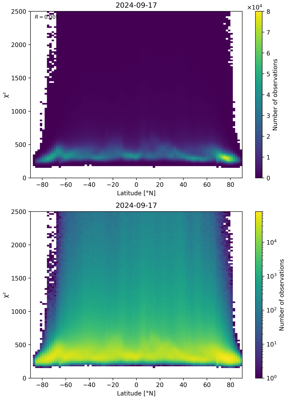
Figure 86: Scatter density plot of “Latitude” against “ \chi^2 ” for 2024-09-17 to 2024-09-18.
