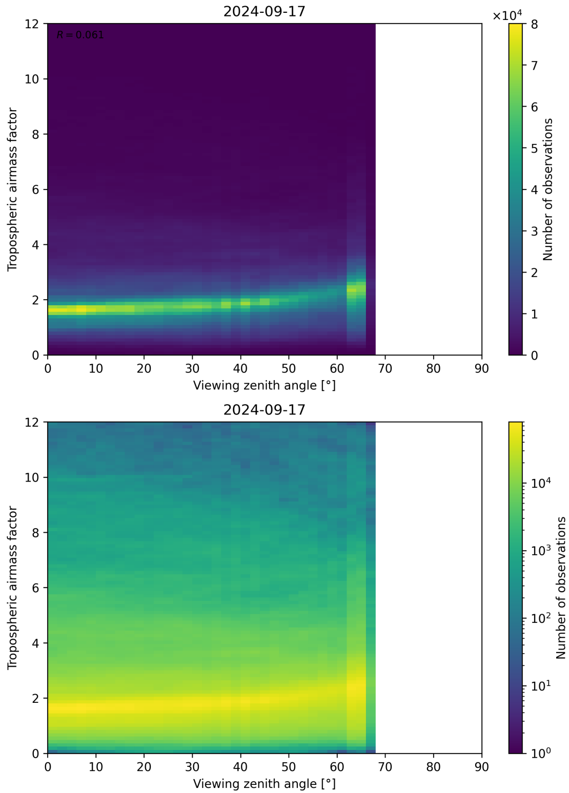
Figure 161: Scatter density plot of “Viewing zenith angle” against “Tropospheric airmass factor” for 2024-09-17 to 2024-09-18.
