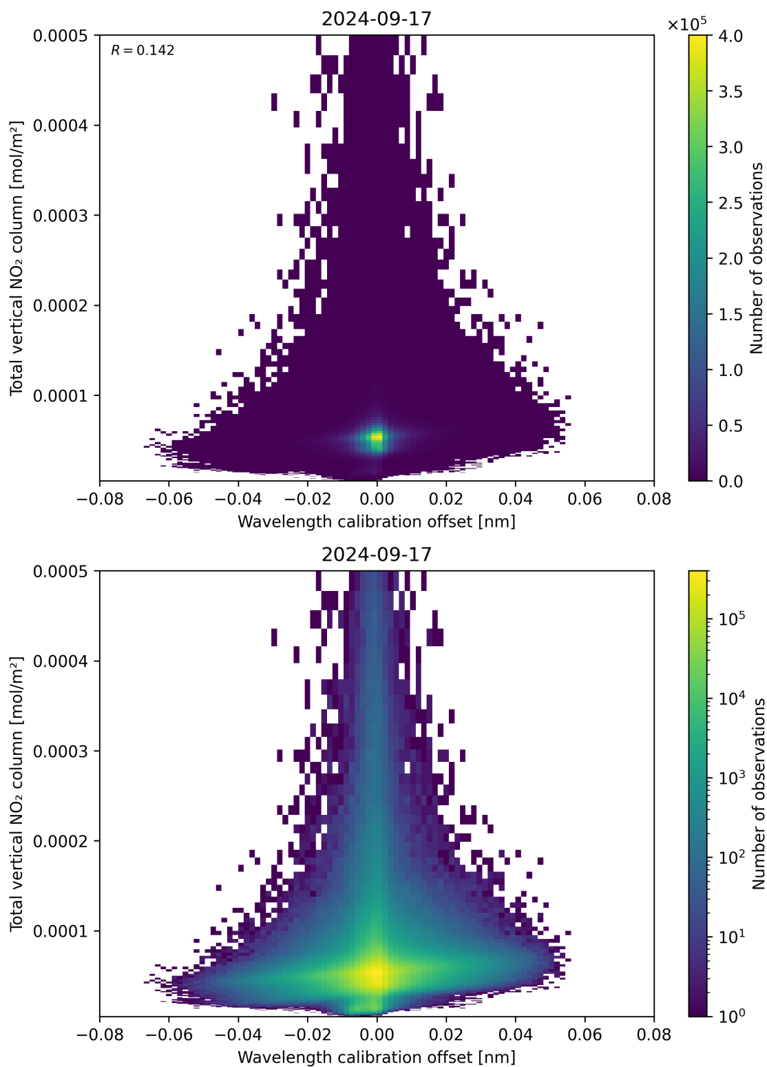
Figure 179: Scatter density plot of “Wavelength calibration offset” against “Total vertical NO 2 column” for 2024-09-17 to 2024-09-18.
