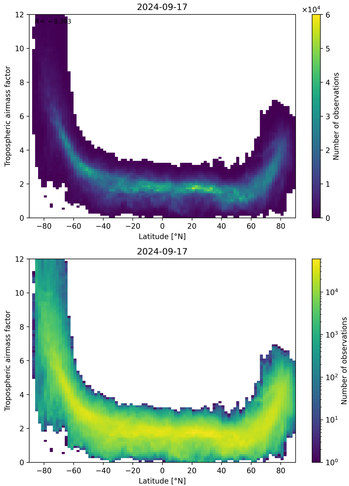
Figure 85: Scatter density plot of “Latitude” against “Tropospheric airmass factor” for 2024-09-17 to 2024-09-18.
