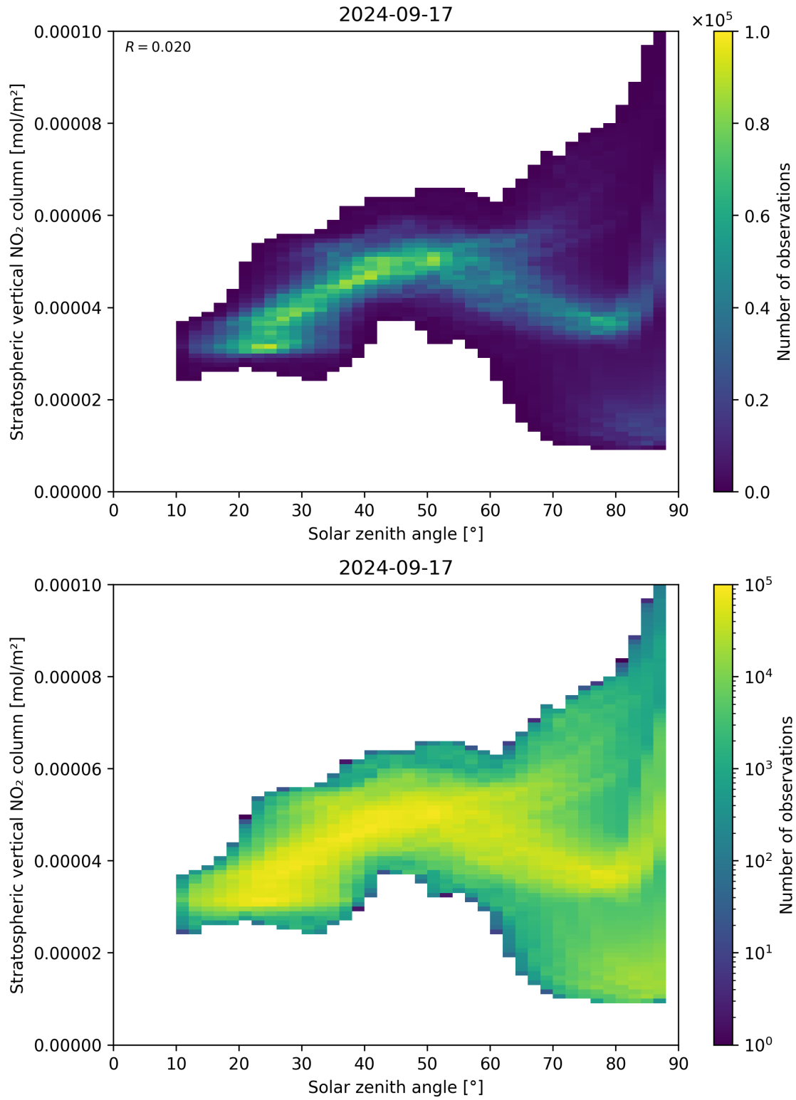
Figure 150: Scatter density plot of “Solar zenith angle” against “Stratospheric vertical NO 2 column” for 2024-09-17 to 2024-09-18.
