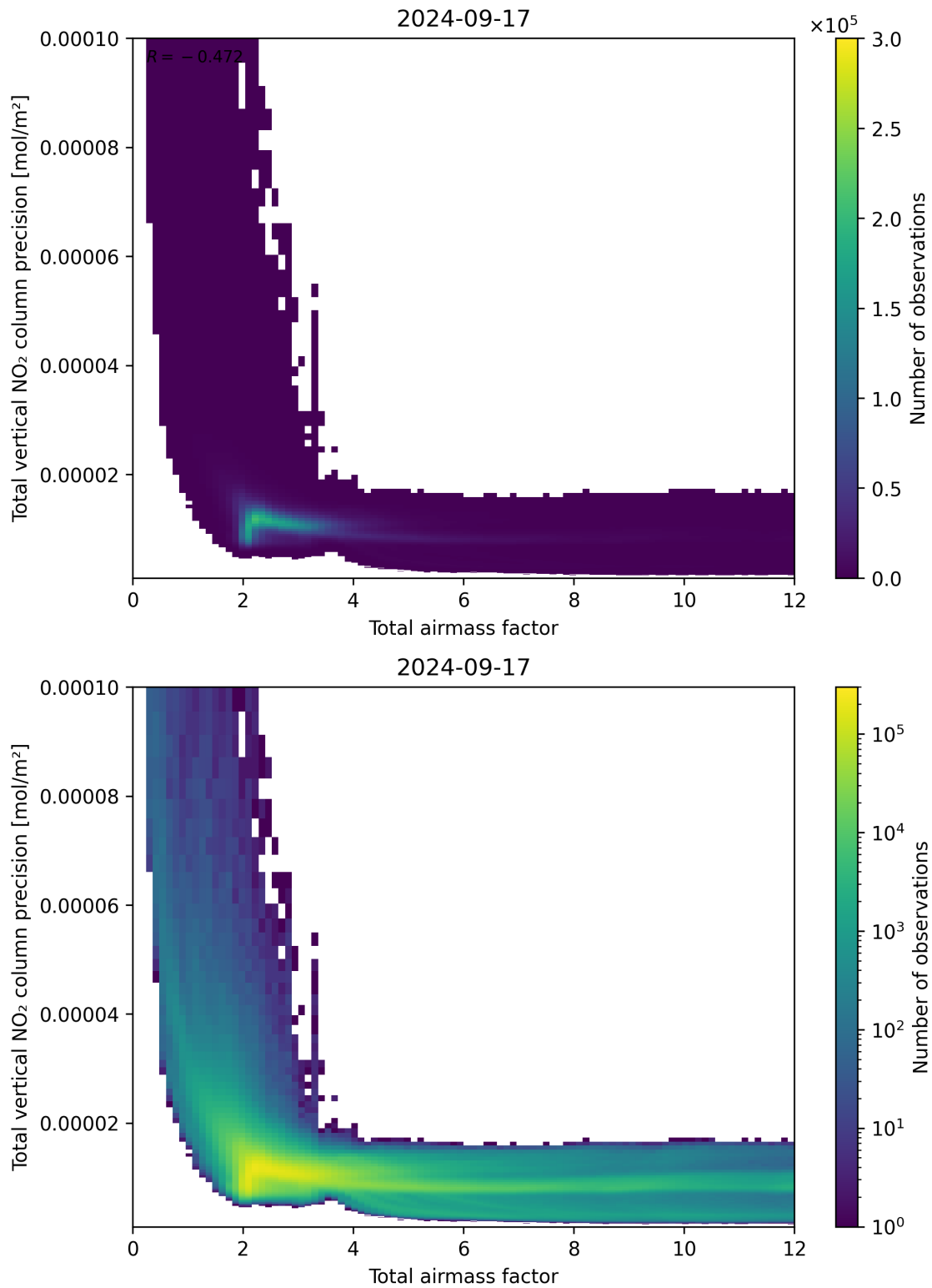
Figure 68: Scatter density plot of “Total airmass factor” against “Total vertical NO 2 column precision” for 2024-09-17 to 2024-09-18.
