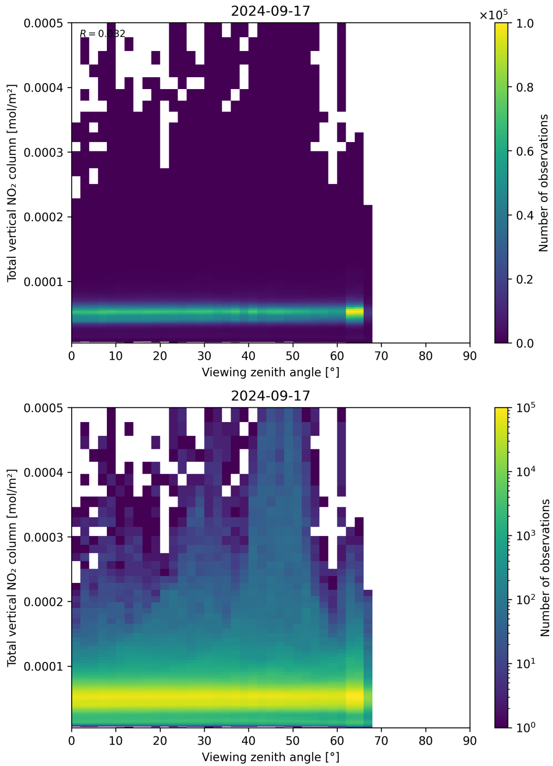
Figure 167: Scatter density plot of “Viewing zenith angle” against “Total vertical NO 2 column” for 2024-09-17 to 2024-09-18.
