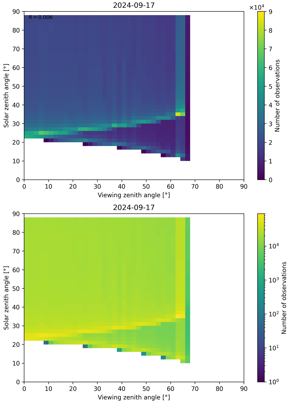
Figure 172: Scatter density plot of “Viewing zenith angle” against “Solar zenith angle” for 2024-09-17 to 2024-09-18.
