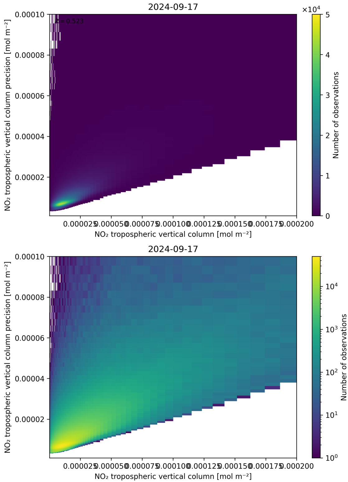
Figure 130: Scatter density plot of “NO 2 tropospheric vertical column” against “NO 2 tropospheric vertical column precision” for 2024-09-17 to 2024-09-18.
