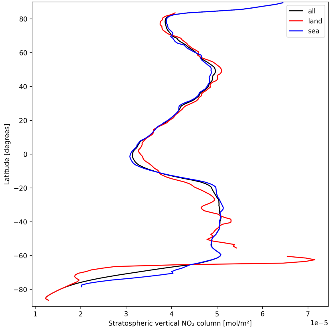
Figure 19: Zonal average of “Stratospheric vertical NO 2 column” for 2024-09-17 to 2024-09-18.
