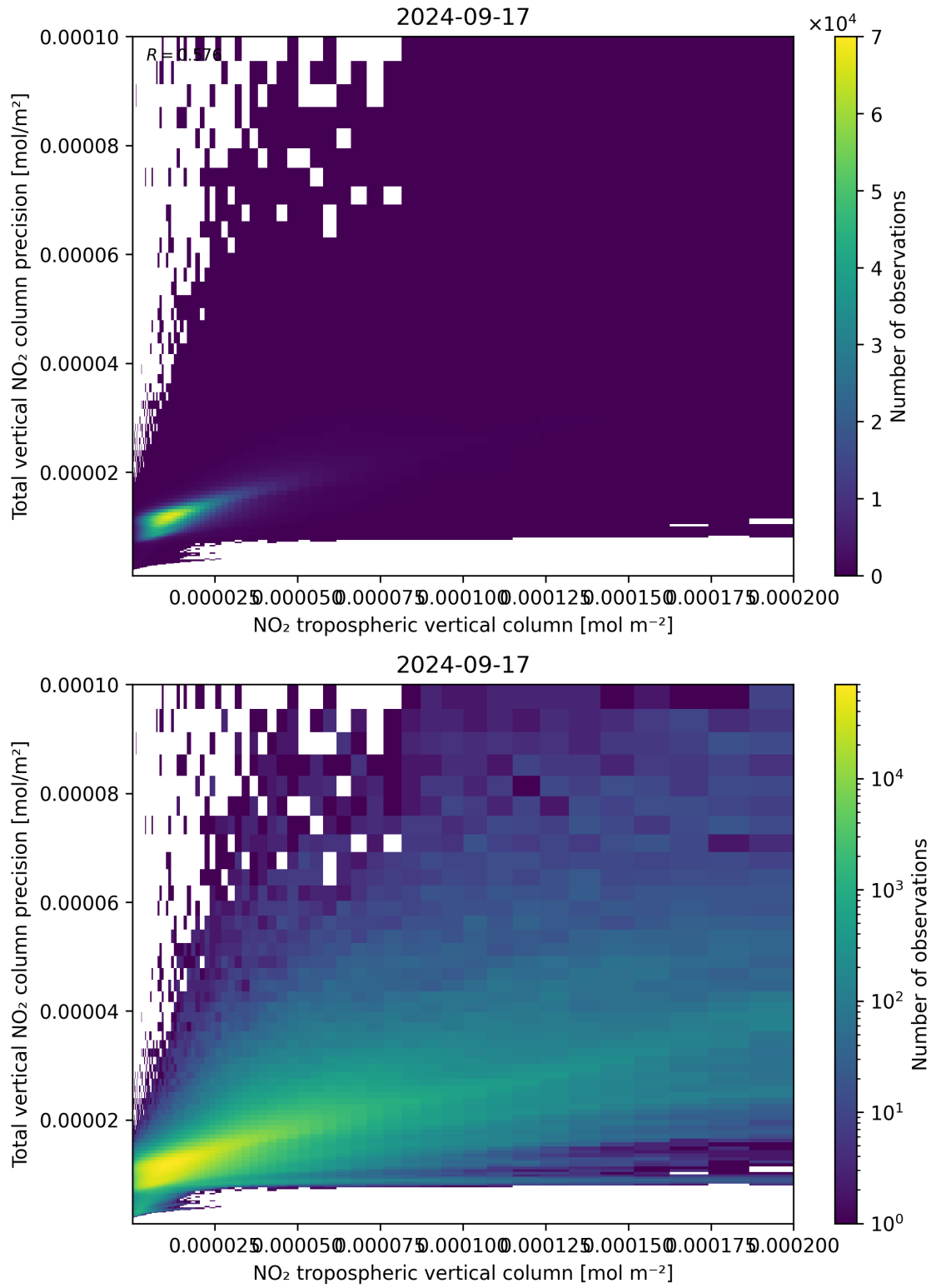
Figure 129: Scatter density plot of “NO 2 tropospheric vertical column” against “Total vertical NO 2 column precision” for 2024-09-17 to 2024-09-18.
