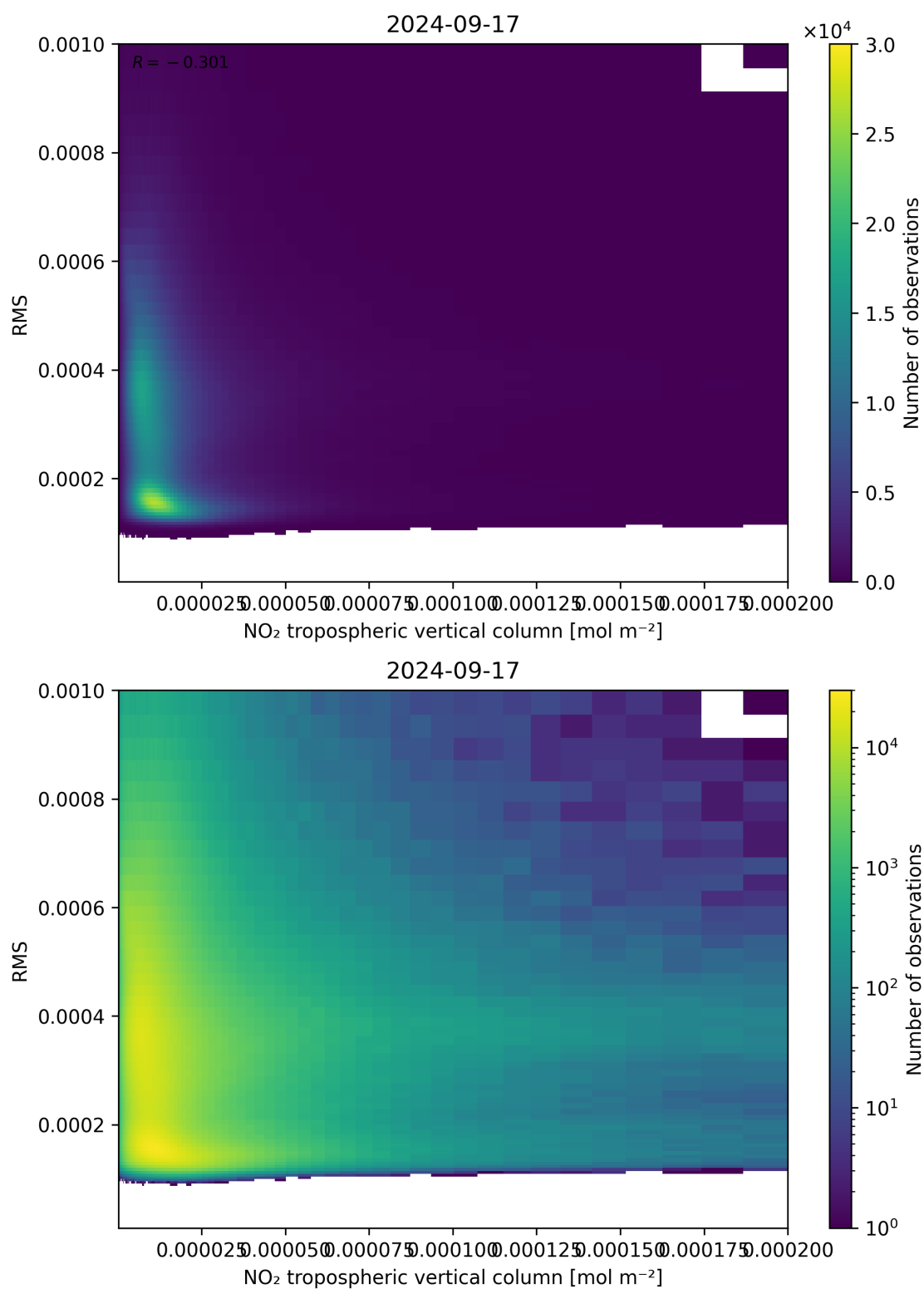
Figure 142: Scatter density plot of “NO 2 tropospheric vertical column” against “RMS” for 2024-09-17 to 2024-09-18.
