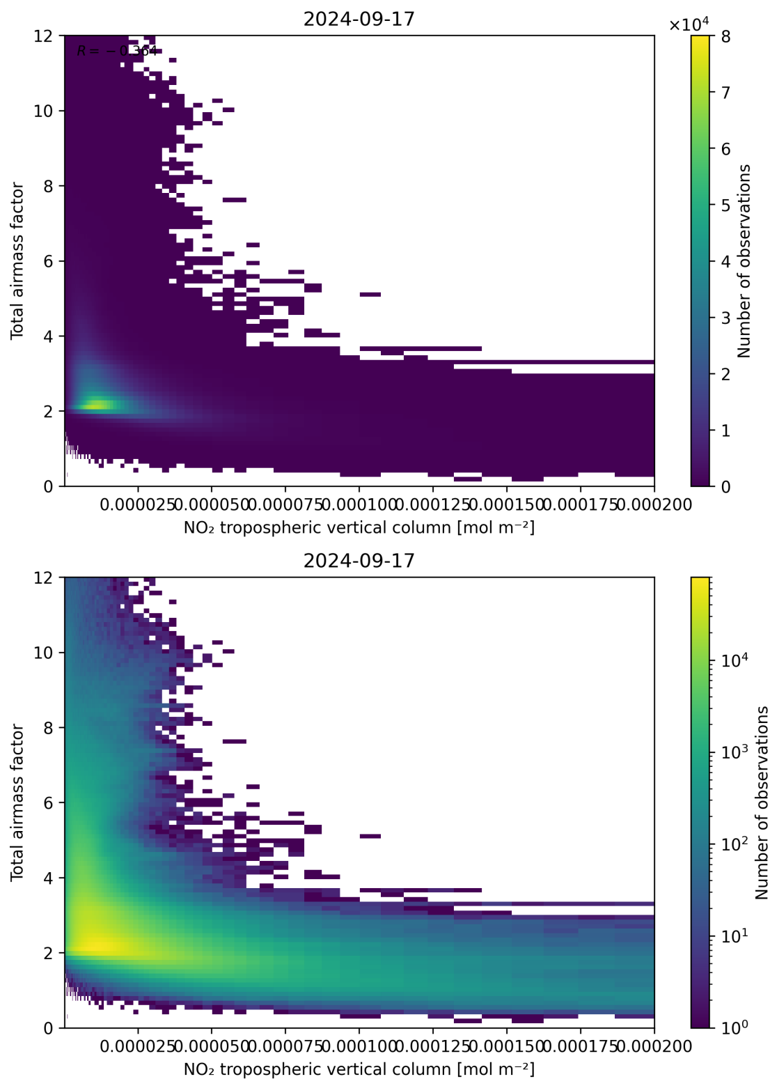
Figure 122: Scatter density plot of “NO 2 tropospheric vertical column” against “Total air mass factor” for 2024-09-17 to 2024-09-18.
