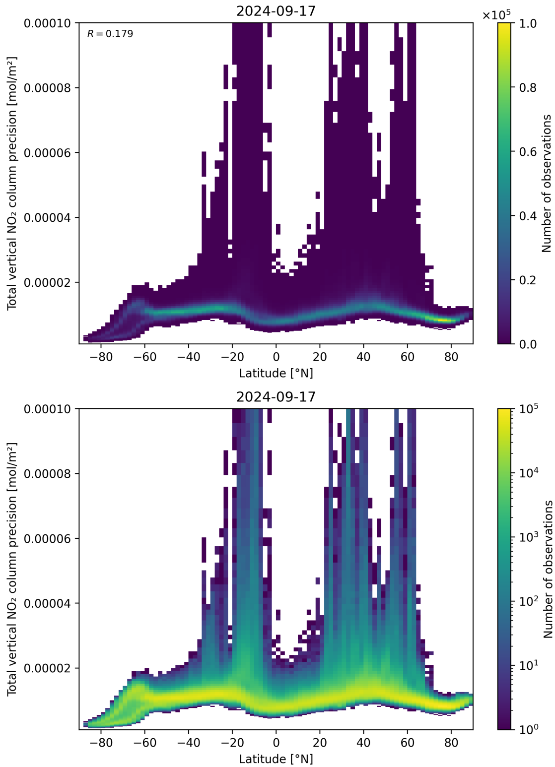
Figure 91: Scatter density plot of “Latitude” against “Total vertical NO 2 column precision” for 2024-09-17 to 2024-09-18.
