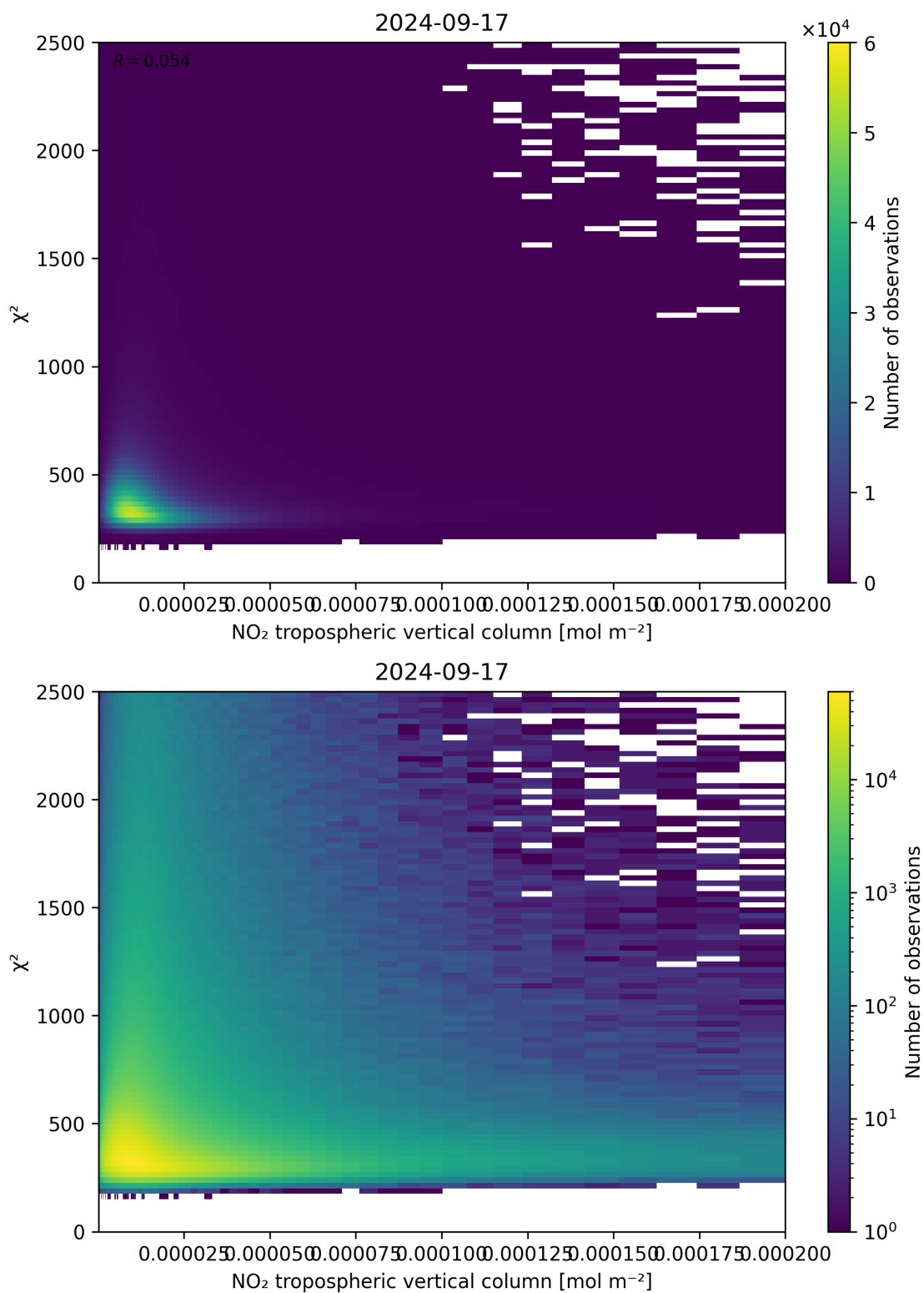
Figure 124: Scatter density plot of “NO 2 tropospheric vertical column” against “ \chi^2 ” for 2024-09-17 to 2024-09-18.
