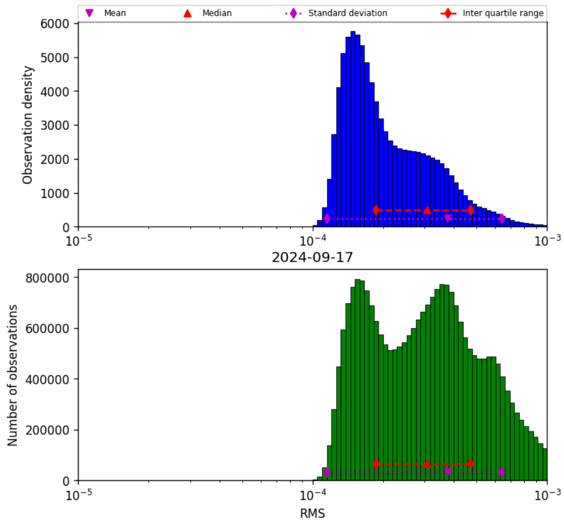
Figure 43: Histogram of “RMS” for 2024-09-17 to 2024-09-18
