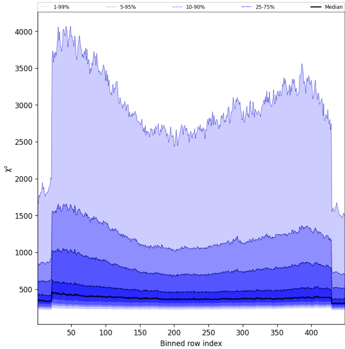
Figure 59: Along track statistics of “ \chi^2 ” for 2024-09-17 to 2024-09-18
