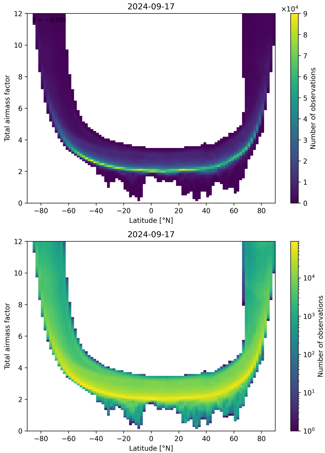
Figure 84: Scatter density plot of “Latitude” against “Total airmass factor” for 2024-09-17 to 2024-09-18.
