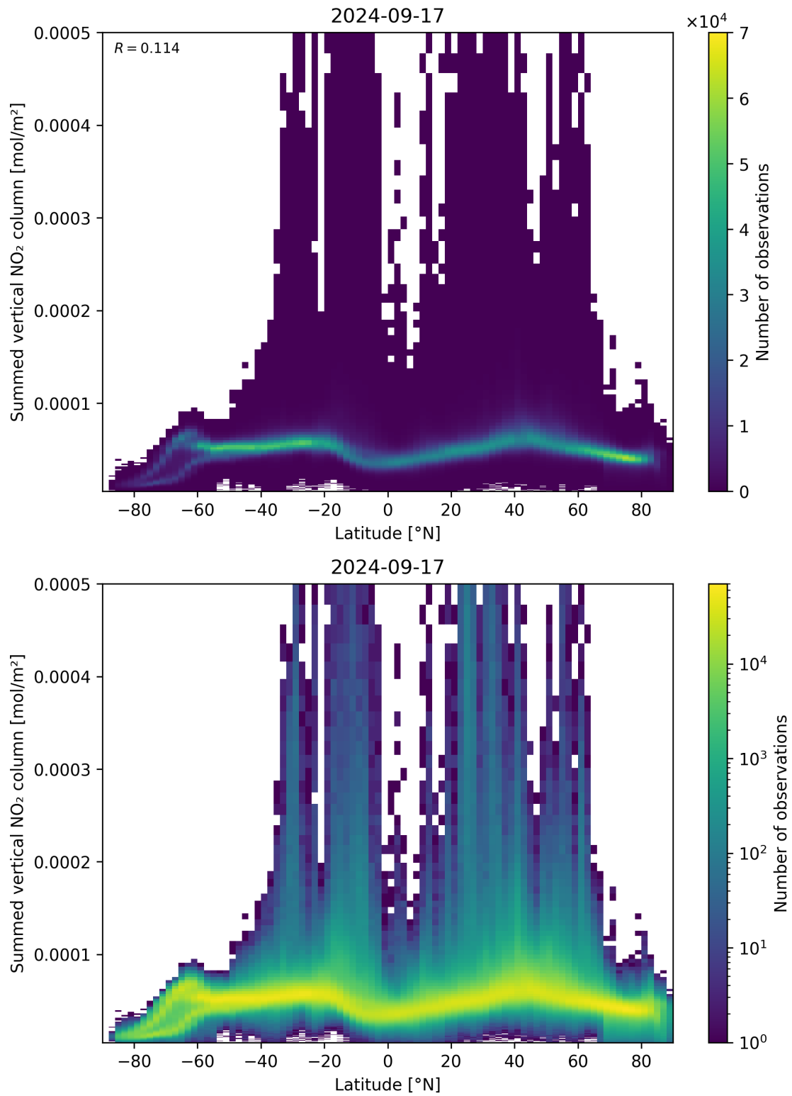
Figure 88: Scatter density plot of “Latitude” against “Summed vertical NO 2 column” for 2024-09-17 to 2024-09-18.
