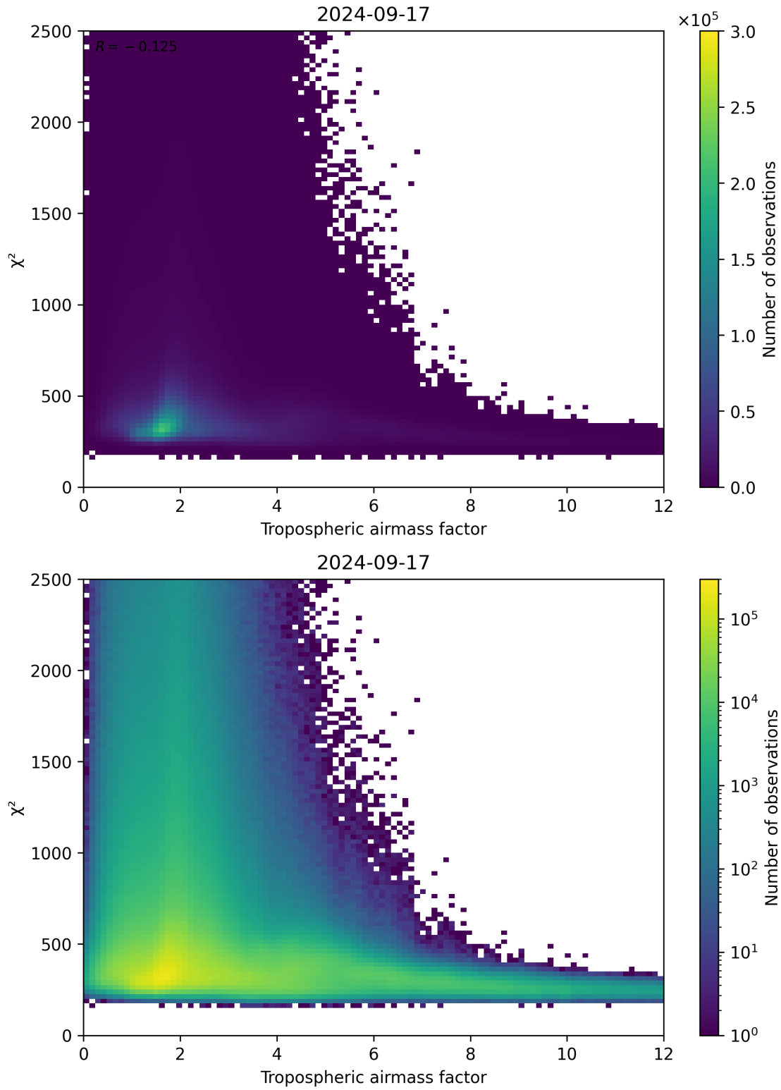
Figure 73: Scatter density plot of “Tropospheric airmass factor” against “ \chi^2 ” for 2024-09-17 to 2024-09-18.
