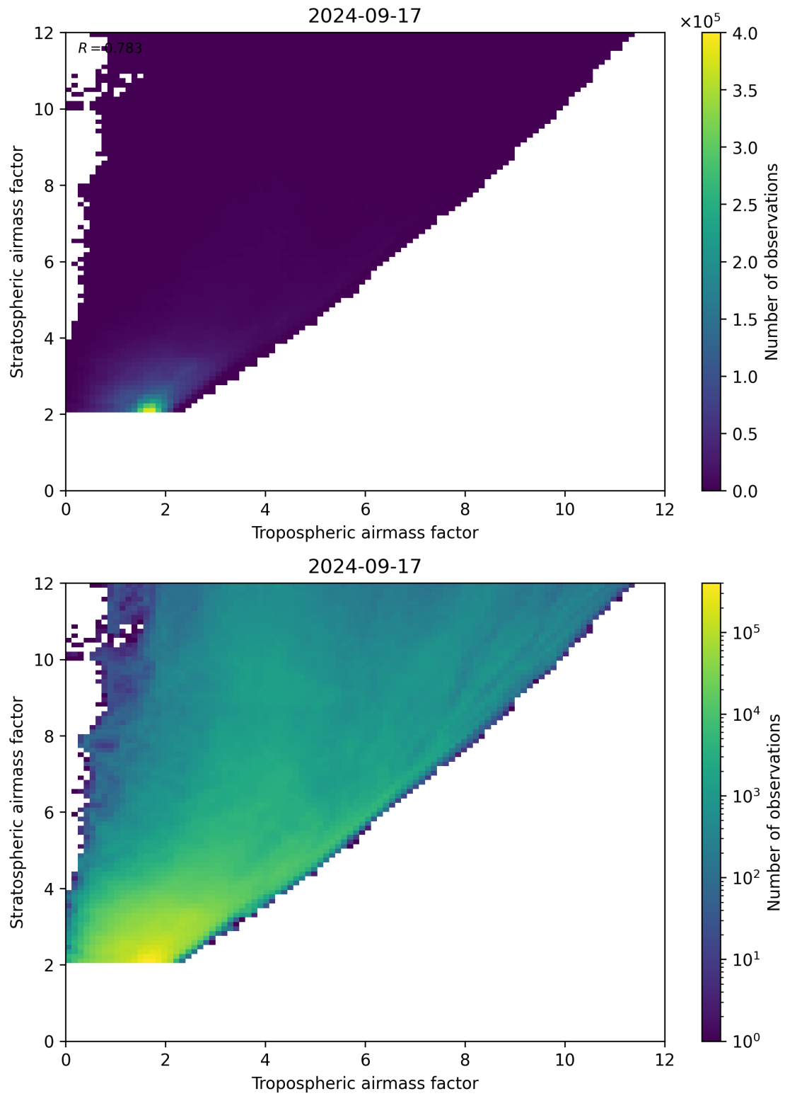
Figure 71: Scatter density plot of “Tropospheric airmass factor” against “Stratospheric airmass factor” for 2024-09-17 to 2024-09-18.
