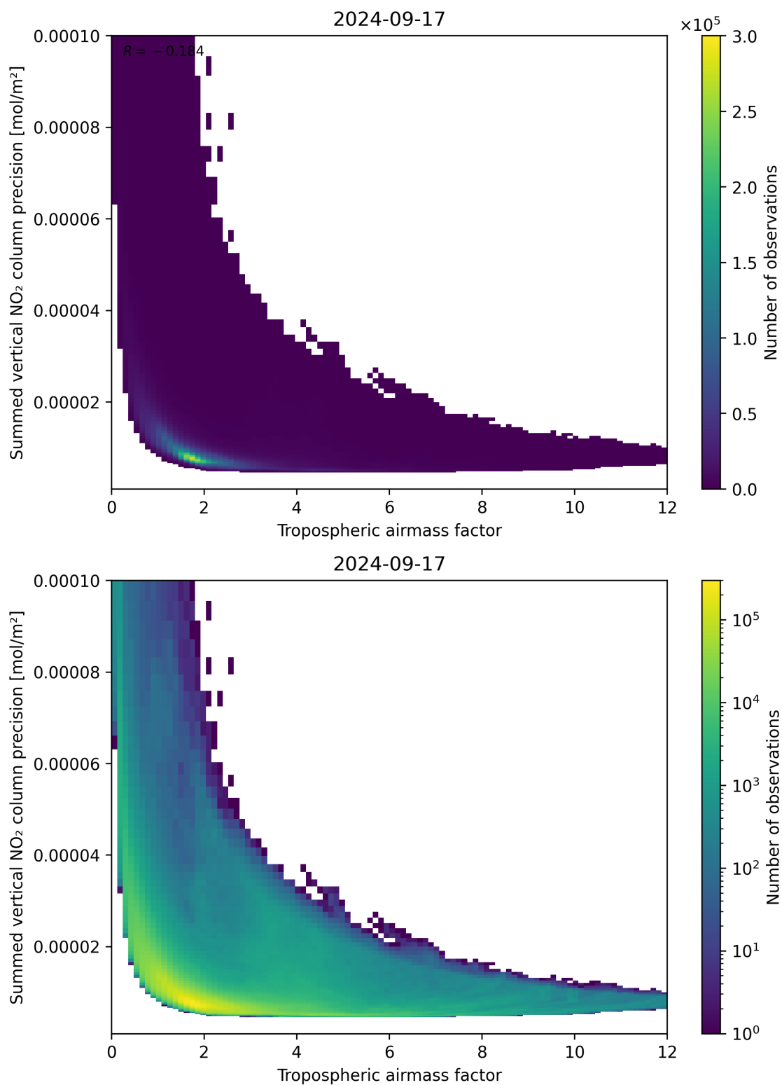
Figure 76: Scatter density plot of “Tropospheric airmass factor” against “Summed vertical NO 2 column precision” for 2024-09-17 to 2024-09-18.
