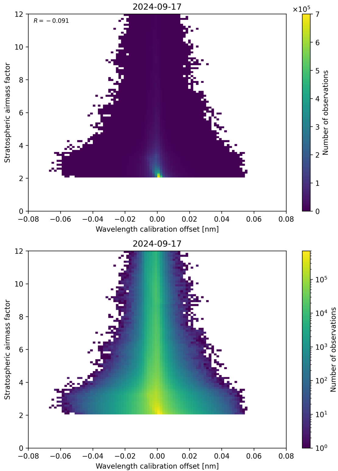
Figure 174: Scatter density plot of “Wavelength calibration offset” against “Stratospheric air mass factor” for 2024-09-17 to 2024-09-18.
