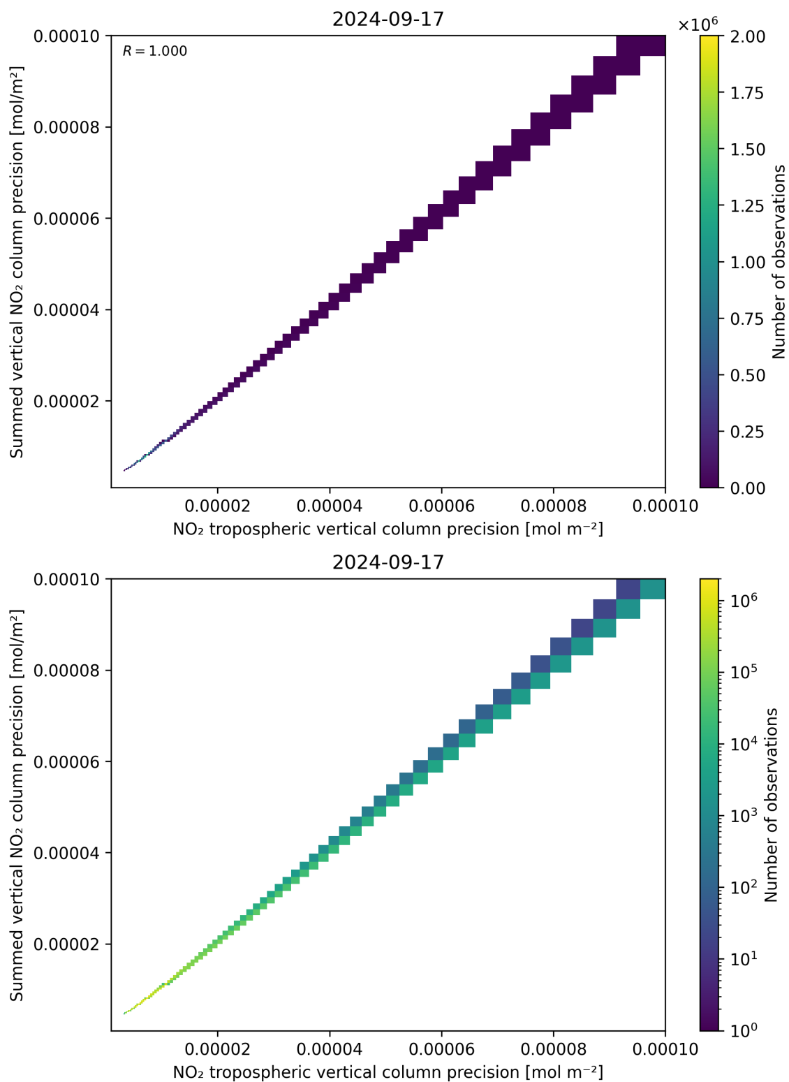
Figure 137: Scatter density plot of “NO 2 tropospheric vertical column precision” against “Summed vertical NO 2 column precision” for 2024-09-17 to 2024-09-18.
