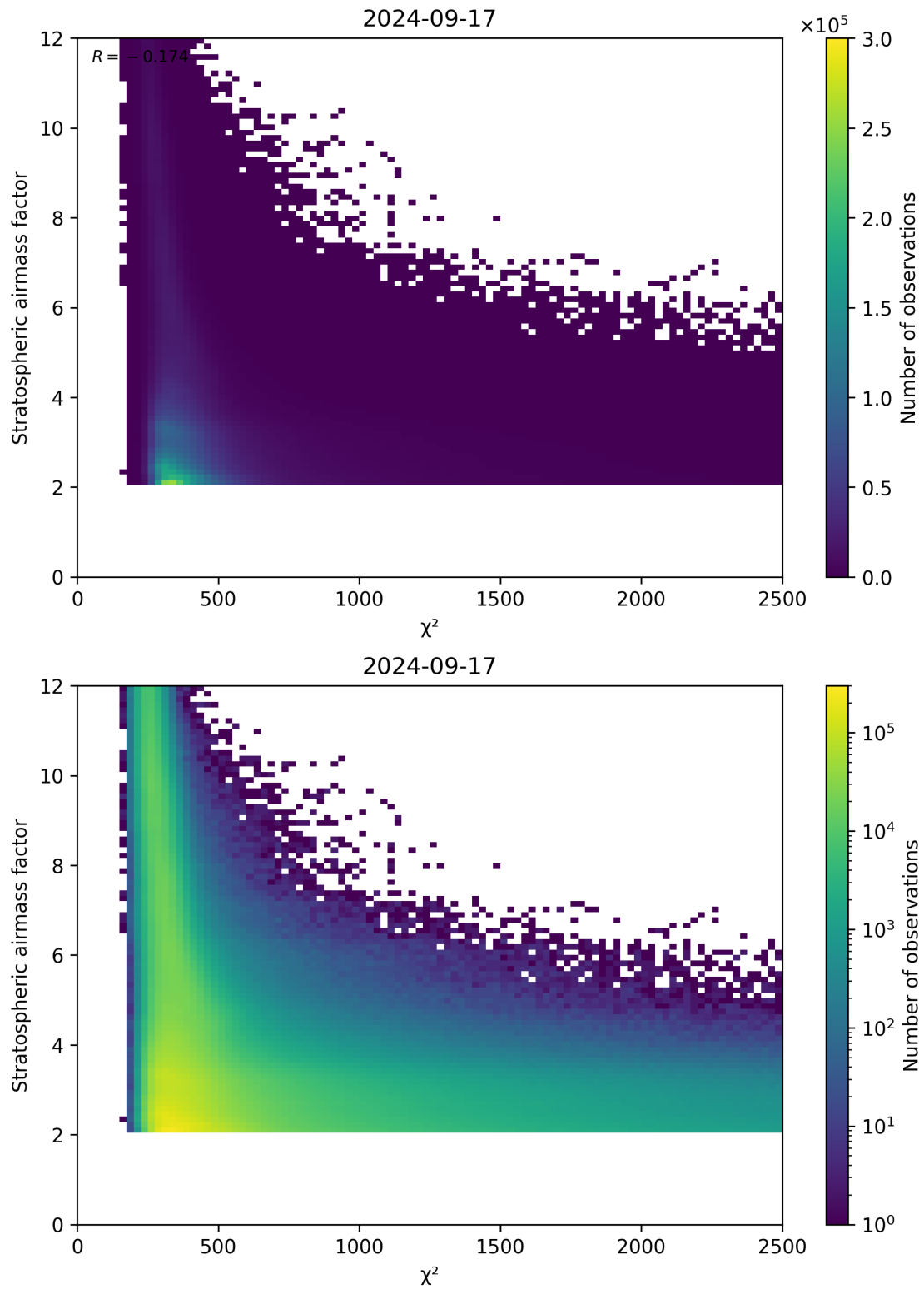
Figure 81: Scatter density plot of “ \chi^2 ” against “Stratospheric airmass factor” for 2024-09-17 to 2024-09-18.
