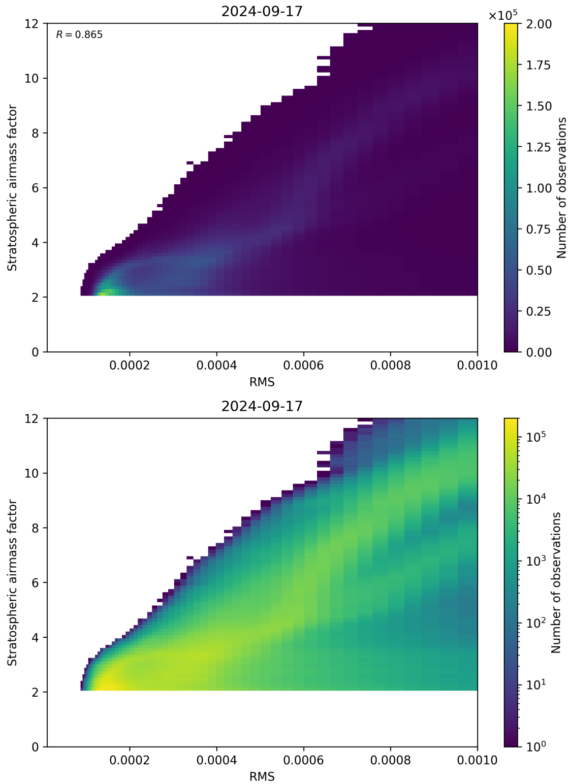
Figure 144: Scatter density plot of “RMS” against “Stratospheric airmass factor” for 2024-09-17 to 2024-09-18.
