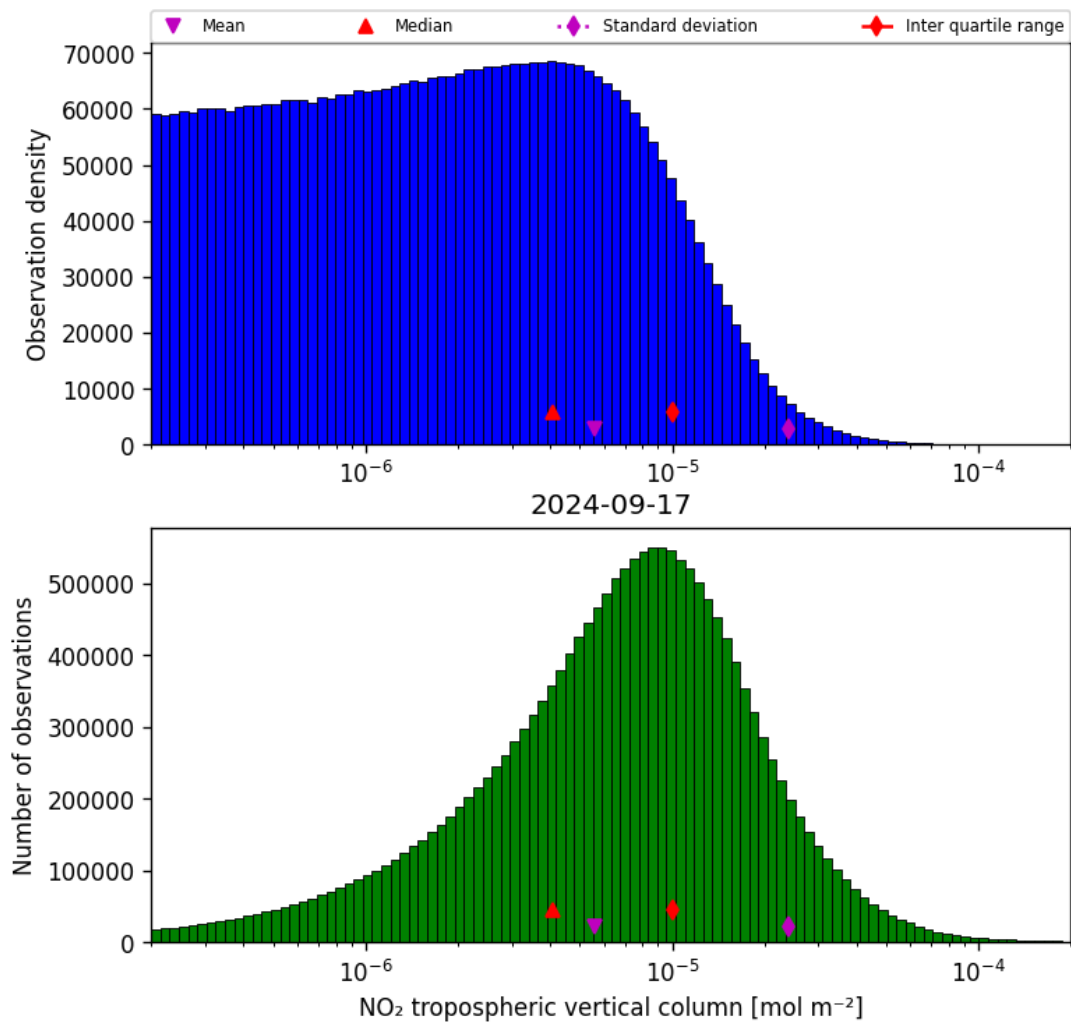
Figure 29: Histogram of “NO 2 tropospheric vertical column” for 2024-09-17 to 2024-09-18
