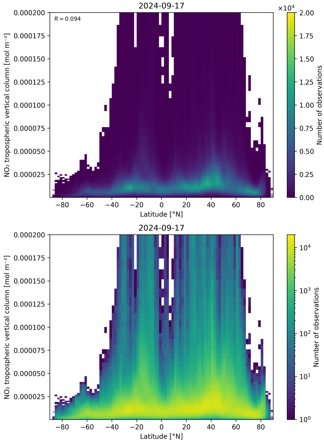
Figure 92: Scatter density plot of “Latitude” against “NO 2 tropospheric vertical column” for 2024-09-17 to 2024-09-18.
