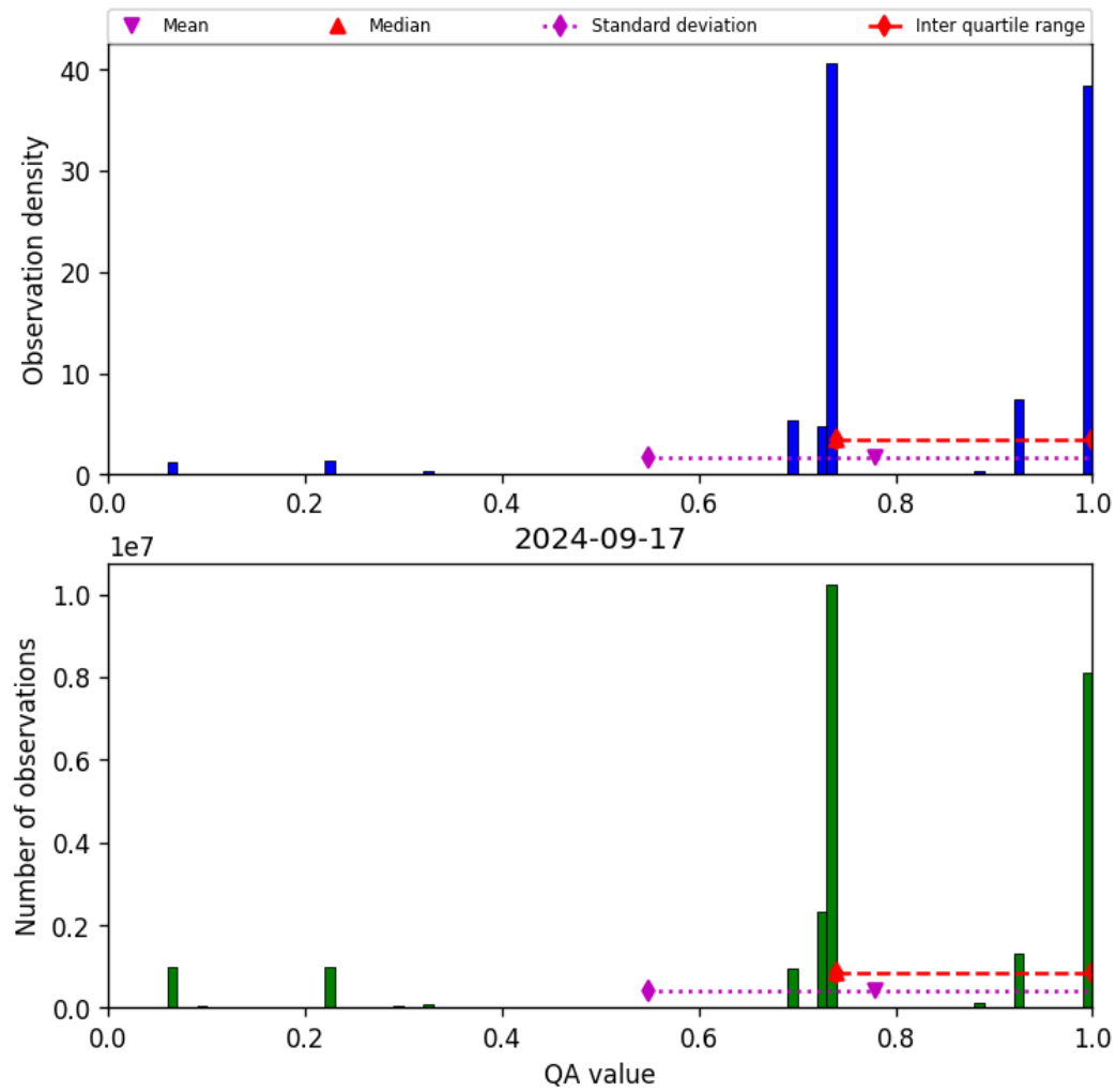
Figure 28: Histogram of “QA value” for 2024-09-17 to 2024-09-18
