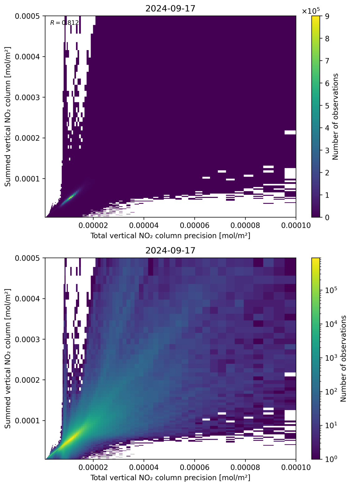
Figure 117: Scatter density plot of “Total vertical NO 2 column precision” against “Summed vertical NO 2 column” for 2024-09-17 to 2024-09-18.
