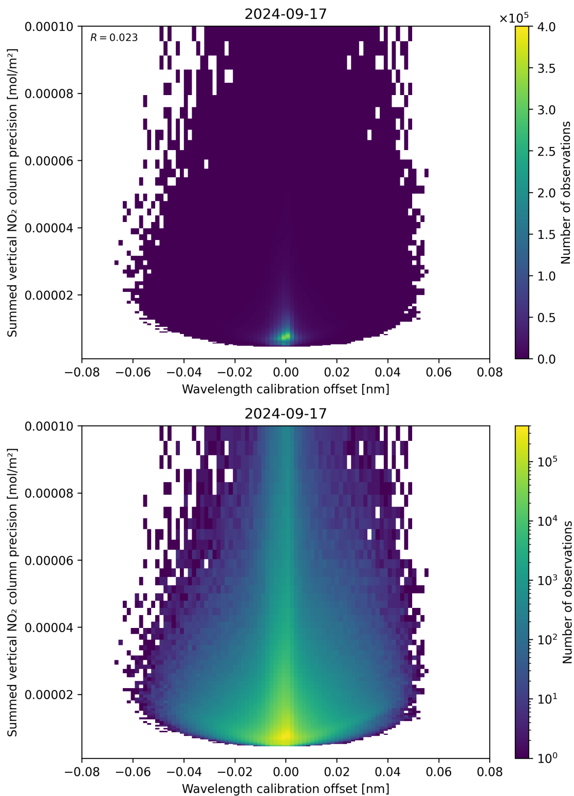
Figure 178: Scatter density plot of “Wavelength calibration offset” against “Summed vertical NO 2 column precision” for 2024-09-17 to 2024-09-18.
