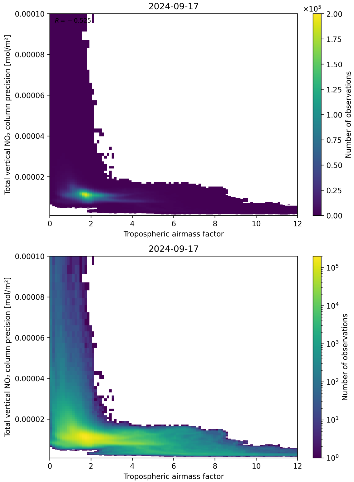
Figure 78: Scatter density plot of “Tropospheric air mass factor” against “Total vertical NO 2 column precision” for 2024-09-17 to 2024-09-18.
