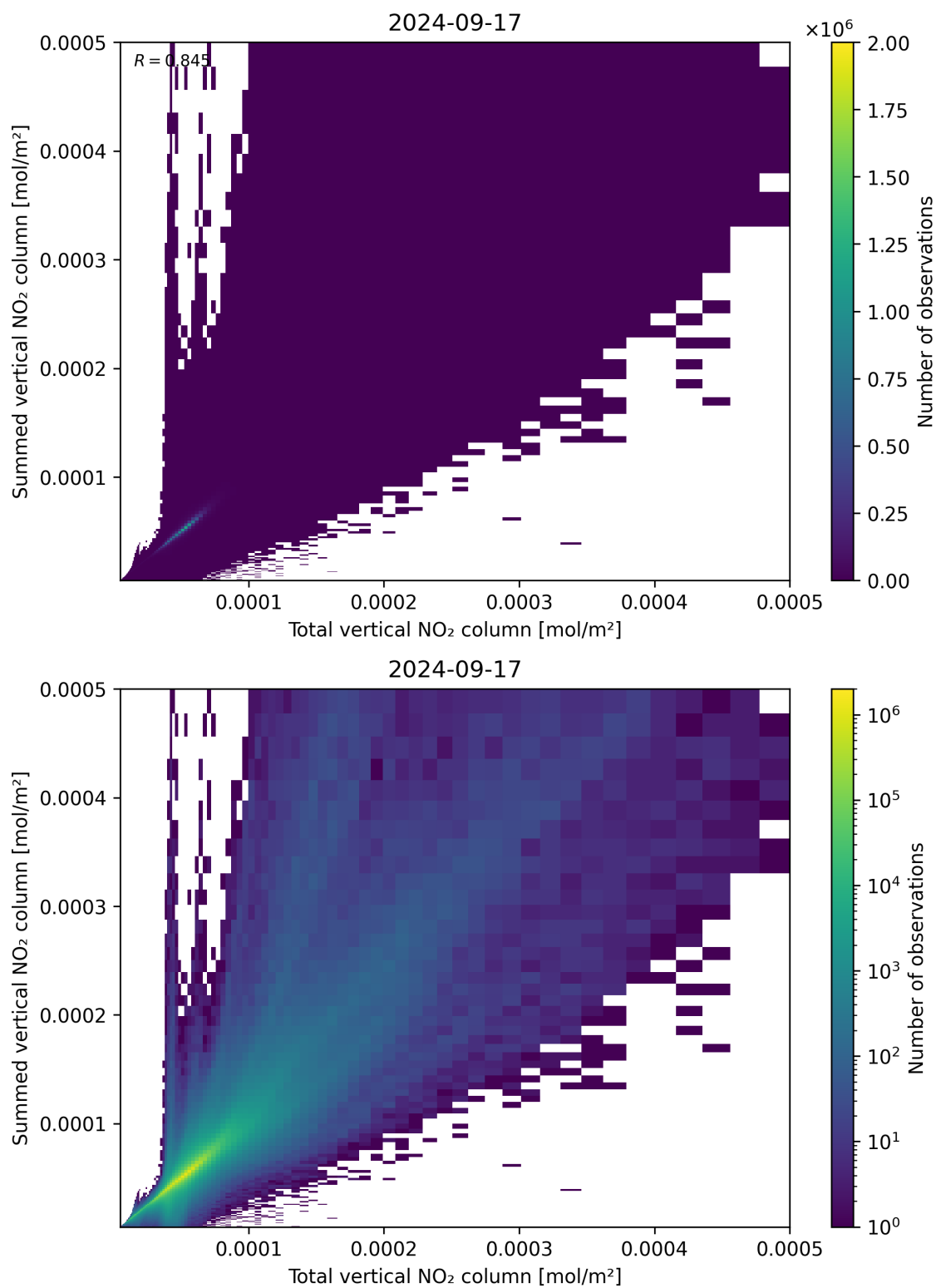
Figure 112: Scatter density plot of “Total vertical NO 2 column” against “Summed vertical NO 2 column” for 2024-09-17 to 2024-09-18.
