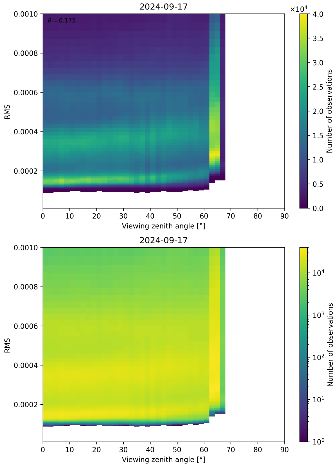
Figure 171: Scatter density plot of “Viewing zenith angle” against “RMS” for 2024-09-17 to 2024-09-18.
