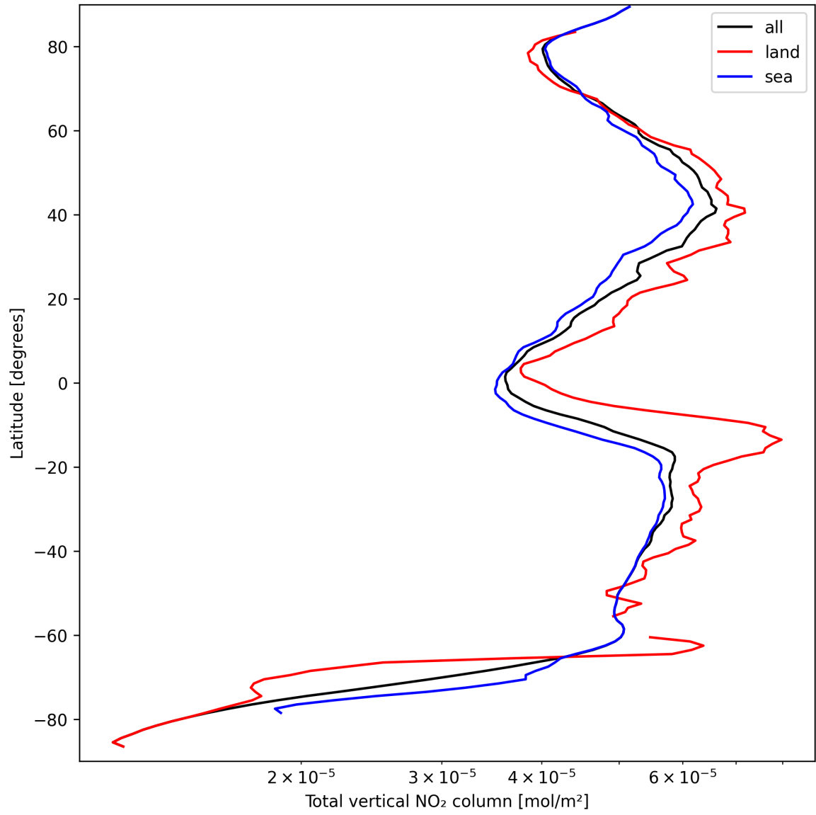
Figure 21: Zonal average of “Total vertical NO 2 column” for 2024-09-17 to 2024-09-18.
