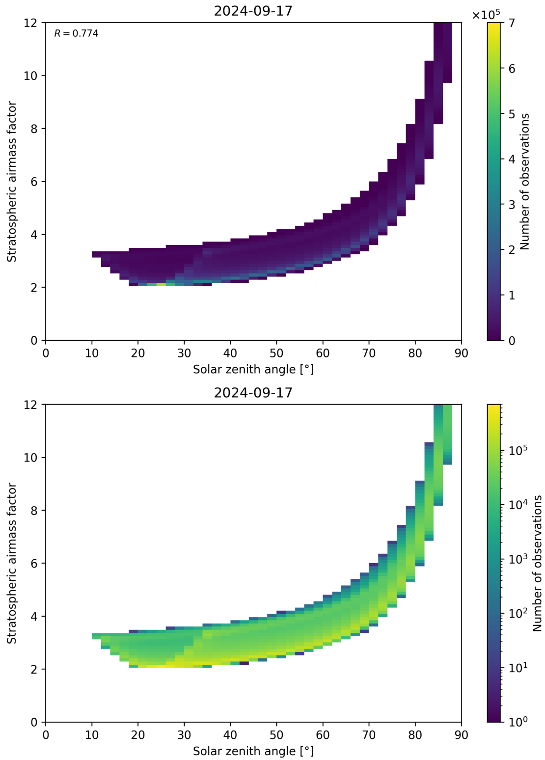
Figure 145: Scatter density plot of “Solar zenith angle” against “Stratospheric airmass factor” for 2024-09-17 to 2024-09-18.
