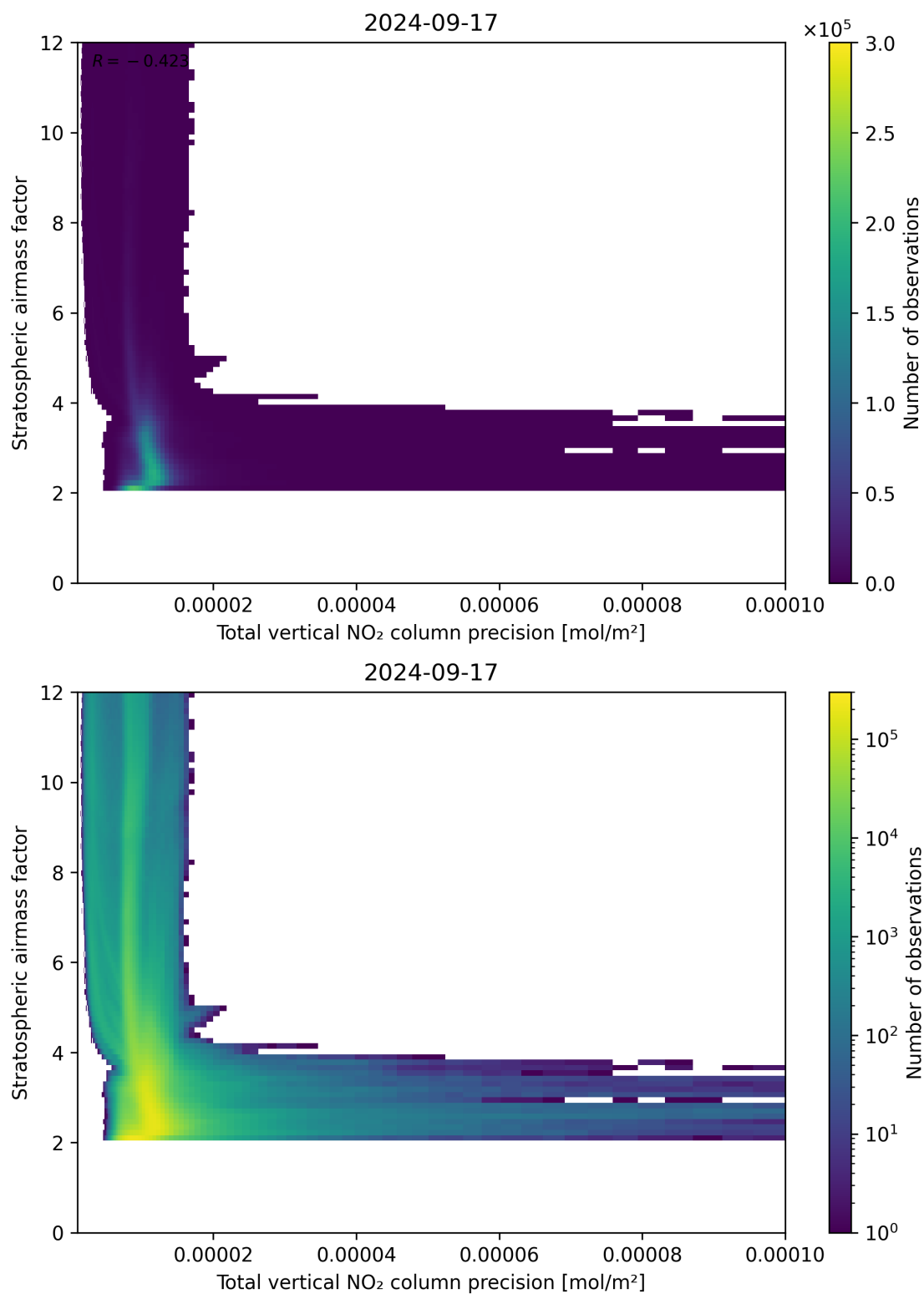
Figure 115: Scatter density plot of “Total vertical NO 2 column precision” against “Stratospheric air mass factor” for 2024-09-17 to 2024-09-18.
