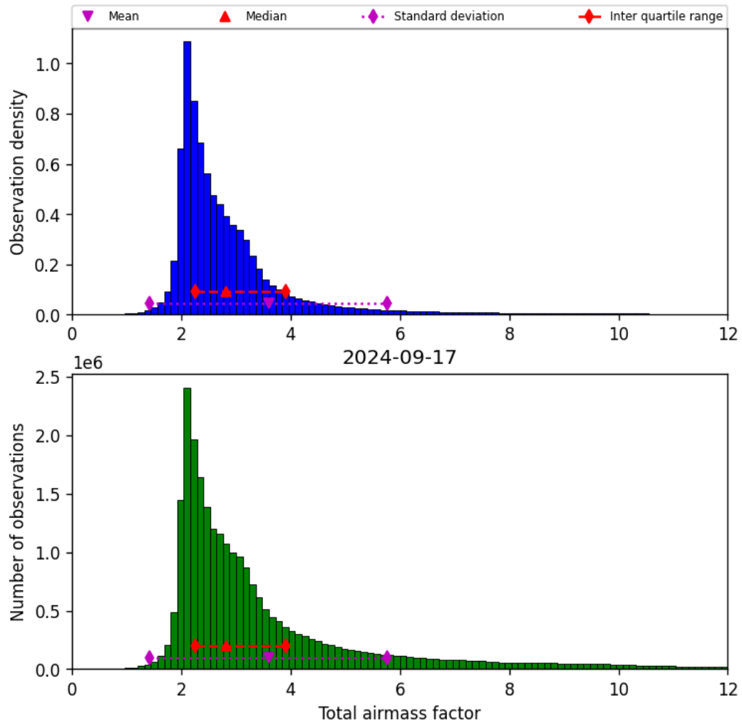
Figure 32: Histogram of “Total airmass factor” for 2024-09-17 to 2024-09-18
