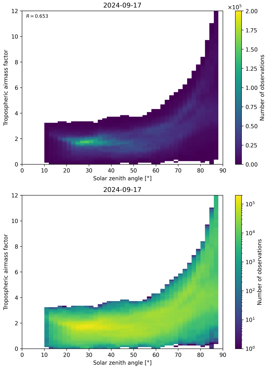
Figure 147: Scatter density plot of “Solar zenith angle” against “Tropospheric airmass factor” for 2024-09-17 to 2024-09-18.
