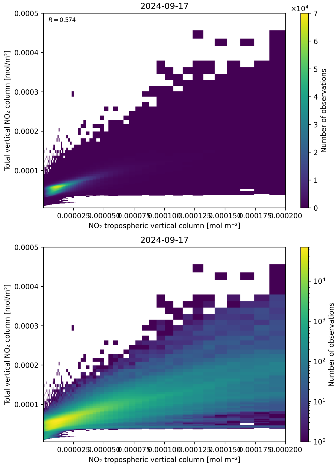
Figure 128: Scatter density plot of “NO 2 tropospheric vertical column” against “Total vertical NO 2 column” for 2024-09-17 to 2024-09-18.
