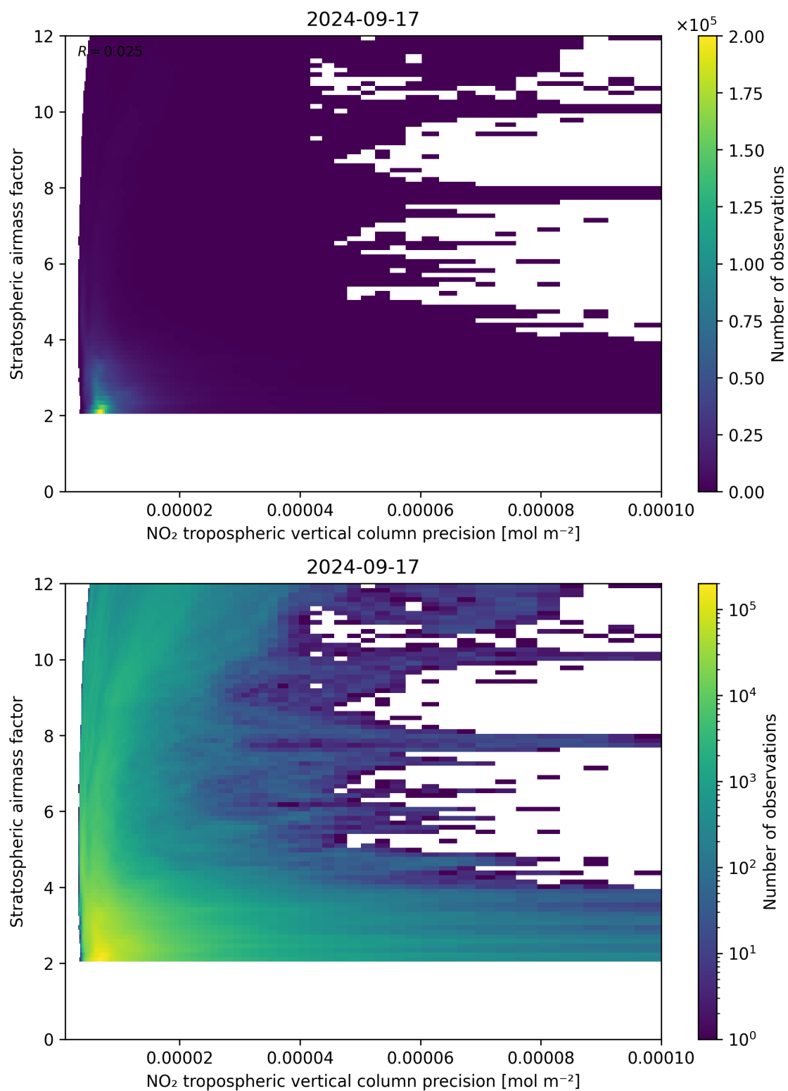
Figure 131: Scatter density plot of “NO 2 tropospheric vertical column precision” against “Stratospheric airmass factor” for 2024-09-17 to 2024-09-18.
