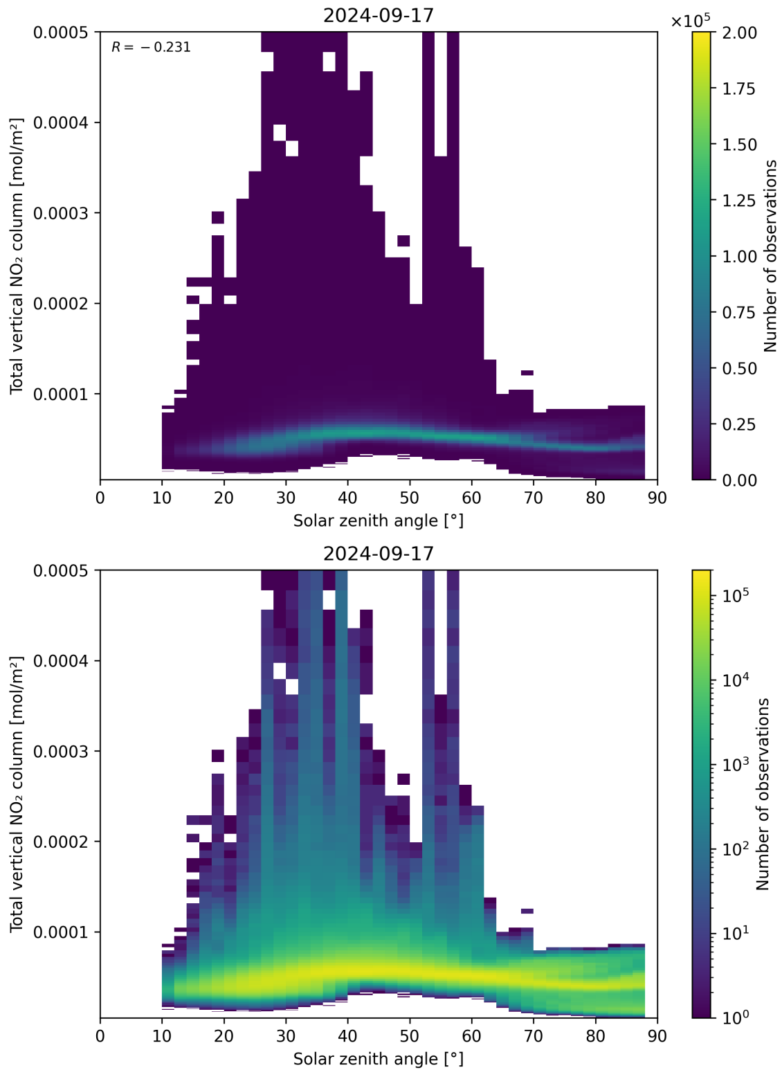
Figure 153: Scatter density plot of “Solar zenith angle” against “Total vertical NO 2 column” for 2024-09-17 to 2024-09-18.
