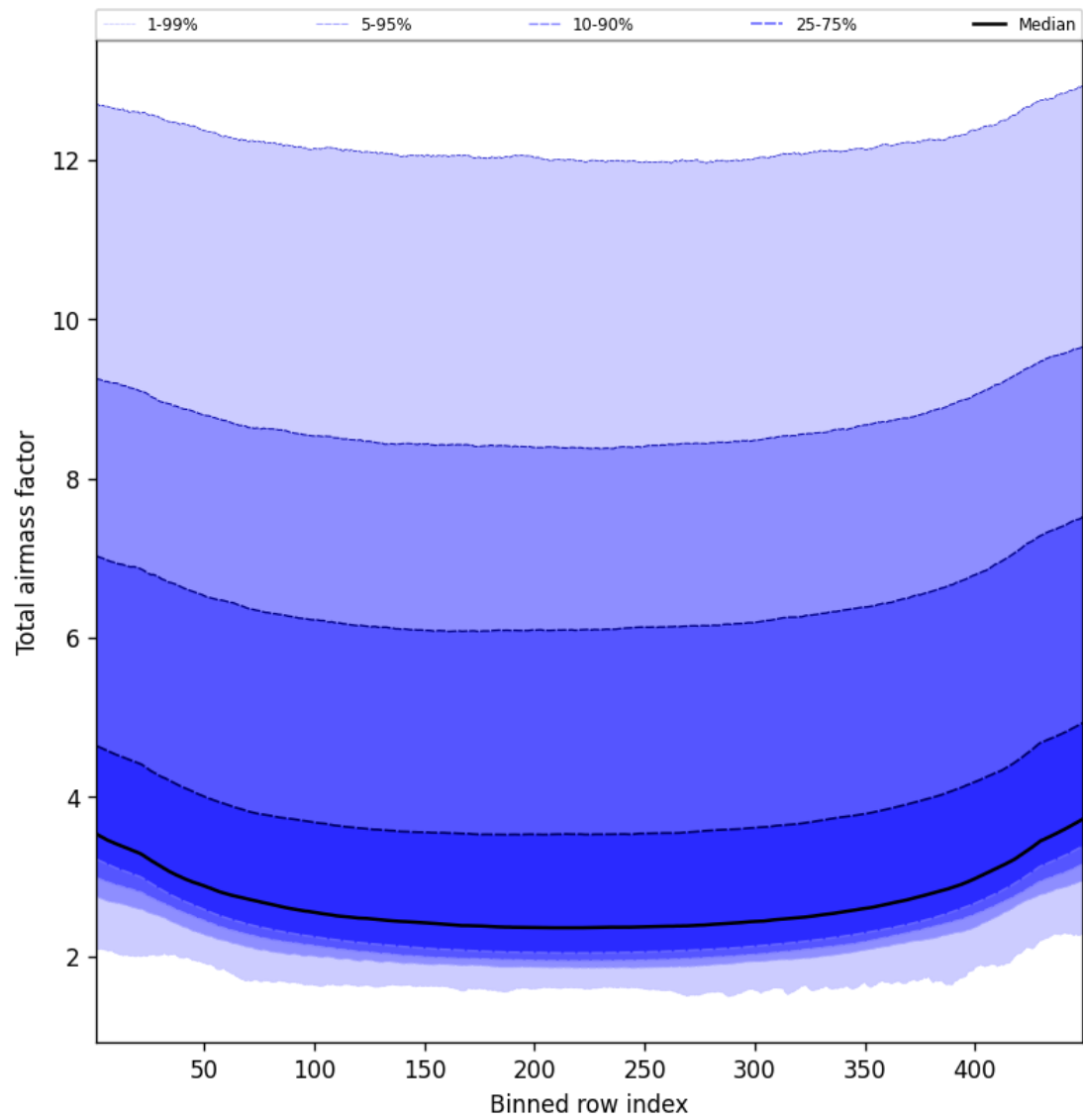
Figure 49: Along track statistics of “Total airmass factor” for 2024-09-17 to 2024-09-18
