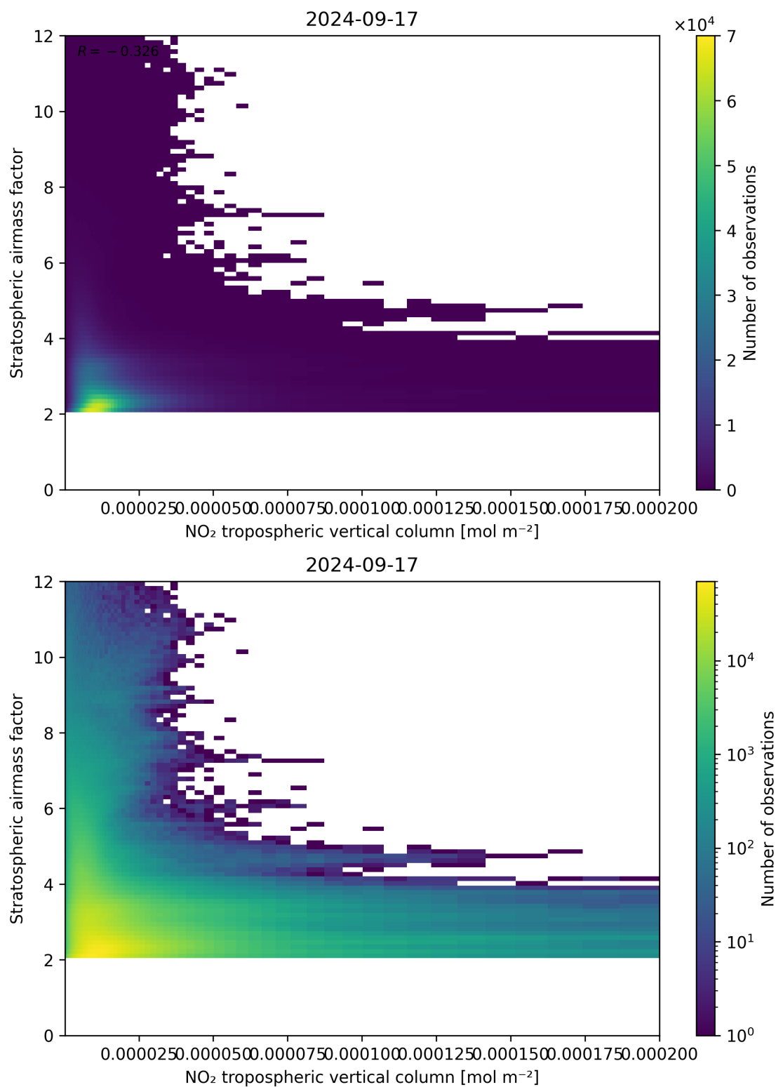
Figure 121: Scatter density plot of “NO 2 tropospheric vertical column” against “Stratospheric air mass factor” for 2024-09-17 to 2024-09-18.
