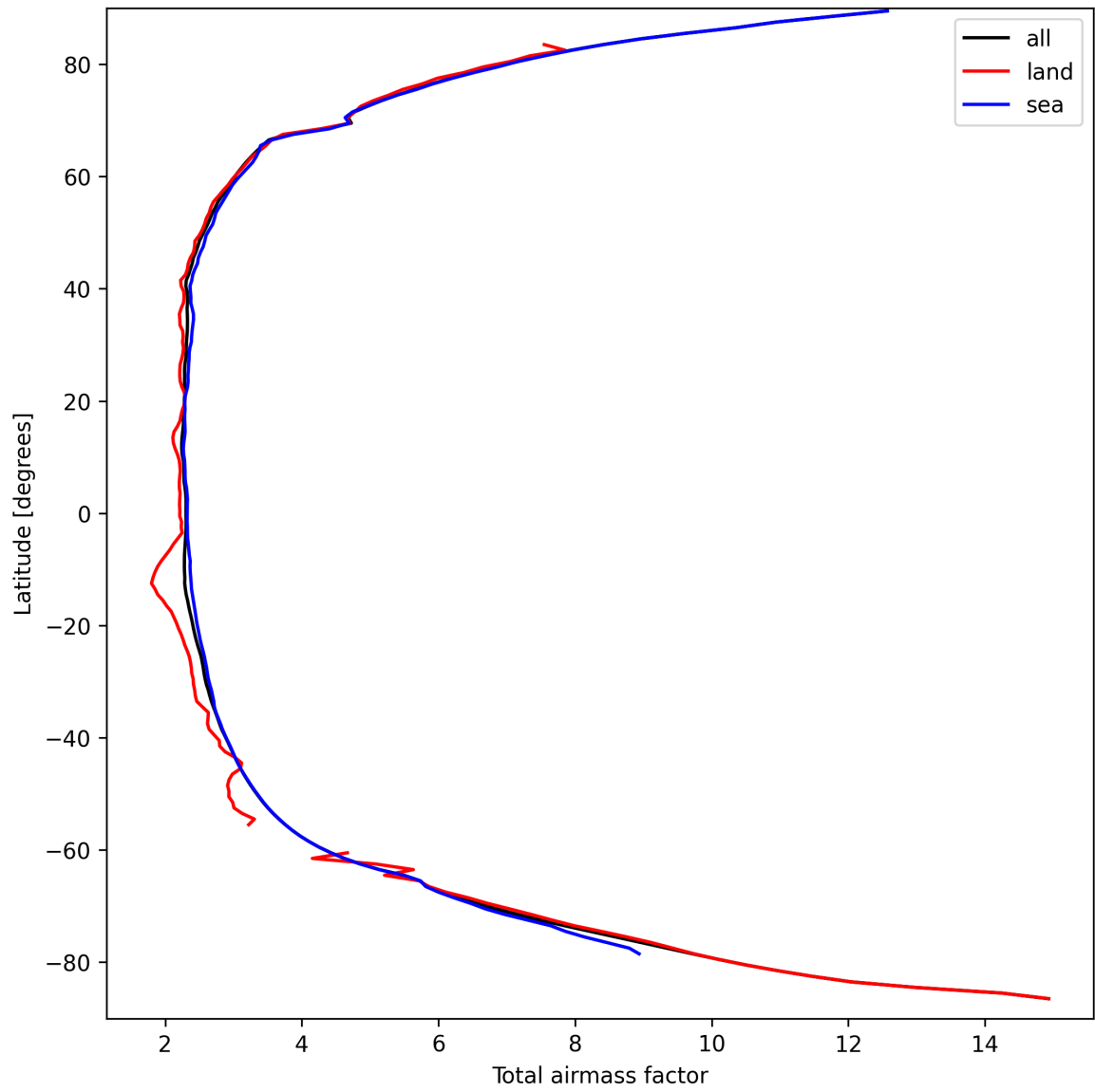
Figure 15: Zonal average of “Total airmass factor” for 2024-09-17 to 2024-09-18.
