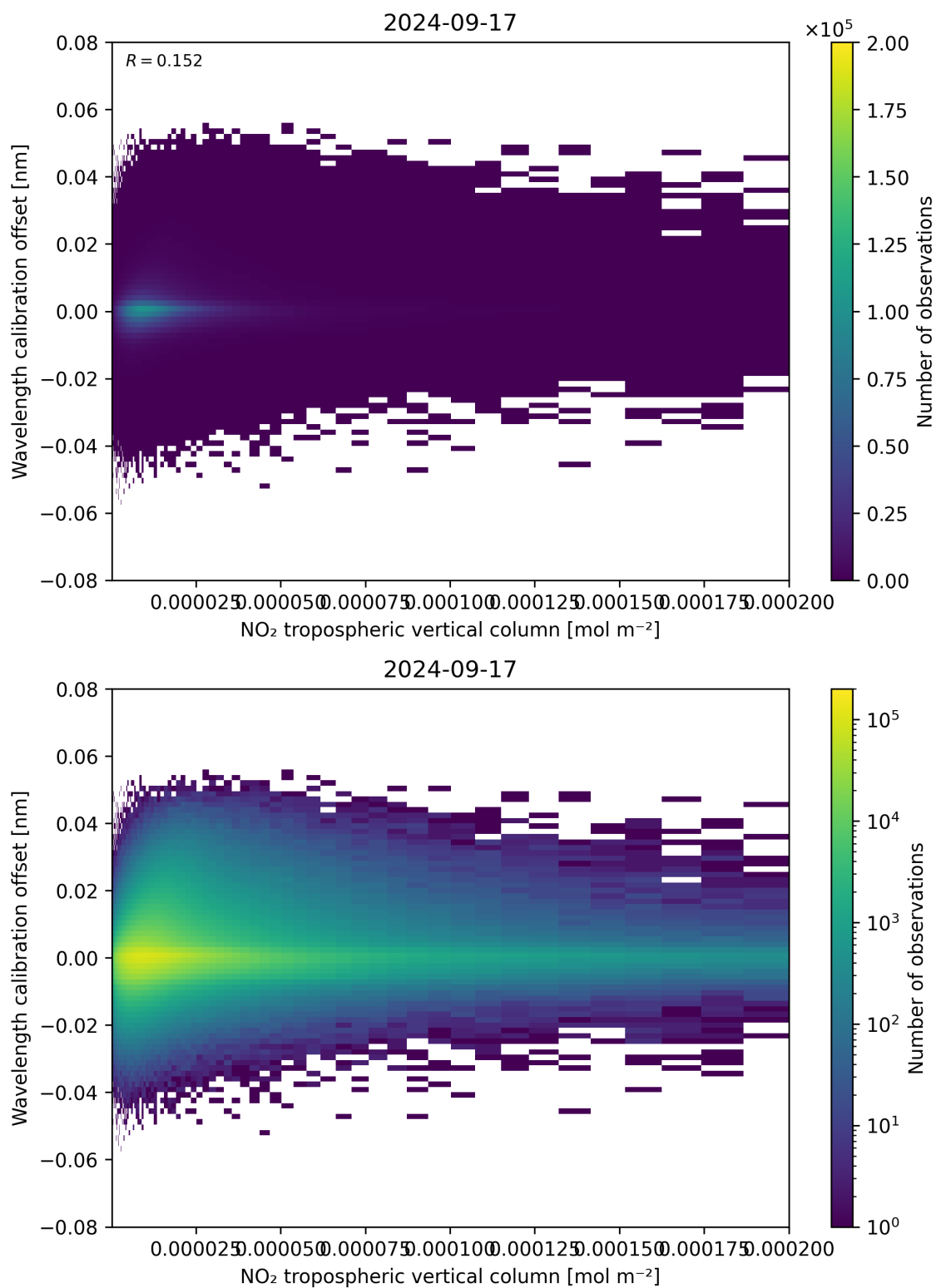
Figure 143: Scatter density plot of “NO 2 tropospheric vertical column” against “Wavelength calibration offset” for 2024-09-17 to 2024-09-18.
