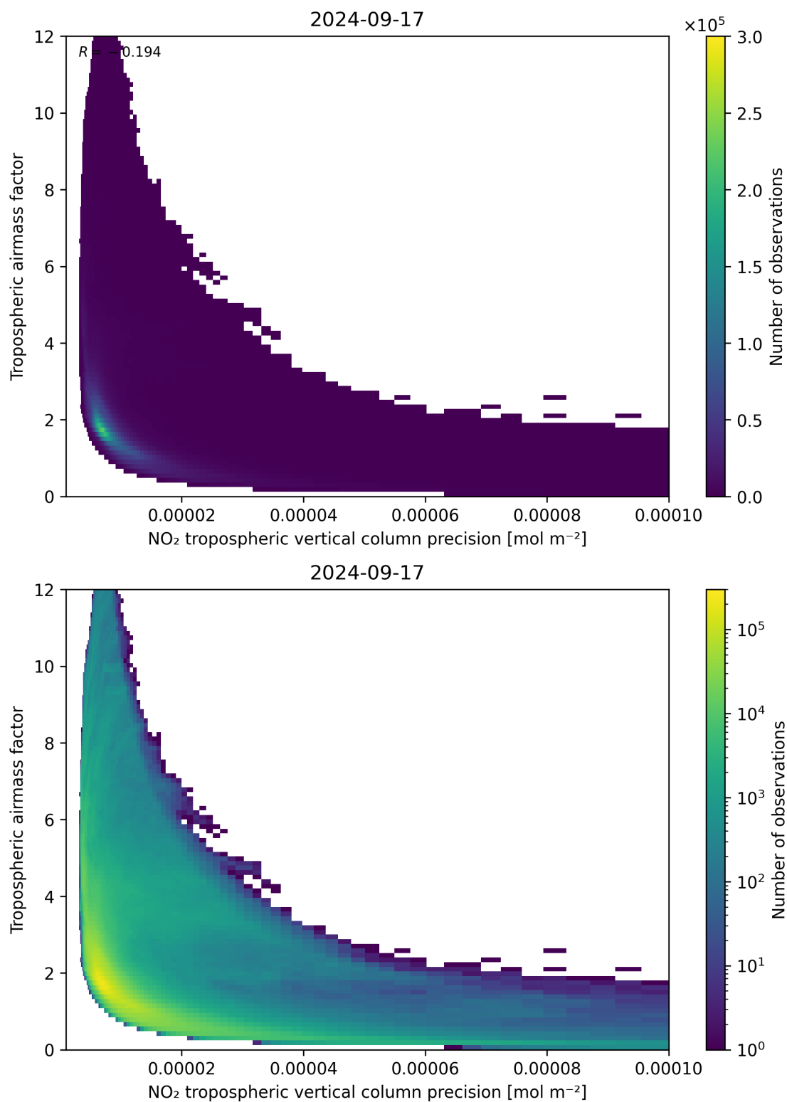
Figure 133: Scatter density plot of “NO 2 tropospheric vertical column precision” against “Tropospheric airmass factor” for 2024-09-17 to 2024-09-18.
