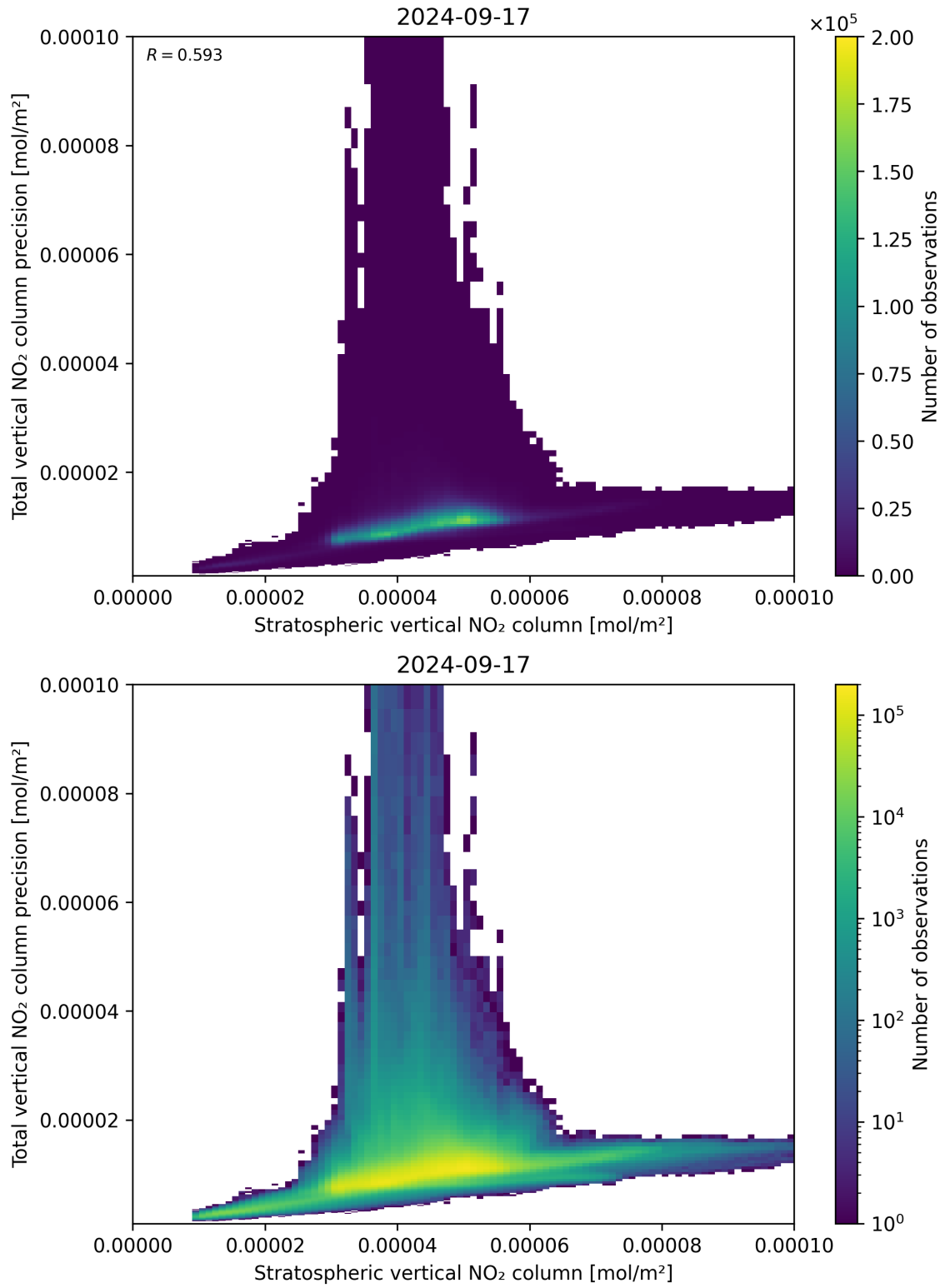
Figure 101: Scatter density plot of “Stratospheric vertical NO 2 column” against “Total vertical NO 2 column precision” for 2024-09-17 to 2024-09-18.
