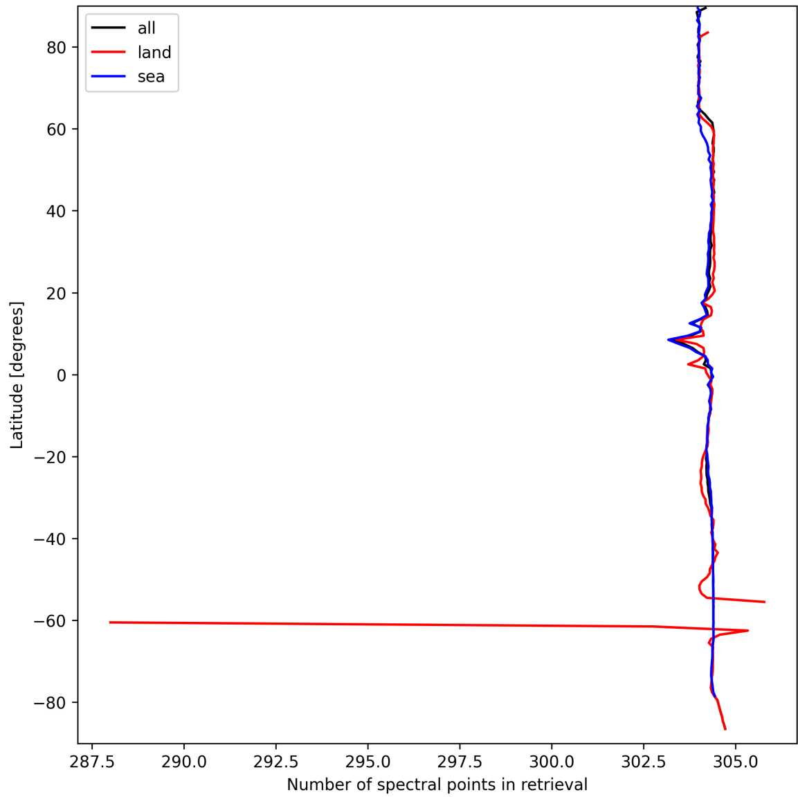
Figure 16: Zonal average of “Number of spectral points in retrieval” for 2024-09-17 to 2024-09-18.
