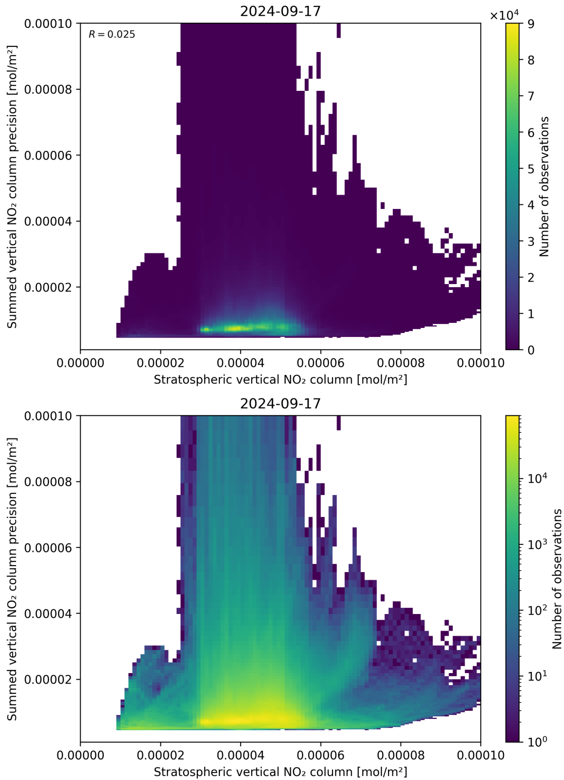
Figure 99: Scatter density plot of “Stratospheric vertical NO 2 column” against “Summed vertical NO 2 column precision” for 2024-09-17 to 2024-09-18.
