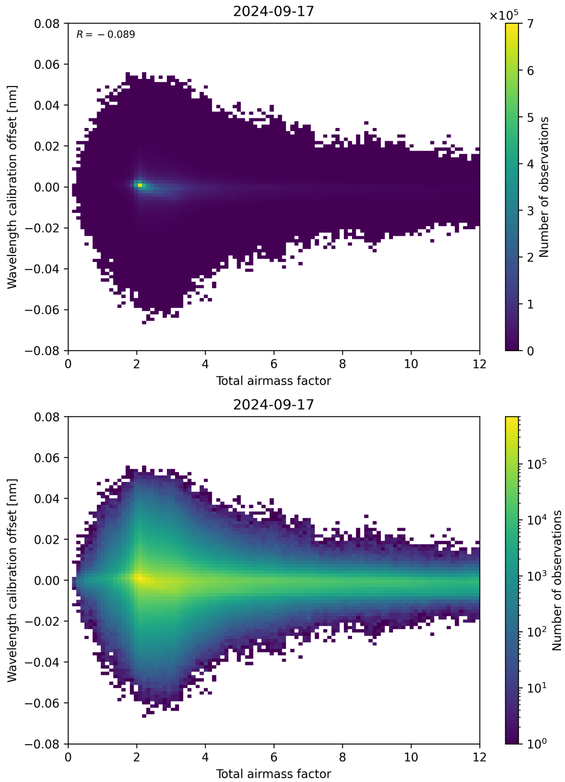
Figure 70: Scatter density plot of “Total airmass factor” against “Wavelength calibration offset” for 2024-09-17 to 2024-09-18.
