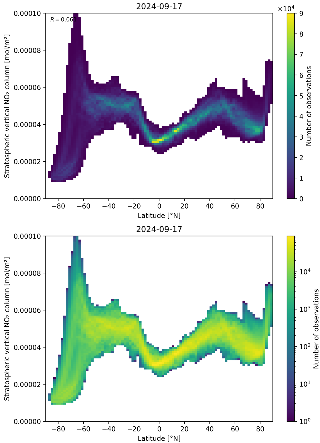
Figure 87: Scatter density plot of “Latitude” against “Stratospheric vertical NO 2 column” for 2024-09-17 to 2024-09-18.
