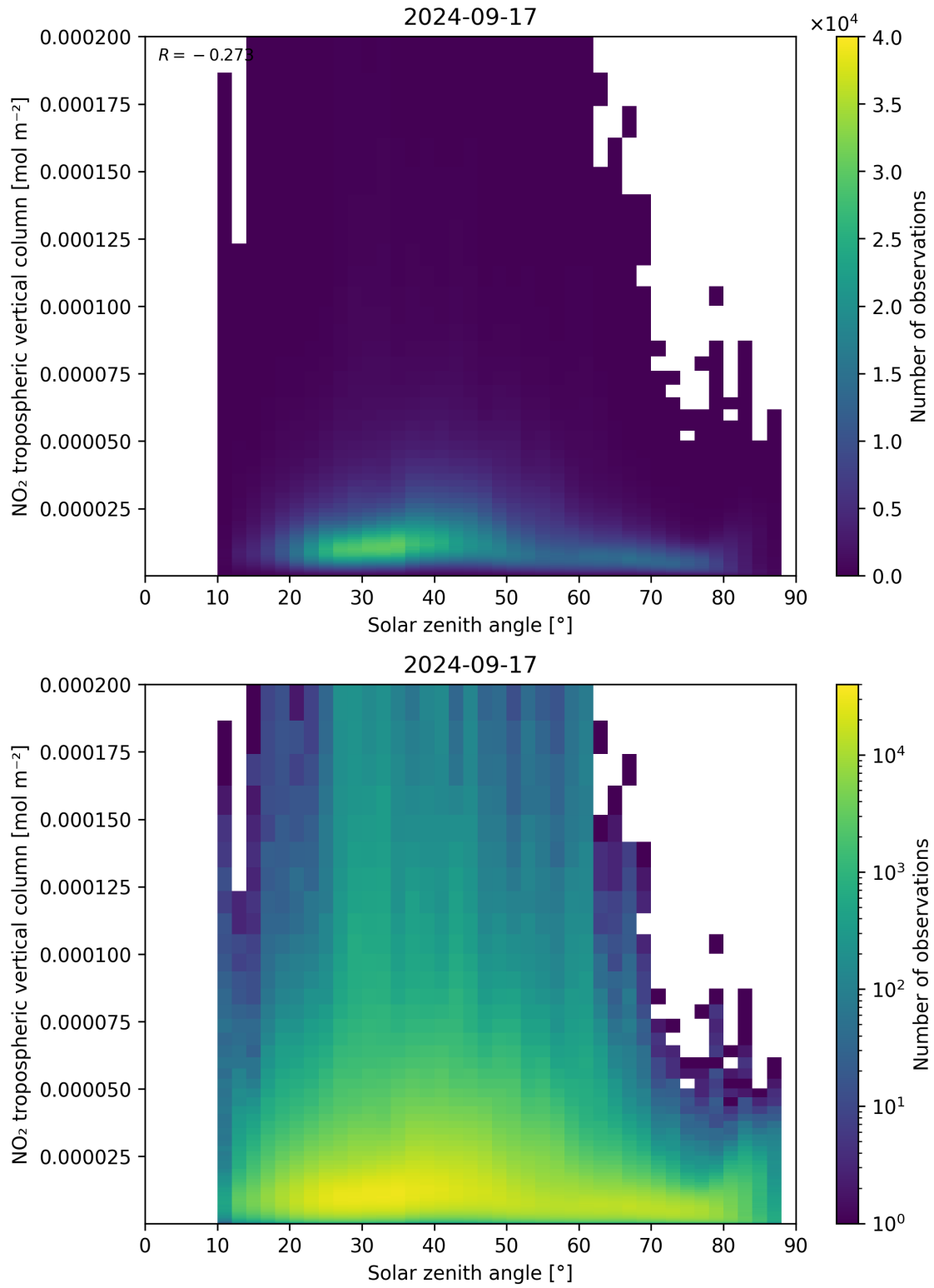
Figure 155: Scatter density plot of “Solar zenith angle” against “NO 2 tropospheric vertical column” for 2024-09-17 to 2024-09-18.
