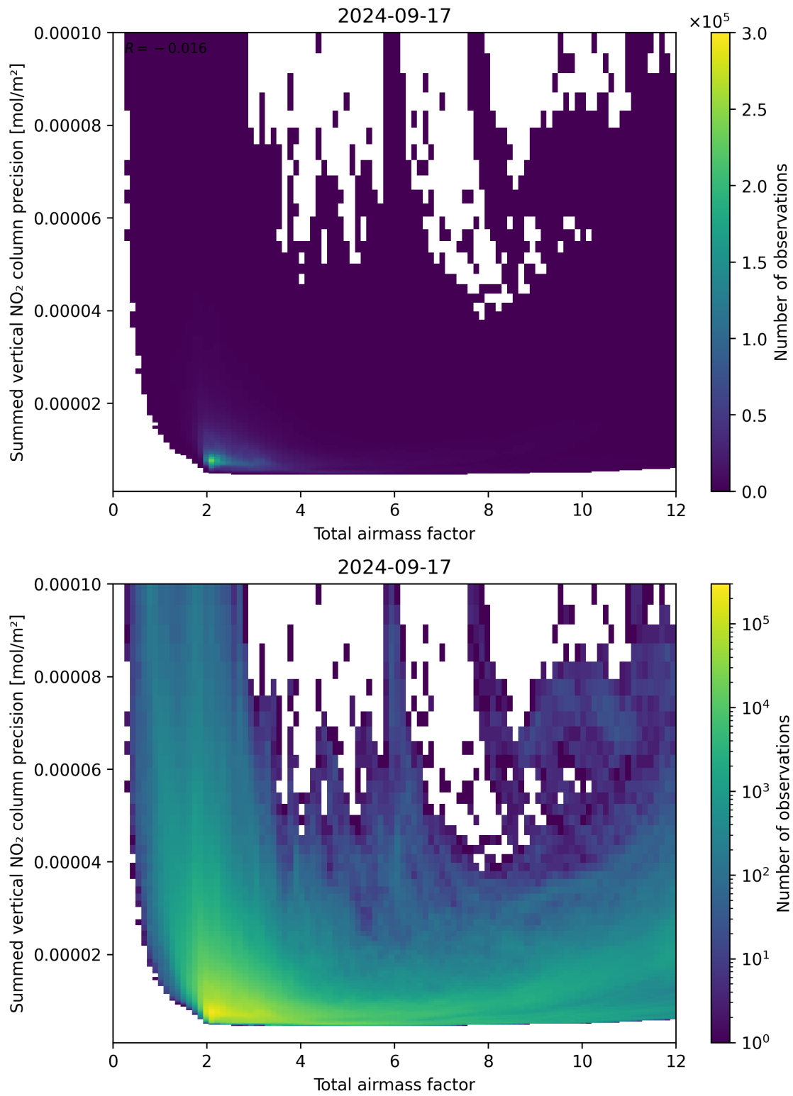
Figure 66: Scatter density plot of “Total airmass factor” against “Summed vertical NO 2 column precision” for 2024-09-17 to 2024-09-18.
