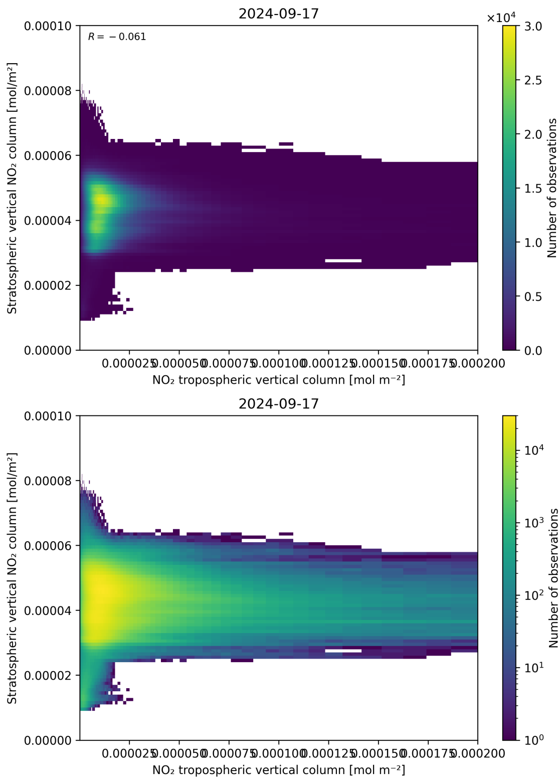
Figure 125: Scatter density plot of “NO 2 tropospheric vertical column” against “Stratospheric vertical NO 2 column” for 2024-09-17 to 2024-09-18.
