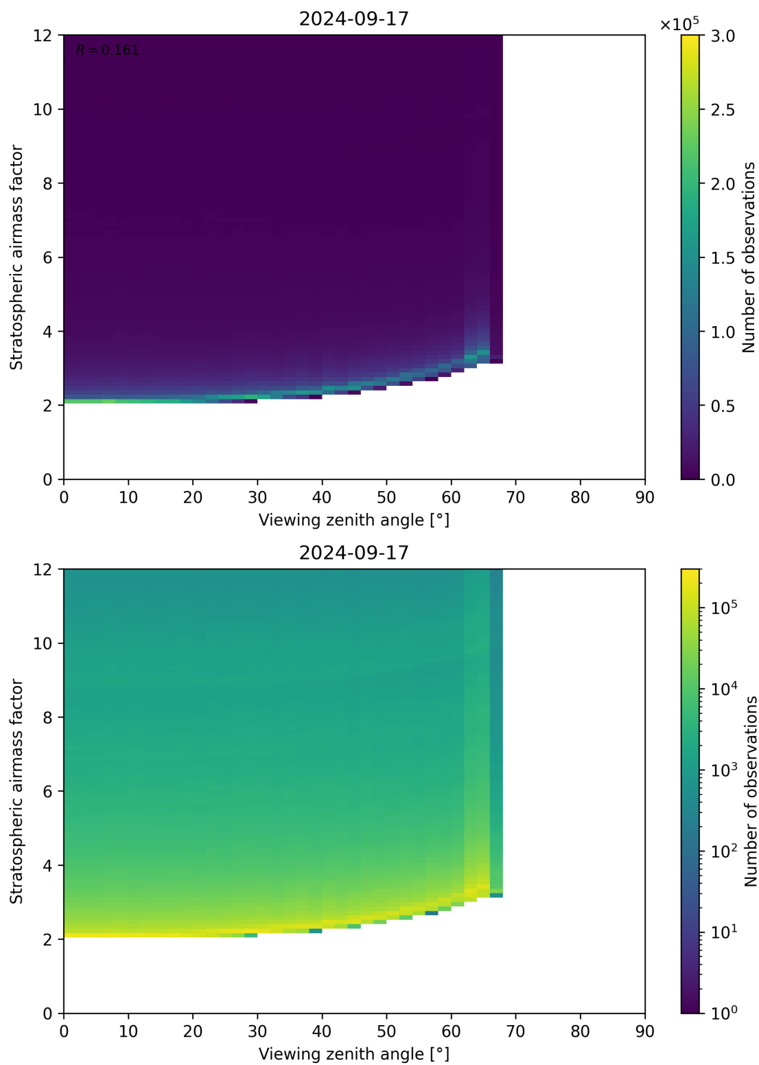
Figure 159: Scatter density plot of “Viewing zenith angle” against “Stratospheric airmass factor” for 2024-09-17 to 2024-09-18.
