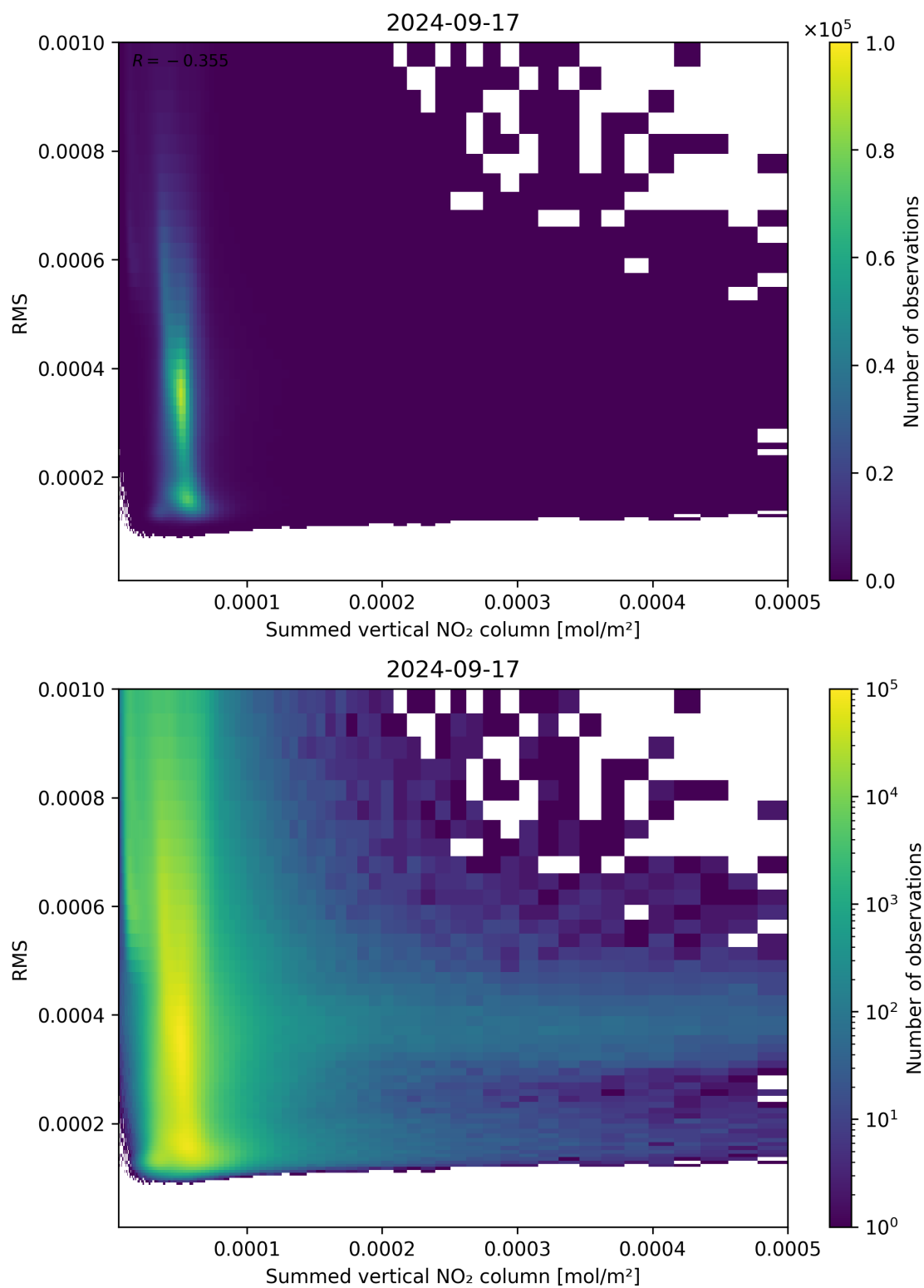
Figure 109: Scatter density plot of “Summed vertical NO 2 column” against “RMS” for 2024-09-17 to 2024-09-18.
