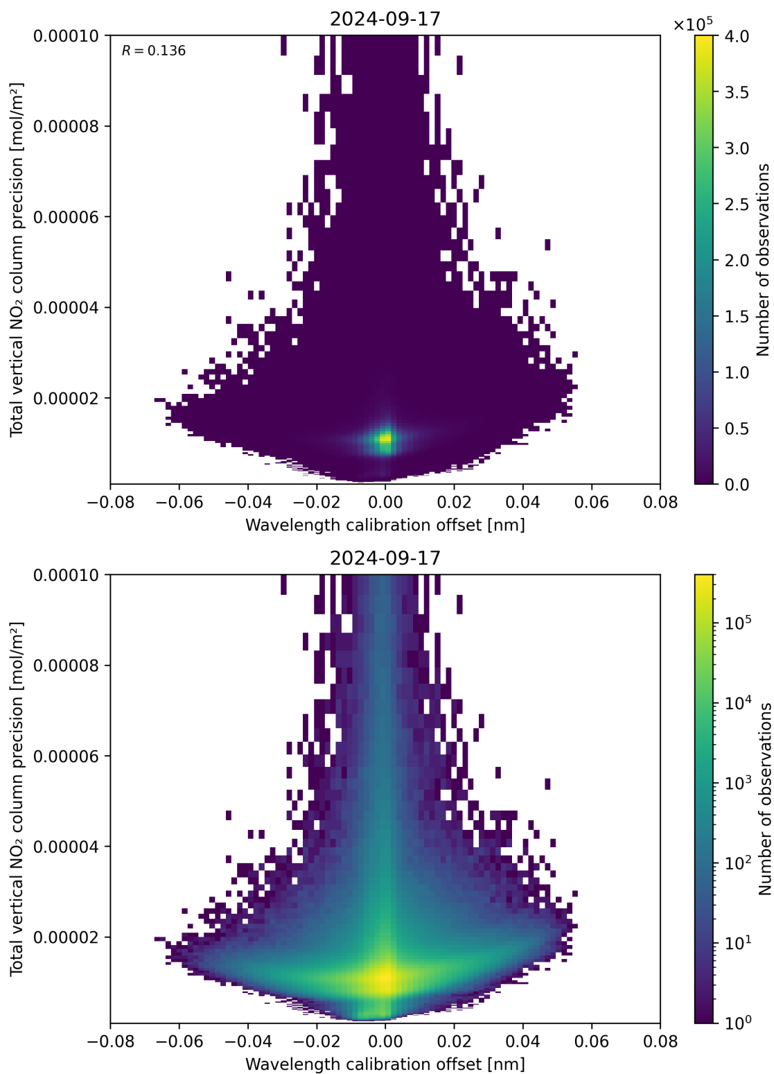
Figure 180: Scatter density plot of “Wavelength calibration offset” against “Total vertical NO 2 column precision” for 2024-09-17 to 2024-09-18.
