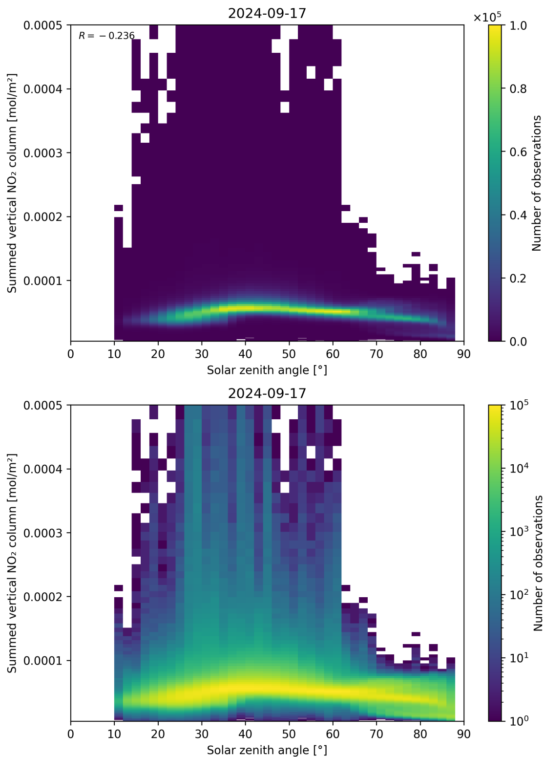
Figure 151: Scatter density plot of “Solar zenith angle” against “Summed vertical NO 2 column” for 2024-09-17 to 2024-09-18.
