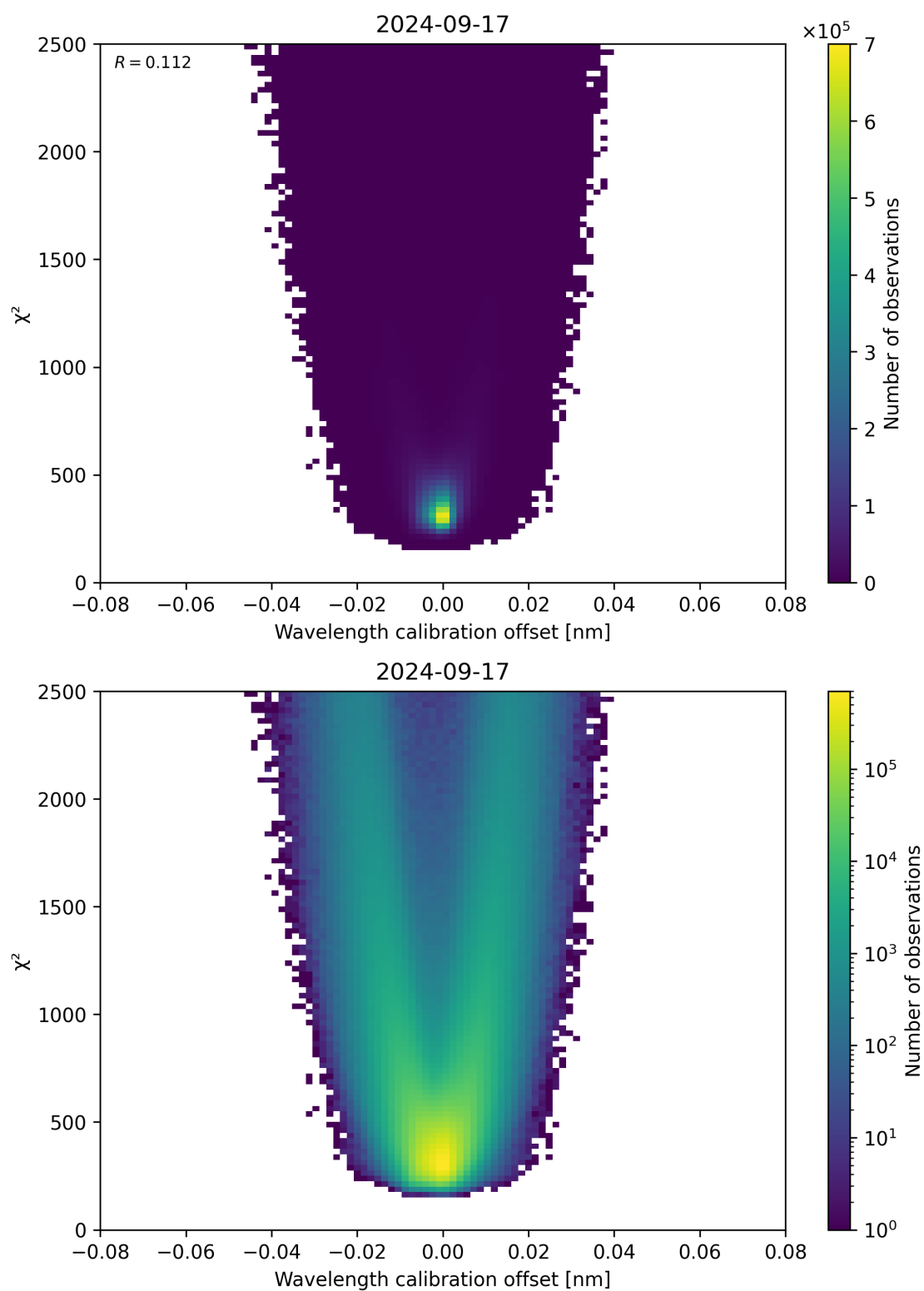
Figure 175: Scatter density plot of “Wavelength calibration offset” against “ \chi^2 ” for 2024-09-17 to 2024-09-18.
