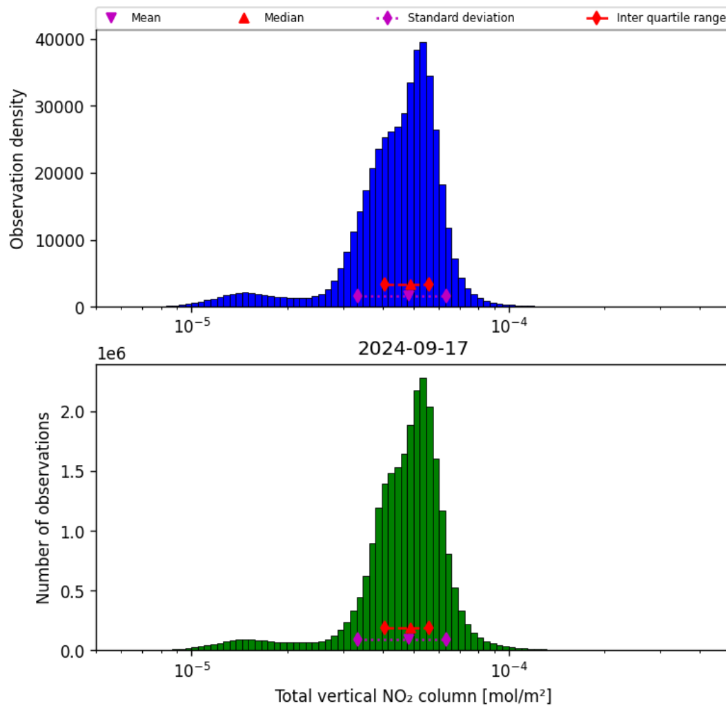
Figure 38: Histogram of “Total vertical NO 2 column” for 2024-09-17 to 2024-09-18
