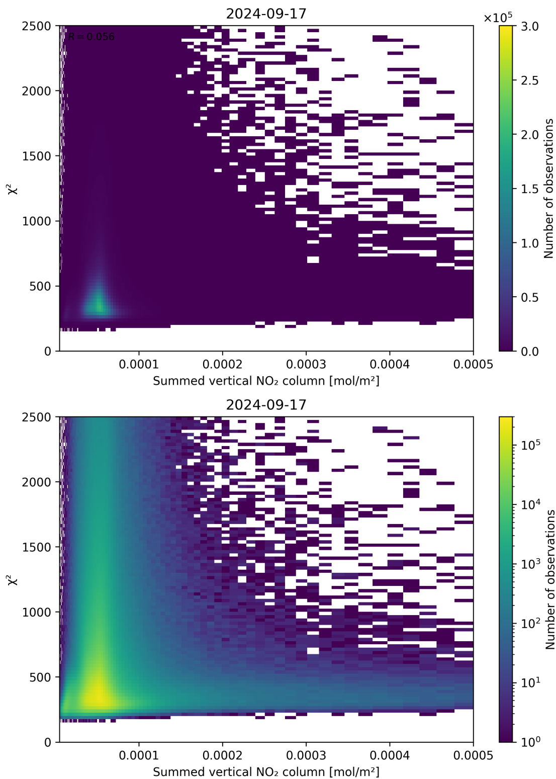
Figure 104: Scatter density plot of “Summed vertical NO 2 column” against “ \chi^2 ” for 2024-09-17 to 2024-09-18.
