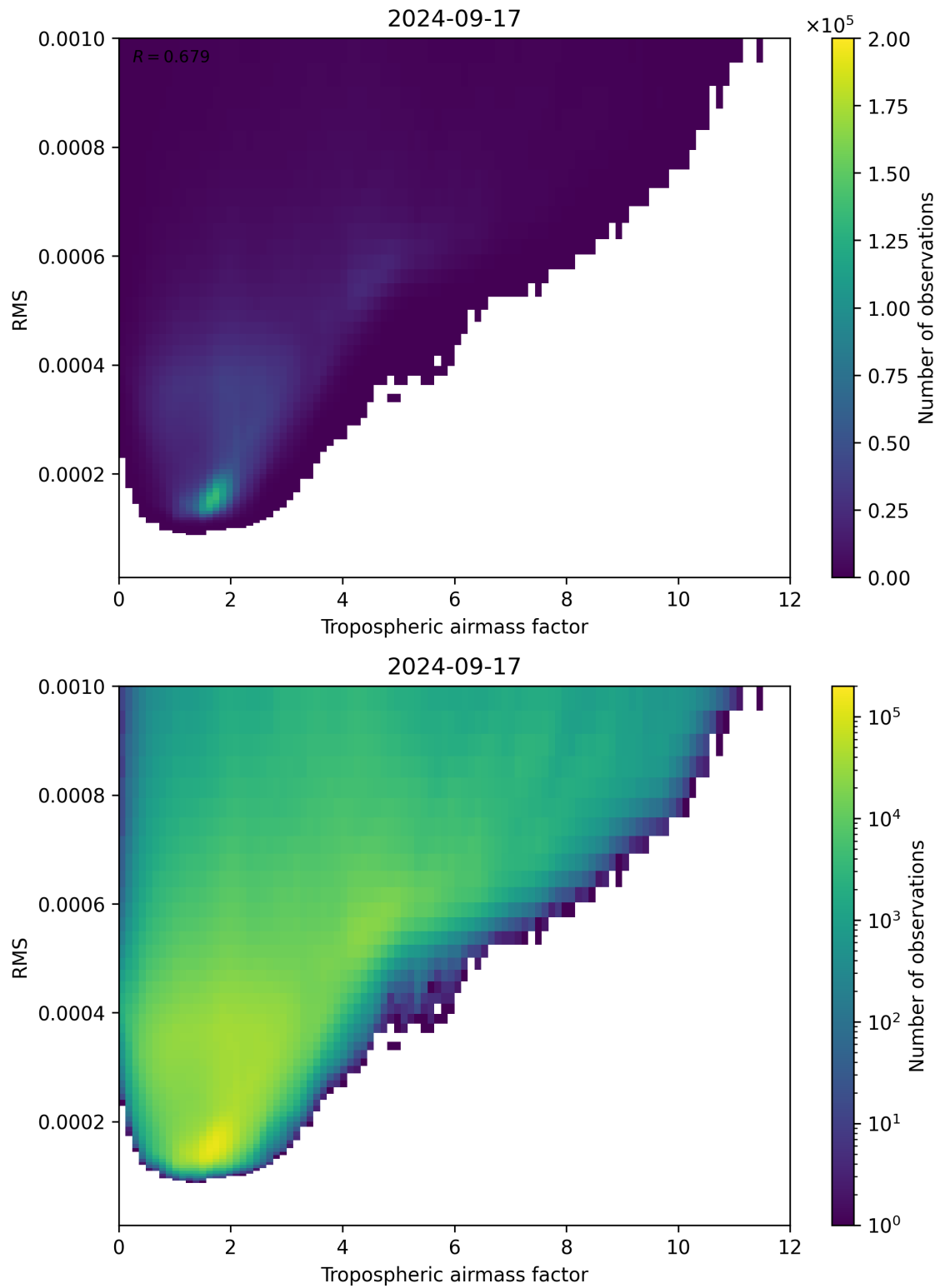
Figure 79: Scatter density plot of “Tropospheric airmass factor” against “RMS” for 2024-09-17 to 2024-09-18.
