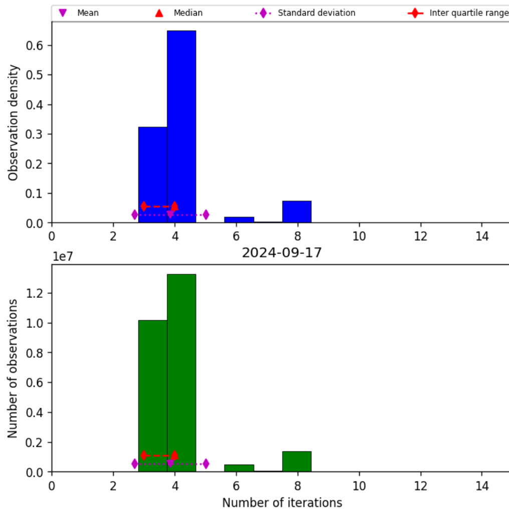
Figure 34: Histogram of “Number of iterations” for 2024-09-17 to 2024-09-18
