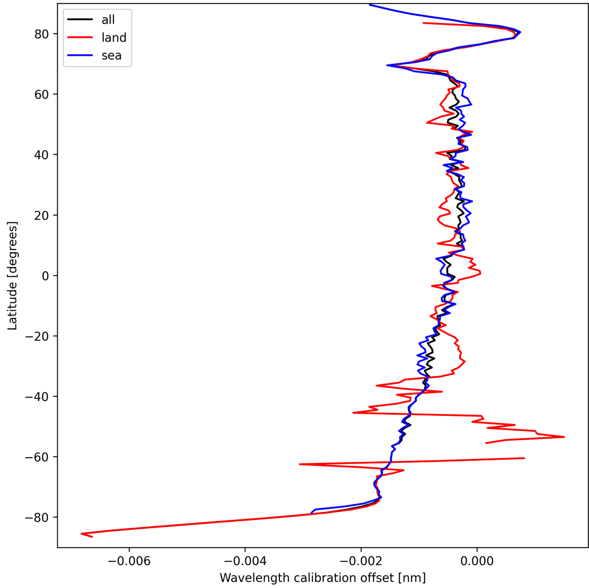
Figure 18: Zonal average of “Wavelength calibration offset” for 2024-09-17 to 2024-09-18.
