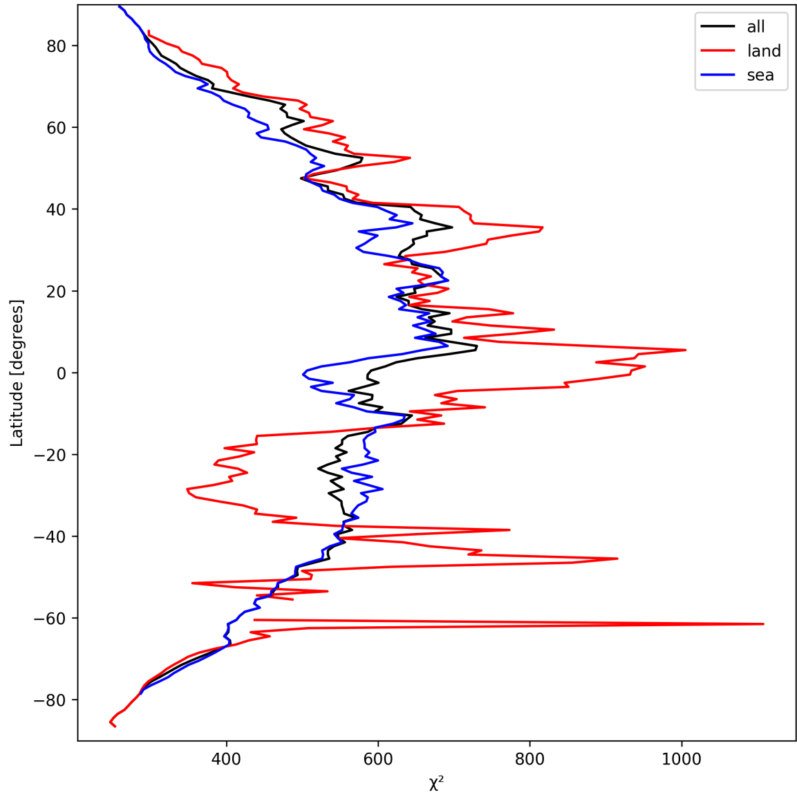
Figure 25: Zonal average of “ \chi^2 ” for 2024-09-17 to 2024-09-18.
