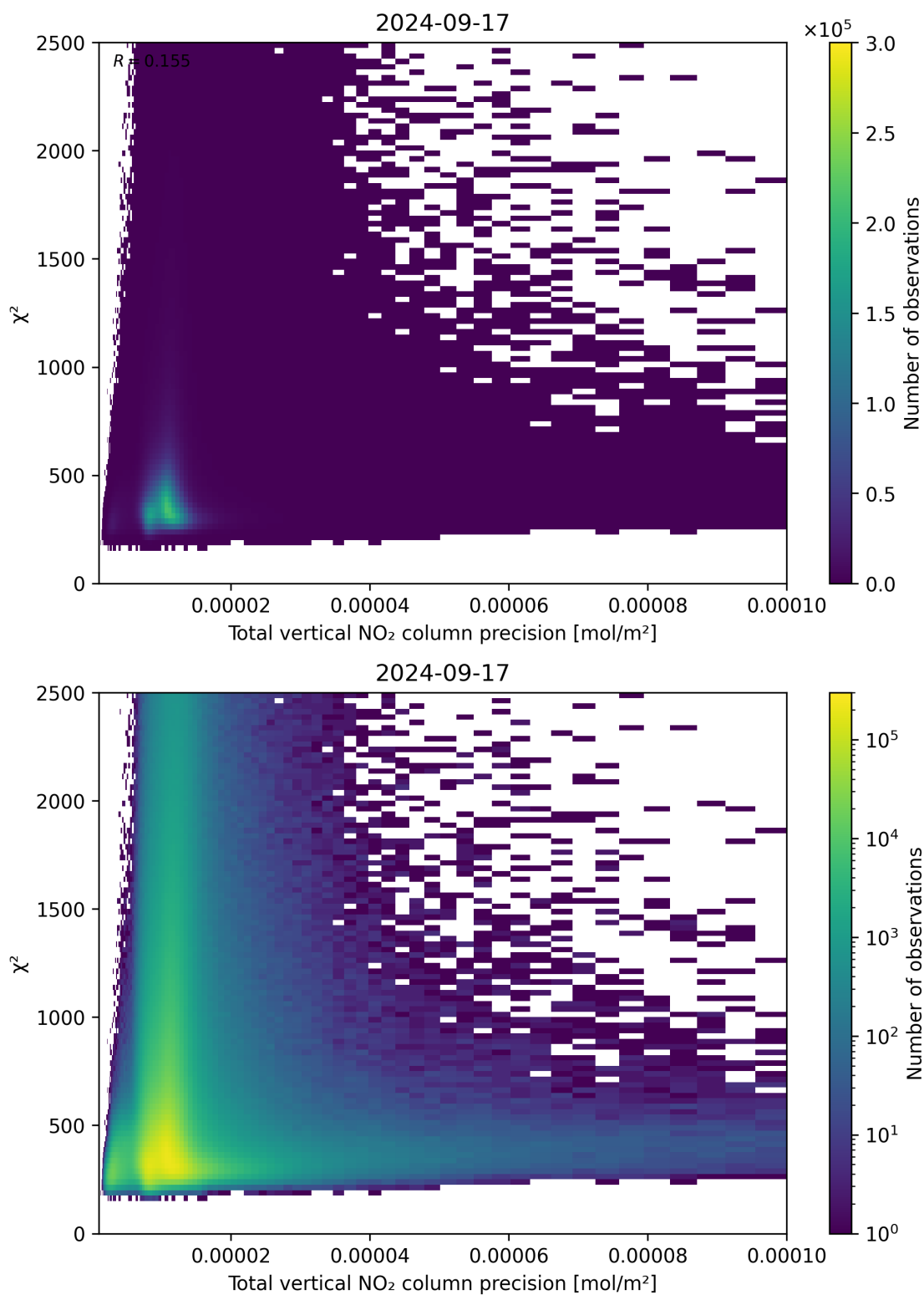
Figure 116: Scatter density plot of “Total vertical NO 2 column precision” against “ \chi^2 ” for 2024-09-17 to 2024-09-18.
