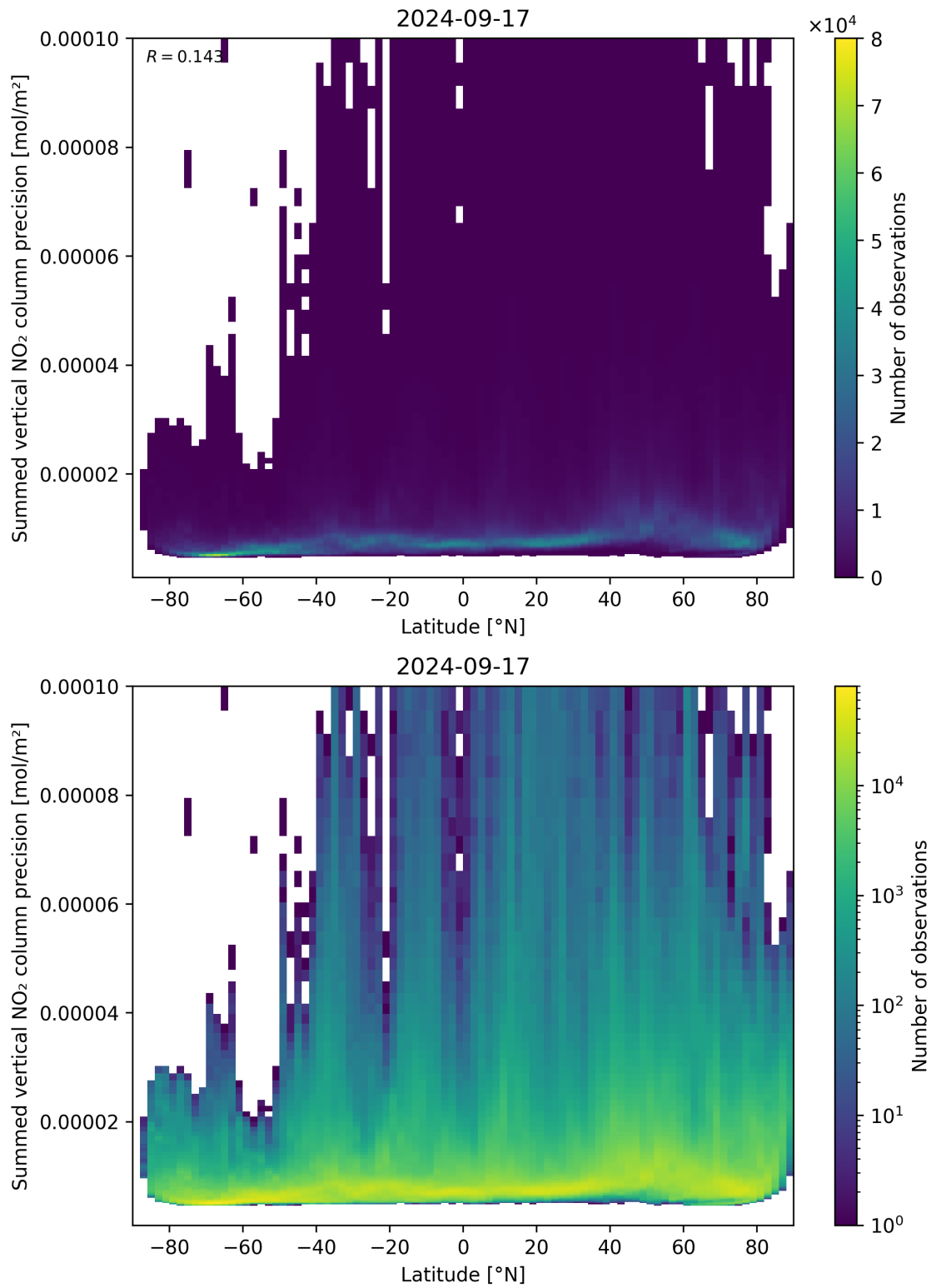
Figure 89: Scatter density plot of “Latitude” against “Summed vertical NO 2 column precision” for 2024-09-17 to 2024-09-18.
