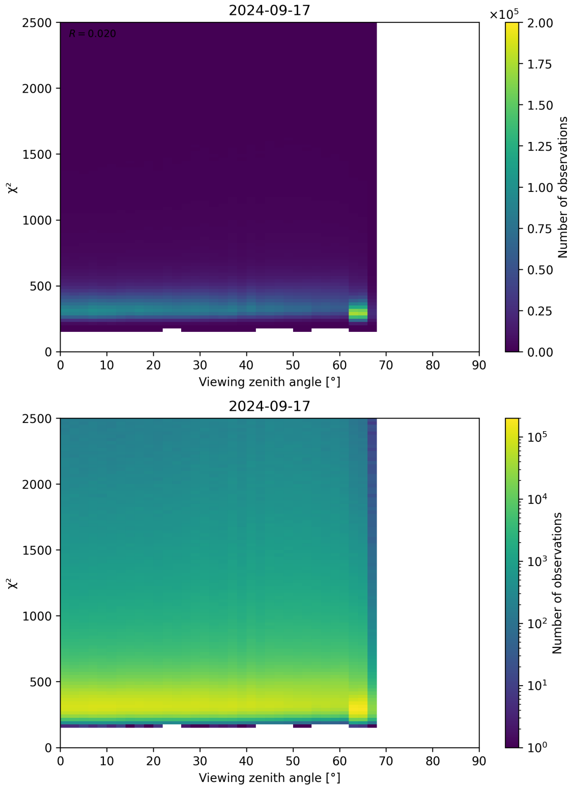
Figure 162: Scatter density plot of “Viewing zenith angle” against “ \chi^2 ” for 2024-09-17 to 2024-09-18.
