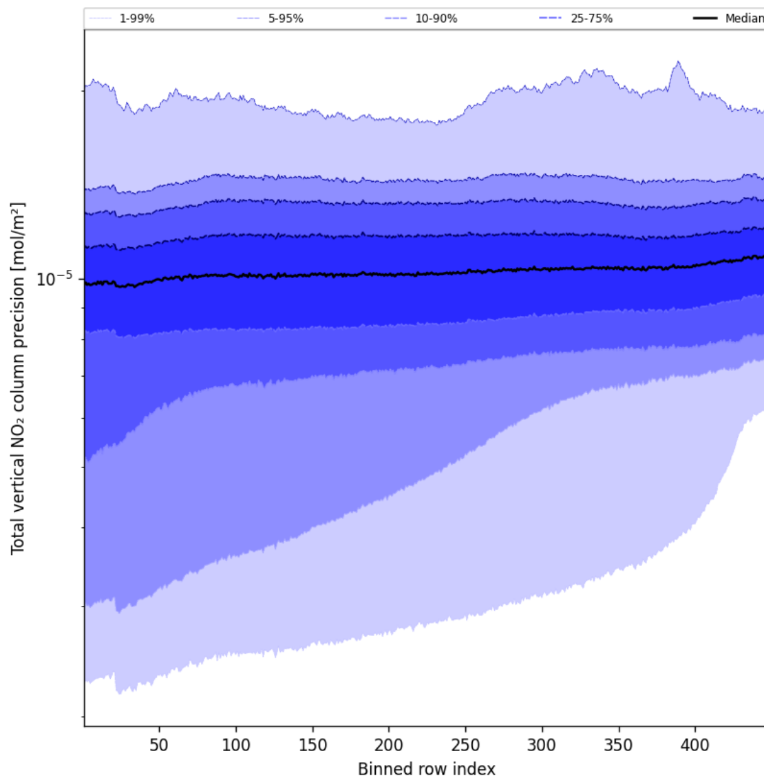
Figure 56: Along track statistics of “Total vertical NO 2 column precision” for 2024-09-17 to 2024-09-18
