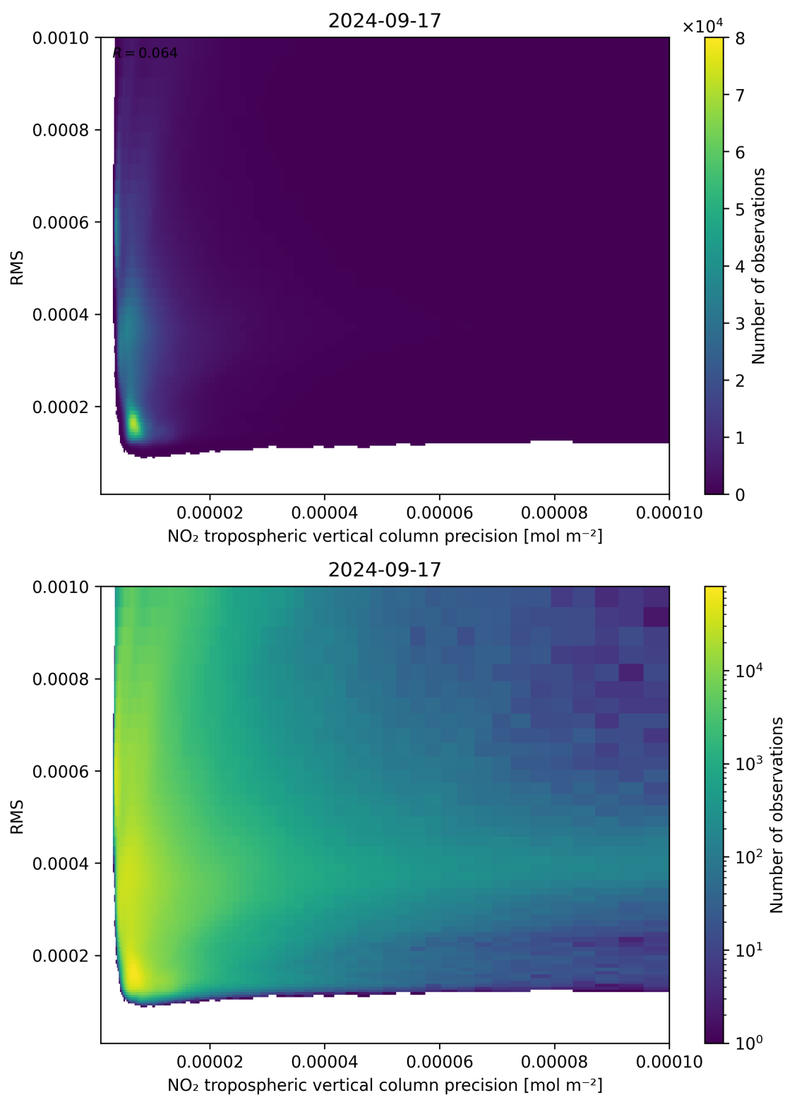
Figure 140: Scatter density plot of “NO 2 tropospheric vertical column precision” against “RMS” for 2024-09-17 to 2024-09-18.
