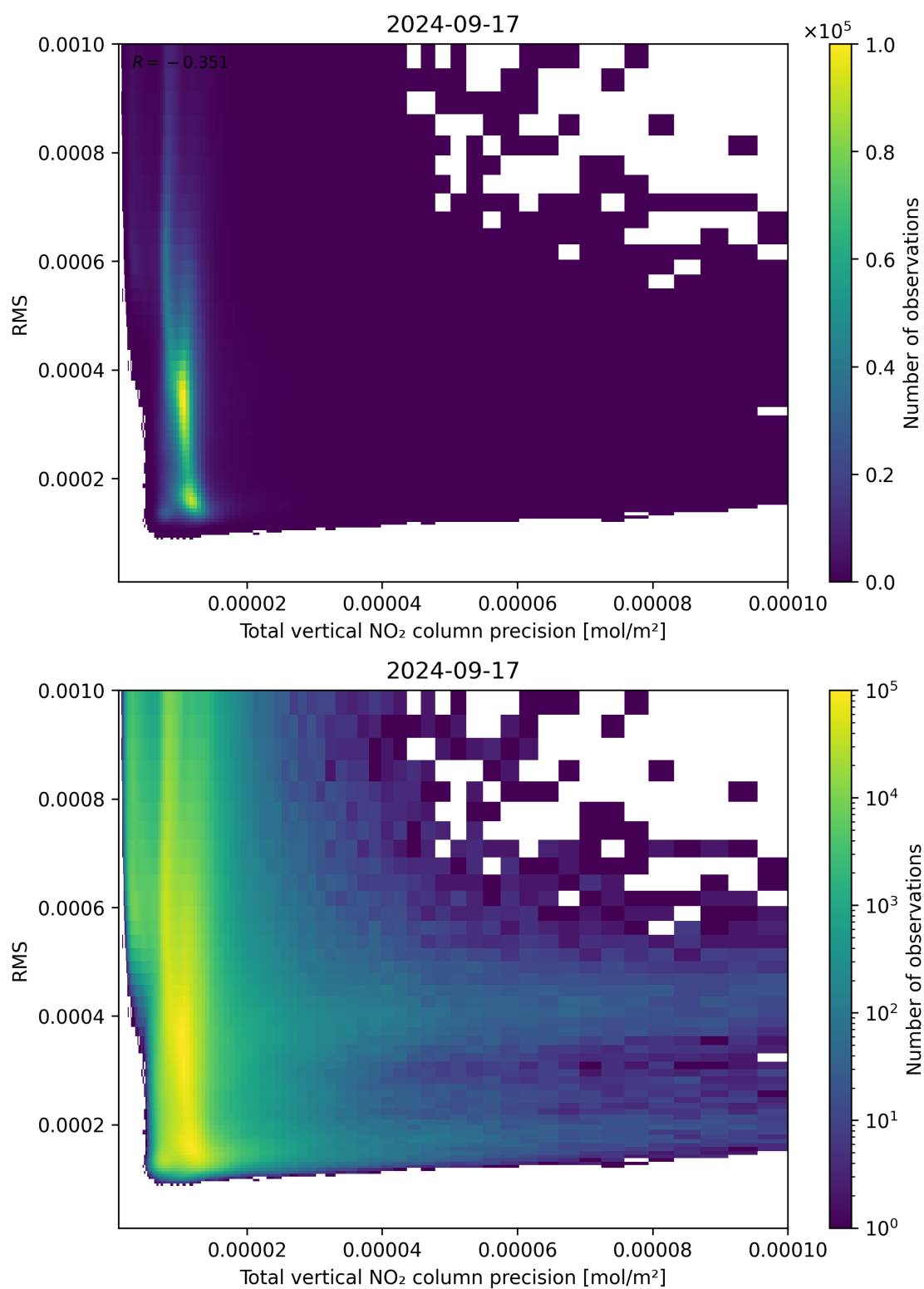
Figure 119: Scatter density plot of “Total vertical NO 2 column precision” against “RMS” for 2024-09-17 to 2024-09-18.
