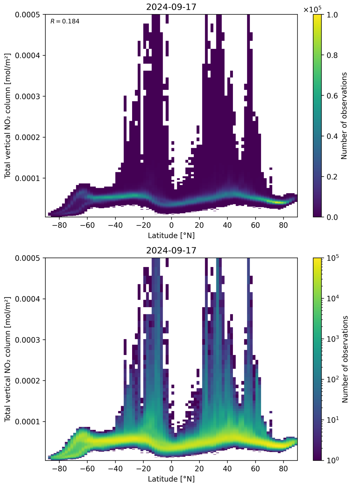
Figure 90: Scatter density plot of “Latitude” against “Total vertical NO 2 column” for 2024-09-17 to 2024-09-18.
