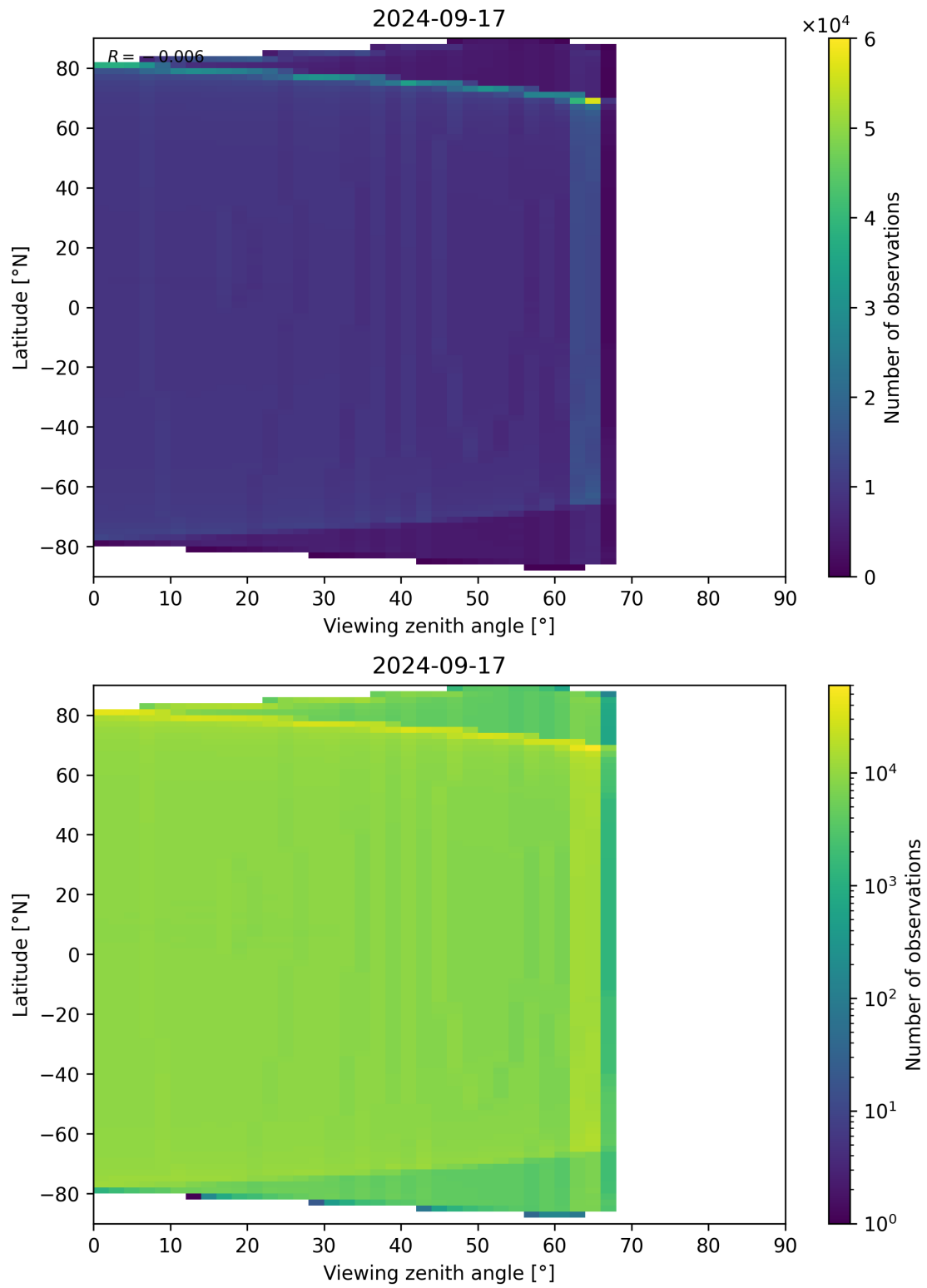
Figure 163: Scatter density plot of “Viewing zenith angle” against “Latitude” for 2024-09-17 to 2024-09-18.
