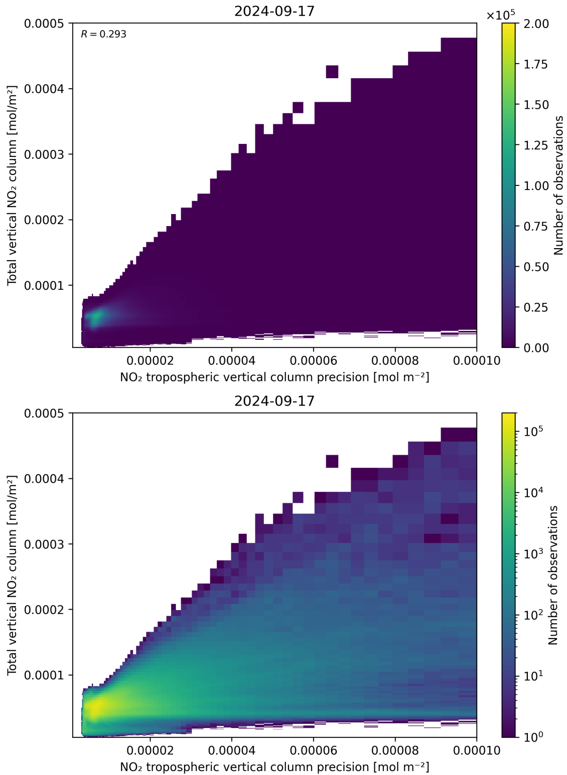
Figure 138: Scatter density plot of “NO 2 tropospheric vertical column precision” against “Total vertical NO 2 column” for 2024-09-17 to 2024-09-18.
