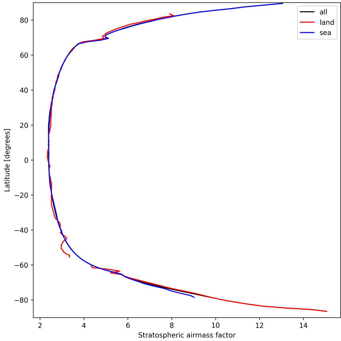
Figure 27: Zonal average of “Stratospheric airmass factor” for 2024-09-17 to 2024-09-18.
