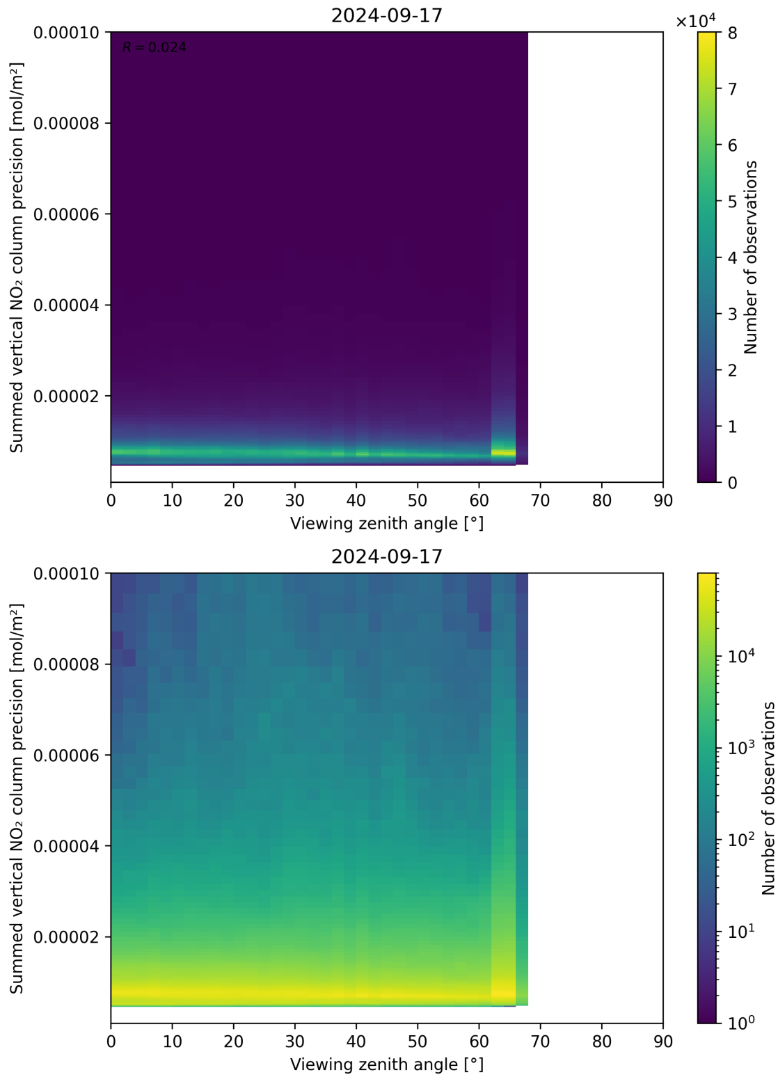
Figure 166: Scatter density plot of “Viewing zenith angle” against “Summed vertical NO 2 column precision” for 2024-09-17 to 2024-09-18.
