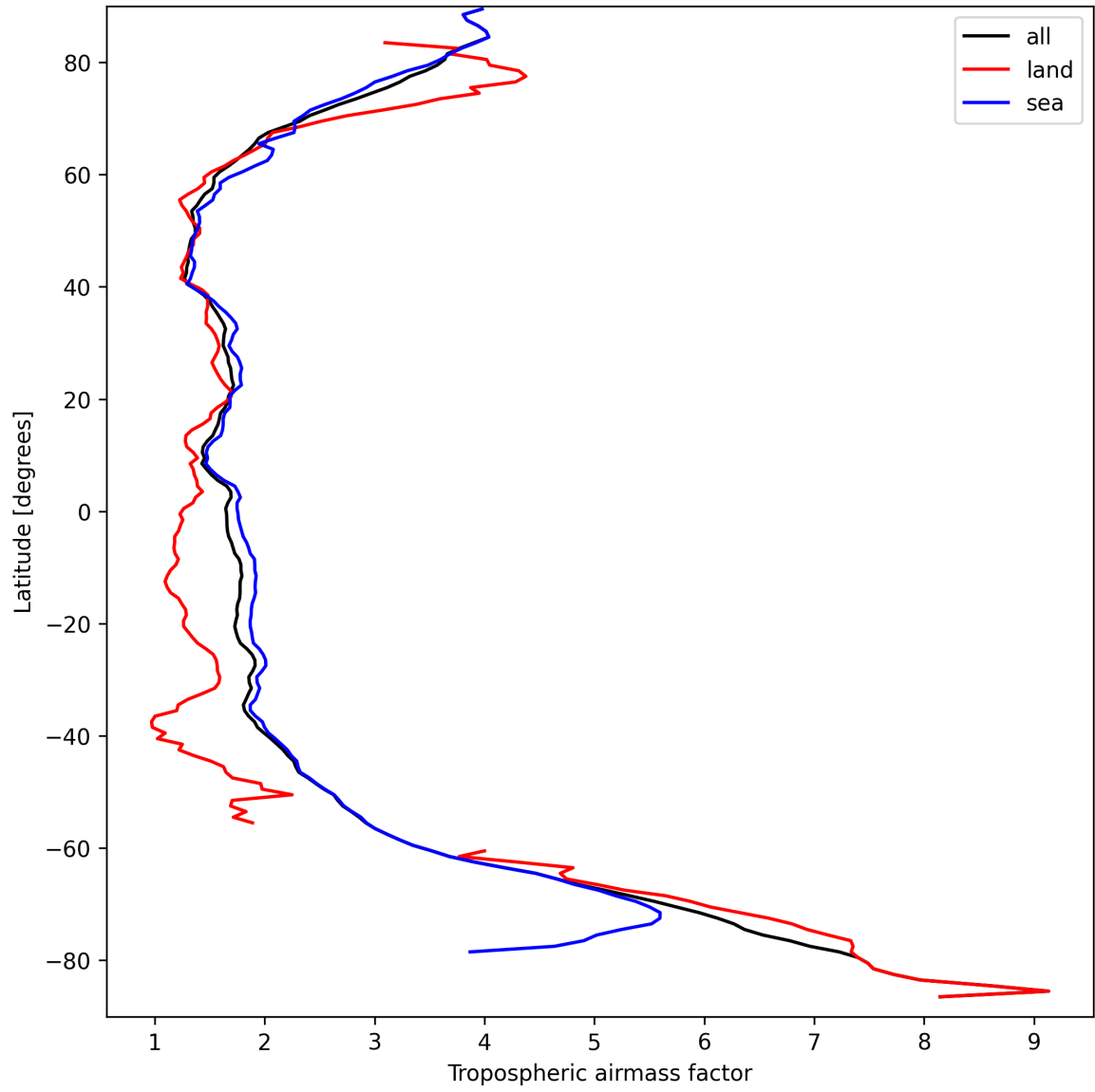
Figure 14: Zonal average of “Tropospheric air mass factor” for 2024-09-17 to 2024-09-18.
