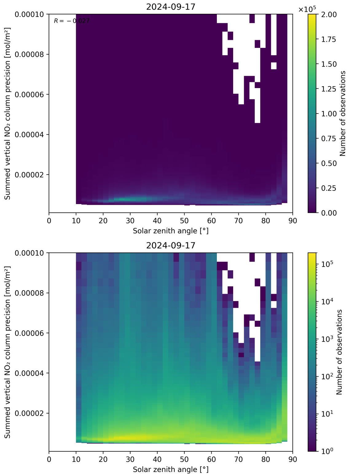
Figure 152: Scatter density plot of “Solar zenith angle” against “Summed vertical NO 2 column precision” for 2024-09-17 to 2024-09-18.
