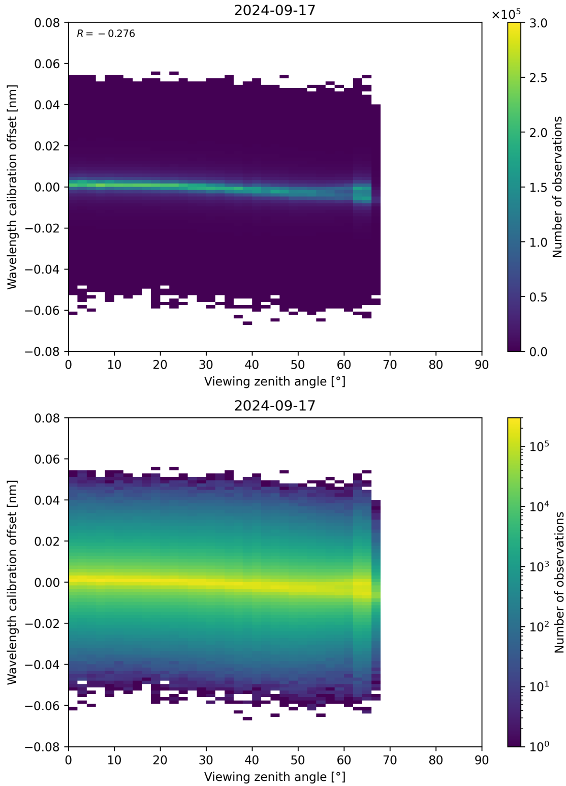
Figure 173: Scatter density plot of “Viewing zenith angle” against “Wavelength calibration offset” for 2024-09-17 to 2024-09-18.
