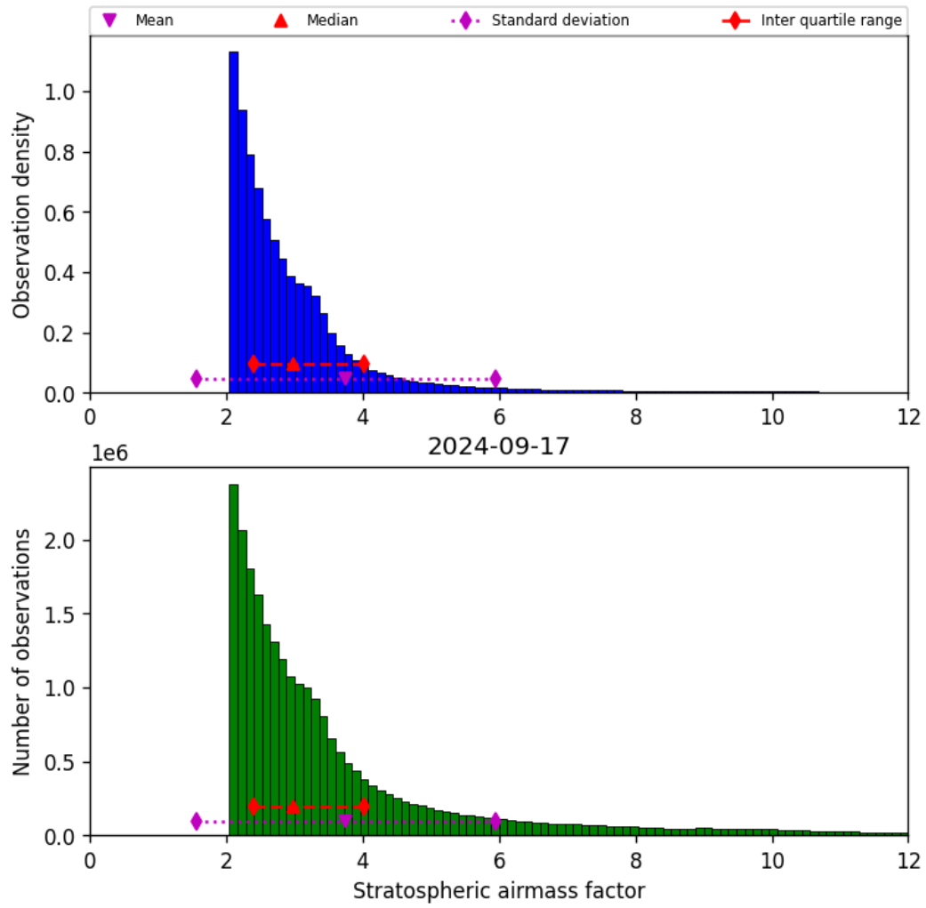
Figure 44: Histogram of “Stratospheric airmass factor” for 2024-09-17 to 2024-09-18
