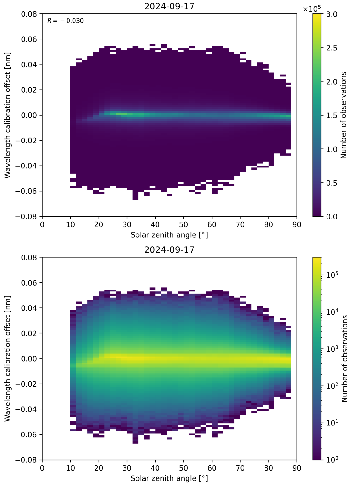
Figure 158: Scatter density plot of “Solar zenith angle” against “Wavelength calibration offset” for 2024-09-17 to 2024-09-18.
