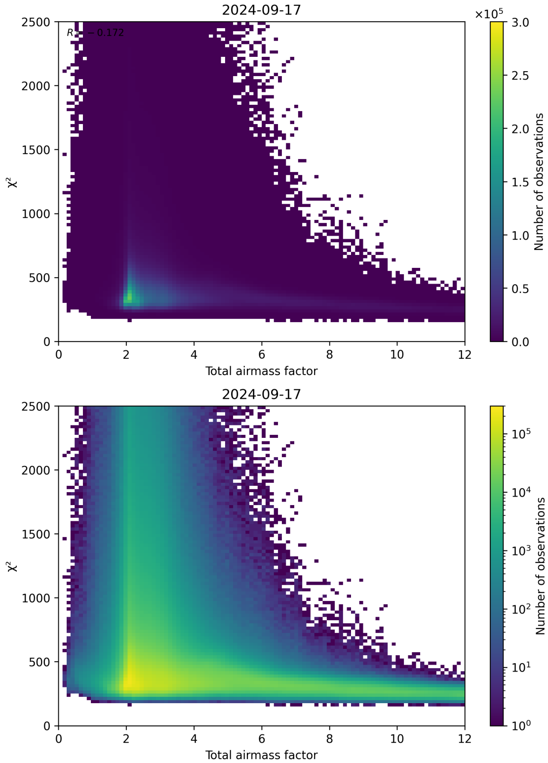
Figure 63: Scatter density plot of “Total airmass factor” against “ \chi^2 ” for 2024-09-17 to 2024-09-18.
