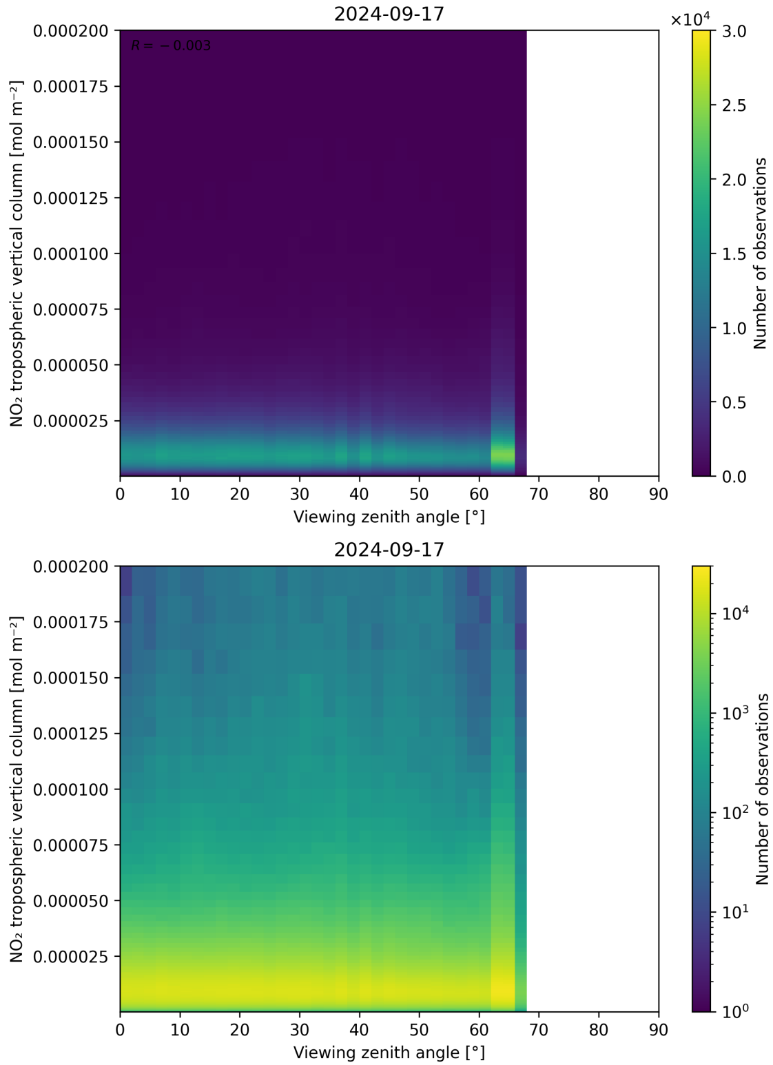
Figure 169: Scatter density plot of “Viewing zenith angle” against “NO 2 tropospheric vertical column” for 2024-09-17 to 2024-09-18.
