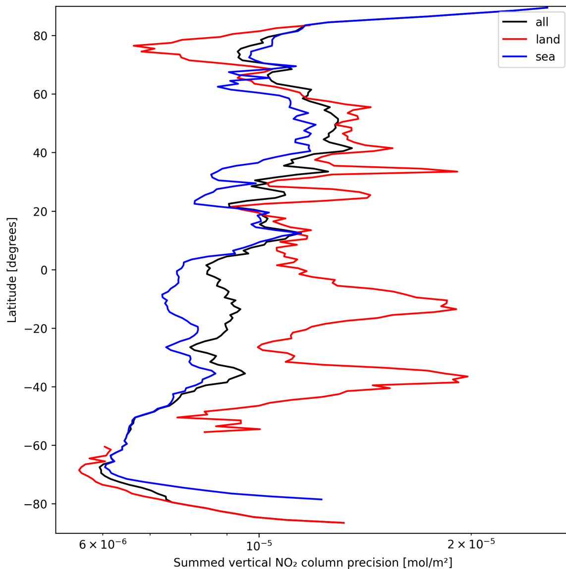
Figure 24: Zonal average of “Summed vertical NO 2 column precision” for 2024-09-17 to 2024-09-18.
