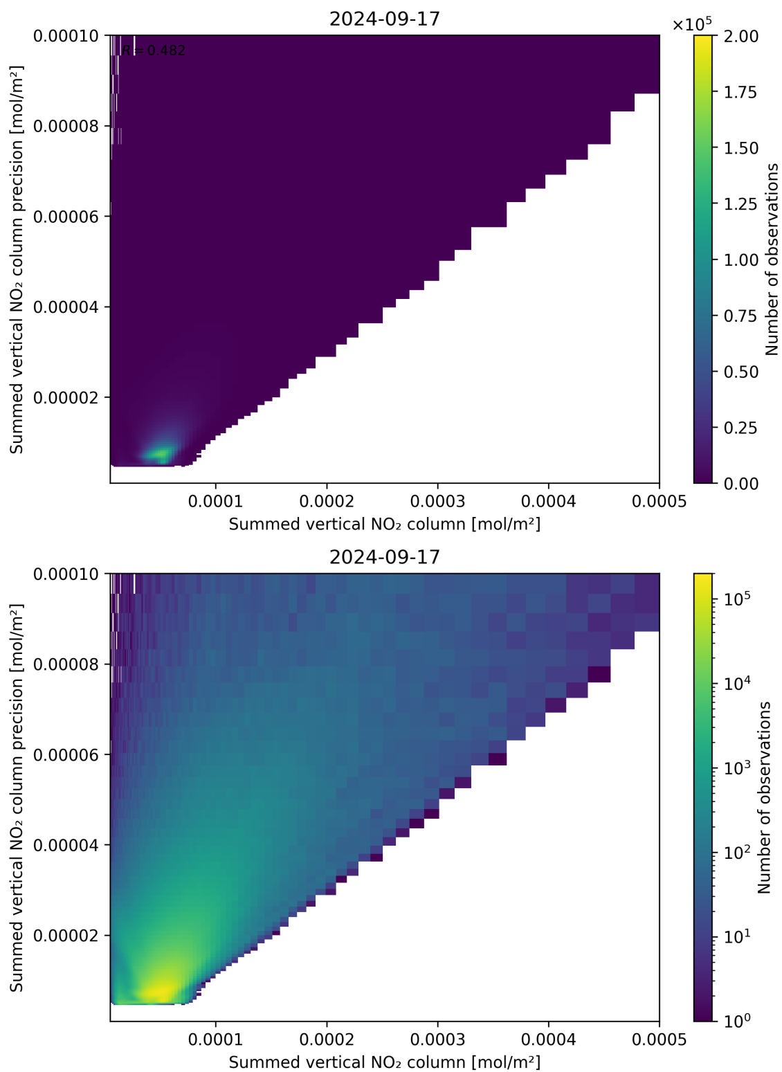
Figure 105: Scatter density plot of “Summed vertical NO 2 column” against “Summed vertical NO 2 column precision” for 2024-09-17 to 2024-09-18.
