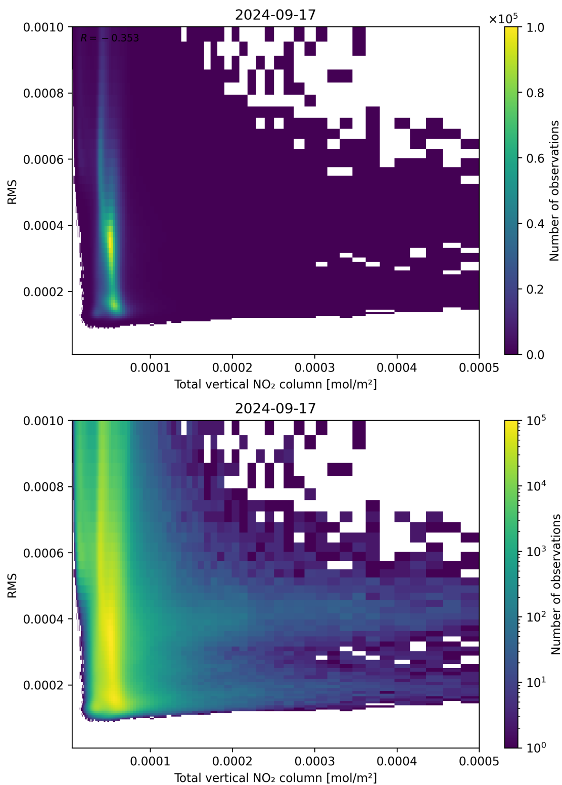
Figure 120: Scatter density plot of “Total vertical NO 2 column” against “RMS” for 2024-09-17 to 2024-09-18.
