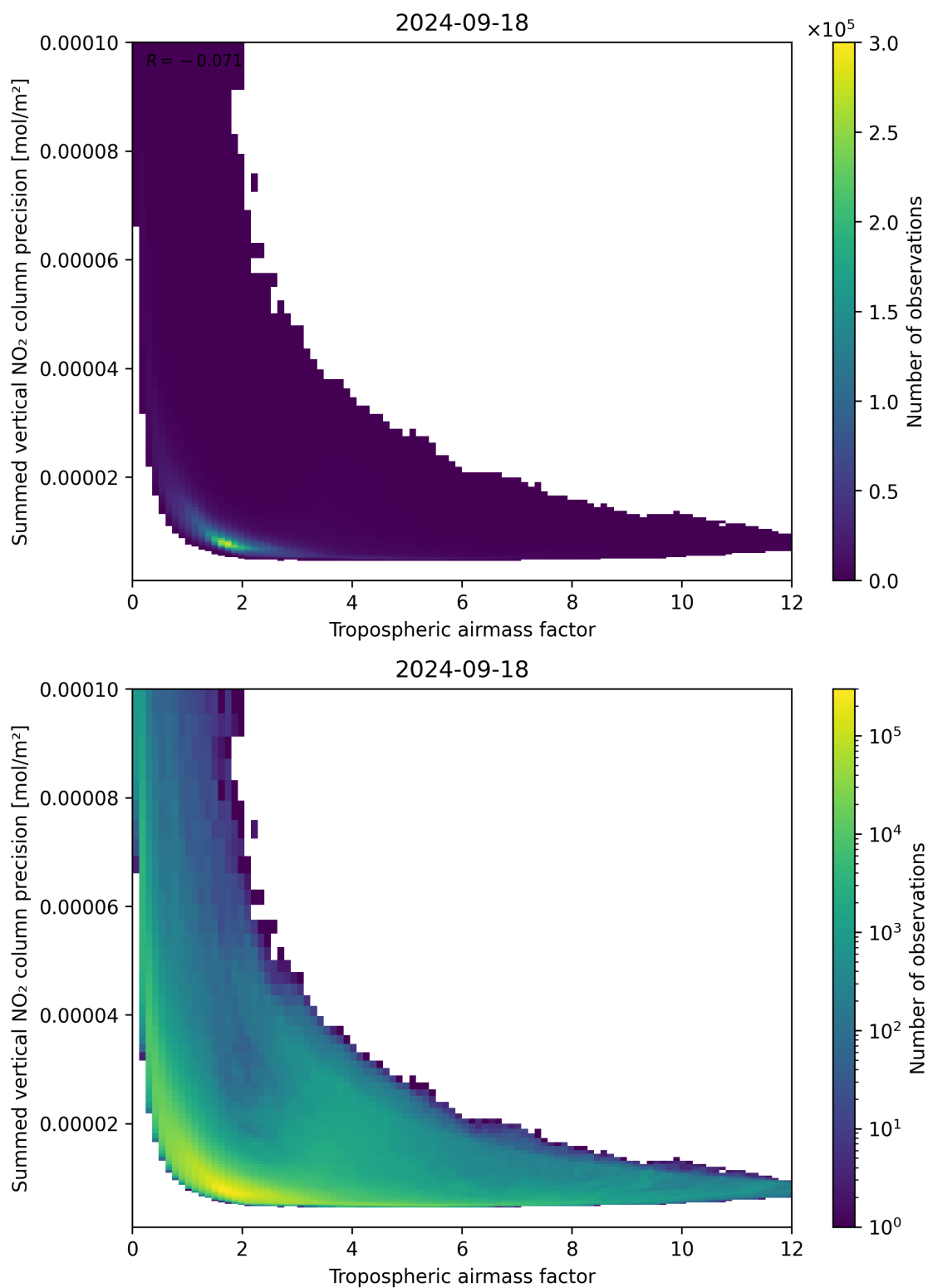
Figure 76: Scatter density plot of “Tropospheric air mass factor” against “Summed vertical NO 2 column precision” for 2024-09-17 to 2024-09-19.
