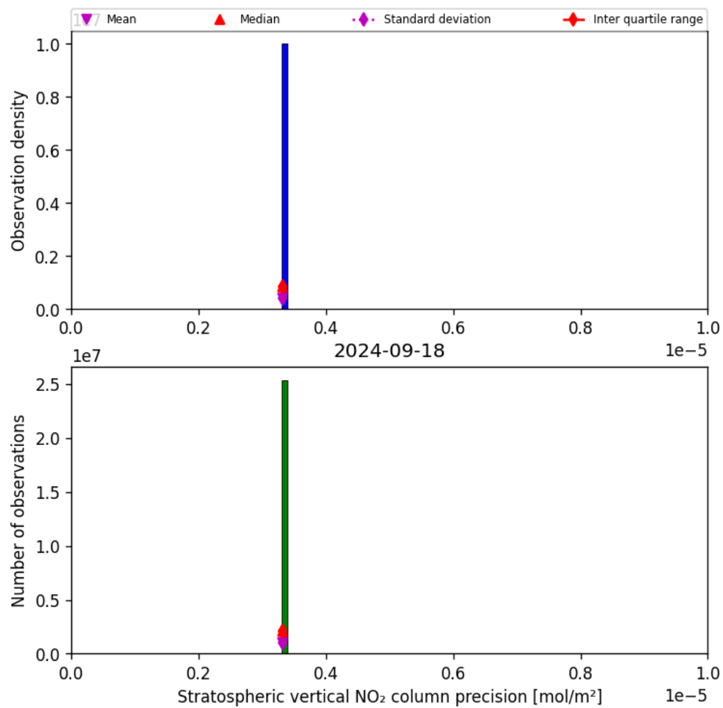
Figure 37: Histogram of “Stratospheric vertical NO 2 column precision” for 2024-09-17 to 2024-09-19
