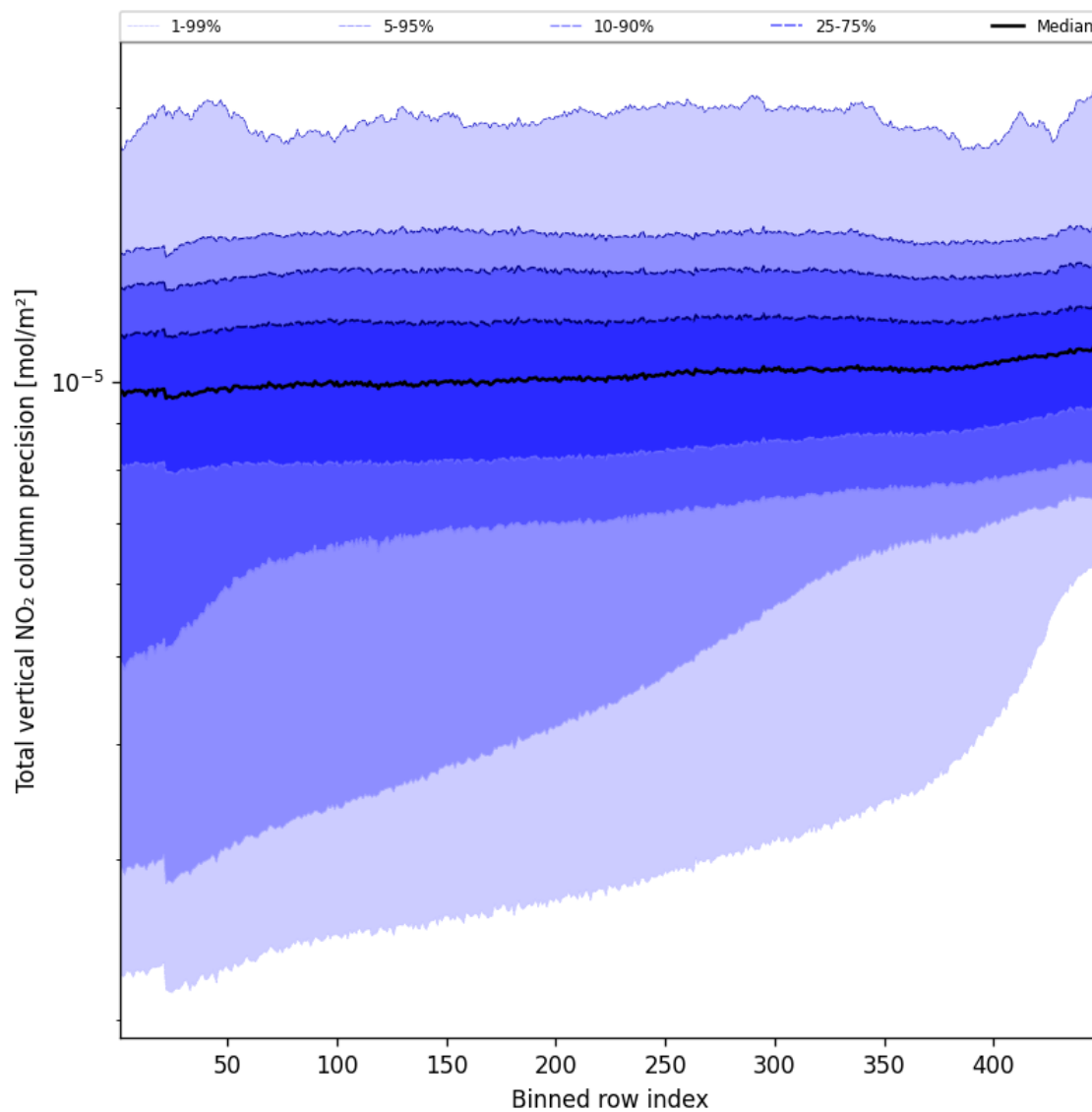
Figure 56: Along track statistics of “Total vertical NO 2 column precision” for 2024-09-17 to 2024-09-19
