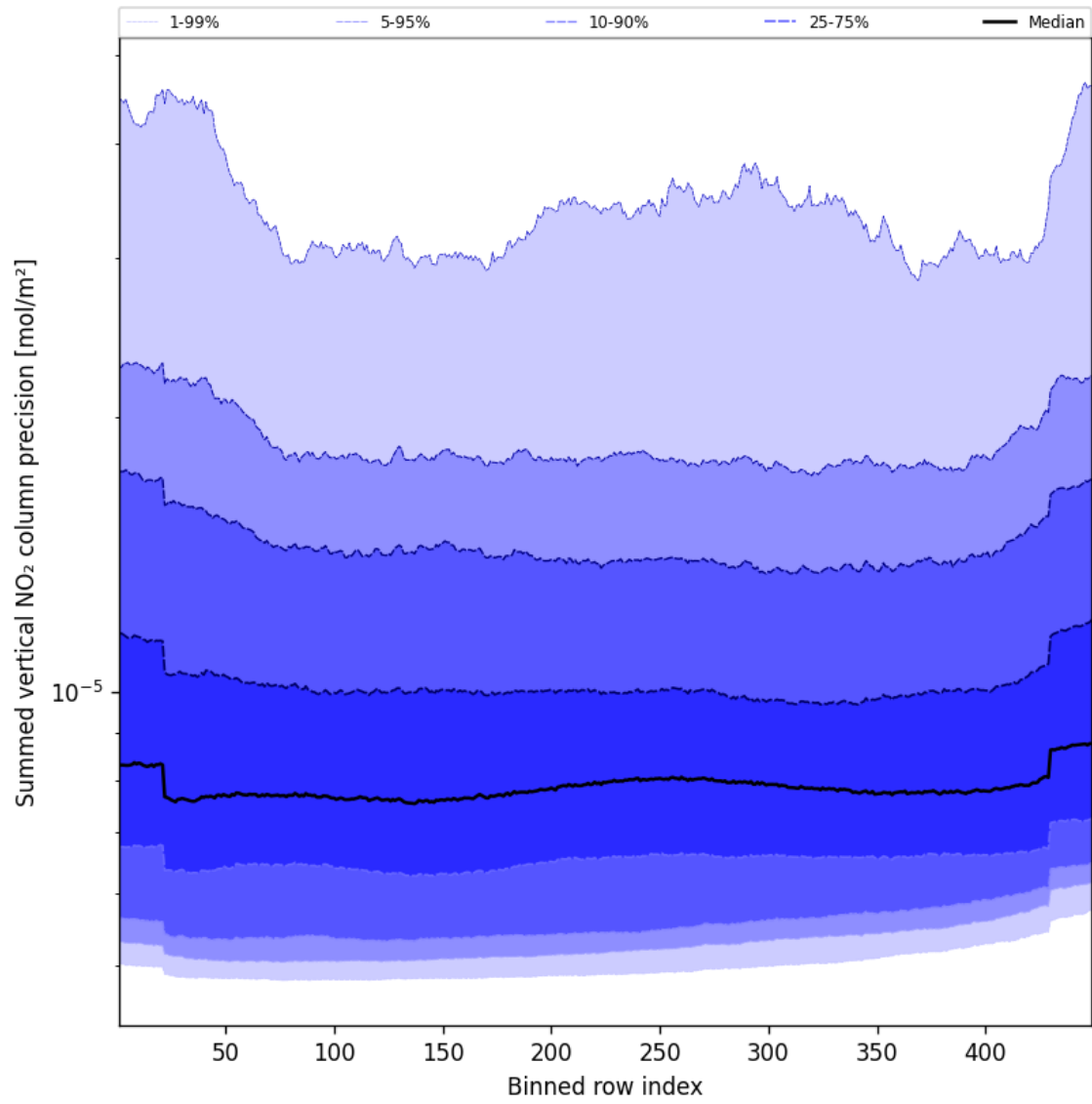
Figure 58: Along track statistics of “Summed vertical NO 2 column precision” for 2024-09-17 to 2024-09-19
