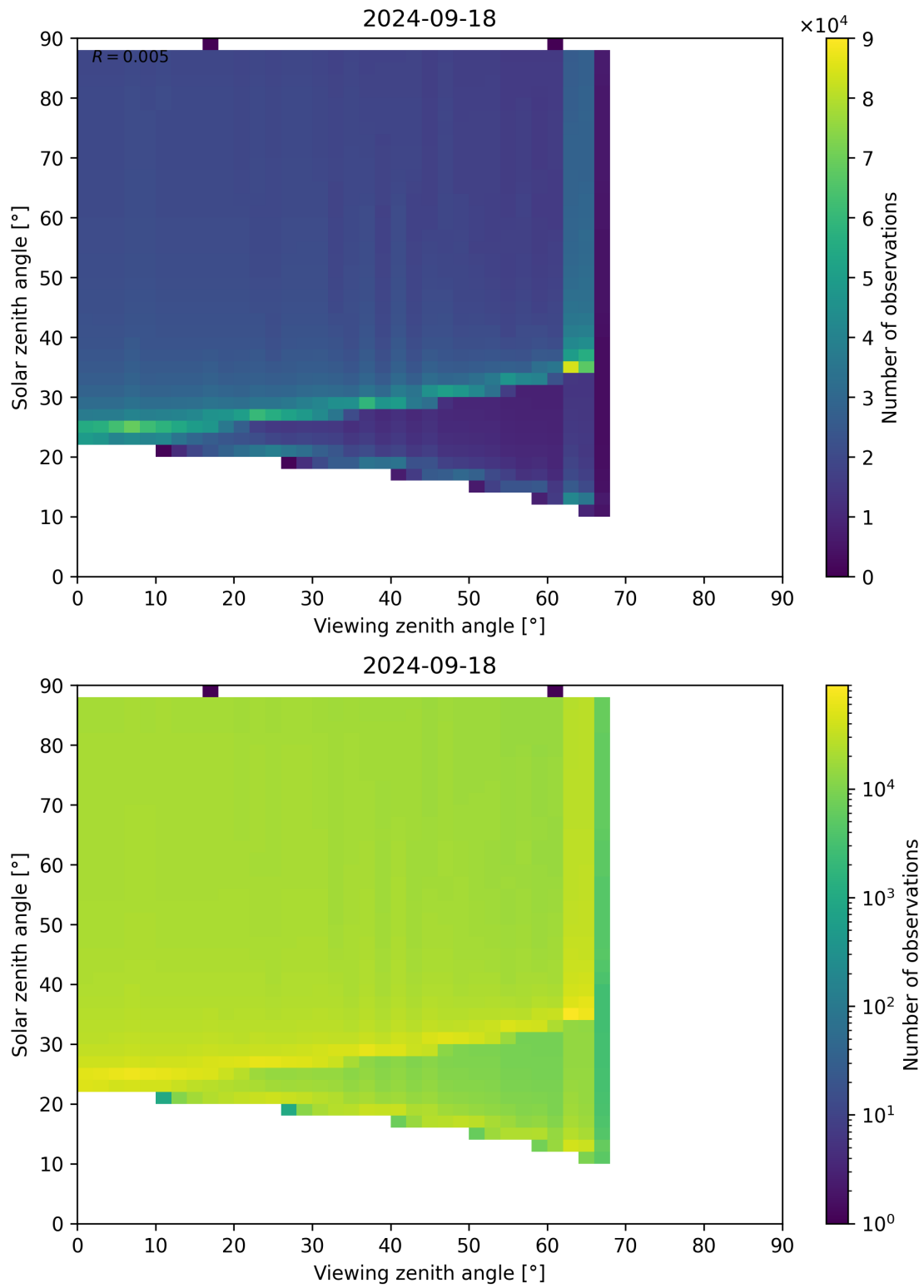
Figure 172: Scatter density plot of “Viewing zenith angle” against “Solar zenith angle” for 2024-09-17 to 2024-09-19.
