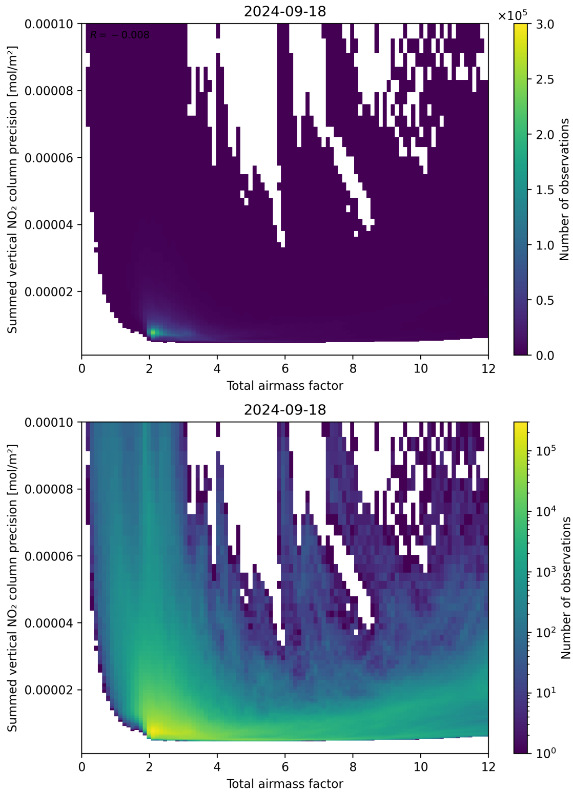
Figure 66: Scatter density plot of “Total airmass factor” against “Summed vertical NO 2 column precision” for 2024-09-17 to 2024-09-19.
