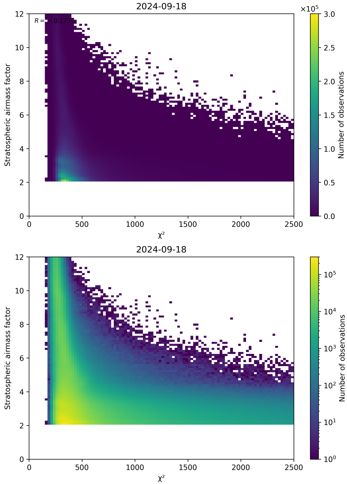
Figure 81: Scatter density plot of “ \chi^2 ” against “Stratospheric airmass factor” for 2024-09-17 to 2024-09-19.
