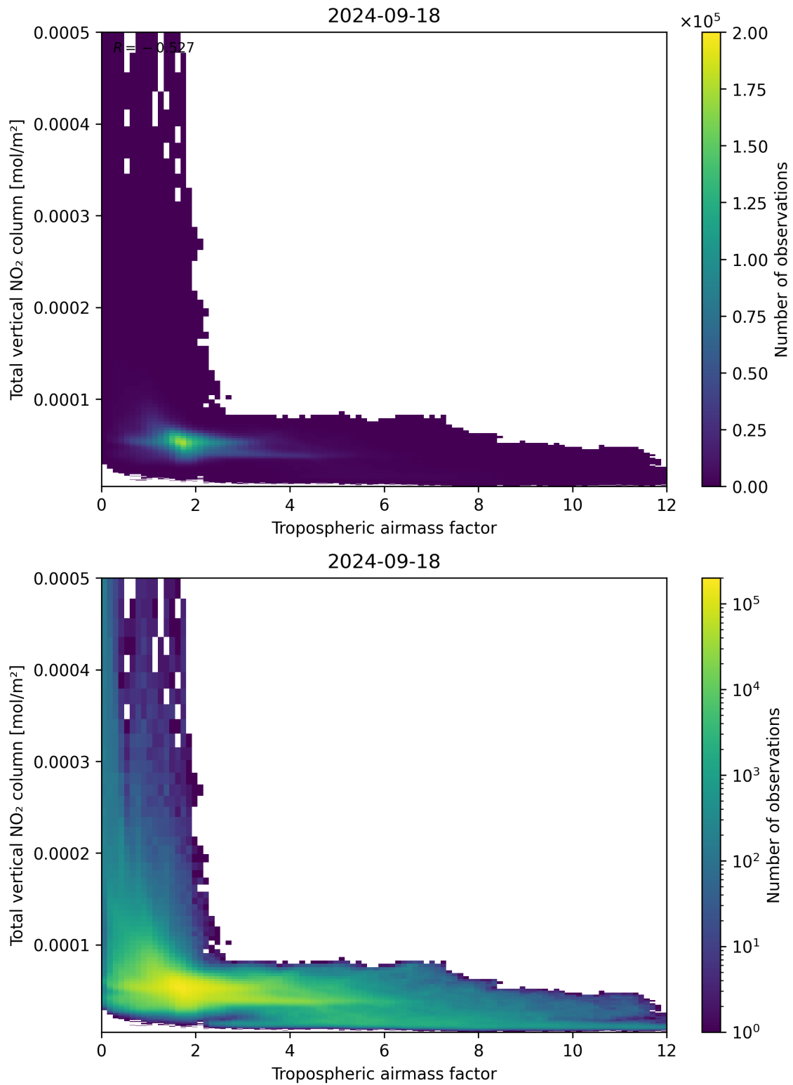
Figure 77: Scatter density plot of “Tropospheric airmass factor” against “Total vertical NO 2 column” for 2024-09-17 to 2024-09-19.
