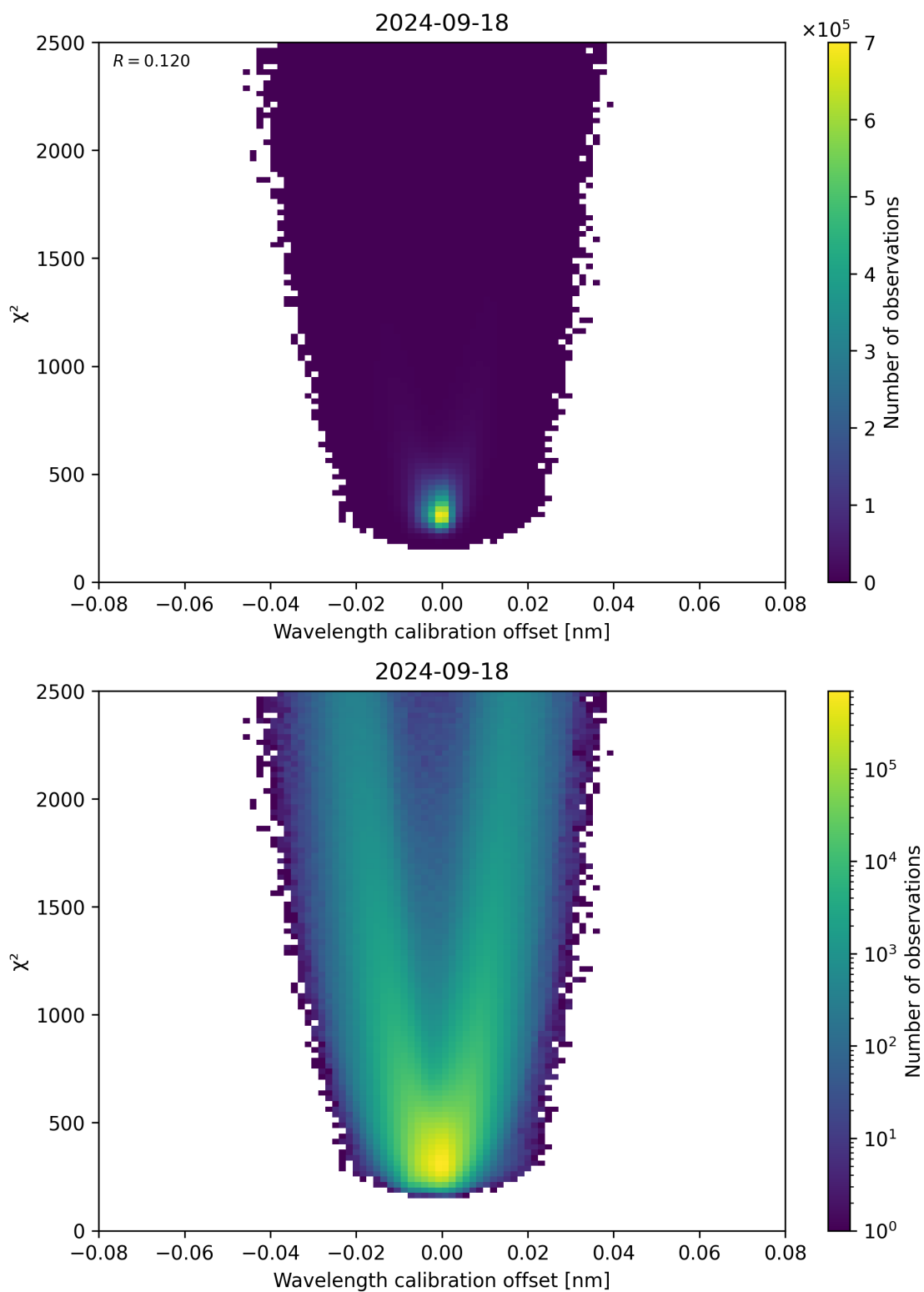
Figure 175: Scatter density plot of “Wavelength calibration offset” against “ \chi^2 ” for 2024-09-17 to 2024-09-19.
