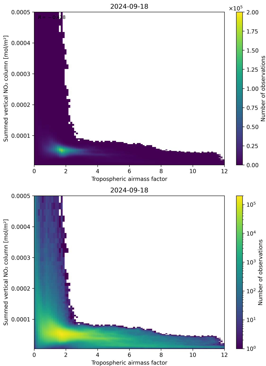
Figure 75: Scatter density plot of “Tropospheric air mass factor” against “Summed vertical NO 2 column” for 2024-09-17 to 2024-09-19.
