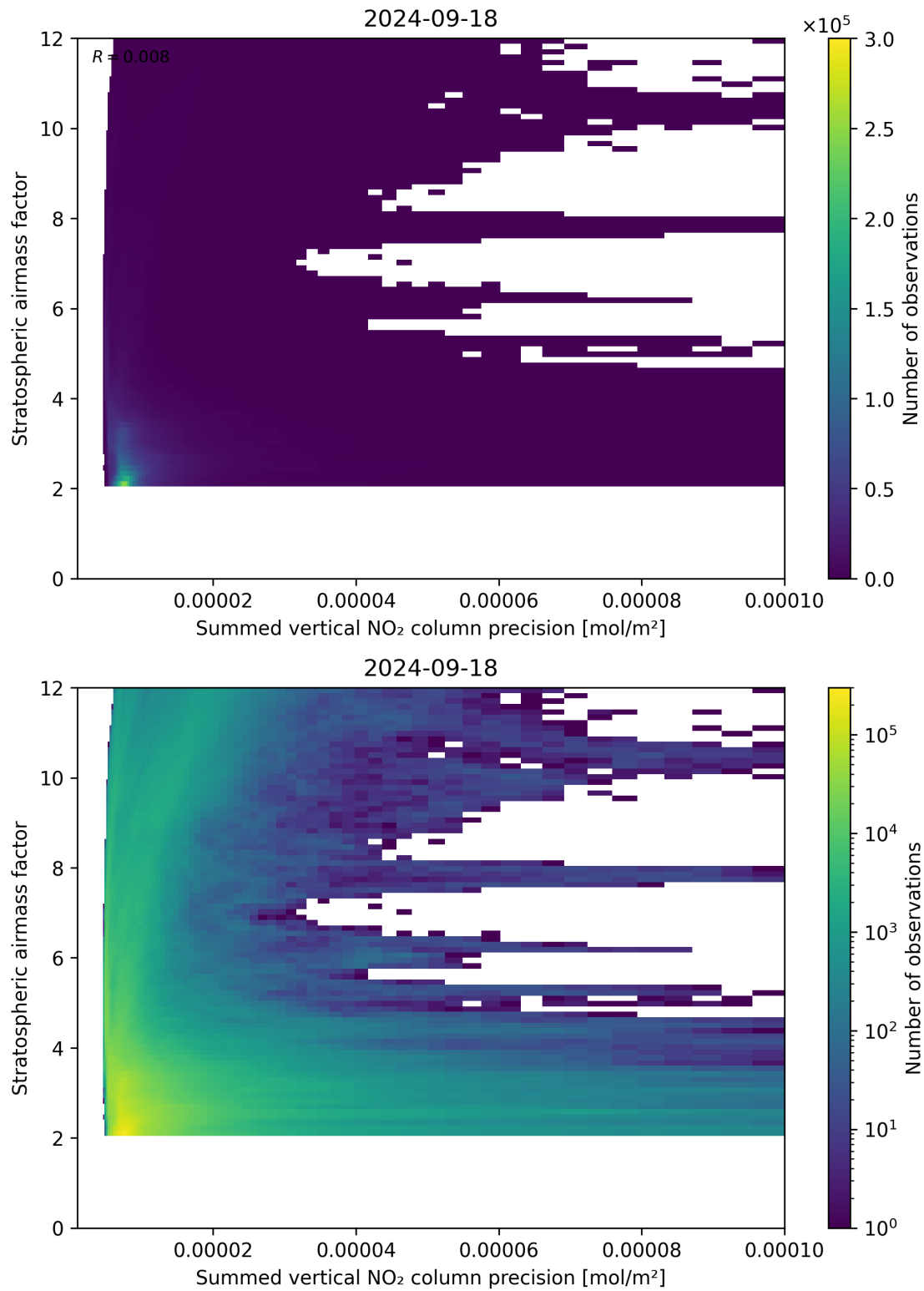
Figure 106: Scatter density plot of “Summed vertical NO 2 column precision” against “Stratospheric airmass factor” for 2024-09-17 to 2024-09-19.
