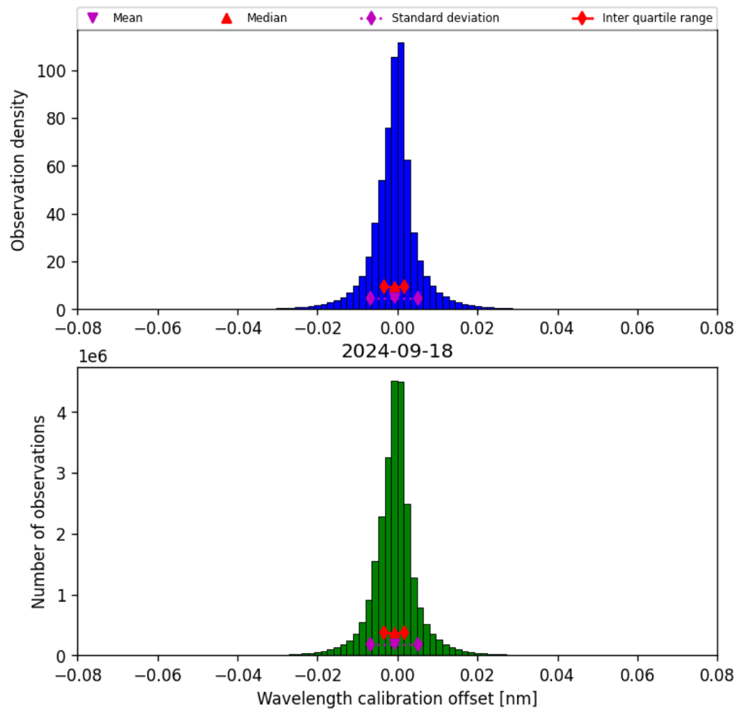
Figure 35: Histogram of “Wavelength calibration offset” for 2024-09-17 to 2024-09-19
