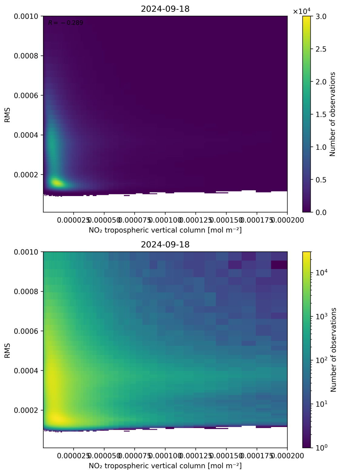
Figure 142: Scatter density plot of “NO 2 tropospheric vertical column” against “RMS” for 2024-09-17 to 2024-09-19.
