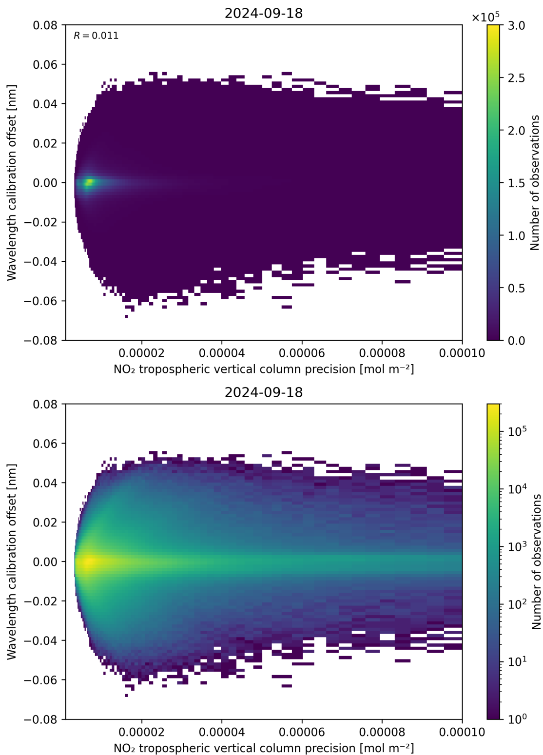
Figure 141: Scatter density plot of “NO 2 tropospheric vertical column precision” against “Wavelength calibration offset” for 2024-09-17 to 2024-09-19.
