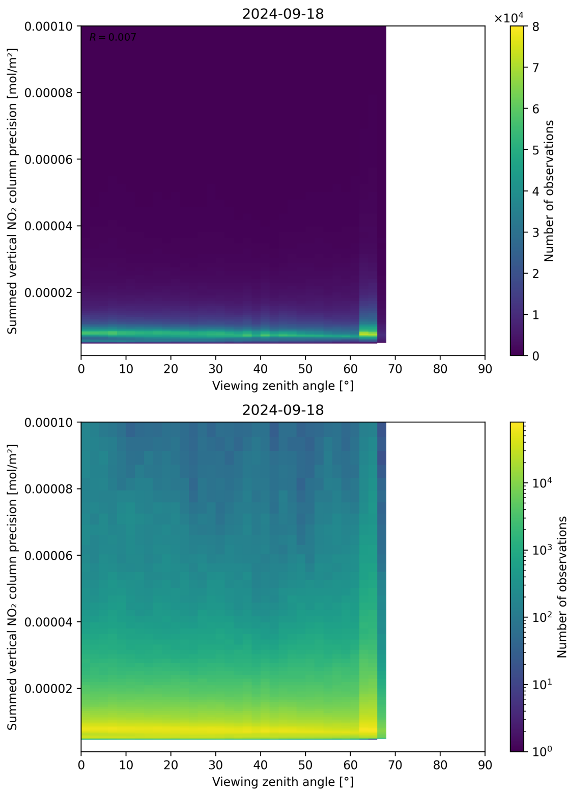
Figure 166: Scatter density plot of “Viewing zenith angle” against “Summed vertical NO 2 column precision” for 2024-09-17 to 2024-09-19.
