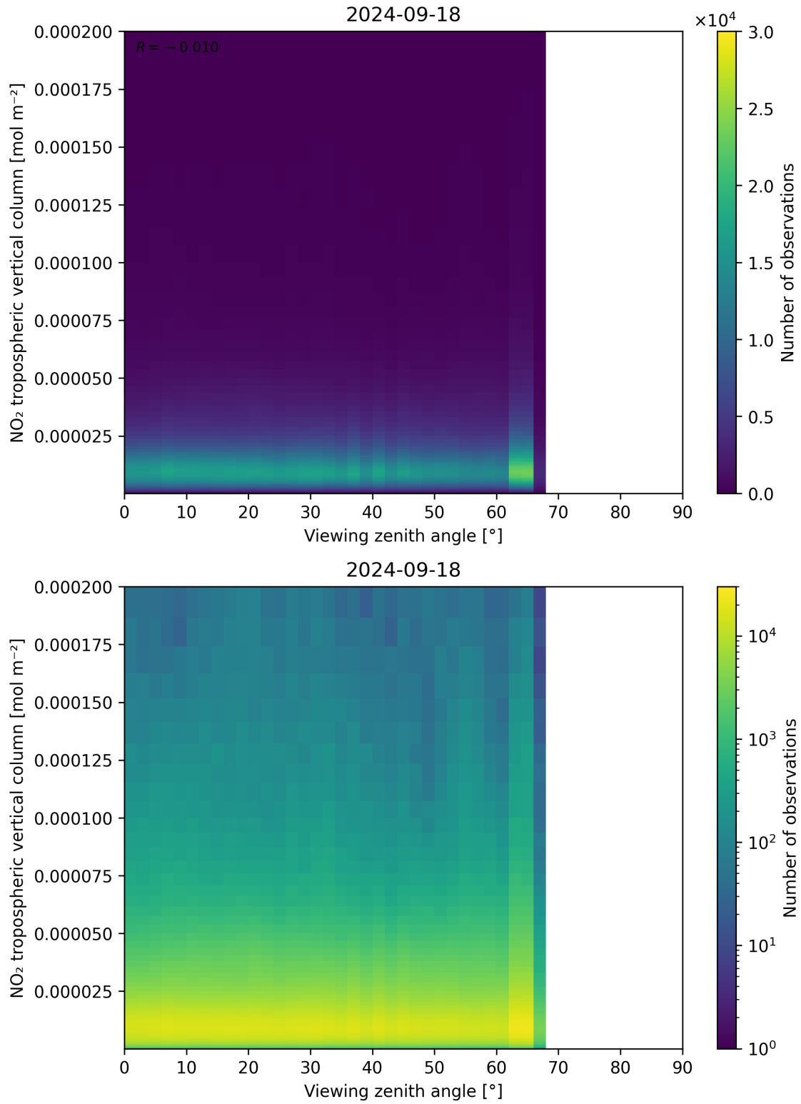
Figure 169: Scatter density plot of “Viewing zenith angle” against “NO 2 tropospheric vertical column” for 2024-09-17 to 2024-09-19.
