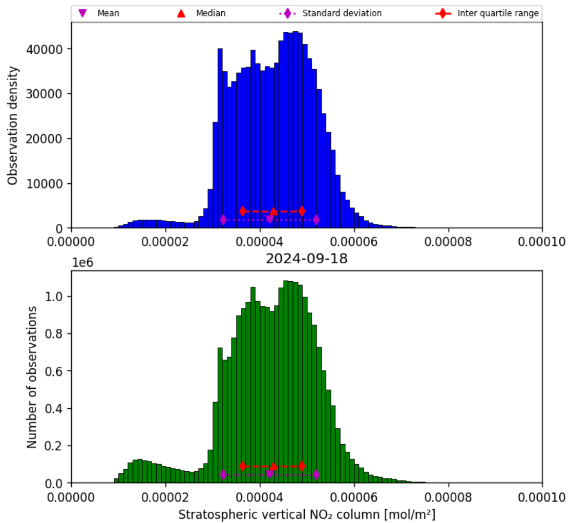
Figure 36: Histogram of “Stratospheric vertical NO 2 column” for 2024-09-17 to 2024-09-19
