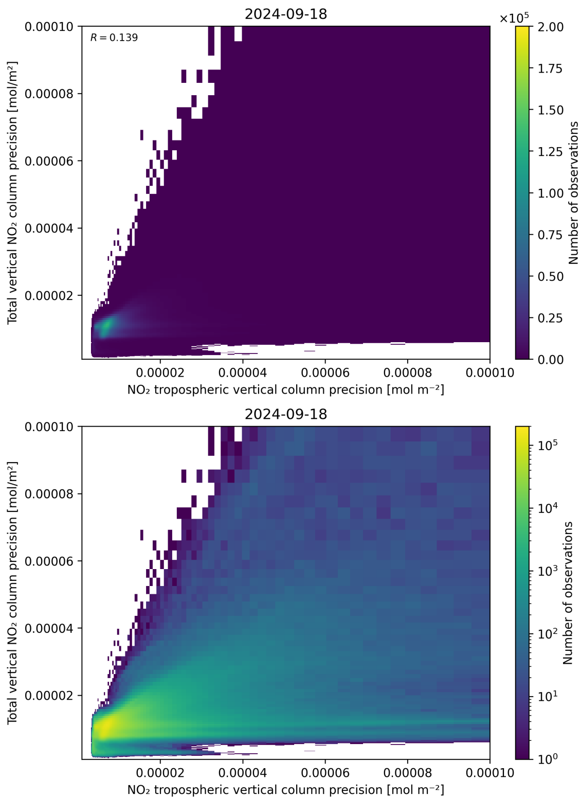
Figure 139: Scatter density plot of “NO 2 tropospheric vertical column precision” against “Total vertical NO 2 column precision” for 2024-09-17 to 2024-09-19.
