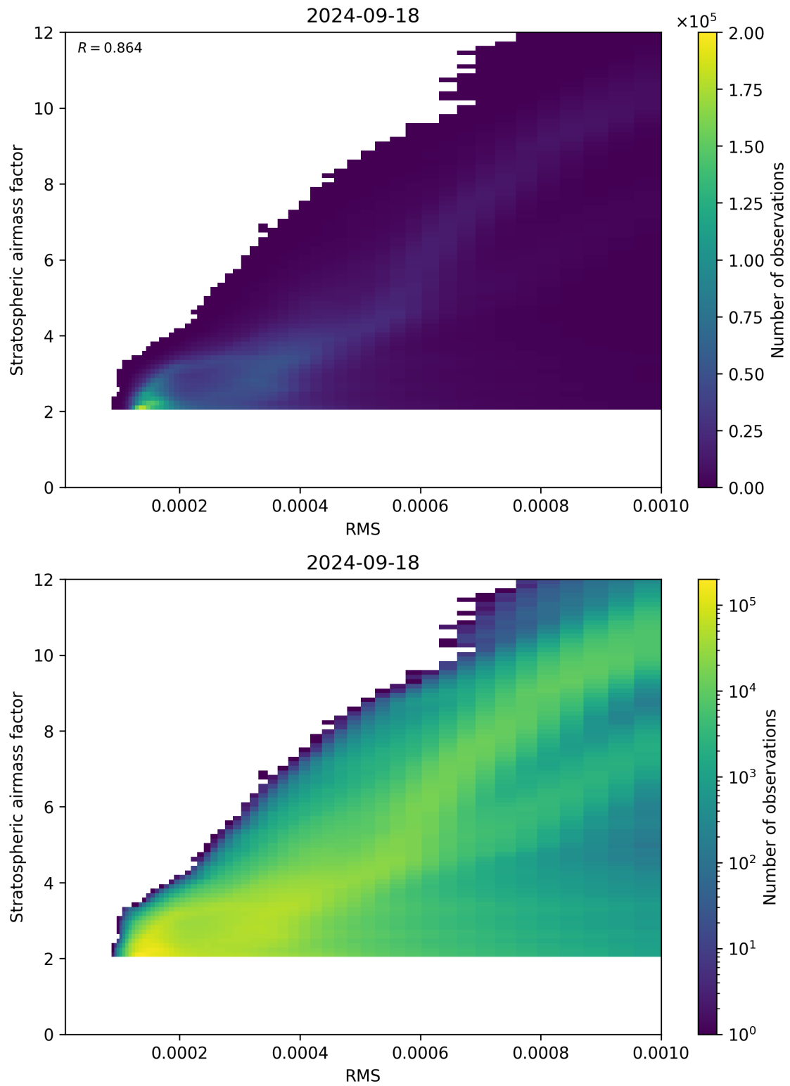
Figure 144: Scatter density plot of “RMS” against “Stratospheric airmass factor” for 2024-09-17 to 2024-09-19.
