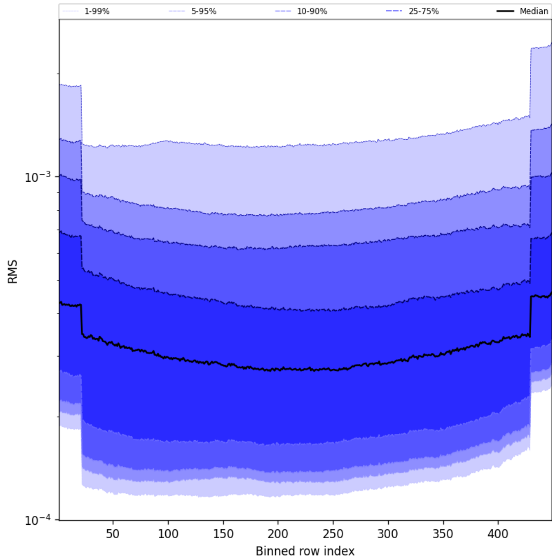
Figure 60: Along track statistics of “RMS” for 2024-09-17 to 2024-09-19
