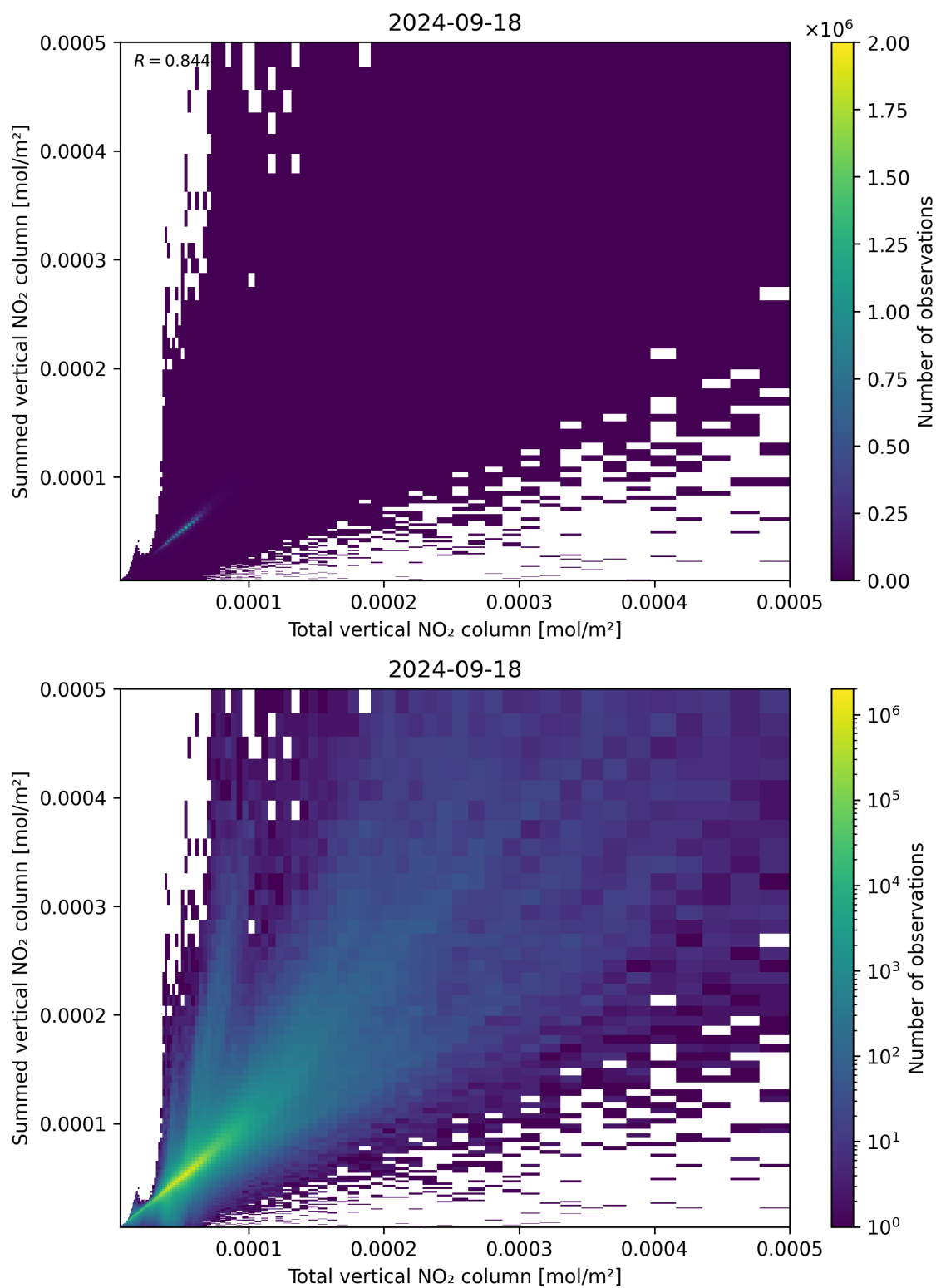
Figure 112: Scatter density plot of “Total vertical NO 2 column” against “Summed vertical NO 2 column” for 2024-09-17 to 2024-09-19.
