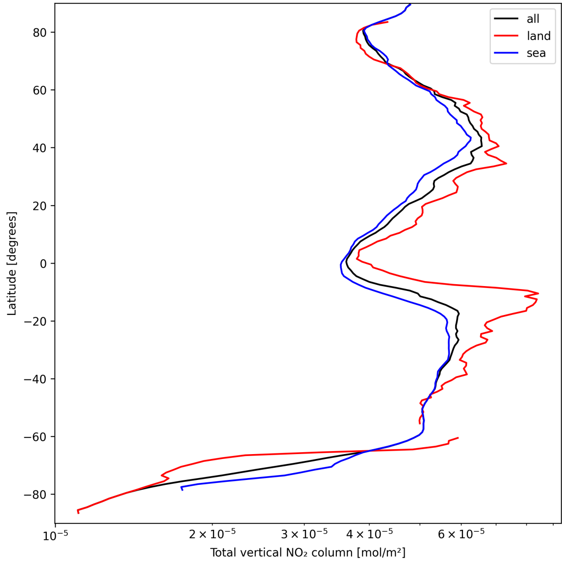
Figure 21: Zonal average of “Total vertical NO 2 column” for 2024-09-17 to 2024-09-19.
