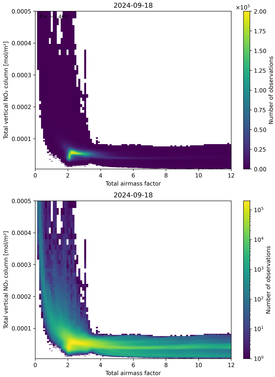
Figure 67: Scatter density plot of “Total air mass factor” against “Total vertical NO 2 column” for 2024-09-17 to 2024-09-19.
