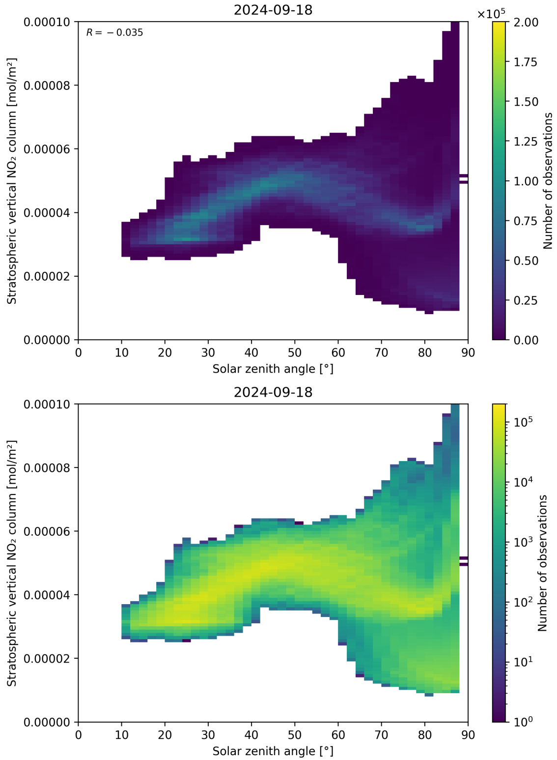
Figure 150: Scatter density plot of “Solar zenith angle” against “Stratospheric vertical NO 2 column” for 2024-09-17 to 2024-09-19.
