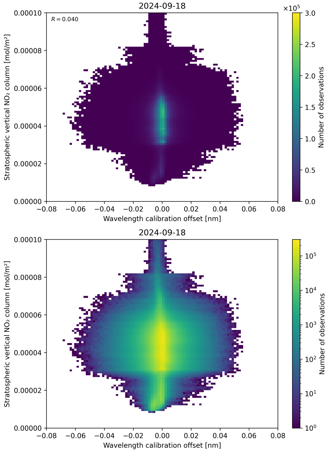
Figure 176: Scatter density plot of “Wavelength calibration offset” against “Stratospheric vertical NO 2 column” for 2024-09-17 to 2024-09-19.
