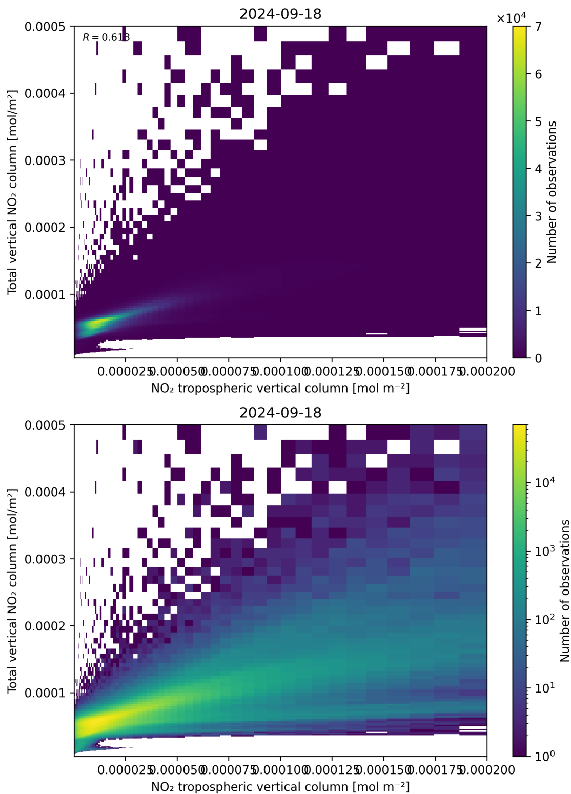
Figure 128: Scatter density plot of “NO 2 tropospheric vertical column” against “Total vertical NO 2 column” for 2024-09-17 to 2024-09-19.
