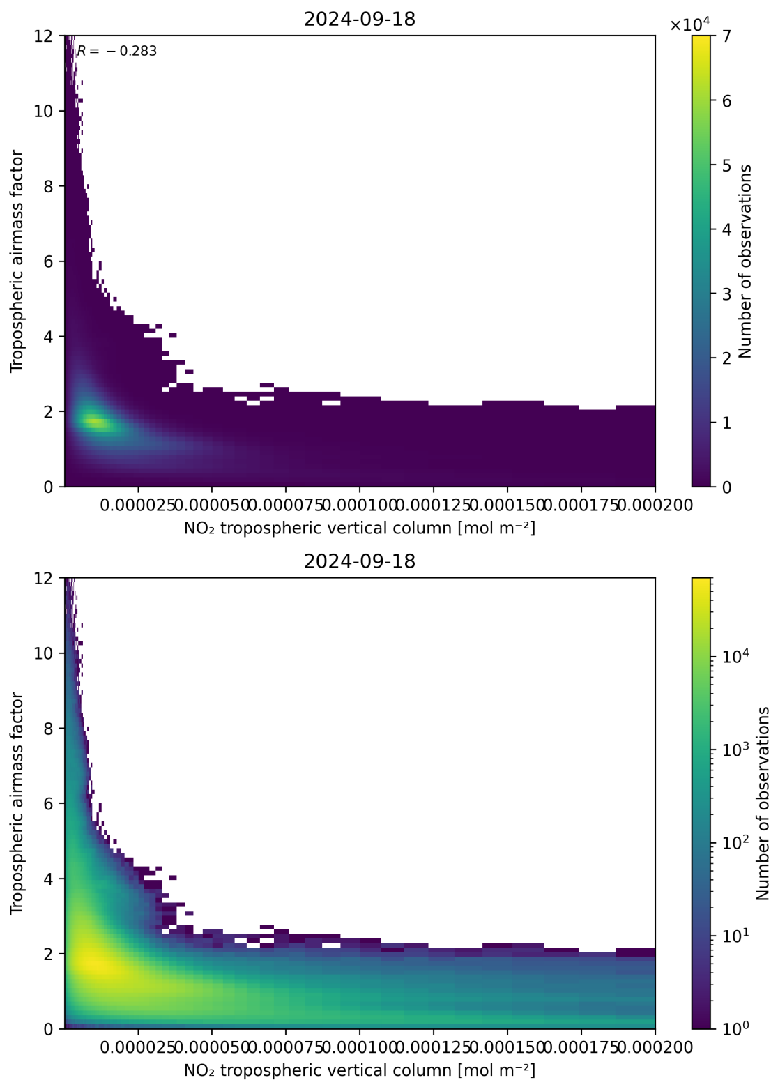
Figure 123: Scatter density plot of “NO 2 tropospheric vertical column” against “Tropospheric air mass factor” for 2024-09-17 to 2024-09-19.
