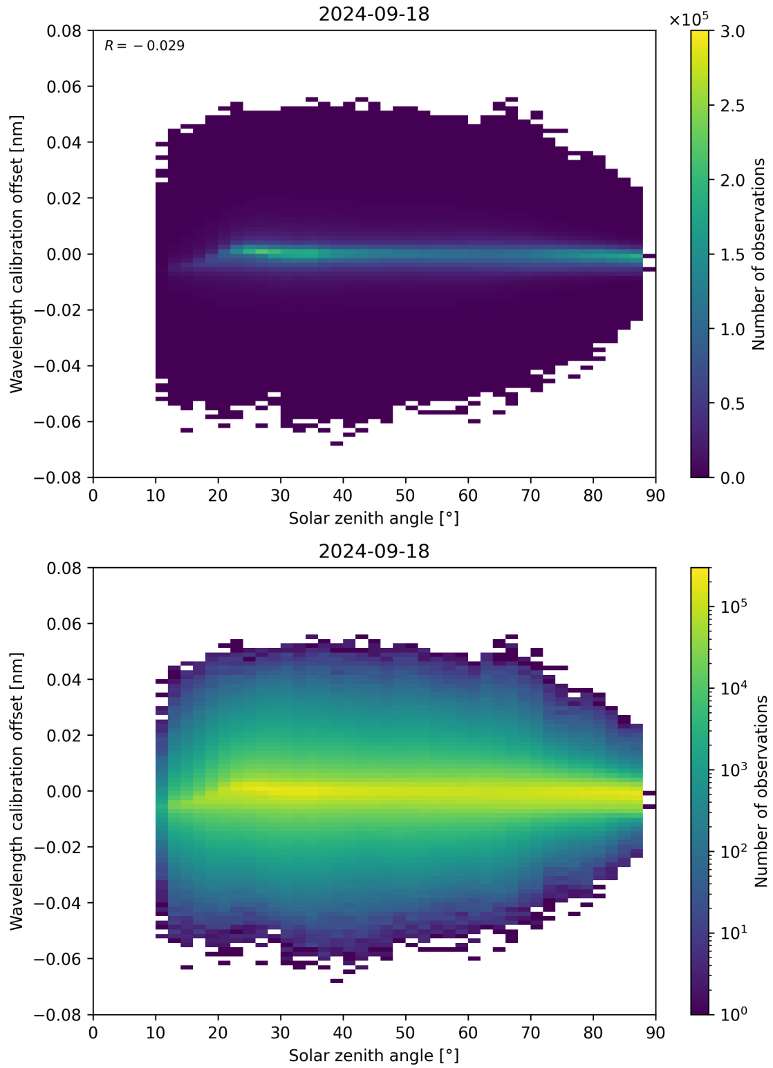
Figure 158: Scatter density plot of “Solar zenith angle” against “Wavelength calibration offset” for 2024-09-17 to 2024-09-19.
