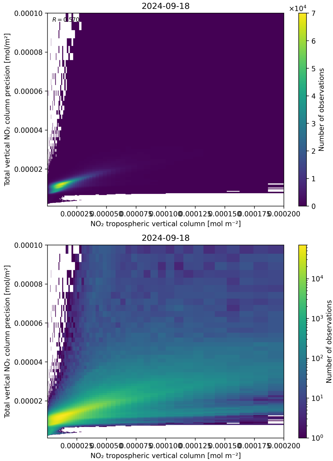
Figure 129: Scatter density plot of “NO 2 tropospheric vertical column” against “Total vertical NO 2 column precision” for 2024-09-17 to 2024-09-19.
