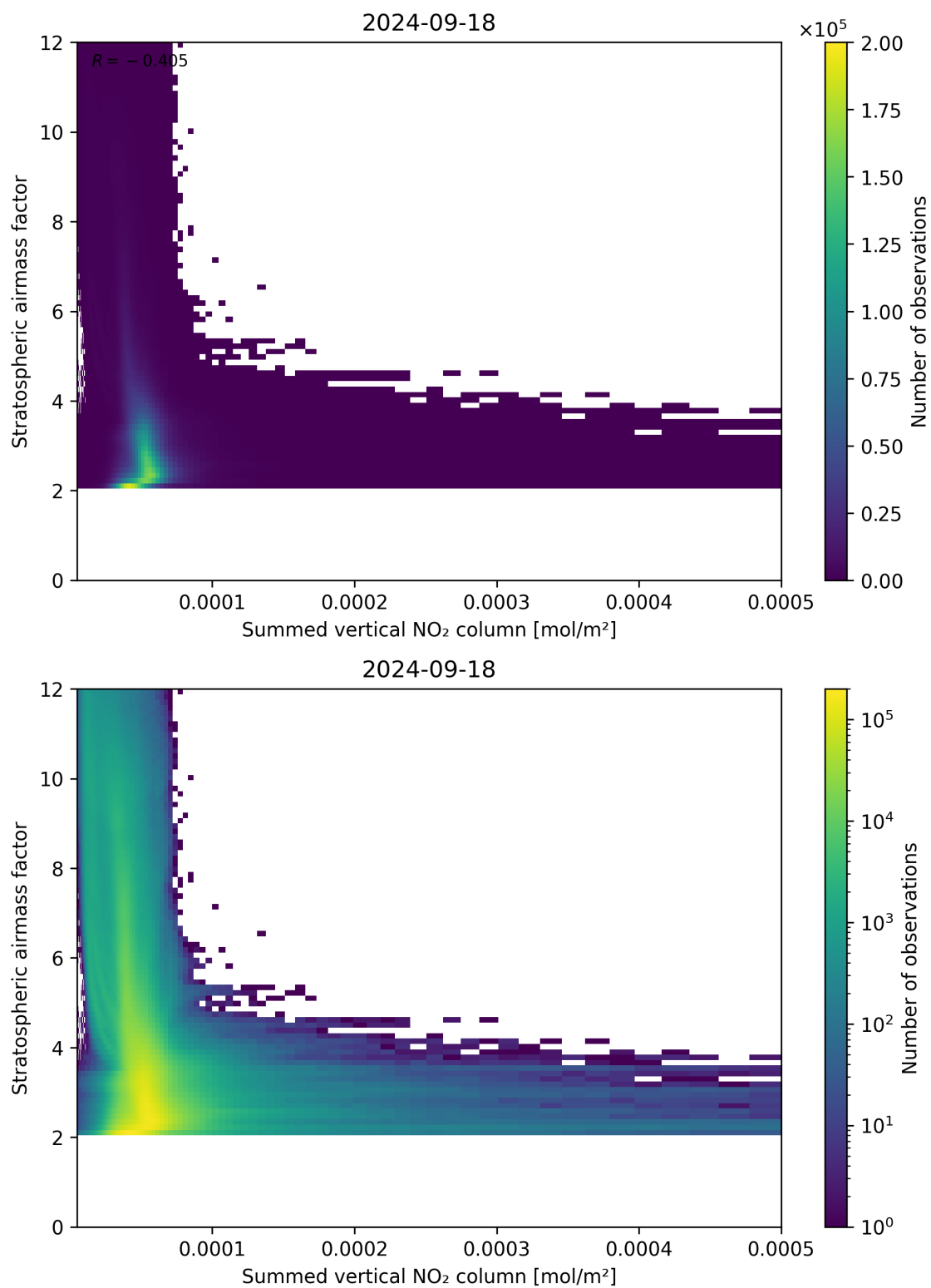
Figure 103: Scatter density plot of “Summed vertical NO 2 column” against “Stratospheric airmass factor” for 2024-09-17 to 2024-09-19.
