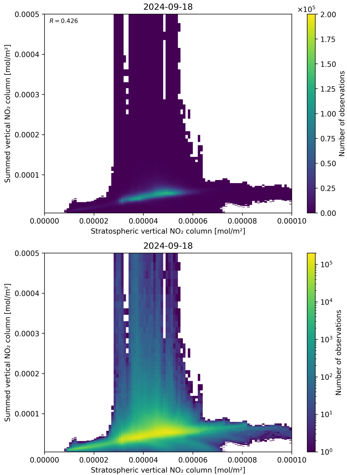
Figure 98: Scatter density plot of “Stratospheric vertical NO 2 column” against “Summed vertical NO 2 column” for 2024-09-17 to 2024-09-19.
