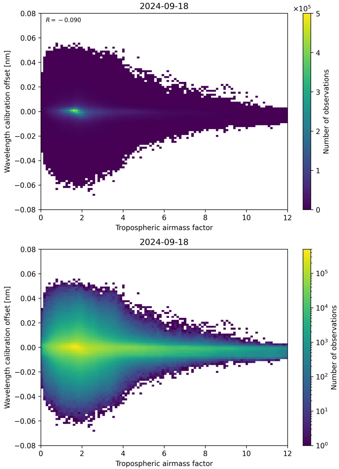
Figure 80: Scatter density plot of “Tropospheric airmass factor” against “Wavelength calibration offset” for 2024-09-17 to 2024-09-19.
