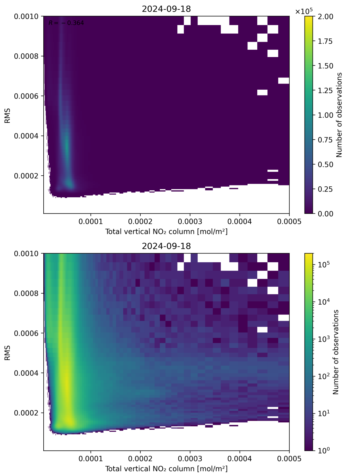
Figure 120: Scatter density plot of “Total vertical NO 2 column” against “RMS” for 2024-09-17 to 2024-09-19.
