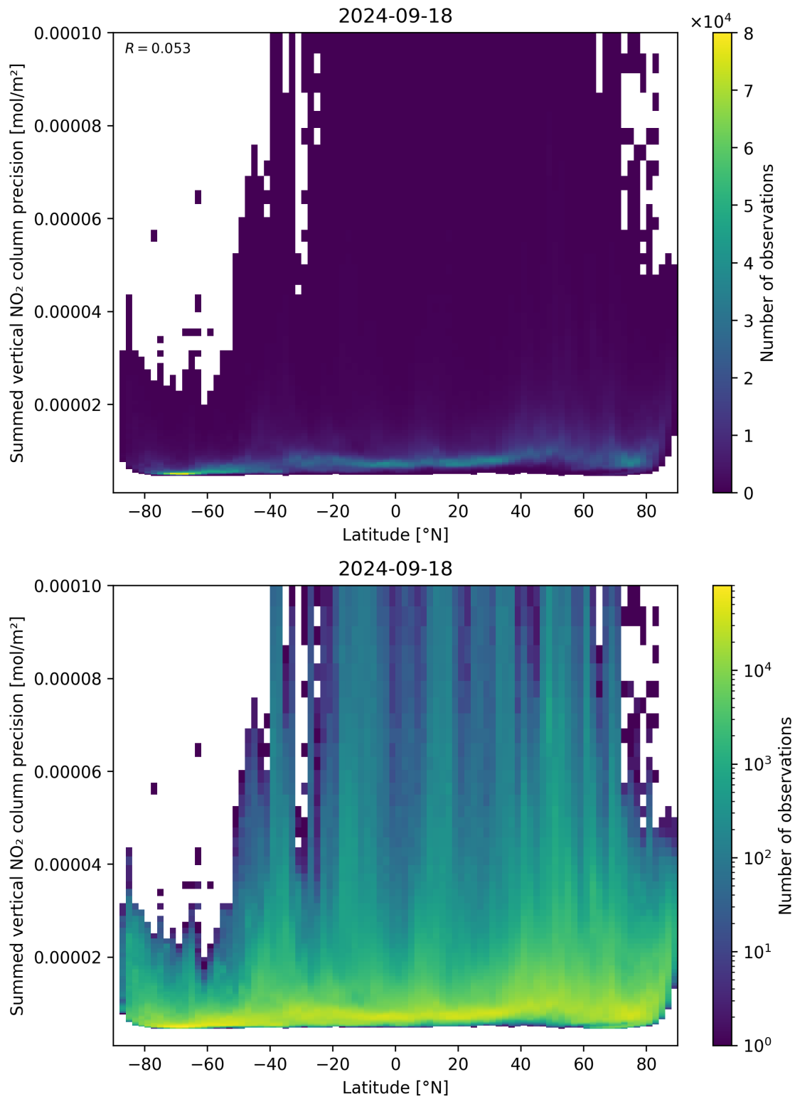
Figure 89: Scatter density plot of “Latitude” against “Summed vertical NO 2 column precision” for 2024-09-17 to 2024-09-19.
