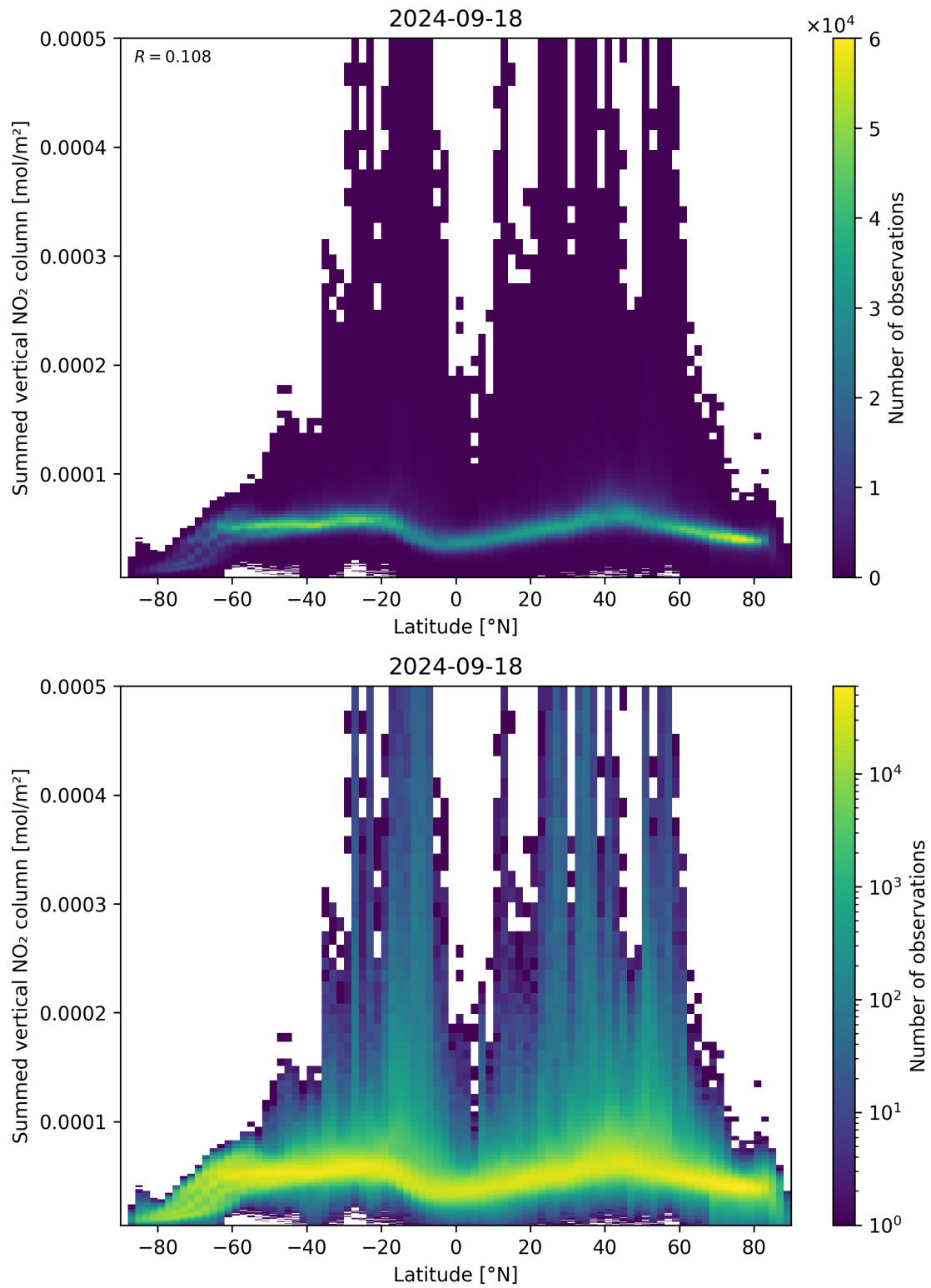
Figure 88: Scatter density plot of “Latitude” against “Summed vertical NO 2 column” for 2024-09-17 to 2024-09-19.
