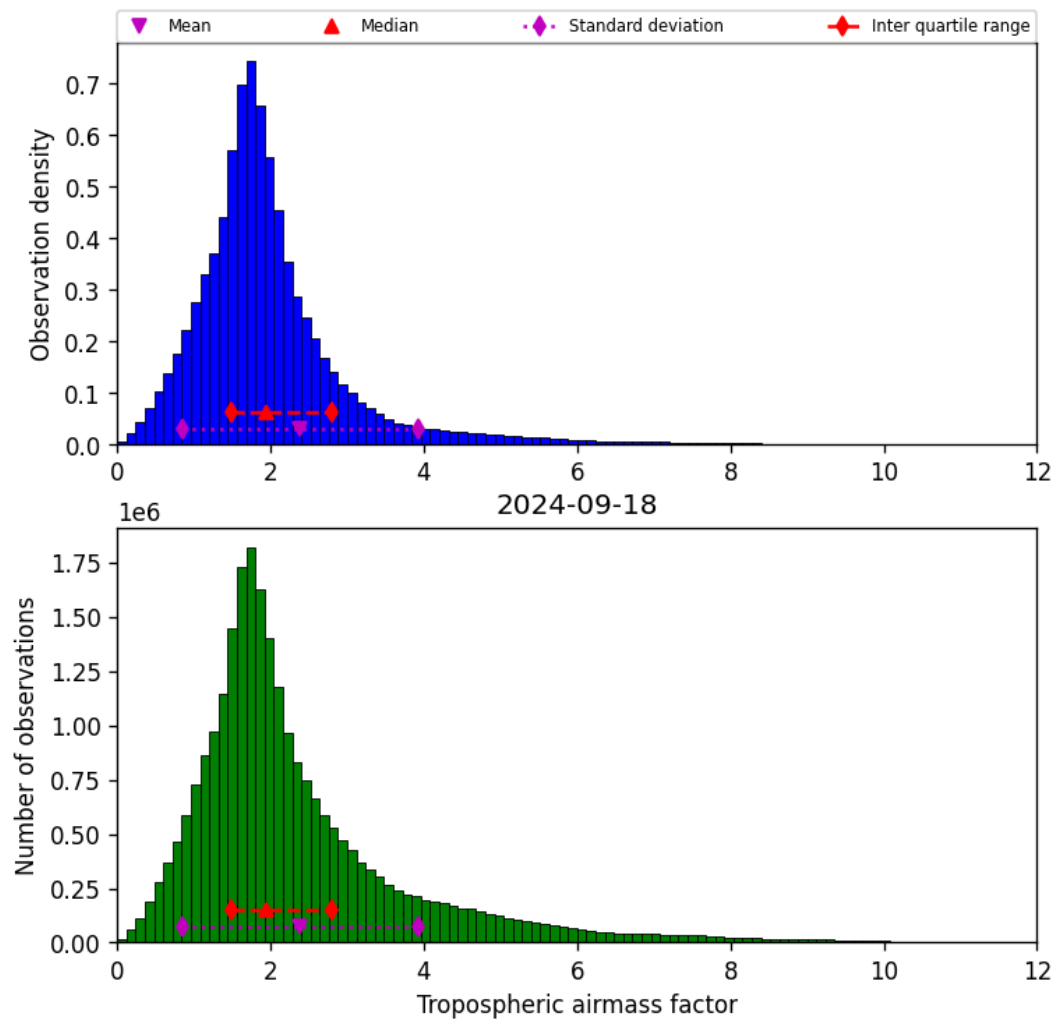
Figure 31: Histogram of “Tropospheric airmass factor” for 2024-09-17 to 2024-09-19
