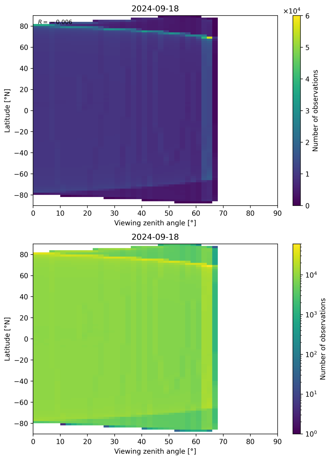
Figure 163: Scatter density plot of “Viewing zenith angle” against “Latitude” for 2024-09-17 to 2024-09-19.
