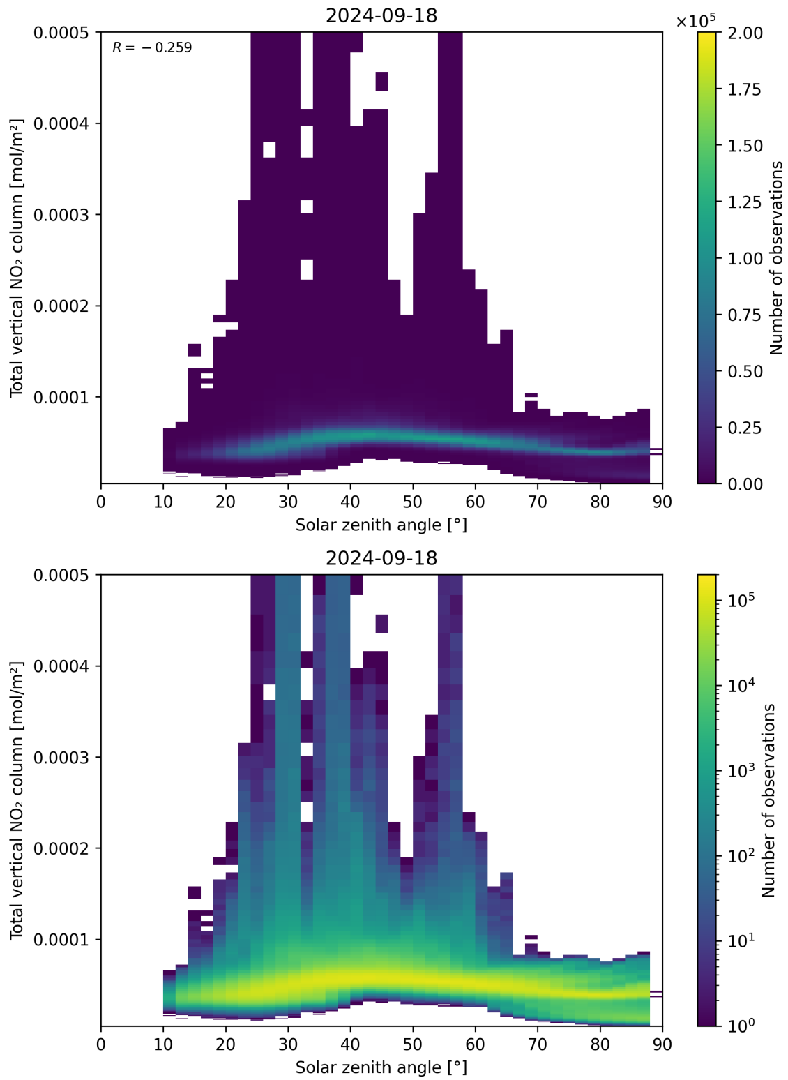
Figure 153: Scatter density plot of “Solar zenith angle” against “Total vertical NO 2 column” for 2024-09-17 to 2024-09-19.
