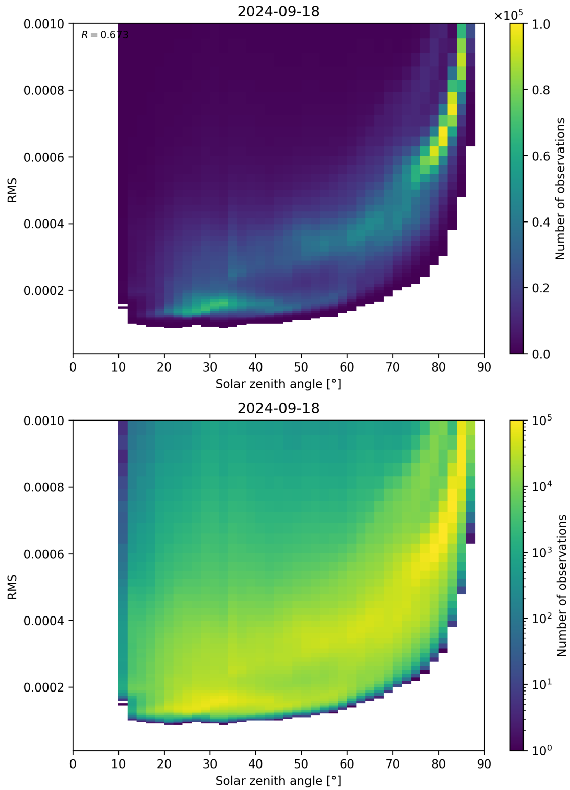
Figure 157: Scatter density plot of “Solar zenith angle” against “RMS” for 2024-09-17 to 2024-09-19.
