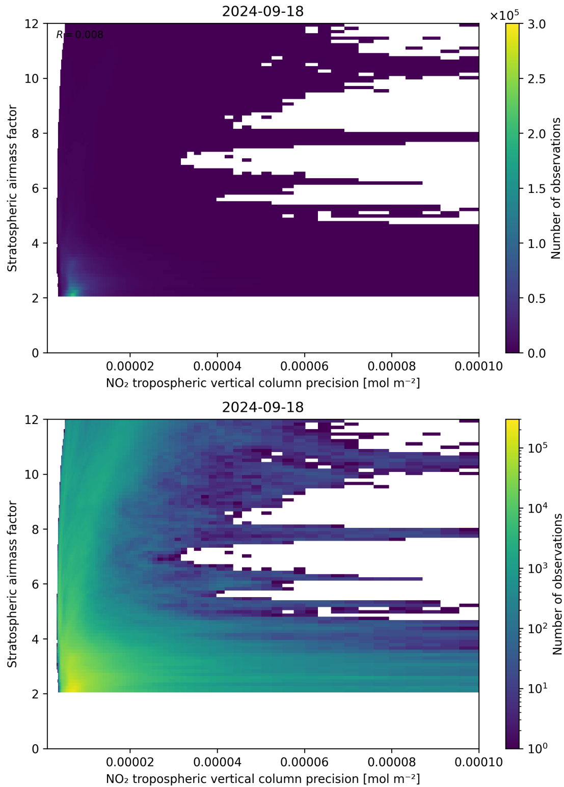
Figure 131: Scatter density plot of “NO 2 tropospheric vertical column precision” against “Stratospheric airmass factor” for 2024-09-17 to 2024-09-19.
