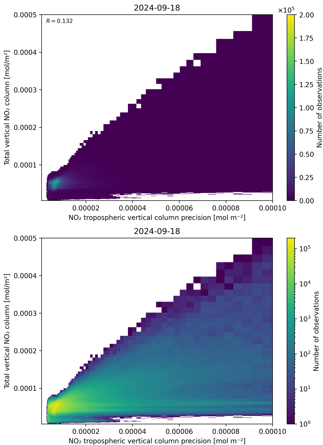
Figure 138: Scatter density plot of “NO 2 tropospheric vertical column precision” against “Total vertical NO 2 column” for 2024-09-17 to 2024-09-19.
