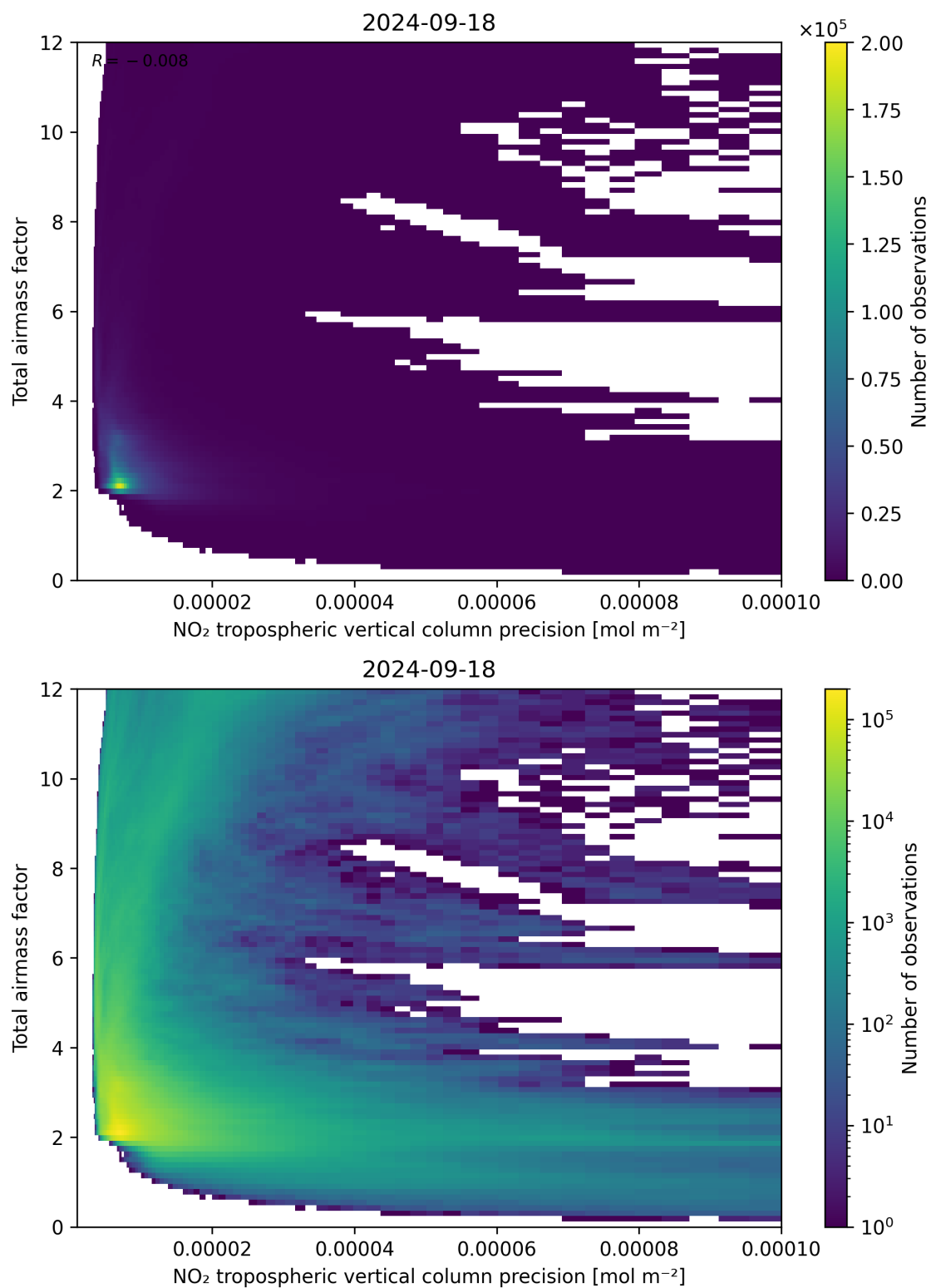
Figure 132: Scatter density plot of “NO 2 tropospheric vertical column precision” against “Total airmass factor” for 2024-09-17 to 2024-09-19.
