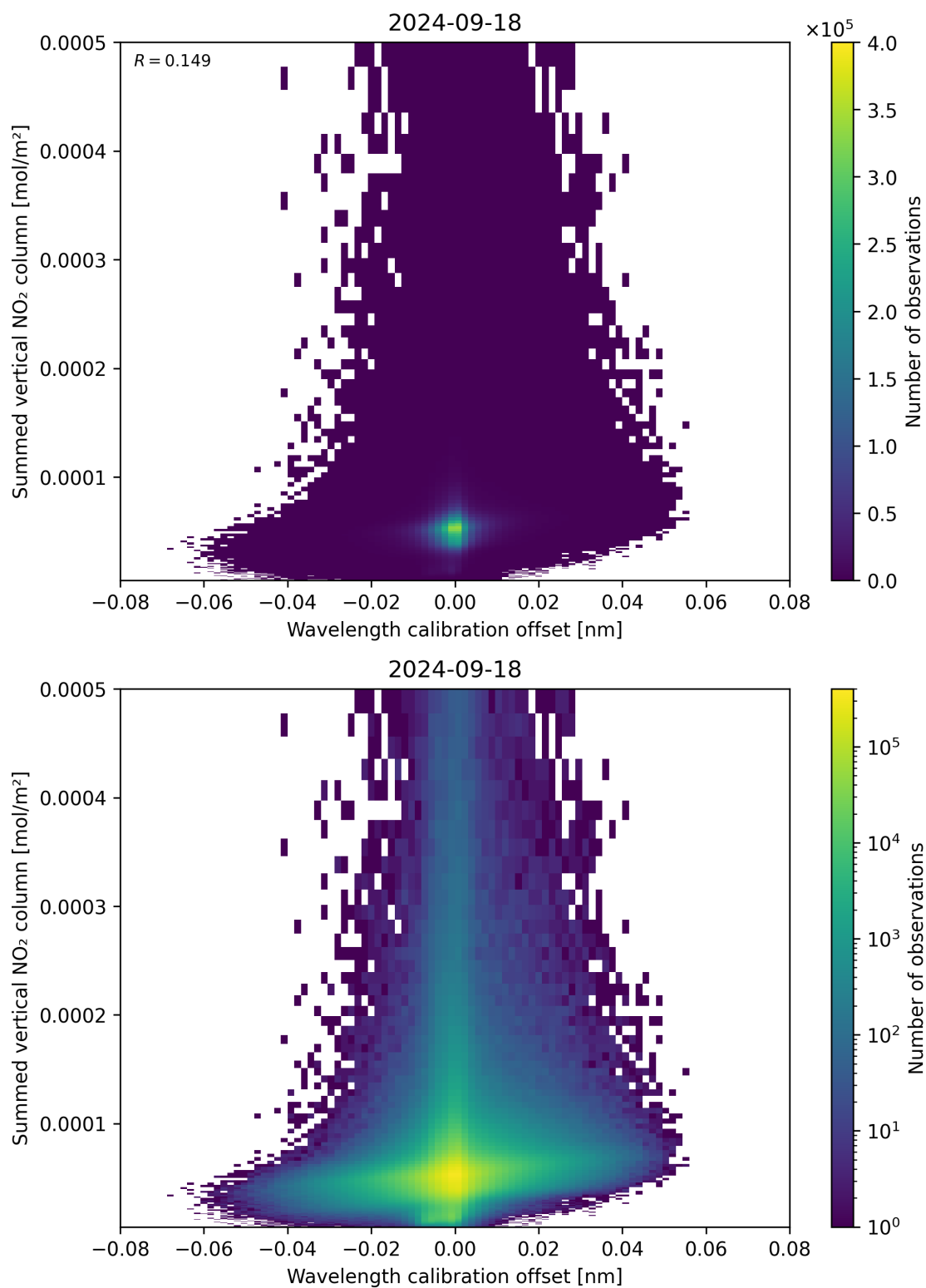
Figure 177: Scatter density plot of “Wavelength calibration offset” against “Summed vertical NO 2 column” for 2024-09-17 to 2024-09-19.
