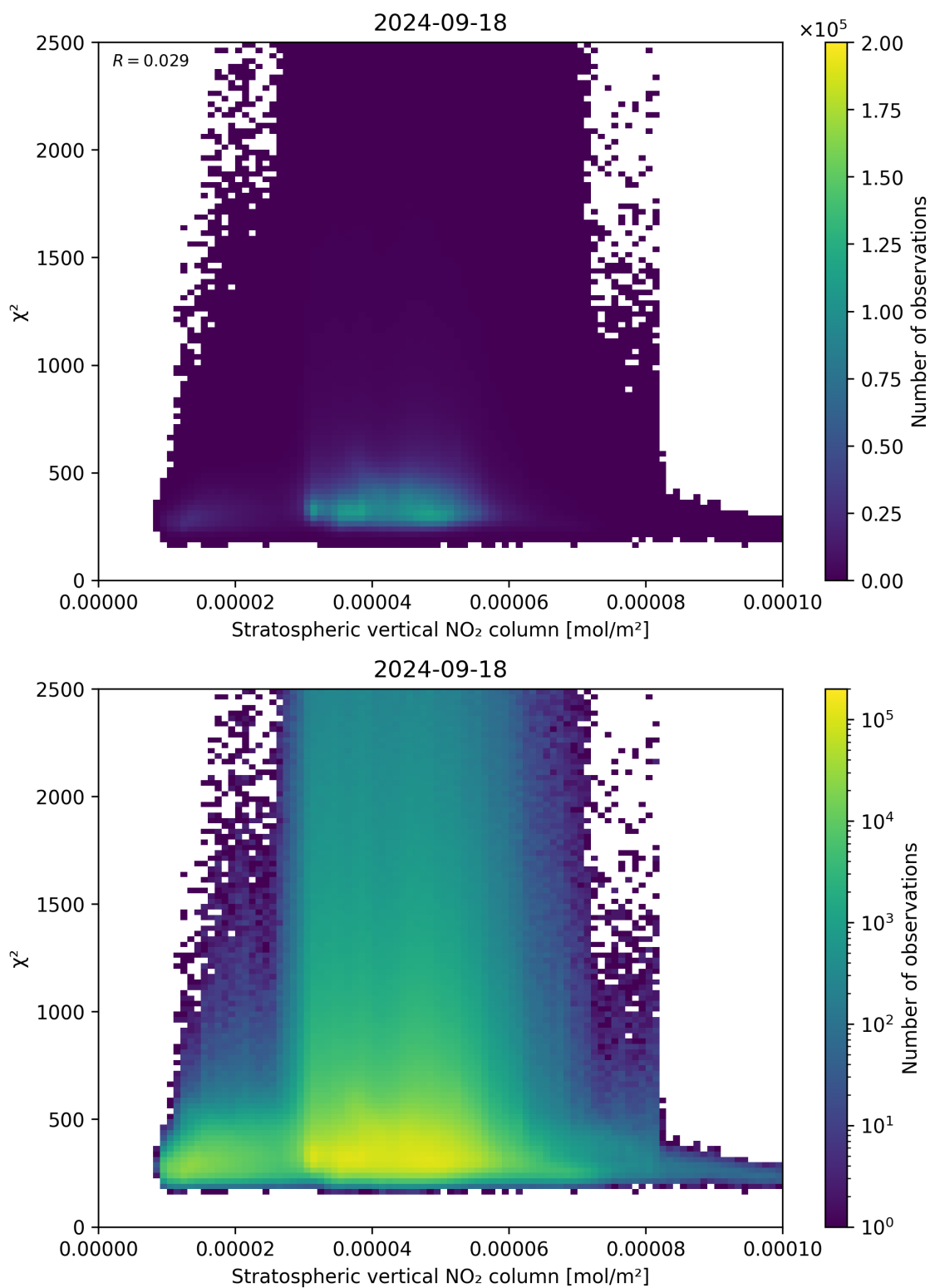
Figure 97: Scatter density plot of “Stratospheric vertical NO 2 column” against “ \chi^2 ” for 2024-09-17 to 2024-09-19.
