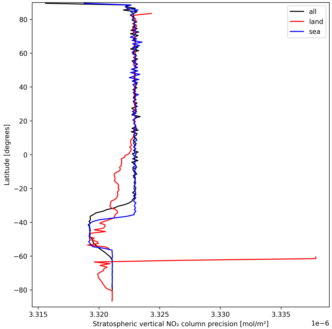
Figure 20: Zonal average of “Stratospheric vertical NO 2 column precision” for 2024-09-17 to 2024-09-19.
