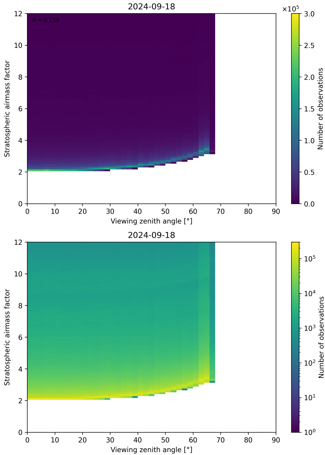
Figure 159: Scatter density plot of “Viewing zenith angle” against “Stratospheric airmass factor” for 2024-09-17 to 2024-09-19.
