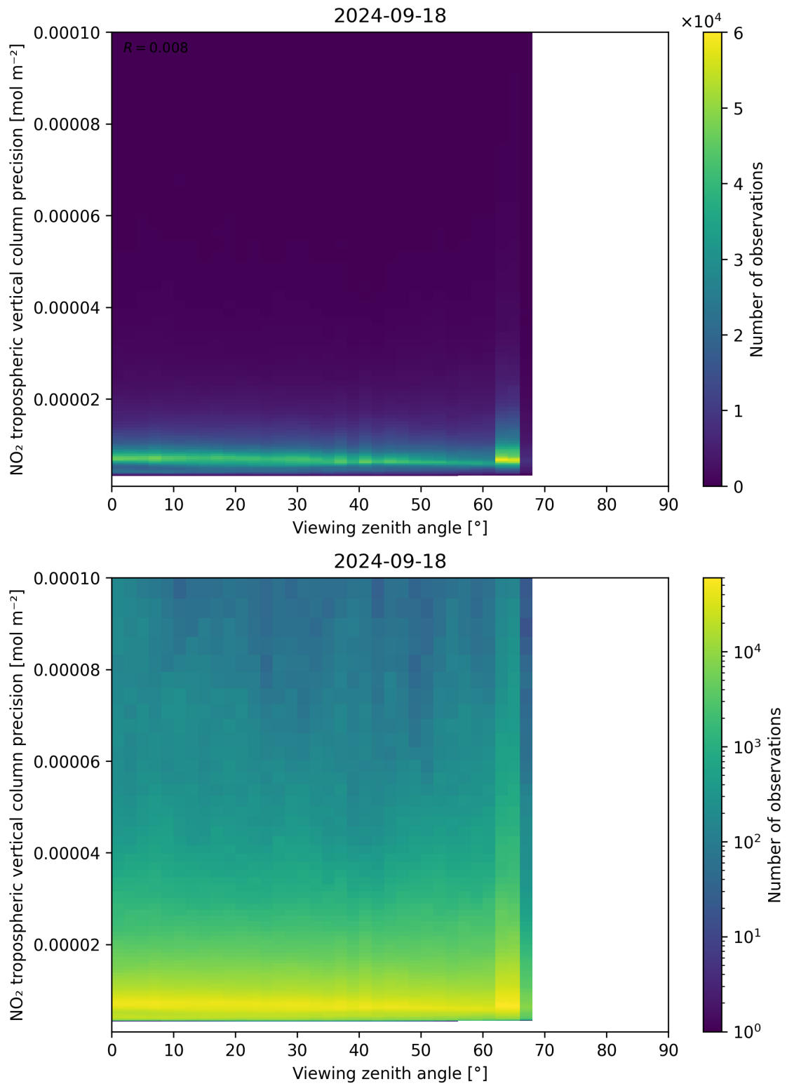
Figure 170: Scatter density plot of “Viewing zenith angle” against “NO 2 tropospheric vertical column precision” for 2024-09-17 to 2024-09-19.
