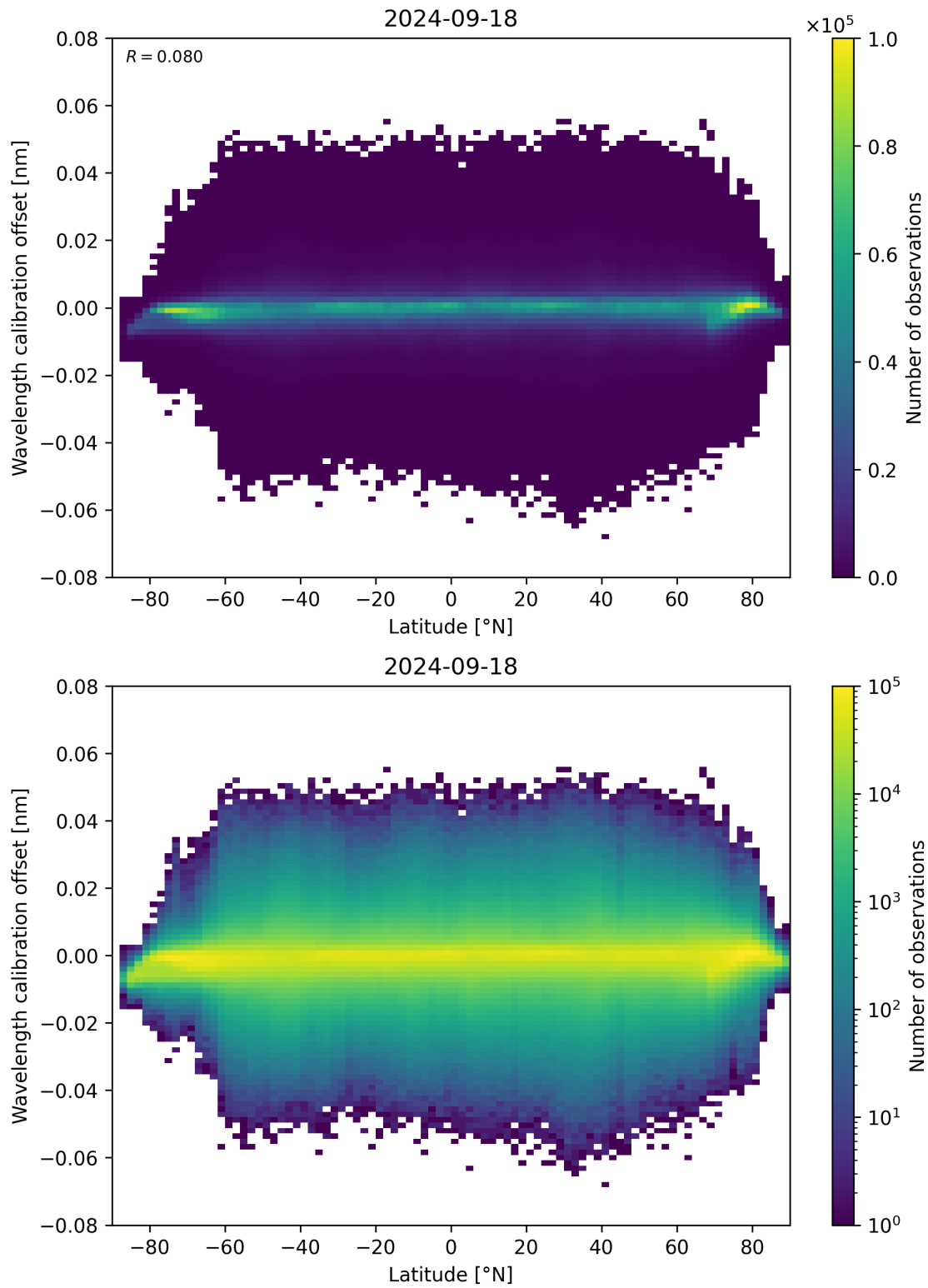
Figure 95: Scatter density plot of “Latitude” against “Wavelength calibration offset” for 2024-09-17 to 2024-09-19.
