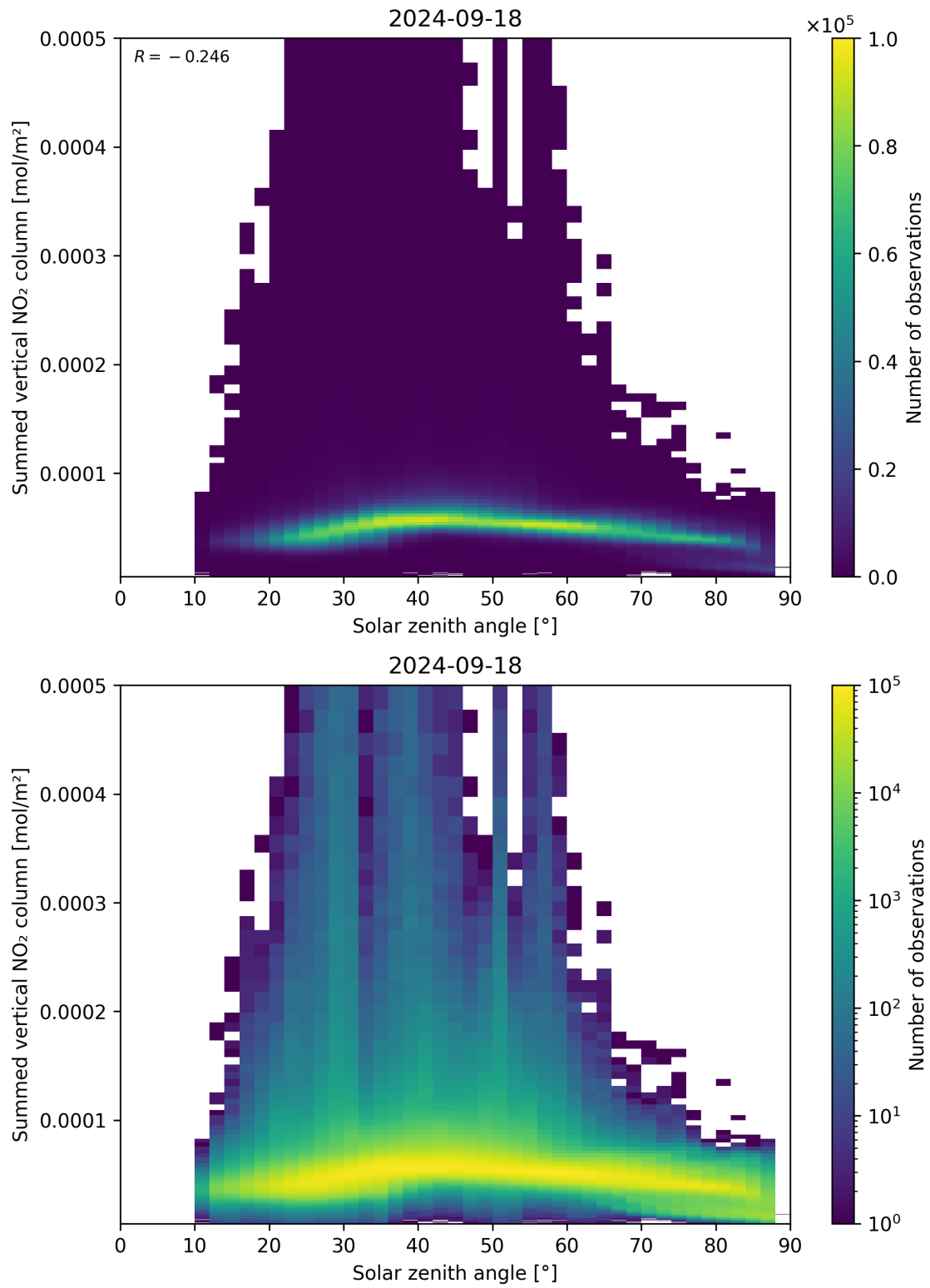
Figure 151: Scatter density plot of “Solar zenith angle” against “Summed vertical NO 2 column” for 2024-09-17 to 2024-09-19.
