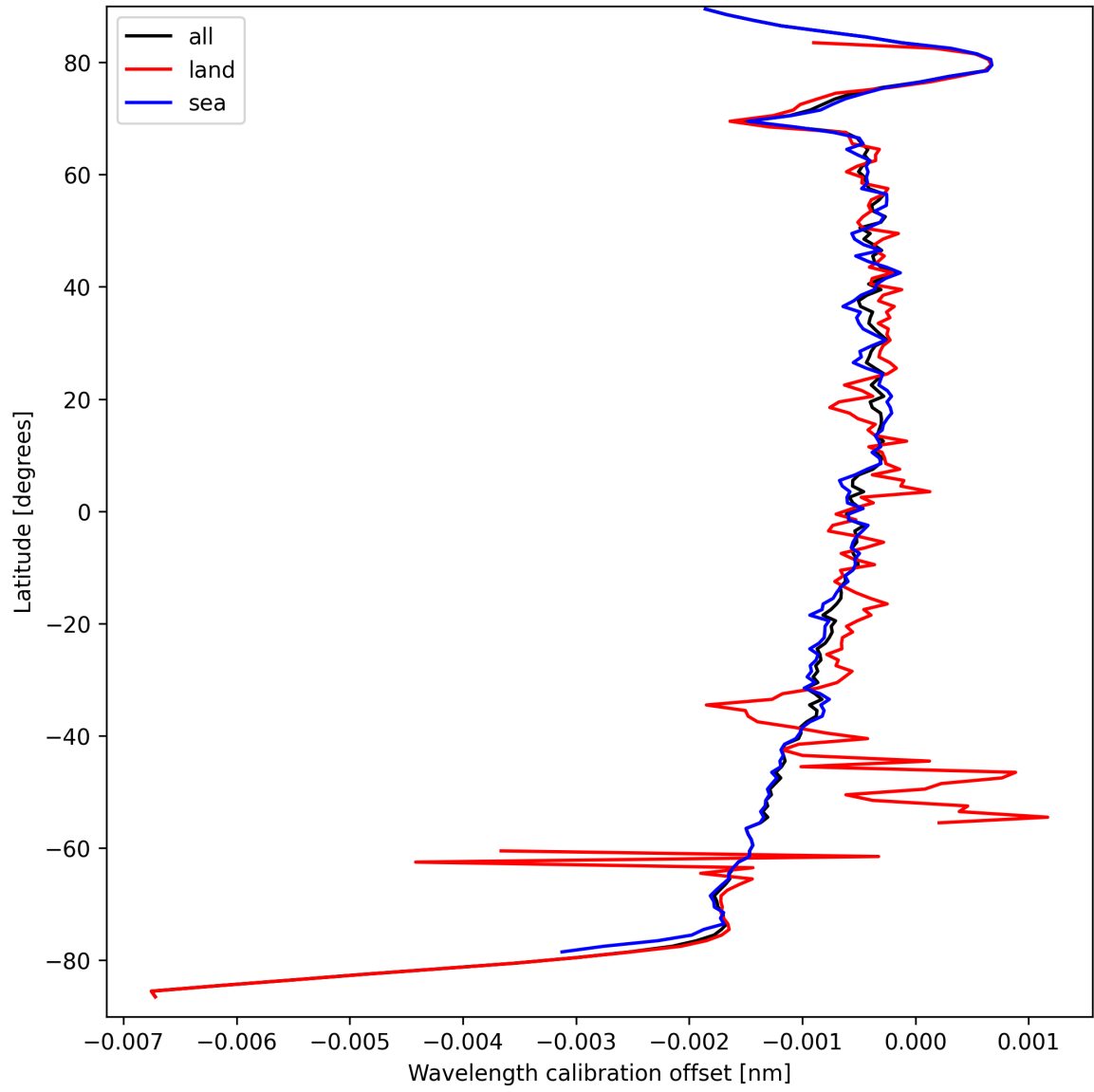
Figure 18: Zonal average of “Wavelength calibration offset” for 2024-09-17 to 2024-09-19.
