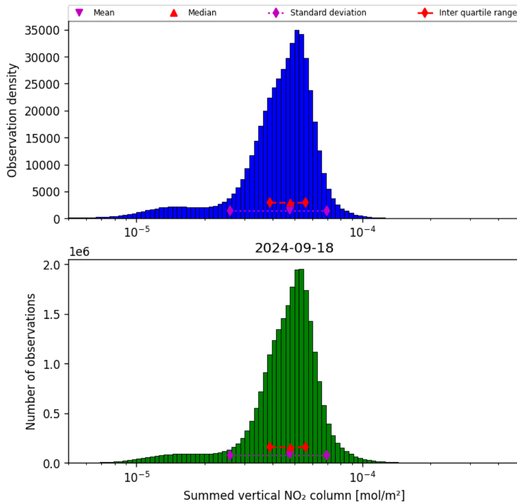
Figure 40: Histogram of “Summed vertical NO 2 column” for 2024-09-17 to 2024-09-19
