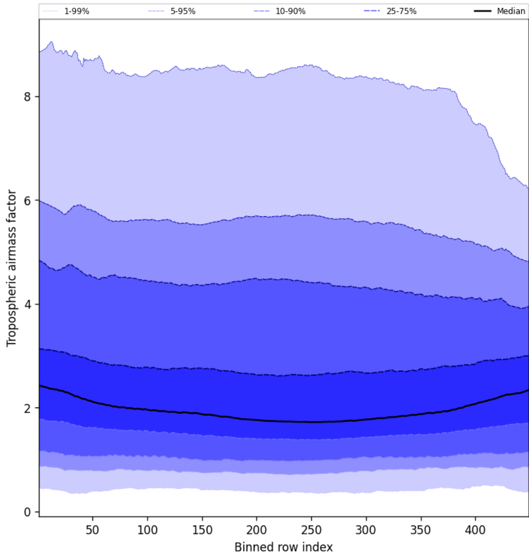
Figure 48: Along track statistics of “Tropospheric air mass factor” for 2024-09-17 to 2024-09-19
