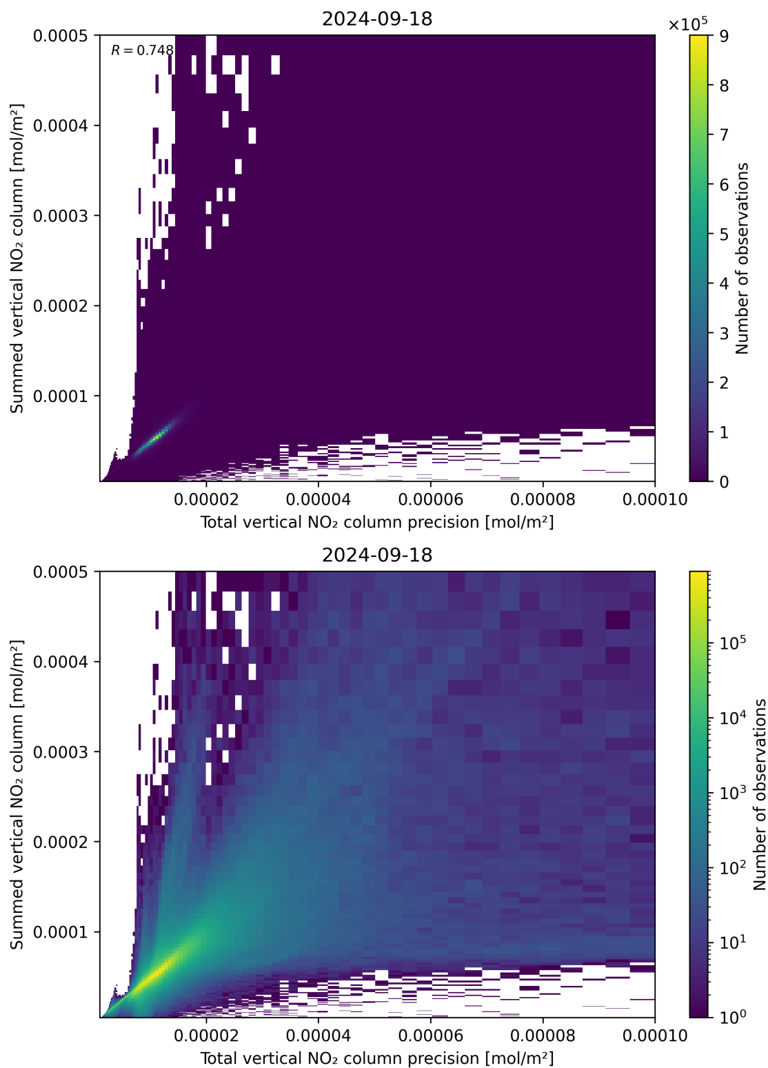
Figure 117: Scatter density plot of “Total vertical NO 2 column precision” against “Summed vertical NO 2 column” for 2024-09-17 to 2024-09-19.
