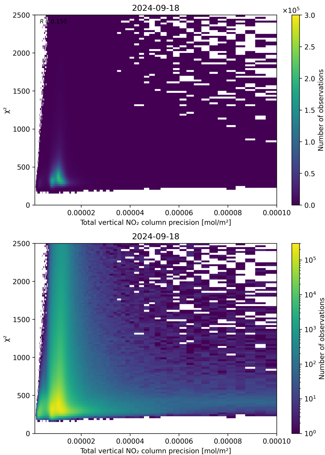
Figure 116: Scatter density plot of “Total vertical NO 2 column precision” against “ \chi^2 ” for 2024-09-17 to 2024-09-19.
