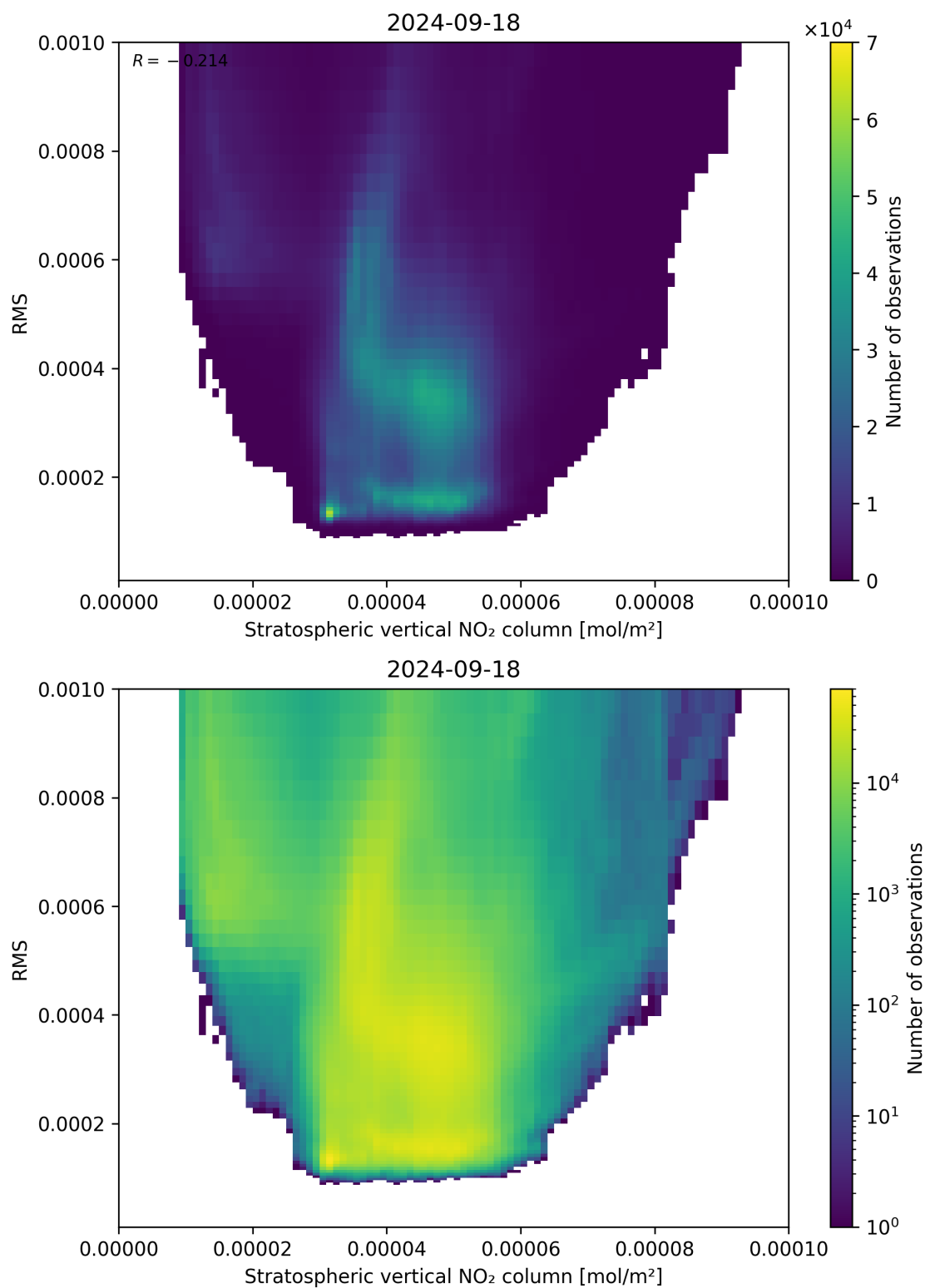
Figure 102: Scatter density plot of “Stratospheric vertical NO 2 column” against “RMS” for 2024-09-17 to 2024-09-19.
