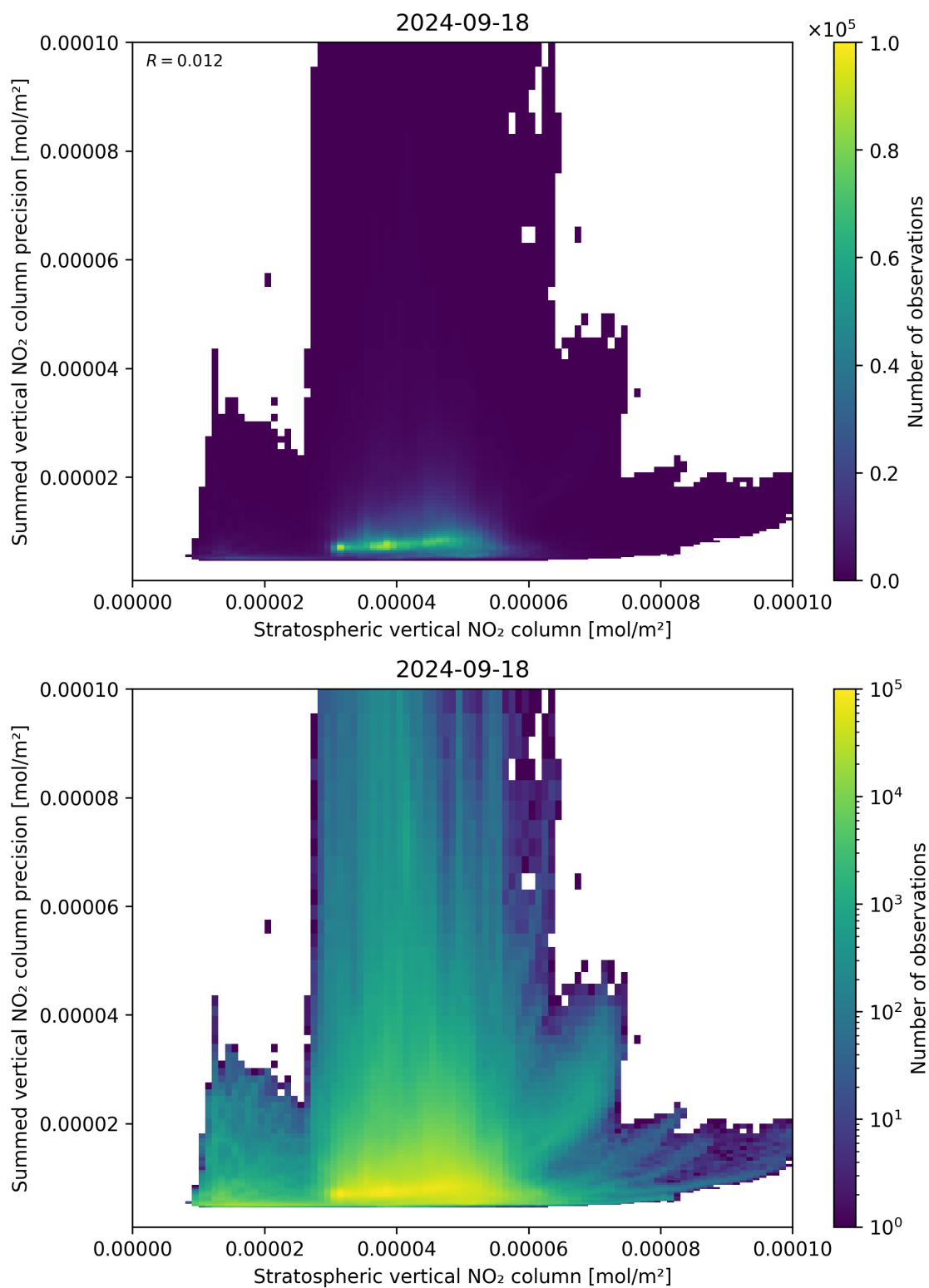
Figure 99: Scatter density plot of “Stratospheric vertical NO 2 column” against “Summed vertical NO 2 column precision” for 2024-09-17 to 2024-09-19.
