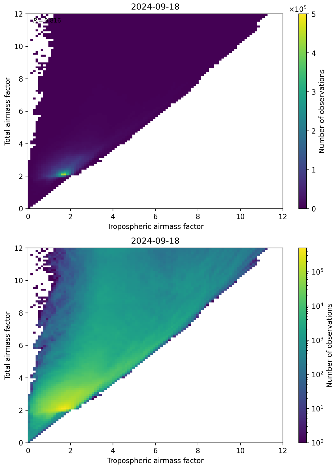
Figure 72: Scatter density plot of “Tropospheric airmass factor” against “Total airmass factor” for 2024-09-17 to 2024-09-19.
