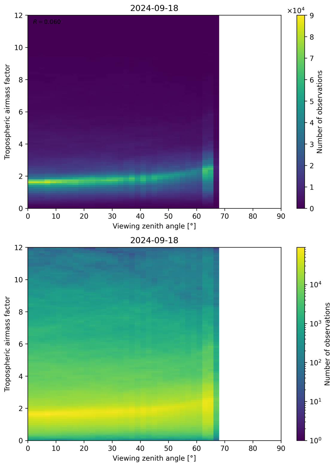
Figure 161: Scatter density plot of “Viewing zenith angle” against “Tropospheric air mass factor” for 2024-09-17 to 2024-09-19.
