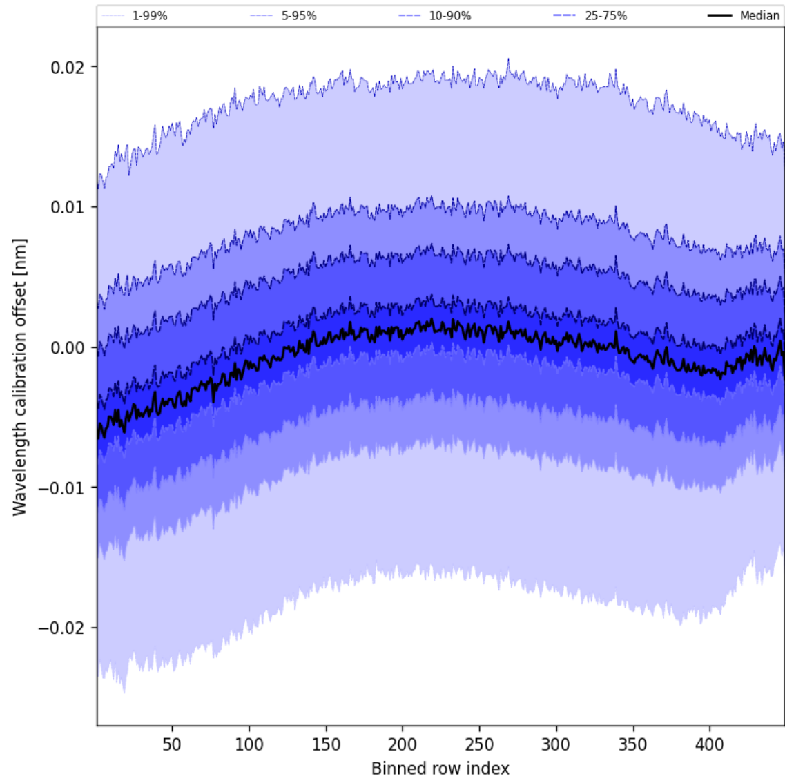
Figure 52: Along track statistics of “Wavelength calibration offset” for 2024-09-17 to 2024-09-19
