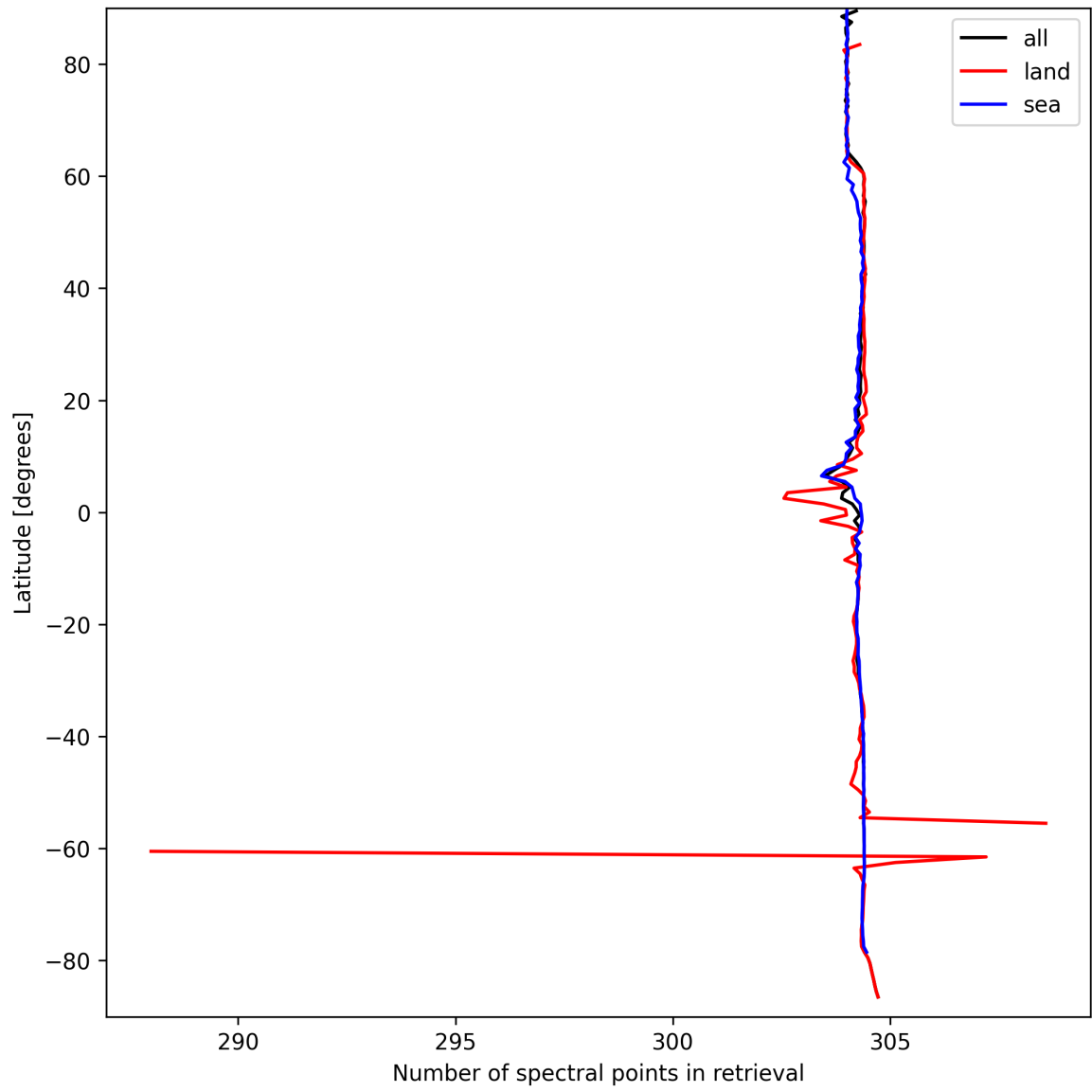
Figure 16: Zonal average of “Number of spectral points in retrieval” for 2024-09-17 to 2024-09-19.
