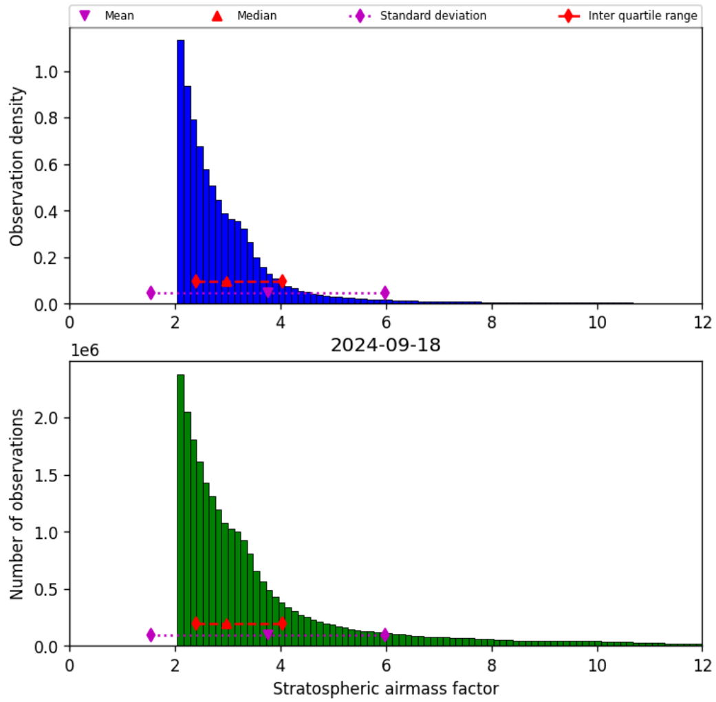
Figure 44: Histogram of “Stratospheric airmass factor” for 2024-09-17 to 2024-09-19
