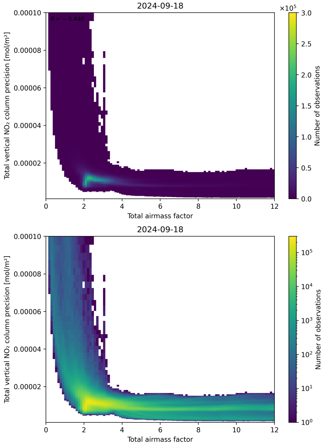
Figure 68: Scatter density plot of “Total airmass factor” against “Total vertical NO 2 column precision” for 2024-09-17 to 2024-09-19.
