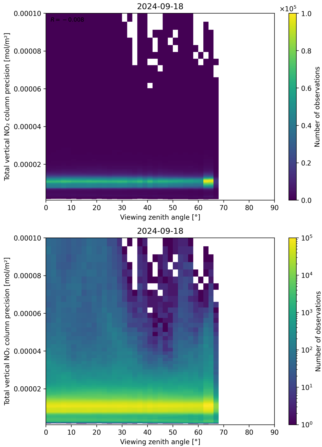
Figure 168: Scatter density plot of “Viewing zenith angle” against “Total vertical NO 2 column precision” for 2024-09-17 to 2024-09-19.
