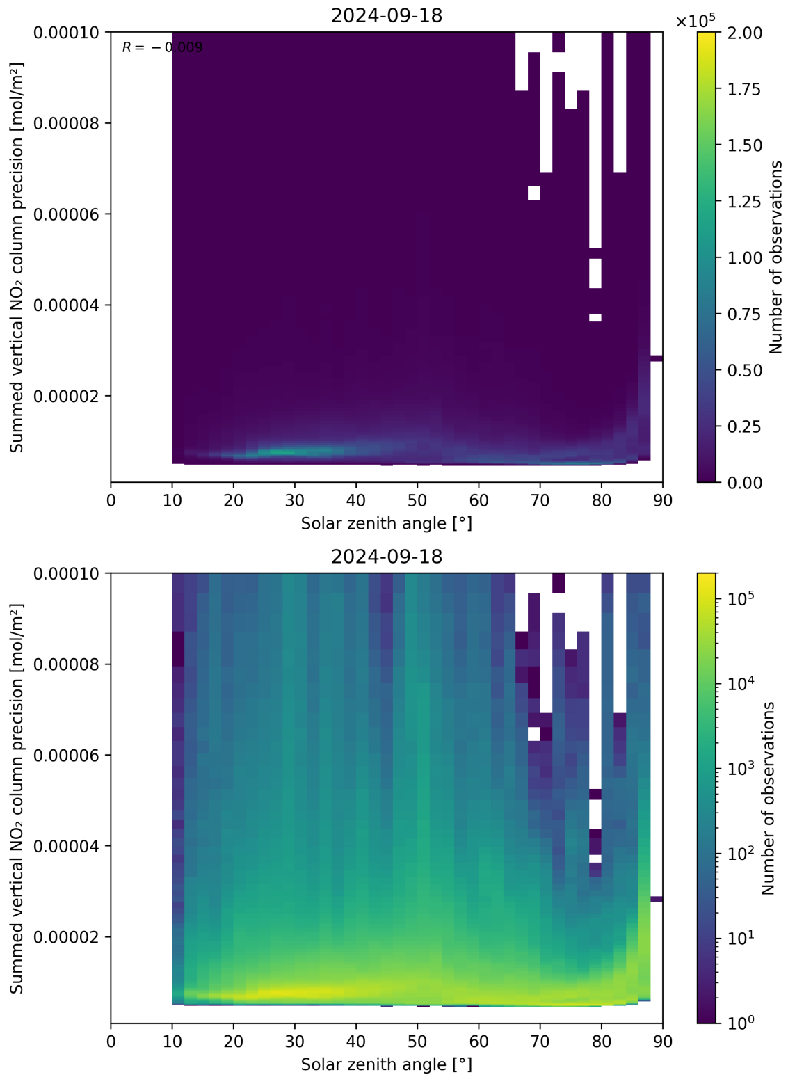
Figure 152: Scatter density plot of “Solar zenith angle” against “Summed vertical NO 2 column precision” for 2024-09-17 to 2024-09-19.
