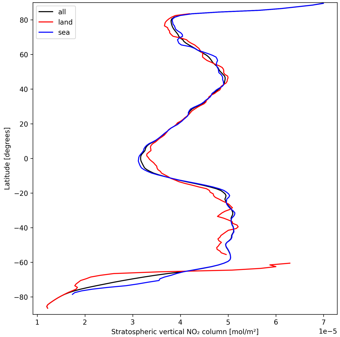
Figure 19: Zonal average of “Stratospheric vertical NO 2 column” for 2024-09-17 to 2024-09-19.
