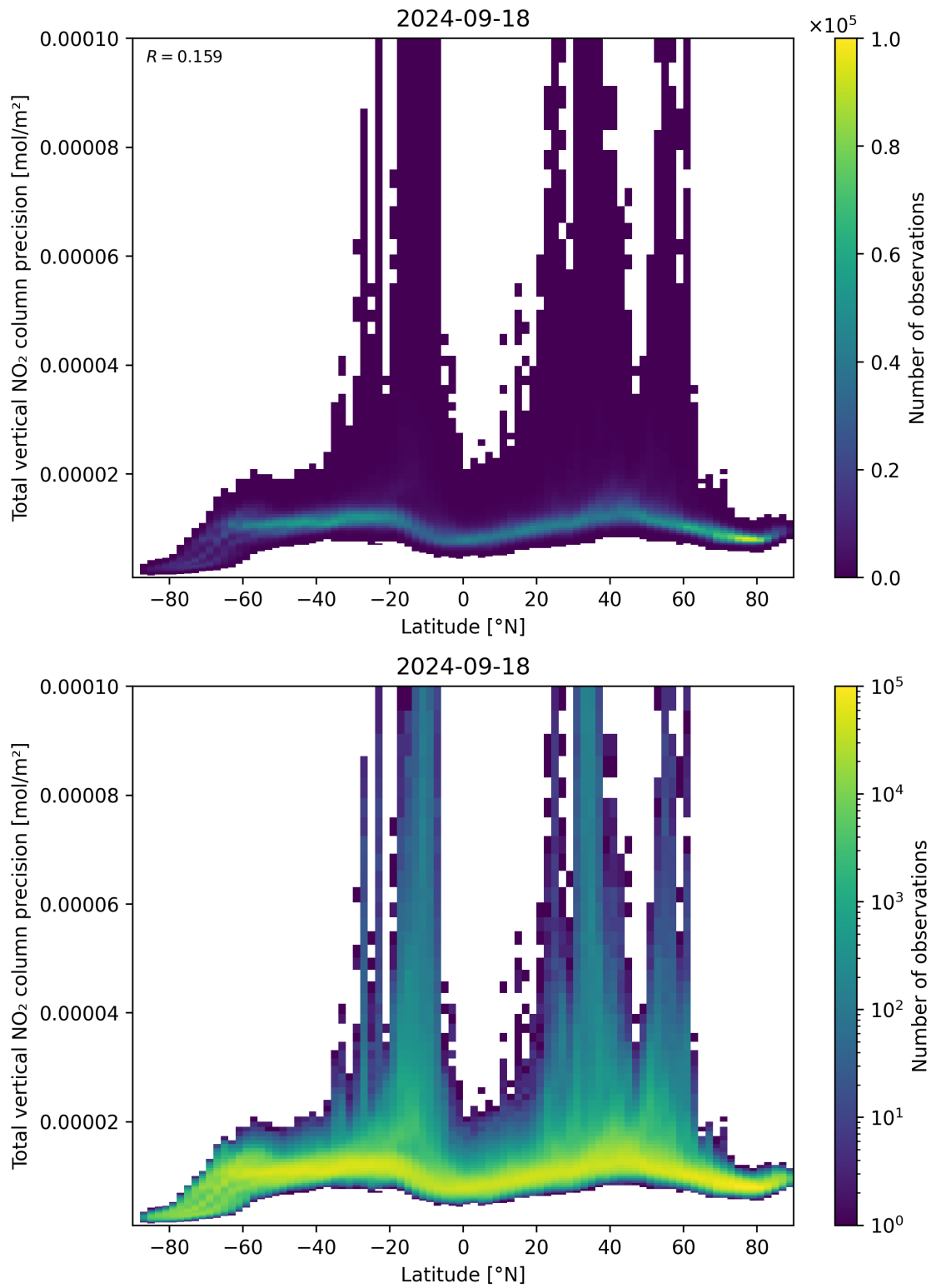
Figure 91: Scatter density plot of “Latitude” against “Total vertical NO 2 column precision” for 2024-09-17 to 2024-09-19.
