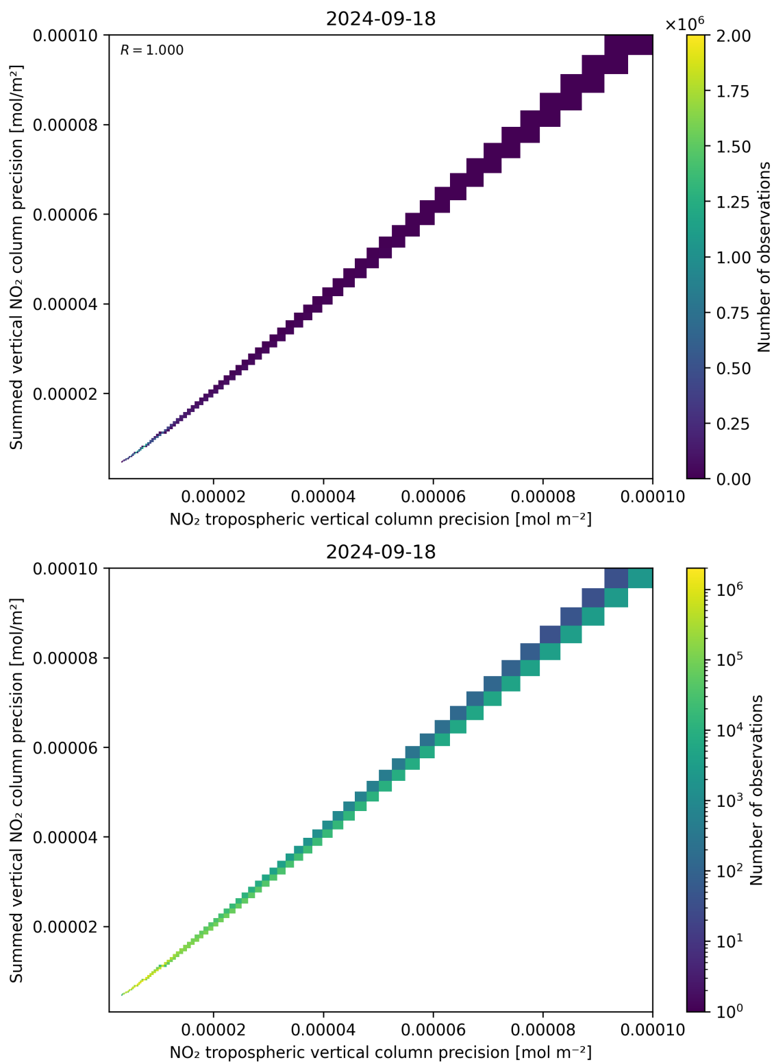
Figure 137: Scatter density plot of “NO 2 tropospheric vertical column precision” against “Summed vertical NO 2 column precision” for 2024-09-17 to 2024-09-19.
