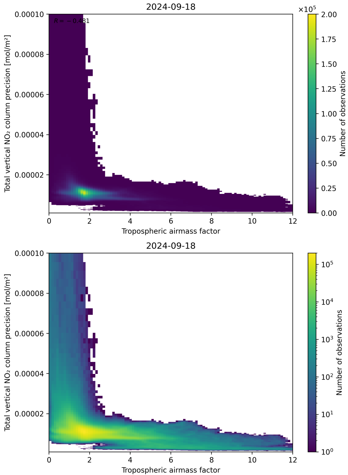
Figure 78: Scatter density plot of “Tropospheric air mass factor” against “Total vertical NO 2 column precision” for 2024-09-17 to 2024-09-19.
