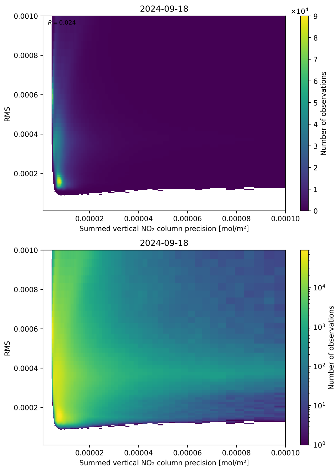
Figure 108: Scatter density plot of “Summed vertical NO 2 column precision” against “RMS” for 2024-09-17 to 2024-09-19.
