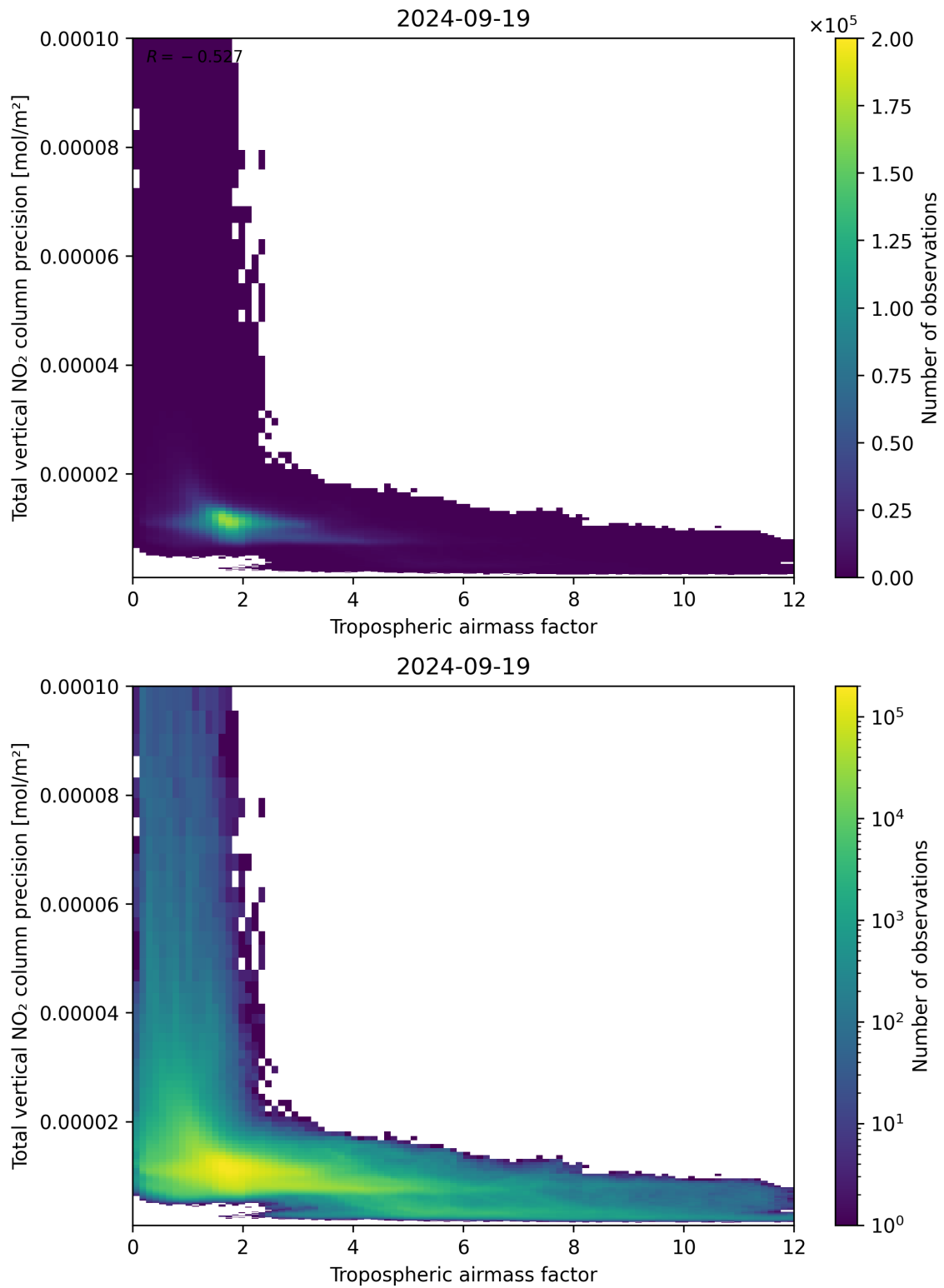
Figure 78: Scatter density plot of “Tropospheric air mass factor” against “Total vertical NO 2 column precision” for 2024-09-18 to 2024-09-20.
