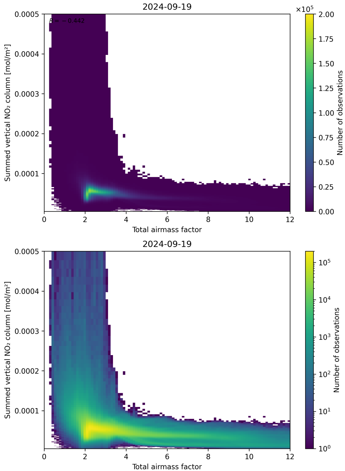
Figure 65: Scatter density plot of “Total airmass factor” against “Summed vertical NO 2 column” for 2024-09-18 to 2024-09-20.
