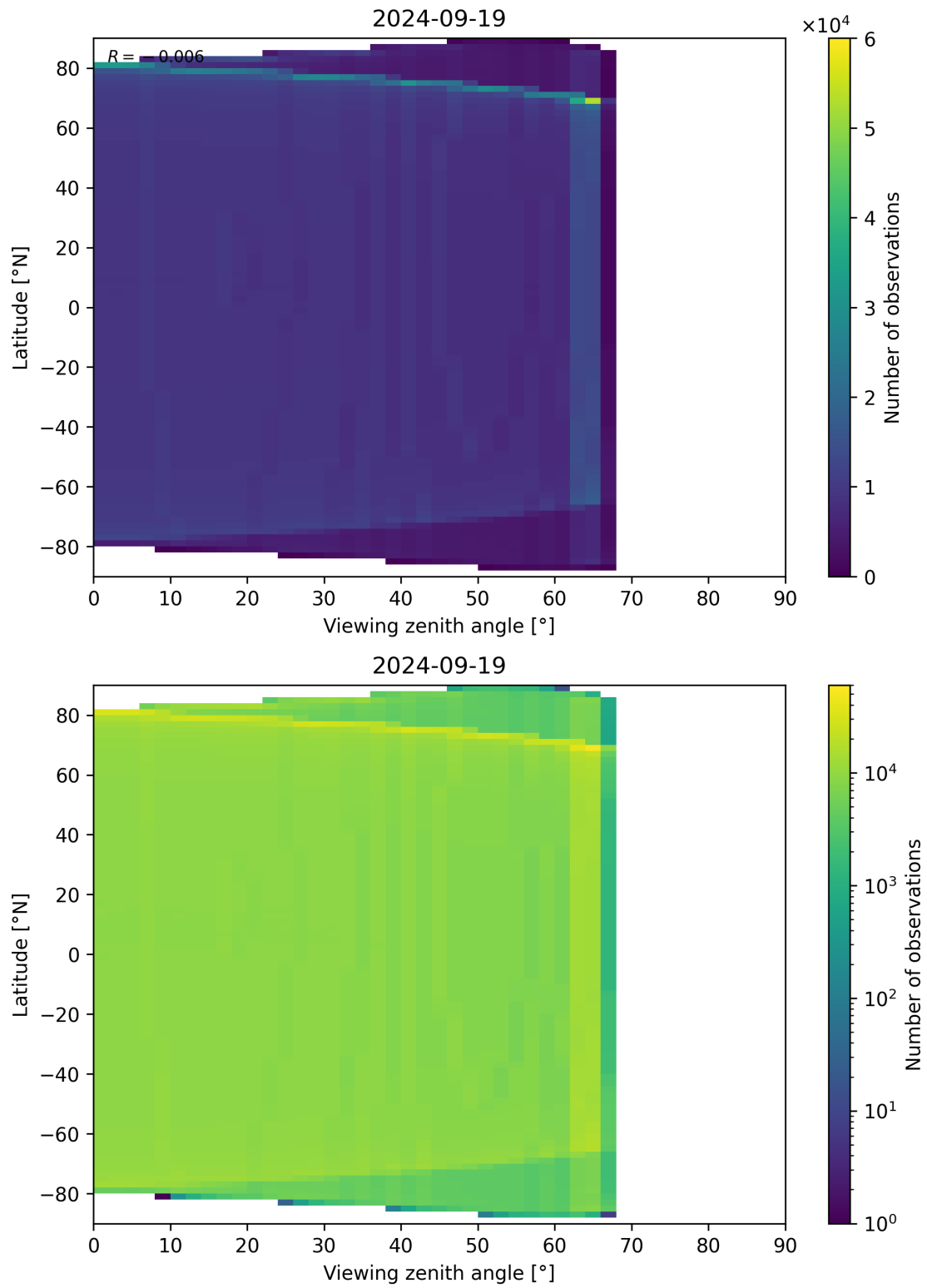
Figure 163: Scatter density plot of “Viewing zenith angle” against “Latitude” for 2024-09-18 to 2024-09-20.
