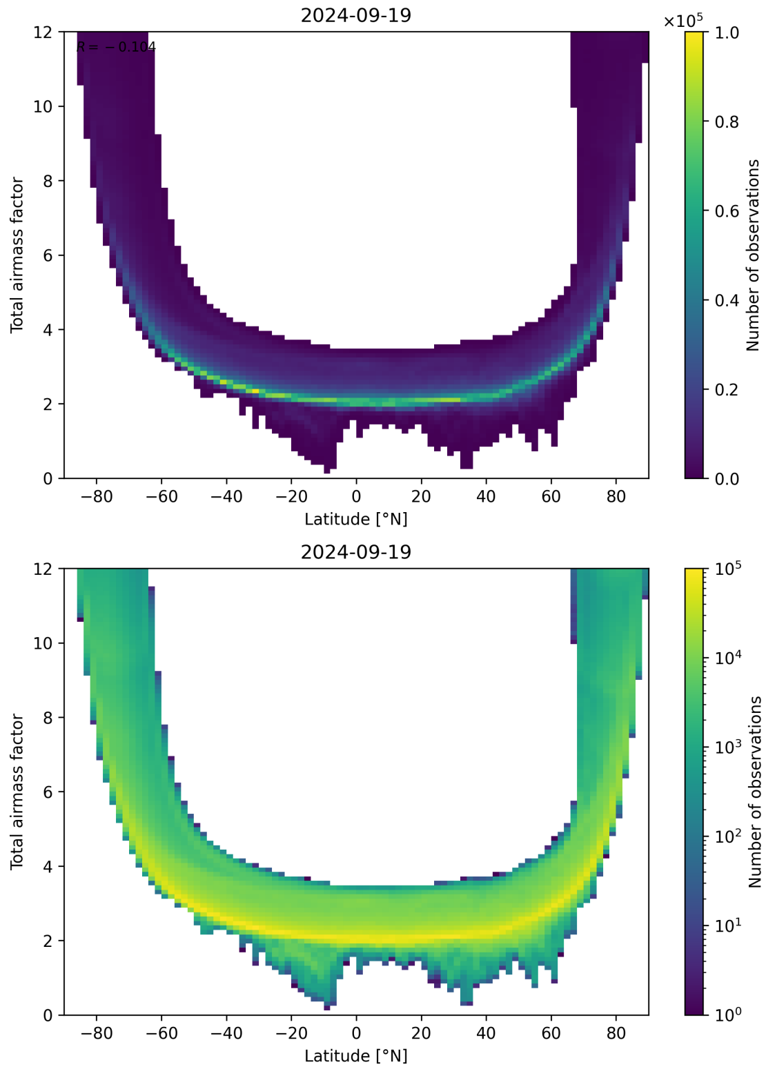
Figure 84: Scatter density plot of “Latitude” against “Total airmass factor” for 2024-09-18 to 2024-09-20.
