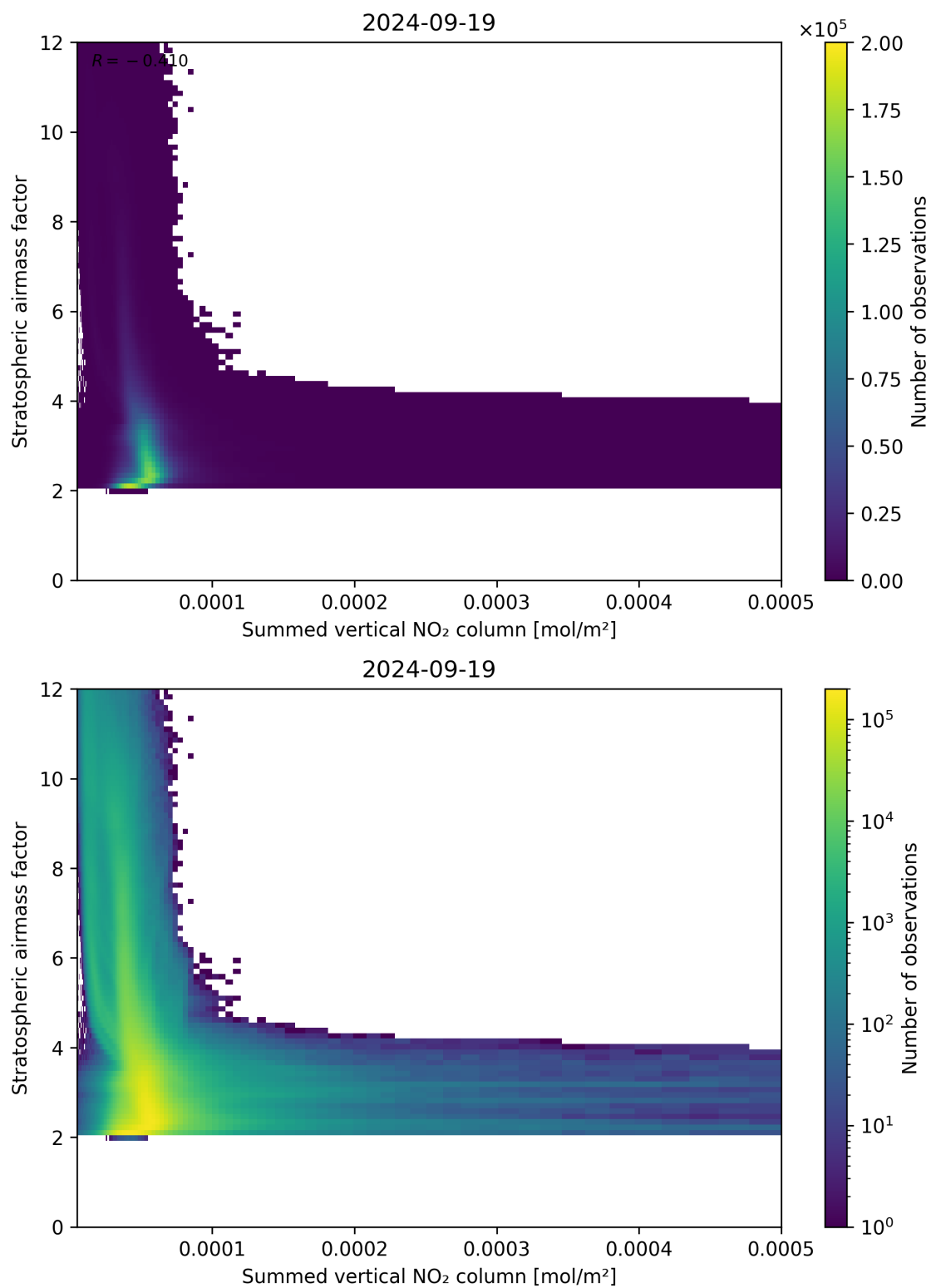
Figure 103: Scatter density plot of “Summed vertical NO 2 column” against “Stratospheric airmass factor” for 2024-09-18 to 2024-09-20.
