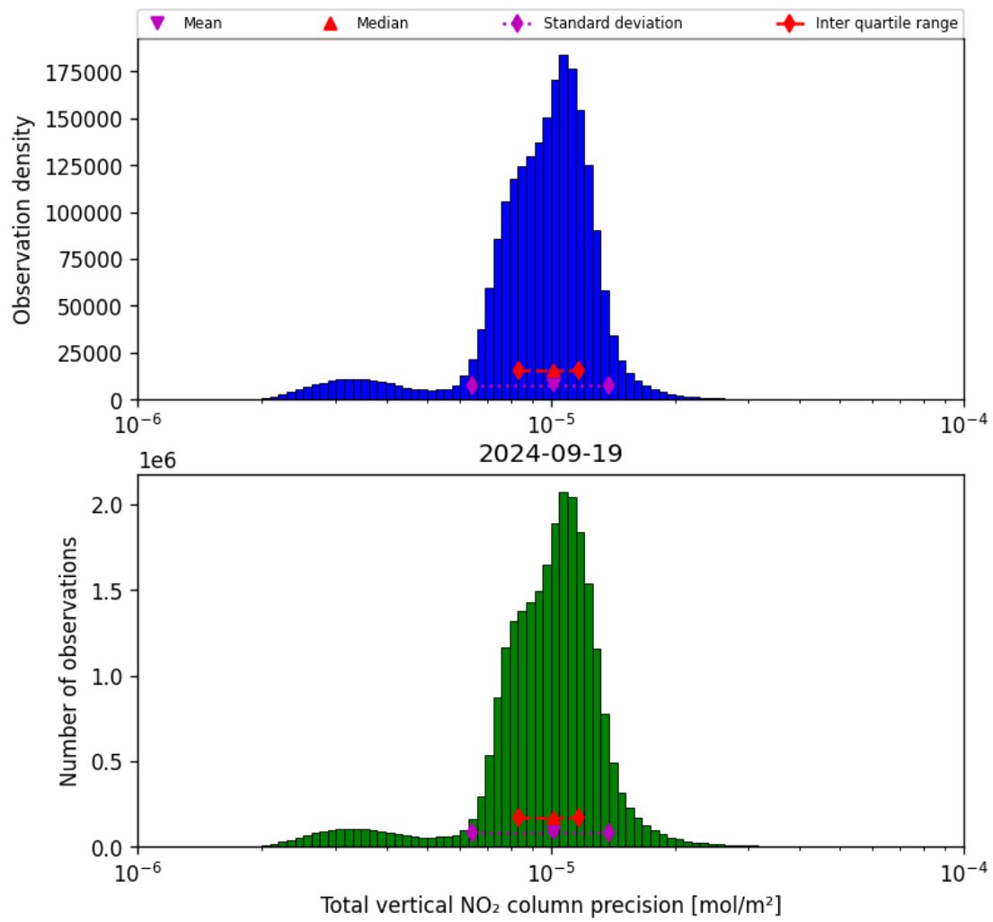
Figure 39: Histogram of “Total vertical NO 2 column precision” for 2024-09-18 to 2024-09-20
