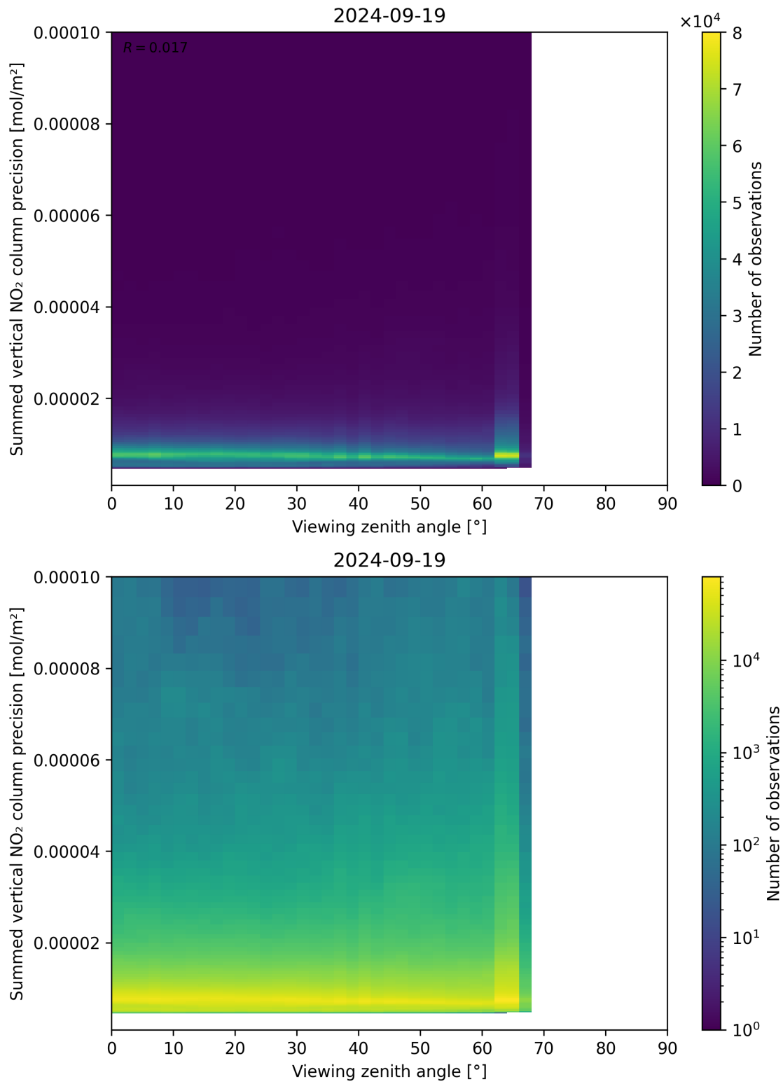
Figure 166: Scatter density plot of “Viewing zenith angle” against “Summed vertical NO 2 column precision” for 2024-09-18 to 2024-09-20.
