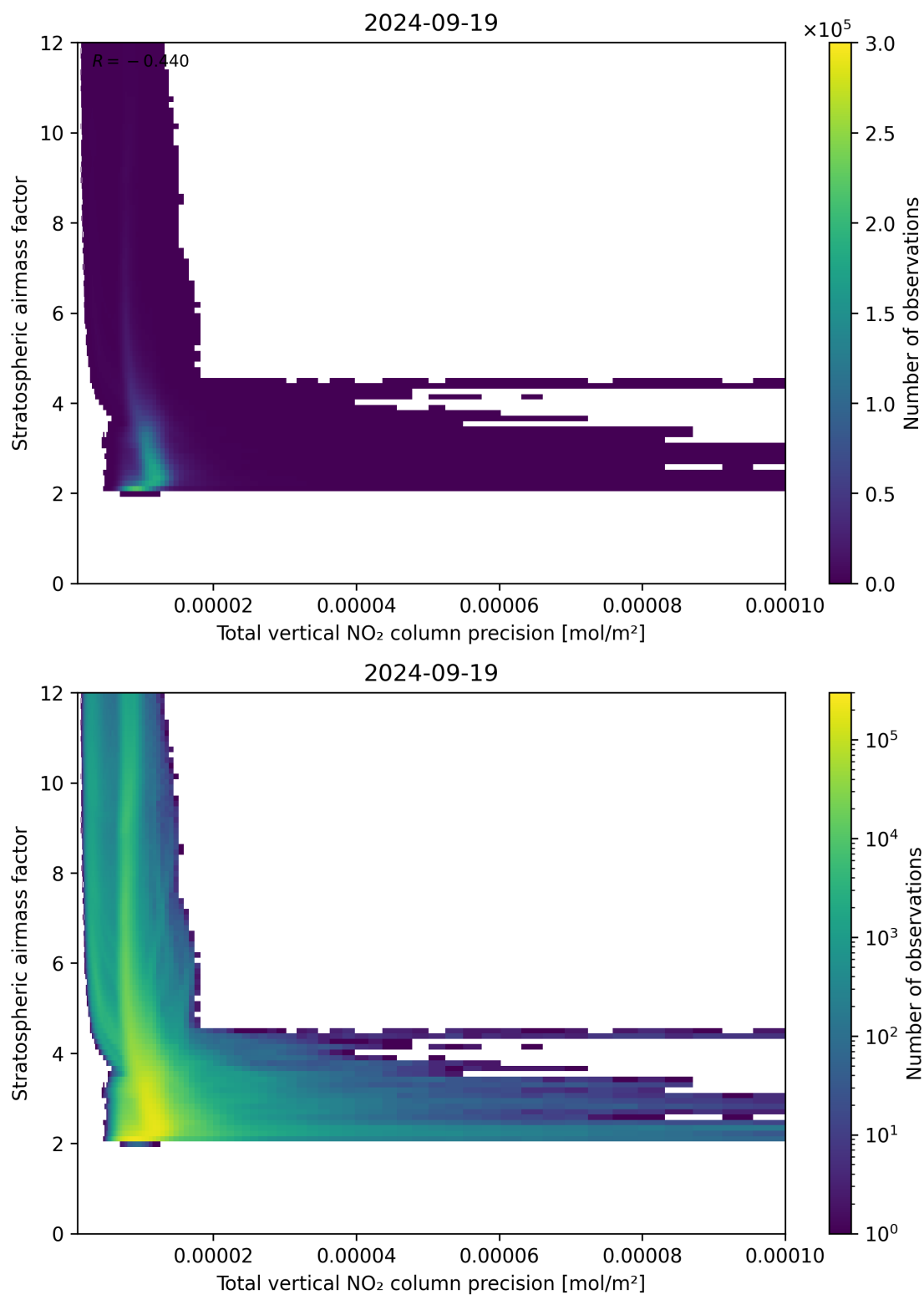
Figure 115: Scatter density plot of “Total vertical NO 2 column precision” against “Stratospheric air mass factor” for 2024-09-18 to 2024-09-20.
