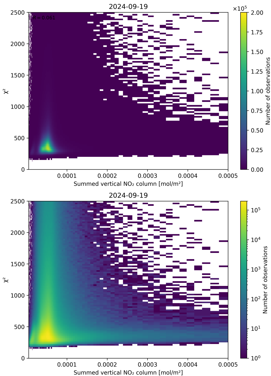
Figure 104: Scatter density plot of “Summed vertical NO 2 column” against “ \chi^2 ” for 2024-09-18 to 2024-09-20.
