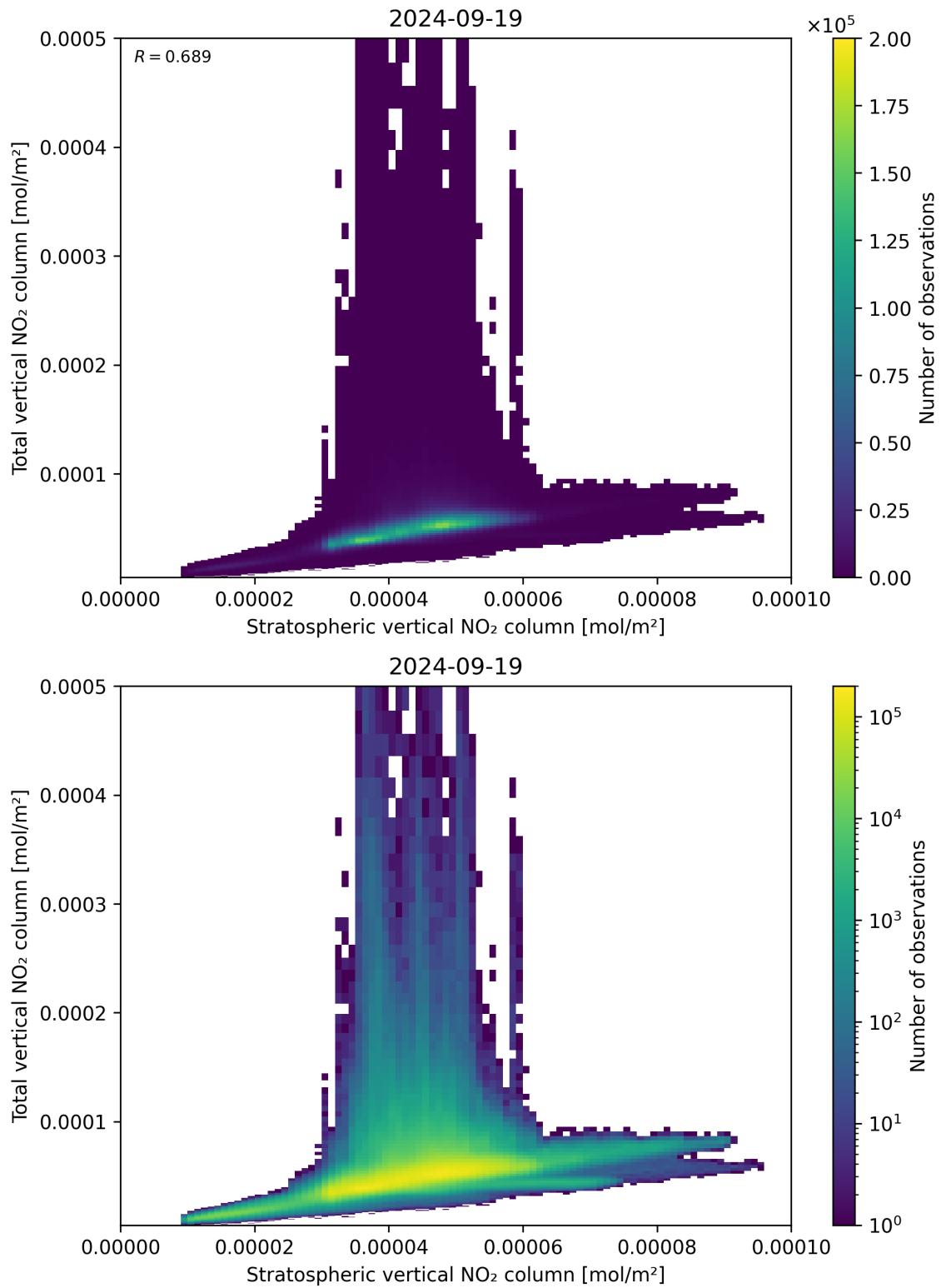
Figure 100: Scatter density plot of “Stratospheric vertical NO 2 column” against “Total vertical NO 2 column” for 2024-09-18 to 2024-09-20.
