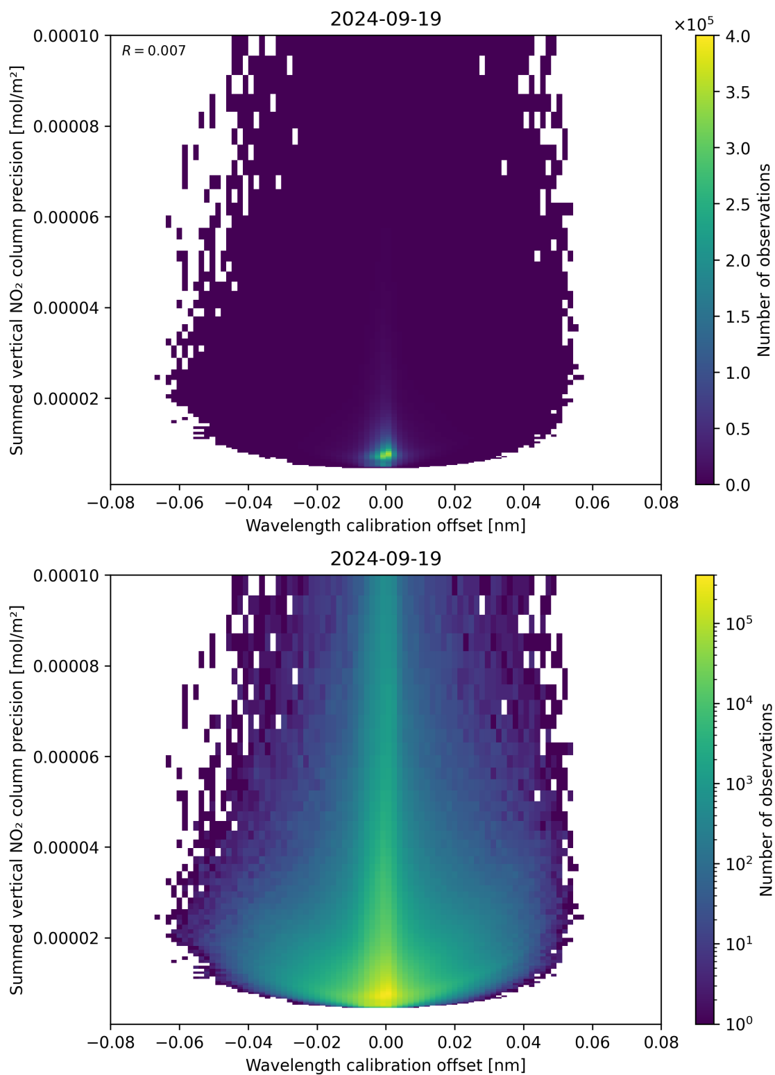
Figure 178: Scatter density plot of “Wavelength calibration offset” against “Summed vertical NO 2 column precision” for 2024-09-18 to 2024-09-20.
