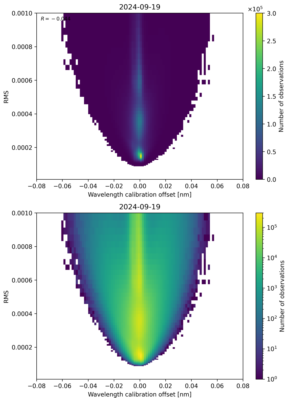
Figure 181: Scatter density plot of “Wavelength calibration offset” against “RMS” for 2024-09-18 to 2024-09-20.
