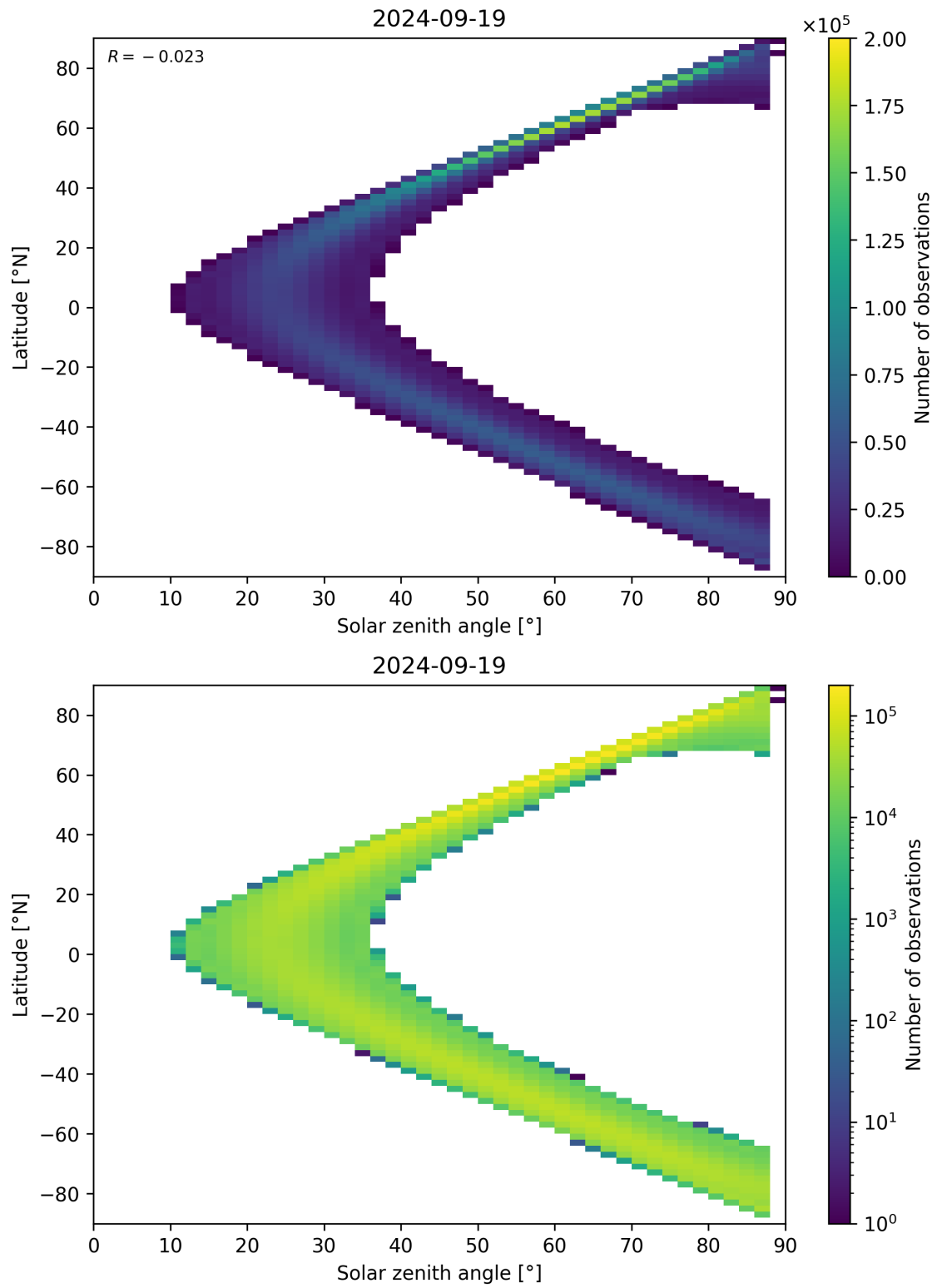
Figure 149: Scatter density plot of “Solar zenith angle” against “Latitude” for 2024-09-18 to 2024-09-20.
