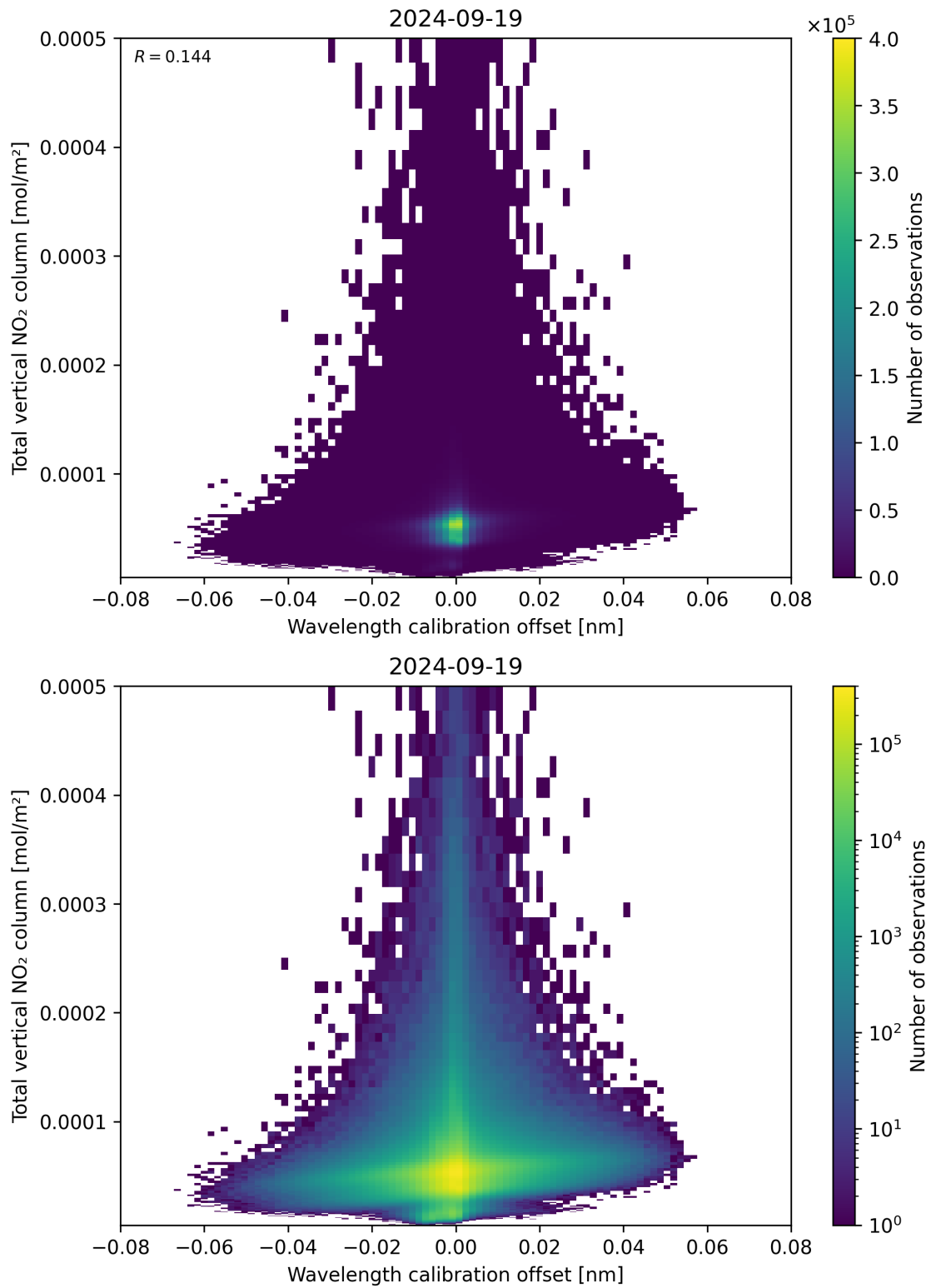
Figure 179: Scatter density plot of “Wavelength calibration offset” against “Total vertical NO 2 column” for 2024-09-18 to 2024-09-20.
