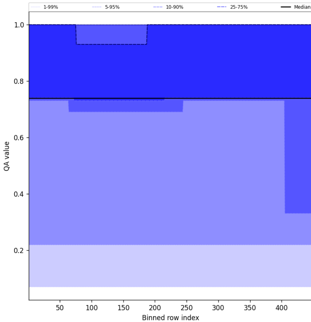
Figure 45: Along track statistics of “QA value” for 2024-09-18 to 2024-09-20
