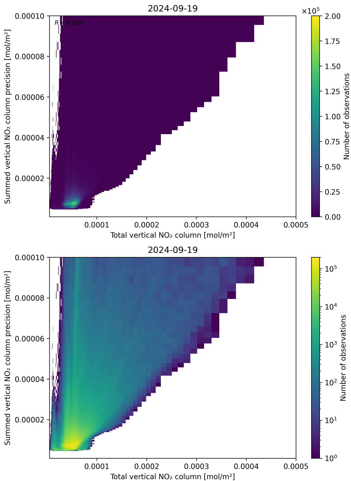
Figure 113: Scatter density plot of “Total vertical NO 2 column” against “Summed vertical NO 2 column precision” for 2024-09-18 to 2024-09-20.
