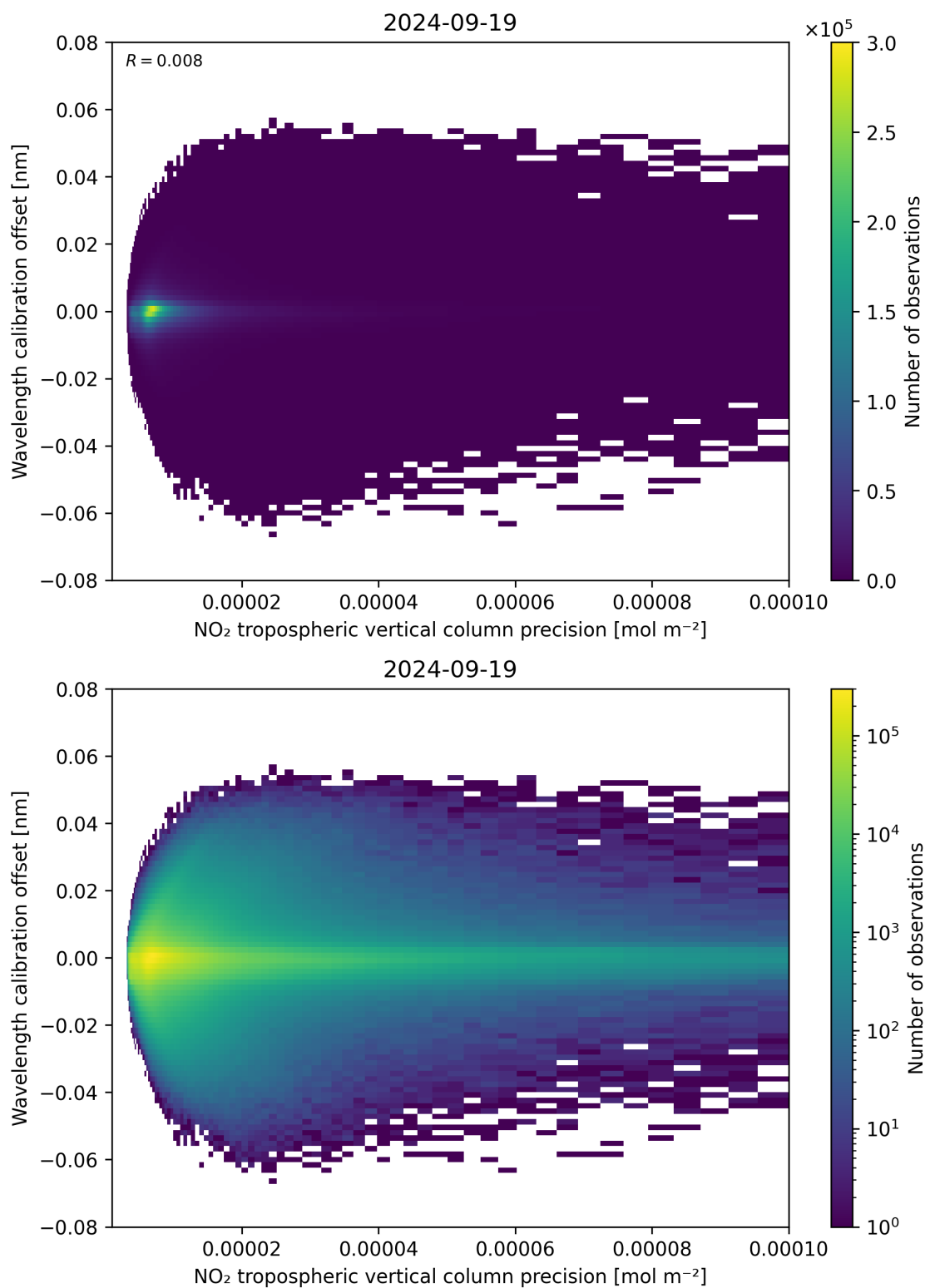
Figure 141: Scatter density plot of “NO 2 tropospheric vertical column precision” against “Wavelength calibration offset” for 2024-09-18 to 2024-09-20.
