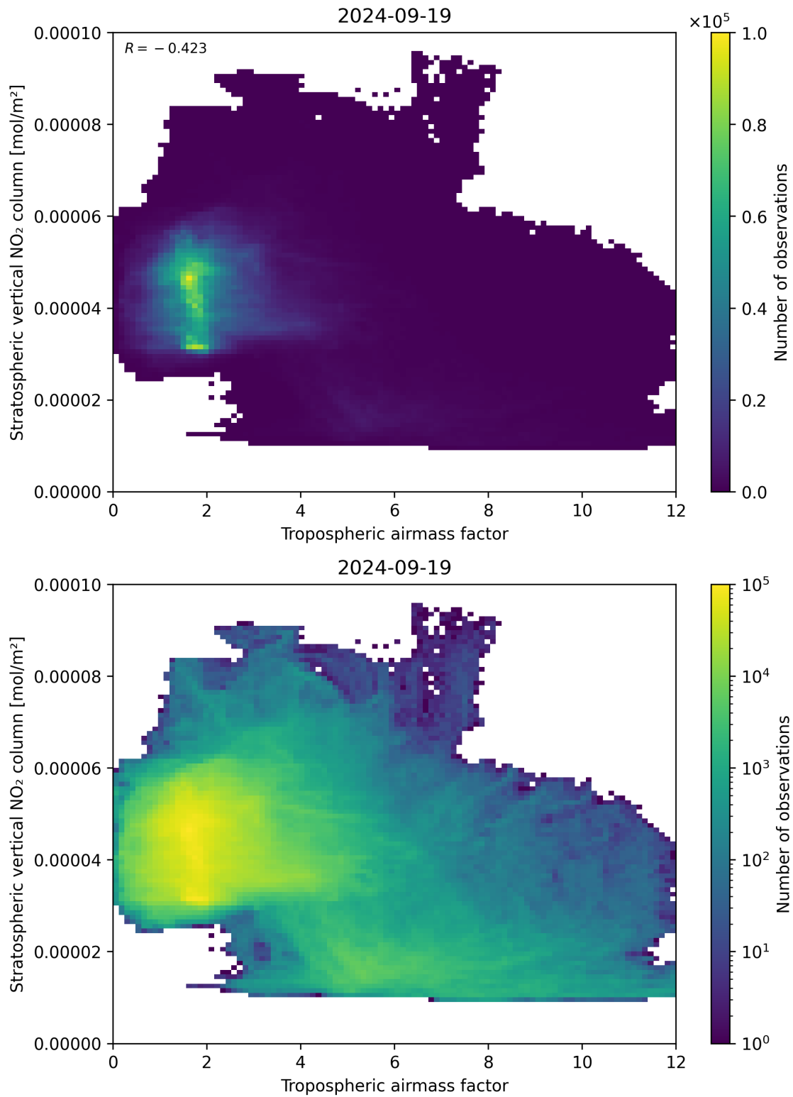
Figure 74: Scatter density plot of “Tropospheric air mass factor” against “Stratospheric vertical NO 2 column” for 2024-09-18 to 2024-09-20.
