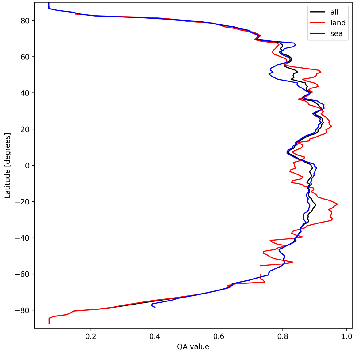
Figure 11: Zonal average of “QA value” for 2024-09-18 to 2024-09-20.
