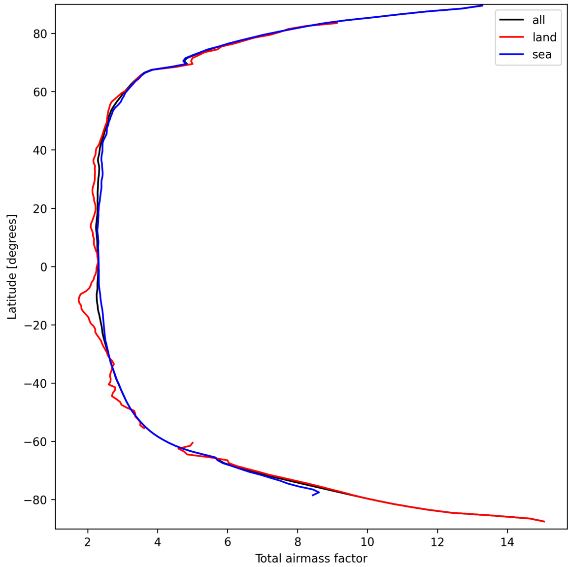
Figure 15: Zonal average of “Total airmass factor” for 2024-09-18 to 2024-09-20.
