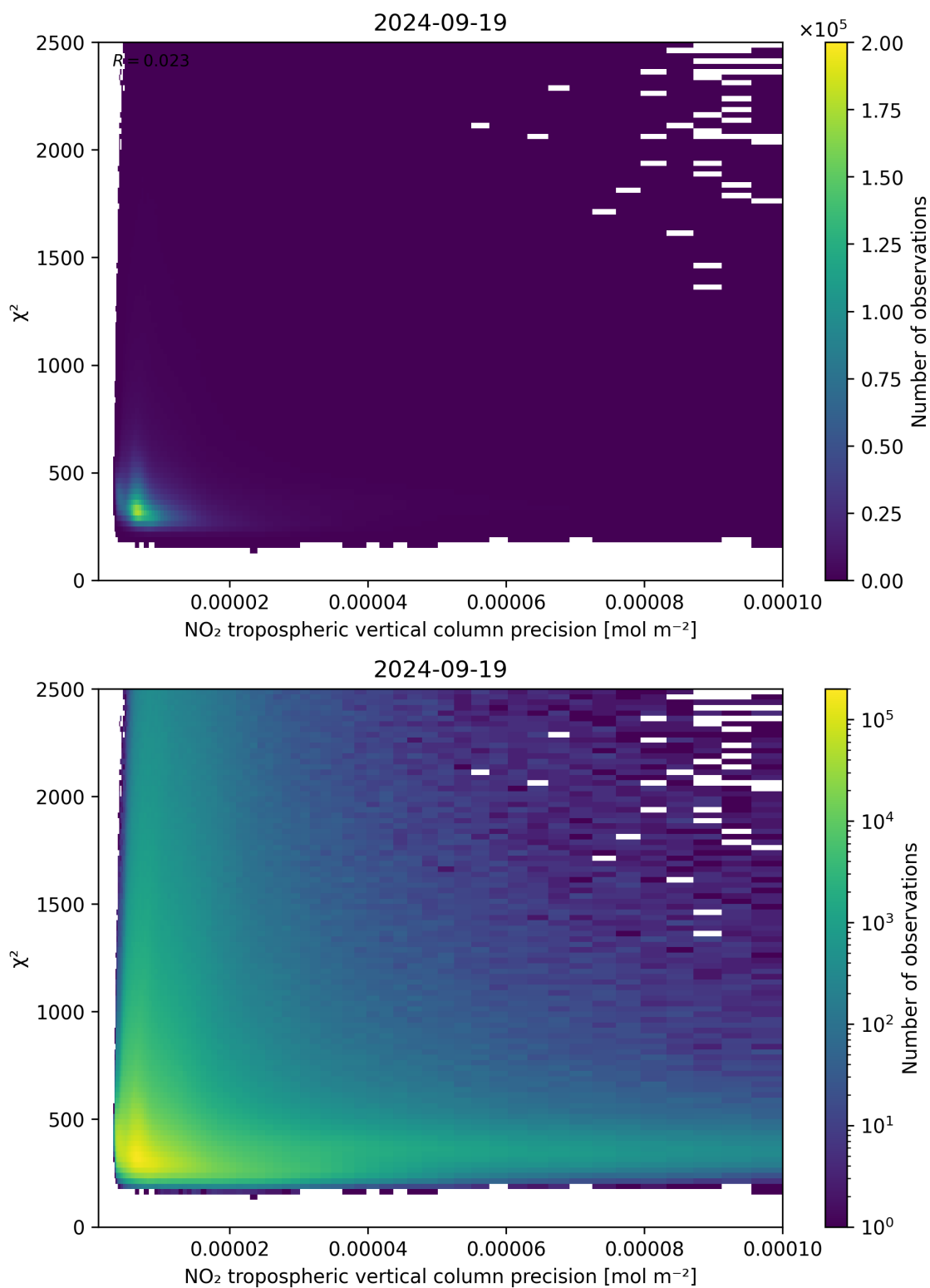
Figure 134: Scatter density plot of “NO 2 tropospheric vertical column precision” against “ \chi^2 ” for 2024-09-18 to 2024-09-20.
