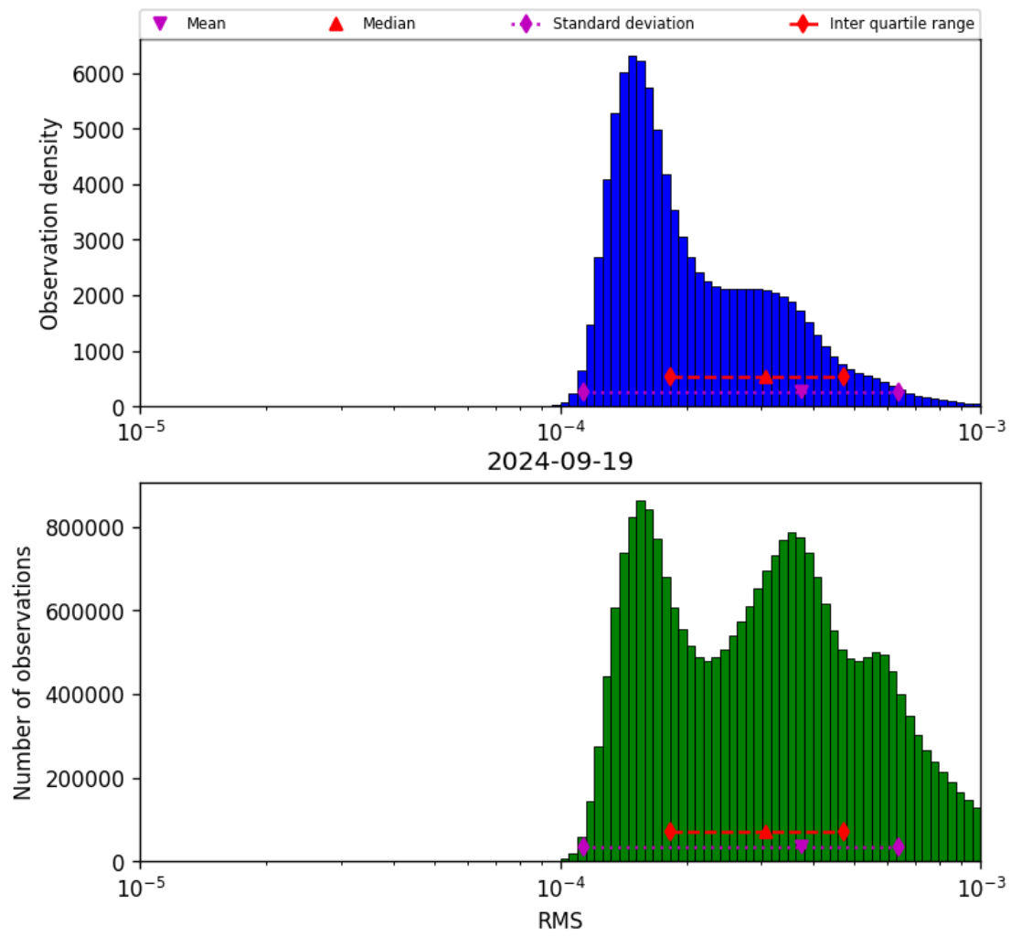
Figure 43: Histogram of “RMS” for 2024-09-18 to 2024-09-20
