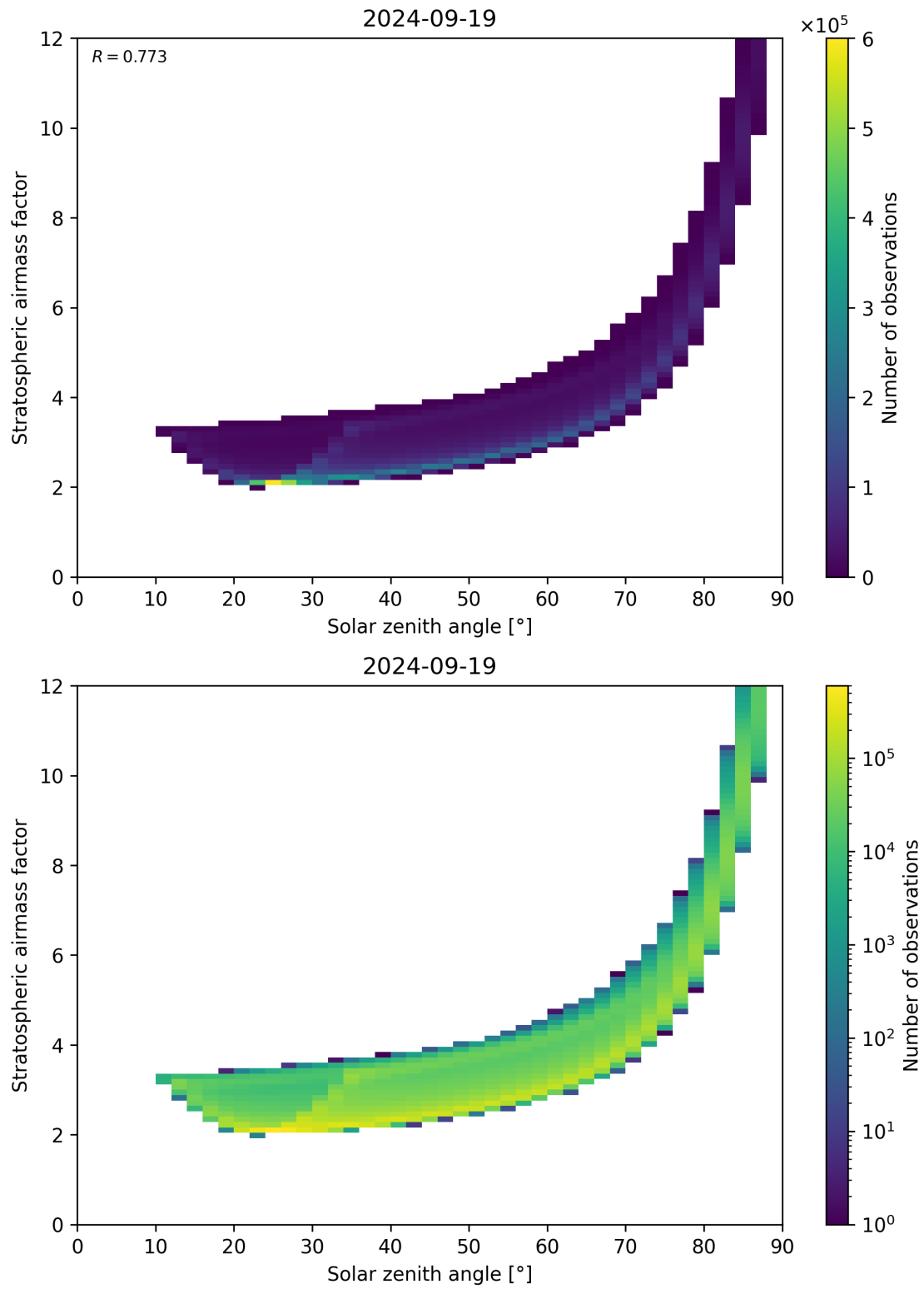
Figure 145: Scatter density plot of “Solar zenith angle” against “Stratospheric airmass factor” for 2024-09-18 to 2024-09-20.
