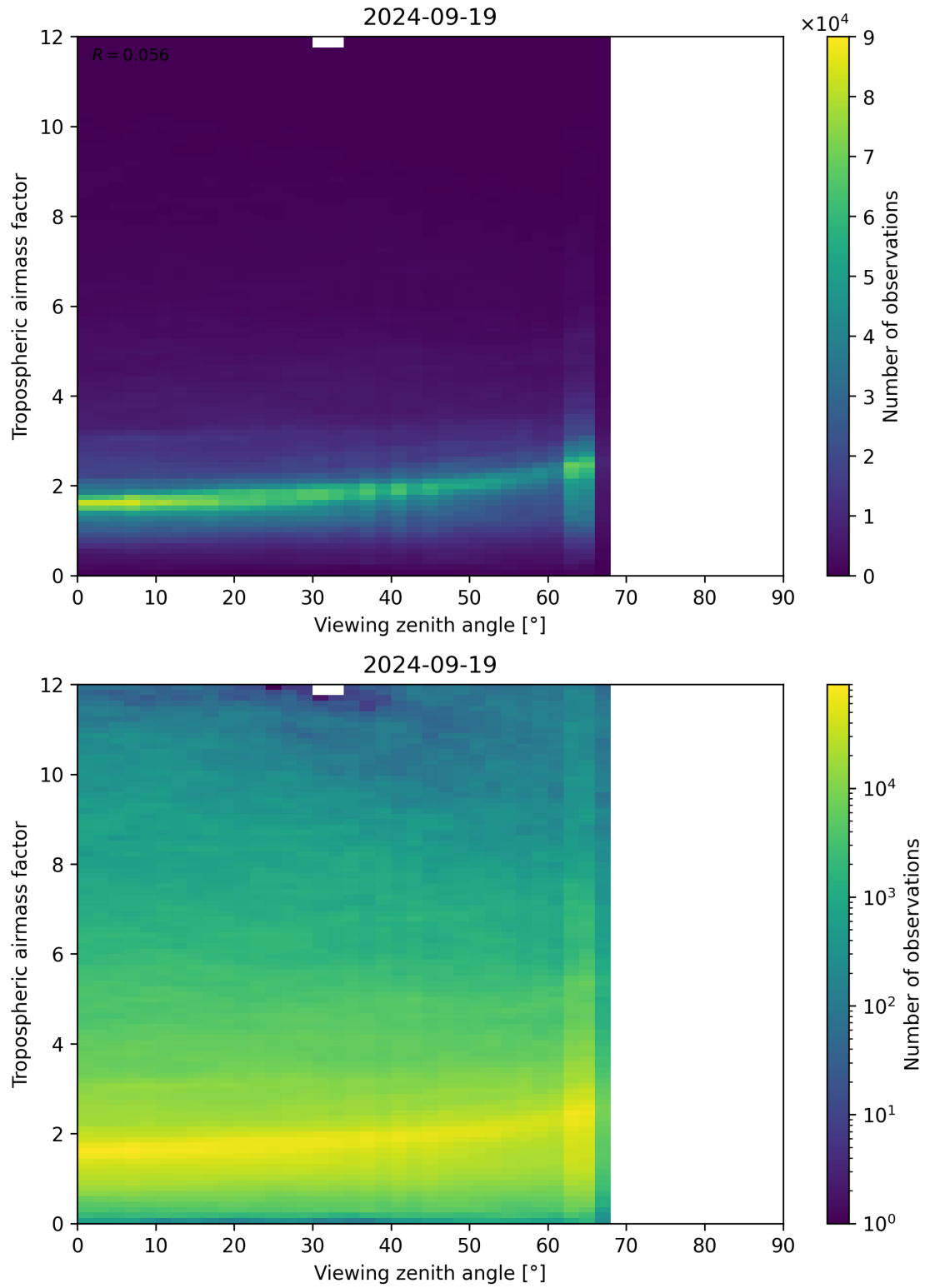
Figure 161: Scatter density plot of “Viewing zenith angle” against “Tropospheric airmass factor” for 2024-09-18 to 2024-09-20.
