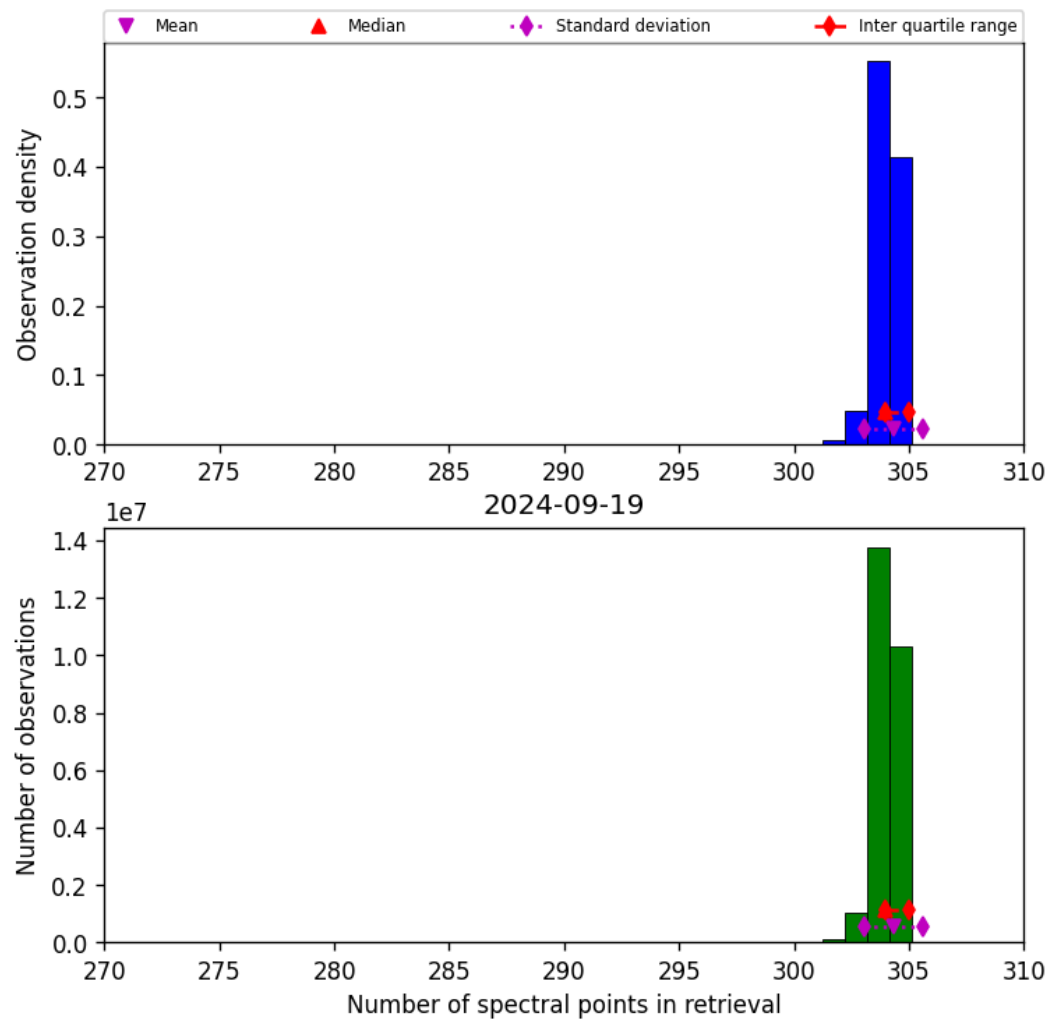
Figure 33: Histogram of “Number of spectral points in retrieval” for 2024-09-18 to 2024-09-20
