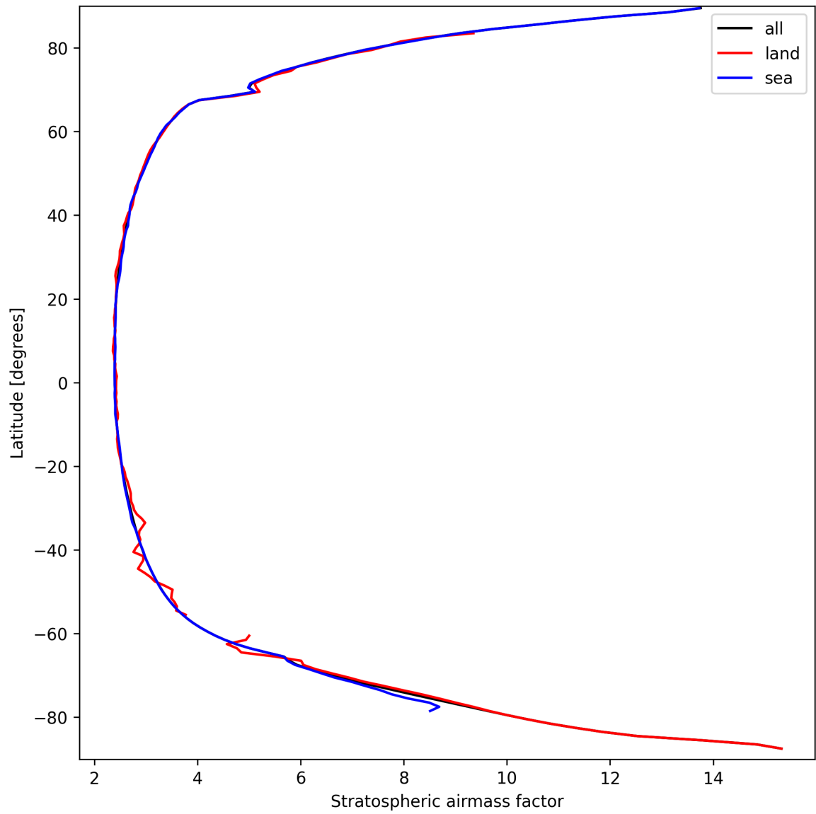
Figure 27: Zonal average of “Stratospheric airmass factor” for 2024-09-18 to 2024-09-20.
