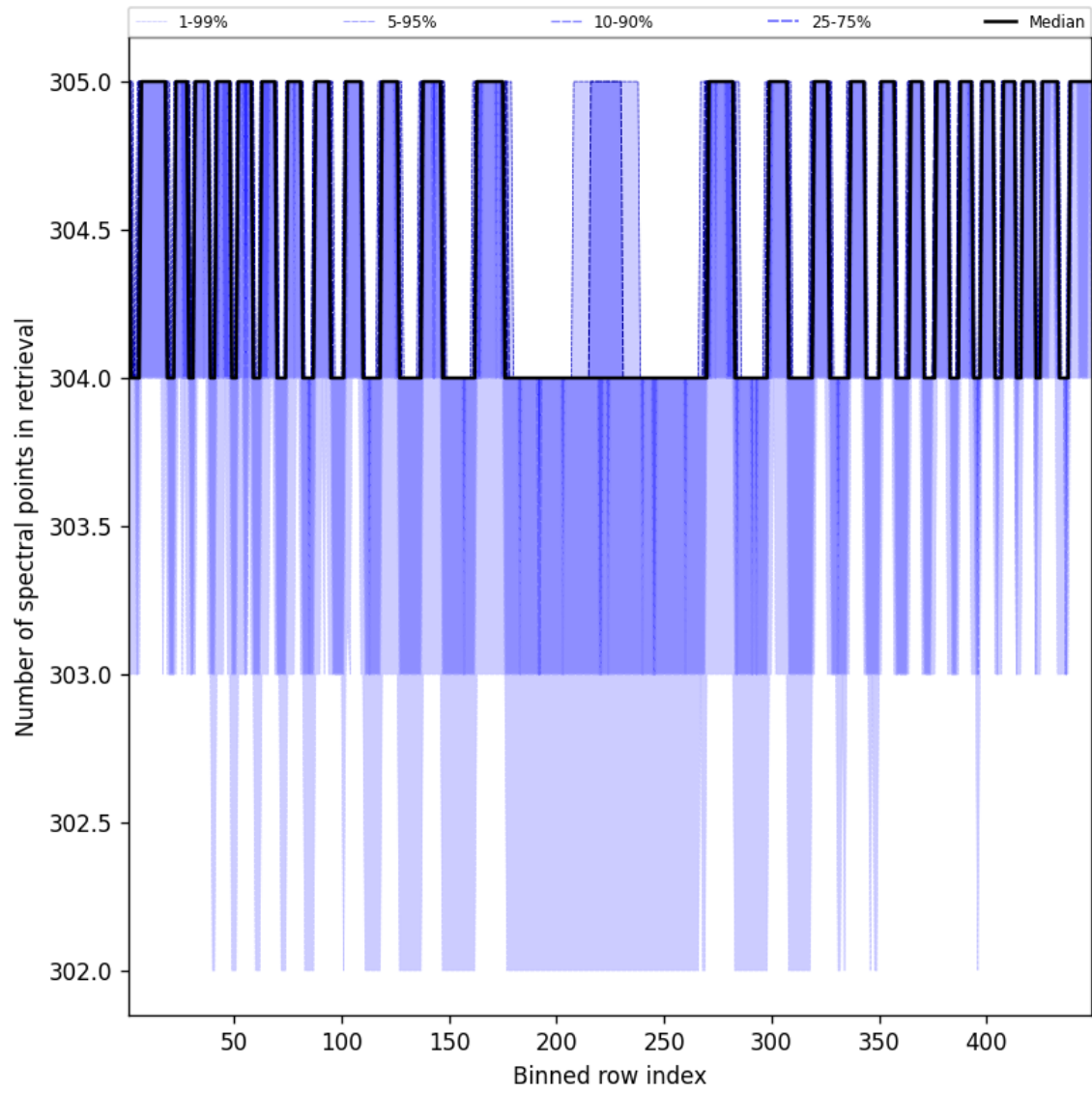
Figure 50: Along track statistics of “Number of spectral points in retrieval” for 2024-09-18 to 2024-09-20
