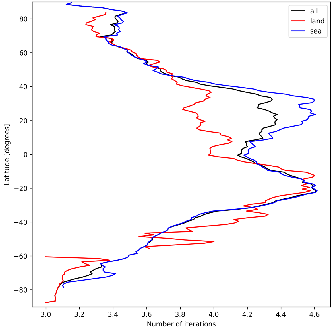
Figure 17: Zonal average of “Number of iterations” for 2024-09-18 to 2024-09-20.
