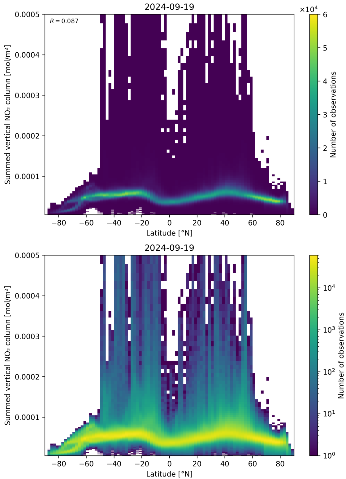
Figure 88: Scatter density plot of “Latitude” against “Summed vertical NO 2 column” for 2024-09-18 to 2024-09-20.
