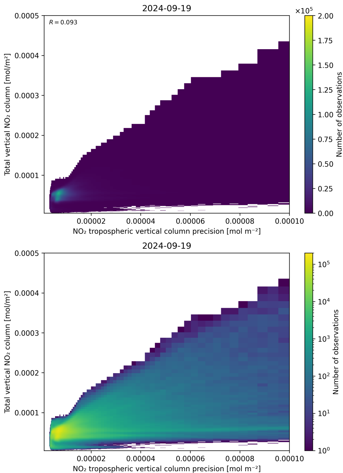
Figure 138: Scatter density plot of “NO 2 tropospheric vertical column precision” against “Total vertical NO 2 column” for 2024-09-18 to 2024-09-20.
