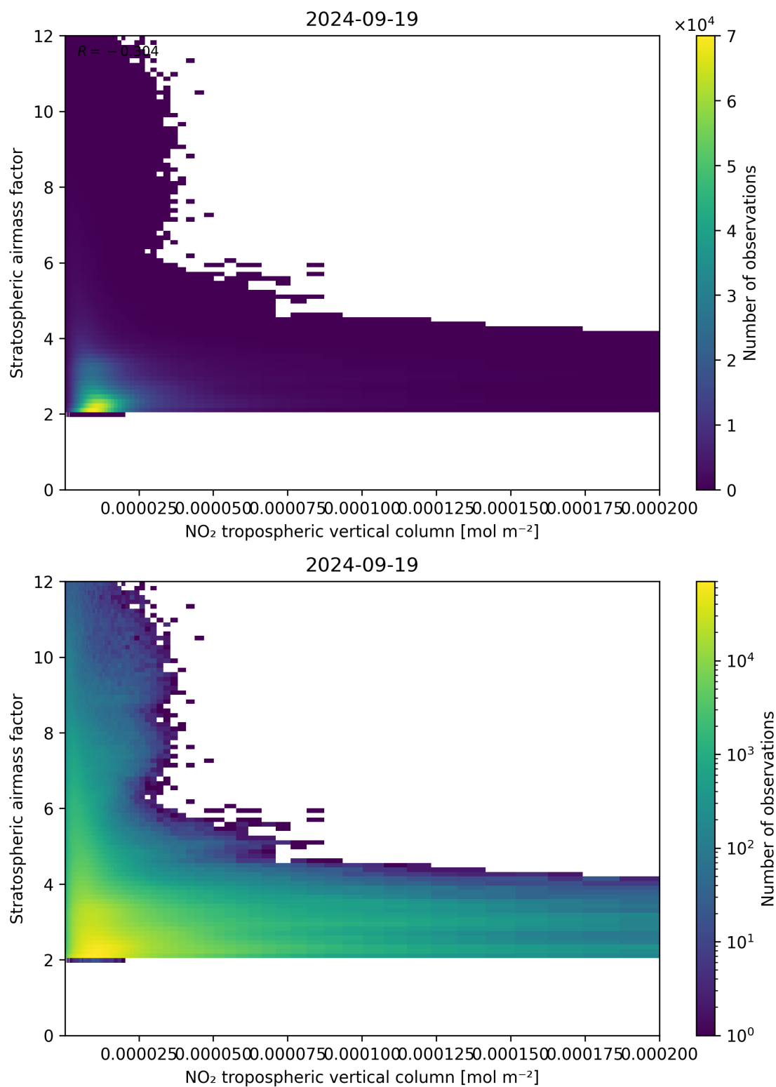
Figure 121: Scatter density plot of “NO 2 tropospheric vertical column” against “Stratospheric air mass factor” for 2024-09-18 to 2024-09-20.
