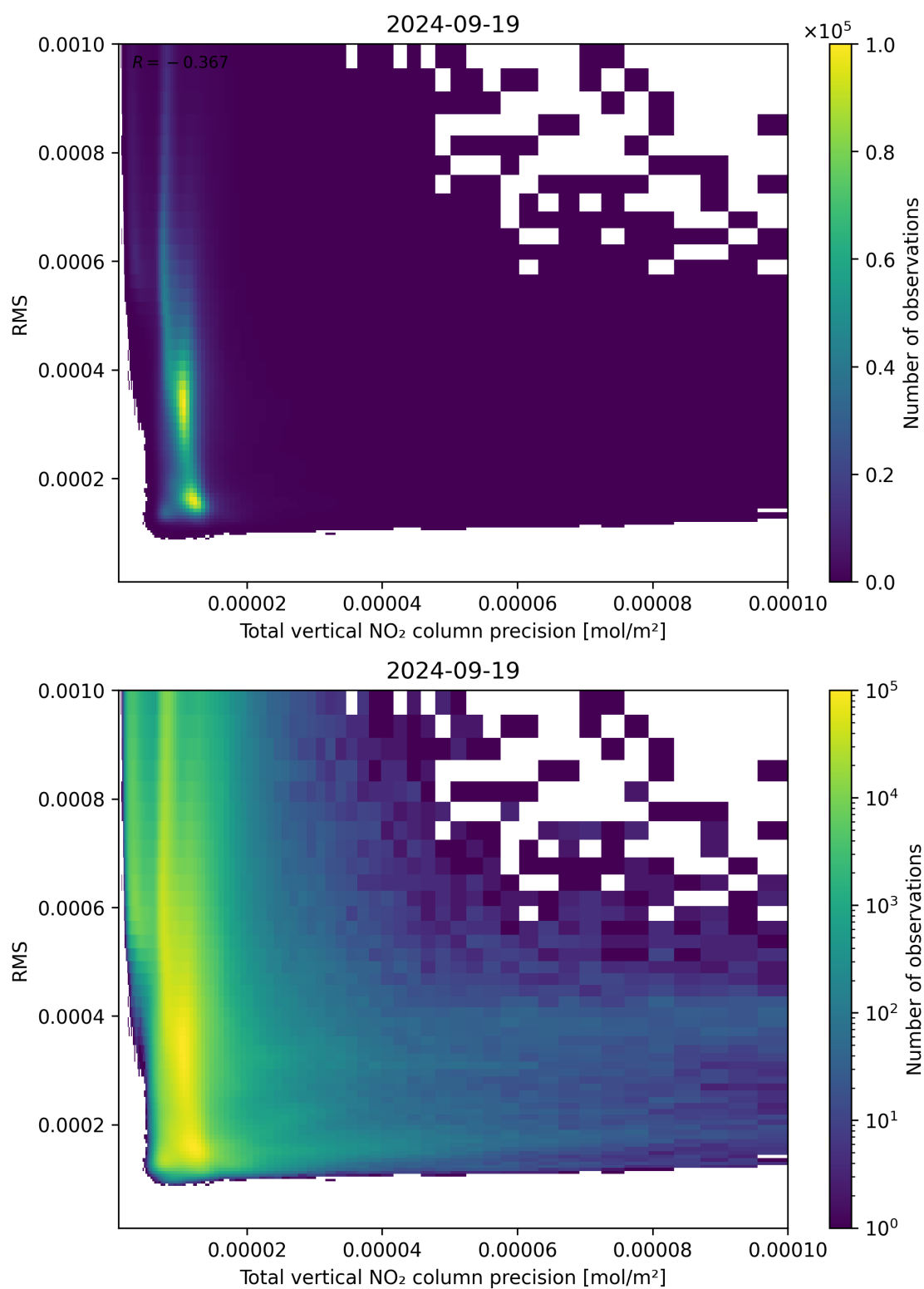
Figure 119: Scatter density plot of “Total vertical NO 2 column precision” against “RMS” for 2024-09-18 to 2024-09-20.
