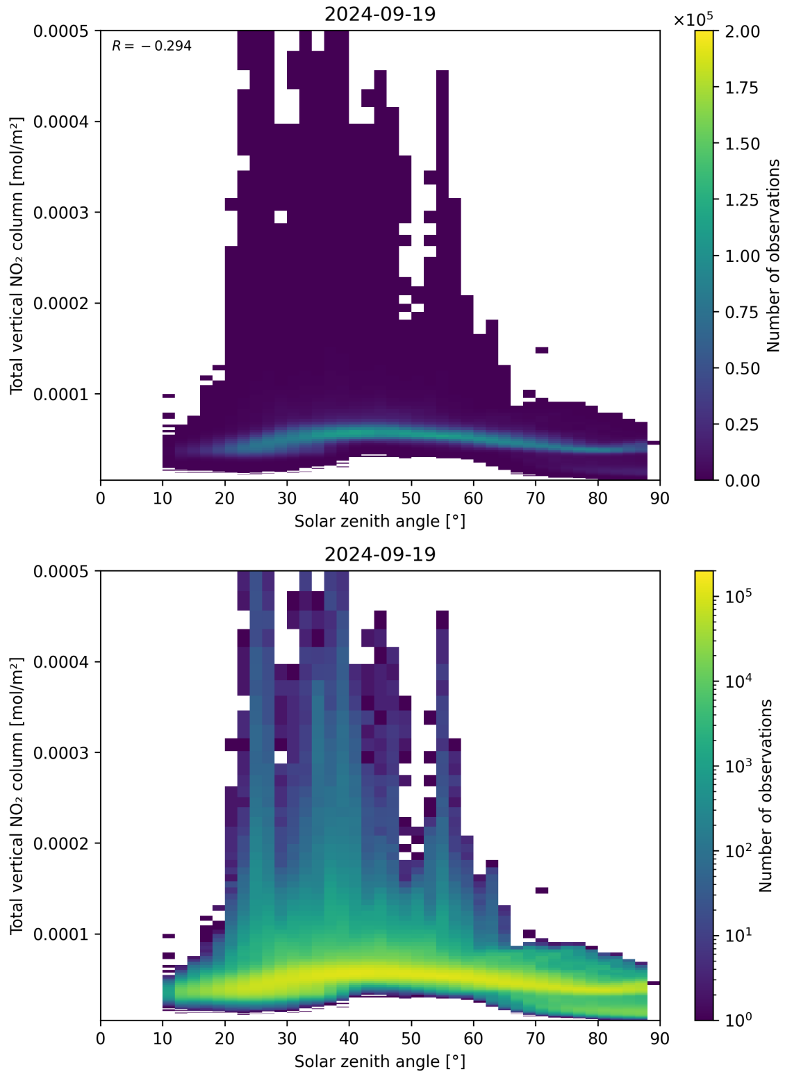
Figure 153: Scatter density plot of “Solar zenith angle” against “Total vertical NO 2 column” for 2024-09-18 to 2024-09-20.
