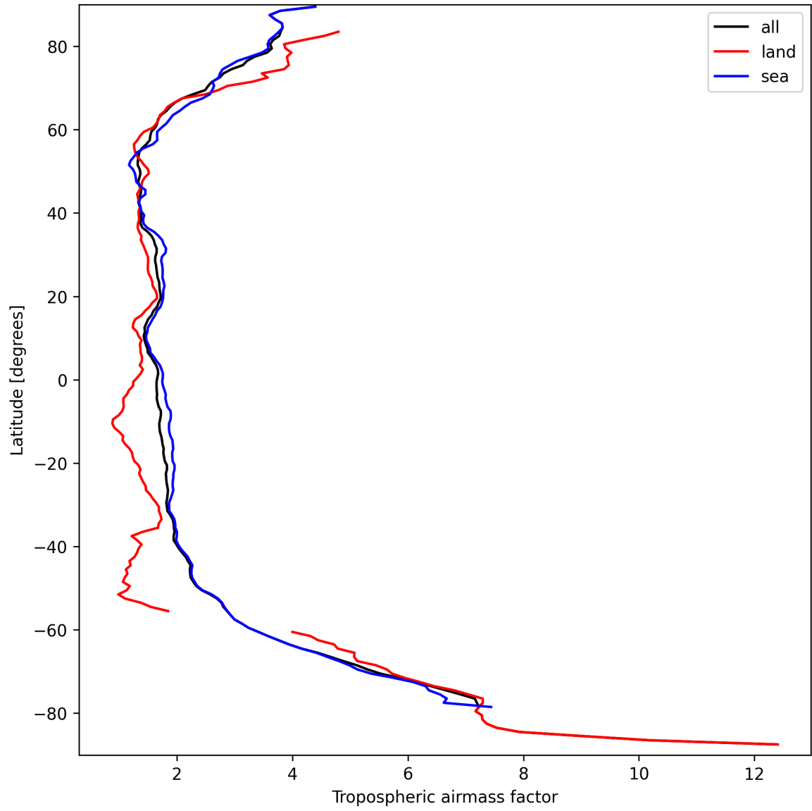
Figure 14: Zonal average of “Tropospheric airmass factor” for 2024-09-18 to 2024-09-20.
