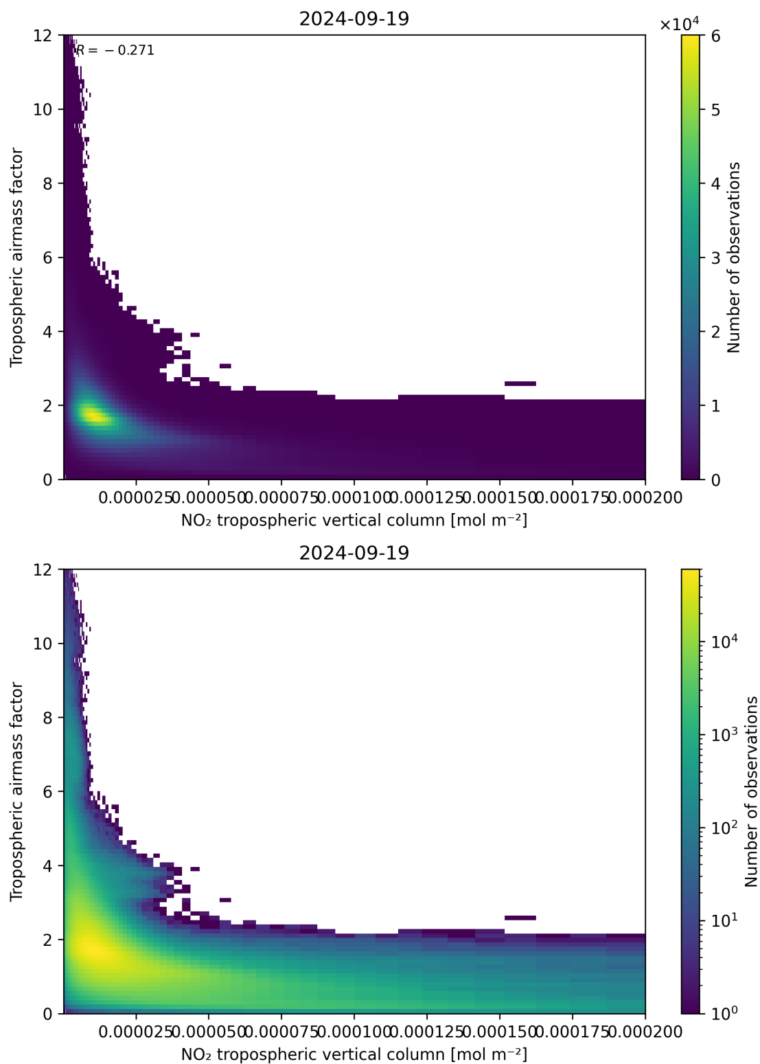
Figure 123: Scatter density plot of “NO 2 tropospheric vertical column” against “Tropospheric air mass factor” for 2024-09-18 to 2024-09-20.
