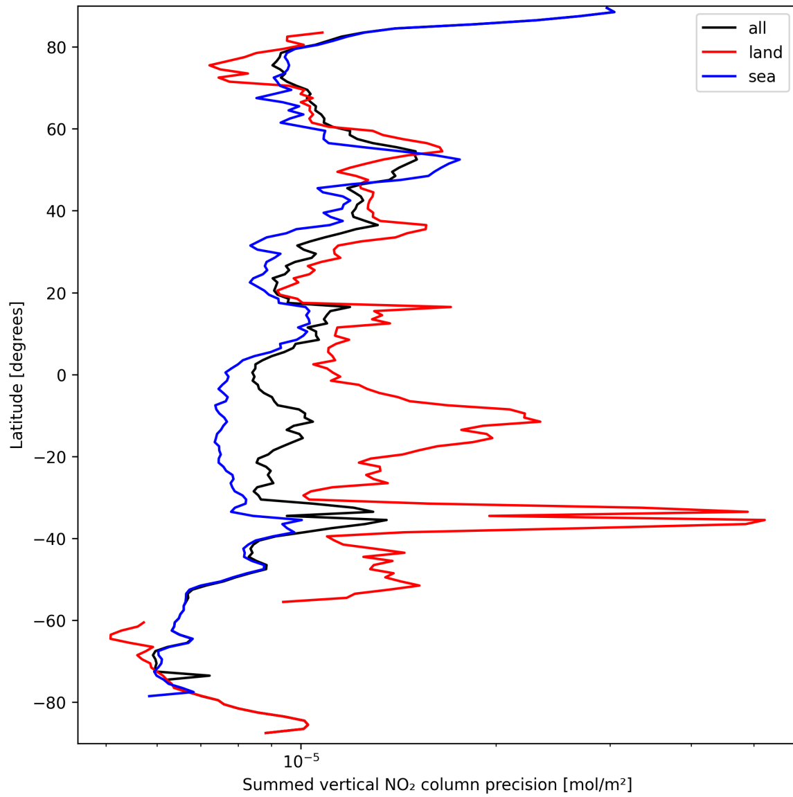
Figure 24: Zonal average of “Summed vertical NO 2 column precision” for 2024-09-18 to 2024-09-20.
