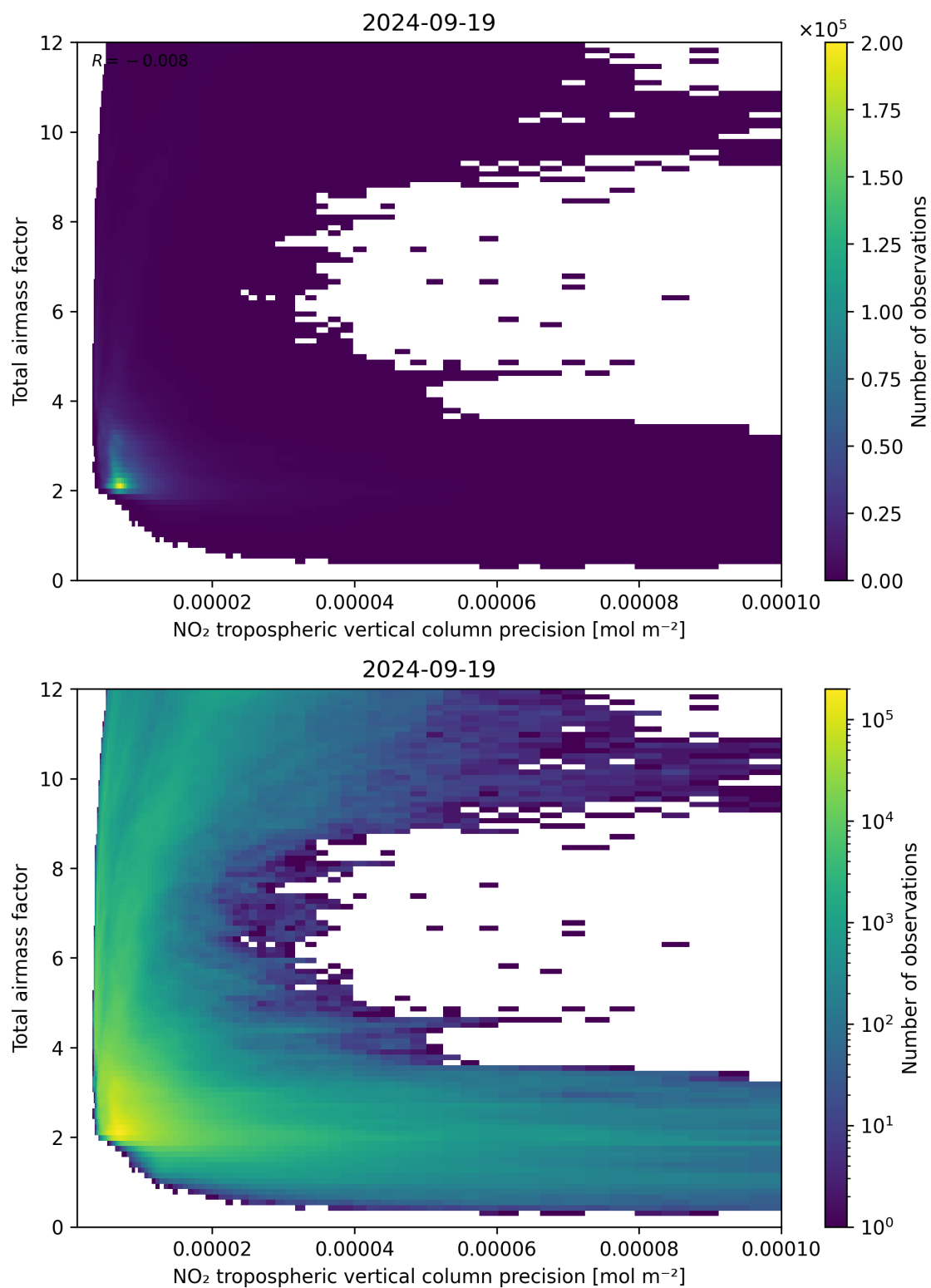
Figure 132: Scatter density plot of “NO 2 tropospheric vertical column precision” against “Total air mass factor” for 2024-09-18 to 2024-09-20.
