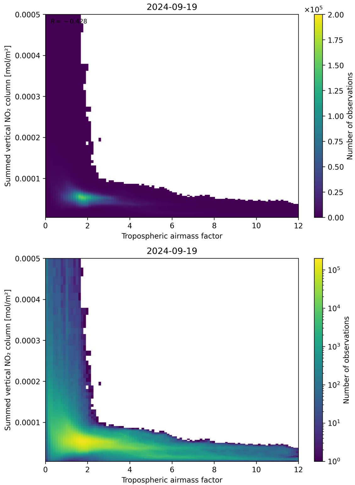
Figure 75: Scatter density plot of “Tropospheric air mass factor” against “Summed vertical NO 2 column” for 2024-09-18 to 2024-09-20.
