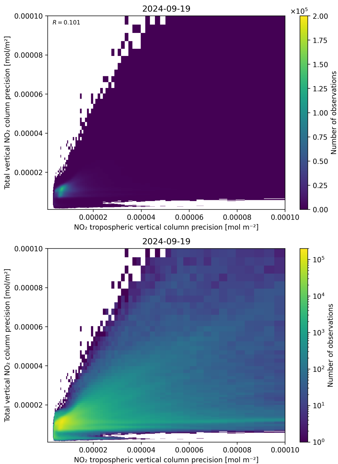
Figure 139: Scatter density plot of “NO 2 tropospheric vertical column precision” against “Total vertical NO 2 column precision” for 2024-09-18 to 2024-09-20.
