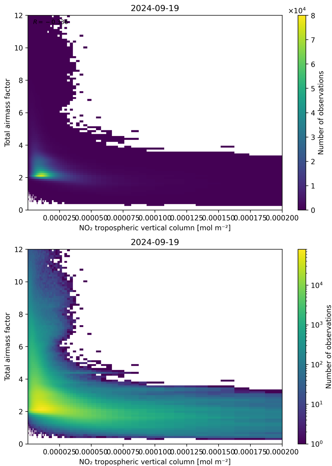
Figure 122: Scatter density plot of “NO 2 tropospheric vertical column” against “Total air mass factor” for 2024-09-18 to 2024-09-20.
