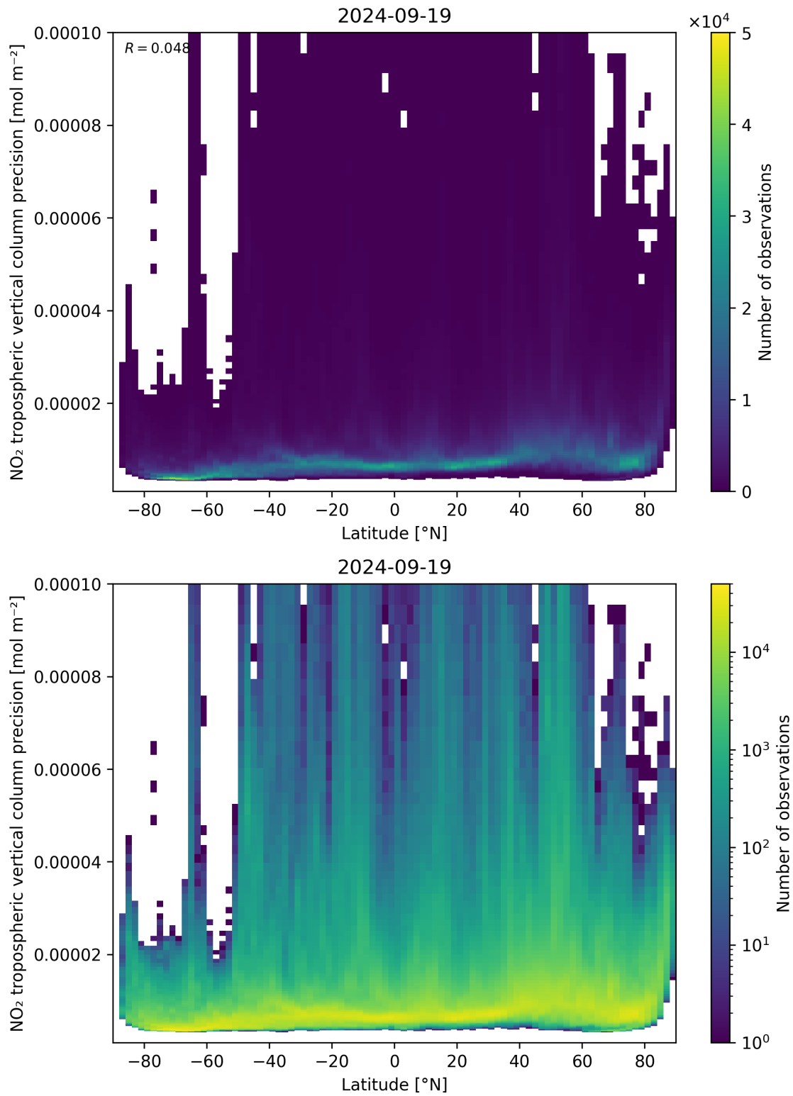
Figure 93: Scatter density plot of “Latitude” against “NO 2 tropospheric vertical column precision” for 2024-09-18 to 2024-09-20.
