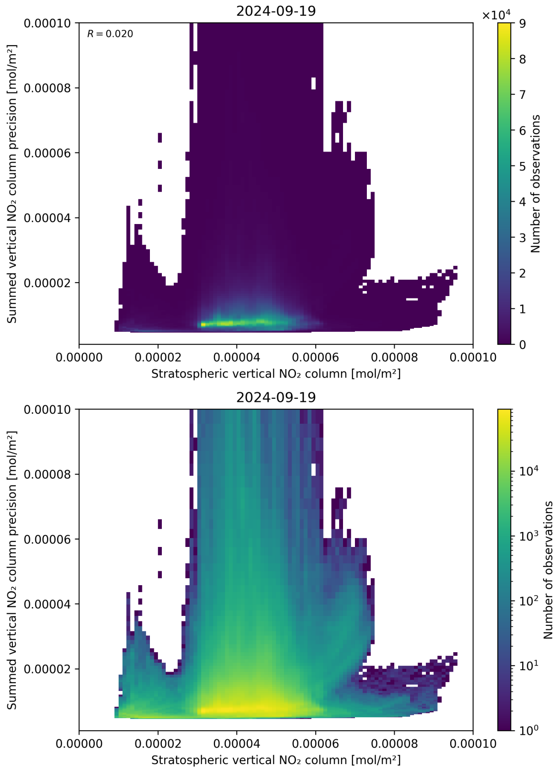
Figure 99: Scatter density plot of “Stratospheric vertical NO 2 column” against “Summed vertical NO 2 column precision” for 2024-09-18 to 2024-09-20.
