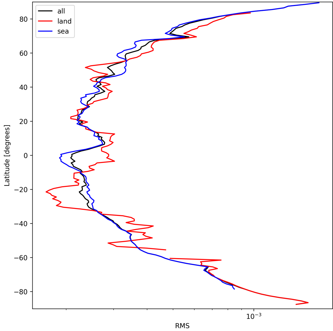
Figure 26: Zonal average of “RMS” for 2024-09-18 to 2024-09-20.
