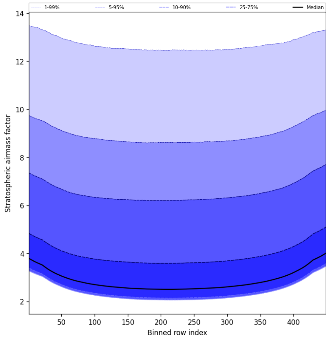
Figure 61: Along track statistics of “Stratospheric airmass factor” for 2024-09-18 to 2024-09-20
