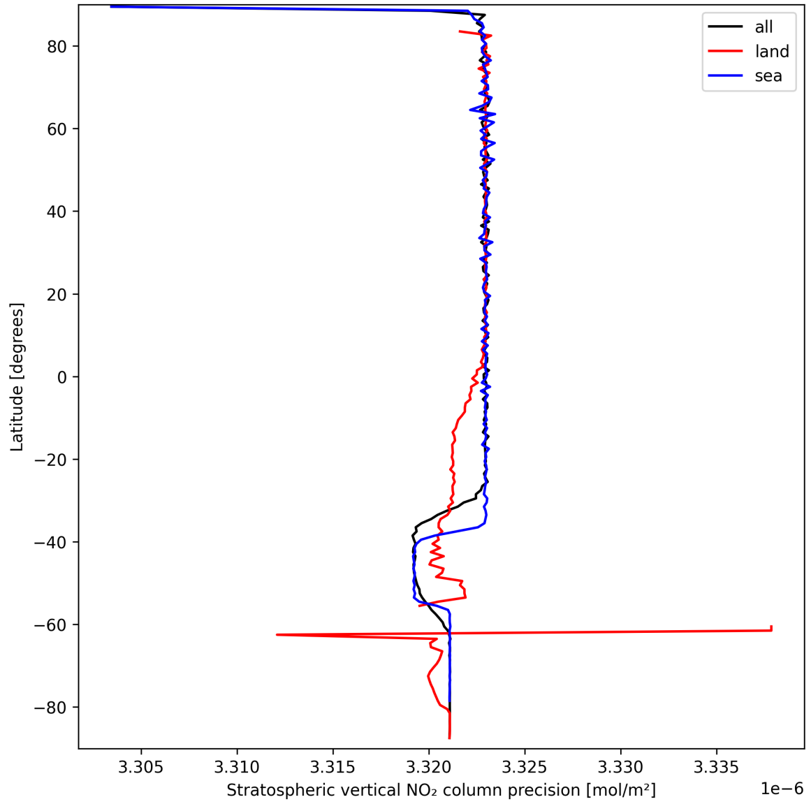
Figure 20: Zonal average of “Stratospheric vertical NO 2 column precision” for 2024-09-18 to 2024-09-20.
