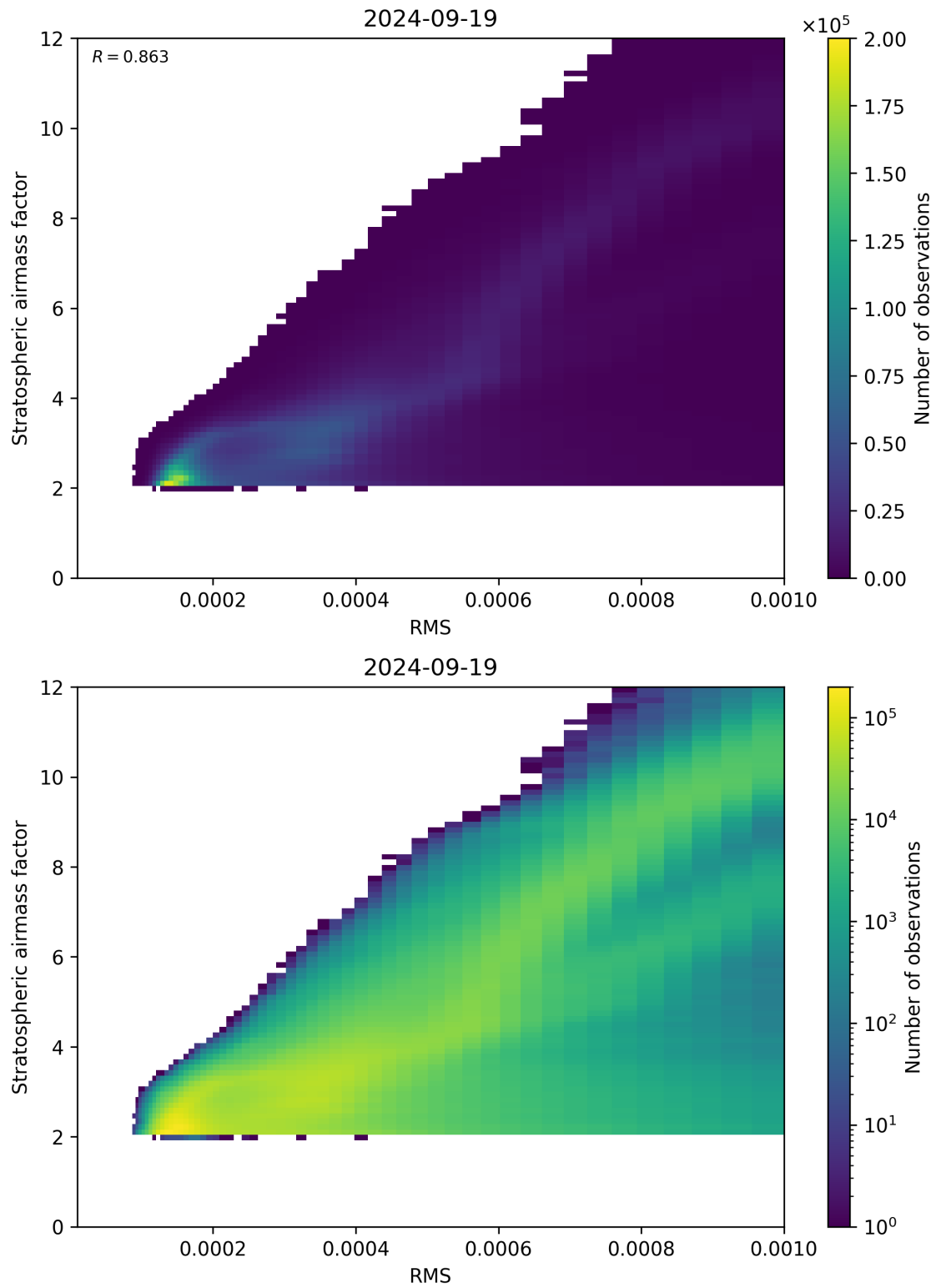
Figure 144: Scatter density plot of “RMS” against “Stratospheric airmass factor” for 2024-09-18 to 2024-09-20.
