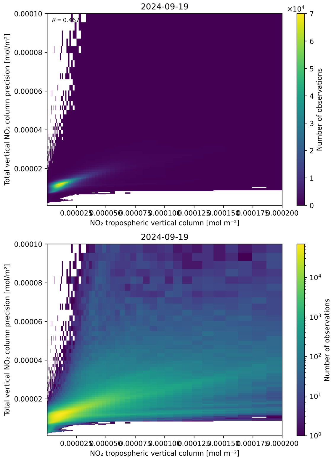
Figure 129: Scatter density plot of “NO 2 tropospheric vertical column” against “Total vertical NO 2 column precision” for 2024-09-18 to 2024-09-20.
