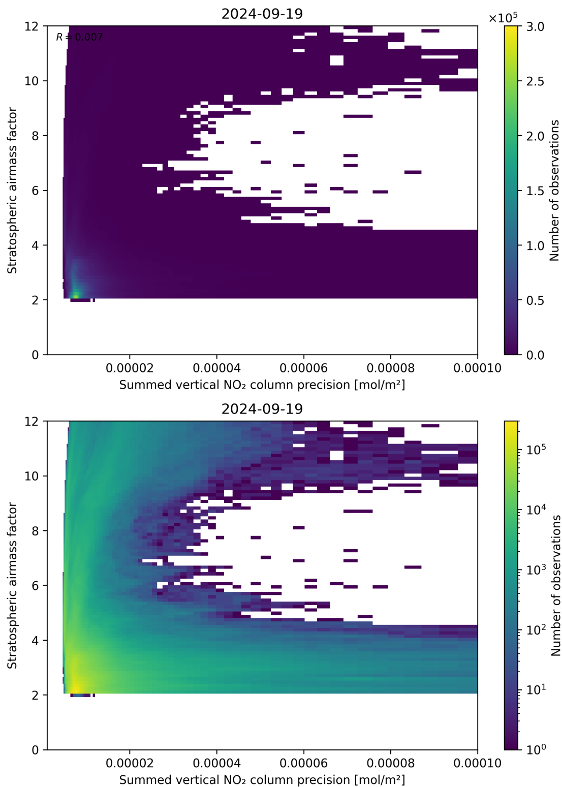
Figure 106: Scatter density plot of “Summed vertical NO 2 column precision” against “Stratospheric airmass factor” for 2024-09-18 to 2024-09-20.
