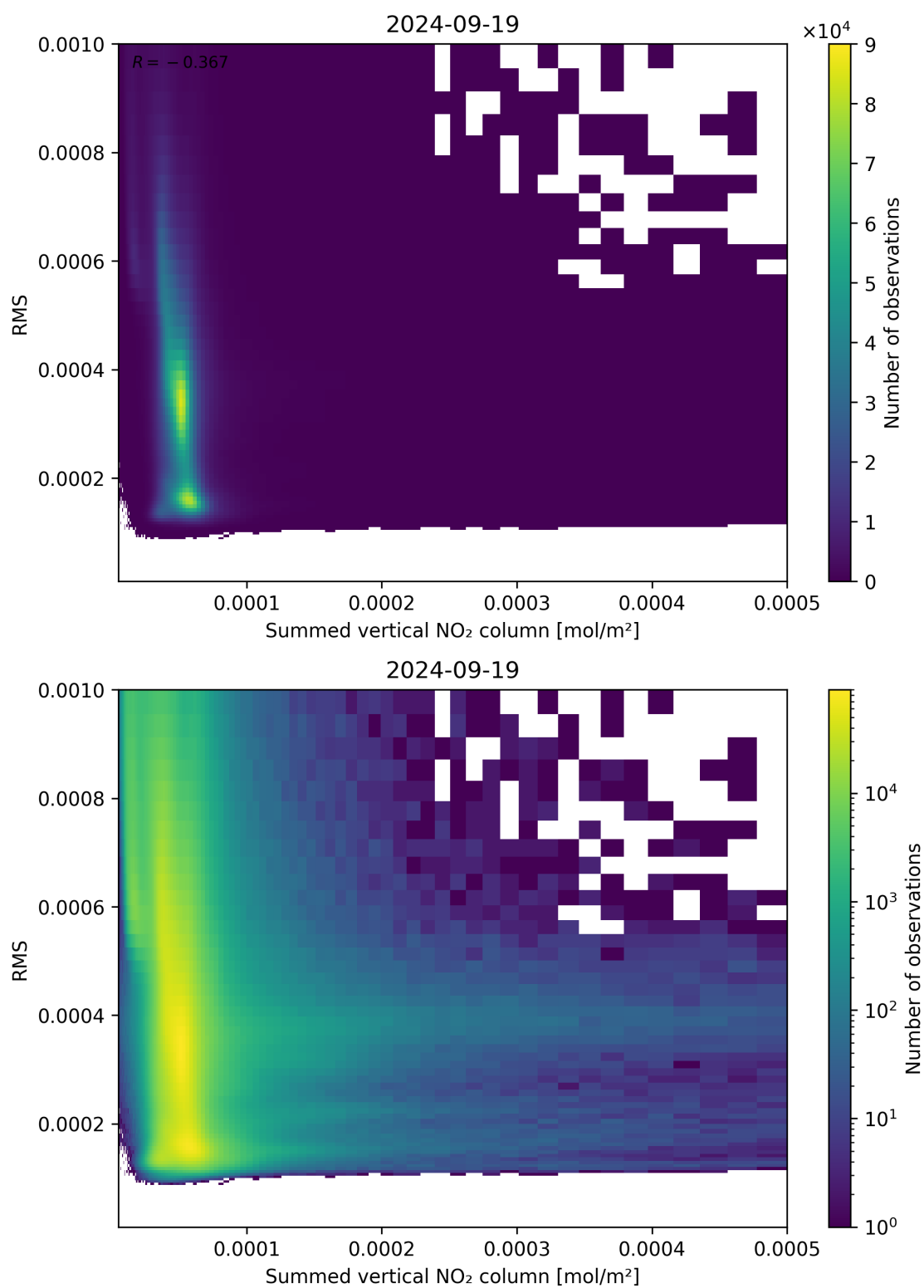
Figure 109: Scatter density plot of “Summed vertical NO 2 column” against “RMS” for 2024-09-18 to 2024-09-20.
