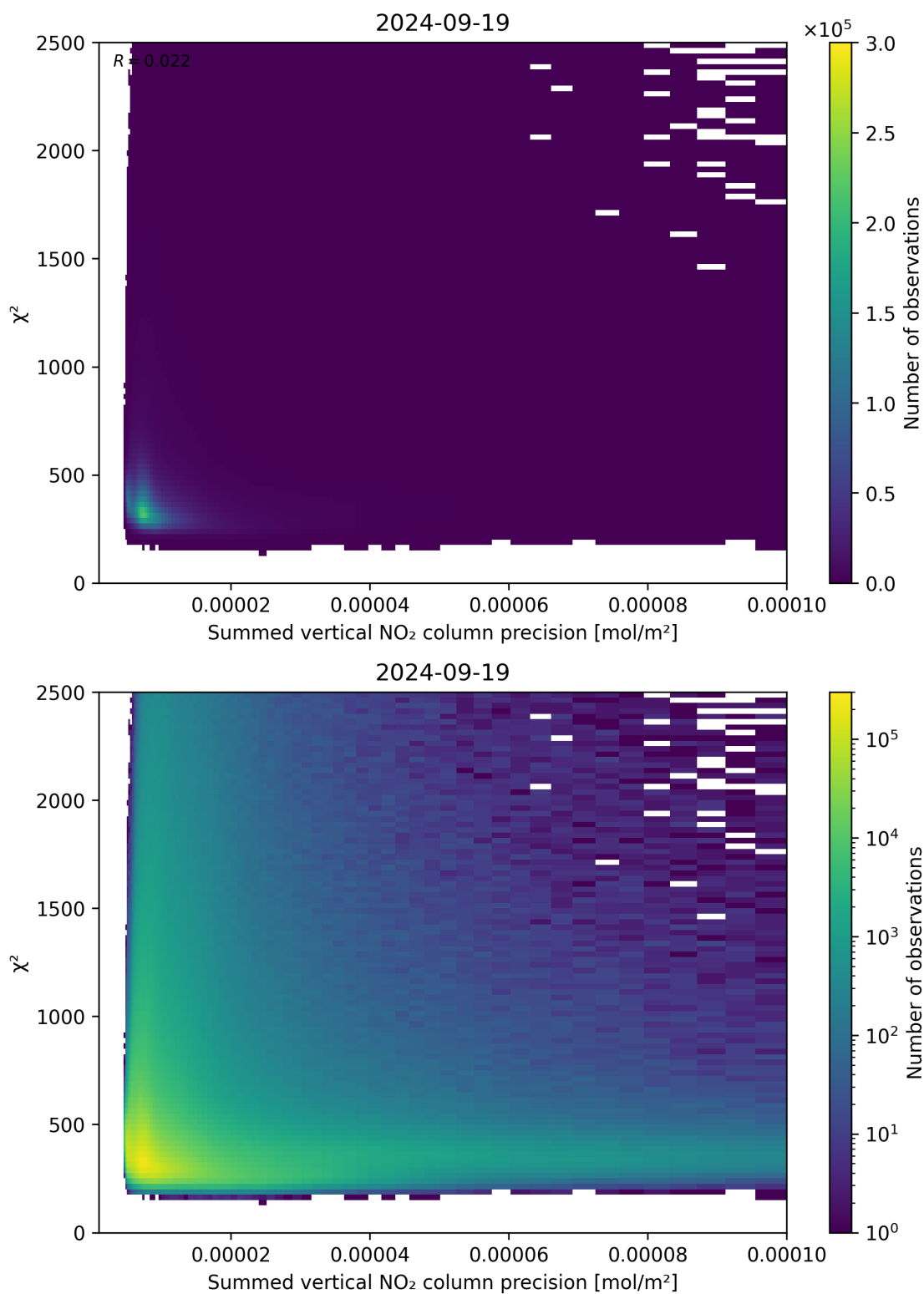
Figure 107: Scatter density plot of “Summed vertical NO 2 column precision” against “ \chi^2 ” for 2024-09-18 to 2024-09-20.
