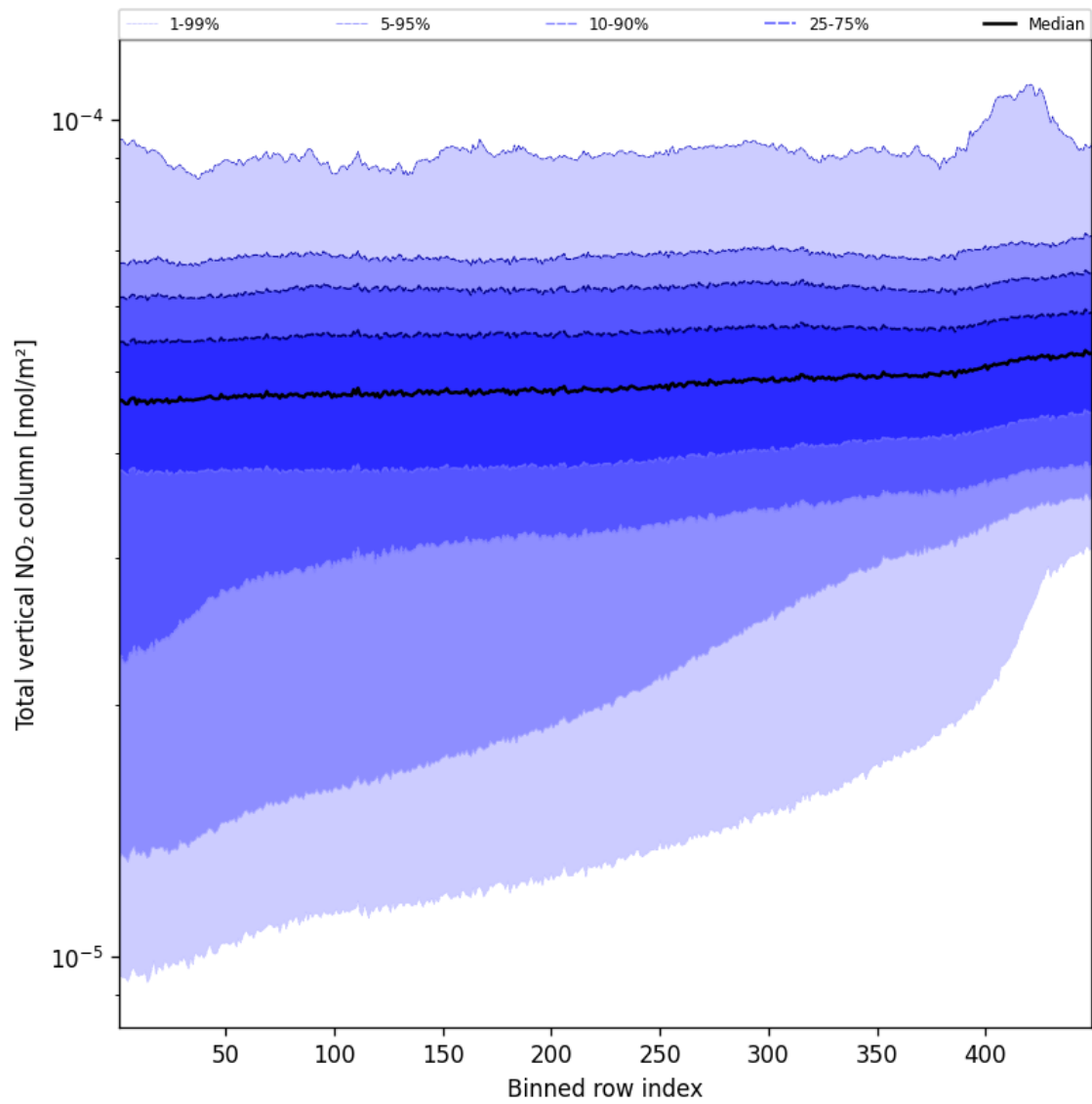
Figure 55: Along track statistics of “Total vertical NO 2 column” for 2024-09-18 to 2024-09-20
