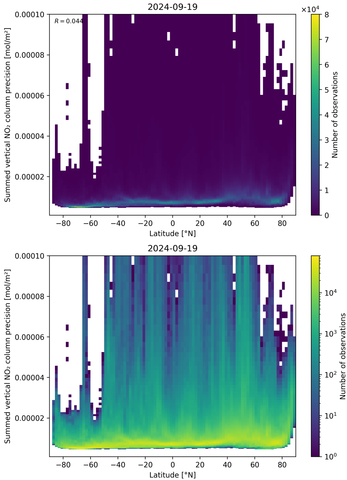
Figure 89: Scatter density plot of “Latitude” against “Summed vertical NO 2 column precision” for 2024-09-18 to 2024-09-20.
