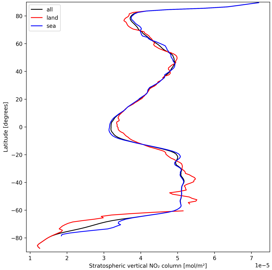
Figure 19: Zonal average of “Stratospheric vertical NO 2 column” for 2024-09-18 to 2024-09-20.
