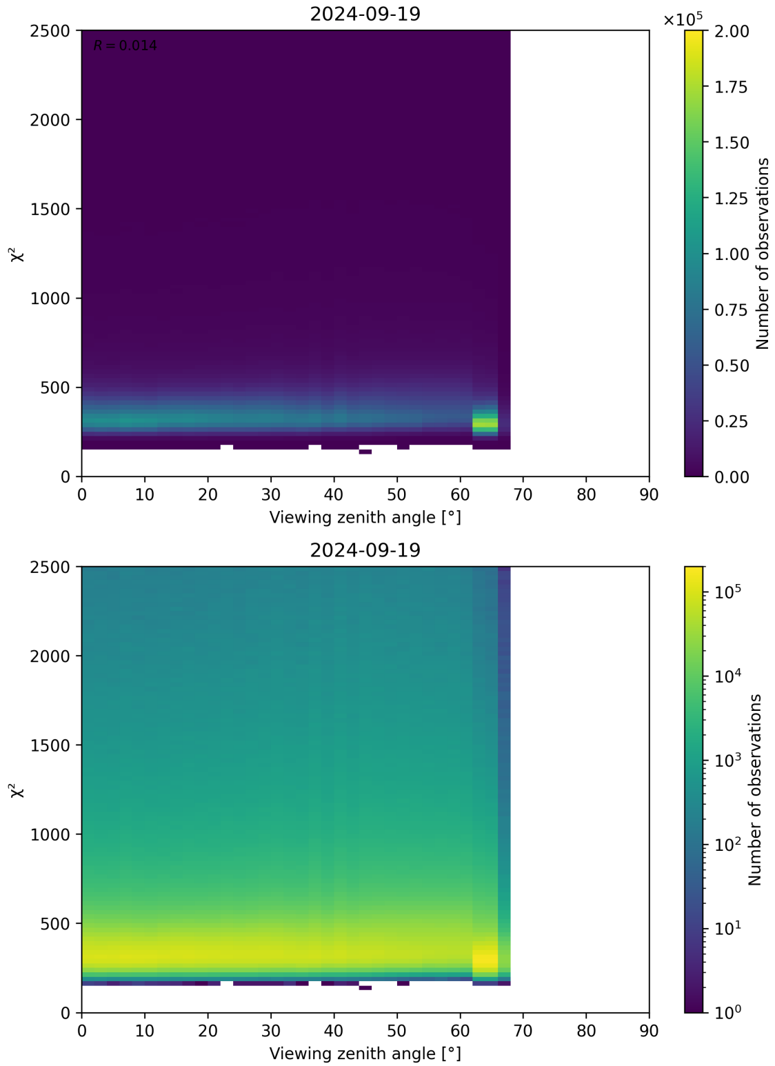
Figure 162: Scatter density plot of “Viewing zenith angle” against “ \chi^2 ” for 2024-09-18 to 2024-09-20.
