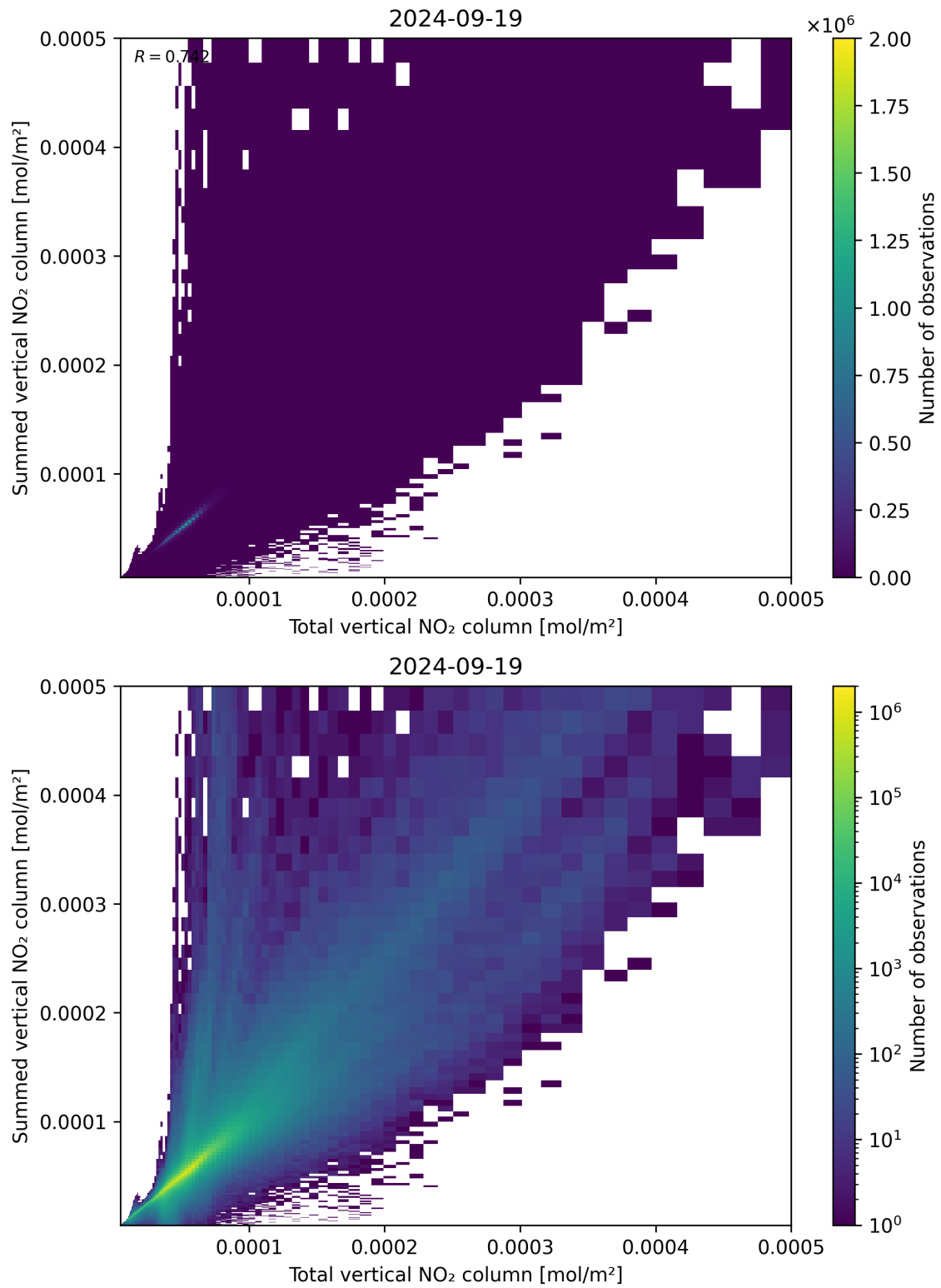
Figure 112: Scatter density plot of “Total vertical NO 2 column” against “Summed vertical NO 2 column” for 2024-09-18 to 2024-09-20.
