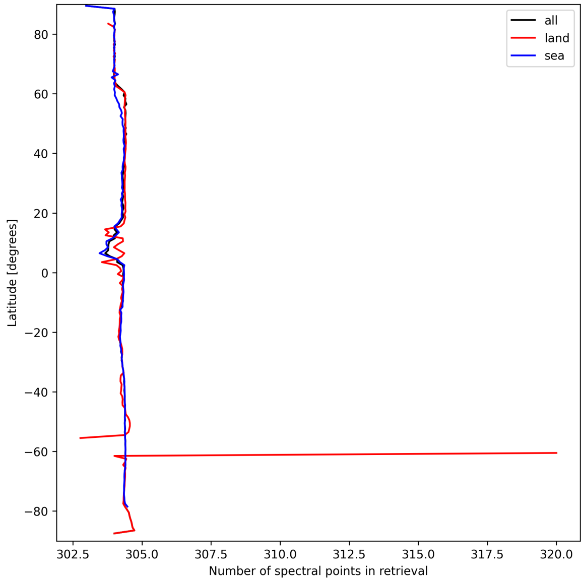
Figure 16: Zonal average of “Number of spectral points in retrieval” for 2024-09-18 to 2024-09-20.
