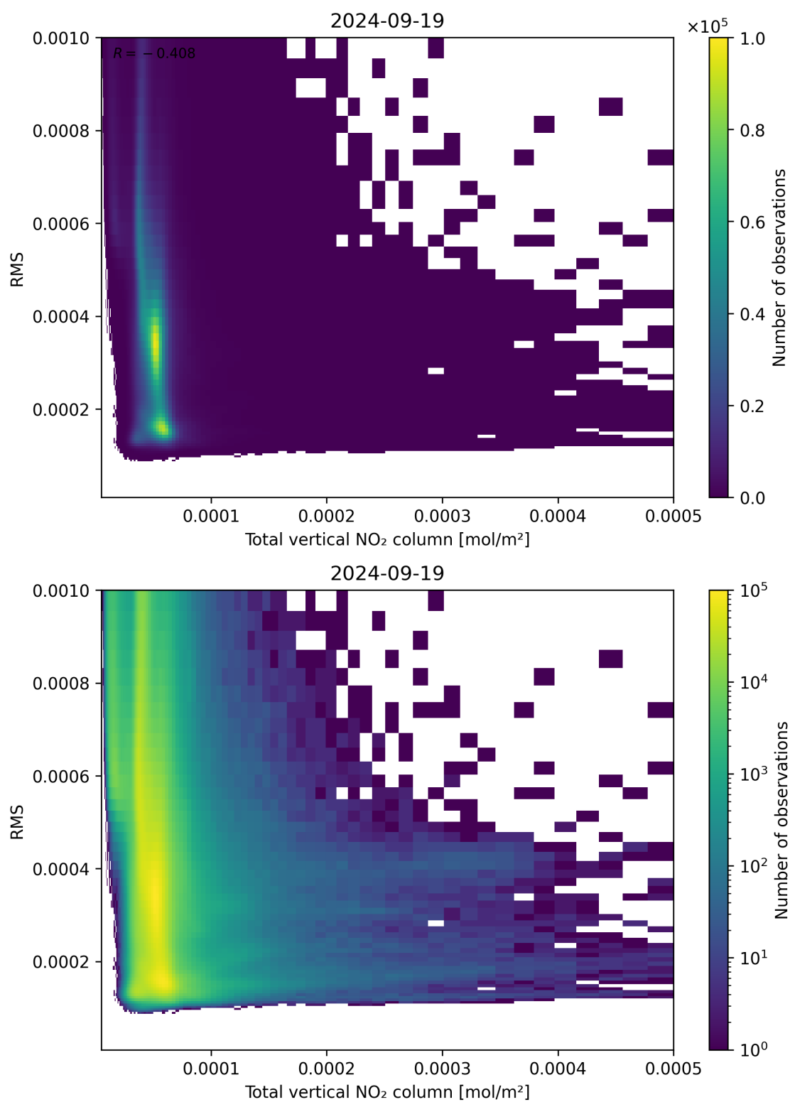
Figure 120: Scatter density plot of “Total vertical NO 2 column” against “RMS” for 2024-09-18 to 2024-09-20.
