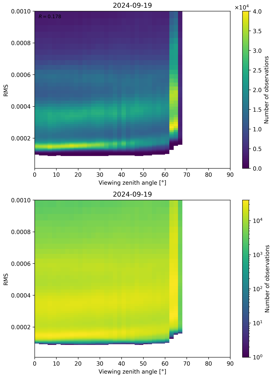
Figure 171: Scatter density plot of “Viewing zenith angle” against “RMS” for 2024-09-18 to 2024-09-20.
