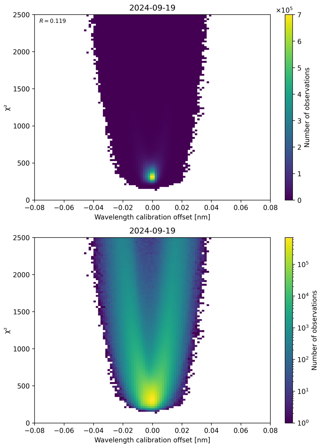
Figure 175: Scatter density plot of “Wavelength calibration offset” against “ \chi^2 ” for 2024-09-18 to 2024-09-20.
