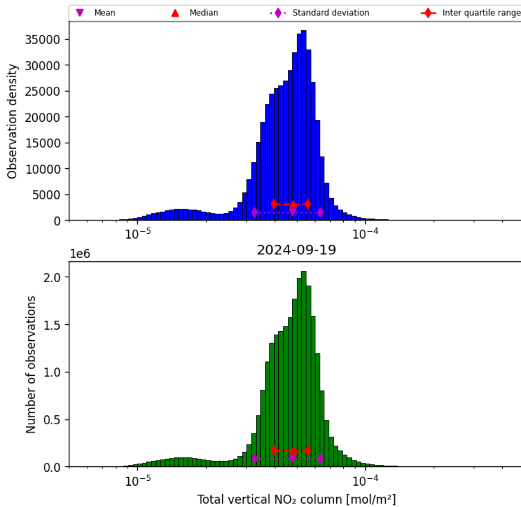
Figure 38: Histogram of “Total vertical NO 2 column” for 2024-09-18 to 2024-09-20
