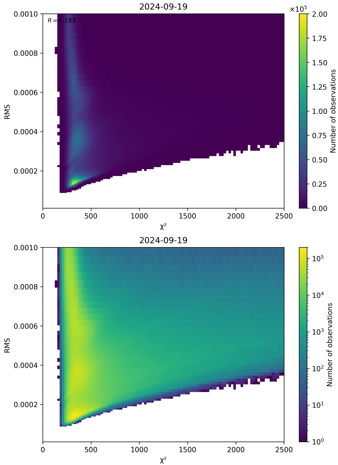
Figure 82: Scatter density plot of “ \chi^2 ” against “RMS” for 2024-09-18 to 2024-09-20.
