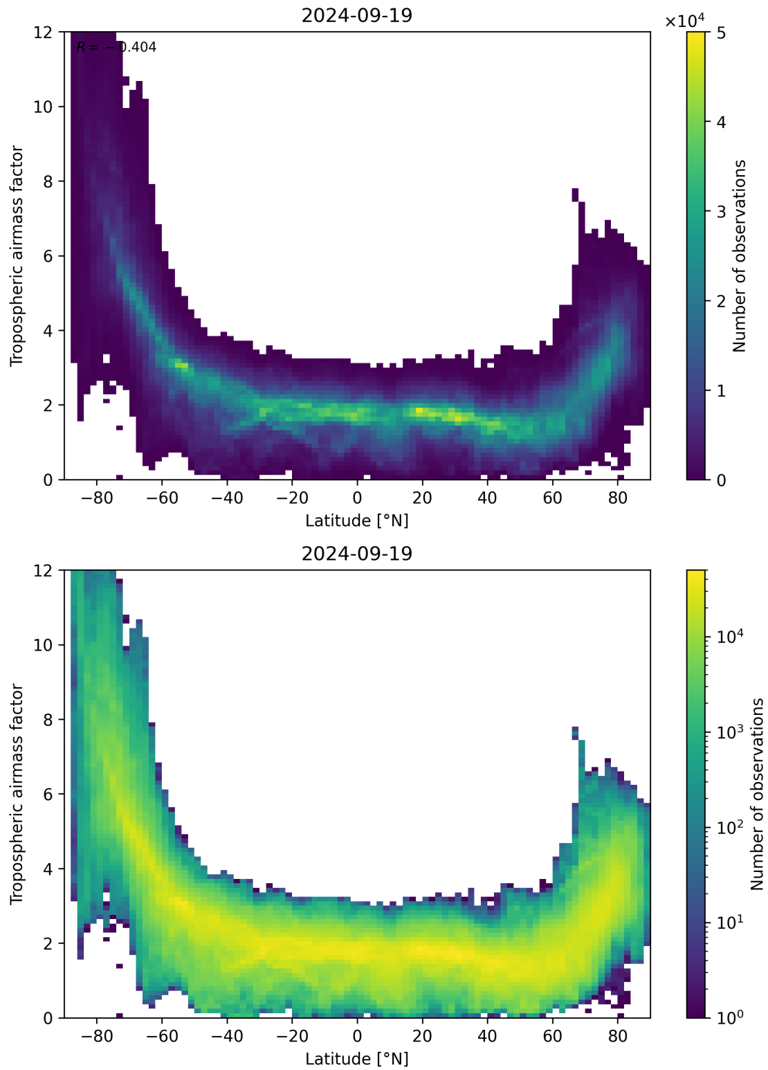
Figure 85: Scatter density plot of “Latitude” against “Tropospheric airmass factor” for 2024-09-18 to 2024-09-20.
