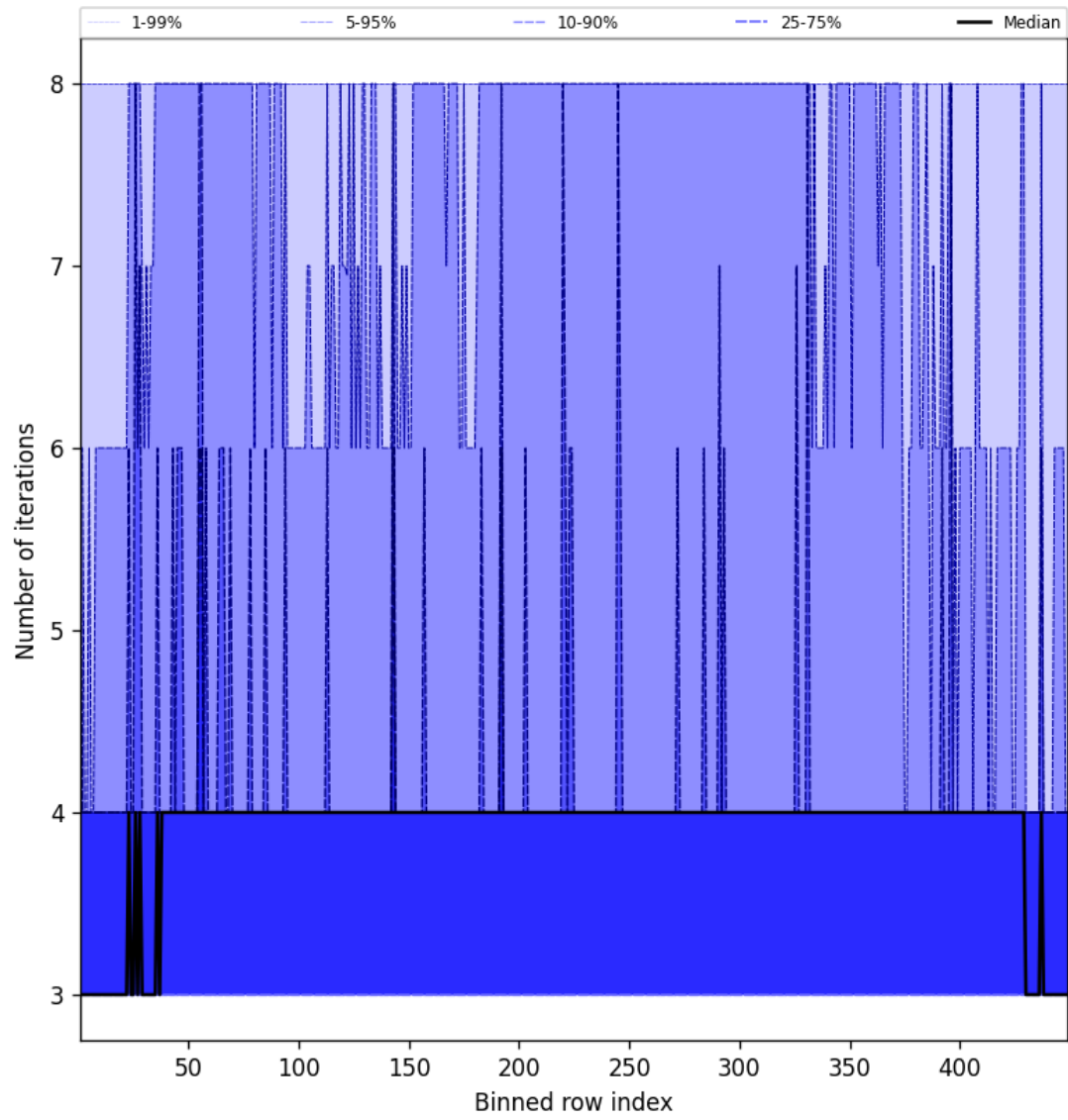
Figure 51: Along track statistics of “Number of iterations” for 2024-09-18 to 2024-09-20
