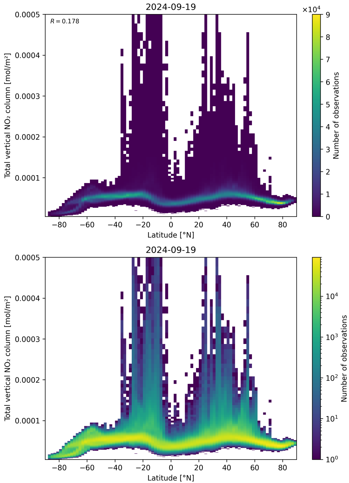
Figure 90: Scatter density plot of “Latitude” against “Total vertical NO 2 column” for 2024-09-18 to 2024-09-20.
