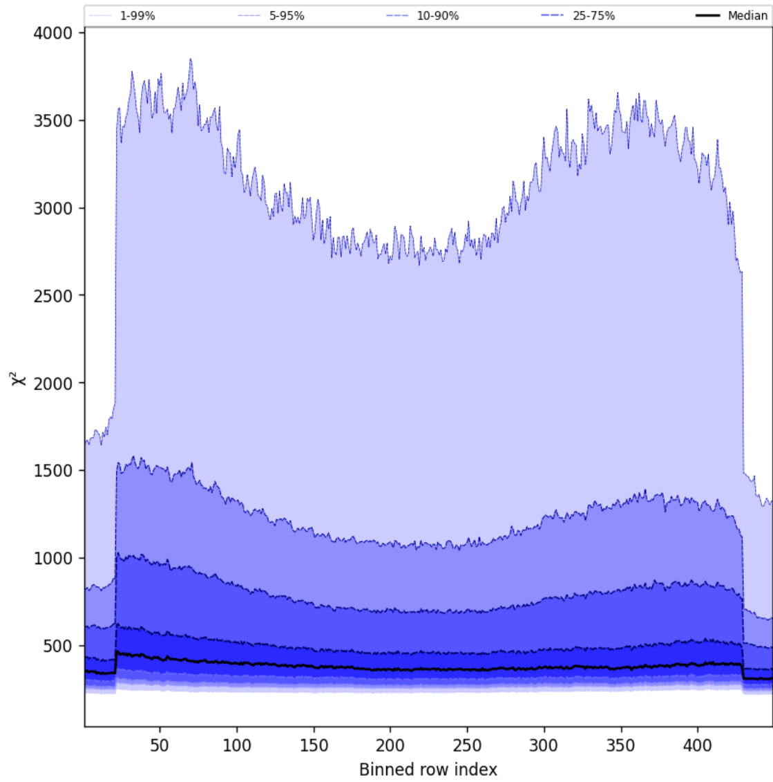
Figure 59: Along track statistics of “ \chi^2 ” for 2024-09-18 to 2024-09-20
