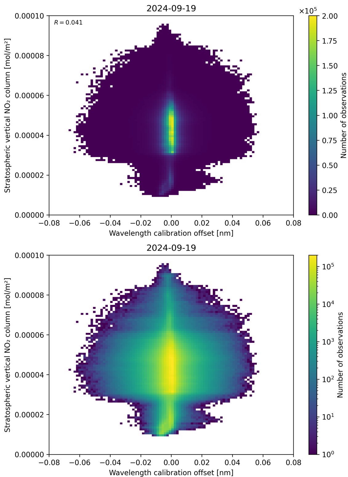
Figure 176: Scatter density plot of “Wavelength calibration offset” against “Stratospheric vertical NO 2 column” for 2024-09-18 to 2024-09-20.
