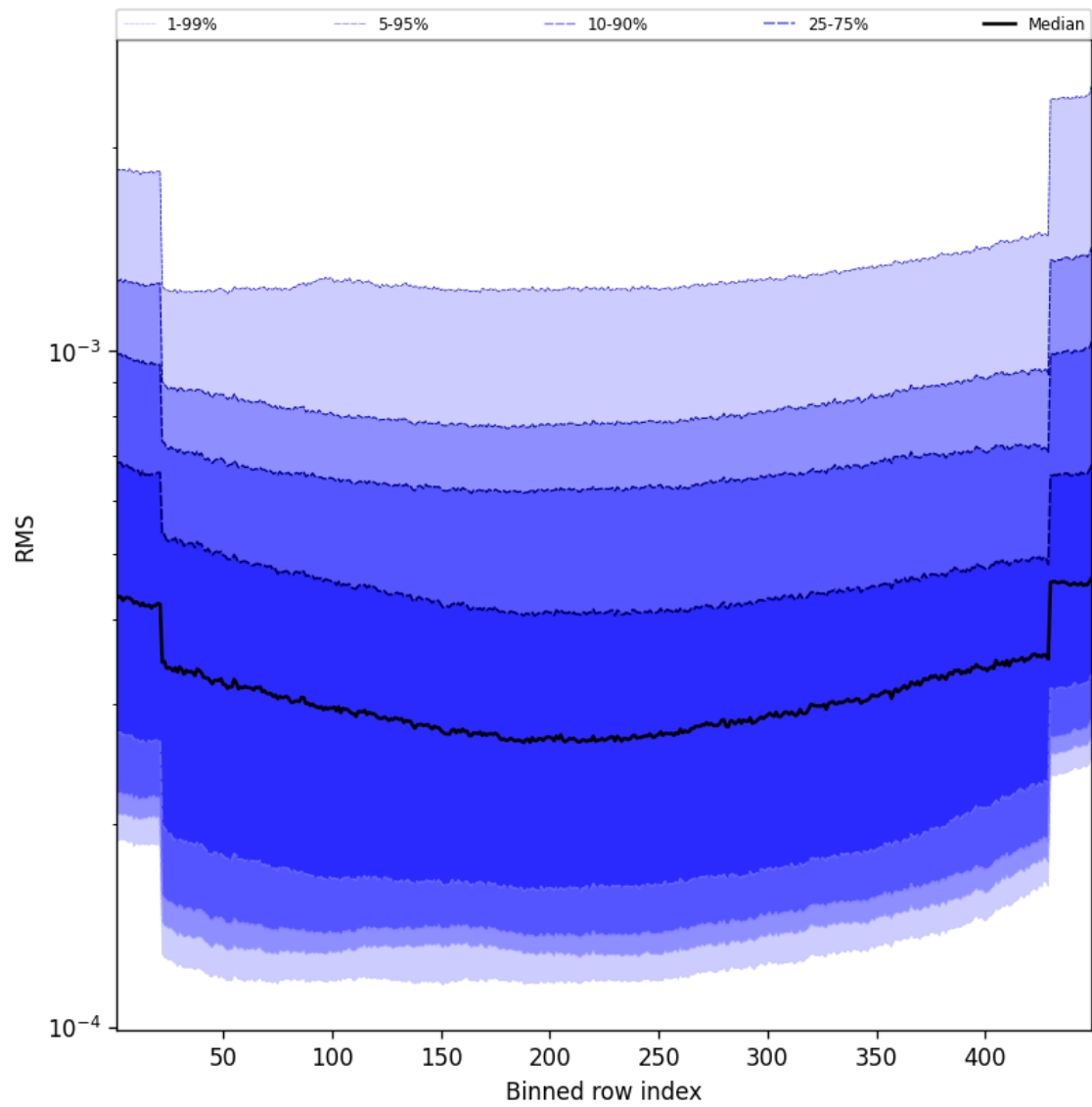
Figure 60: Along track statistics of “RMS” for 2024-09-18 to 2024-09-20
