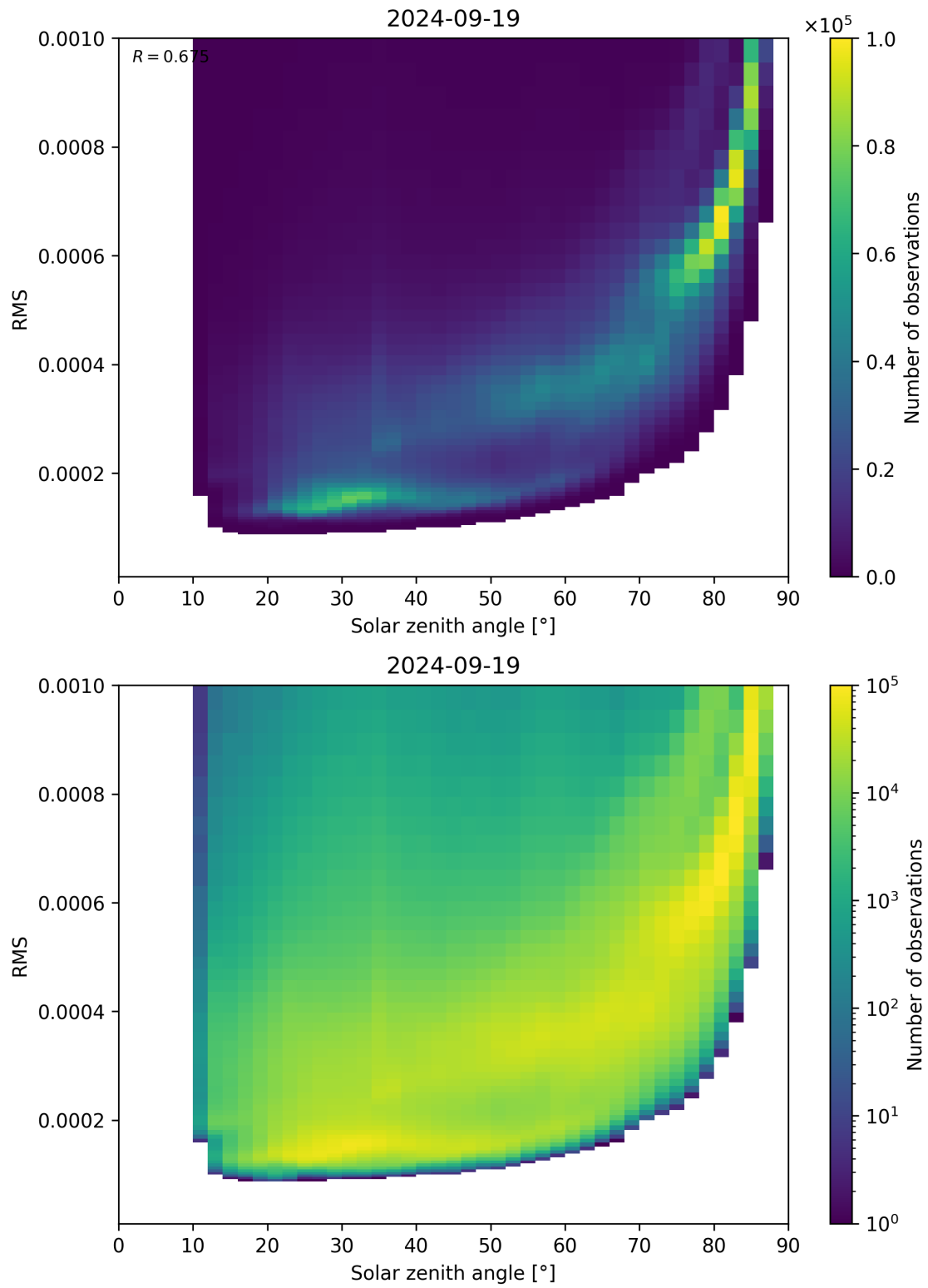
Figure 157: Scatter density plot of “Solar zenith angle” against “RMS” for 2024-09-18 to 2024-09-20.
