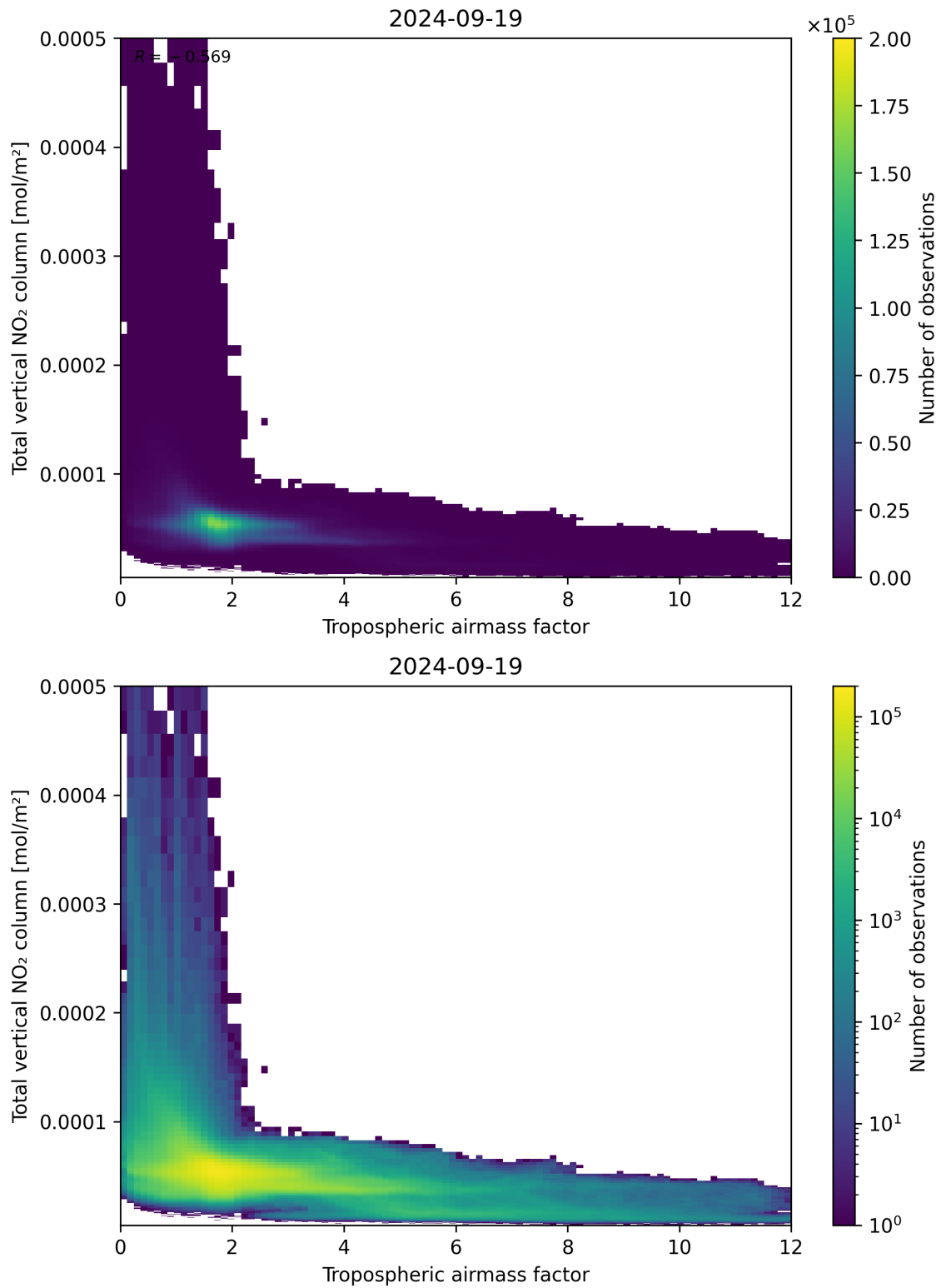
Figure 77: Scatter density plot of “Tropospheric airmass factor” against “Total vertical NO 2 column” for 2024-09-18 to 2024-09-20.
