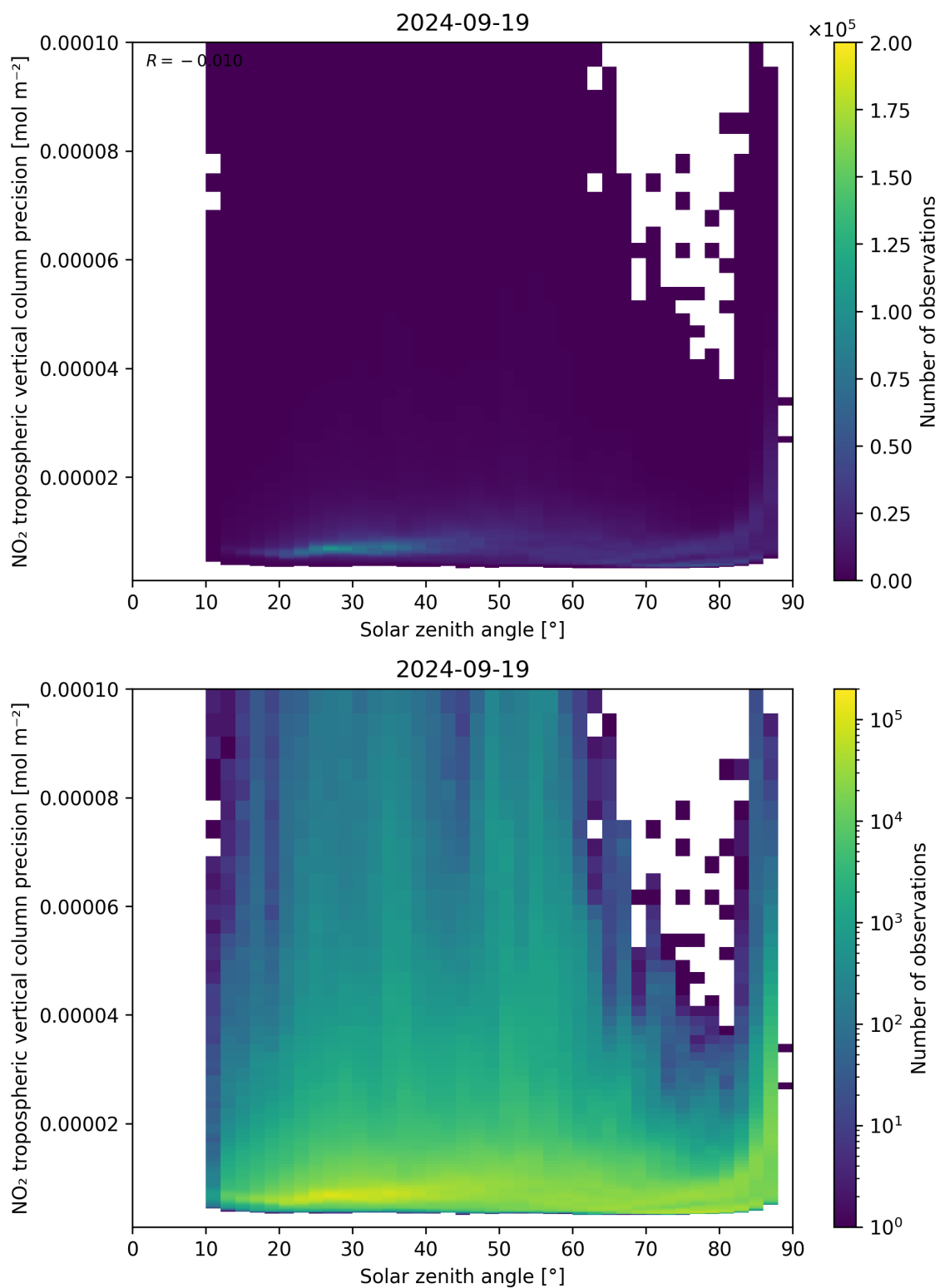
Figure 156: Scatter density plot of “Solar zenith angle” against “NO 2 tropospheric vertical column precision” for 2024-09-18 to 2024-09-20.
