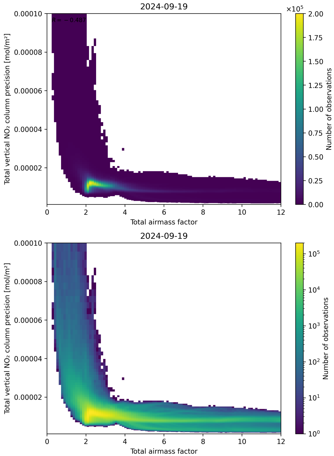
Figure 68: Scatter density plot of “Total airmass factor” against “Total vertical NO 2 column precision” for 2024-09-18 to 2024-09-20.
