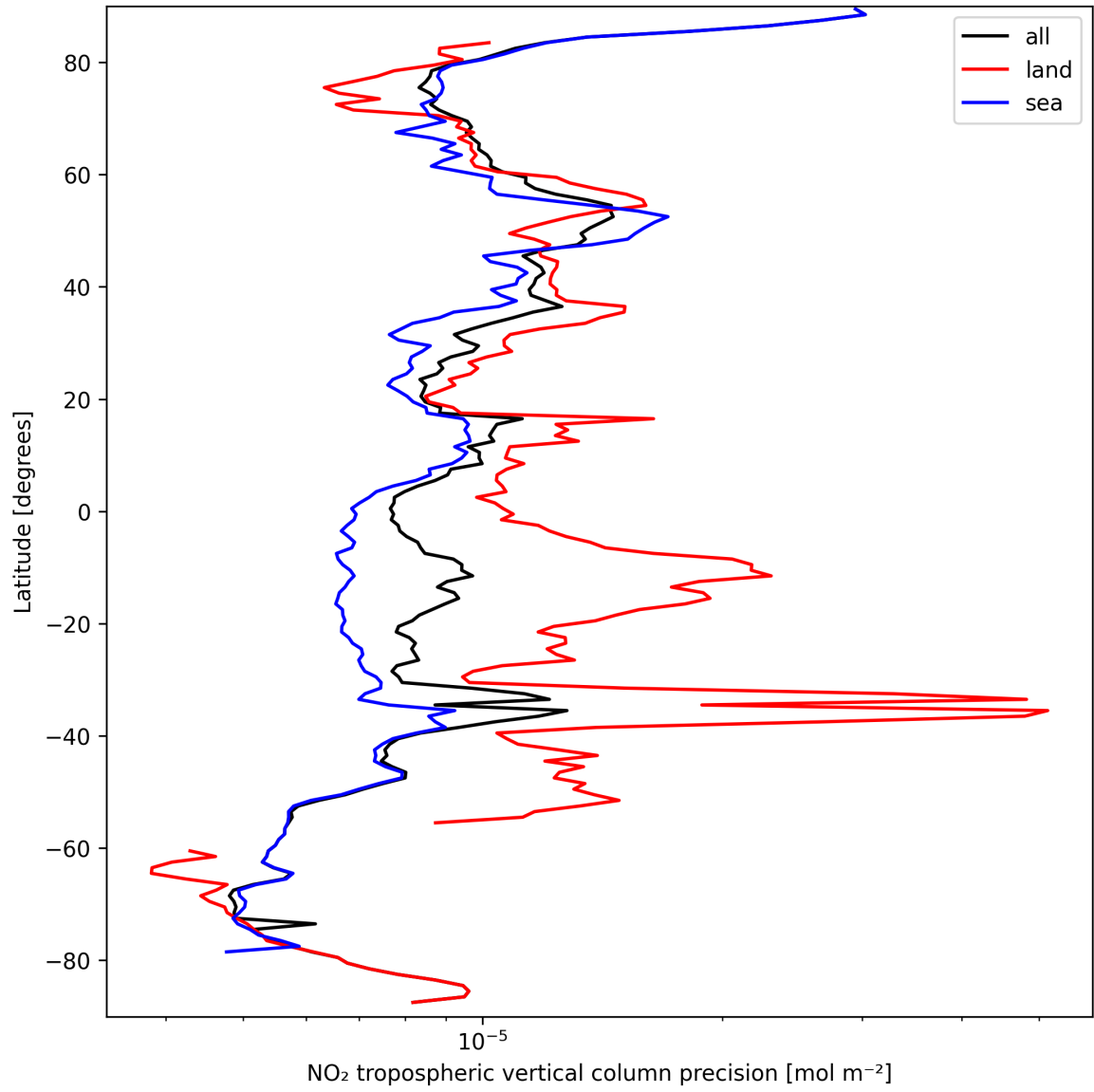
Figure 13: Zonal average of “NO 2 tropospheric vertical column precision” for 2024-09-18 to 2024-09-20.
