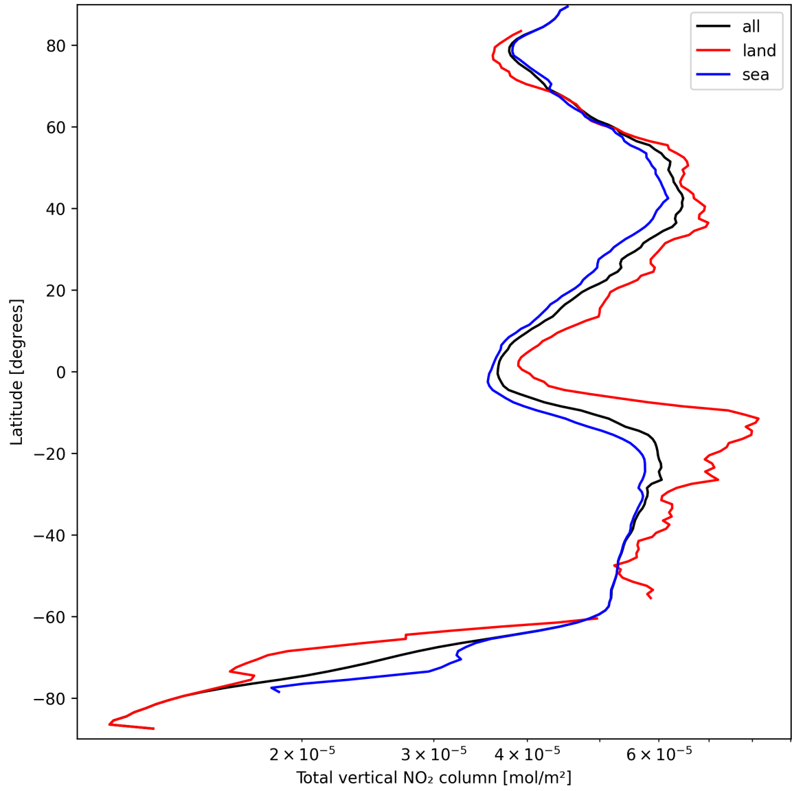
Figure 21: Zonal average of “Total vertical NO 2 column” for 2024-09-18 to 2024-09-20.
