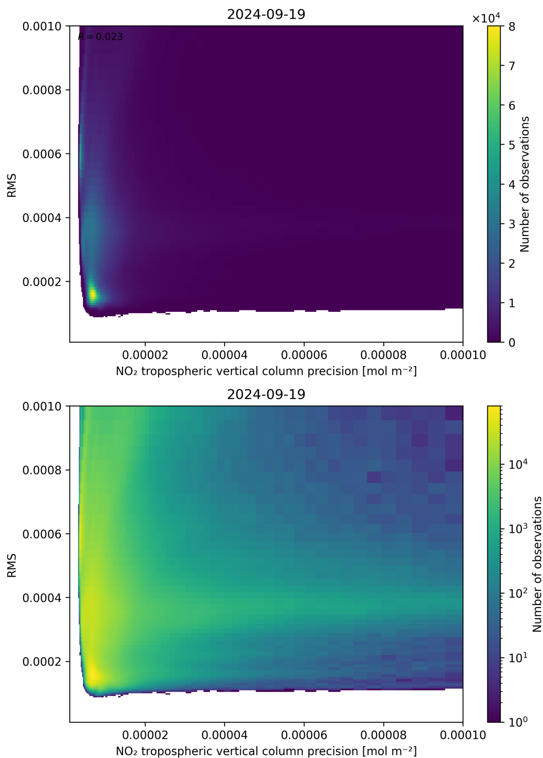
Figure 140: Scatter density plot of “NO 2 tropospheric vertical column precision” against “RMS” for 2024-09-18 to 2024-09-20.
