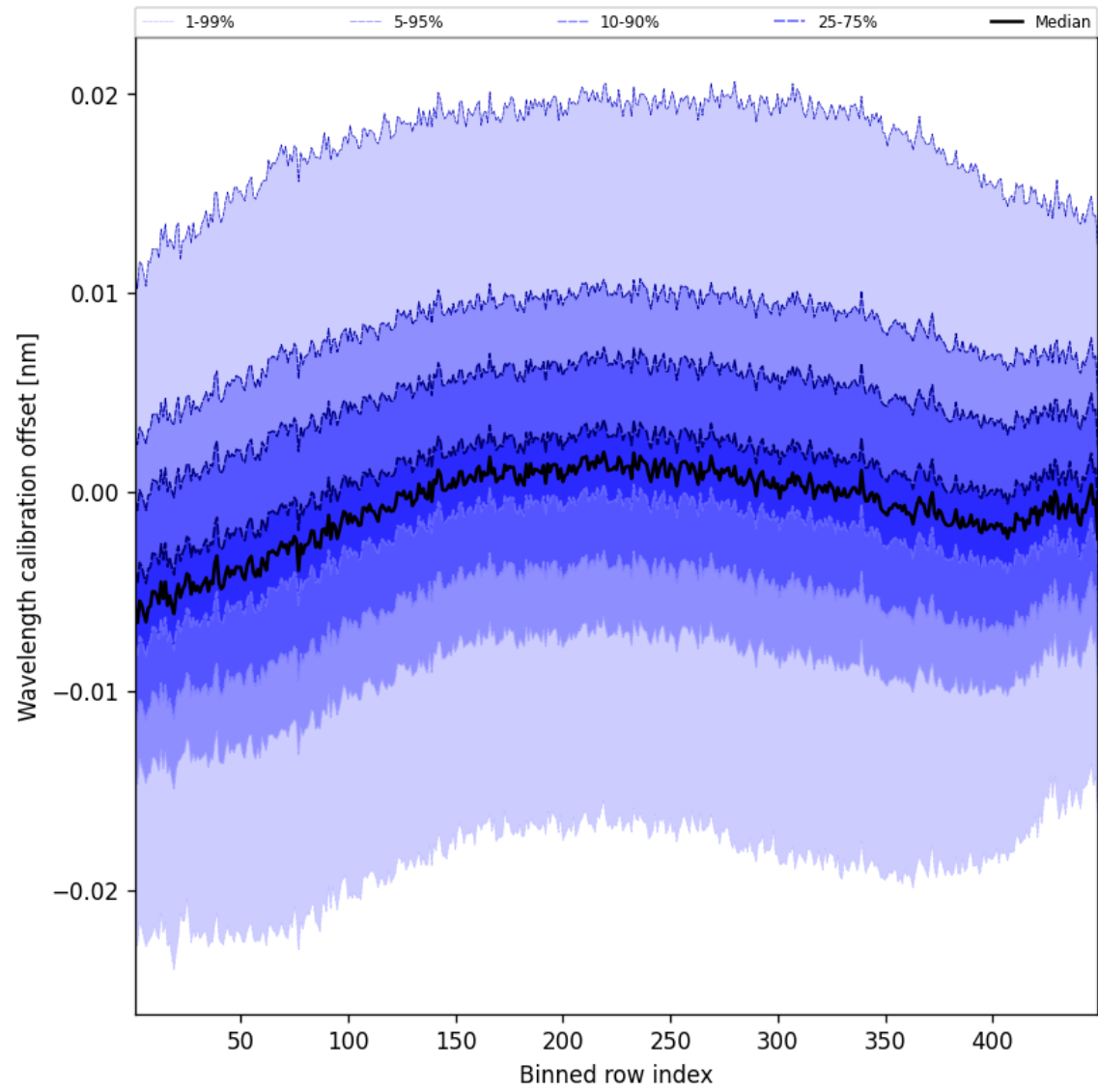
Figure 52: Along track statistics of “Wavelength calibration offset” for 2024-09-18 to 2024-09-20
