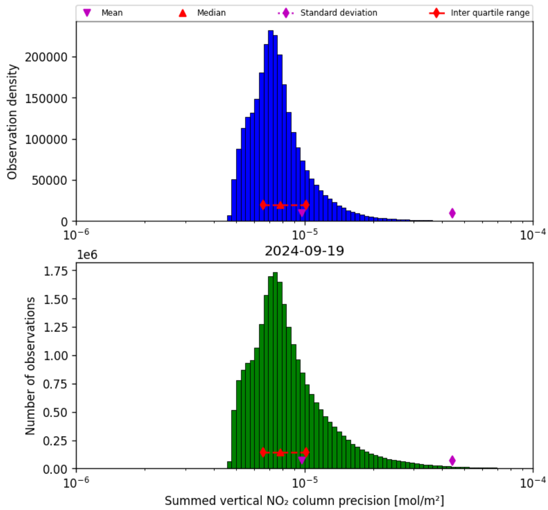
Figure 41: Histogram of "Summed vertical NO 2 column precision" for 2024-09-18 to 2024-09-20
