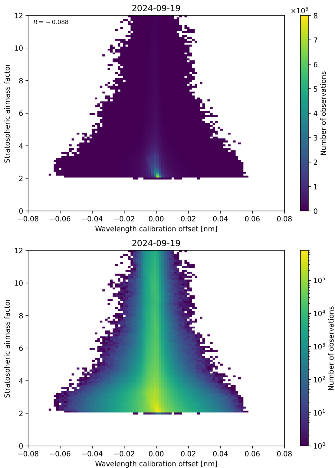
Figure 174: Scatter density plot of “Wavelength calibration offset” against “Stratospheric airmass factor” for 2024-09-18 to 2024-09-20.
