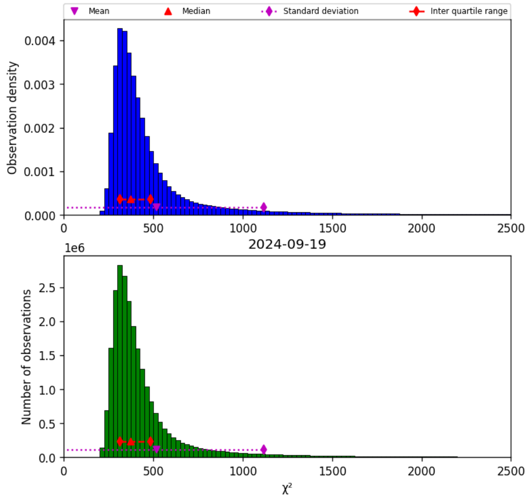
Figure 42: Histogram of “ \chi^2 ” for 2024-09-18 to 2024-09-20
