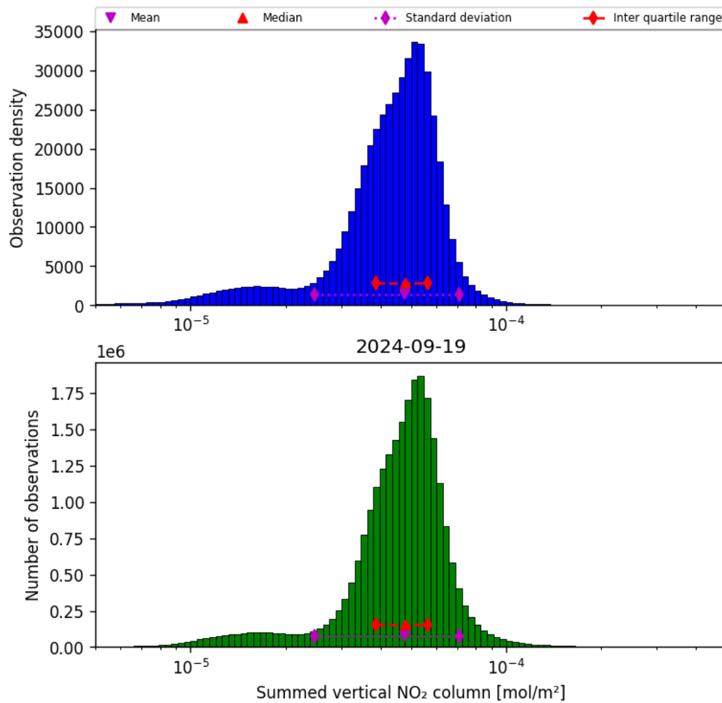
Figure 40: Histogram of “Summed vertical NO 2 column” for 2024-09-18 to 2024-09-20
