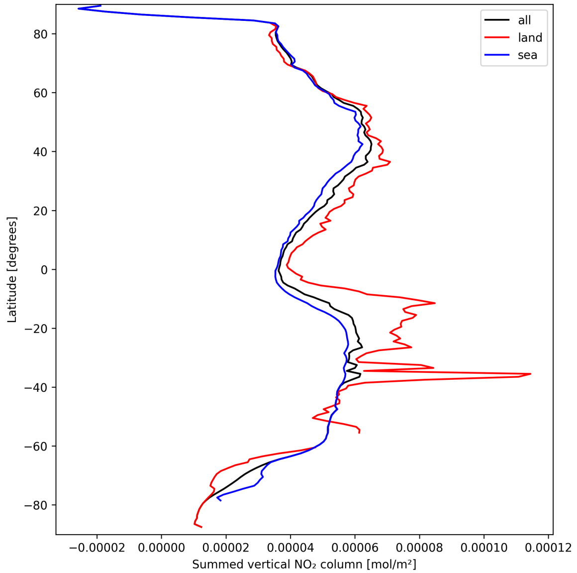
Figure 23: Zonal average of “Summed vertical NO 2 column” for 2024-09-18 to 2024-09-20.
