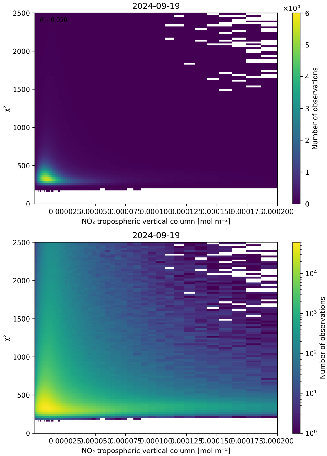
Figure 124: Scatter density plot of “NO 2 tropospheric vertical column” against “ \chi^2 ” for 2024-09-18 to 2024-09-20.
