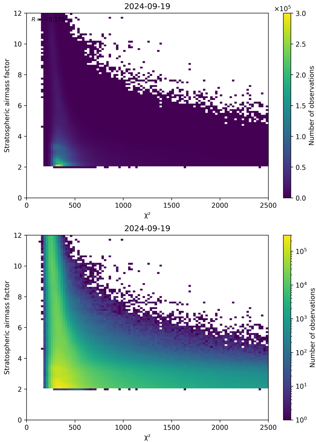
Figure 81: Scatter density plot of “ \chi^2 ” against “Stratospheric airmass factor” for 2024-09-18 to 2024-09-20.
