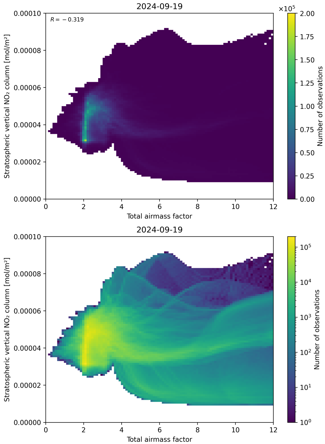
Figure 64: Scatter density plot of “Total airmass factor” against “Stratospheric vertical NO 2 column” for 2024-09-18 to 2024-09-20.
