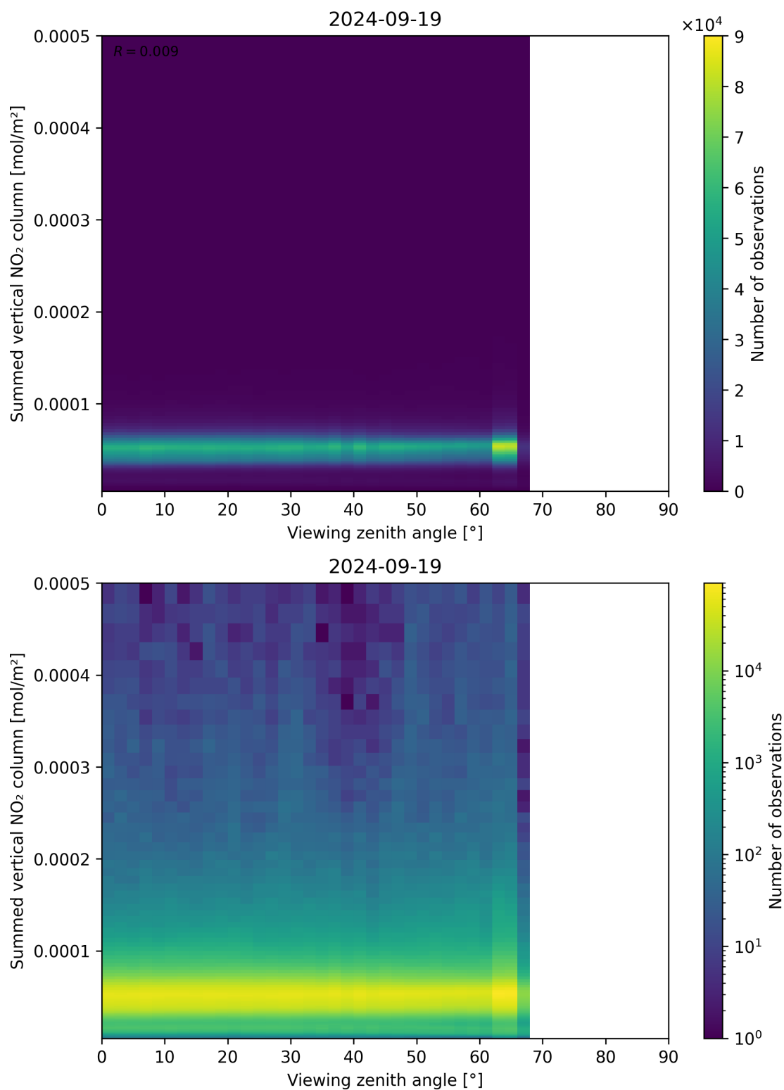
Figure 165: Scatter density plot of “Viewing zenith angle” against “Summed vertical NO 2 column” for 2024-09-18 to 2024-09-20.
