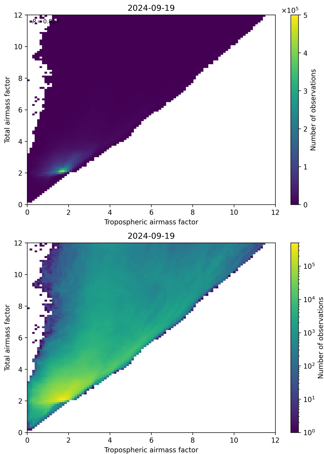
Figure 72: Scatter density plot of “Tropospheric airmass factor” against “Total airmass factor” for 2024-09-18 to 2024-09-20.
