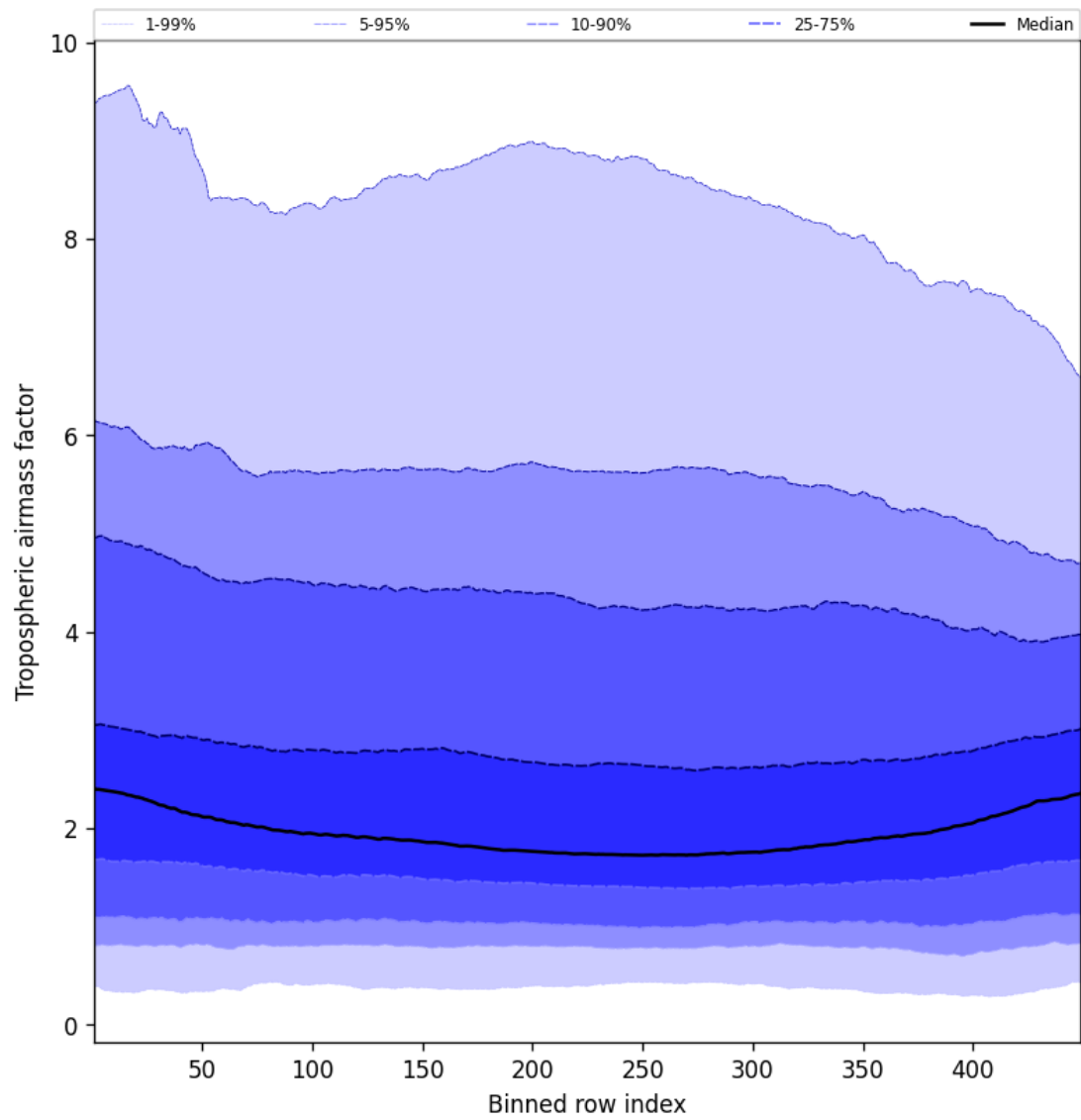
Figure 48: Along track statistics of “Tropospheric air mass factor” for 2024-09-18 to 2024-09-20
