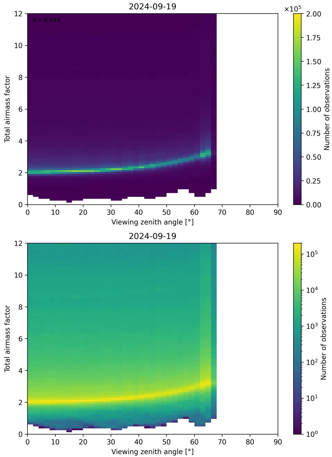
Figure 160: Scatter density plot of “Viewing zenith angle” against “Total airmass factor” for 2024-09-18 to 2024-09-20.
