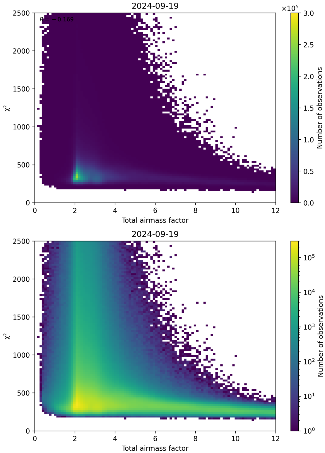
Figure 63: Scatter density plot of “Total airmass factor” against “ \chi^2 ” for 2024-09-18 to 2024-09-20.
