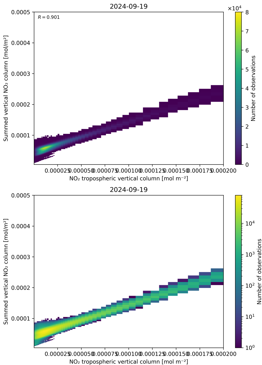
Figure 126: Scatter density plot of “NO 2 tropospheric vertical column” against “Summed vertical NO 2 column” for 2024-09-18 to 2024-09-20.
