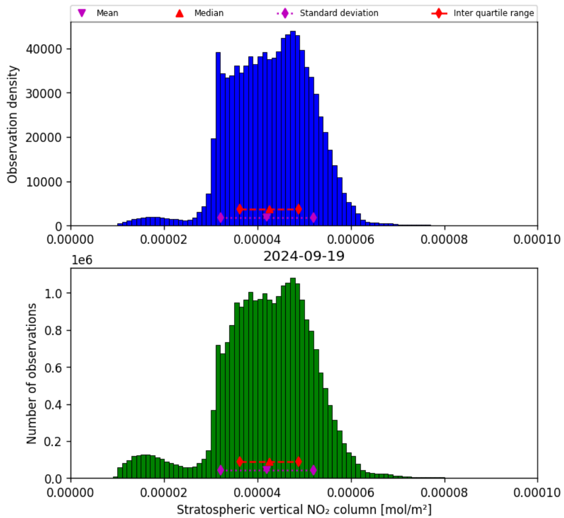
Figure 36: Histogram of “Stratospheric vertical NO 2 column” for 2024-09-18 to 2024-09-20
