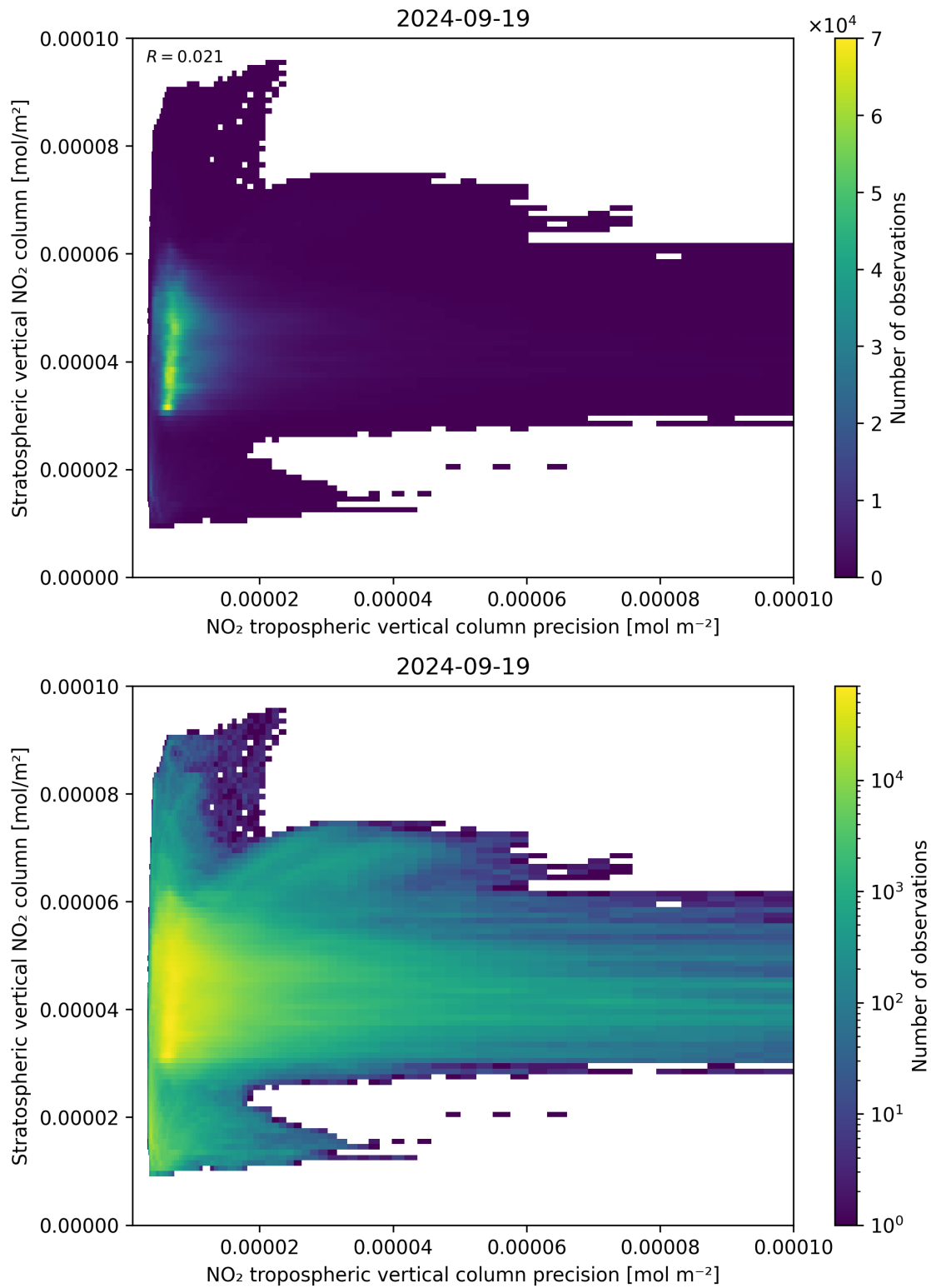
Figure 135: Scatter density plot of “NO 2 tropospheric vertical column precision” against “Stratospheric vertical NO 2 column” for 2024-09-18 to 2024-09-20.
