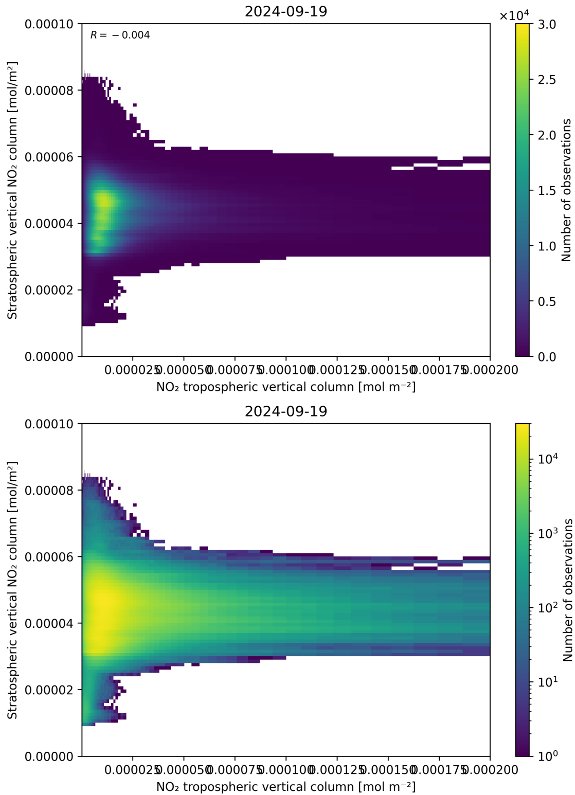
Figure 125: Scatter density plot of “NO 2 tropospheric vertical column” against “Stratospheric vertical NO 2 column” for 2024-09-18 to 2024-09-20.
