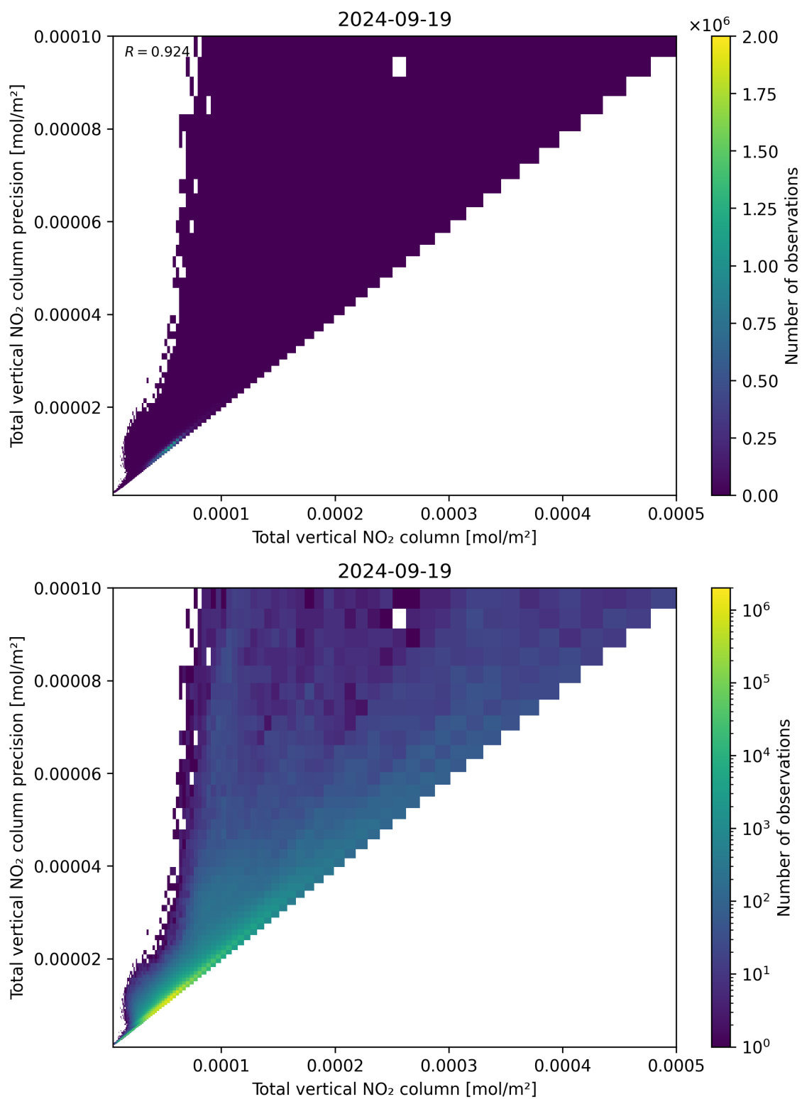
Figure 114: Scatter density plot of “Total vertical NO 2 column” against “Total vertical NO 2 column precision” for 2024-09-18 to 2024-09-20.
