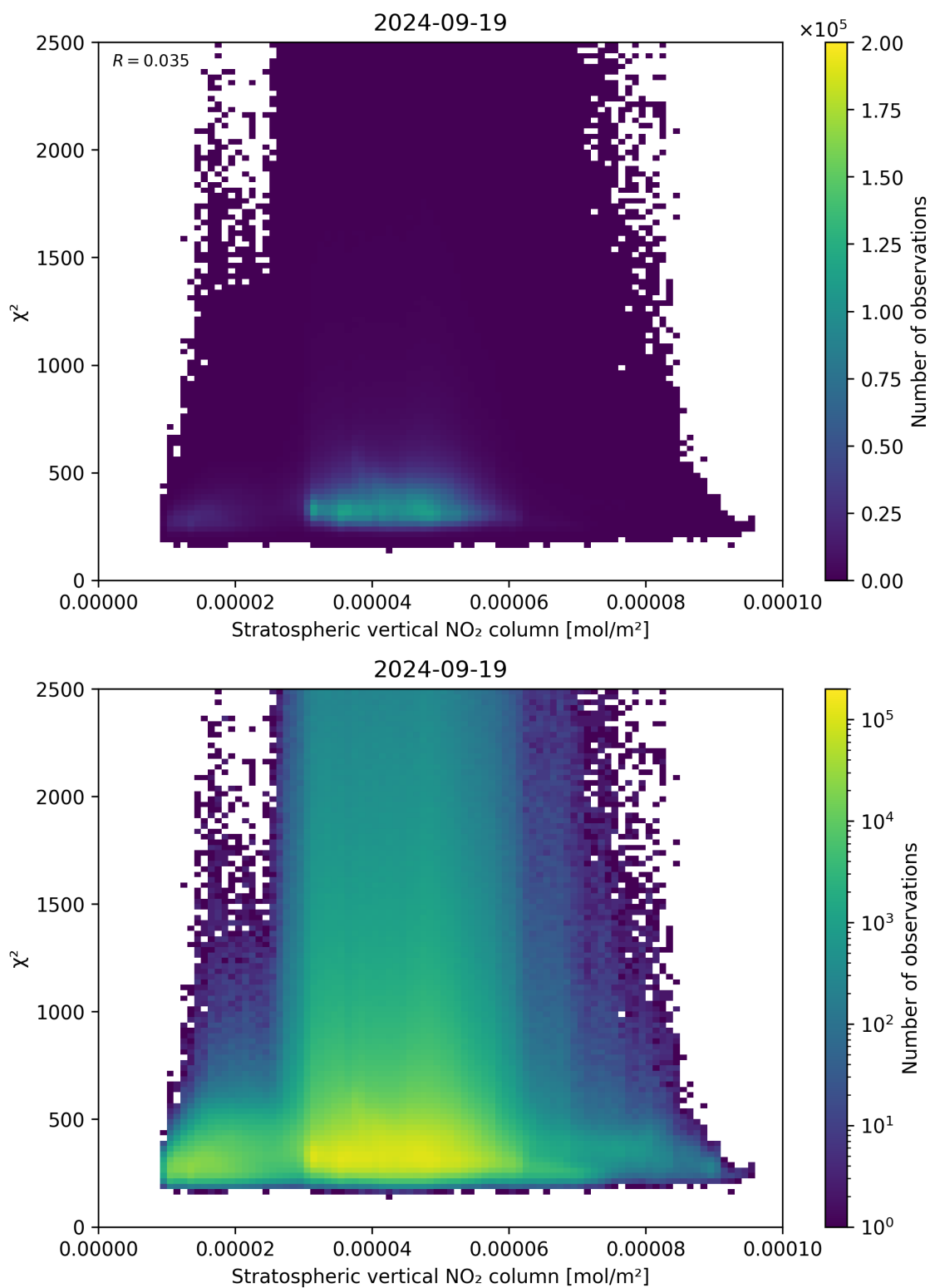
Figure 97: Scatter density plot of “Stratospheric vertical NO 2 column” against “ \chi^2 ” for 2024-09-18 to 2024-09-20.
