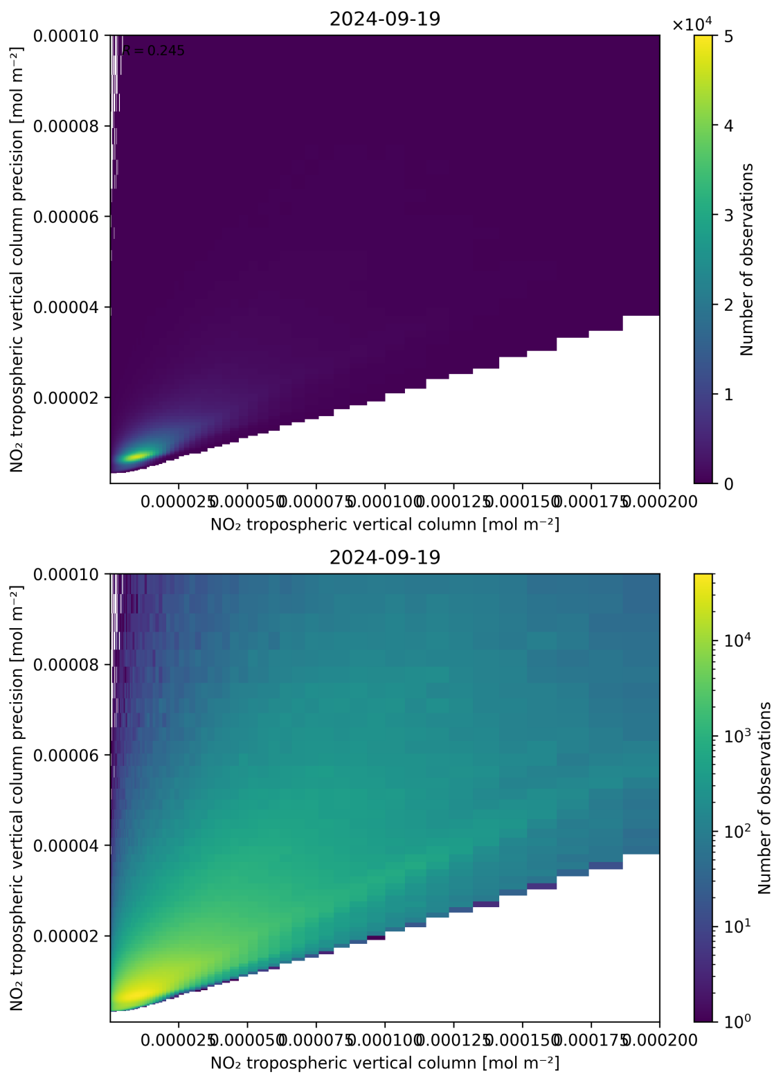
Figure 130: Scatter density plot of “NO 2 tropospheric vertical column” against “NO 2 tropospheric vertical column precision” for 2024-09-18 to 2024-09-20.
