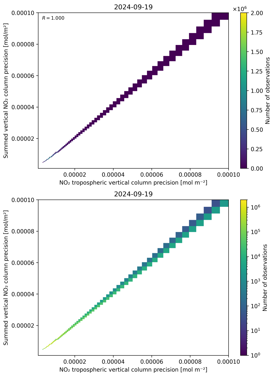
Figure 137: Scatter density plot of “NO 2 tropospheric vertical column precision” against “Summed vertical NO 2 column precision” for 2024-09-18 to 2024-09-20.
