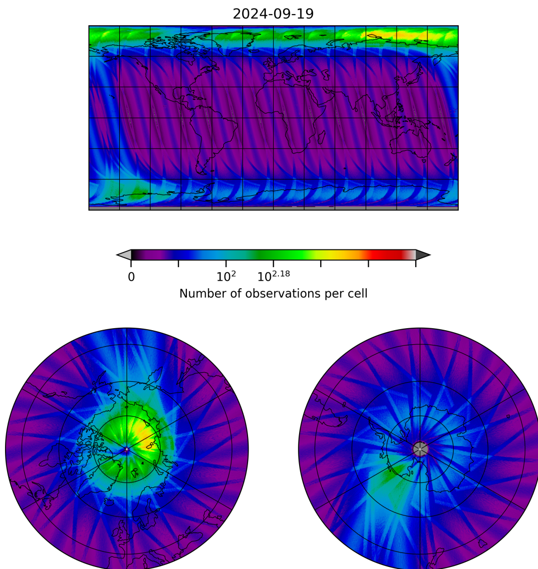
Figure 10: Map of the number of observations for 2024-09-18 to 2024-09-20
