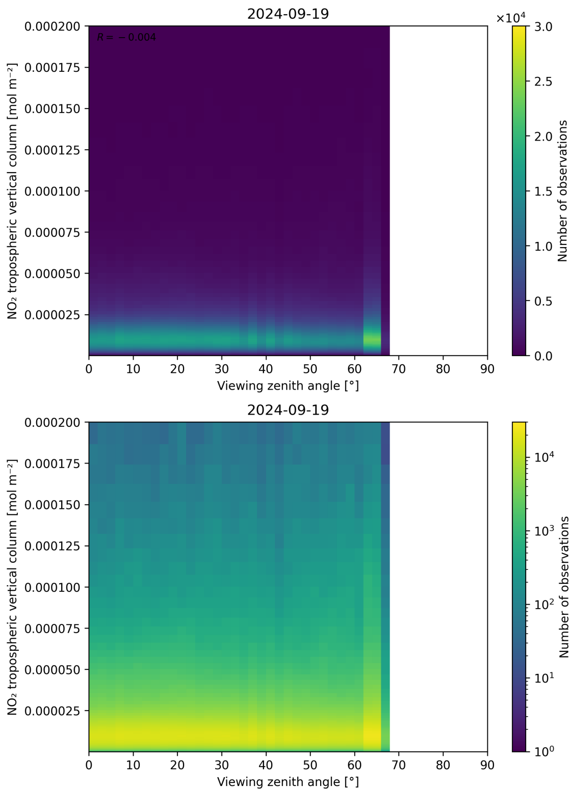
Figure 169: Scatter density plot of “Viewing zenith angle” against “NO 2 tropospheric vertical column” for 2024-09-18 to 2024-09-20.
