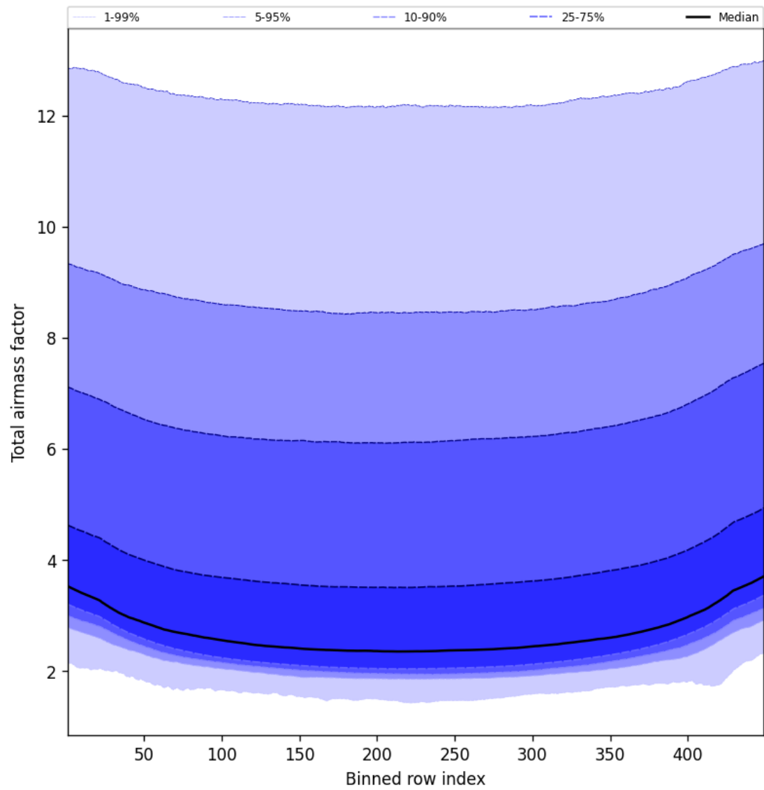
Figure 49: Along track statistics of “Total airmass factor” for 2024-09-18 to 2024-09-20
