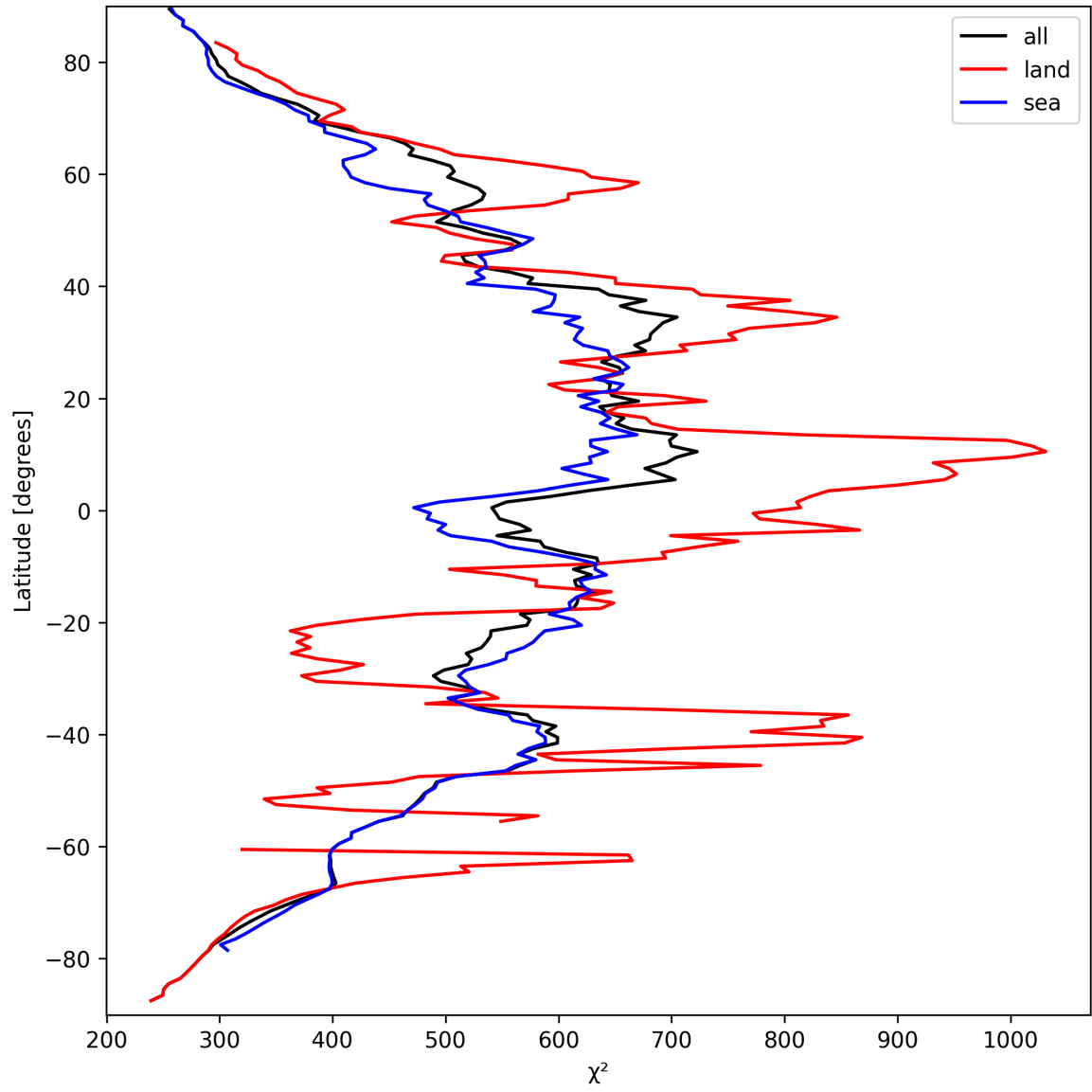
Figure 25: Zonal average of " \chi^2 " for 2024-09-18 to 2024-09-20.
