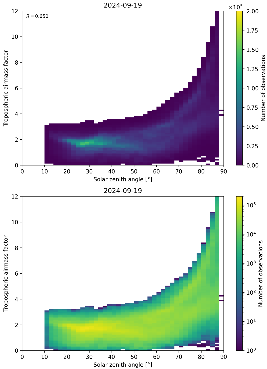
Figure 147: Scatter density plot of “Solar zenith angle” against “Tropospheric airmass factor” for 2024-09-18 to 2024-09-20.
