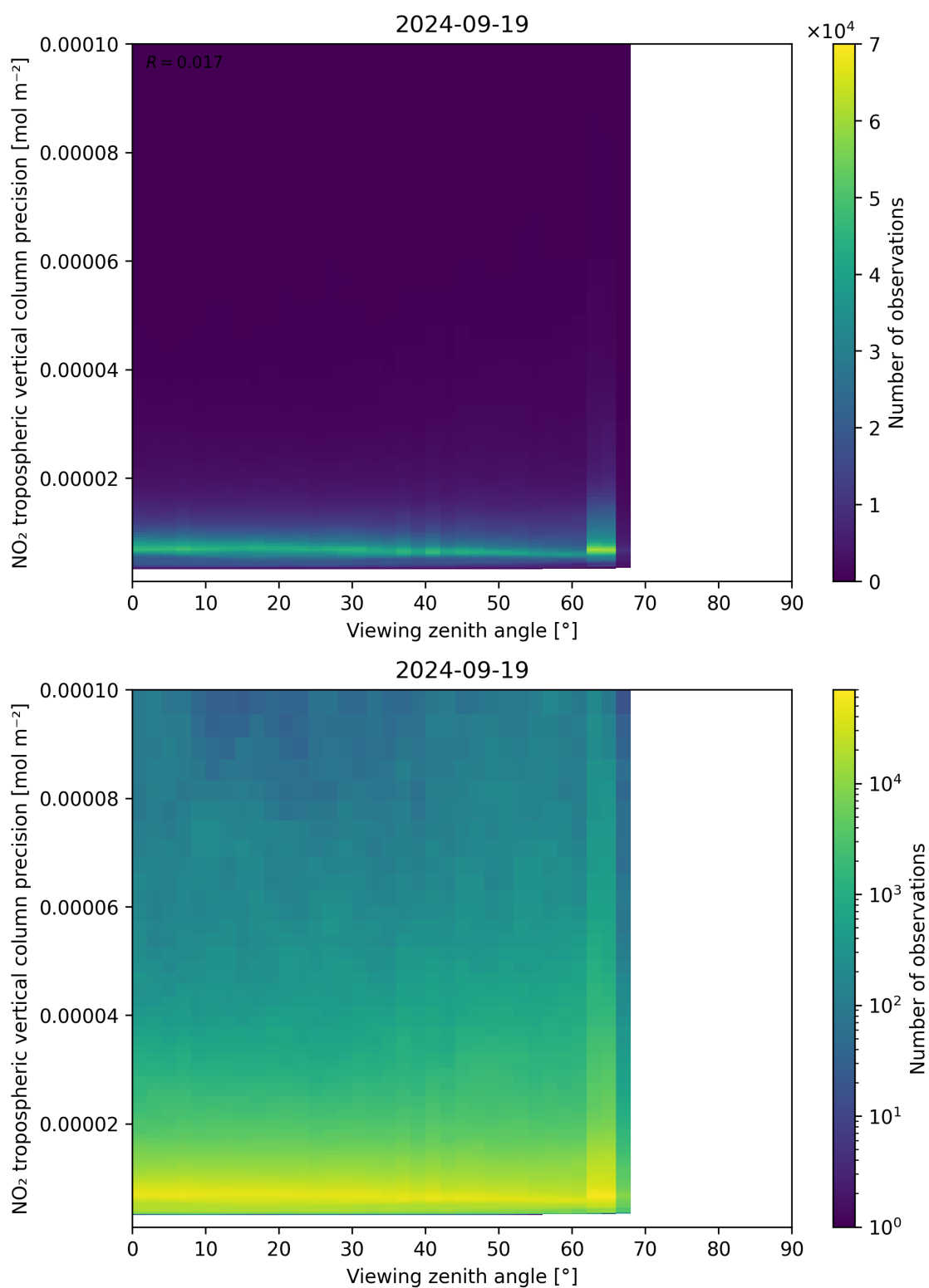
Figure 170: Scatter density plot of “Viewing zenith angle” against “NO 2 tropospheric vertical column precision” for 2024-09-18 to 2024-09-20.
