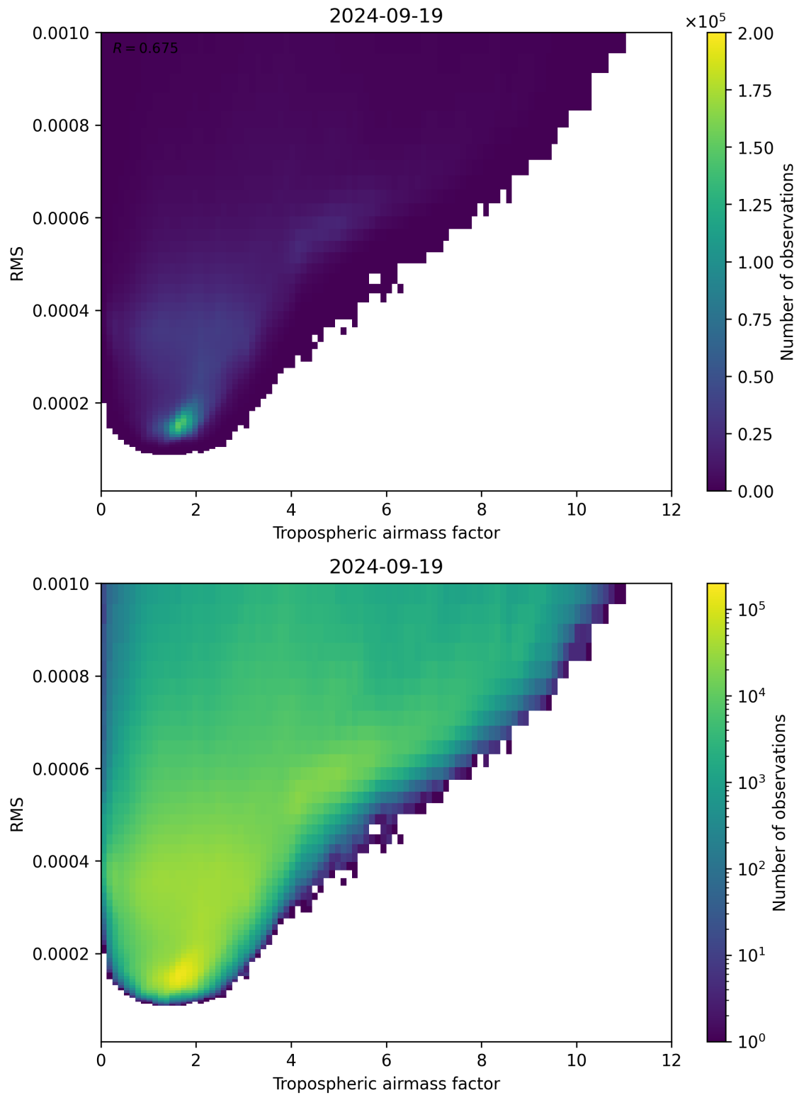
Figure 79: Scatter density plot of “Tropospheric airmass factor” against “RMS” for 2024-09-18 to 2024-09-20.
