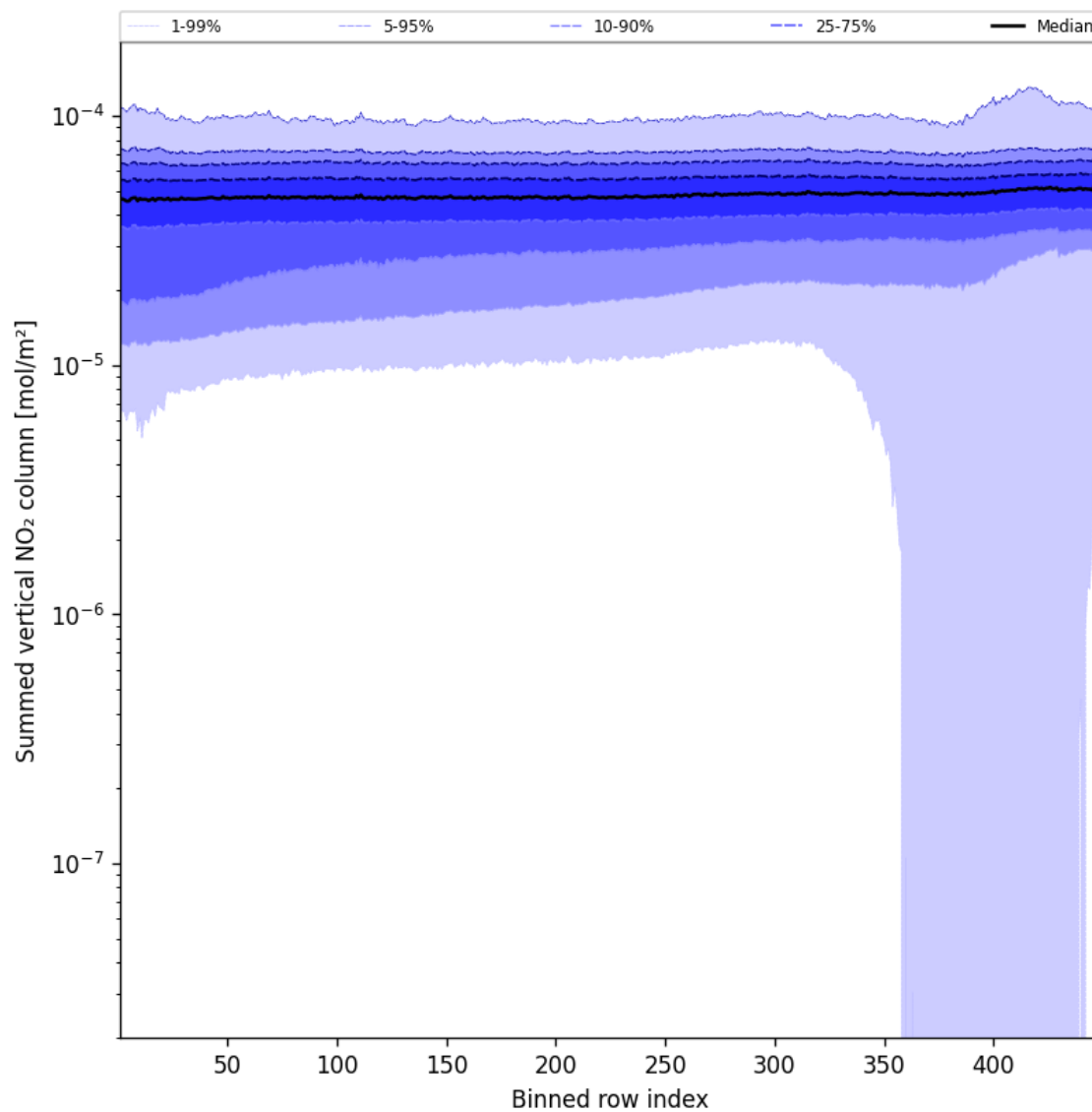
Figure 57: Along track statistics of “Summed vertical NO 2 column” for 2024-09-18 to 2024-09-20
