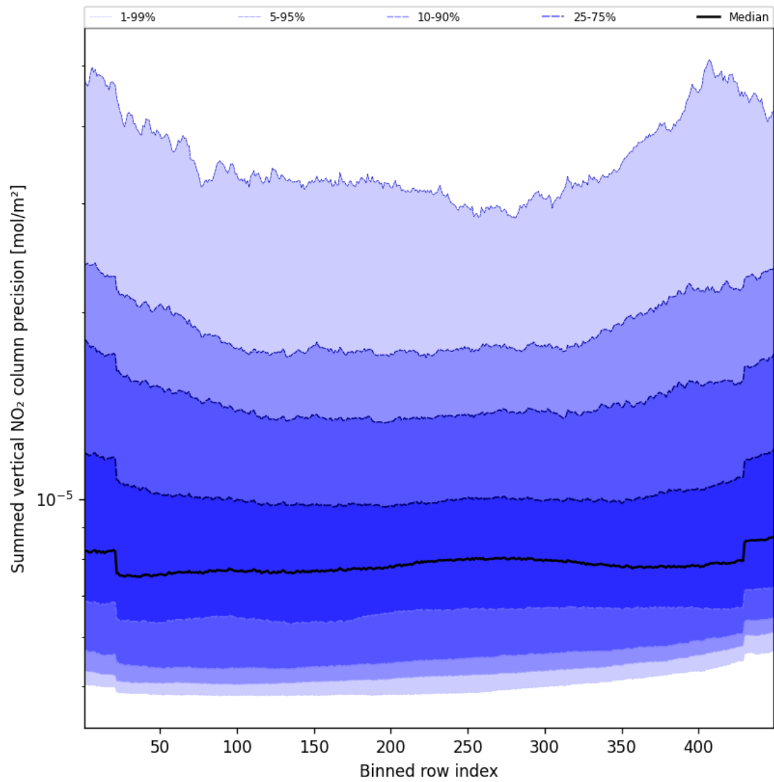
Figure 58: Along track statistics of “Summed vertical NO 2 column precision” for 2024-09-18 to 2024-09-20
