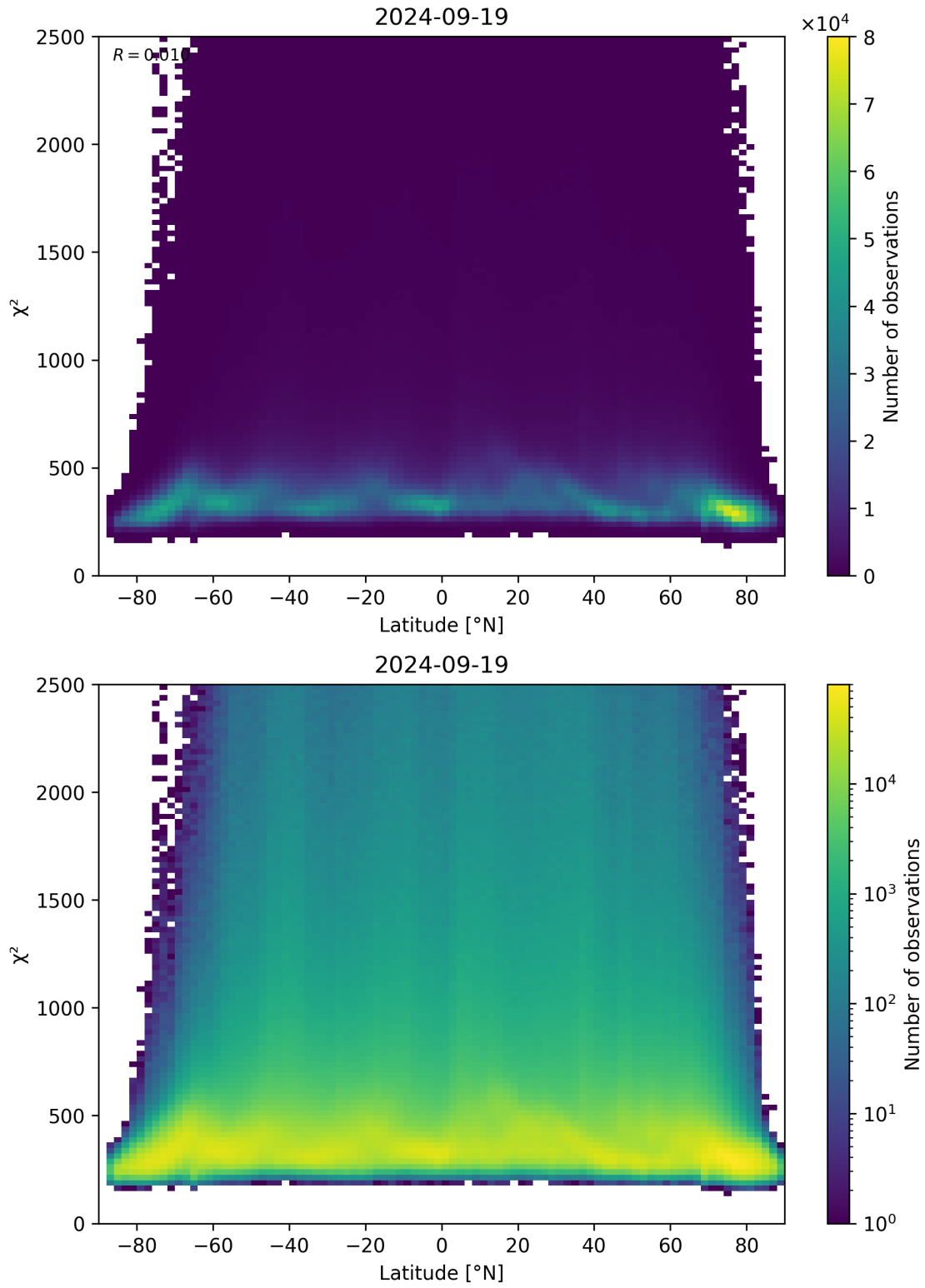
Figure 86: Scatter density plot of “Latitude” against “ \chi^2 ” for 2024-09-18 to 2024-09-20.
