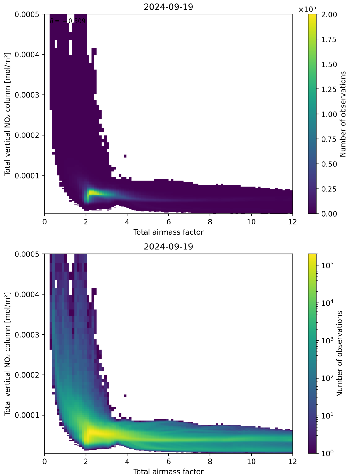
Figure 67: Scatter density plot of “Total airmass factor” against “Total vertical NO 2 column” for 2024-09-18 to 2024-09-20.
