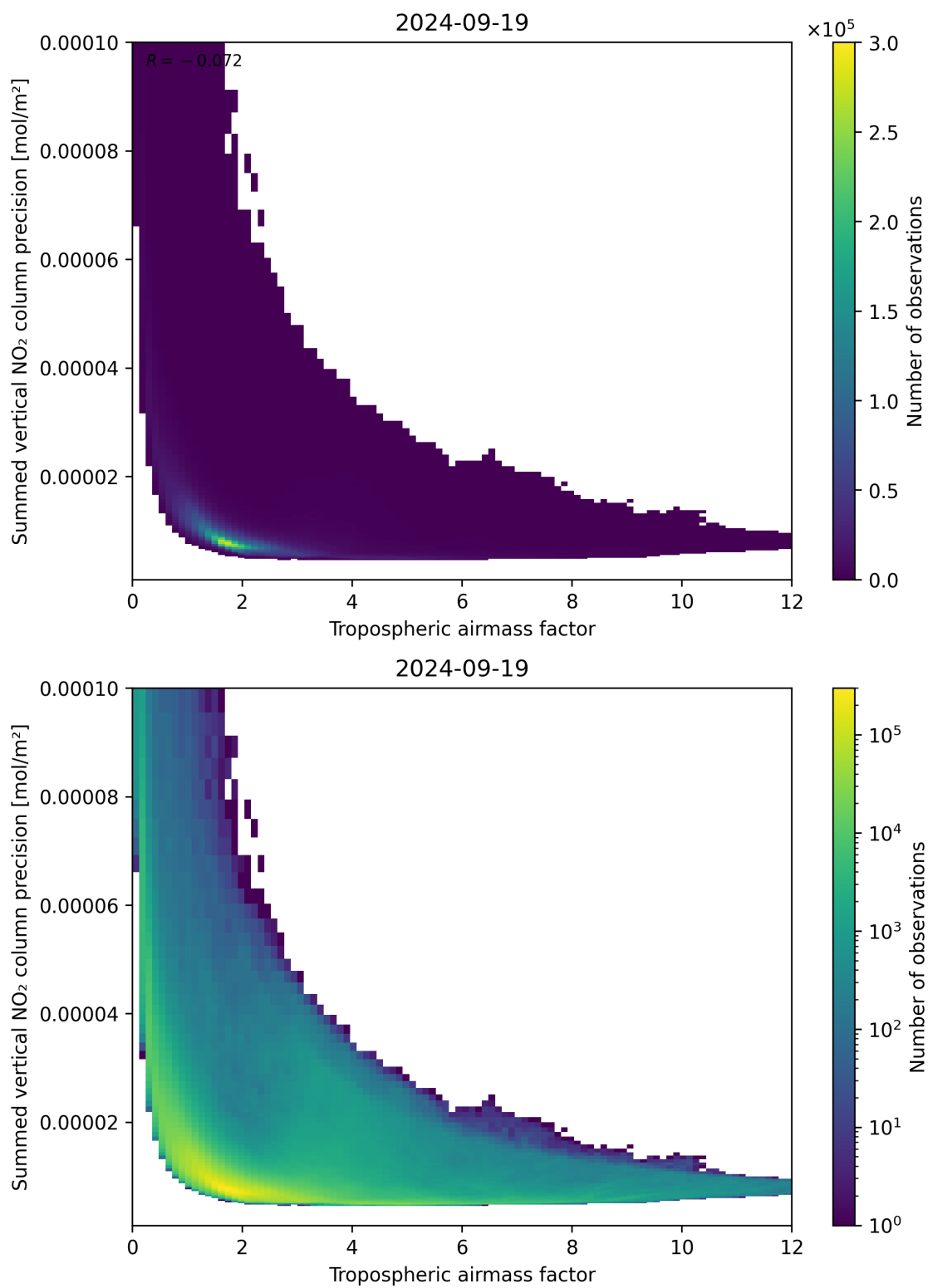
Figure 76: Scatter density plot of “Tropospheric air mass factor” against “Summed vertical NO 2 column precision” for 2024-09-18 to 2024-09-20.
