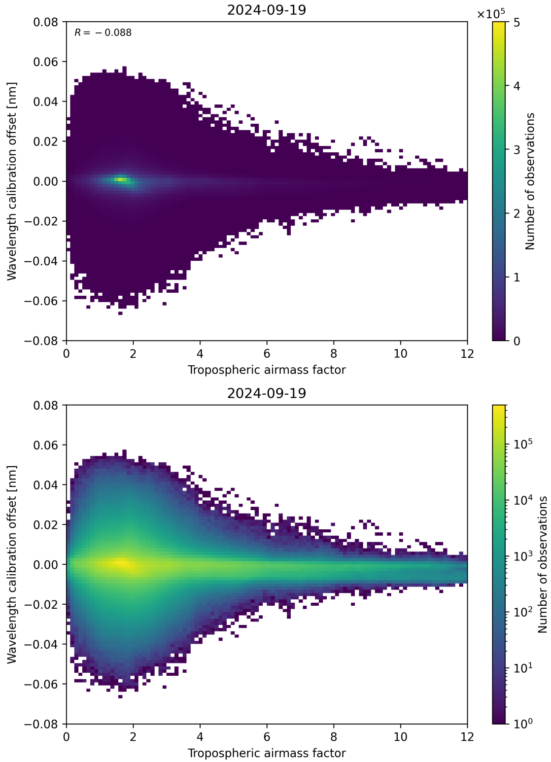
Figure 80: Scatter density plot of “Tropospheric airmass factor” against “Wavelength calibration offset” for 2024-09-18 to 2024-09-20.
