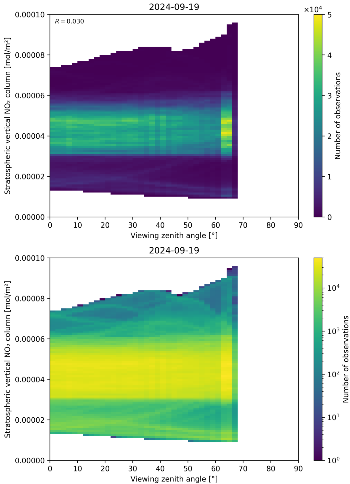
Figure 164: Scatter density plot of “Viewing zenith angle” against “Stratospheric vertical NO 2 column” for 2024-09-18 to 2024-09-20.
