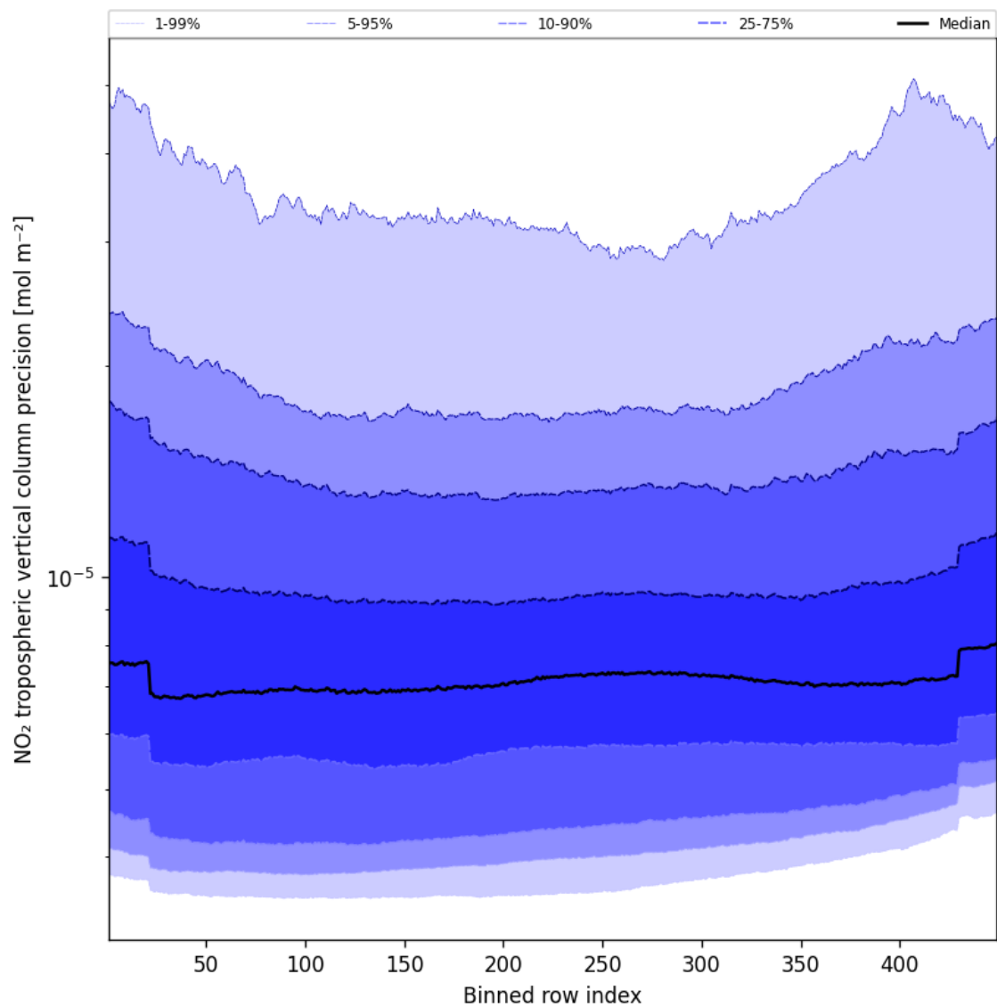
Figure 47: Along track statistics of “NO 2 tropospheric vertical column precision” for 2024-09-18 to 2024-09-20
