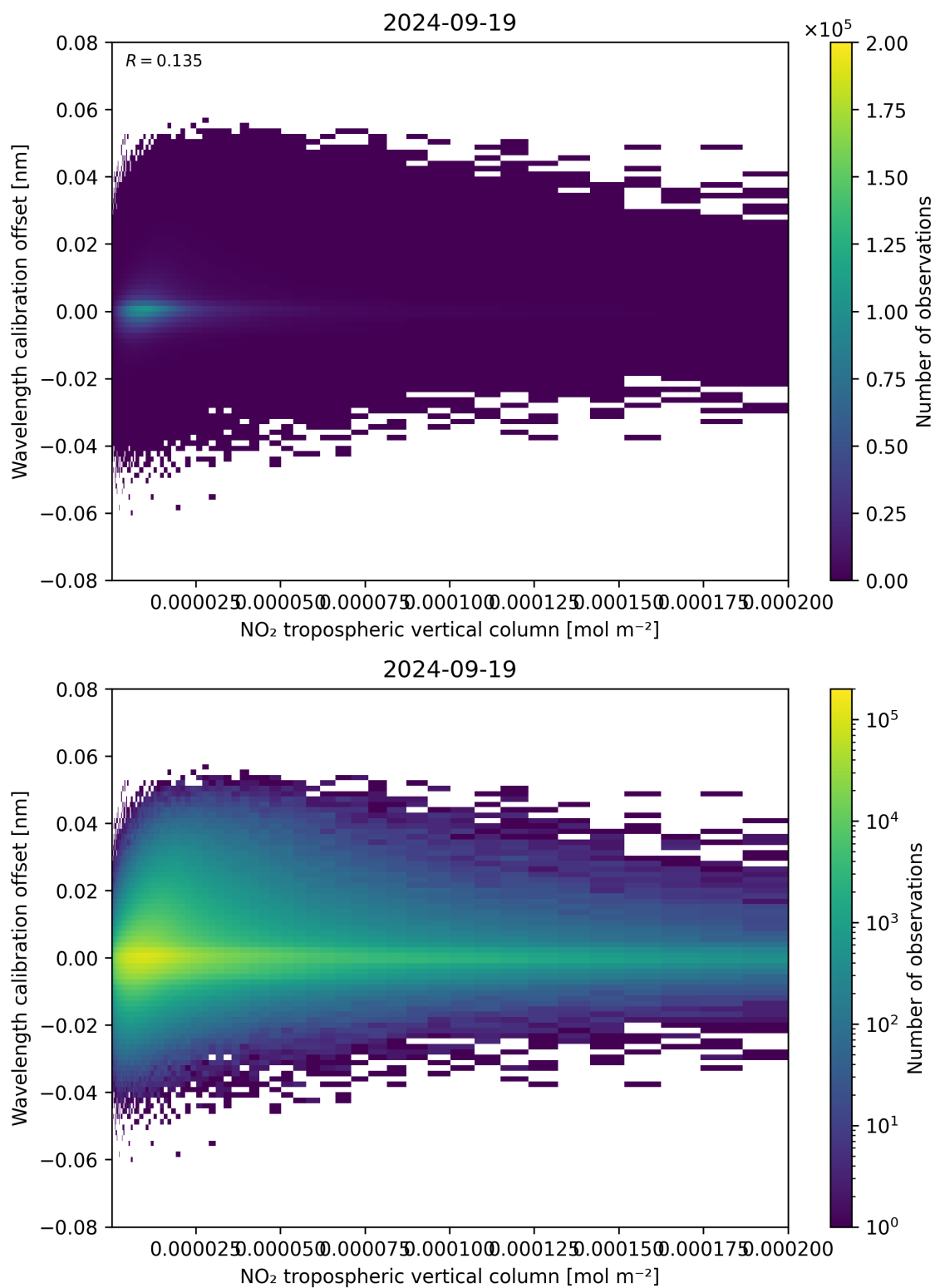
Figure 143: Scatter density plot of “NO 2 tropospheric vertical column” against “Wavelength calibration offset” for 2024-09-18 to 2024-09-20.
