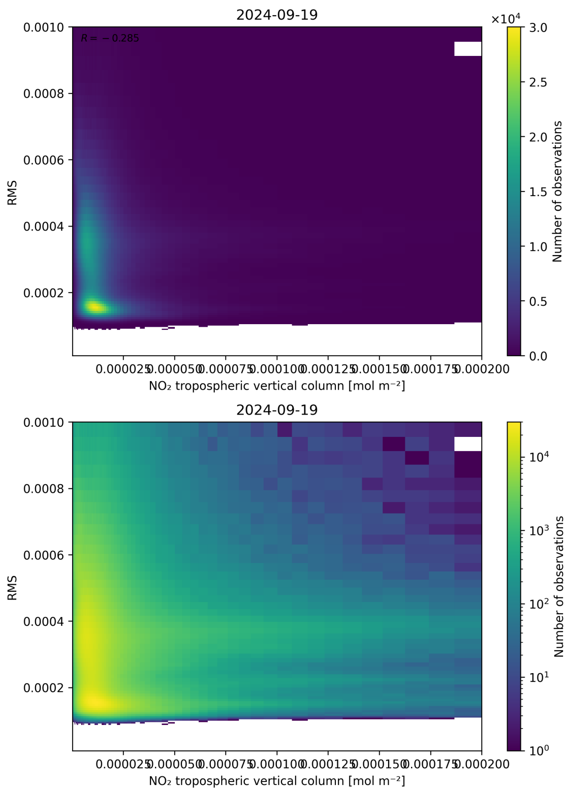
Figure 142: Scatter density plot of “NO 2 tropospheric vertical column” against “RMS” for 2024-09-18 to 2024-09-20.
