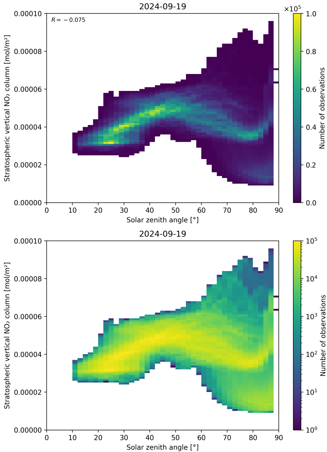
Figure 150: Scatter density plot of “Solar zenith angle” against “Stratospheric vertical NO 2 column” for 2024-09-18 to 2024-09-20.
