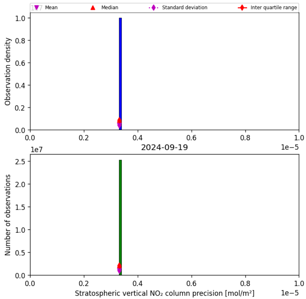
Figure 37: Histogram of “Stratospheric vertical NO 2 column precision” for 2024-09-18 to 2024-09-20
