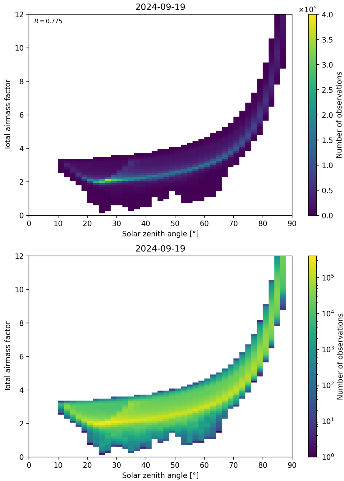
Figure 146: Scatter density plot of “Solar zenith angle” against “Total air mass factor” for 2024-09-18 to 2024-09-20.
