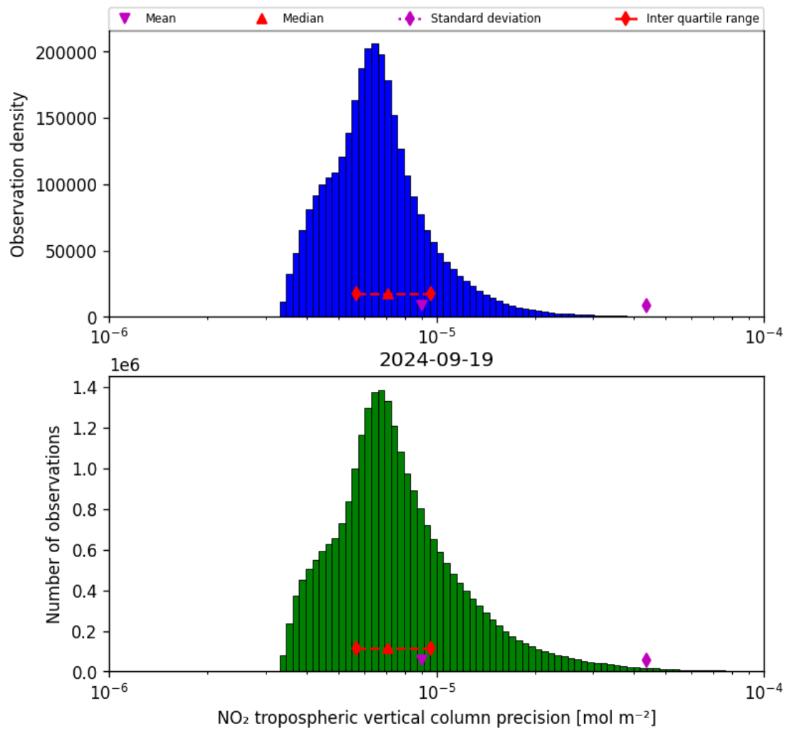
Figure 30: Histogram of “NO 2 tropospheric vertical column precision” for 2024-09-18 to 2024-09-20
