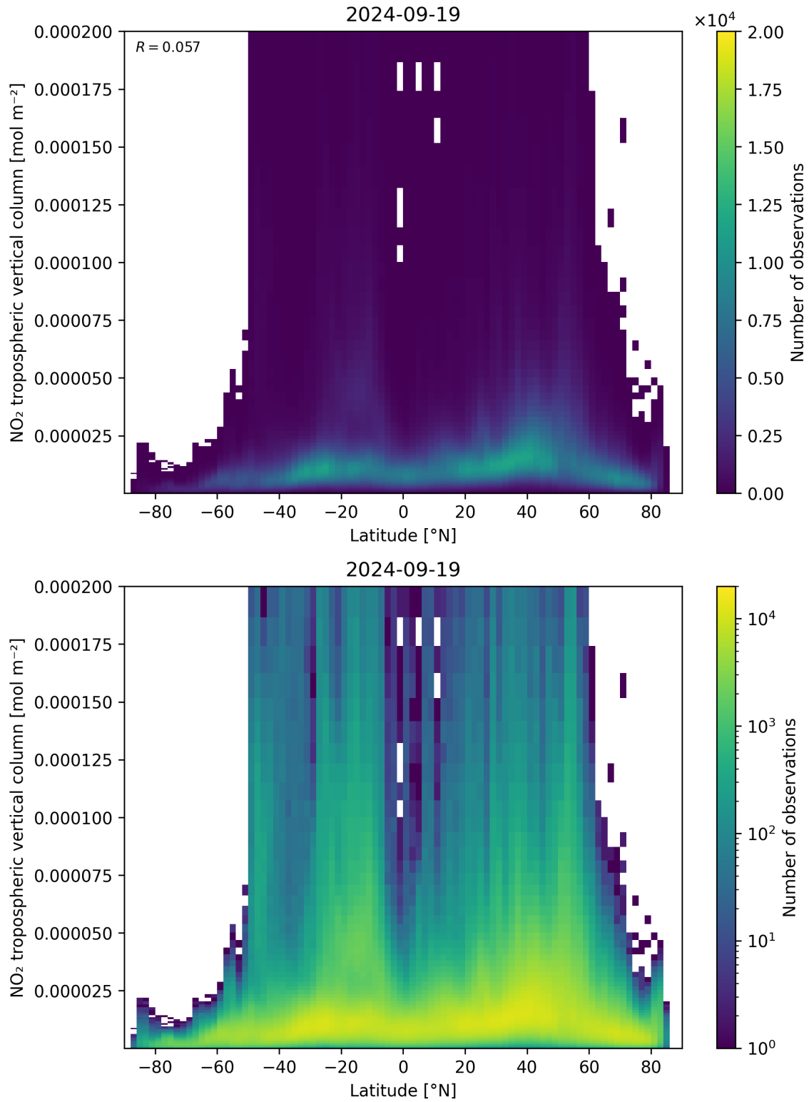
Figure 92: Scatter density plot of “Latitude” against “NO 2 tropospheric vertical column” for 2024-09-18 to 2024-09-20.
