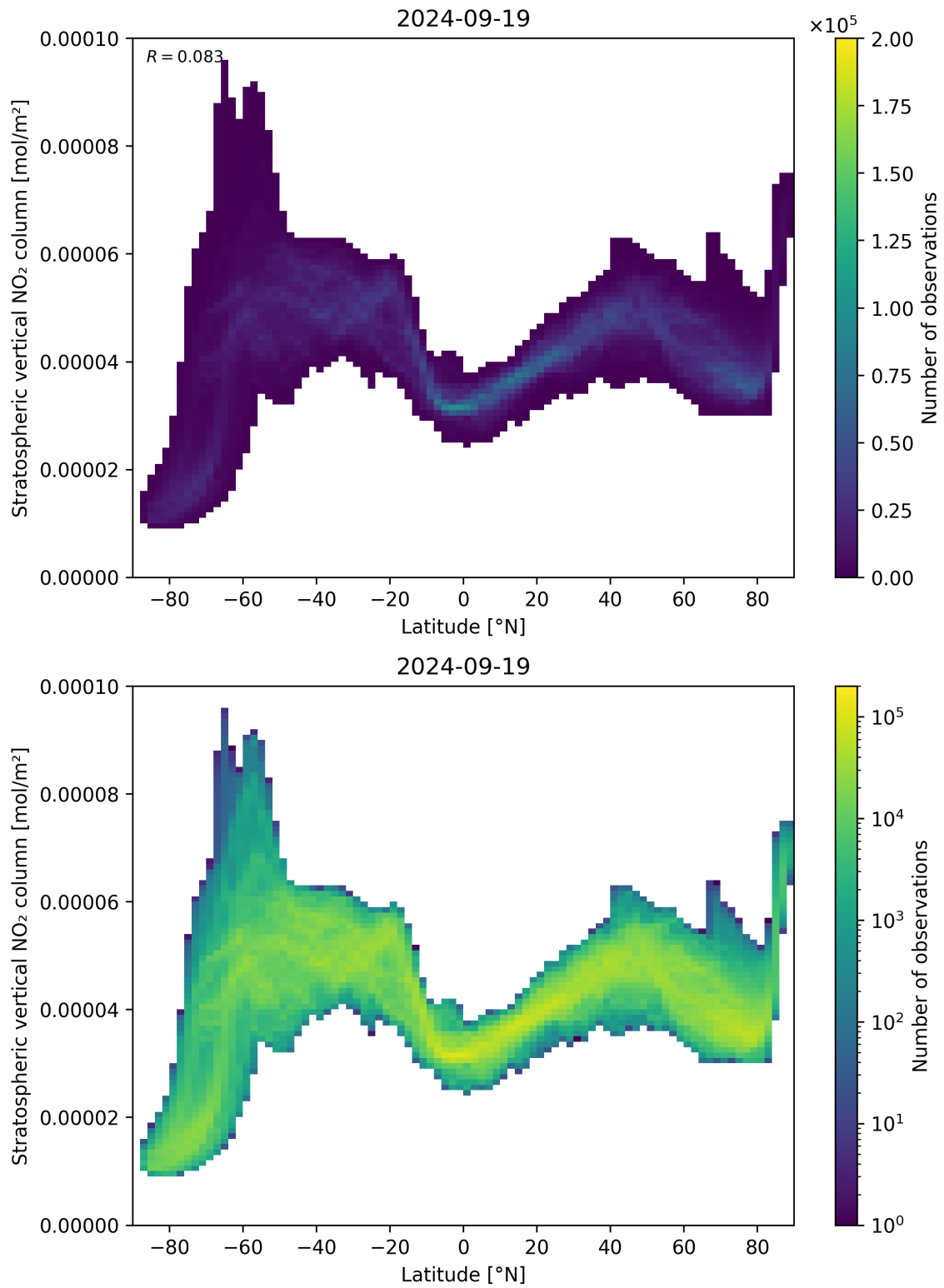
Figure 87: Scatter density plot of “Latitude” against “Stratospheric vertical NO 2 column” for 2024-09-18 to 2024-09-20.
