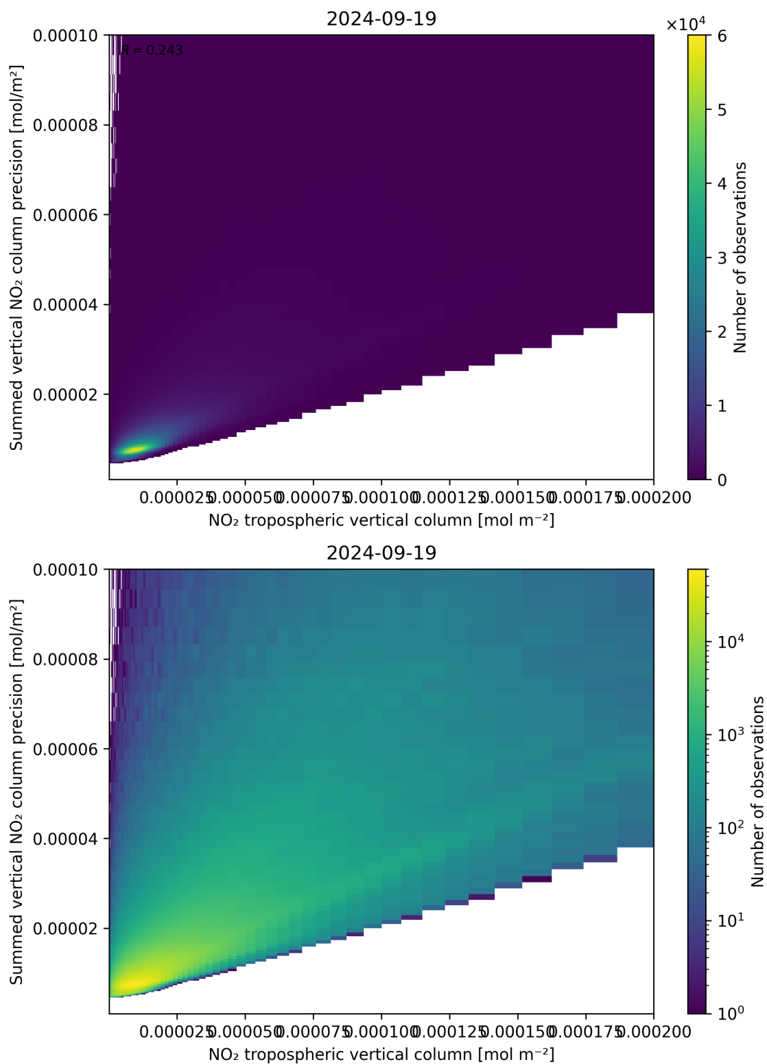
Figure 127: Scatter density plot of “NO 2 tropospheric vertical column” against “Summed vertical NO 2 column precision” for 2024-09-18 to 2024-09-20.
