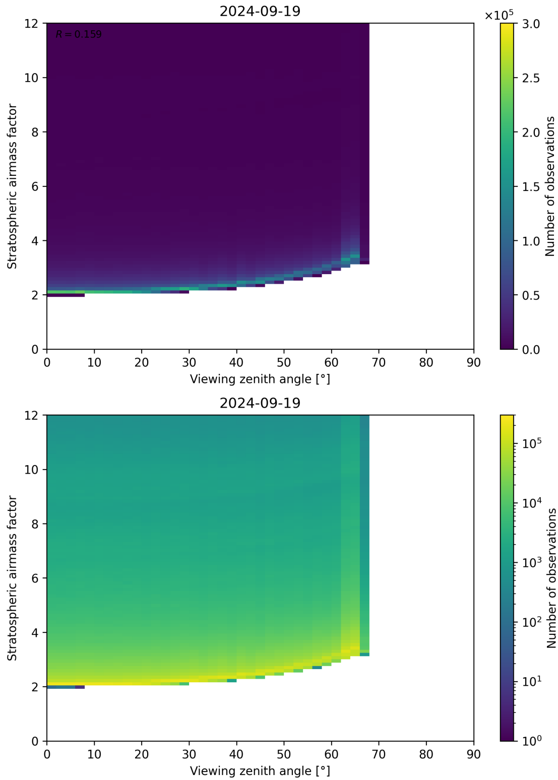
Figure 159: Scatter density plot of “Viewing zenith angle” against “Stratospheric airmass factor” for 2024-09-18 to 2024-09-20.
