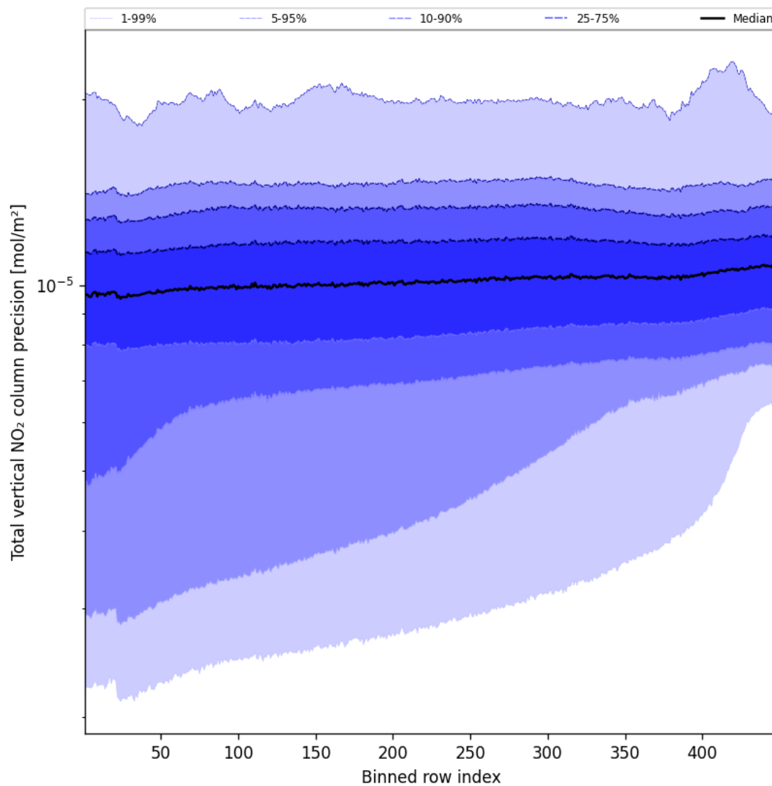
Figure 56: Along track statistics of “Total vertical NO 2 column precision” for 2024-09-18 to 2024-09-20
