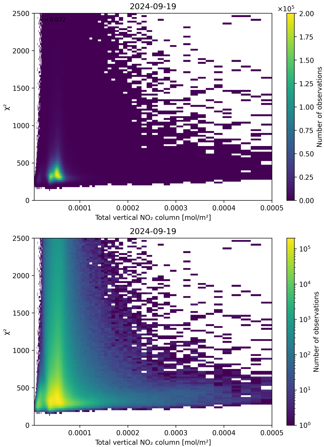
Figure 111: Scatter density plot of “Total vertical NO 2 column” against “ \chi^2 ” for 2024-09-18 to 2024-09-20.
