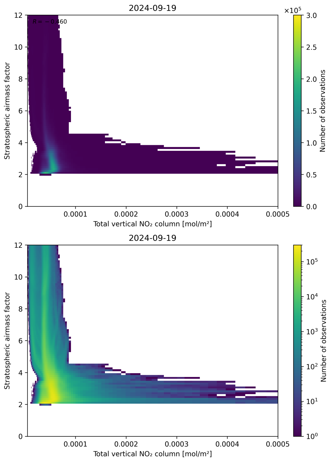
Figure 110: Scatter density plot of “Total vertical NO 2 column” against “Stratospheric airmass factor” for 2024-09-18 to 2024-09-20.
