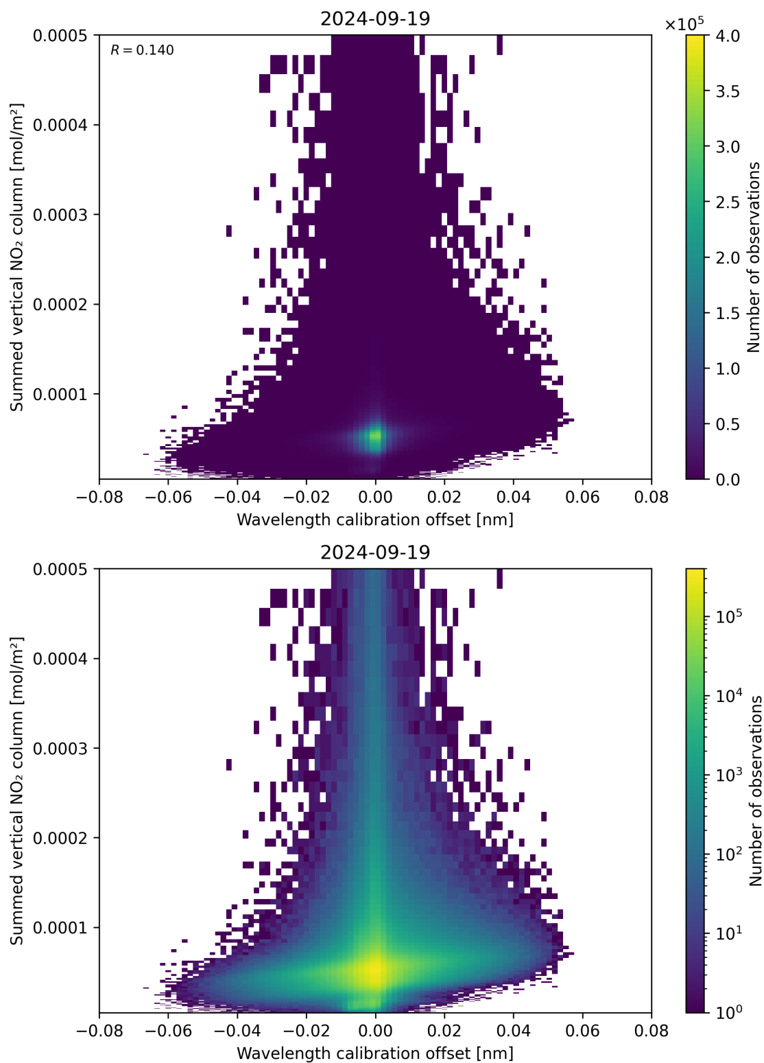
Figure 177: Scatter density plot of “Wavelength calibration offset” against “Summed vertical NO 2 column” for 2024-09-18 to 2024-09-20.
