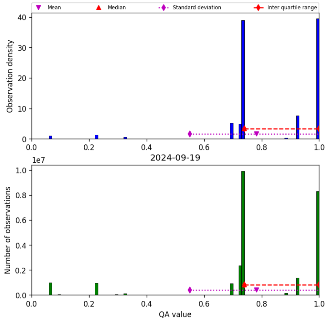
Figure 28: Histogram of “QA value” for 2024-09-18 to 2024-09-20
