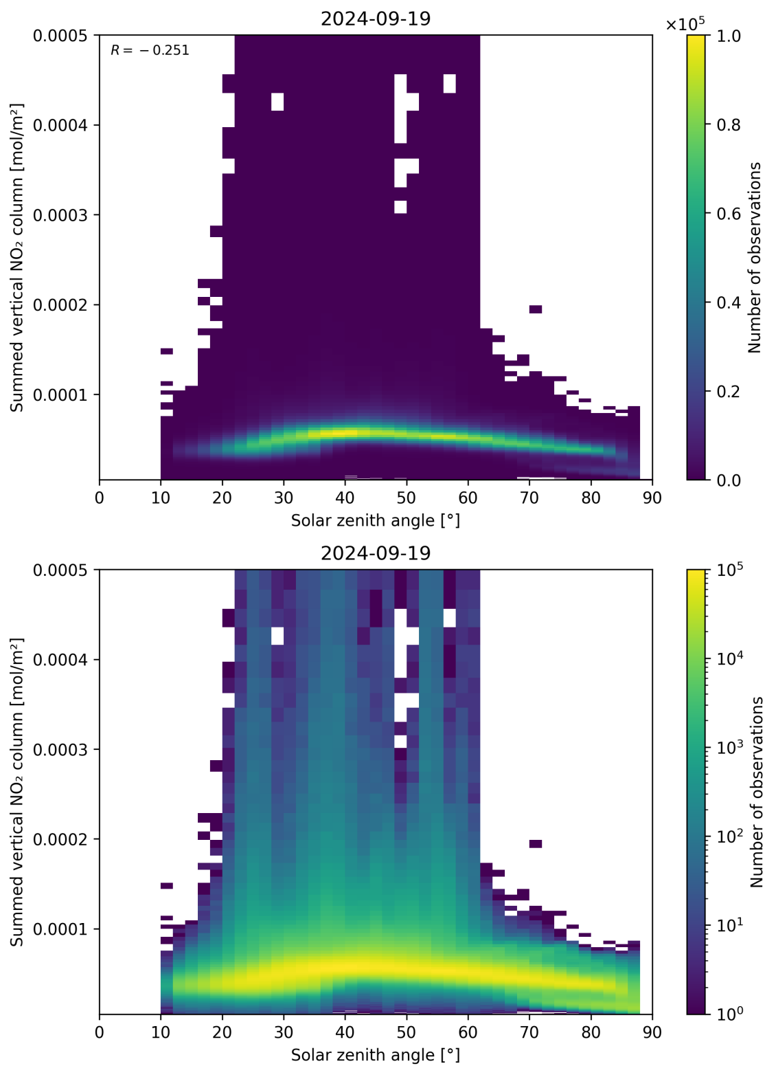
Figure 151: Scatter density plot of “Solar zenith angle” against “Summed vertical NO 2 column” for 2024-09-18 to 2024-09-20.
