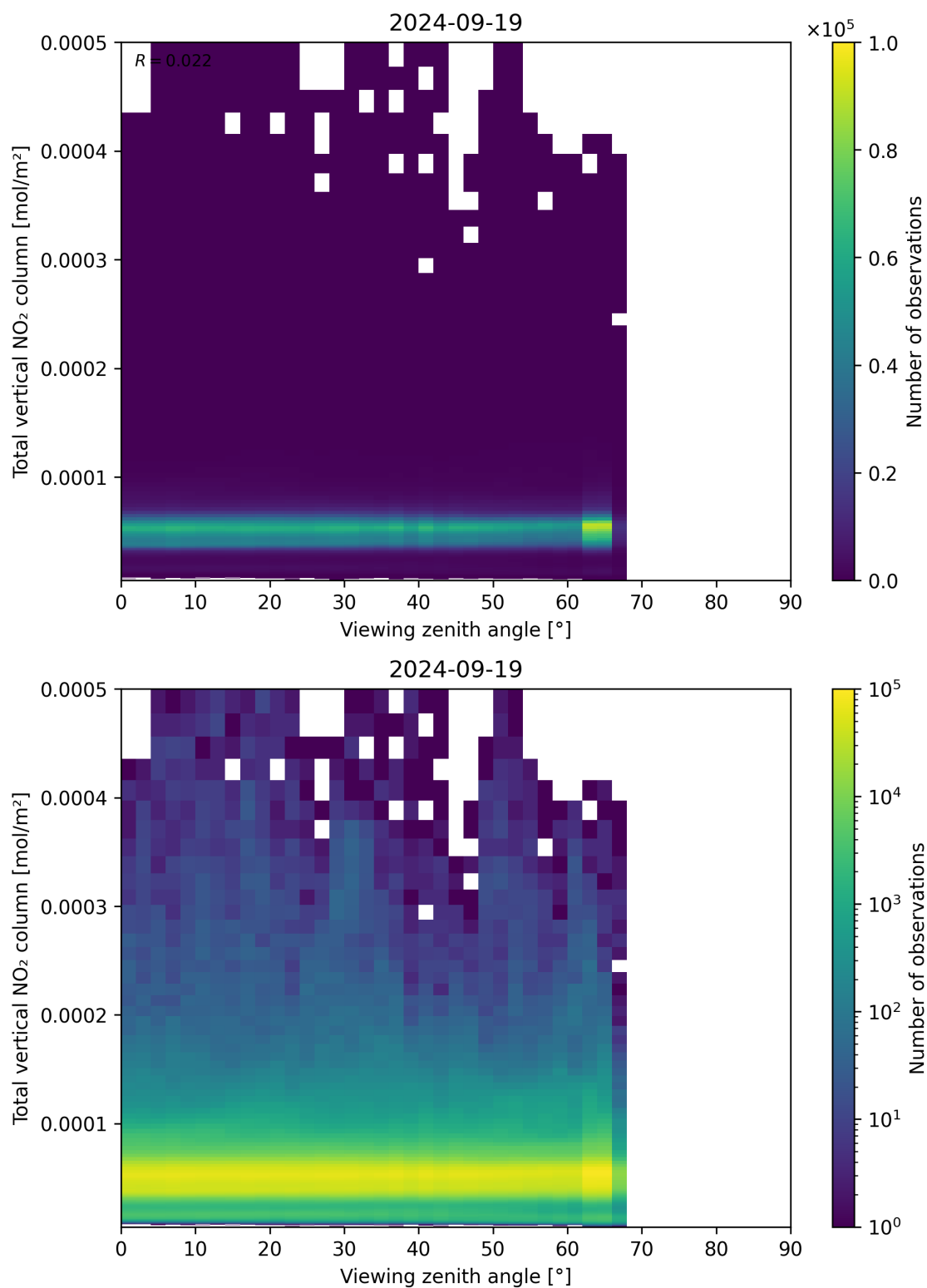
Figure 167: Scatter density plot of “Viewing zenith angle” against “Total vertical NO 2 column” for 2024-09-18 to 2024-09-20.
