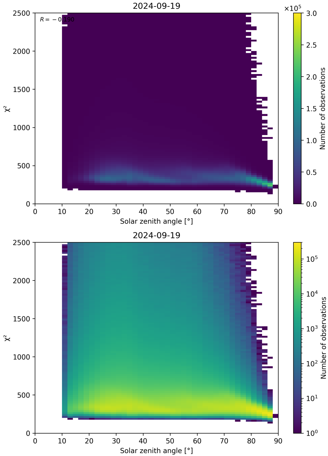
Figure 148: Scatter density plot of “Solar zenith angle” against “ \chi^2 ” for 2024-09-18 to 2024-09-20.
