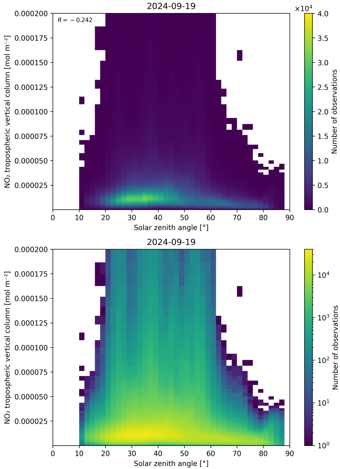
Figure 155: Scatter density plot of “Solar zenith angle” against “NO 2 tropospheric vertical column” for 2024-09-18 to 2024-09-20.
