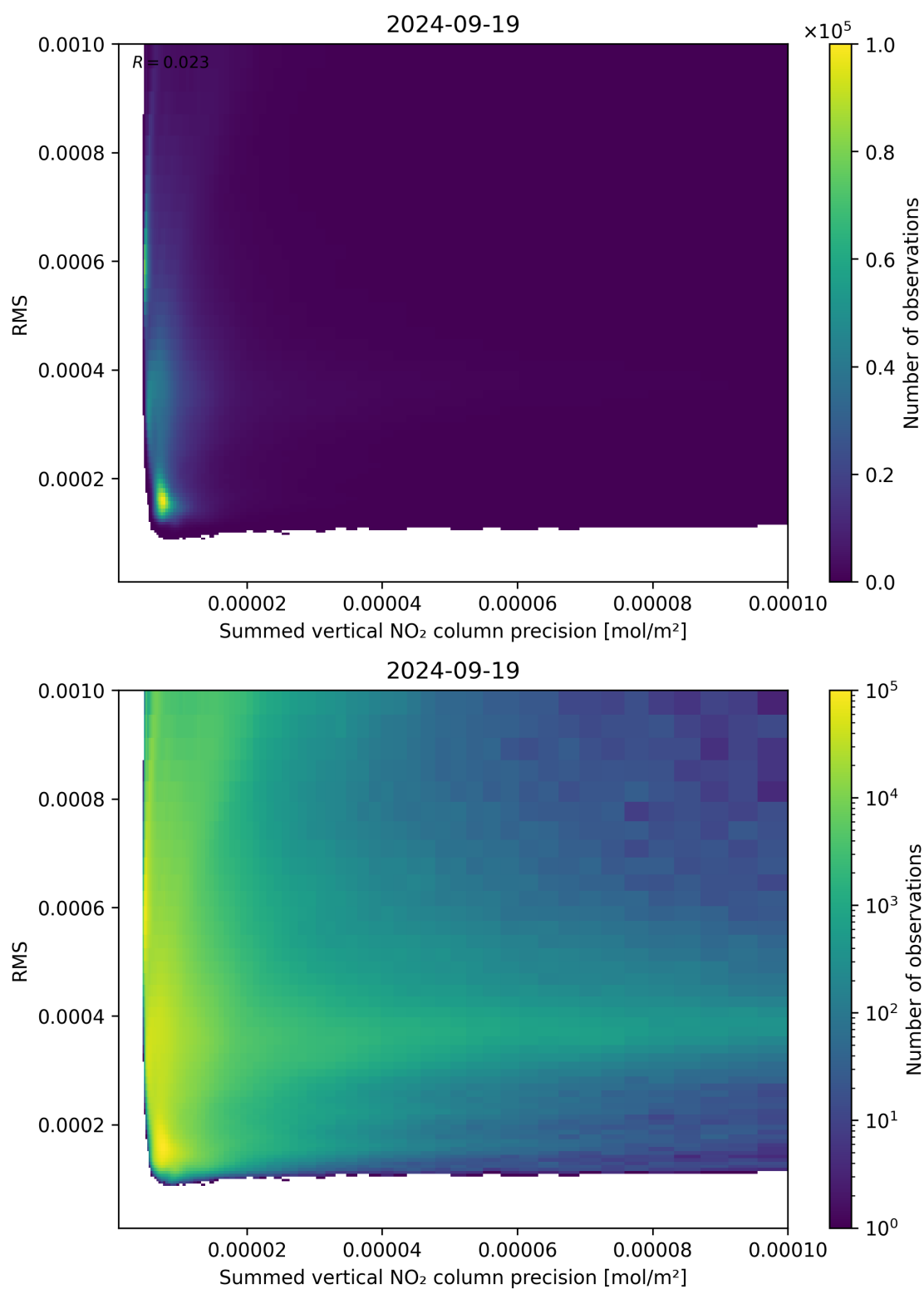
Figure 108: Scatter density plot of “Summed vertical NO 2 column precision” against “RMS” for 2024-09-18 to 2024-09-20.
