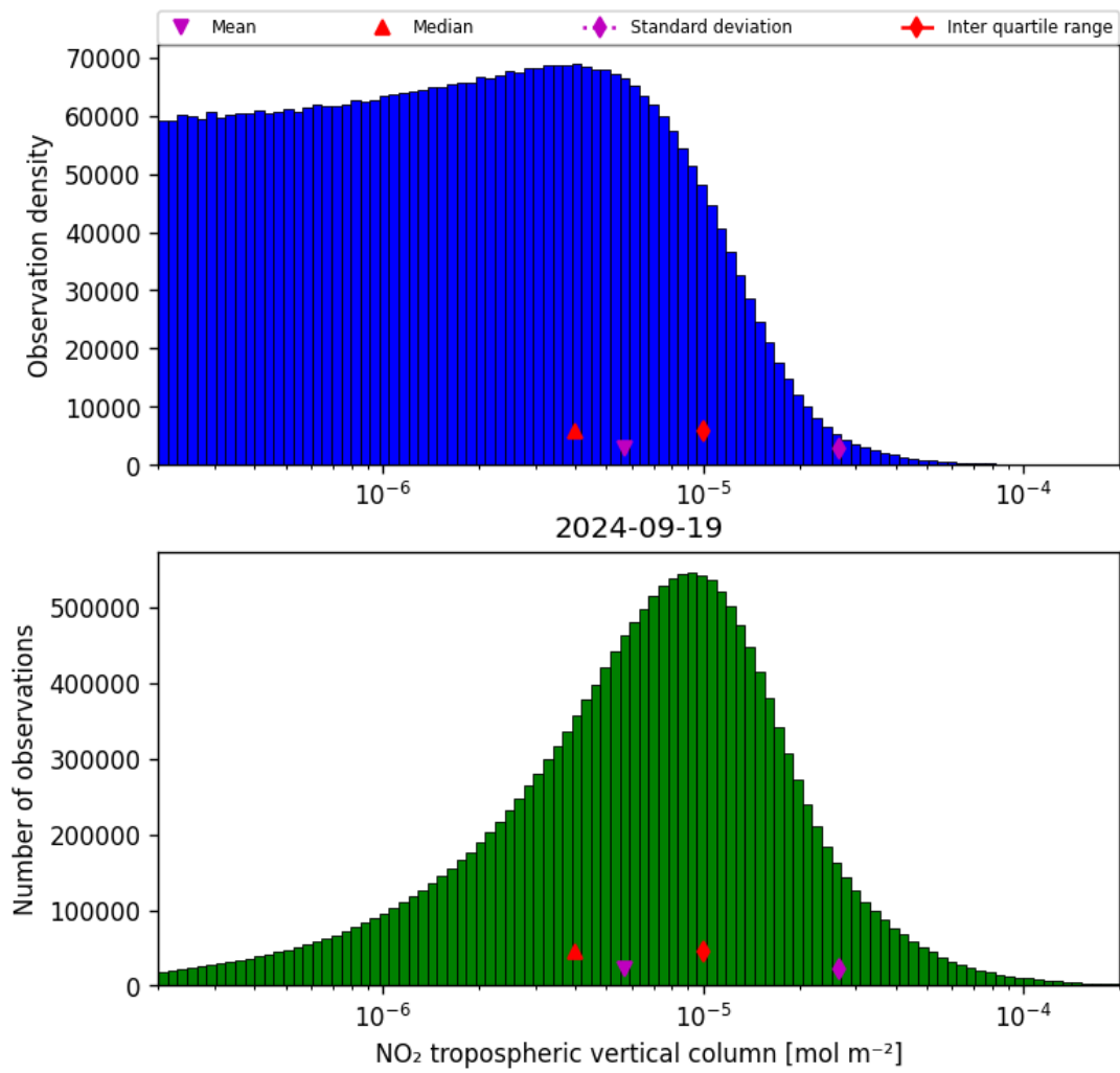
Figure 29: Histogram of “NO 2 tropospheric vertical column” for 2024-09-18 to 2024-09-20
