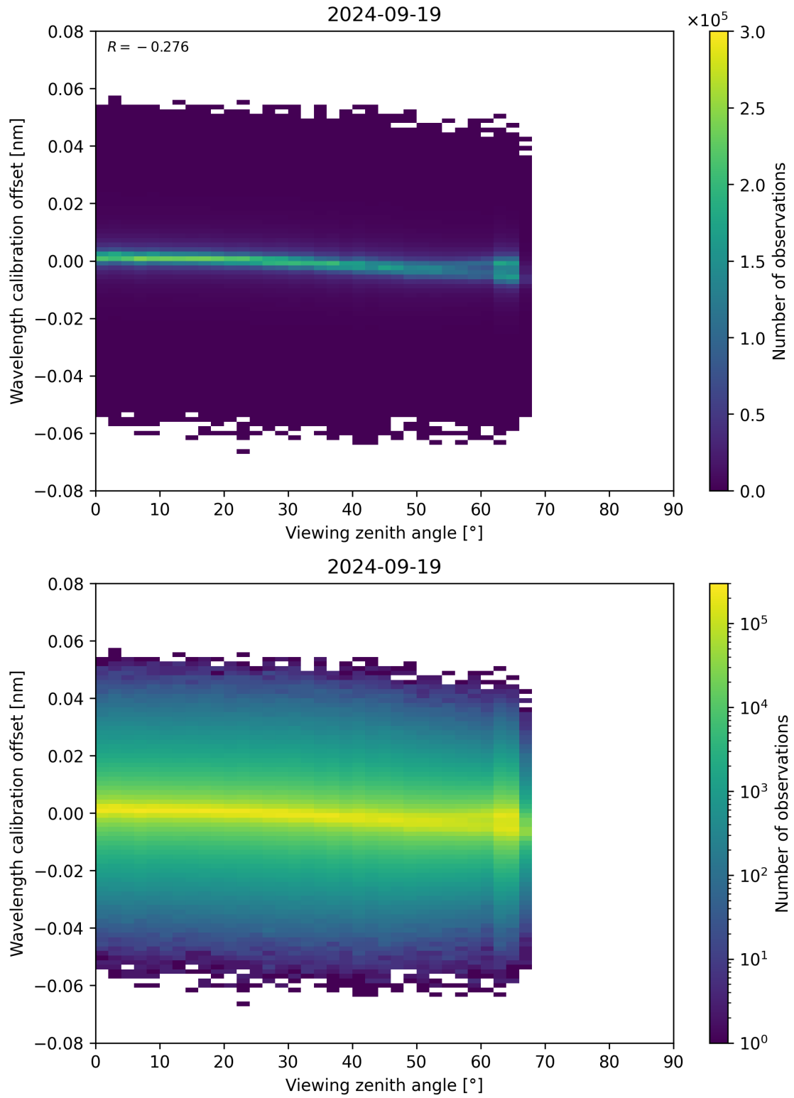
Figure 173: Scatter density plot of “Viewing zenith angle” against “Wavelength calibration offset” for 2024-09-18 to 2024-09-20.
