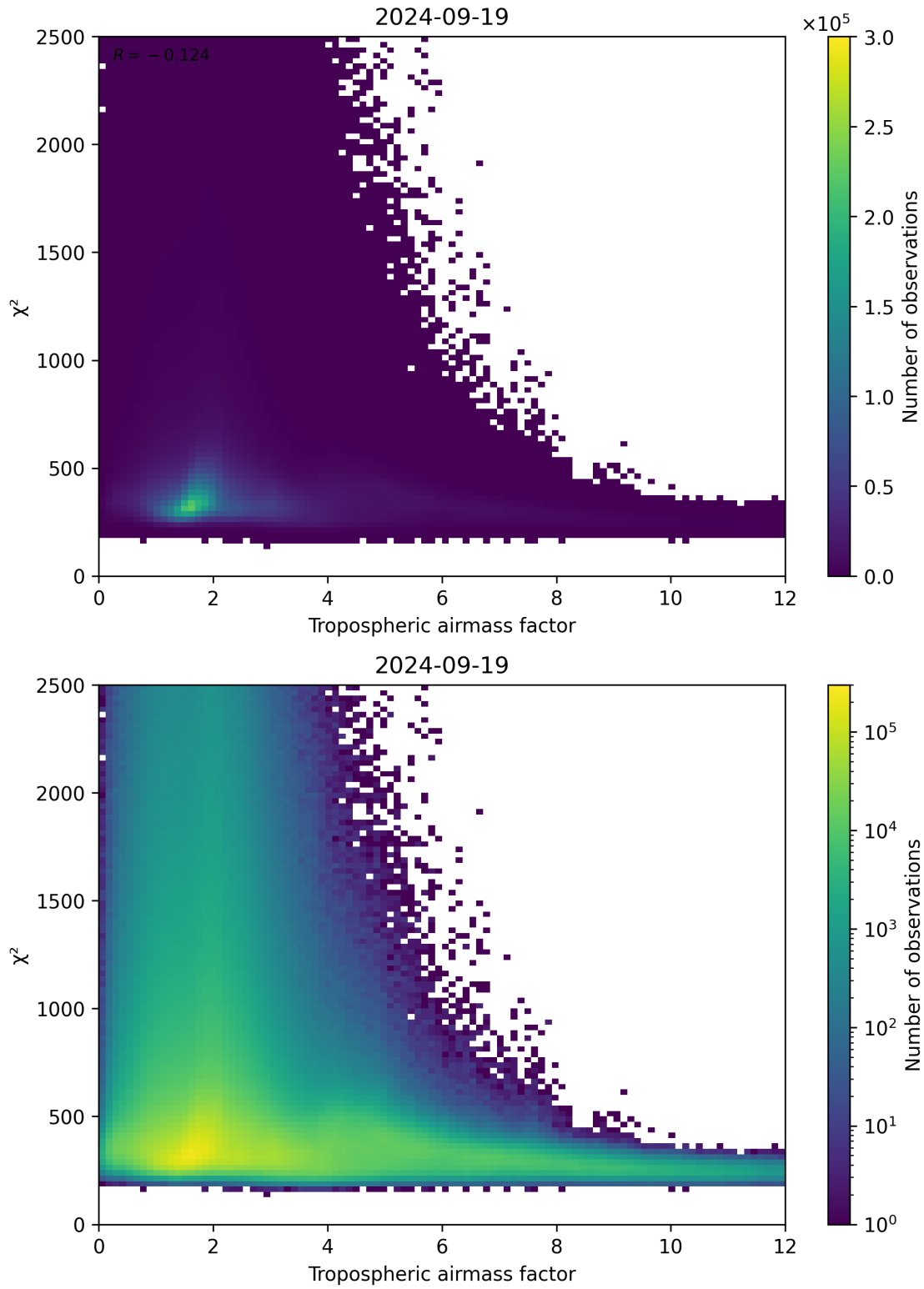
Figure 73: Scatter density plot of “Tropospheric airmass factor” against “ \chi^2 ” for 2024-09-18 to 2024-09-20.
