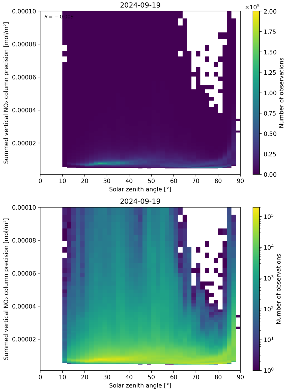
Figure 152: Scatter density plot of “Solar zenith angle” against “Summed vertical NO 2 column precision” for 2024-09-18 to 2024-09-20.
