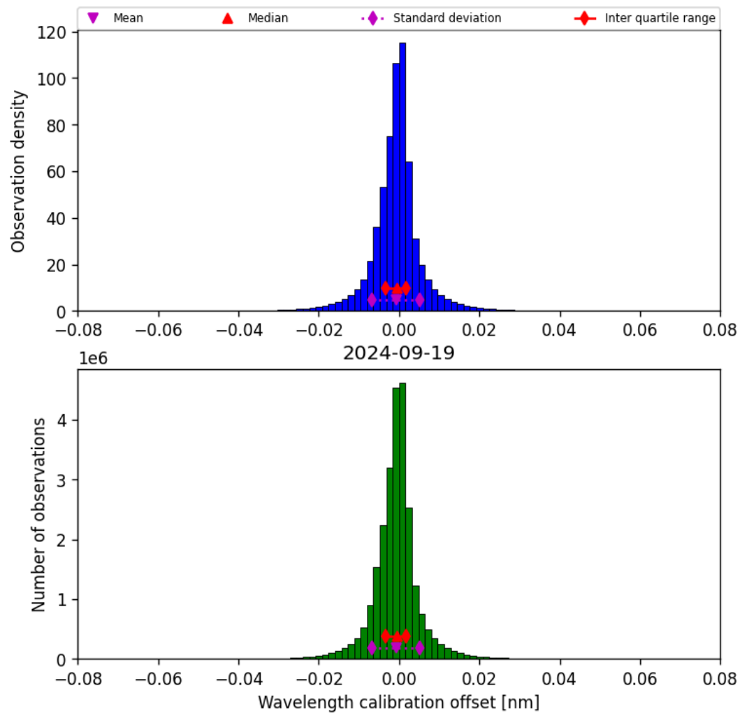
Figure 35: Histogram of “Wavelength calibration offset” for 2024-09-18 to 2024-09-20
