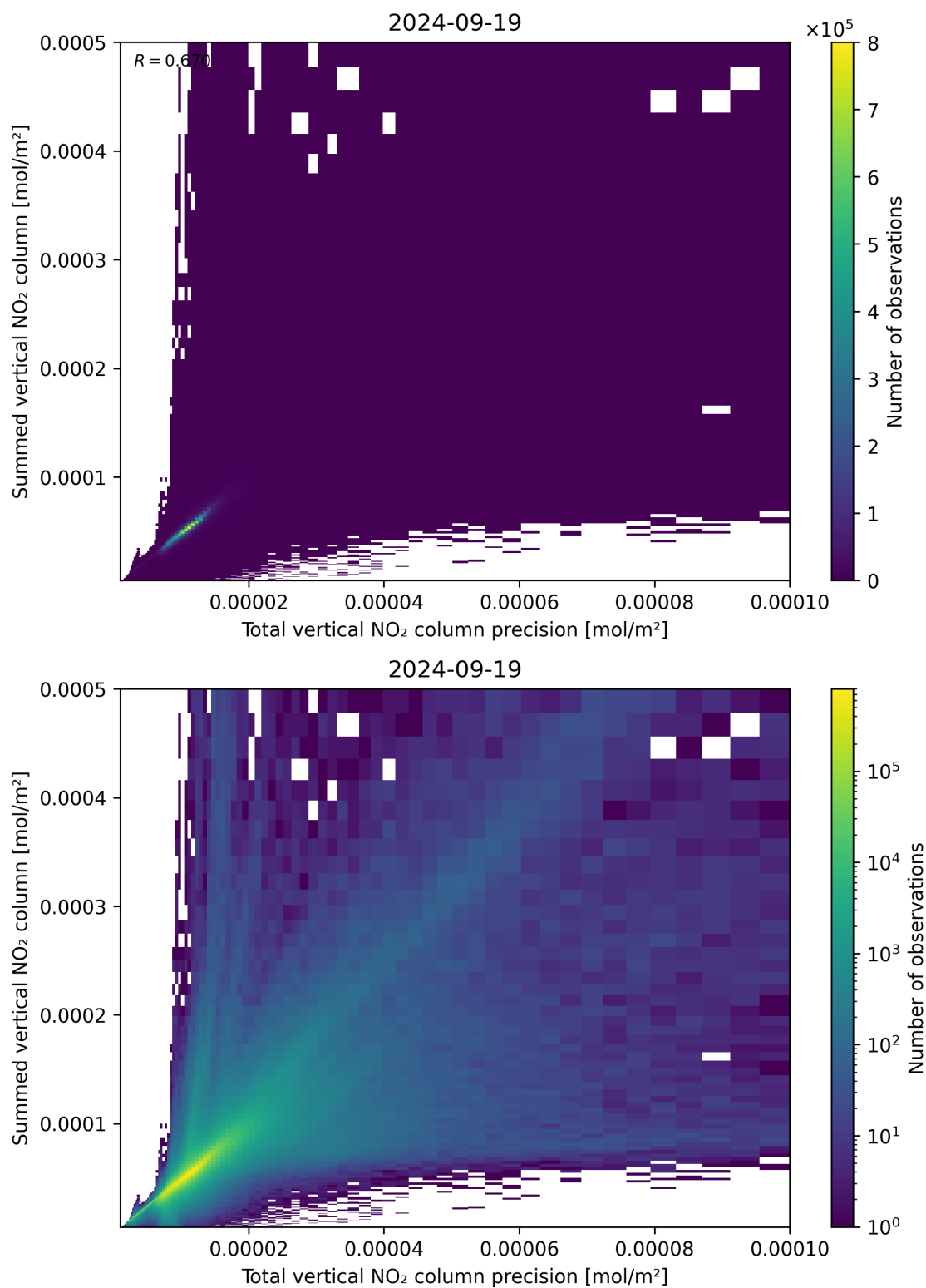
Figure 117: Scatter density plot of “Total vertical NO 2 column precision” against “Summed vertical NO 2 column” for 2024-09-18 to 2024-09-20.
