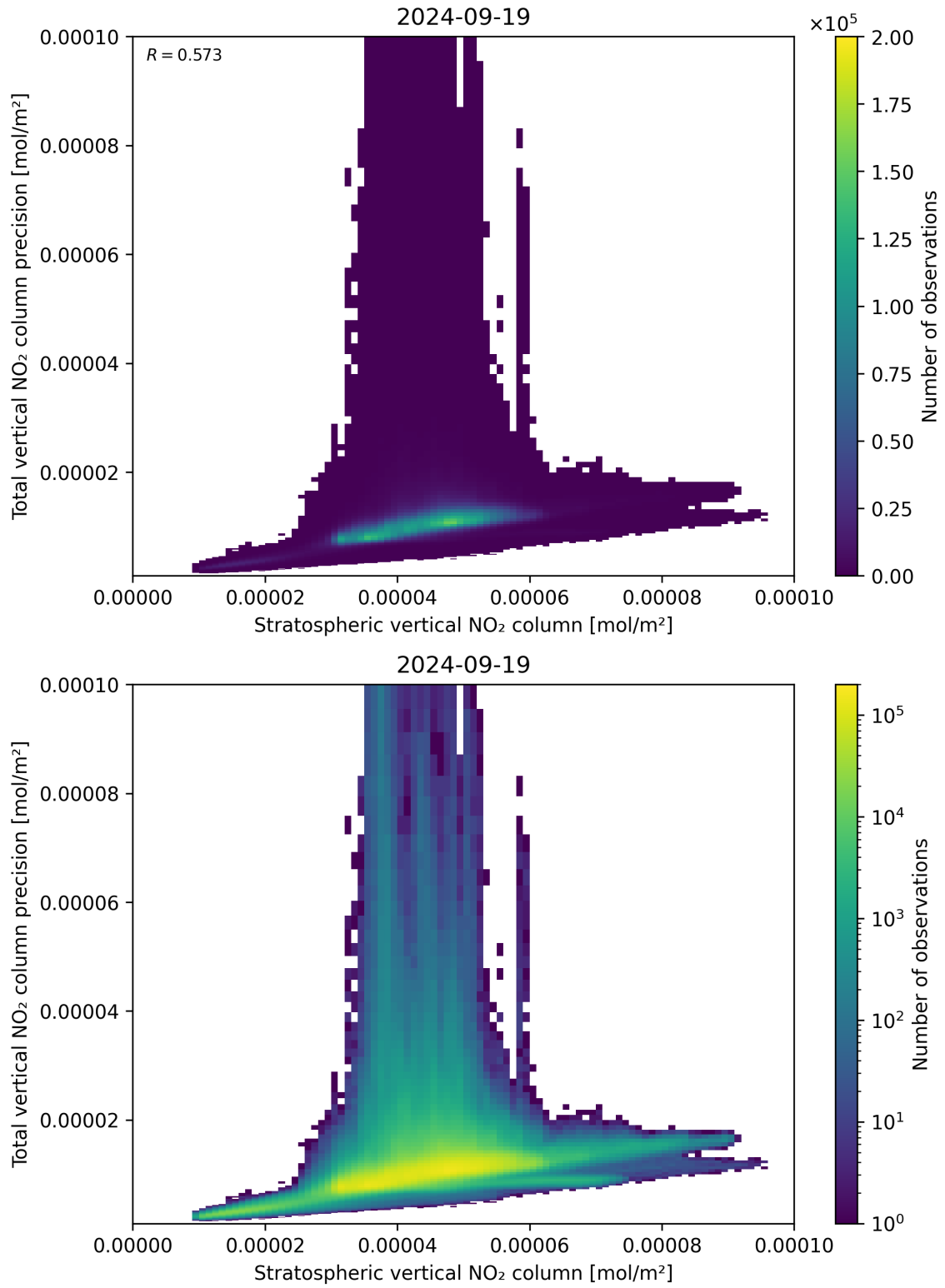
Figure 101: Scatter density plot of “Stratospheric vertical NO 2 column” against “Total vertical NO 2 column precision” for 2024-09-18 to 2024-09-20.
