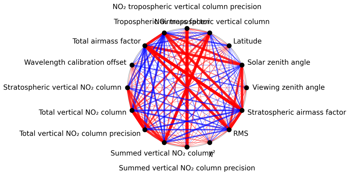
Figure 1: Map of correlation graph for 2024-09-18 to 2024-09-20.
