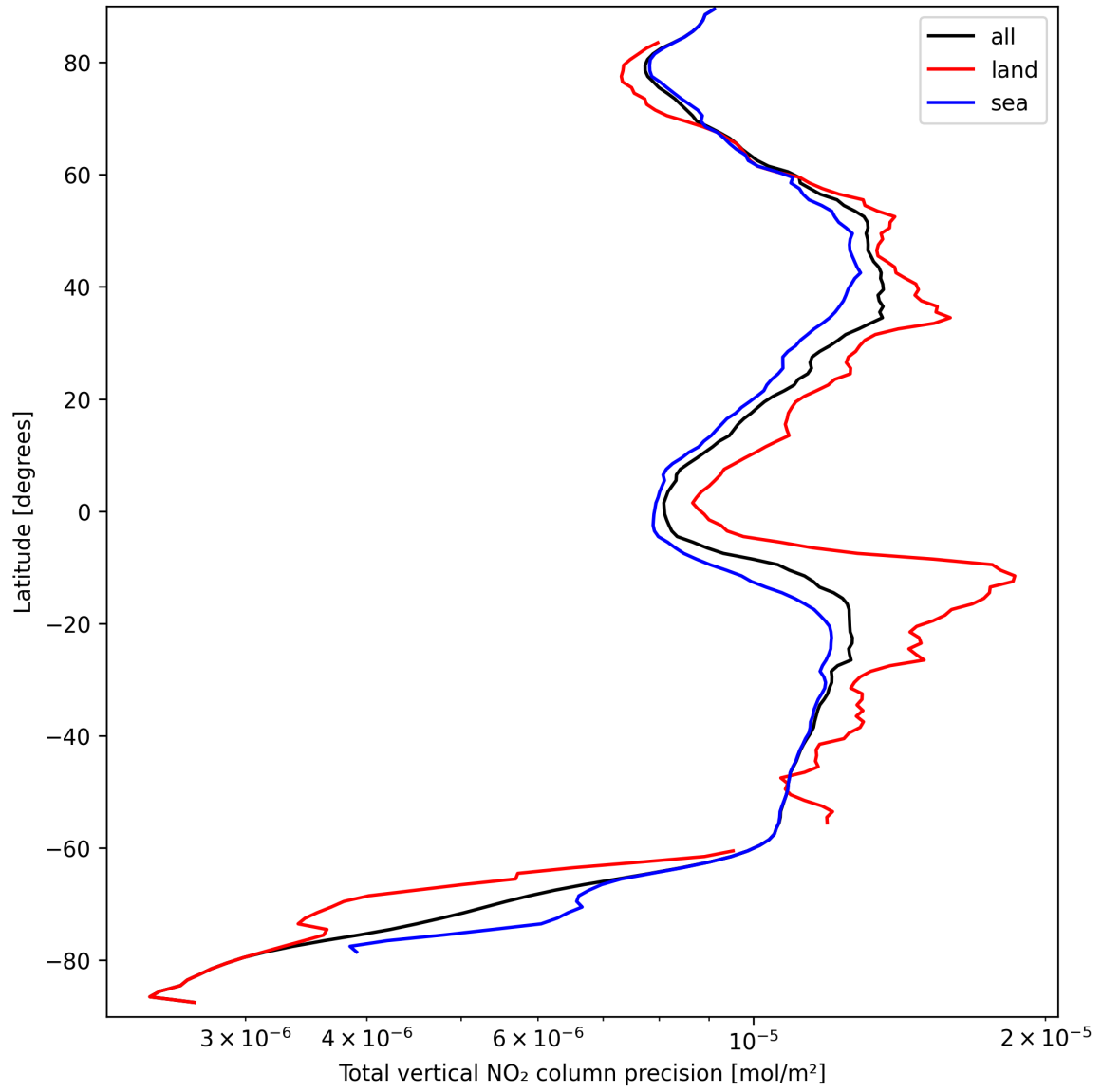
Figure 22: Zonal average of “Total vertical NO 2 column precision” for 2024-09-18 to 2024-09-20.
