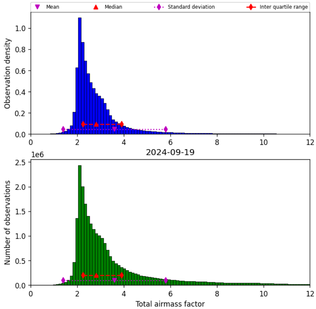
Figure 32: Histogram of “Total airmass factor” for 2024-09-18 to 2024-09-20
