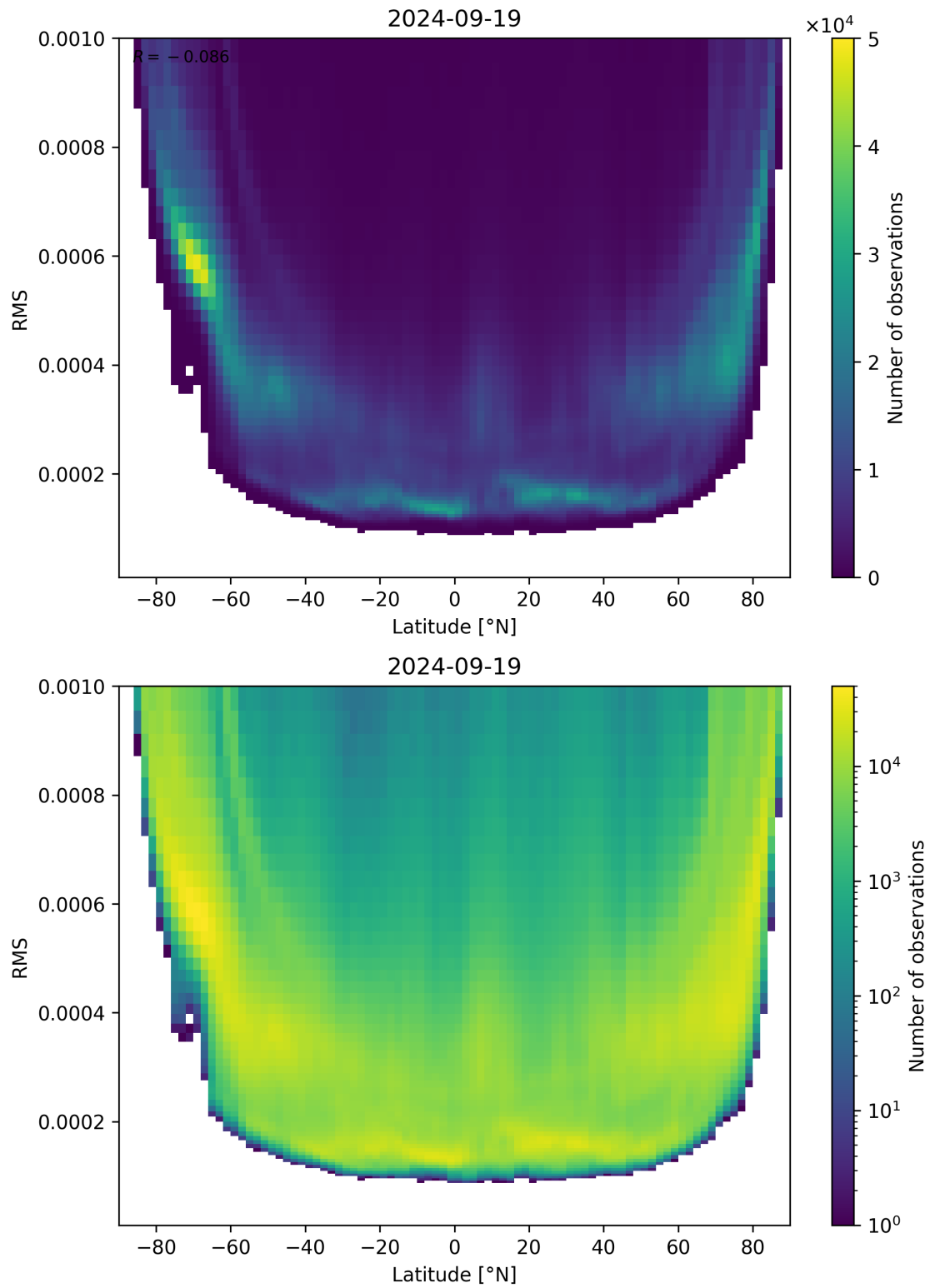
Figure 94: Scatter density plot of “Latitude” against “RMS” for 2024-09-18 to 2024-09-20.
