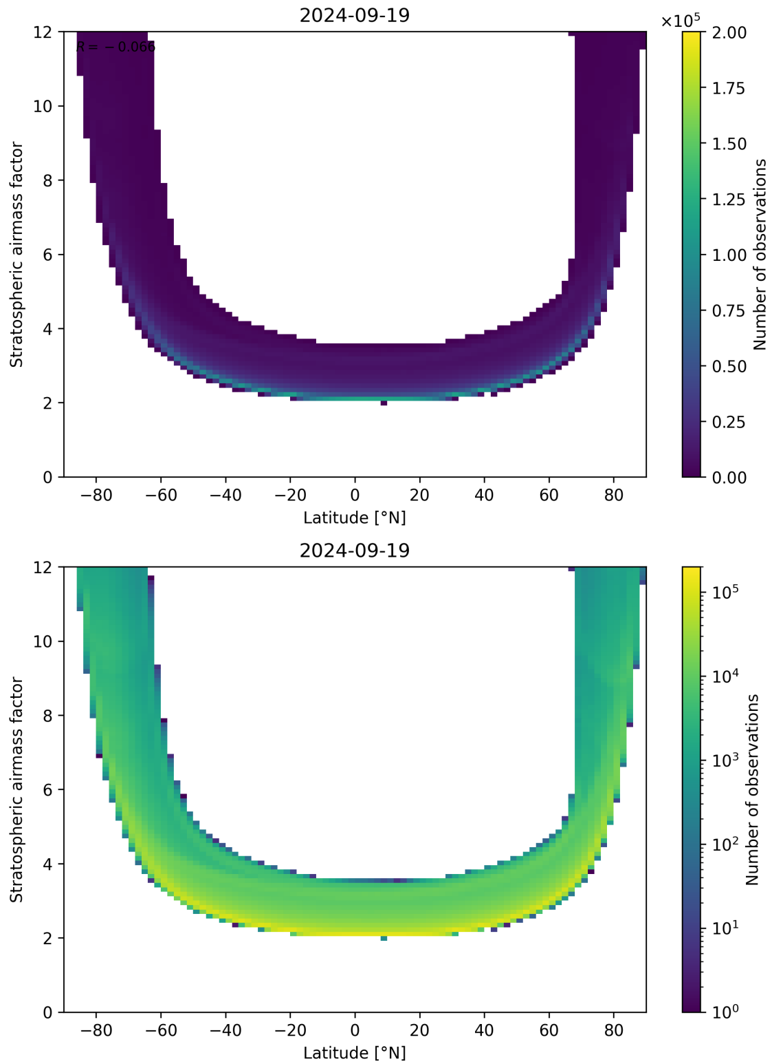
Figure 83: Scatter density plot of “Latitude” against “Stratospheric air mass factor” for 2024-09-18 to 2024-09-20.
