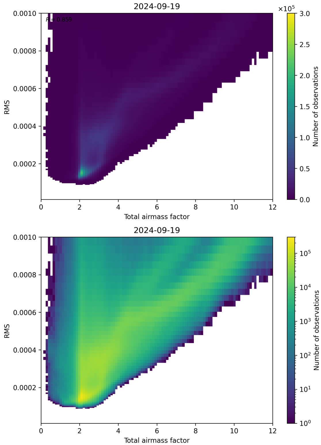
Figure 69: Scatter density plot of “Total airmass factor” against “RMS” for 2024-09-18 to 2024-09-20.
