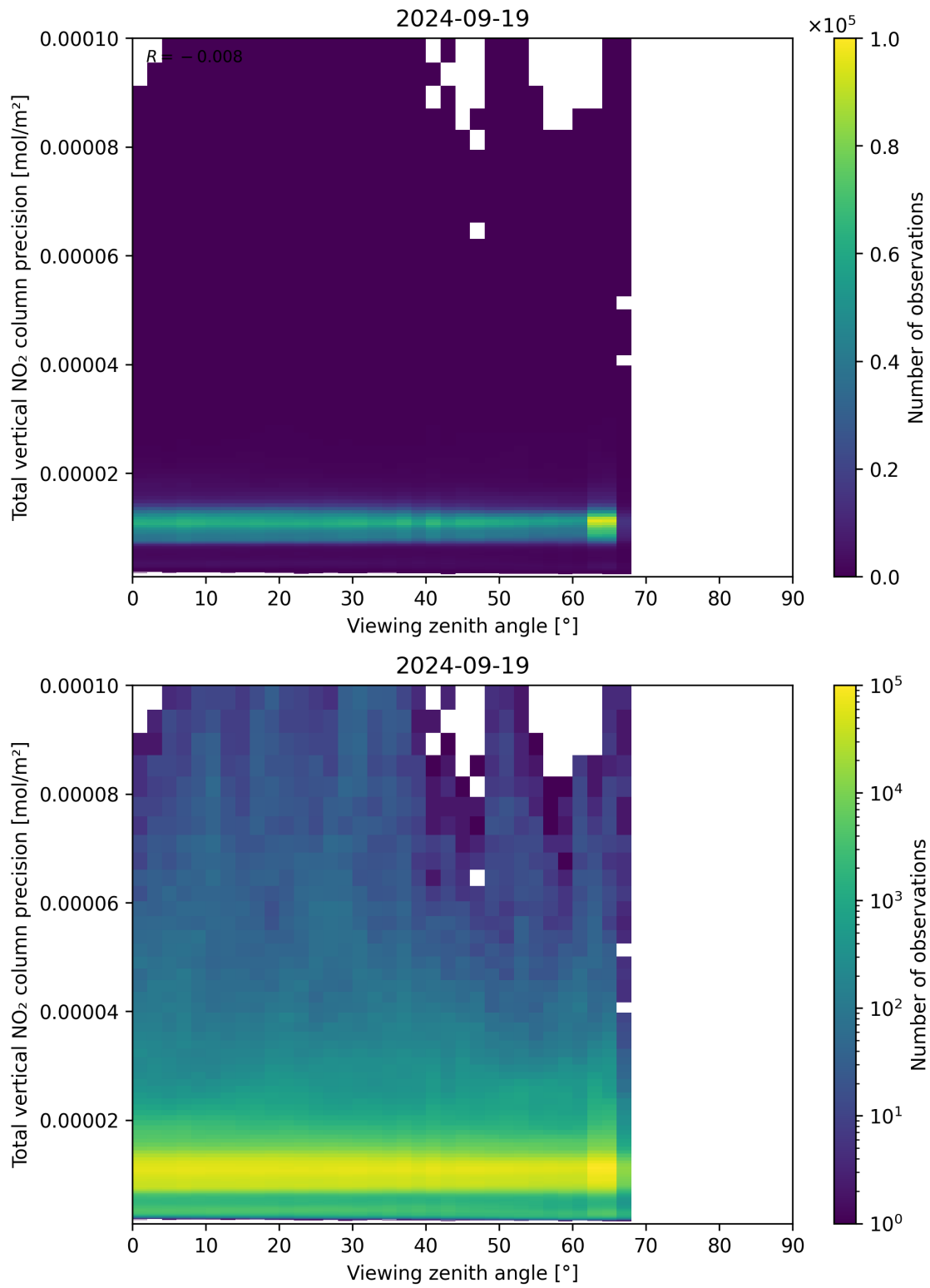
Figure 168: Scatter density plot of “Viewing zenith angle” against “Total vertical NO 2 column precision” for 2024-09-18 to 2024-09-20.
