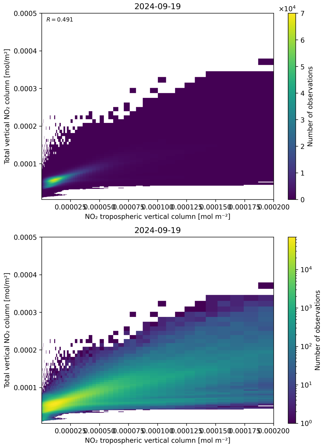
Figure 128: Scatter density plot of “NO 2 tropospheric vertical column” against “Total vertical NO 2 column” for 2024-09-18 to 2024-09-20.
