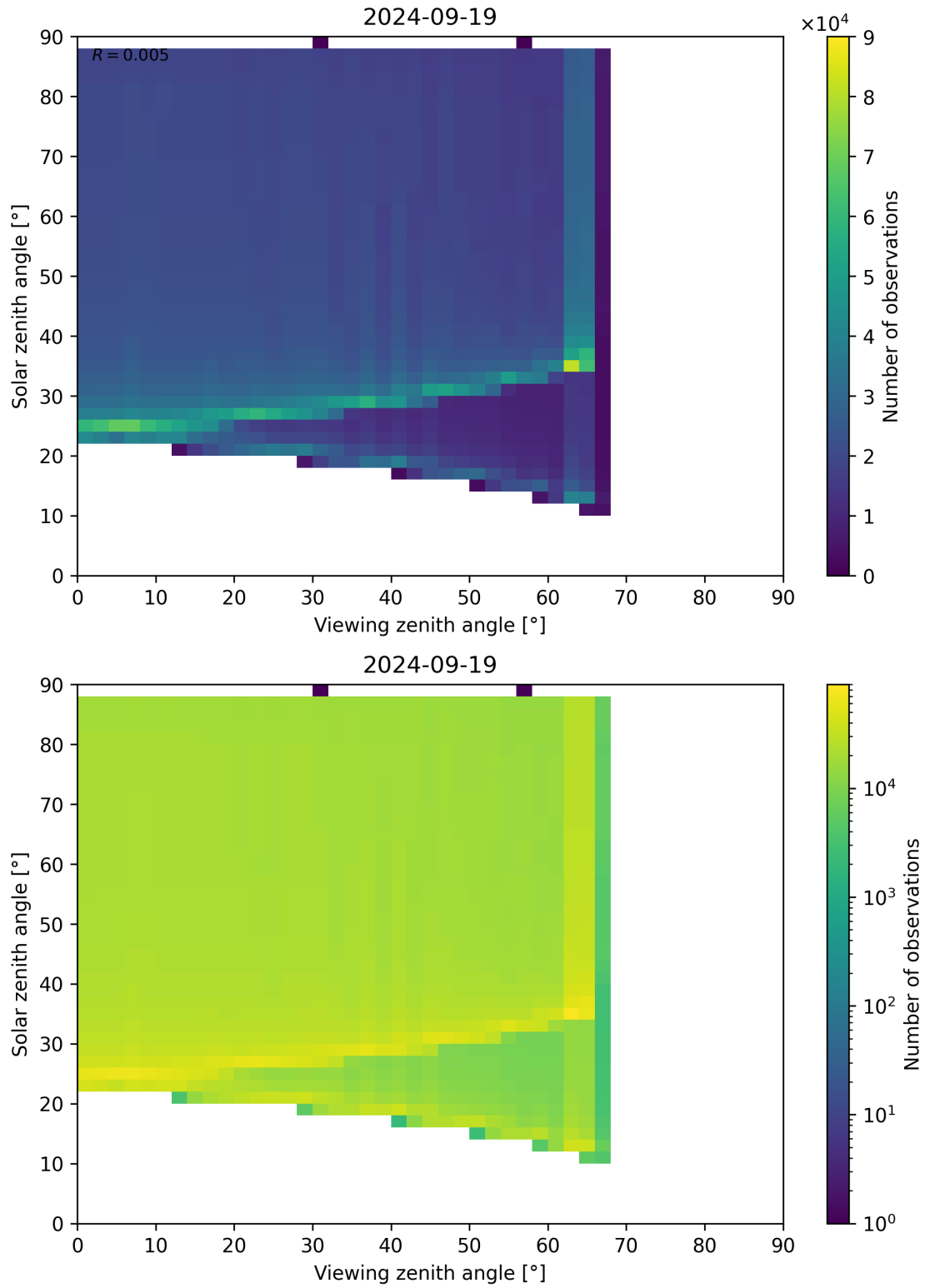
Figure 172: Scatter density plot of “Viewing zenith angle” against “Solar zenith angle” for 2024-09-18 to 2024-09-20.
