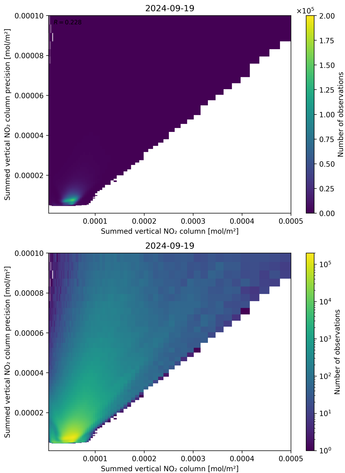
Figure 105: Scatter density plot of “Summed vertical NO 2 column” against “Summed vertical NO 2 column precision” for 2024-09-18 to 2024-09-20.
