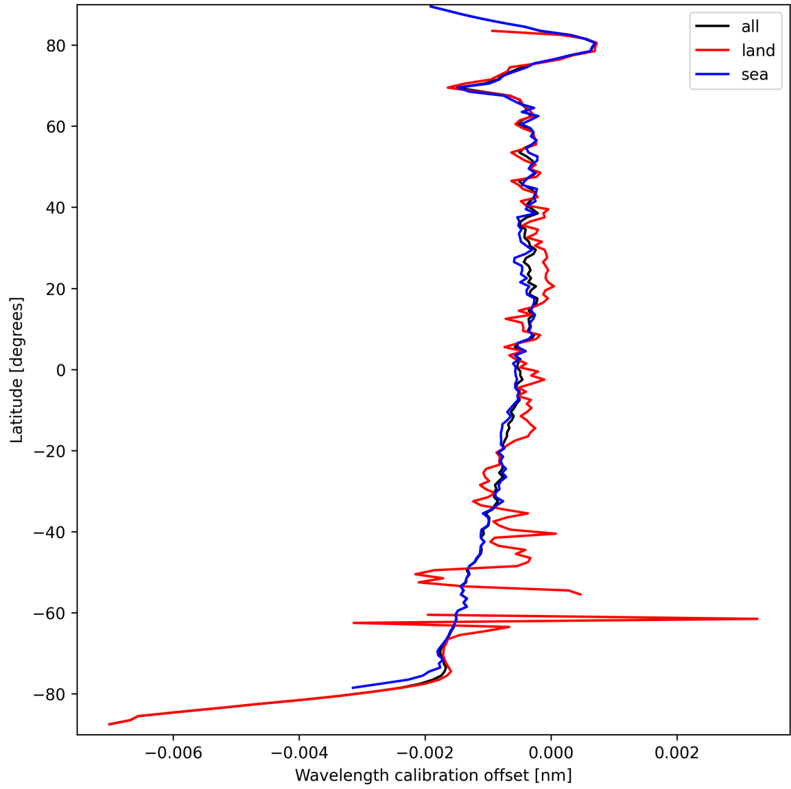
Figure 18: Zonal average of “Wavelength calibration offset” for 2024-09-18 to 2024-09-20.
