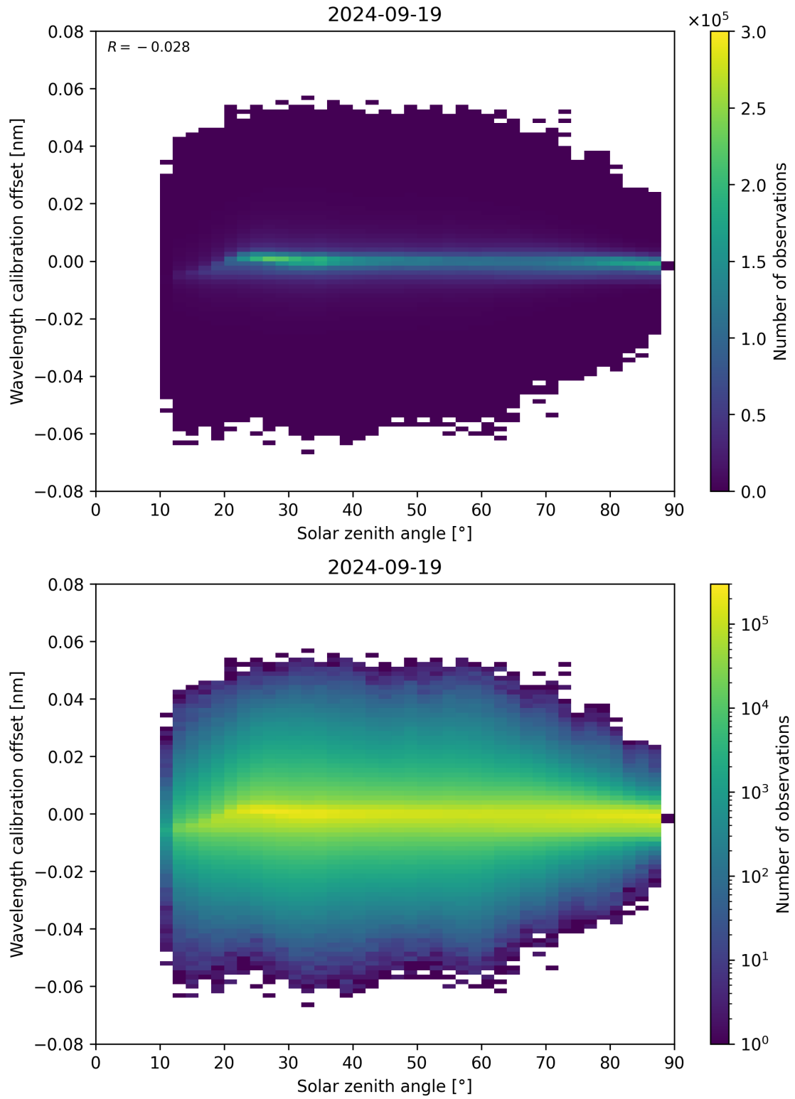
Figure 158: Scatter density plot of “Solar zenith angle” against “Wavelength calibration offset” for 2024-09-18 to 2024-09-20.
