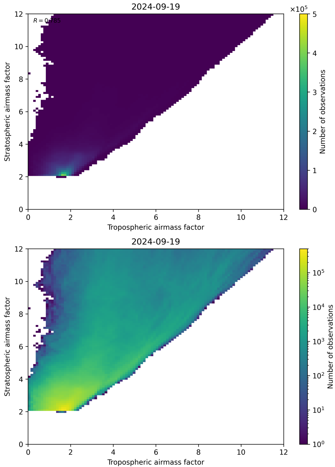
Figure 71: Scatter density plot of “Tropospheric airmass factor” against “Stratospheric airmass factor” for 2024-09-18 to 2024-09-20.
