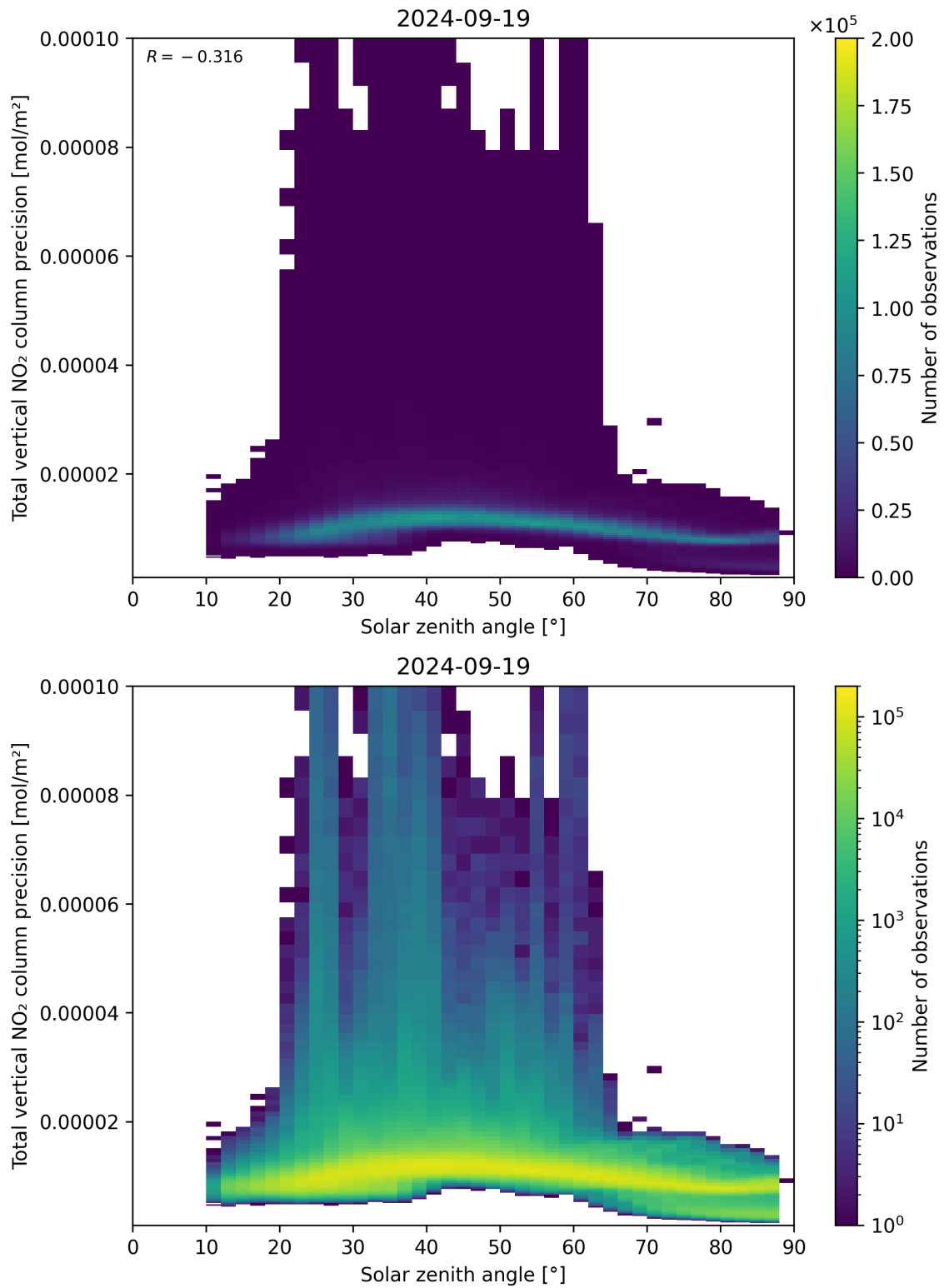
Figure 154: Scatter density plot of “Solar zenith angle” against “Total vertical NO 2 column precision” for 2024-09-18 to 2024-09-20.
