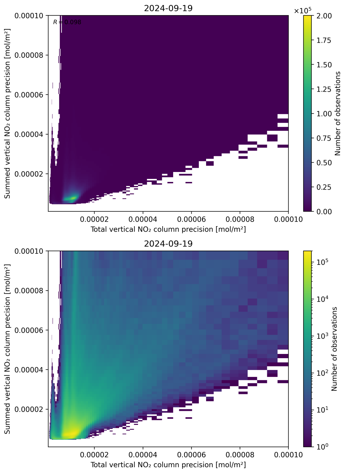
Figure 118: Scatter density plot of “Total vertical NO 2 column precision” against “Summed vertical NO 2 column precision” for 2024-09-18 to 2024-09-20.
