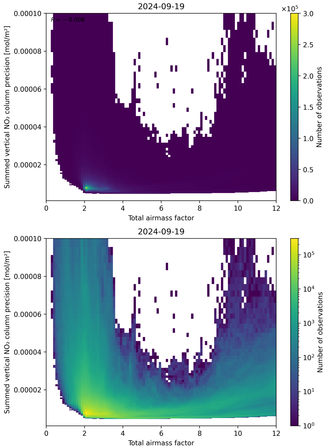
Figure 66: Scatter density plot of “Total airmass factor” against “Summed vertical NO 2 column precision” for 2024-09-18 to 2024-09-20.
