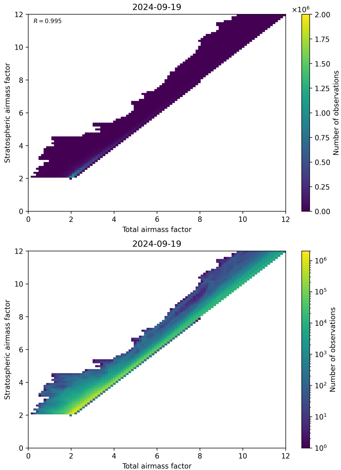
Figure 62: Scatter density plot of “Total airmass factor” against “Stratospheric airmass factor” for 2024-09-18 to 2024-09-20.
