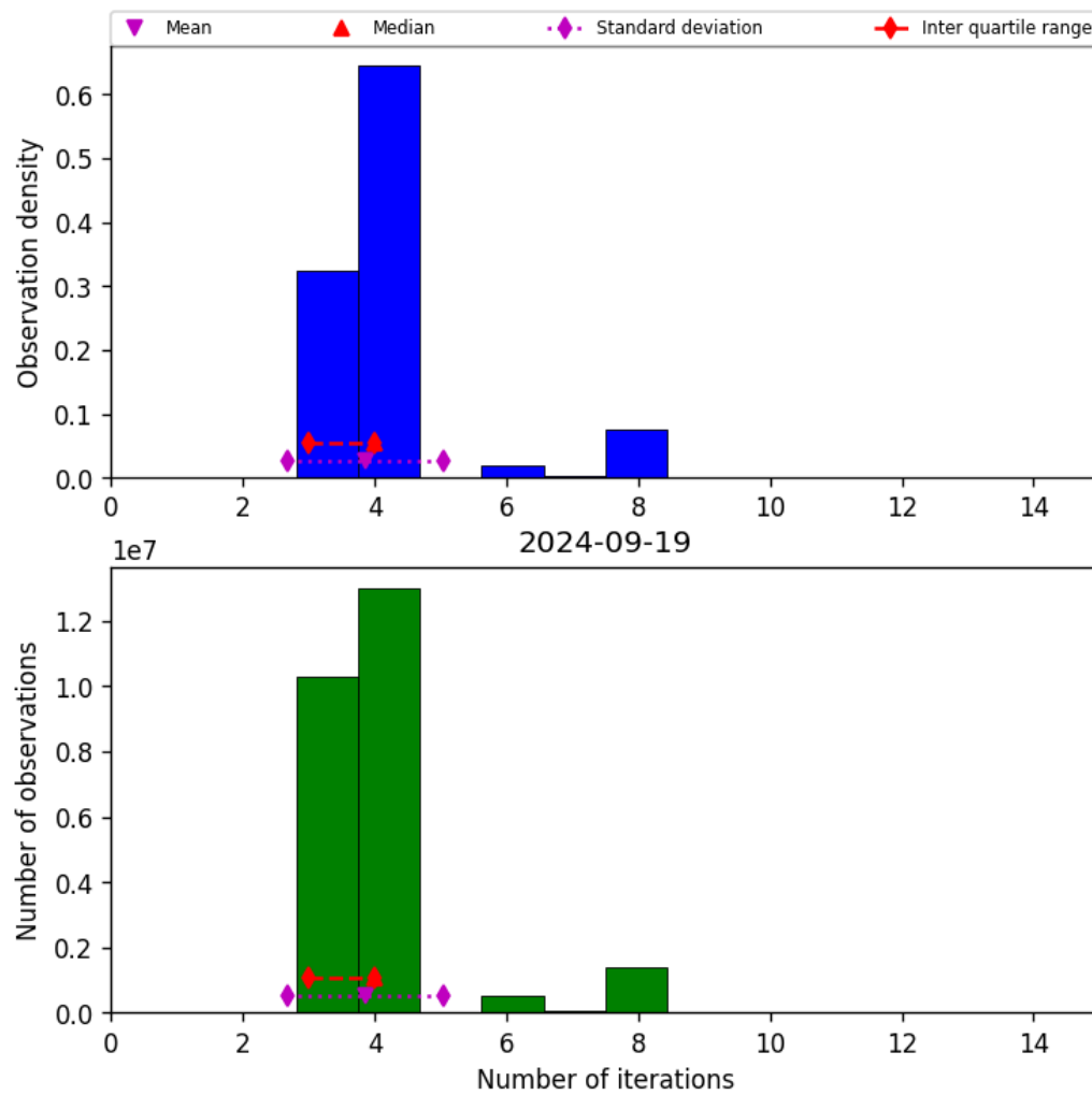
Figure 34: Histogram of “Number of iterations” for 2024-09-18 to 2024-09-20
