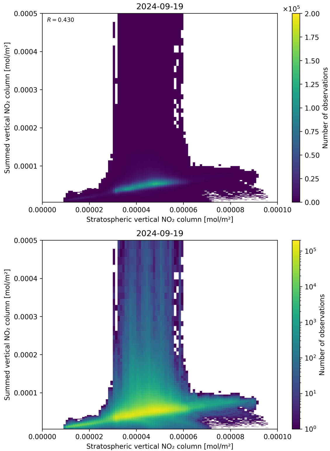
Figure 98: Scatter density plot of “Stratospheric vertical NO 2 column” against “Summed vertical NO 2 column” for 2024-09-18 to 2024-09-20.
