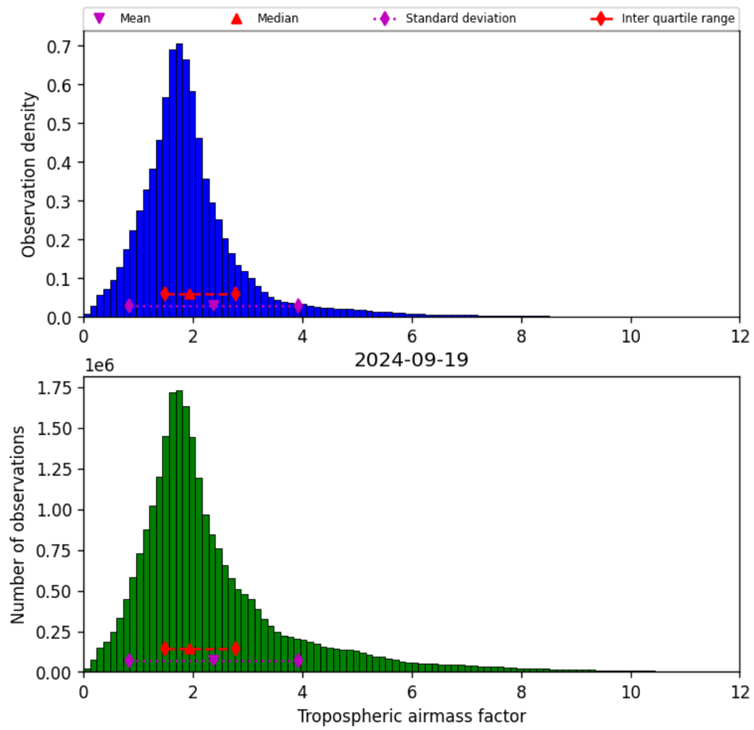
Figure 31: Histogram of “Tropospheric air mass factor” for 2024-09-18 to 2024-09-20
