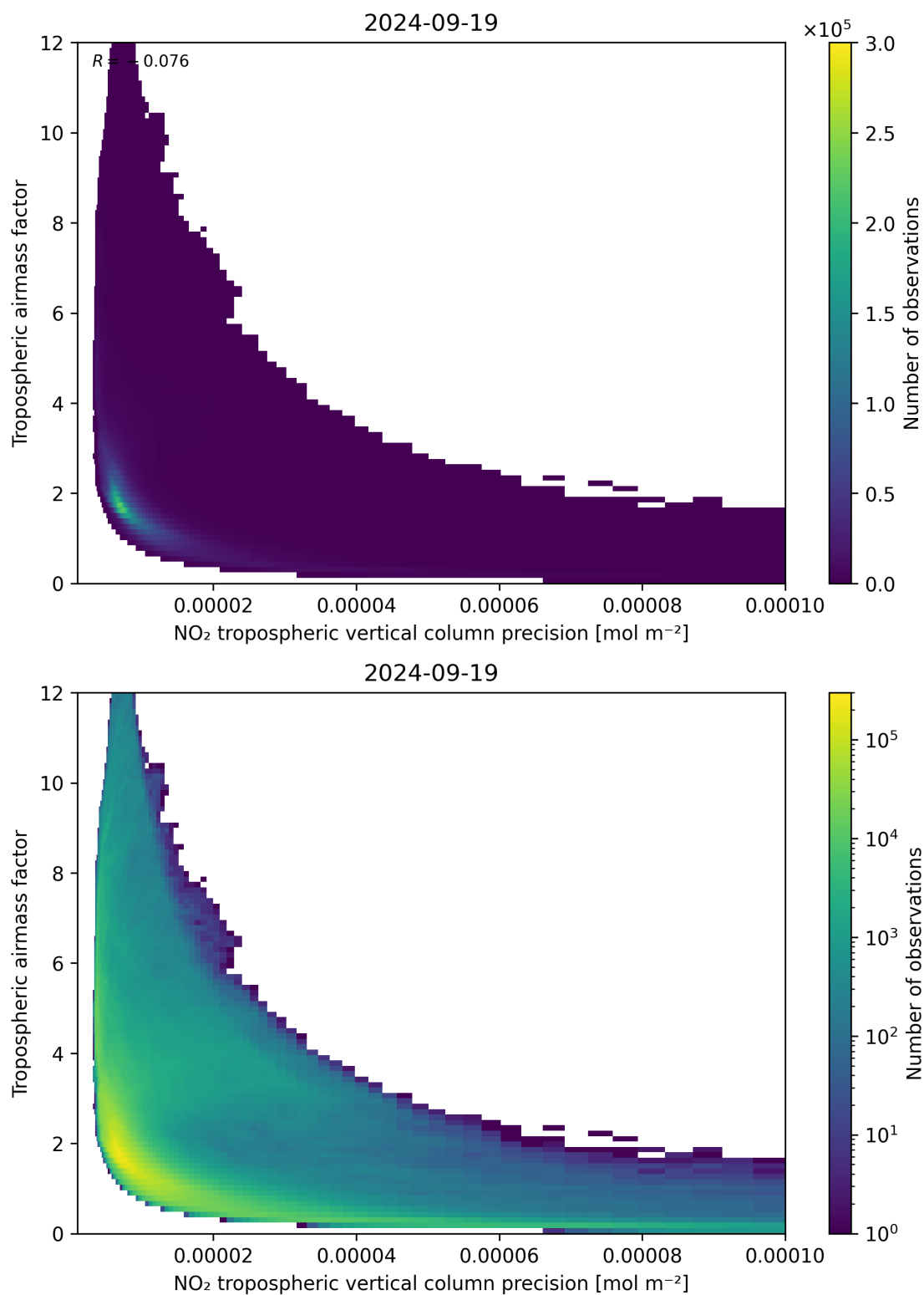
Figure 133: Scatter density plot of “NO 2 tropospheric vertical column precision” against “Tropospheric airmass factor” for 2024-09-18 to 2024-09-20.
