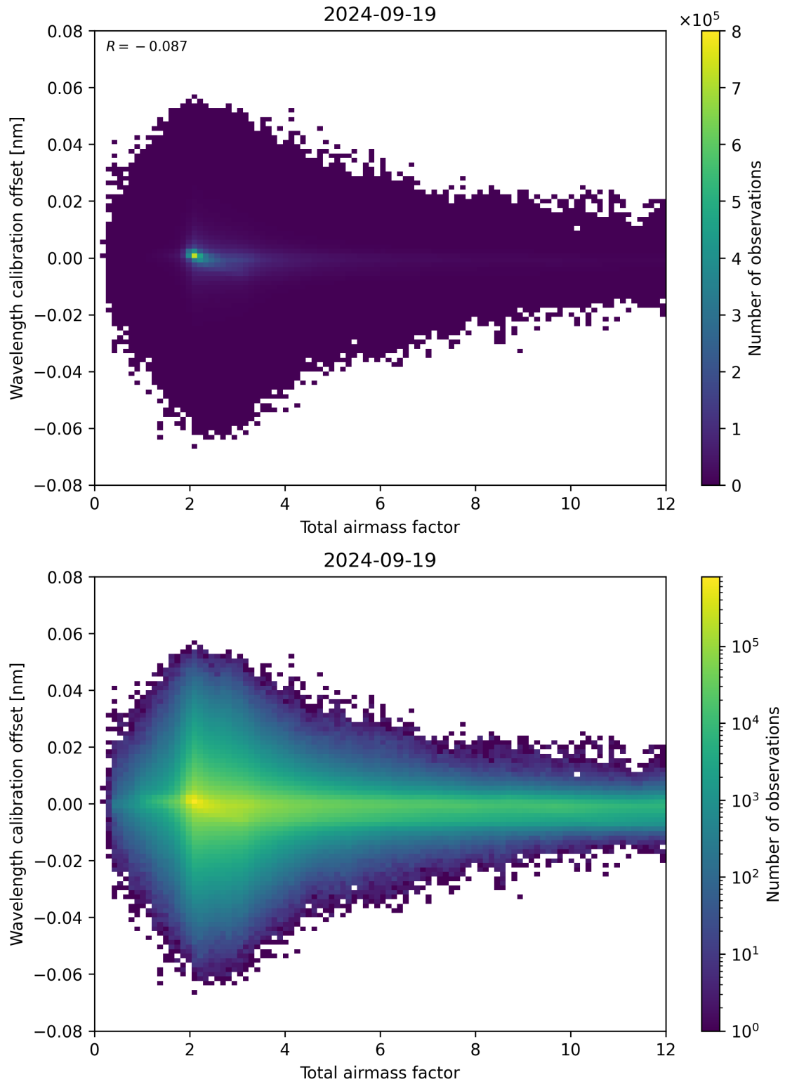
Figure 70: Scatter density plot of “Total airmass factor” against “Wavelength calibration offset” for 2024-09-18 to 2024-09-20.
