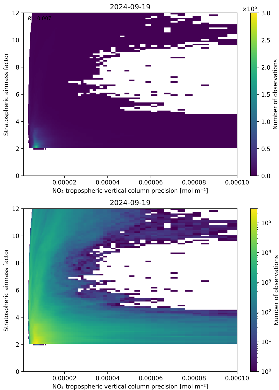
Figure 131: Scatter density plot of “NO 2 tropospheric vertical column precision” against “Stratospheric airmass factor” for 2024-09-18 to 2024-09-20.
