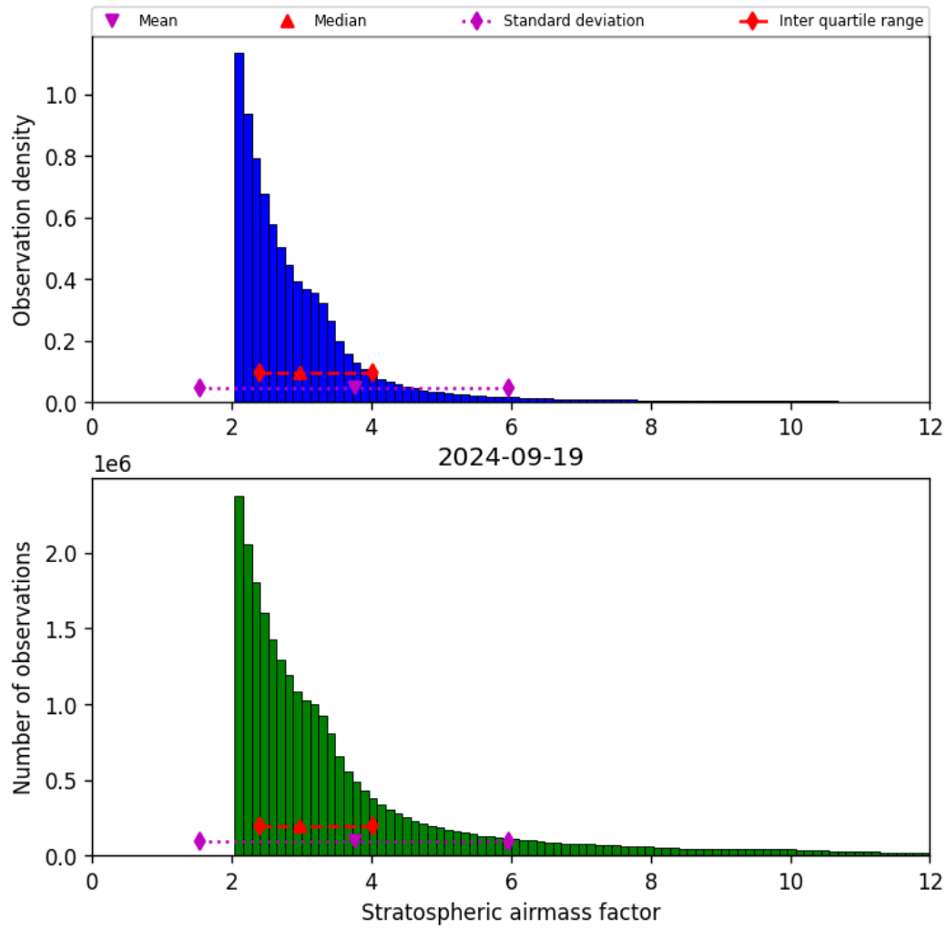
Figure 44: Histogram of “Stratospheric airmass factor” for 2024-09-18 to 2024-09-20
