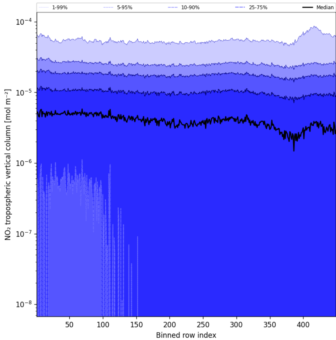
Figure 46: Along track statistics of “NO 2 tropospheric vertical column” for 2024-09-18 to 2024-09-20
