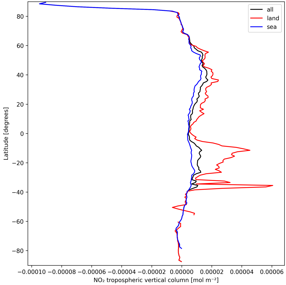
Figure 12: Zonal average of “NO 2 tropospheric vertical column” for 2024-09-18 to 2024-09-20.
