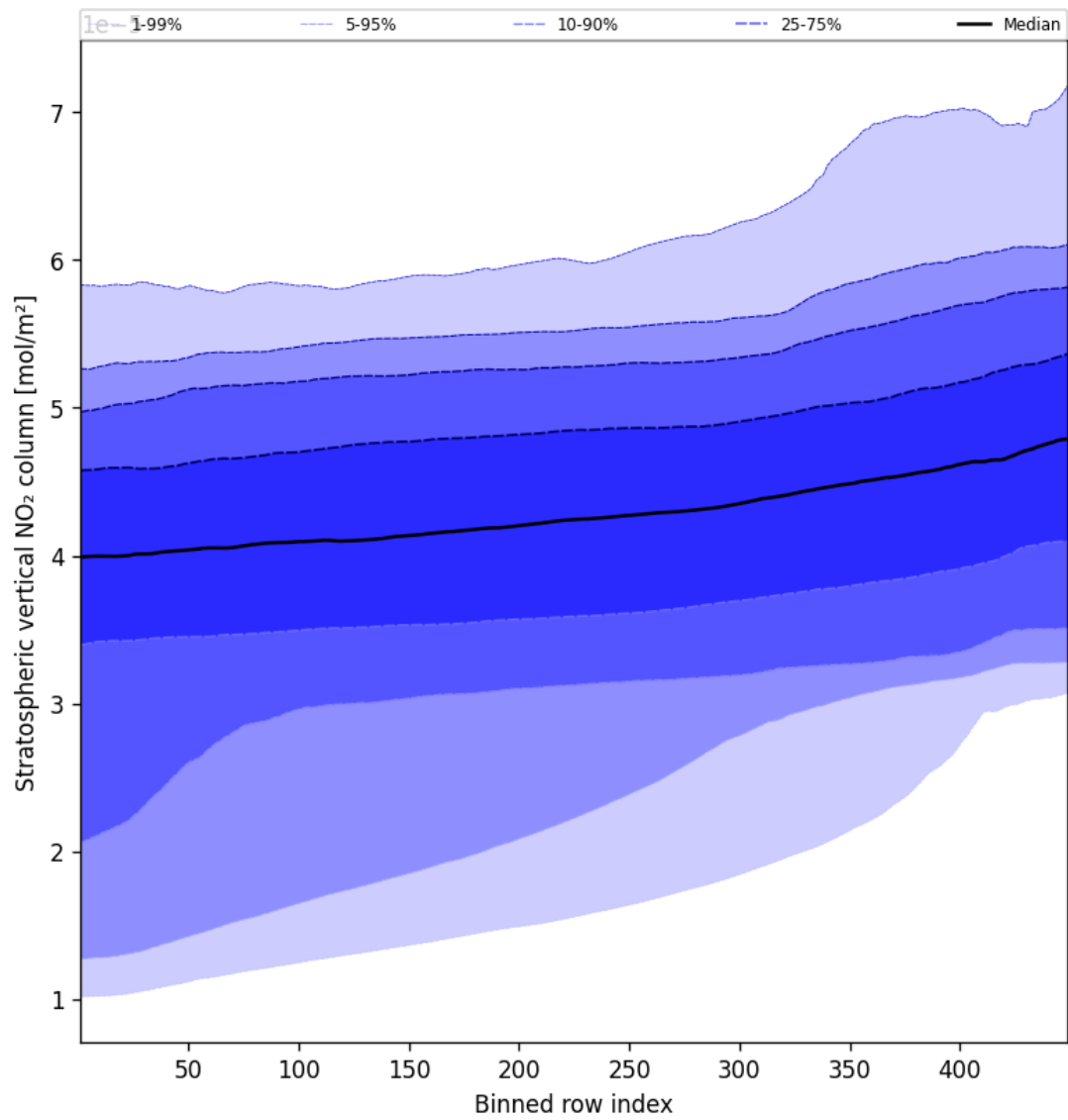
Figure 53: Along track statistics of “Stratospheric vertical NO 2 column” for 2024-09-18 to 2024-09-20
