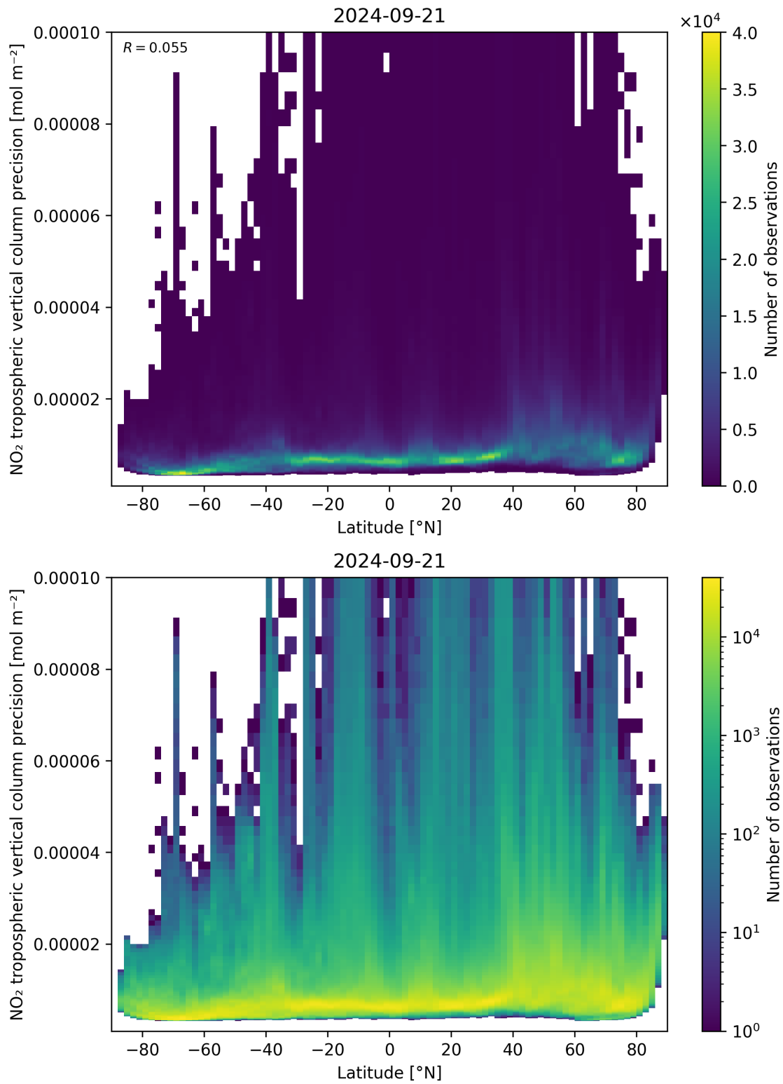
Figure 93: Scatter density plot of “Latitude” against “NO 2 tropospheric vertical column precision” for 2024-09-20 to 2024-09-22.
