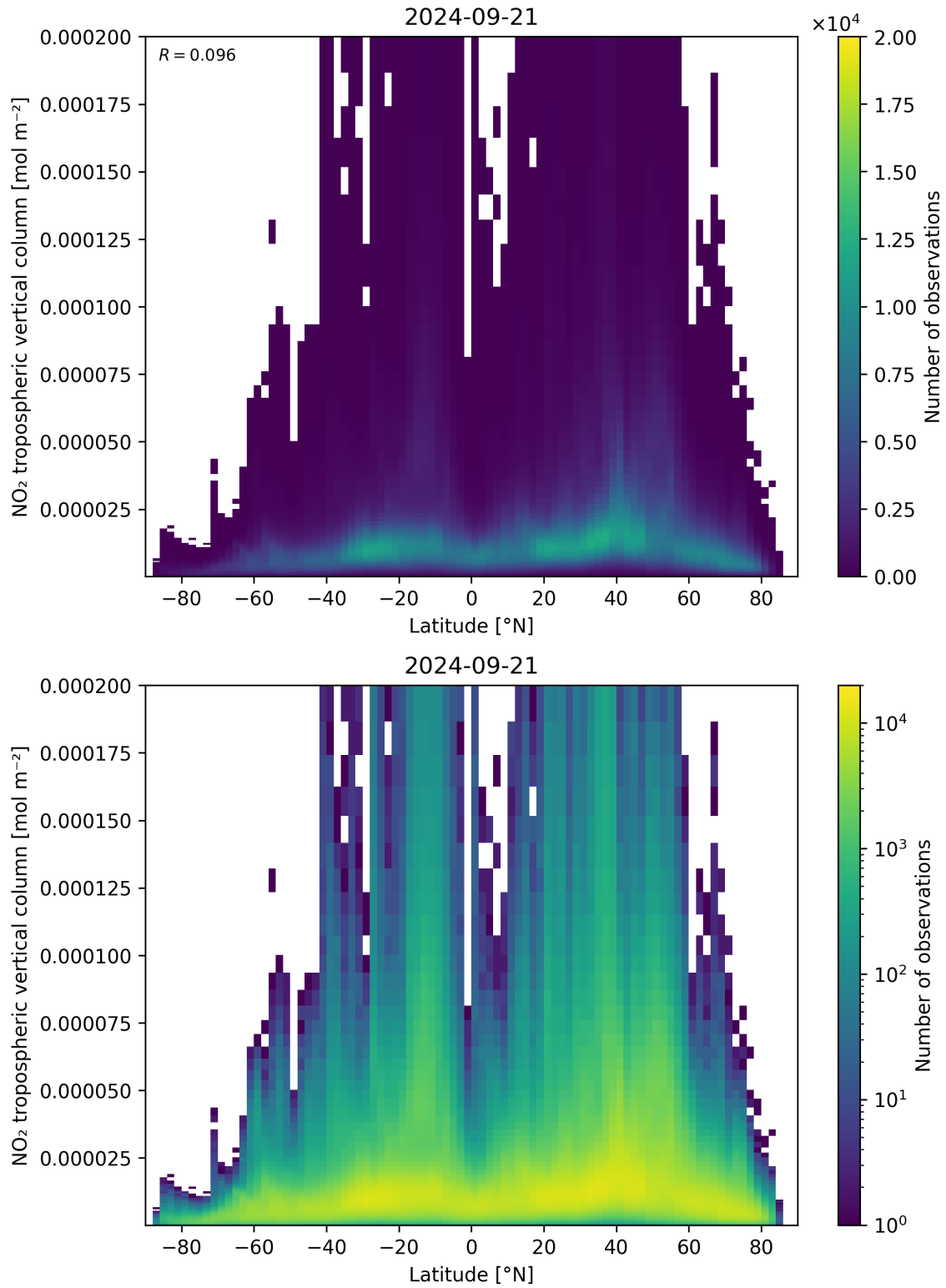
Figure 92: Scatter density plot of “Latitude” against “NO 2 tropospheric vertical column” for 2024-09-20 to 2024-09-22.
