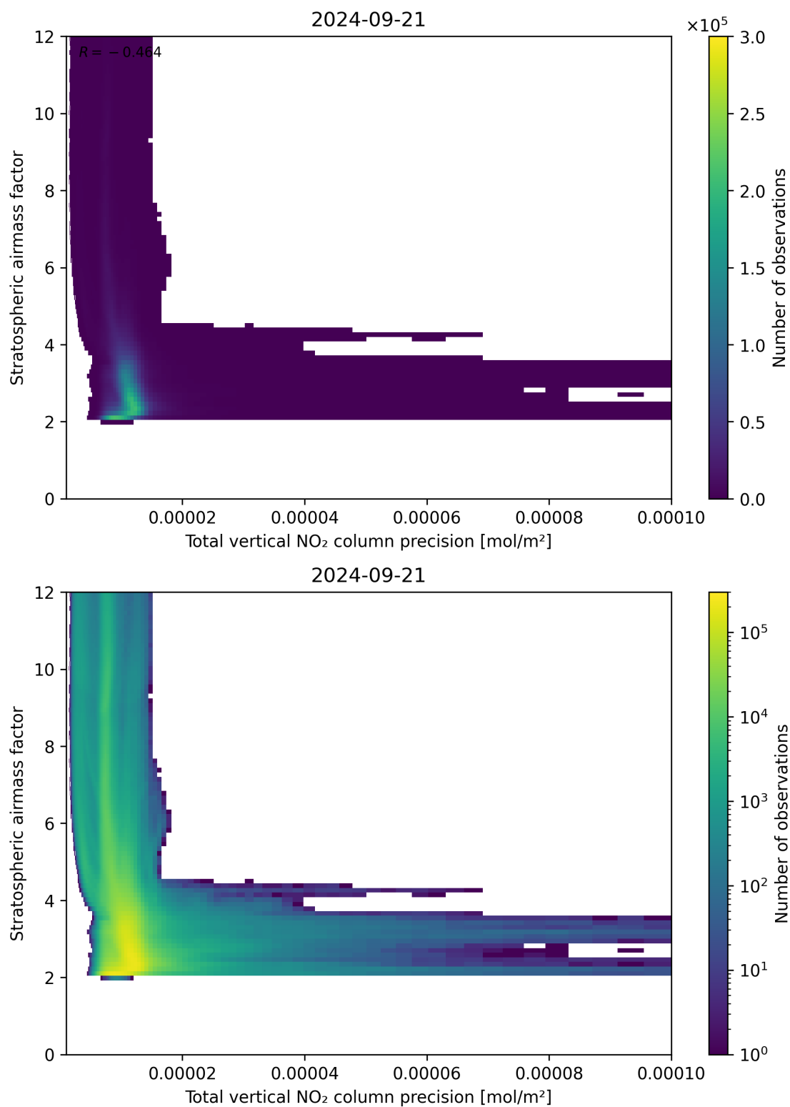
Figure 115: Scatter density plot of “Total vertical NO 2 column precision” against “Stratospheric airmass factor” for 2024-09-20 to 2024-09-22.
