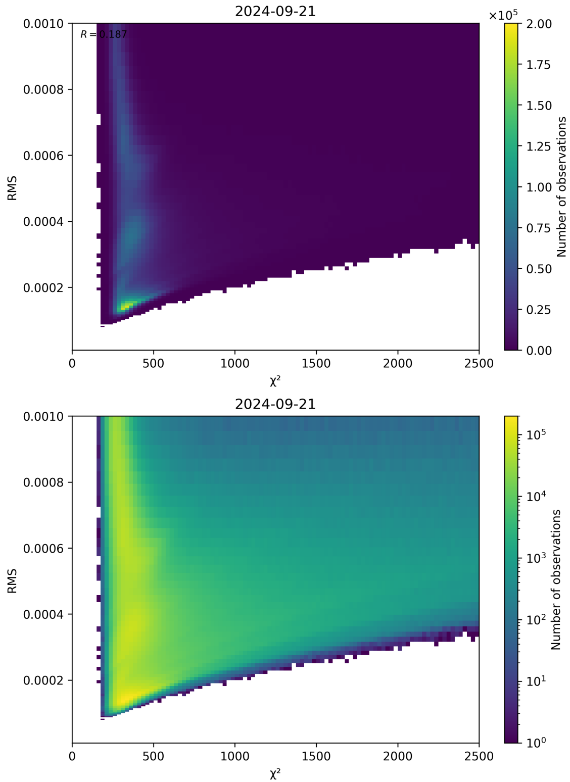
Figure 82: Scatter density plot of “ \chi^2 ” against “RMS” for 2024-09-20 to 2024-09-22.
