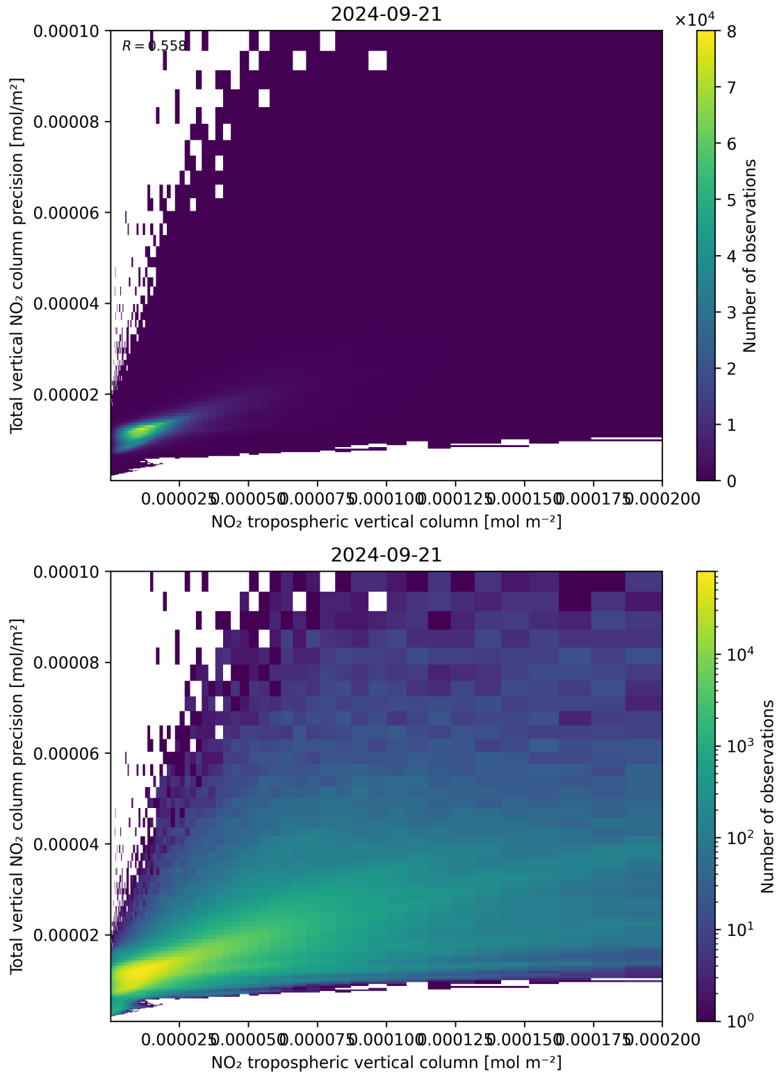
Figure 129: Scatter density plot of “NO 2 tropospheric vertical column” against “Total vertical NO 2 column precision” for 2024-09-20 to 2024-09-22.
