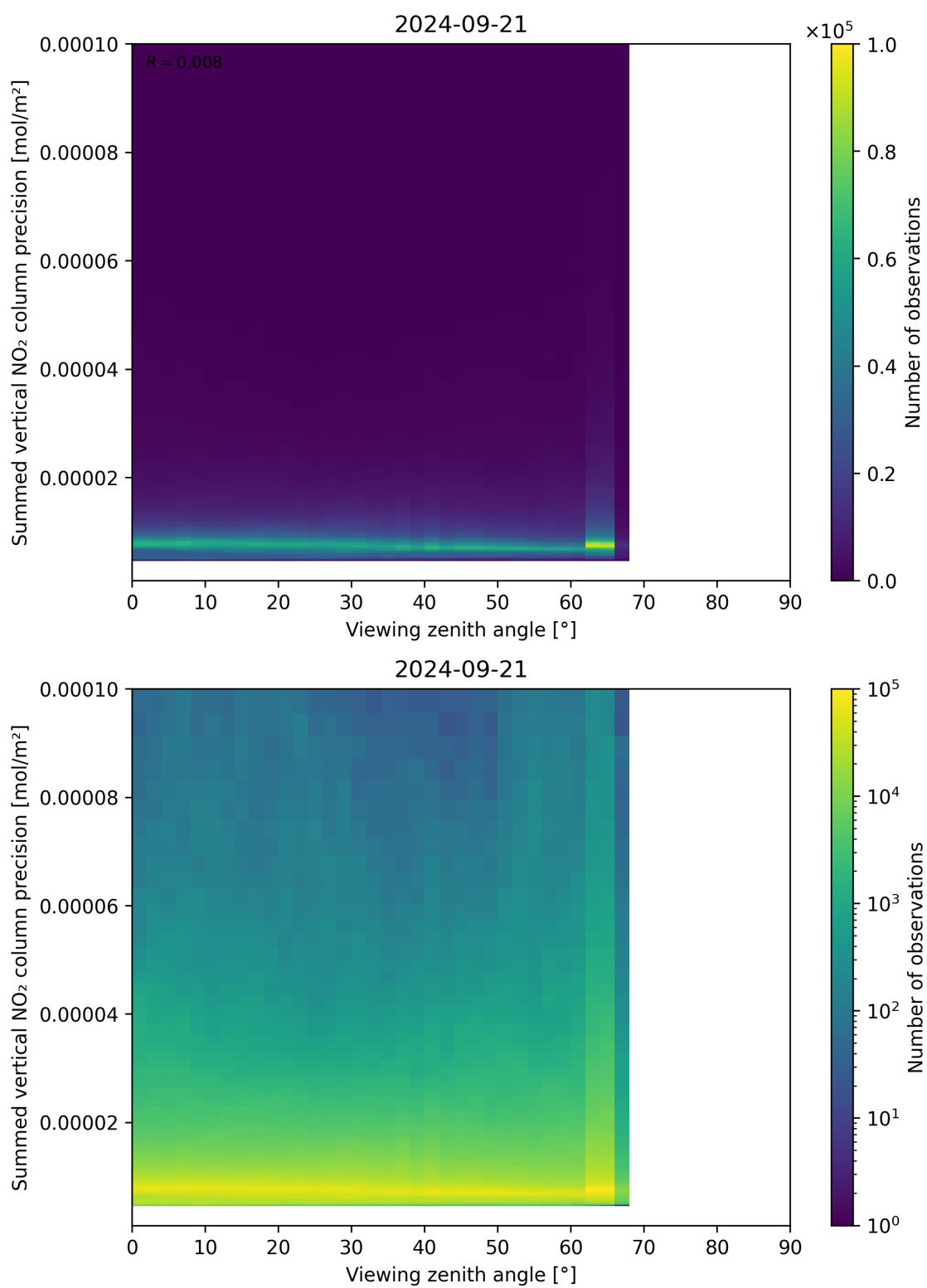
Figure 166: Scatter density plot of “Viewing zenith angle” against “Summed vertical NO 2 column precision” for 2024-09-20 to 2024-09-22.
