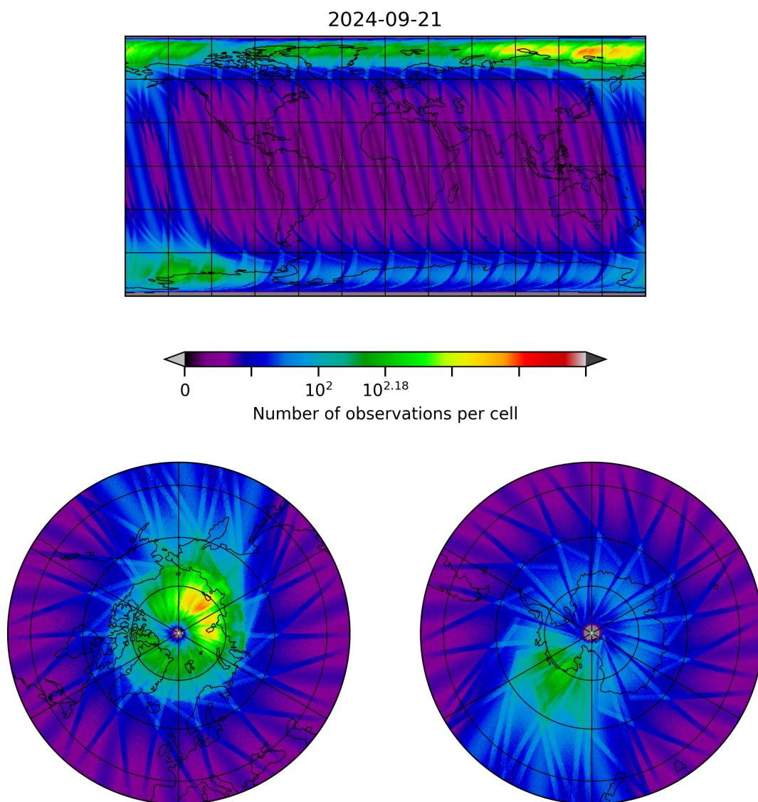
Figure 10: Map of the number of observations for 2024-09-20 to 2024-09-22
