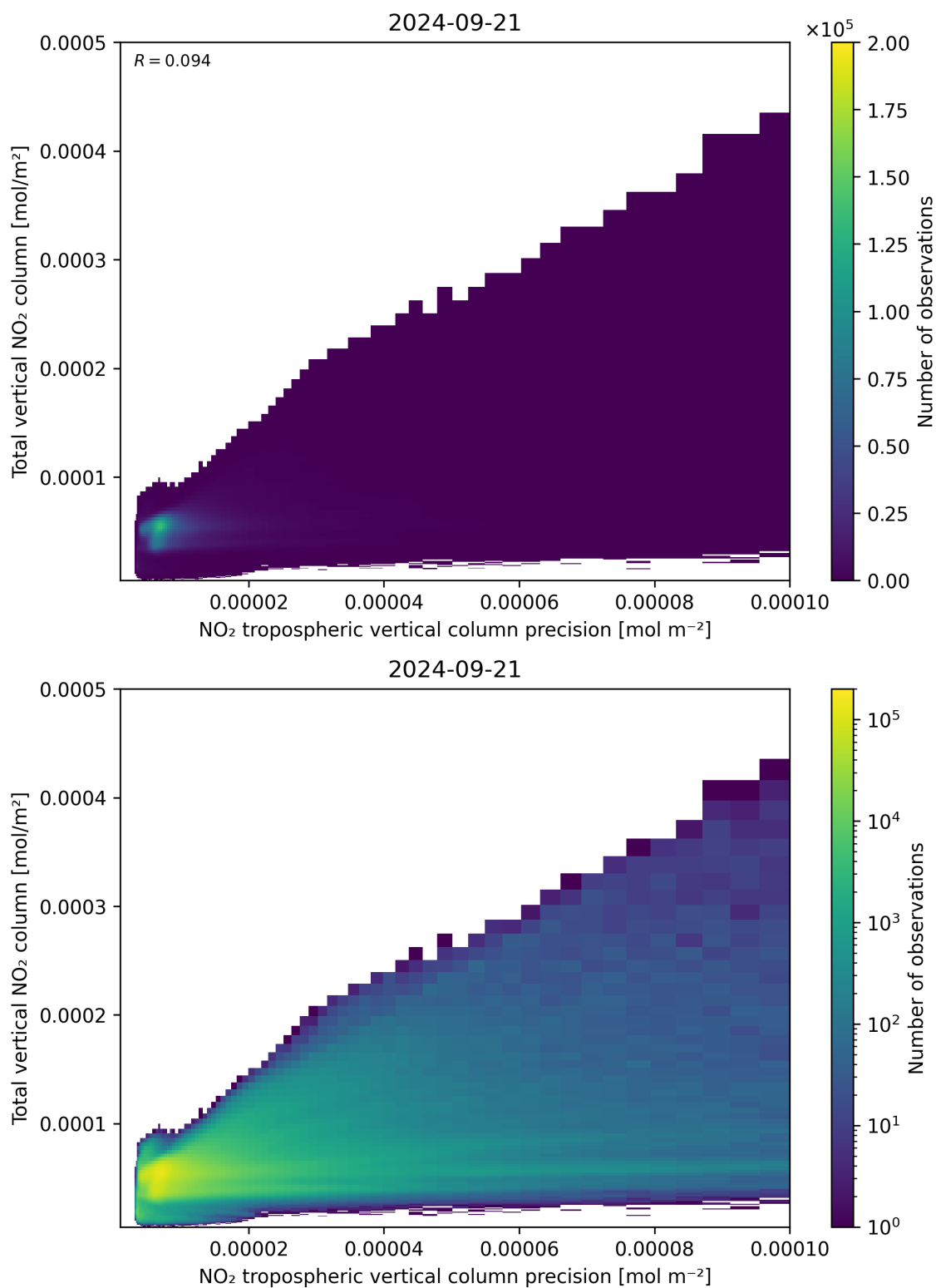
Figure 138: Scatter density plot of “NO 2 tropospheric vertical column precision” against “Total vertical NO 2 column” for 2024-09-20 to 2024-09-22.
