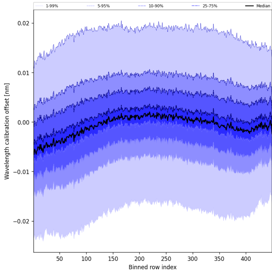
Figure 52: Along track statistics of “Wavelength calibration offset” for 2024-09-20 to 2024-09-22
