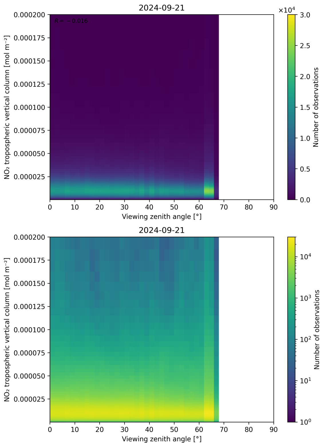
Figure 169: Scatter density plot of “Viewing zenith angle” against “NO 2 tropospheric vertical column” for 2024-09-20 to 2024-09-22.
