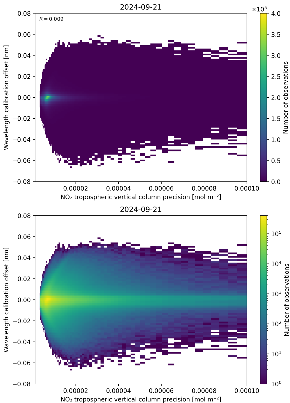
Figure 141: Scatter density plot of “NO 2 tropospheric vertical column precision” against “Wavelength calibration offset” for 2024-09-20 to 2024-09-22.
