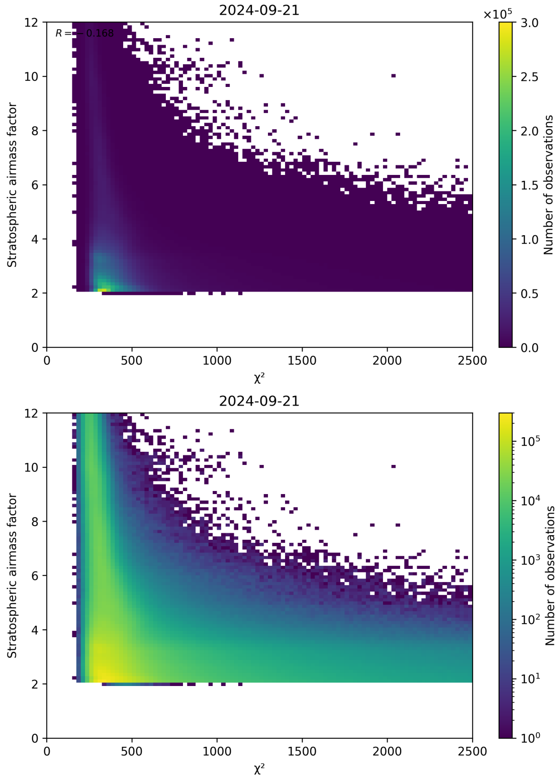
Figure 81: Scatter density plot of “ \chi^2 ” against “Stratospheric airmass factor” for 2024-09-20 to 2024-09-22.
