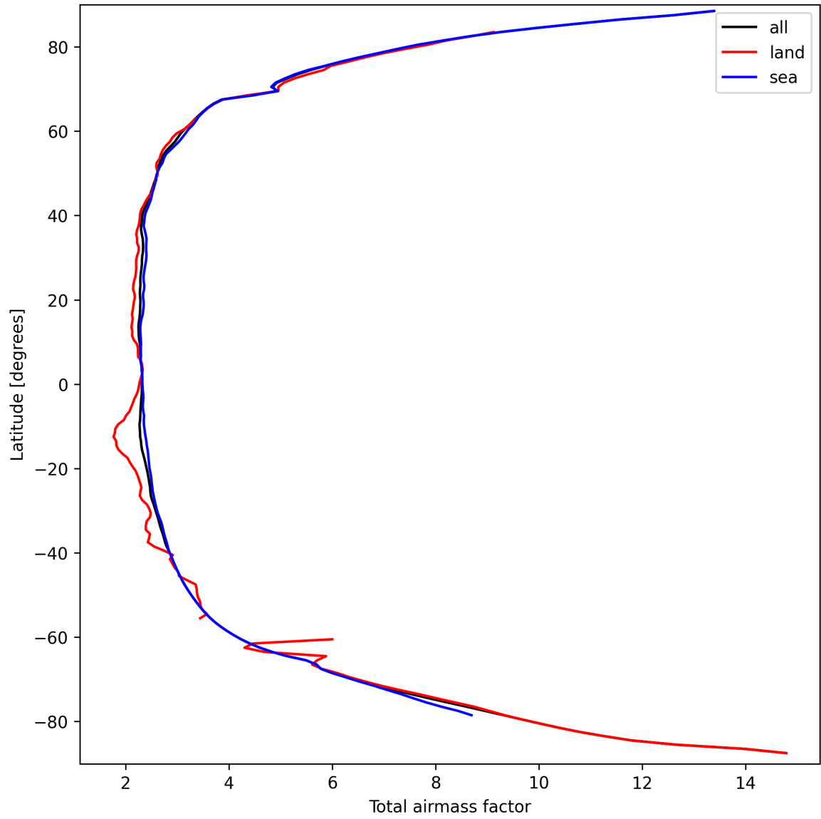
Figure 15: Zonal average of “Total airmass factor” for 2024-09-20 to 2024-09-22.
