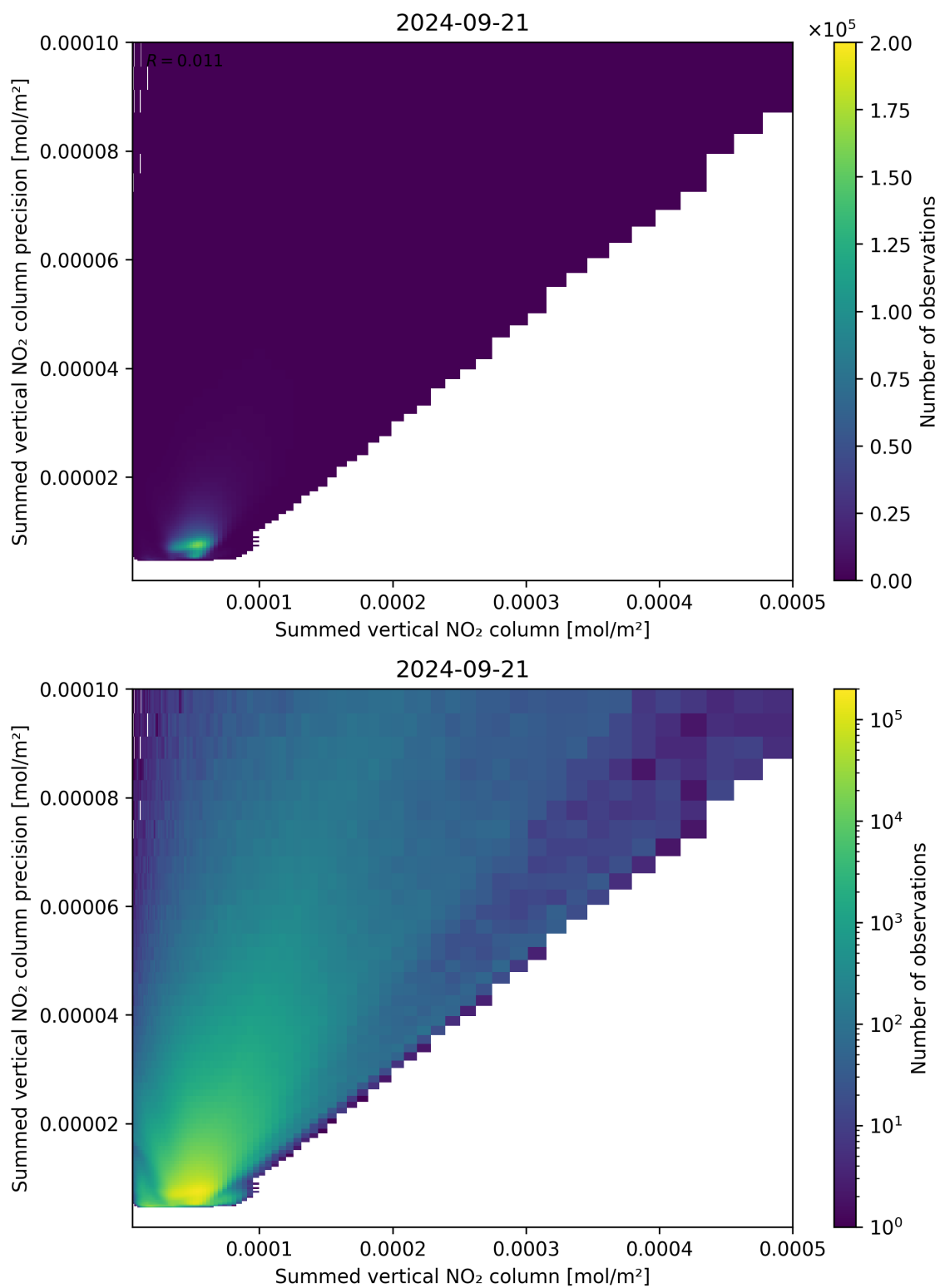
Figure 105: Scatter density plot of “Summed vertical NO 2 column” against “Summed vertical NO 2 column precision” for 2024-09-20 to 2024-09-22.
