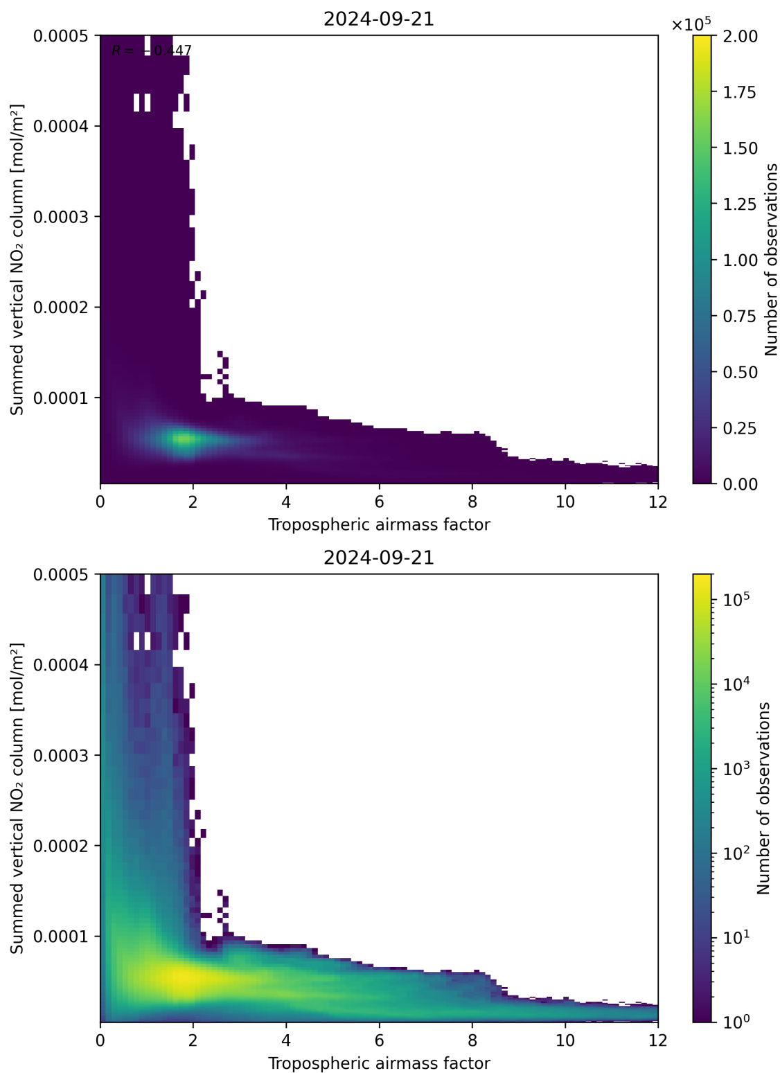
Figure 75: Scatter density plot of “Tropospheric airmass factor” against “Summed vertical NO 2 column” for 2024-09-20 to 2024-09-22.
