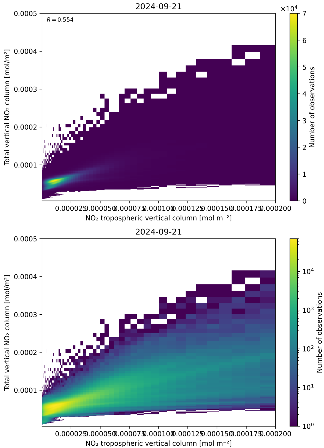
Figure 128: Scatter density plot of “NO 2 tropospheric vertical column” against “Total vertical NO 2 column” for 2024-09-20 to 2024-09-22.
