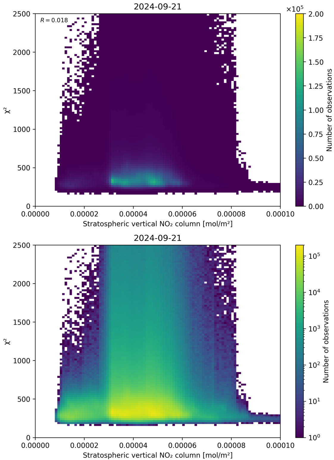
Figure 97: Scatter density plot of “Stratospheric vertical NO 2 column” against “ \chi^2 ” for 2024-09-20 to 2024-09-22.
