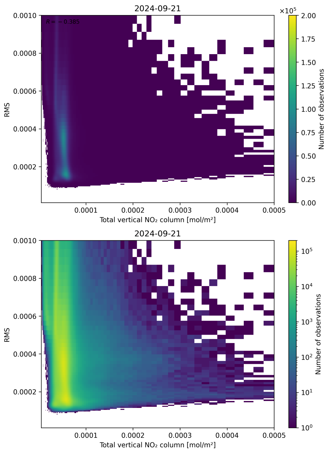
Figure 120: Scatter density plot of “Total vertical NO 2 column” against “RMS” for 2024-09-20 to 2024-09-22.
