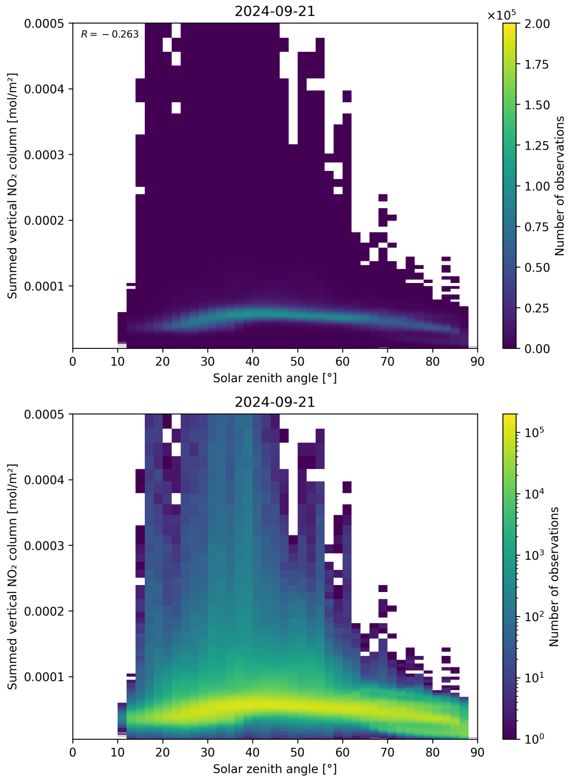
Figure 151: Scatter density plot of “Solar zenith angle” against “Summed vertical NO 2 column” for 2024-09-20 to 2024-09-22.
