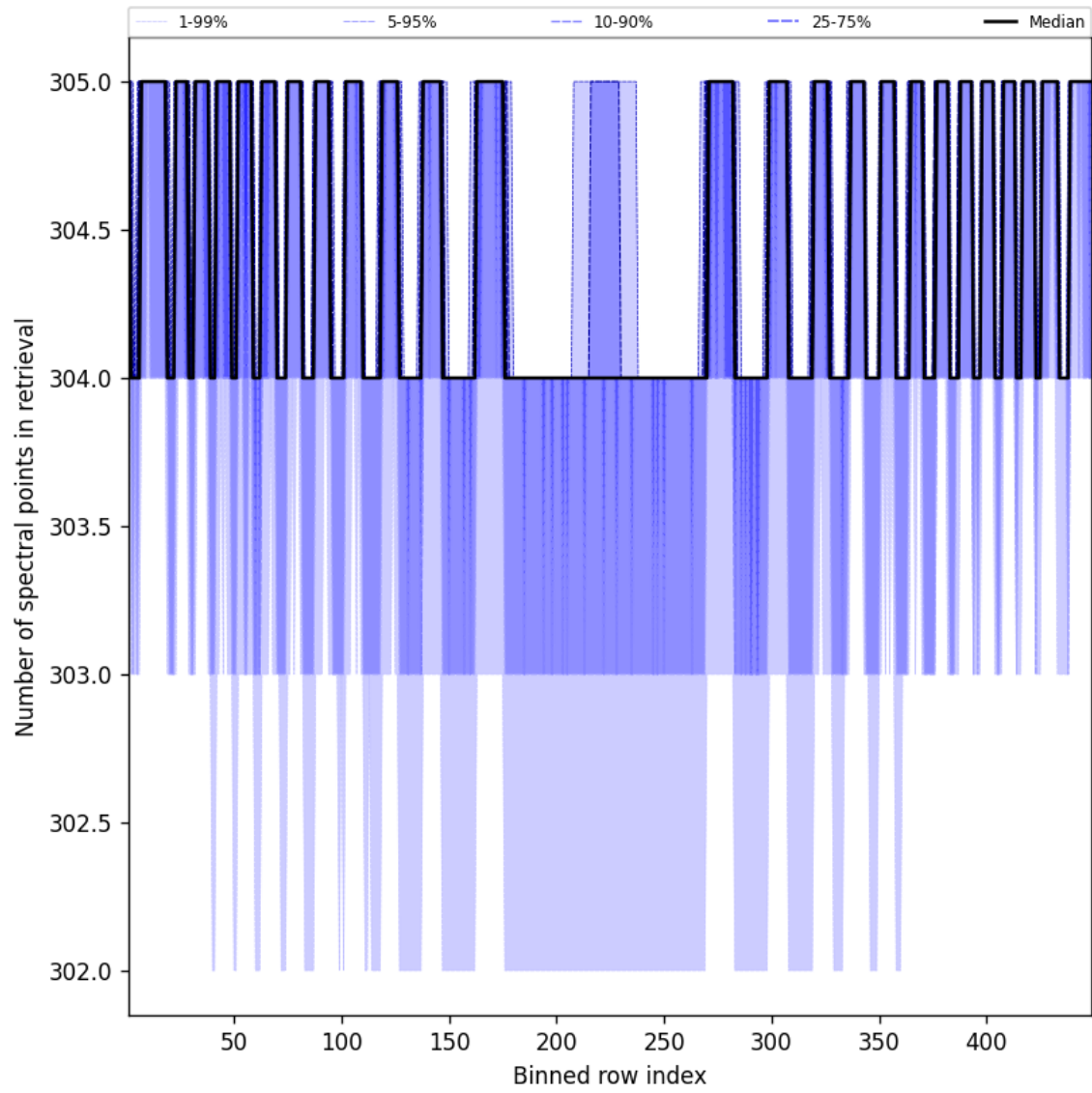
Figure 50: Along track statistics of “Number of spectral points in retrieval” for 2024-09-20 to 2024-09-22
