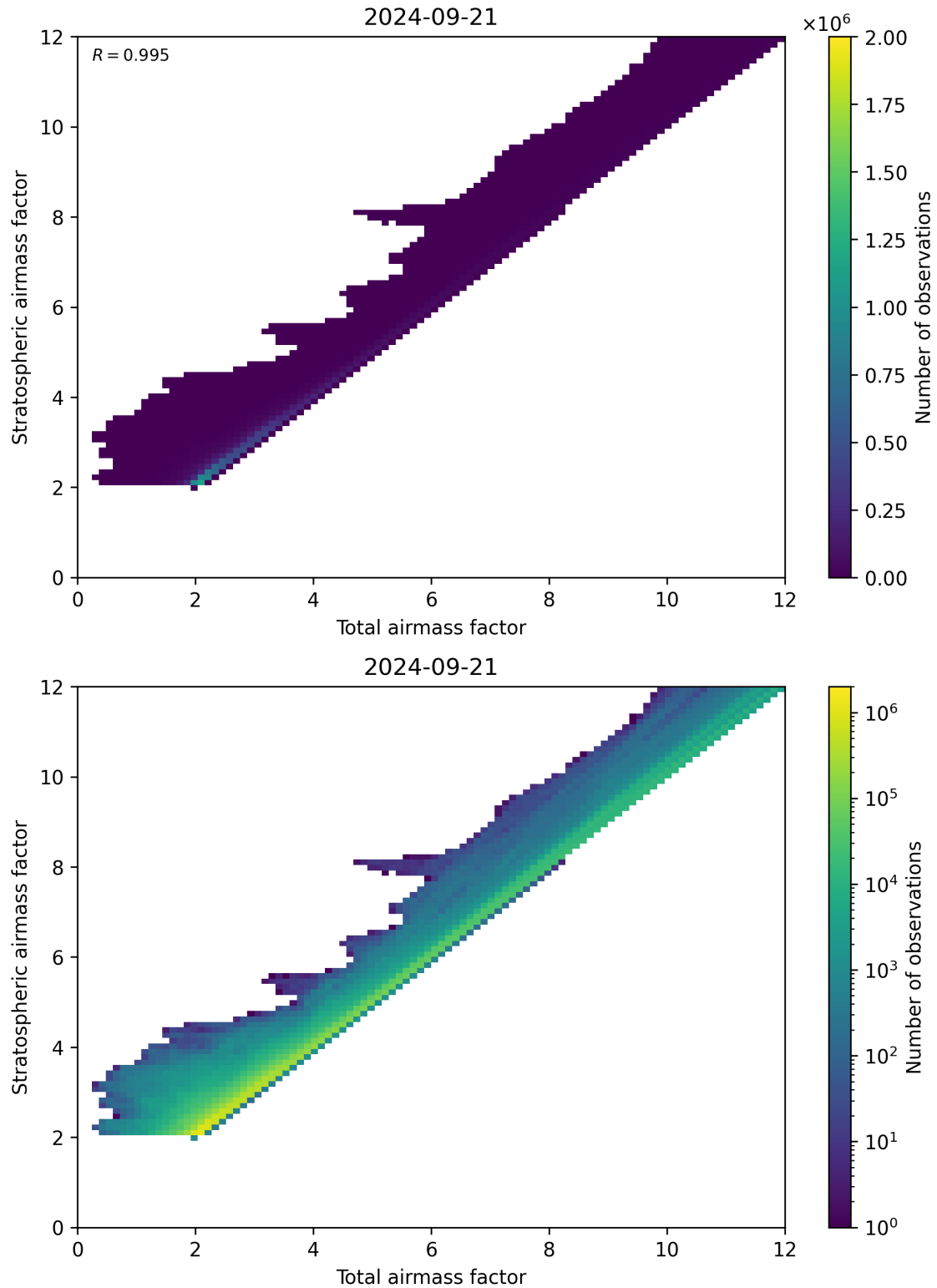
Figure 62: Scatter density plot of “Total airmass factor” against “Stratospheric airmass factor” for 2024-09-20 to 2024-09-22.
