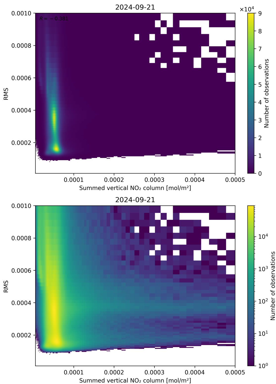
Figure 109: Scatter density plot of “Summed vertical NO 2 column” against “RMS” for 2024-09-20 to 2024-09-22.
