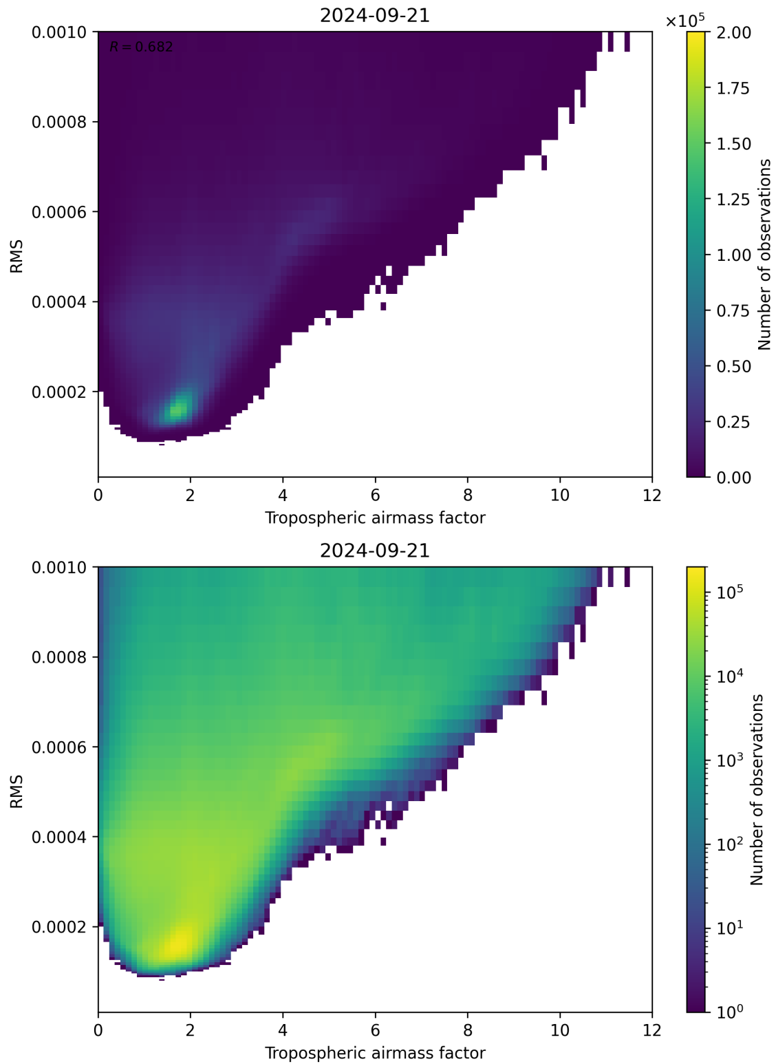
Figure 79: Scatter density plot of “Tropospheric airmass factor” against “RMS” for 2024-09-20 to 2024-09-22.
