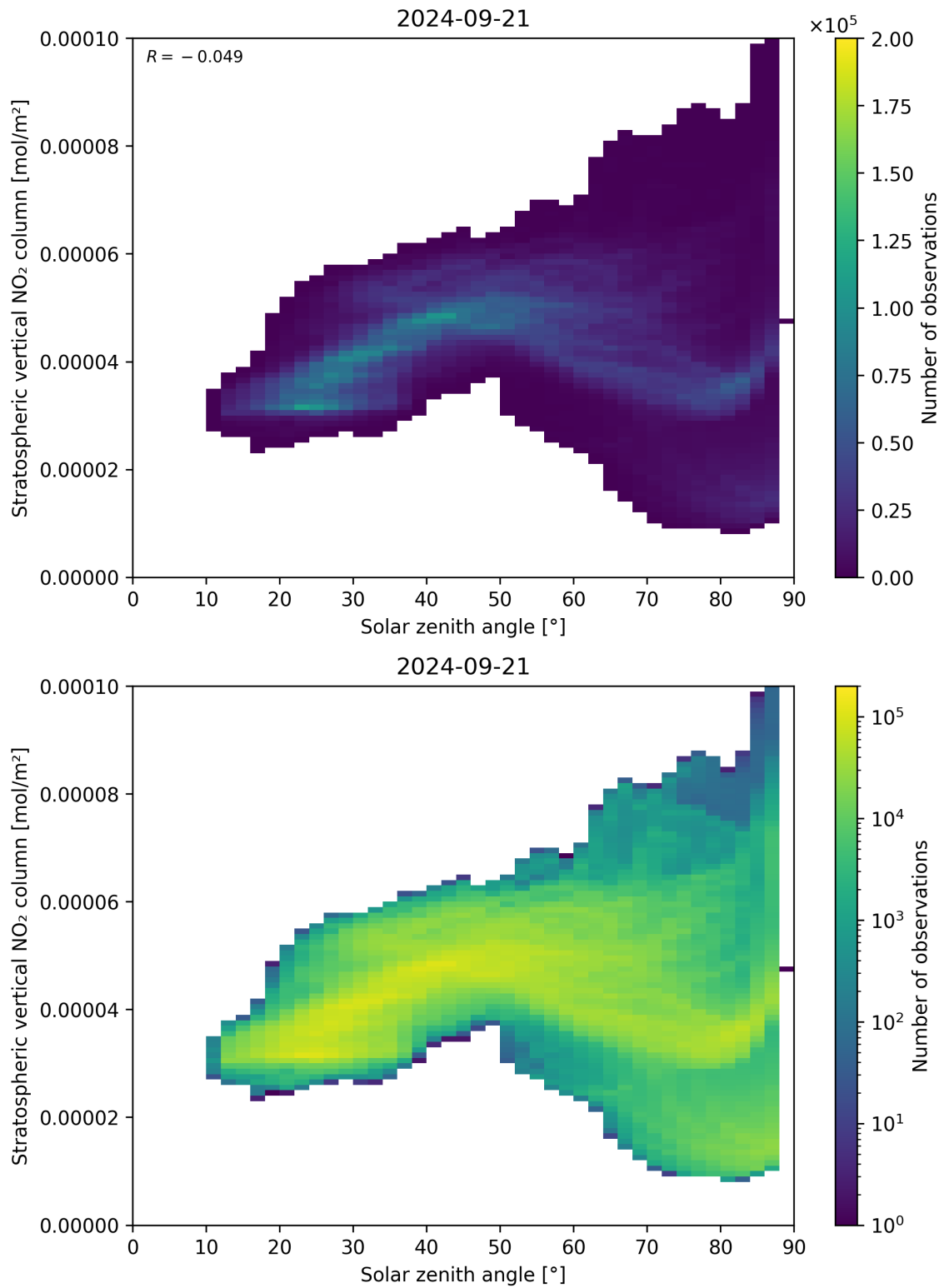
Figure 150: Scatter density plot of “Solar zenith angle” against “Stratospheric vertical NO 2 column” for 2024-09-20 to 2024-09-22.
