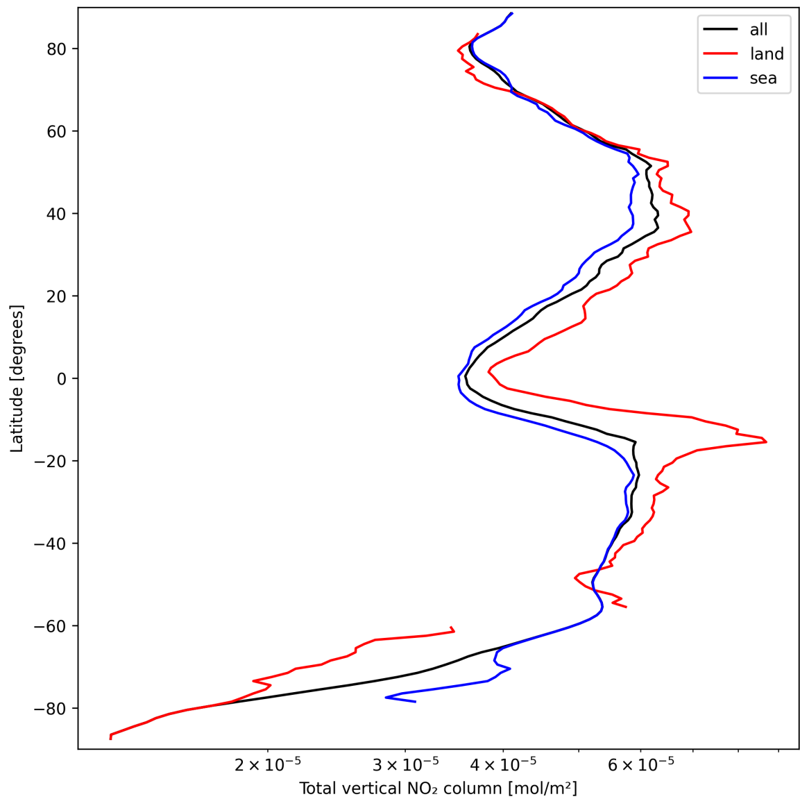
Figure 21: Zonal average of “Total vertical NO 2 column” for 2024-09-20 to 2024-09-22.
