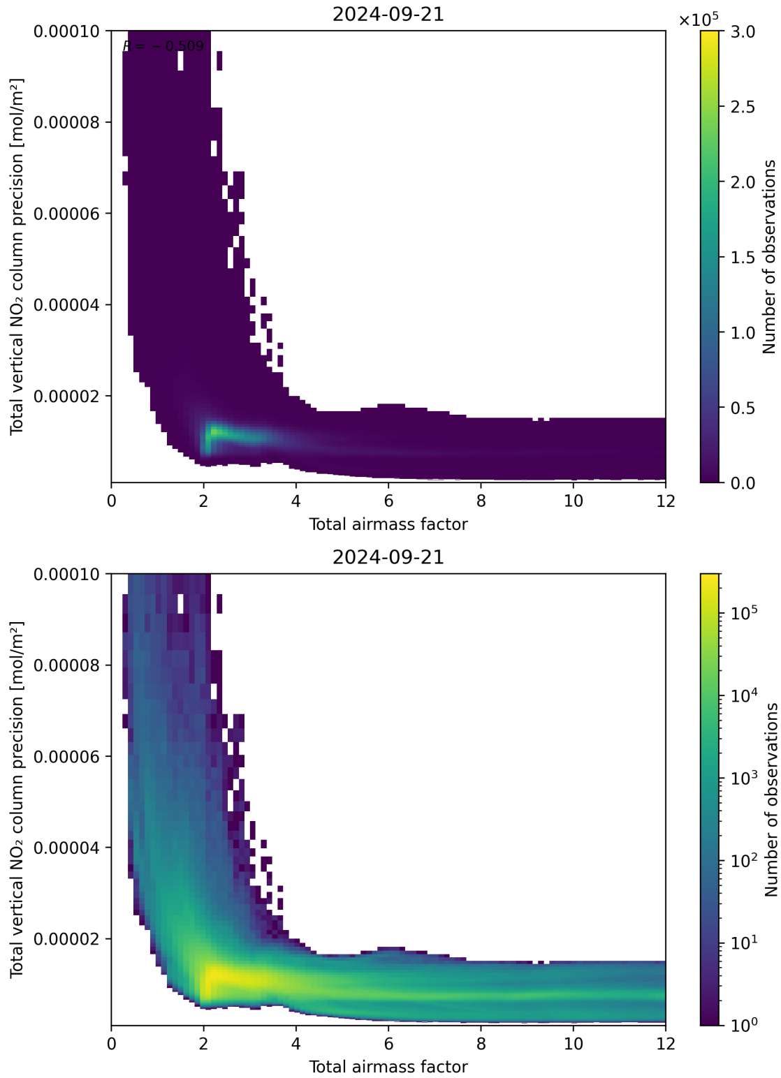
Figure 68: Scatter density plot of “Total airmass factor” against “Total vertical NO 2 column precision” for 2024-09-20 to 2024-09-22.
