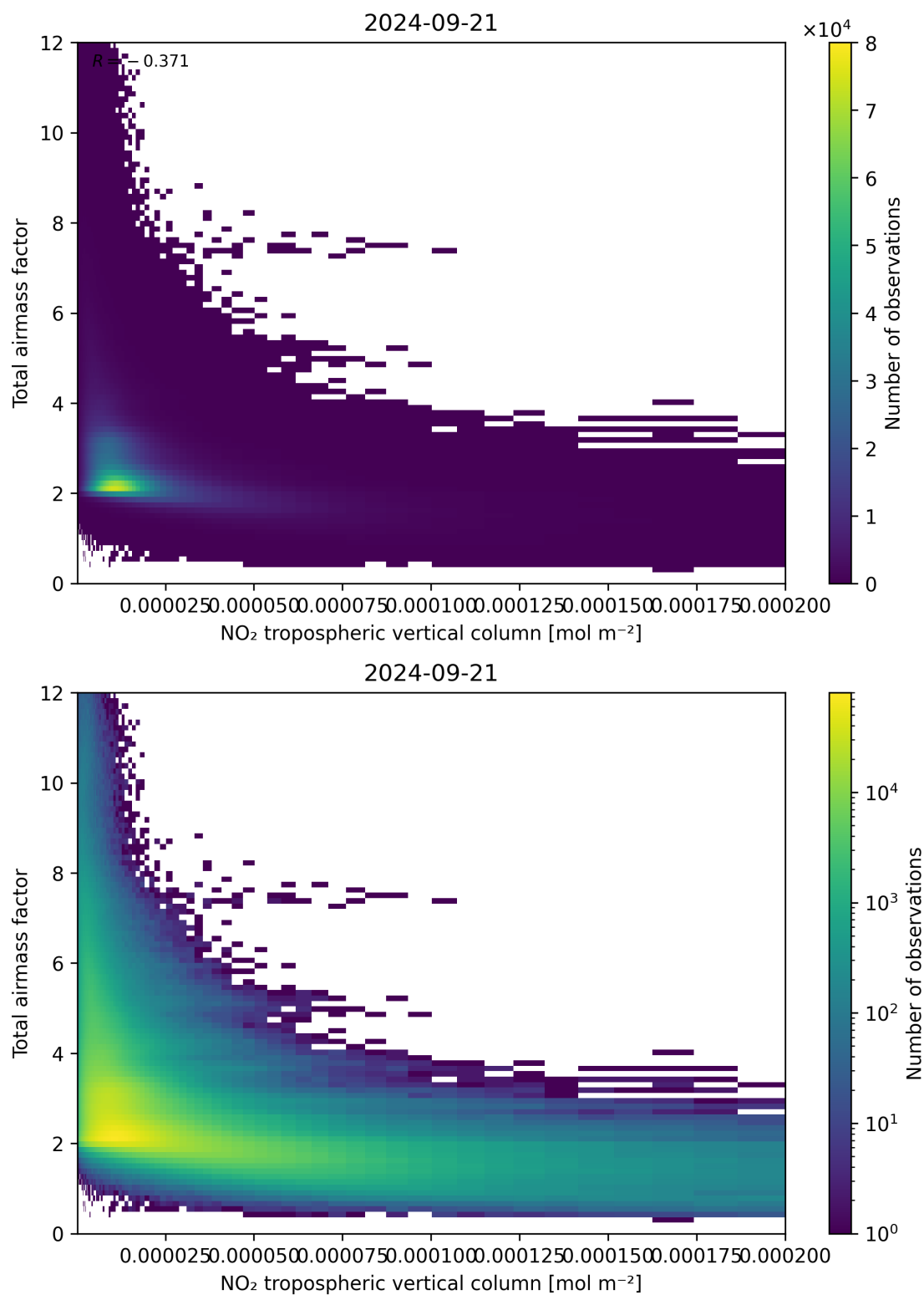
Figure 122: Scatter density plot of “NO 2 tropospheric vertical column” against “Total air mass factor” for 2024-09-20 to 2024-09-22.
