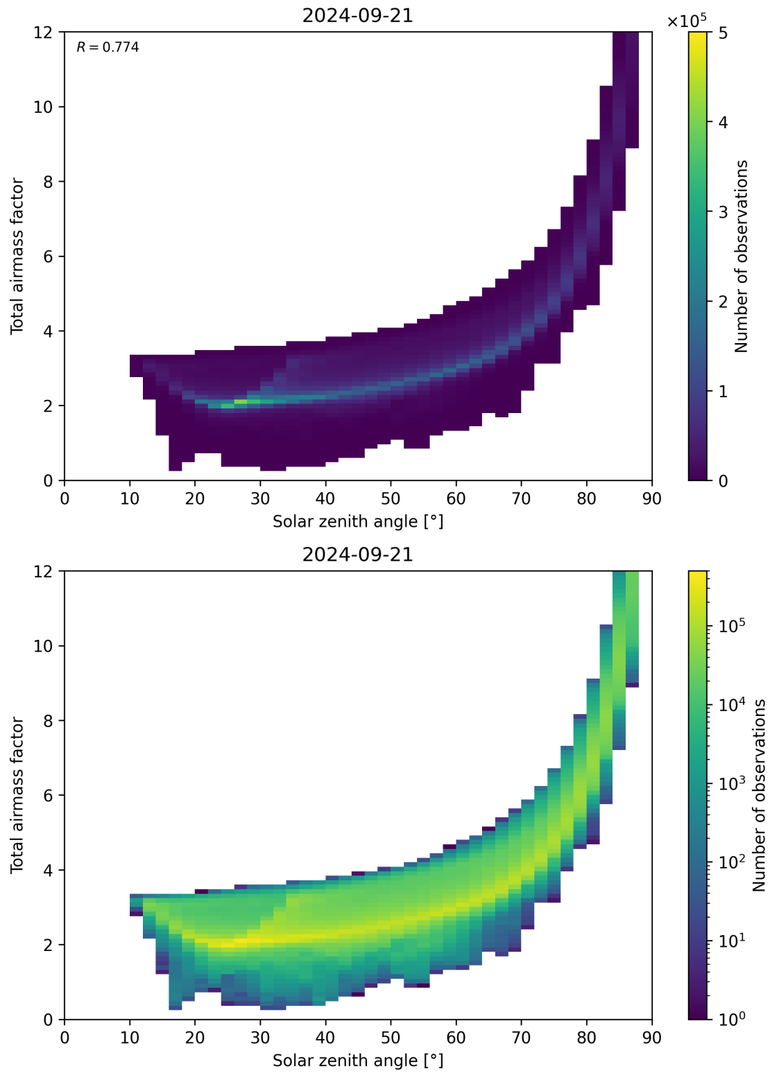
Figure 146: Scatter density plot of “Solar zenith angle” against “Total airmass factor” for 2024-09-20 to 2024-09-22.
