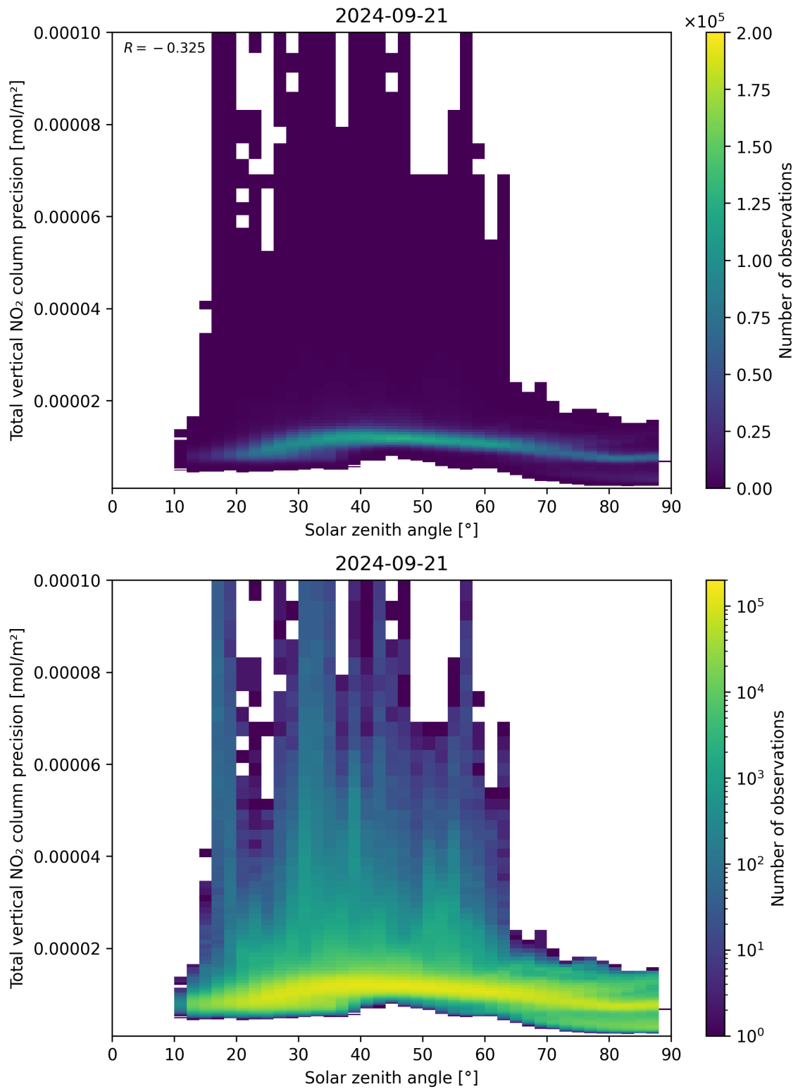
Figure 154: Scatter density plot of “Solar zenith angle” against “Total vertical NO 2 column precision” for 2024-09-20 to 2024-09-22.
