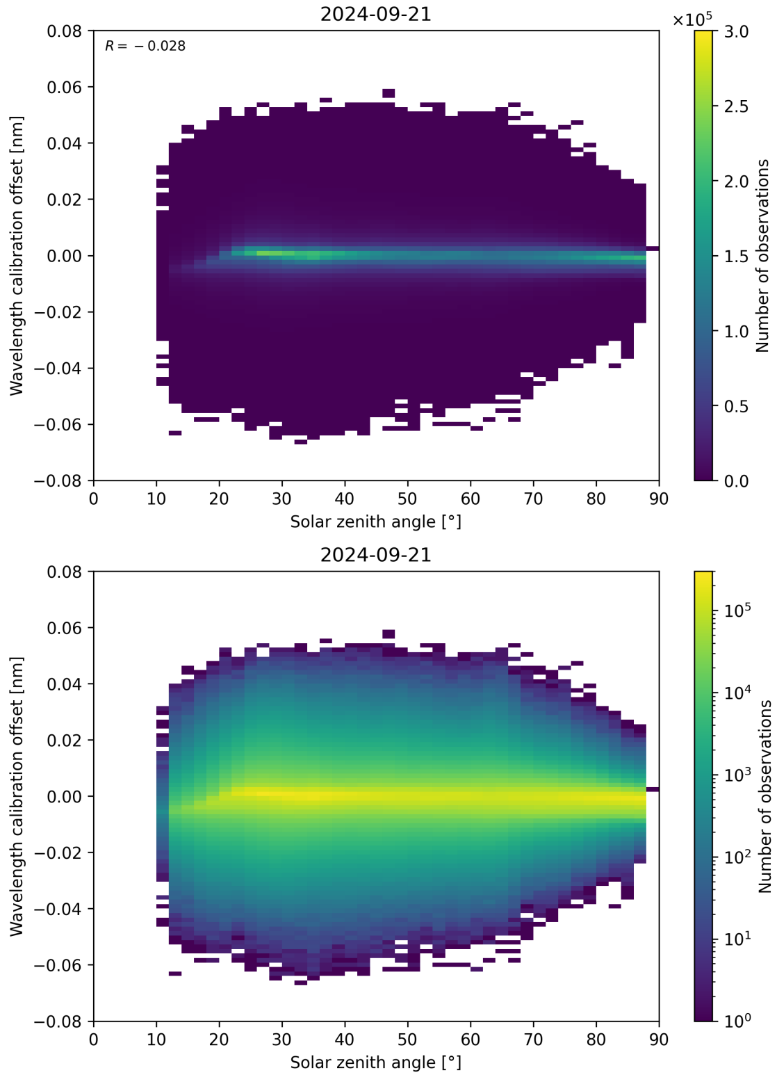
Figure 158: Scatter density plot of “Solar zenith angle” against “Wavelength calibration offset” for 2024-09-20 to 2024-09-22.
