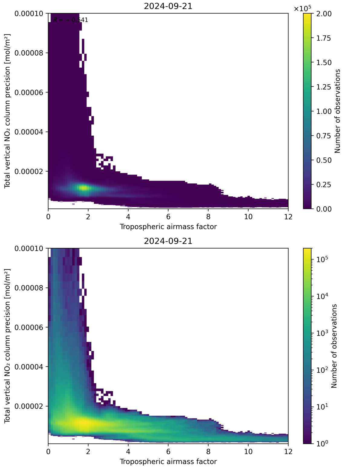
Figure 78: Scatter density plot of “Tropospheric airmass factor” against “Total vertical NO 2 column precision” for 2024-09-20 to 2024-09-22.
