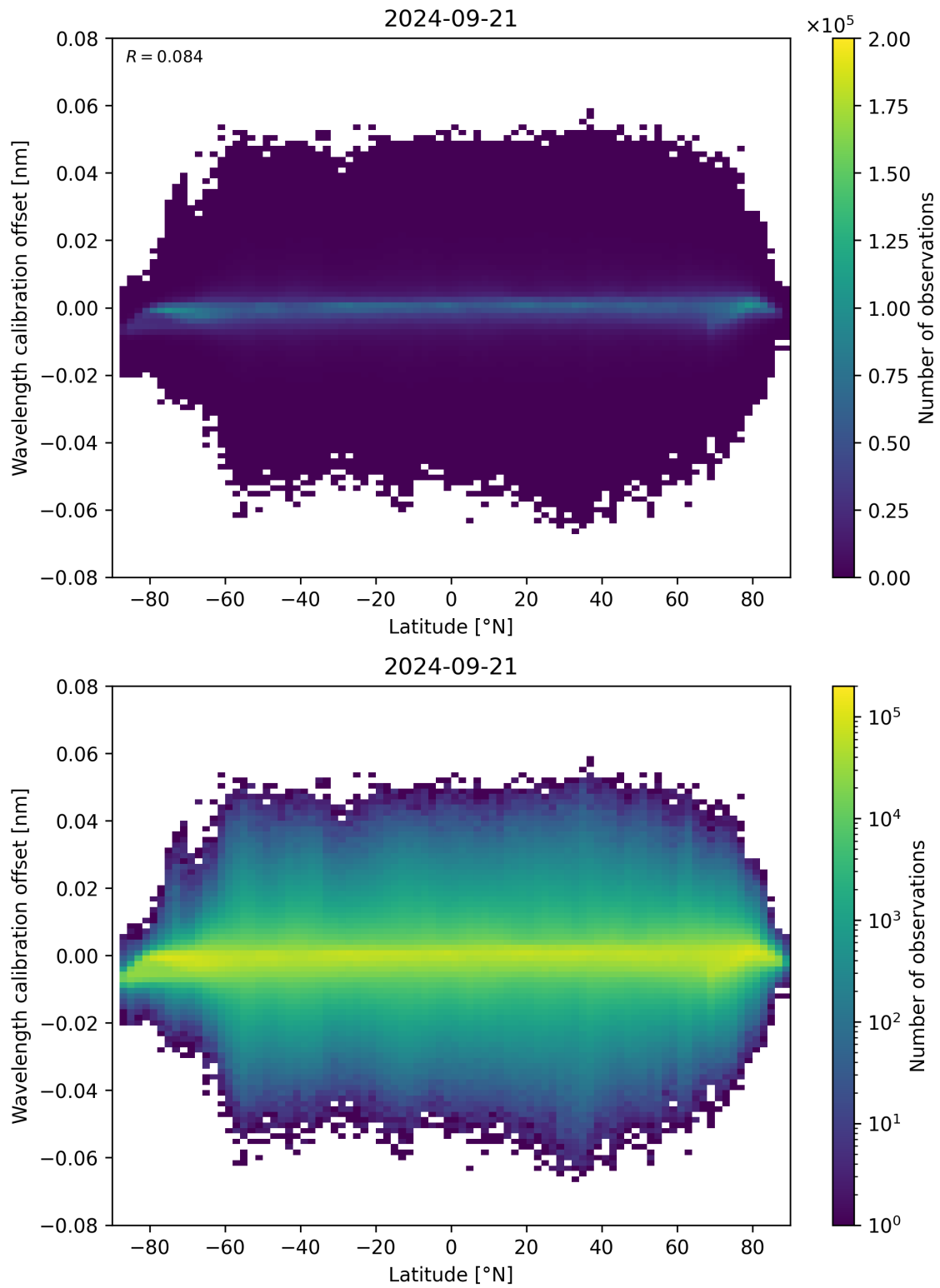
Figure 95: Scatter density plot of “Latitude” against “Wavelength calibration offset” for 2024-09-20 to 2024-09-22.
