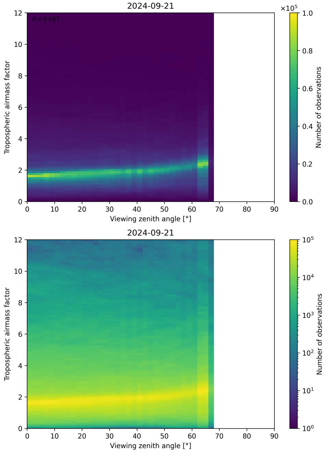
Figure 161: Scatter density plot of “Viewing zenith angle” against “Tropospheric airmass factor” for 2024-09-20 to 2024-09-22.
