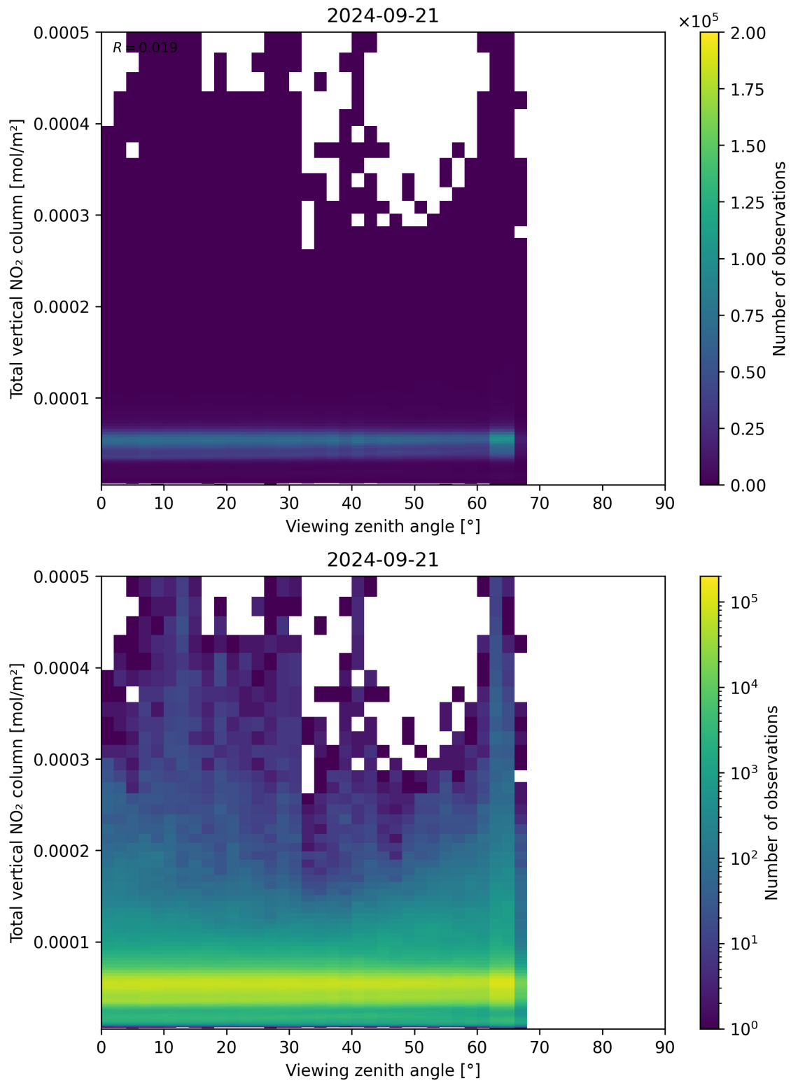
Figure 167: Scatter density plot of “Viewing zenith angle” against “Total vertical NO 2 column” for 2024-09-20 to 2024-09-22.
