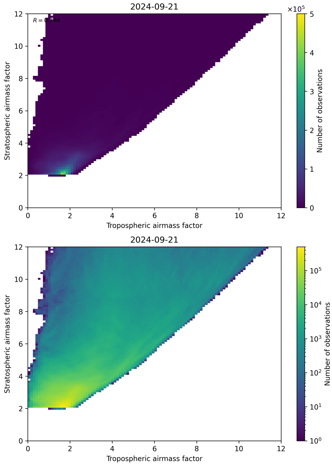
Figure 71: Scatter density plot of “Tropospheric airmass factor” against “Stratospheric airmass factor” for 2024-09-20 to 2024-09-22.
