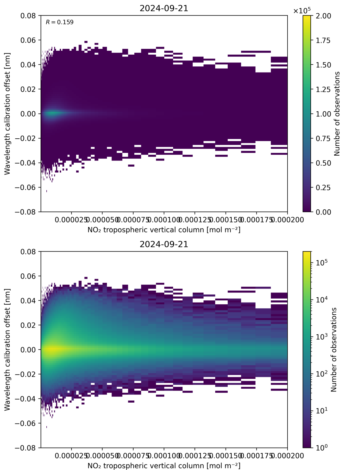
Figure 143: Scatter density plot of “NO 2 tropospheric vertical column” against “Wavelength calibration offset” for 2024-09-20 to 2024-09-22.
