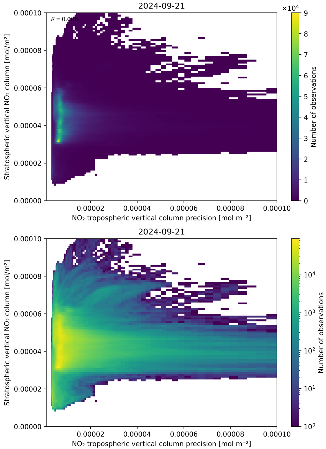
Figure 135: Scatter density plot of “NO 2 tropospheric vertical column precision” against “Stratospheric vertical NO 2 column” for 2024-09-20 to 2024-09-22.
