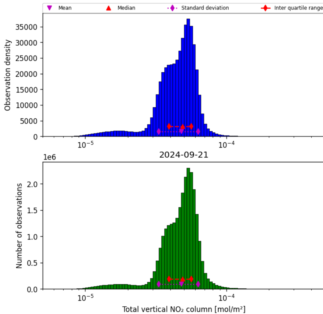
Figure 38: Histogram of “Total vertical NO 2 column” for 2024-09-20 to 2024-09-22
