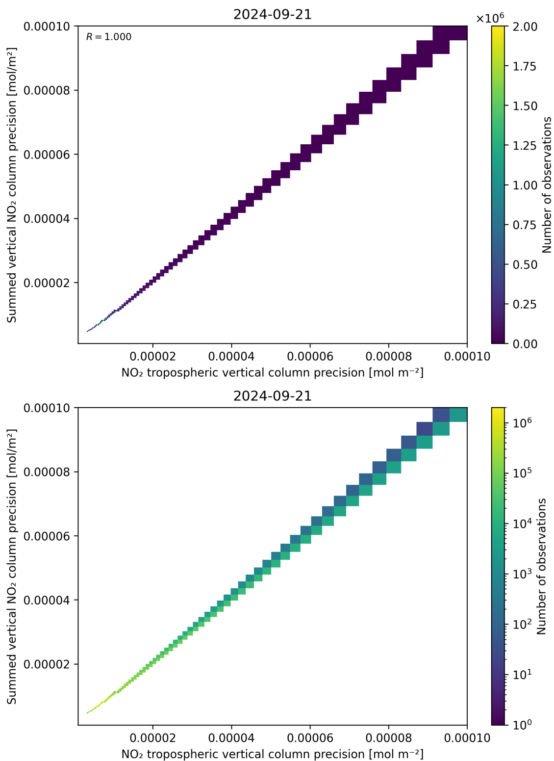
Figure 137: Scatter density plot of “NO 2 tropospheric vertical column precision” against “Summed vertical NO 2 column precision” for 2024-09-20 to 2024-09-22.
