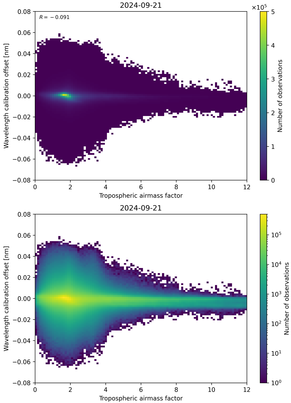
Figure 80: Scatter density plot of “Tropospheric airmass factor” against “Wavelength calibration offset” for 2024-09-20 to 2024-09-22.
