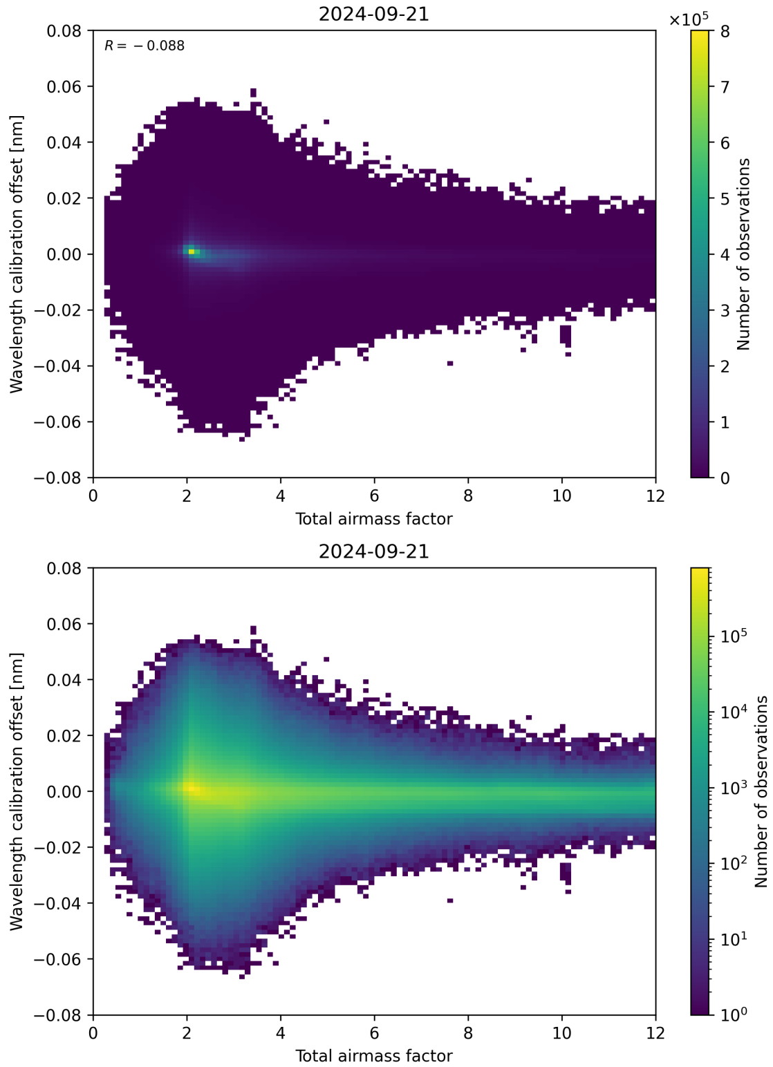
Figure 70: Scatter density plot of “Total airmass factor” against “Wavelength calibration offset” for 2024-09-20 to 2024-09-22.
