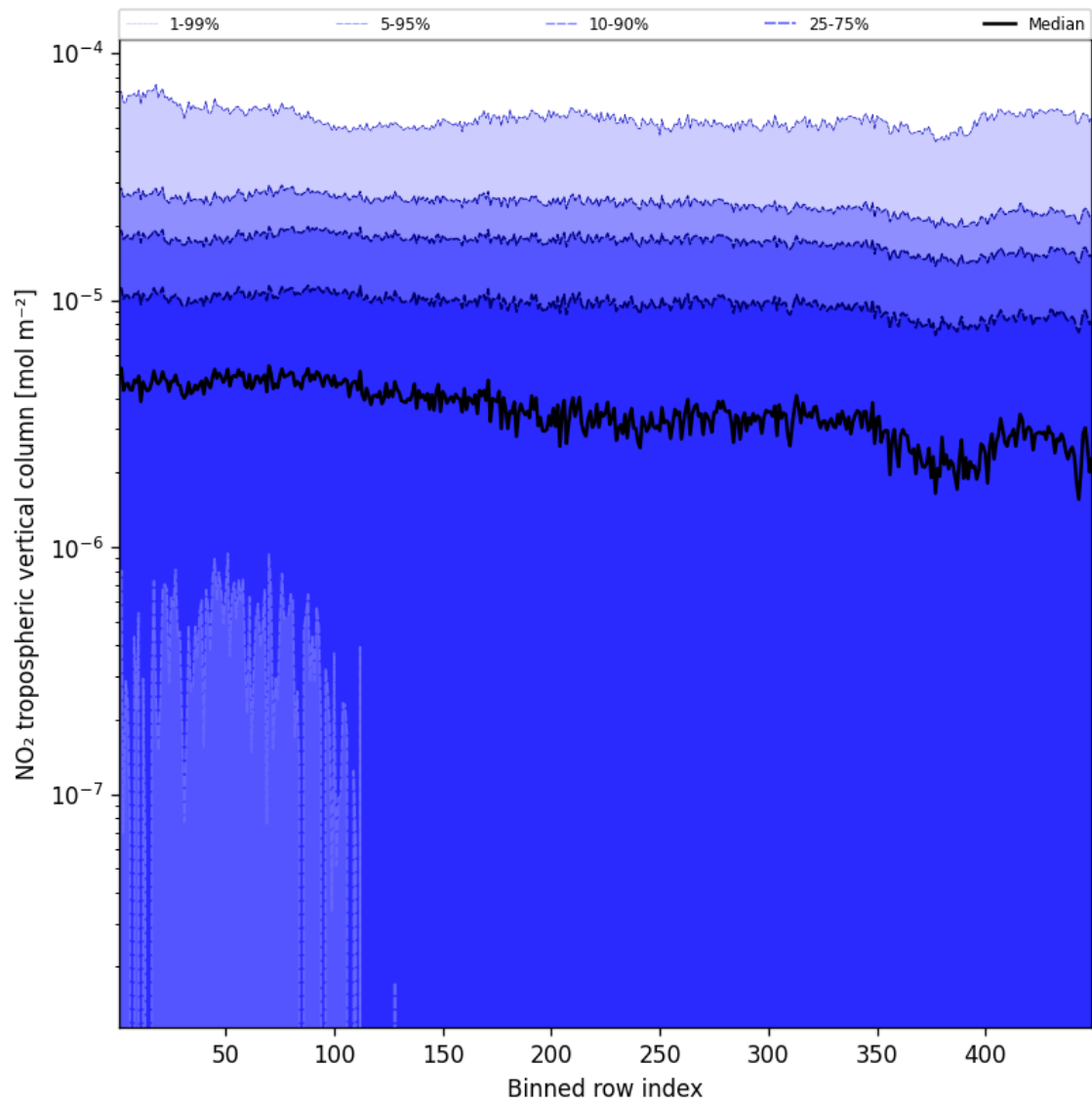
Figure 46: Along track statistics of “NO 2 tropospheric vertical column” for 2024-09-20 to 2024-09-22
