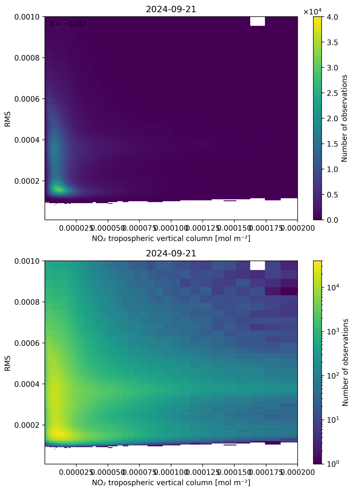
Figure 142: Scatter density plot of “NO 2 tropospheric vertical column” against “RMS” for 2024-09-20 to 2024-09-22.
