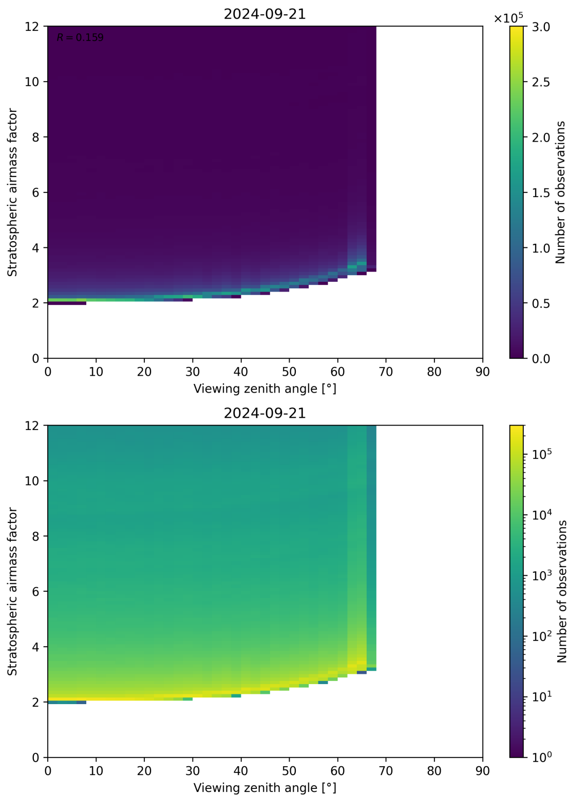
Figure 159: Scatter density plot of “Viewing zenith angle” against “Stratospheric airmass factor” for 2024-09-20 to 2024-09-22.
