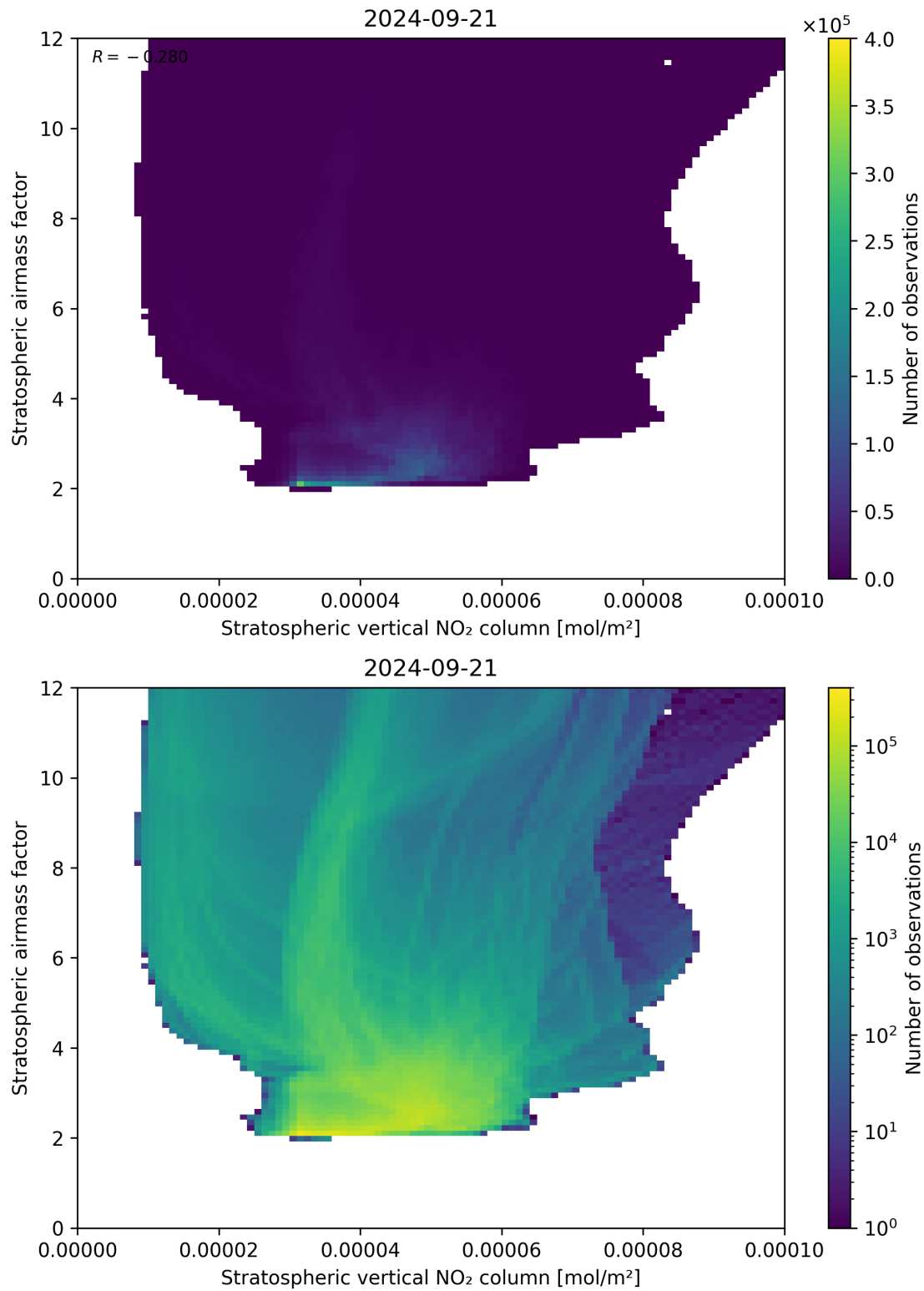
Figure 96: Scatter density plot of “Stratospheric vertical NO 2 column” against “Stratospheric airmass factor” for 2024-09-20 to 2024-09-22.
