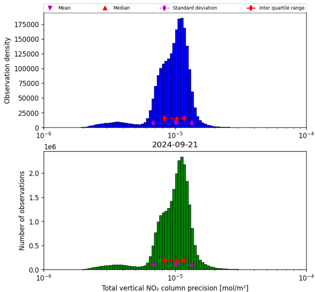
Figure 39: Histogram of “Total vertical NO 2 column precision” for 2024-09-20 to 2024-09-22
