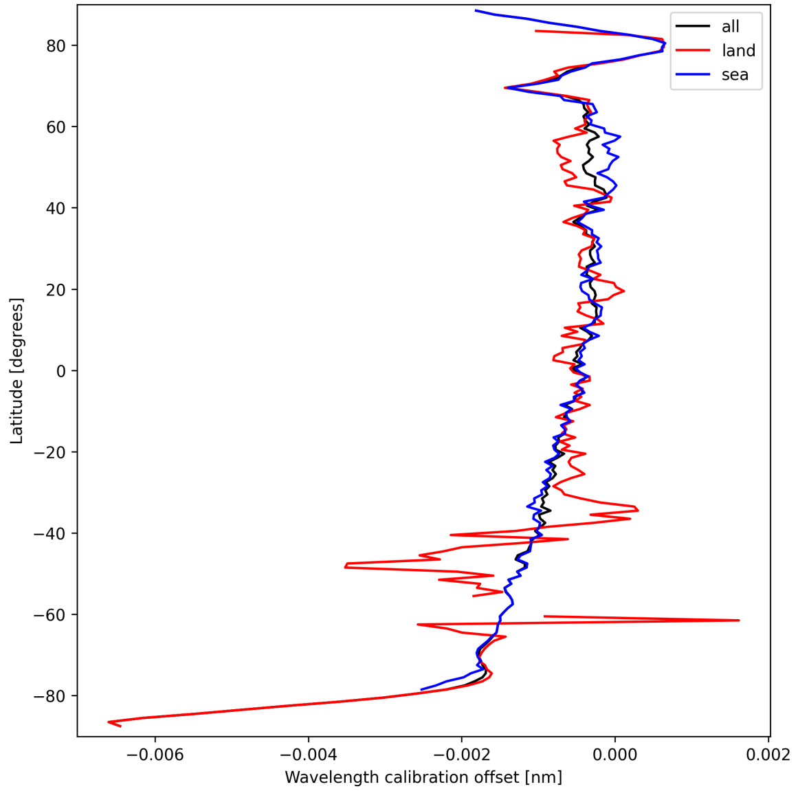
Figure 18: Zonal average of “Wavelength calibration offset” for 2024-09-20 to 2024-09-22.
