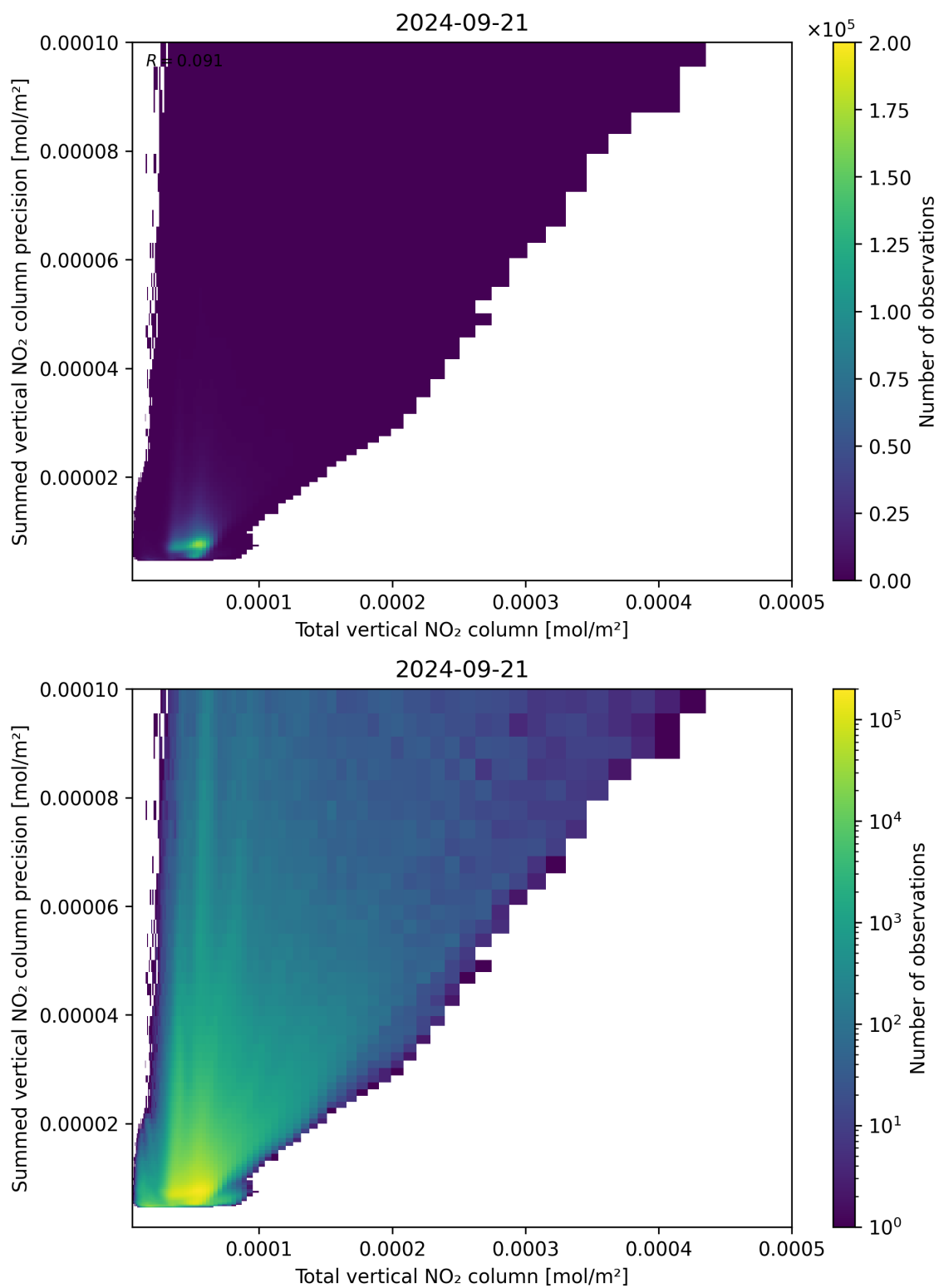
Figure 113: Scatter density plot of “Total vertical NO 2 column” against “Summed vertical NO 2 column precision” for 2024-09-20 to 2024-09-22.
