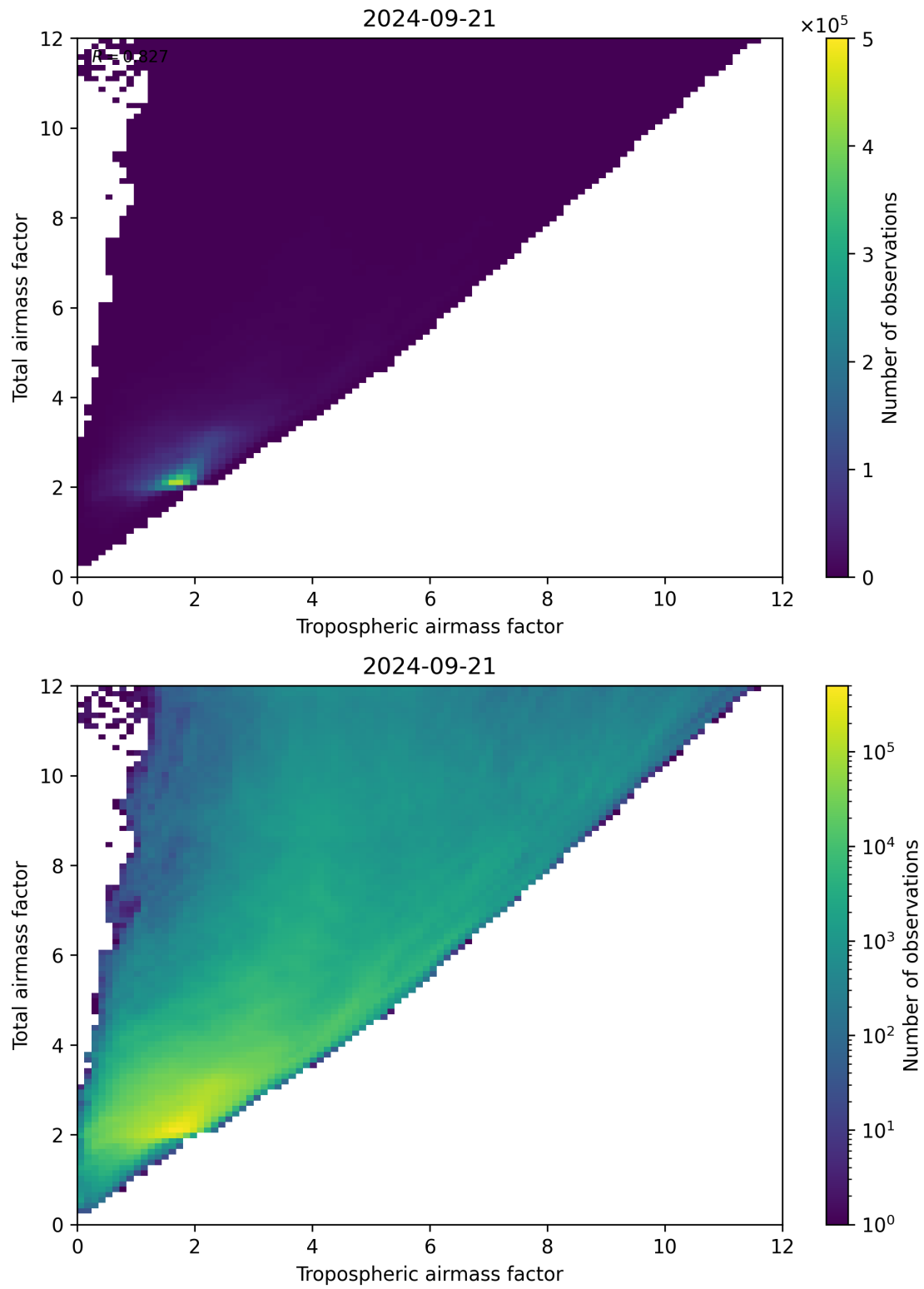
Figure 72: Scatter density plot of “Tropospheric airmass factor” against “Total airmass factor” for 2024-09-20 to 2024-09-22.
