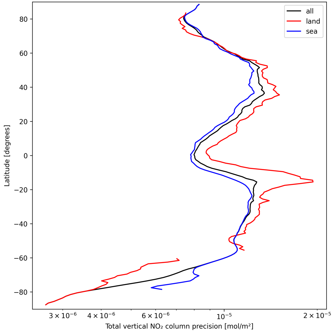
Figure 22: Zonal average of “Total vertical NO 2 column precision” for 2024-09-20 to 2024-09-22.
