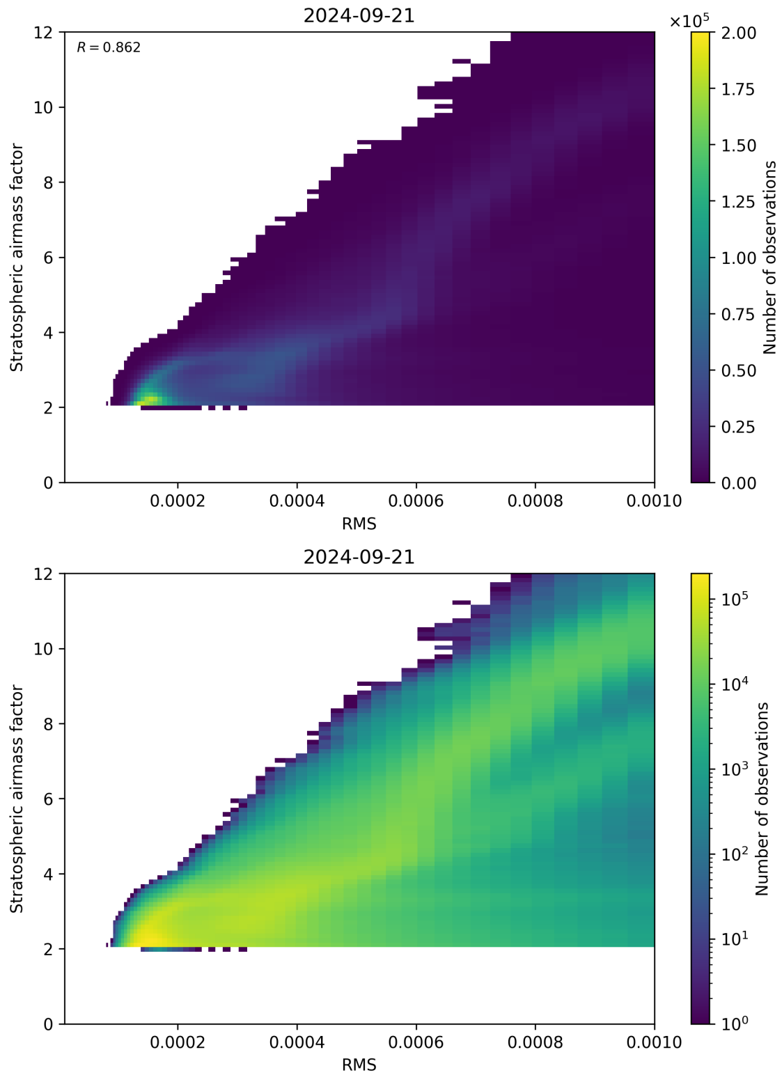
Figure 144: Scatter density plot of “RMS” against “Stratospheric airmass factor” for 2024-09-20 to 2024-09-22.
