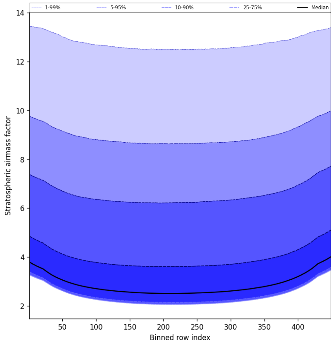
Figure 61: Along track statistics of “Stratospheric airmass factor” for 2024-09-20 to 2024-09-22
