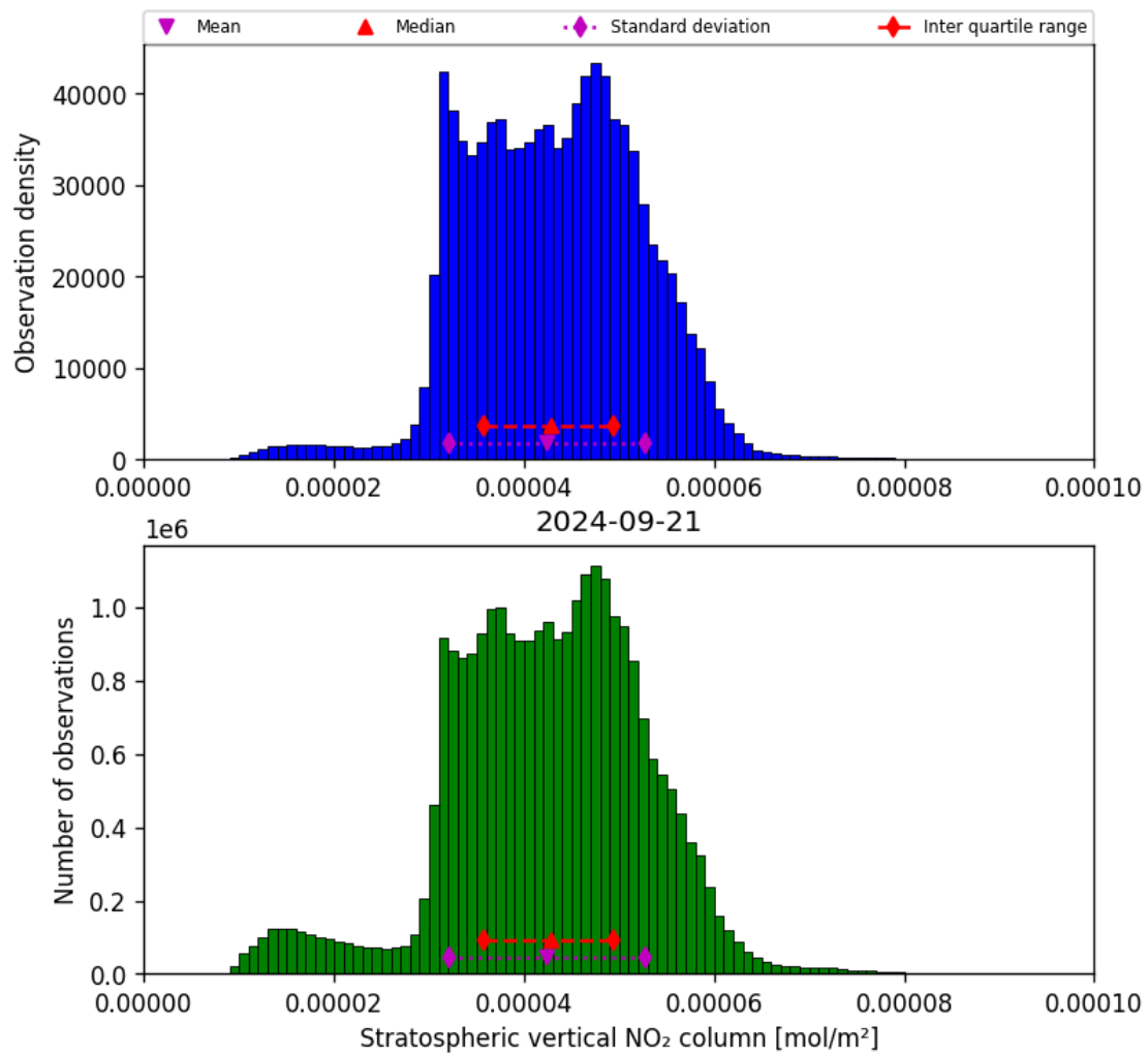
Figure 36: Histogram of “Stratospheric vertical NO 2 column” for 2024-09-20 to 2024-09-22
