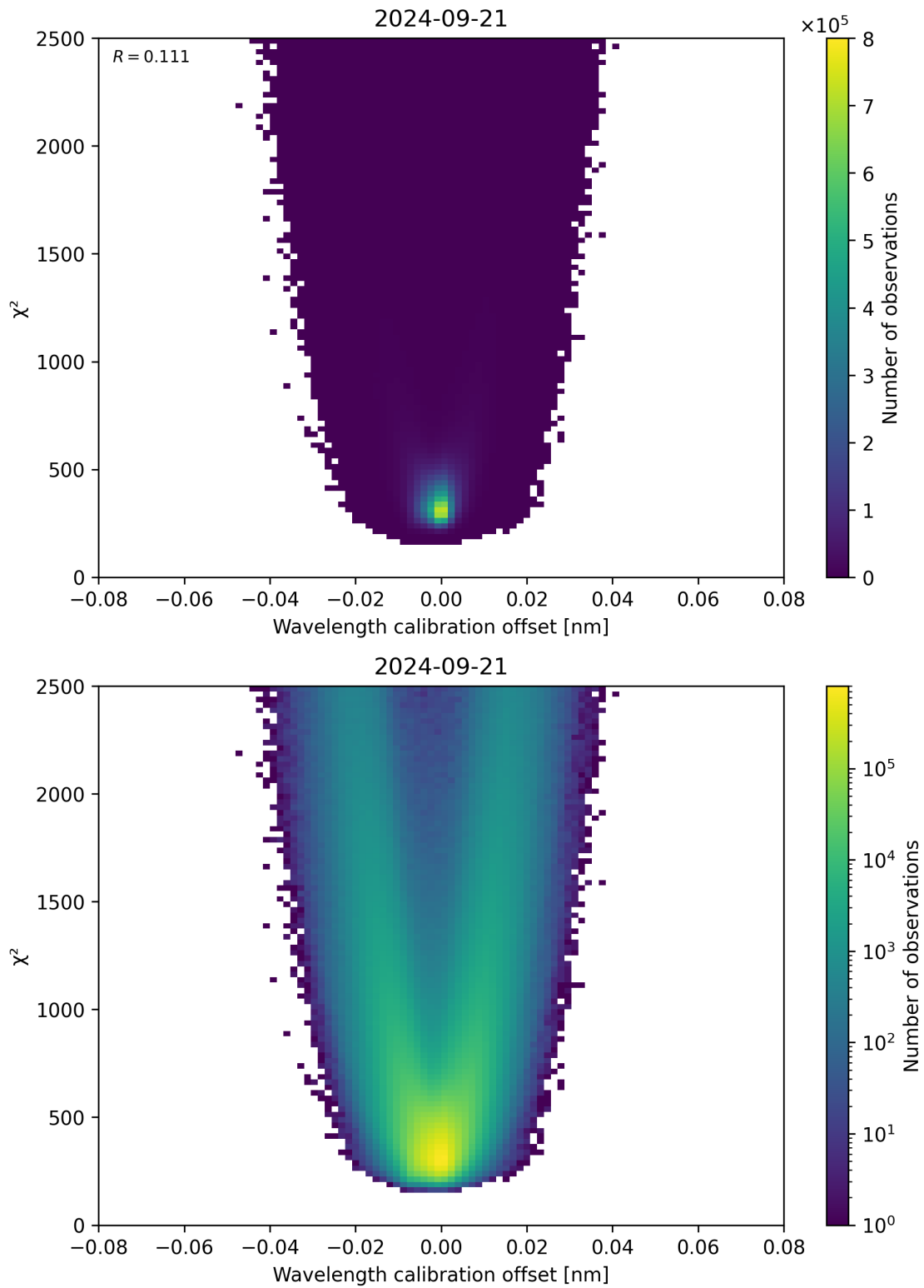
Figure 175: Scatter density plot of “Wavelength calibration offset” against “ \chi^2 ” for 2024-09-20 to 2024-09-22.
