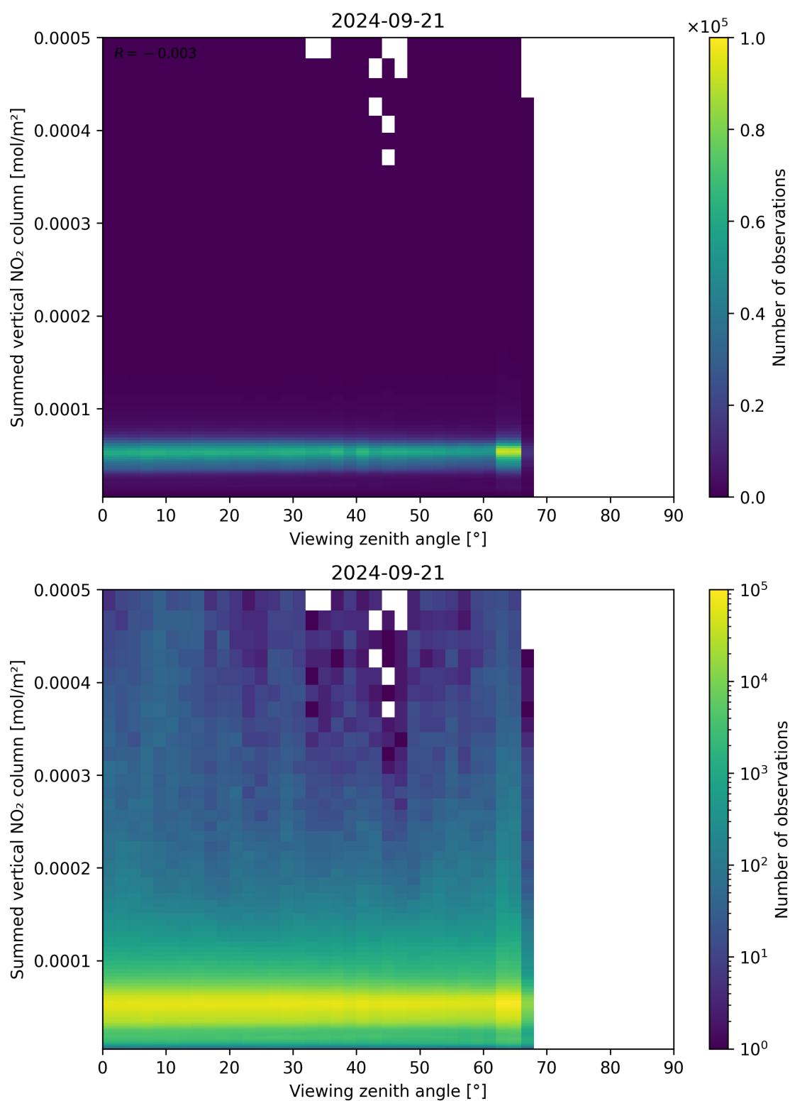
Figure 165: Scatter density plot of “Viewing zenith angle” against “Summed vertical NO 2 column” for 2024-09-20 to 2024-09-22.
