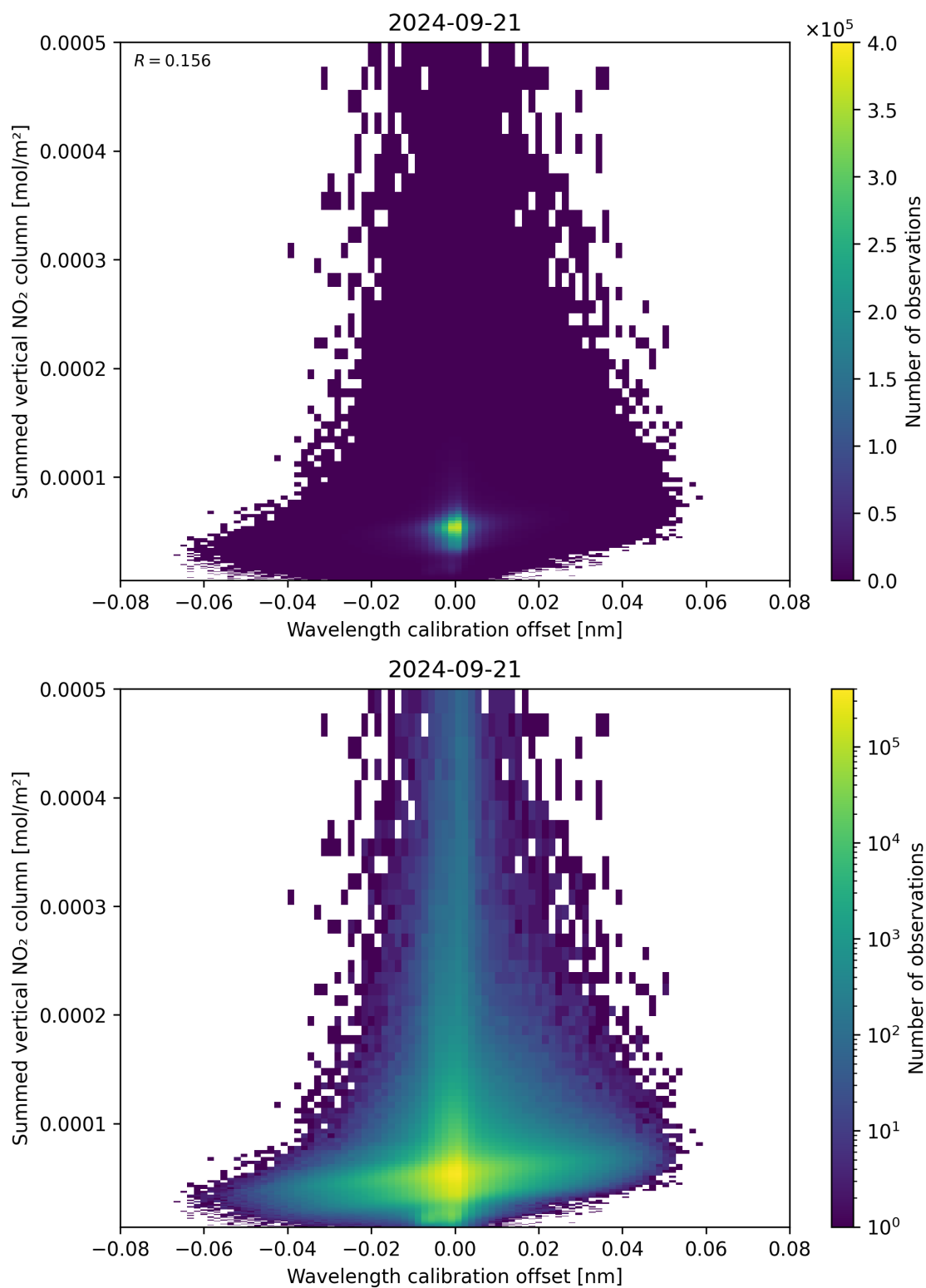
Figure 177: Scatter density plot of “Wavelength calibration offset” against “Summed vertical NO 2 column” for 2024-09-20 to 2024-09-22.
