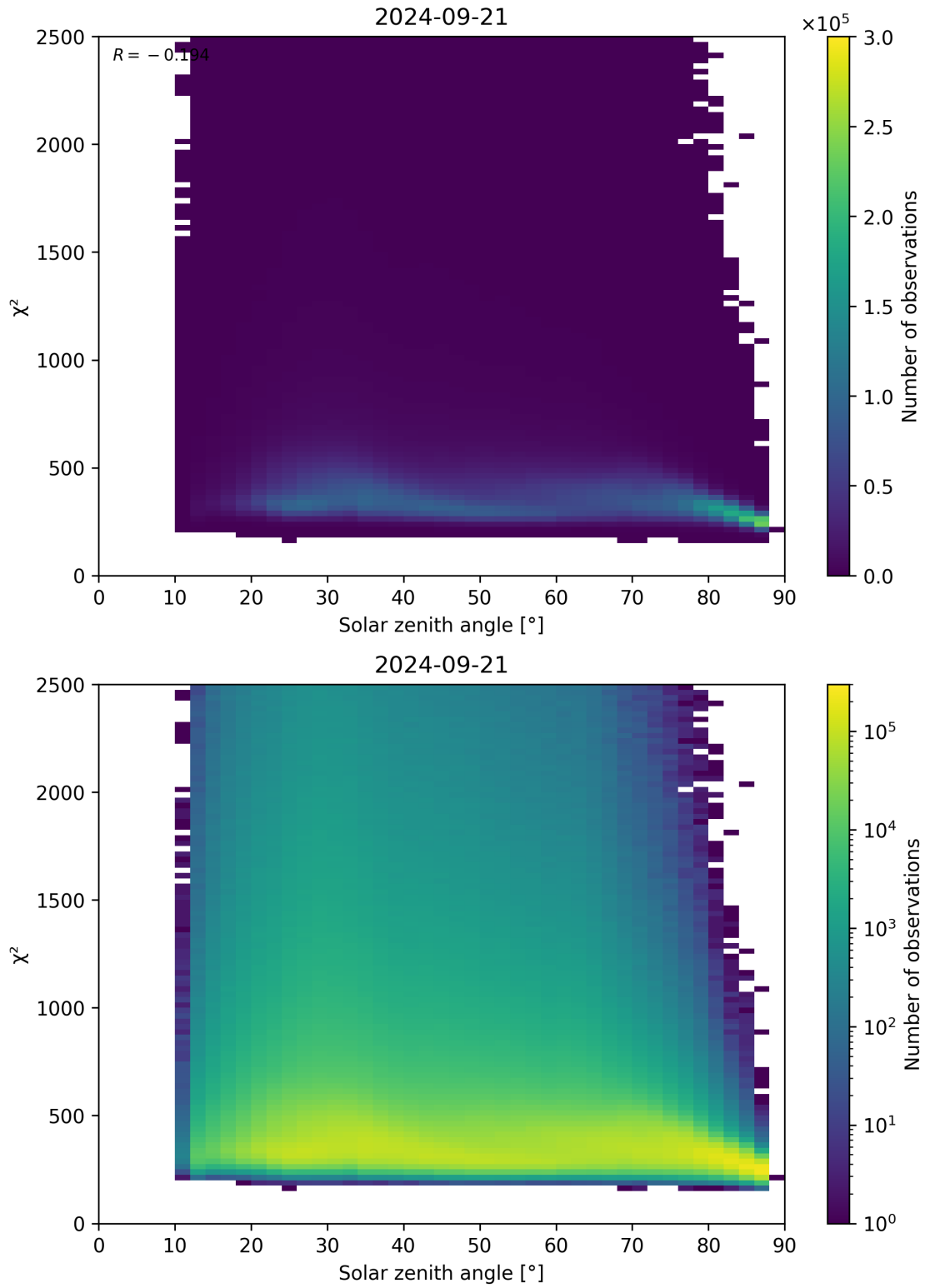
Figure 148: Scatter density plot of “Solar zenith angle” against “ \chi^2 ” for 2024-09-20 to 2024-09-22.
