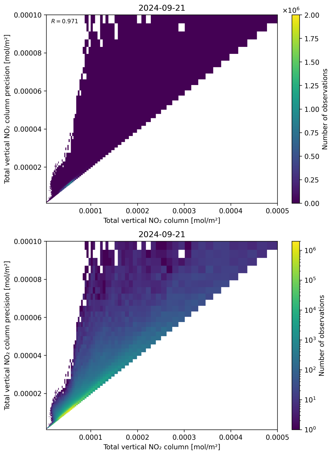
Figure 114: Scatter density plot of “Total vertical NO 2 column” against “Total vertical NO 2 column precision” for 2024-09-20 to 2024-09-22.
