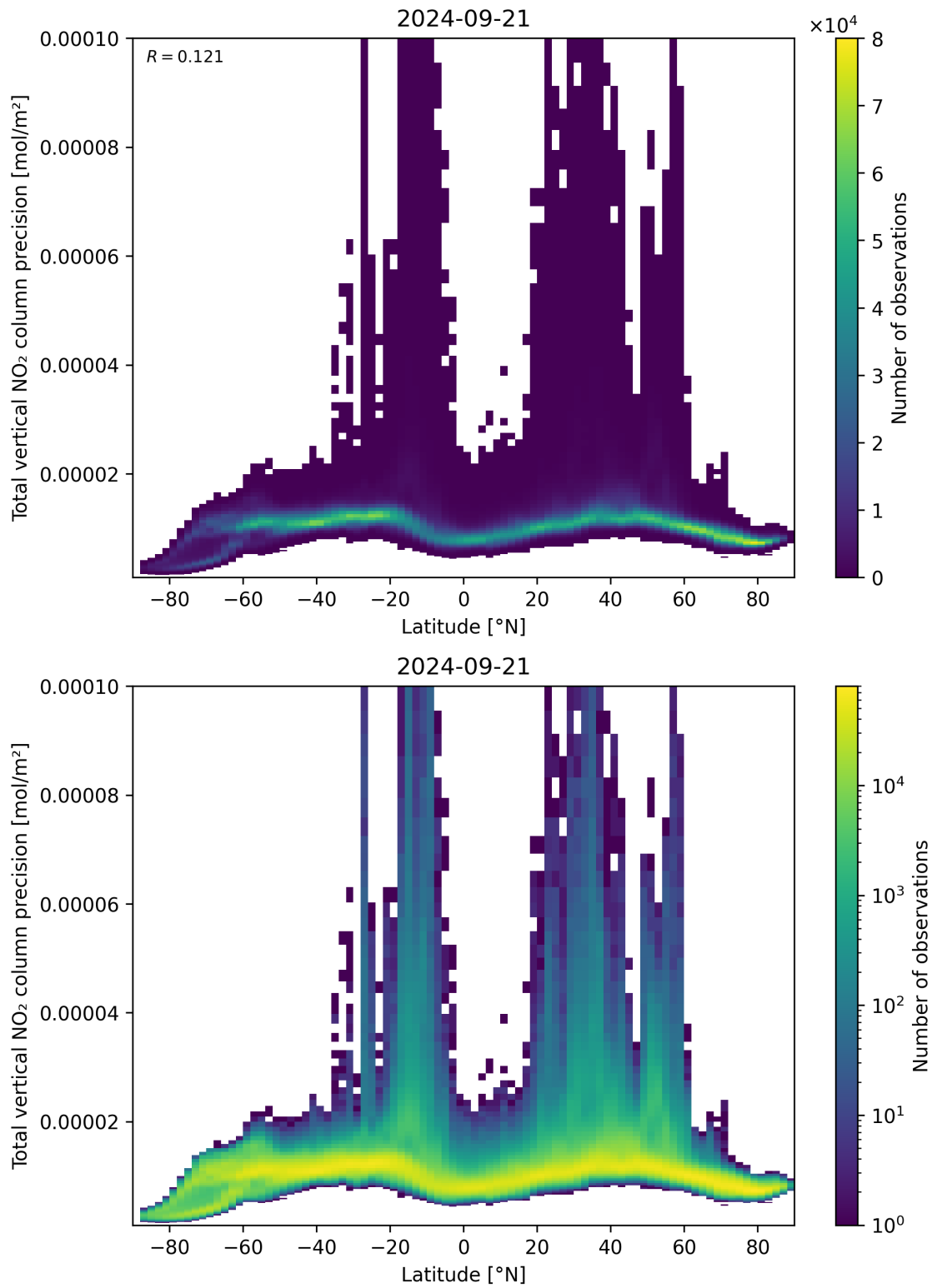
Figure 91: Scatter density plot of “Latitude” against “Total vertical NO 2 column precision” for 2024-09-20 to 2024-09-22.
