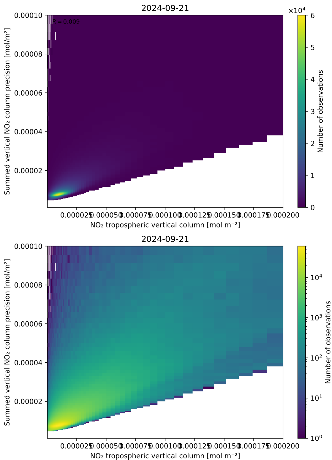
Figure 127: Scatter density plot of “NO 2 tropospheric vertical column” against “Summed vertical NO 2 column precision” for 2024-09-20 to 2024-09-22.
