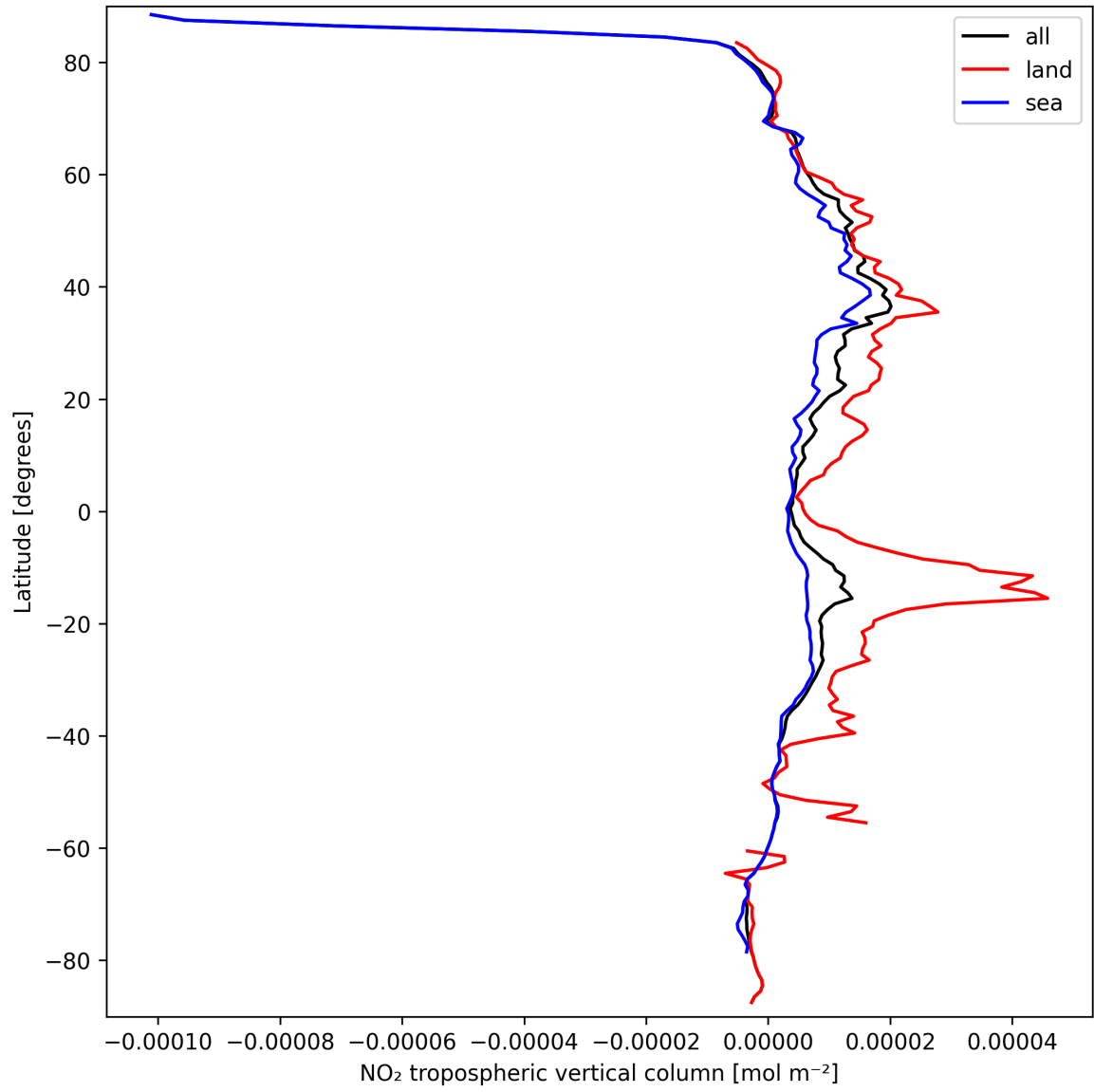
Figure 12: Zonal average of “NO 2 tropospheric vertical column” for 2024-09-20 to 2024-09-22.
