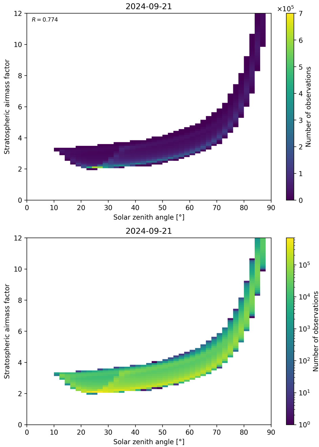
Figure 145: Scatter density plot of “Solar zenith angle” against “Stratospheric airmass factor” for 2024-09-20 to 2024-09-22.
