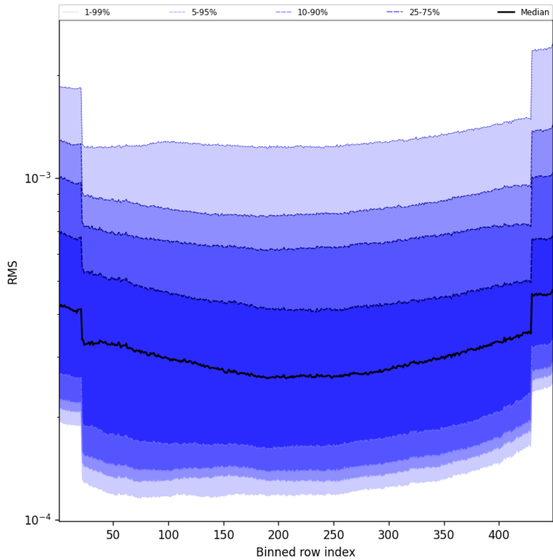
Figure 60: Along track statistics of “RMS” for 2024-09-20 to 2024-09-22
