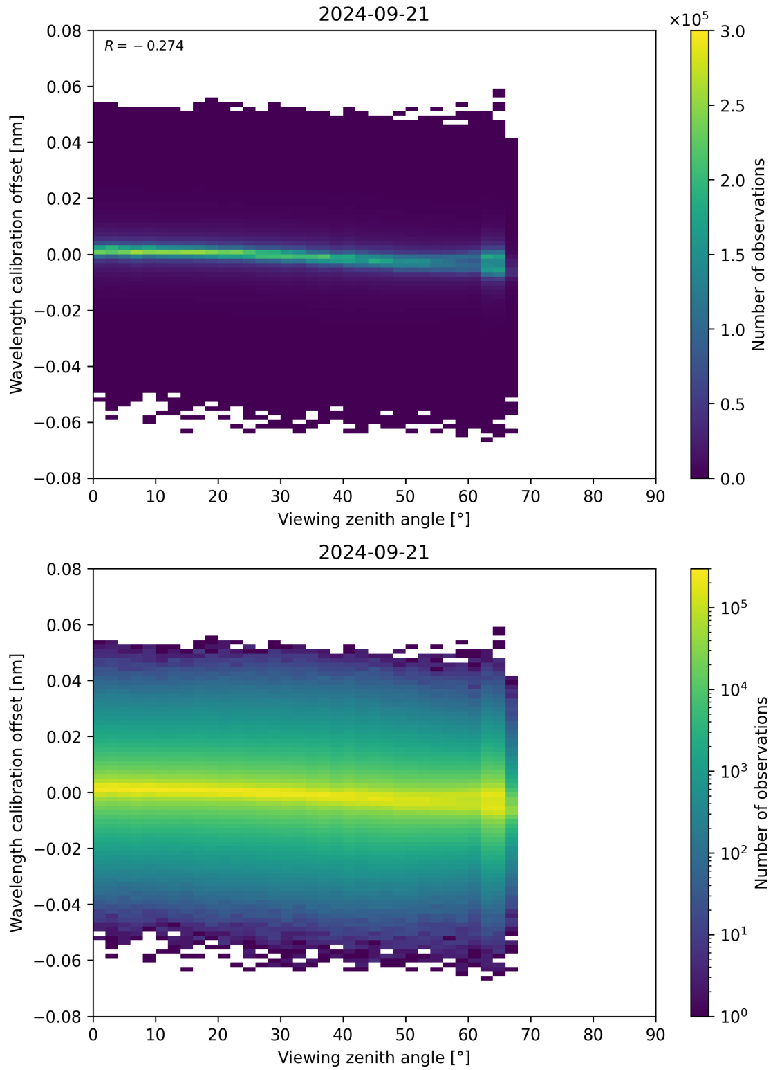
Figure 173: Scatter density plot of “Viewing zenith angle” against “Wavelength calibration offset” for 2024-09-20 to 2024-09-22.
