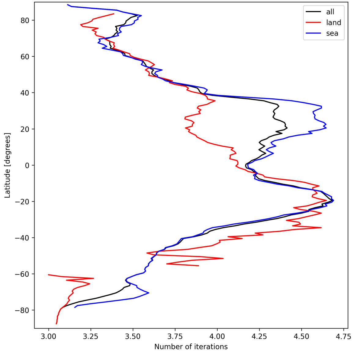
Figure 17: Zonal average of “Number of iterations” for 2024-09-20 to 2024-09-22.
