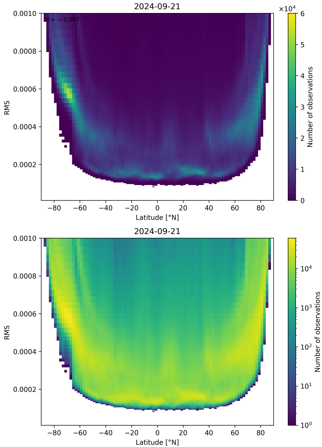
Figure 94: Scatter density plot of “Latitude” against “RMS” for 2024-09-20 to 2024-09-22.
