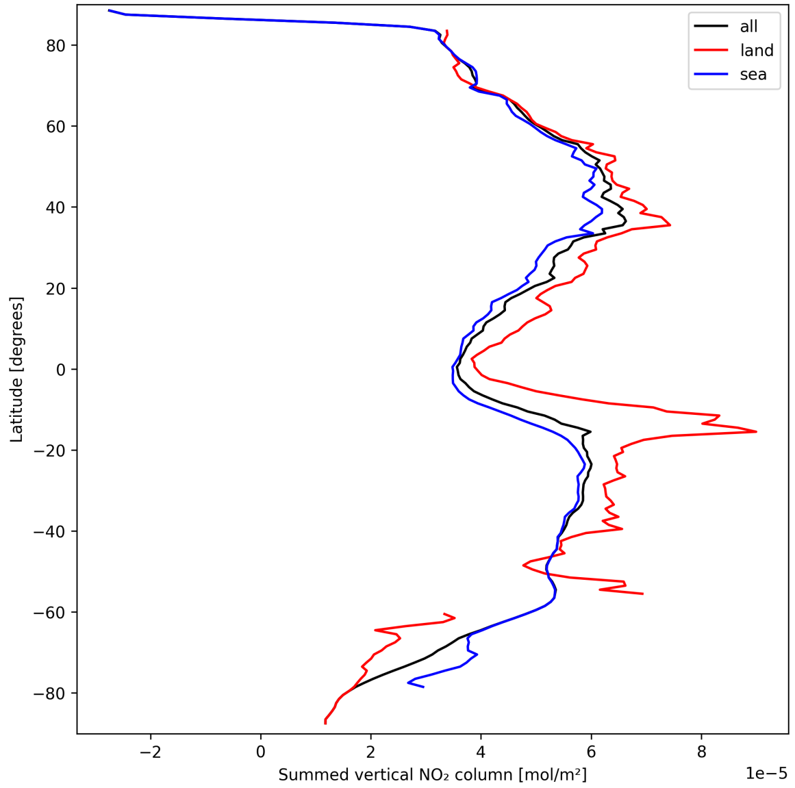
Figure 23: Zonal average of “Summed vertical NO 2 column” for 2024-09-20 to 2024-09-22.
