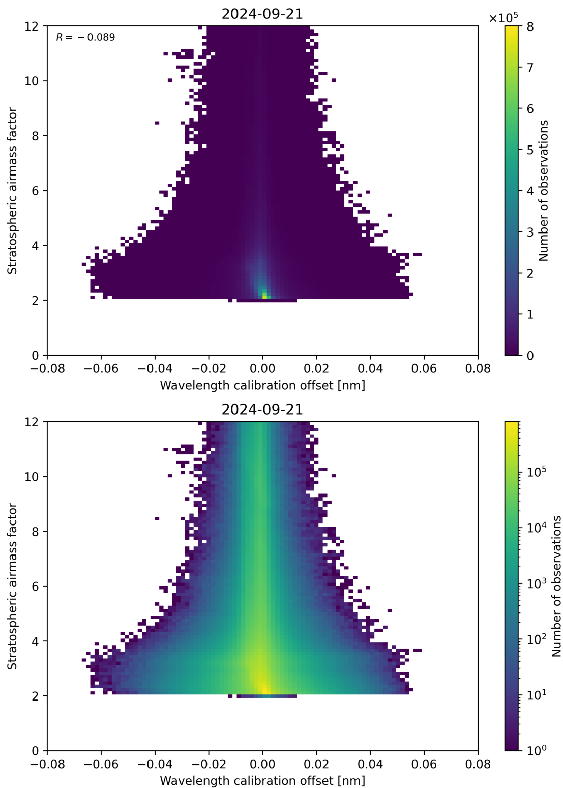
Figure 174: Scatter density plot of “Wavelength calibration offset” against “Stratospheric air mass factor” for 2024-09-20 to 2024-09-22.
