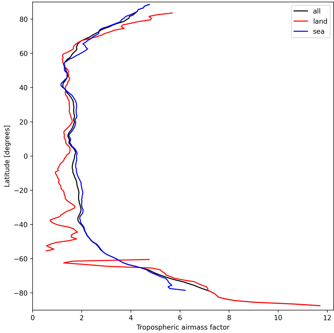
Figure 14: Zonal average of “Tropospheric airmass factor” for 2024-09-20 to 2024-09-22.
