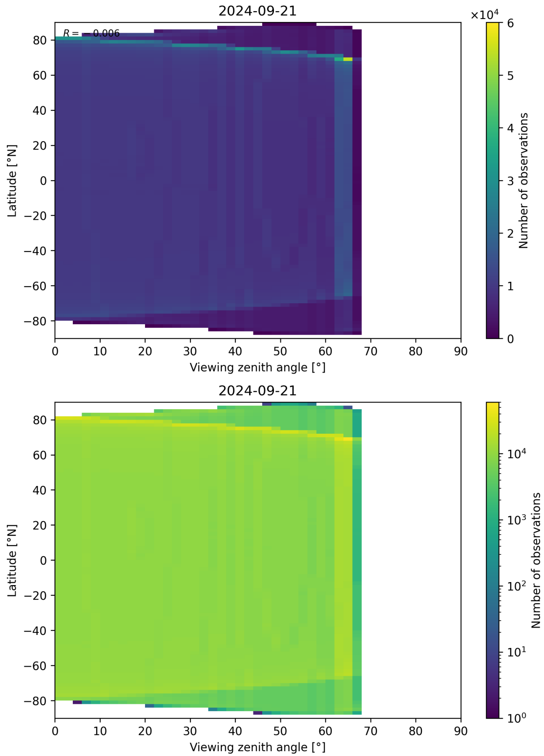
Figure 163: Scatter density plot of “Viewing zenith angle” against “Latitude” for 2024-09-20 to 2024-09-22.
