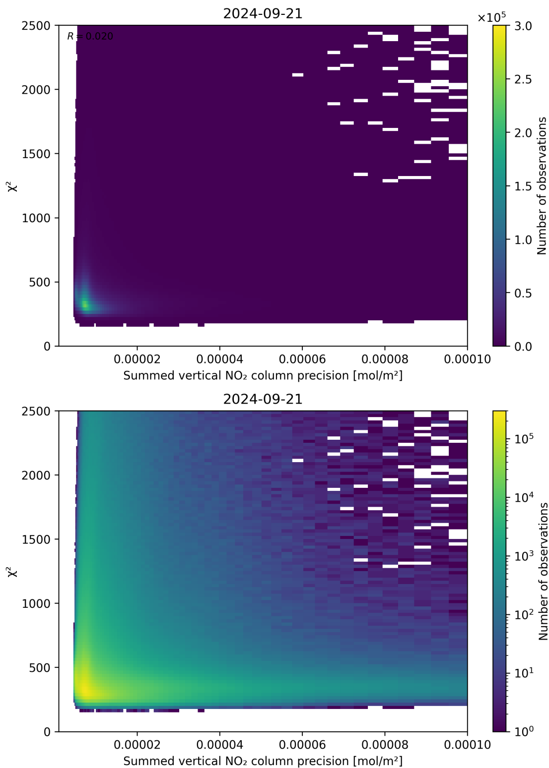
Figure 107: Scatter density plot of “Summed vertical NO 2 column precision” against “ \chi^2 ” for 2024-09-20 to 2024-09-22.
