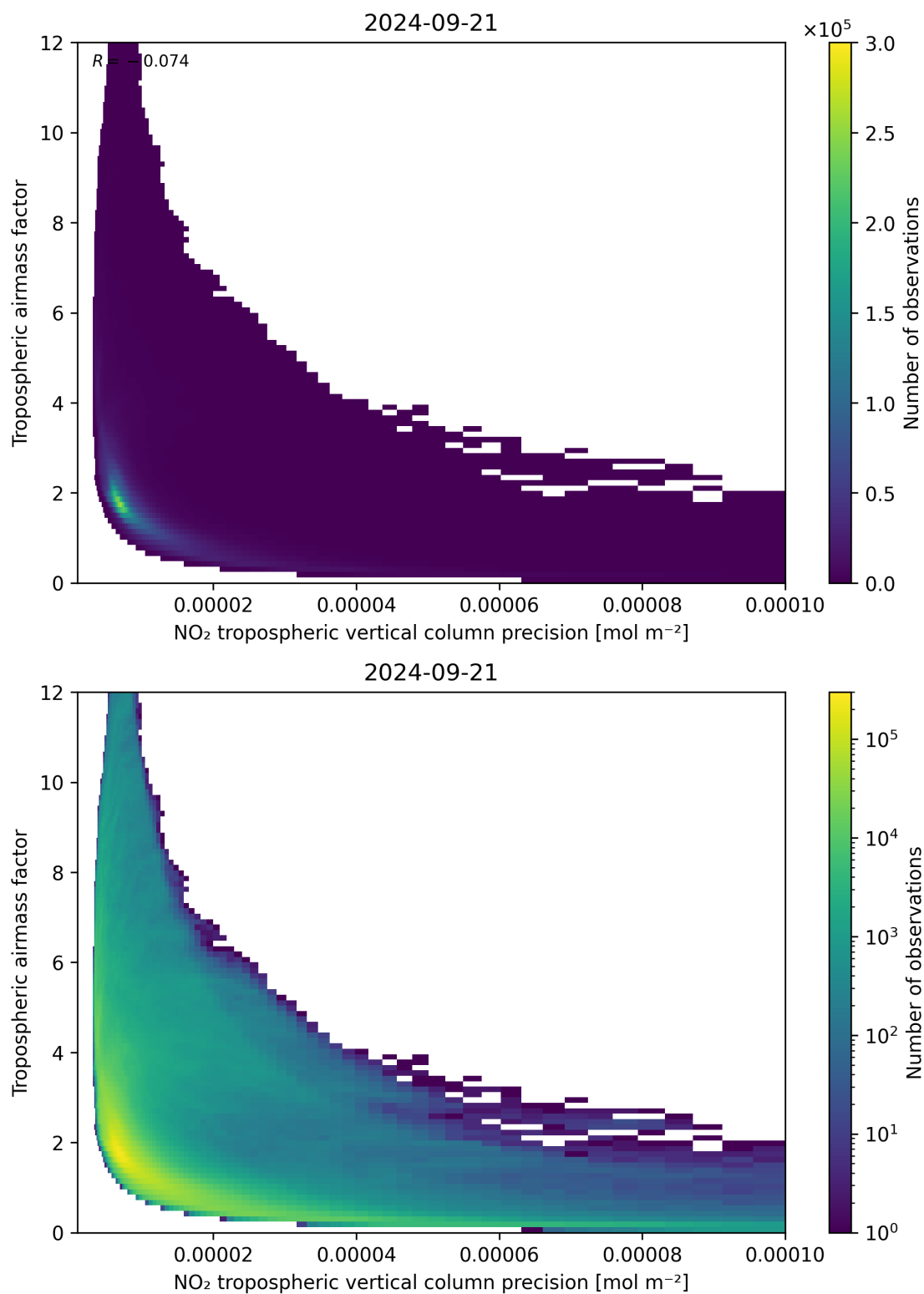
Figure 133: Scatter density plot of “NO 2 tropospheric vertical column precision” against “Tropospheric airmass factor” for 2024-09-20 to 2024-09-22.
