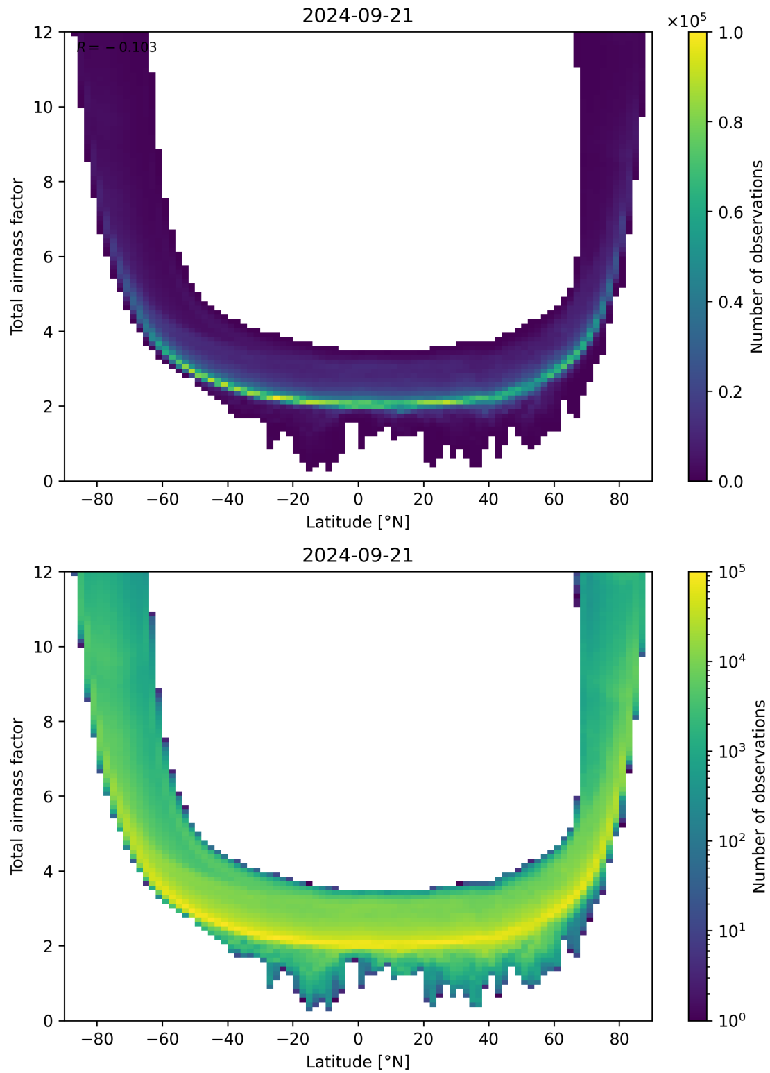
Figure 84: Scatter density plot of “Latitude” against “Total airmass factor” for 2024-09-20 to 2024-09-22.
