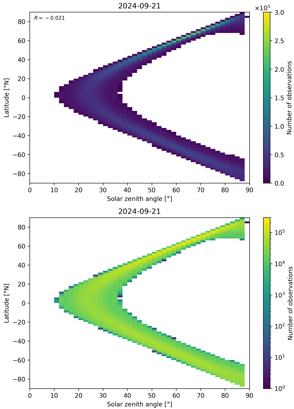
Figure 149: Scatter density plot of “Solar zenith angle” against “Latitude” for 2024-09-20 to 2024-09-22.
