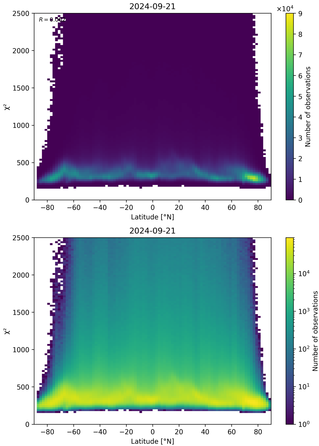
Figure 86: Scatter density plot of “Latitude” against “ \chi^2 ” for 2024-09-20 to 2024-09-22.
