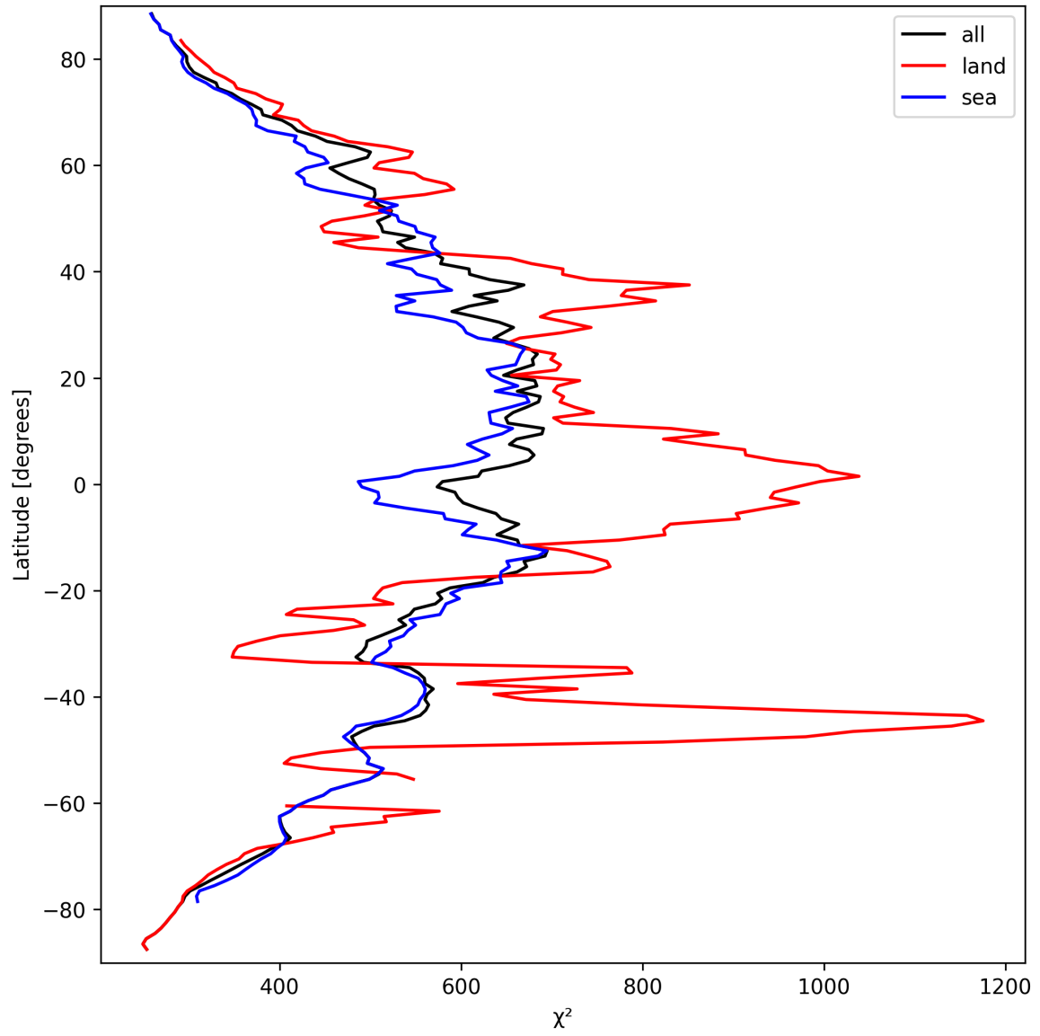
Figure 25: Zonal average of “ \chi^2 ” for 2024-09-20 to 2024-09-22.
