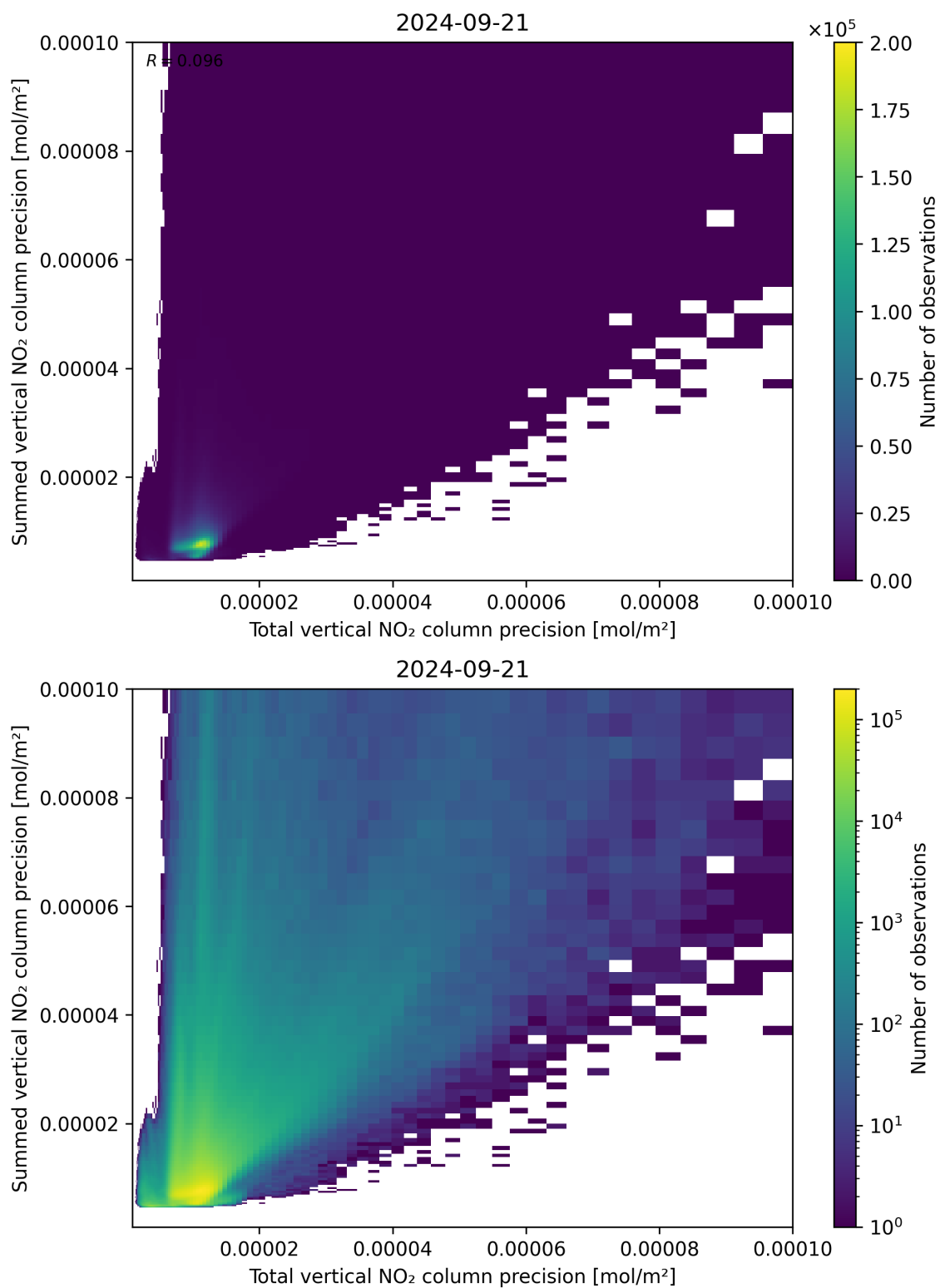
Figure 118: Scatter density plot of “Total vertical NO 2 column precision” against “Summed vertical NO 2 column precision” for 2024-09-20 to 2024-09-22.
