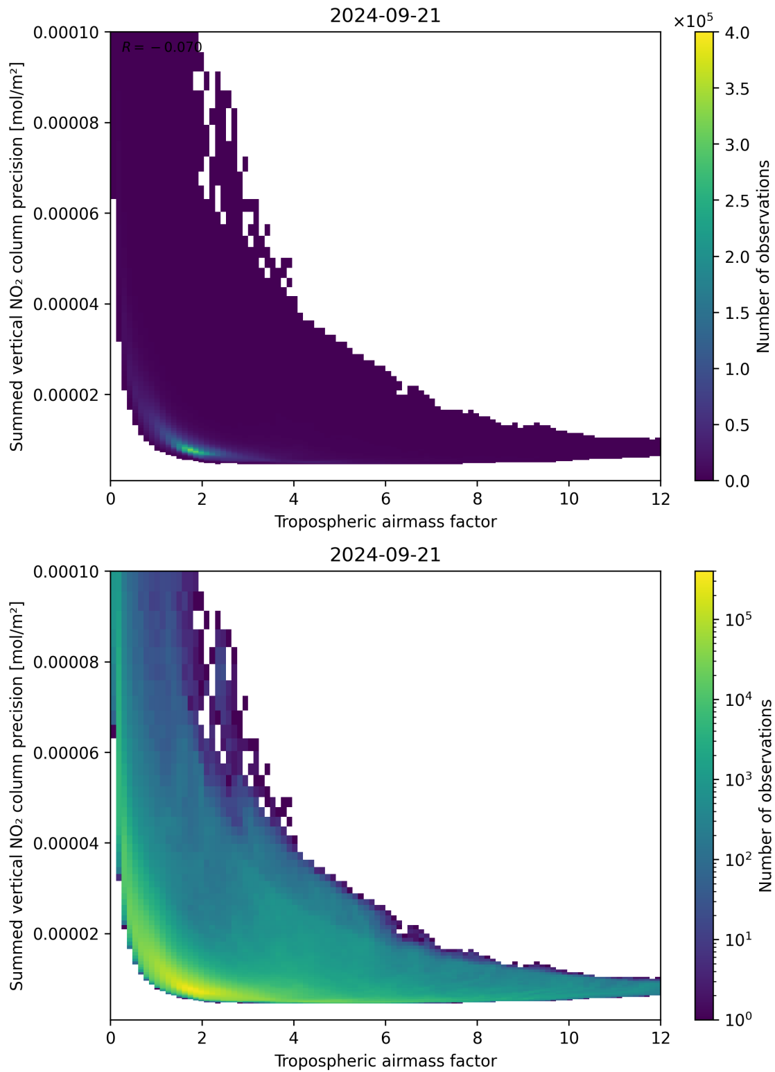
Figure 76: Scatter density plot of “Tropospheric air mass factor” against “Summed vertical NO 2 column precision” for 2024-09-20 to 2024-09-22.
