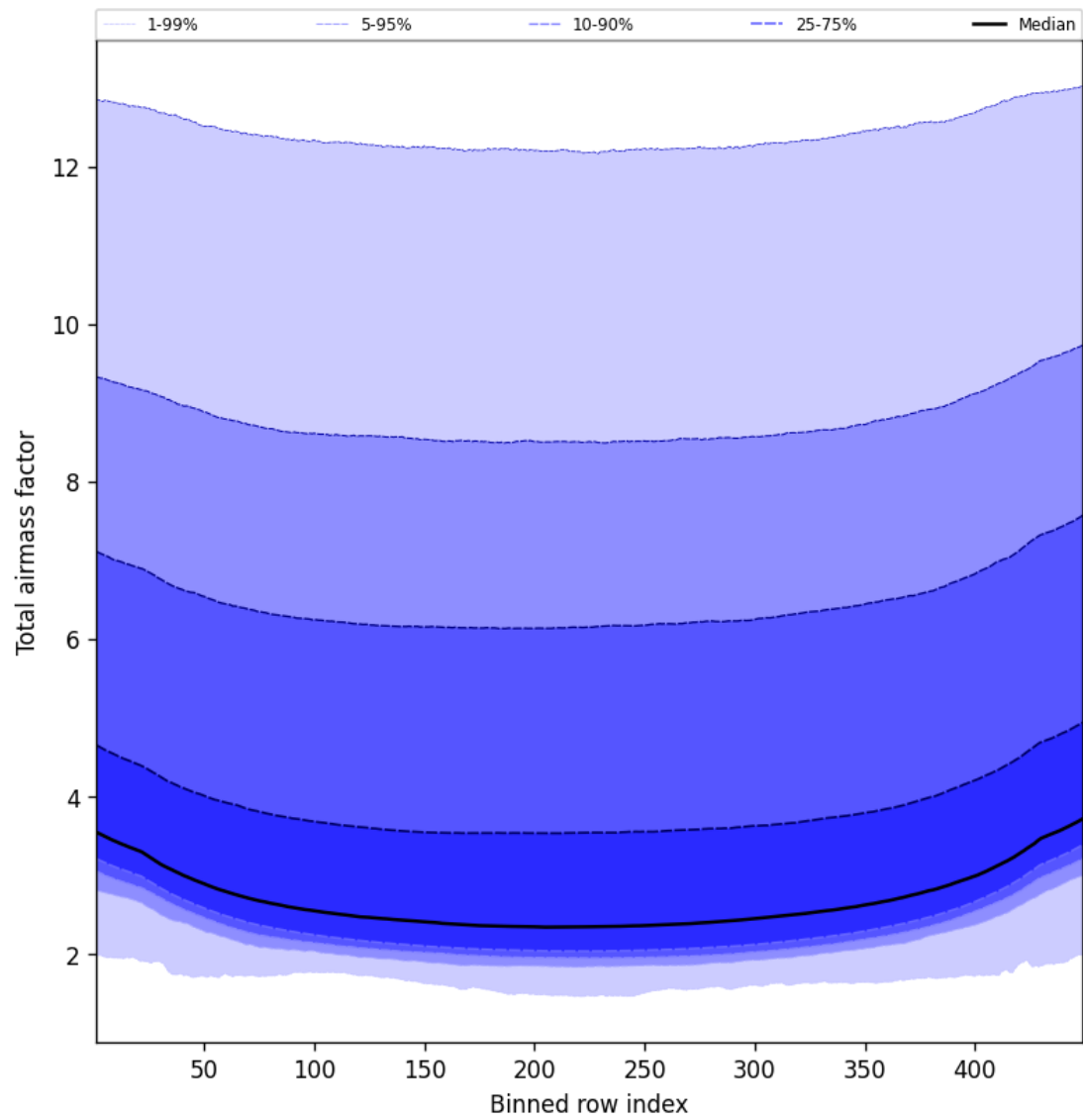
Figure 49: Along track statistics of “Total airmass factor” for 2024-09-20 to 2024-09-22
