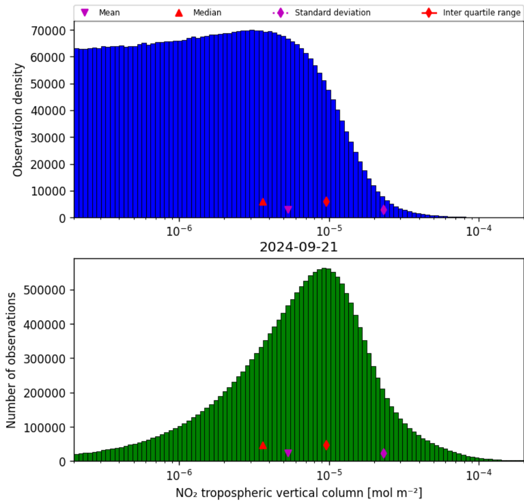
Figure 29: Histogram of “NO 2 tropospheric vertical column” for 2024-09-20 to 2024-09-22
