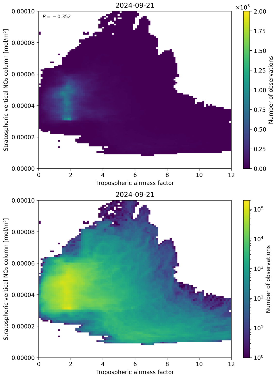
Figure 74: Scatter density plot of “Tropospheric air mass factor” against “Stratospheric vertical NO 2 column” for 2024-09-20 to 2024-09-22.
