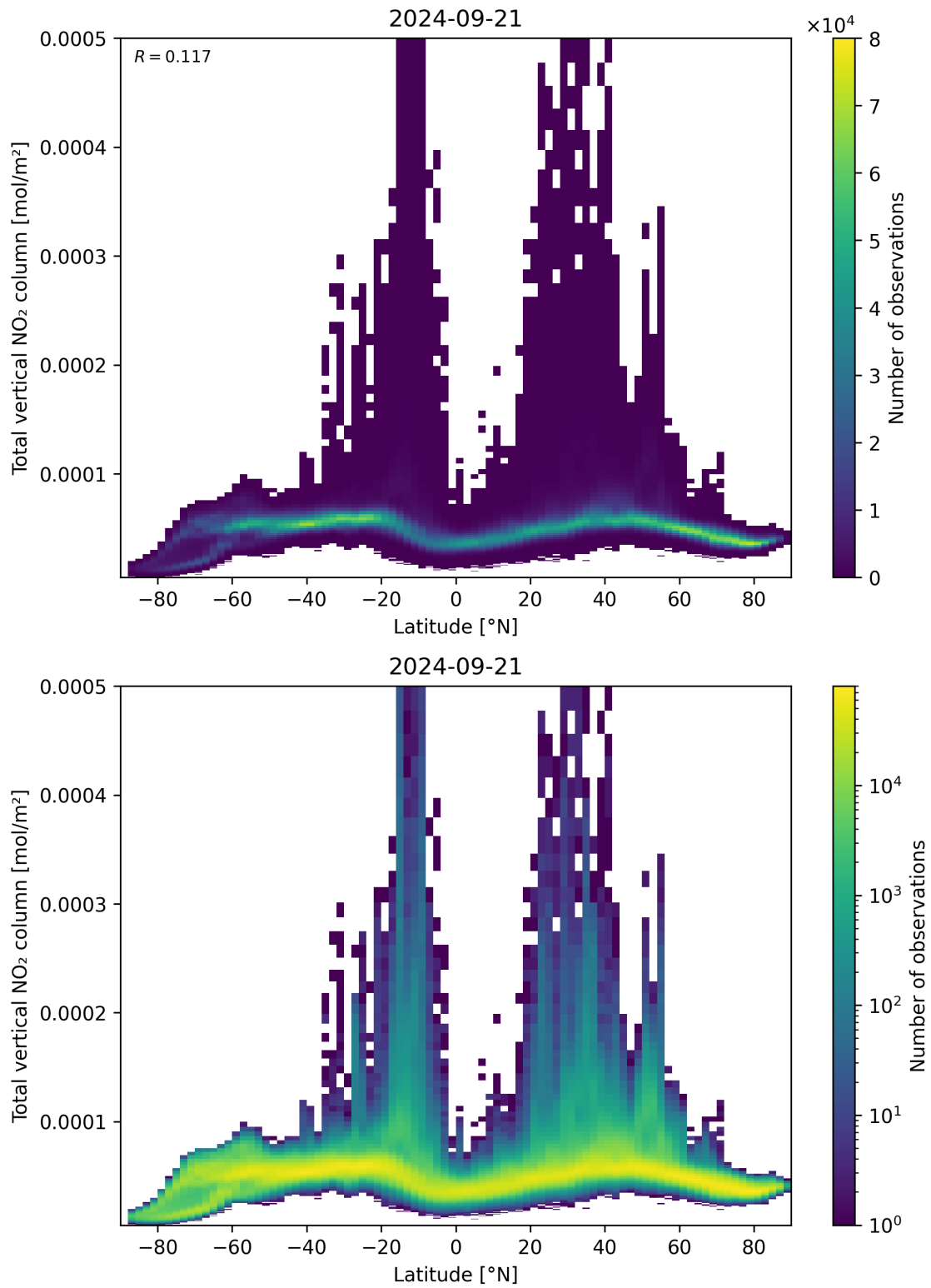
Figure 90: Scatter density plot of “Latitude” against “Total vertical NO 2 column” for 2024-09-20 to 2024-09-22.
