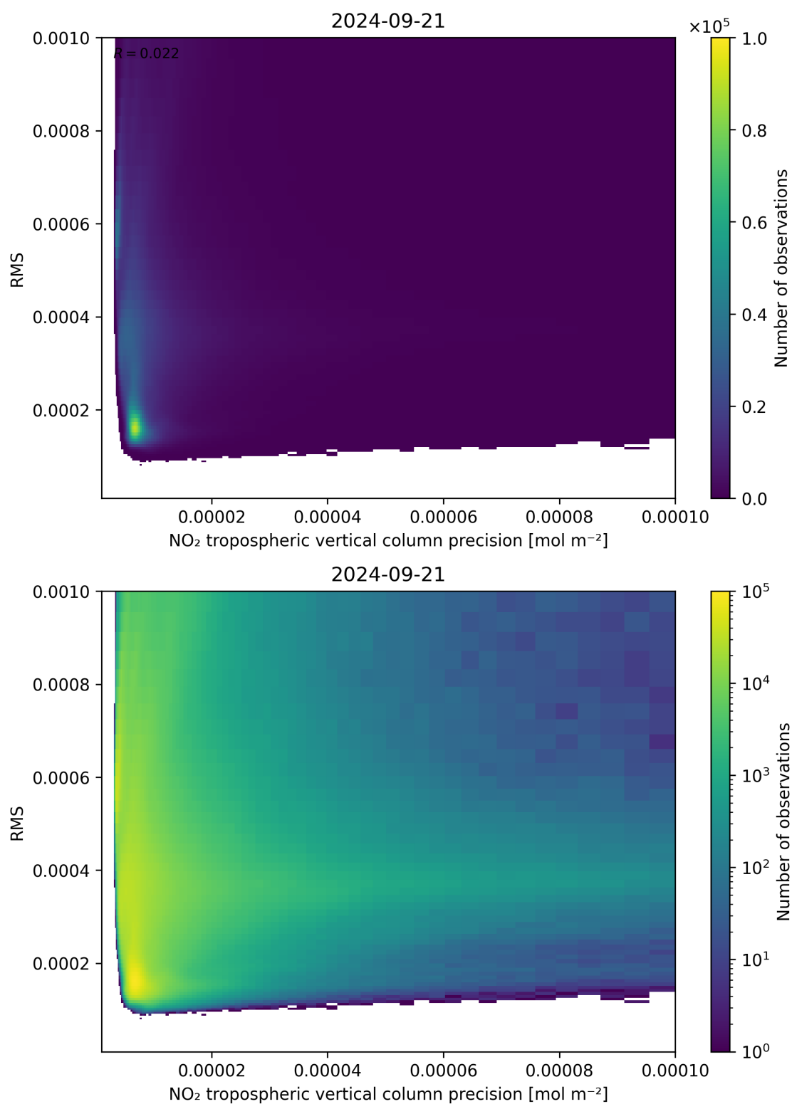
Figure 140: Scatter density plot of “NO 2 tropospheric vertical column precision” against “RMS” for 2024-09-20 to 2024-09-22.
