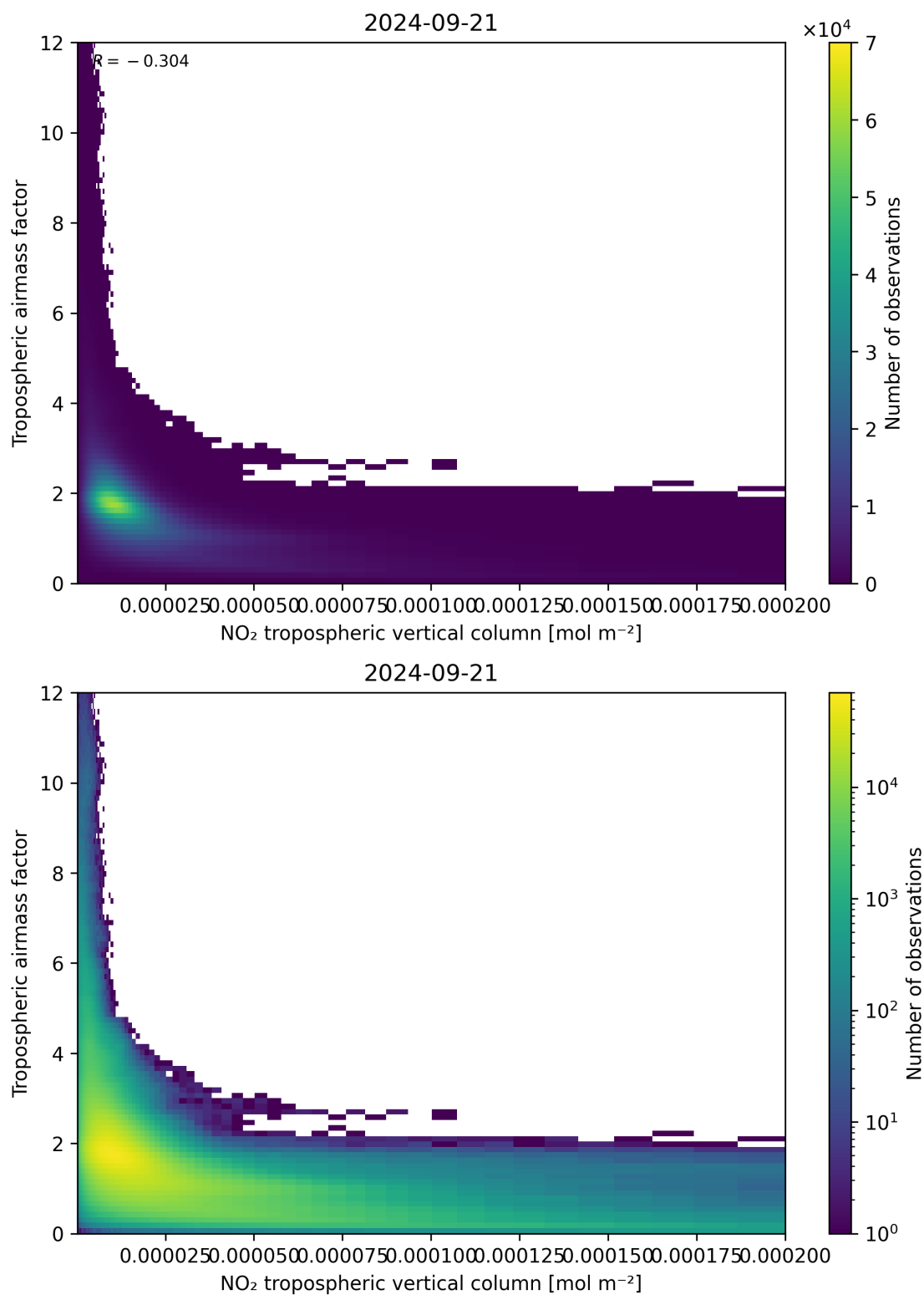
Figure 123: Scatter density plot of “NO 2 tropospheric vertical column” against “Tropospheric airmass factor” for 2024-09-20 to 2024-09-22.
