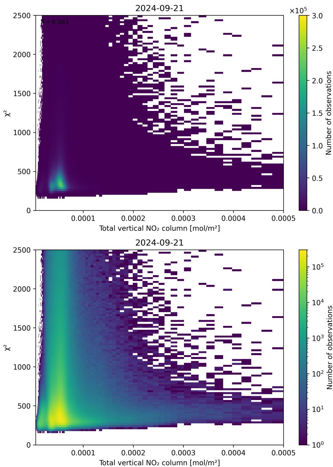
Figure 111: Scatter density plot of “Total vertical NO 2 column” against “ \chi^2 ” for 2024-09-20 to 2024-09-22.
