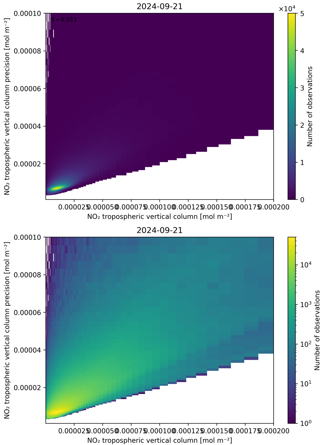
Figure 130: Scatter density plot of “NO 2 tropospheric vertical column” against “NO 2 tropospheric vertical column precision” for 2024-09-20 to 2024-09-22.
