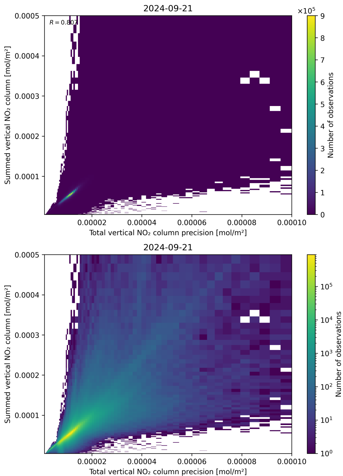
Figure 117: Scatter density plot of “Total vertical NO 2 column precision” against “Summed vertical NO 2 column” for 2024-09-20 to 2024-09-22.
