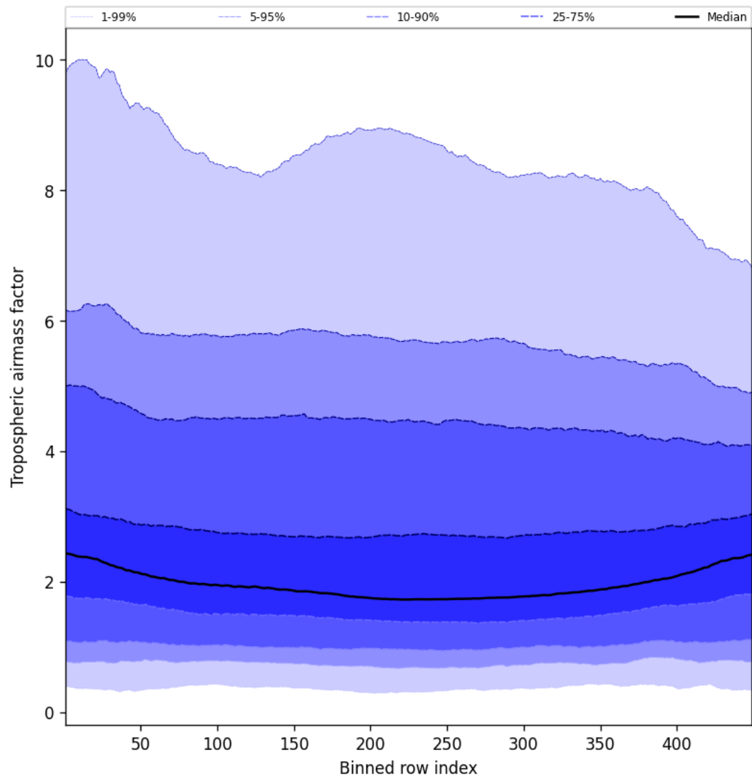
Figure 48: Along track statistics of “Tropospheric air mass factor” for 2024-09-20 to 2024-09-22
