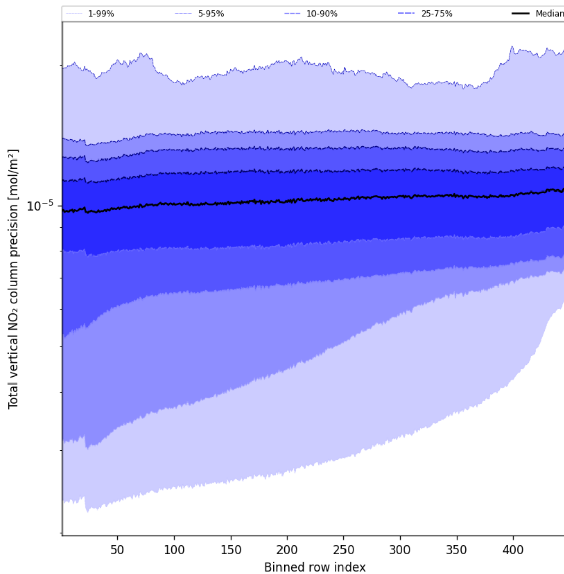
Figure 56: Along track statistics of “Total vertical NO 2 column precision” for 2024-09-20 to 2024-09-22
