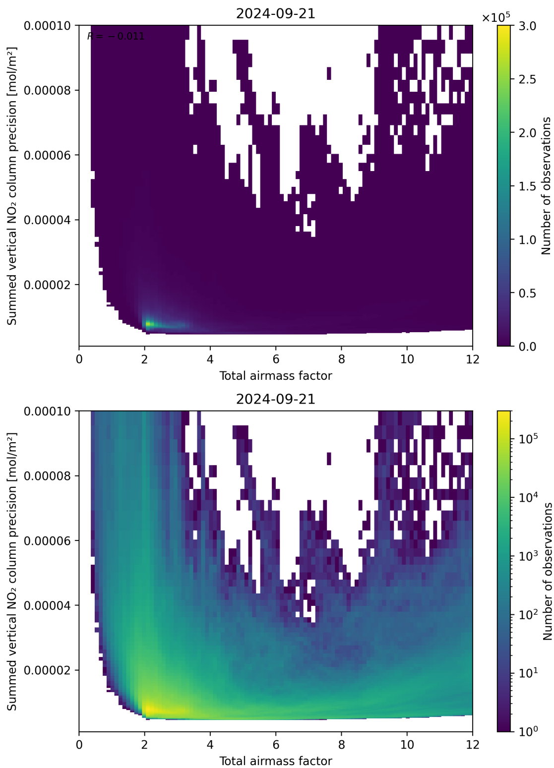
Figure 66: Scatter density plot of “Total airmass factor” against “Summed vertical NO 2 column precision” for 2024-09-20 to 2024-09-22.
