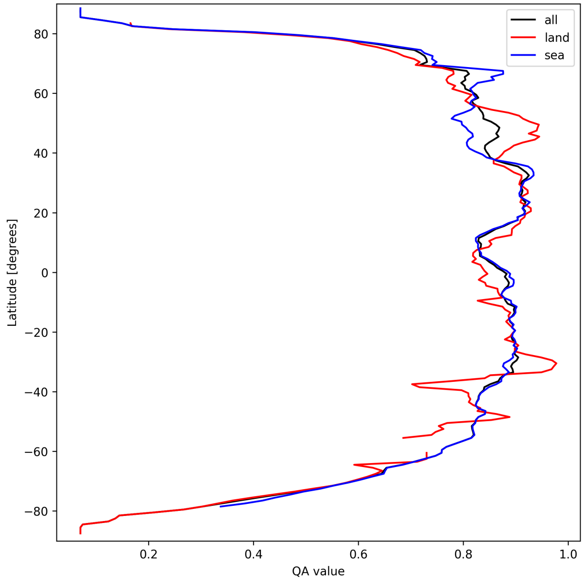
Figure 11: Zonal average of “QA value” for 2024-09-20 to 2024-09-22.
