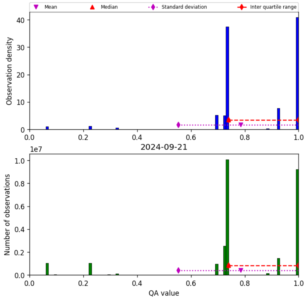
Figure 28: Histogram of “QA value” for 2024-09-20 to 2024-09-22
