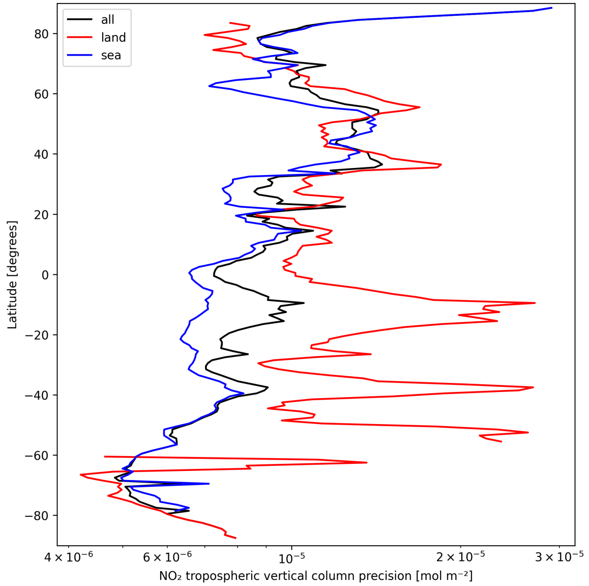
Figure 13: Zonal average of “NO 2 tropospheric vertical column precision” for 2024-09-20 to 2024-09-22.
