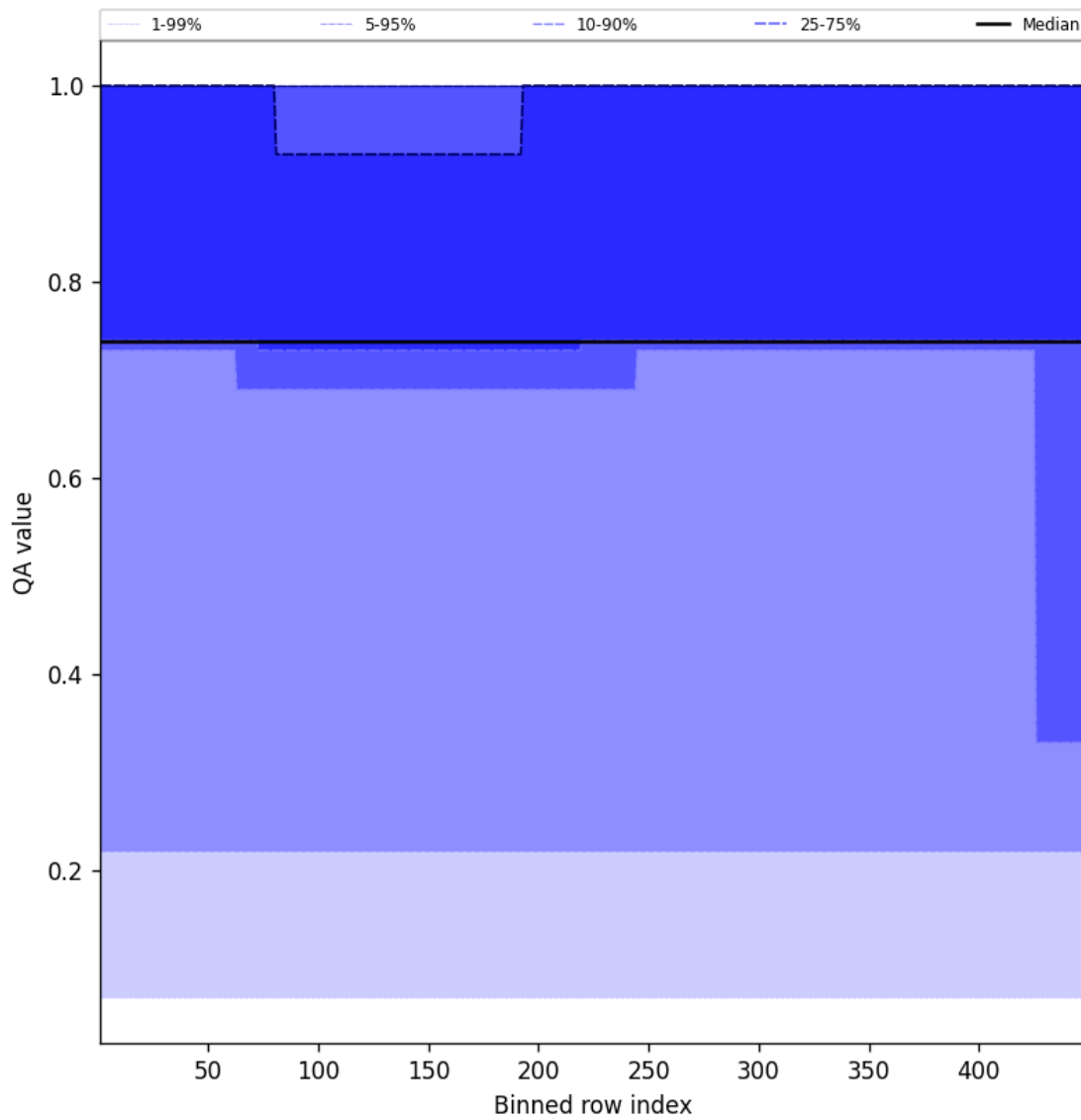
Figure 45: Along track statistics of “QA value” for 2024-09-20 to 2024-09-22
