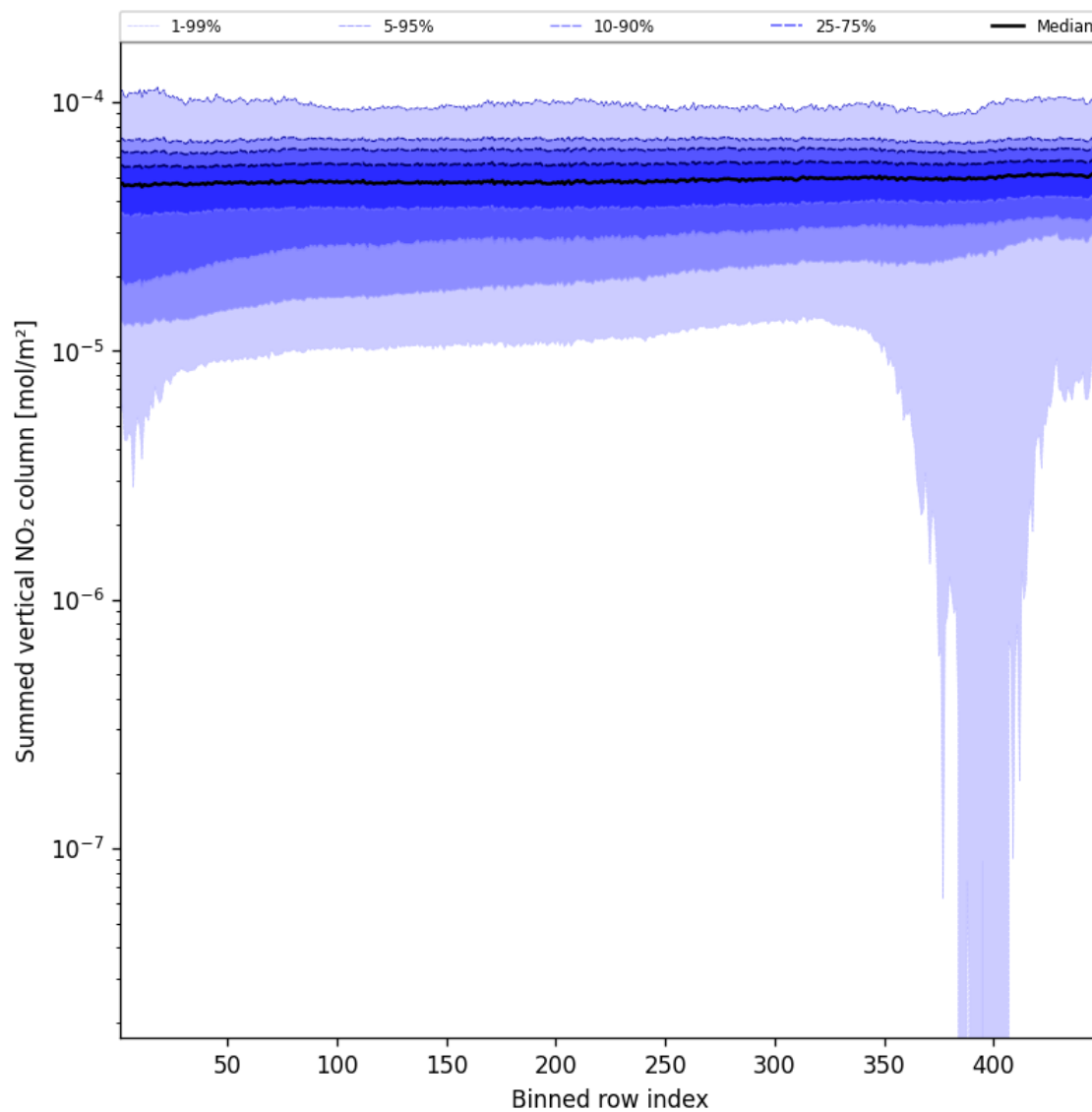
Figure 57: Along track statistics of “Summed vertical NO 2 column” for 2024-09-20 to 2024-09-22
