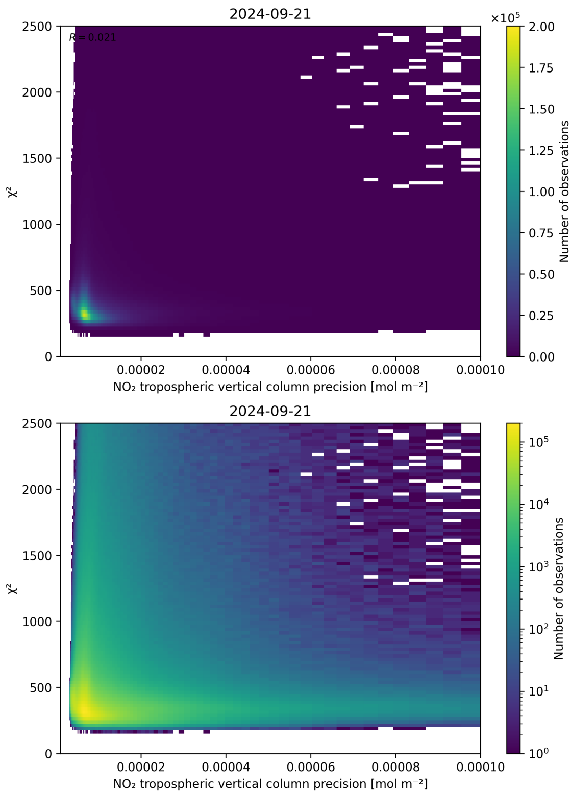
Figure 134: Scatter density plot of “NO 2 tropospheric vertical column precision” against “ \chi^2 ” for 2024-09-20 to 2024-09-22.
