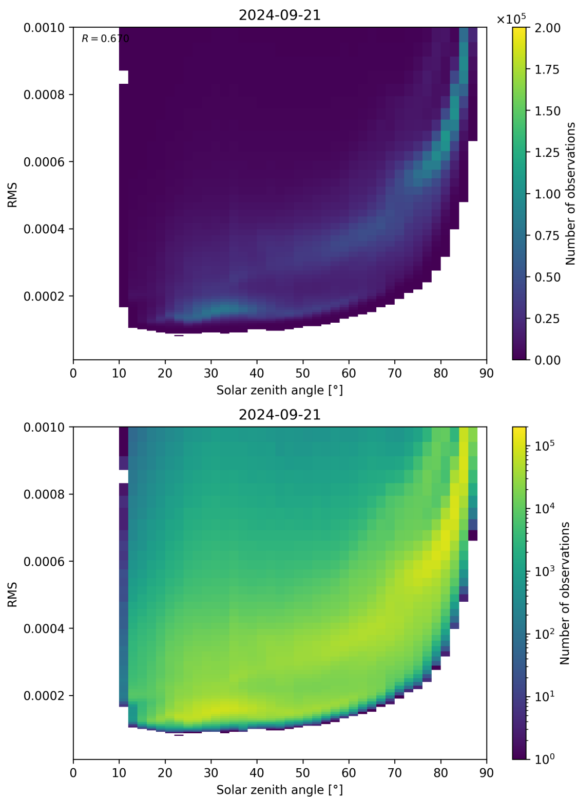
Figure 157: Scatter density plot of “Solar zenith angle” against “RMS” for 2024-09-20 to 2024-09-22.
