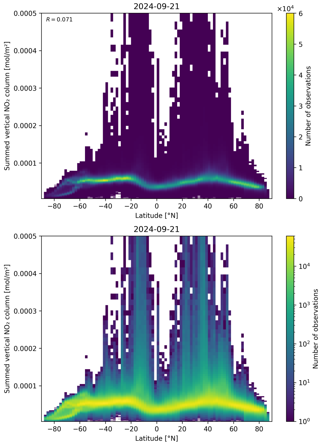
Figure 88: Scatter density plot of “Latitude” against “Summed vertical NO 2 column” for 2024-09-20 to 2024-09-22.
