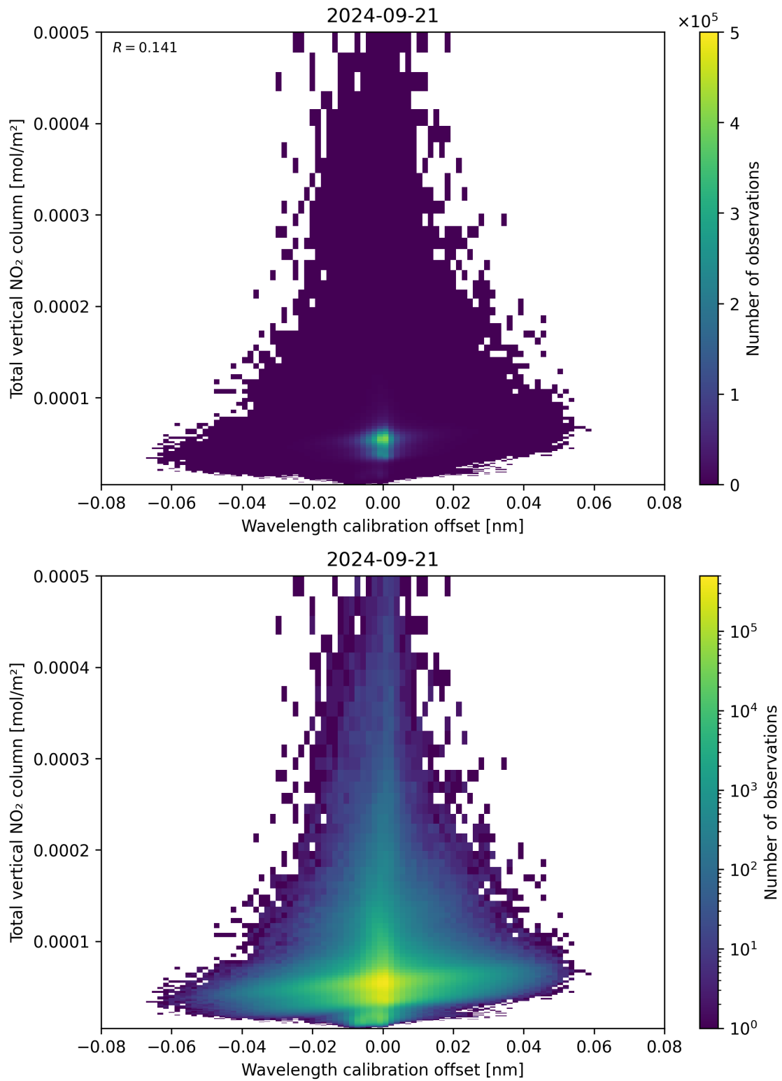
Figure 179: Scatter density plot of “Wavelength calibration offset” against “Total vertical NO 2 column” for 2024-09-20 to 2024-09-22.
