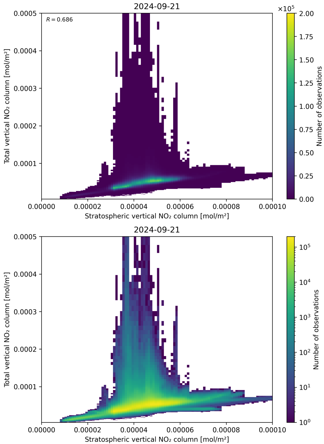
Figure 100: Scatter density plot of “Stratospheric vertical NO 2 column” against “Total vertical NO 2 column” for 2024-09-20 to 2024-09-22.
