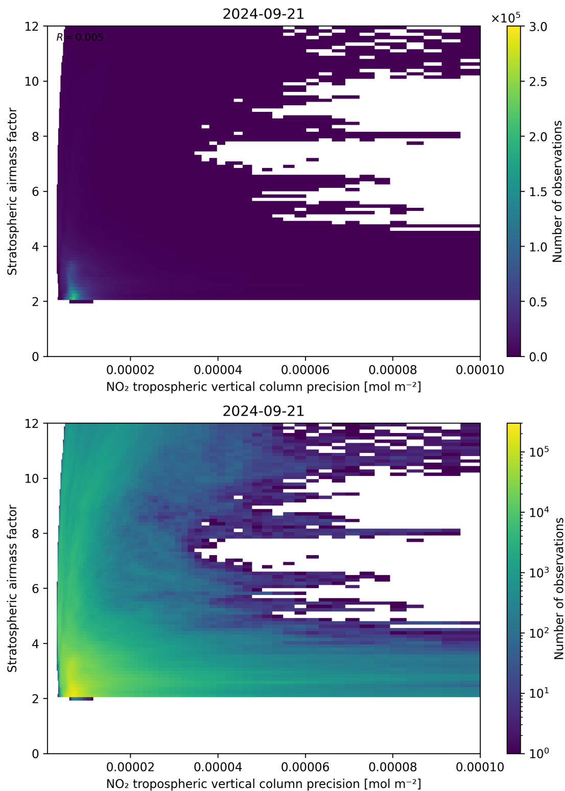
Figure 131: Scatter density plot of “NO 2 tropospheric vertical column precision” against “Stratospheric airmass factor” for 2024-09-20 to 2024-09-22.
