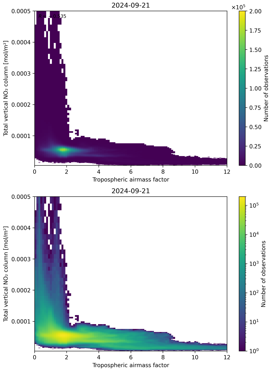
Figure 77: Scatter density plot of “Tropospheric airmass factor” against “Total vertical NO 2 column” for 2024-09-20 to 2024-09-22.
