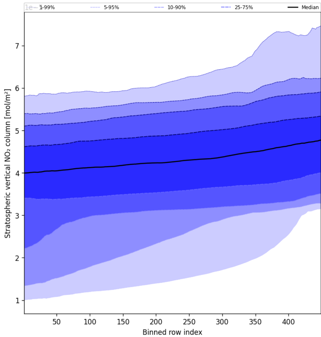
Figure 53: Along track statistics of “Stratospheric vertical NO 2 column” for 2024-09-20 to 2024-09-22
