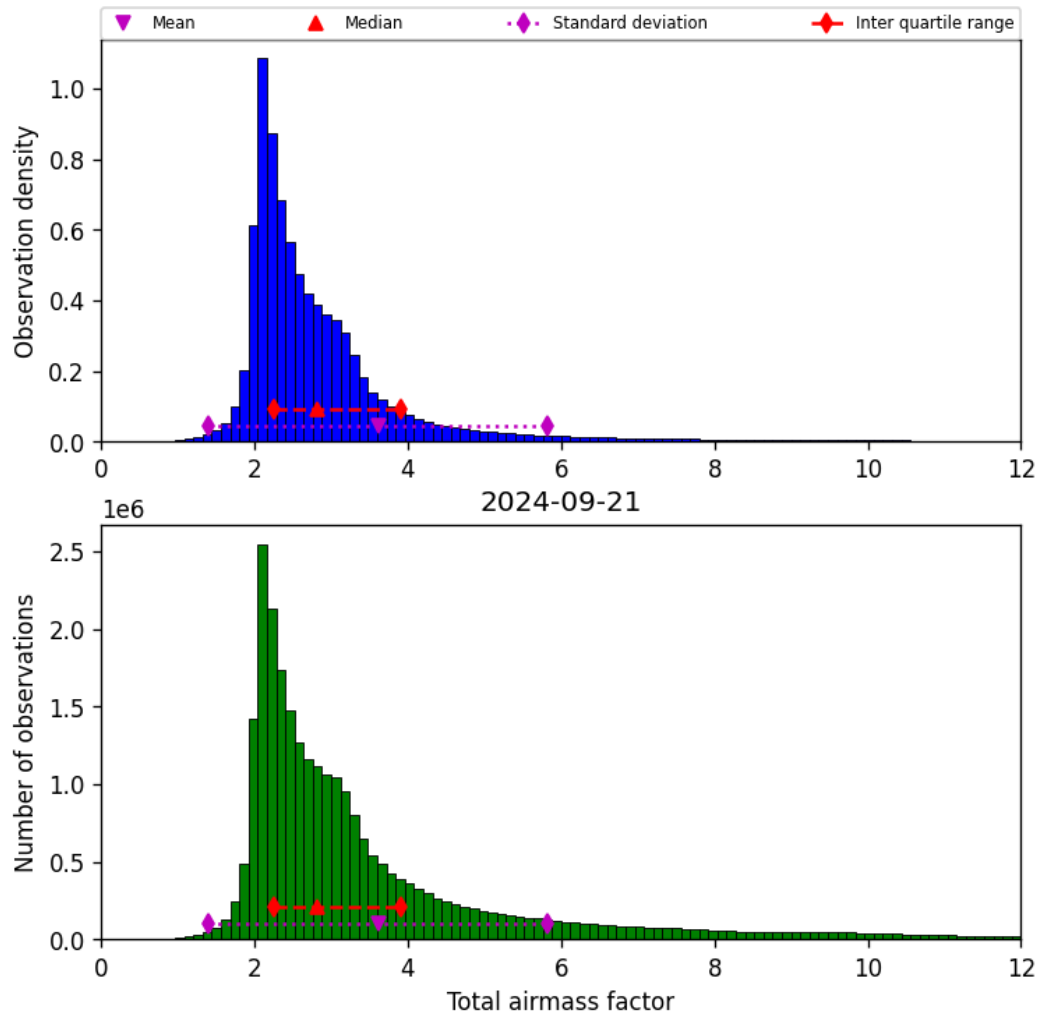
Figure 32: Histogram of “Total airmass factor” for 2024-09-20 to 2024-09-22
