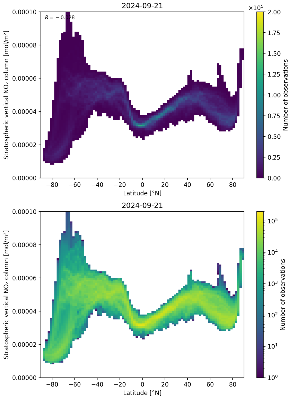
Figure 87: Scatter density plot of “Latitude” against “Stratospheric vertical NO 2 column” for 2024-09-20 to 2024-09-22.
