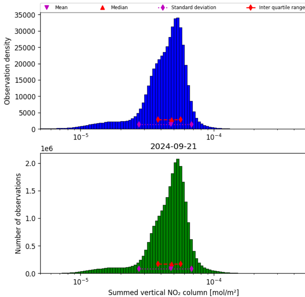
Figure 40: Histogram of “Summed vertical NO 2 column” for 2024-09-20 to 2024-09-22
