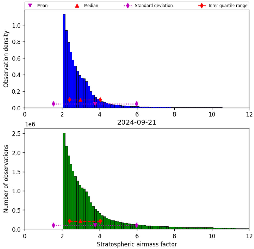
Figure 44: Histogram of “Stratospheric airmass factor” for 2024-09-20 to 2024-09-22
