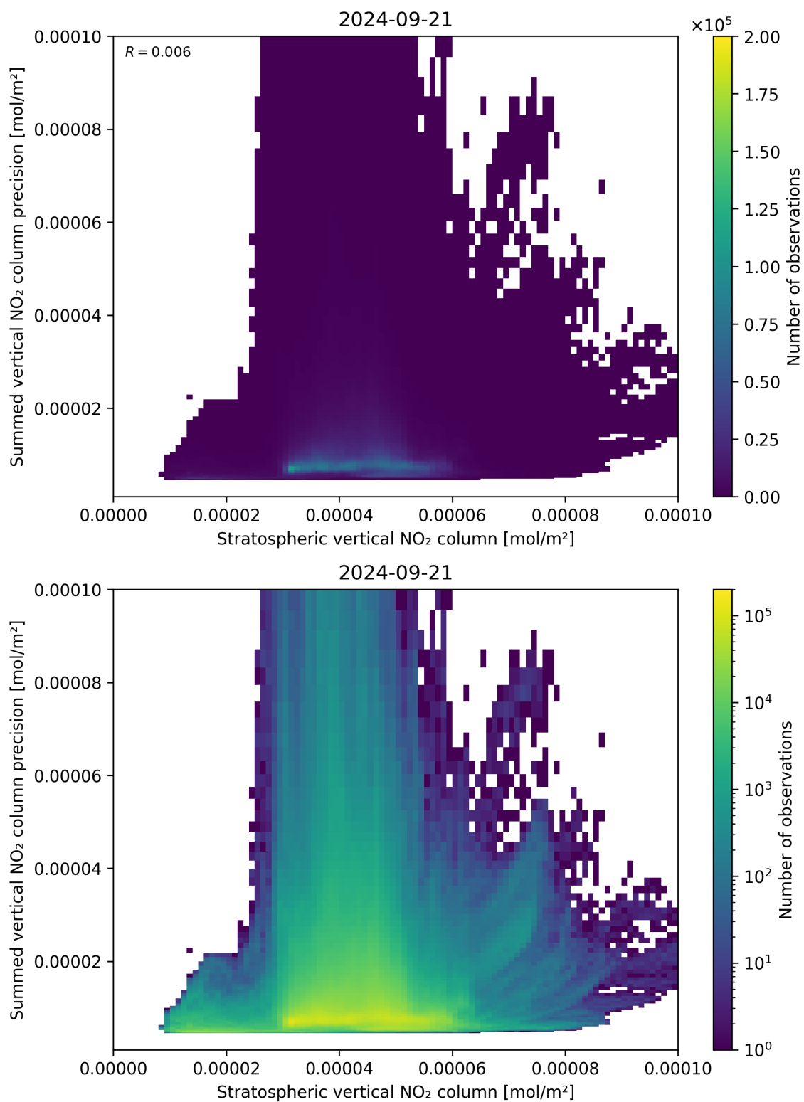
Figure 99: Scatter density plot of “Stratospheric vertical NO 2 column” against “Summed vertical NO 2 column precision” for 2024-09-20 to 2024-09-22.
