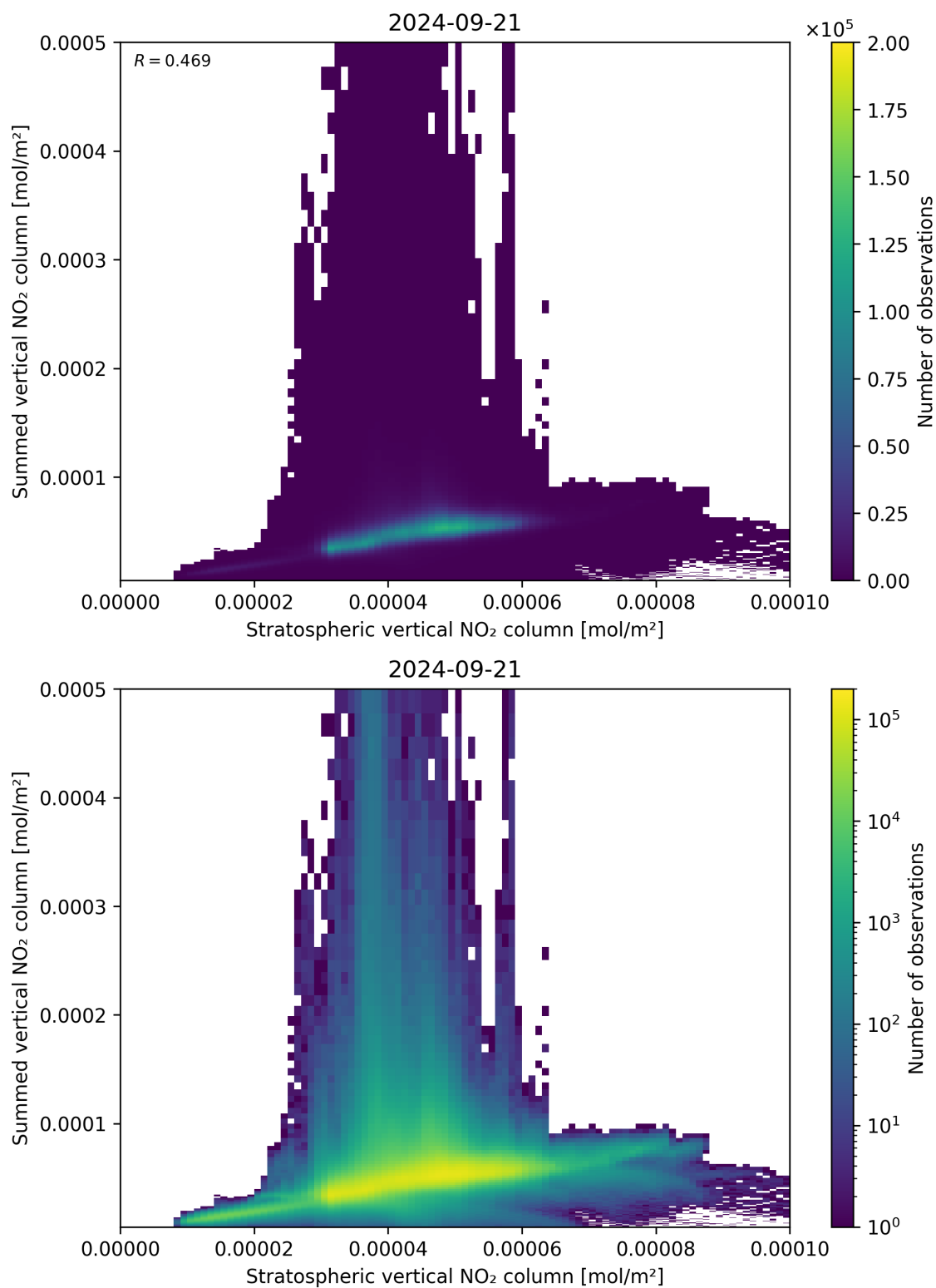
Figure 98: Scatter density plot of “Stratospheric vertical NO 2 column” against “Summed vertical NO 2 column” for 2024-09-20 to 2024-09-22.
