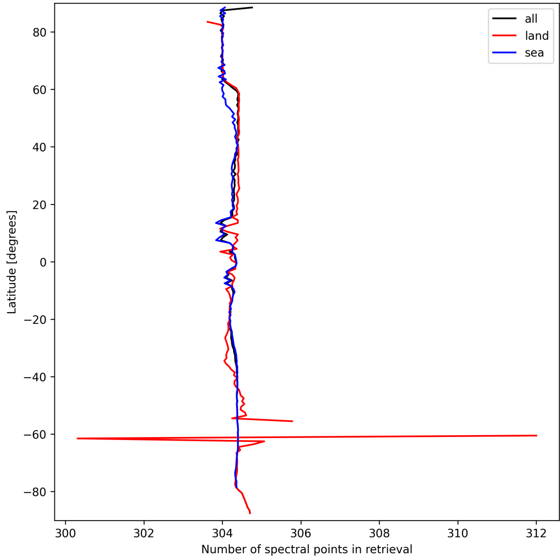
Figure 16: Zonal average of “Number of spectral points in retrieval” for 2024-09-20 to 2024-09-22.
