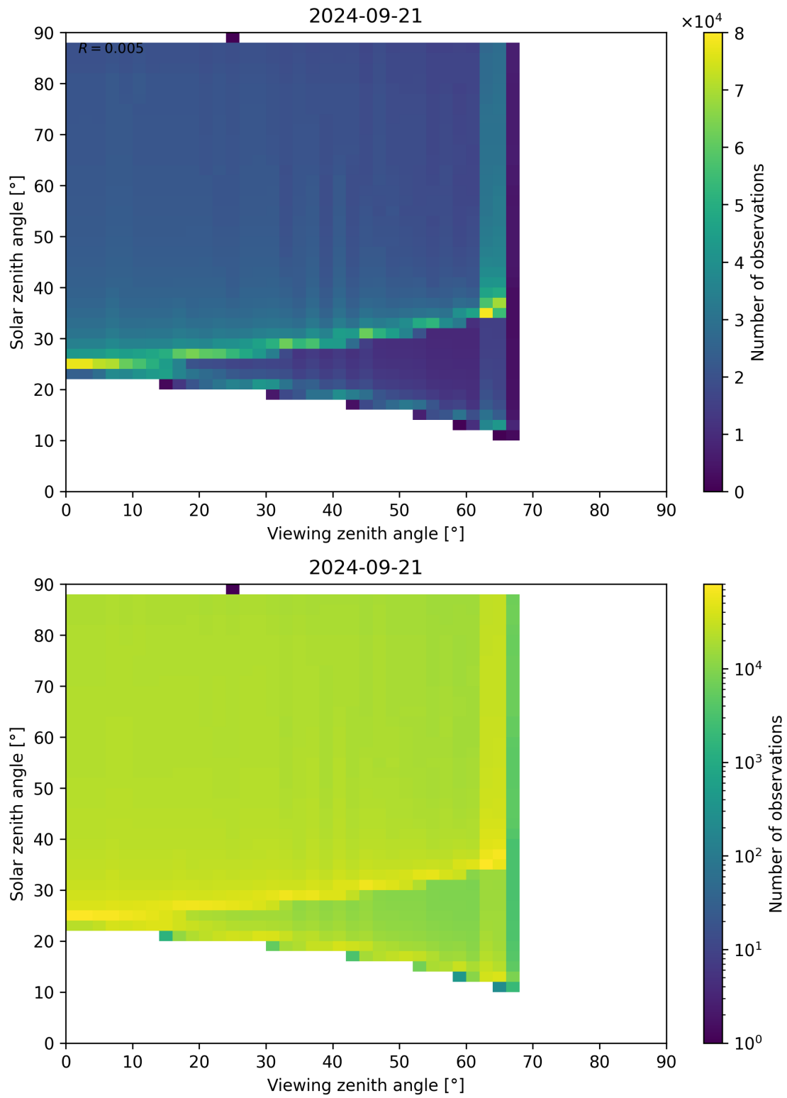
Figure 172: Scatter density plot of “Viewing zenith angle” against “Solar zenith angle” for 2024-09-20 to 2024-09-22.
