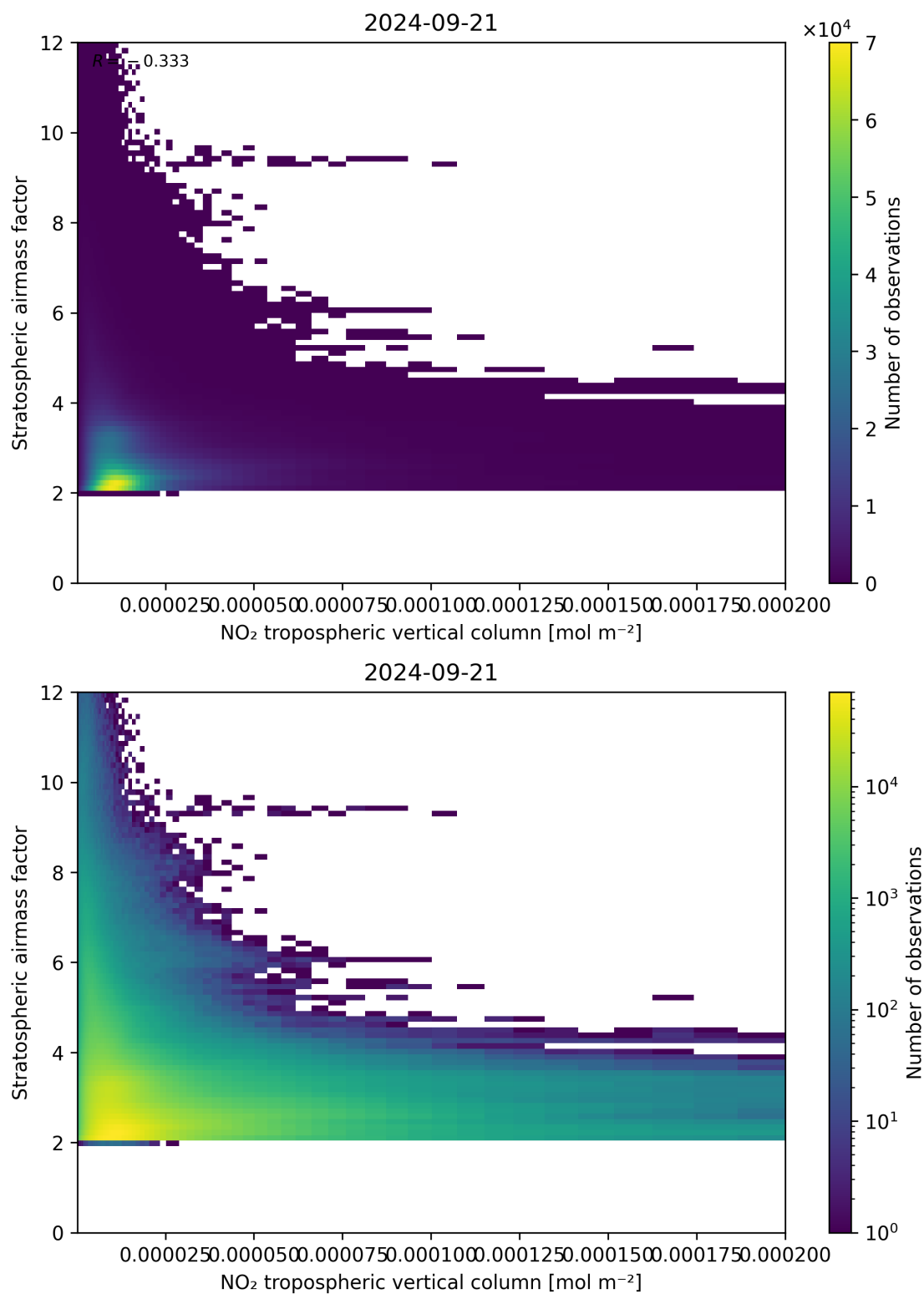
Figure 121: Scatter density plot of “NO 2 tropospheric vertical column” against “Stratospheric air mass factor” for 2024-09-20 to 2024-09-22.
