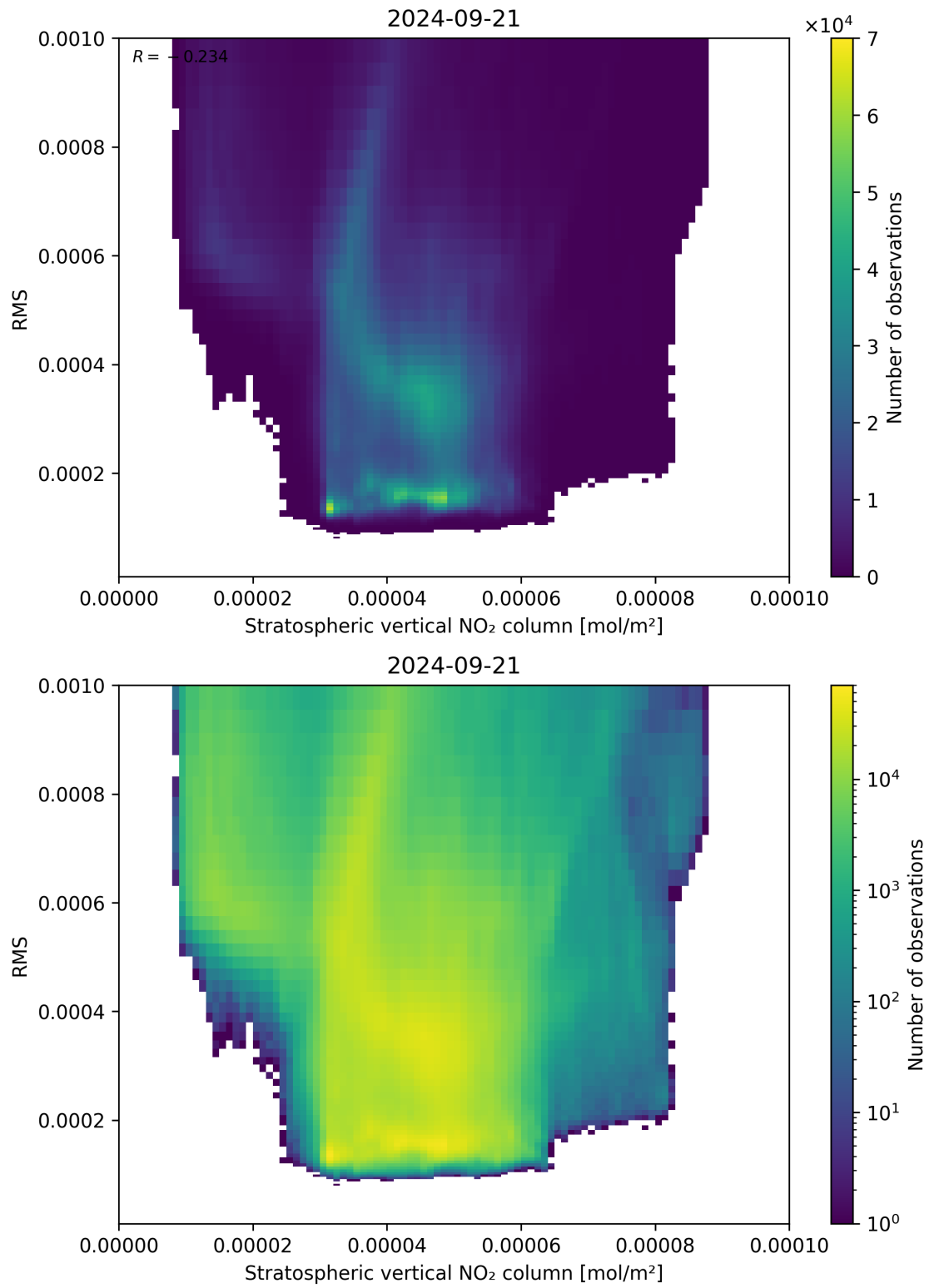
Figure 102: Scatter density plot of “Stratospheric vertical NO 2 column” against “RMS” for 2024-09-20 to 2024-09-22.
