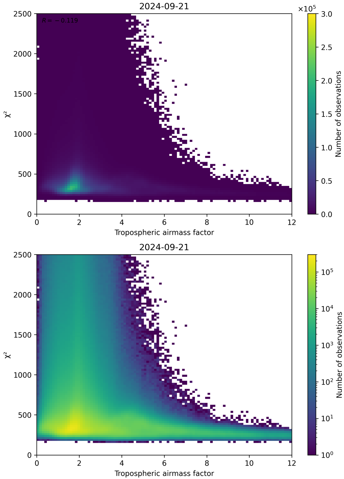
Figure 73: Scatter density plot of “Tropospheric airmass factor” against “ \chi^2 ” for 2024-09-20 to 2024-09-22.
