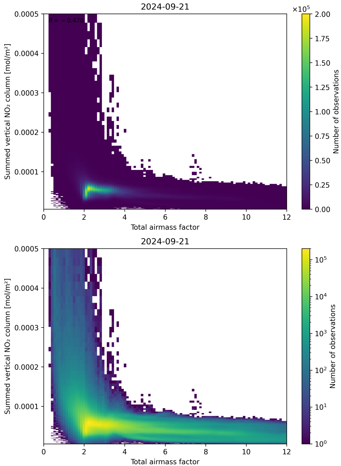
Figure 65: Scatter density plot of “Total airmass factor” against “Summed vertical NO 2 column” for 2024-09-20 to 2024-09-22.
