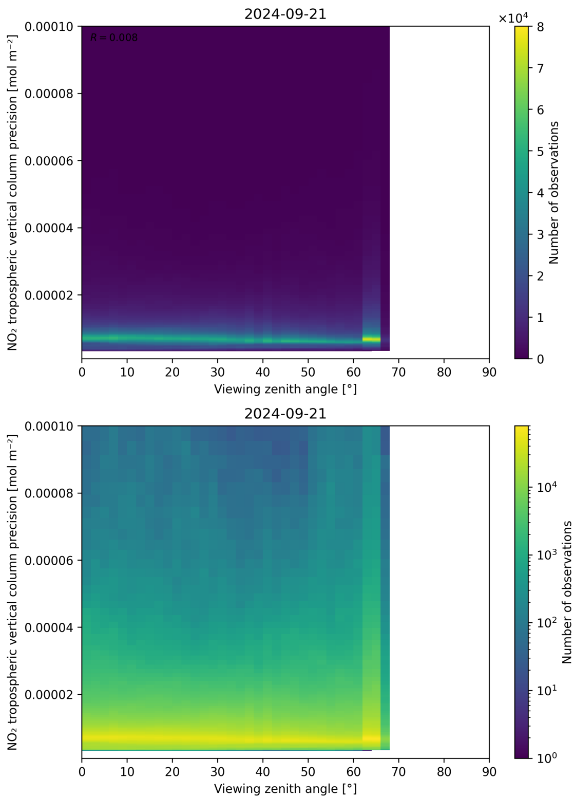
Figure 170: Scatter density plot of “Viewing zenith angle” against “NO 2 tropospheric vertical column precision” for 2024-09-20 to 2024-09-22.
