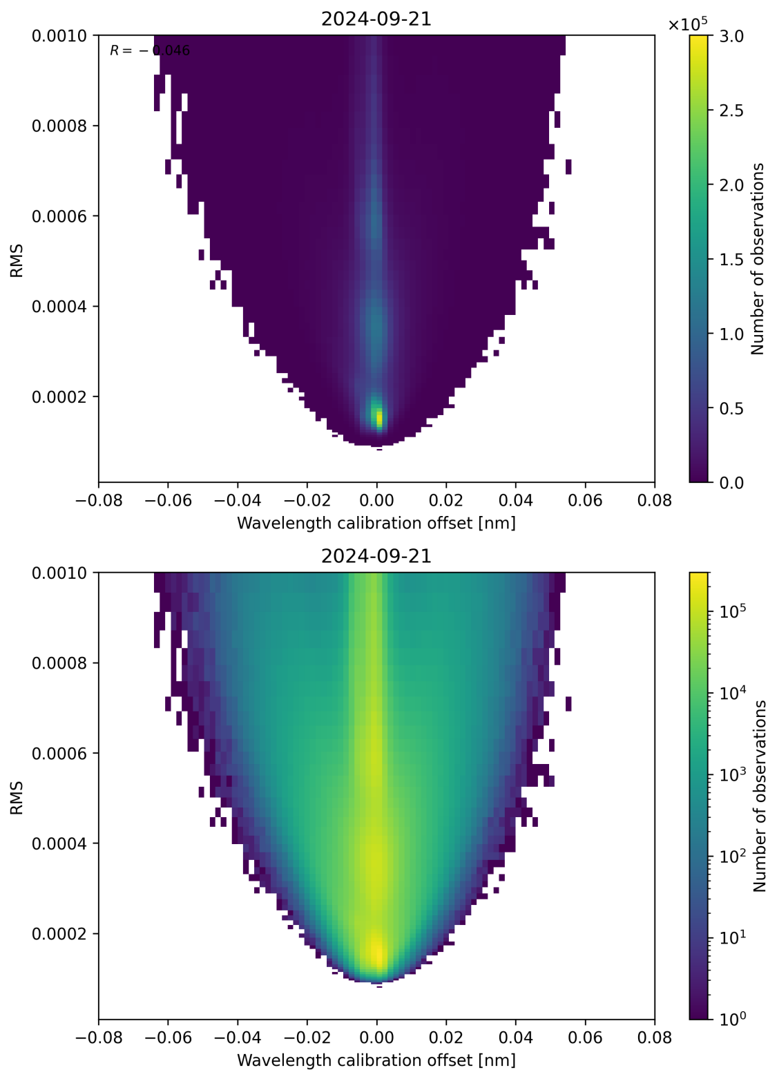
Figure 181: Scatter density plot of “Wavelength calibration offset” against “RMS” for 2024-09-20 to 2024-09-22.
