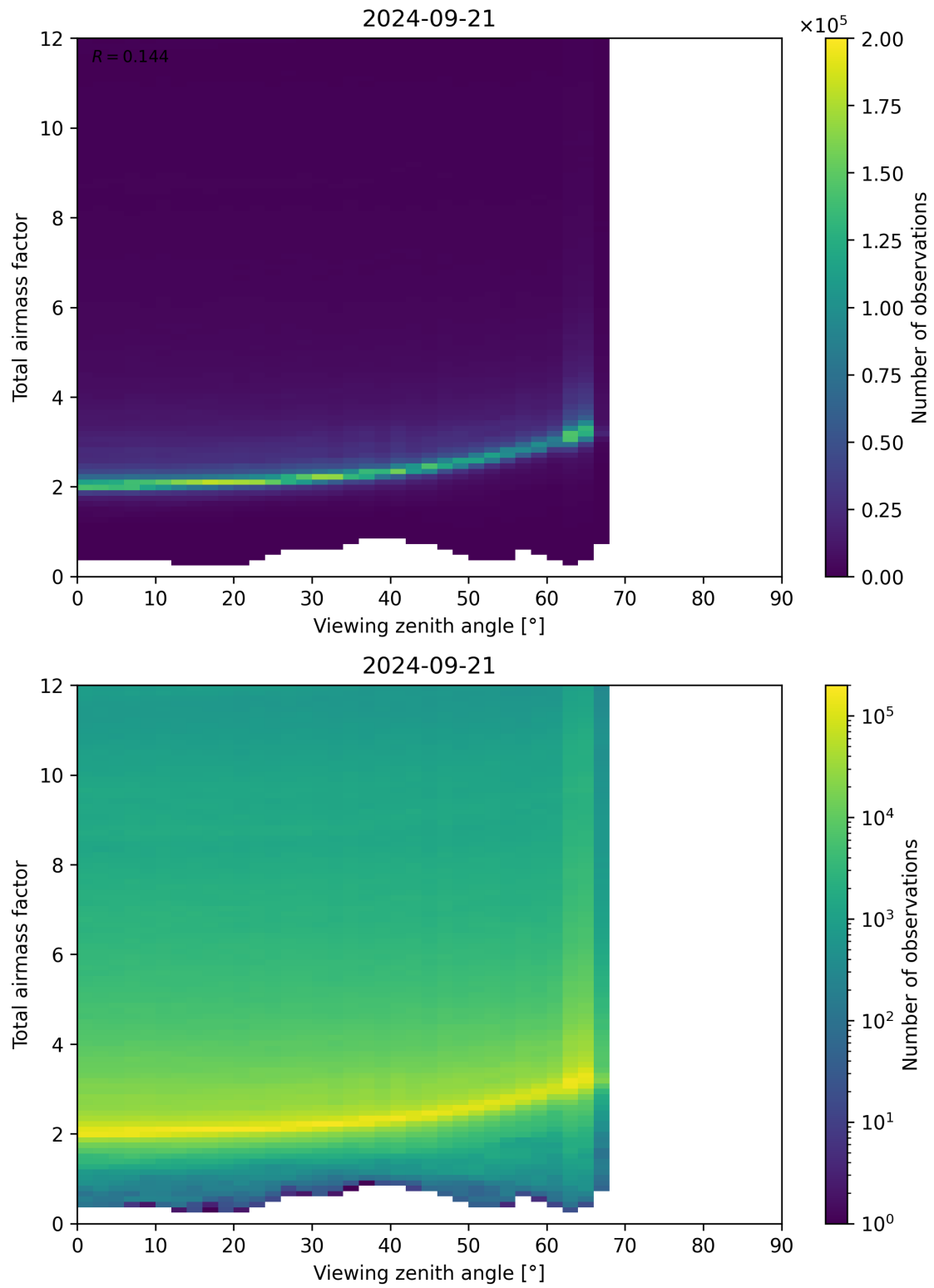
Figure 160: Scatter density plot of “Viewing zenith angle” against “Total airmass factor” for 2024-09-20 to 2024-09-22.
