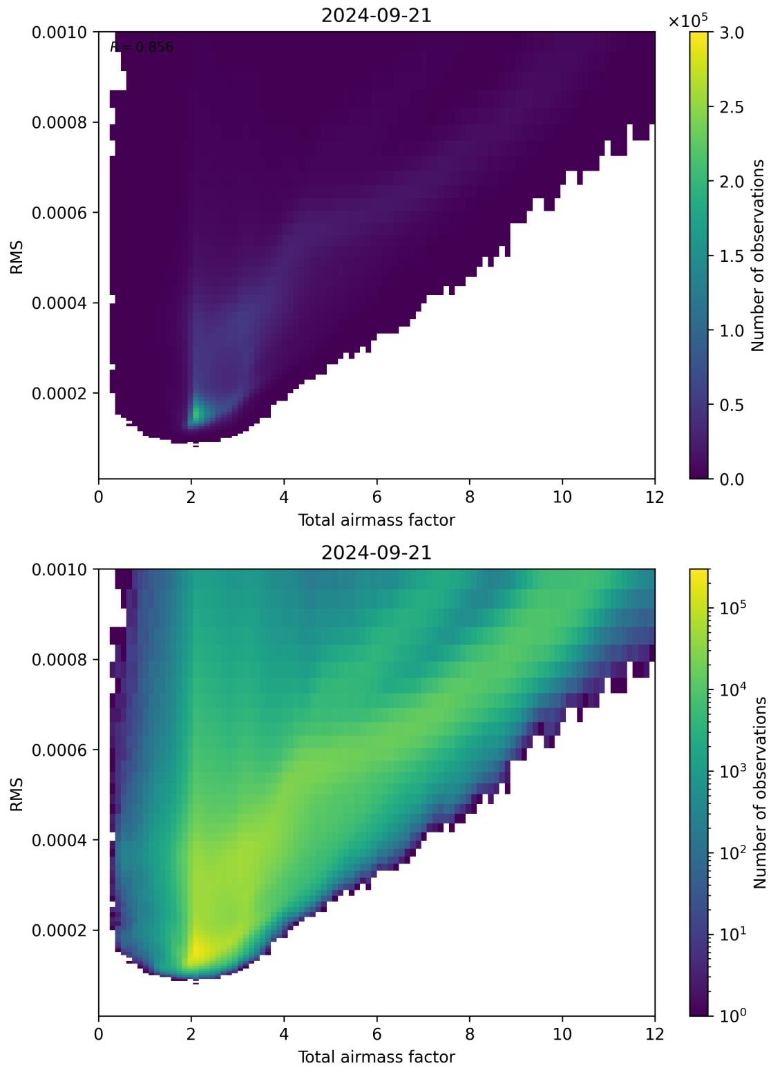
Figure 69: Scatter density plot of “Total airmass factor” against “RMS” for 2024-09-20 to 2024-09-22.
