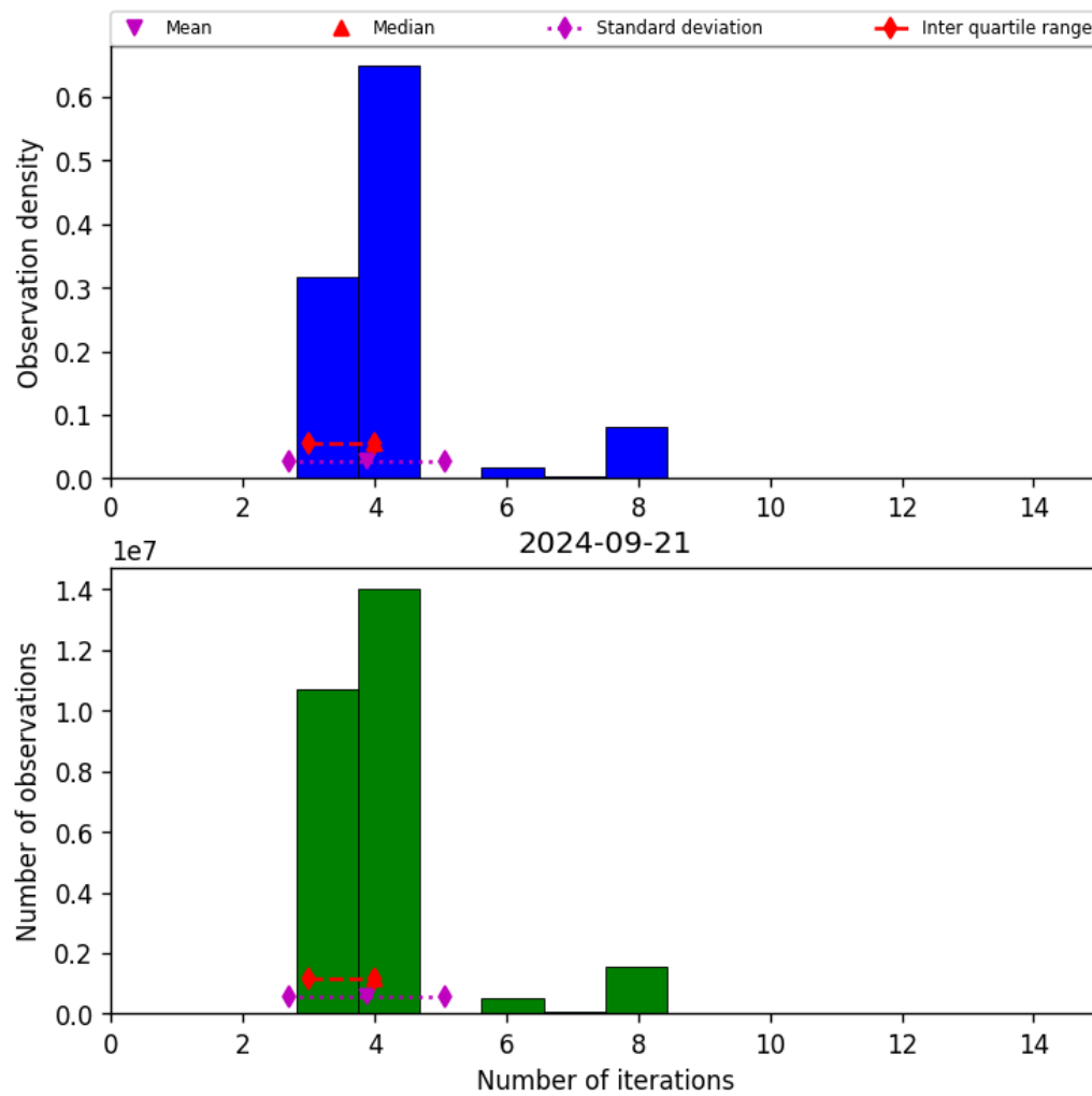
Figure 34: Histogram of “Number of iterations” for 2024-09-20 to 2024-09-22
