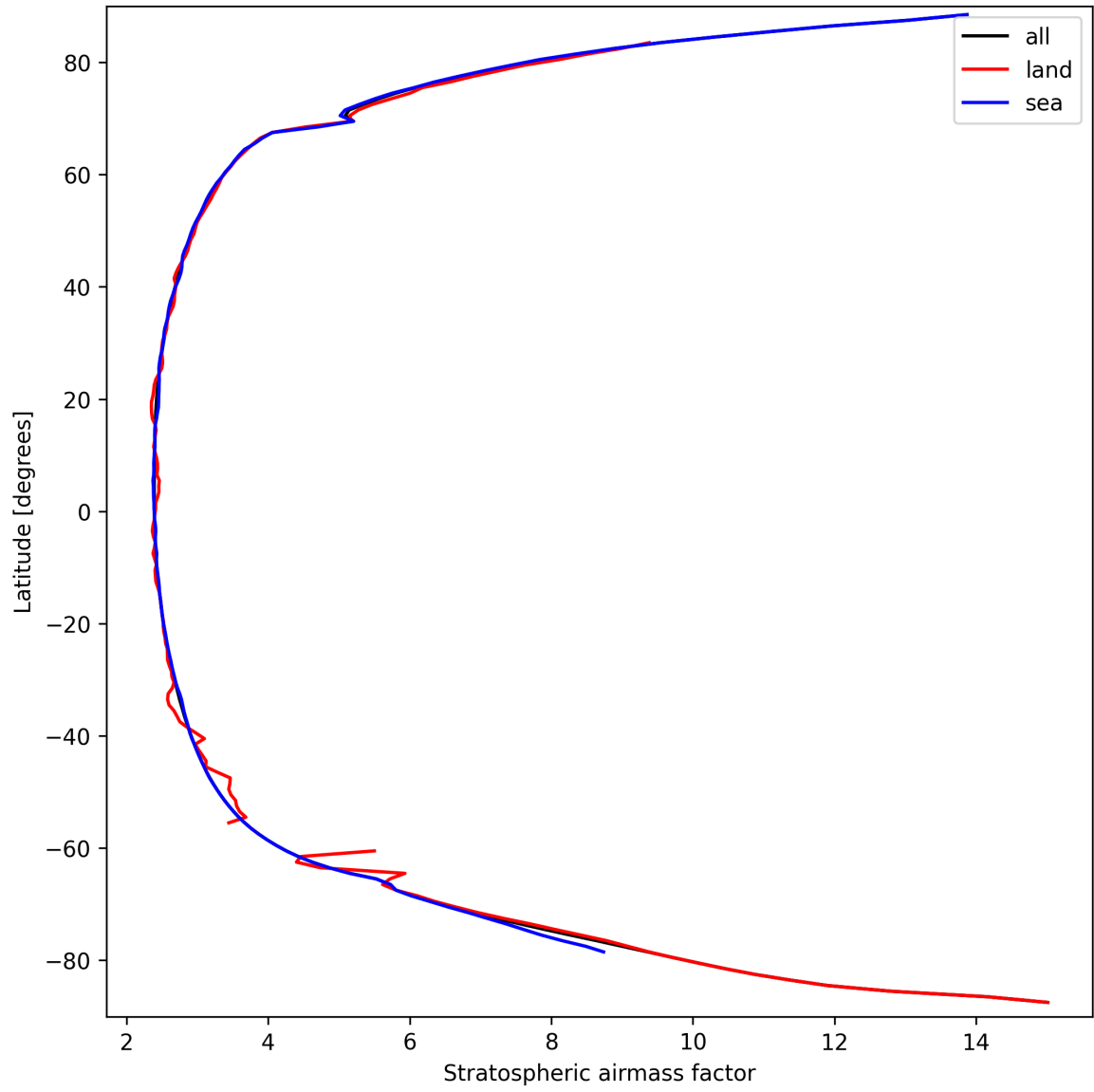
Figure 27: Zonal average of “Stratospheric airmass factor” for 2024-09-20 to 2024-09-22.
