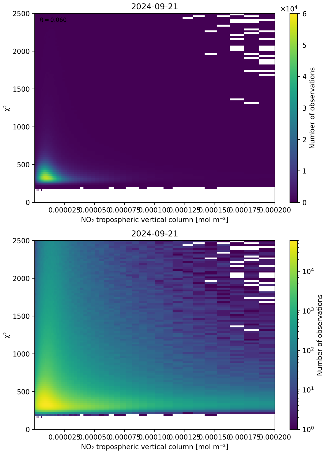
Figure 124: Scatter density plot of “NO 2 tropospheric vertical column” against “ \chi^2 ” for 2024-09-20 to 2024-09-22.
