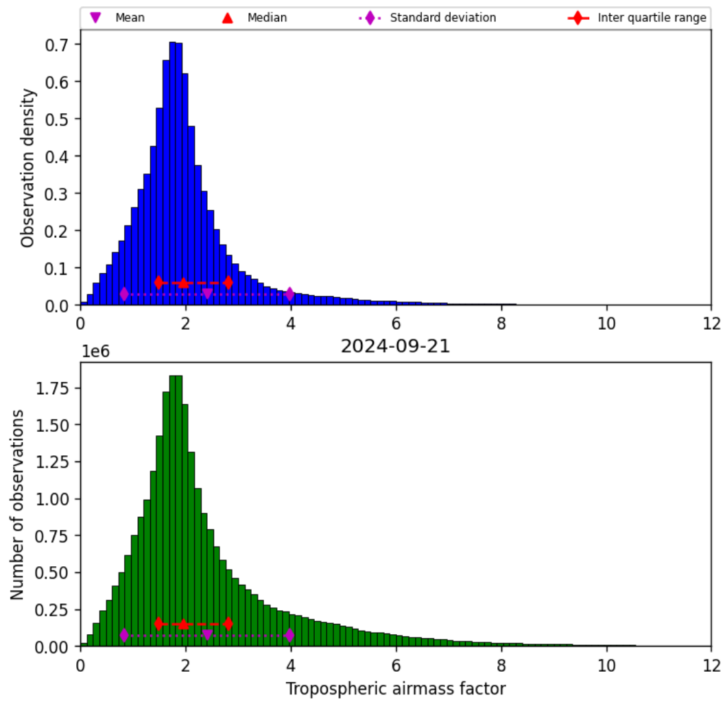
Figure 31: Histogram of “Tropospheric airmass factor” for 2024-09-20 to 2024-09-22
