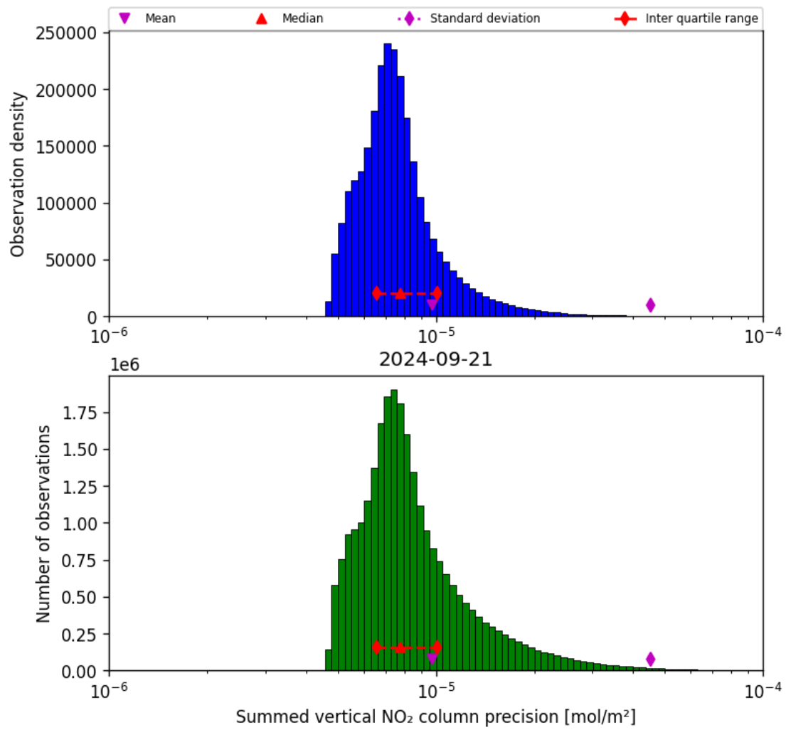
Figure 41: Histogram of “Summed vertical NO 2 column precision” for 2024-09-20 to 2024-09-22
