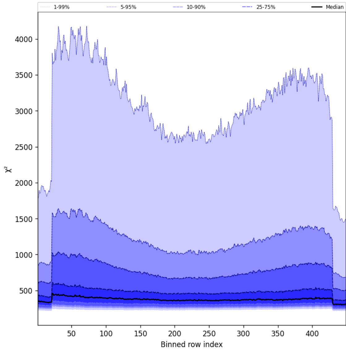
Figure 59: Along track statistics of “ \chi^2 ” for 2024-09-20 to 2024-09-22
