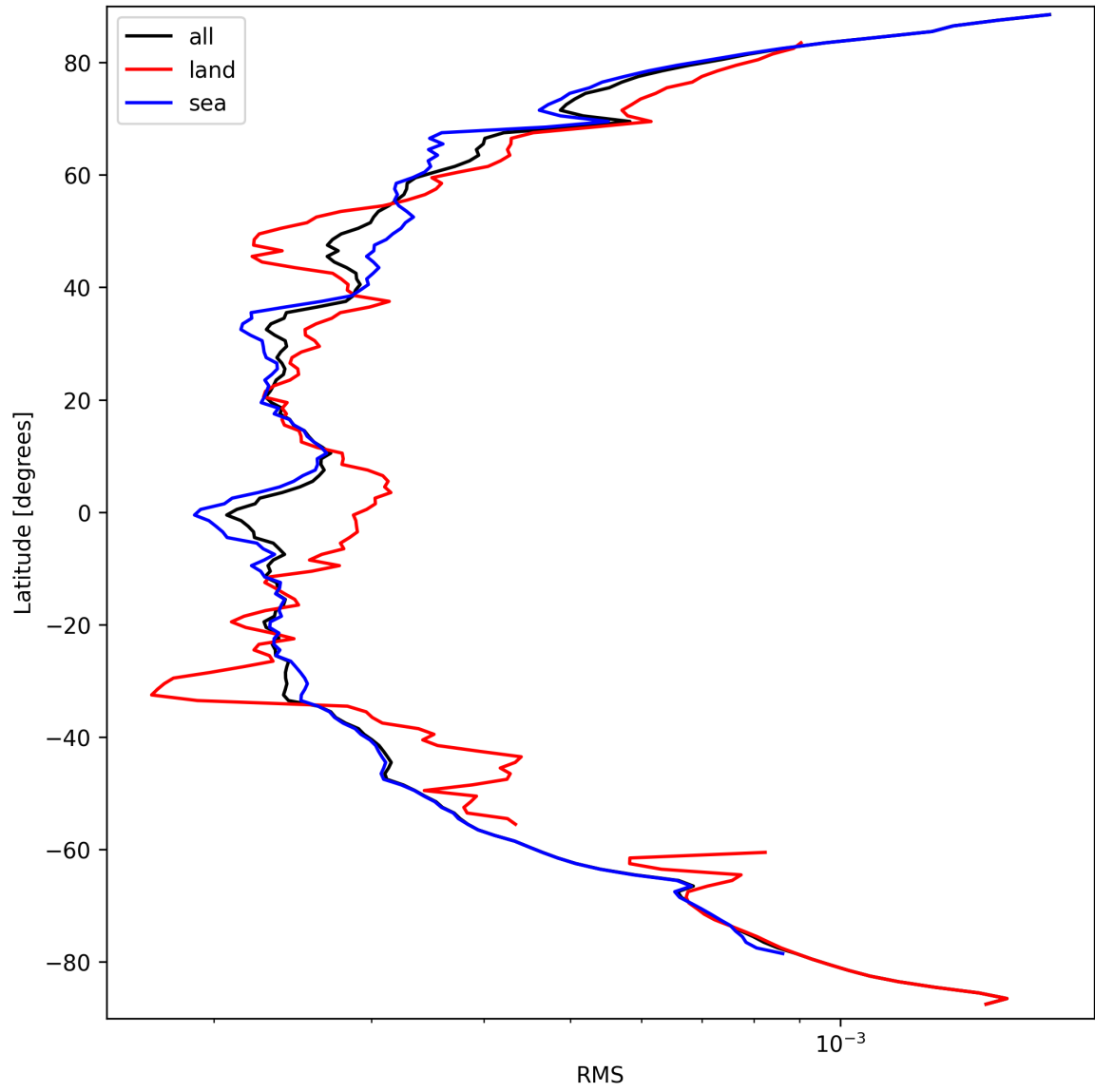
Figure 26: Zonal average of “RMS” for 2024-09-20 to 2024-09-22.
