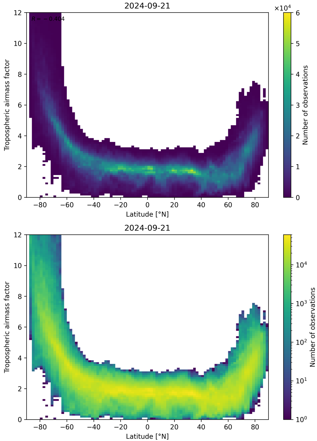
Figure 85: Scatter density plot of “Latitude” against “Tropospheric airmass factor” for 2024-09-20 to 2024-09-22.
