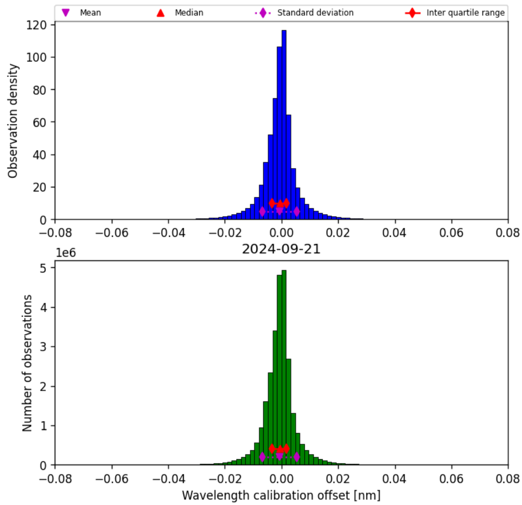
Figure 35: Histogram of “Wavelength calibration offset” for 2024-09-20 to 2024-09-22
