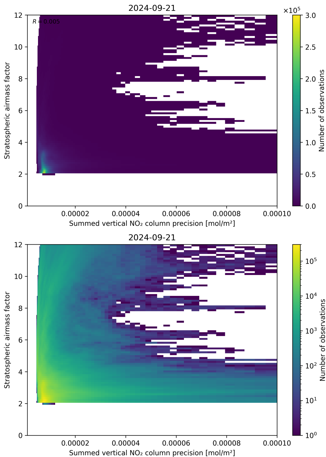
Figure 106: Scatter density plot of “Summed vertical NO 2 column precision” against “Stratospheric airmass factor” for 2024-09-20 to 2024-09-22.
