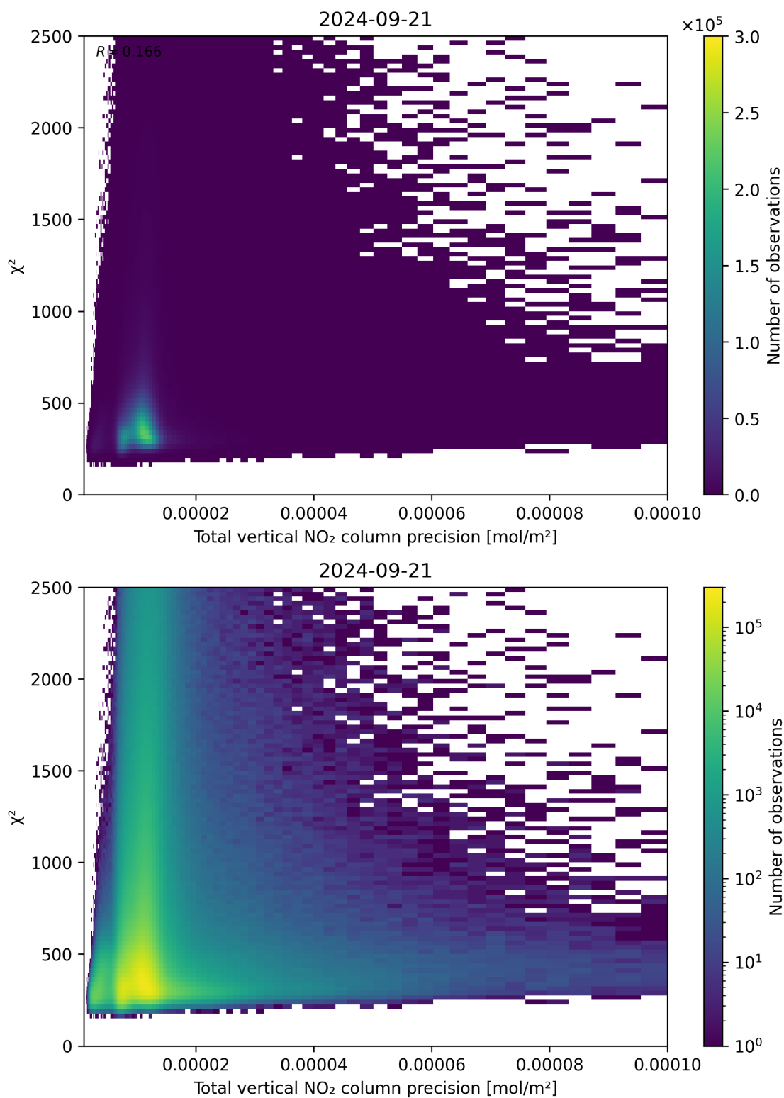
Figure 116: Scatter density plot of “Total vertical NO 2 column precision” against “ \chi^2 ” for 2024-09-20 to 2024-09-22.
