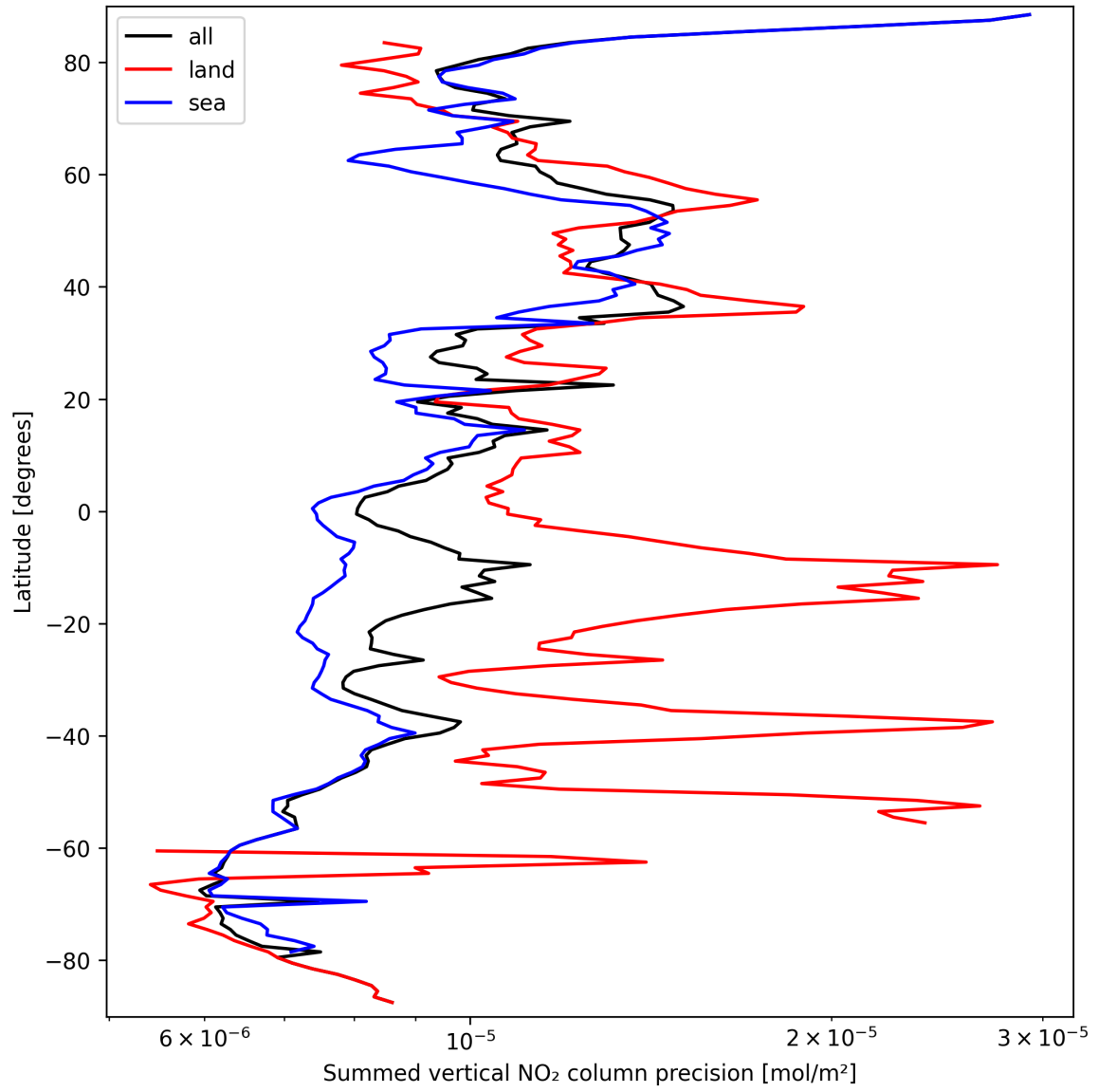
Figure 24: Zonal average of “Summed vertical NO 2 column precision” for 2024-09-20 to 2024-09-22.
