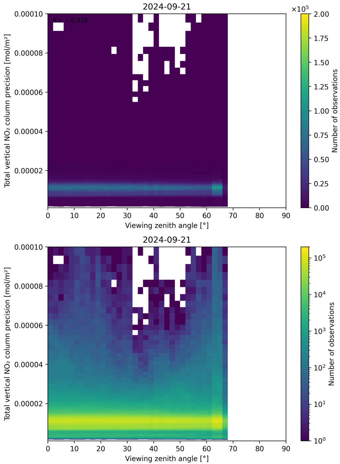
Figure 168: Scatter density plot of “Viewing zenith angle” against “Total vertical NO 2 column precision” for 2024-09-20 to 2024-09-22.
