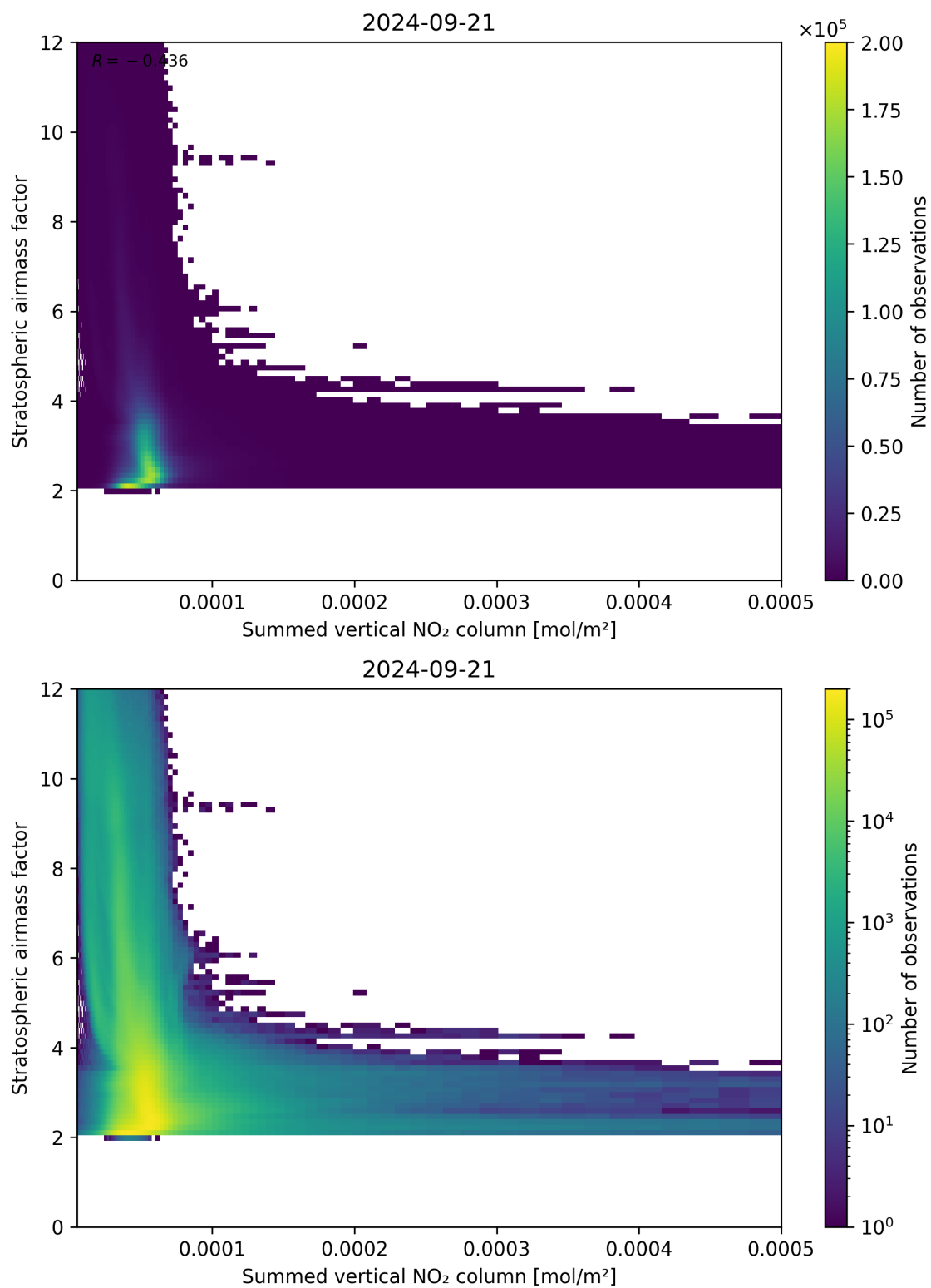
Figure 103: Scatter density plot of “Summed vertical NO 2 column” against “Stratospheric airmass factor” for 2024-09-20 to 2024-09-22.
