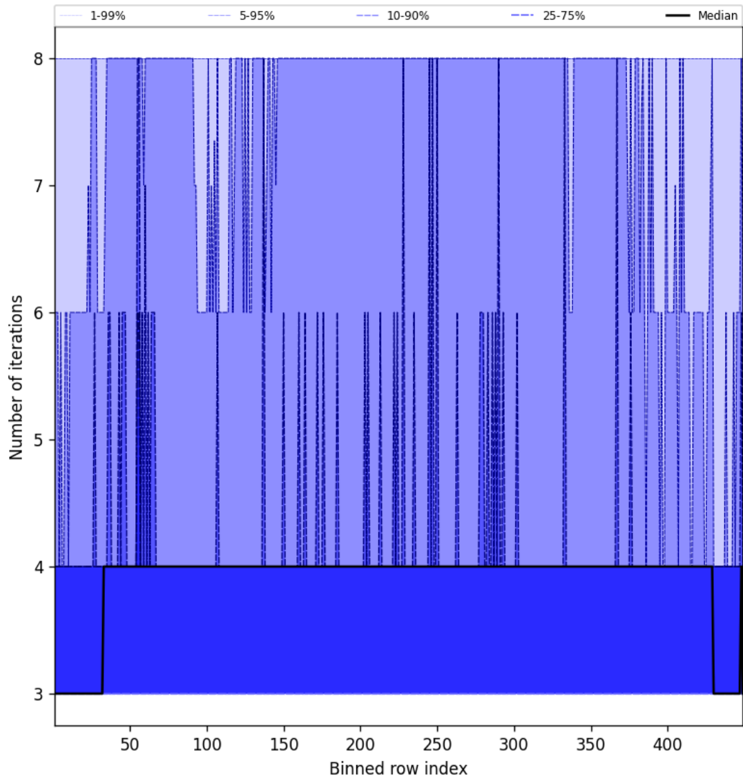
Figure 51: Along track statistics of “Number of iterations” for 2024-09-20 to 2024-09-22
