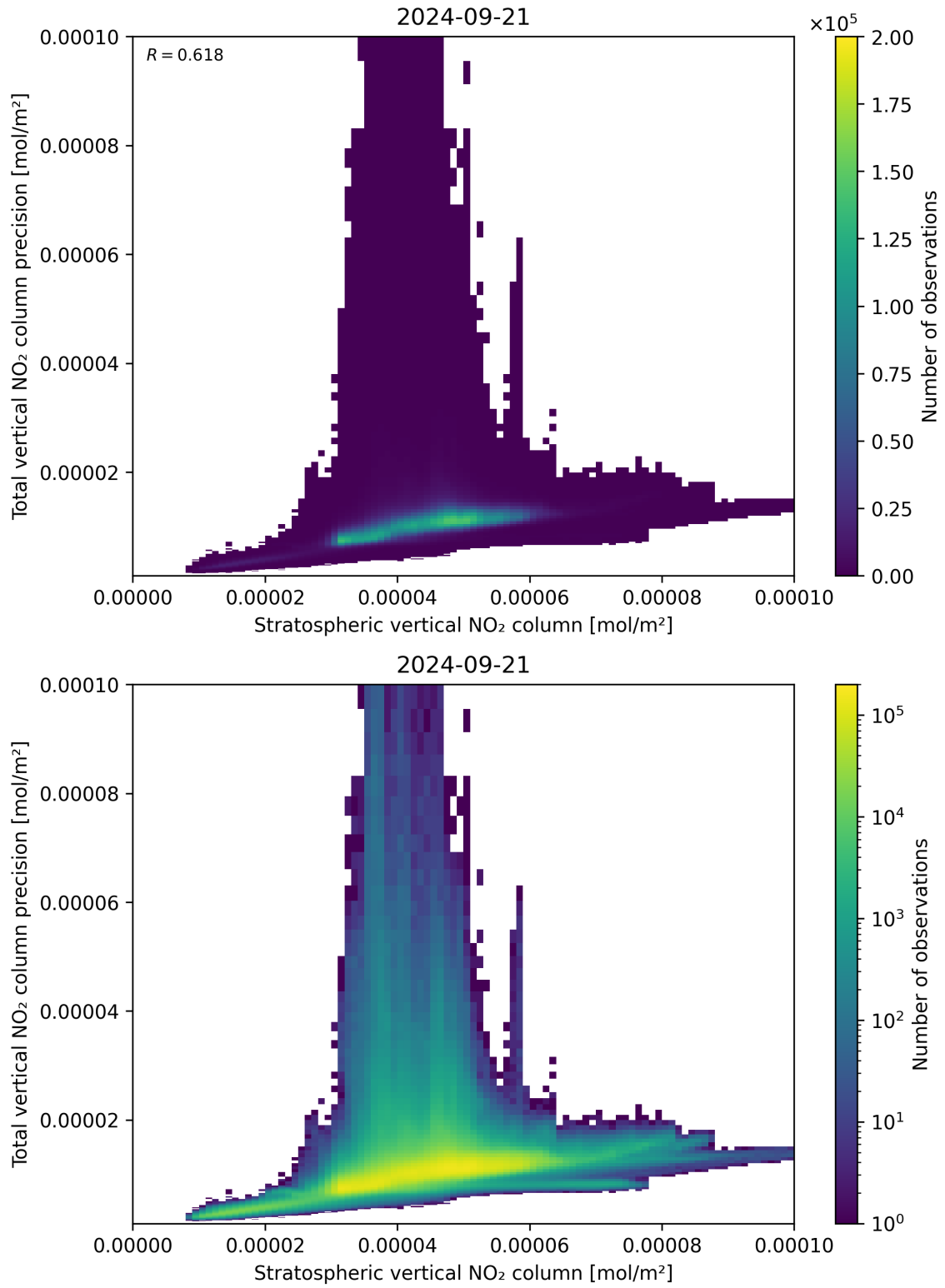
Figure 101: Scatter density plot of “Stratospheric vertical NO 2 column” against “Total vertical NO 2 column precision” for 2024-09-20 to 2024-09-22.
