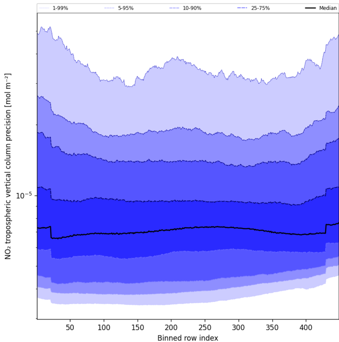
Figure 47: Along track statistics of “NO 2 tropospheric vertical column precision” for 2024-09-20 to 2024-09-22
