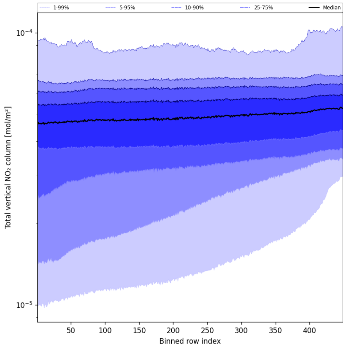
Figure 55: Along track statistics of “Total vertical NO 2 column” for 2024-09-20 to 2024-09-22
