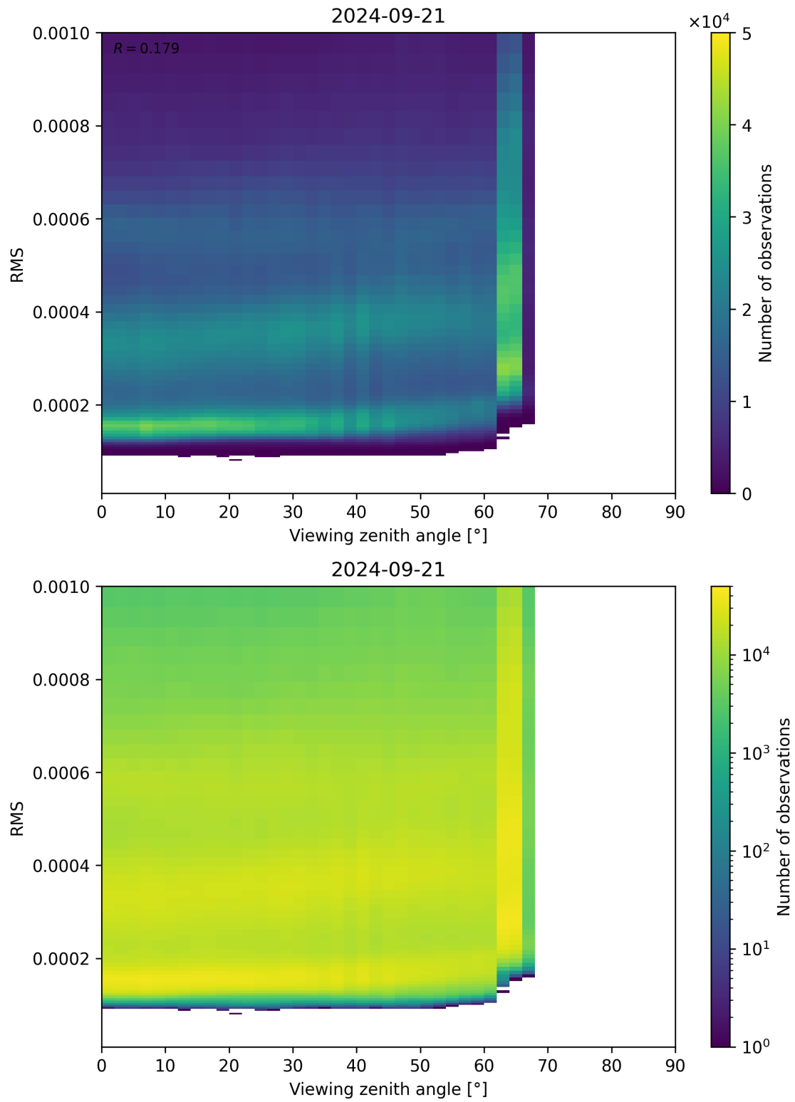
Figure 171: Scatter density plot of “Viewing zenith angle” against “RMS” for 2024-09-20 to 2024-09-22.
