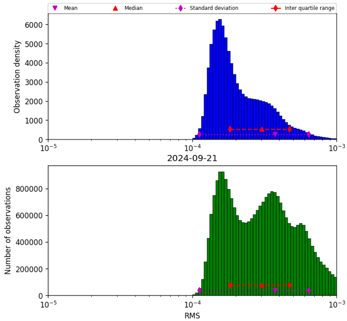
Figure 43: Histogram of “RMS” for 2024-09-20 to 2024-09-22
