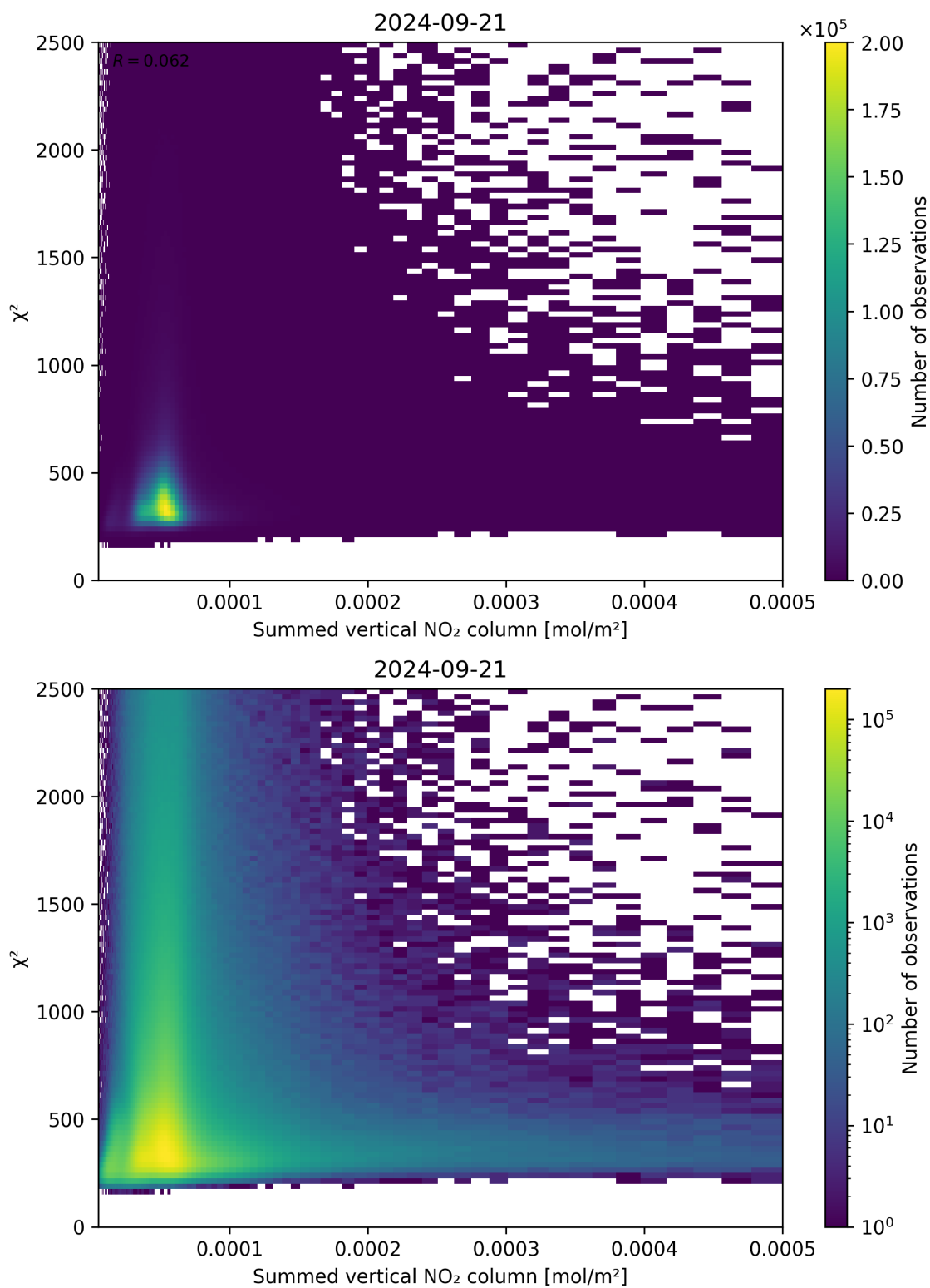
Figure 104: Scatter density plot of “Summed vertical NO 2 column” against “ \chi^2 ” for 2024-09-20 to 2024-09-22.
