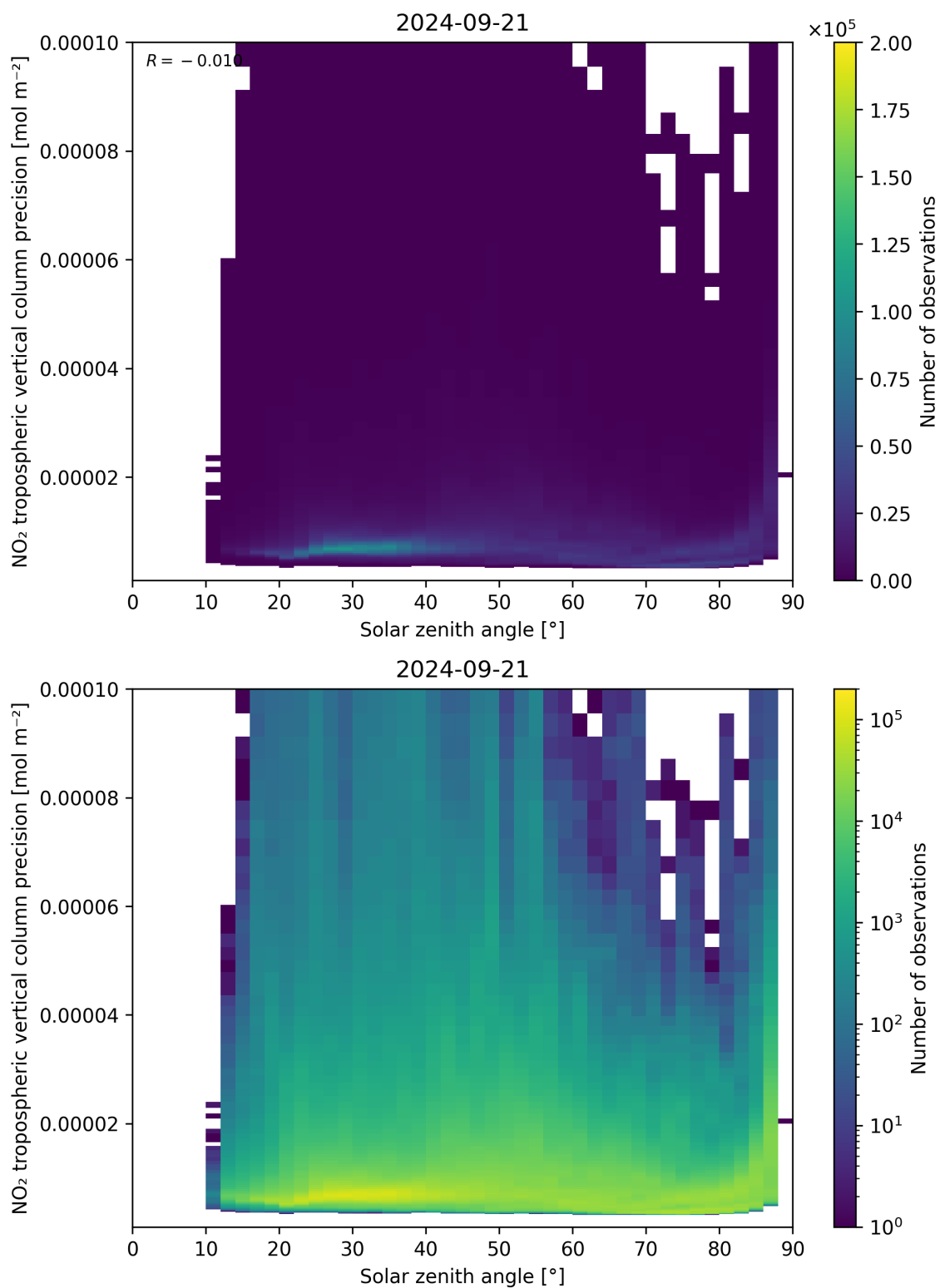
Figure 156: Scatter density plot of “Solar zenith angle” against “NO 2 tropospheric vertical column precision” for 2024-09-20 to 2024-09-22.
