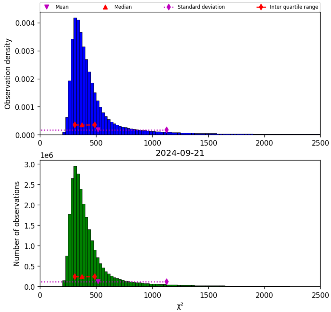
Figure 42: Histogram of " \chi^2 " for 2024-09-20 to 2024-09-22
