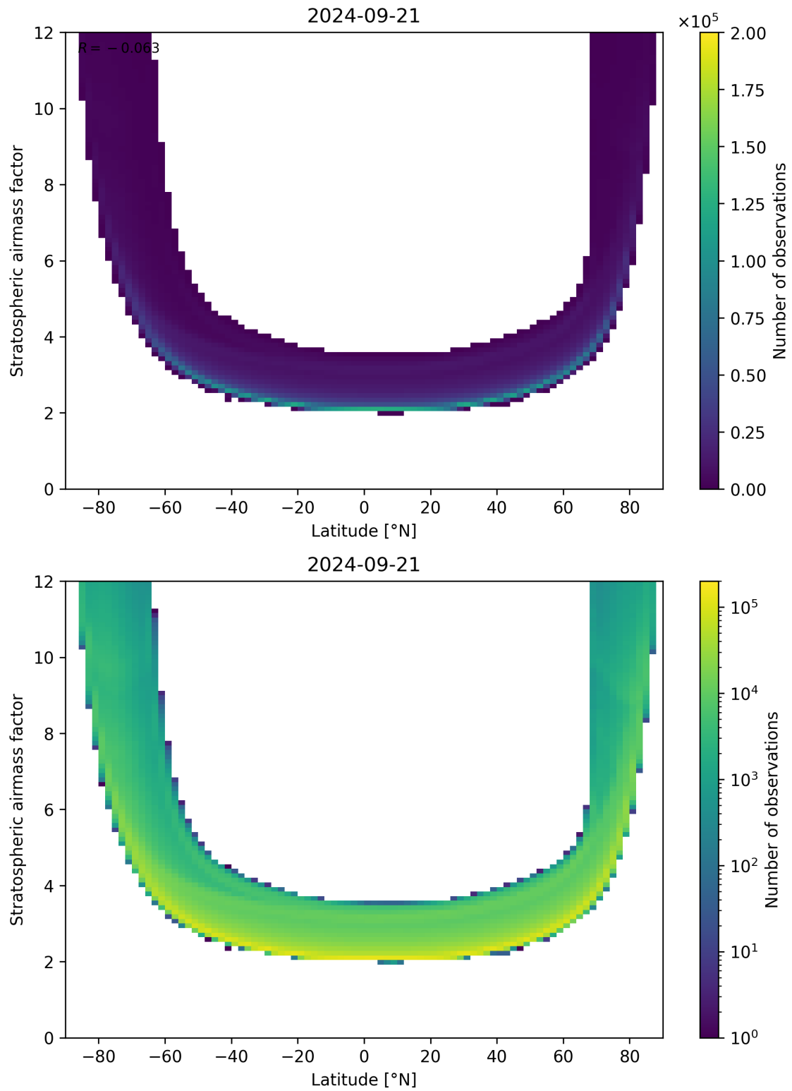
Figure 83: Scatter density plot of “Latitude” against “Stratospheric air mass factor” for 2024-09-20 to 2024-09-22.
