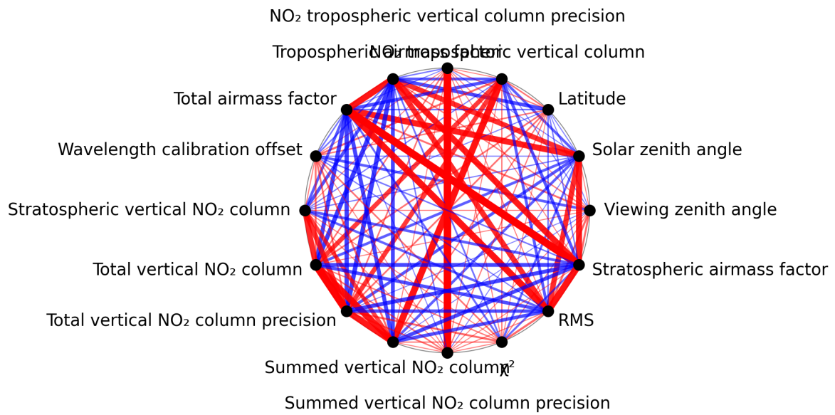
Figure 1: Map of correlation graph for 2024-09-20 to 2024-09-22.
