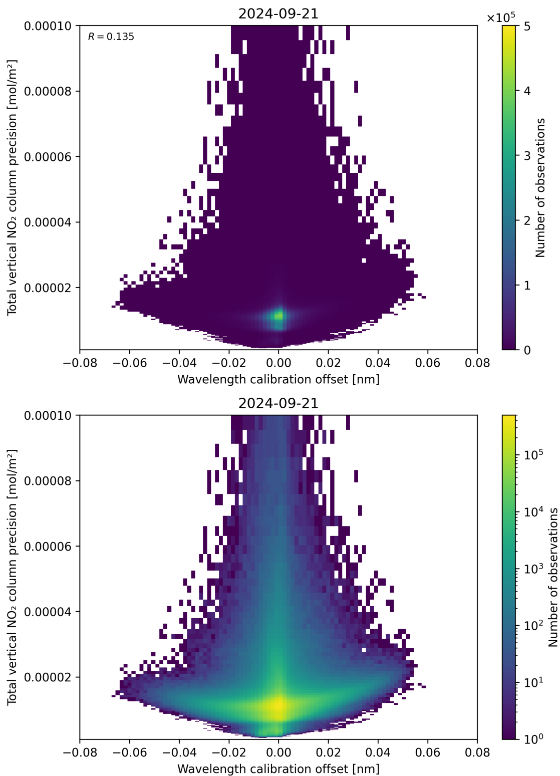
Figure 180: Scatter density plot of “Wavelength calibration offset” against “Total vertical NO 2 column precision” for 2024-09-20 to 2024-09-22.
