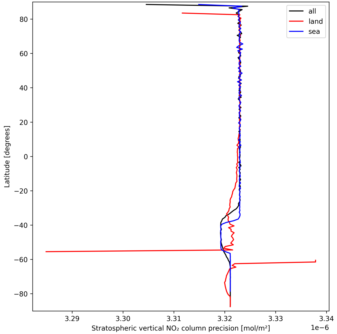
Figure 20: Zonal average of “Stratospheric vertical NO 2 column precision” for 2024-09-20 to 2024-09-22.
