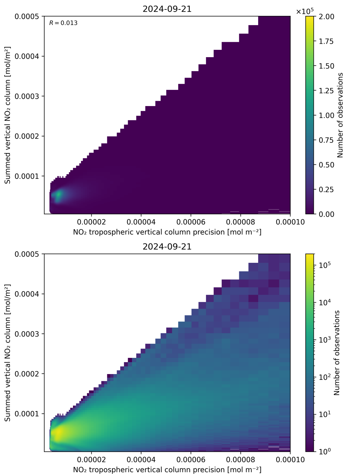
Figure 136: Scatter density plot of “NO 2 tropospheric vertical column precision” against “Summed vertical NO 2 column” for 2024-09-20 to 2024-09-22.
