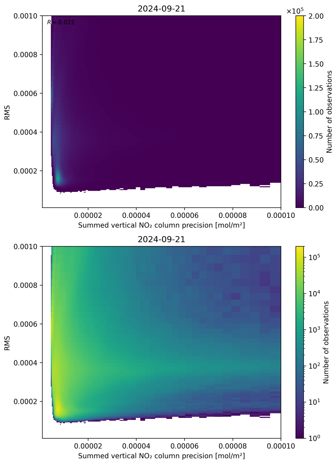
Figure 108: Scatter density plot of “Summed vertical NO 2 column precision” against “RMS” for 2024-09-20 to 2024-09-22.
