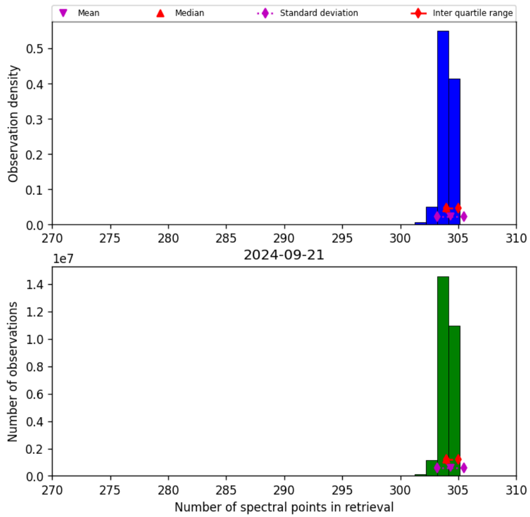
Figure 33: Histogram of “Number of spectral points in retrieval” for 2024-09-20 to 2024-09-22
