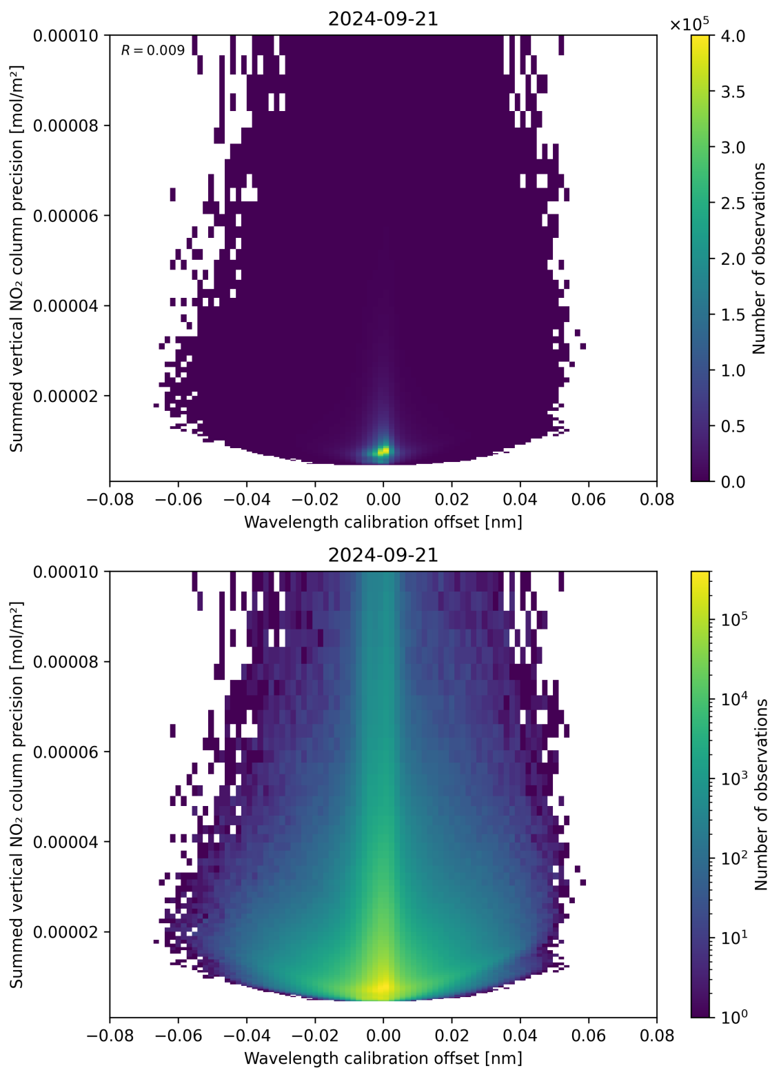
Figure 178: Scatter density plot of “Wavelength calibration offset” against “Summed vertical NO 2 column precision” for 2024-09-20 to 2024-09-22.
