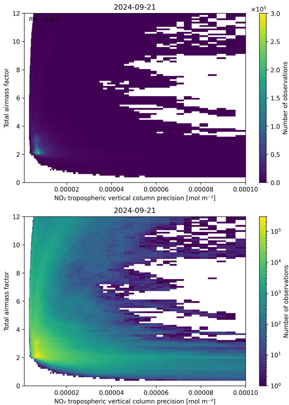
Figure 132: Scatter density plot of “NO 2 tropospheric vertical column precision” against “Total air mass factor” for 2024-09-20 to 2024-09-22.
