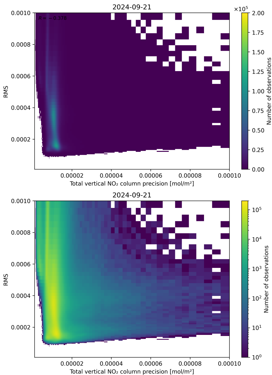
Figure 119: Scatter density plot of “Total vertical NO 2 column precision” against “RMS” for 2024-09-20 to 2024-09-22.
