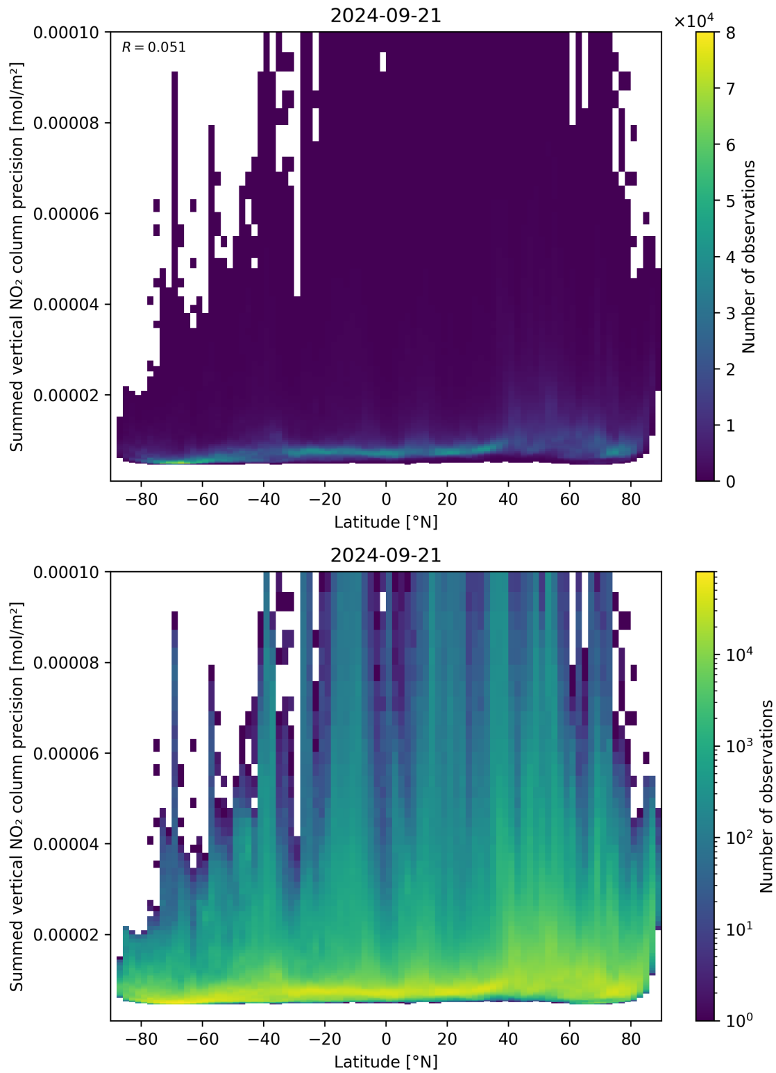
Figure 89: Scatter density plot of “Latitude” against “Summed vertical NO 2 column precision” for 2024-09-20 to 2024-09-22.
