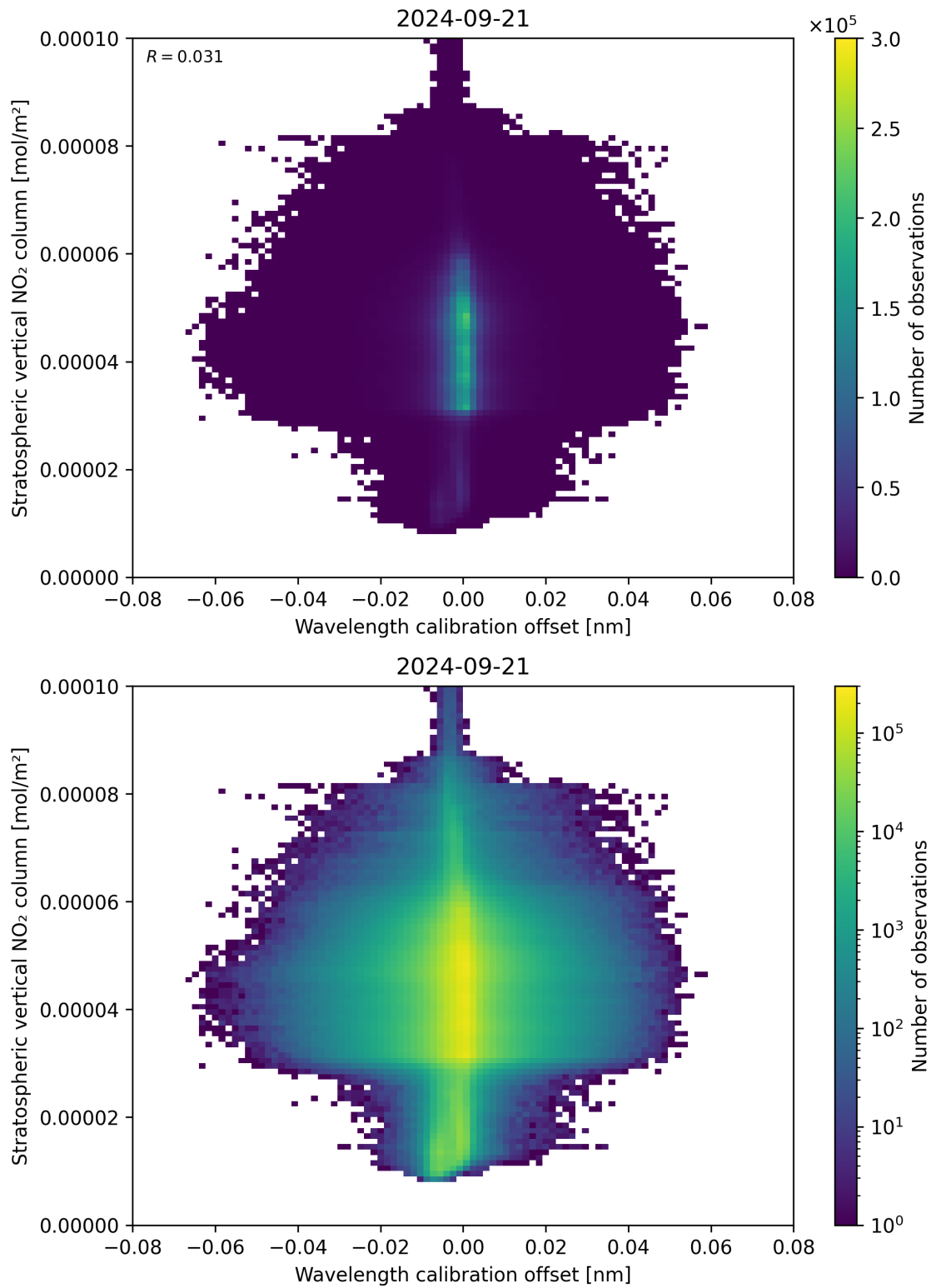
Figure 176: Scatter density plot of “Wavelength calibration offset” against “Stratospheric vertical NO 2 column” for 2024-09-20 to 2024-09-22.
