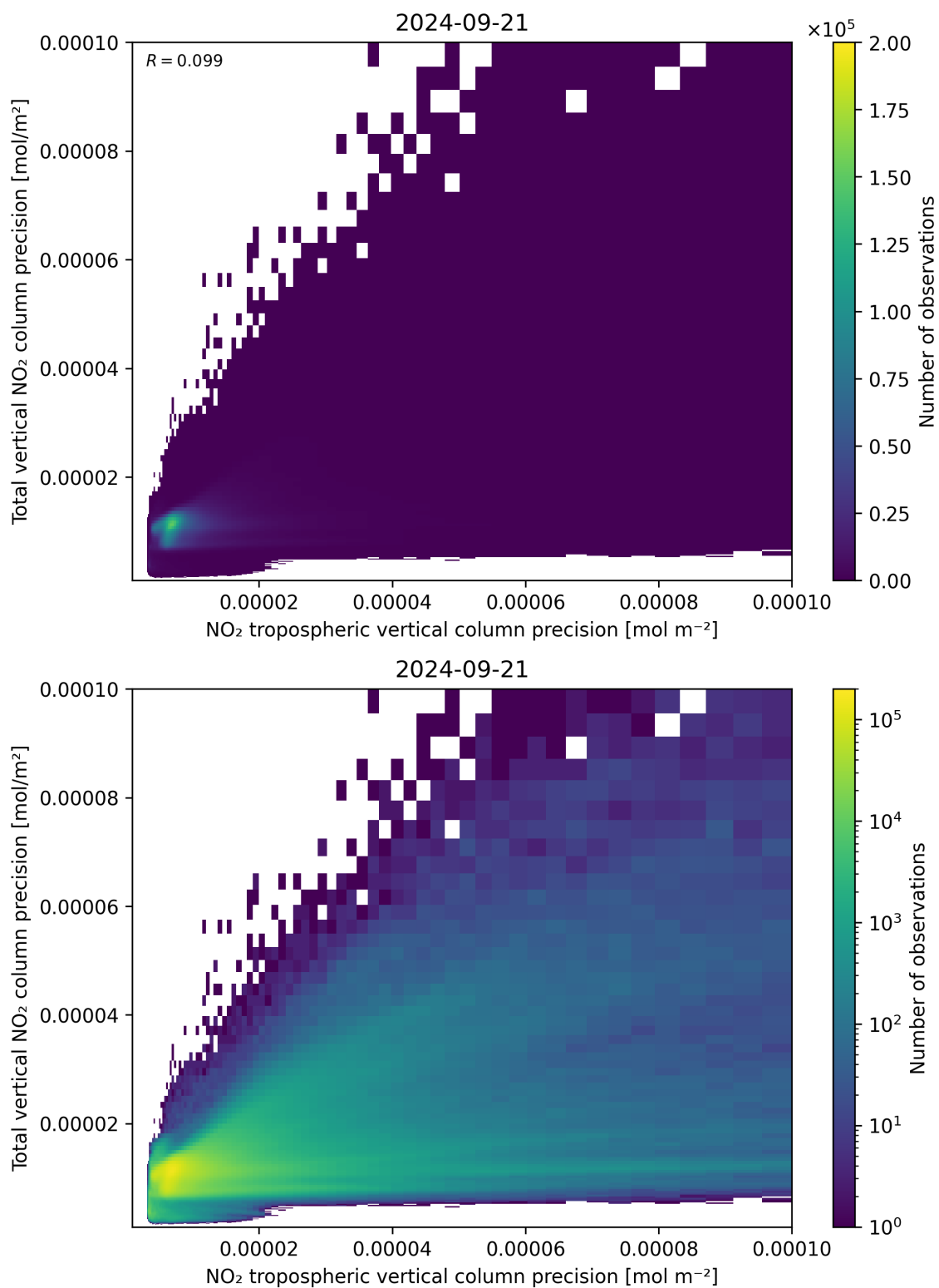
Figure 139: Scatter density plot of “NO 2 tropospheric vertical column precision” against “Total vertical NO 2 column precision” for 2024-09-20 to 2024-09-22.
