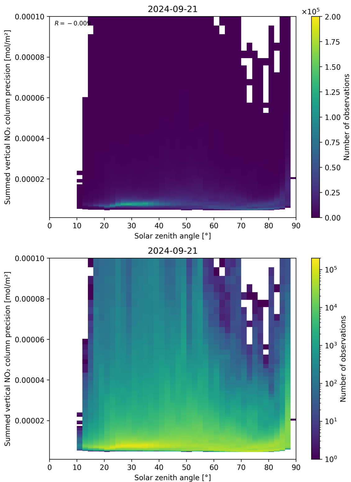
Figure 152: Scatter density plot of “Solar zenith angle” against “Summed vertical NO 2 column precision” for 2024-09-20 to 2024-09-22.
