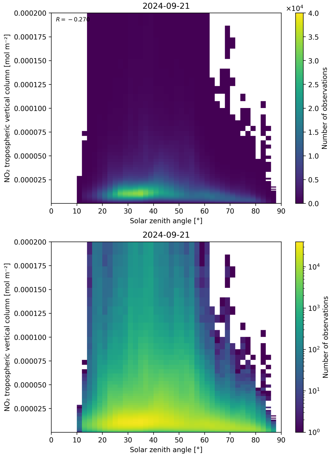
Figure 155: Scatter density plot of “Solar zenith angle” against “NO 2 tropospheric vertical column” for 2024-09-20 to 2024-09-22.
