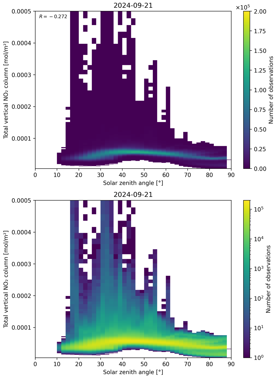
Figure 153: Scatter density plot of “Solar zenith angle” against “Total vertical NO 2 column” for 2024-09-20 to 2024-09-22.
