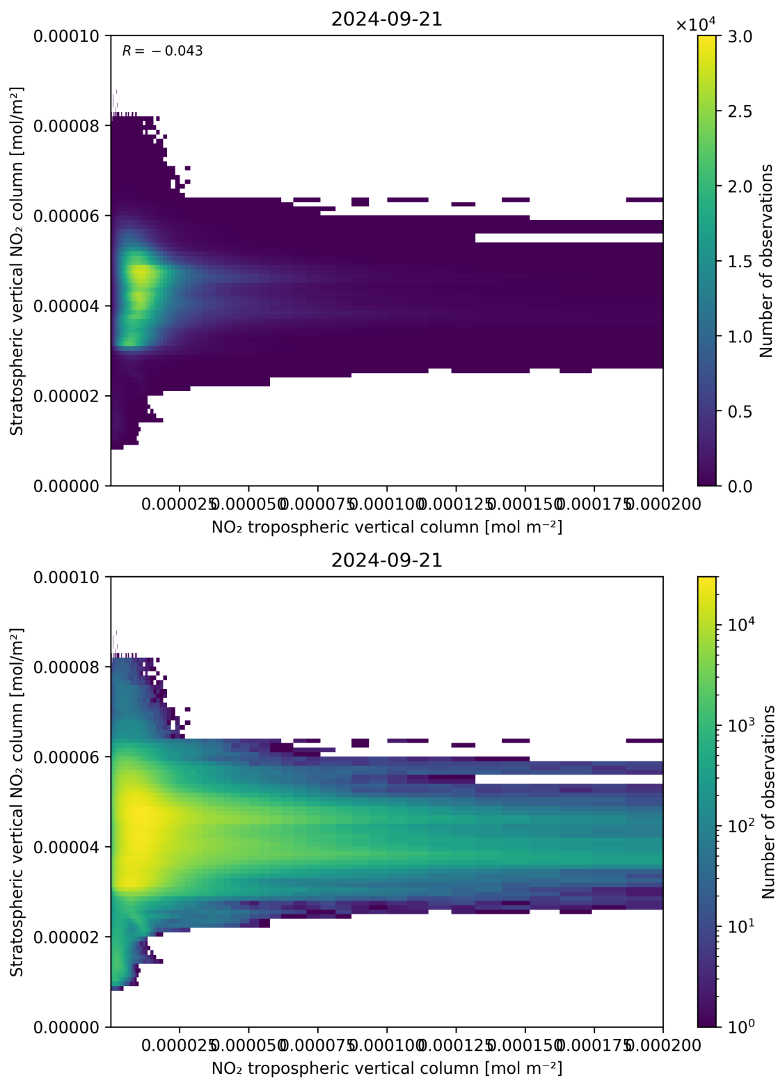
Figure 125: Scatter density plot of “NO 2 tropospheric vertical column” against “Stratospheric vertical NO 2 column” for 2024-09-20 to 2024-09-22.
