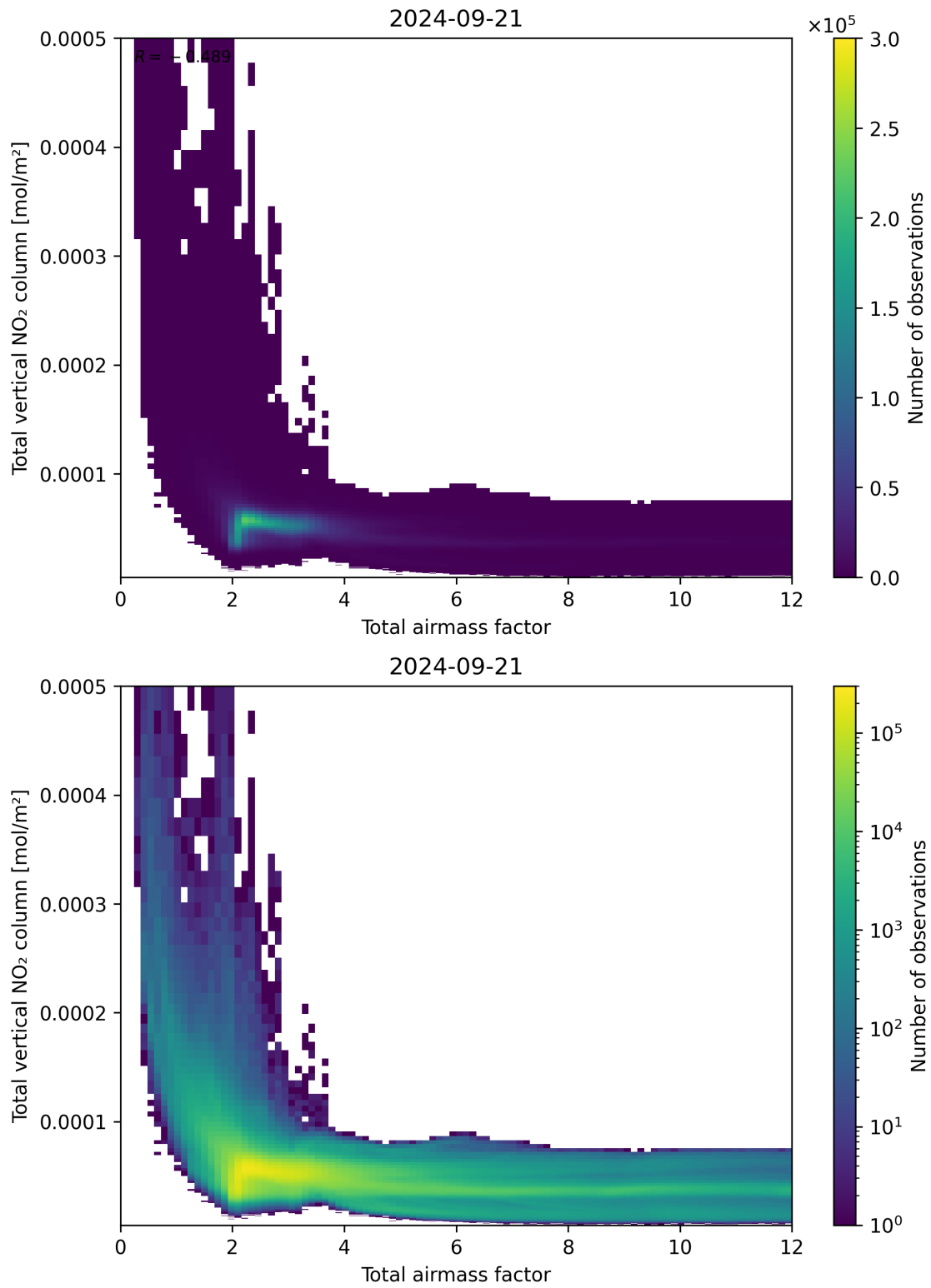
Figure 67: Scatter density plot of “Total airmass factor” against “Total vertical NO 2 column” for 2024-09-20 to 2024-09-22.
