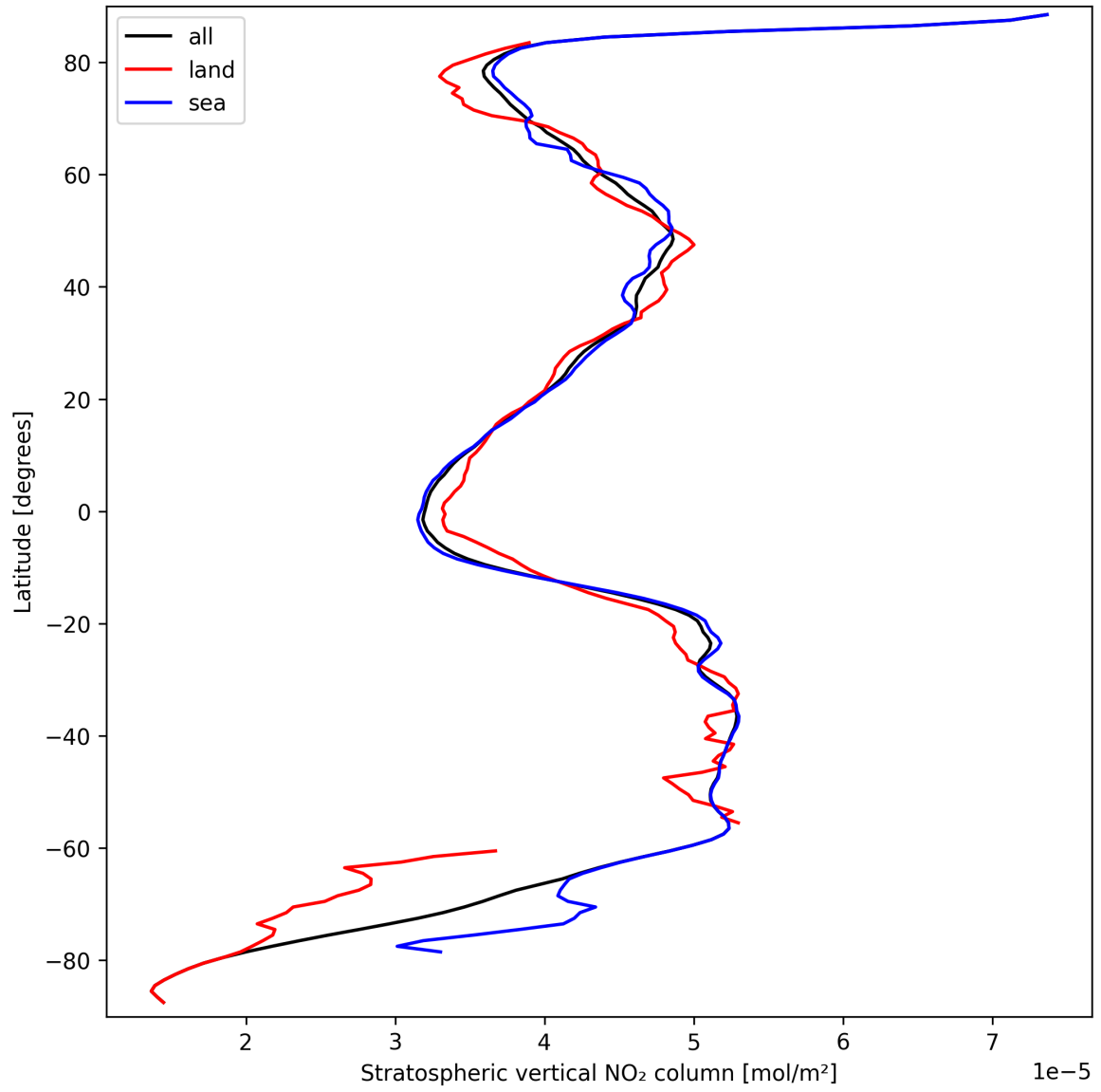
Figure 19: Zonal average of “Stratospheric vertical NO 2 column” for 2024-09-20 to 2024-09-22.
