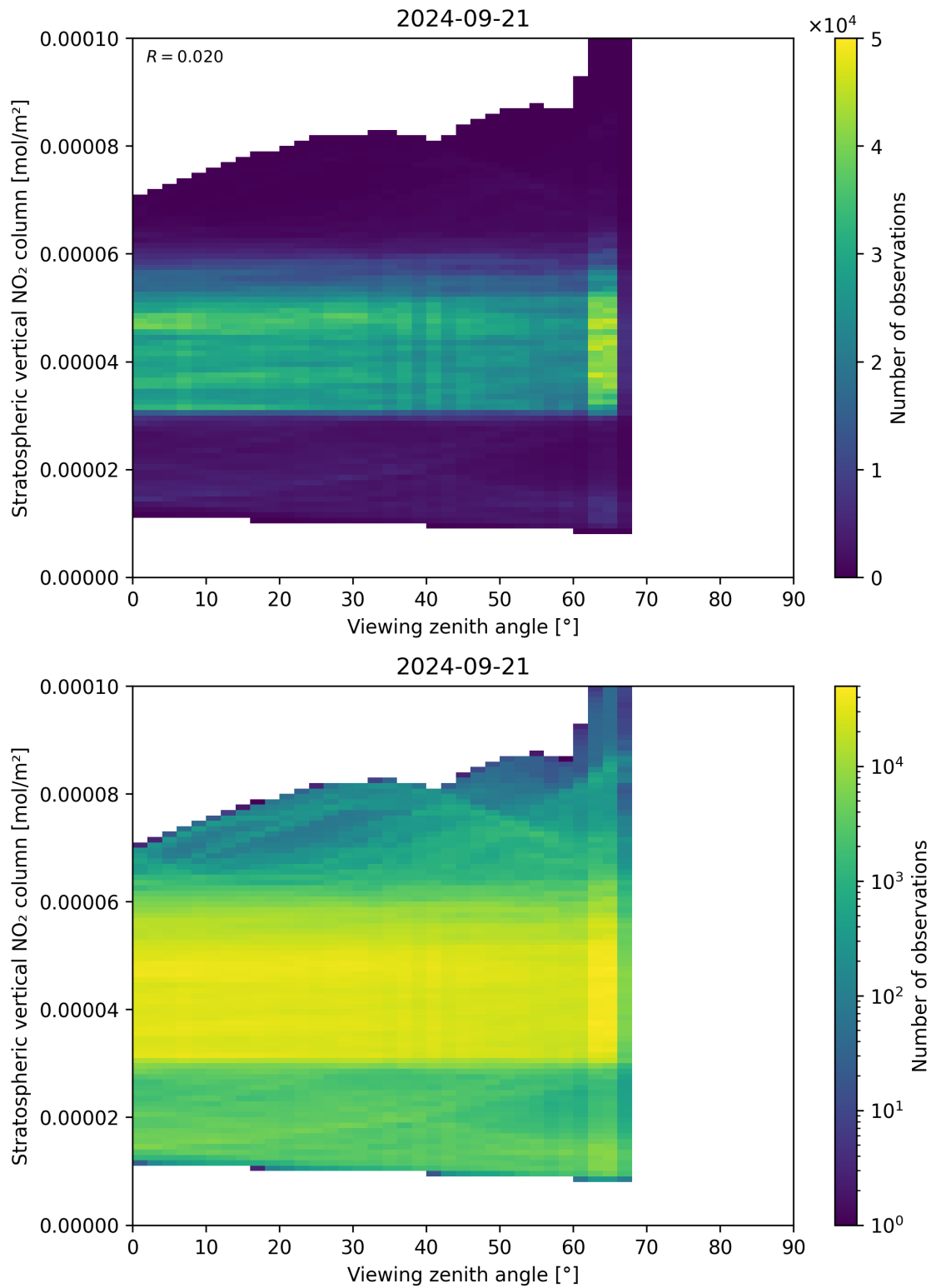
Figure 164: Scatter density plot of “Viewing zenith angle” against “Stratospheric vertical NO 2 column” for 2024-09-20 to 2024-09-22.
