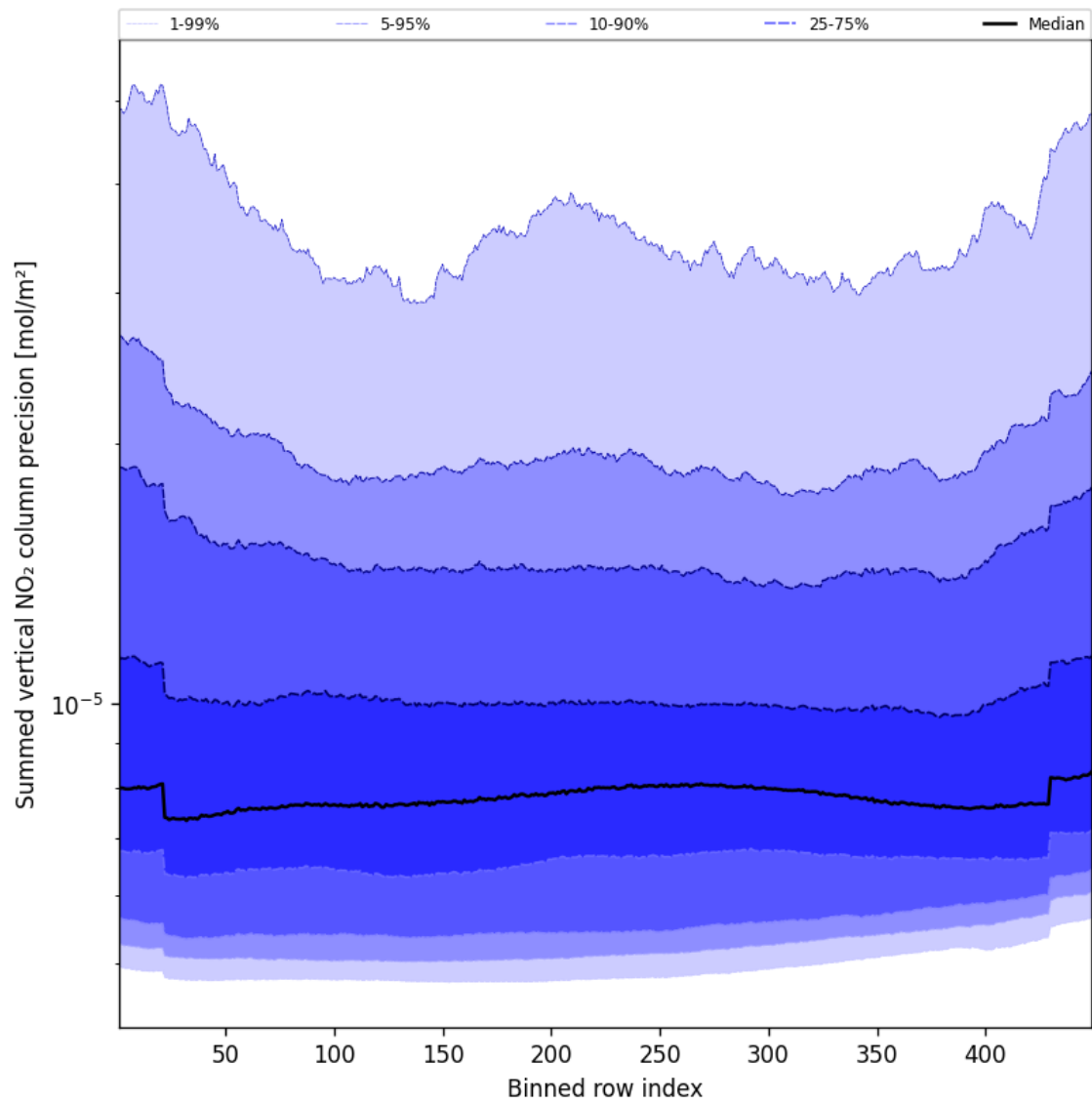
Figure 58: Along track statistics of “Summed vertical NO 2 column precision” for 2024-09-20 to 2024-09-22
