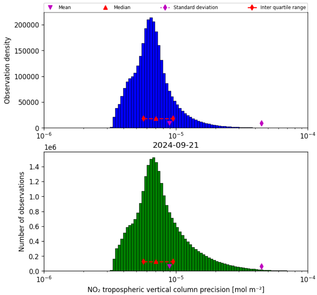
Figure 30: Histogram of “NO 2 tropospheric vertical column precision” for 2024-09-20 to 2024-09-22
