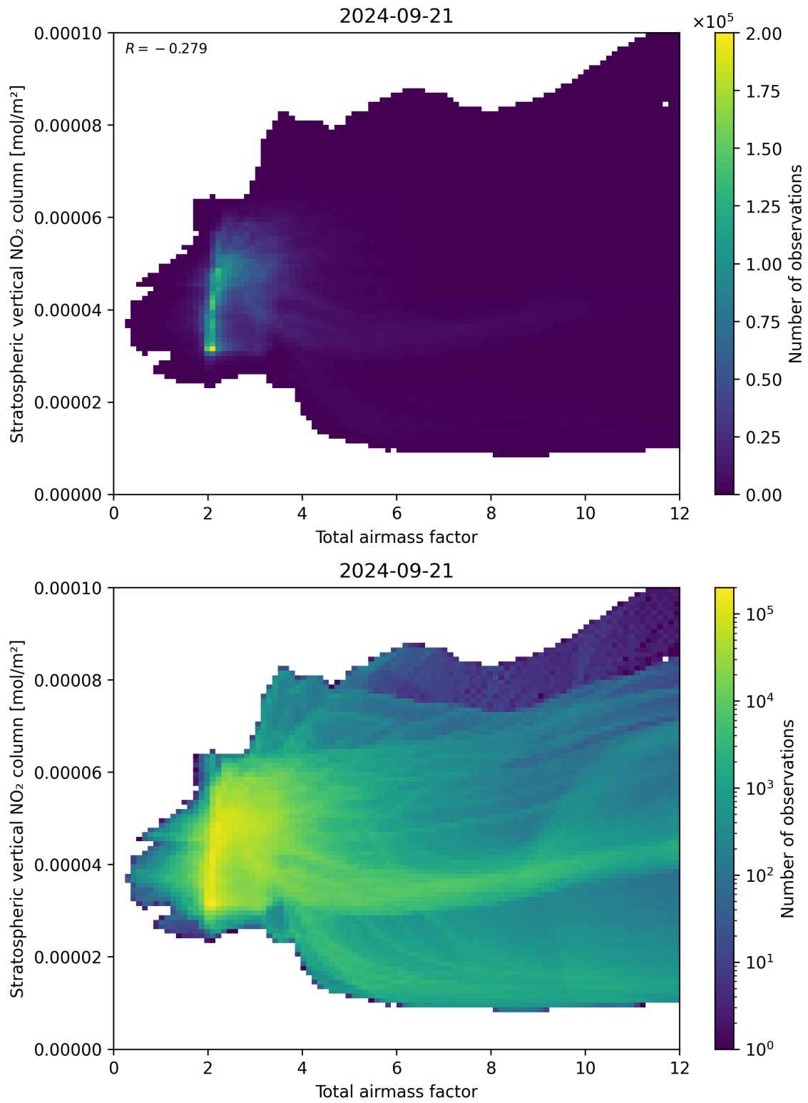
Figure 64: Scatter density plot of “Total airmass factor” against “Stratospheric vertical NO 2 column” for 2024-09-20 to 2024-09-22.
