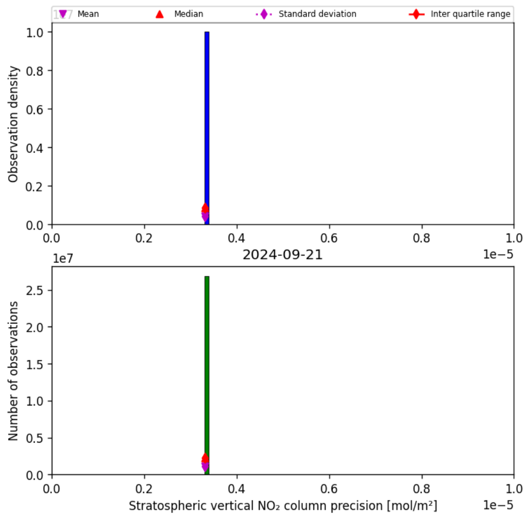
Figure 37: Histogram of “Stratospheric vertical NO 2 column precision” for 2024-09-20 to 2024-09-22
