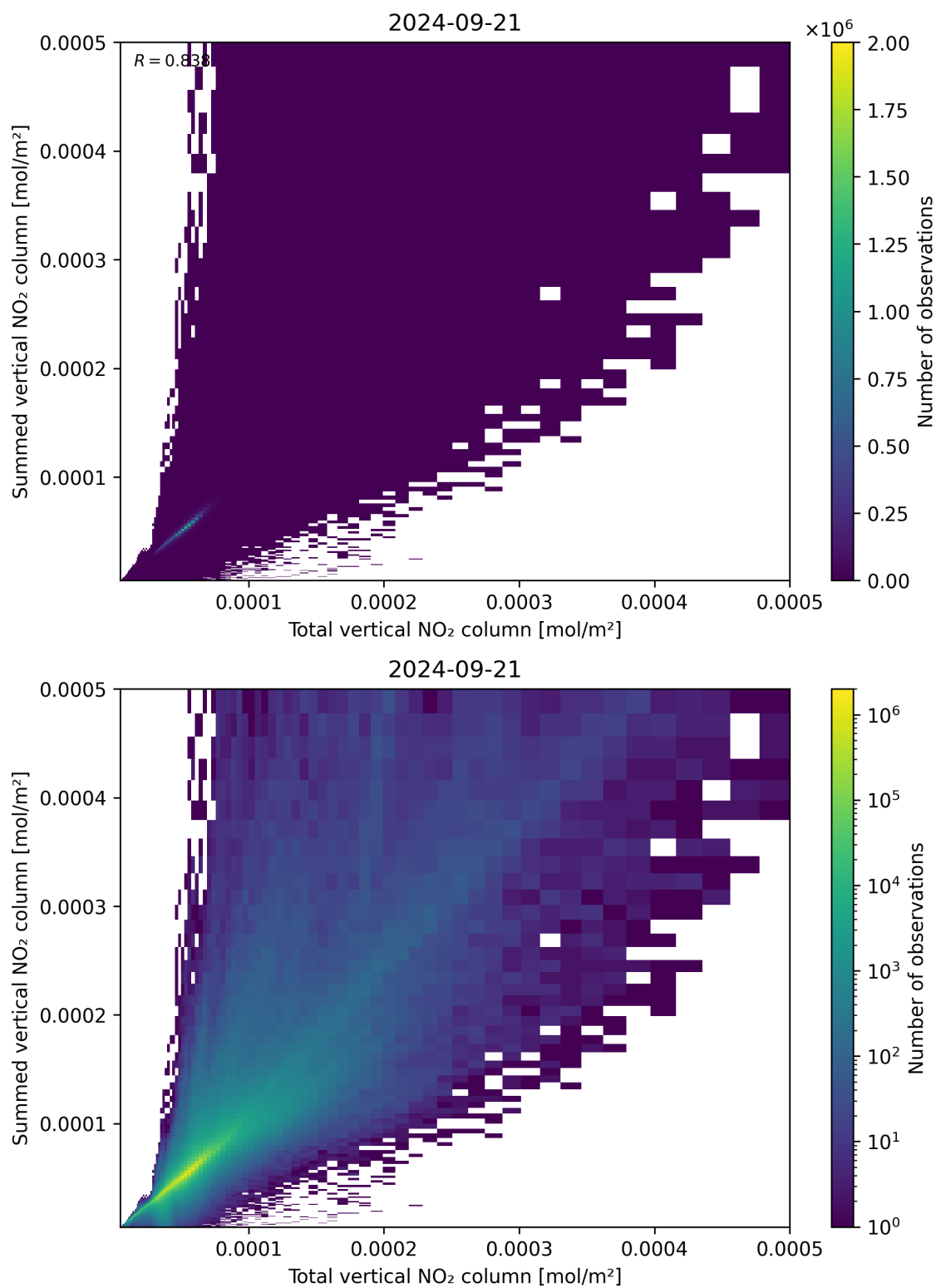
Figure 112: Scatter density plot of “Total vertical NO 2 column” against “Summed vertical NO 2 column” for 2024-09-20 to 2024-09-22.
