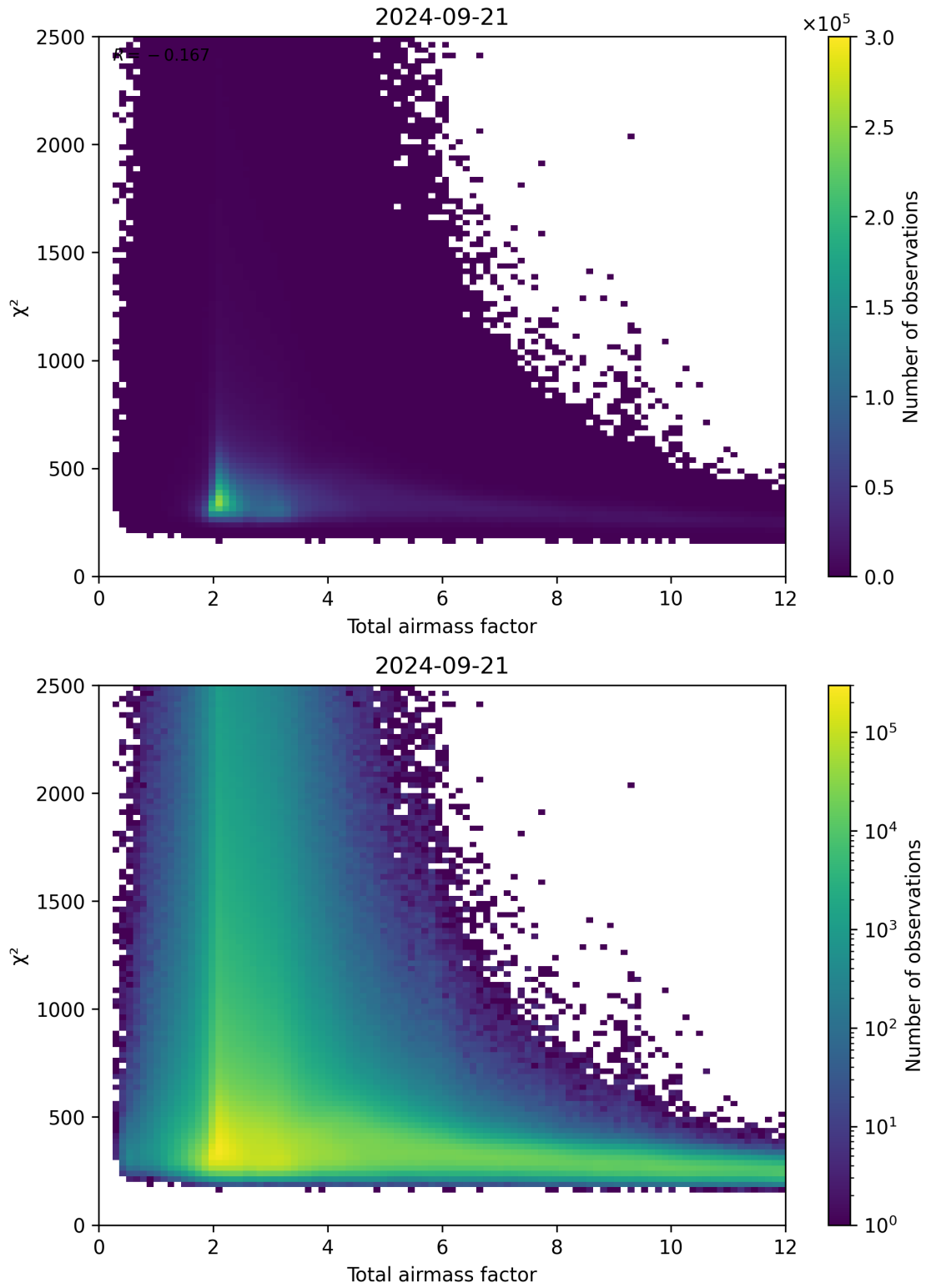
Figure 63: Scatter density plot of “Total airmass factor” against “ \chi^2 ” for 2024-09-20 to 2024-09-22.
