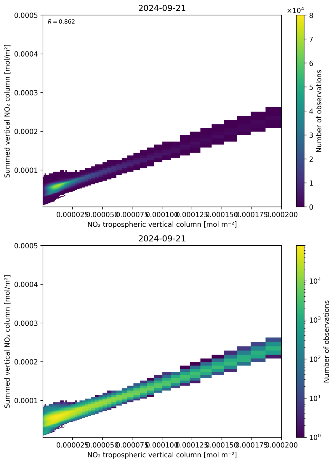
Figure 126: Scatter density plot of “NO 2 tropospheric vertical column” against “Summed vertical NO 2 column” for 2024-09-20 to 2024-09-22.
