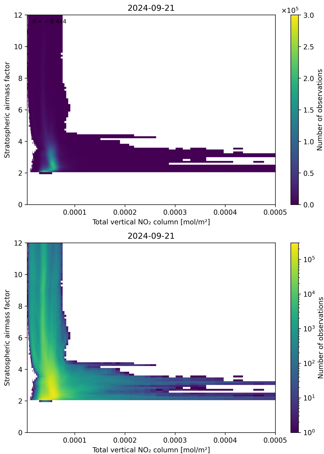
Figure 110: Scatter density plot of “Total vertical NO 2 column” against “Stratospheric airmass factor” for 2024-09-20 to 2024-09-22.
