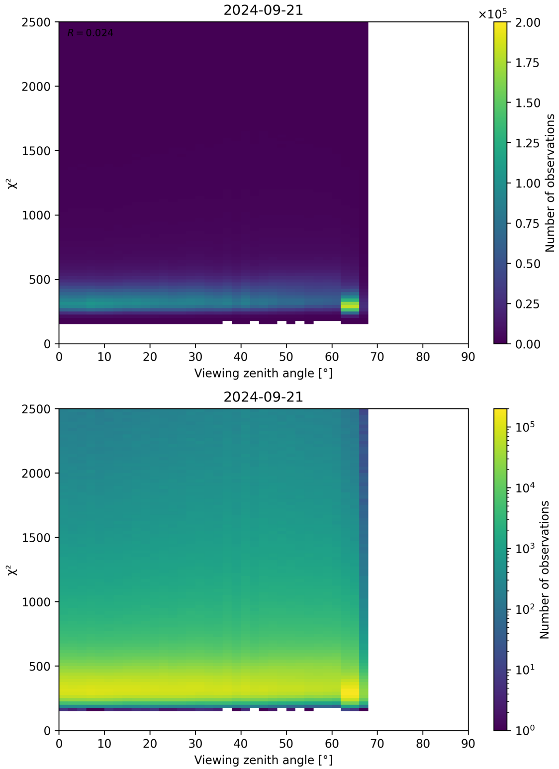
Figure 162: Scatter density plot of “Viewing zenith angle” against “ \chi^2 ” for 2024-09-20 to 2024-09-22.
