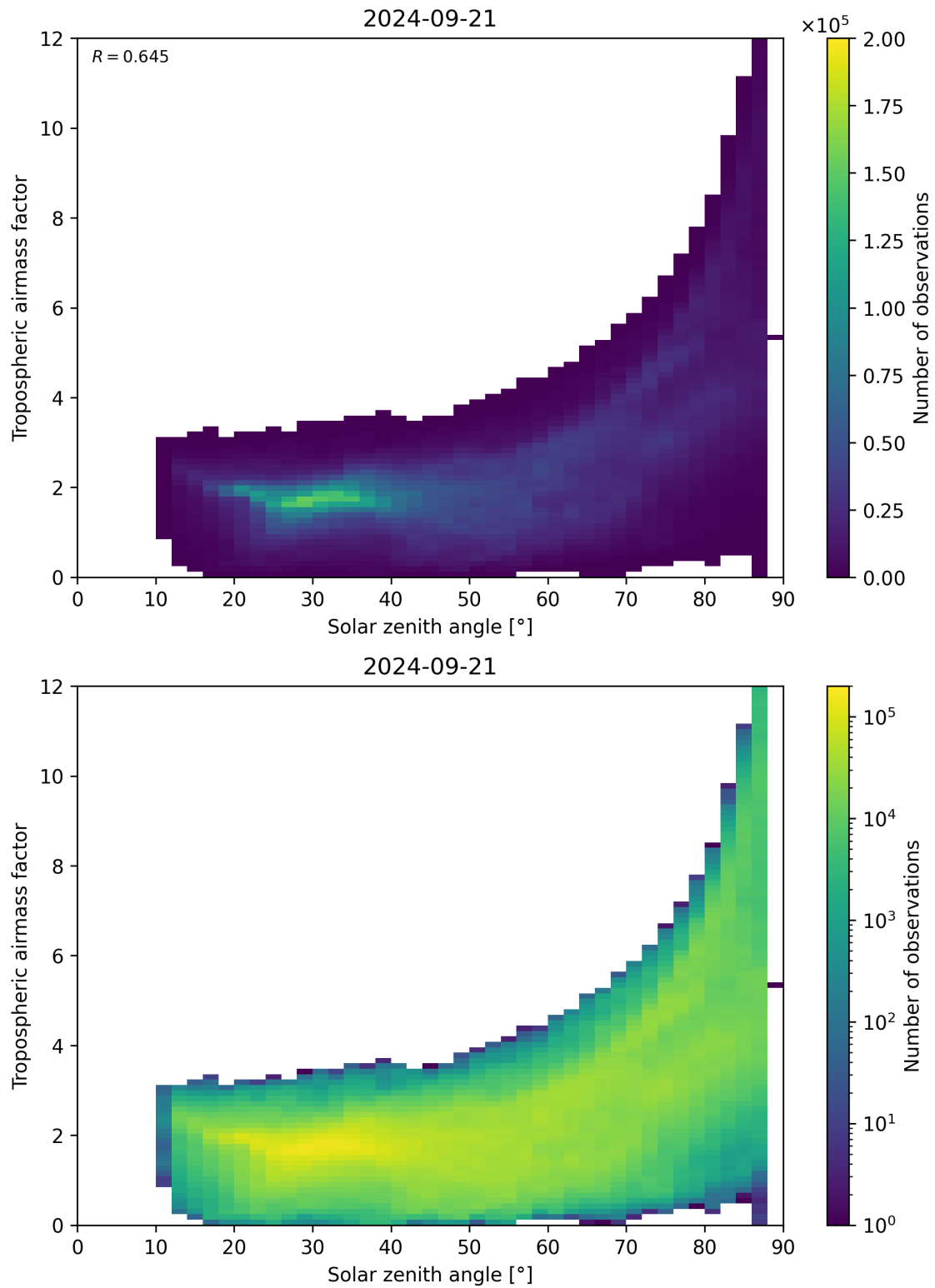
Figure 147: Scatter density plot of “Solar zenith angle” against “Tropospheric airmass factor” for 2024-09-20 to 2024-09-22.
