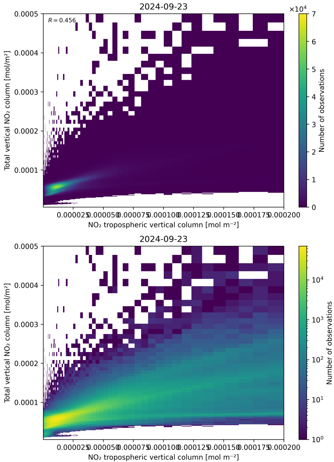
Figure 128: Scatter density plot of “NO 2 tropospheric vertical column” against “Total vertical NO 2 column” for 2024-09-22 to 2024-09-24.
