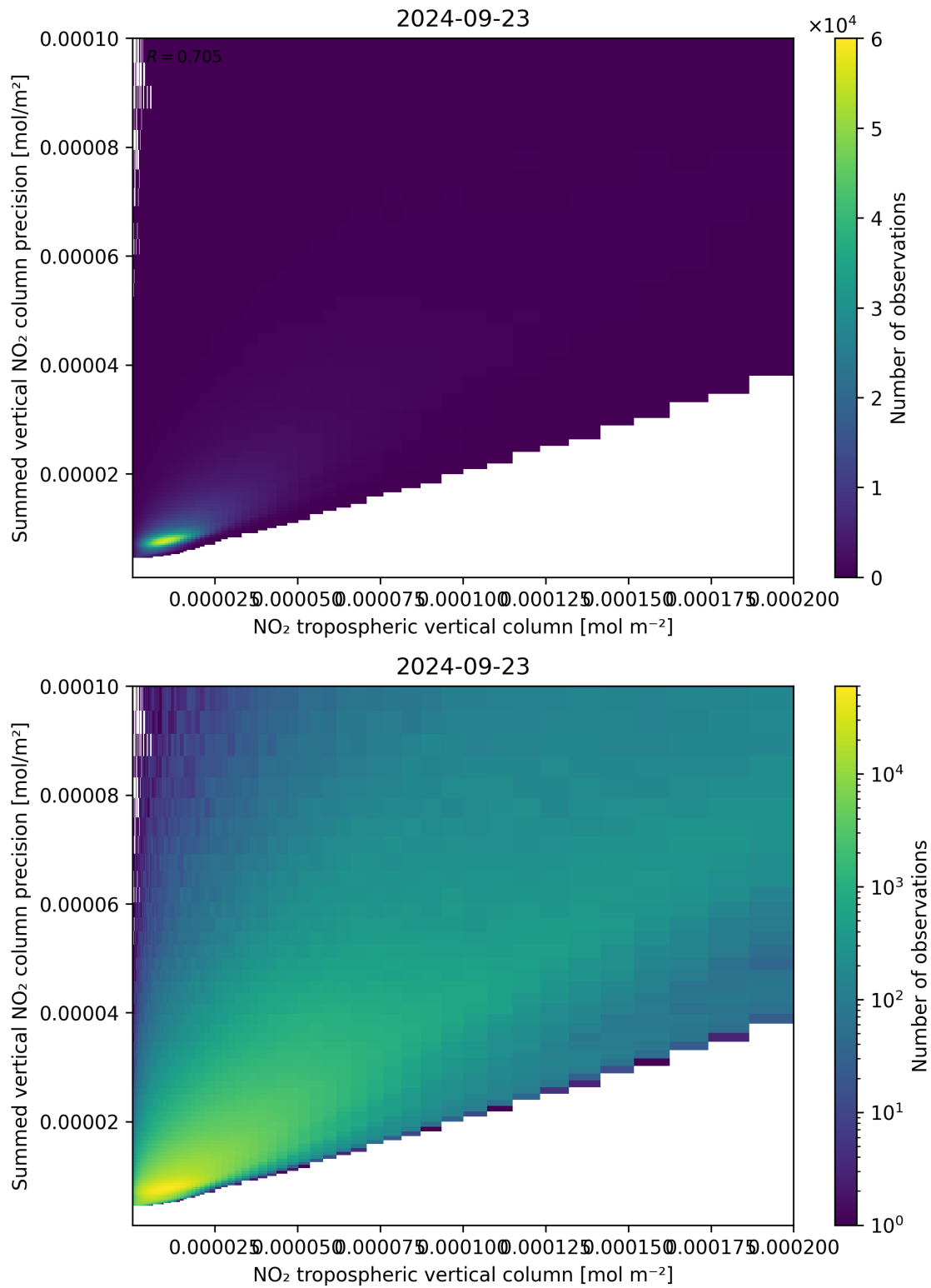
Figure 127: Scatter density plot of “NO 2 tropospheric vertical column” against “Summed vertical NO 2 column precision” for 2024-09-22 to 2024-09-24.
