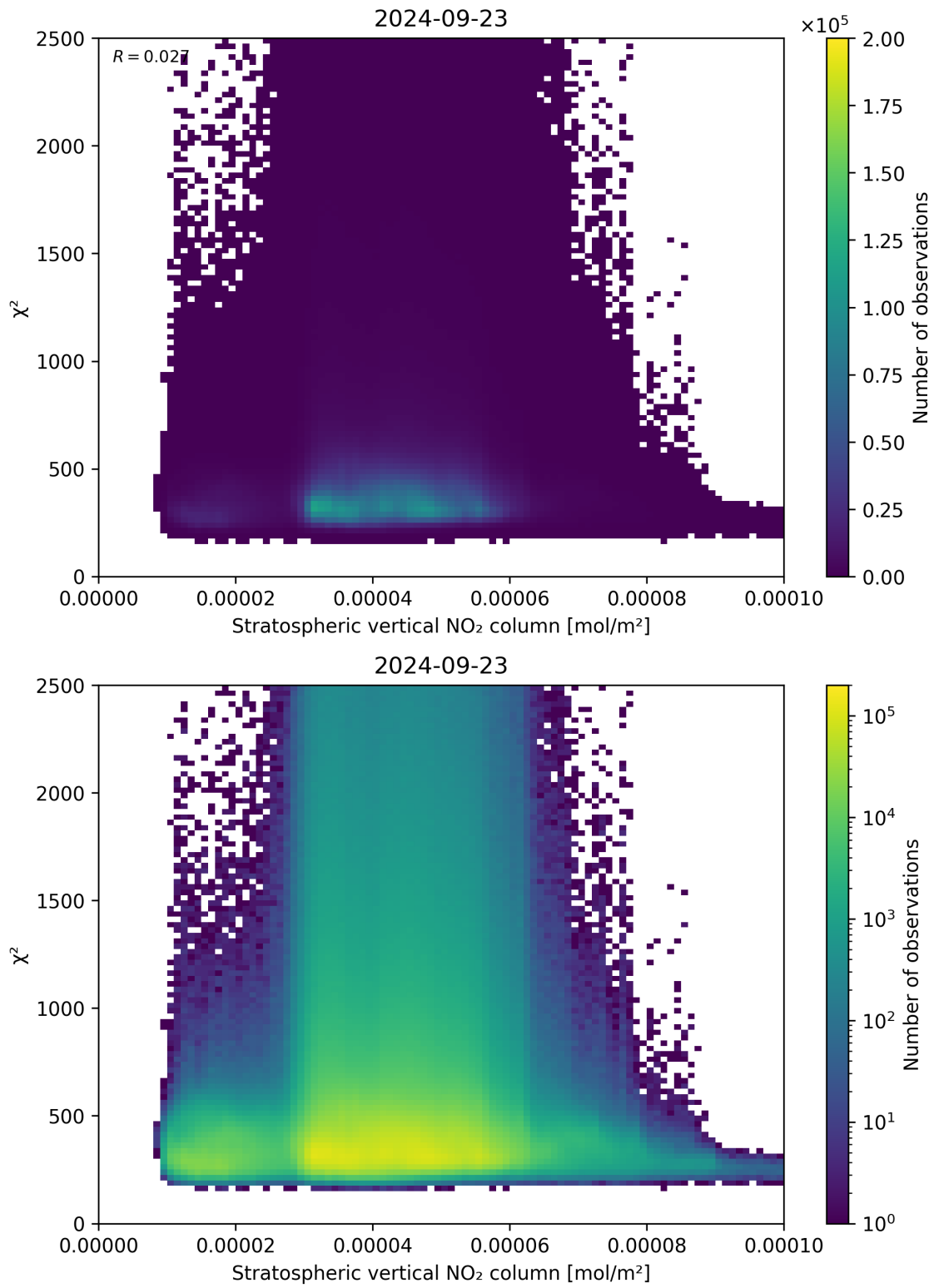
Figure 97: Scatter density plot of “Stratospheric vertical NO 2 column” against “ \chi^2 ” for 2024-09-22 to 2024-09-24.
