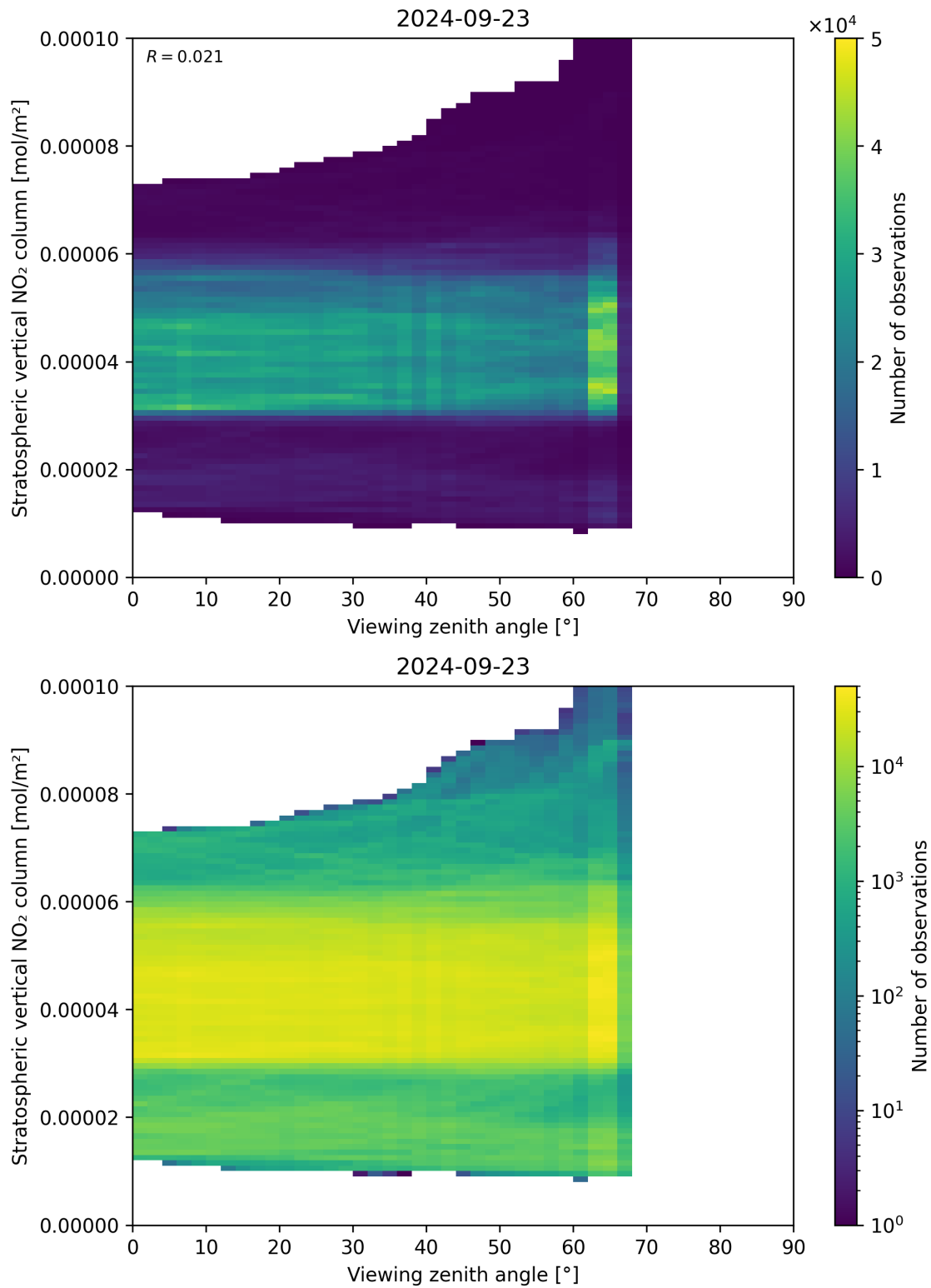
Figure 164: Scatter density plot of “Viewing zenith angle” against “Stratospheric vertical NO 2 column” for 2024-09-22 to 2024-09-24.
