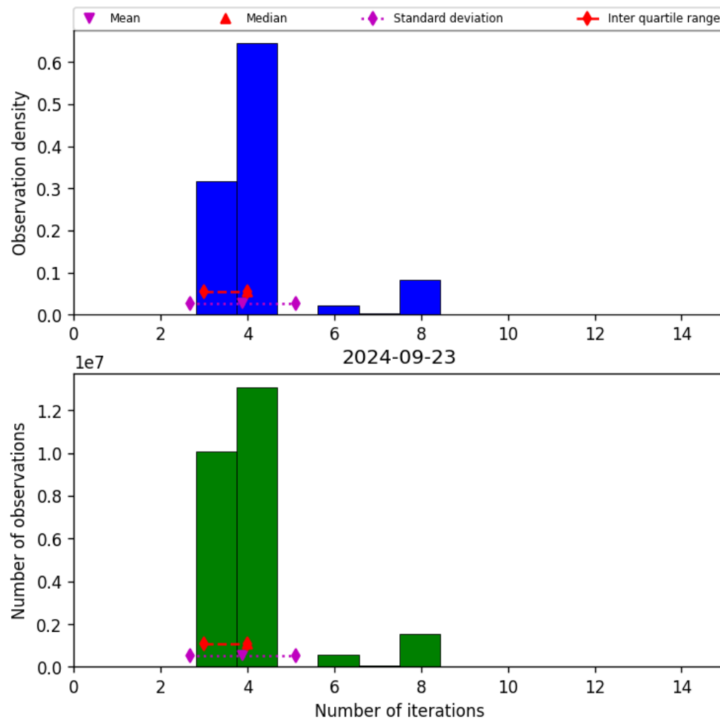
Figure 34: Histogram of “Number of iterations” for 2024-09-22 to 2024-09-24
