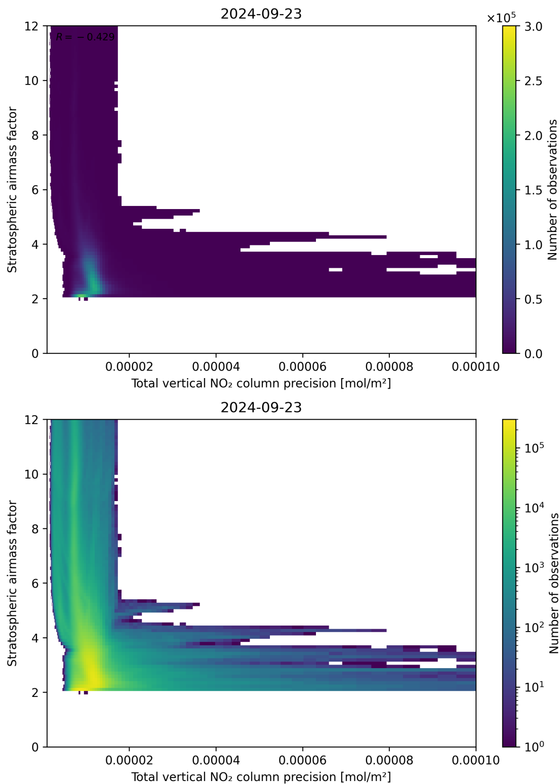
Figure 115: Scatter density plot of “Total vertical NO 2 column precision” against “Stratospheric airmass factor” for 2024-09-22 to 2024-09-24.
