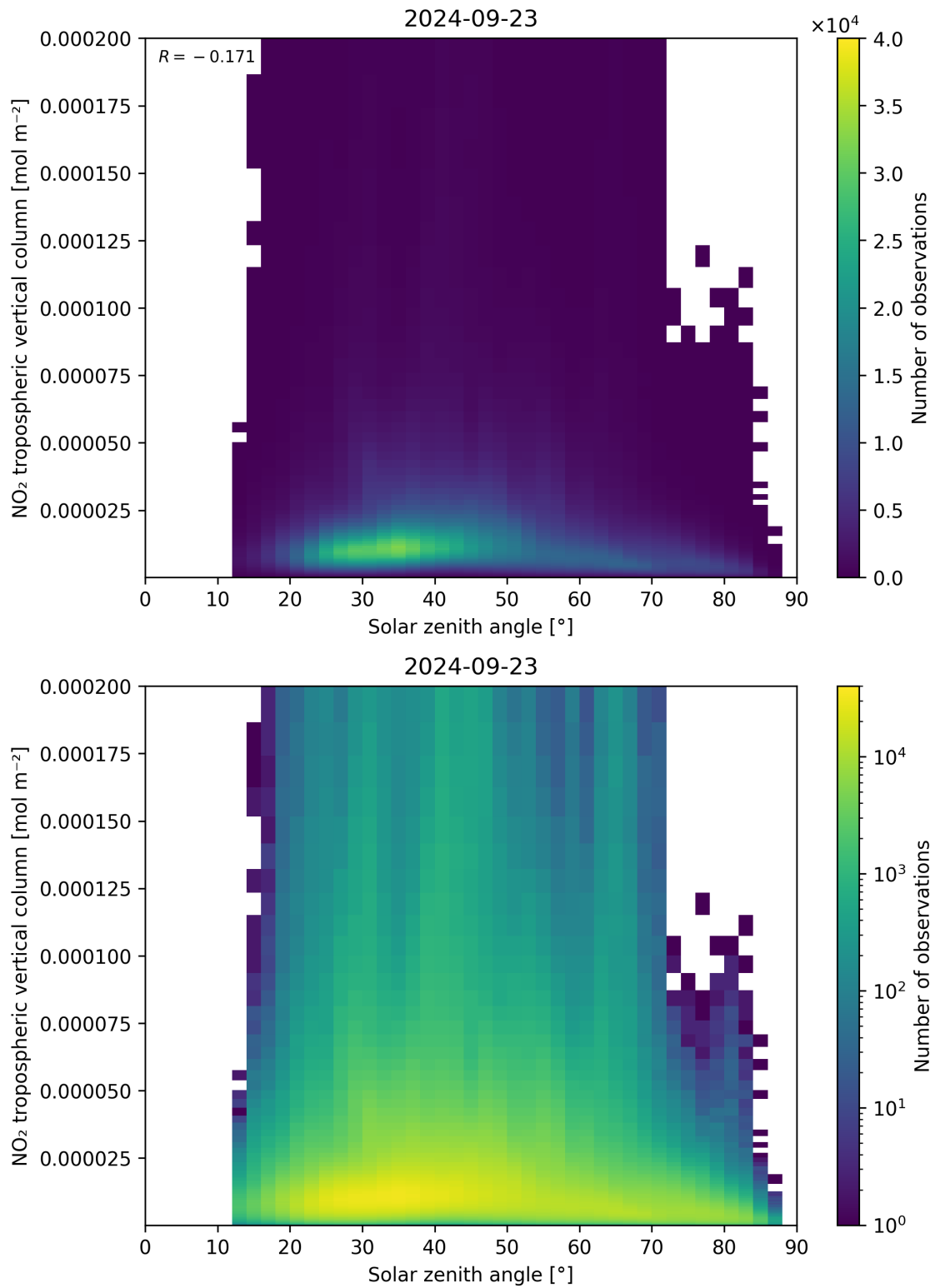
Figure 155: Scatter density plot of “Solar zenith angle” against “NO 2 tropospheric vertical column” for 2024-09-22 to 2024-09-24.
