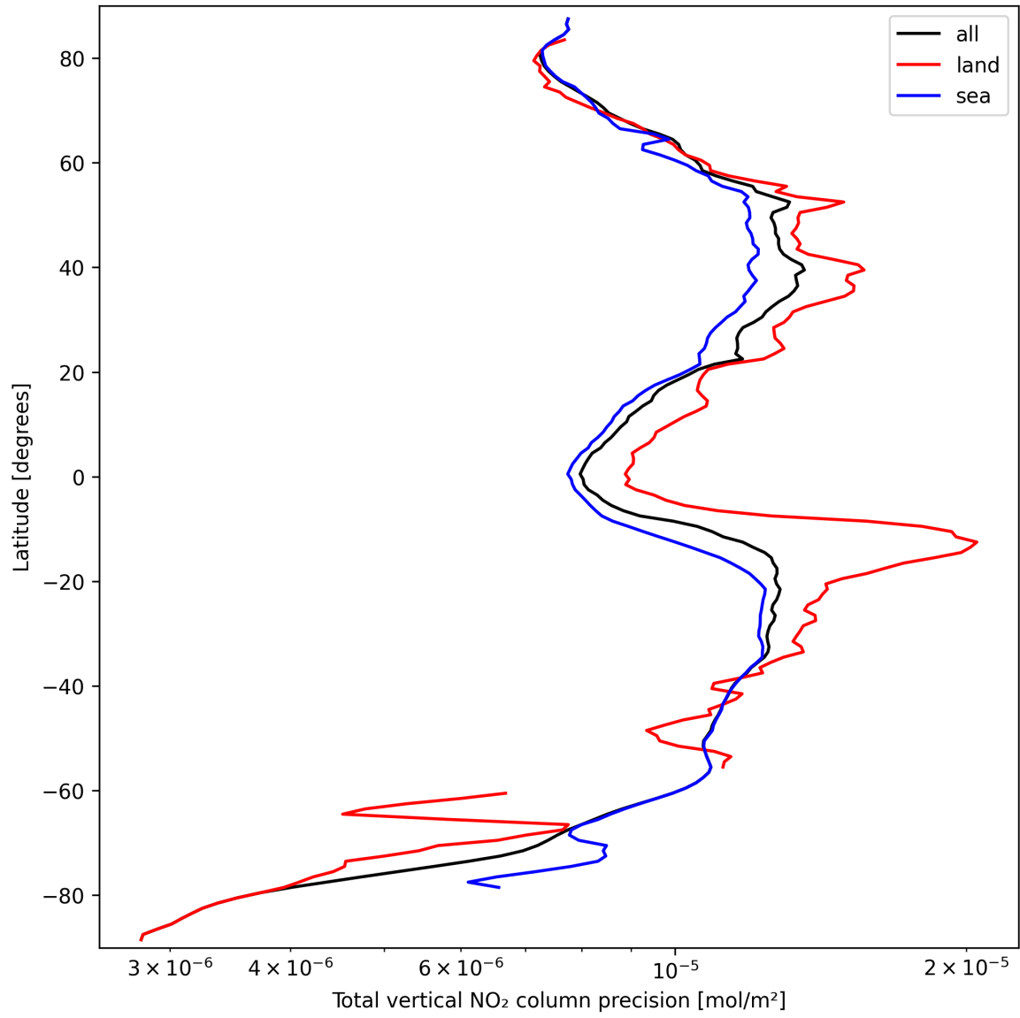
Figure 22: Zonal average of “Total vertical NO 2 column precision” for 2024-09-22 to 2024-09-24.
