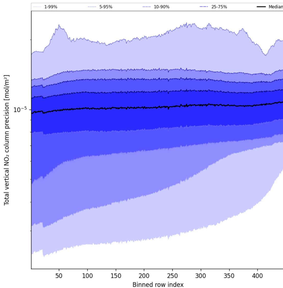
Figure 56: Along track statistics of “Total vertical NO 2 column precision” for 2024-09-22 to 2024-09-24
