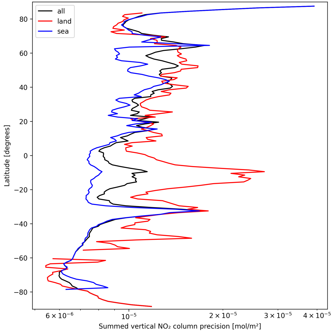
Figure 24: Zonal average of “Summed vertical NO 2 column precision” for 2024-09-22 to 2024-09-24.
