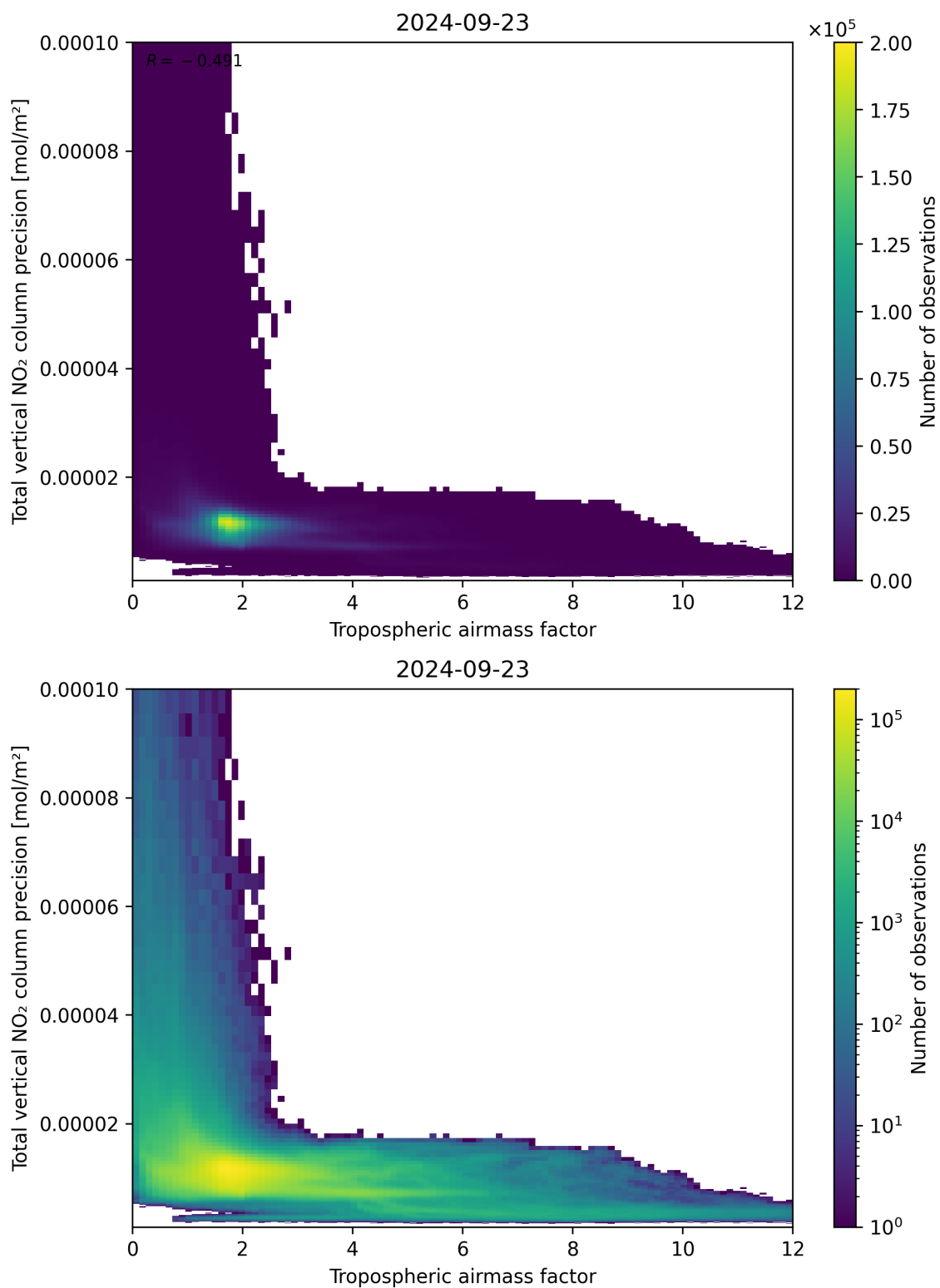
Figure 78: Scatter density plot of “Tropospheric air mass factor” against “Total vertical NO 2 column precision” for 2024-09-22 to 2024-09-24.
