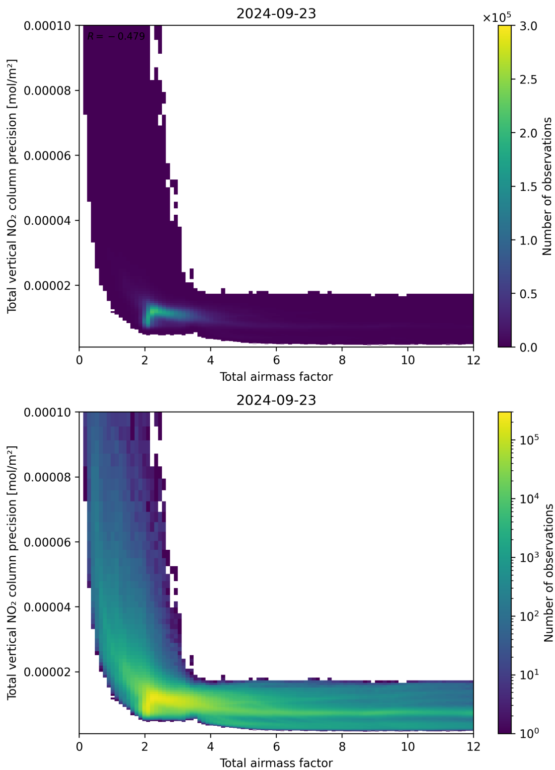
Figure 68: Scatter density plot of “Total airmass factor” against “Total vertical NO 2 column precision” for 2024-09-22 to 2024-09-24.
