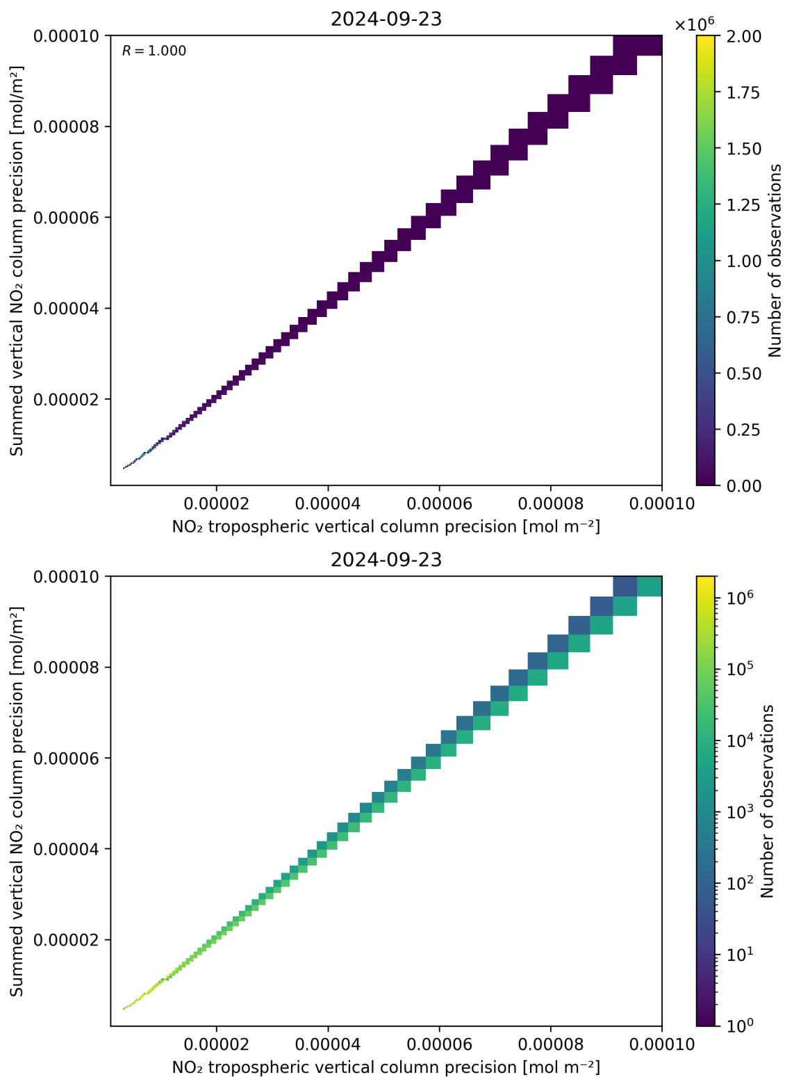
Figure 137: Scatter density plot of “NO 2 tropospheric vertical column precision” against “Summed vertical NO 2 column precision” for 2024-09-22 to 2024-09-24.
