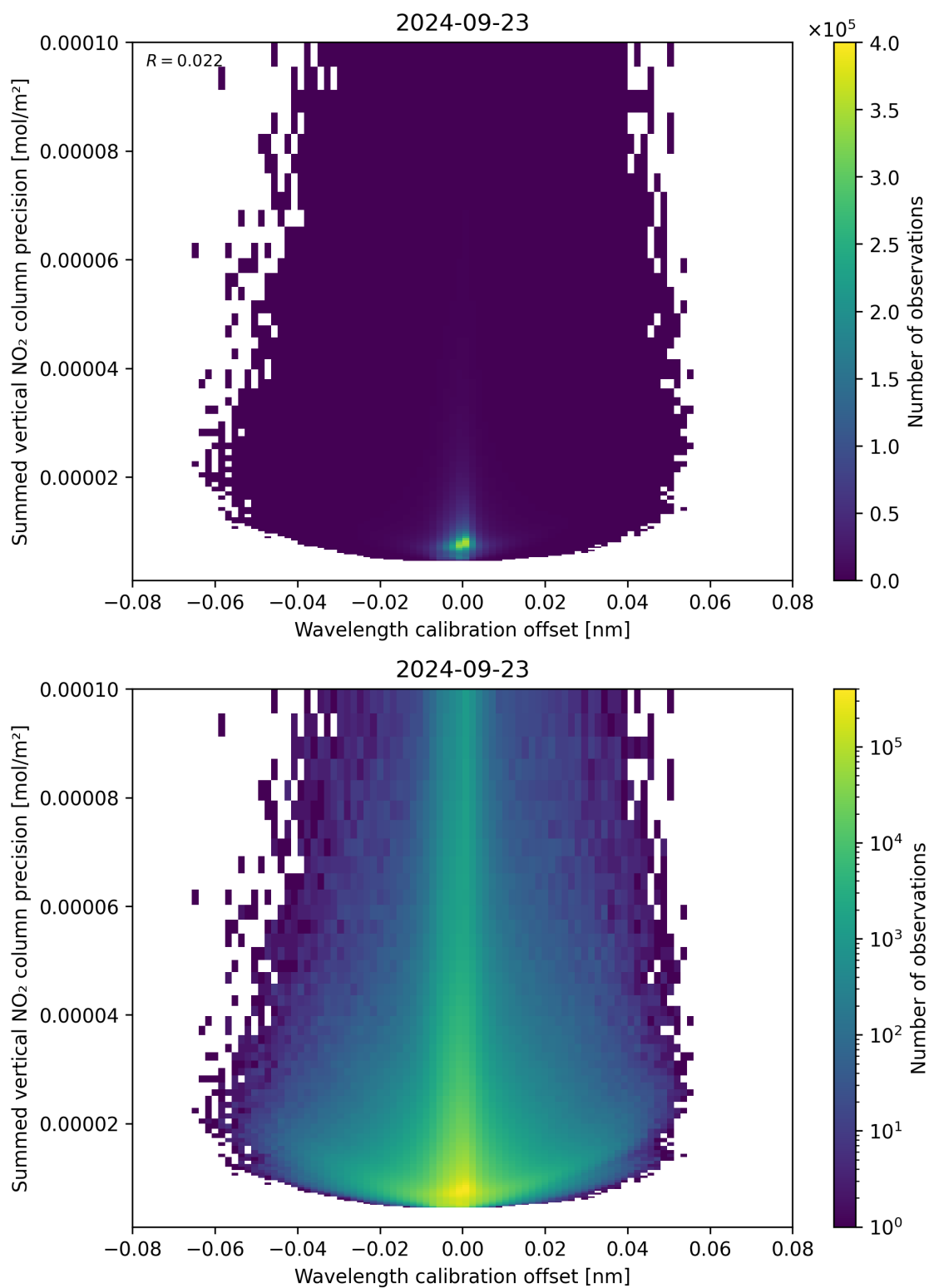
Figure 178: Scatter density plot of “Wavelength calibration offset” against “Summed vertical NO 2 column precision” for 2024-09-22 to 2024-09-24.
