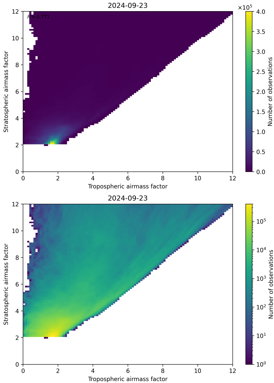
Figure 71: Scatter density plot of “Tropospheric airmass factor” against “Stratospheric airmass factor” for 2024-09-22 to 2024-09-24.
