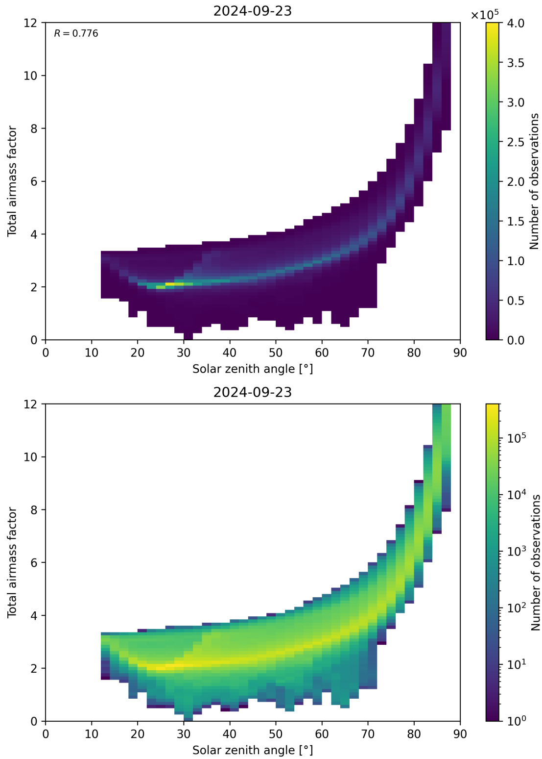
Figure 146: Scatter density plot of “Solar zenith angle” against “Total air mass factor” for 2024-09-22 to 2024-09-24.
