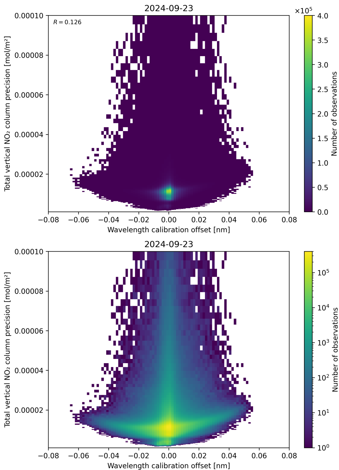
Figure 180: Scatter density plot of “Wavelength calibration offset” against “Total vertical NO 2 column precision” for 2024-09-22 to 2024-09-24.
