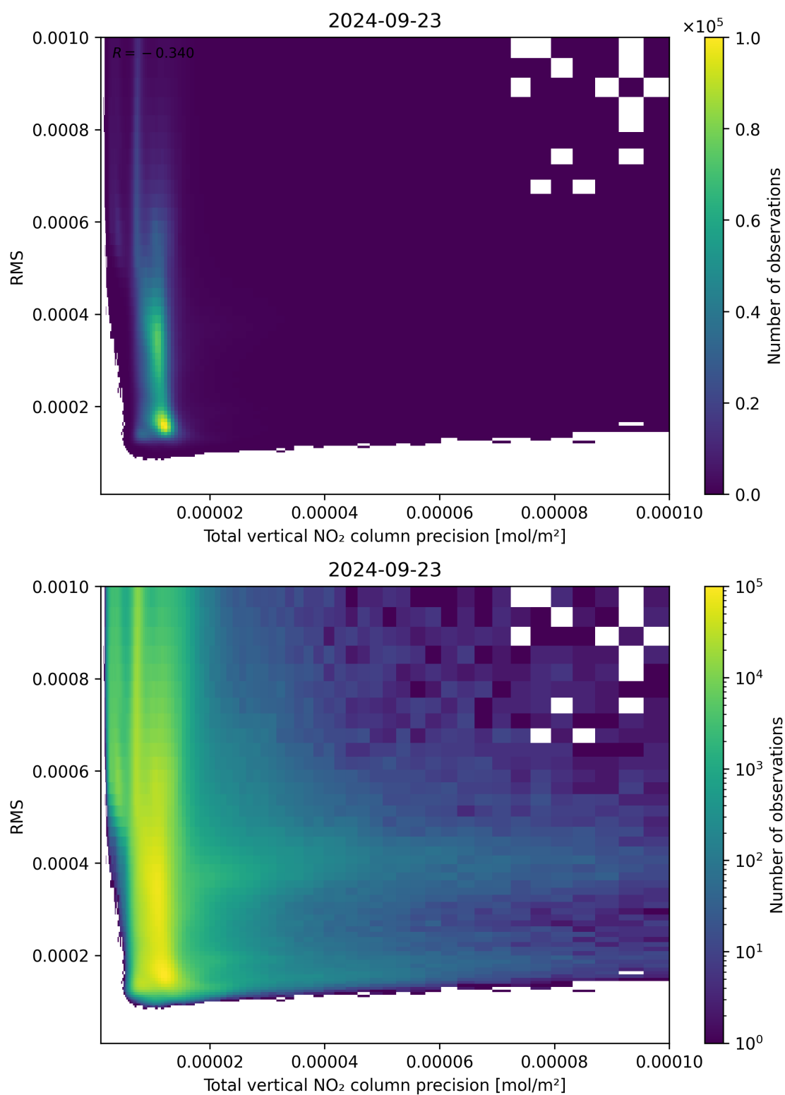
Figure 119: Scatter density plot of “Total vertical NO 2 column precision” against “RMS” for 2024-09-22 to 2024-09-24.
