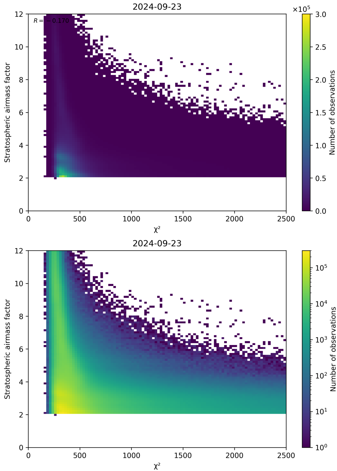
Figure 81: Scatter density plot of “ \chi^2 ” against “Stratospheric airmass factor” for 2024-09-22 to 2024-09-24.
