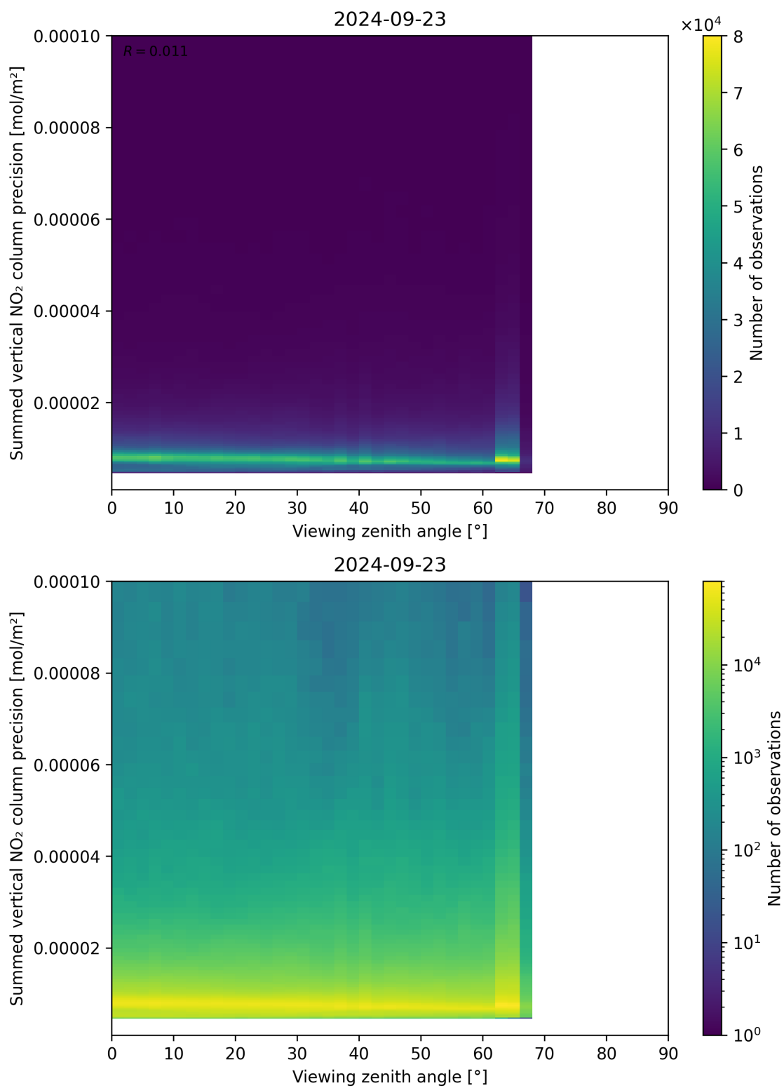
Figure 166: Scatter density plot of “Viewing zenith angle” against “Summed vertical NO 2 column precision” for 2024-09-22 to 2024-09-24.
