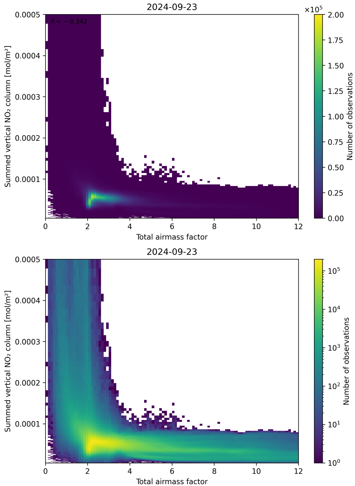
Figure 65: Scatter density plot of “Total airmass factor” against “Summed vertical NO 2 column” for 2024-09-22 to 2024-09-24.
