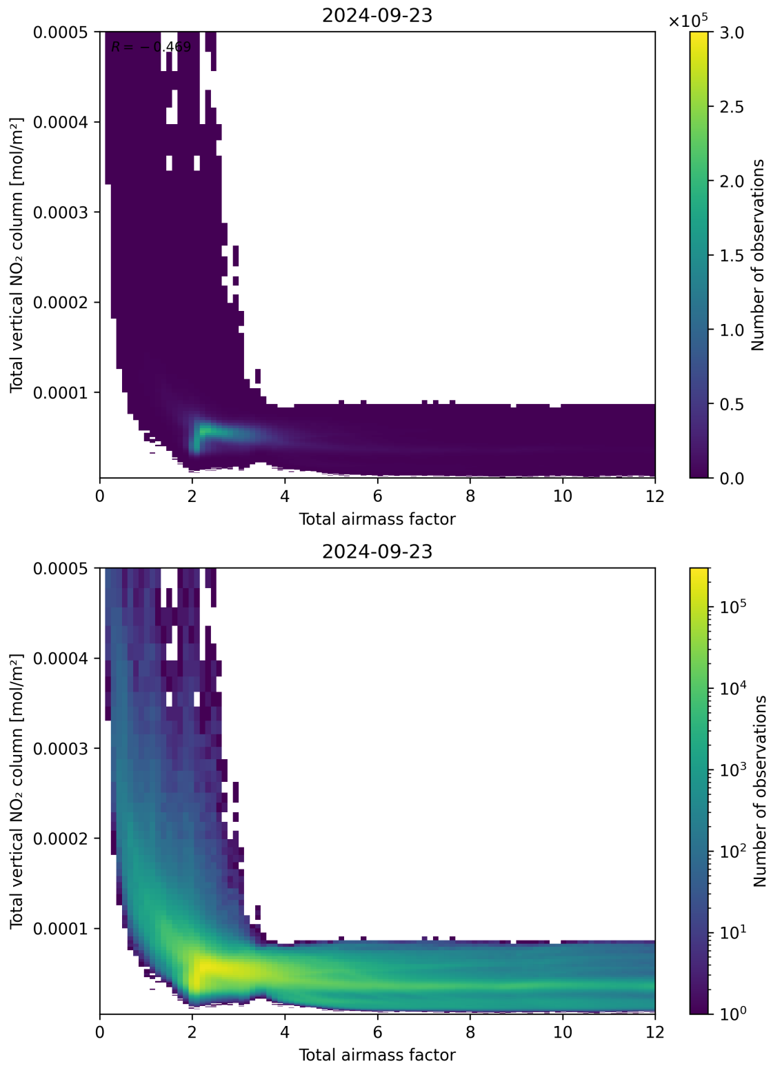
Figure 67: Scatter density plot of “Total airmass factor” against “Total vertical NO 2 column” for 2024-09-22 to 2024-09-24.
