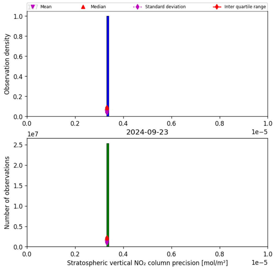
Figure 37: Histogram of “Stratospheric vertical NO 2 column precision” for 2024-09-22 to 2024-09-24
