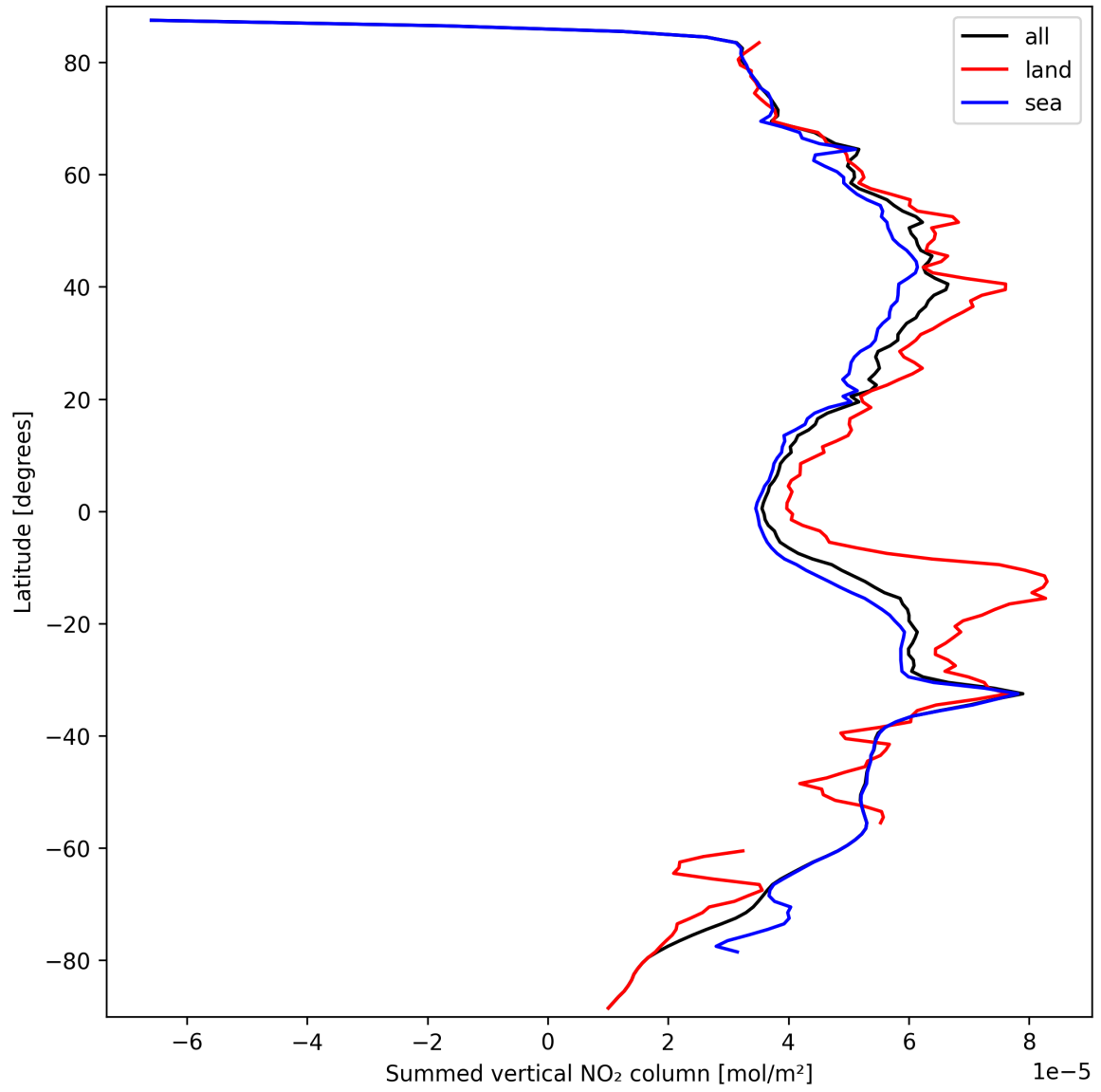
Figure 23: Zonal average of “Summed vertical NO 2 column” for 2024-09-22 to 2024-09-24.
