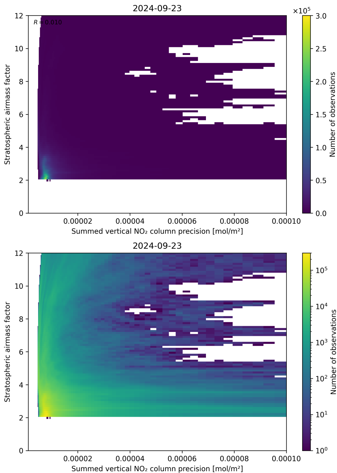
Figure 106: Scatter density plot of “Summed vertical NO 2 column precision” against “Stratospheric airmass factor” for 2024-09-22 to 2024-09-24.
