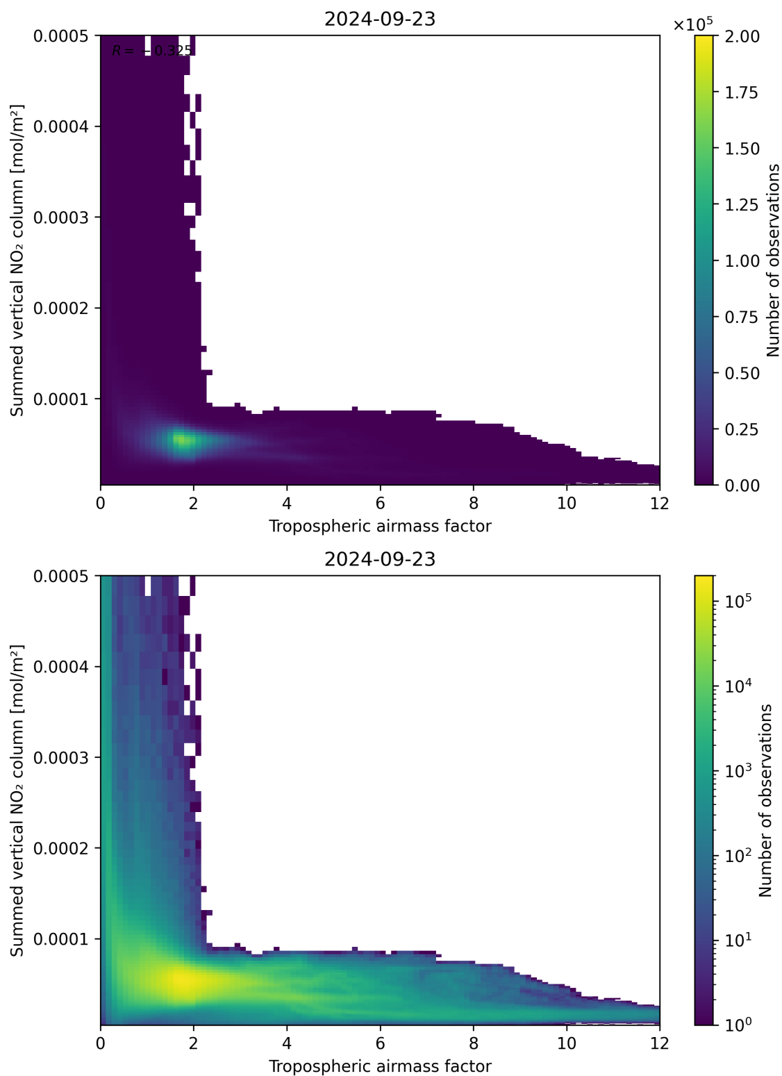
Figure 75: Scatter density plot of “Tropospheric air mass factor” against “Summed vertical NO 2 column” for 2024-09-22 to 2024-09-24.
