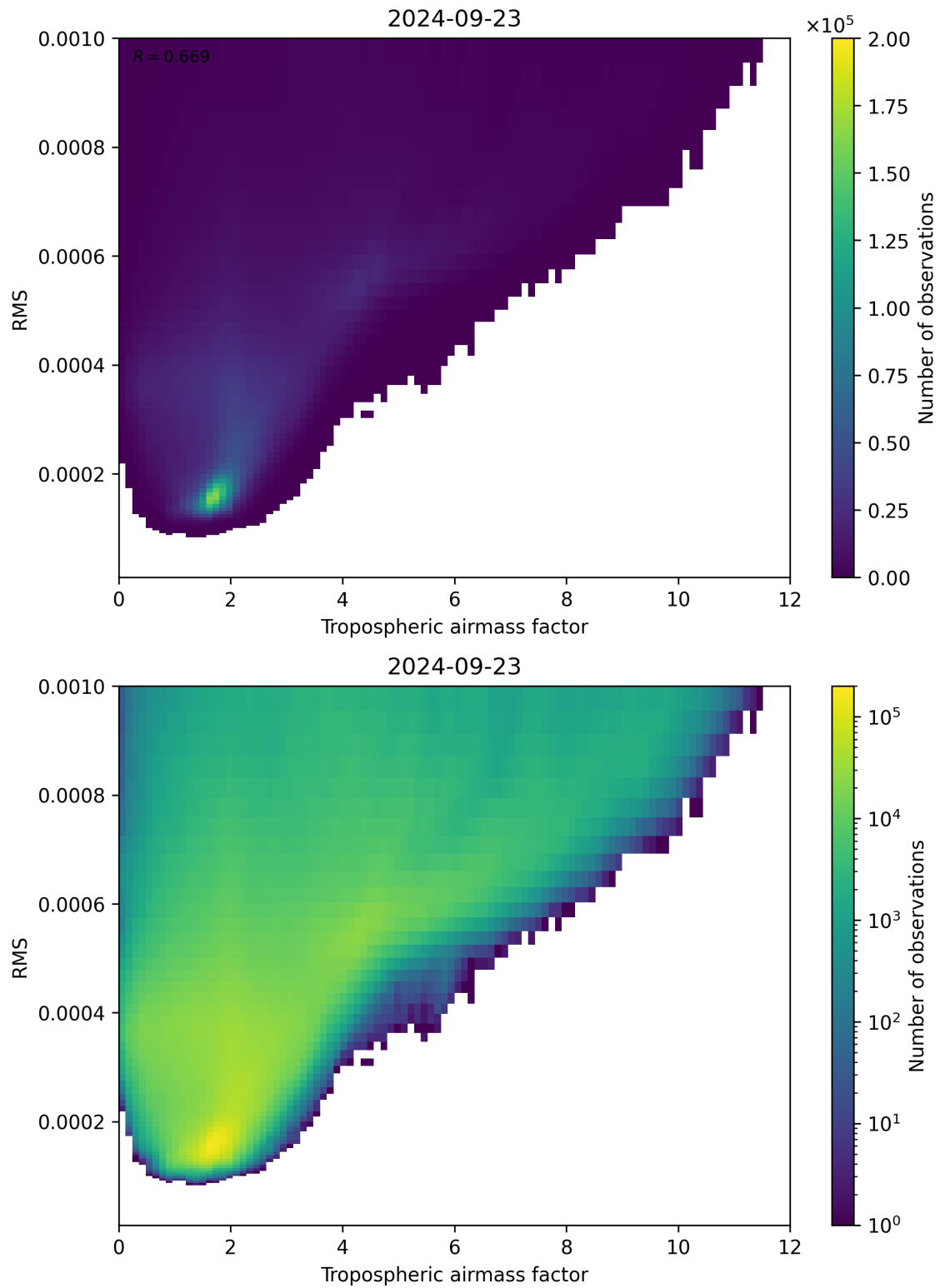
Figure 79: Scatter density plot of “Tropospheric airmass factor” against “RMS” for 2024-09-22 to 2024-09-24.
