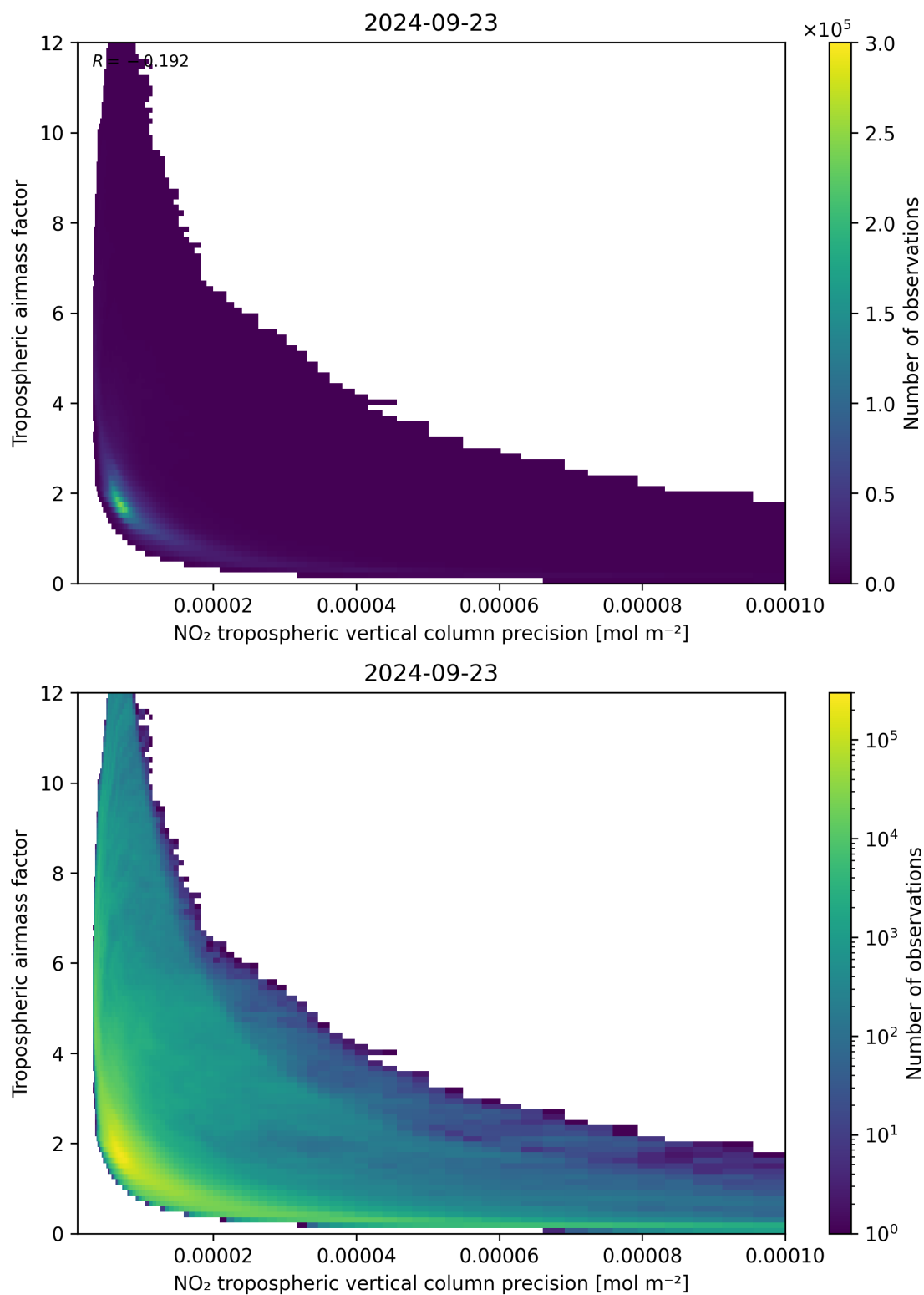
Figure 133: Scatter density plot of “NO 2 tropospheric vertical column precision” against “Tropospheric air mass factor” for 2024-09-22 to 2024-09-24.
