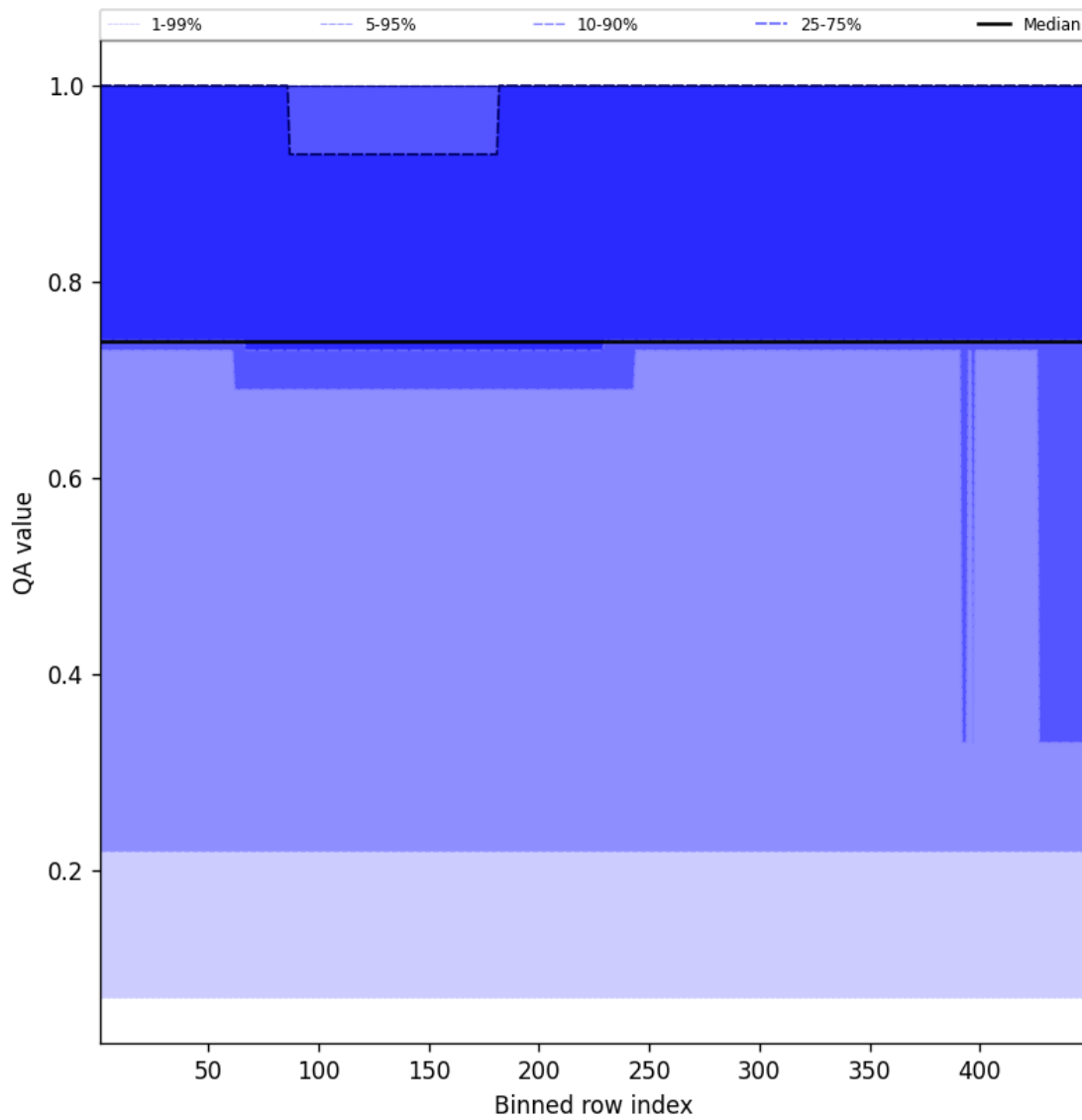
Figure 45: Along track statistics of “QA value” for 2024-09-22 to 2024-09-24
