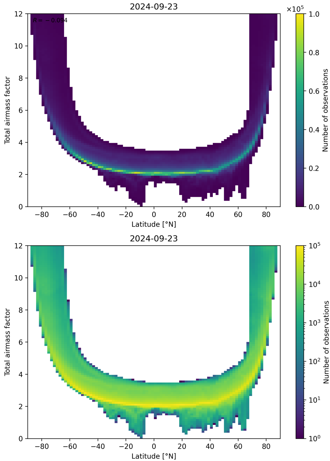
Figure 84: Scatter density plot of “Latitude” against “Total airmass factor” for 2024-09-22 to 2024-09-24.
