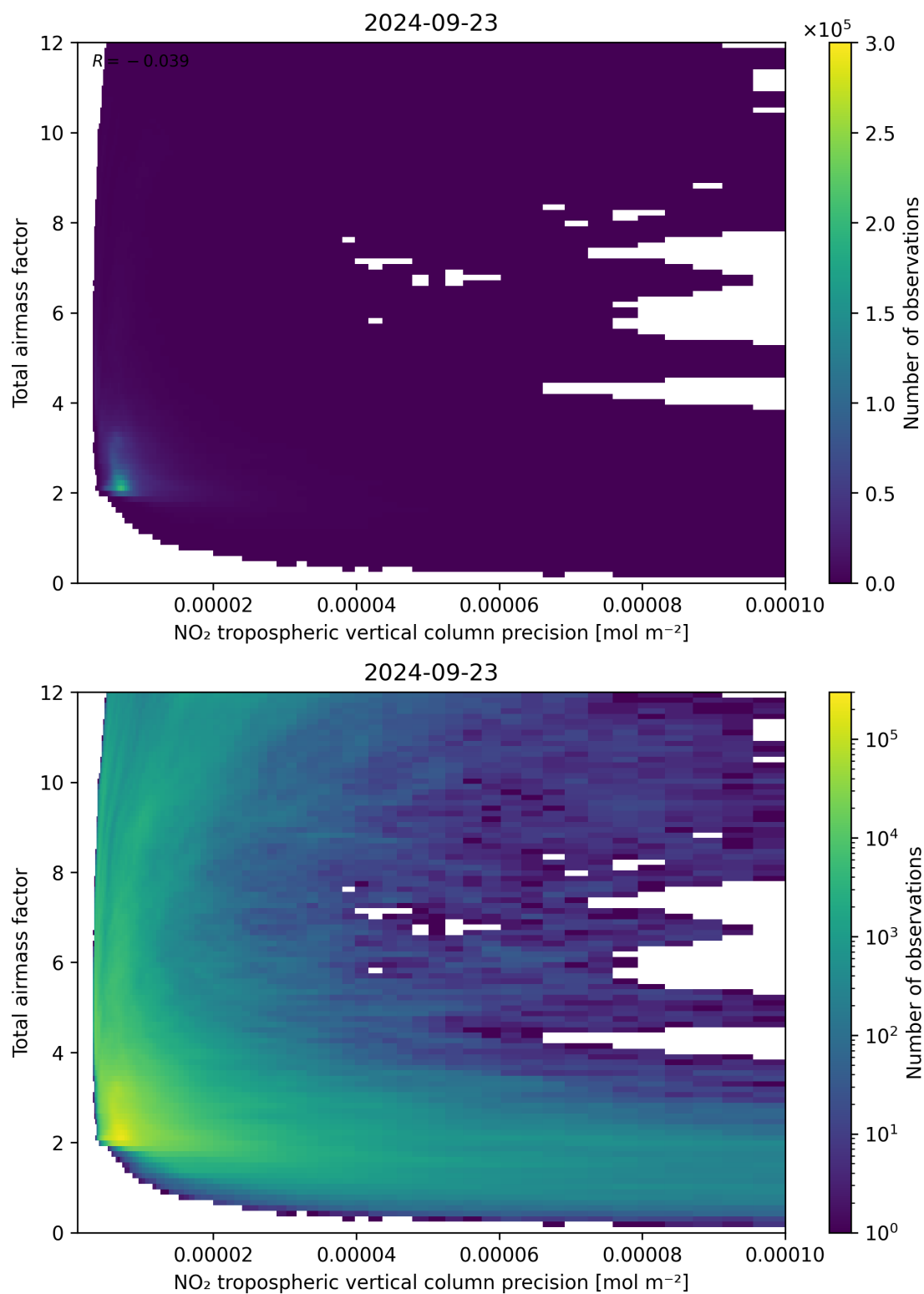
Figure 132: Scatter density plot of “NO 2 tropospheric vertical column precision” against “Total air mass factor” for 2024-09-22 to 2024-09-24.
