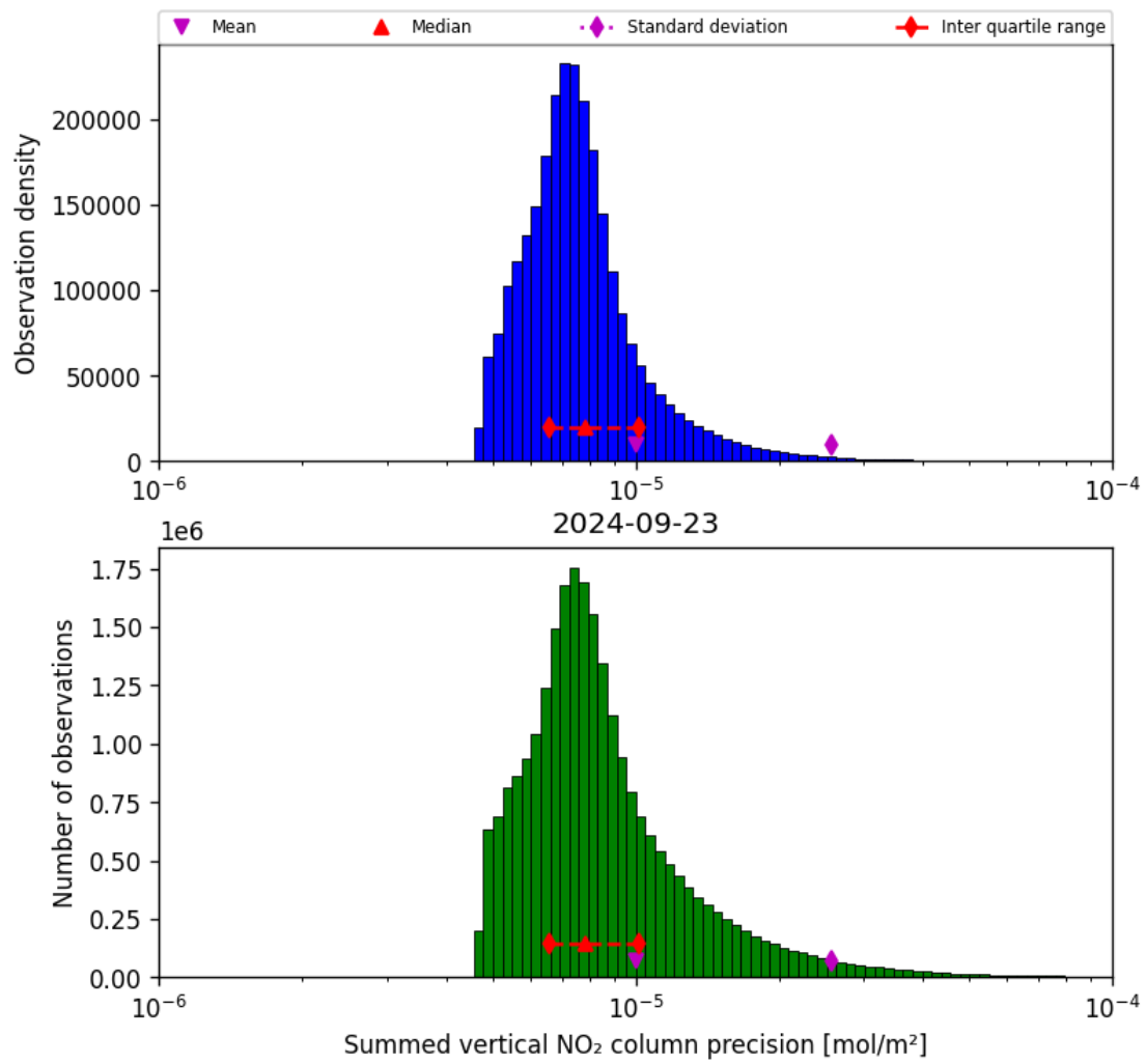
Figure 41: Histogram of “Summed vertical NO 2 column precision” for 2024-09-22 to 2024-09-24
