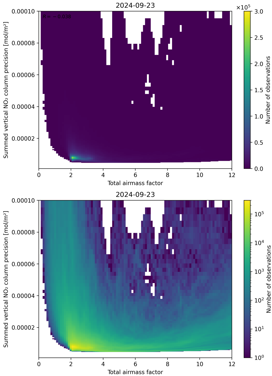
Figure 66: Scatter density plot of “Total airmass factor” against “Summed vertical NO 2 column precision” for 2024-09-22 to 2024-09-24.
