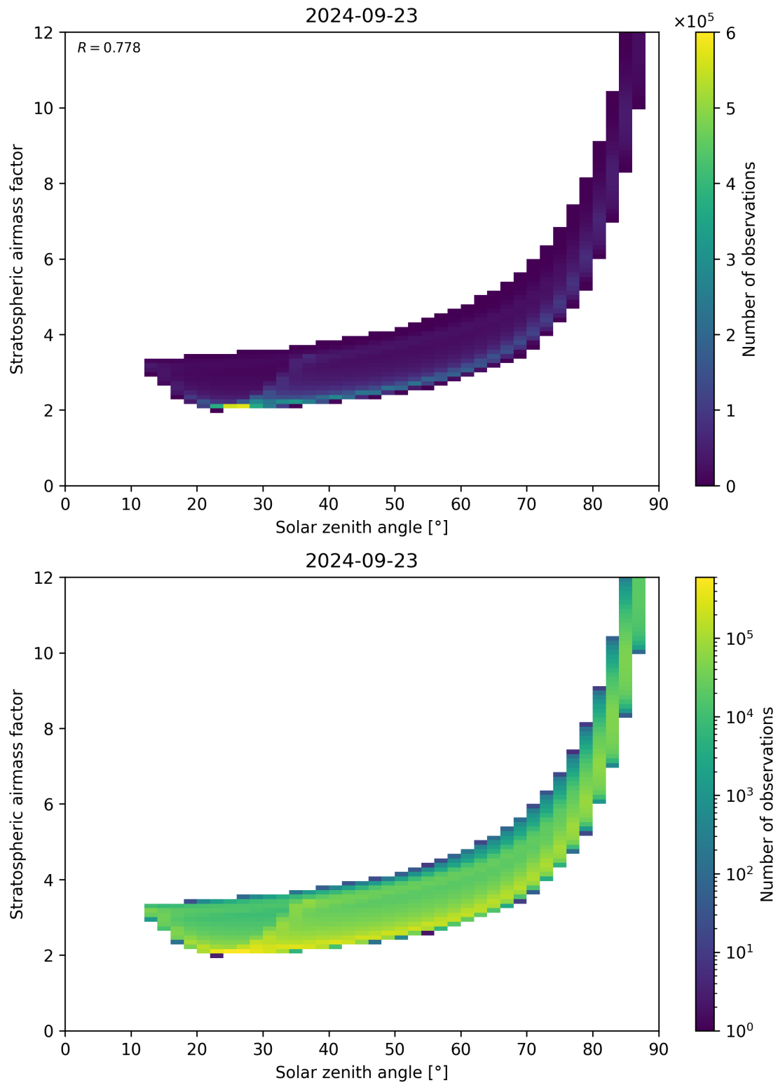
Figure 145: Scatter density plot of “Solar zenith angle” against “Stratospheric airmass factor” for 2024-09-22 to 2024-09-24.
