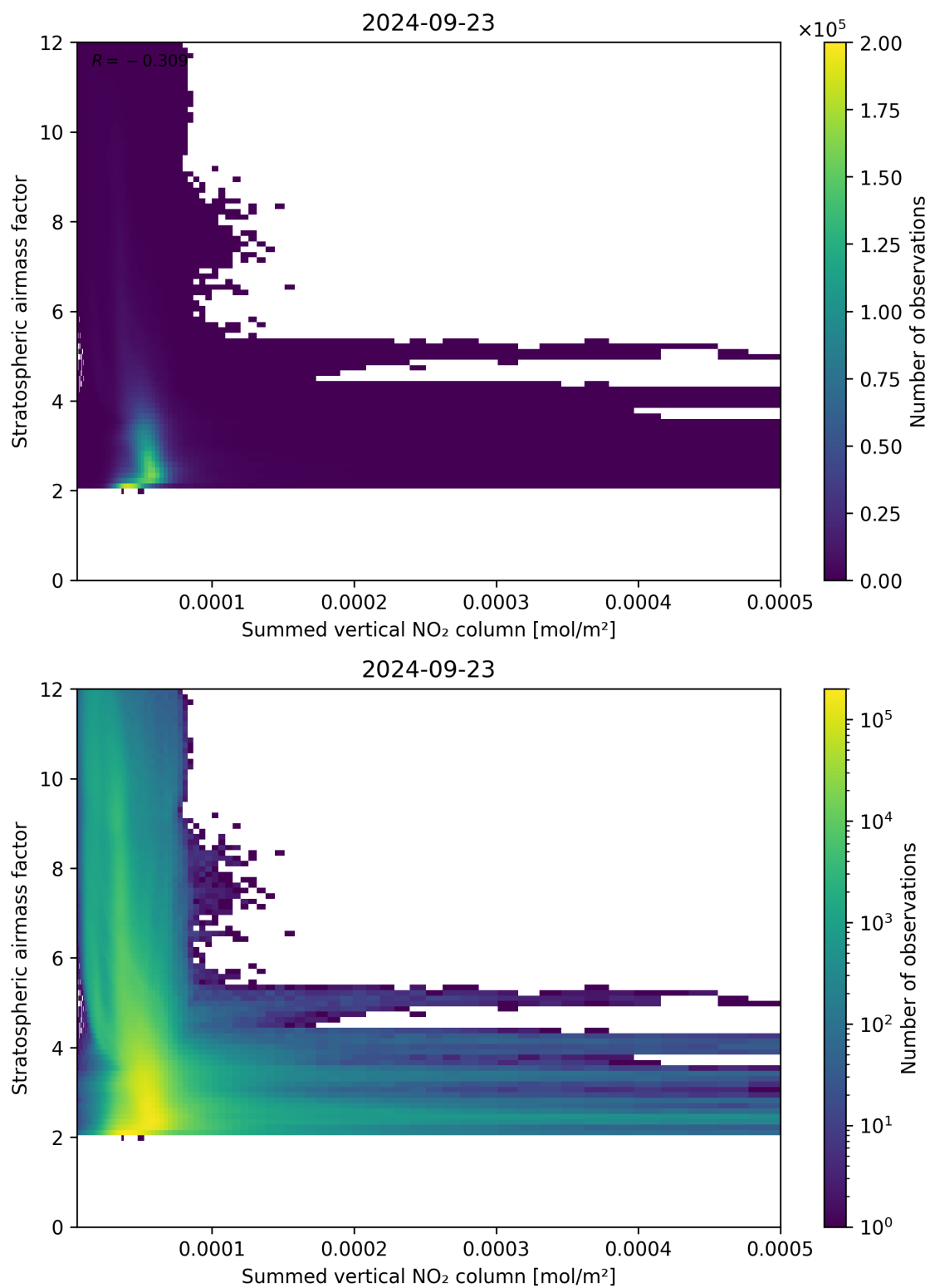
Figure 103: Scatter density plot of “Summed vertical NO 2 column” against “Stratospheric air mass factor” for 2024-09-22 to 2024-09-24.
