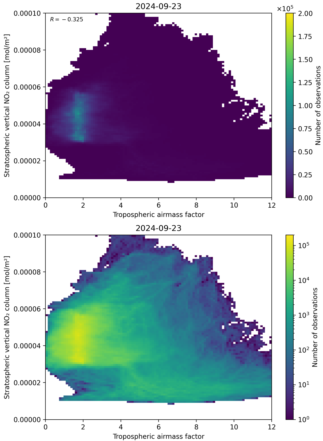
Figure 74: Scatter density plot of “Tropospheric air mass factor” against “Stratospheric vertical NO 2 column” for 2024-09-22 to 2024-09-24.
