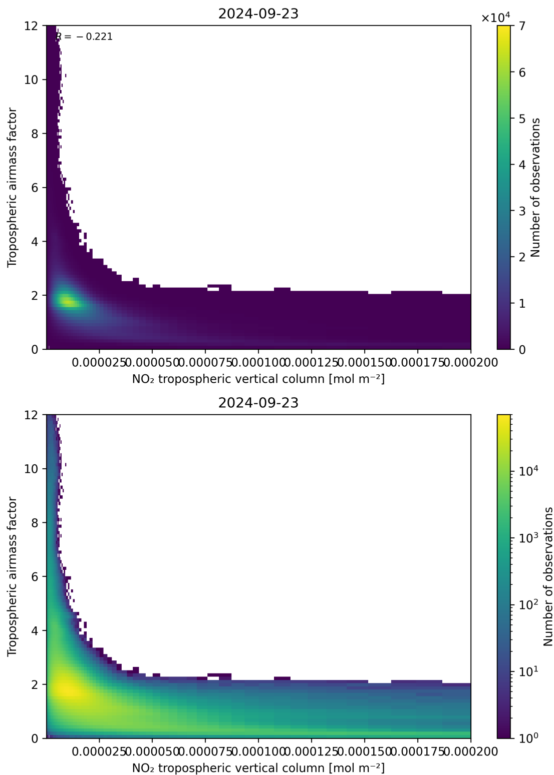
Figure 123: Scatter density plot of “NO 2 tropospheric vertical column” against “Tropospheric air mass factor” for 2024-09-22 to 2024-09-24.
