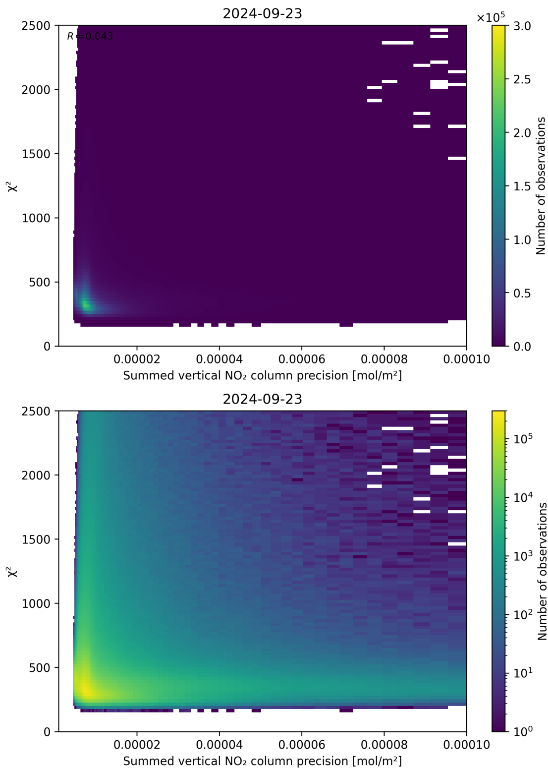
Figure 107: Scatter density plot of “Summed vertical NO 2 column precision” against “ \chi^2 ” for 2024-09-22 to 2024-09-24.
