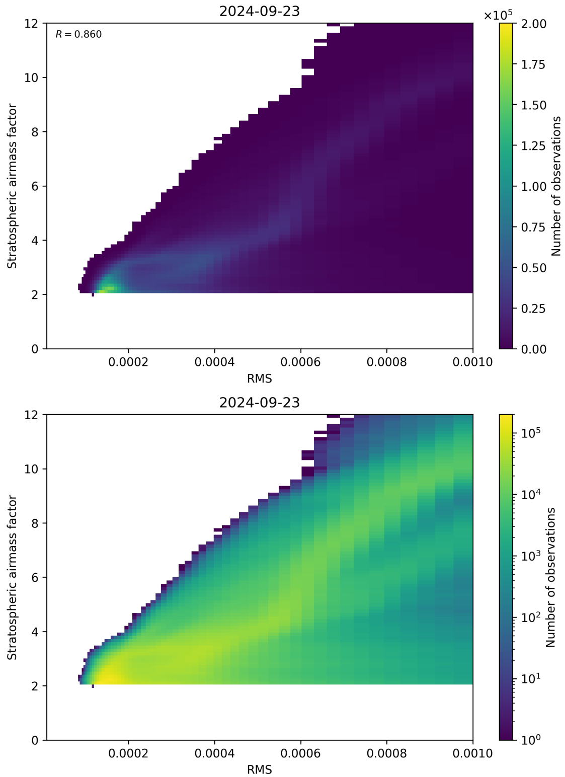
Figure 144: Scatter density plot of “RMS” against “Stratospheric airmass factor” for 2024-09-22 to 2024-09-24.
