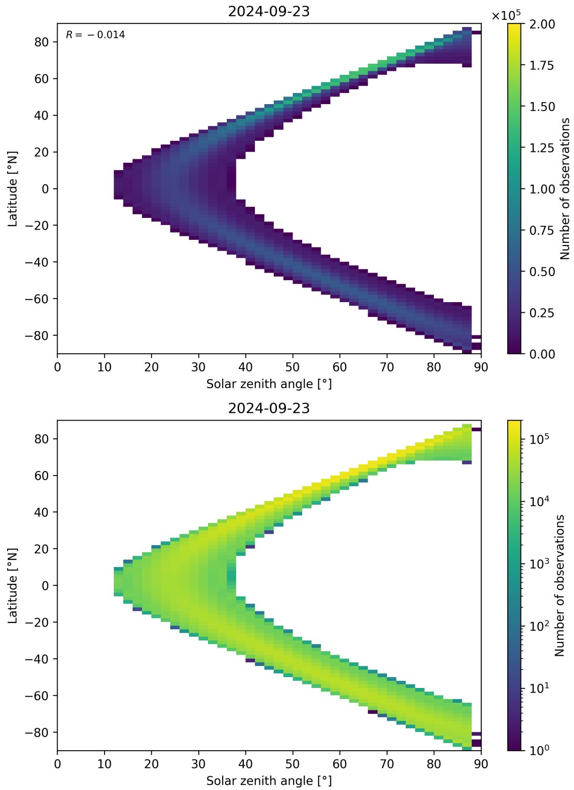
Figure 149: Scatter density plot of “Solar zenith angle” against “Latitude” for 2024-09-22 to 2024-09-24.
