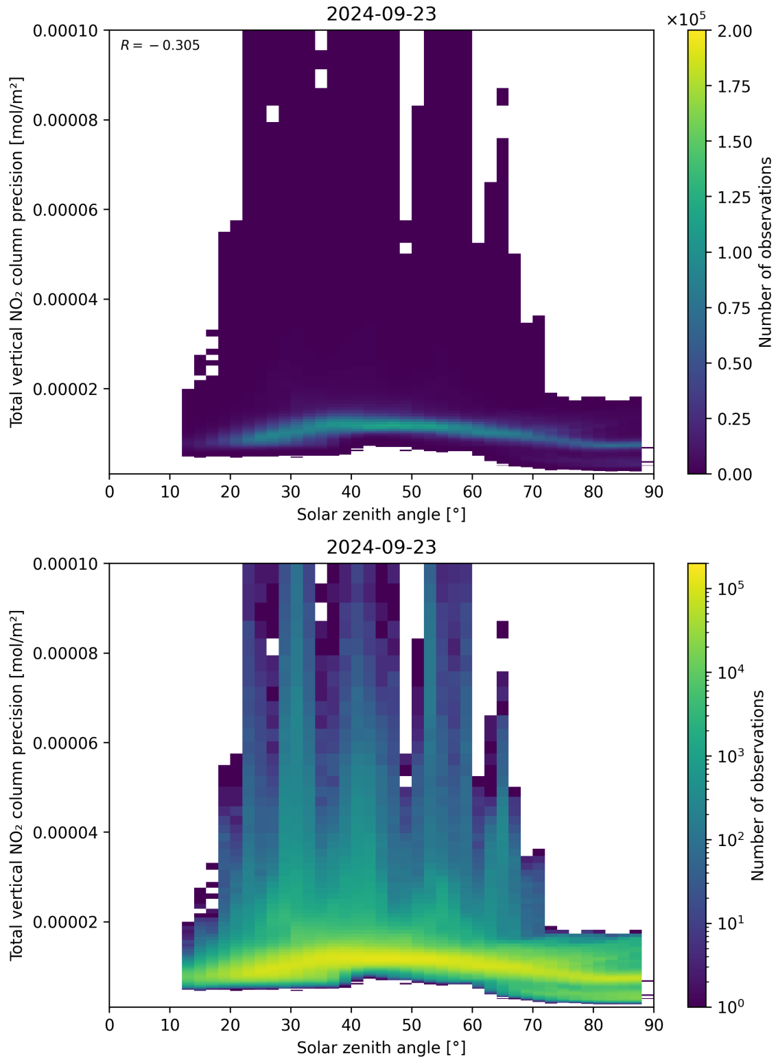
Figure 154: Scatter density plot of “Solar zenith angle” against “Total vertical NO 2 column precision” for 2024-09-22 to 2024-09-24.
