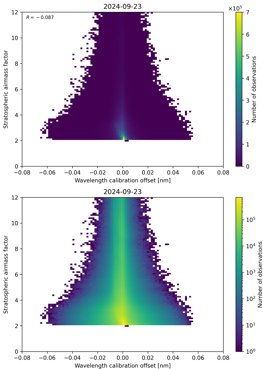
Figure 174: Scatter density plot of “Wavelength calibration offset” against “Stratospheric airmass factor” for 2024-09-22 to 2024-09-24.
