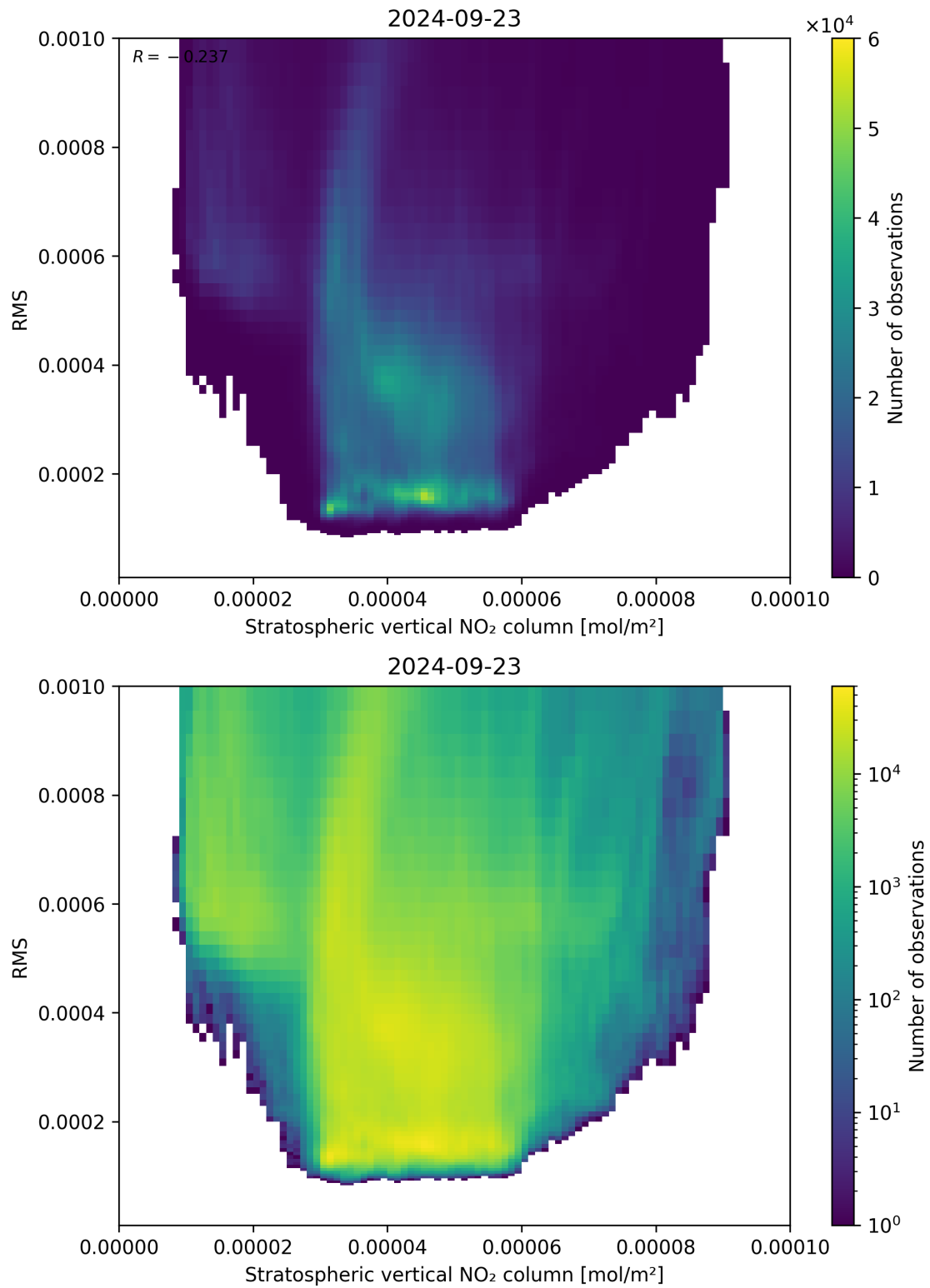
Figure 102: Scatter density plot of “Stratospheric vertical NO 2 column” against “RMS” for 2024-09-22 to 2024-09-24.
