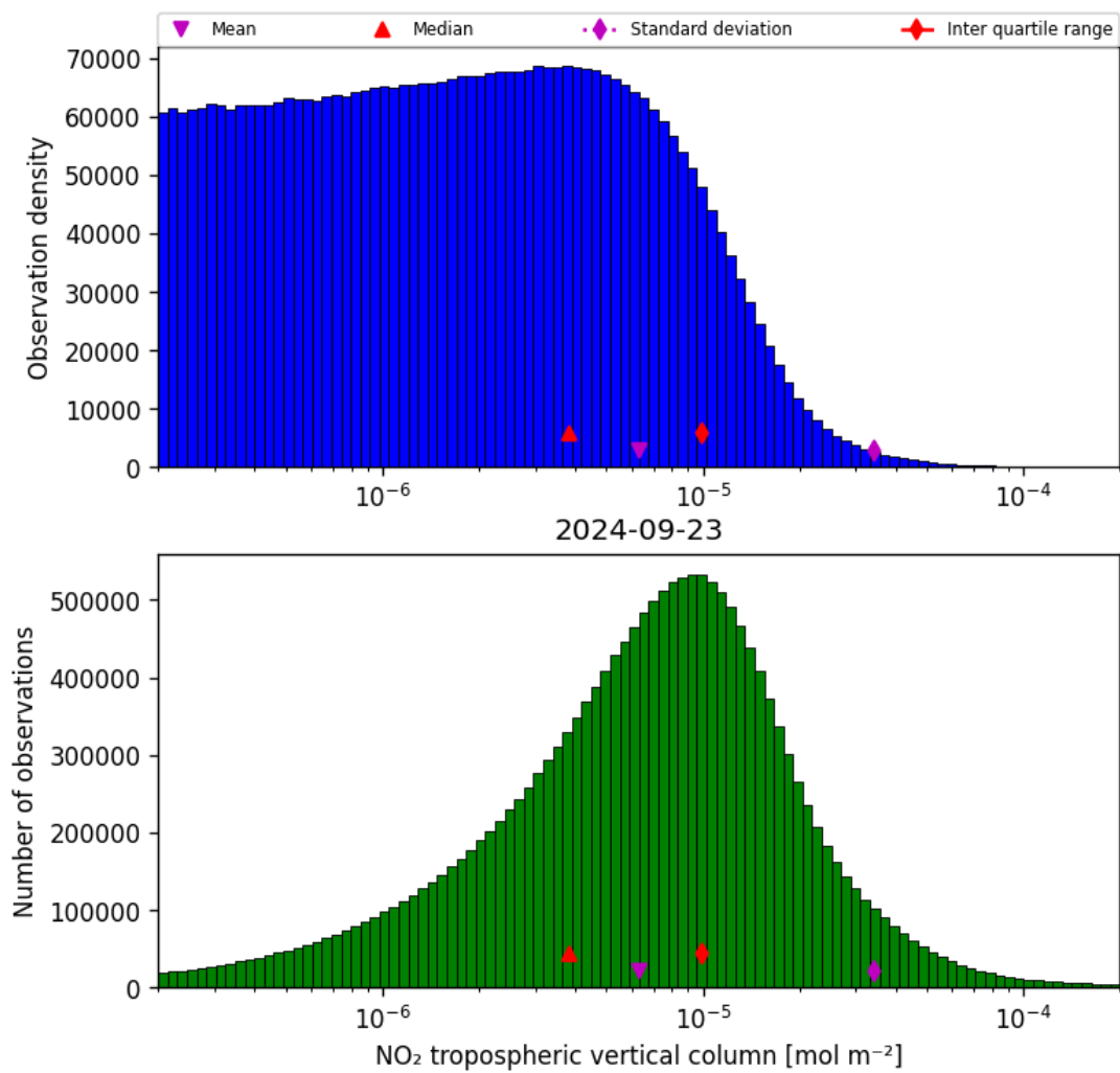
Figure 29: Histogram of “NO 2 tropospheric vertical column” for 2024-09-22 to 2024-09-24
