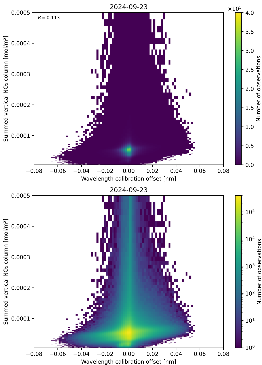
Figure 177: Scatter density plot of “Wavelength calibration offset” against “Summed vertical NO 2 column” for 2024-09-22 to 2024-09-24.
