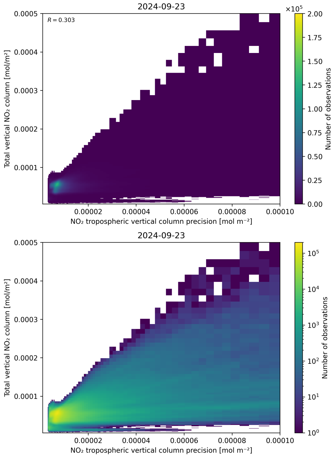
Figure 138: Scatter density plot of “NO 2 tropospheric vertical column precision” against “Total vertical NO 2 column” for 2024-09-22 to 2024-09-24.
