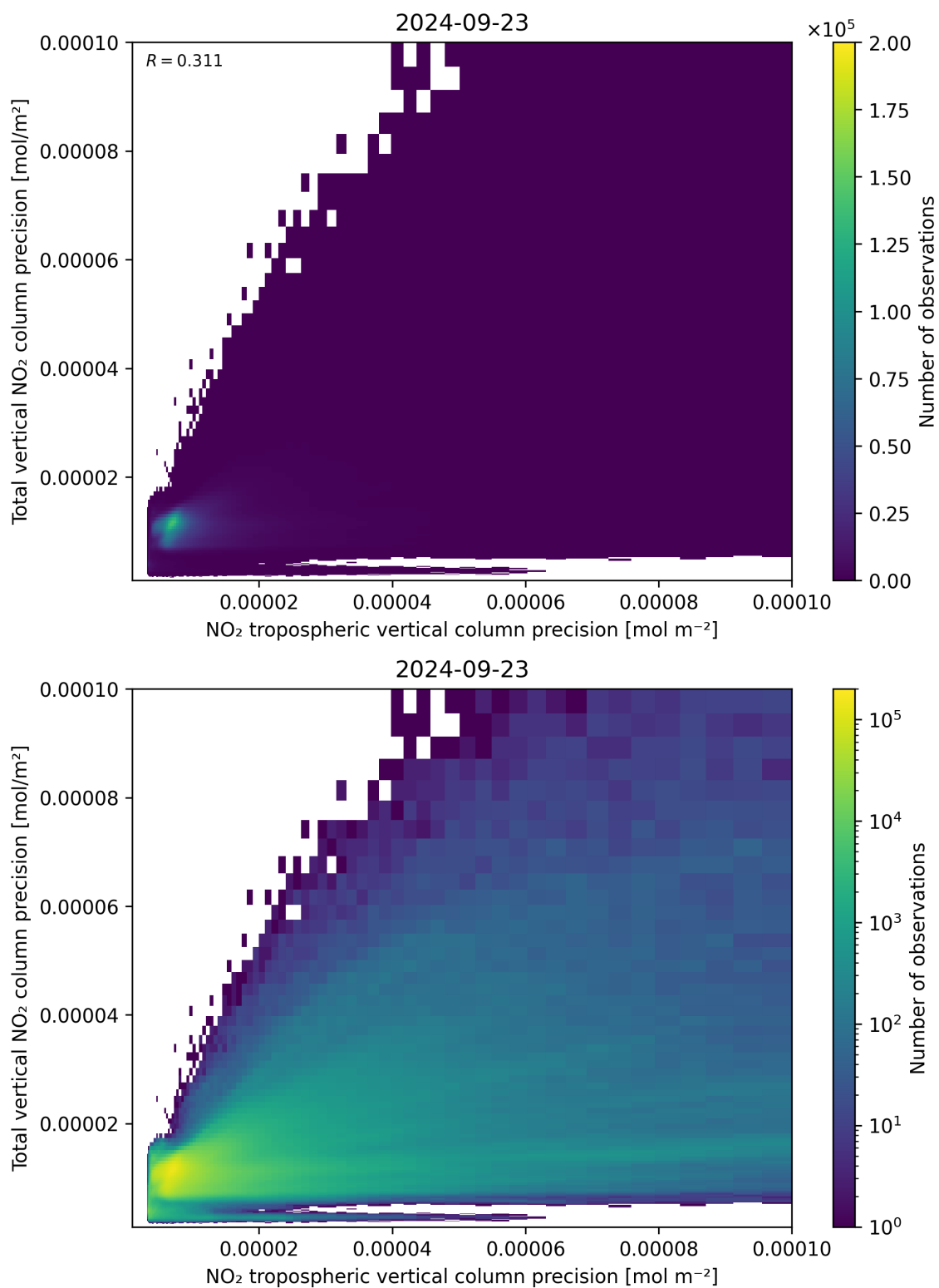
Figure 139: Scatter density plot of “NO 2 tropospheric vertical column precision” against “Total vertical NO 2 column precision” for 2024-09-22 to 2024-09-24.
