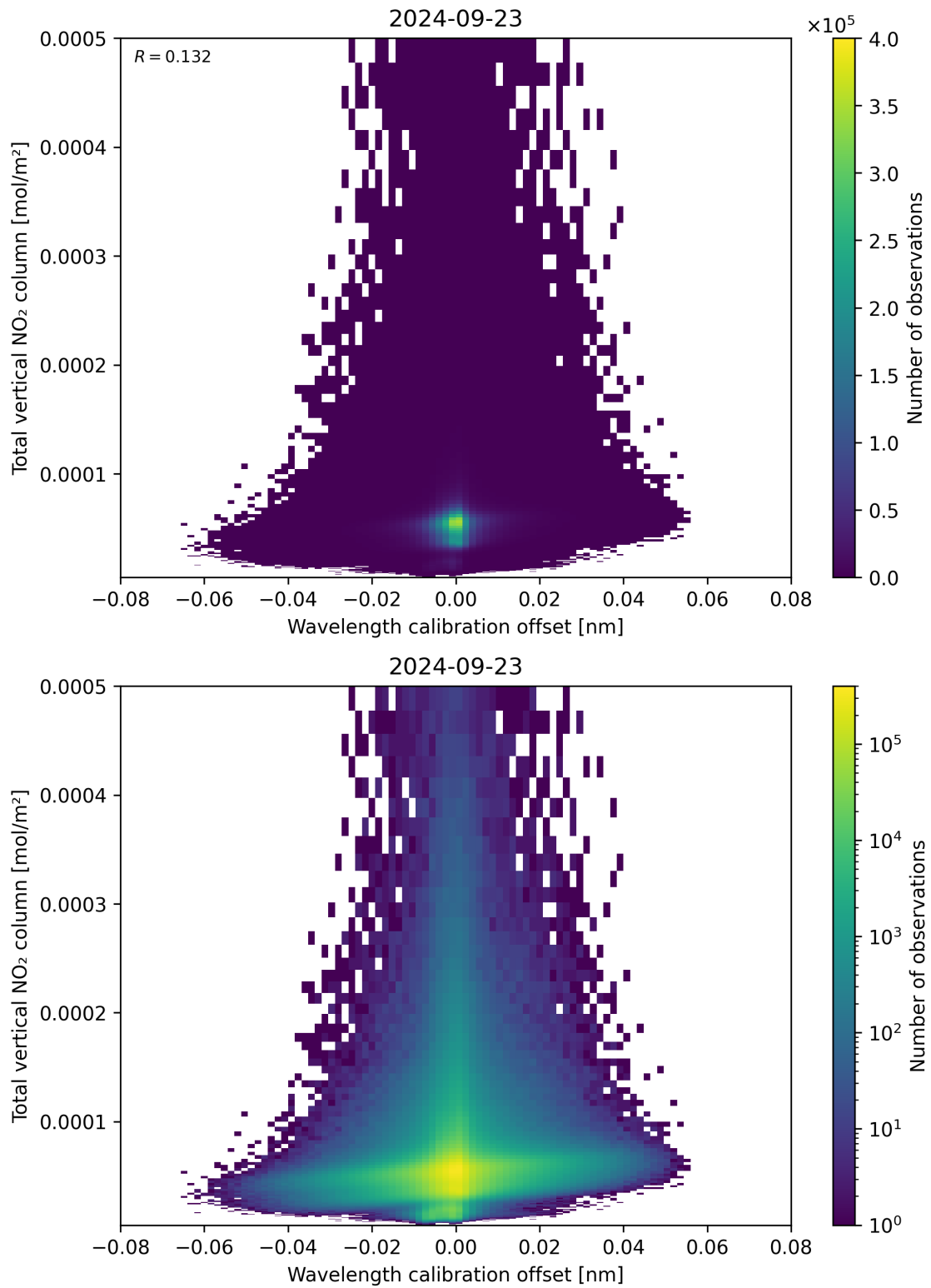
Figure 179: Scatter density plot of “Wavelength calibration offset” against “Total vertical NO 2 column” for 2024-09-22 to 2024-09-24.
