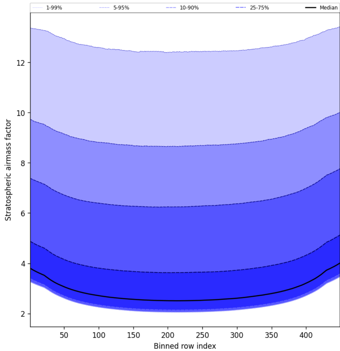
Figure 61: Along track statistics of “Stratospheric air mass factor” for 2024-09-22 to 2024-09-24
