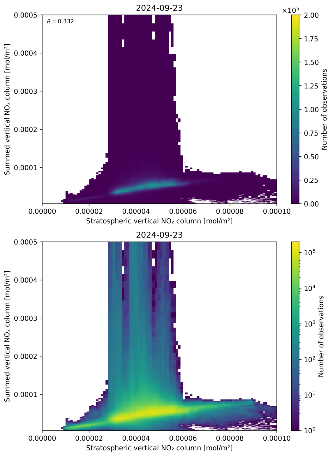
Figure 98: Scatter density plot of “Stratospheric vertical NO 2 column” against “Summed vertical NO 2 column” for 2024-09-22 to 2024-09-24.
