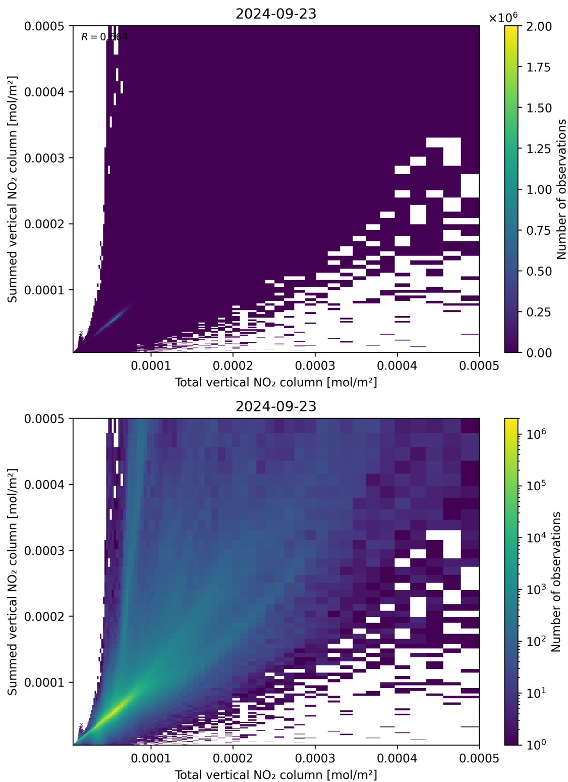
Figure 112: Scatter density plot of “Total vertical NO 2 column” against “Summed vertical NO 2 column” for 2024-09-22 to 2024-09-24.
