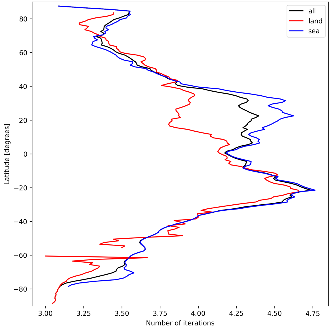
Figure 17: Zonal average of “Number of iterations” for 2024-09-22 to 2024-09-24.
