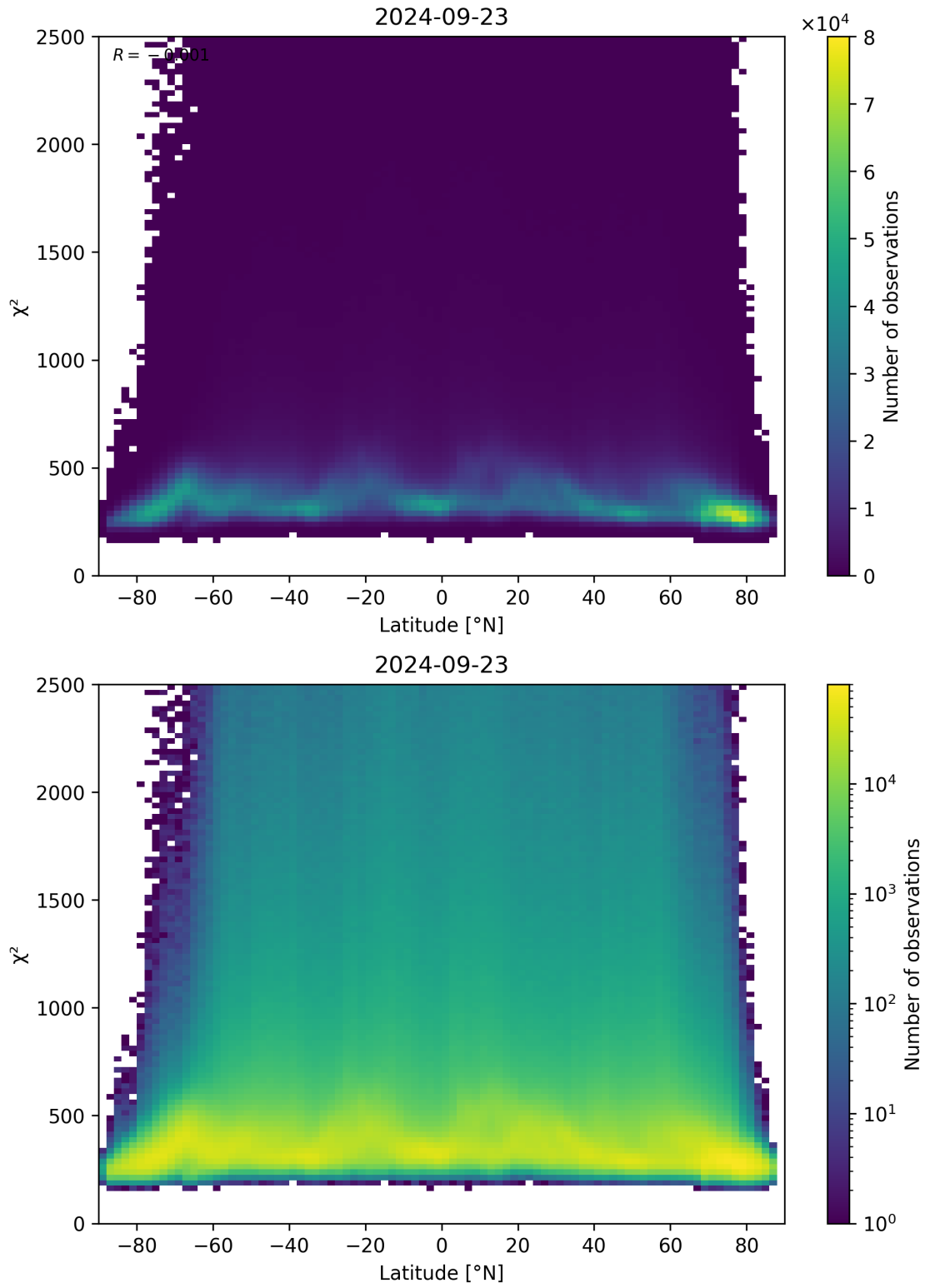
Figure 86: Scatter density plot of “Latitude” against “ \chi^2 ” for 2024-09-22 to 2024-09-24.
