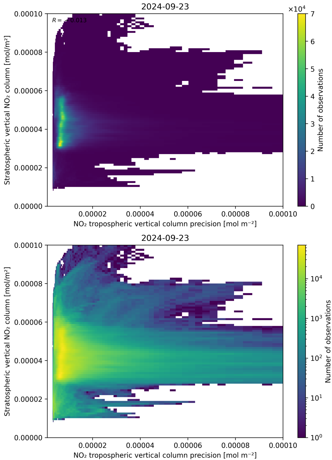
Figure 135: Scatter density plot of “NO 2 tropospheric vertical column precision” against “Stratospheric vertical NO 2 column” for 2024-09-22 to 2024-09-24.
