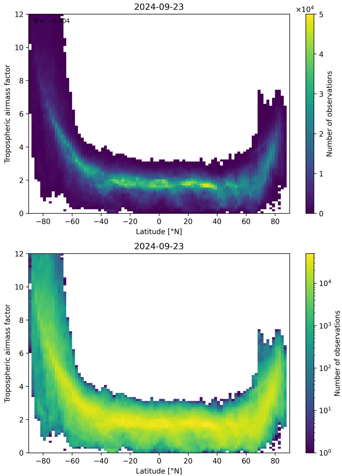
Figure 85: Scatter density plot of “Latitude” against “Tropospheric airmass factor” for 2024-09-22 to 2024-09-24.
