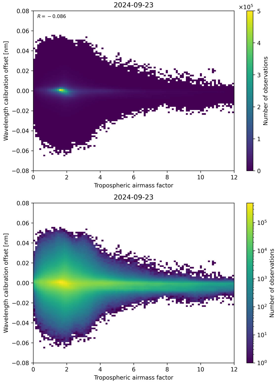
Figure 80: Scatter density plot of “Tropospheric airmass factor” against “Wavelength calibration offset” for 2024-09-22 to 2024-09-24.
