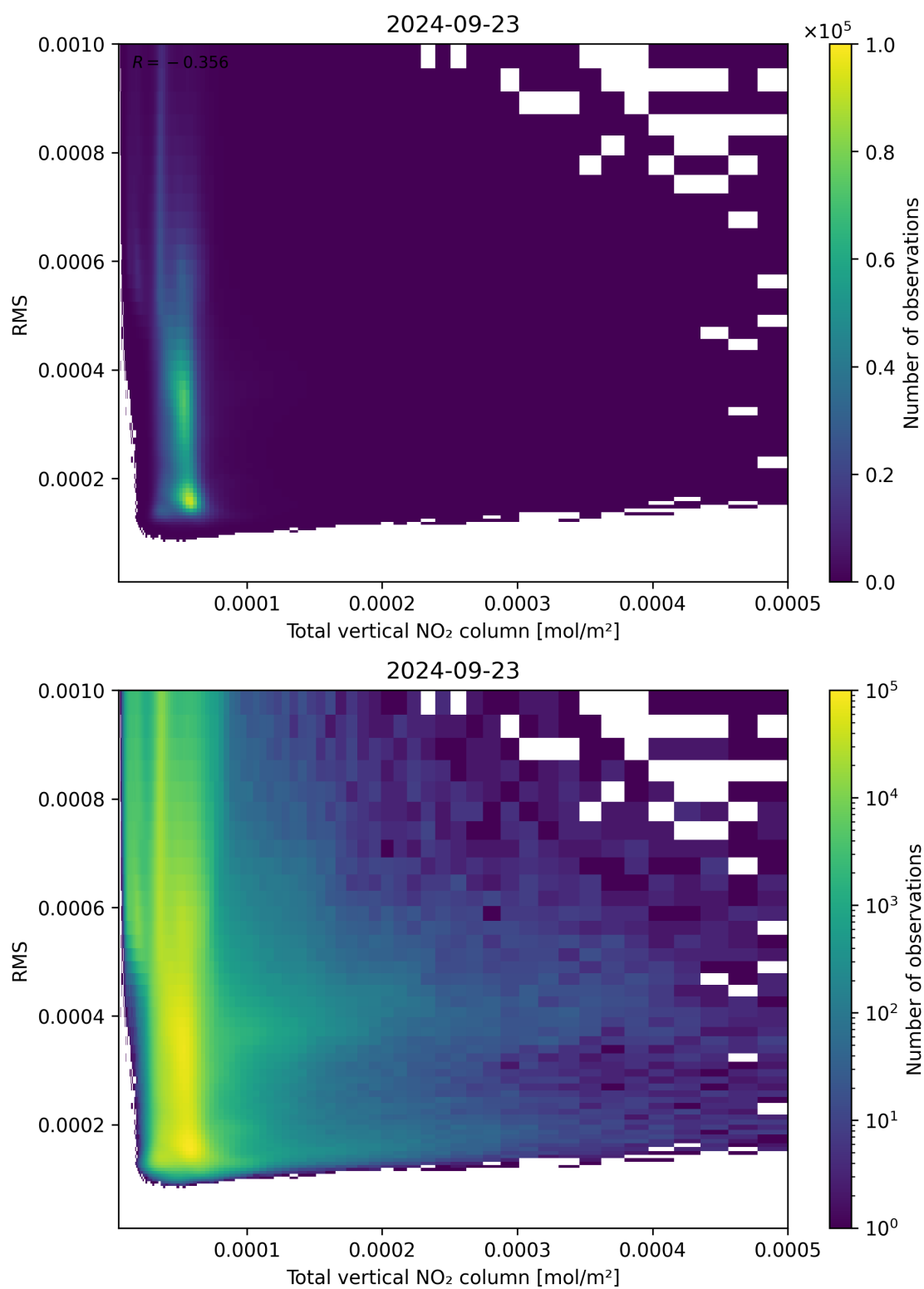
Figure 120: Scatter density plot of “Total vertical NO 2 column” against “RMS” for 2024-09-22 to 2024-09-24.
