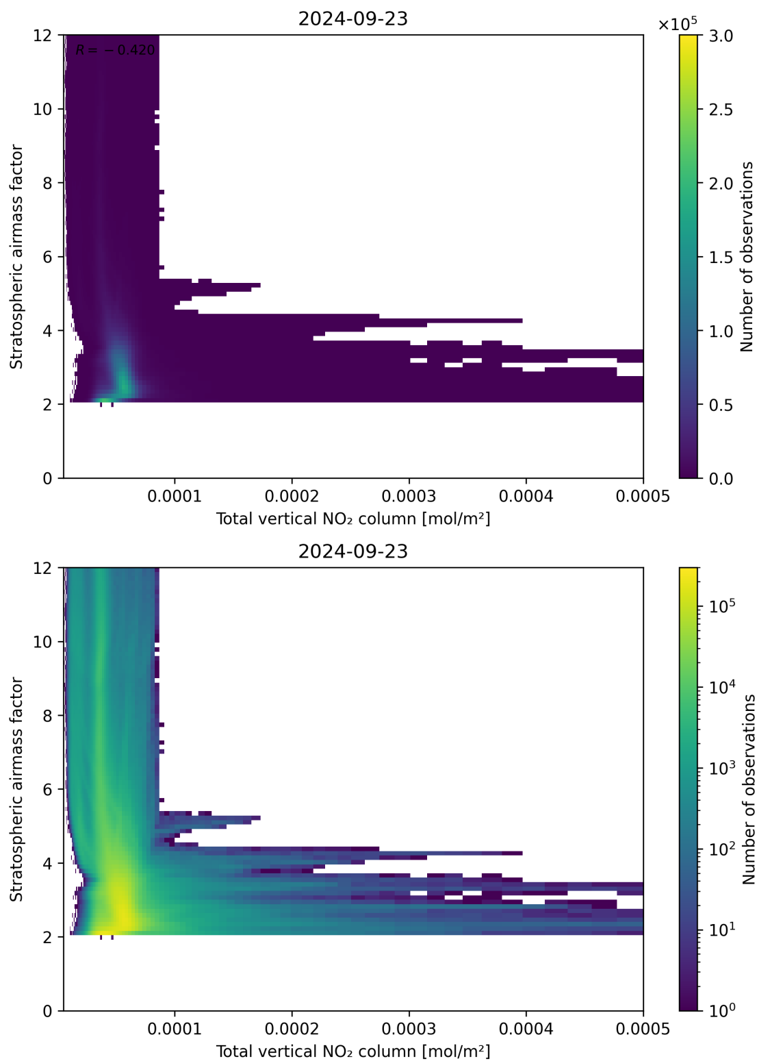
Figure 110: Scatter density plot of “Total vertical NO 2 column” against “Stratospheric airmass factor” for 2024-09-22 to 2024-09-24.
