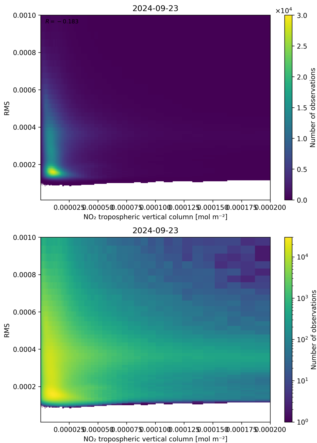
Figure 142: Scatter density plot of “NO 2 tropospheric vertical column” against “RMS” for 2024-09-22 to 2024-09-24.
