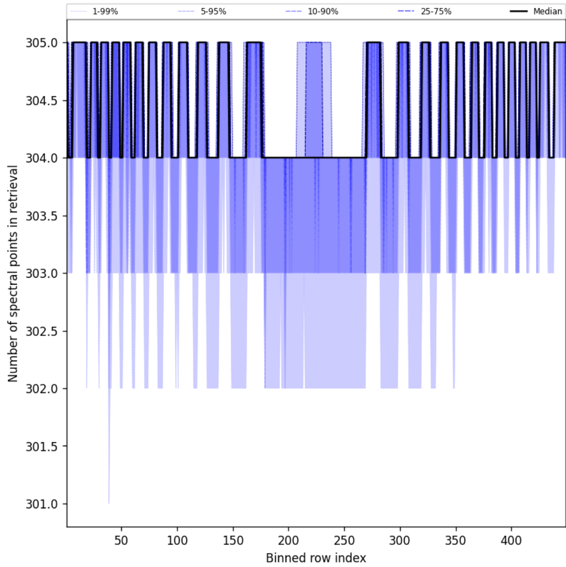
Figure 50: Along track statistics of “Number of spectral points in retrieval” for 2024-09-22 to 2024-09-24
