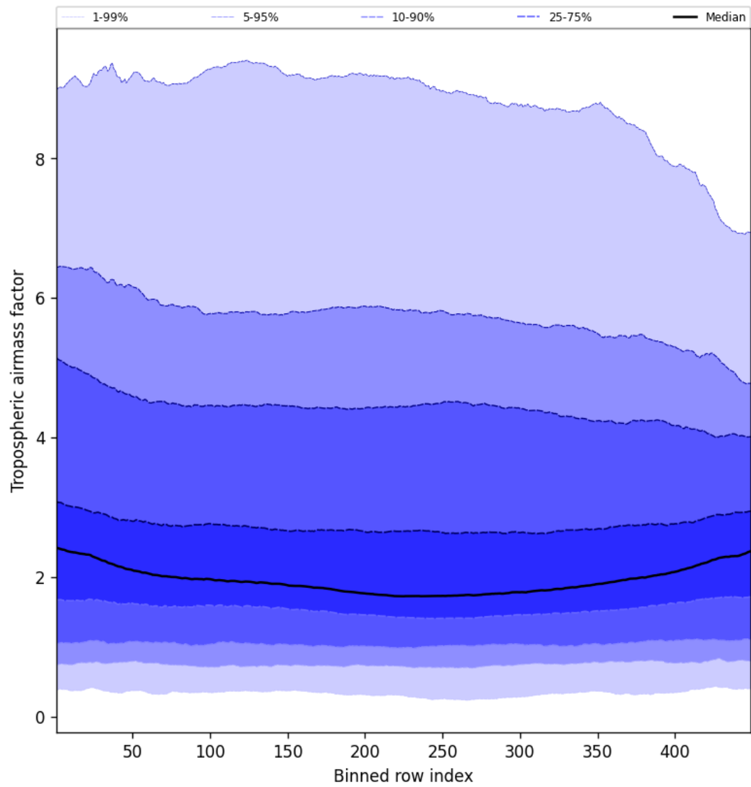
Figure 48: Along track statistics of “Tropospheric air mass factor” for 2024-09-22 to 2024-09-24
