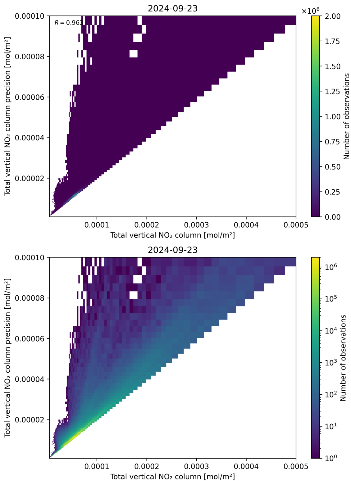
Figure 114: Scatter density plot of “Total vertical NO 2 column” against “Total vertical NO 2 column precision” for 2024-09-22 to 2024-09-24.
