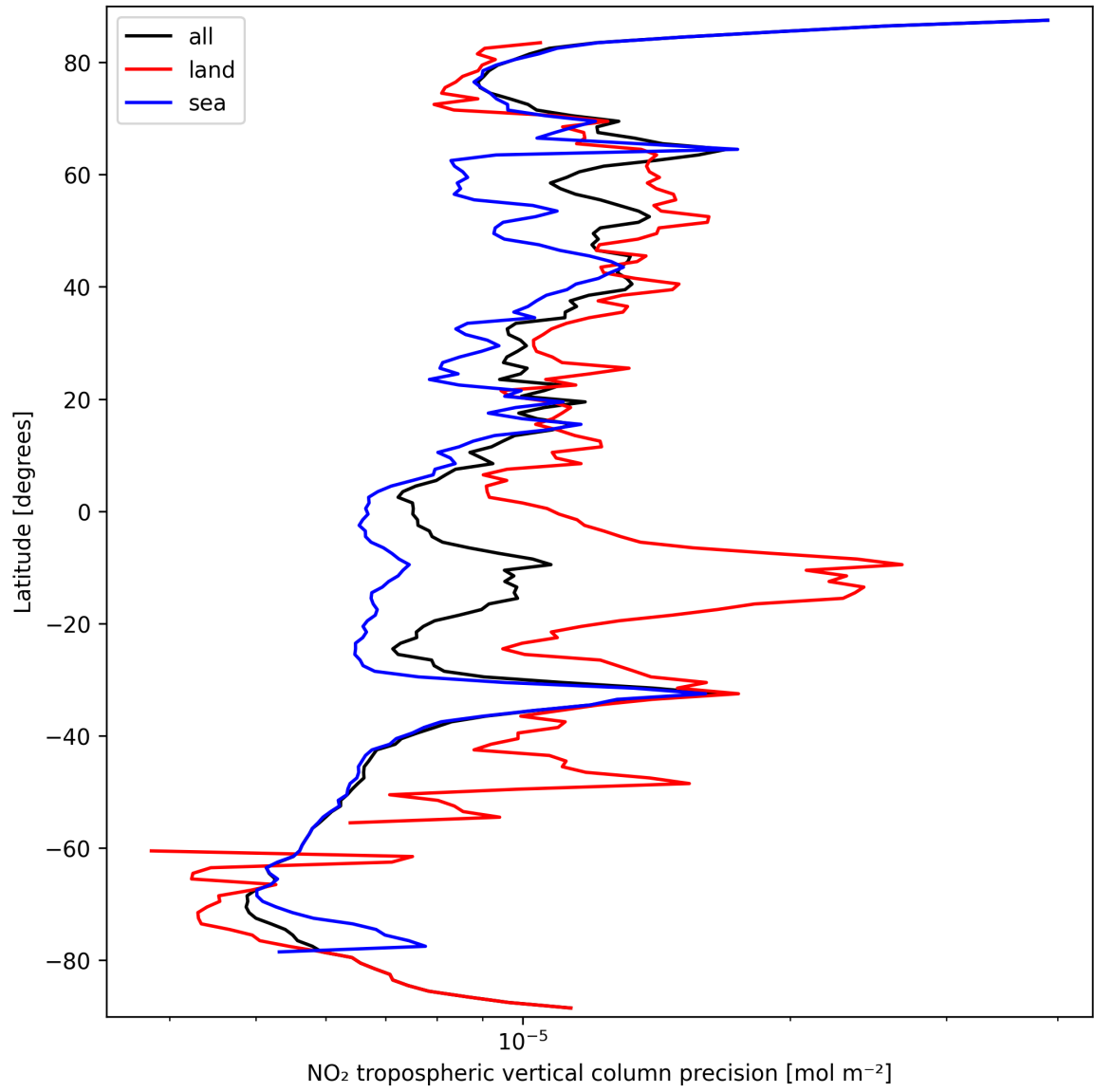
Figure 13: Zonal average of “NO 2 tropospheric vertical column precision” for 2024-09-22 to 2024-09-24.
