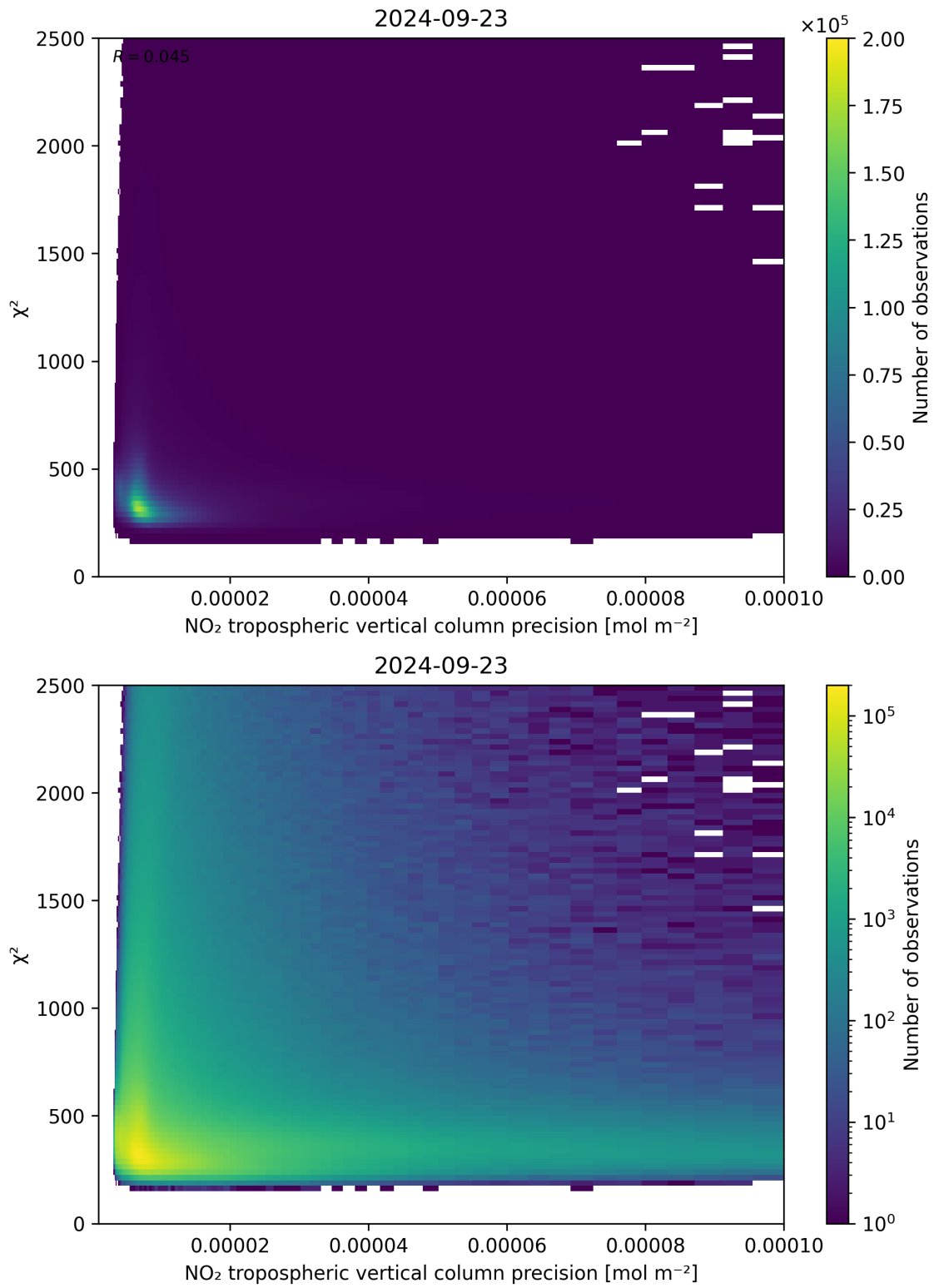
Figure 134: Scatter density plot of “NO 2 tropospheric vertical column precision” against “ \chi^2 ” for 2024-09-22 to 2024-09-24.
