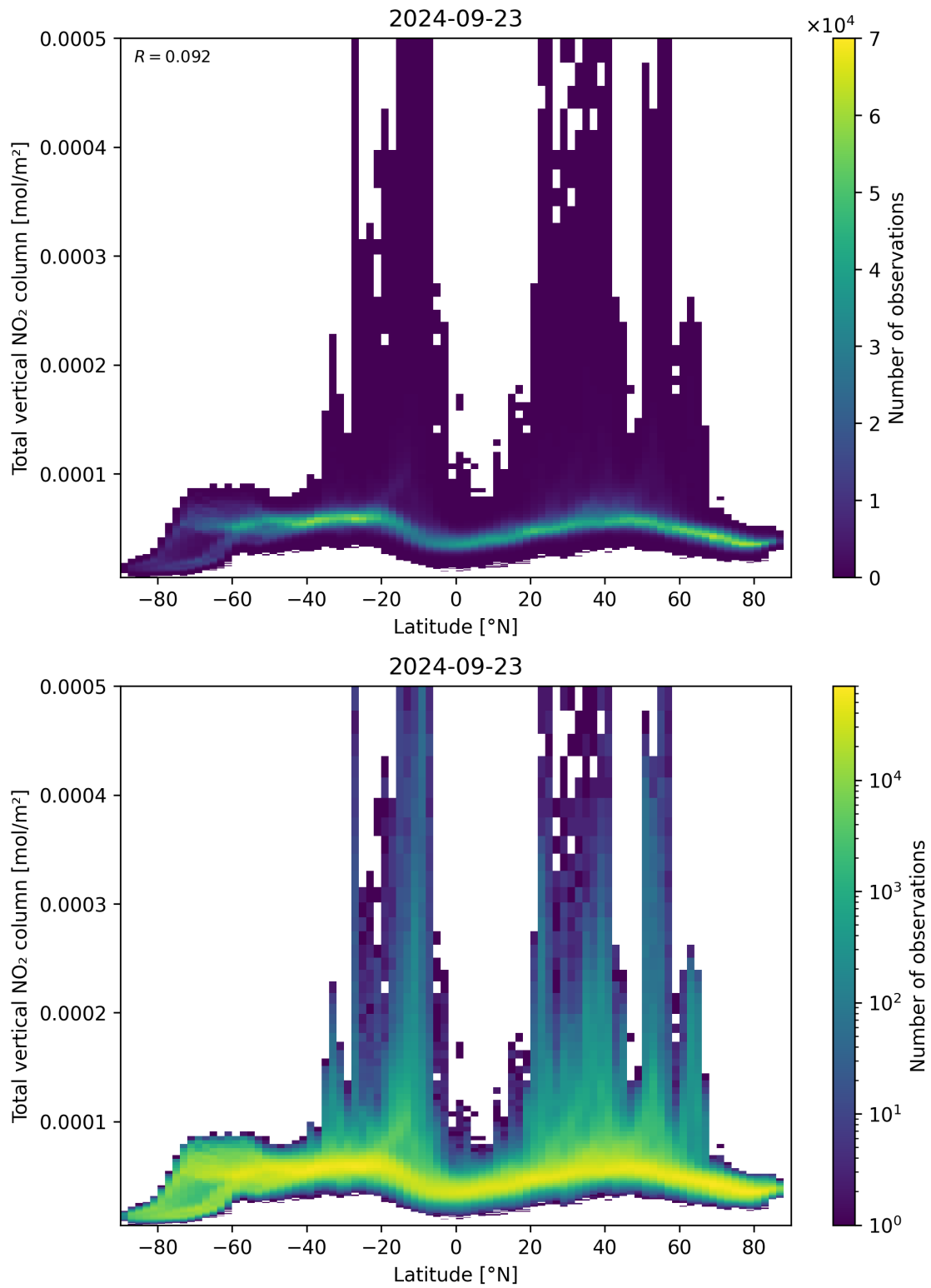
Figure 90: Scatter density plot of “Latitude” against “Total vertical NO 2 column” for 2024-09-22 to 2024-09-24.
