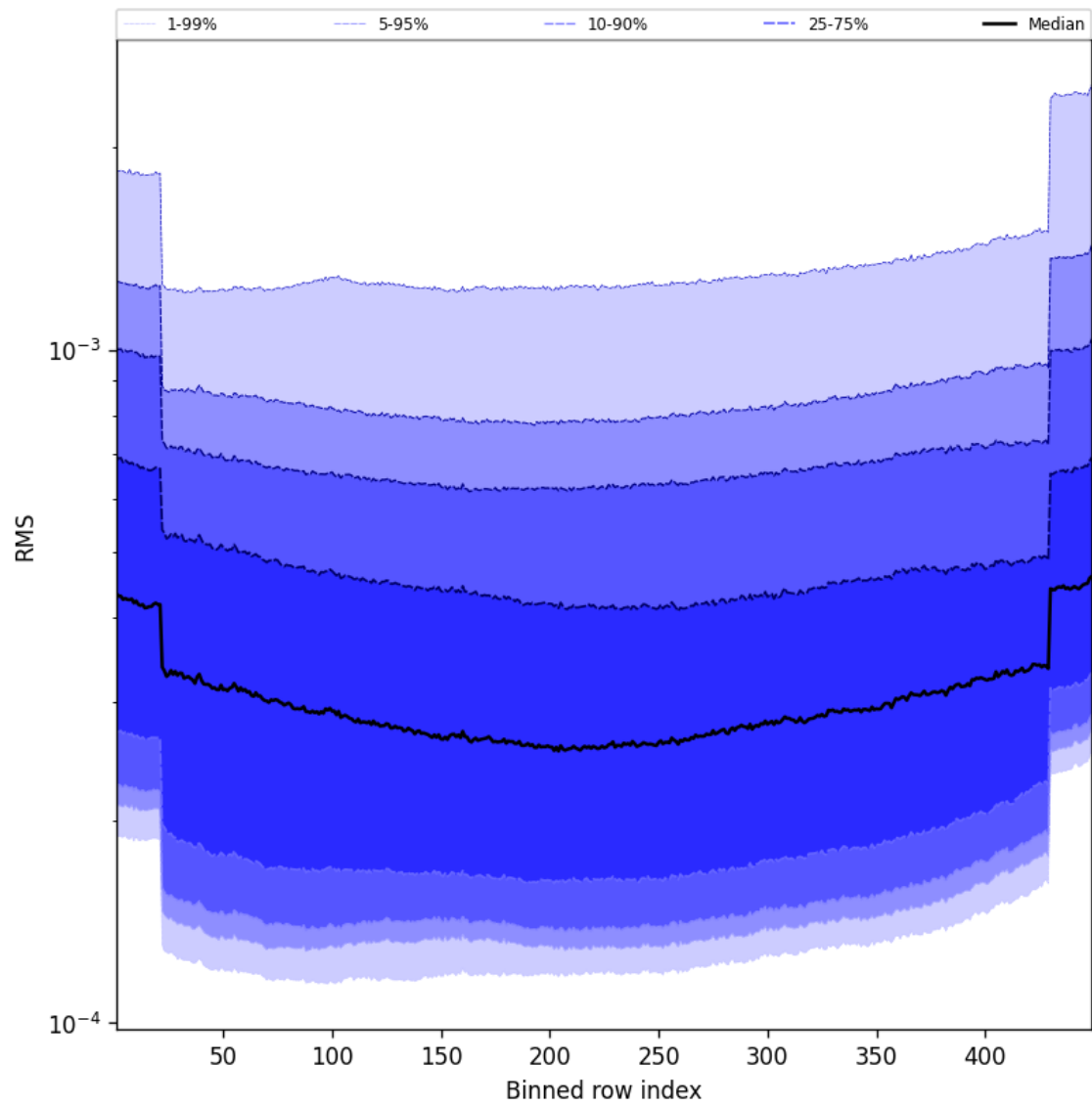
Figure 60: Along track statistics of “RMS” for 2024-09-22 to 2024-09-24
