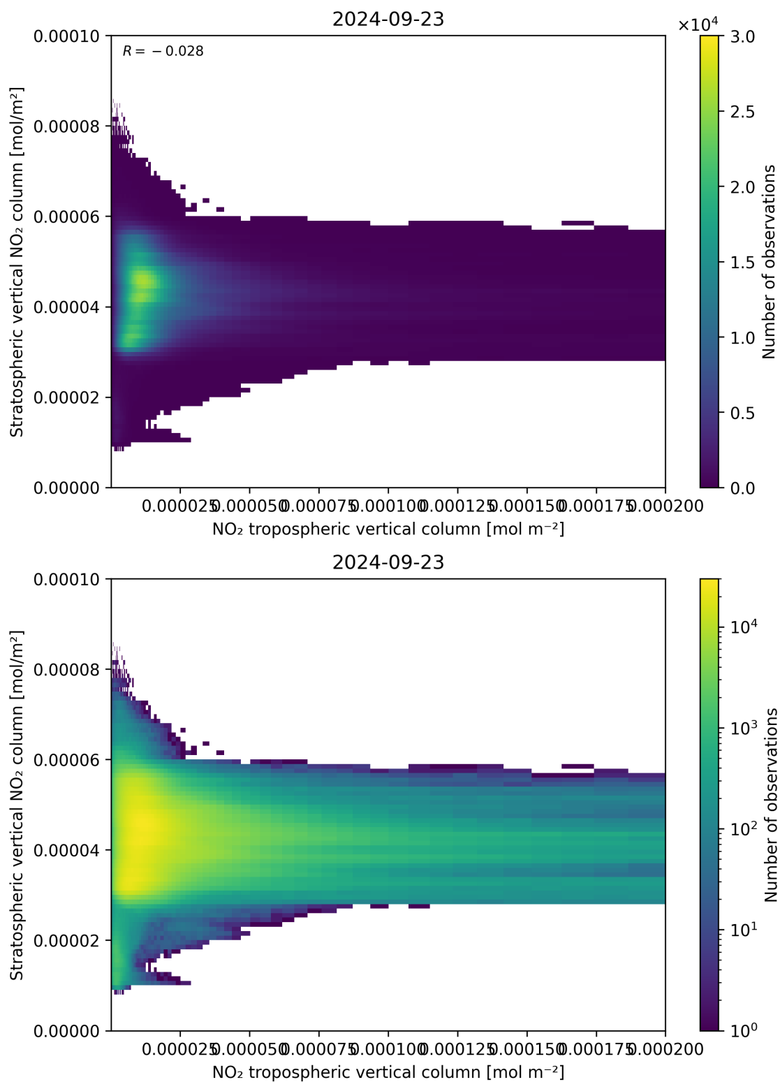
Figure 125: Scatter density plot of “NO 2 tropospheric vertical column” against “Stratospheric vertical NO 2 column” for 2024-09-22 to 2024-09-24.
