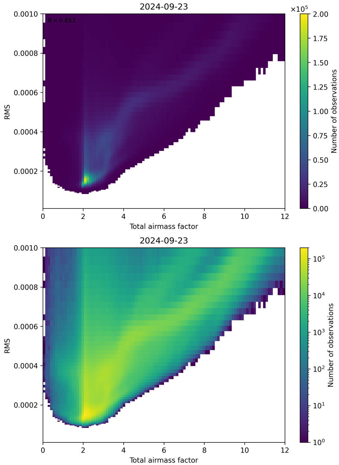
Figure 69: Scatter density plot of “Total airmass factor” against “RMS” for 2024-09-22 to 2024-09-24.
