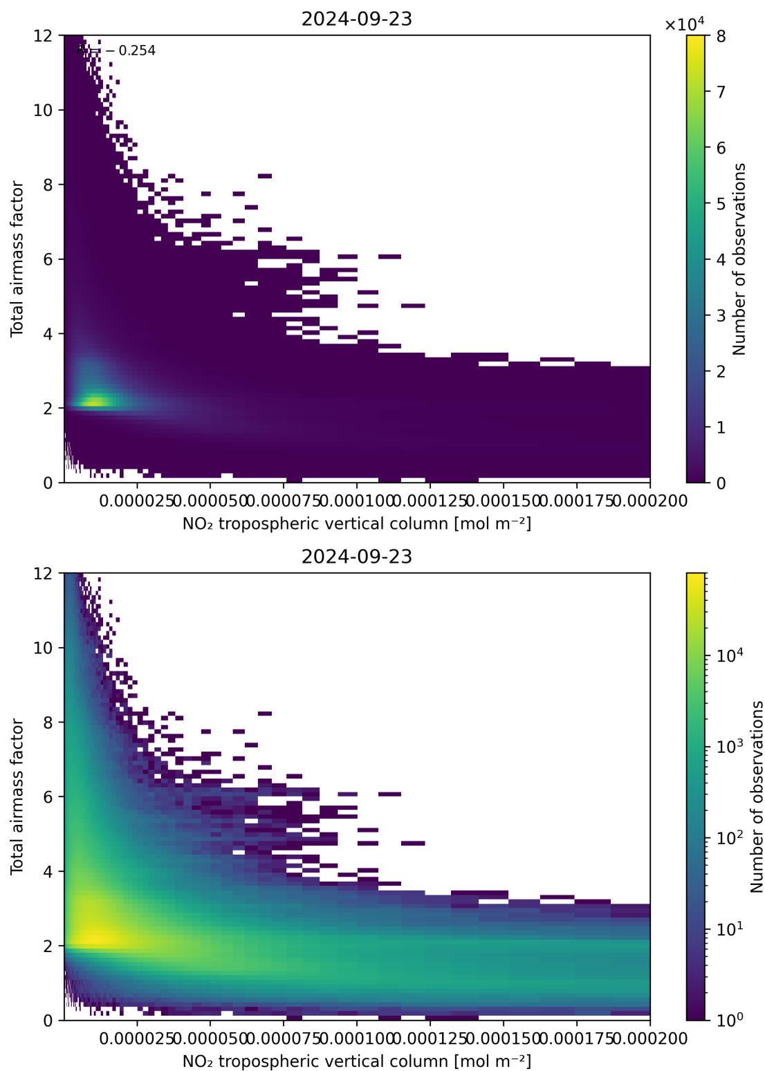
Figure 122: Scatter density plot of “NO 2 tropospheric vertical column” against “Total airmass factor” for 2024-09-22 to 2024-09-24.
