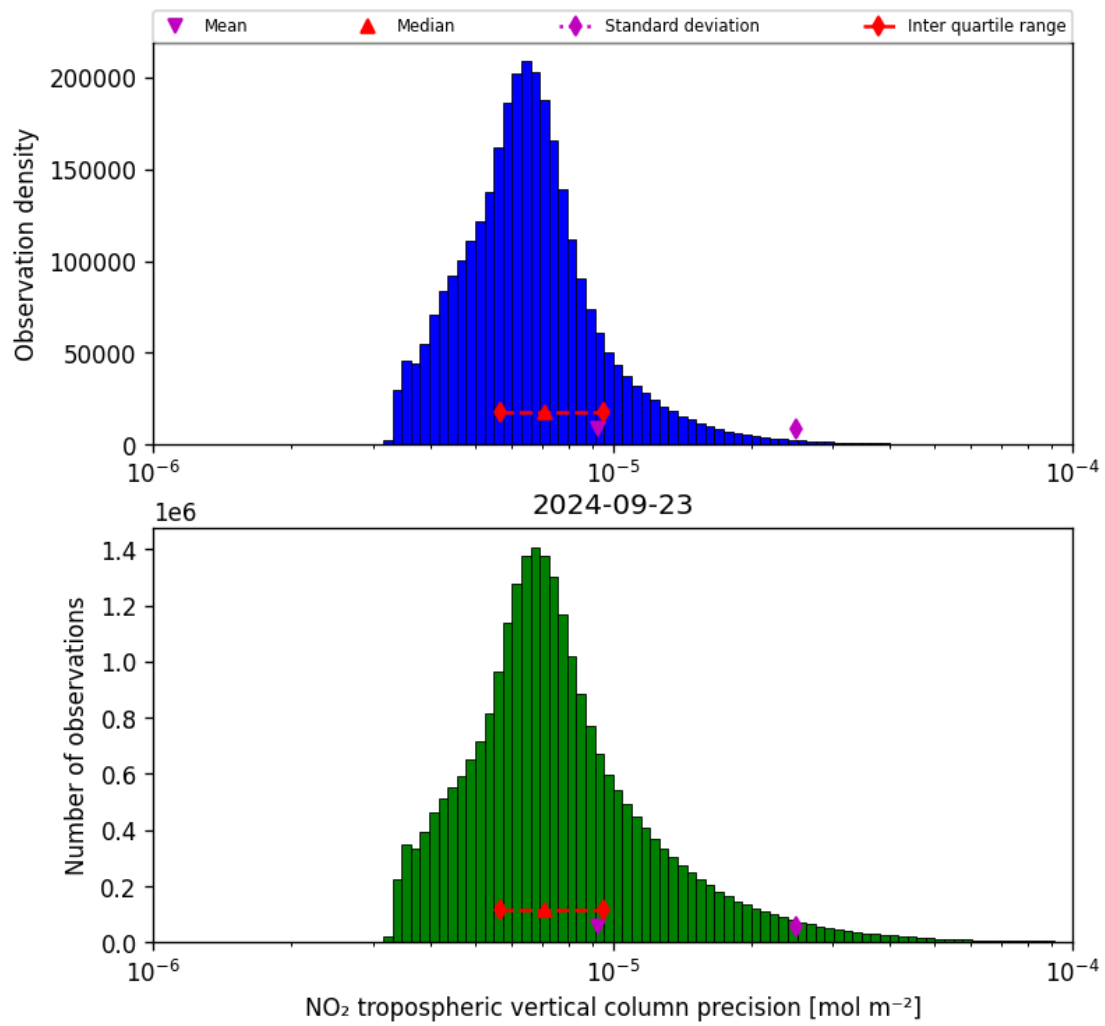
Figure 30: Histogram of “NO 2 tropospheric vertical column precision” for 2024-09-22 to 2024-09-24
