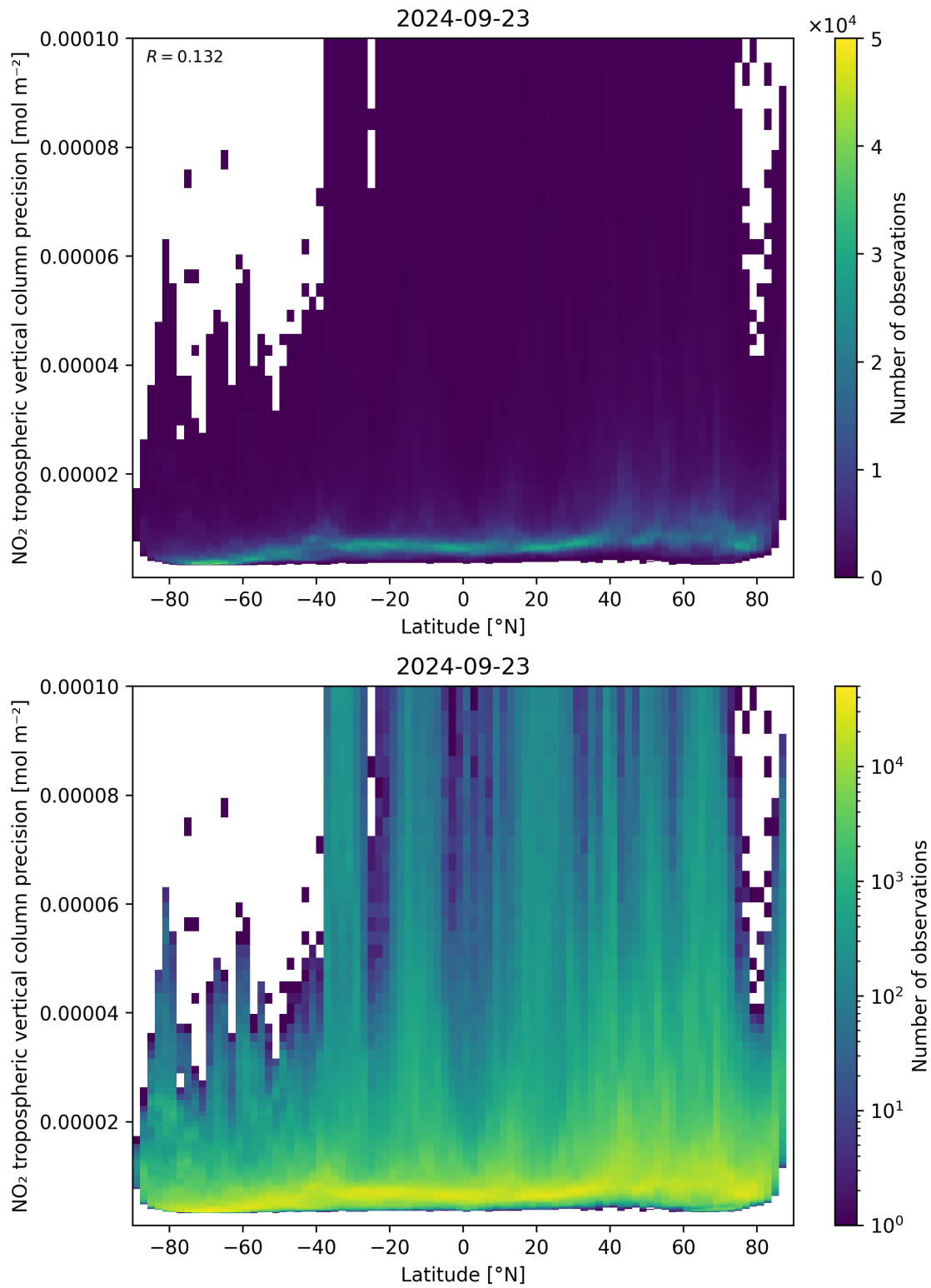
Figure 93: Scatter density plot of “Latitude” against “NO 2 tropospheric vertical column precision” for 2024-09-22 to 2024-09-24.
