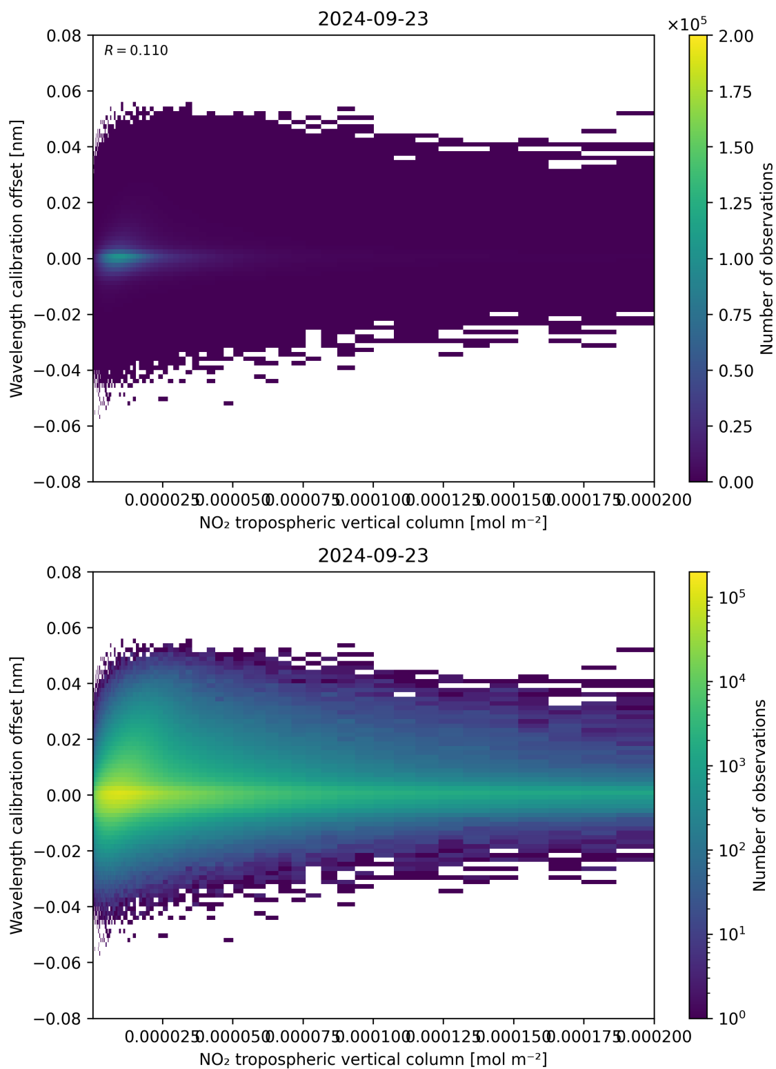
Figure 143: Scatter density plot of “NO 2 tropospheric vertical column” against “Wavelength calibration offset” for 2024-09-22 to 2024-09-24.
