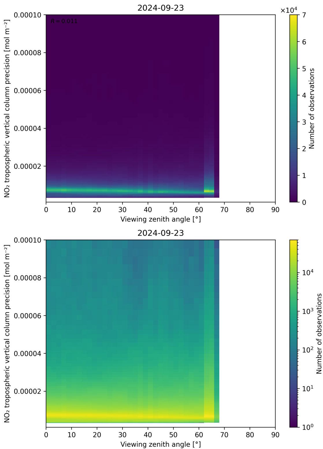
Figure 170: Scatter density plot of “Viewing zenith angle” against “NO 2 tropospheric vertical column precision” for 2024-09-22 to 2024-09-24.
