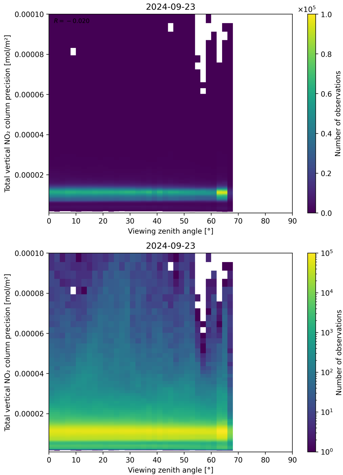
Figure 168: Scatter density plot of “Viewing zenith angle” against “Total vertical NO 2 column precision” for 2024-09-22 to 2024-09-24.
