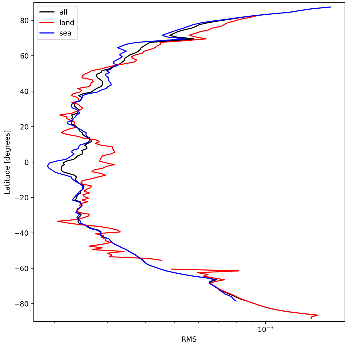
Figure 26: Zonal average of “RMS” for 2024-09-22 to 2024-09-24.
