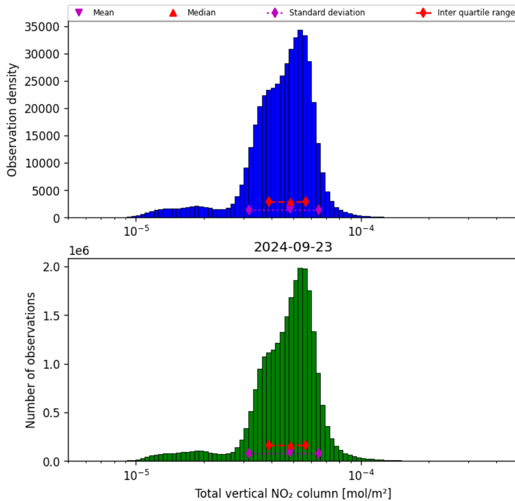
Figure 38: Histogram of “Total vertical NO 2 column” for 2024-09-22 to 2024-09-24
