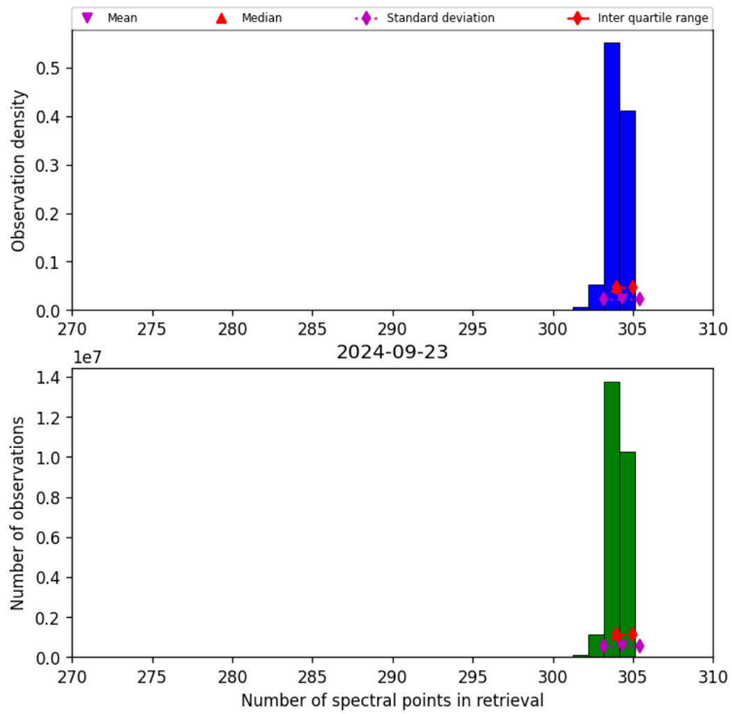
Figure 33: Histogram of “Number of spectral points in retrieval” for 2024-09-22 to 2024-09-24
