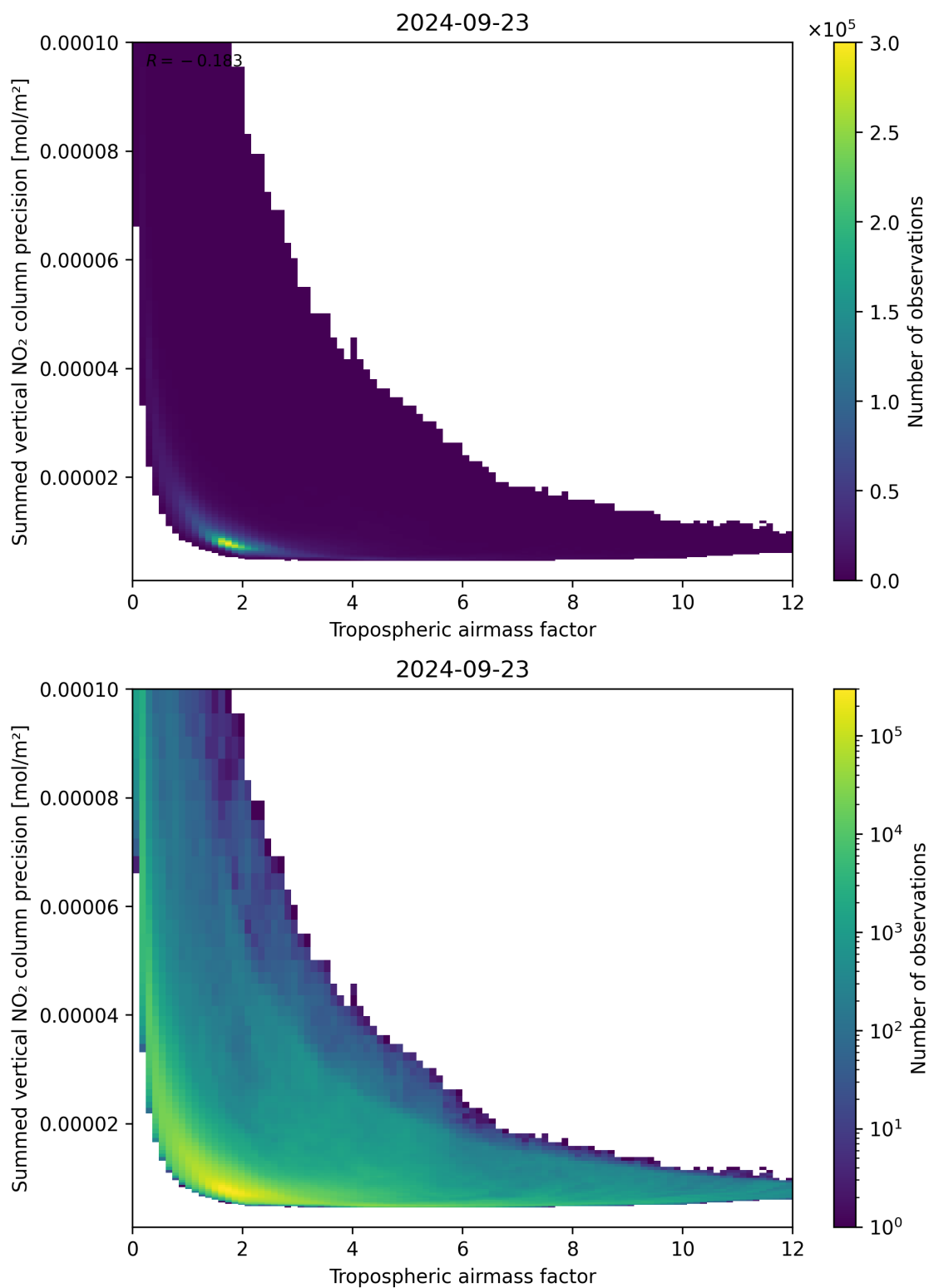
Figure 76: Scatter density plot of “Tropospheric airmass factor” against “Summed vertical NO 2 column precision” for 2024-09-22 to 2024-09-24.
