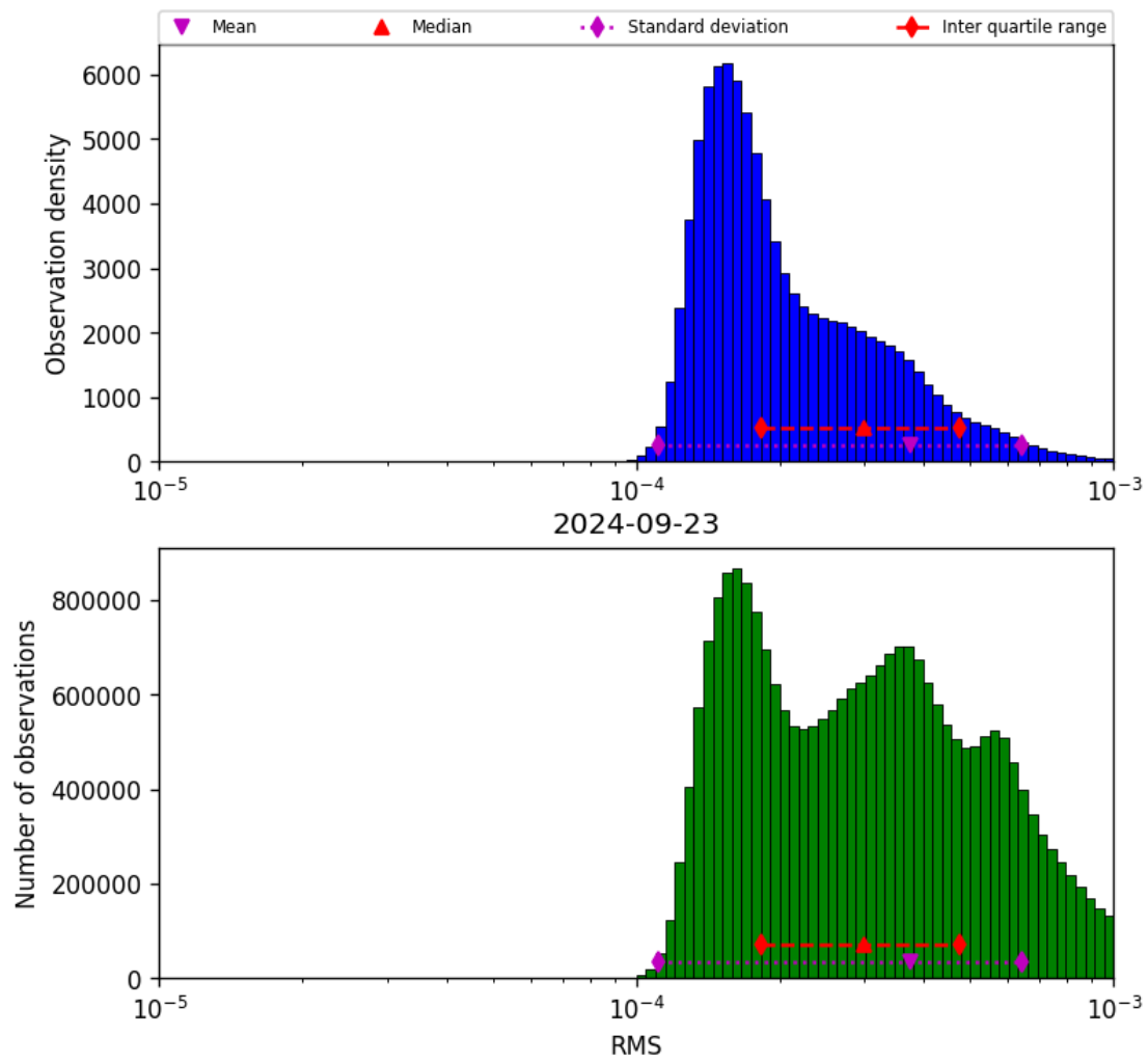
Figure 43: Histogram of “RMS” for 2024-09-22 to 2024-09-24
