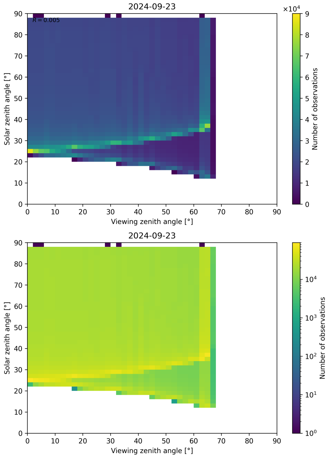
Figure 172: Scatter density plot of “Viewing zenith angle” against “Solar zenith angle” for 2024-09-22 to 2024-09-24.
