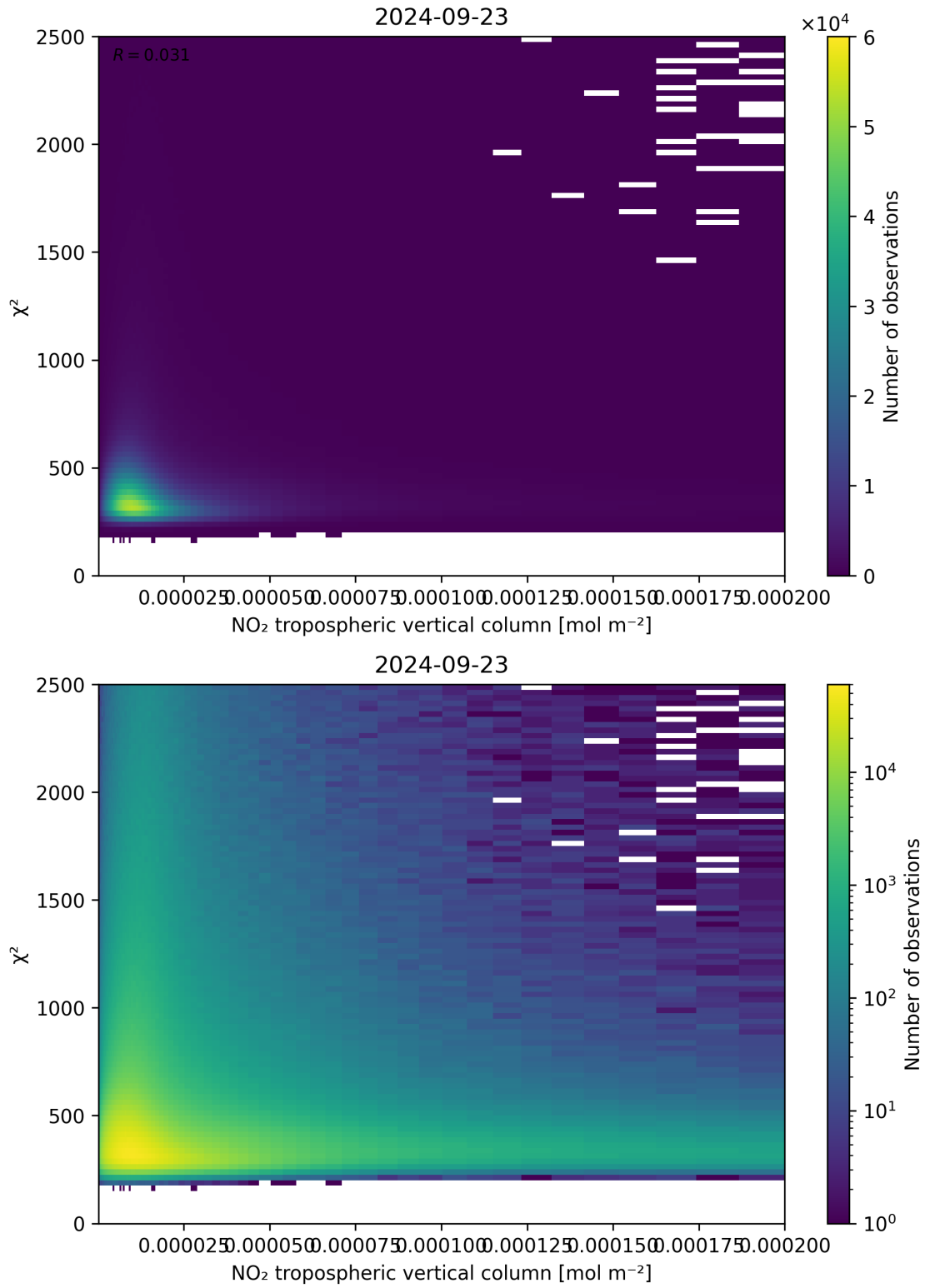
Figure 124: Scatter density plot of “NO 2 tropospheric vertical column” against “ \chi^2 ” for 2024-09-22 to 2024-09-24.
