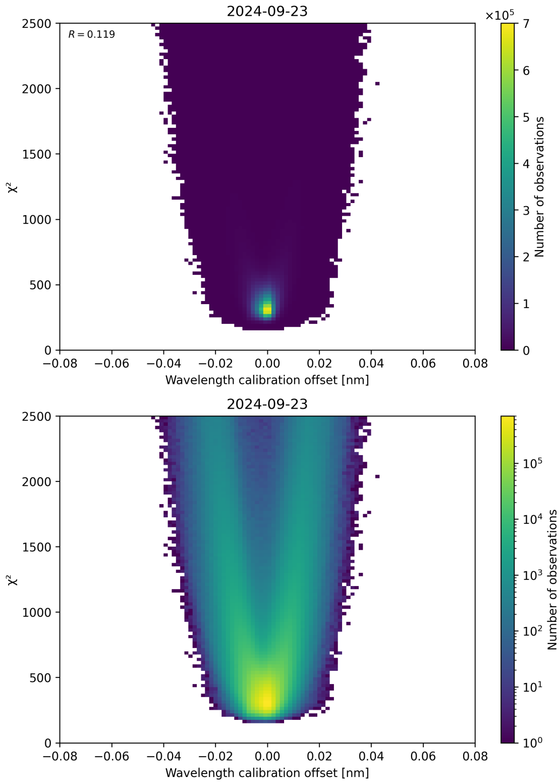
Figure 175: Scatter density plot of “Wavelength calibration offset” against “ \chi^2 ” for 2024-09-22 to 2024-09-24.
