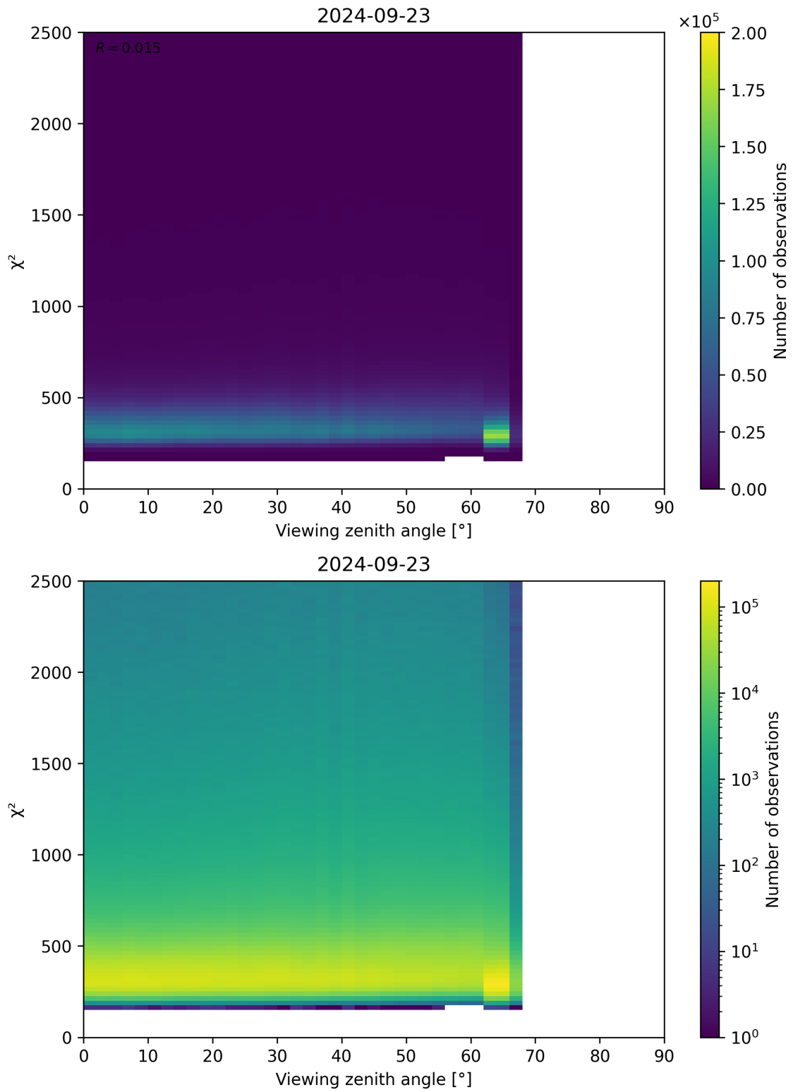
Figure 162: Scatter density plot of “Viewing zenith angle” against “ \chi^2 ” for 2024-09-22 to 2024-09-24.
