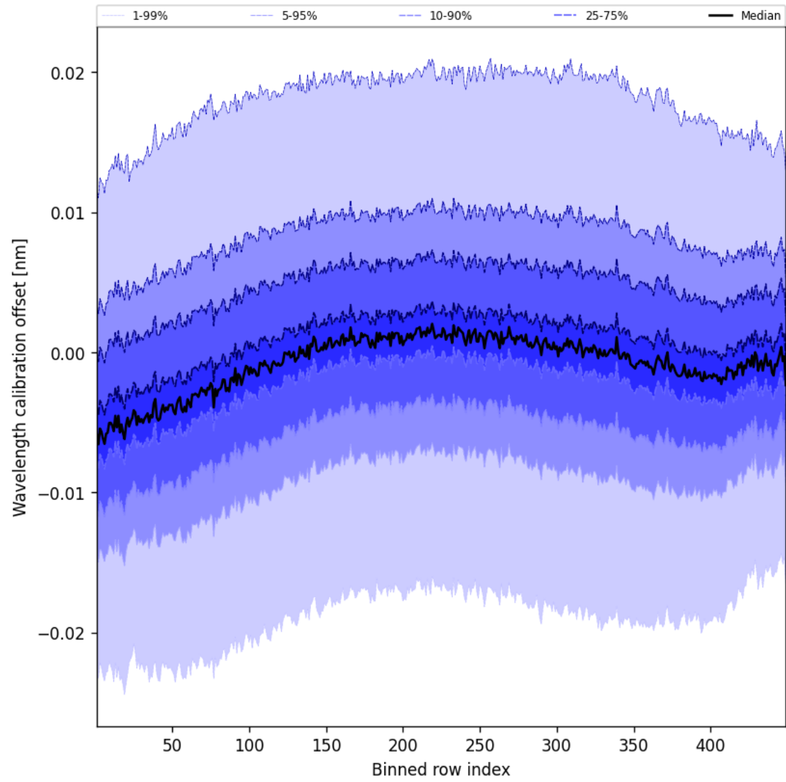
Figure 52: Along track statistics of “Wavelength calibration offset” for 2024-09-22 to 2024-09-24
