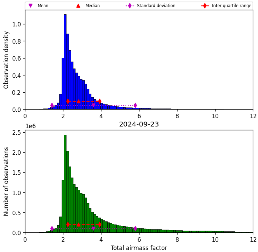
Figure 32: Histogram of “Total airmass factor” for 2024-09-22 to 2024-09-24
