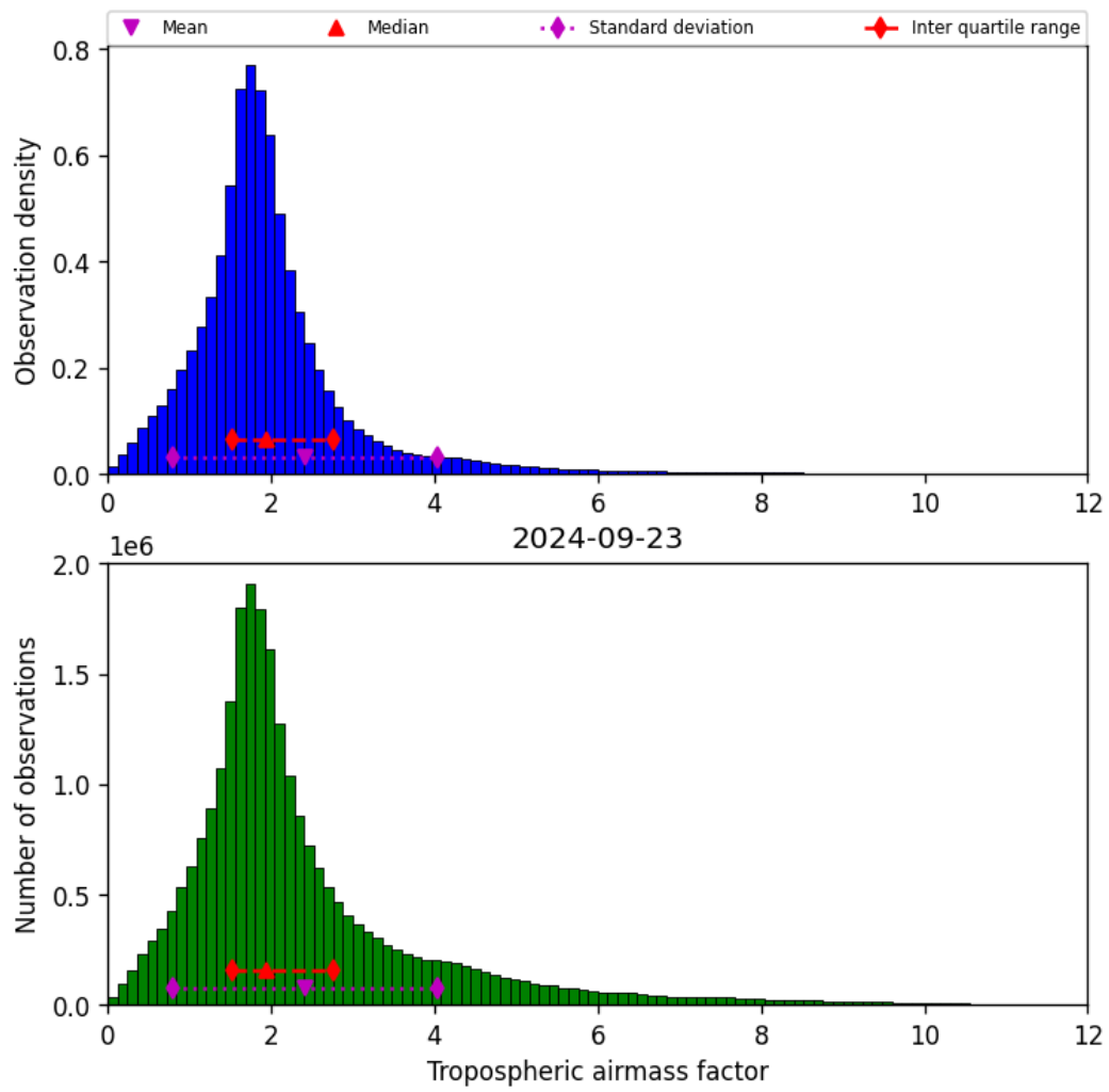
Figure 31: Histogram of “Tropospheric airmass factor” for 2024-09-22 to 2024-09-24
