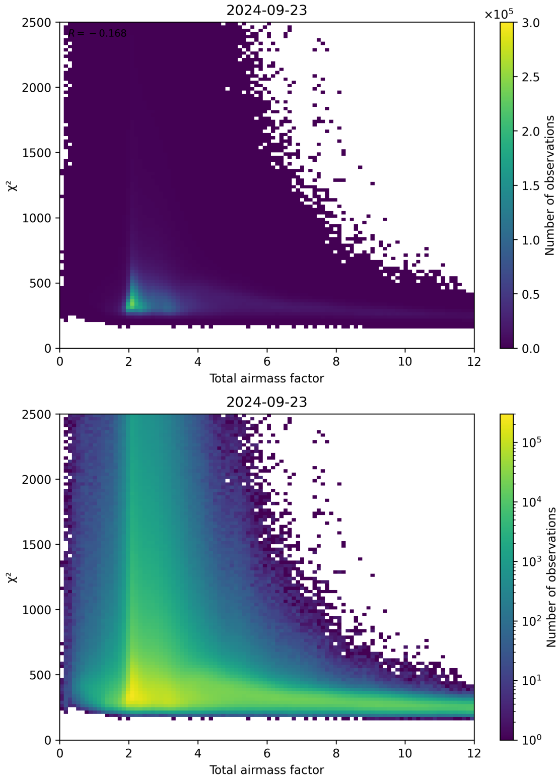
Figure 63: Scatter density plot of “Total airmass factor” against “ \chi^2 ” for 2024-09-22 to 2024-09-24.
