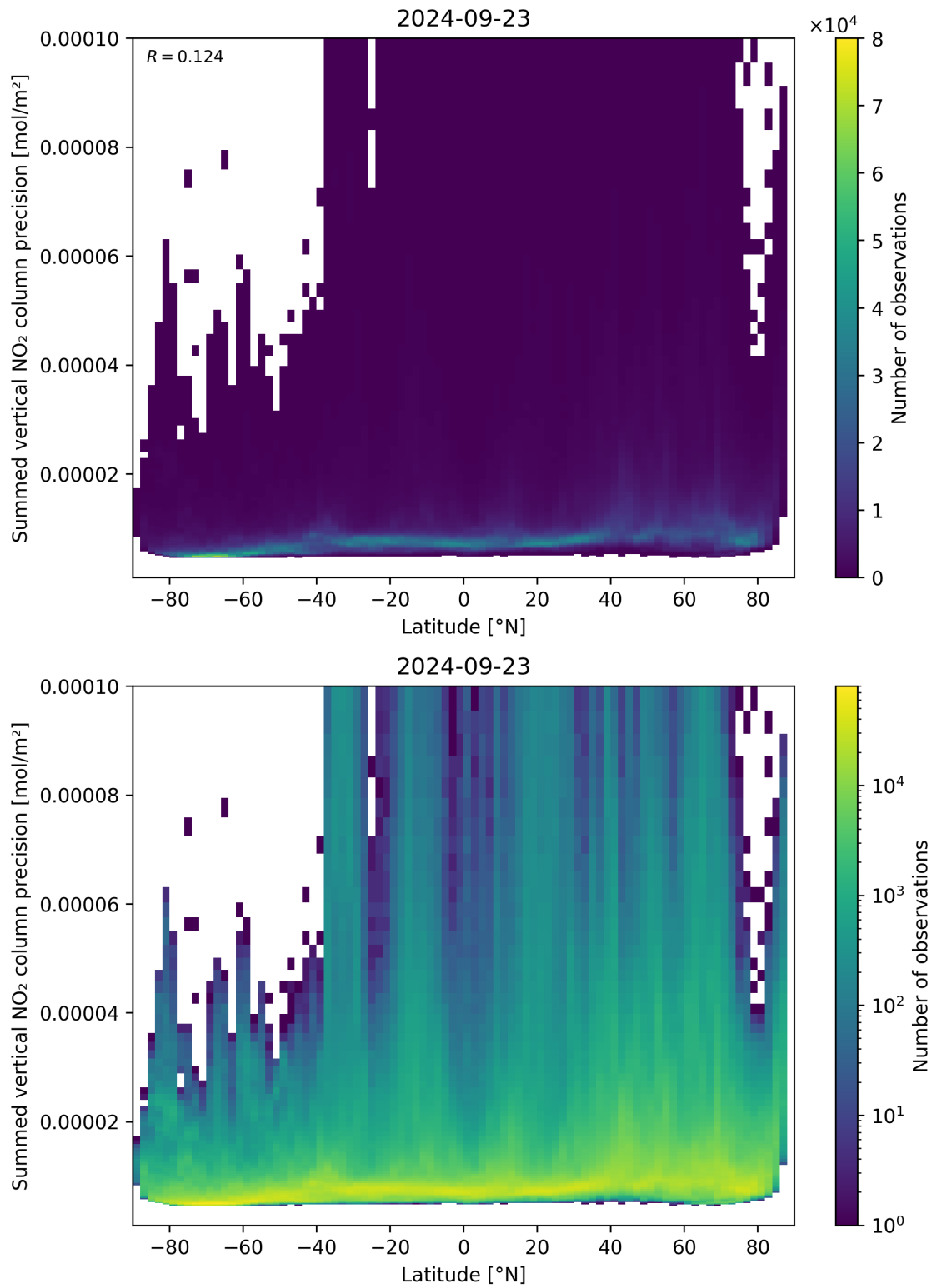
Figure 89: Scatter density plot of “Latitude” against “Summed vertical NO 2 column precision” for 2024-09-22 to 2024-09-24.
