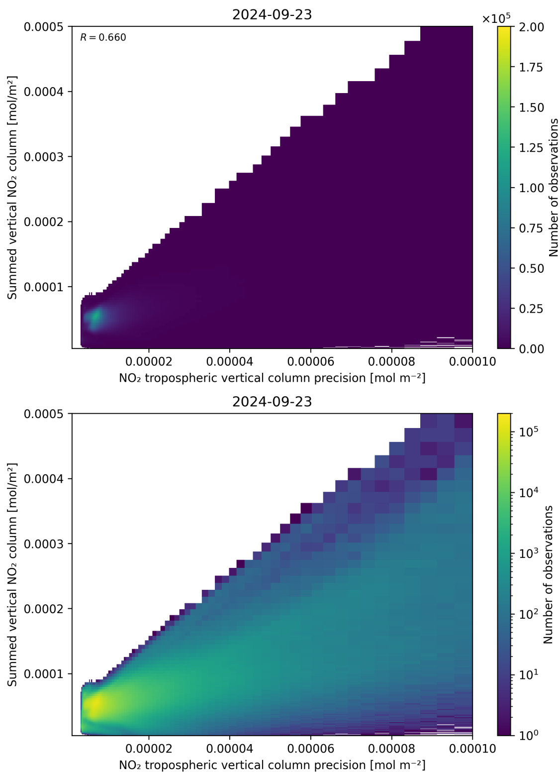
Figure 136: Scatter density plot of “NO 2 tropospheric vertical column precision” against “Summed vertical NO 2 column” for 2024-09-22 to 2024-09-24.
