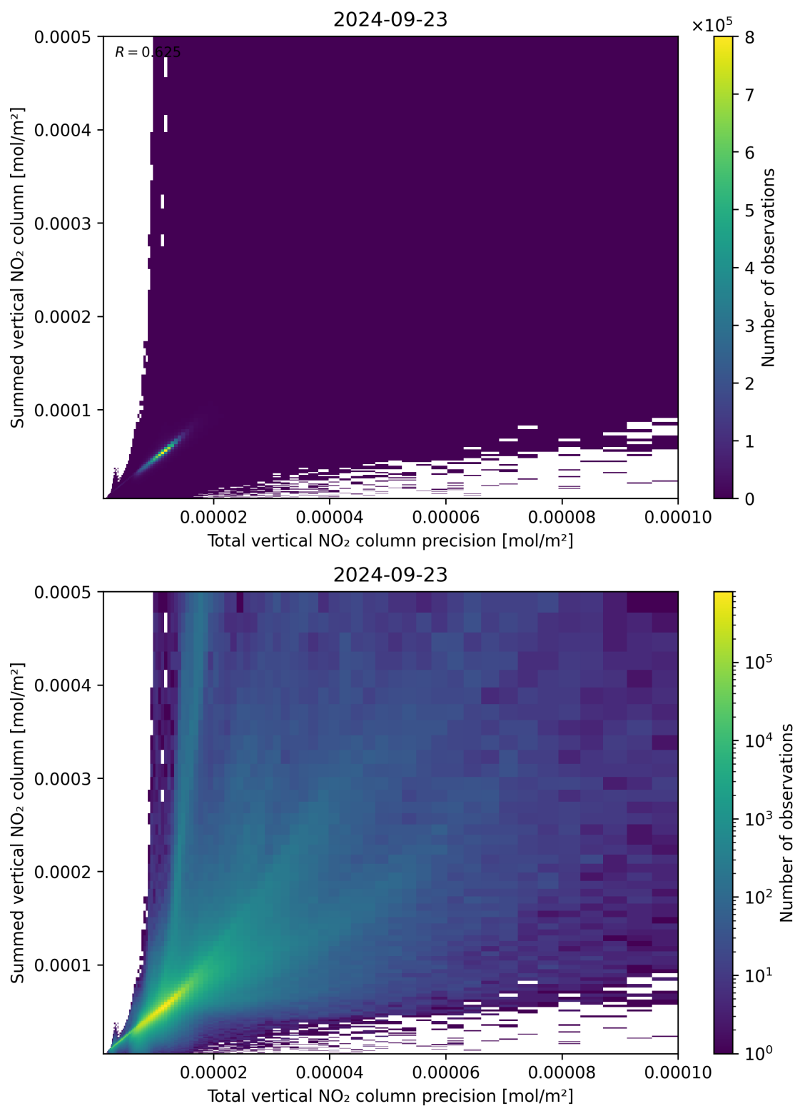
Figure 117: Scatter density plot of “Total vertical NO 2 column precision” against “Summed vertical NO 2 column” for 2024-09-22 to 2024-09-24.
