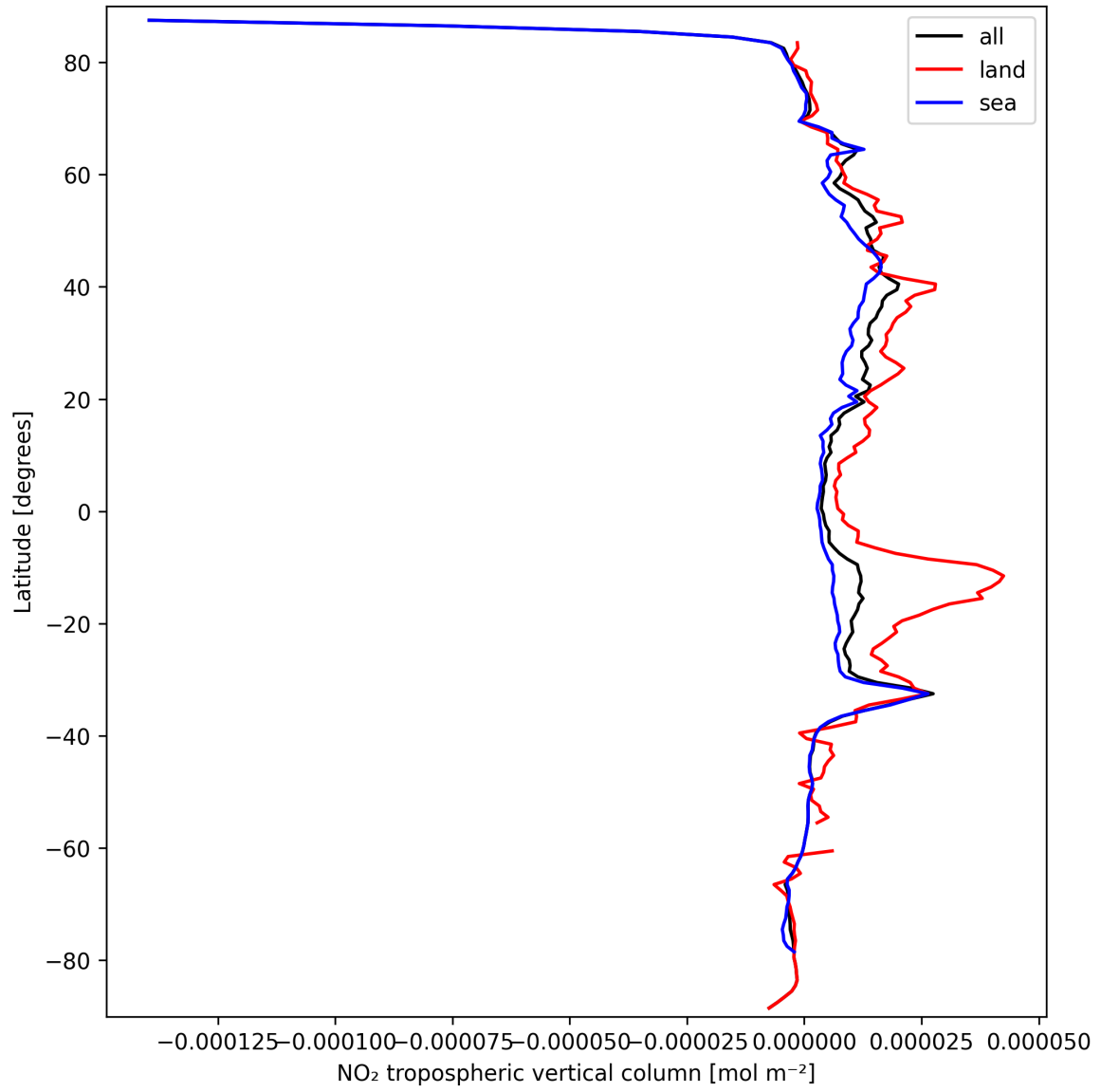
Figure 12: Zonal average of “NO 2 tropospheric vertical column” for 2024-09-22 to 2024-09-24.
