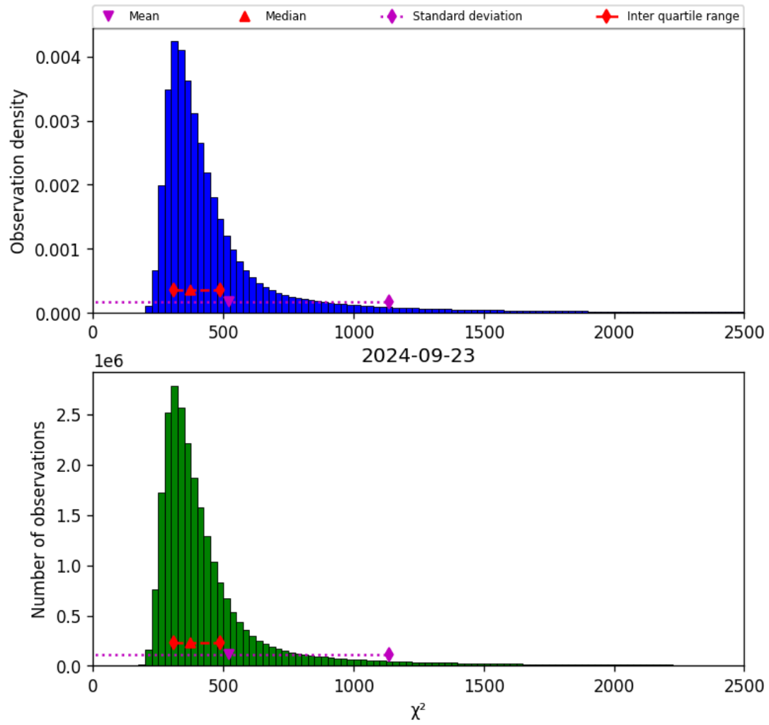
Figure 42: Histogram of “ \chi^2 ” for 2024-09-22 to 2024-09-24
