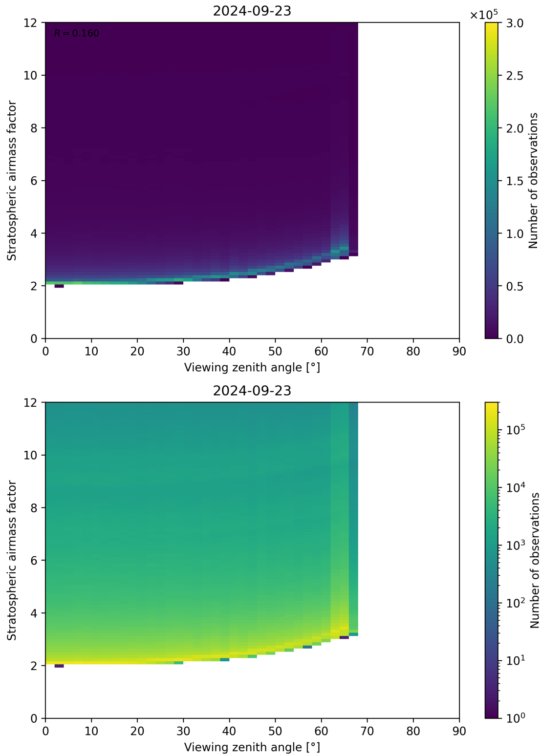
Figure 159: Scatter density plot of “Viewing zenith angle” against “Stratospheric airmass factor” for 2024-09-22 to 2024-09-24.
