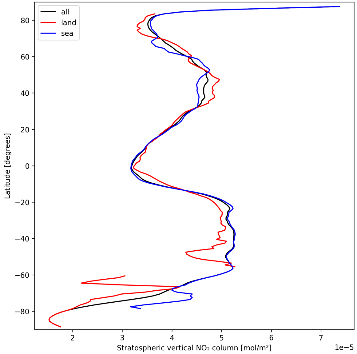
Figure 19: Zonal average of “Stratospheric vertical NO 2 column” for 2024-09-22 to 2024-09-24.
