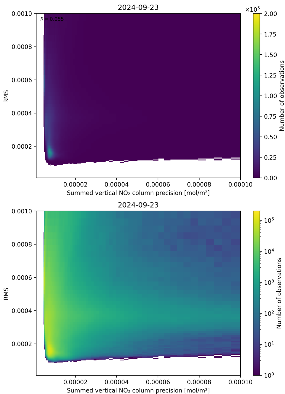
Figure 108: Scatter density plot of “Summed vertical NO 2 column precision” against “RMS” for 2024-09-22 to 2024-09-24.
