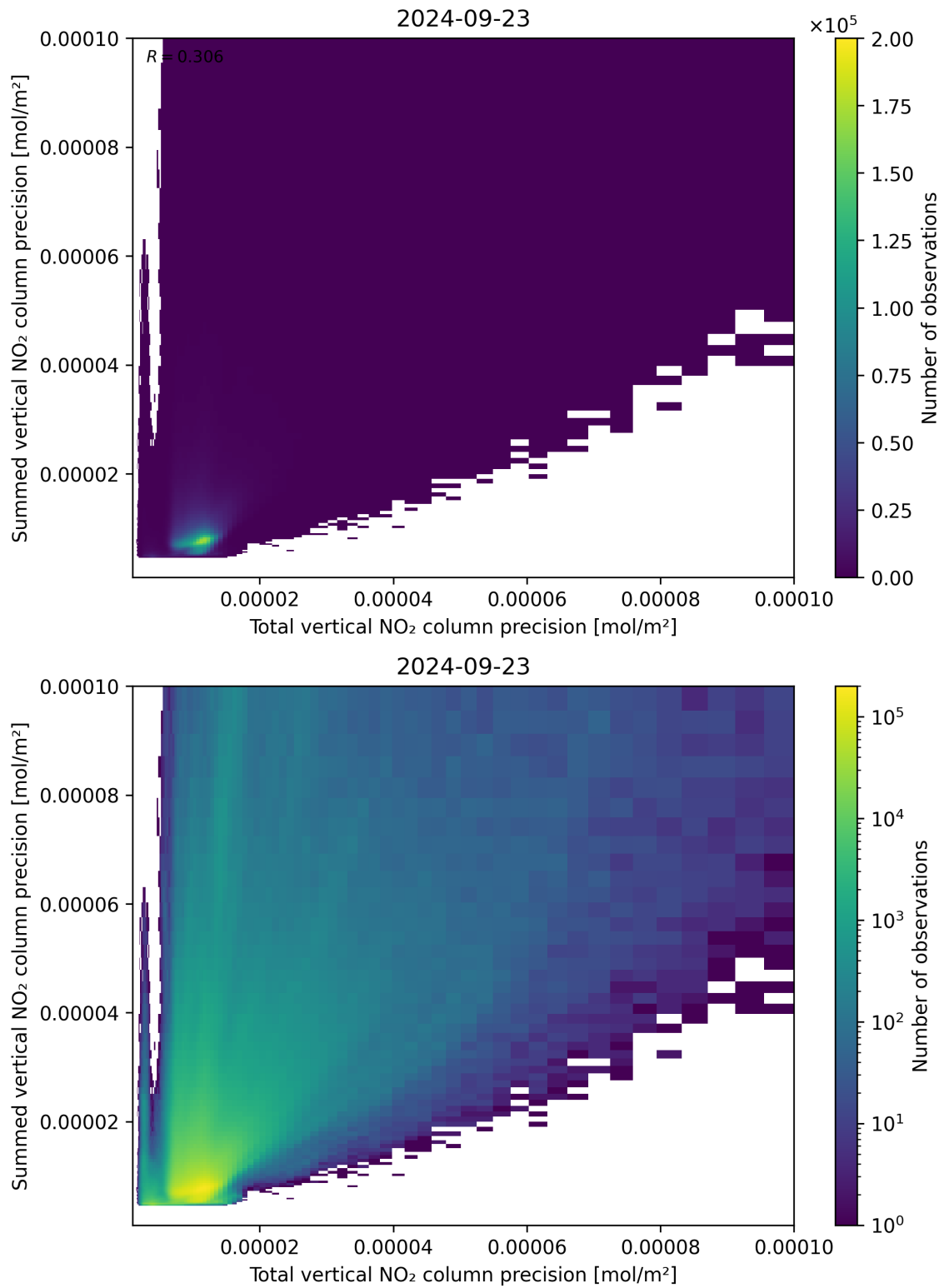
Figure 118: Scatter density plot of “Total vertical NO 2 column precision” against “Summed vertical NO 2 column precision” for 2024-09-22 to 2024-09-24.
