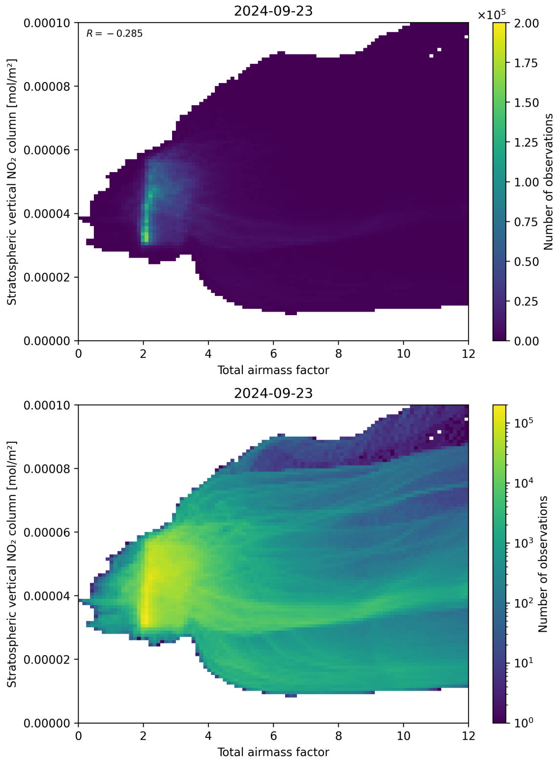
Figure 64: Scatter density plot of “Total airmass factor” against “Stratospheric vertical \text{NO}_2 column” for 2024-09-22 to 2024-09-24.
