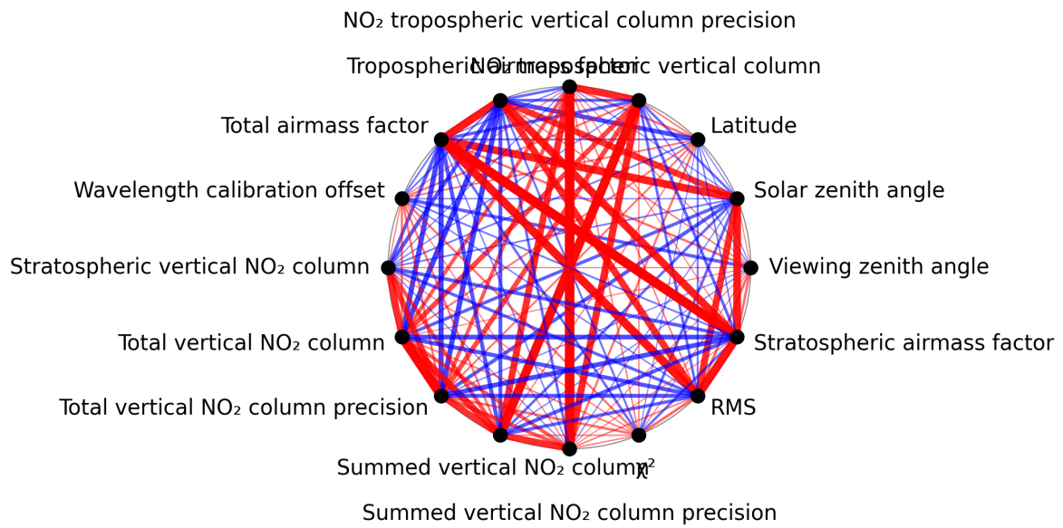
Figure 1: Map of correlation graph for 2024-09-22 to 2024-09-24.
