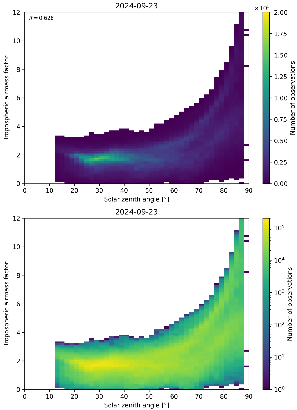
Figure 147: Scatter density plot of “Solar zenith angle” against “Tropospheric airmass factor” for 2024-09-22 to 2024-09-24.
