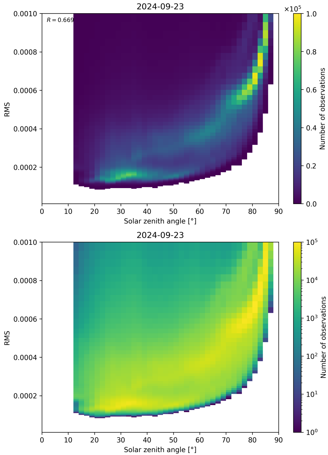
Figure 157: Scatter density plot of “Solar zenith angle” against “RMS” for 2024-09-22 to 2024-09-24.
