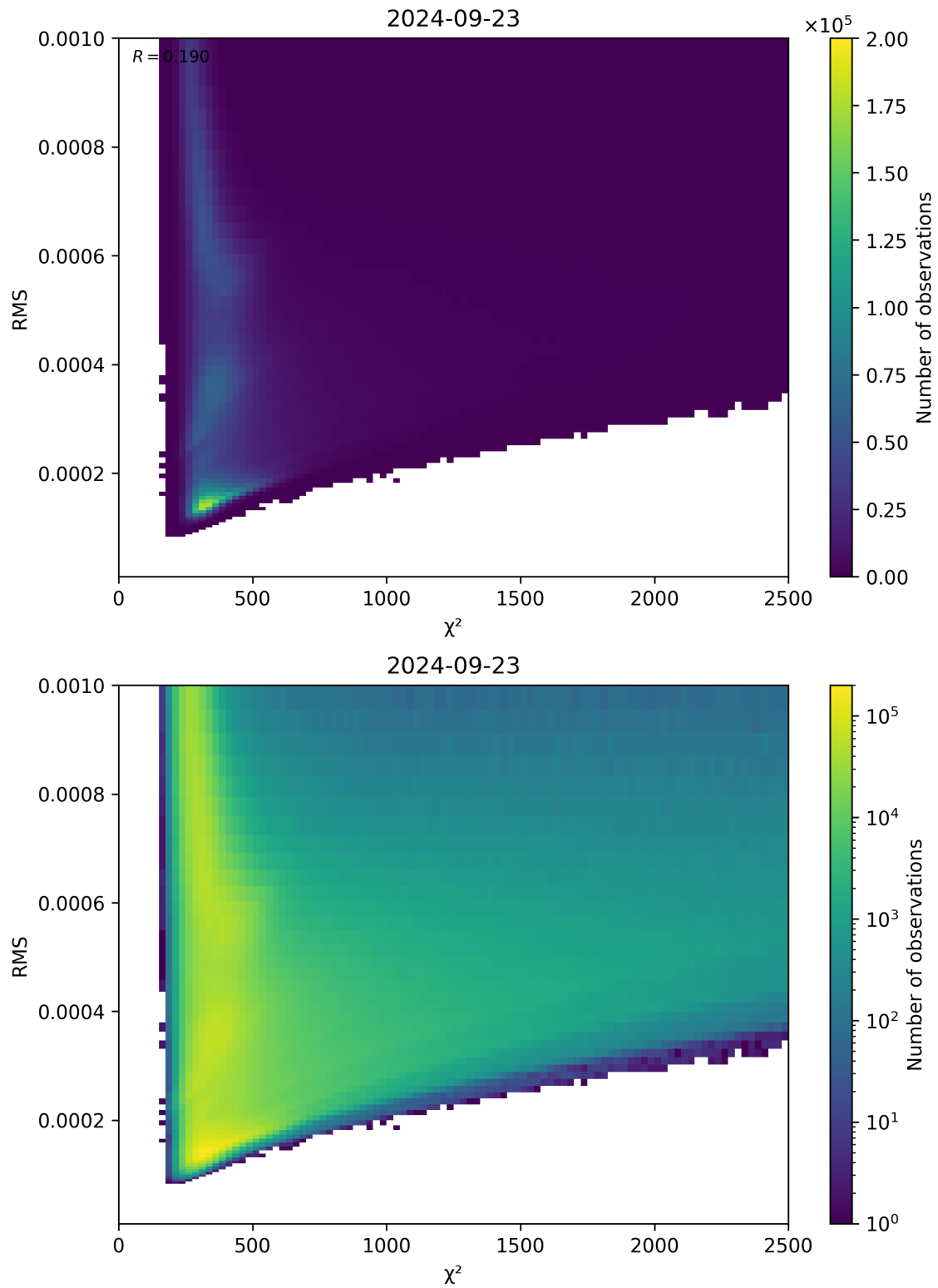
Figure 82: Scatter density plot of “ \chi^2 ” against “RMS” for 2024-09-22 to 2024-09-24.
