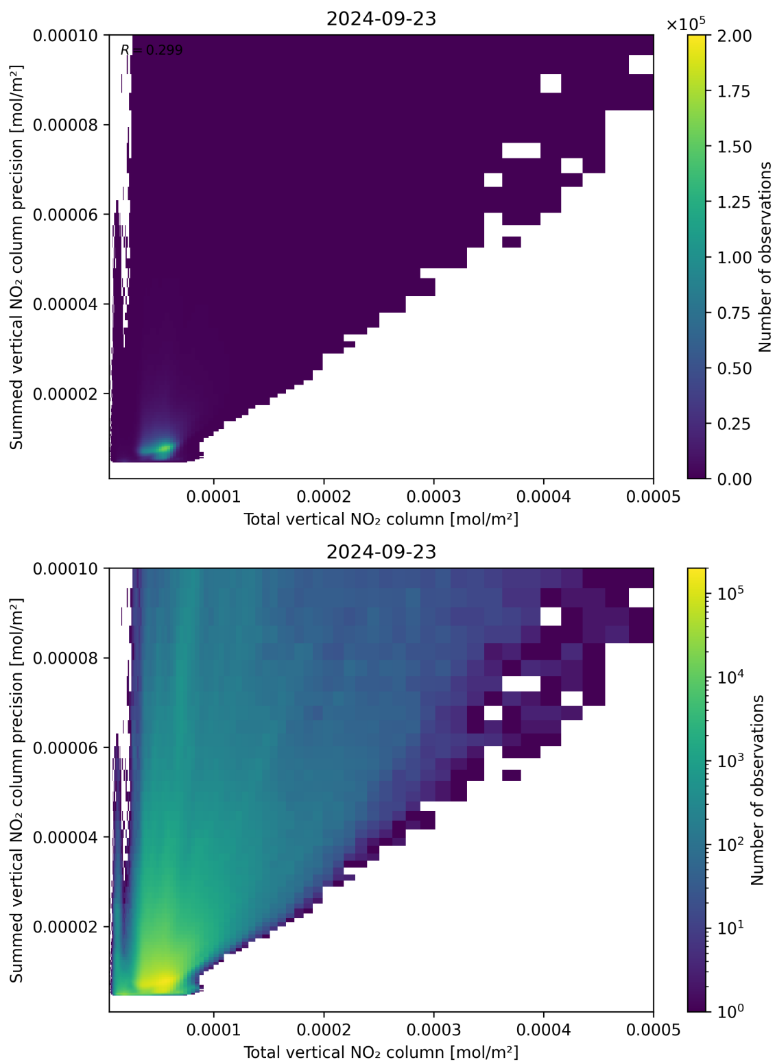
Figure 113: Scatter density plot of “Total vertical NO 2 column” against “Summed vertical NO 2 column precision” for 2024-09-22 to 2024-09-24.
