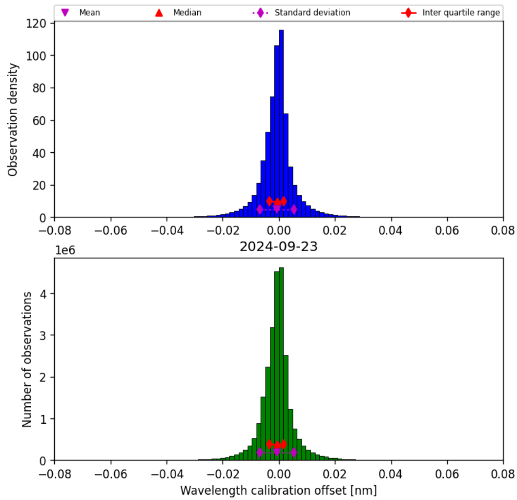
Figure 35: Histogram of “Wavelength calibration offset” for 2024-09-22 to 2024-09-24
