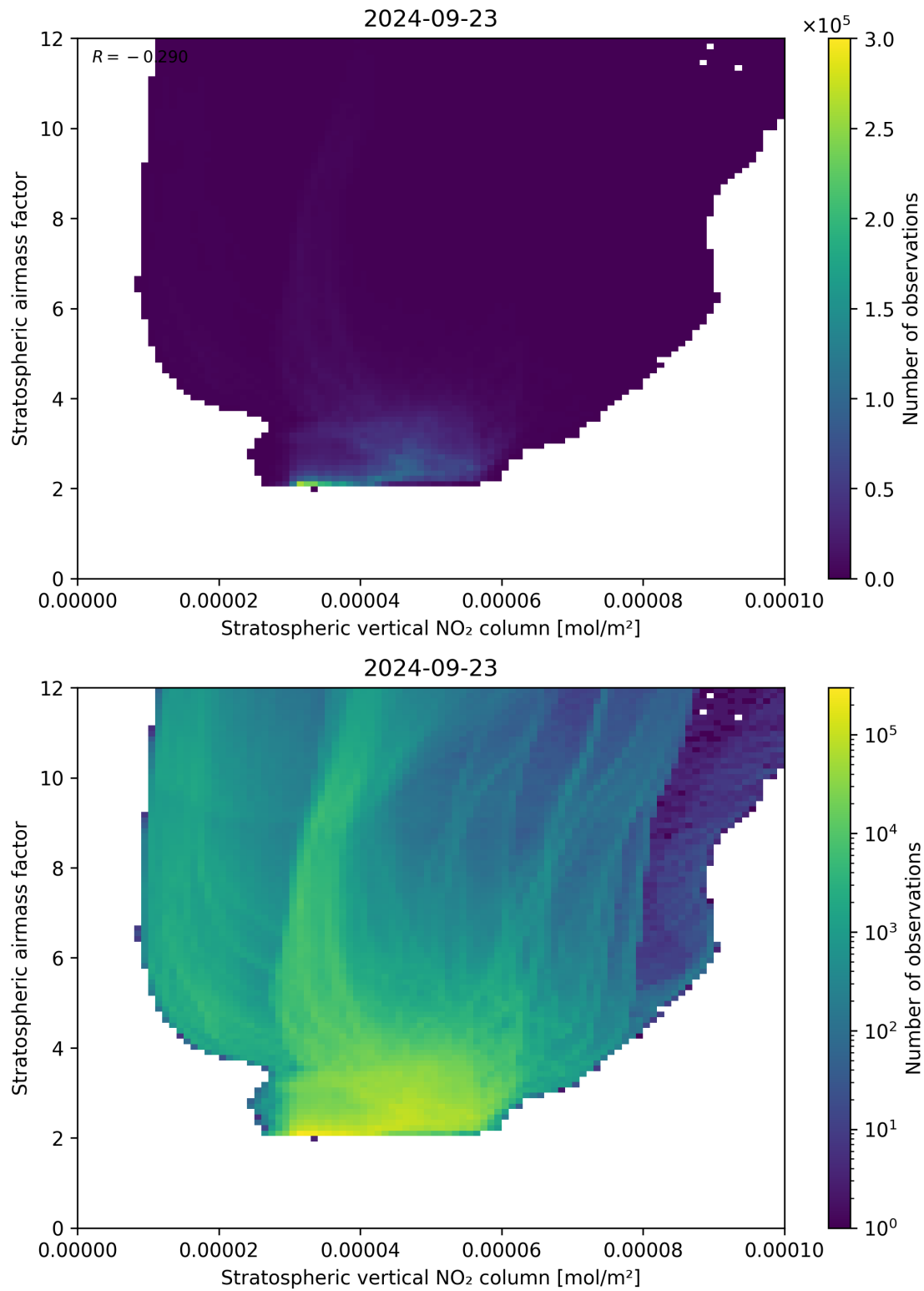
Figure 96: Scatter density plot of “Stratospheric vertical NO 2 column” against “Stratospheric airmass factor” for 2024-09-22 to 2024-09-24.
