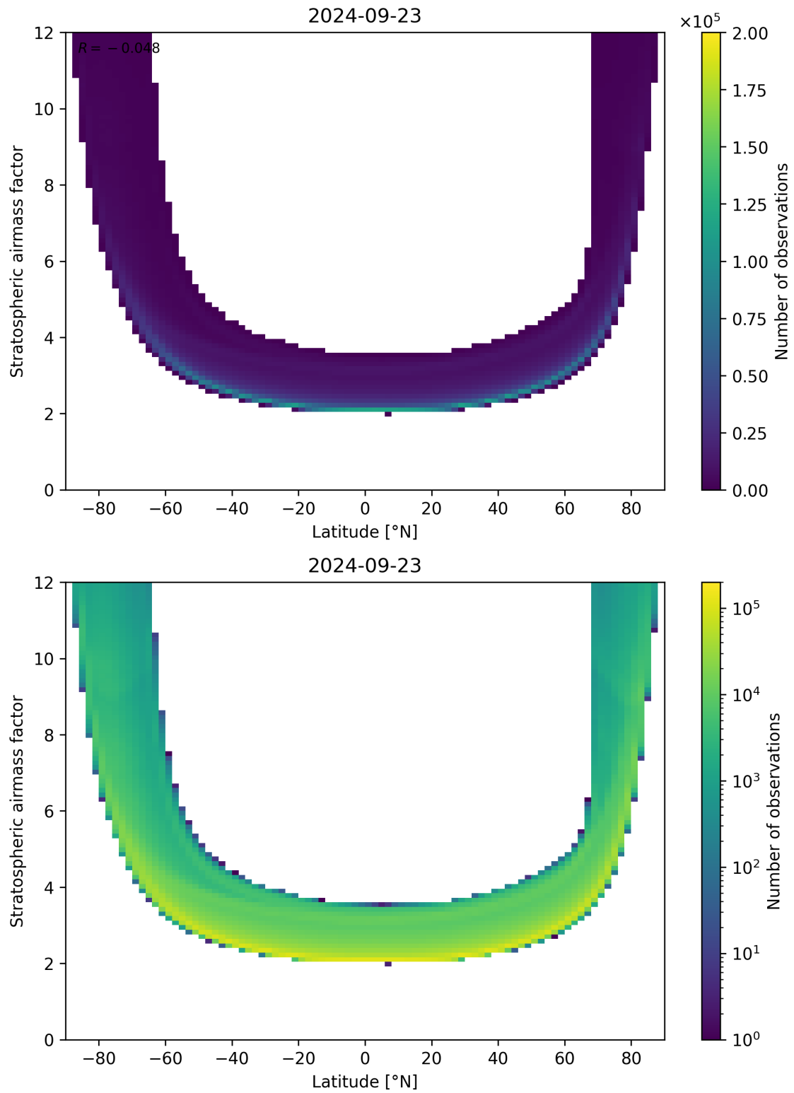
Figure 83: Scatter density plot of “Latitude” against “Stratospheric airmass factor” for 2024-09-22 to 2024-09-24.
