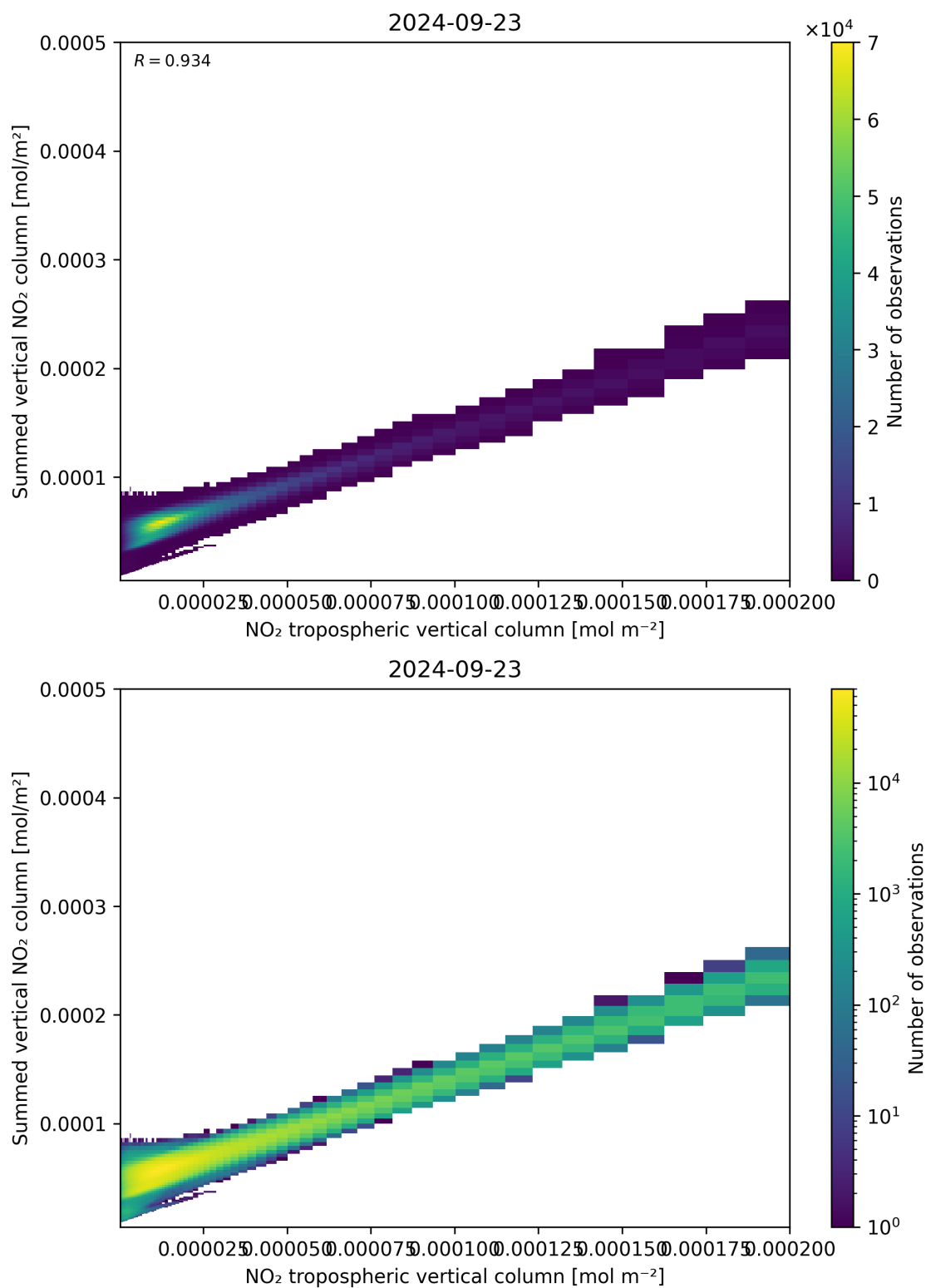
Figure 126: Scatter density plot of “NO 2 tropospheric vertical column” against “Summed vertical NO 2 column” for 2024-09-22 to 2024-09-24.
