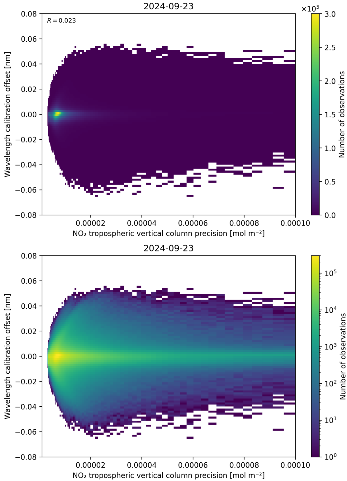
Figure 141: Scatter density plot of “NO 2 tropospheric vertical column precision” against “Wavelength calibration offset” for 2024-09-22 to 2024-09-24.
