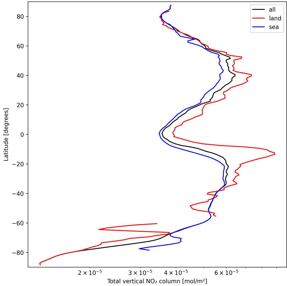
Figure 21: Zonal average of “Total vertical NO 2 column” for 2024-09-22 to 2024-09-24.
