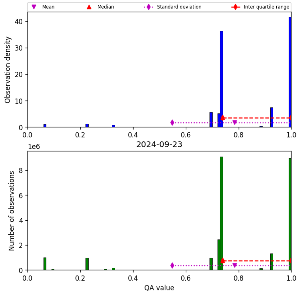
Figure 28: Histogram of “QA value” for 2024-09-22 to 2024-09-24
