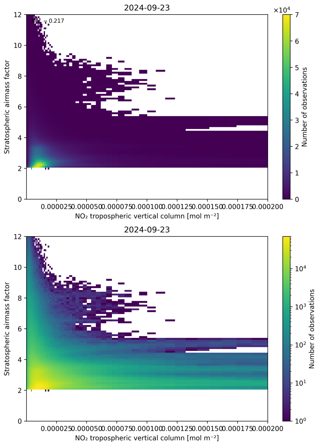
Figure 121: Scatter density plot of “NO 2 tropospheric vertical column” against “Stratospheric air mass factor” for 2024-09-22 to 2024-09-24.
