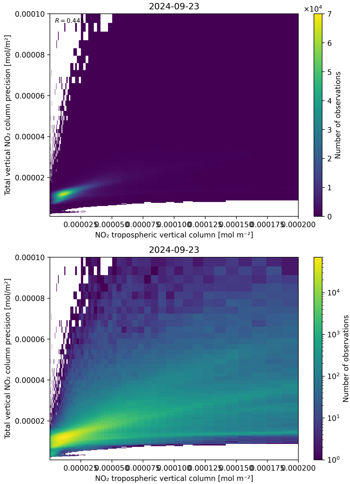
Figure 129: Scatter density plot of “NO 2 tropospheric vertical column” against “Total vertical NO 2 column precision” for 2024-09-22 to 2024-09-24.
