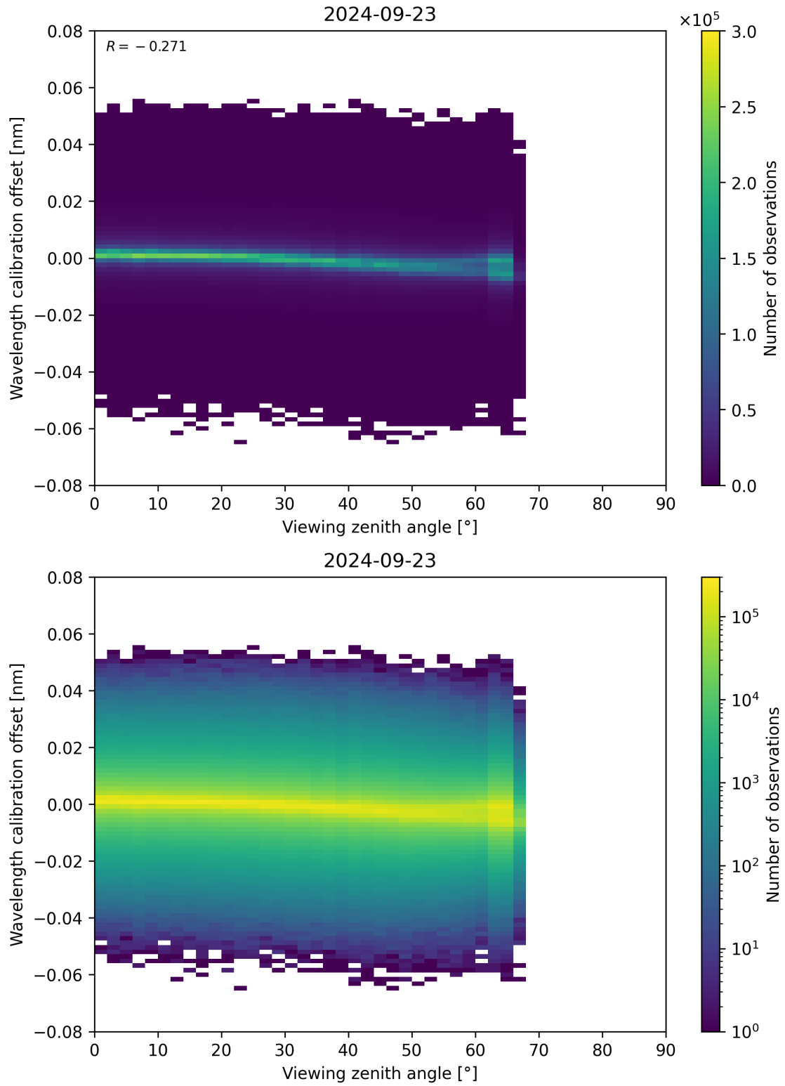
Figure 173: Scatter density plot of “Viewing zenith angle” against “Wavelength calibration offset” for 2024-09-22 to 2024-09-24.
