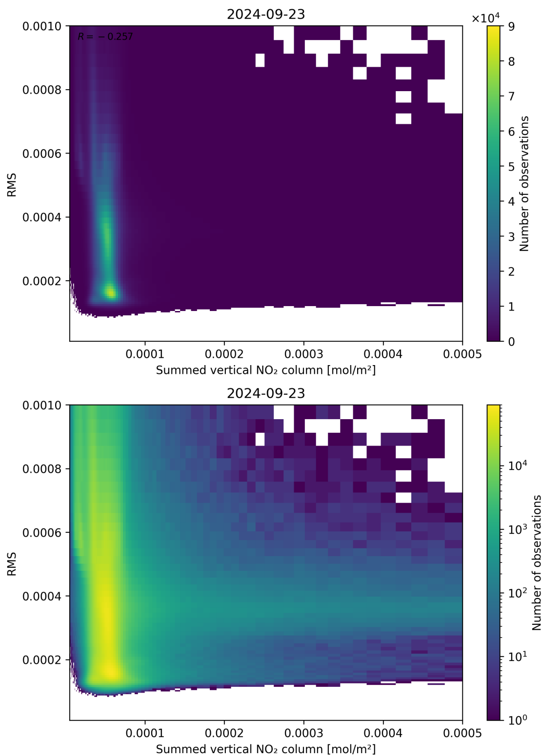
Figure 109: Scatter density plot of “Summed vertical NO 2 column” against “RMS” for 2024-09-22 to 2024-09-24.
