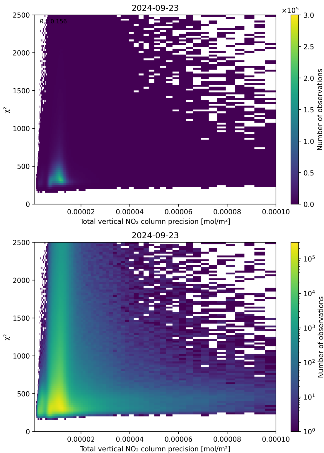
Figure 116: Scatter density plot of “Total vertical NO 2 column precision” against “ \chi^2 ” for 2024-09-22 to 2024-09-24.
