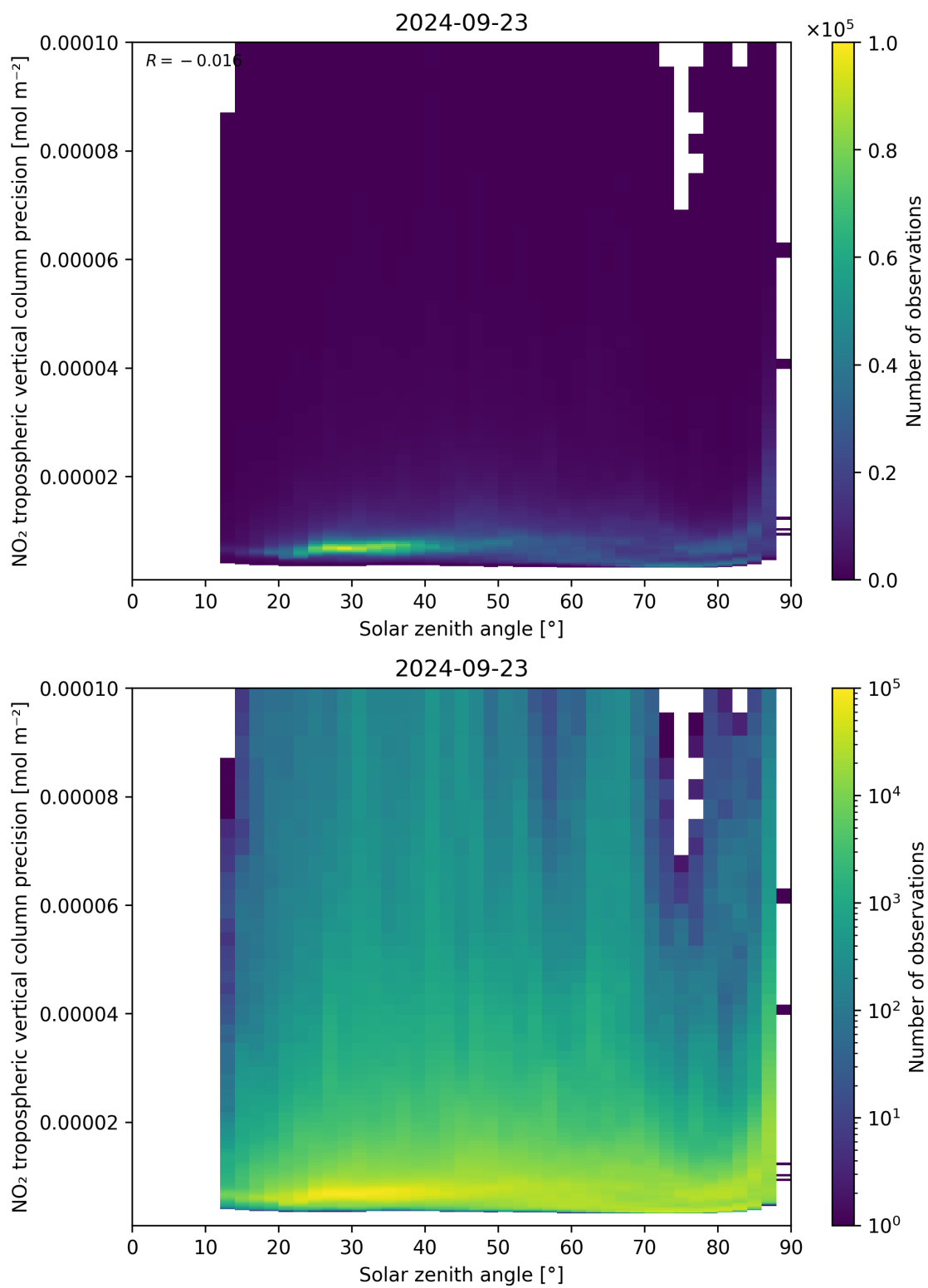
Figure 156: Scatter density plot of “Solar zenith angle” against “NO 2 tropospheric vertical column precision” for 2024-09-22 to 2024-09-24.
