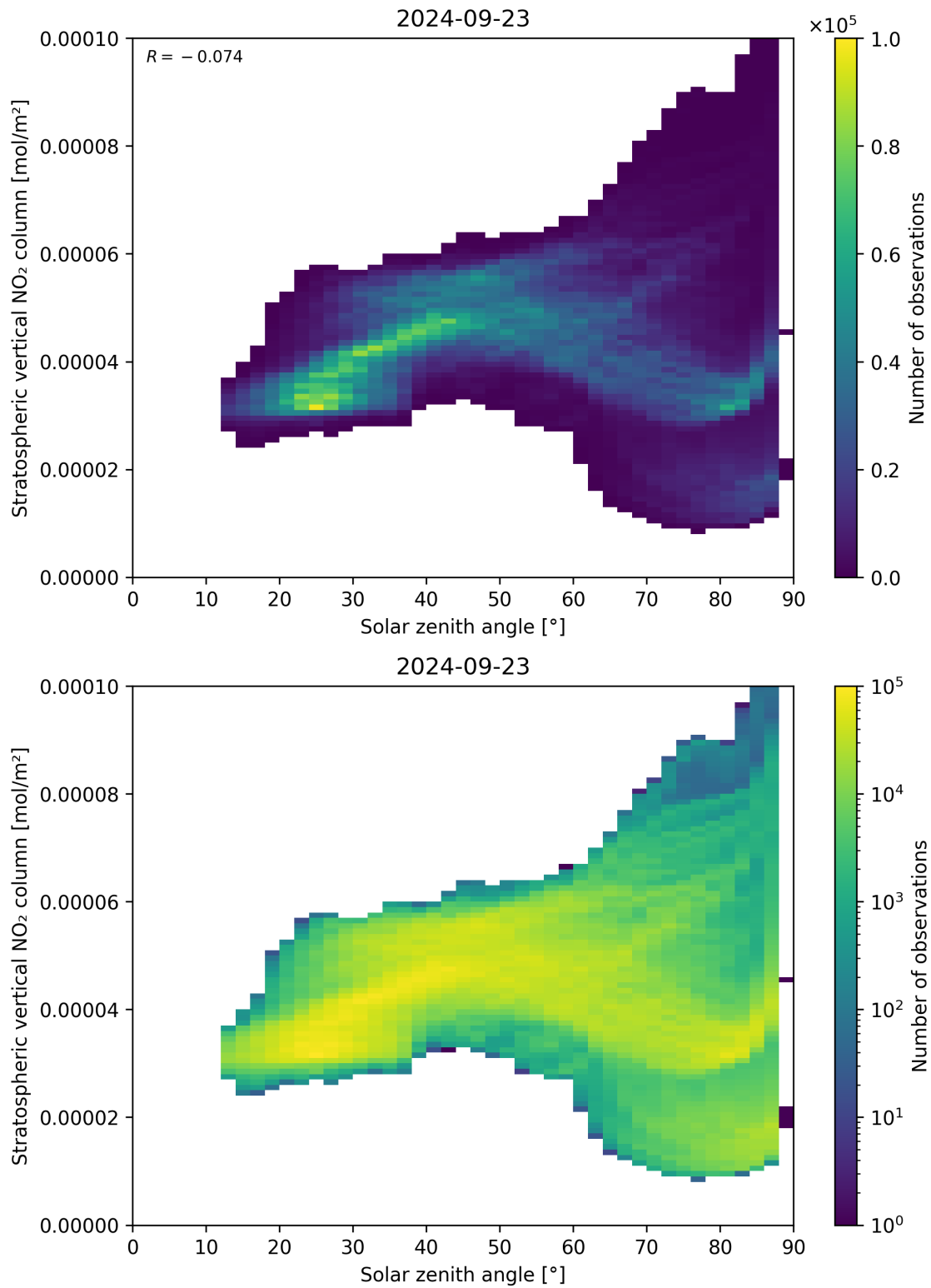
Figure 150: Scatter density plot of “Solar zenith angle” against “Stratospheric vertical NO 2 column” for 2024-09-22 to 2024-09-24.
