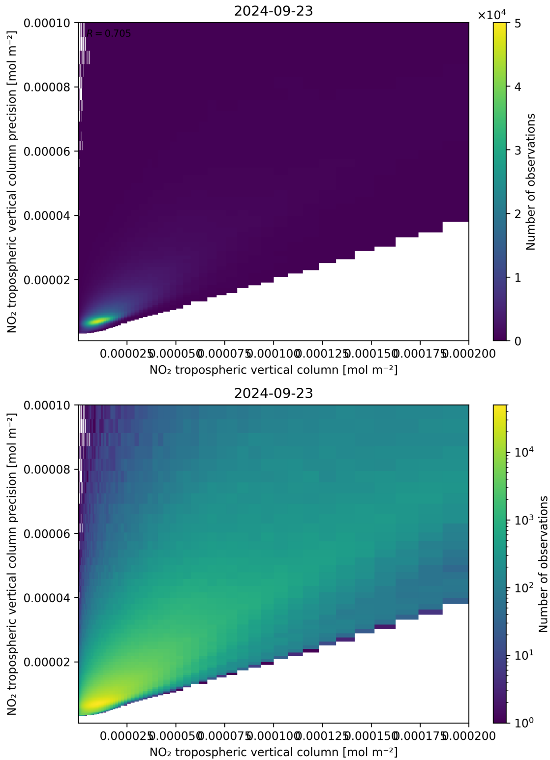
Figure 130: Scatter density plot of “NO 2 tropospheric vertical column” against “NO 2 tropospheric vertical column precision” for 2024-09-22 to 2024-09-24.
