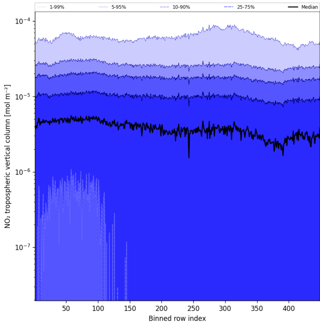
Figure 46: Along track statistics of “NO 2 tropospheric vertical column” for 2024-09-22 to 2024-09-24
