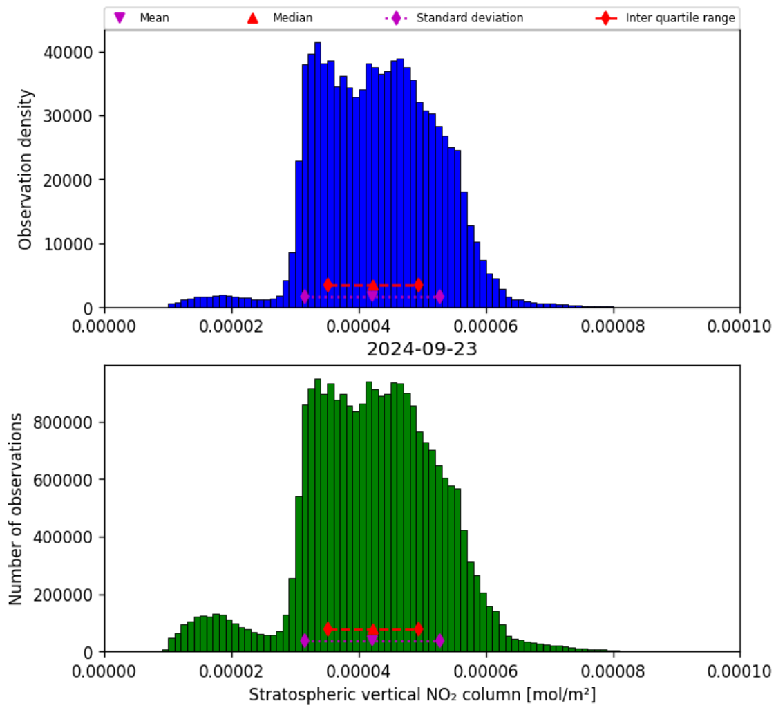
Figure 36: Histogram of “Stratospheric vertical NO 2 column” for 2024-09-22 to 2024-09-24
