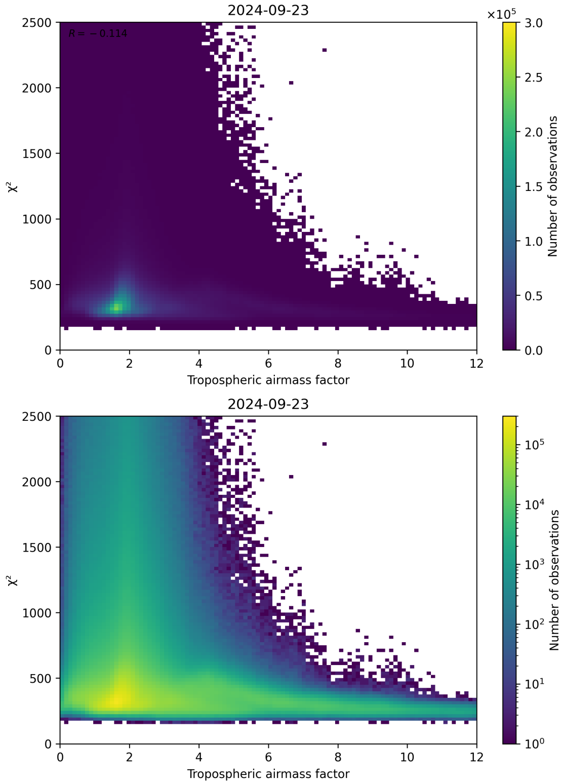
Figure 73: Scatter density plot of “Tropospheric airmass factor” against “ \chi^2 ” for 2024-09-22 to 2024-09-24.
