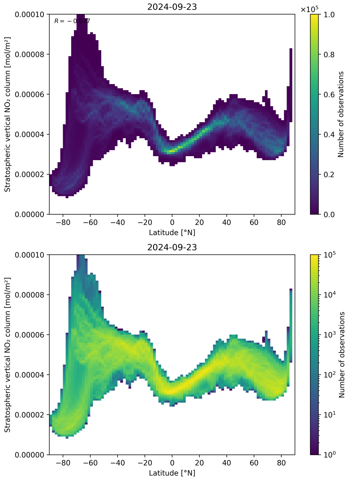
Figure 87: Scatter density plot of “Latitude” against “Stratospheric vertical NO 2 column” for 2024-09-22 to 2024-09-24.
