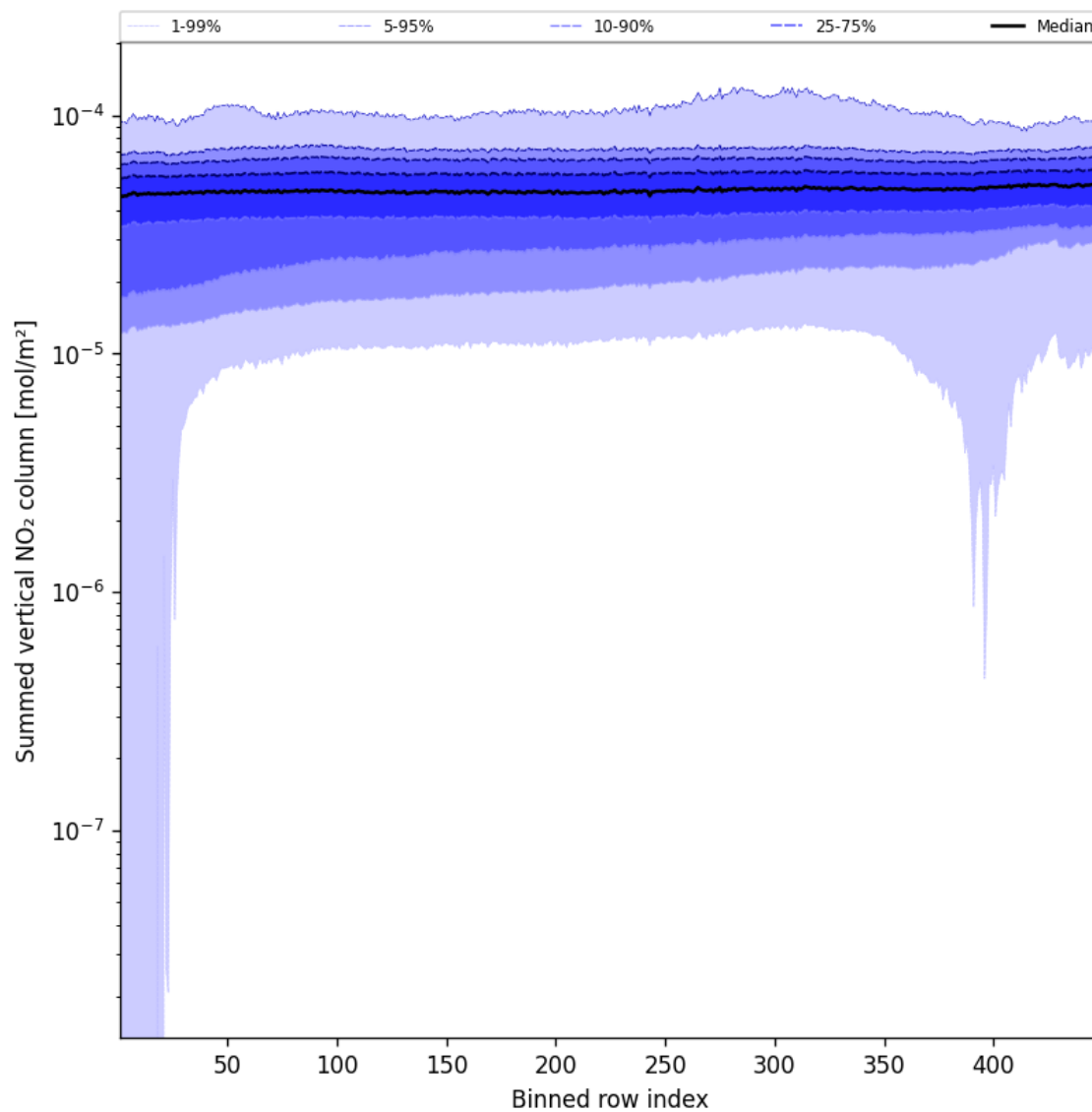
Figure 57: Along track statistics of “Summed vertical NO 2 column” for 2024-09-22 to 2024-09-24
