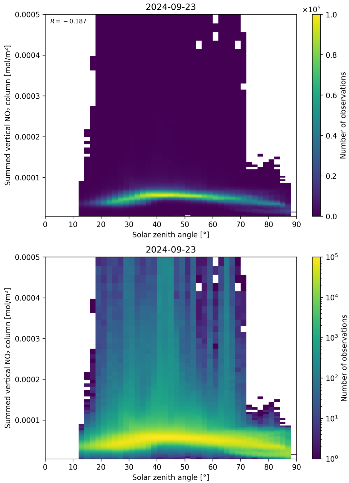
Figure 151: Scatter density plot of “Solar zenith angle” against “Summed vertical NO 2 column” for 2024-09-22 to 2024-09-24.
