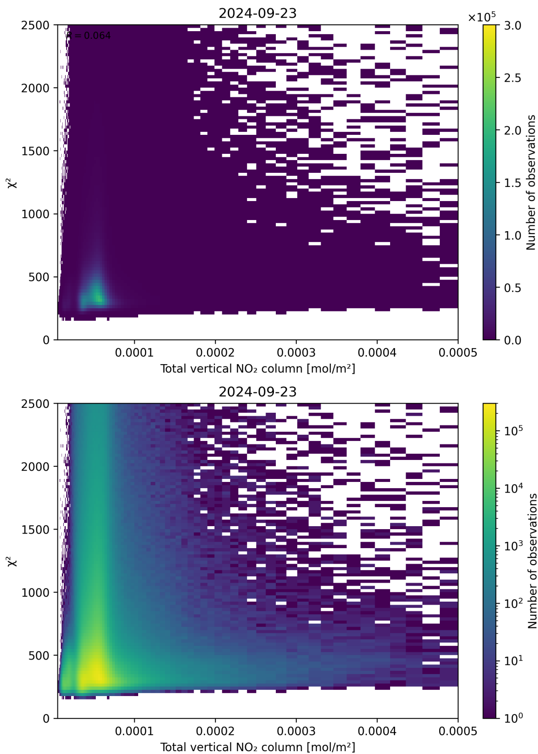
Figure 111: Scatter density plot of “Total vertical NO 2 column” against “ \chi^2 ” for 2024-09-22 to 2024-09-24.
