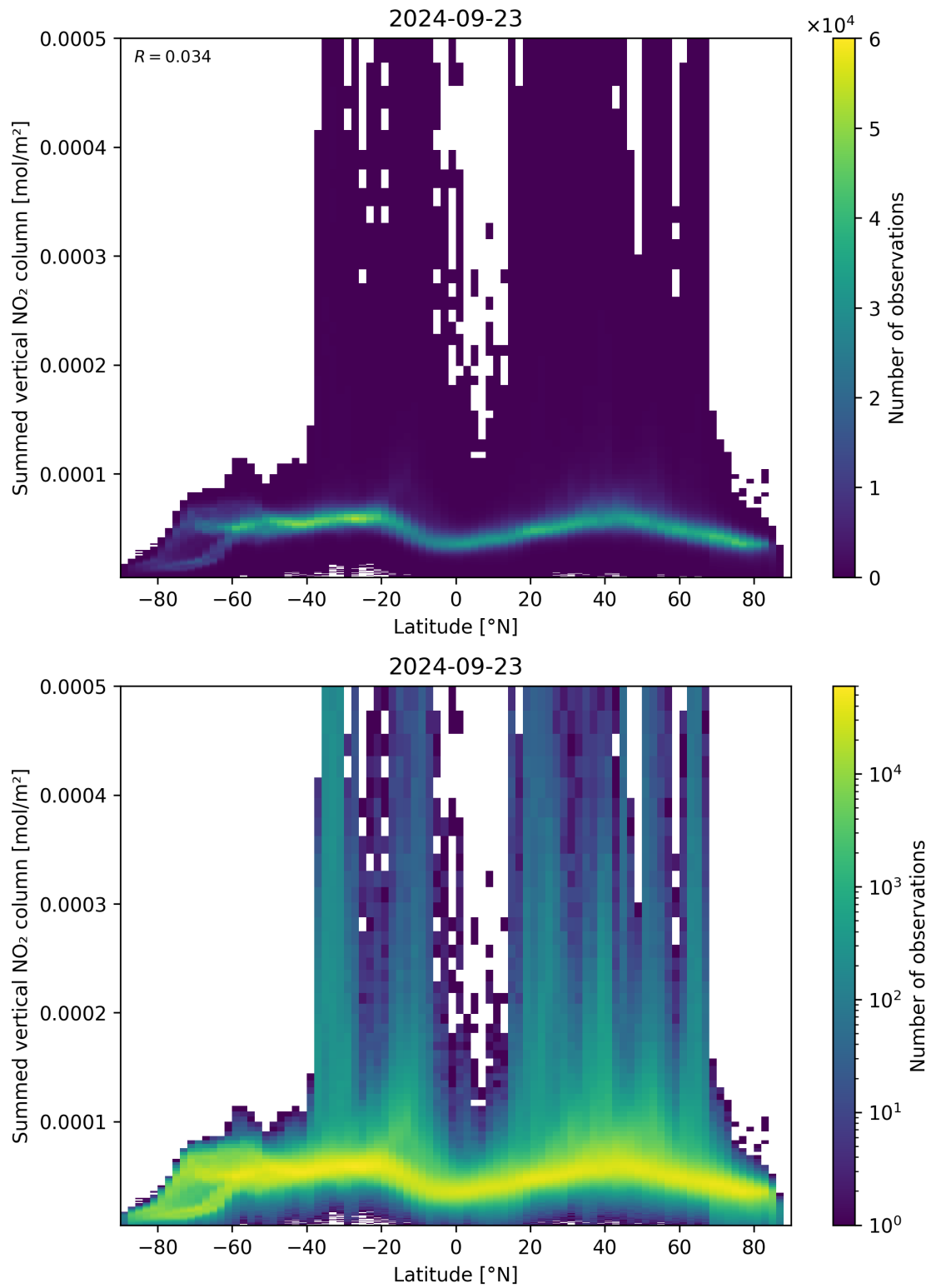
Figure 88: Scatter density plot of “Latitude” against “Summed vertical NO 2 column” for 2024-09-22 to 2024-09-24.
