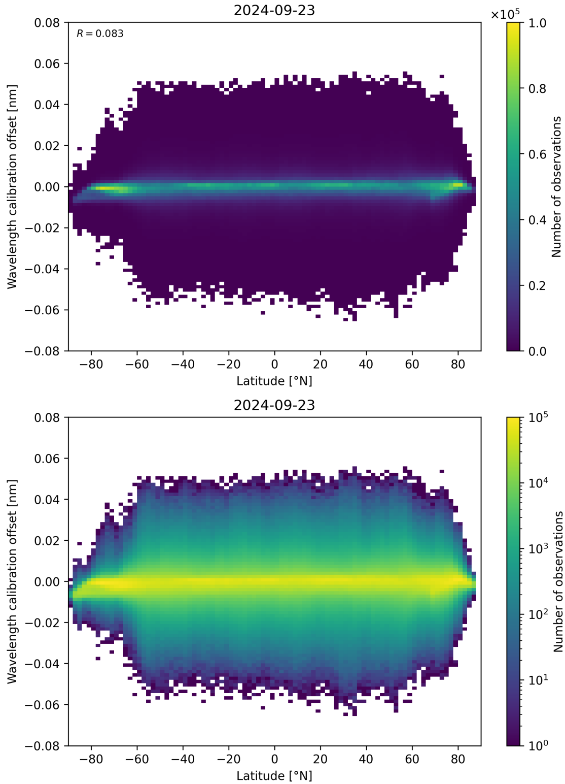
Figure 95: Scatter density plot of “Latitude” against “Wavelength calibration offset” for 2024-09-22 to 2024-09-24.
