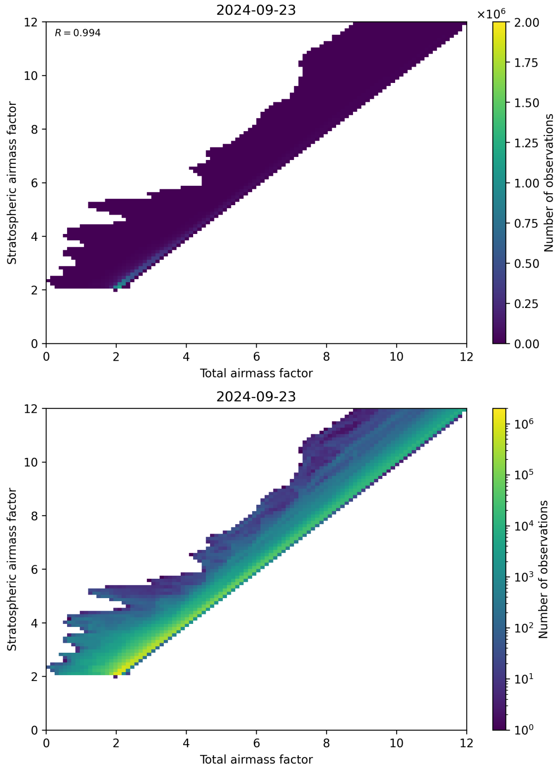
Figure 62: Scatter density plot of “Total airmass factor” against “Stratospheric airmass factor” for 2024-09-22 to 2024-09-24.
