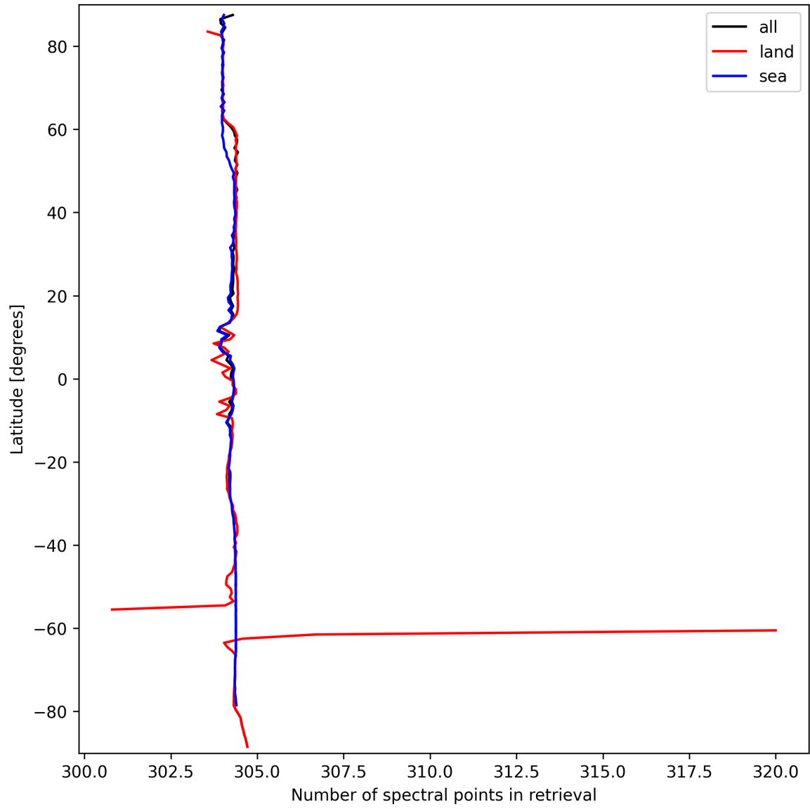
Figure 16: Zonal average of “Number of spectral points in retrieval” for 2024-09-22 to 2024-09-24.
