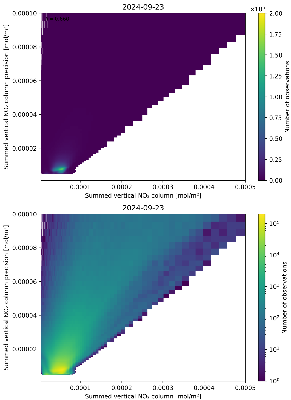
Figure 105: Scatter density plot of “Summed vertical NO 2 column” against “Summed vertical NO 2 column precision” for 2024-09-22 to 2024-09-24.
