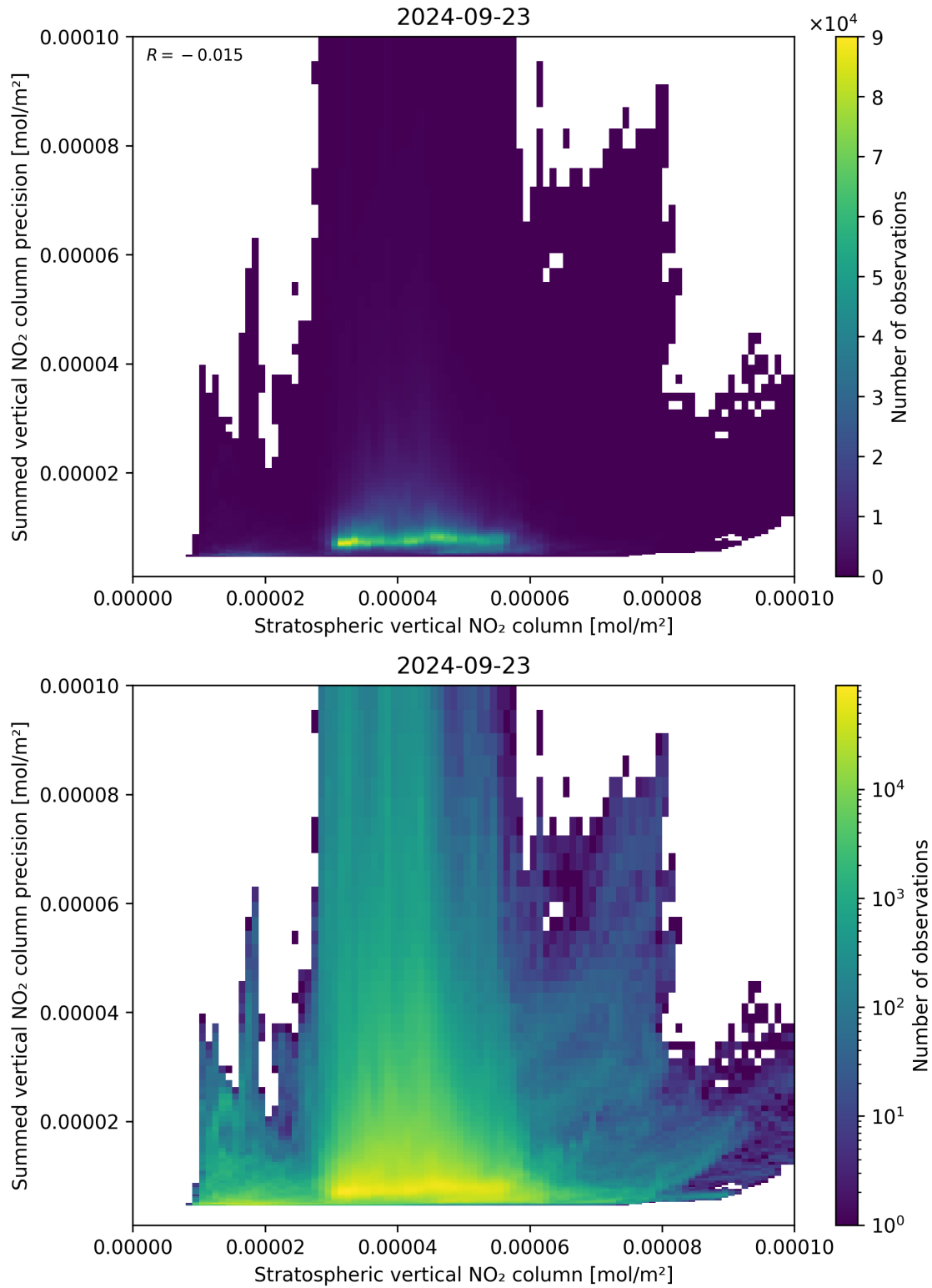
Figure 99: Scatter density plot of “Stratospheric vertical NO 2 column” against “Summed vertical NO 2 column precision” for 2024-09-22 to 2024-09-24.
