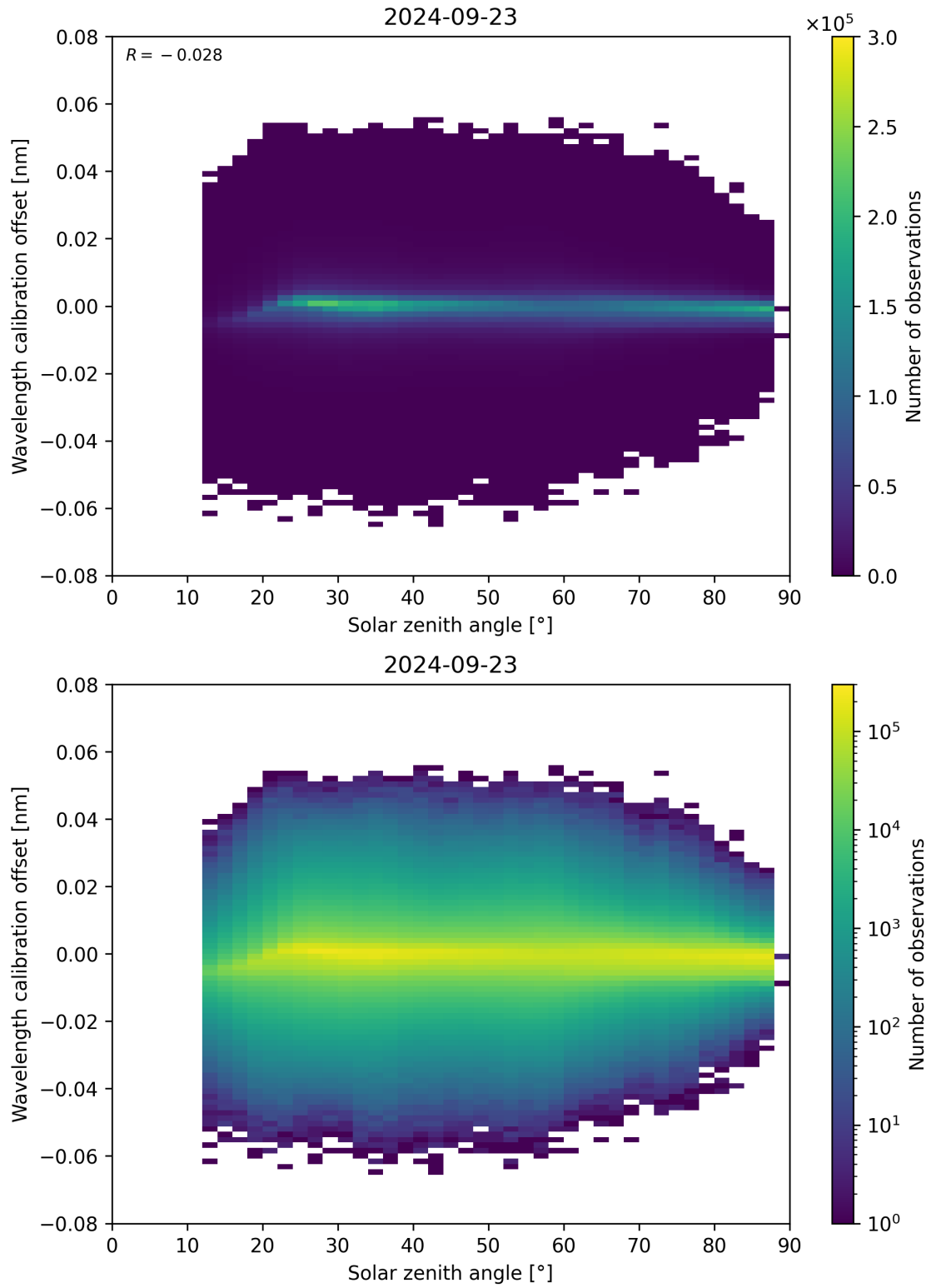
Figure 158: Scatter density plot of “Solar zenith angle” against “Wavelength calibration offset” for 2024-09-22 to 2024-09-24.
