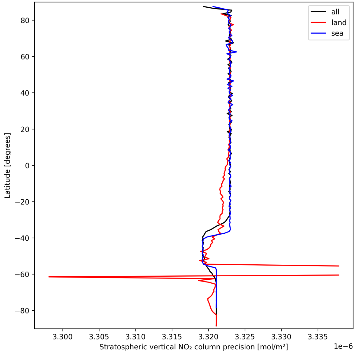
Figure 20: Zonal average of “Stratospheric vertical NO 2 column precision” for 2024-09-22 to 2024-09-24.
