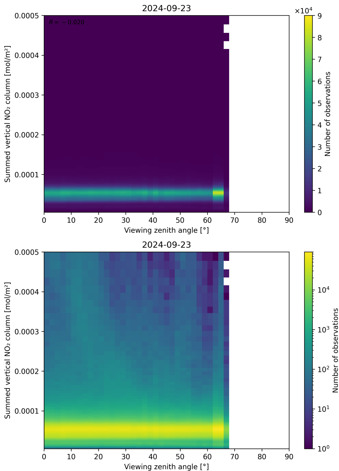
Figure 165: Scatter density plot of “Viewing zenith angle” against “Summed vertical NO 2 column” for 2024-09-22 to 2024-09-24.
