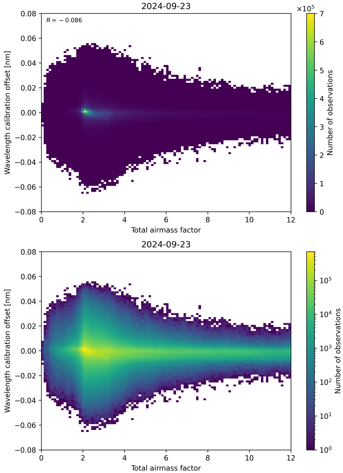
Figure 70: Scatter density plot of “Total airmass factor” against “Wavelength calibration offset” for 2024-09-22 to 2024-09-24.
