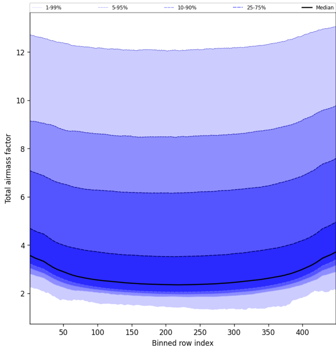
Figure 49: Along track statistics of “Total airmass factor” for 2024-09-22 to 2024-09-24
