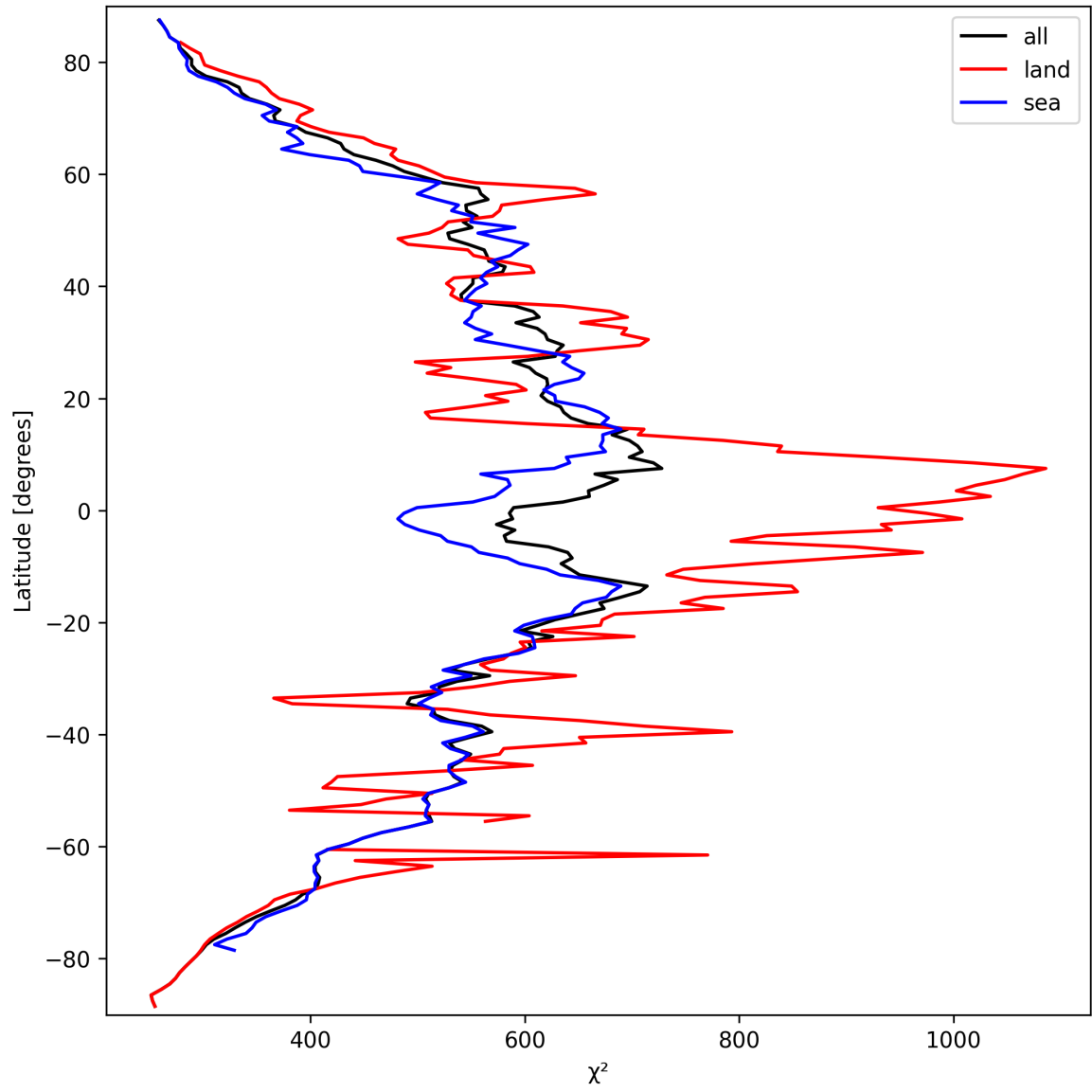
Figure 25: Zonal average of “ \chi^2 ” for 2024-09-22 to 2024-09-24.
