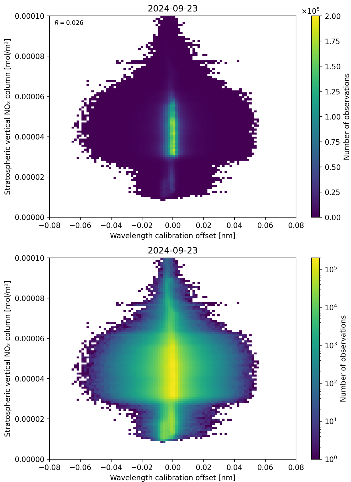
Figure 176: Scatter density plot of “Wavelength calibration offset” against “Stratospheric vertical NO 2 column” for 2024-09-22 to 2024-09-24.
