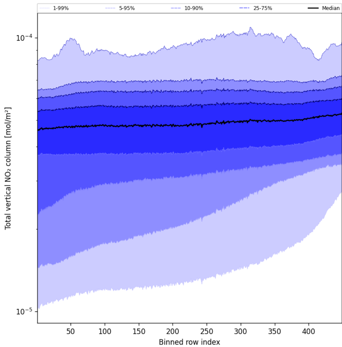
Figure 55: Along track statistics of “Total vertical NO 2 column” for 2024-09-22 to 2024-09-24
