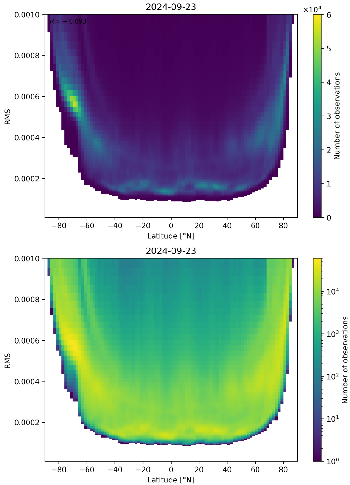
Figure 94: Scatter density plot of “Latitude” against “RMS” for 2024-09-22 to 2024-09-24.
