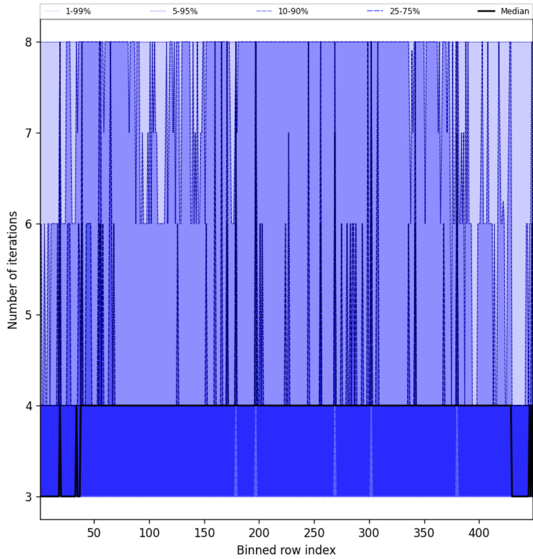
Figure 51: Along track statistics of “Number of iterations” for 2024-09-22 to 2024-09-24
