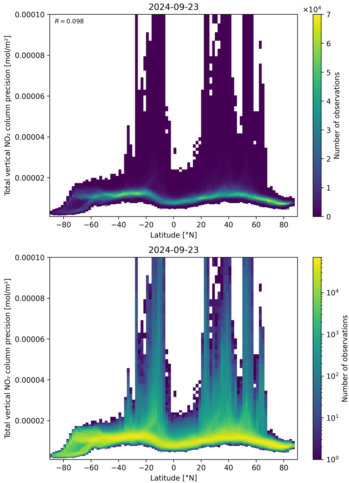
Figure 91: Scatter density plot of “Latitude” against “Total vertical NO 2 column precision” for 2024-09-22 to 2024-09-24.
