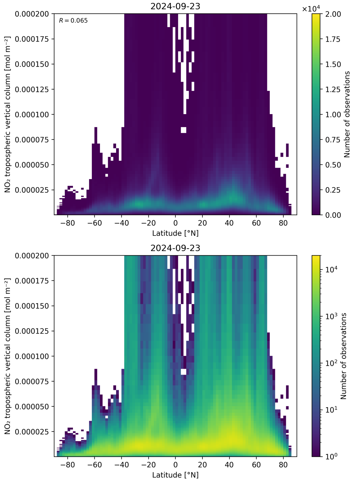
Figure 92: Scatter density plot of “Latitude” against “NO 2 tropospheric vertical column” for 2024-09-22 to 2024-09-24.
