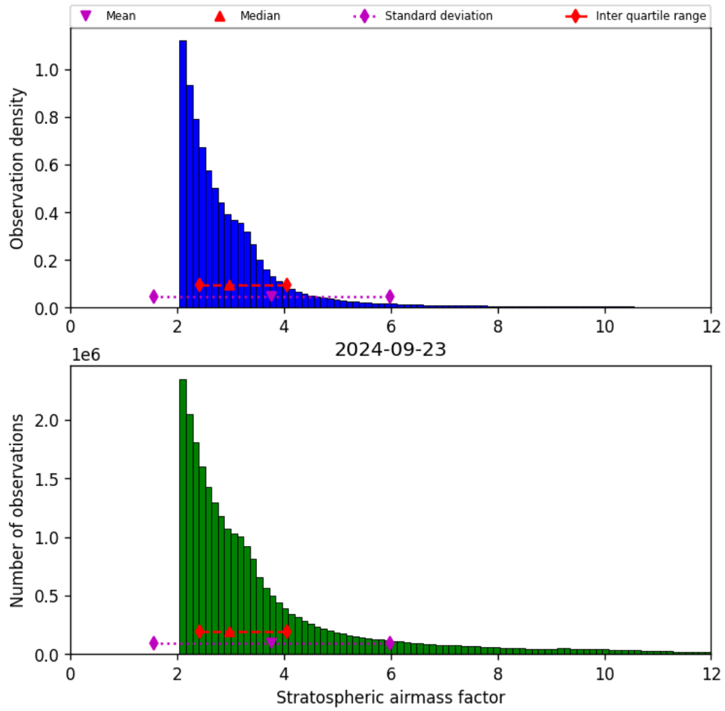
Figure 44: Histogram of “Stratospheric airmass factor” for 2024-09-22 to 2024-09-24
