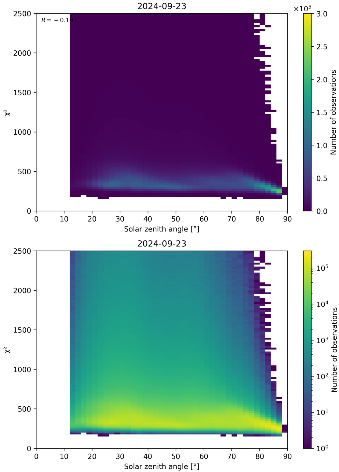
Figure 148: Scatter density plot of “Solar zenith angle” against “ \chi^2 ” for 2024-09-22 to 2024-09-24.
