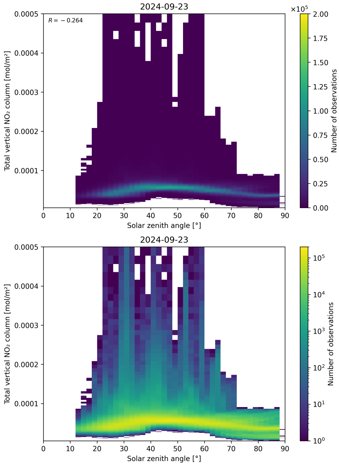
Figure 153: Scatter density plot of “Solar zenith angle” against “Total vertical NO 2 column” for 2024-09-22 to 2024-09-24.
