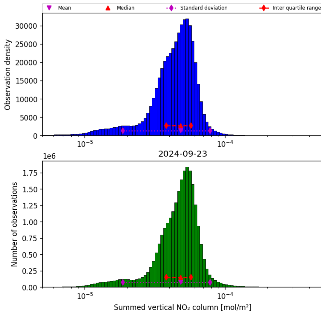
Figure 40: Histogram of “Summed vertical NO 2 column” for 2024-09-22 to 2024-09-24
