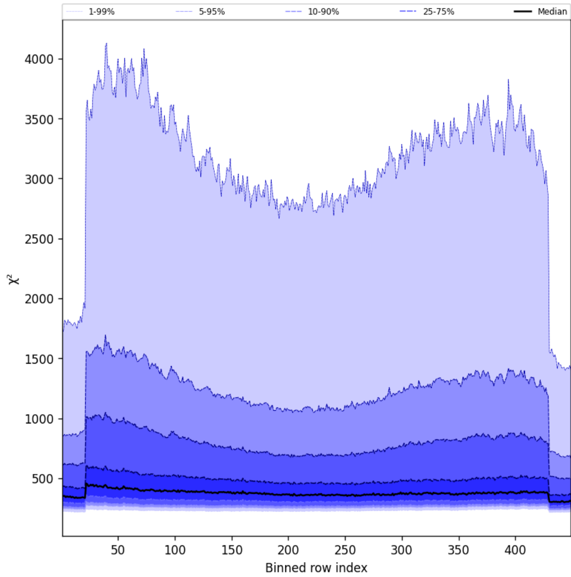
Figure 59: Along track statistics of “ \chi^2 ” for 2024-09-22 to 2024-09-24
