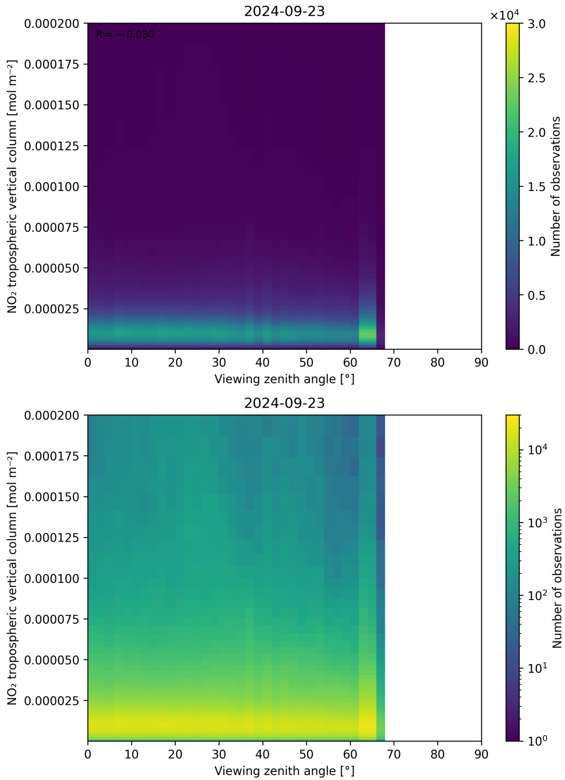
Figure 169: Scatter density plot of “Viewing zenith angle” against “NO 2 tropospheric vertical column” for 2024-09-22 to 2024-09-24.
