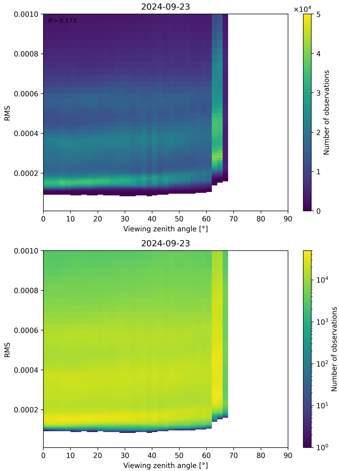
Figure 171: Scatter density plot of “Viewing zenith angle” against “RMS” for 2024-09-22 to 2024-09-24.
