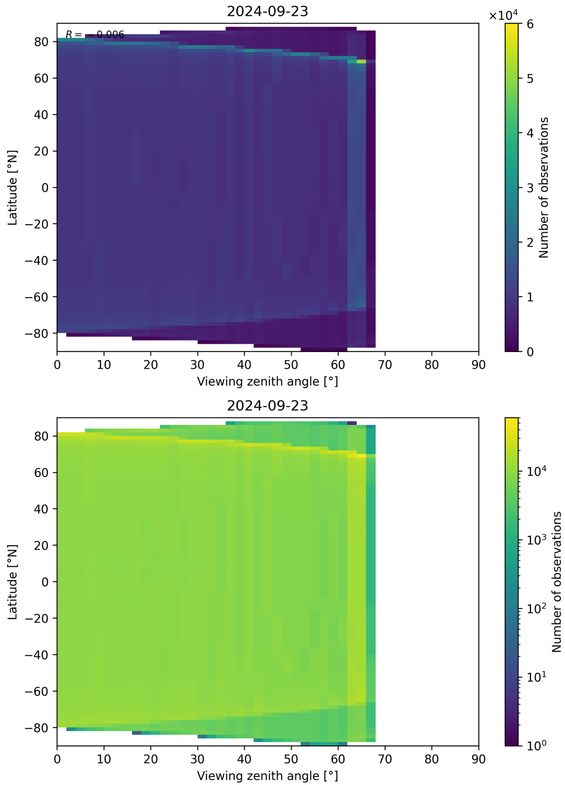
Figure 163: Scatter density plot of “Viewing zenith angle” against “Latitude” for 2024-09-22 to 2024-09-24.
