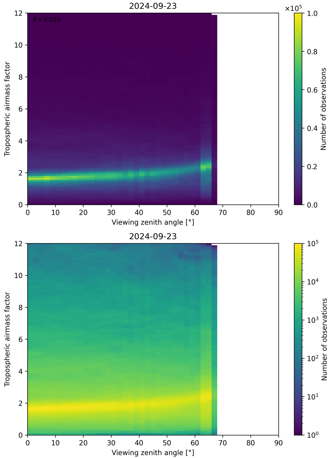
Figure 161: Scatter density plot of “Viewing zenith angle” against “Tropospheric airmass factor” for 2024-09-22 to 2024-09-24.
