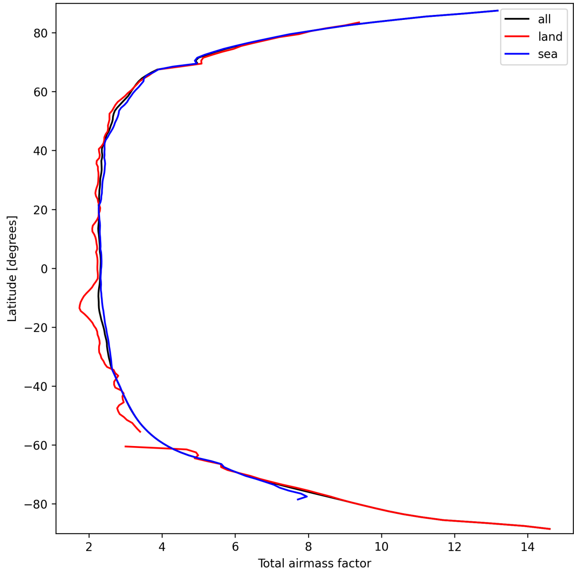
Figure 15: Zonal average of “Total airmass factor” for 2024-09-22 to 2024-09-24.
