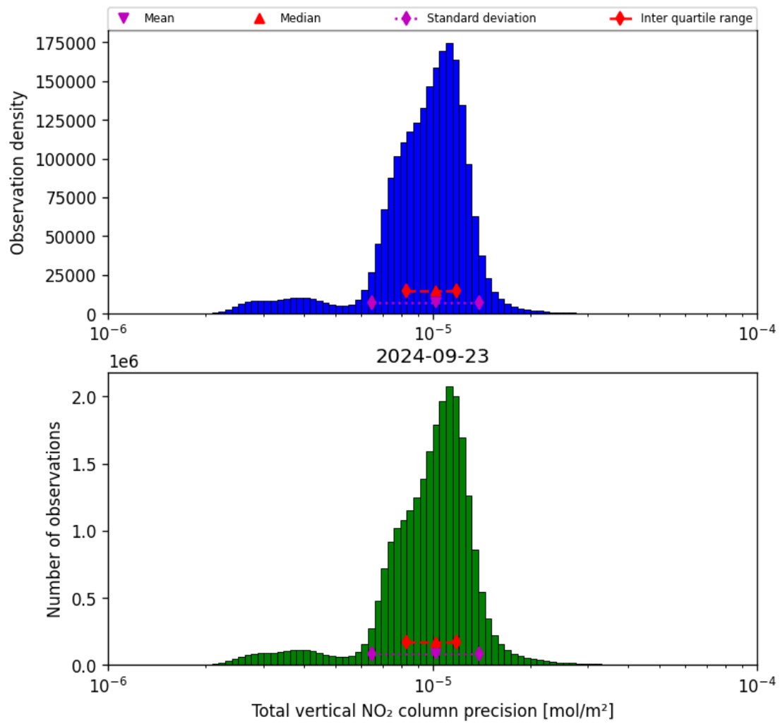
Figure 39: Histogram of “Total vertical NO 2 column precision” for 2024-09-22 to 2024-09-24
