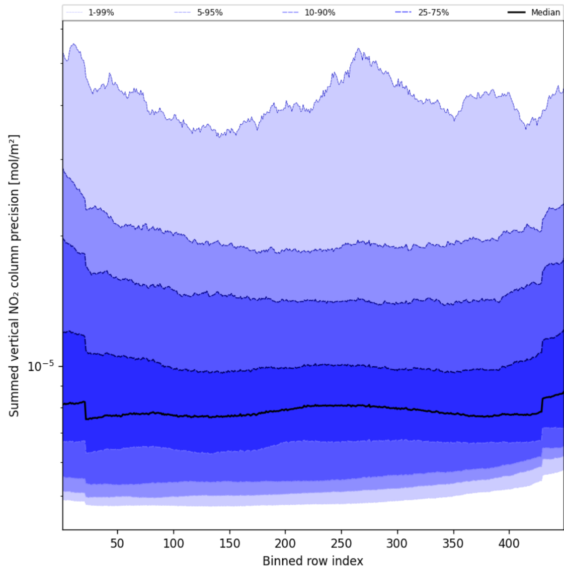
Figure 58: Along track statistics of “Summed vertical NO 2 column precision” for 2024-09-22 to 2024-09-24
