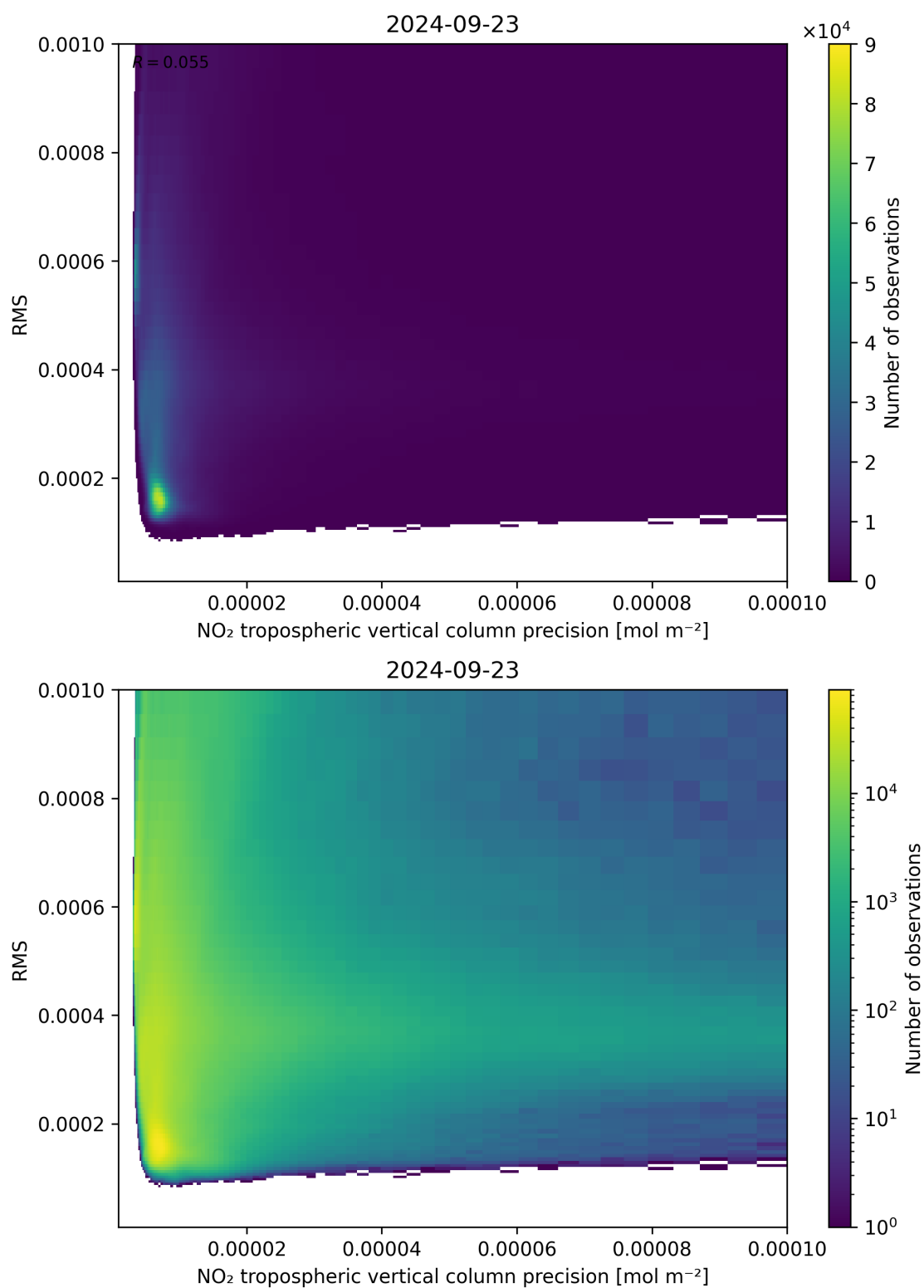
Figure 140: Scatter density plot of “NO 2 tropospheric vertical column precision” against “RMS” for 2024-09-22 to 2024-09-24.
