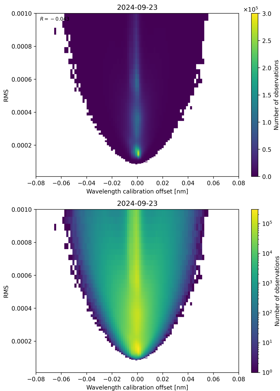
Figure 181: Scatter density plot of “Wavelength calibration offset” against “RMS” for 2024-09-22 to 2024-09-24.
