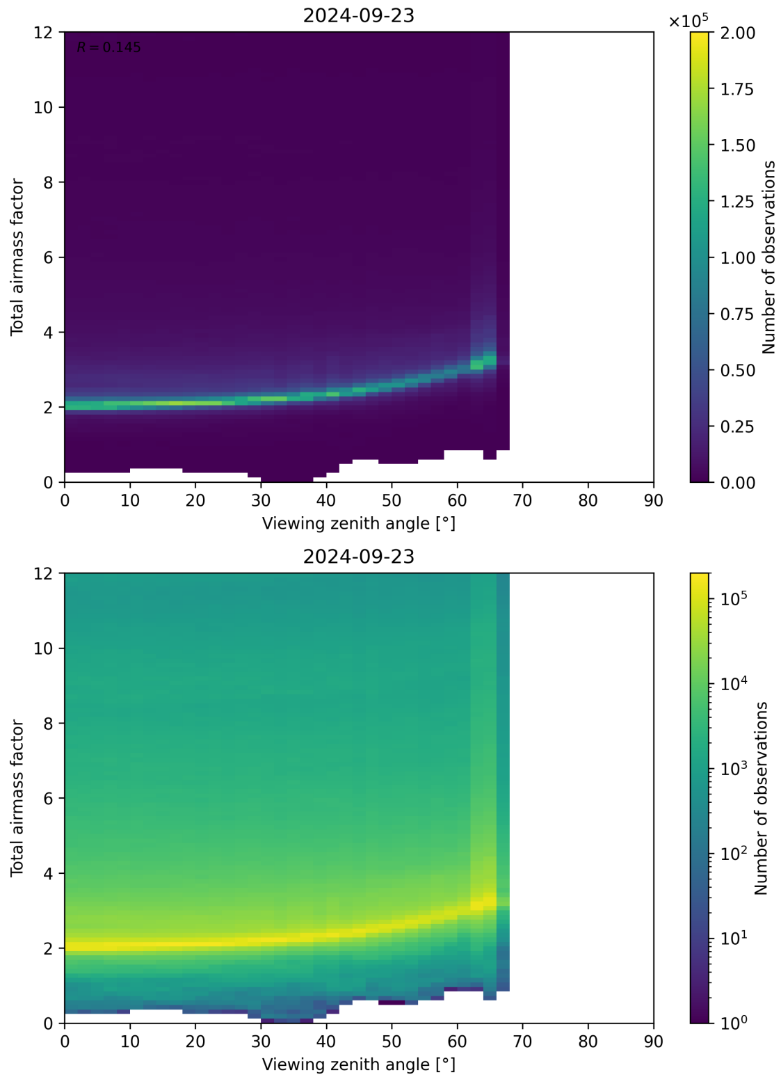
Figure 160: Scatter density plot of “Viewing zenith angle” against “Total airmass factor” for 2024-09-22 to 2024-09-24.
