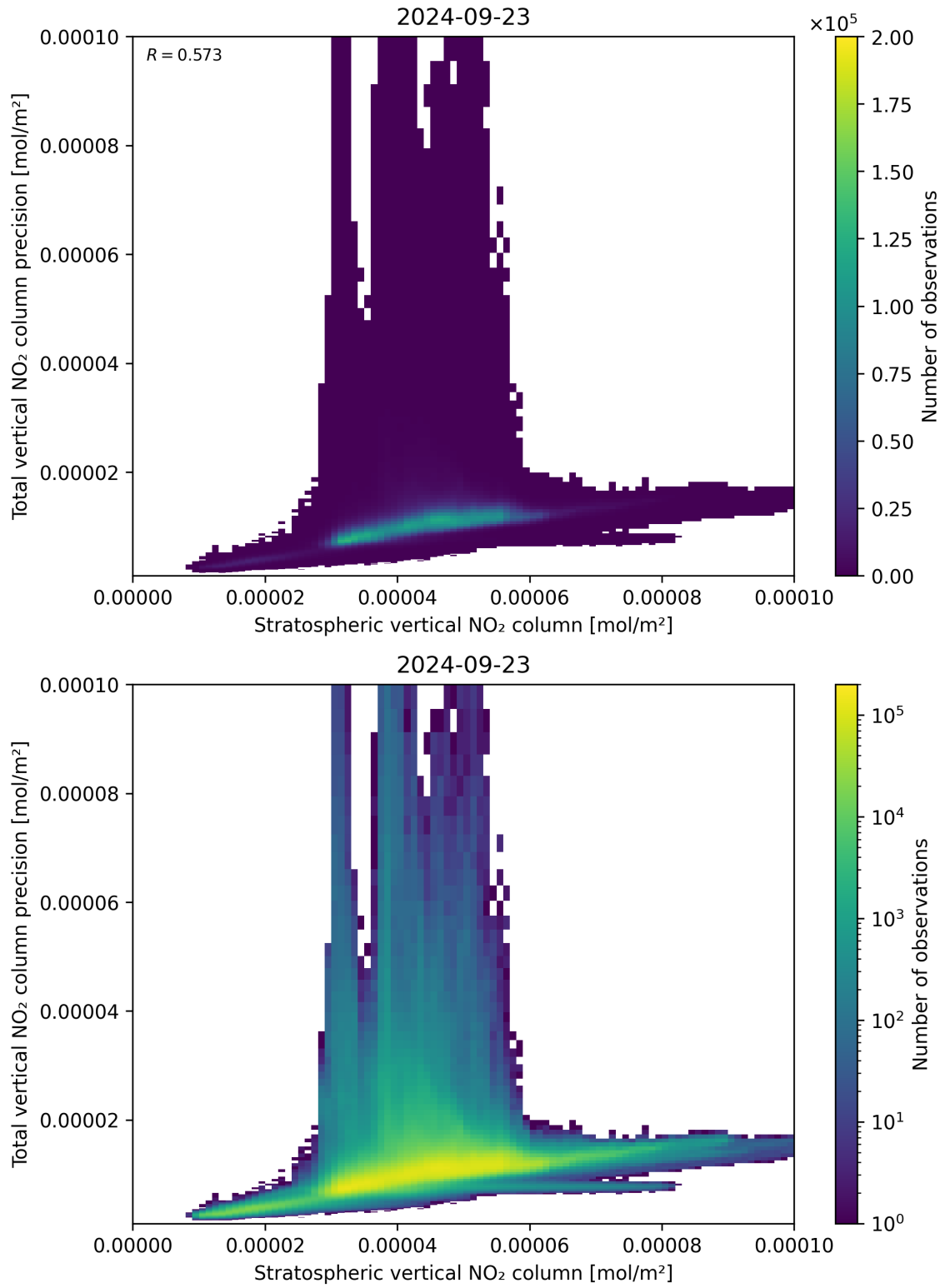
Figure 101: Scatter density plot of “Stratospheric vertical NO 2 column” against “Total vertical NO 2 column precision” for 2024-09-22 to 2024-09-24.
