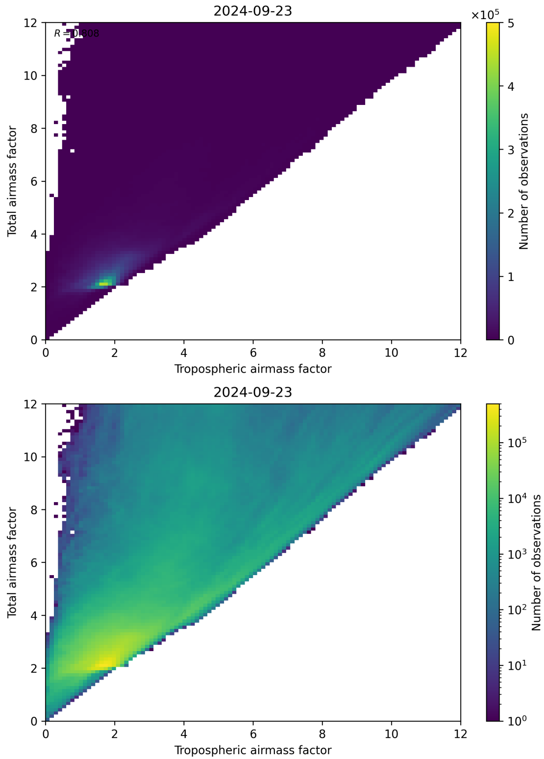
Figure 72: Scatter density plot of “Tropospheric airmass factor” against “Total airmass factor” for 2024-09-22 to 2024-09-24.
