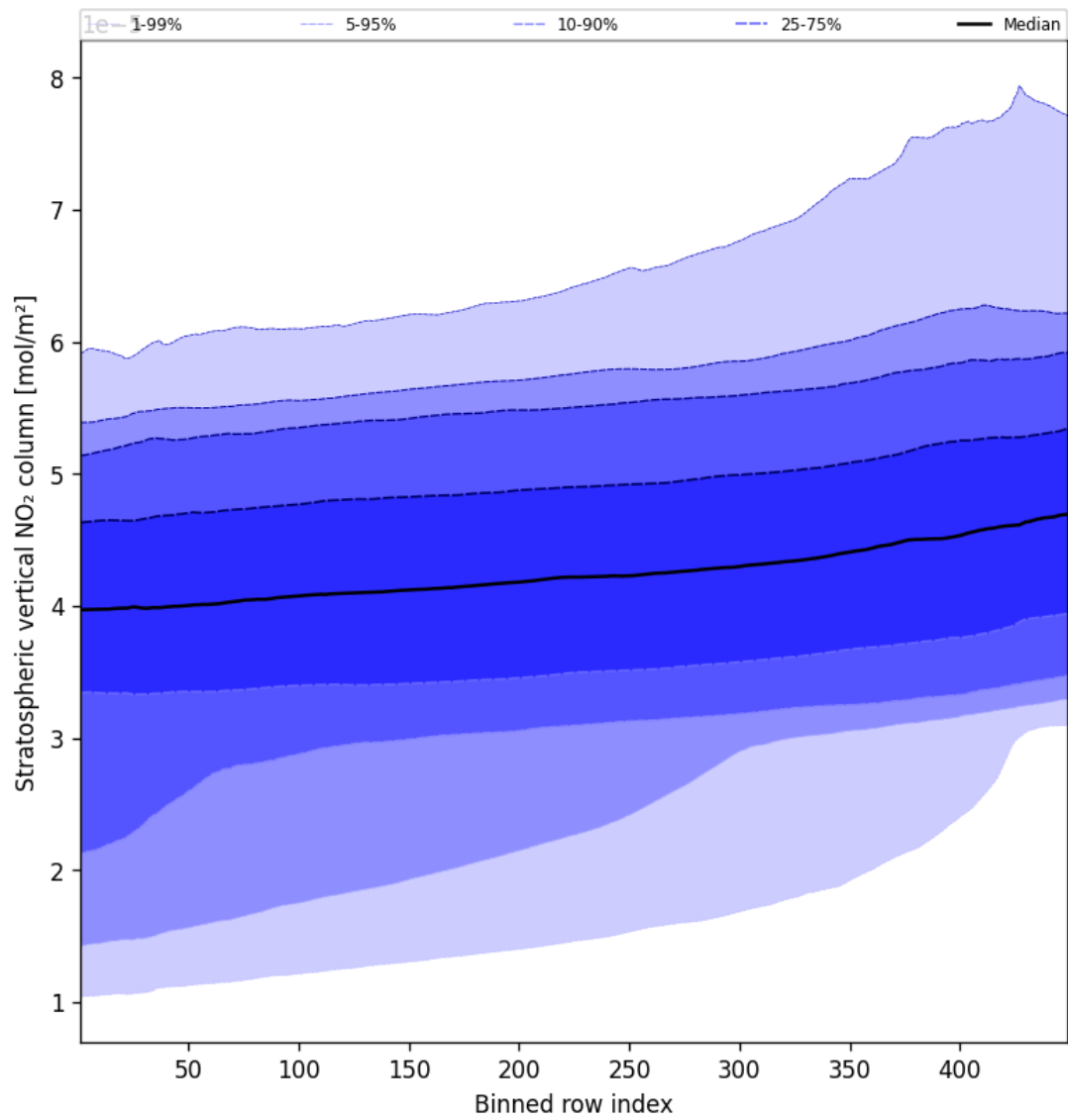
Figure 53: Along track statistics of “Stratospheric vertical NO 2 column” for 2024-09-22 to 2024-09-24
