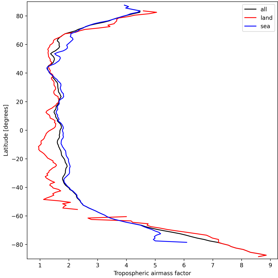
Figure 14: Zonal average of “Tropospheric airmass factor” for 2024-09-22 to 2024-09-24.
