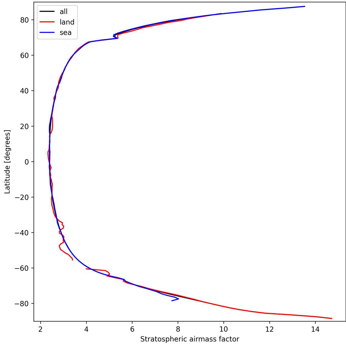
Figure 27: Zonal average of “Stratospheric air mass factor” for 2024-09-22 to 2024-09-24.
