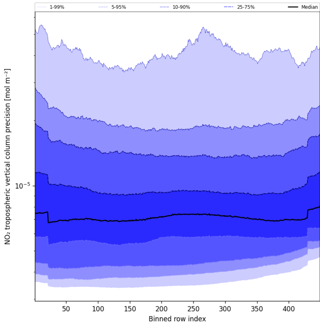
Figure 47: Along track statistics of “NO 2 tropospheric vertical column precision” for 2024-09-22 to 2024-09-24
