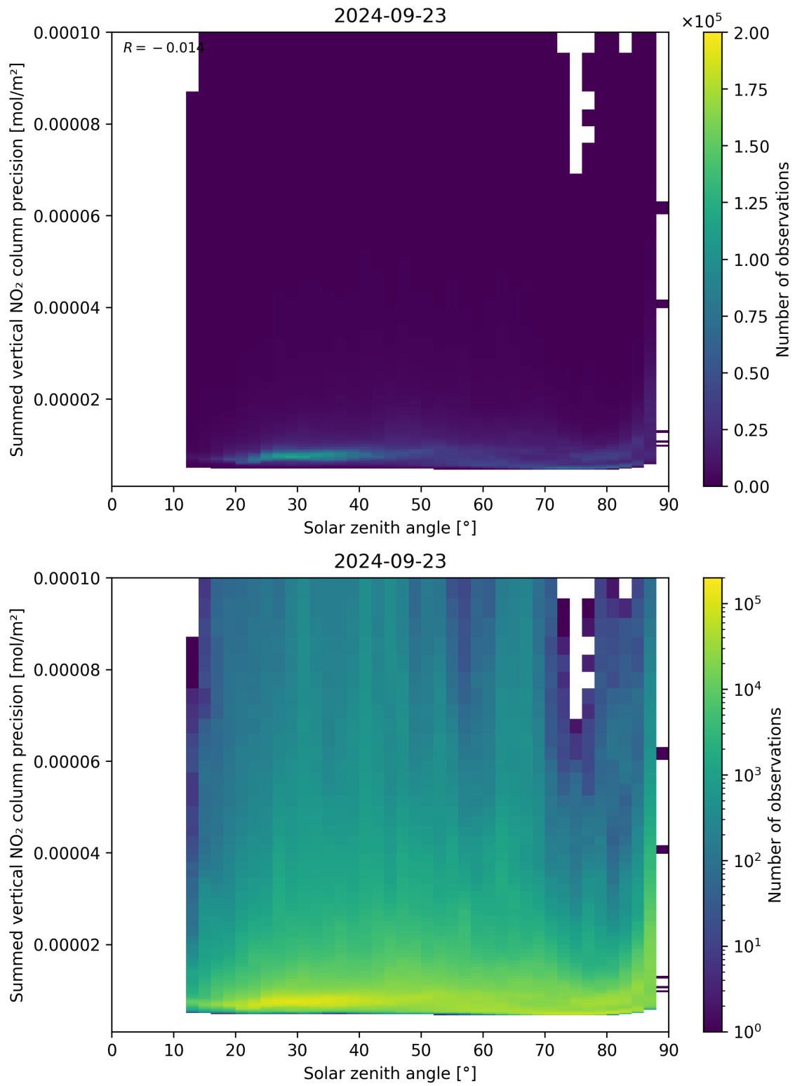
Figure 152: Scatter density plot of “Solar zenith angle” against “Summed vertical NO 2 column precision” for 2024-09-22 to 2024-09-24.
