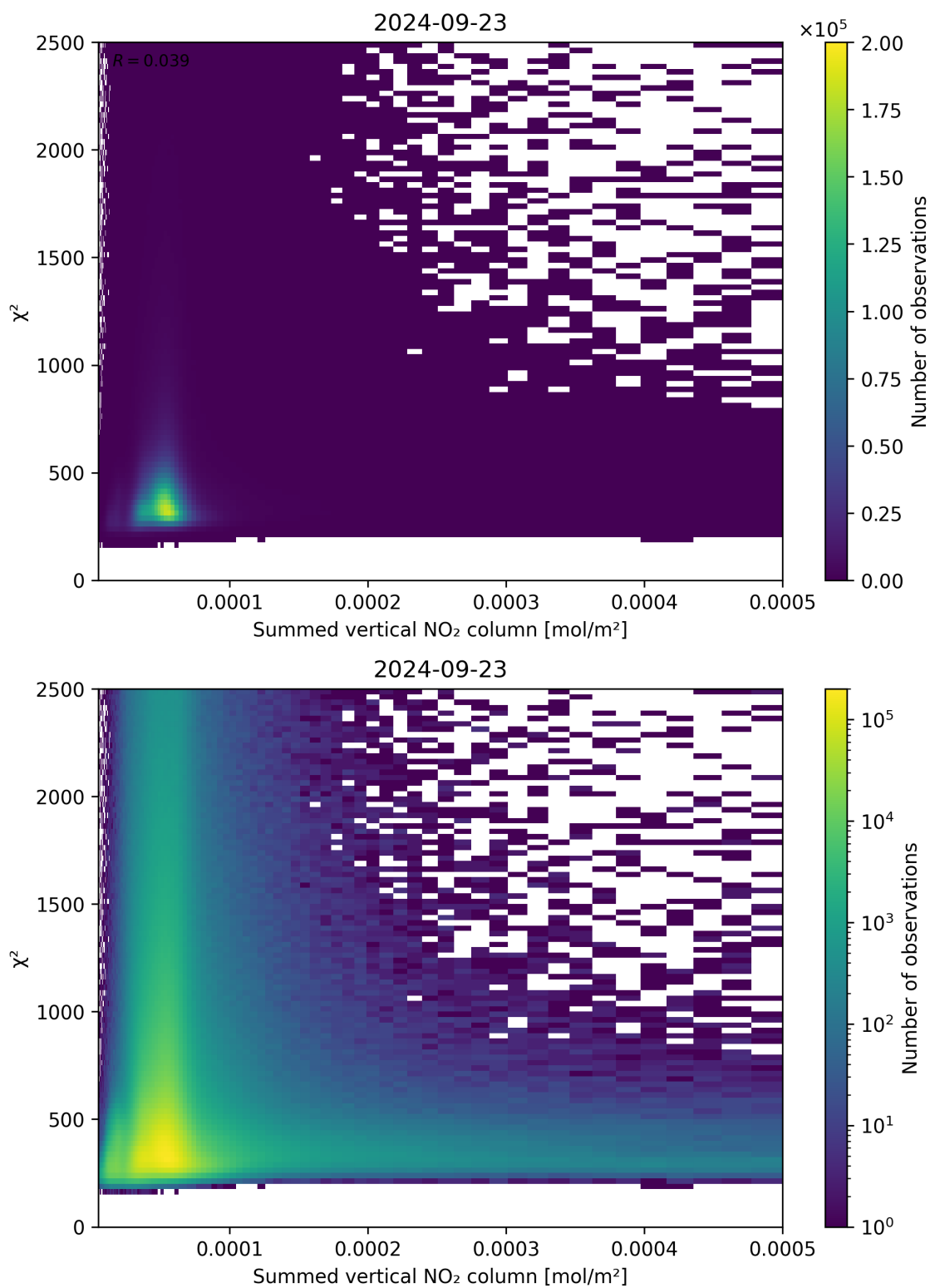
Figure 104: Scatter density plot of “Summed vertical NO 2 column” against “ \chi^2 ” for 2024-09-22 to 2024-09-24.
