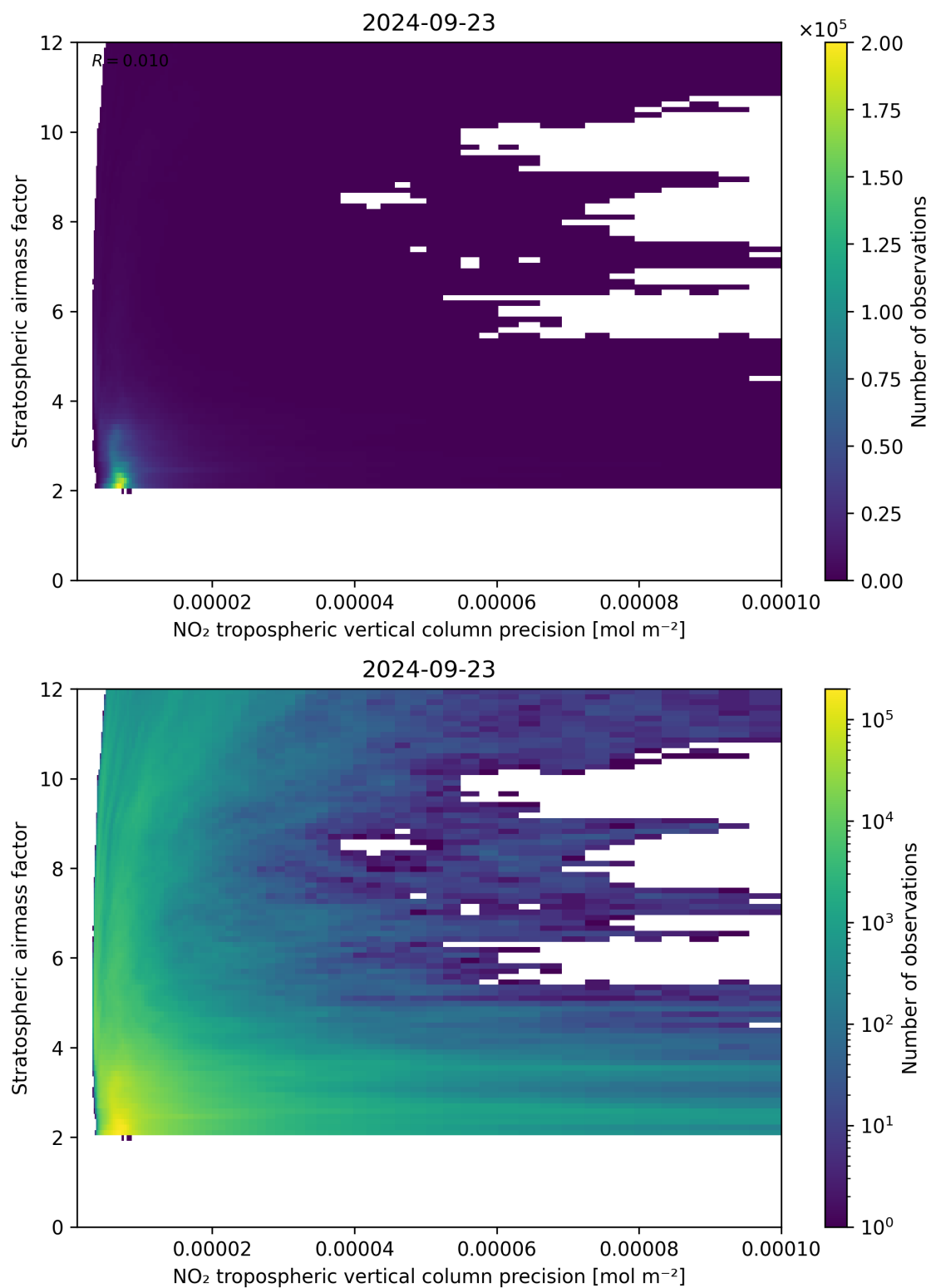
Figure 131: Scatter density plot of “NO 2 tropospheric vertical column precision” against “Stratospheric airmass factor” for 2024-09-22 to 2024-09-24.
