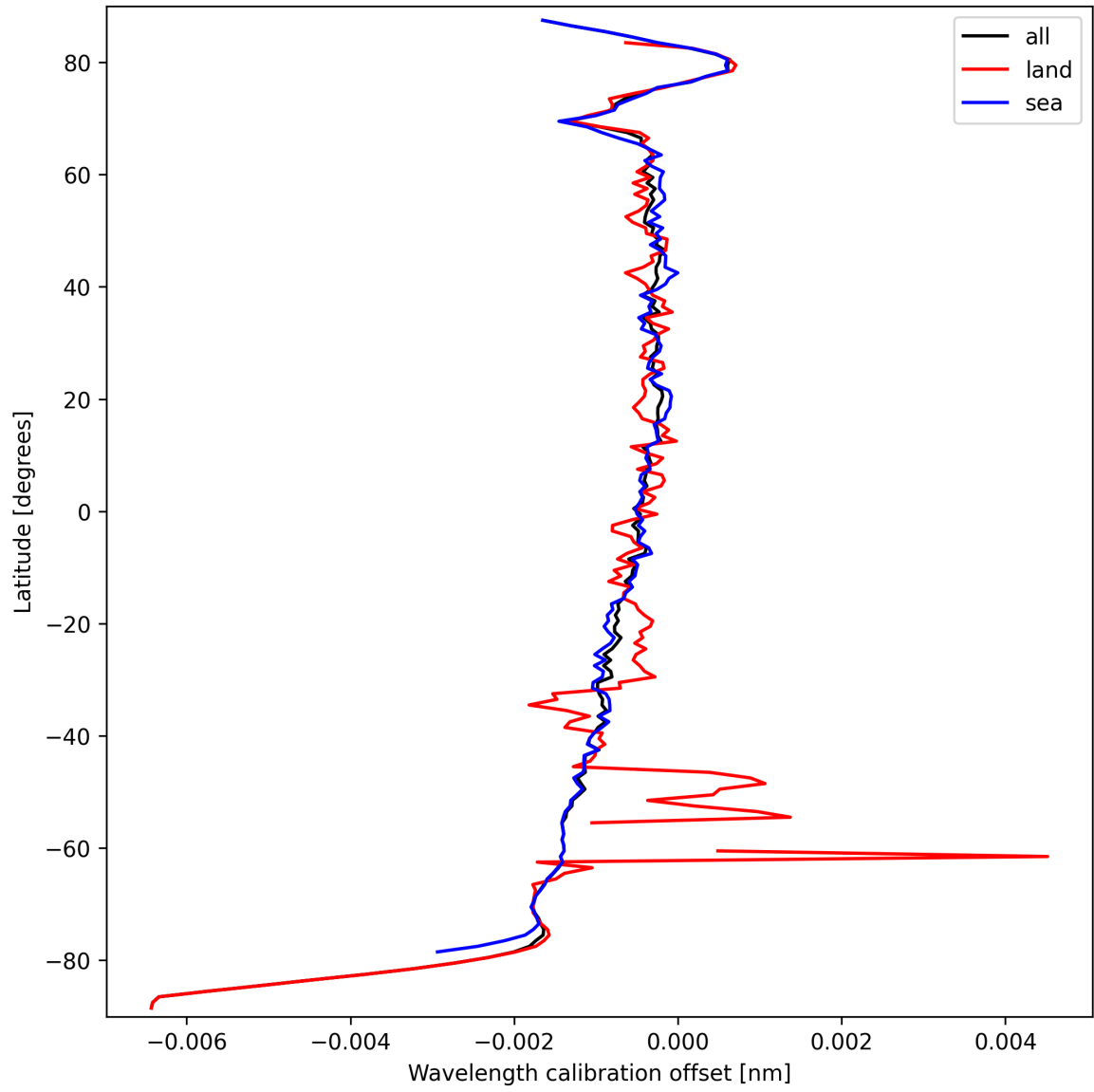
Figure 18: Zonal average of “Wavelength calibration offset” for 2024-09-22 to 2024-09-24.
