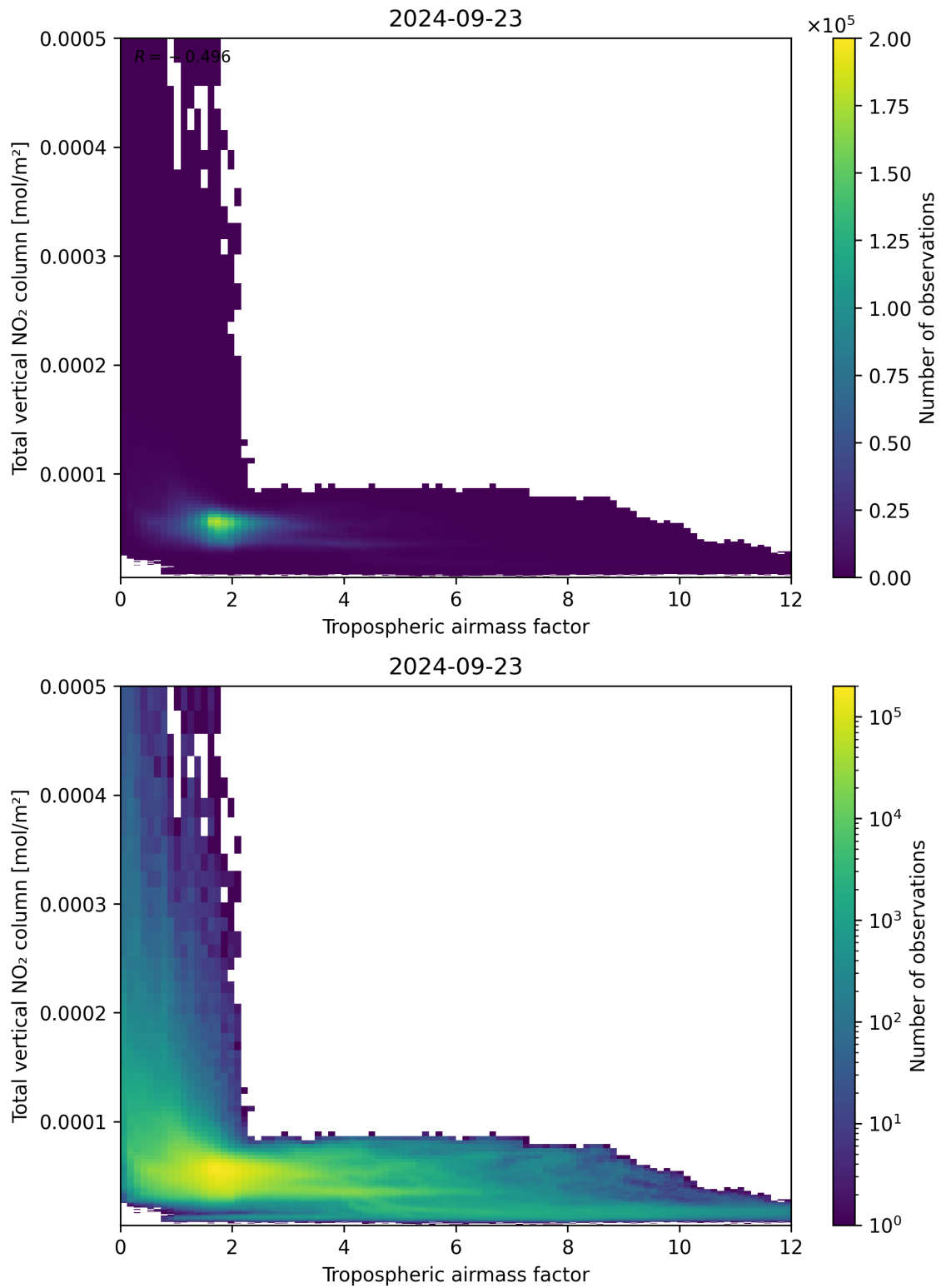
Figure 77: Scatter density plot of “Tropospheric airmass factor” against “Total vertical NO 2 column” for 2024-09-22 to 2024-09-24.
