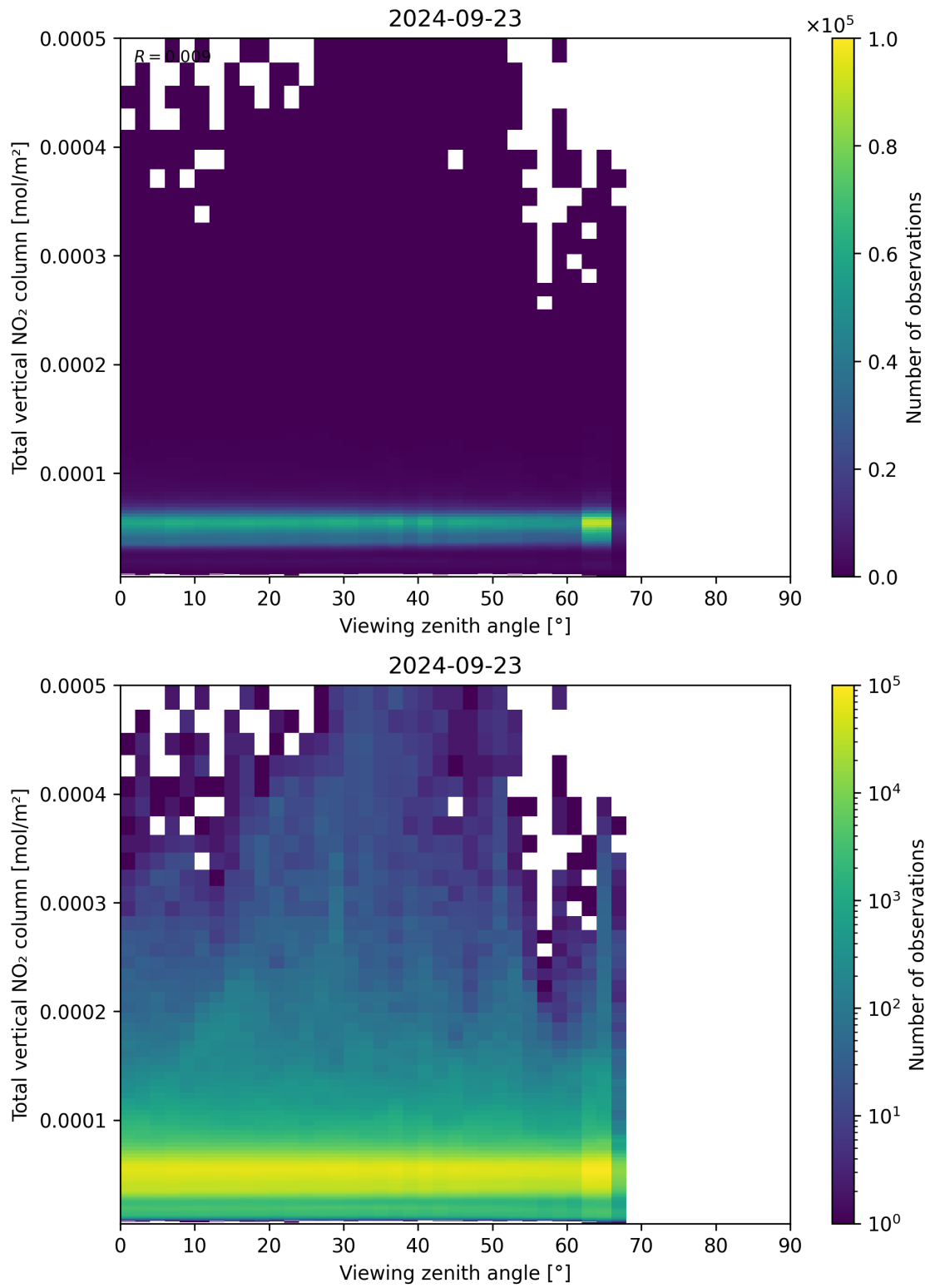
Figure 167: Scatter density plot of “Viewing zenith angle” against “Total vertical NO 2 column” for 2024-09-22 to 2024-09-24.
