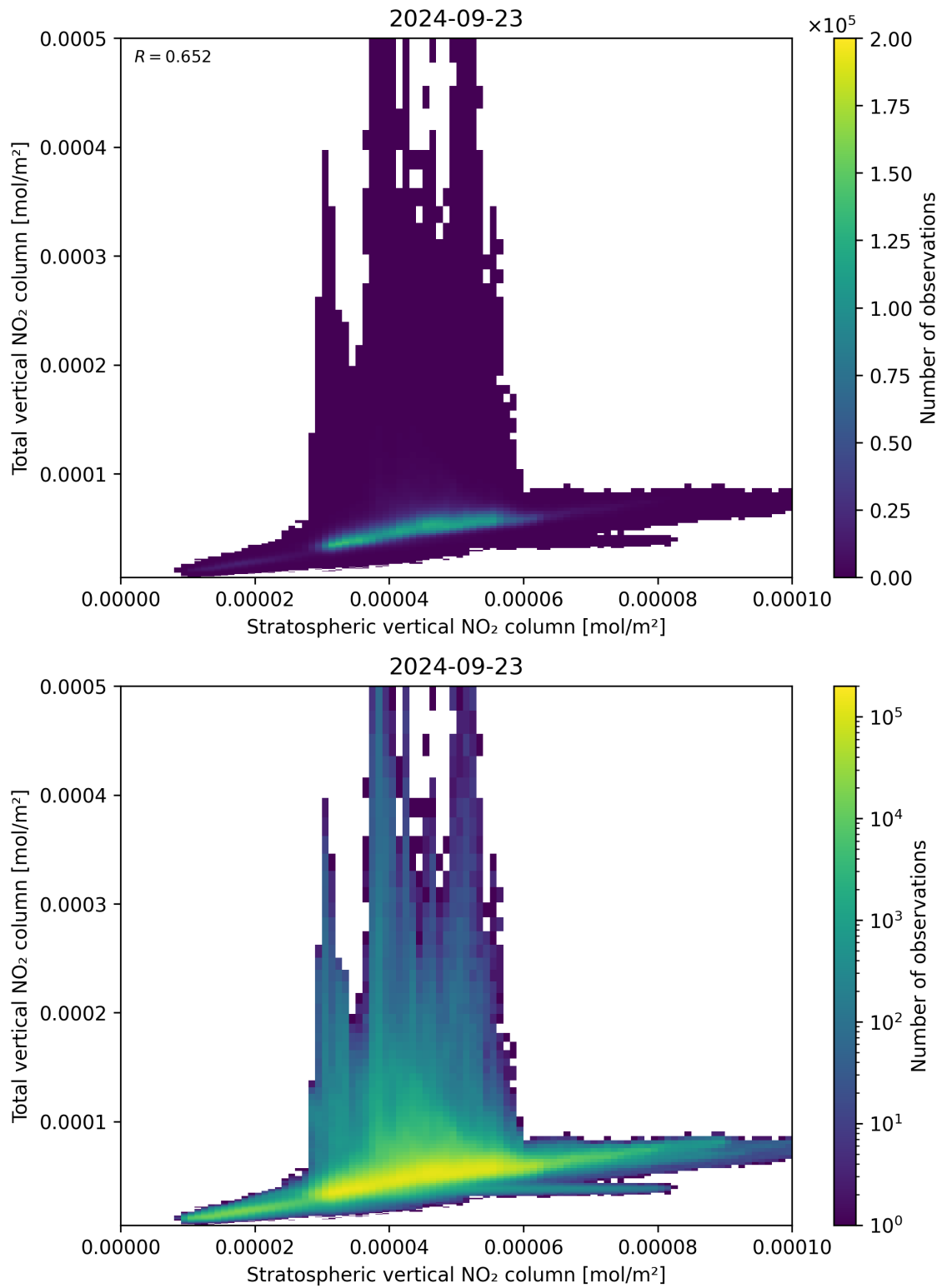
Figure 100: Scatter density plot of “Stratospheric vertical NO 2 column” against “Total vertical NO 2 column” for 2024-09-22 to 2024-09-24.
