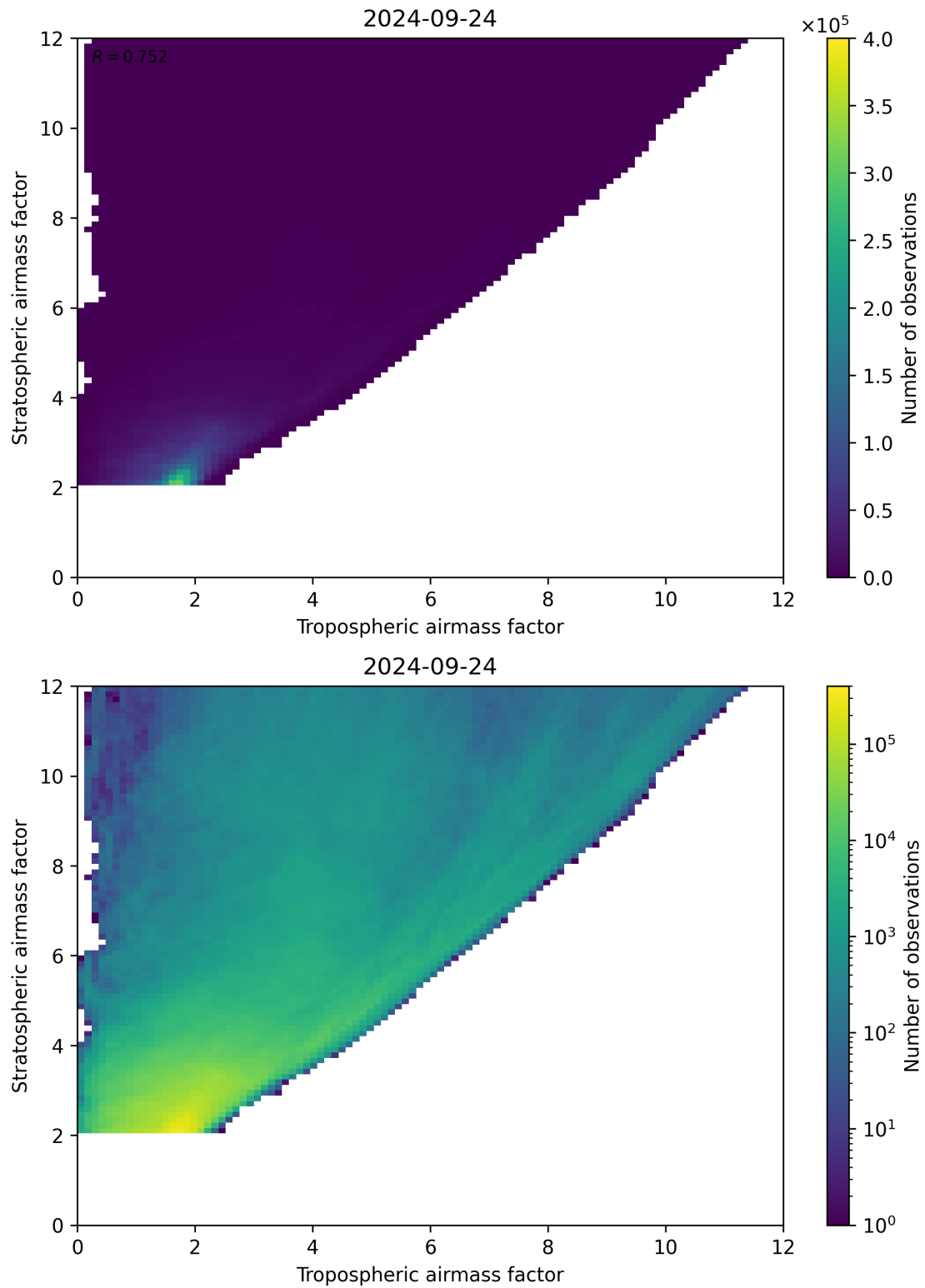
Figure 71: Scatter density plot of “Tropospheric airmass factor” against “Stratospheric airmass factor” for 2024-09-23 to 2024-09-25.
