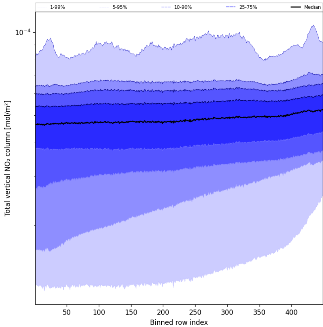
Figure 55: Along track statistics of “Total vertical NO 2 column” for 2024-09-23 to 2024-09-25
