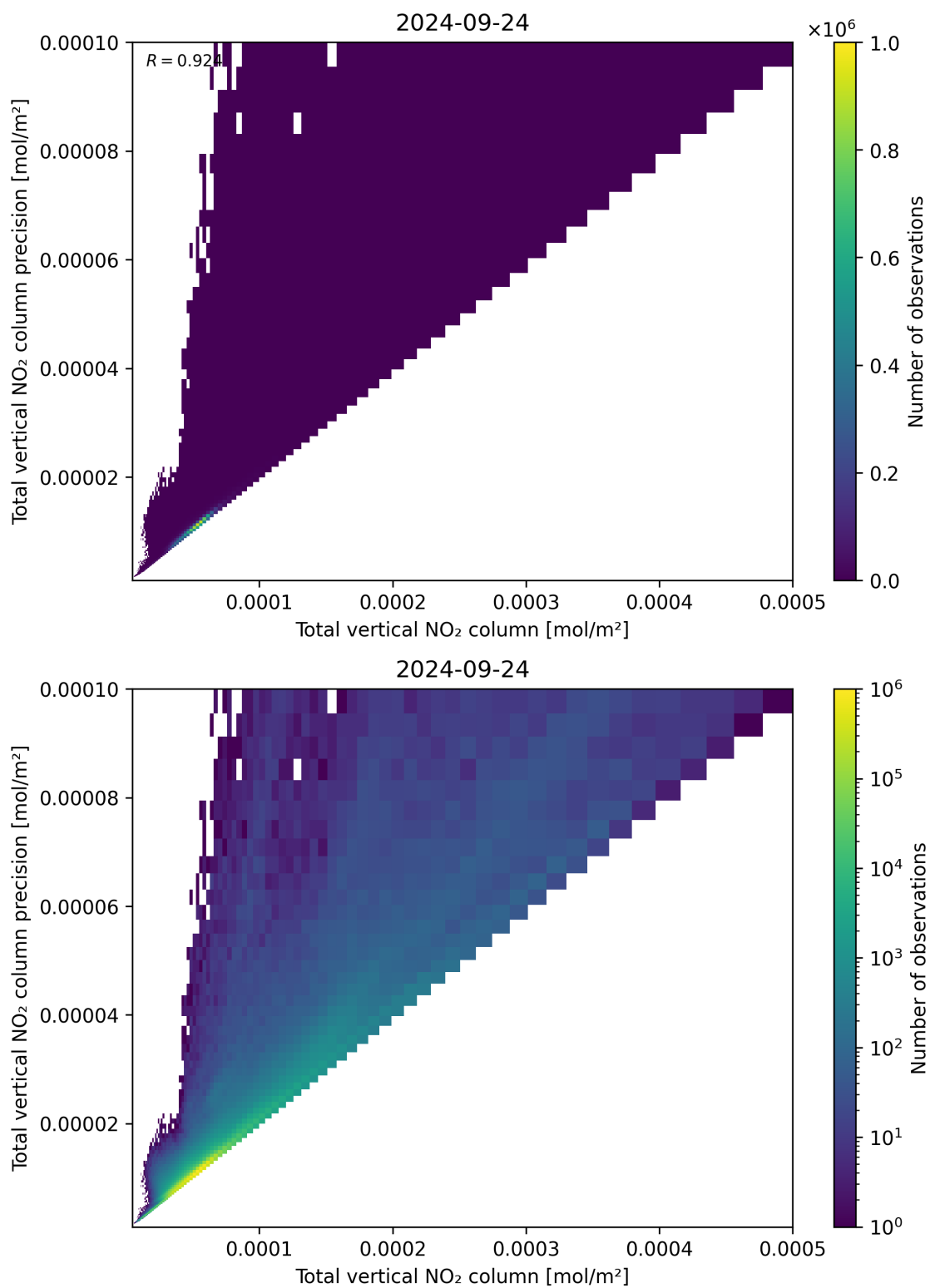
Figure 114: Scatter density plot of “Total vertical NO 2 column” against “Total vertical NO 2 column precision” for 2024-09-23 to 2024-09-25.
