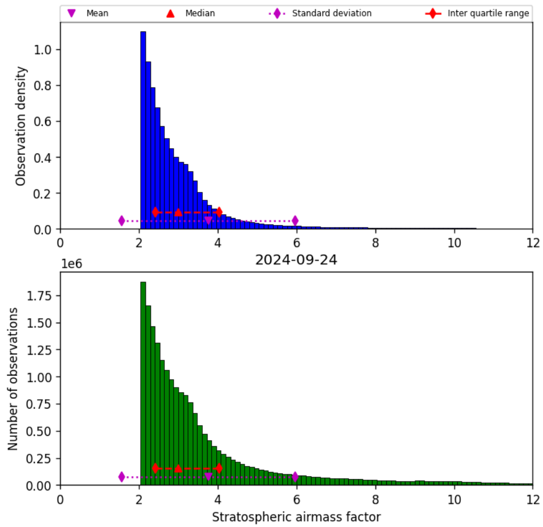
Figure 44: Histogram of “Stratospheric airmass factor” for 2024-09-23 to 2024-09-25
