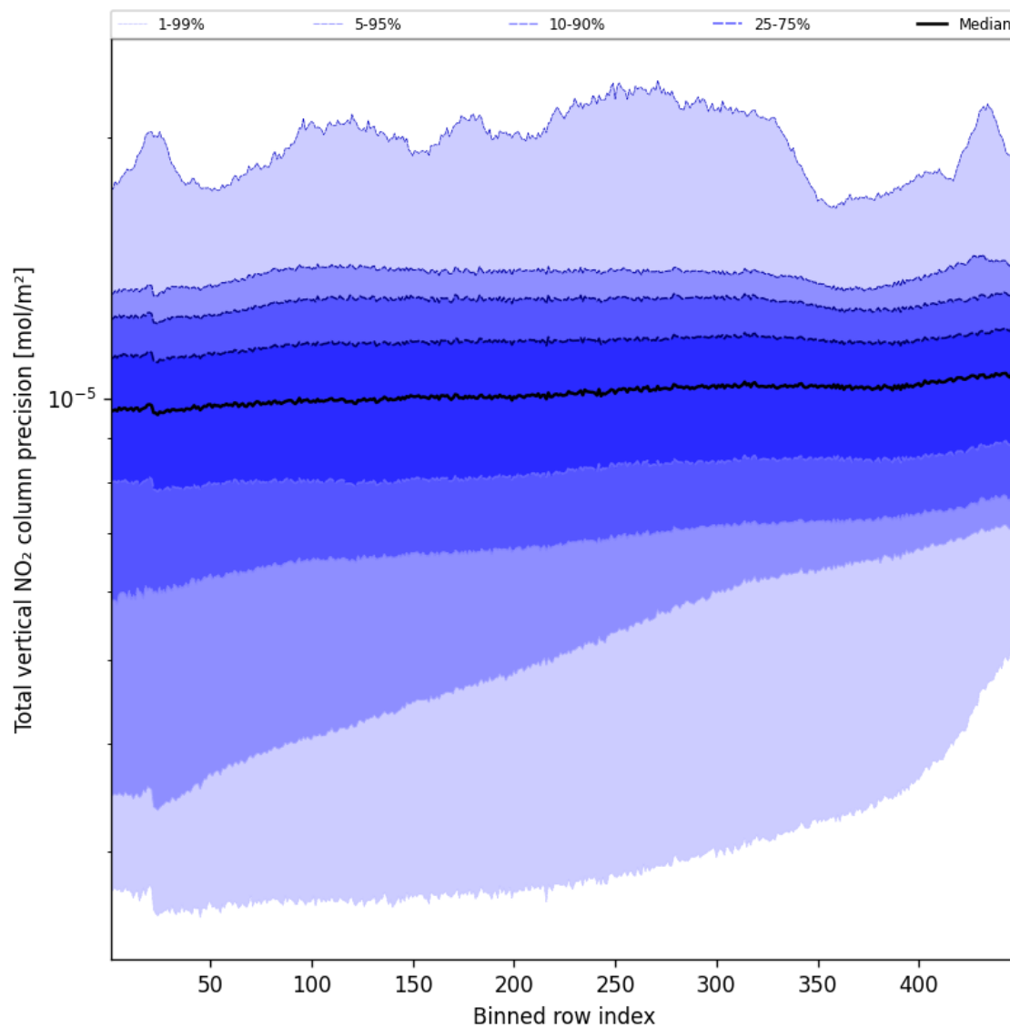
Figure 56: Along track statistics of “Total vertical NO 2 column precision” for 2024-09-23 to 2024-09-25
