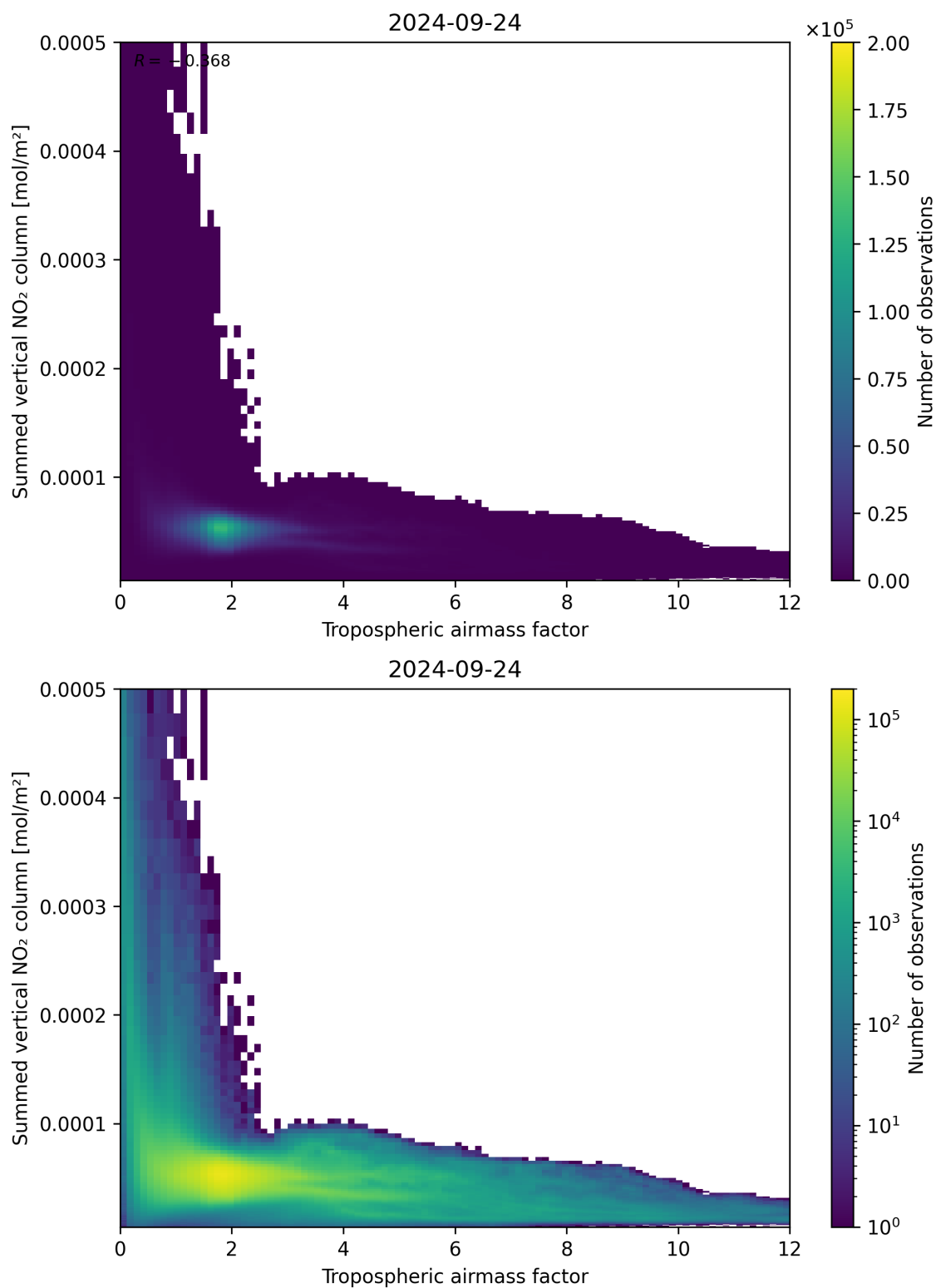
Figure 75: Scatter density plot of “Tropospheric airmass factor” against “Summed vertical NO 2 column” for 2024-09-23 to 2024-09-25.
