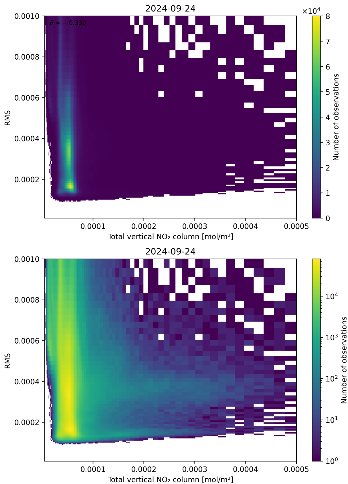
Figure 120: Scatter density plot of “Total vertical NO 2 column” against “RMS” for 2024-09-23 to 2024-09-25.
