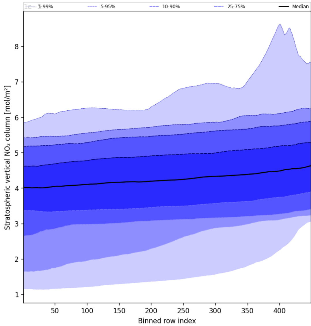
Figure 53: Along track statistics of “Stratospheric vertical NO 2 column” for 2024-09-23 to 2024-09-25
