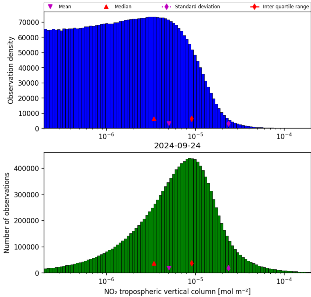
Figure 29: Histogram of “NO 2 tropospheric vertical column” for 2024-09-23 to 2024-09-25
