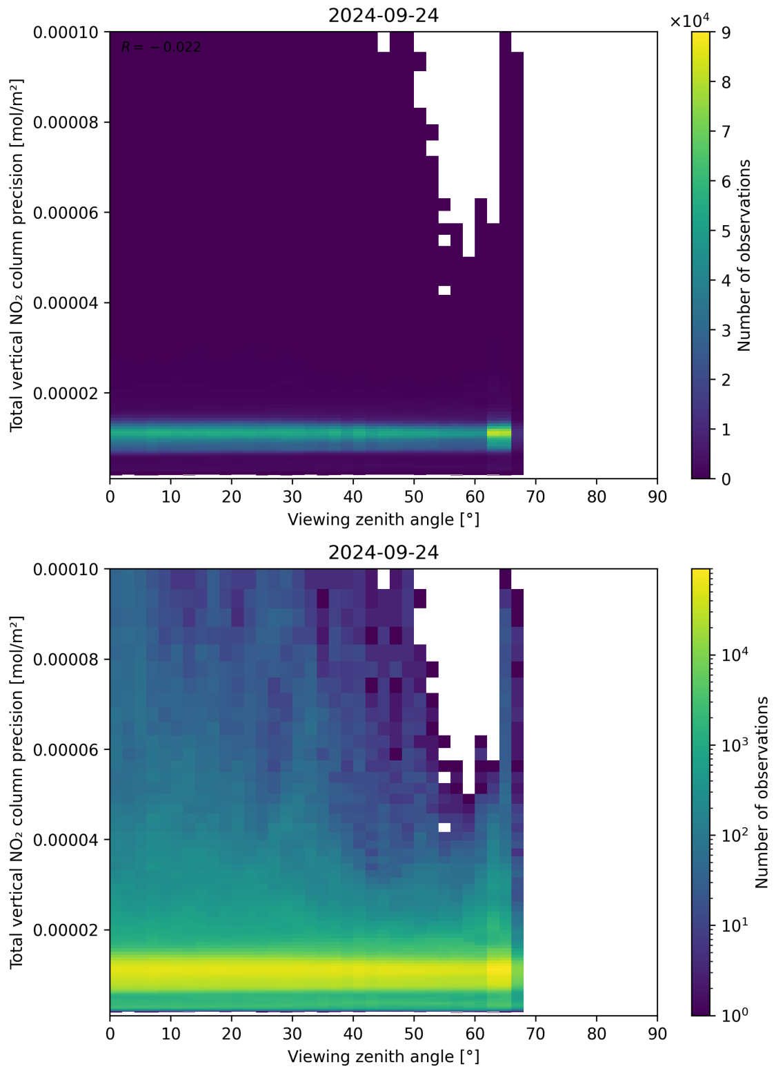
Figure 168: Scatter density plot of “Viewing zenith angle” against “Total vertical NO 2 column precision” for 2024-09-23 to 2024-09-25.
