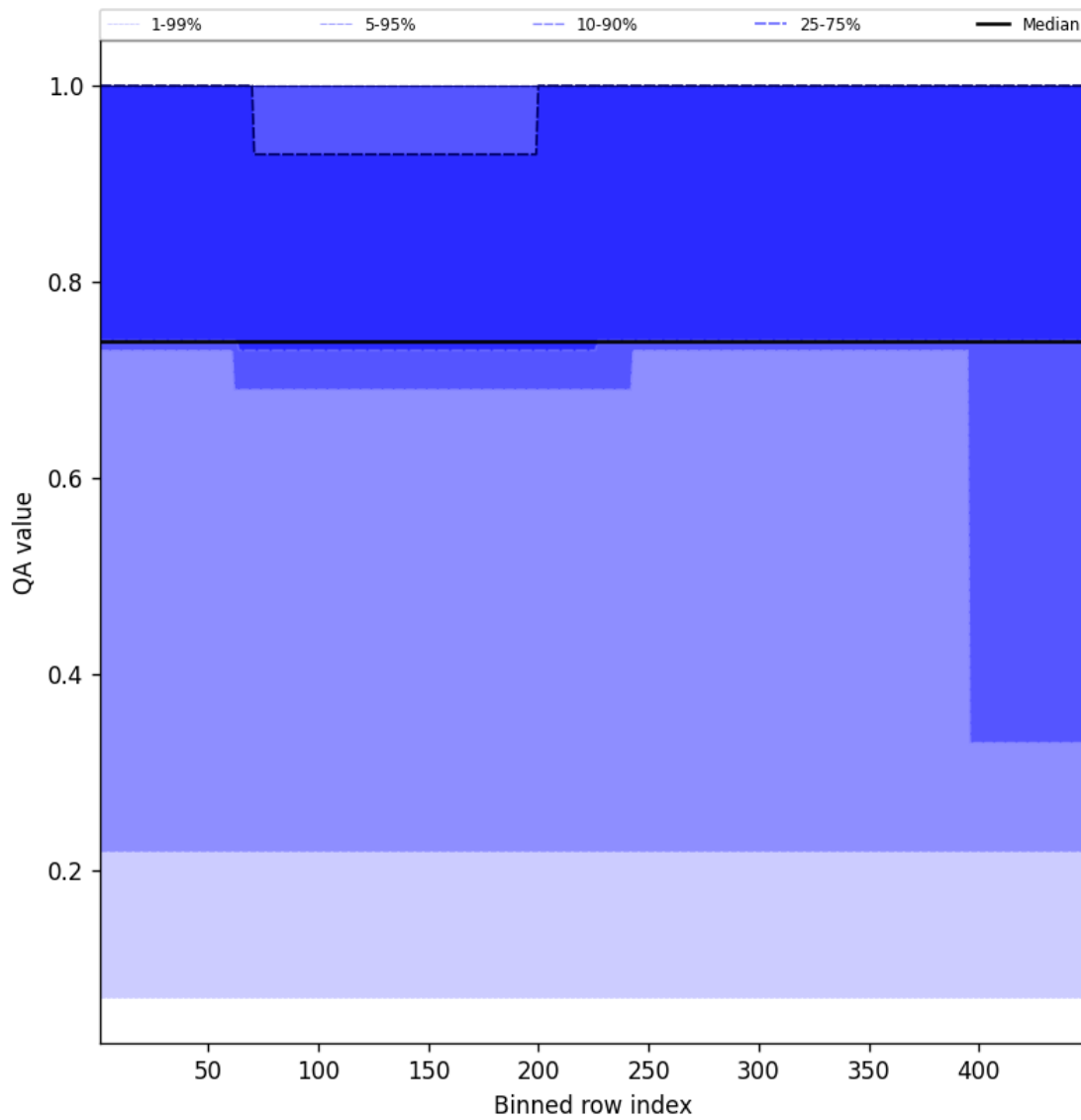
Figure 45: Along track statistics of “QA value” for 2024-09-23 to 2024-09-25
