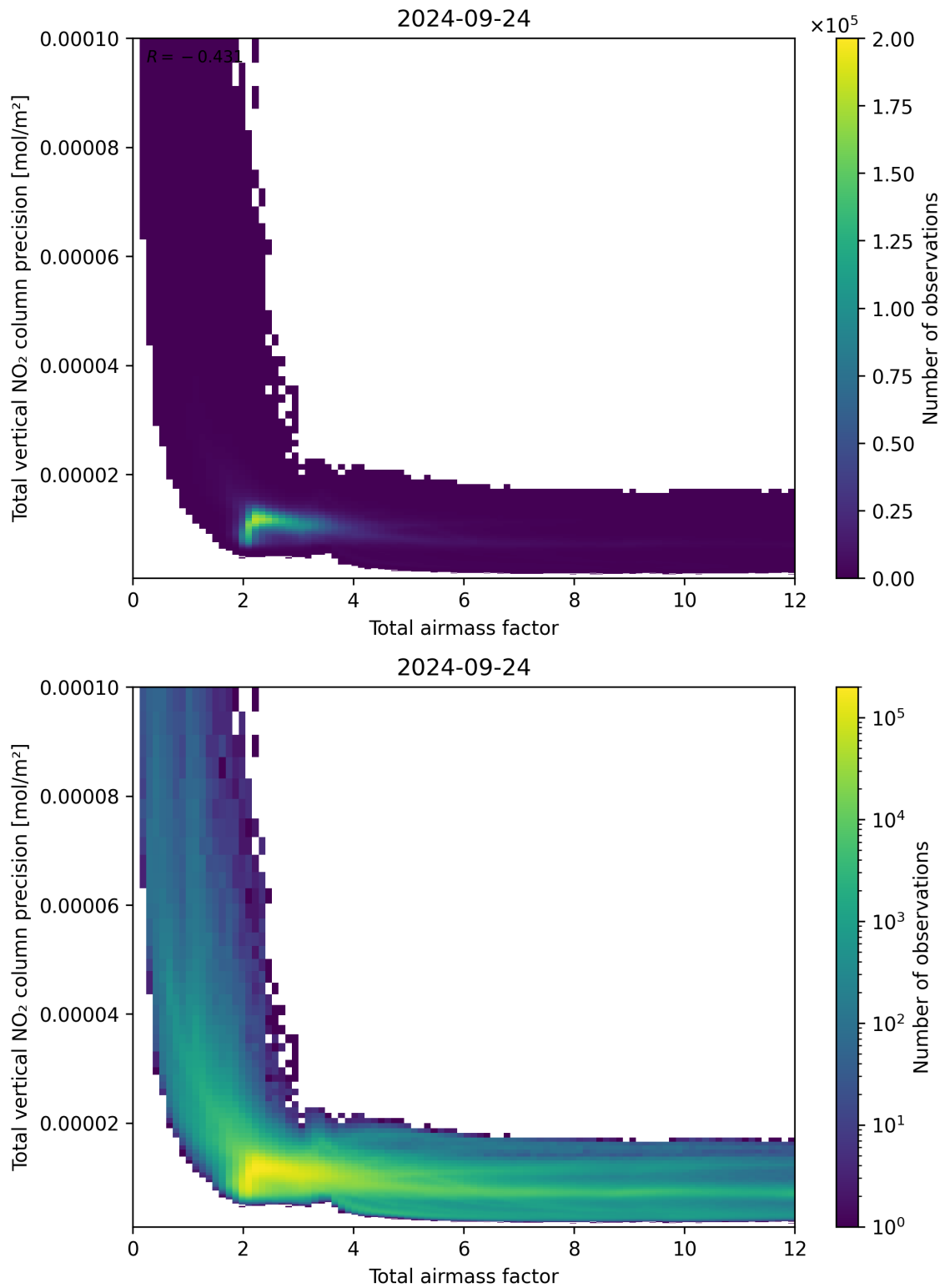
Figure 68: Scatter density plot of “Total airmass factor” against “Total vertical NO 2 column precision” for 2024-09-23 to 2024-09-25.
