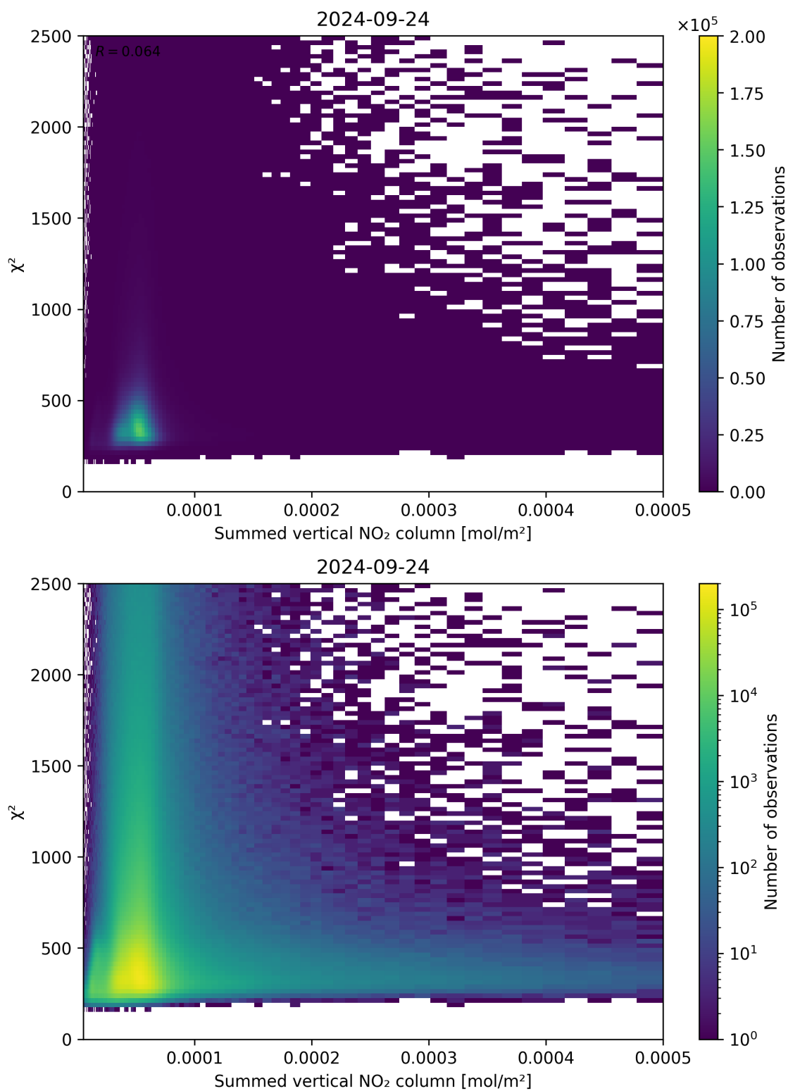
Figure 104: Scatter density plot of “Summed vertical NO 2 column” against “ \chi^2 ” for 2024-09-23 to 2024-09-25.
