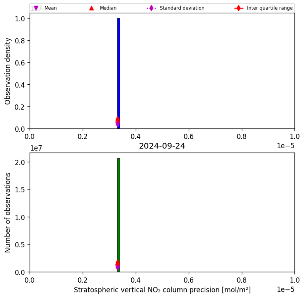
Figure 37: Histogram of “Stratospheric vertical NO 2 column precision” for 2024-09-23 to 2024-09-25
