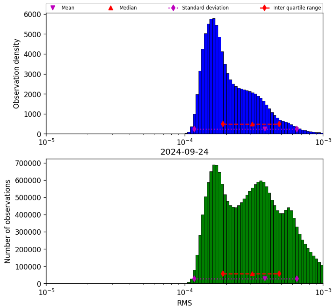
Figure 43: Histogram of “RMS” for 2024-09-23 to 2024-09-25
