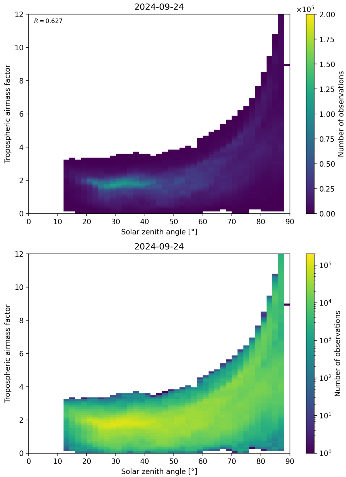
Figure 147: Scatter density plot of “Solar zenith angle” against “Tropospheric airmass factor” for 2024-09-23 to 2024-09-25.
