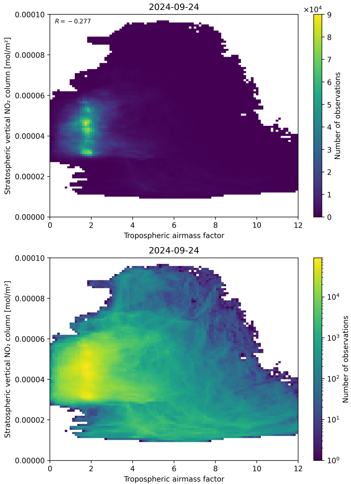
Figure 74: Scatter density plot of “Tropospheric air mass factor” against “Stratospheric vertical NO 2 column” for 2024-09-23 to 2024-09-25.
