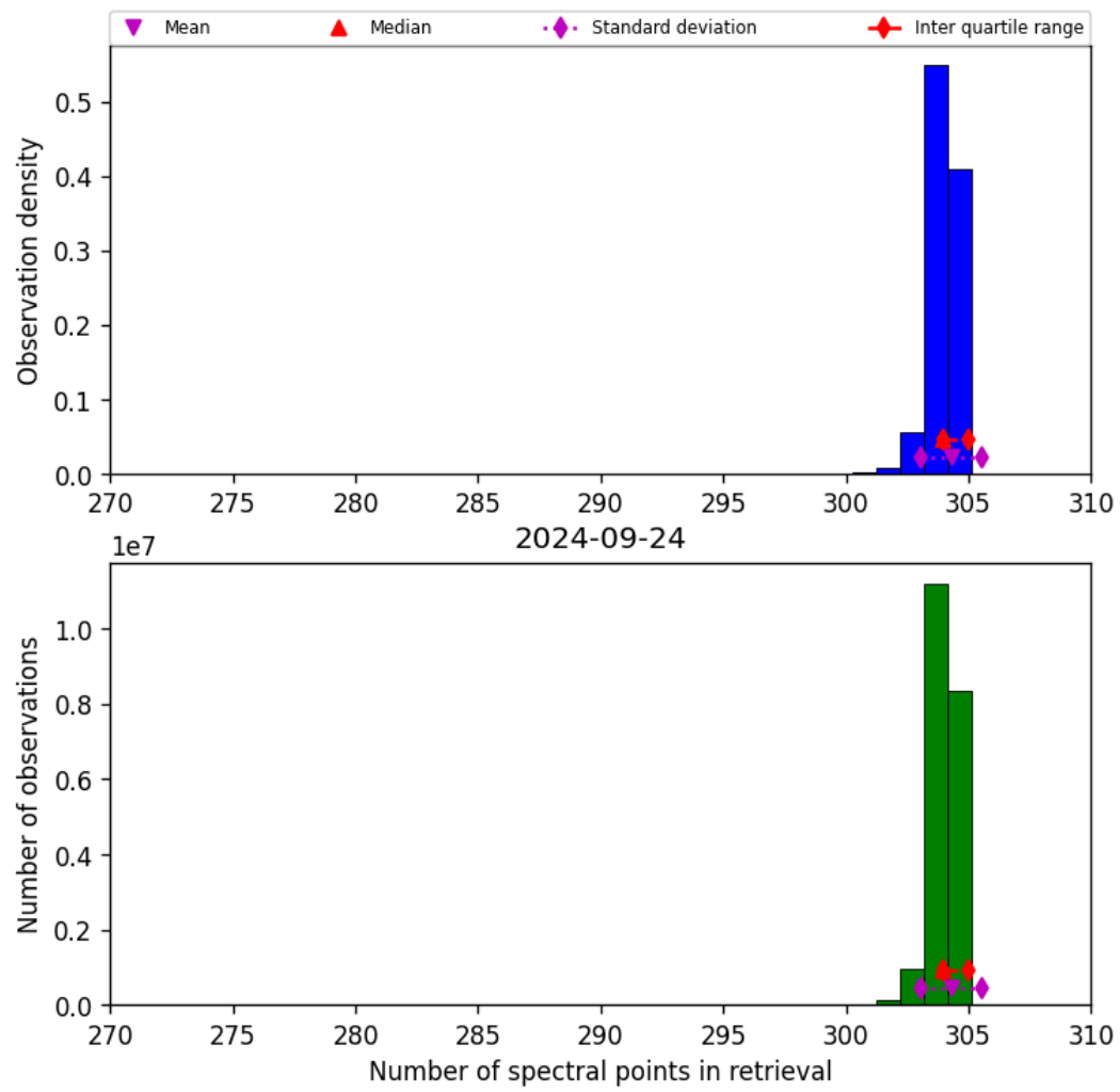
Figure 33: Histogram of “Number of spectral points in retrieval” for 2024-09-23 to 2024-09-25
