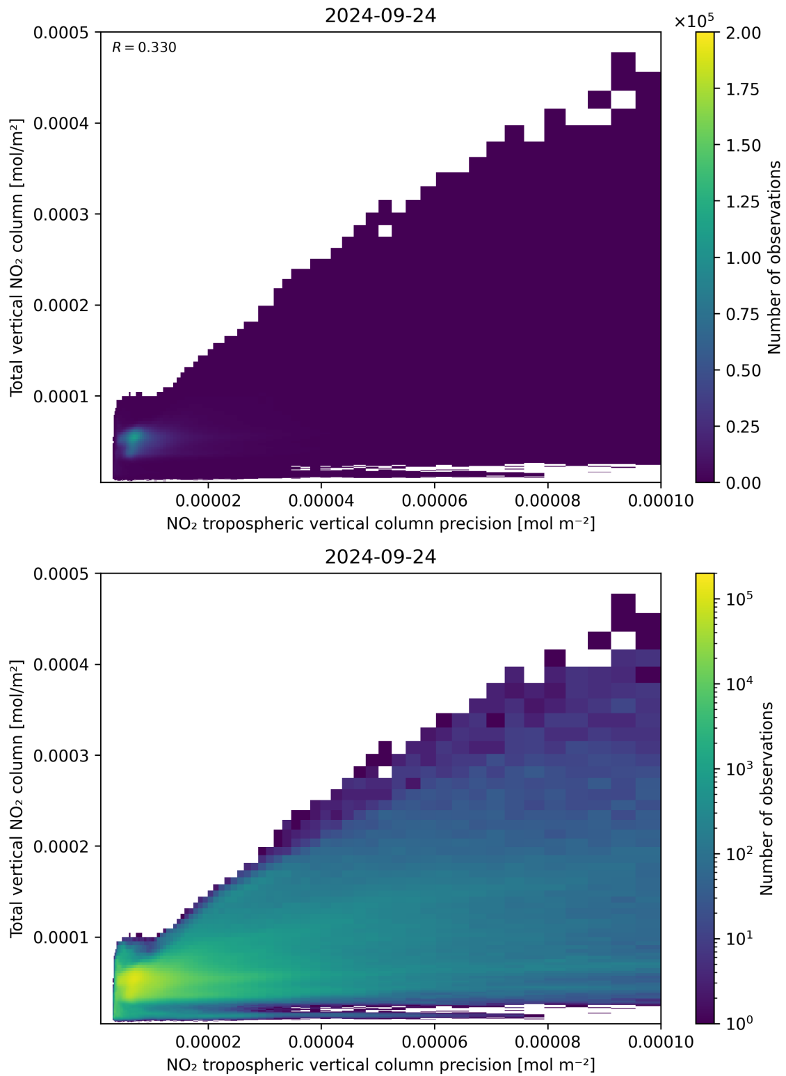
Figure 138: Scatter density plot of “NO 2 tropospheric vertical column precision” against “Total vertical NO 2 column” for 2024-09-23 to 2024-09-25.
