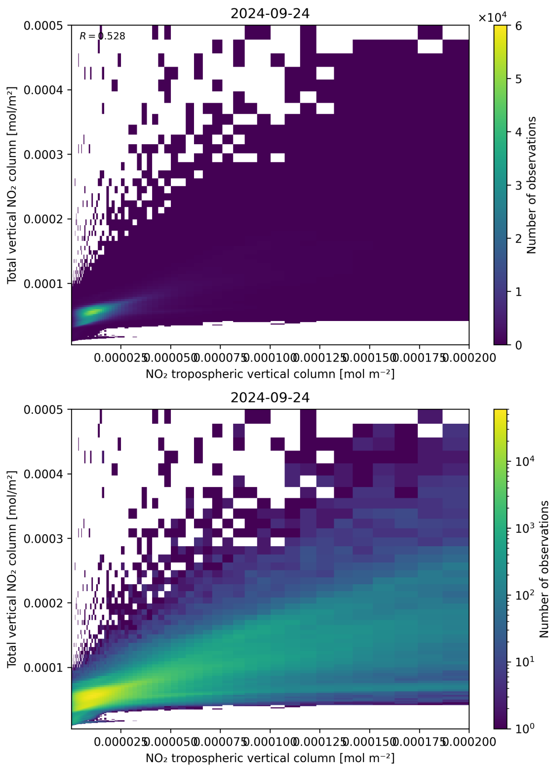
Figure 128: Scatter density plot of “NO 2 tropospheric vertical column” against “Total vertical NO 2 column” for 2024-09-23 to 2024-09-25.
