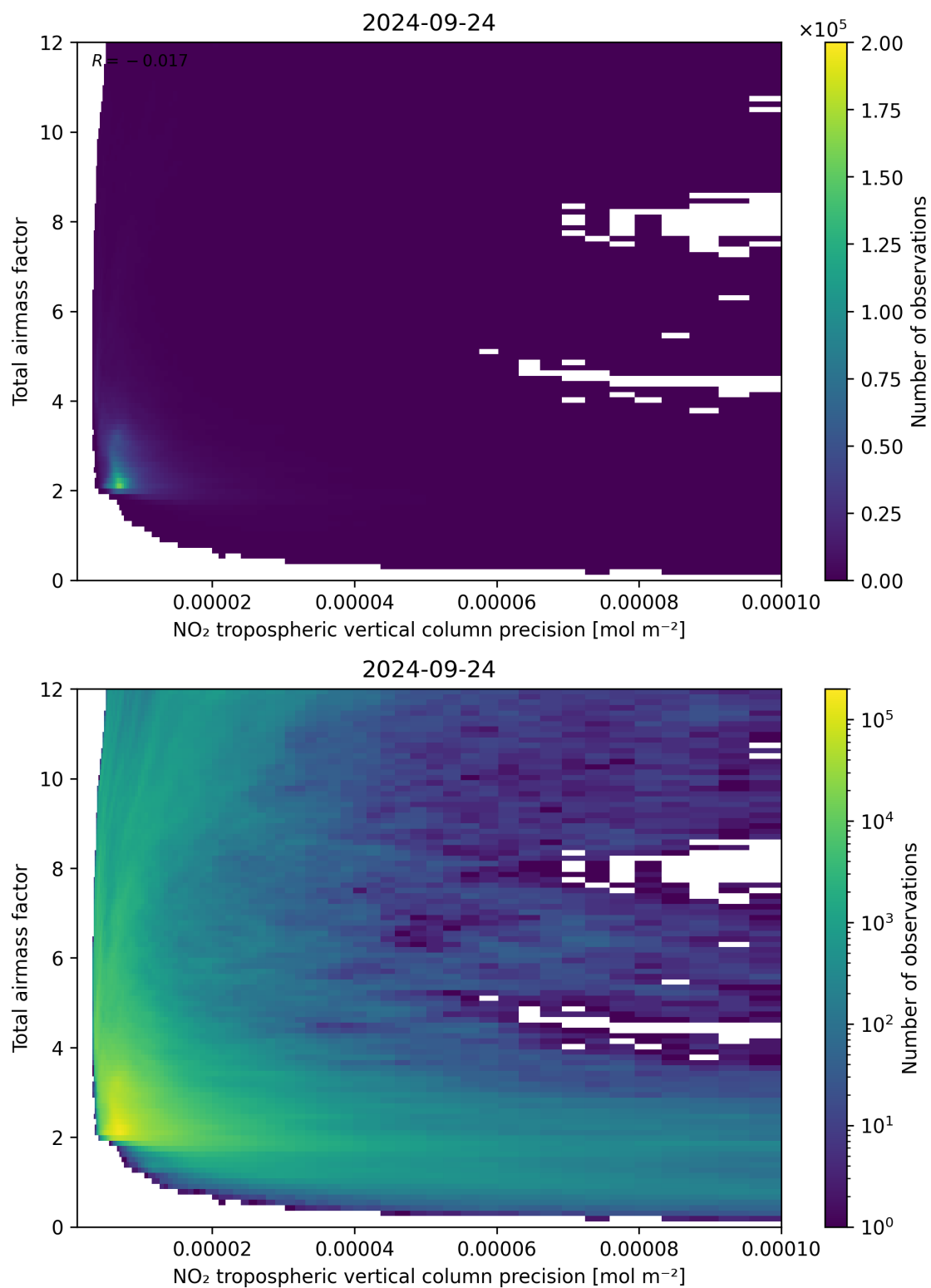
Figure 132: Scatter density plot of “NO 2 tropospheric vertical column precision” against “Total air mass factor” for 2024-09-23 to 2024-09-25.
