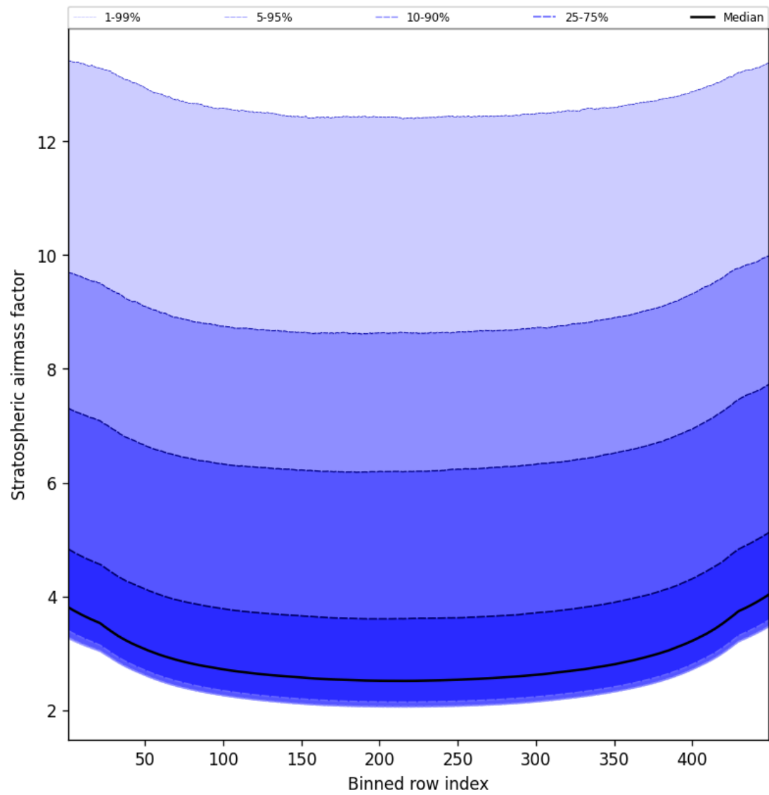
Figure 61: Along track statistics of “Stratospheric airmass factor” for 2024-09-23 to 2024-09-25
