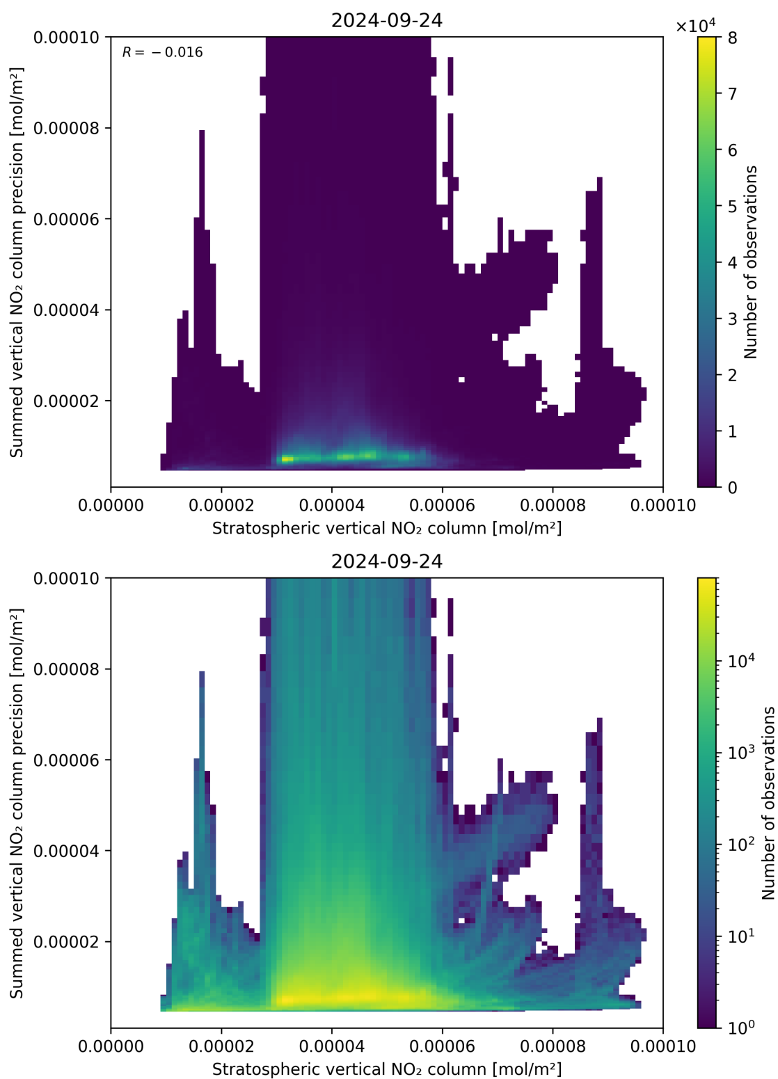
Figure 99: Scatter density plot of “Stratospheric vertical NO 2 column” against “Summed vertical NO 2 column precision” for 2024-09-23 to 2024-09-25.
