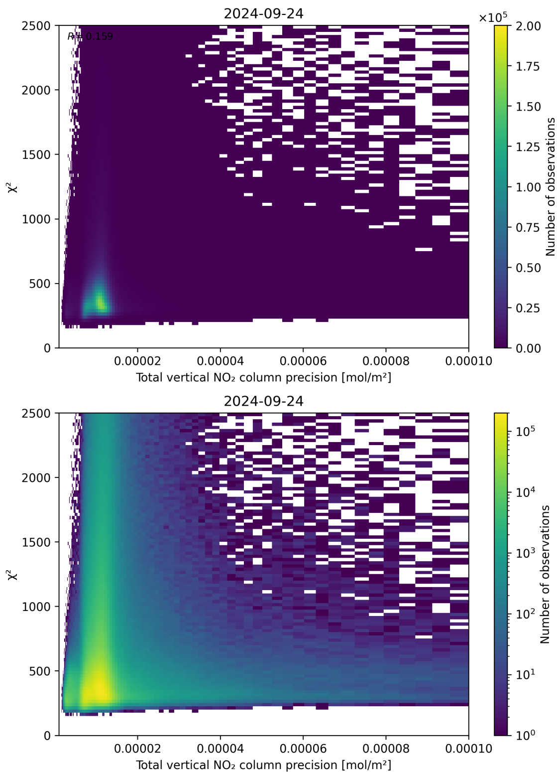
Figure 116: Scatter density plot of “Total vertical NO 2 column precision” against “ \chi^2 ” for 2024-09-23 to 2024-09-25.
