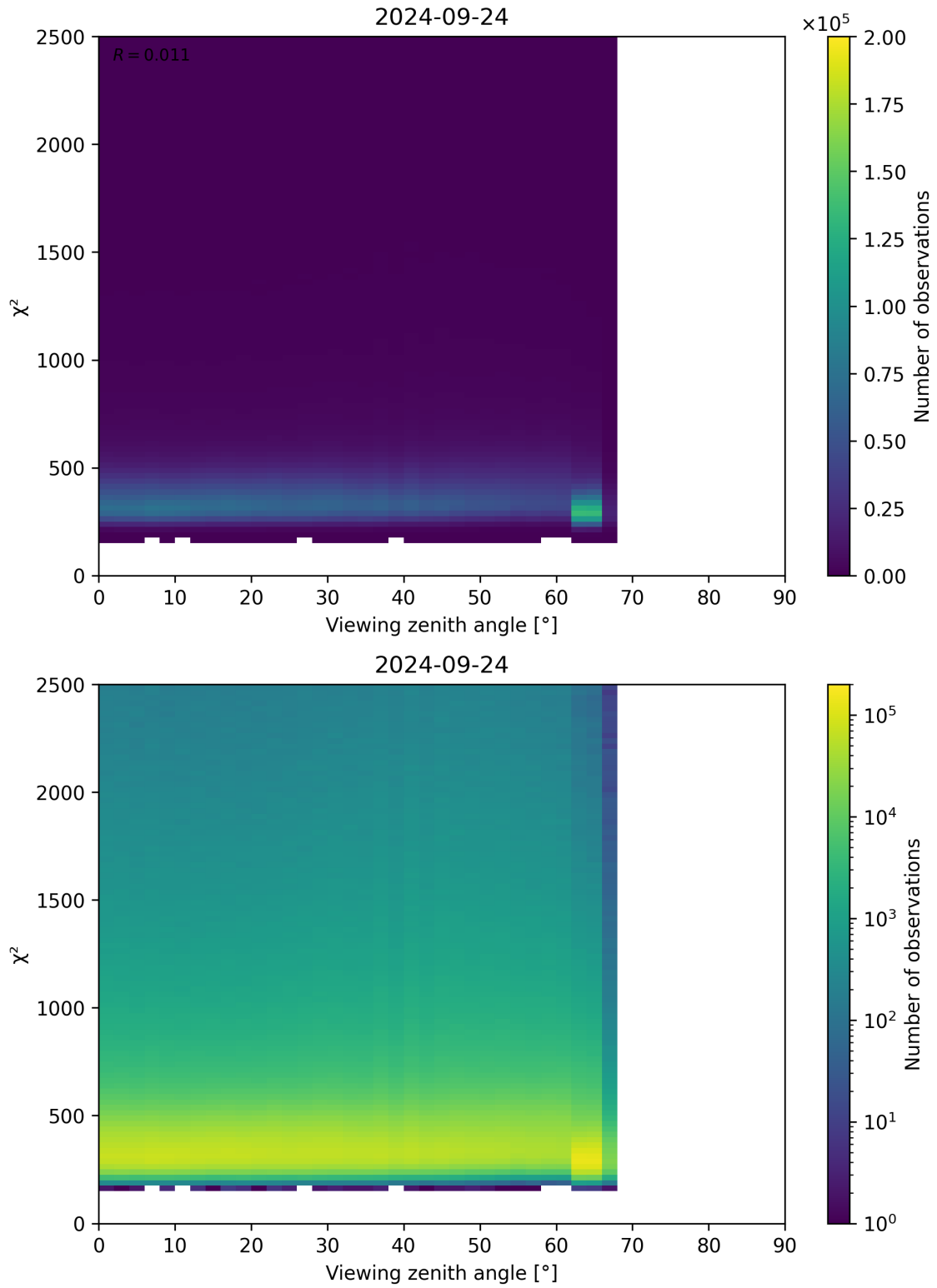
Figure 162: Scatter density plot of “Viewing zenith angle” against “ \chi^2 ” for 2024-09-23 to 2024-09-25.
