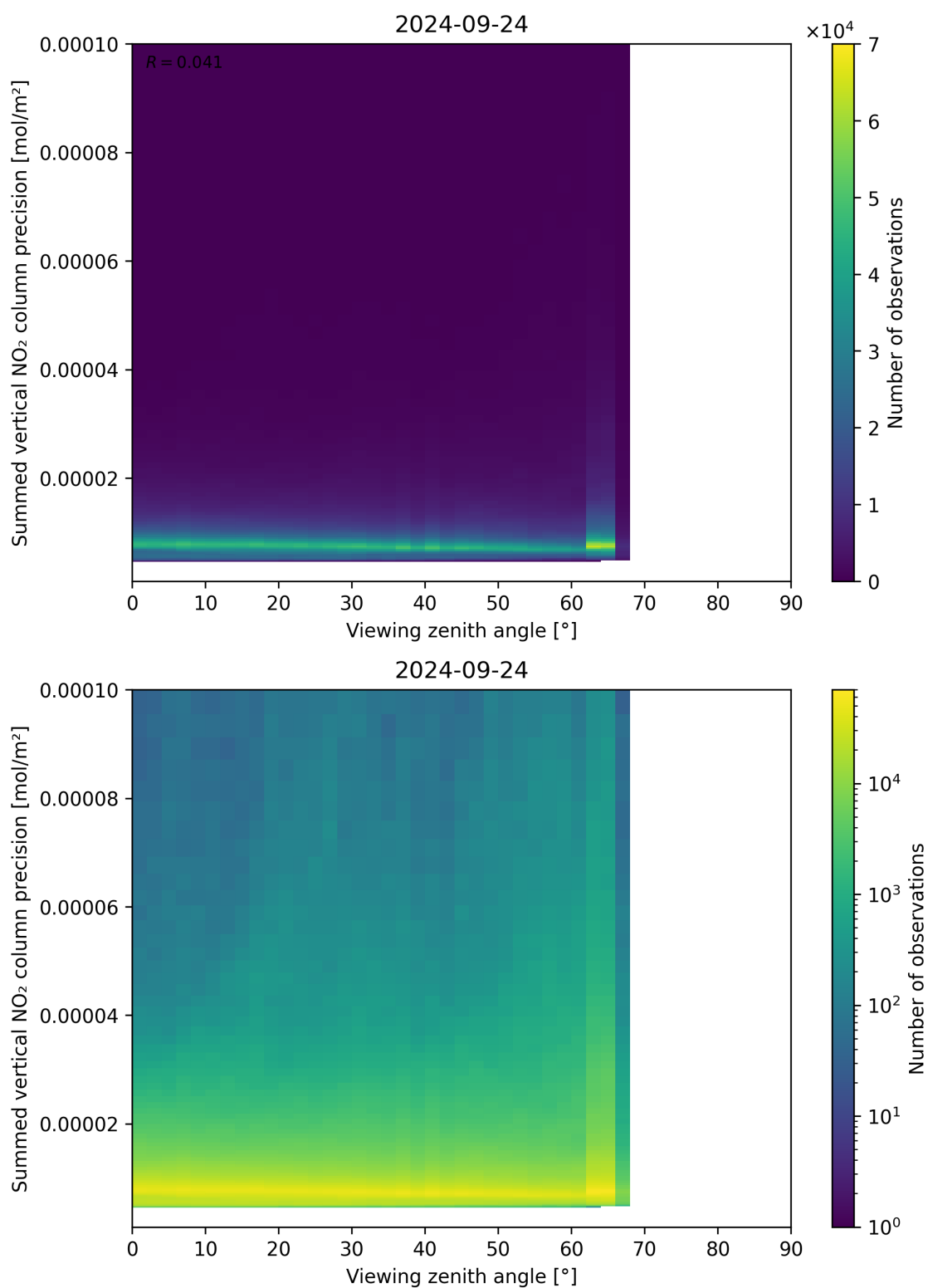
Figure 166: Scatter density plot of “Viewing zenith angle” against “Summed vertical NO 2 column precision” for 2024-09-23 to 2024-09-25.
