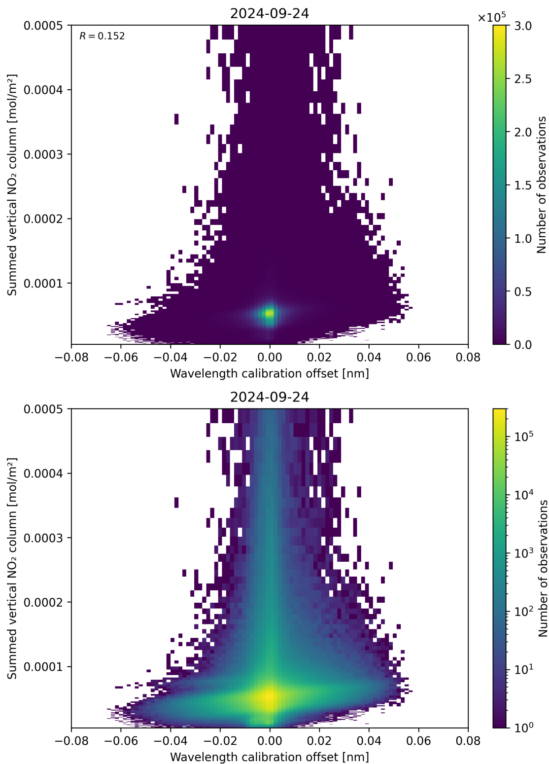
Figure 177: Scatter density plot of “Wavelength calibration offset” against “Summed vertical NO 2 column” for 2024-09-23 to 2024-09-25.
