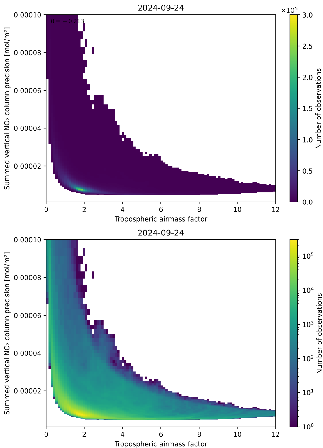
Figure 76: Scatter density plot of “Tropospheric airmass factor” against “Summed vertical NO 2 column precision” for 2024-09-23 to 2024-09-25.
