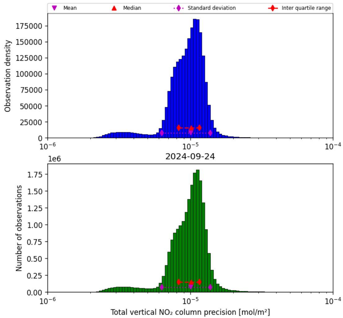
Figure 39: Histogram of “Total vertical NO 2 column precision” for 2024-09-23 to 2024-09-25
