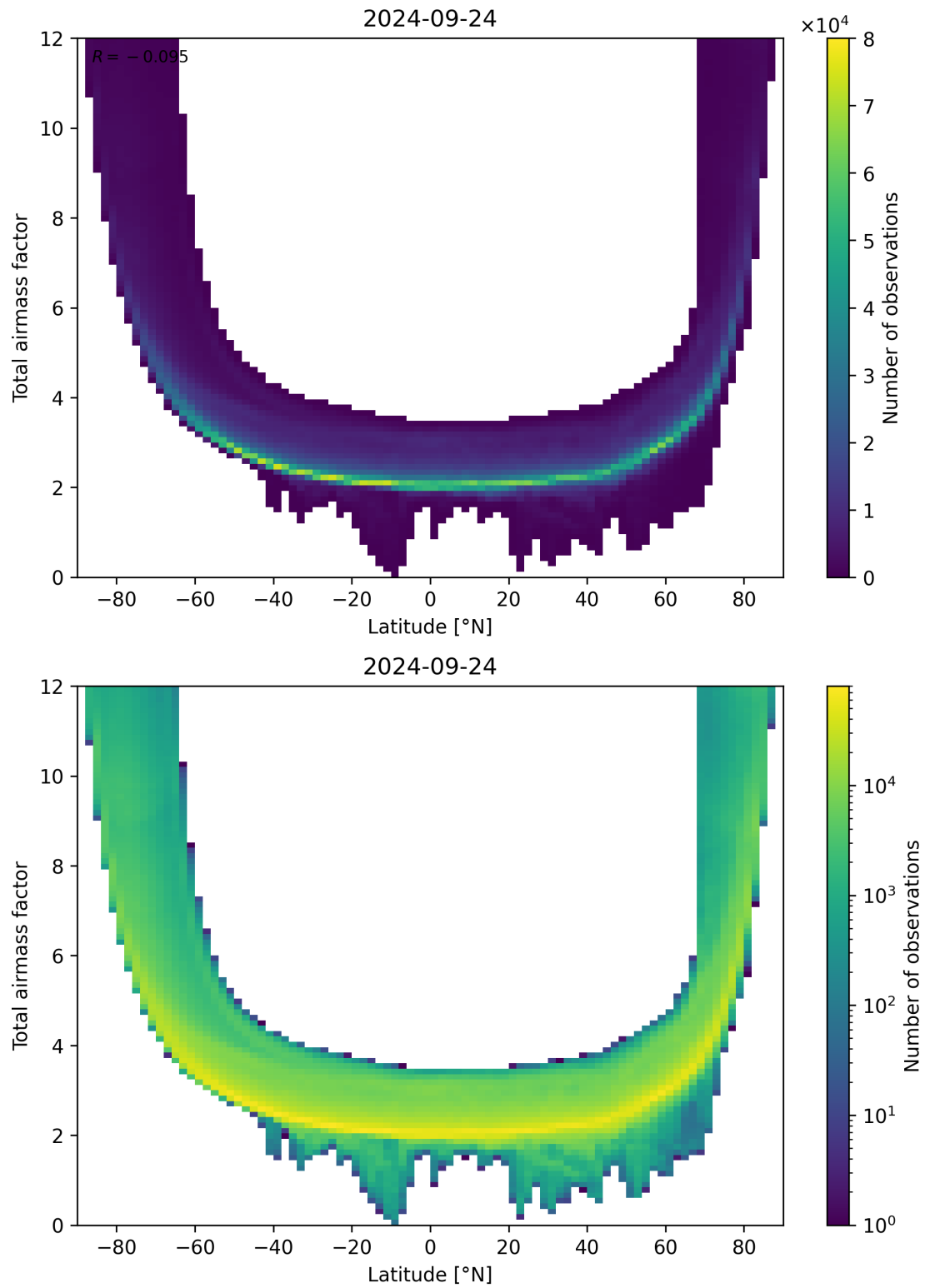
Figure 84: Scatter density plot of “Latitude” against “Total airmass factor” for 2024-09-23 to 2024-09-25.
