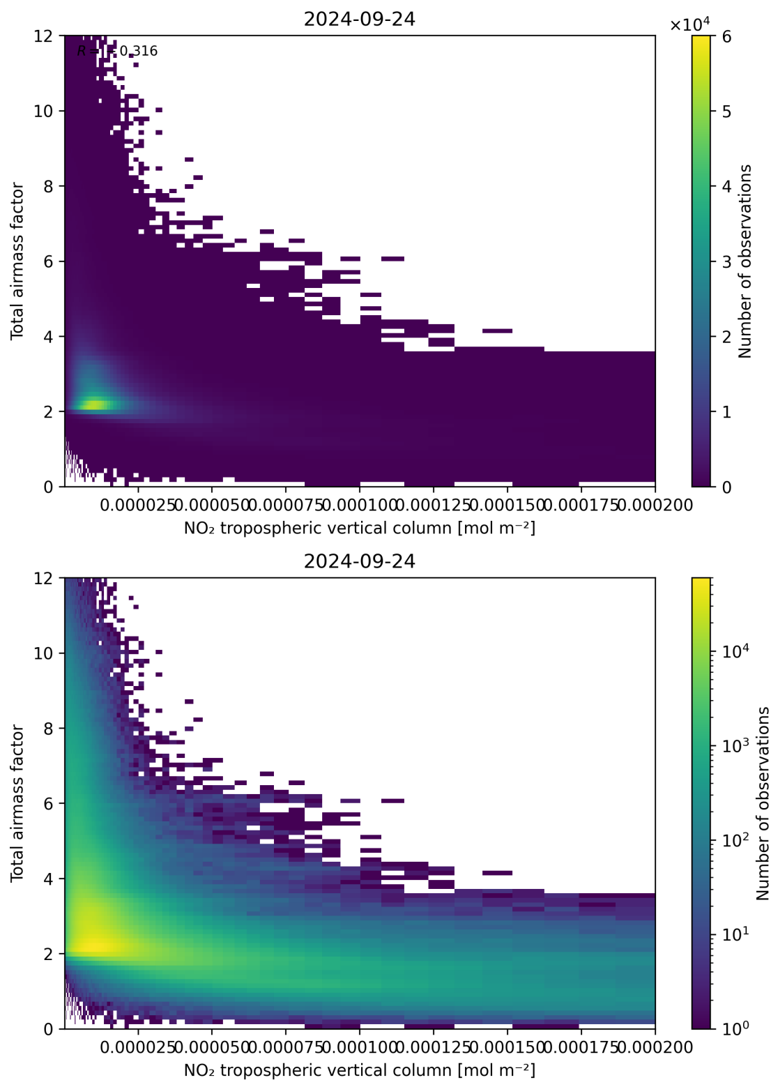
Figure 122: Scatter density plot of “NO 2 tropospheric vertical column” against “Total air mass factor” for 2024-09-23 to 2024-09-25.
