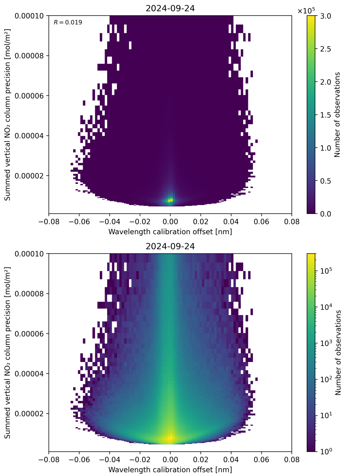
Figure 178: Scatter density plot of “Wavelength calibration offset” against “Summed vertical NO 2 column precision” for 2024-09-23 to 2024-09-25.
