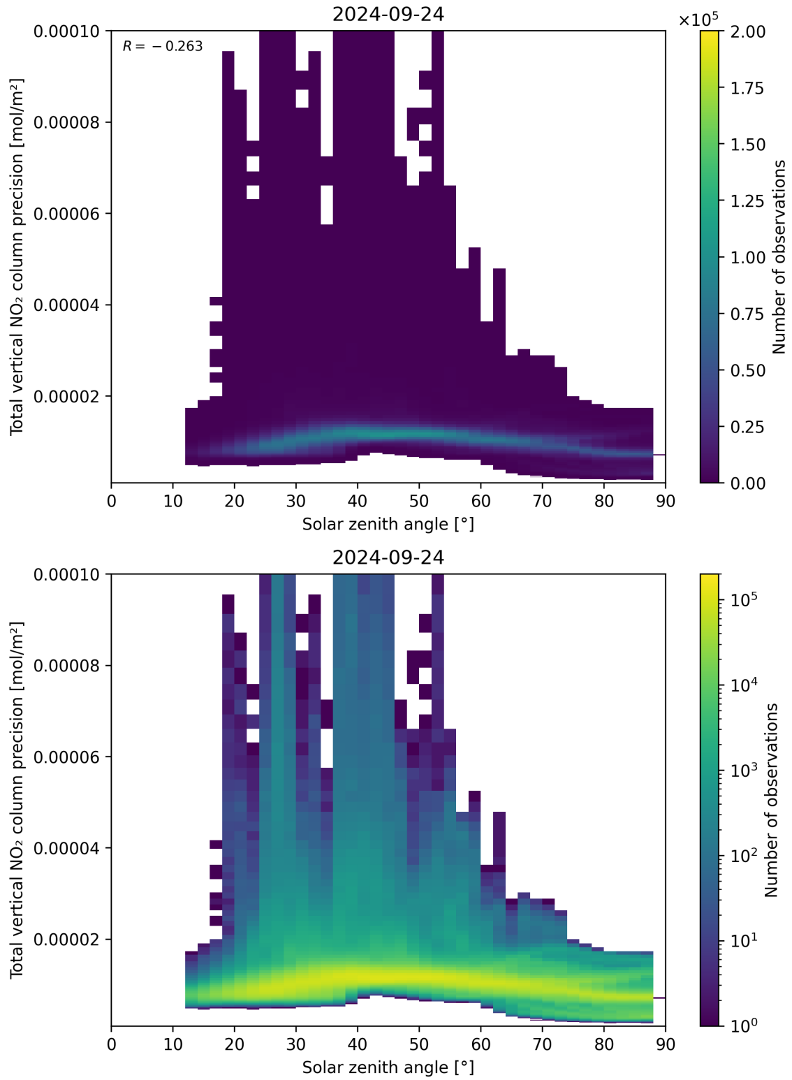
Figure 154: Scatter density plot of “Solar zenith angle” against “Total vertical NO 2 column precision” for 2024-09-23 to 2024-09-25.
