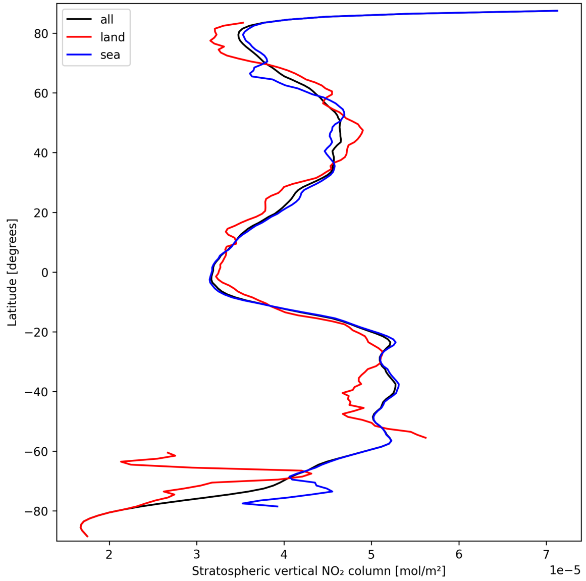
Figure 19: Zonal average of “Stratospheric vertical NO 2 column” for 2024-09-23 to 2024-09-25.
