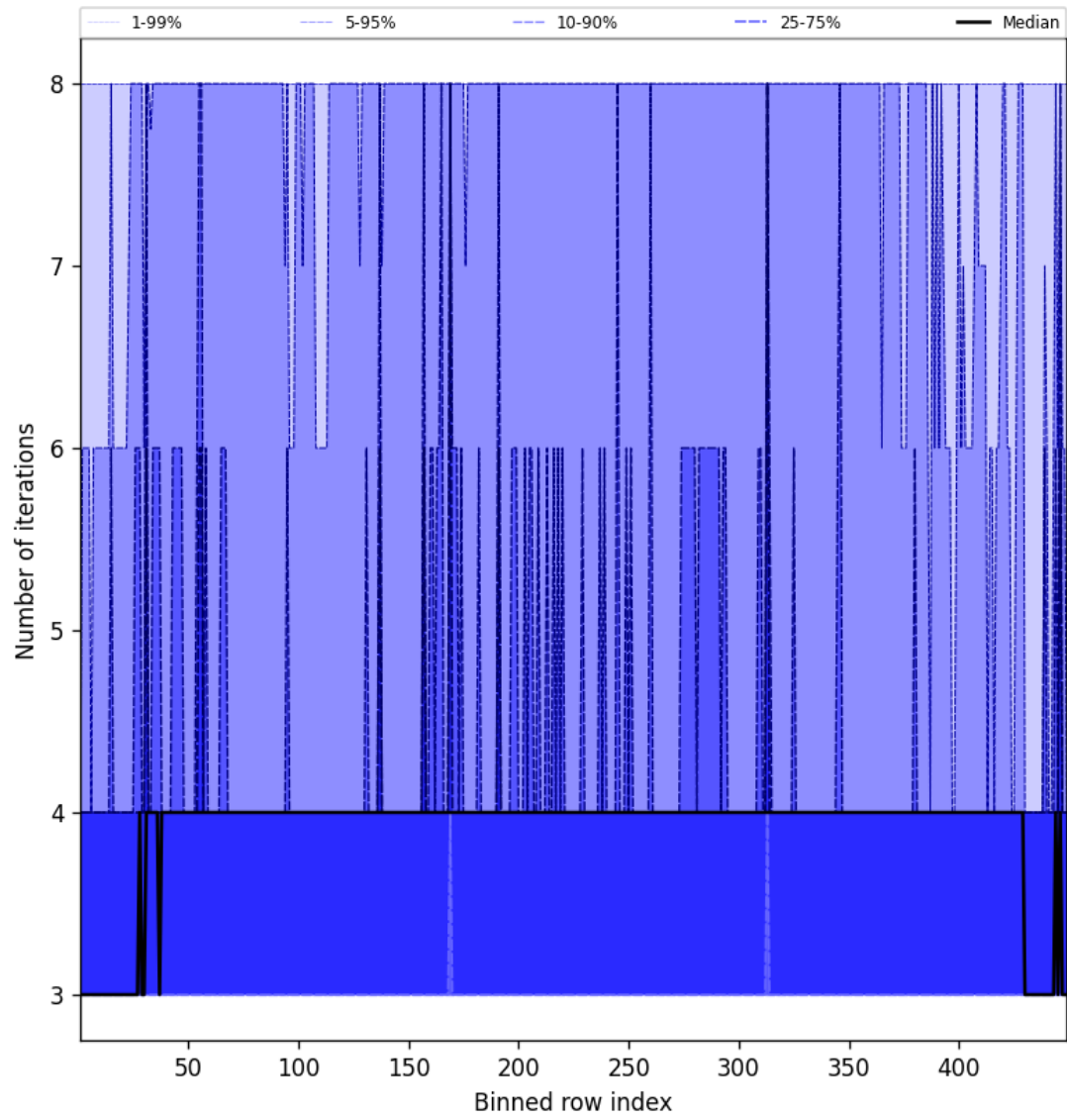
Figure 51: Along track statistics of “Number of iterations” for 2024-09-23 to 2024-09-25
