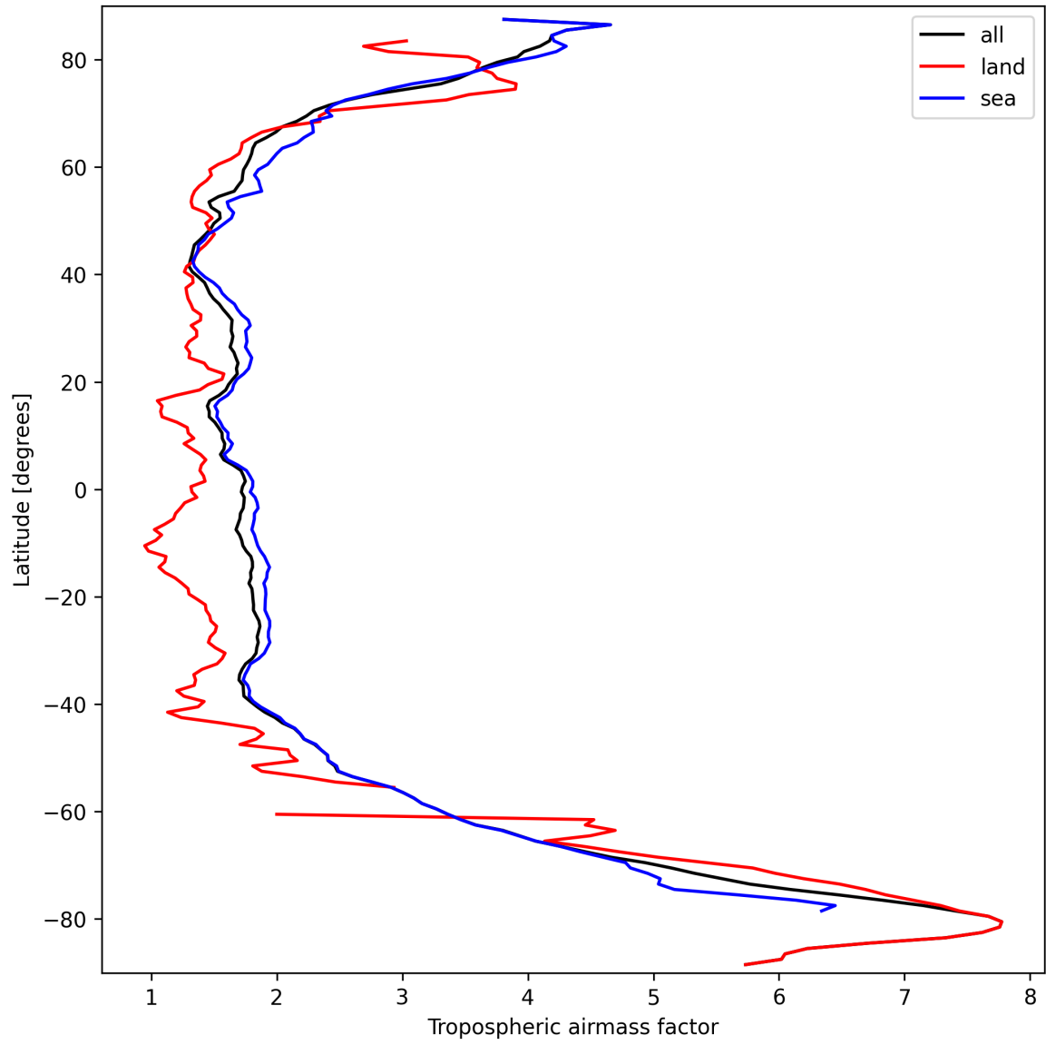
Figure 14: Zonal average of “Tropospheric airmass factor” for 2024-09-23 to 2024-09-25.
