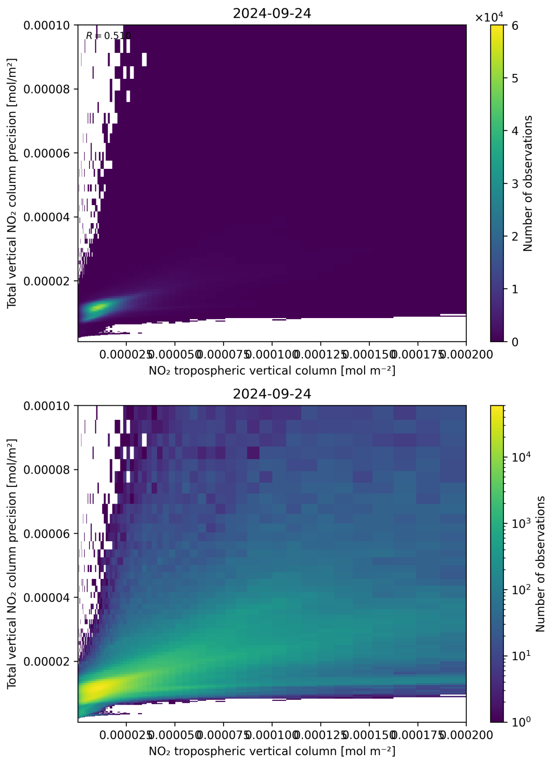
Figure 129: Scatter density plot of “NO 2 tropospheric vertical column” against “Total vertical NO 2 column precision” for 2024-09-23 to 2024-09-25.
