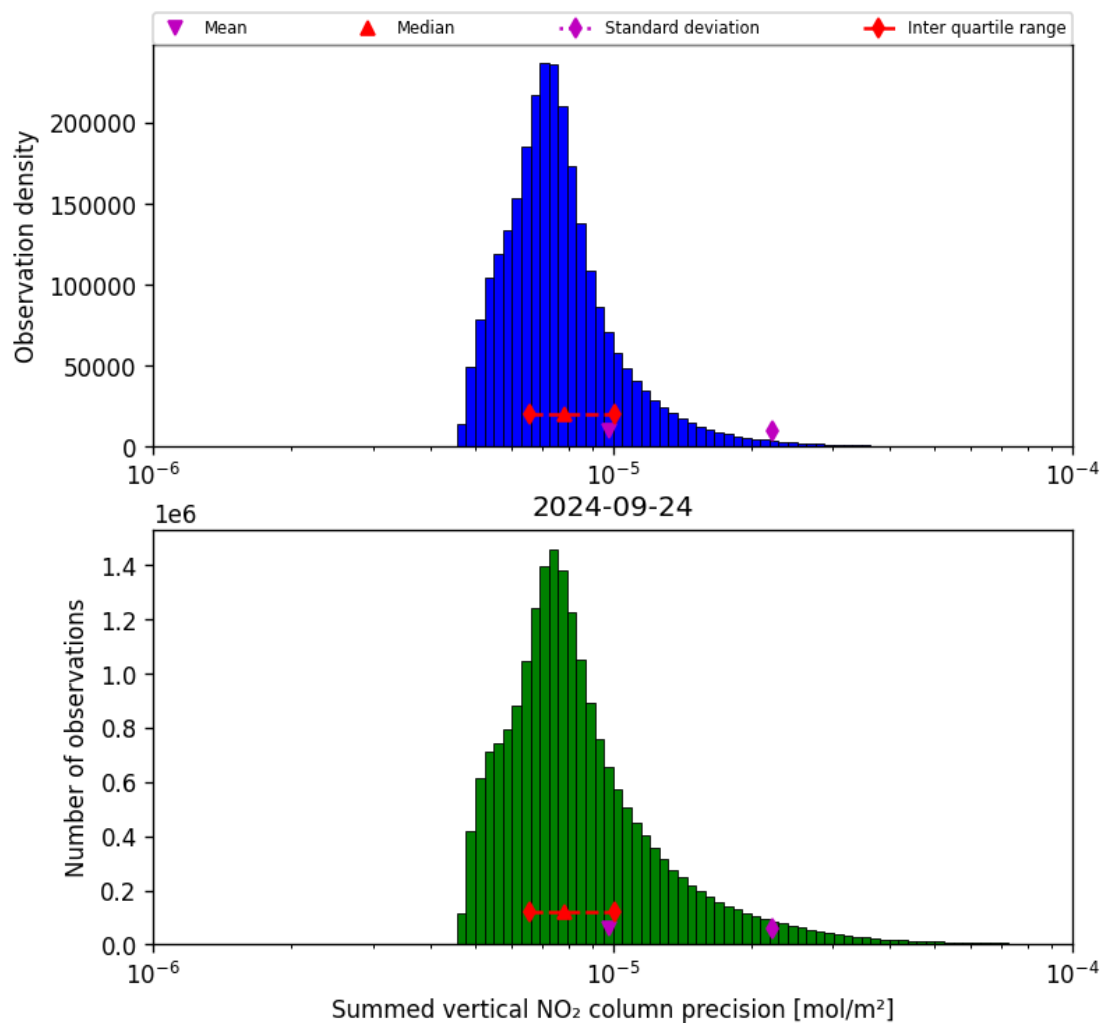
Figure 41: Histogram of “Summed vertical NO 2 column precision” for 2024-09-23 to 2024-09-25
