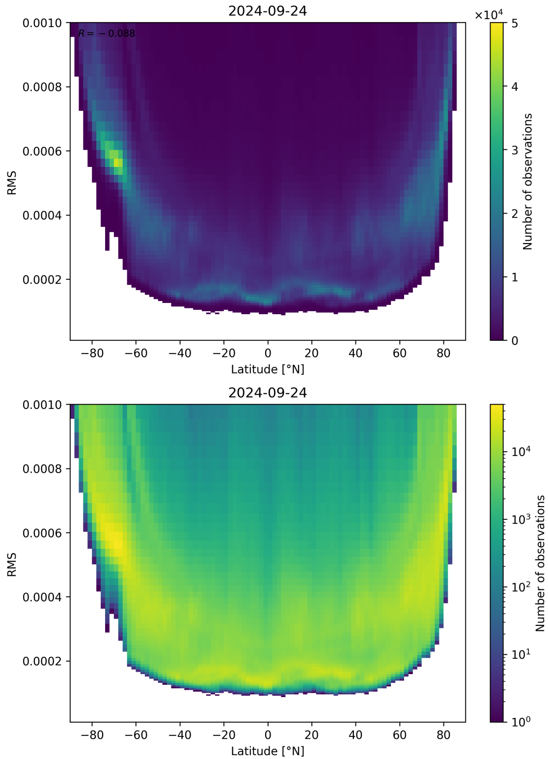
Figure 94: Scatter density plot of “Latitude” against “RMS” for 2024-09-23 to 2024-09-25.
