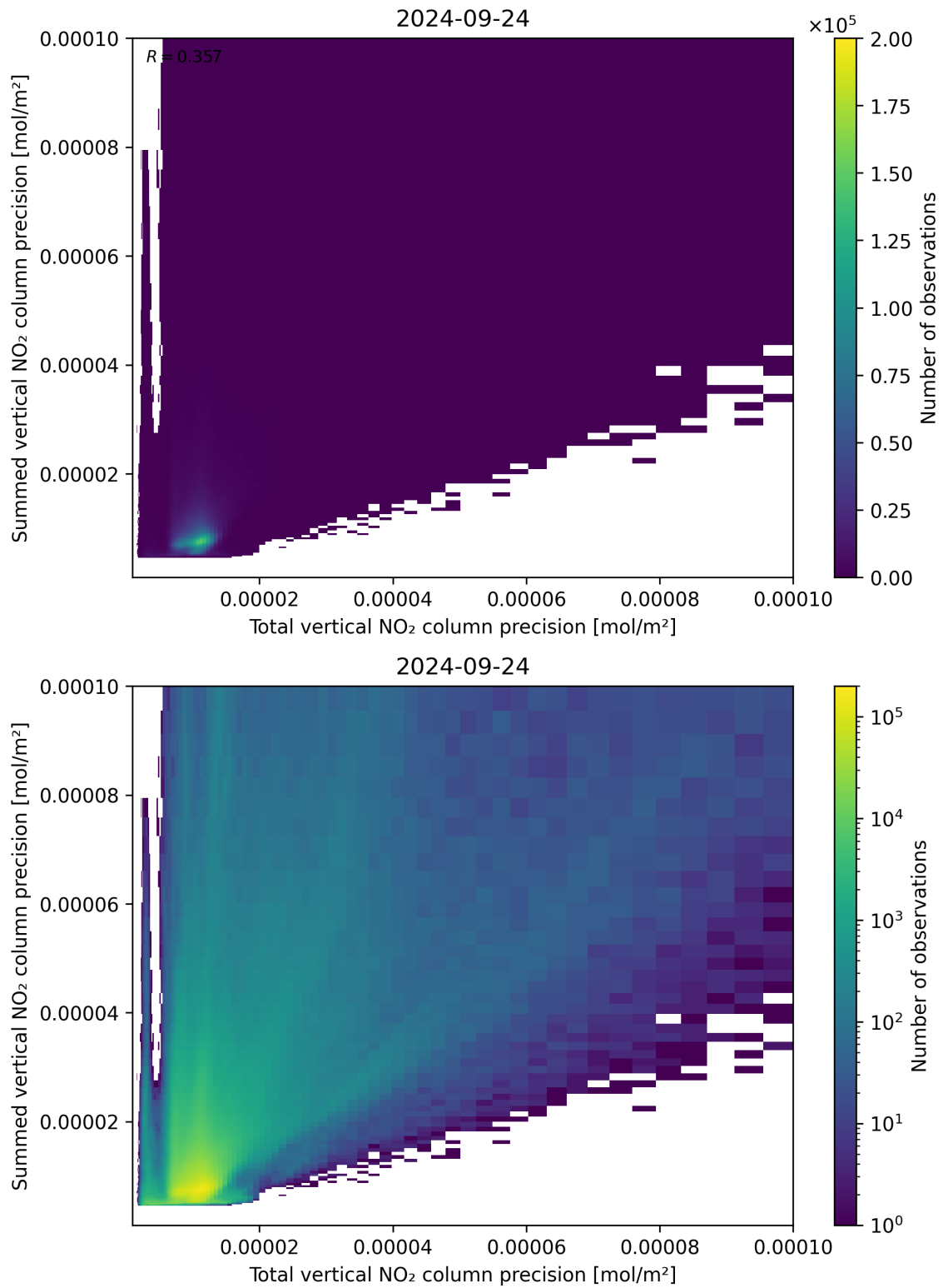
Figure 118: Scatter density plot of “Total vertical NO 2 column precision” against “Summed vertical NO 2 column precision” for 2024-09-23 to 2024-09-25.
