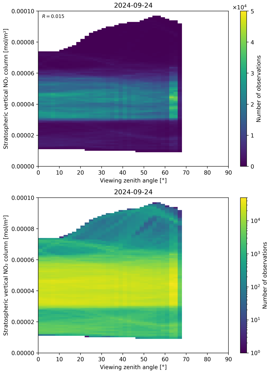
Figure 164: Scatter density plot of “Viewing zenith angle” against “Stratospheric vertical NO 2 column” for 2024-09-23 to 2024-09-25.
