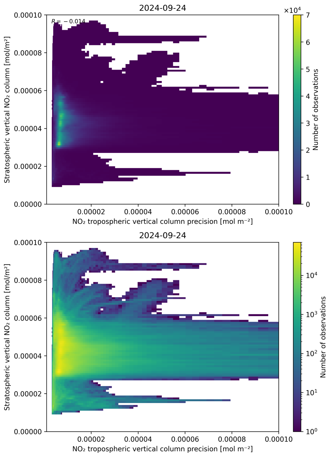
Figure 135: Scatter density plot of “NO 2 tropospheric vertical column precision” against “Stratospheric vertical NO 2 column” for 2024-09-23 to 2024-09-25.
