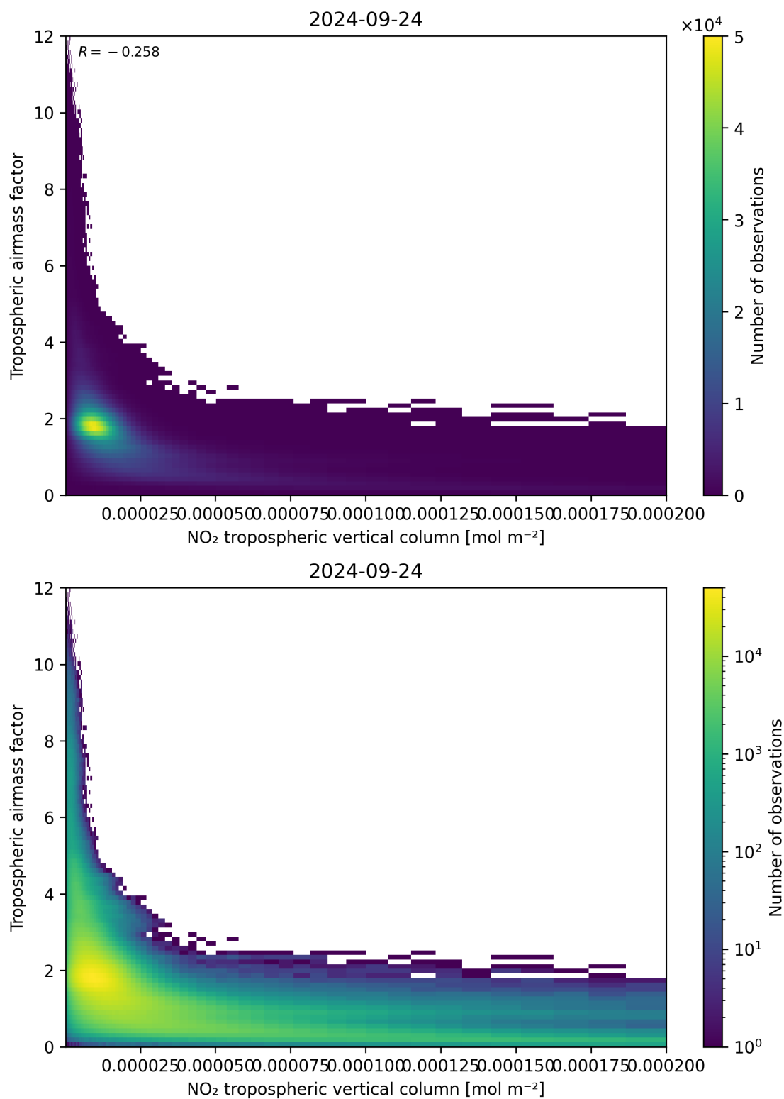
Figure 123: Scatter density plot of “NO 2 tropospheric vertical column” against “Tropospheric airmass factor” for 2024-09-23 to 2024-09-25.
