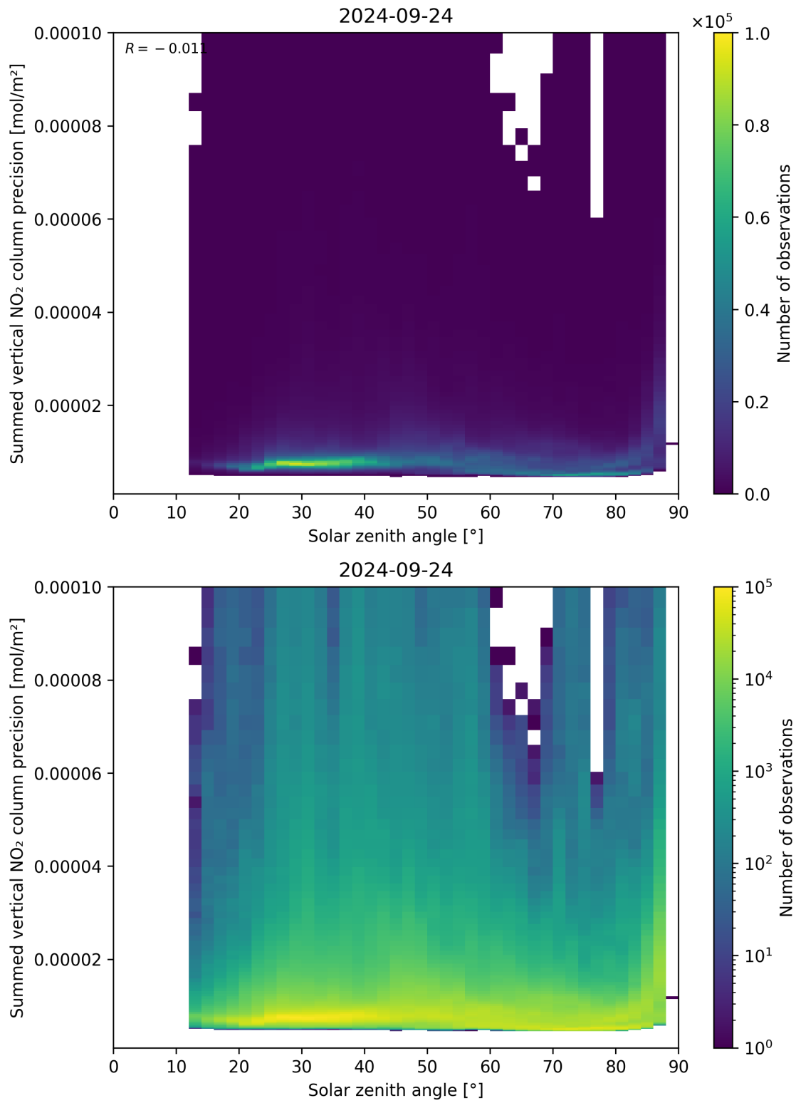
Figure 152: Scatter density plot of “Solar zenith angle” against “Summed vertical NO 2 column precision” for 2024-09-23 to 2024-09-25.
