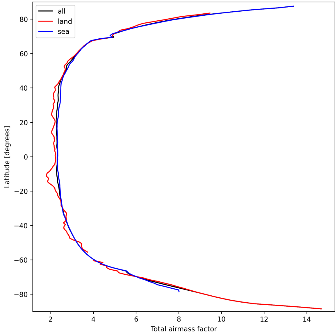
Figure 15: Zonal average of “Total airmass factor” for 2024-09-23 to 2024-09-25.
