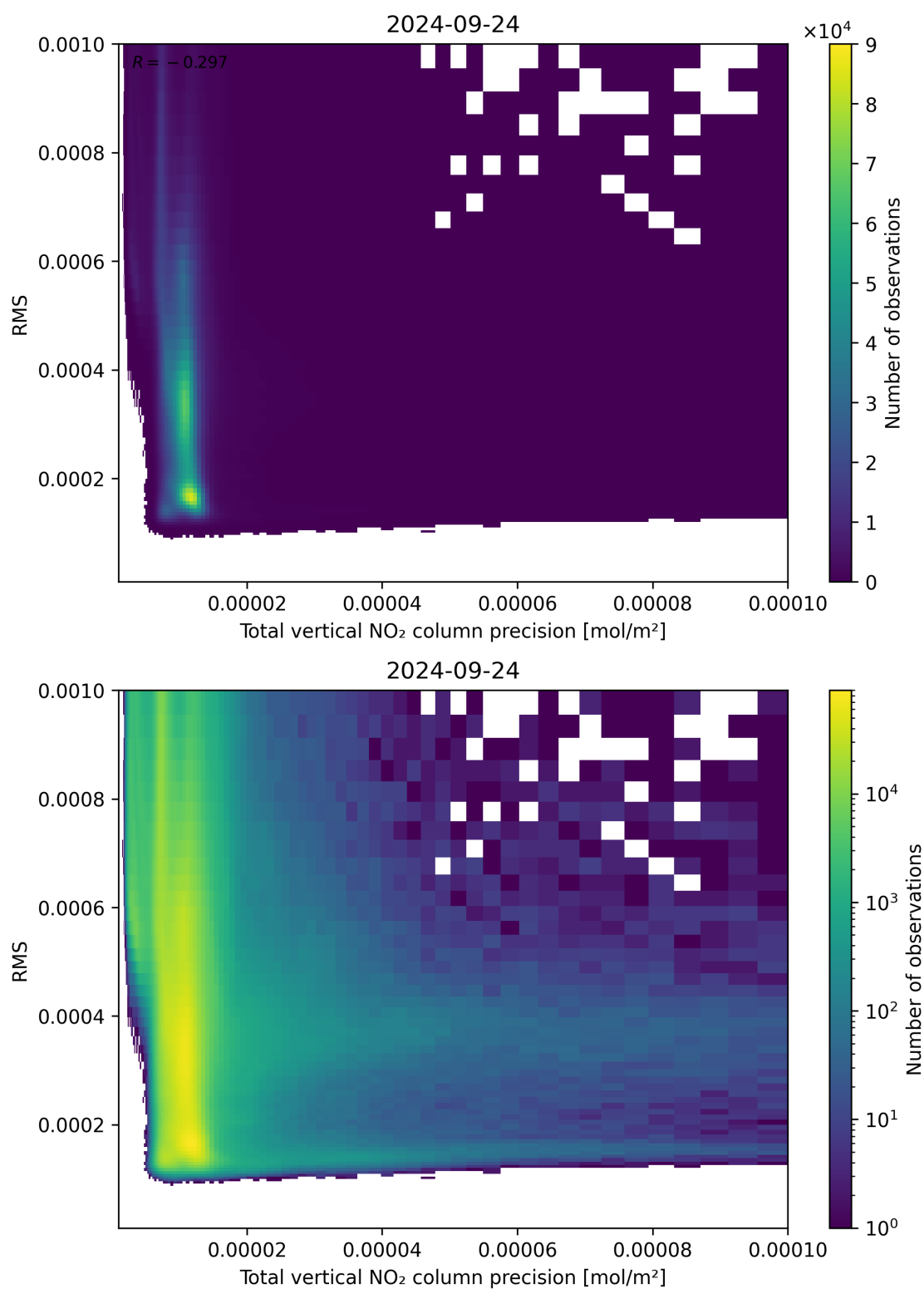
Figure 119: Scatter density plot of “Total vertical NO 2 column precision” against “RMS” for 2024-09-23 to 2024-09-25.
