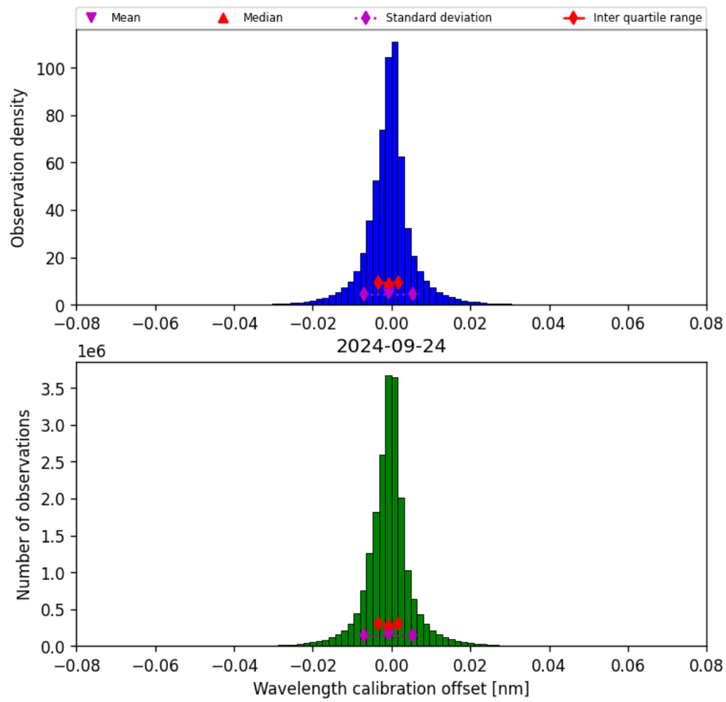
Figure 35: Histogram of “Wavelength calibration offset” for 2024-09-23 to 2024-09-25
