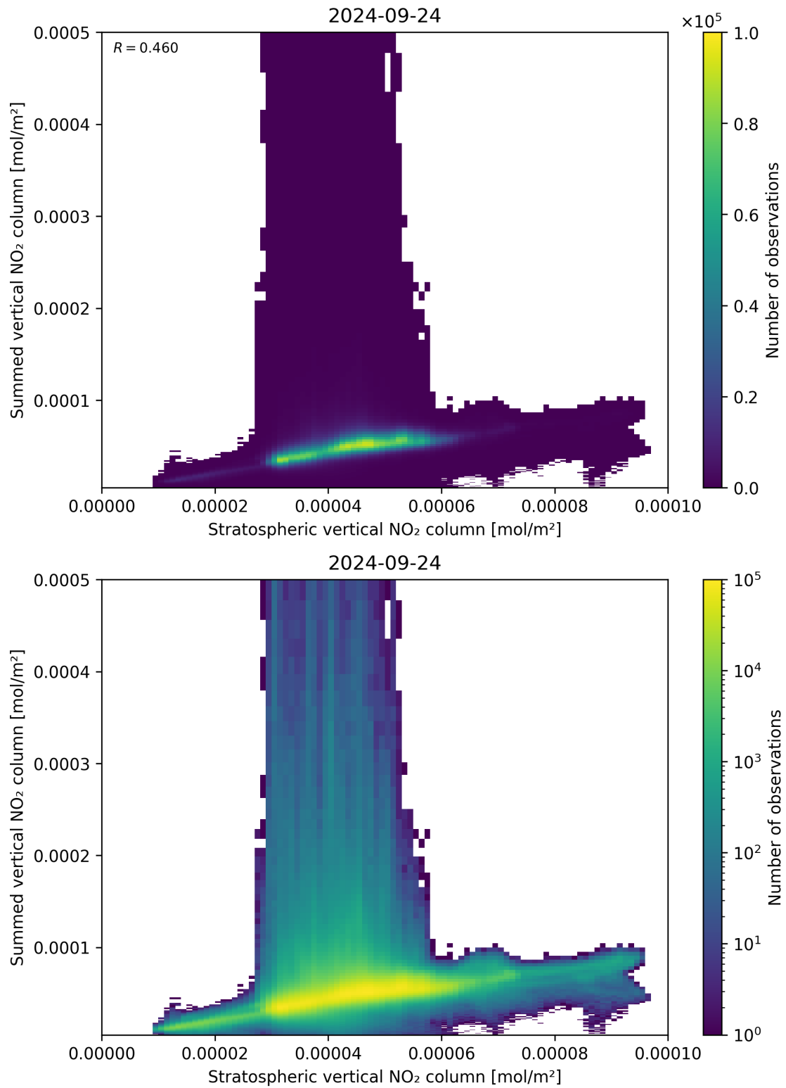
Figure 98: Scatter density plot of “Stratospheric vertical NO 2 column” against “Summed vertical NO 2 column” for 2024-09-23 to 2024-09-25.
