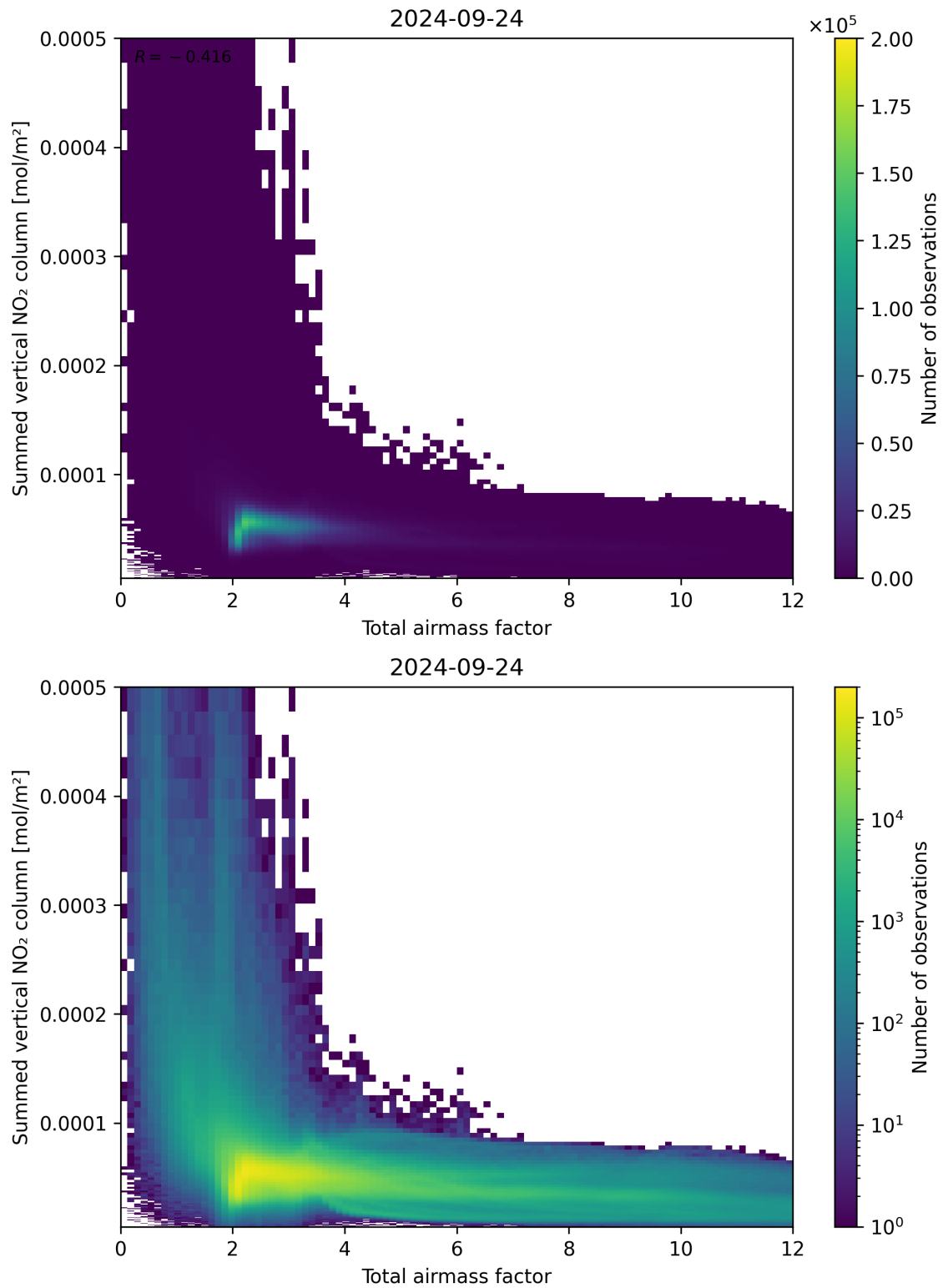
Figure 65: Scatter density plot of “Total airmass factor” against “Summed vertical NO 2 column” for 2024-09-23 to 2024-09-25.
