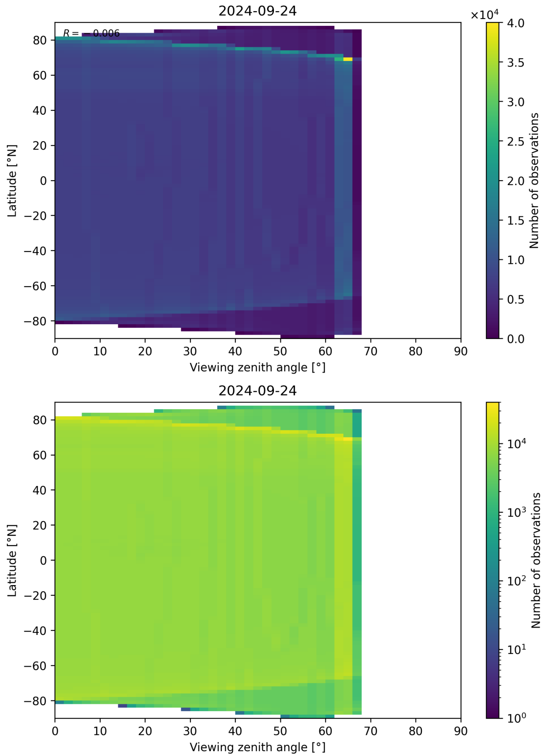
Figure 163: Scatter density plot of “Viewing zenith angle” against “Latitude” for 2024-09-23 to 2024-09-25.
