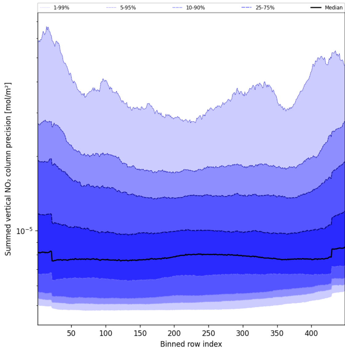
Figure 58: Along track statistics of “Summed vertical NO 2 column precision” for 2024-09-23 to 2024-09-25
