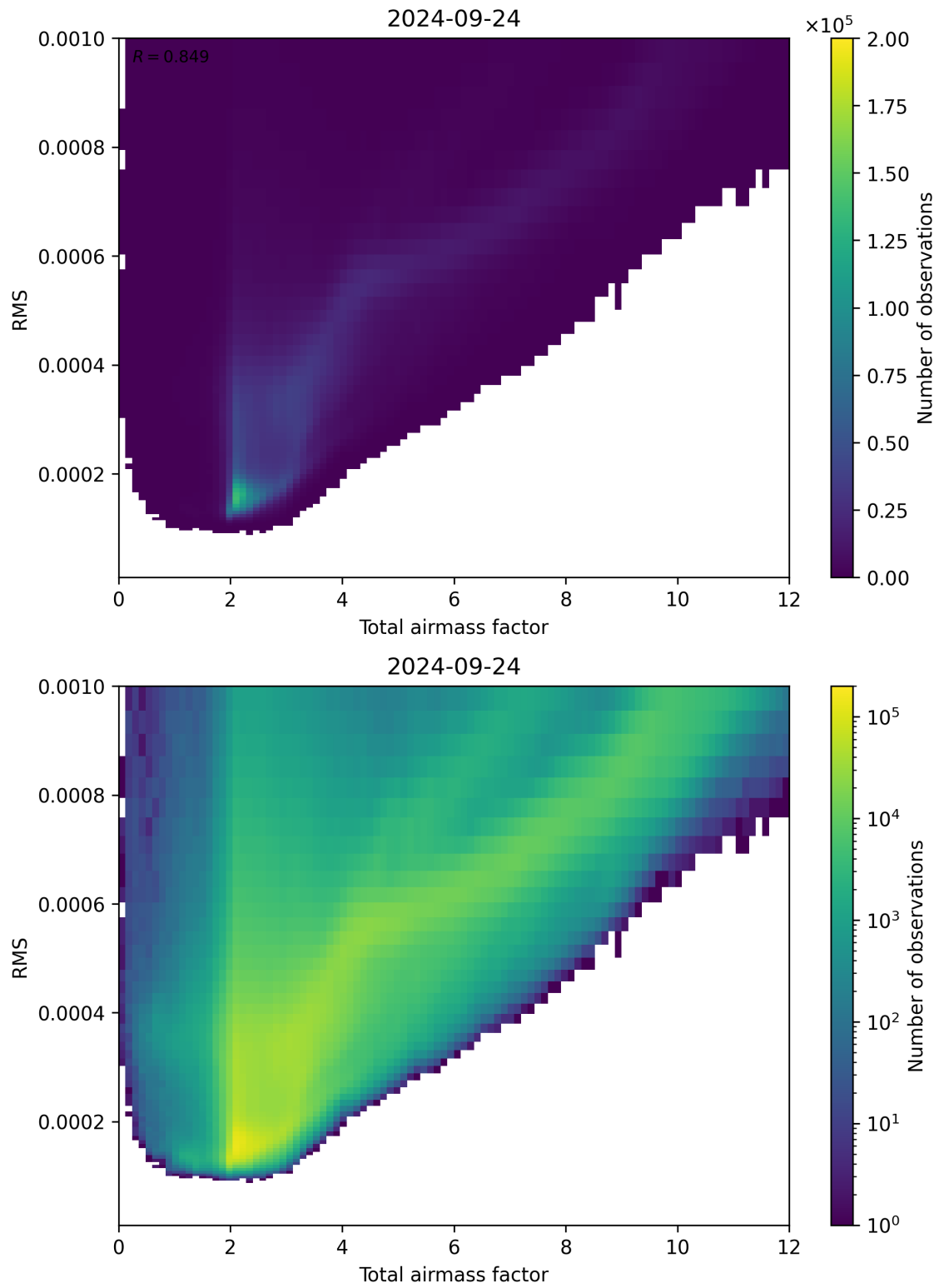
Figure 69: Scatter density plot of “Total airmass factor” against “RMS” for 2024-09-23 to 2024-09-25.
