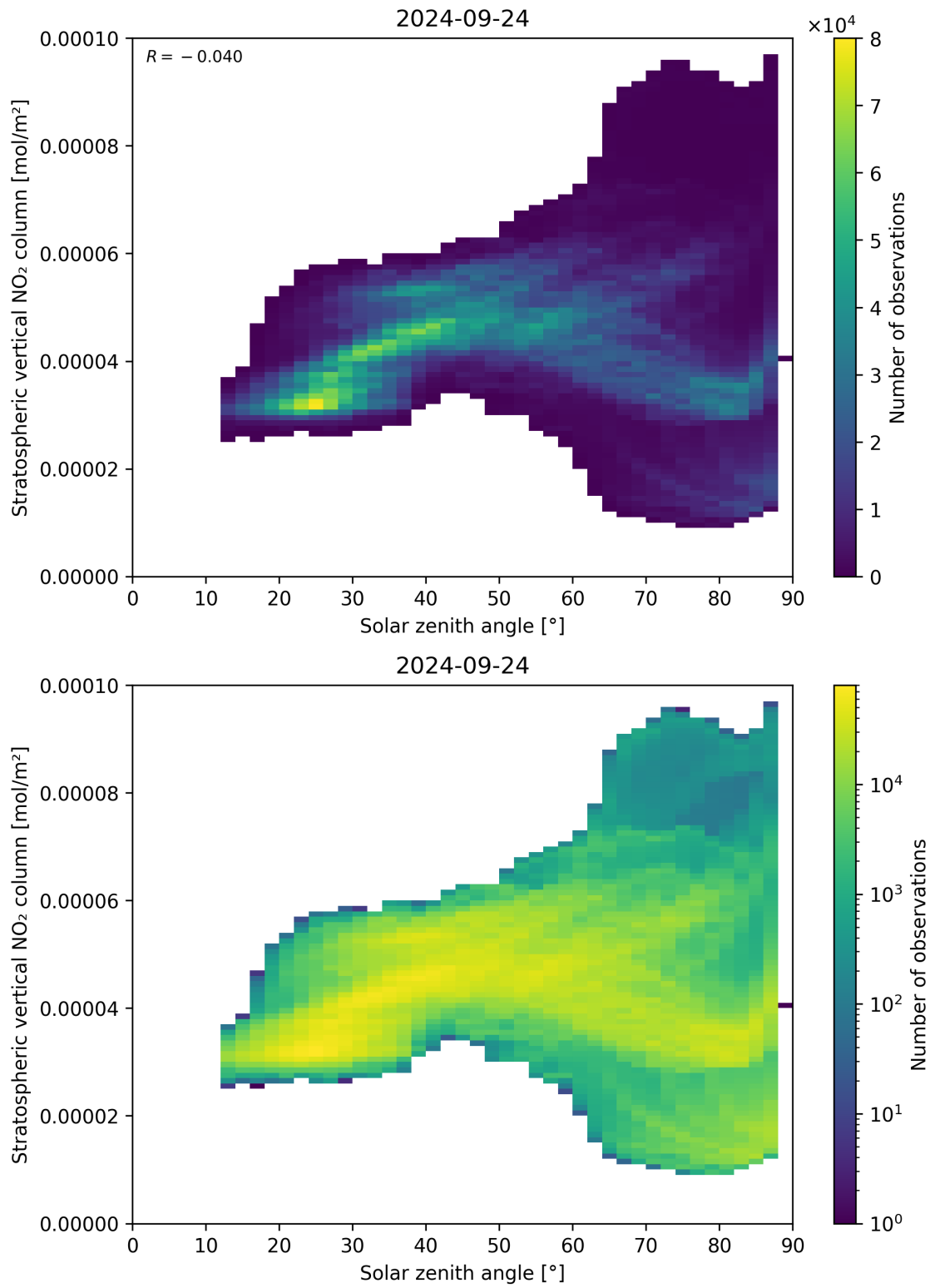
Figure 150: Scatter density plot of “Solar zenith angle” against “Stratospheric vertical NO 2 column” for 2024-09-23 to 2024-09-25.
