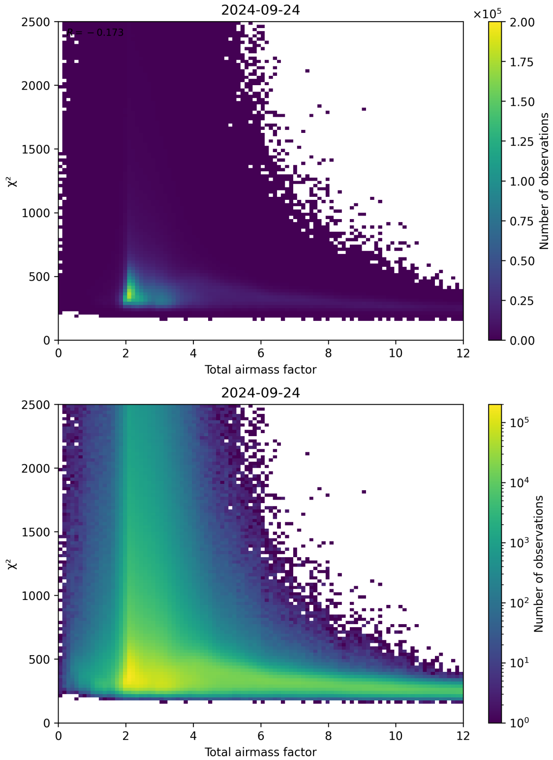
Figure 63: Scatter density plot of “Total airmass factor” against “ \chi^2 ” for 2024-09-23 to 2024-09-25.
