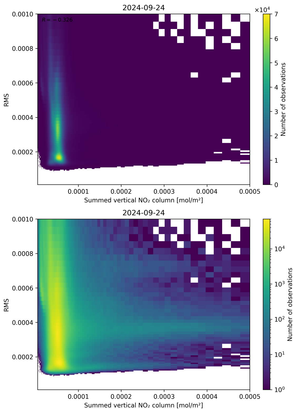
Figure 109: Scatter density plot of “Summed vertical NO 2 column” against “RMS” for 2024-09-23 to 2024-09-25.
