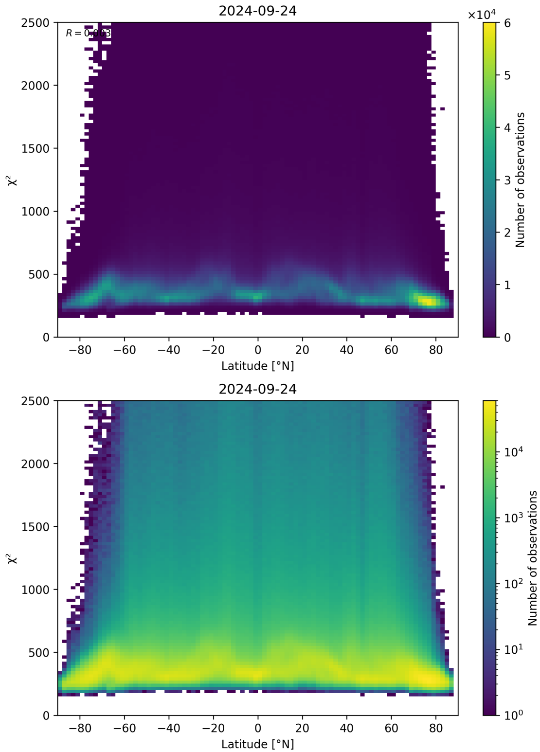
Figure 86: Scatter density plot of “Latitude” against “ \chi^2 ” for 2024-09-23 to 2024-09-25.
