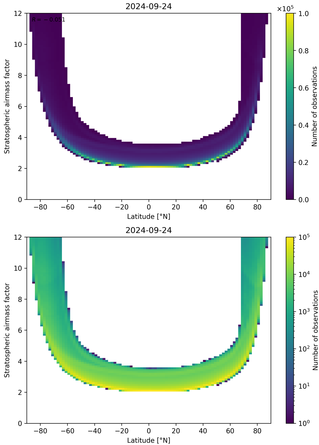
Figure 83: Scatter density plot of “Latitude” against “Stratospheric air mass factor” for 2024-09-23 to 2024-09-25.
