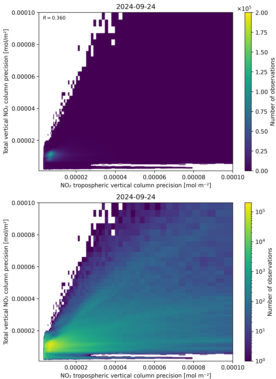
Figure 139: Scatter density plot of “NO 2 tropospheric vertical column precision” against “Total vertical NO 2 column precision” for 2024-09-23 to 2024-09-25.
