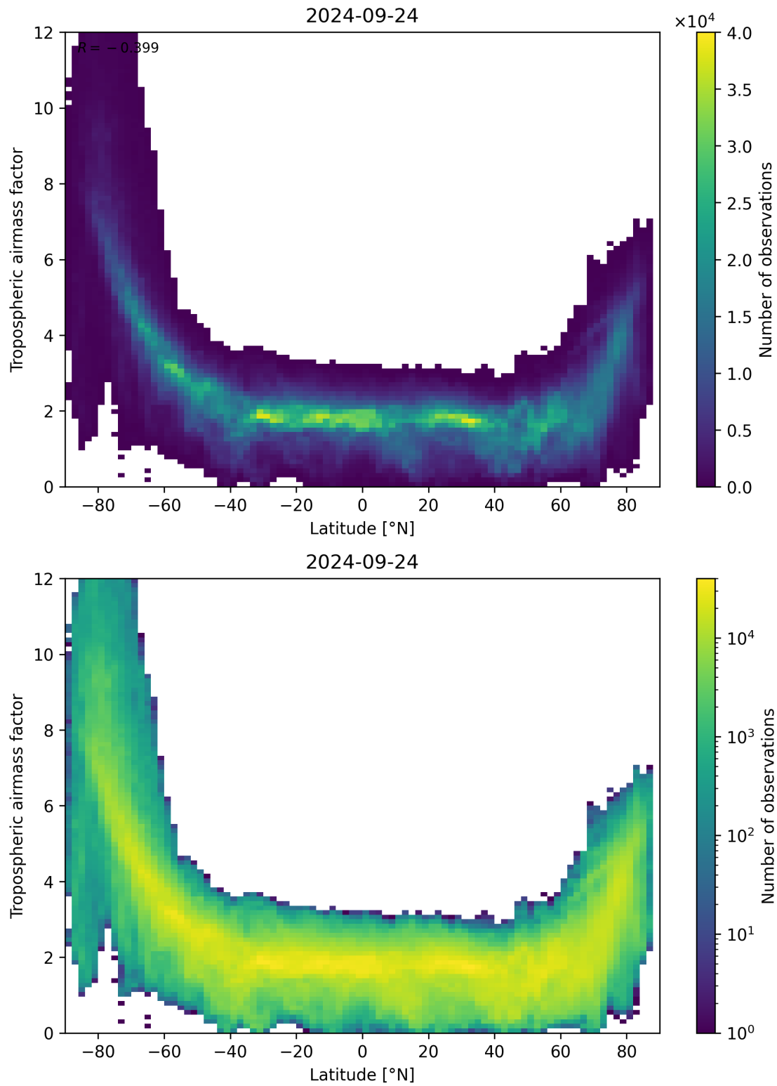
Figure 85: Scatter density plot of “Latitude” against “Tropospheric air mass factor” for 2024-09-23 to 2024-09-25.
