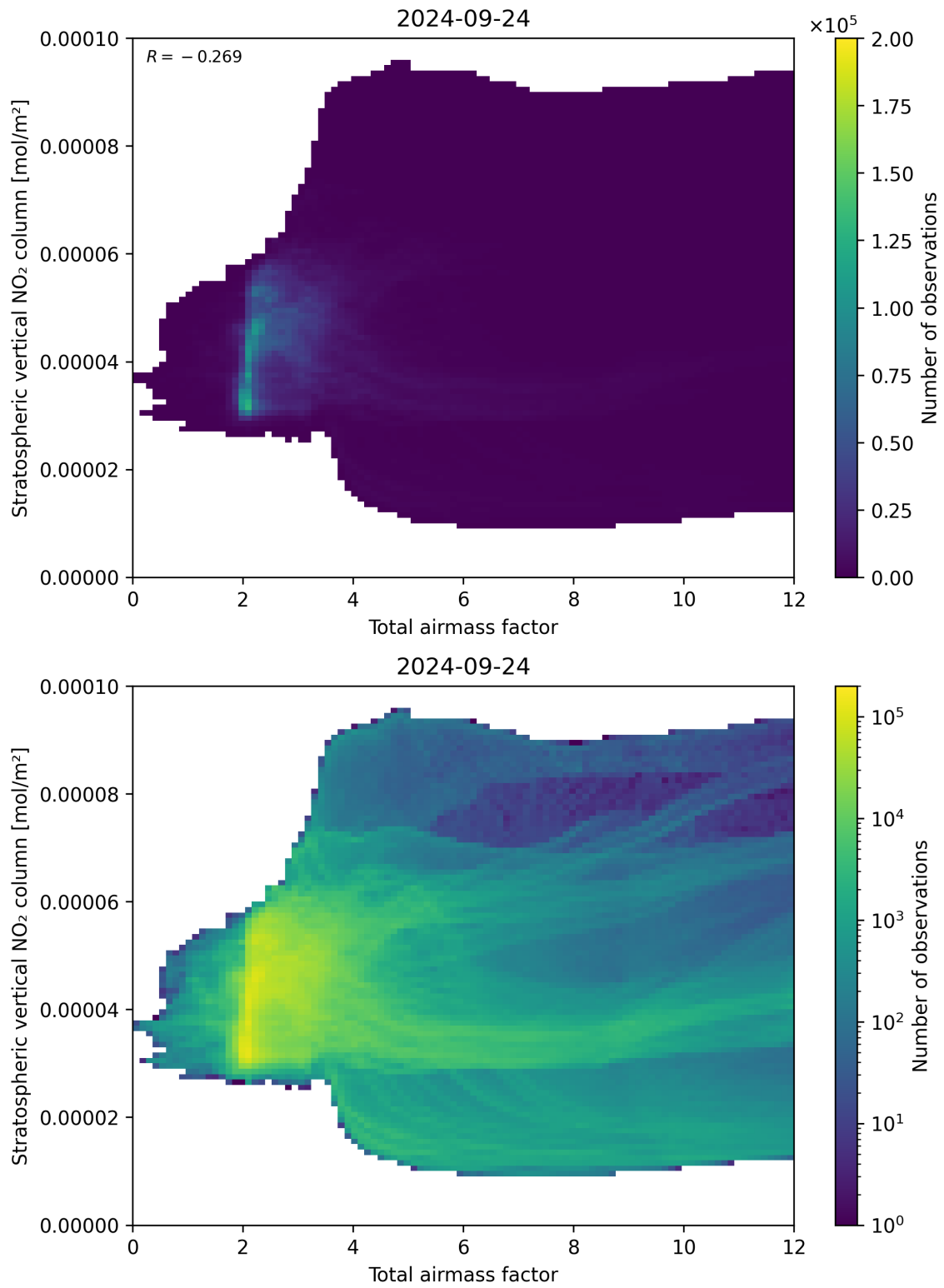
Figure 64: Scatter density plot of “Total airmass factor” against “Stratospheric vertical \text{NO}_2 column” for 2024-09-23 to 2024-09-25.
