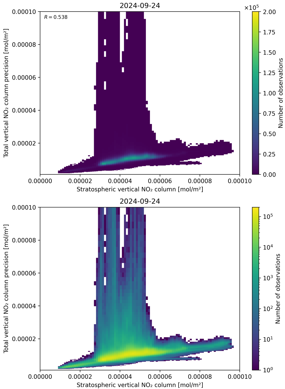
Figure 101: Scatter density plot of “Stratospheric vertical NO 2 column” against “Total vertical NO 2 column precision” for 2024-09-23 to 2024-09-25.
