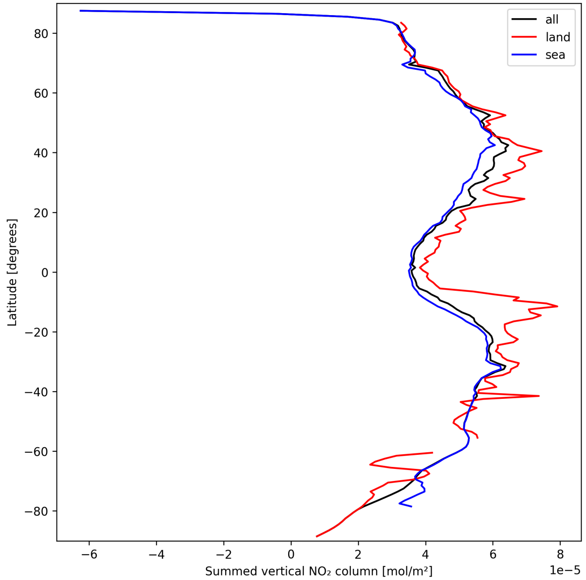
Figure 23: Zonal average of “Summed vertical NO 2 column” for 2024-09-23 to 2024-09-25.
