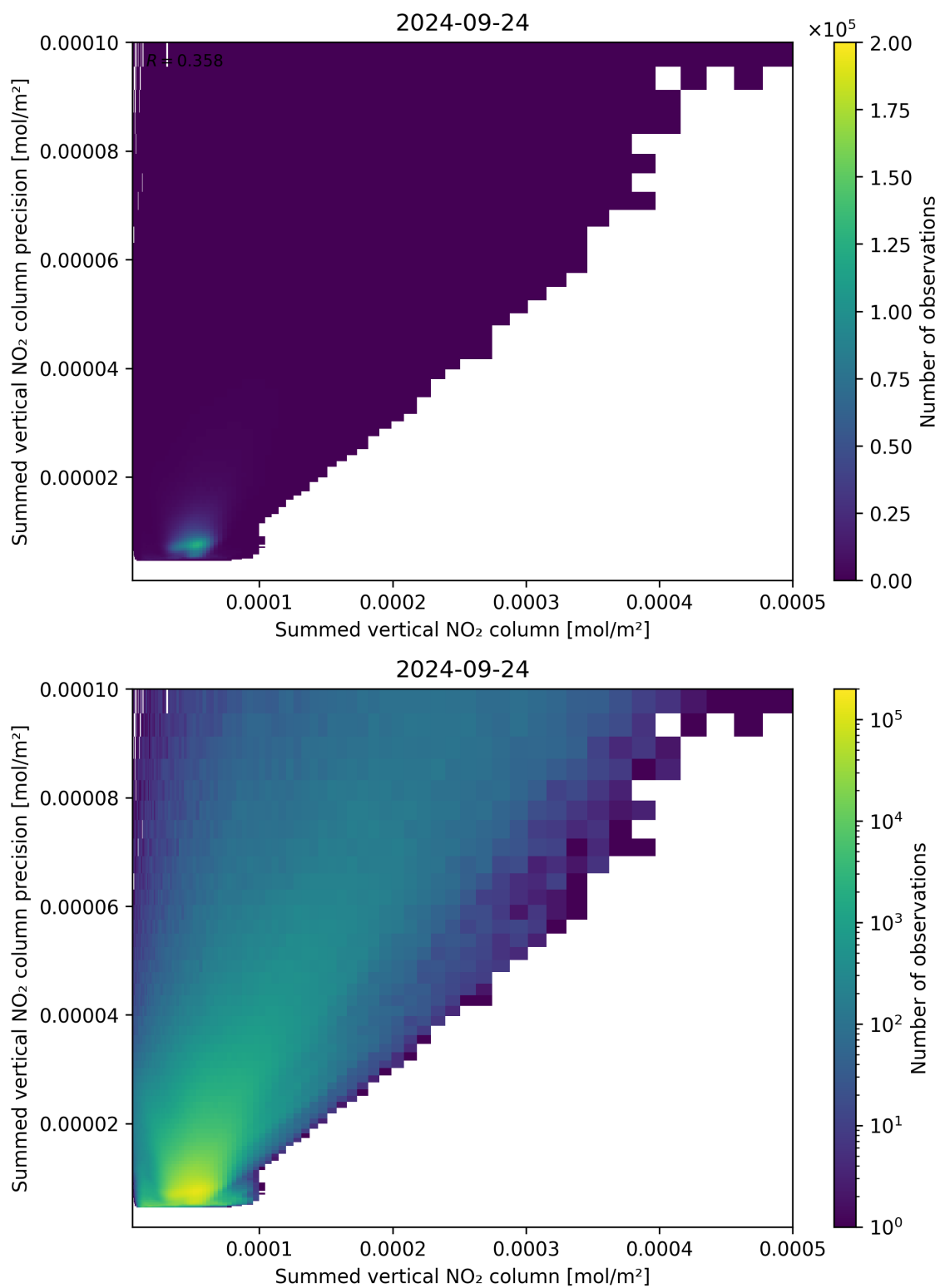
Figure 105: Scatter density plot of “Summed vertical NO 2 column” against “Summed vertical NO 2 column precision” for 2024-09-23 to 2024-09-25.
