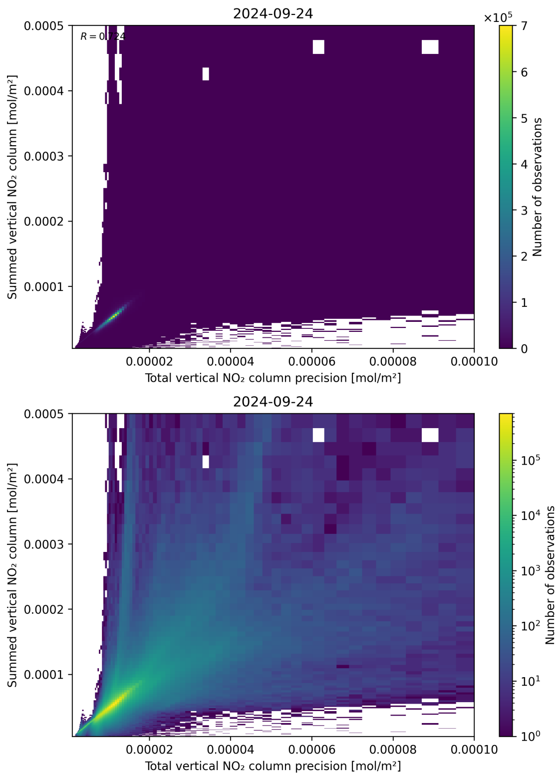
Figure 117: Scatter density plot of “Total vertical NO 2 column precision” against “Summed vertical NO 2 column” for 2024-09-23 to 2024-09-25.
