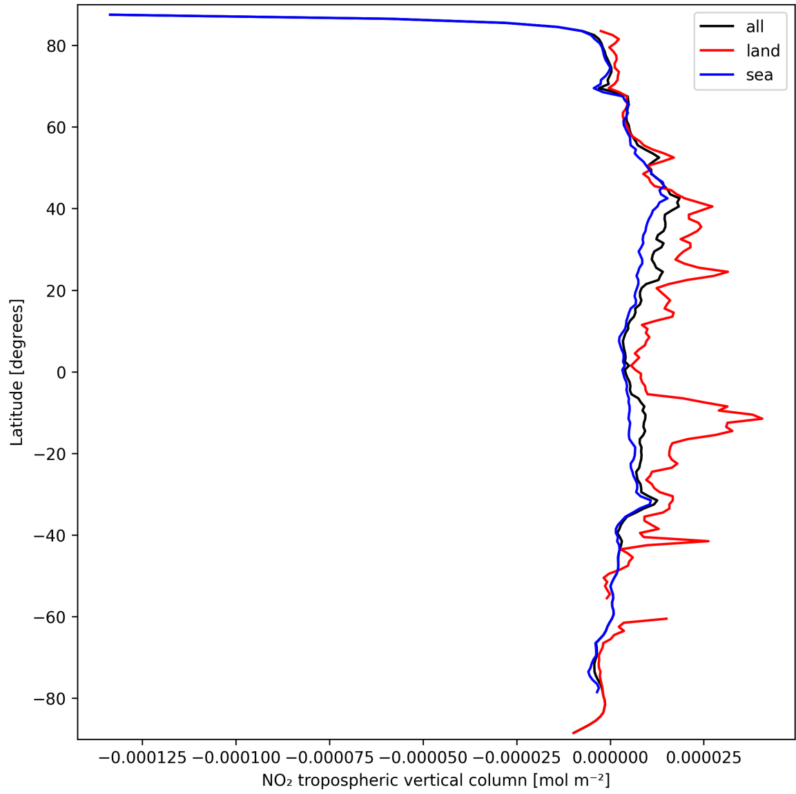
Figure 12: Zonal average of “NO 2 tropospheric vertical column” for 2024-09-23 to 2024-09-25.
