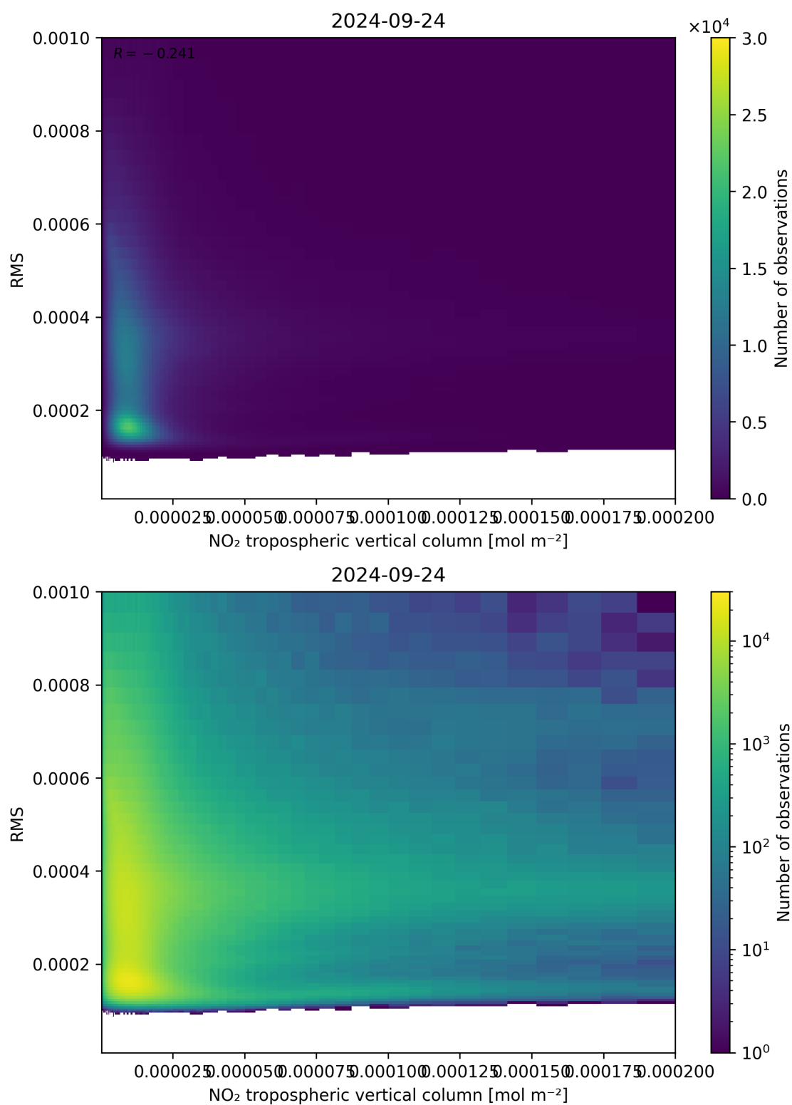
Figure 142: Scatter density plot of “NO 2 tropospheric vertical column” against “RMS” for 2024-09-23 to 2024-09-25.
