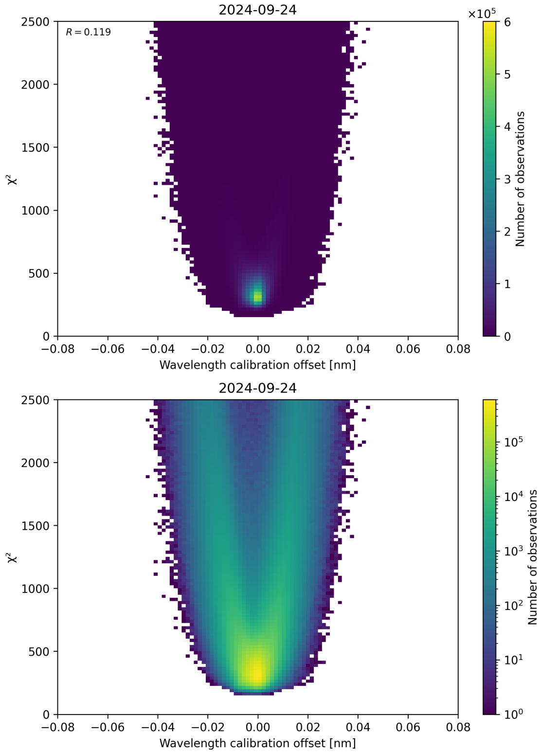
Figure 175: Scatter density plot of “Wavelength calibration offset” against “ \chi^2 ” for 2024-09-23 to 2024-09-25.
