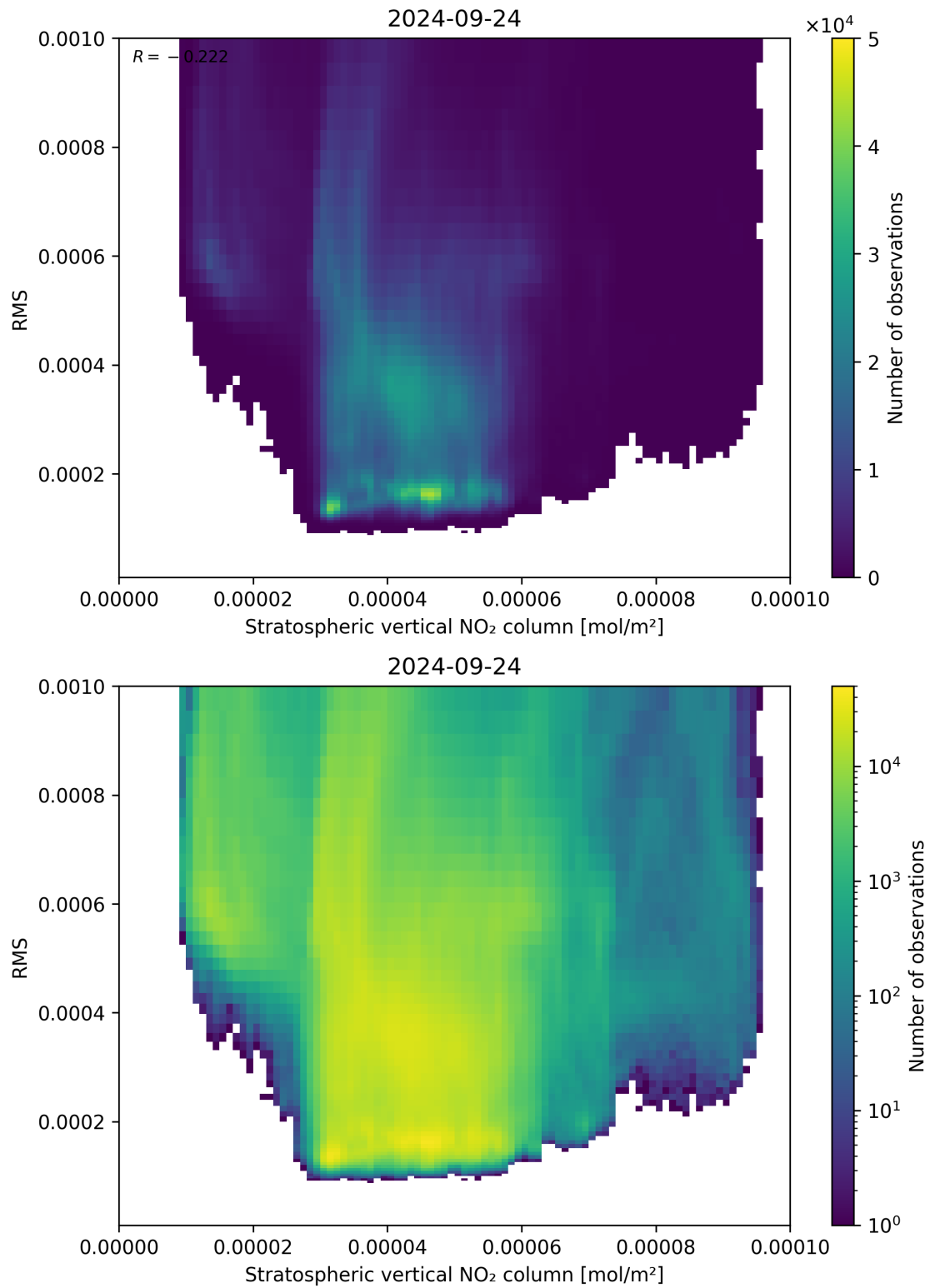
Figure 102: Scatter density plot of “Stratospheric vertical NO 2 column” against “RMS” for 2024-09-23 to 2024-09-25.
