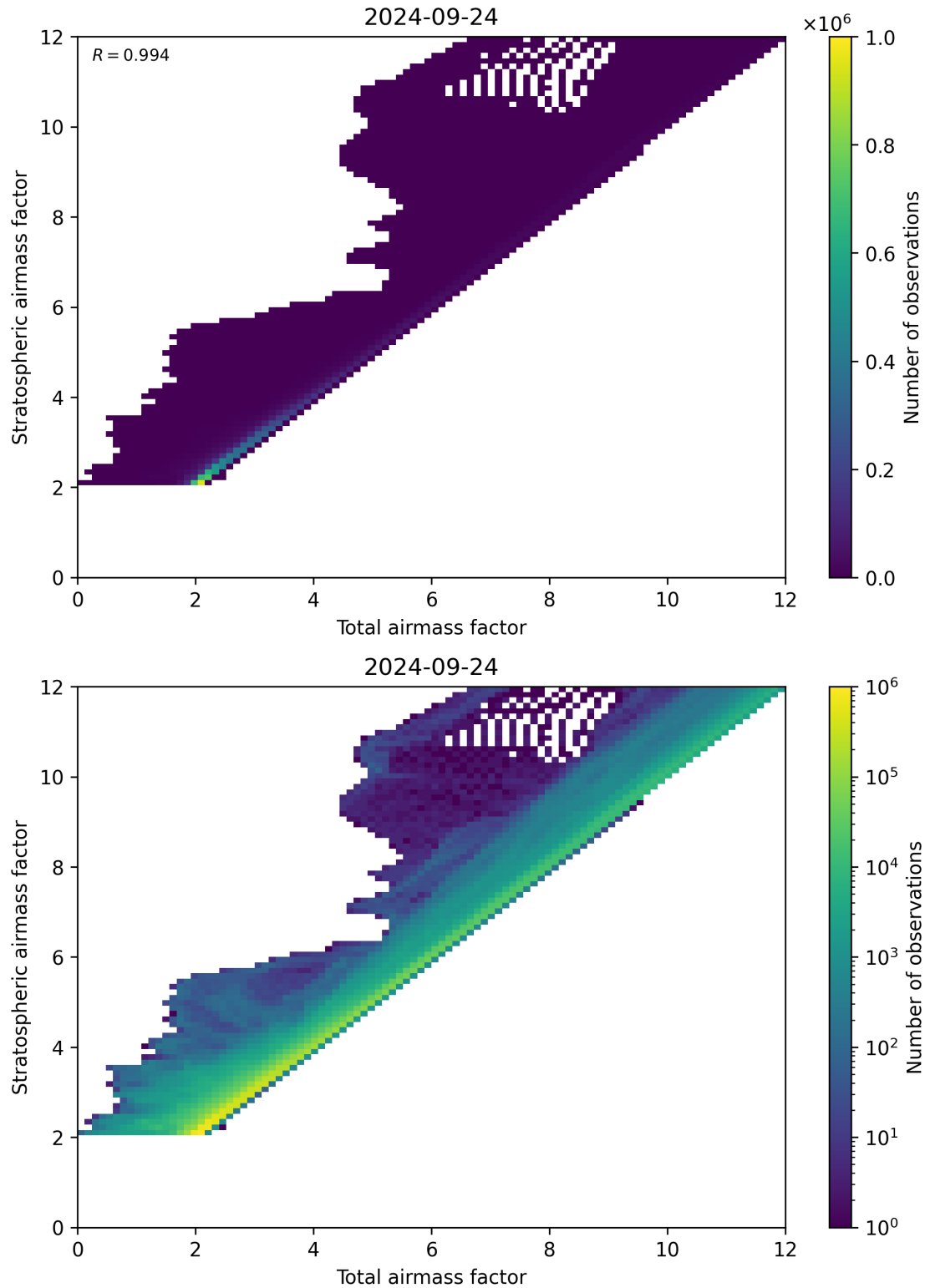
Figure 62: Scatter density plot of “Total airmass factor” against “Stratospheric airmass factor” for 2024-09-23 to 2024-09-25.
