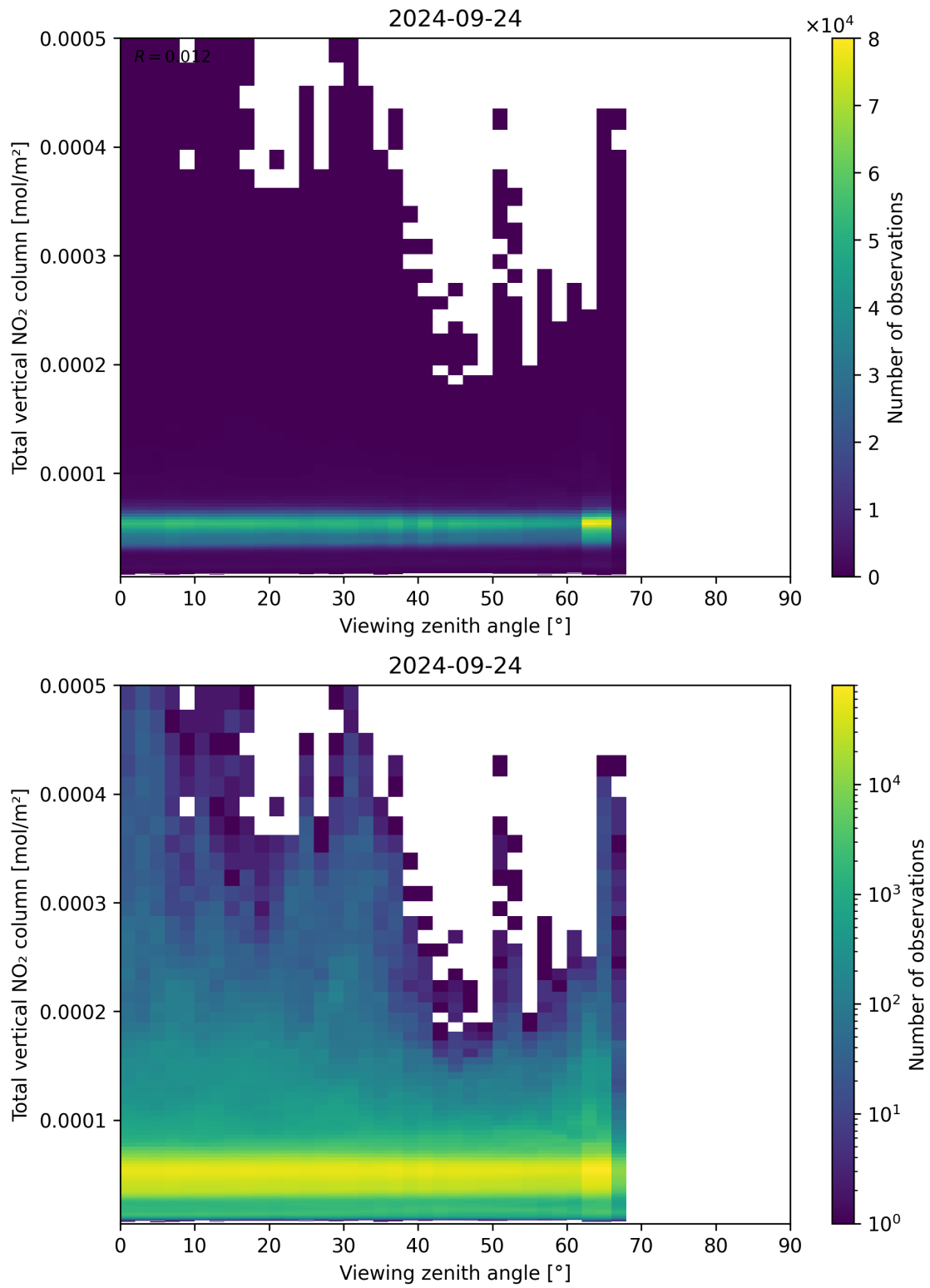
Figure 167: Scatter density plot of “Viewing zenith angle” against “Total vertical NO 2 column” for 2024-09-23 to 2024-09-25.
