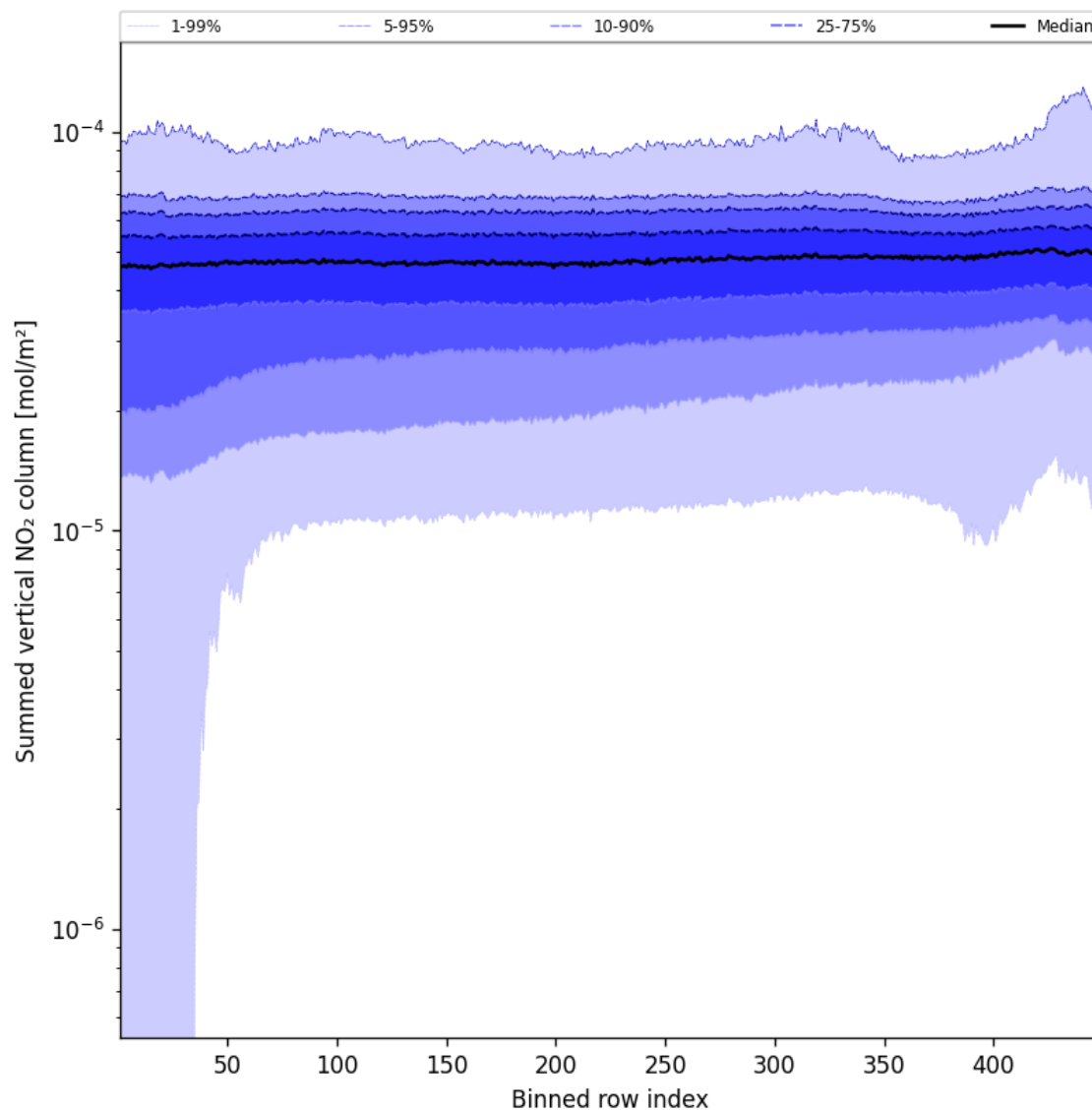
Figure 57: Along track statistics of “Summed vertical NO 2 column” for 2024-09-23 to 2024-09-25
