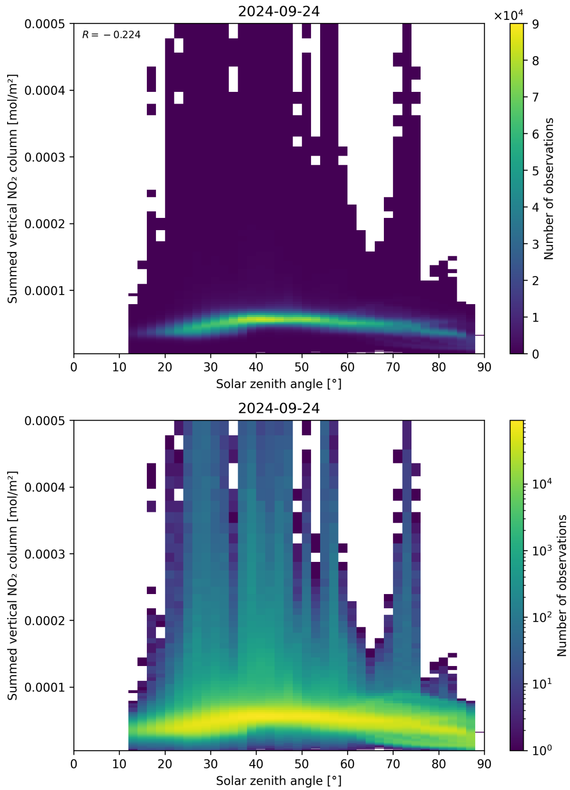
Figure 151: Scatter density plot of “Solar zenith angle” against “Summed vertical NO 2 column” for 2024-09-23 to 2024-09-25.
