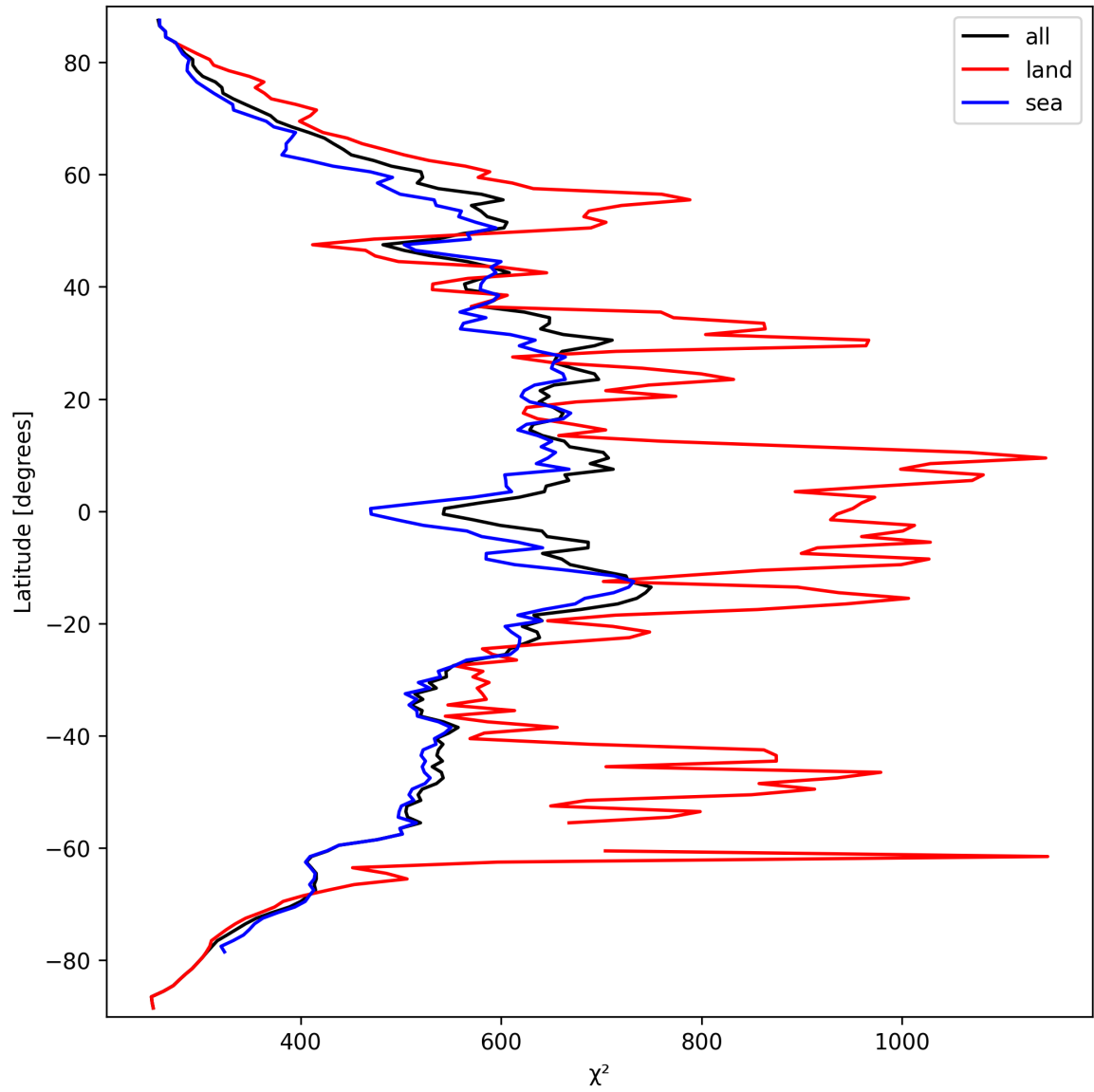
Figure 25: Zonal average of “ \chi^2 ” for 2024-09-23 to 2024-09-25.
