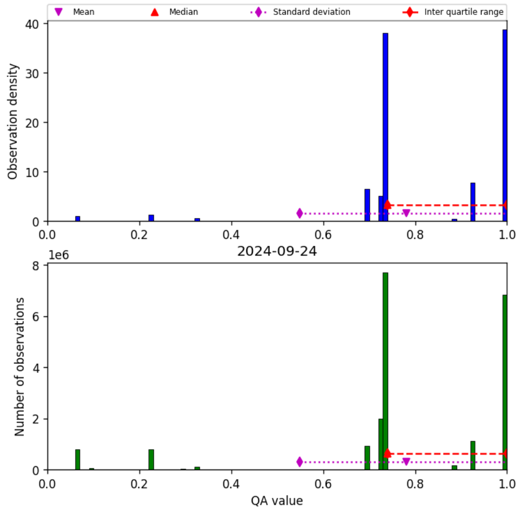
Figure 28: Histogram of “QA value” for 2024-09-23 to 2024-09-25
