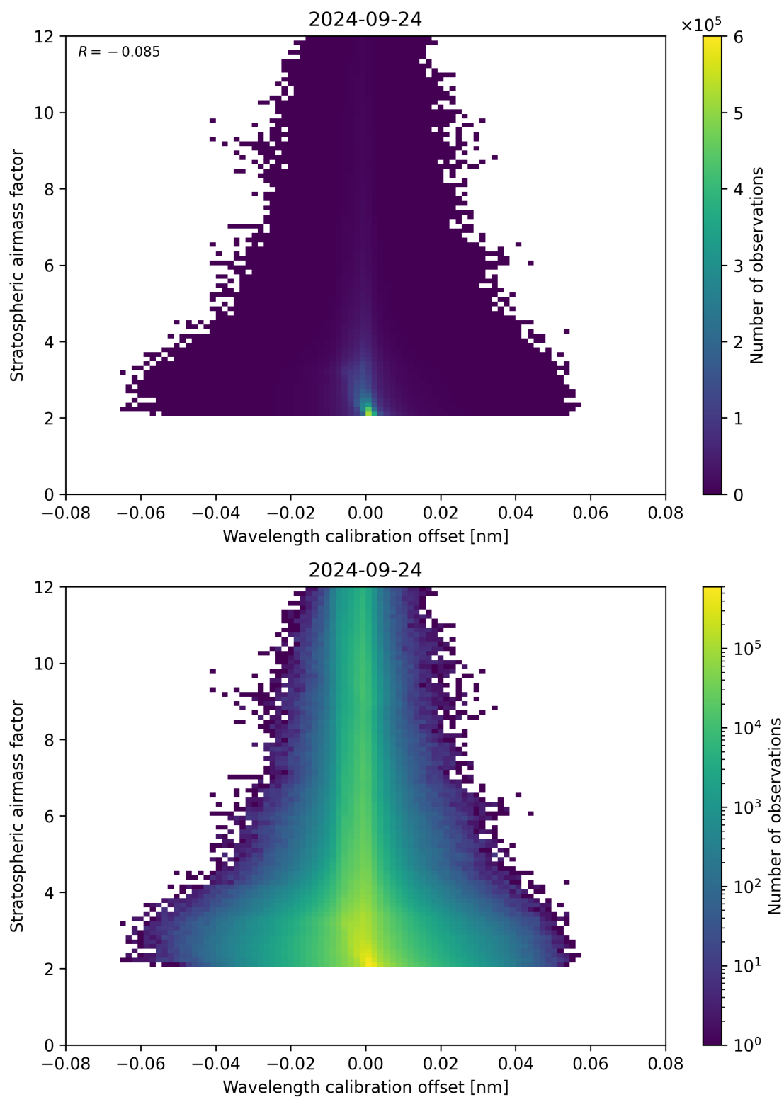
Figure 174: Scatter density plot of “Wavelength calibration offset” against “Stratospheric airmass factor” for 2024-09-23 to 2024-09-25.
