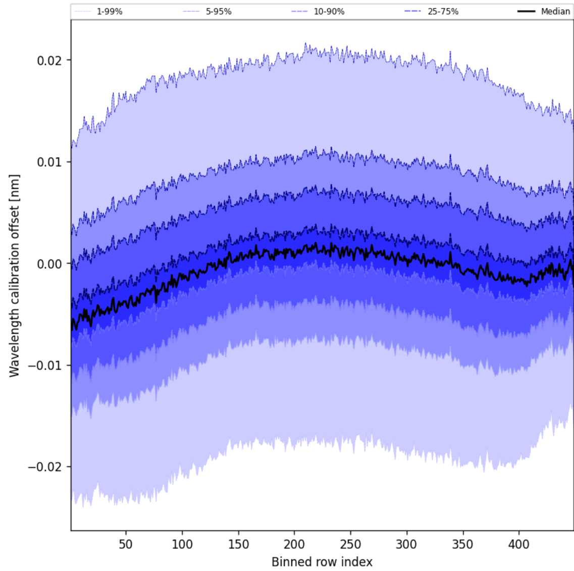
Figure 52: Along track statistics of “Wavelength calibration offset” for 2024-09-23 to 2024-09-25
