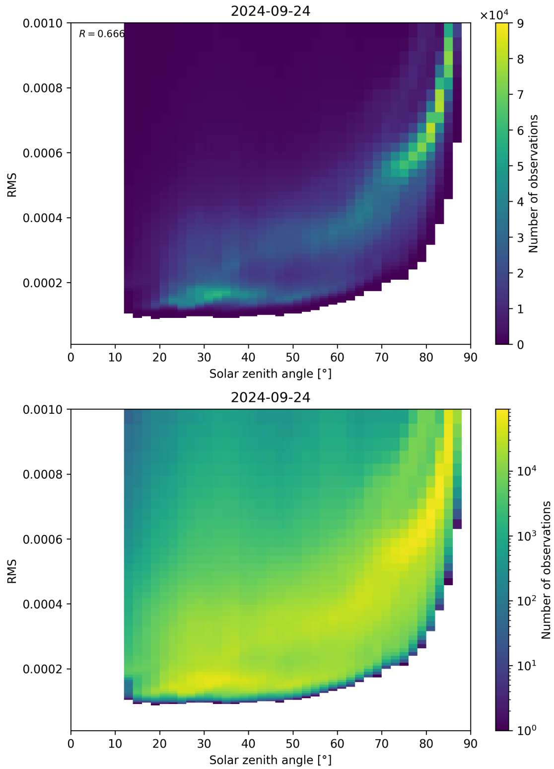
Figure 157: Scatter density plot of “Solar zenith angle” against “RMS” for 2024-09-23 to 2024-09-25.
