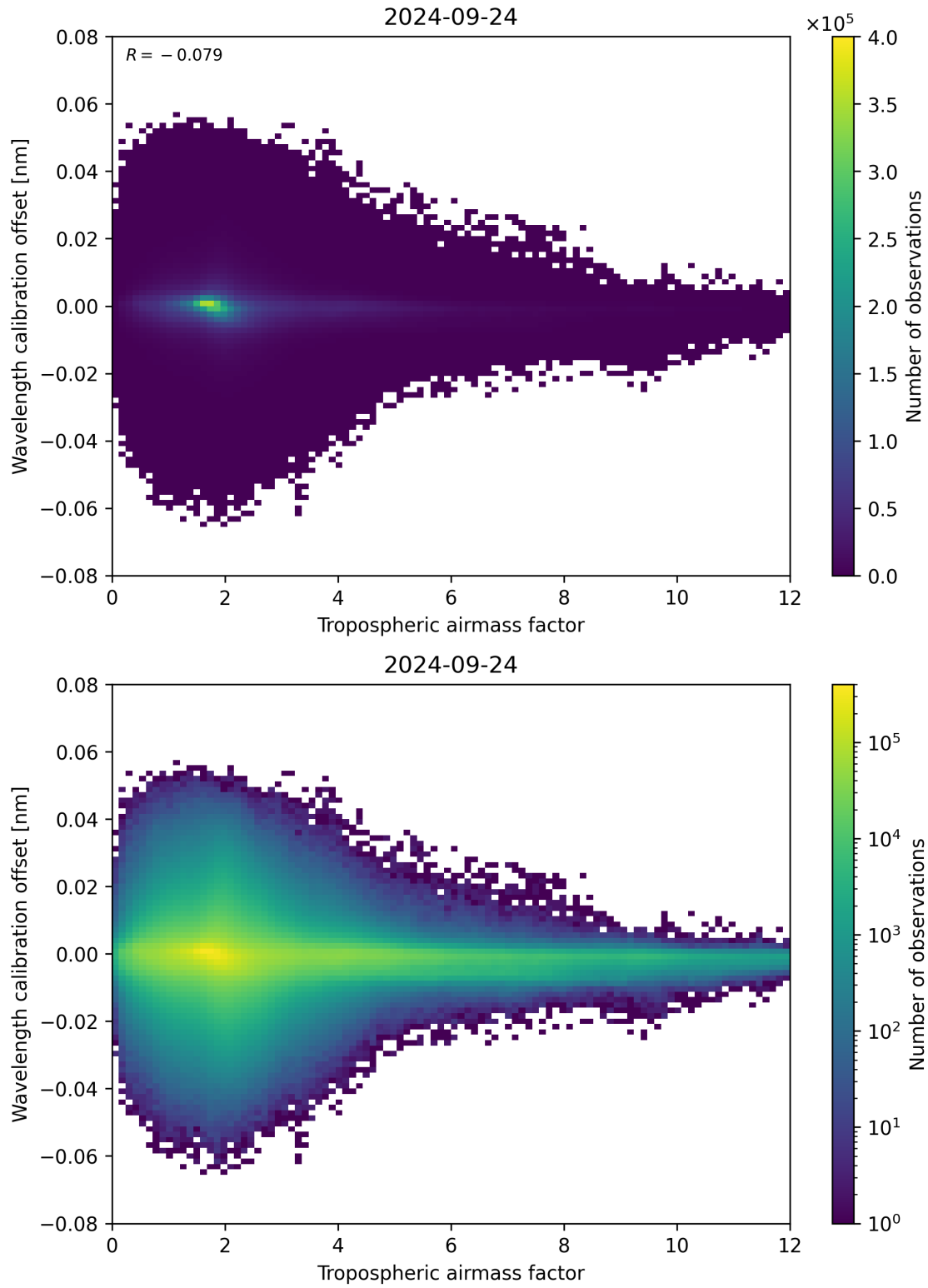
Figure 80: Scatter density plot of “Tropospheric airmass factor” against “Wavelength calibration offset” for 2024-09-23 to 2024-09-25.
