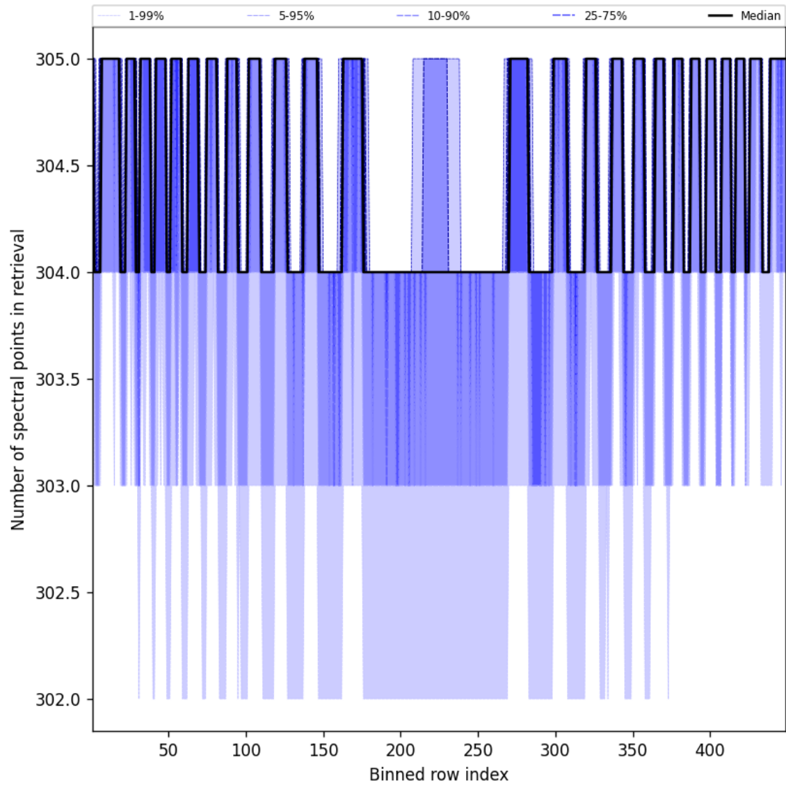
Figure 50: Along track statistics of “Number of spectral points in retrieval” for 2024-09-23 to 2024-09-25
