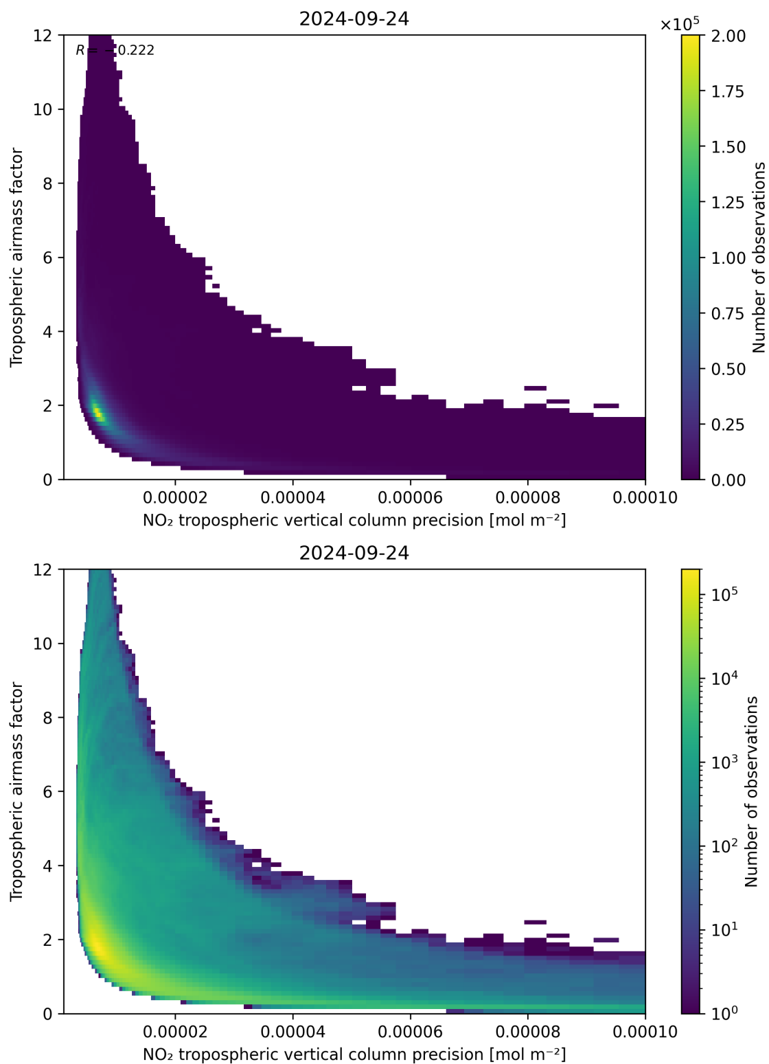
Figure 133: Scatter density plot of “NO 2 tropospheric vertical column precision” against “Tropospheric air mass factor” for 2024-09-23 to 2024-09-25.
