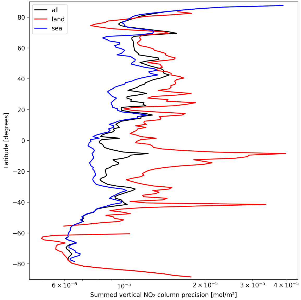
Figure 24: Zonal average of “Summed vertical NO 2 column precision” for 2024-09-23 to 2024-09-25.
