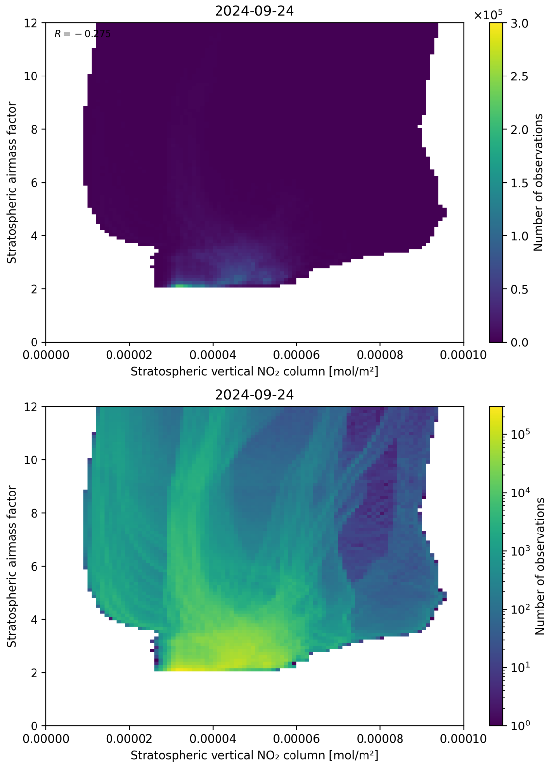
Figure 96: Scatter density plot of “Stratospheric vertical NO 2 column” against “Stratospheric airmass factor” for 2024-09-23 to 2024-09-25.
