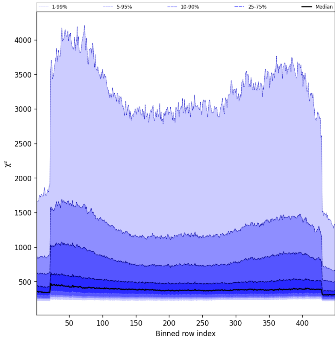
Figure 59: Along track statistics of “ \chi^2 ” for 2024-09-23 to 2024-09-25
