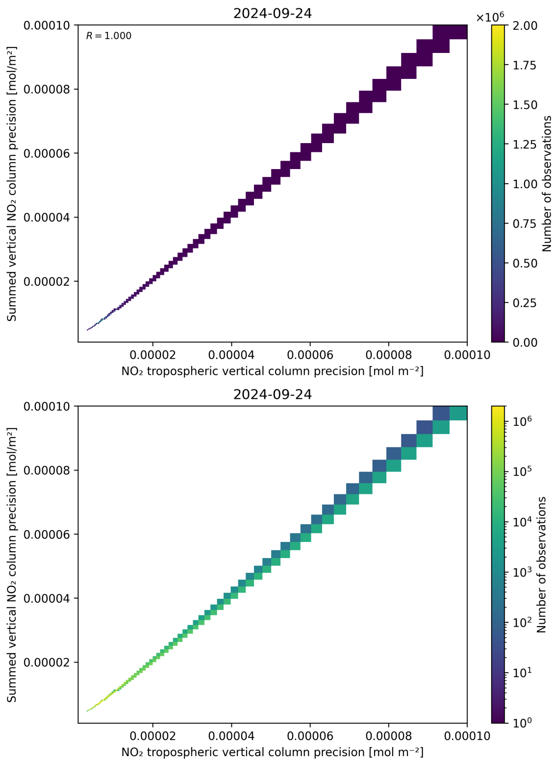
Figure 137: Scatter density plot of “NO 2 tropospheric vertical column precision” against “Summed vertical NO 2 column precision” for 2024-09-23 to 2024-09-25.
