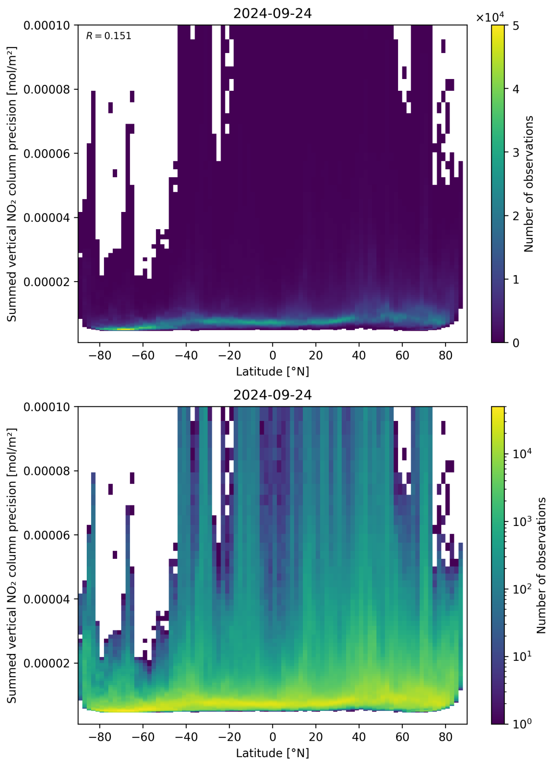
Figure 89: Scatter density plot of “Latitude” against “Summed vertical NO 2 column precision” for 2024-09-23 to 2024-09-25.
