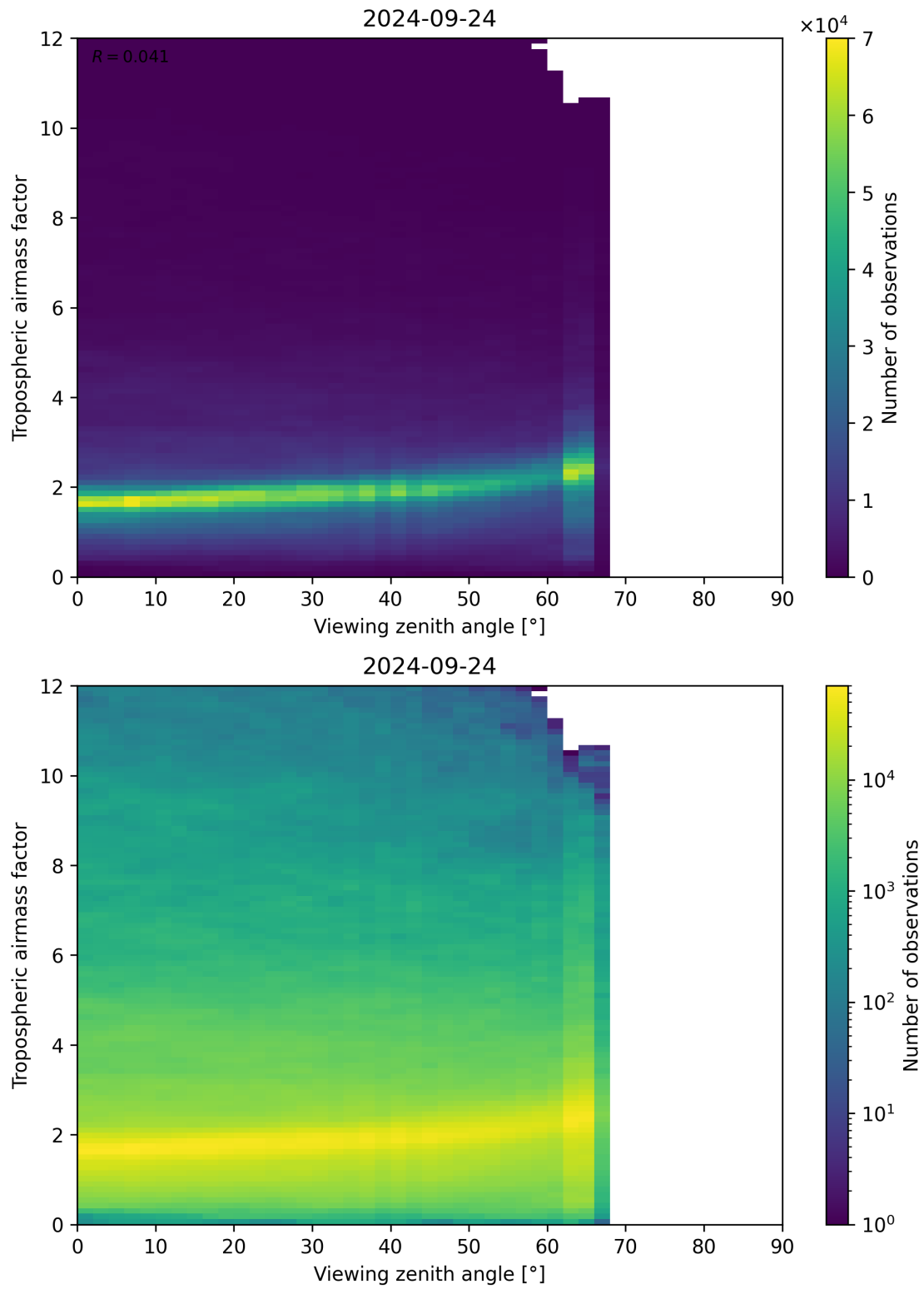
Figure 161: Scatter density plot of “Viewing zenith angle” against “Tropospheric airmass factor” for 2024-09-23 to 2024-09-25.
