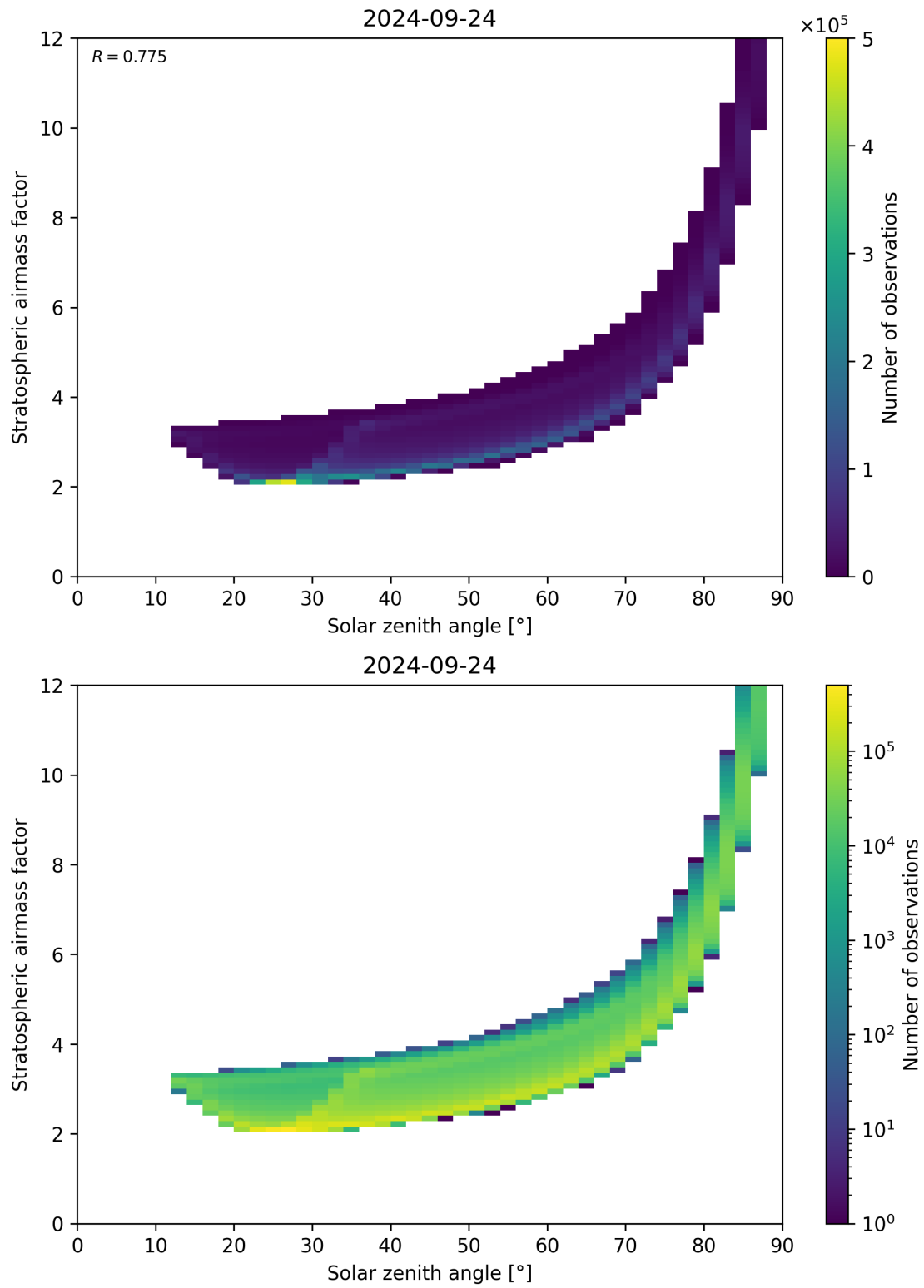
Figure 145: Scatter density plot of “Solar zenith angle” against “Stratospheric airmass factor” for 2024-09-23 to 2024-09-25.
