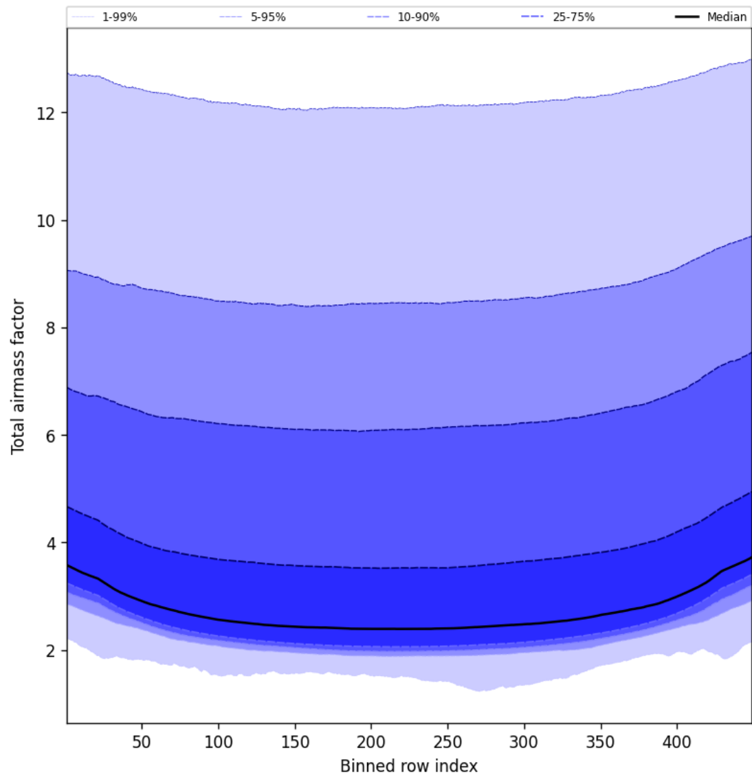
Figure 49: Along track statistics of “Total airmass factor” for 2024-09-23 to 2024-09-25
