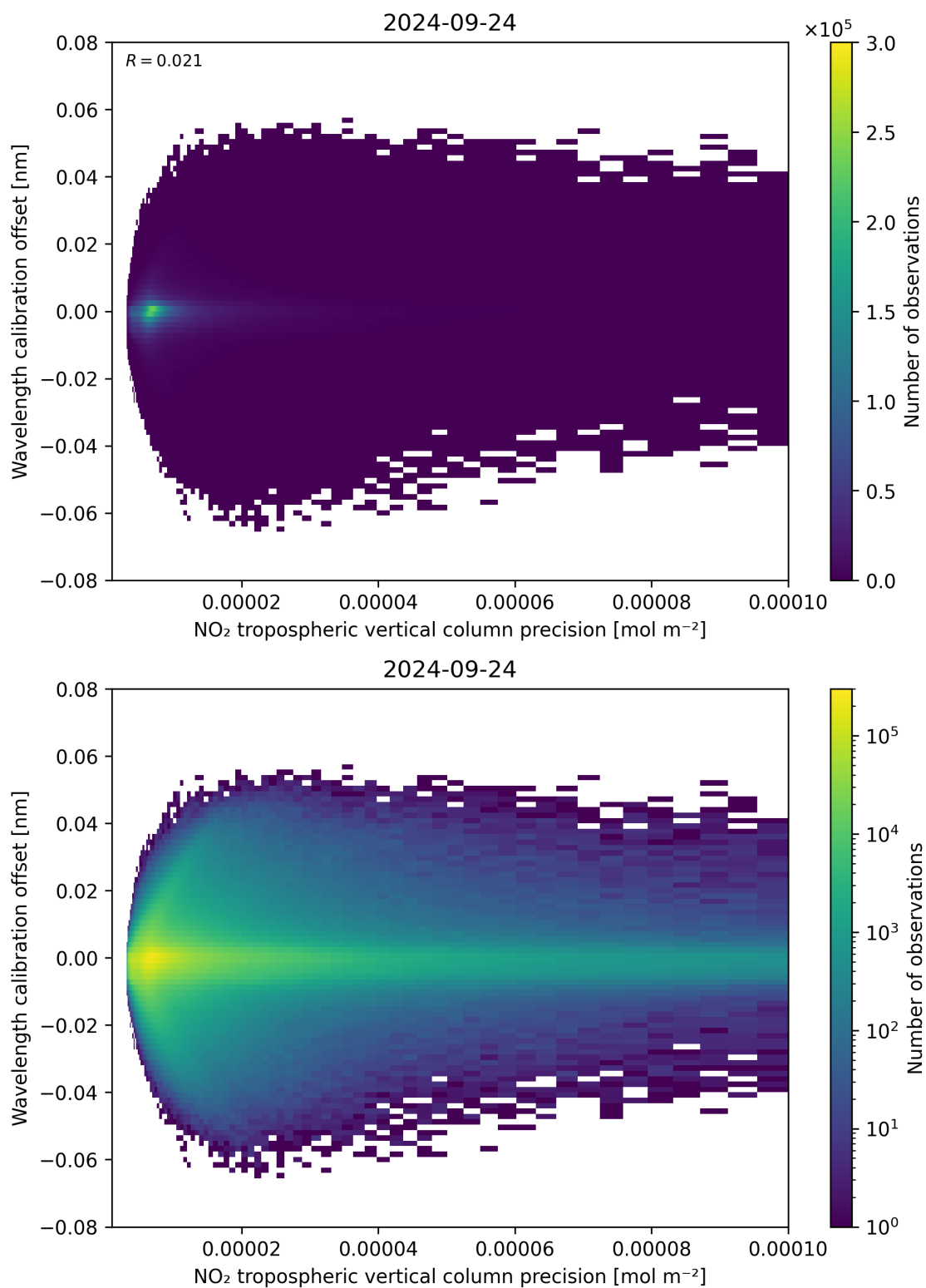
Figure 141: Scatter density plot of “NO 2 tropospheric vertical column precision” against “Wavelength calibration offset” for 2024-09-23 to 2024-09-25.
