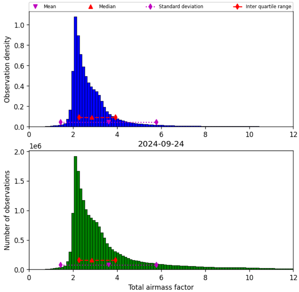
Figure 32: Histogram of “Total airmass factor” for 2024-09-23 to 2024-09-25
