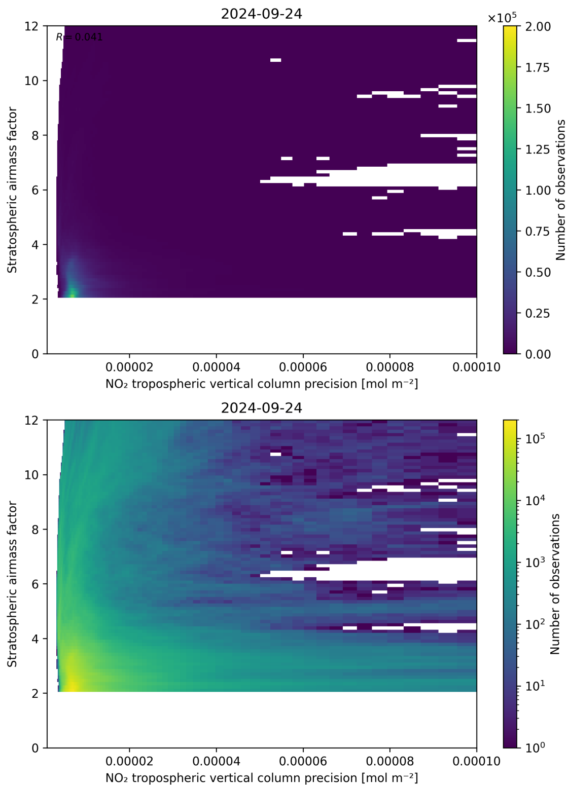
Figure 131: Scatter density plot of “NO 2 tropospheric vertical column precision” against “Stratospheric airmass factor” for 2024-09-23 to 2024-09-25.
