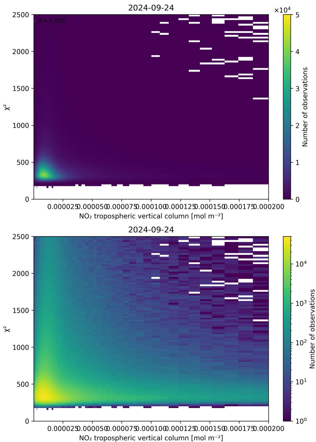
Figure 124: Scatter density plot of “NO 2 tropospheric vertical column” against “ \chi^2 ” for 2024-09-23 to 2024-09-25.
