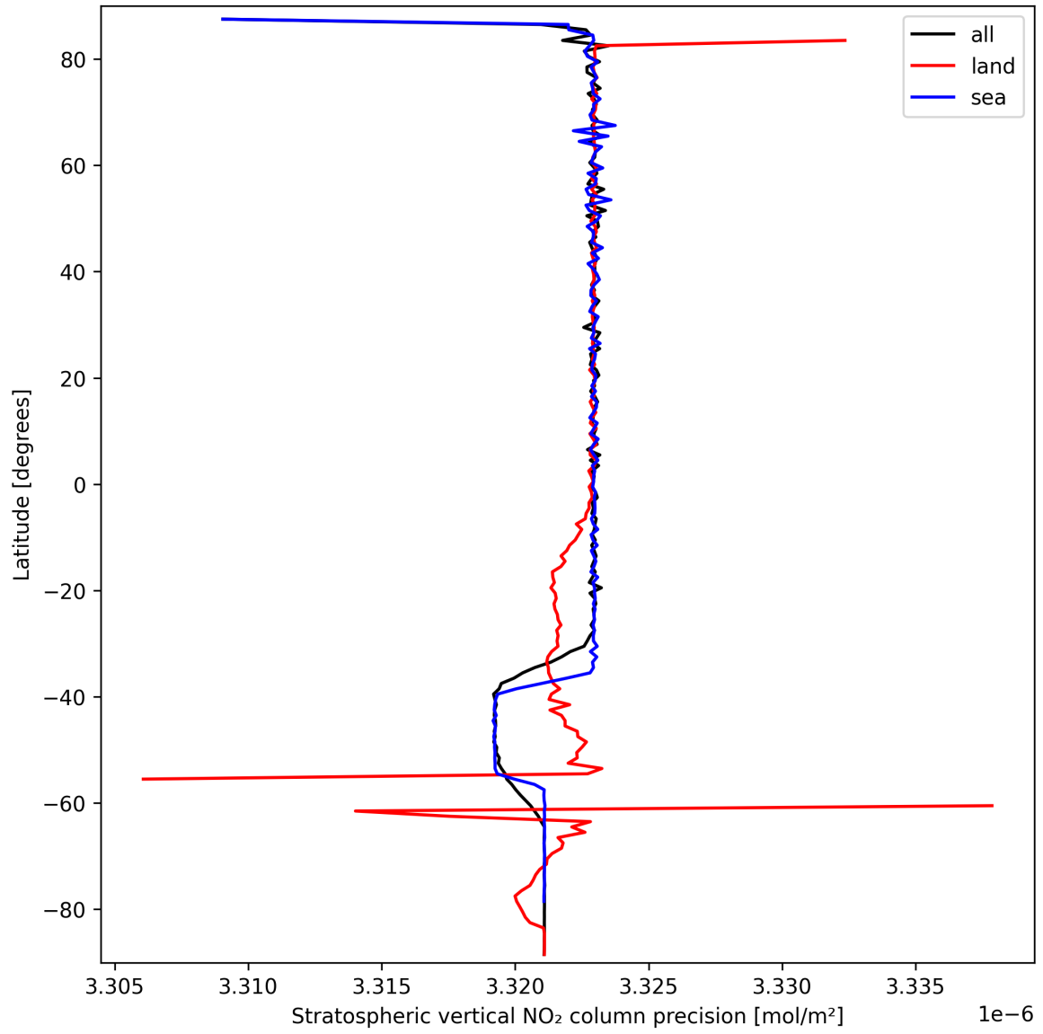
Figure 20: Zonal average of “Stratospheric vertical NO 2 column precision” for 2024-09-23 to 2024-09-25.
