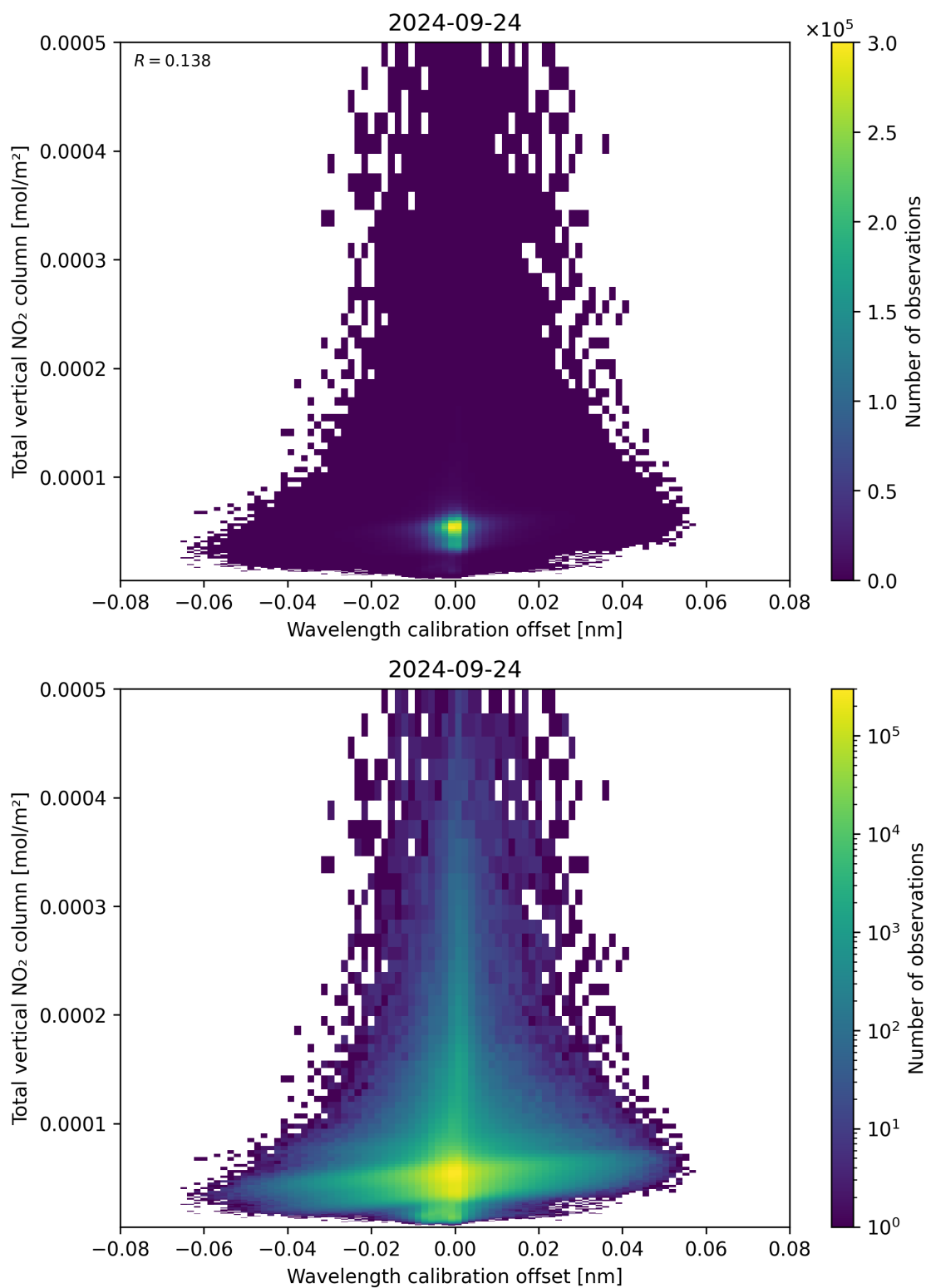
Figure 179: Scatter density plot of “Wavelength calibration offset” against “Total vertical NO 2 column” for 2024-09-23 to 2024-09-25.
