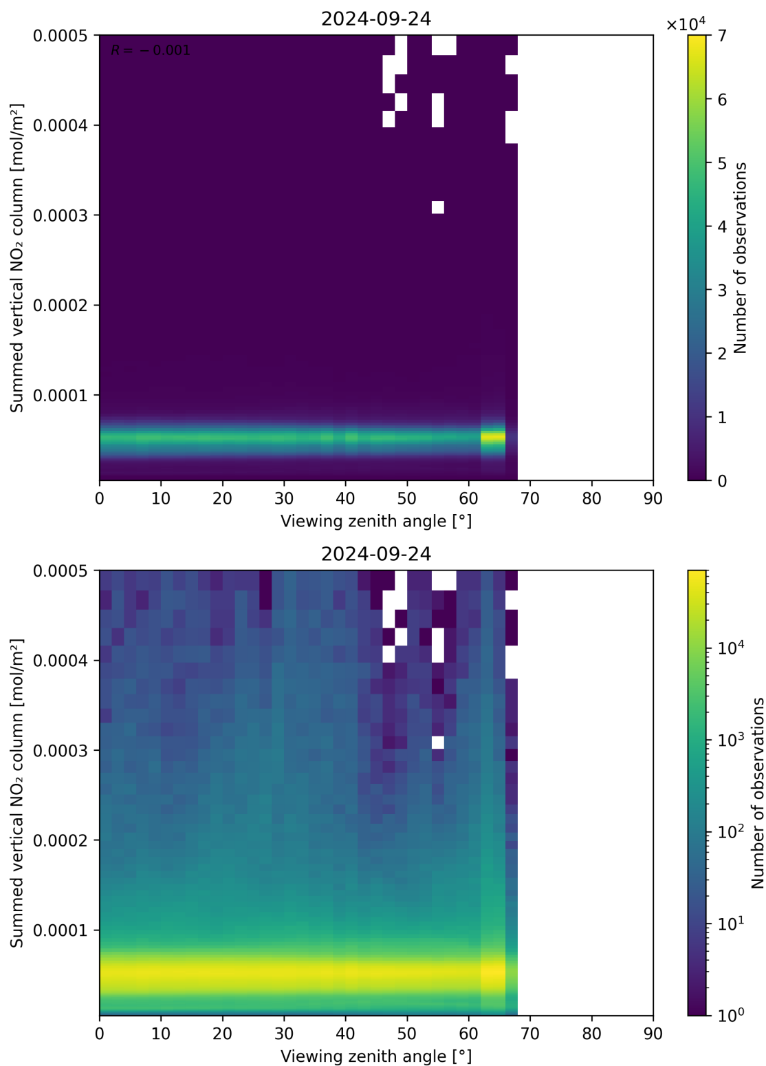
Figure 165: Scatter density plot of “Viewing zenith angle” against “Summed vertical NO 2 column” for 2024-09-23 to 2024-09-25.
