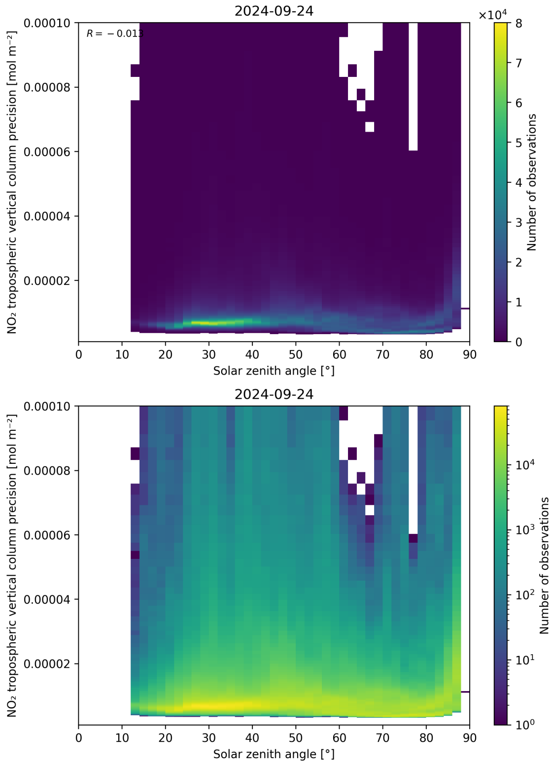
Figure 156: Scatter density plot of “Solar zenith angle” against “NO 2 tropospheric vertical column precision” for 2024-09-23 to 2024-09-25.
