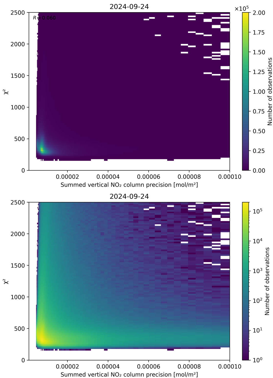
Figure 107: Scatter density plot of “Summed vertical NO 2 column precision” against “ \chi^2 ” for 2024-09-23 to 2024-09-25.
