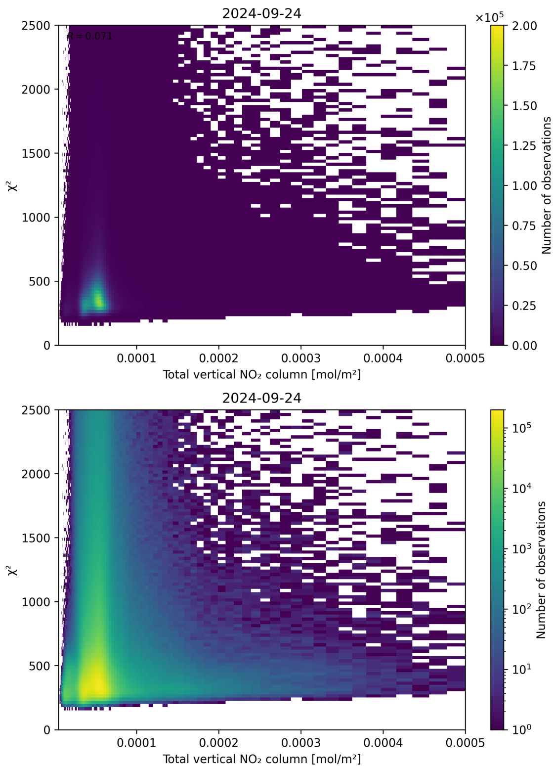
Figure 111: Scatter density plot of “Total vertical NO 2 column” against “ \chi^2 ” for 2024-09-23 to 2024-09-25.
