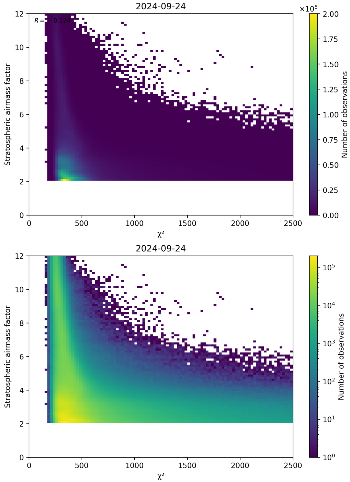
Figure 81: Scatter density plot of “ \chi^2 ” against “Stratospheric airmass factor” for 2024-09-23 to 2024-09-25.
