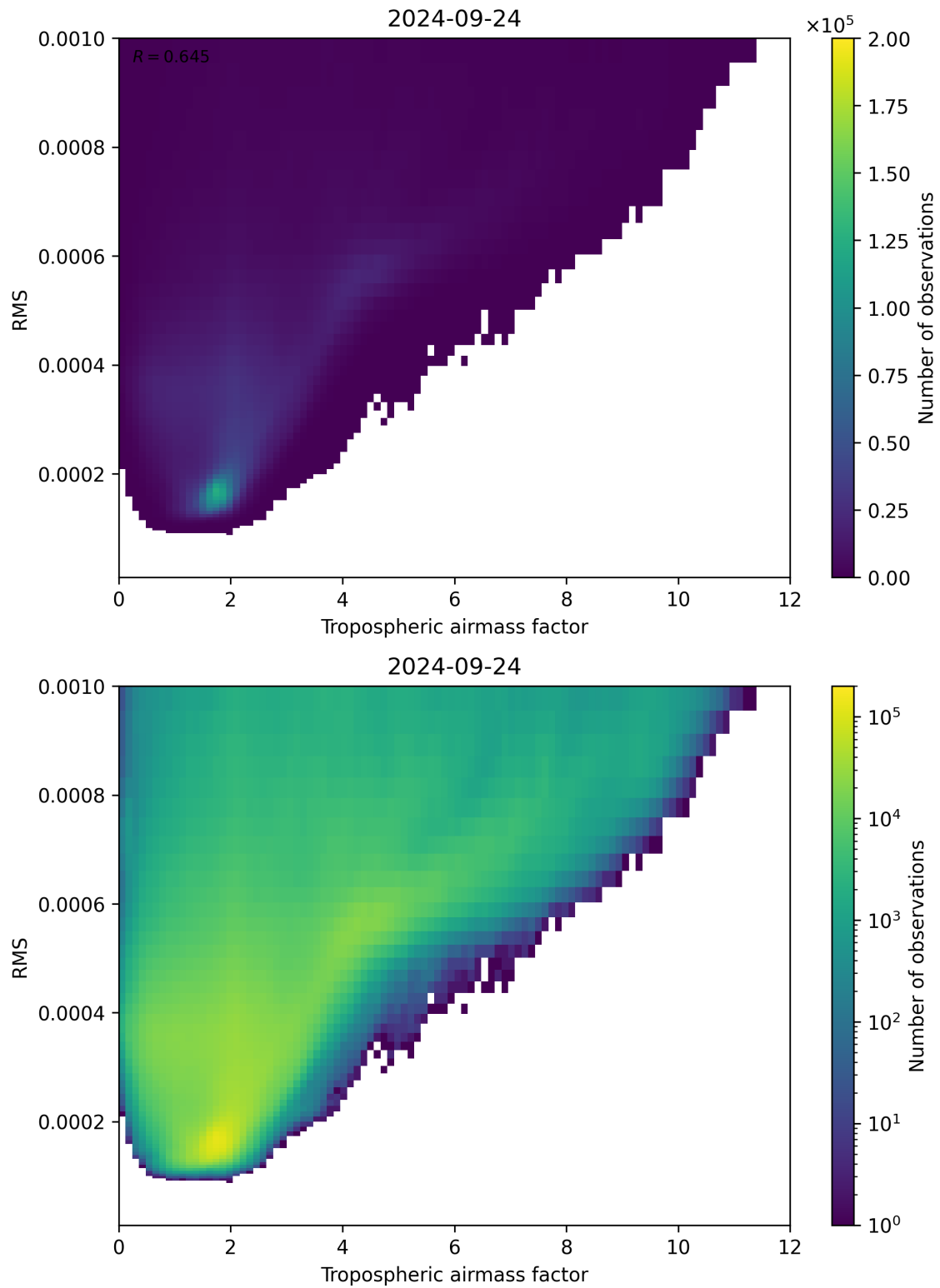
Figure 79: Scatter density plot of “Tropospheric airmass factor” against “RMS” for 2024-09-23 to 2024-09-25.
