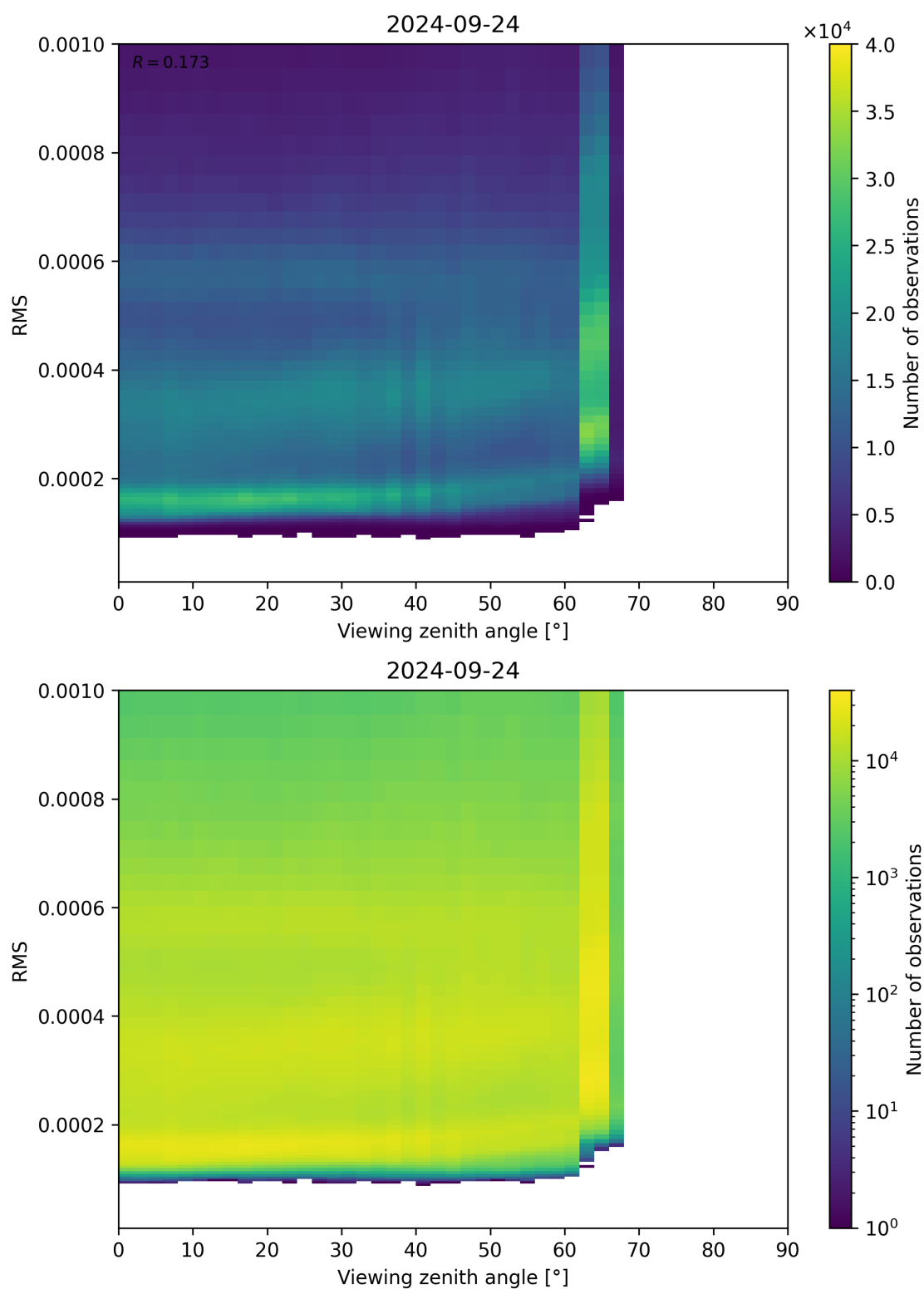
Figure 171: Scatter density plot of “Viewing zenith angle” against “RMS” for 2024-09-23 to 2024-09-25.
