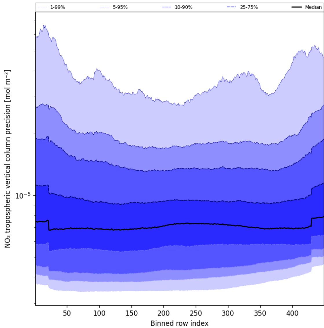
Figure 47: Along track statistics of “NO 2 tropospheric vertical column precision” for 2024-09-23 to 2024-09-25
