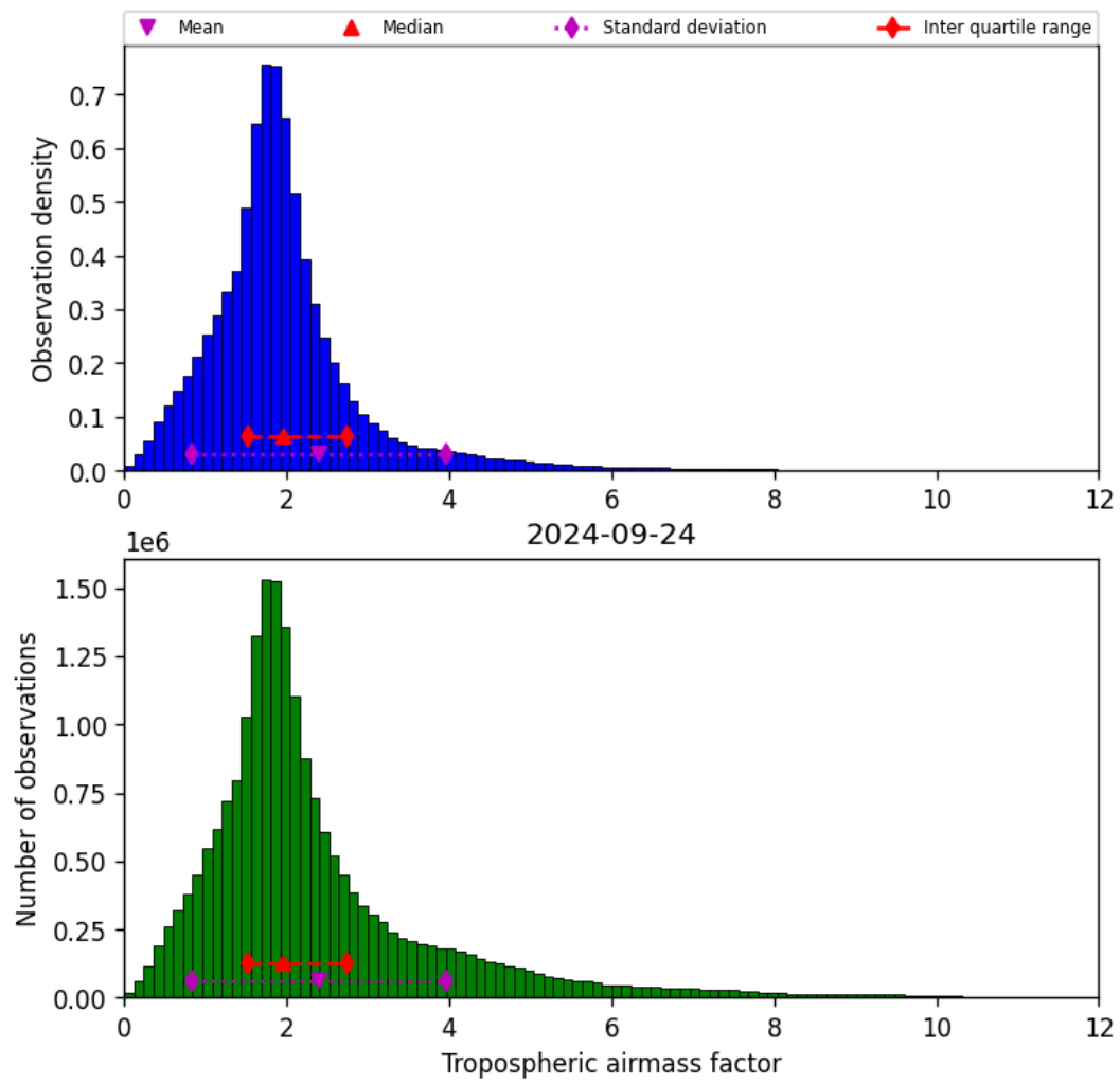
Figure 31: Histogram of “Tropospheric airmass factor” for 2024-09-23 to 2024-09-25
