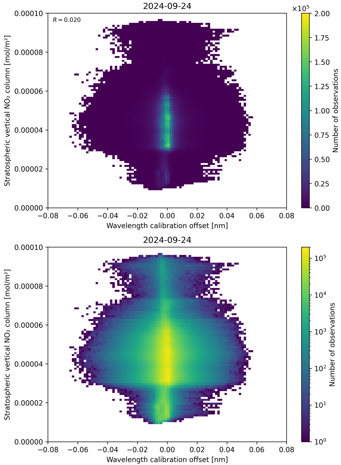
Figure 176: Scatter density plot of “Wavelength calibration offset” against “Stratospheric vertical NO 2 column” for 2024-09-23 to 2024-09-25.
