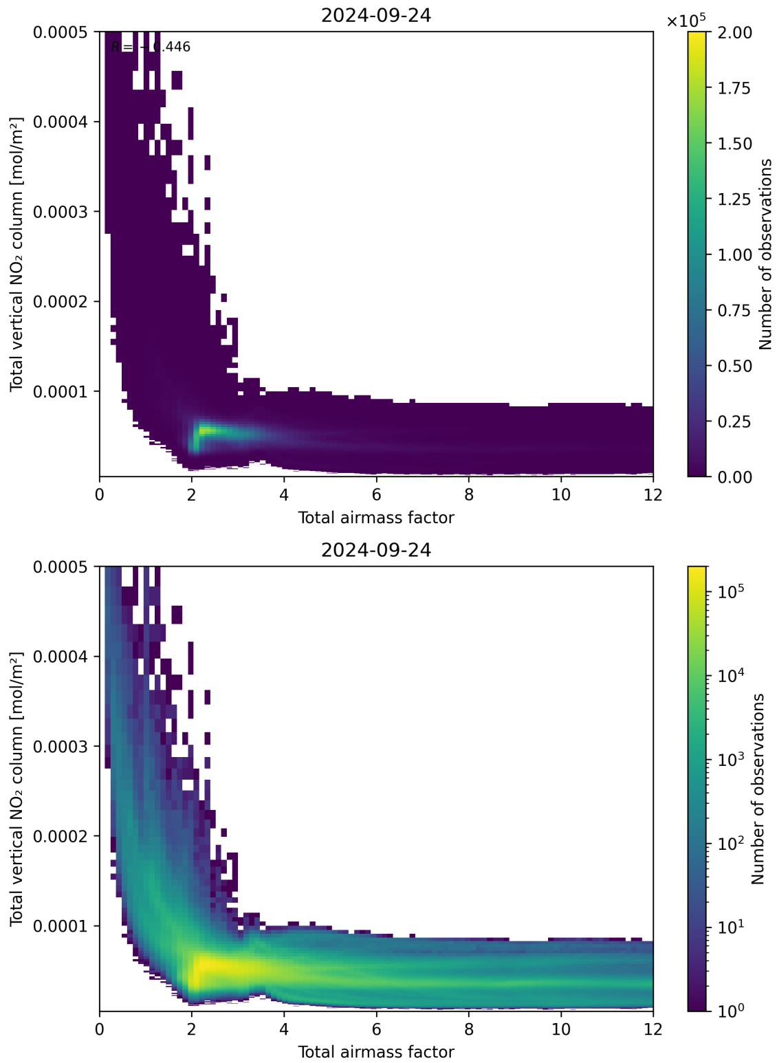
Figure 67: Scatter density plot of “Total airmass factor” against “Total vertical NO 2 column” for 2024-09-23 to 2024-09-25.
