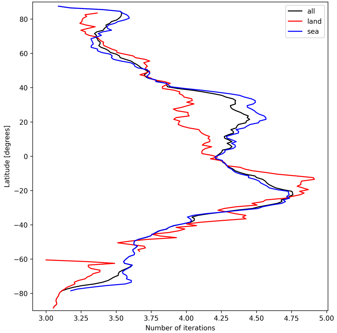
Figure 17: Zonal average of “Number of iterations” for 2024-09-23 to 2024-09-25.
