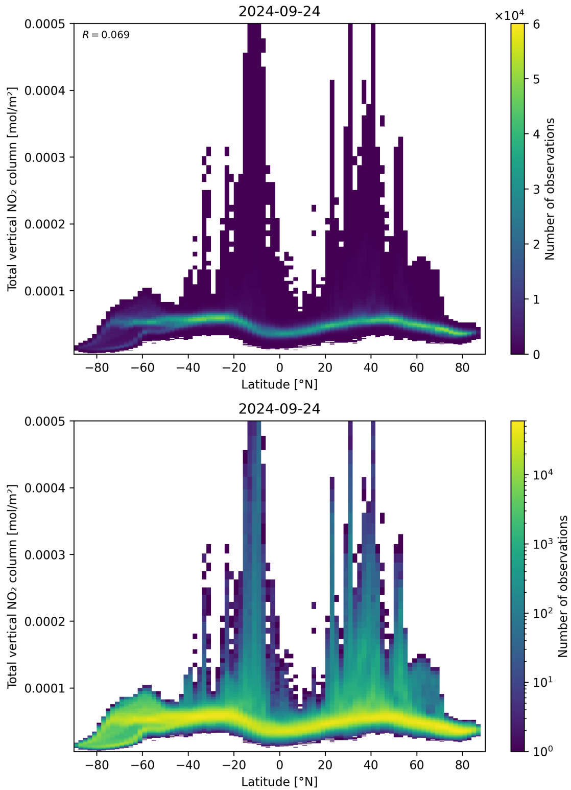
Figure 90: Scatter density plot of “Latitude” against “Total vertical NO 2 column” for 2024-09-23 to 2024-09-25.
