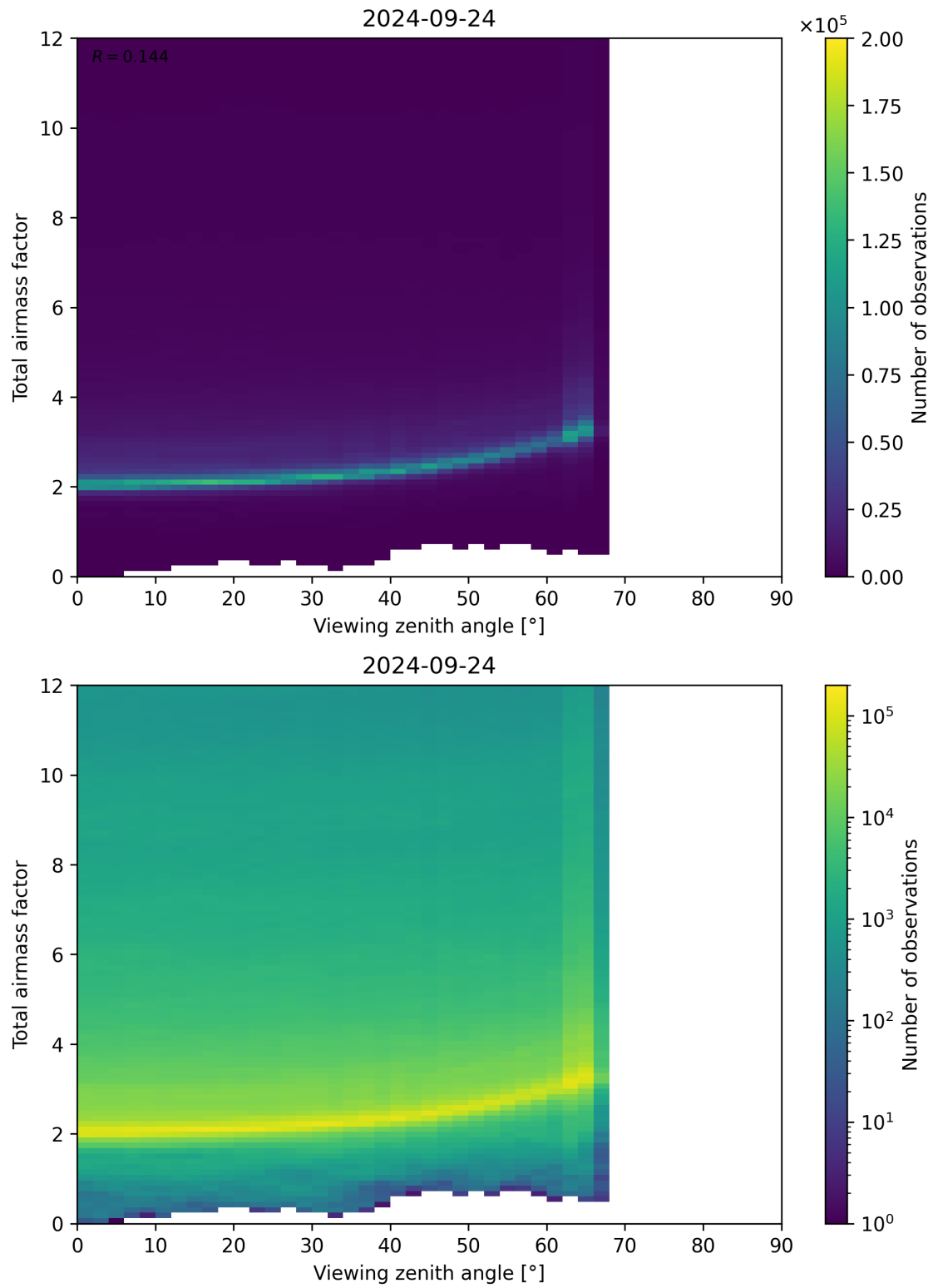
Figure 160: Scatter density plot of “Viewing zenith angle” against “Total airmass factor” for 2024-09-23 to 2024-09-25.
