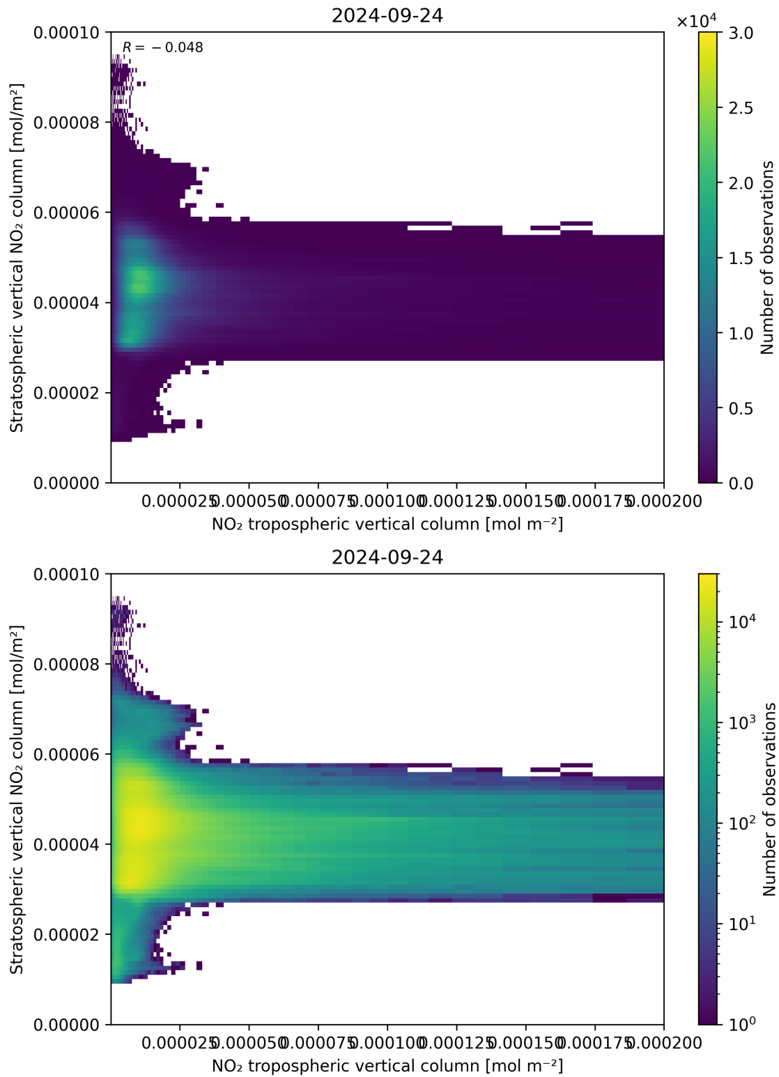
Figure 125: Scatter density plot of “NO 2 tropospheric vertical column” against “Stratospheric vertical NO 2 column” for 2024-09-23 to 2024-09-25.
