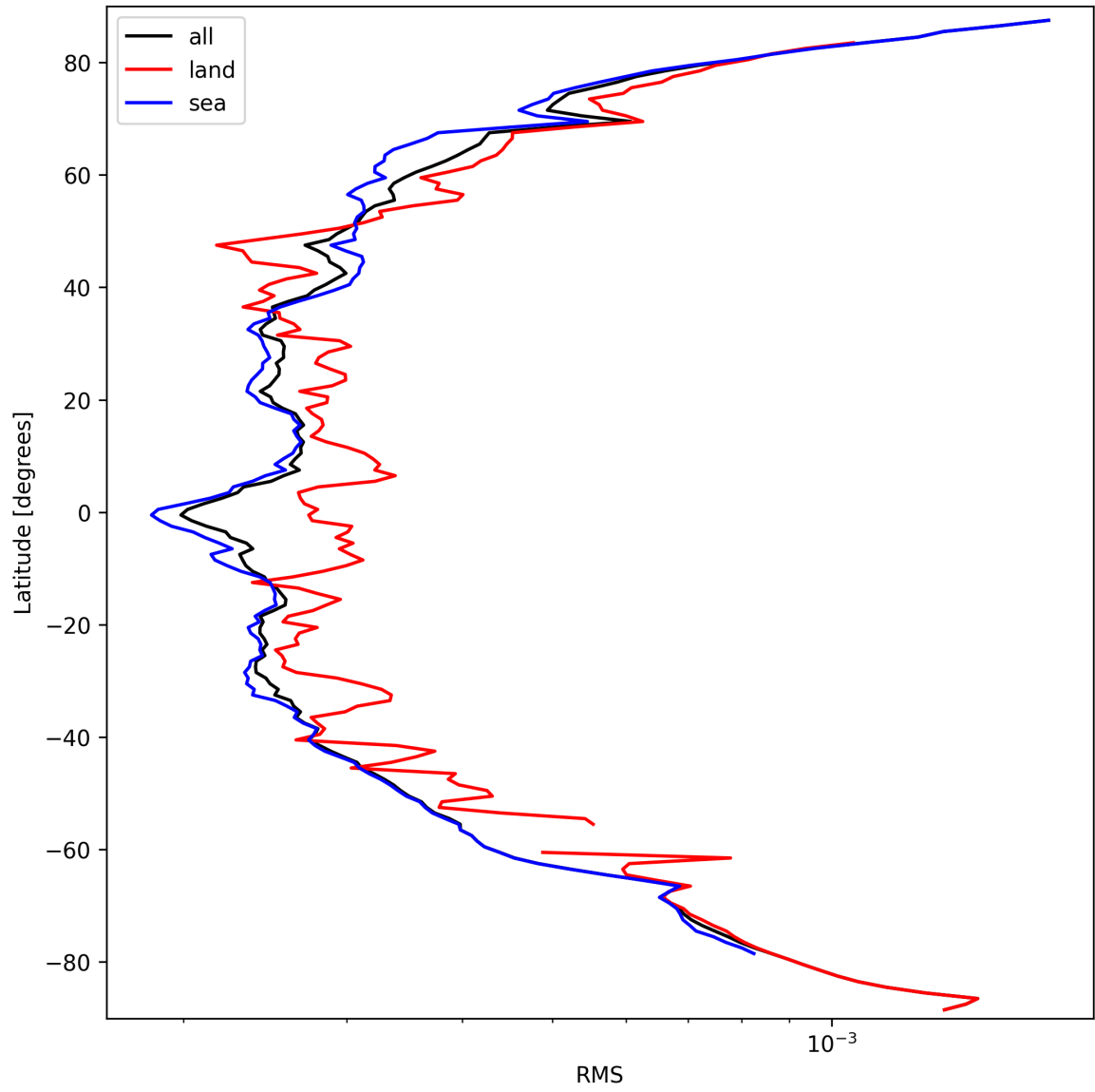
Figure 26: Zonal average of “RMS” for 2024-09-23 to 2024-09-25.
