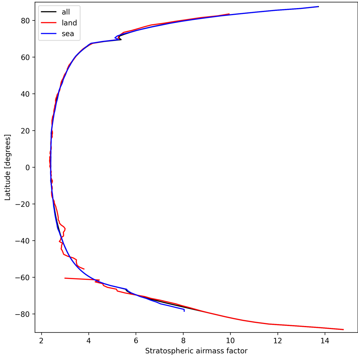
Figure 27: Zonal average of “Stratospheric air mass factor” for 2024-09-23 to 2024-09-25.
