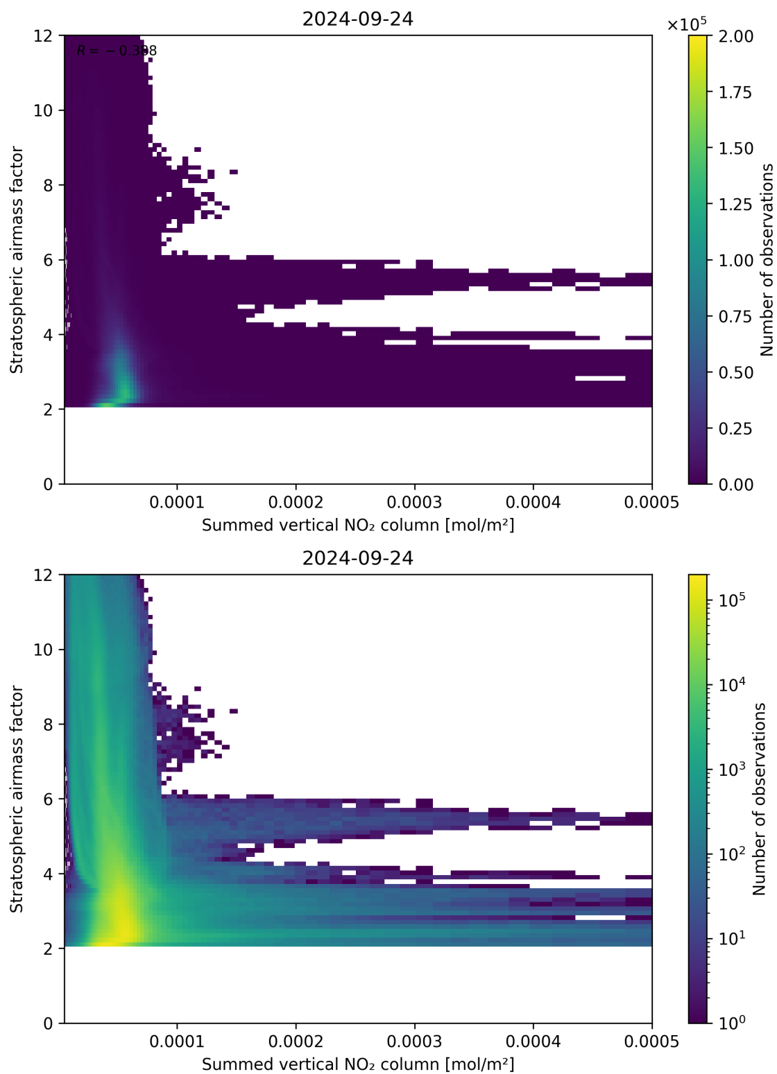
Figure 103: Scatter density plot of “Summed vertical NO 2 column” against “Stratospheric airmass factor” for 2024-09-23 to 2024-09-25.
