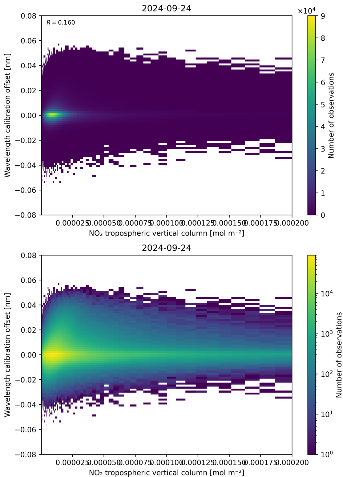
Figure 143: Scatter density plot of “NO 2 tropospheric vertical column” against “Wavelength calibration offset” for 2024-09-23 to 2024-09-25.
