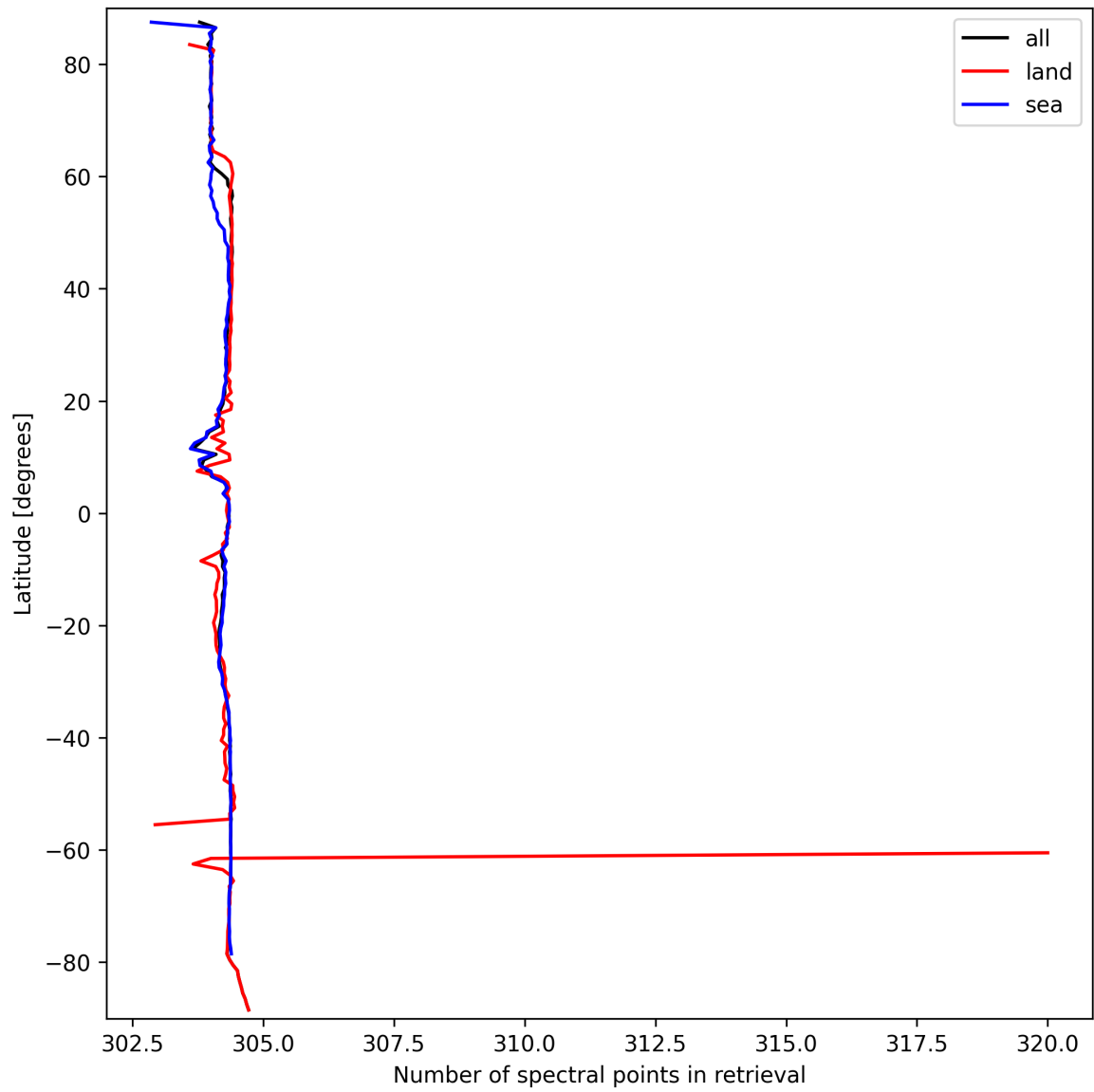
Figure 16: Zonal average of “Number of spectral points in retrieval” for 2024-09-23 to 2024-09-25.
