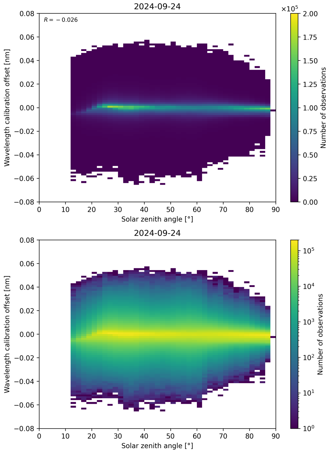
Figure 158: Scatter density plot of “Solar zenith angle” against “Wavelength calibration offset” for 2024-09-23 to 2024-09-25.
