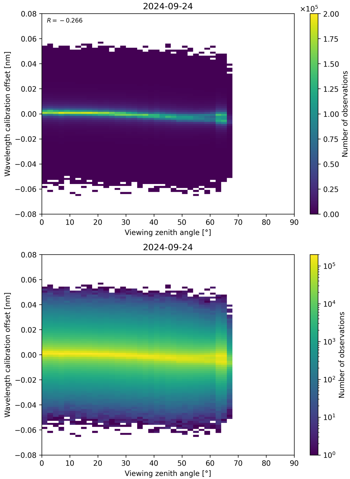
Figure 173: Scatter density plot of “Viewing zenith angle” against “Wavelength calibration offset” for 2024-09-23 to 2024-09-25.
