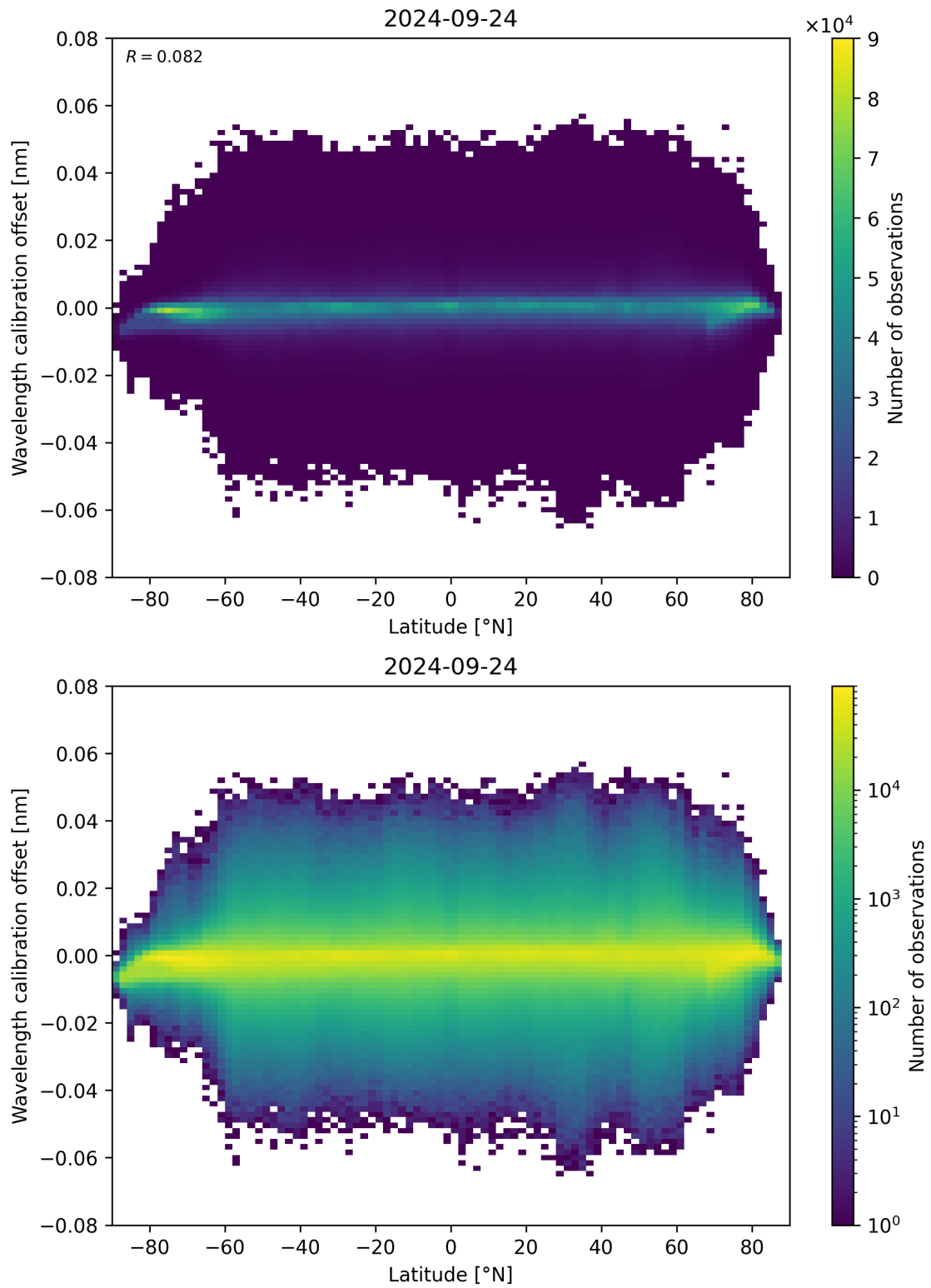
Figure 95: Scatter density plot of “Latitude” against “Wavelength calibration offset” for 2024-09-23 to 2024-09-25.
