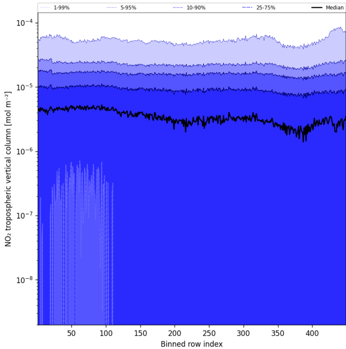
Figure 46: Along track statistics of “NO 2 tropospheric vertical column” for 2024-09-23 to 2024-09-25
