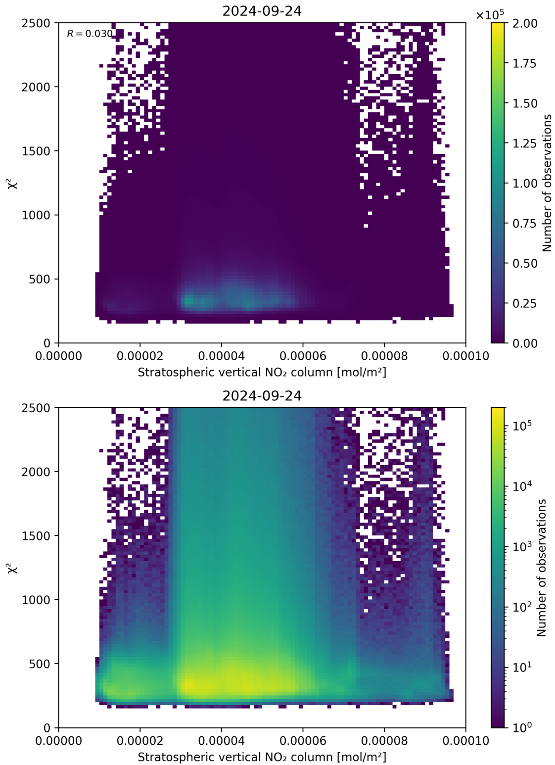
Figure 97: Scatter density plot of “Stratospheric vertical NO 2 column” against “ \chi^2 ” for 2024-09-23 to 2024-09-25.
