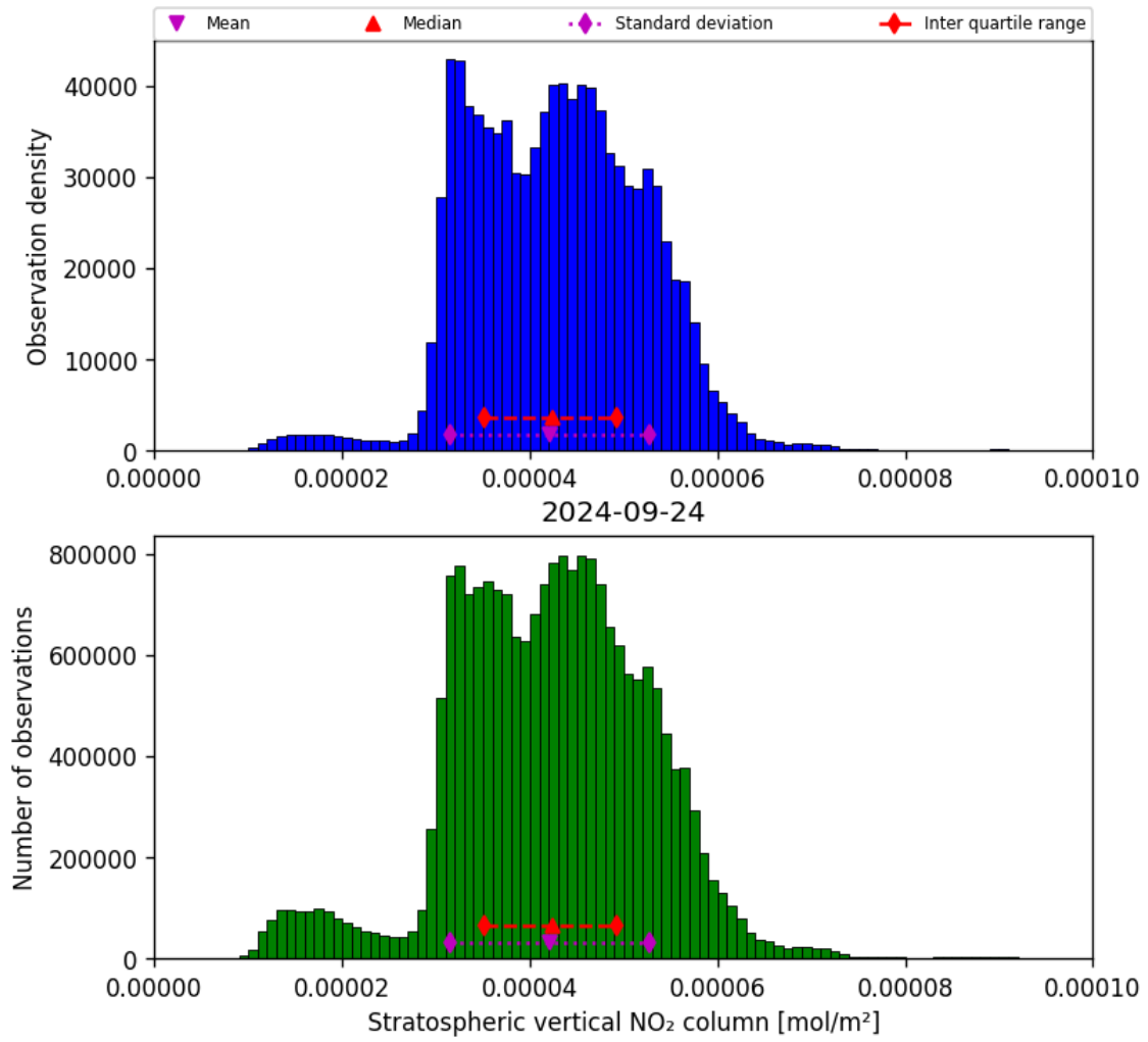
Figure 36: Histogram of “Stratospheric vertical NO 2 column” for 2024-09-23 to 2024-09-25
