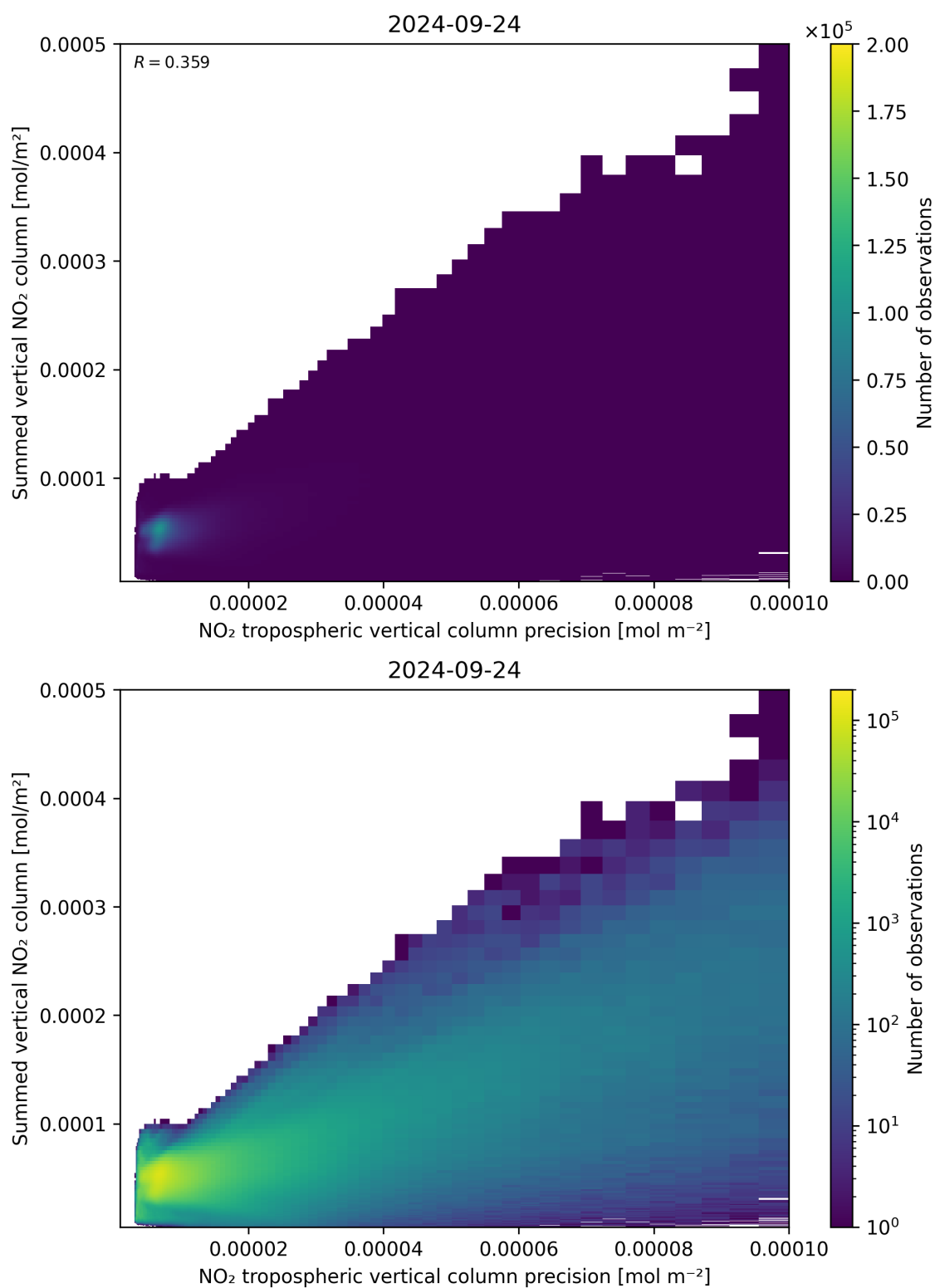
Figure 136: Scatter density plot of “NO 2 tropospheric vertical column precision” against “Summed vertical NO 2 column” for 2024-09-23 to 2024-09-25.
