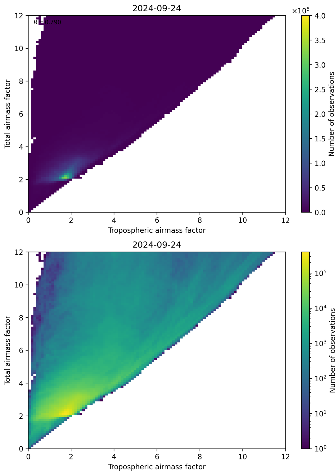
Figure 72: Scatter density plot of “Tropospheric airmass factor” against “Total airmass factor” for 2024-09-23 to 2024-09-25.
