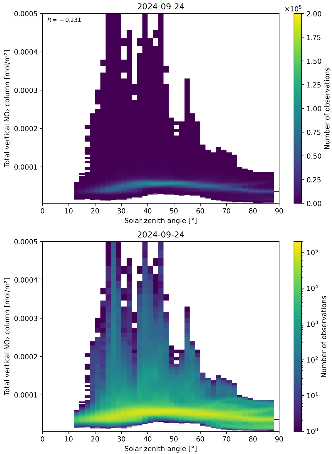
Figure 153: Scatter density plot of “Solar zenith angle” against “Total vertical NO 2 column” for 2024-09-23 to 2024-09-25.
