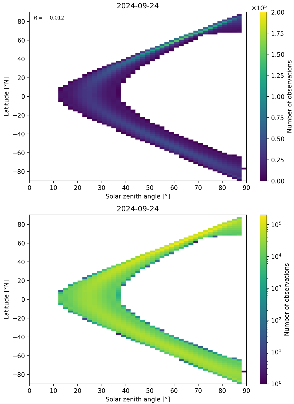
Figure 149: Scatter density plot of “Solar zenith angle” against “Latitude” for 2024-09-23 to 2024-09-25.
