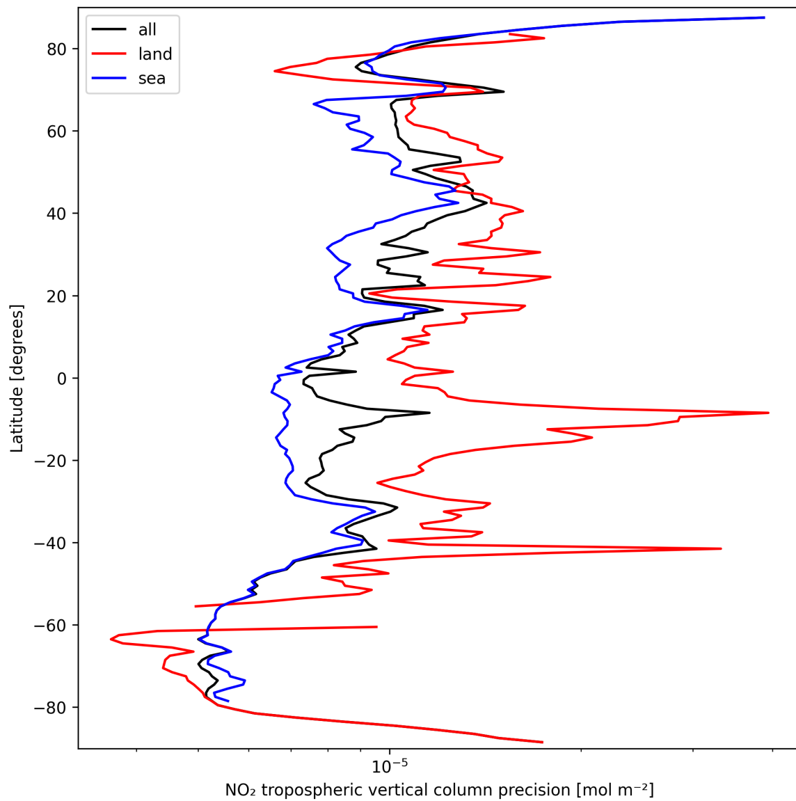
Figure 13: Zonal average of “NO 2 tropospheric vertical column precision” for 2024-09-23 to 2024-09-25.
