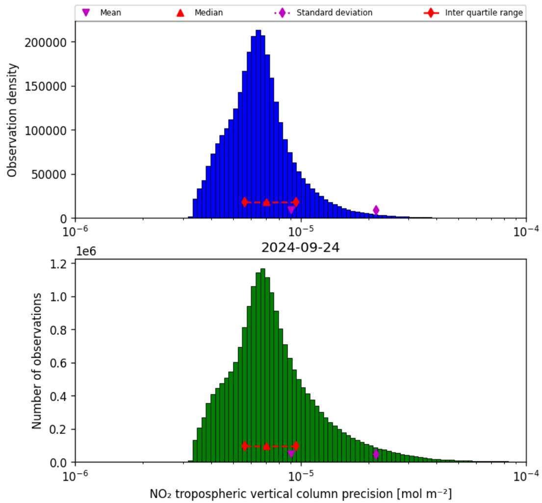
Figure 30: Histogram of “NO 2 tropospheric vertical column precision” for 2024-09-23 to 2024-09-25
