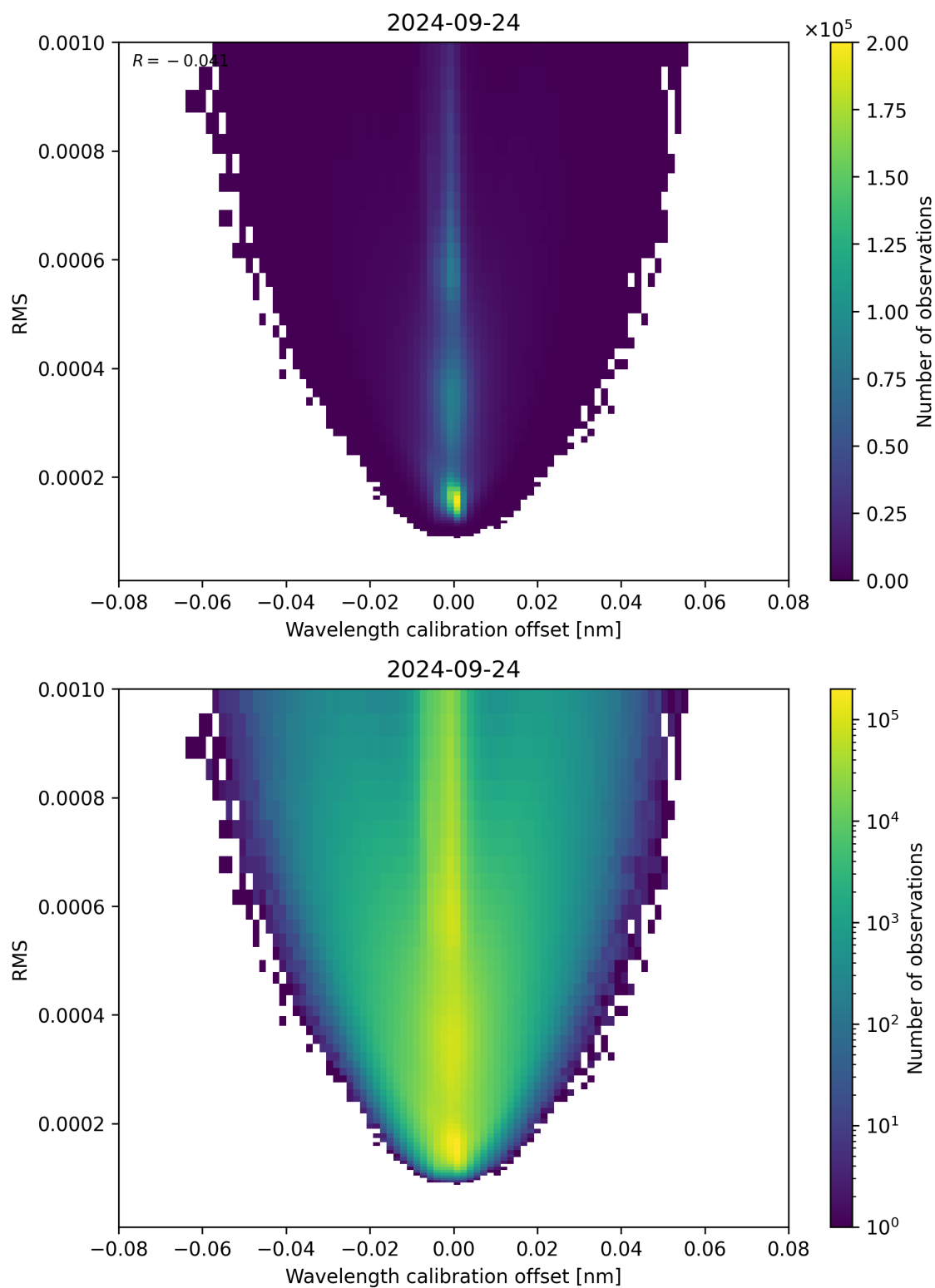
Figure 181: Scatter density plot of “Wavelength calibration offset” against “RMS” for 2024-09-23 to 2024-09-25.
