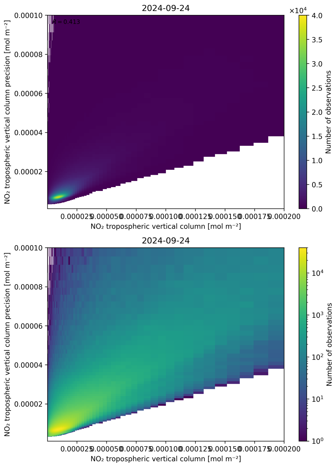
Figure 130: Scatter density plot of “NO 2 tropospheric vertical column” against “NO 2 tropospheric vertical column precision” for 2024-09-23 to 2024-09-25.
