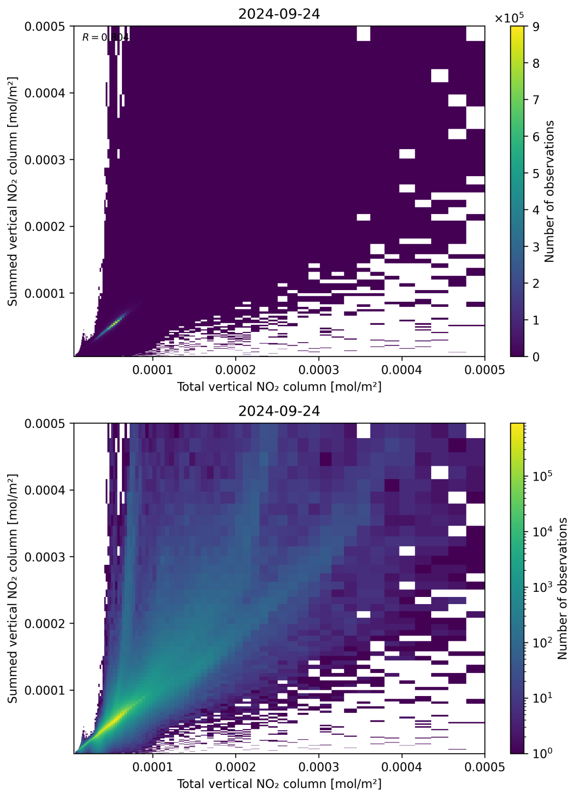
Figure 112: Scatter density plot of “Total vertical NO 2 column” against “Summed vertical NO 2 column” for 2024-09-23 to 2024-09-25.
