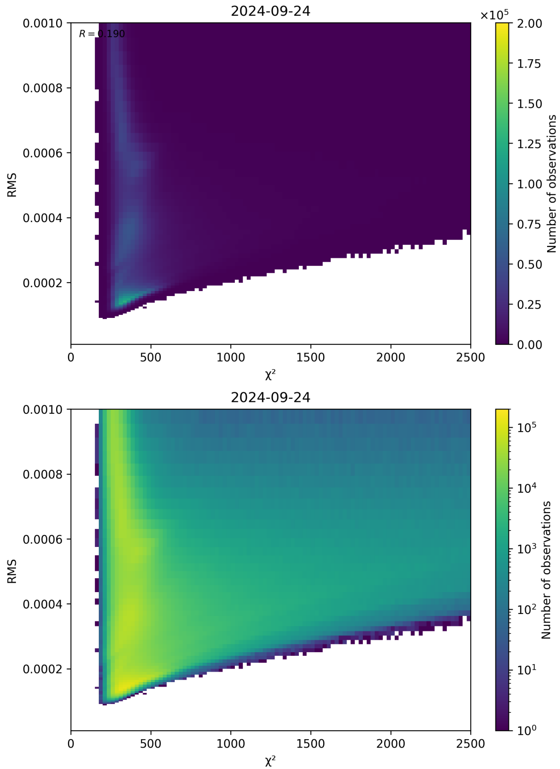
Figure 82: Scatter density plot of “ \chi^2 ” against “RMS” for 2024-09-23 to 2024-09-25.
