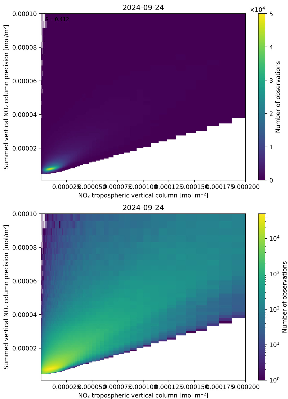
Figure 127: Scatter density plot of “NO 2 tropospheric vertical column” against “Summed vertical NO 2 column precision” for 2024-09-23 to 2024-09-25.
