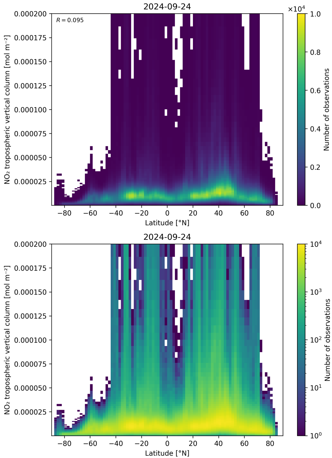
Figure 92: Scatter density plot of “Latitude” against “NO 2 tropospheric vertical column” for 2024-09-23 to 2024-09-25.
