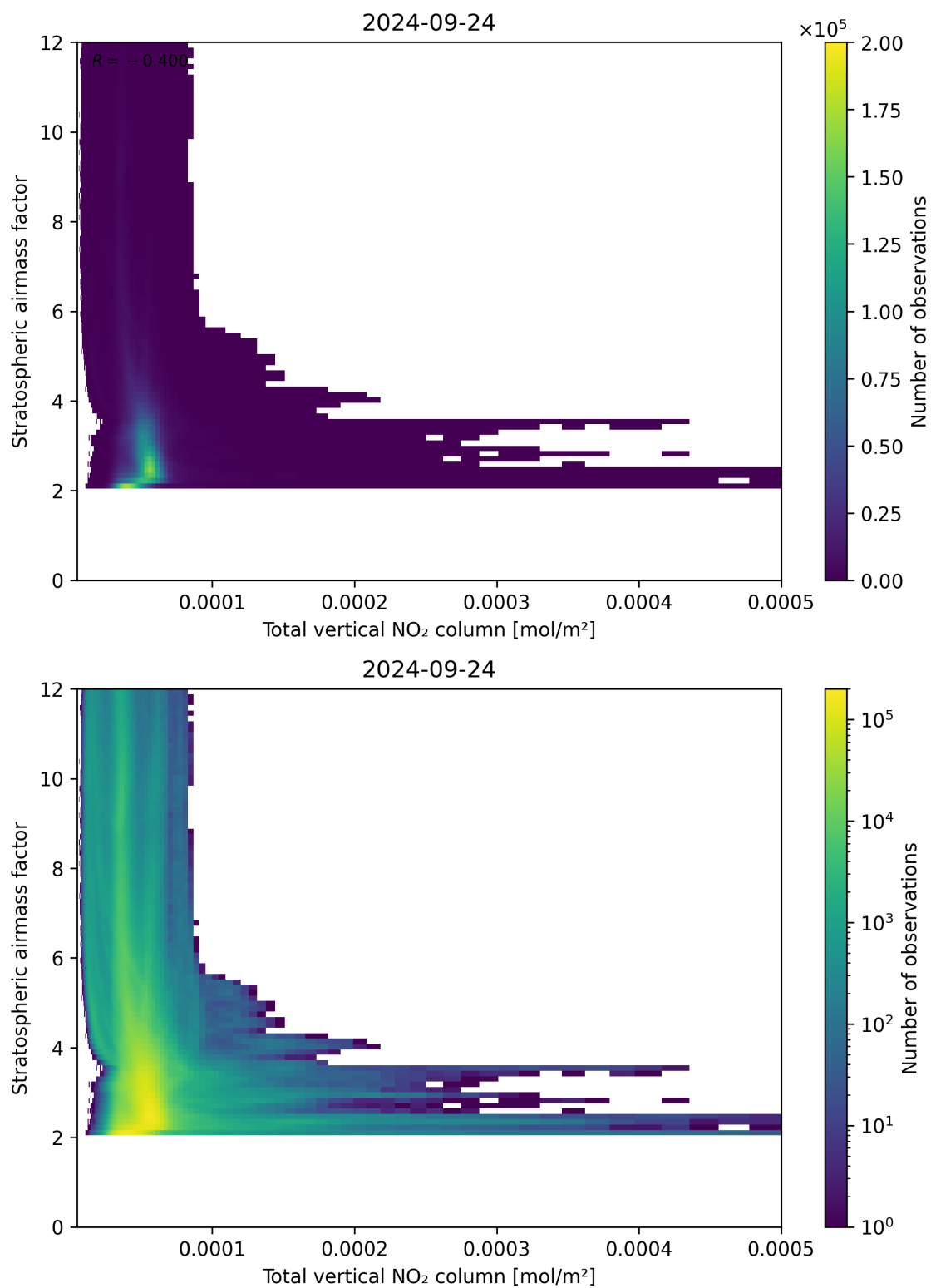
Figure 110: Scatter density plot of “Total vertical NO 2 column” against “Stratospheric airmass factor” for 2024-09-23 to 2024-09-25.
