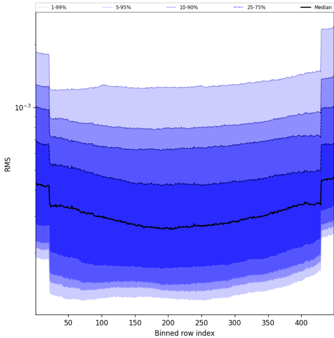
Figure 60: Along track statistics of “RMS” for 2024-09-23 to 2024-09-25
