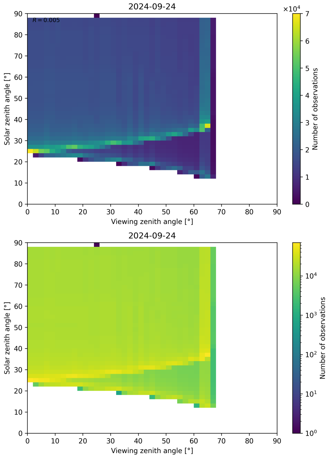
Figure 172: Scatter density plot of “Viewing zenith angle” against “Solar zenith angle” for 2024-09-23 to 2024-09-25.
