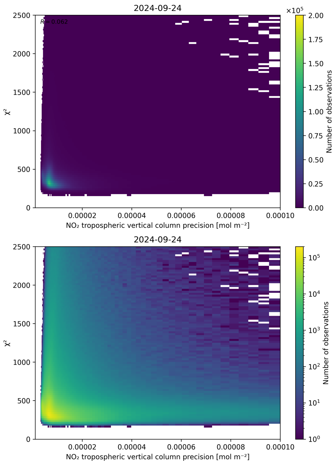
Figure 134: Scatter density plot of “NO 2 tropospheric vertical column precision” against “ \chi^2 ” for 2024-09-23 to 2024-09-25.
