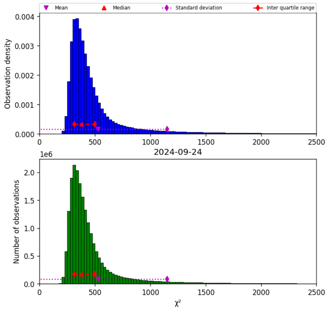
Figure 42: Histogram of “ \chi^2 ” for 2024-09-23 to 2024-09-25
