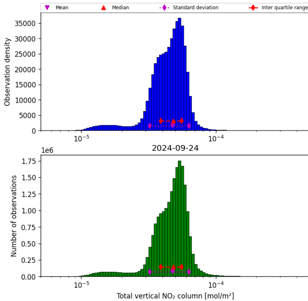
Figure 38: Histogram of “Total vertical NO 2 column” for 2024-09-23 to 2024-09-25
