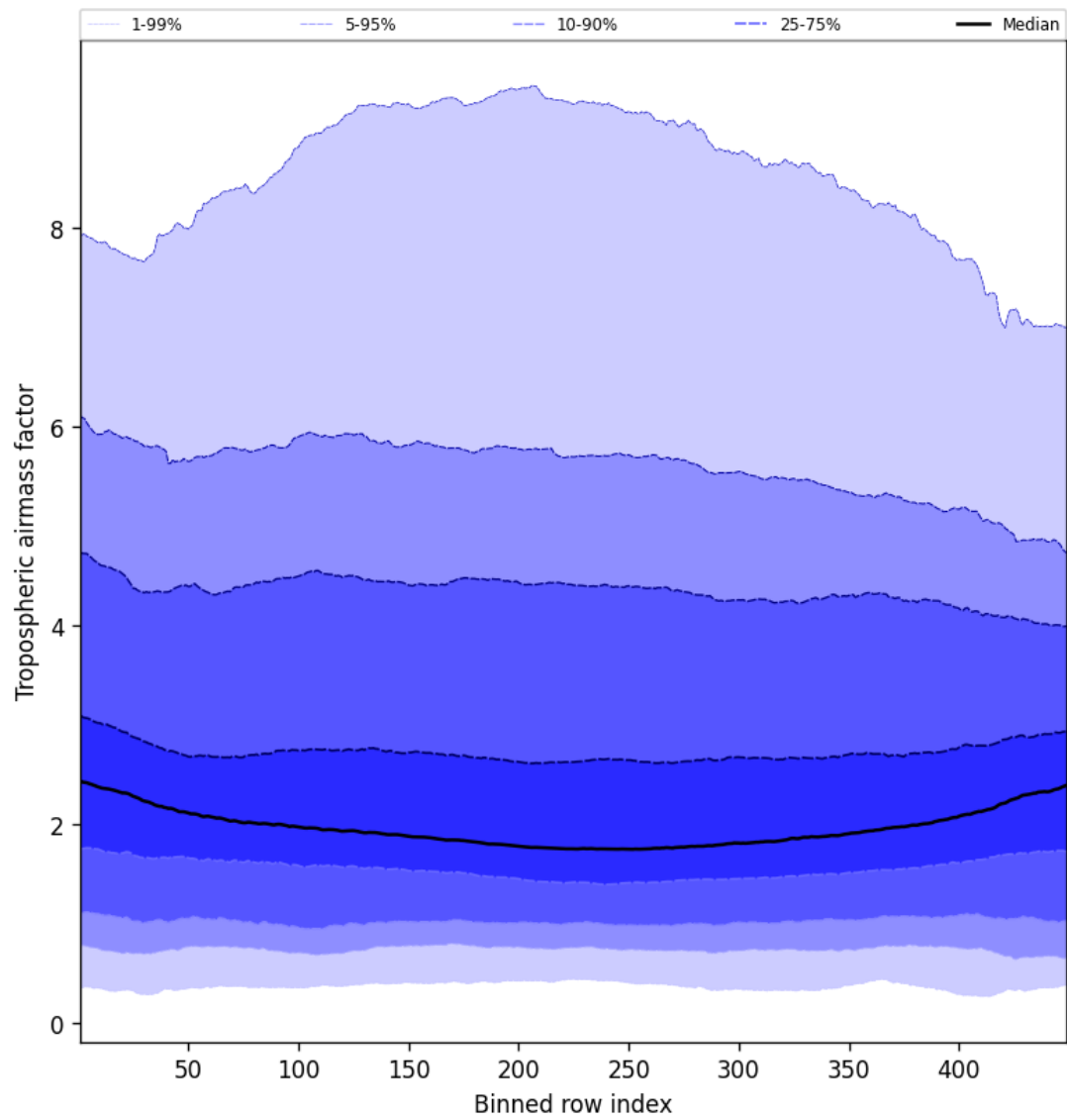
Figure 48: Along track statistics of “Tropospheric air mass factor” for 2024-09-23 to 2024-09-25
