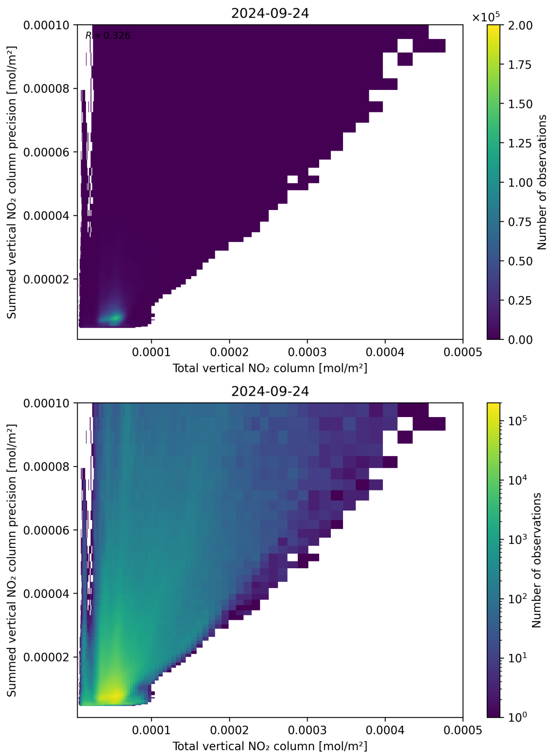
Figure 113: Scatter density plot of “Total vertical NO 2 column” against “Summed vertical NO 2 column precision” for 2024-09-23 to 2024-09-25.
