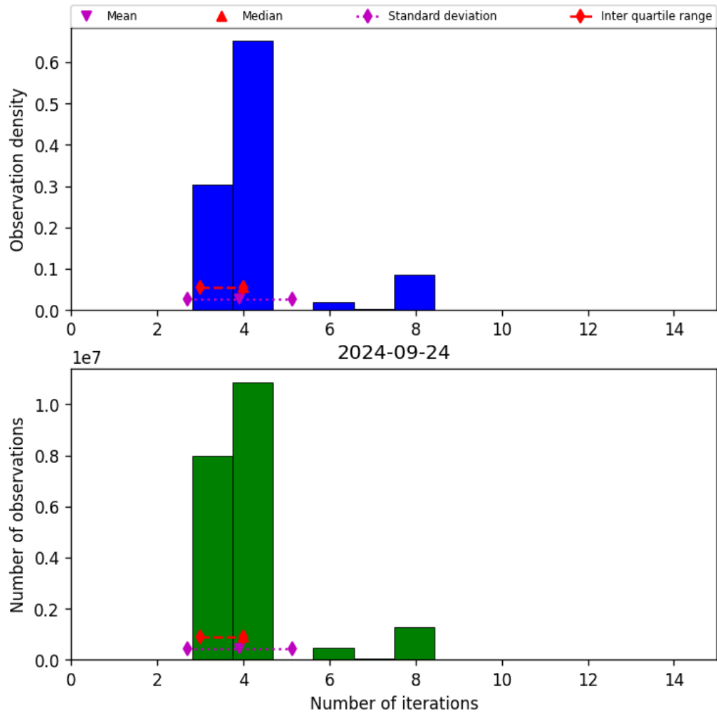
Figure 34: Histogram of “Number of iterations” for 2024-09-23 to 2024-09-25
