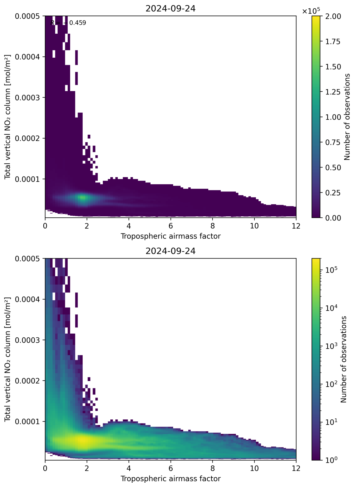
Figure 77: Scatter density plot of “Tropospheric airmass factor” against “Total vertical NO 2 column” for 2024-09-23 to 2024-09-25.
