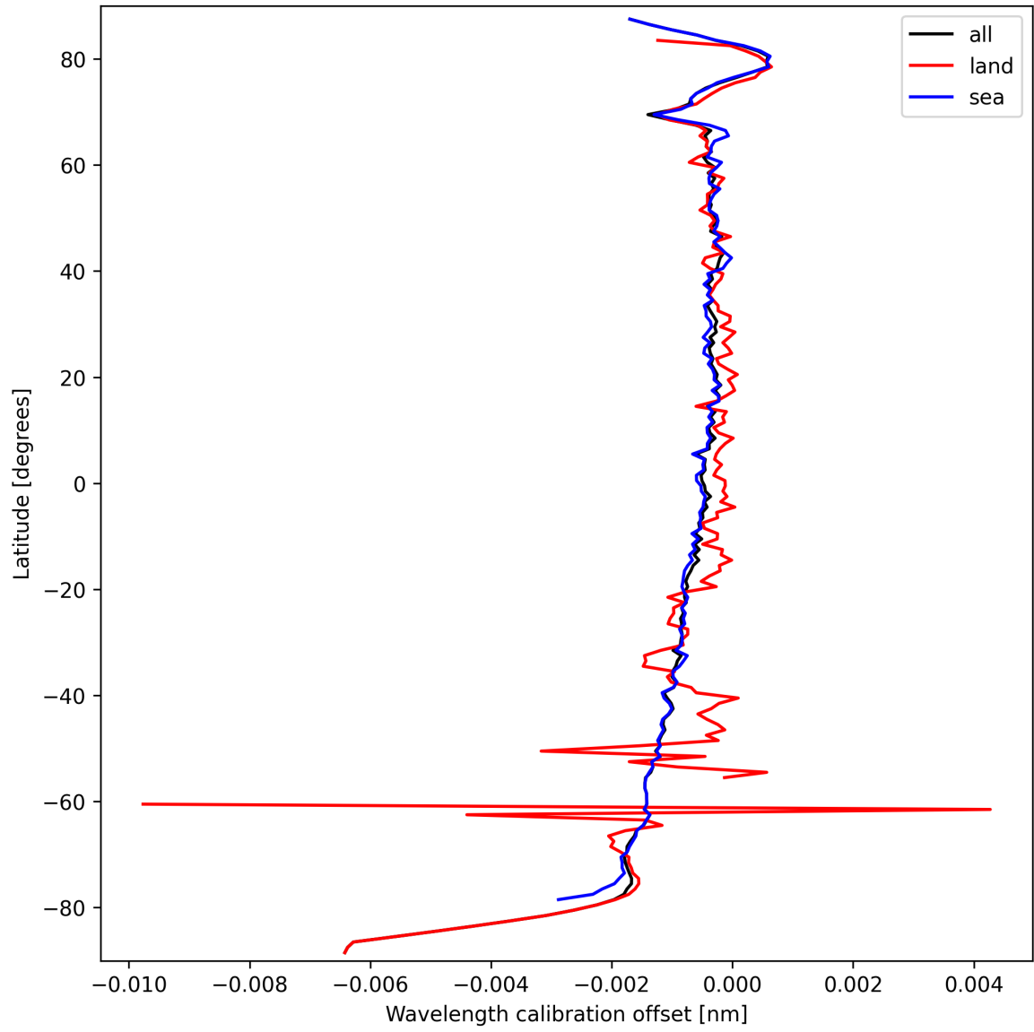
Figure 18: Zonal average of “Wavelength calibration offset” for 2024-09-23 to 2024-09-25.
