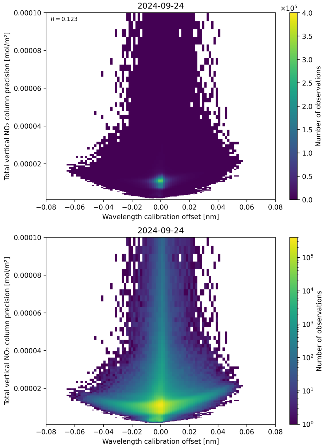
Figure 180: Scatter density plot of “Wavelength calibration offset” against “Total vertical NO 2 column precision” for 2024-09-23 to 2024-09-25.
