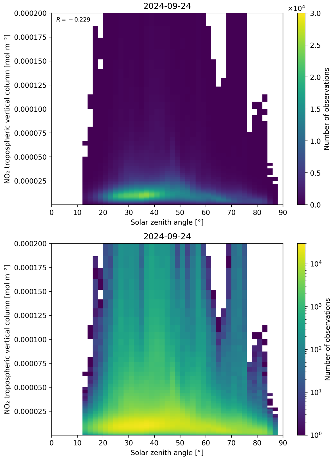
Figure 155: Scatter density plot of “Solar zenith angle” against “NO 2 tropospheric vertical column” for 2024-09-23 to 2024-09-25.
