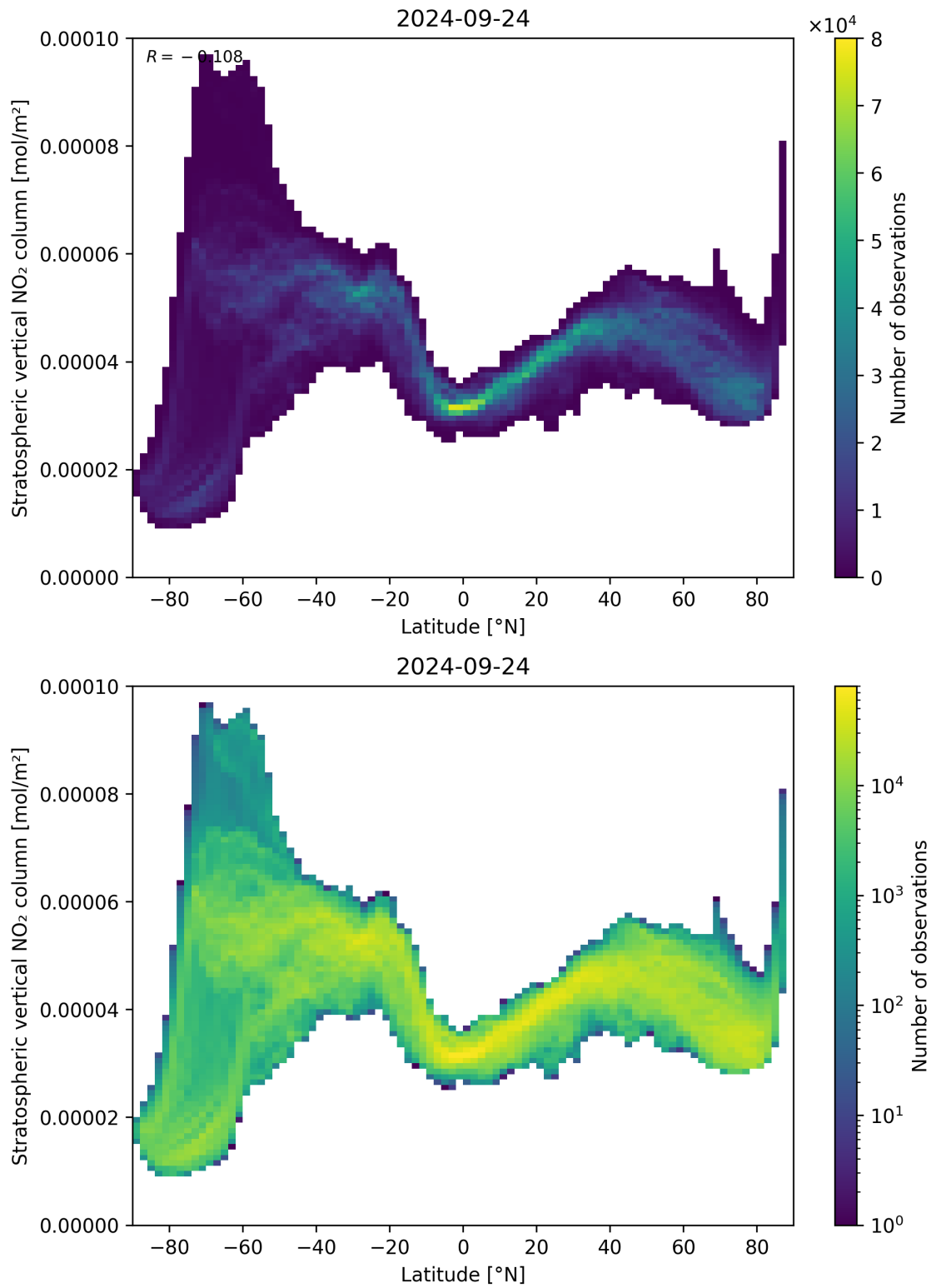
Figure 87: Scatter density plot of “Latitude” against “Stratospheric vertical NO 2 column” for 2024-09-23 to 2024-09-25.
