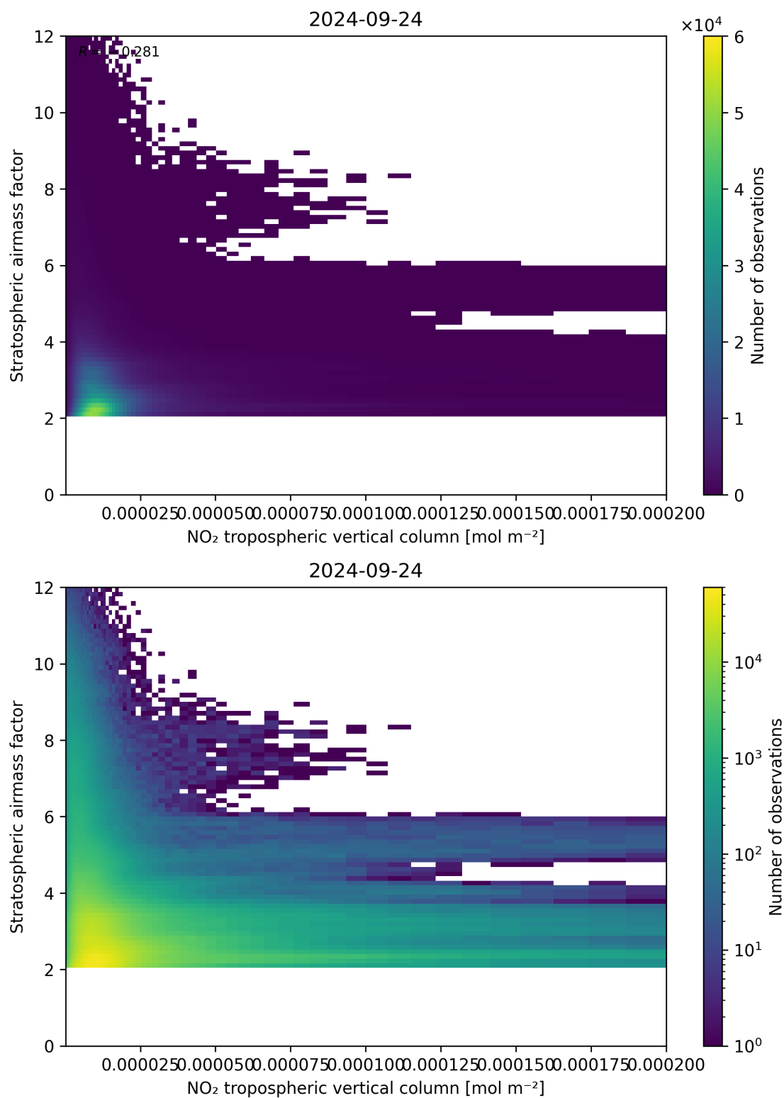
Figure 121: Scatter density plot of “NO 2 tropospheric vertical column” against “Stratospheric air mass factor” for 2024-09-23 to 2024-09-25.
