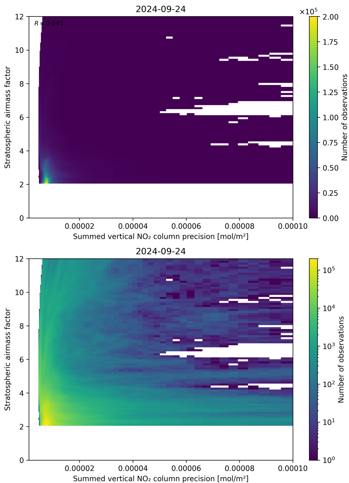
Figure 106: Scatter density plot of “Summed vertical NO 2 column precision” against “Stratospheric airmass factor” for 2024-09-23 to 2024-09-25.
