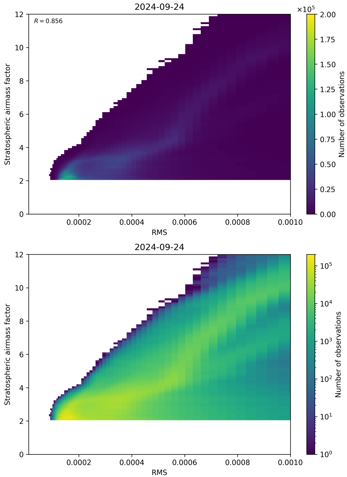
Figure 144: Scatter density plot of “RMS” against “Stratospheric airmass factor” for 2024-09-23 to 2024-09-25.
