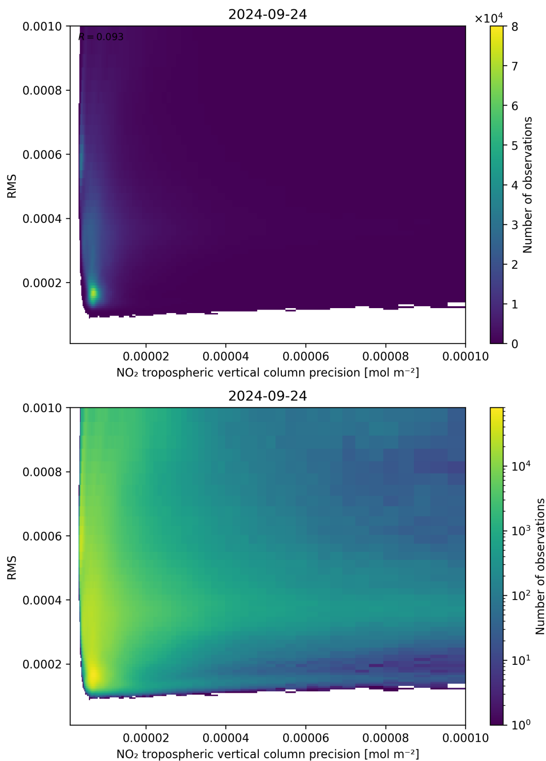
Figure 140: Scatter density plot of “NO 2 tropospheric vertical column precision” against “RMS” for 2024-09-23 to 2024-09-25.
