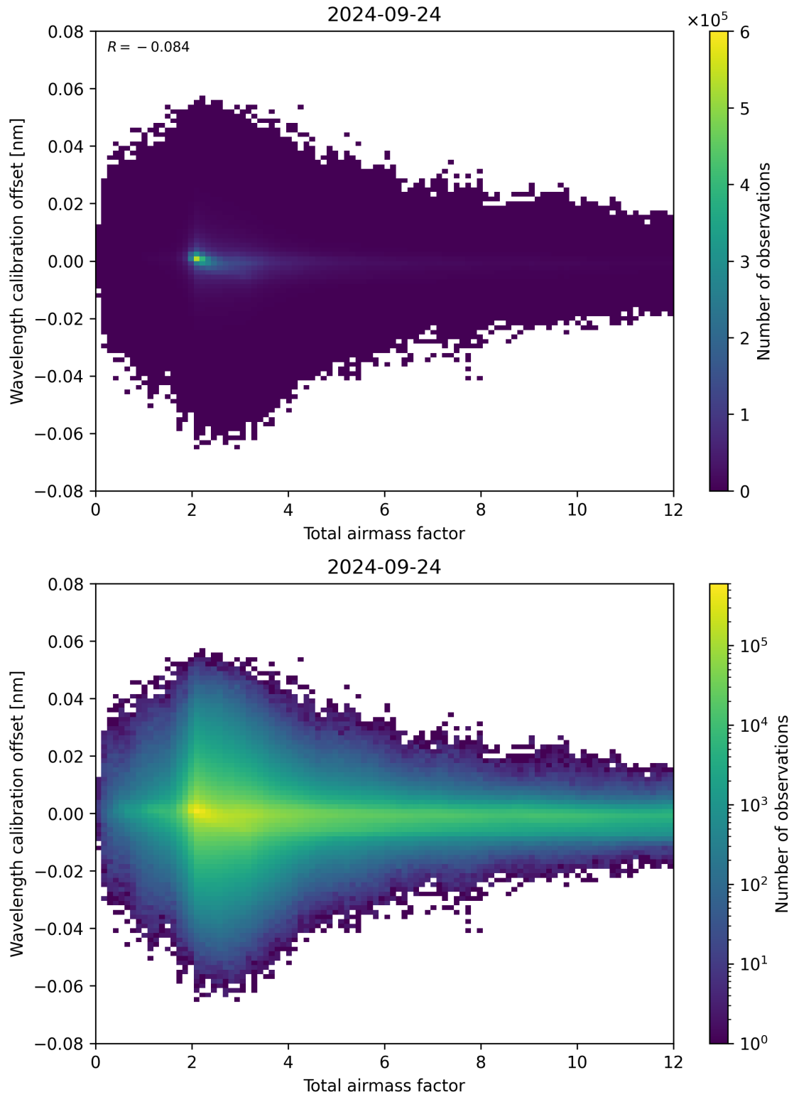
Figure 70: Scatter density plot of “Total airmass factor” against “Wavelength calibration offset” for 2024-09-23 to 2024-09-25.
