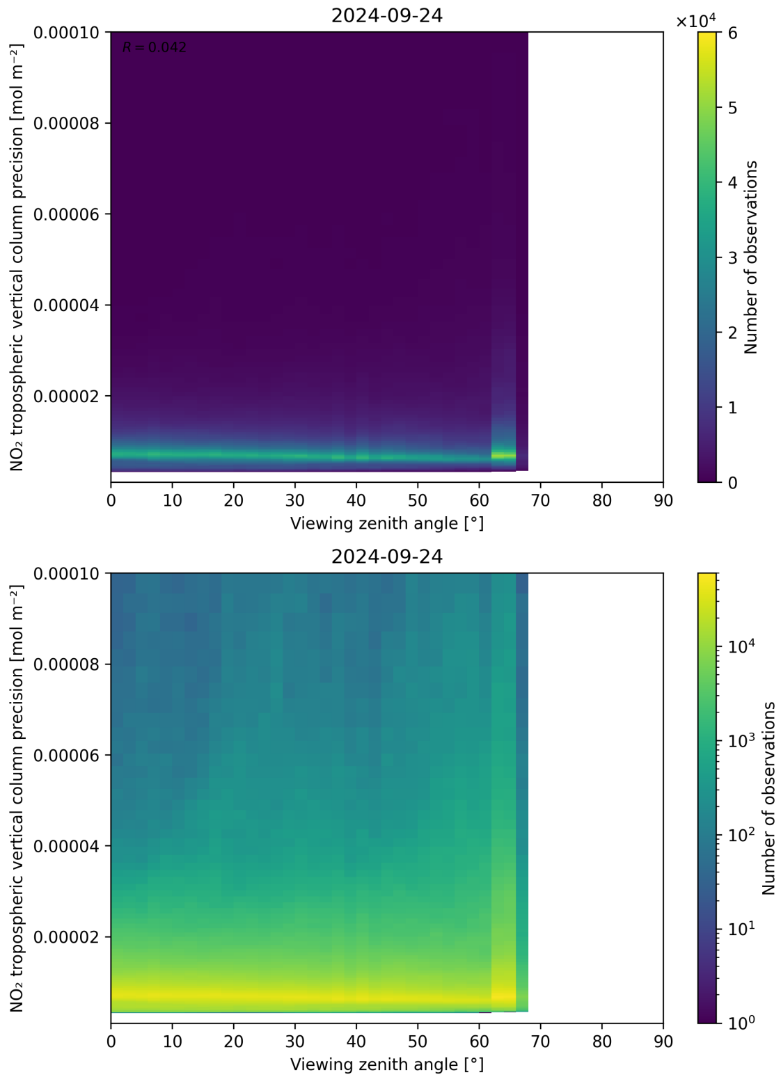
Figure 170: Scatter density plot of “Viewing zenith angle” against “NO 2 tropospheric vertical column precision” for 2024-09-23 to 2024-09-25.
