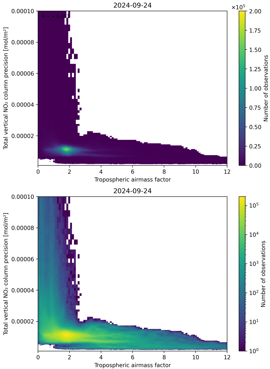
Figure 78: Scatter density plot of “Tropospheric air mass factor” against “Total vertical NO 2 column precision” for 2024-09-23 to 2024-09-25.
