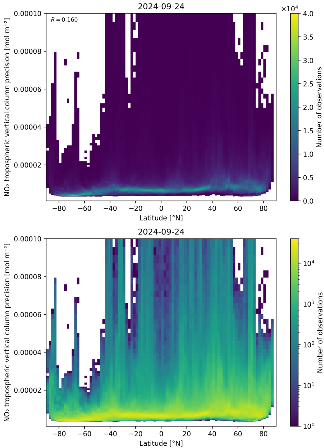
Figure 93: Scatter density plot of “Latitude” against “NO 2 tropospheric vertical column precision” for 2024-09-23 to 2024-09-25.
