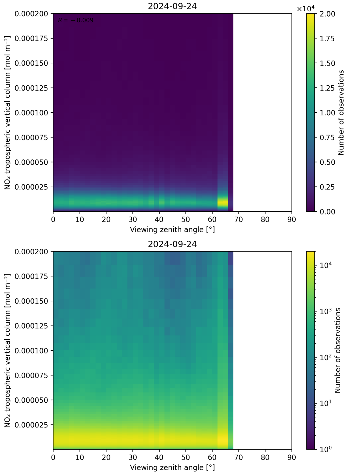
Figure 169: Scatter density plot of “Viewing zenith angle” against “NO 2 tropospheric vertical column” for 2024-09-23 to 2024-09-25.
