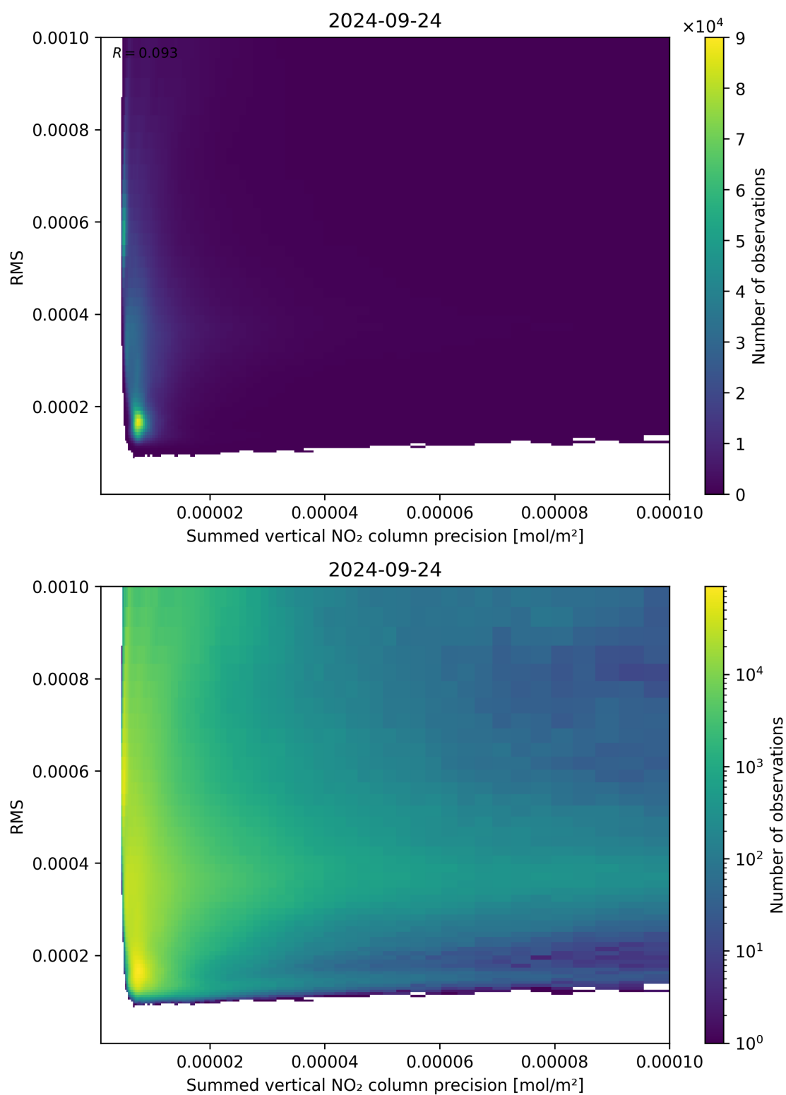
Figure 108: Scatter density plot of “Summed vertical NO 2 column precision” against “RMS” for 2024-09-23 to 2024-09-25.
