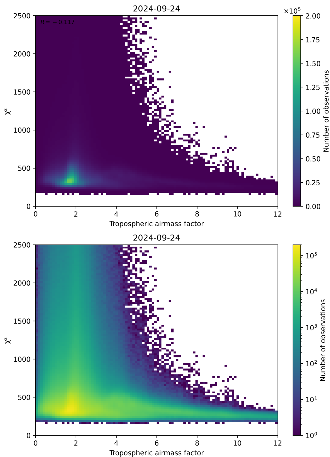
Figure 73: Scatter density plot of “Tropospheric airmass factor” against “ \chi^2 ” for 2024-09-23 to 2024-09-25.
