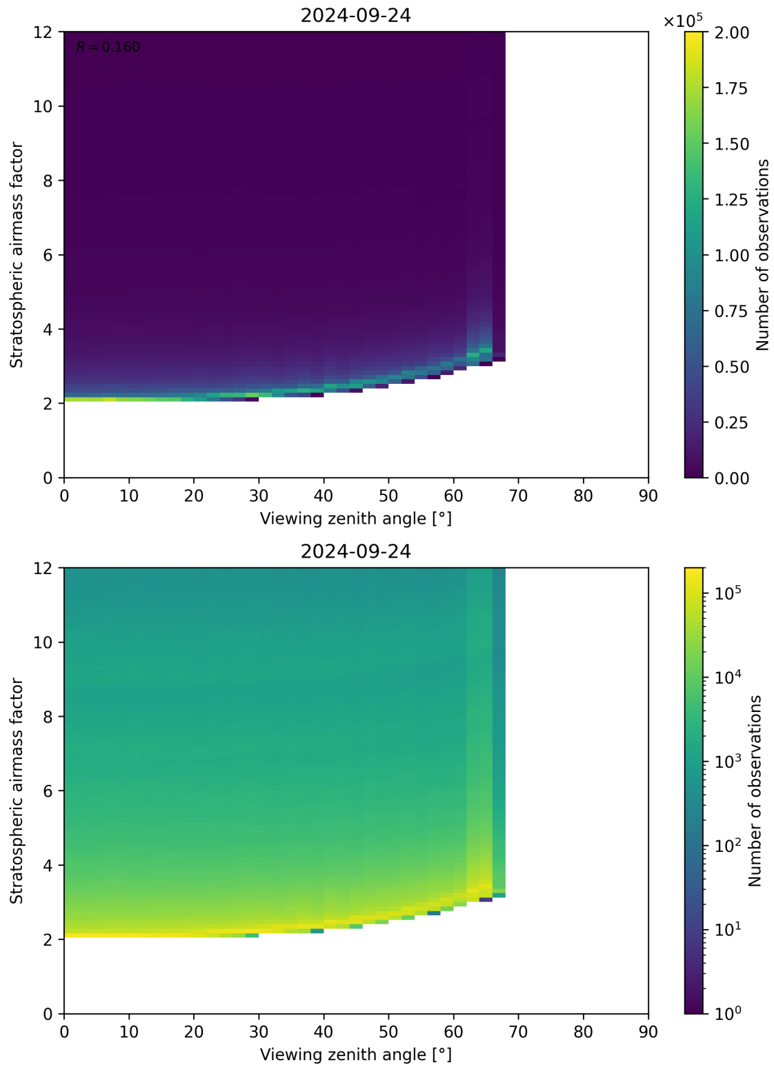
Figure 159: Scatter density plot of “Viewing zenith angle” against “Stratospheric airmass factor” for 2024-09-23 to 2024-09-25.
