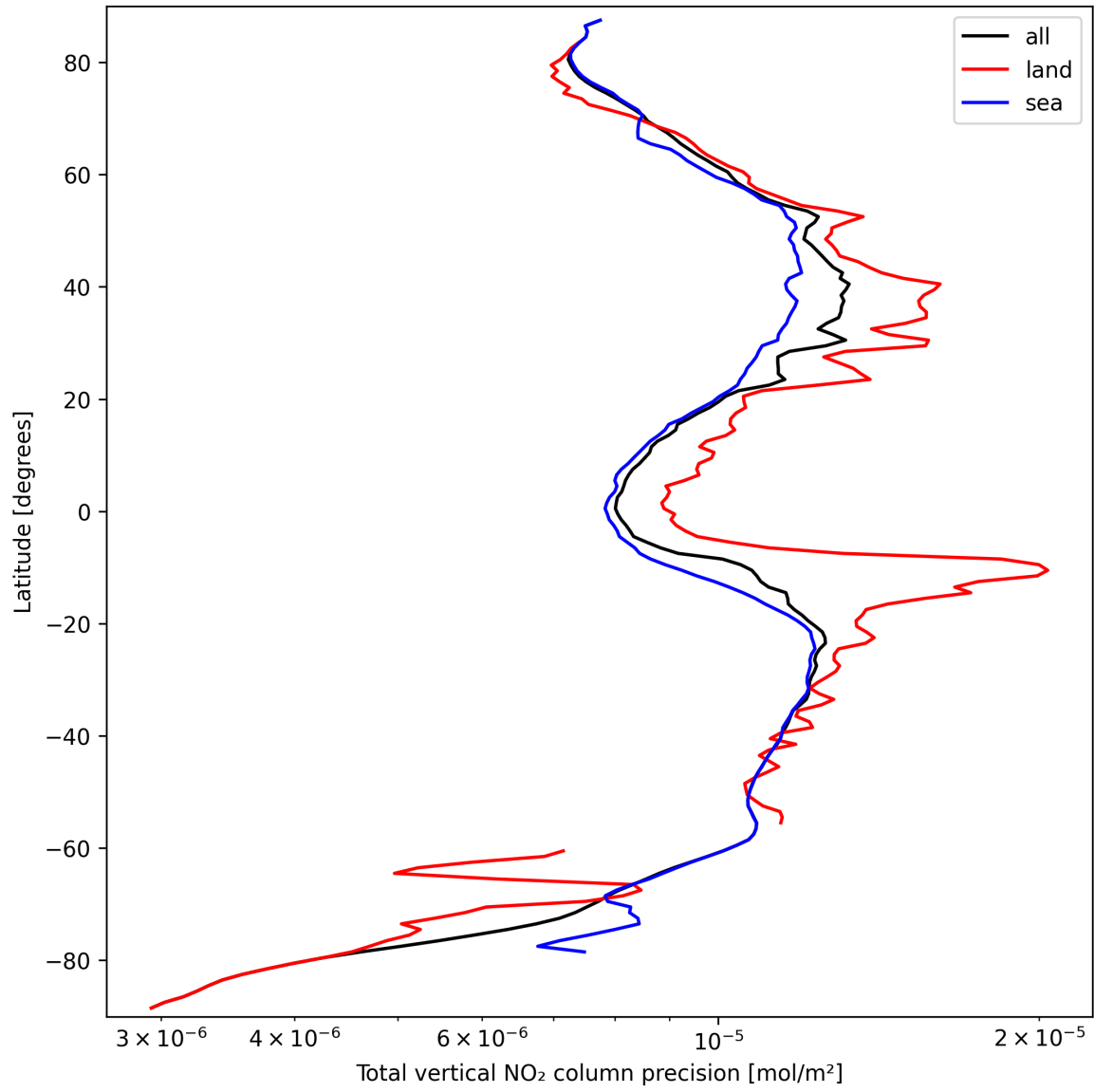
Figure 22: Zonal average of “Total vertical NO 2 column precision” for 2024-09-23 to 2024-09-25.
