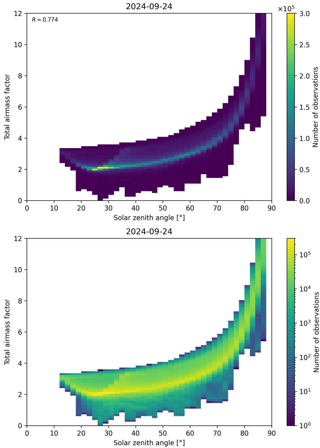
Figure 146: Scatter density plot of “Solar zenith angle” against “Total airmass factor” for 2024-09-23 to 2024-09-25.
