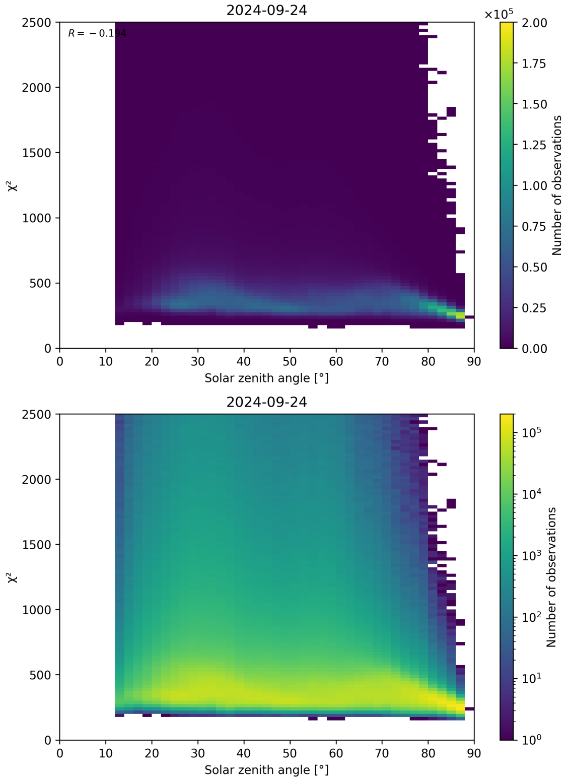
Figure 148: Scatter density plot of “Solar zenith angle” against “ \chi^2 ” for 2024-09-23 to 2024-09-25.
