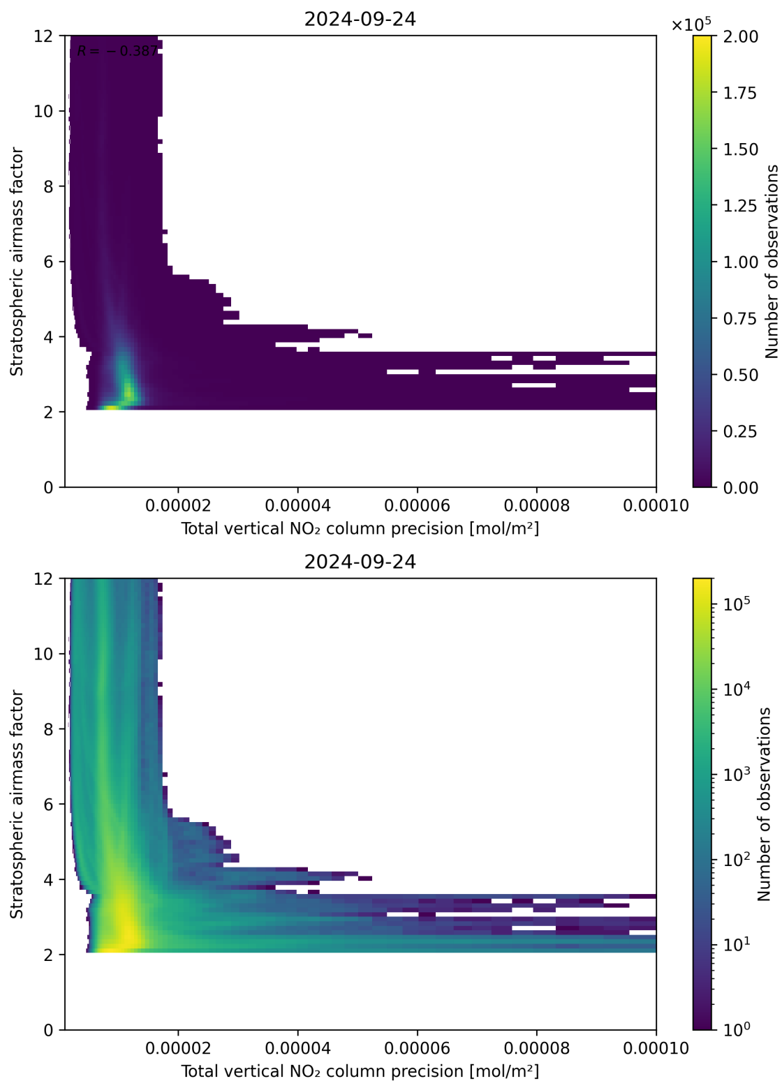
Figure 115: Scatter density plot of “Total vertical NO 2 column precision” against “Stratospheric air mass factor” for 2024-09-23 to 2024-09-25.
