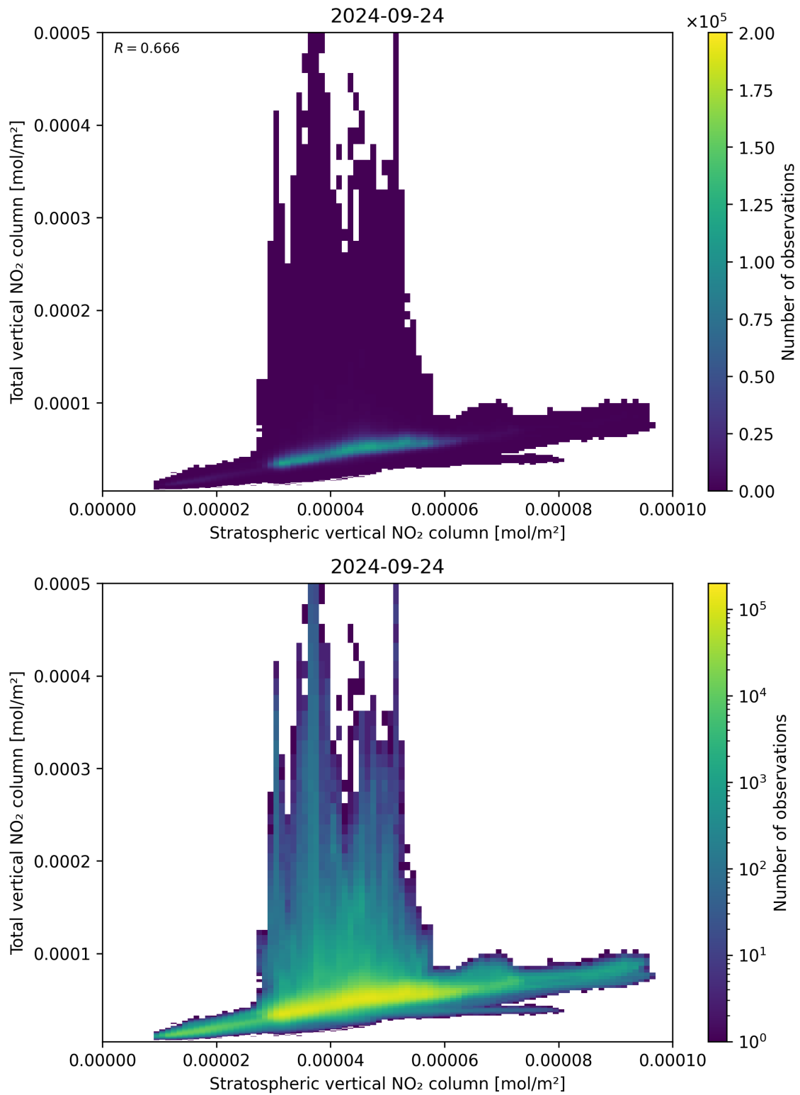
Figure 100: Scatter density plot of “Stratospheric vertical NO 2 column” against “Total vertical NO 2 column” for 2024-09-23 to 2024-09-25.
