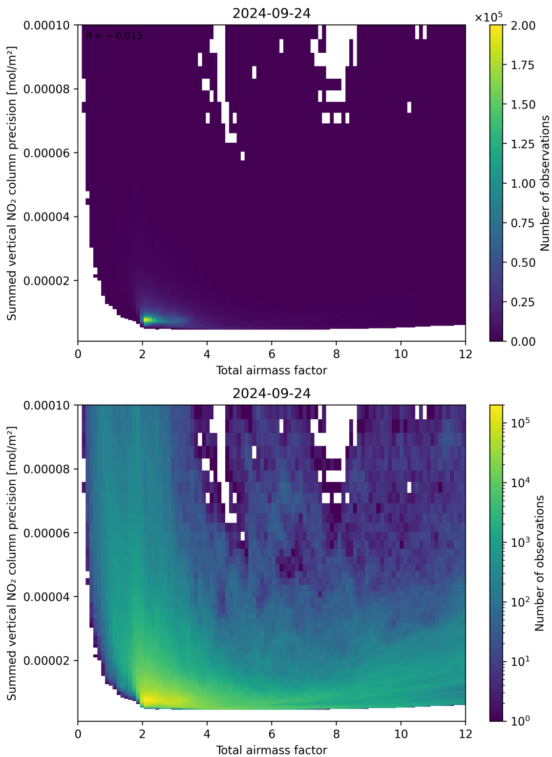
Figure 66: Scatter density plot of “Total airmass factor” against “Summed vertical NO 2 column precision” for 2024-09-23 to 2024-09-25.
