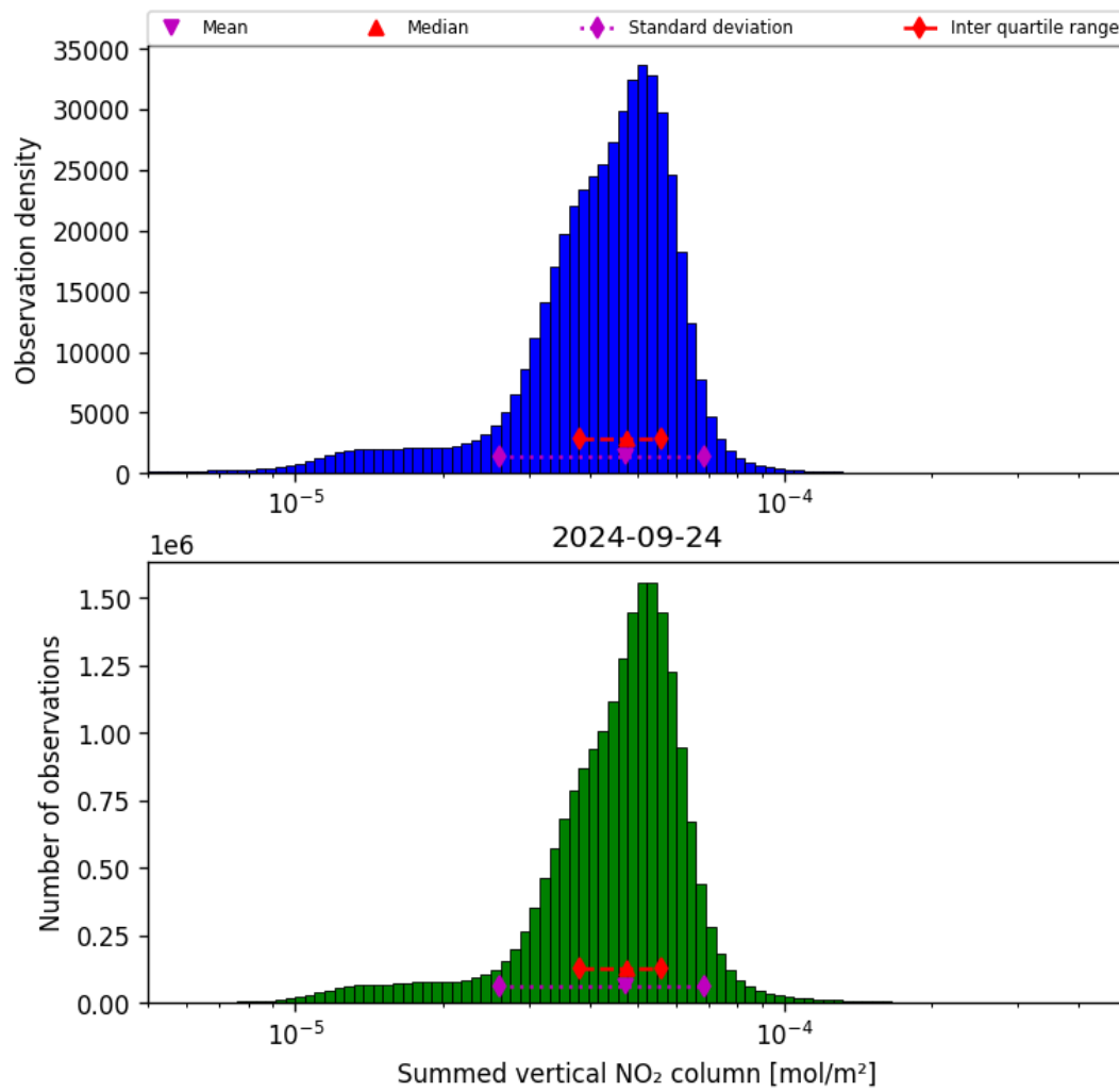
Figure 40: Histogram of “Summed vertical NO 2 column” for 2024-09-23 to 2024-09-25
