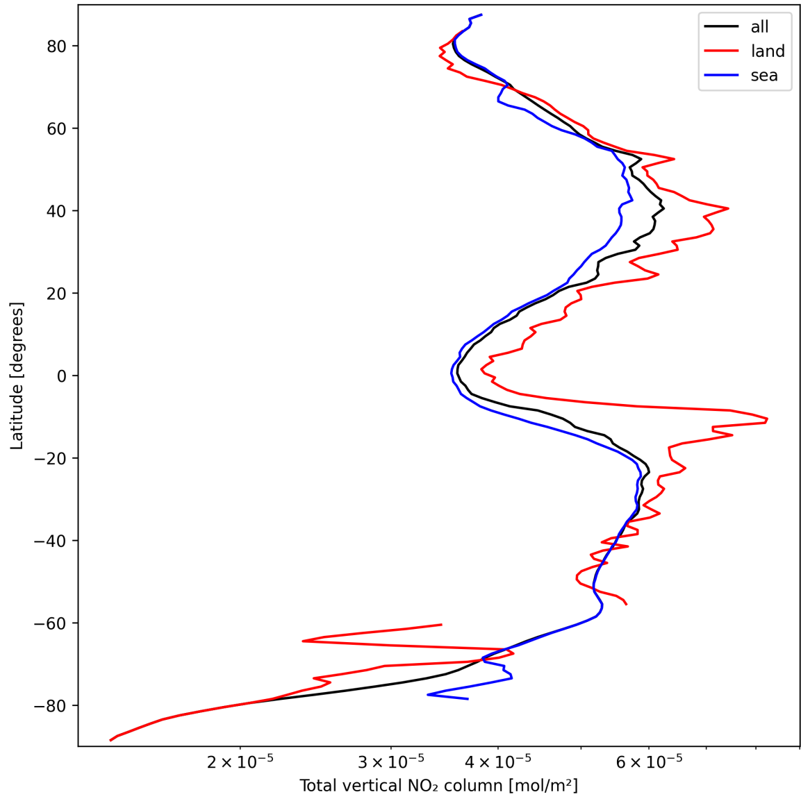
Figure 21: Zonal average of “Total vertical NO 2 column” for 2024-09-23 to 2024-09-25.
