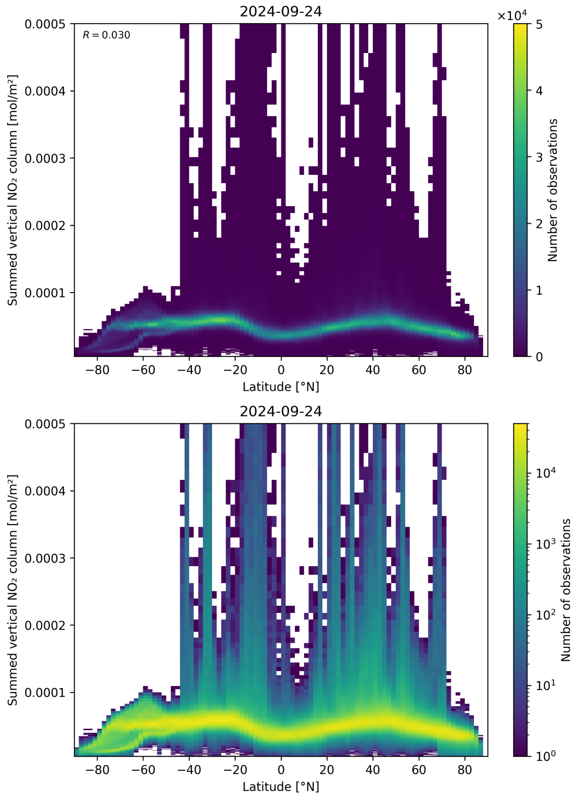
Figure 88: Scatter density plot of “Latitude” against “Summed vertical NO 2 column” for 2024-09-23 to 2024-09-25.
