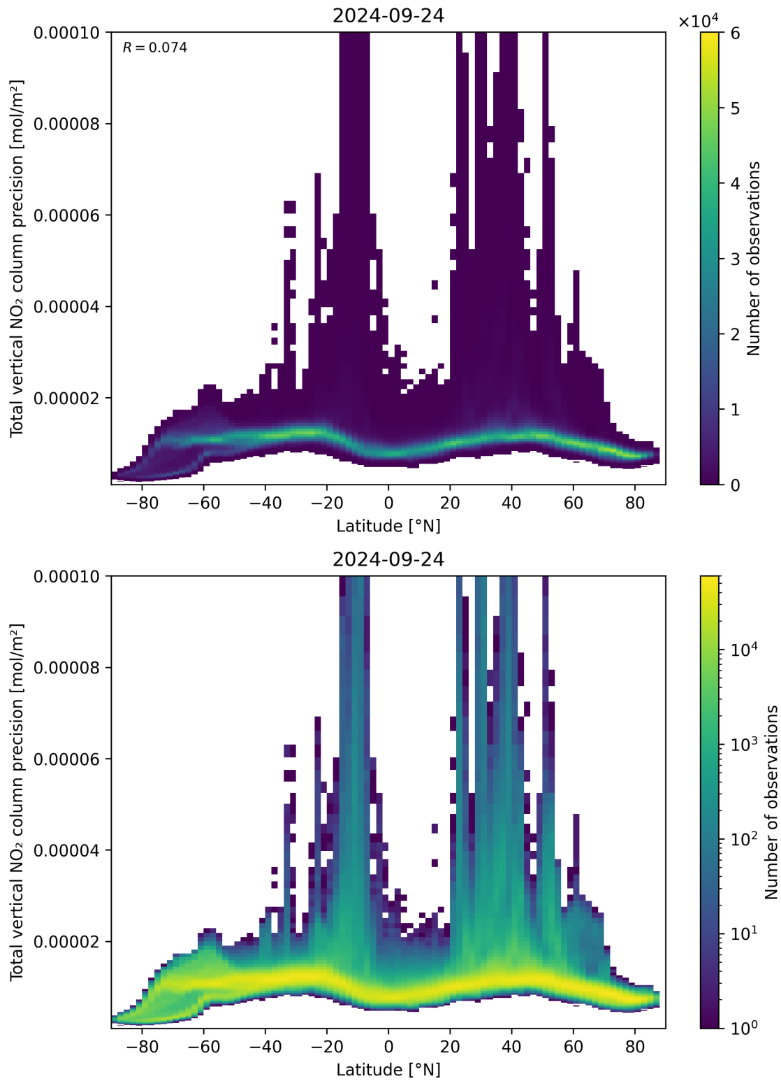
Figure 91: Scatter density plot of “Latitude” against “Total vertical NO 2 column precision” for 2024-09-23 to 2024-09-25.
