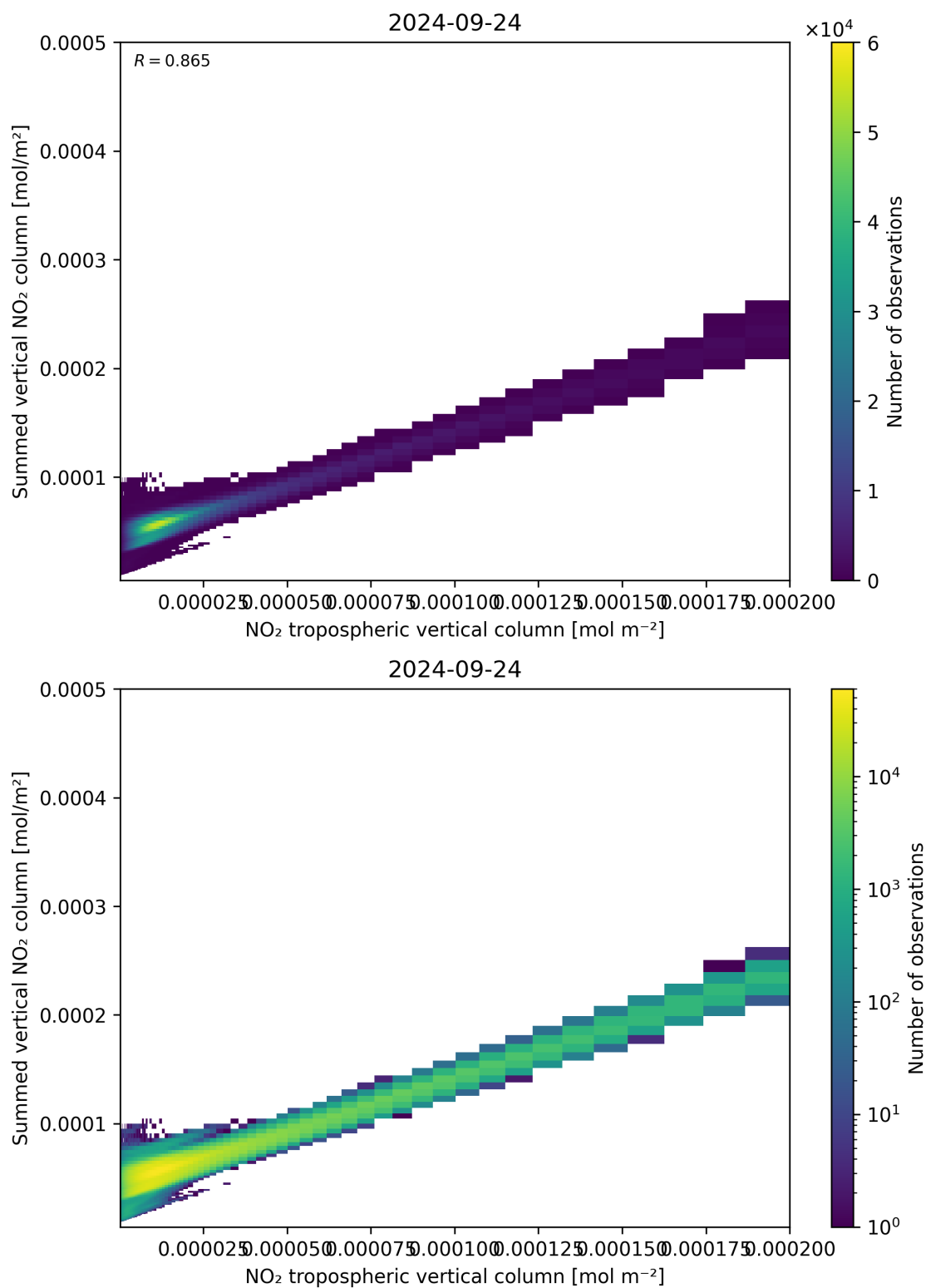
Figure 126: Scatter density plot of “NO 2 tropospheric vertical column” against “Summed vertical NO 2 column” for 2024-09-23 to 2024-09-25.
