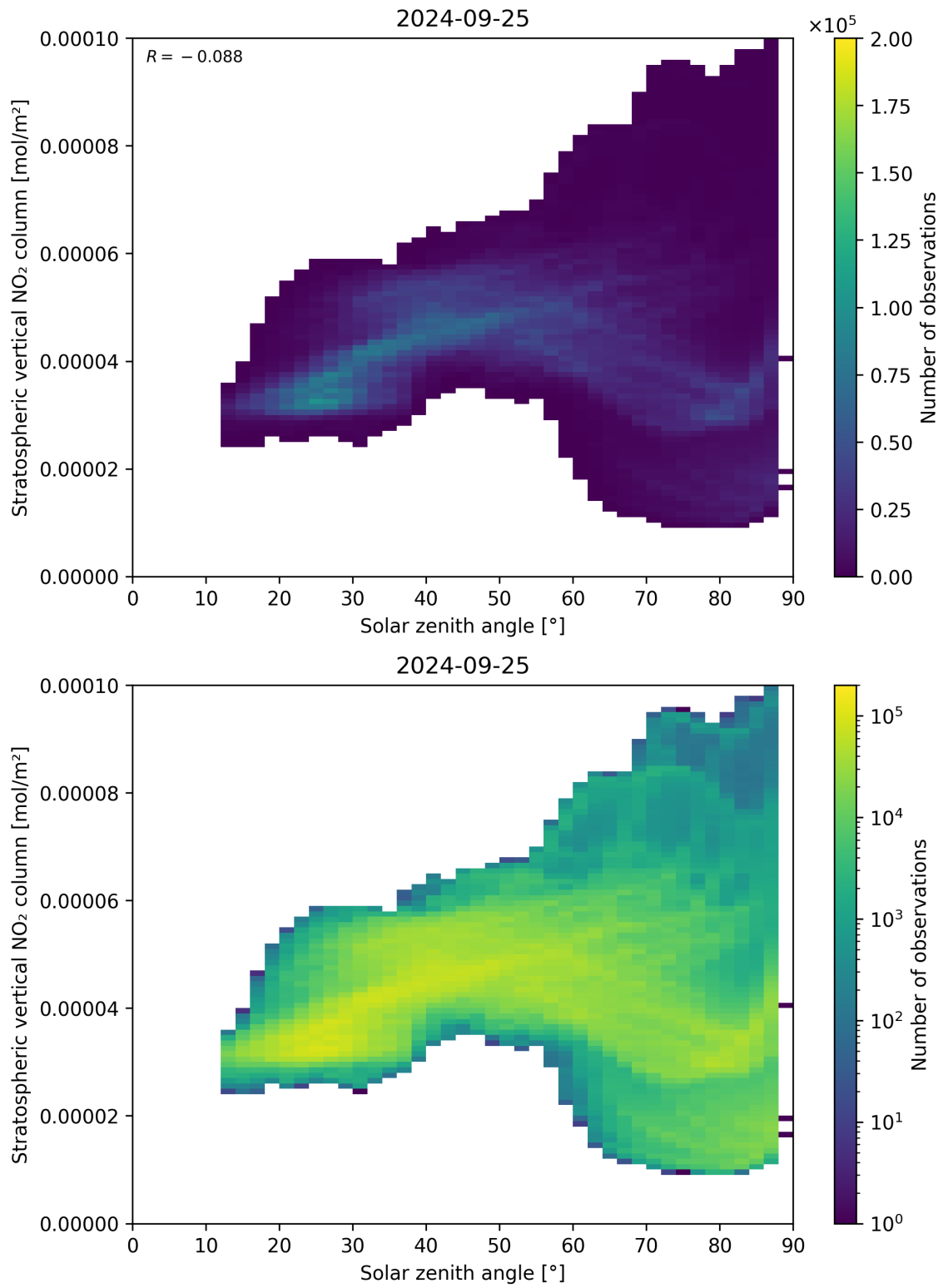
Figure 150: Scatter density plot of “Solar zenith angle” against “Stratospheric vertical NO 2 column” for 2024-09-24 to 2024-09-26.
