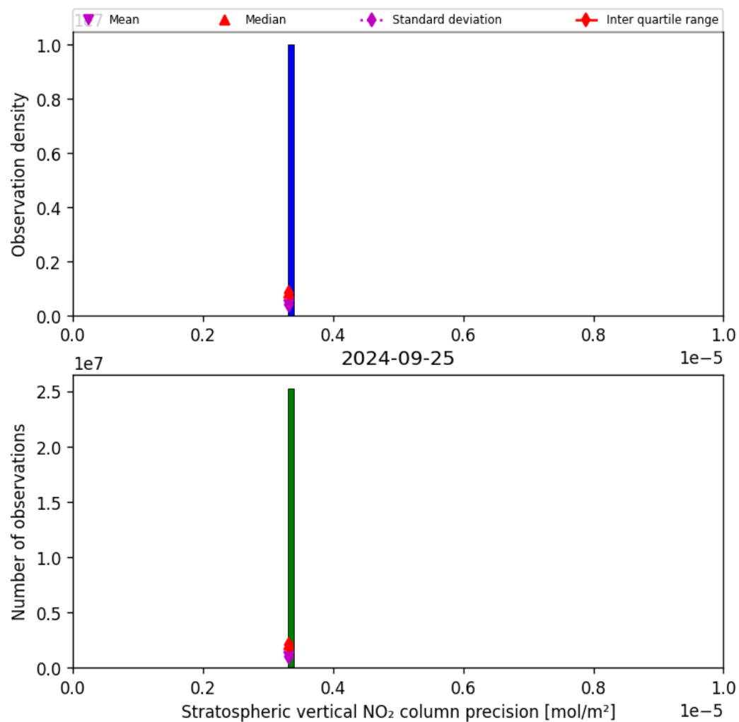
Figure 37: Histogram of “Stratospheric vertical NO 2 column precision” for 2024-09-24 to 2024-09-26
