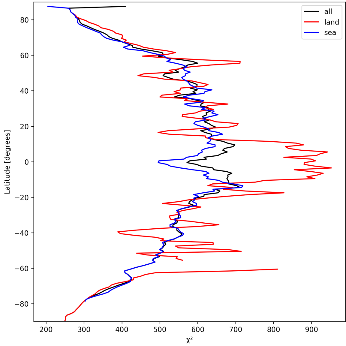
Figure 25: Zonal average of “ \chi^2 ” for 2024-09-24 to 2024-09-26.
