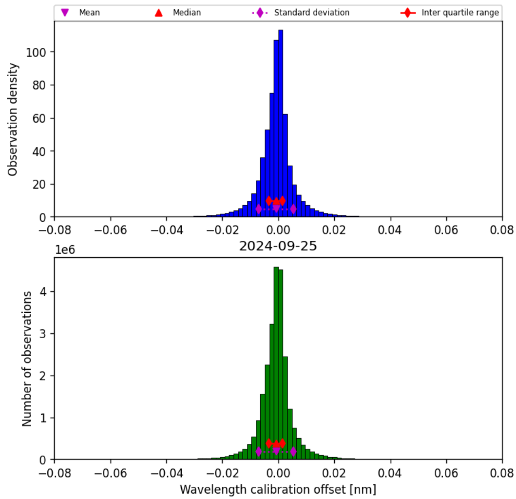
Figure 35: Histogram of “Wavelength calibration offset” for 2024-09-24 to 2024-09-26
