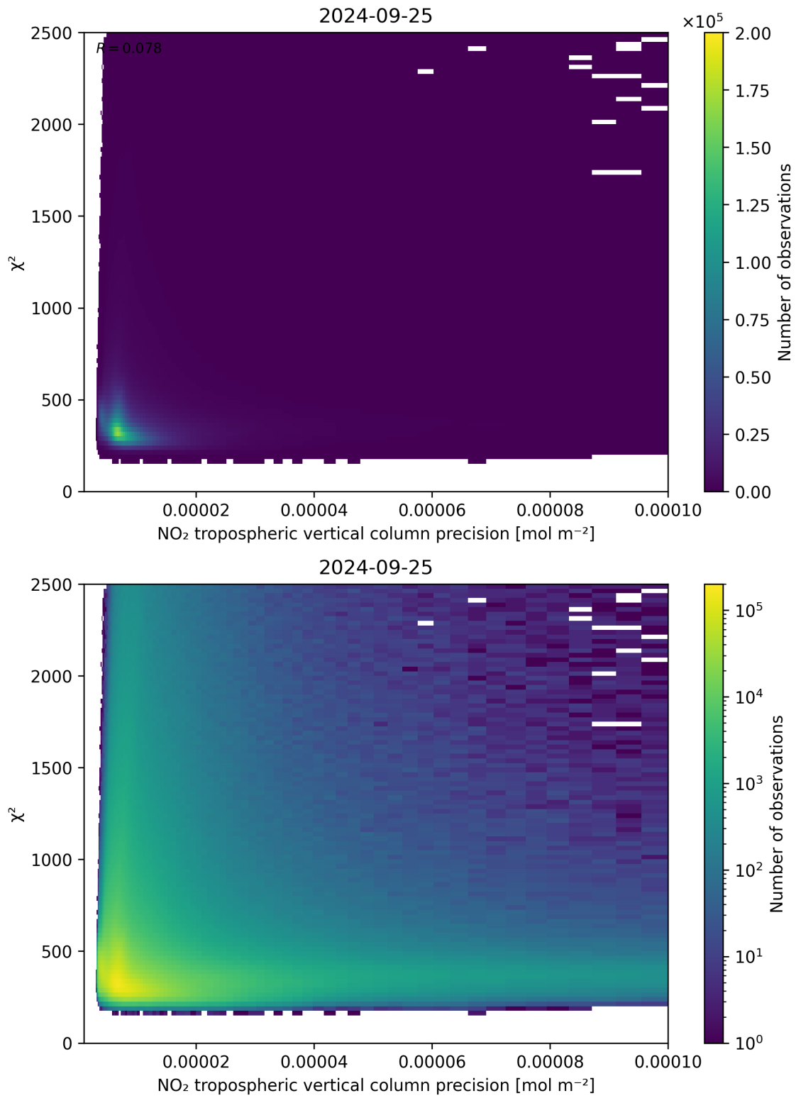
Figure 134: Scatter density plot of “NO 2 tropospheric vertical column precision” against “ \chi^2 ” for 2024-09-24 to 2024-09-26.
