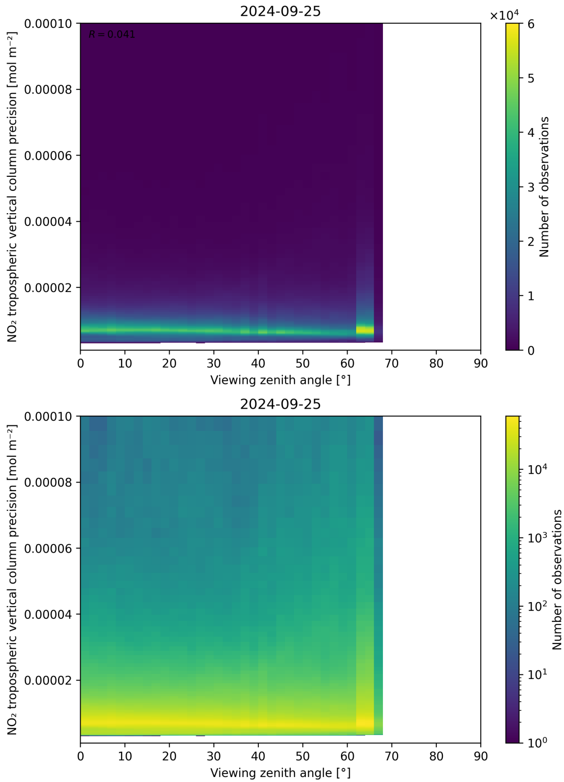
Figure 170: Scatter density plot of “Viewing zenith angle” against “NO 2 tropospheric vertical column precision” for 2024-09-24 to 2024-09-26.
