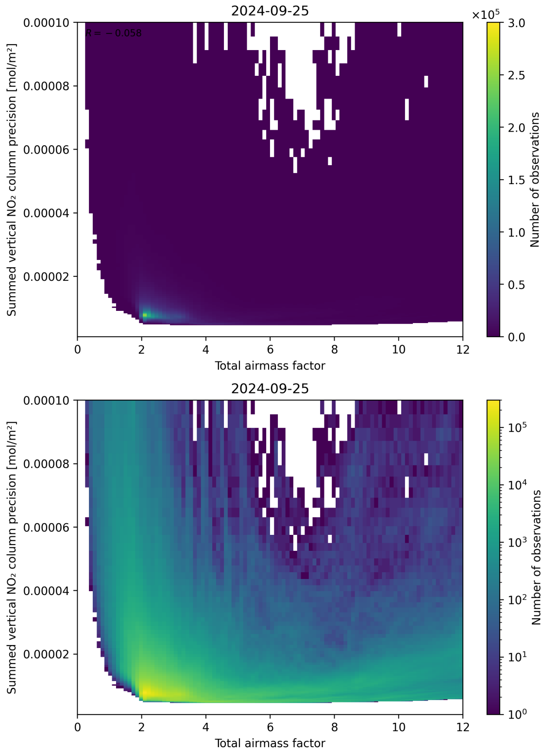
Figure 66: Scatter density plot of “Total airmass factor” against “Summed vertical NO 2 column precision” for 2024-09-24 to 2024-09-26.
