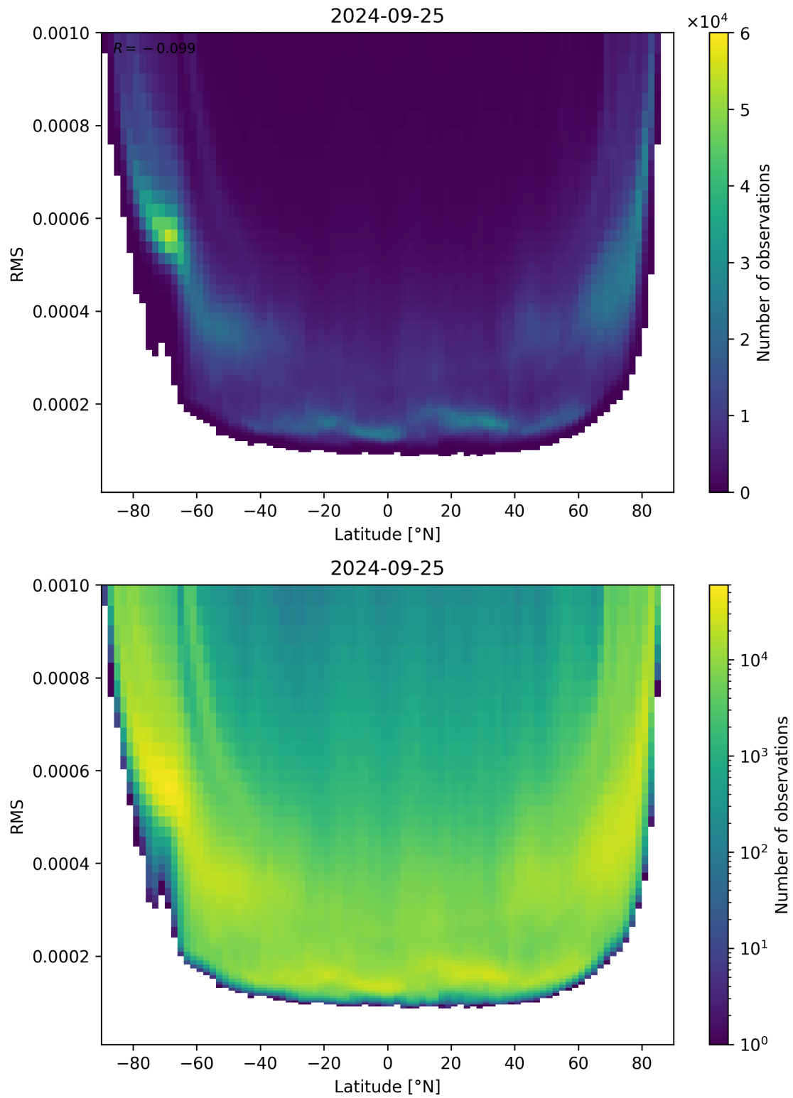
Figure 94: Scatter density plot of “Latitude” against “RMS” for 2024-09-24 to 2024-09-26.
