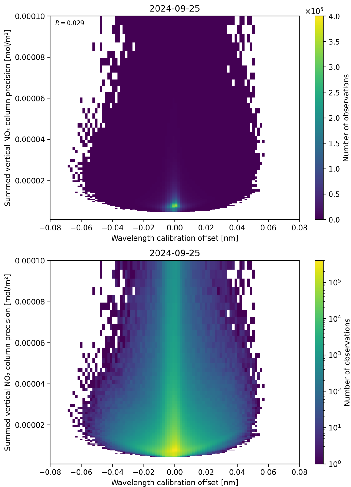
Figure 178: Scatter density plot of “Wavelength calibration offset” against “Summed vertical NO 2 column precision” for 2024-09-24 to 2024-09-26.
