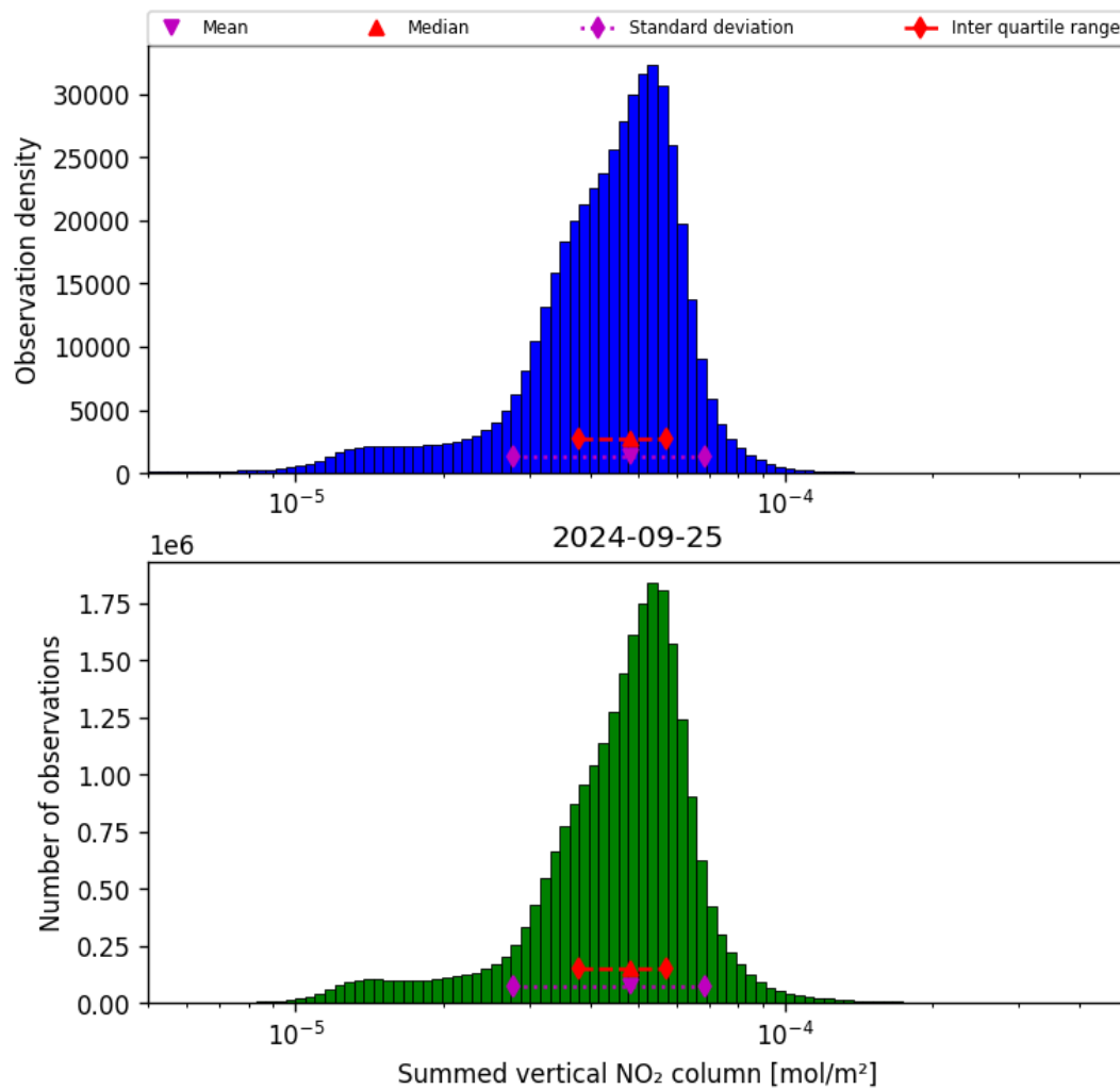
Figure 40: Histogram of “Summed vertical NO 2 column” for 2024-09-24 to 2024-09-26
