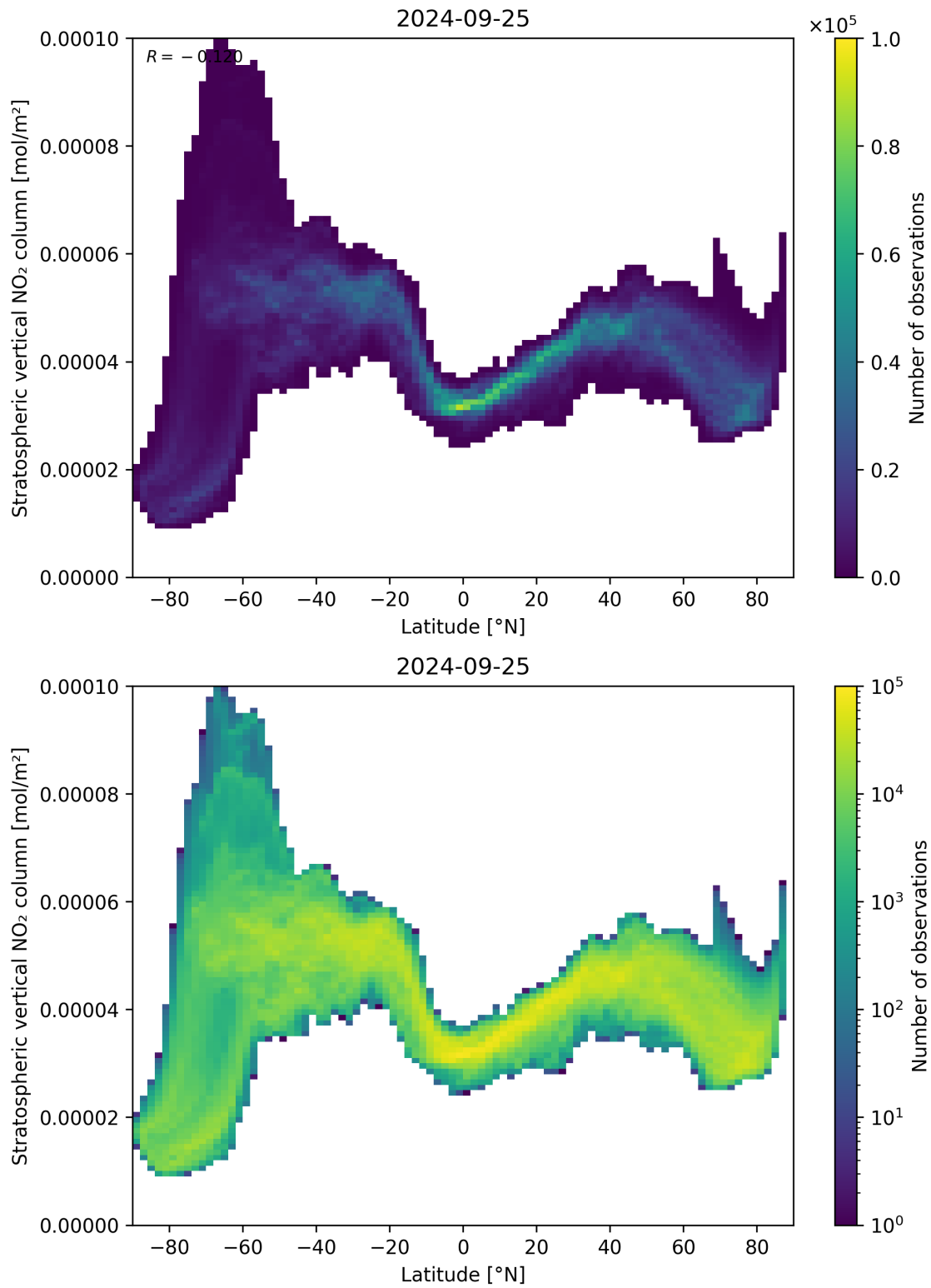
Figure 87: Scatter density plot of “Latitude” against “Stratospheric vertical NO 2 column” for 2024-09-24 to 2024-09-26.
