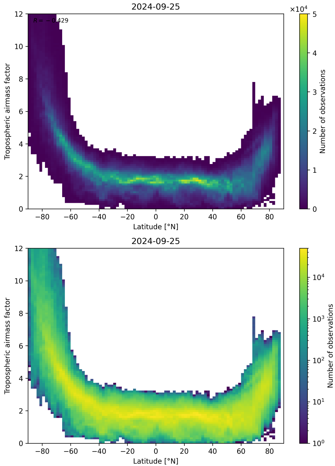
Figure 85: Scatter density plot of “Latitude” against “Tropospheric air mass factor” for 2024-09-24 to 2024-09-26.
