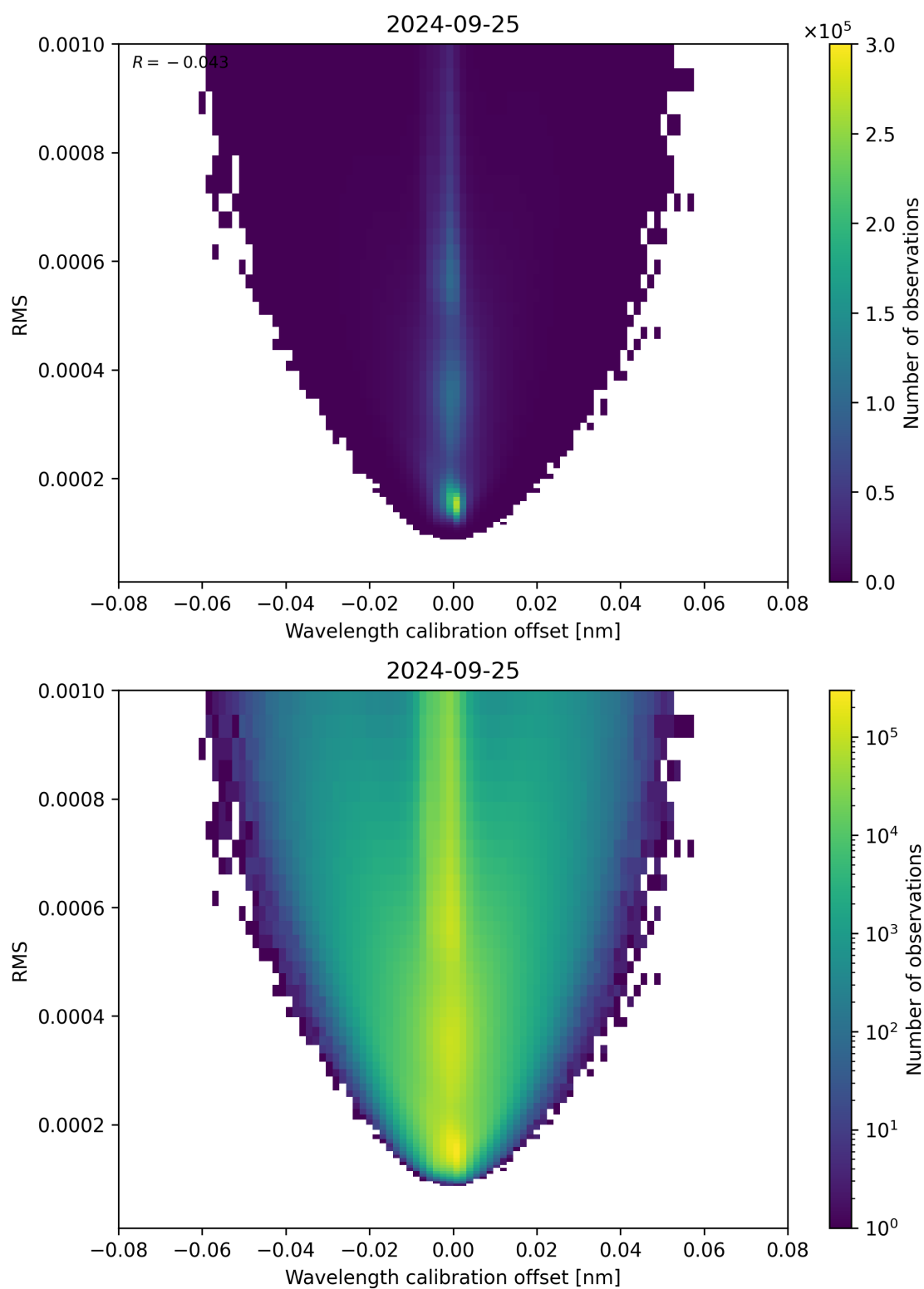
Figure 181: Scatter density plot of “Wavelength calibration offset” against “RMS” for 2024-09-24 to 2024-09-26.
