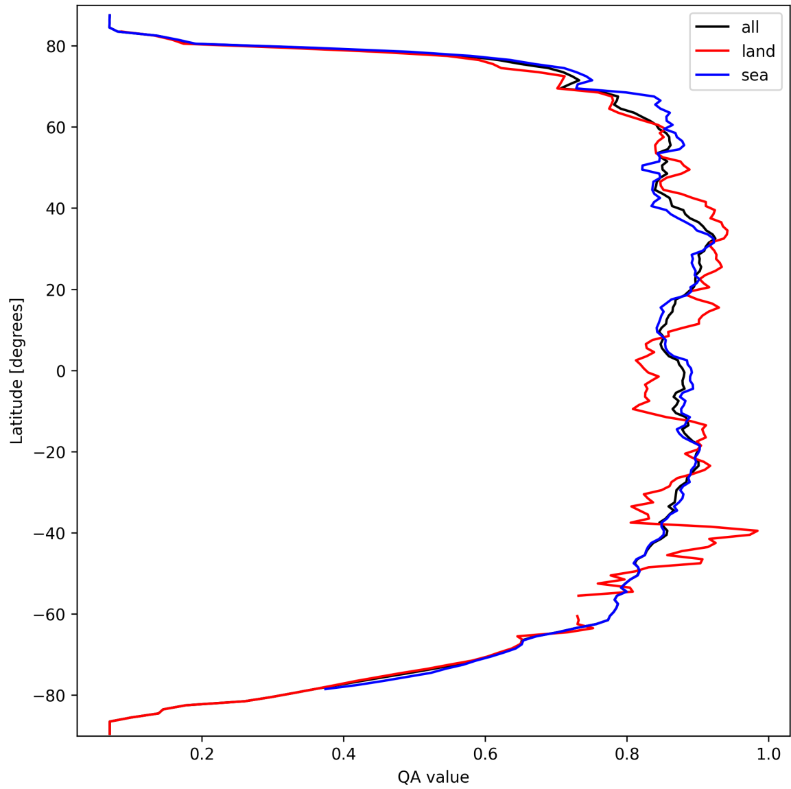
Figure 11: Zonal average of “QA value” for 2024-09-24 to 2024-09-26.
