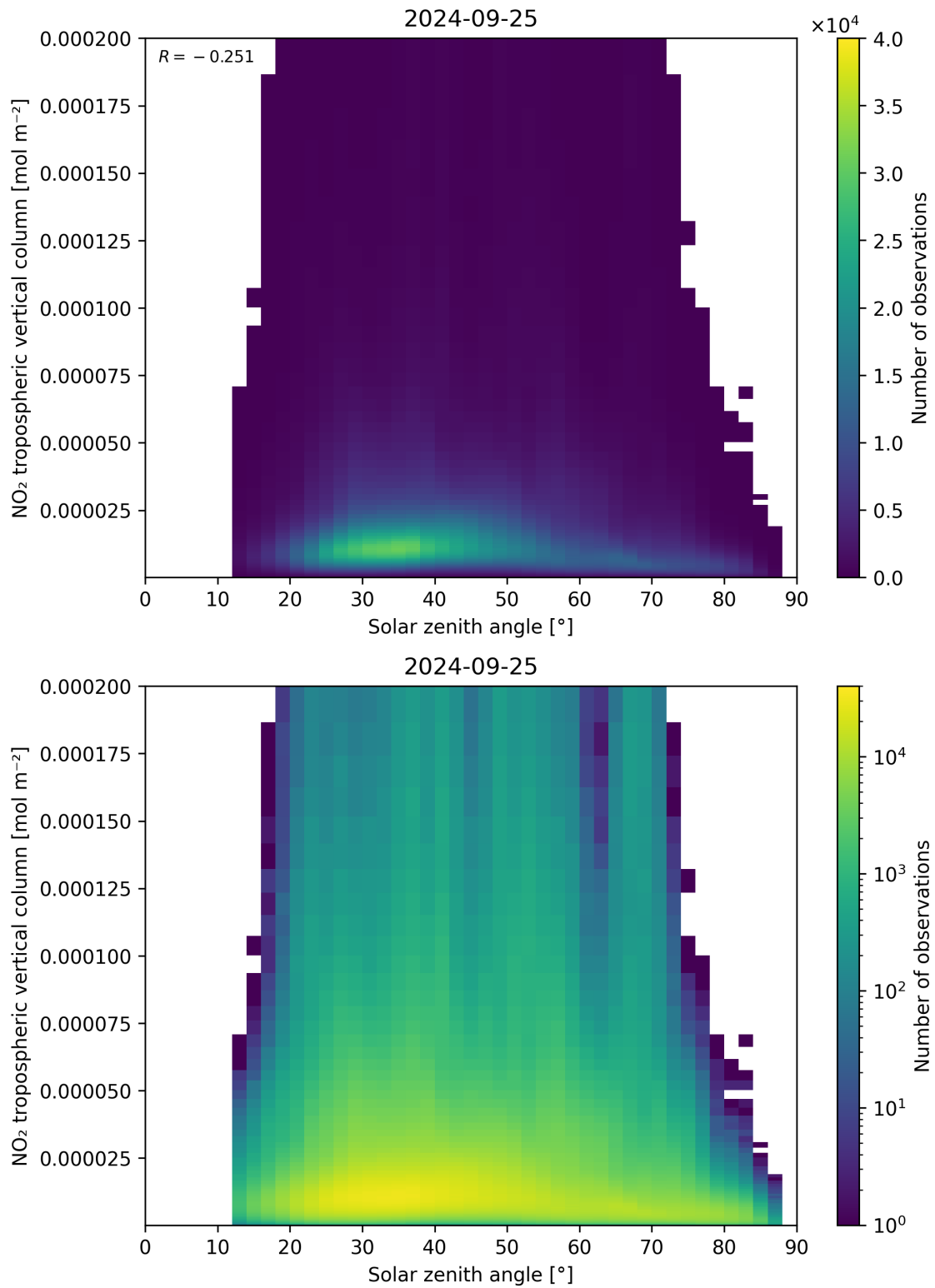
Figure 155: Scatter density plot of “Solar zenith angle” against “NO 2 tropospheric vertical column” for 2024-09-24 to 2024-09-26.
