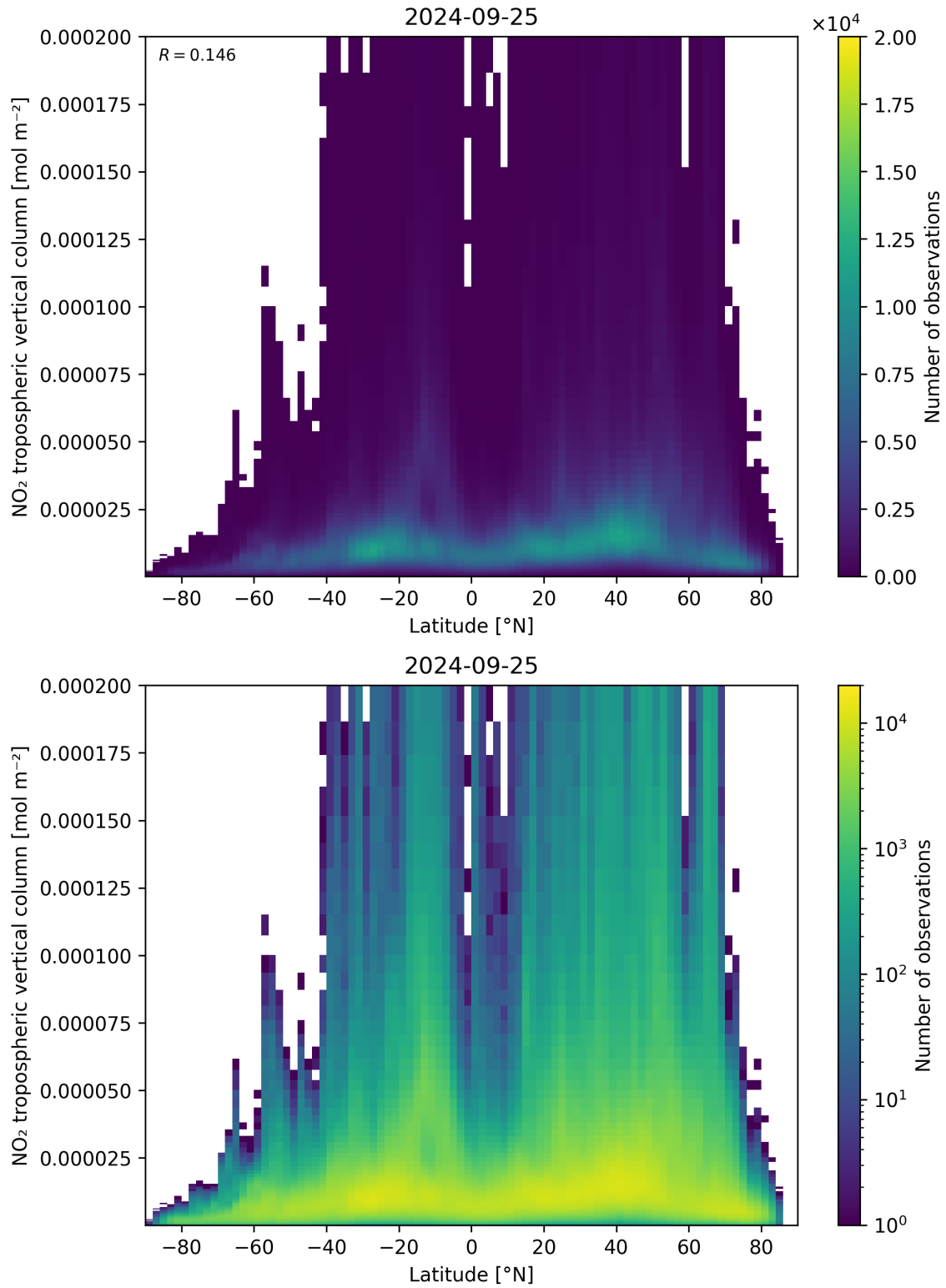
Figure 92: Scatter density plot of “Latitude” against “NO 2 tropospheric vertical column” for 2024-09-24 to 2024-09-26.
