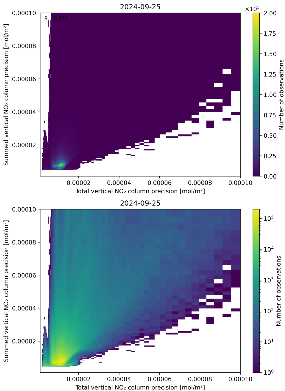
Figure 118: Scatter density plot of “Total vertical NO 2 column precision” against “Summed vertical NO 2 column precision” for 2024-09-24 to 2024-09-26.
