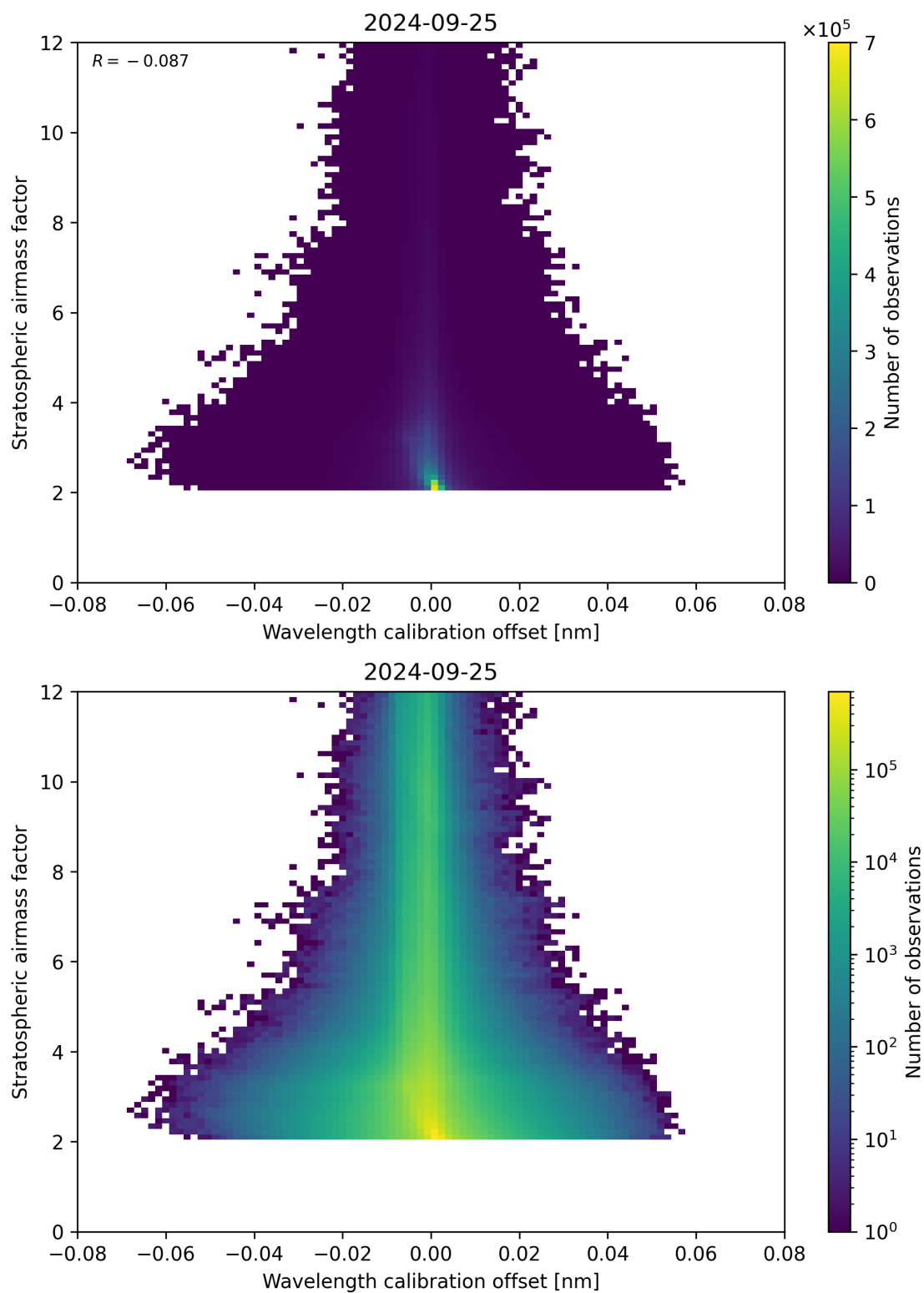
Figure 174: Scatter density plot of “Wavelength calibration offset” against “Stratospheric airmass factor” for 2024-09-24 to 2024-09-26.
