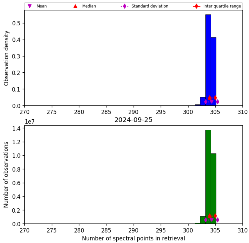
Figure 33: Histogram of “Number of spectral points in retrieval” for 2024-09-24 to 2024-09-26
