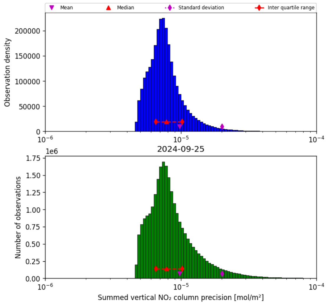
Figure 41: Histogram of "Summed vertical NO 2 column precision" for 2024-09-24 to 2024-09-26
