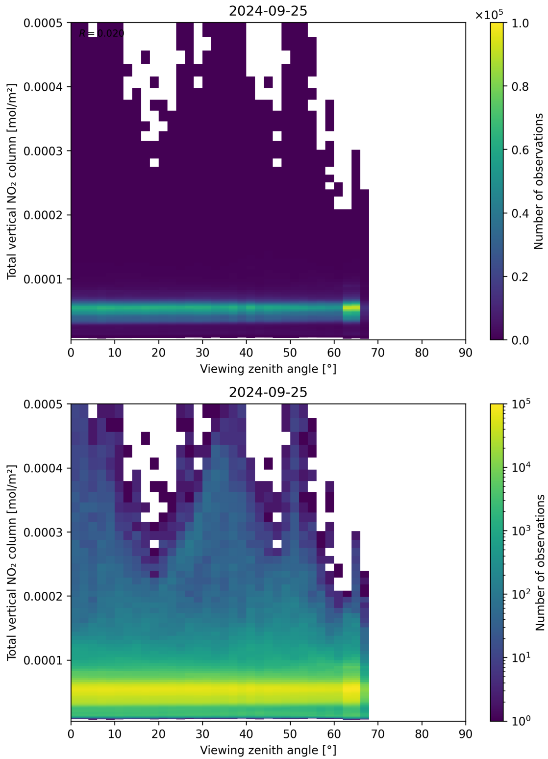
Figure 167: Scatter density plot of “Viewing zenith angle” against “Total vertical NO 2 column” for 2024-09-24 to 2024-09-26.
