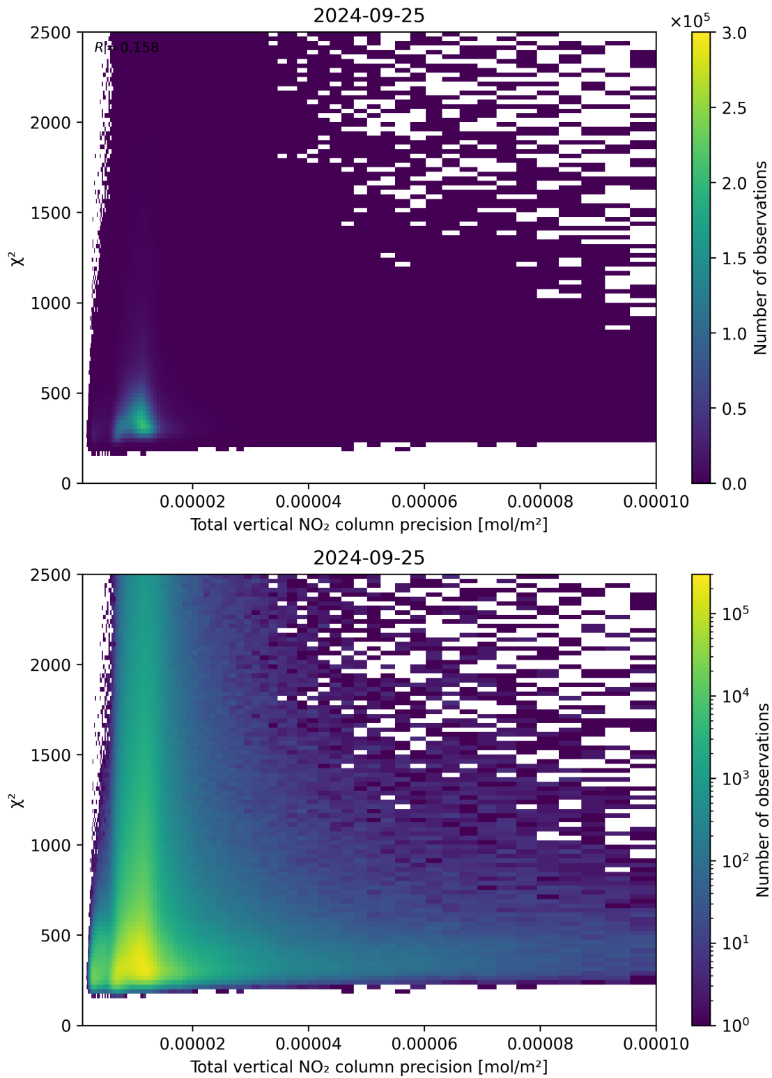
Figure 116: Scatter density plot of “Total vertical NO 2 column precision” against “ \chi^2 ” for 2024-09-24 to 2024-09-26.
