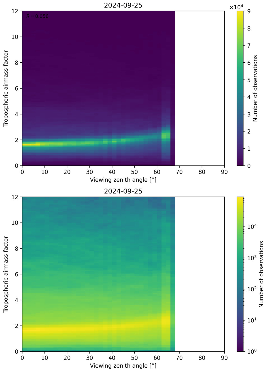
Figure 161: Scatter density plot of “Viewing zenith angle” against “Tropospheric airmass factor” for 2024-09-24 to 2024-09-26.
