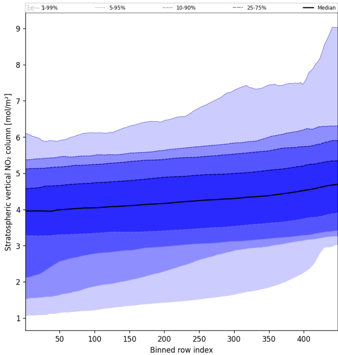
Figure 53: Along track statistics of “Stratospheric vertical NO 2 column” for 2024-09-24 to 2024-09-26
