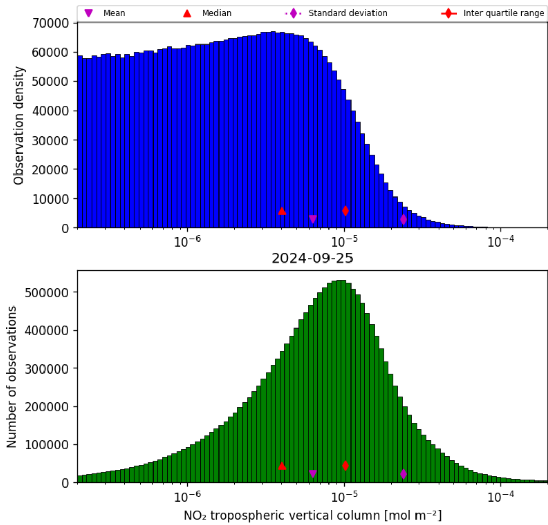
Figure 29: Histogram of “NO 2 tropospheric vertical column” for 2024-09-24 to 2024-09-26
