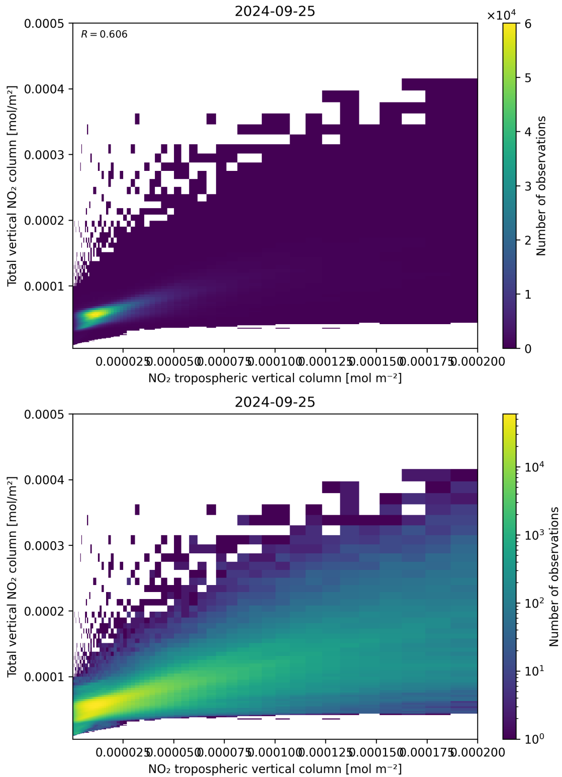
Figure 128: Scatter density plot of “NO 2 tropospheric vertical column” against “Total vertical NO 2 column” for 2024-09-24 to 2024-09-26.
