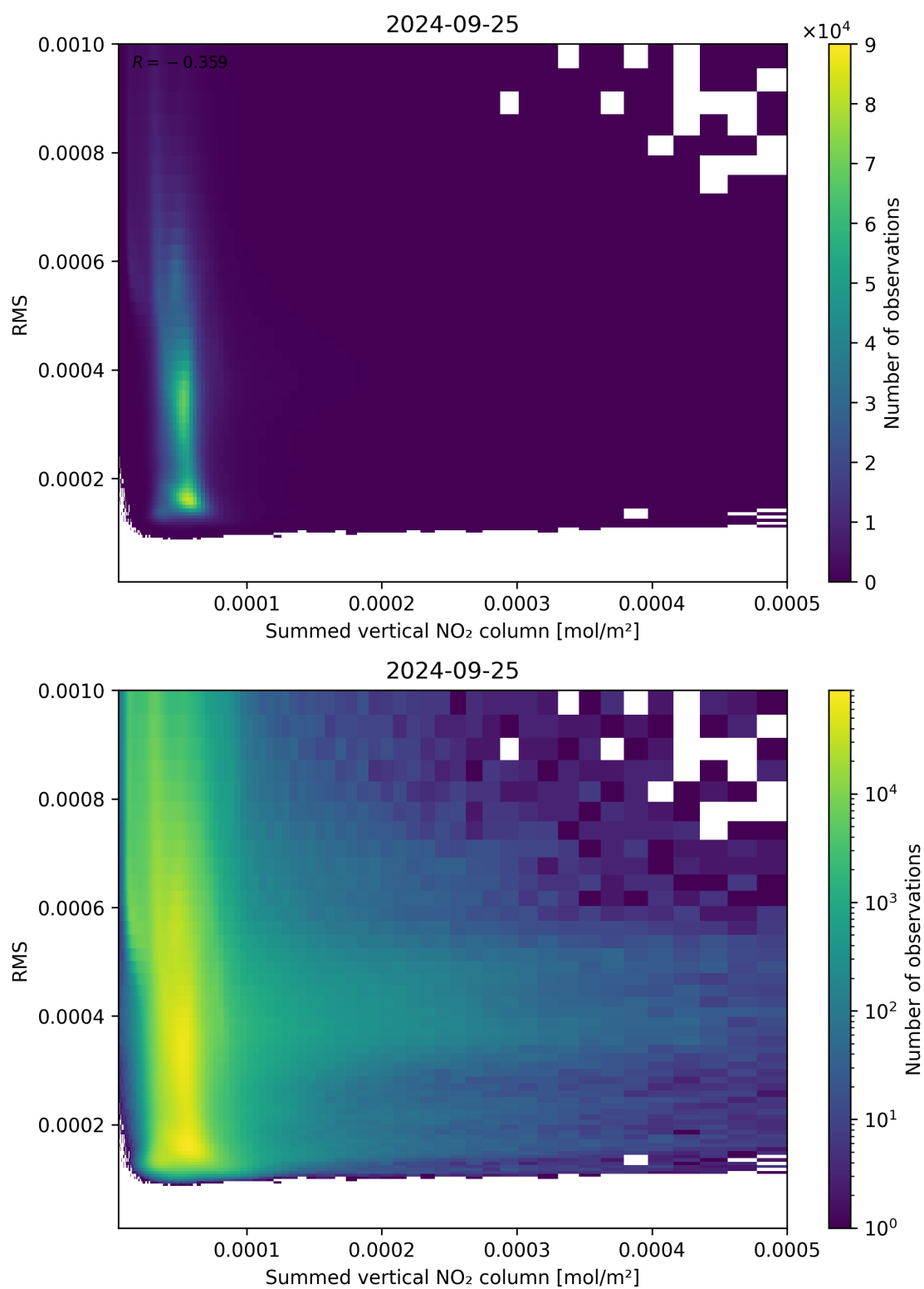
Figure 109: Scatter density plot of “Summed vertical NO 2 column” against “RMS” for 2024-09-24 to 2024-09-26.
