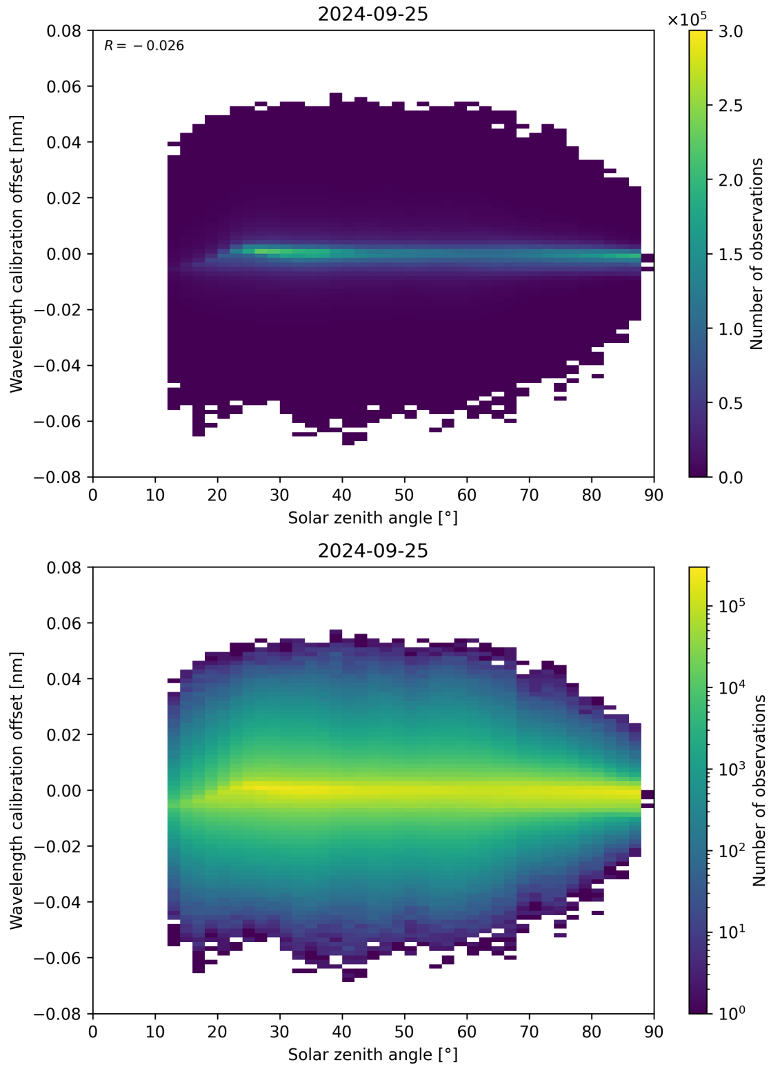
Figure 158: Scatter density plot of “Solar zenith angle” against “Wavelength calibration offset” for 2024-09-24 to 2024-09-26.
