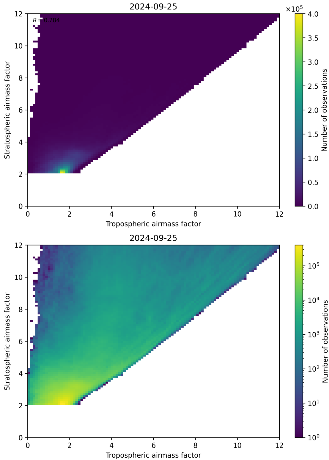
Figure 71: Scatter density plot of “Tropospheric airmass factor” against “Stratospheric airmass factor” for 2024-09-24 to 2024-09-26.
