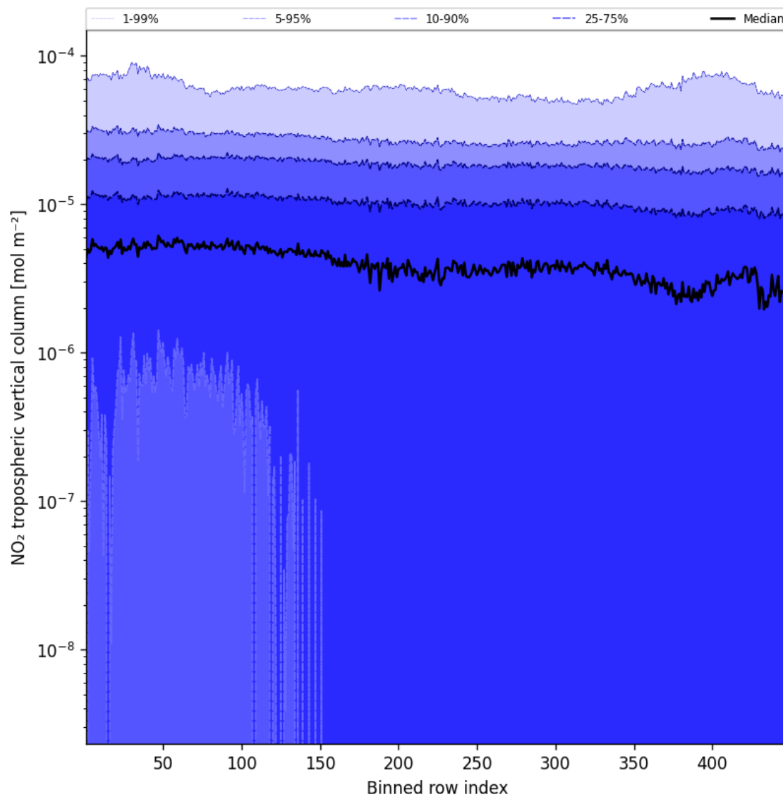
Figure 46: Along track statistics of “NO 2 tropospheric vertical column” for 2024-09-24 to 2024-09-26
