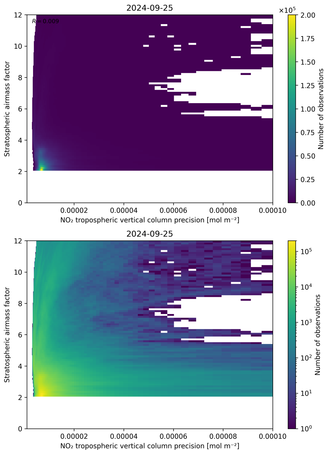
Figure 131: Scatter density plot of “NO 2 tropospheric vertical column precision” against “Stratospheric airmass factor” for 2024-09-24 to 2024-09-26.
