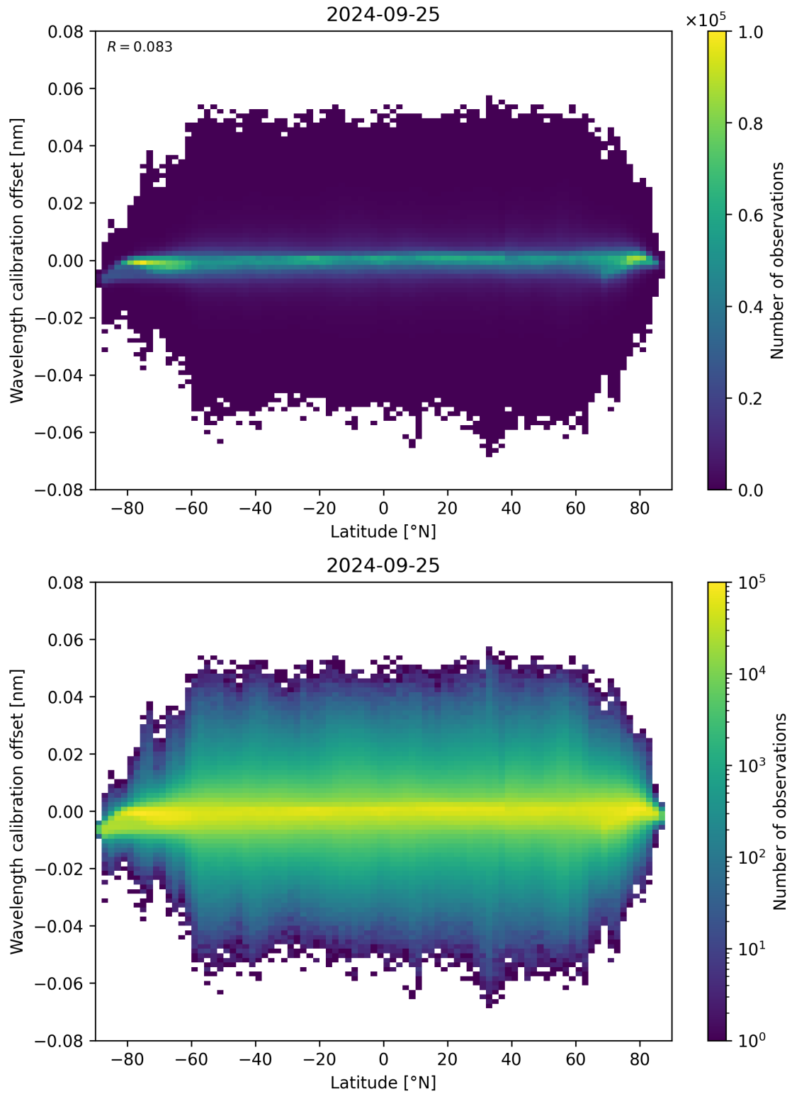
Figure 95: Scatter density plot of “Latitude” against “Wavelength calibration offset” for 2024-09-24 to 2024-09-26.
