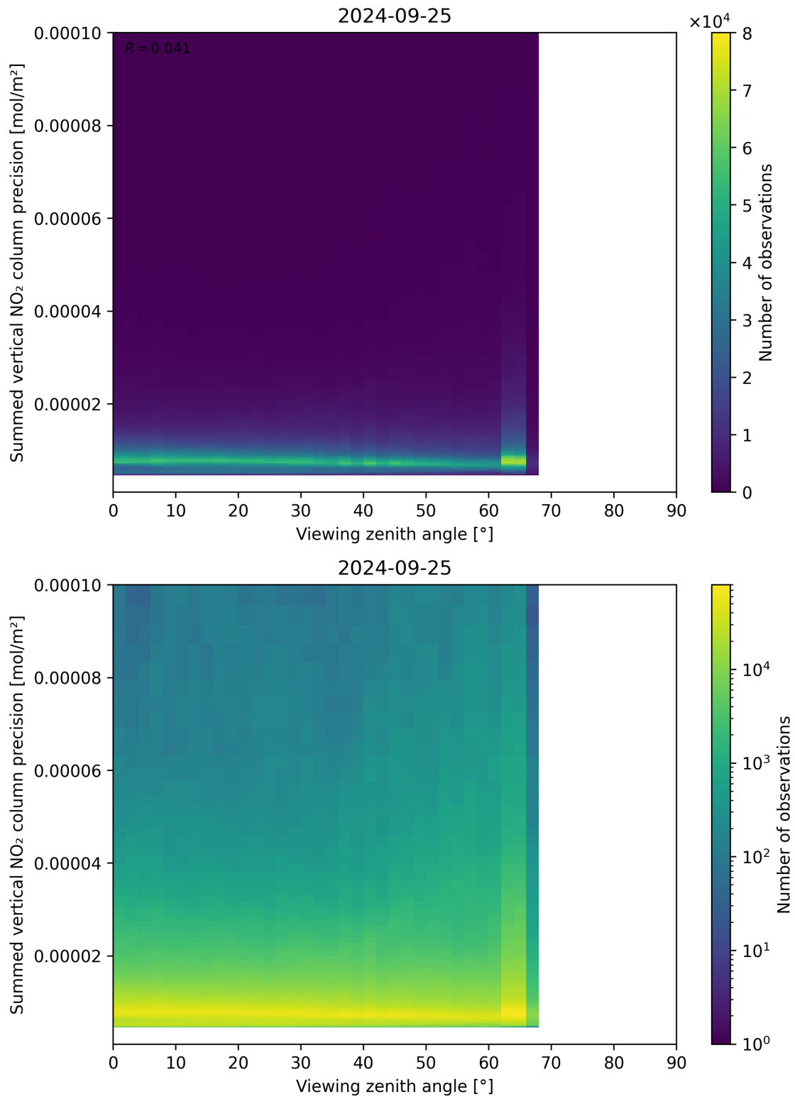
Figure 166: Scatter density plot of “Viewing zenith angle” against “Summed vertical NO 2 column precision” for 2024-09-24 to 2024-09-26.
