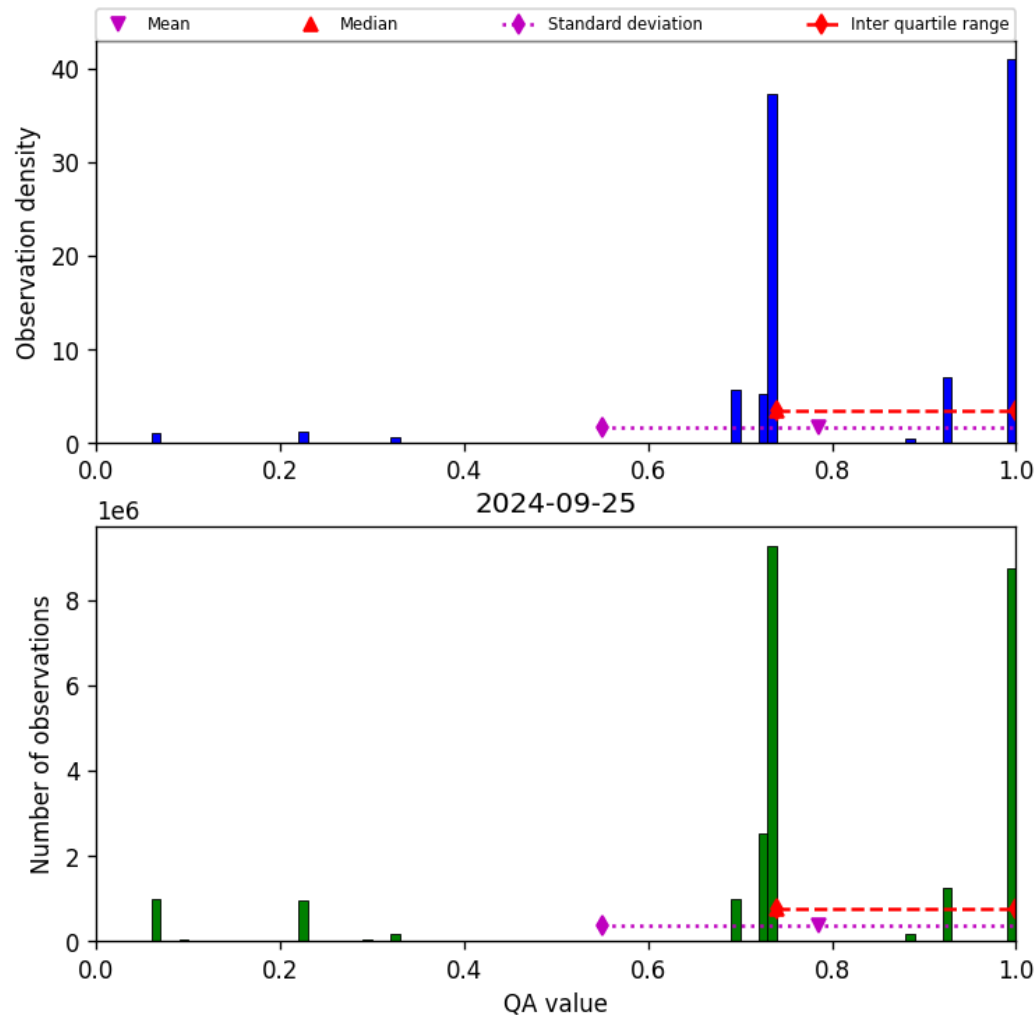
Figure 28: Histogram of “QA value” for 2024-09-24 to 2024-09-26
