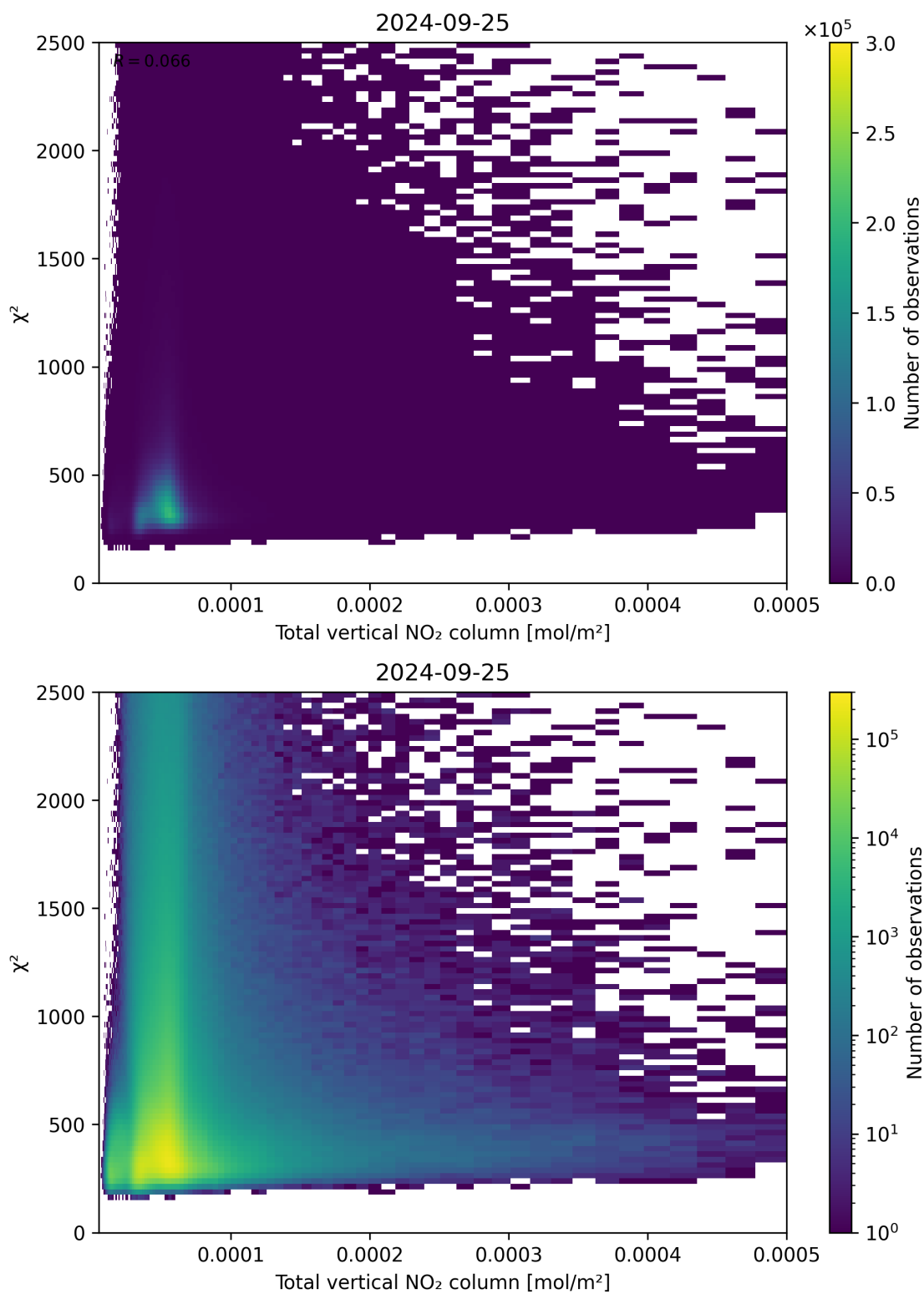
Figure 111: Scatter density plot of “Total vertical NO 2 column” against “ \chi^2 ” for 2024-09-24 to 2024-09-26.
