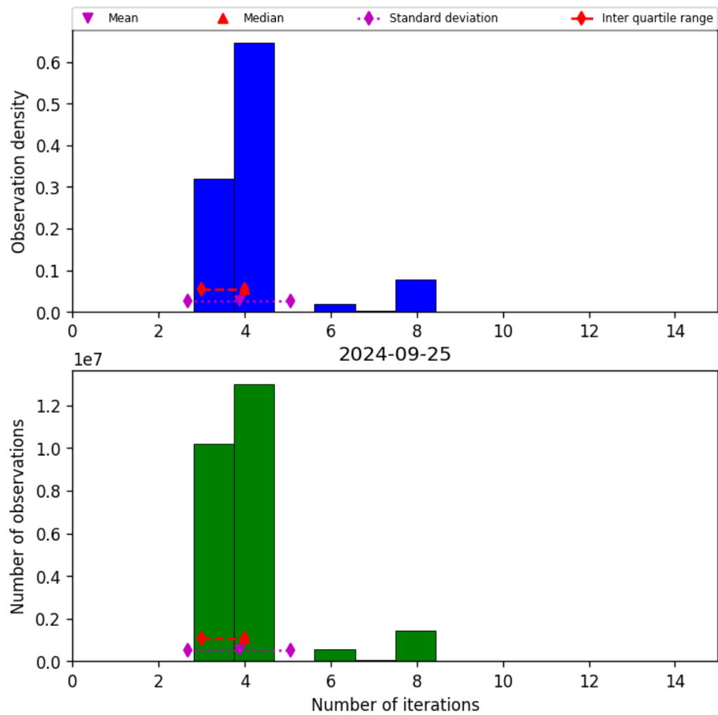
Figure 34: Histogram of “Number of iterations” for 2024-09-24 to 2024-09-26
