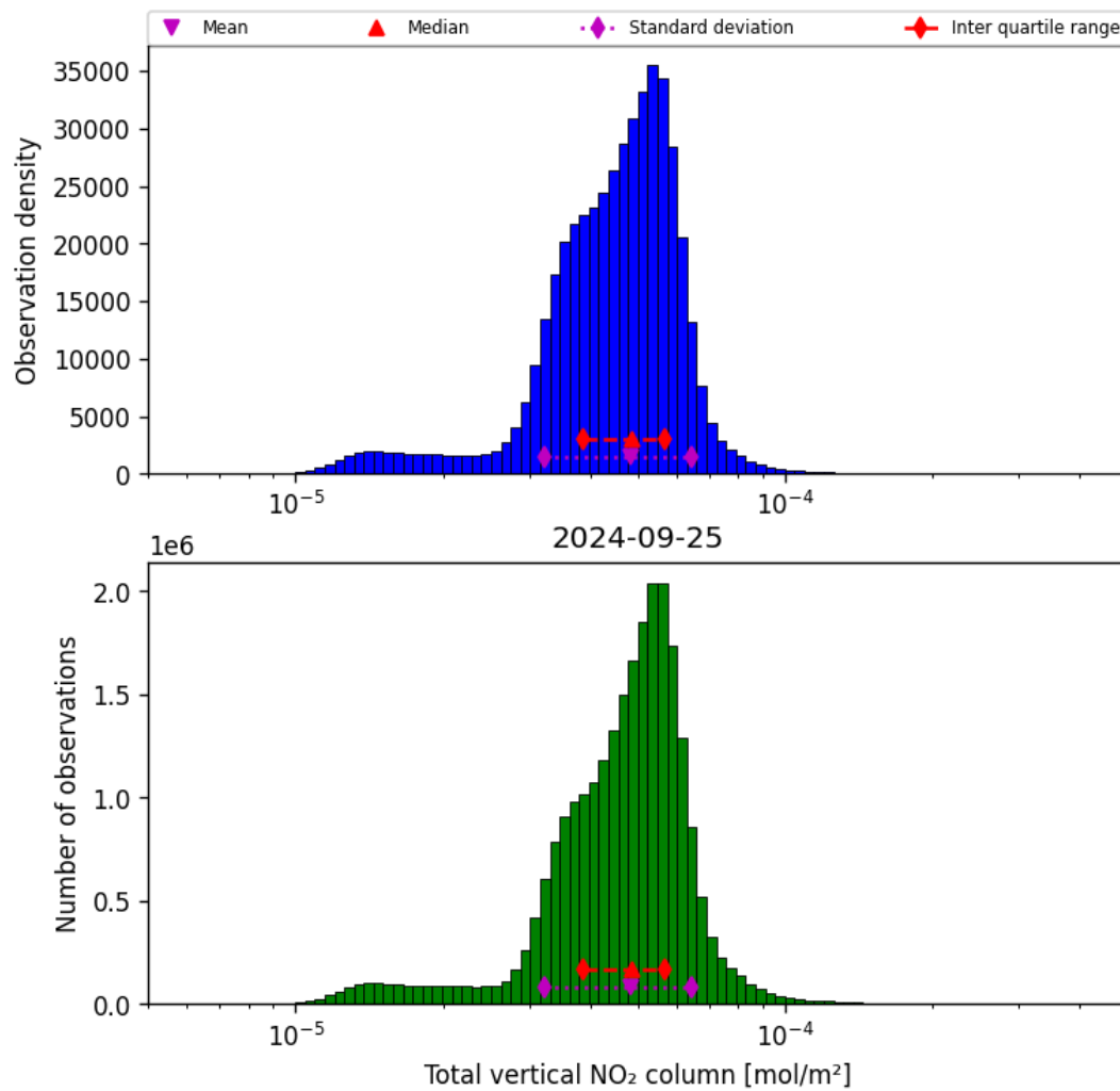
Figure 38: Histogram of “Total vertical NO 2 column” for 2024-09-24 to 2024-09-26
