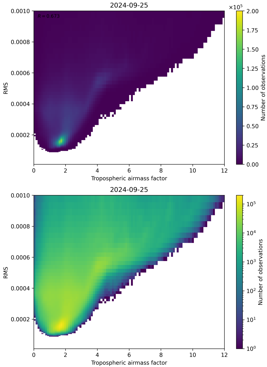
Figure 79: Scatter density plot of “Tropospheric airmass factor” against “RMS” for 2024-09-24 to 2024-09-26.
