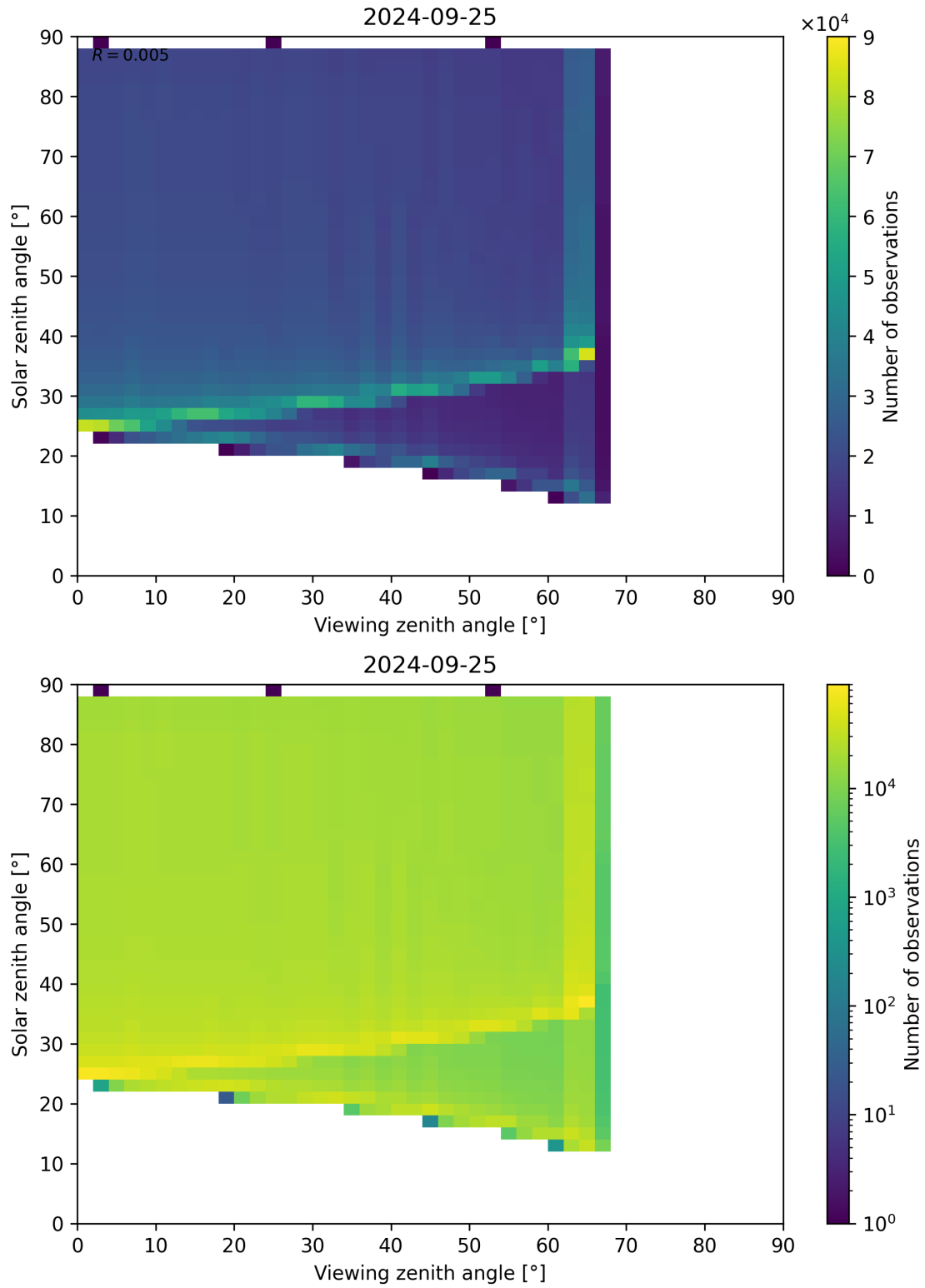
Figure 172: Scatter density plot of “Viewing zenith angle” against “Solar zenith angle” for 2024-09-24 to 2024-09-26.
