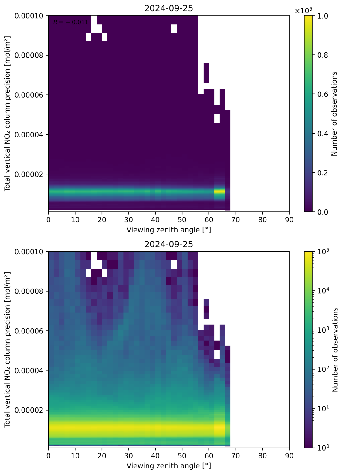
Figure 168: Scatter density plot of “Viewing zenith angle” against “Total vertical NO 2 column precision” for 2024-09-24 to 2024-09-26.
