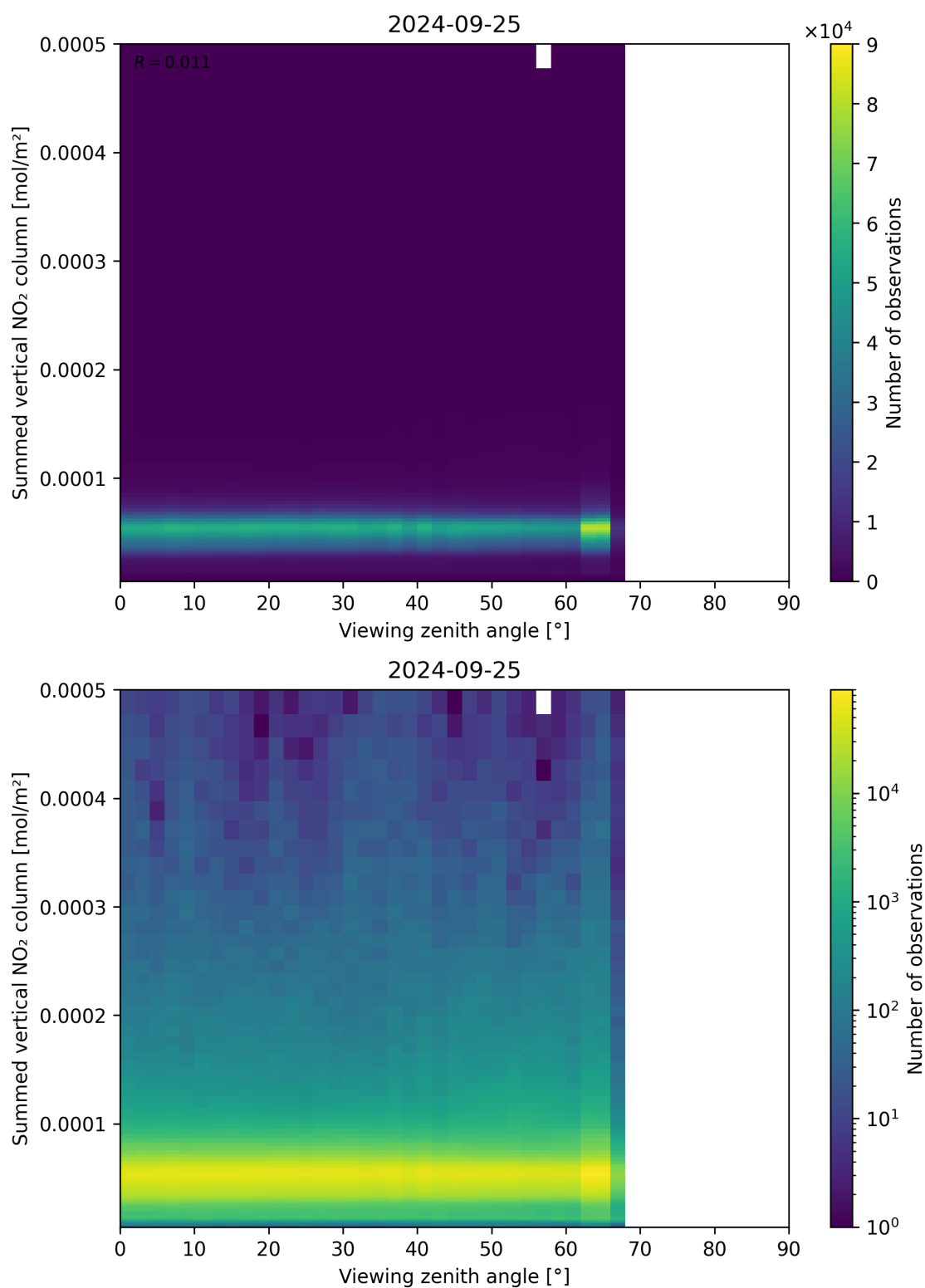
Figure 165: Scatter density plot of “Viewing zenith angle” against “Summed vertical NO 2 column” for 2024-09-24 to 2024-09-26.
