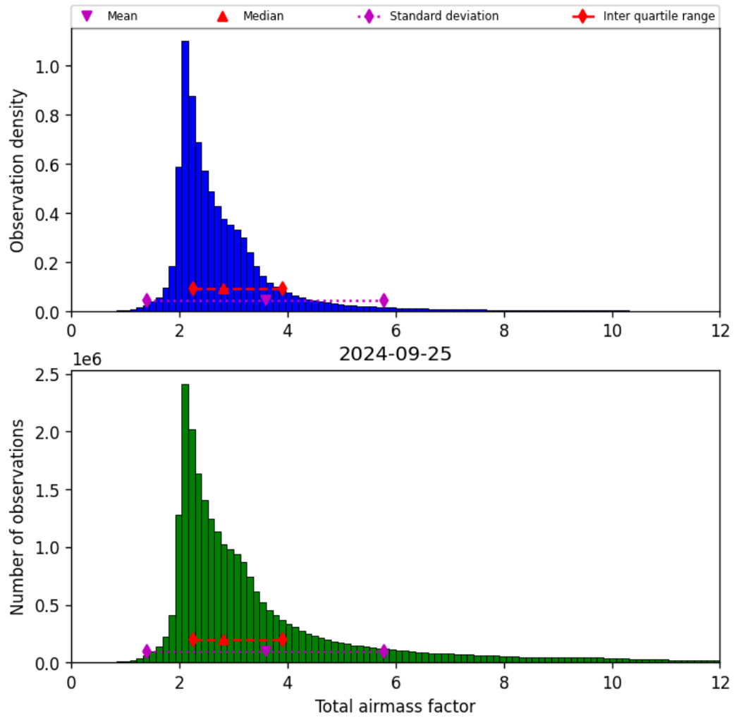
Figure 32: Histogram of “Total airmass factor” for 2024-09-24 to 2024-09-26
