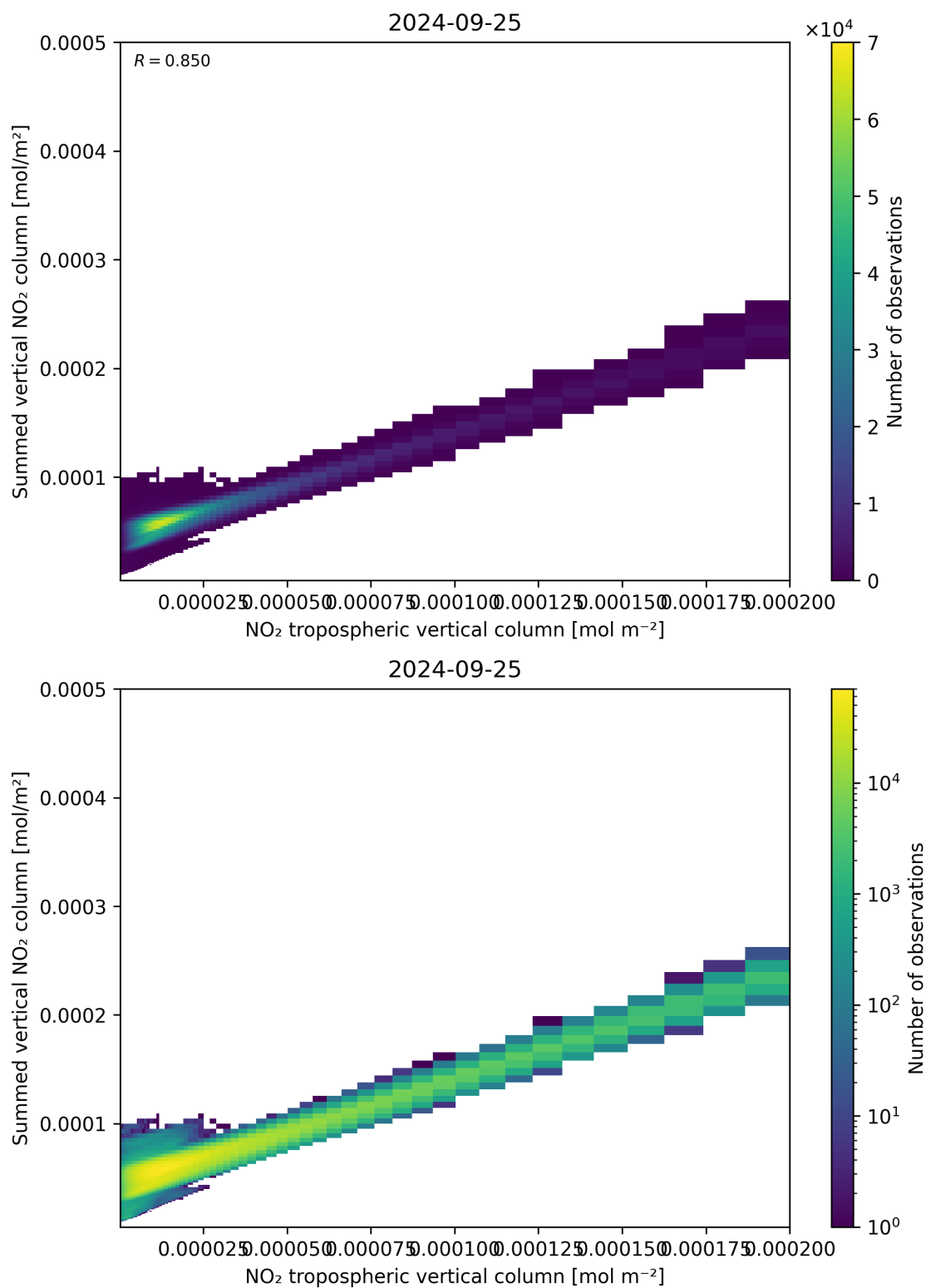
Figure 126: Scatter density plot of “NO 2 tropospheric vertical column” against “Summed vertical NO 2 column” for 2024-09-24 to 2024-09-26.
