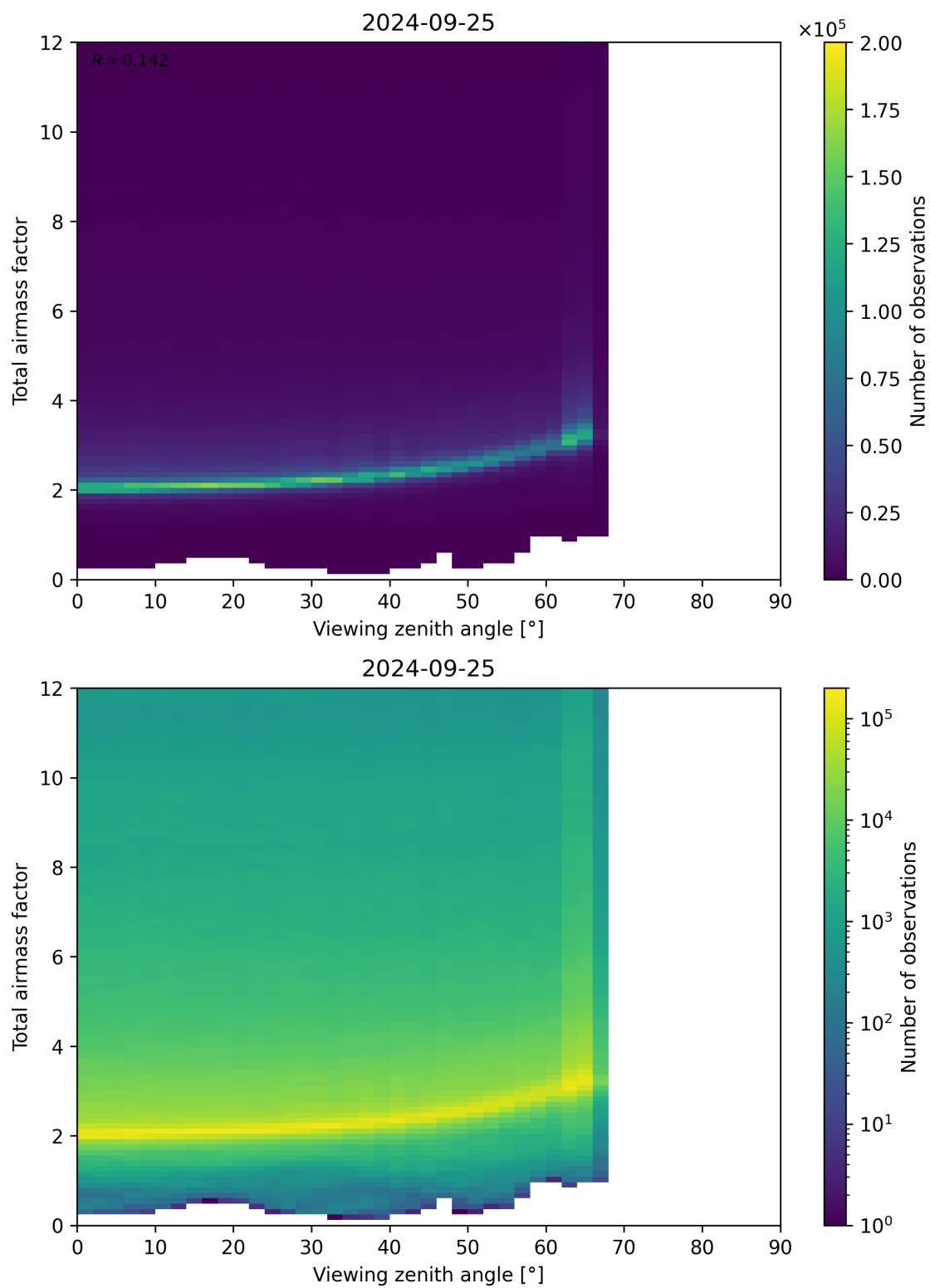
Figure 160: Scatter density plot of “Viewing zenith angle” against “Total airmass factor” for 2024-09-24 to 2024-09-26.
