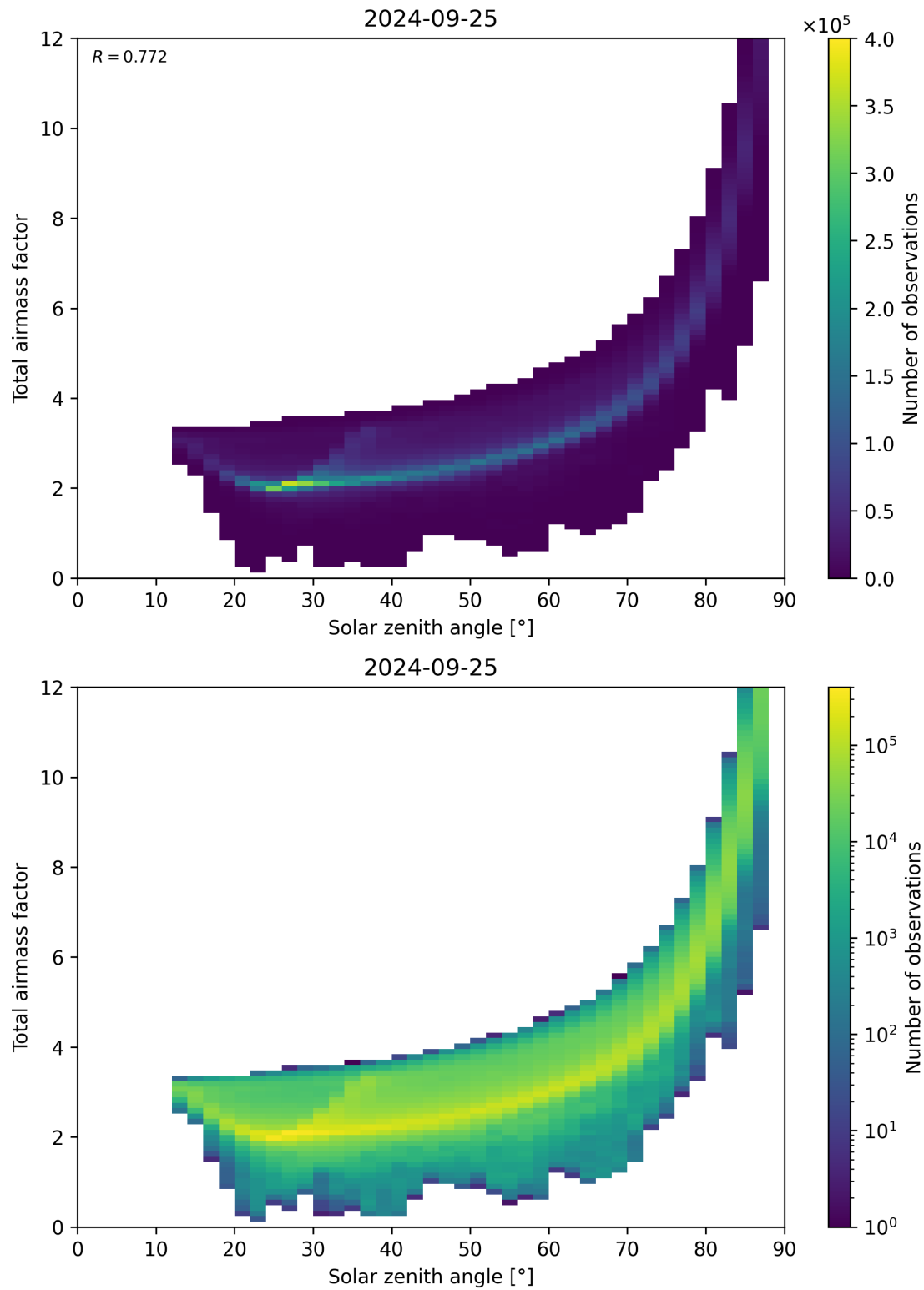
Figure 146: Scatter density plot of “Solar zenith angle” against “Total air mass factor” for 2024-09-24 to 2024-09-26.
