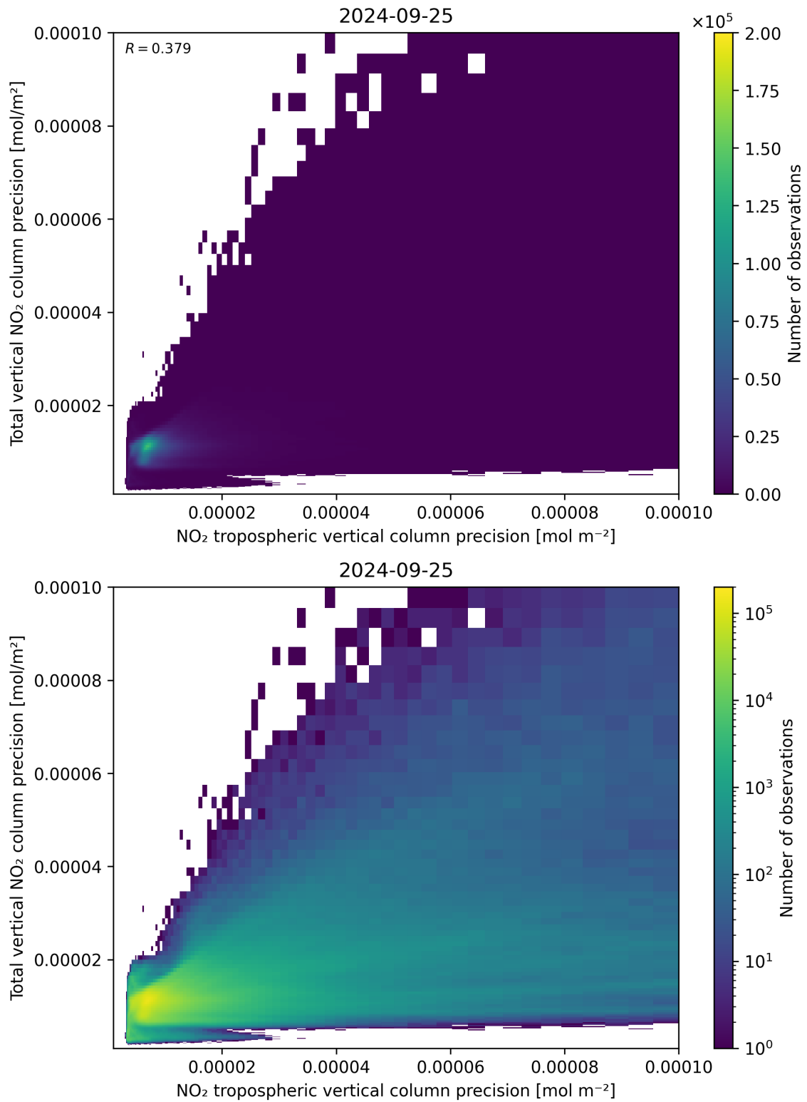
Figure 139: Scatter density plot of “NO 2 tropospheric vertical column precision” against “Total vertical NO 2 column precision” for 2024-09-24 to 2024-09-26.
