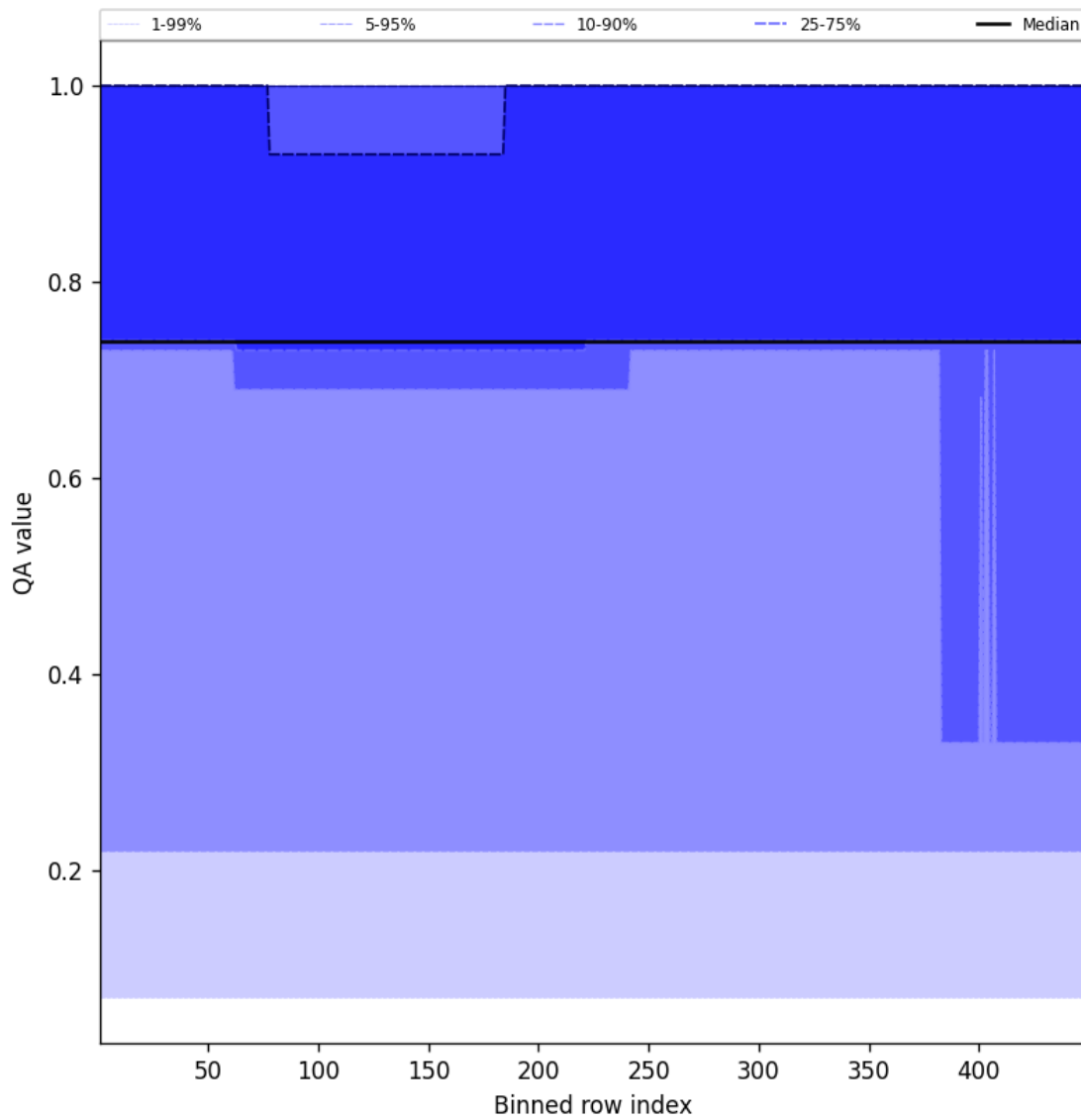
Figure 45: Along track statistics of "QA value" for 2024-09-24 to 2024-09-26
