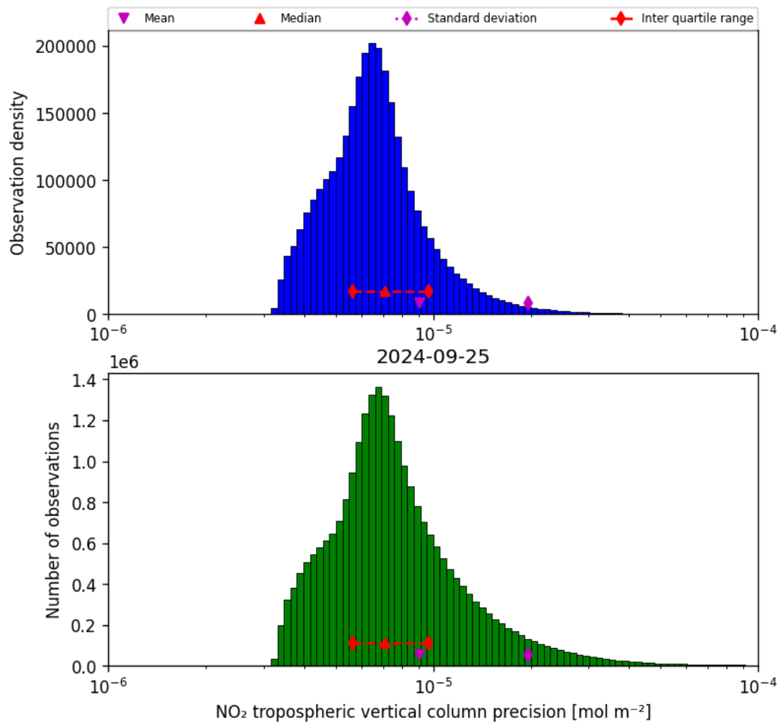
Figure 30: Histogram of “NO 2 tropospheric vertical column precision” for 2024-09-24 to 2024-09-26
