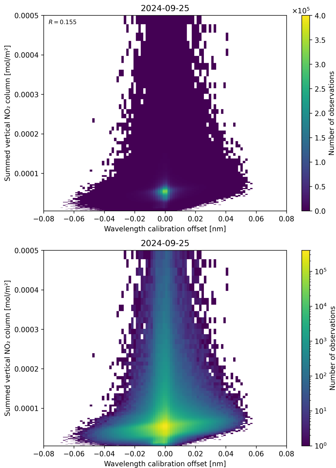
Figure 177: Scatter density plot of “Wavelength calibration offset” against “Summed vertical NO 2 column” for 2024-09-24 to 2024-09-26.
