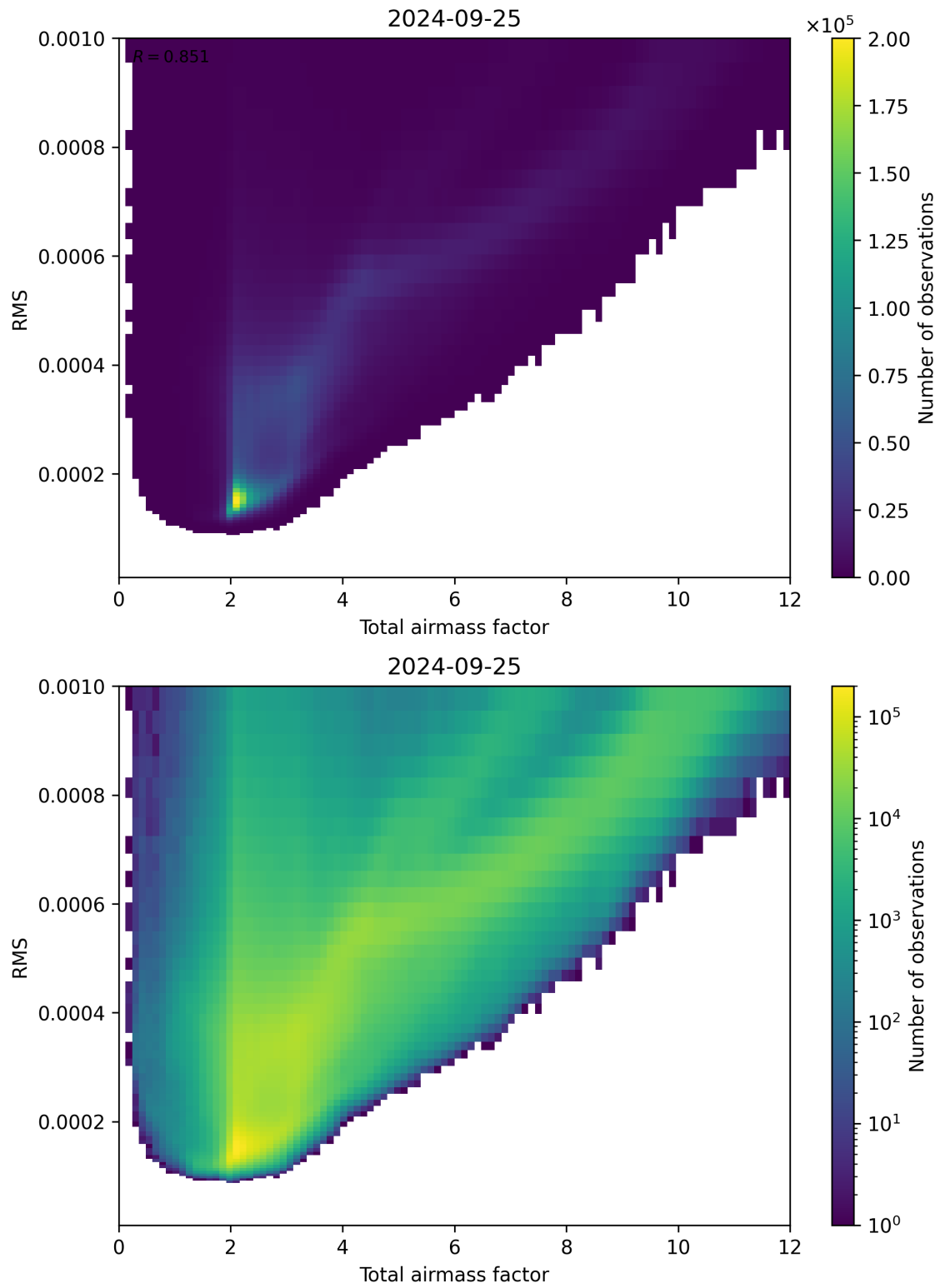
Figure 69: Scatter density plot of “Total airmass factor” against “RMS” for 2024-09-24 to 2024-09-26.
