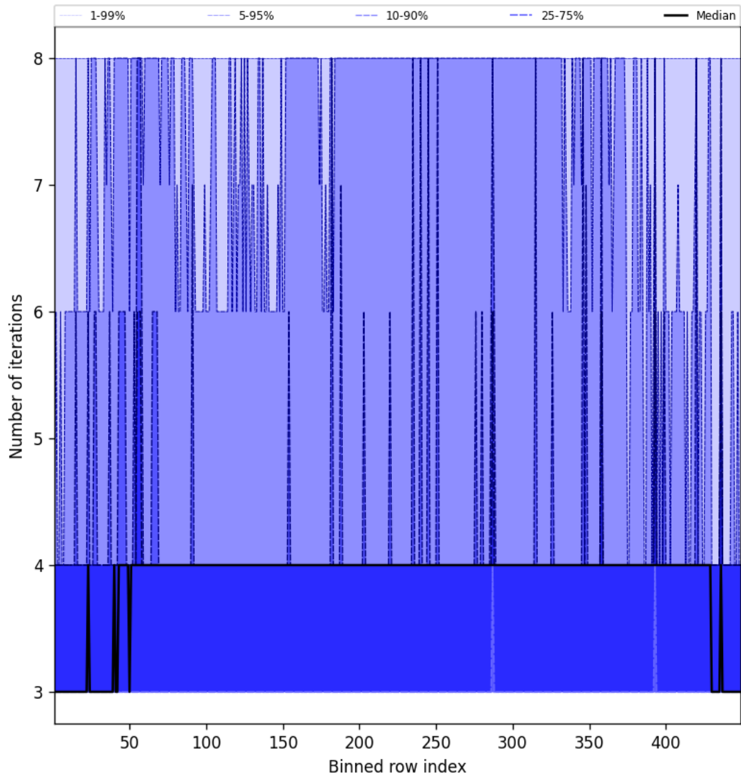
Figure 51: Along track statistics of “Number of iterations” for 2024-09-24 to 2024-09-26
