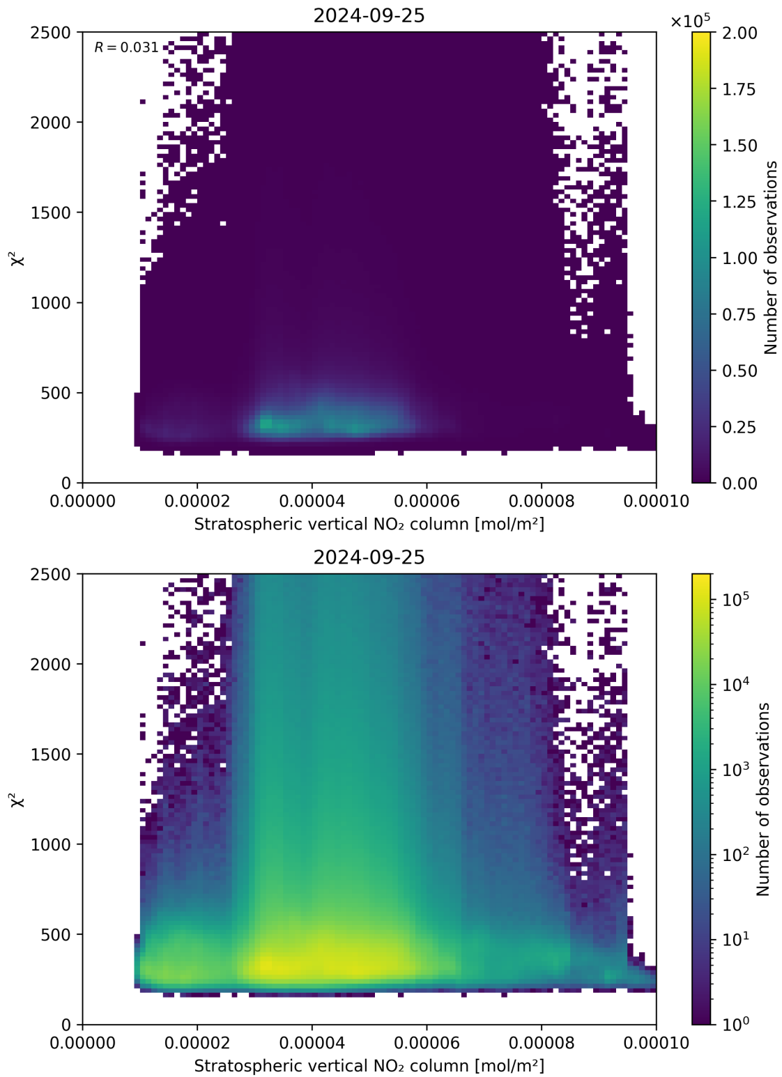
Figure 97: Scatter density plot of “Stratospheric vertical NO 2 column” against “ \chi^2 ” for 2024-09-24 to 2024-09-26.
