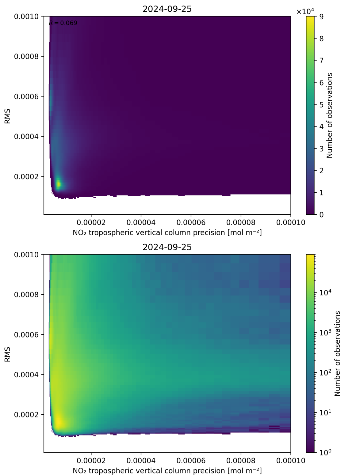
Figure 140: Scatter density plot of “NO 2 tropospheric vertical column precision” against “RMS” for 2024-09-24 to 2024-09-26.
