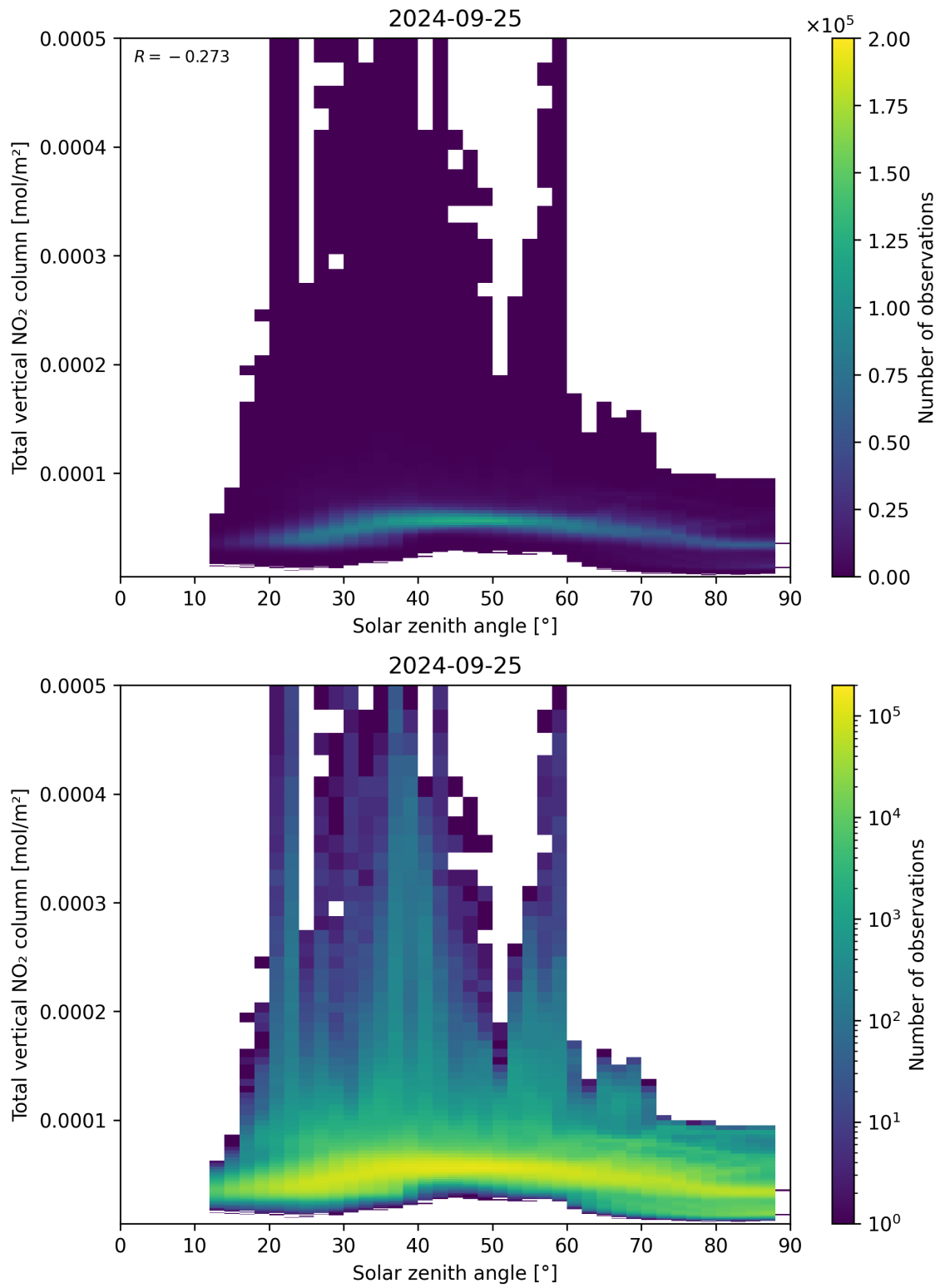
Figure 153: Scatter density plot of “Solar zenith angle” against “Total vertical NO 2 column” for 2024-09-24 to 2024-09-26.
