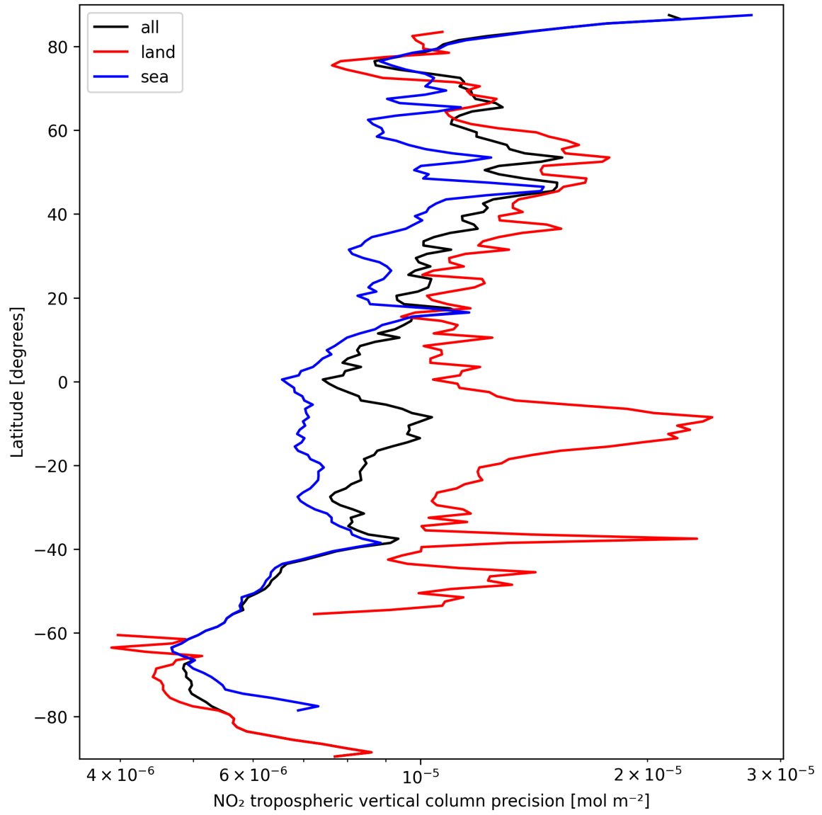
Figure 13: Zonal average of “NO 2 tropospheric vertical column precision” for 2024-09-24 to 2024-09-26.
