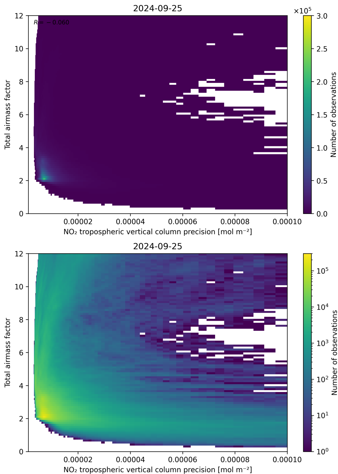
Figure 132: Scatter density plot of “NO 2 tropospheric vertical column precision” against “Total air mass factor” for 2024-09-24 to 2024-09-26.
