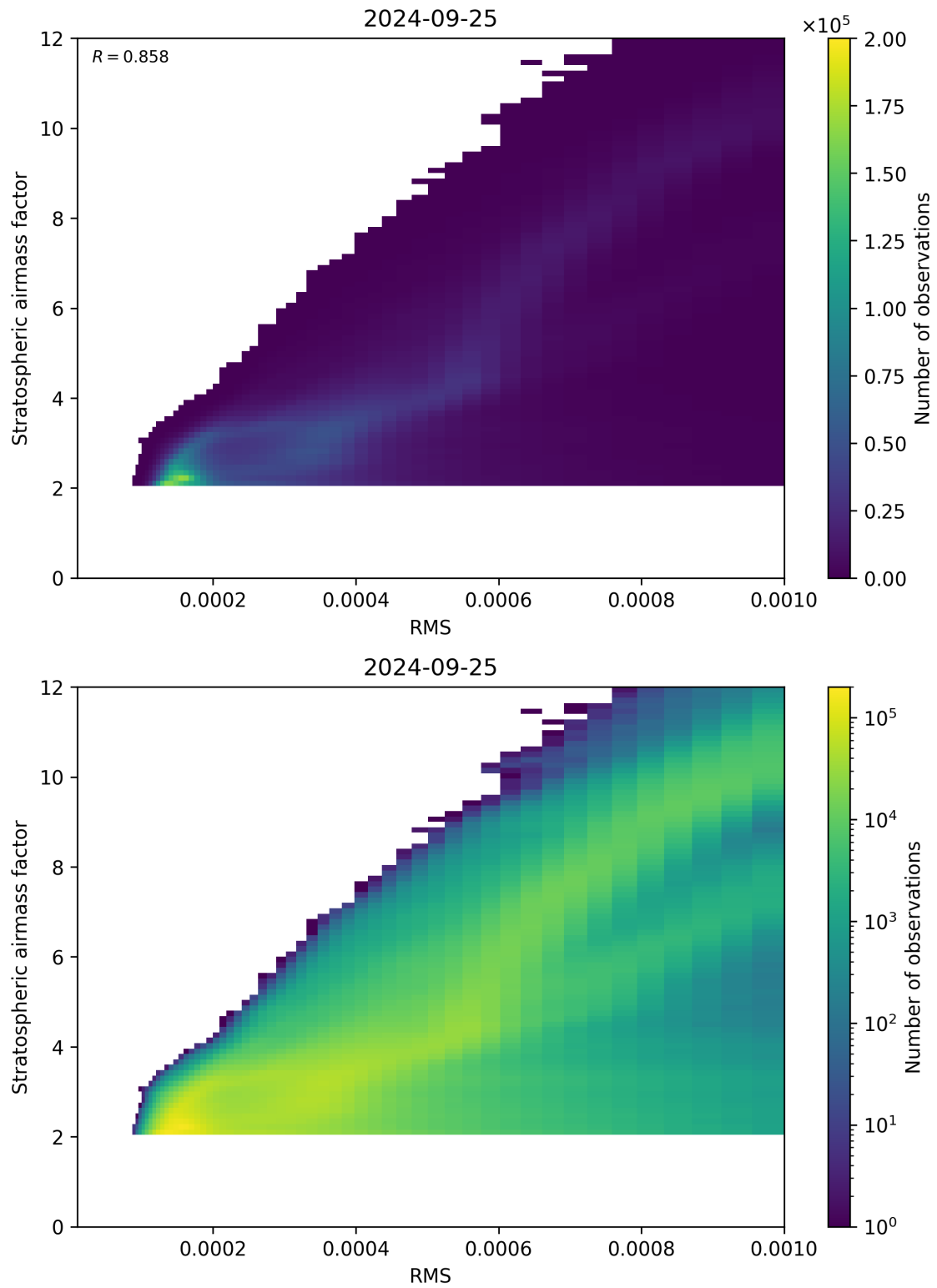
Figure 144: Scatter density plot of “RMS” against “Stratospheric airmass factor” for 2024-09-24 to 2024-09-26.
