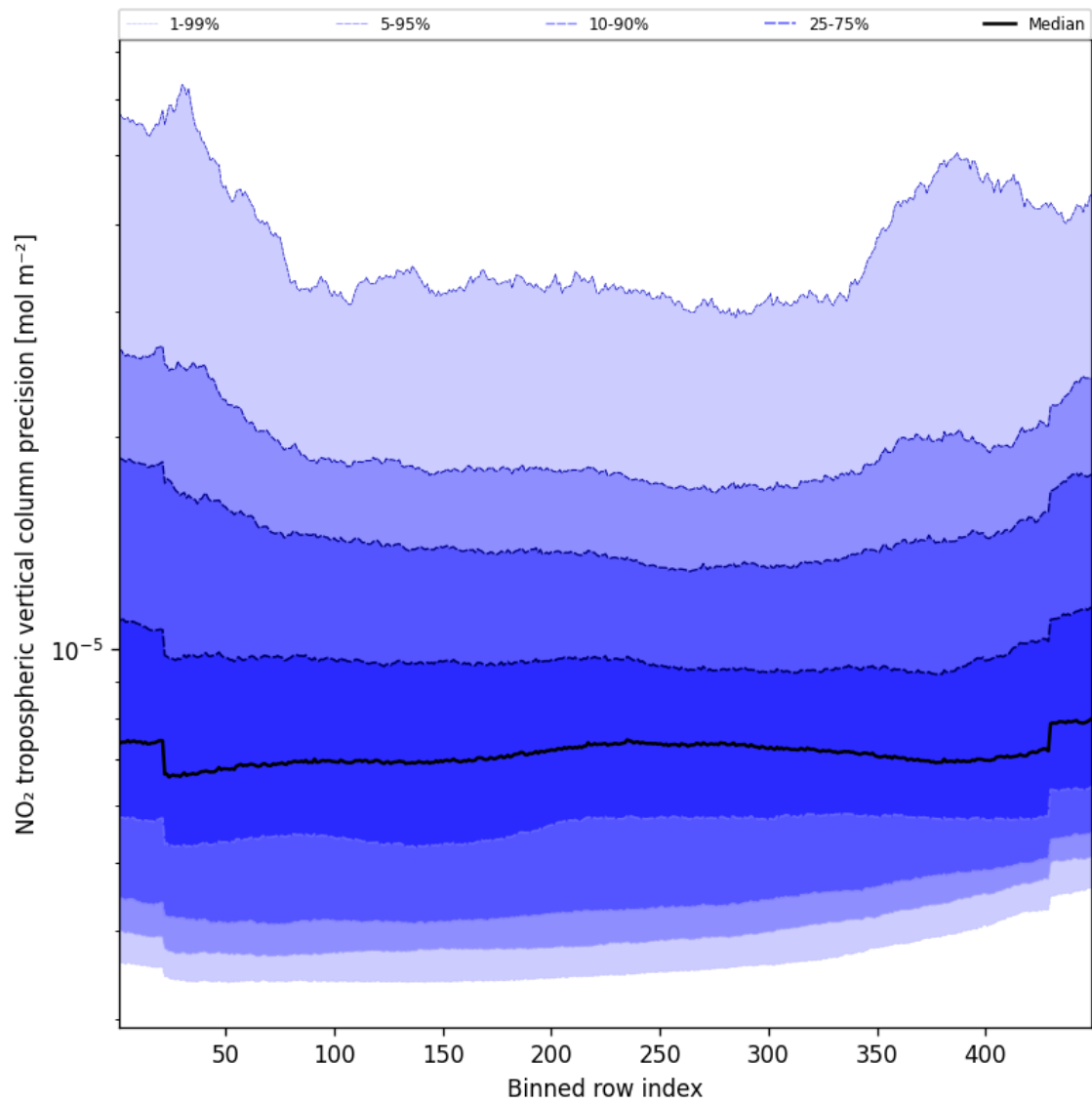
Figure 47: Along track statistics of “NO 2 tropospheric vertical column precision” for 2024-09-24 to 2024-09-26
