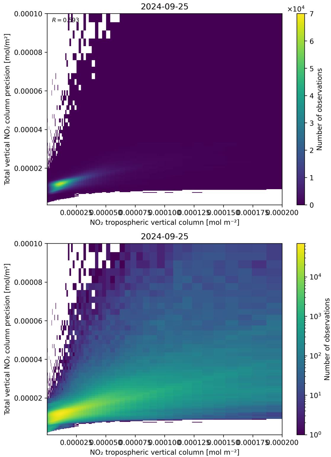
Figure 129: Scatter density plot of “NO 2 tropospheric vertical column” against “Total vertical NO 2 column precision” for 2024-09-24 to 2024-09-26.
