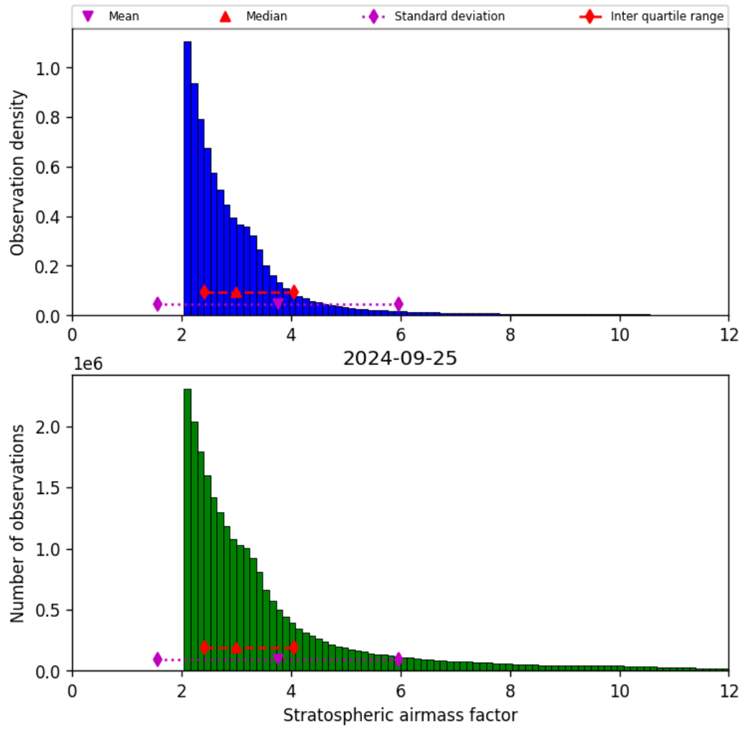
Figure 44: Histogram of “Stratospheric airmass factor” for 2024-09-24 to 2024-09-26
