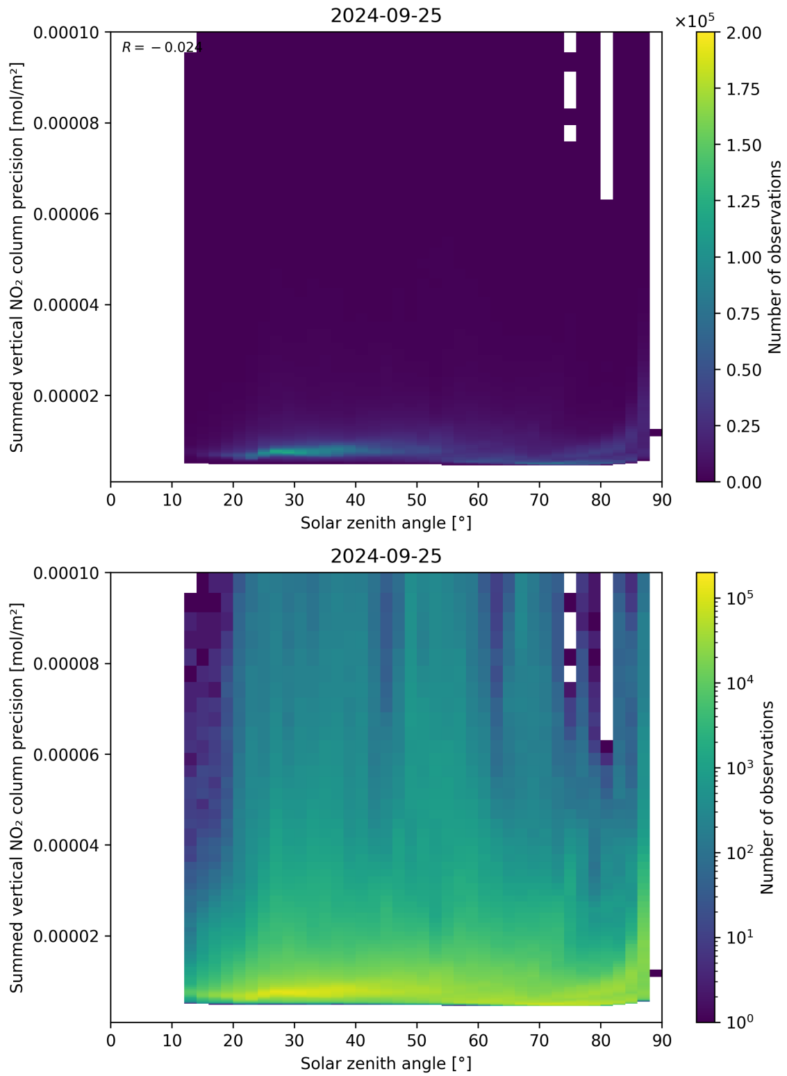
Figure 152: Scatter density plot of “Solar zenith angle” against “Summed vertical NO 2 column precision” for 2024-09-24 to 2024-09-26.
