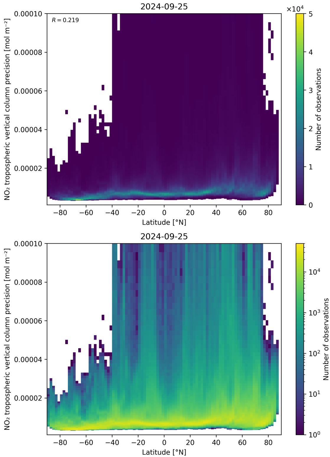
Figure 93: Scatter density plot of “Latitude” against “NO 2 tropospheric vertical column precision” for 2024-09-24 to 2024-09-26.
