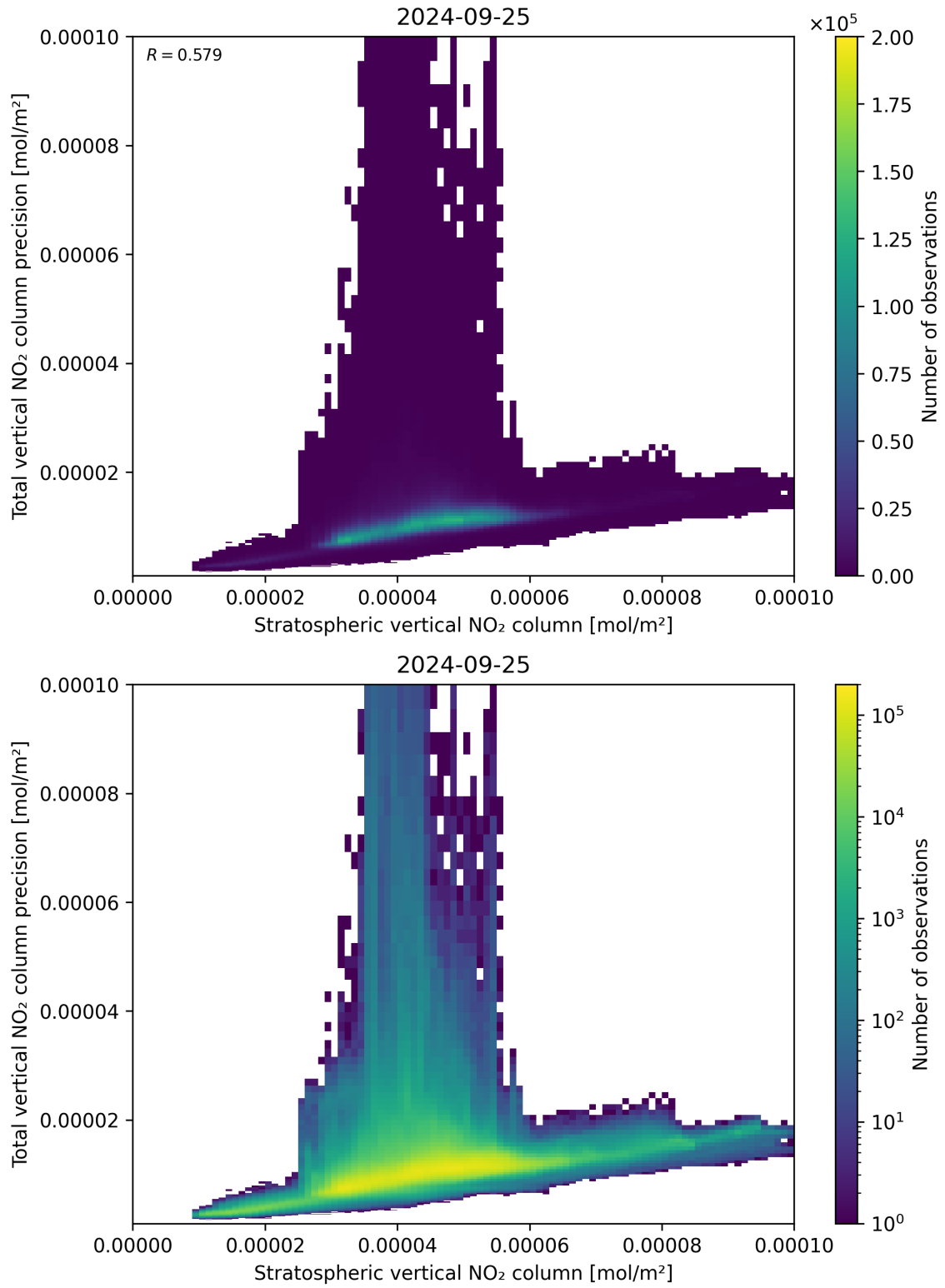
Figure 101: Scatter density plot of “Stratospheric vertical NO 2 column” against “Total vertical NO 2 column precision” for 2024-09-24 to 2024-09-26.
