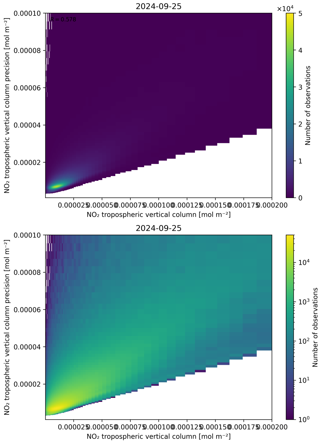
Figure 130: Scatter density plot of “NO 2 tropospheric vertical column” against “NO 2 tropospheric vertical column precision” for 2024-09-24 to 2024-09-26.
