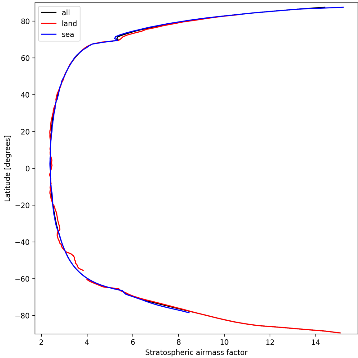
Figure 27: Zonal average of “Stratospheric airmass factor” for 2024-09-24 to 2024-09-26.
