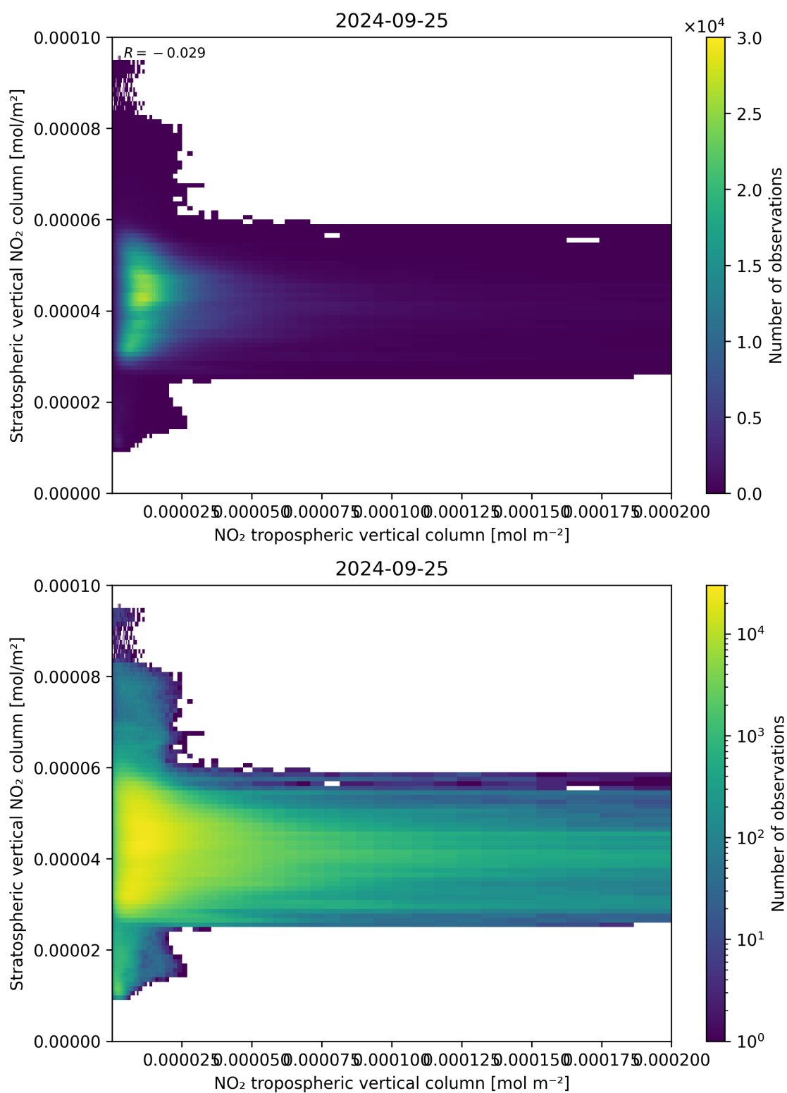
Figure 125: Scatter density plot of “NO 2 tropospheric vertical column” against “Stratospheric vertical NO 2 column” for 2024-09-24 to 2024-09-26.
