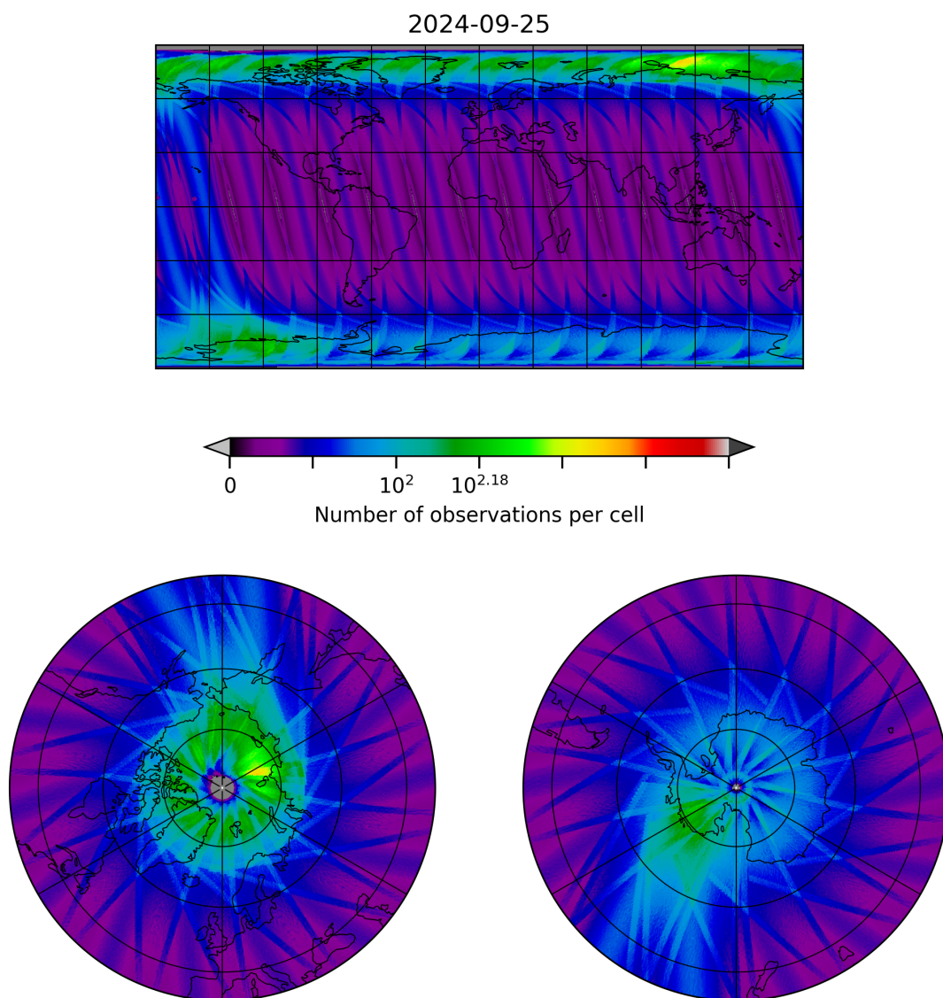
Figure 10: Map of the number of observations for 2024-09-24 to 2024-09-26
