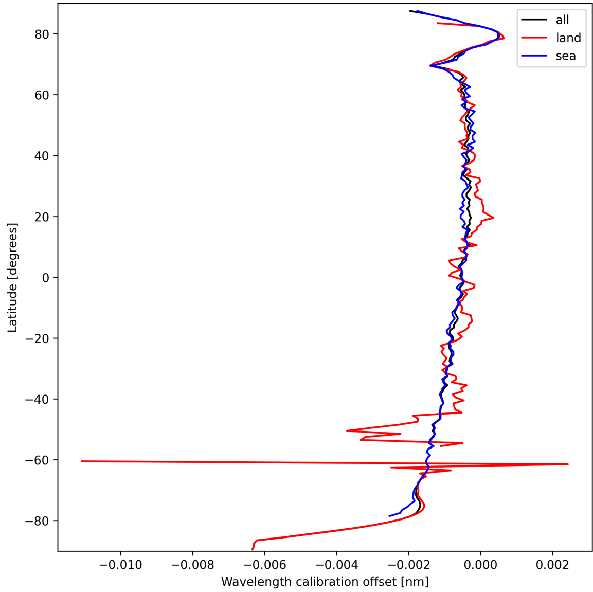
Figure 18: Zonal average of “Wavelength calibration offset” for 2024-09-24 to 2024-09-26.
