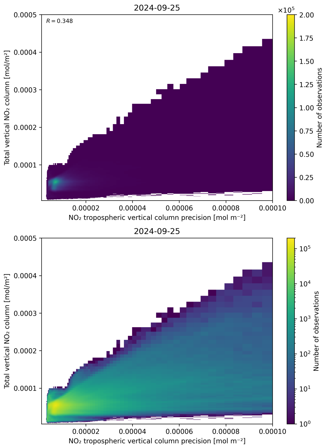
Figure 138: Scatter density plot of “NO 2 tropospheric vertical column precision” against “Total vertical NO 2 column” for 2024-09-24 to 2024-09-26.
