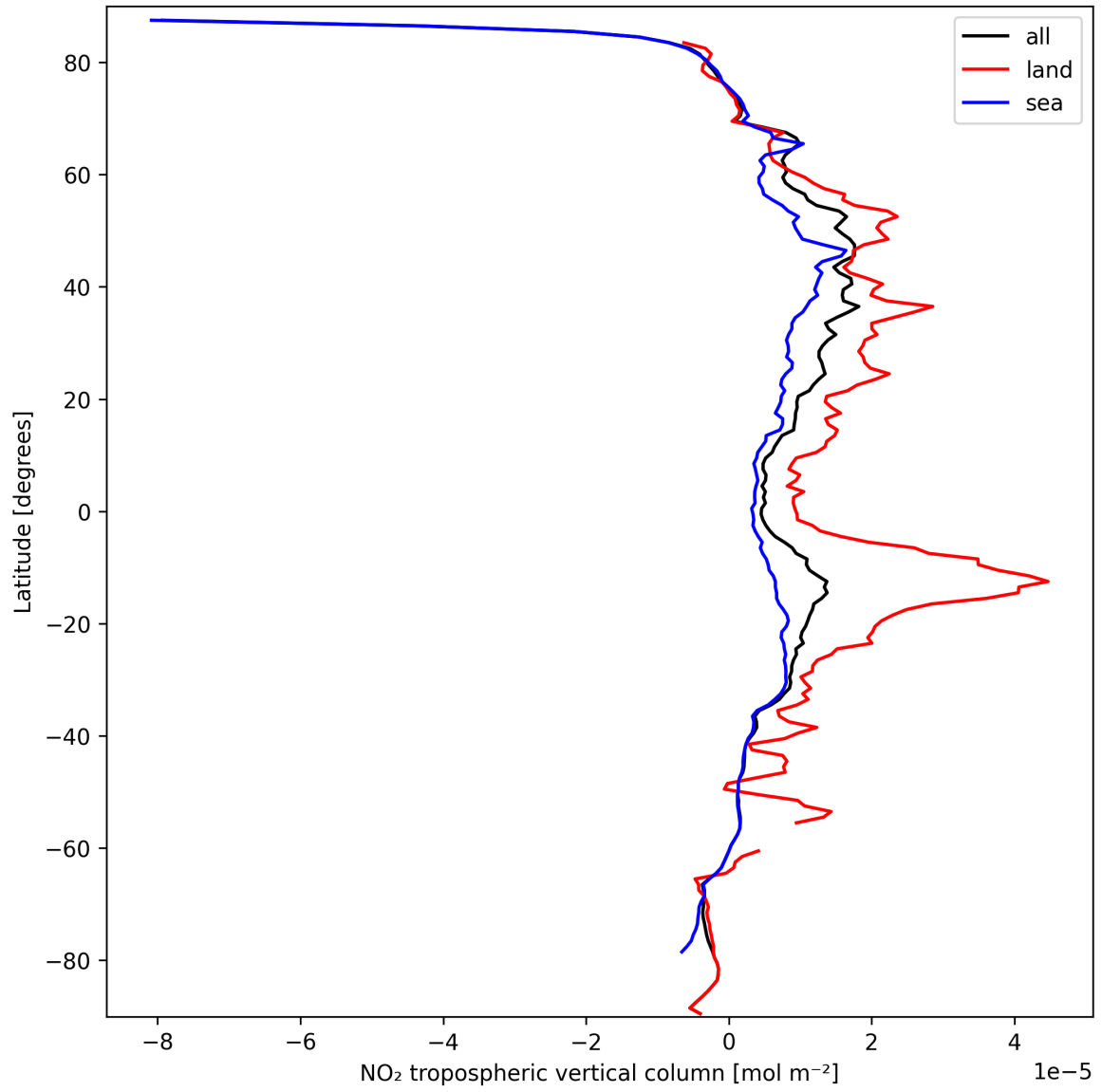
Figure 12: Zonal average of “NO 2 tropospheric vertical column” for 2024-09-24 to 2024-09-26.
