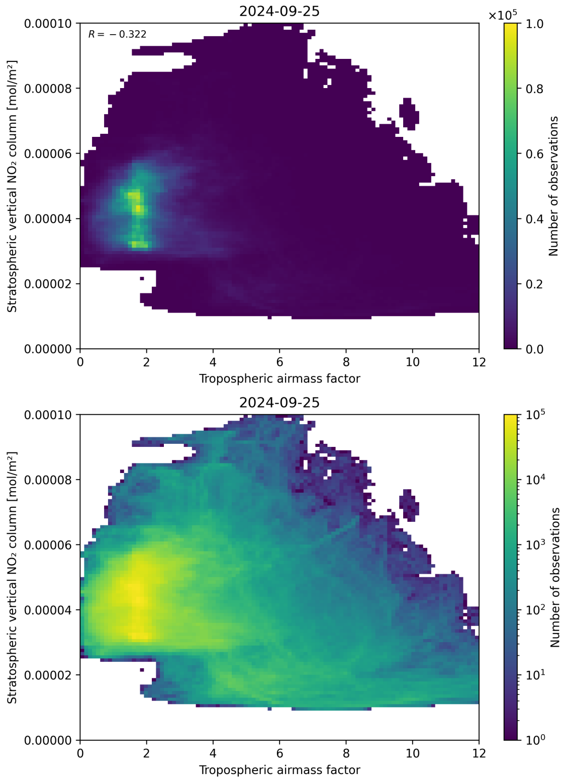
Figure 74: Scatter density plot of “Tropospheric air mass factor” against “Stratospheric vertical NO 2 column” for 2024-09-24 to 2024-09-26.
