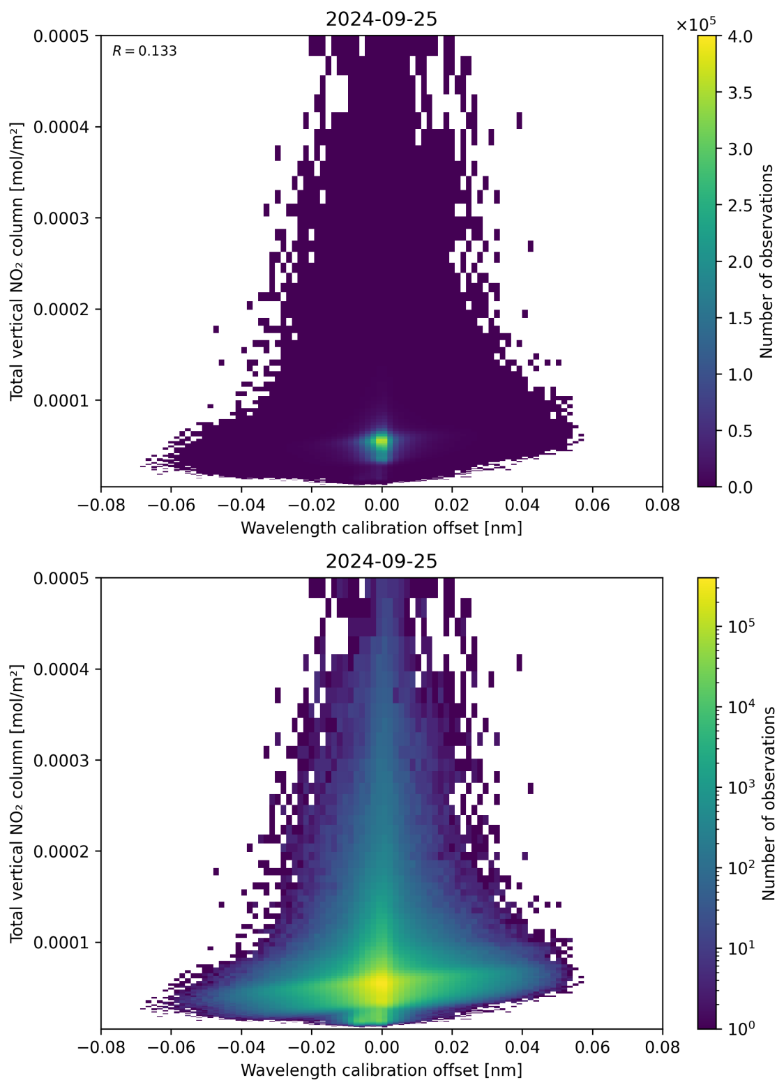
Figure 179: Scatter density plot of “Wavelength calibration offset” against “Total vertical NO 2 column” for 2024-09-24 to 2024-09-26.
