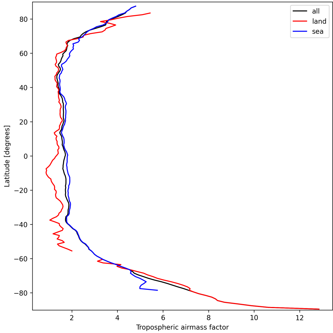
Figure 14: Zonal average of “Tropospheric airmass factor” for 2024-09-24 to 2024-09-26.
