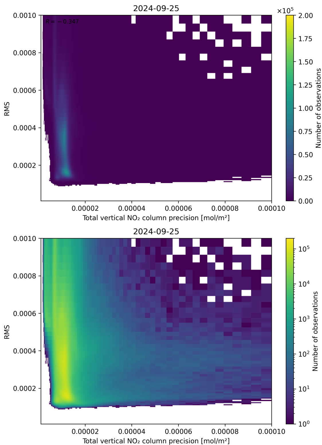
Figure 119: Scatter density plot of “Total vertical NO 2 column precision” against “RMS” for 2024-09-24 to 2024-09-26.
