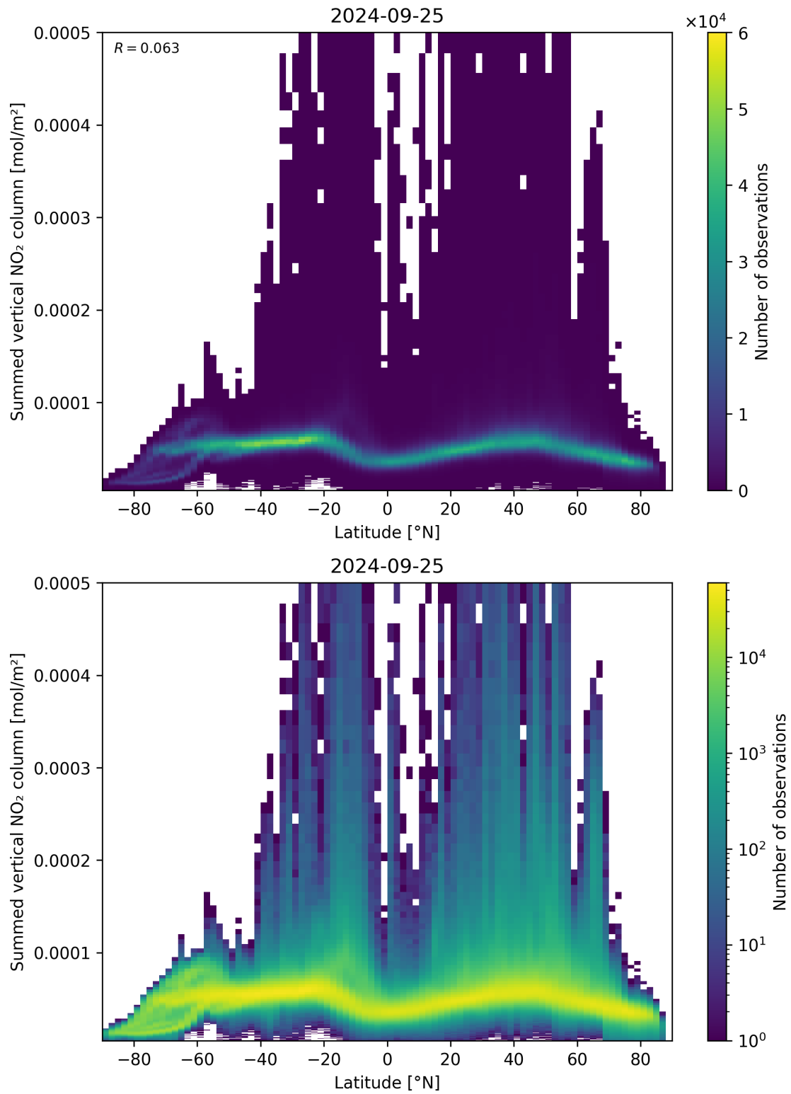
Figure 88: Scatter density plot of “Latitude” against “Summed vertical NO 2 column” for 2024-09-24 to 2024-09-26.
