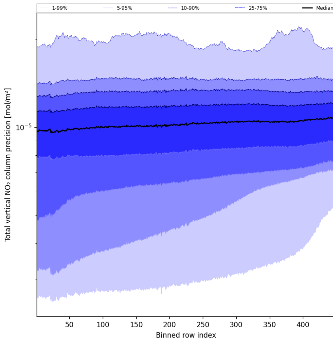
Figure 56: Along track statistics of “Total vertical NO 2 column precision” for 2024-09-24 to 2024-09-26
