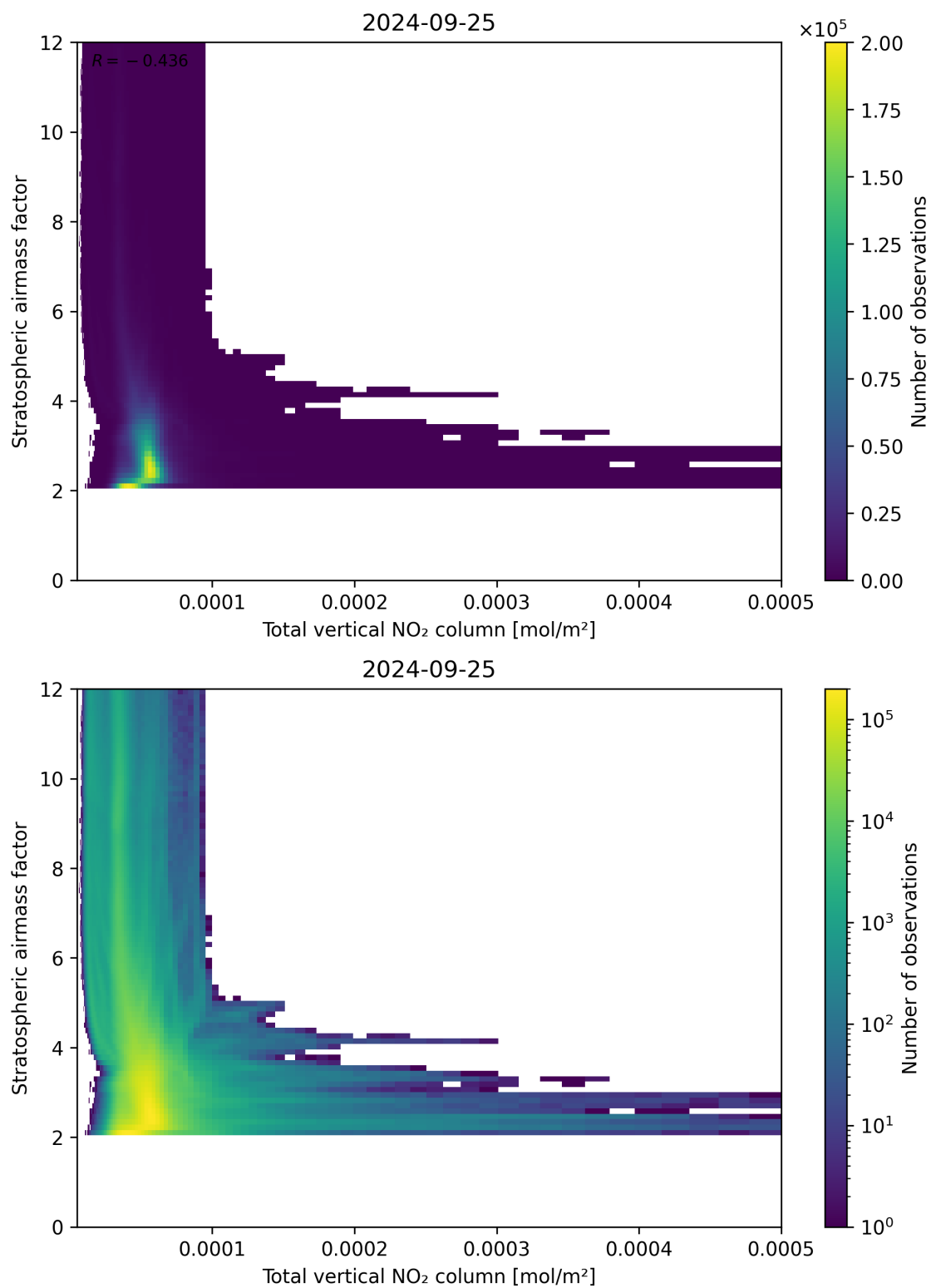
Figure 110: Scatter density plot of “Total vertical NO 2 column” against “Stratospheric airmass factor” for 2024-09-24 to 2024-09-26.
