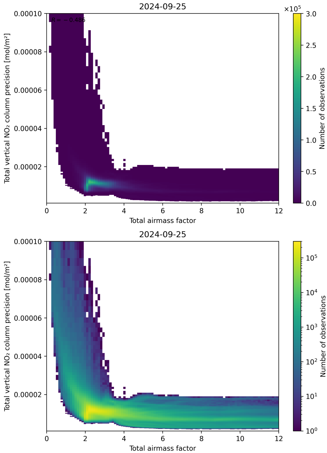
Figure 68: Scatter density plot of “Total airmass factor” against “Total vertical NO 2 column precision” for 2024-09-24 to 2024-09-26.
