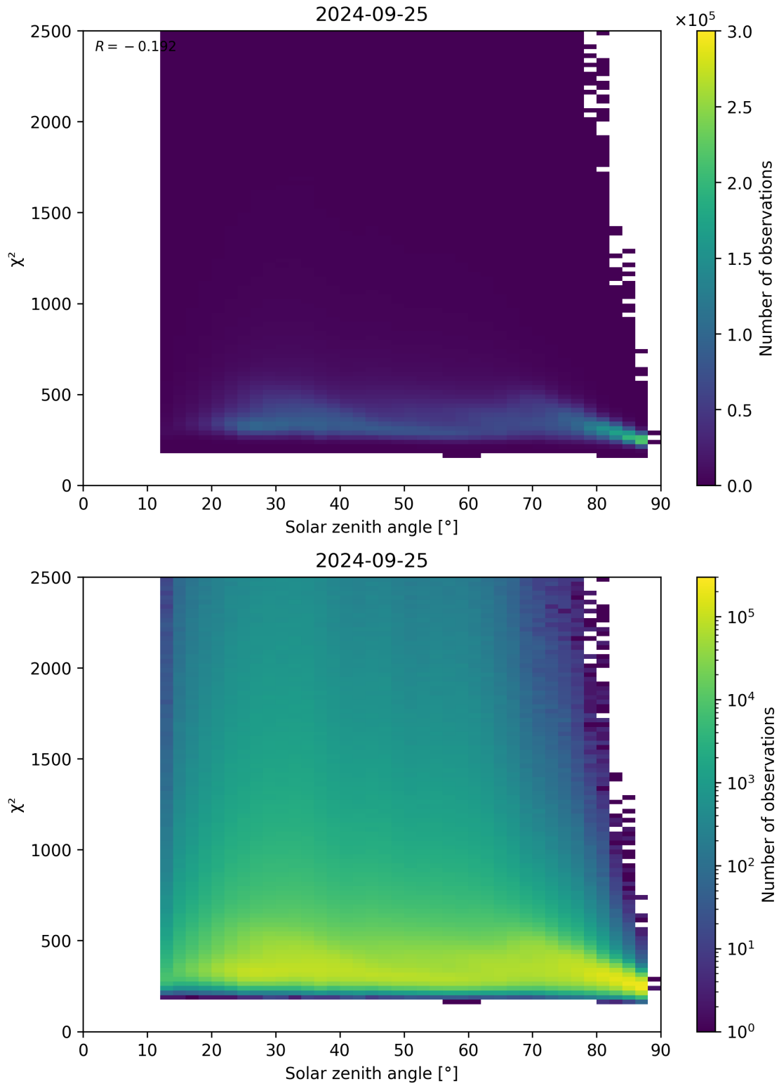
Figure 148: Scatter density plot of “Solar zenith angle” against “ \chi^2 ” for 2024-09-24 to 2024-09-26.
