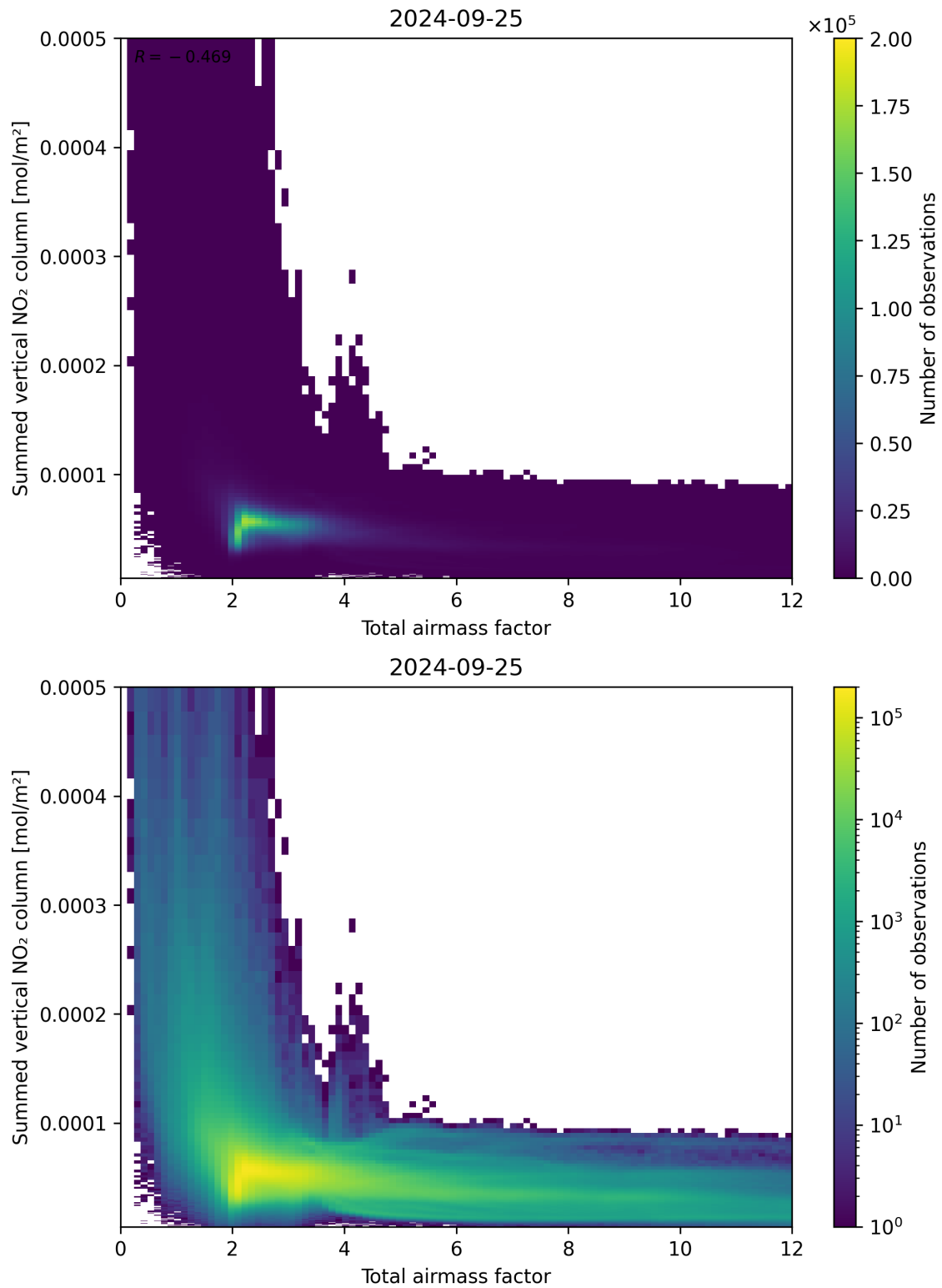
Figure 65: Scatter density plot of “Total airmass factor” against “Summed vertical NO 2 column” for 2024-09-24 to 2024-09-26.
