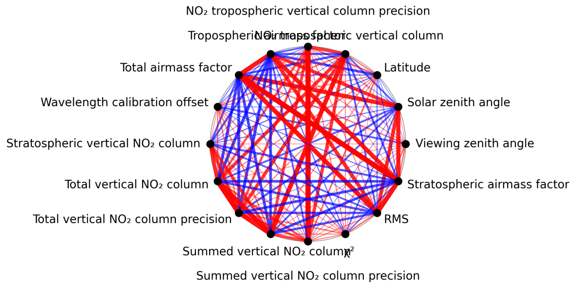
Figure 1: Map of correlation graph for 2024-09-24 to 2024-09-26.
