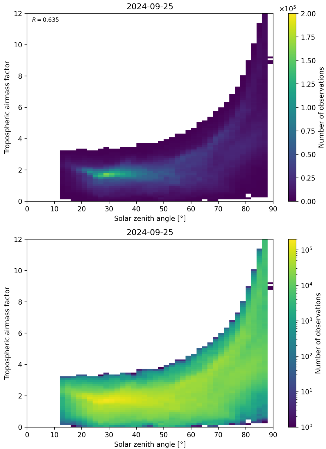
Figure 147: Scatter density plot of “Solar zenith angle” against “Tropospheric airmass factor” for 2024-09-24 to 2024-09-26.
