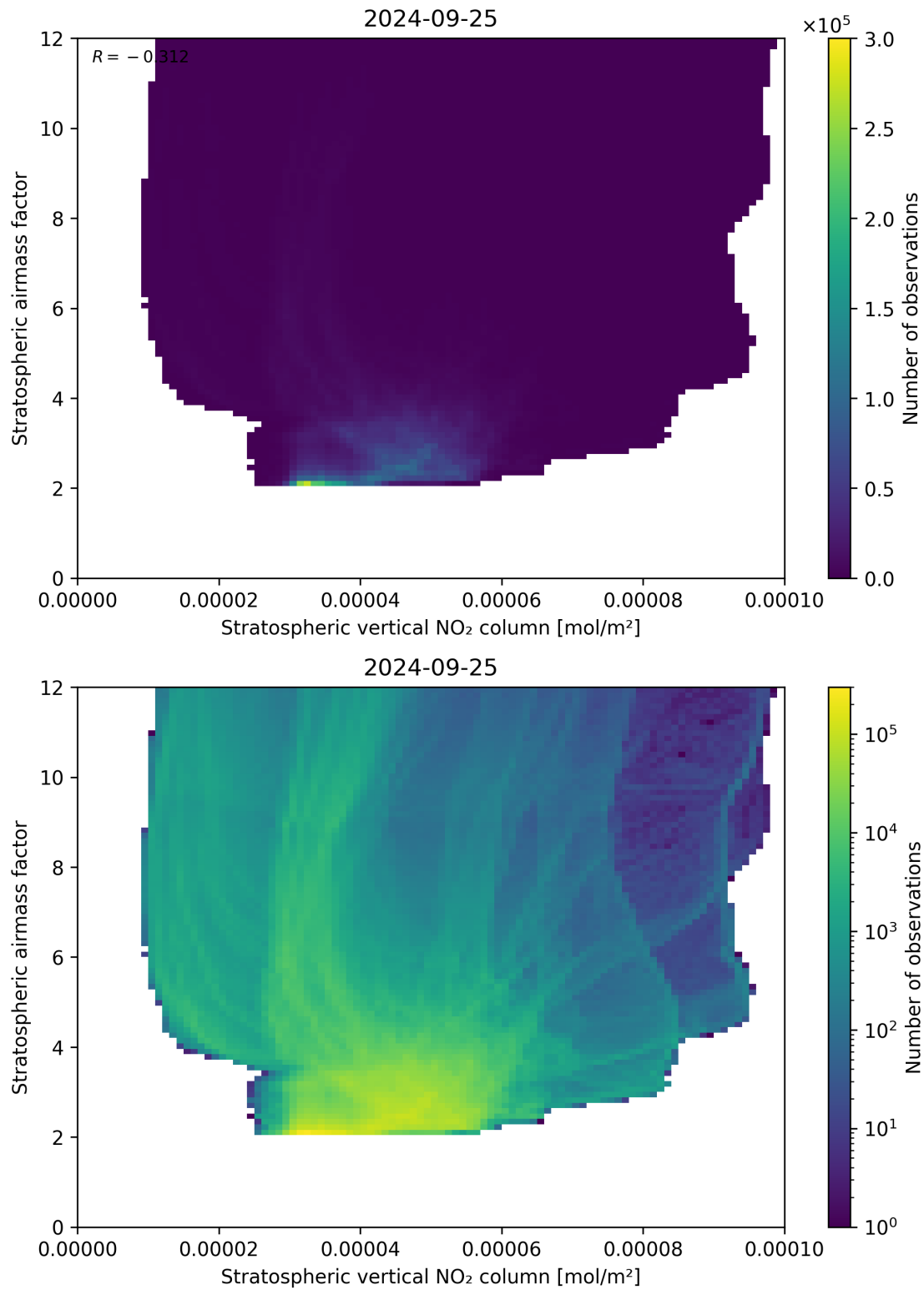
Figure 96: Scatter density plot of “Stratospheric vertical NO 2 column” against “Stratospheric airmass factor” for 2024-09-24 to 2024-09-26.
