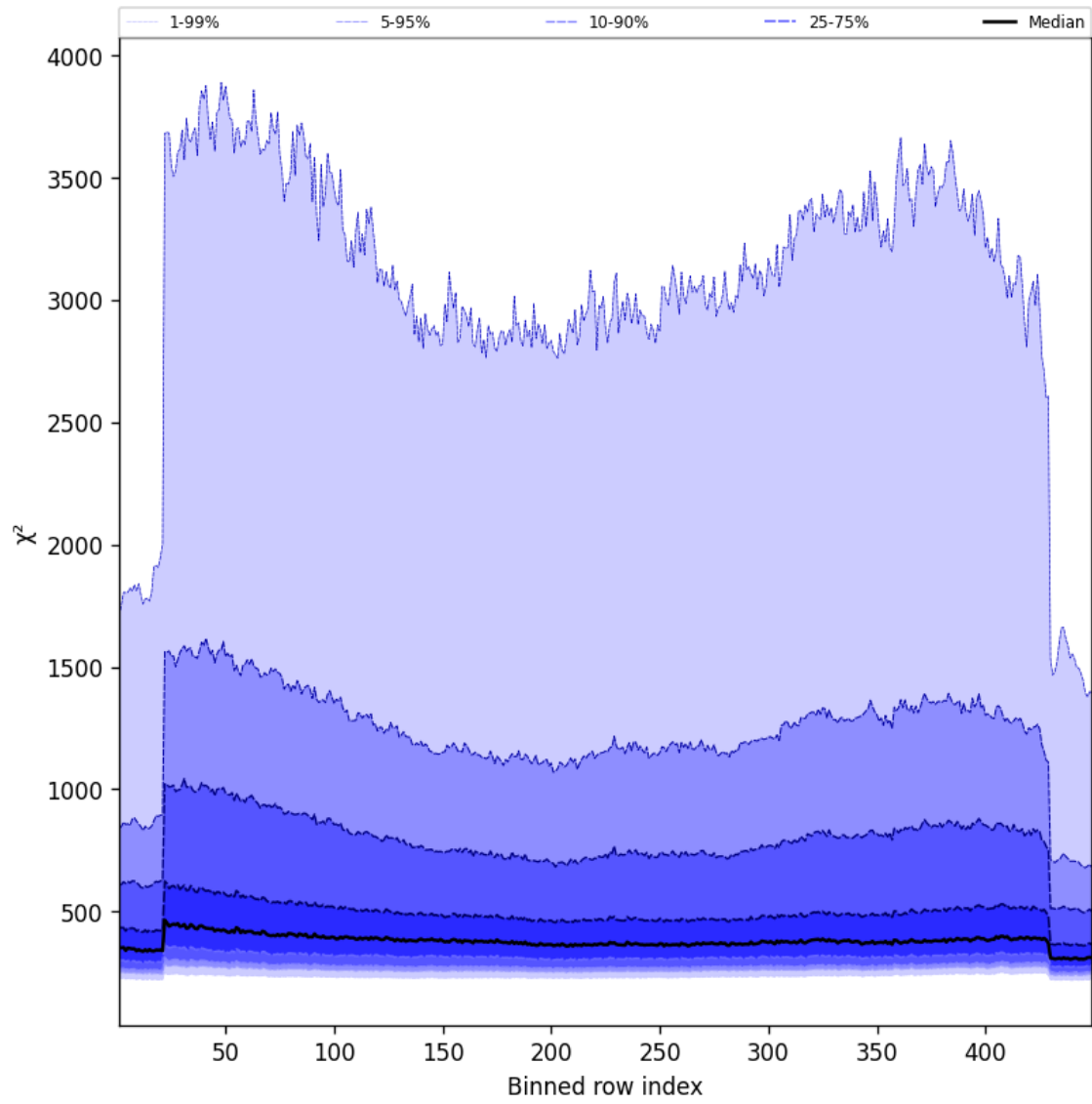
Figure 59: Along track statistics of “ \chi^2 ” for 2024-09-24 to 2024-09-26
