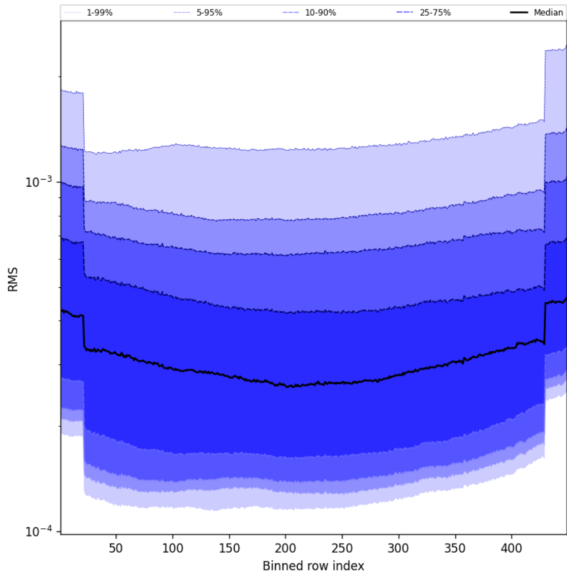
Figure 60: Along track statistics of “RMS” for 2024-09-24 to 2024-09-26
