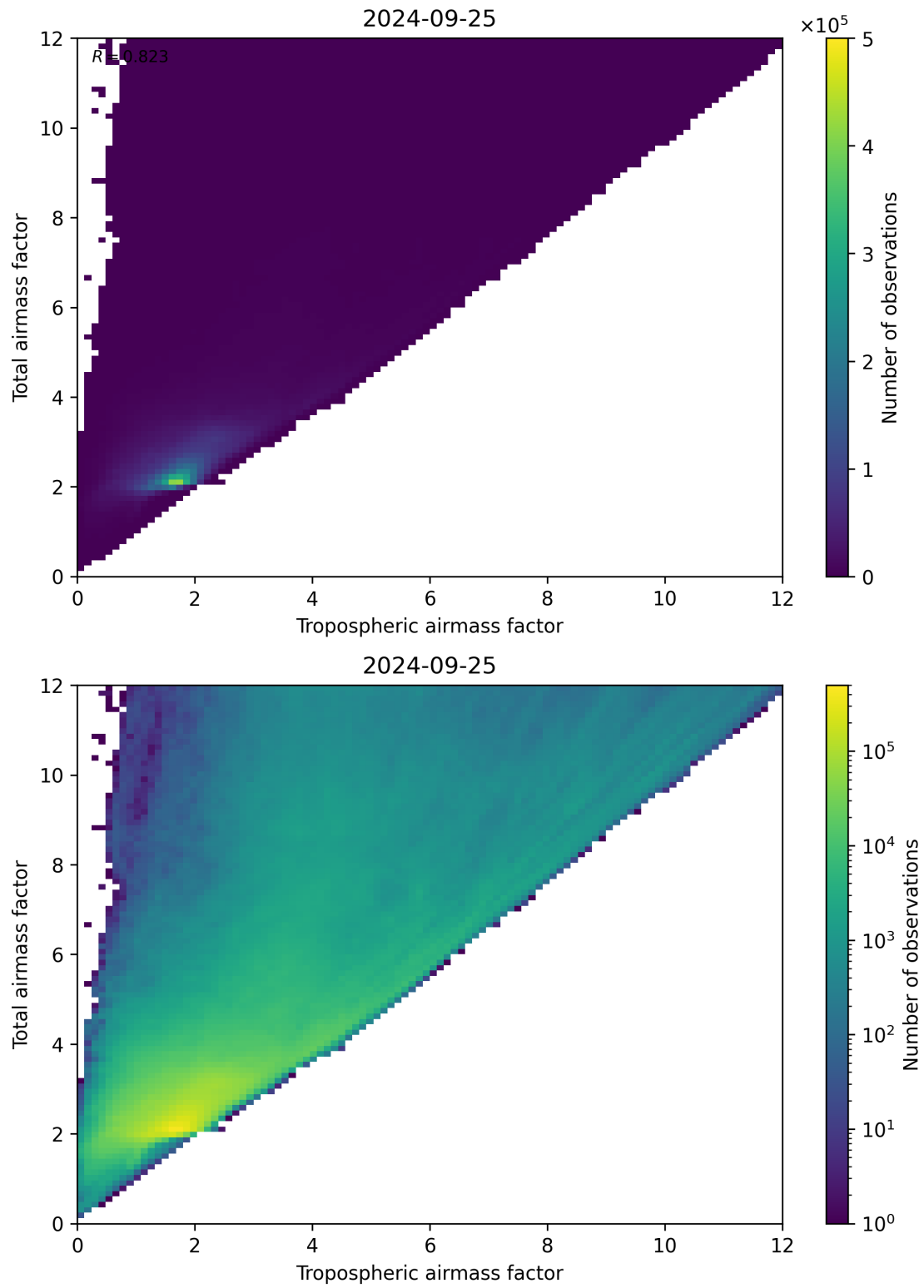
Figure 72: Scatter density plot of “Tropospheric airmass factor” against “Total airmass factor” for 2024-09-24 to 2024-09-26.
