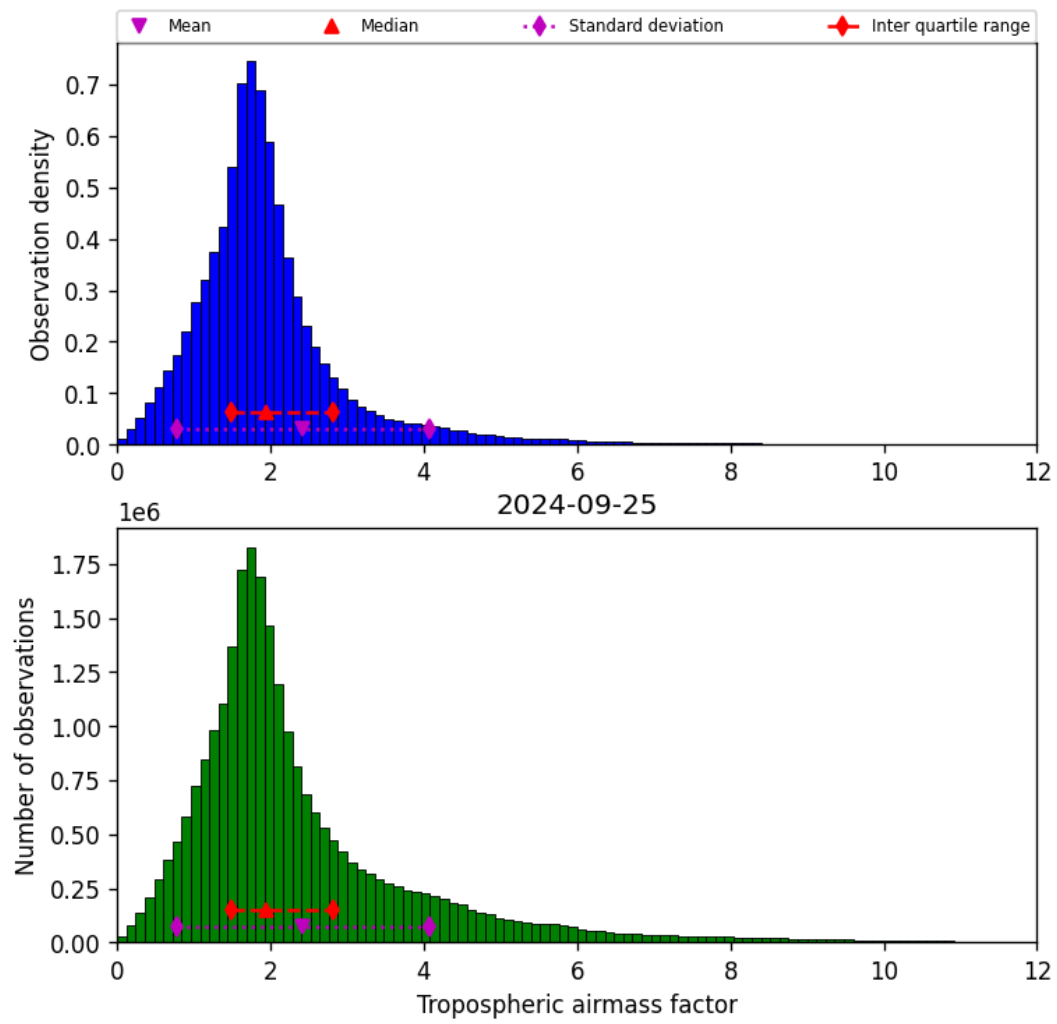
Figure 31: Histogram of “Tropospheric airmass factor” for 2024-09-24 to 2024-09-26
