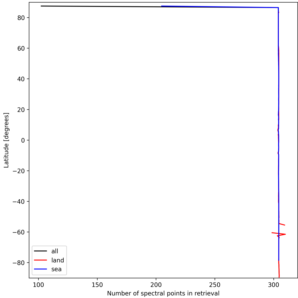
Figure 16: Zonal average of “Number of spectral points in retrieval” for 2024-09-24 to 2024-09-26.
