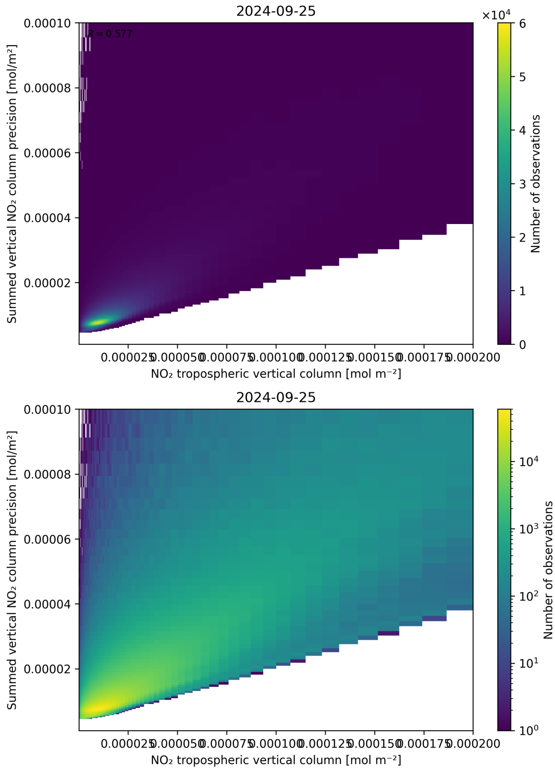
Figure 127: Scatter density plot of “NO 2 tropospheric vertical column” against “Summed vertical NO 2 column precision” for 2024-09-24 to 2024-09-26.
