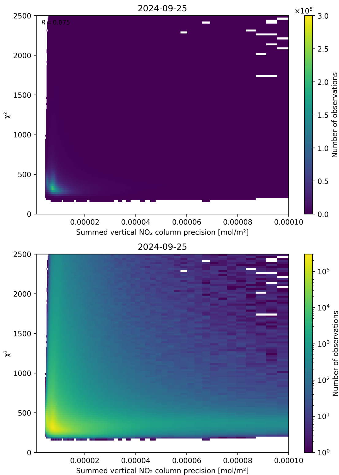
Figure 107: Scatter density plot of “Summed vertical NO 2 column precision” against “ \chi^2 ” for 2024-09-24 to 2024-09-26.
