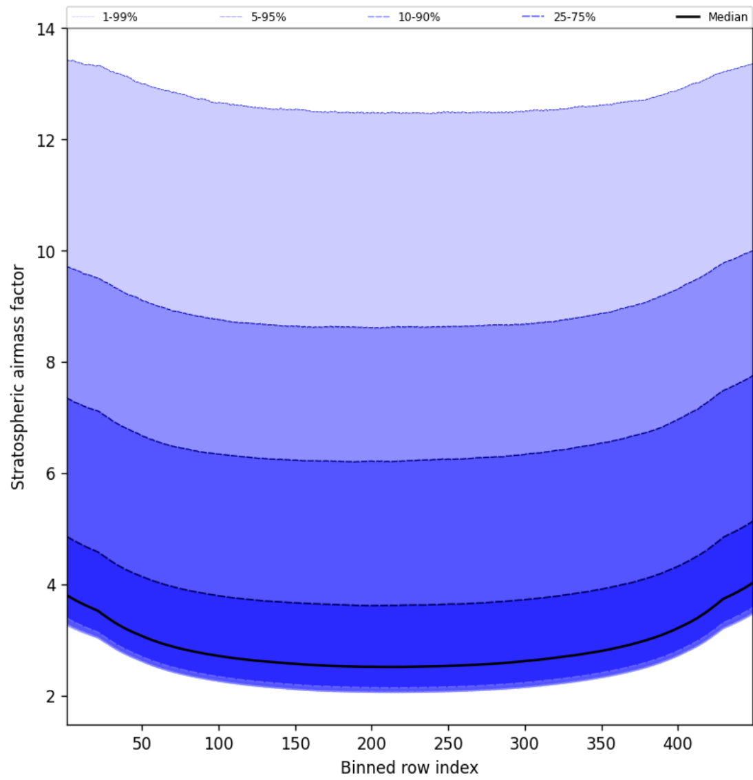
Figure 61: Along track statistics of “Stratospheric airmass factor” for 2024-09-24 to 2024-09-26
