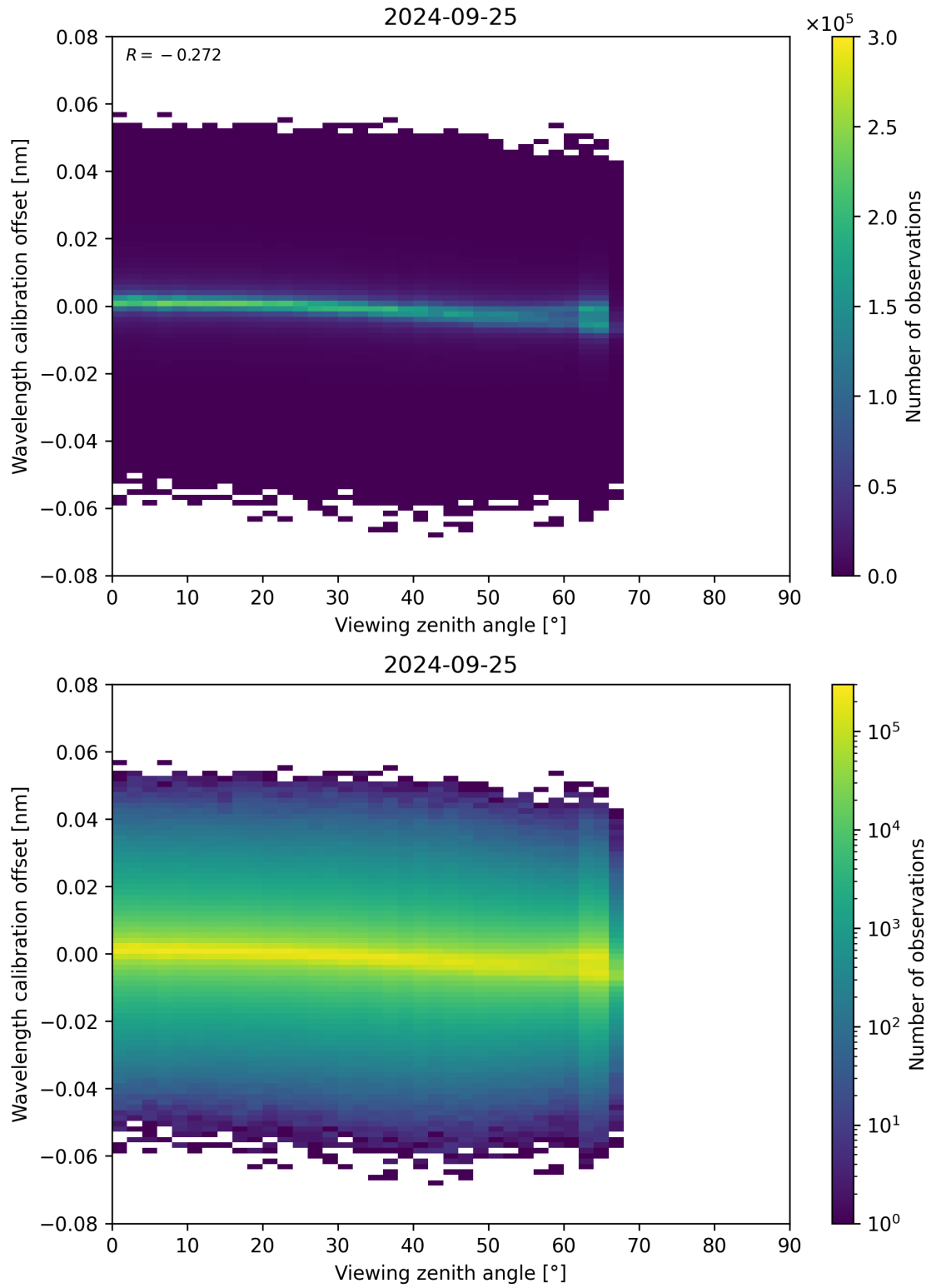
Figure 173: Scatter density plot of “Viewing zenith angle” against “Wavelength calibration offset” for 2024-09-24 to 2024-09-26.
