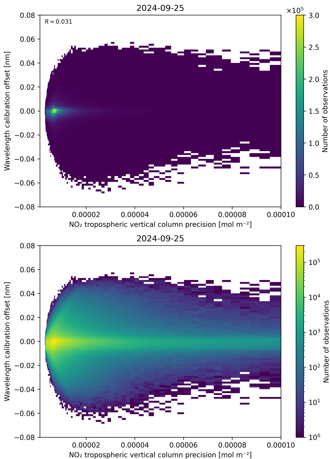
Figure 141: Scatter density plot of “NO 2 tropospheric vertical column precision” against “Wavelength calibration offset” for 2024-09-24 to 2024-09-26.
