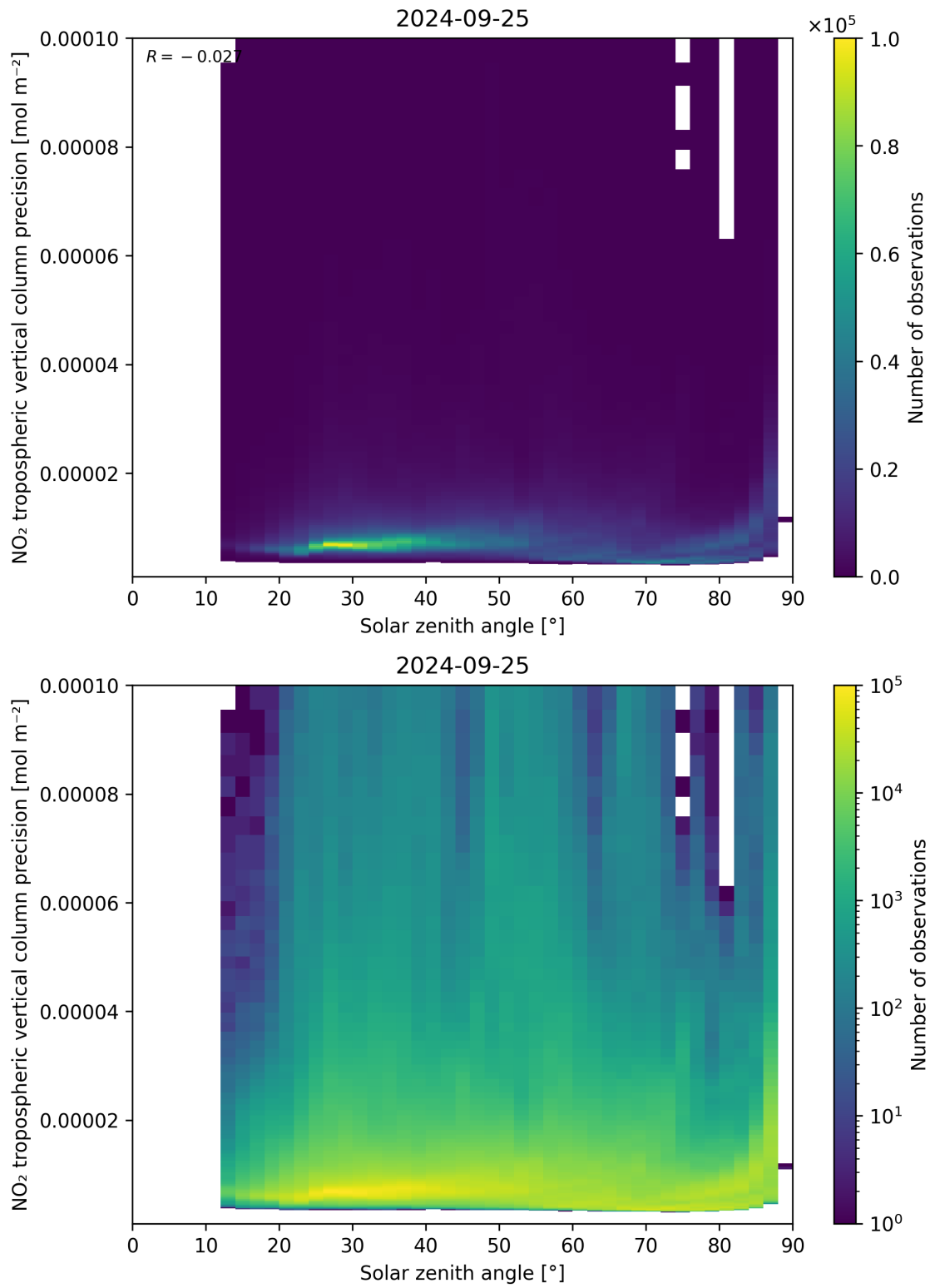
Figure 156: Scatter density plot of “Solar zenith angle” against “NO 2 tropospheric vertical column precision” for 2024-09-24 to 2024-09-26.
