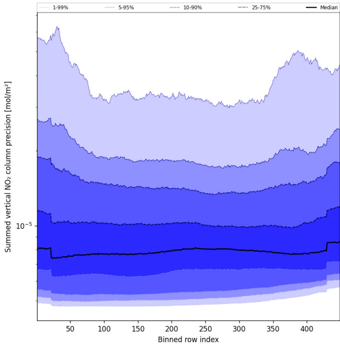
Figure 58: Along track statistics of “Summed vertical NO 2 column precision” for 2024-09-24 to 2024-09-26
