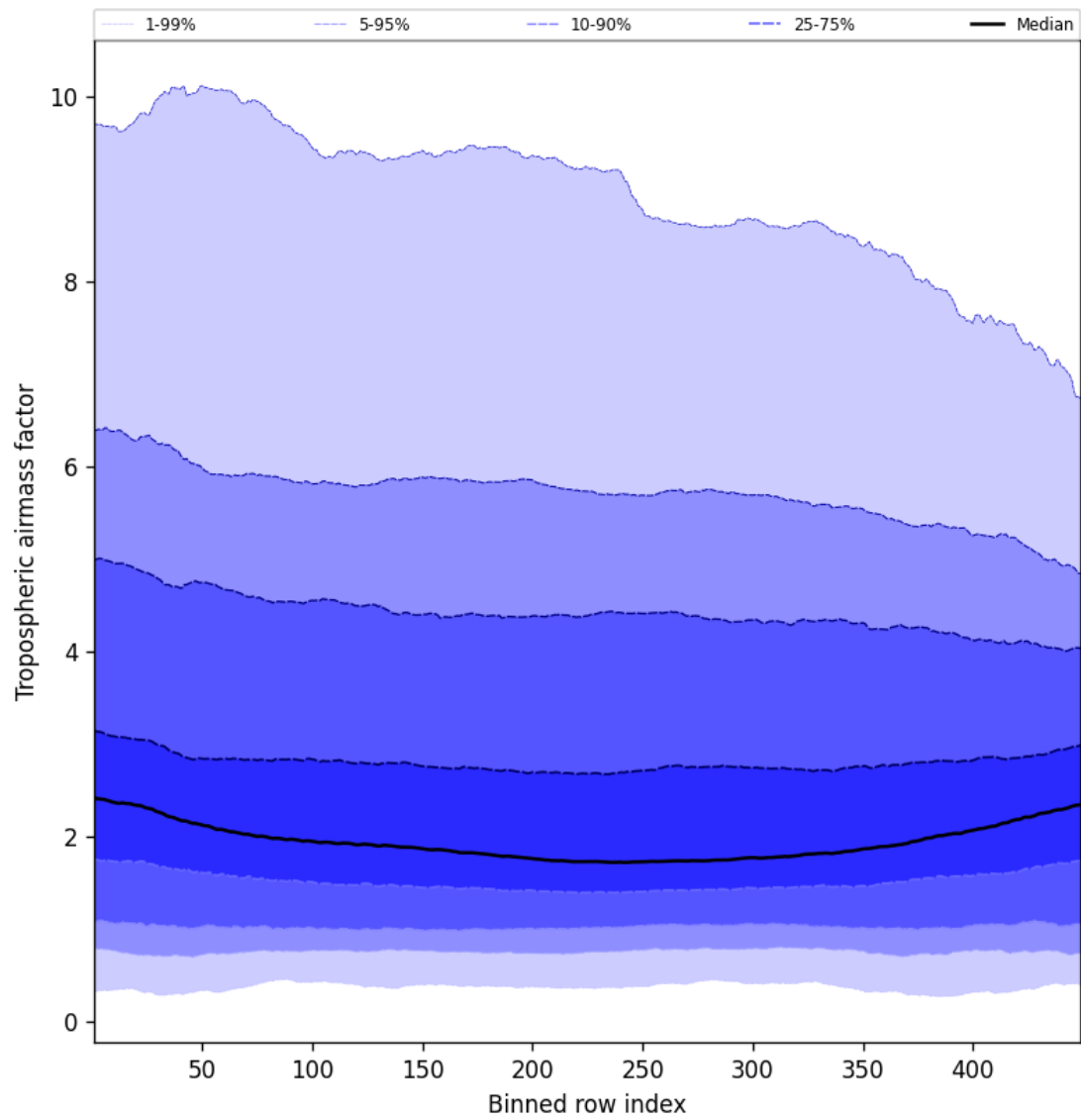
Figure 48: Along track statistics of “Tropospheric air mass factor” for 2024-09-24 to 2024-09-26
