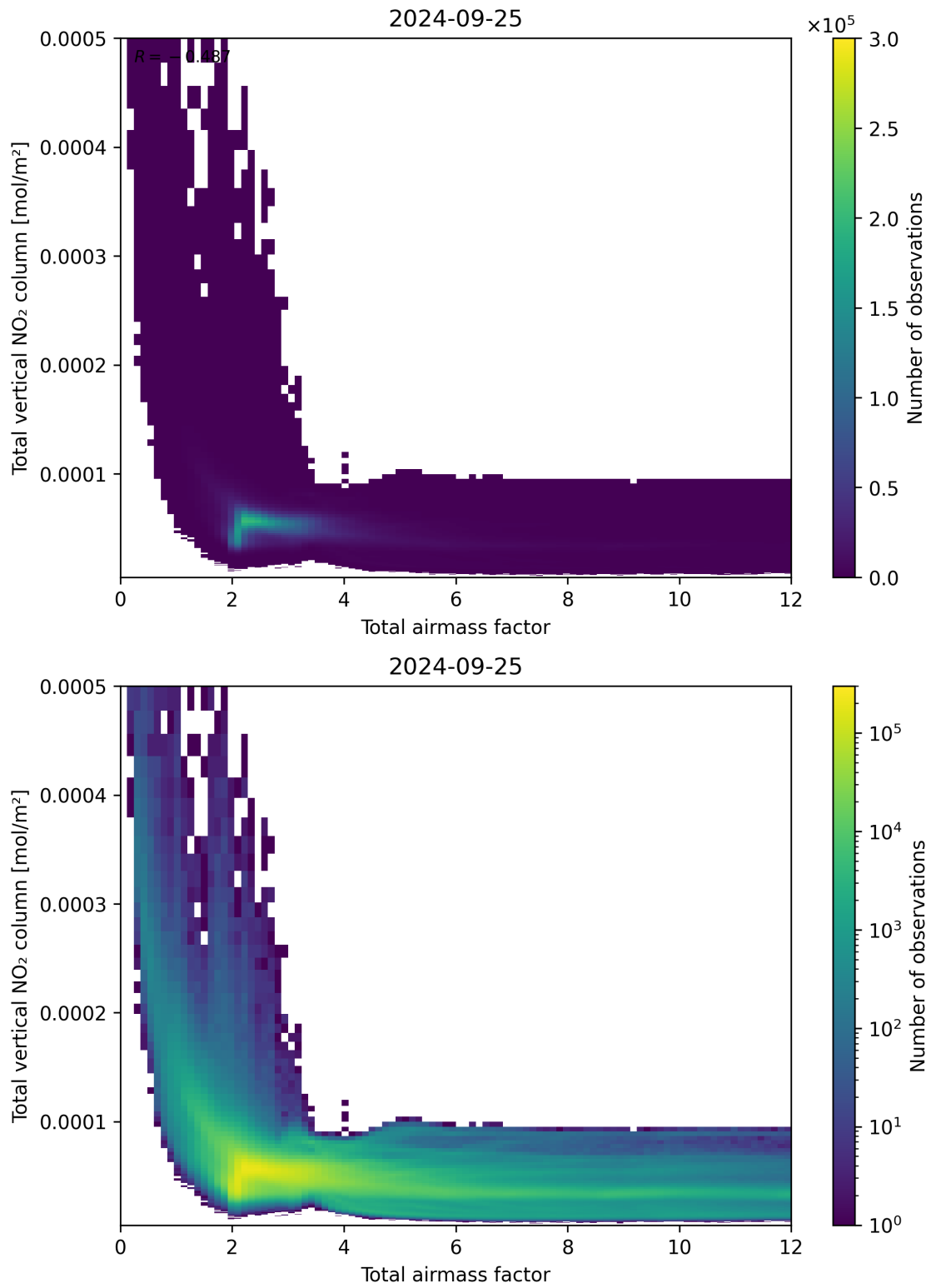
Figure 67: Scatter density plot of “Total airmass factor” against “Total vertical NO 2 column” for 2024-09-24 to 2024-09-26.
