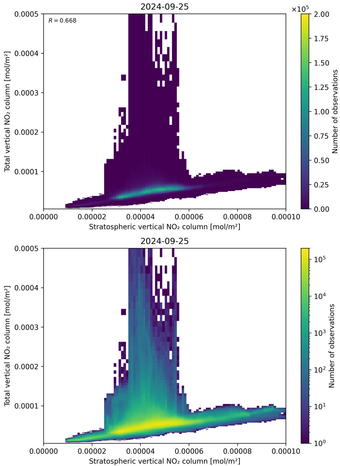
Figure 100: Scatter density plot of “Stratospheric vertical NO 2 column” against “Total vertical NO 2 column” for 2024-09-24 to 2024-09-26.
