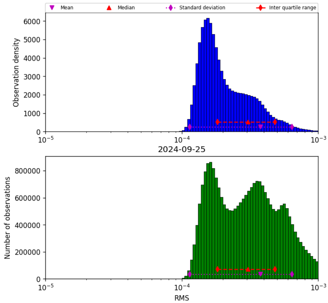
Figure 43: Histogram of “RMS” for 2024-09-24 to 2024-09-26
