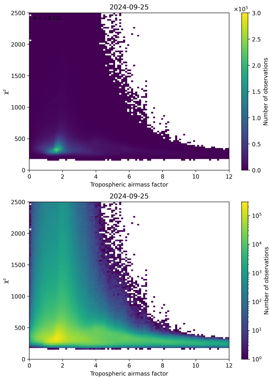
Figure 73: Scatter density plot of “Tropospheric airmass factor” against “ \chi^2 ” for 2024-09-24 to 2024-09-26.
