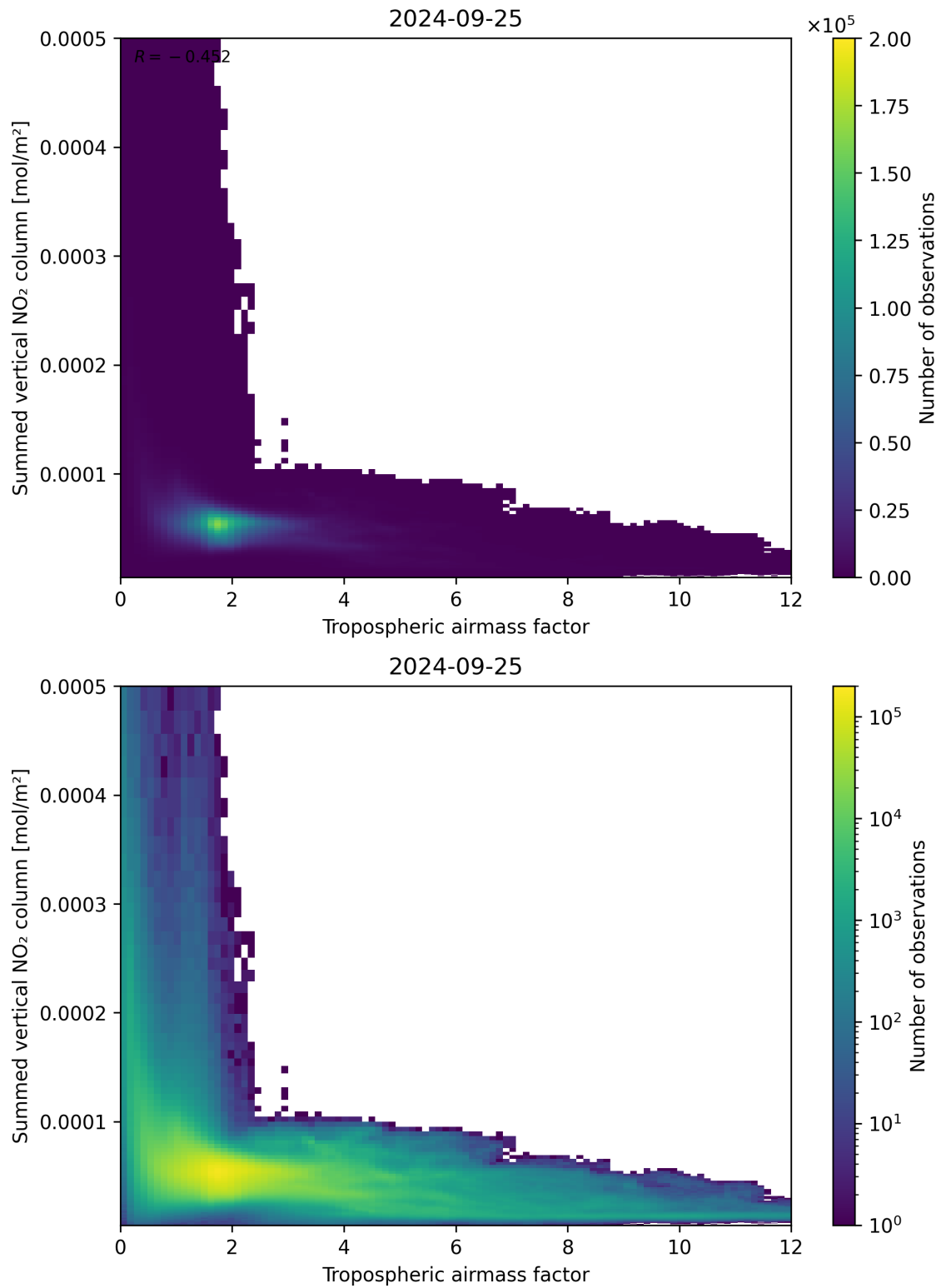
Figure 75: Scatter density plot of “Tropospheric air mass factor” against “Summed vertical NO 2 column” for 2024-09-24 to 2024-09-26.
