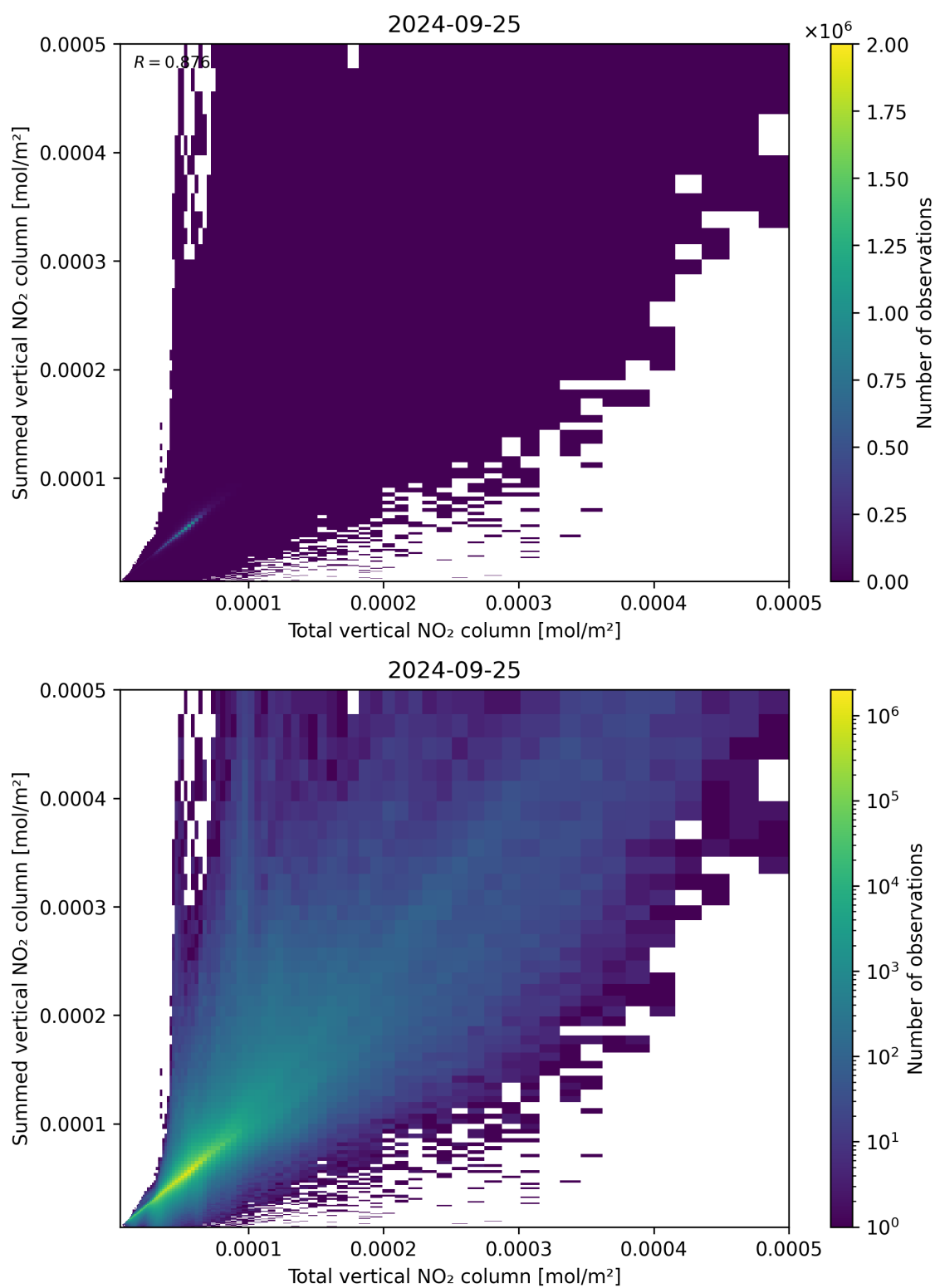
Figure 112: Scatter density plot of “Total vertical NO 2 column” against “Summed vertical NO 2 column” for 2024-09-24 to 2024-09-26.
