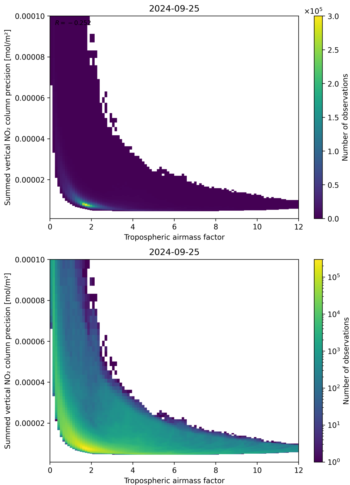
Figure 76: Scatter density plot of “Tropospheric airmass factor” against “Summed vertical NO 2 column precision” for 2024-09-24 to 2024-09-26.
