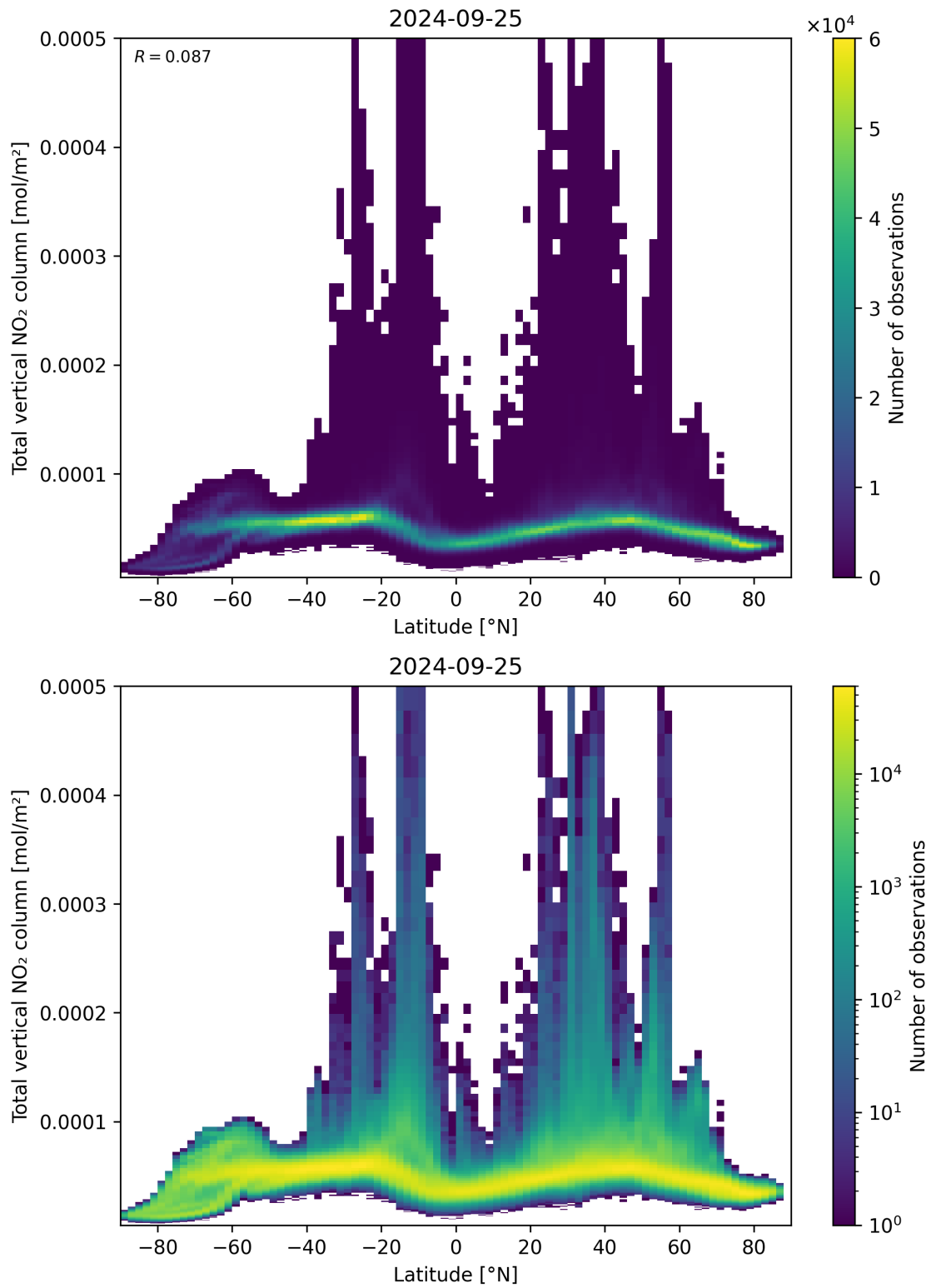
Figure 90: Scatter density plot of “Latitude” against “Total vertical NO 2 column” for 2024-09-24 to 2024-09-26.
