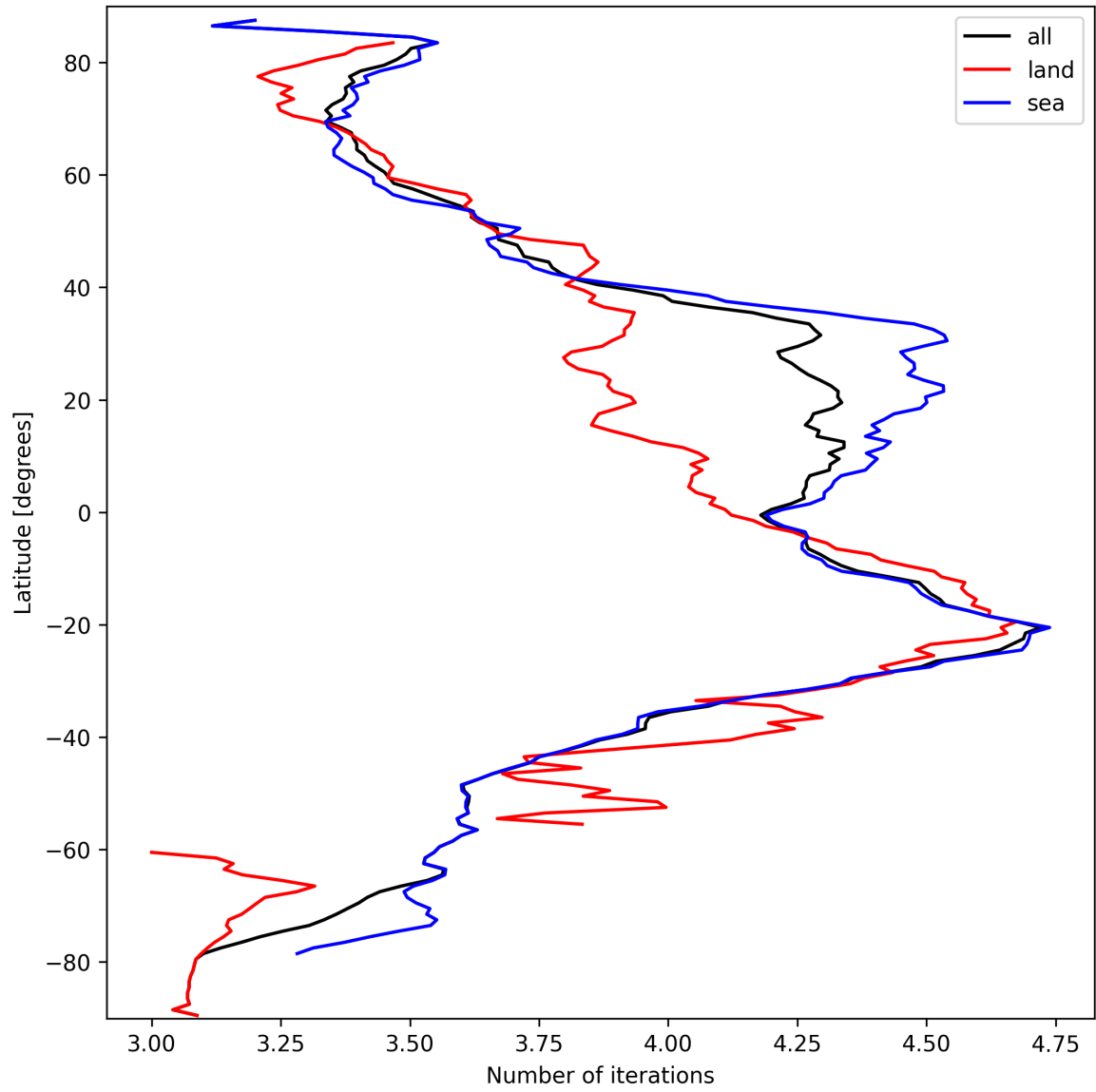
Figure 17: Zonal average of “Number of iterations” for 2024-09-24 to 2024-09-26.
