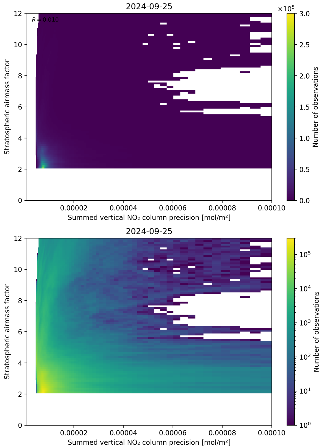
Figure 106: Scatter density plot of “Summed vertical NO 2 column precision” against “Stratospheric airmass factor” for 2024-09-24 to 2024-09-26.
