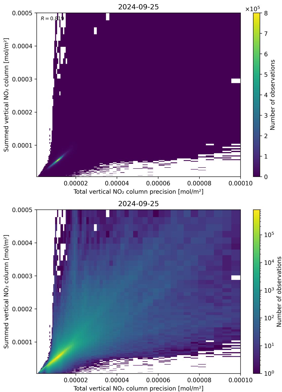
Figure 117: Scatter density plot of “Total vertical NO 2 column precision” against “Summed vertical NO 2 column” for 2024-09-24 to 2024-09-26.
