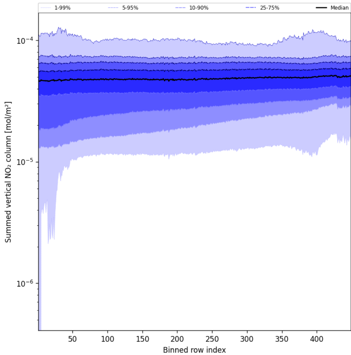
Figure 57: Along track statistics of “Summed vertical NO 2 column” for 2024-09-24 to 2024-09-26
