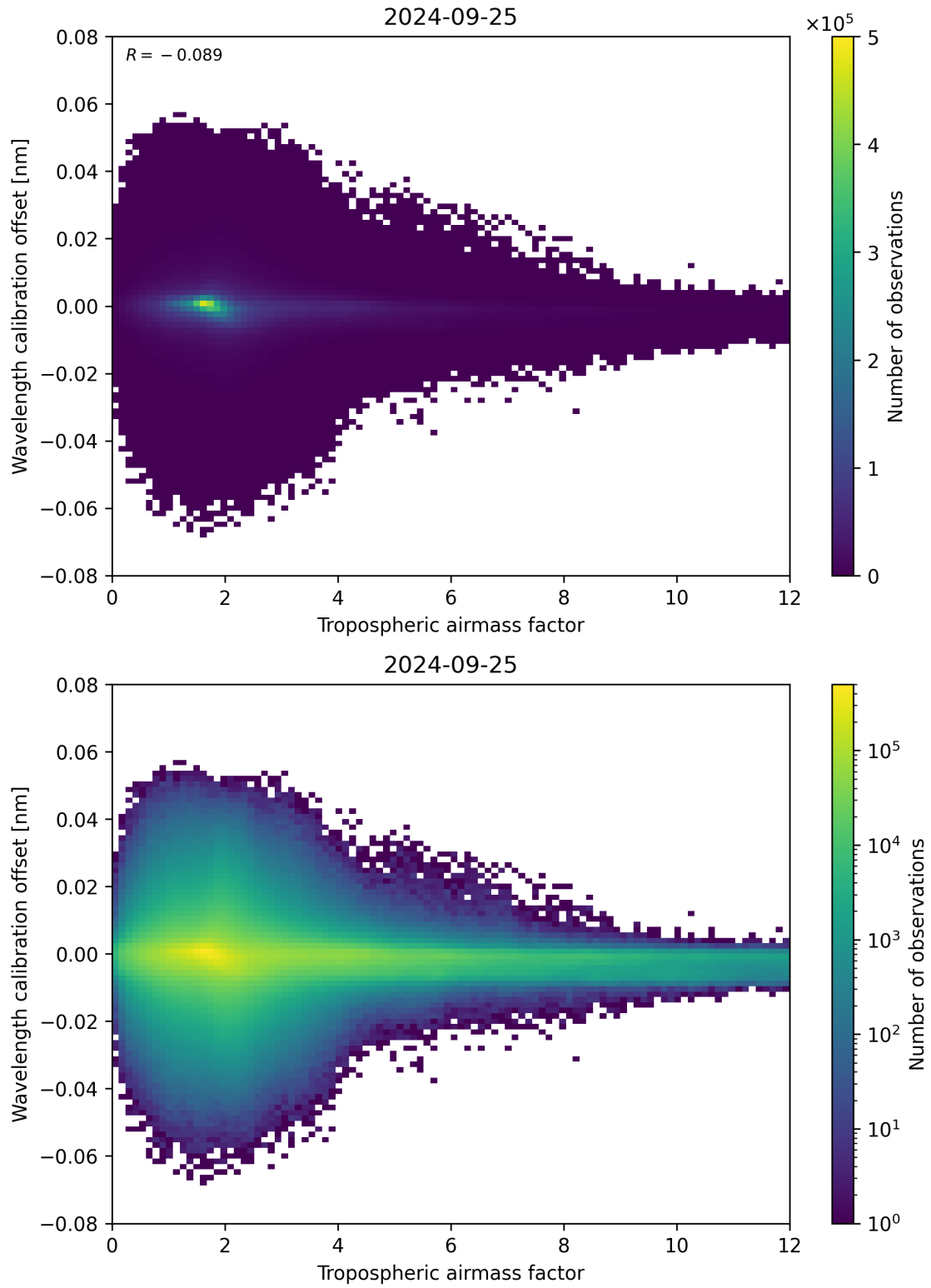
Figure 80: Scatter density plot of “Tropospheric airmass factor” against “Wavelength calibration offset” for 2024-09-24 to 2024-09-26.
