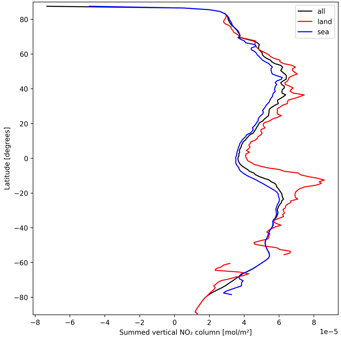
Figure 23: Zonal average of “Summed vertical NO 2 column” for 2024-09-24 to 2024-09-26.
