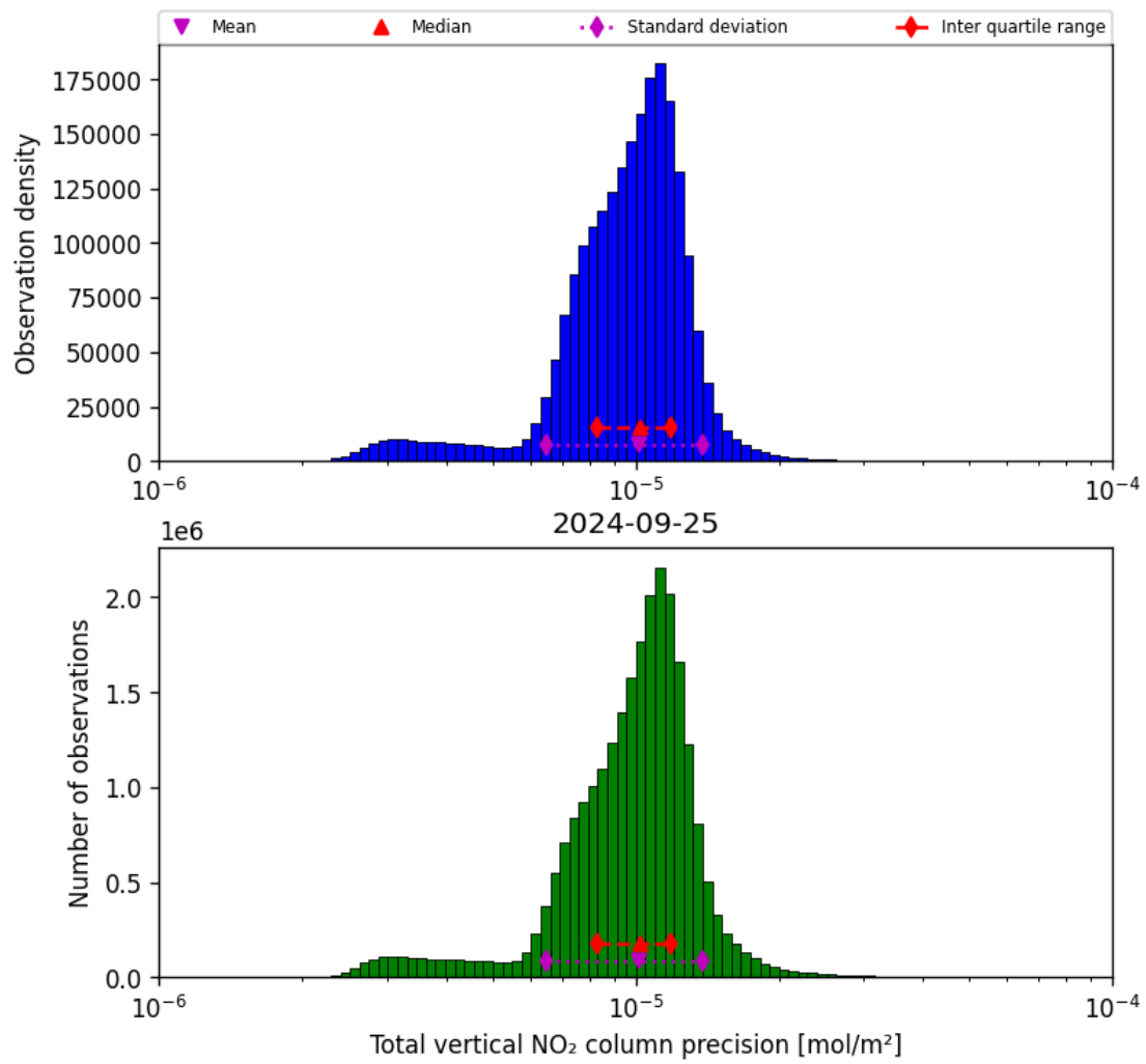
Figure 39: Histogram of “Total vertical NO 2 column precision” for 2024-09-24 to 2024-09-26
