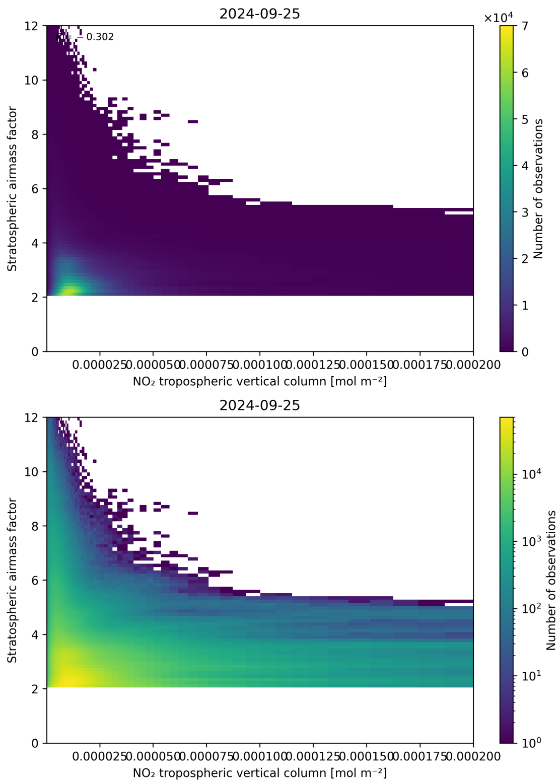
Figure 121: Scatter density plot of “NO 2 tropospheric vertical column” against “Stratospheric air mass factor” for 2024-09-24 to 2024-09-26.
