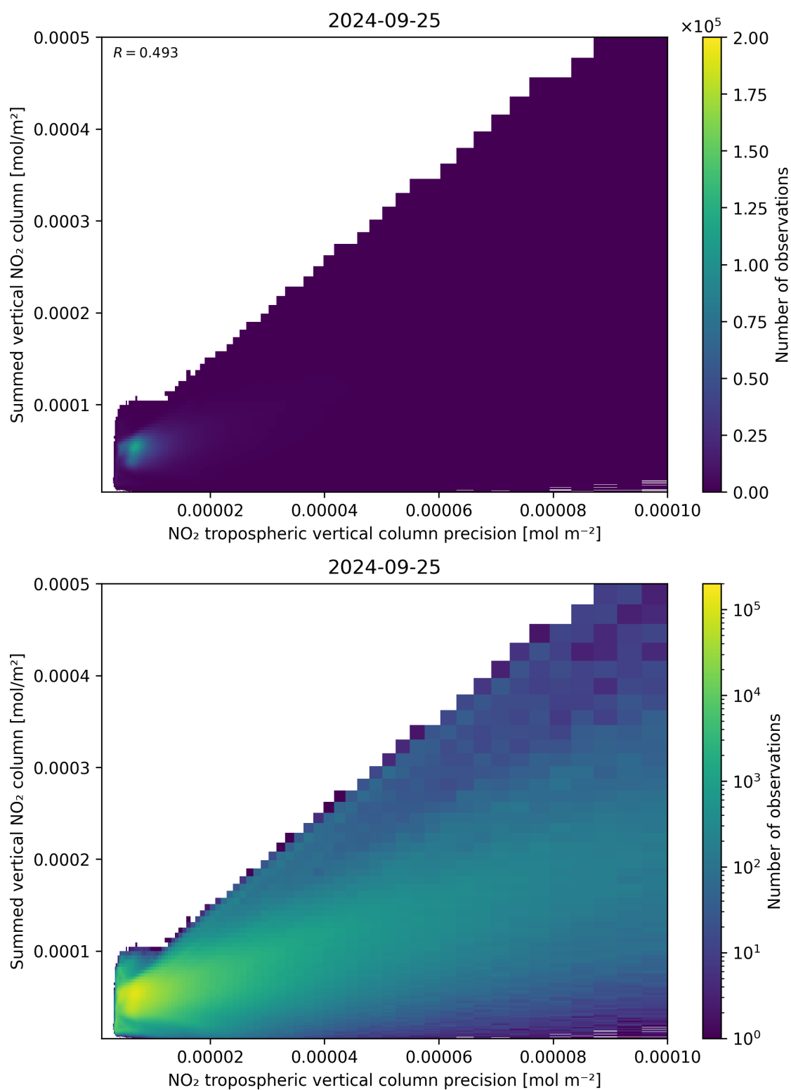
Figure 136: Scatter density plot of “NO 2 tropospheric vertical column precision” against “Summed vertical NO 2 column” for 2024-09-24 to 2024-09-26.
