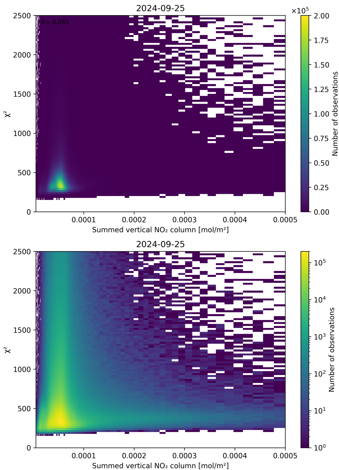
Figure 104: Scatter density plot of “Summed vertical NO 2 column” against “ \chi^2 ” for 2024-09-24 to 2024-09-26.
