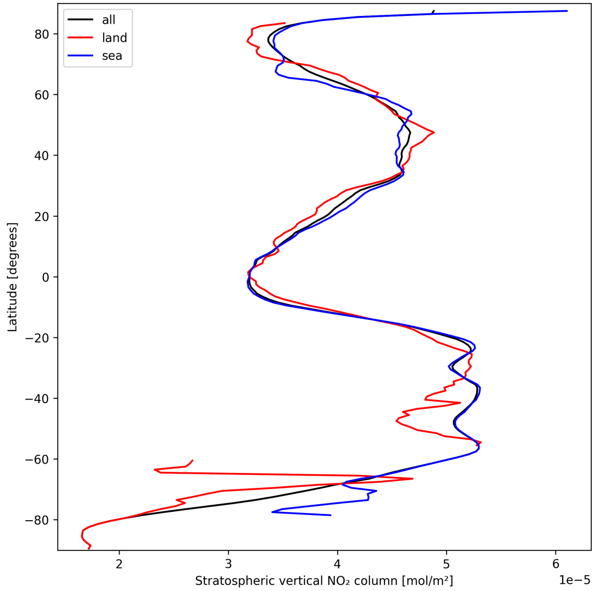
Figure 19: Zonal average of “Stratospheric vertical NO 2 column” for 2024-09-24 to 2024-09-26.
