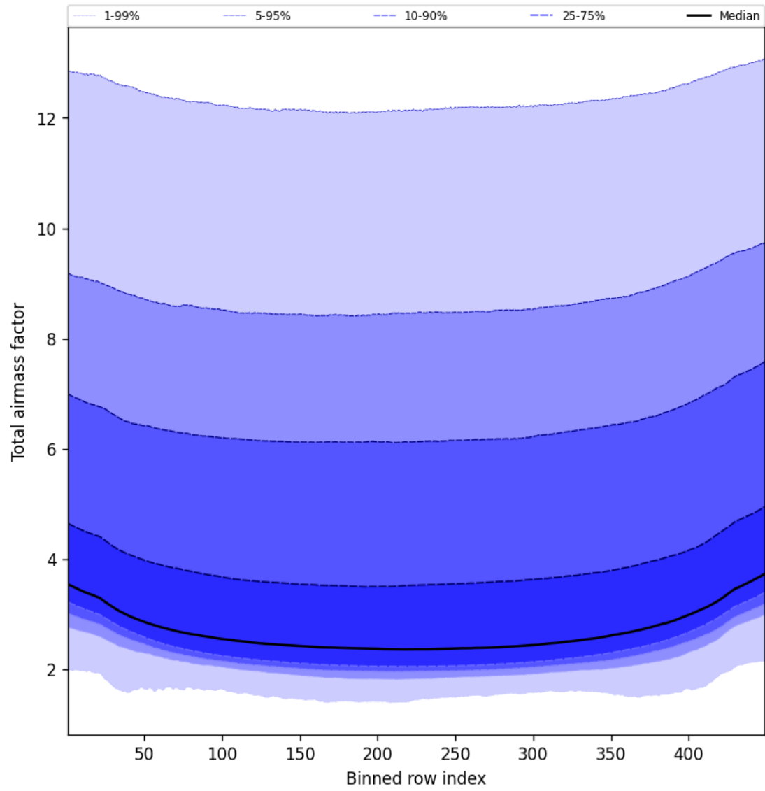
Figure 49: Along track statistics of “Total airmass factor” for 2024-09-24 to 2024-09-26
