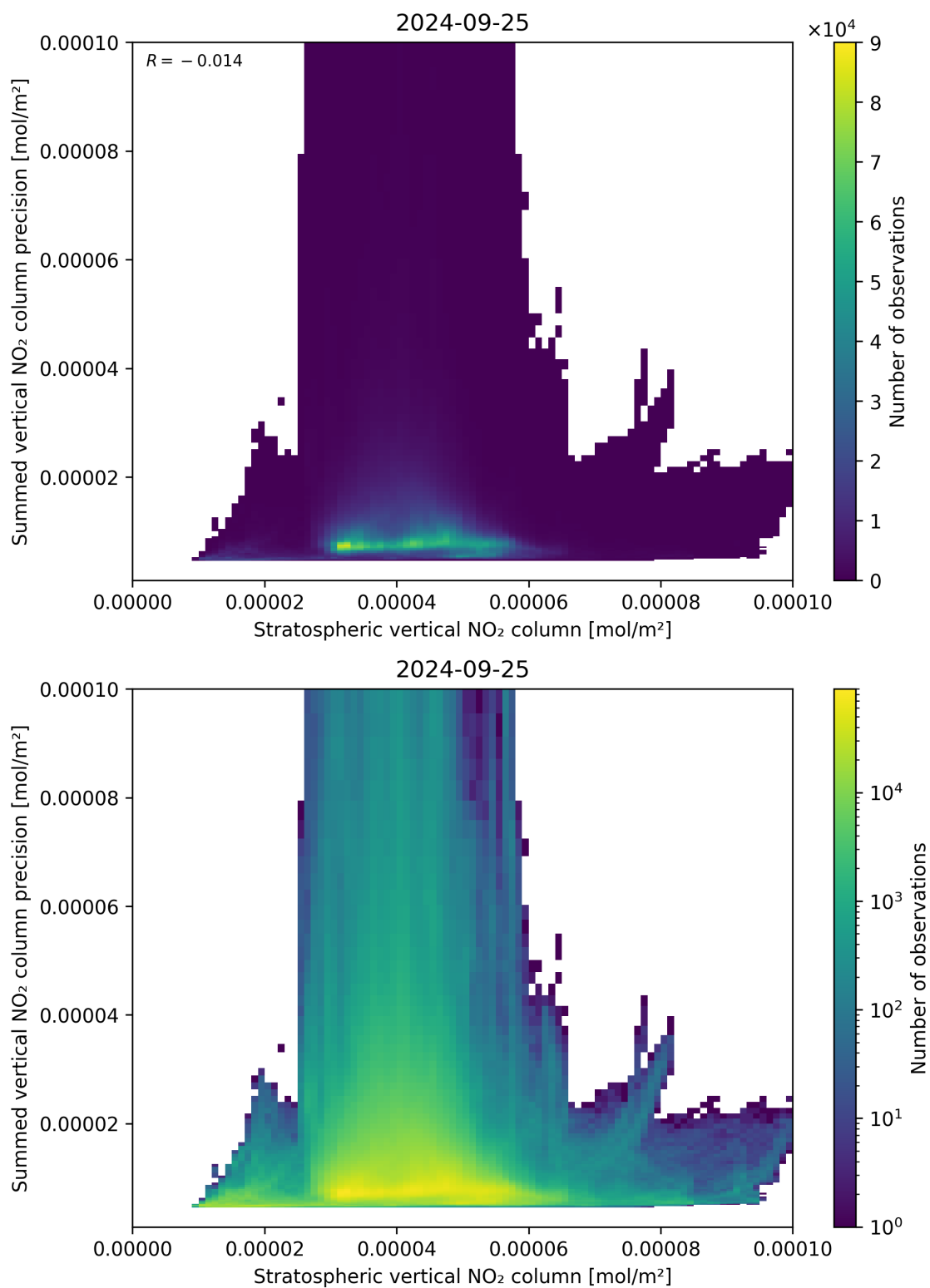
Figure 99: Scatter density plot of “Stratospheric vertical NO 2 column” against “Summed vertical NO 2 column precision” for 2024-09-24 to 2024-09-26.
