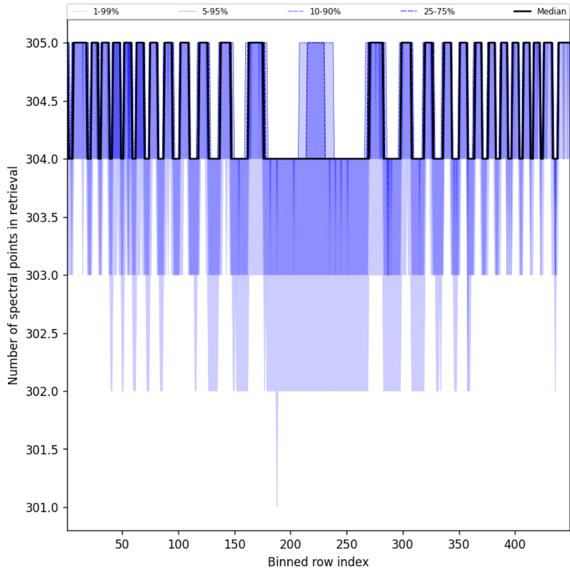
Figure 50: Along track statistics of “Number of spectral points in retrieval” for 2024-09-24 to 2024-09-26
