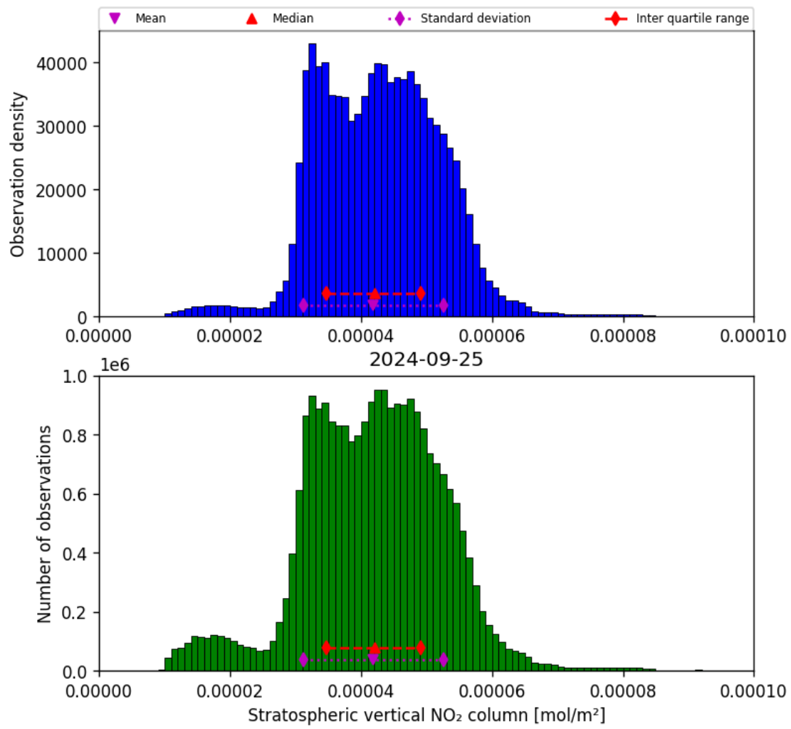
Figure 36: Histogram of “Stratospheric vertical NO 2 column” for 2024-09-24 to 2024-09-26
