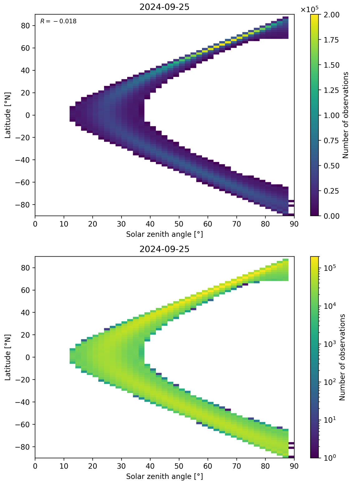
Figure 149: Scatter density plot of “Solar zenith angle” against “Latitude” for 2024-09-24 to 2024-09-26.
