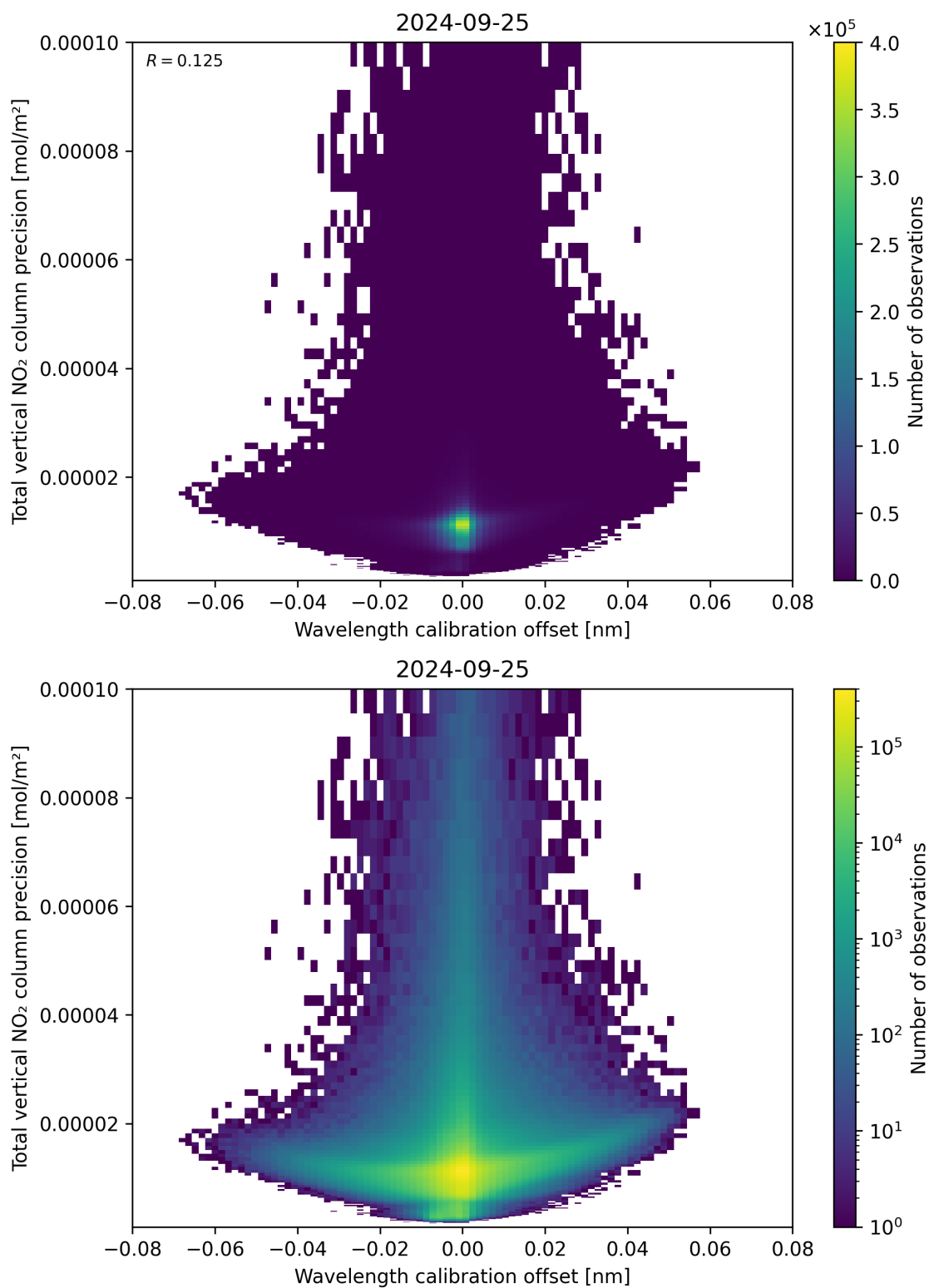
Figure 180: Scatter density plot of “Wavelength calibration offset” against “Total vertical NO 2 column precision” for 2024-09-24 to 2024-09-26.
