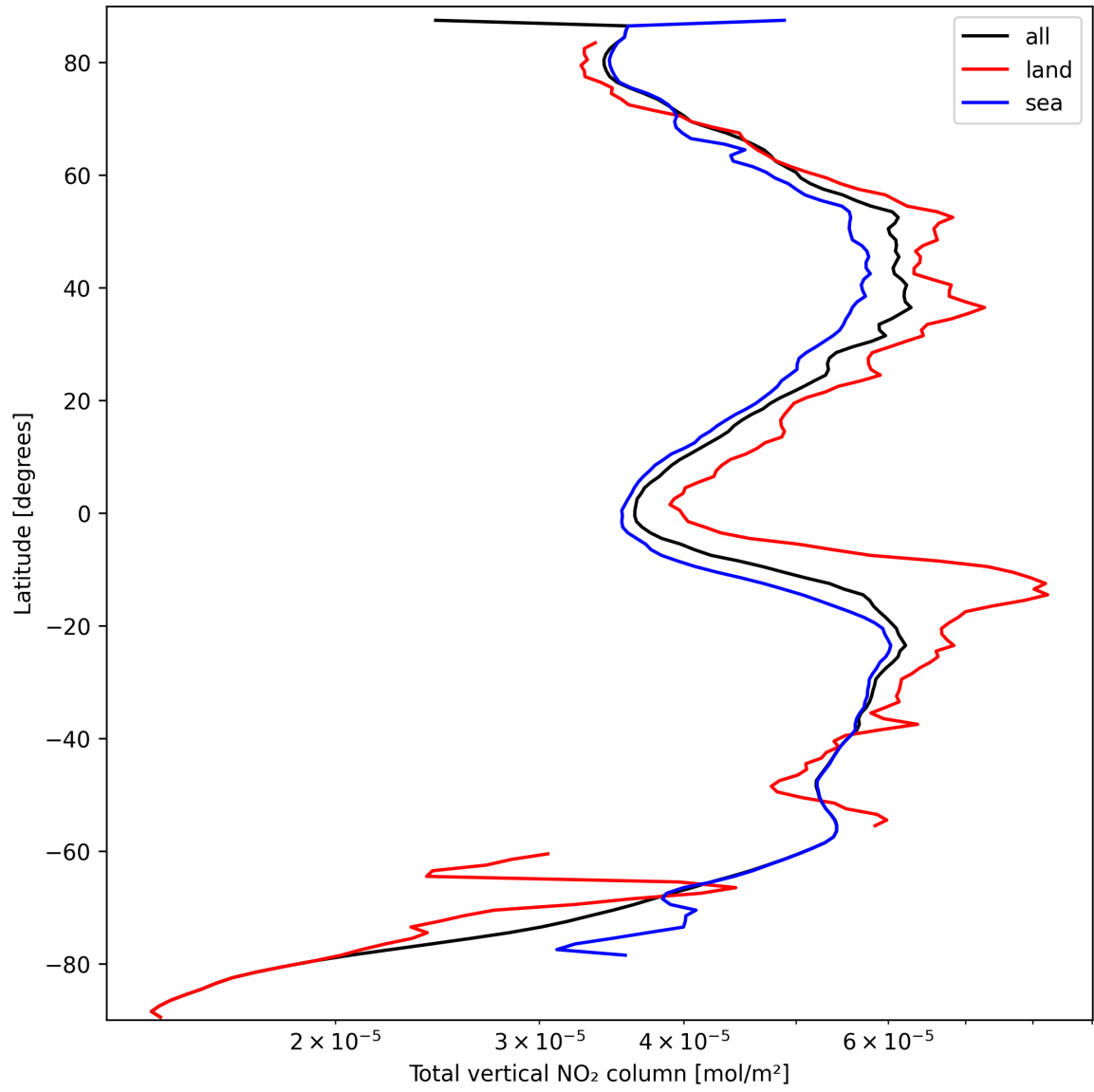
Figure 21: Zonal average of “Total vertical NO 2 column” for 2024-09-24 to 2024-09-26.
