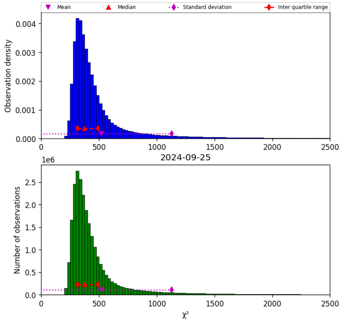
Figure 42: Histogram of “ \chi^2 ” for 2024-09-24 to 2024-09-26
