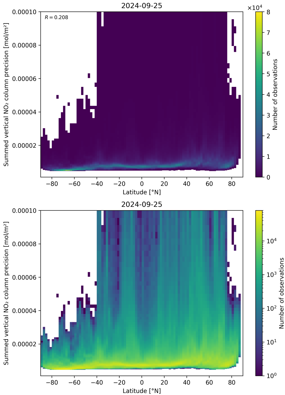
Figure 89: Scatter density plot of “Latitude” against “Summed vertical NO 2 column precision” for 2024-09-24 to 2024-09-26.
