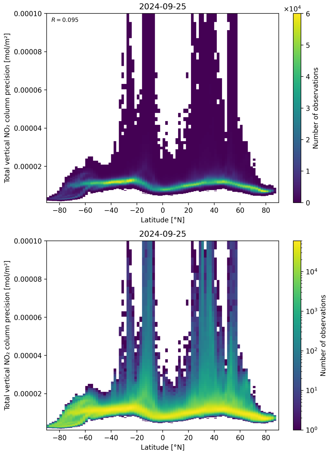
Figure 91: Scatter density plot of “Latitude” against “Total vertical NO 2 column precision” for 2024-09-24 to 2024-09-26.
