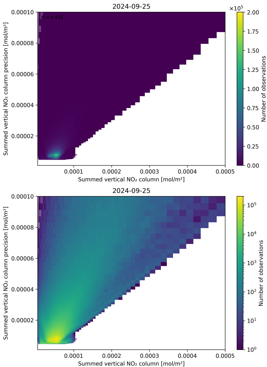
Figure 105: Scatter density plot of “Summed vertical NO 2 column” against “Summed vertical NO 2 column precision” for 2024-09-24 to 2024-09-26.
