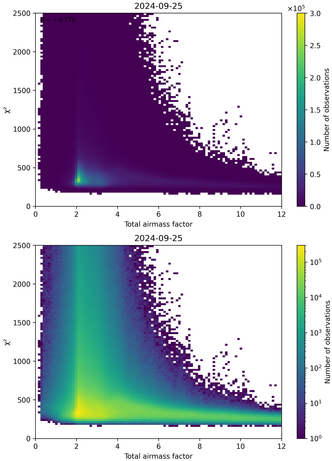
Figure 63: Scatter density plot of “Total airmass factor” against “ \chi^2 ” for 2024-09-24 to 2024-09-26.
