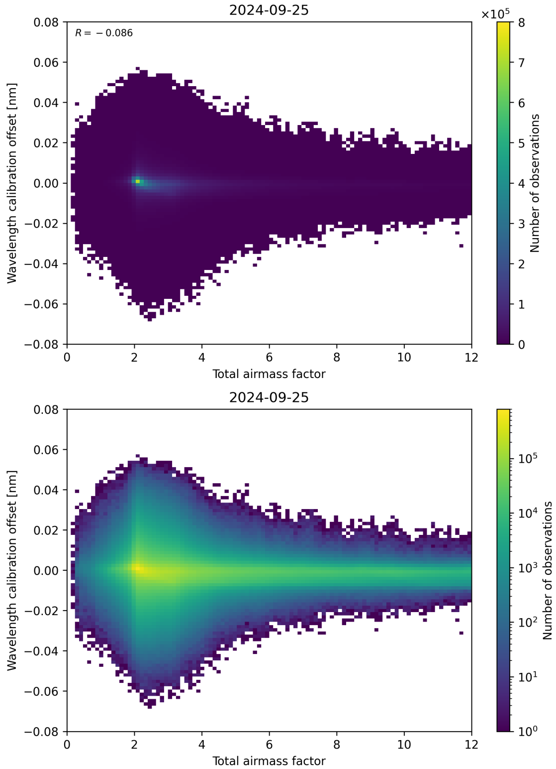
Figure 70: Scatter density plot of “Total airmass factor” against “Wavelength calibration offset” for 2024-09-24 to 2024-09-26.
