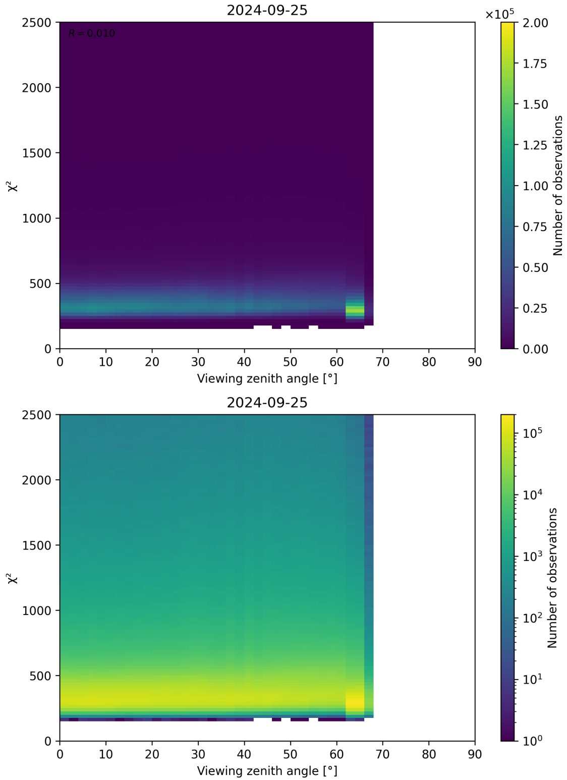
Figure 162: Scatter density plot of “Viewing zenith angle” against “ \chi^2 ” for 2024-09-24 to 2024-09-26.
