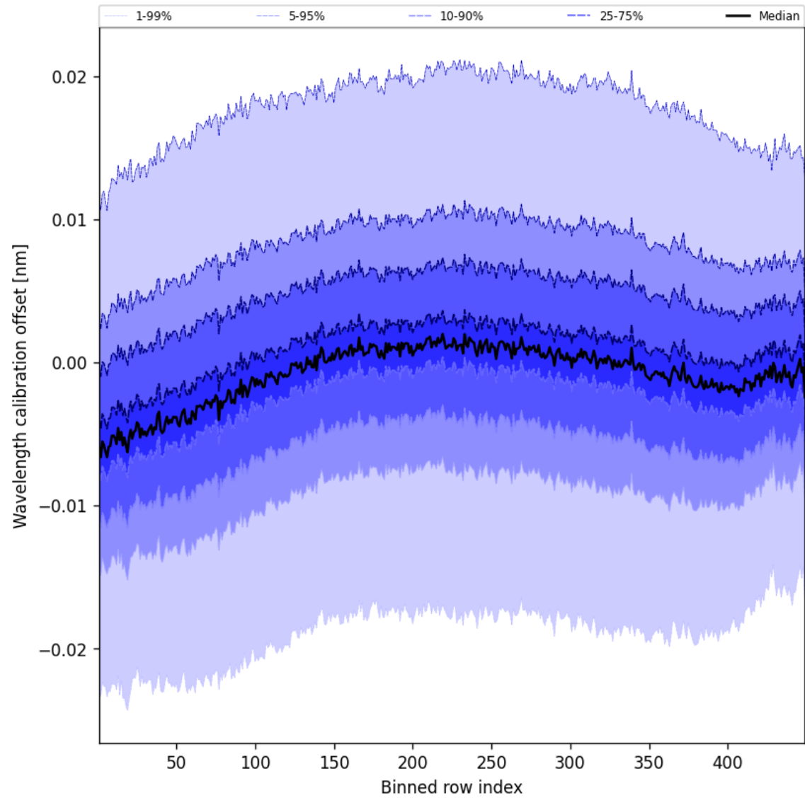
Figure 52: Along track statistics of “Wavelength calibration offset” for 2024-09-24 to 2024-09-26
