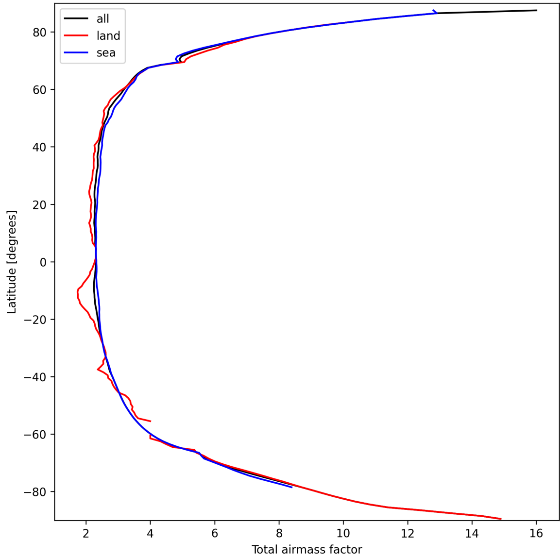
Figure 15: Zonal average of “Total airmass factor” for 2024-09-24 to 2024-09-26.
