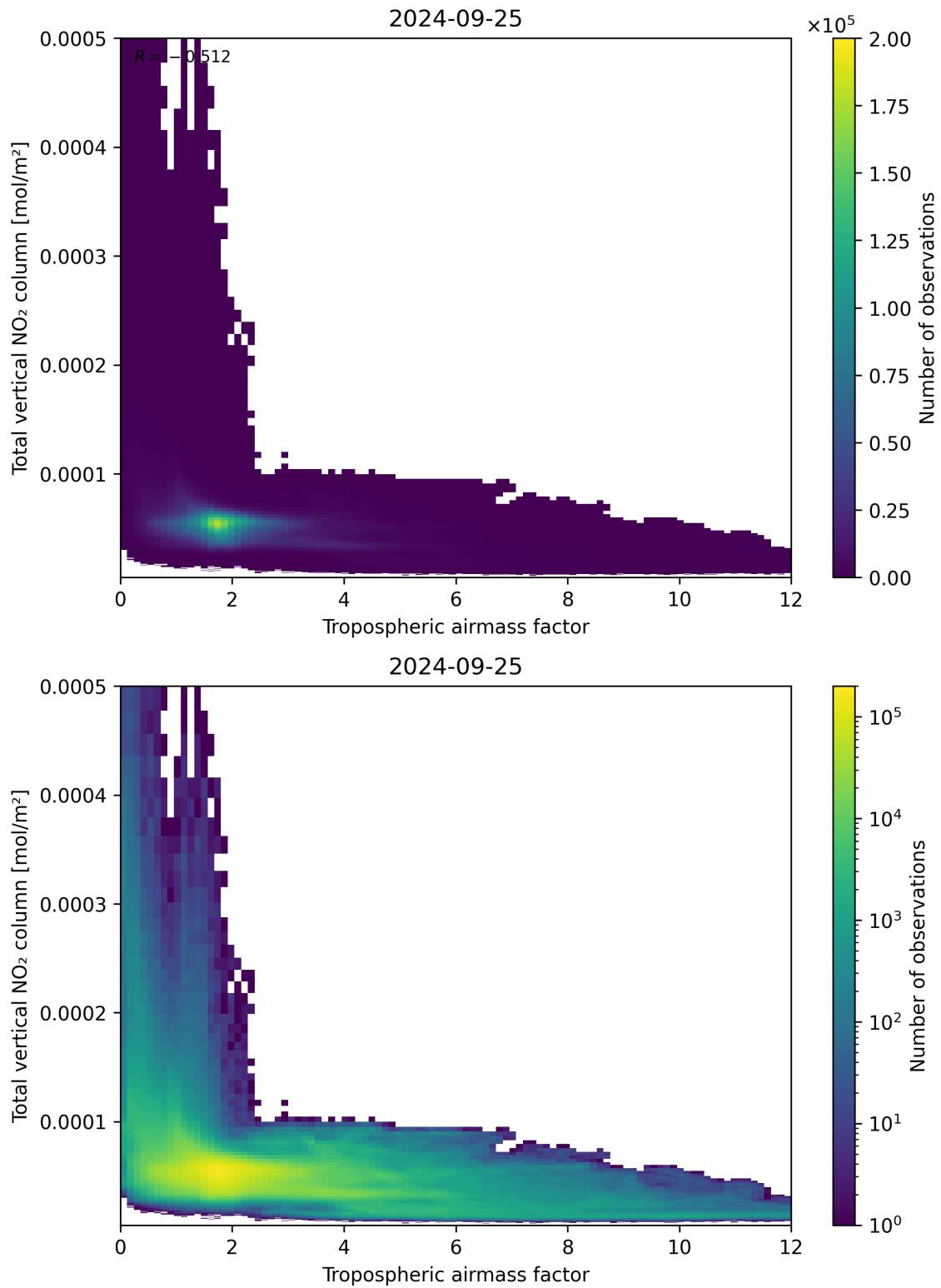
Figure 77: Scatter density plot of “Tropospheric airmass factor” against “Total vertical NO 2 column” for 2024-09-24 to 2024-09-26.
