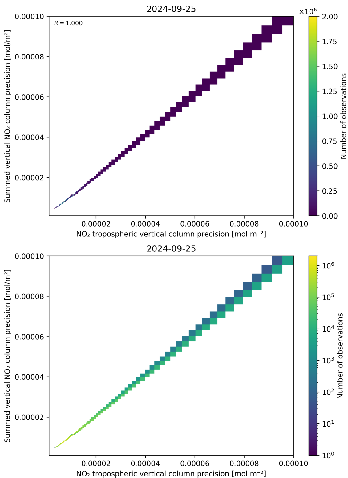
Figure 137: Scatter density plot of “NO 2 tropospheric vertical column precision” against “Summed vertical NO 2 column precision” for 2024-09-24 to 2024-09-26.
