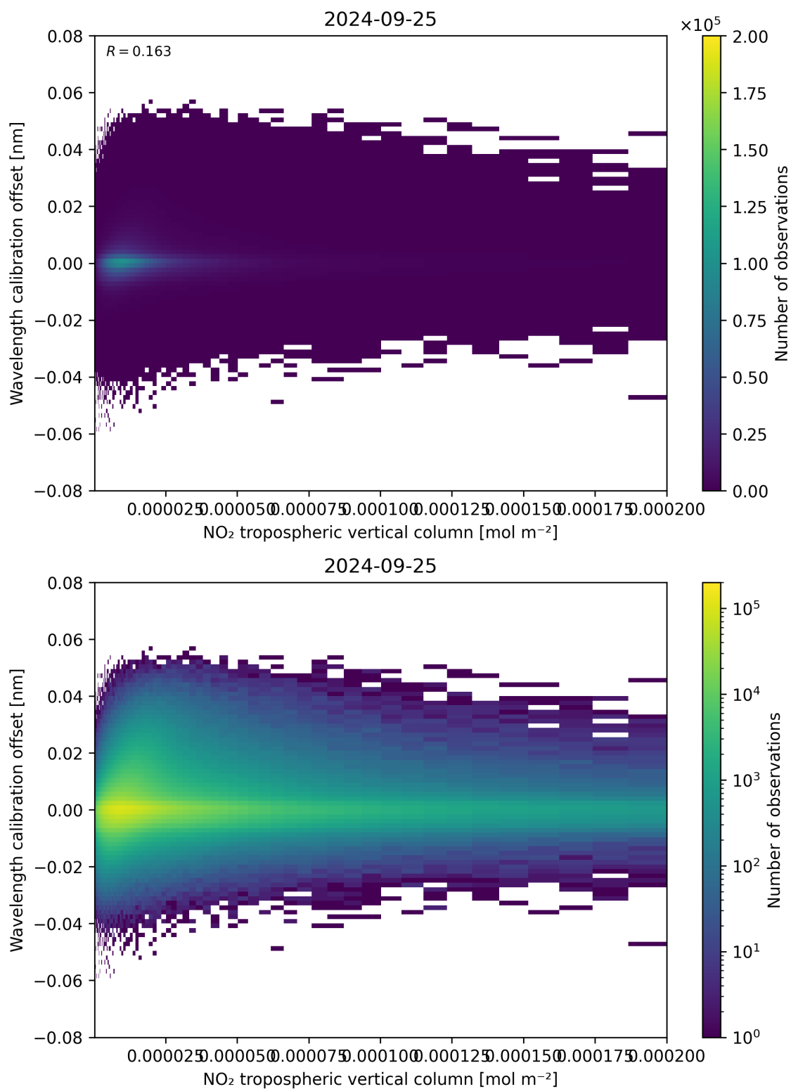
Figure 143: Scatter density plot of “NO 2 tropospheric vertical column” against “Wavelength calibration offset” for 2024-09-24 to 2024-09-26.
