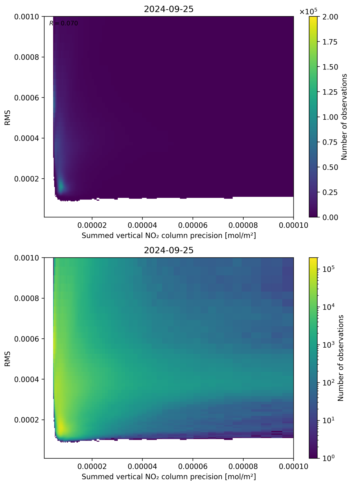
Figure 108: Scatter density plot of “Summed vertical NO 2 column precision” against “RMS” for 2024-09-24 to 2024-09-26.
