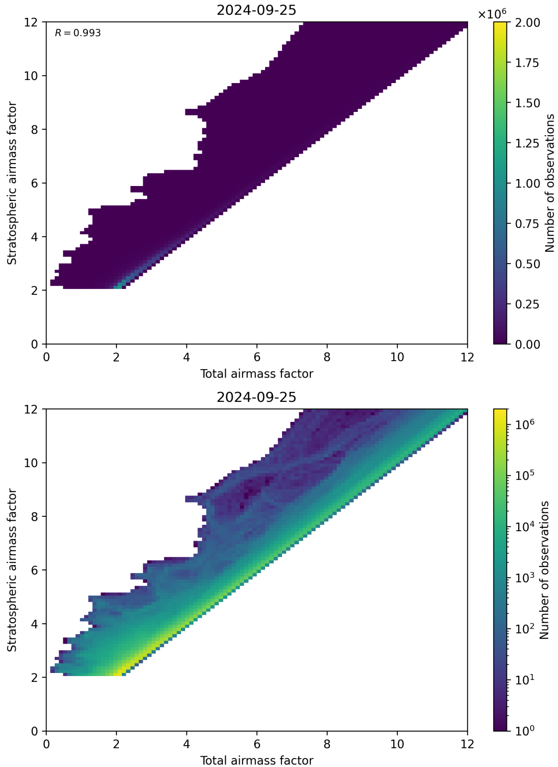
Figure 62: Scatter density plot of “Total airmass factor” against “Stratospheric airmass factor” for 2024-09-24 to 2024-09-26.
