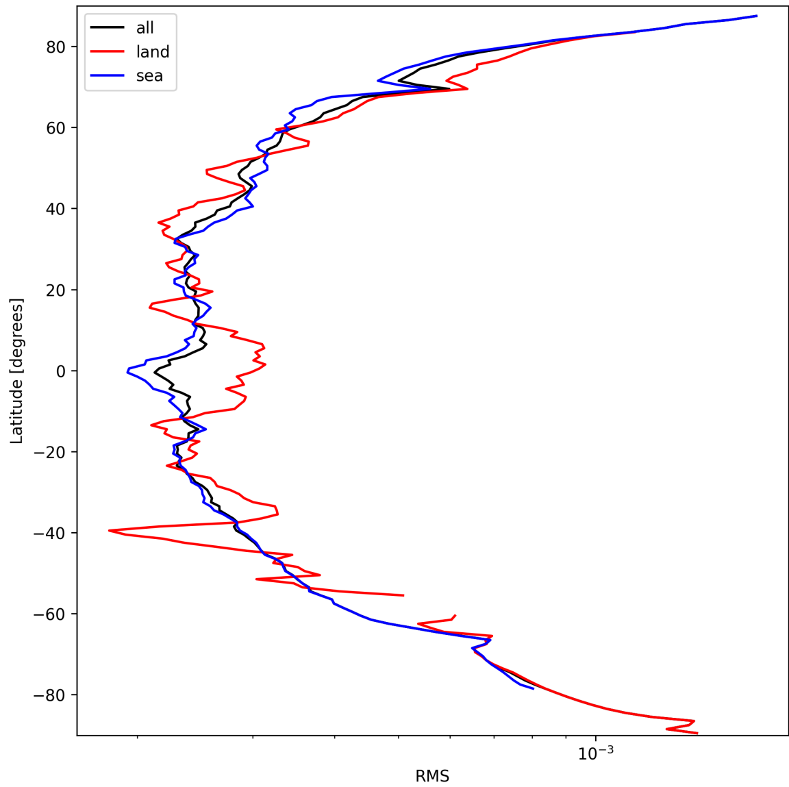
Figure 26: Zonal average of “RMS” for 2024-09-24 to 2024-09-26.
