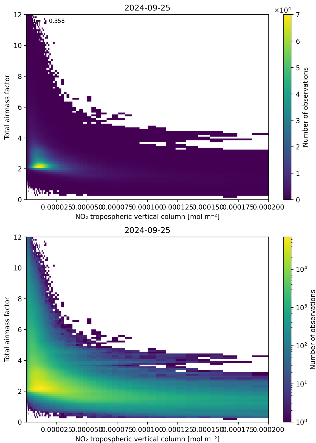
Figure 122: Scatter density plot of “NO 2 tropospheric vertical column” against “Total air mass factor” for 2024-09-24 to 2024-09-26.
