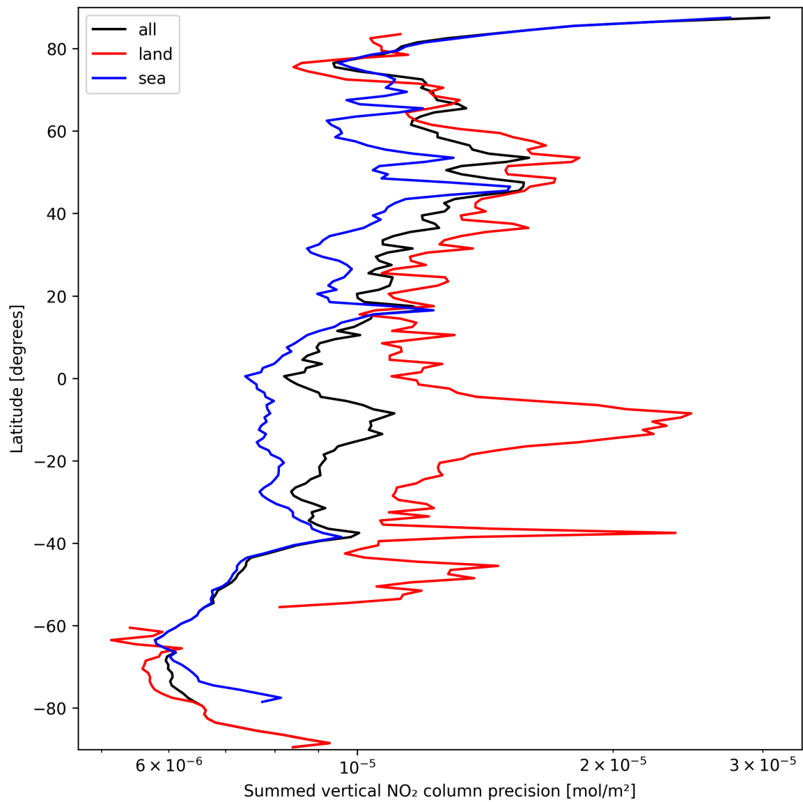
Figure 24: Zonal average of “Summed vertical NO 2 column precision” for 2024-09-24 to 2024-09-26.
