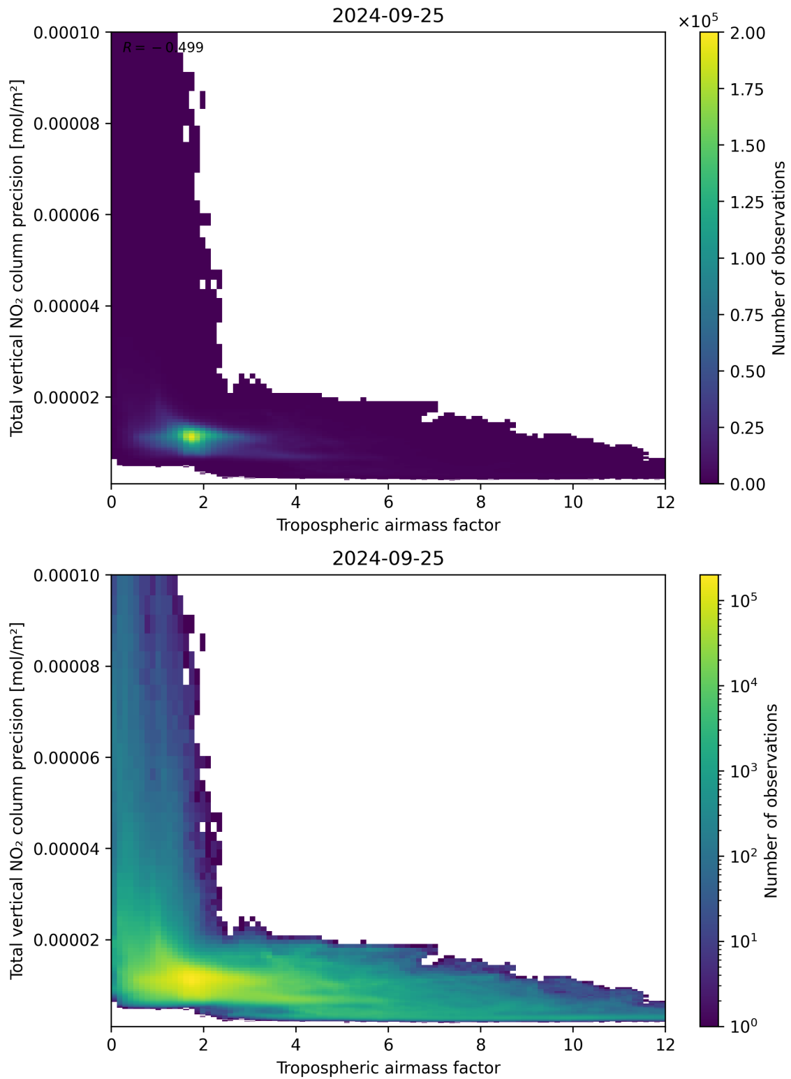
Figure 78: Scatter density plot of “Tropospheric air mass factor” against “Total vertical NO 2 column precision” for 2024-09-24 to 2024-09-26.
