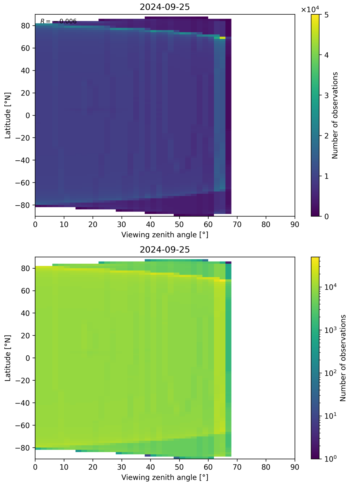
Figure 163: Scatter density plot of “Viewing zenith angle” against “Latitude” for 2024-09-24 to 2024-09-26.
