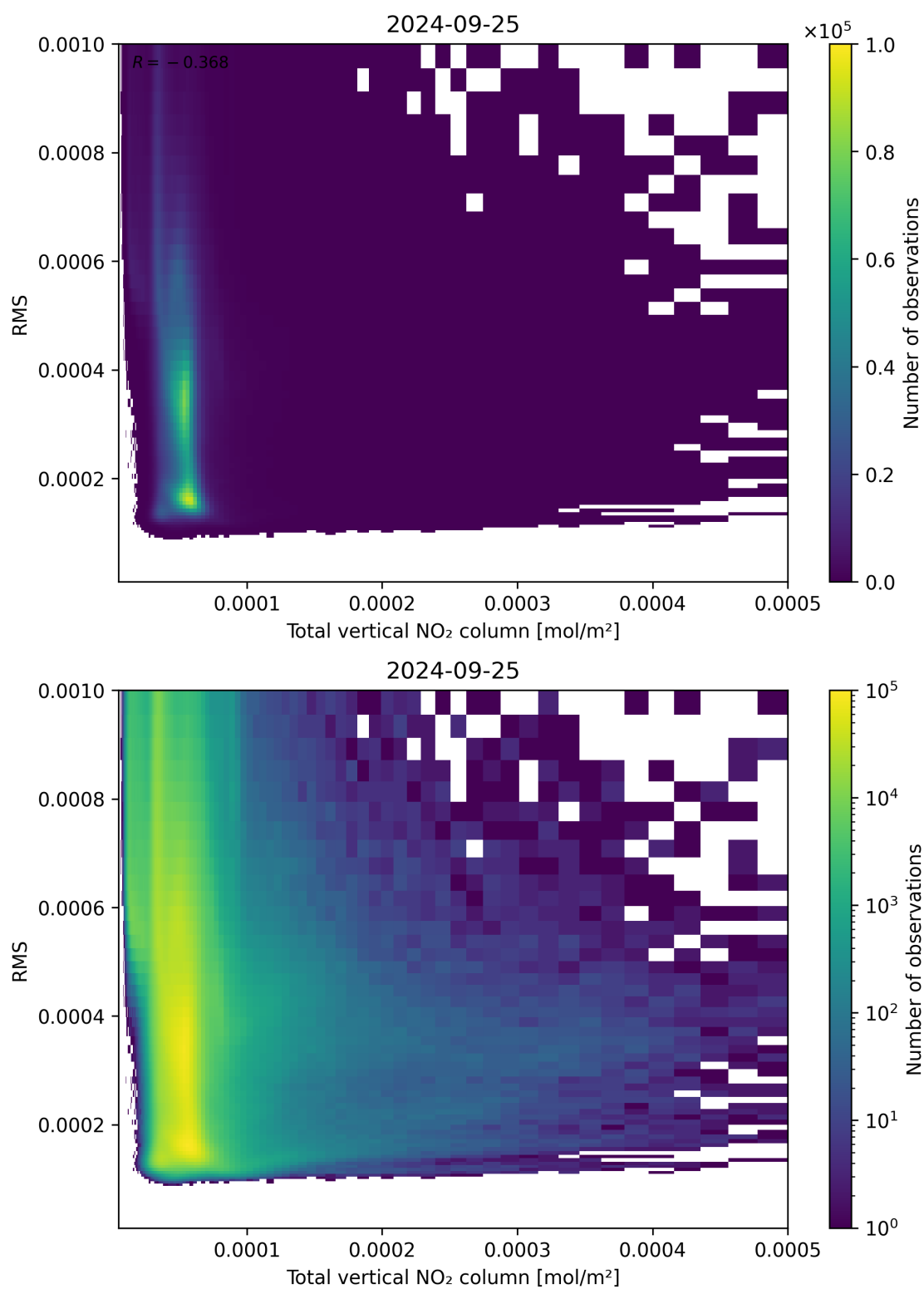
Figure 120: Scatter density plot of “Total vertical NO 2 column” against “RMS” for 2024-09-24 to 2024-09-26.
