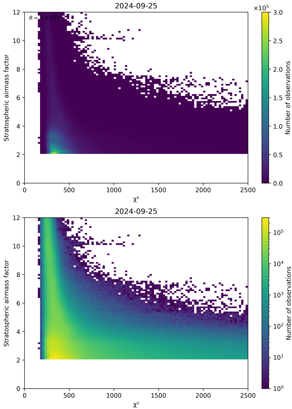
Figure 81: Scatter density plot of “ \chi^2 ” against “Stratospheric airmass factor” for 2024-09-24 to 2024-09-26.
