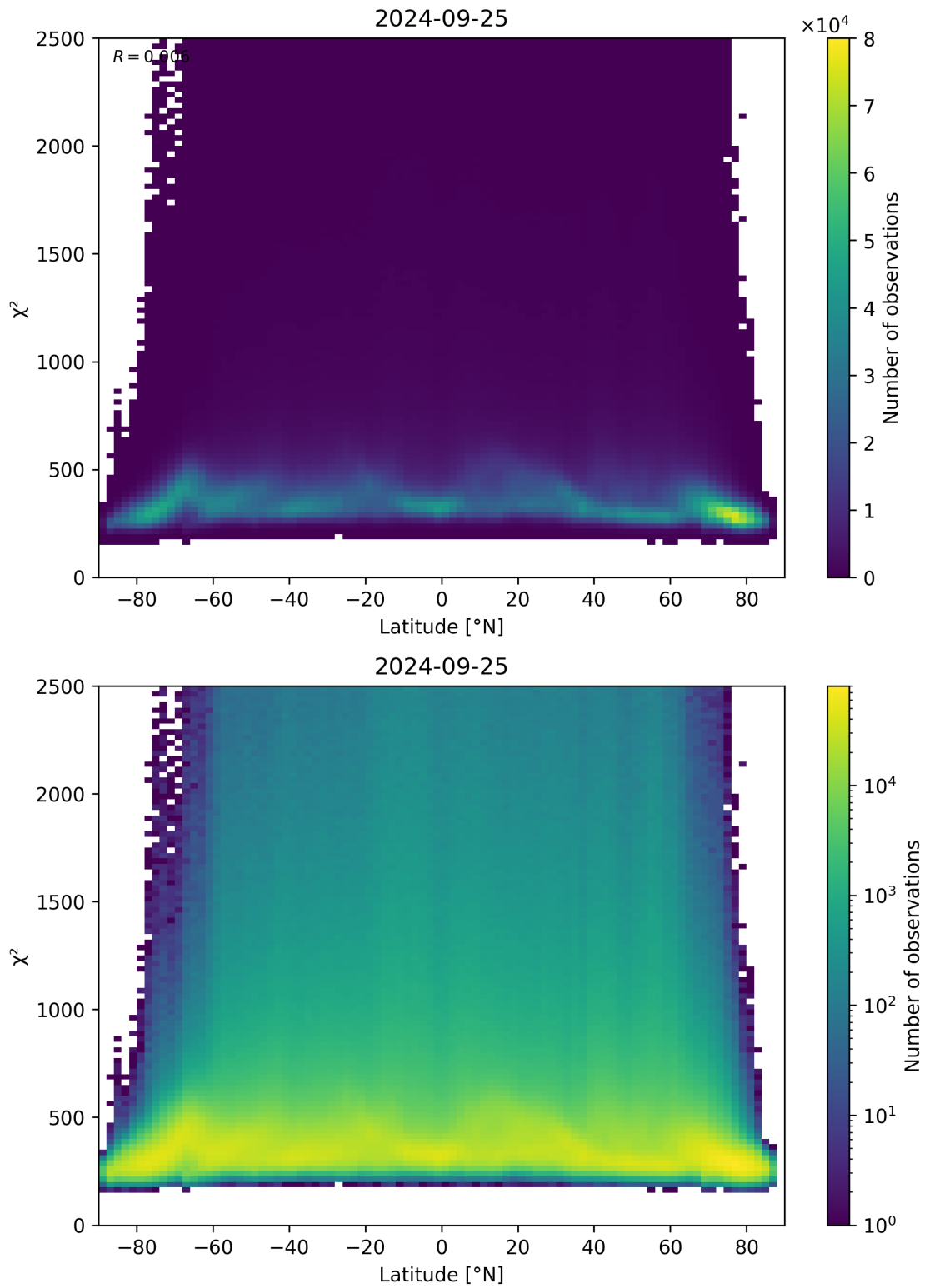
Figure 86: Scatter density plot of “Latitude” against “ \chi^2 ” for 2024-09-24 to 2024-09-26.
