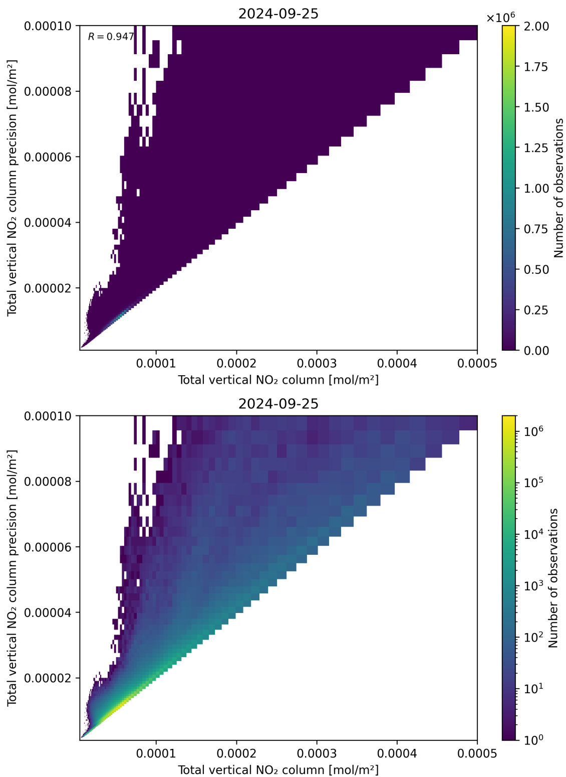
Figure 114: Scatter density plot of “Total vertical NO 2 column” against “Total vertical NO 2 column precision” for 2024-09-24 to 2024-09-26.
