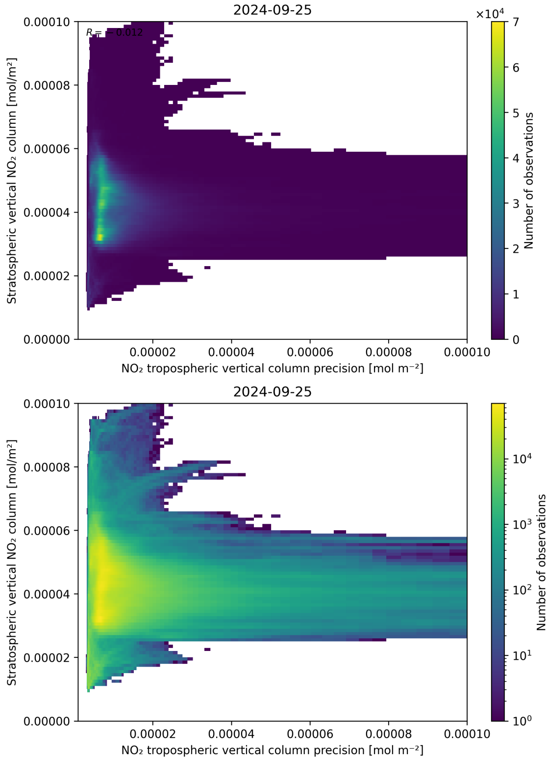
Figure 135: Scatter density plot of “NO 2 tropospheric vertical column precision” against “Stratospheric vertical NO 2 column” for 2024-09-24 to 2024-09-26.
