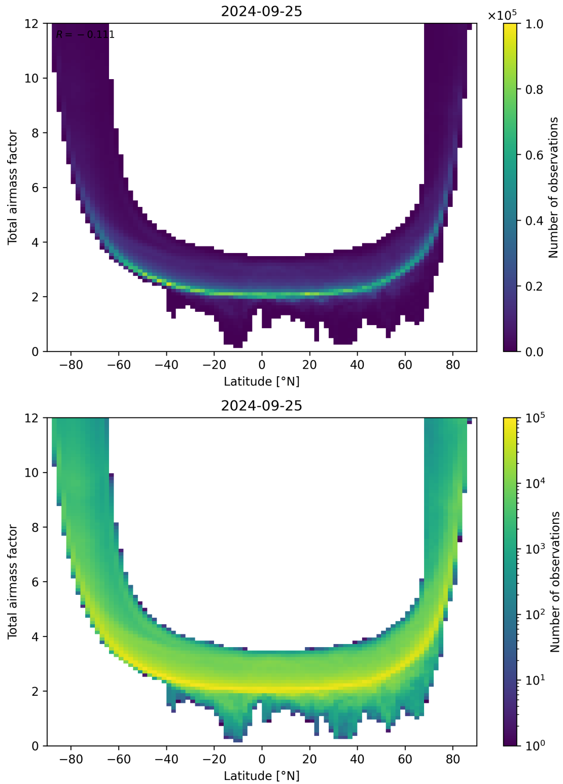
Figure 84: Scatter density plot of “Latitude” against “Total airmass factor” for 2024-09-24 to 2024-09-26.
