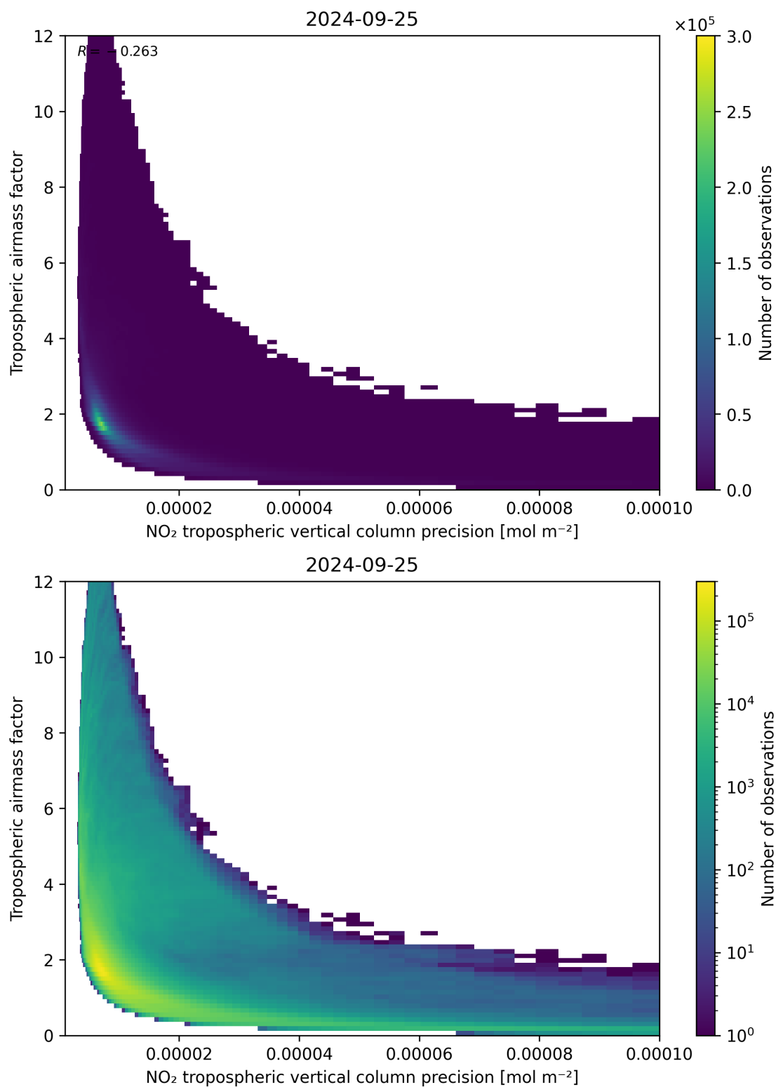
Figure 133: Scatter density plot of “NO 2 tropospheric vertical column precision” against “Tropospheric airmass factor” for 2024-09-24 to 2024-09-26.
