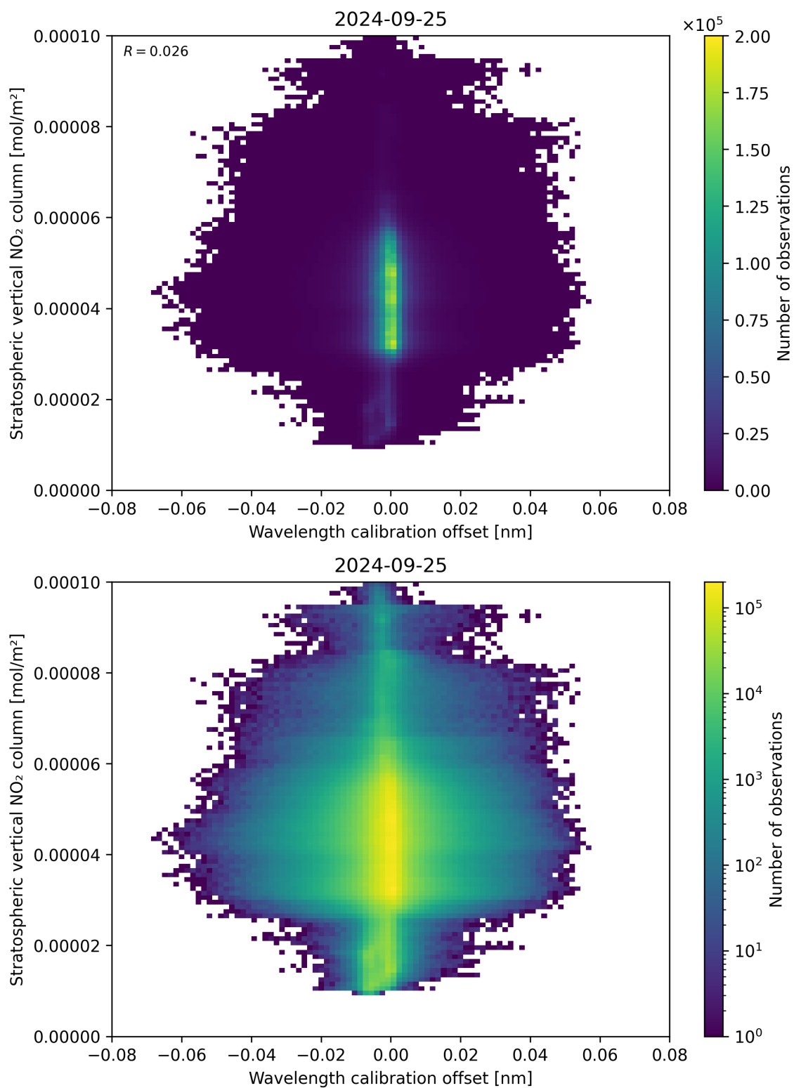
Figure 176: Scatter density plot of “Wavelength calibration offset” against “Stratospheric vertical NO 2 column” for 2024-09-24 to 2024-09-26.
