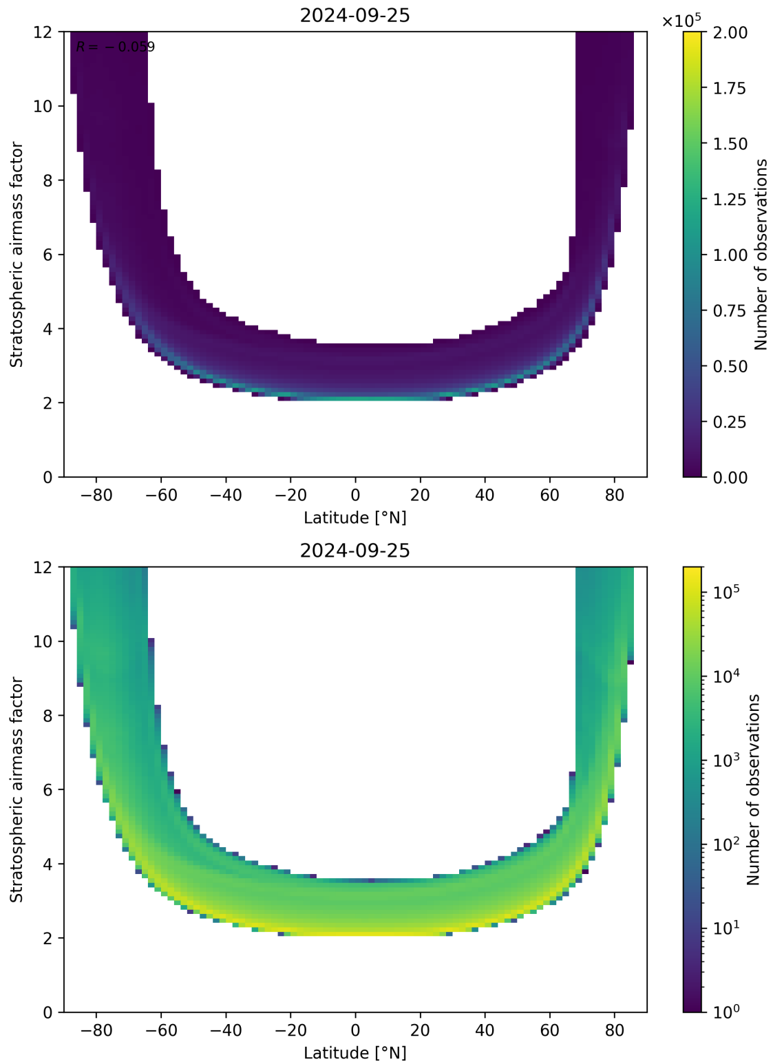
Figure 83: Scatter density plot of “Latitude” against “Stratospheric airmass factor” for 2024-09-24 to 2024-09-26.
