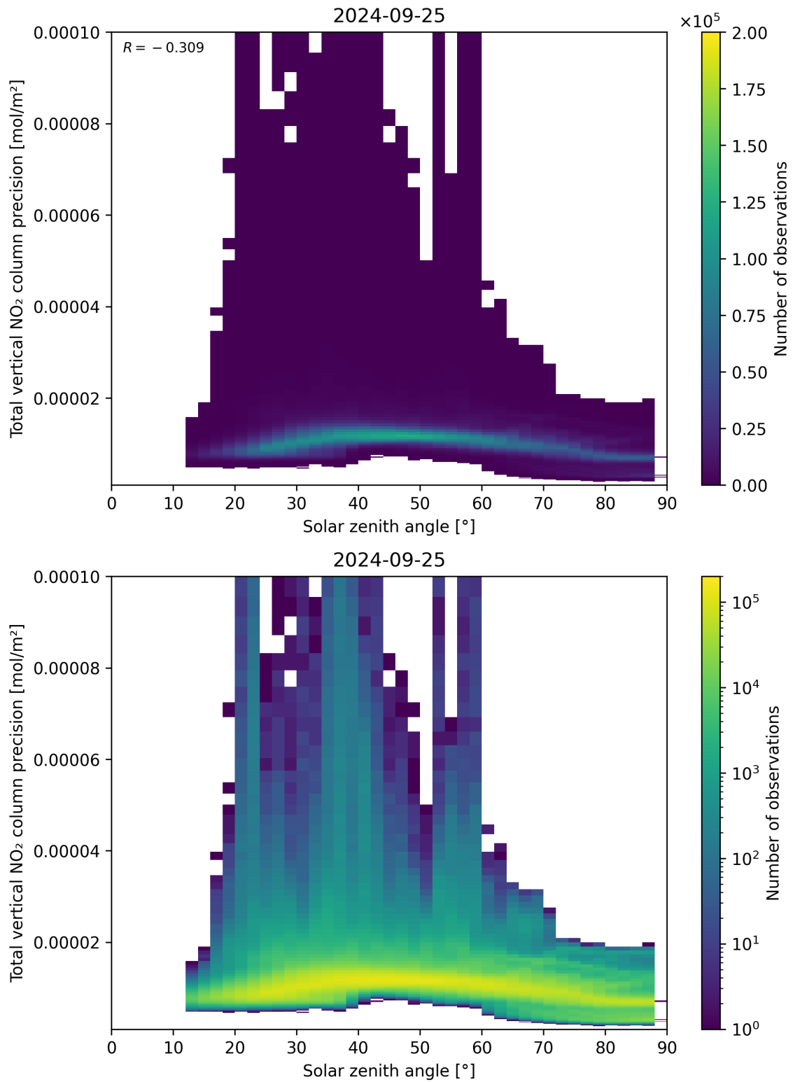
Figure 154: Scatter density plot of “Solar zenith angle” against “Total vertical NO 2 column precision” for 2024-09-24 to 2024-09-26.
