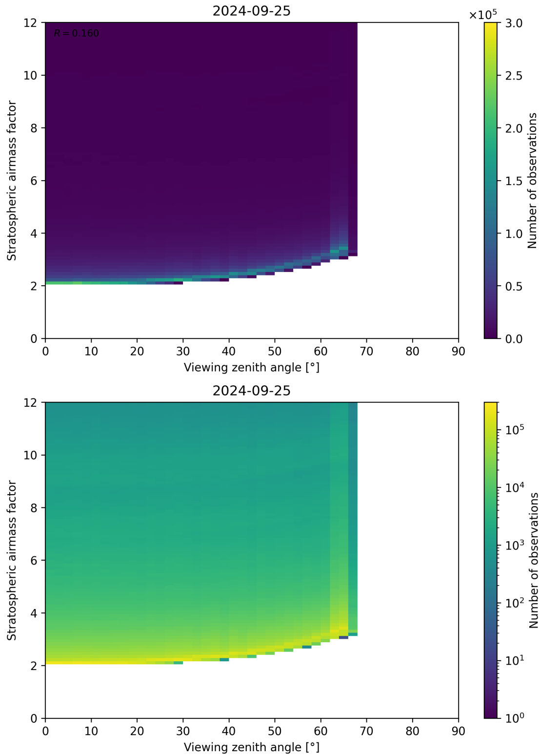
Figure 159: Scatter density plot of “Viewing zenith angle” against “Stratospheric airmass factor” for 2024-09-24 to 2024-09-26.
