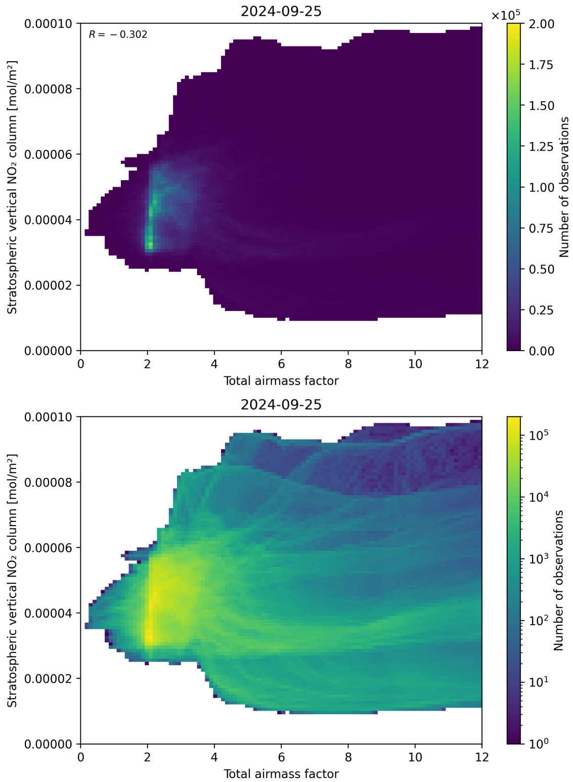
Figure 64: Scatter density plot of “Total airmass factor” against “Stratospheric vertical NO 2 column” for 2024-09-24 to 2024-09-26.
