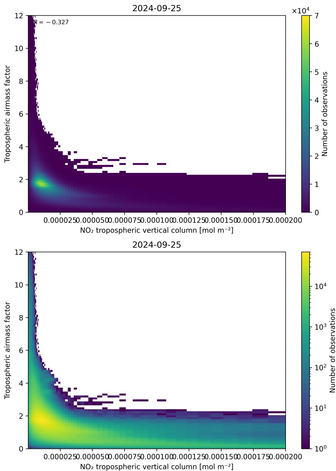
Figure 123: Scatter density plot of “NO 2 tropospheric vertical column” against “Tropospheric air mass factor” for 2024-09-24 to 2024-09-26.
