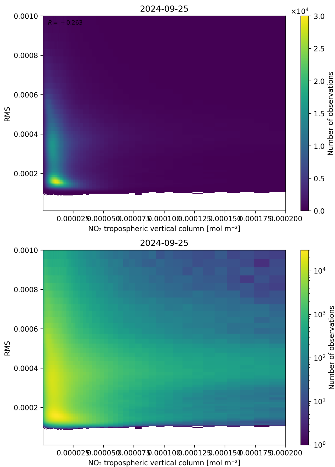
Figure 142: Scatter density plot of “NO 2 tropospheric vertical column” against “RMS” for 2024-09-24 to 2024-09-26.
