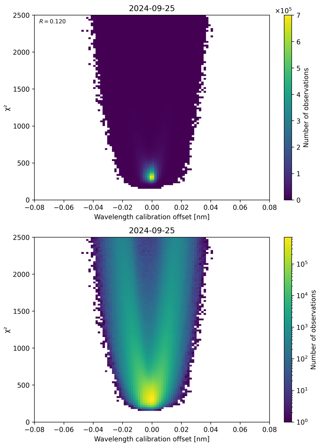
Figure 175: Scatter density plot of “Wavelength calibration offset” against “ \chi^2 ” for 2024-09-24 to 2024-09-26.
