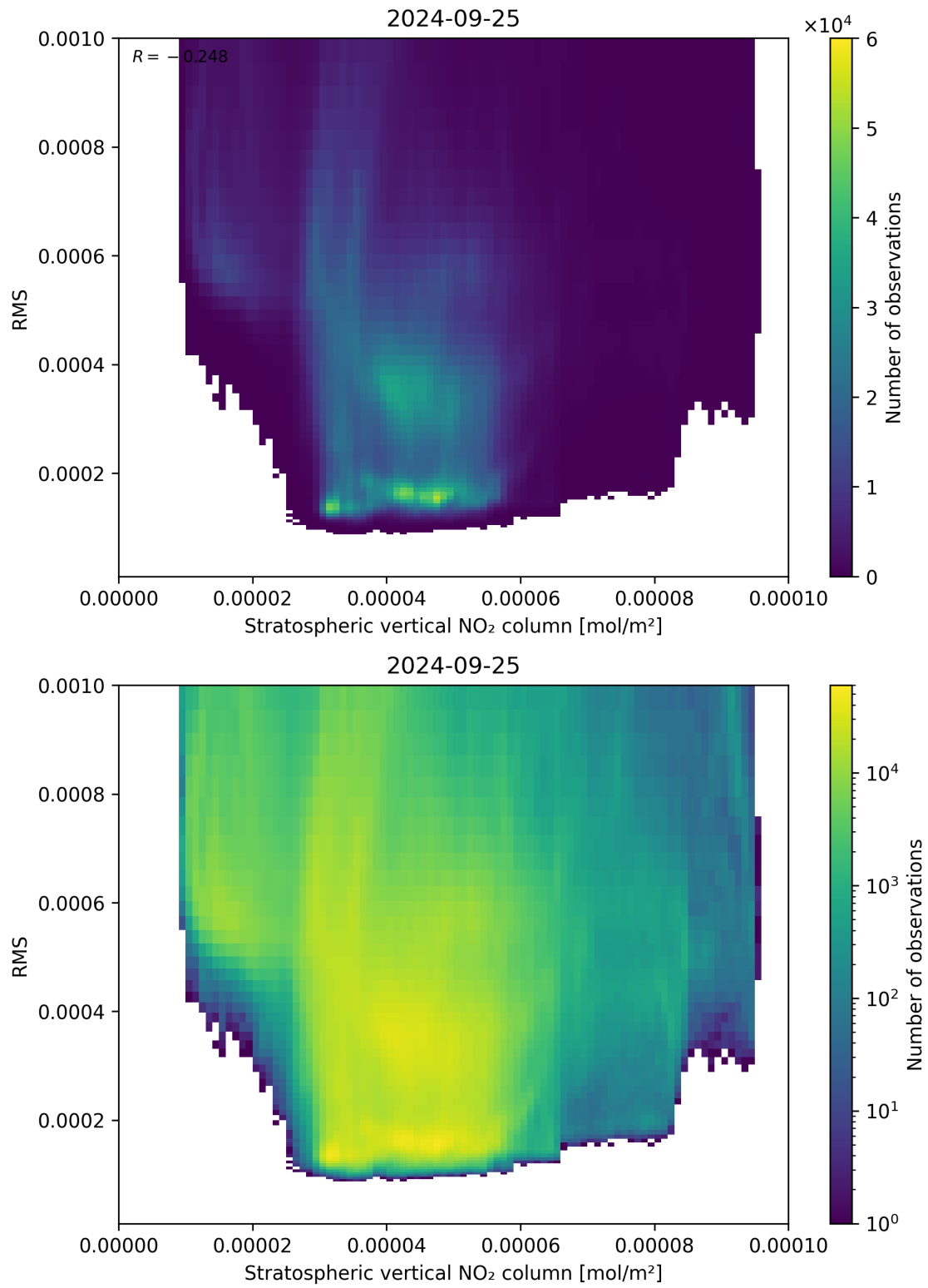
Figure 102: Scatter density plot of “Stratospheric vertical NO 2 column” against “RMS” for 2024-09-24 to 2024-09-26.
