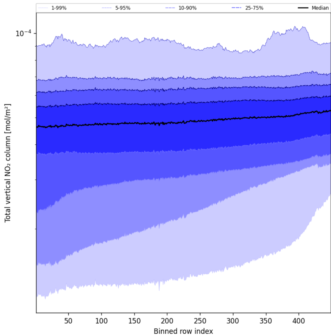
Figure 55: Along track statistics of “Total vertical NO 2 column” for 2024-09-24 to 2024-09-26
