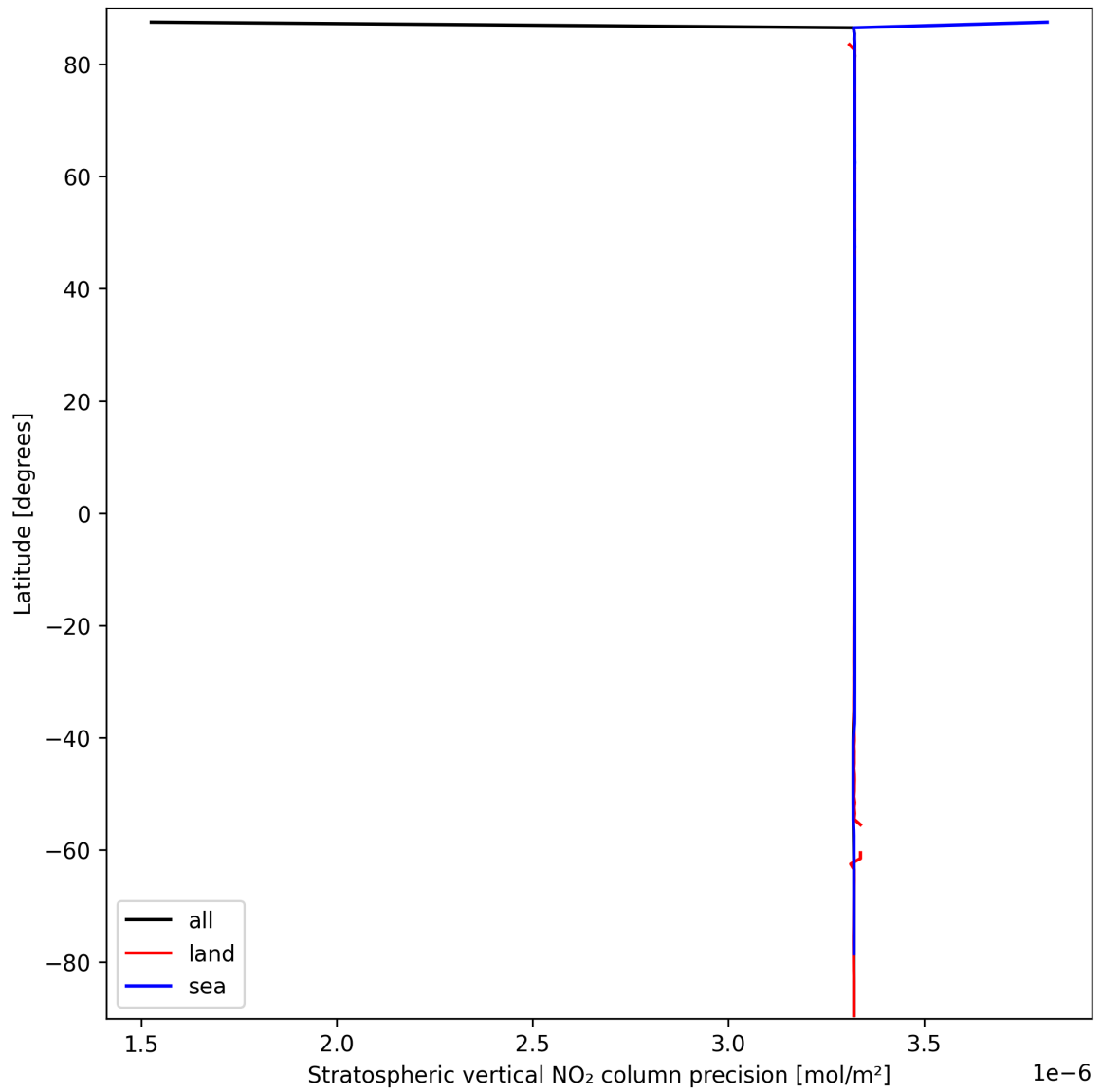
Figure 20: Zonal average of “Stratospheric vertical NO 2 column precision” for 2024-09-24 to 2024-09-26.
