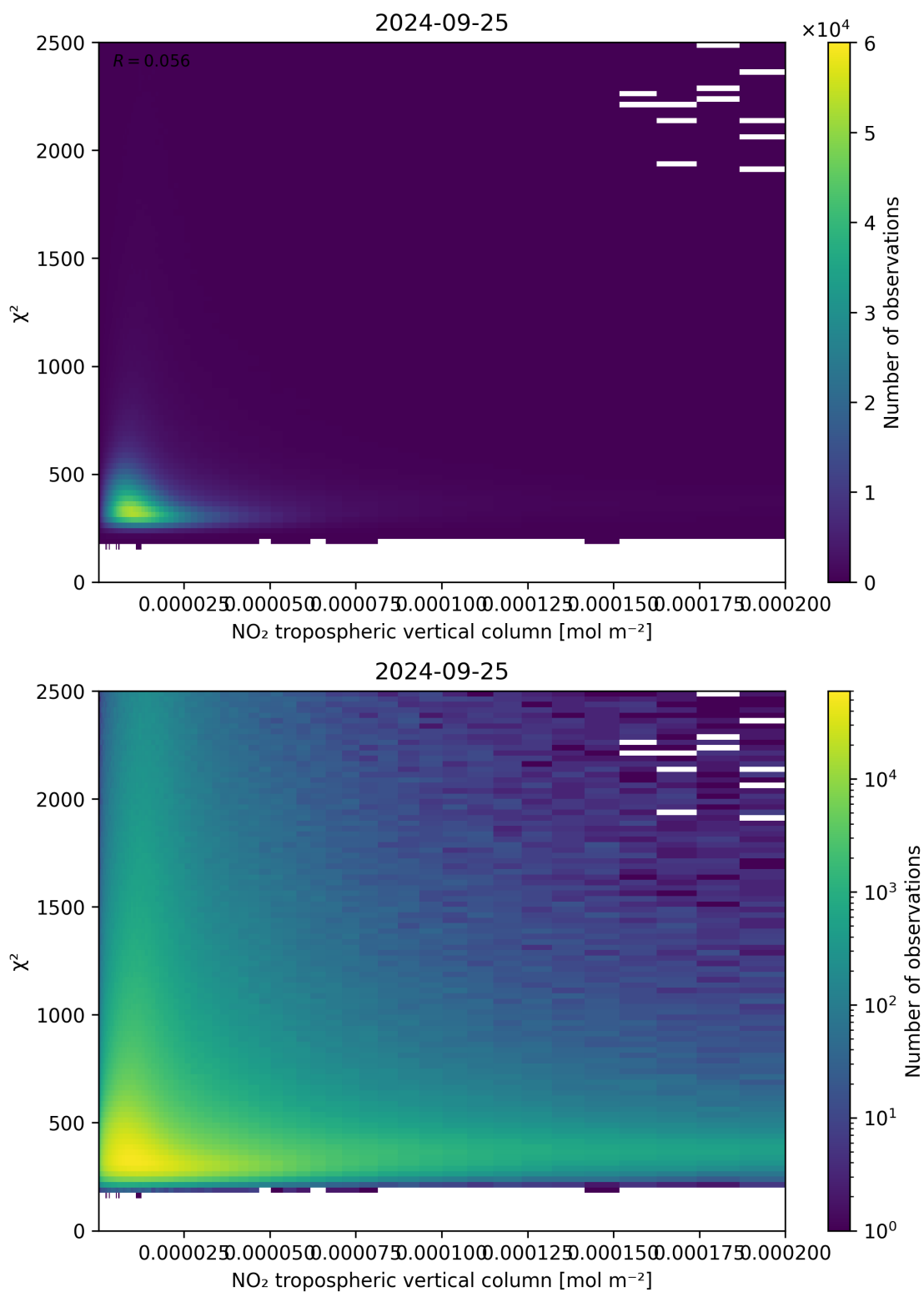
Figure 124: Scatter density plot of “NO 2 tropospheric vertical column” against “ \chi^2 ” for 2024-09-24 to 2024-09-26.
