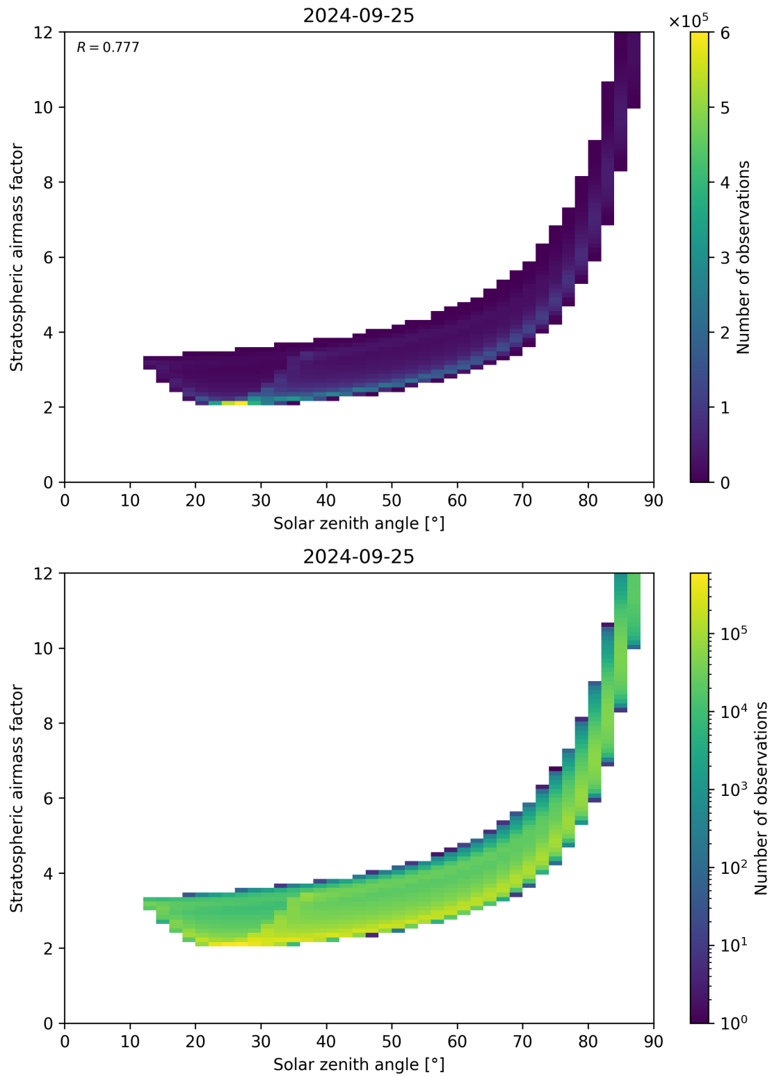
Figure 145: Scatter density plot of “Solar zenith angle” against “Stratospheric airmass factor” for 2024-09-24 to 2024-09-26.
