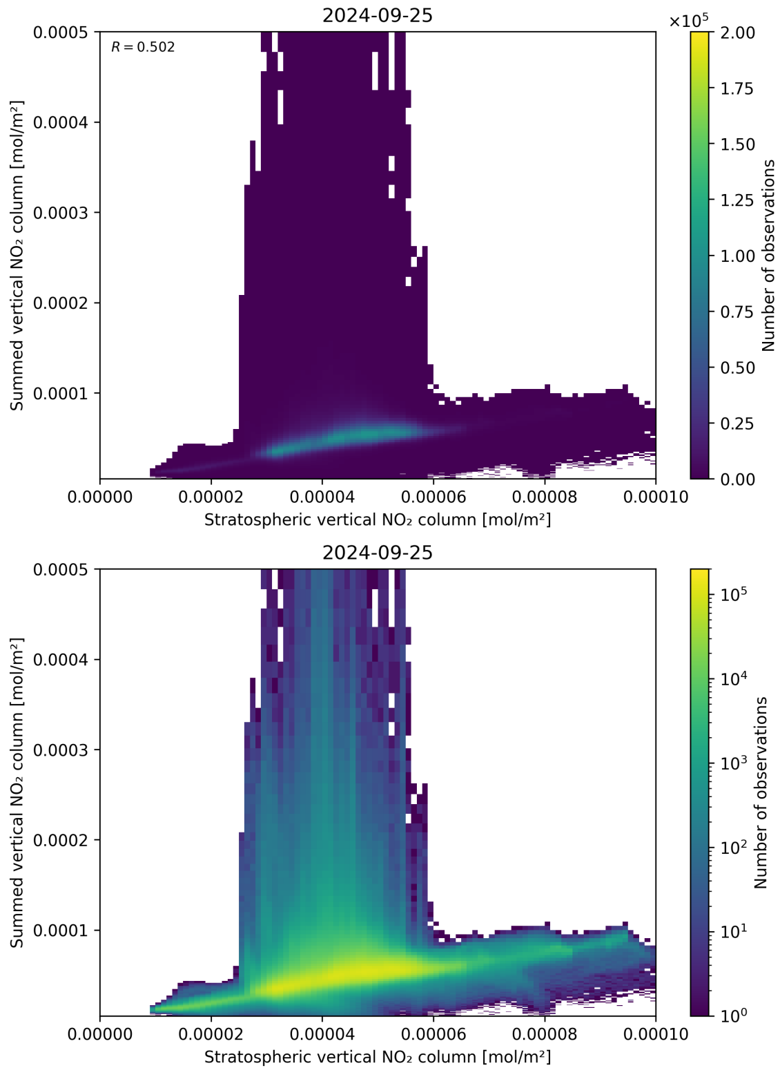
Figure 98: Scatter density plot of “Stratospheric vertical NO 2 column” against “Summed vertical NO 2 column” for 2024-09-24 to 2024-09-26.
