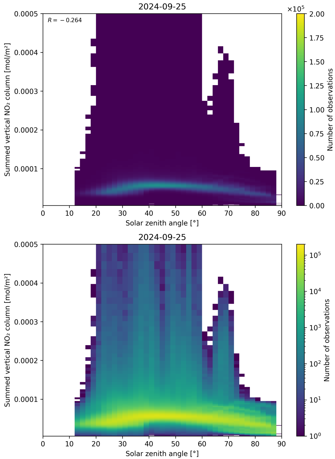
Figure 151: Scatter density plot of “Solar zenith angle” against “Summed vertical NO 2 column” for 2024-09-24 to 2024-09-26.
