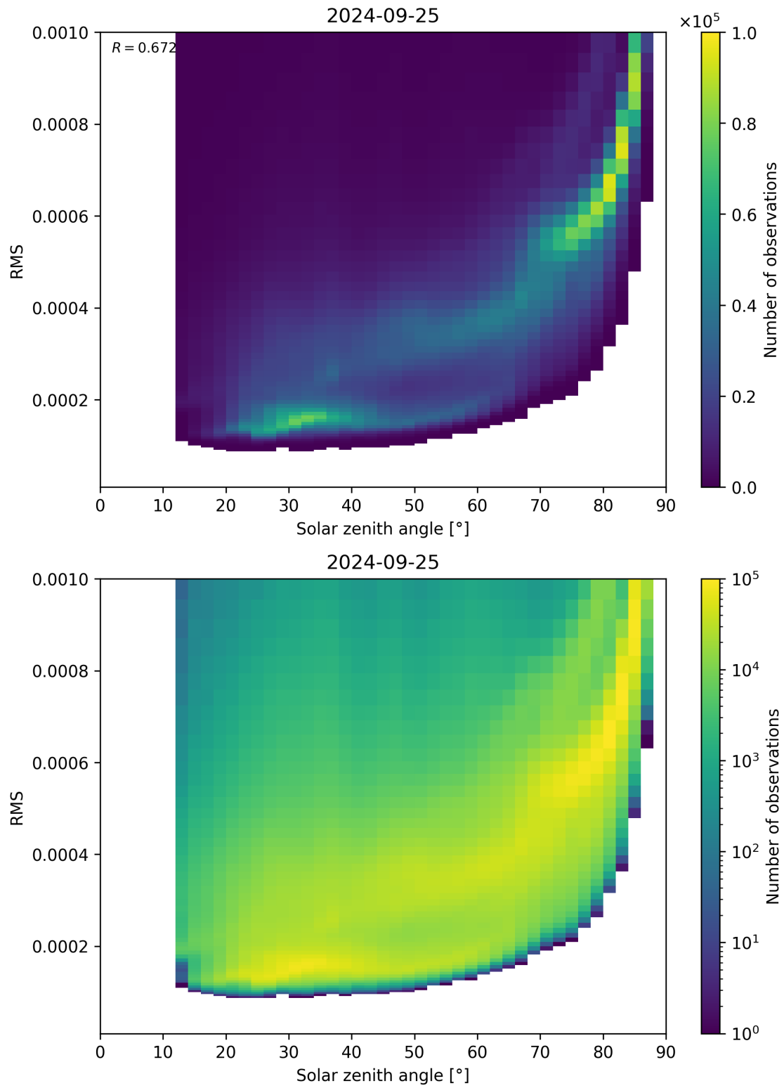
Figure 157: Scatter density plot of “Solar zenith angle” against “RMS” for 2024-09-24 to 2024-09-26.
