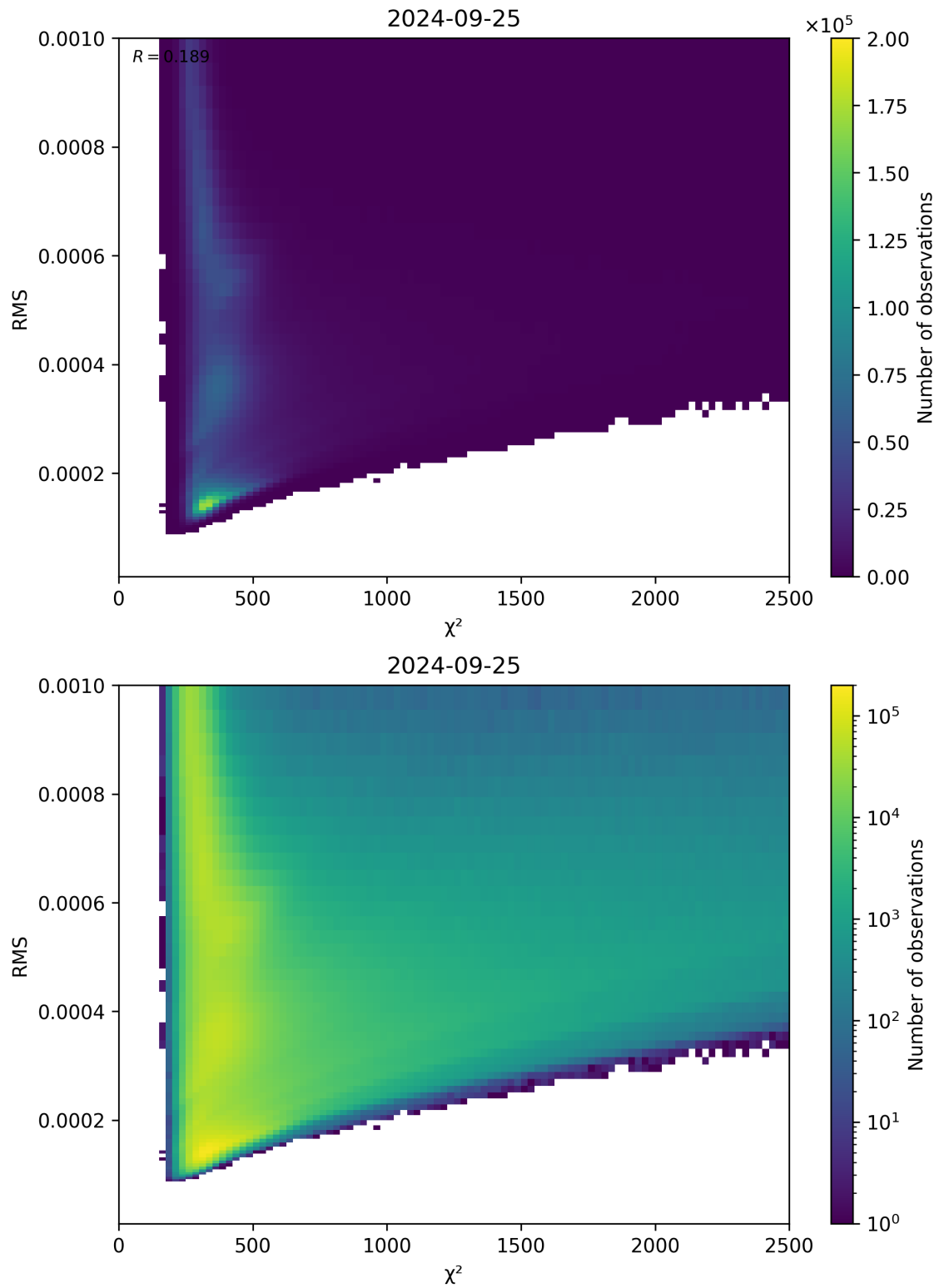
Figure 82: Scatter density plot of “ \chi^2 ” against “RMS” for 2024-09-24 to 2024-09-26.
