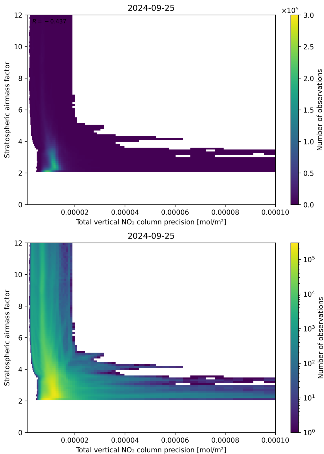
Figure 115: Scatter density plot of “Total vertical NO 2 column precision” against “Stratospheric airmass factor” for 2024-09-24 to 2024-09-26.
