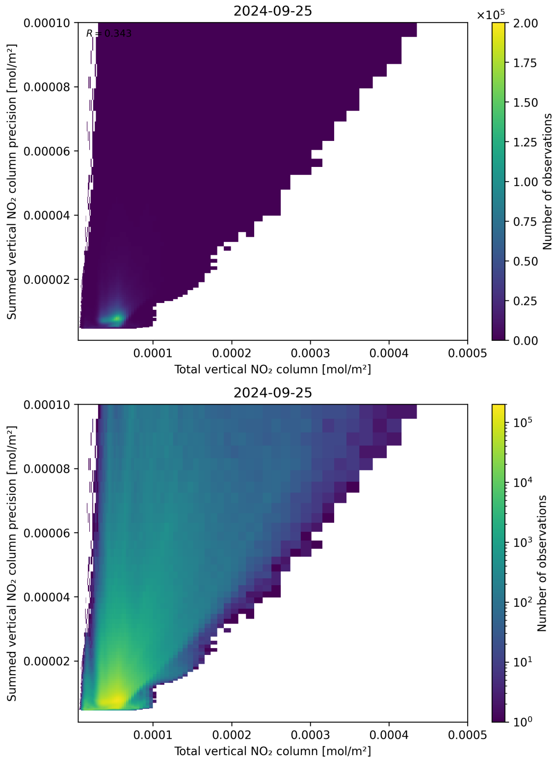
Figure 113: Scatter density plot of “Total vertical NO 2 column” against “Summed vertical NO 2 column precision” for 2024-09-24 to 2024-09-26.
