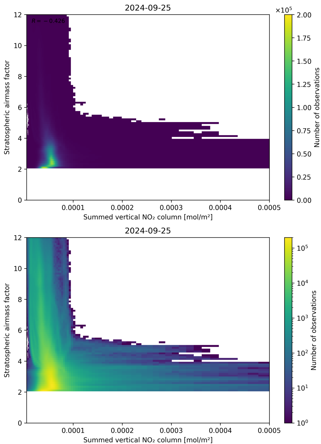
Figure 103: Scatter density plot of “Summed vertical NO 2 column” against “Stratospheric airmass factor” for 2024-09-24 to 2024-09-26.
