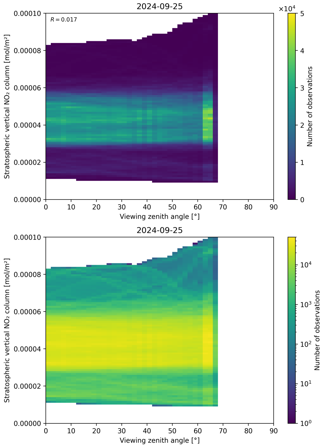
Figure 164: Scatter density plot of “Viewing zenith angle” against “Stratospheric vertical NO 2 column” for 2024-09-24 to 2024-09-26.
