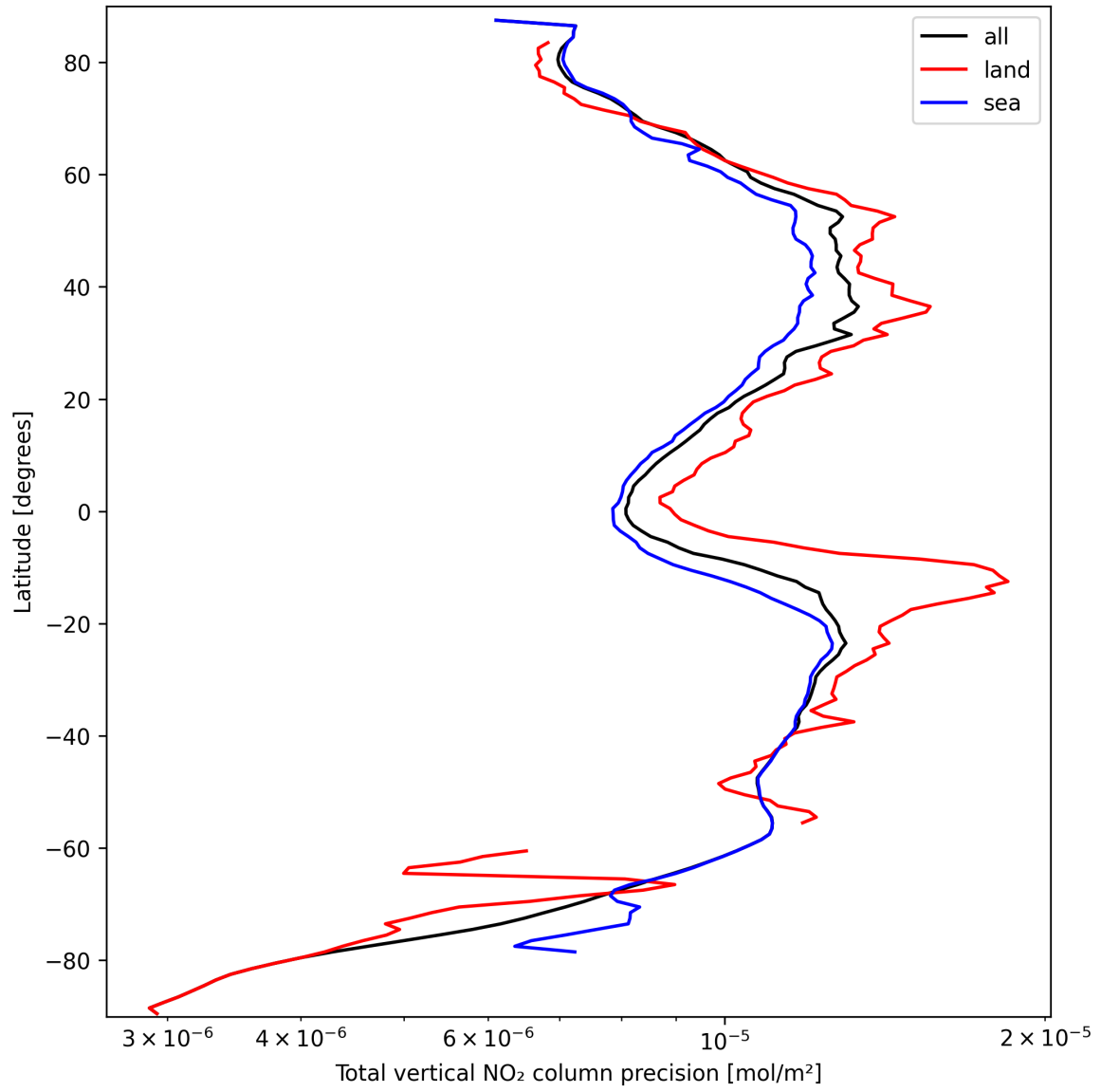
Figure 22: Zonal average of “Total vertical NO 2 column precision” for 2024-09-24 to 2024-09-26.
