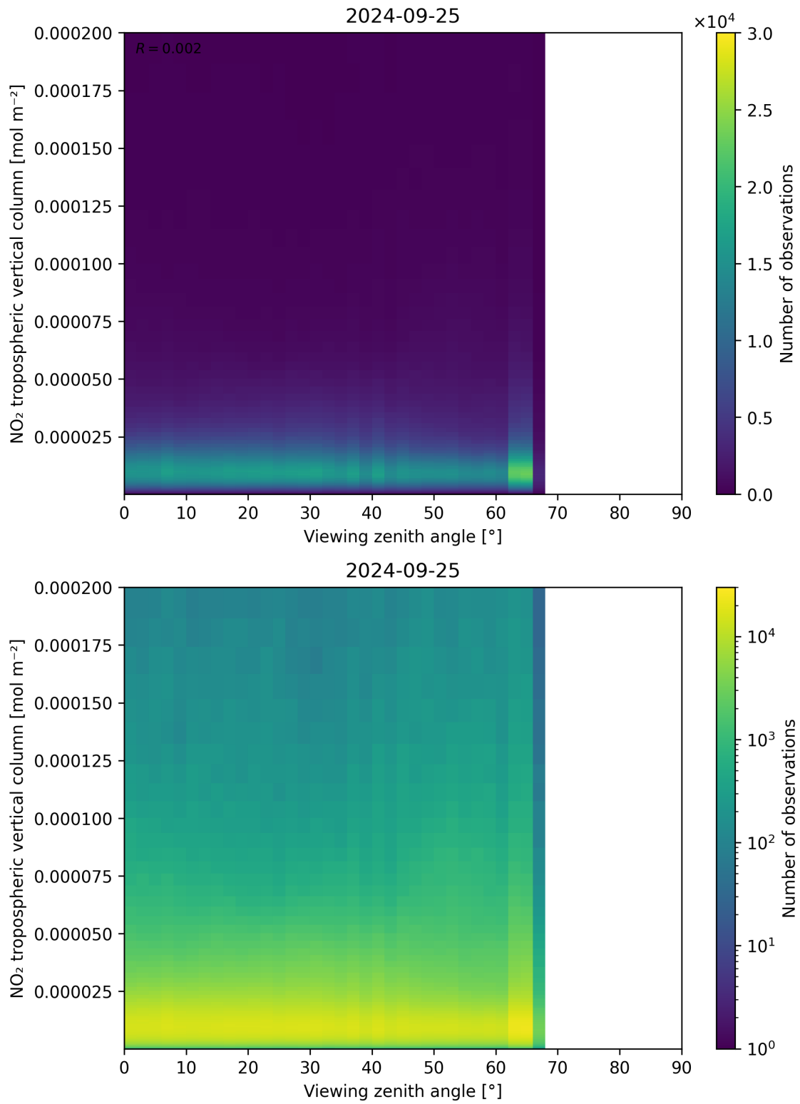
Figure 169: Scatter density plot of “Viewing zenith angle” against “NO 2 tropospheric vertical column” for 2024-09-24 to 2024-09-26.
