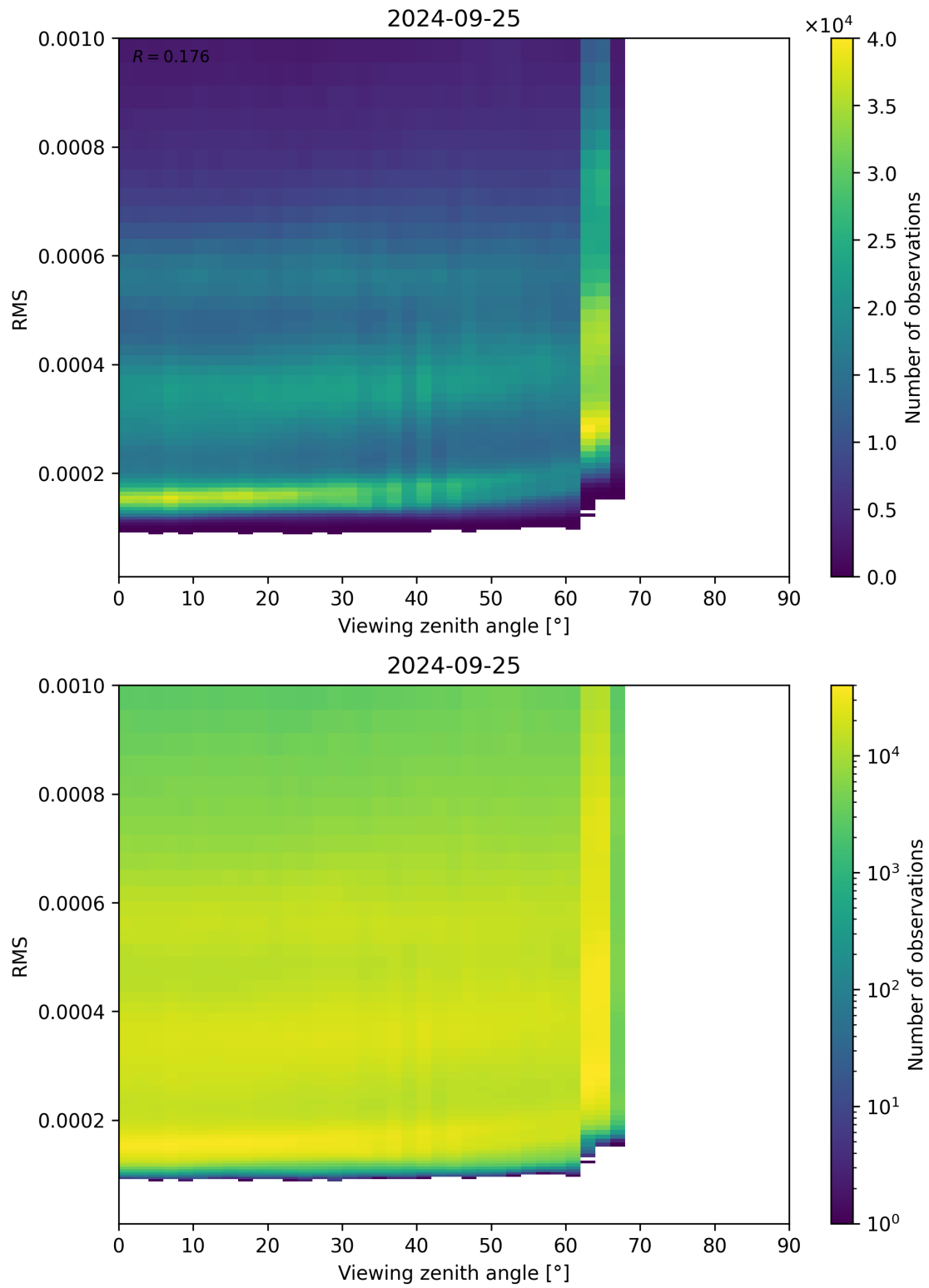
Figure 171: Scatter density plot of “Viewing zenith angle” against “RMS” for 2024-09-24 to 2024-09-26.
