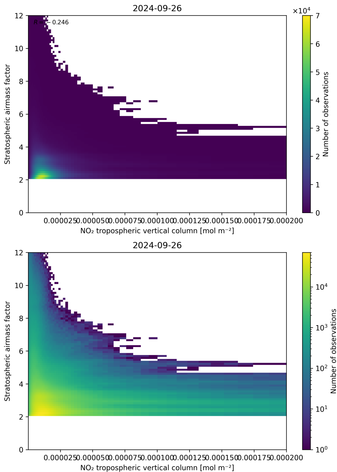
Figure 121: Scatter density plot of “NO 2 tropospheric vertical column” against “Stratospheric air mass factor” for 2024-09-25 to 2024-09-27.
