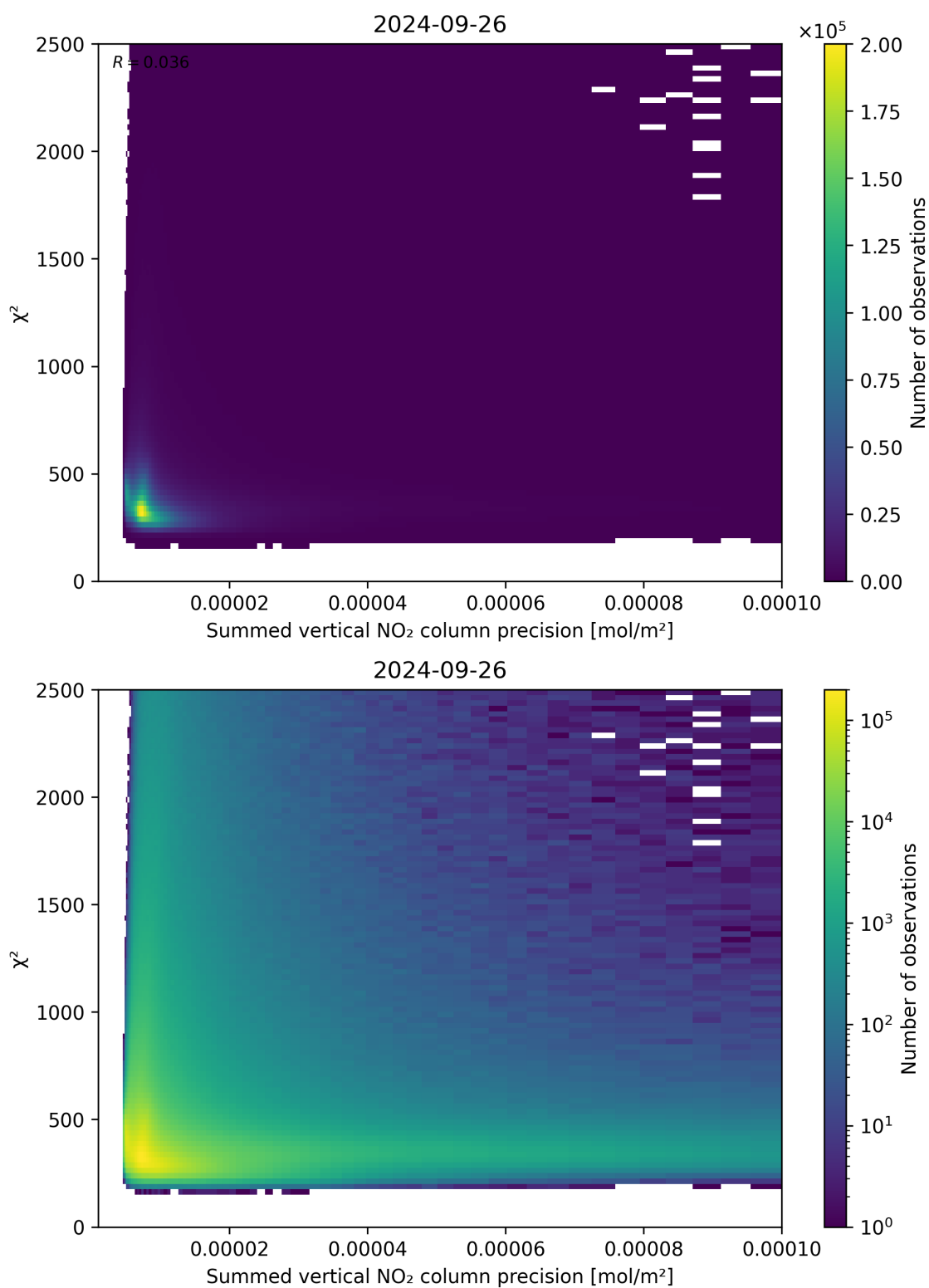
Figure 107: Scatter density plot of “Summed vertical NO 2 column precision” against “ \chi^2 ” for 2024-09-25 to 2024-09-27.
