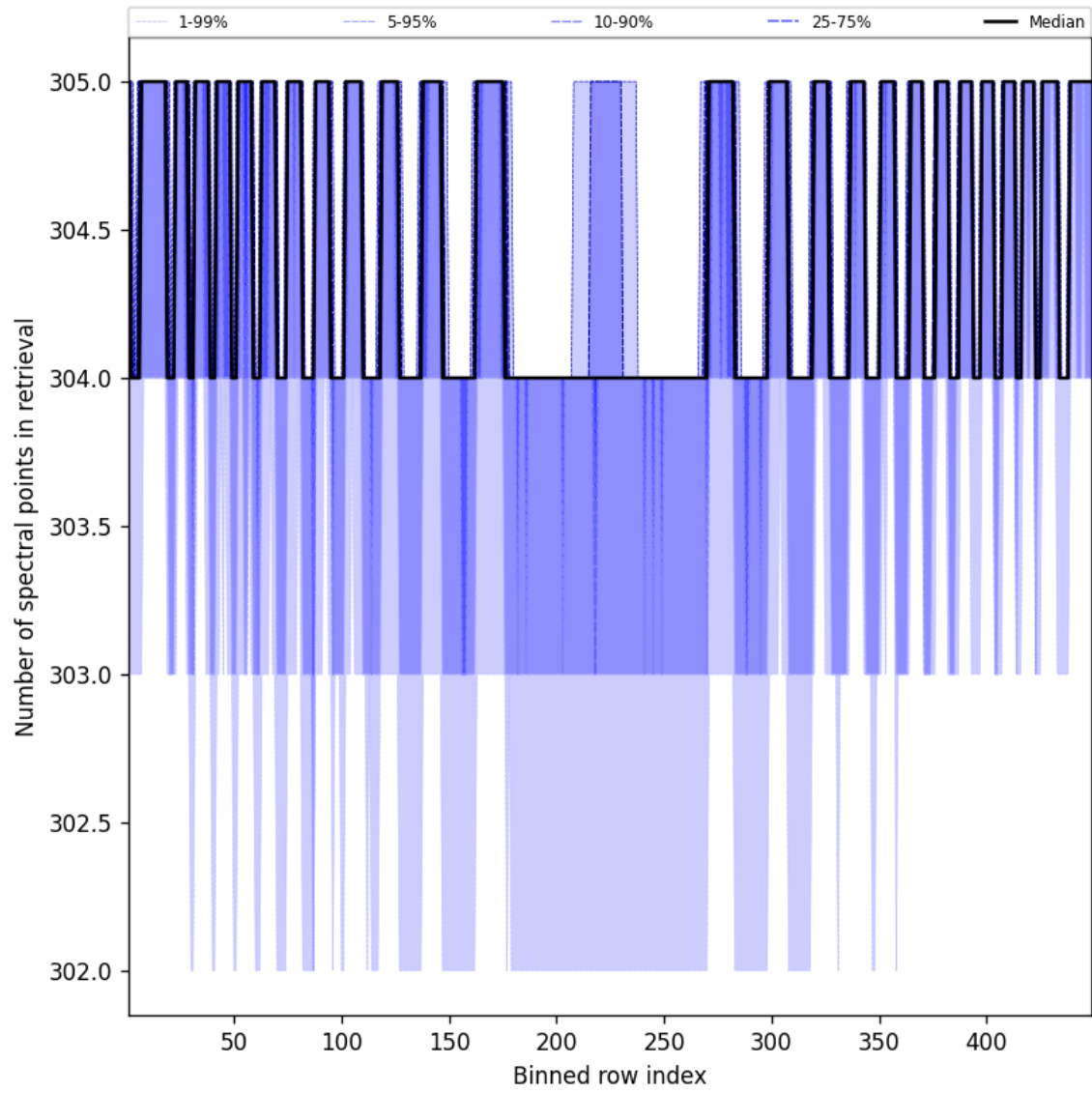
Figure 50: Along track statistics of “Number of spectral points in retrieval” for 2024-09-25 to 2024-09-27
