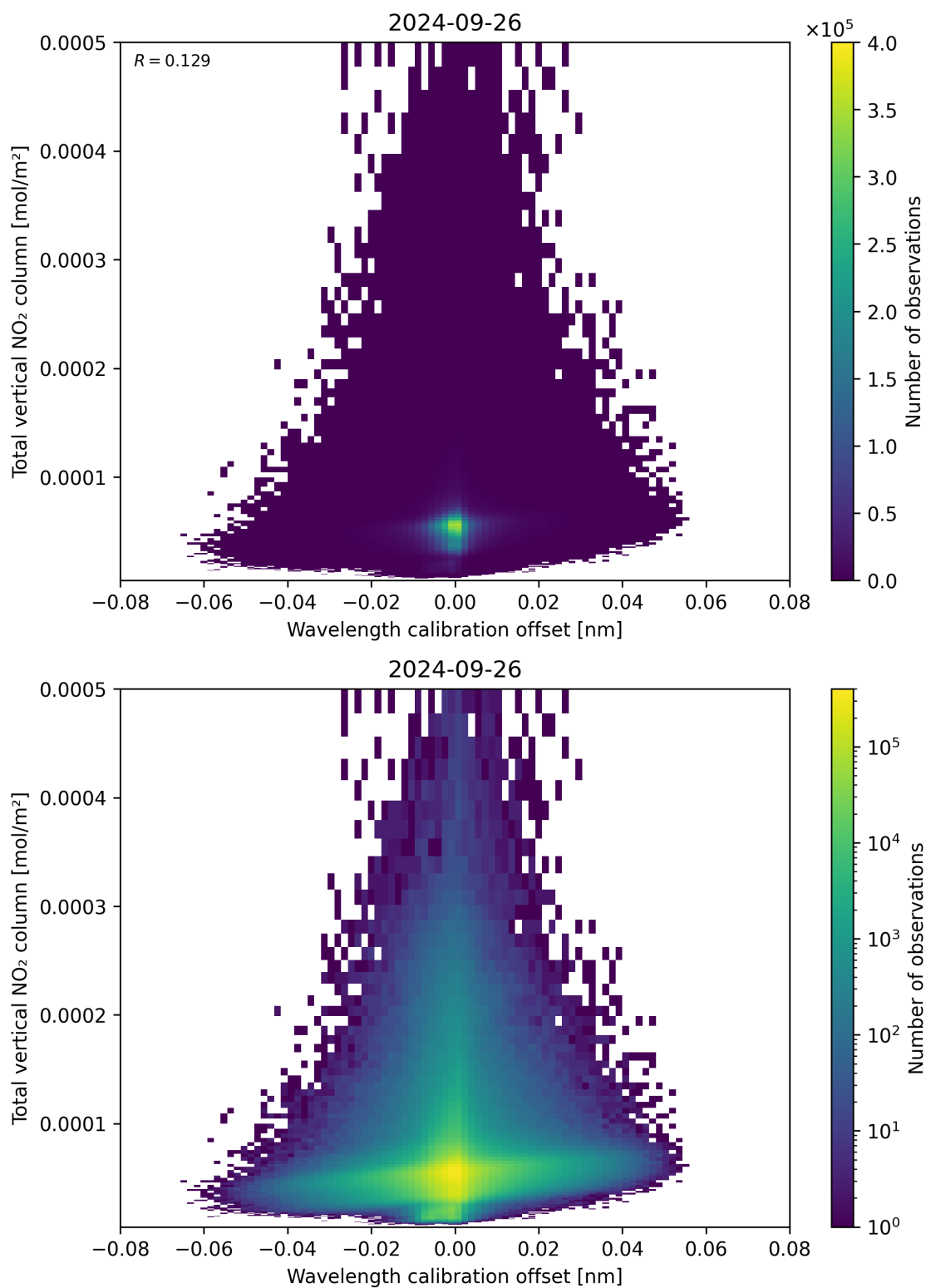
Figure 179: Scatter density plot of “Wavelength calibration offset” against “Total vertical NO 2 column” for 2024-09-25 to 2024-09-27.
