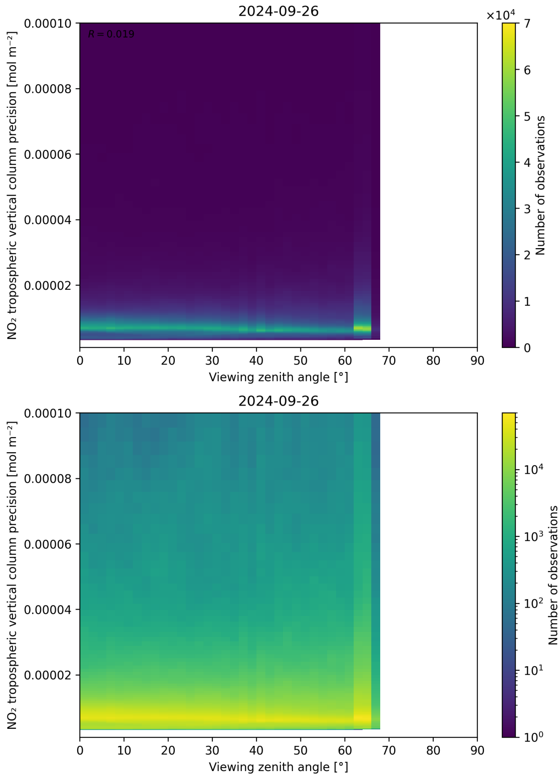
Figure 170: Scatter density plot of “Viewing zenith angle” against “NO 2 tropospheric vertical column precision” for 2024-09-25 to 2024-09-27.
