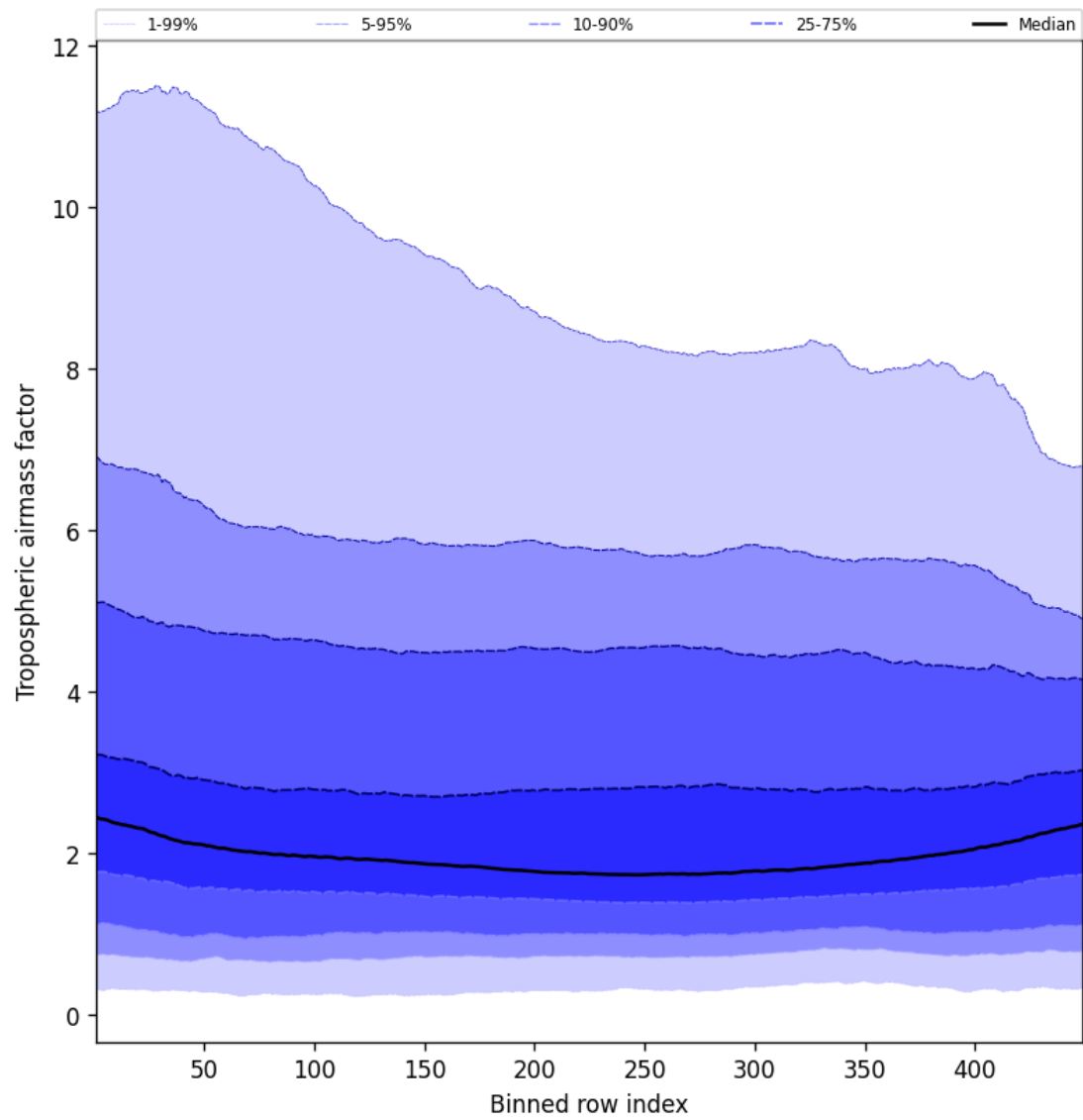
Figure 48: Along track statistics of “Tropospheric air mass factor” for 2024-09-25 to 2024-09-27
