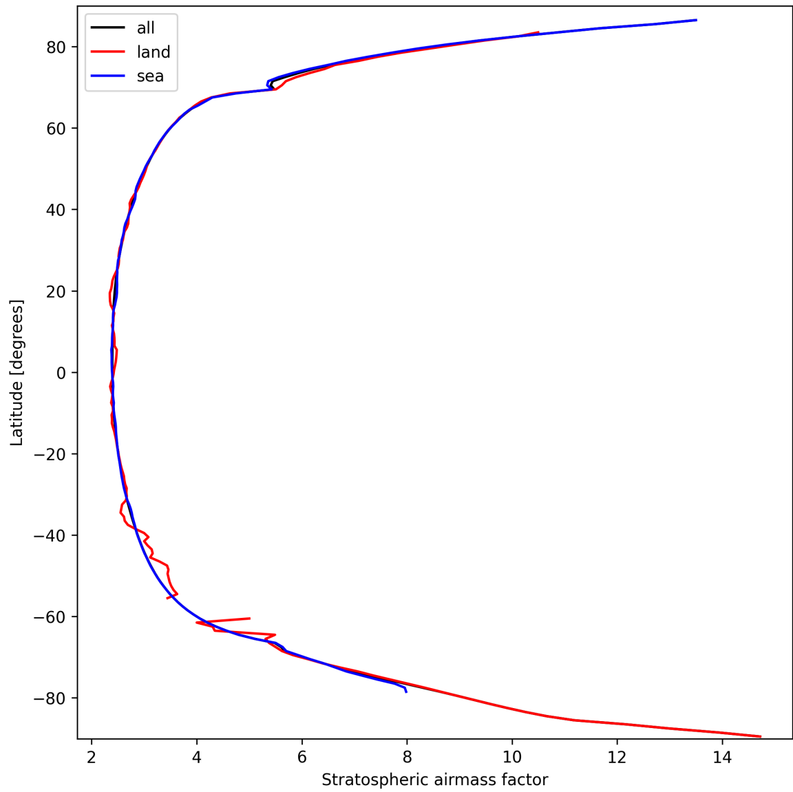
Figure 27: Zonal average of “Stratospheric air mass factor” for 2024-09-25 to 2024-09-27.
