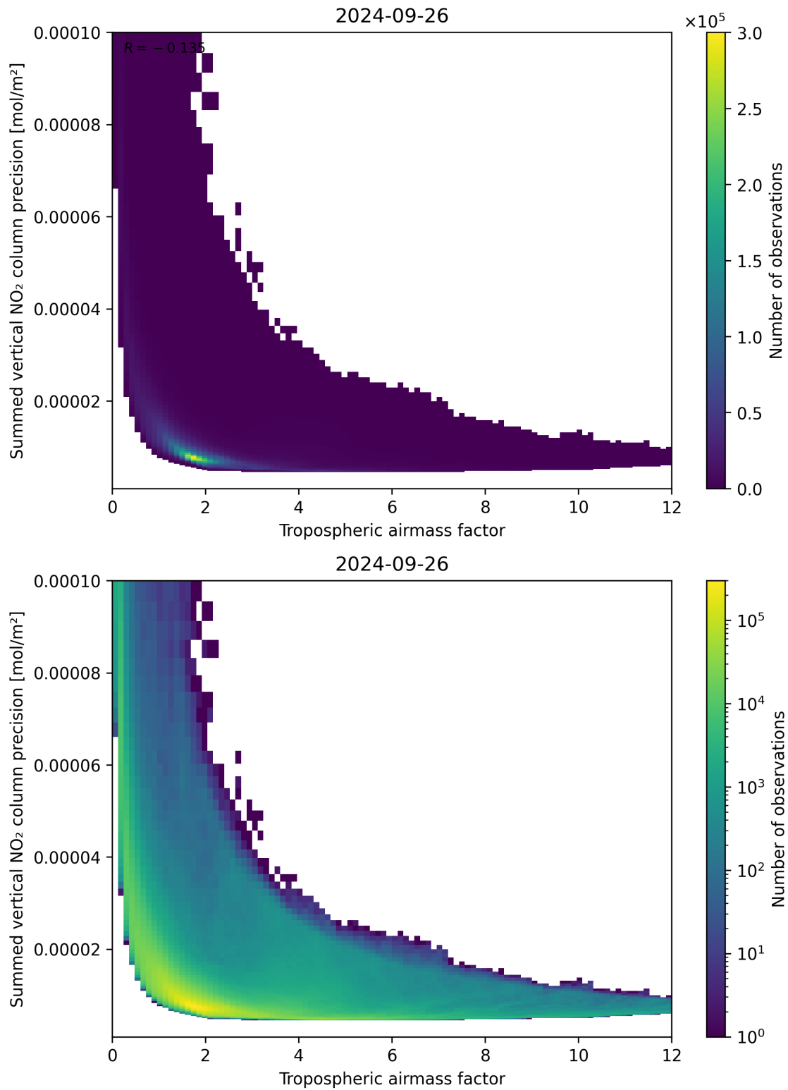
Figure 76: Scatter density plot of “Tropospheric airmass factor” against “Summed vertical NO 2 column precision” for 2024-09-25 to 2024-09-27.
