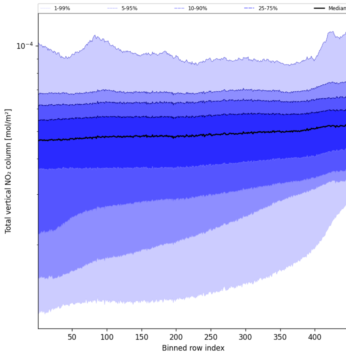
Figure 55: Along track statistics of “Total vertical NO 2 column” for 2024-09-25 to 2024-09-27
