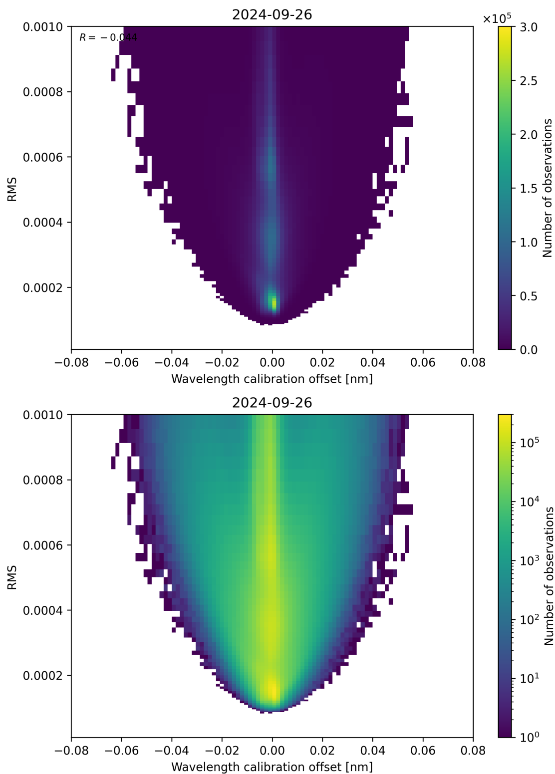
Figure 181: Scatter density plot of “Wavelength calibration offset” against “RMS” for 2024-09-25 to 2024-09-27.
