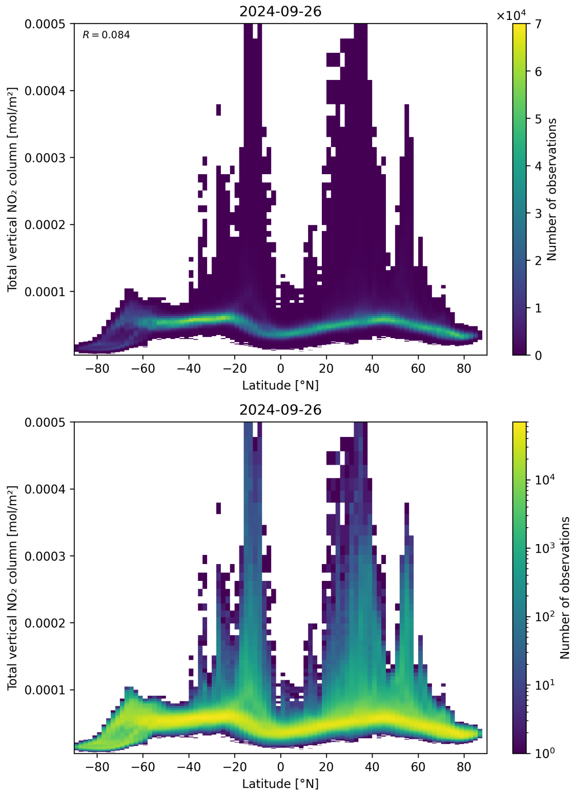
Figure 90: Scatter density plot of “Latitude” against “Total vertical NO 2 column” for 2024-09-25 to 2024-09-27.
