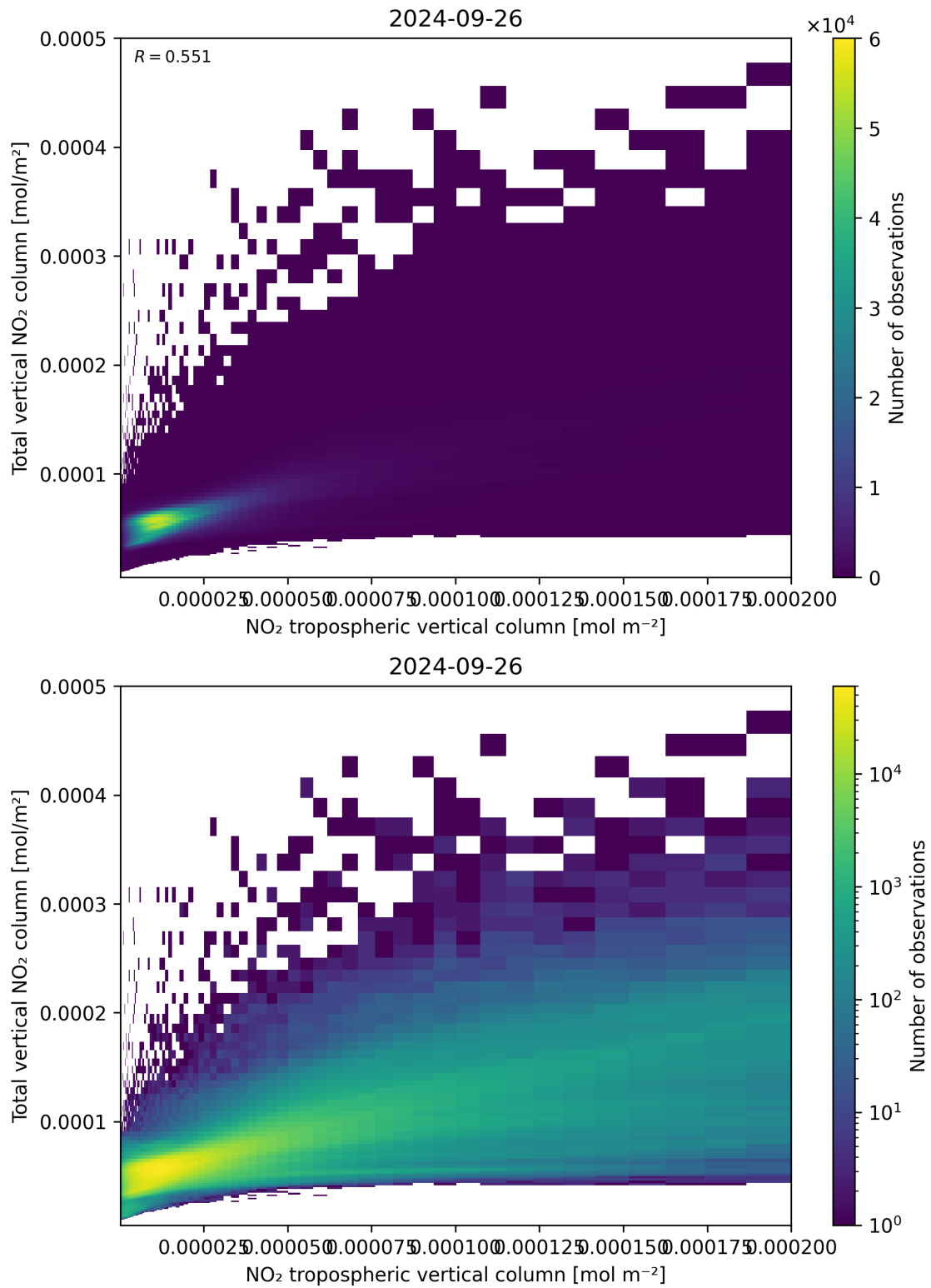
Figure 128: Scatter density plot of “NO 2 tropospheric vertical column” against “Total vertical NO 2 column” for 2024-09-25 to 2024-09-27.
