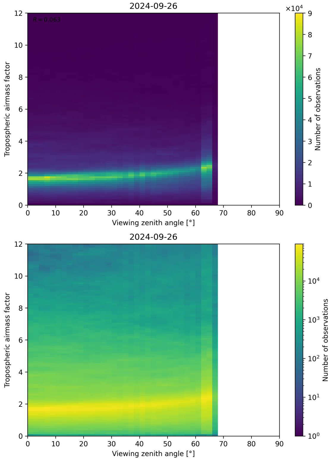
Figure 161: Scatter density plot of “Viewing zenith angle” against “Tropospheric airmass factor” for 2024-09-25 to 2024-09-27.
