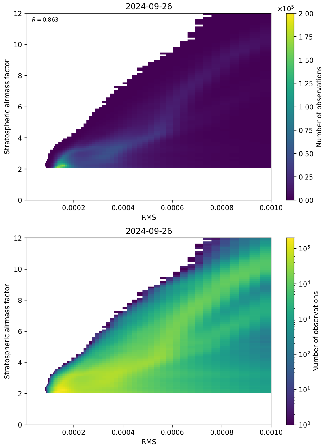
Figure 144: Scatter density plot of “RMS” against “Stratospheric airmass factor” for 2024-09-25 to 2024-09-27.
