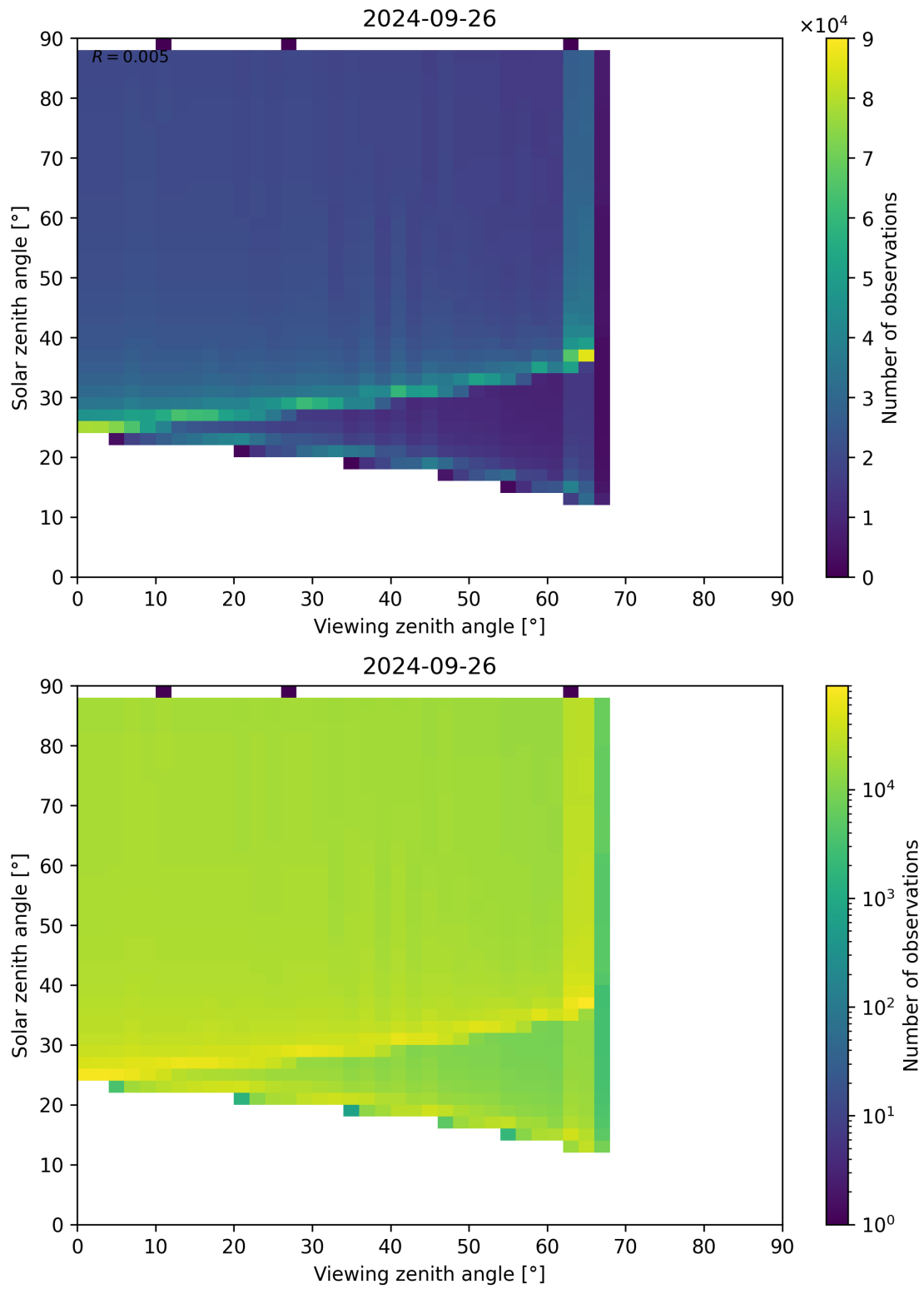
Figure 172: Scatter density plot of “Viewing zenith angle” against “Solar zenith angle” for 2024-09-25 to 2024-09-27.
