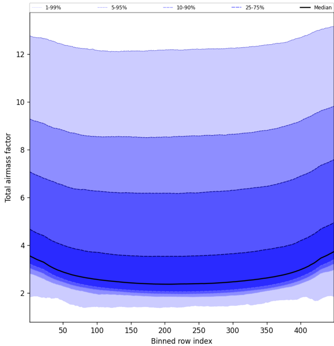
Figure 49: Along track statistics of “Total airmass factor” for 2024-09-25 to 2024-09-27
