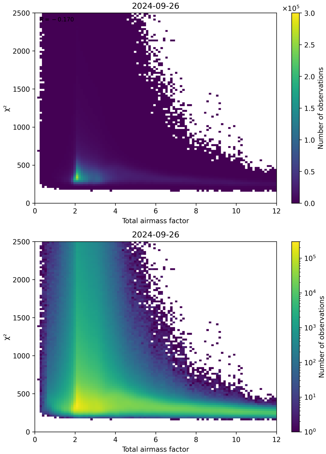
Figure 63: Scatter density plot of “Total airmass factor” against “ \chi^2 ” for 2024-09-25 to 2024-09-27.
