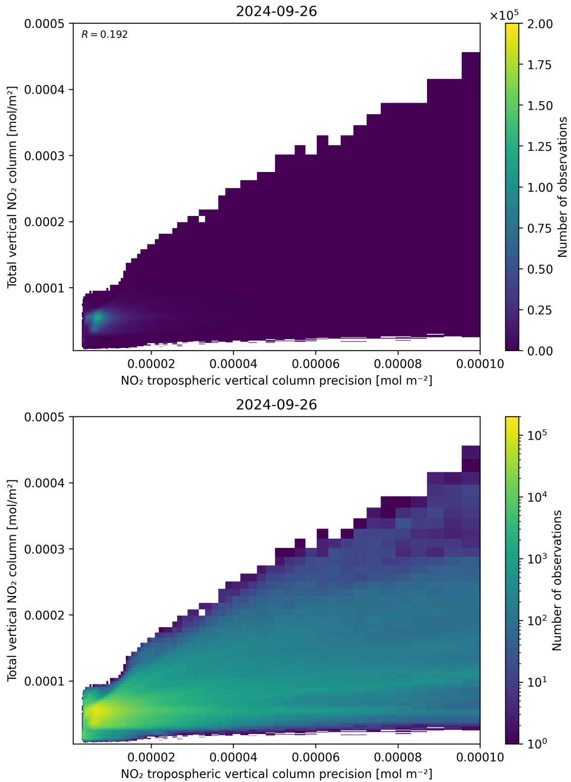
Figure 138: Scatter density plot of “NO 2 tropospheric vertical column precision” against “Total vertical NO 2 column” for 2024-09-25 to 2024-09-27.
