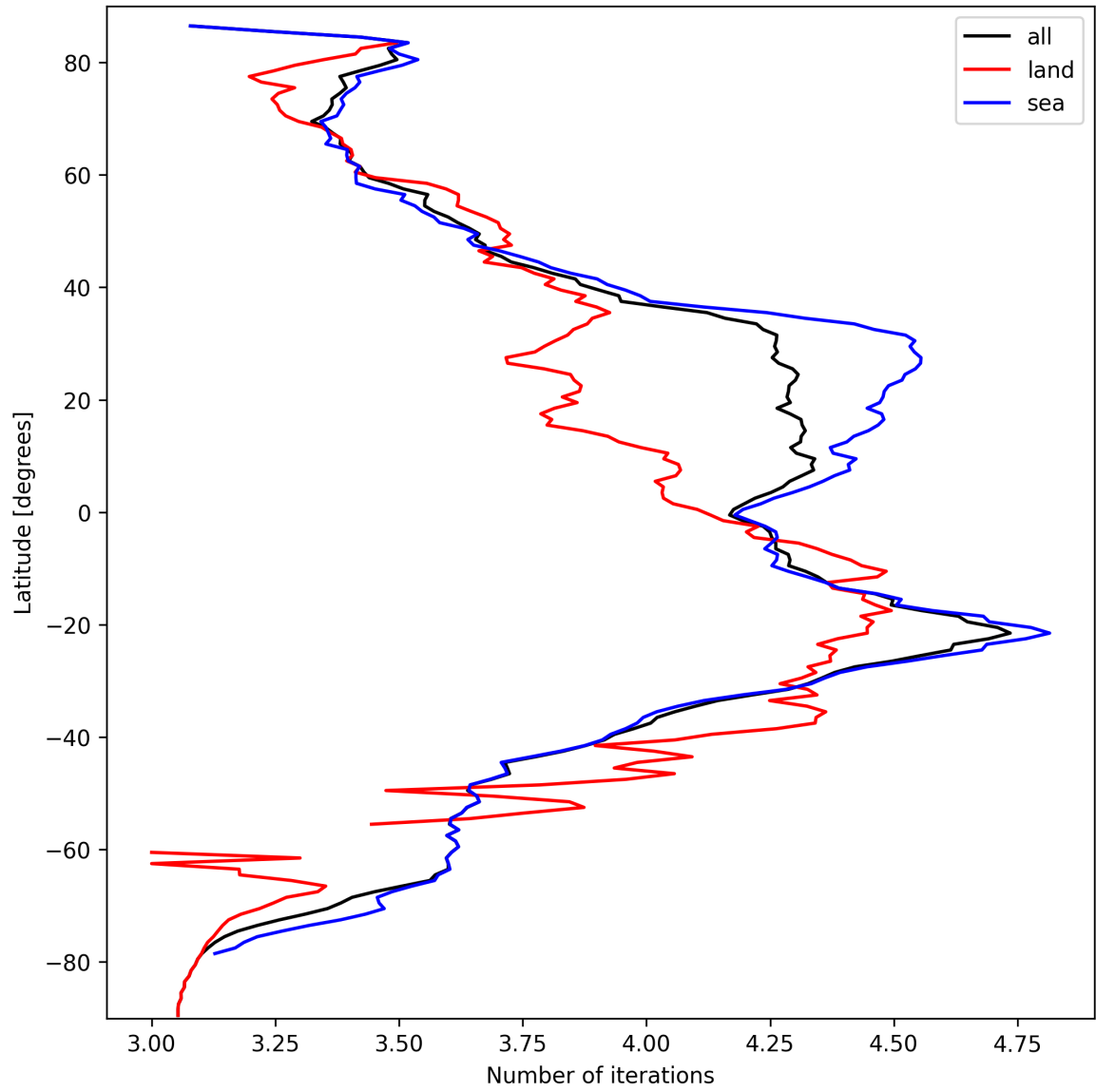
Figure 17: Zonal average of “Number of iterations” for 2024-09-25 to 2024-09-27.
