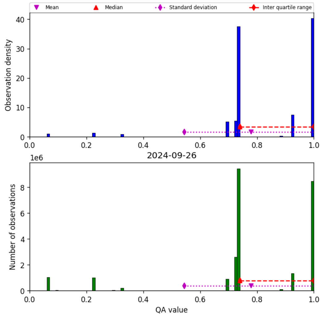
Figure 28: Histogram of “QA value” for 2024-09-25 to 2024-09-27
