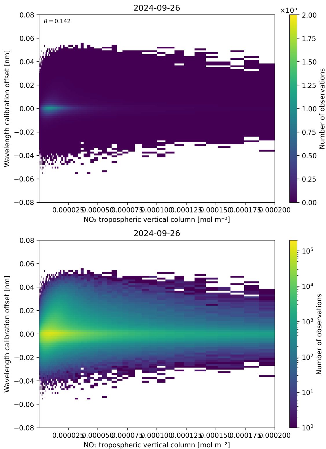
Figure 143: Scatter density plot of “NO 2 tropospheric vertical column” against “Wavelength calibration offset” for 2024-09-25 to 2024-09-27.
