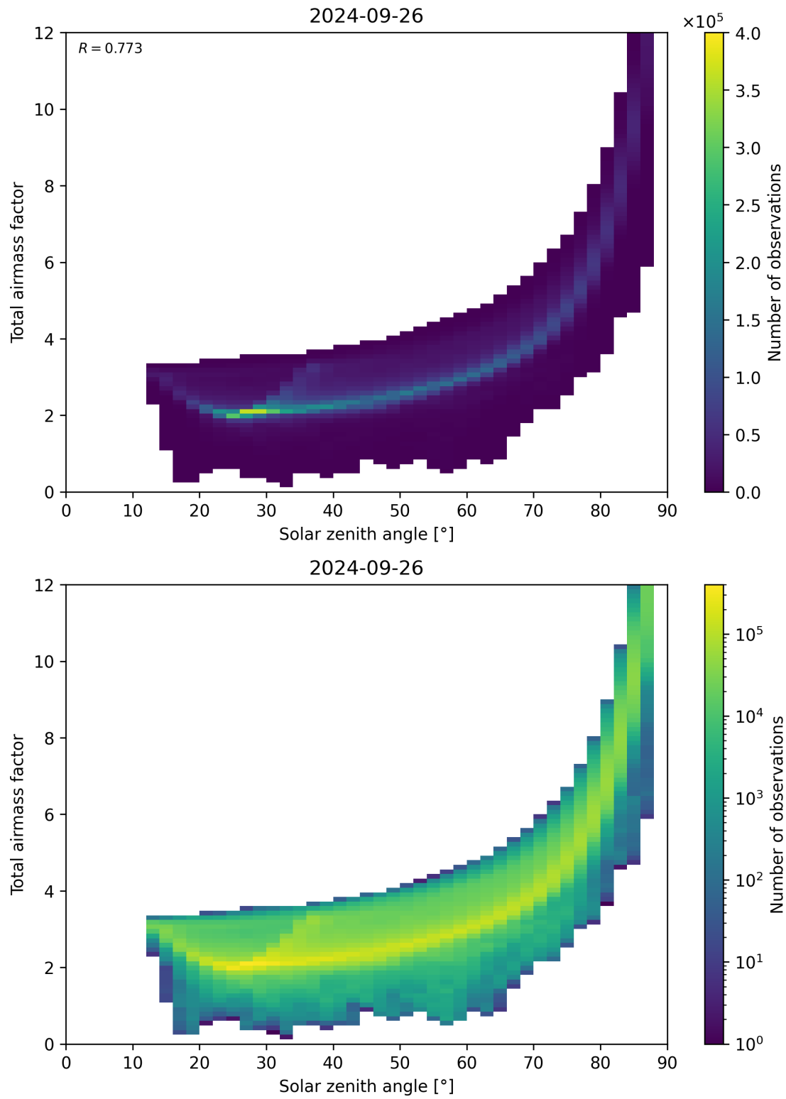
Figure 146: Scatter density plot of “Solar zenith angle” against “Total airmass factor” for 2024-09-25 to 2024-09-27.
