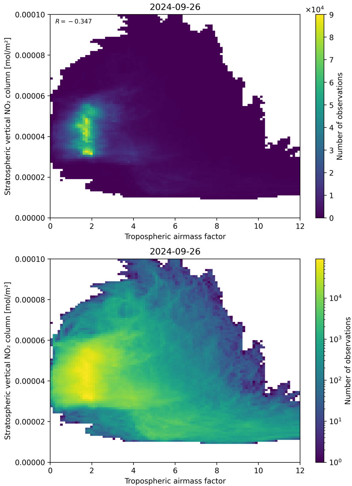
Figure 74: Scatter density plot of “Tropospheric air mass factor” against “Stratospheric vertical NO 2 column” for 2024-09-25 to 2024-09-27.
