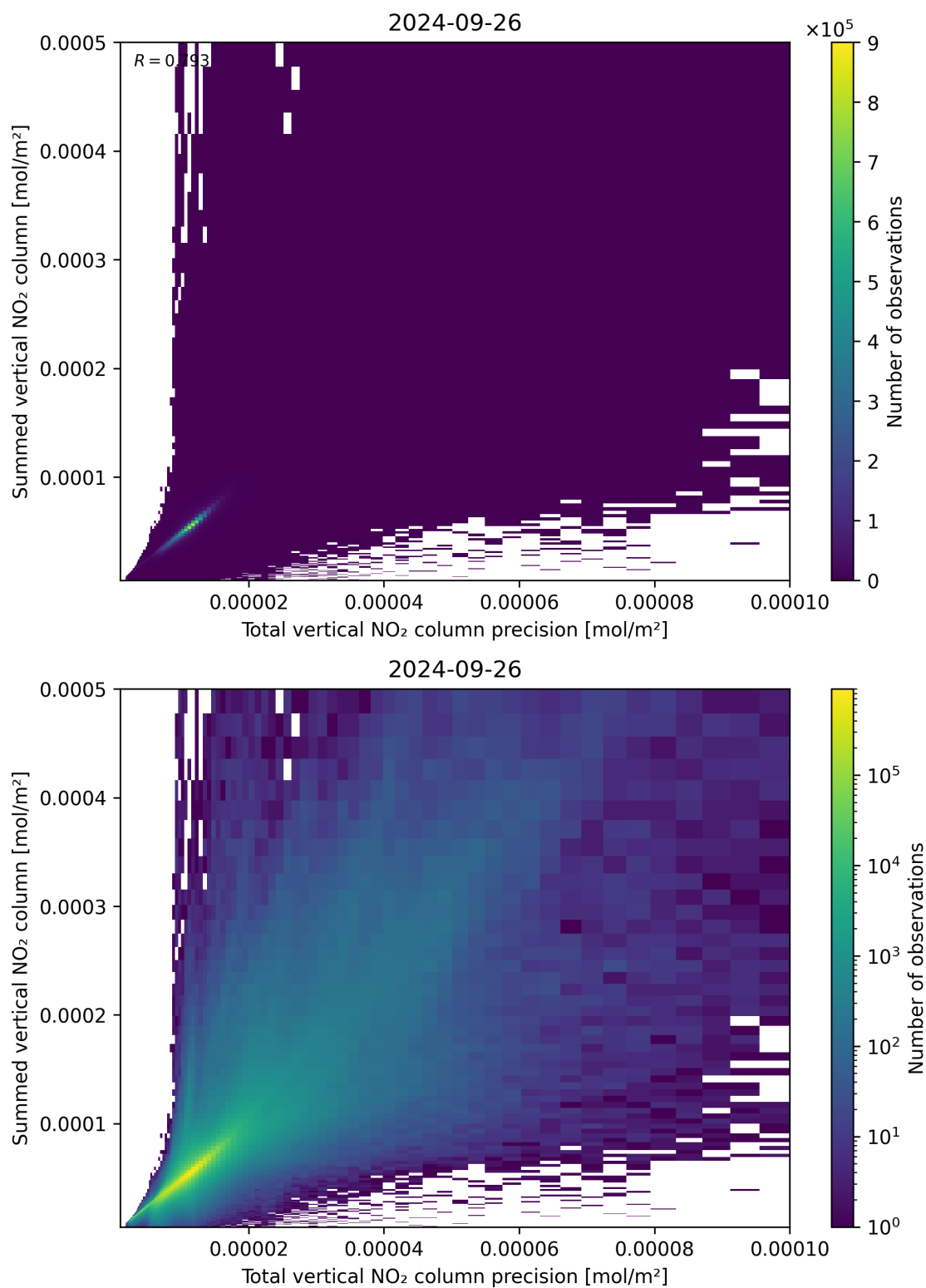
Figure 117: Scatter density plot of “Total vertical NO 2 column precision” against “Summed vertical NO 2 column” for 2024-09-25 to 2024-09-27.
