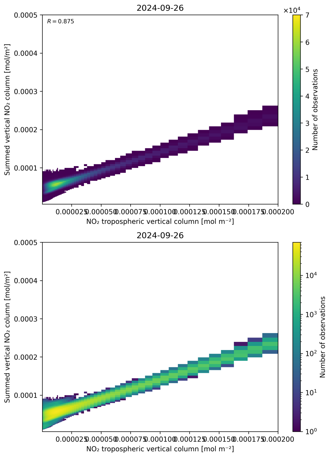
Figure 126: Scatter density plot of “NO 2 tropospheric vertical column” against “Summed vertical NO 2 column” for 2024-09-25 to 2024-09-27.
