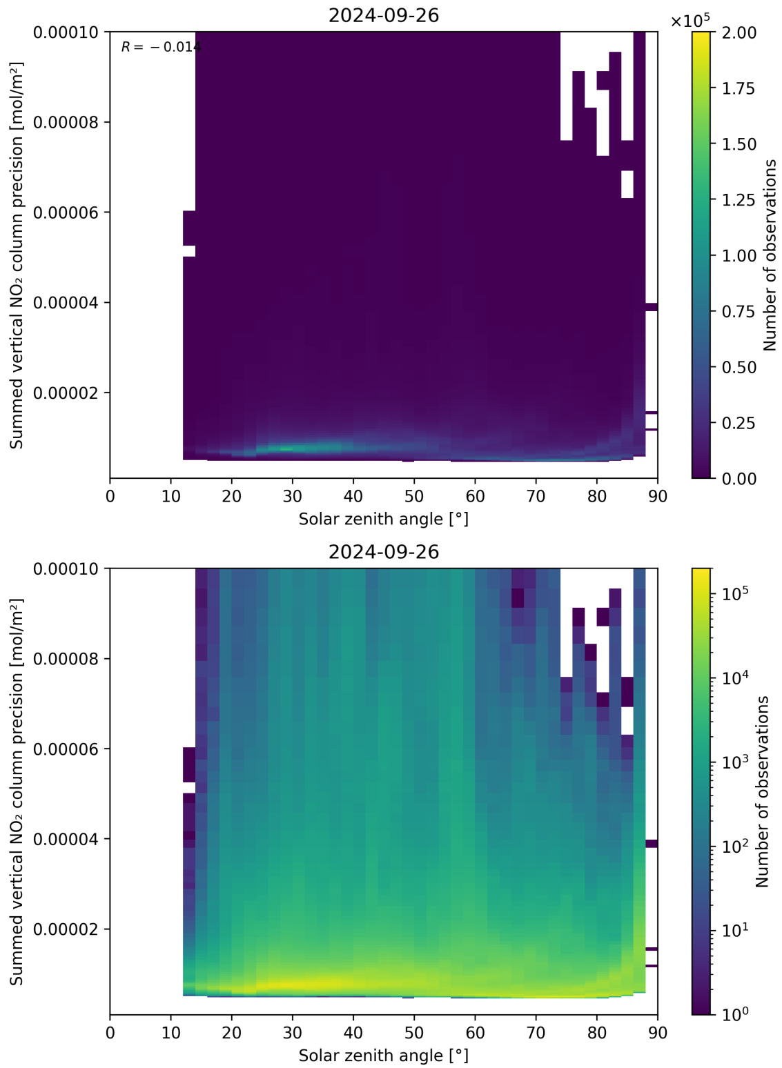
Figure 152: Scatter density plot of “Solar zenith angle” against “Summed vertical NO 2 column precision” for 2024-09-25 to 2024-09-27.
