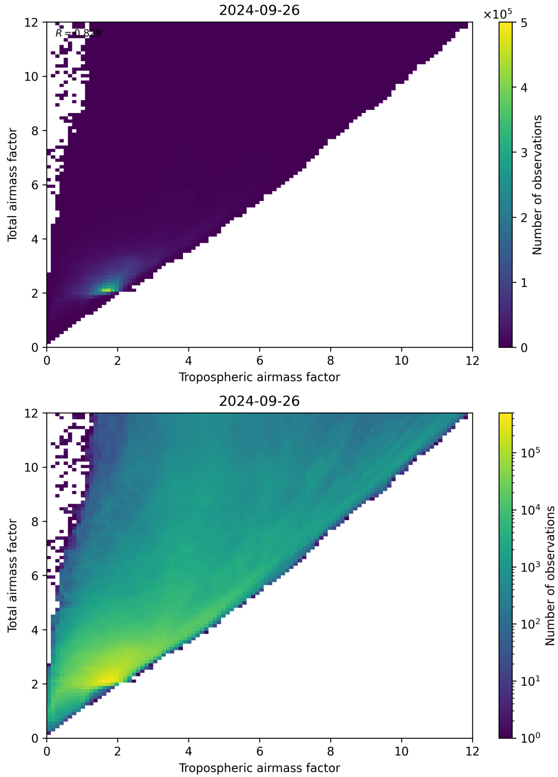
Figure 72: Scatter density plot of “Tropospheric airmass factor” against “Total airmass factor” for 2024-09-25 to 2024-09-27.
