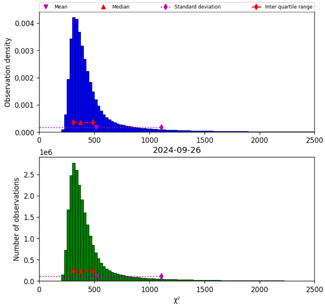
Figure 42: Histogram of “ \chi^2 ” for 2024-09-25 to 2024-09-27
