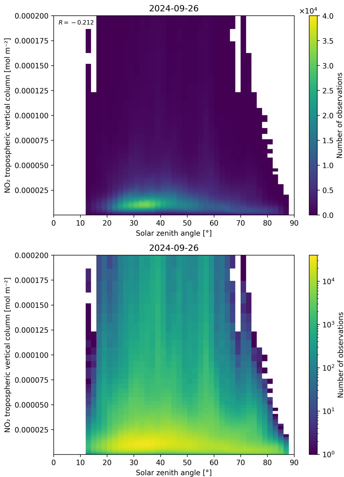
Figure 155: Scatter density plot of “Solar zenith angle” against “NO 2 tropospheric vertical column” for 2024-09-25 to 2024-09-27.
