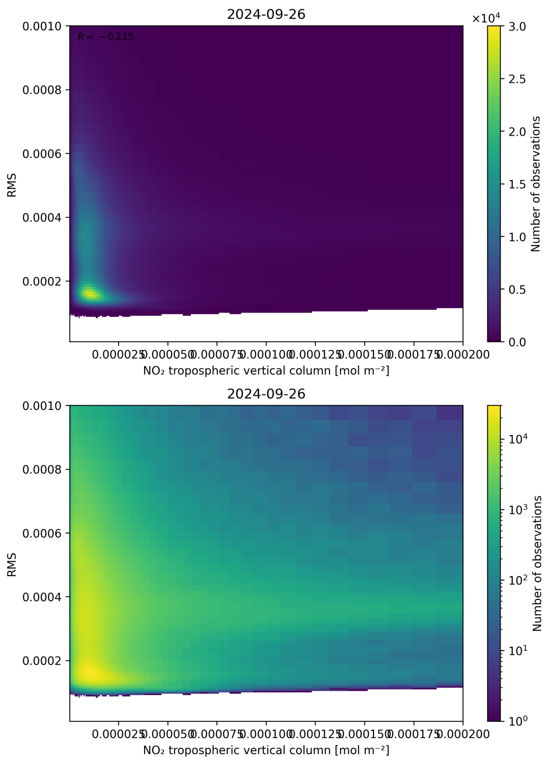
Figure 142: Scatter density plot of “NO 2 tropospheric vertical column” against “RMS” for 2024-09-25 to 2024-09-27.
