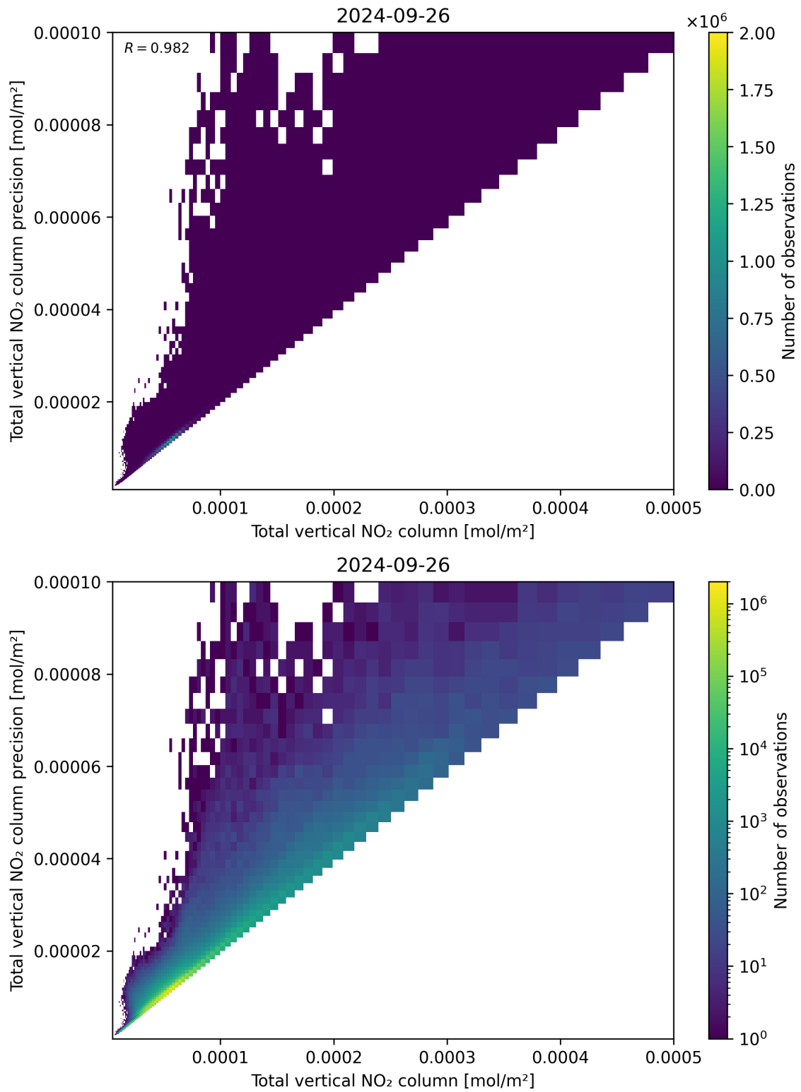
Figure 114: Scatter density plot of “Total vertical NO 2 column” against “Total vertical NO 2 column precision” for 2024-09-25 to 2024-09-27.
