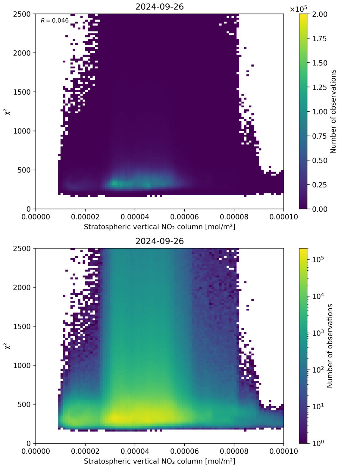
Figure 97: Scatter density plot of “Stratospheric vertical NO 2 column” against “ \chi^2 ” for 2024-09-25 to 2024-09-27.
