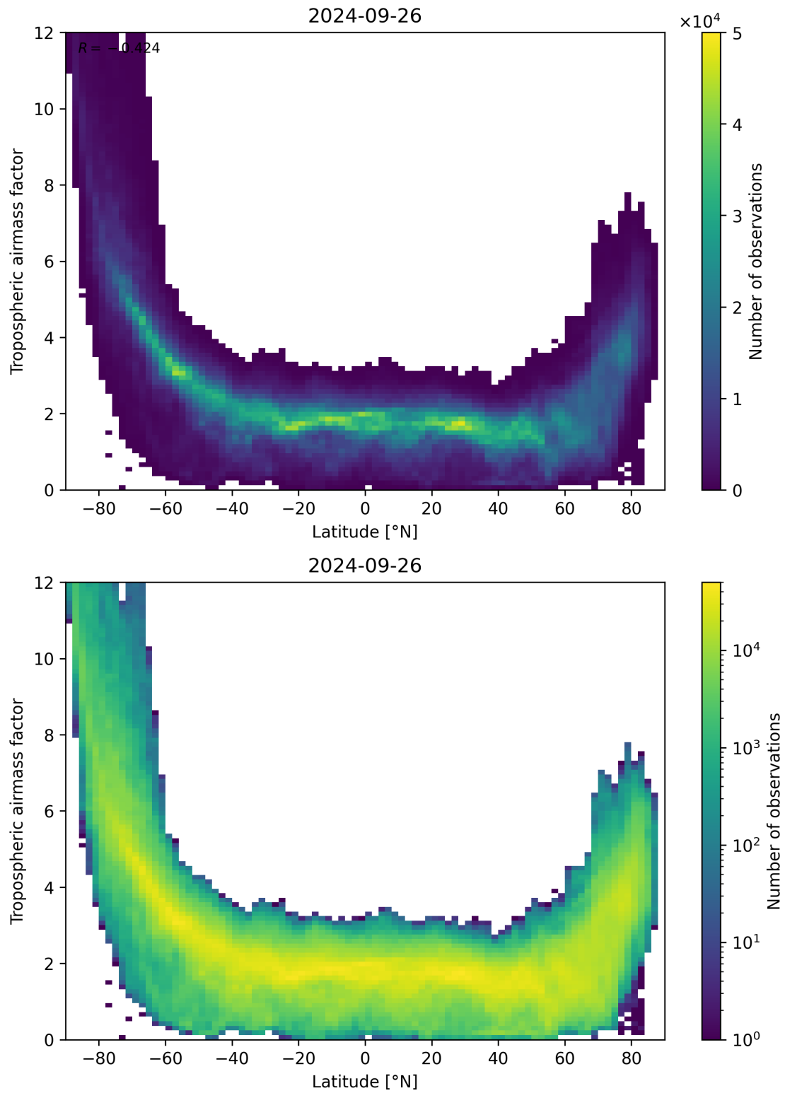
Figure 85: Scatter density plot of “Latitude” against “Tropospheric air mass factor” for 2024-09-25 to 2024-09-27.
