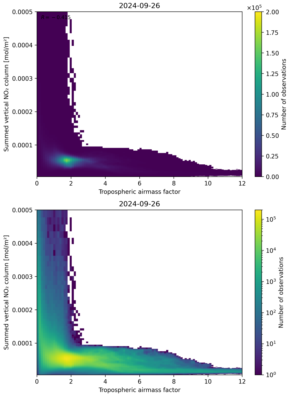
Figure 75: Scatter density plot of “Tropospheric air mass factor” against “Summed vertical NO 2 column” for 2024-09-25 to 2024-09-27.
