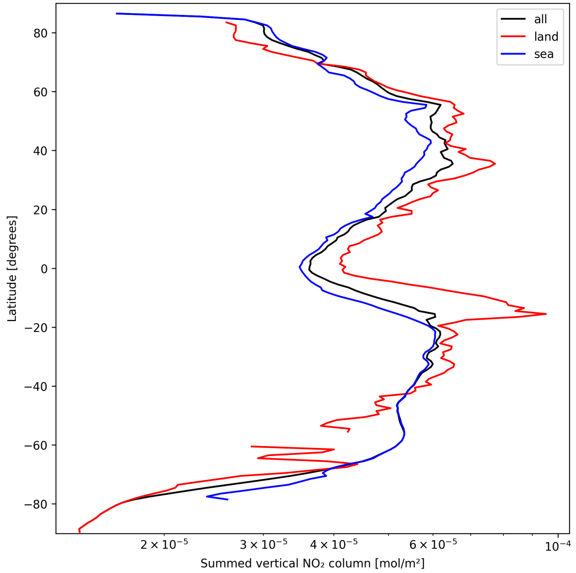
Figure 23: Zonal average of “Summed vertical NO 2 column” for 2024-09-25 to 2024-09-27.
