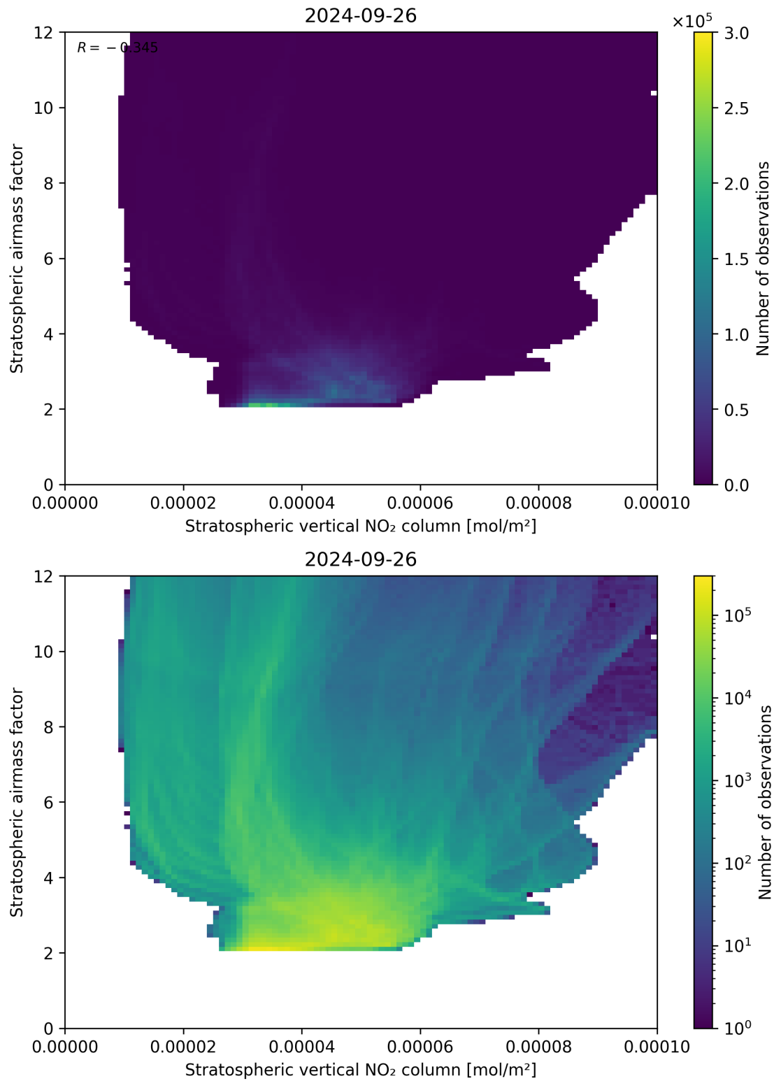
Figure 96: Scatter density plot of “Stratospheric vertical NO 2 column” against “Stratospheric airmass factor” for 2024-09-25 to 2024-09-27.
