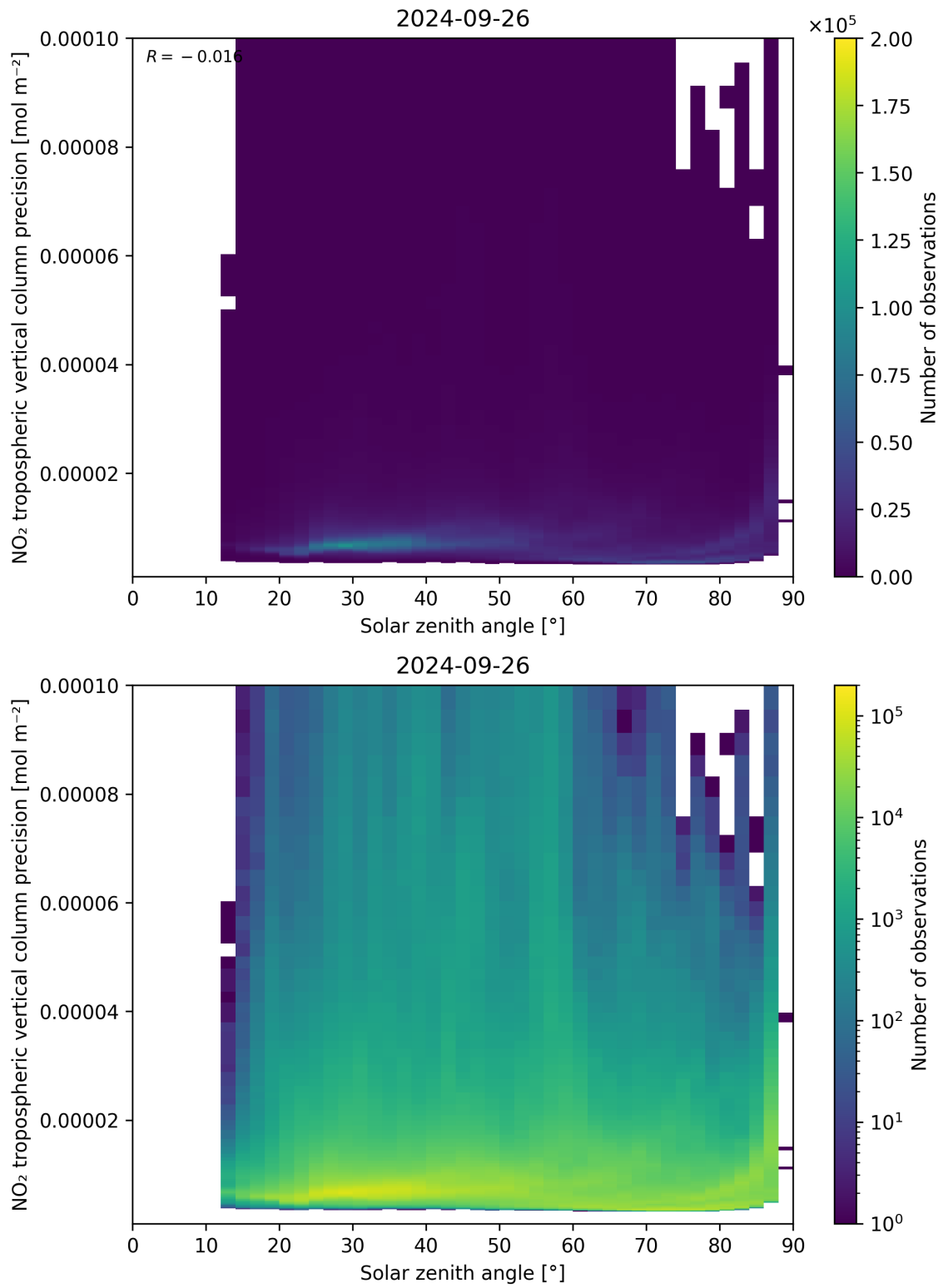
Figure 156: Scatter density plot of “Solar zenith angle” against “NO 2 tropospheric vertical column precision” for 2024-09-25 to 2024-09-27.
