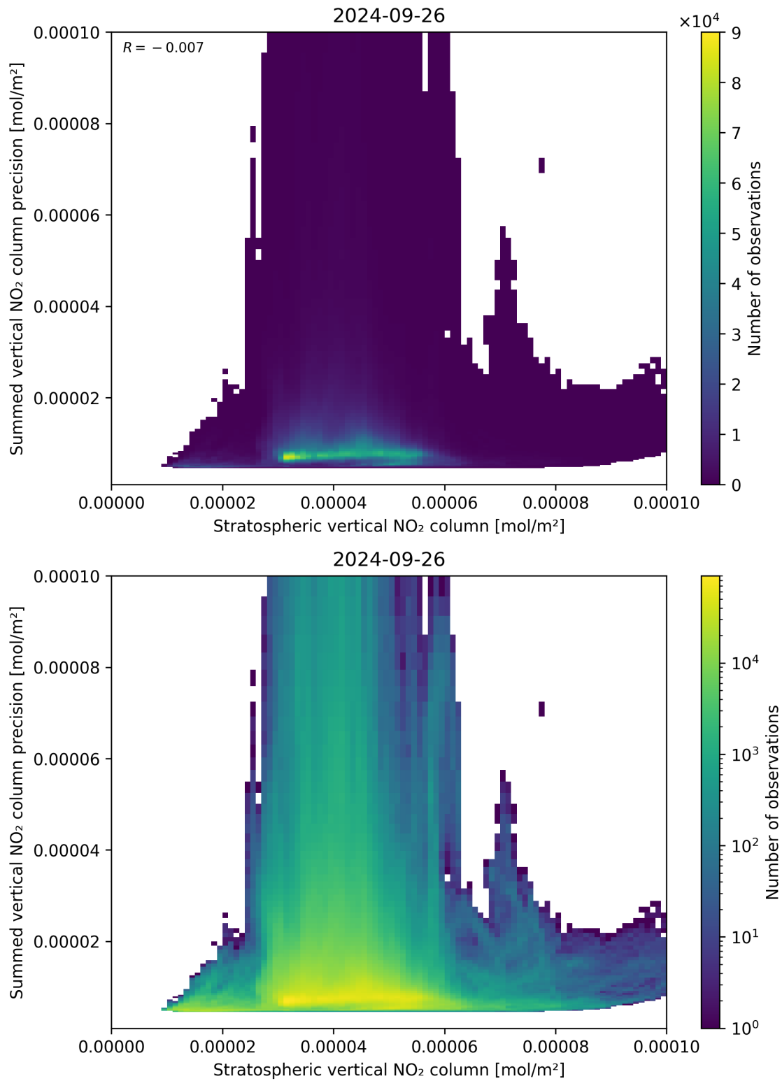
Figure 99: Scatter density plot of “Stratospheric vertical NO 2 column” against “Summed vertical NO 2 column precision” for 2024-09-25 to 2024-09-27.
