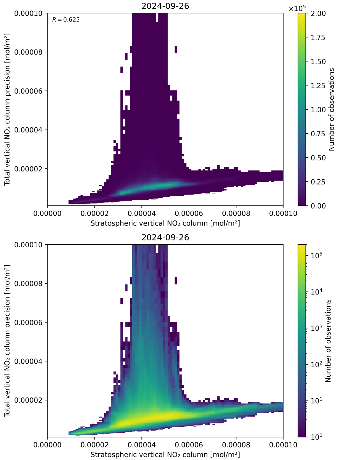
Figure 101: Scatter density plot of “Stratospheric vertical NO 2 column” against “Total vertical NO 2 column precision” for 2024-09-25 to 2024-09-27.
