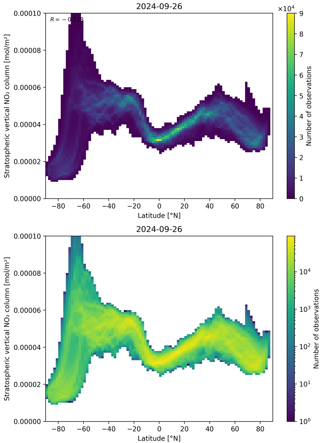
Figure 87: Scatter density plot of “Latitude” against “Stratospheric vertical NO 2 column” for 2024-09-25 to 2024-09-27.
