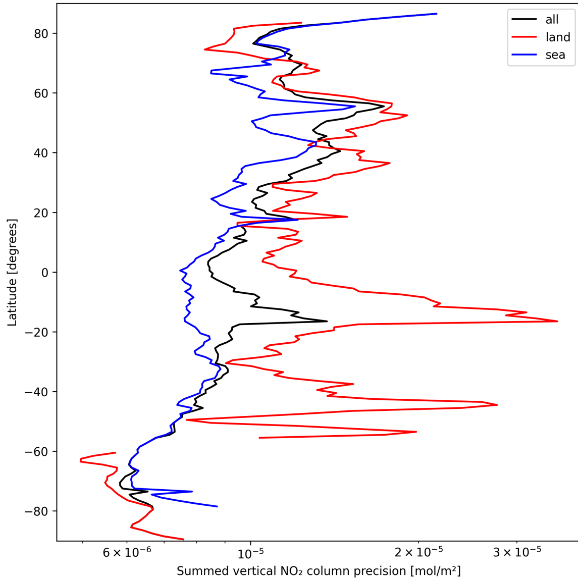
Figure 24: Zonal average of “Summed vertical NO 2 column precision” for 2024-09-25 to 2024-09-27.
