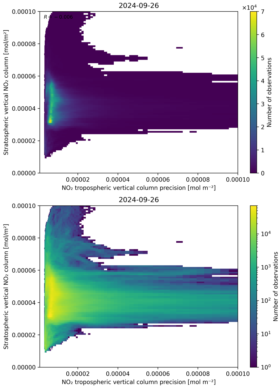
Figure 135: Scatter density plot of “NO 2 tropospheric vertical column precision” against “Stratospheric vertical NO 2 column” for 2024-09-25 to 2024-09-27.
