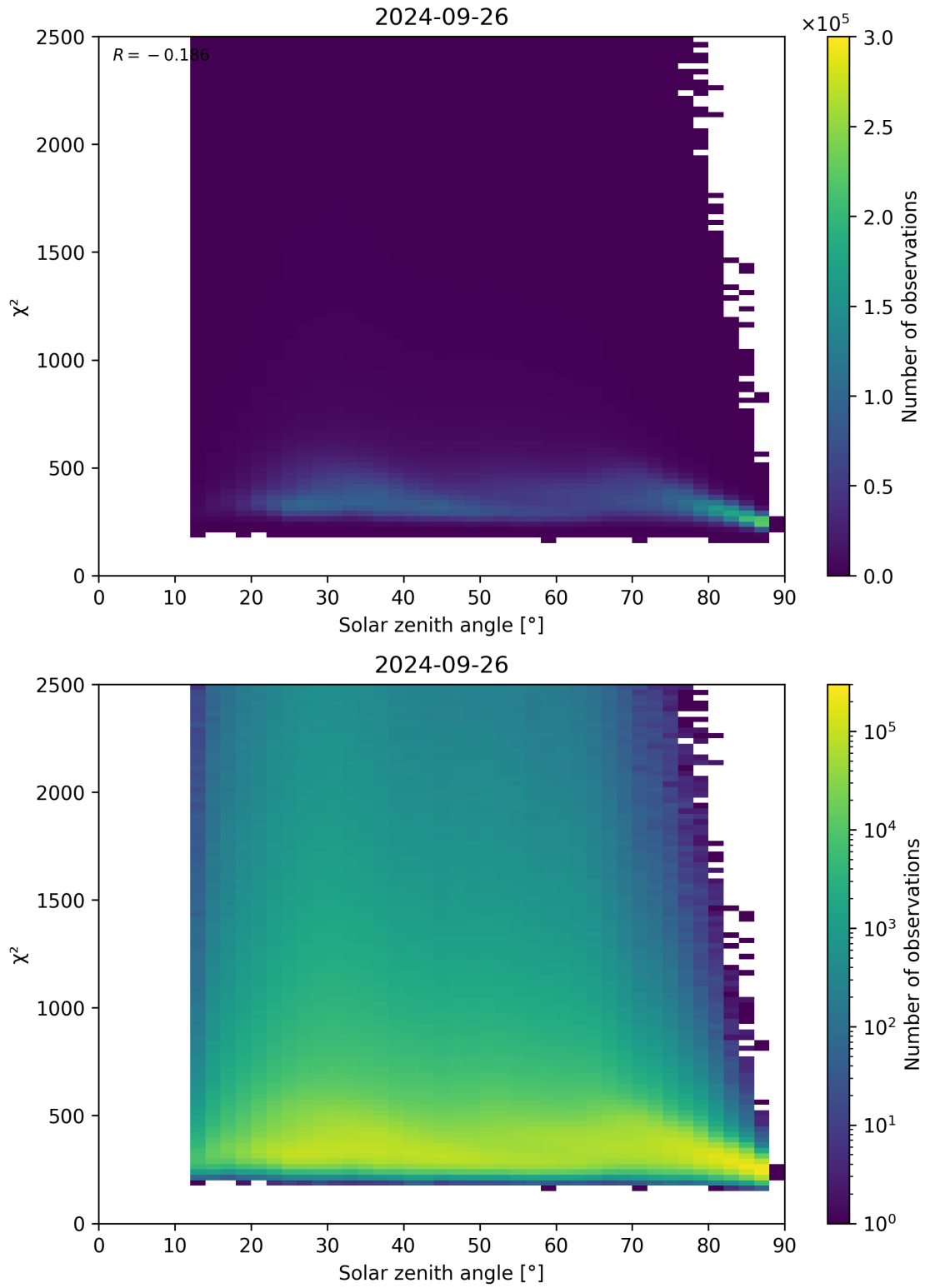
Figure 148: Scatter density plot of “Solar zenith angle” against “ \chi^2 ” for 2024-09-25 to 2024-09-27.
