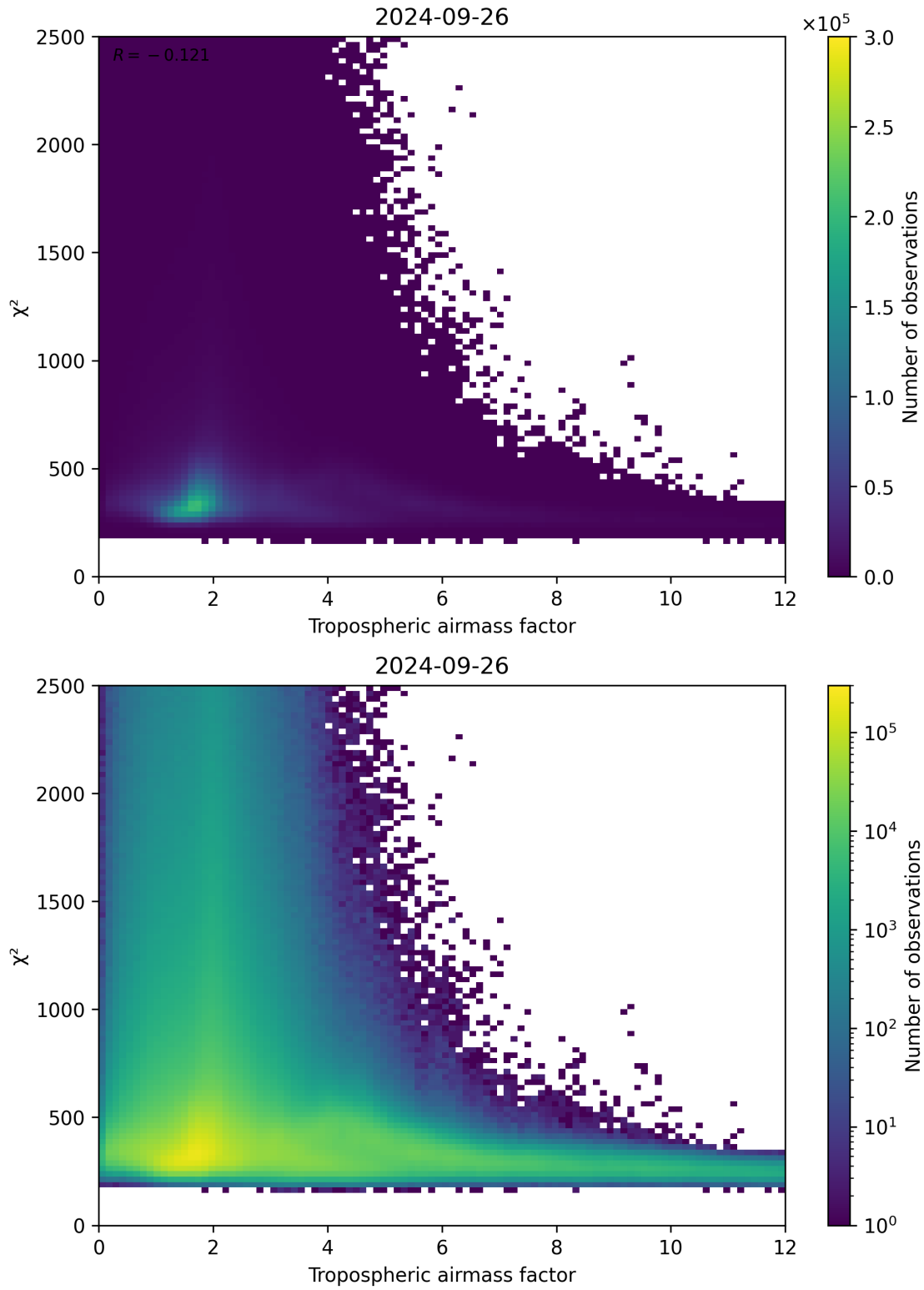
Figure 73: Scatter density plot of “Tropospheric airmass factor” against “ \chi^2 ” for 2024-09-25 to 2024-09-27.
