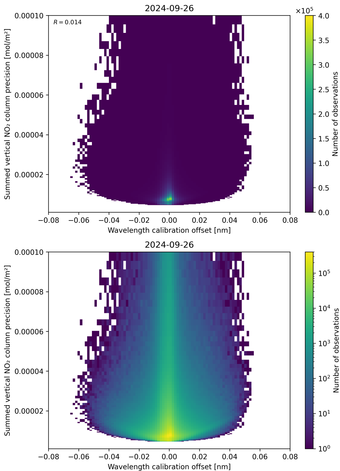
Figure 178: Scatter density plot of “Wavelength calibration offset” against “Summed vertical NO 2 column precision” for 2024-09-25 to 2024-09-27.
