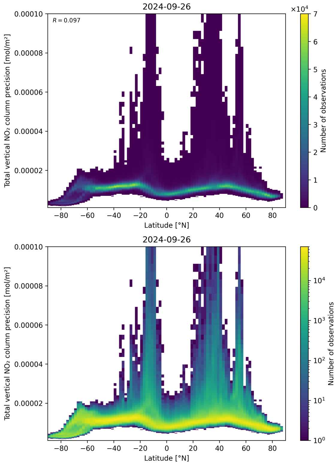
Figure 91: Scatter density plot of “Latitude” against “Total vertical NO 2 column precision” for 2024-09-25 to 2024-09-27.
