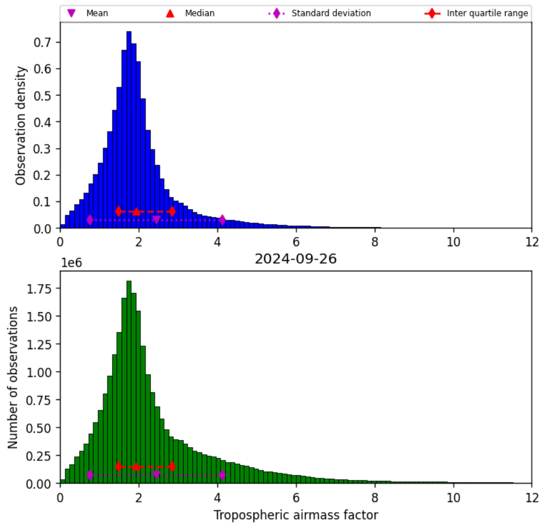
Figure 31: Histogram of “Tropospheric airmass factor” for 2024-09-25 to 2024-09-27
