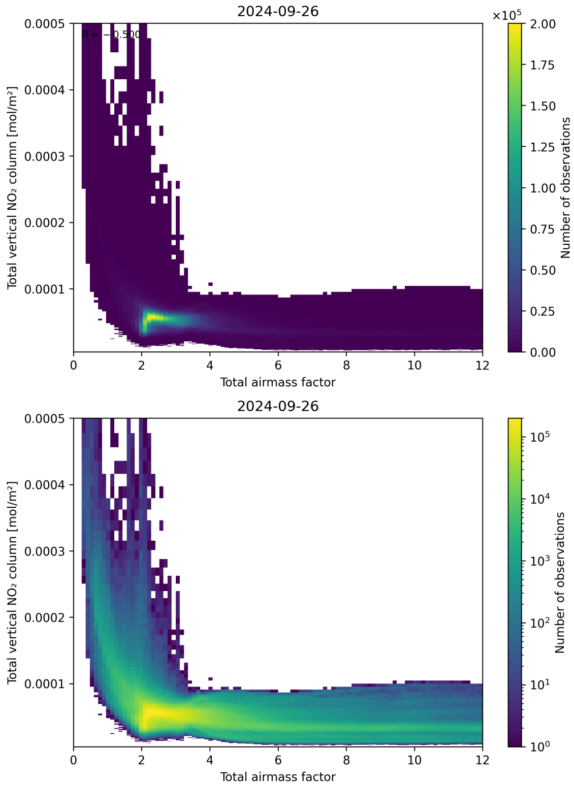
Figure 67: Scatter density plot of “Total airmass factor” against “Total vertical NO 2 column” for 2024-09-25 to 2024-09-27.
