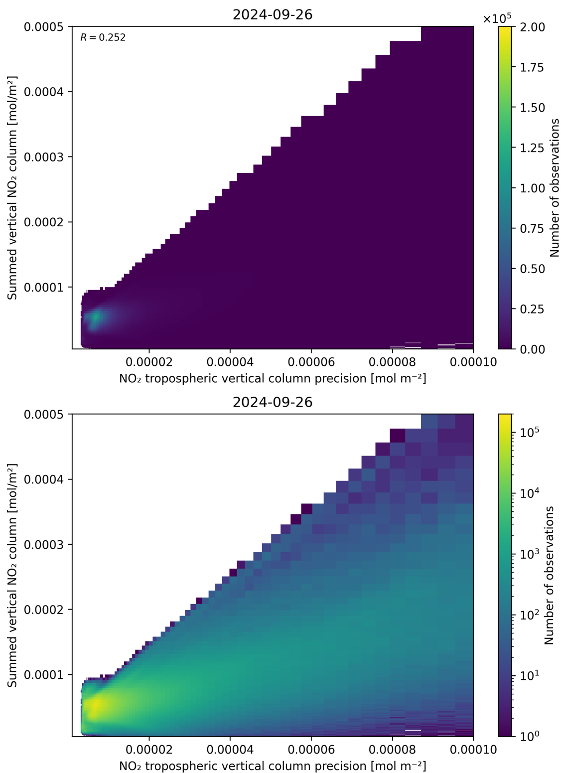
Figure 136: Scatter density plot of “NO 2 tropospheric vertical column precision” against “Summed vertical NO 2 column” for 2024-09-25 to 2024-09-27.
