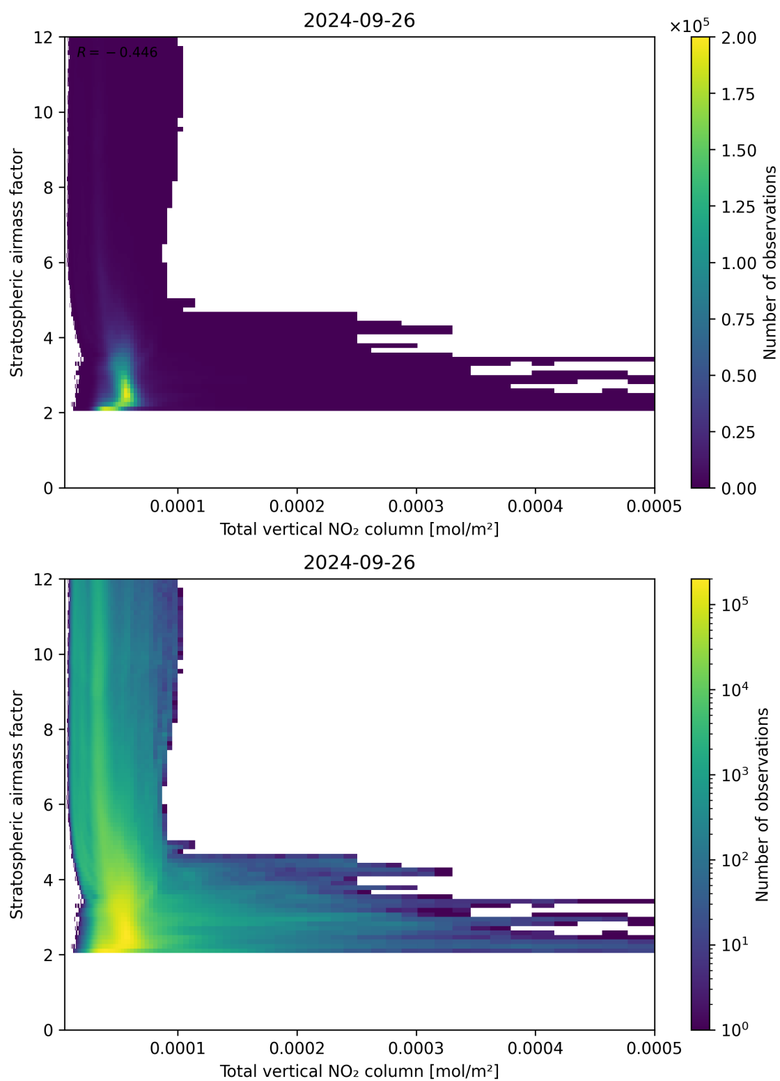
Figure 110: Scatter density plot of “Total vertical NO 2 column” against “Stratospheric airmass factor” for 2024-09-25 to 2024-09-27.
