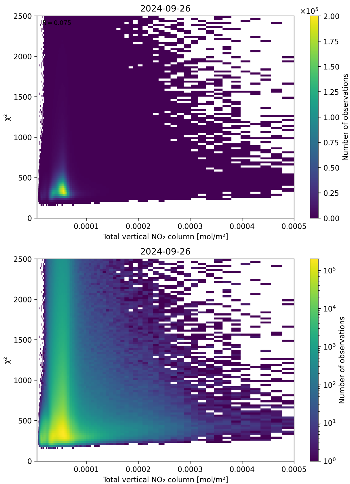
Figure 111: Scatter density plot of “Total vertical NO 2 column” against “ \chi^2 ” for 2024-09-25 to 2024-09-27.
