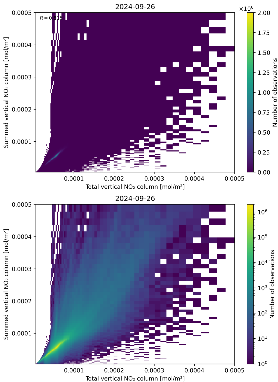
Figure 112: Scatter density plot of “Total vertical NO 2 column” against “Summed vertical NO 2 column” for 2024-09-25 to 2024-09-27.
