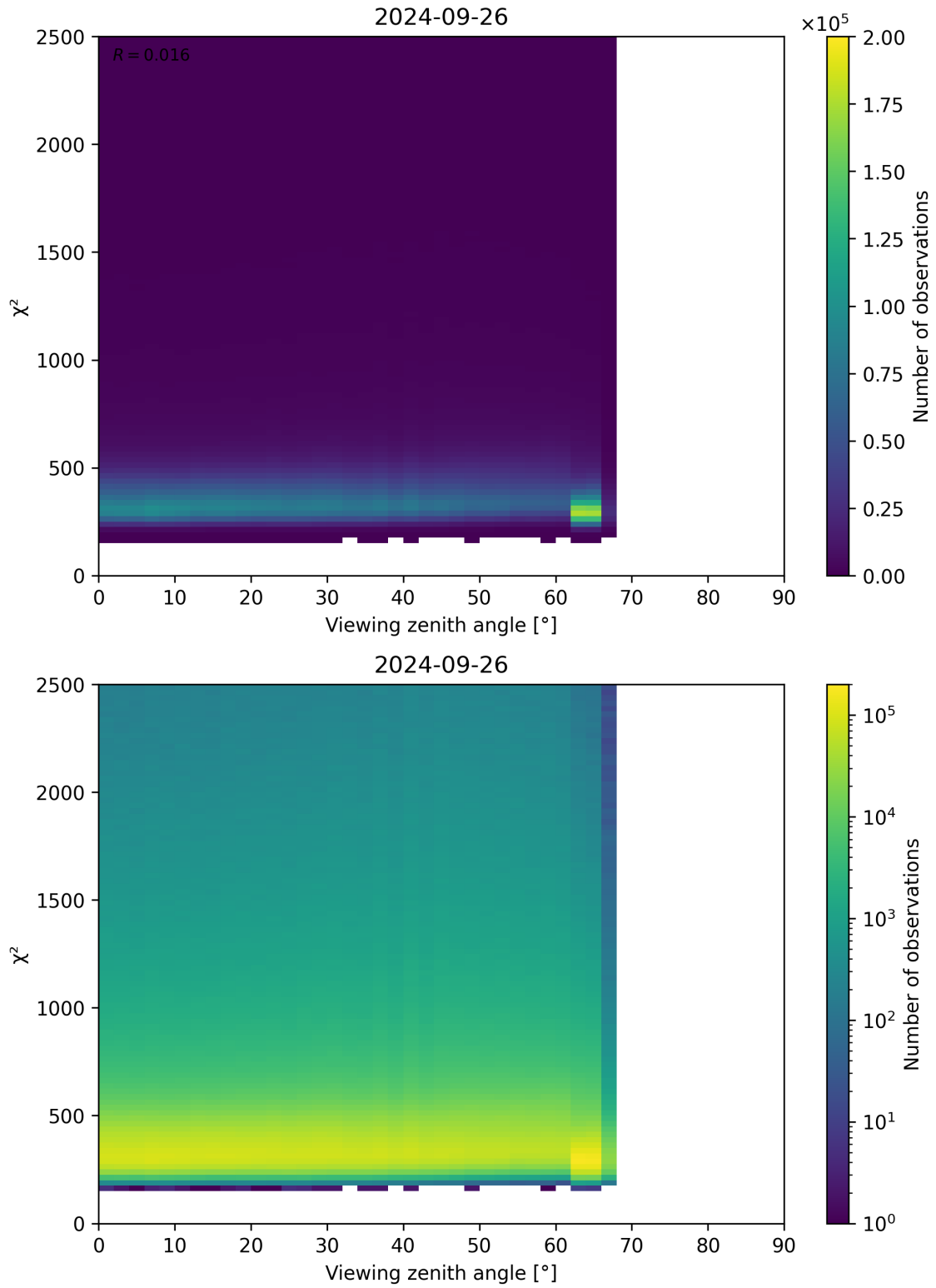
Figure 162: Scatter density plot of “Viewing zenith angle” against “ \chi^2 ” for 2024-09-25 to 2024-09-27.
