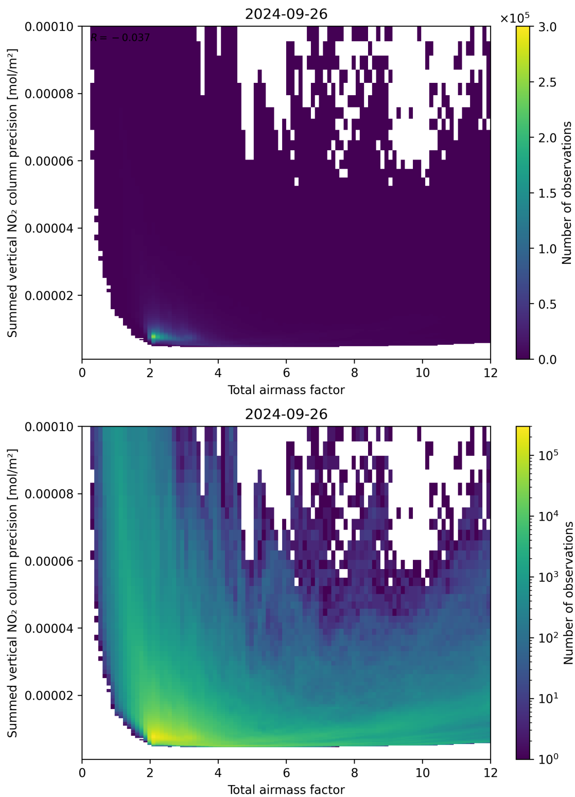
Figure 66: Scatter density plot of “Total airmass factor” against “Summed vertical NO 2 column precision” for 2024-09-25 to 2024-09-27.
