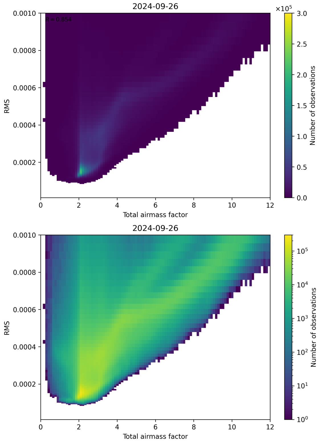
Figure 69: Scatter density plot of “Total airmass factor” against “RMS” for 2024-09-25 to 2024-09-27.
