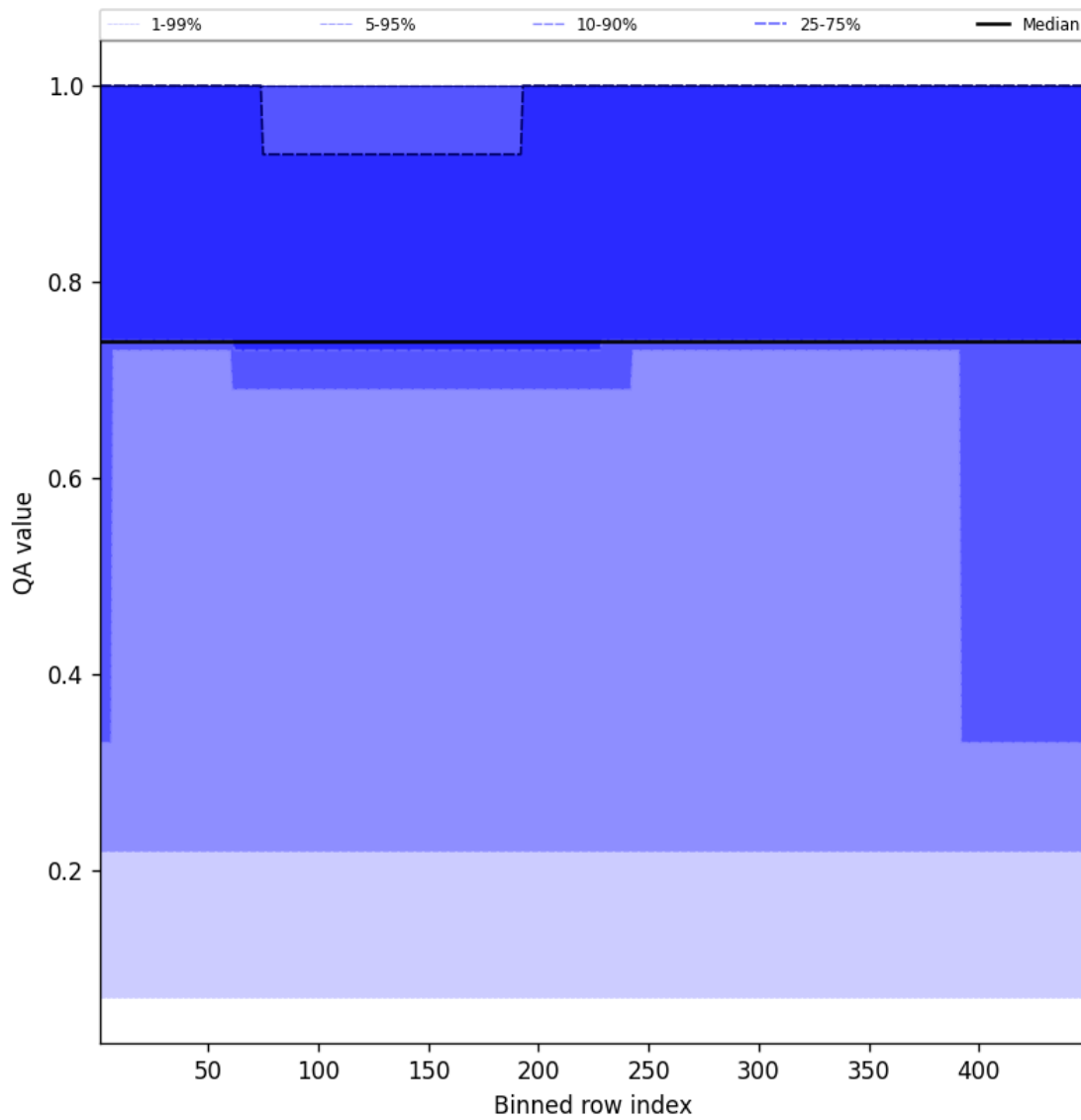
Figure 45: Along track statistics of "QA value" for 2024-09-25 to 2024-09-27
