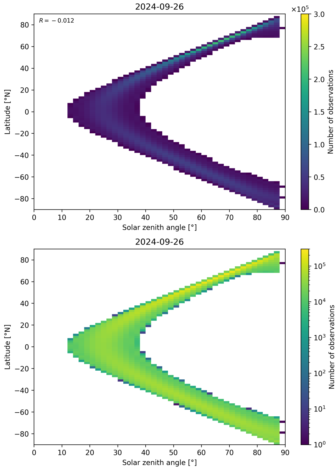
Figure 149: Scatter density plot of “Solar zenith angle” against “Latitude” for 2024-09-25 to 2024-09-27.
