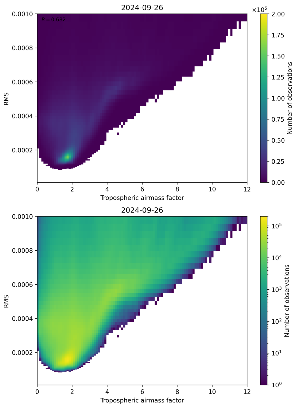
Figure 79: Scatter density plot of “Tropospheric airmass factor” against “RMS” for 2024-09-25 to 2024-09-27.
