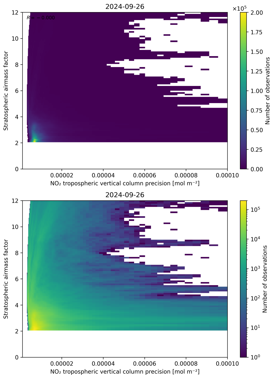
Figure 131: Scatter density plot of “NO 2 tropospheric vertical column precision” against “Stratospheric airmass factor” for 2024-09-25 to 2024-09-27.
