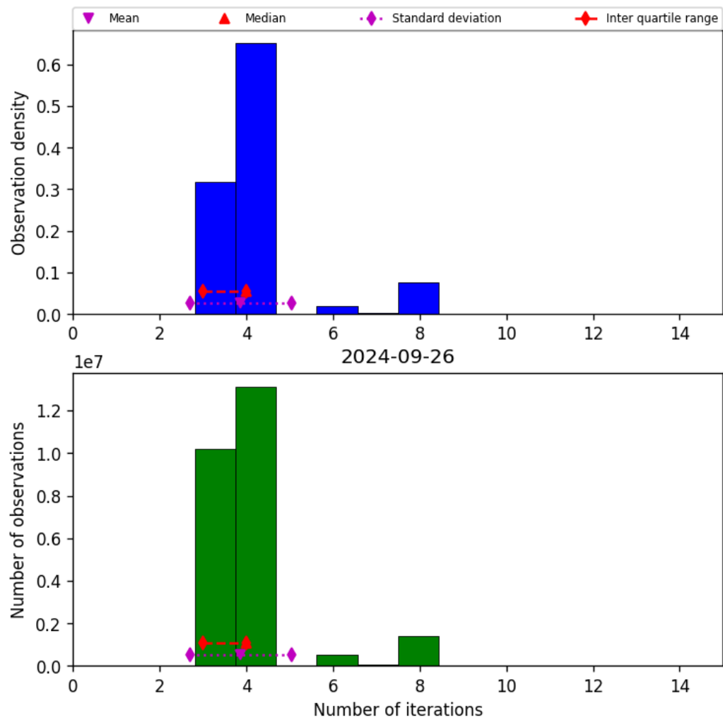
Figure 34: Histogram of “Number of iterations” for 2024-09-25 to 2024-09-27
