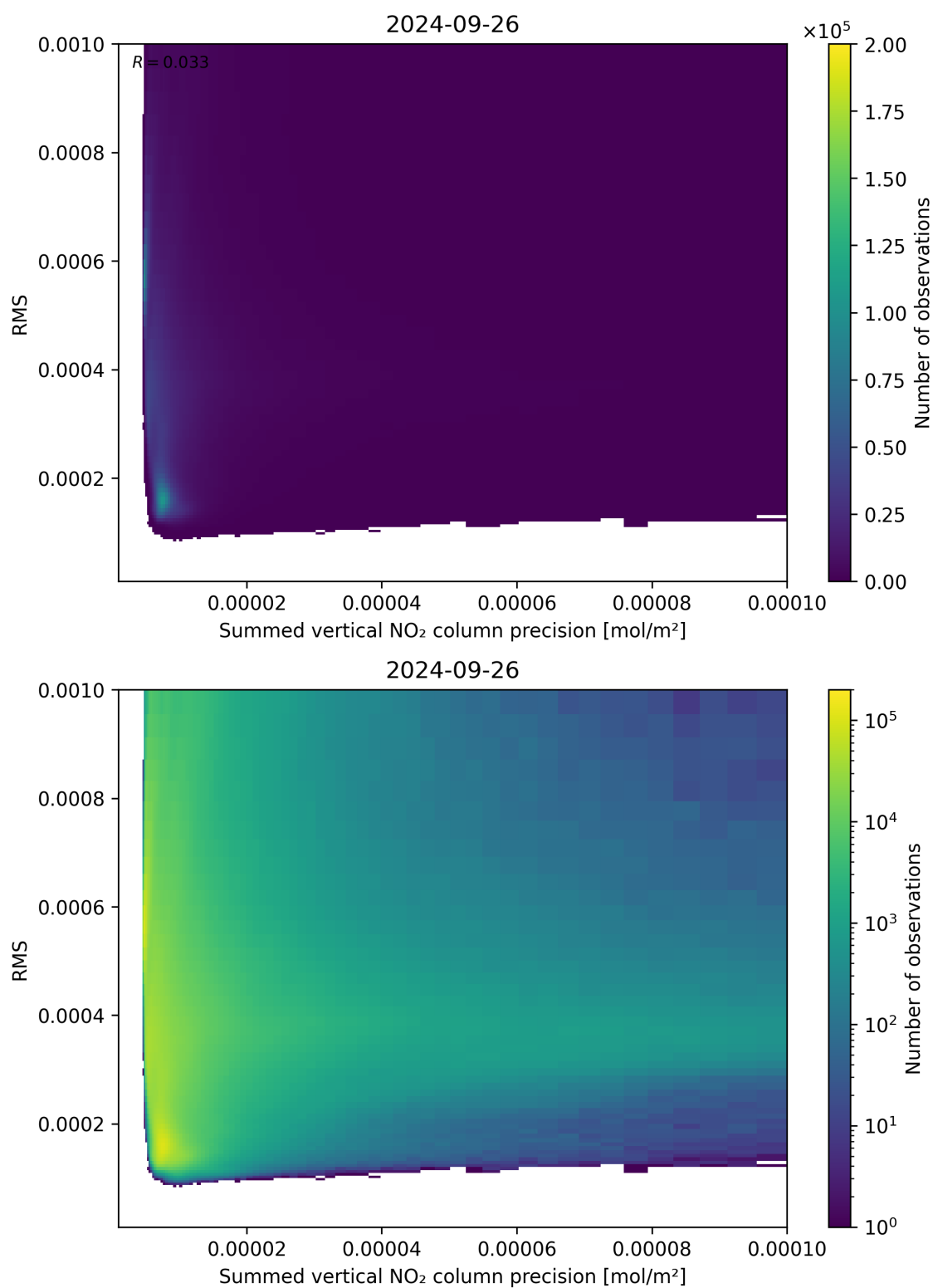
Figure 108: Scatter density plot of “Summed vertical NO 2 column precision” against “RMS” for 2024-09-25 to 2024-09-27.
