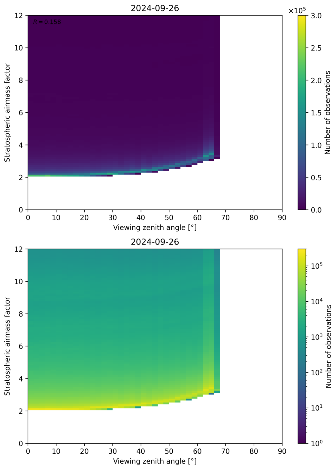
Figure 159: Scatter density plot of “Viewing zenith angle” against “Stratospheric airmass factor” for 2024-09-25 to 2024-09-27.
