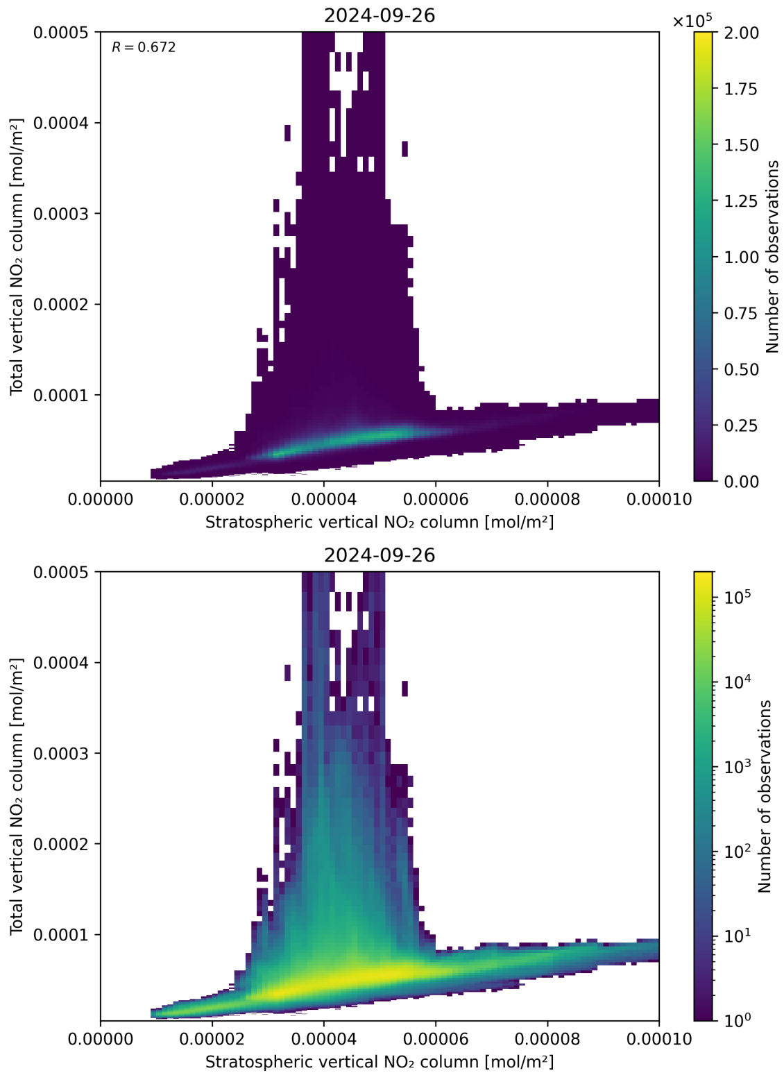
Figure 100: Scatter density plot of “Stratospheric vertical NO 2 column” against “Total vertical NO 2 column” for 2024-09-25 to 2024-09-27.
