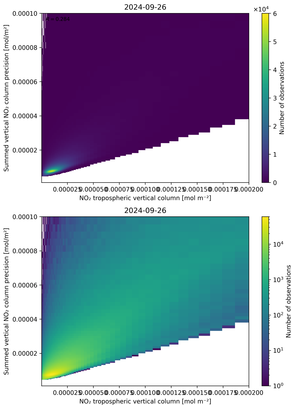
Figure 127: Scatter density plot of “NO 2 tropospheric vertical column” against “Summed vertical NO 2 column precision” for 2024-09-25 to 2024-09-27.
