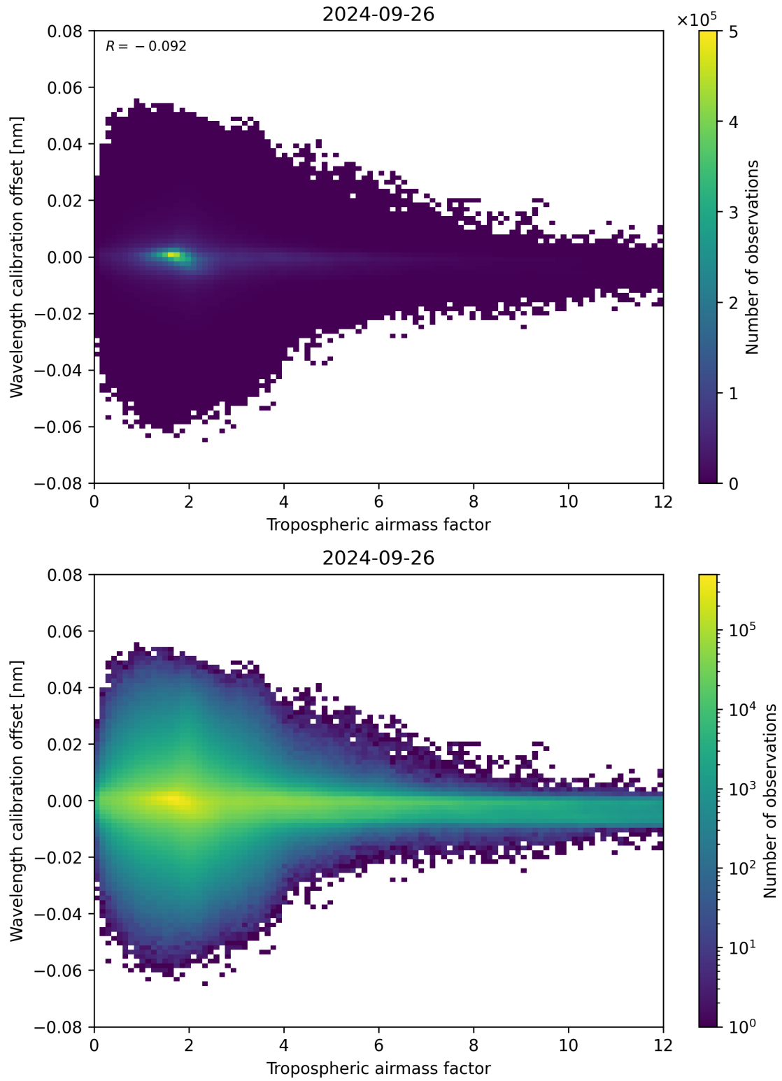
Figure 80: Scatter density plot of “Tropospheric airmass factor” against “Wavelength calibration offset” for 2024-09-25 to 2024-09-27.
