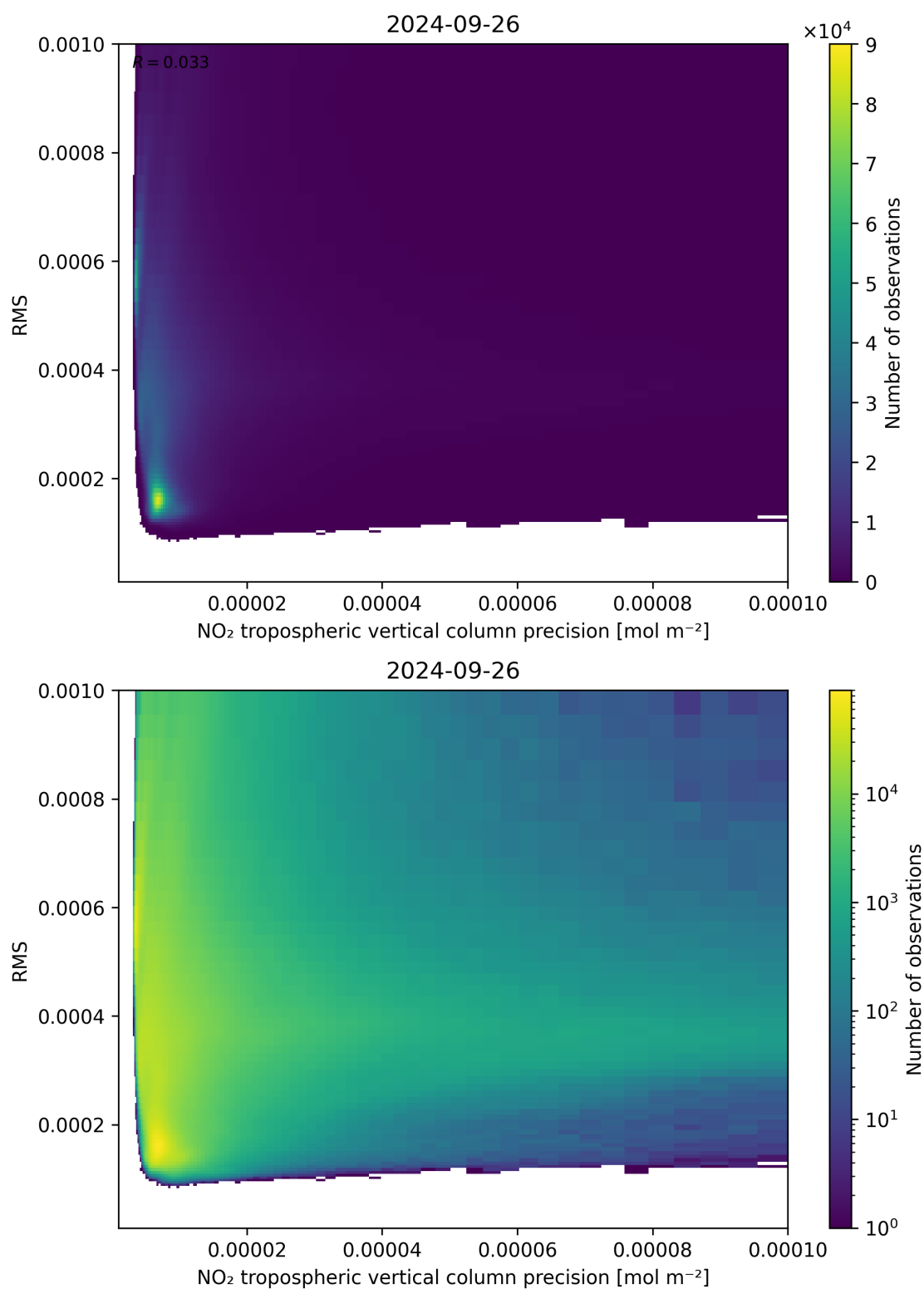
Figure 140: Scatter density plot of “NO 2 tropospheric vertical column precision” against “RMS” for 2024-09-25 to 2024-09-27.
