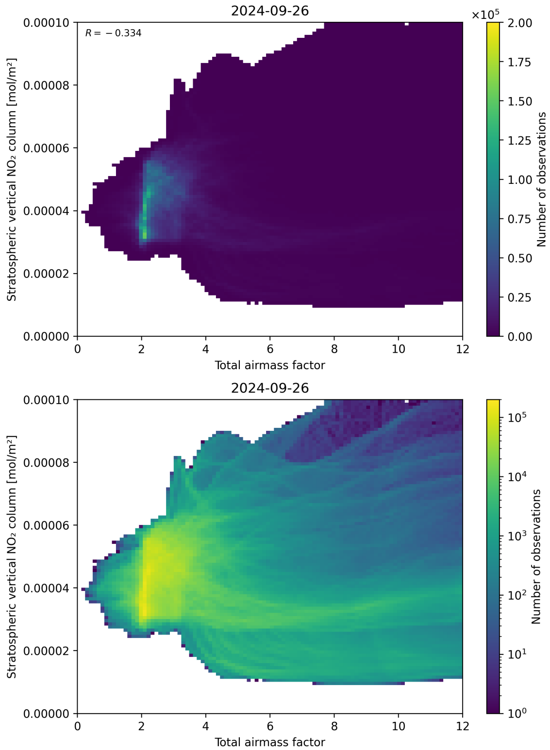
Figure 64: Scatter density plot of “Total airmass factor” against “Stratospheric vertical \text{NO}_2 column” for 2024-09-25 to 2024-09-27.
