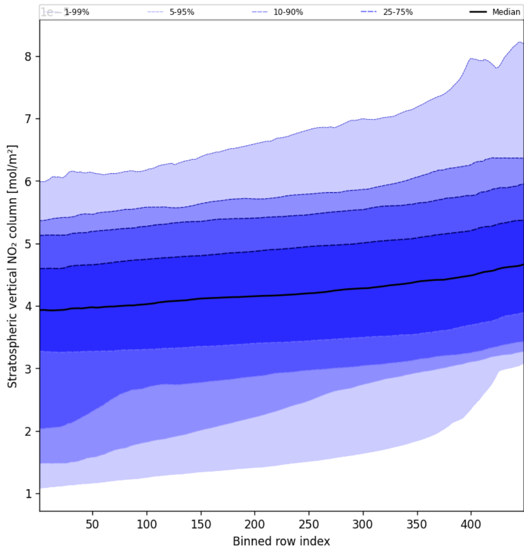
Figure 53: Along track statistics of “Stratospheric vertical NO 2 column” for 2024-09-25 to 2024-09-27
