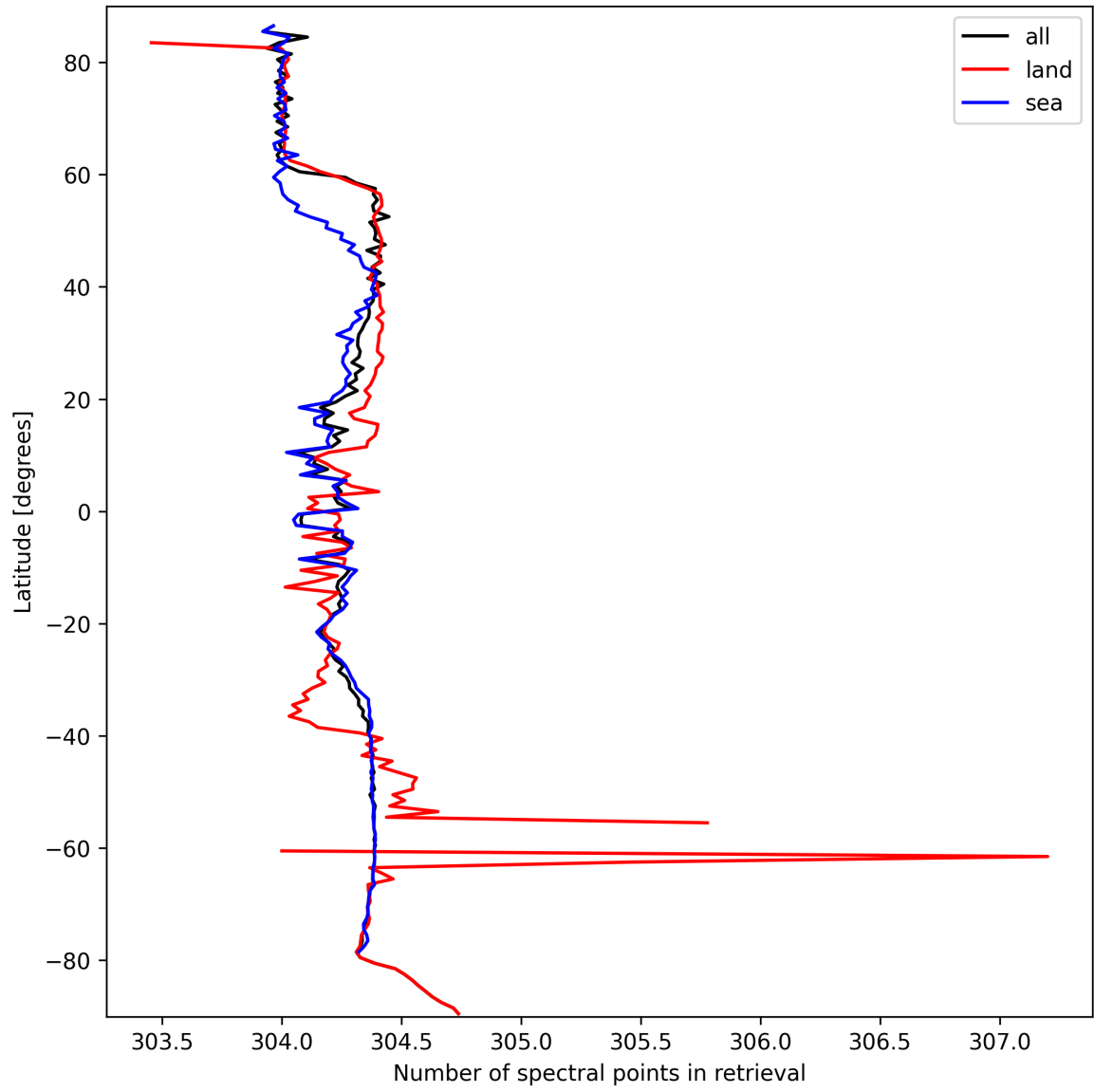
Figure 16: Zonal average of “Number of spectral points in retrieval” for 2024-09-25 to 2024-09-27.
