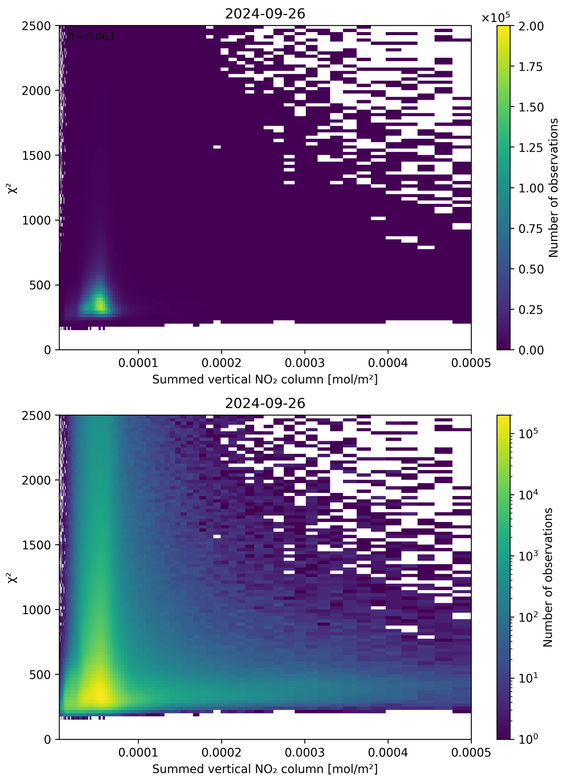
Figure 104: Scatter density plot of “Summed vertical NO 2 column” against “ \chi^2 ” for 2024-09-25 to 2024-09-27.
