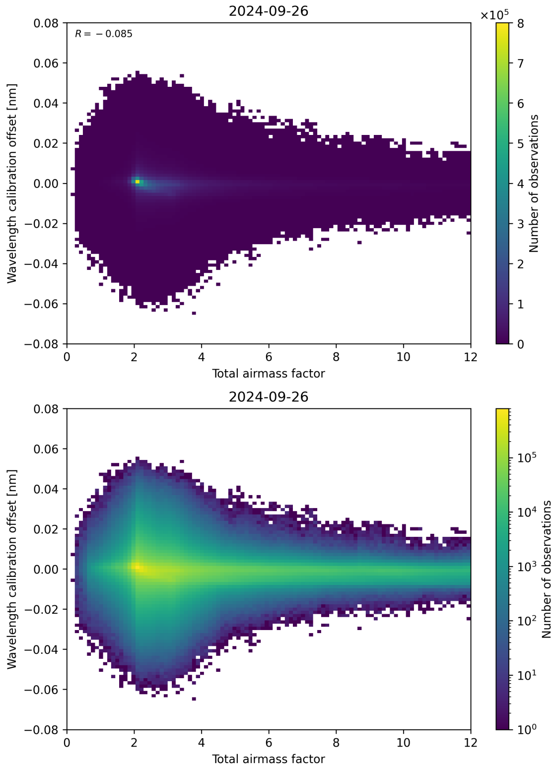
Figure 70: Scatter density plot of “Total airmass factor” against “Wavelength calibration offset” for 2024-09-25 to 2024-09-27.
