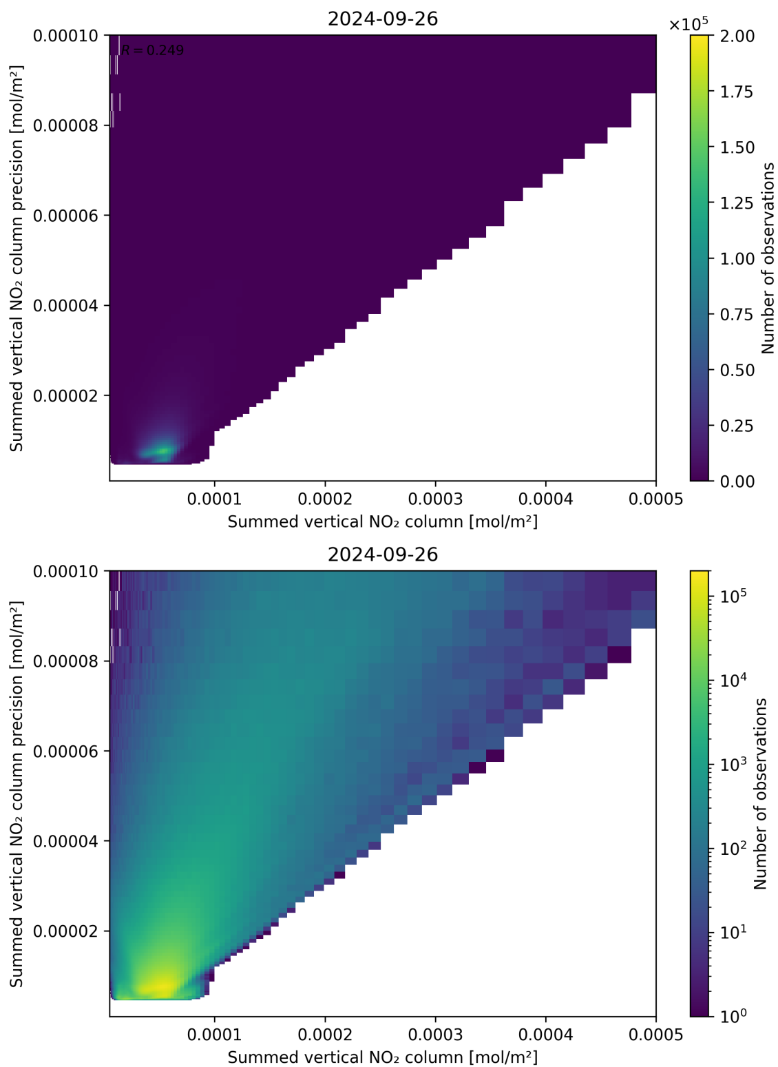
Figure 105: Scatter density plot of “Summed vertical NO 2 column” against “Summed vertical NO 2 column precision” for 2024-09-25 to 2024-09-27.
