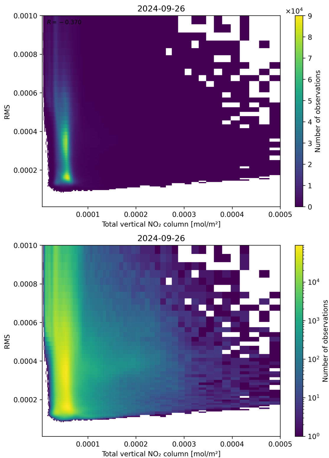
Figure 120: Scatter density plot of “Total vertical NO 2 column” against “RMS” for 2024-09-25 to 2024-09-27.
