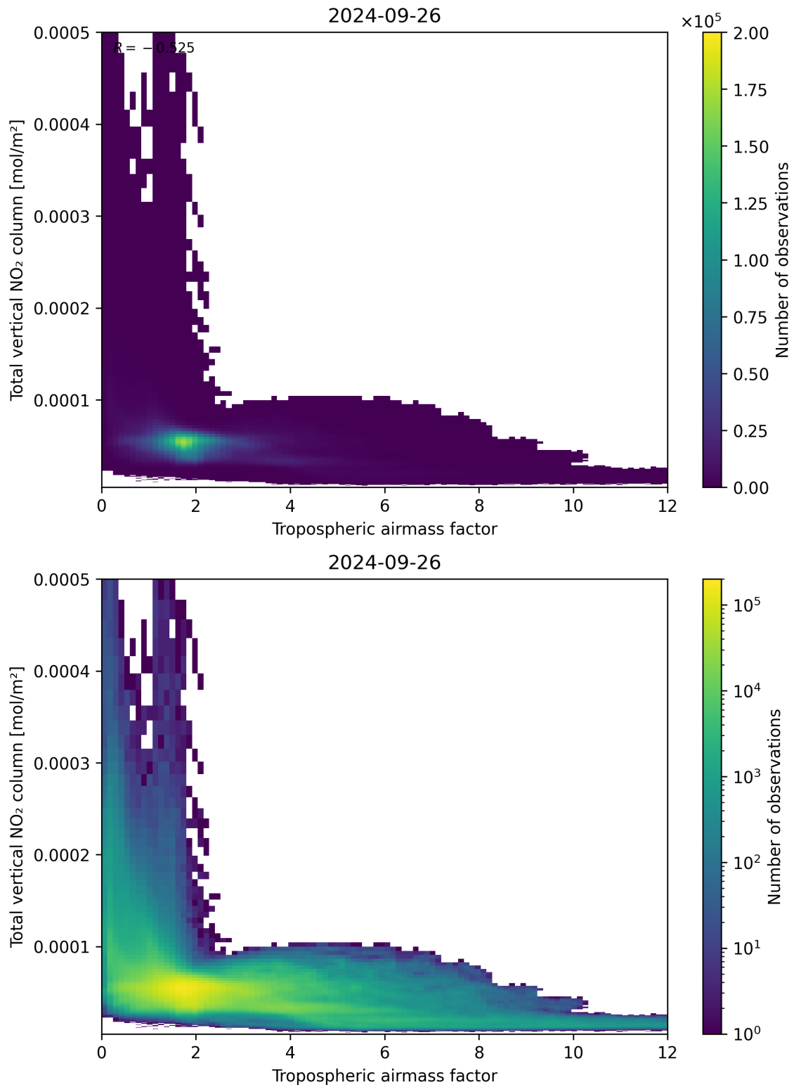
Figure 77: Scatter density plot of “Tropospheric airmass factor” against “Total vertical NO 2 column” for 2024-09-25 to 2024-09-27.
