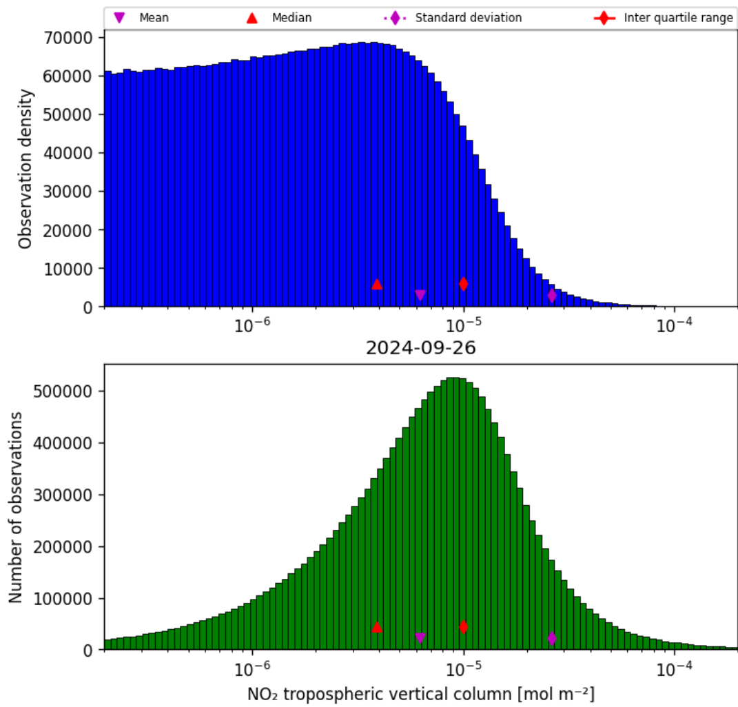
Figure 29: Histogram of “NO 2 tropospheric vertical column” for 2024-09-25 to 2024-09-27
