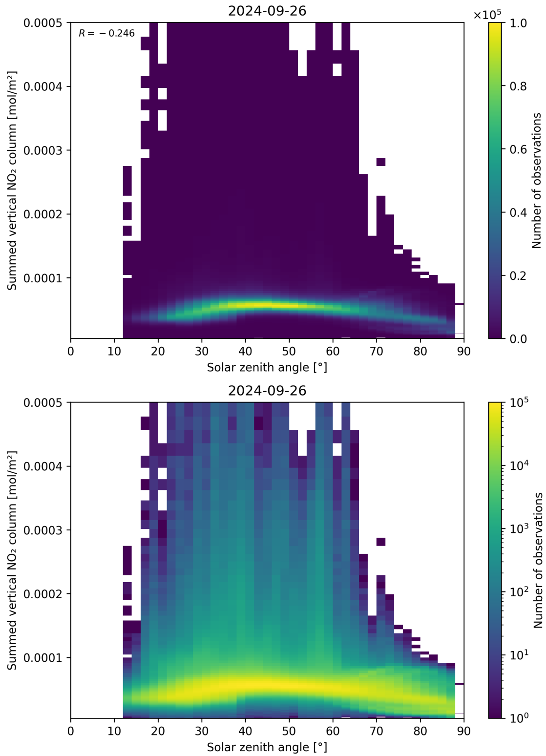
Figure 151: Scatter density plot of “Solar zenith angle” against “Summed vertical NO 2 column” for 2024-09-25 to 2024-09-27.
