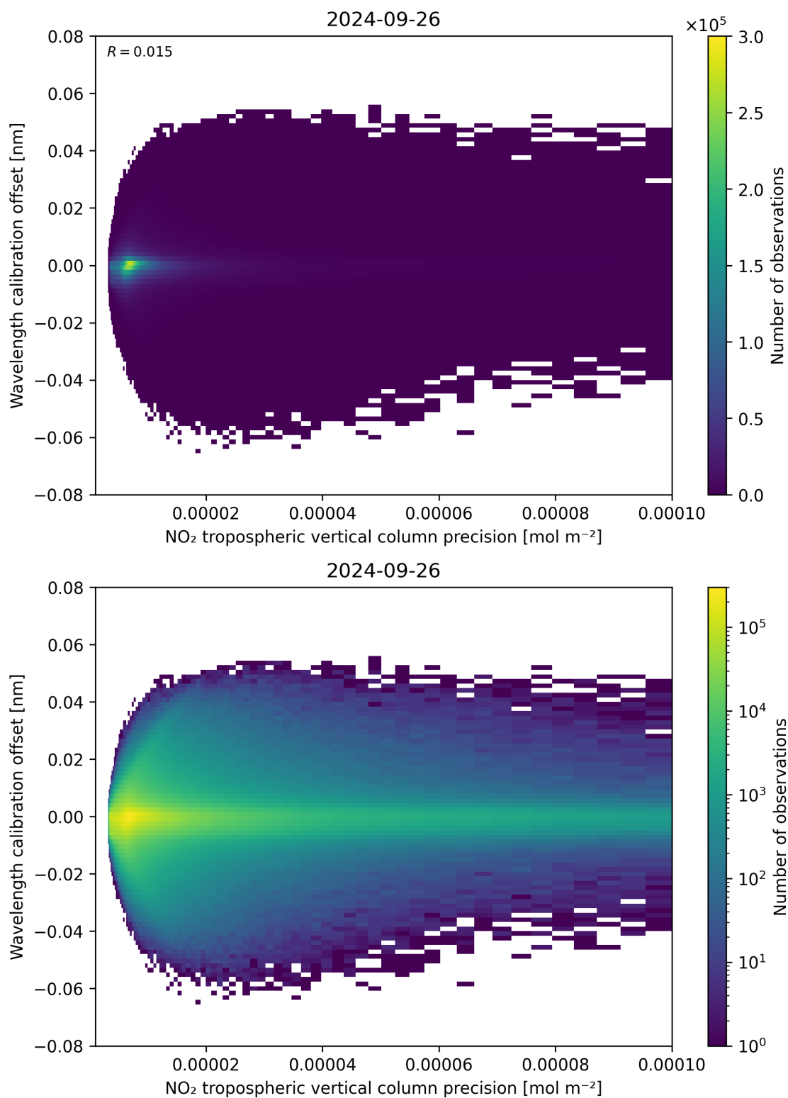
Figure 141: Scatter density plot of “NO 2 tropospheric vertical column precision” against “Wavelength calibration offset” for 2024-09-25 to 2024-09-27.
