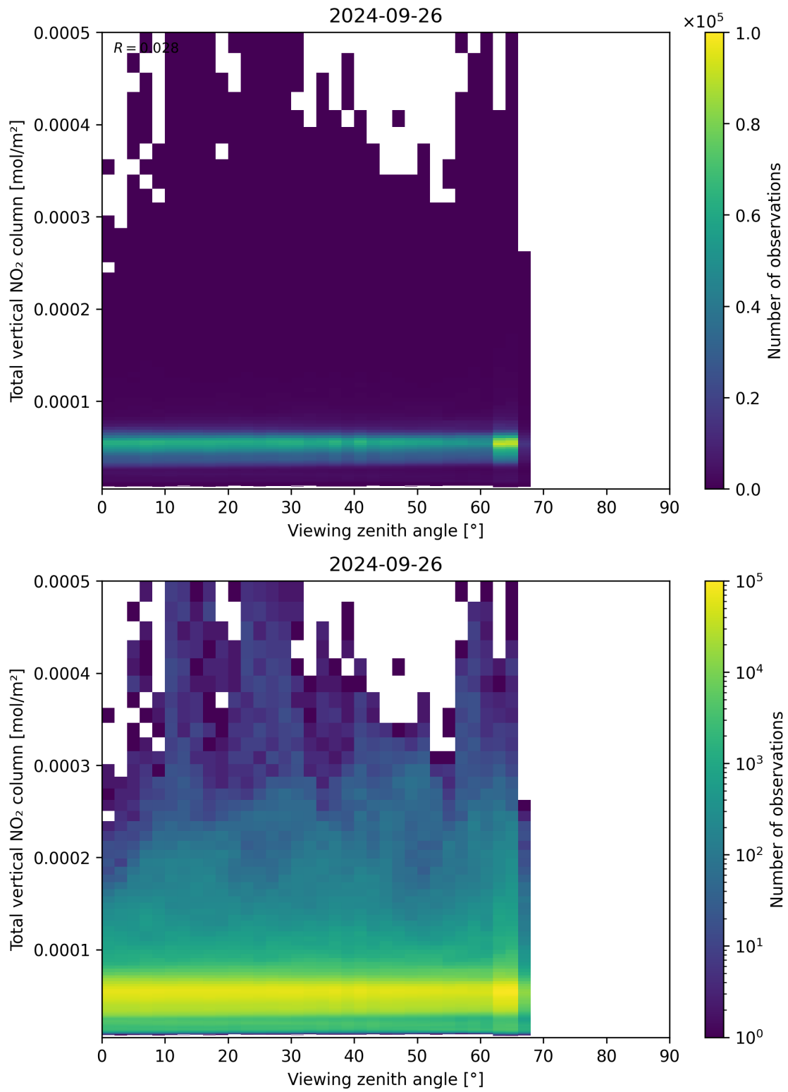
Figure 167: Scatter density plot of “Viewing zenith angle” against “Total vertical NO 2 column” for 2024-09-25 to 2024-09-27.
