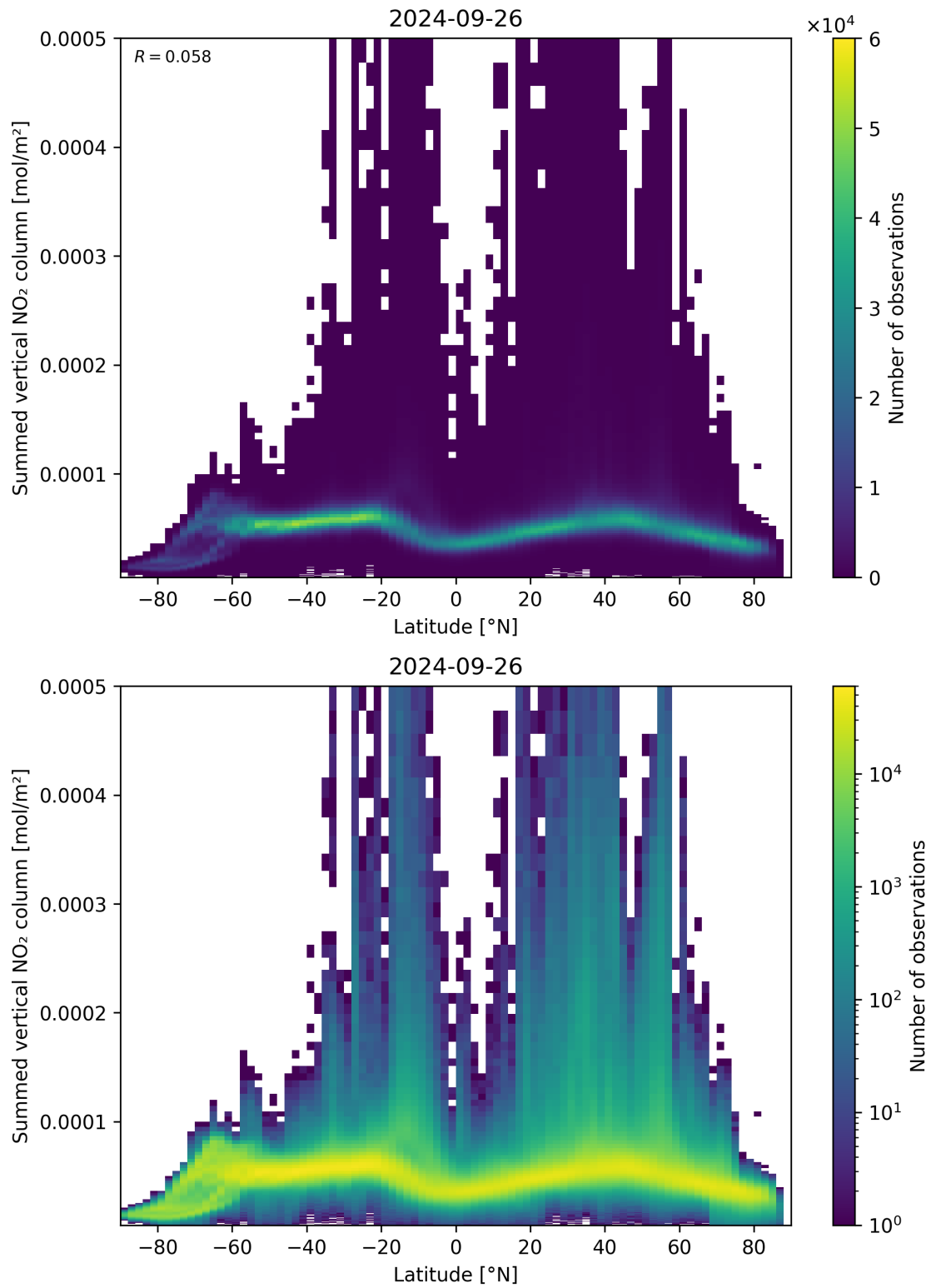
Figure 88: Scatter density plot of “Latitude” against “Summed vertical NO 2 column” for 2024-09-25 to 2024-09-27.
