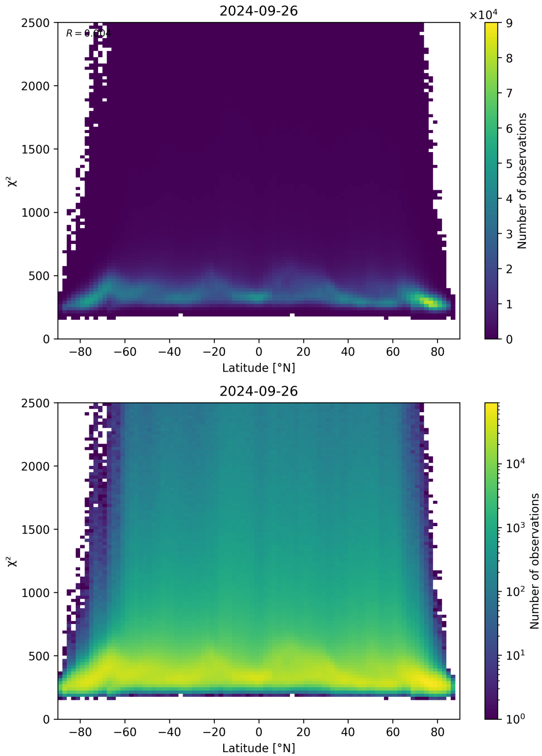
Figure 86: Scatter density plot of “Latitude” against “ \chi^2 ” for 2024-09-25 to 2024-09-27.
