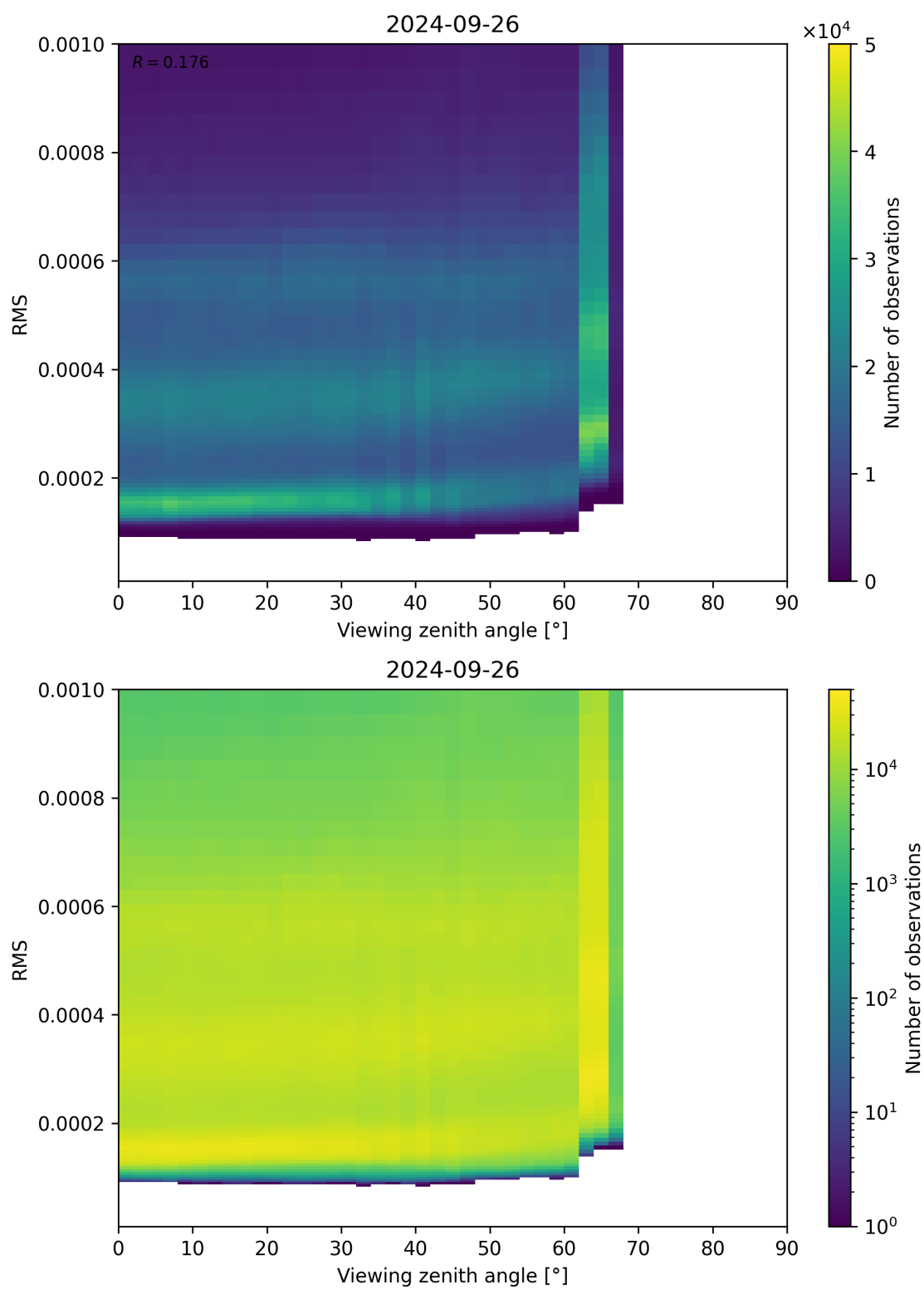
Figure 171: Scatter density plot of “Viewing zenith angle” against “RMS” for 2024-09-25 to 2024-09-27.
