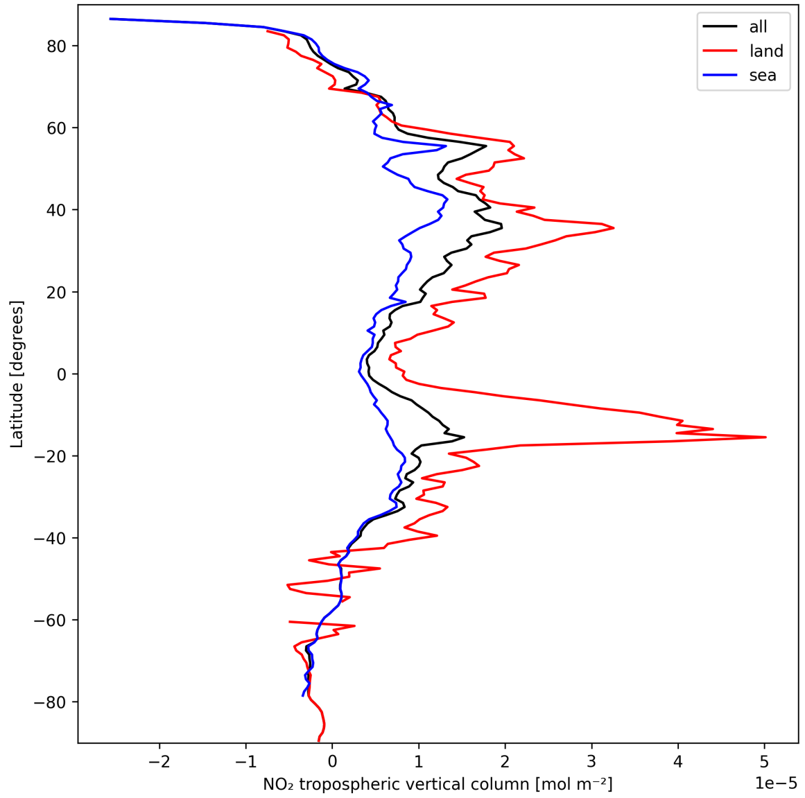
Figure 12: Zonal average of “NO 2 tropospheric vertical column” for 2024-09-25 to 2024-09-27.
