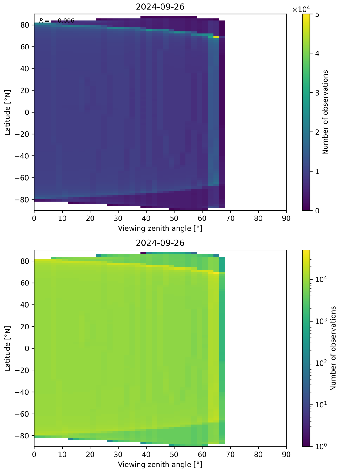
Figure 163: Scatter density plot of “Viewing zenith angle” against “Latitude” for 2024-09-25 to 2024-09-27.
