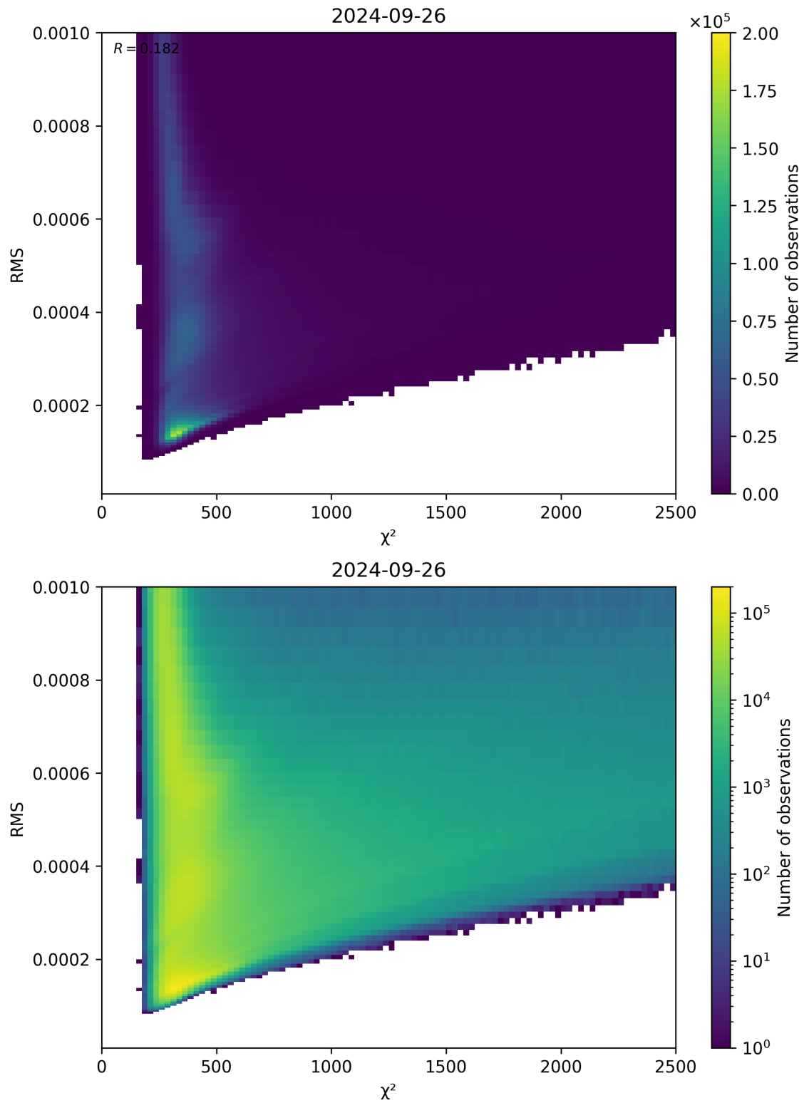
Figure 82: Scatter density plot of “ \chi^2 ” against “RMS” for 2024-09-25 to 2024-09-27.
