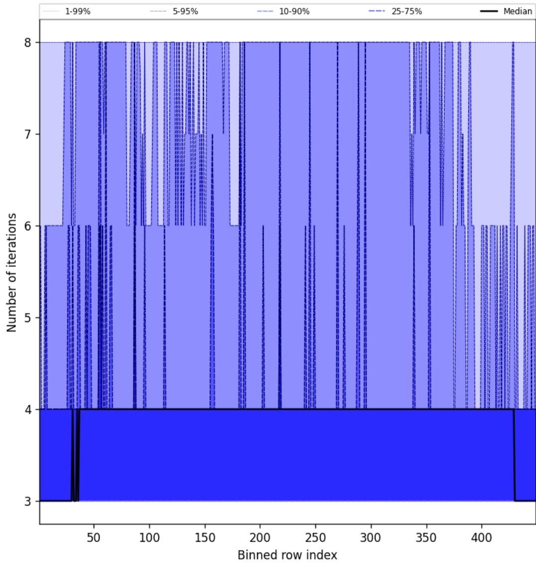
Figure 51: Along track statistics of “Number of iterations” for 2024-09-25 to 2024-09-27
