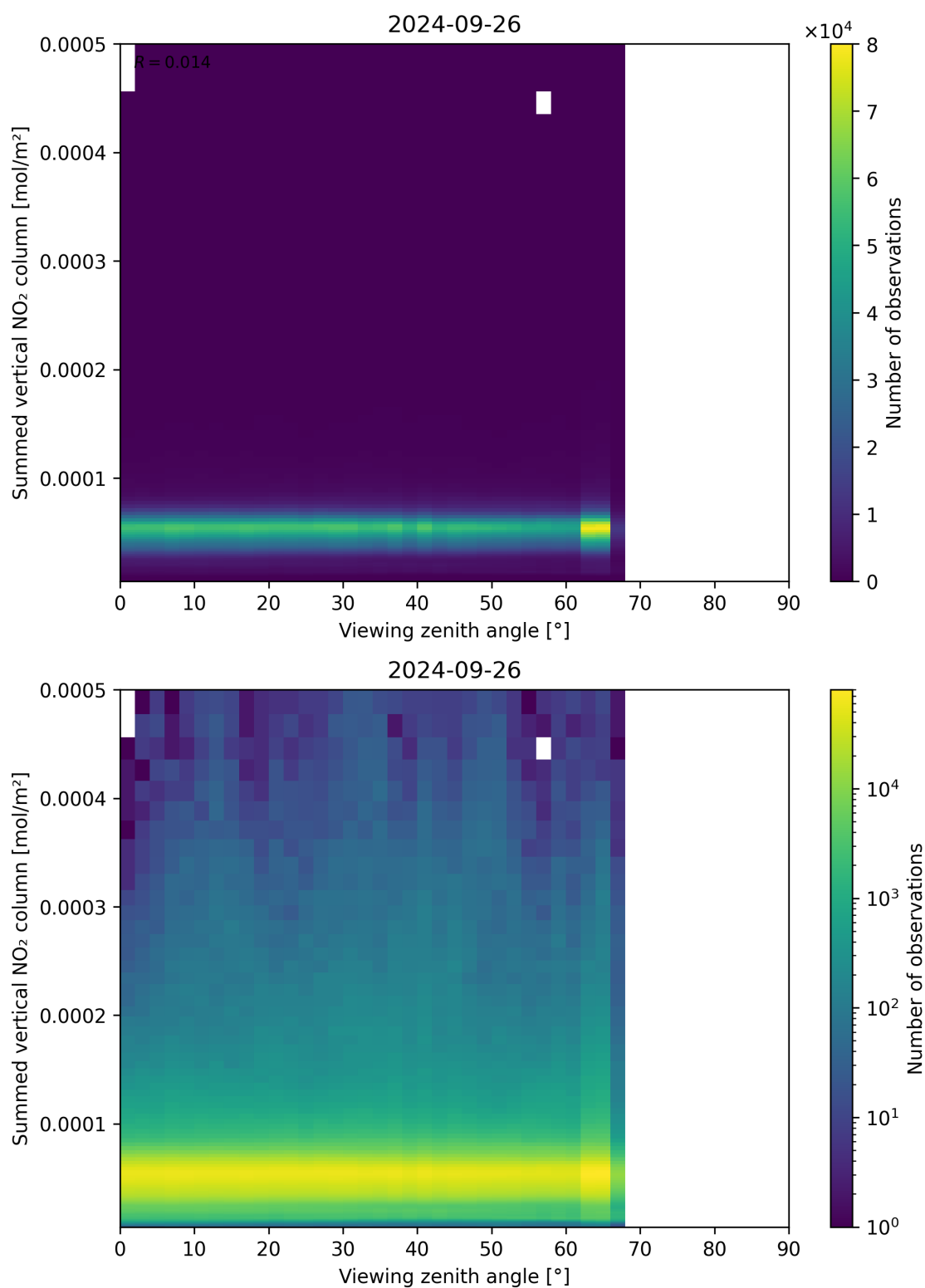
Figure 165: Scatter density plot of “Viewing zenith angle” against “Summed vertical NO 2 column” for 2024-09-25 to 2024-09-27.
