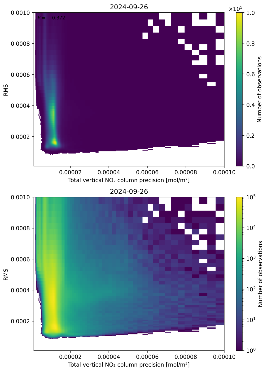
Figure 119: Scatter density plot of “Total vertical NO 2 column precision” against “RMS” for 2024-09-25 to 2024-09-27.
