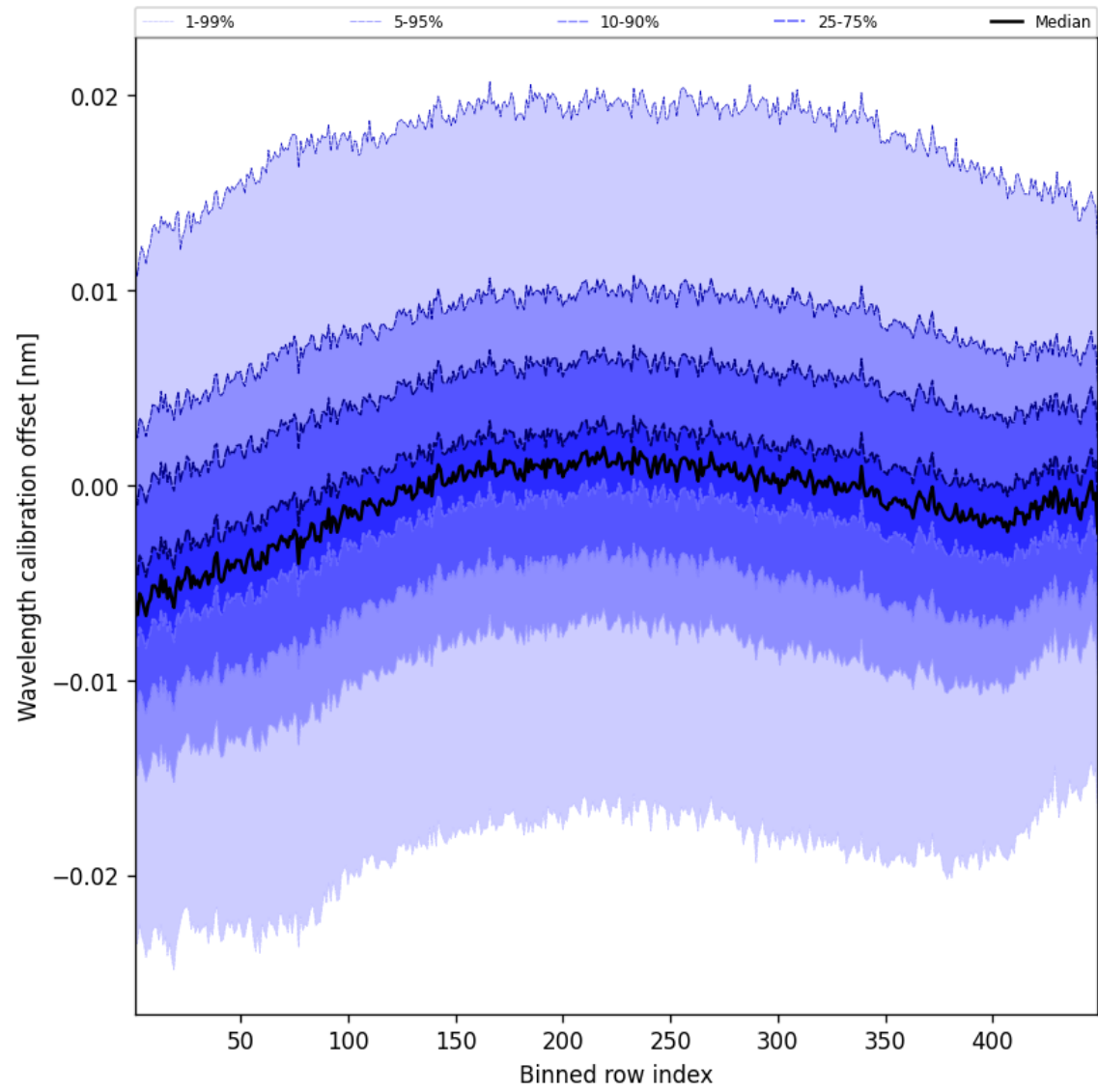
Figure 52: Along track statistics of “Wavelength calibration offset” for 2024-09-25 to 2024-09-27
