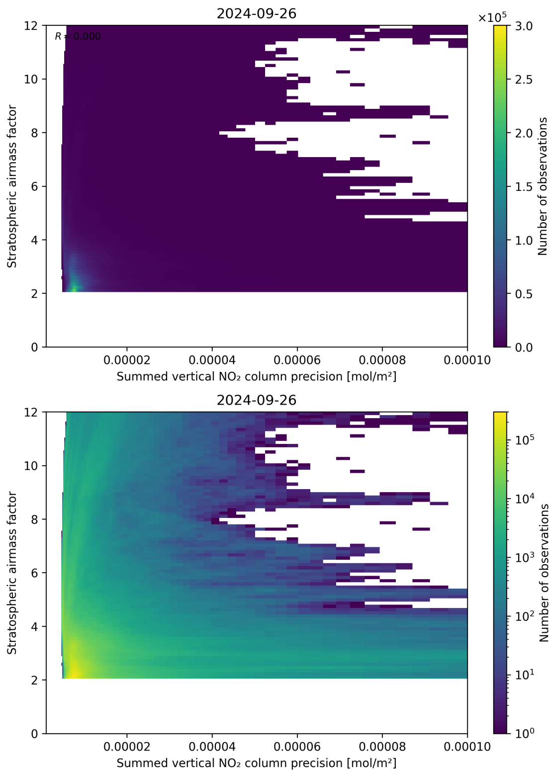
Figure 106: Scatter density plot of “Summed vertical NO 2 column precision” against “Stratospheric airmass factor” for 2024-09-25 to 2024-09-27.
