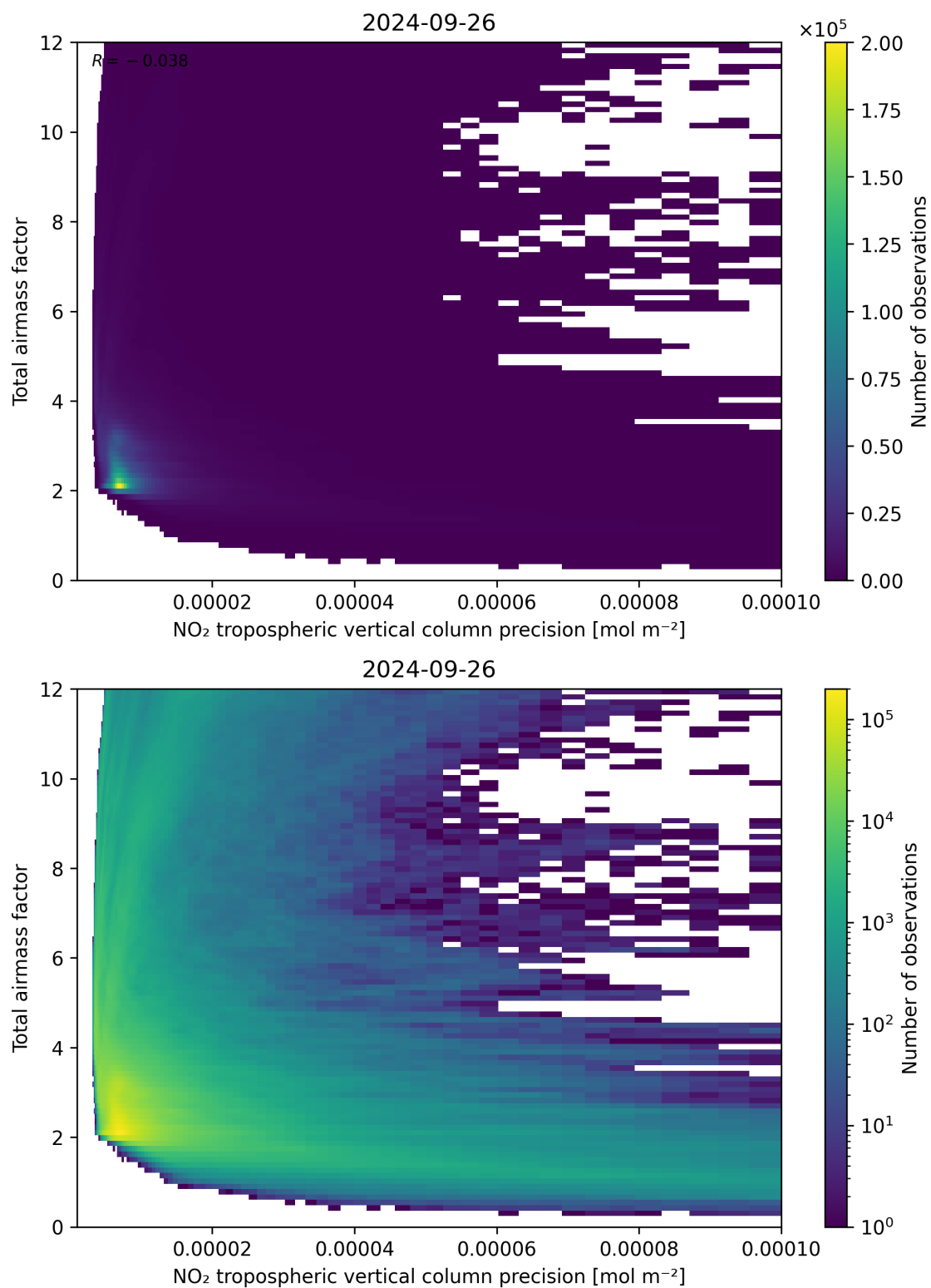
Figure 132: Scatter density plot of “NO 2 tropospheric vertical column precision” against “Total air mass factor” for 2024-09-25 to 2024-09-27.
