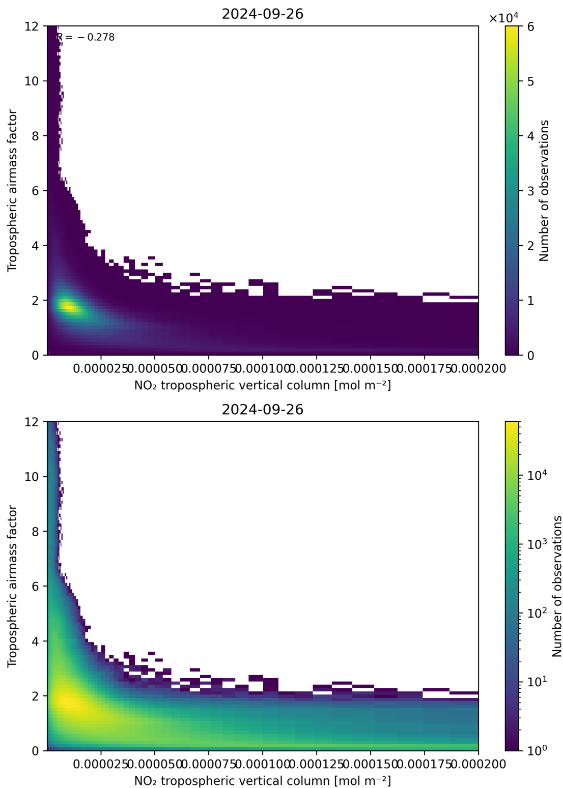
Figure 123: Scatter density plot of “NO 2 tropospheric vertical column” against “Tropospheric air mass factor” for 2024-09-25 to 2024-09-27.
