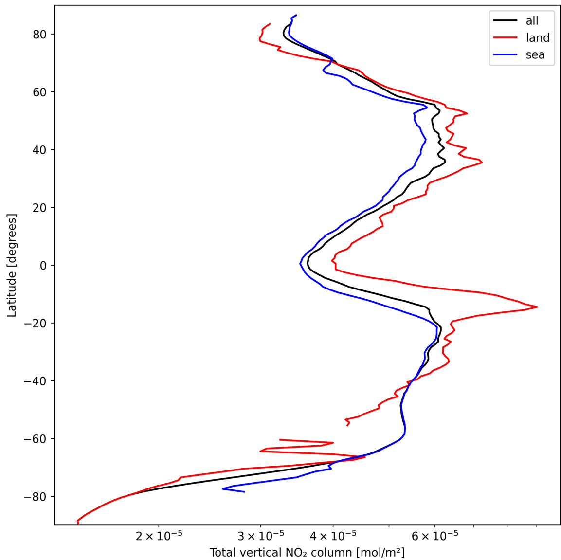
Figure 21: Zonal average of “Total vertical NO 2 column” for 2024-09-25 to 2024-09-27.
