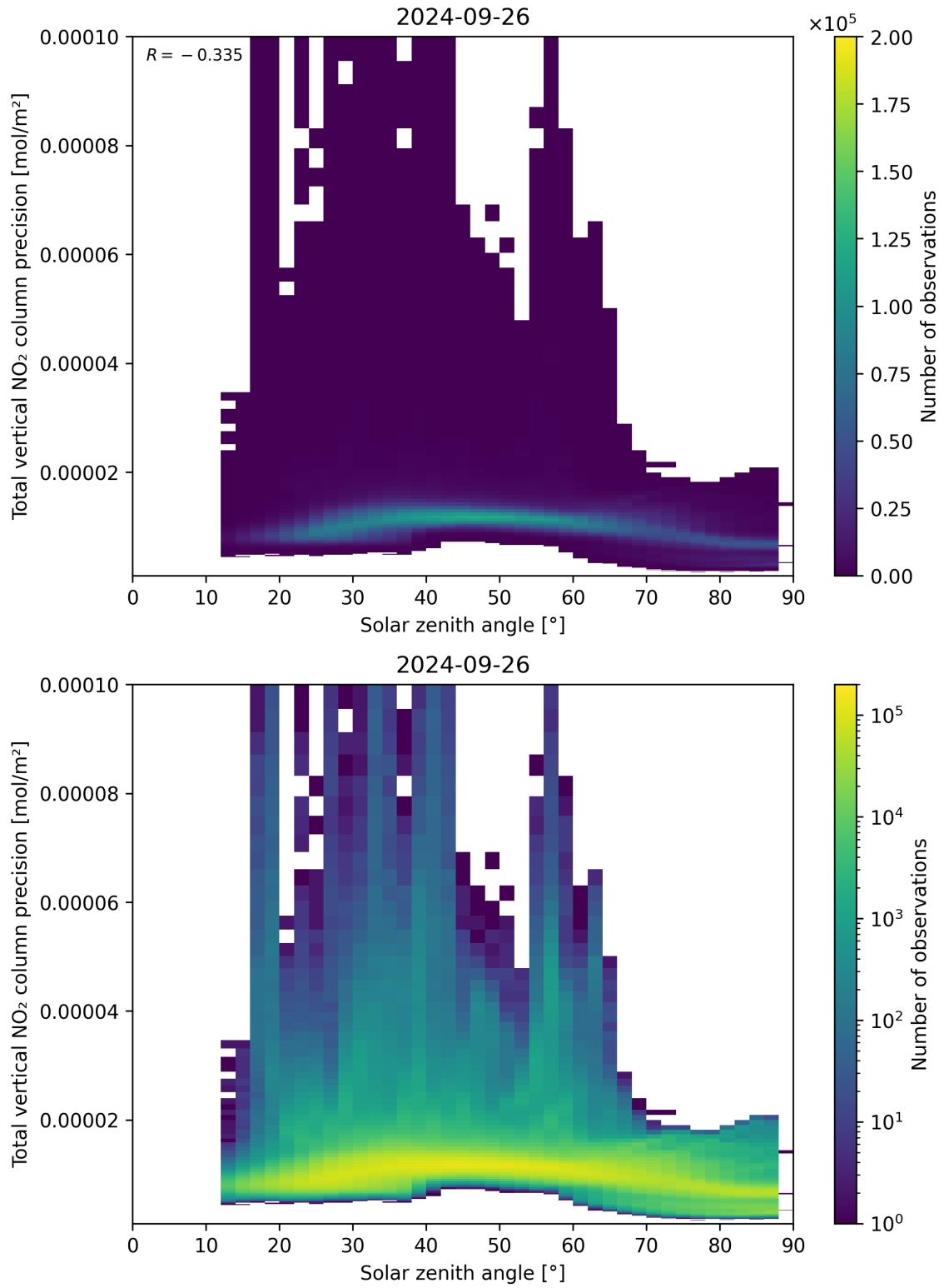
Figure 154: Scatter density plot of “Solar zenith angle” against “Total vertical NO 2 column precision” for 2024-09-25 to 2024-09-27.
