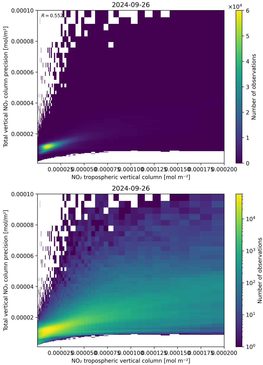
Figure 129: Scatter density plot of “NO 2 tropospheric vertical column” against “Total vertical NO 2 column precision” for 2024-09-25 to 2024-09-27.
