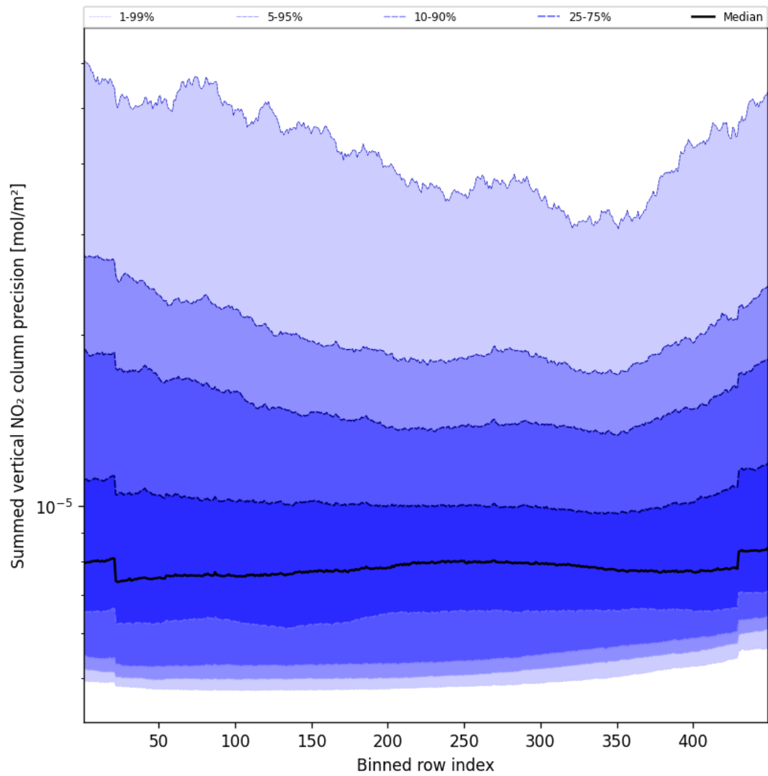
Figure 58: Along track statistics of “Summed vertical NO 2 column precision” for 2024-09-25 to 2024-09-27
