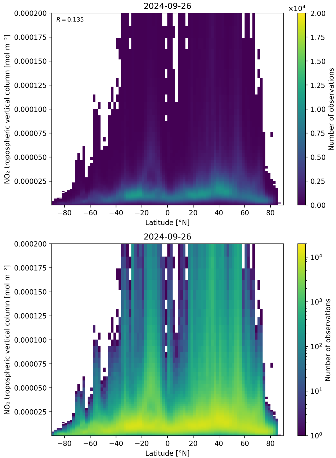
Figure 92: Scatter density plot of “Latitude” against “NO 2 tropospheric vertical column” for 2024-09-25 to 2024-09-27.
