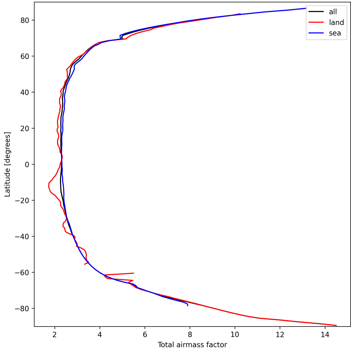
Figure 15: Zonal average of “Total airmass factor” for 2024-09-25 to 2024-09-27.
