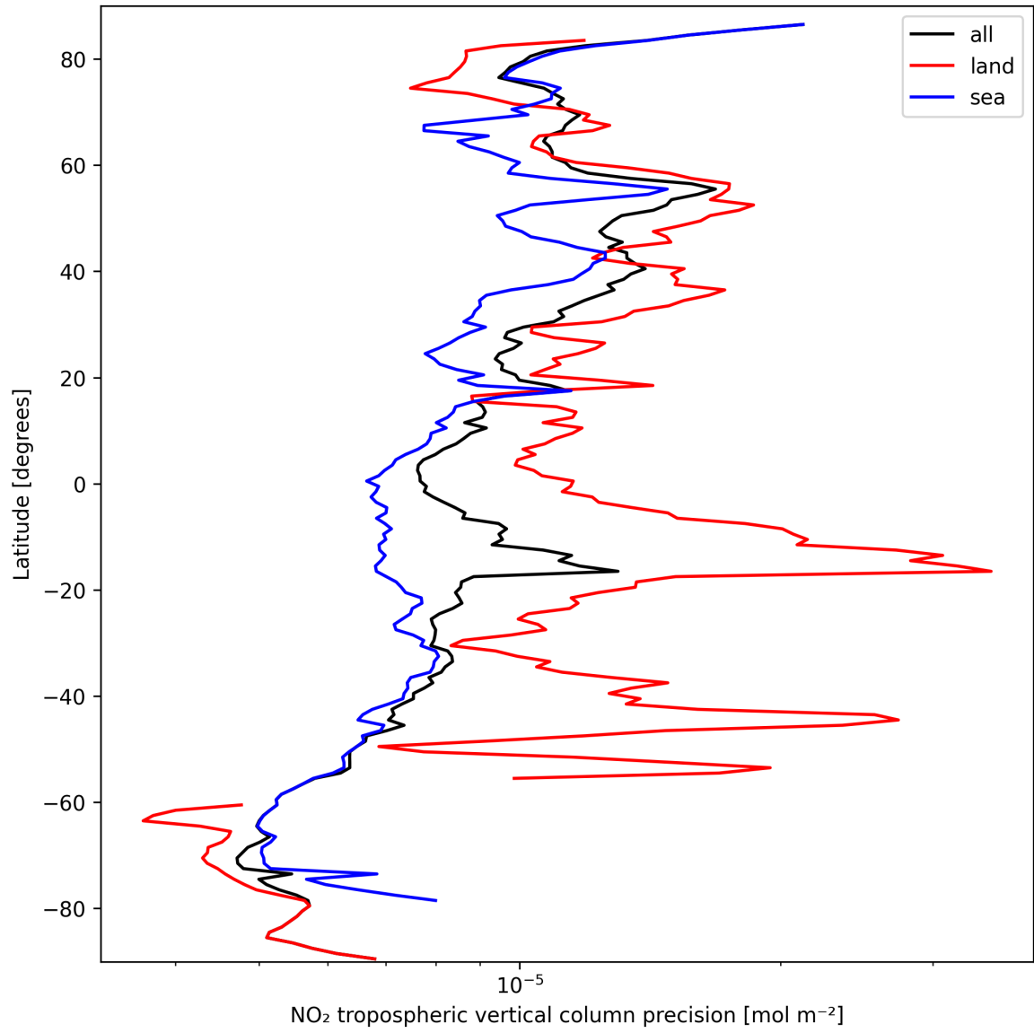
Figure 13: Zonal average of “NO 2 tropospheric vertical column precision” for 2024-09-25 to 2024-09-27.
