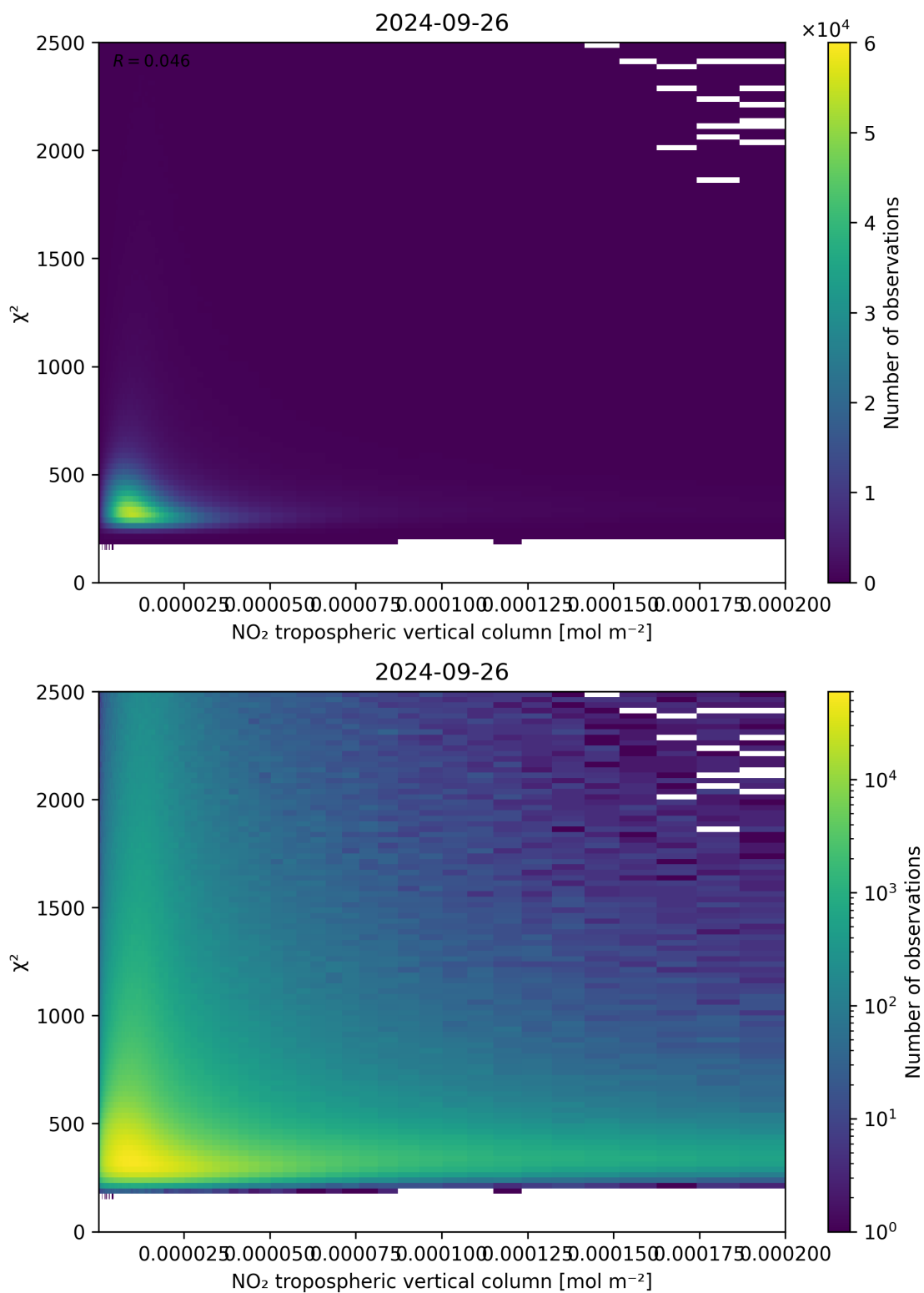
Figure 124: Scatter density plot of “NO 2 tropospheric vertical column” against “ \chi^2 ” for 2024-09-25 to 2024-09-27.
