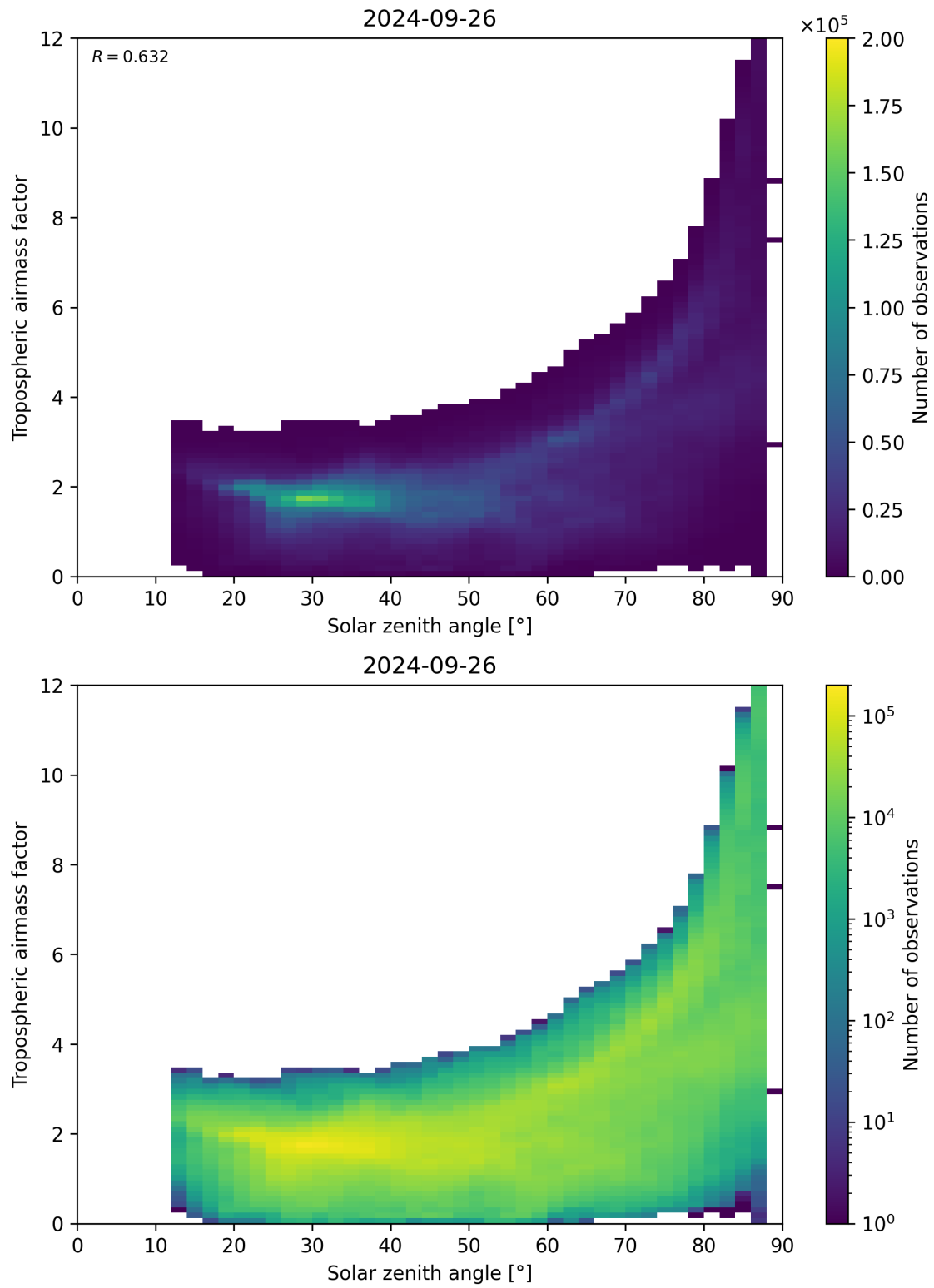
Figure 147: Scatter density plot of “Solar zenith angle” against “Tropospheric airmass factor” for 2024-09-25 to 2024-09-27.
