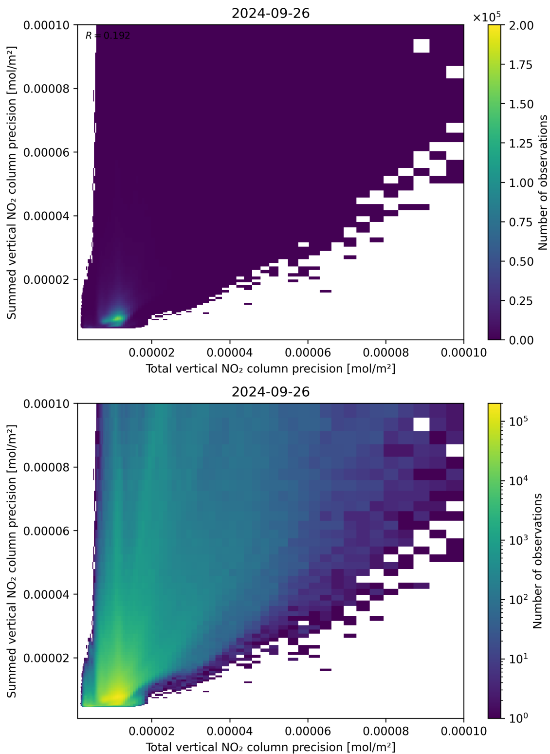
Figure 118: Scatter density plot of “Total vertical NO 2 column precision” against “Summed vertical NO 2 column precision” for 2024-09-25 to 2024-09-27.
