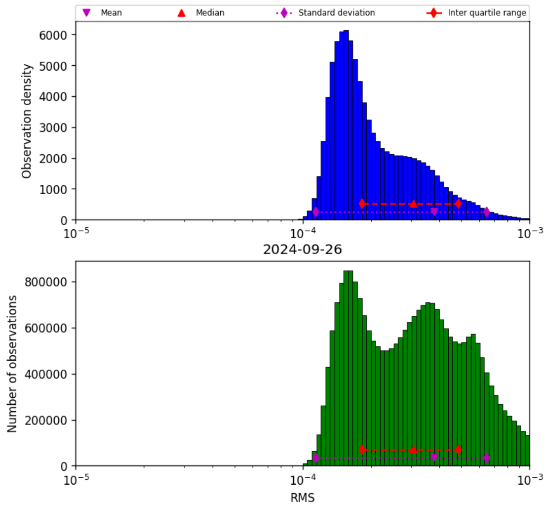
Figure 43: Histogram of “RMS” for 2024-09-25 to 2024-09-27
