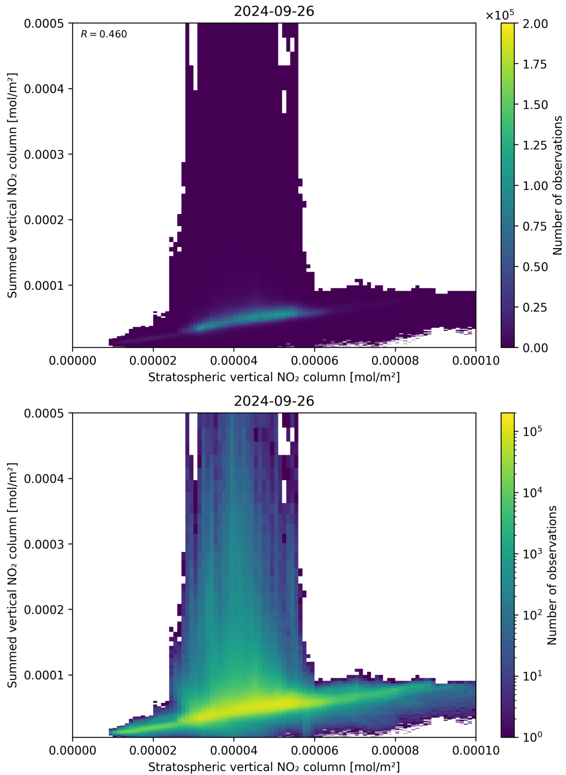
Figure 98: Scatter density plot of “Stratospheric vertical NO 2 column” against “Summed vertical NO 2 column” for 2024-09-25 to 2024-09-27.
