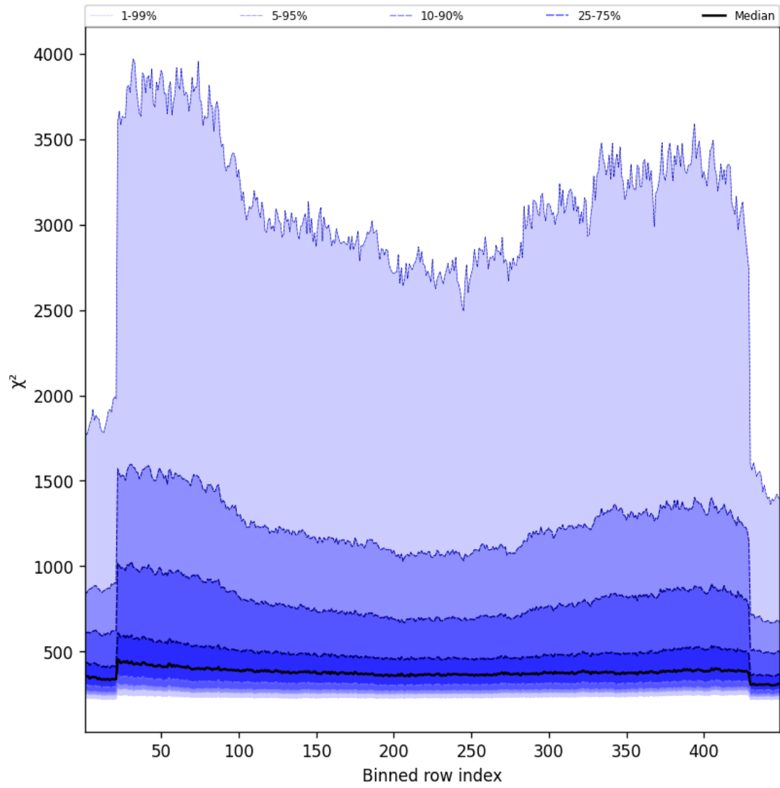
Figure 59: Along track statistics of “ \chi^2 ” for 2024-09-25 to 2024-09-27
