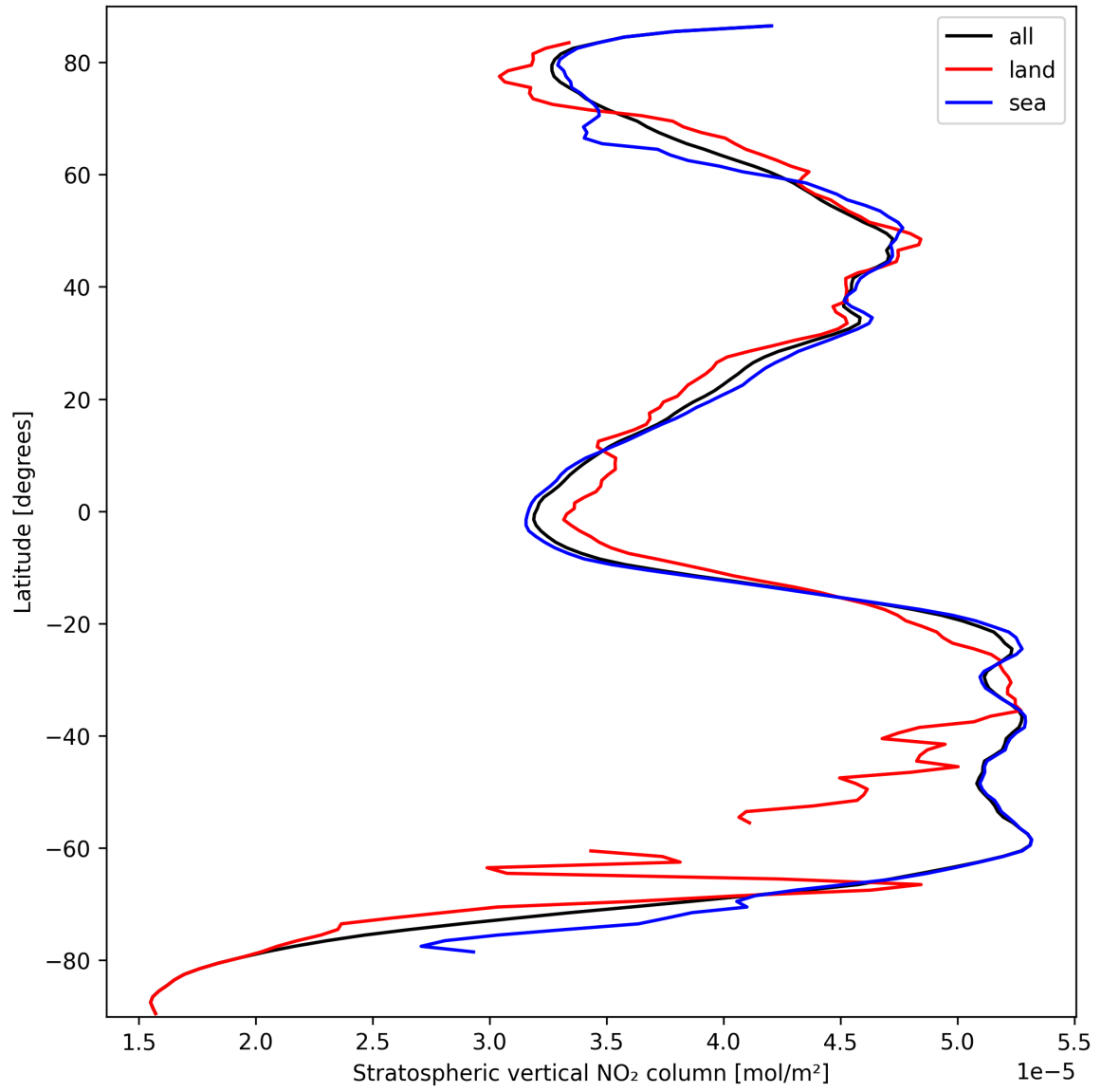
Figure 19: Zonal average of “Stratospheric vertical NO 2 column” for 2024-09-25 to 2024-09-27.
