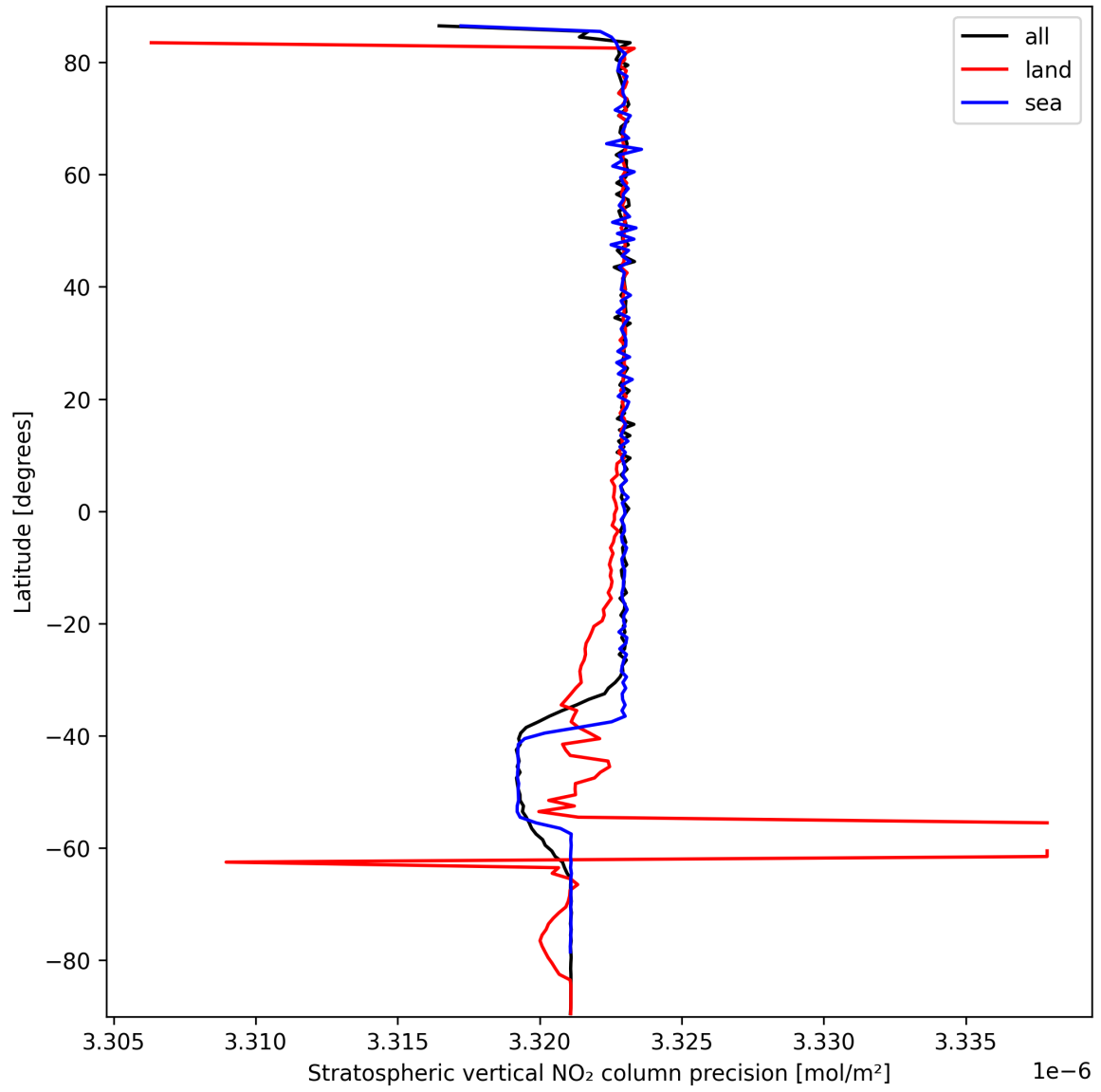
Figure 20: Zonal average of “Stratospheric vertical NO 2 column precision” for 2024-09-25 to 2024-09-27.
