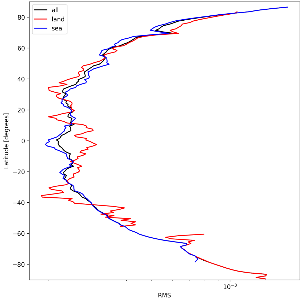
Figure 26: Zonal average of “RMS” for 2024-09-25 to 2024-09-27.
