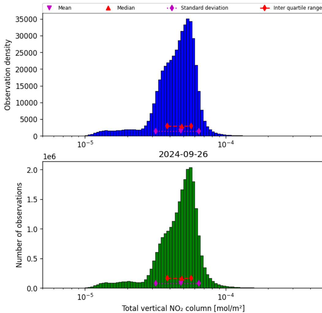
Figure 38: Histogram of “Total vertical NO 2 column” for 2024-09-25 to 2024-09-27
