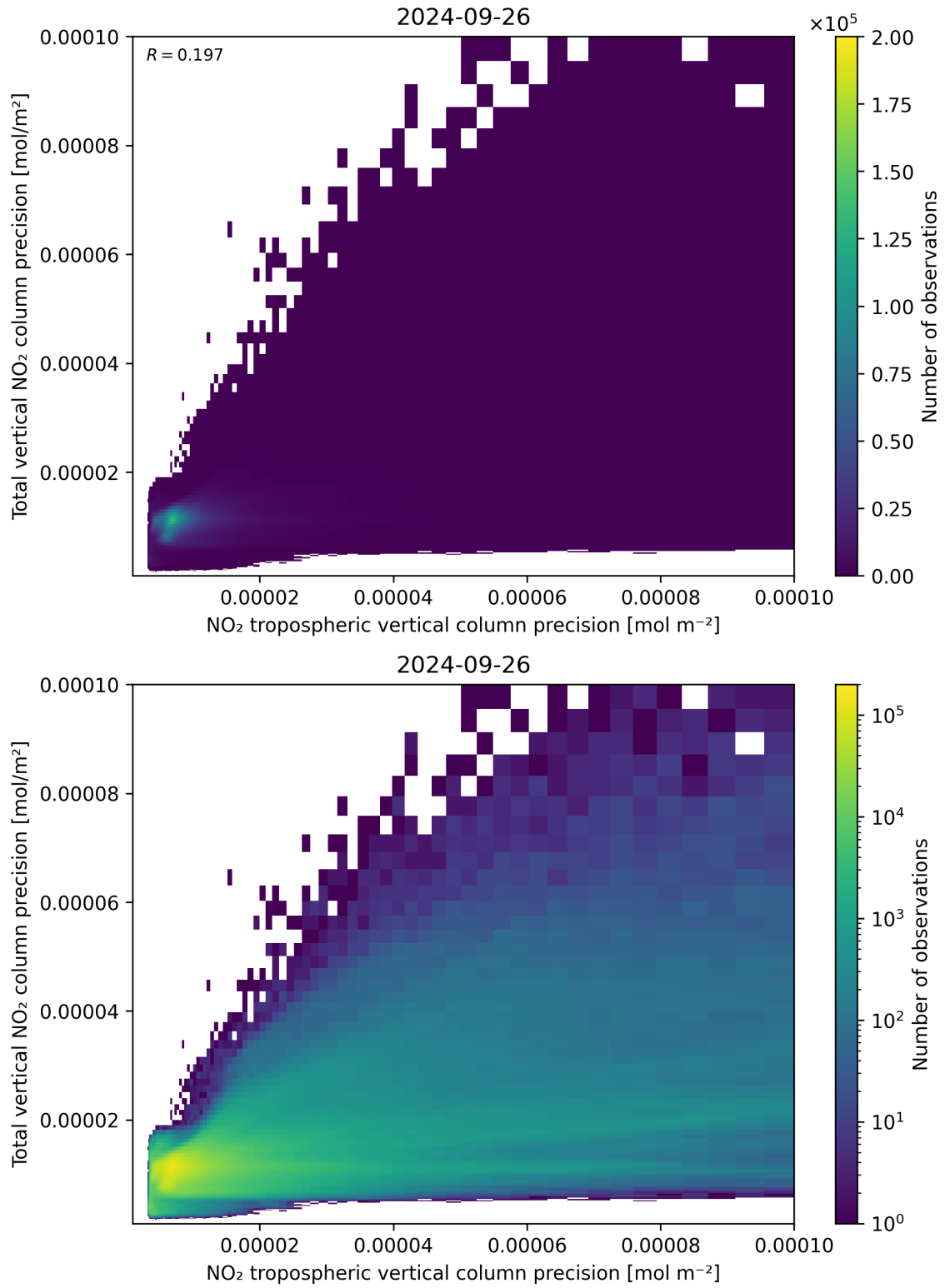
Figure 139: Scatter density plot of “NO 2 tropospheric vertical column precision” against “Total vertical NO 2 column precision” for 2024-09-25 to 2024-09-27.
