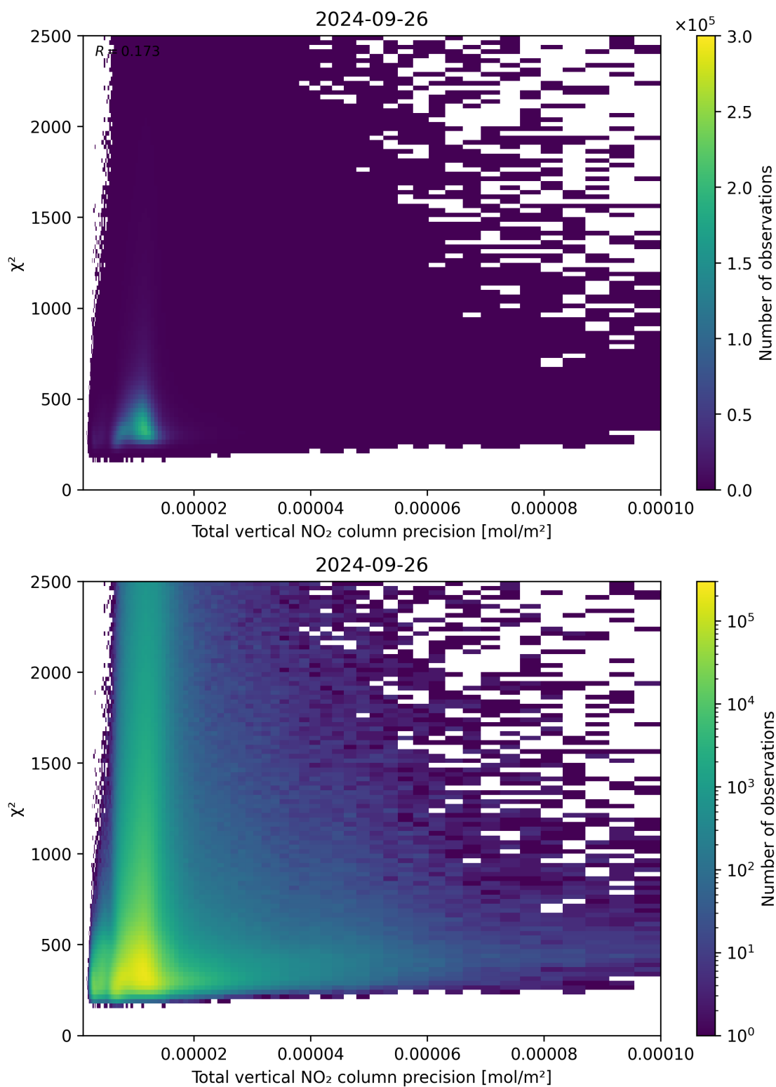
Figure 116: Scatter density plot of “Total vertical NO 2 column precision” against “ \chi^2 ” for 2024-09-25 to 2024-09-27.
