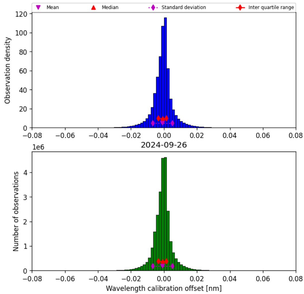
Figure 35: Histogram of “Wavelength calibration offset” for 2024-09-25 to 2024-09-27
