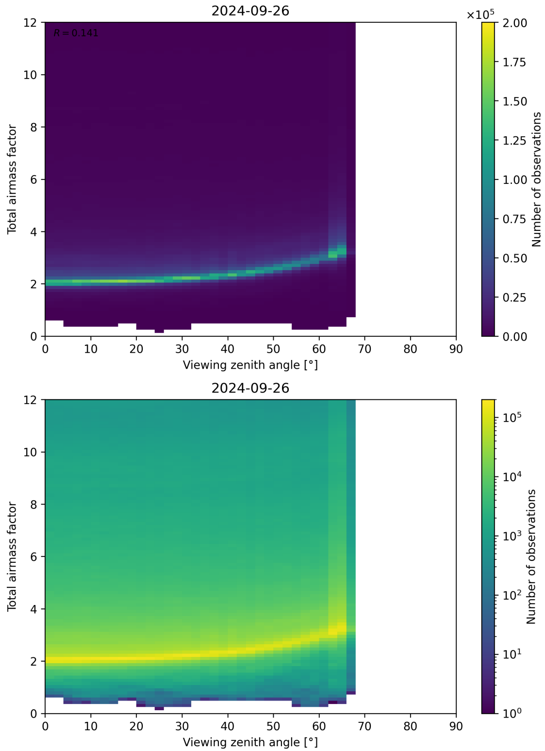
Figure 160: Scatter density plot of “Viewing zenith angle” against “Total airmass factor” for 2024-09-25 to 2024-09-27.
