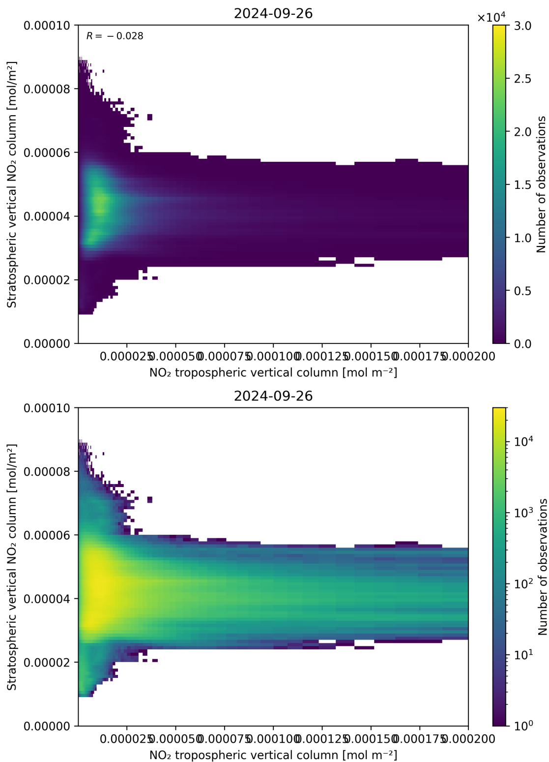
Figure 125: Scatter density plot of “NO 2 tropospheric vertical column” against “Stratospheric vertical NO 2 column” for 2024-09-25 to 2024-09-27.
