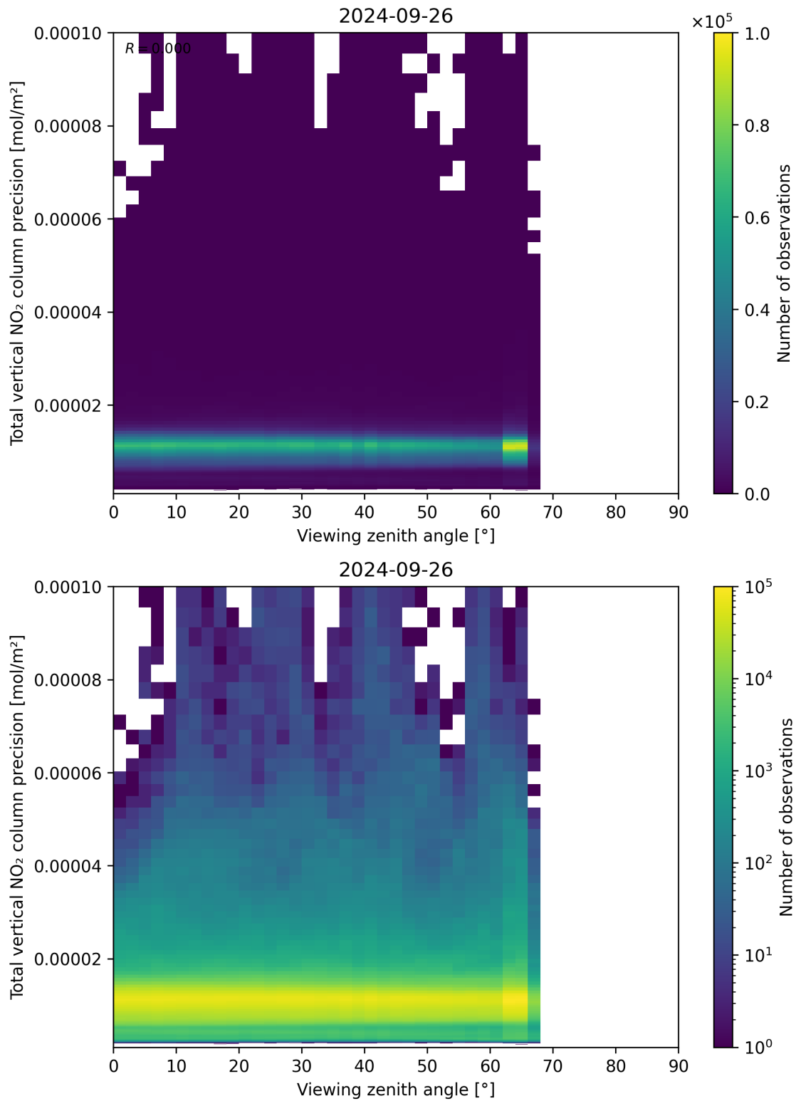
Figure 168: Scatter density plot of “Viewing zenith angle” against “Total vertical NO 2 column precision” for 2024-09-25 to 2024-09-27.
