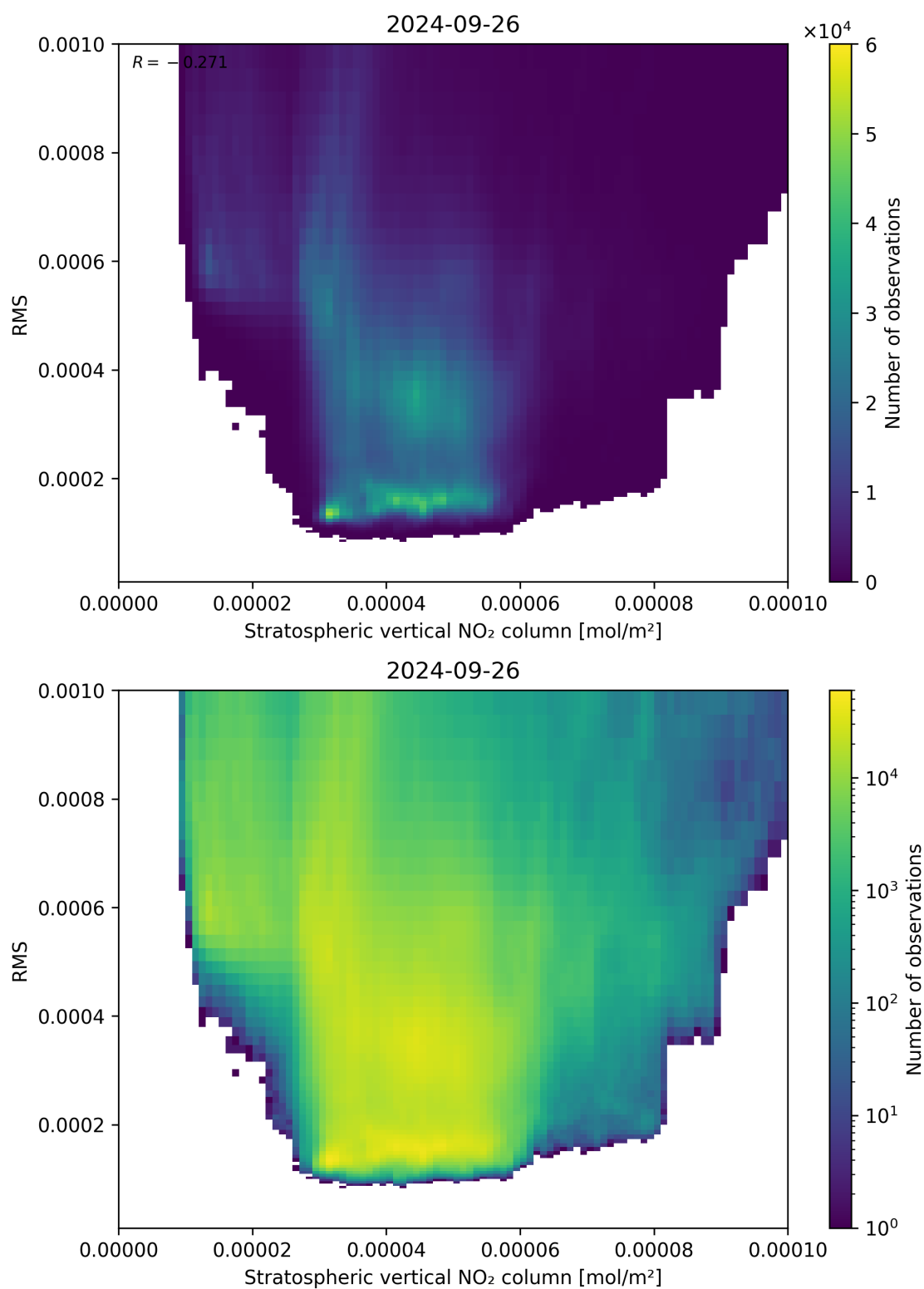
Figure 102: Scatter density plot of “Stratospheric vertical NO 2 column” against “RMS” for 2024-09-25 to 2024-09-27.
