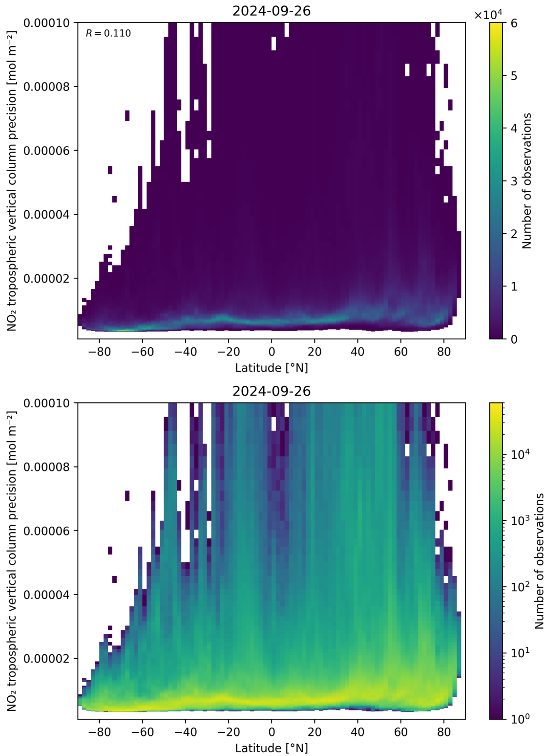
Figure 93: Scatter density plot of “Latitude” against “NO 2 tropospheric vertical column precision” for 2024-09-25 to 2024-09-27.
