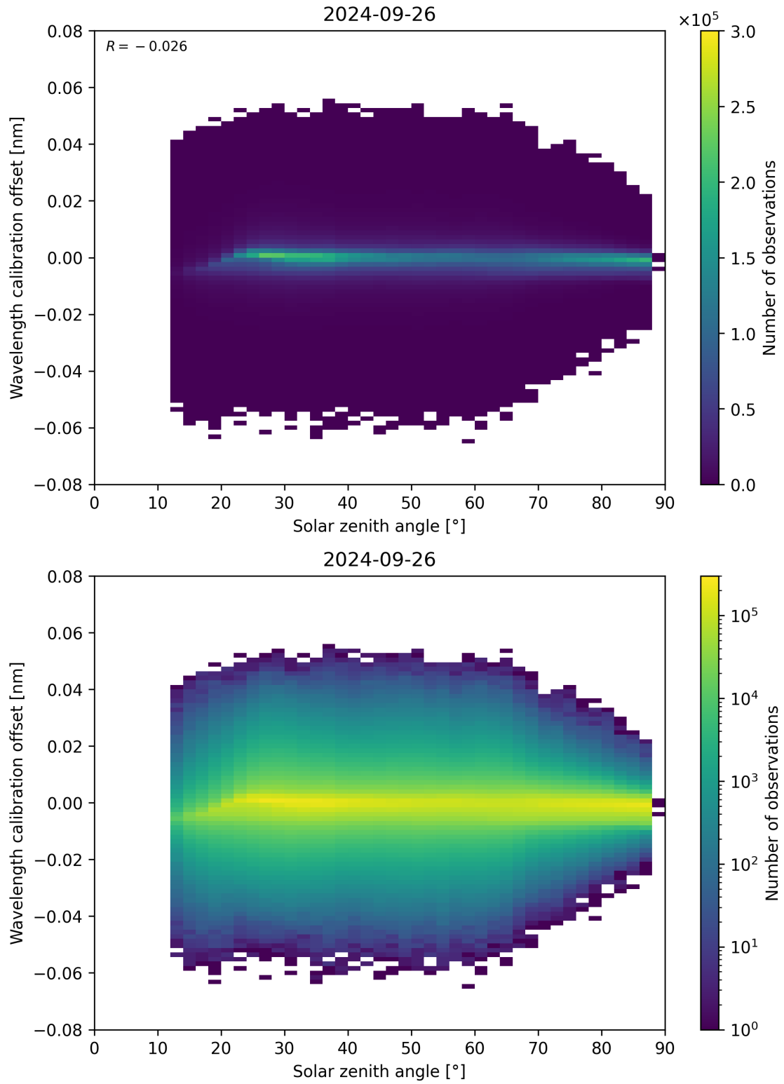
Figure 158: Scatter density plot of “Solar zenith angle” against “Wavelength calibration offset” for 2024-09-25 to 2024-09-27.
