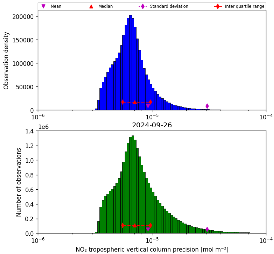
Figure 30: Histogram of “NO 2 tropospheric vertical column precision” for 2024-09-25 to 2024-09-27
