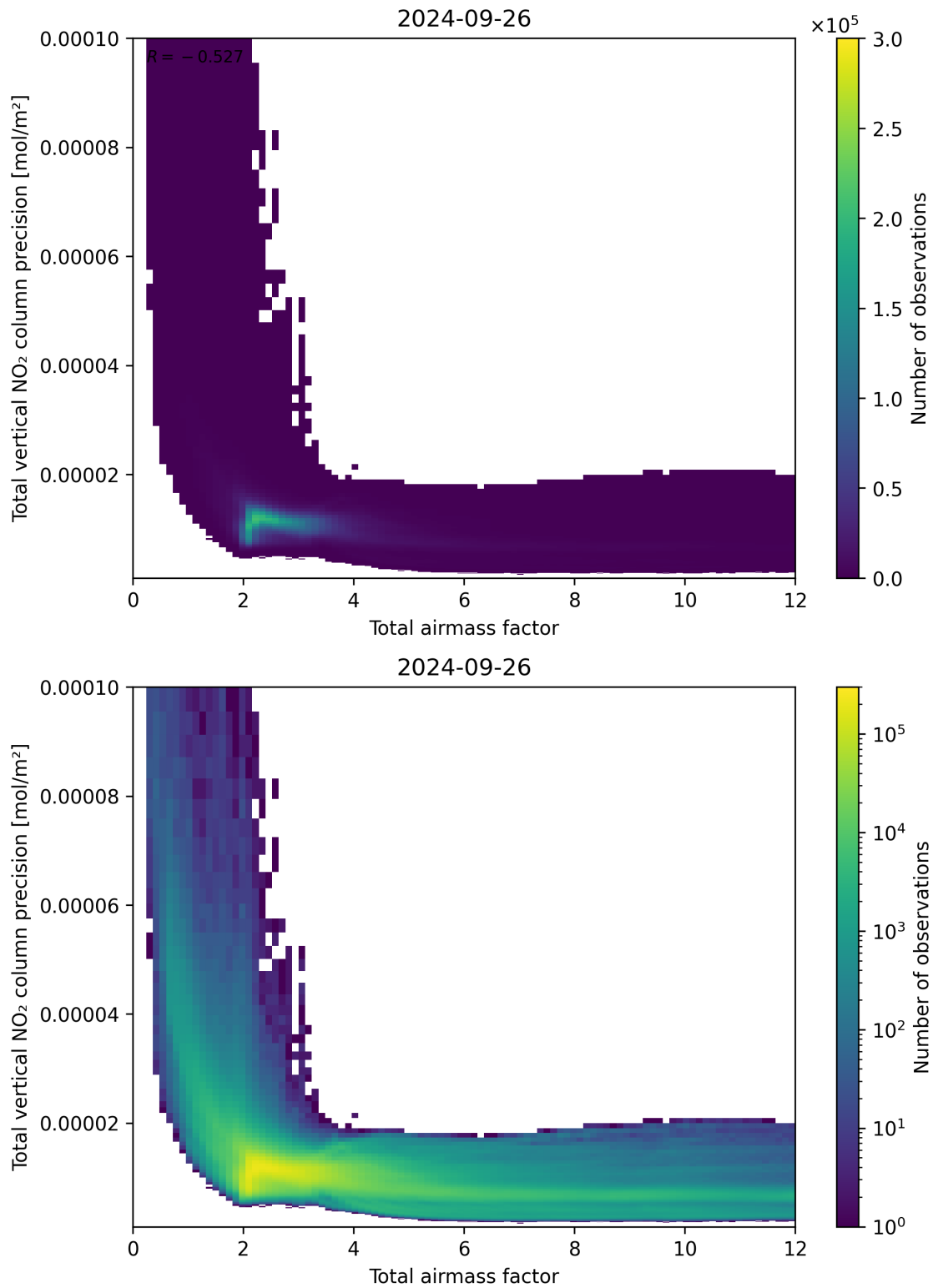
Figure 68: Scatter density plot of “Total airmass factor” against “Total vertical NO 2 column precision” for 2024-09-25 to 2024-09-27.
