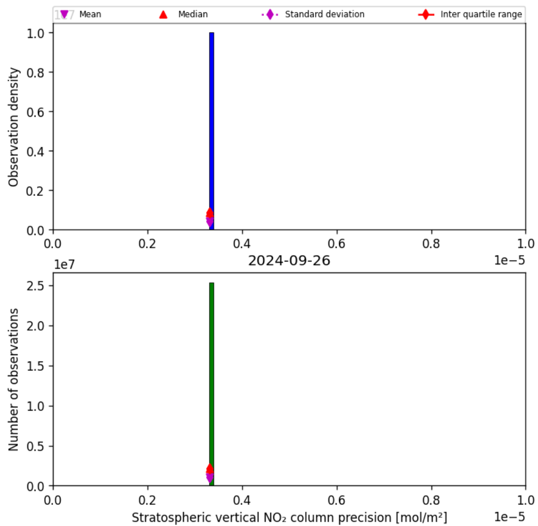
Figure 37: Histogram of “Stratospheric vertical NO 2 column precision” for 2024-09-25 to 2024-09-27
