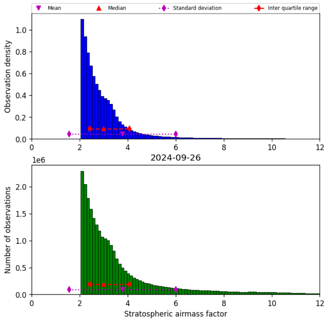
Figure 44: Histogram of “Stratospheric airmass factor” for 2024-09-25 to 2024-09-27
