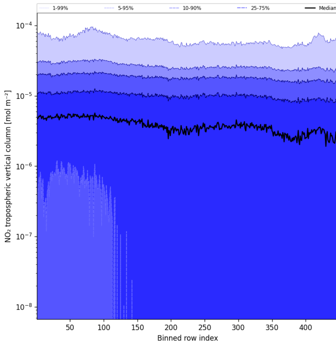
Figure 46: Along track statistics of “NO 2 tropospheric vertical column” for 2024-09-25 to 2024-09-27
