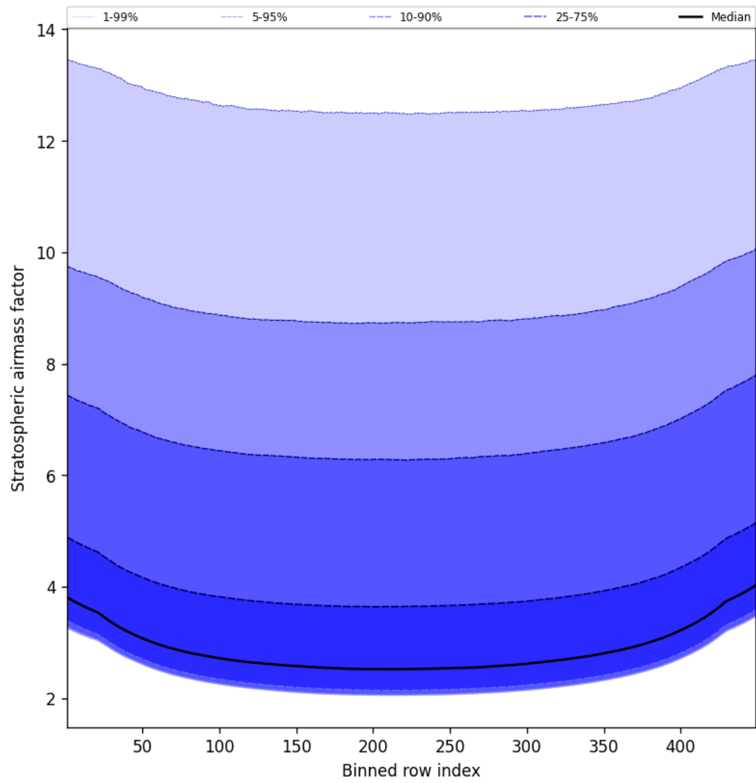
Figure 61: Along track statistics of “Stratospheric airmass factor” for 2024-09-25 to 2024-09-27
