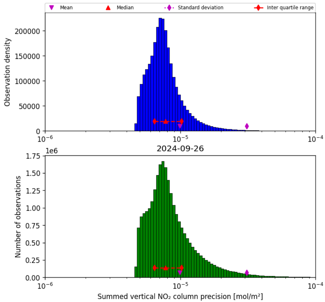
Figure 41: Histogram of "Summed vertical NO 2 column precision" for 2024-09-25 to 2024-09-27
