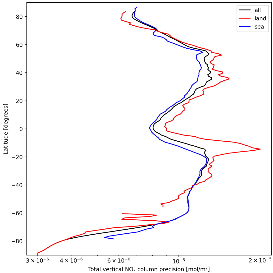
Figure 22: Zonal average of “Total vertical NO 2 column precision” for 2024-09-25 to 2024-09-27.
