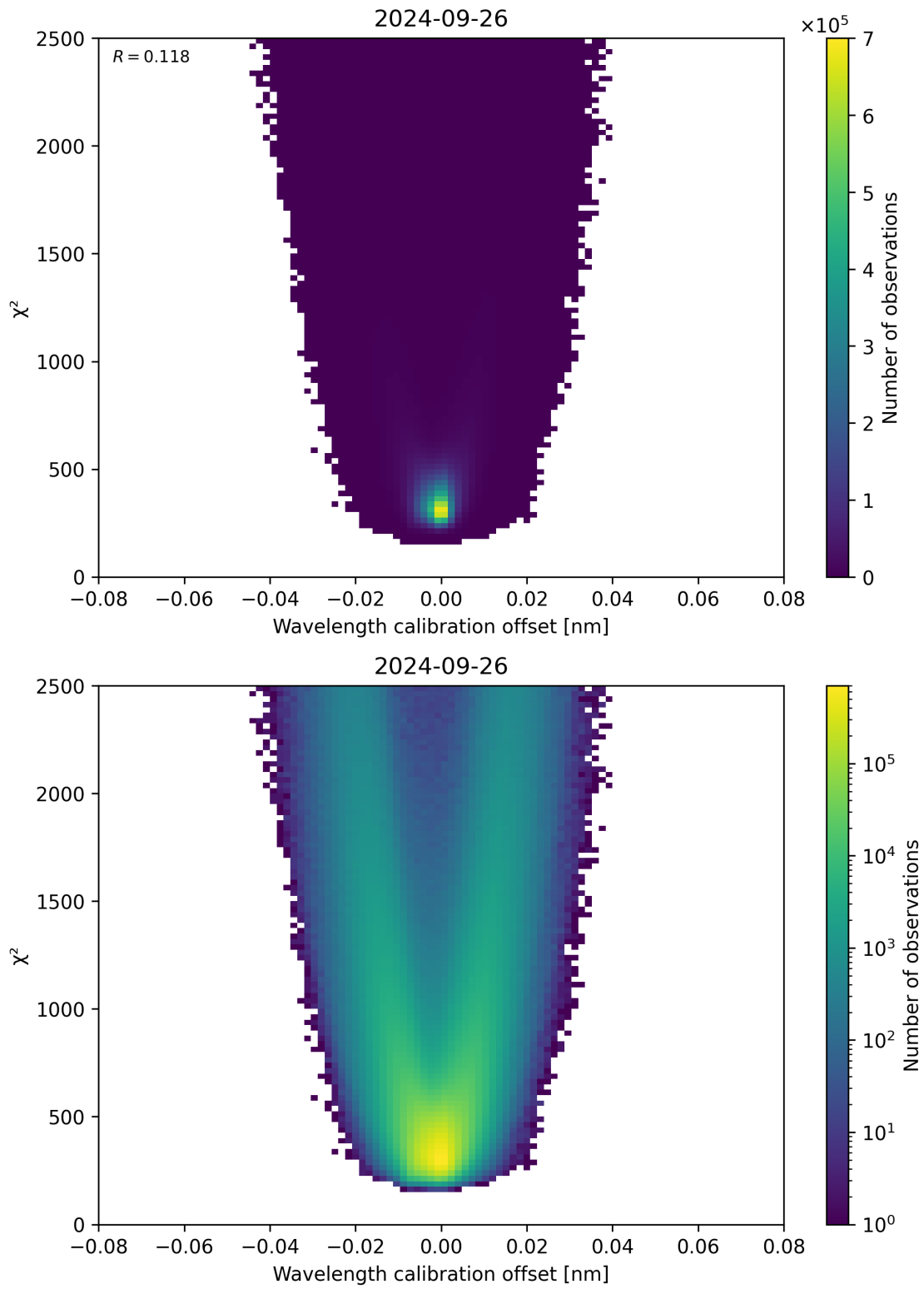
Figure 175: Scatter density plot of “Wavelength calibration offset” against “ \chi^2 ” for 2024-09-25 to 2024-09-27.
