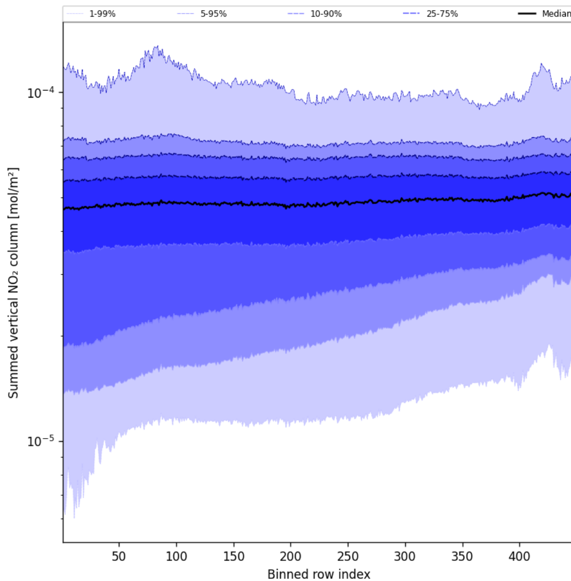
Figure 57: Along track statistics of “Summed vertical NO 2 column” for 2024-09-25 to 2024-09-27
