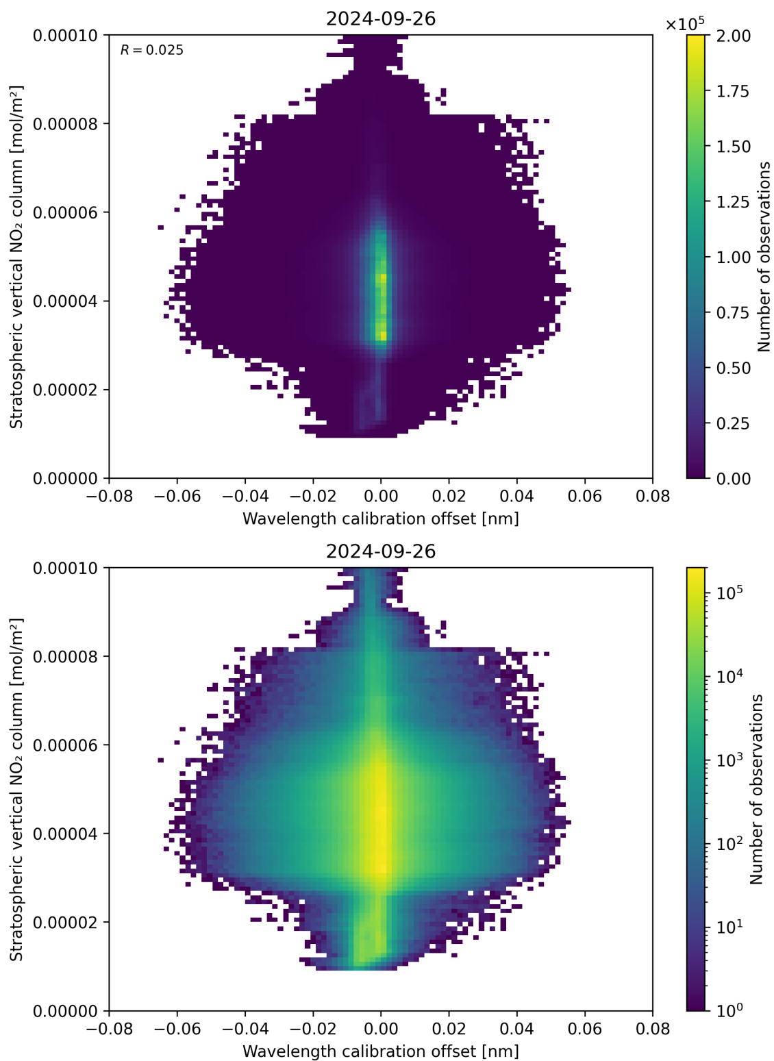
Figure 176: Scatter density plot of “Wavelength calibration offset” against “Stratospheric vertical NO 2 column” for 2024-09-25 to 2024-09-27.
