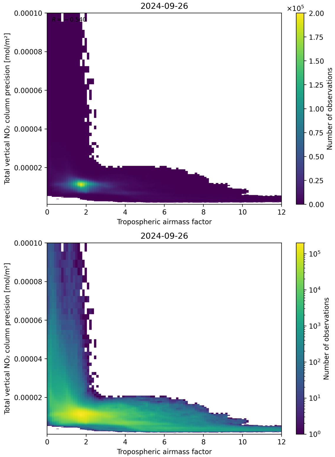
Figure 78: Scatter density plot of “Tropospheric air mass factor” against “Total vertical NO 2 column precision” for 2024-09-25 to 2024-09-27.
