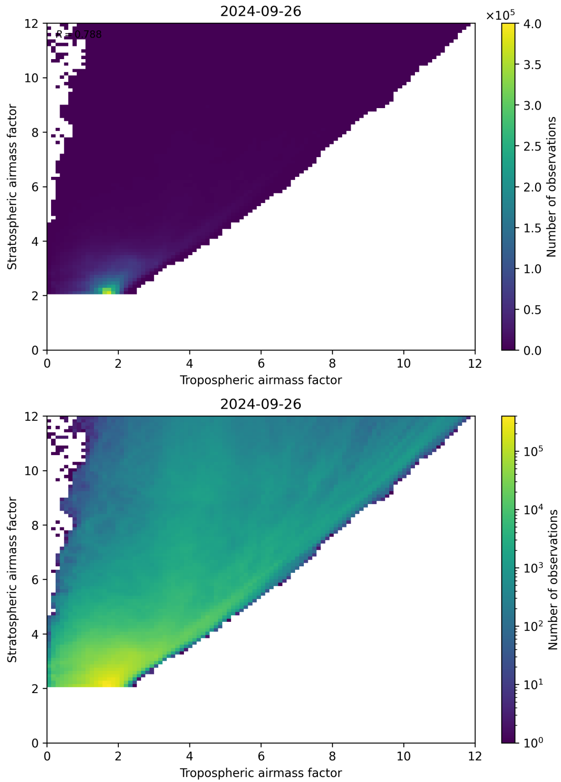
Figure 71: Scatter density plot of “Tropospheric airmass factor” against “Stratospheric airmass factor” for 2024-09-25 to 2024-09-27.
