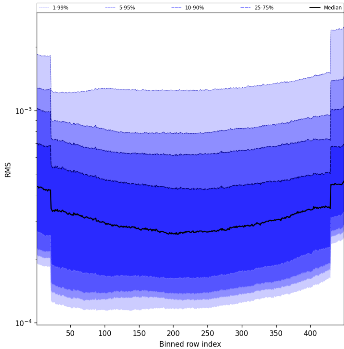
Figure 60: Along track statistics of “RMS” for 2024-09-25 to 2024-09-27
