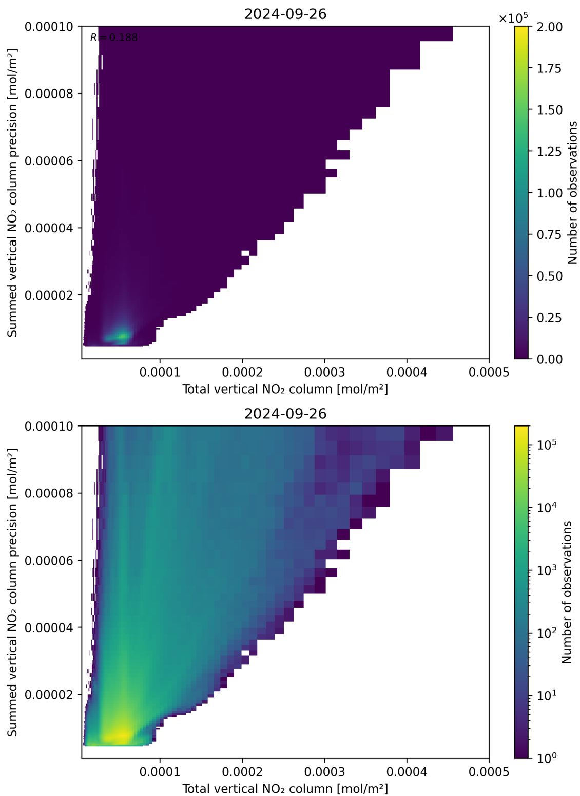
Figure 113: Scatter density plot of “Total vertical NO 2 column” against “Summed vertical NO 2 column precision” for 2024-09-25 to 2024-09-27.
