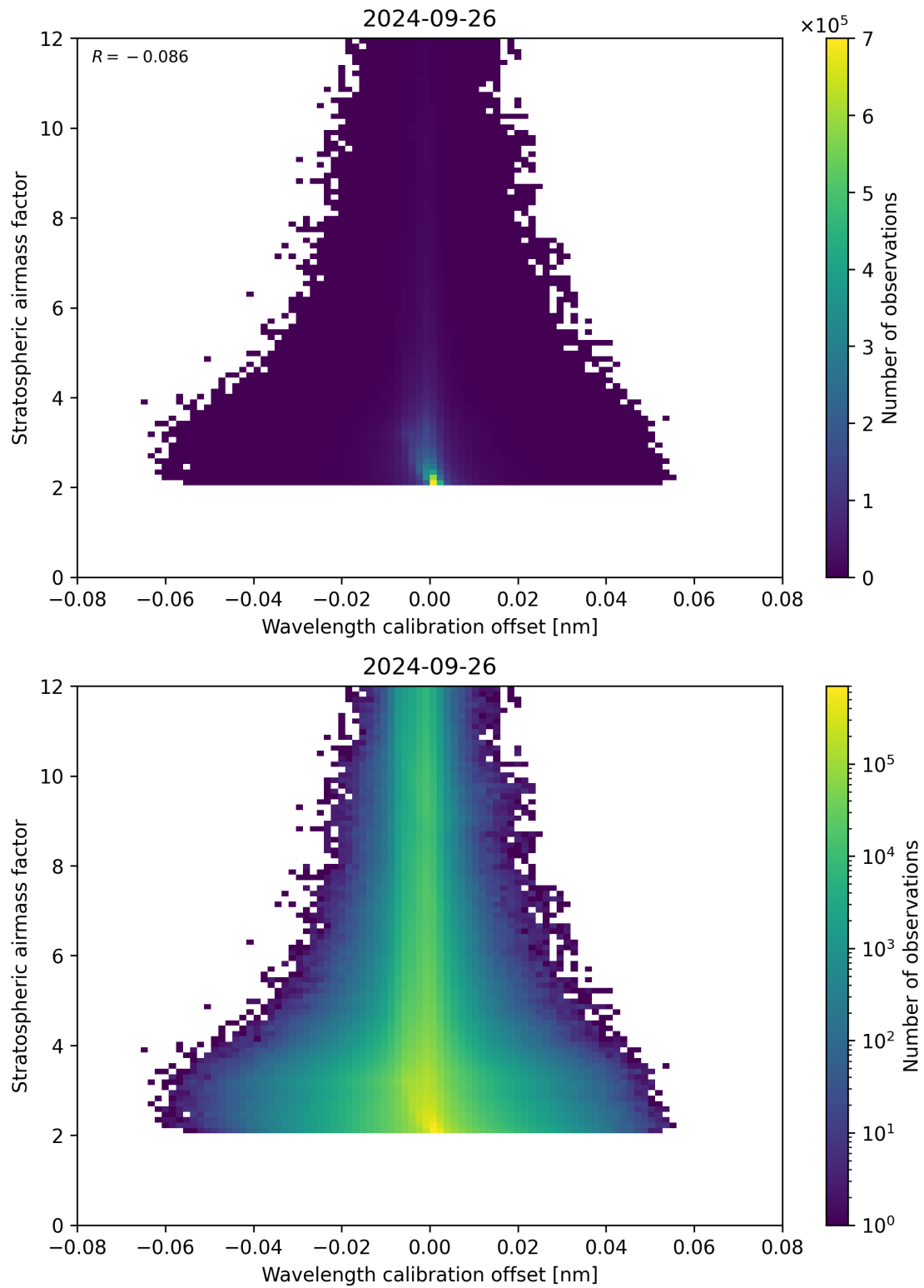
Figure 174: Scatter density plot of “Wavelength calibration offset” against “Stratospheric air mass factor” for 2024-09-25 to 2024-09-27.
