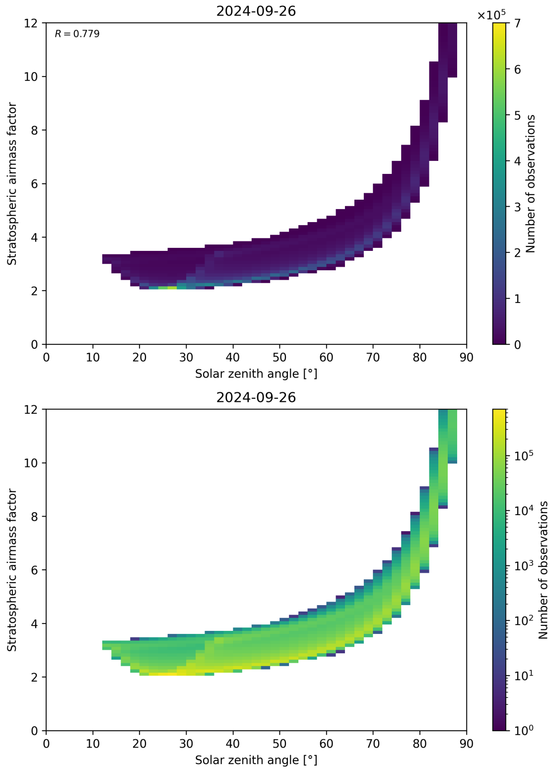
Figure 145: Scatter density plot of “Solar zenith angle” against “Stratospheric airmass factor” for 2024-09-25 to 2024-09-27.
