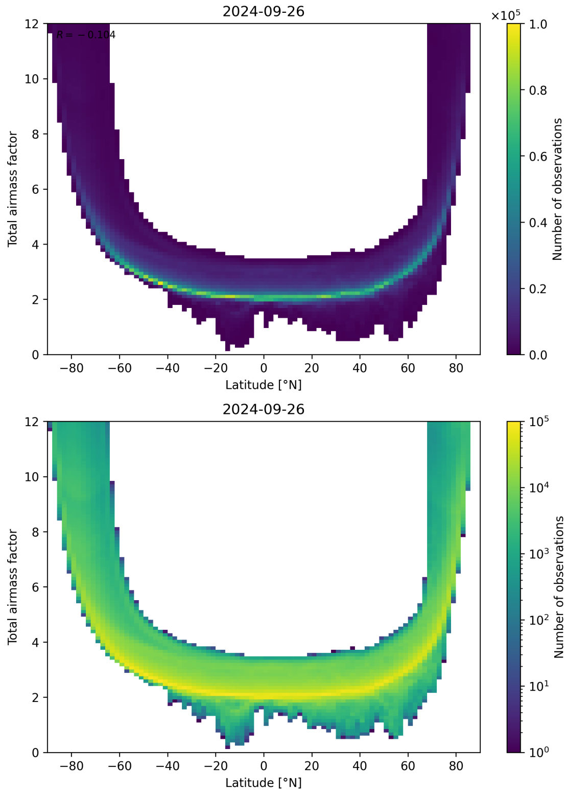
Figure 84: Scatter density plot of “Latitude” against “Total airmass factor” for 2024-09-25 to 2024-09-27.
