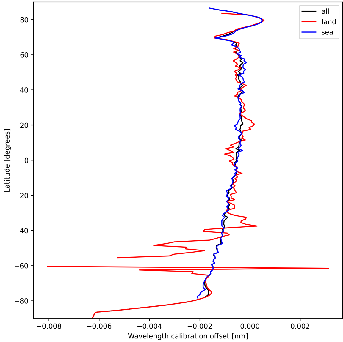
Figure 18: Zonal average of “Wavelength calibration offset” for 2024-09-25 to 2024-09-27.
