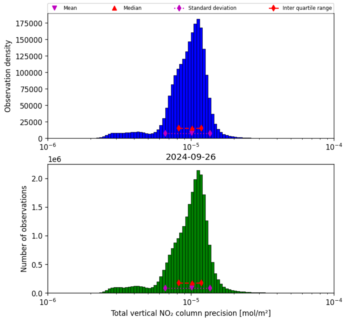
Figure 39: Histogram of “Total vertical NO 2 column precision” for 2024-09-25 to 2024-09-27
