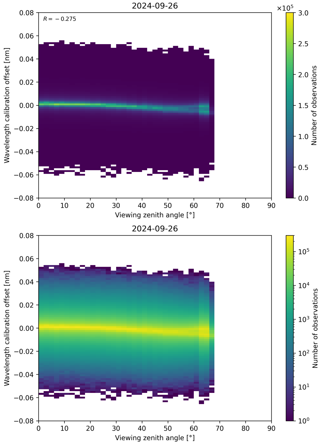
Figure 173: Scatter density plot of “Viewing zenith angle” against “Wavelength calibration offset” for 2024-09-25 to 2024-09-27.
