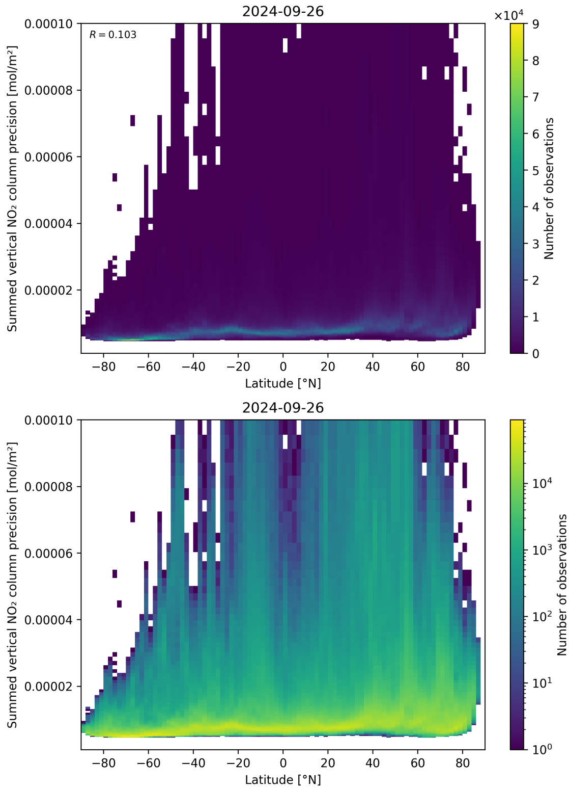
Figure 89: Scatter density plot of “Latitude” against “Summed vertical NO 2 column precision” for 2024-09-25 to 2024-09-27.
