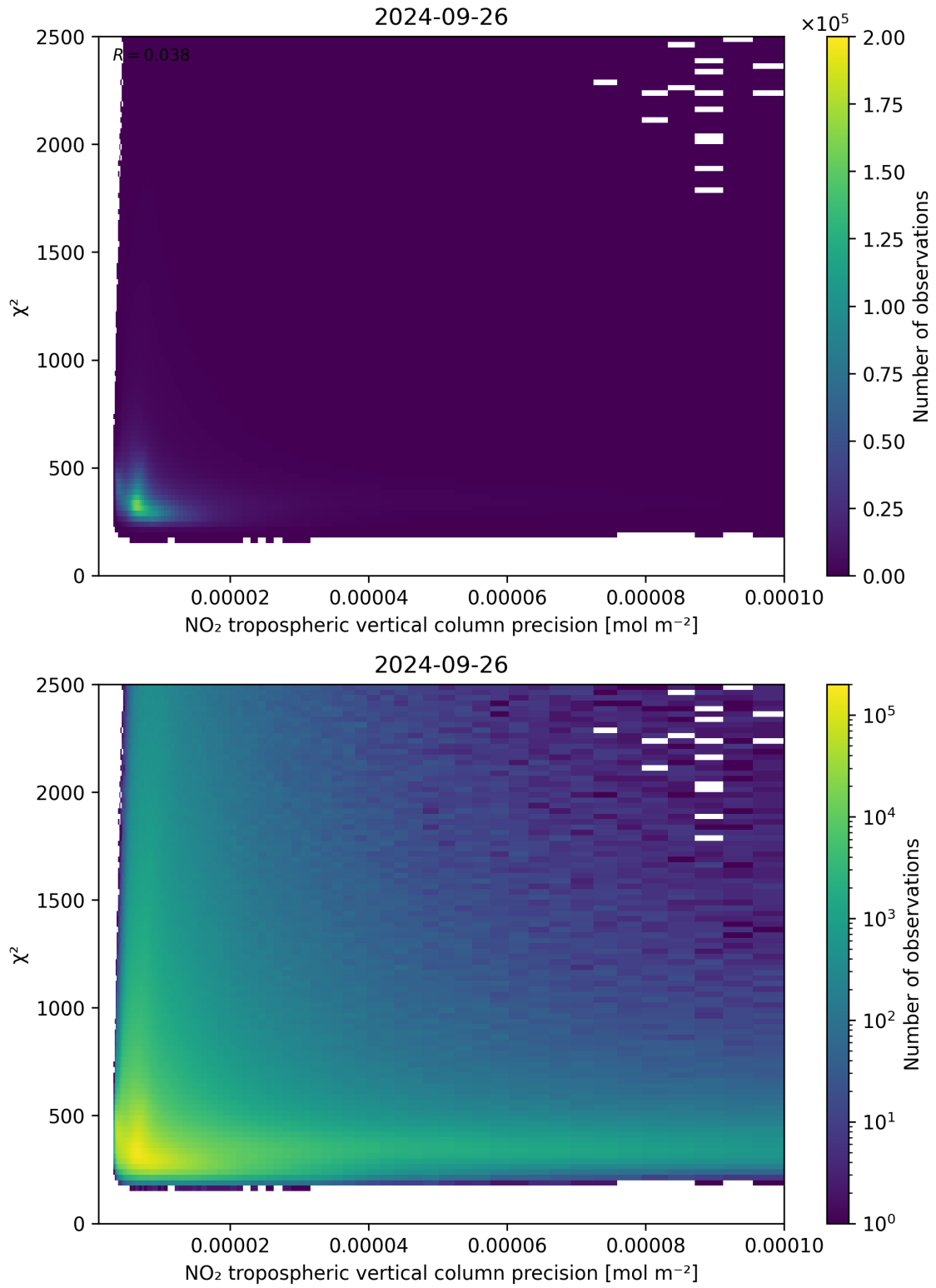
Figure 134: Scatter density plot of “NO 2 tropospheric vertical column precision” against “ \chi^2 ” for 2024-09-25 to 2024-09-27.
