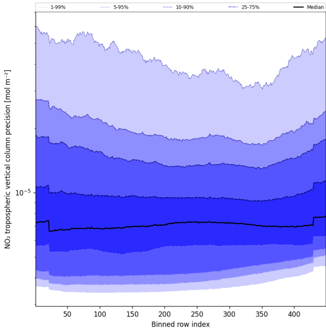
Figure 47: Along track statistics of “NO 2 tropospheric vertical column precision” for 2024-09-25 to 2024-09-27
