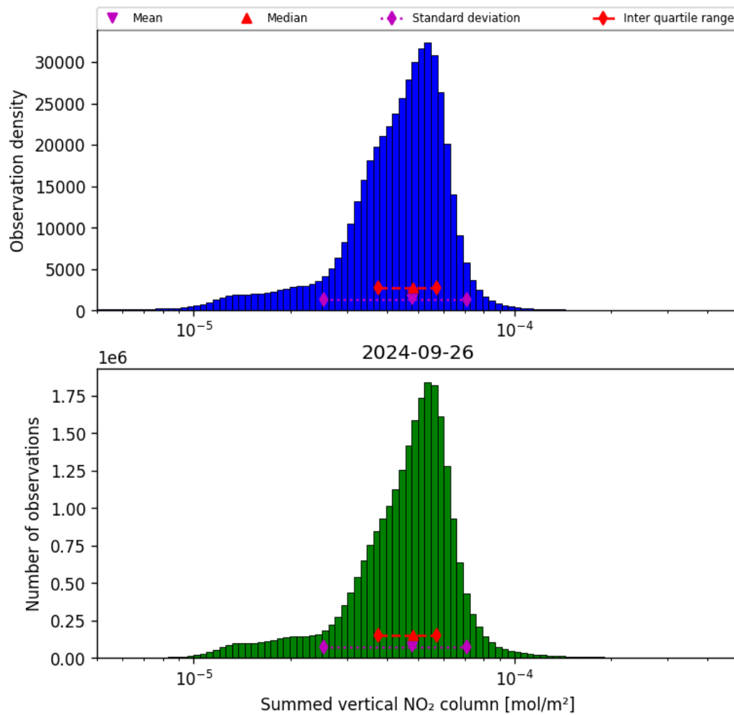
Figure 40: Histogram of “Summed vertical NO 2 column” for 2024-09-25 to 2024-09-27
