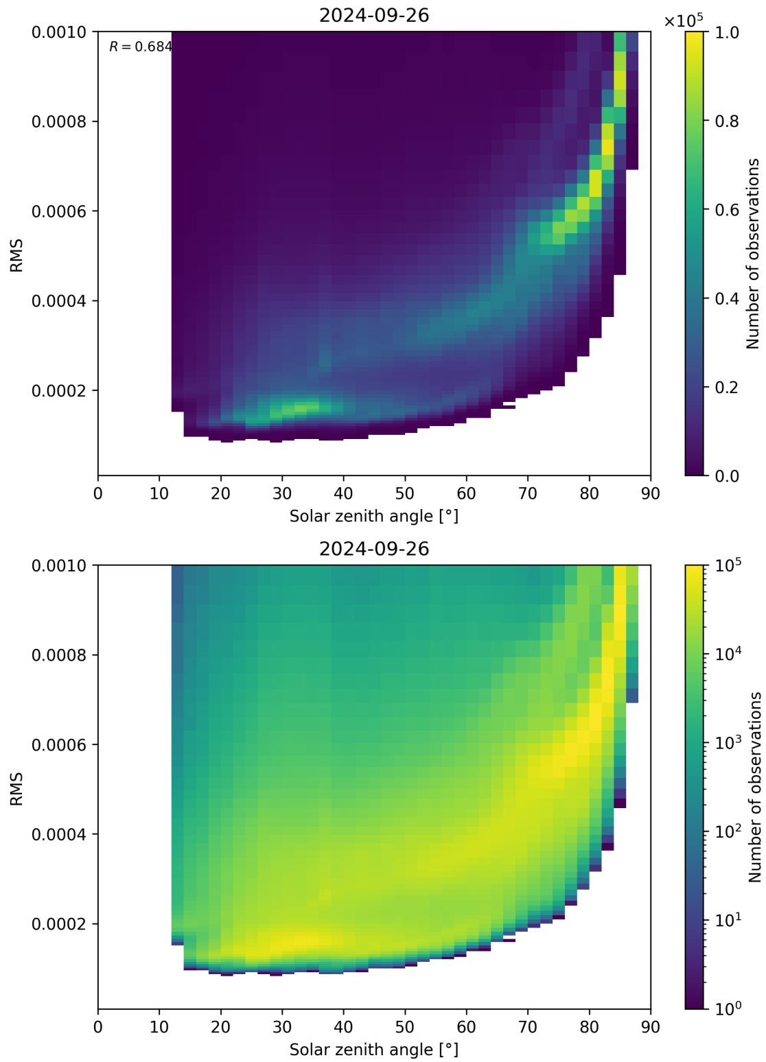
Figure 157: Scatter density plot of “Solar zenith angle” against “RMS” for 2024-09-25 to 2024-09-27.
