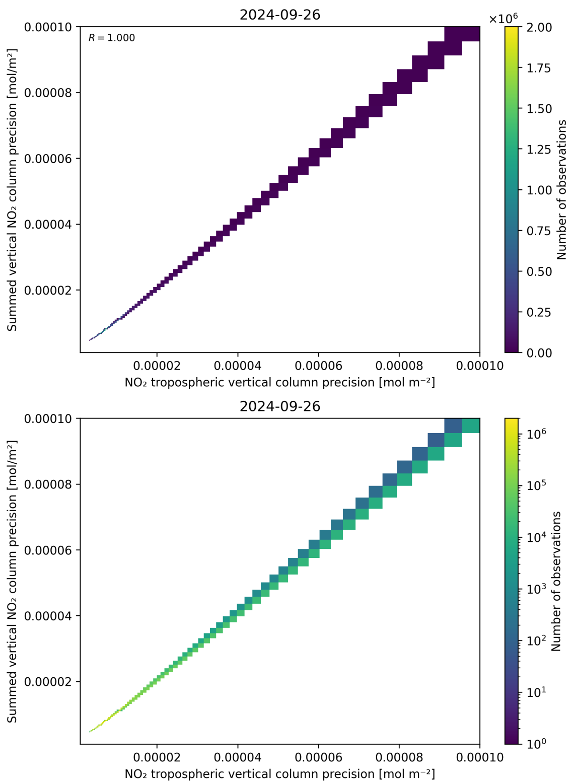
Figure 137: Scatter density plot of “NO 2 tropospheric vertical column precision” against “Summed vertical NO 2 column precision” for 2024-09-25 to 2024-09-27.
