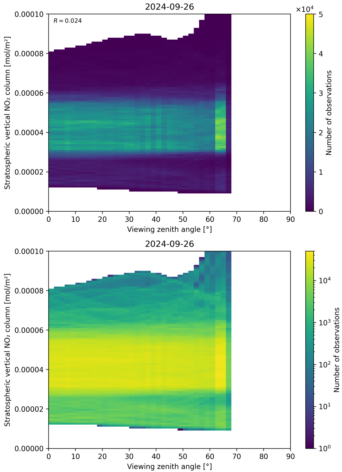
Figure 164: Scatter density plot of “Viewing zenith angle” against “Stratospheric vertical NO 2 column” for 2024-09-25 to 2024-09-27.
