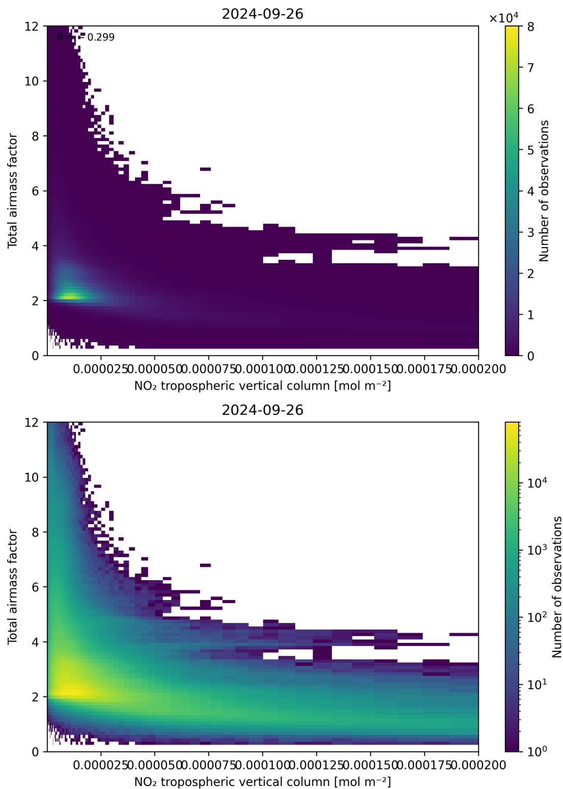
Figure 122: Scatter density plot of “NO 2 tropospheric vertical column” against “Total air mass factor” for 2024-09-25 to 2024-09-27.
