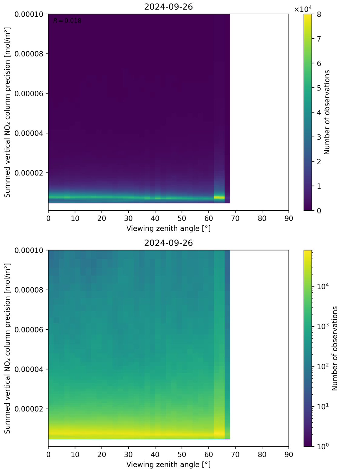
Figure 166: Scatter density plot of “Viewing zenith angle” against “Summed vertical NO 2 column precision” for 2024-09-25 to 2024-09-27.
