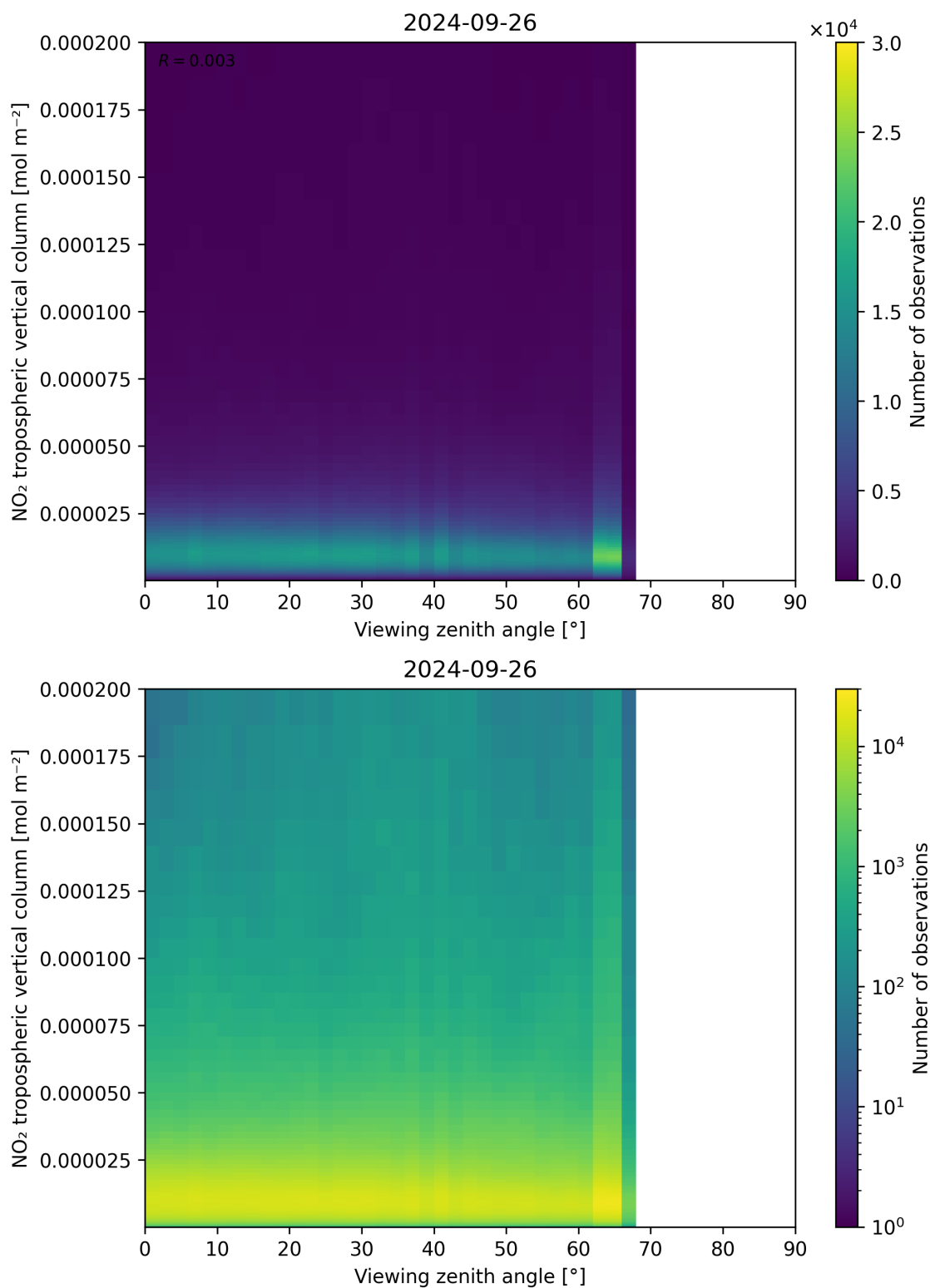
Figure 169: Scatter density plot of “Viewing zenith angle” against “NO 2 tropospheric vertical column” for 2024-09-25 to 2024-09-27.
