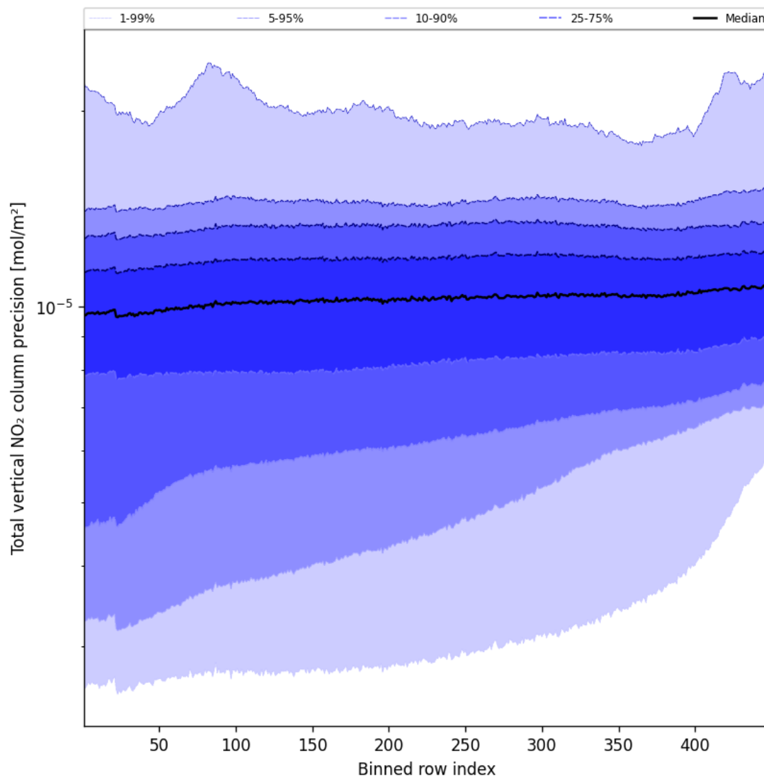
Figure 56: Along track statistics of “Total vertical NO 2 column precision” for 2024-09-25 to 2024-09-27
