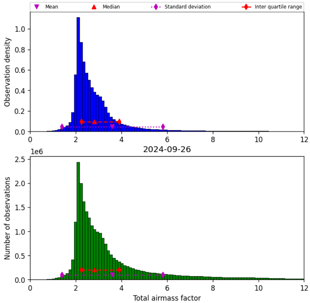
Figure 32: Histogram of “Total airmass factor” for 2024-09-25 to 2024-09-27
