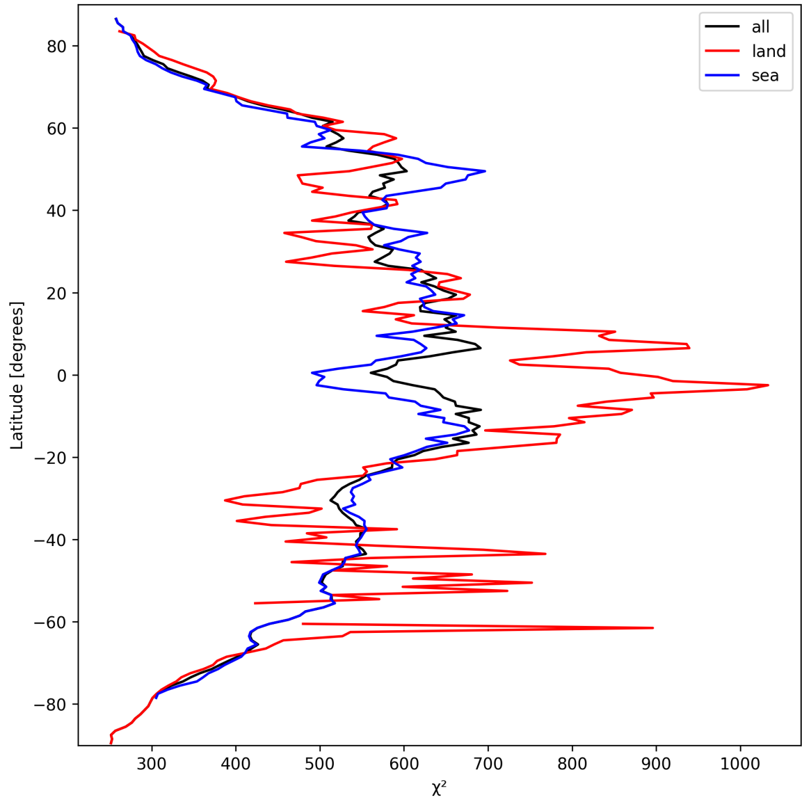
Figure 25: Zonal average of “ \chi^2 ” for 2024-09-25 to 2024-09-27.
