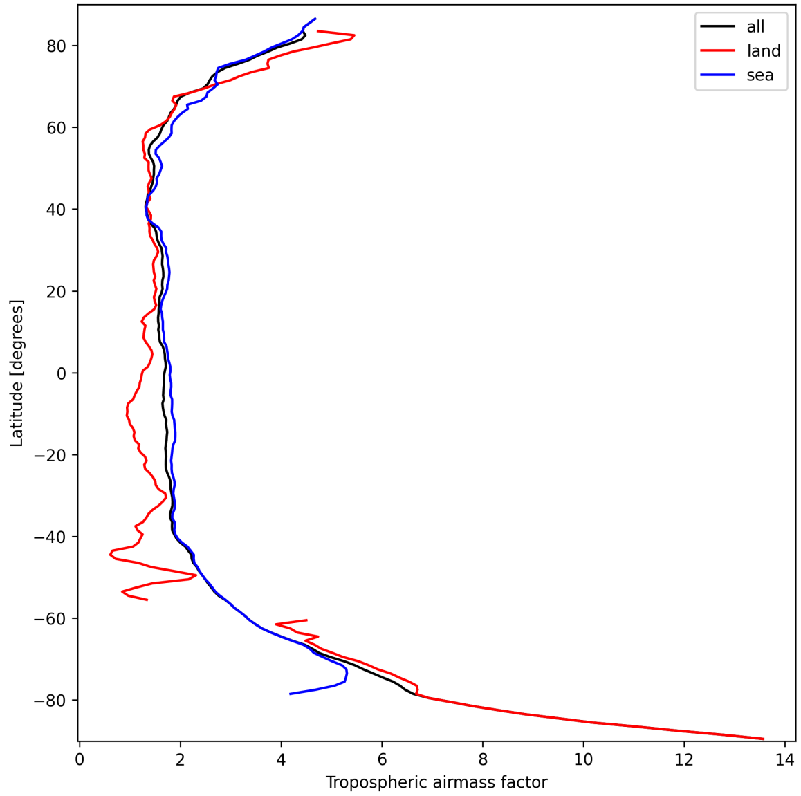
Figure 14: Zonal average of “Tropospheric airmass factor” for 2024-09-25 to 2024-09-27.
