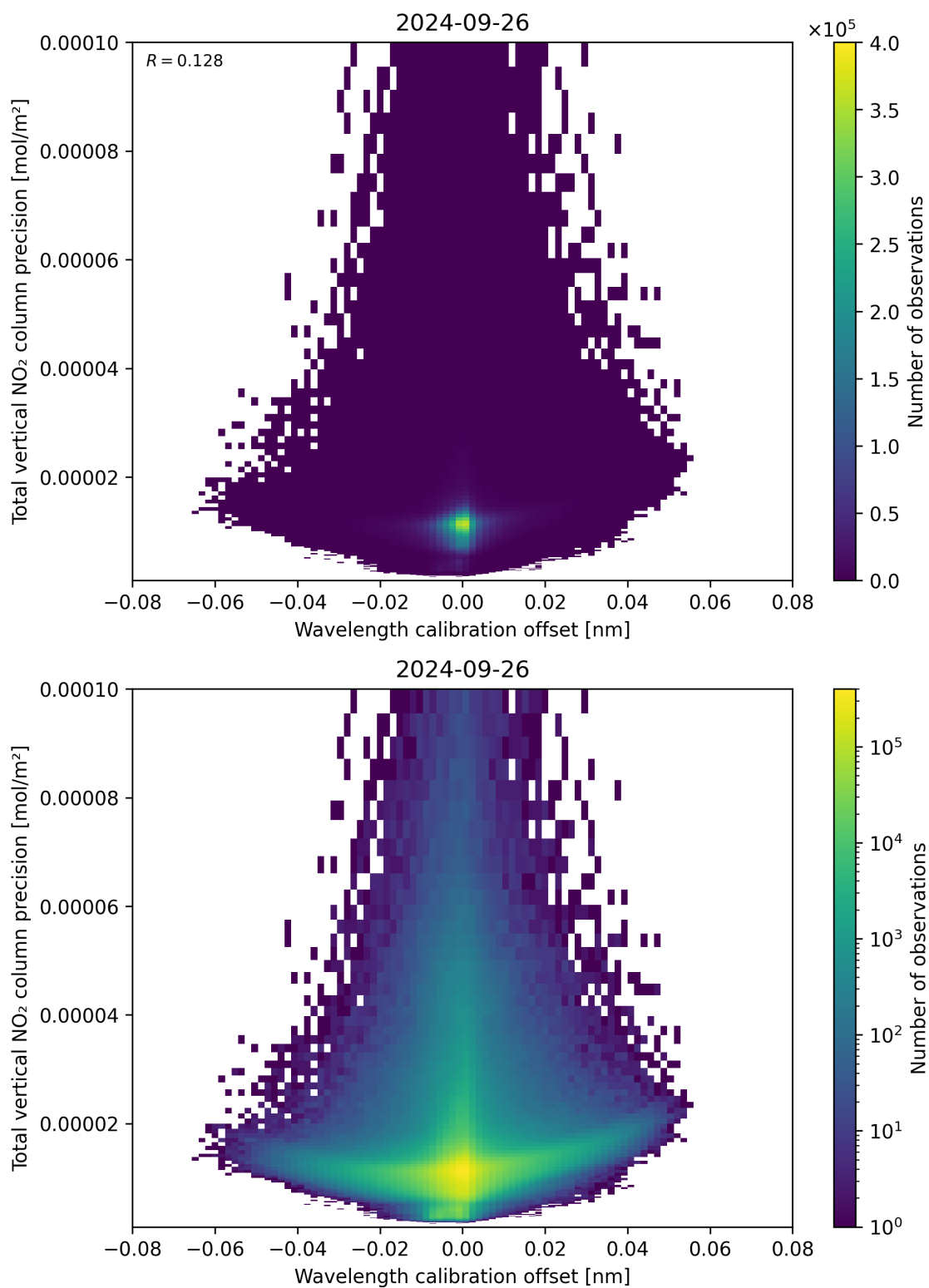
Figure 180: Scatter density plot of “Wavelength calibration offset” against “Total vertical NO 2 column precision” for 2024-09-25 to 2024-09-27.
