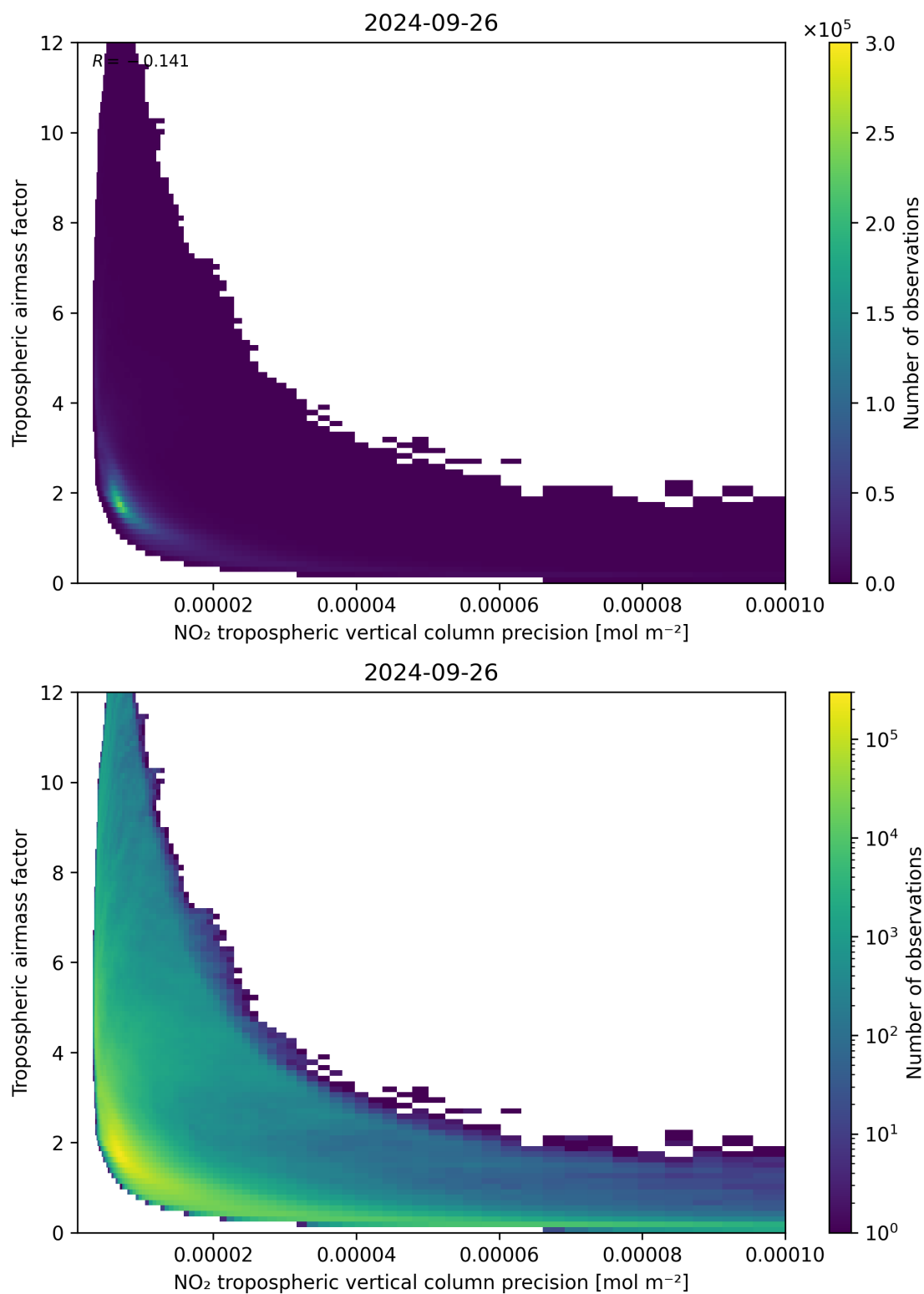
Figure 133: Scatter density plot of “NO 2 tropospheric vertical column precision” against “Tropospheric air mass factor” for 2024-09-25 to 2024-09-27.
