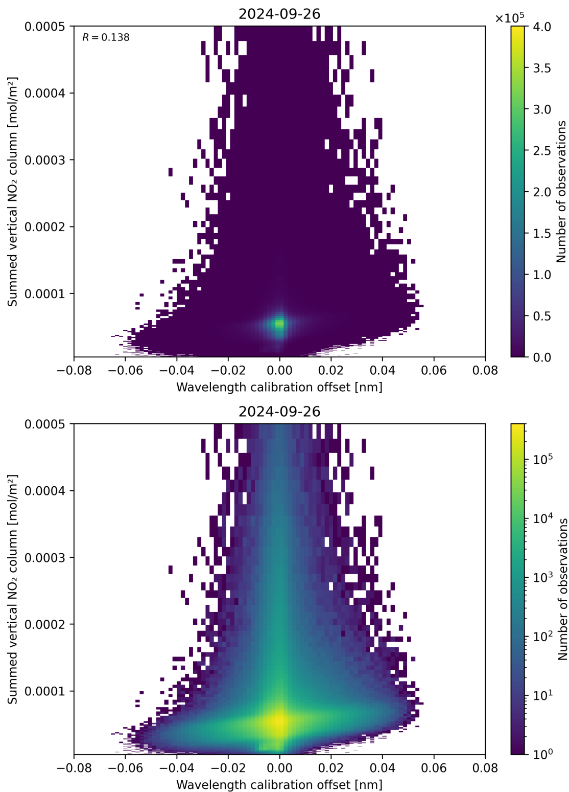
Figure 177: Scatter density plot of “Wavelength calibration offset” against “Summed vertical NO 2 column” for 2024-09-25 to 2024-09-27.
