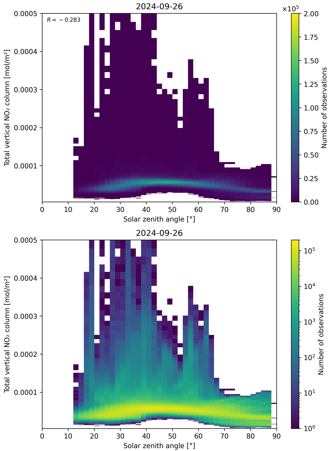
Figure 153: Scatter density plot of “Solar zenith angle” against “Total vertical NO 2 column” for 2024-09-25 to 2024-09-27.
