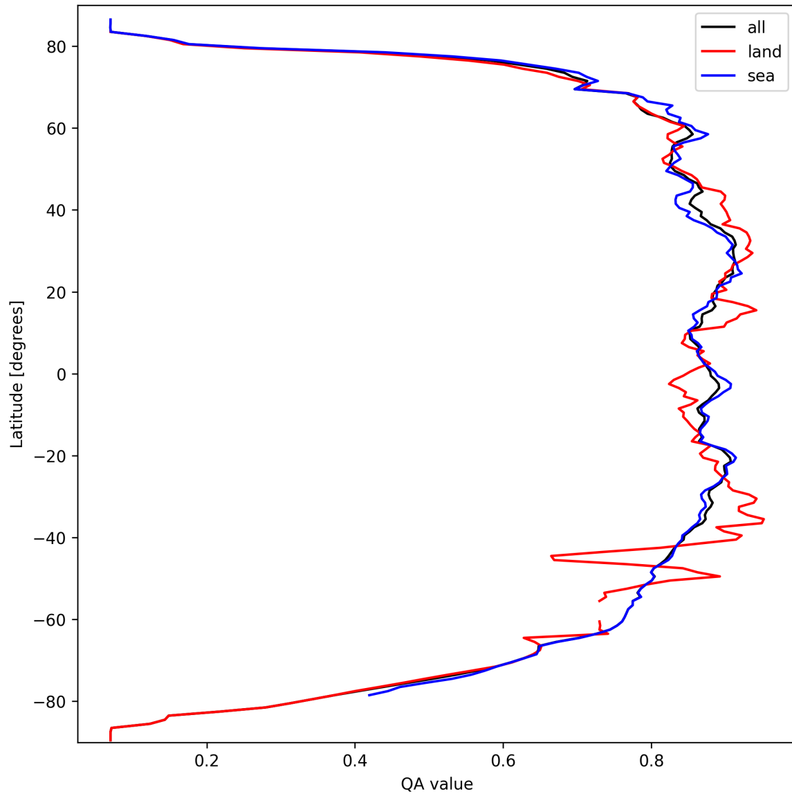
Figure 11: Zonal average of “QA value” for 2024-09-25 to 2024-09-27.
