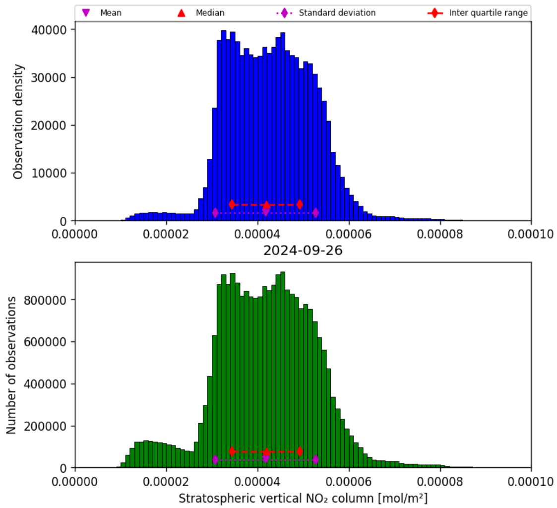
Figure 36: Histogram of “Stratospheric vertical NO 2 column” for 2024-09-25 to 2024-09-27
