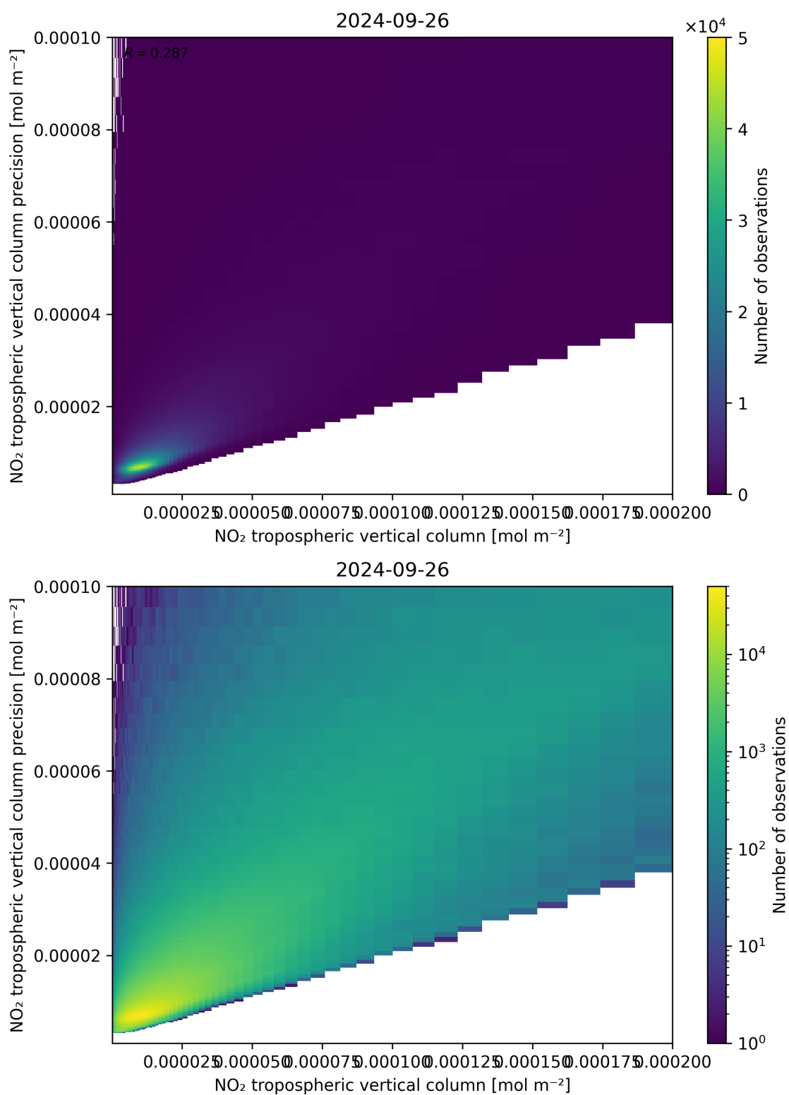
Figure 130: Scatter density plot of “NO 2 tropospheric vertical column” against “NO 2 tropospheric vertical column precision” for 2024-09-25 to 2024-09-27.
