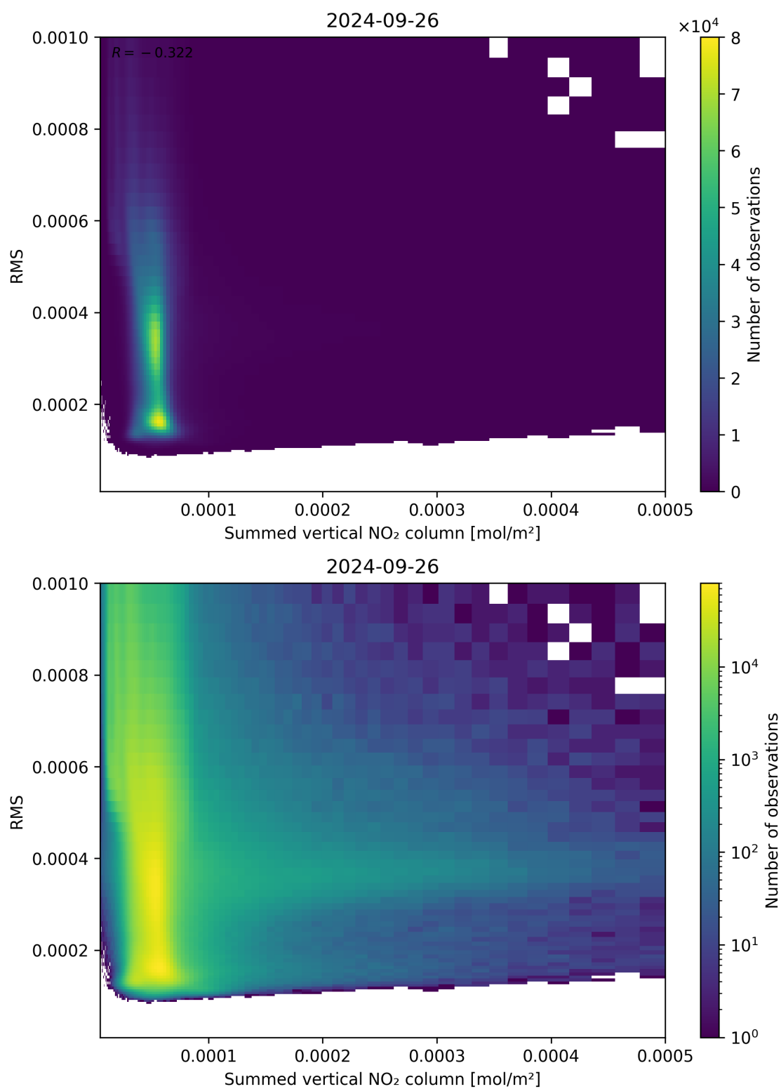
Figure 109: Scatter density plot of “Summed vertical NO 2 column” against “RMS” for 2024-09-25 to 2024-09-27.
