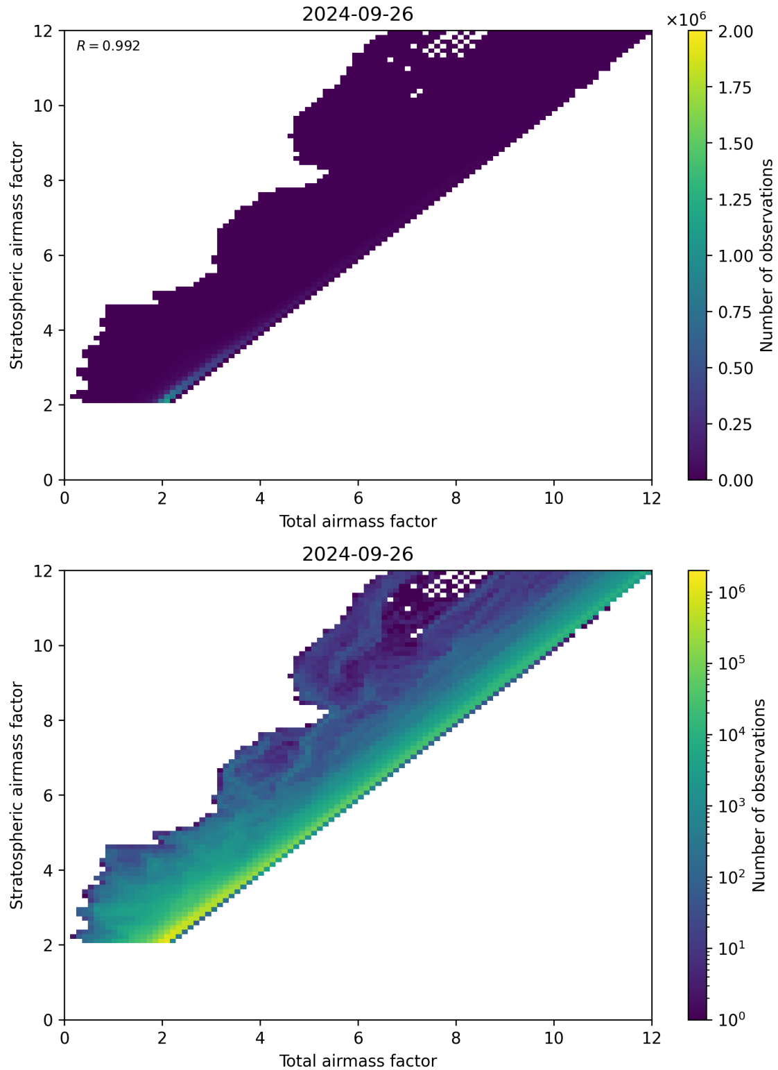
Figure 62: Scatter density plot of “Total airmass factor” against “Stratospheric airmass factor” for 2024-09-25 to 2024-09-27.
