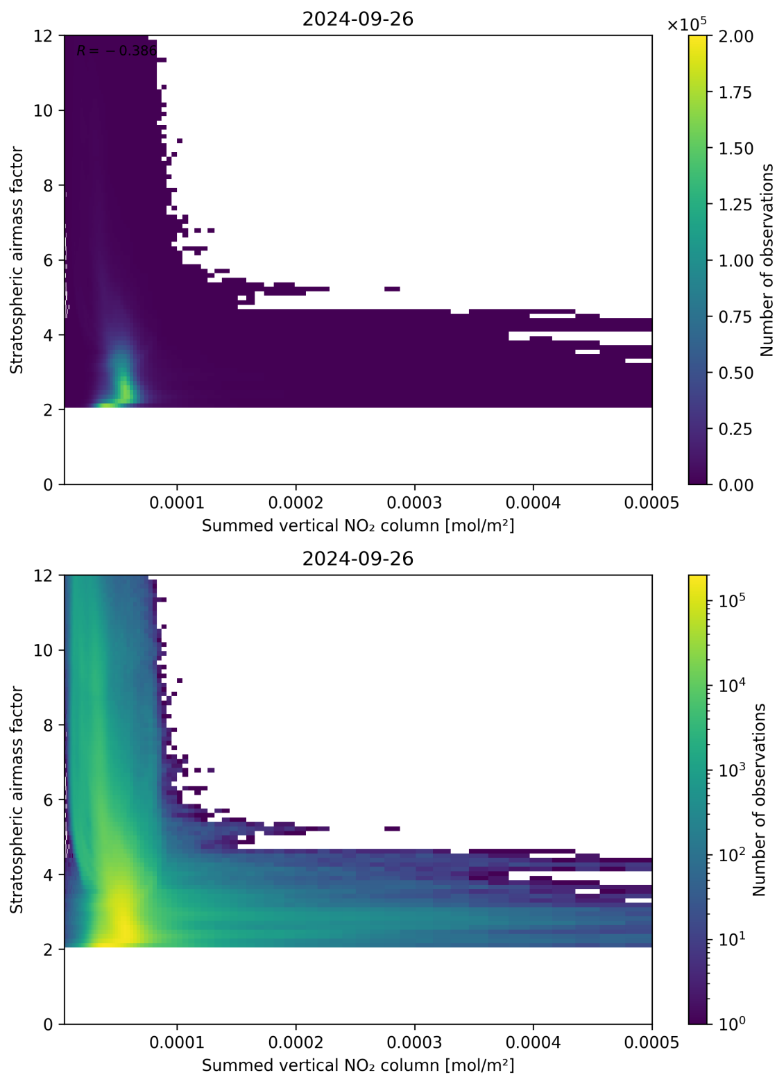
Figure 103: Scatter density plot of “Summed vertical NO 2 column” against “Stratospheric airmass factor” for 2024-09-25 to 2024-09-27.
