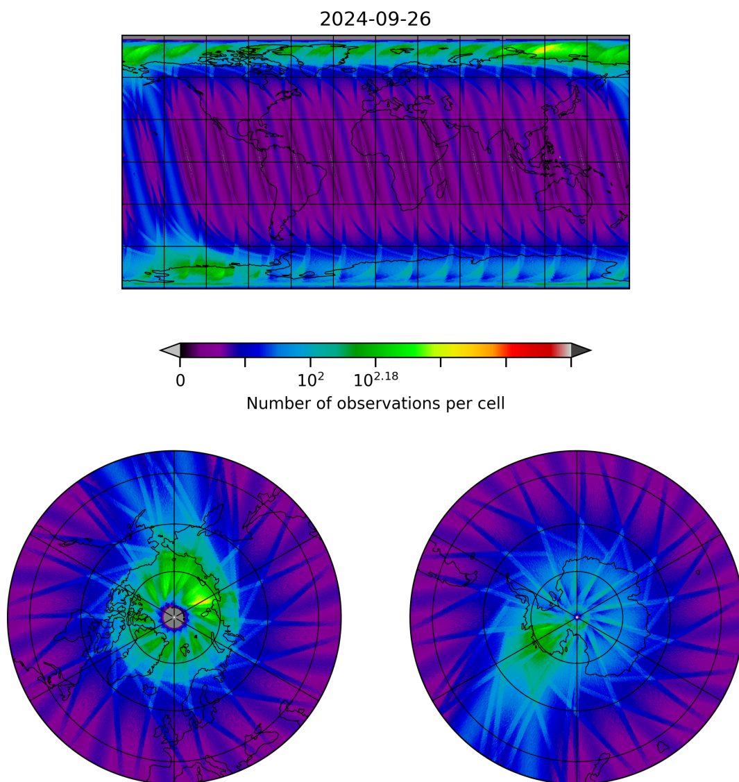
Figure 10: Map of the number of observations for 2024-09-25 to 2024-09-27
