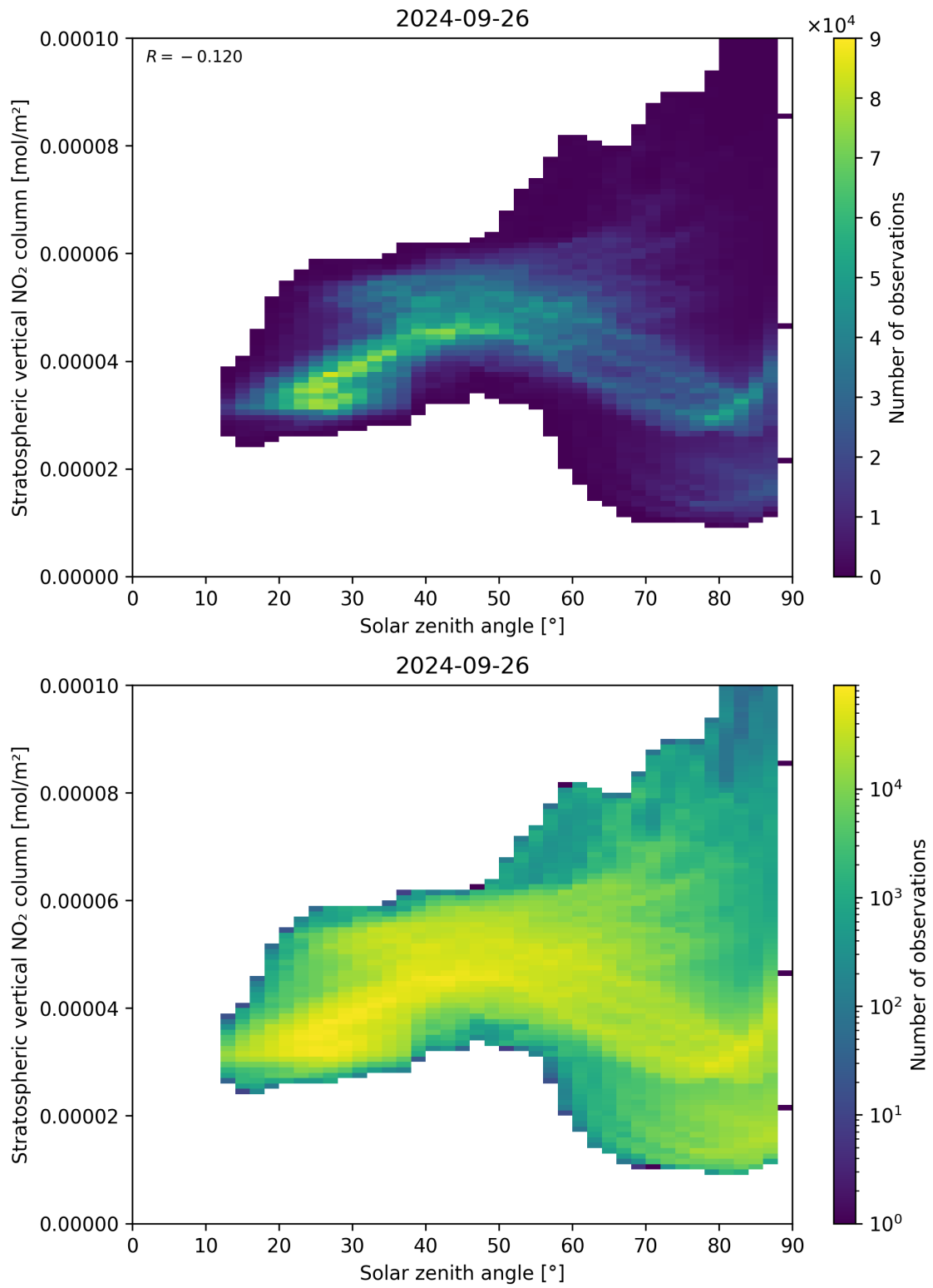
Figure 150: Scatter density plot of “Solar zenith angle” against “Stratospheric vertical NO 2 column” for 2024-09-25 to 2024-09-27.
