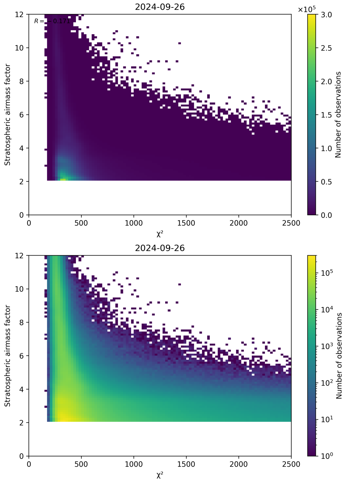
Figure 81: Scatter density plot of “ \chi^2 ” against “Stratospheric airmass factor” for 2024-09-25 to 2024-09-27.
