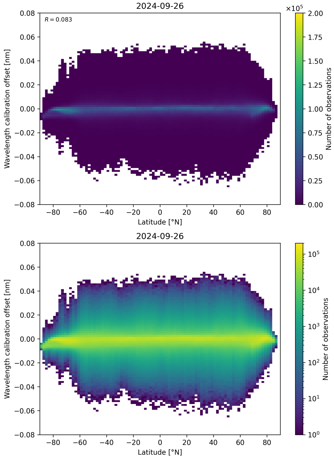
Figure 95: Scatter density plot of “Latitude” against “Wavelength calibration offset” for 2024-09-25 to 2024-09-27.
