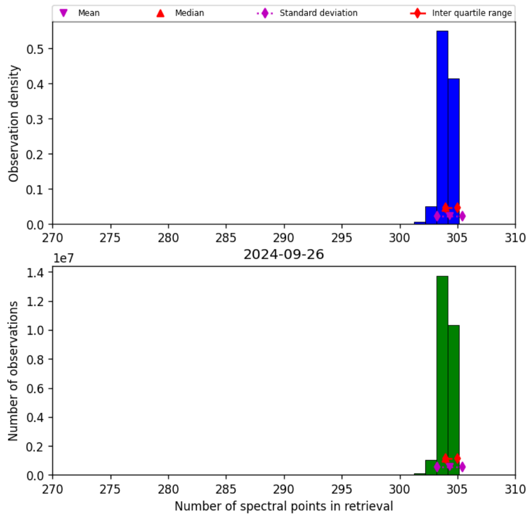
Figure 33: Histogram of “Number of spectral points in retrieval” for 2024-09-25 to 2024-09-27
