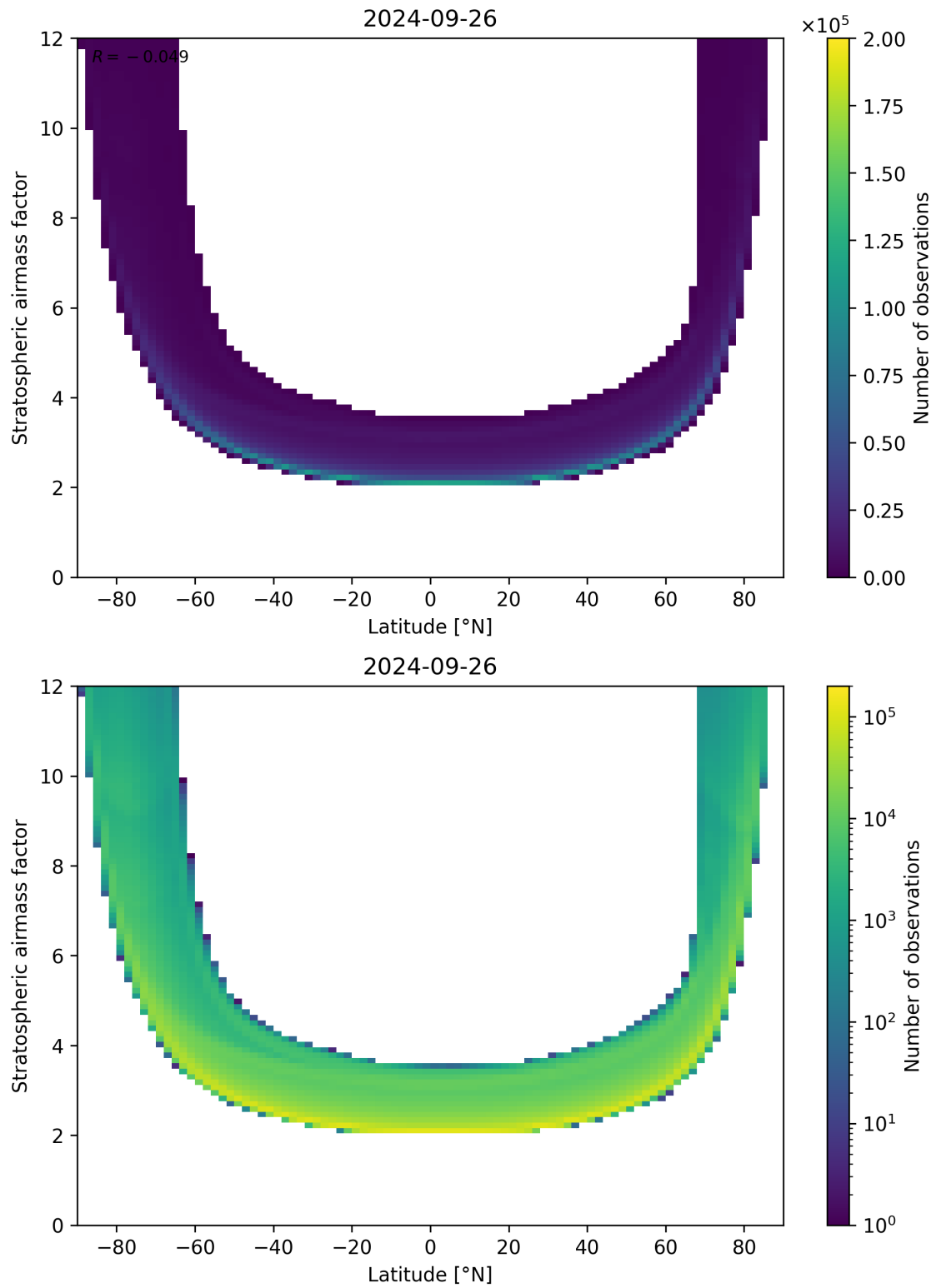
Figure 83: Scatter density plot of “Latitude” against “Stratospheric air mass factor” for 2024-09-25 to 2024-09-27.
