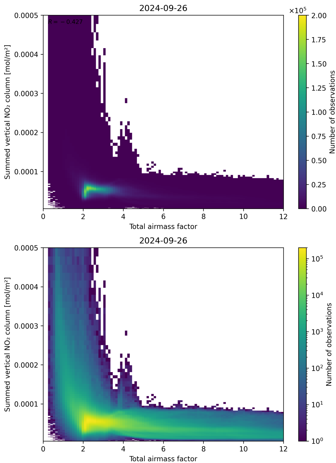
Figure 65: Scatter density plot of “Total airmass factor” against “Summed vertical NO 2 column” for 2024-09-25 to 2024-09-27.
