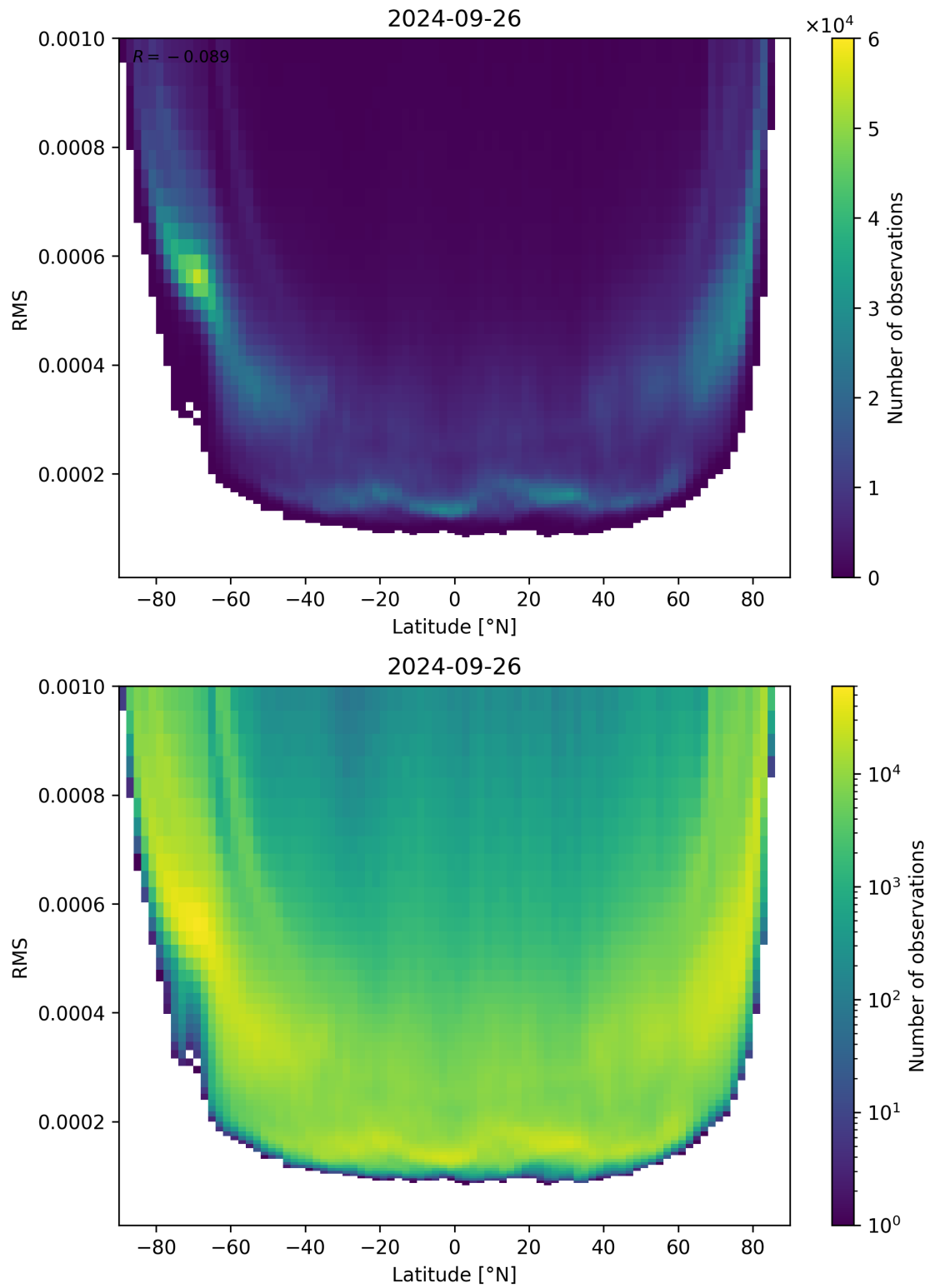
Figure 94: Scatter density plot of “Latitude” against “RMS” for 2024-09-25 to 2024-09-27.
