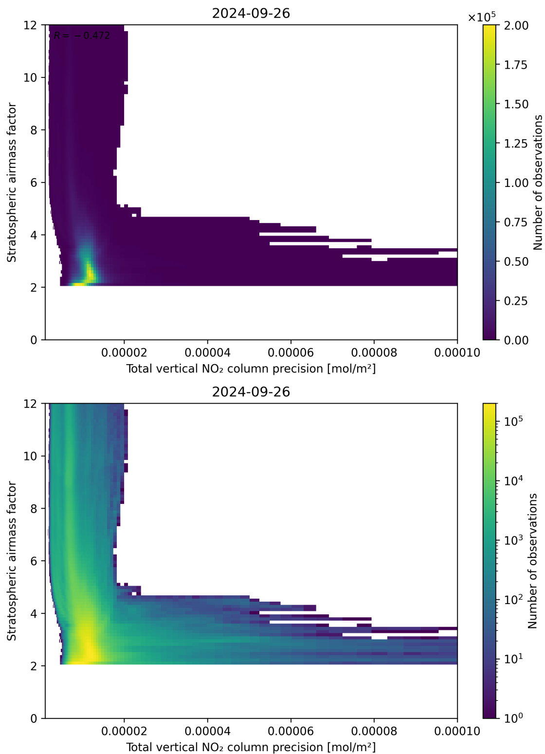
Figure 115: Scatter density plot of “Total vertical NO 2 column precision” against “Stratospheric air mass factor” for 2024-09-25 to 2024-09-27.
