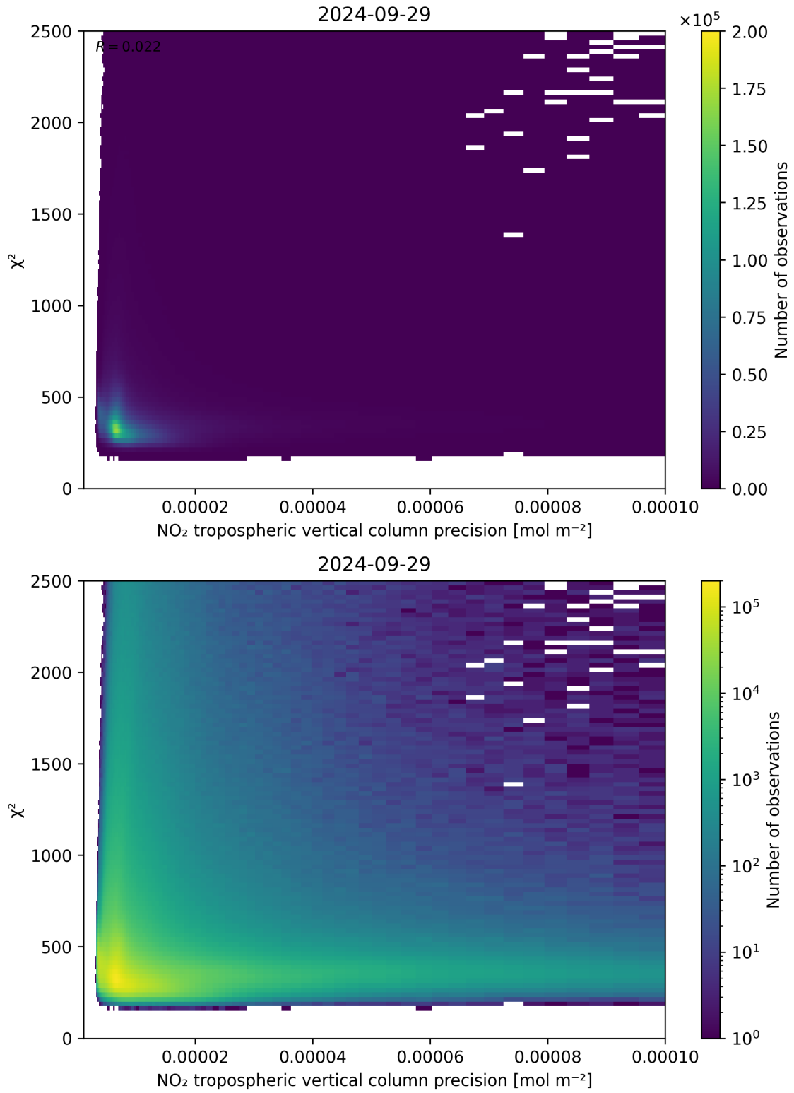
Figure 134: Scatter density plot of “NO 2 tropospheric vertical column precision” against “ \chi^2 ” for 2024-09-28 to 2024-09-30.
