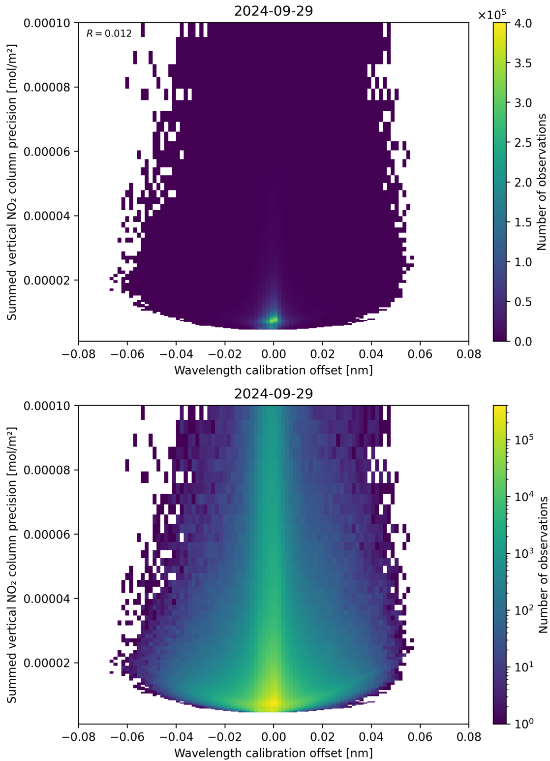
Figure 178: Scatter density plot of “Wavelength calibration offset” against “Summed vertical NO 2 column precision” for 2024-09-28 to 2024-09-30.
