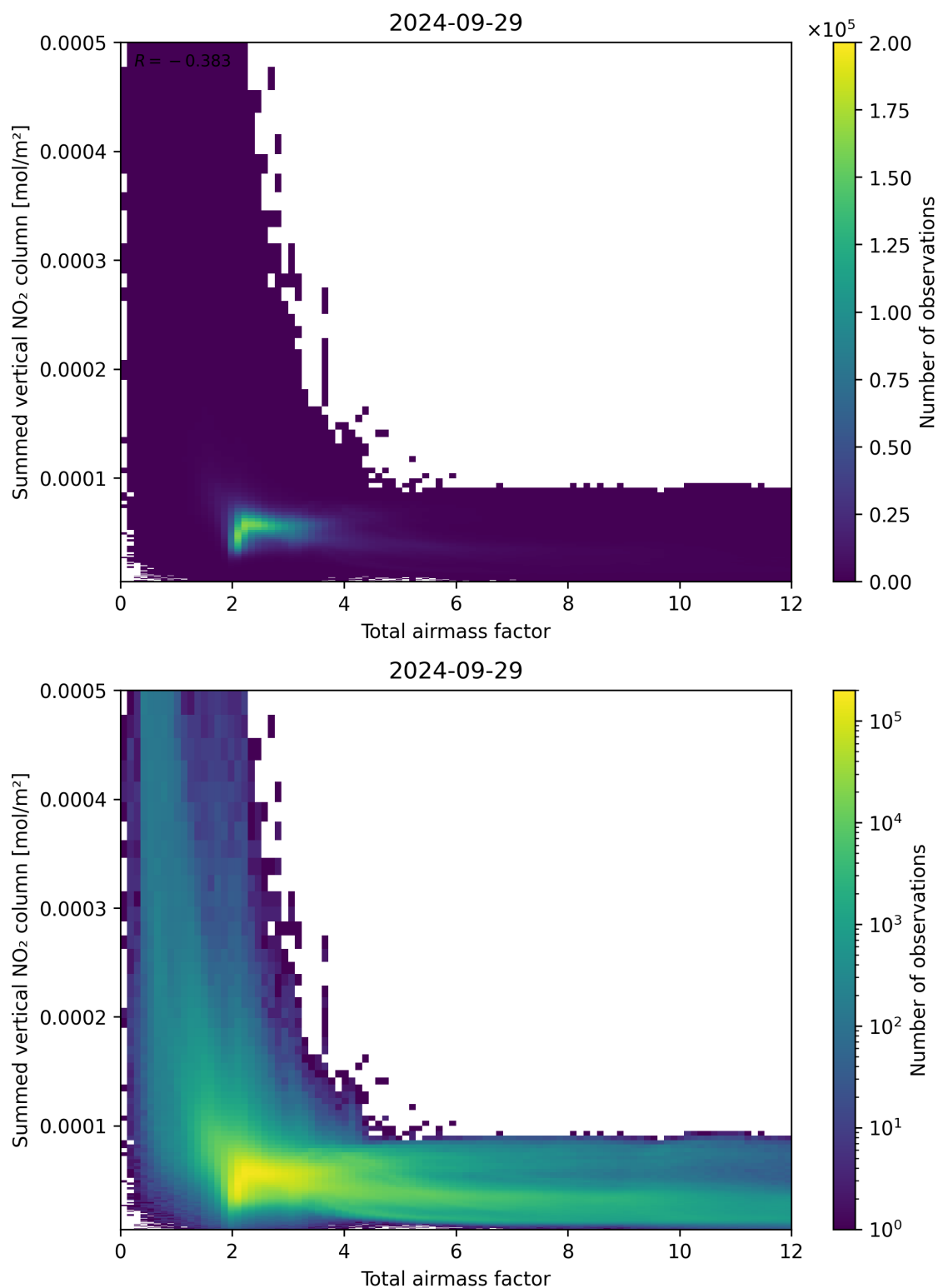
Figure 65: Scatter density plot of “Total airmass factor” against “Summed vertical NO 2 column” for 2024-09-28 to 2024-09-30.
