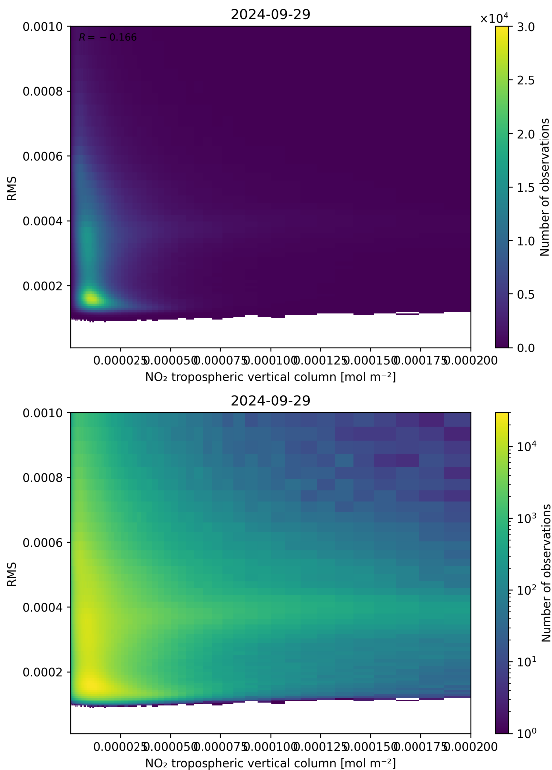
Figure 142: Scatter density plot of “NO 2 tropospheric vertical column” against “RMS” for 2024-09-28 to 2024-09-30.
