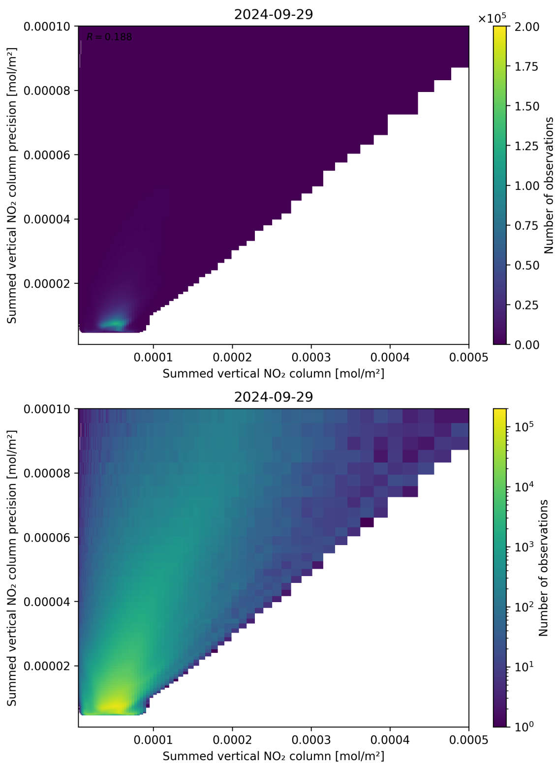
Figure 105: Scatter density plot of “Summed vertical NO 2 column” against “Summed vertical NO 2 column precision” for 2024-09-28 to 2024-09-30.
