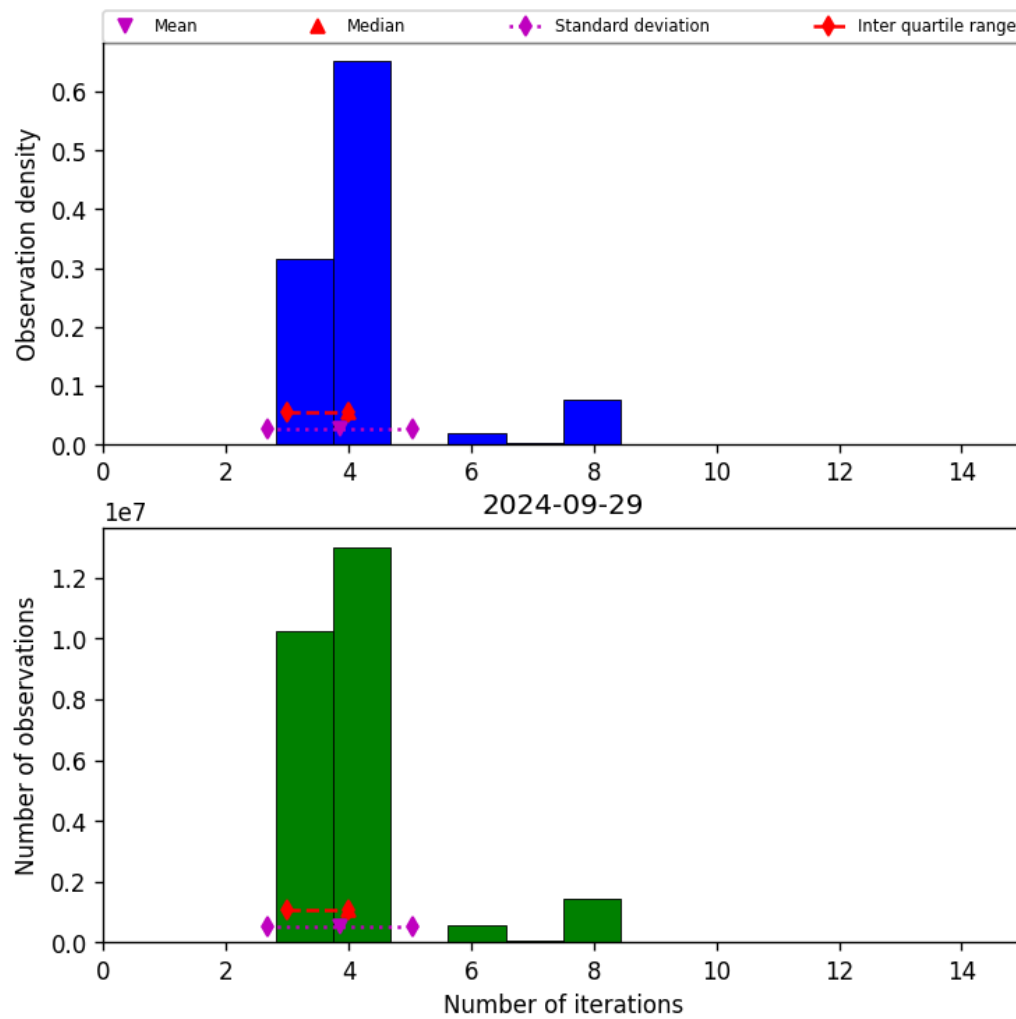
Figure 34: Histogram of “Number of iterations” for 2024-09-28 to 2024-09-30
