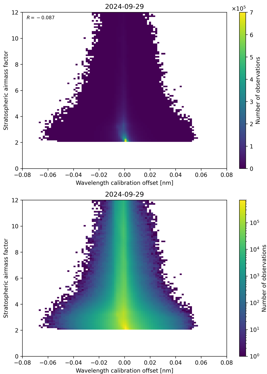
Figure 174: Scatter density plot of “Wavelength calibration offset” against “Stratospheric air mass factor” for 2024-09-28 to 2024-09-30.
