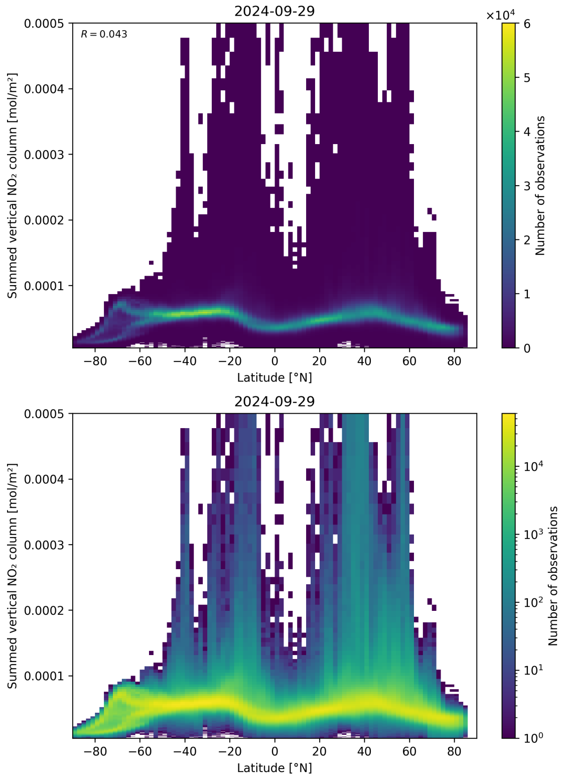
Figure 88: Scatter density plot of “Latitude” against “Summed vertical NO 2 column” for 2024-09-28 to 2024-09-30.
