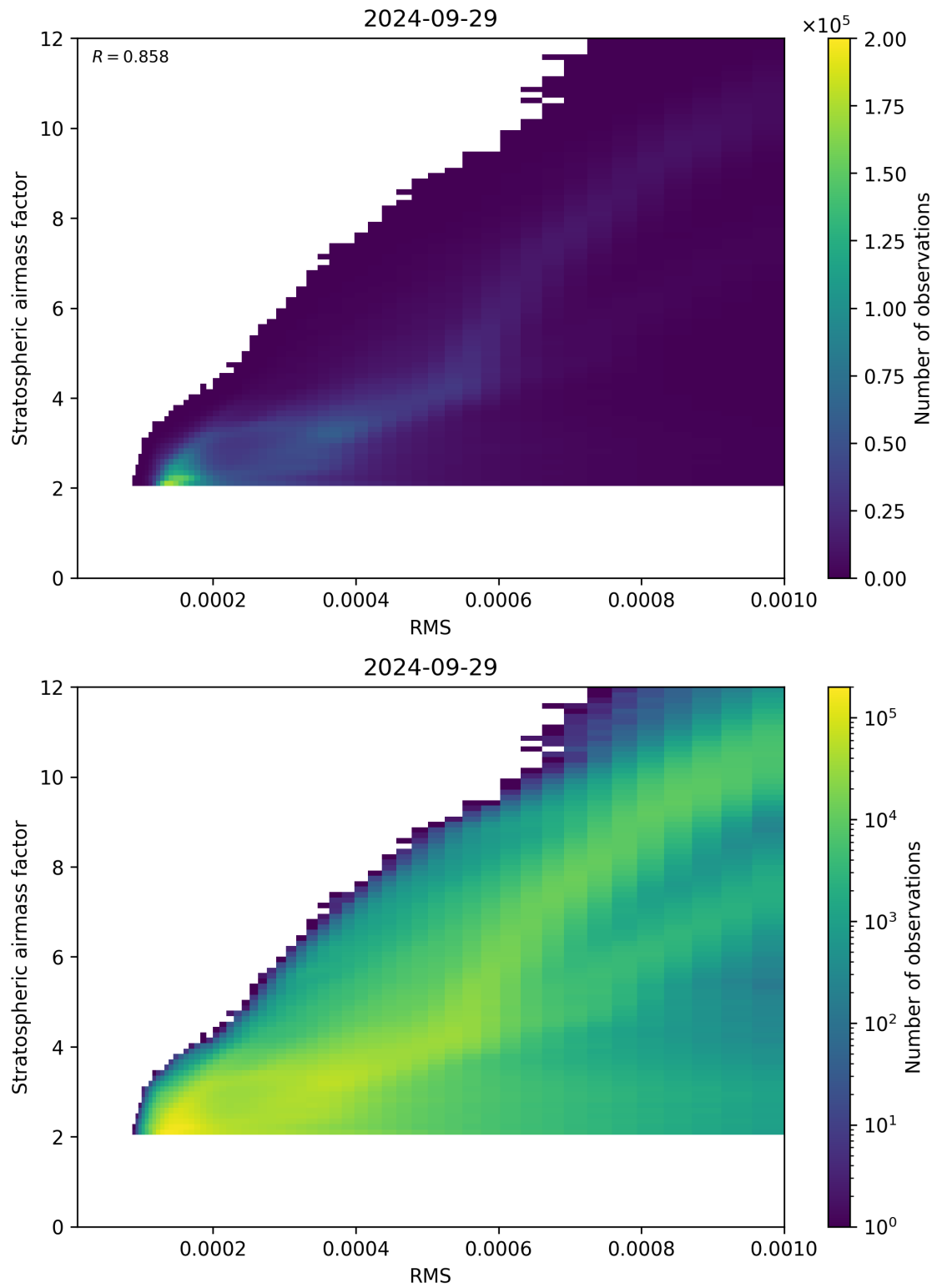
Figure 144: Scatter density plot of “RMS” against “Stratospheric airmass factor” for 2024-09-28 to 2024-09-30.
