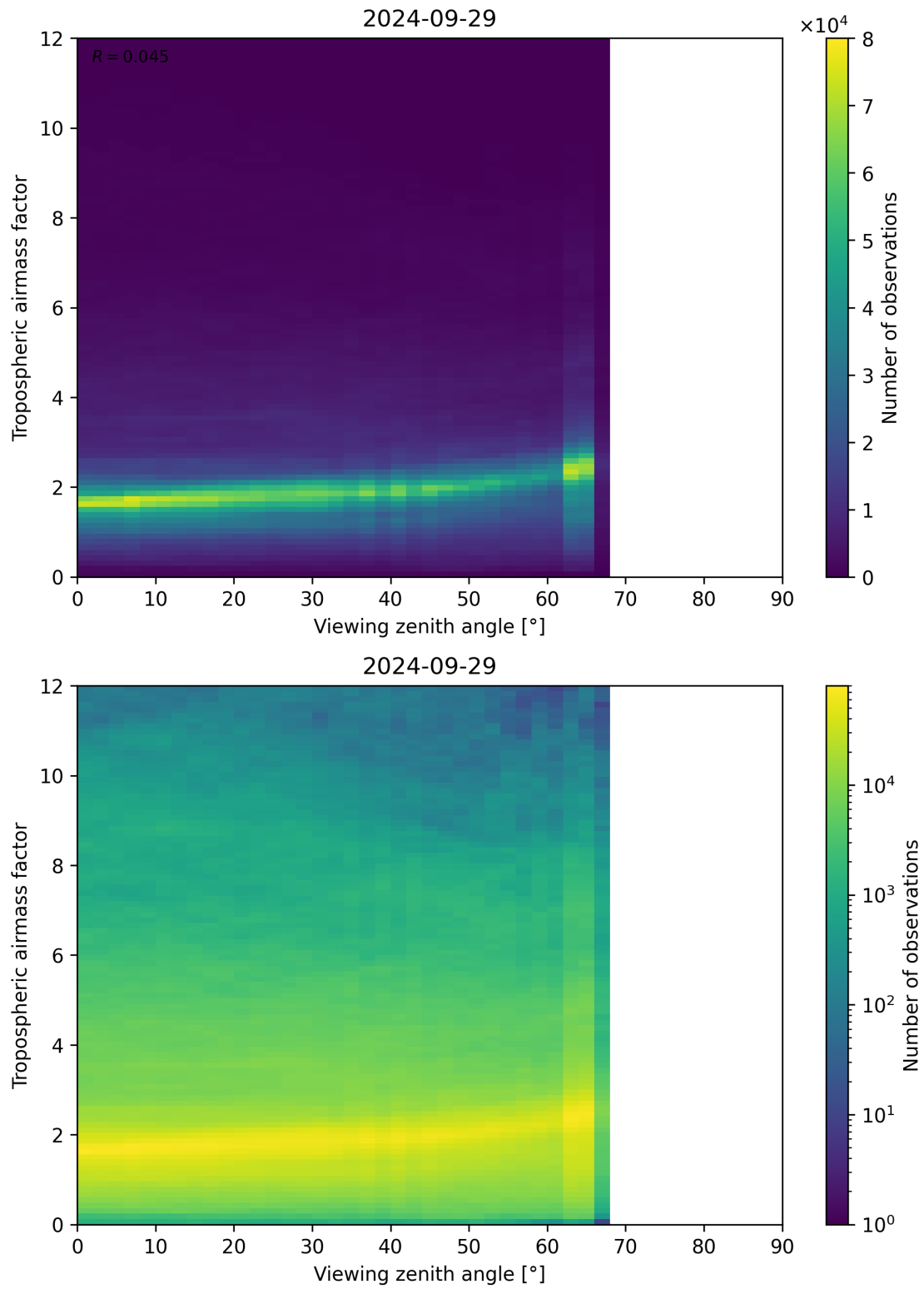
Figure 161: Scatter density plot of “Viewing zenith angle” against “Tropospheric airmass factor” for 2024-09-28 to 2024-09-30.
