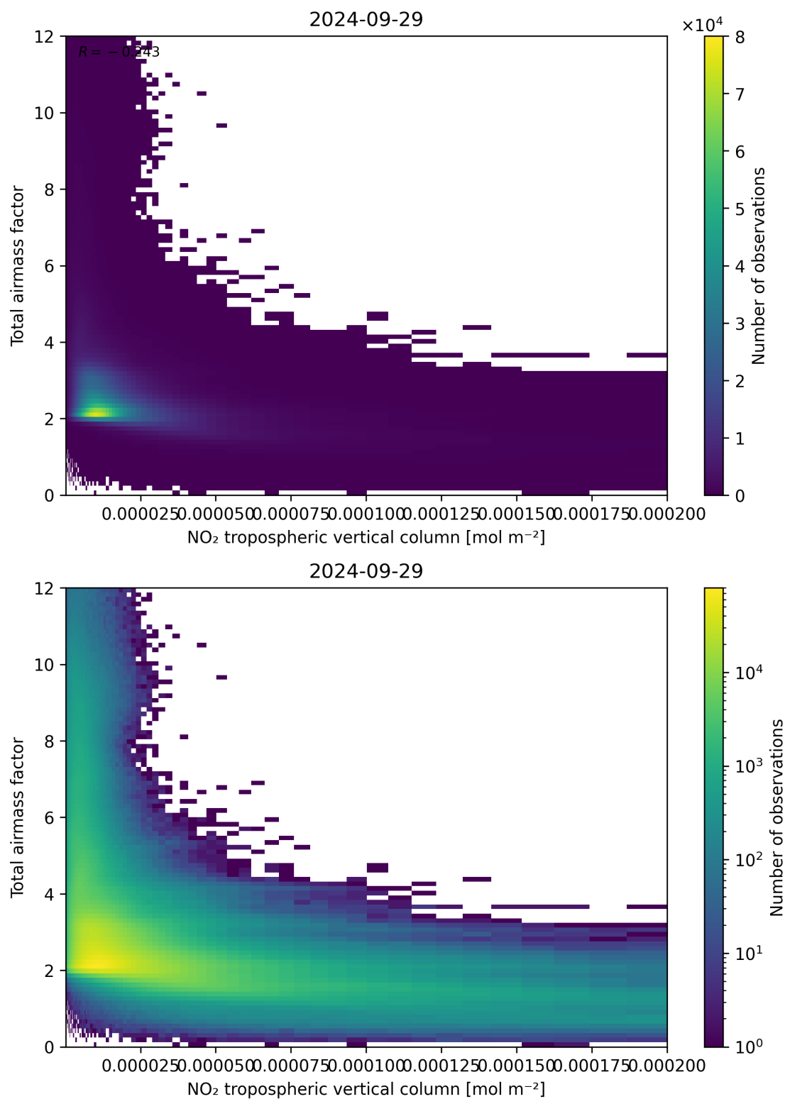
Figure 122: Scatter density plot of “NO 2 tropospheric vertical column” against “Total air mass factor” for 2024-09-28 to 2024-09-30.
