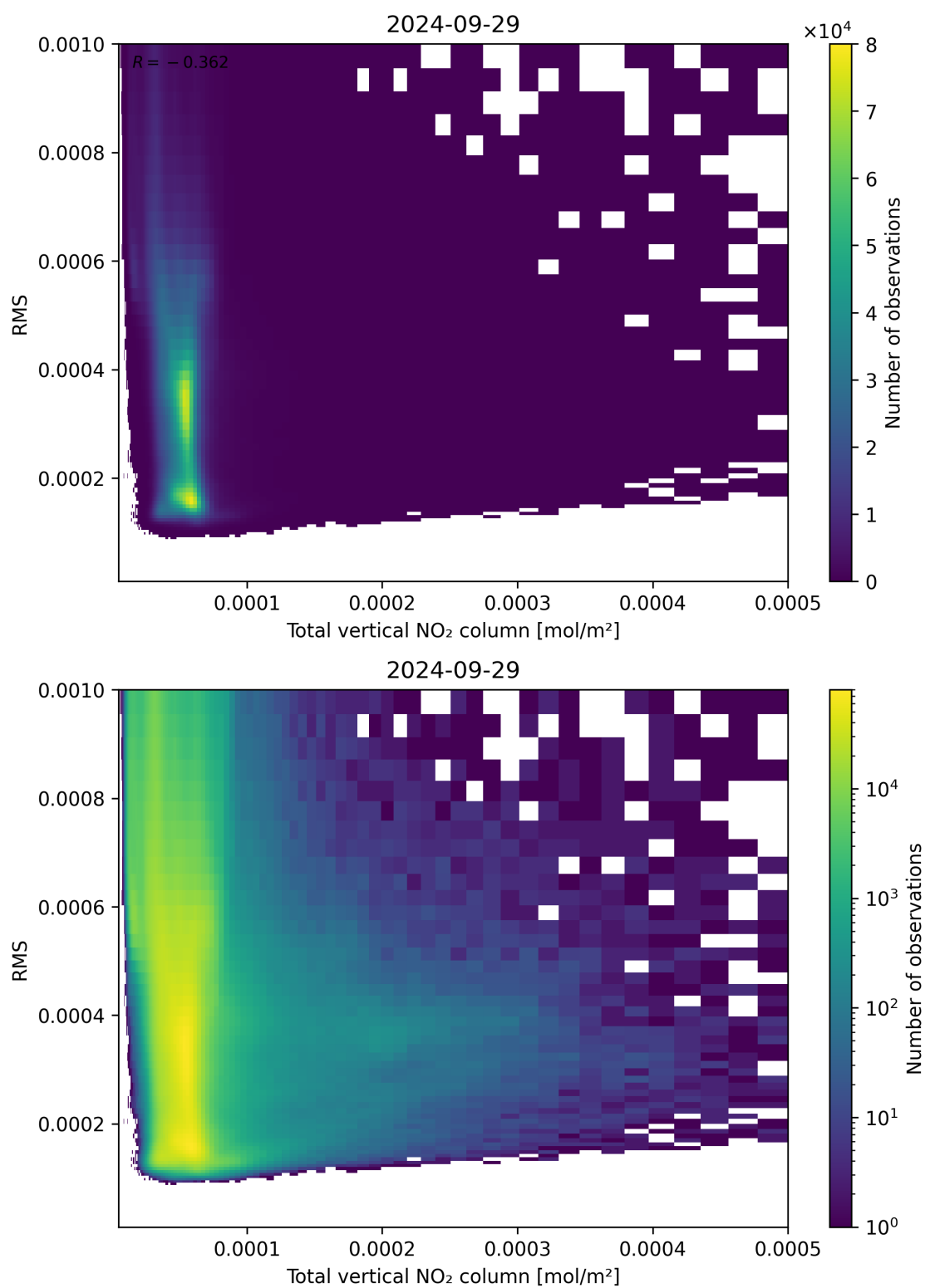
Figure 120: Scatter density plot of “Total vertical NO 2 column” against “RMS” for 2024-09-28 to 2024-09-30.
