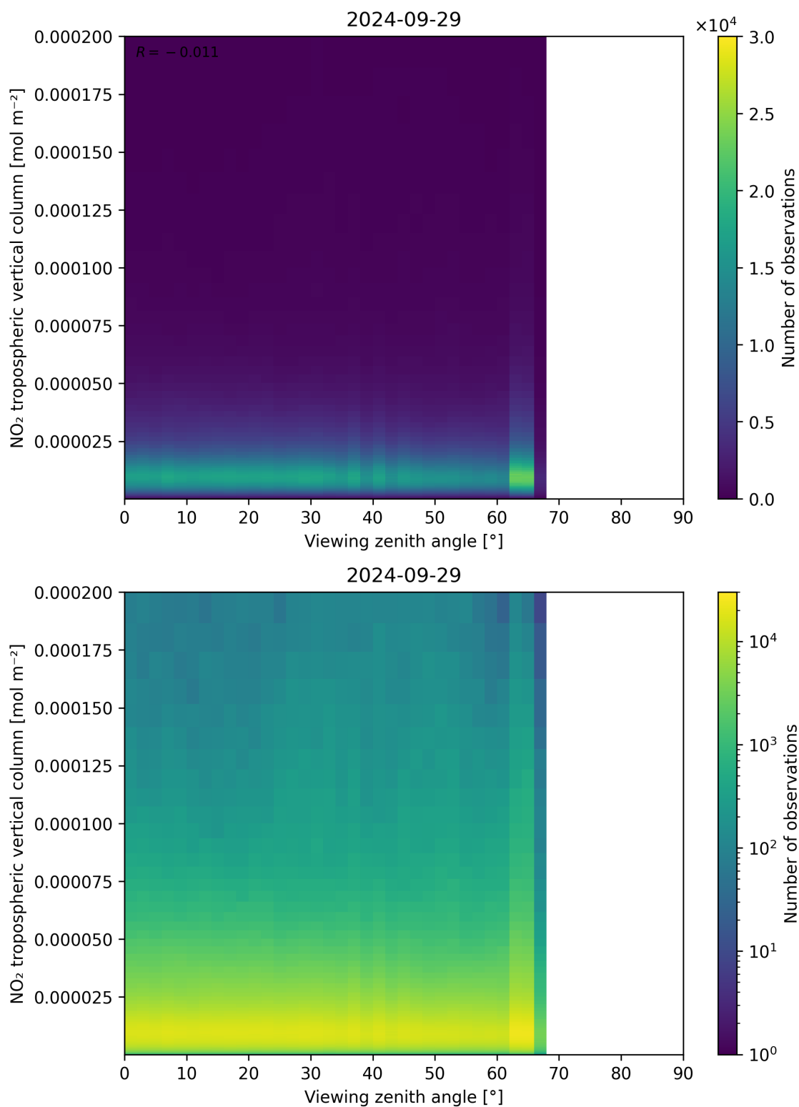
Figure 169: Scatter density plot of “Viewing zenith angle” against “NO 2 tropospheric vertical column” for 2024-09-28 to 2024-09-30.
