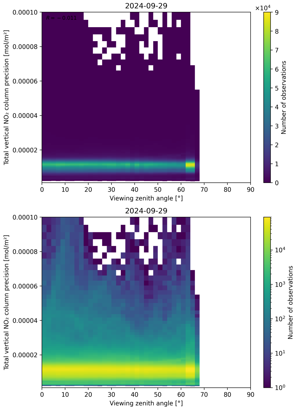
Figure 168: Scatter density plot of “Viewing zenith angle” against “Total vertical NO 2 column precision” for 2024-09-28 to 2024-09-30.
