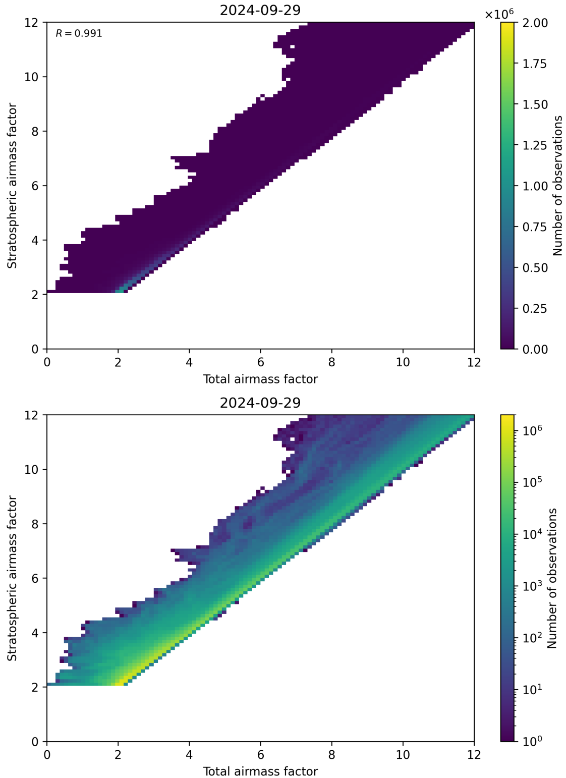
Figure 62: Scatter density plot of “Total airmass factor” against “Stratospheric airmass factor” for 2024-09-28 to 2024-09-30.
