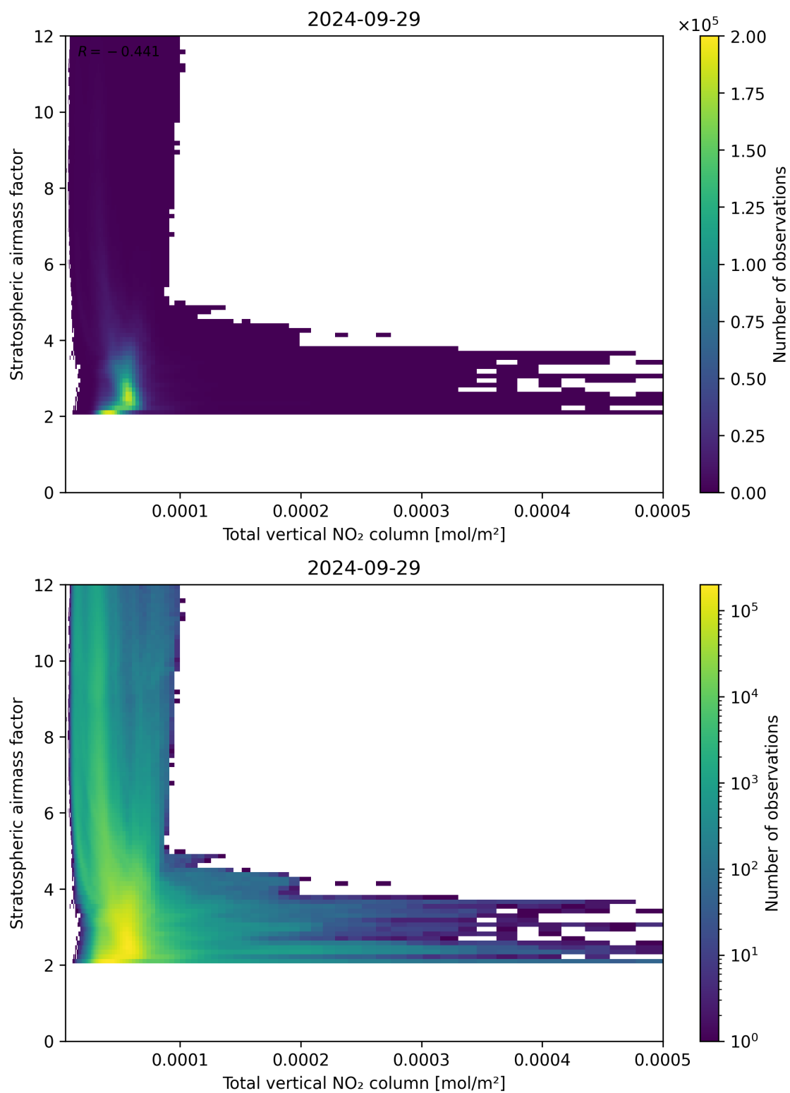
Figure 110: Scatter density plot of “Total vertical NO 2 column” against “Stratospheric airmass factor” for 2024-09-28 to 2024-09-30.
