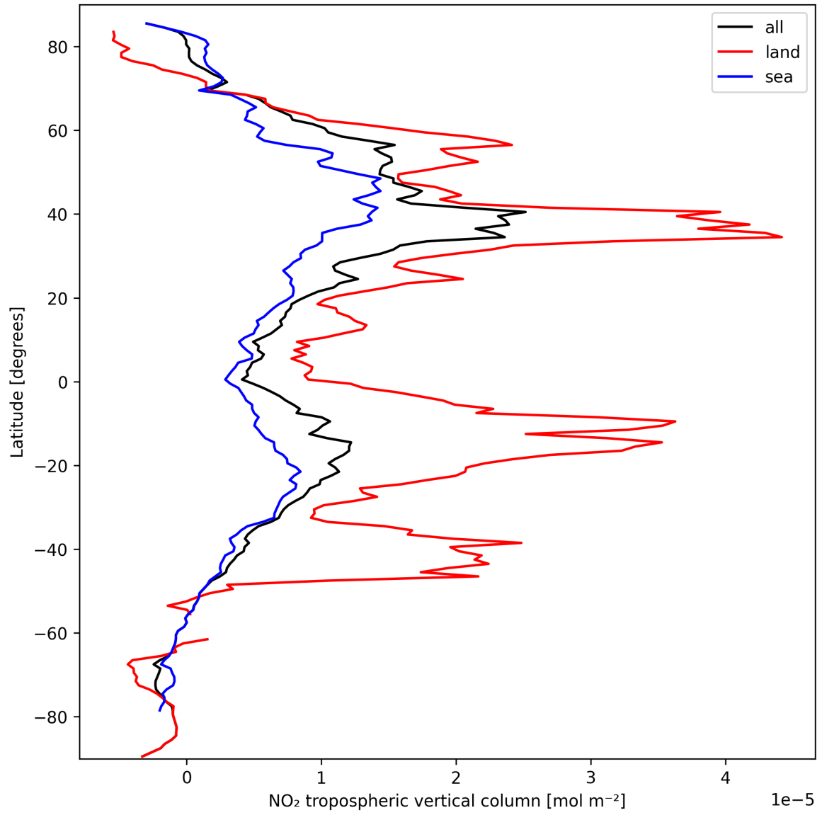
Figure 12: Zonal average of “NO 2 tropospheric vertical column” for 2024-09-28 to 2024-09-30.
