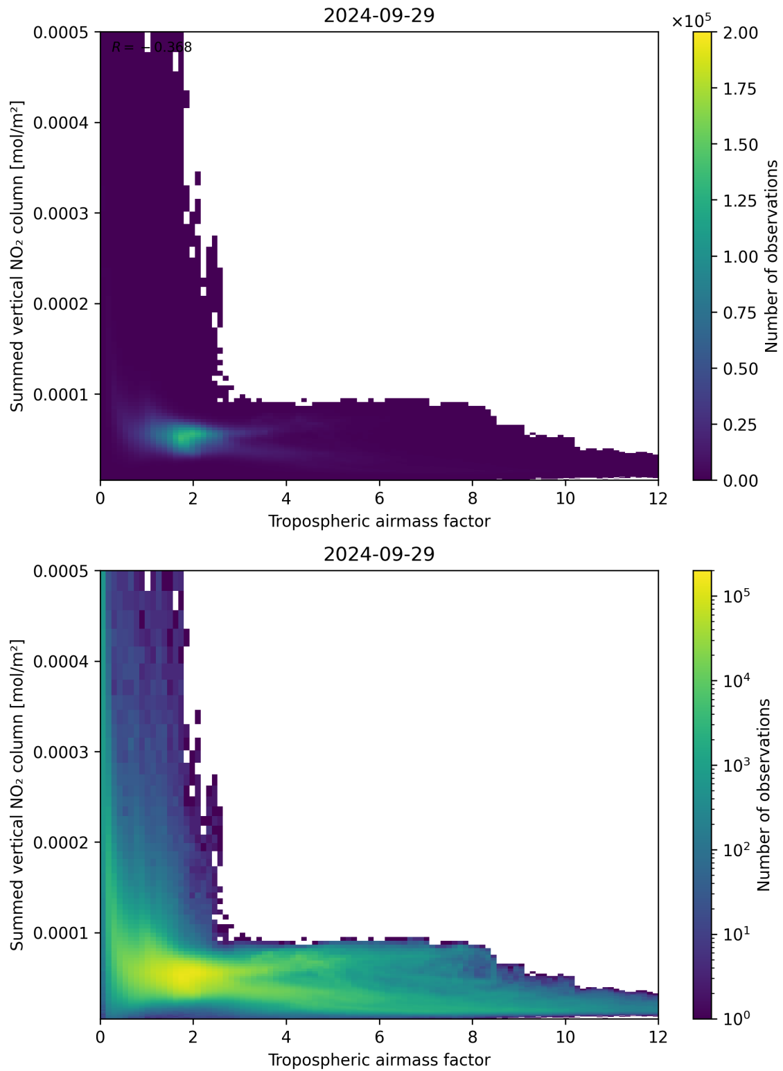
Figure 75: Scatter density plot of “Tropospheric air mass factor” against “Summed vertical NO 2 column” for 2024-09-28 to 2024-09-30.
