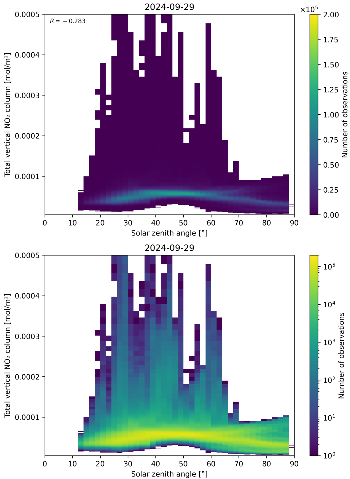
Figure 153: Scatter density plot of “Solar zenith angle” against “Total vertical NO 2 column” for 2024-09-28 to 2024-09-30.
