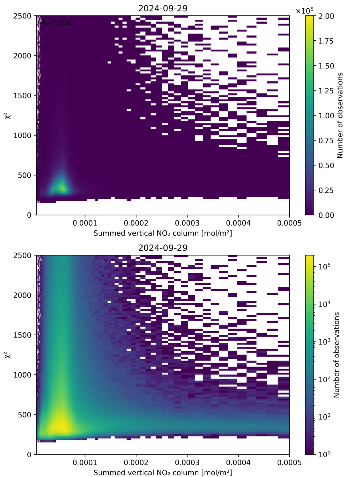
Figure 104: Scatter density plot of “Summed vertical NO 2 column” against “ \chi^2 ” for 2024-09-28 to 2024-09-30.
