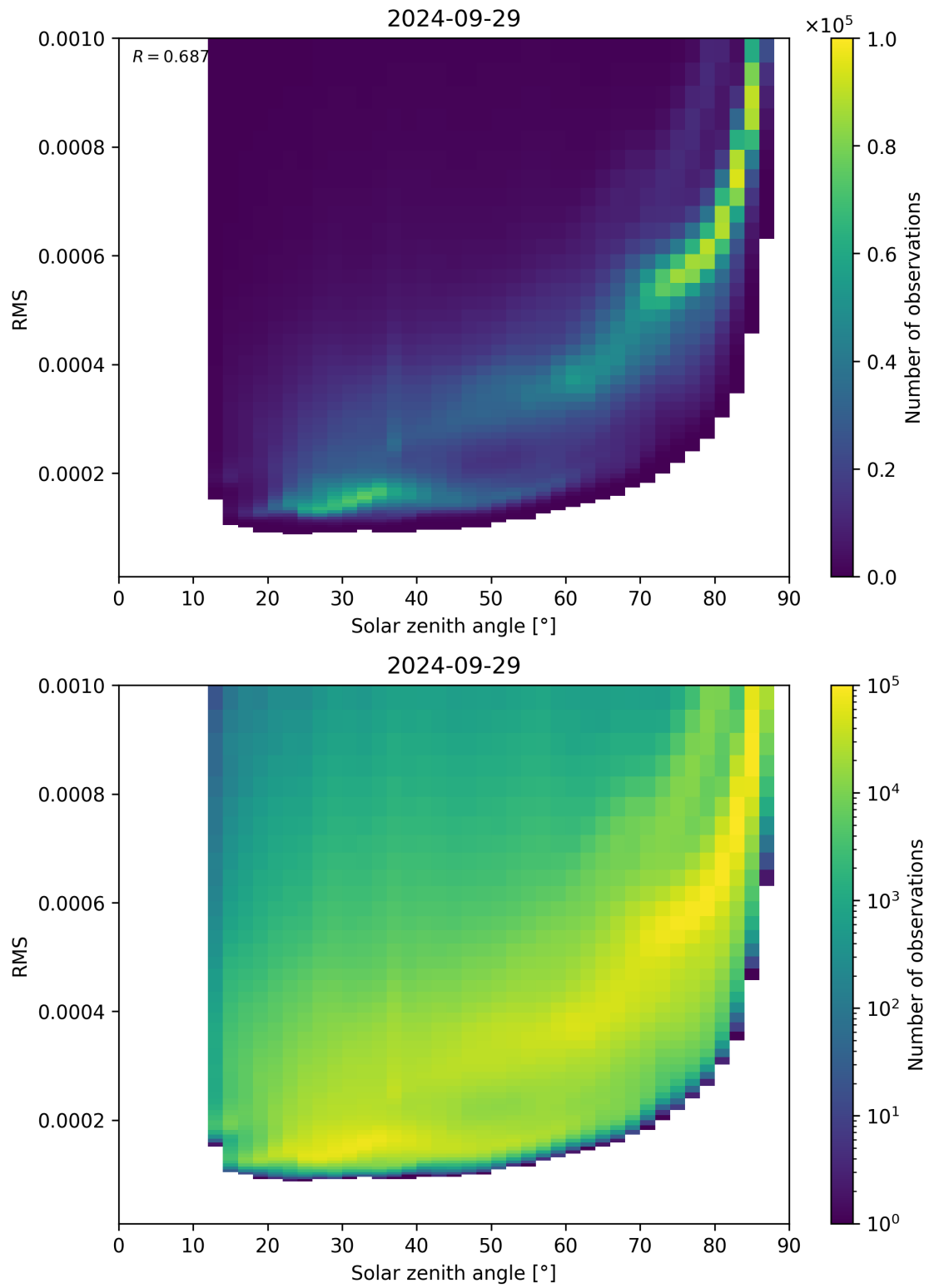
Figure 157: Scatter density plot of “Solar zenith angle” against “RMS” for 2024-09-28 to 2024-09-30.
