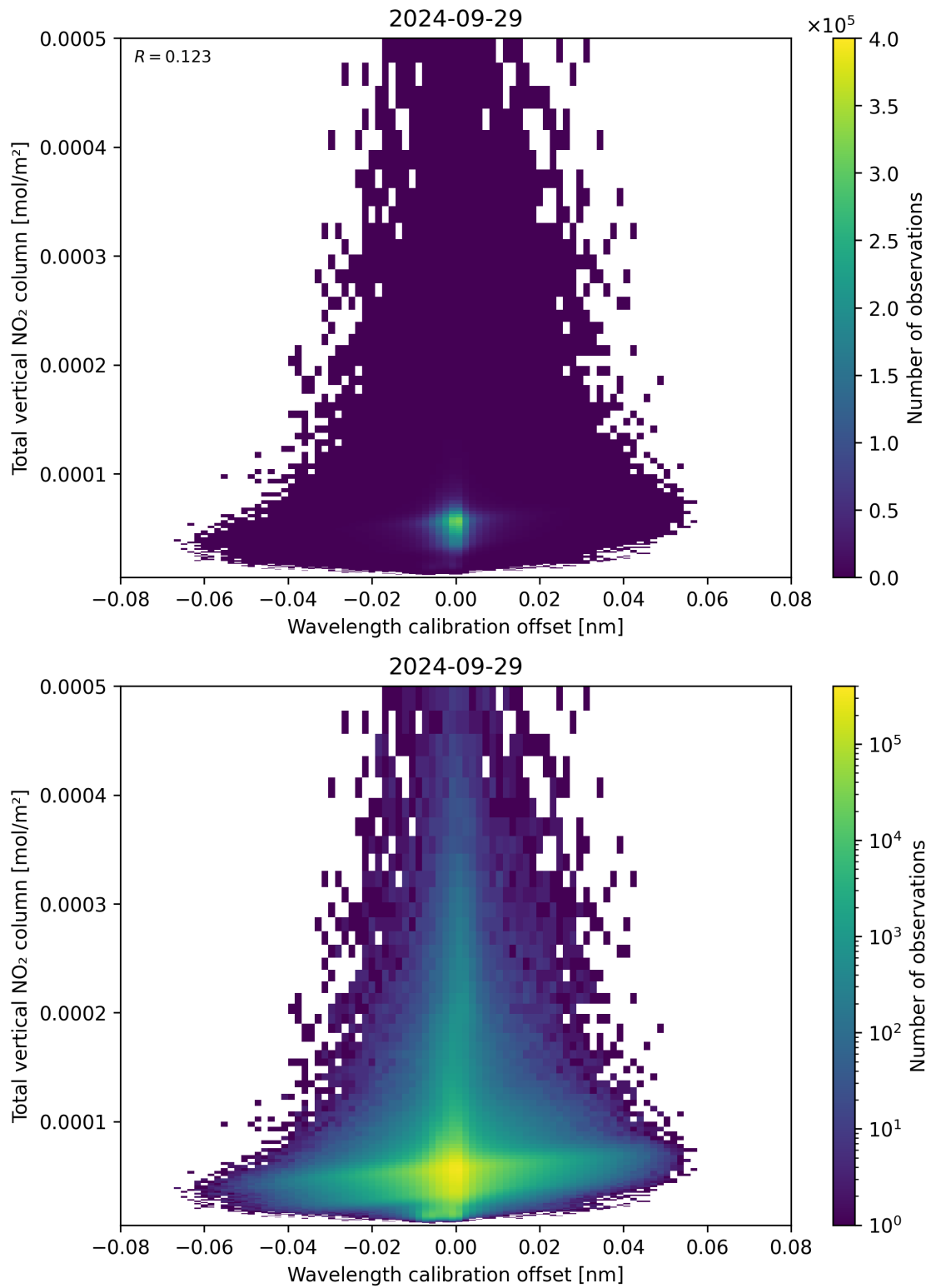
Figure 179: Scatter density plot of “Wavelength calibration offset” against “Total vertical NO 2 column” for 2024-09-28 to 2024-09-30.
