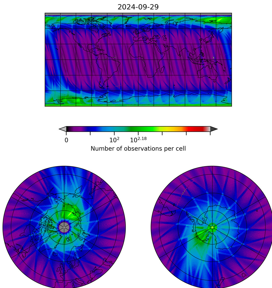
Figure 10: Map of the number of observations for 2024-09-28 to 2024-09-30
