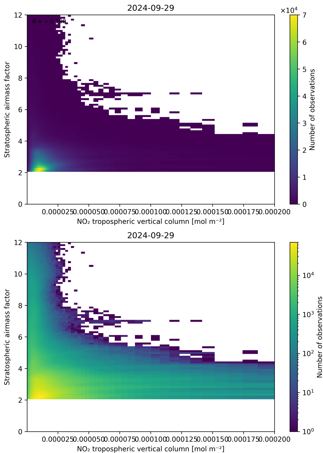
Figure 121: Scatter density plot of “NO 2 tropospheric vertical column” against “Stratospheric air mass factor” for 2024-09-28 to 2024-09-30.
