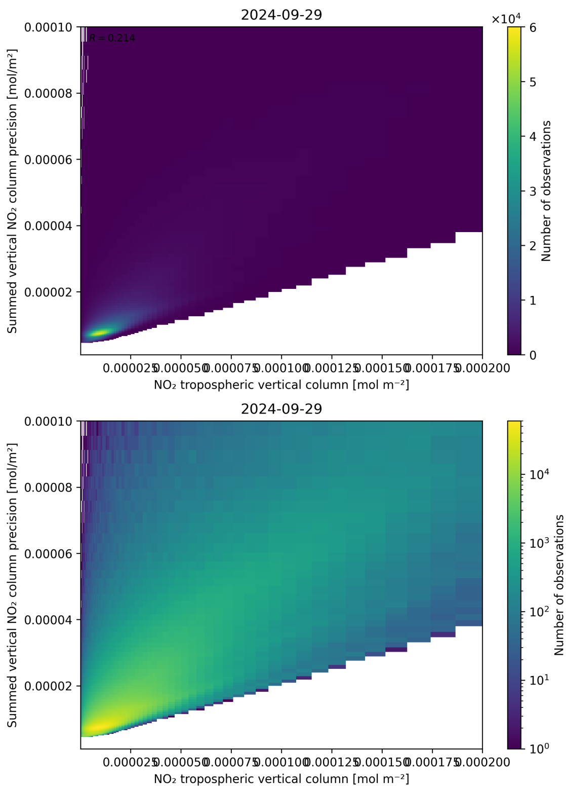
Figure 127: Scatter density plot of “NO 2 tropospheric vertical column” against “Summed vertical NO 2 column precision” for 2024-09-28 to 2024-09-30.
