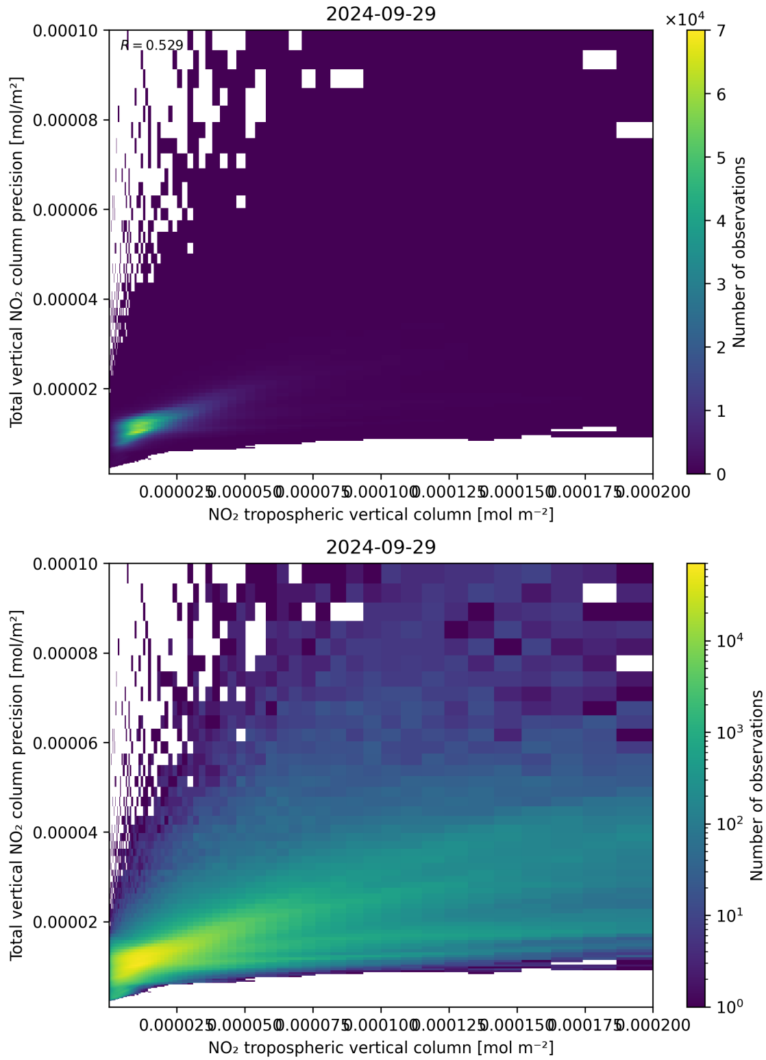
Figure 129: Scatter density plot of “NO 2 tropospheric vertical column” against “Total vertical NO 2 column precision” for 2024-09-28 to 2024-09-30.
