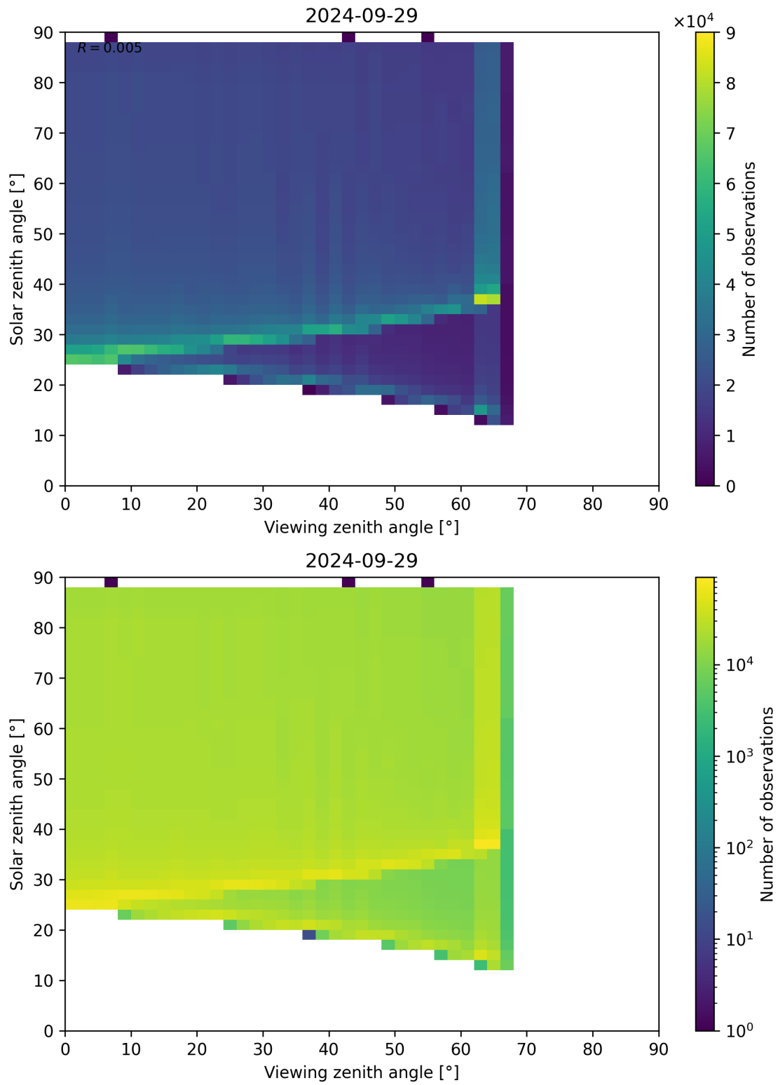
Figure 172: Scatter density plot of “Viewing zenith angle” against “Solar zenith angle” for 2024-09-28 to 2024-09-30.
