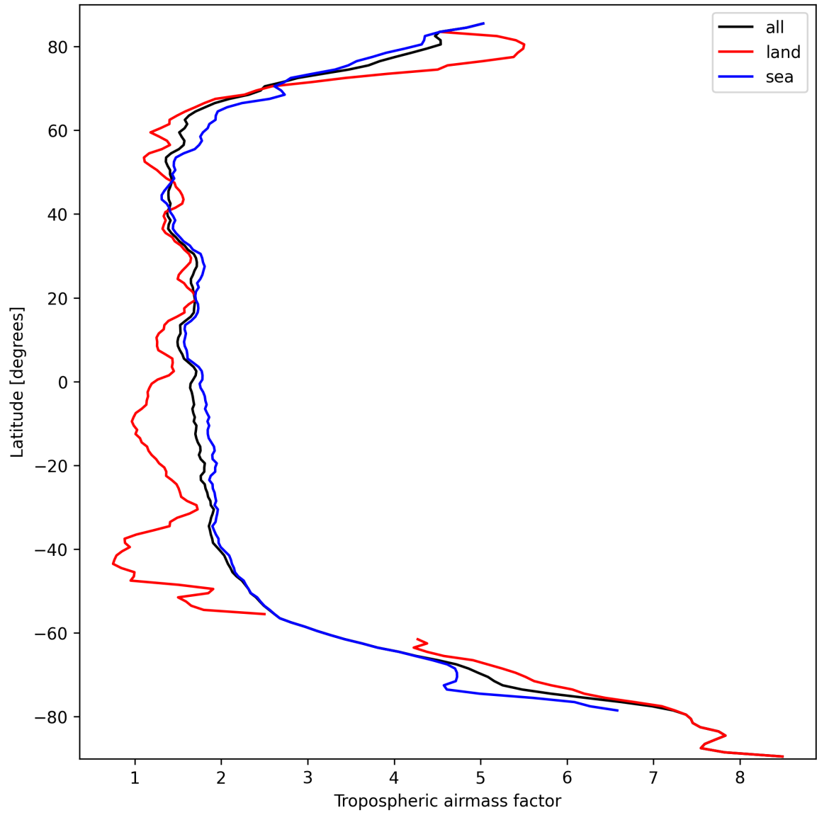
Figure 14: Zonal average of “Tropospheric airmass factor” for 2024-09-28 to 2024-09-30.
