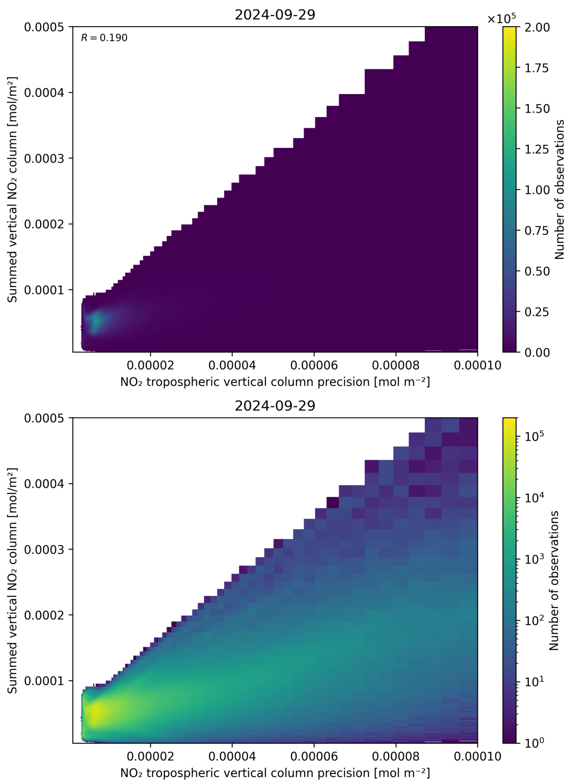
Figure 136: Scatter density plot of “NO 2 tropospheric vertical column precision” against “Summed vertical NO 2 column” for 2024-09-28 to 2024-09-30.
