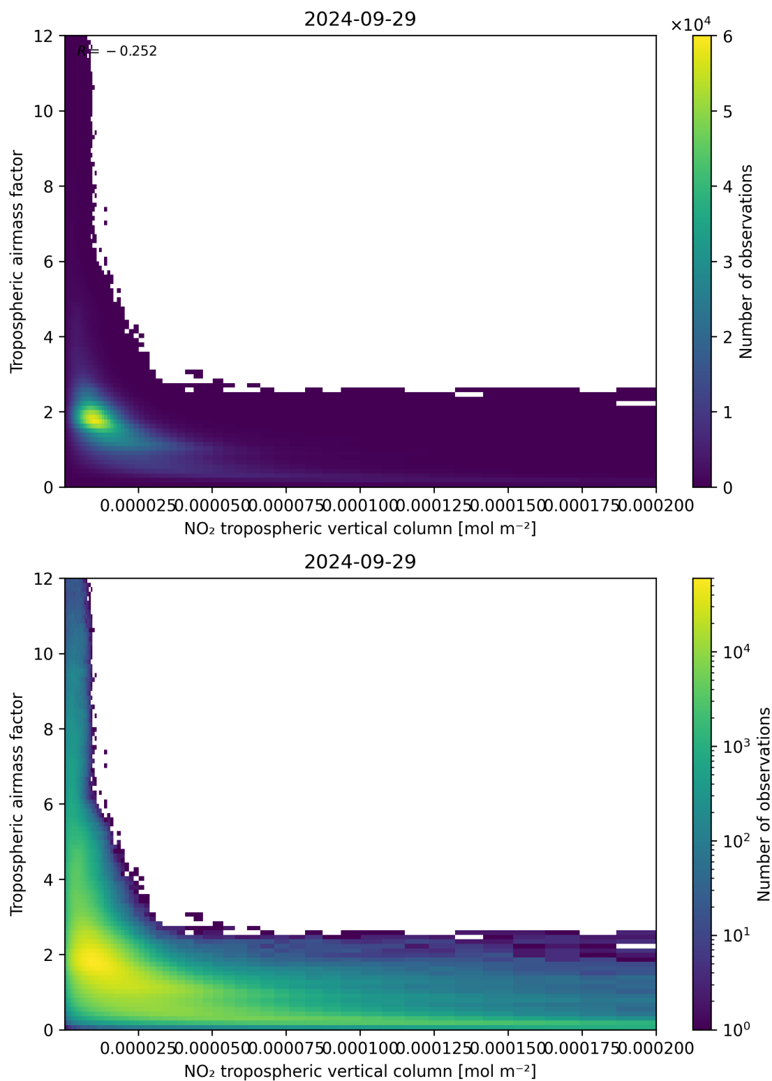
Figure 123: Scatter density plot of “NO 2 tropospheric vertical column” against “Tropospheric air mass factor” for 2024-09-28 to 2024-09-30.
