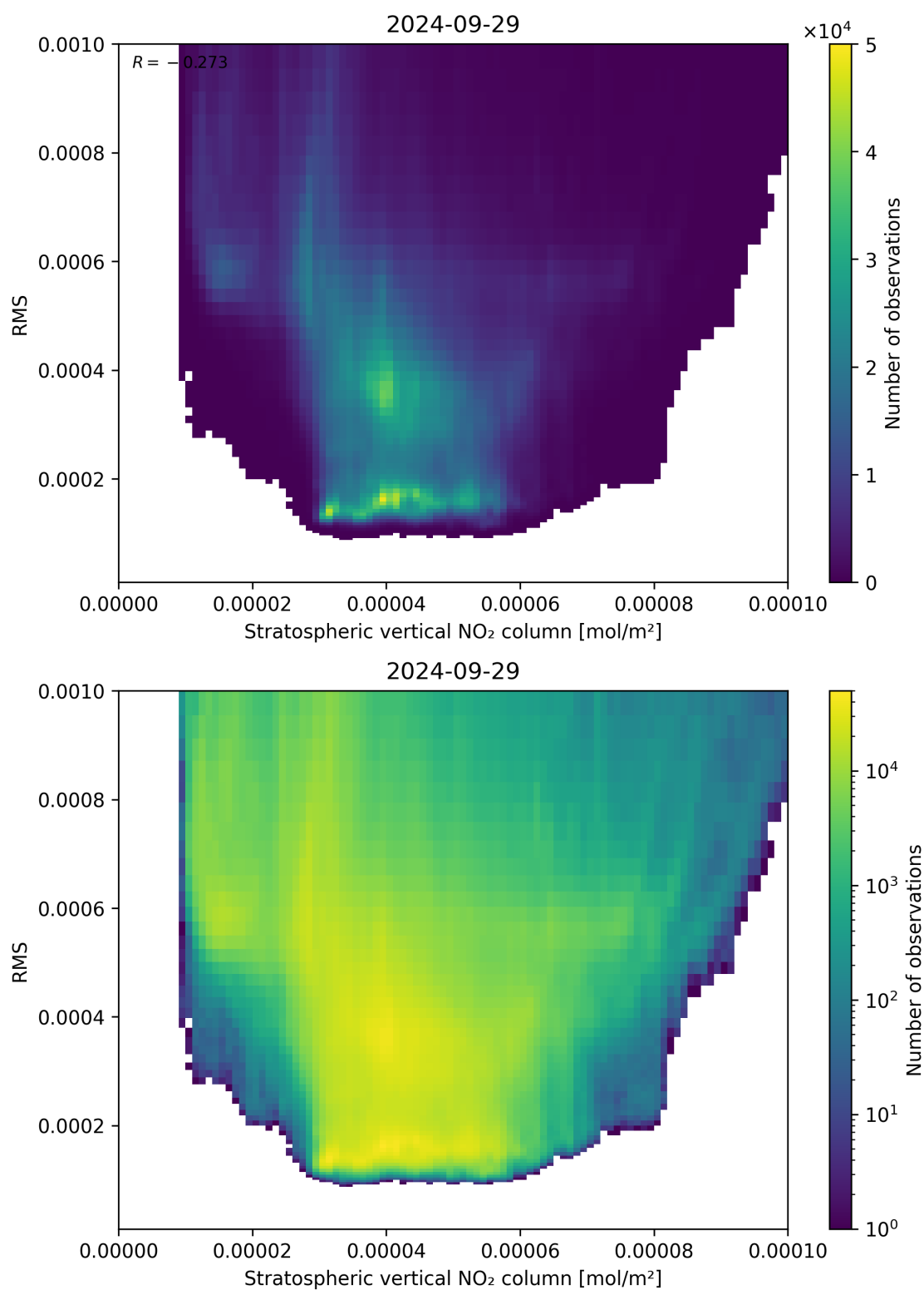
Figure 102: Scatter density plot of “Stratospheric vertical NO 2 column” against “RMS” for 2024-09-28 to 2024-09-30.
