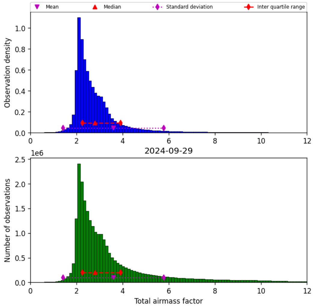
Figure 32: Histogram of “Total airmass factor” for 2024-09-28 to 2024-09-30
