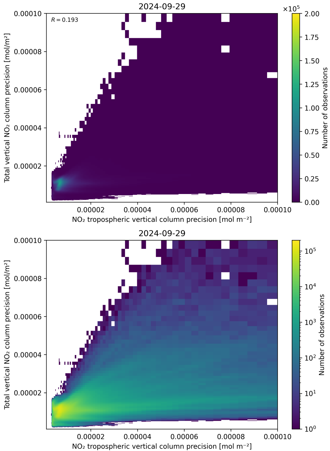
Figure 139: Scatter density plot of “NO 2 tropospheric vertical column precision” against “Total vertical NO 2 column precision” for 2024-09-28 to 2024-09-30.
