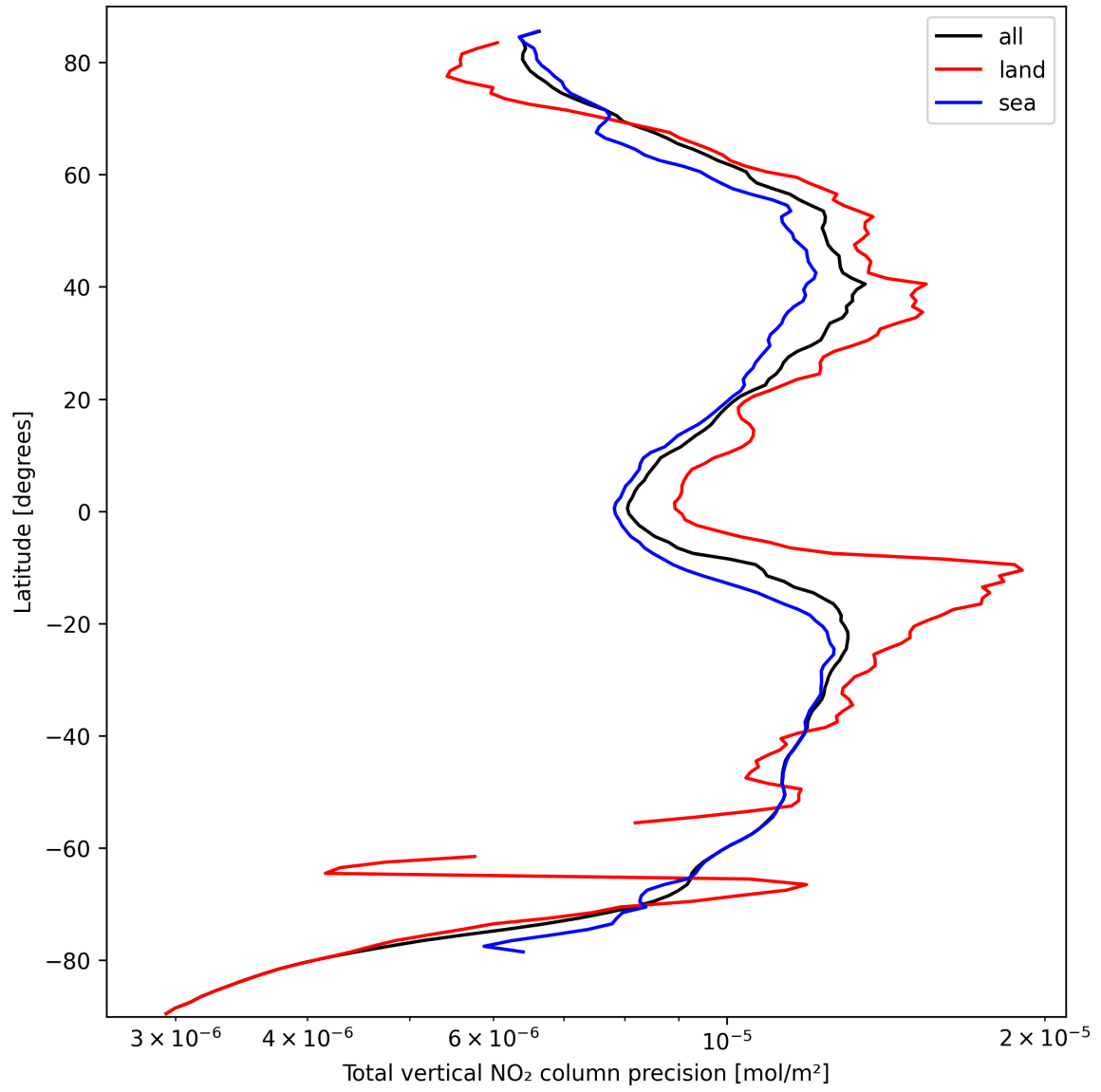
Figure 22: Zonal average of “Total vertical NO 2 column precision” for 2024-09-28 to 2024-09-30.
