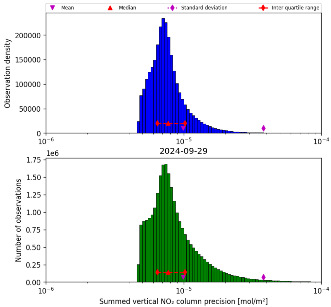
Figure 41: Histogram of "Summed vertical NO 2 column precision" for 2024-09-28 to 2024-09-30
