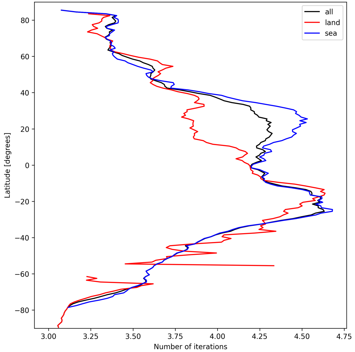
Figure 17: Zonal average of “Number of iterations” for 2024-09-28 to 2024-09-30.
