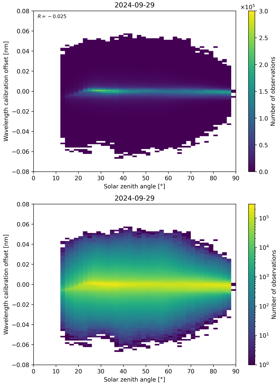
Figure 158: Scatter density plot of “Solar zenith angle” against “Wavelength calibration offset” for 2024-09-28 to 2024-09-30.
