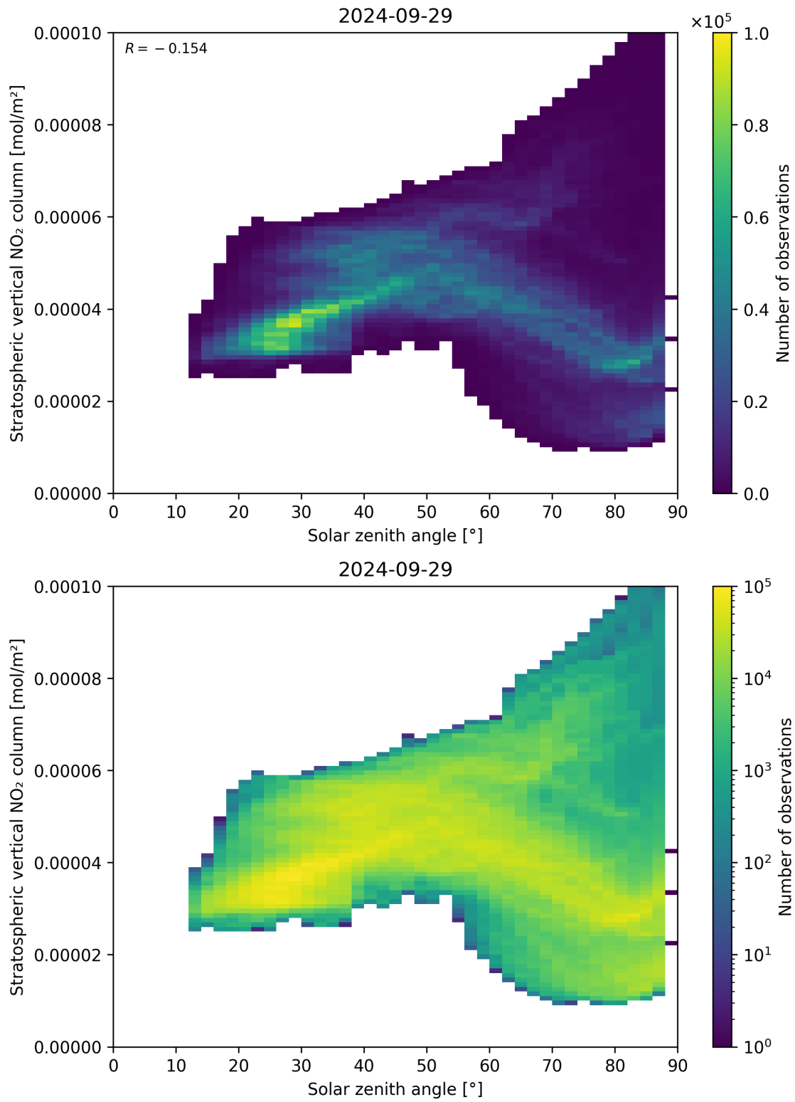
Figure 150: Scatter density plot of “Solar zenith angle” against “Stratospheric vertical \text{NO}_2 column” for 2024-09-28 to 2024-09-30.
