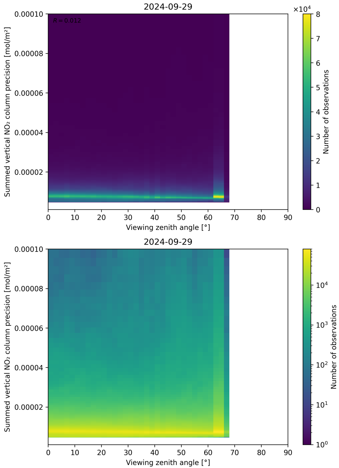
Figure 166: Scatter density plot of “Viewing zenith angle” against “Summed vertical NO 2 column precision” for 2024-09-28 to 2024-09-30.
