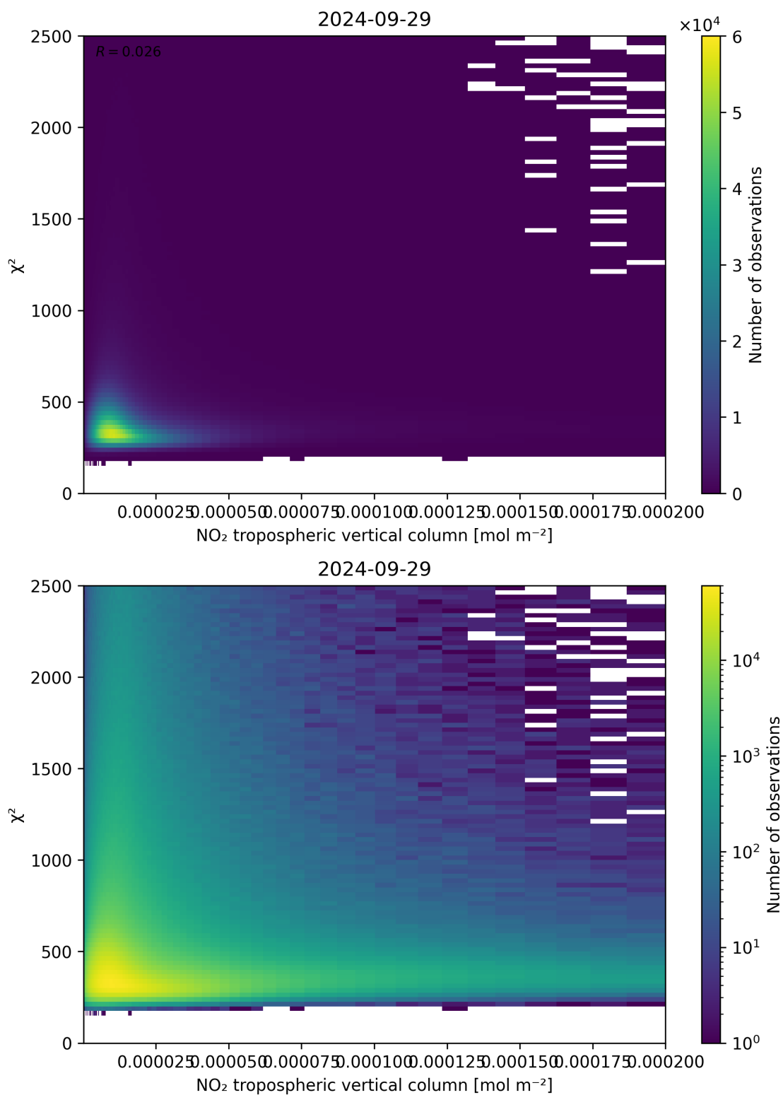
Figure 124: Scatter density plot of “NO 2 tropospheric vertical column” against “ \chi^2 ” for 2024-09-28 to 2024-09-30.
