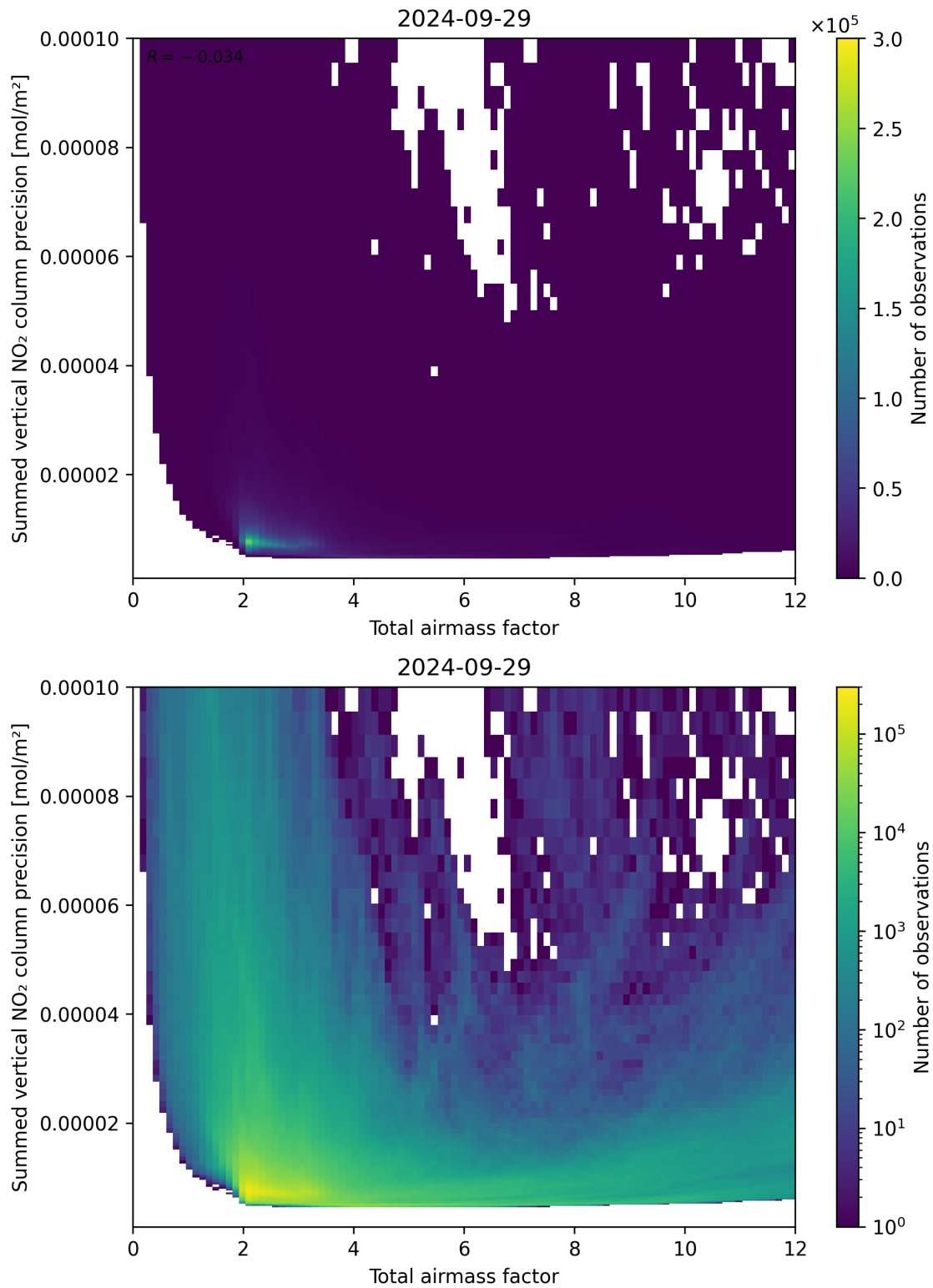
Figure 66: Scatter density plot of “Total airmass factor” against “Summed vertical NO 2 column precision” for 2024-09-28 to 2024-09-30.
