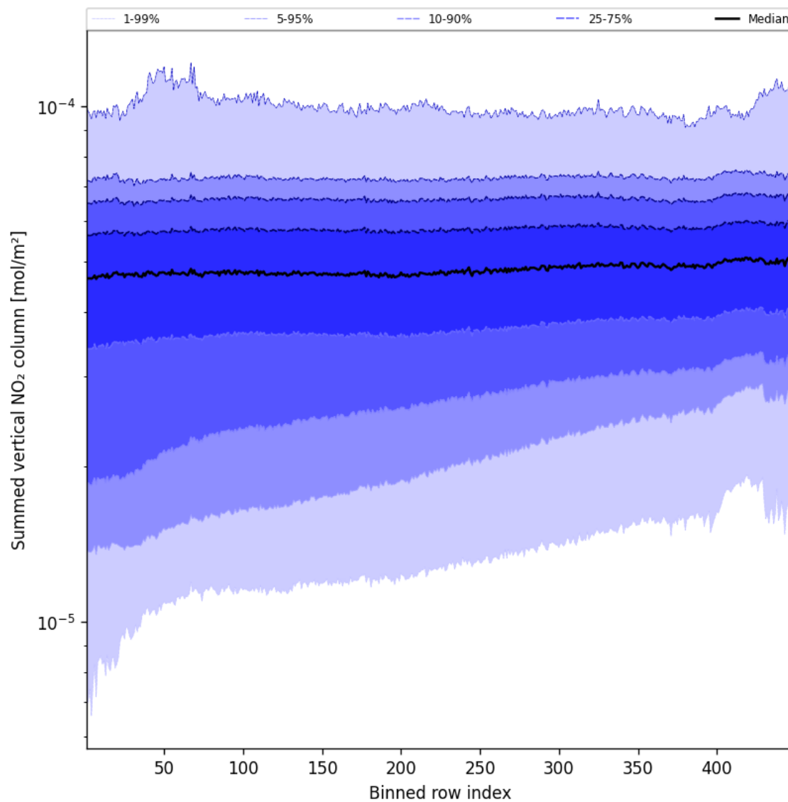
Figure 57: Along track statistics of “Summed vertical NO 2 column” for 2024-09-28 to 2024-09-30
