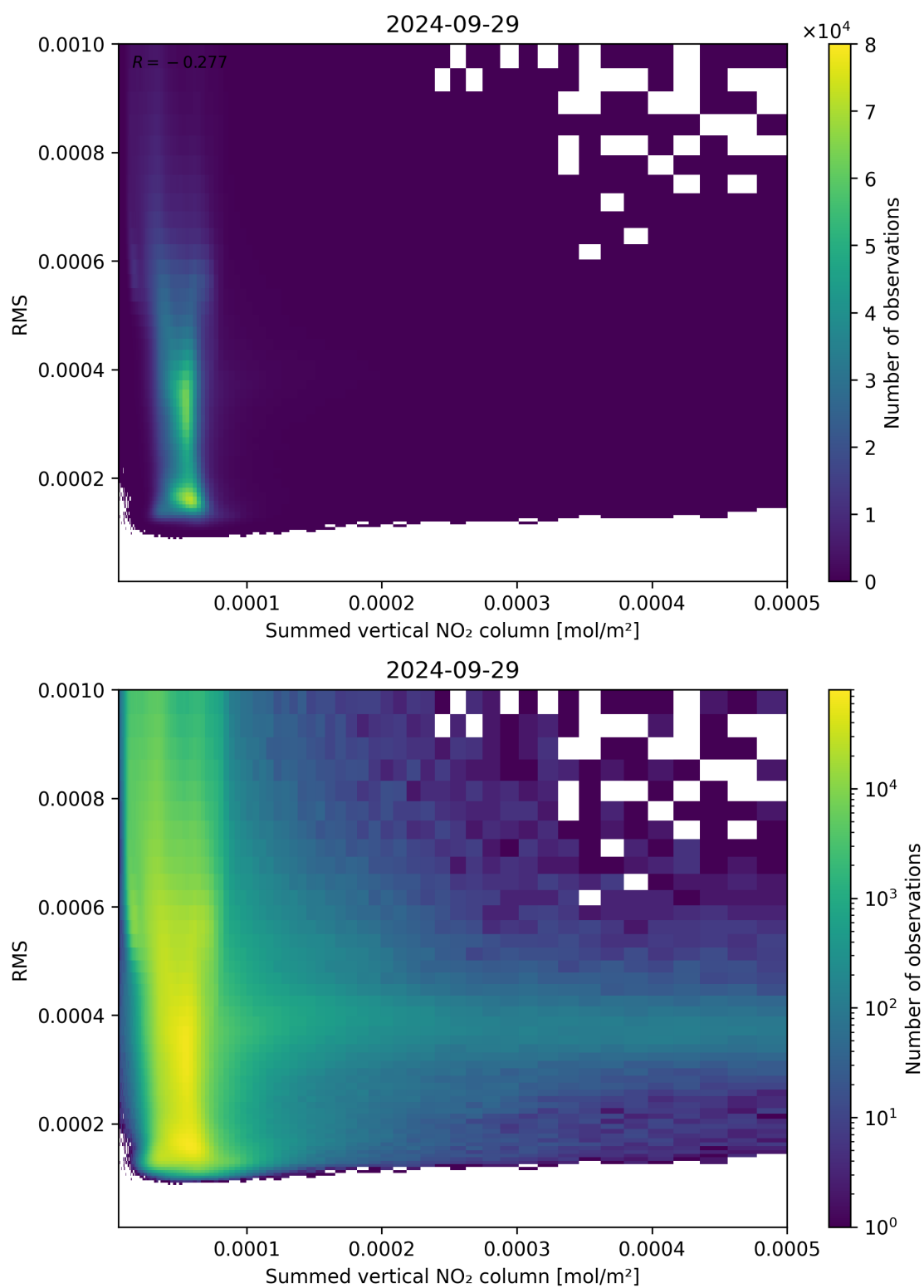
Figure 109: Scatter density plot of “Summed vertical NO 2 column” against “RMS” for 2024-09-28 to 2024-09-30.
