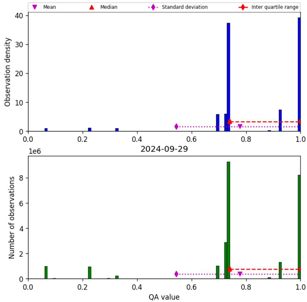
Figure 28: Histogram of “QA value” for 2024-09-28 to 2024-09-30
