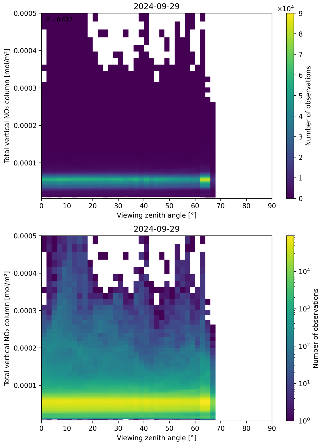
Figure 167: Scatter density plot of “Viewing zenith angle” against “Total vertical NO 2 column” for 2024-09-28 to 2024-09-30.
