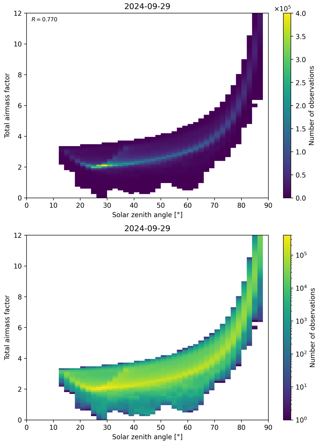
Figure 146: Scatter density plot of “Solar zenith angle” against “Total air mass factor” for 2024-09-28 to 2024-09-30.
