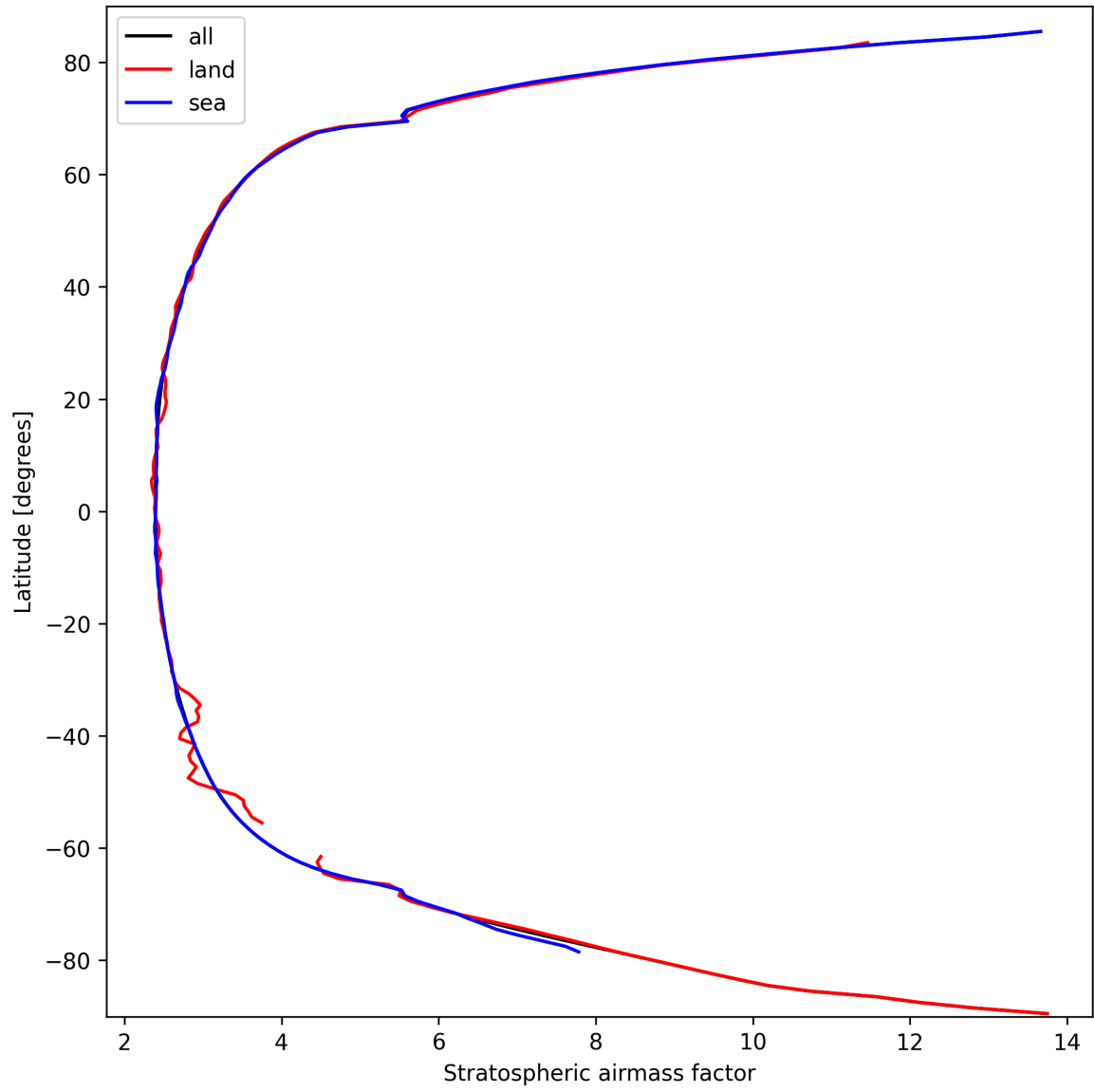
Figure 27: Zonal average of “Stratospheric airmass factor” for 2024-09-28 to 2024-09-30.
