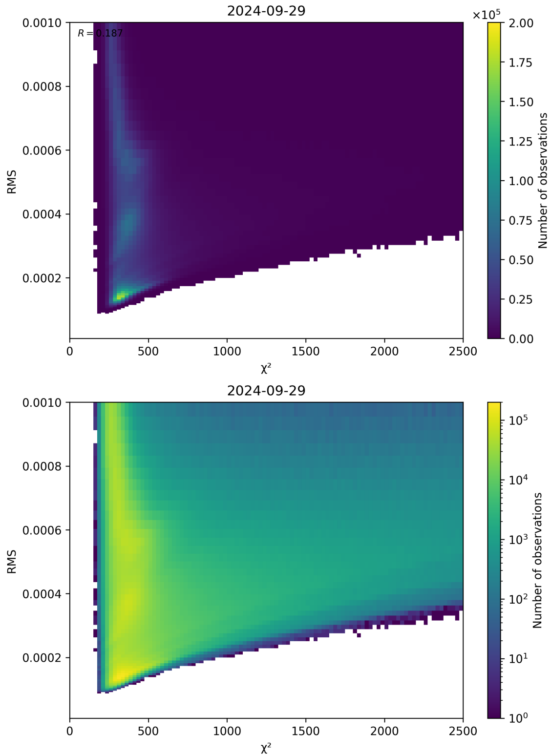
Figure 82: Scatter density plot of “ \chi^2 ” against “RMS” for 2024-09-28 to 2024-09-30.
