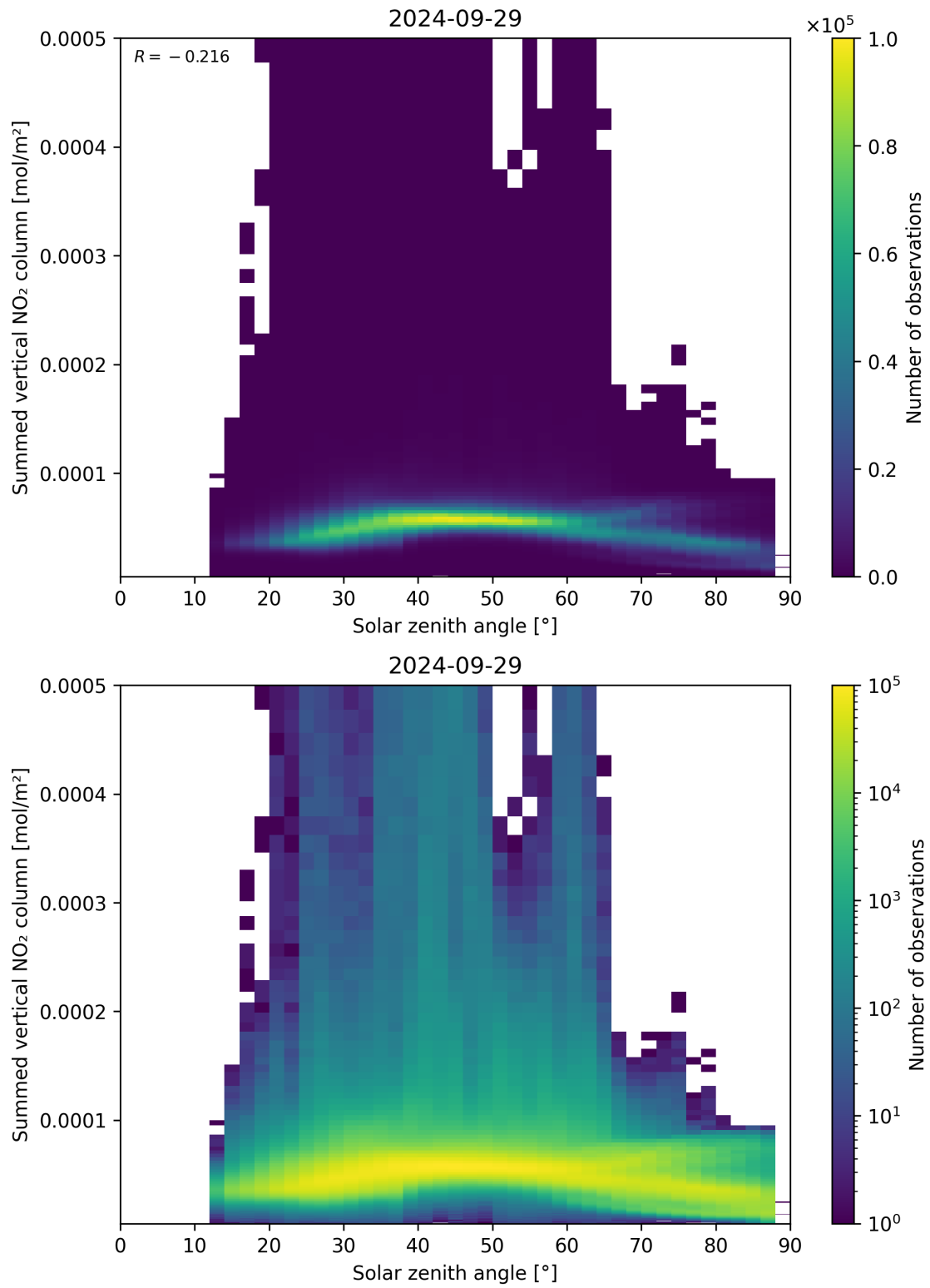
Figure 151: Scatter density plot of “Solar zenith angle” against “Summed vertical NO 2 column” for 2024-09-28 to 2024-09-30.
