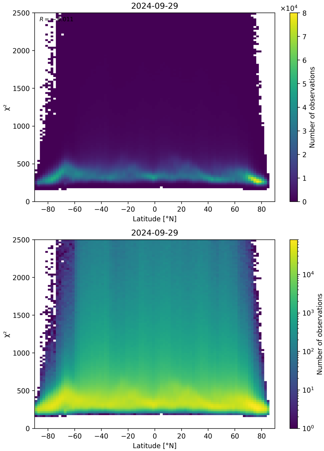
Figure 86: Scatter density plot of “Latitude” against “ \chi^2 ” for 2024-09-28 to 2024-09-30.
