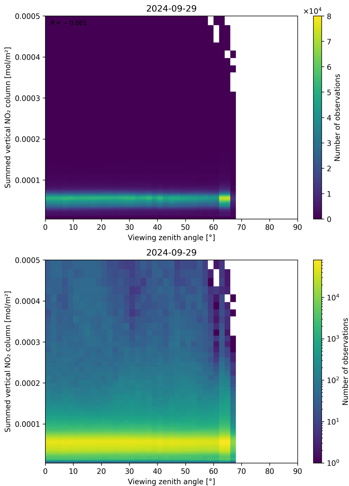
Figure 165: Scatter density plot of “Viewing zenith angle” against “Summed vertical NO 2 column” for 2024-09-28 to 2024-09-30.
