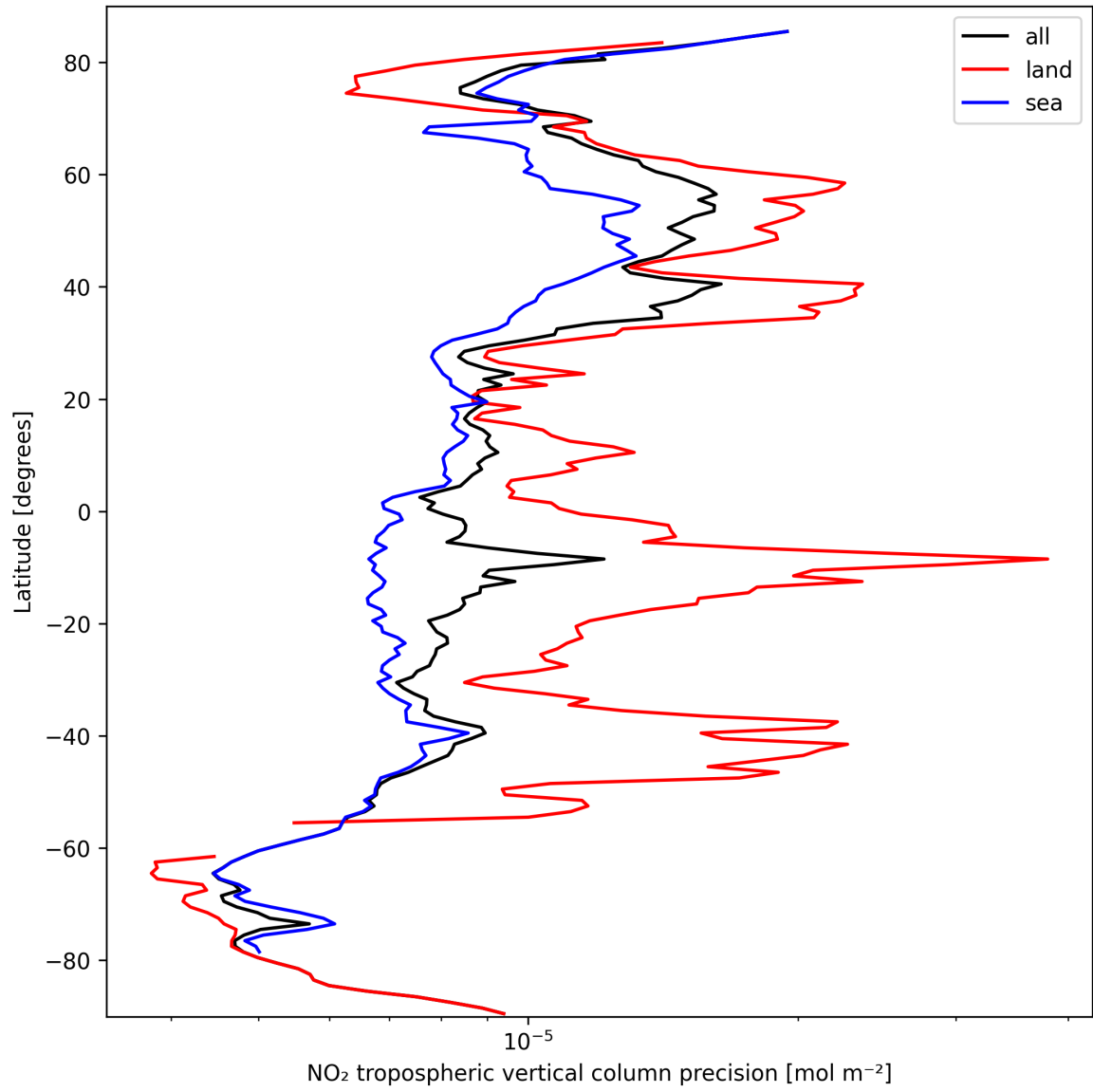
Figure 13: Zonal average of “NO 2 tropospheric vertical column precision” for 2024-09-28 to 2024-09-30.
