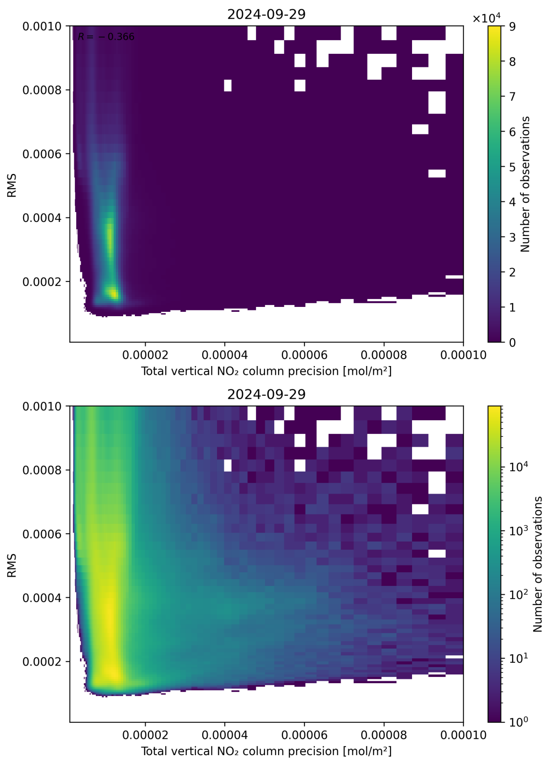
Figure 119: Scatter density plot of “Total vertical NO 2 column precision” against “RMS” for 2024-09-28 to 2024-09-30.
