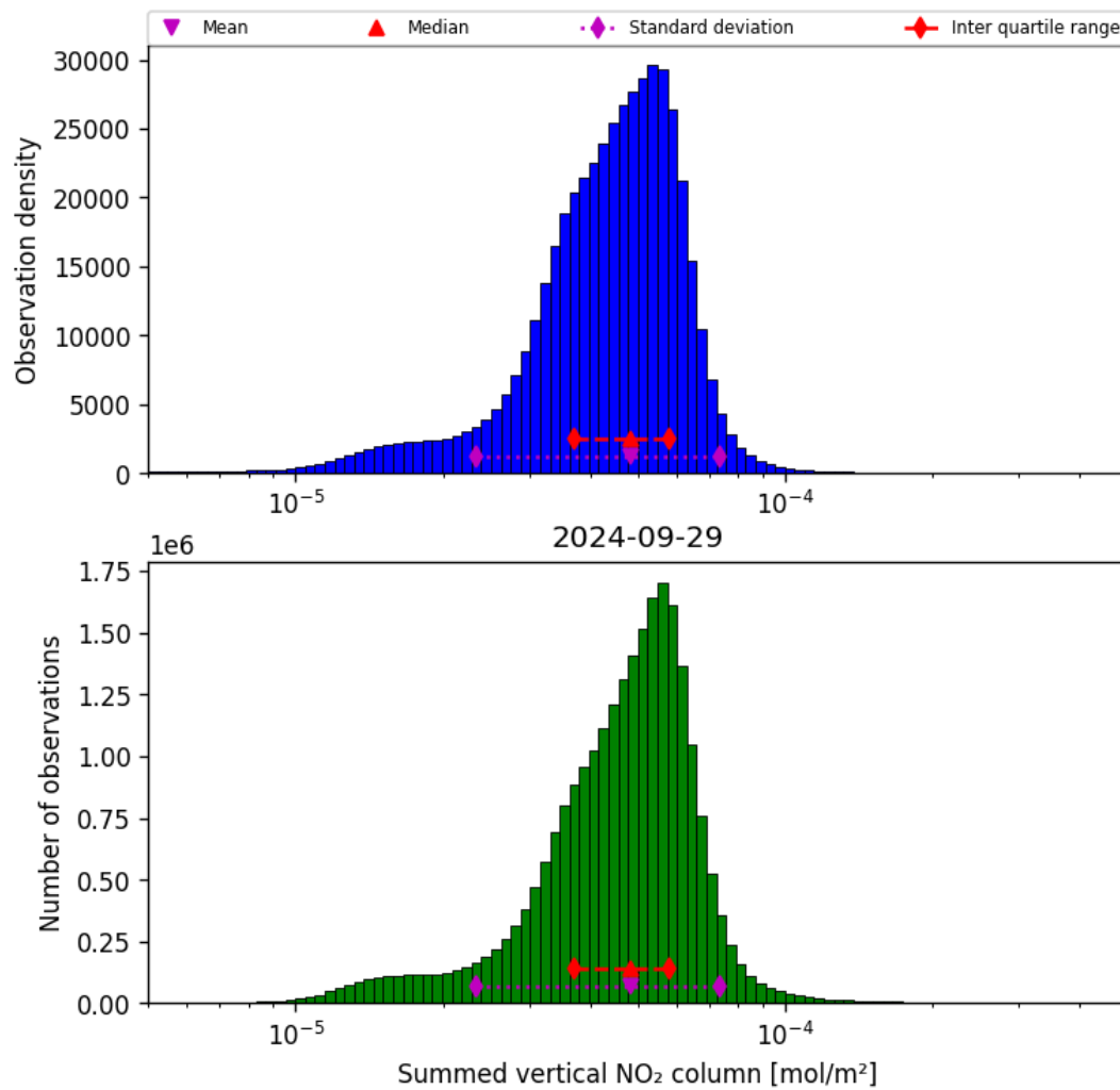
Figure 40: Histogram of “Summed vertical NO 2 column” for 2024-09-28 to 2024-09-30
