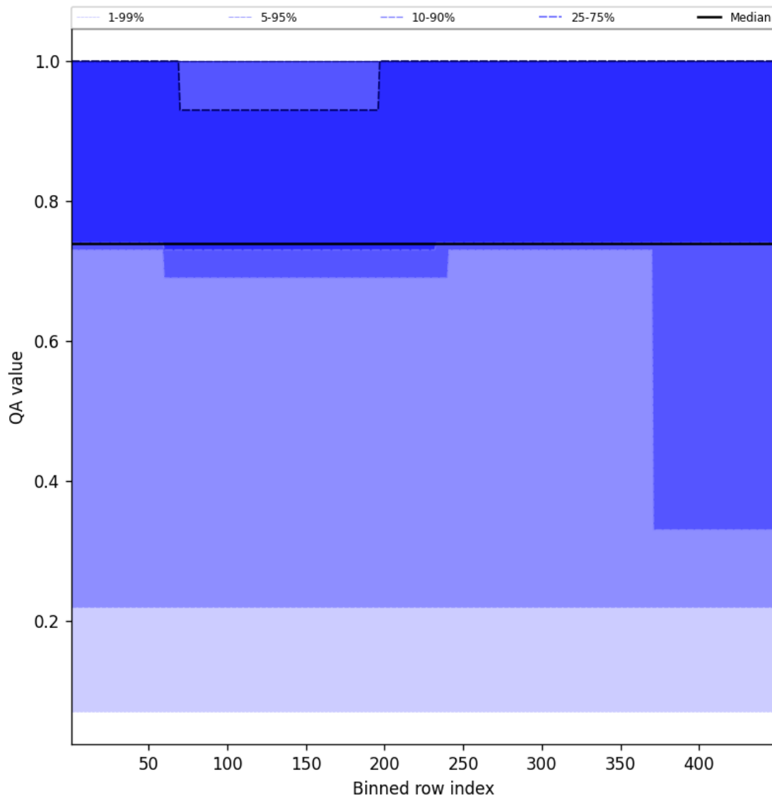
Figure 45: Along track statistics of “QA value” for 2024-09-28 to 2024-09-30
