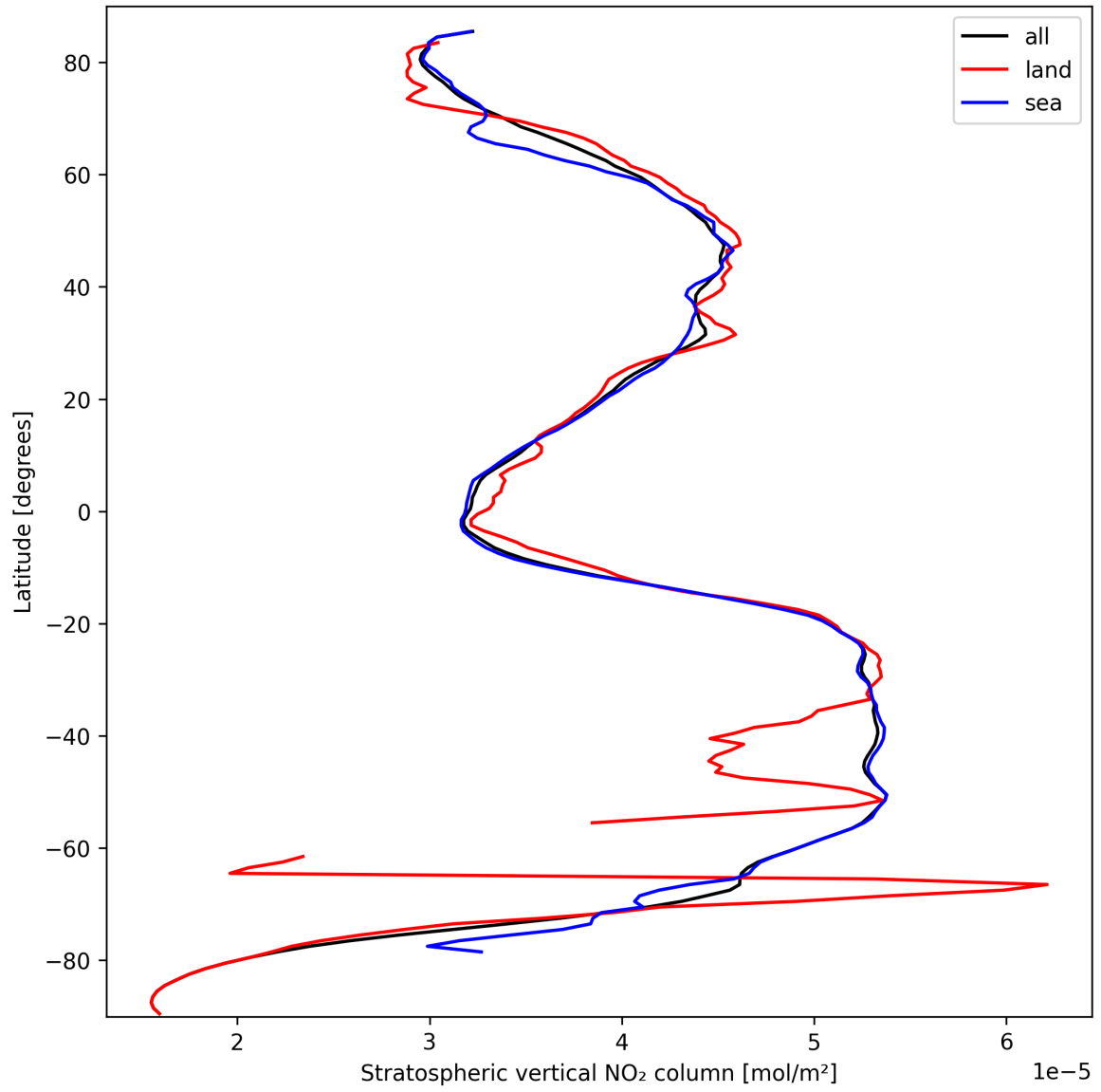
Figure 19: Zonal average of “Stratospheric vertical NO 2 column” for 2024-09-28 to 2024-09-30.
