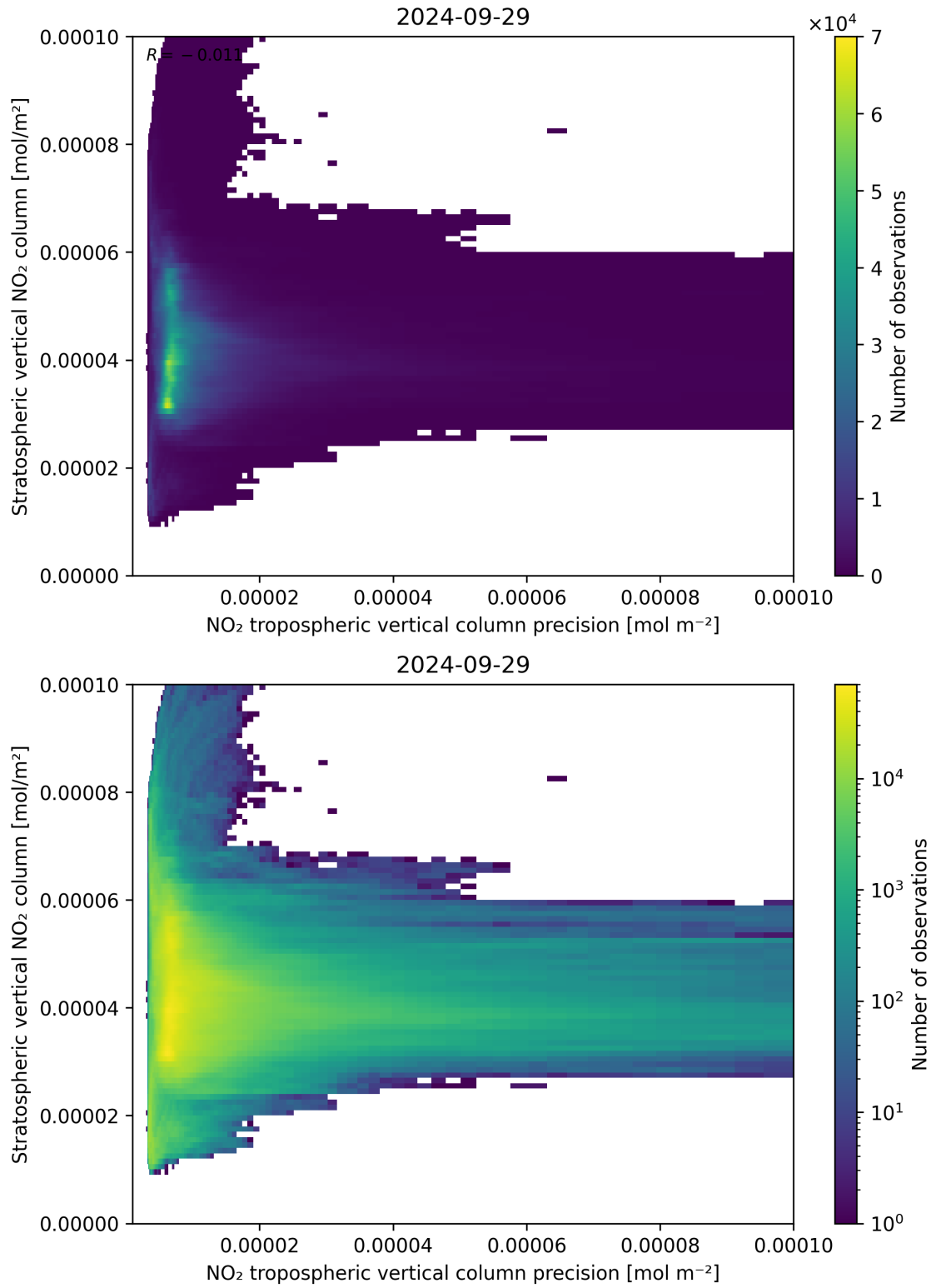
Figure 135: Scatter density plot of “NO 2 tropospheric vertical column precision” against “Stratospheric vertical NO 2 column” for 2024-09-28 to 2024-09-30.
