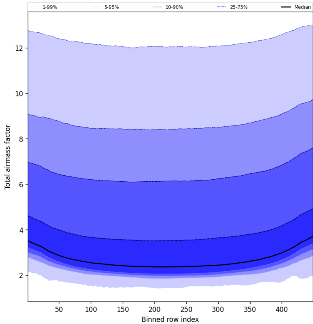
Figure 49: Along track statistics of “Total airmass factor” for 2024-09-28 to 2024-09-30
