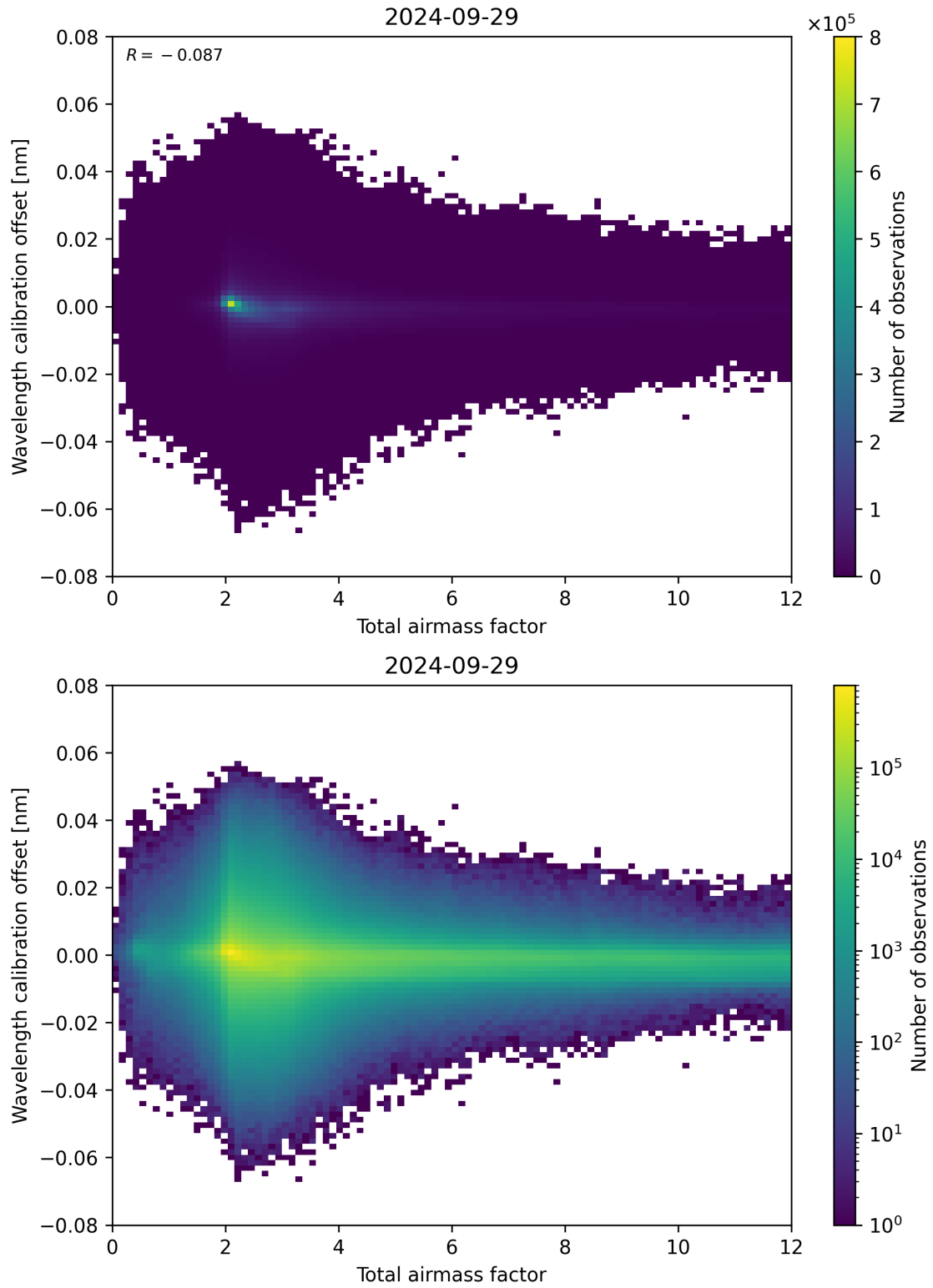
Figure 70: Scatter density plot of “Total airmass factor” against “Wavelength calibration offset” for 2024-09-28 to 2024-09-30.
