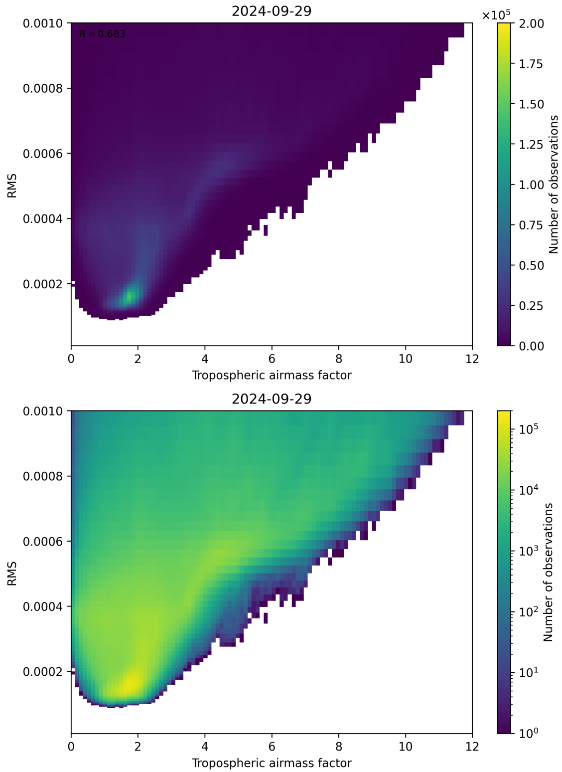
Figure 79: Scatter density plot of “Tropospheric airmass factor” against “RMS” for 2024-09-28 to 2024-09-30.
