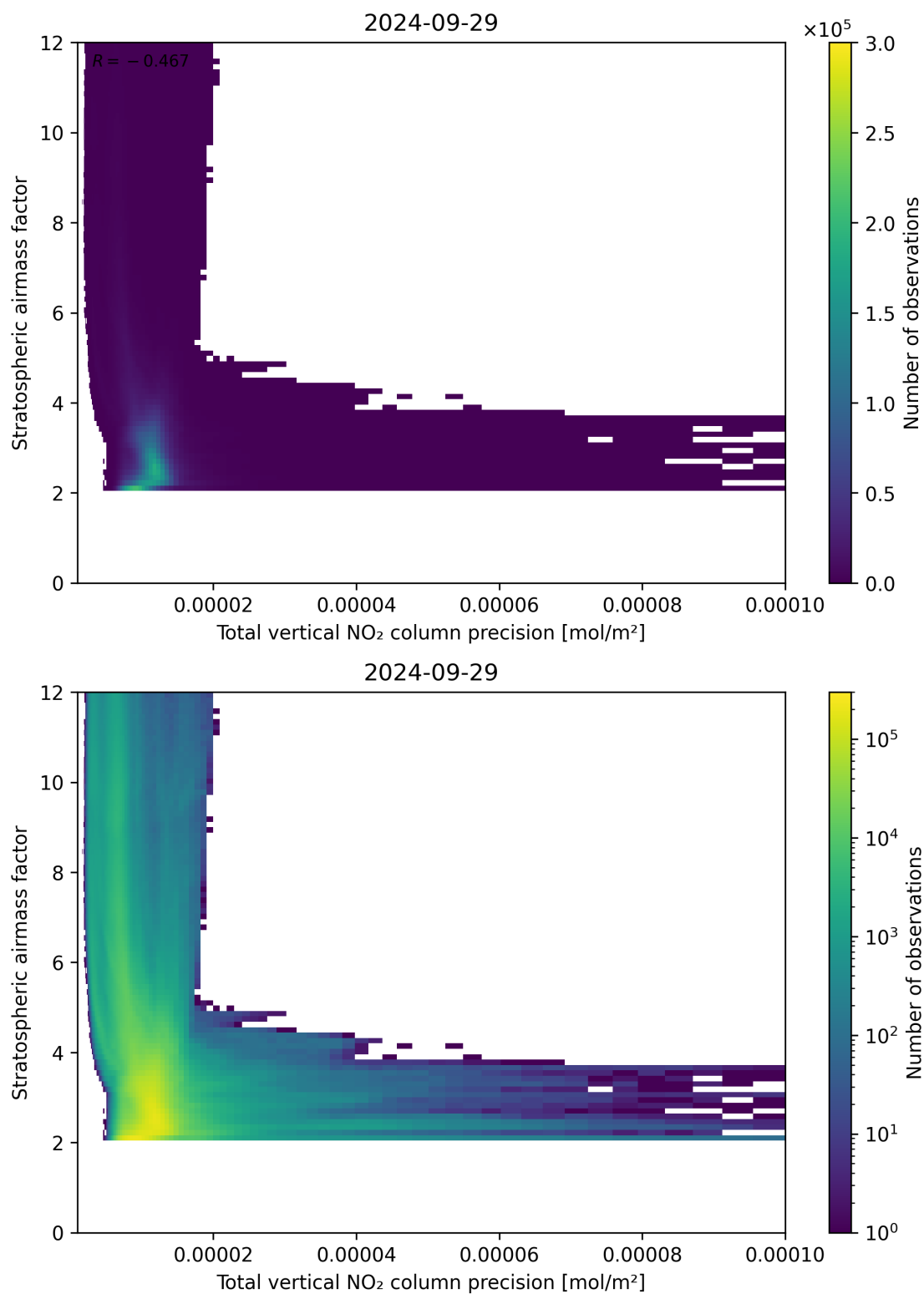
Figure 115: Scatter density plot of “Total vertical NO 2 column precision” against “Stratospheric air mass factor” for 2024-09-28 to 2024-09-30.
