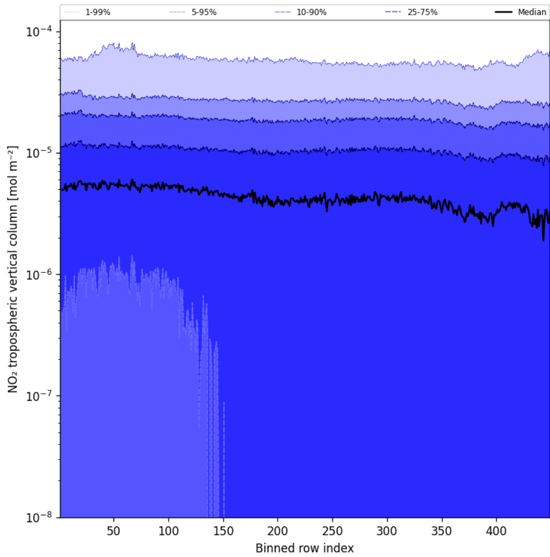
Figure 46: Along track statistics of “NO 2 tropospheric vertical column” for 2024-09-28 to 2024-09-30
