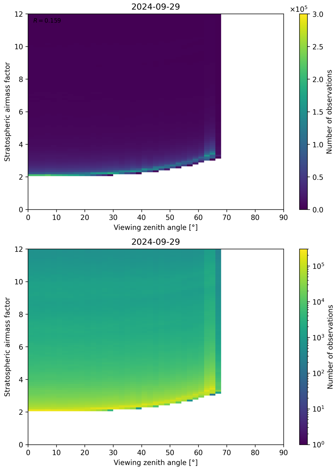
Figure 159: Scatter density plot of “Viewing zenith angle” against “Stratospheric airmass factor” for 2024-09-28 to 2024-09-30.
