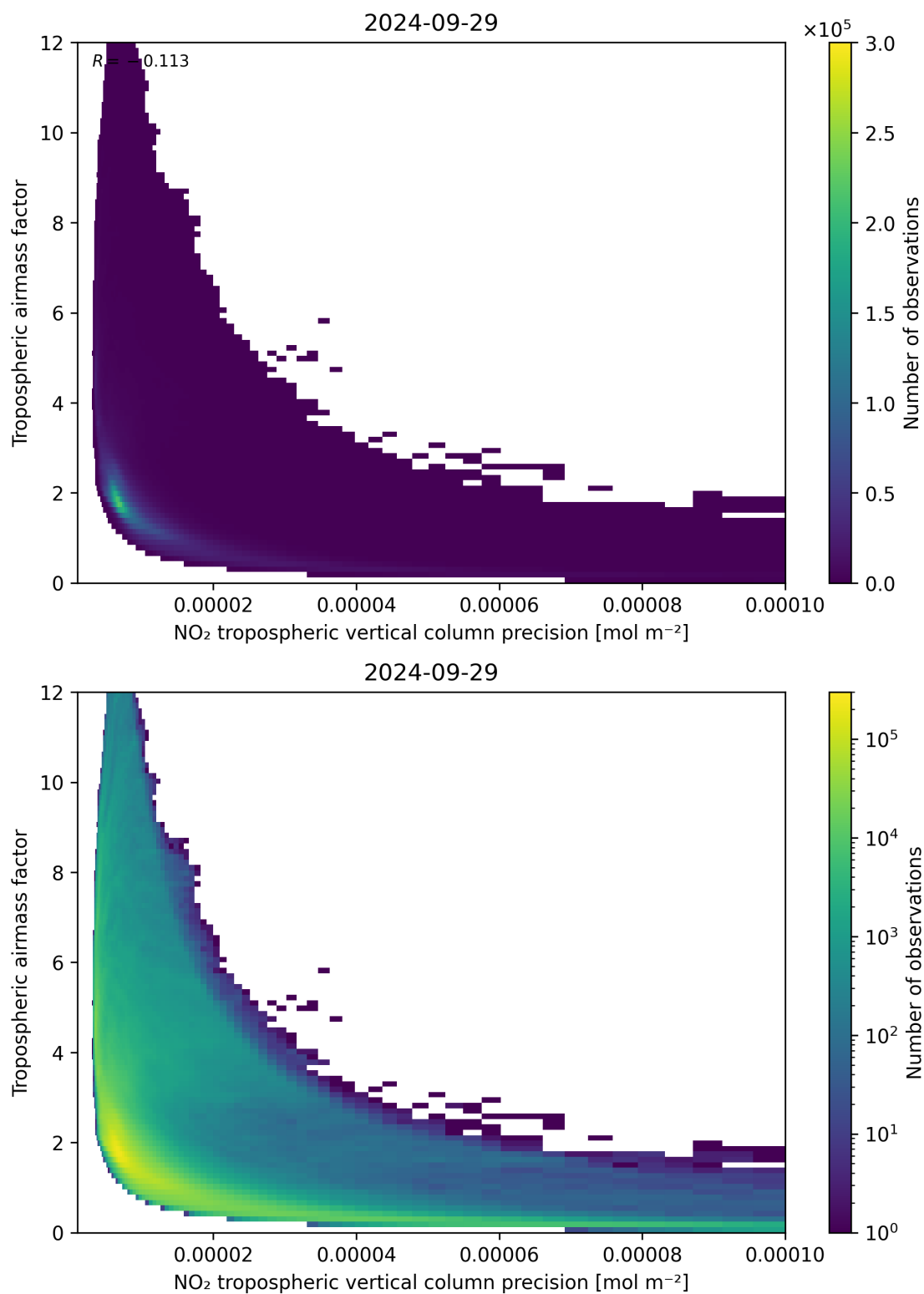
Figure 133: Scatter density plot of “NO 2 tropospheric vertical column precision” against “Tropospheric air mass factor” for 2024-09-28 to 2024-09-30.
