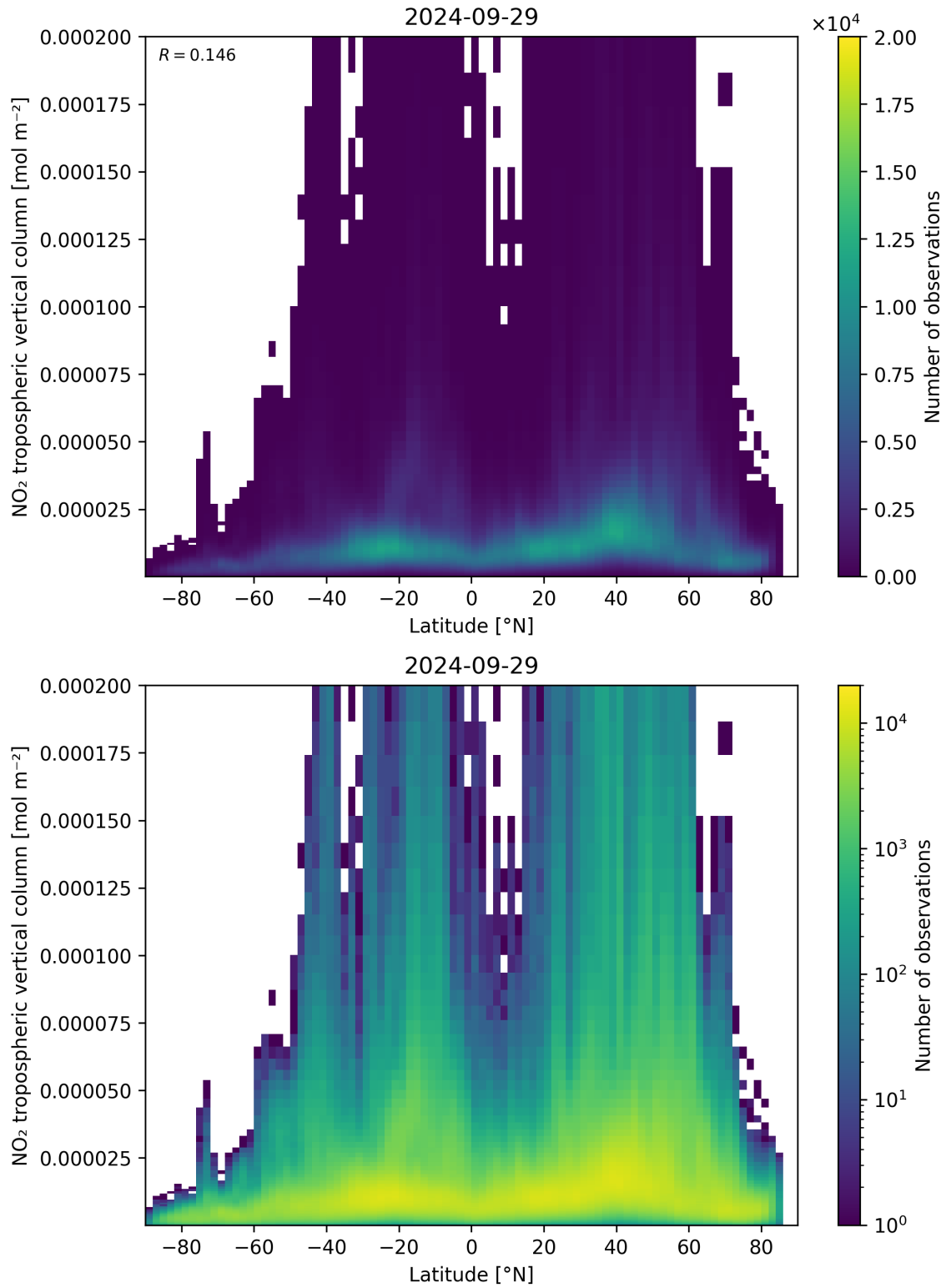
Figure 92: Scatter density plot of “Latitude” against “NO 2 tropospheric vertical column” for 2024-09-28 to 2024-09-30.
