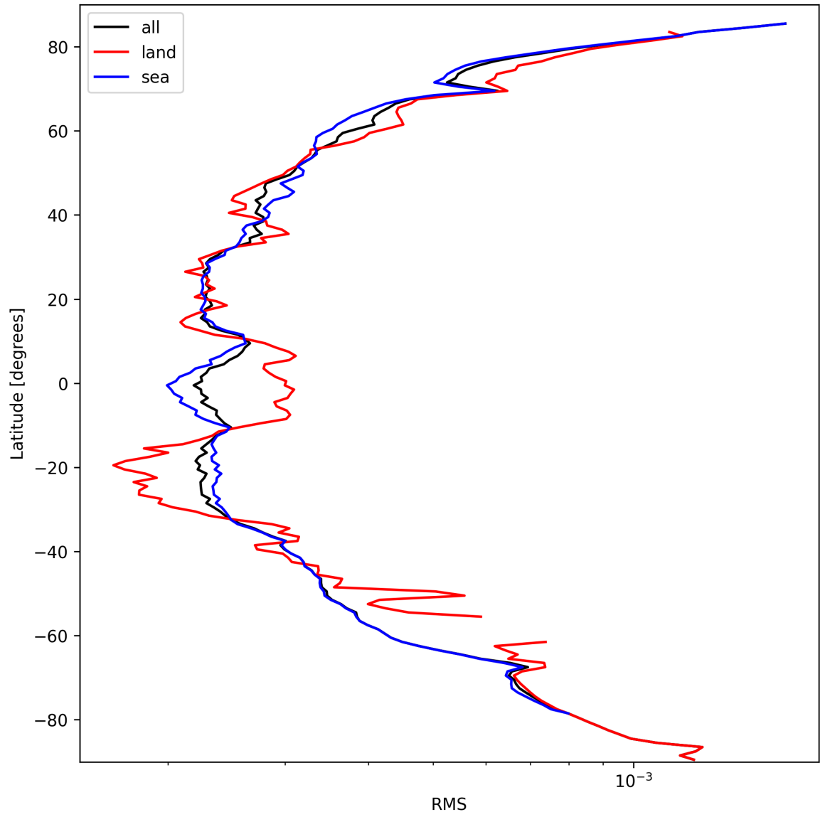
Figure 26: Zonal average of “RMS” for 2024-09-28 to 2024-09-30.
