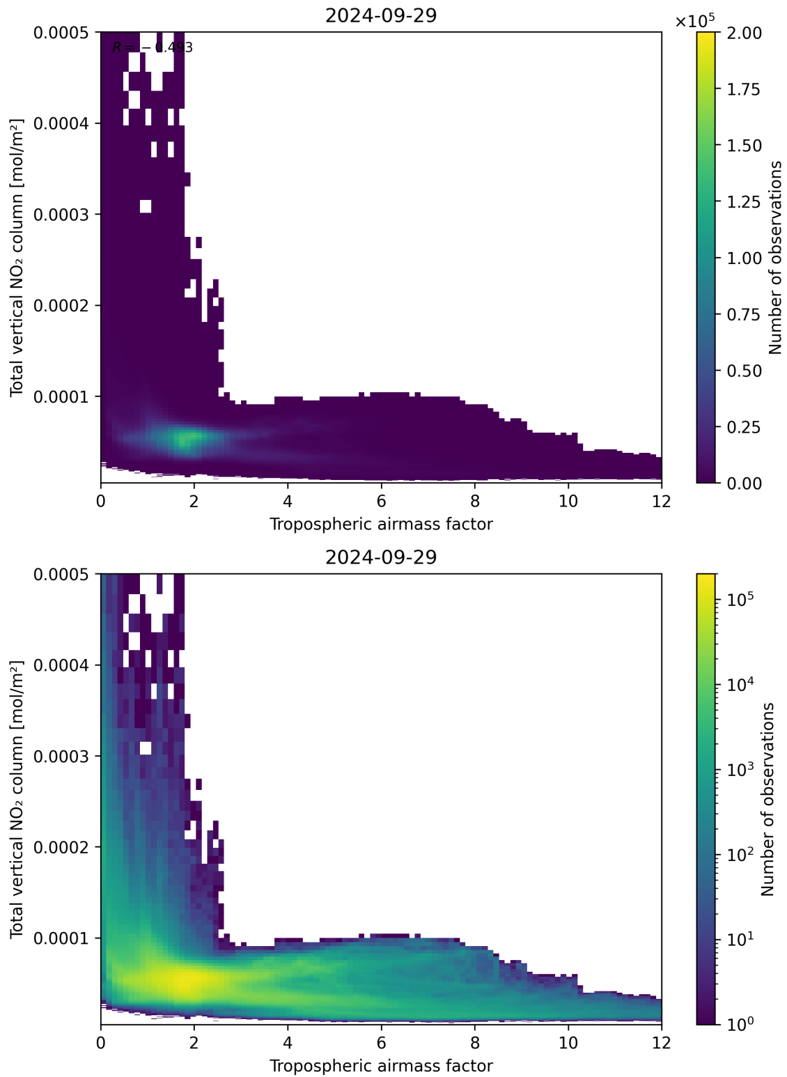
Figure 77: Scatter density plot of “Tropospheric airmass factor” against “Total vertical NO 2 column” for 2024-09-28 to 2024-09-30.
