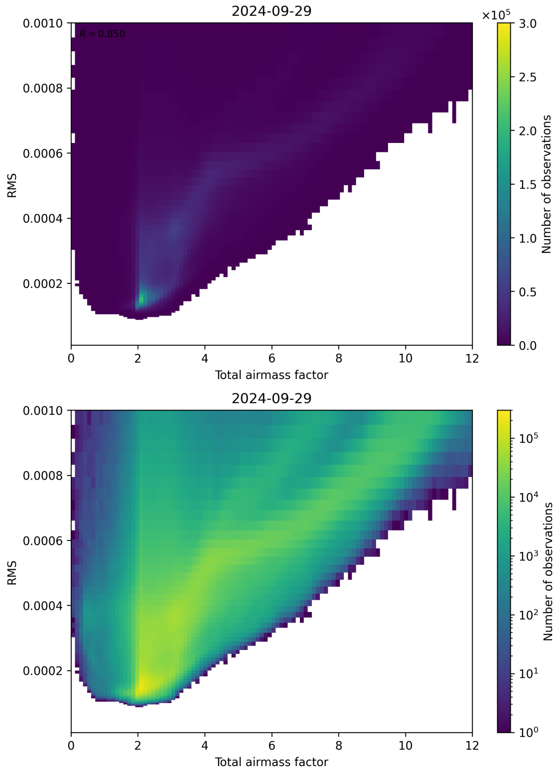
Figure 69: Scatter density plot of “Total airmass factor” against “RMS” for 2024-09-28 to 2024-09-30.
