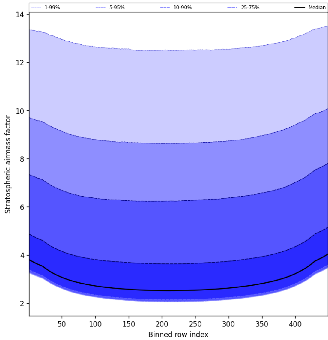
Figure 61: Along track statistics of “Stratospheric airmass factor” for 2024-09-28 to 2024-09-30
