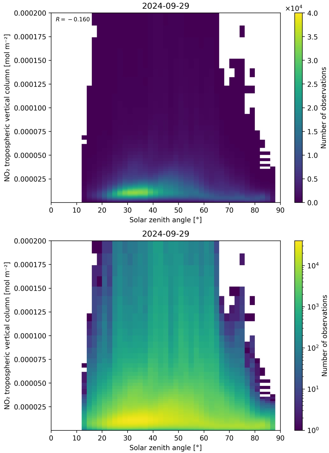
Figure 155: Scatter density plot of “Solar zenith angle” against “NO 2 tropospheric vertical column” for 2024-09-28 to 2024-09-30.
