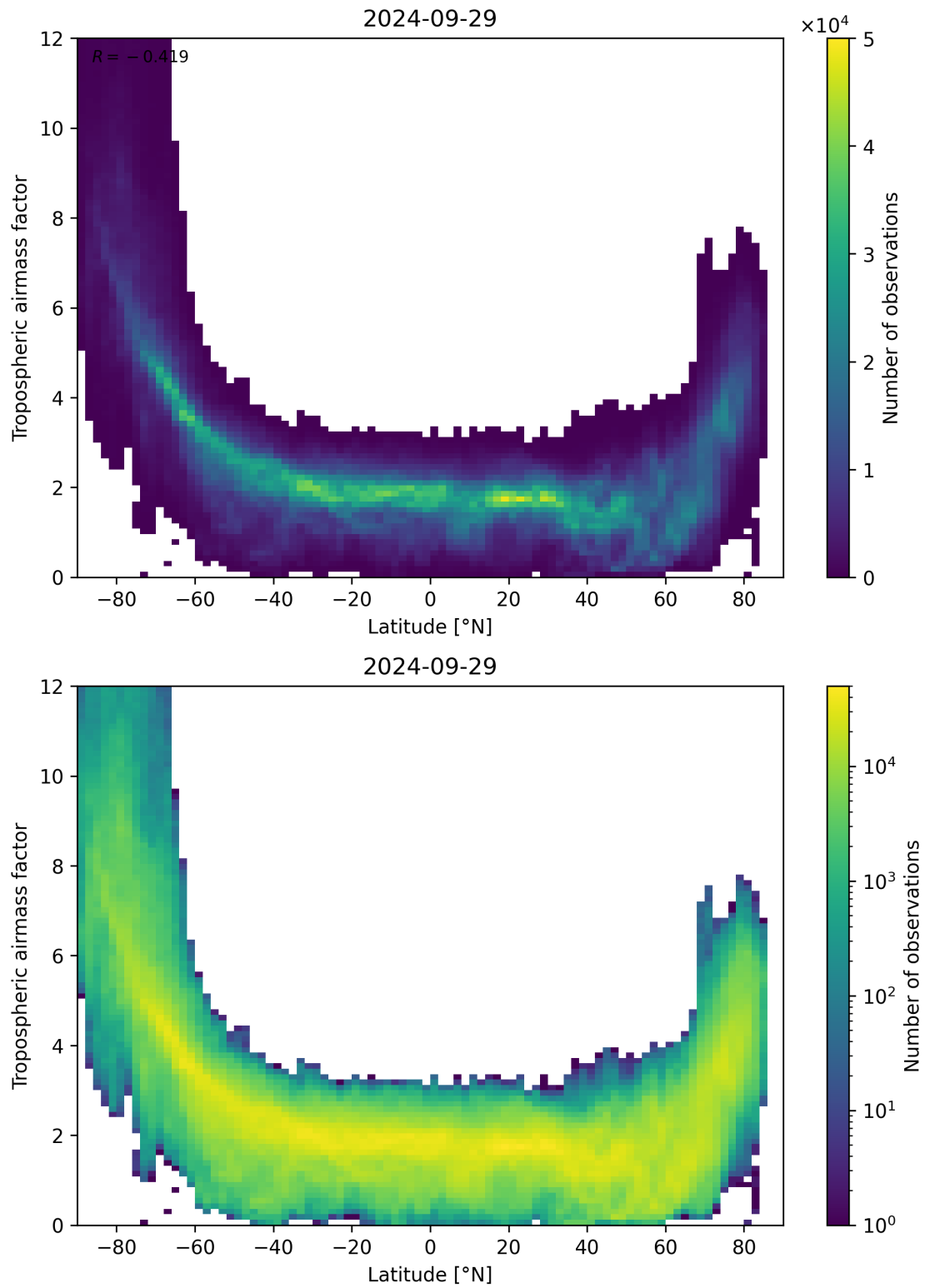
Figure 85: Scatter density plot of “Latitude” against “Tropospheric airmass factor” for 2024-09-28 to 2024-09-30.
