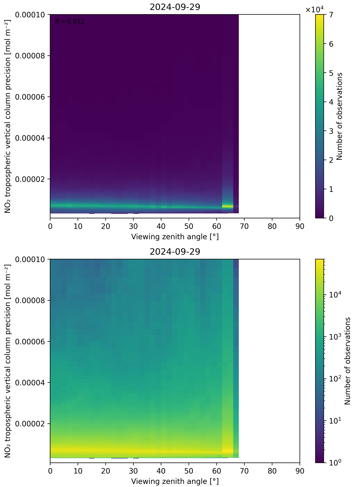
Figure 170: Scatter density plot of “Viewing zenith angle” against “NO 2 tropospheric vertical column precision” for 2024-09-28 to 2024-09-30.
