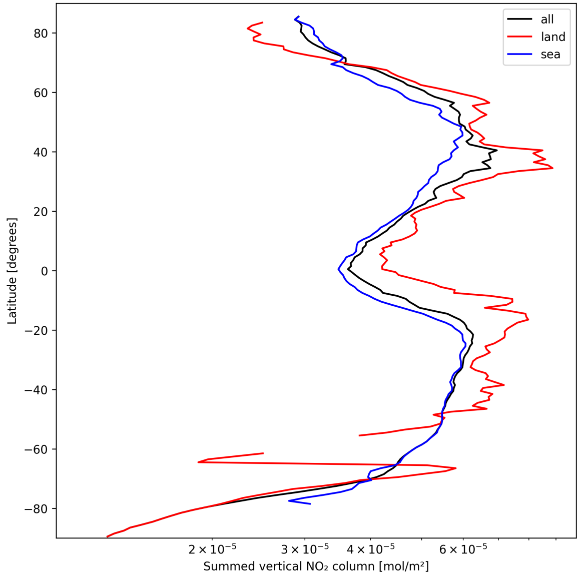
Figure 23: Zonal average of “Summed vertical NO 2 column” for 2024-09-28 to 2024-09-30.
