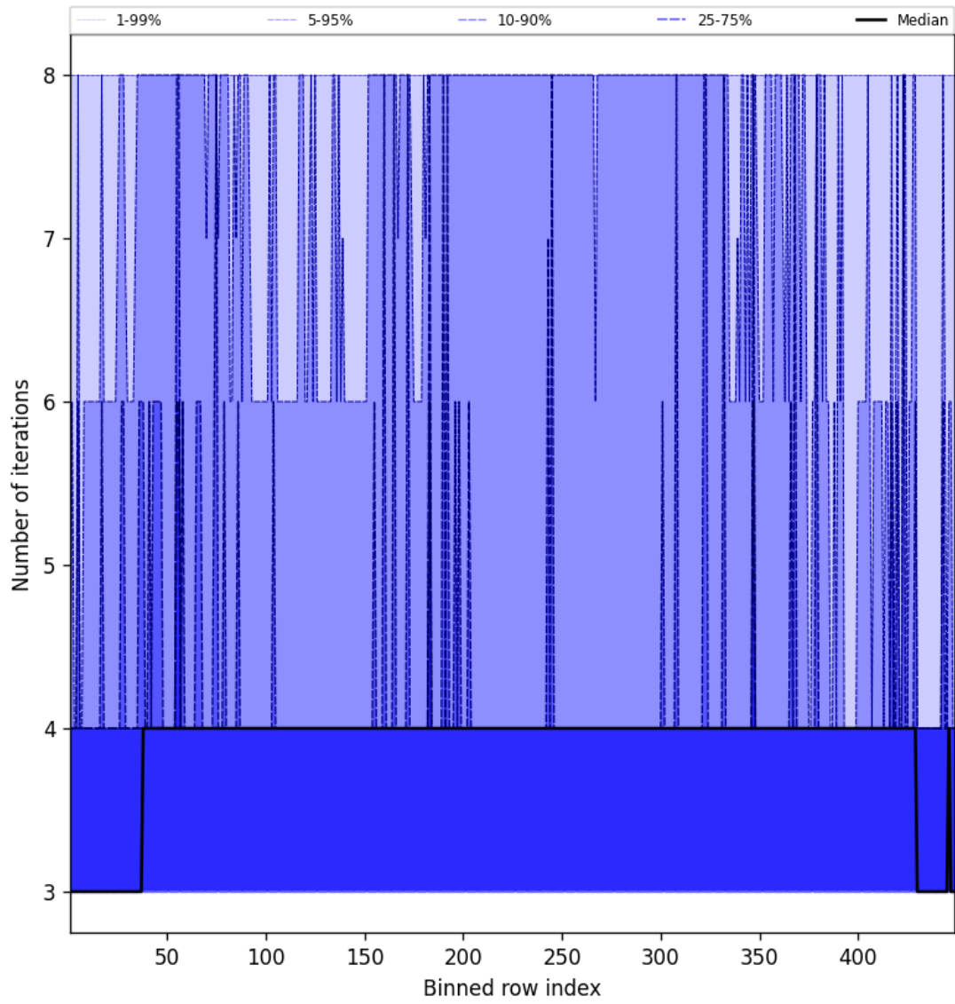
Figure 51: Along track statistics of “Number of iterations” for 2024-09-28 to 2024-09-30
