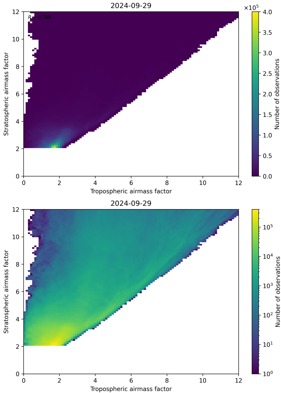
Figure 71: Scatter density plot of “Tropospheric airmass factor” against “Stratospheric airmass factor” for 2024-09-28 to 2024-09-30.
