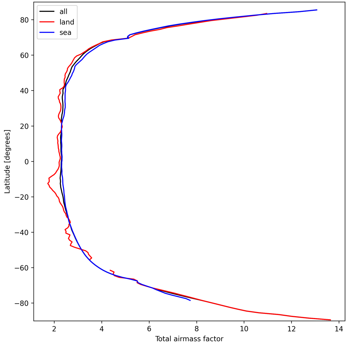
Figure 15: Zonal average of “Total airmass factor” for 2024-09-28 to 2024-09-30.
