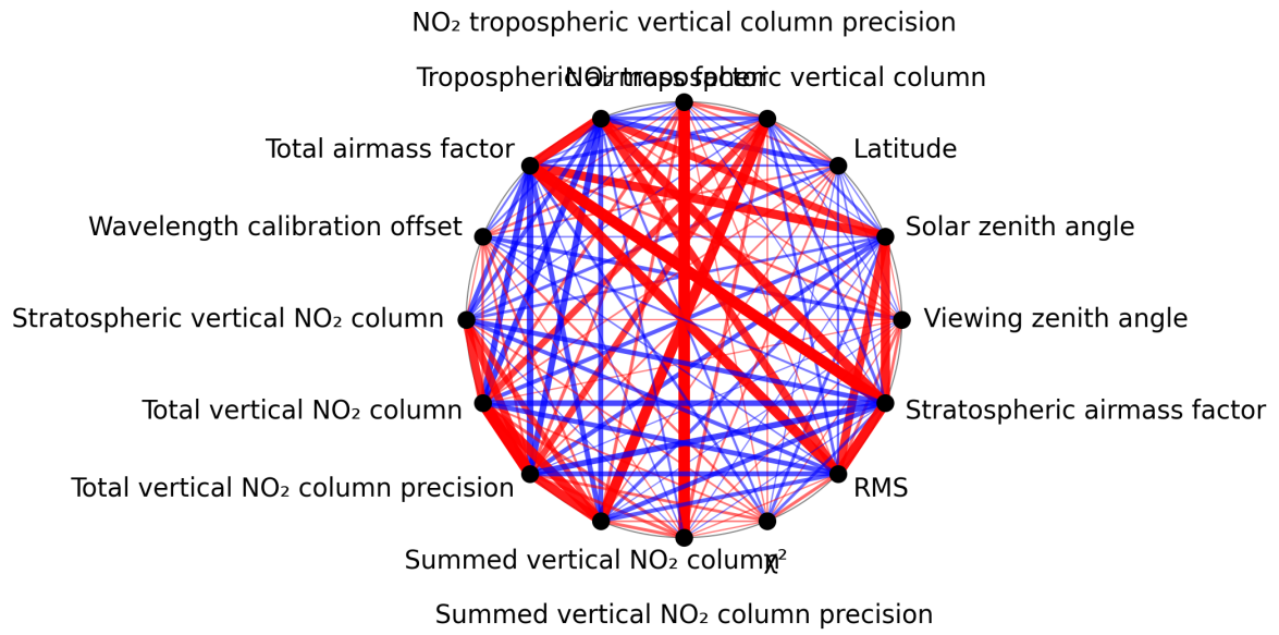
Figure 1: Map of correlation graph for 2024-09-28 to 2024-09-30.
