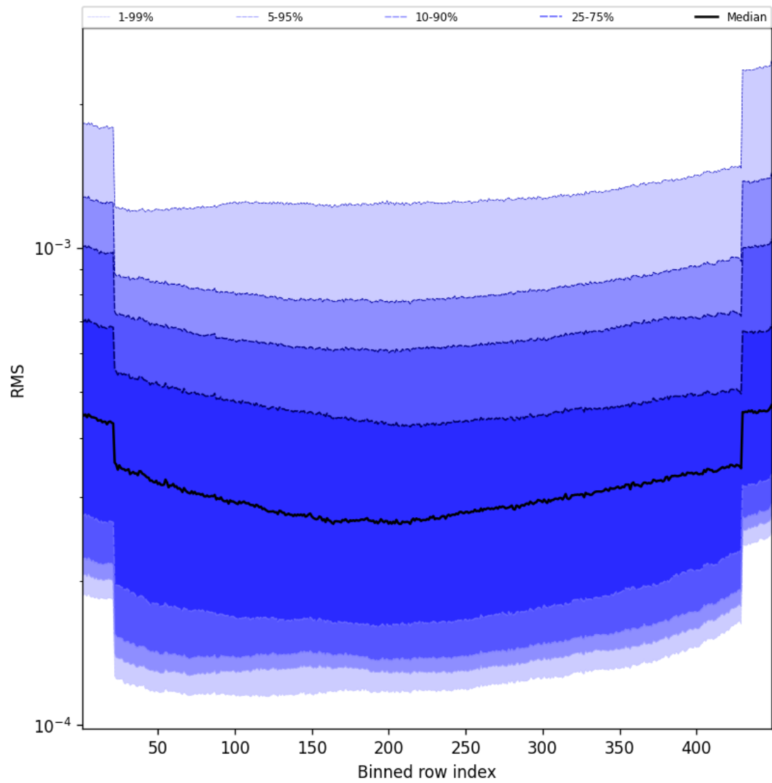
Figure 60: Along track statistics of “RMS” for 2024-09-28 to 2024-09-30
