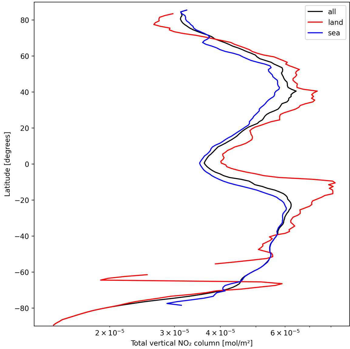
Figure 21: Zonal average of “Total vertical NO 2 column” for 2024-09-28 to 2024-09-30.
