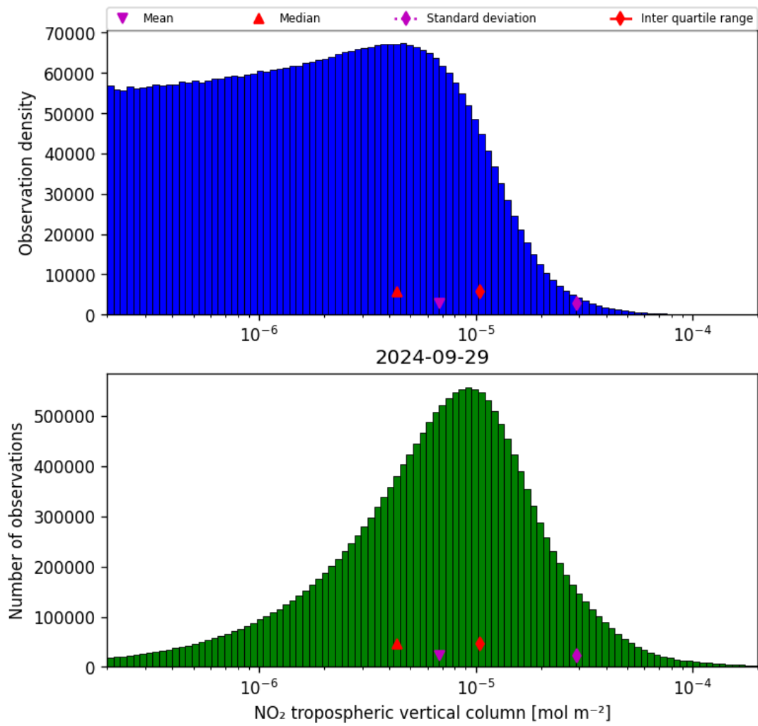
Figure 29: Histogram of “NO 2 tropospheric vertical column” for 2024-09-28 to 2024-09-30
