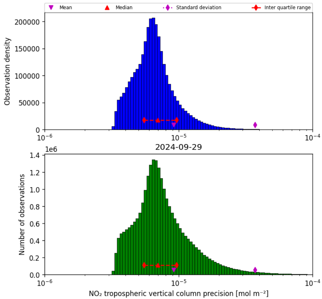
Figure 30: Histogram of “NO 2 tropospheric vertical column precision” for 2024-09-28 to 2024-09-30
