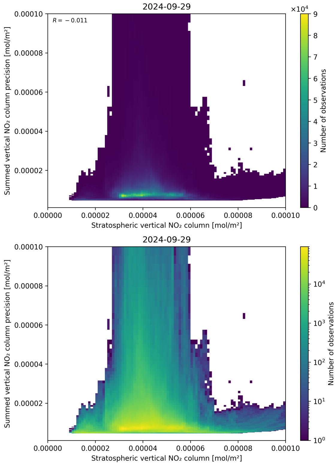
Figure 99: Scatter density plot of “Stratospheric vertical NO 2 column” against “Summed vertical NO 2 column precision” for 2024-09-28 to 2024-09-30.
