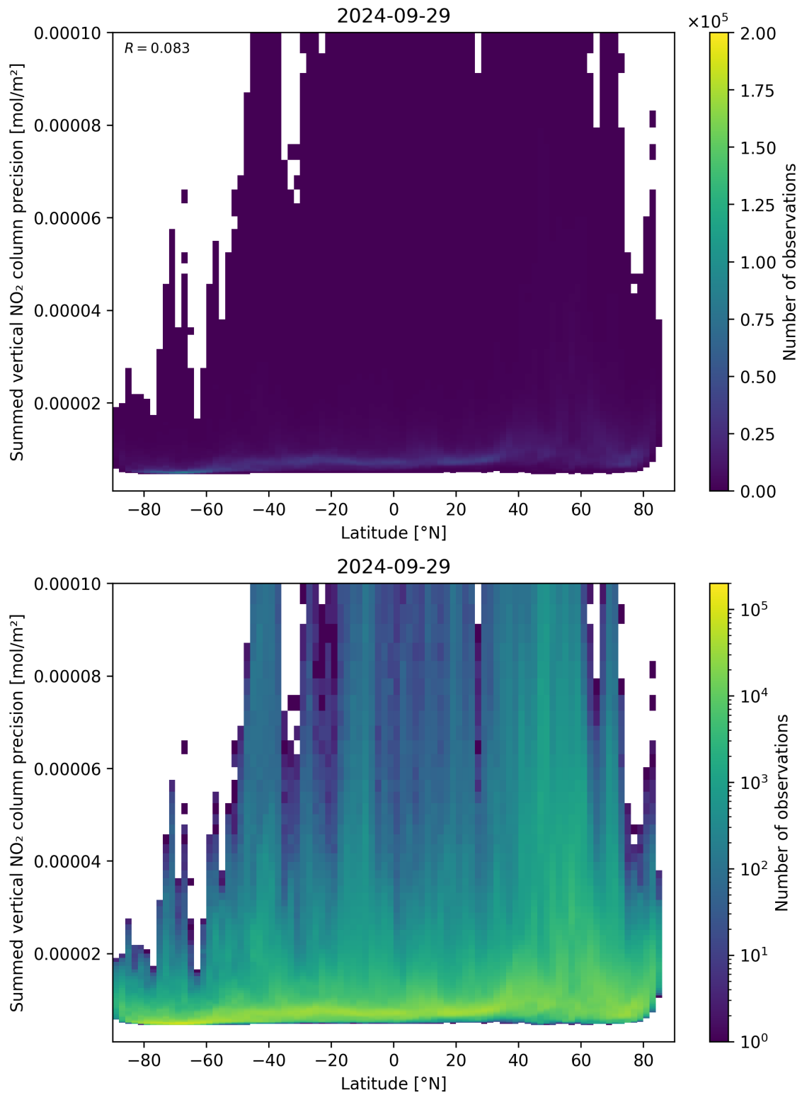
Figure 89: Scatter density plot of “Latitude” against “Summed vertical NO 2 column precision” for 2024-09-28 to 2024-09-30.
