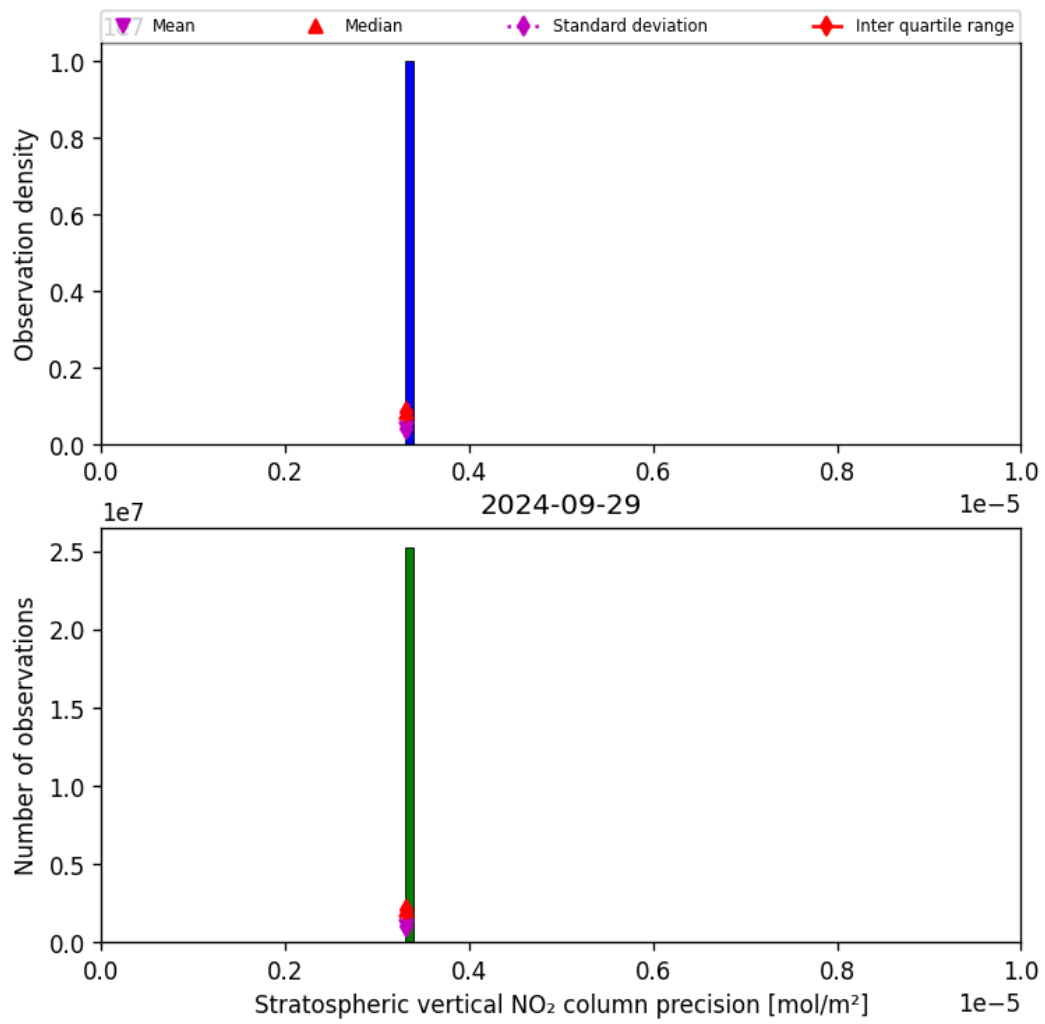
Figure 37: Histogram of “Stratospheric vertical NO 2 column precision” for 2024-09-28 to 2024-09-30
