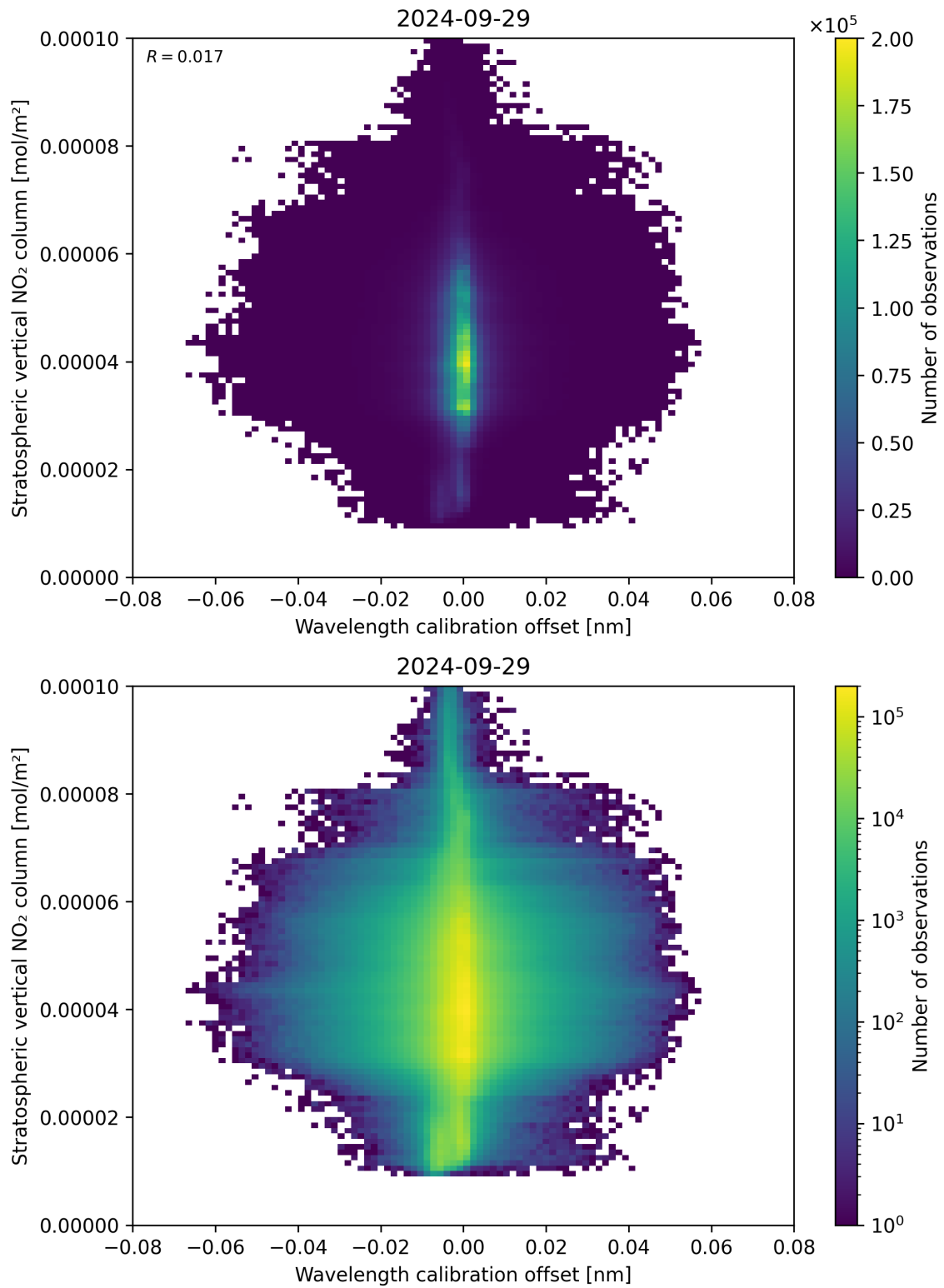
Figure 176: Scatter density plot of “Wavelength calibration offset” against “Stratospheric vertical NO 2 column” for 2024-09-28 to 2024-09-30.
