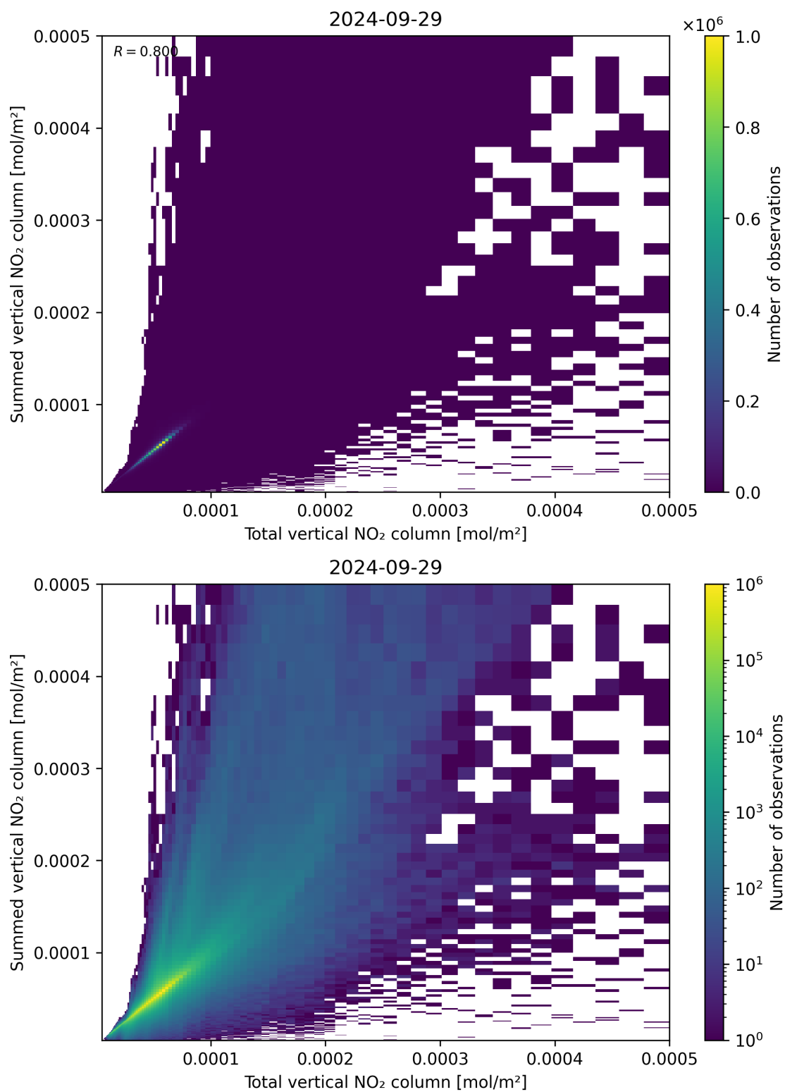
Figure 112: Scatter density plot of “Total vertical NO 2 column” against “Summed vertical NO 2 column” for 2024-09-28 to 2024-09-30.
