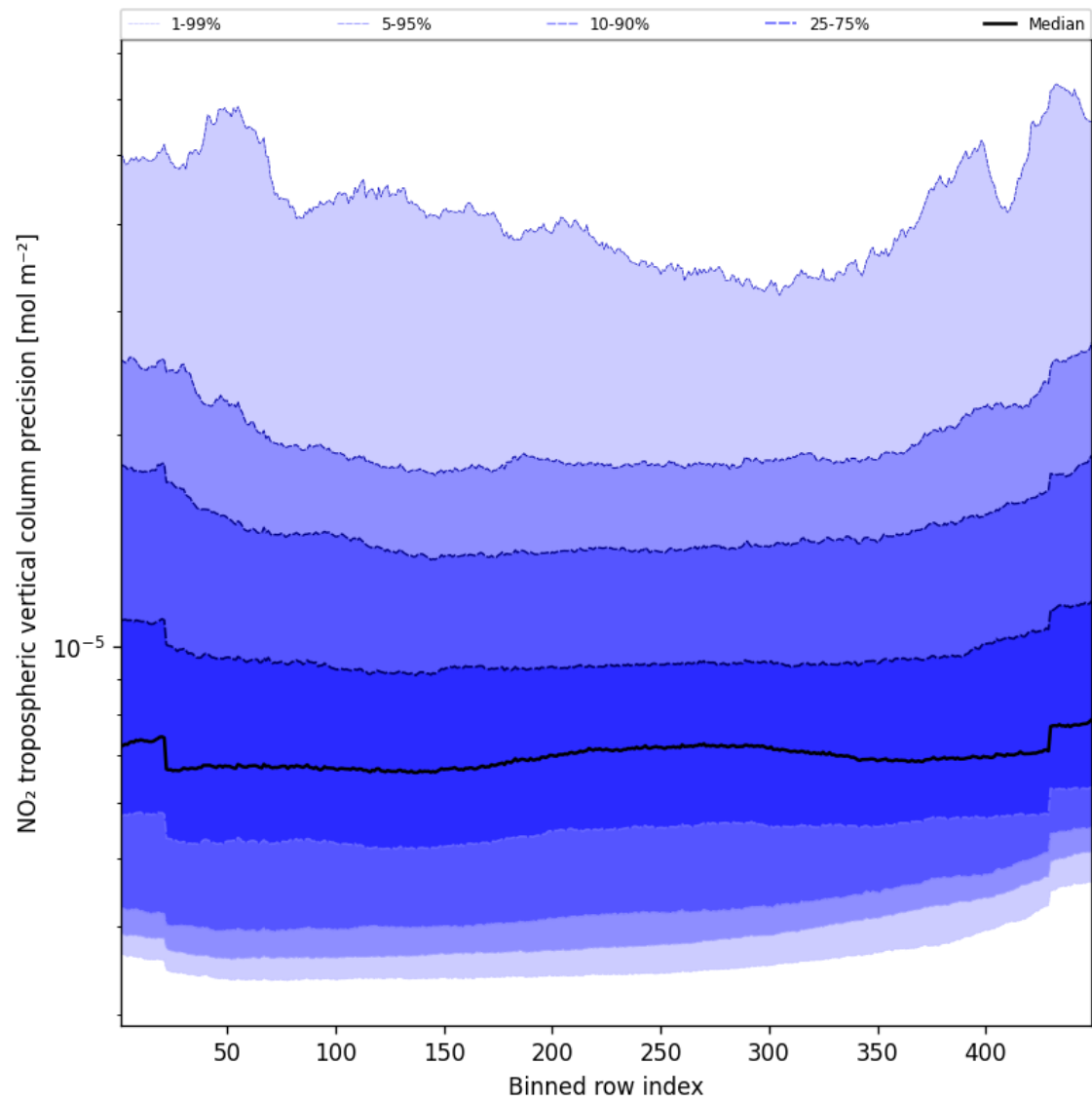
Figure 47: Along track statistics of “NO 2 tropospheric vertical column precision” for 2024-09-28 to 2024-09-30
