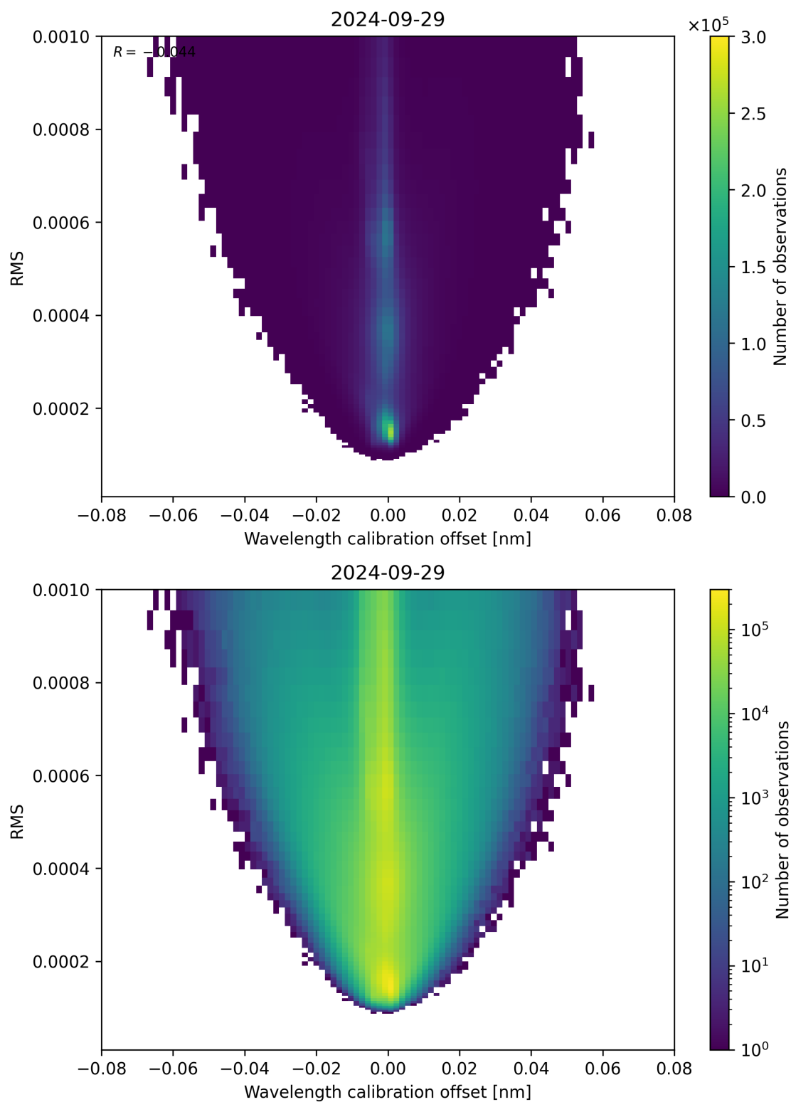
Figure 181: Scatter density plot of “Wavelength calibration offset” against “RMS” for 2024-09-28 to 2024-09-30.
