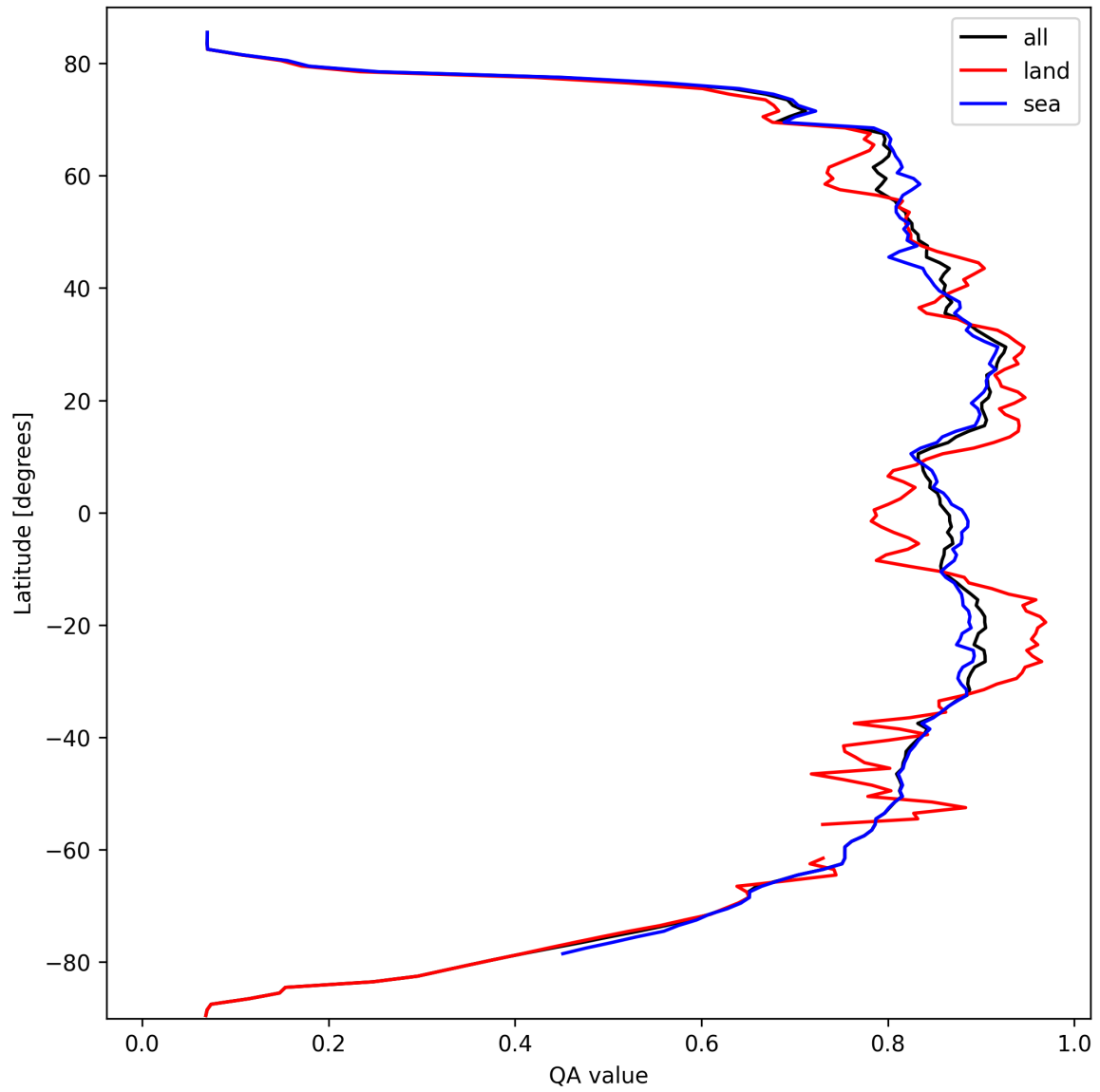
Figure 11: Zonal average of “QA value” for 2024-09-28 to 2024-09-30.
