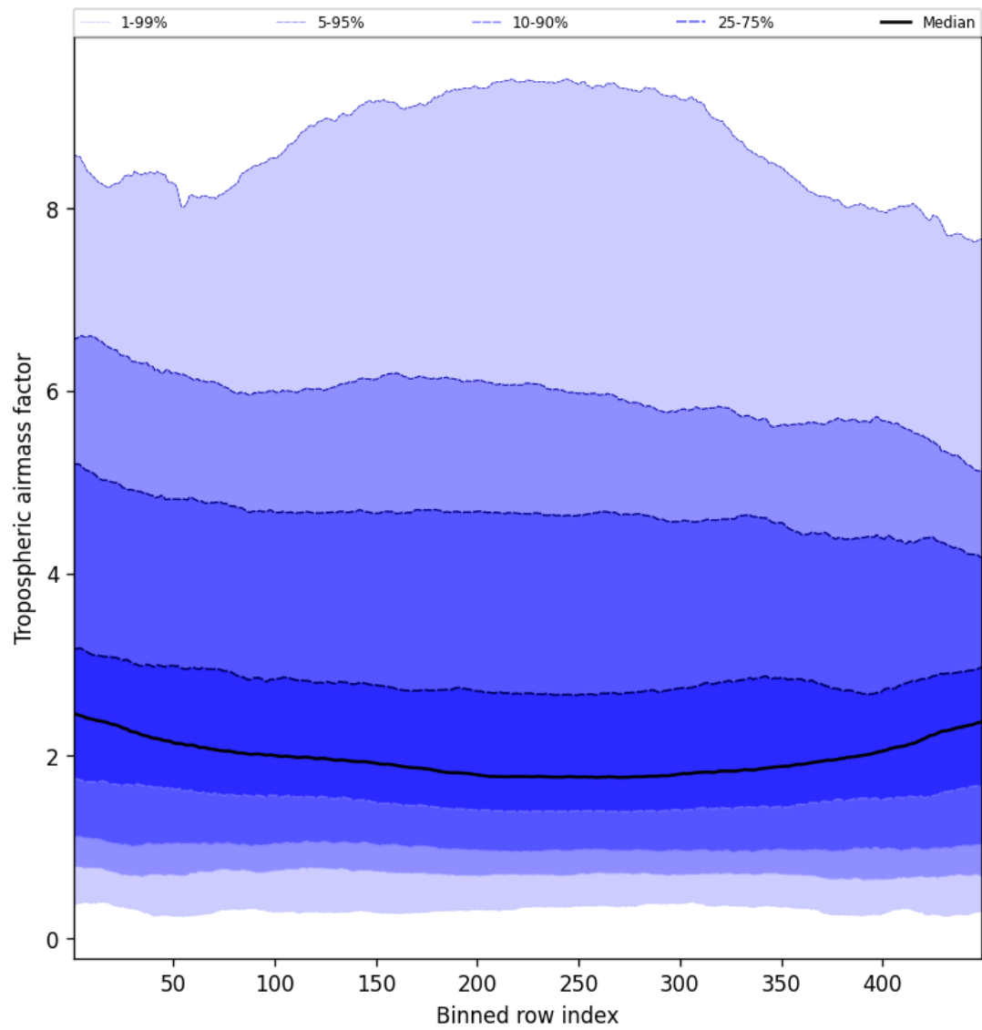
Figure 48: Along track statistics of “Tropospheric air mass factor” for 2024-09-28 to 2024-09-30
