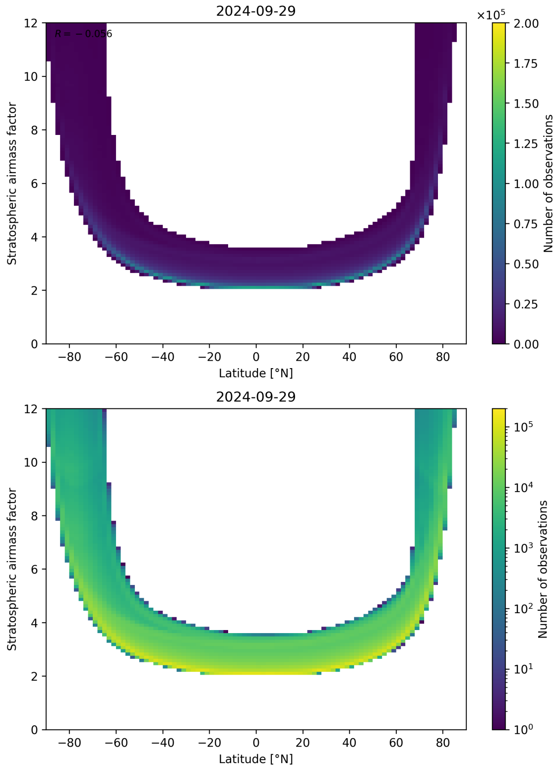
Figure 83: Scatter density plot of “Latitude” against “Stratospheric air mass factor” for 2024-09-28 to 2024-09-30.
