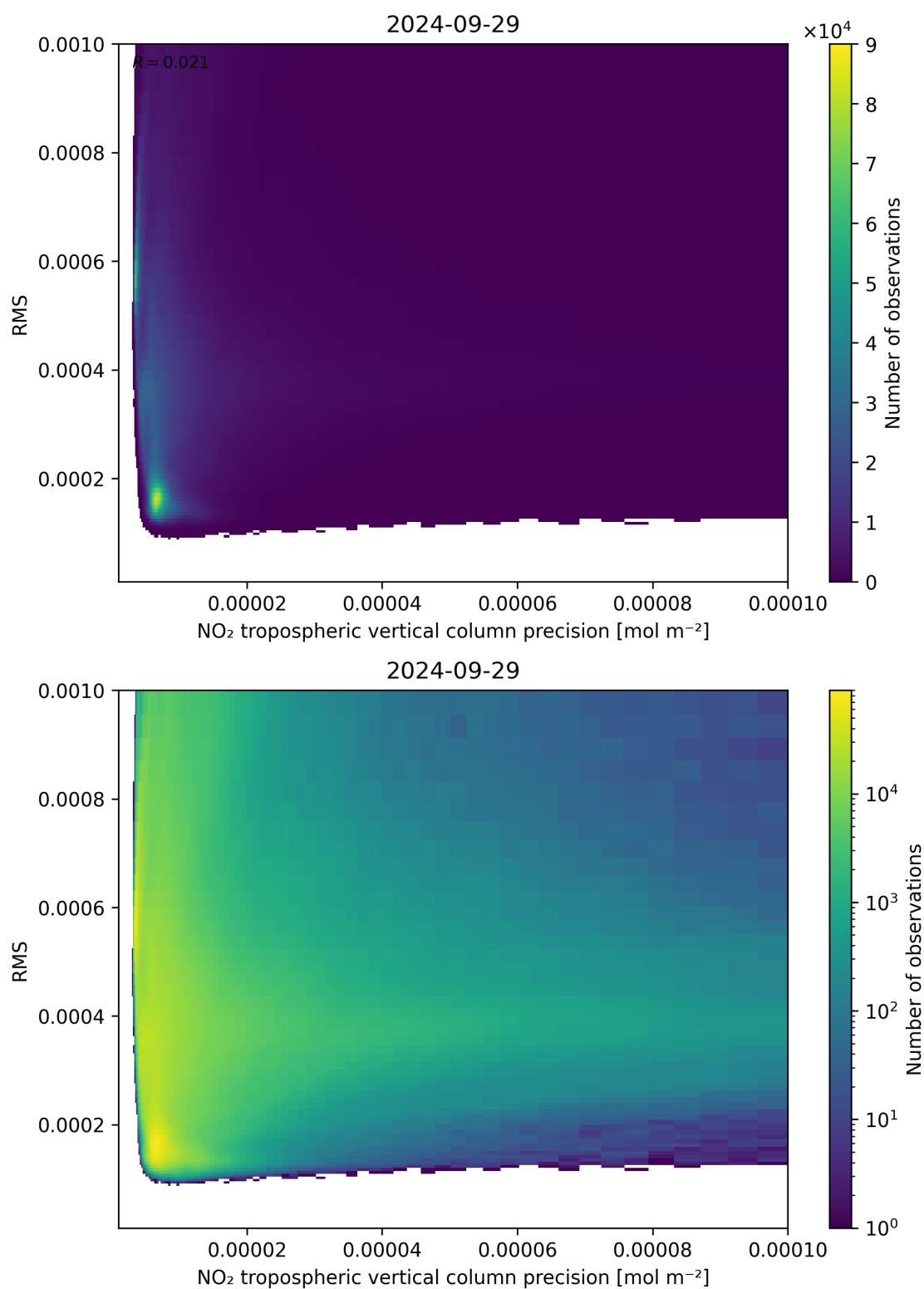
Figure 140: Scatter density plot of “NO 2 tropospheric vertical column precision” against “RMS” for 2024-09-28 to 2024-09-30.
