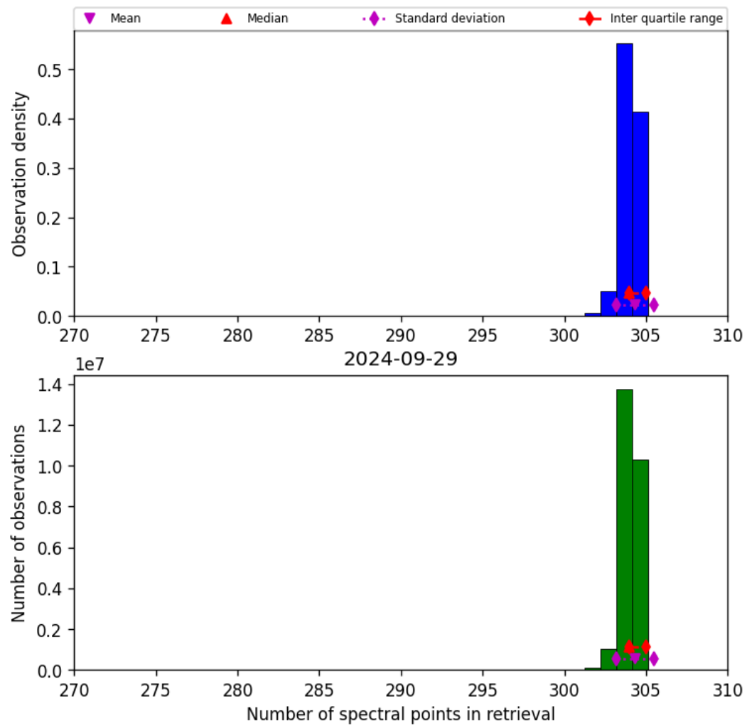
Figure 33: Histogram of “Number of spectral points in retrieval” for 2024-09-28 to 2024-09-30
