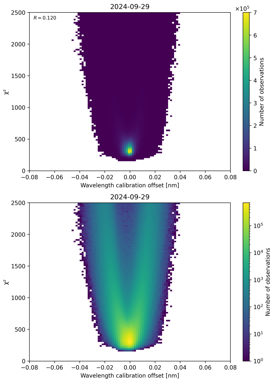
Figure 175: Scatter density plot of “Wavelength calibration offset” against “ \chi^2 ” for 2024-09-28 to 2024-09-30.
