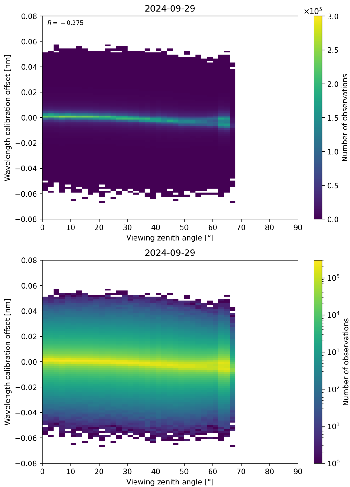
Figure 173: Scatter density plot of “Viewing zenith angle” against “Wavelength calibration offset” for 2024-09-28 to 2024-09-30.
