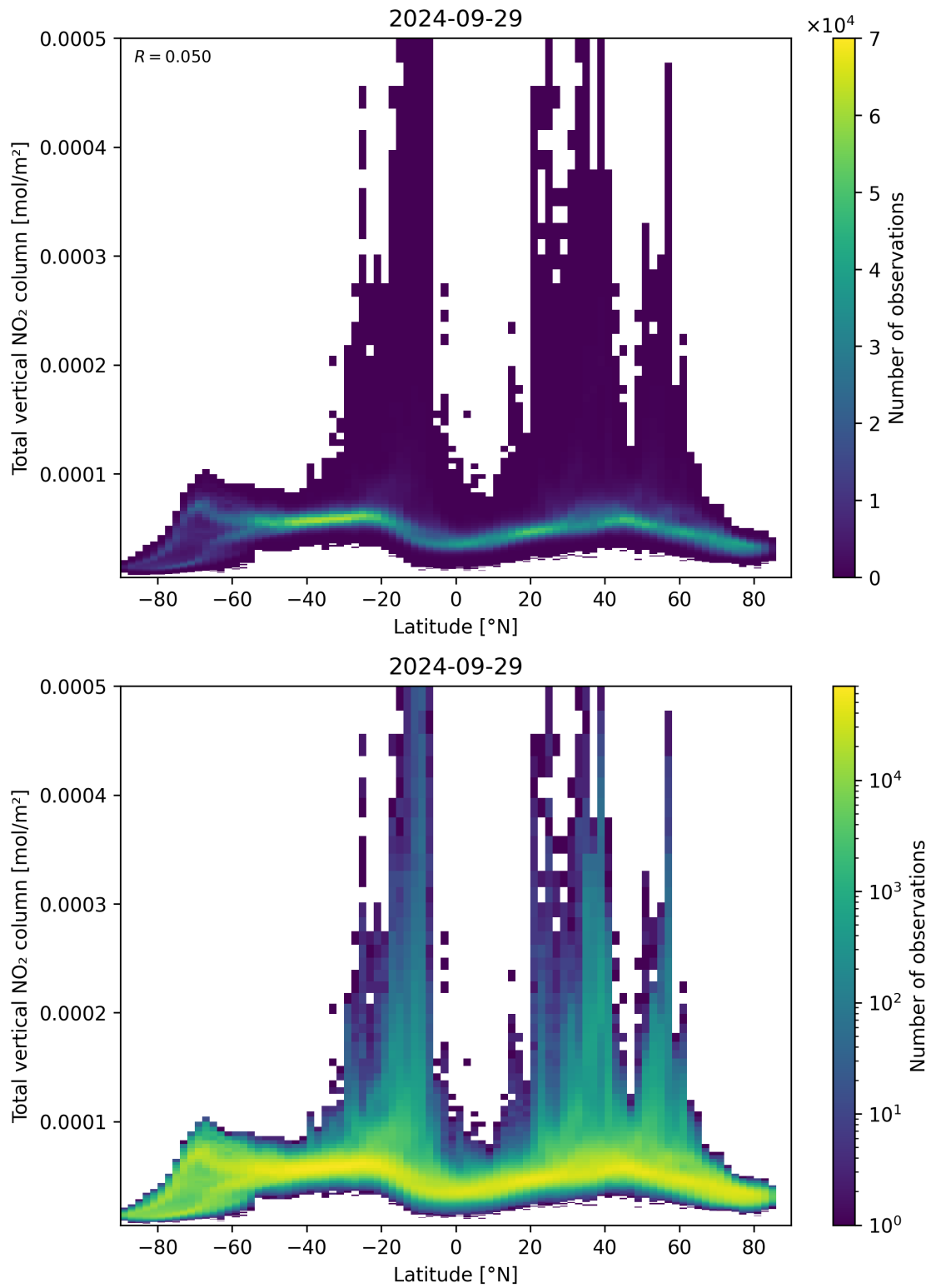
Figure 90: Scatter density plot of “Latitude” against “Total vertical NO 2 column” for 2024-09-28 to 2024-09-30.
