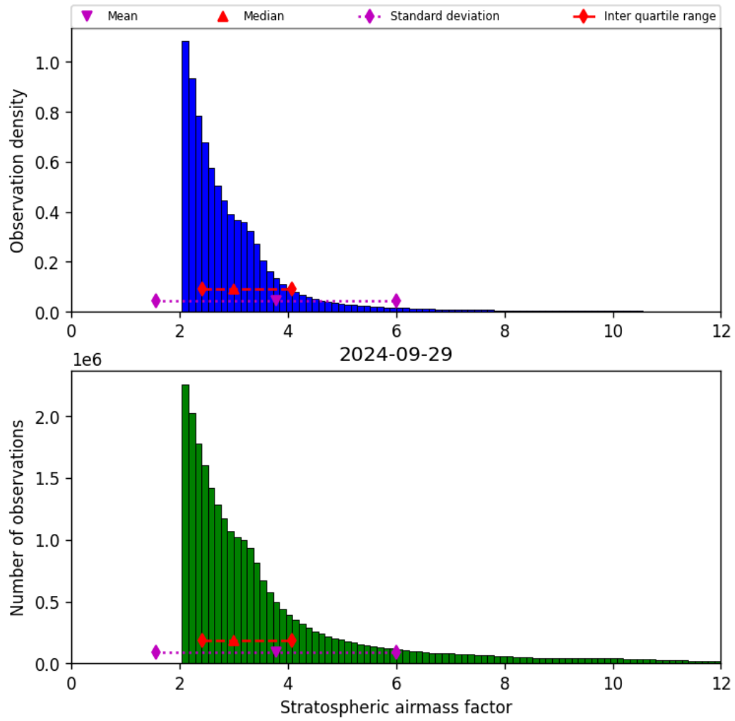
Figure 44: Histogram of “Stratospheric airmass factor” for 2024-09-28 to 2024-09-30
