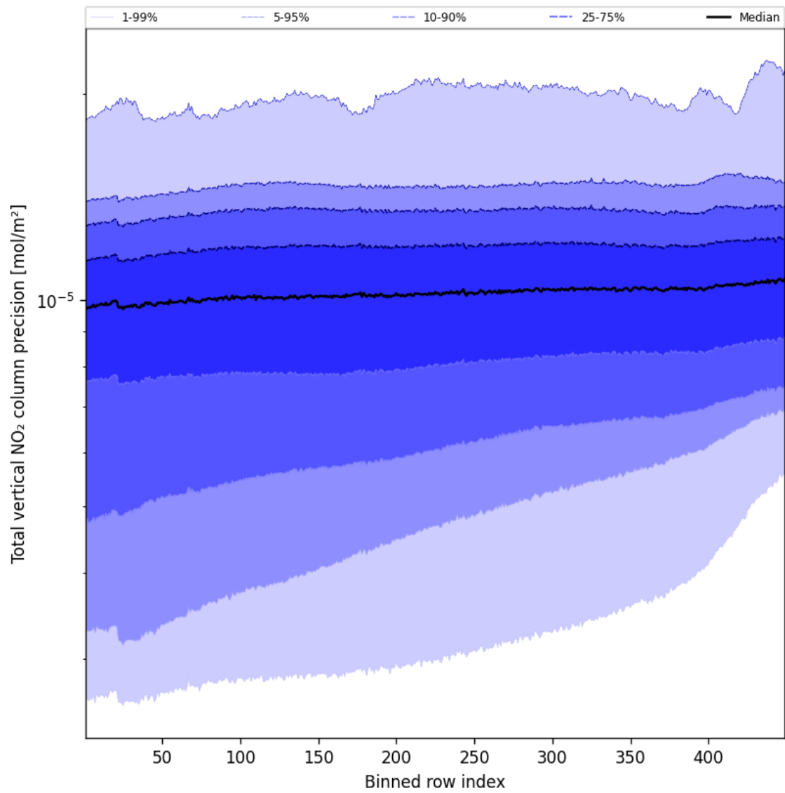
Figure 56: Along track statistics of “Total vertical NO 2 column precision” for 2024-09-28 to 2024-09-30
