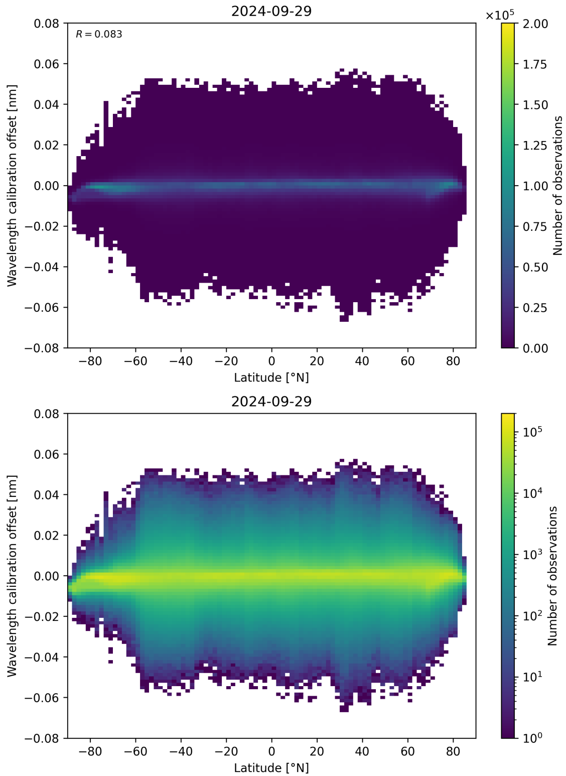
Figure 95: Scatter density plot of “Latitude” against “Wavelength calibration offset” for 2024-09-28 to 2024-09-30.
