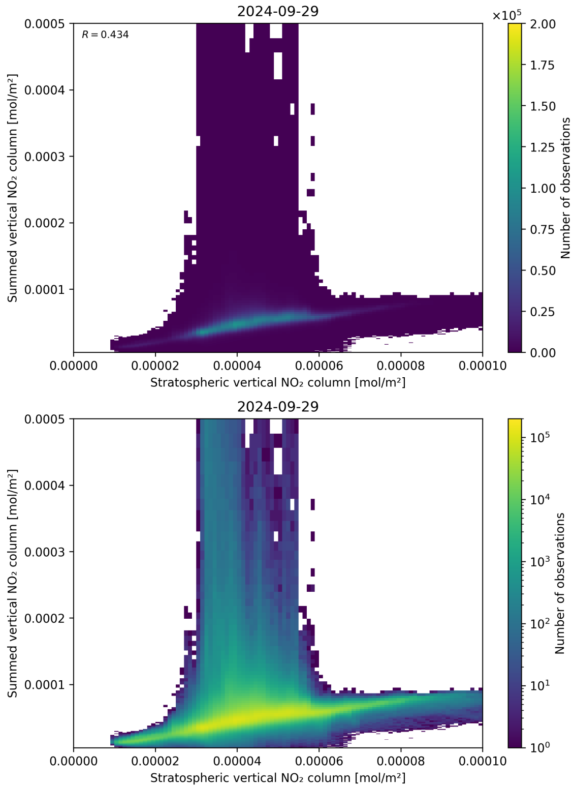
Figure 98: Scatter density plot of “Stratospheric vertical NO 2 column” against “Summed vertical NO 2 column” for 2024-09-28 to 2024-09-30.
