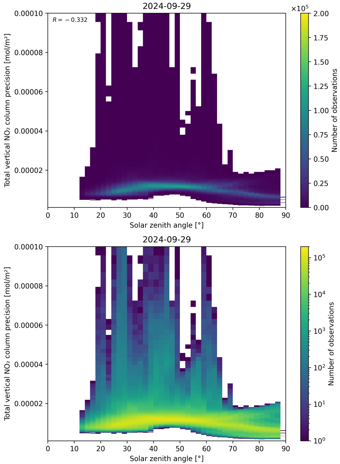
Figure 154: Scatter density plot of “Solar zenith angle” against “Total vertical NO 2 column precision” for 2024-09-28 to 2024-09-30.
