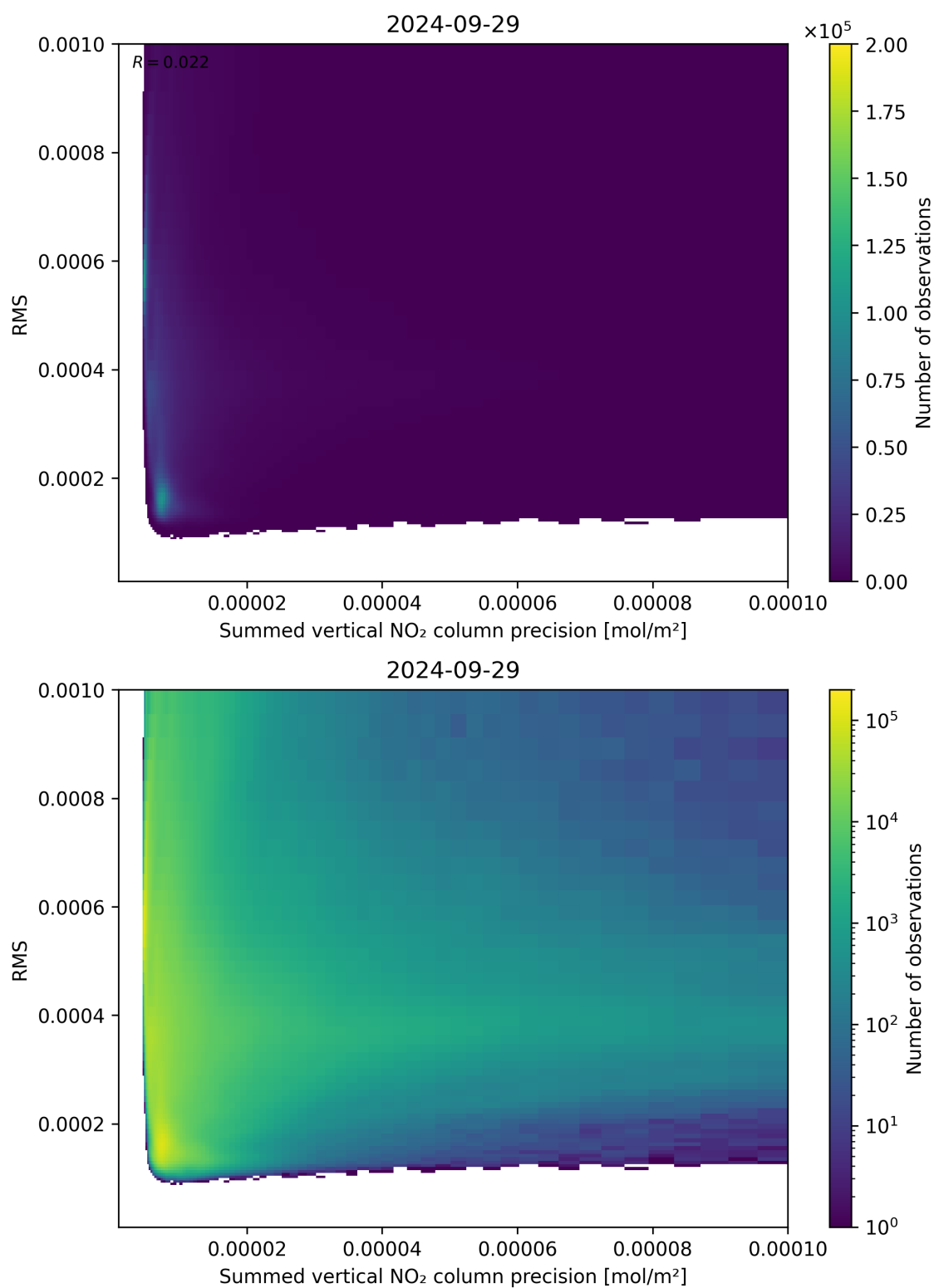
Figure 108: Scatter density plot of “Summed vertical NO 2 column precision” against “RMS” for 2024-09-28 to 2024-09-30.
