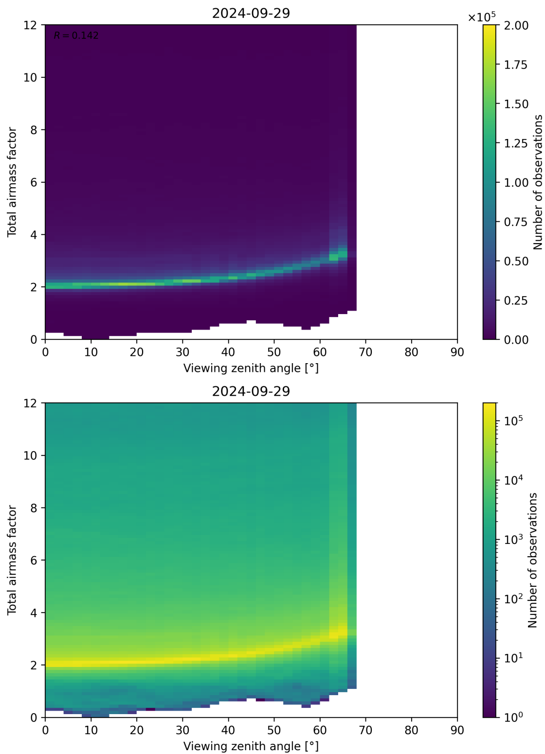
Figure 160: Scatter density plot of “Viewing zenith angle” against “Total airmass factor” for 2024-09-28 to 2024-09-30.
