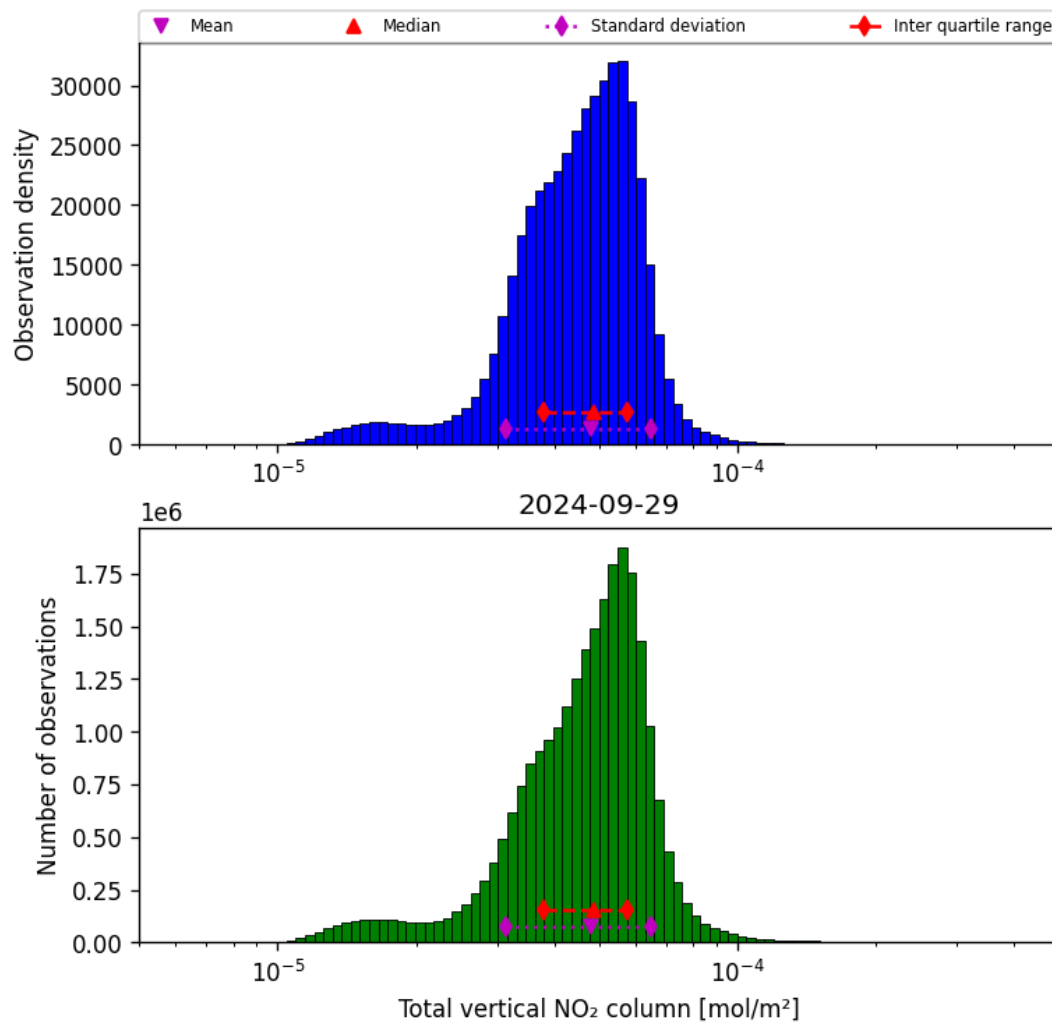
Figure 38: Histogram of "Total vertical NO 2 column" for 2024-09-28 to 2024-09-30
