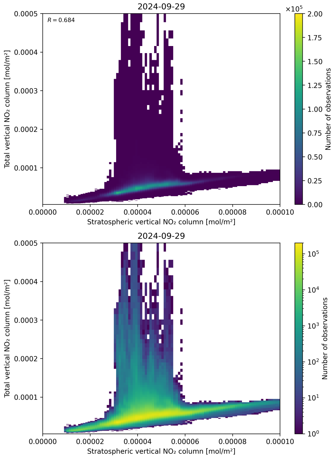
Figure 100: Scatter density plot of “Stratospheric vertical NO 2 column” against “Total vertical NO 2 column” for 2024-09-28 to 2024-09-30.
