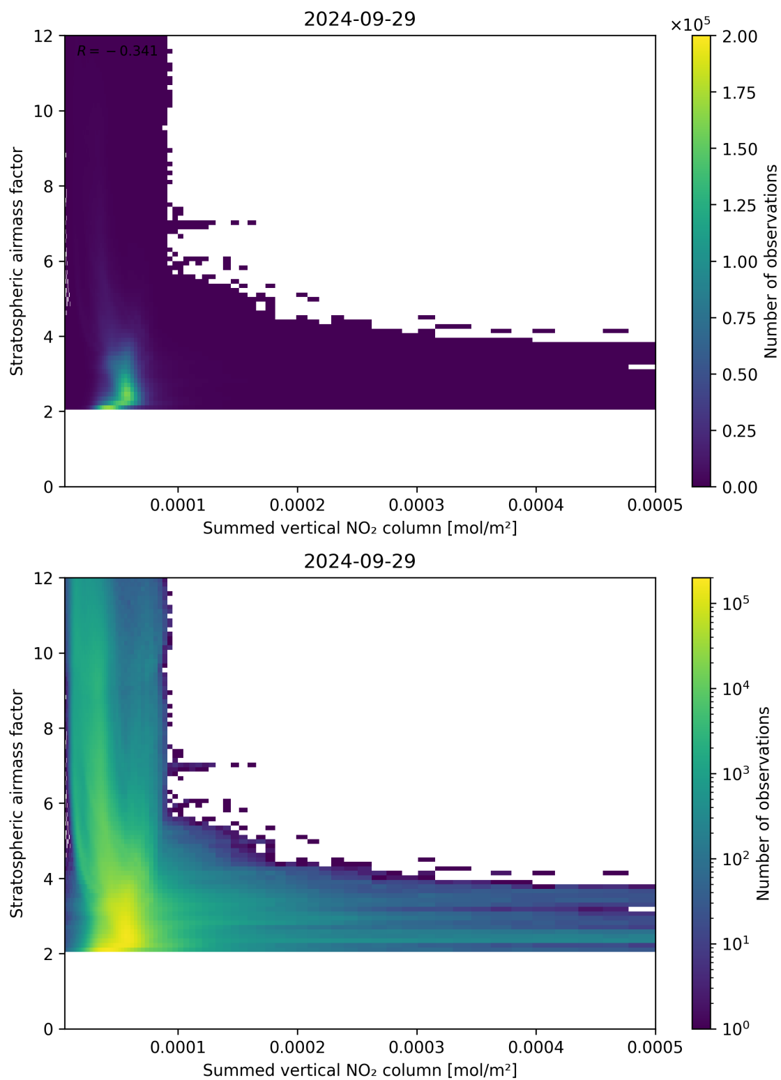
Figure 103: Scatter density plot of “Summed vertical NO 2 column” against “Stratospheric airmass factor” for 2024-09-28 to 2024-09-30.
