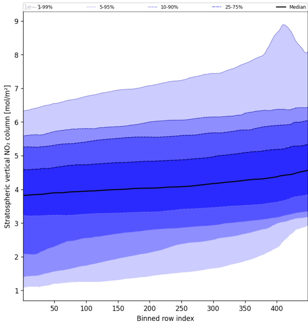
Figure 53: Along track statistics of “Stratospheric vertical NO 2 column” for 2024-09-28 to 2024-09-30
