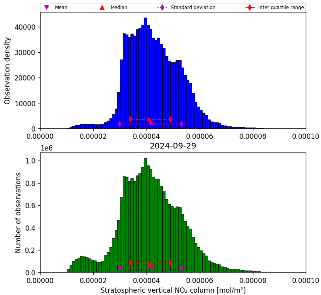
Figure 36: Histogram of “Stratospheric vertical NO 2 column” for 2024-09-28 to 2024-09-30
