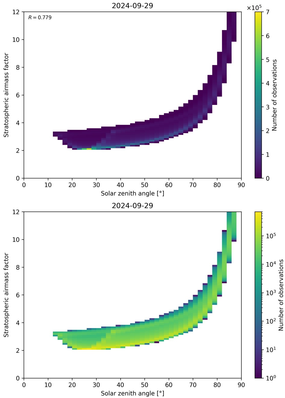
Figure 145: Scatter density plot of “Solar zenith angle” against “Stratospheric airmass factor” for 2024-09-28 to 2024-09-30.
