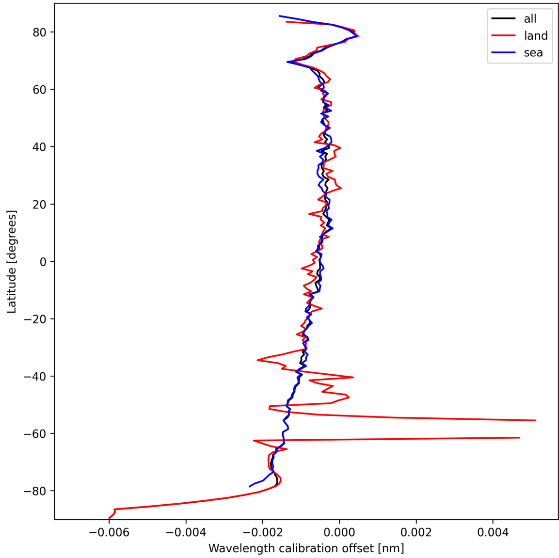
Figure 18: Zonal average of “Wavelength calibration offset” for 2024-09-28 to 2024-09-30.
