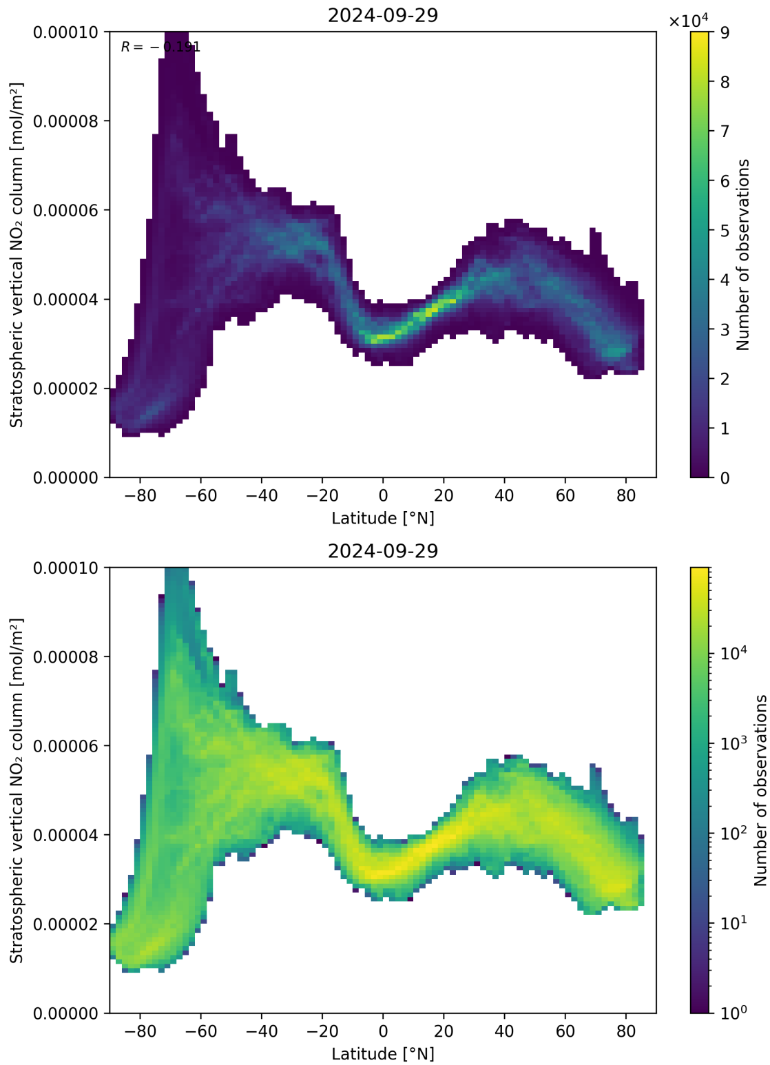
Figure 87: Scatter density plot of “Latitude” against “Stratospheric vertical NO 2 column” for 2024-09-28 to 2024-09-30.
