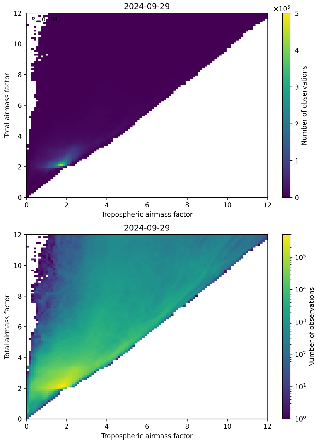
Figure 72: Scatter density plot of “Tropospheric airmass factor” against “Total airmass factor” for 2024-09-28 to 2024-09-30.
