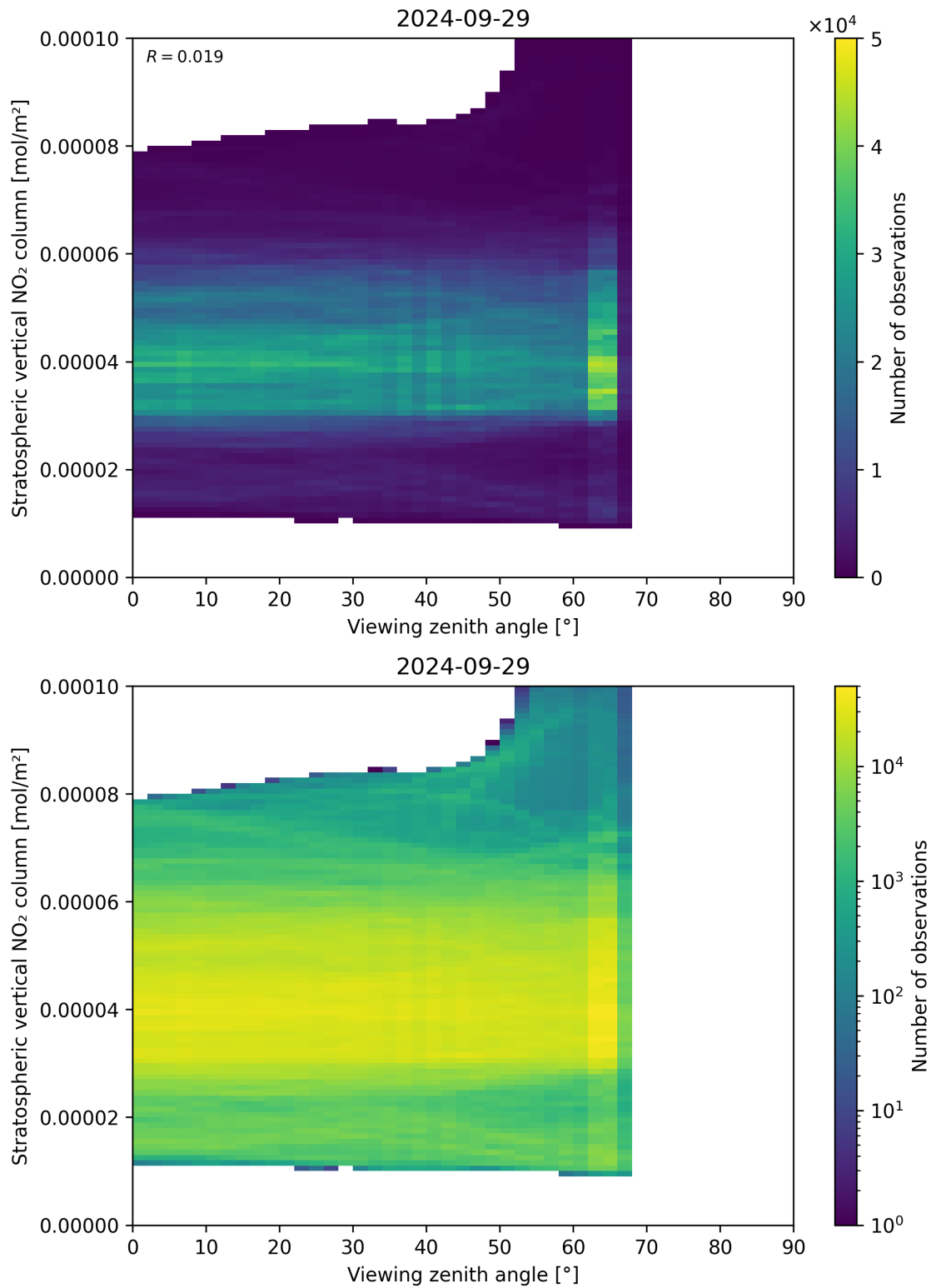
Figure 164: Scatter density plot of “Viewing zenith angle” against “Stratospheric vertical NO 2 column” for 2024-09-28 to 2024-09-30.
