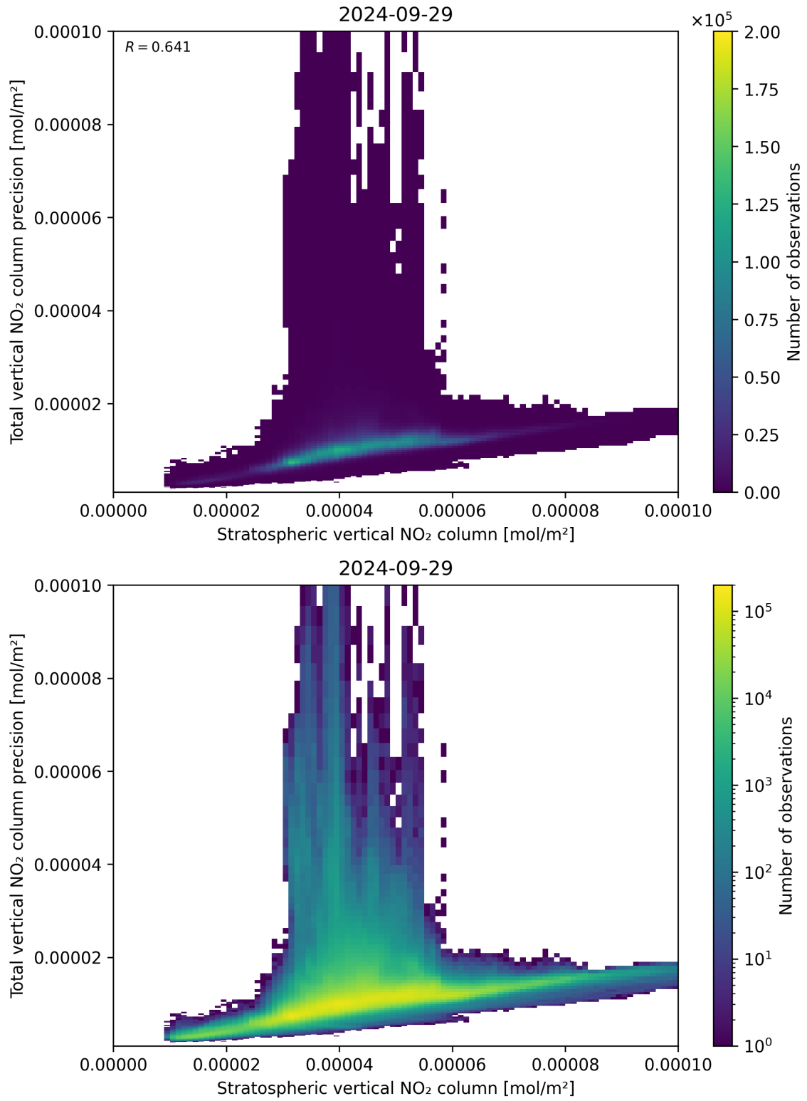
Figure 101: Scatter density plot of “Stratospheric vertical NO 2 column” against “Total vertical NO 2 column precision” for 2024-09-28 to 2024-09-30.
