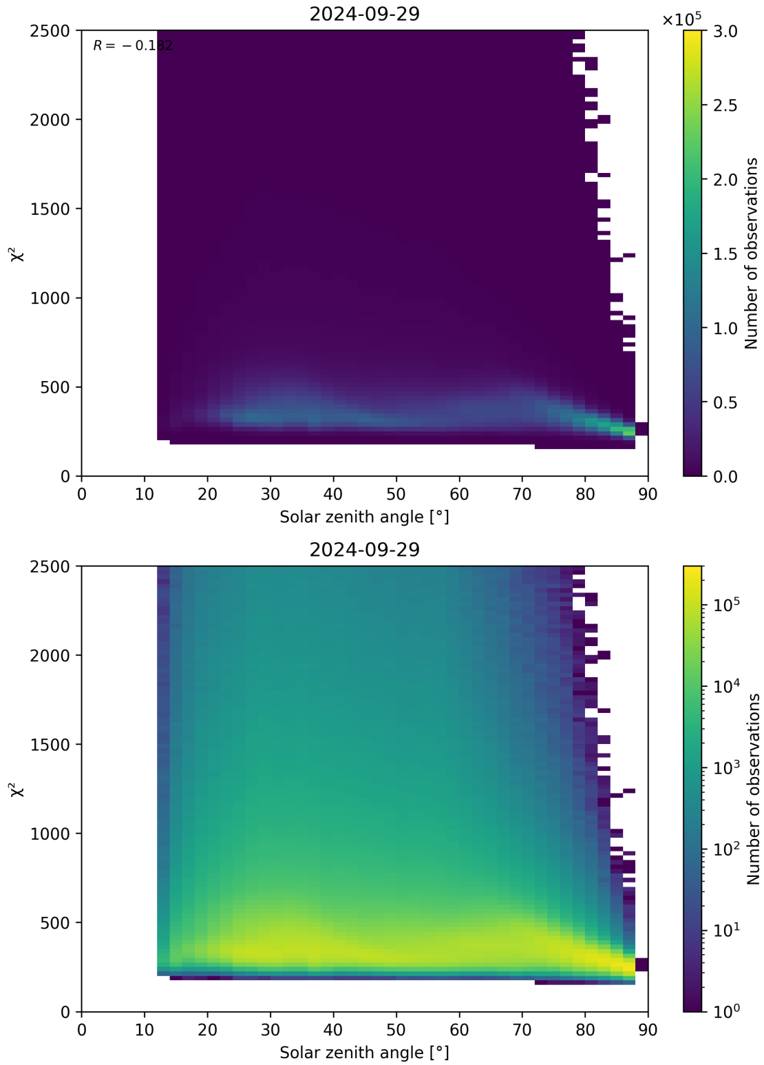
Figure 148: Scatter density plot of “Solar zenith angle” against “ \chi^2 ” for 2024-09-28 to 2024-09-30.
