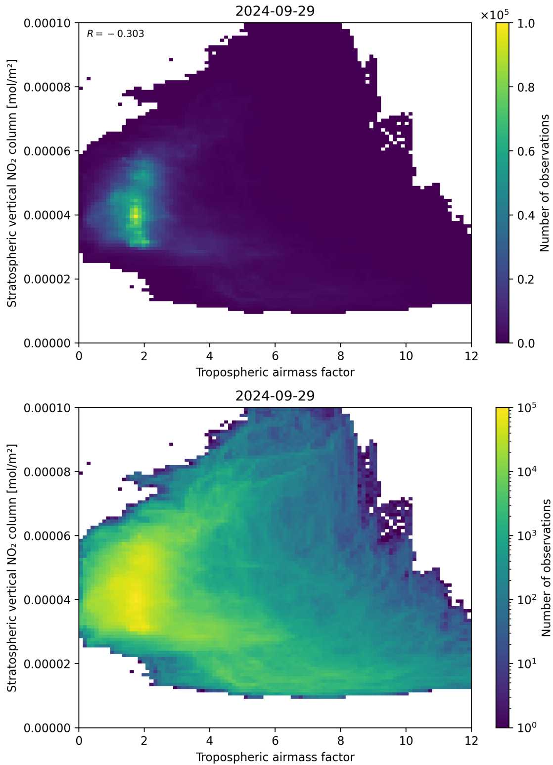
Figure 74: Scatter density plot of “Tropospheric air mass factor” against “Stratospheric vertical NO 2 column” for 2024-09-28 to 2024-09-30.
