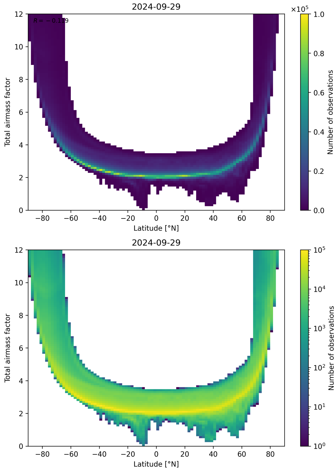
Figure 84: Scatter density plot of “Latitude” against “Total airmass factor” for 2024-09-28 to 2024-09-30.
