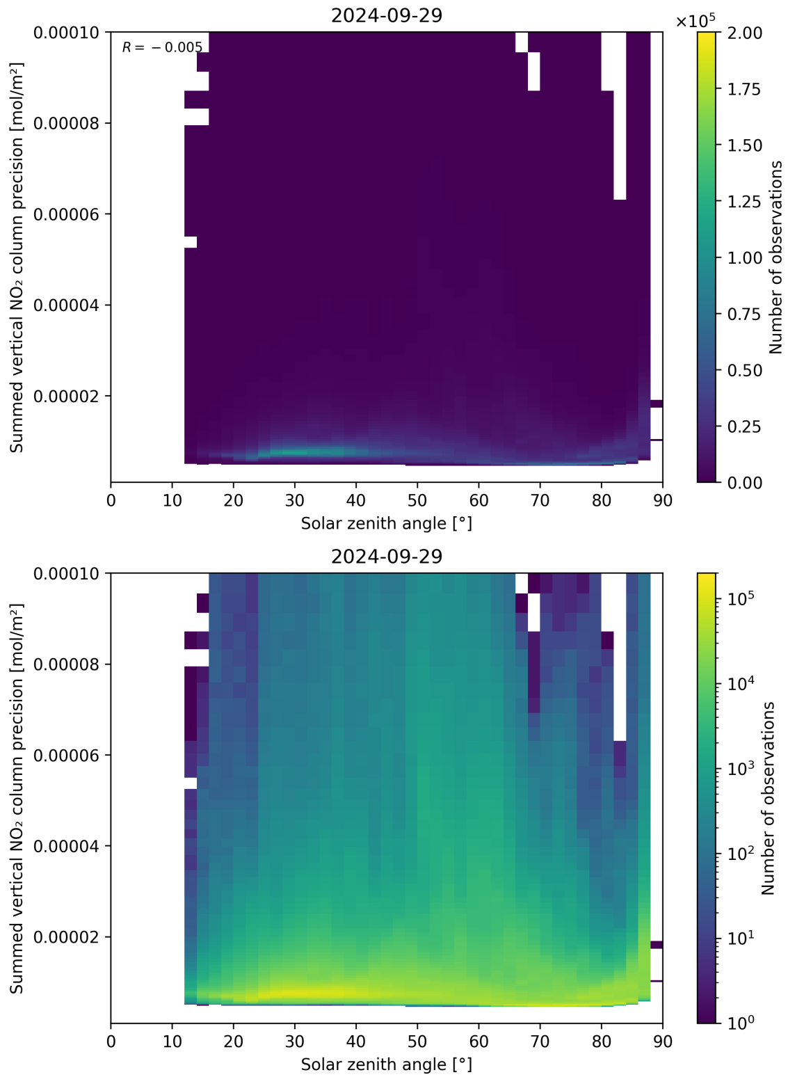
Figure 152: Scatter density plot of “Solar zenith angle” against “Summed vertical NO 2 column precision” for 2024-09-28 to 2024-09-30.
