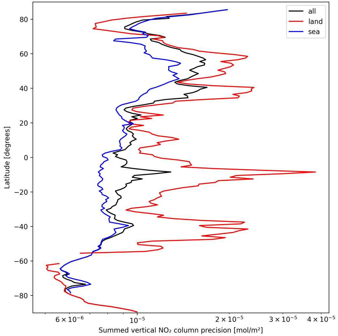
Figure 24: Zonal average of “Summed vertical NO 2 column precision” for 2024-09-28 to 2024-09-30.
