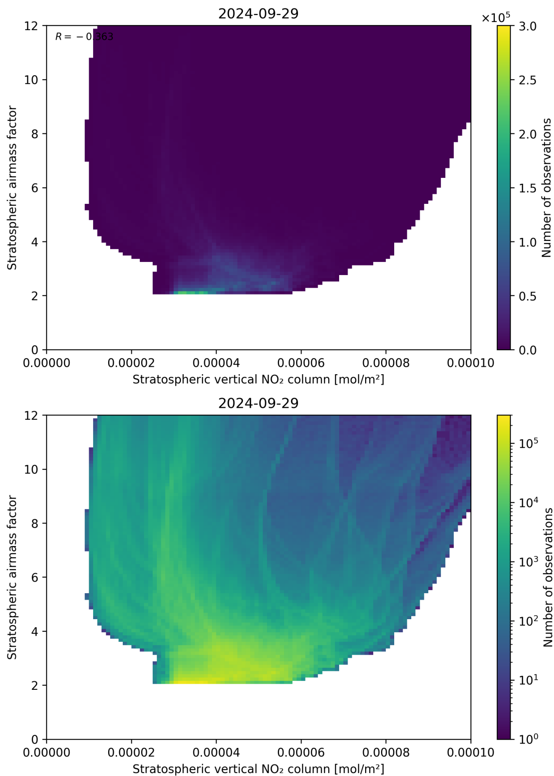
Figure 96: Scatter density plot of “Stratospheric vertical NO 2 column” against “Stratospheric airmass factor” for 2024-09-28 to 2024-09-30.
