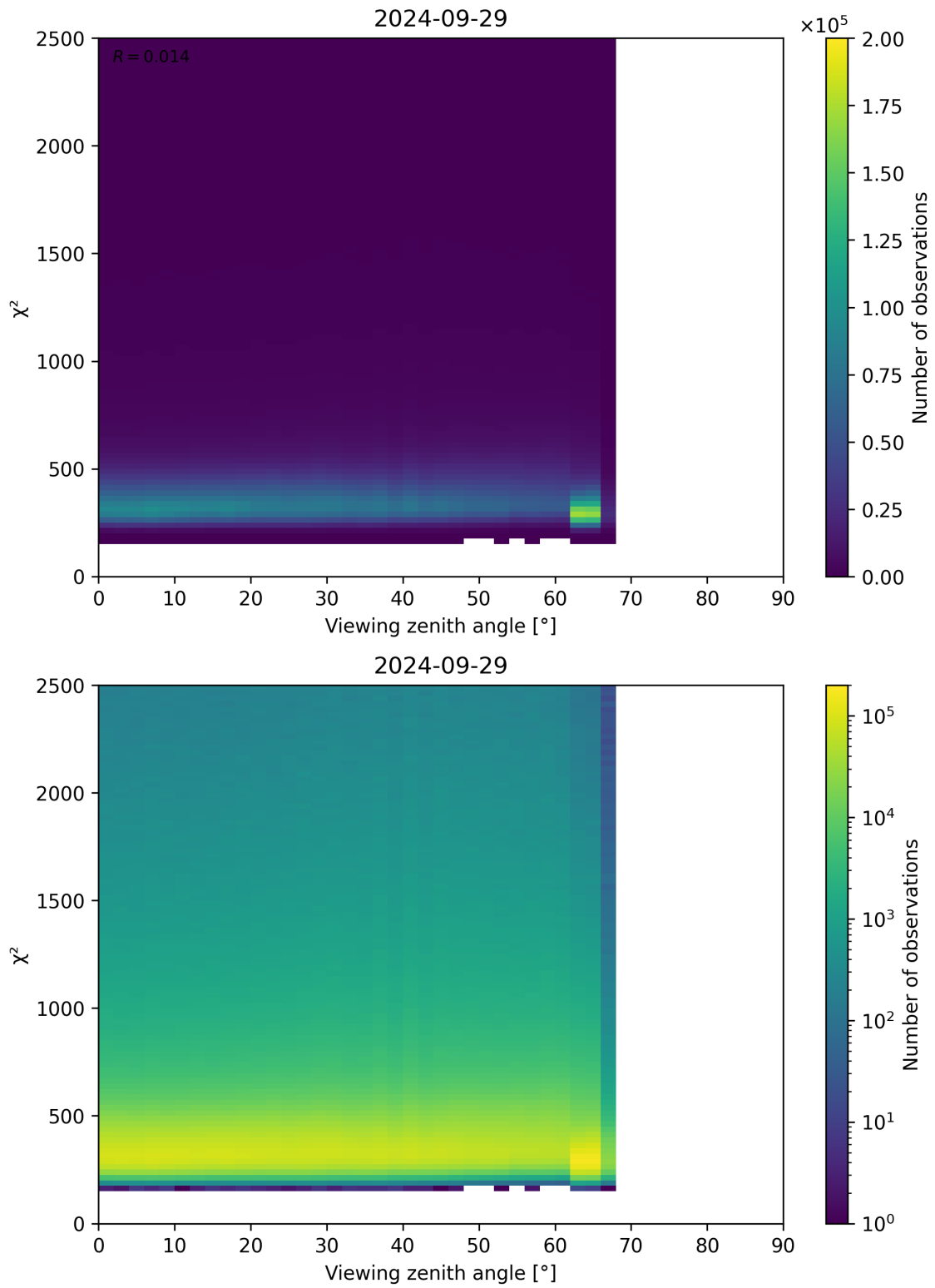
Figure 162: Scatter density plot of “Viewing zenith angle” against “ \chi^2 ” for 2024-09-28 to 2024-09-30.
