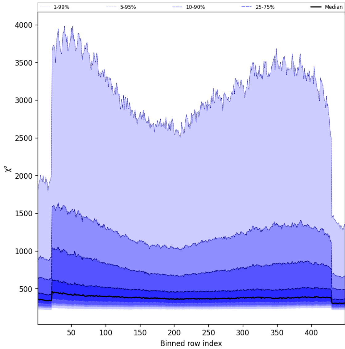
Figure 59: Along track statistics of “ \chi^2 ” for 2024-09-28 to 2024-09-30
