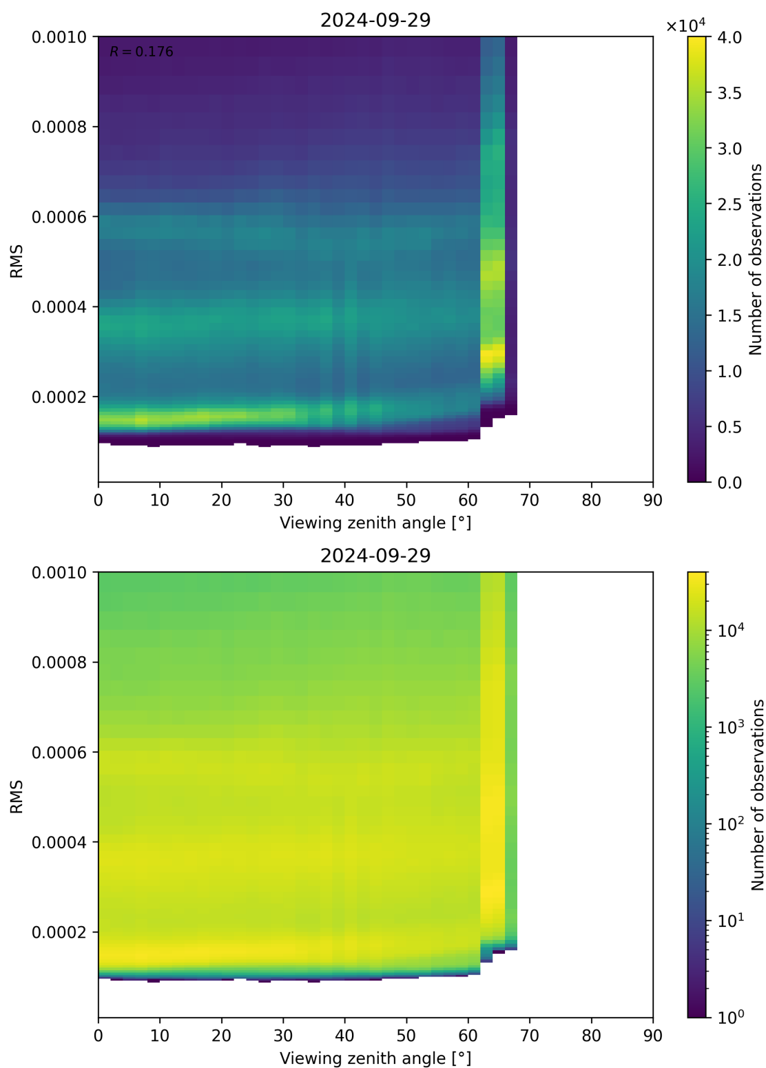
Figure 171: Scatter density plot of “Viewing zenith angle” against “RMS” for 2024-09-28 to 2024-09-30.
