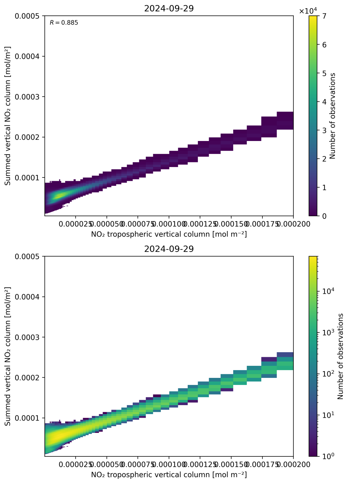
Figure 126: Scatter density plot of “NO 2 tropospheric vertical column” against “Summed vertical NO 2 column” for 2024-09-28 to 2024-09-30.
