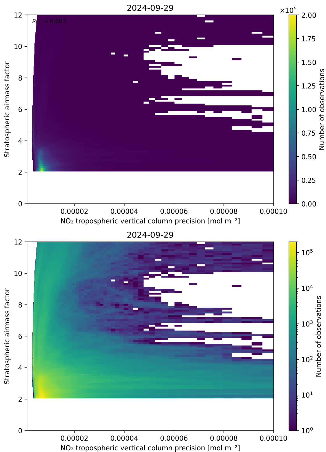
Figure 131: Scatter density plot of “NO 2 tropospheric vertical column precision” against “Stratospheric airmass factor” for 2024-09-28 to 2024-09-30.
