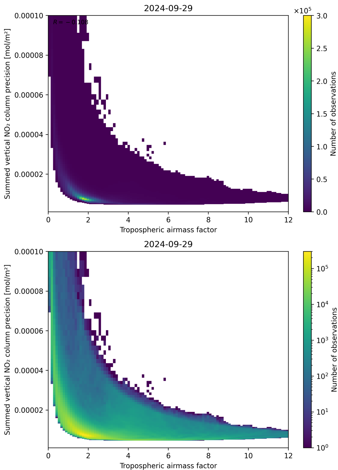
Figure 76: Scatter density plot of “Tropospheric air mass factor” against “Summed vertical NO 2 column precision” for 2024-09-28 to 2024-09-30.
