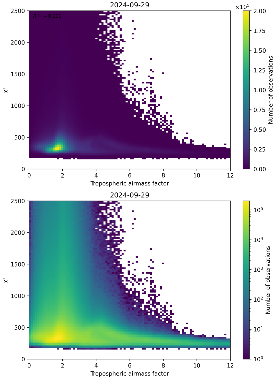
Figure 73: Scatter density plot of “Tropospheric airmass factor” against “ \chi^2 ” for 2024-09-28 to 2024-09-30.
