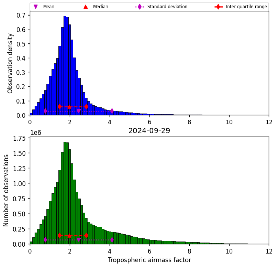
Figure 31: Histogram of “Tropospheric airmass factor” for 2024-09-28 to 2024-09-30
