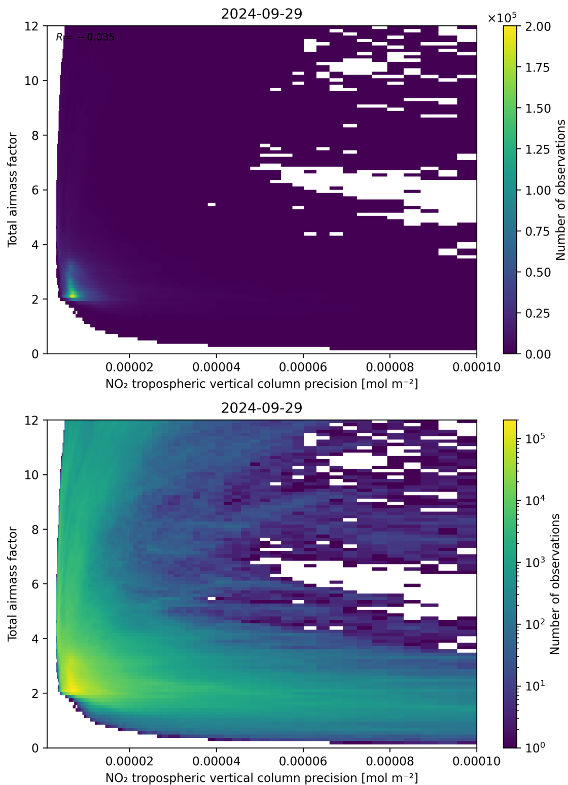
Figure 132: Scatter density plot of “NO 2 tropospheric vertical column precision” against “Total air mass factor” for 2024-09-28 to 2024-09-30.
