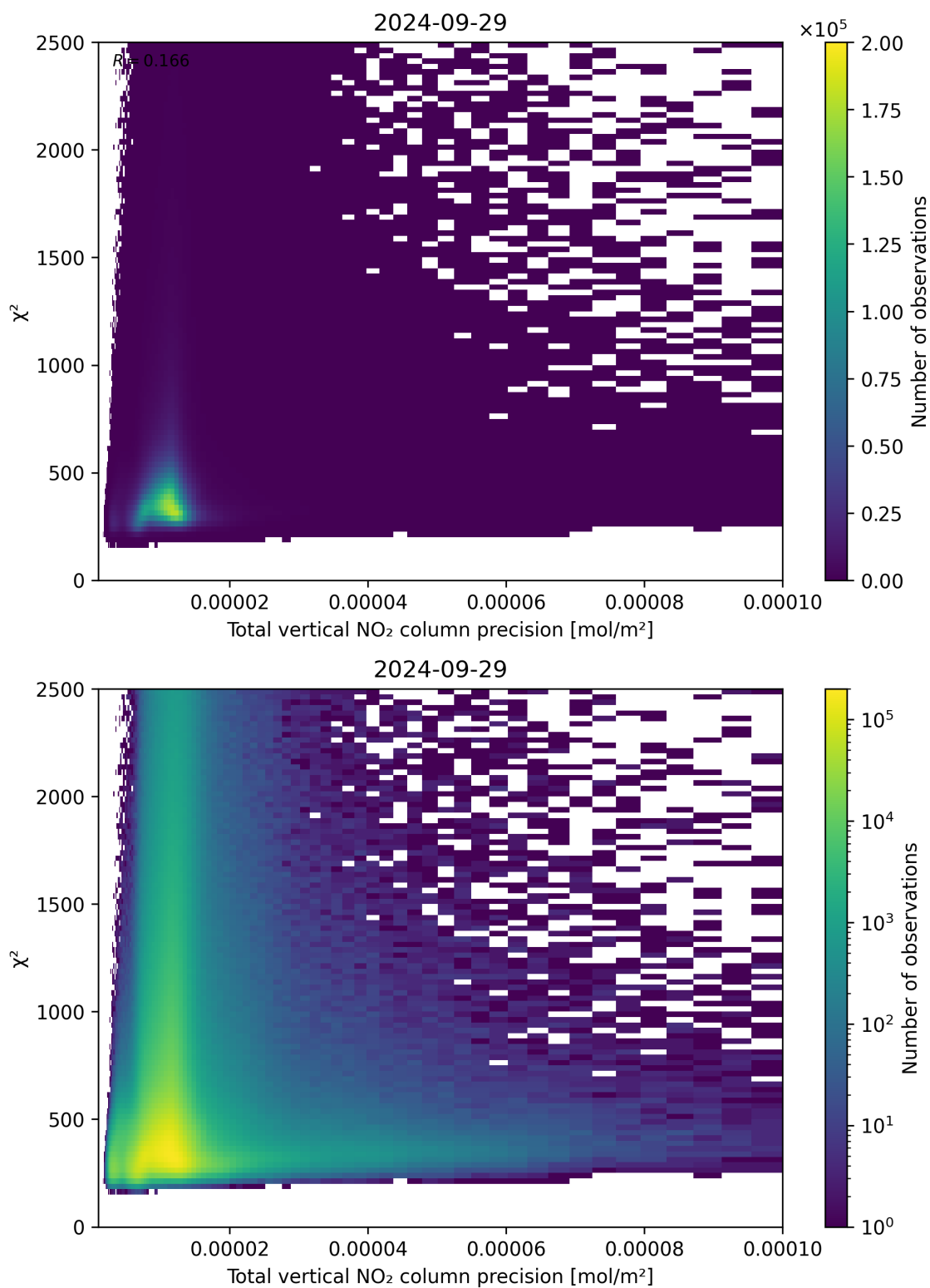
Figure 116: Scatter density plot of “Total vertical NO 2 column precision” against “ \chi^2 ” for 2024-09-28 to 2024-09-30.
