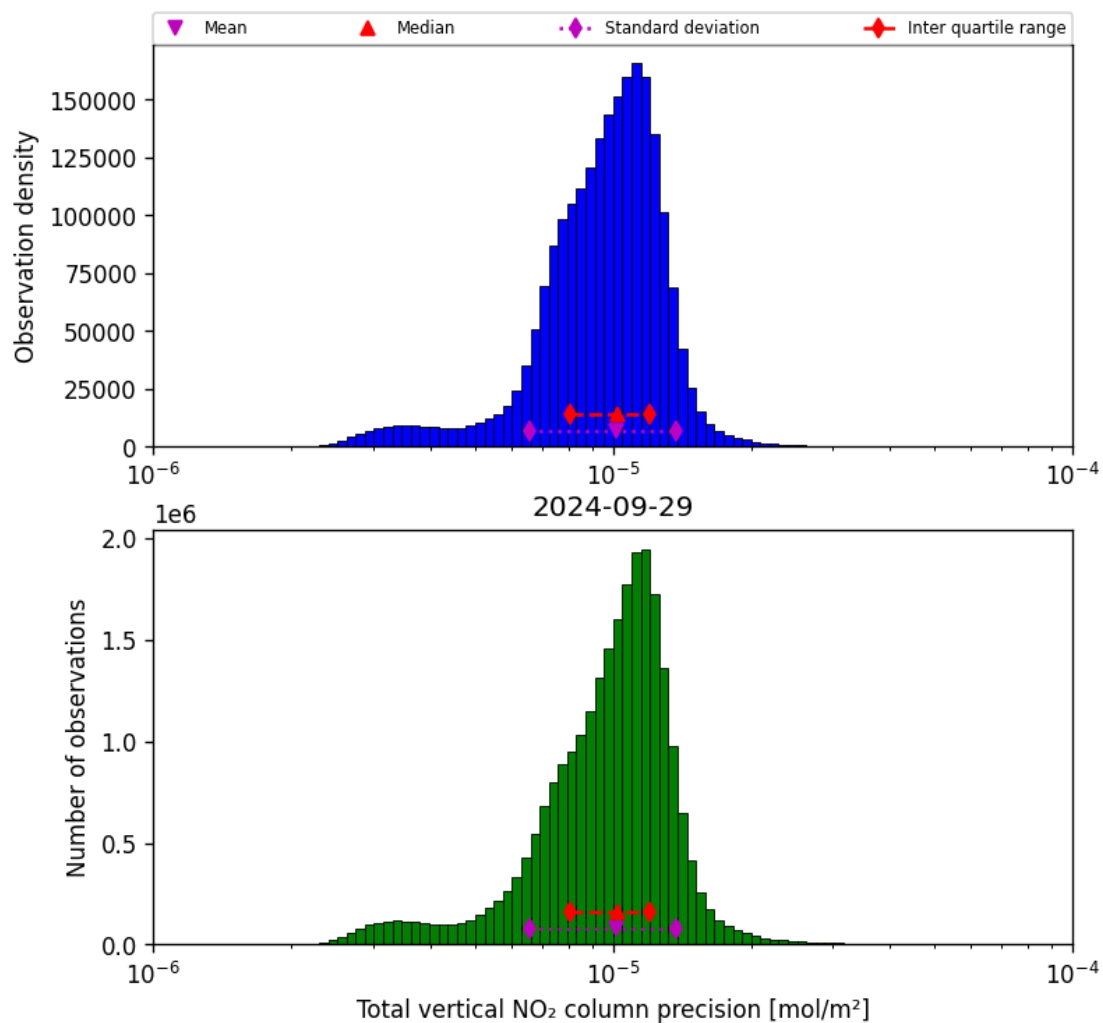
Figure 39: Histogram of “Total vertical NO 2 column precision” for 2024-09-28 to 2024-09-30
