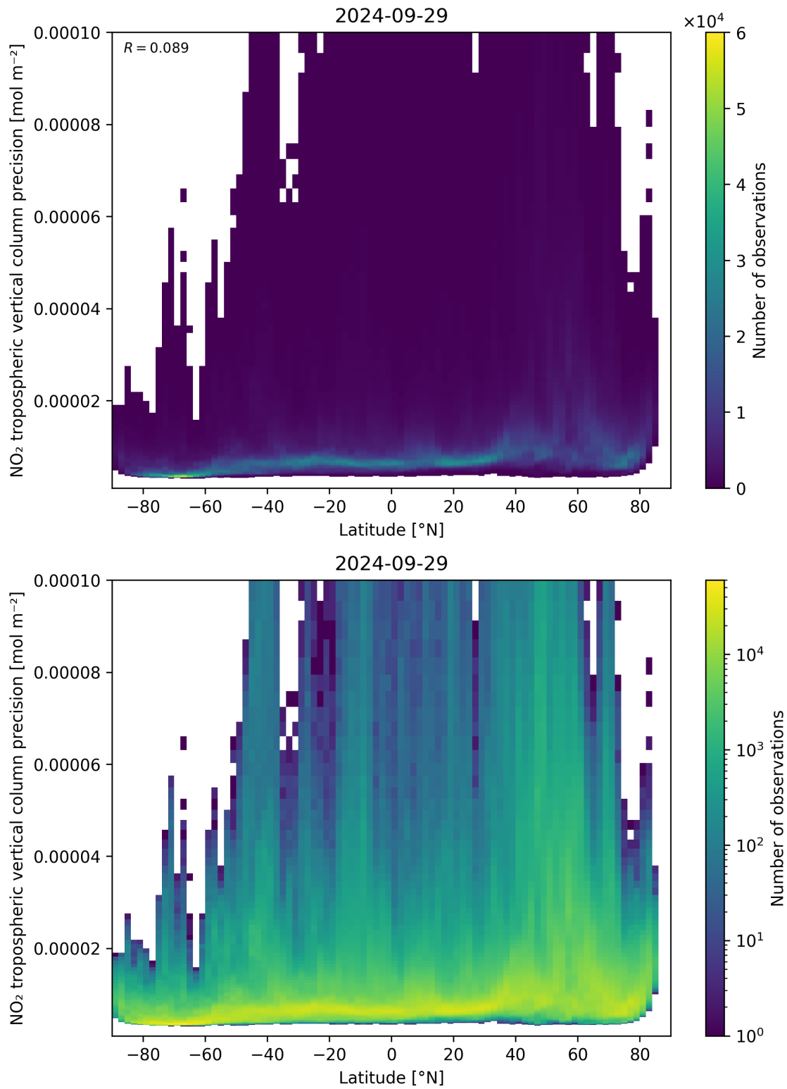
Figure 93: Scatter density plot of “Latitude” against “NO 2 tropospheric vertical column precision” for 2024-09-28 to 2024-09-30.
