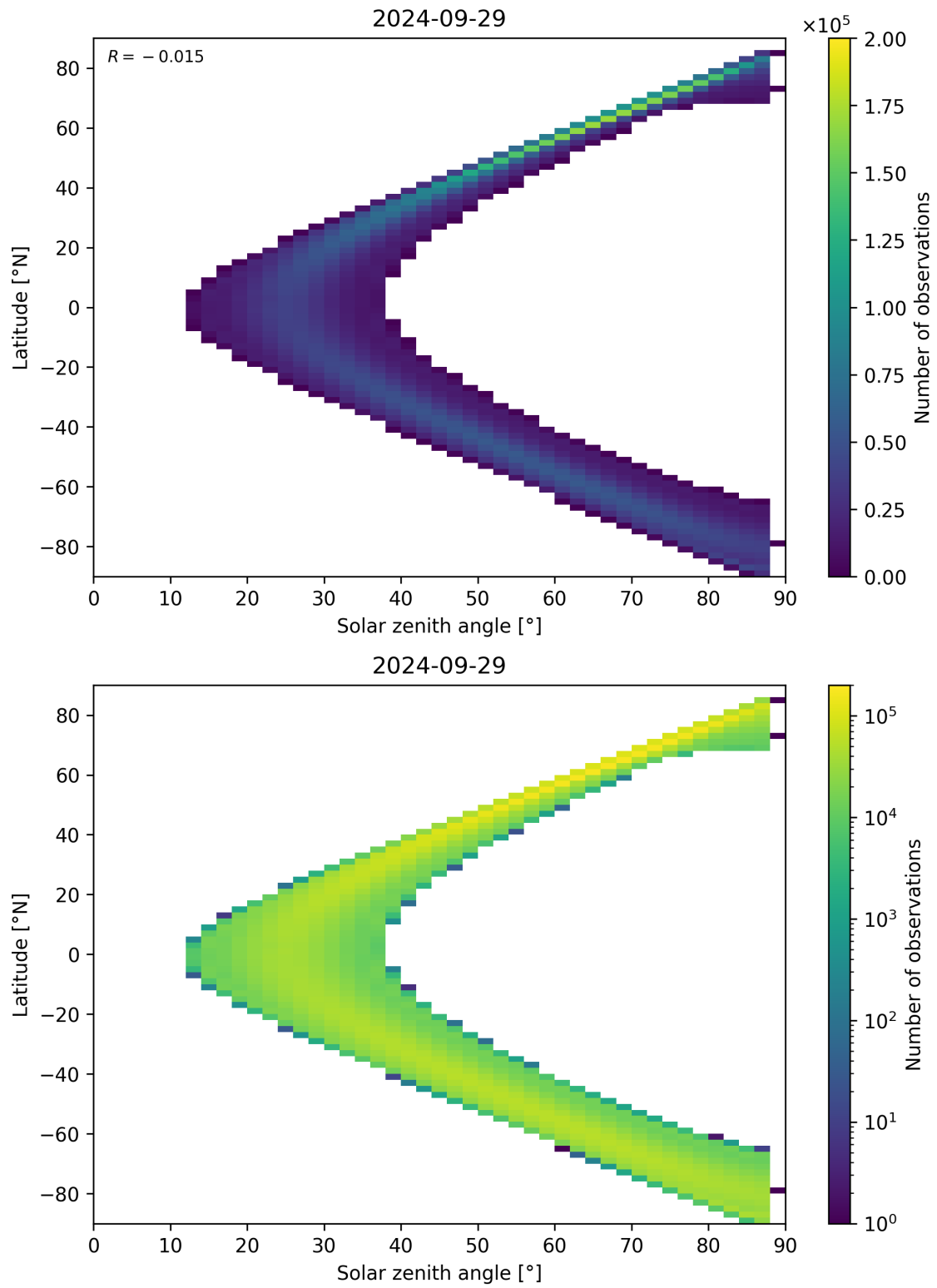
Figure 149: Scatter density plot of “Solar zenith angle” against “Latitude” for 2024-09-28 to 2024-09-30.
