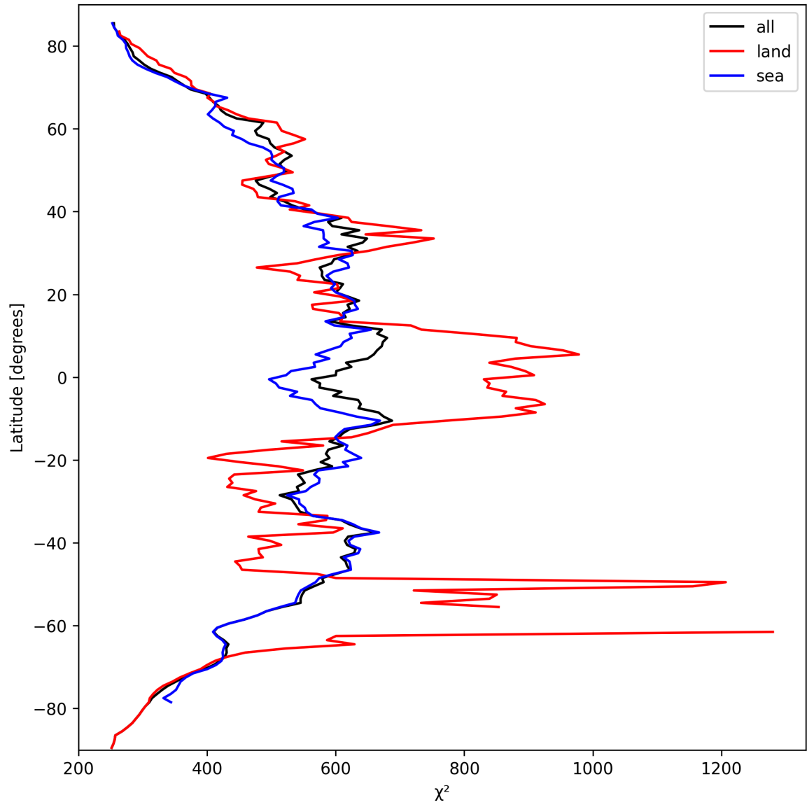
Figure 25: Zonal average of “ \chi^2 ” for 2024-09-28 to 2024-09-30.
