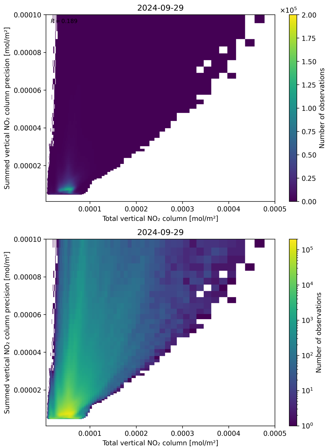
Figure 113: Scatter density plot of “Total vertical NO 2 column” against “Summed vertical NO 2 column precision” for 2024-09-28 to 2024-09-30.
