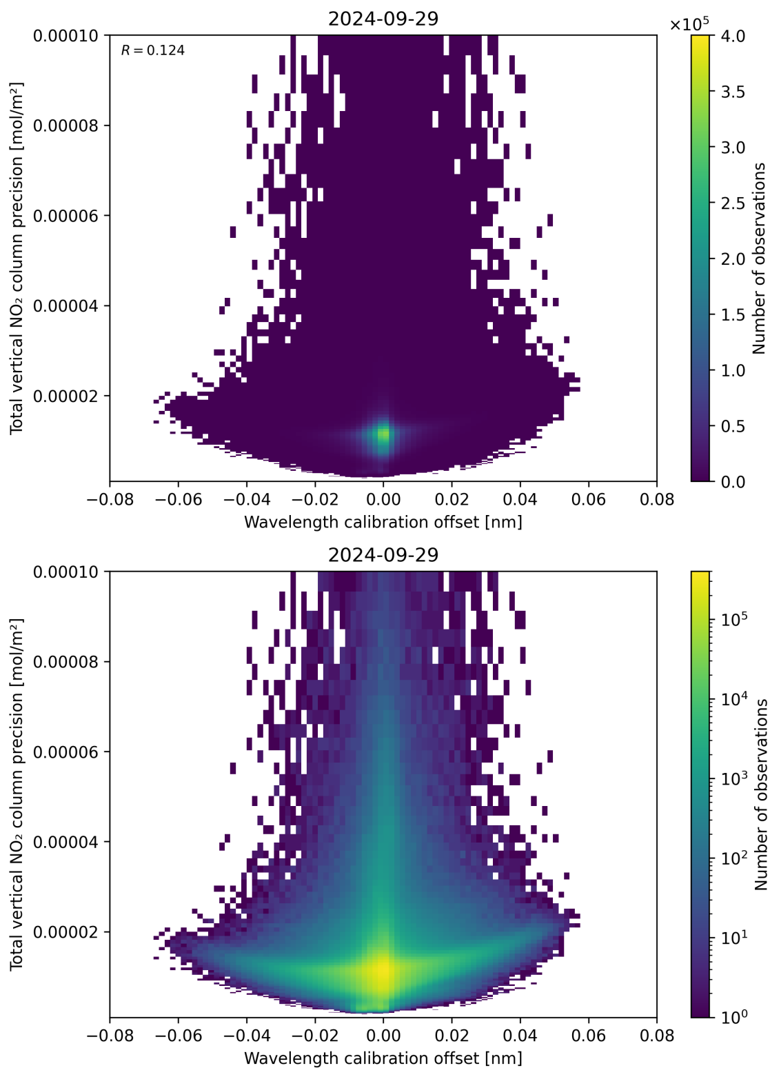
Figure 180: Scatter density plot of “Wavelength calibration offset” against “Total vertical NO 2 column precision” for 2024-09-28 to 2024-09-30.
