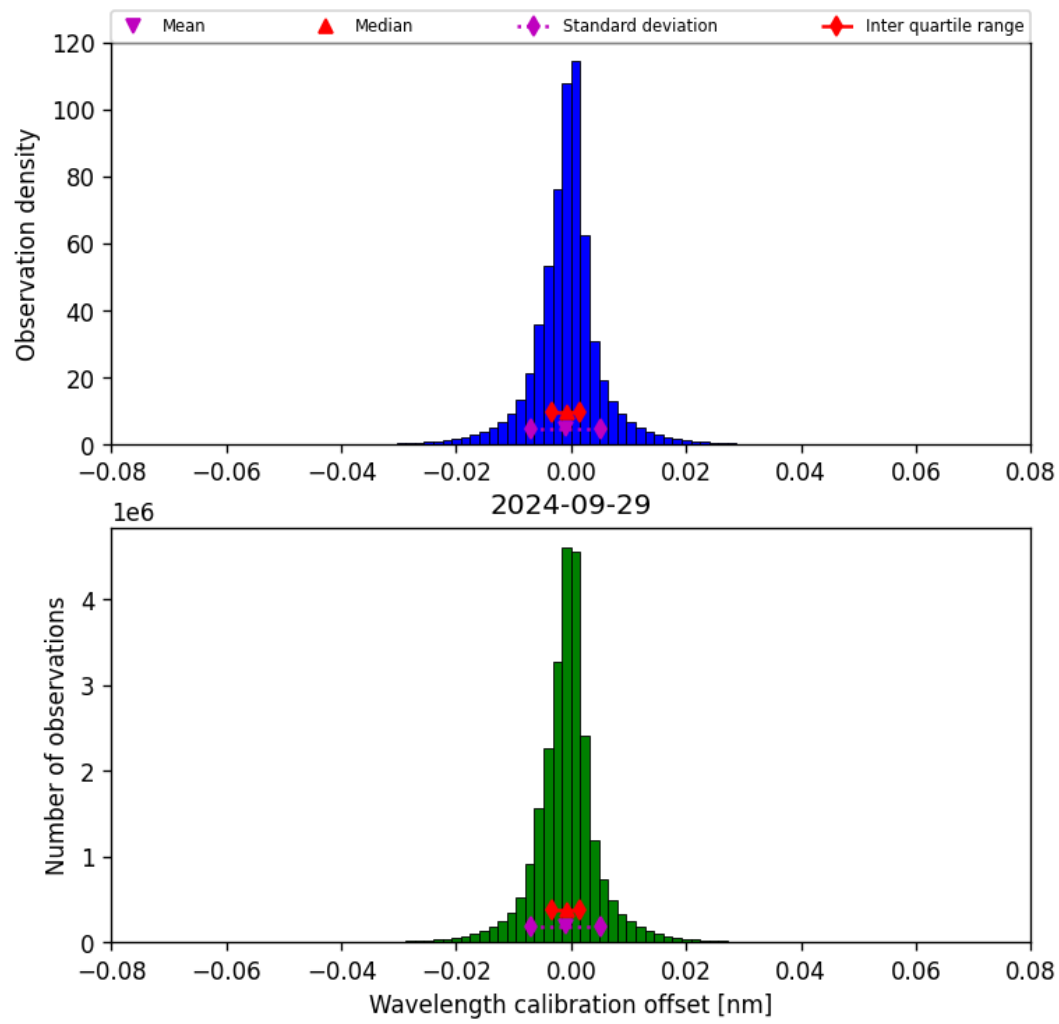
Figure 35: Histogram of “Wavelength calibration offset” for 2024-09-28 to 2024-09-30
