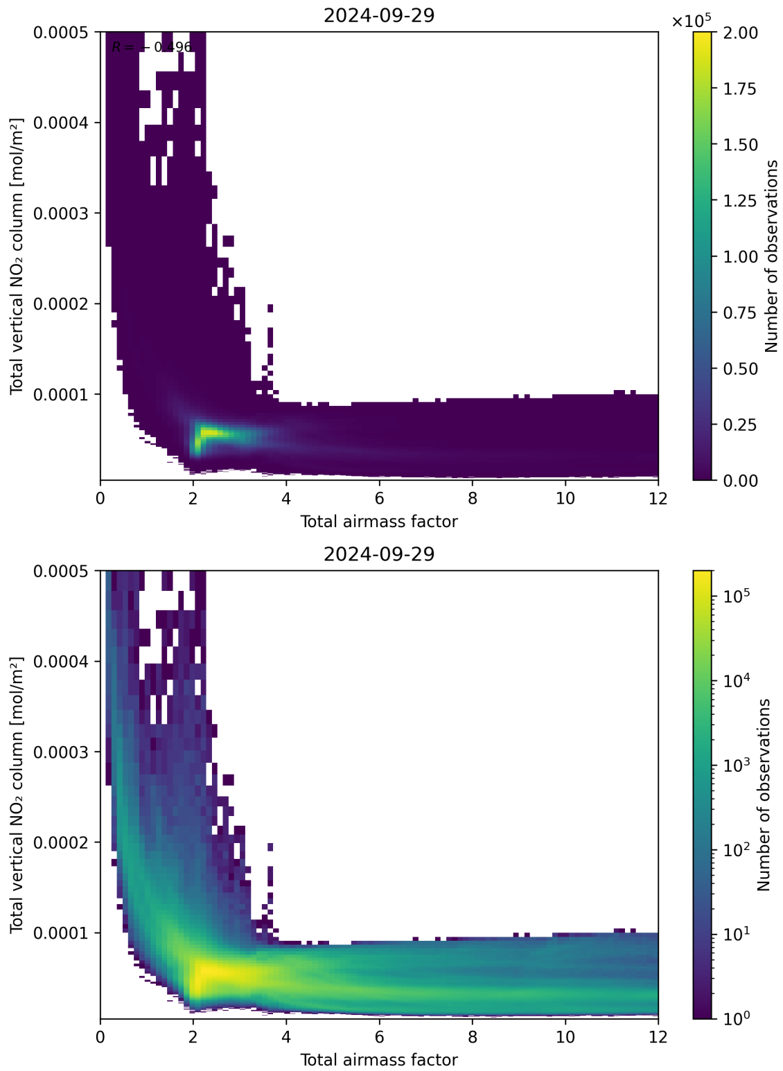
Figure 67: Scatter density plot of “Total airmass factor” against “Total vertical NO 2 column” for 2024-09-28 to 2024-09-30.
