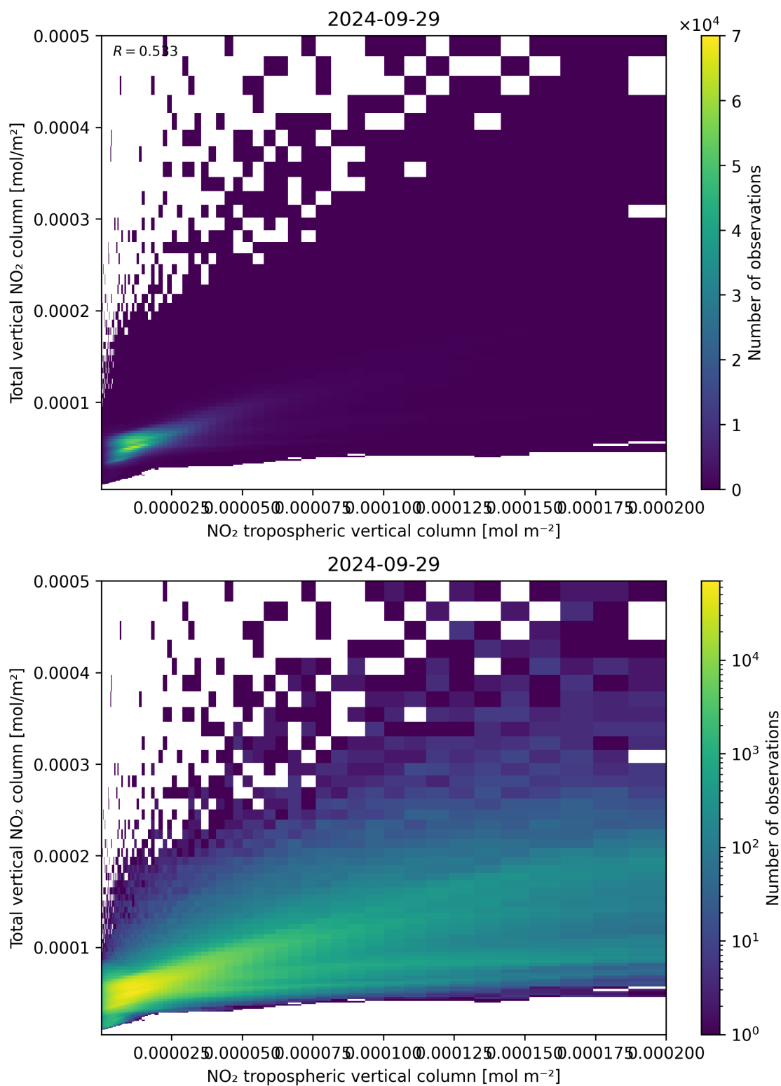
Figure 128: Scatter density plot of “NO 2 tropospheric vertical column” against “Total vertical NO 2 column” for 2024-09-28 to 2024-09-30.
