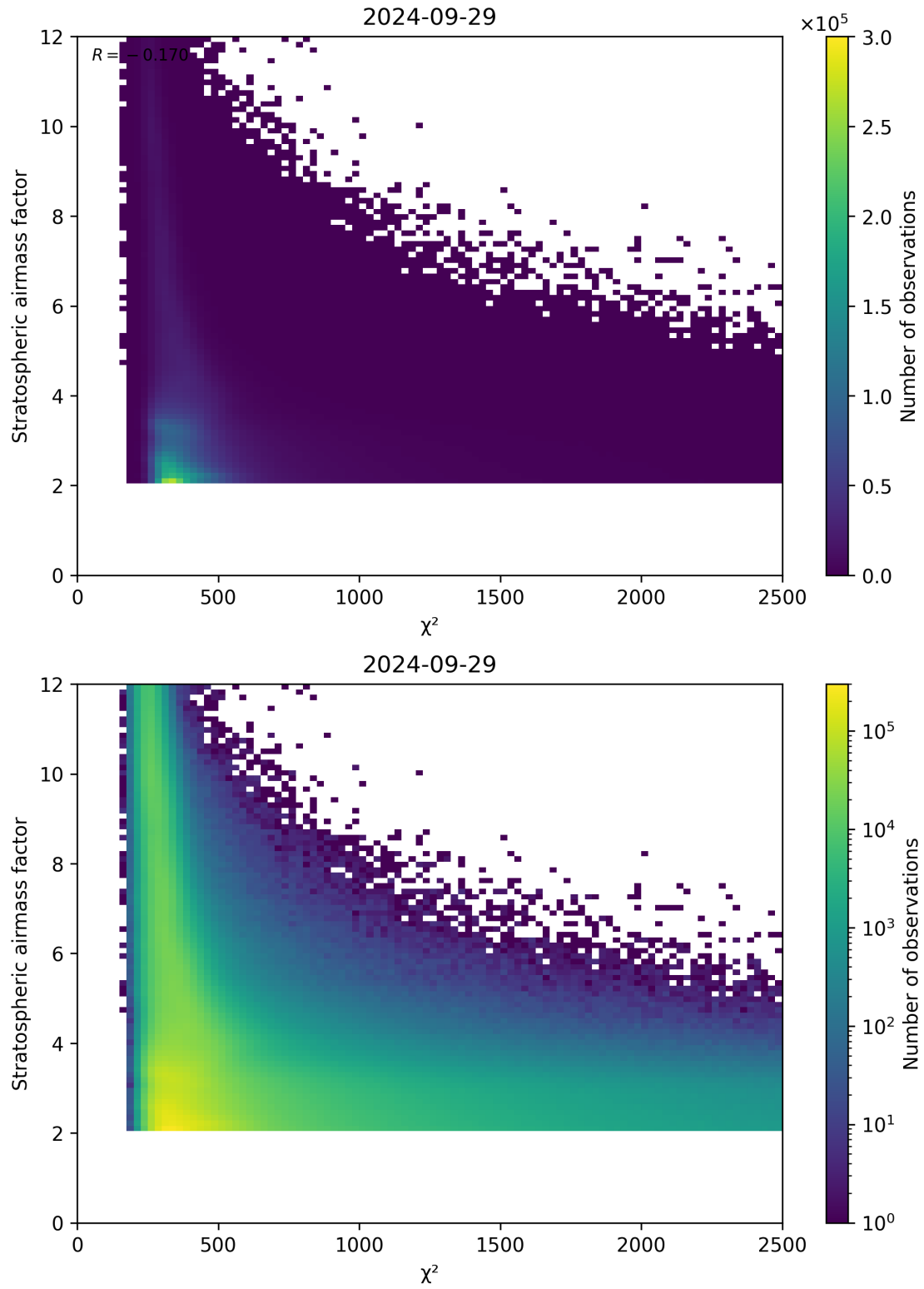
Figure 81: Scatter density plot of “ \chi^2 ” against “Stratospheric airmass factor” for 2024-09-28 to 2024-09-30.
