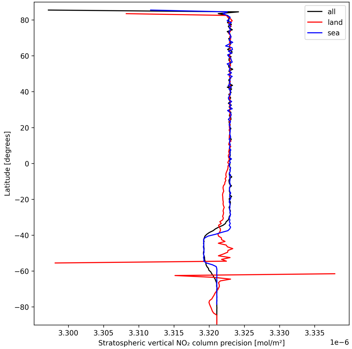
Figure 20: Zonal average of “Stratospheric vertical NO 2 column precision” for 2024-09-28 to 2024-09-30.
