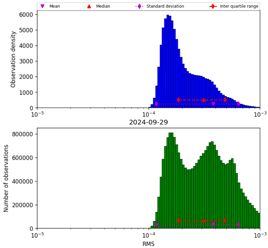
Figure 43: Histogram of “RMS” for 2024-09-28 to 2024-09-30
