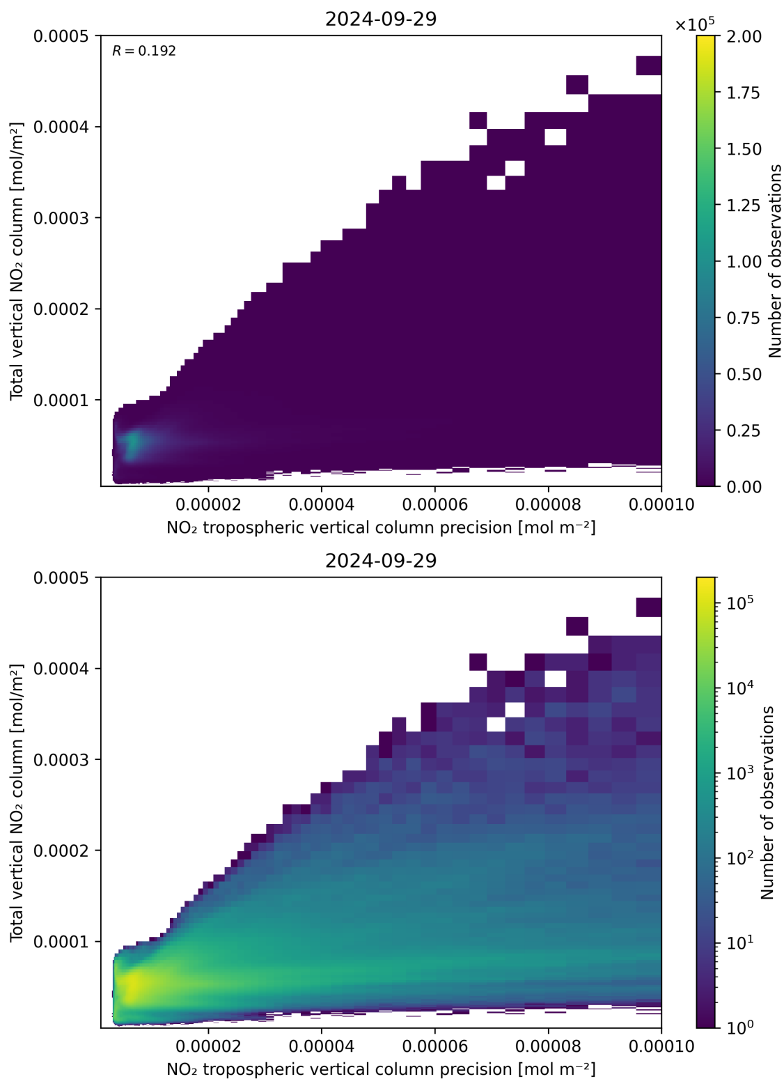
Figure 138: Scatter density plot of “NO 2 tropospheric vertical column precision” against “Total vertical NO 2 column” for 2024-09-28 to 2024-09-30.
