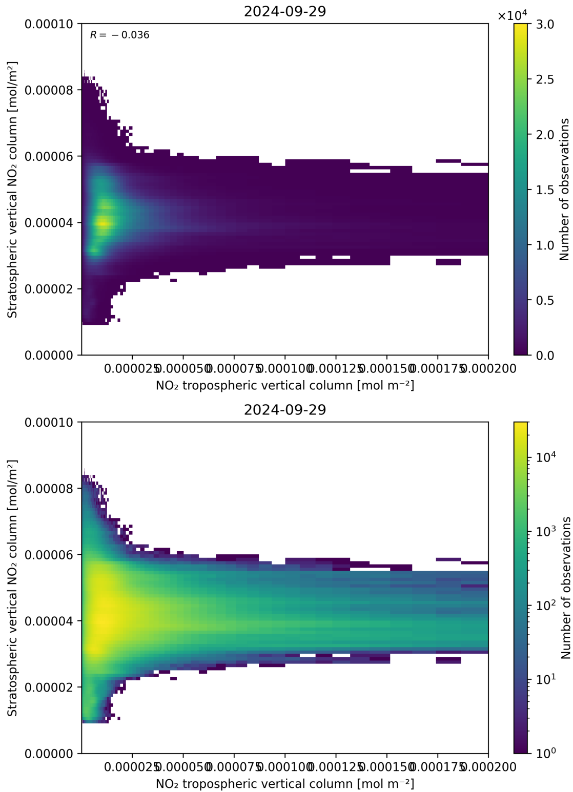
Figure 125: Scatter density plot of “NO 2 tropospheric vertical column” against “Stratospheric vertical NO 2 column” for 2024-09-28 to 2024-09-30.
