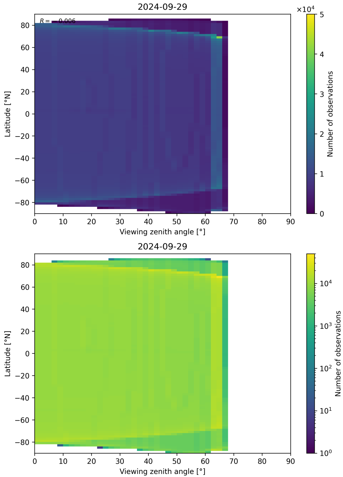
Figure 163: Scatter density plot of “Viewing zenith angle” against “Latitude” for 2024-09-28 to 2024-09-30.
