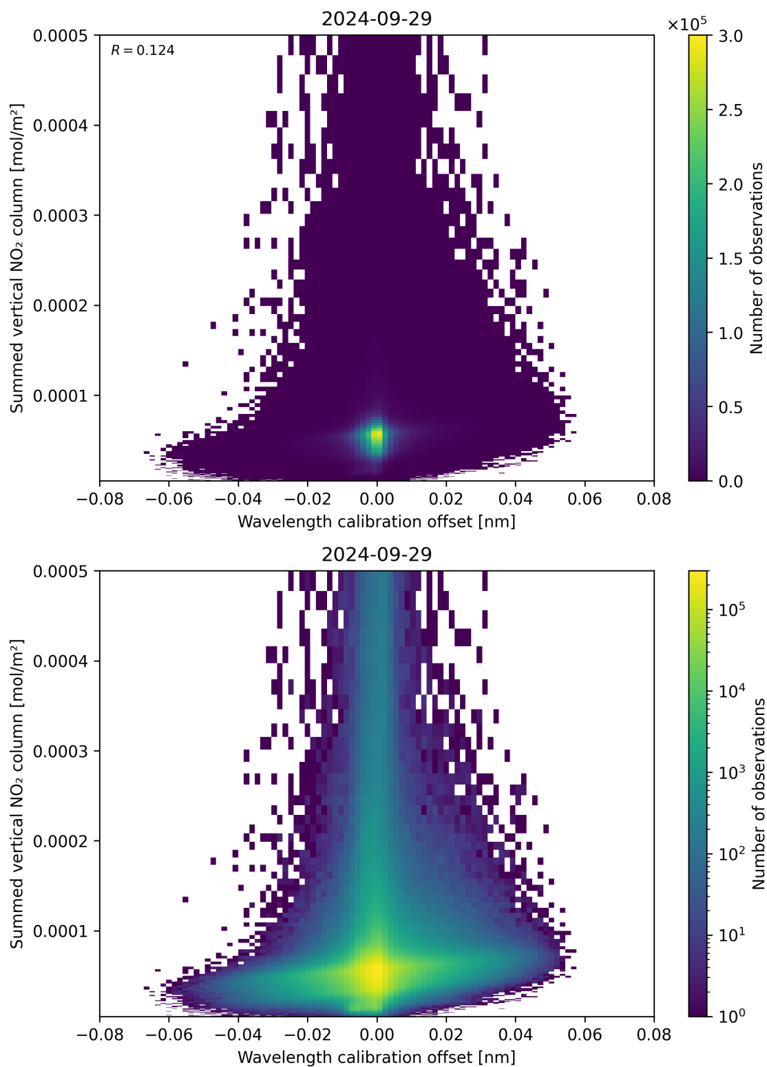
Figure 177: Scatter density plot of “Wavelength calibration offset” against “Summed vertical NO 2 column” for 2024-09-28 to 2024-09-30.
