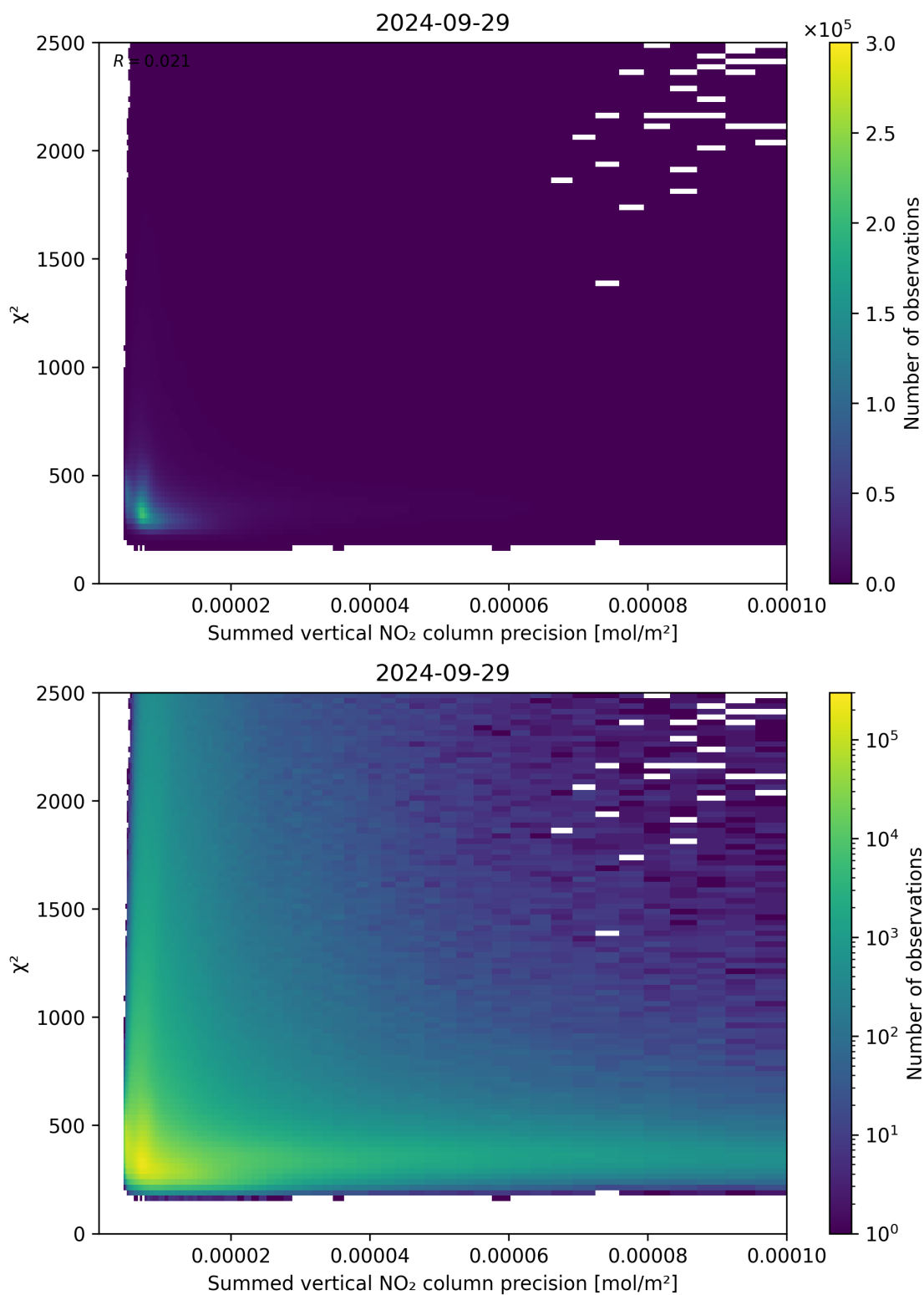
Figure 107: Scatter density plot of “Summed vertical NO 2 column precision” against “ \chi^2 ” for 2024-09-28 to 2024-09-30.
