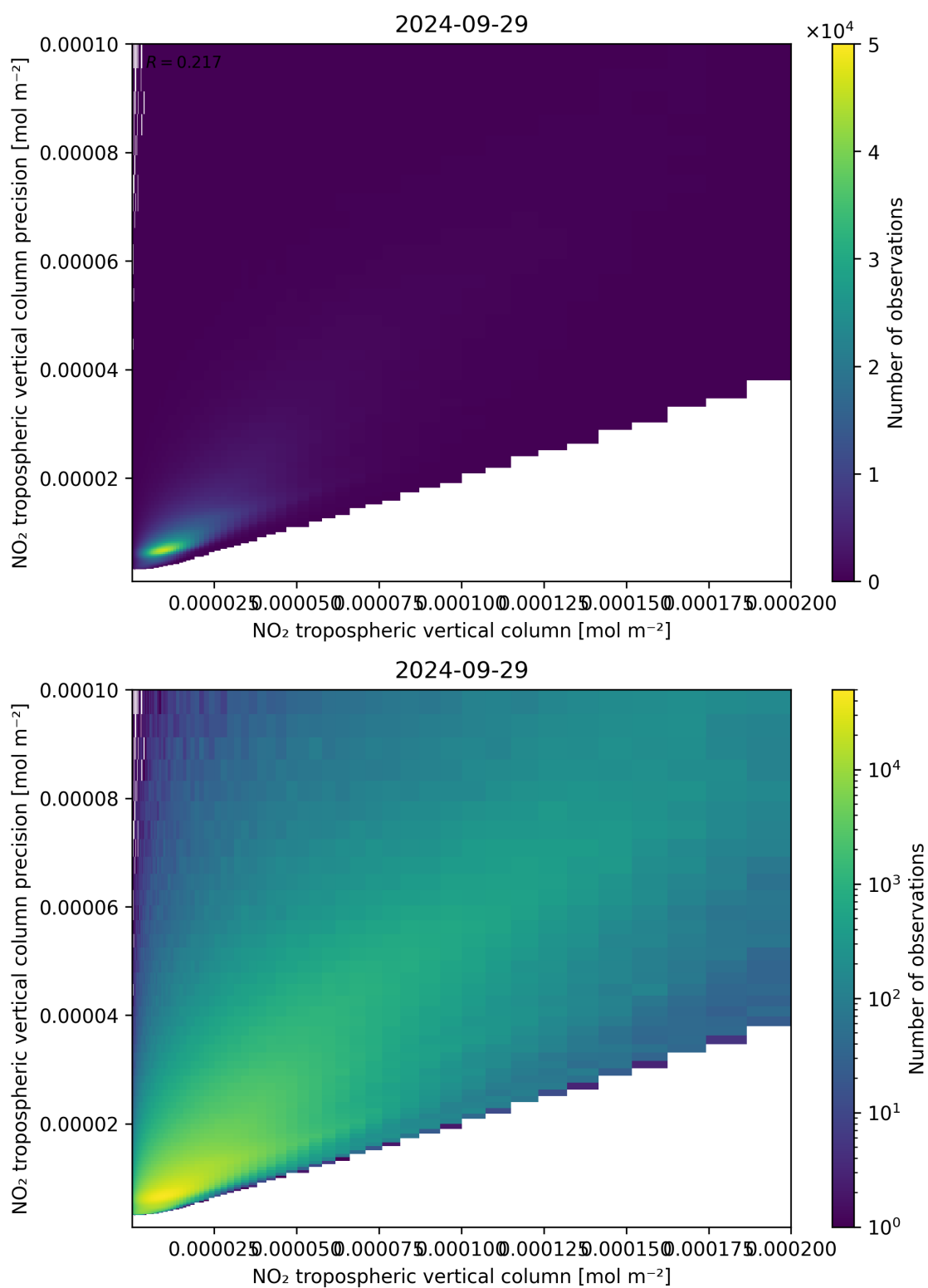
Figure 130: Scatter density plot of “NO 2 tropospheric vertical column” against “NO 2 tropospheric vertical column precision” for 2024-09-28 to 2024-09-30.
