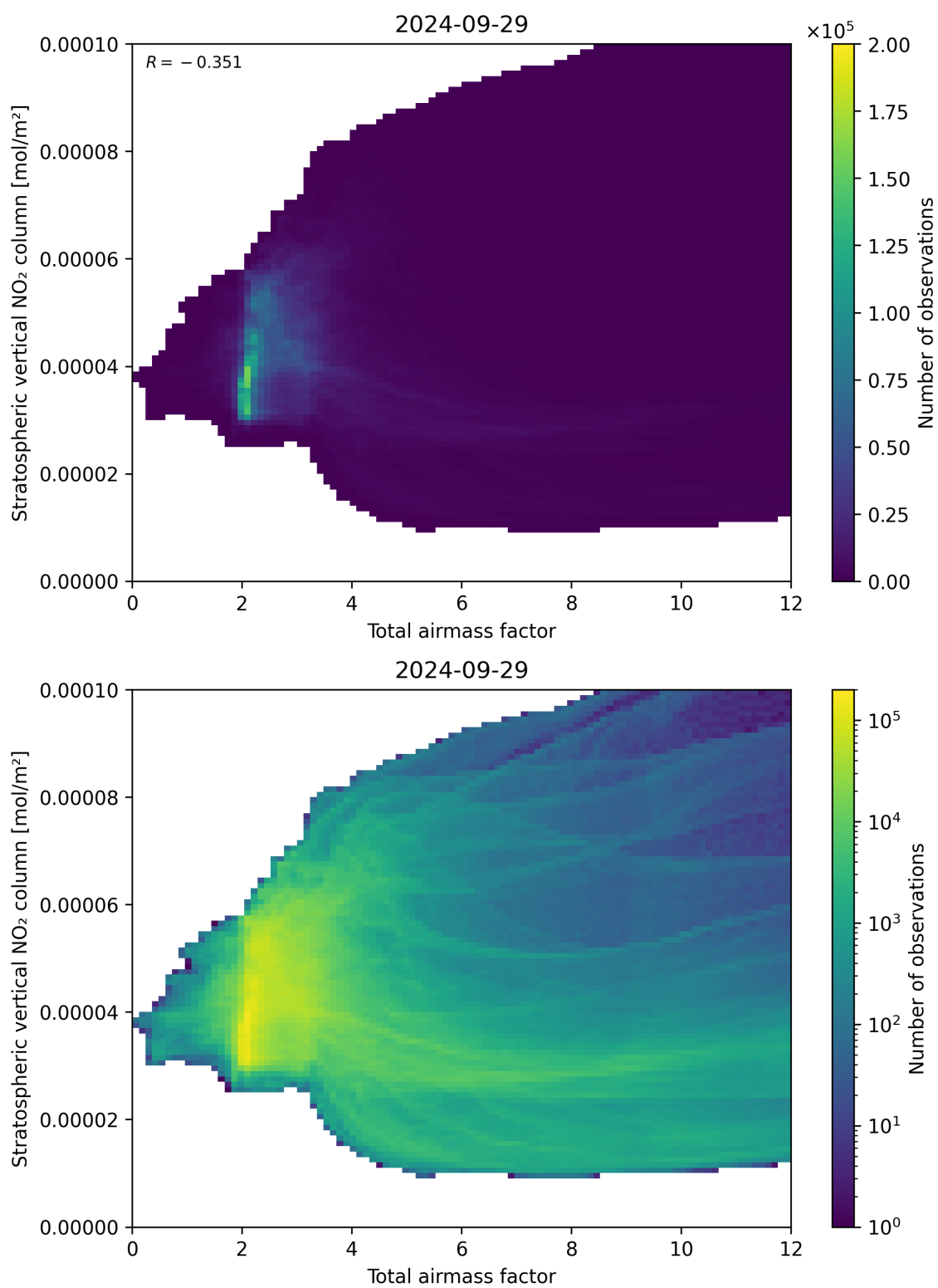
Figure 64: Scatter density plot of “Total airmass factor” against “Stratospheric vertical NO 2 column” for 2024-09-28 to 2024-09-30.
