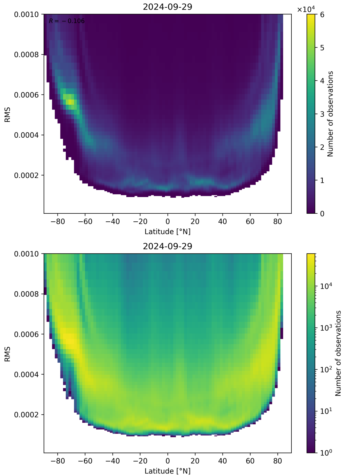
Figure 94: Scatter density plot of “Latitude” against “RMS” for 2024-09-28 to 2024-09-30.
