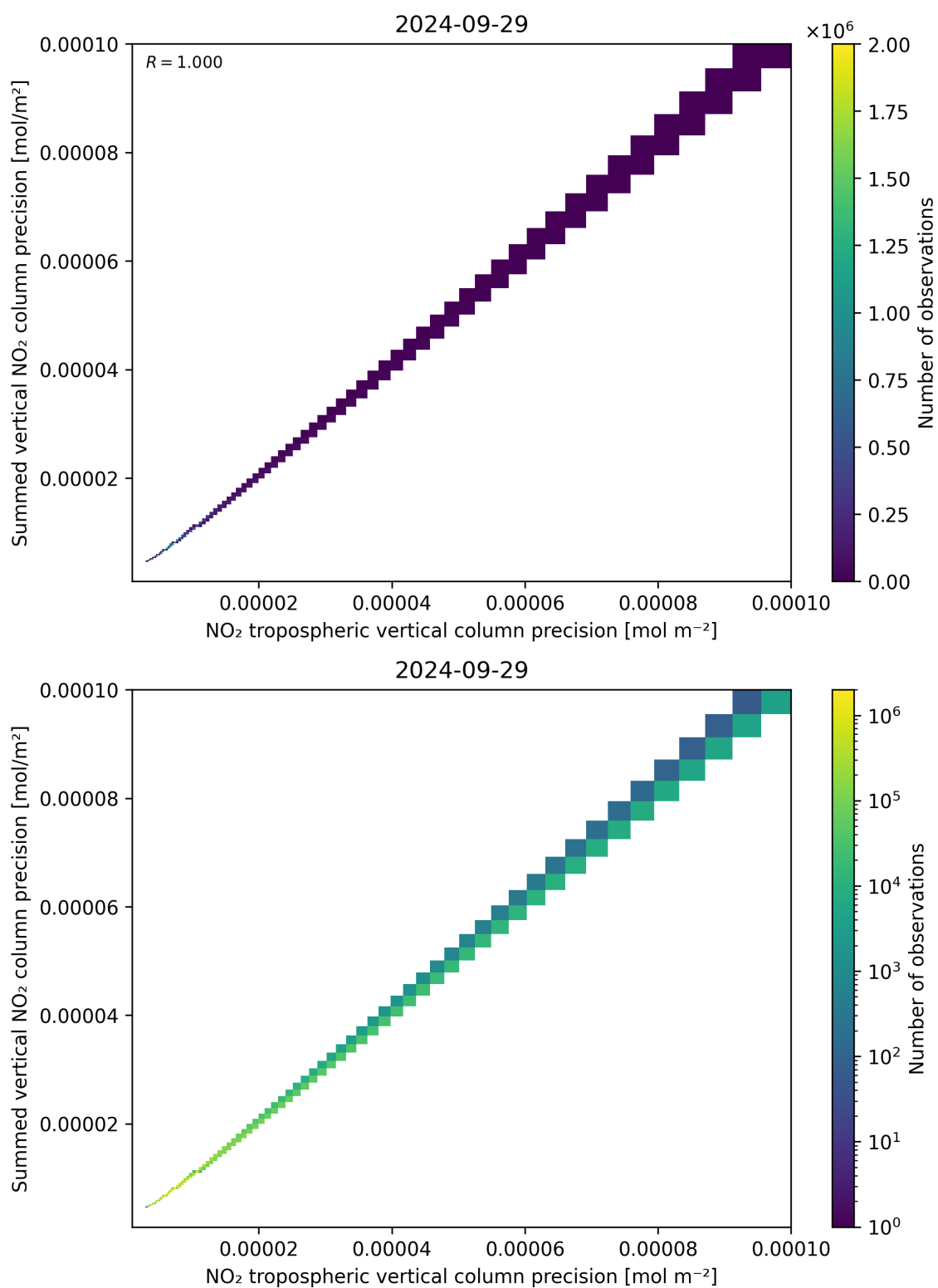
Figure 137: Scatter density plot of “NO 2 tropospheric vertical column precision” against “Summed vertical NO 2 column precision” for 2024-09-28 to 2024-09-30.
