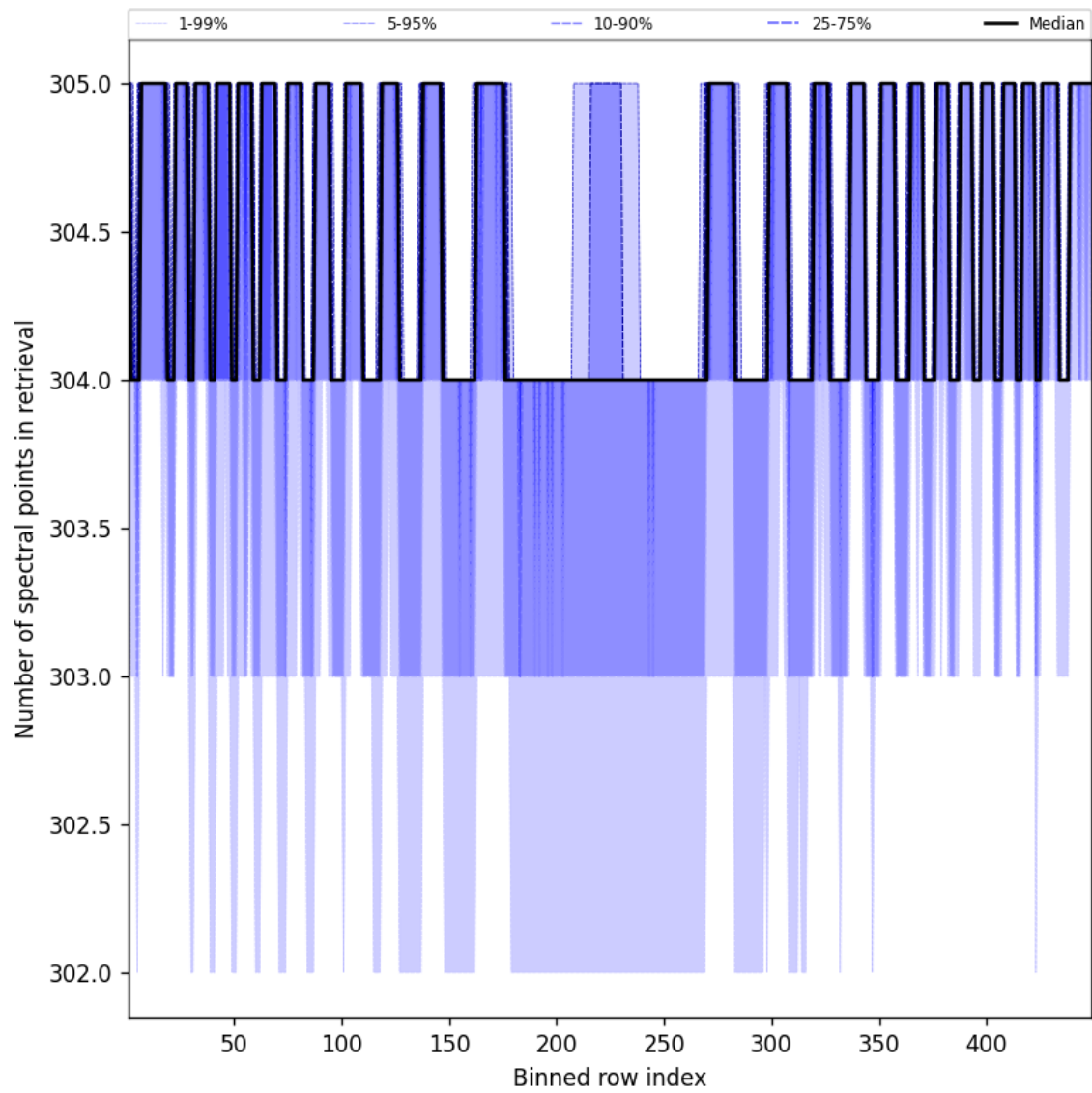
Figure 50: Along track statistics of “Number of spectral points in retrieval” for 2024-09-28 to 2024-09-30
