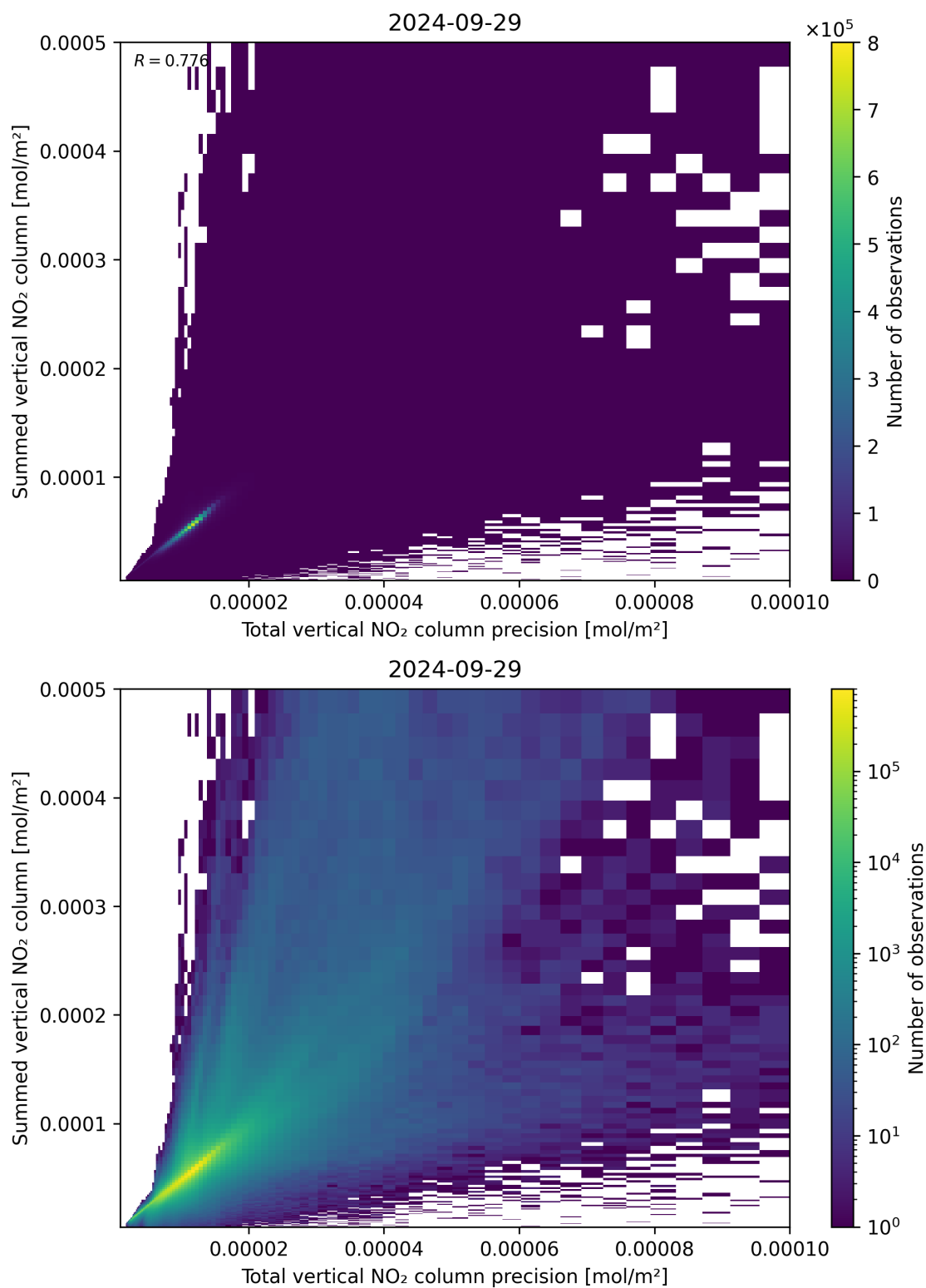
Figure 117: Scatter density plot of “Total vertical NO 2 column precision” against “Summed vertical NO 2 column” for 2024-09-28 to 2024-09-30.
