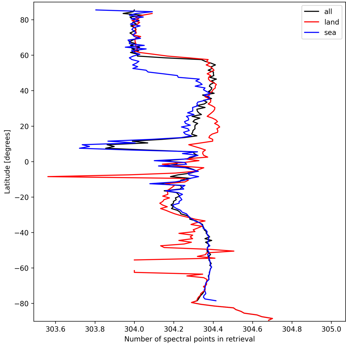
Figure 16: Zonal average of “Number of spectral points in retrieval” for 2024-09-28 to 2024-09-30.
