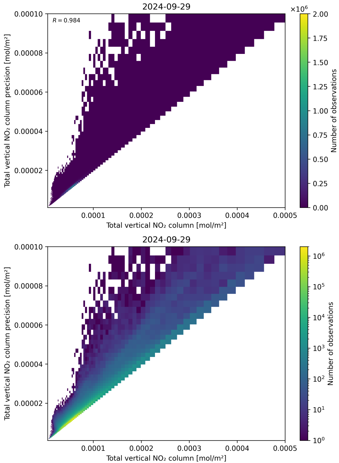
Figure 114: Scatter density plot of “Total vertical NO 2 column” against “Total vertical NO 2 column precision” for 2024-09-28 to 2024-09-30.
