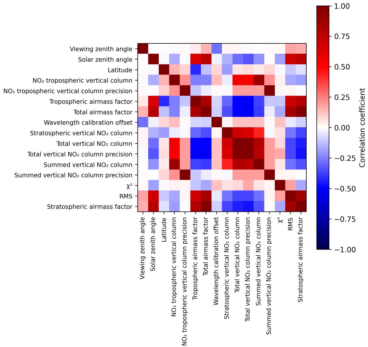
Figure 2: Map of correlation matrix for 2024-09-28 to 2024-09-30.
