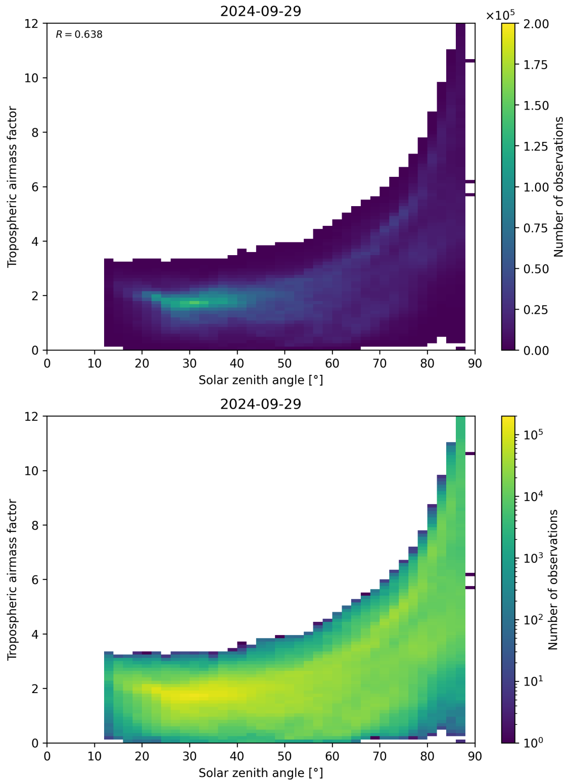
Figure 147: Scatter density plot of “Solar zenith angle” against “Tropospheric airmass factor” for 2024-09-28 to 2024-09-30.
