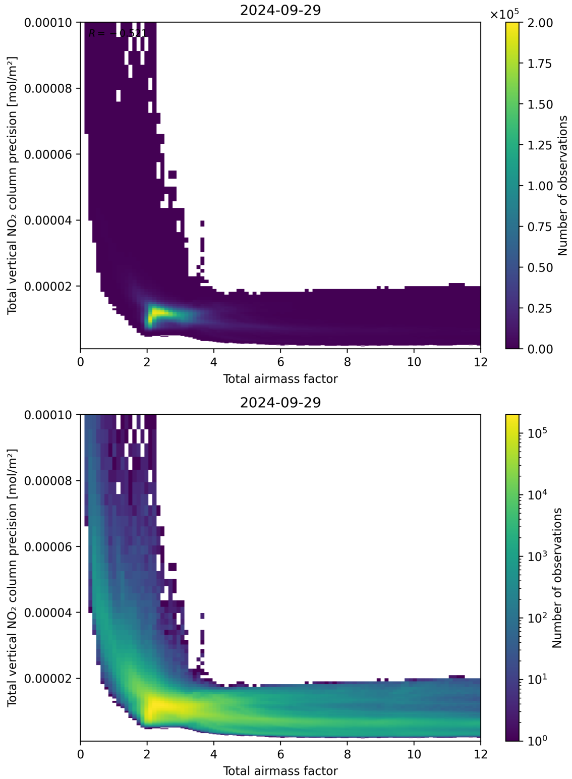
Figure 68: Scatter density plot of “Total airmass factor” against “Total vertical NO 2 column precision” for 2024-09-28 to 2024-09-30.
