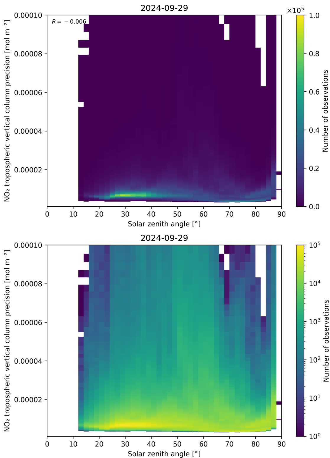
Figure 156: Scatter density plot of “Solar zenith angle” against “NO 2 tropospheric vertical column precision” for 2024-09-28 to 2024-09-30.
