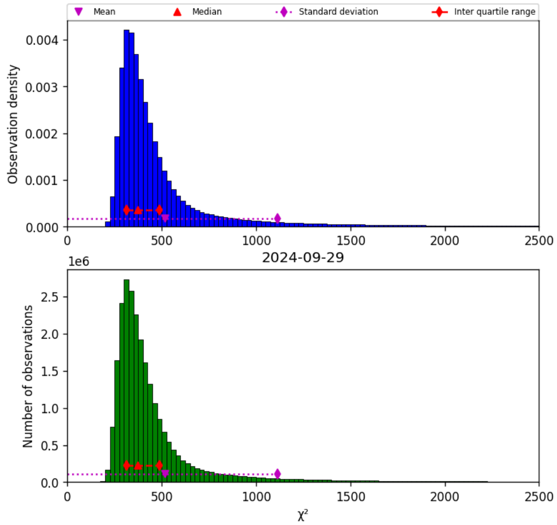
Figure 42: Histogram of “ \chi^2 ” for 2024-09-28 to 2024-09-30
