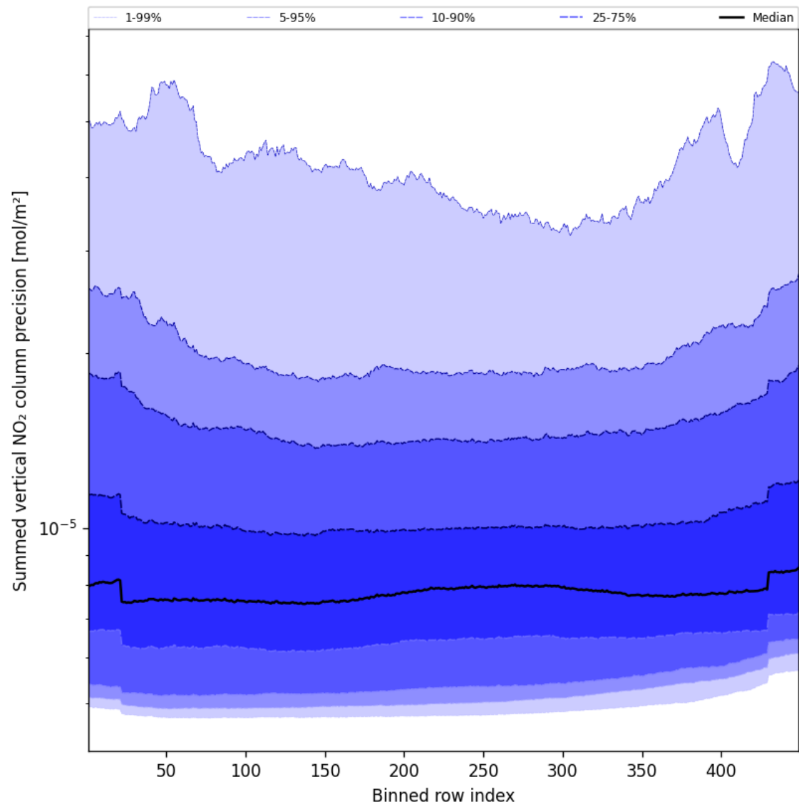
Figure 58: Along track statistics of “Summed vertical NO 2 column precision” for 2024-09-28 to 2024-09-30
