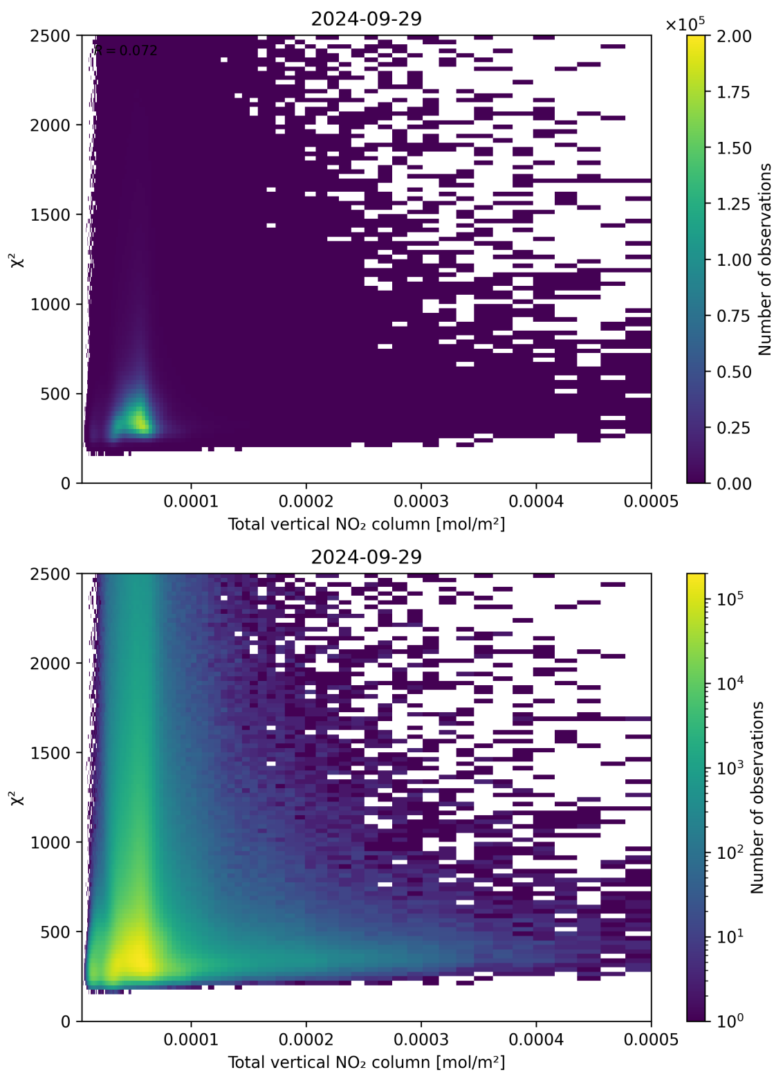
Figure 111: Scatter density plot of “Total vertical NO 2 column” against “ \chi^2 ” for 2024-09-28 to 2024-09-30.
