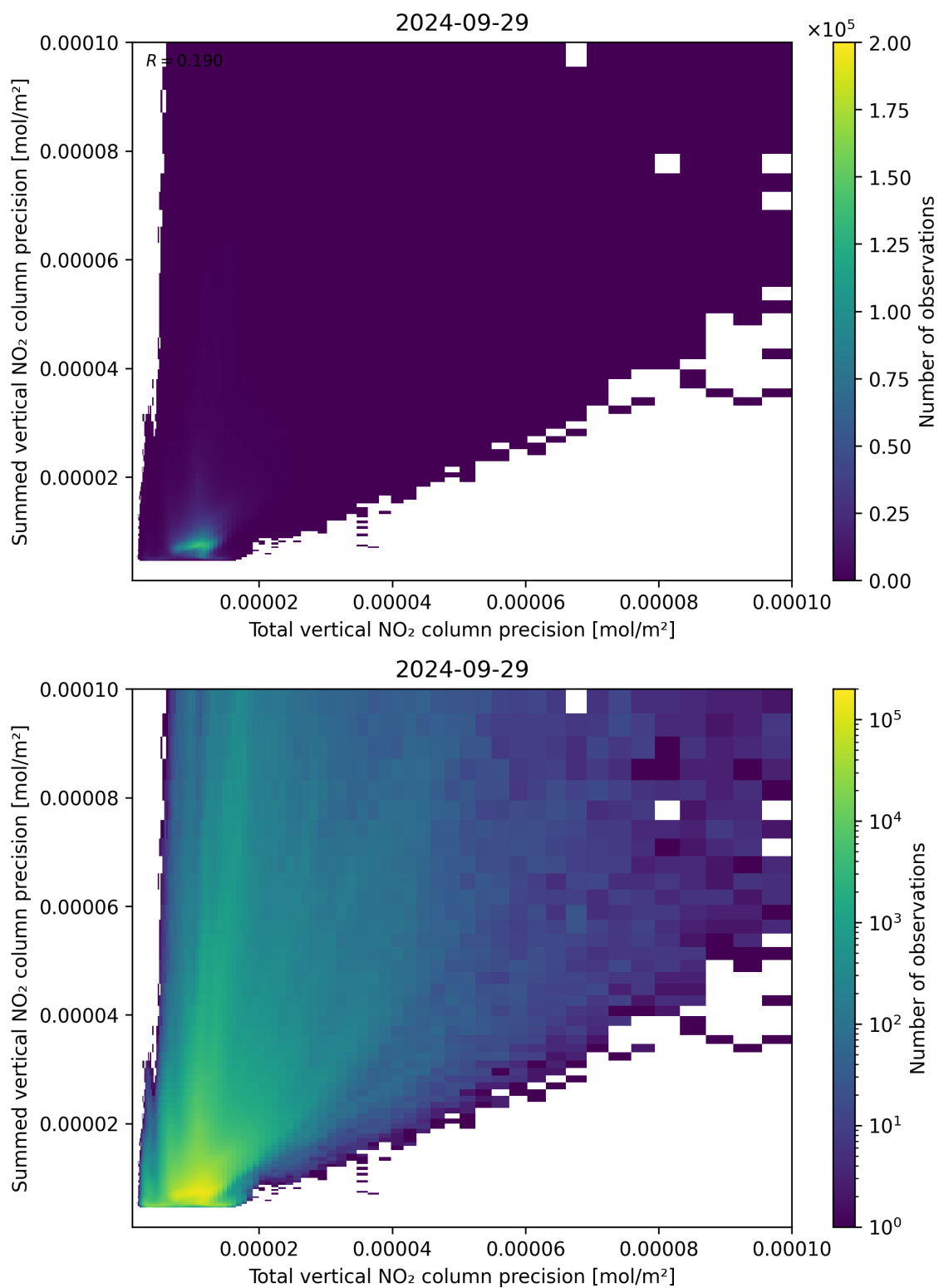
Figure 118: Scatter density plot of “Total vertical NO 2 column precision” against “Summed vertical NO 2 column precision” for 2024-09-28 to 2024-09-30.
