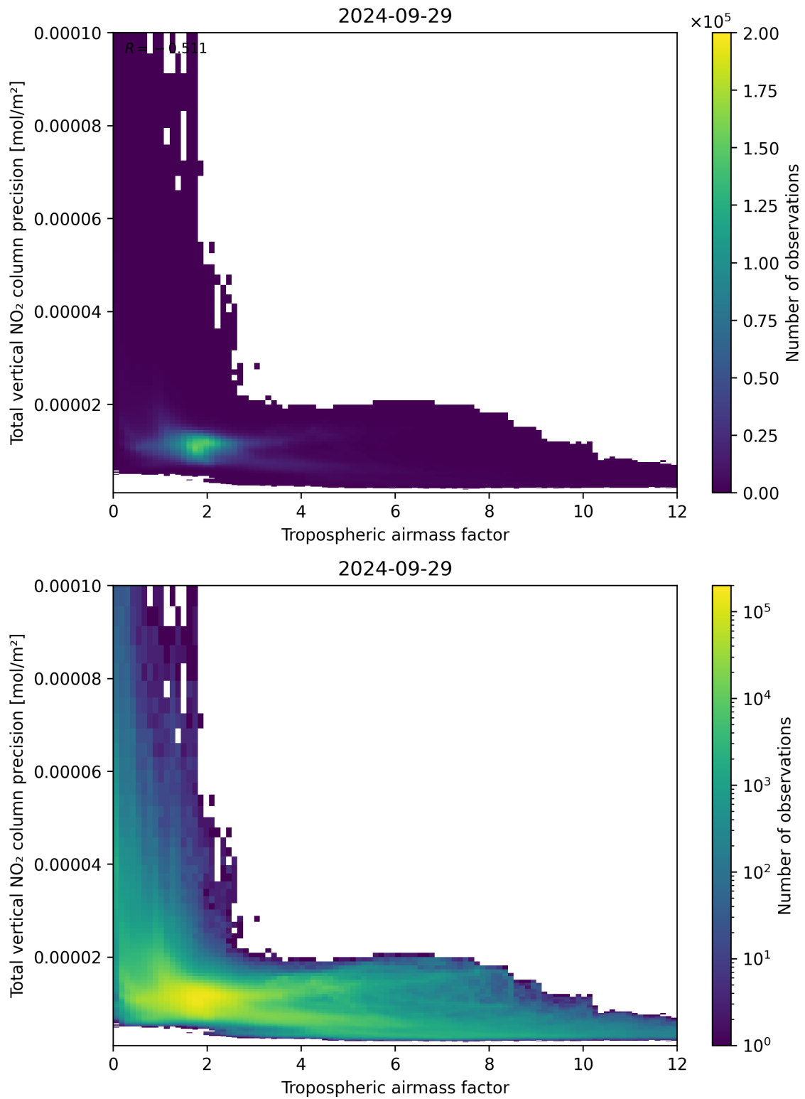
Figure 78: Scatter density plot of “Tropospheric airmass factor” against “Total vertical NO 2 column precision” for 2024-09-28 to 2024-09-30.
