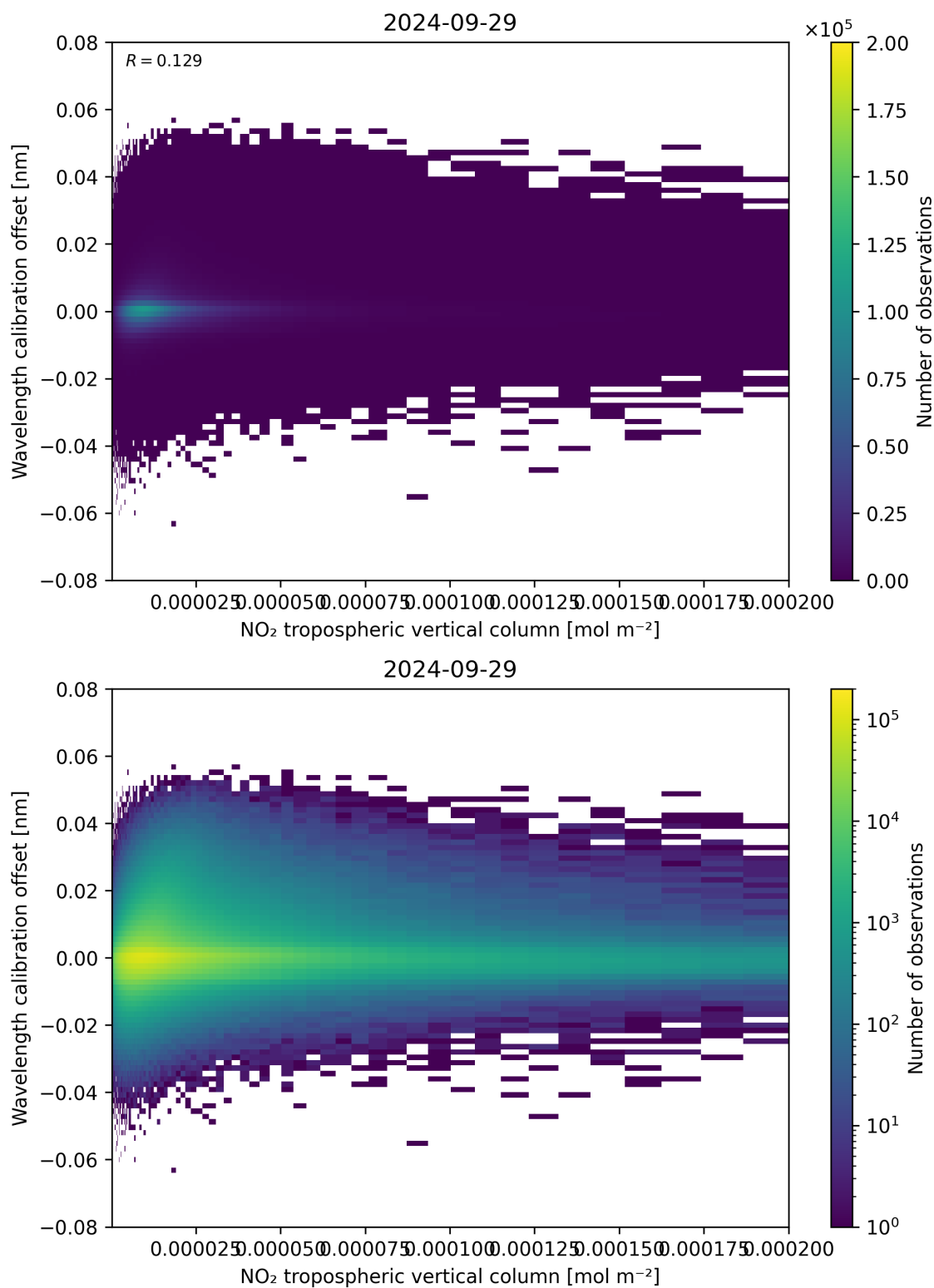
Figure 143: Scatter density plot of “NO 2 tropospheric vertical column” against “Wavelength calibration offset” for 2024-09-28 to 2024-09-30.
