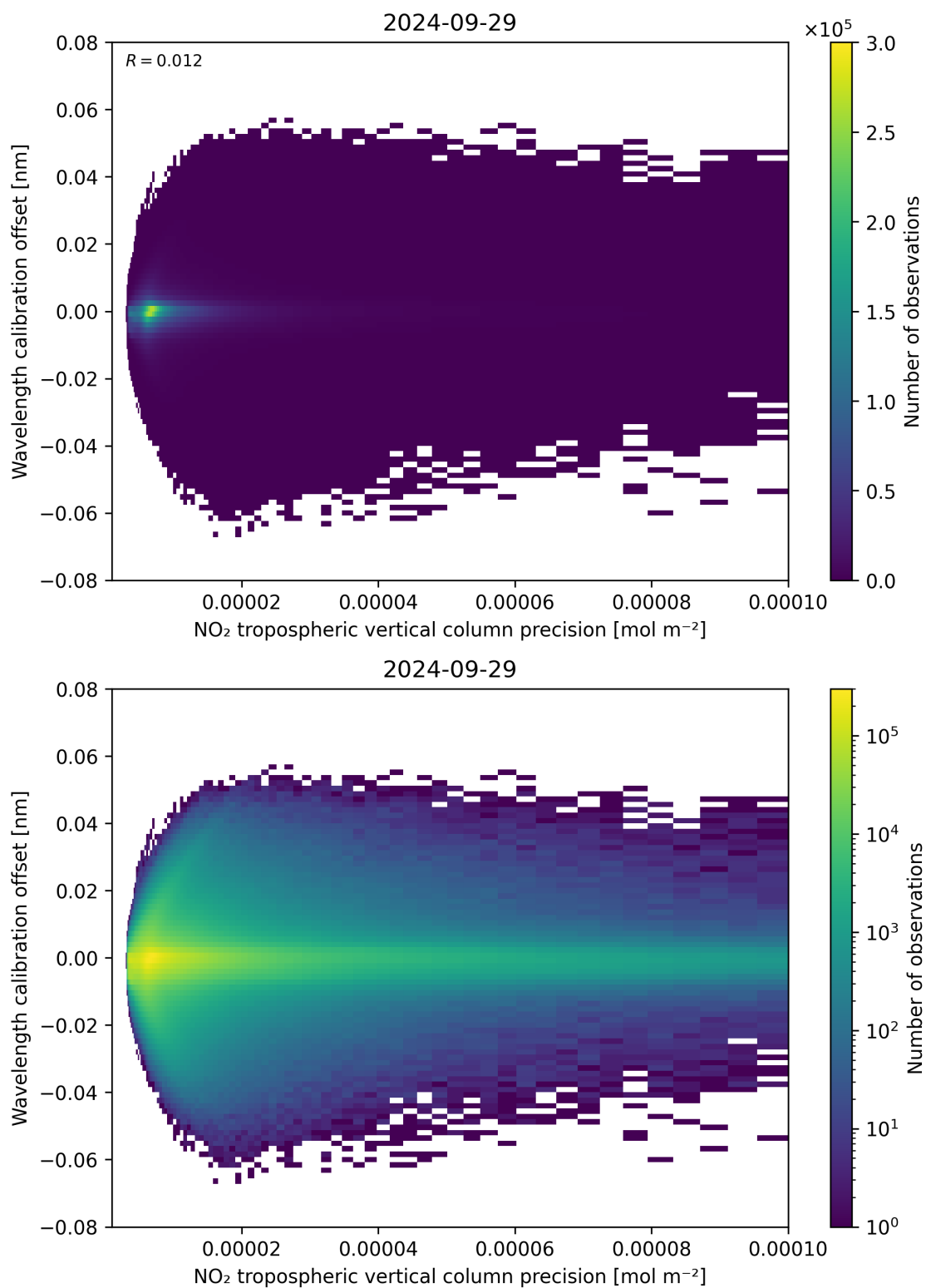
Figure 141: Scatter density plot of “NO 2 tropospheric vertical column precision” against “Wavelength calibration offset” for 2024-09-28 to 2024-09-30.
