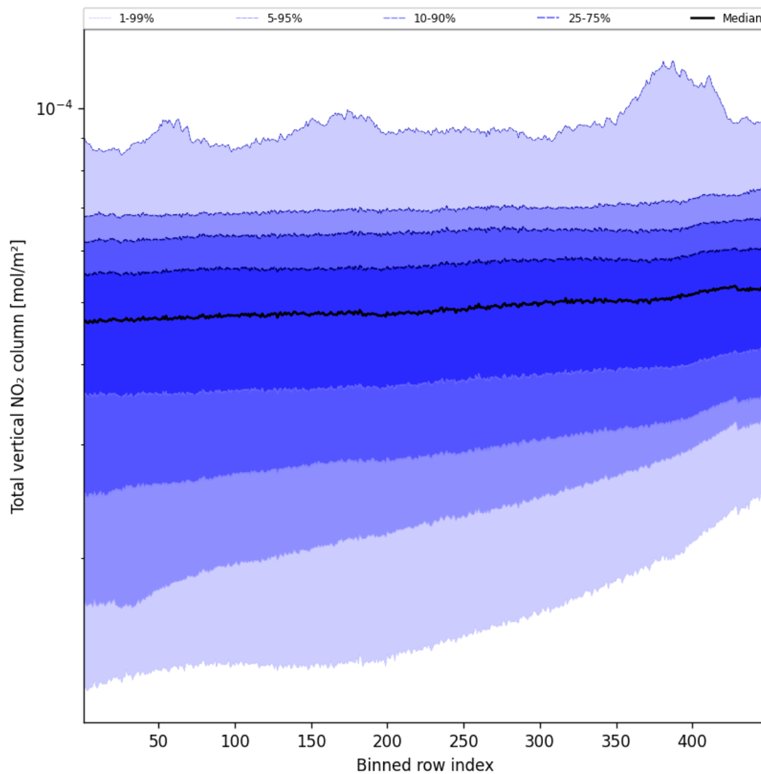
Figure 55: Along track statistics of “Total vertical NO 2 column” for 2024-09-29 to 2024-10-01
