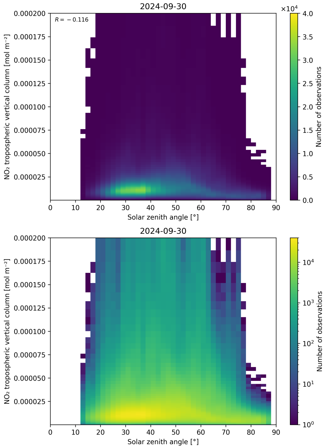
Figure 155: Scatter density plot of “Solar zenith angle” against “NO 2 tropospheric vertical column” for 2024-09-29 to 2024-10-01.
