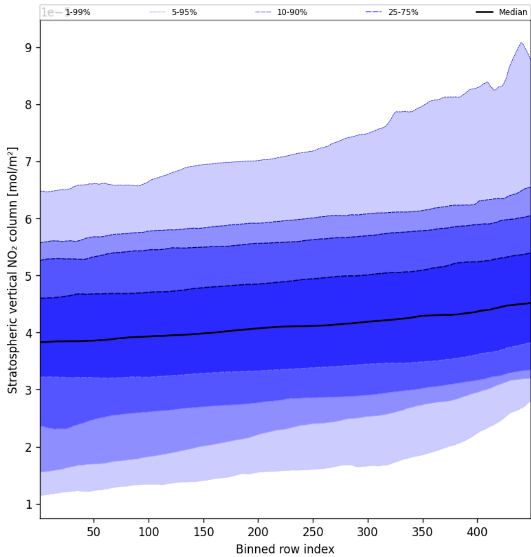
Figure 53: Along track statistics of “Stratospheric vertical NO 2 column” for 2024-09-29 to 2024-10-01
