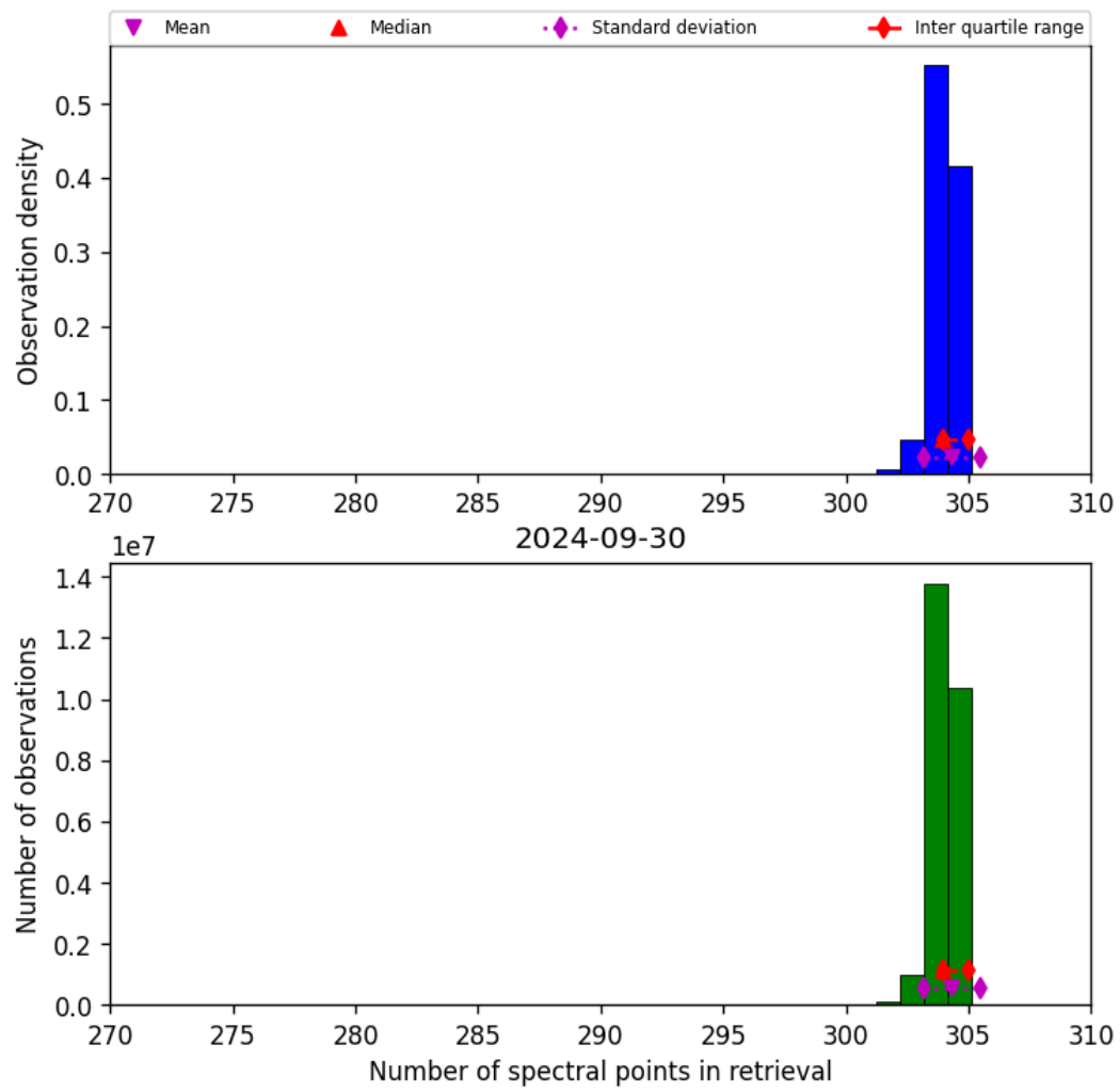
Figure 33: Histogram of “Number of spectral points in retrieval” for 2024-09-29 to 2024-10-01
