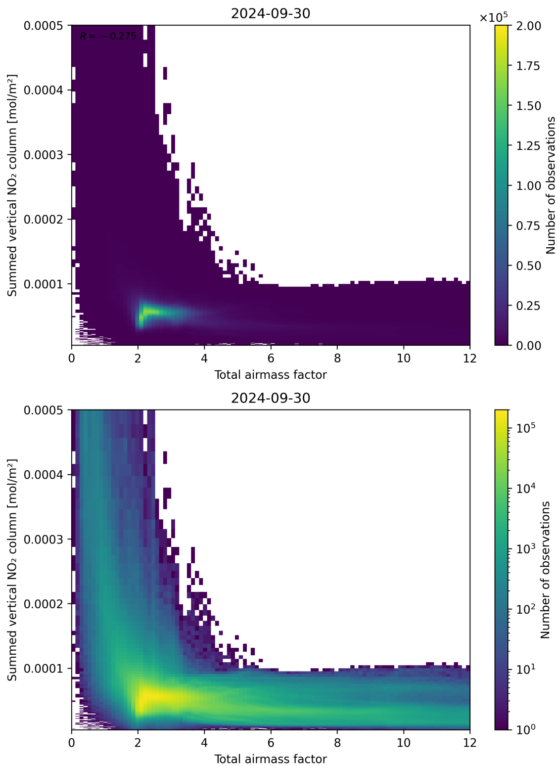
Figure 65: Scatter density plot of “Total airmass factor” against “Summed vertical NO 2 column” for 2024-09-29 to 2024-10-01.
