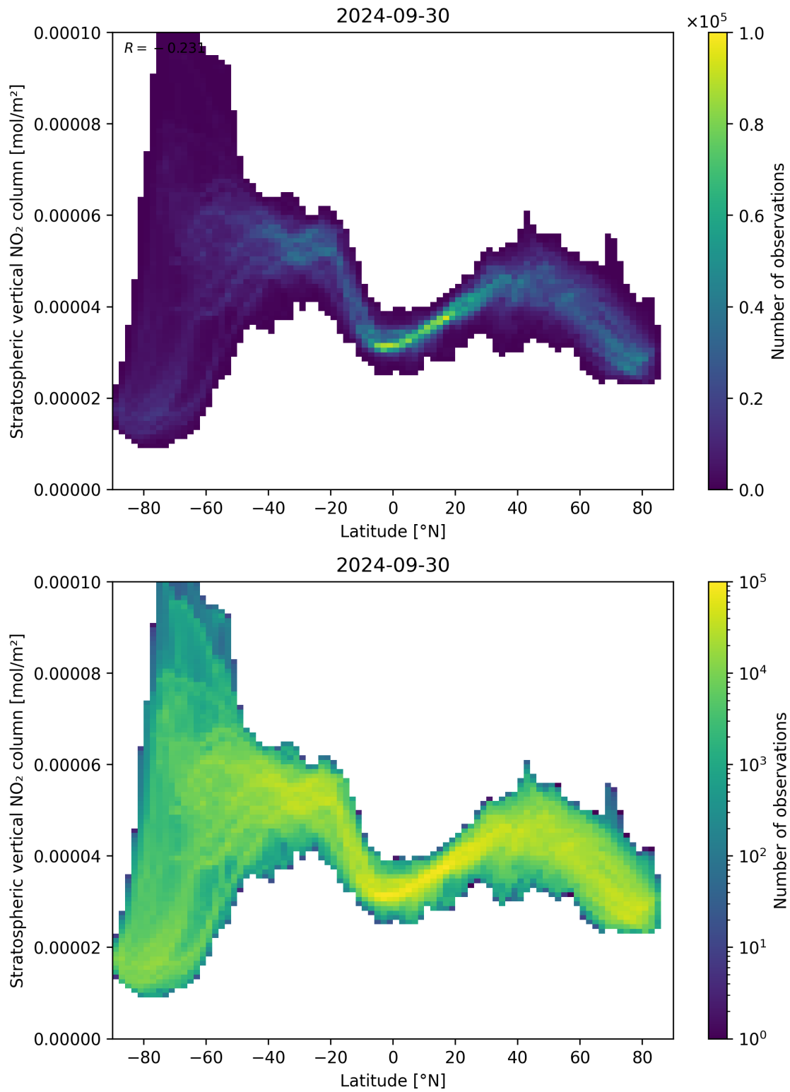
Figure 87: Scatter density plot of “Latitude” against “Stratospheric vertical NO 2 column” for 2024-09-29 to 2024-10-01.
