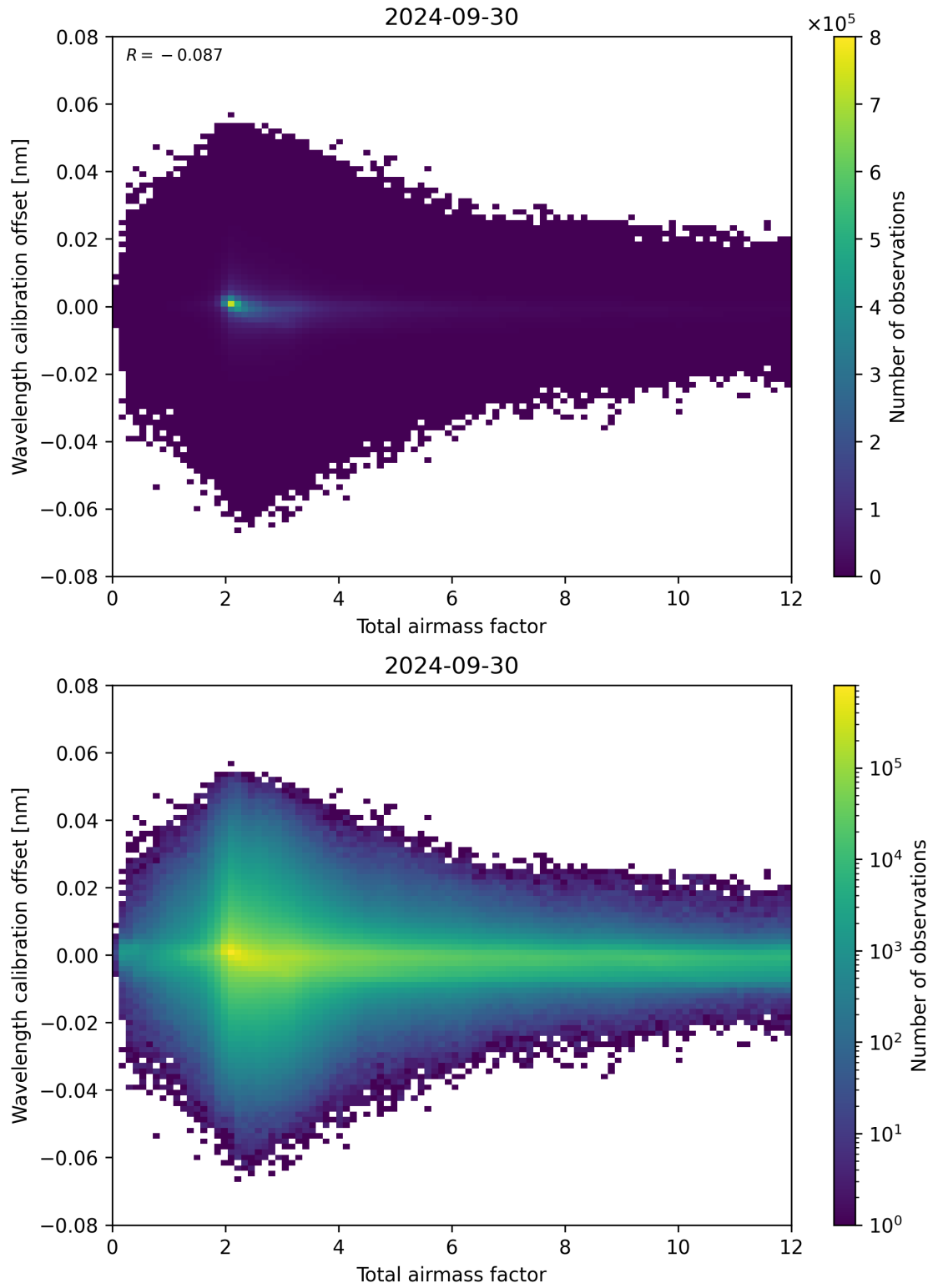
Figure 70: Scatter density plot of “Total airmass factor” against “Wavelength calibration offset” for 2024-09-29 to 2024-10-01.
