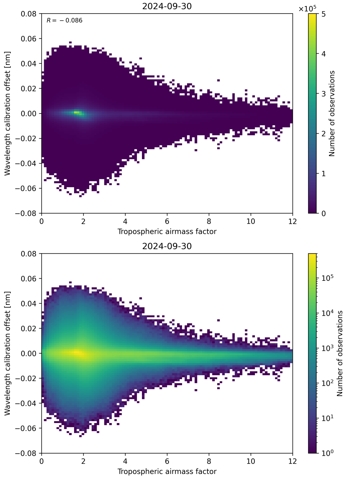
Figure 80: Scatter density plot of “Tropospheric airmass factor” against “Wavelength calibration offset” for 2024-09-29 to 2024-10-01.
