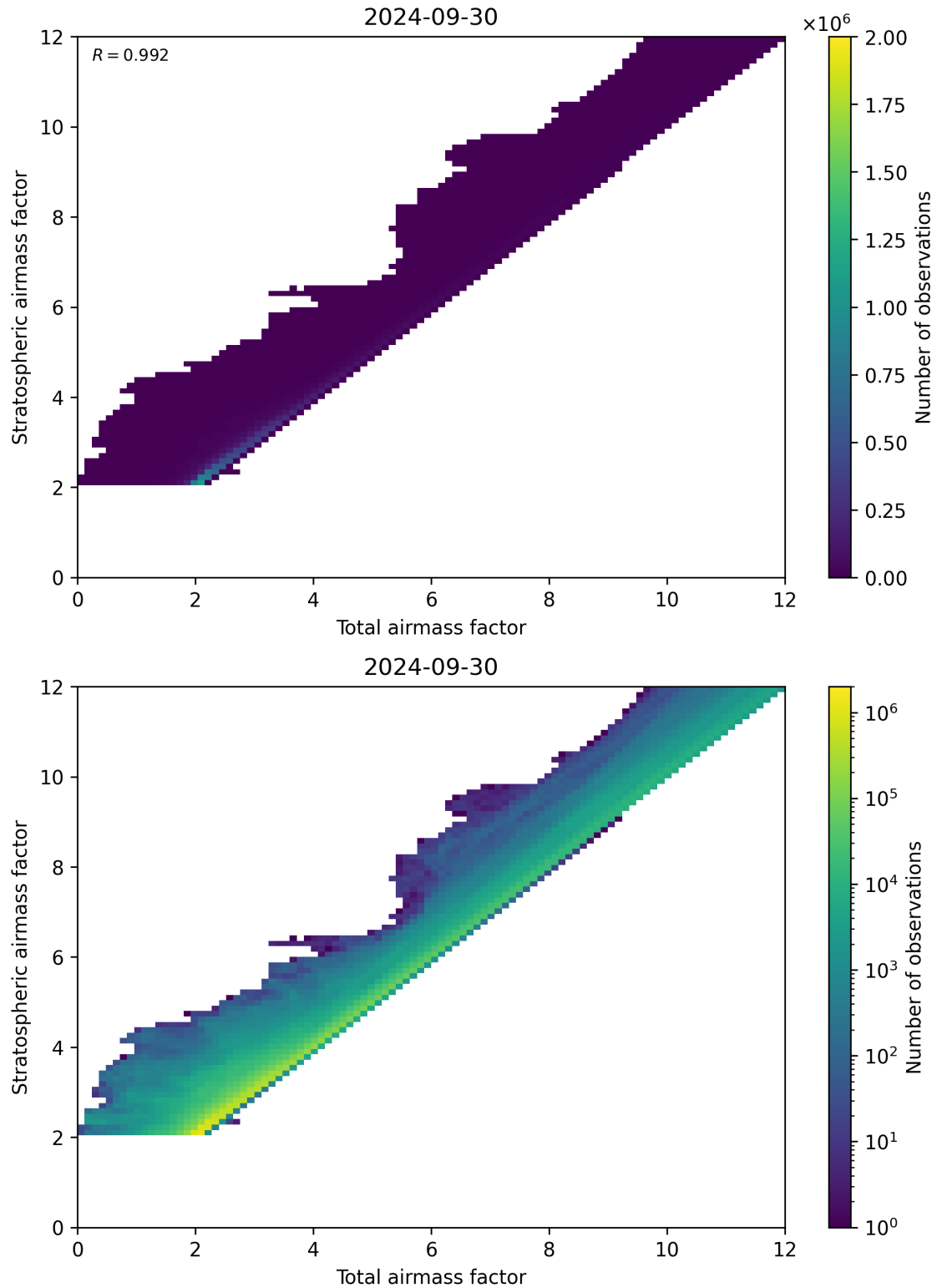
Figure 62: Scatter density plot of “Total airmass factor” against “Stratospheric airmass factor” for 2024-09-29 to 2024-10-01.
