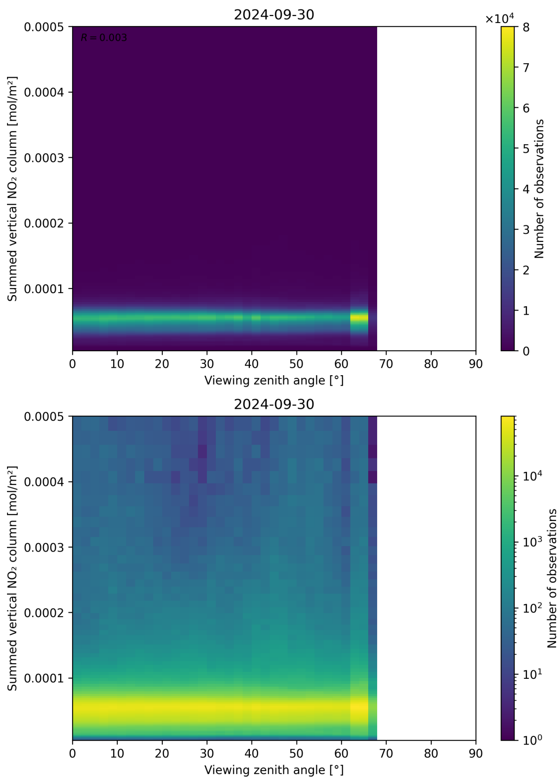
Figure 165: Scatter density plot of “Viewing zenith angle” against “Summed vertical NO 2 column” for 2024-09-29 to 2024-10-01.
