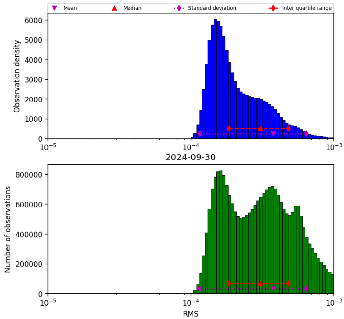
Figure 43: Histogram of “RMS” for 2024-09-29 to 2024-10-01
