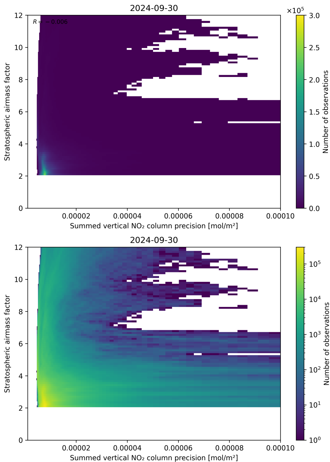
Figure 106: Scatter density plot of “Summed vertical NO 2 column precision” against “Stratospheric airmass factor” for 2024-09-29 to 2024-10-01.
