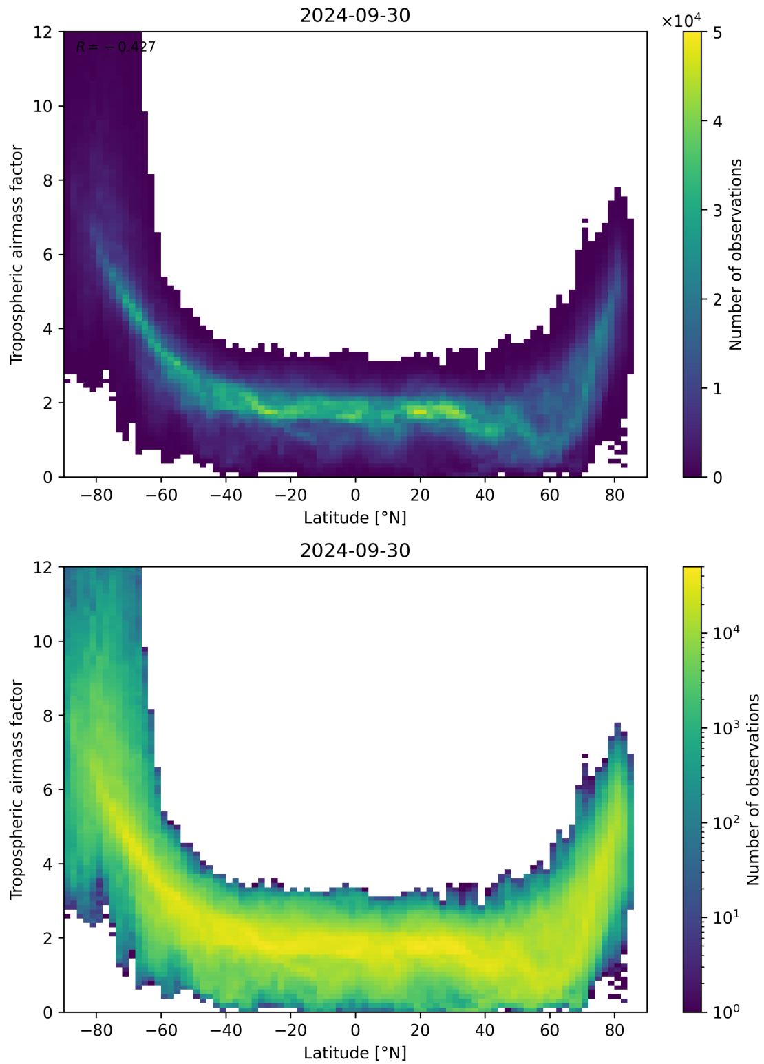
Figure 85: Scatter density plot of “Latitude” against “Tropospheric air mass factor” for 2024-09-29 to 2024-10-01.
