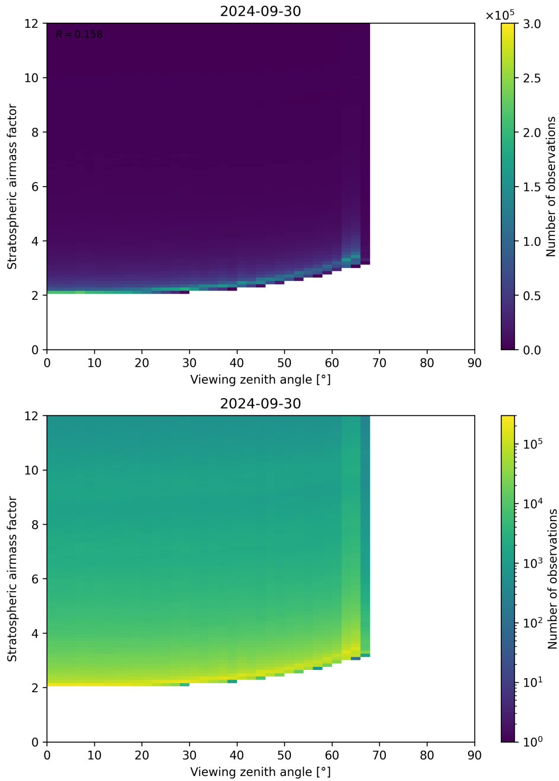
Figure 159: Scatter density plot of “Viewing zenith angle” against “Stratospheric airmass factor” for 2024-09-29 to 2024-10-01.
