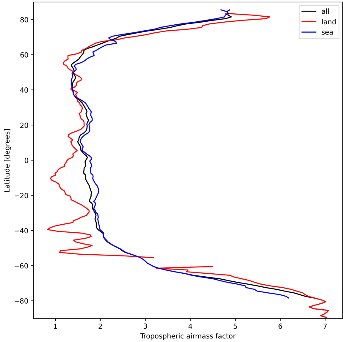
Figure 14: Zonal average of “Tropospheric airmass factor” for 2024-09-29 to 2024-10-01.
