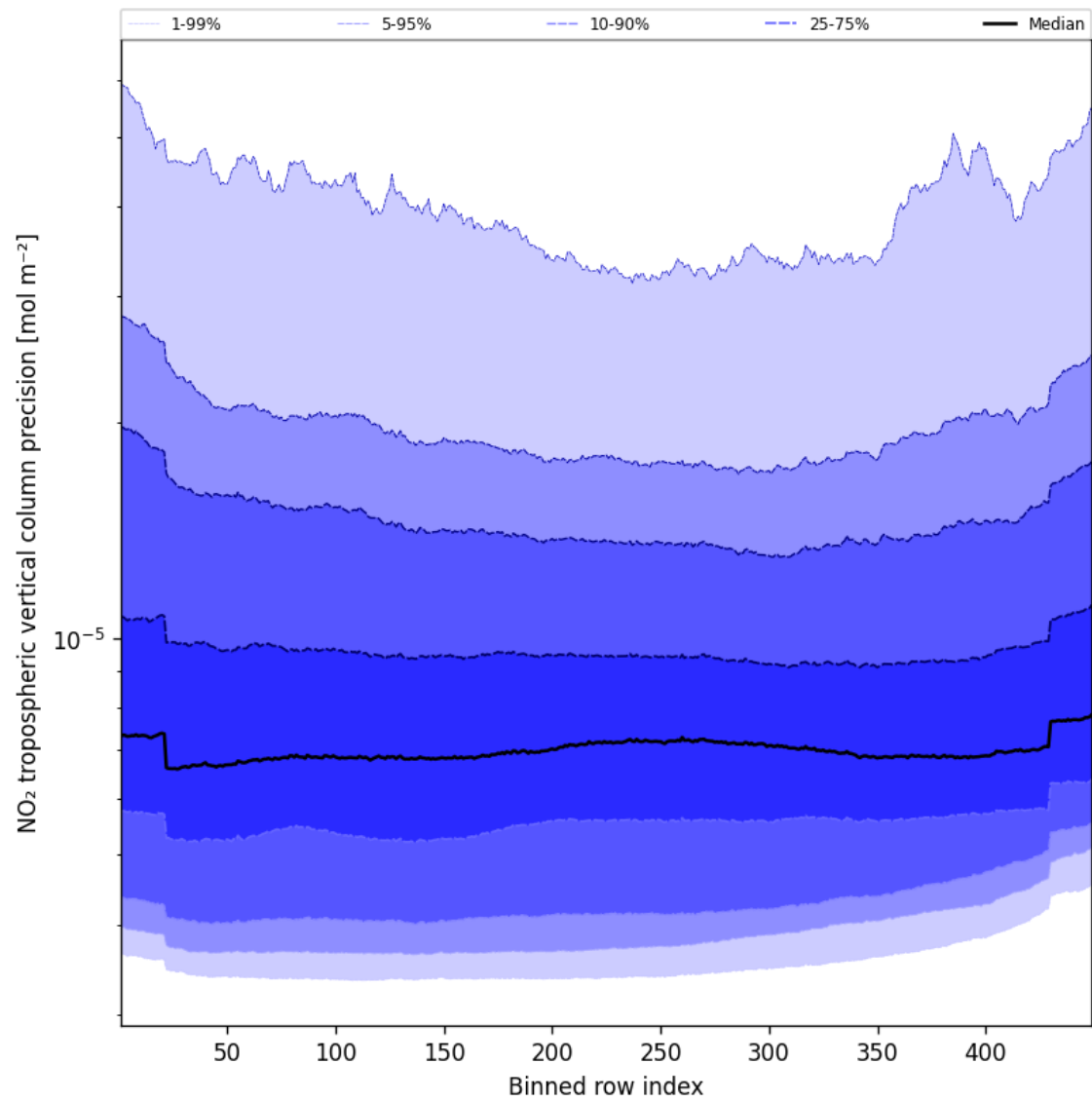
Figure 47: Along track statistics of “NO 2 tropospheric vertical column precision” for 2024-09-29 to 2024-10-01
