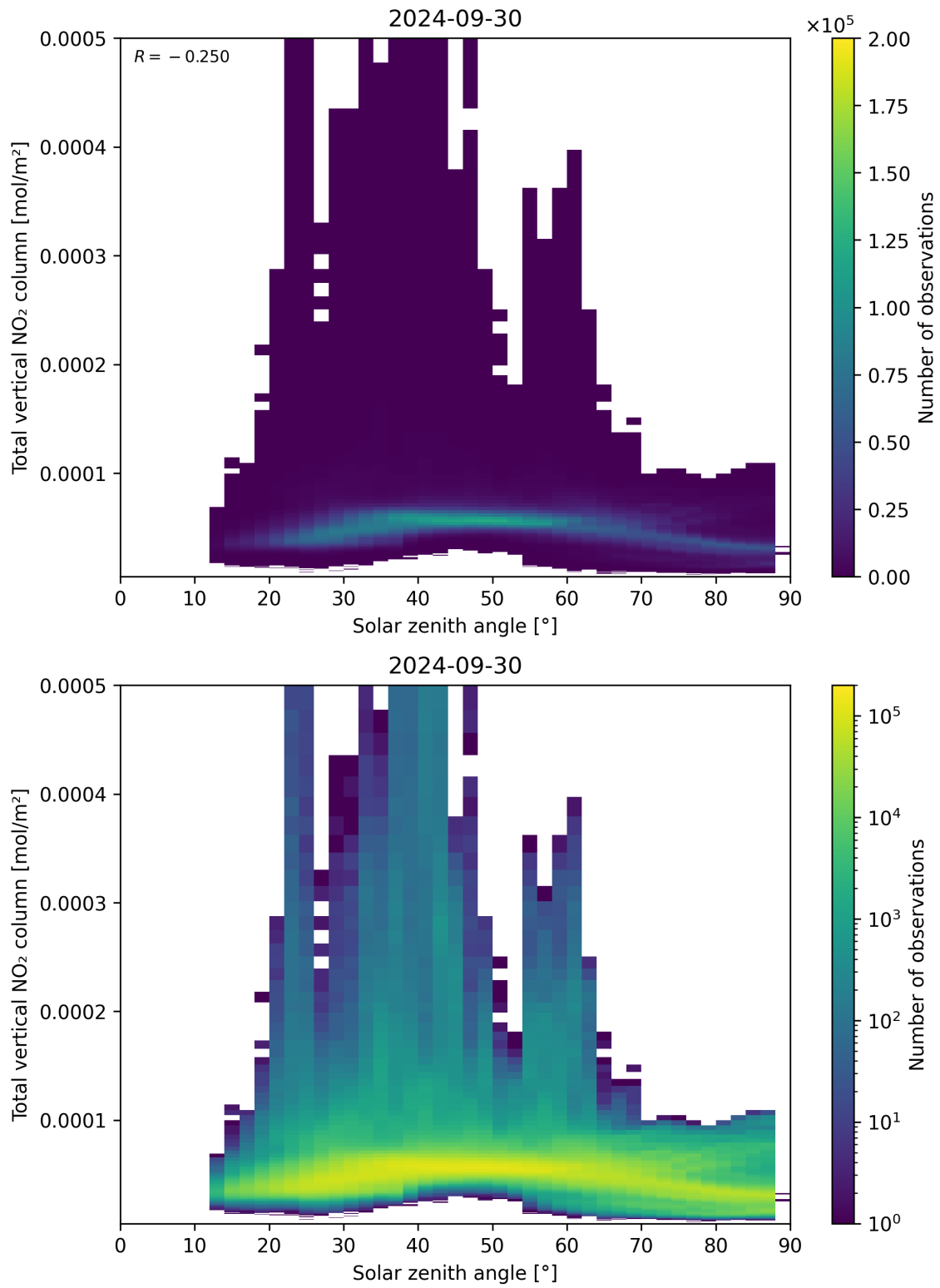
Figure 153: Scatter density plot of “Solar zenith angle” against “Total vertical NO 2 column” for 2024-09-29 to 2024-10-01.
