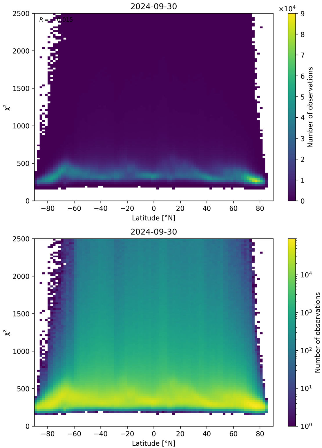
Figure 86: Scatter density plot of “Latitude” against “ \chi^2 ” for 2024-09-29 to 2024-10-01.
