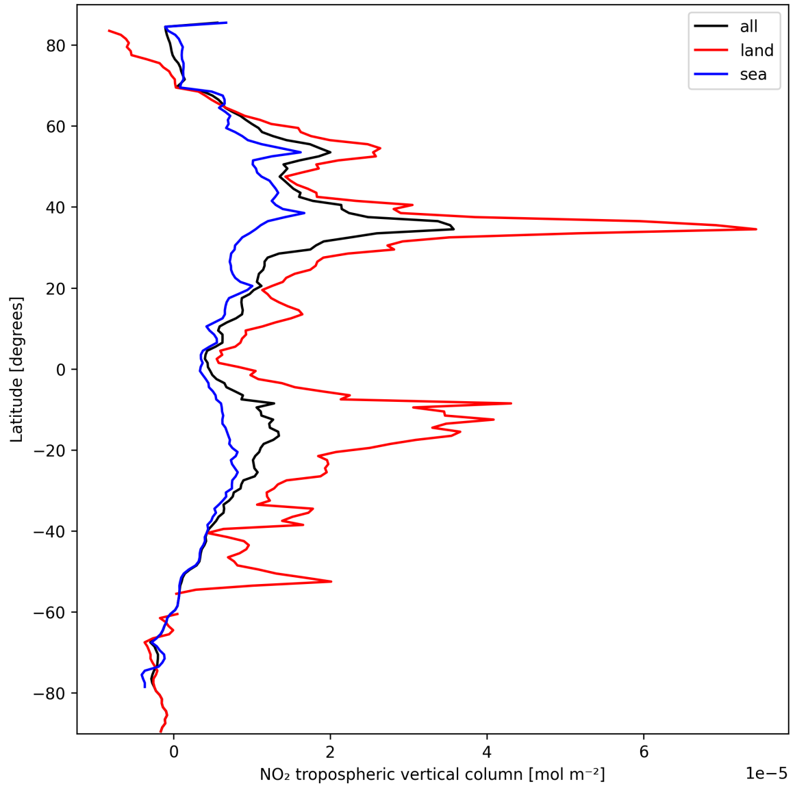
Figure 12: Zonal average of “NO 2 tropospheric vertical column” for 2024-09-29 to 2024-10-01.
