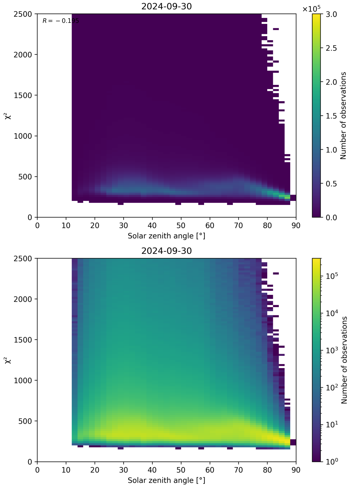
Figure 148: Scatter density plot of “Solar zenith angle” against “ \chi^2 ” for 2024-09-29 to 2024-10-01.
