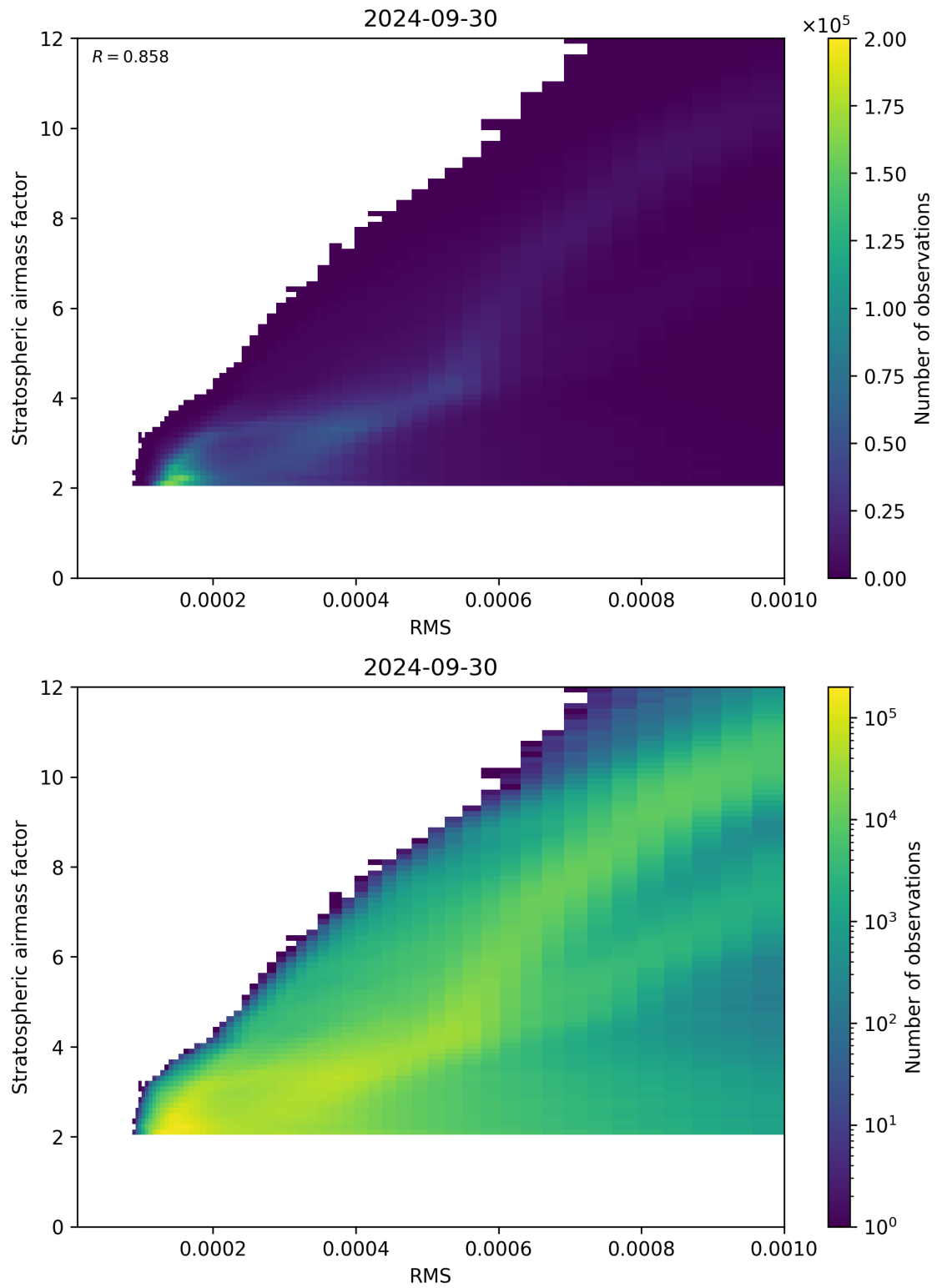
Figure 144: Scatter density plot of “RMS” against “Stratospheric airmass factor” for 2024-09-29 to 2024-10-01.
