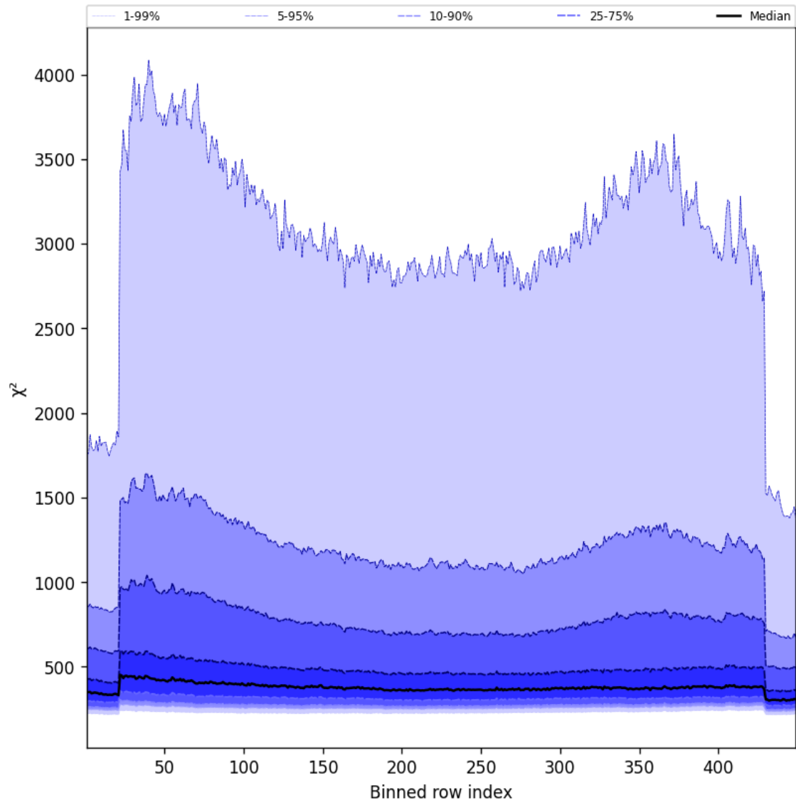
Figure 59: Along track statistics of “ \chi^2 ” for 2024-09-29 to 2024-10-01
