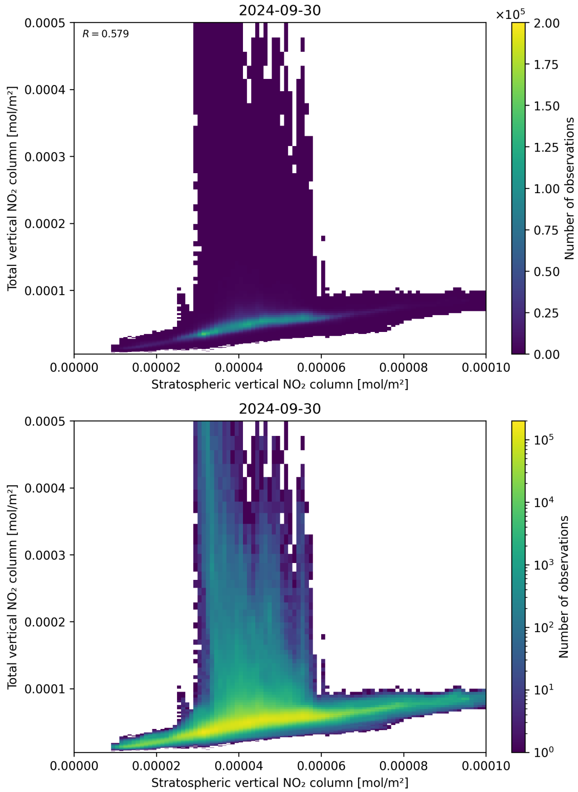
Figure 100: Scatter density plot of “Stratospheric vertical NO 2 column” against “Total vertical NO 2 column” for 2024-09-29 to 2024-10-01.
