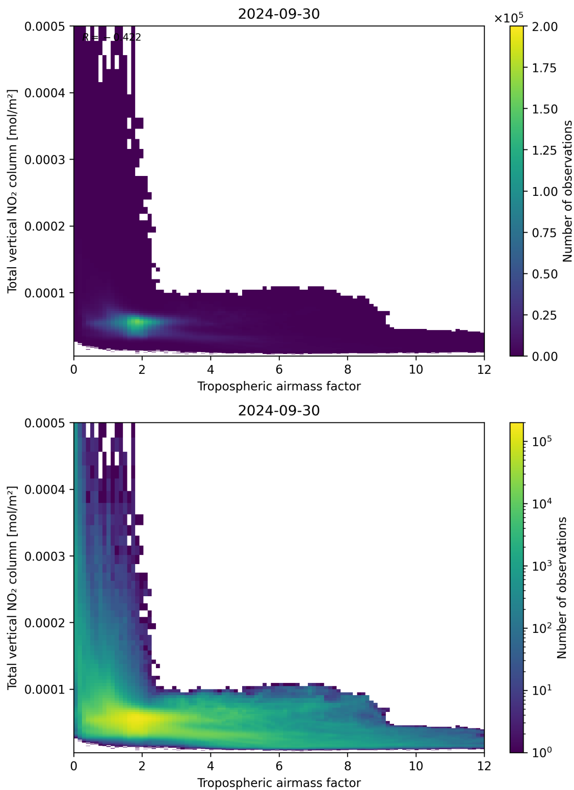
Figure 77: Scatter density plot of “Tropospheric airmass factor” against “Total vertical NO 2 column” for 2024-09-29 to 2024-10-01.
