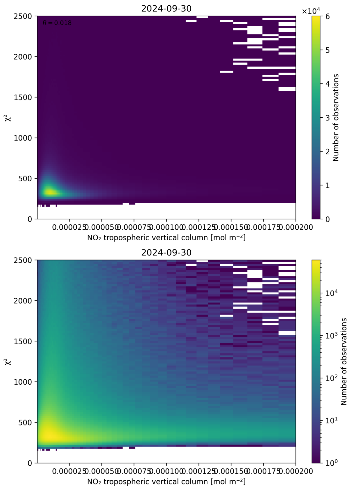
Figure 124: Scatter density plot of “NO 2 tropospheric vertical column” against “ \chi^2 ” for 2024-09-29 to 2024-10-01.
