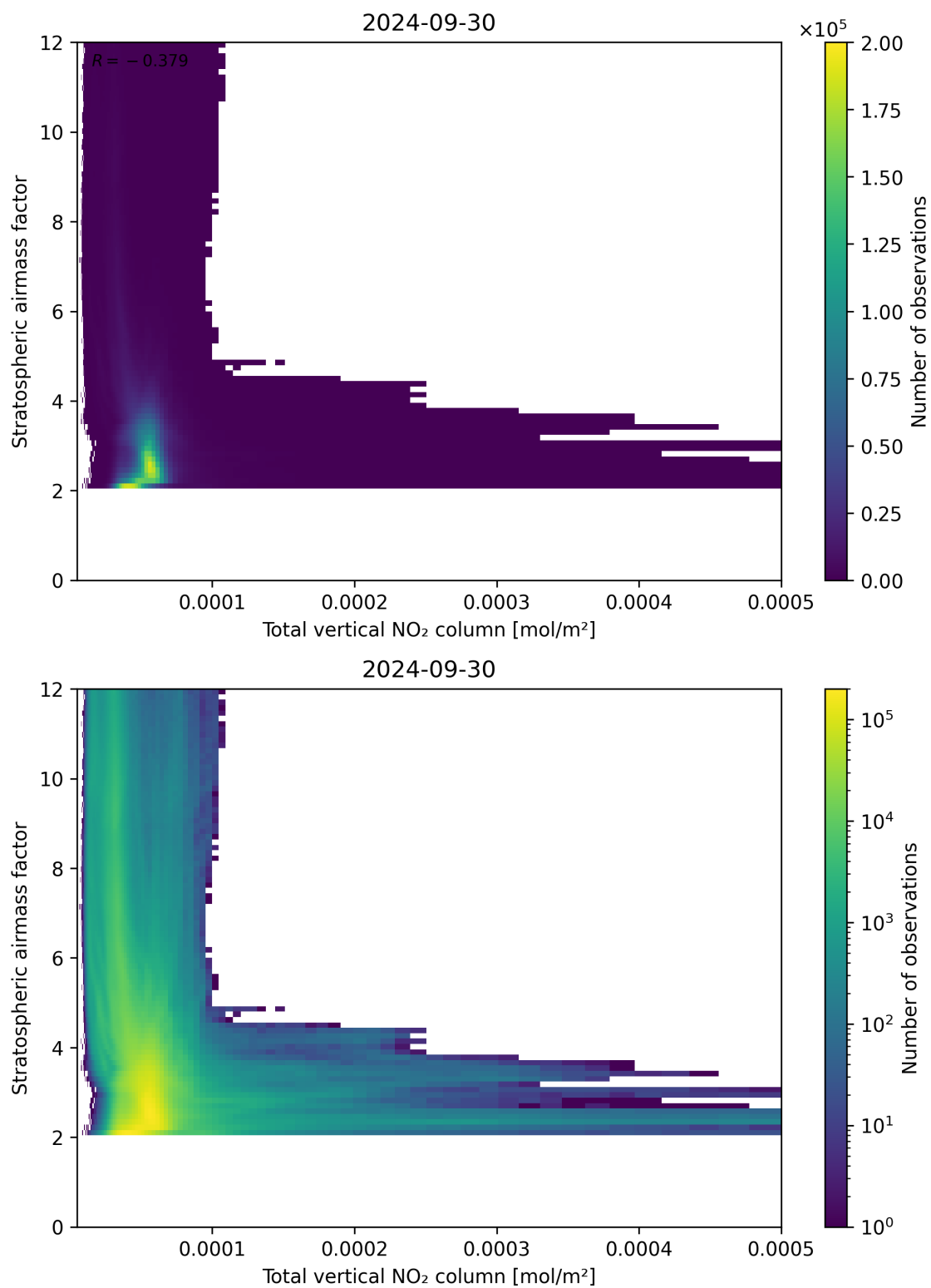
Figure 110: Scatter density plot of “Total vertical NO 2 column” against “Stratospheric airmass factor” for 2024-09-29 to 2024-10-01.
