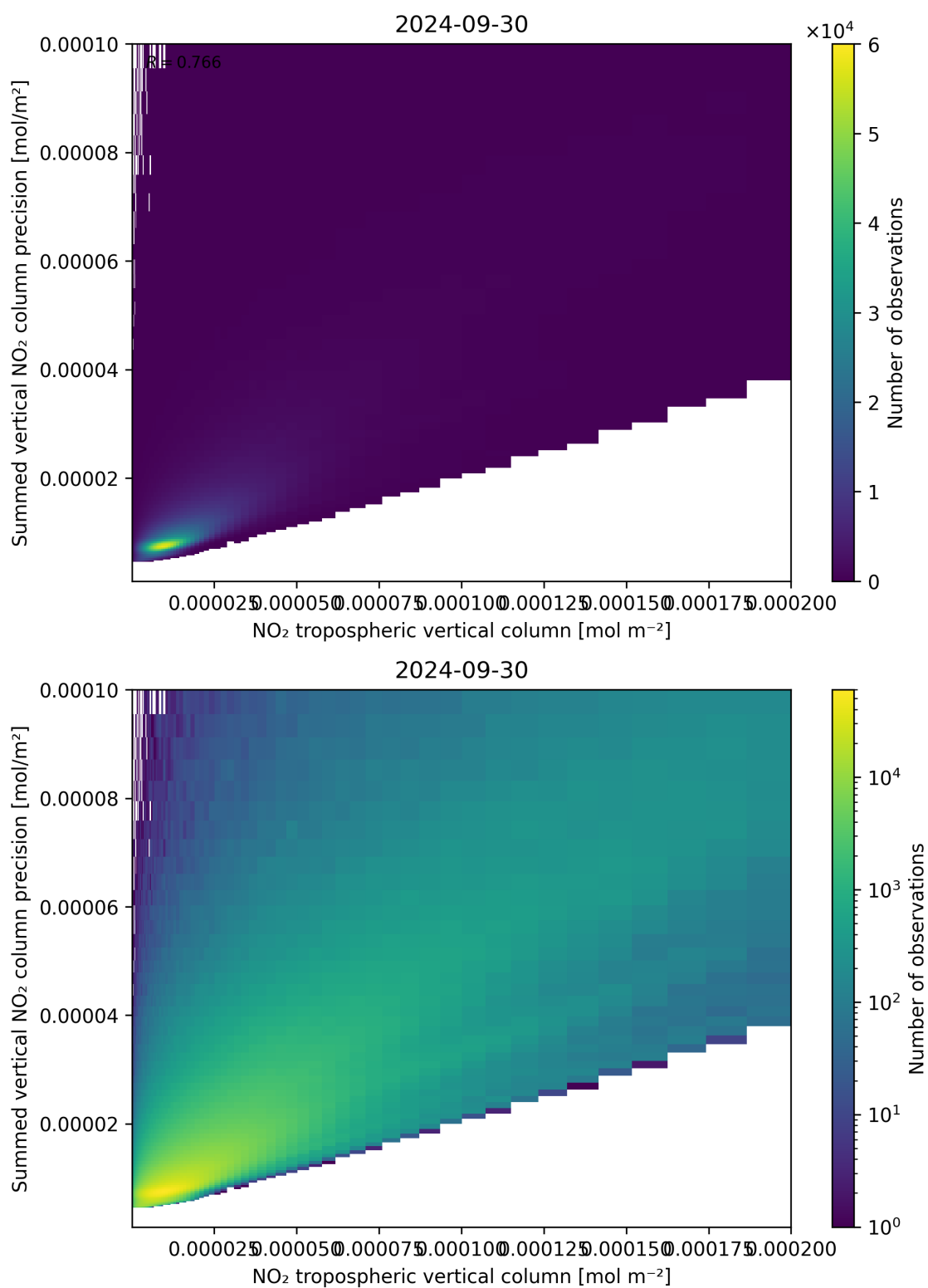
Figure 127: Scatter density plot of “NO 2 tropospheric vertical column” against “Summed vertical NO 2 column precision” for 2024-09-29 to 2024-10-01.
