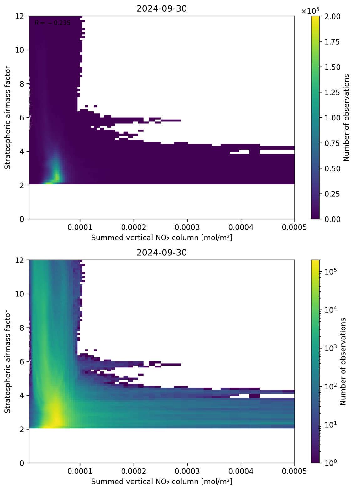
Figure 103: Scatter density plot of “Summed vertical NO 2 column” against “Stratospheric airmass factor” for 2024-09-29 to 2024-10-01.
