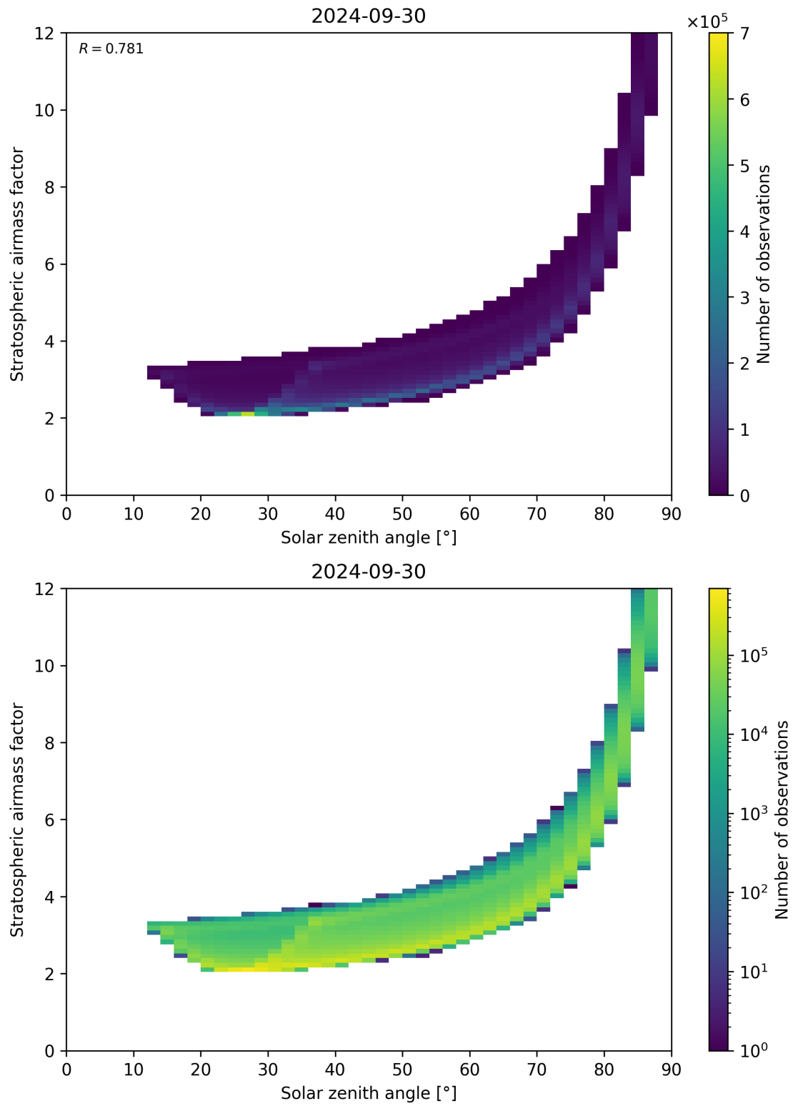
Figure 145: Scatter density plot of “Solar zenith angle” against “Stratospheric airmass factor” for 2024-09-29 to 2024-10-01.
