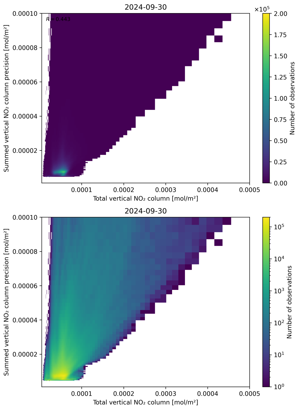
Figure 113: Scatter density plot of “Total vertical NO 2 column” against “Summed vertical NO 2 column precision” for 2024-09-29 to 2024-10-01.
