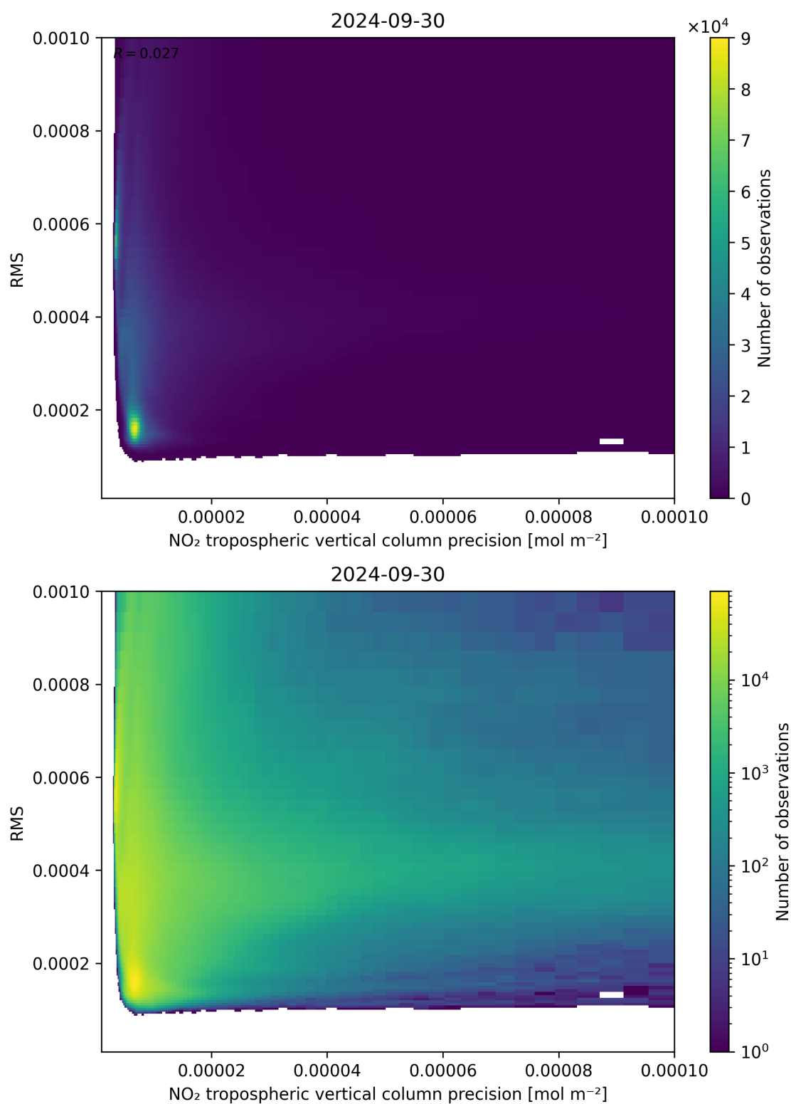
Figure 140: Scatter density plot of “NO 2 tropospheric vertical column precision” against “RMS” for 2024-09-29 to 2024-10-01.
