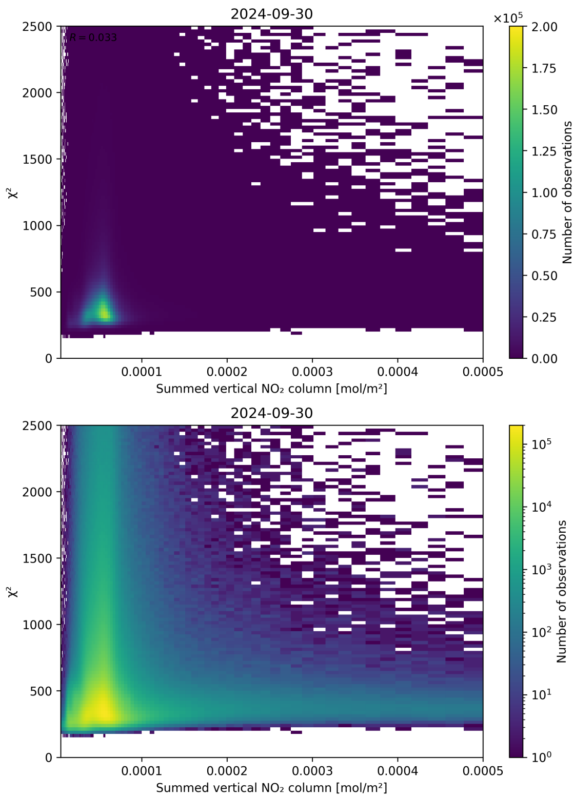
Figure 104: Scatter density plot of “Summed vertical NO 2 column” against “ \chi^2 ” for 2024-09-29 to 2024-10-01.
