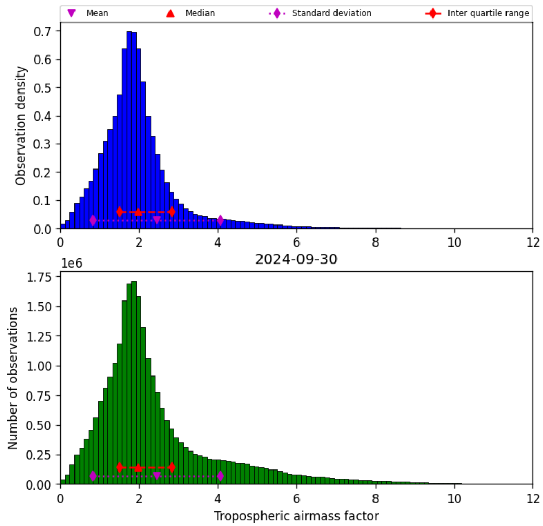
Figure 31: Histogram of “Tropospheric airmass factor” for 2024-09-29 to 2024-10-01
