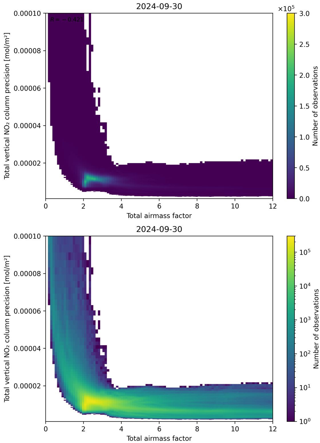
Figure 68: Scatter density plot of “Total airmass factor” against “Total vertical NO 2 column precision” for 2024-09-29 to 2024-10-01.
