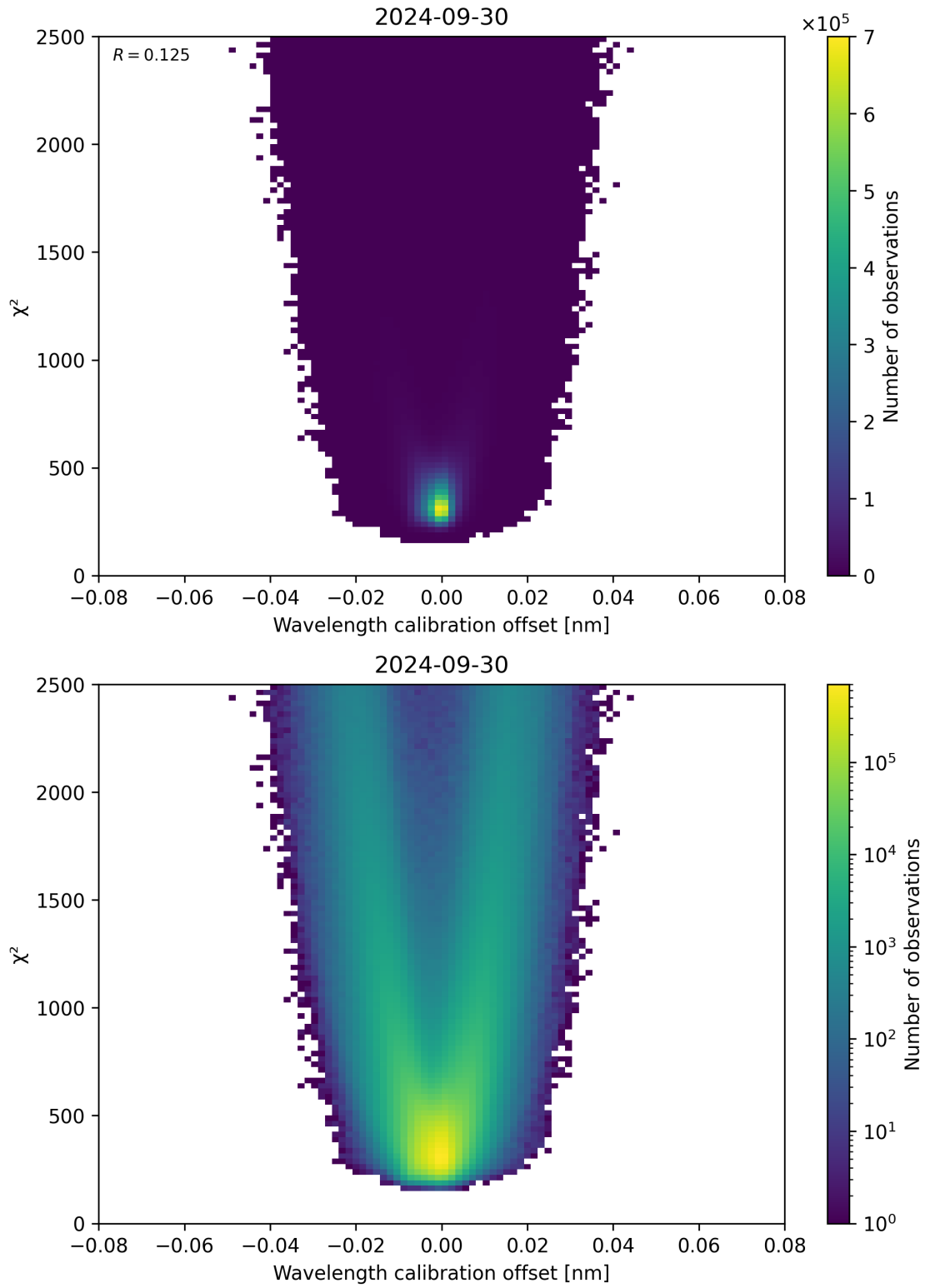
Figure 175: Scatter density plot of “Wavelength calibration offset” against “ \chi^2 ” for 2024-09-29 to 2024-10-01.
