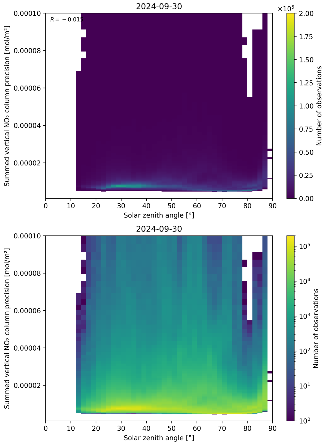
Figure 152: Scatter density plot of “Solar zenith angle” against “Summed vertical NO 2 column precision” for 2024-09-29 to 2024-10-01.
