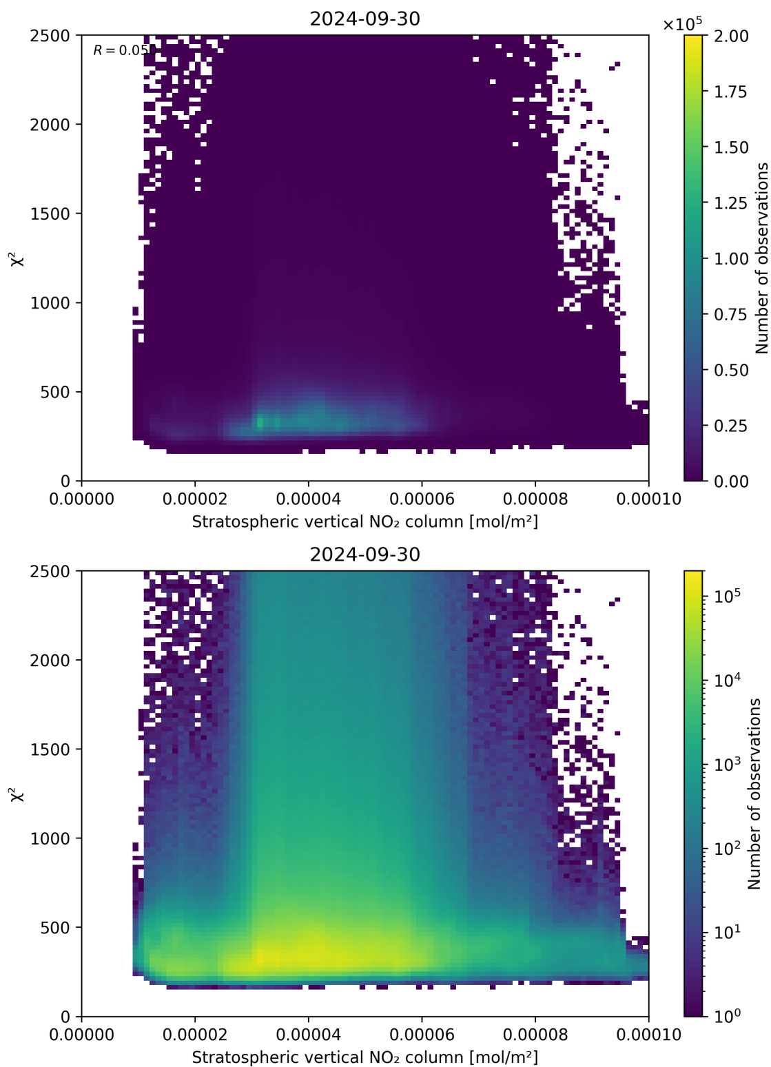
Figure 97: Scatter density plot of “Stratospheric vertical NO 2 column” against “ \chi^2 ” for 2024-09-29 to 2024-10-01.
