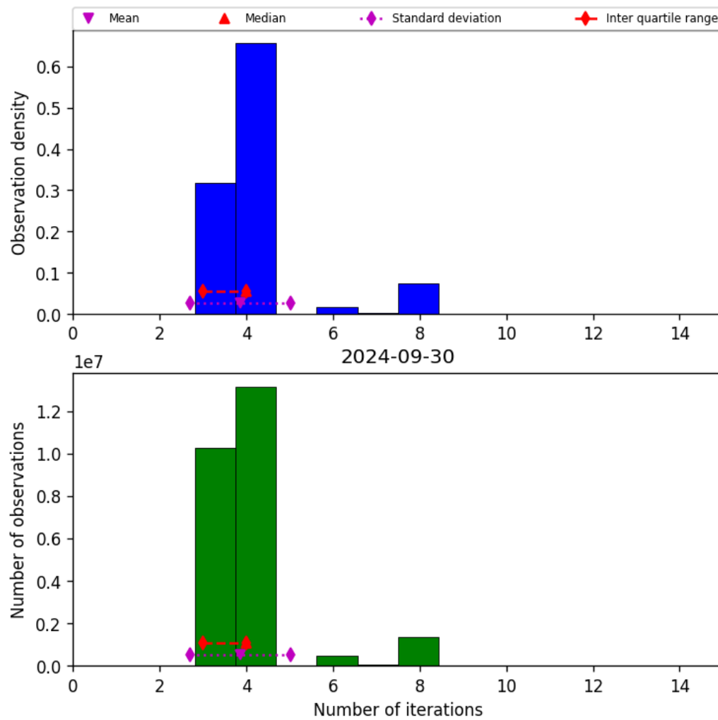
Figure 34: Histogram of “Number of iterations” for 2024-09-29 to 2024-10-01
