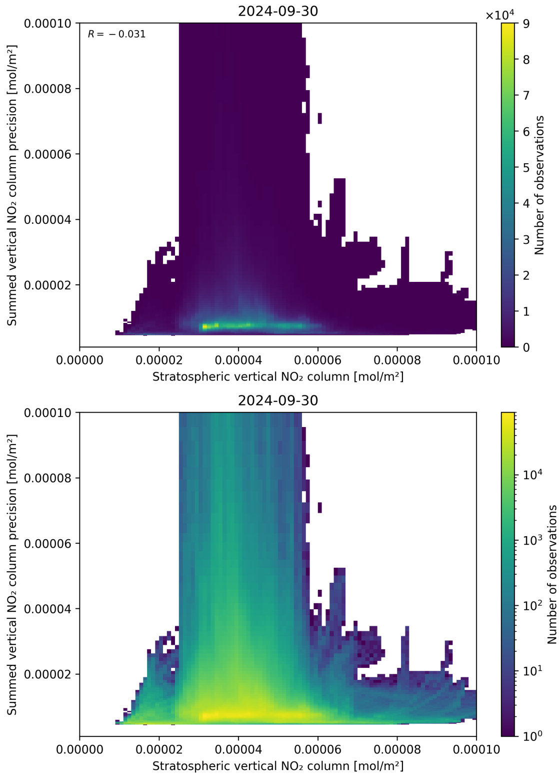
Figure 99: Scatter density plot of “Stratospheric vertical NO 2 column” against “Summed vertical NO 2 column precision” for 2024-09-29 to 2024-10-01.
