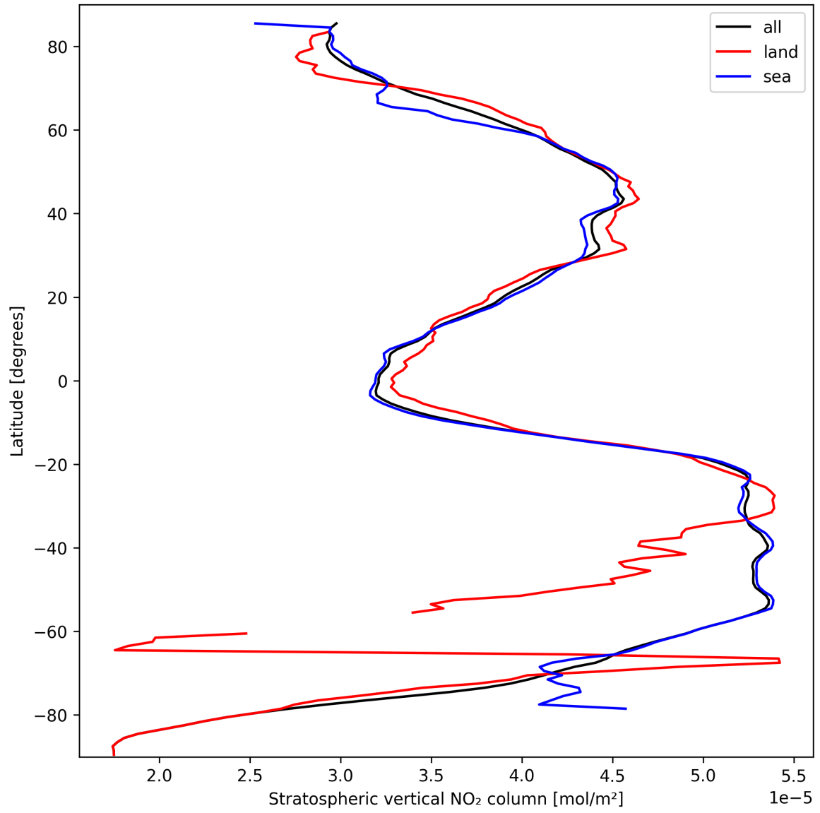
Figure 19: Zonal average of “Stratospheric vertical NO 2 column” for 2024-09-29 to 2024-10-01.
