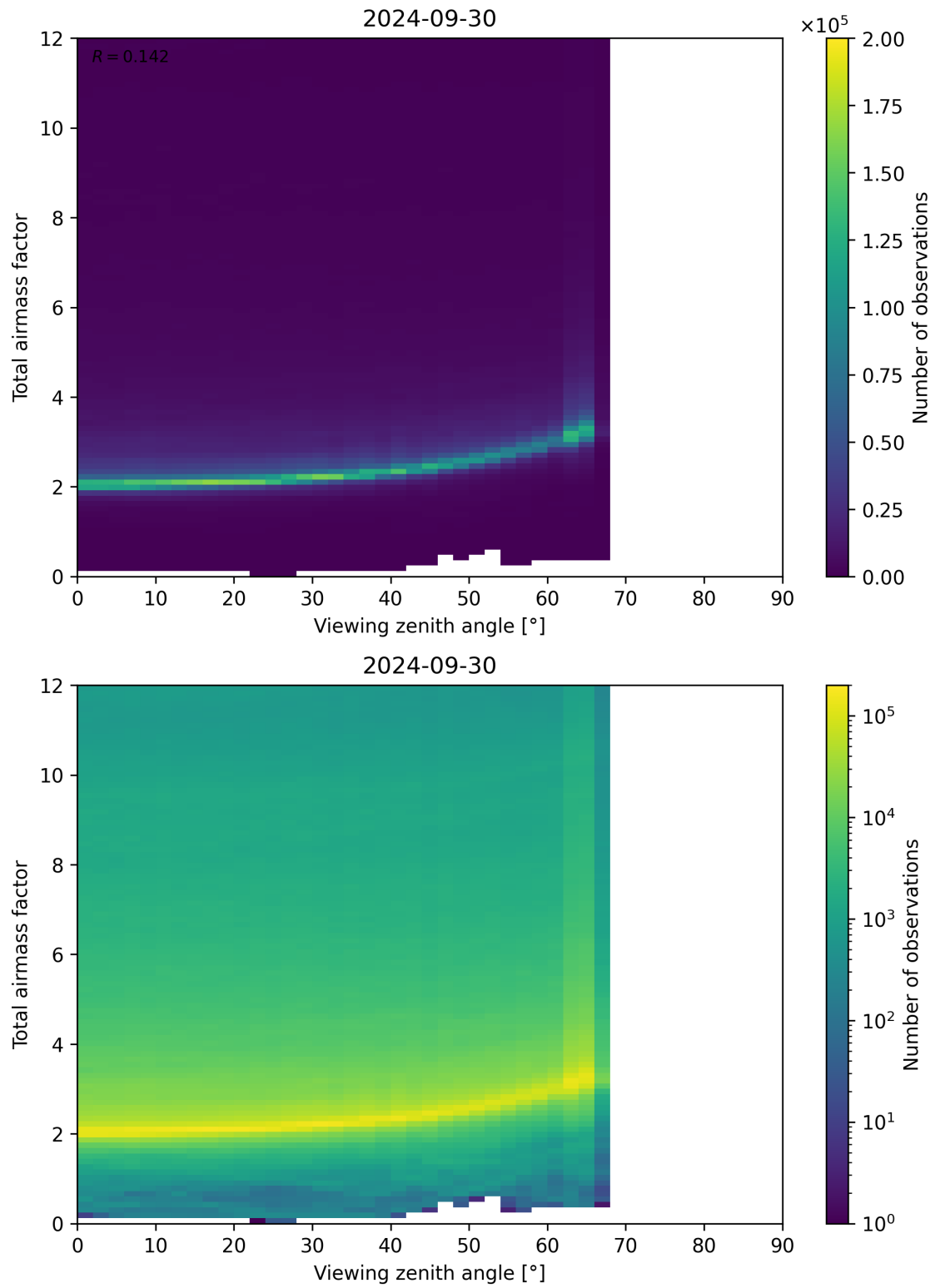
Figure 160: Scatter density plot of “Viewing zenith angle” against “Total airmass factor” for 2024-09-29 to 2024-10-01.
