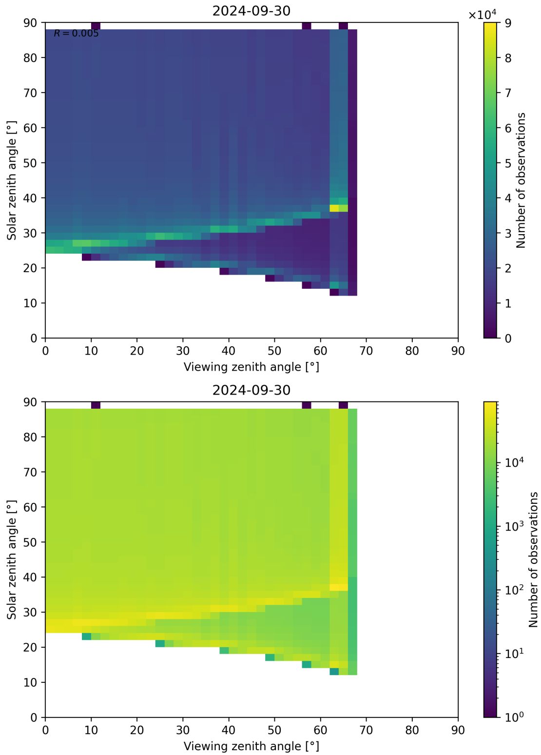
Figure 172: Scatter density plot of “Viewing zenith angle” against “Solar zenith angle” for 2024-09-29 to 2024-10-01.
