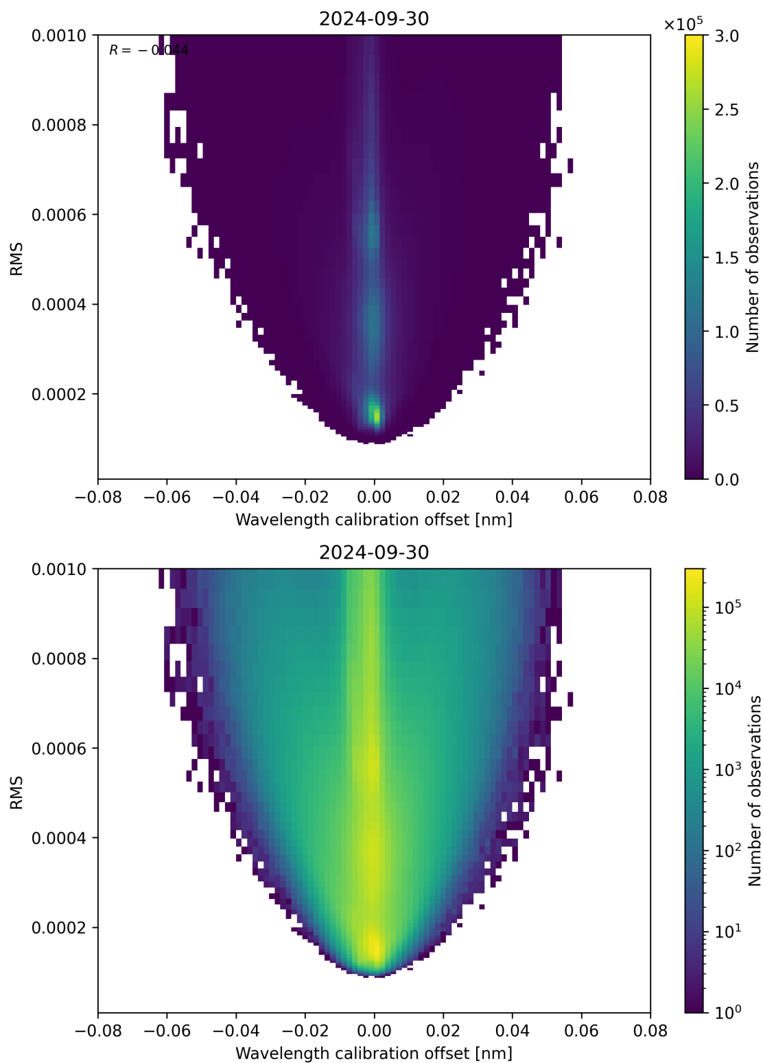
Figure 181: Scatter density plot of “Wavelength calibration offset” against “RMS” for 2024-09-29 to 2024-10-01.
