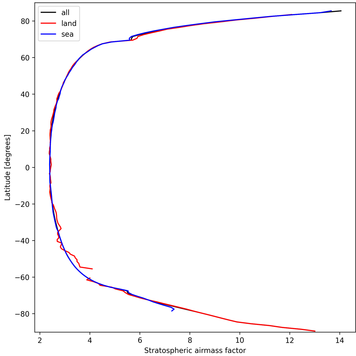
Figure 27: Zonal average of “Stratospheric air mass factor” for 2024-09-29 to 2024-10-01.
