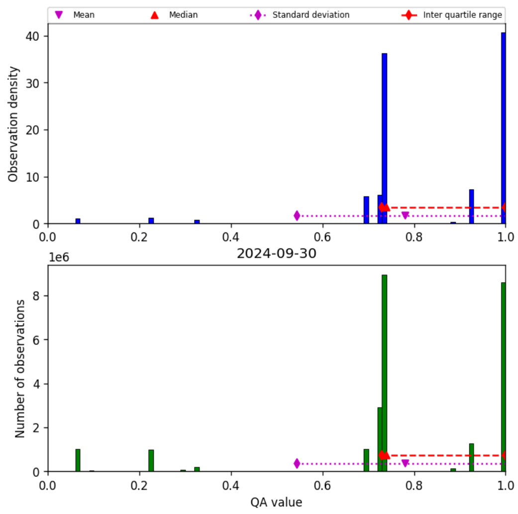
Figure 28: Histogram of “QA value” for 2024-09-29 to 2024-10-01
