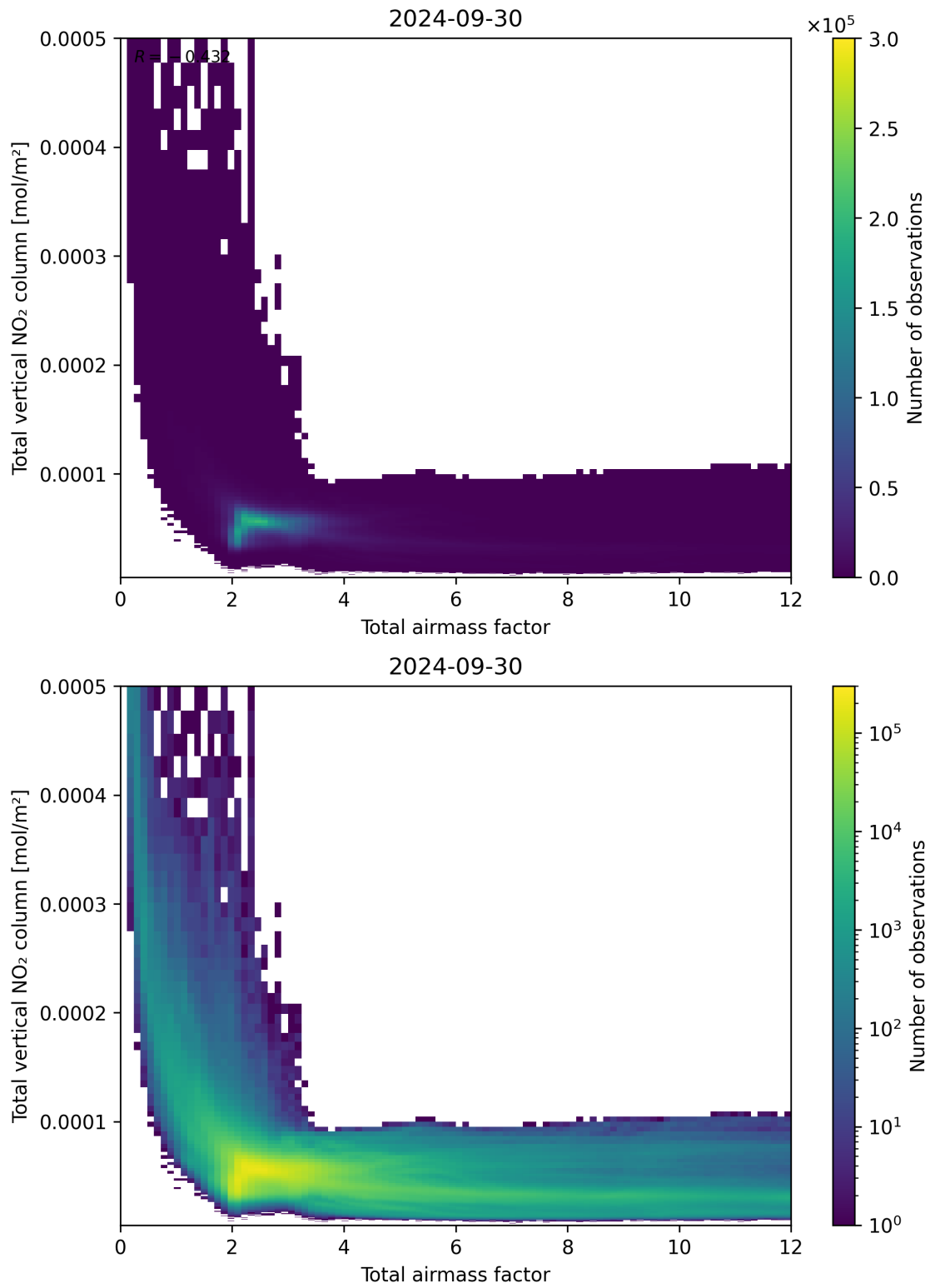
Figure 67: Scatter density plot of “Total airmass factor” against “Total vertical NO 2 column” for 2024-09-29 to 2024-10-01.
