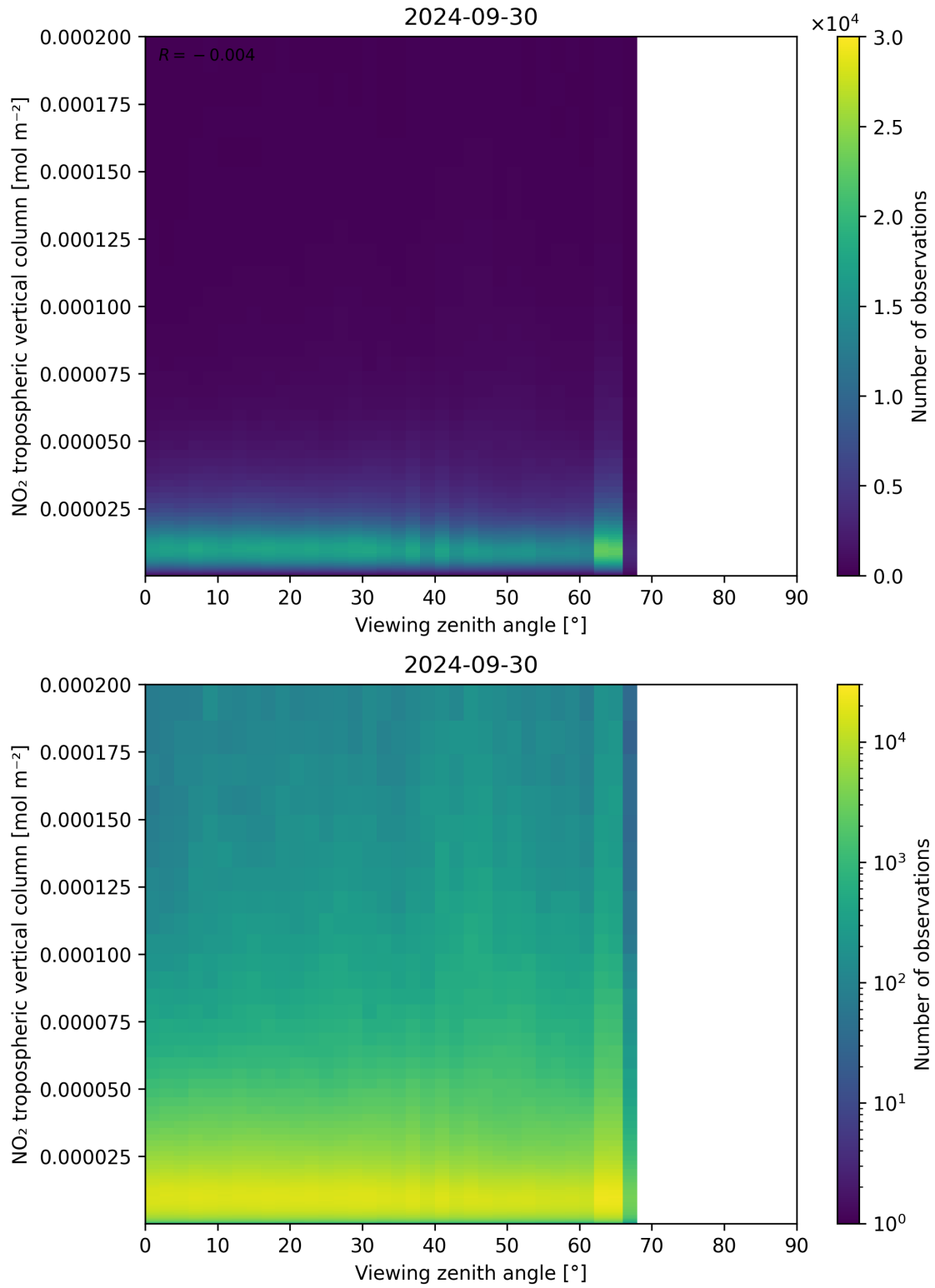
Figure 169: Scatter density plot of “Viewing zenith angle” against “NO 2 tropospheric vertical column” for 2024-09-29 to 2024-10-01.
