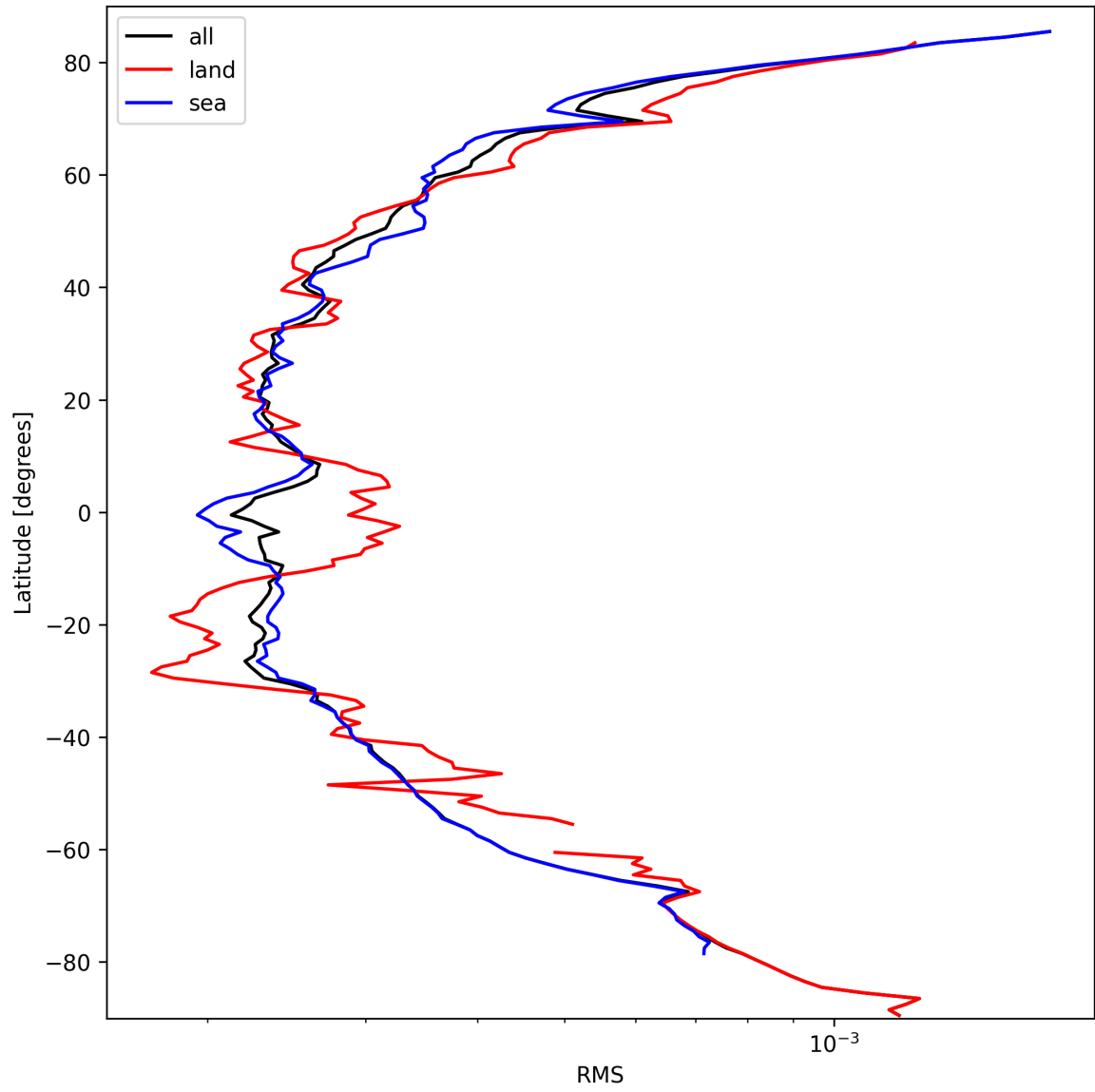
Figure 26: Zonal average of “RMS” for 2024-09-29 to 2024-10-01.
