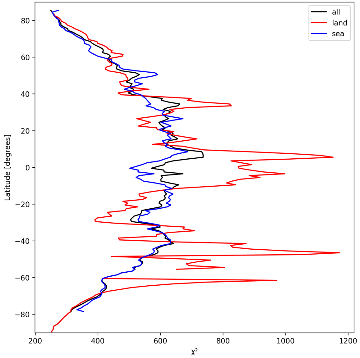
Figure 25: Zonal average of “ \chi^2 ” for 2024-09-29 to 2024-10-01.
