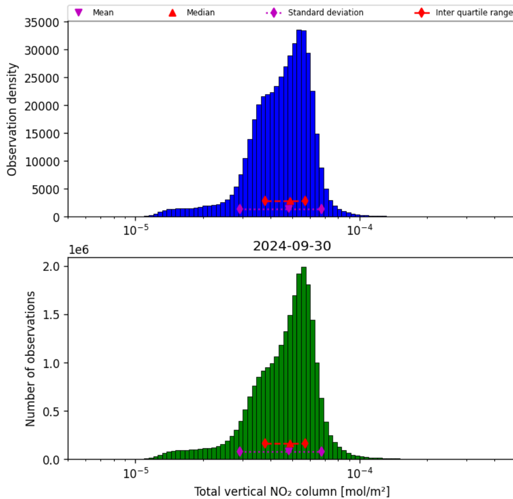
Figure 38: Histogram of “Total vertical NO 2 column” for 2024-09-29 to 2024-10-01
