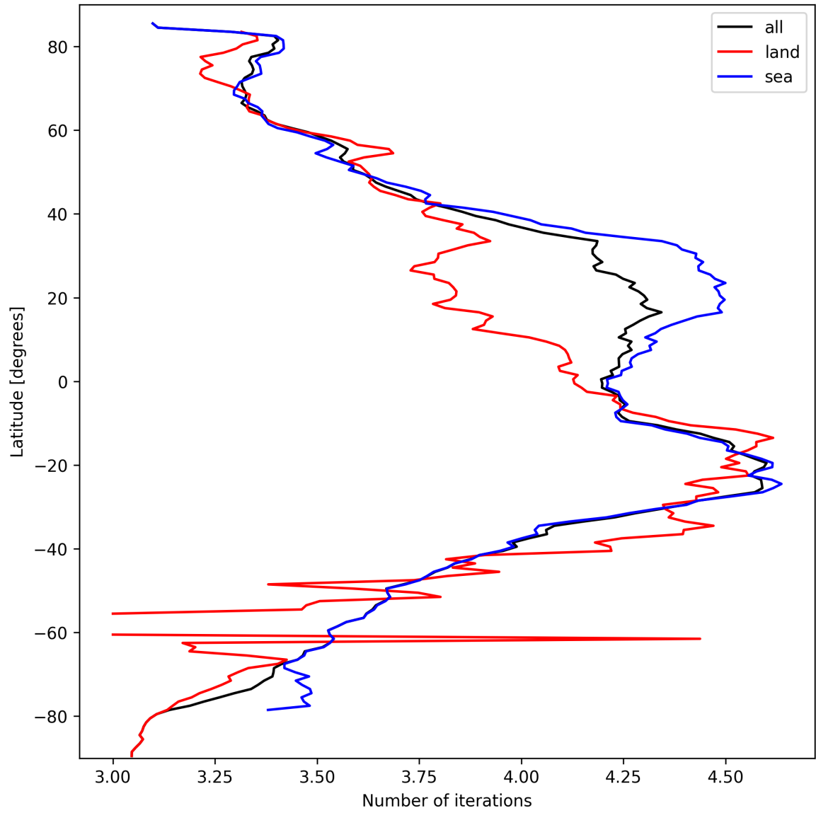
Figure 17: Zonal average of “Number of iterations” for 2024-09-29 to 2024-10-01.
