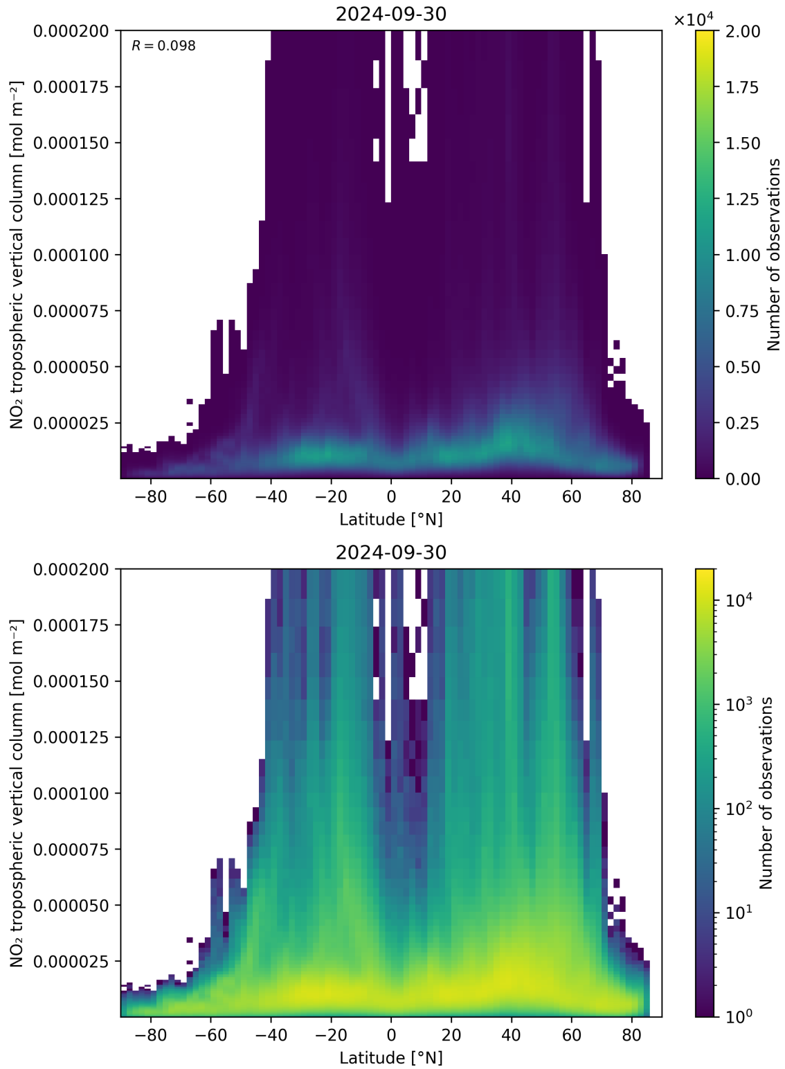
Figure 92: Scatter density plot of “Latitude” against “NO 2 tropospheric vertical column” for 2024-09-29 to 2024-10-01.
