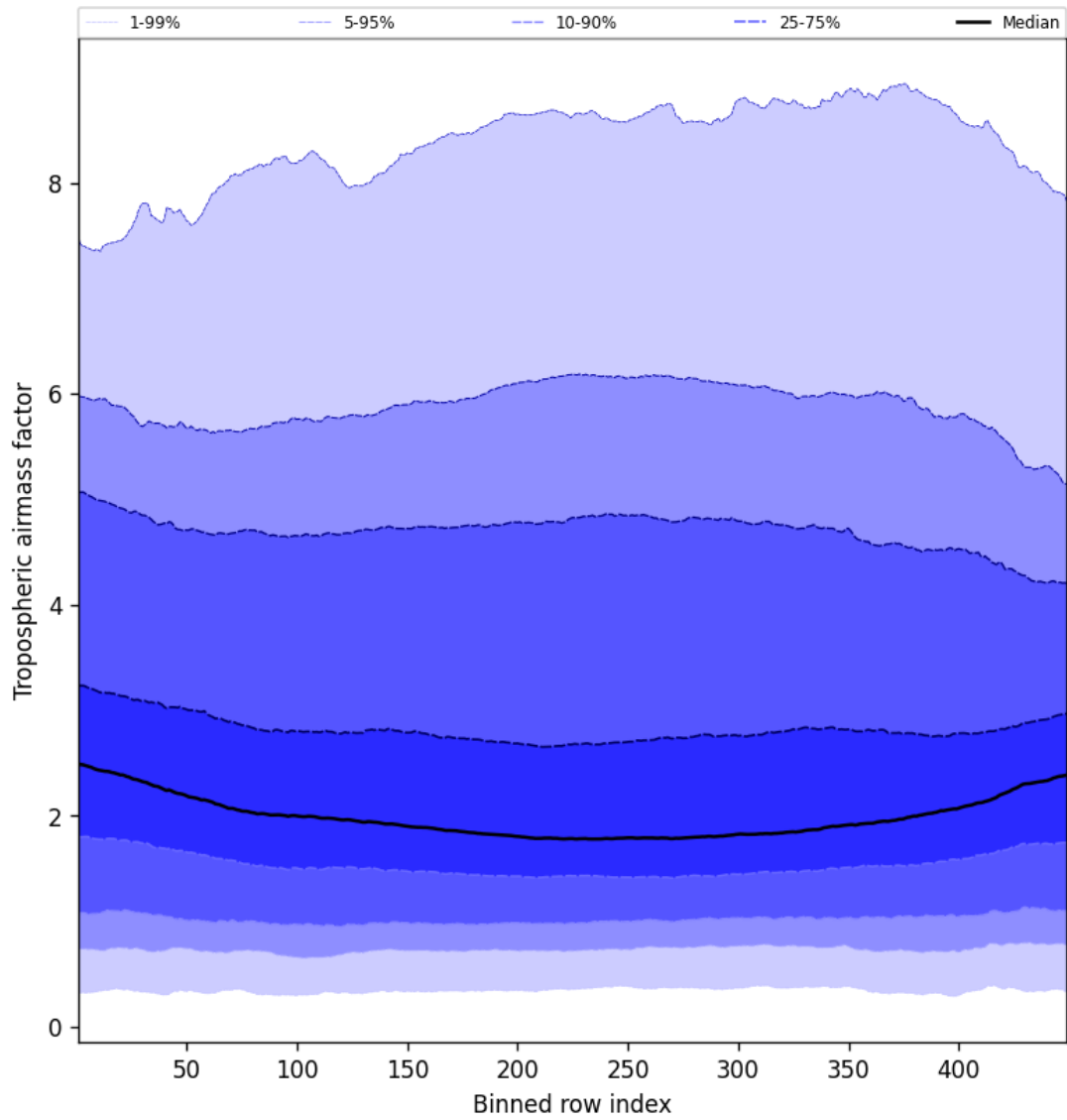
Figure 48: Along track statistics of “Tropospheric airmass factor” for 2024-09-29 to 2024-10-01
