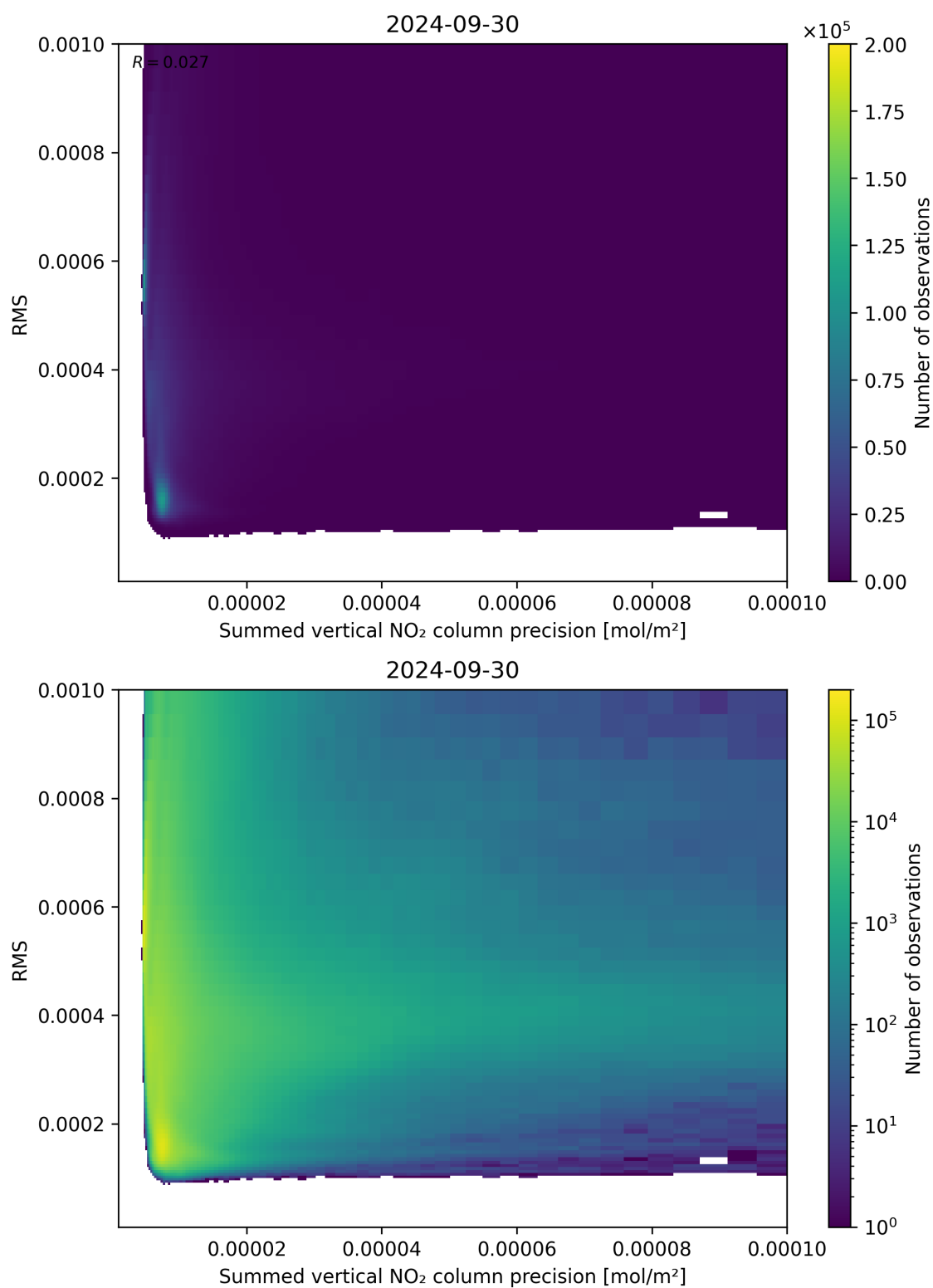
Figure 108: Scatter density plot of “Summed vertical NO 2 column precision” against “RMS” for 2024-09-29 to 2024-10-01.
