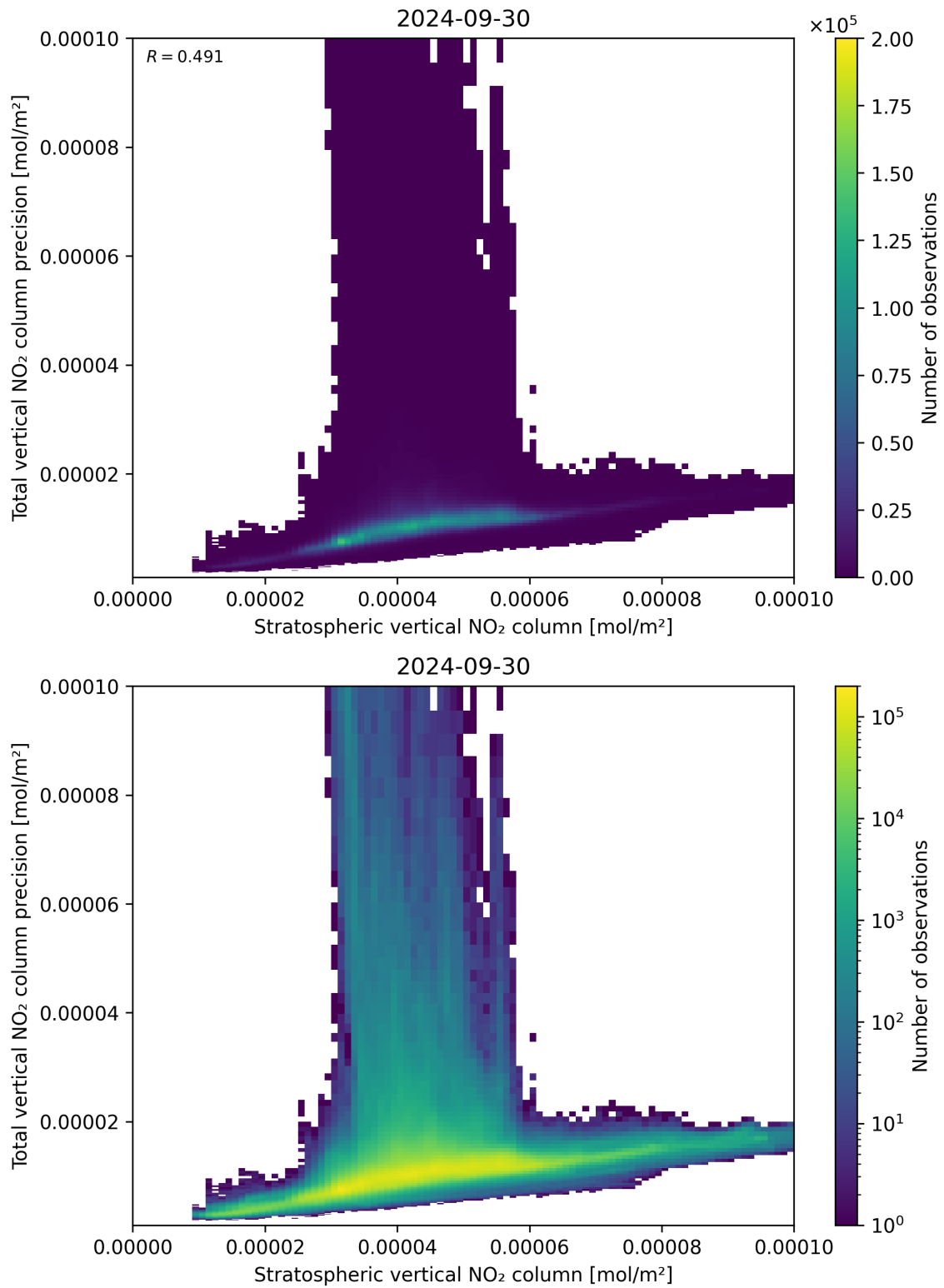
Figure 101: Scatter density plot of “Stratospheric vertical NO 2 column” against “Total vertical NO 2 column precision” for 2024-09-29 to 2024-10-01.
