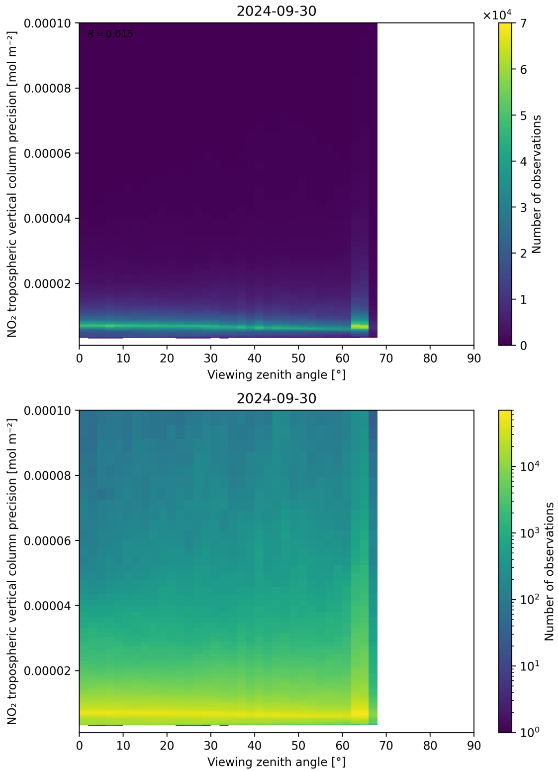
Figure 170: Scatter density plot of “Viewing zenith angle” against “NO 2 tropospheric vertical column precision” for 2024-09-29 to 2024-10-01.
