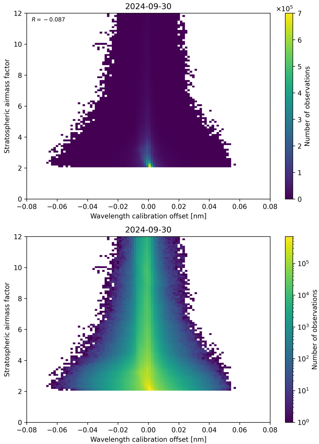
Figure 174: Scatter density plot of “Wavelength calibration offset” against “Stratospheric airmass factor” for 2024-09-29 to 2024-10-01.
