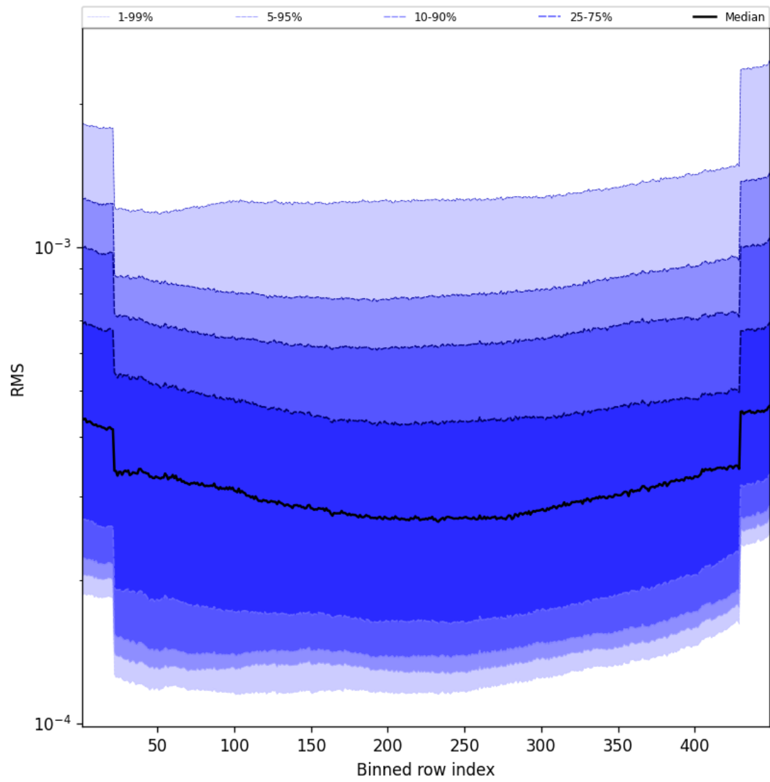
Figure 60: Along track statistics of “RMS” for 2024-09-29 to 2024-10-01
