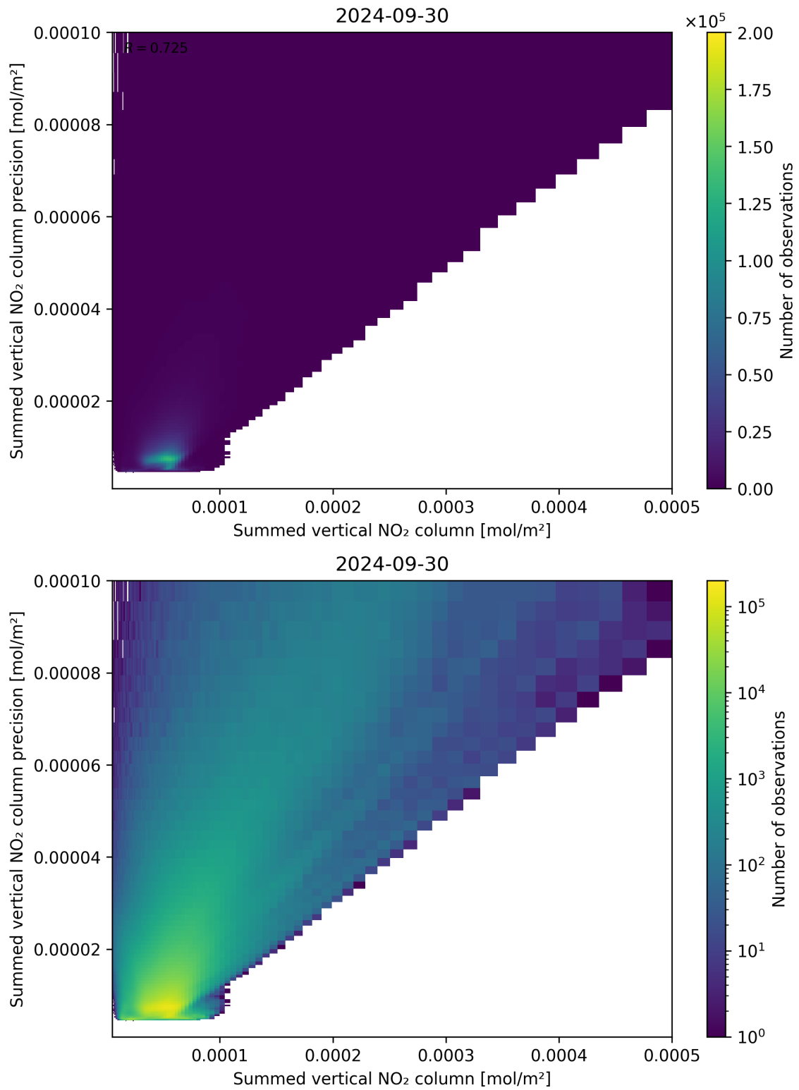
Figure 105: Scatter density plot of “Summed vertical NO 2 column” against “Summed vertical NO 2 column precision” for 2024-09-29 to 2024-10-01.
