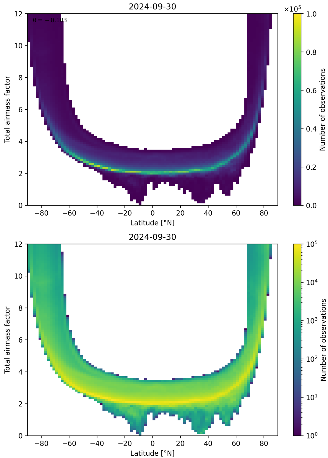
Figure 84: Scatter density plot of “Latitude” against “Total airmass factor” for 2024-09-29 to 2024-10-01.
