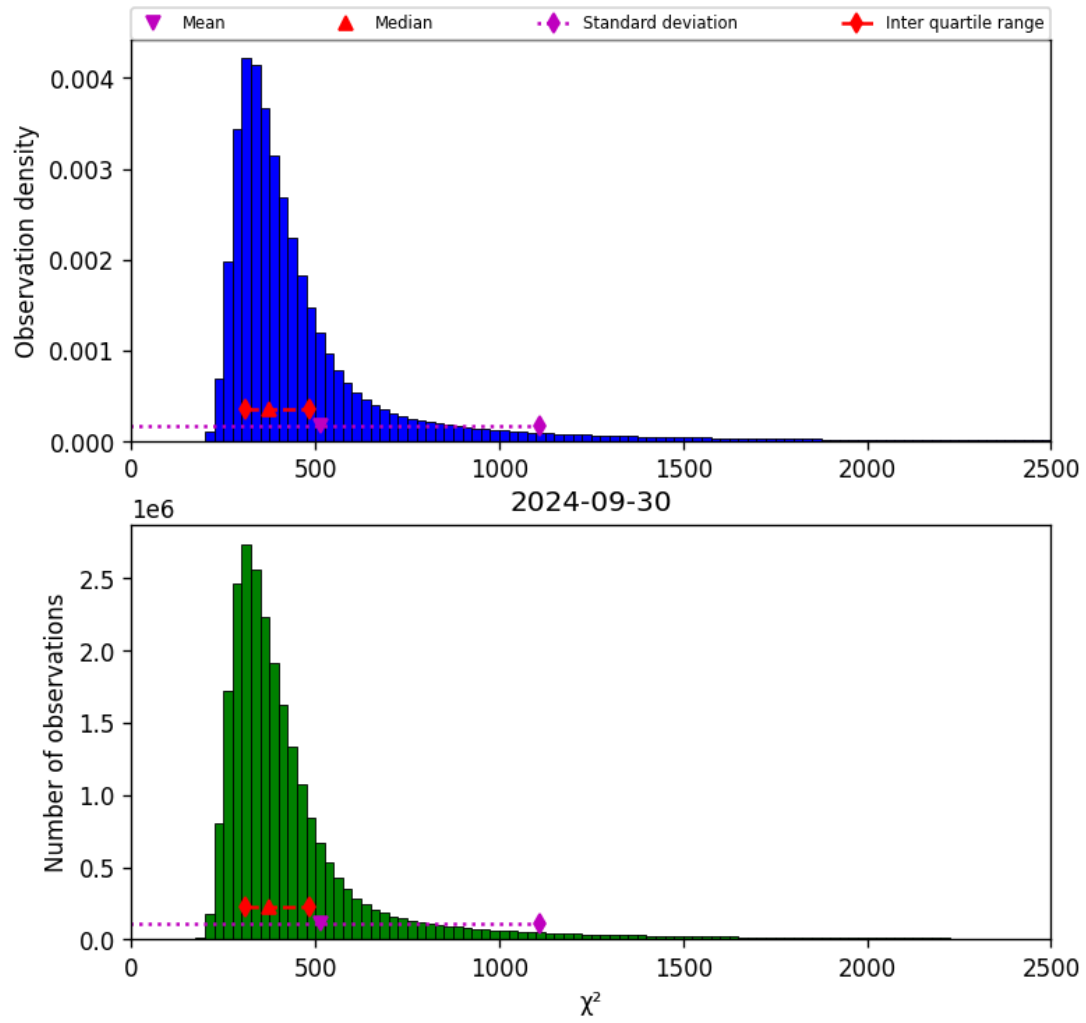
Figure 42: Histogram of “ \chi^2 ” for 2024-09-29 to 2024-10-01
