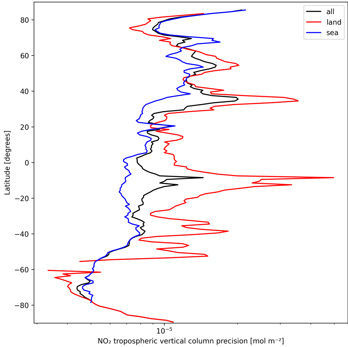
Figure 13: Zonal average of “NO 2 tropospheric vertical column precision” for 2024-09-29 to 2024-10-01.
