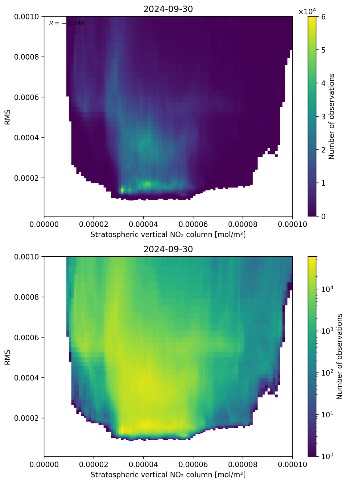
Figure 102: Scatter density plot of “Stratospheric vertical NO 2 column” against “RMS” for 2024-09-29 to 2024-10-01.
