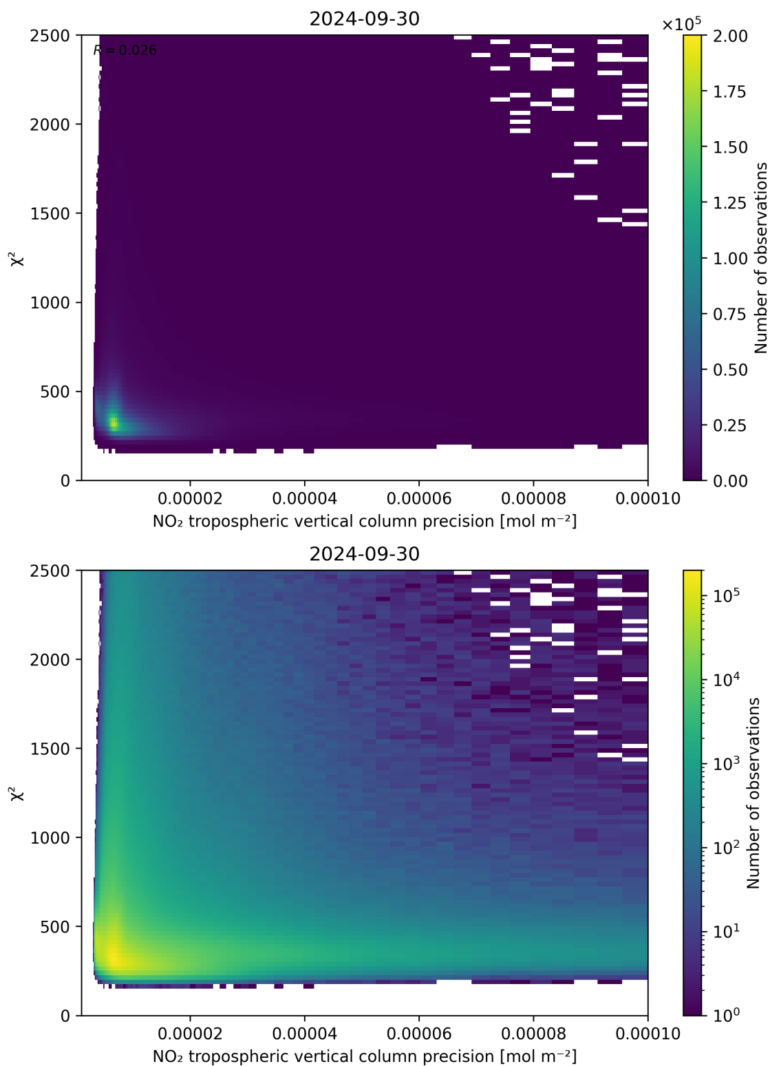
Figure 134: Scatter density plot of “NO 2 tropospheric vertical column precision” against “ \chi^2 ” for 2024-09-29 to 2024-10-01.
