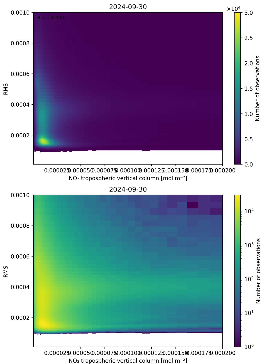
Figure 142: Scatter density plot of “NO 2 tropospheric vertical column” against “RMS” for 2024-09-29 to 2024-10-01.
