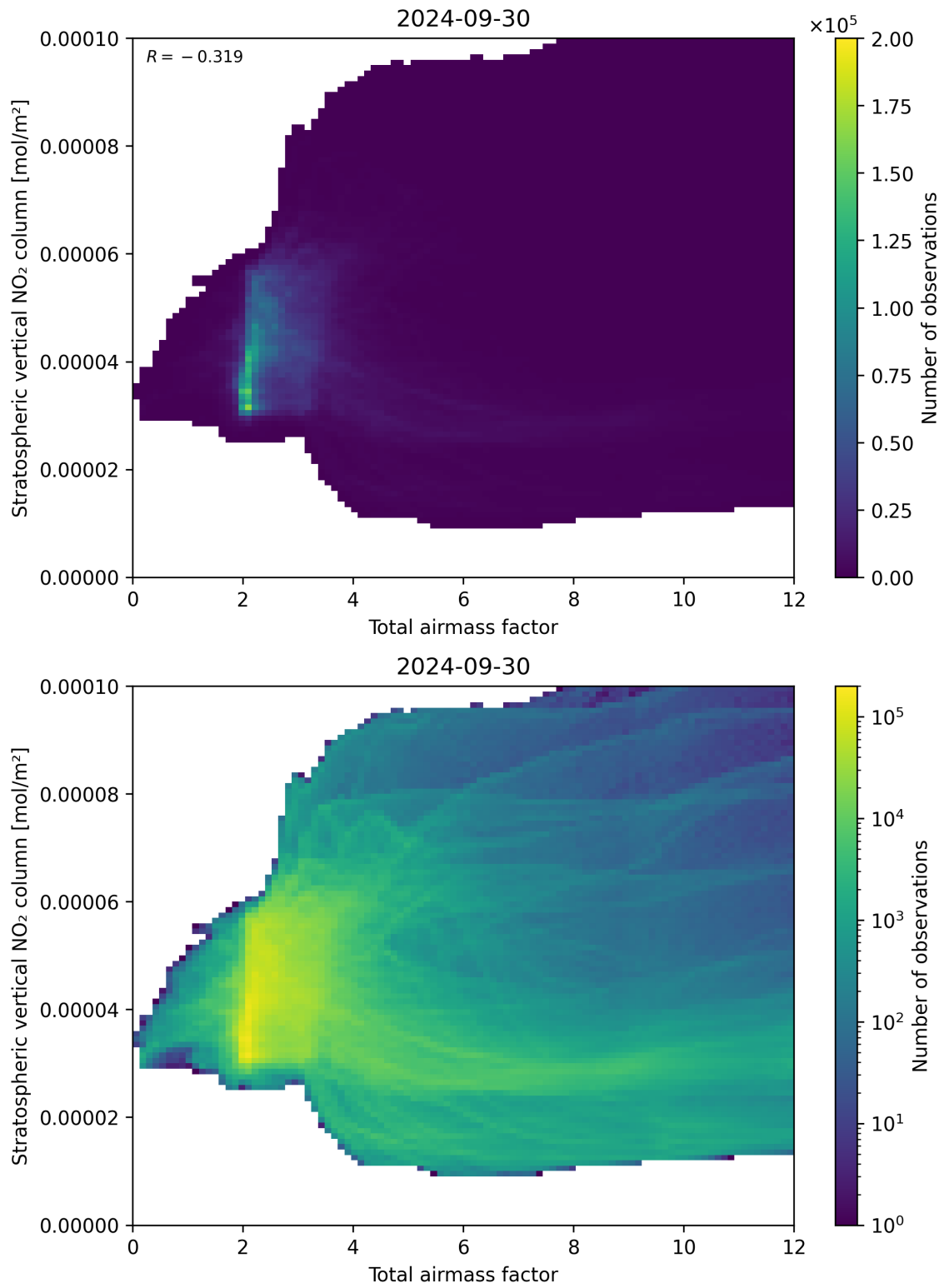
Figure 64: Scatter density plot of “Total airmass factor” against “Stratospheric vertical NO 2 column” for 2024-09-29 to 2024-10-01.
