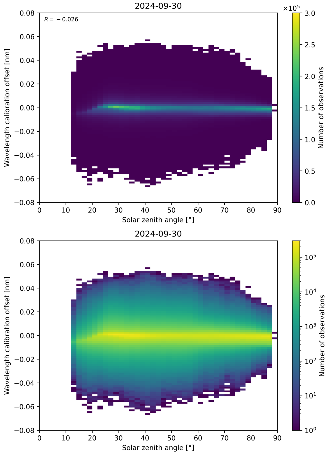
Figure 158: Scatter density plot of “Solar zenith angle” against “Wavelength calibration offset” for 2024-09-29 to 2024-10-01.
