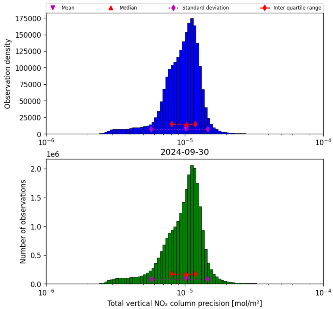
Figure 39: Histogram of “Total vertical NO 2 column precision” for 2024-09-29 to 2024-10-01
