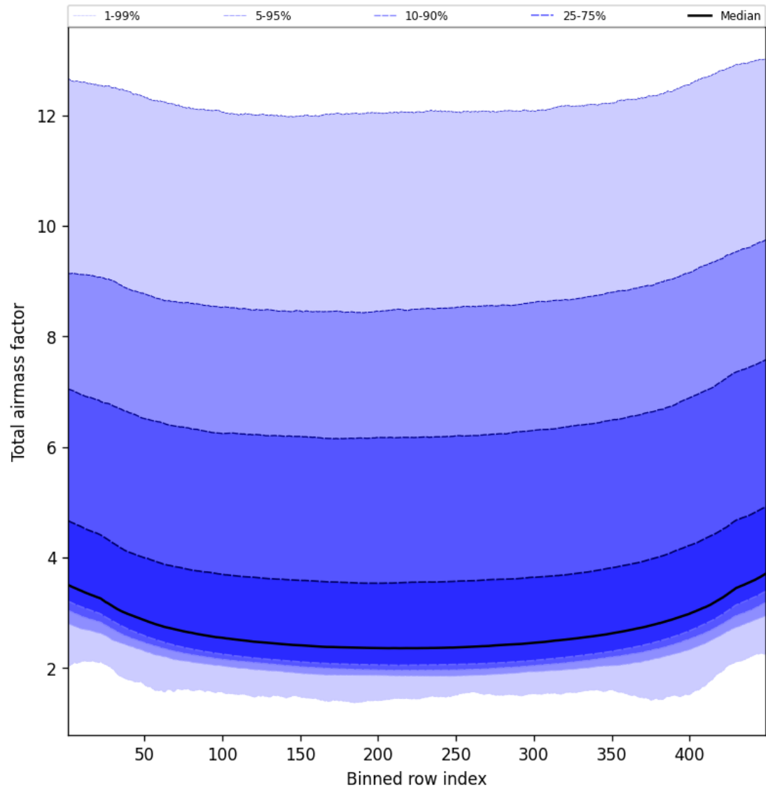
Figure 49: Along track statistics of “Total airmass factor” for 2024-09-29 to 2024-10-01
