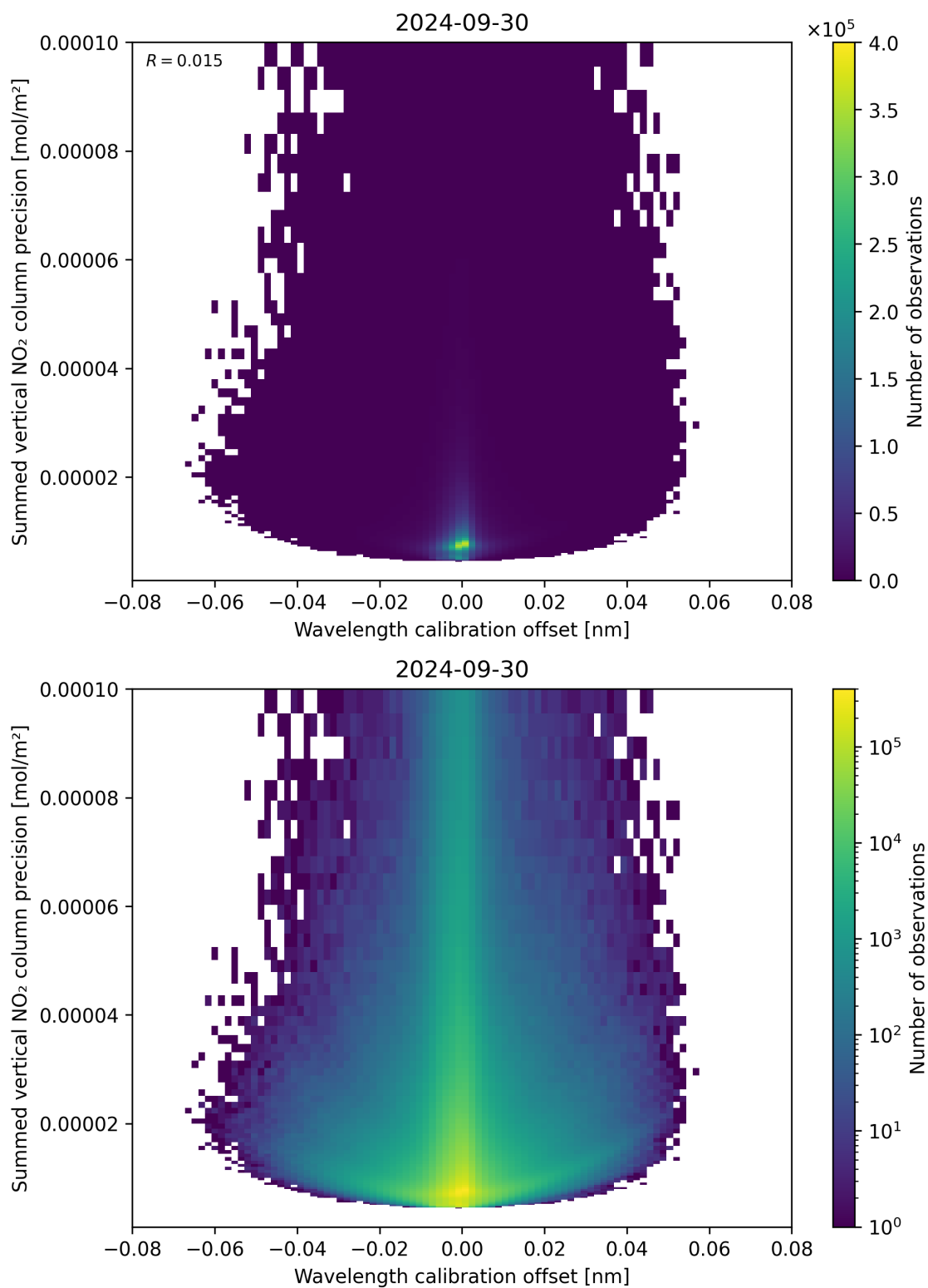
Figure 178: Scatter density plot of “Wavelength calibration offset” against “Summed vertical NO 2 column precision” for 2024-09-29 to 2024-10-01.
