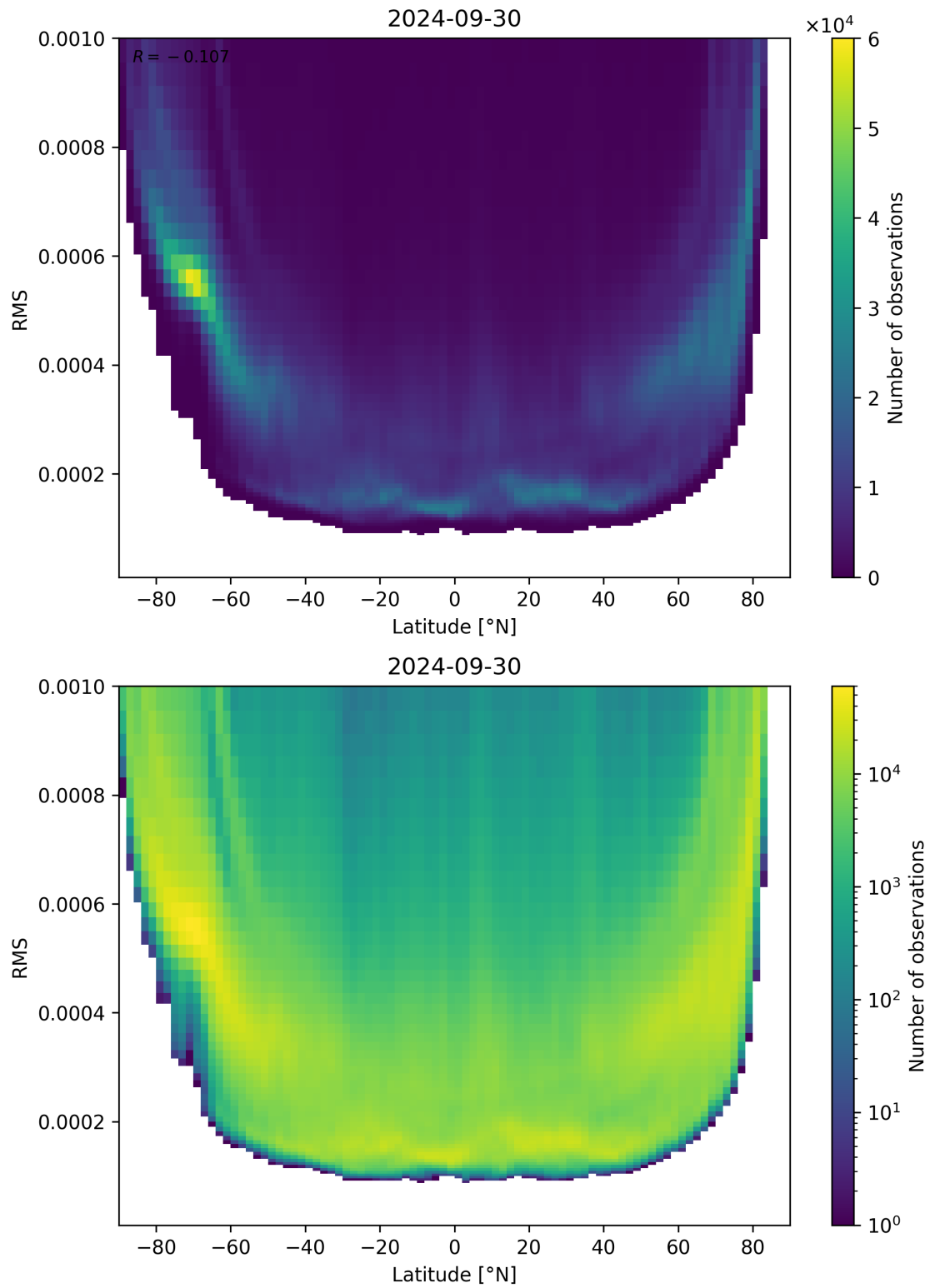
Figure 94: Scatter density plot of “Latitude” against “RMS” for 2024-09-29 to 2024-10-01.
