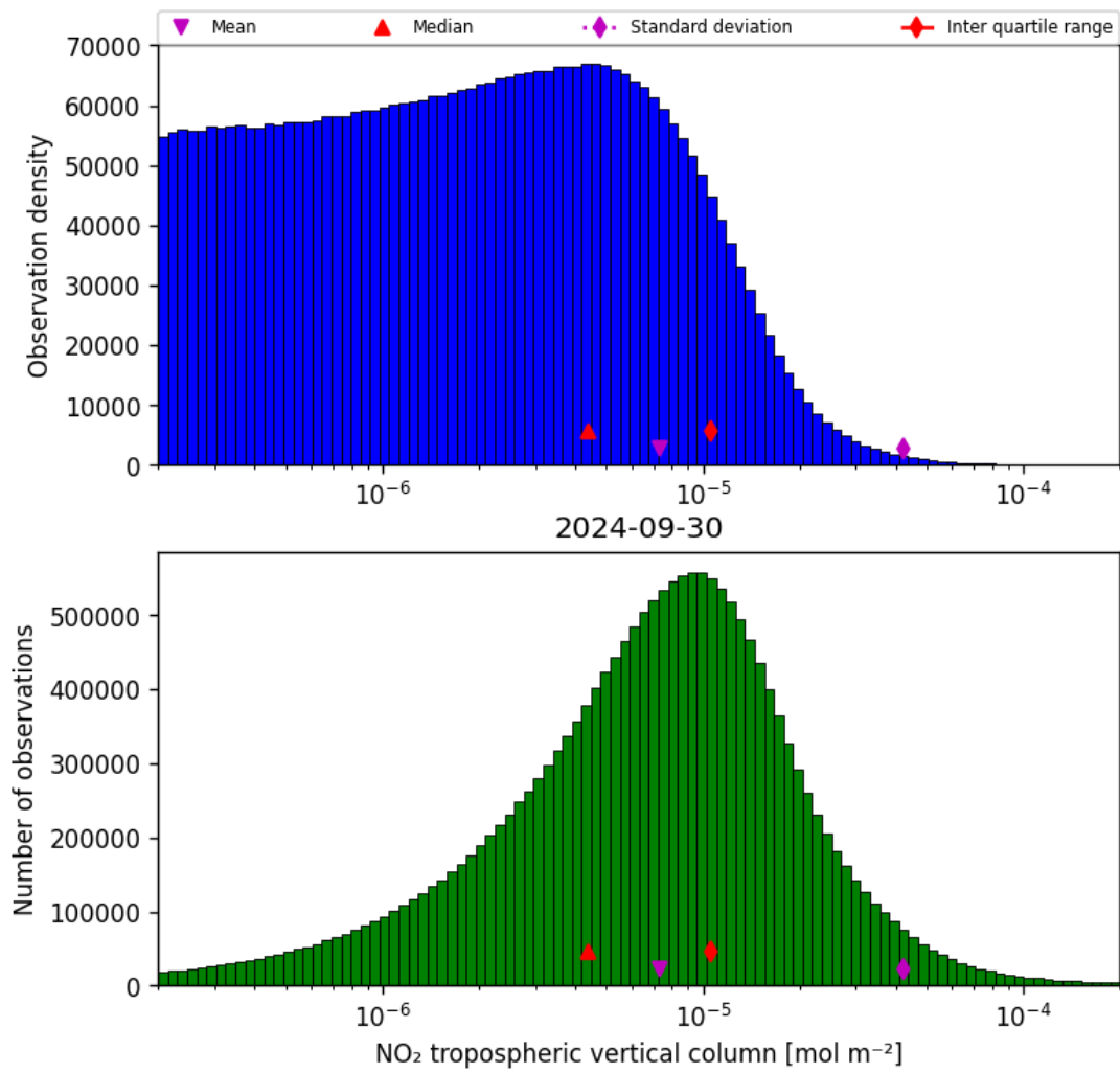
Figure 29: Histogram of “NO 2 tropospheric vertical column” for 2024-09-29 to 2024-10-01
