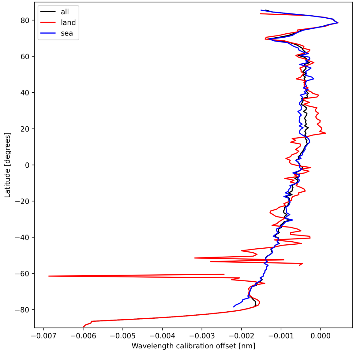
Figure 18: Zonal average of “Wavelength calibration offset” for 2024-09-29 to 2024-10-01.
