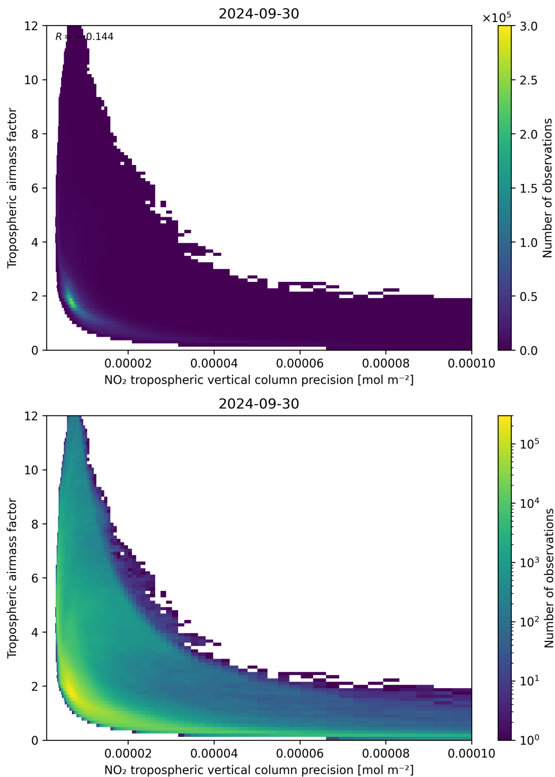
Figure 133: Scatter density plot of “NO 2 tropospheric vertical column precision” against “Tropospheric air mass factor” for 2024-09-29 to 2024-10-01.
