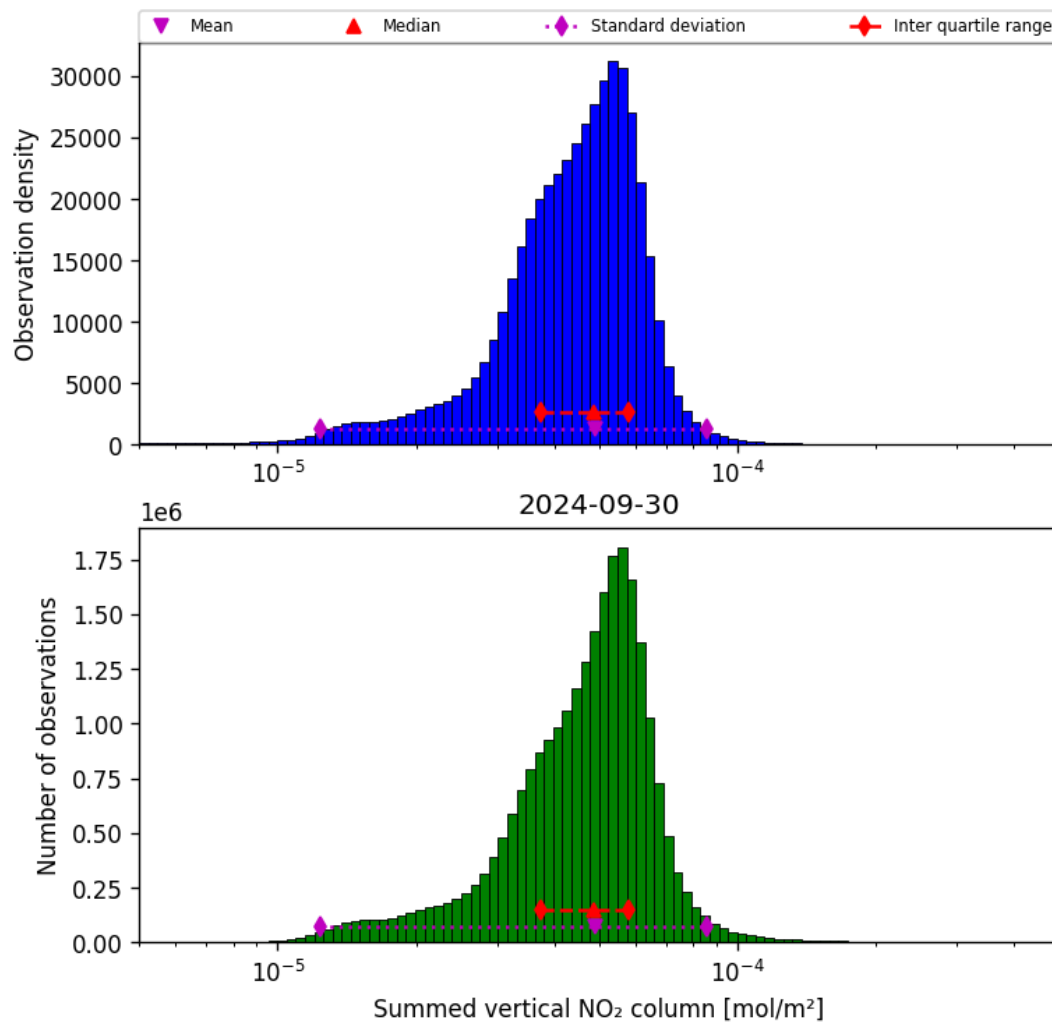
Figure 40: Histogram of “Summed vertical NO 2 column” for 2024-09-29 to 2024-10-01
