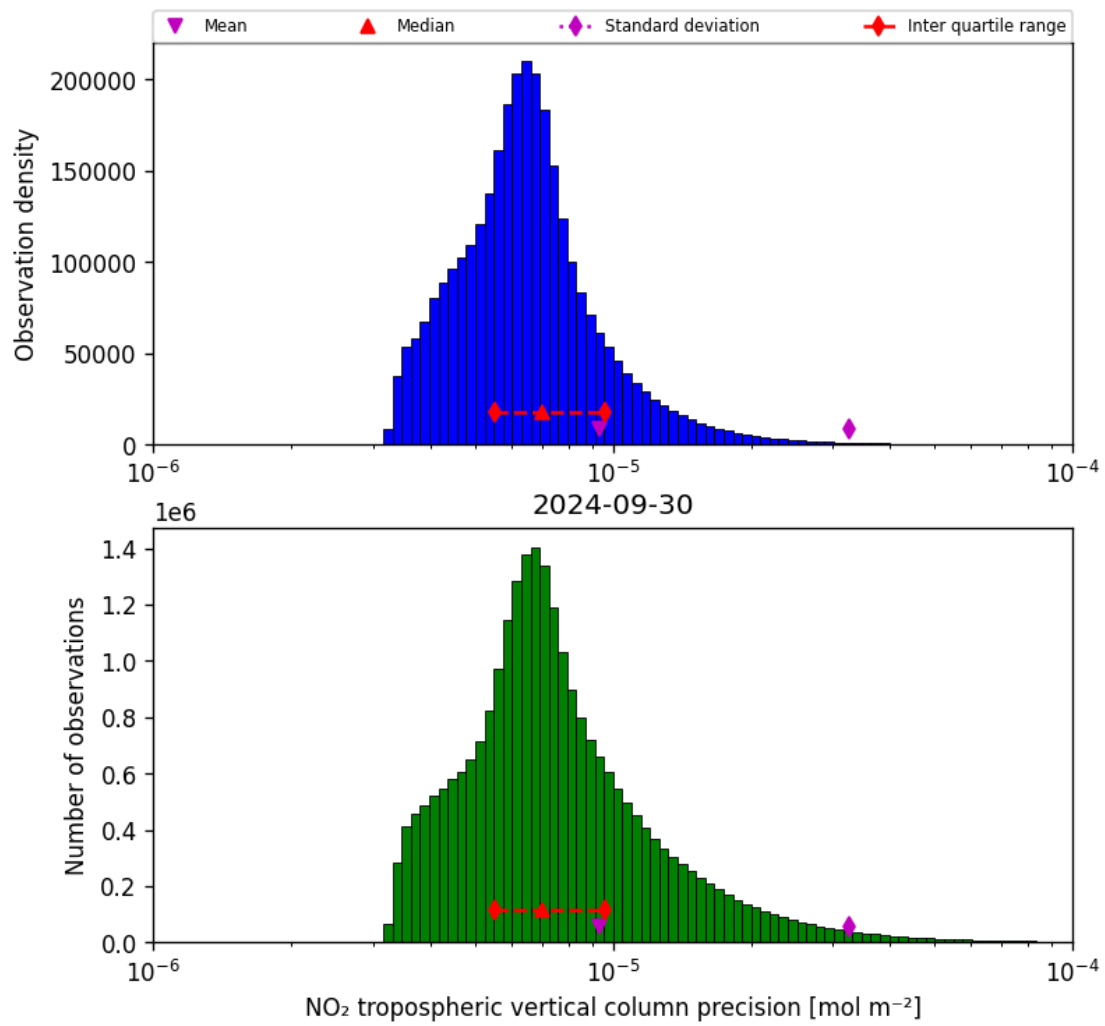
Figure 30: Histogram of “NO 2 tropospheric vertical column precision” for 2024-09-29 to 2024-10-01
