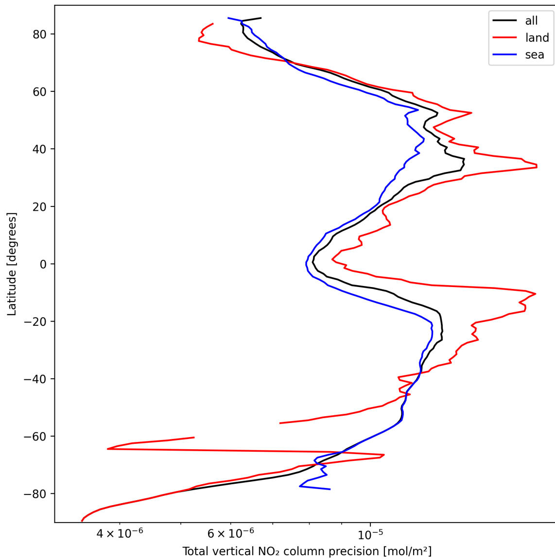
Figure 22: Zonal average of “Total vertical NO 2 column precision” for 2024-09-29 to 2024-10-01.
