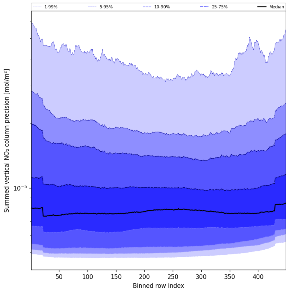
Figure 58: Along track statistics of “Summed vertical NO 2 column precision” for 2024-09-29 to 2024-10-01
