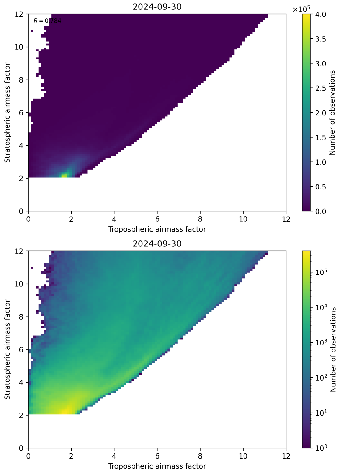
Figure 71: Scatter density plot of “Tropospheric airmass factor” against “Stratospheric airmass factor” for 2024-09-29 to 2024-10-01.
