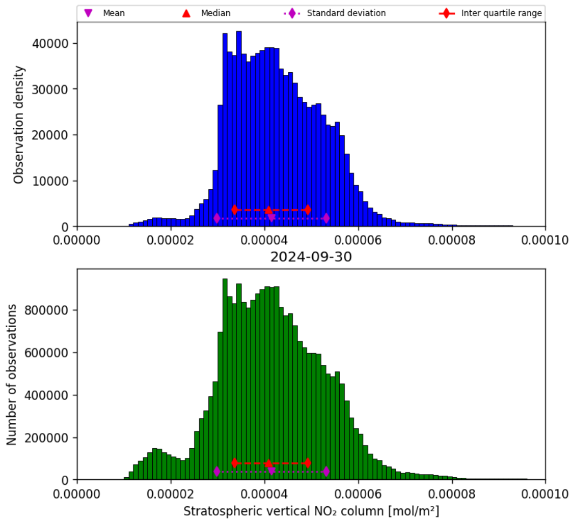
Figure 36: Histogram of “Stratospheric vertical NO 2 column” for 2024-09-29 to 2024-10-01
