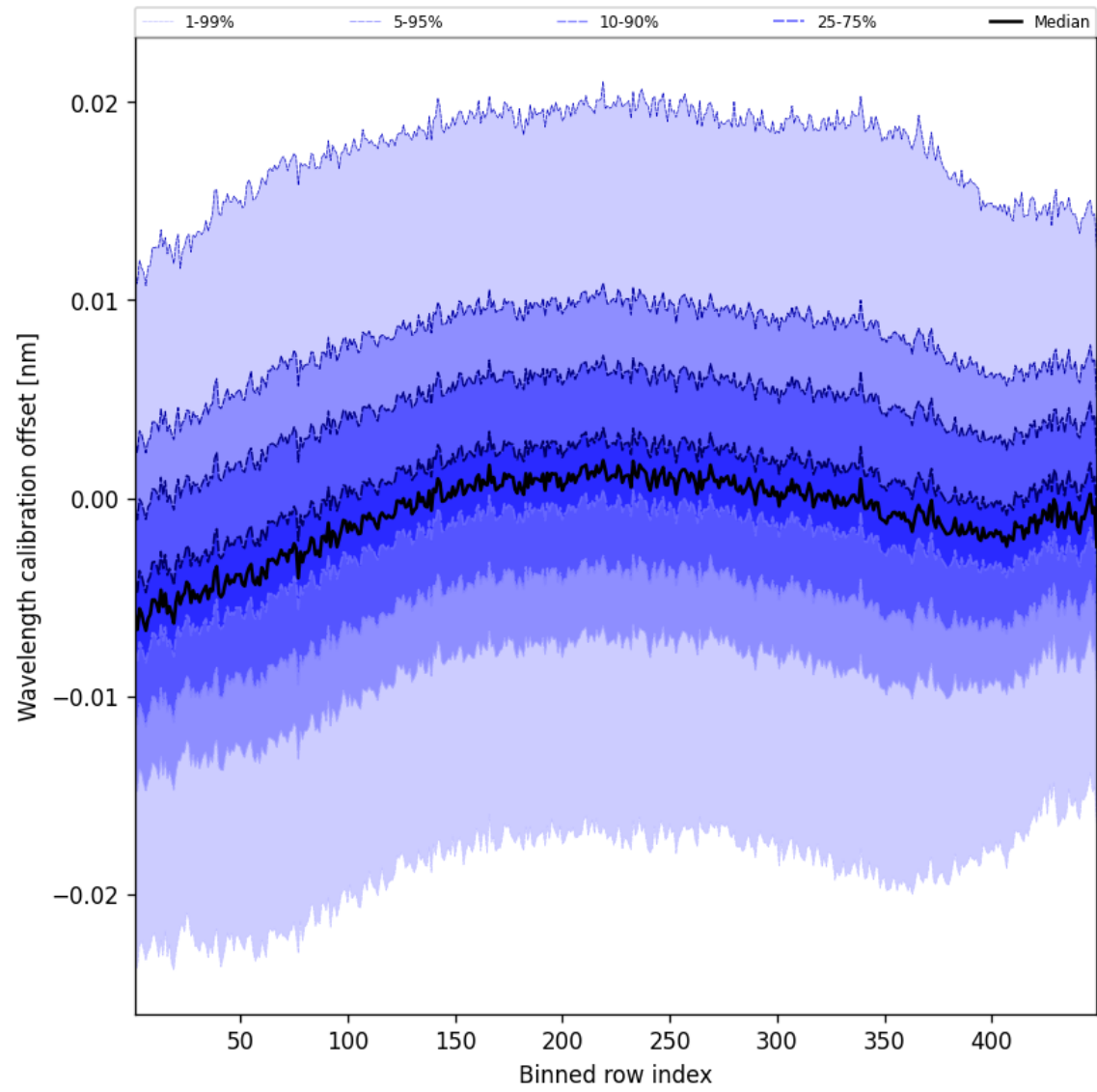
Figure 52: Along track statistics of “Wavelength calibration offset” for 2024-09-29 to 2024-10-01
