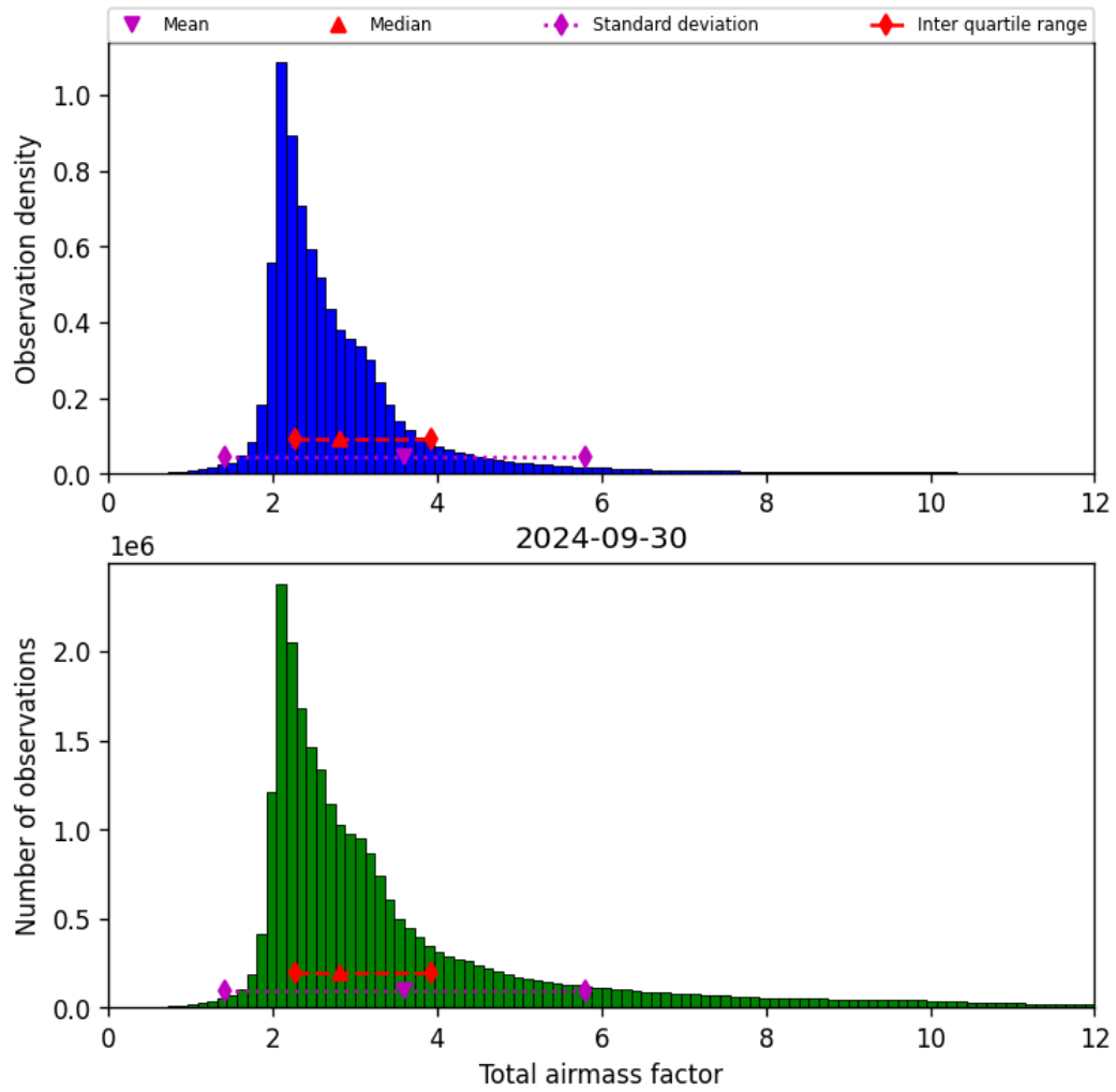
Figure 32: Histogram of “Total airmass factor” for 2024-09-29 to 2024-10-01
