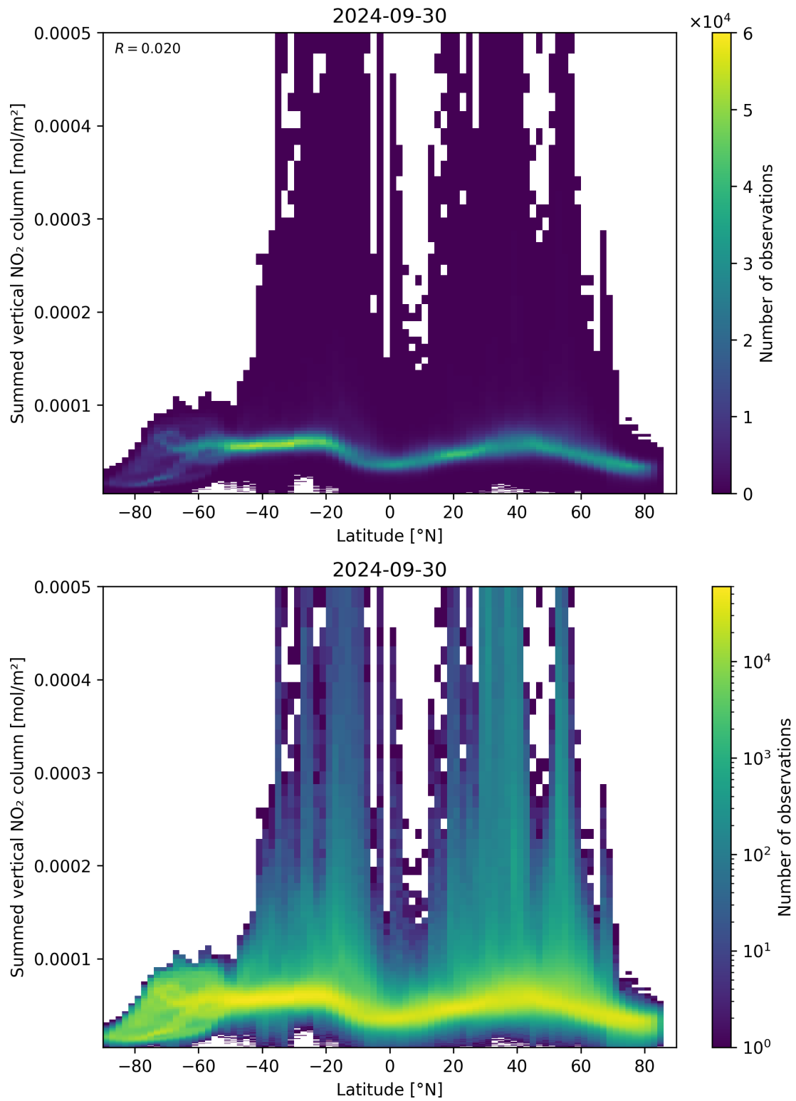
Figure 88: Scatter density plot of “Latitude” against “Summed vertical NO 2 column” for 2024-09-29 to 2024-10-01.
