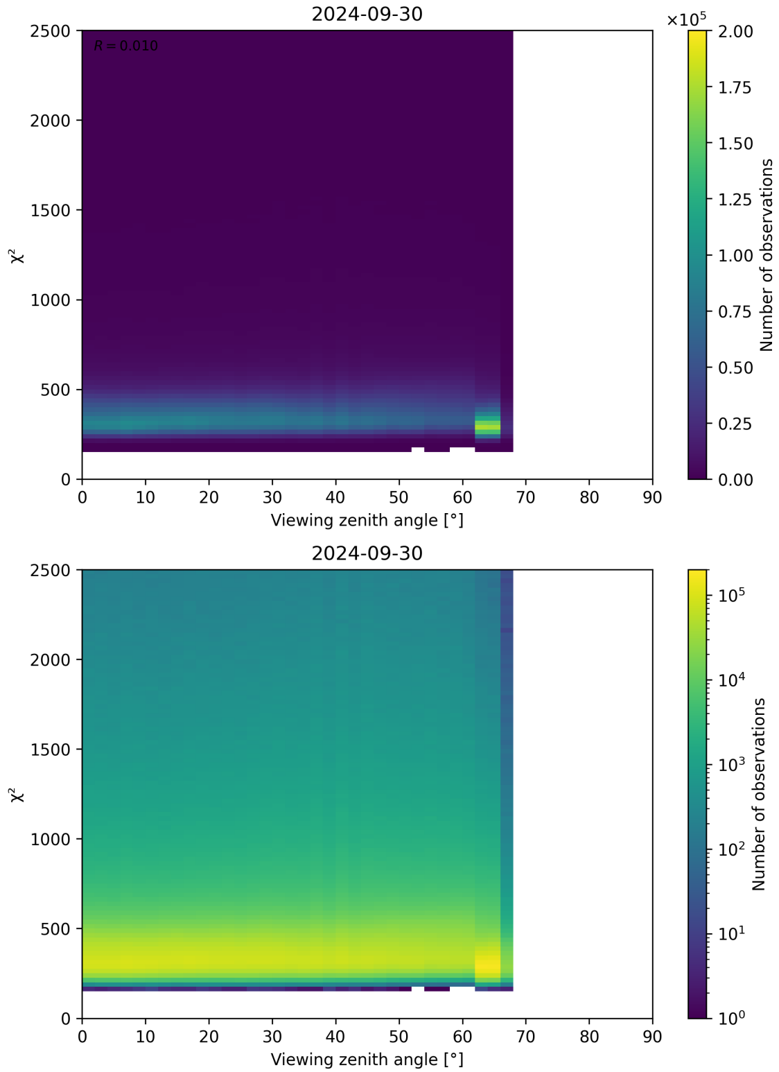
Figure 162: Scatter density plot of “Viewing zenith angle” against “ \chi^2 ” for 2024-09-29 to 2024-10-01.
