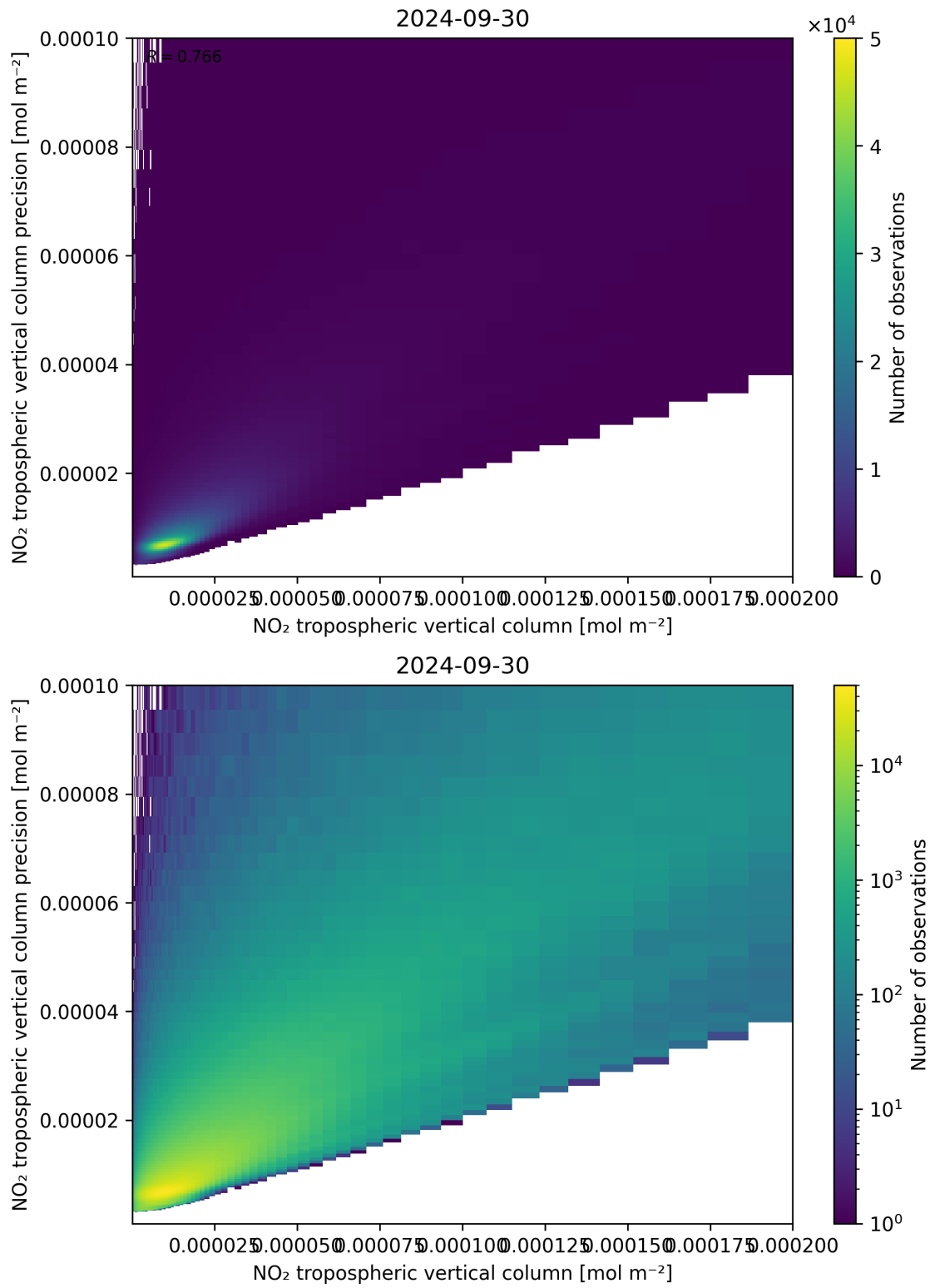
Figure 130: Scatter density plot of “NO 2 tropospheric vertical column” against “NO 2 tropospheric vertical column precision” for 2024-09-29 to 2024-10-01.
