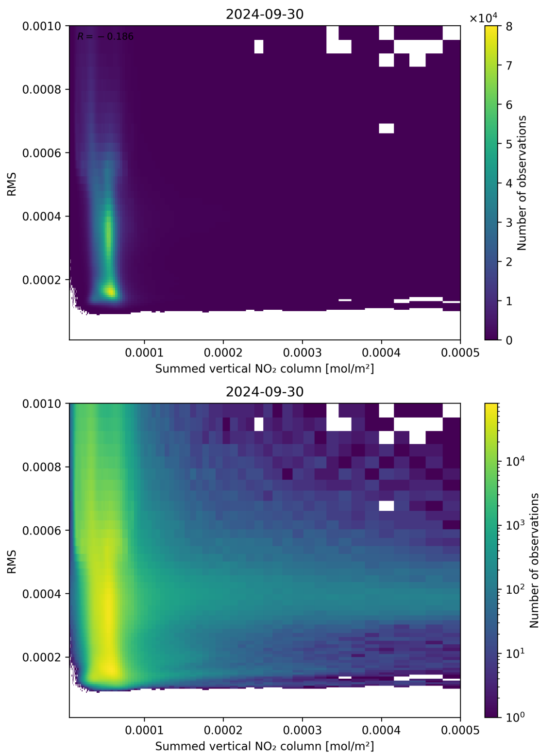
Figure 109: Scatter density plot of “Summed vertical NO 2 column” against “RMS” for 2024-09-29 to 2024-10-01.
