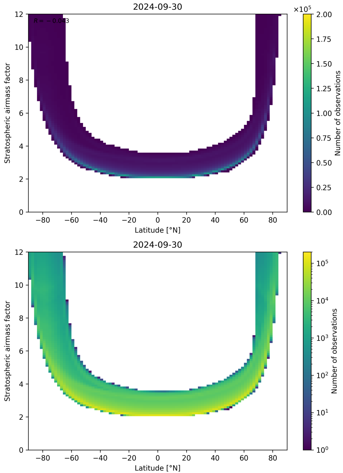
Figure 83: Scatter density plot of “Latitude” against “Stratospheric airmass factor” for 2024-09-29 to 2024-10-01.
