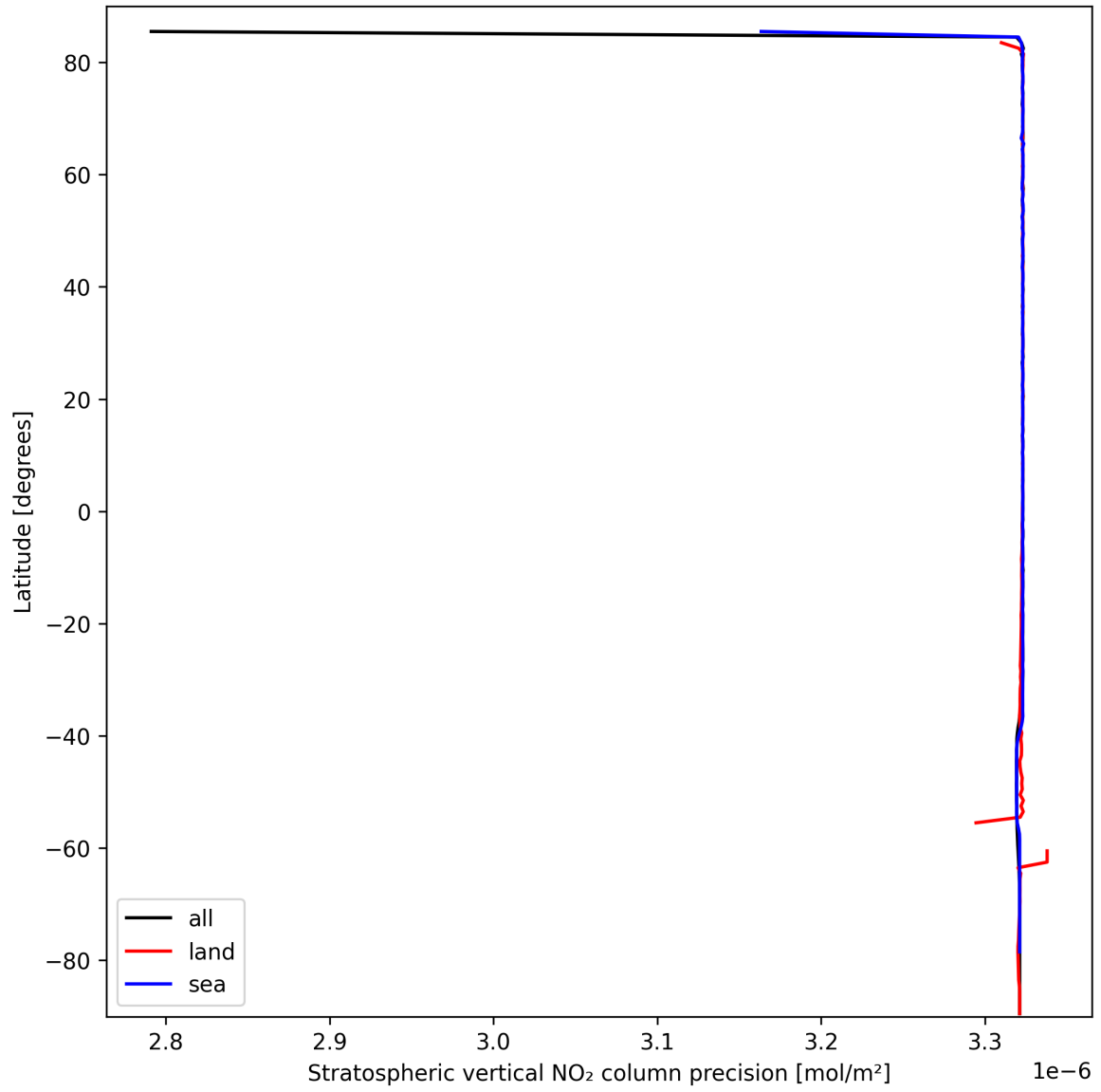
Figure 20: Zonal average of “Stratospheric vertical NO 2 column precision” for 2024-09-29 to 2024-10-01.
