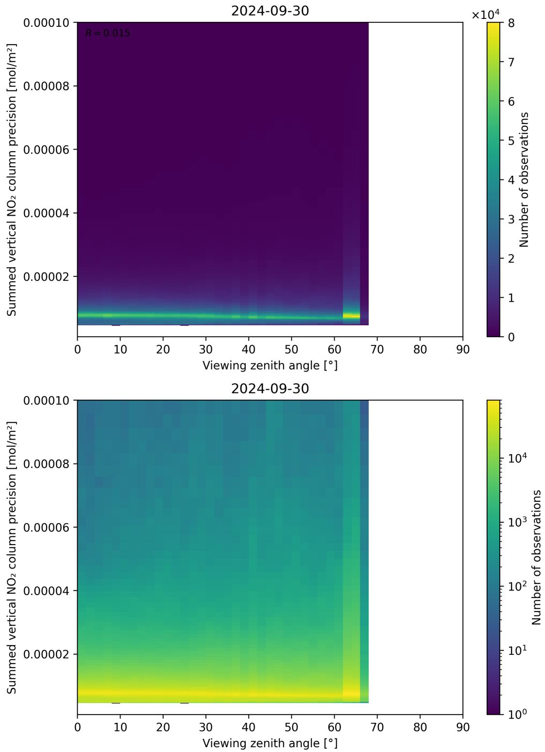
Figure 166: Scatter density plot of “Viewing zenith angle” against “Summed vertical NO 2 column precision” for 2024-09-29 to 2024-10-01.
