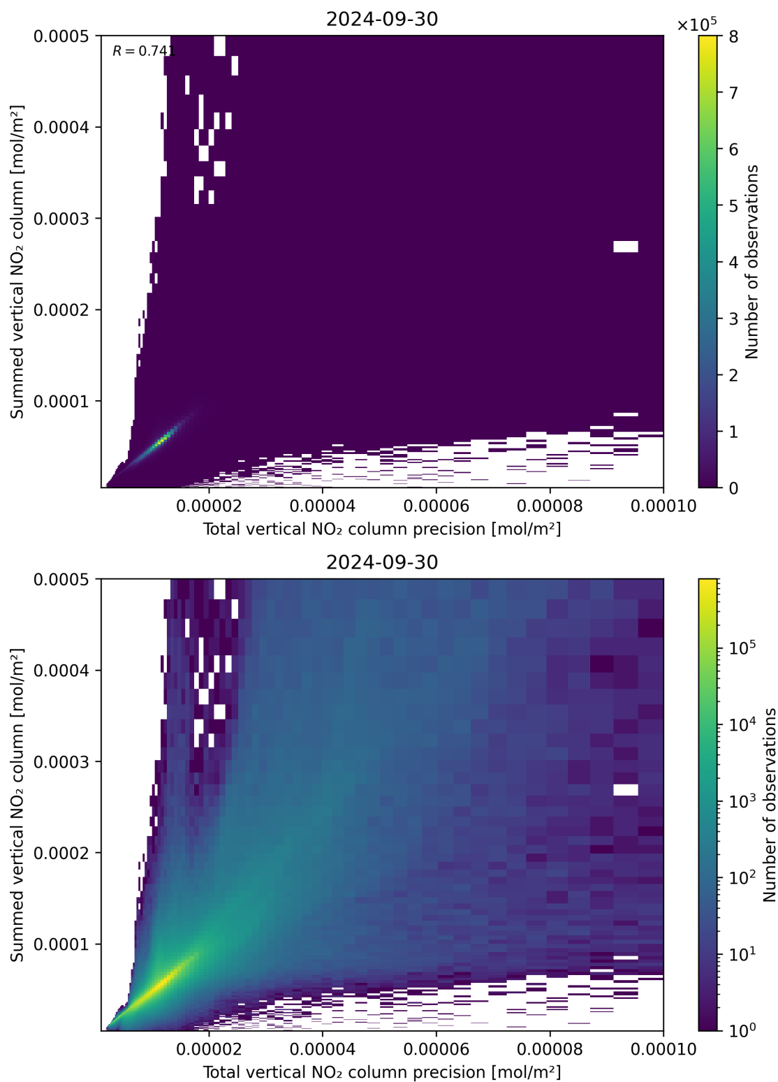
Figure 117: Scatter density plot of “Total vertical NO 2 column precision” against “Summed vertical NO 2 column” for 2024-09-29 to 2024-10-01.
