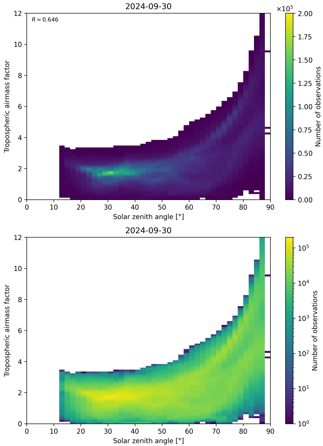
Figure 147: Scatter density plot of “Solar zenith angle” against “Tropospheric airmass factor” for 2024-09-29 to 2024-10-01.
