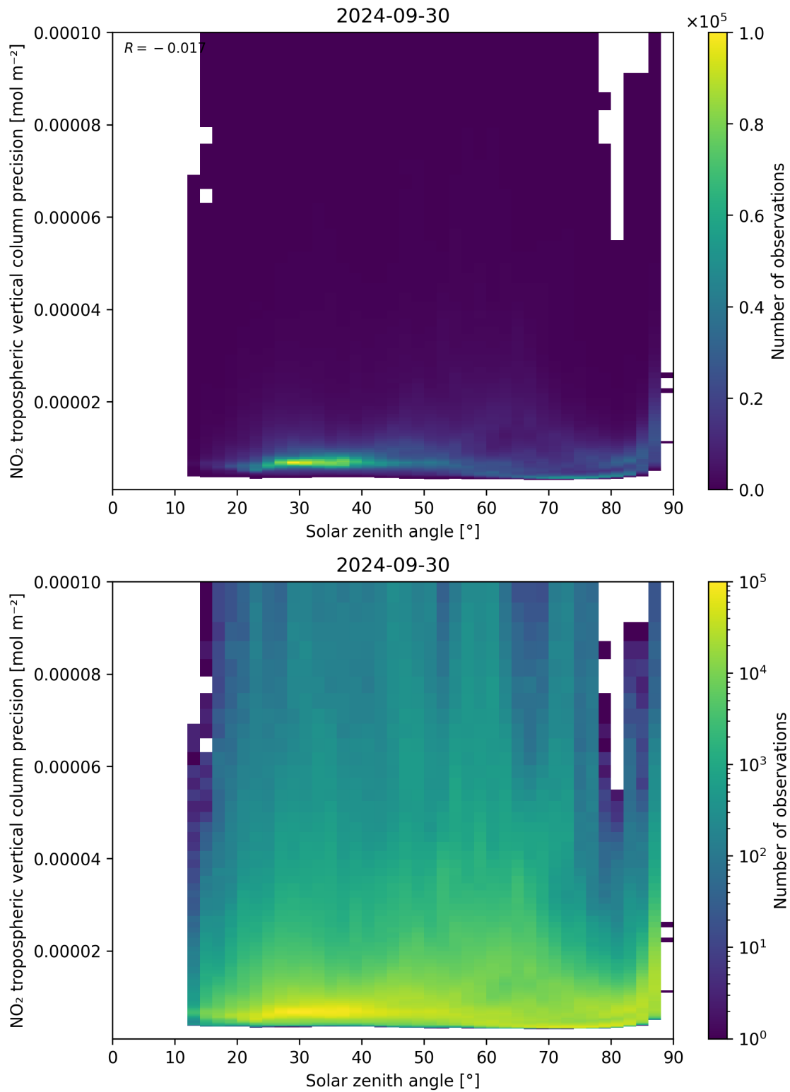
Figure 156: Scatter density plot of “Solar zenith angle” against “NO 2 tropospheric vertical column precision” for 2024-09-29 to 2024-10-01.
