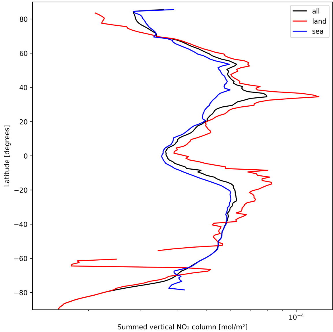
Figure 23: Zonal average of “Summed vertical NO 2 column” for 2024-09-29 to 2024-10-01.
