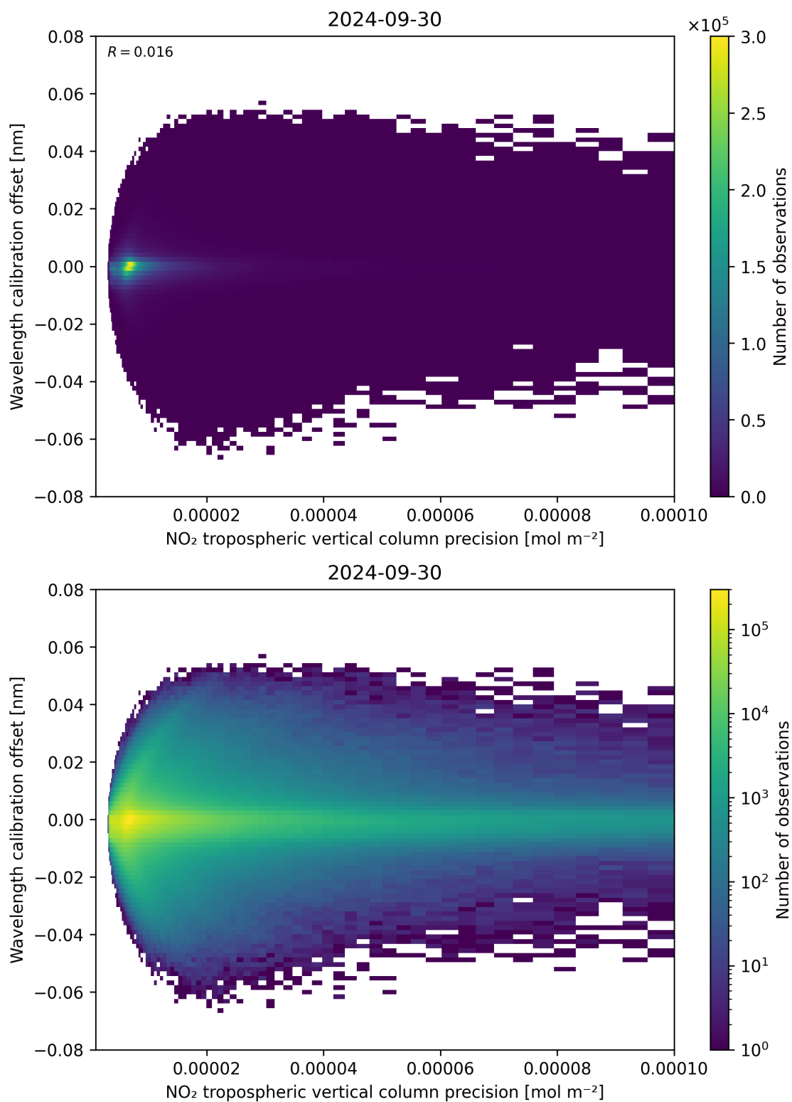
Figure 141: Scatter density plot of “NO 2 tropospheric vertical column precision” against “Wavelength calibration offset” for 2024-09-29 to 2024-10-01.
