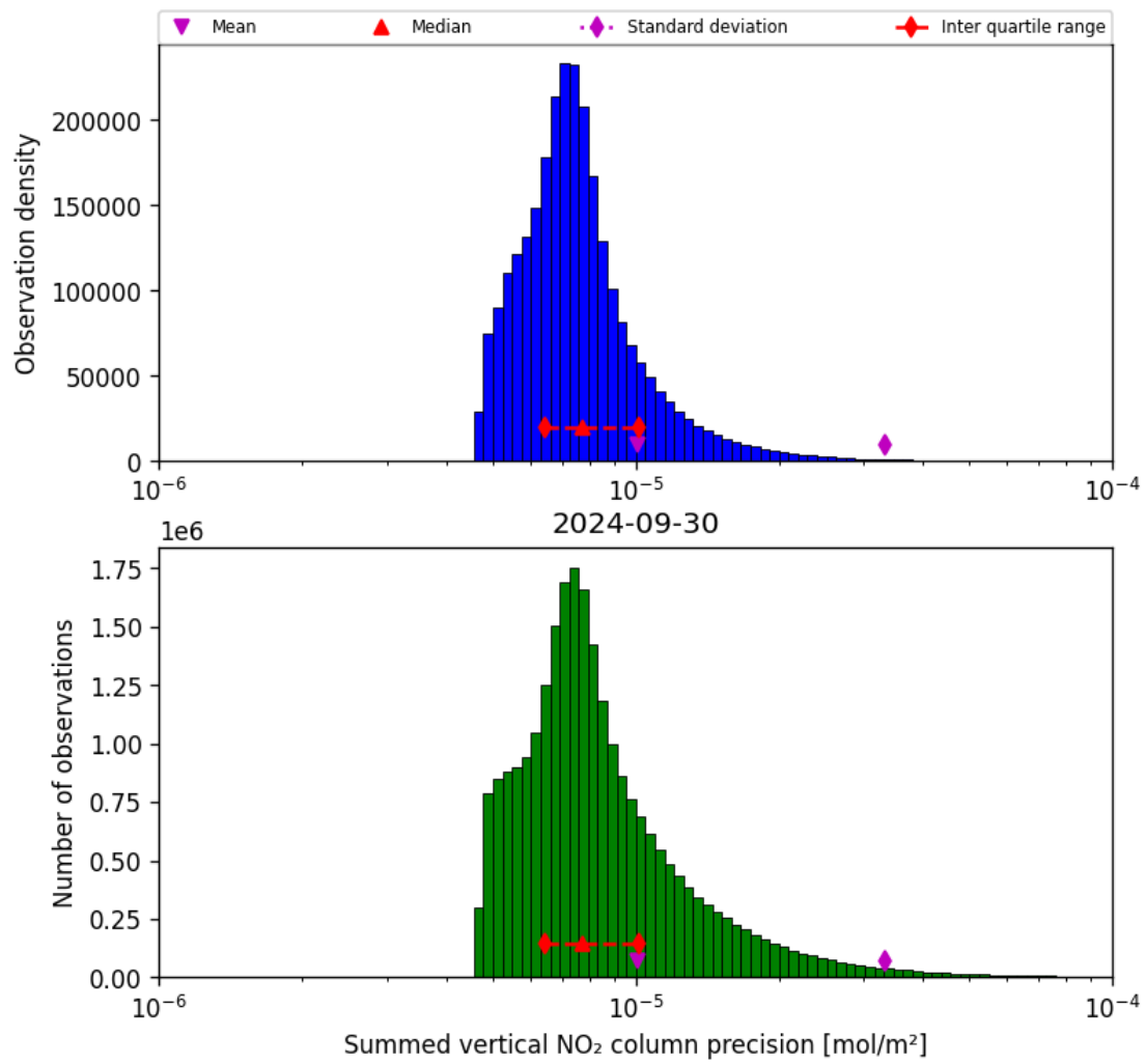
Figure 41: Histogram of “Summed vertical NO 2 column precision” for 2024-09-29 to 2024-10-01
