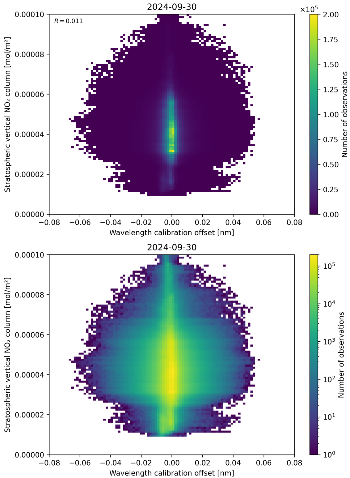
Figure 176: Scatter density plot of “Wavelength calibration offset” against “Stratospheric vertical NO 2 column” for 2024-09-29 to 2024-10-01.
