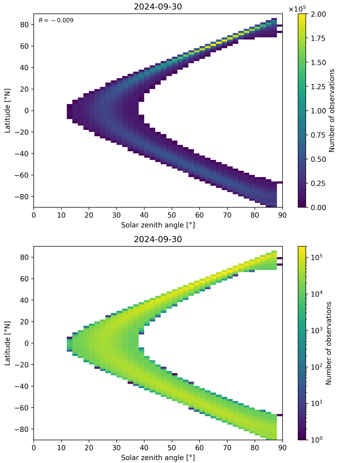
Figure 149: Scatter density plot of “Solar zenith angle” against “Latitude” for 2024-09-29 to 2024-10-01.
