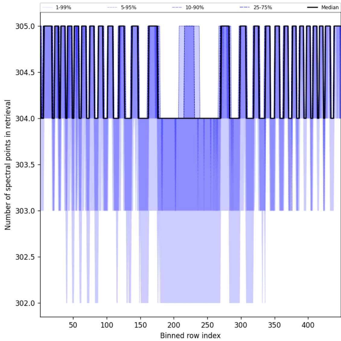
Figure 50: Along track statistics of “Number of spectral points in retrieval” for 2024-09-29 to 2024-10-01
