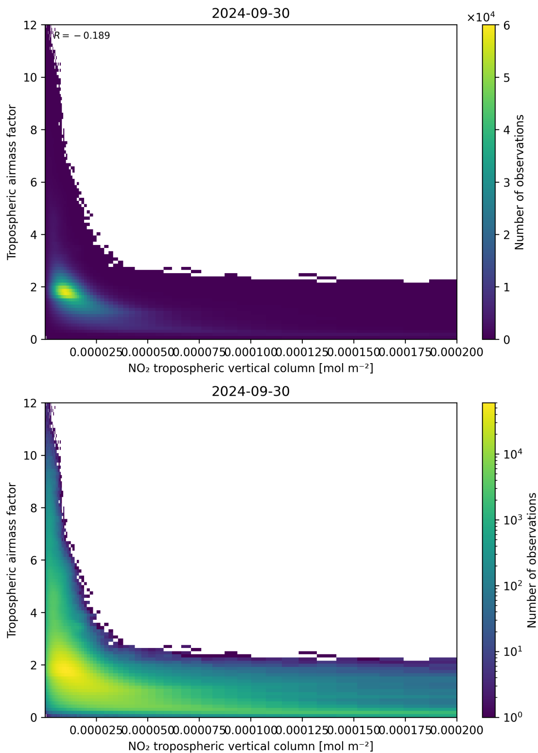
Figure 123: Scatter density plot of “NO 2 tropospheric vertical column” against “Tropospheric air mass factor” for 2024-09-29 to 2024-10-01.
