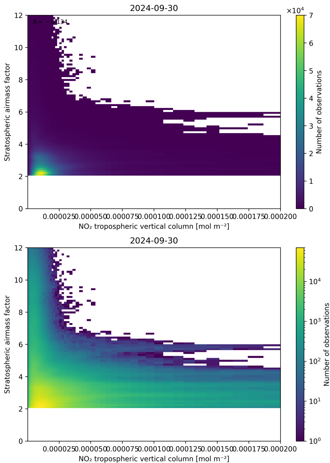
Figure 121: Scatter density plot of “NO 2 tropospheric vertical column” against “Stratospheric airmass factor” for 2024-09-29 to 2024-10-01.
