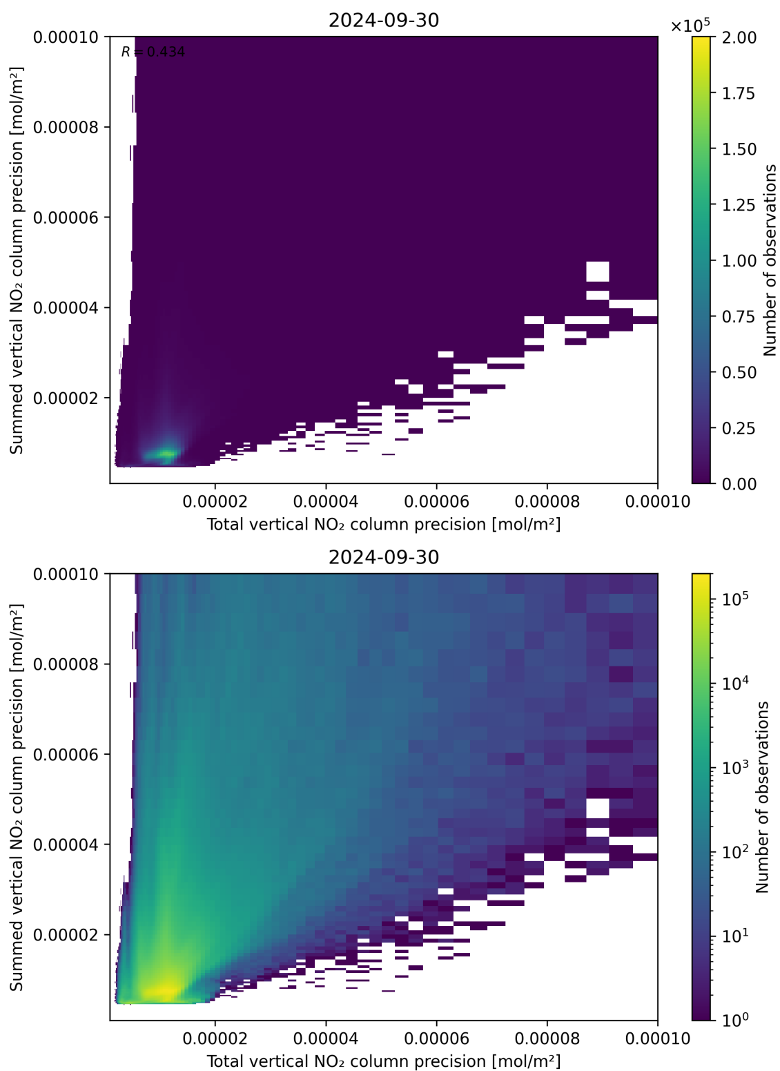
Figure 118: Scatter density plot of “Total vertical NO 2 column precision” against “Summed vertical NO 2 column precision” for 2024-09-29 to 2024-10-01.
