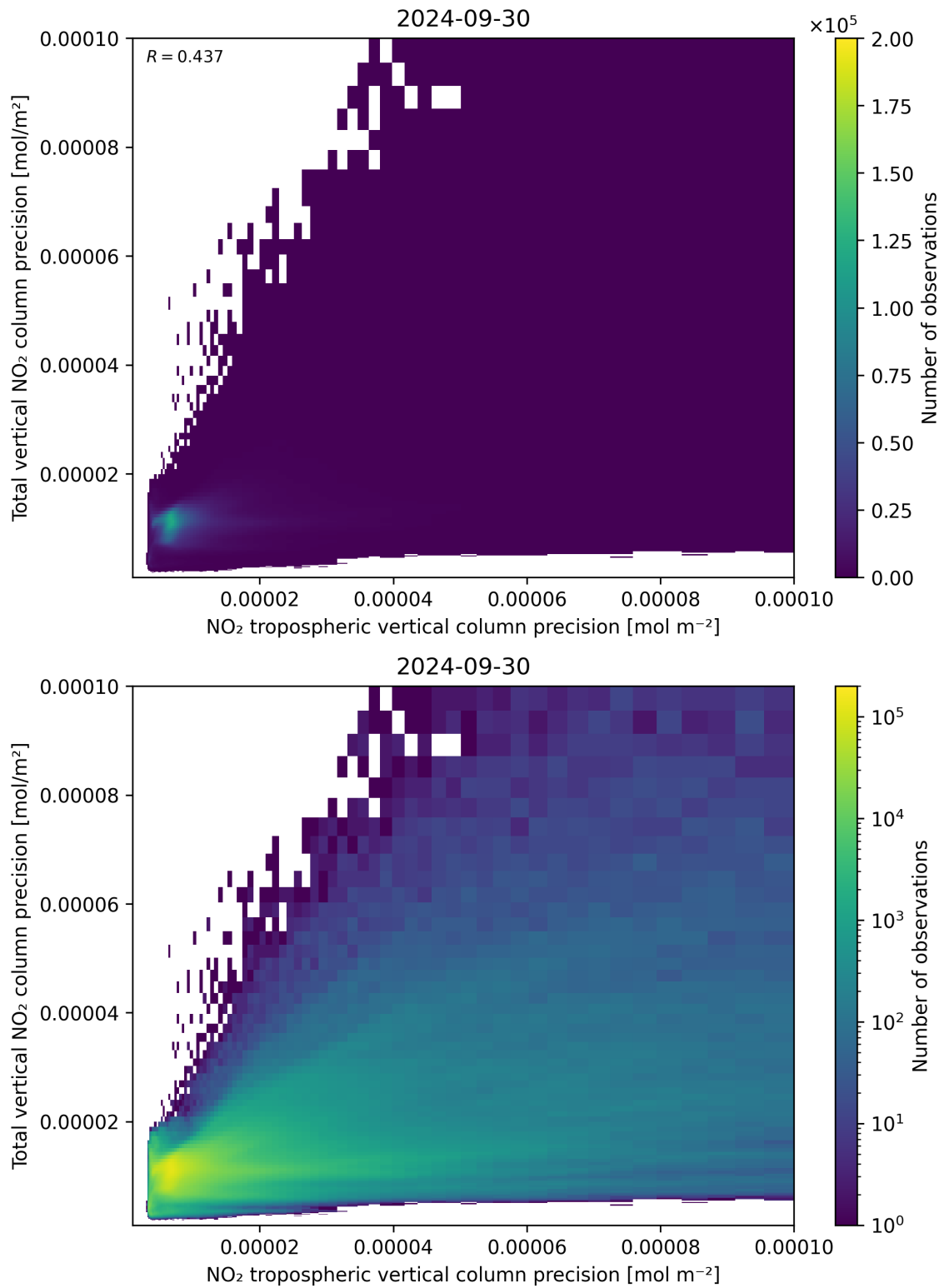
Figure 139: Scatter density plot of “NO 2 tropospheric vertical column precision” against “Total vertical NO 2 column precision” for 2024-09-29 to 2024-10-01.
