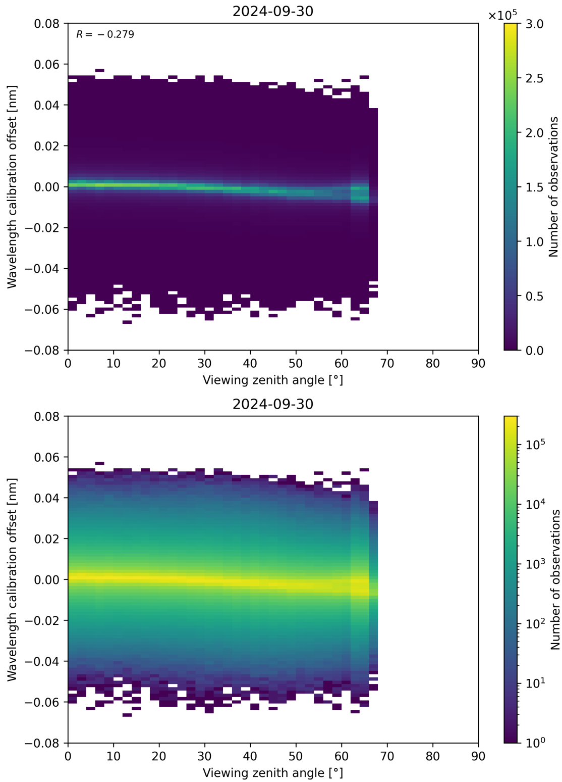
Figure 173: Scatter density plot of “Viewing zenith angle” against “Wavelength calibration offset” for 2024-09-29 to 2024-10-01.
