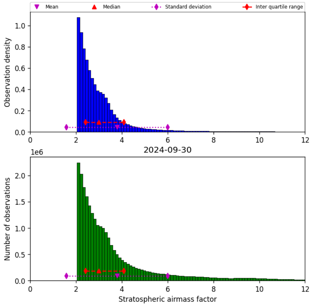
Figure 44: Histogram of “Stratospheric airmass factor” for 2024-09-29 to 2024-10-01
