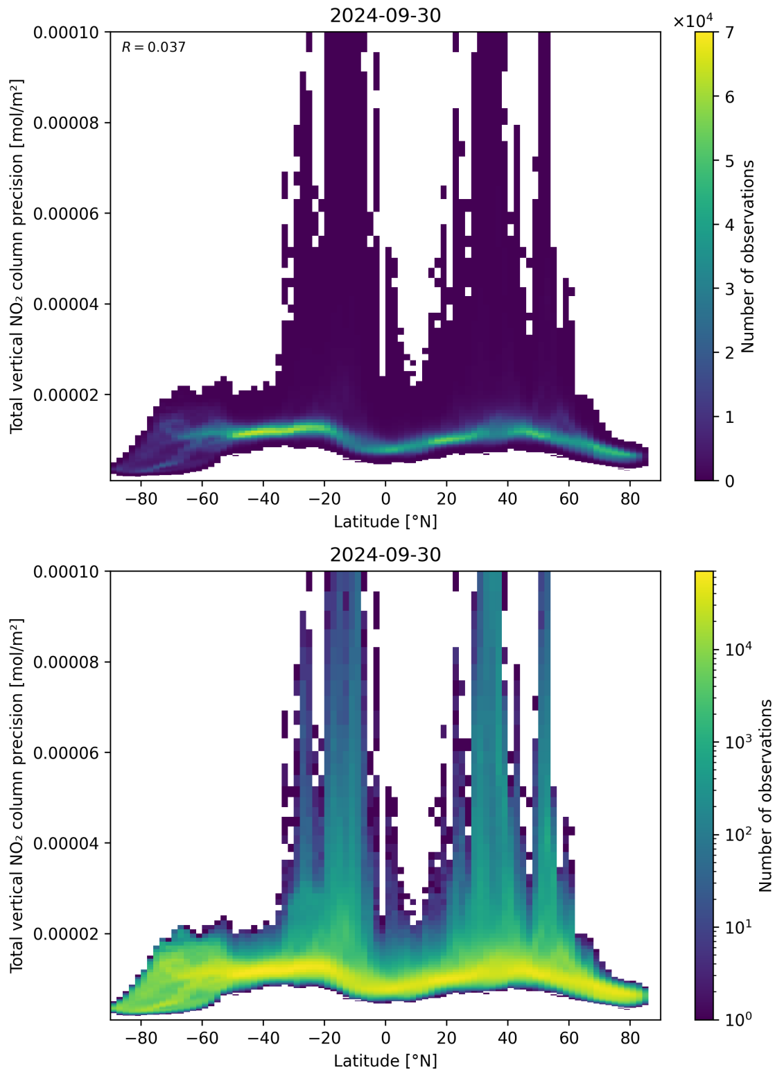
Figure 91: Scatter density plot of “Latitude” against “Total vertical NO 2 column precision” for 2024-09-29 to 2024-10-01.
