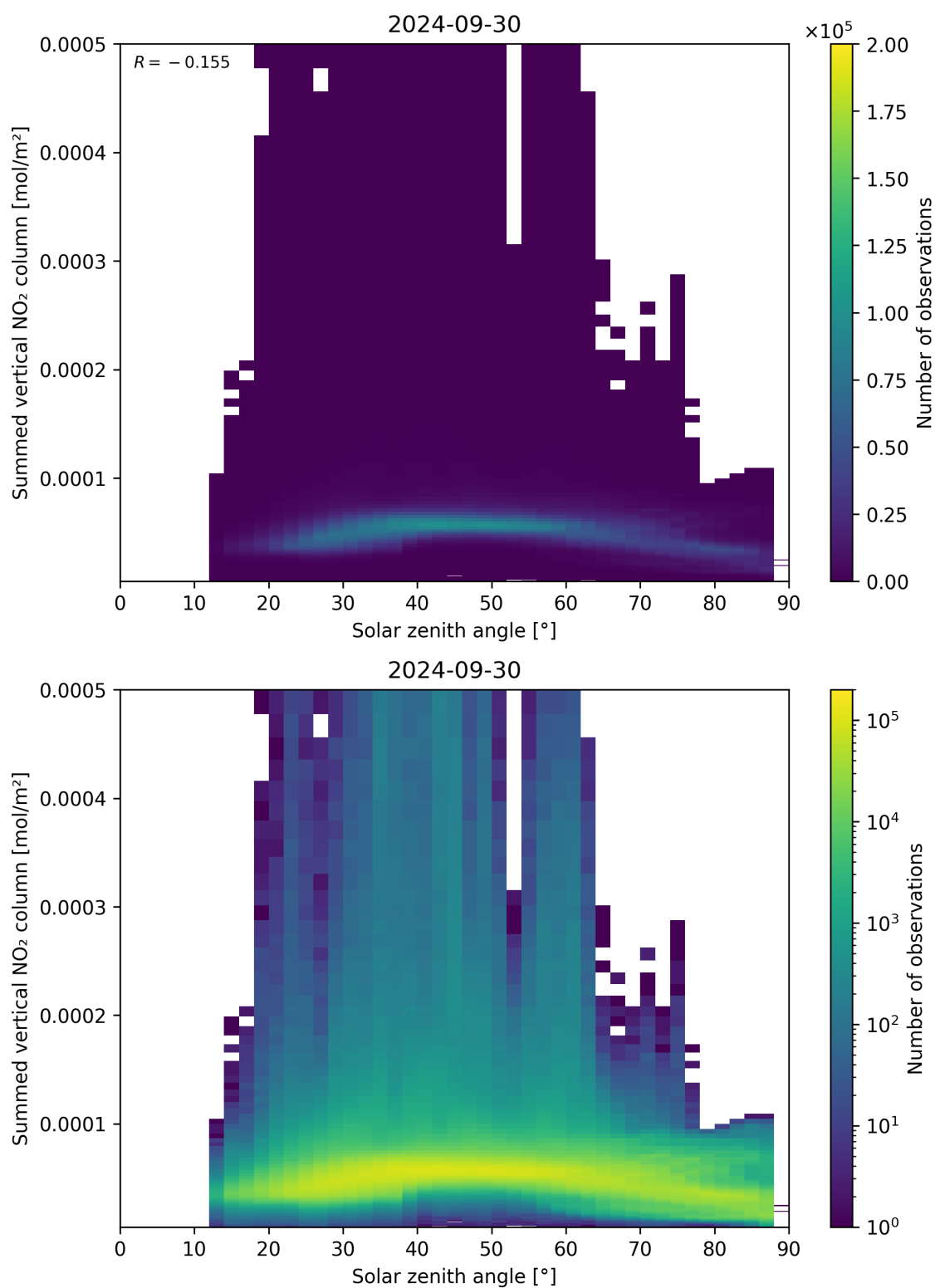
Figure 151: Scatter density plot of “Solar zenith angle” against “Summed vertical NO 2 column” for 2024-09-29 to 2024-10-01.
