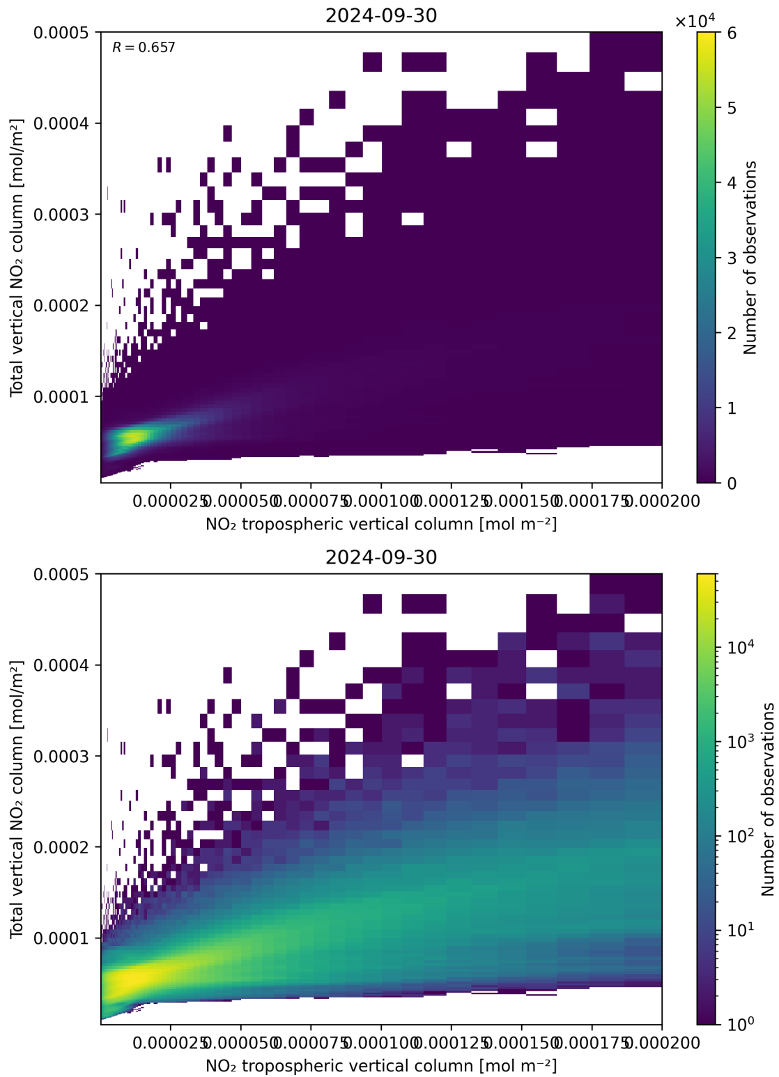
Figure 128: Scatter density plot of “NO 2 tropospheric vertical column” against “Total vertical NO 2 column” for 2024-09-29 to 2024-10-01.
