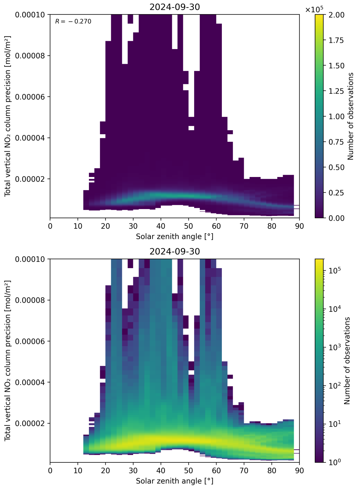
Figure 154: Scatter density plot of “Solar zenith angle” against “Total vertical NO 2 column precision” for 2024-09-29 to 2024-10-01.
