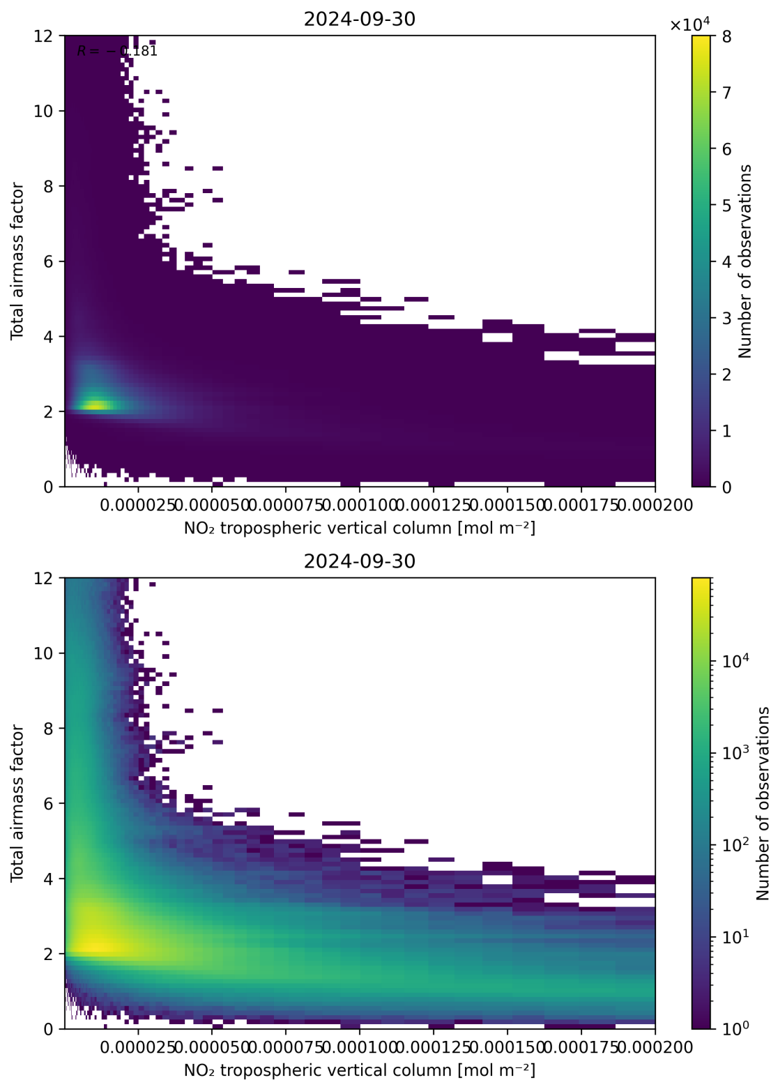
Figure 122: Scatter density plot of “NO 2 tropospheric vertical column” against “Total air mass factor” for 2024-09-29 to 2024-10-01.
