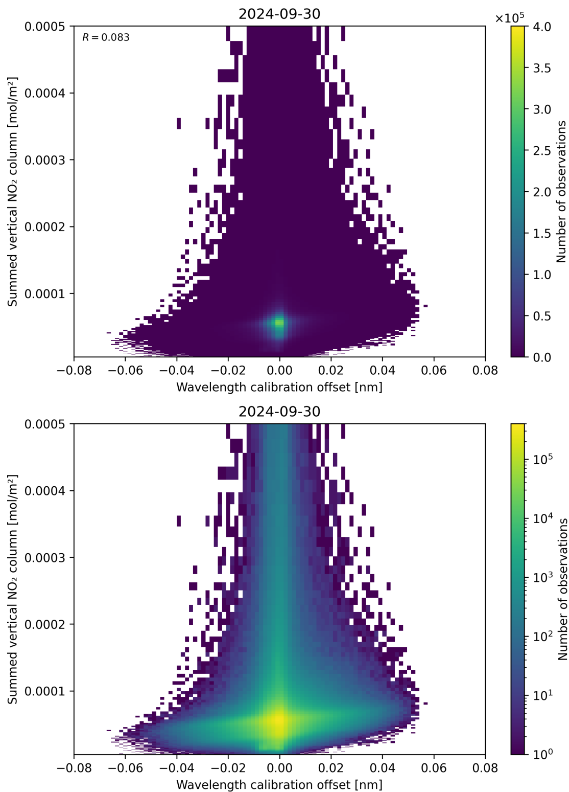
Figure 177: Scatter density plot of “Wavelength calibration offset” against “Summed vertical NO 2 column” for 2024-09-29 to 2024-10-01.
