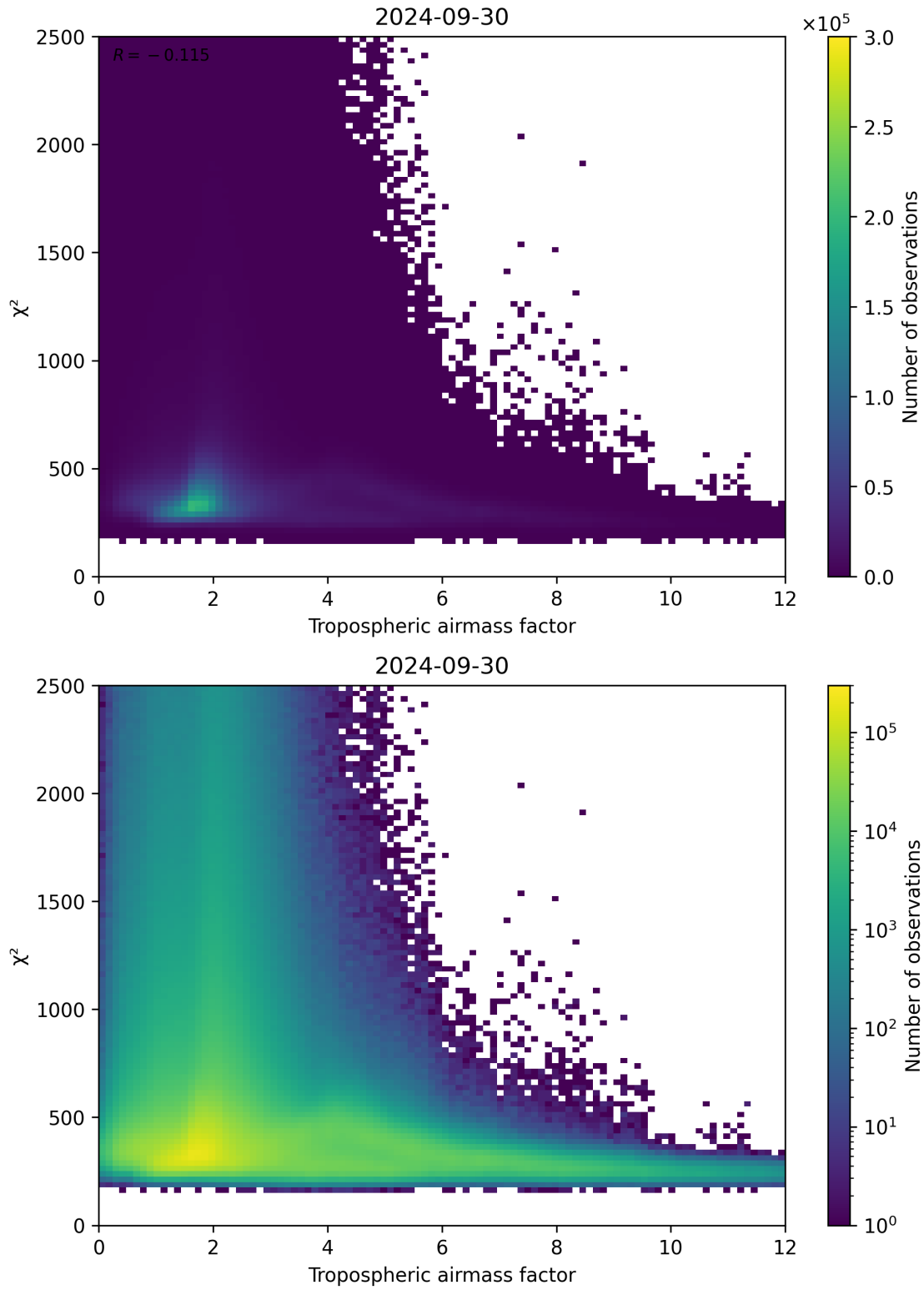
Figure 73: Scatter density plot of “Tropospheric airmass factor” against “ \chi^2 ” for 2024-09-29 to 2024-10-01.
