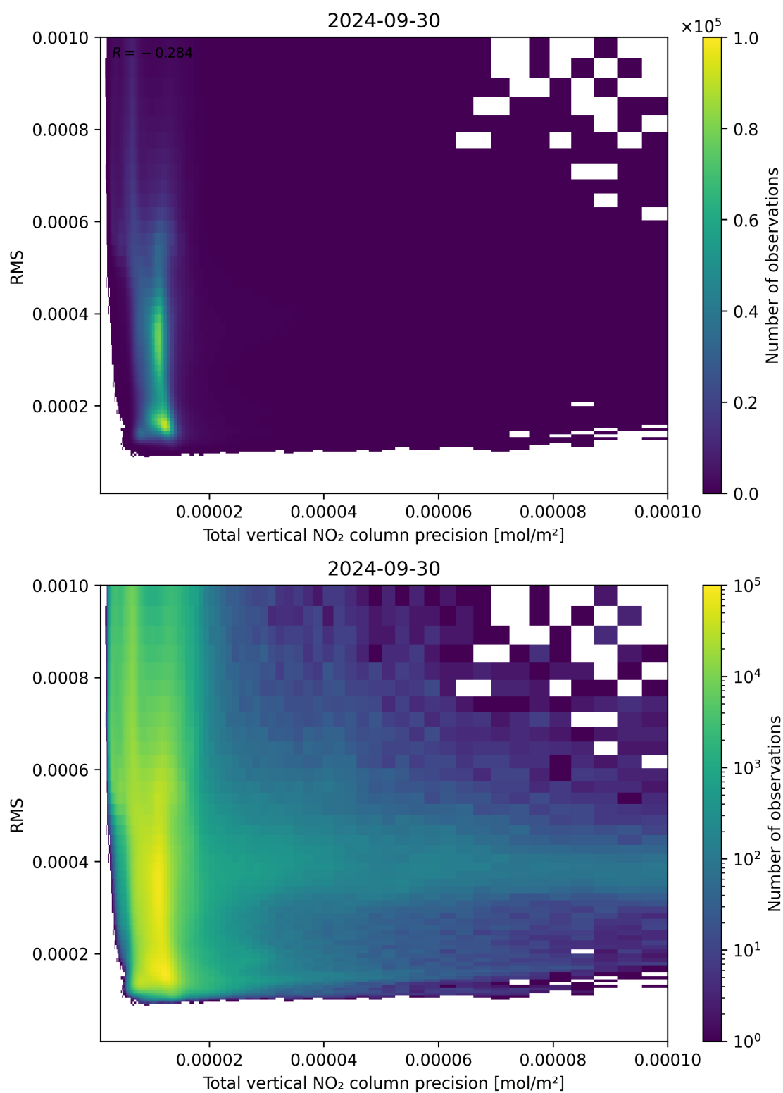
Figure 119: Scatter density plot of “Total vertical NO 2 column precision” against “RMS” for 2024-09-29 to 2024-10-01.
