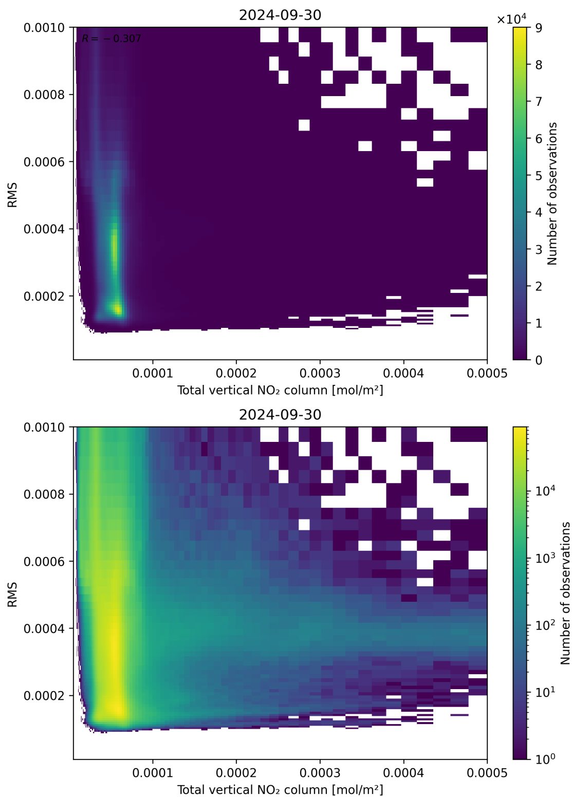
Figure 120: Scatter density plot of “Total vertical NO 2 column” against “RMS” for 2024-09-29 to 2024-10-01.
