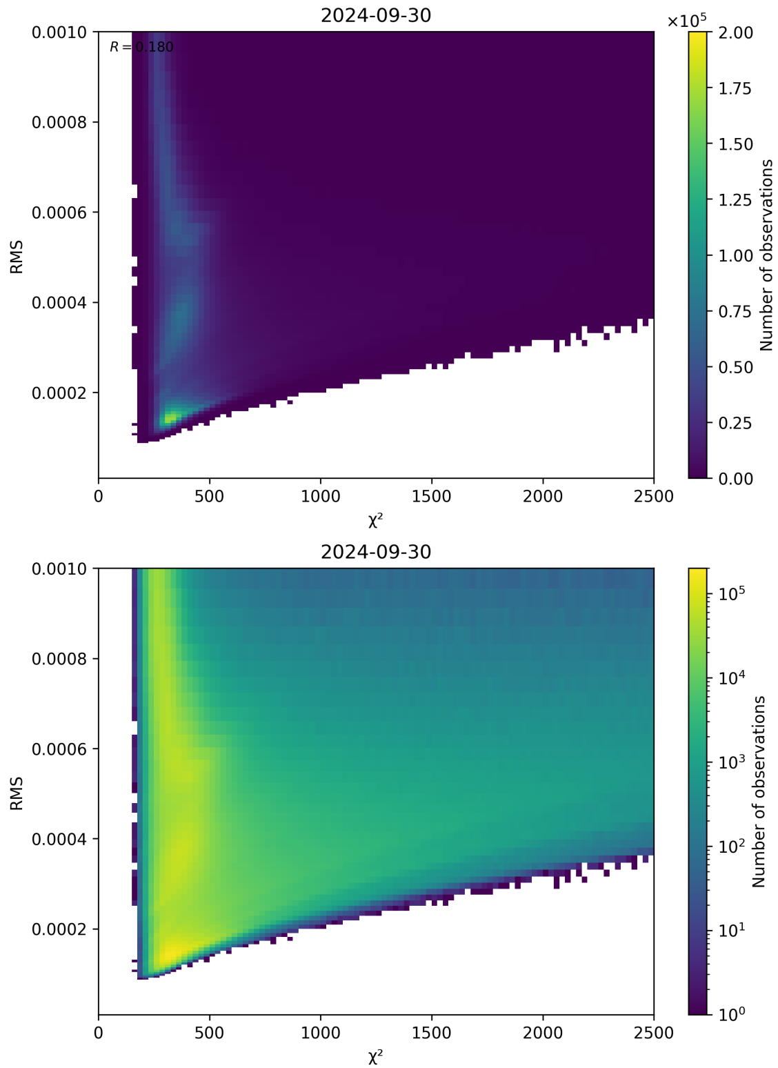
Figure 82: Scatter density plot of “ \chi^2 ” against “RMS” for 2024-09-29 to 2024-10-01.
