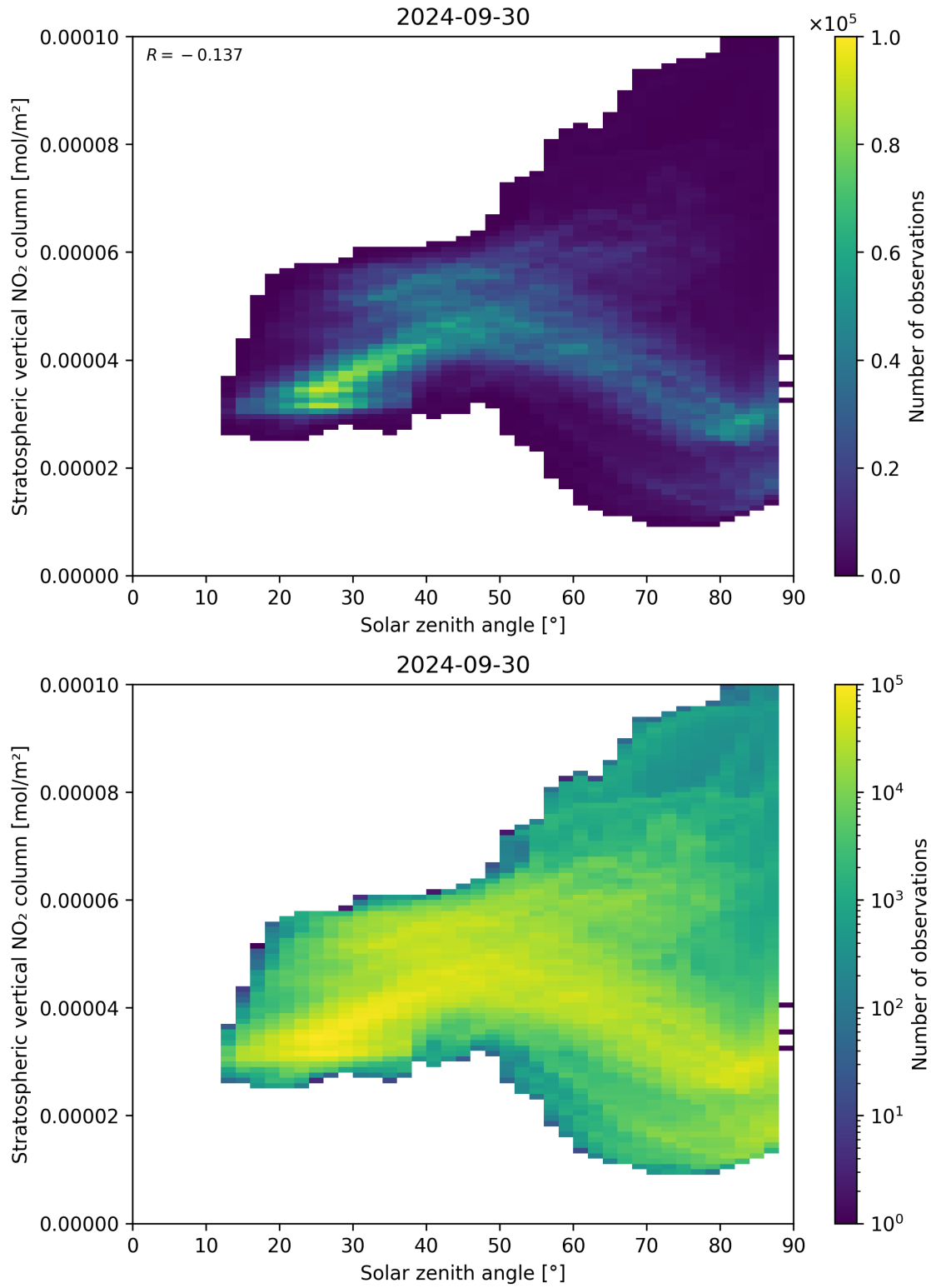
Figure 150: Scatter density plot of “Solar zenith angle” against “Stratospheric vertical NO 2 column” for 2024-09-29 to 2024-10-01.
