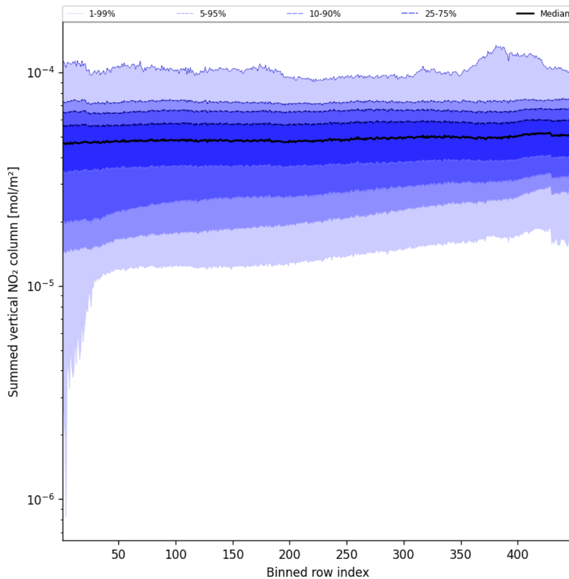
Figure 57: Along track statistics of “Summed vertical NO 2 column” for 2024-09-29 to 2024-10-01
