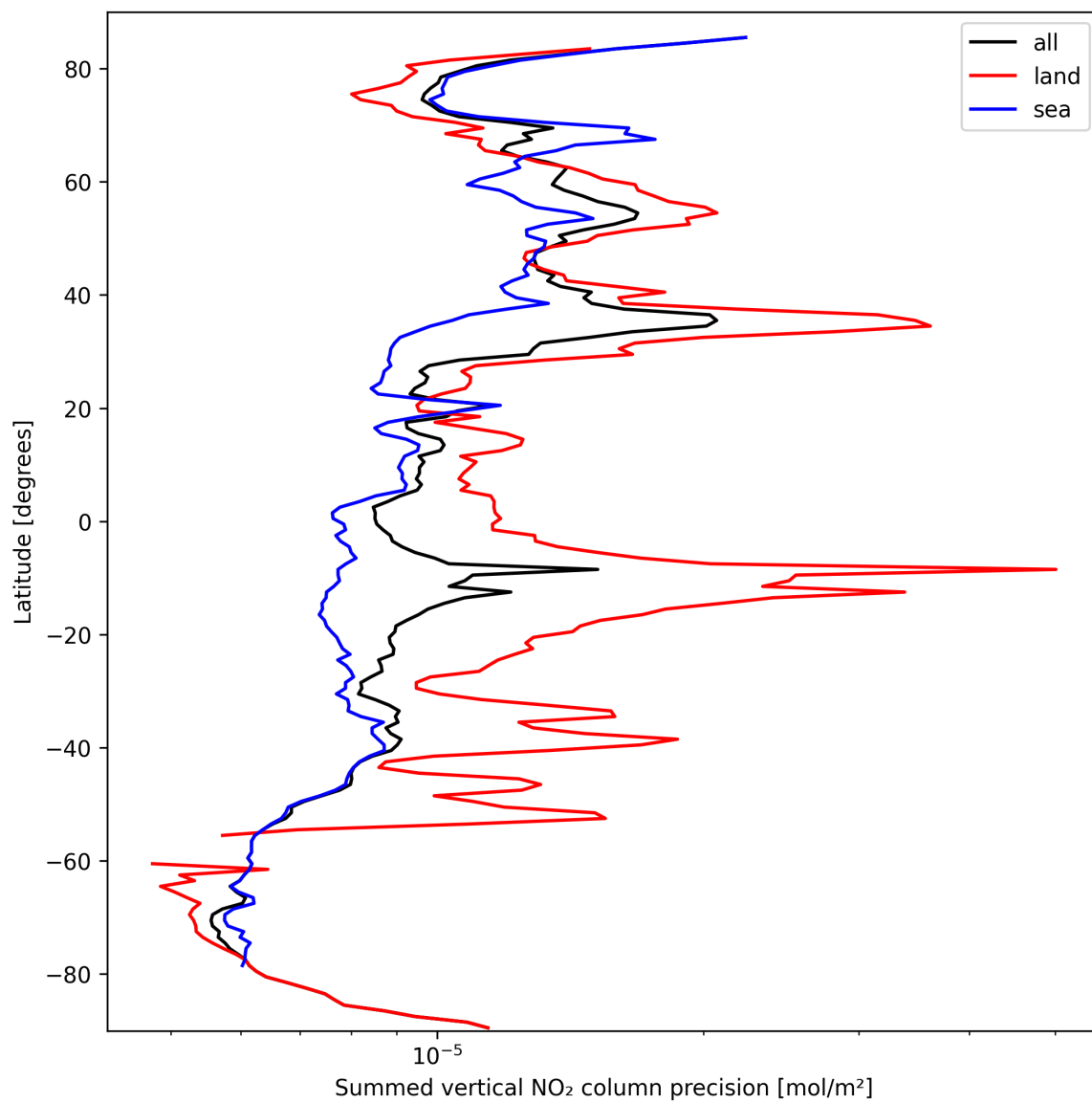
Figure 24: Zonal average of “Summed vertical NO 2 column precision” for 2024-09-29 to 2024-10-01.
