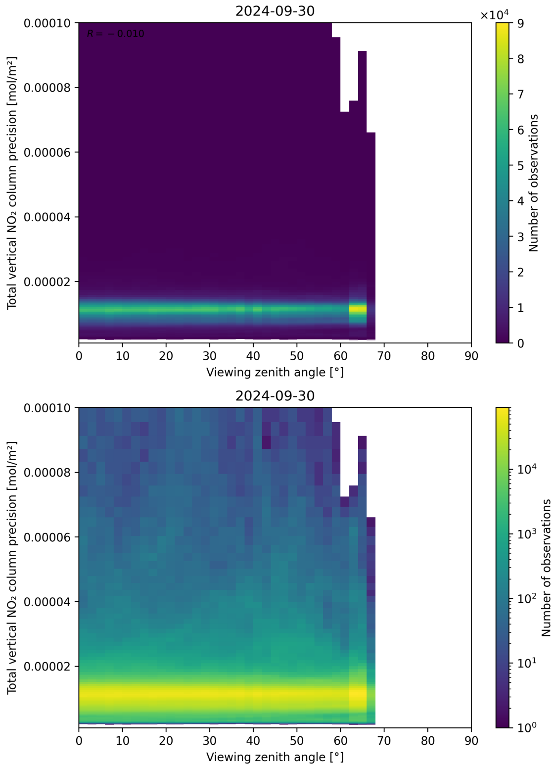
Figure 168: Scatter density plot of “Viewing zenith angle” against “Total vertical NO 2 column precision” for 2024-09-29 to 2024-10-01.
