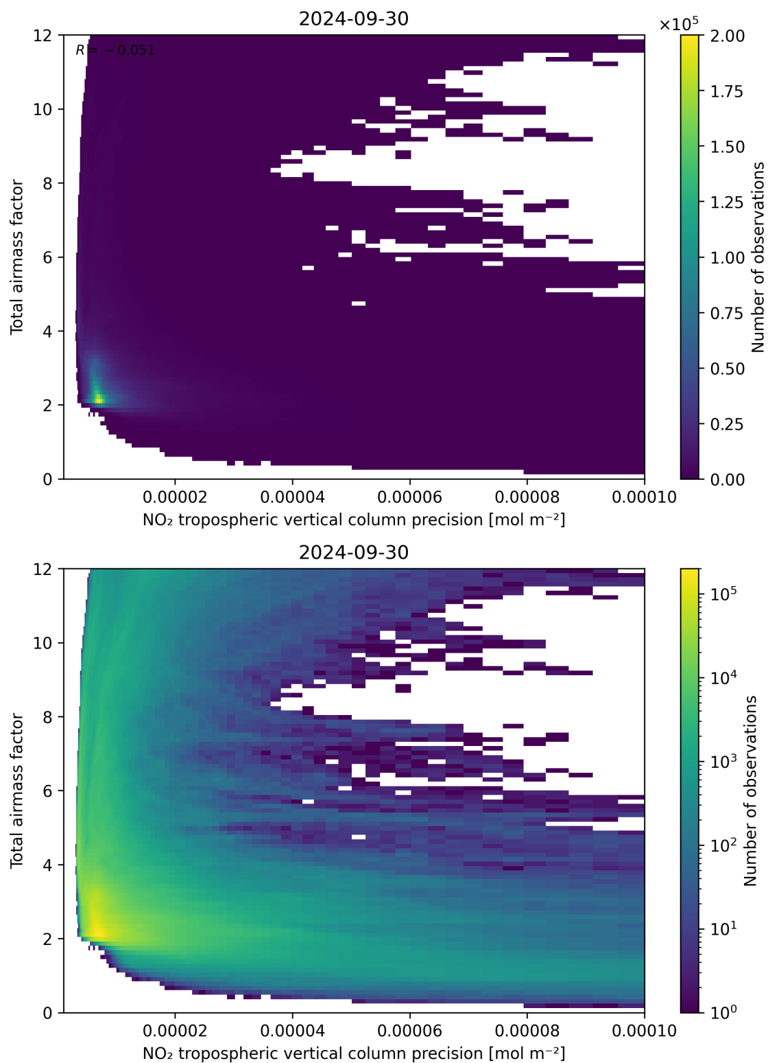
Figure 132: Scatter density plot of “NO 2 tropospheric vertical column precision” against “Total air mass factor” for 2024-09-29 to 2024-10-01.
