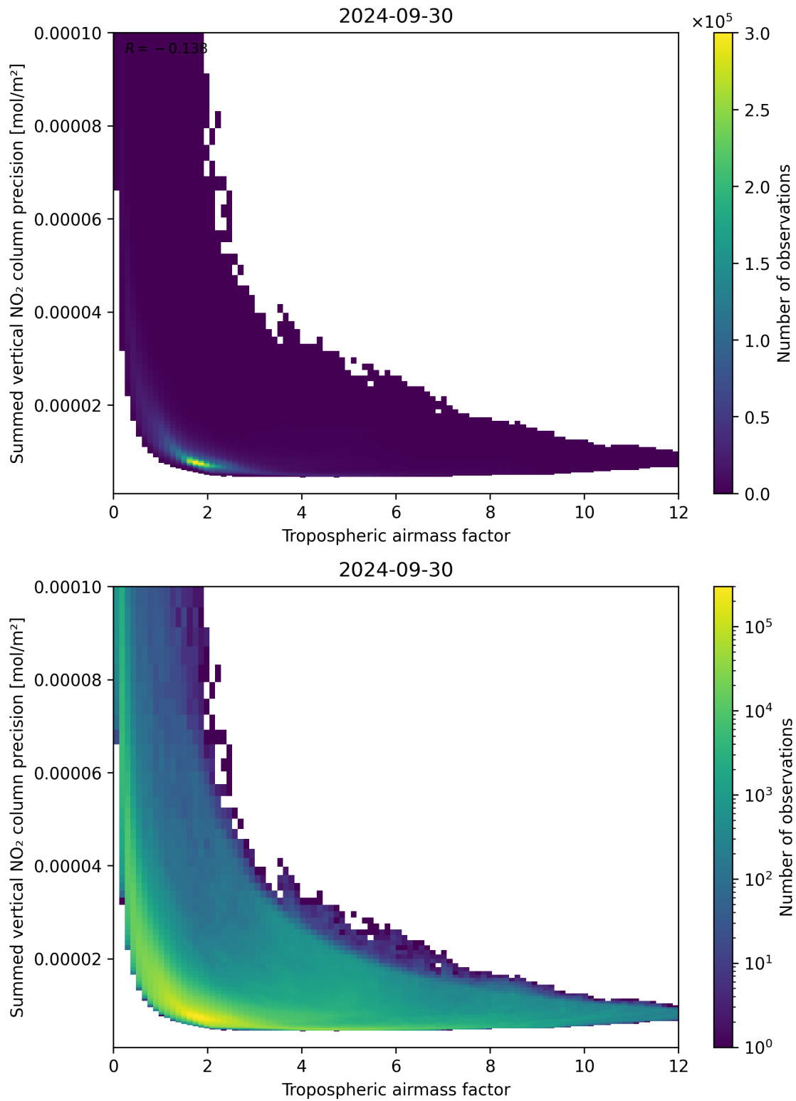
Figure 76: Scatter density plot of “Tropospheric air mass factor” against “Summed vertical NO 2 column precision” for 2024-09-29 to 2024-10-01.
