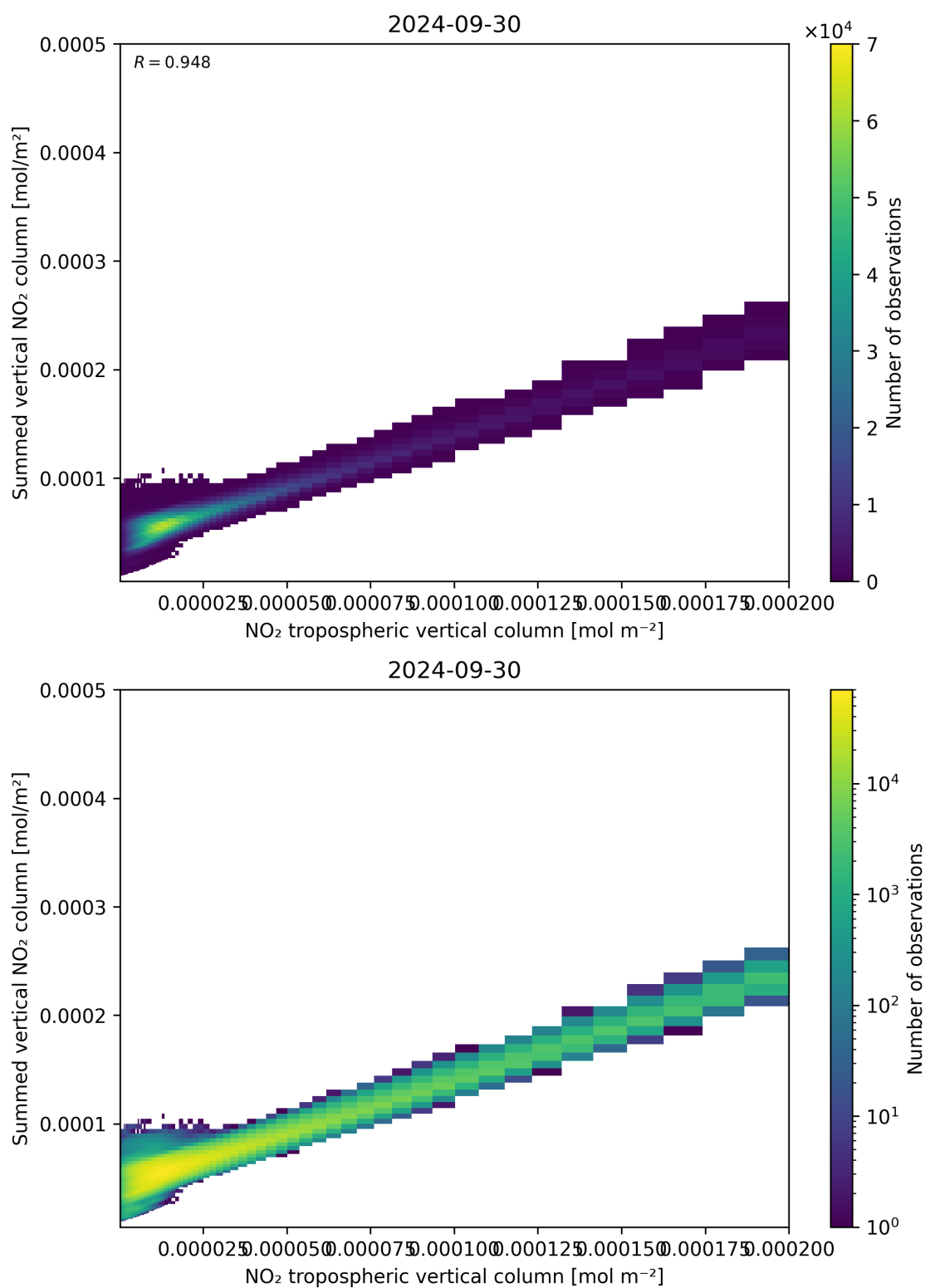
Figure 126: Scatter density plot of “NO 2 tropospheric vertical column” against “Summed vertical NO 2 column” for 2024-09-29 to 2024-10-01.
