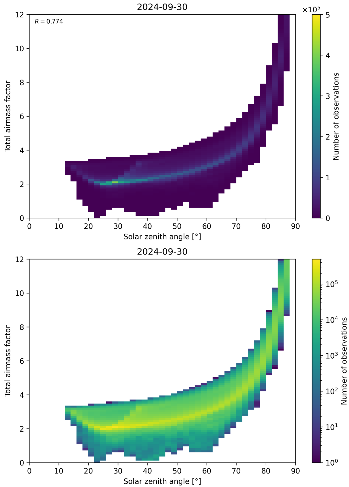
Figure 146: Scatter density plot of “Solar zenith angle” against “Total air mass factor” for 2024-09-29 to 2024-10-01.
