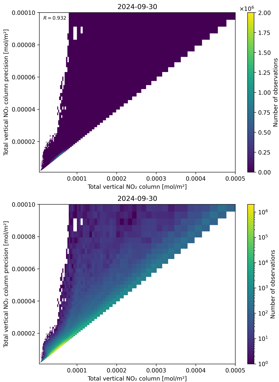
Figure 114: Scatter density plot of “Total vertical NO 2 column” against “Total vertical NO 2 column precision” for 2024-09-29 to 2024-10-01.
