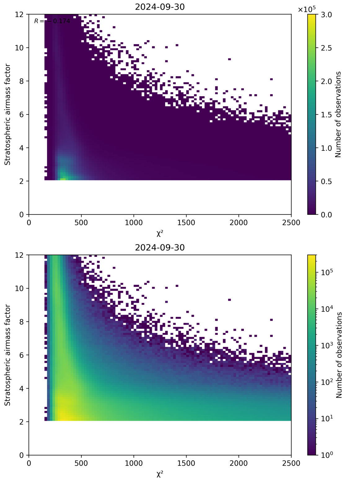
Figure 81: Scatter density plot of “ \chi^2 ” against “Stratospheric airmass factor” for 2024-09-29 to 2024-10-01.
