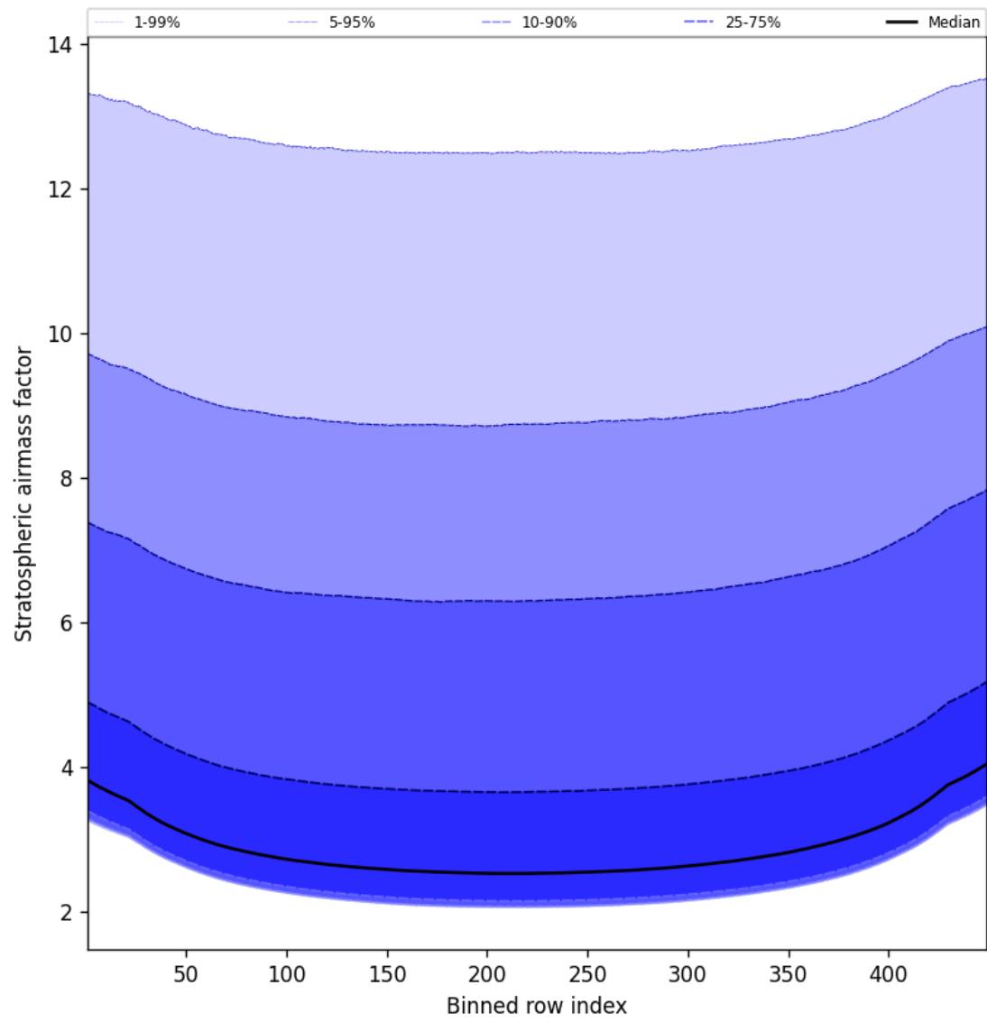
Figure 61: Along track statistics of “Stratospheric air mass factor” for 2024-09-29 to 2024-10-01
