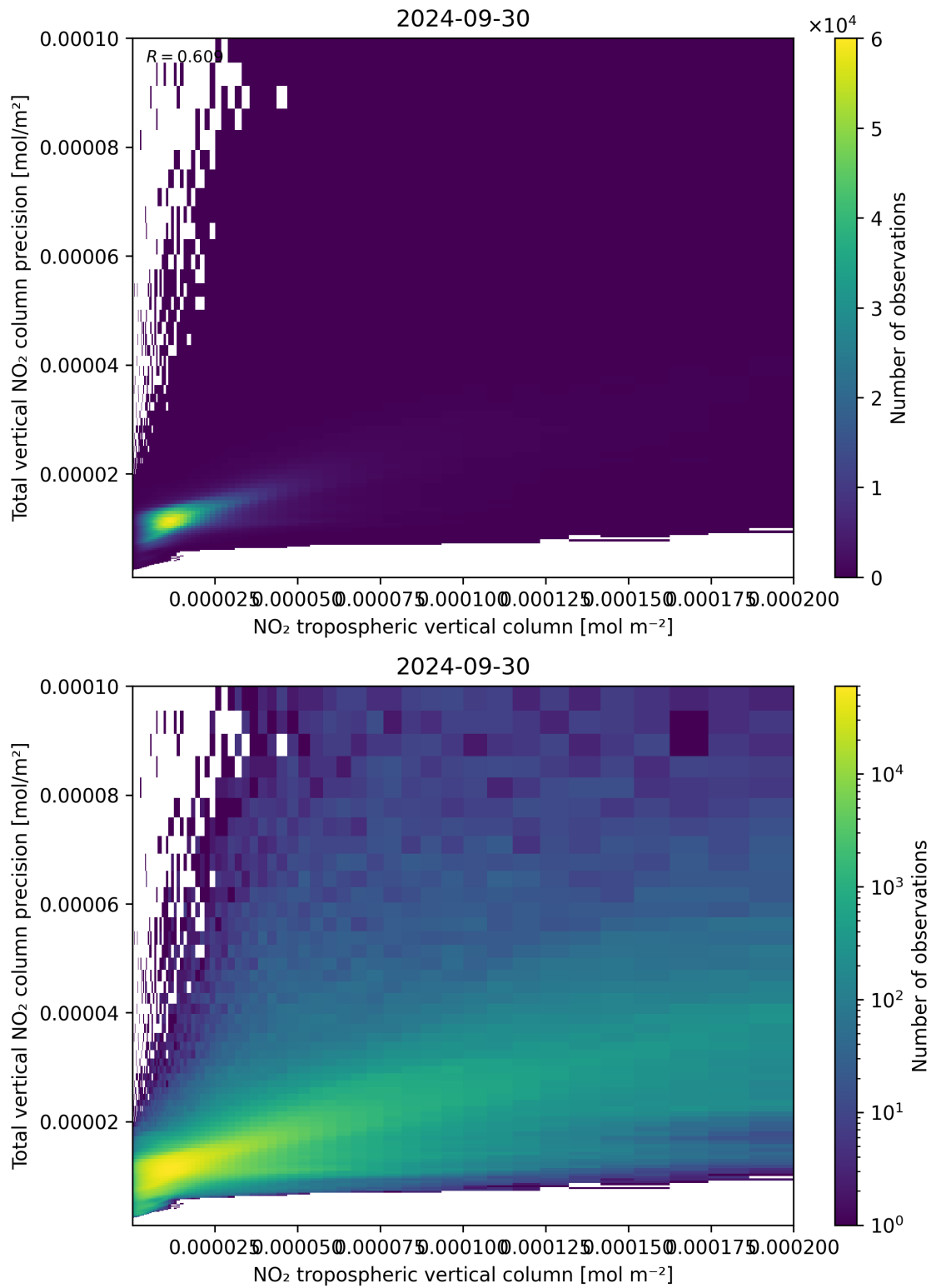
Figure 129: Scatter density plot of “NO 2 tropospheric vertical column” against “Total vertical NO 2 column precision” for 2024-09-29 to 2024-10-01.
