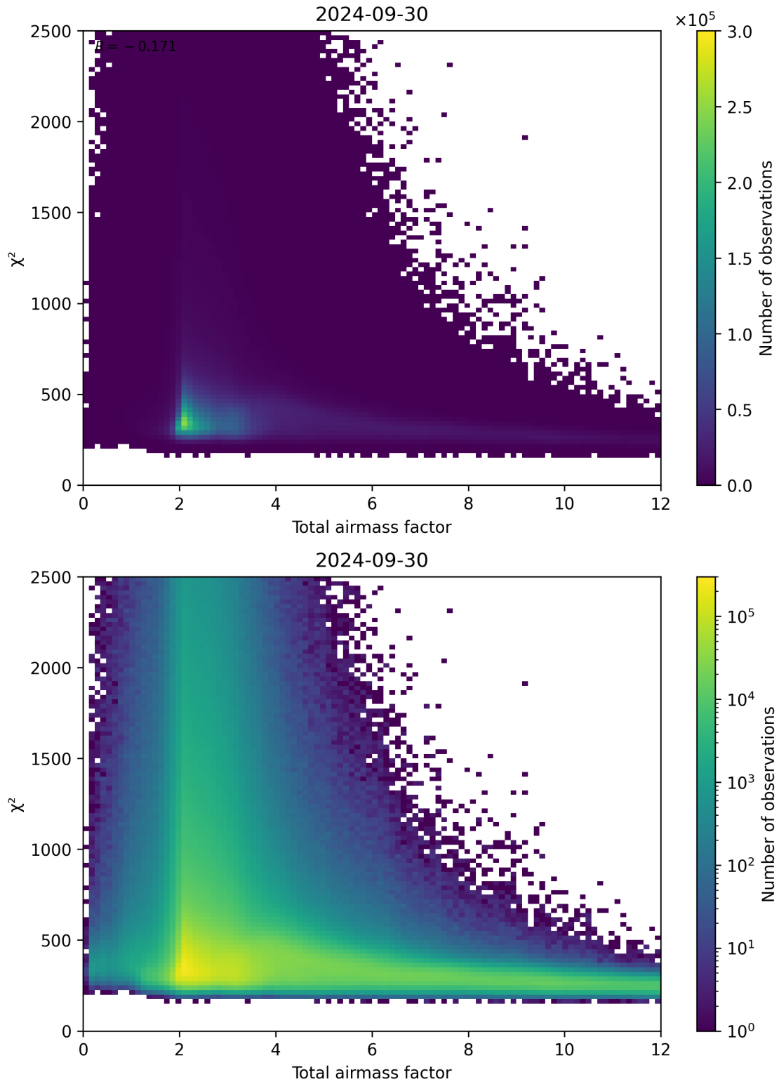
Figure 63: Scatter density plot of “Total airmass factor” against “ \chi^2 ” for 2024-09-29 to 2024-10-01.
