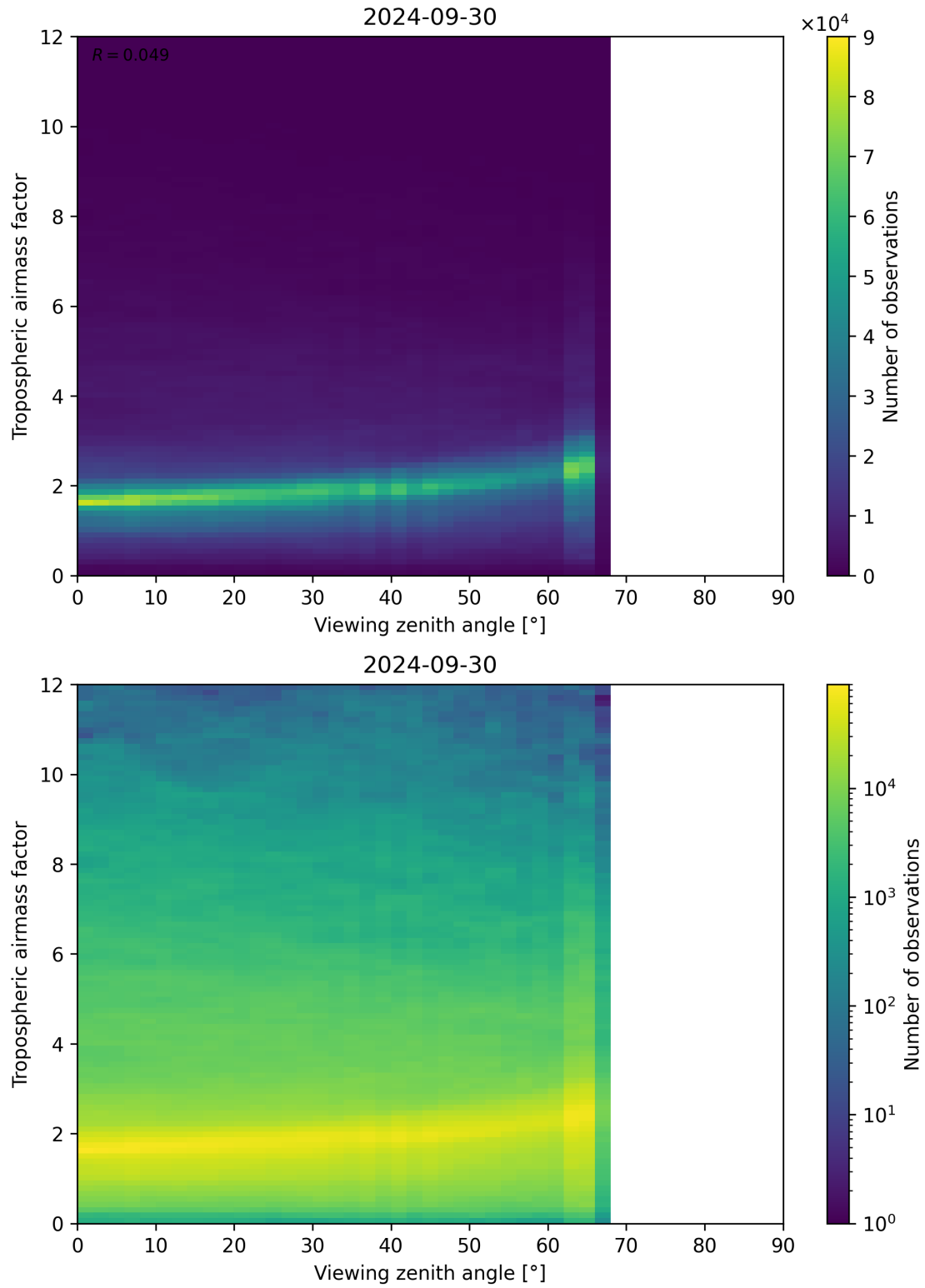
Figure 161: Scatter density plot of “Viewing zenith angle” against “Tropospheric airmass factor” for 2024-09-29 to 2024-10-01.
