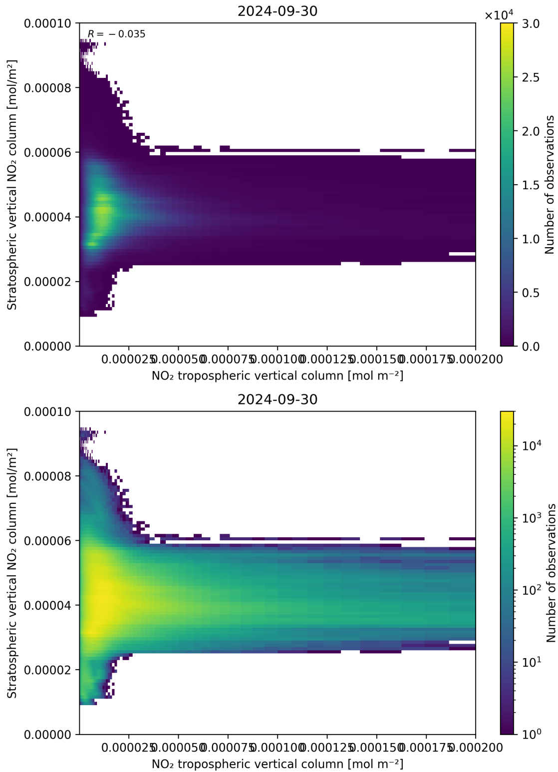
Figure 125: Scatter density plot of “NO 2 tropospheric vertical column” against “Stratospheric vertical NO 2 column” for 2024-09-29 to 2024-10-01.
