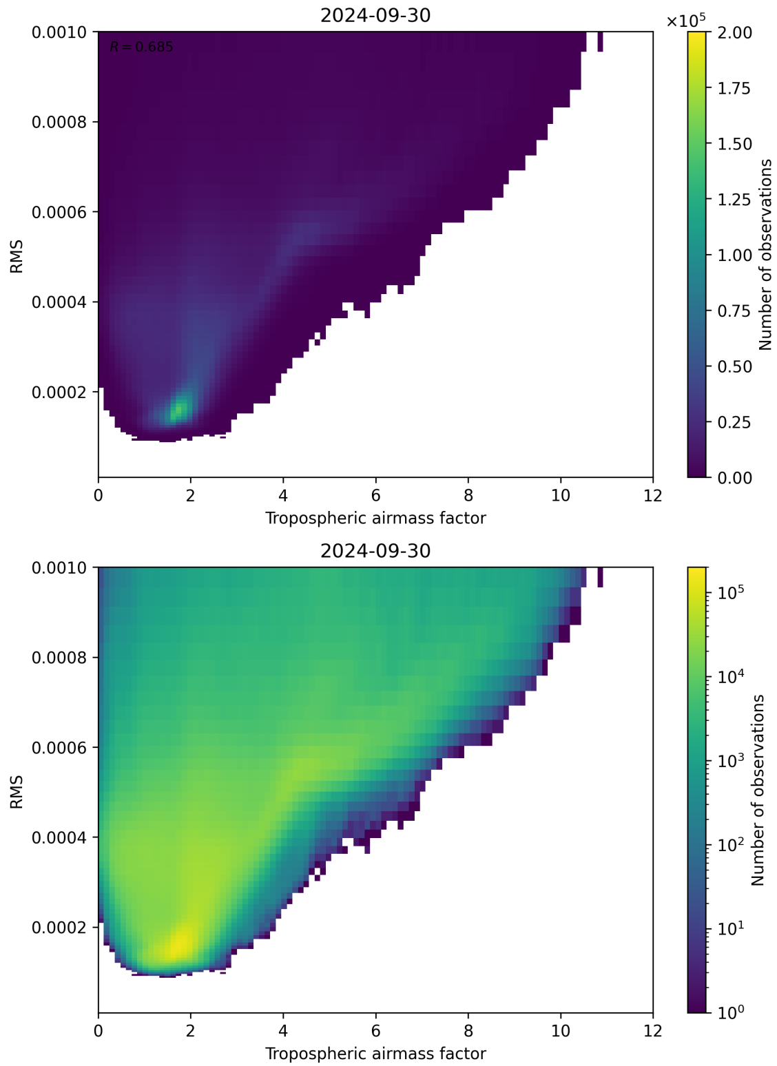
Figure 79: Scatter density plot of “Tropospheric airmass factor” against “RMS” for 2024-09-29 to 2024-10-01.
