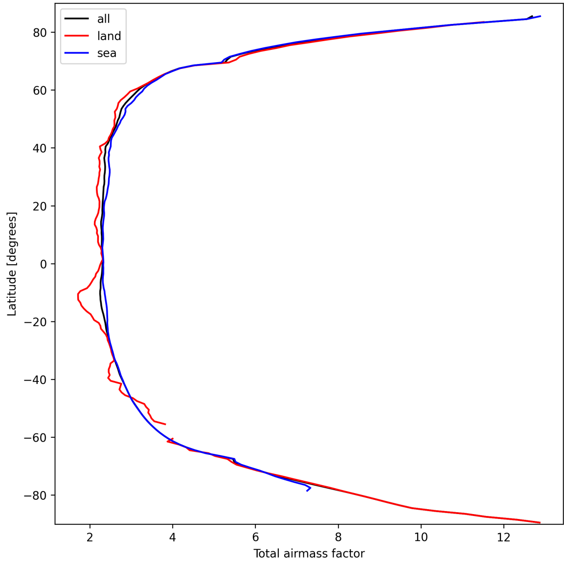
Figure 15: Zonal average of “Total airmass factor” for 2024-09-29 to 2024-10-01.
