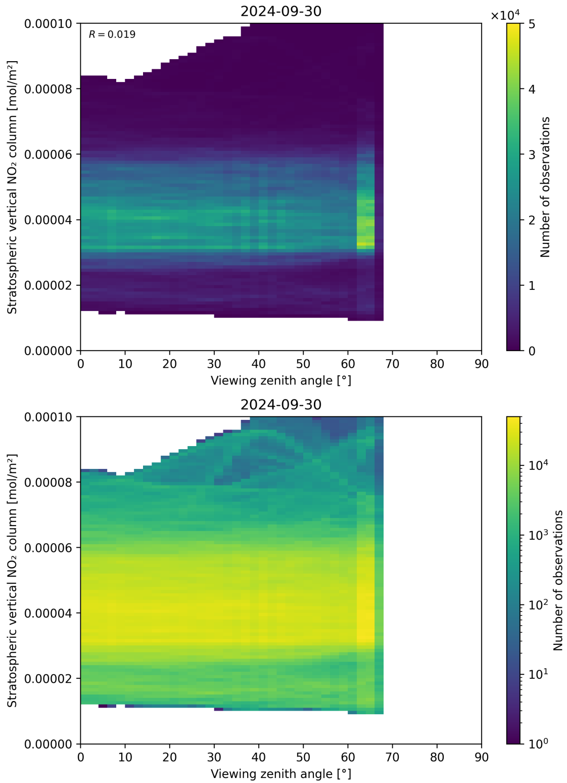
Figure 164: Scatter density plot of “Viewing zenith angle” against “Stratospheric vertical NO 2 column” for 2024-09-29 to 2024-10-01.
