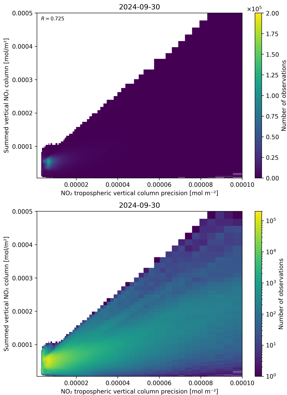
Figure 136: Scatter density plot of “NO 2 tropospheric vertical column precision” against “Summed vertical NO 2 column” for 2024-09-29 to 2024-10-01.
