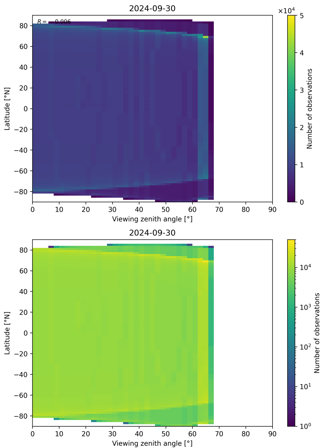
Figure 163: Scatter density plot of “Viewing zenith angle” against “Latitude” for 2024-09-29 to 2024-10-01.
