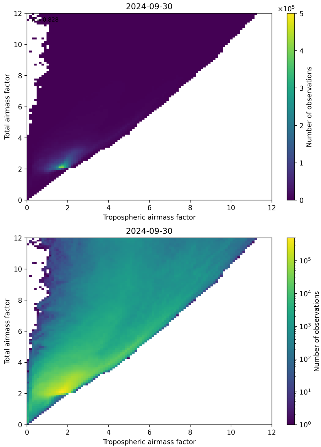
Figure 72: Scatter density plot of “Tropospheric airmass factor” against “Total airmass factor” for 2024-09-29 to 2024-10-01.
