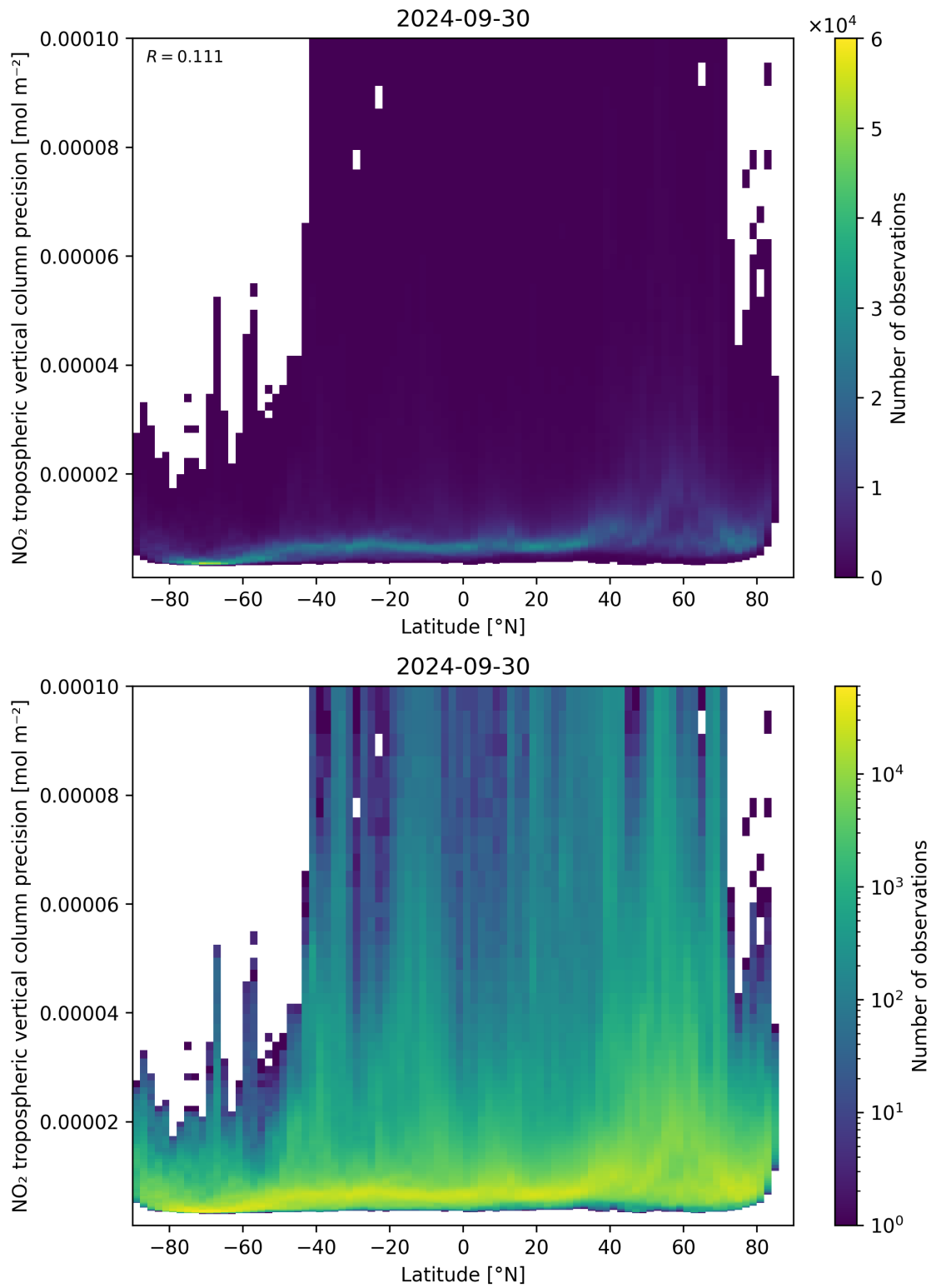
Figure 93: Scatter density plot of “Latitude” against “NO 2 tropospheric vertical column precision” for 2024-09-29 to 2024-10-01.
