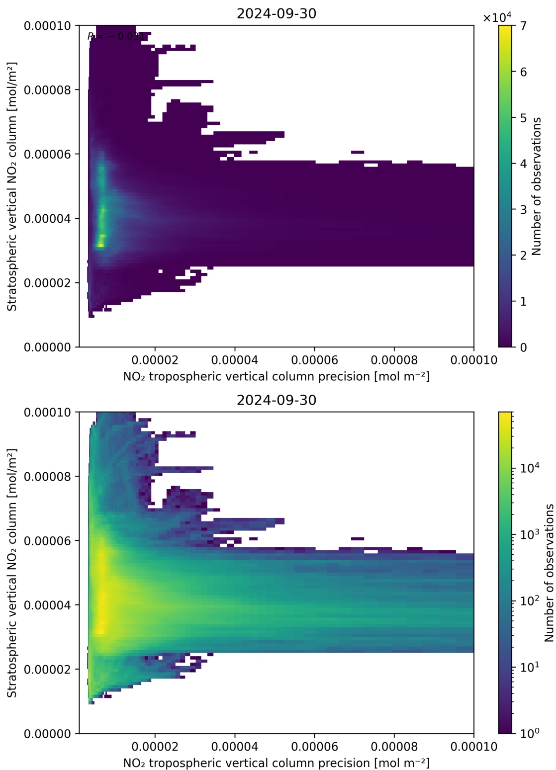
Figure 135: Scatter density plot of “NO 2 tropospheric vertical column precision” against “Stratospheric vertical NO 2 column” for 2024-09-29 to 2024-10-01.
