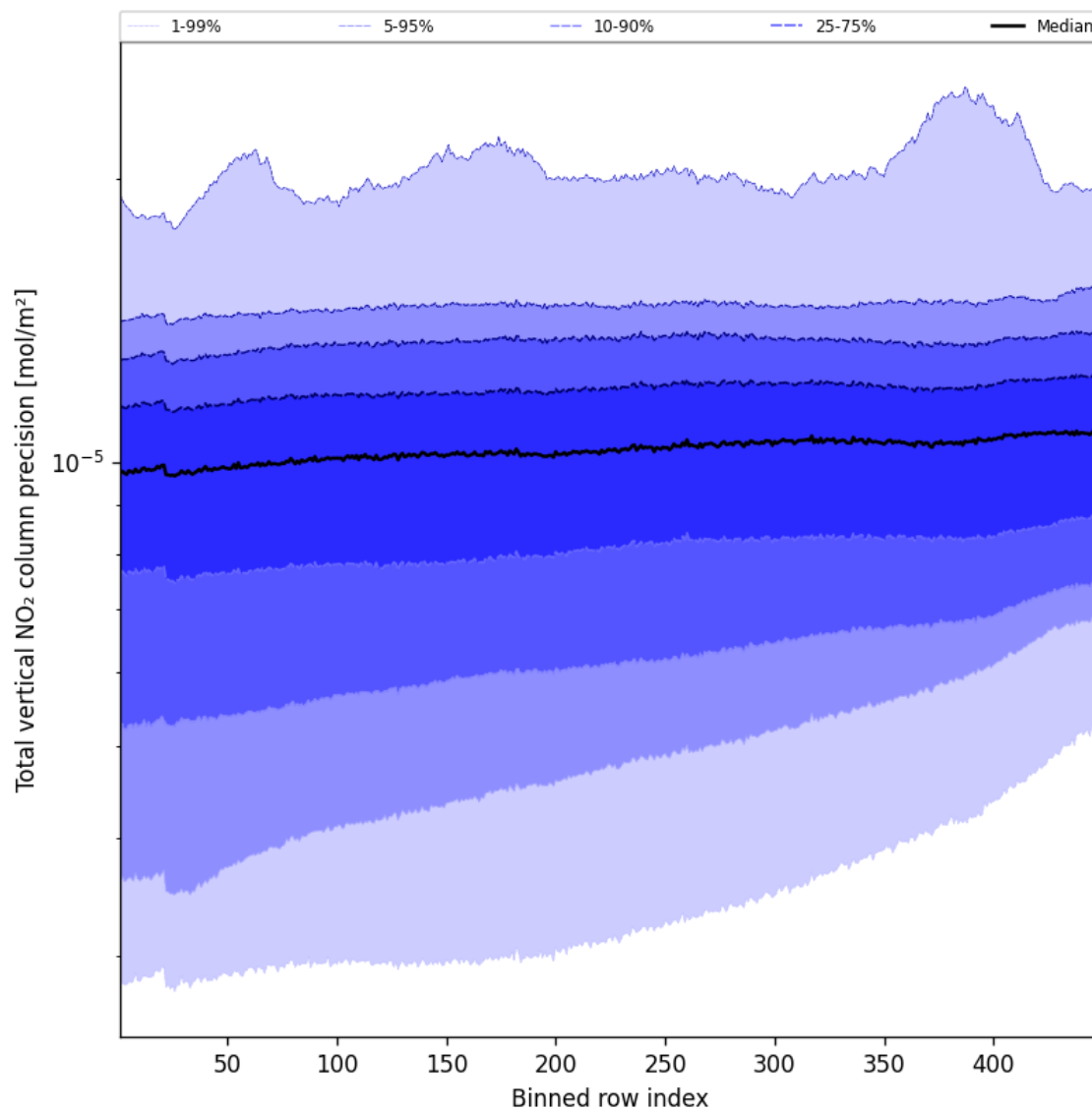
Figure 56: Along track statistics of “Total vertical NO 2 column precision” for 2024-09-29 to 2024-10-01
