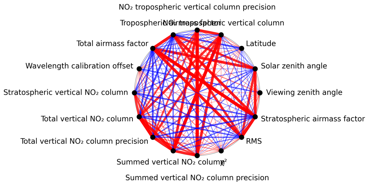
Figure 1: Map of correlation graph for 2024-09-29 to 2024-10-01.
