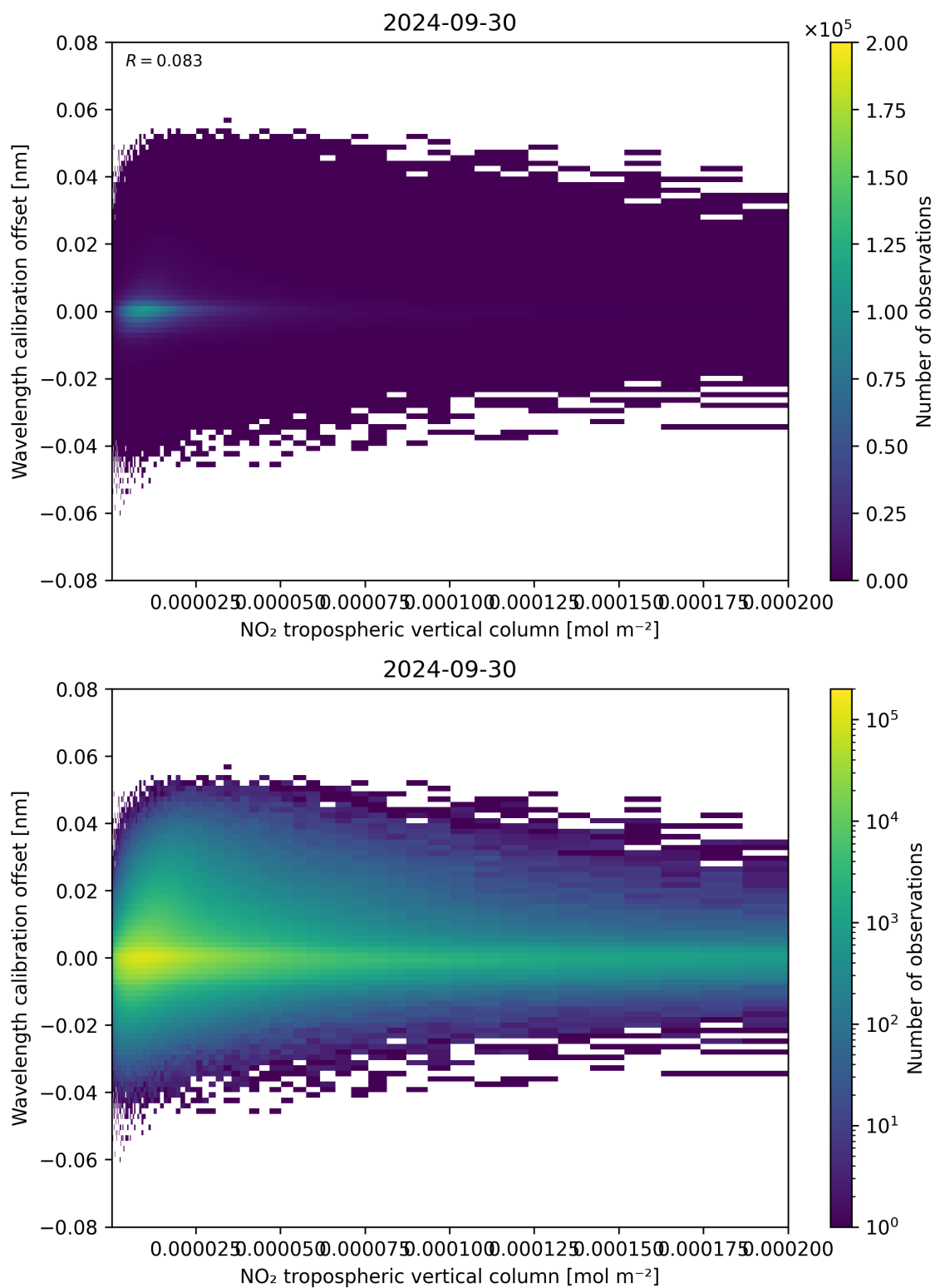
Figure 143: Scatter density plot of “NO 2 tropospheric vertical column” against “Wavelength calibration offset” for 2024-09-29 to 2024-10-01.
