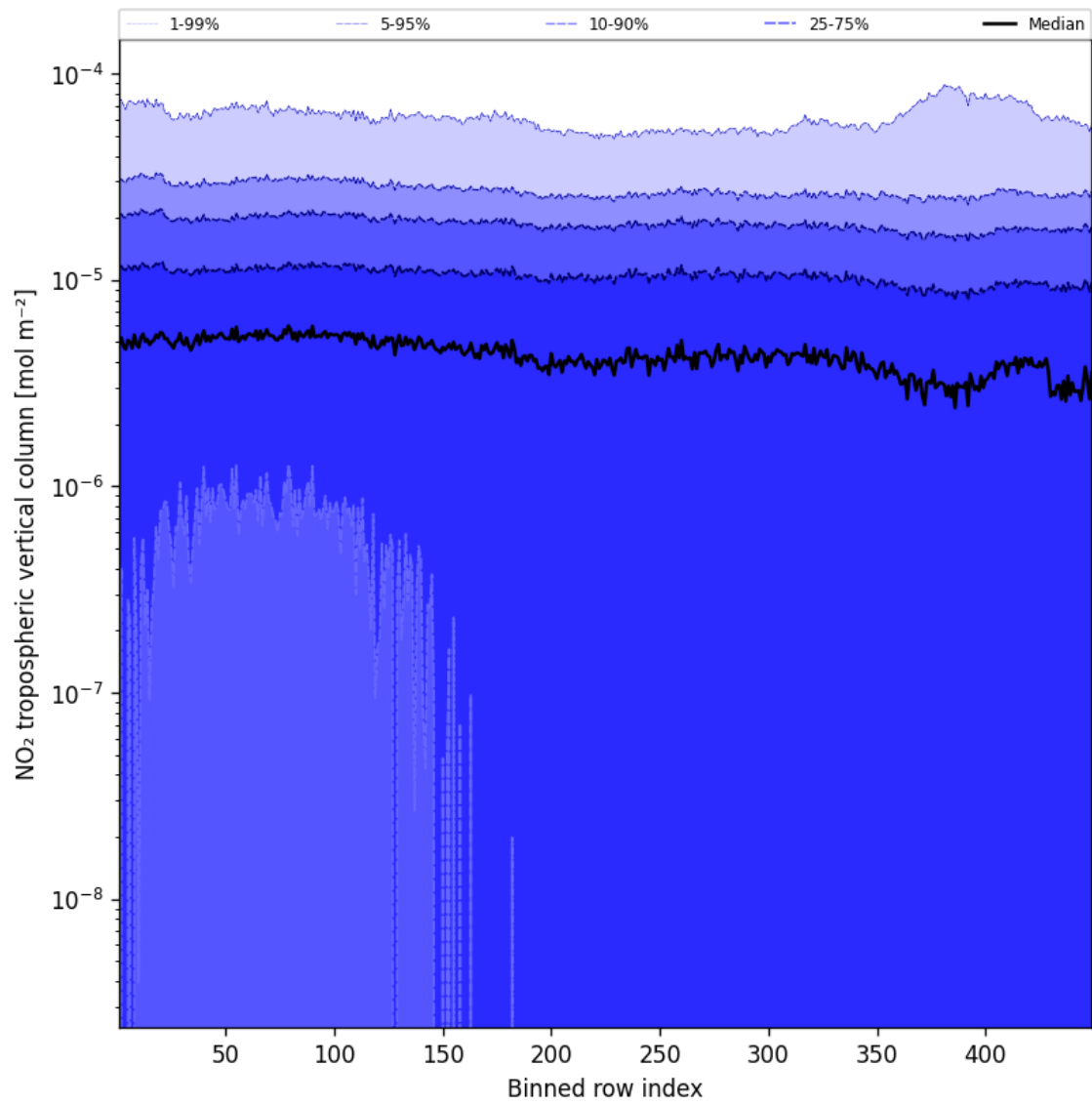
Figure 46: Along track statistics of “NO 2 tropospheric vertical column” for 2024-09-29 to 2024-10-01
