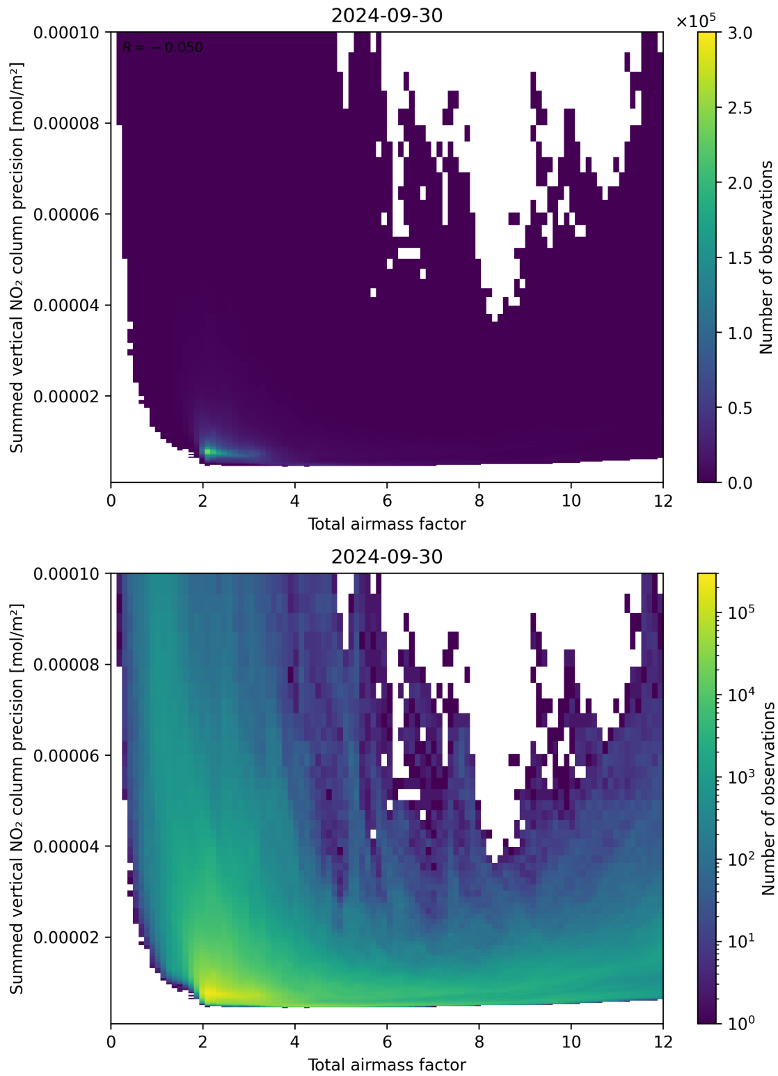
Figure 66: Scatter density plot of “Total airmass factor” against “Summed vertical NO 2 column precision” for 2024-09-29 to 2024-10-01.
