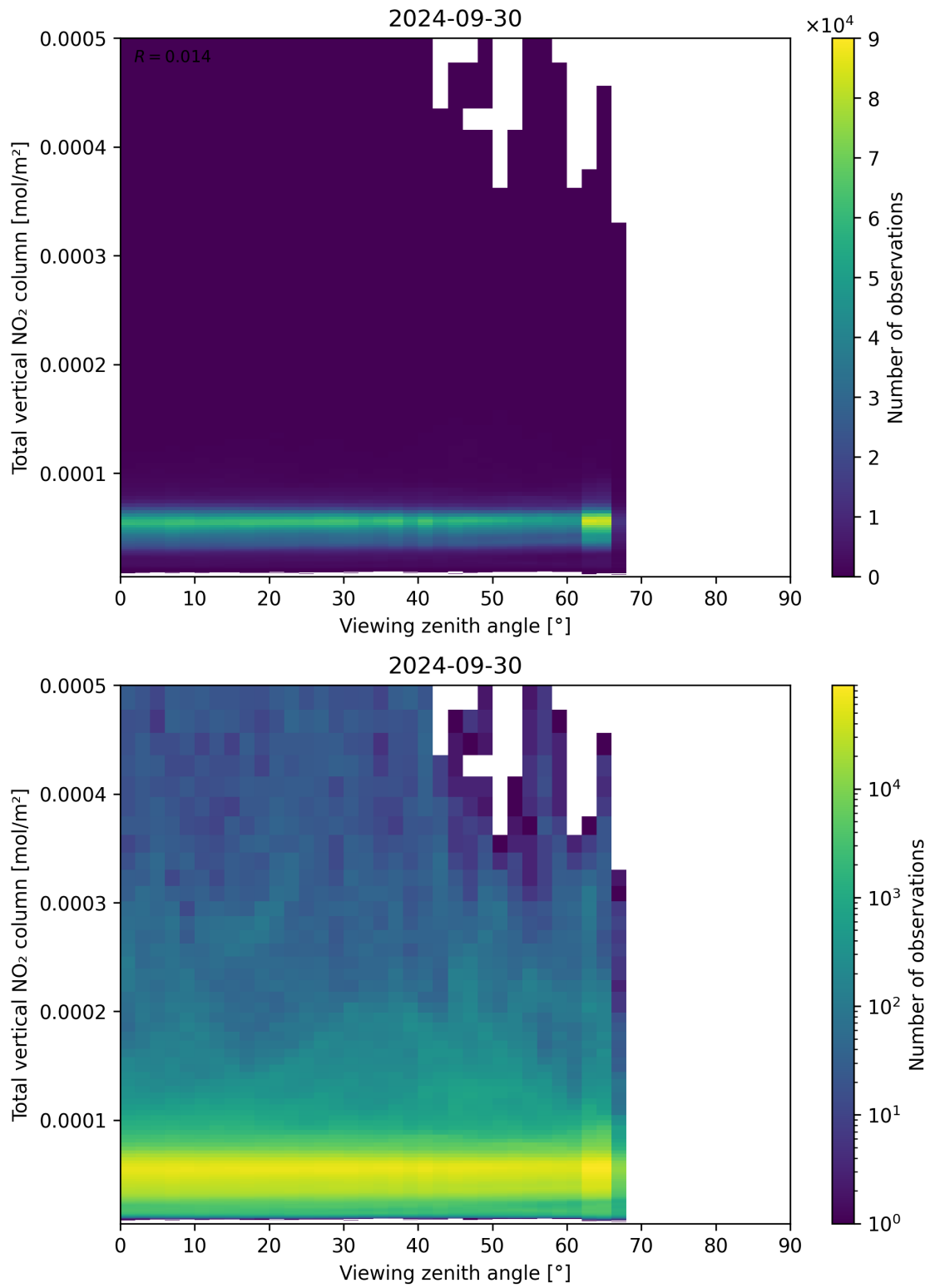
Figure 167: Scatter density plot of “Viewing zenith angle” against “Total vertical NO 2 column” for 2024-09-29 to 2024-10-01.
