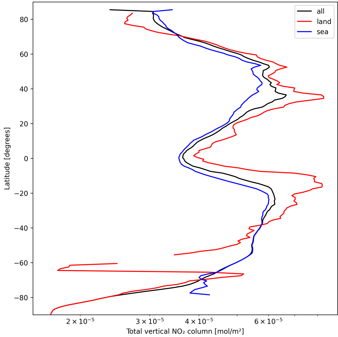
Figure 21: Zonal average of “Total vertical NO 2 column” for 2024-09-29 to 2024-10-01.
