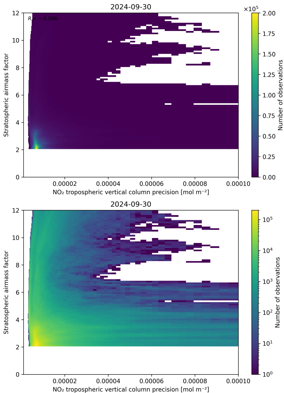
Figure 131: Scatter density plot of “NO 2 tropospheric vertical column precision” against “Stratospheric airmass factor” for 2024-09-29 to 2024-10-01.
