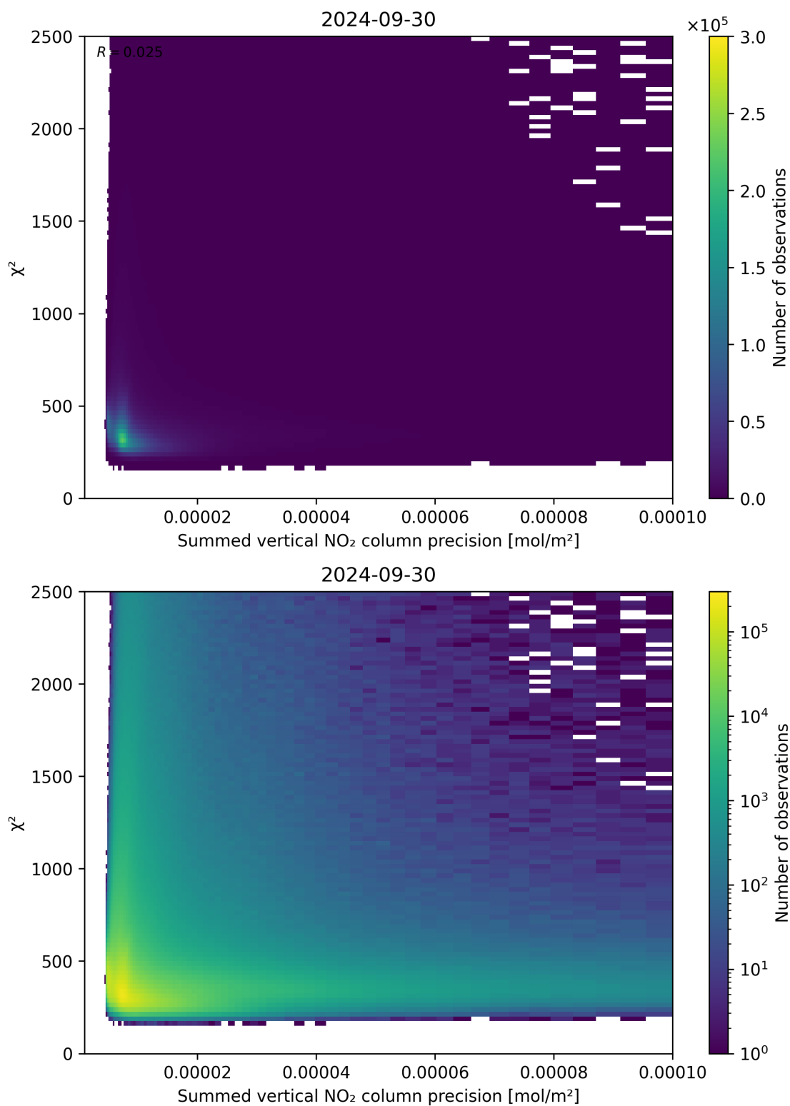
Figure 107: Scatter density plot of “Summed vertical NO 2 column precision” against “ \chi^2 ” for 2024-09-29 to 2024-10-01.
