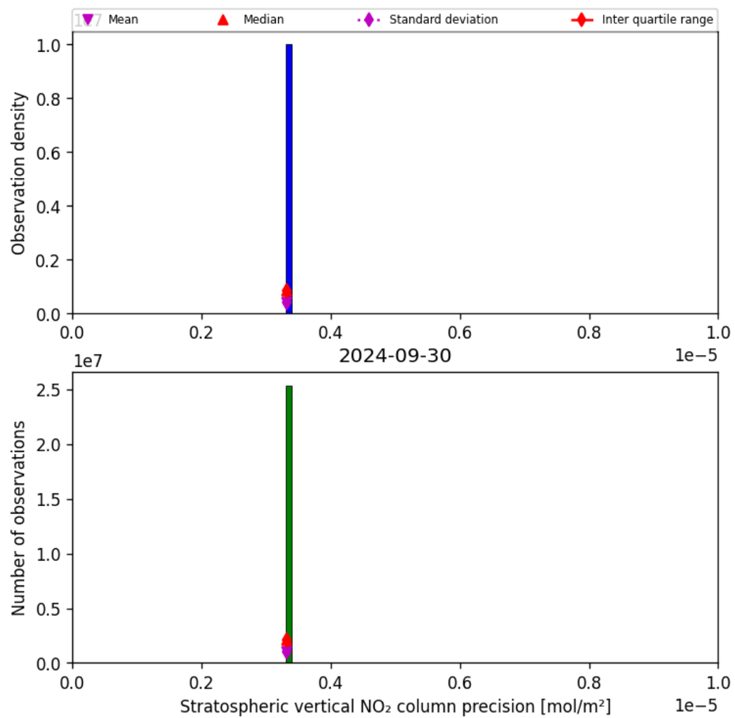
Figure 37: Histogram of “Stratospheric vertical NO 2 column precision” for 2024-09-29 to 2024-10-01
