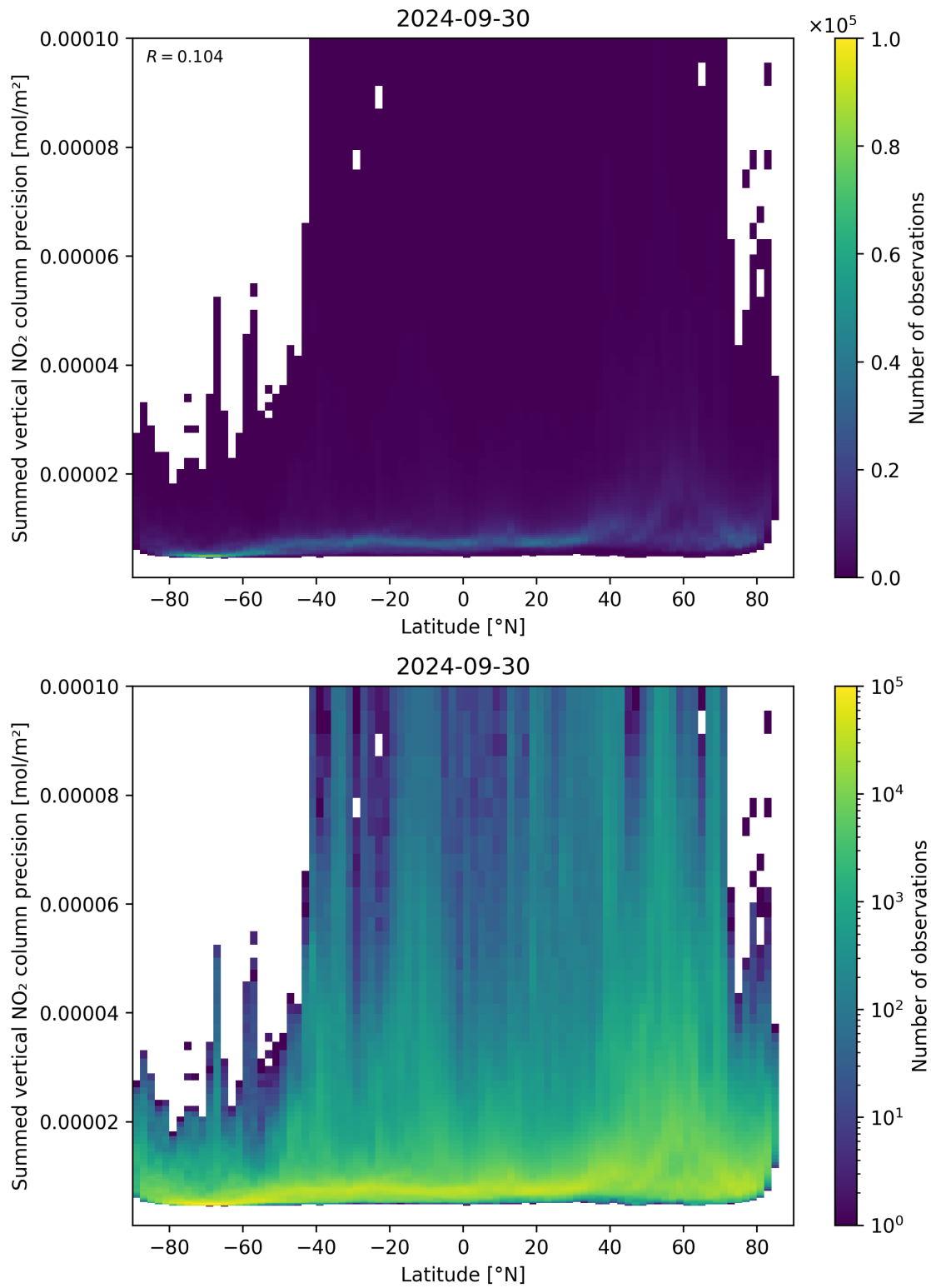
Figure 89: Scatter density plot of “Latitude” against “Summed vertical NO 2 column precision” for 2024-09-29 to 2024-10-01.
