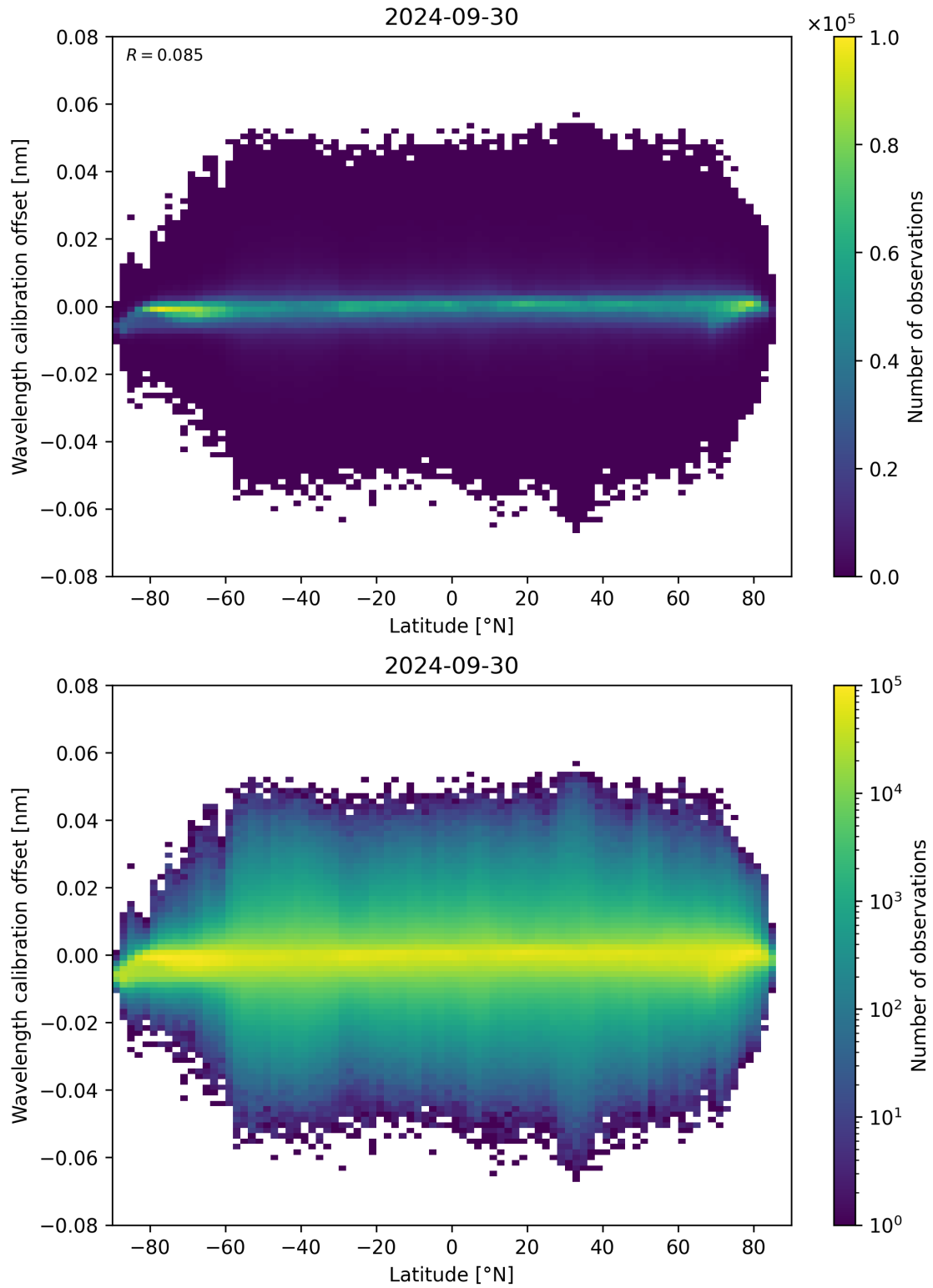
Figure 95: Scatter density plot of “Latitude” against “Wavelength calibration offset” for 2024-09-29 to 2024-10-01.
