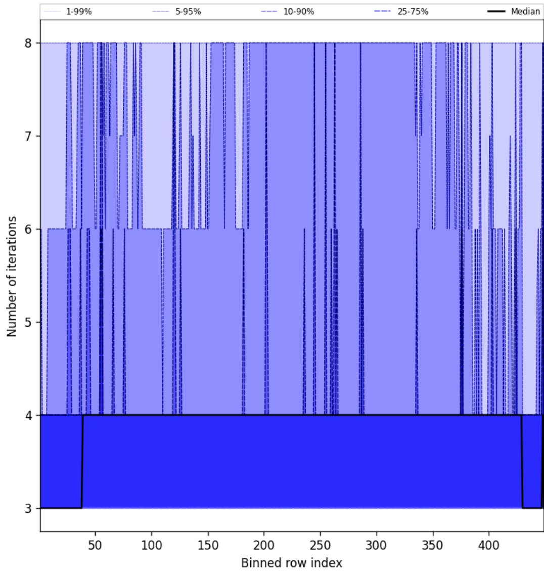
Figure 51: Along track statistics of “Number of iterations” for 2024-09-29 to 2024-10-01
