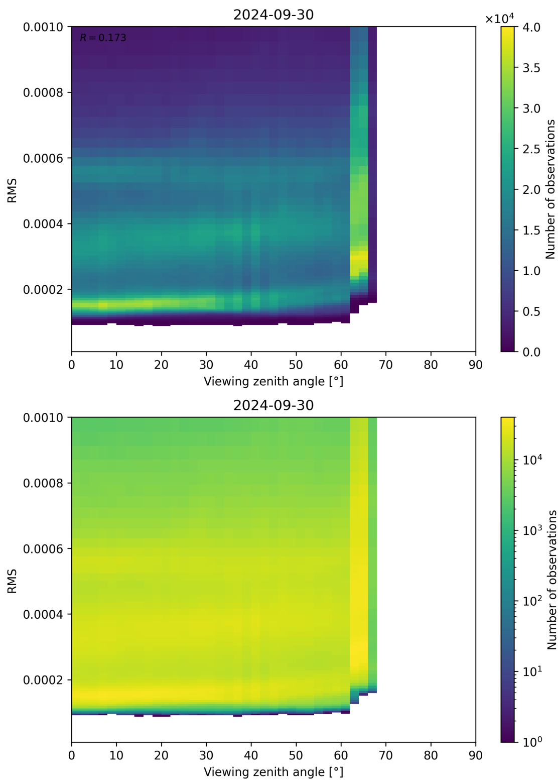
Figure 171: Scatter density plot of “Viewing zenith angle” against “RMS” for 2024-09-29 to 2024-10-01.
