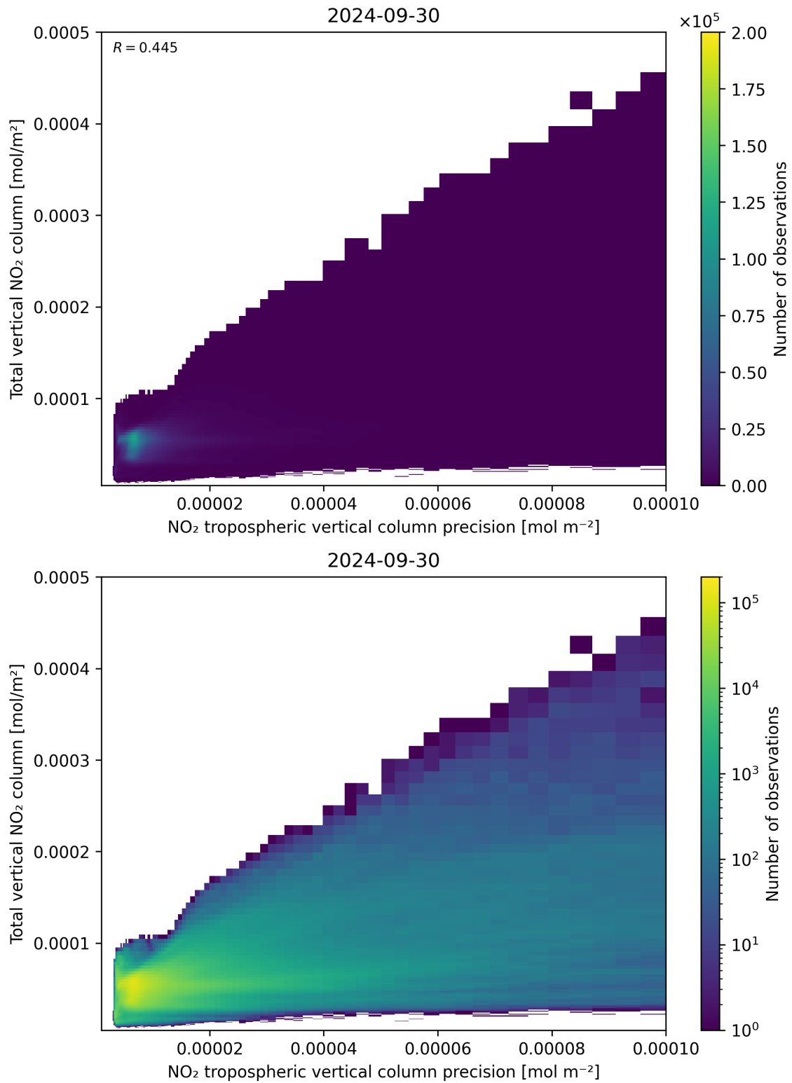
Figure 138: Scatter density plot of “NO 2 tropospheric vertical column precision” against “Total vertical NO 2 column” for 2024-09-29 to 2024-10-01.
