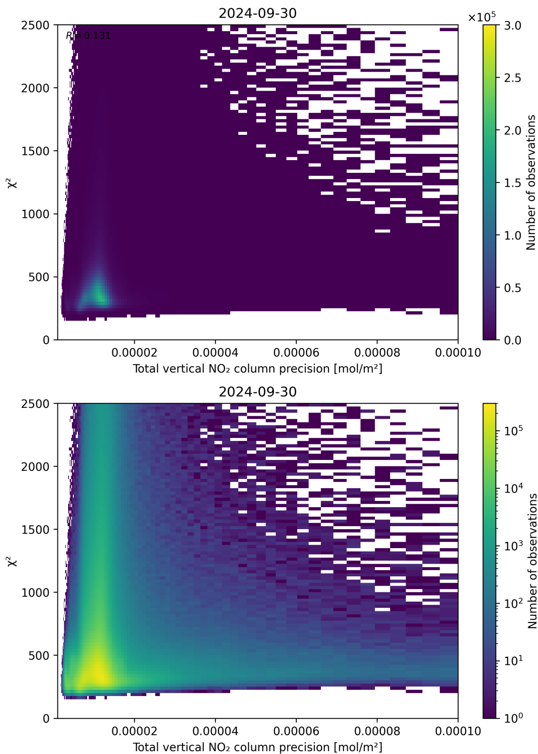
Figure 116: Scatter density plot of “Total vertical NO 2 column precision” against “ \chi^2 ” for 2024-09-29 to 2024-10-01.
