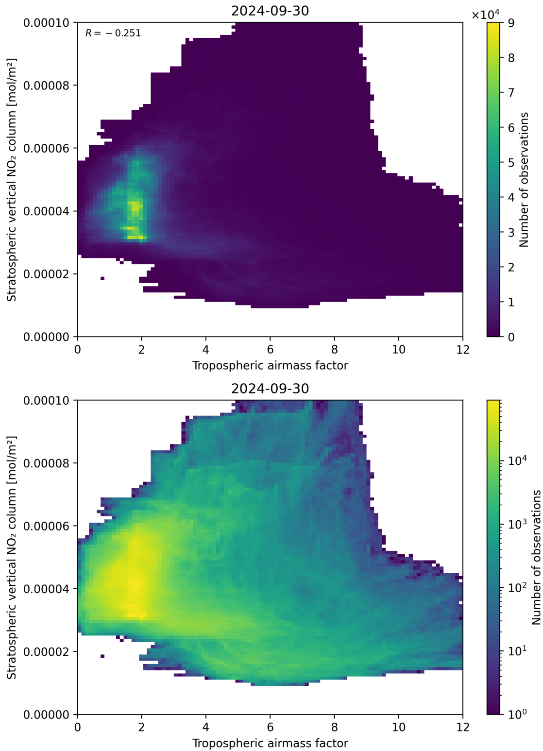
Figure 74: Scatter density plot of “Tropospheric air mass factor” against “Stratospheric vertical NO 2 column” for 2024-09-29 to 2024-10-01.
