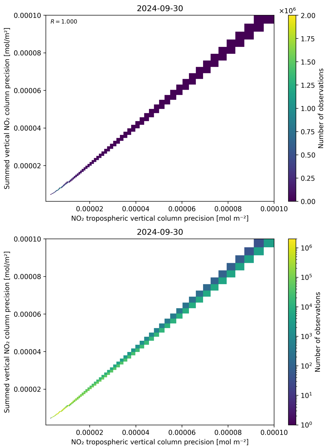
Figure 137: Scatter density plot of “NO 2 tropospheric vertical column precision” against “Summed vertical NO 2 column precision” for 2024-09-29 to 2024-10-01.
