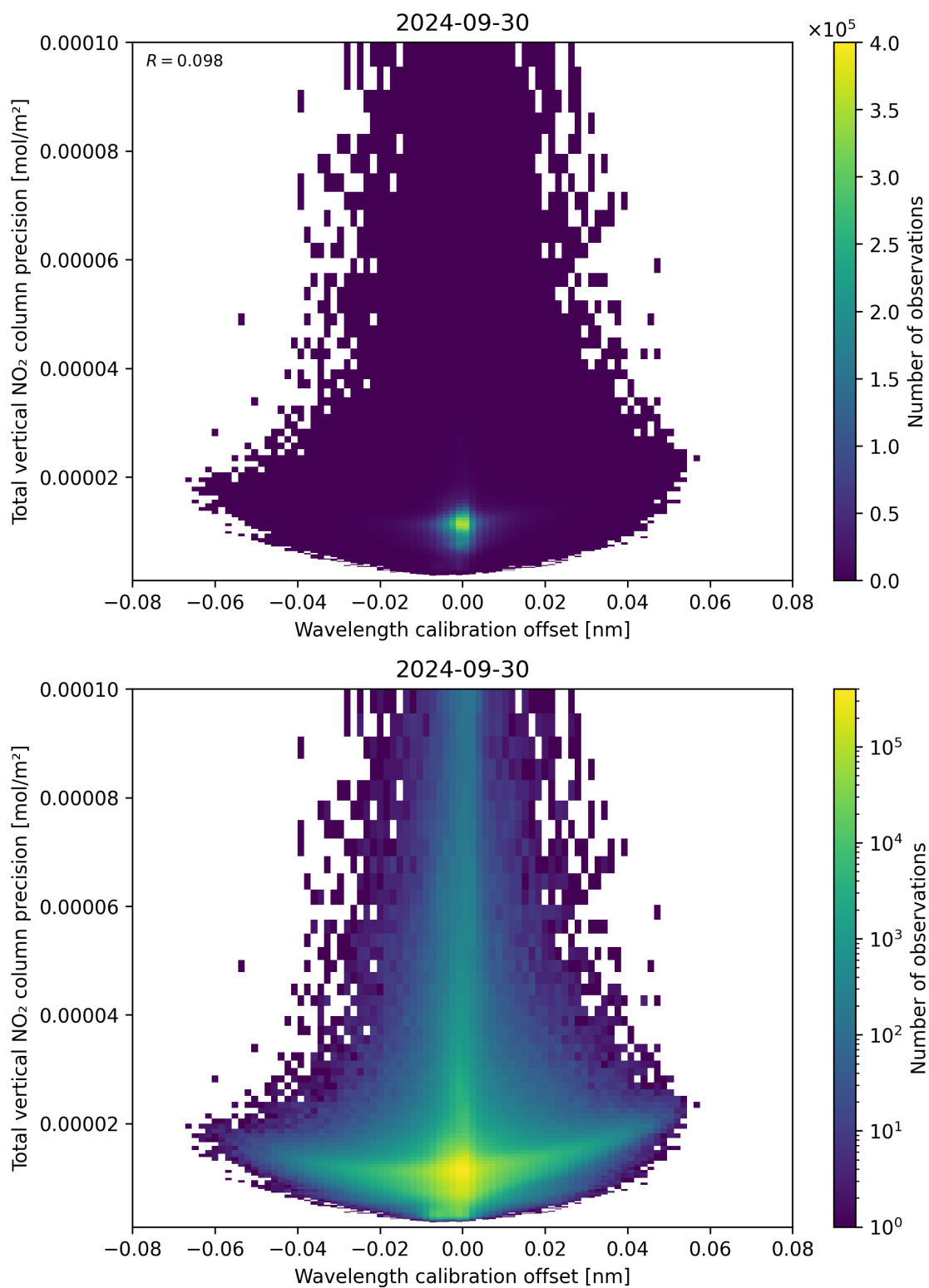
Figure 180: Scatter density plot of “Wavelength calibration offset” against “Total vertical NO 2 column precision” for 2024-09-29 to 2024-10-01.
