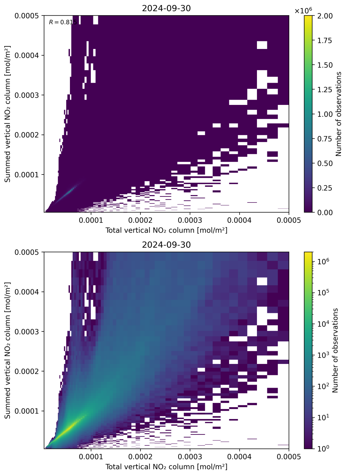
Figure 112: Scatter density plot of “Total vertical NO 2 column” against “Summed vertical NO 2 column” for 2024-09-29 to 2024-10-01.
