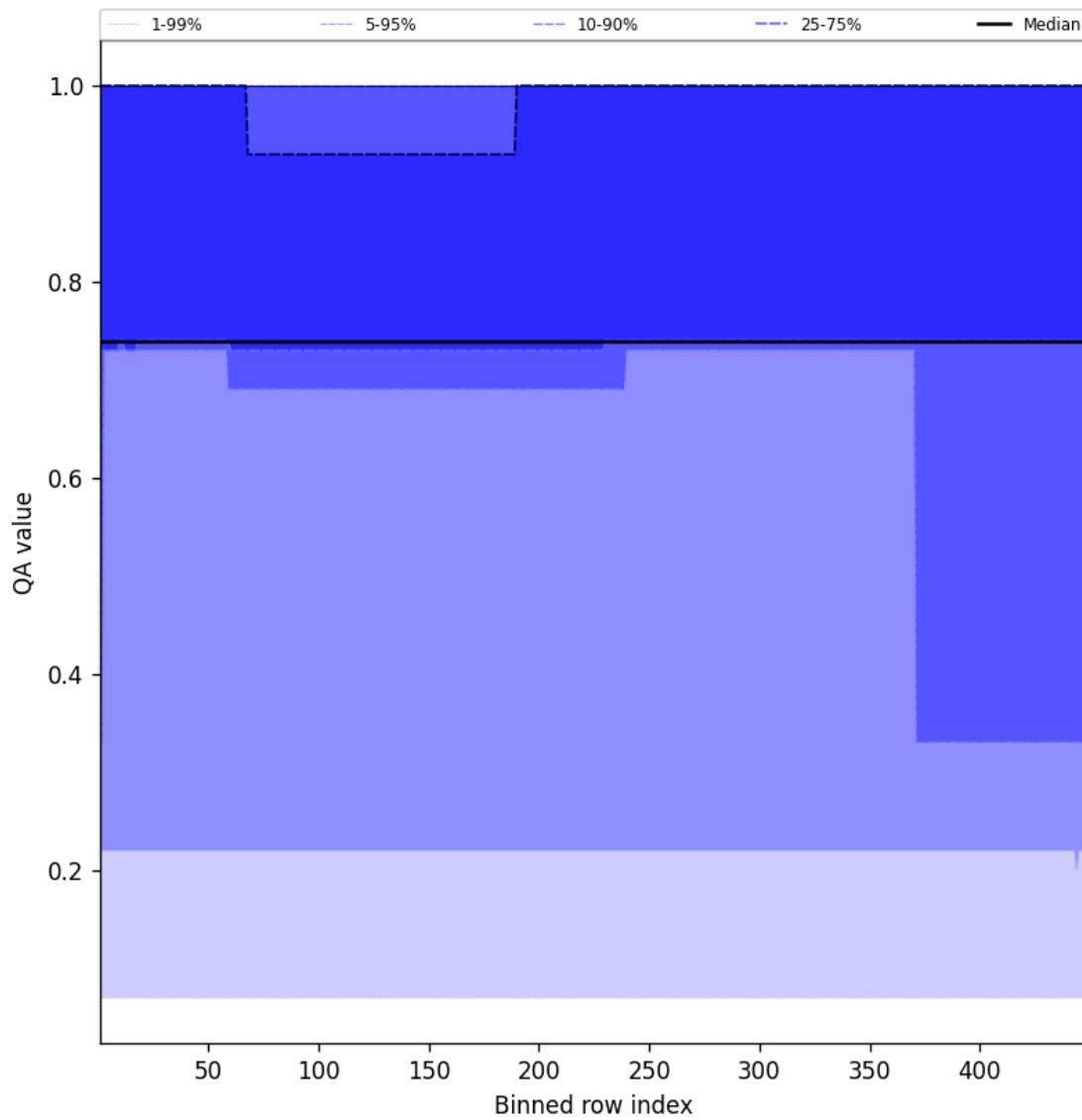
Figure 45: Along track statistics of “QA value” for 2024-09-29 to 2024-10-01
