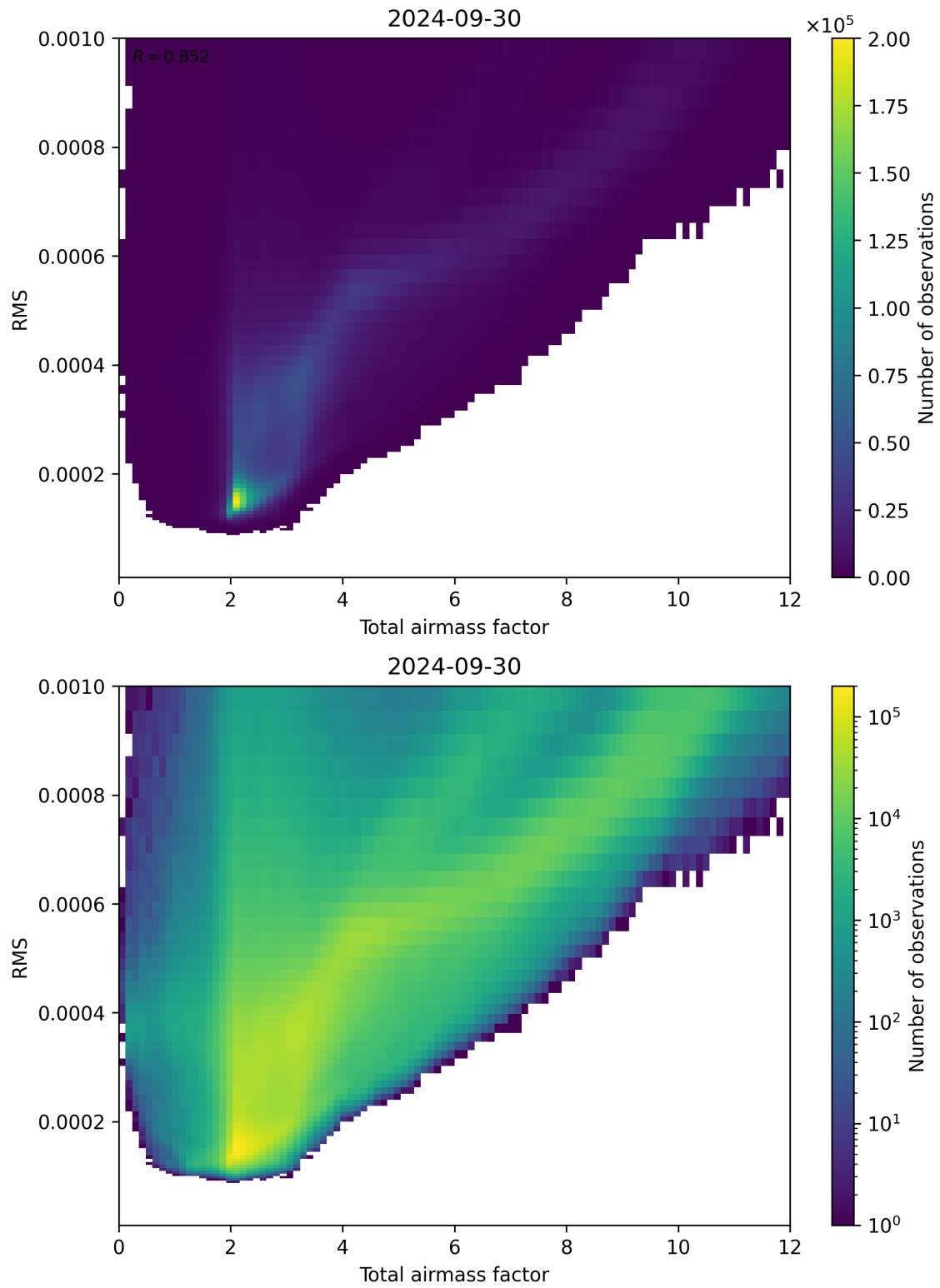
Figure 69: Scatter density plot of “Total airmass factor” against “RMS” for 2024-09-29 to 2024-10-01.
