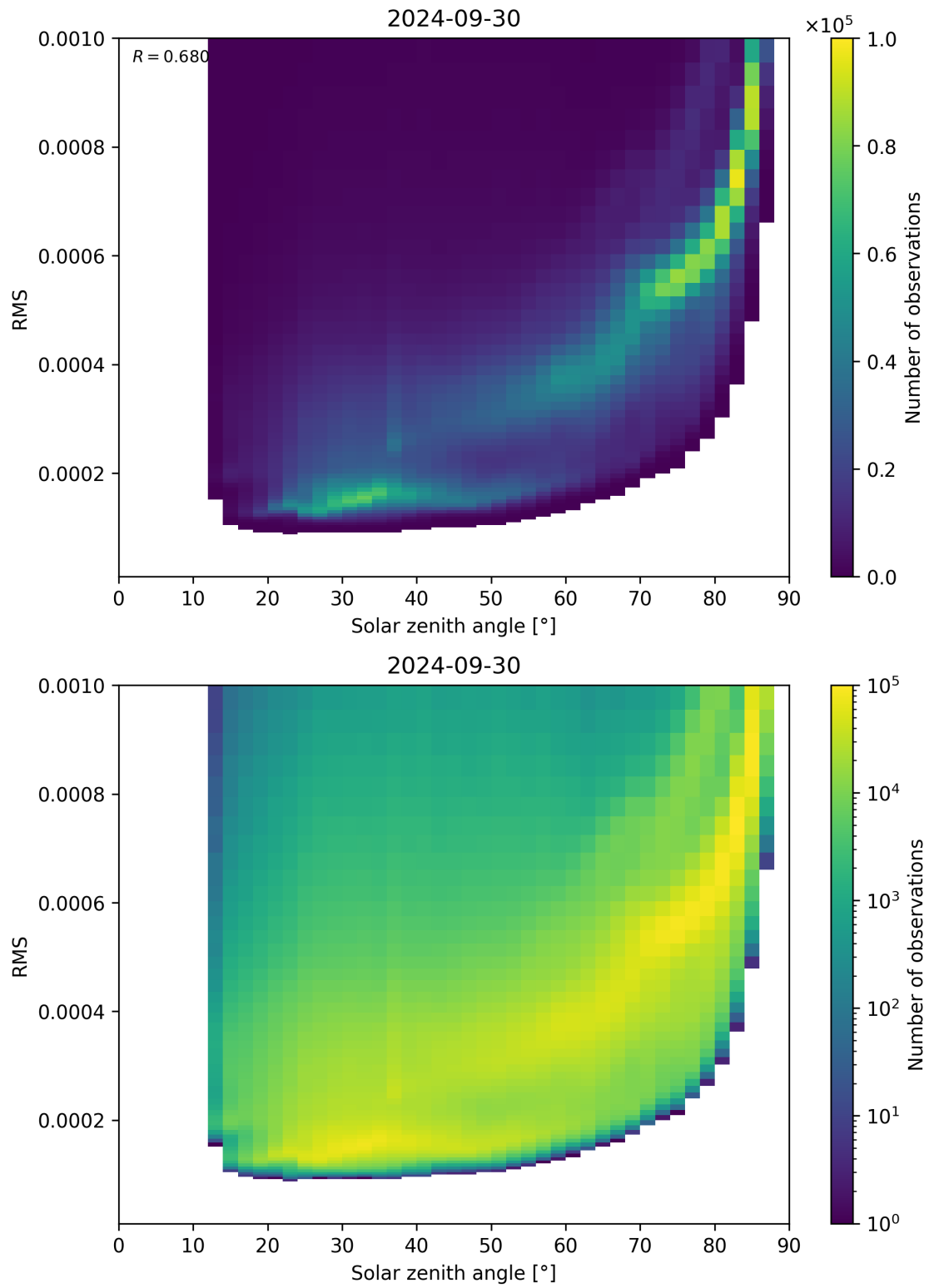
Figure 157: Scatter density plot of “Solar zenith angle” against “RMS” for 2024-09-29 to 2024-10-01.
