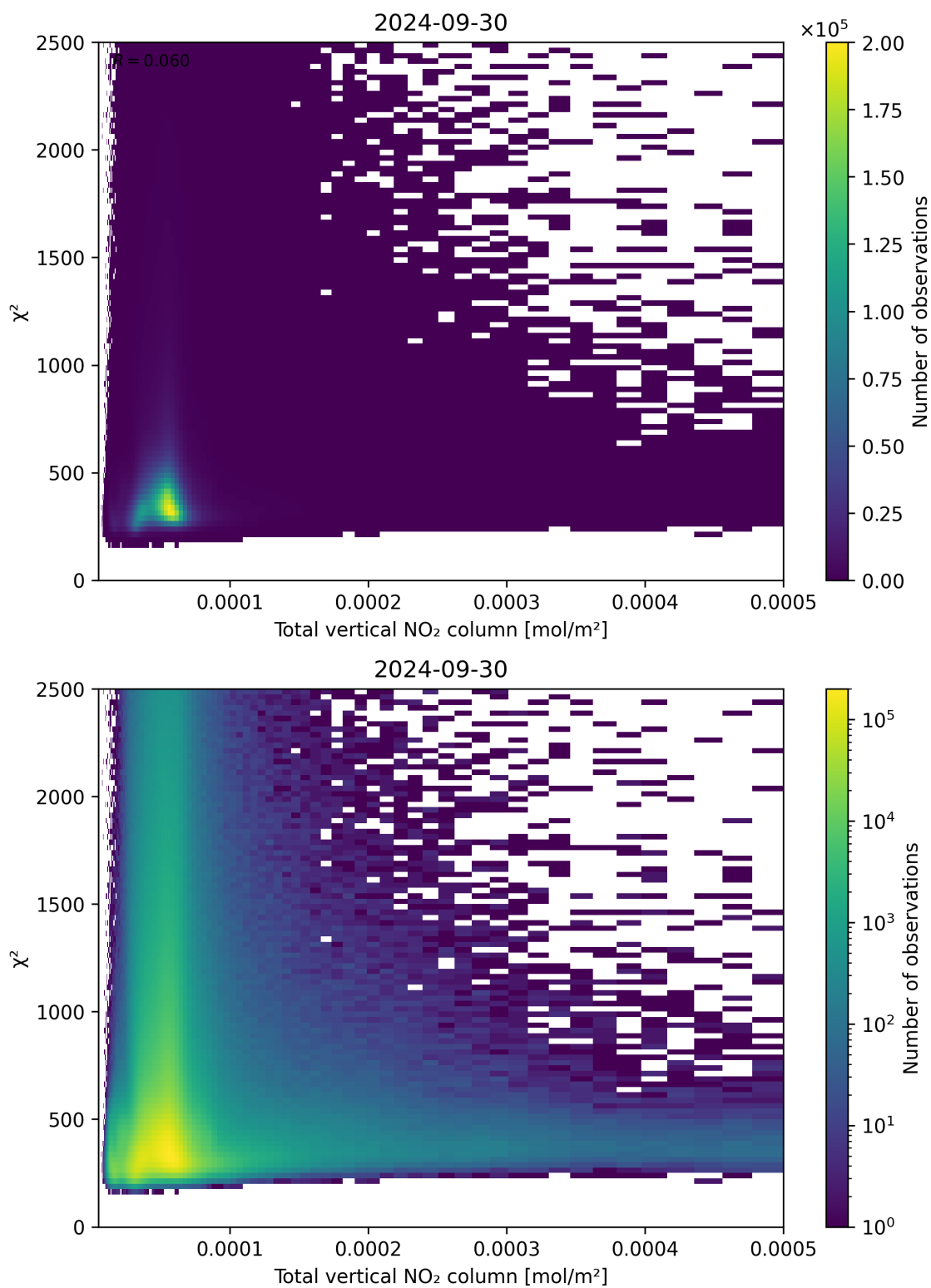
Figure 111: Scatter density plot of “Total vertical NO 2 column” against “ \chi^2 ” for 2024-09-29 to 2024-10-01.
