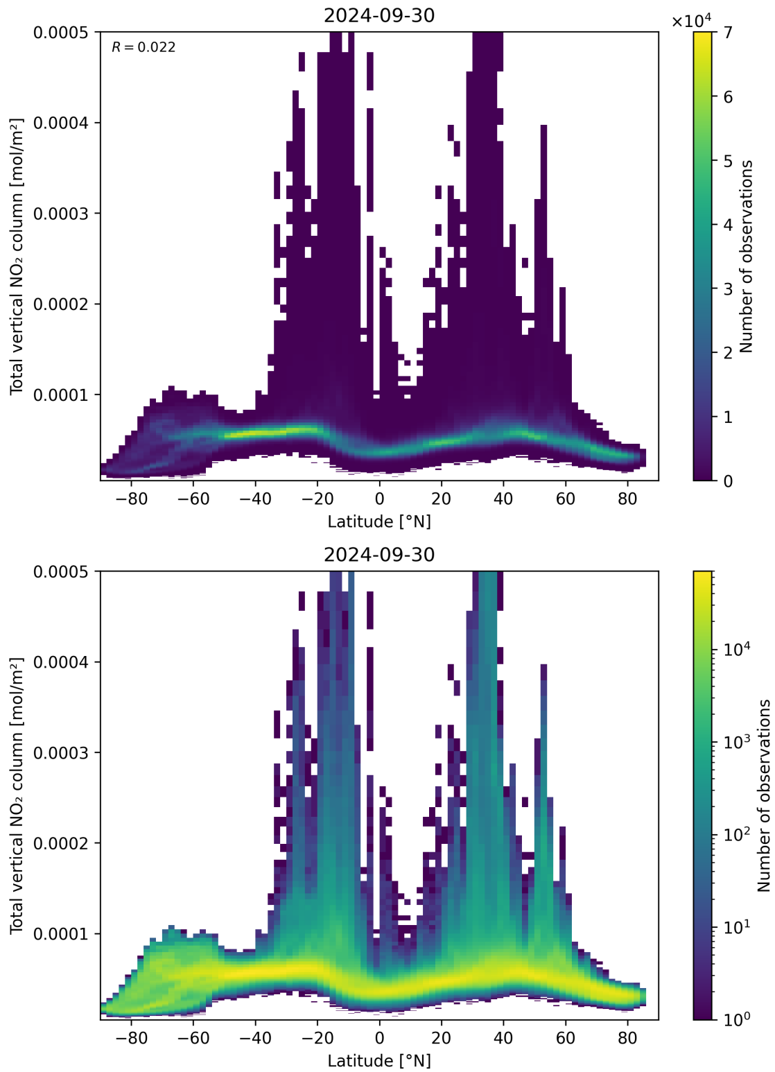
Figure 90: Scatter density plot of “Latitude” against “Total vertical NO 2 column” for 2024-09-29 to 2024-10-01.
