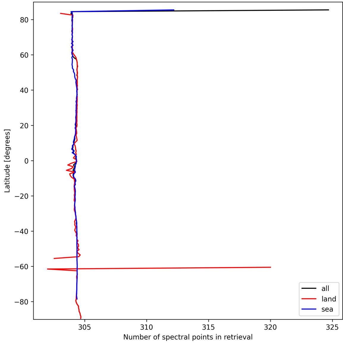
Figure 16: Zonal average of “Number of spectral points in retrieval” for 2024-09-29 to 2024-10-01.
