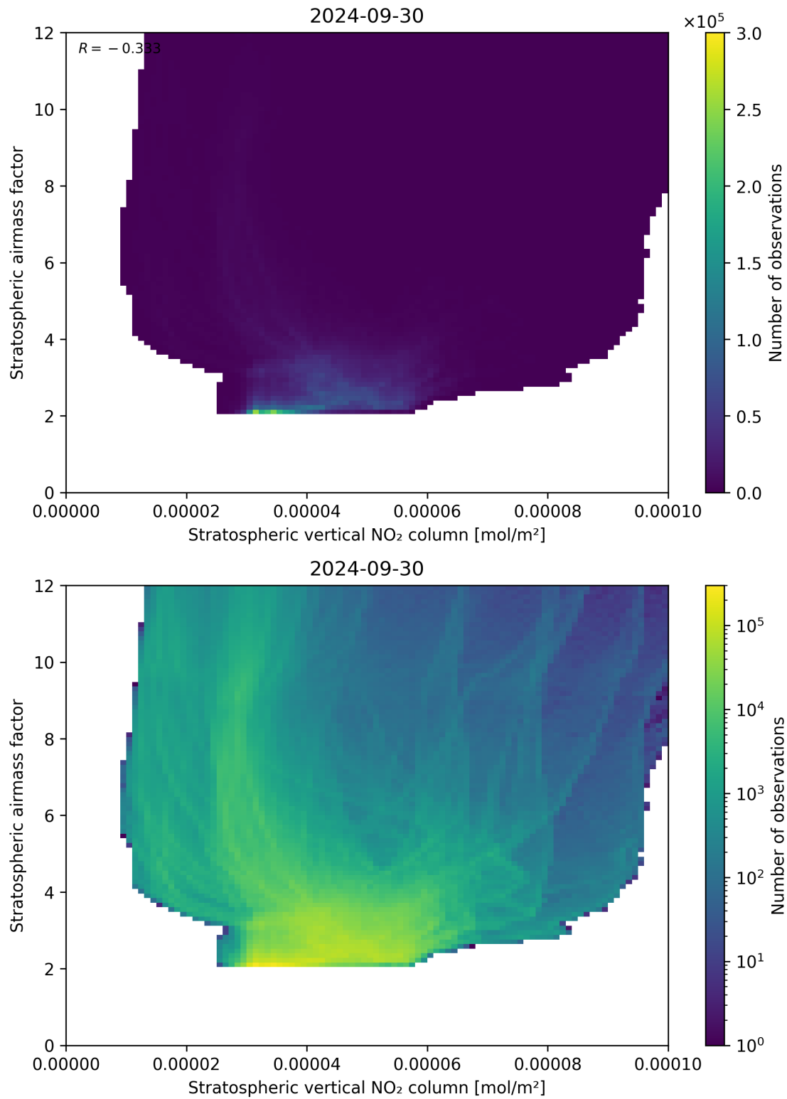
Figure 96: Scatter density plot of “Stratospheric vertical NO 2 column” against “Stratospheric airmass factor” for 2024-09-29 to 2024-10-01.
