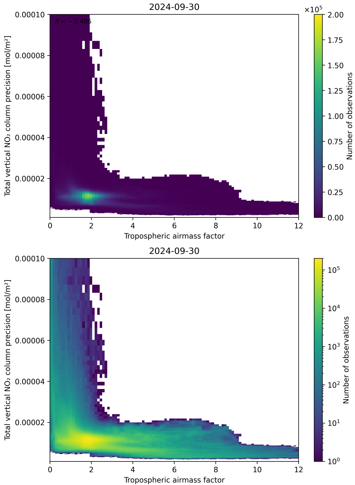
Figure 78: Scatter density plot of “Tropospheric air mass factor” against “Total vertical NO 2 column precision” for 2024-09-29 to 2024-10-01.
