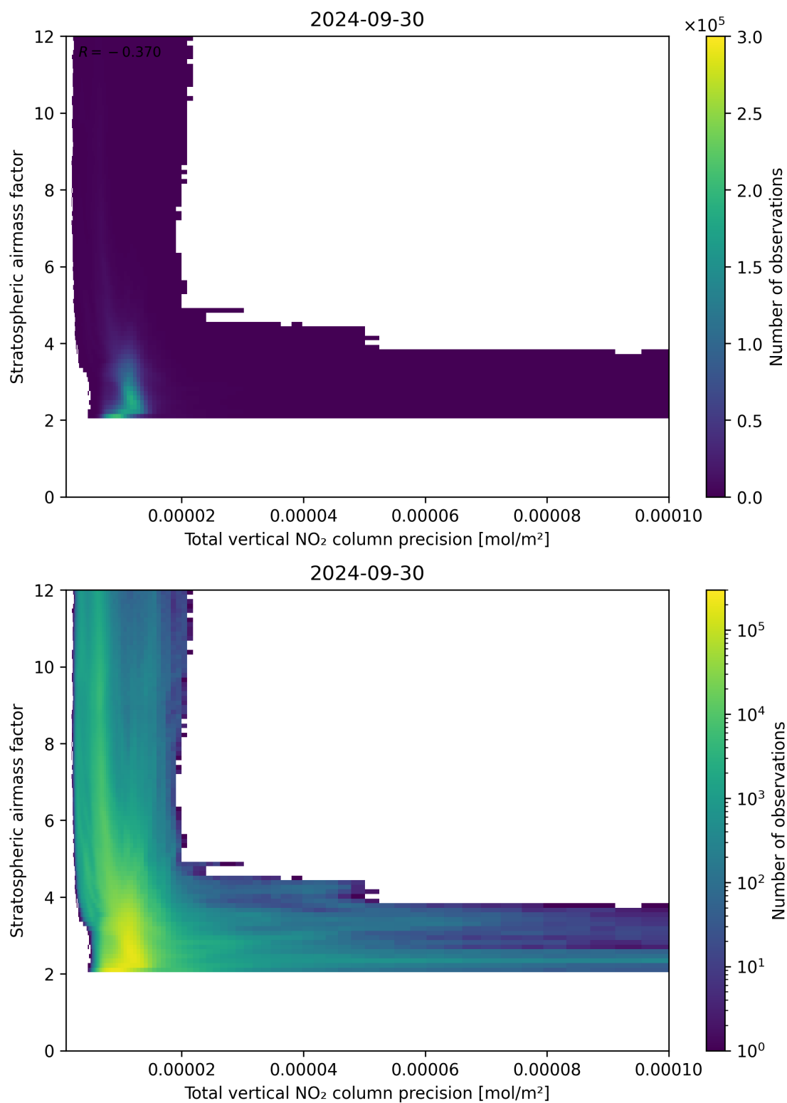
Figure 115: Scatter density plot of “Total vertical NO 2 column precision” against “Stratospheric air mass factor” for 2024-09-29 to 2024-10-01.
