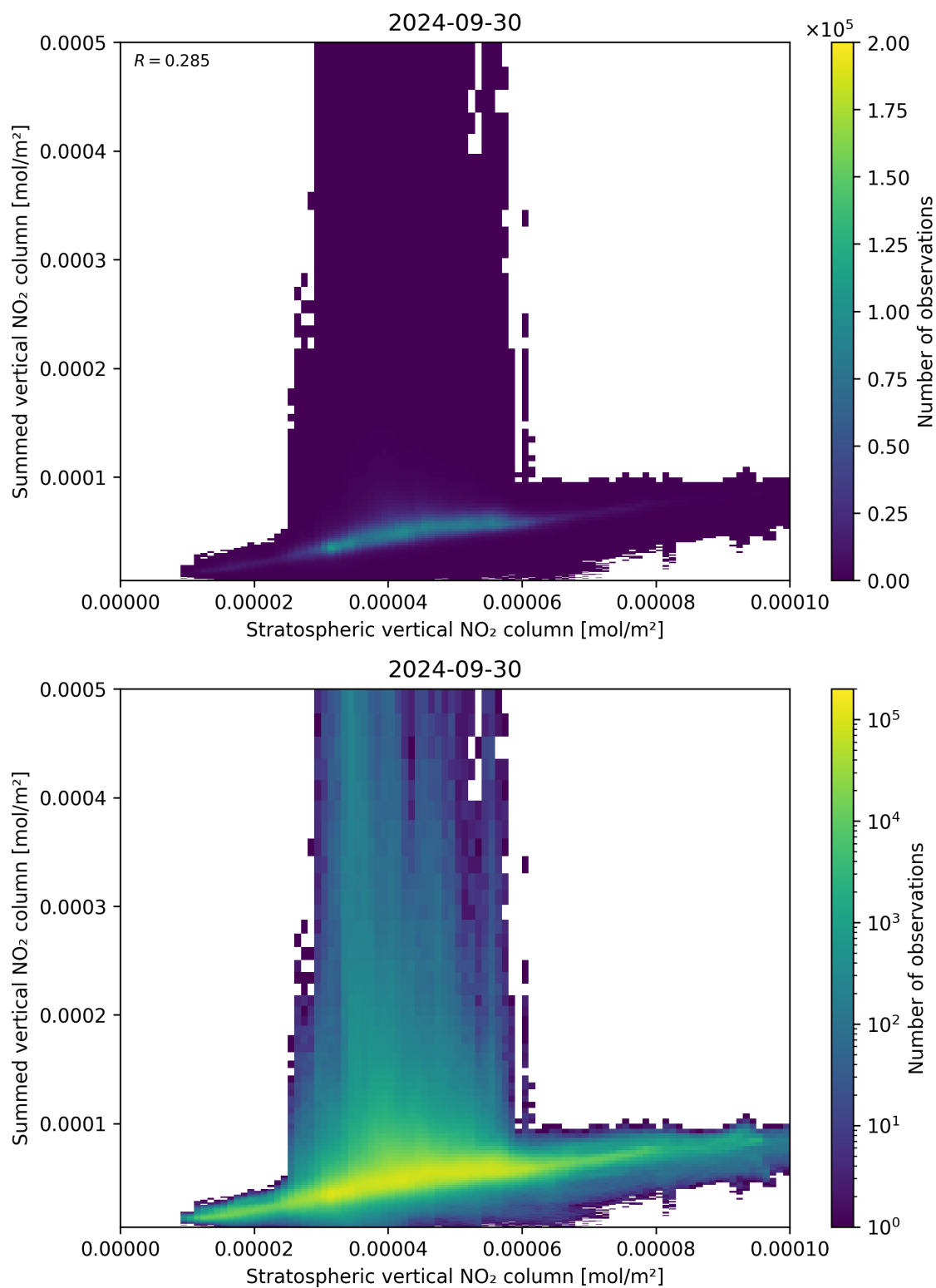
Figure 98: Scatter density plot of “Stratospheric vertical NO 2 column” against “Summed vertical NO 2 column” for 2024-09-29 to 2024-10-01.
