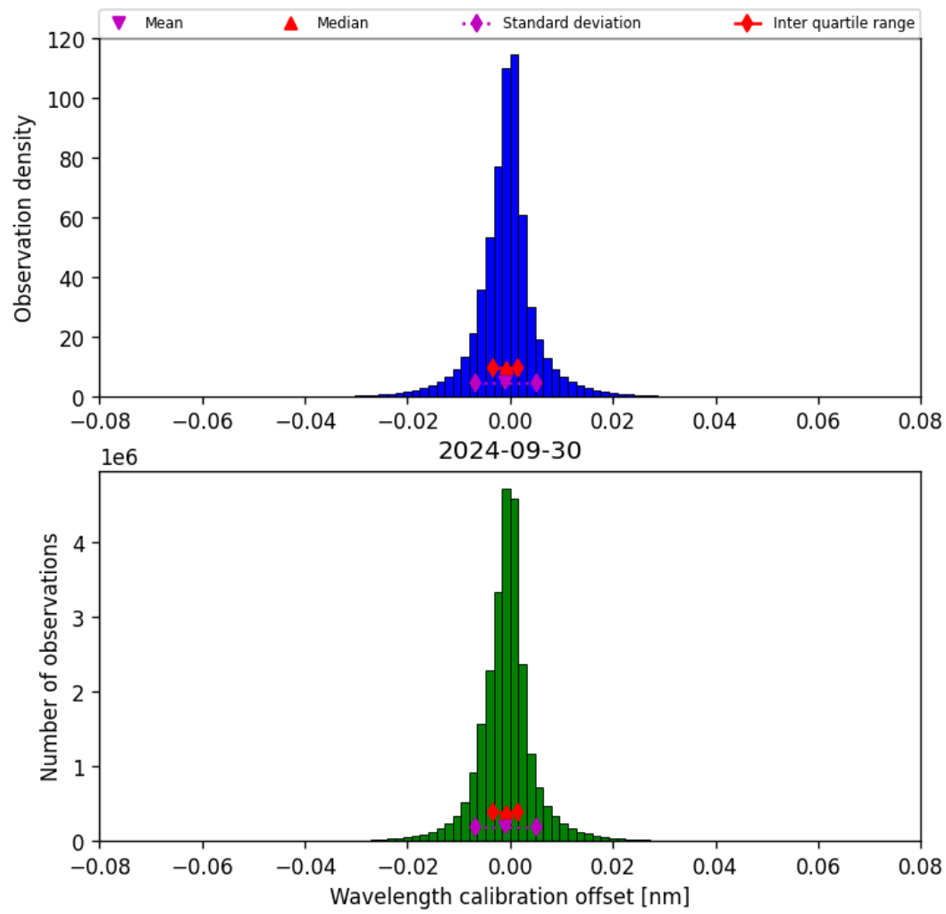
Figure 35: Histogram of “Wavelength calibration offset” for 2024-09-29 to 2024-10-01
