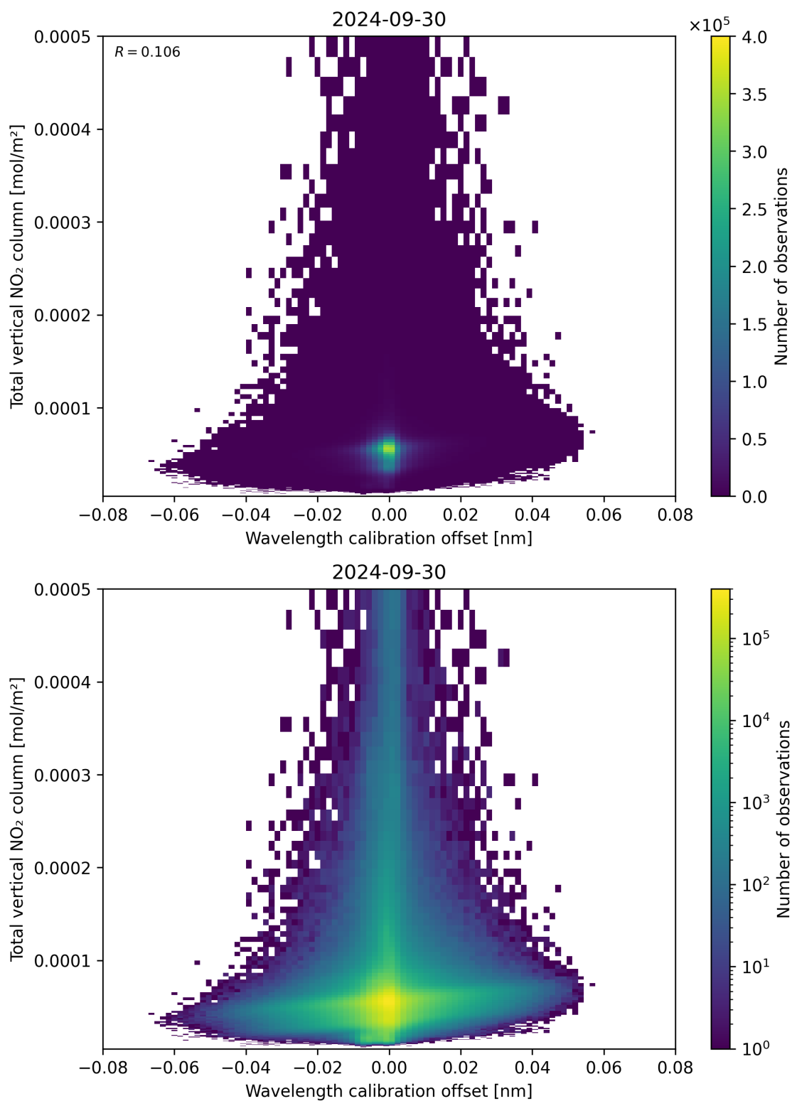
Figure 179: Scatter density plot of “Wavelength calibration offset” against “Total vertical NO 2 column” for 2024-09-29 to 2024-10-01.
