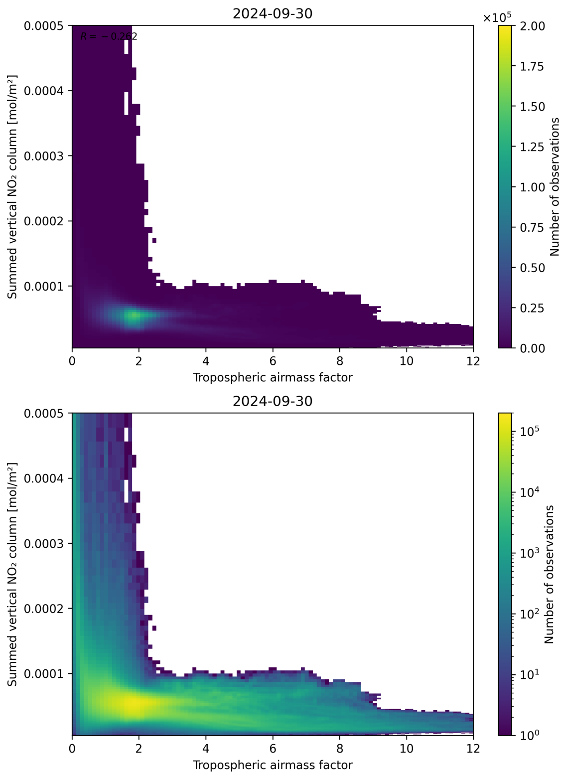
Figure 75: Scatter density plot of “Tropospheric air mass factor” against “Summed vertical NO 2 column” for 2024-09-29 to 2024-10-01.
