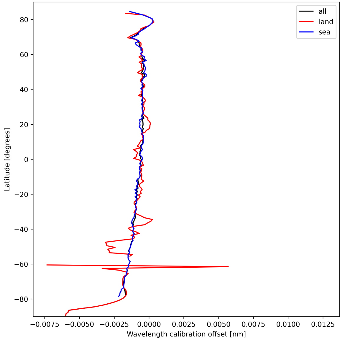
Figure 18: Zonal average of “Wavelength calibration offset” for 2024-09-30 to 2024-10-02.
