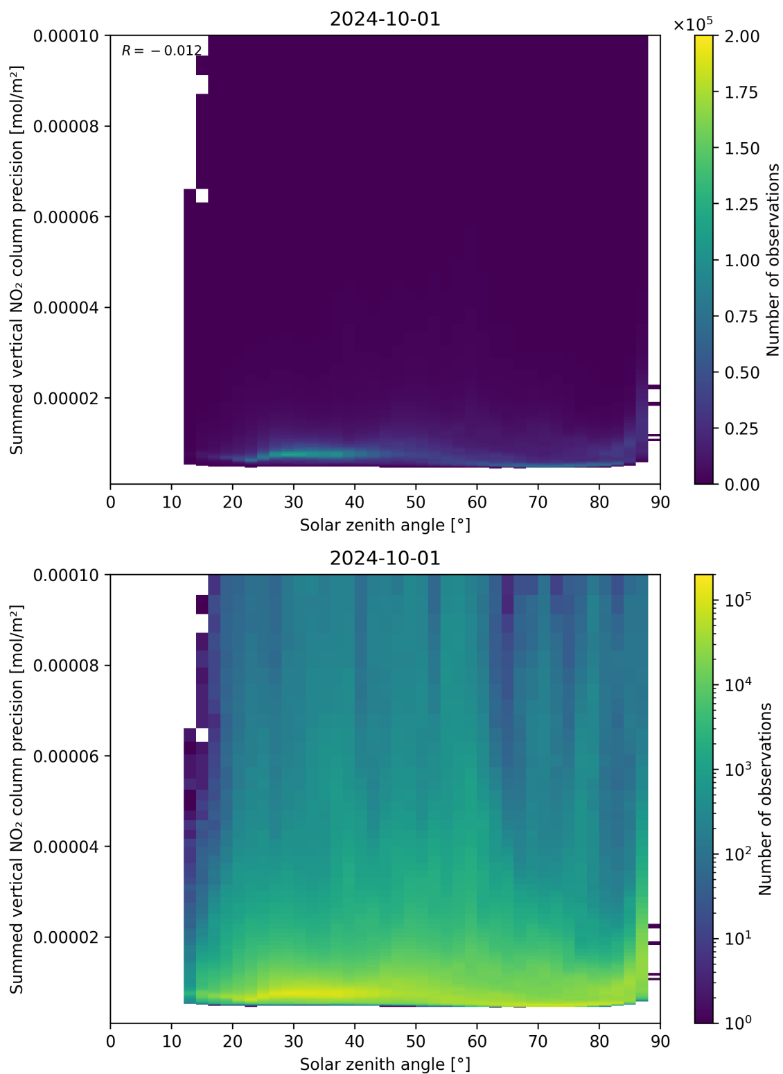
Figure 152: Scatter density plot of “Solar zenith angle” against “Summed vertical NO 2 column precision” for 2024-09-30 to 2024-10-02.
