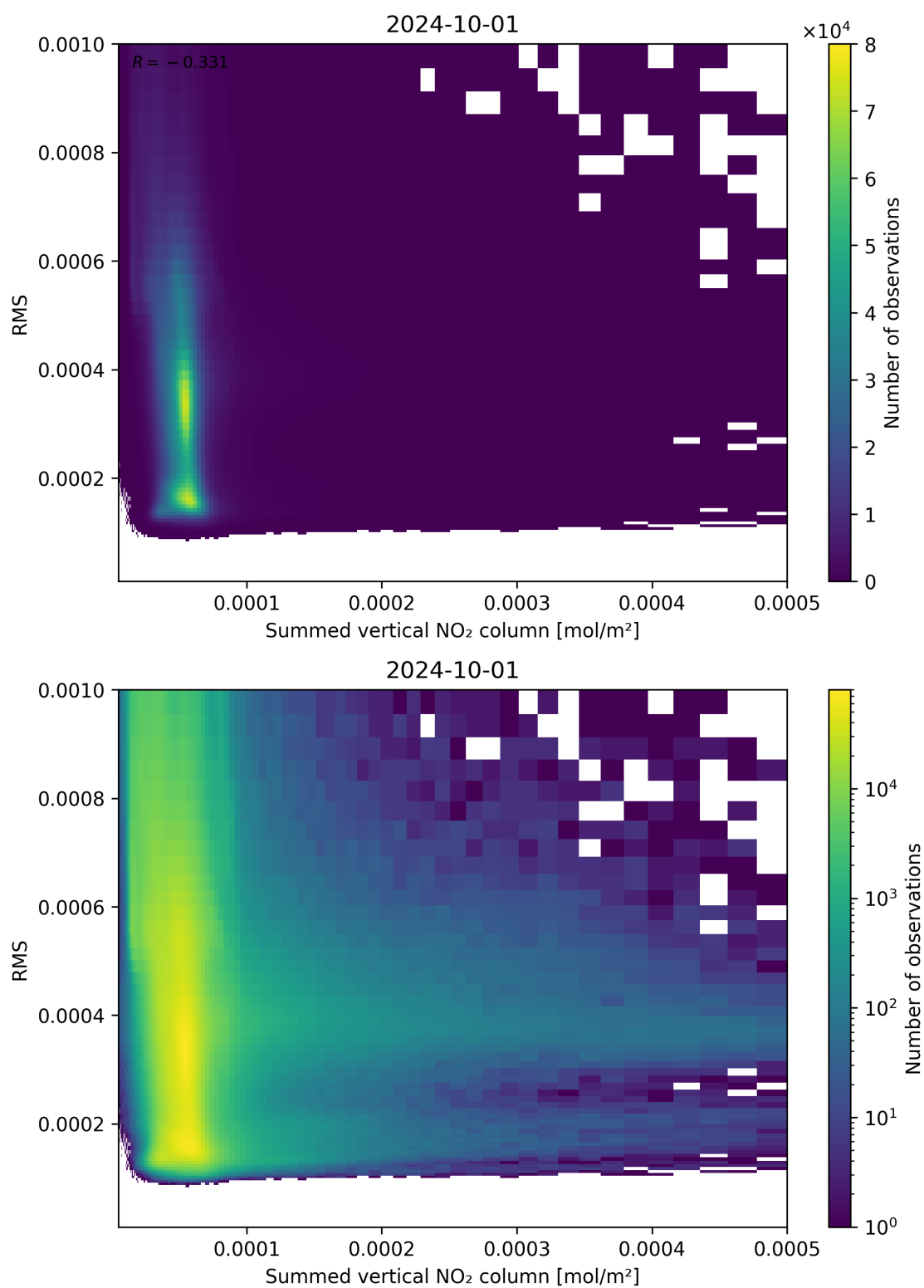
Figure 109: Scatter density plot of “Summed vertical NO 2 column” against “RMS” for 2024-09-30 to 2024-10-02.
