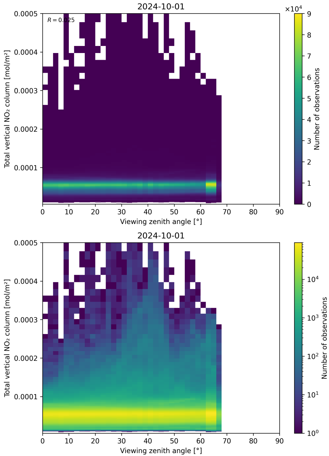
Figure 167: Scatter density plot of “Viewing zenith angle” against “Total vertical NO 2 column” for 2024-09-30 to 2024-10-02.
