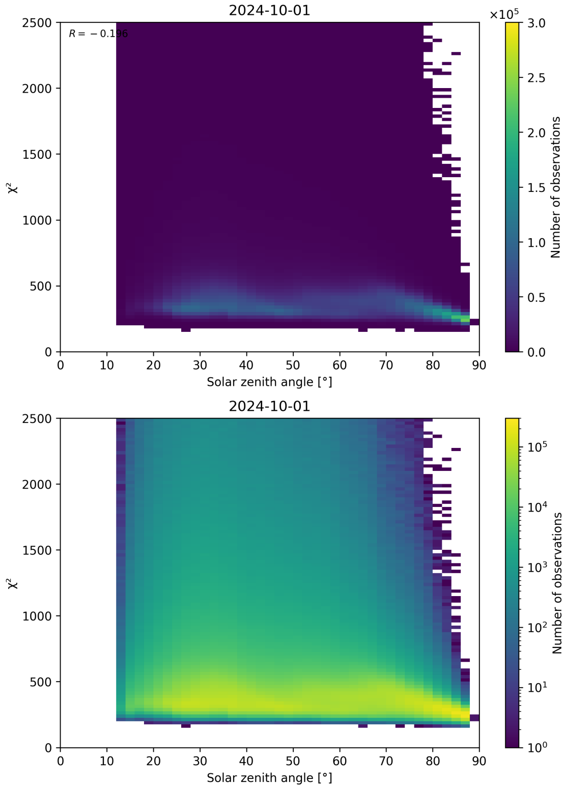
Figure 148: Scatter density plot of “Solar zenith angle” against “ \chi^2 ” for 2024-09-30 to 2024-10-02.
