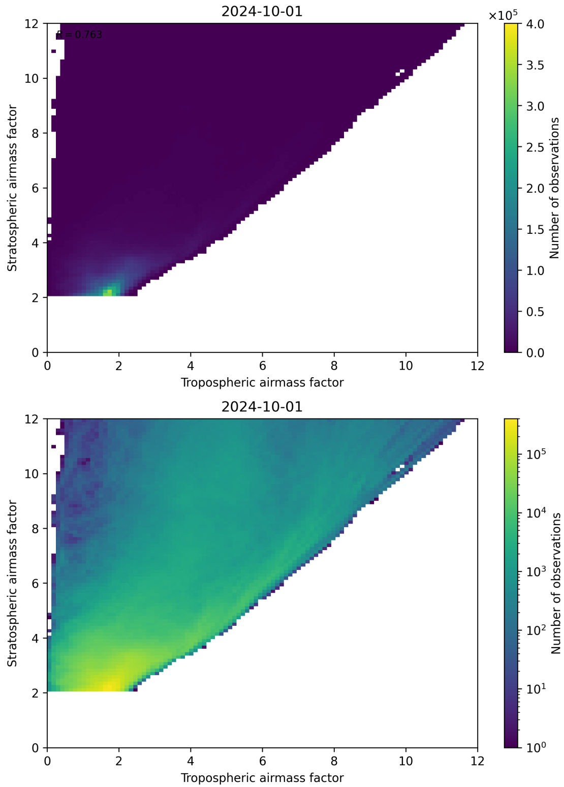
Figure 71: Scatter density plot of “Tropospheric airmass factor” against “Stratospheric airmass factor” for 2024-09-30 to 2024-10-02.
