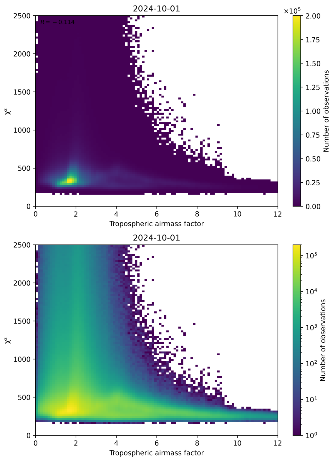
Figure 73: Scatter density plot of “Tropospheric airmass factor” against “ \chi^2 ” for 2024-09-30 to 2024-10-02.
