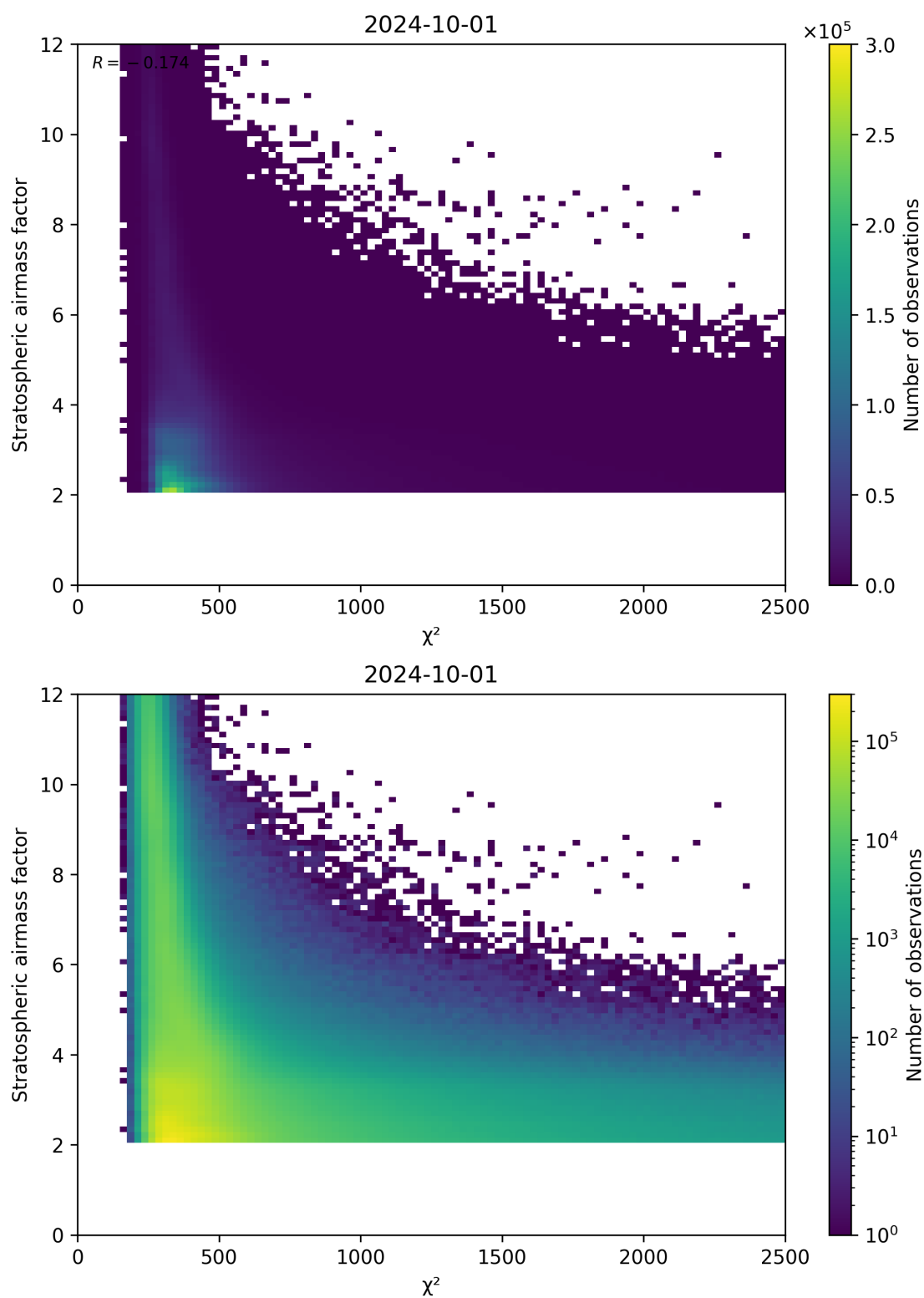
Figure 81: Scatter density plot of “ \chi^2 ” against “Stratospheric airmass factor” for 2024-09-30 to 2024-10-02.
