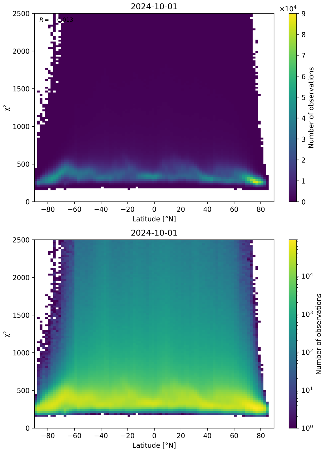
Figure 86: Scatter density plot of “Latitude” against “ \chi^2 ” for 2024-09-30 to 2024-10-02.
