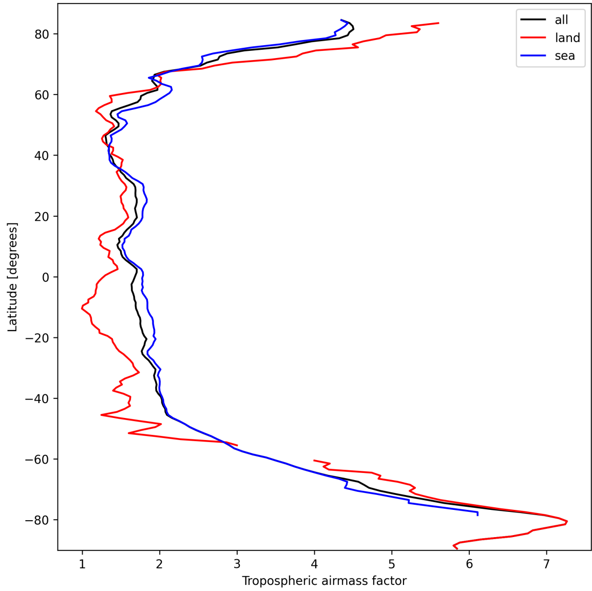
Figure 14: Zonal average of “Tropospheric airmass factor” for 2024-09-30 to 2024-10-02.
