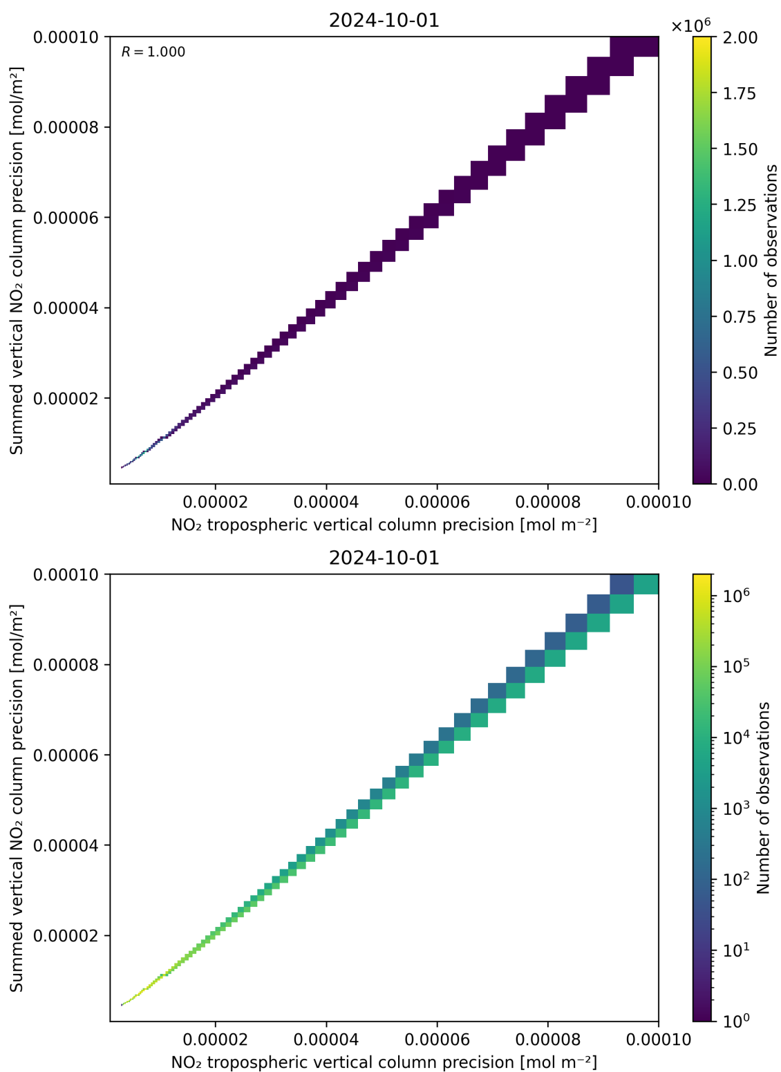
Figure 137: Scatter density plot of “NO 2 tropospheric vertical column precision” against “Summed vertical NO 2 column precision” for 2024-09-30 to 2024-10-02.
