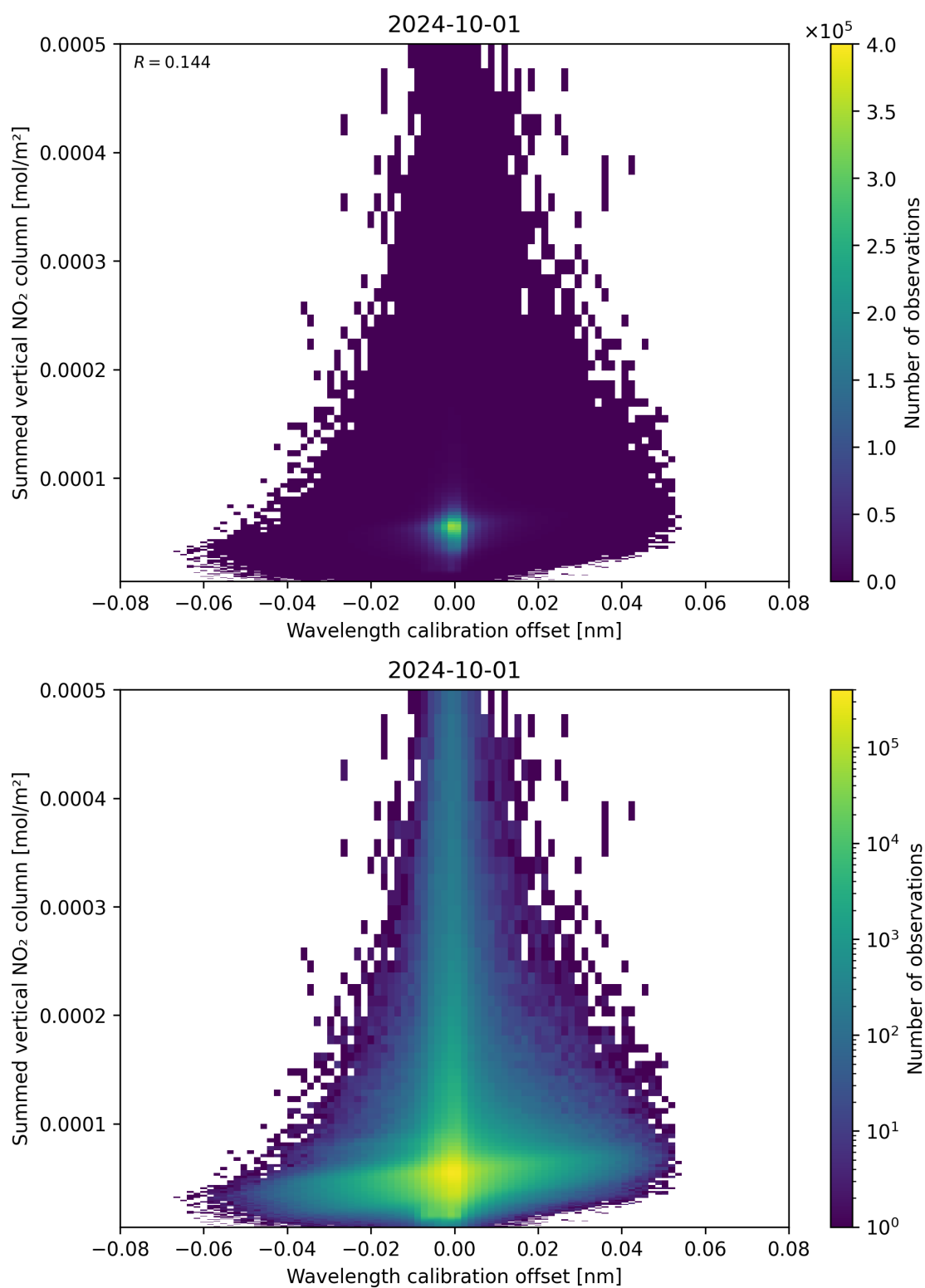
Figure 177: Scatter density plot of “Wavelength calibration offset” against “Summed vertical NO 2 column” for 2024-09-30 to 2024-10-02.
