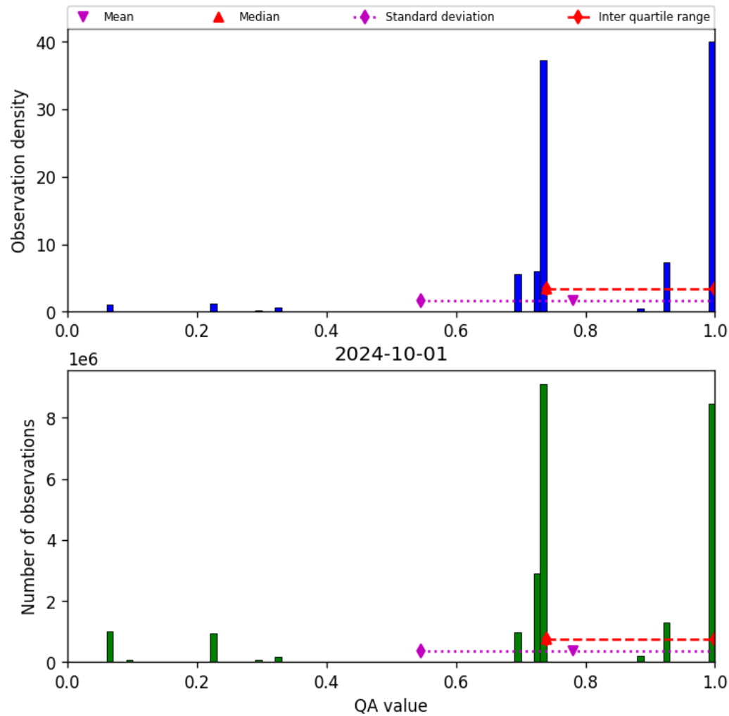
Figure 28: Histogram of “QA value” for 2024-09-30 to 2024-10-02
