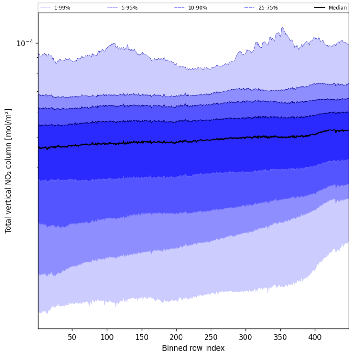
Figure 55: Along track statistics of “Total vertical NO 2 column” for 2024-09-30 to 2024-10-02
