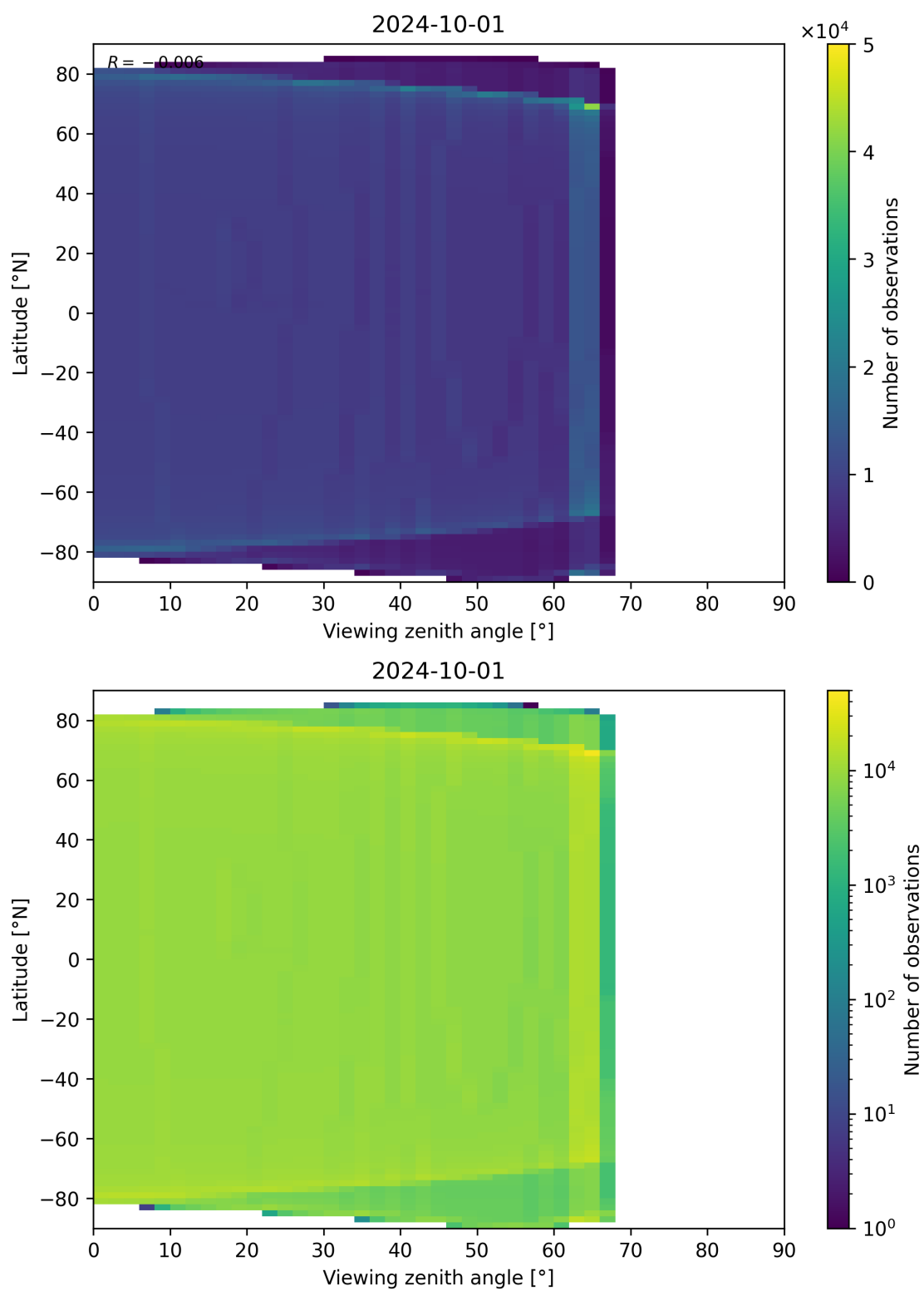
Figure 163: Scatter density plot of “Viewing zenith angle” against “Latitude” for 2024-09-30 to 2024-10-02.
