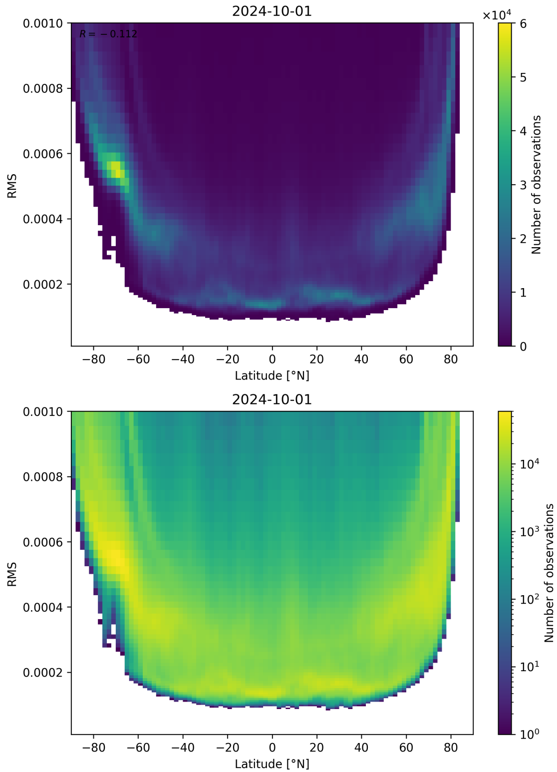
Figure 94: Scatter density plot of “Latitude” against “RMS” for 2024-09-30 to 2024-10-02.
