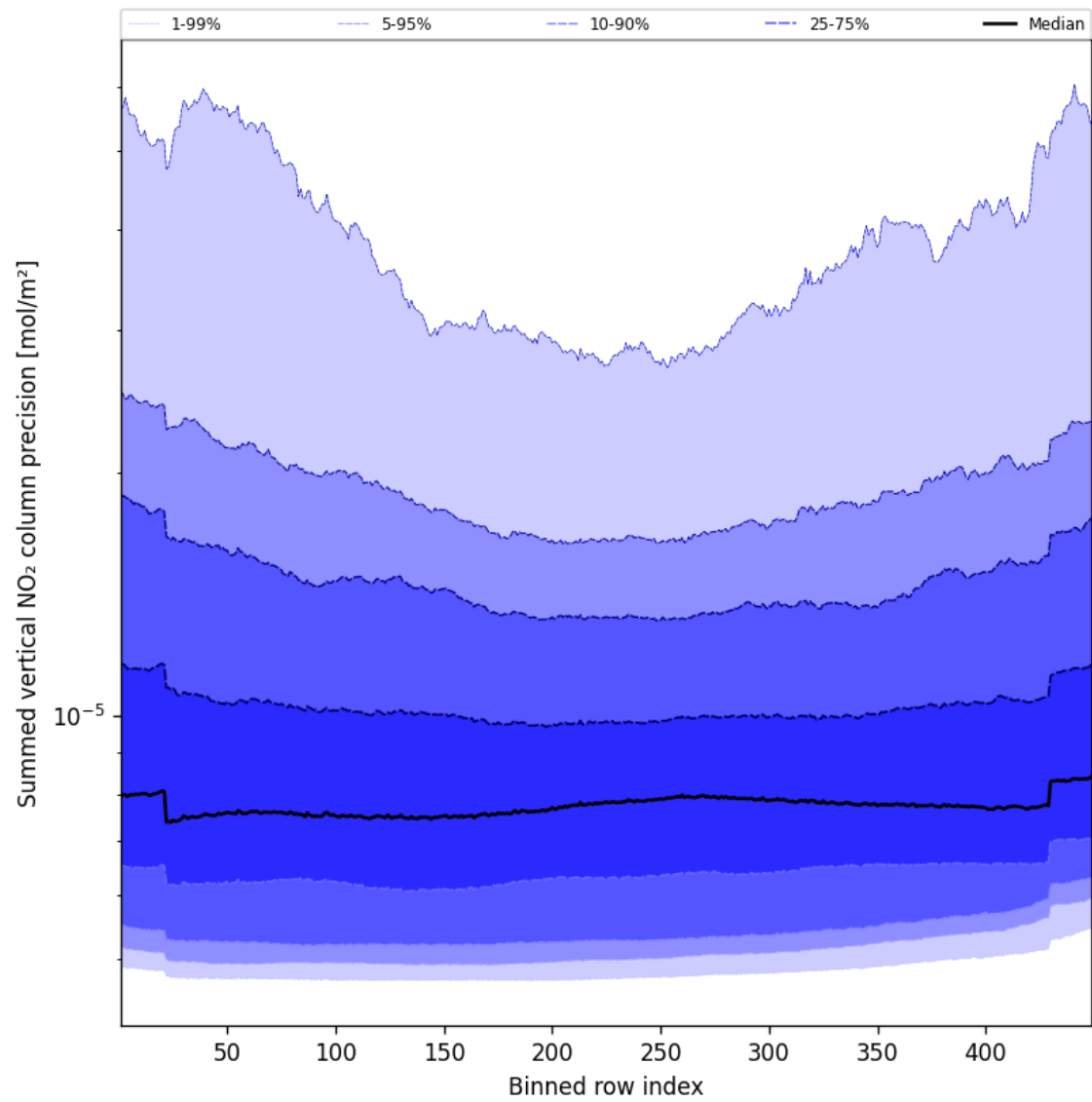
Figure 58: Along track statistics of “Summed vertical NO 2 column precision” for 2024-09-30 to 2024-10-02
