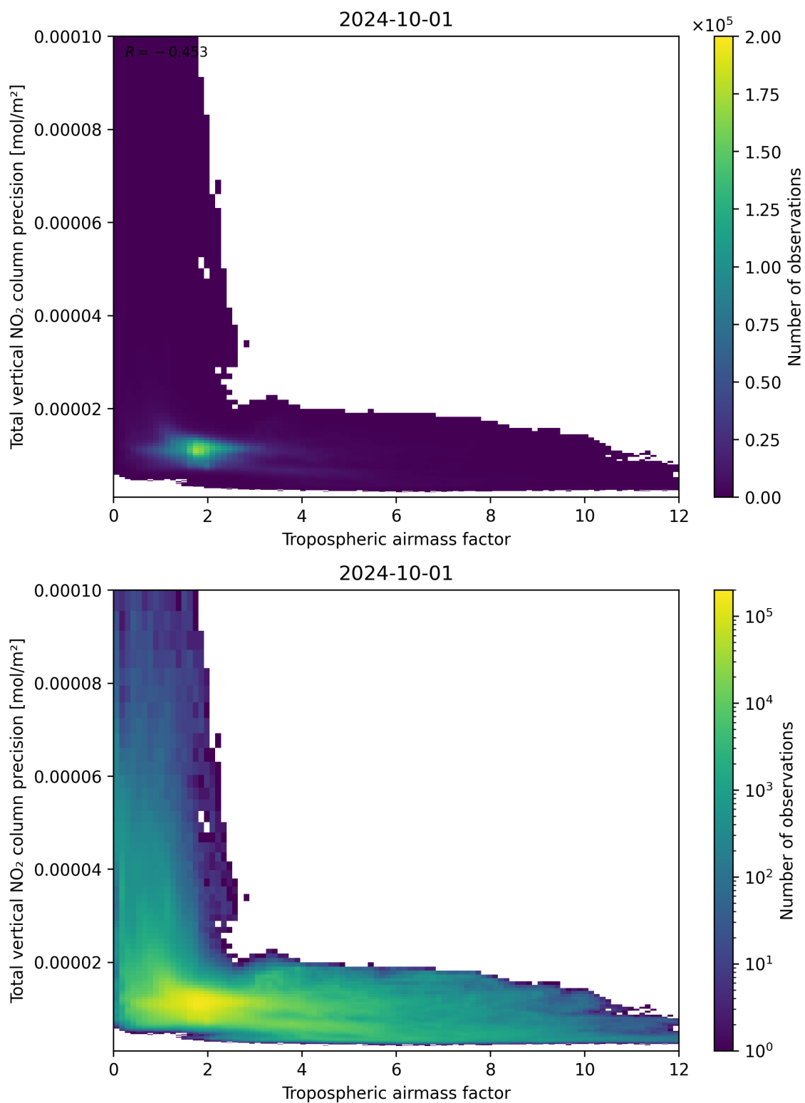
Figure 78: Scatter density plot of “Tropospheric airmass factor” against “Total vertical NO 2 column precision” for 2024-09-30 to 2024-10-02.
