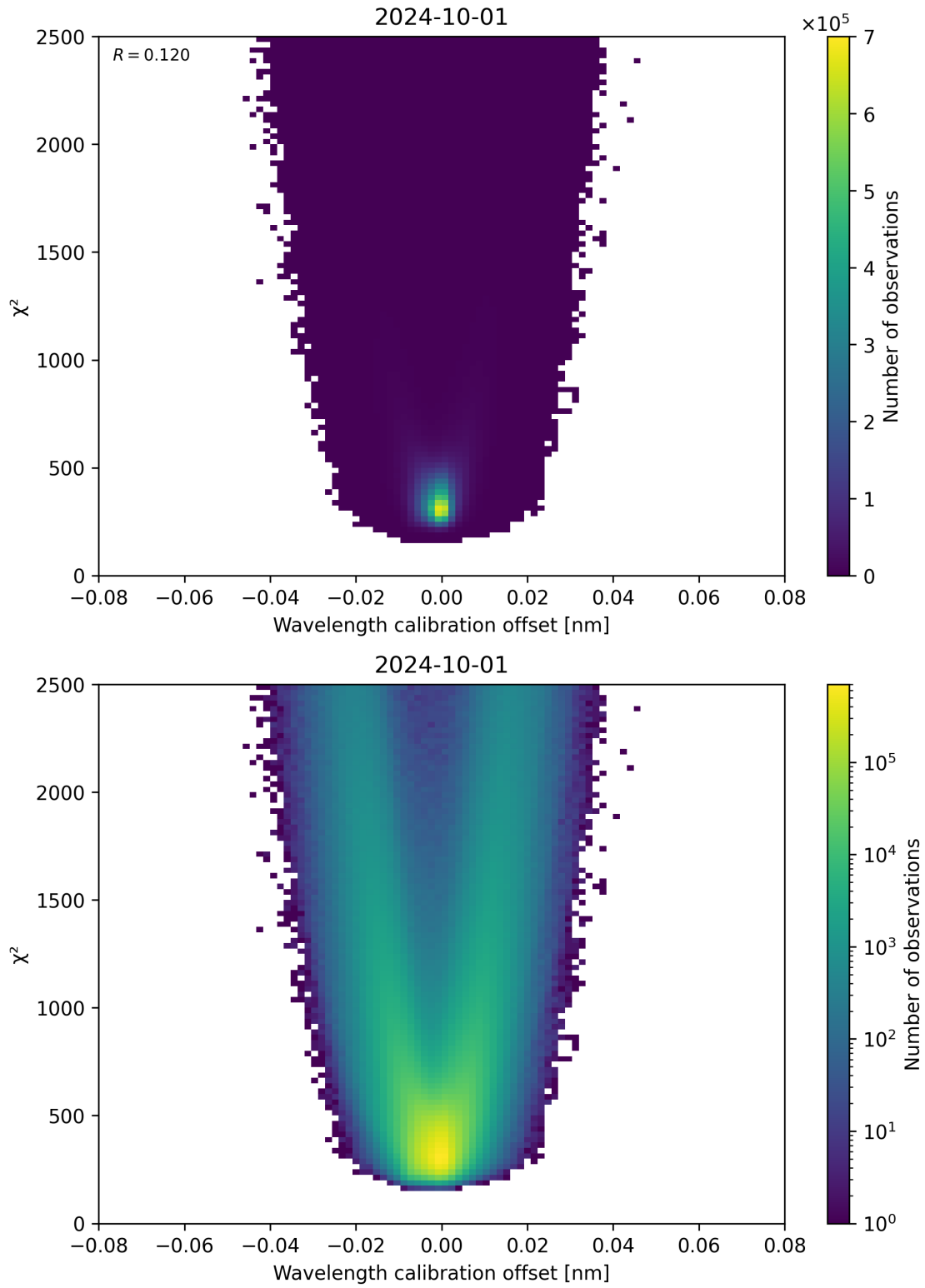
Figure 175: Scatter density plot of “Wavelength calibration offset” against “ \chi^2 ” for 2024-09-30 to 2024-10-02.
