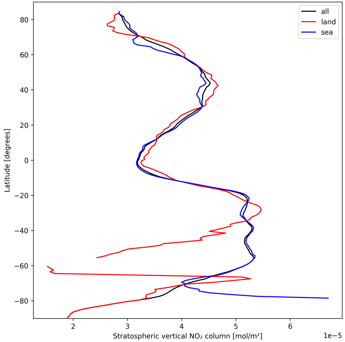
Figure 19: Zonal average of “Stratospheric vertical NO 2 column” for 2024-09-30 to 2024-10-02.
