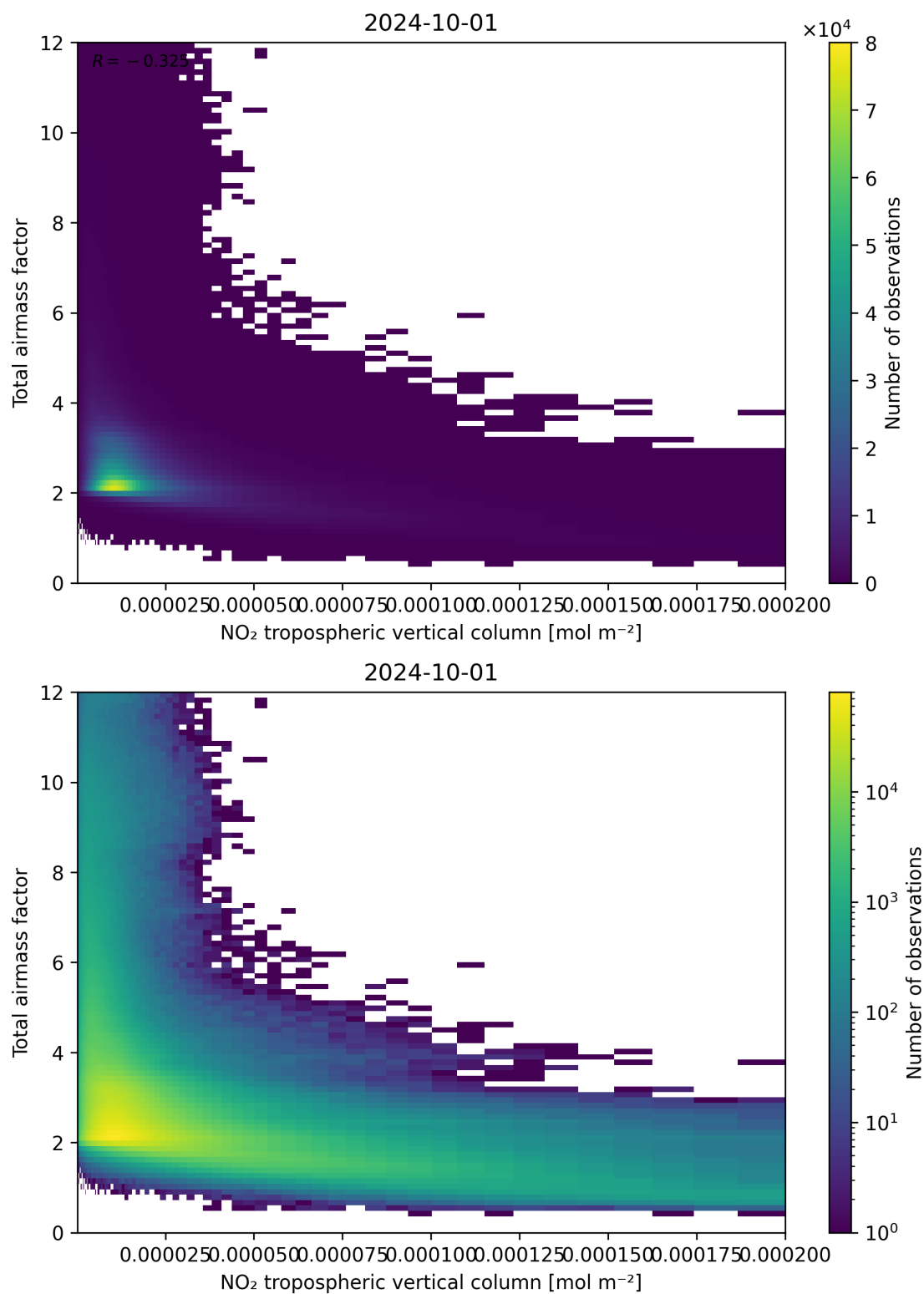
Figure 122: Scatter density plot of “NO 2 tropospheric vertical column” against “Total air mass factor” for 2024-09-30 to 2024-10-02.
