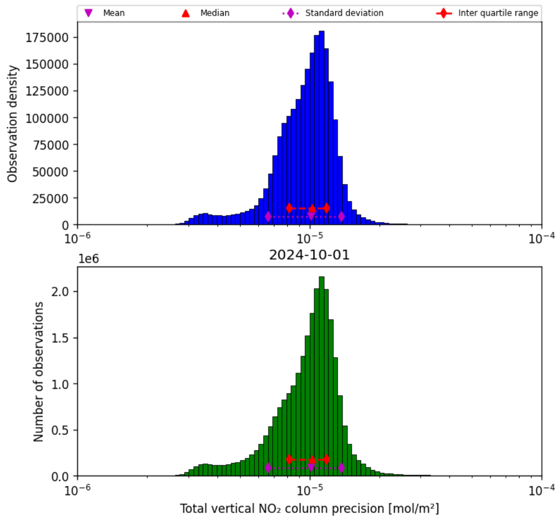
Figure 39: Histogram of “Total vertical NO 2 column precision” for 2024-09-30 to 2024-10-02
