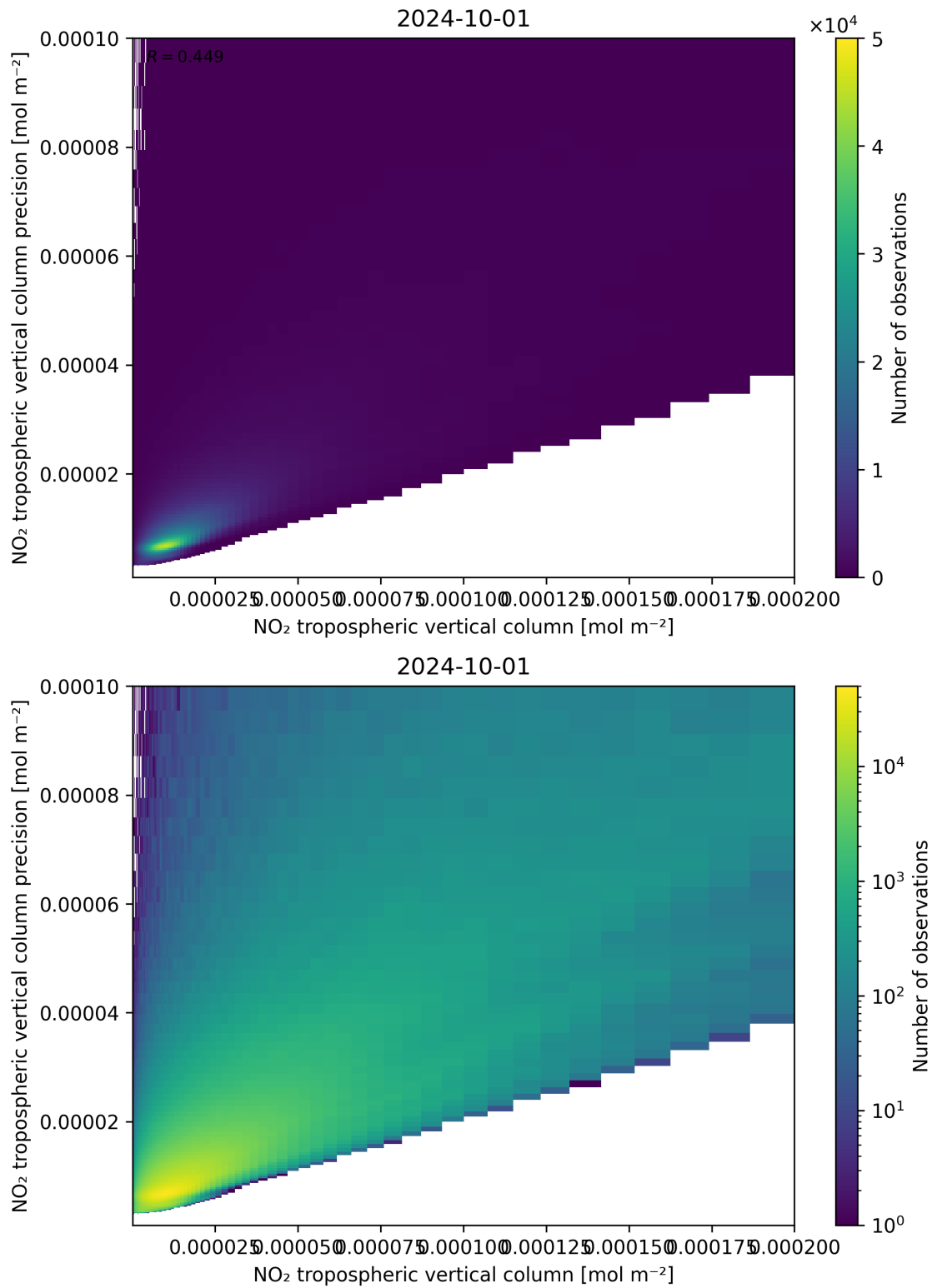
Figure 130: Scatter density plot of “NO 2 tropospheric vertical column” against “NO 2 tropospheric vertical column precision” for 2024-09-30 to 2024-10-02.
