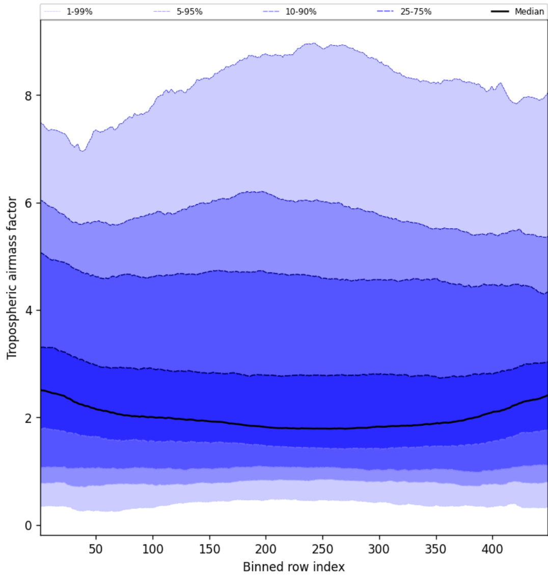
Figure 48: Along track statistics of “Tropospheric air mass factor” for 2024-09-30 to 2024-10-02
