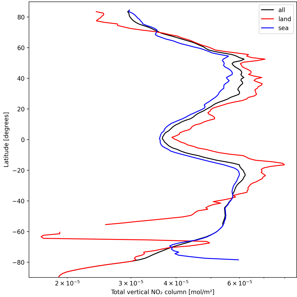
Figure 21: Zonal average of “Total vertical NO 2 column” for 2024-09-30 to 2024-10-02.
