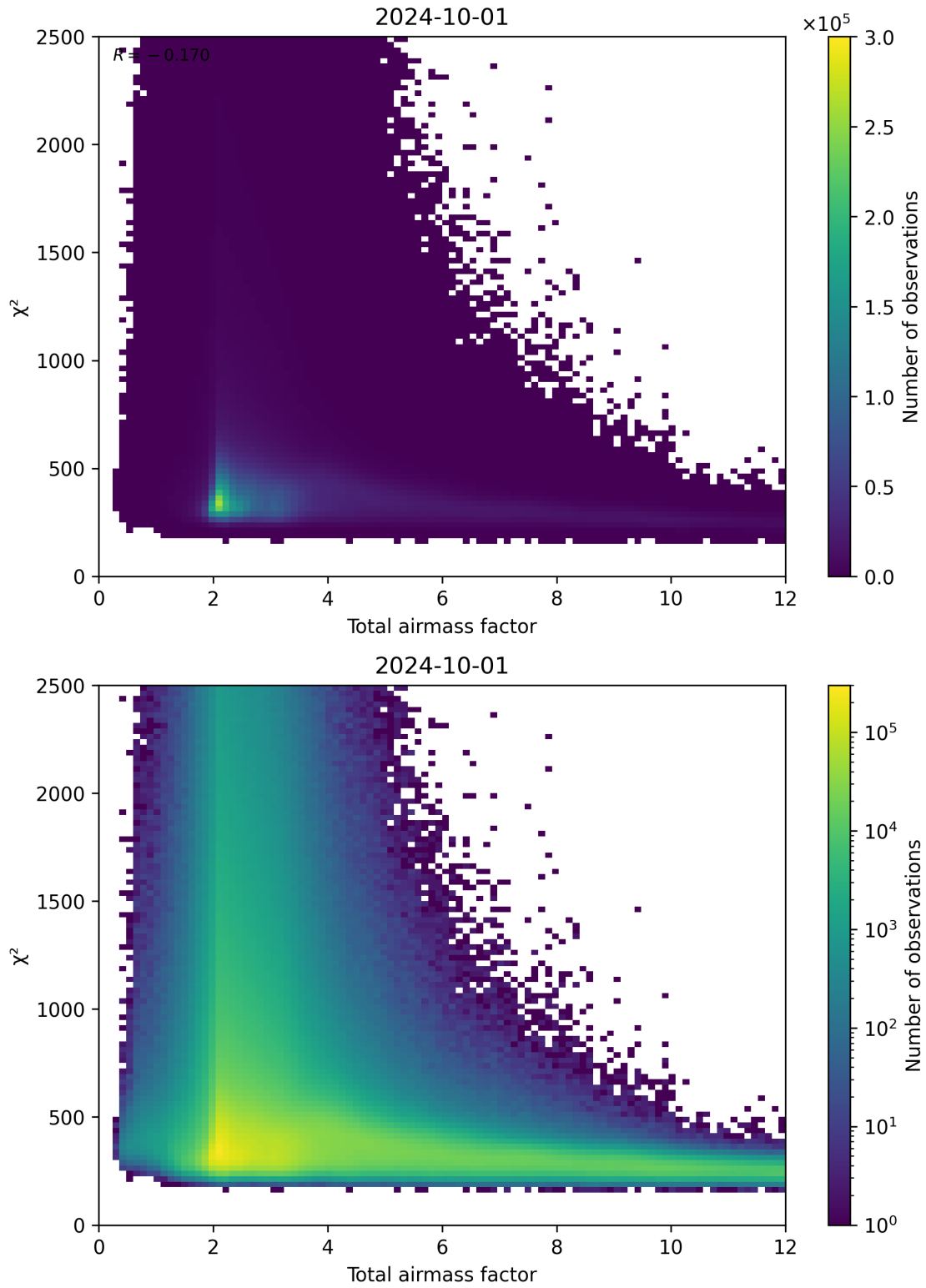
Figure 63: Scatter density plot of “Total airmass factor” against “ \chi^2 ” for 2024-09-30 to 2024-10-02.
