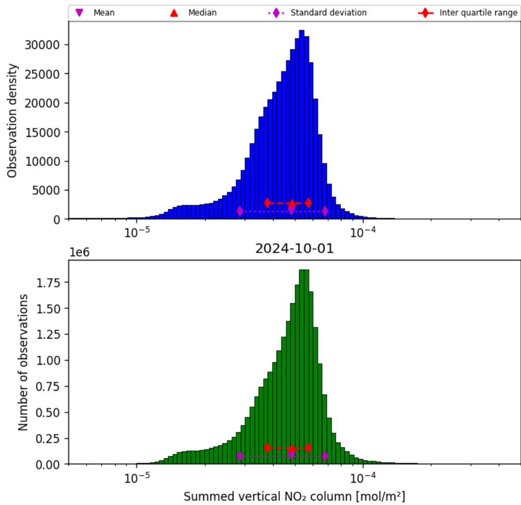
Figure 40: Histogram of “Summed vertical NO 2 column” for 2024-09-30 to 2024-10-02
