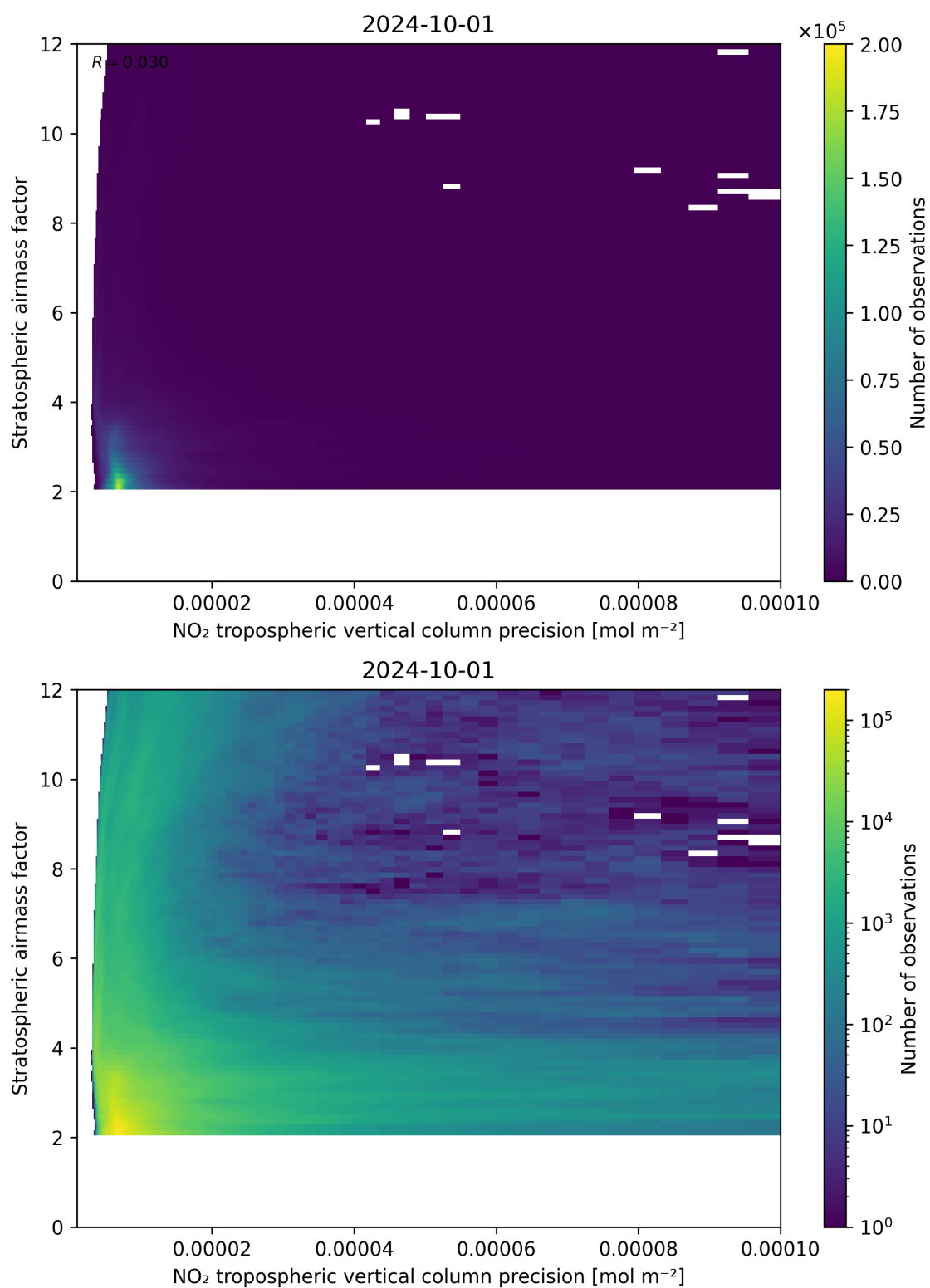
Figure 131: Scatter density plot of “NO 2 tropospheric vertical column precision” against “Stratospheric airmass factor” for 2024-09-30 to 2024-10-02.
