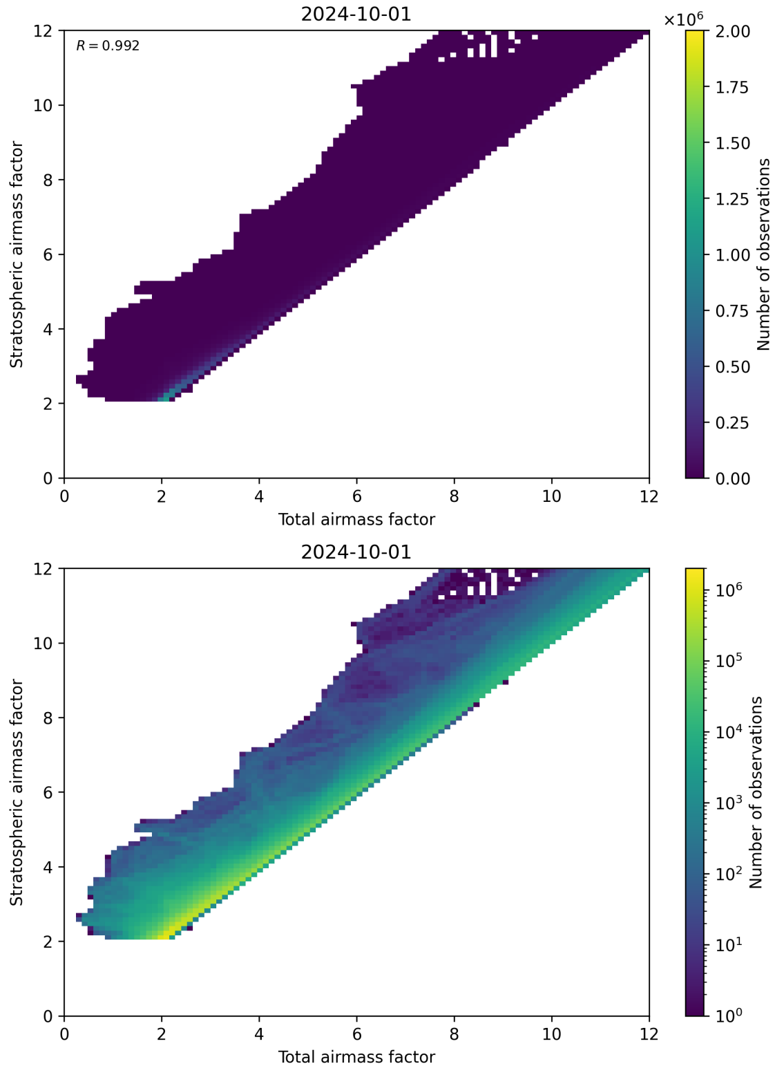
Figure 62: Scatter density plot of “Total airmass factor” against “Stratospheric airmass factor” for 2024-09-30 to 2024-10-02.
