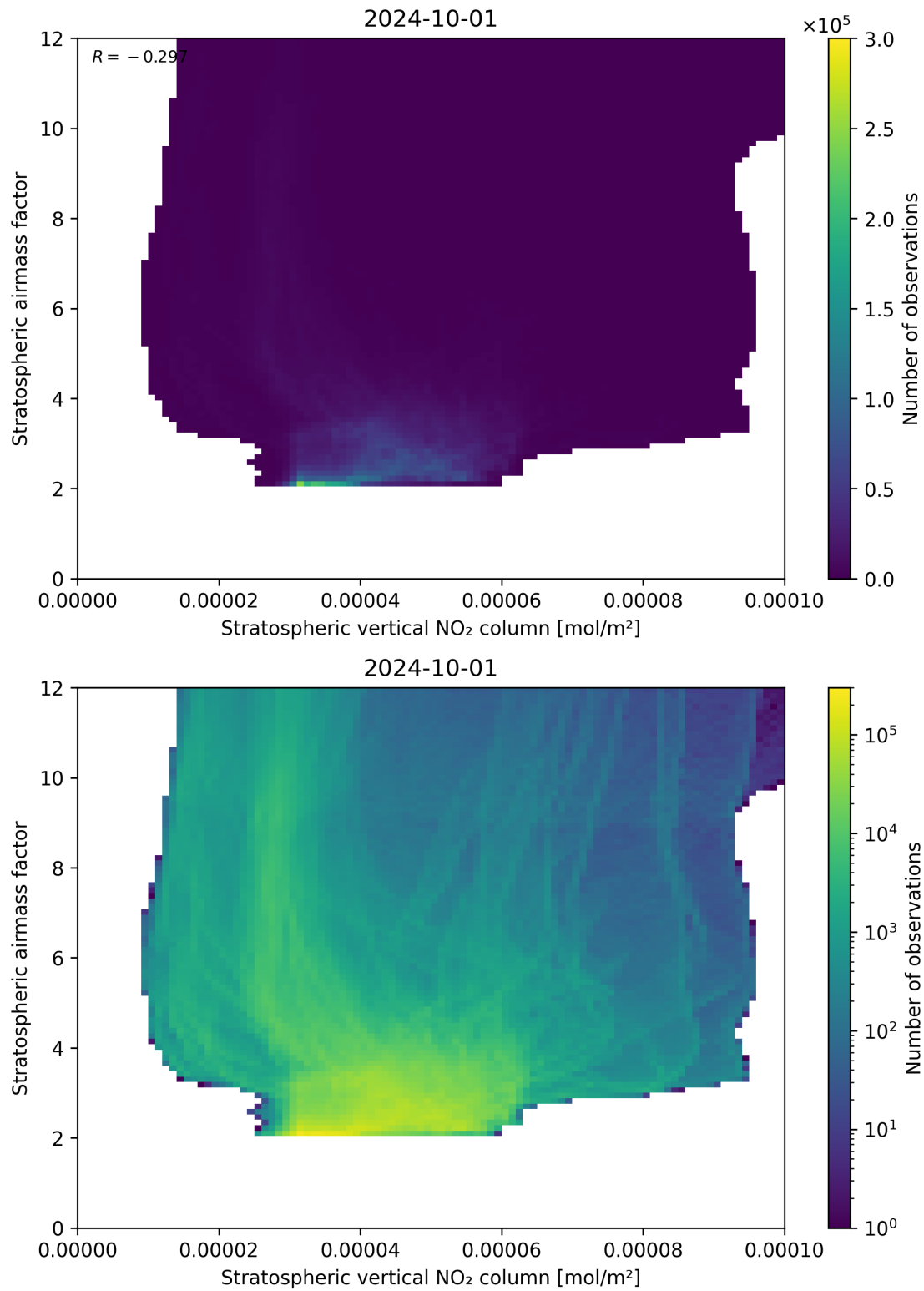
Figure 96: Scatter density plot of “Stratospheric vertical NO 2 column” against “Stratospheric airmass factor” for 2024-09-30 to 2024-10-02.
