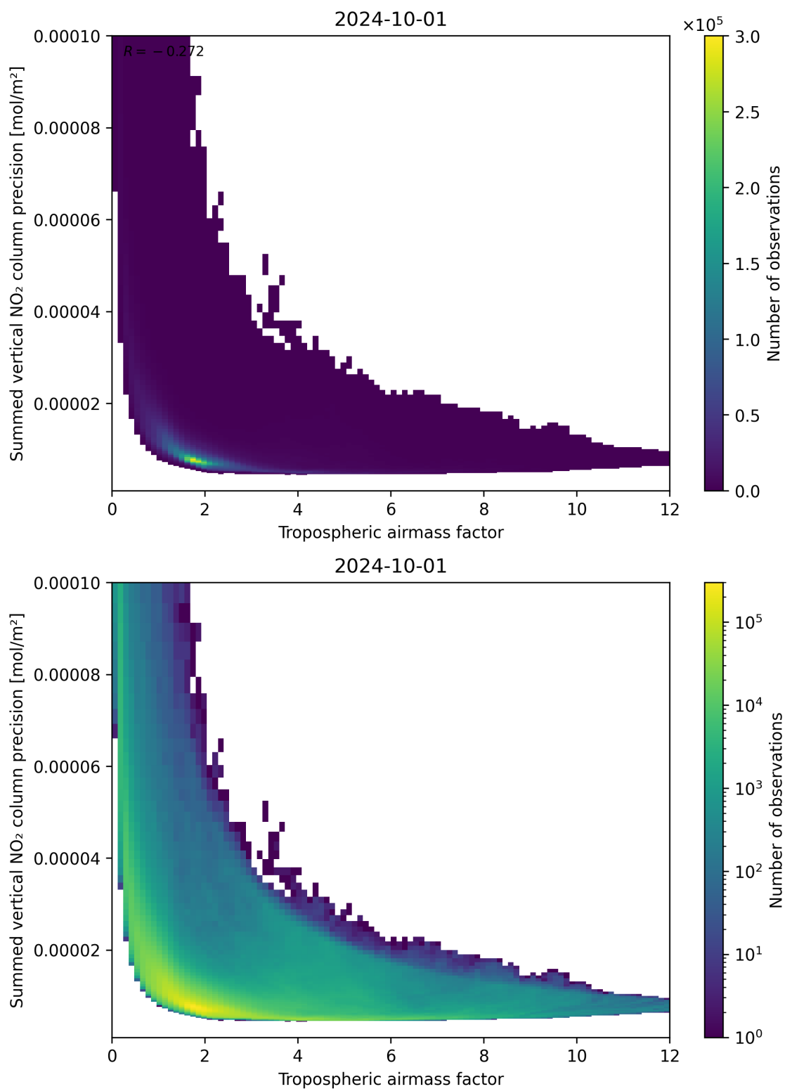
Figure 76: Scatter density plot of “Tropospheric air mass factor” against “Summed vertical NO 2 column precision” for 2024-09-30 to 2024-10-02.
