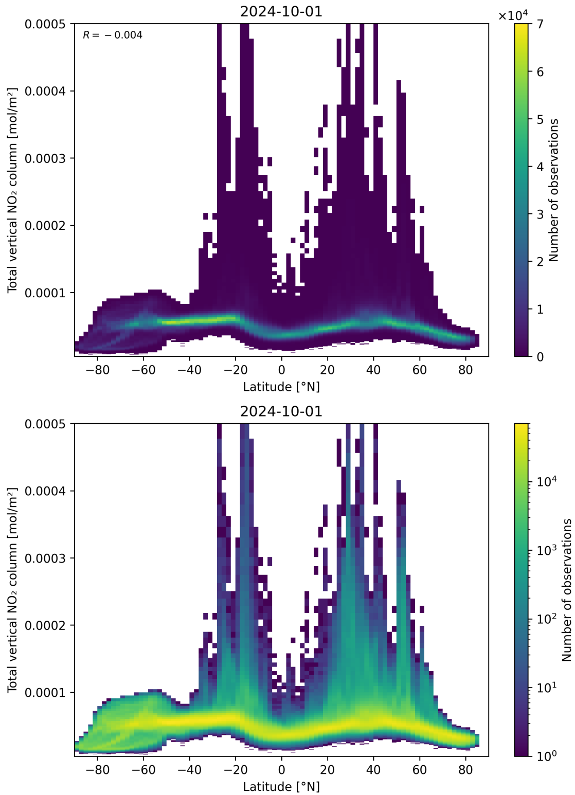
Figure 90: Scatter density plot of “Latitude” against “Total vertical NO 2 column” for 2024-09-30 to 2024-10-02.
