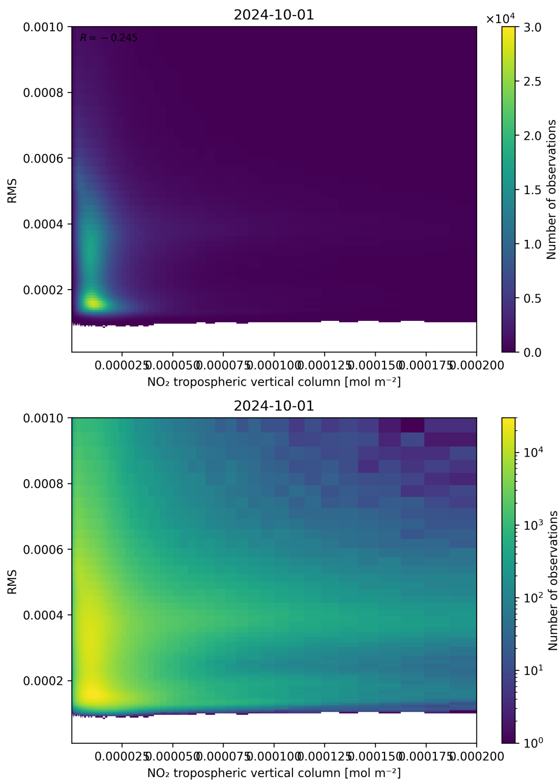
Figure 142: Scatter density plot of “NO 2 tropospheric vertical column” against “RMS” for 2024-09-30 to 2024-10-02.
