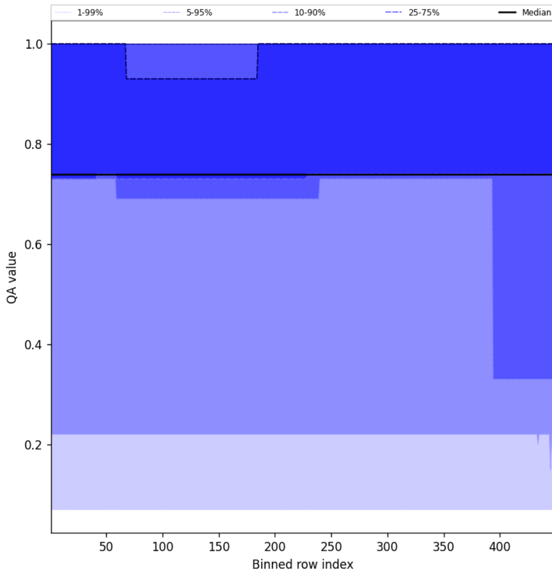
Figure 45: Along track statistics of “QA value” for 2024-09-30 to 2024-10-02
