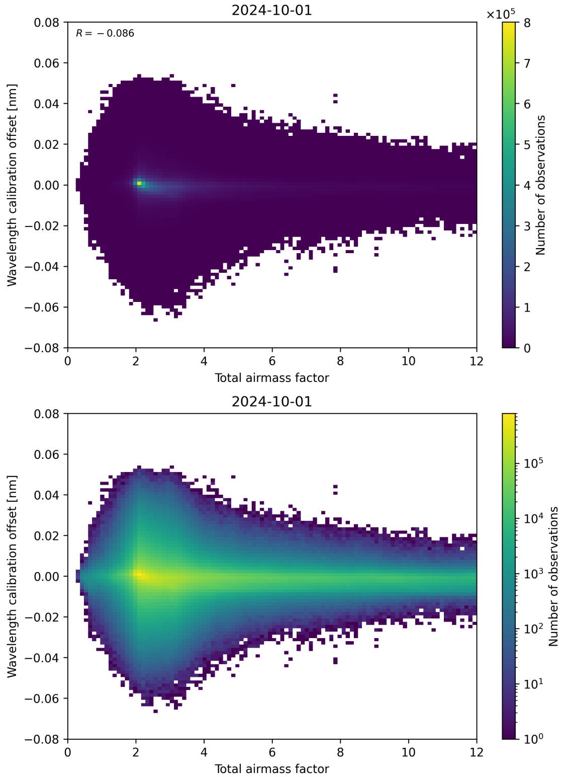
Figure 70: Scatter density plot of “Total airmass factor” against “Wavelength calibration offset” for 2024-09-30 to 2024-10-02.
