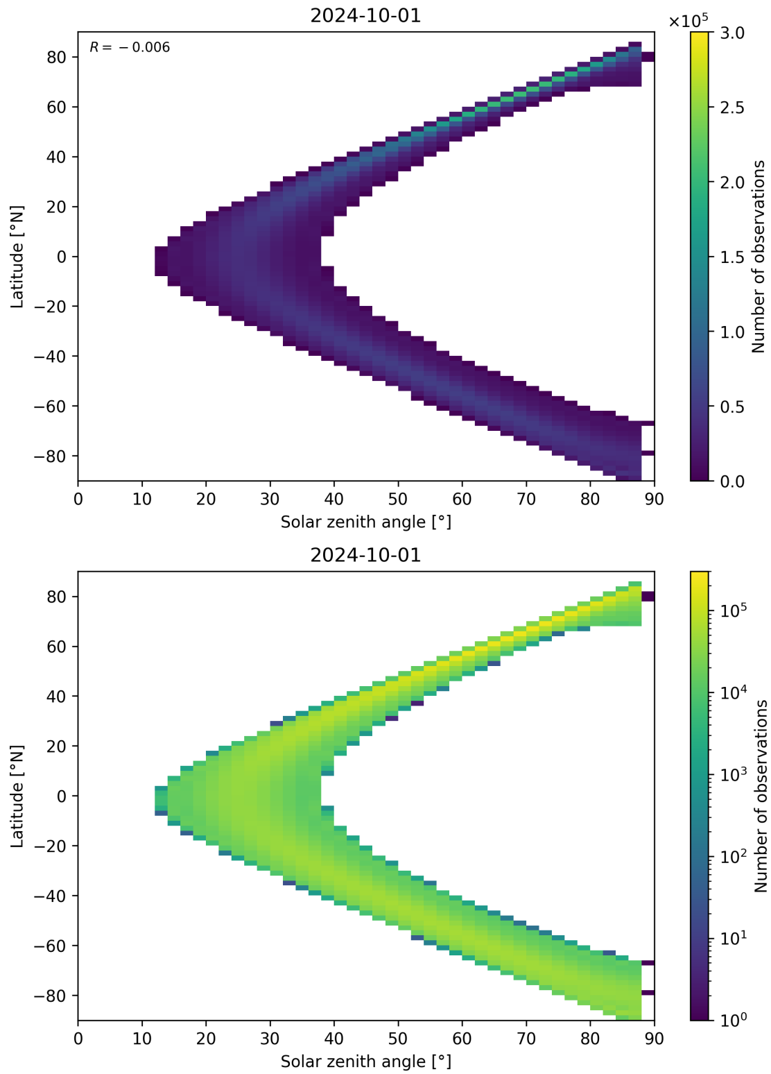
Figure 149: Scatter density plot of “Solar zenith angle” against “Latitude” for 2024-09-30 to 2024-10-02.
