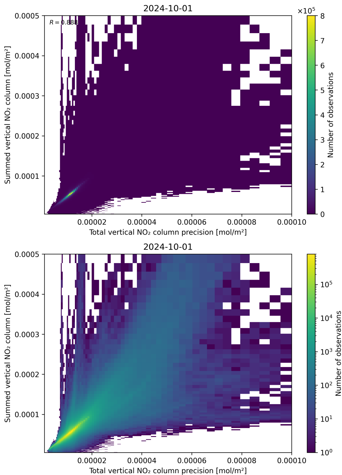
Figure 117: Scatter density plot of “Total vertical NO 2 column precision” against “Summed vertical NO 2 column” for 2024-09-30 to 2024-10-02.
