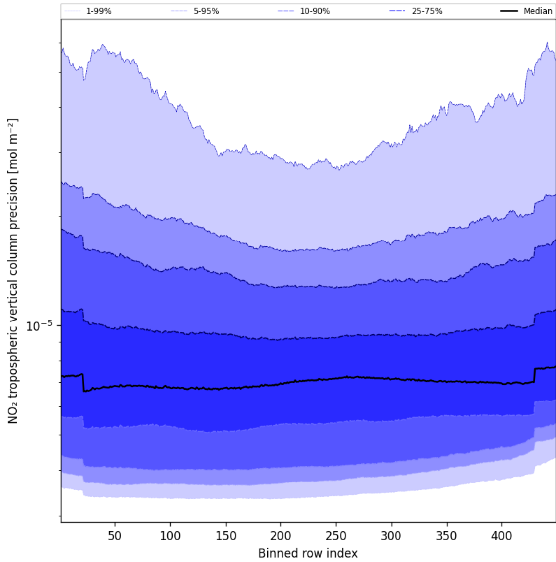
Figure 47: Along track statistics of “NO 2 tropospheric vertical column precision” for 2024-09-30 to 2024-10-02
