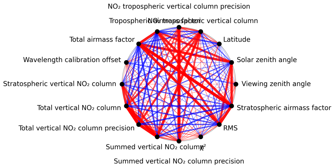
Figure 1: Map of correlation graph for 2024-09-30 to 2024-10-02.
