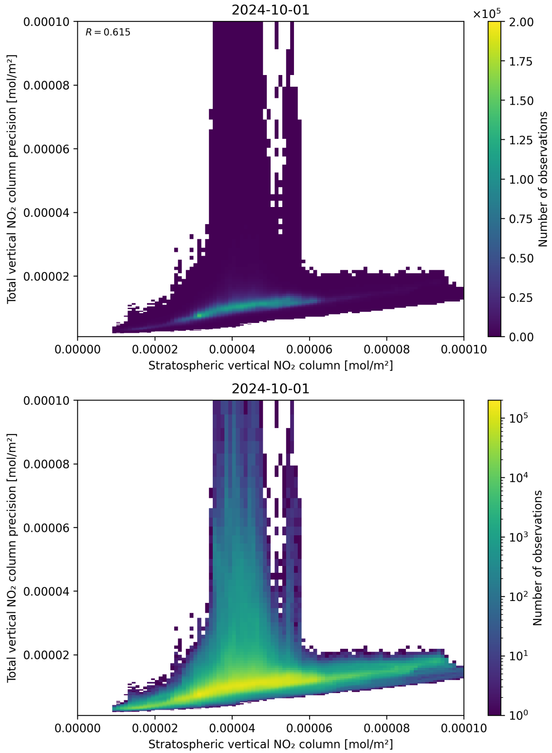
Figure 101: Scatter density plot of “Stratospheric vertical NO 2 column” against “Total vertical NO 2 column precision” for 2024-09-30 to 2024-10-02.
