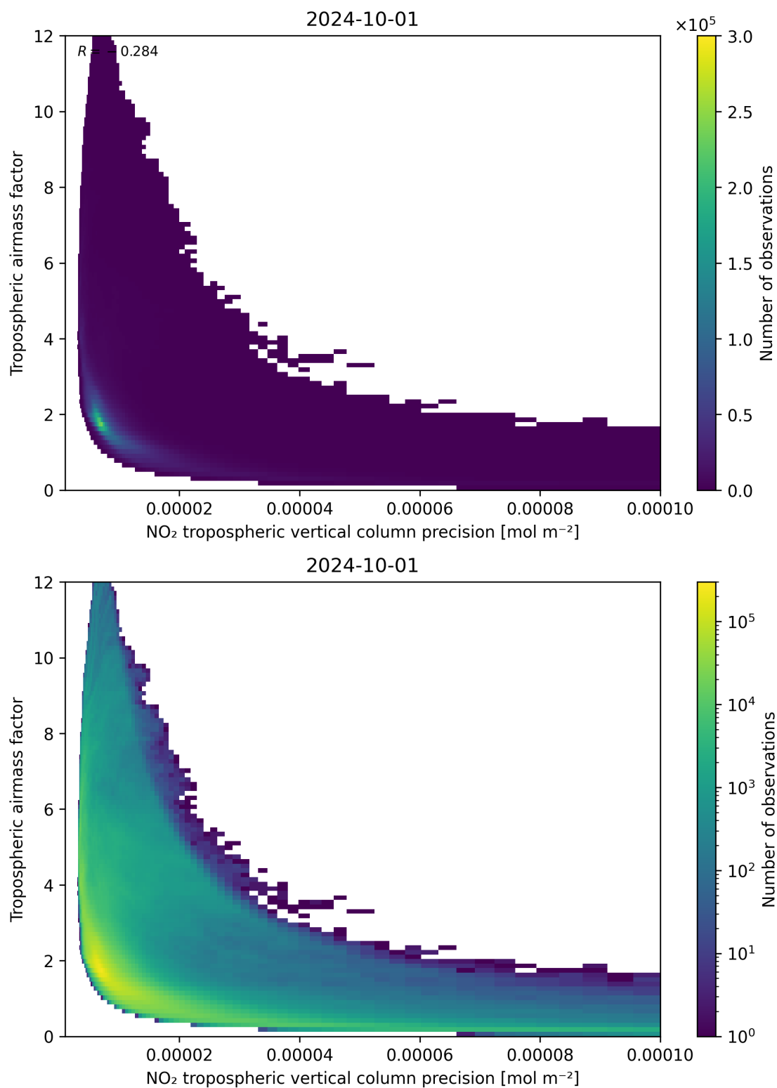
Figure 133: Scatter density plot of “NO 2 tropospheric vertical column precision” against “Tropospheric air mass factor” for 2024-09-30 to 2024-10-02.
