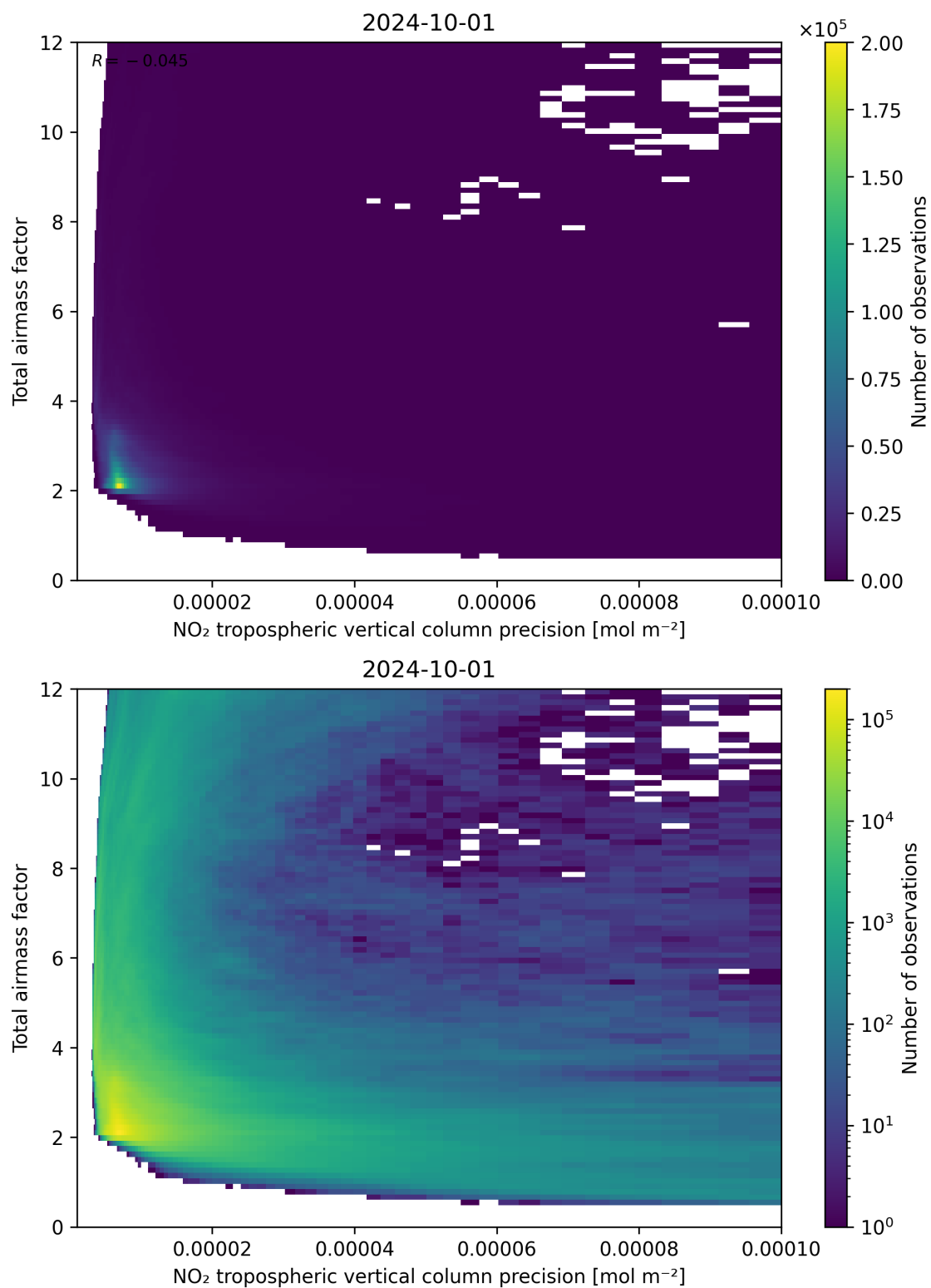
Figure 132: Scatter density plot of “NO 2 tropospheric vertical column precision” against “Total air mass factor” for 2024-09-30 to 2024-10-02.
