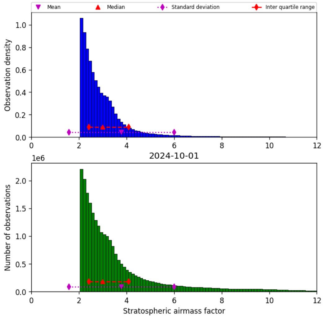
Figure 44: Histogram of “Stratospheric airmass factor” for 2024-09-30 to 2024-10-02
