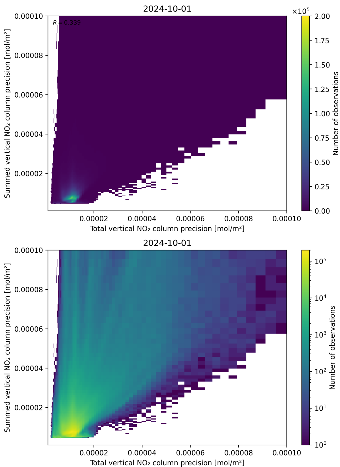
Figure 118: Scatter density plot of “Total vertical NO 2 column precision” against “Summed vertical NO 2 column precision” for 2024-09-30 to 2024-10-02.
