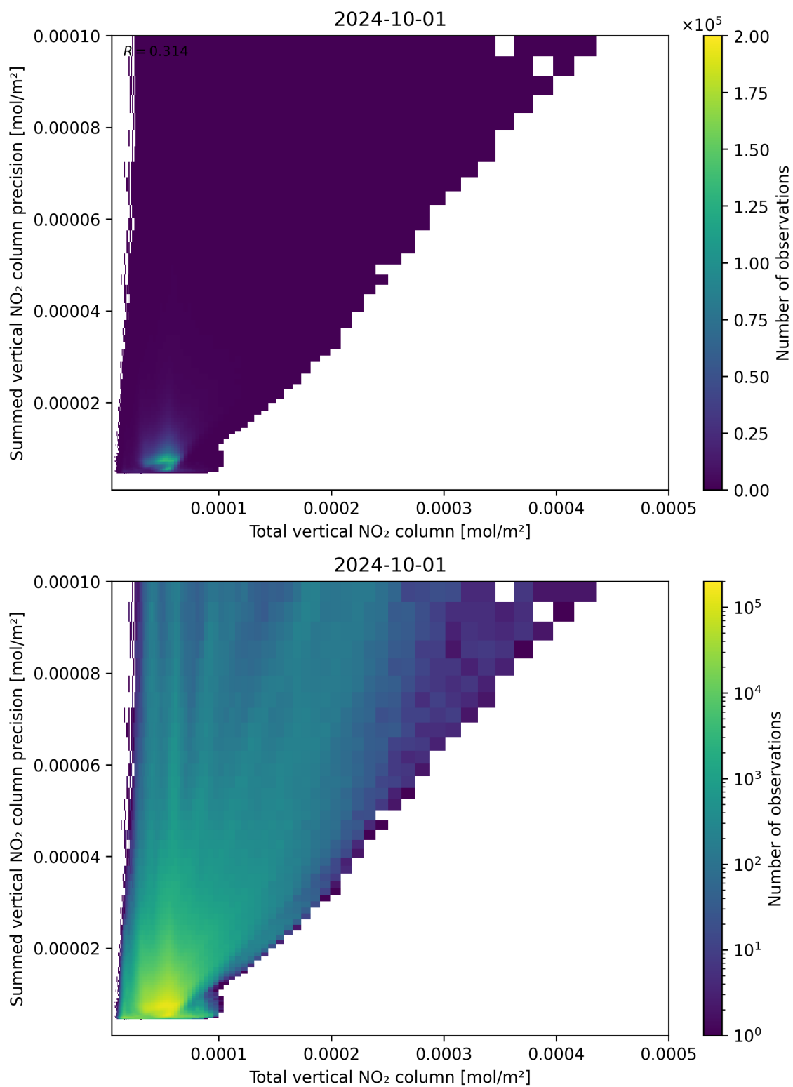
Figure 113: Scatter density plot of “Total vertical NO 2 column” against “Summed vertical NO 2 column precision” for 2024-09-30 to 2024-10-02.
