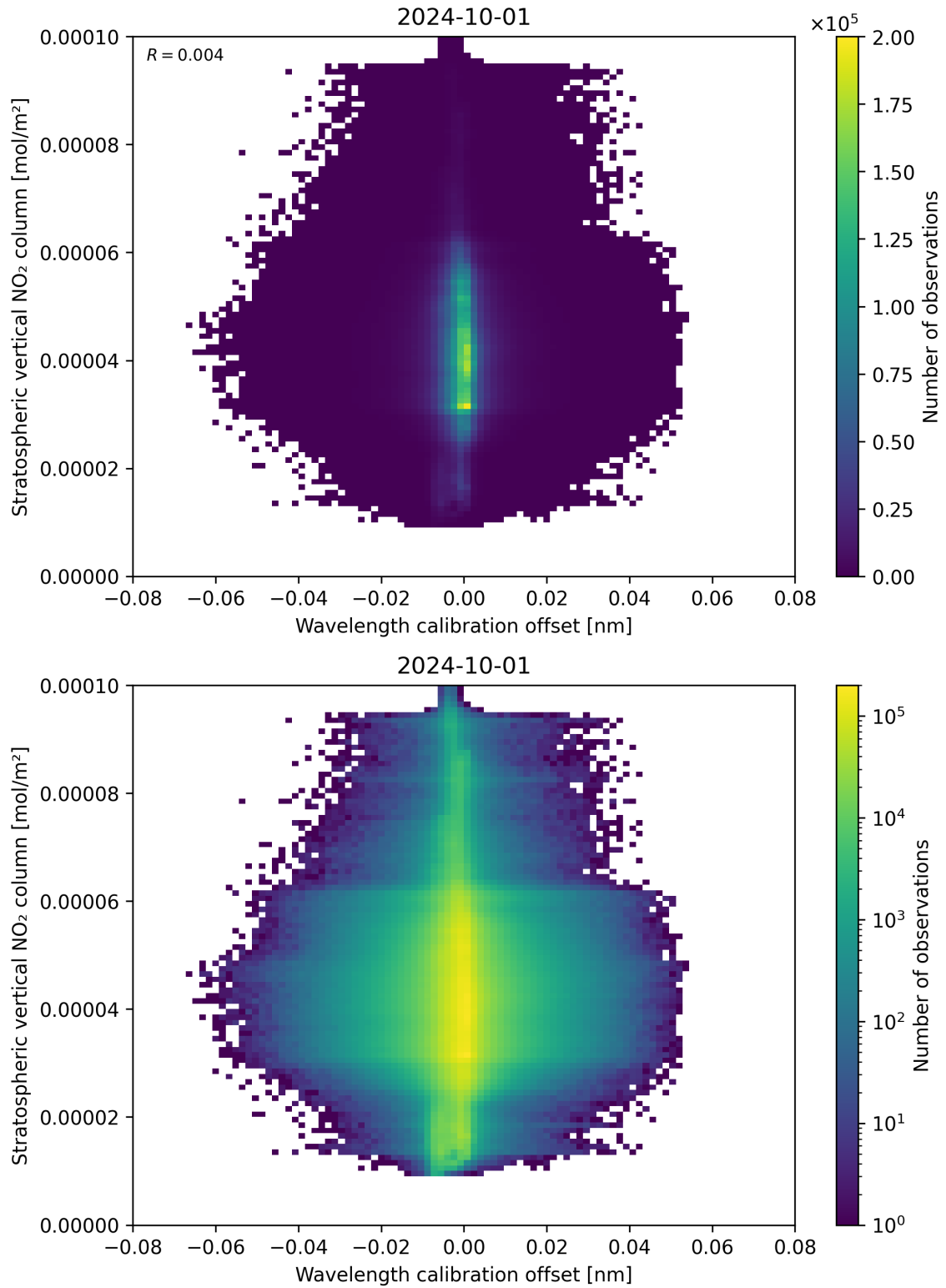
Figure 176: Scatter density plot of “Wavelength calibration offset” against “Stratospheric vertical NO 2 column” for 2024-09-30 to 2024-10-02.
