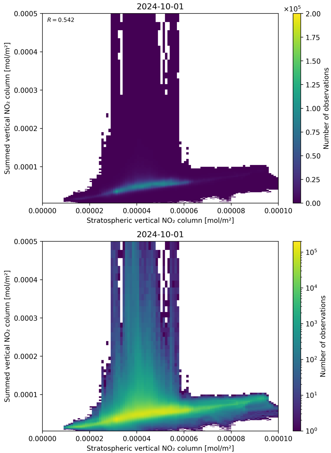
Figure 98: Scatter density plot of “Stratospheric vertical NO 2 column” against “Summed vertical NO 2 column” for 2024-09-30 to 2024-10-02.
