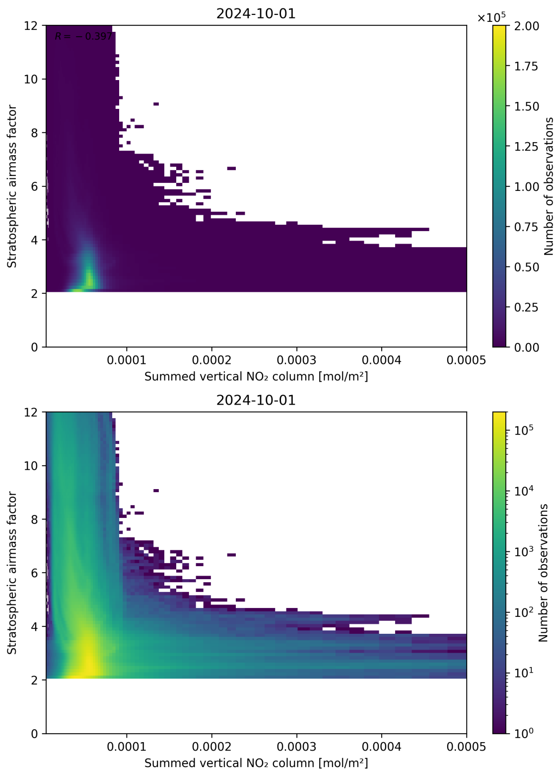
Figure 103: Scatter density plot of “Summed vertical NO 2 column” against “Stratospheric airmass factor” for 2024-09-30 to 2024-10-02.
