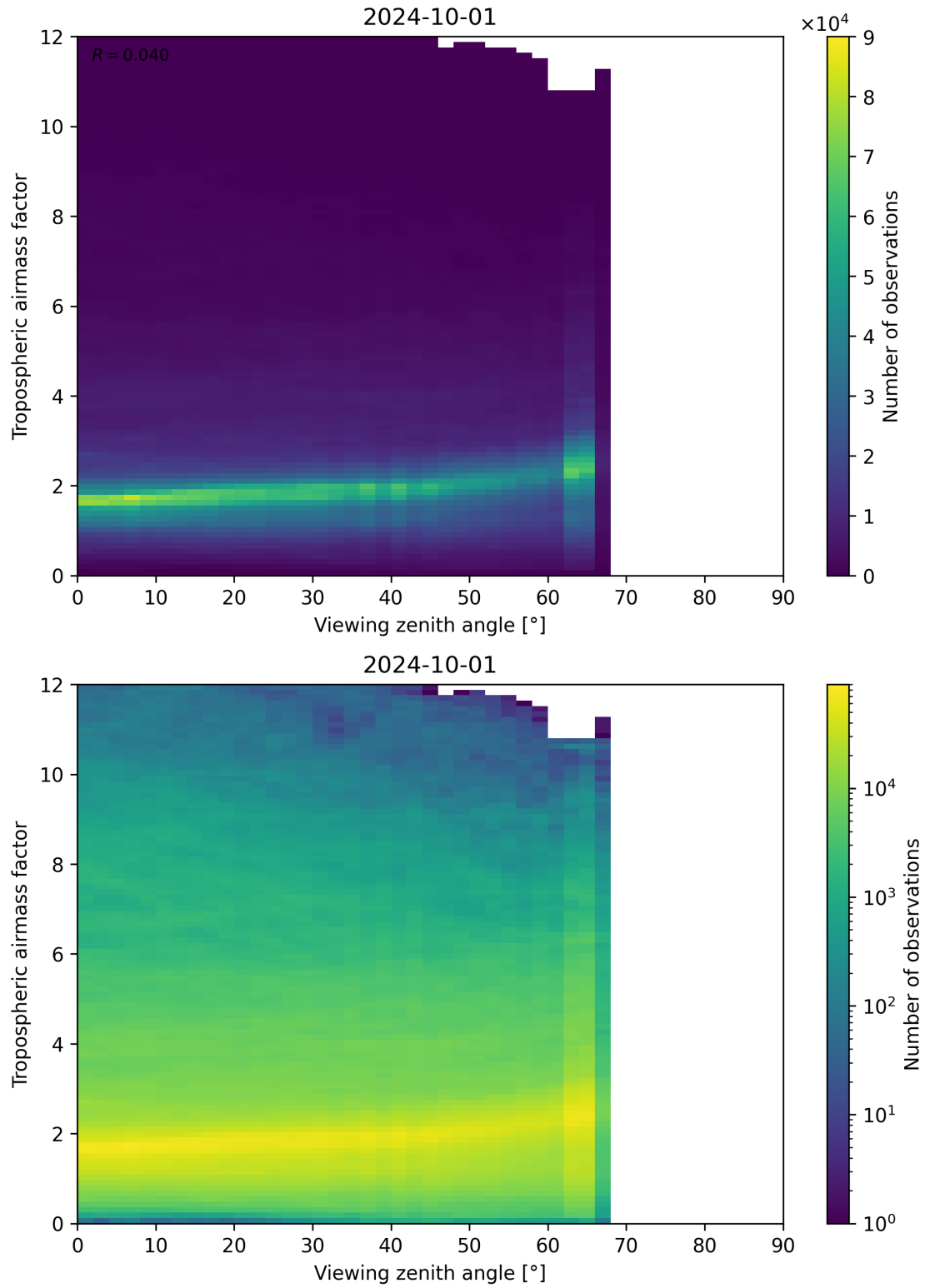
Figure 161: Scatter density plot of “Viewing zenith angle” against “Tropospheric airmass factor” for 2024-09-30 to 2024-10-02.
