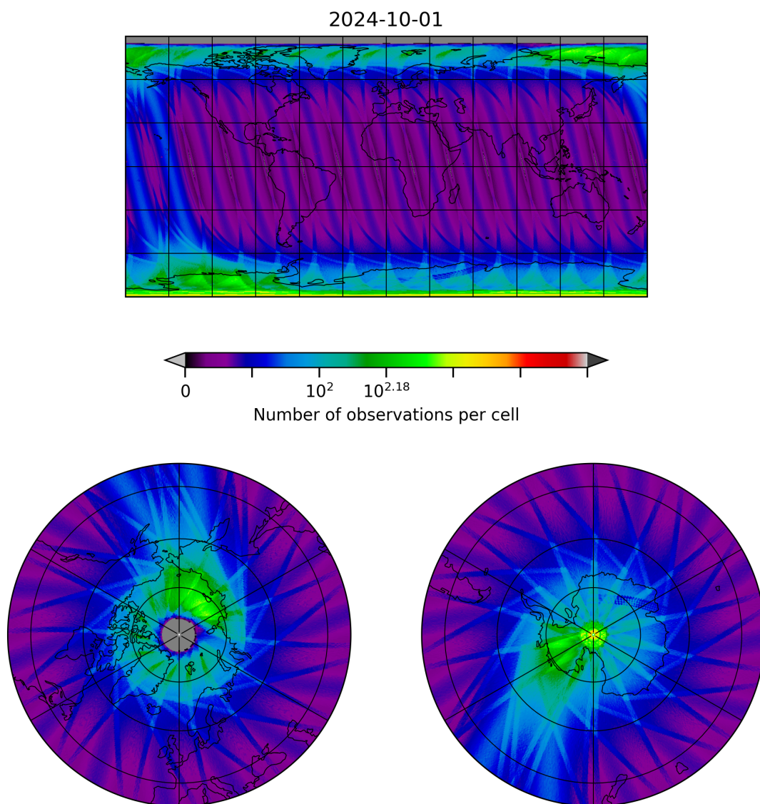
Figure 10: Map of the number of observations for 2024-09-30 to 2024-10-02
