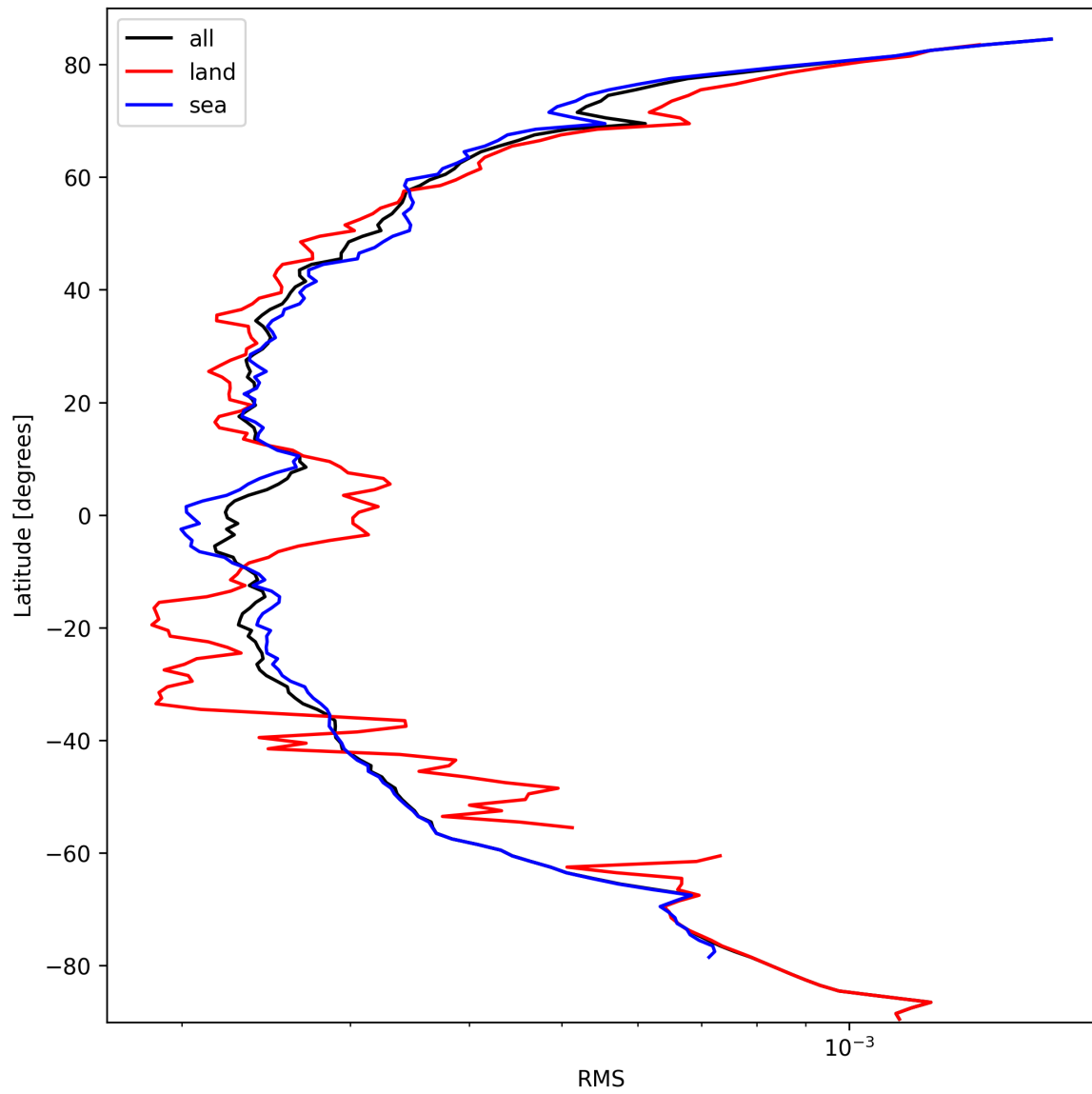
Figure 26: Zonal average of “RMS” for 2024-09-30 to 2024-10-02.
