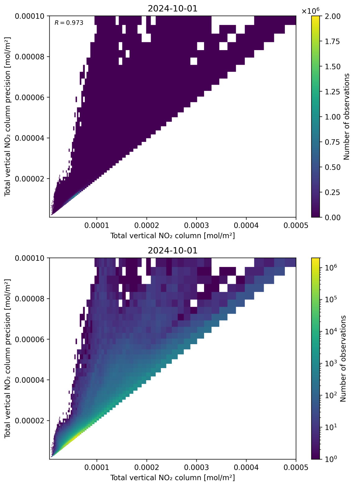
Figure 114: Scatter density plot of “Total vertical NO 2 column” against “Total vertical NO 2 column precision” for 2024-09-30 to 2024-10-02.
