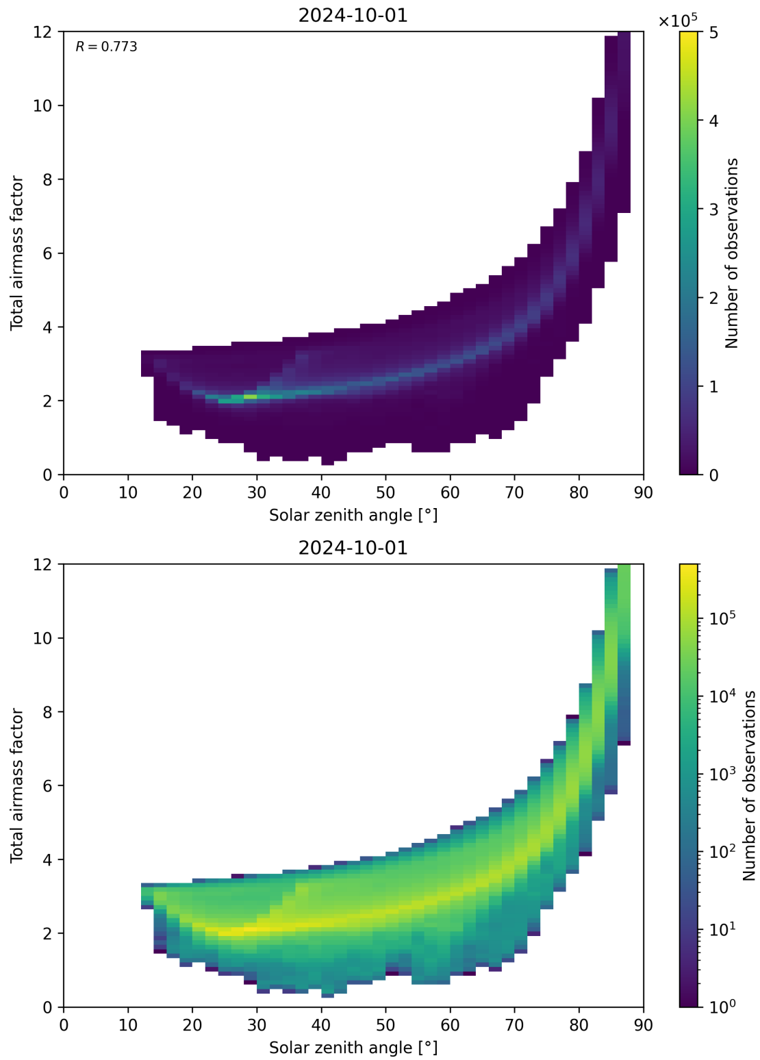
Figure 146: Scatter density plot of “Solar zenith angle” against “Total airmass factor” for 2024-09-30 to 2024-10-02.
