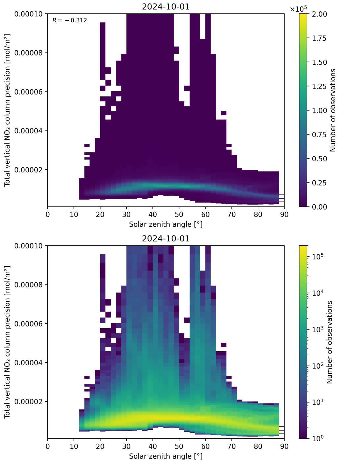
Figure 154: Scatter density plot of “Solar zenith angle” against “Total vertical NO 2 column precision” for 2024-09-30 to 2024-10-02.
