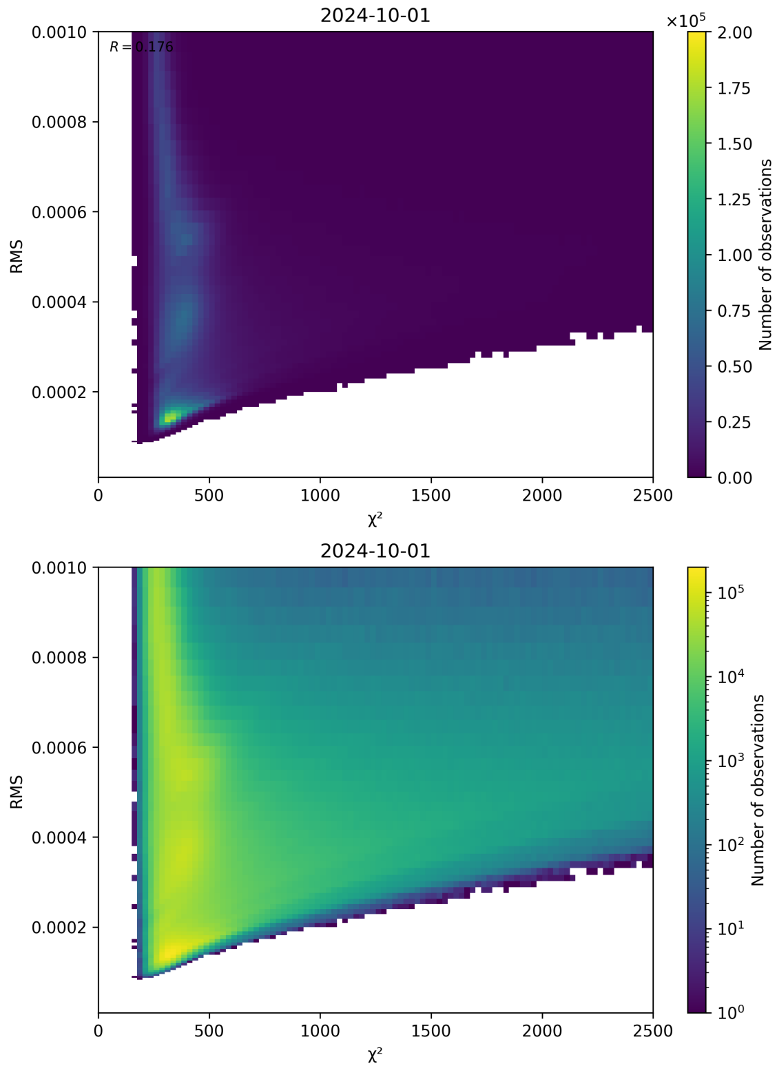
Figure 82: Scatter density plot of “ \chi^2 ” against “RMS” for 2024-09-30 to 2024-10-02.
