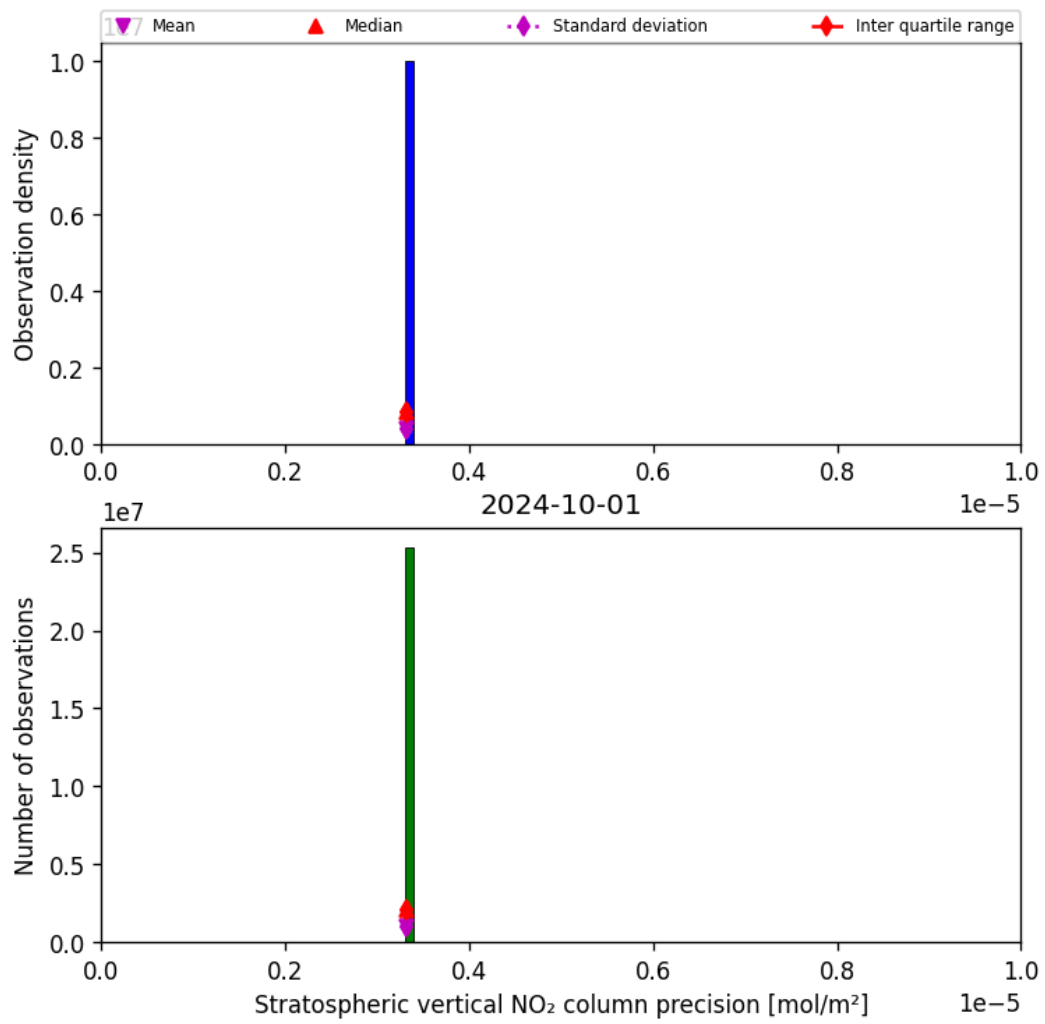
Figure 37: Histogram of “Stratospheric vertical NO 2 column precision” for 2024-09-30 to 2024-10-02
