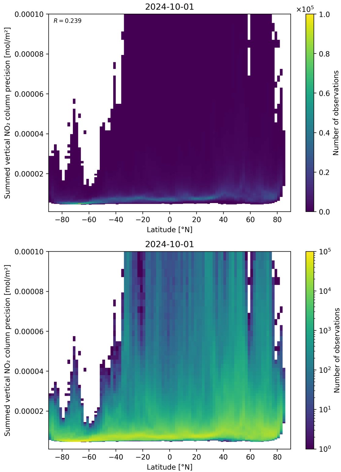
Figure 89: Scatter density plot of “Latitude” against “Summed vertical NO 2 column precision” for 2024-09-30 to 2024-10-02.
