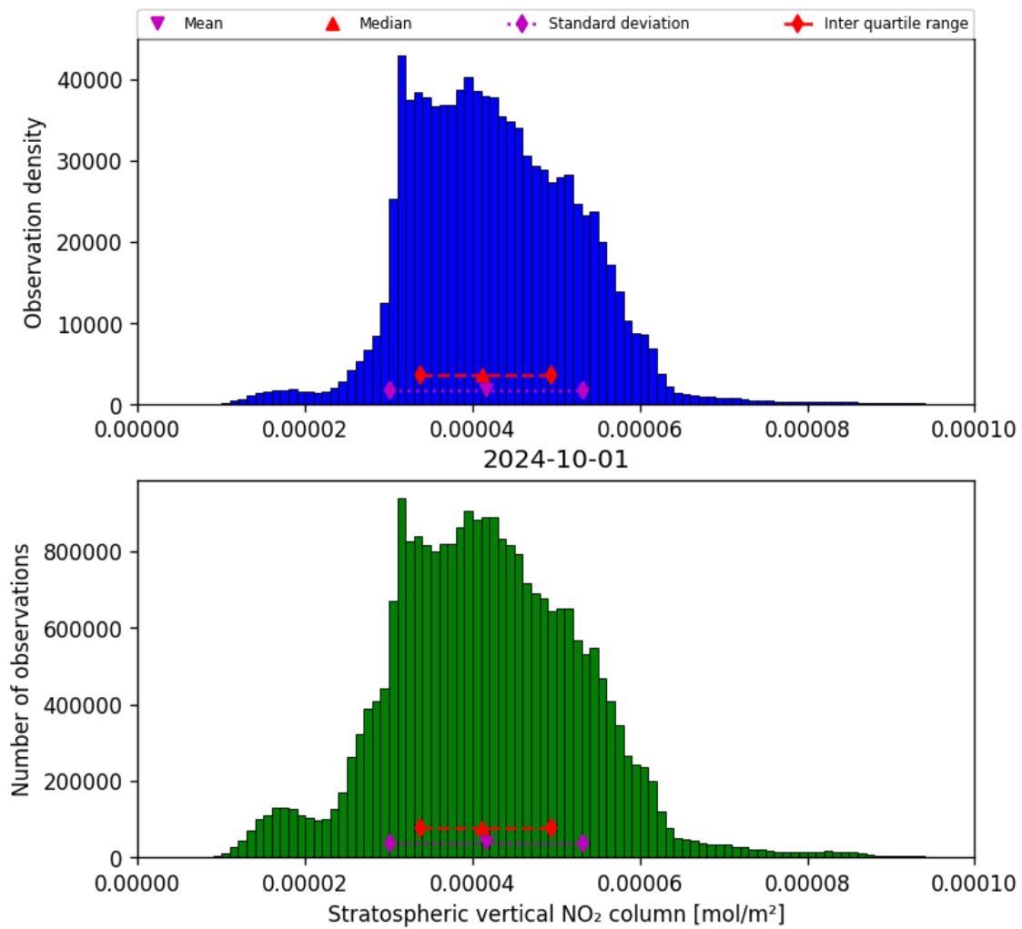
Figure 36: Histogram of “Stratospheric vertical NO 2 column” for 2024-09-30 to 2024-10-02
