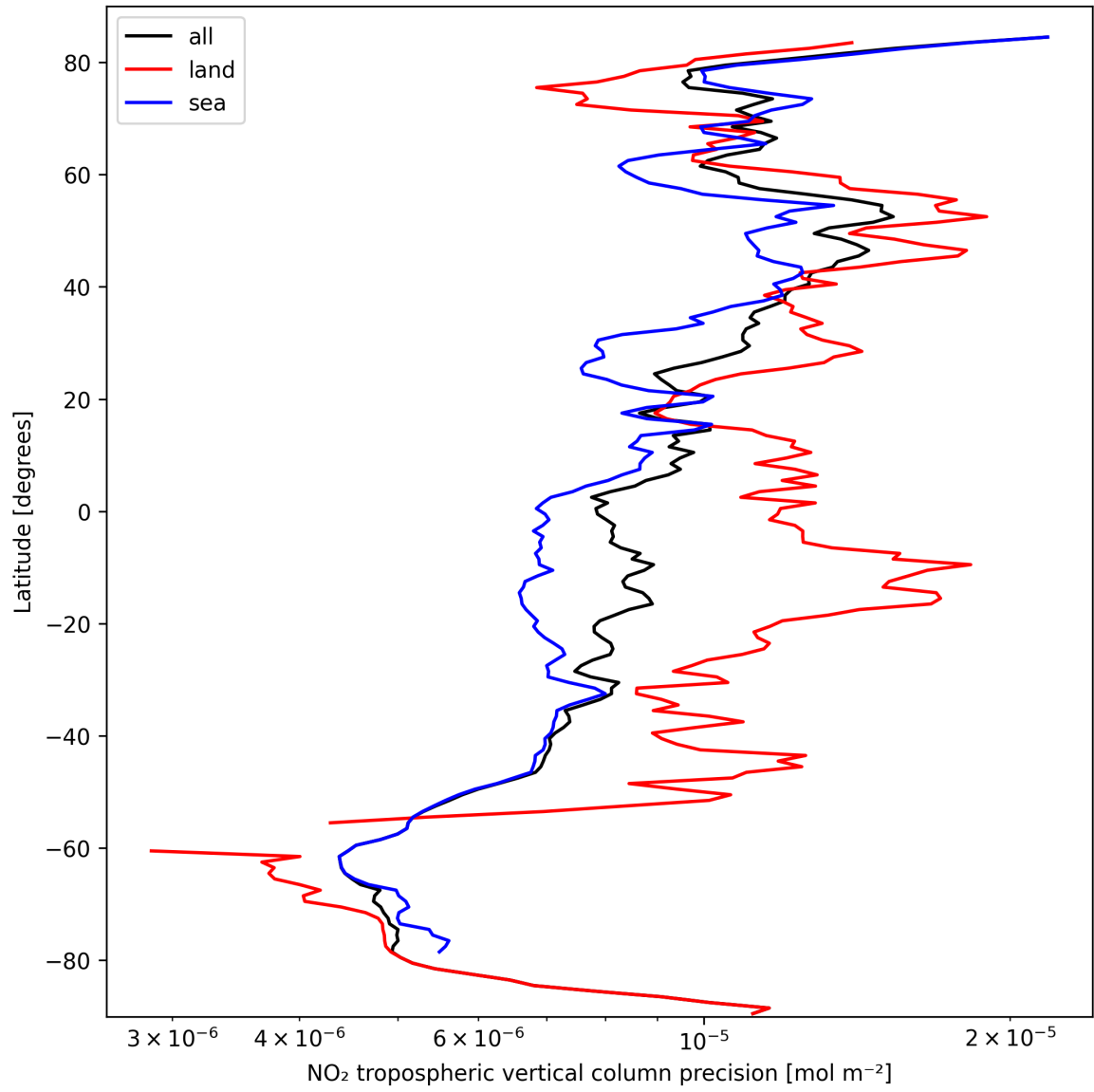
Figure 13: Zonal average of “NO 2 tropospheric vertical column precision” for 2024-09-30 to 2024-10-02.
