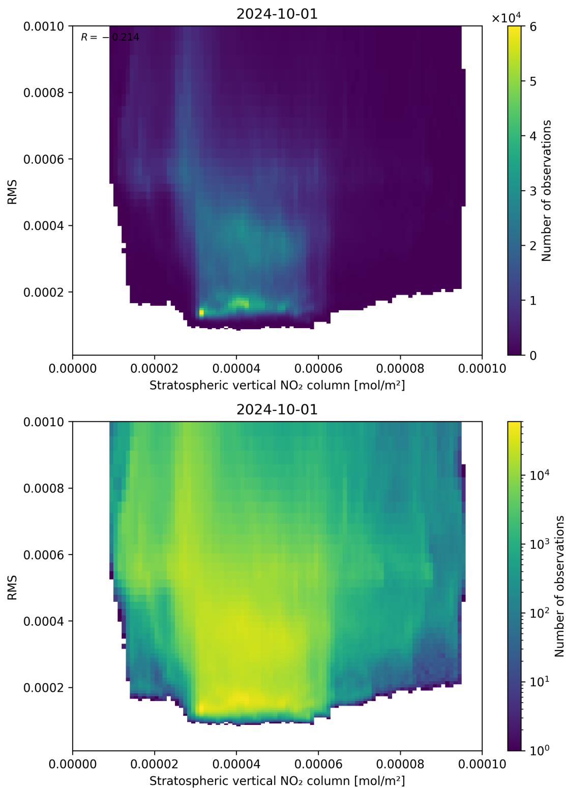
Figure 102: Scatter density plot of “Stratospheric vertical NO 2 column” against “RMS” for 2024-09-30 to 2024-10-02.
