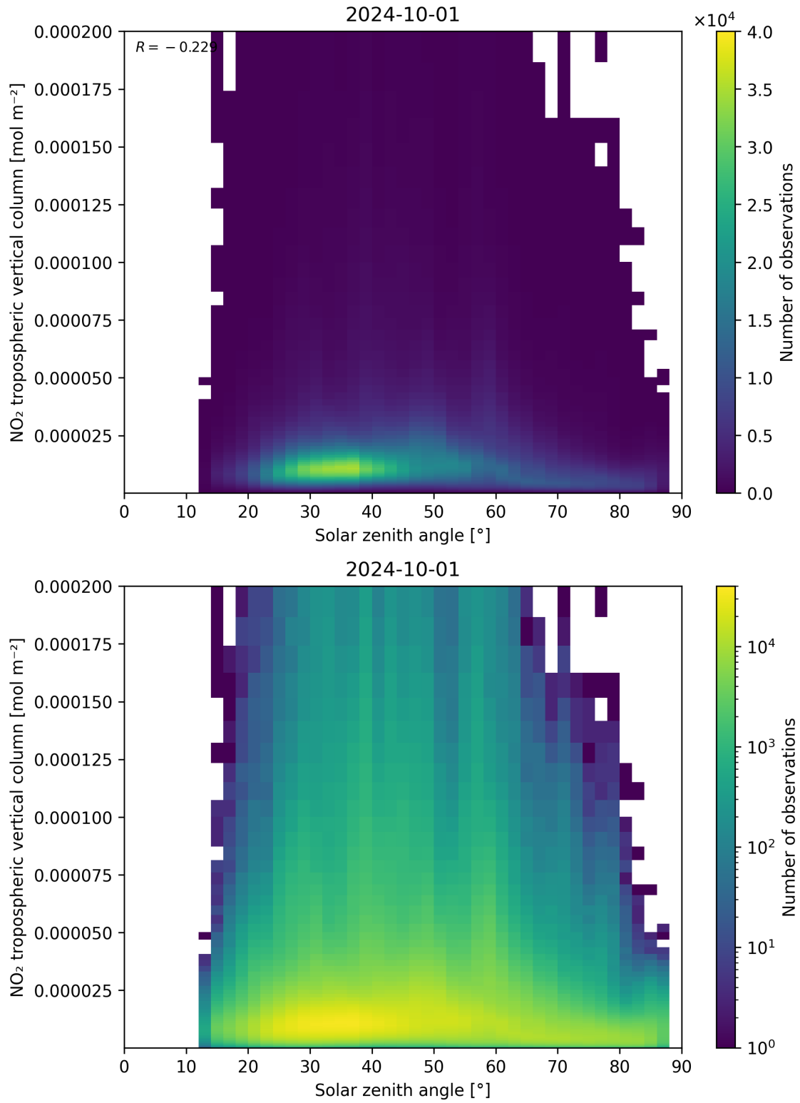
Figure 155: Scatter density plot of “Solar zenith angle” against “NO 2 tropospheric vertical column” for 2024-09-30 to 2024-10-02.
