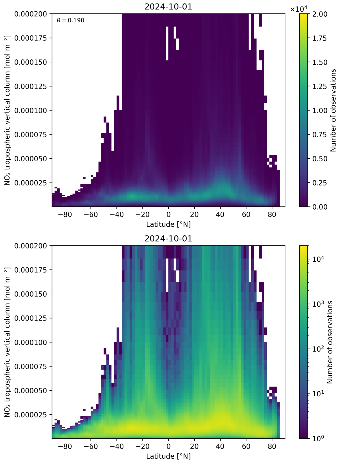
Figure 92: Scatter density plot of “Latitude” against “NO 2 tropospheric vertical column” for 2024-09-30 to 2024-10-02.
