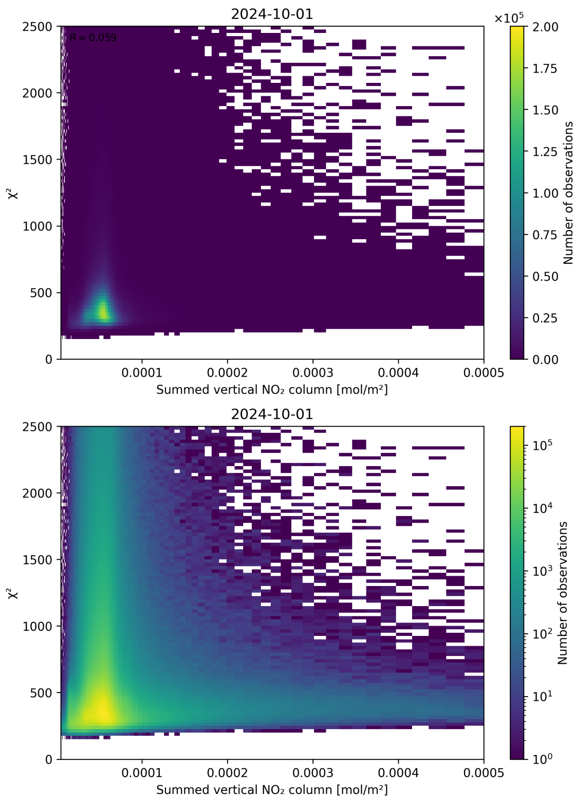
Figure 104: Scatter density plot of “Summed vertical NO 2 column” against “ \chi^2 ” for 2024-09-30 to 2024-10-02.
