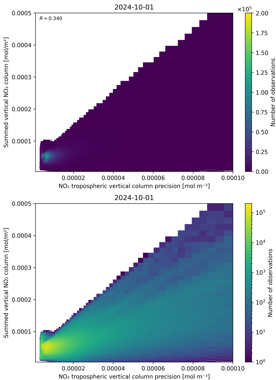
Figure 136: Scatter density plot of “NO 2 tropospheric vertical column precision” against “Summed vertical NO 2 column” for 2024-09-30 to 2024-10-02.
