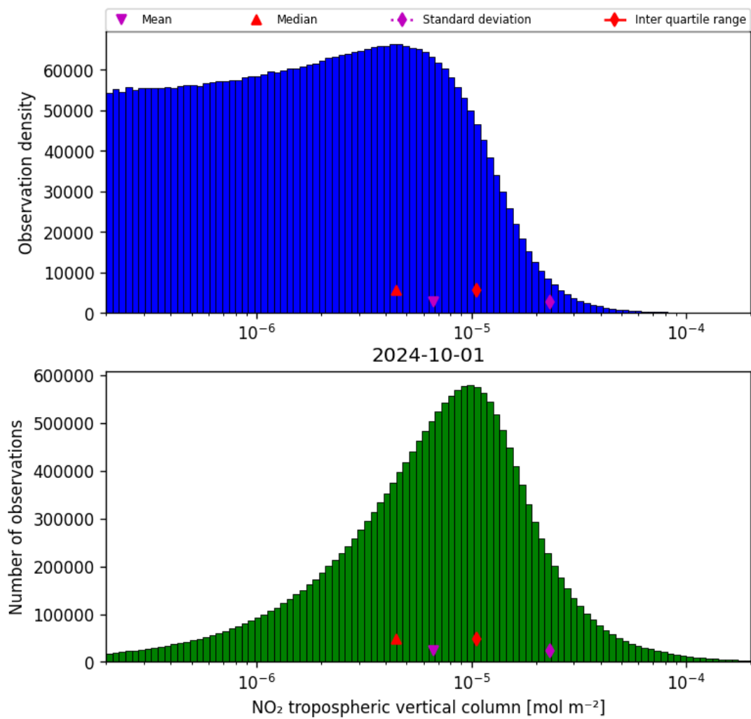
Figure 29: Histogram of “NO 2 tropospheric vertical column” for 2024-09-30 to 2024-10-02
