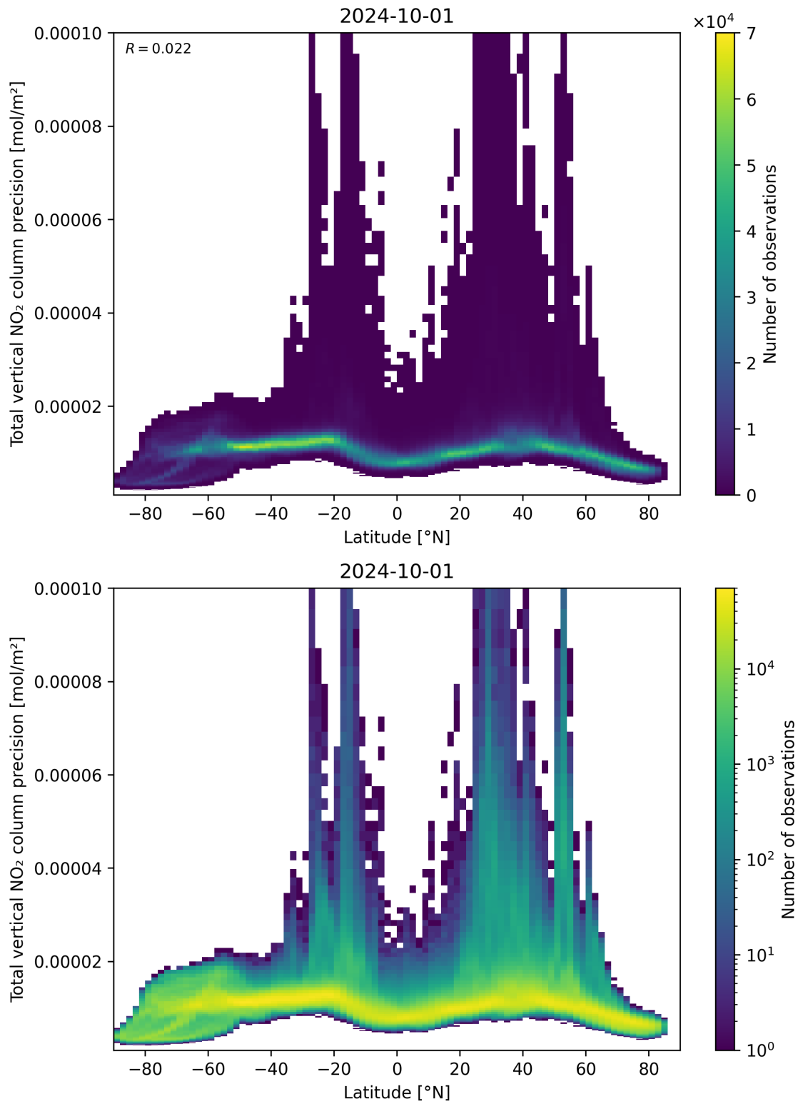
Figure 91: Scatter density plot of “Latitude” against “Total vertical NO 2 column precision” for 2024-09-30 to 2024-10-02.
