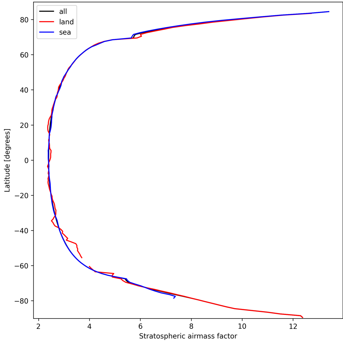
Figure 27: Zonal average of “Stratospheric airmass factor” for 2024-09-30 to 2024-10-02.
