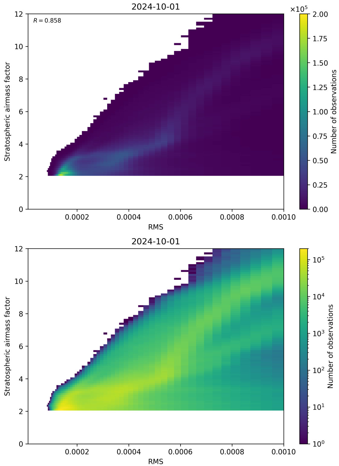
Figure 144: Scatter density plot of “RMS” against “Stratospheric airmass factor” for 2024-09-30 to 2024-10-02.
