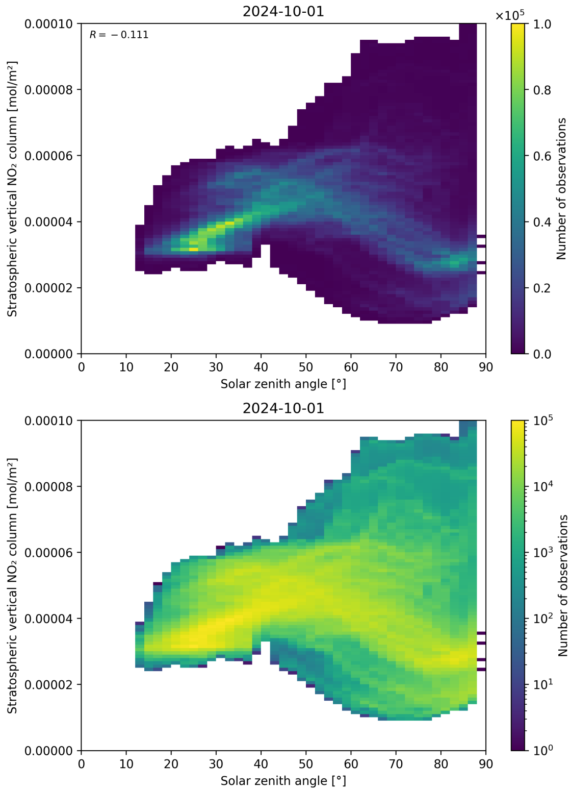
Figure 150: Scatter density plot of “Solar zenith angle” against “Stratospheric vertical NO 2 column” for 2024-09-30 to 2024-10-02.
