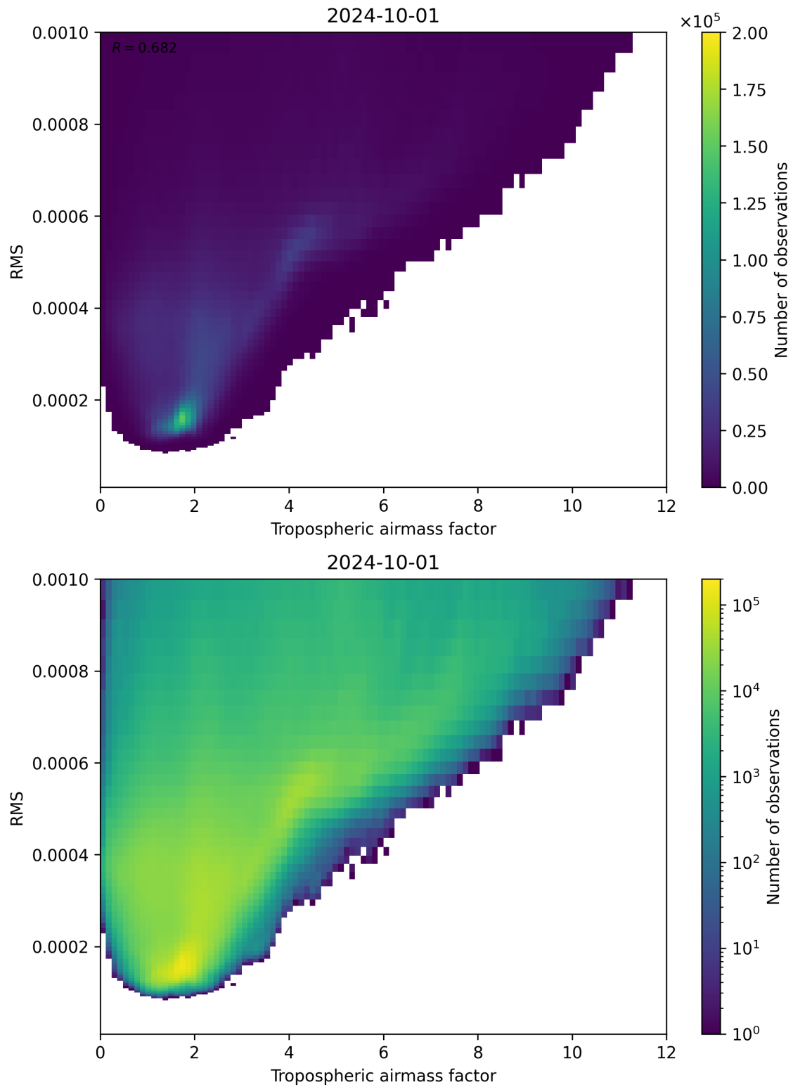
Figure 79: Scatter density plot of “Tropospheric airmass factor” against “RMS” for 2024-09-30 to 2024-10-02.
