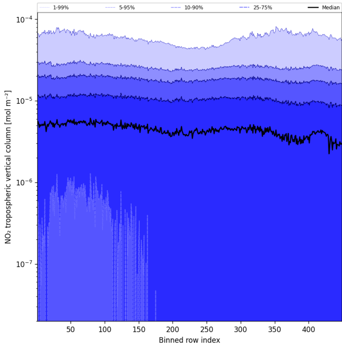
Figure 46: Along track statistics of “NO 2 tropospheric vertical column” for 2024-09-30 to 2024-10-02
