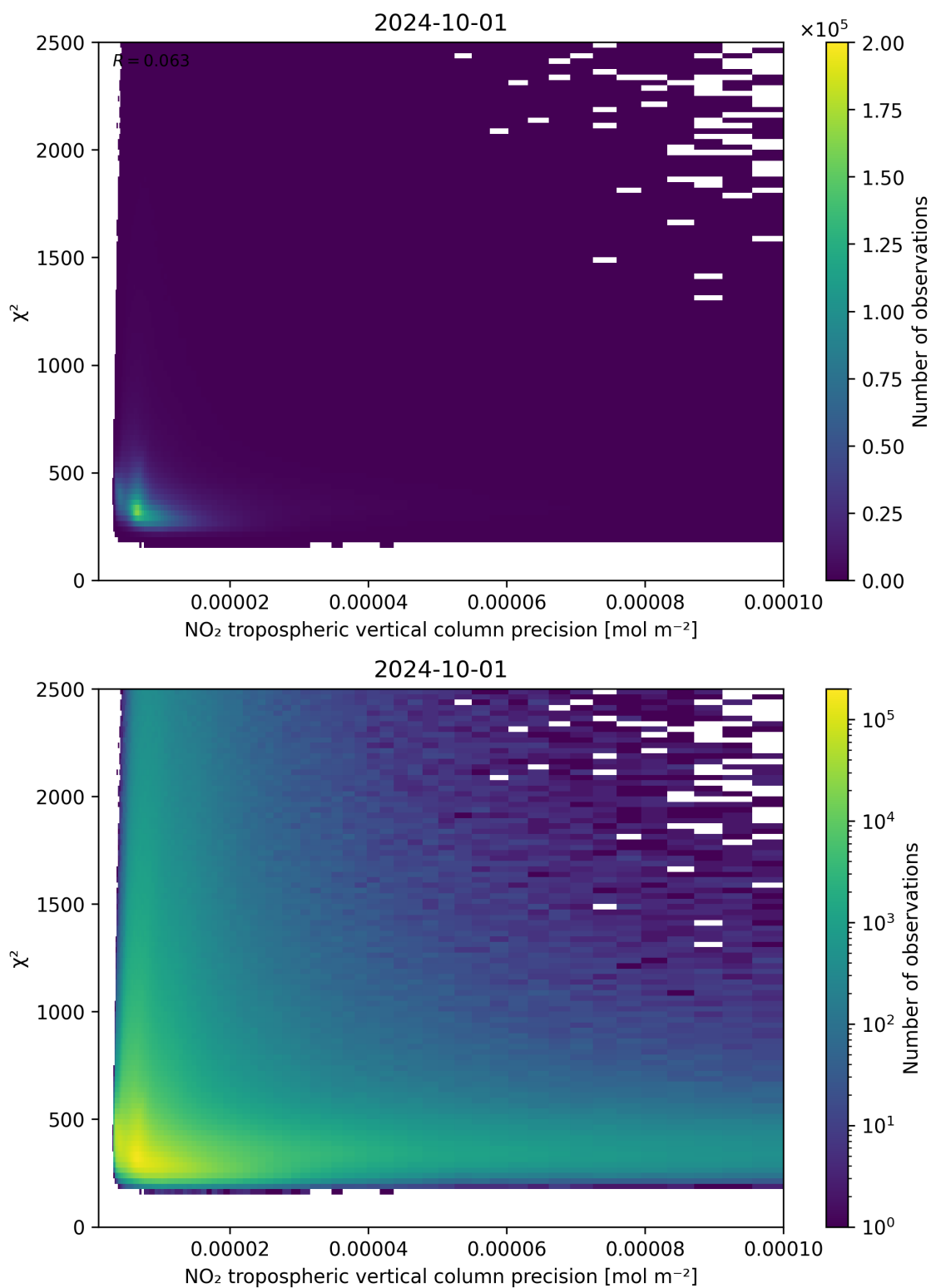
Figure 134: Scatter density plot of “NO 2 tropospheric vertical column precision” against “ \chi^2 ” for 2024-09-30 to 2024-10-02.
