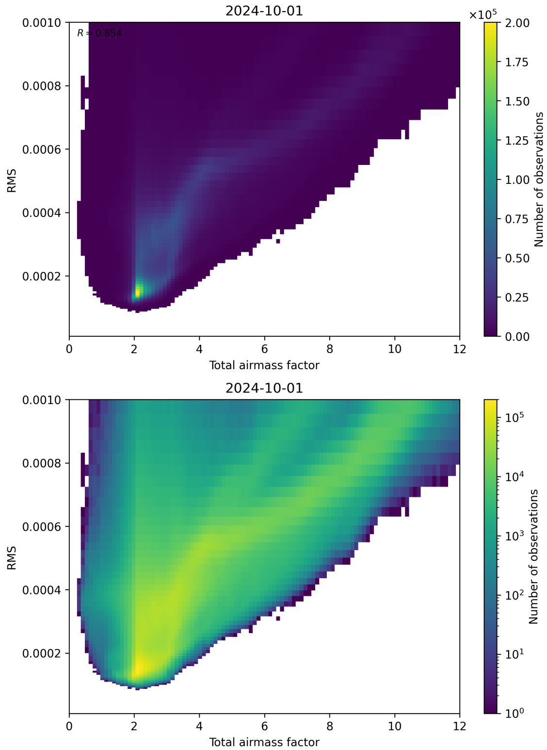
Figure 69: Scatter density plot of “Total airmass factor” against “RMS” for 2024-09-30 to 2024-10-02.
