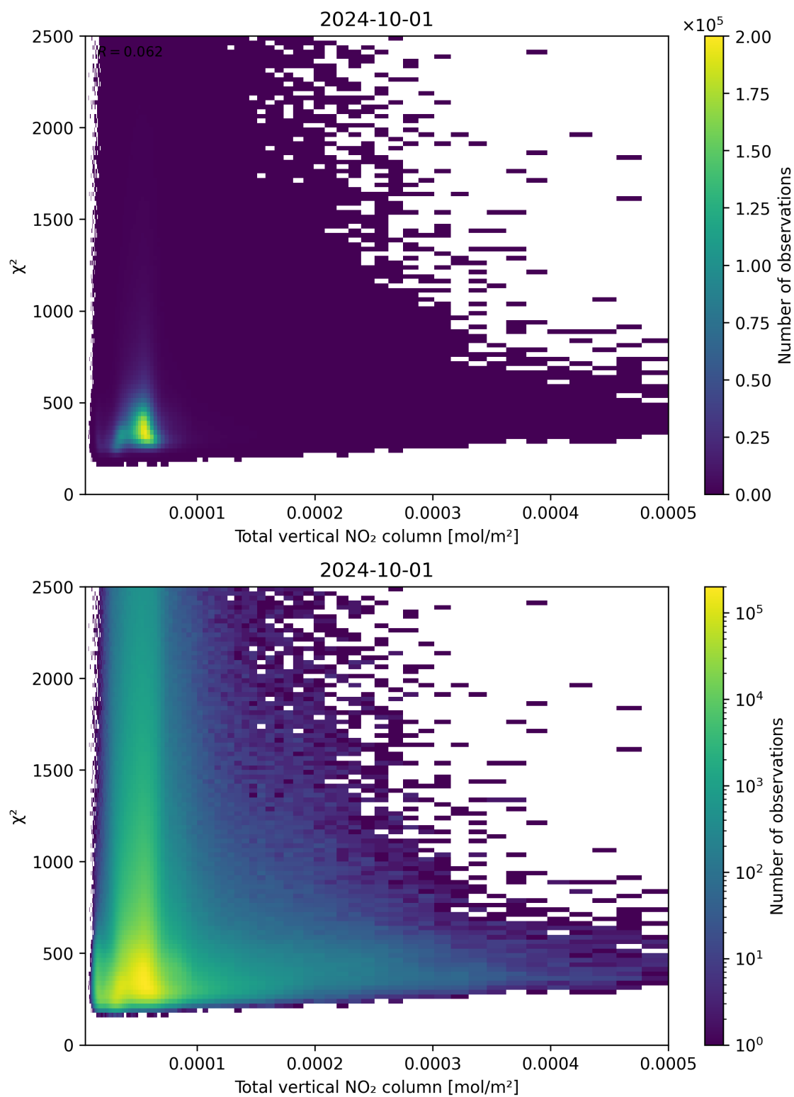
Figure 111: Scatter density plot of “Total vertical NO 2 column” against “ \chi^2 ” for 2024-09-30 to 2024-10-02.
