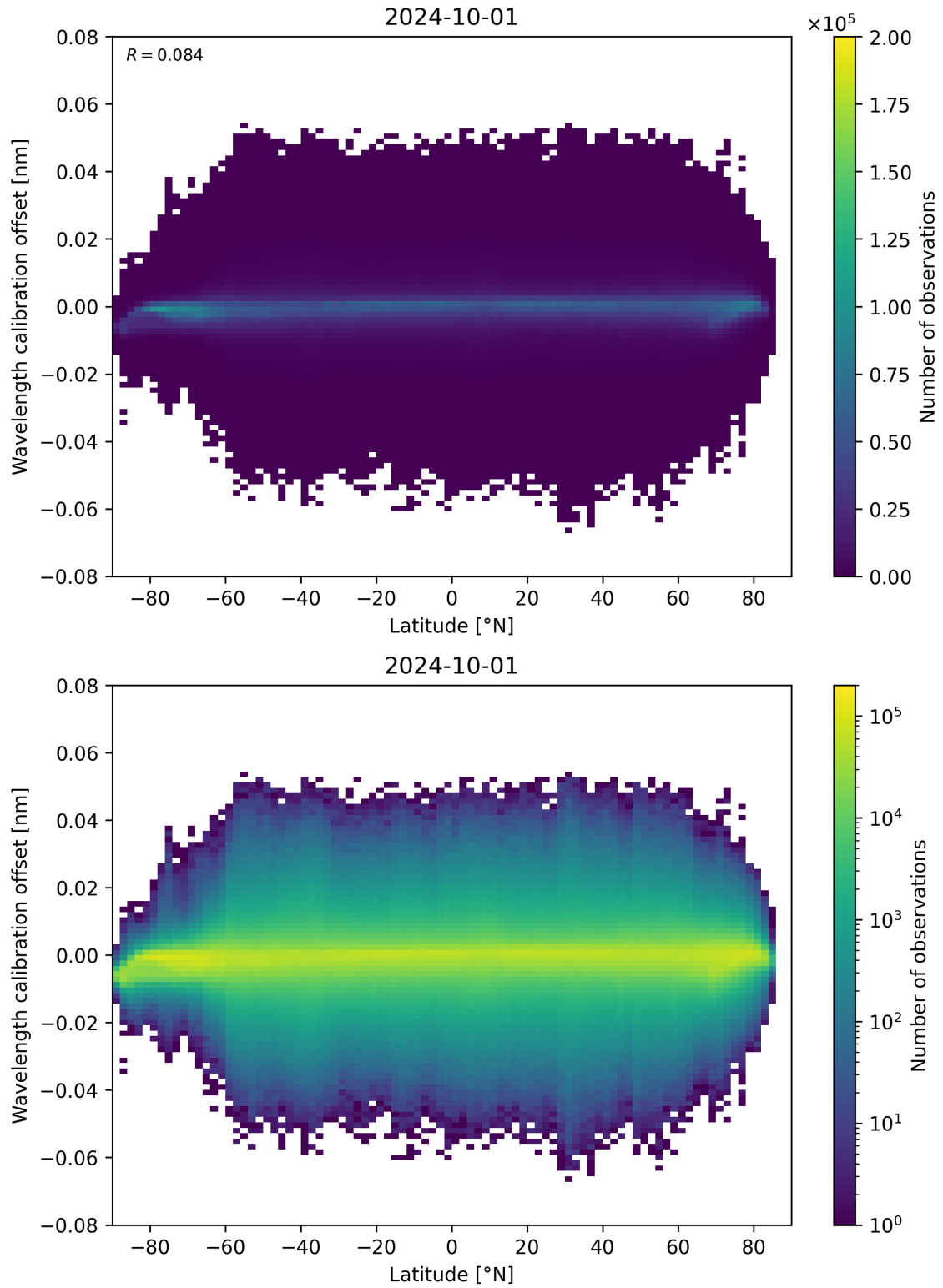
Figure 95: Scatter density plot of “Latitude” against “Wavelength calibration offset” for 2024-09-30 to 2024-10-02.
