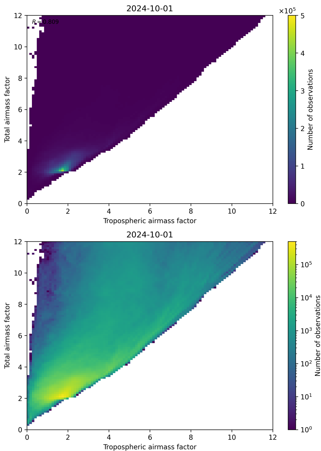
Figure 72: Scatter density plot of “Tropospheric airmass factor” against “Total airmass factor” for 2024-09-30 to 2024-10-02.
