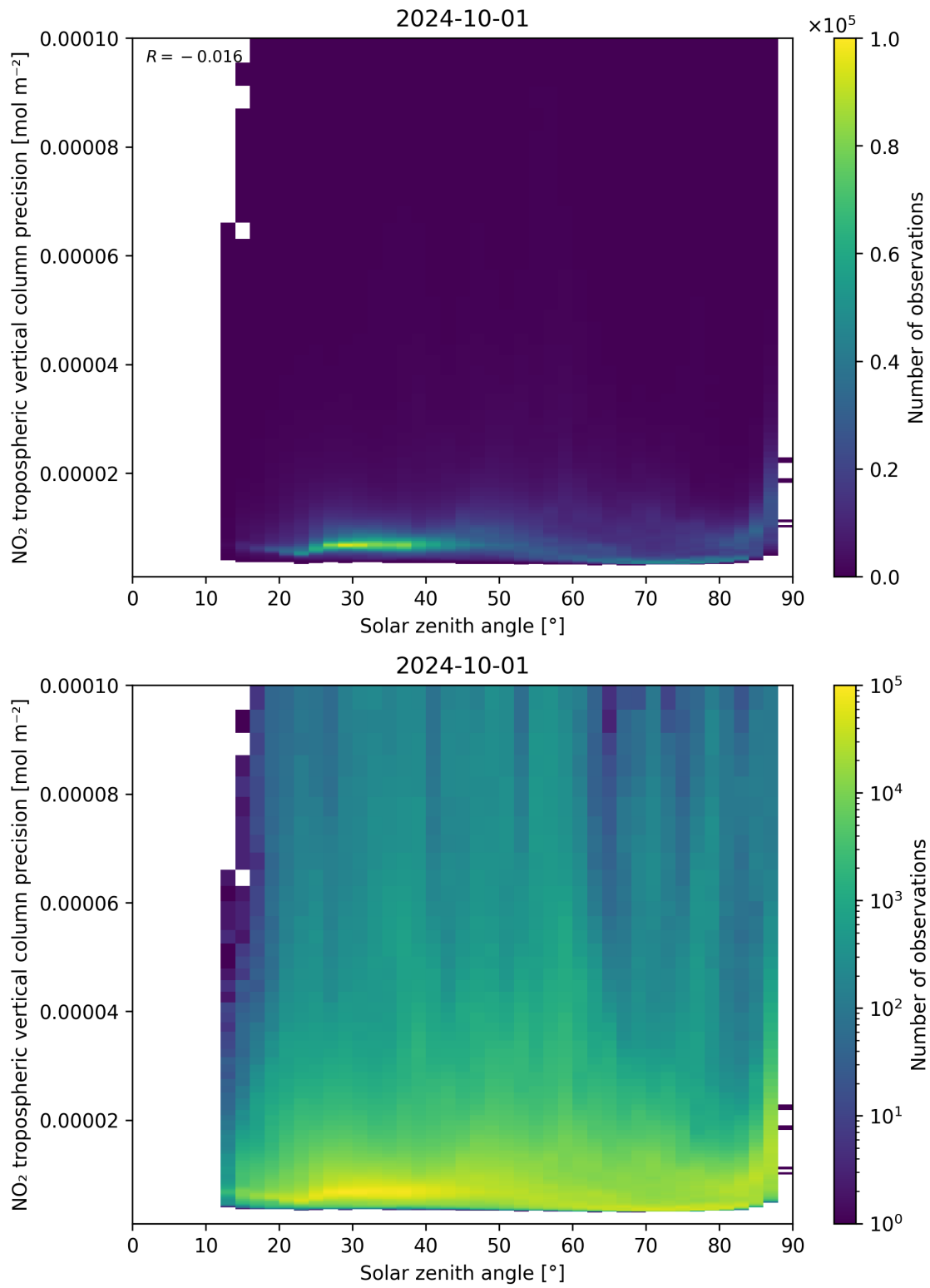
Figure 156: Scatter density plot of “Solar zenith angle” against “NO 2 tropospheric vertical column precision” for 2024-09-30 to 2024-10-02.
