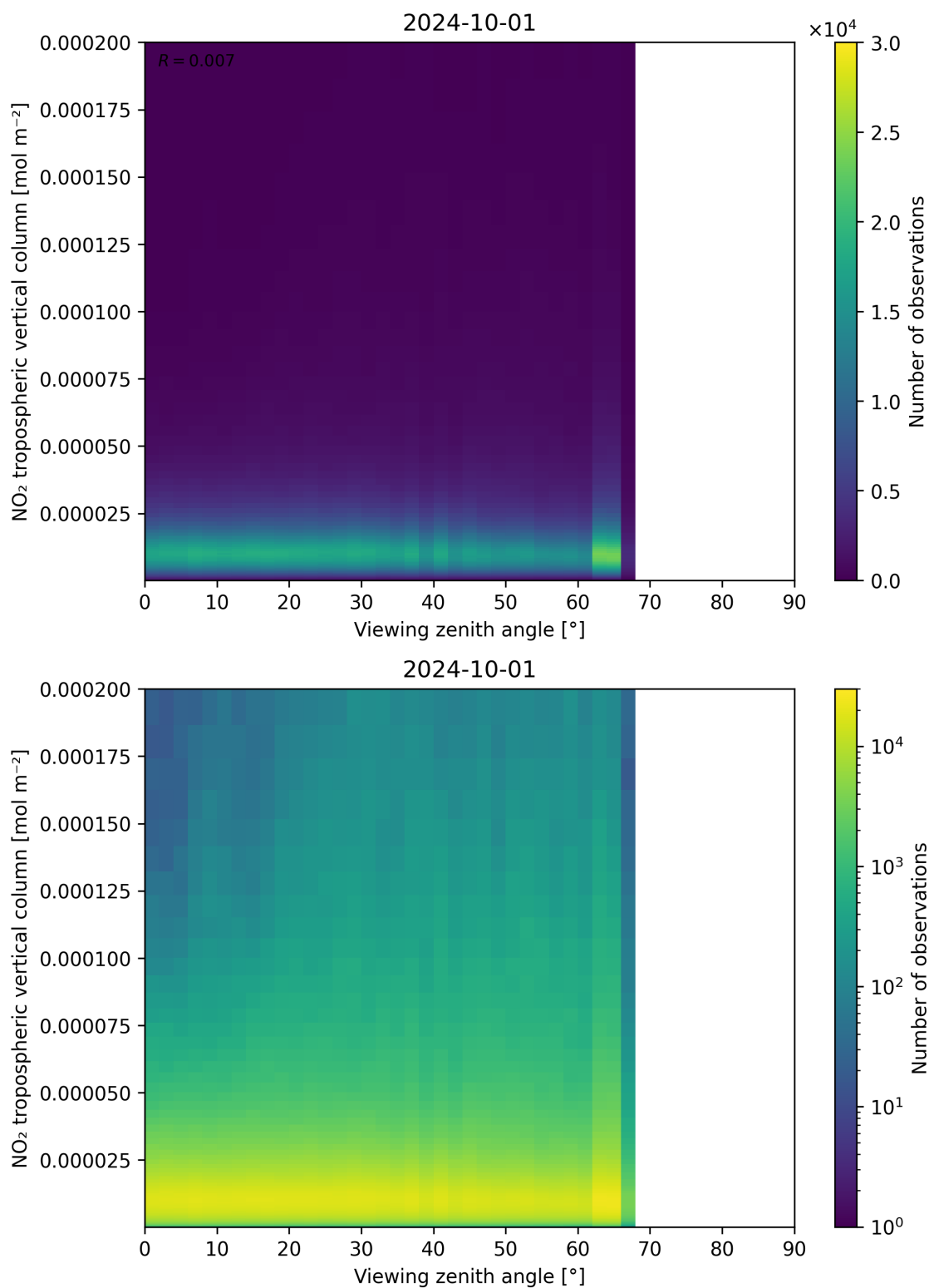
Figure 169: Scatter density plot of “Viewing zenith angle” against “NO 2 tropospheric vertical column” for 2024-09-30 to 2024-10-02.
