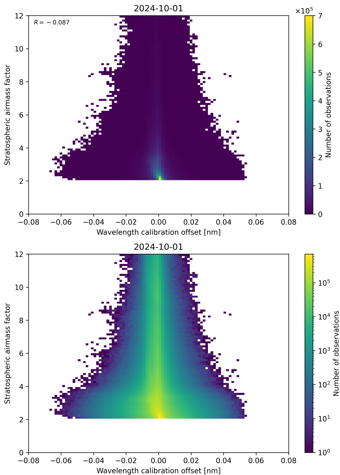
Figure 174: Scatter density plot of “Wavelength calibration offset” against “Stratospheric air mass factor” for 2024-09-30 to 2024-10-02.
