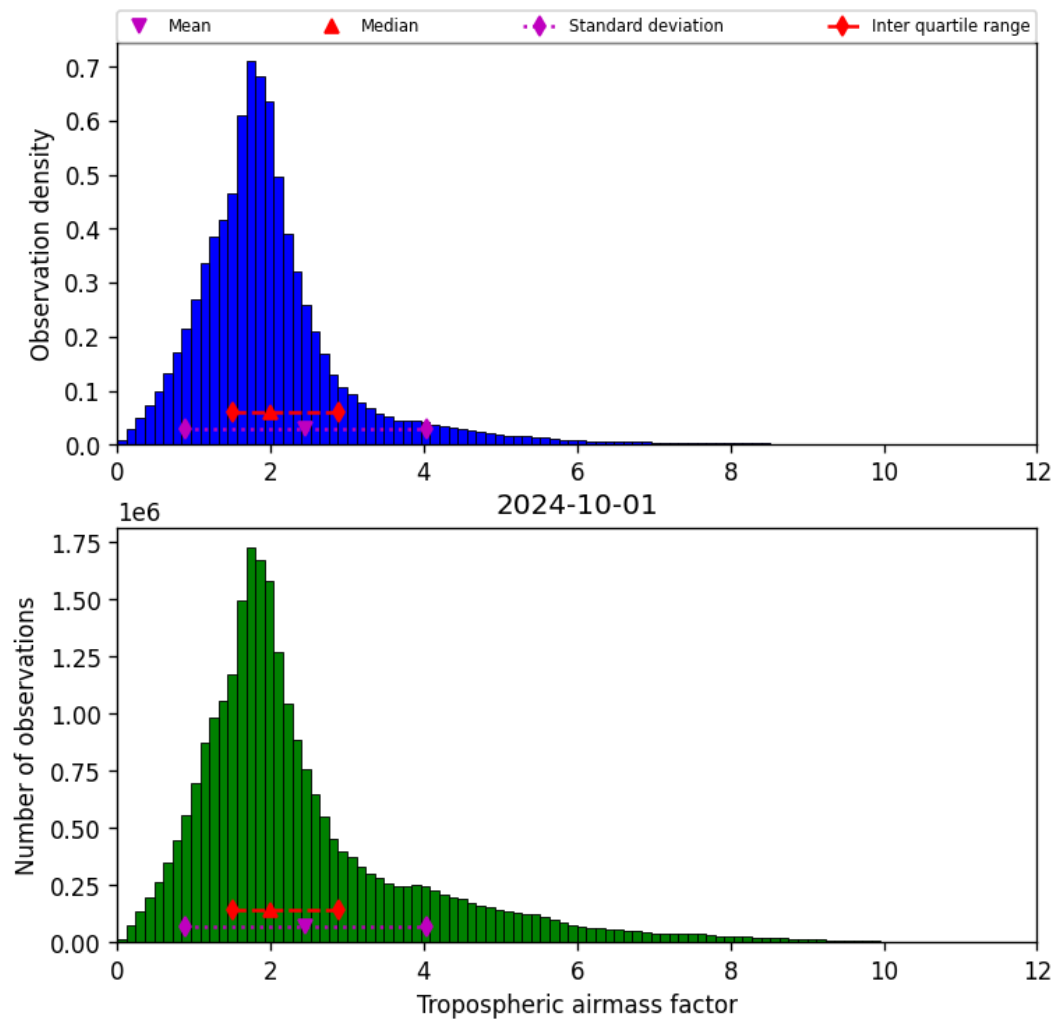
Figure 31: Histogram of “Tropospheric airmass factor” for 2024-09-30 to 2024-10-02
