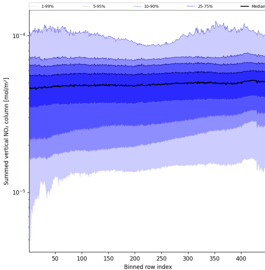
Figure 57: Along track statistics of “Summed vertical NO 2 column” for 2024-09-30 to 2024-10-02
