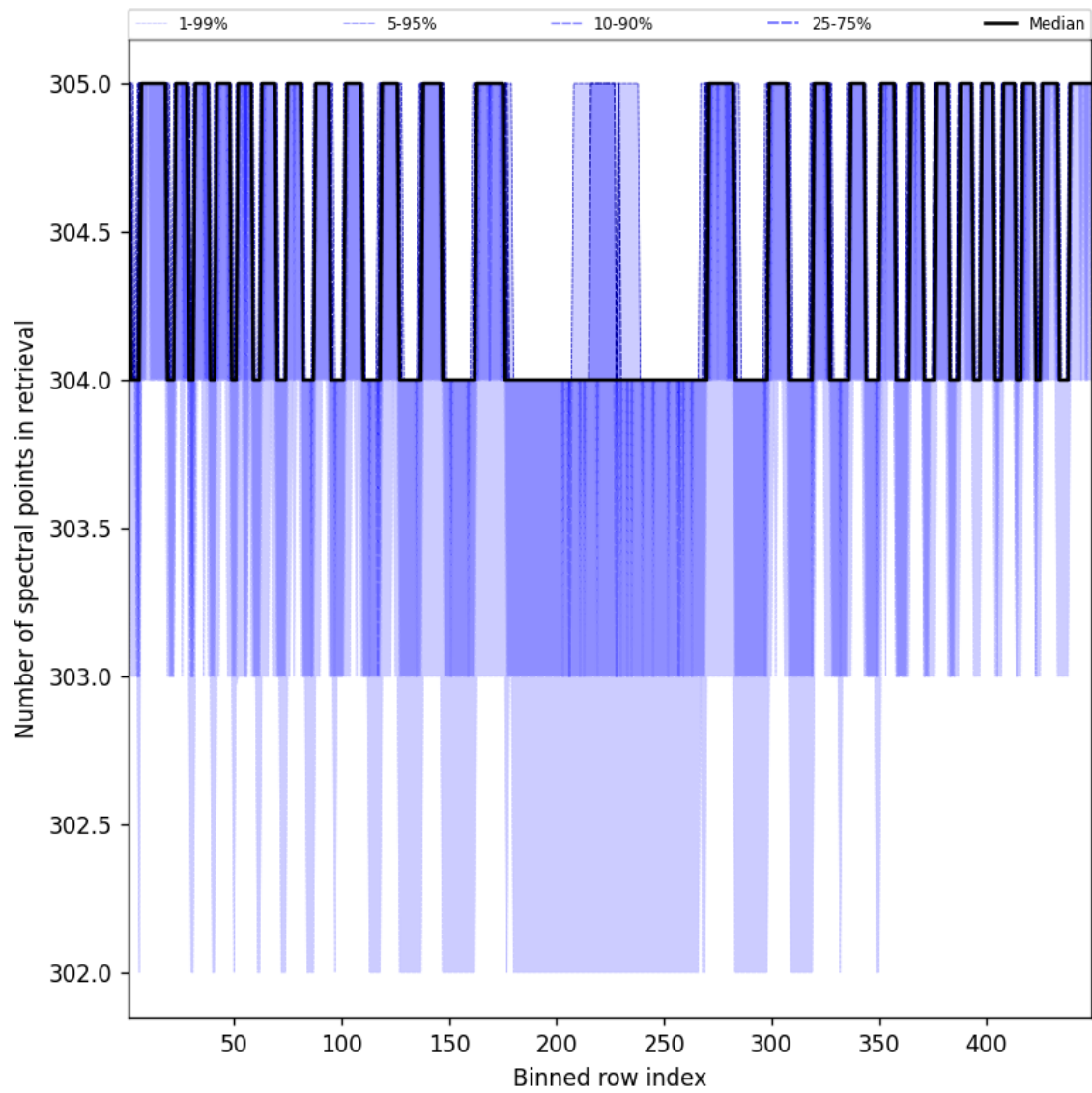
Figure 50: Along track statistics of “Number of spectral points in retrieval” for 2024-09-30 to 2024-10-02
