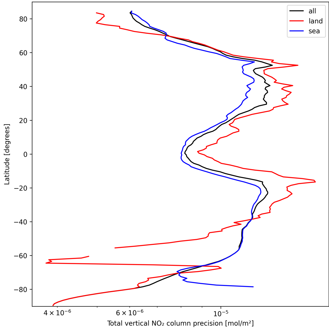
Figure 22: Zonal average of “Total vertical NO 2 column precision” for 2024-09-30 to 2024-10-02.
