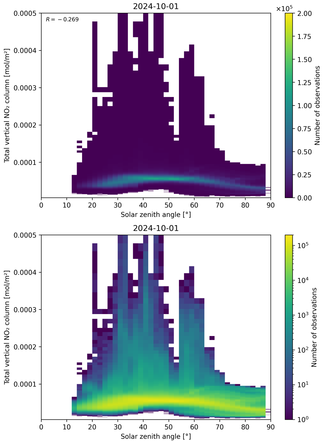
Figure 153: Scatter density plot of “Solar zenith angle” against “Total vertical NO 2 column” for 2024-09-30 to 2024-10-02.
