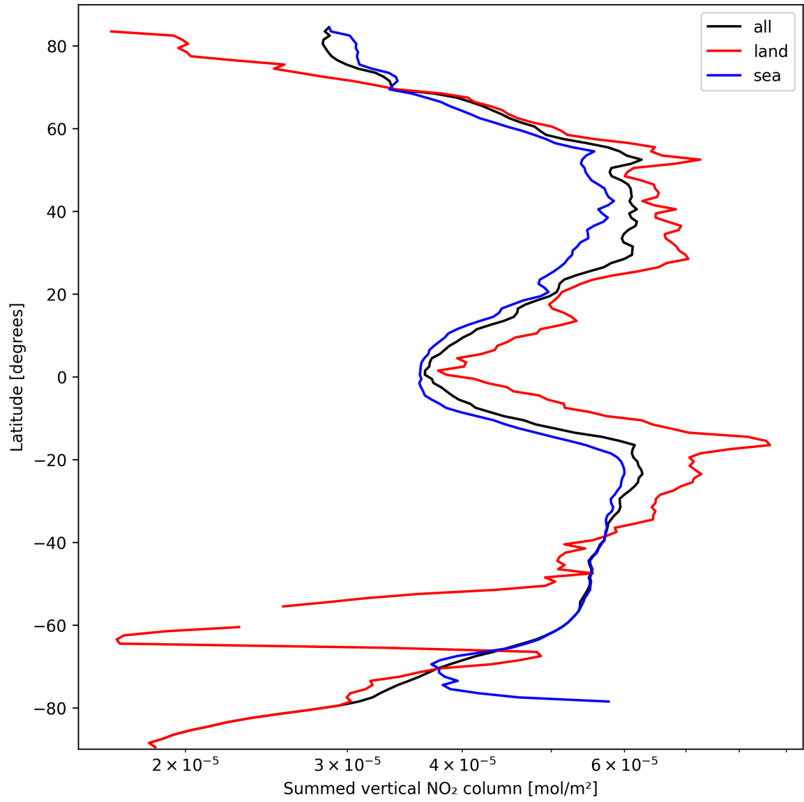
Figure 23: Zonal average of “Summed vertical NO 2 column” for 2024-09-30 to 2024-10-02.
