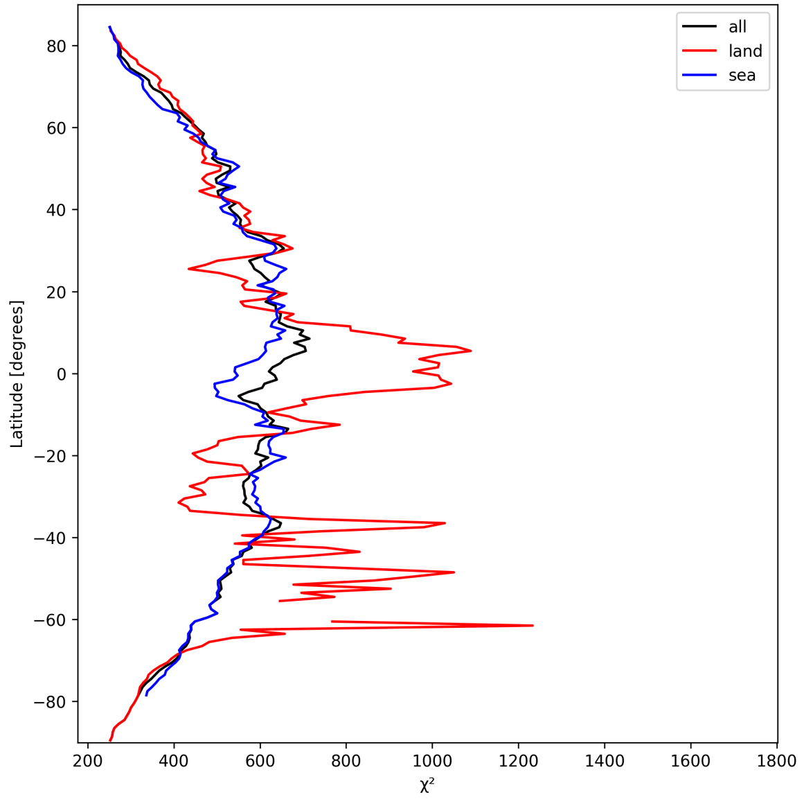
Figure 25: Zonal average of “ \chi^2 ” for 2024-09-30 to 2024-10-02.
