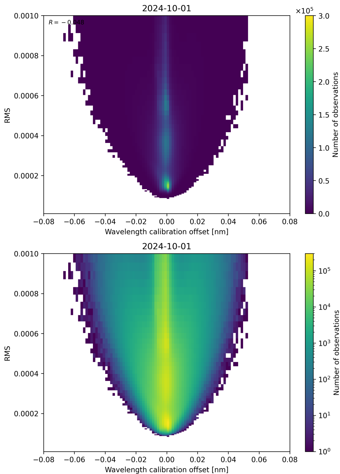
Figure 181: Scatter density plot of “Wavelength calibration offset” against “RMS” for 2024-09-30 to 2024-10-02.
