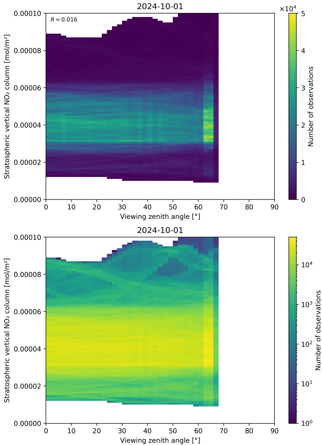
Figure 164: Scatter density plot of “Viewing zenith angle” against “Stratospheric vertical NO 2 column” for 2024-09-30 to 2024-10-02.
