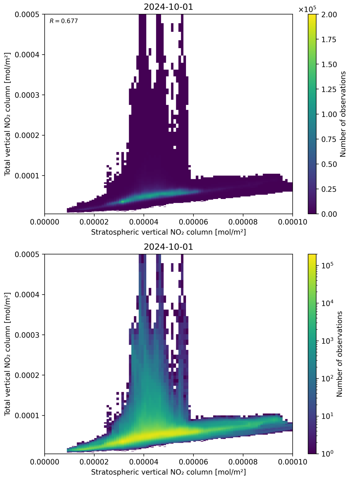
Figure 100: Scatter density plot of “Stratospheric vertical NO 2 column” against “Total vertical NO 2 column” for 2024-09-30 to 2024-10-02.
