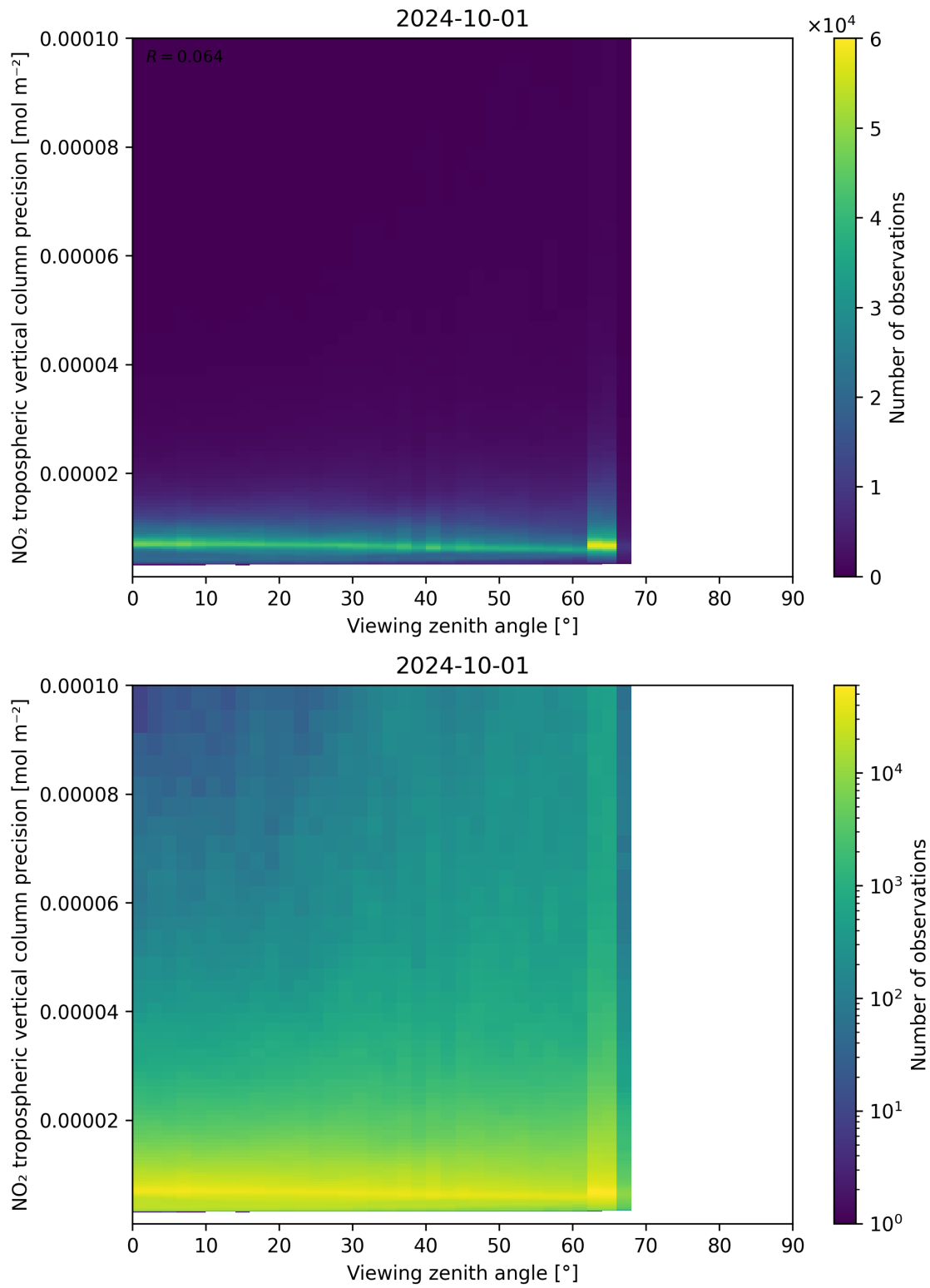
Figure 170: Scatter density plot of “Viewing zenith angle” against “NO 2 tropospheric vertical column precision” for 2024-09-30 to 2024-10-02.
