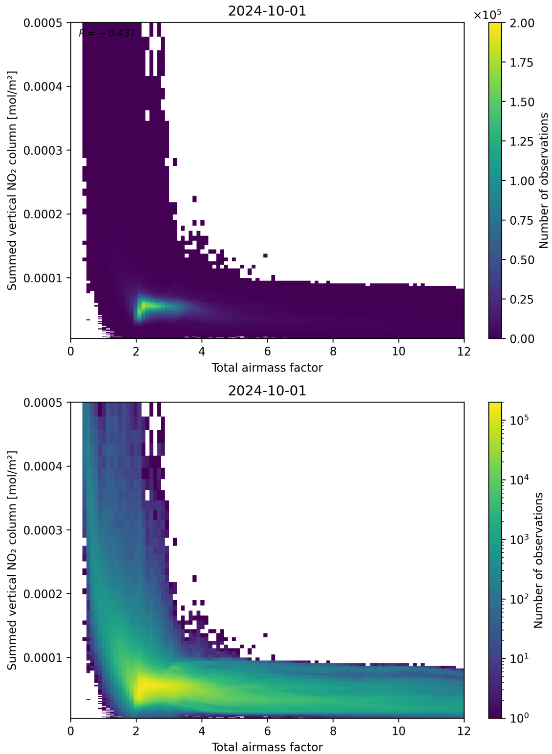
Figure 65: Scatter density plot of “Total airmass factor” against “Summed vertical NO 2 column” for 2024-09-30 to 2024-10-02.
