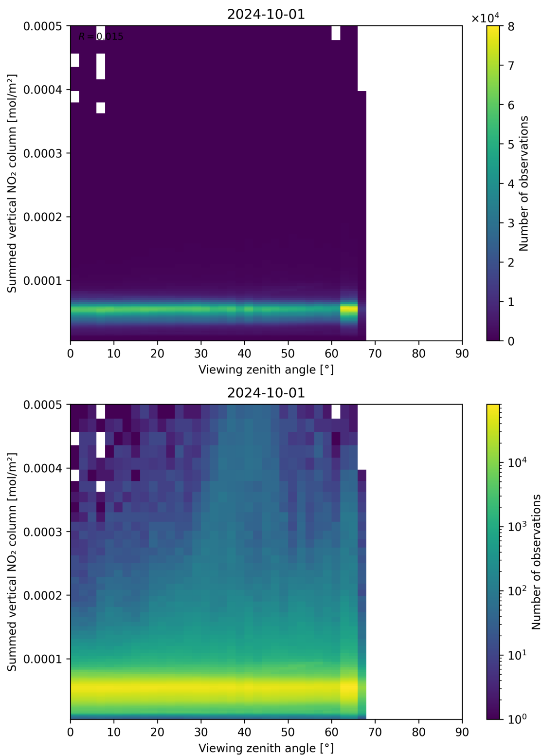
Figure 165: Scatter density plot of “Viewing zenith angle” against “Summed vertical NO 2 column” for 2024-09-30 to 2024-10-02.
