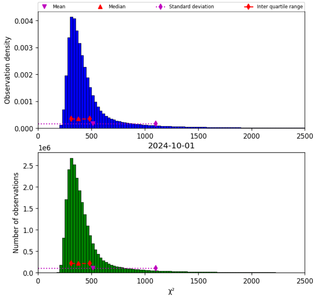
Figure 42: Histogram of " \chi^2 " for 2024-09-30 to 2024-10-02
