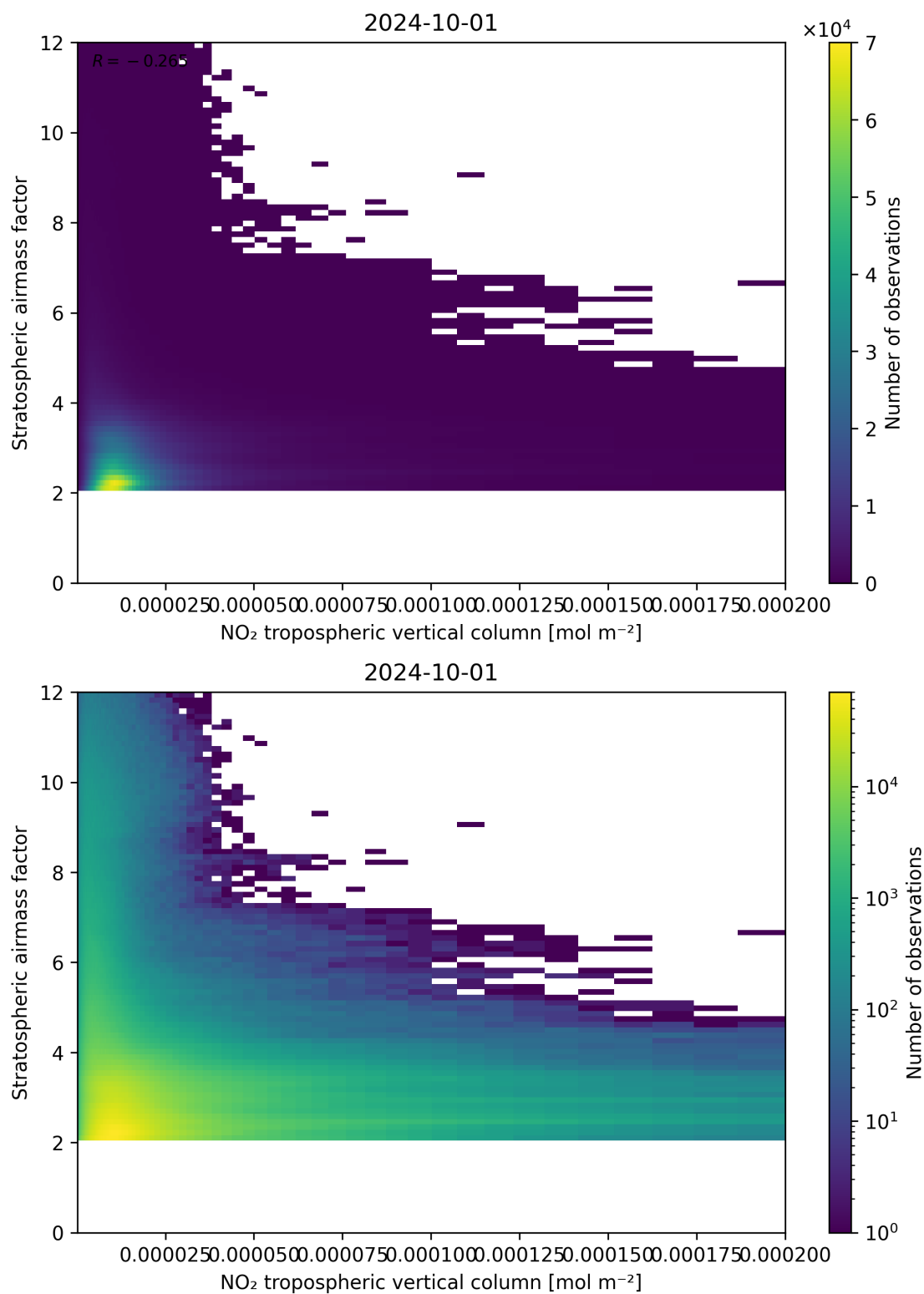
Figure 121: Scatter density plot of “NO 2 tropospheric vertical column” against “Stratospheric air mass factor” for 2024-09-30 to 2024-10-02.
