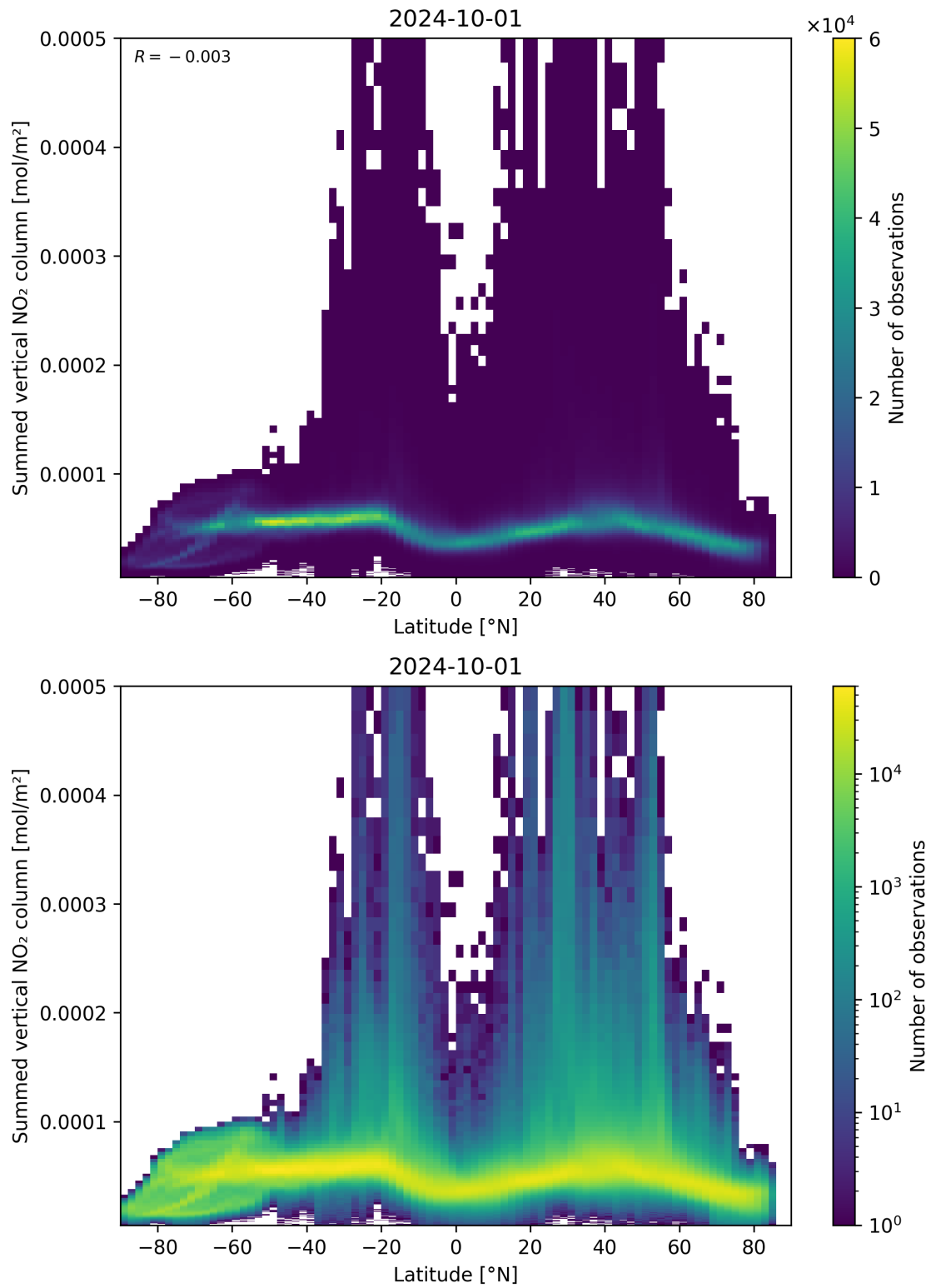
Figure 88: Scatter density plot of “Latitude” against “Summed vertical NO 2 column” for 2024-09-30 to 2024-10-02.
