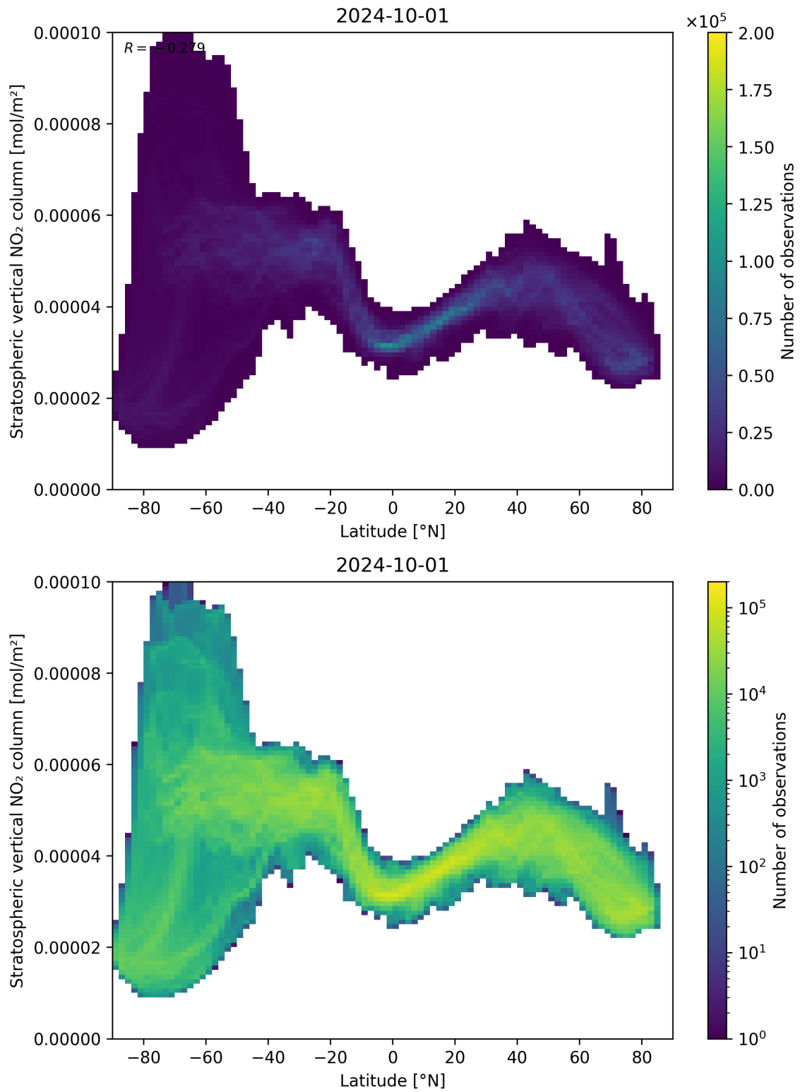
Figure 87: Scatter density plot of “Latitude” against “Stratospheric vertical NO 2 column” for 2024-09-30 to 2024-10-02.
