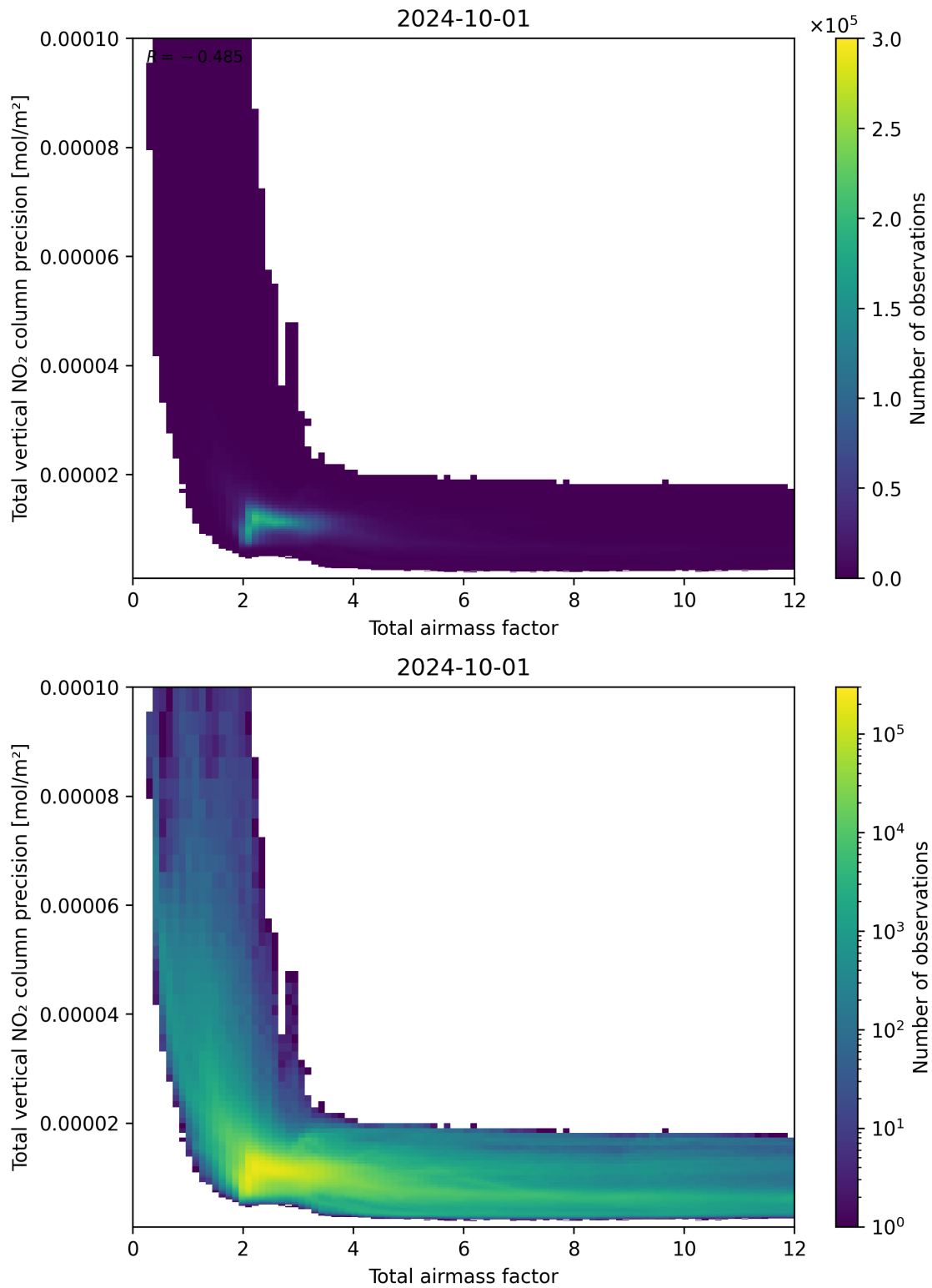
Figure 68: Scatter density plot of “Total airmass factor” against “Total vertical NO 2 column precision” for 2024-09-30 to 2024-10-02.
