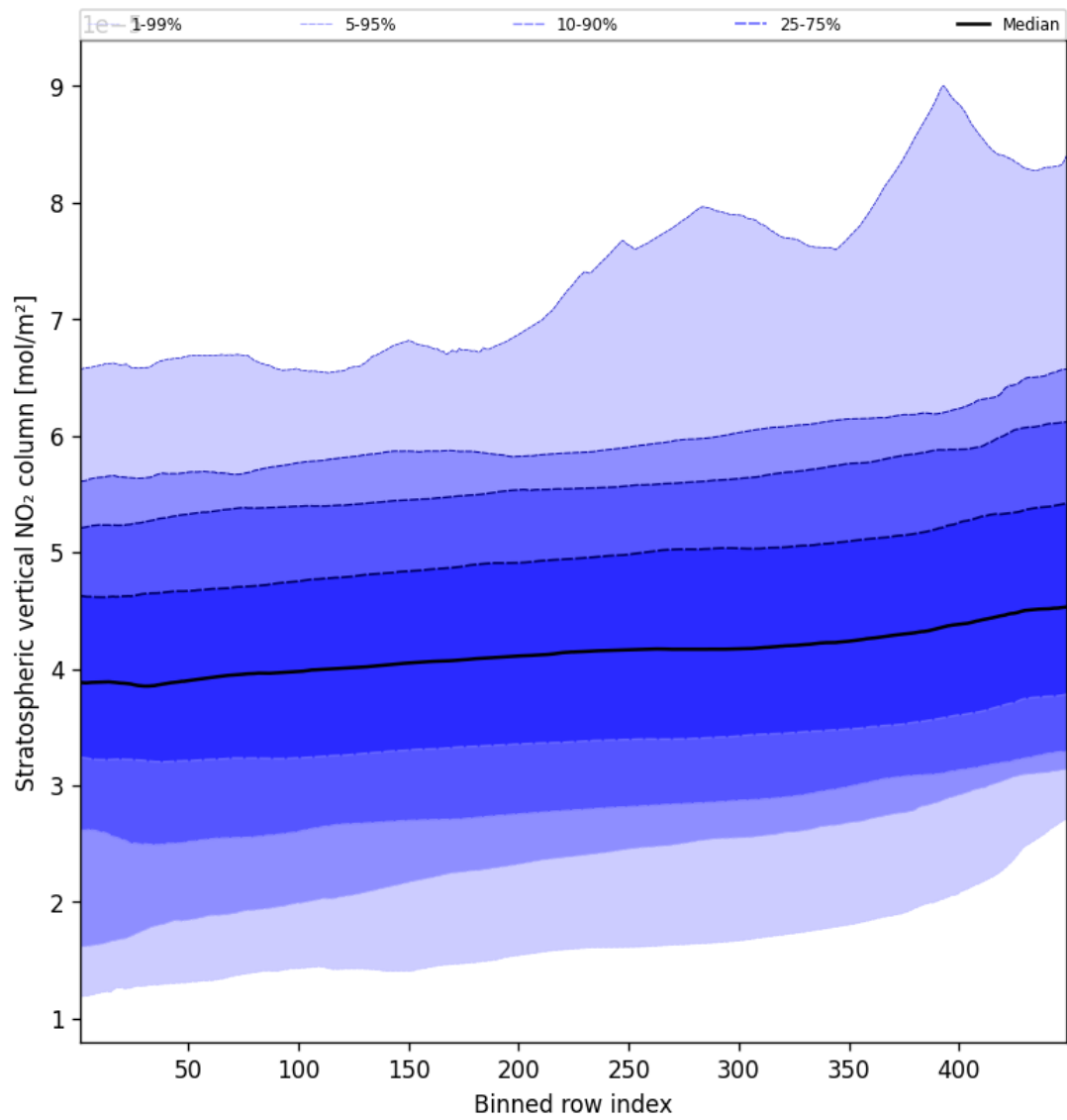
Figure 53: Along track statistics of “Stratospheric vertical NO 2 column” for 2024-09-30 to 2024-10-02
