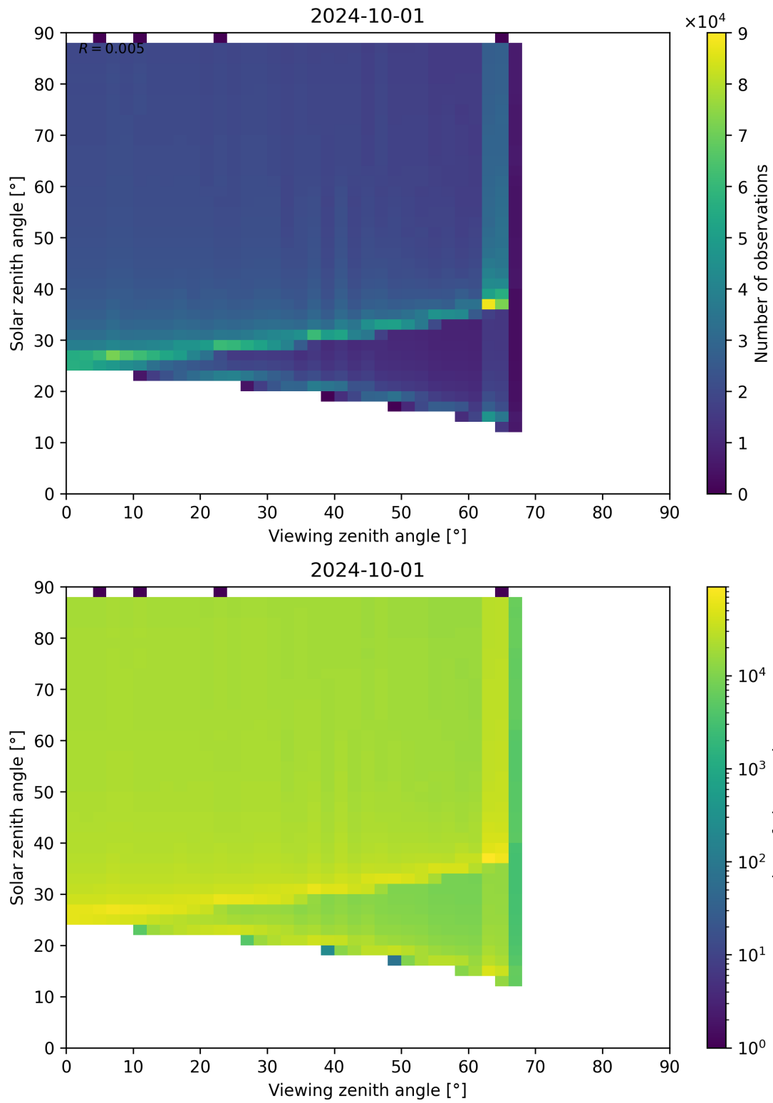
Figure 172: Scatter density plot of “Viewing zenith angle” against “Solar zenith angle” for 2024-09-30 to 2024-10-02.
