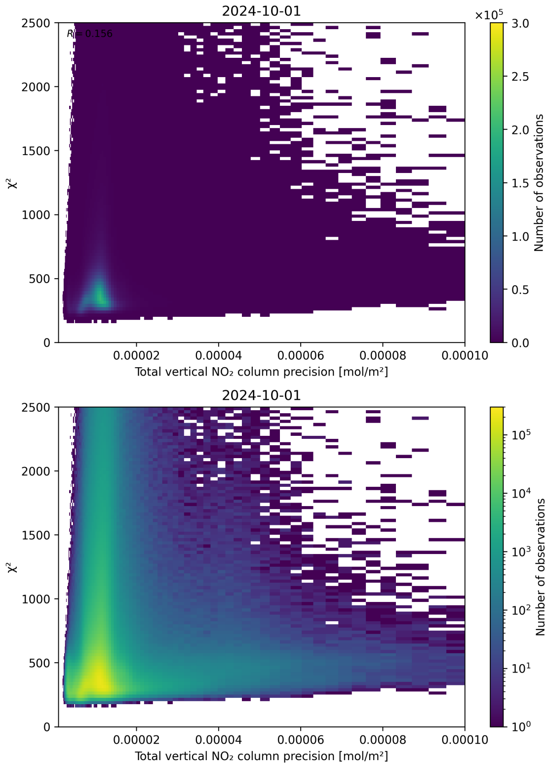
Figure 116: Scatter density plot of “Total vertical NO 2 column precision” against “ \chi^2 ” for 2024-09-30 to 2024-10-02.
