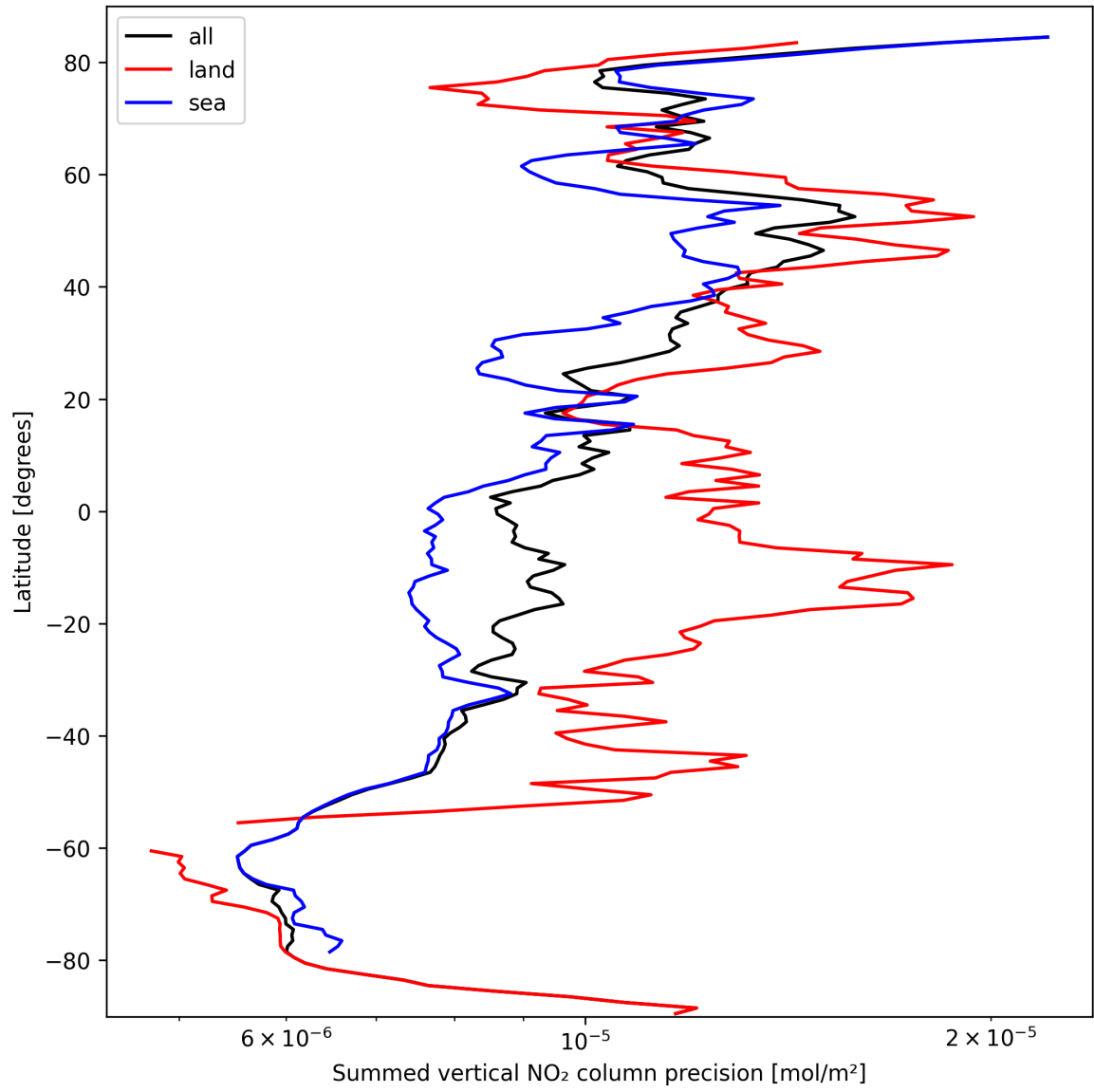
Figure 24: Zonal average of “Summed vertical NO 2 column precision” for 2024-09-30 to 2024-10-02.
