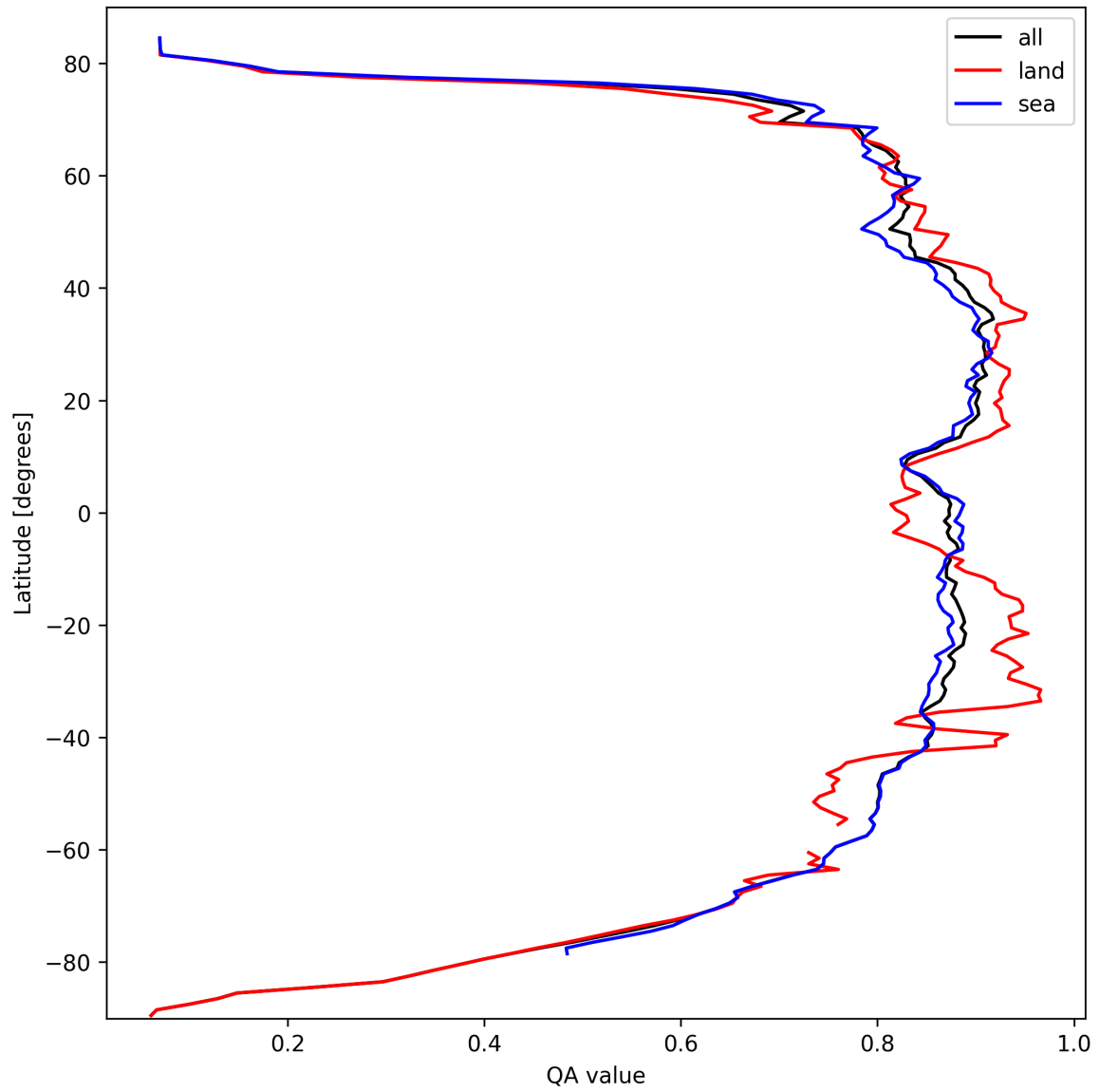
Figure 11: Zonal average of “QA value” for 2024-09-30 to 2024-10-02.
