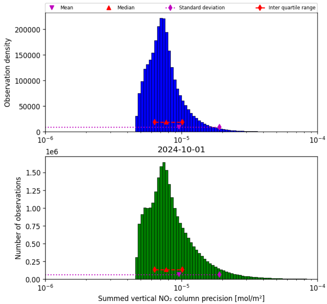
Figure 41: Histogram of “Summed vertical NO 2 column precision” for 2024-09-30 to 2024-10-02
