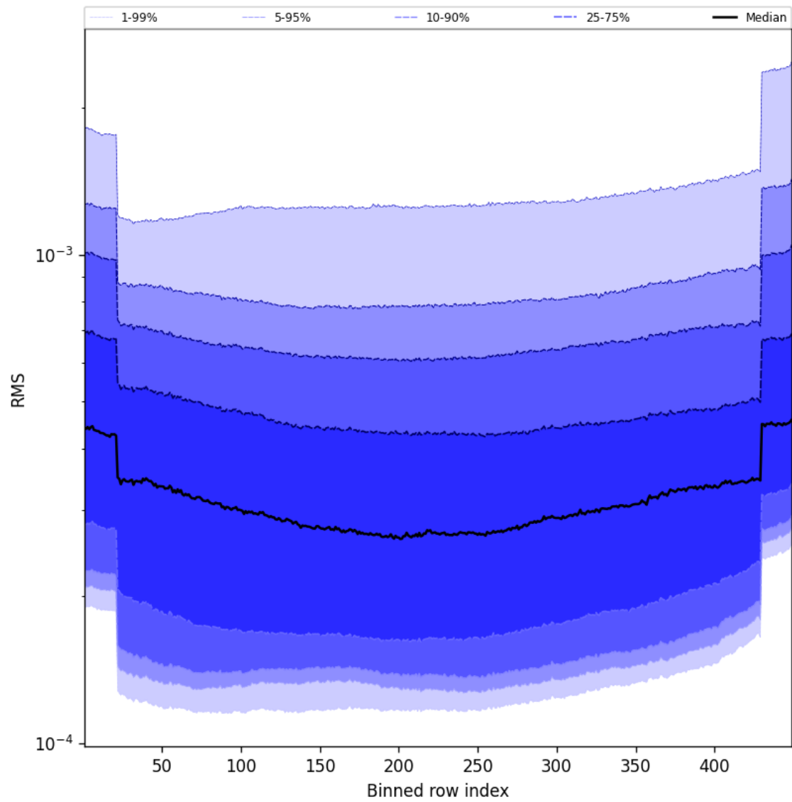
Figure 60: Along track statistics of “RMS” for 2024-09-30 to 2024-10-02
