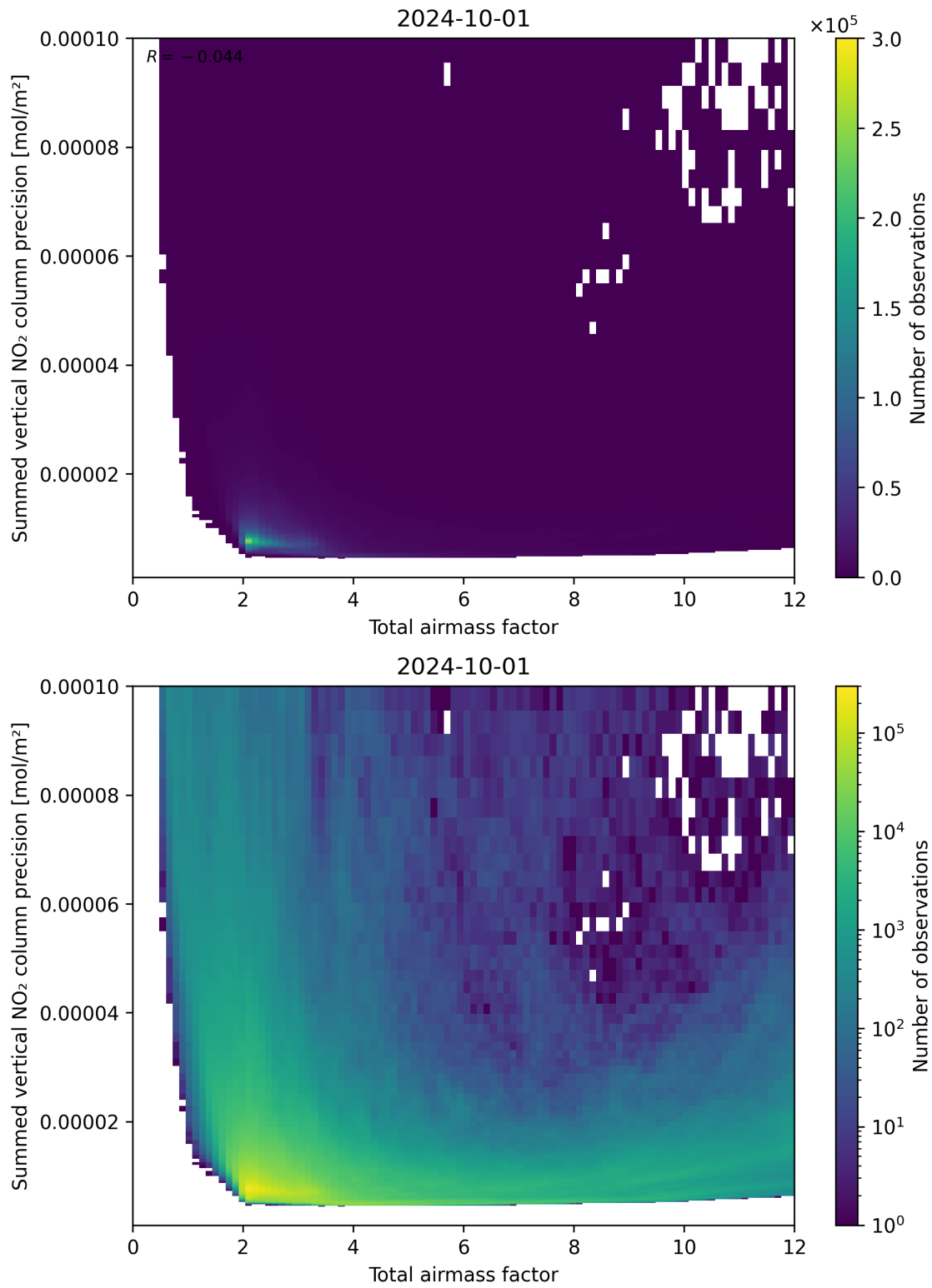
Figure 66: Scatter density plot of “Total airmass factor” against “Summed vertical NO 2 column precision” for 2024-09-30 to 2024-10-02.
