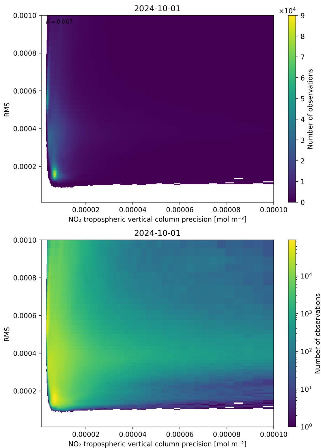
Figure 140: Scatter density plot of “NO 2 tropospheric vertical column precision” against “RMS” for 2024-09-30 to 2024-10-02.
