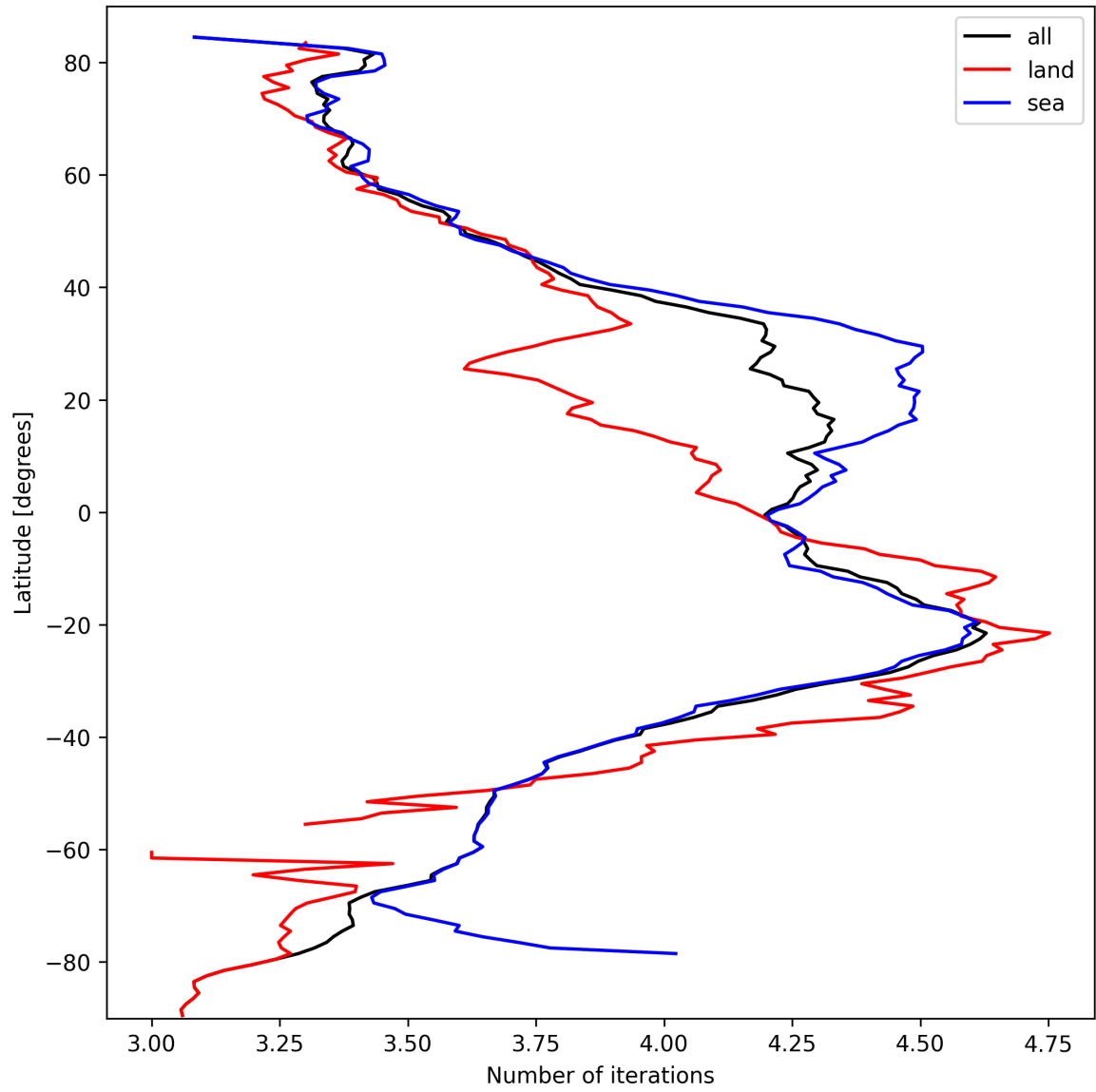
Figure 17: Zonal average of “Number of iterations” for 2024-09-30 to 2024-10-02.
