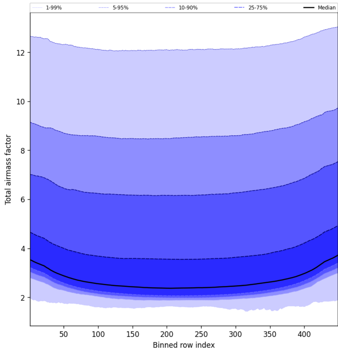
Figure 49: Along track statistics of “Total airmass factor” for 2024-09-30 to 2024-10-02
