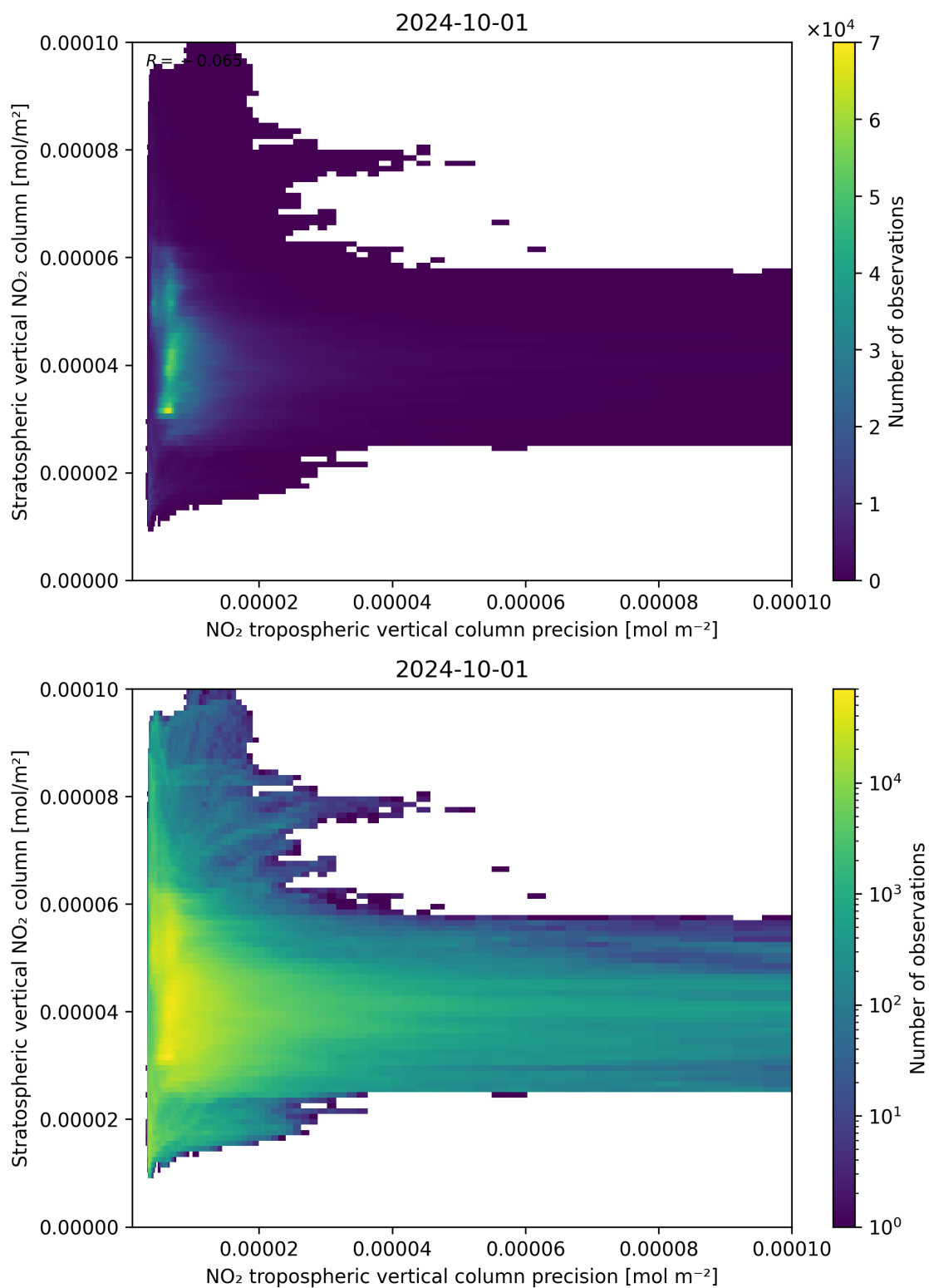
Figure 135: Scatter density plot of “NO 2 tropospheric vertical column precision” against “Stratospheric vertical NO 2 column” for 2024-09-30 to 2024-10-02.
