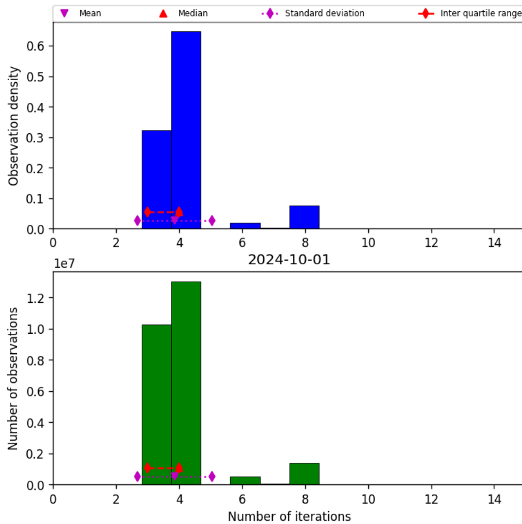
Figure 34: Histogram of “Number of iterations” for 2024-09-30 to 2024-10-02
