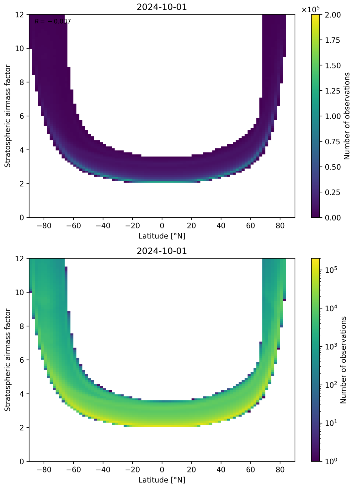
Figure 83: Scatter density plot of “Latitude” against “Stratospheric airmass factor” for 2024-09-30 to 2024-10-02.
