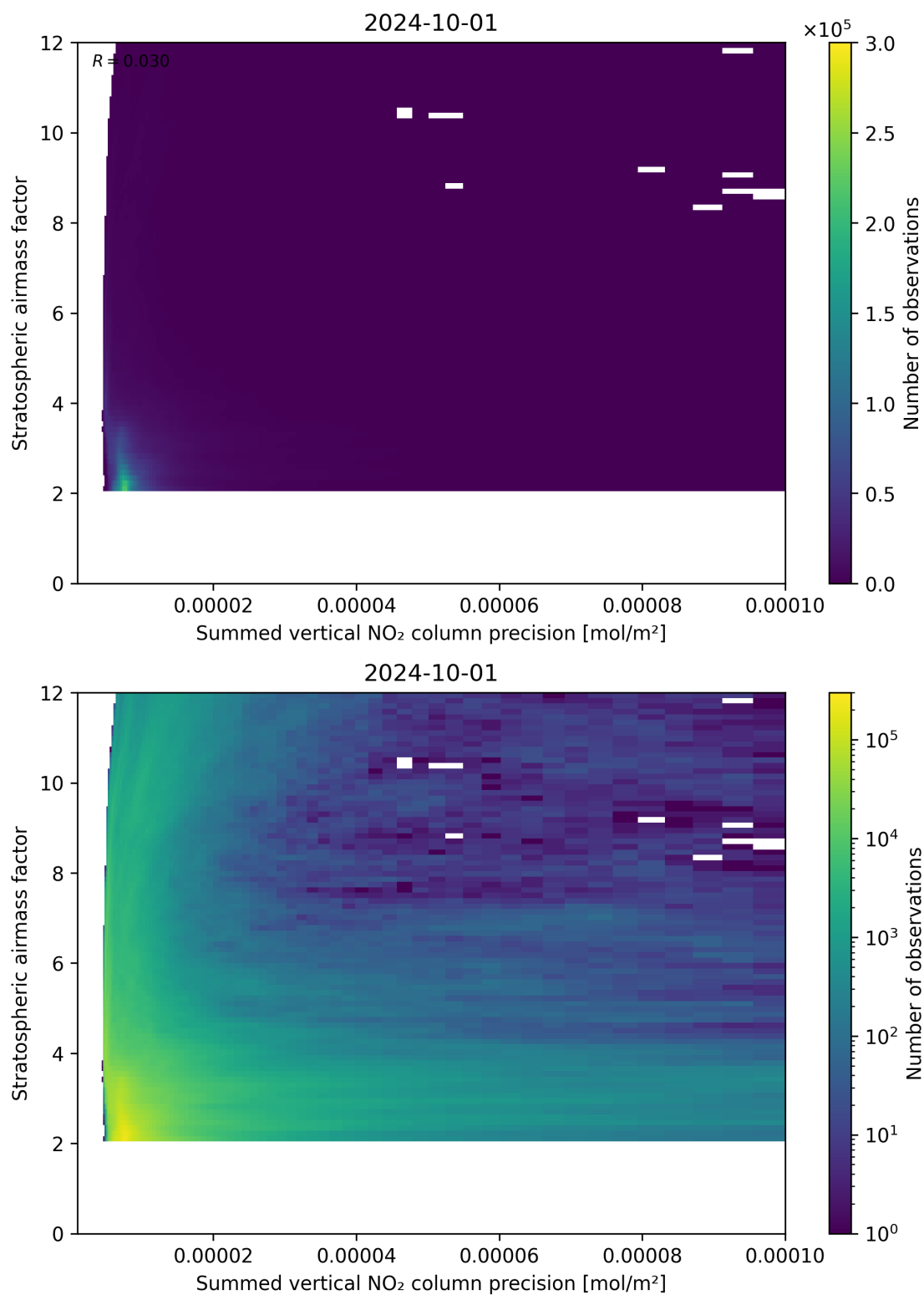
Figure 106: Scatter density plot of “Summed vertical NO 2 column precision” against “Stratospheric airmass factor” for 2024-09-30 to 2024-10-02.
