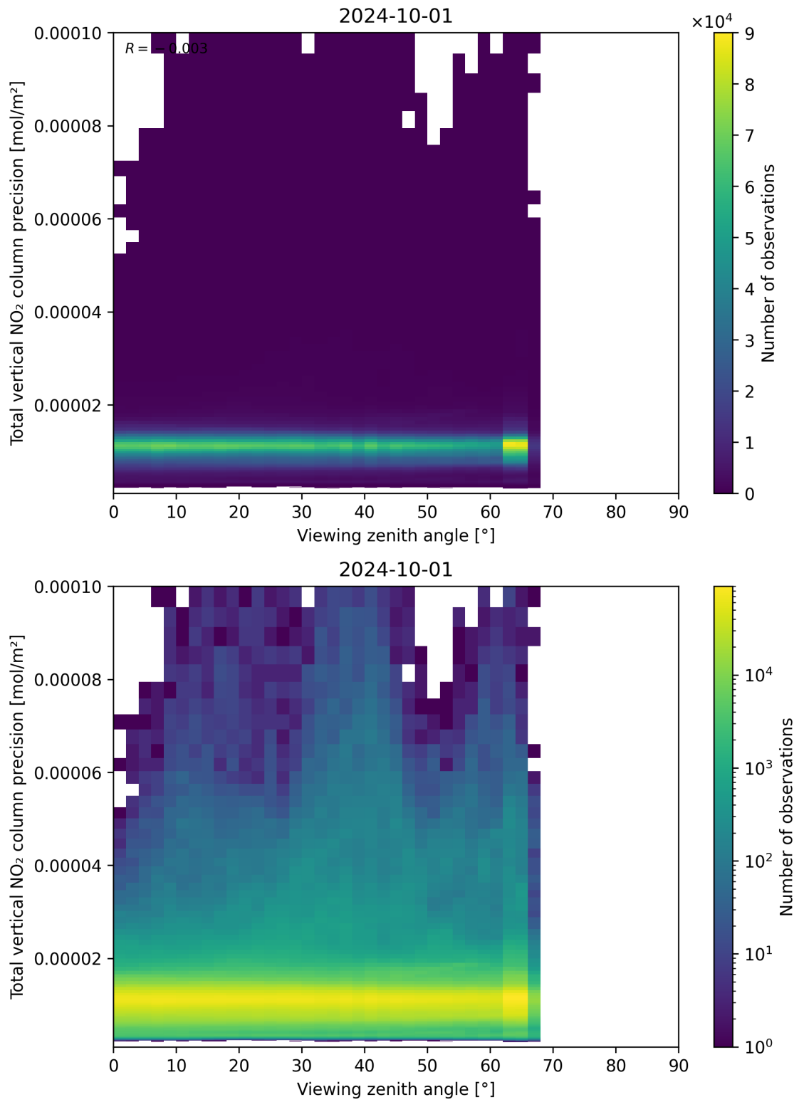
Figure 168: Scatter density plot of “Viewing zenith angle” against “Total vertical NO 2 column precision” for 2024-09-30 to 2024-10-02.
