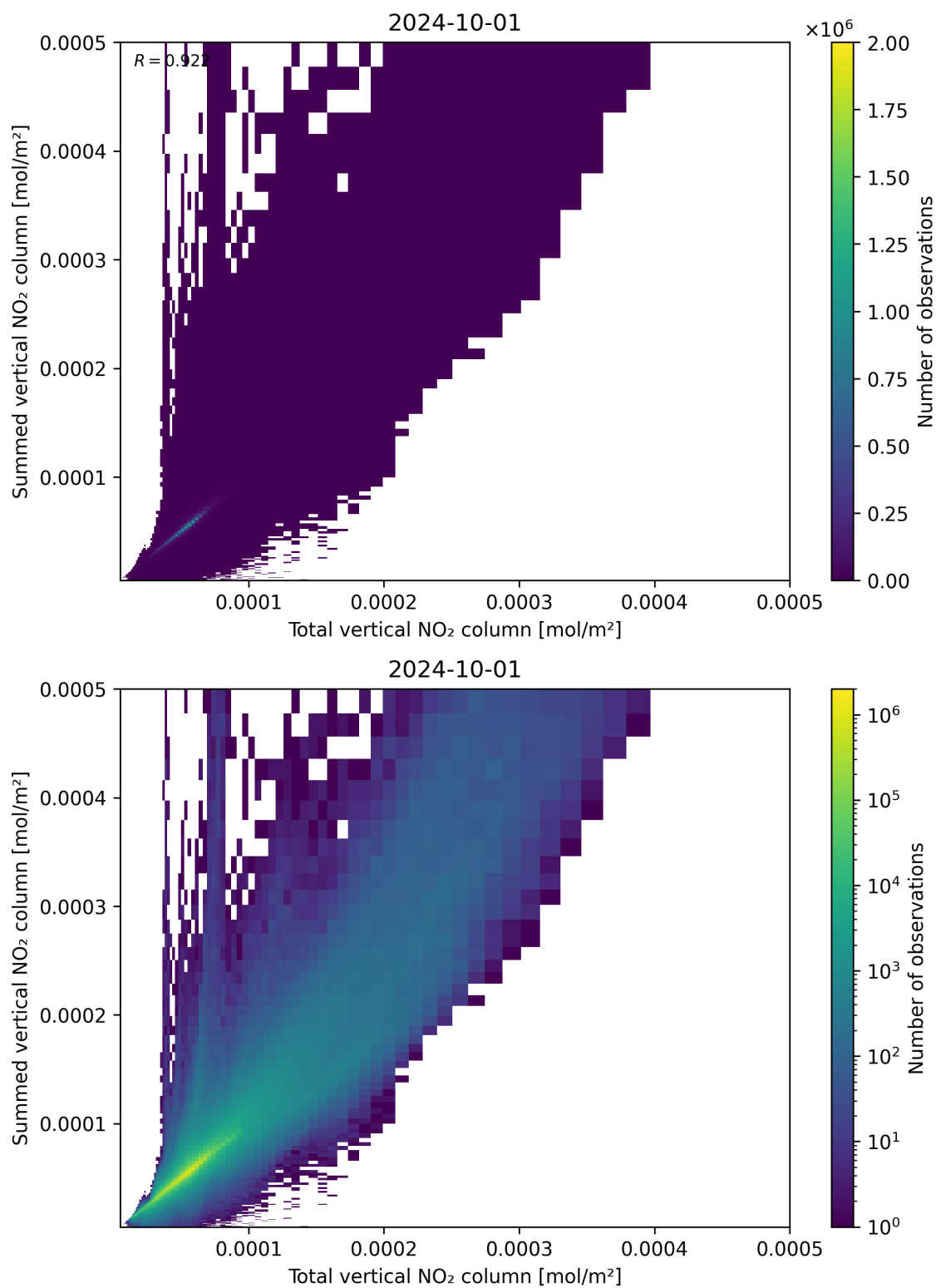
Figure 112: Scatter density plot of “Total vertical NO 2 column” against “Summed vertical NO 2 column” for 2024-09-30 to 2024-10-02.
