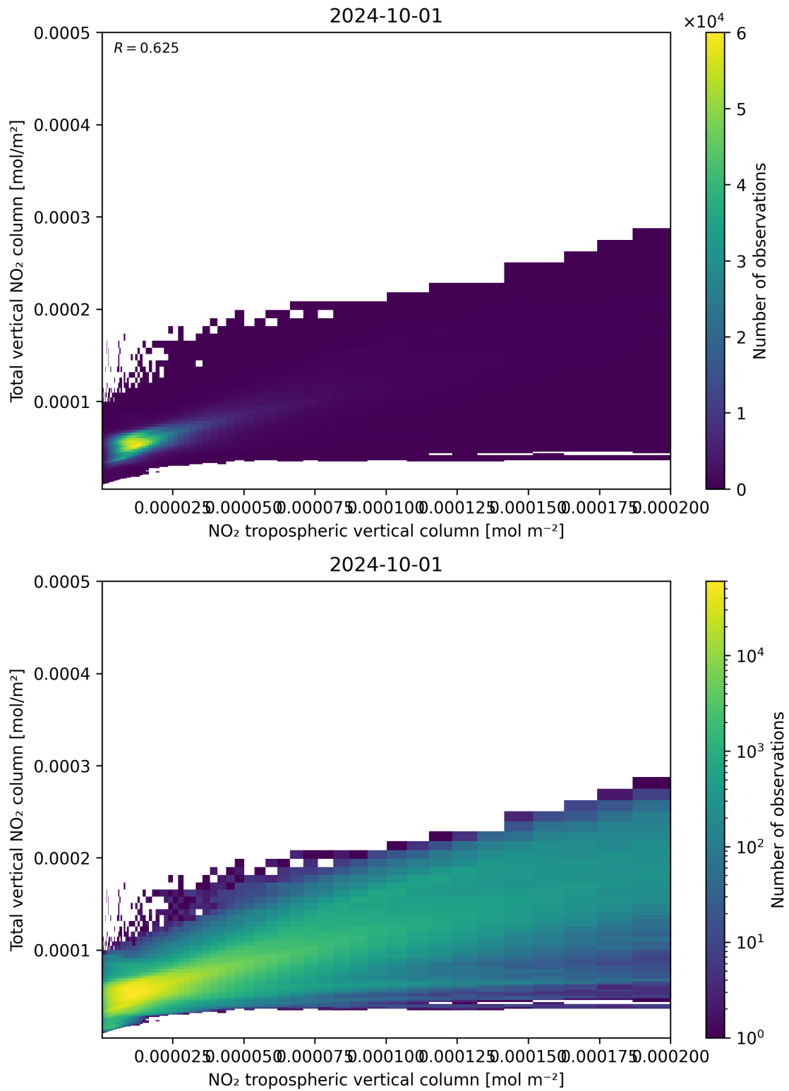
Figure 128: Scatter density plot of “NO 2 tropospheric vertical column” against “Total vertical NO 2 column” for 2024-09-30 to 2024-10-02.
