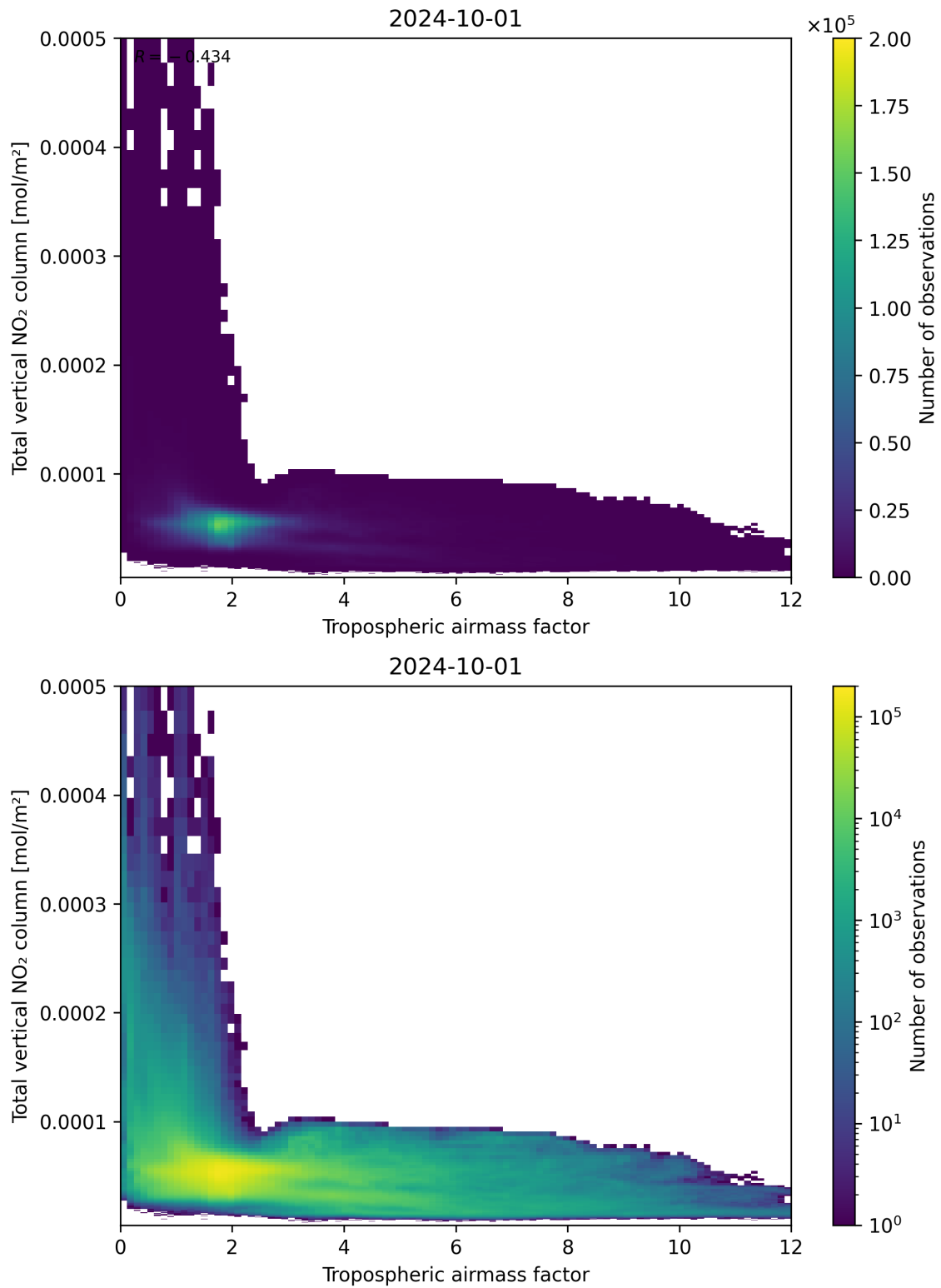
Figure 77: Scatter density plot of “Tropospheric airmass factor” against “Total vertical NO 2 column” for 2024-09-30 to 2024-10-02.
