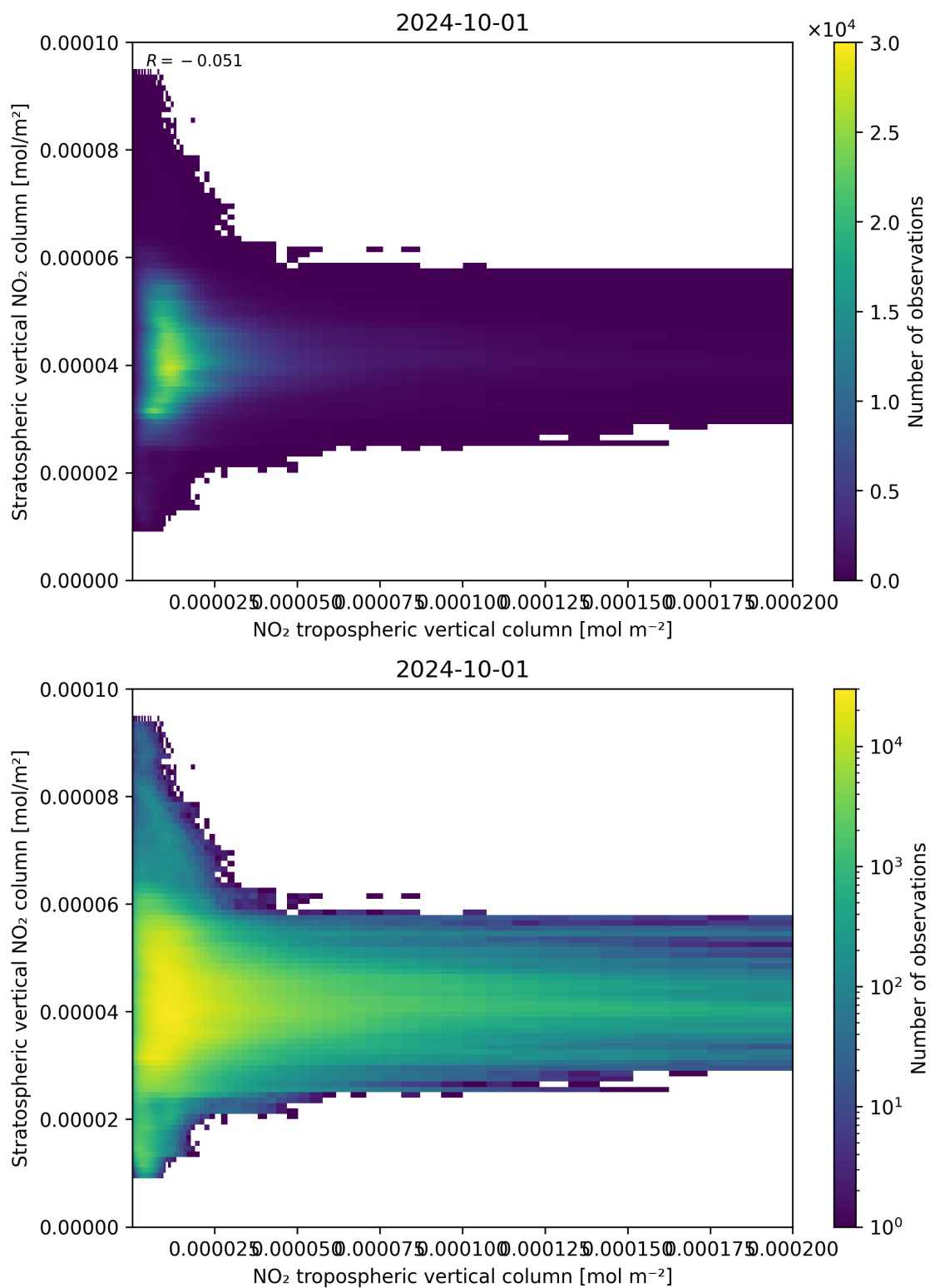
Figure 125: Scatter density plot of “NO 2 tropospheric vertical column” against “Stratospheric vertical NO 2 column” for 2024-09-30 to 2024-10-02.
