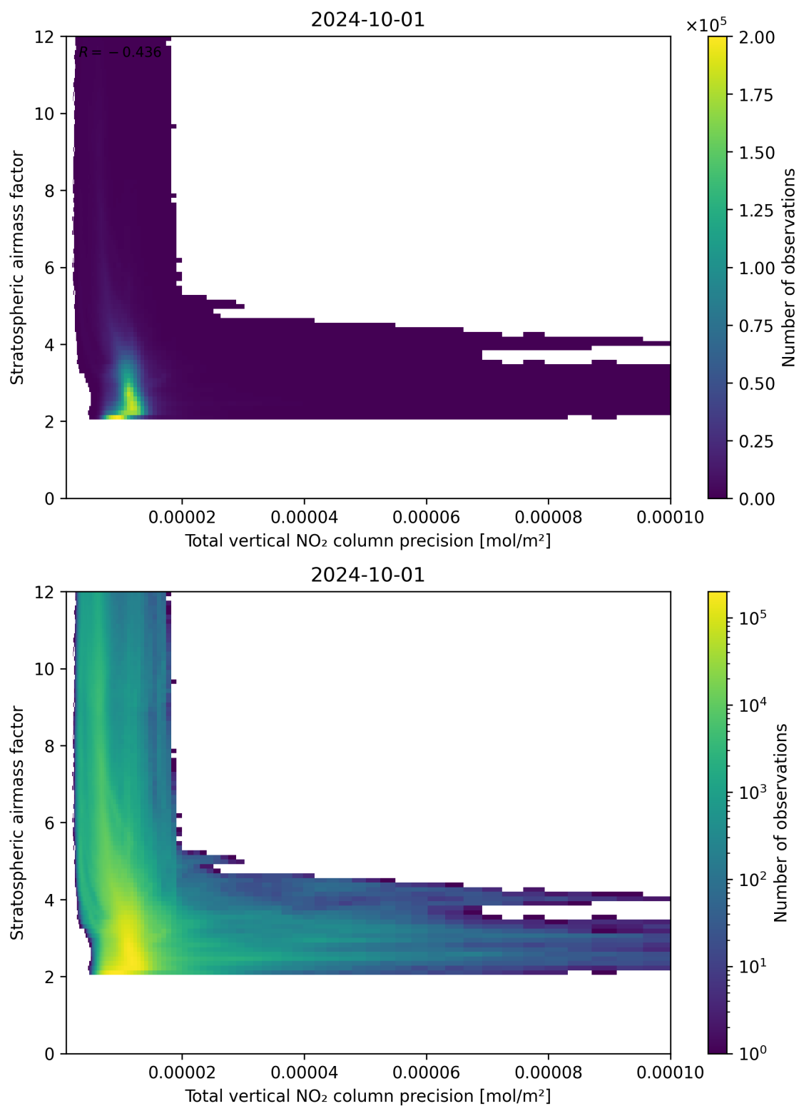
Figure 115: Scatter density plot of “Total vertical NO 2 column precision” against “Stratospheric air mass factor” for 2024-09-30 to 2024-10-02.
