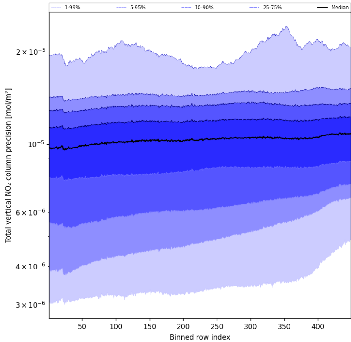
Figure 56: Along track statistics of “Total vertical NO 2 column precision” for 2024-09-30 to 2024-10-02
