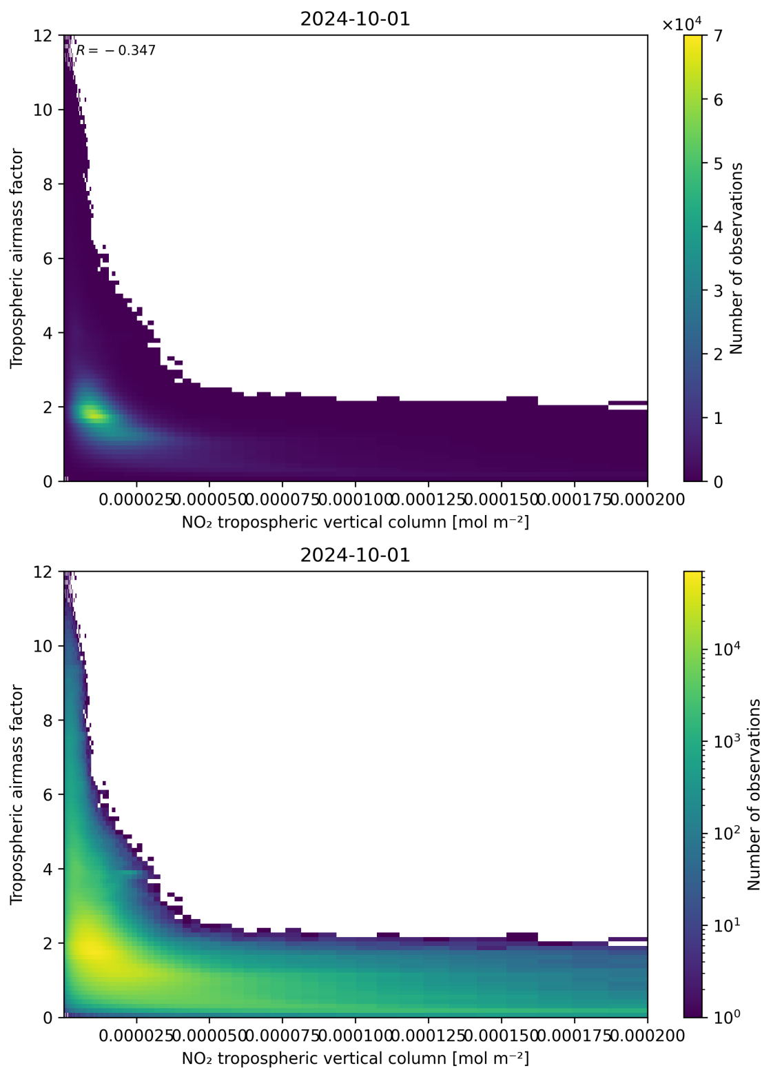
Figure 123: Scatter density plot of “NO 2 tropospheric vertical column” against “Tropospheric air mass factor” for 2024-09-30 to 2024-10-02.
