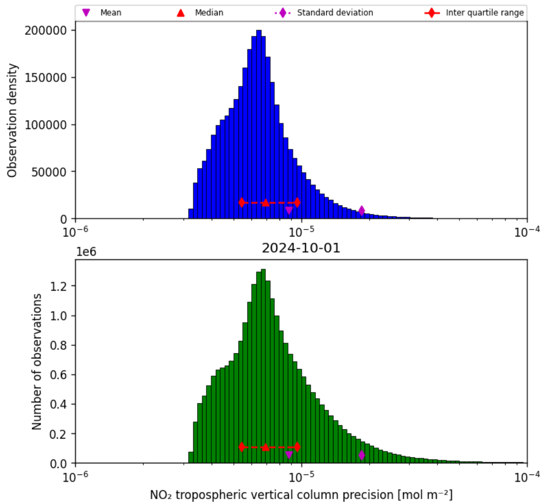
Figure 30: Histogram of “NO 2 tropospheric vertical column precision” for 2024-09-30 to 2024-10-02
