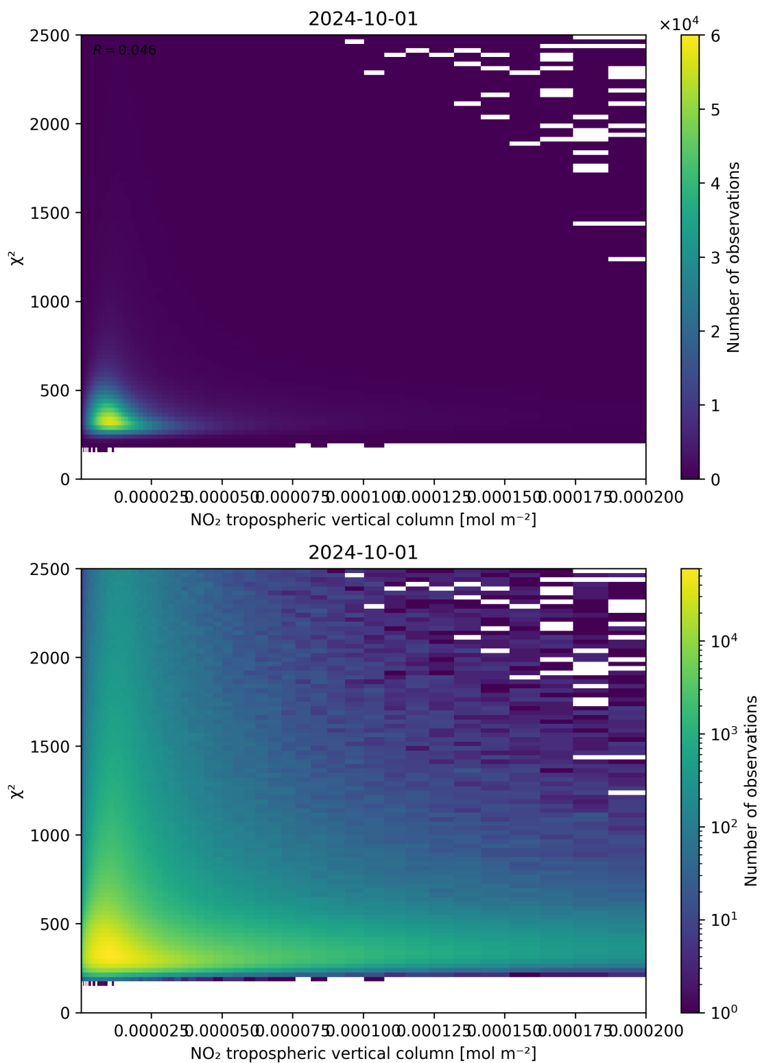
Figure 124: Scatter density plot of “NO 2 tropospheric vertical column” against “ \chi^2 ” for 2024-09-30 to 2024-10-02.
