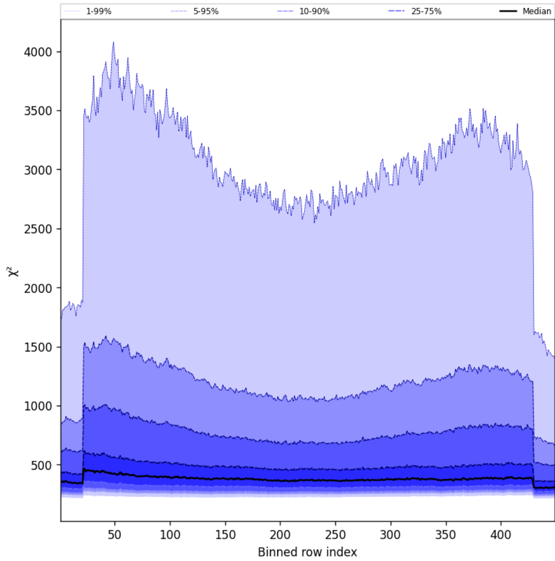
Figure 59: Along track statistics of “ \chi^2 ” for 2024-09-30 to 2024-10-02
