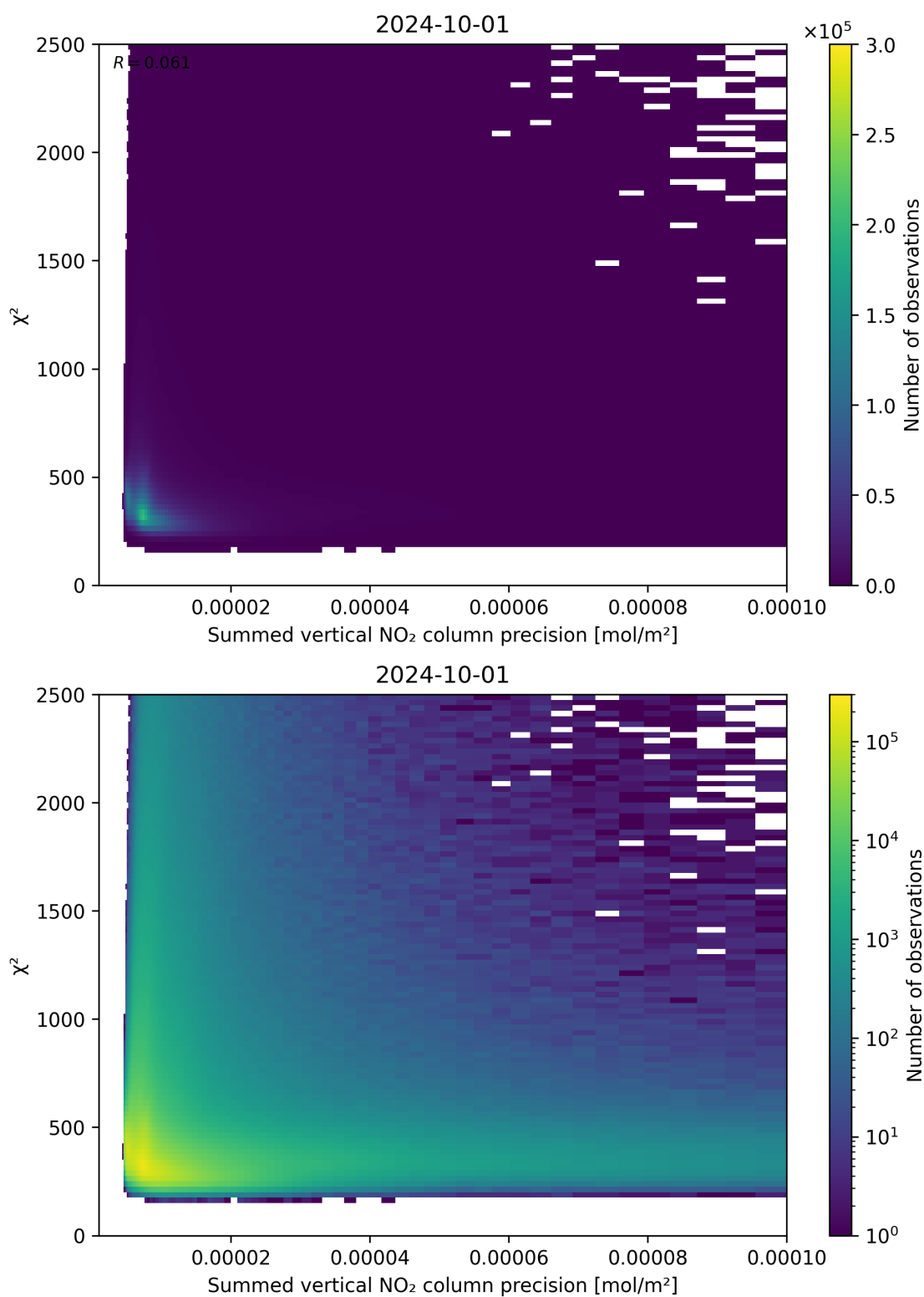
Figure 107: Scatter density plot of “Summed vertical NO 2 column precision” against “ \chi^2 ” for 2024-09-30 to 2024-10-02.
