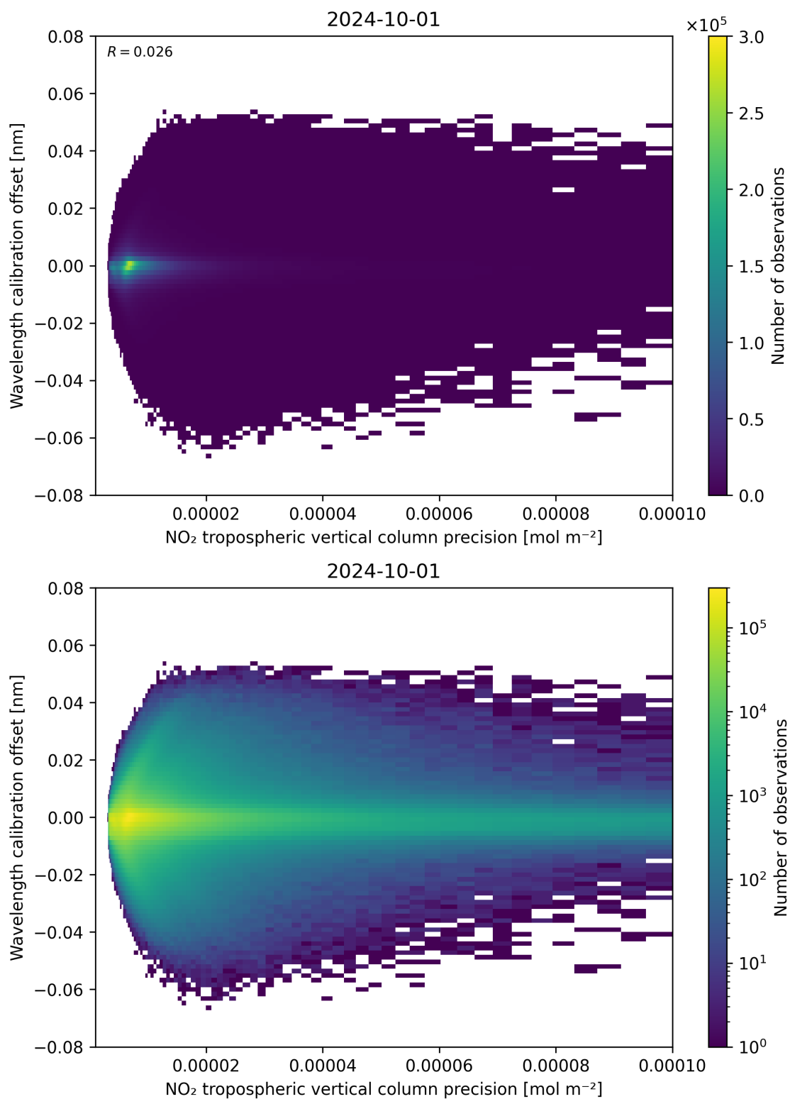
Figure 141: Scatter density plot of “NO 2 tropospheric vertical column precision” against “Wavelength calibration offset” for 2024-09-30 to 2024-10-02.
