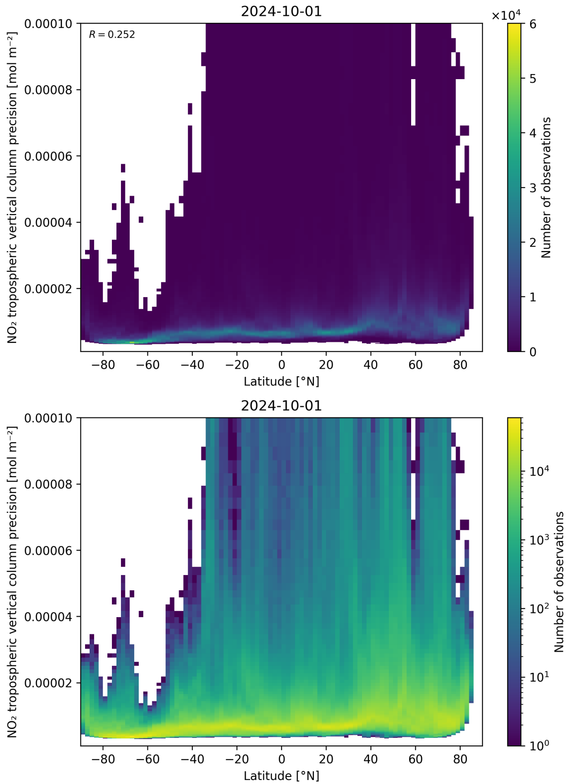
Figure 93: Scatter density plot of “Latitude” against “NO 2 tropospheric vertical column precision” for 2024-09-30 to 2024-10-02.
