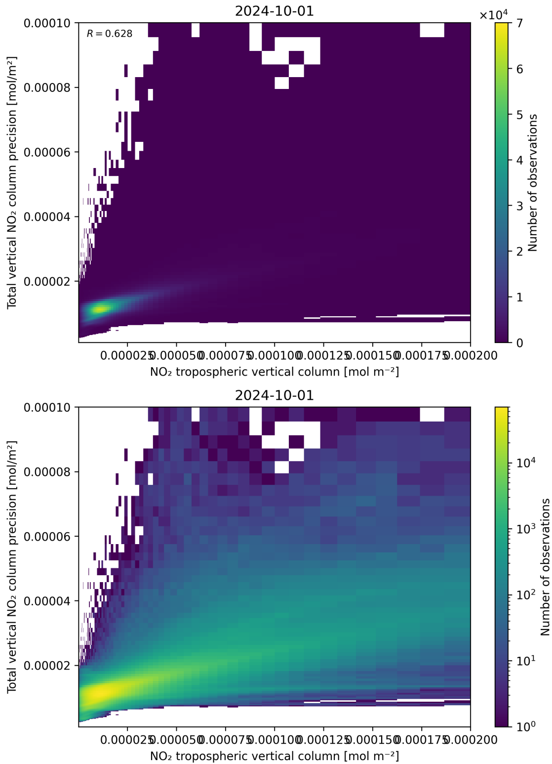
Figure 129: Scatter density plot of “NO 2 tropospheric vertical column” against “Total vertical NO 2 column precision” for 2024-09-30 to 2024-10-02.
