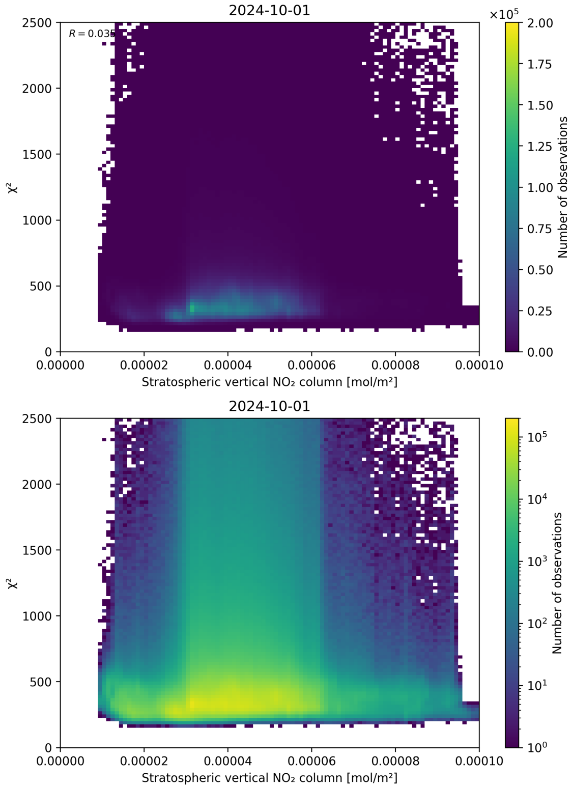
Figure 97: Scatter density plot of “Stratospheric vertical NO 2 column” against “ \chi^2 ” for 2024-09-30 to 2024-10-02.
