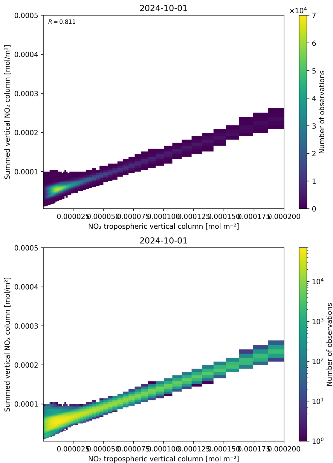
Figure 126: Scatter density plot of “NO 2 tropospheric vertical column” against “Summed vertical NO 2 column” for 2024-09-30 to 2024-10-02.
