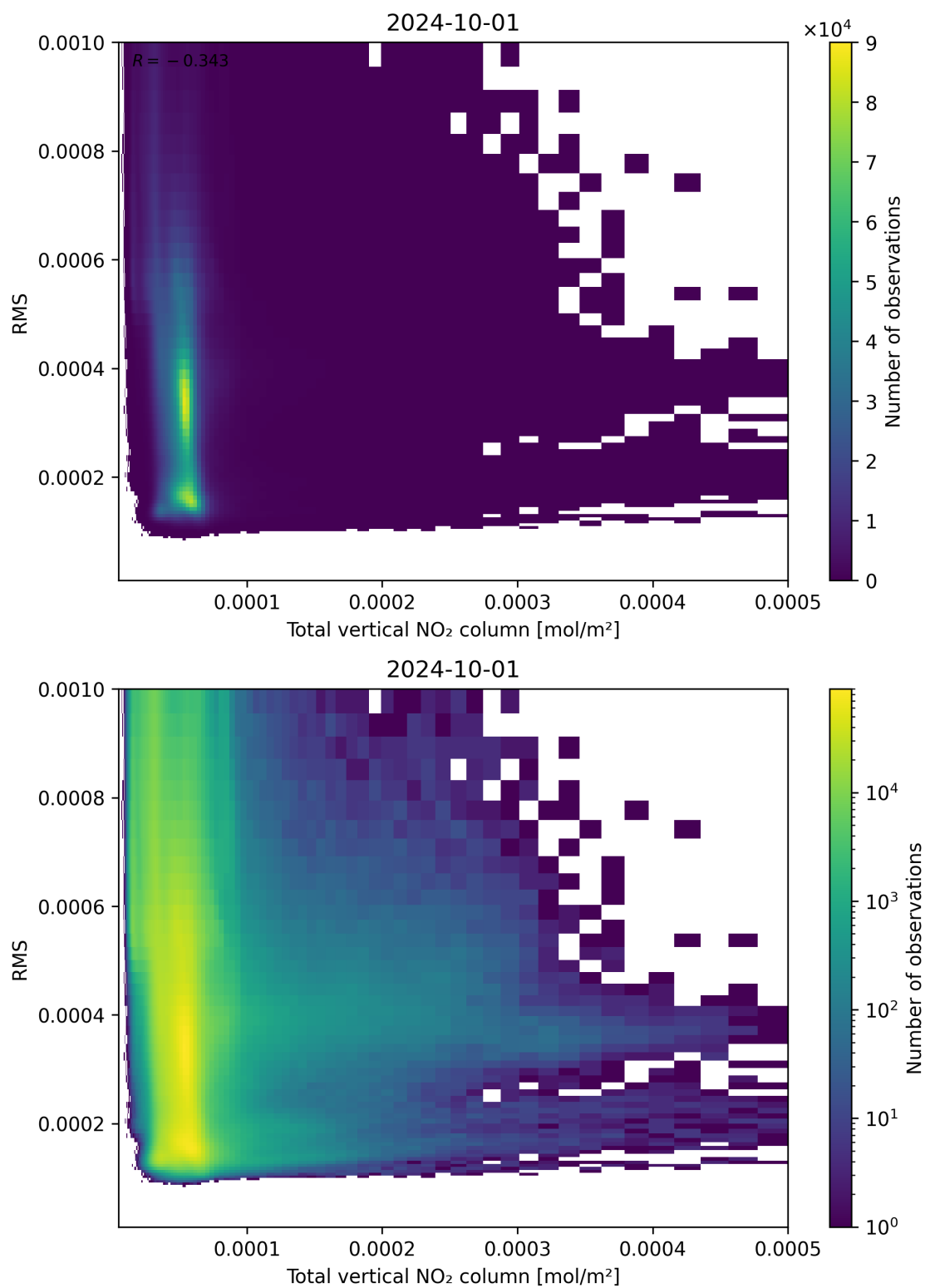
Figure 120: Scatter density plot of “Total vertical NO 2 column” against “RMS” for 2024-09-30 to 2024-10-02.
