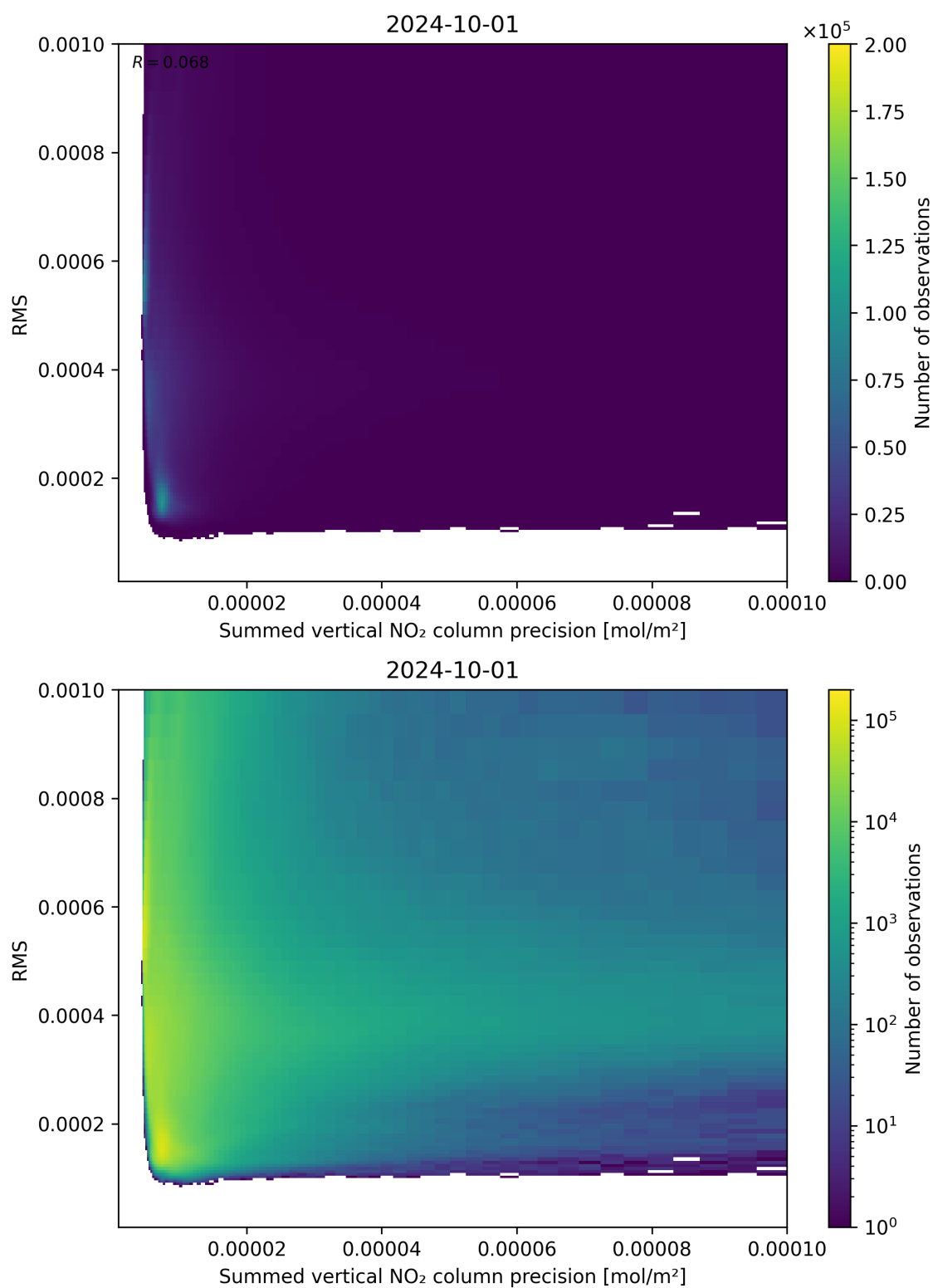
Figure 108: Scatter density plot of “Summed vertical NO 2 column precision” against “RMS” for 2024-09-30 to 2024-10-02.
