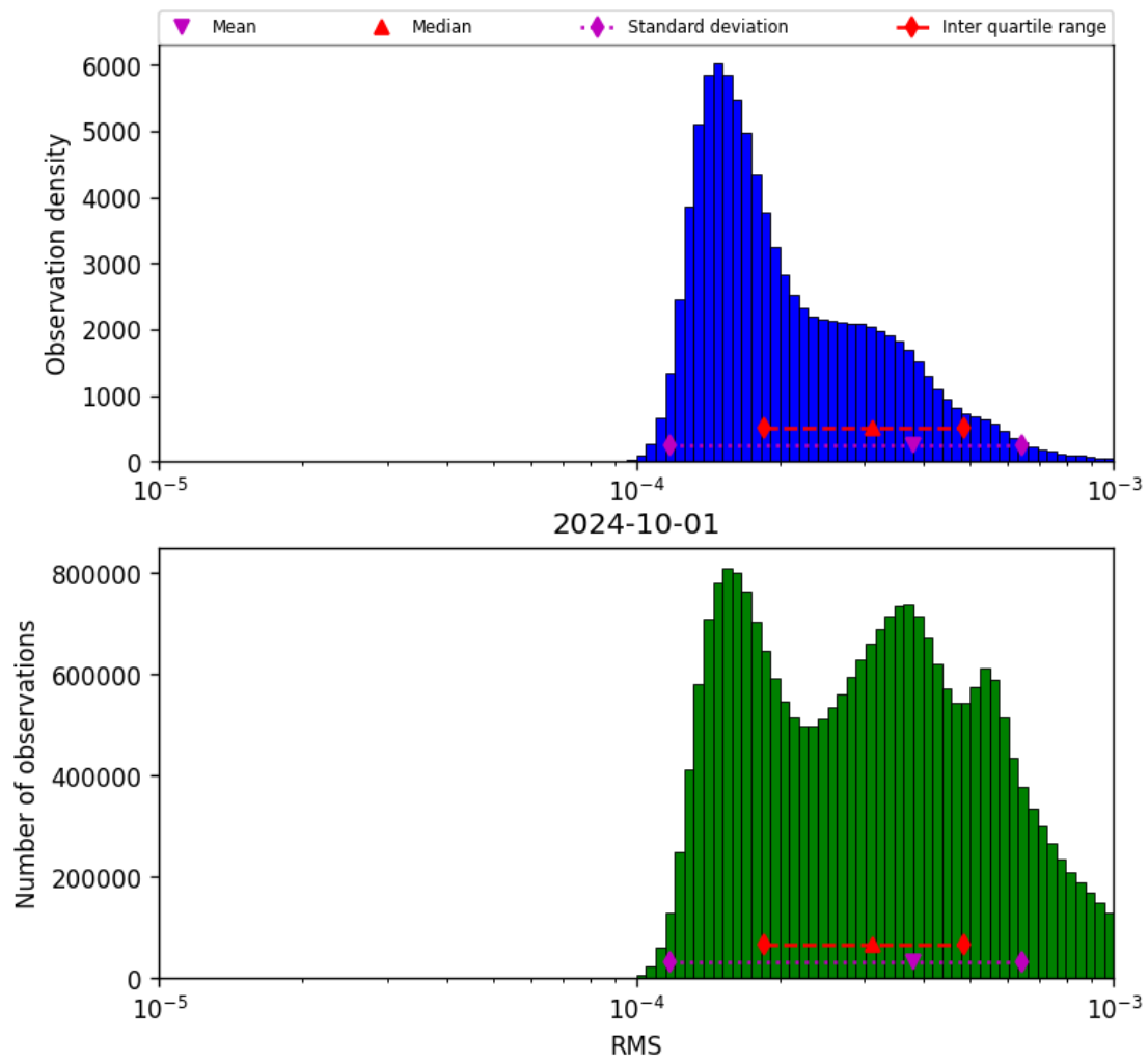
Figure 43: Histogram of “RMS” for 2024-09-30 to 2024-10-02
