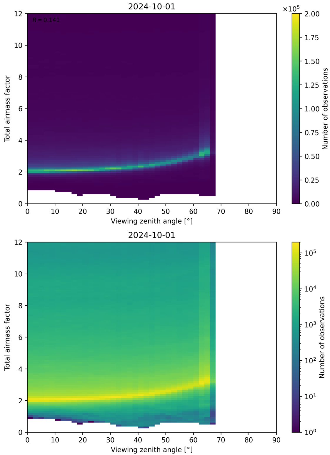
Figure 160: Scatter density plot of “Viewing zenith angle” against “Total airmass factor” for 2024-09-30 to 2024-10-02.
