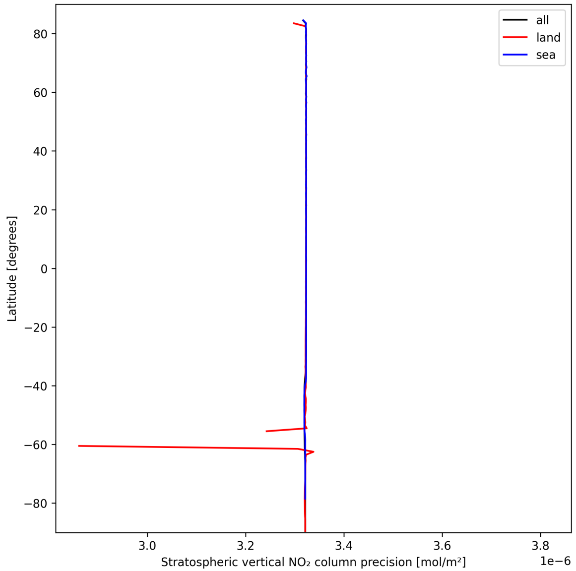
Figure 20: Zonal average of “Stratospheric vertical NO 2 column precision” for 2024-09-30 to 2024-10-02.
