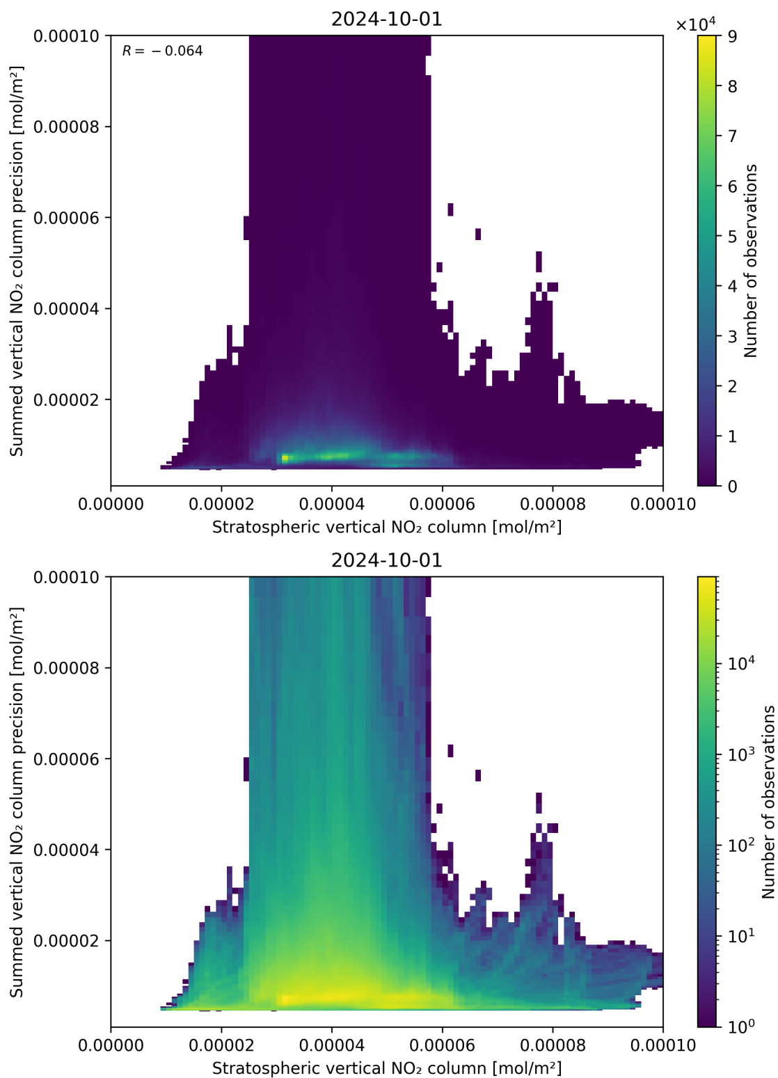
Figure 99: Scatter density plot of “Stratospheric vertical NO 2 column” against “Summed vertical NO 2 column precision” for 2024-09-30 to 2024-10-02.
