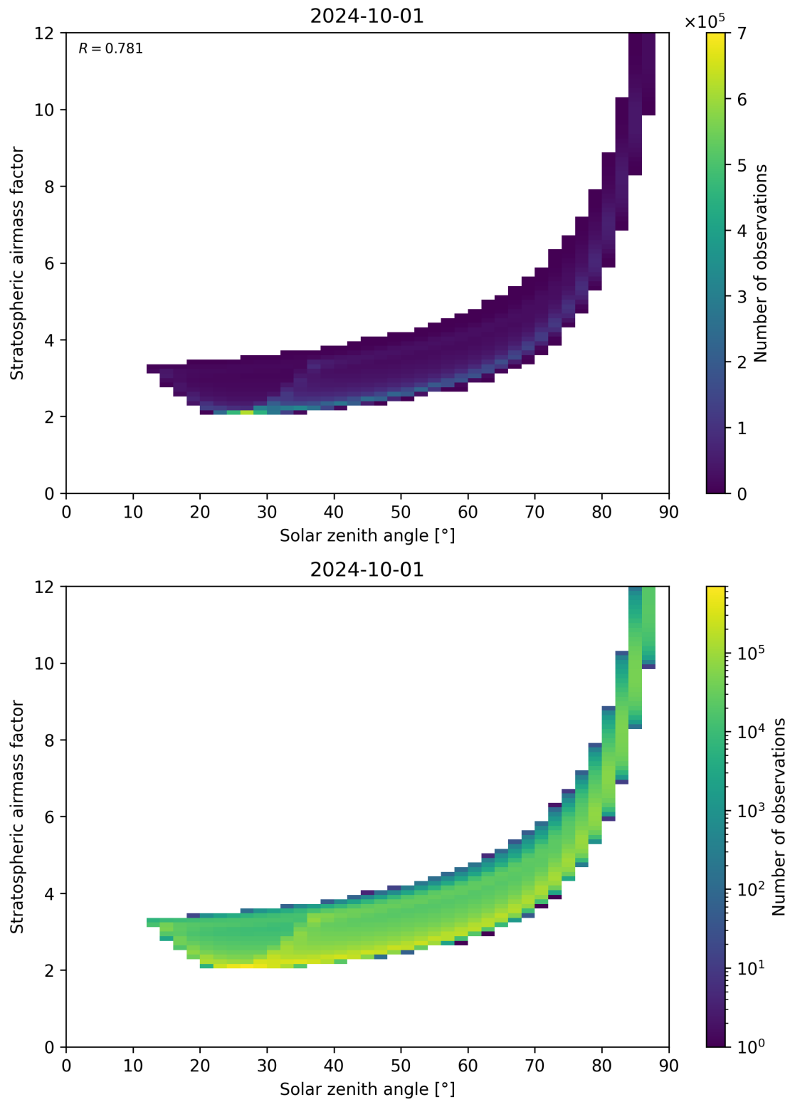
Figure 145: Scatter density plot of “Solar zenith angle” against “Stratospheric airmass factor” for 2024-09-30 to 2024-10-02.
