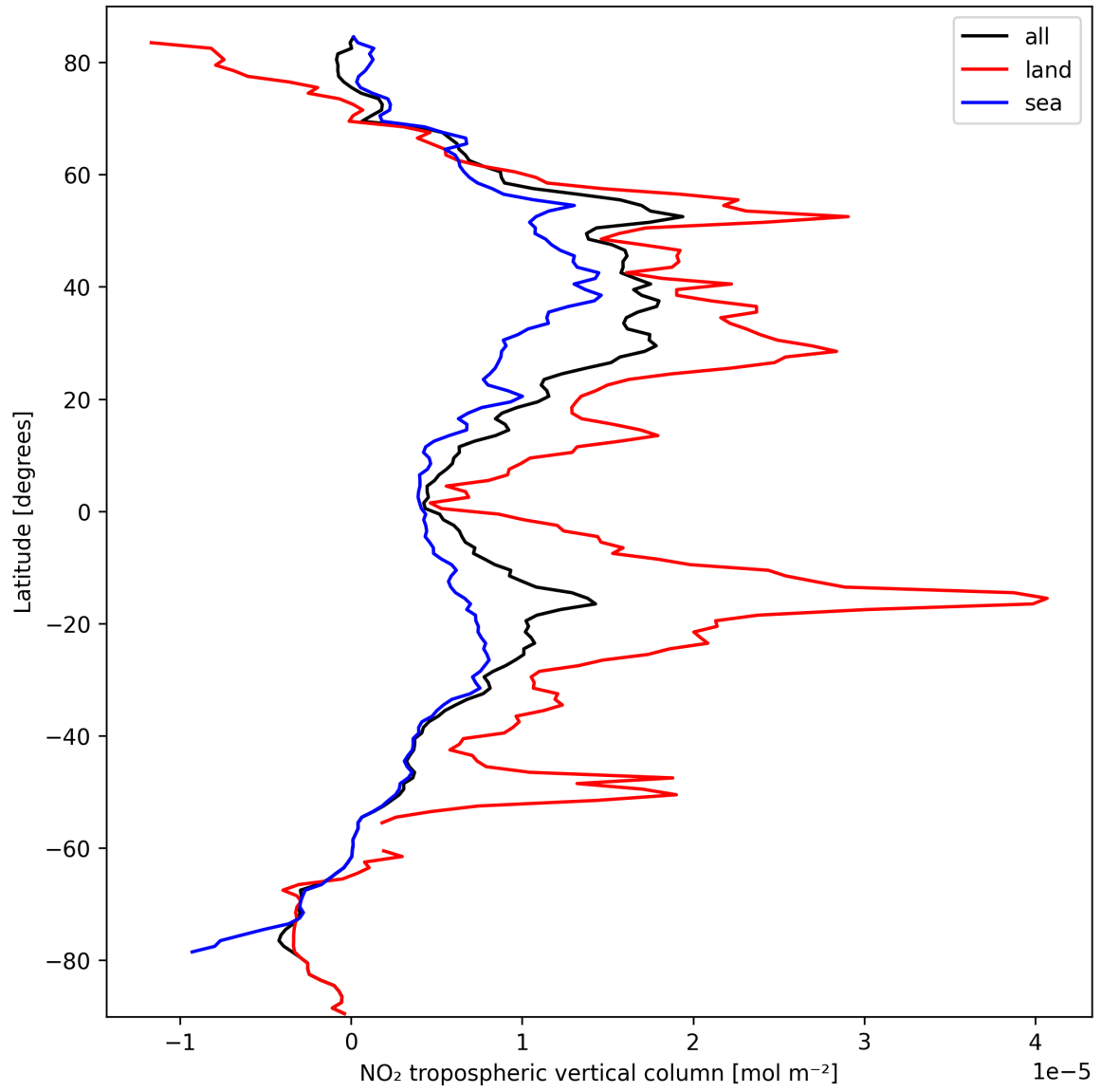
Figure 12: Zonal average of “NO 2 tropospheric vertical column” for 2024-09-30 to 2024-10-02.
