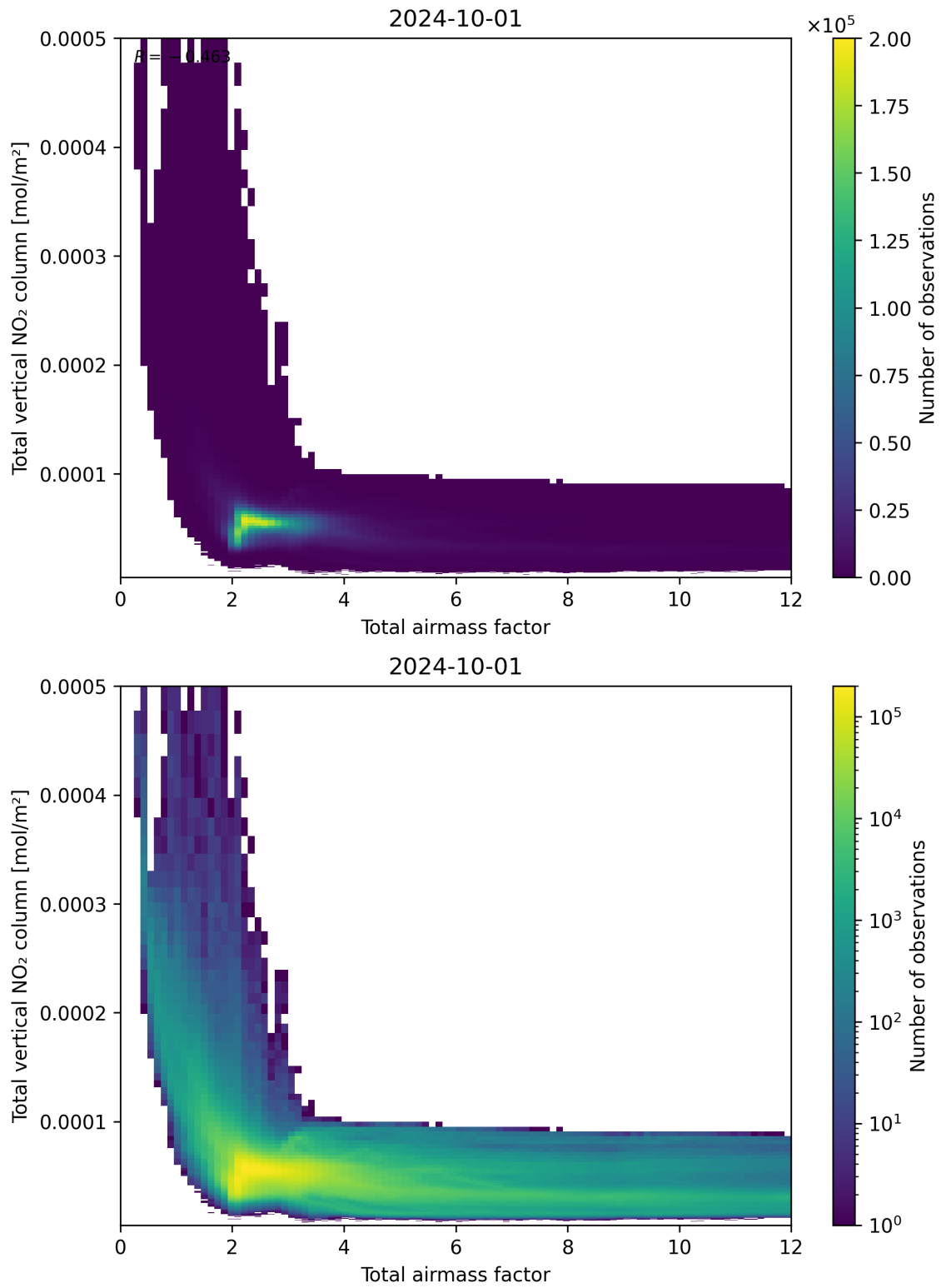
Figure 67: Scatter density plot of “Total airmass factor” against “Total vertical NO 2 column” for 2024-09-30 to 2024-10-02.
