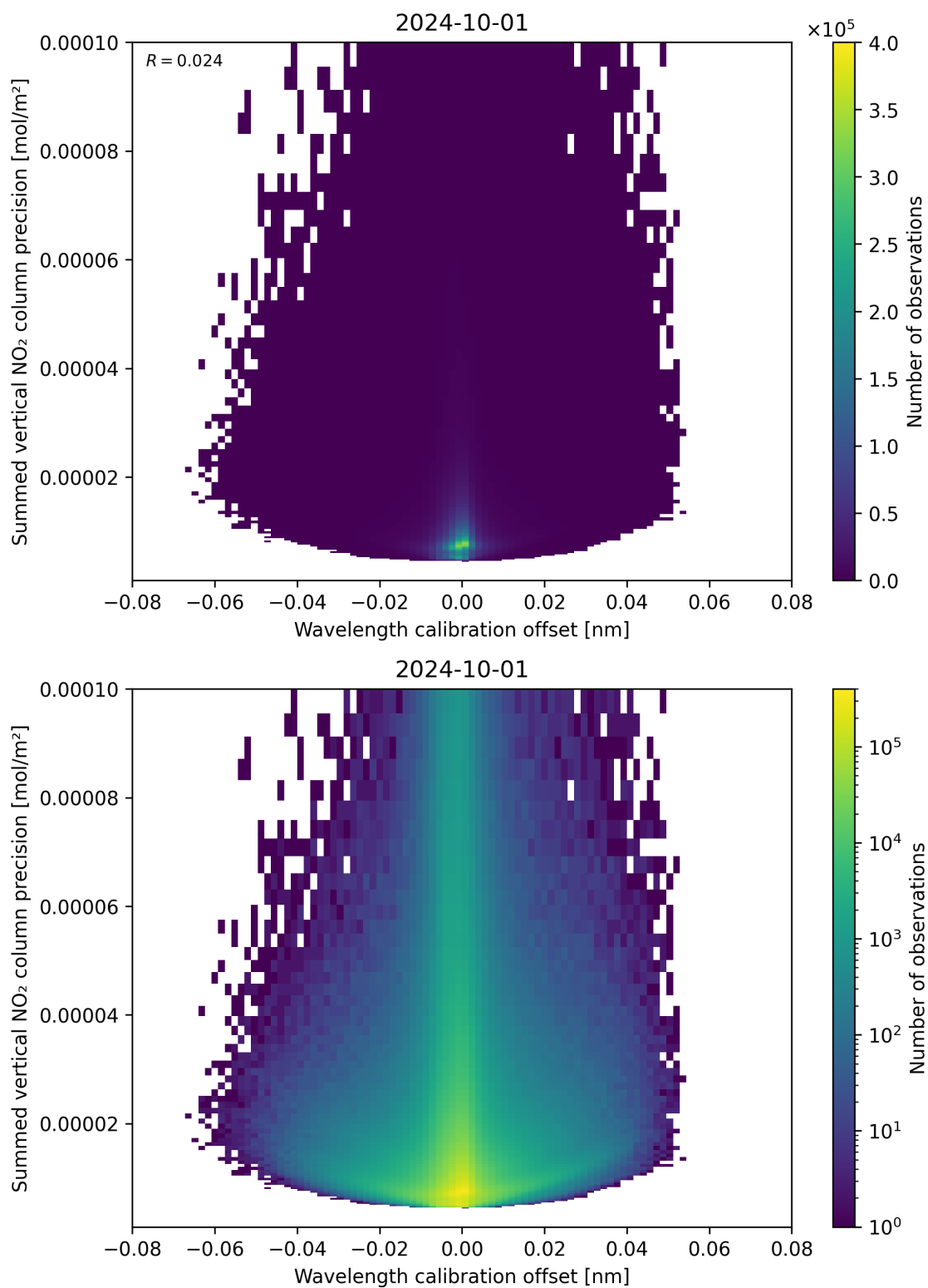
Figure 178: Scatter density plot of “Wavelength calibration offset” against “Summed vertical NO 2 column precision” for 2024-09-30 to 2024-10-02.
