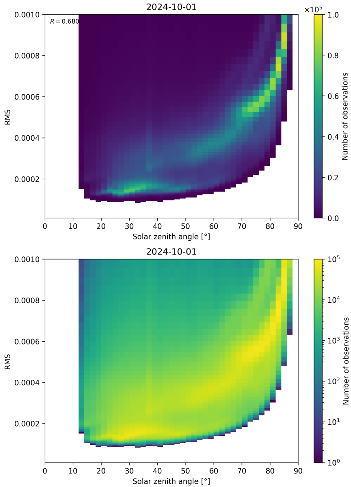
Figure 157: Scatter density plot of “Solar zenith angle” against “RMS” for 2024-09-30 to 2024-10-02.
