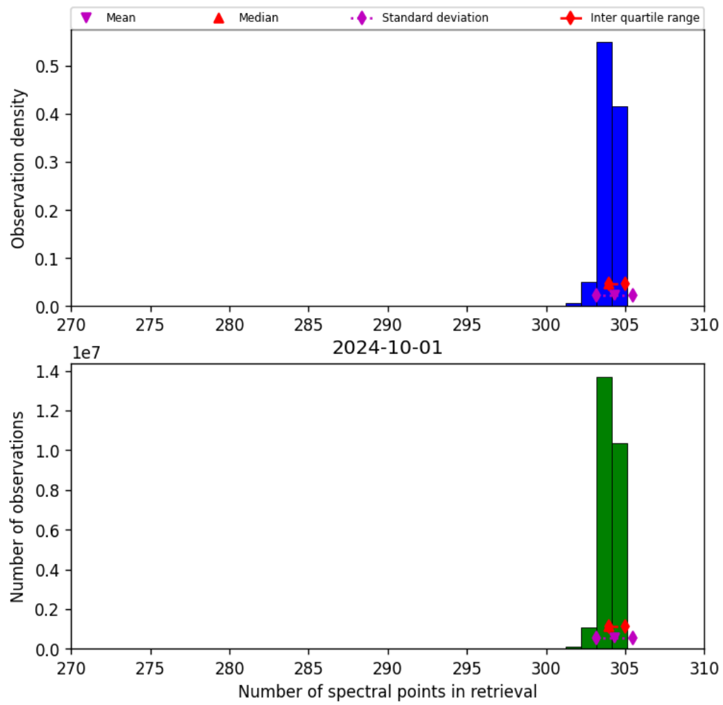
Figure 33: Histogram of “Number of spectral points in retrieval” for 2024-09-30 to 2024-10-02
