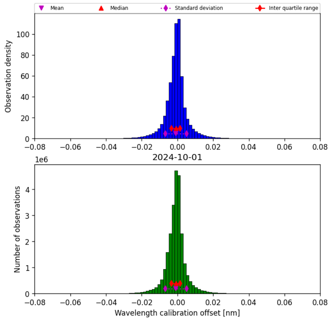
Figure 35: Histogram of “Wavelength calibration offset” for 2024-09-30 to 2024-10-02
