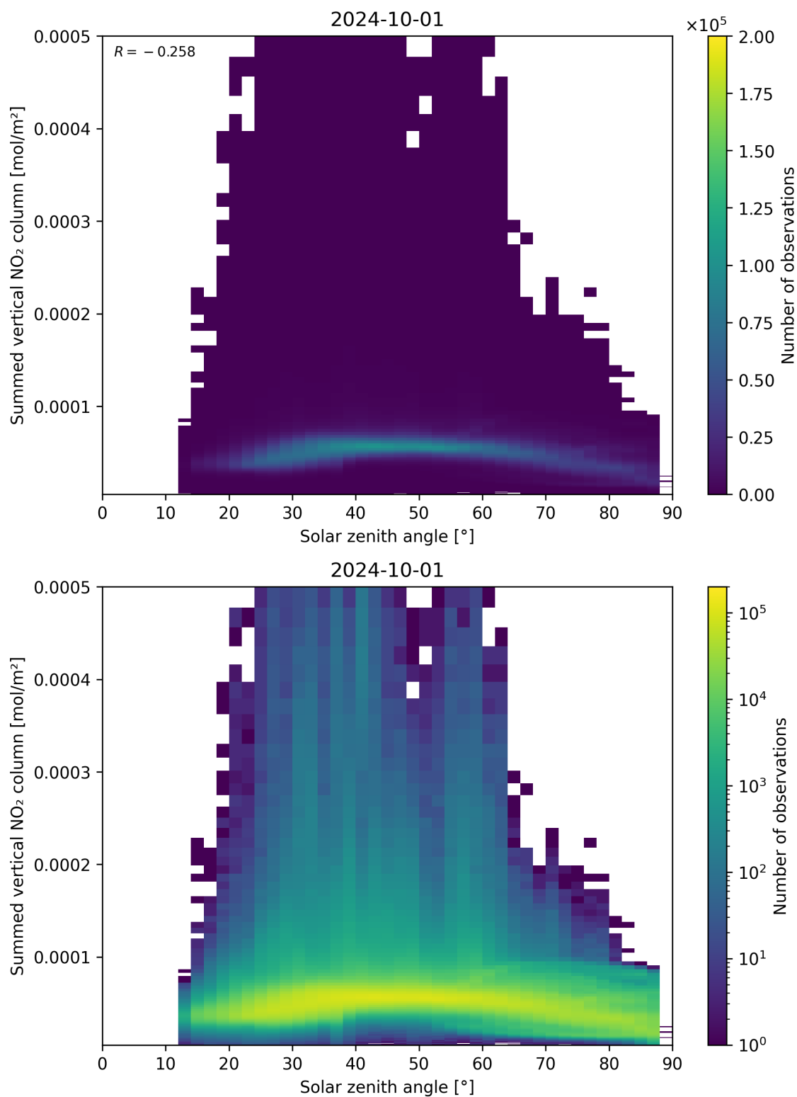
Figure 151: Scatter density plot of “Solar zenith angle” against “Summed vertical NO 2 column” for 2024-09-30 to 2024-10-02.
