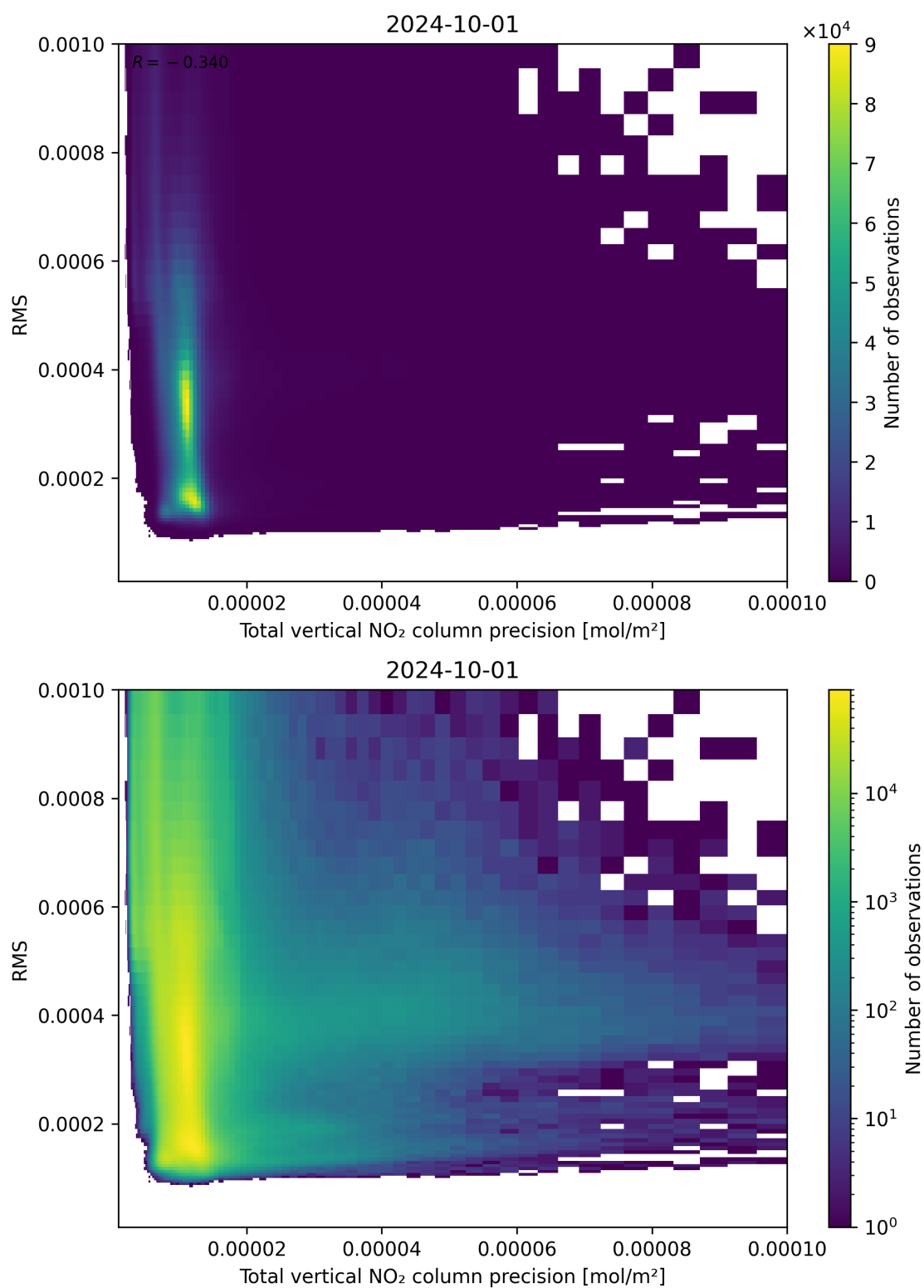
Figure 119: Scatter density plot of “Total vertical NO 2 column precision” against “RMS” for 2024-09-30 to 2024-10-02.
