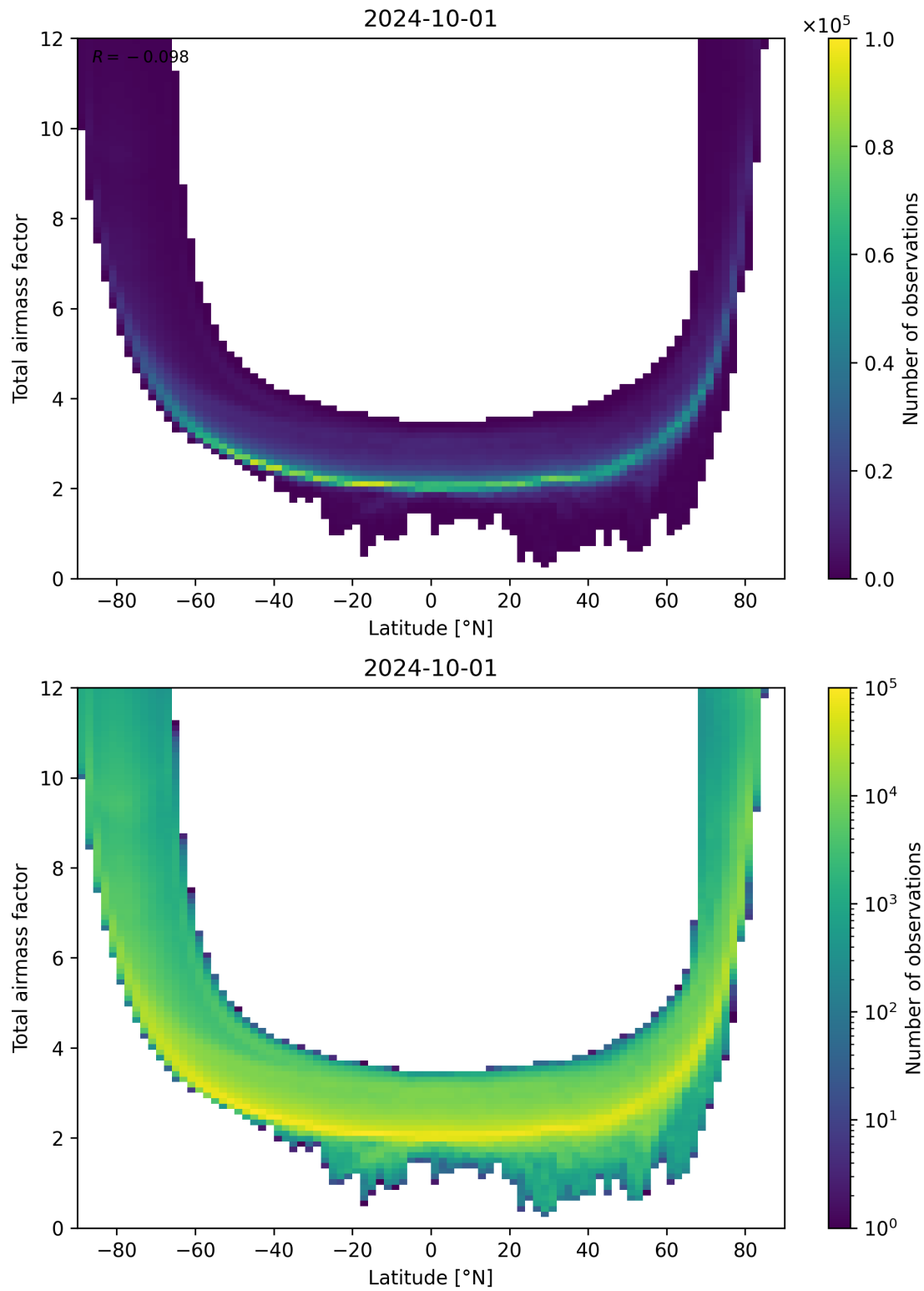
Figure 84: Scatter density plot of “Latitude” against “Total airmass factor” for 2024-09-30 to 2024-10-02.
