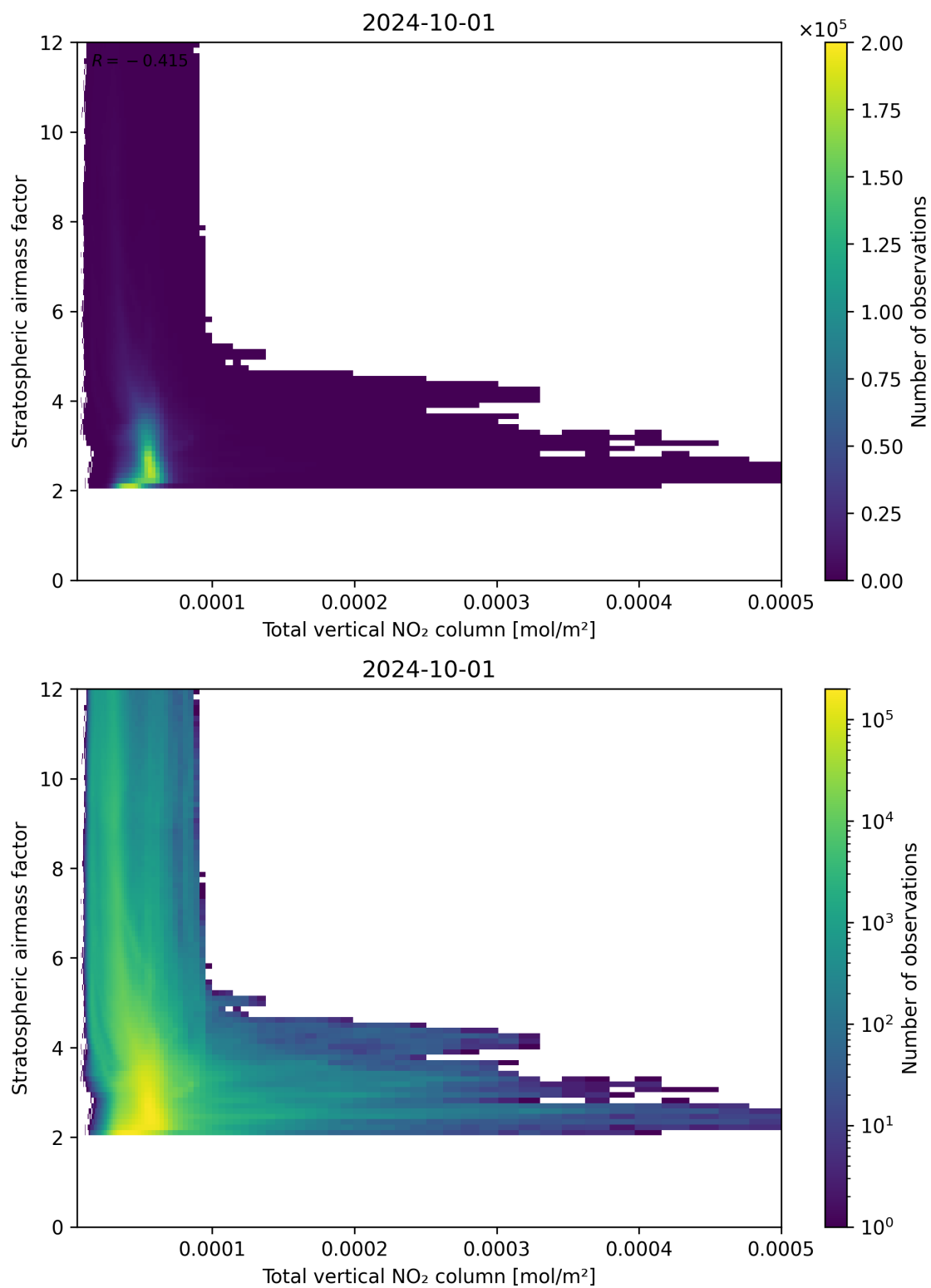
Figure 110: Scatter density plot of “Total vertical NO 2 column” against “Stratospheric airmass factor” for 2024-09-30 to 2024-10-02.
