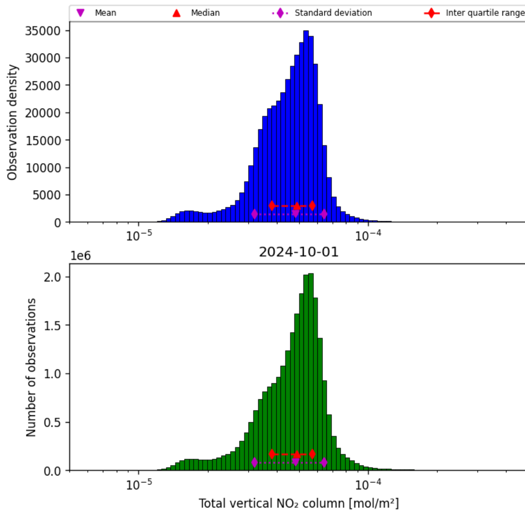
Figure 38: Histogram of “Total vertical NO 2 column” for 2024-09-30 to 2024-10-02
