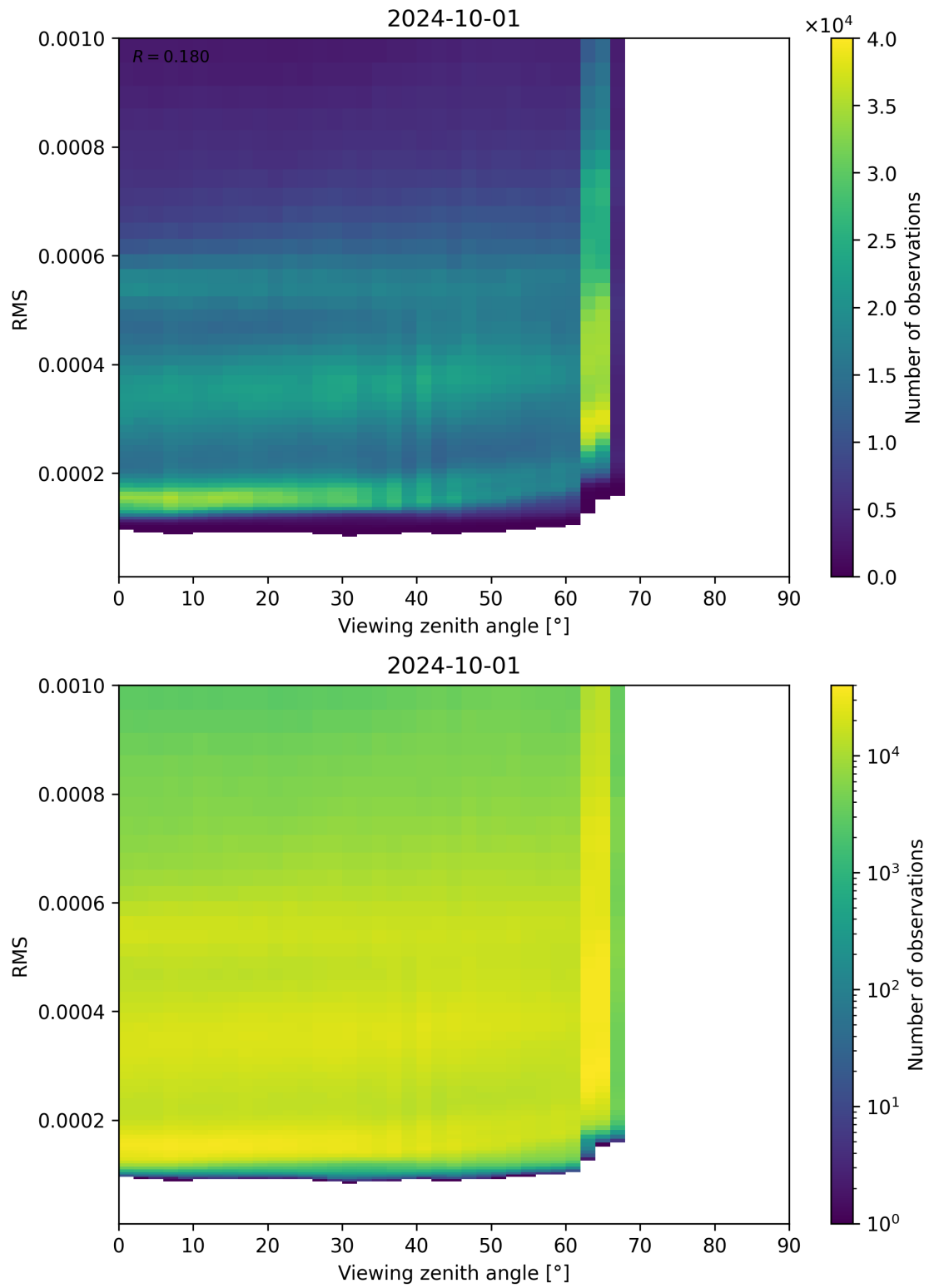
Figure 171: Scatter density plot of “Viewing zenith angle” against “RMS” for 2024-09-30 to 2024-10-02.
