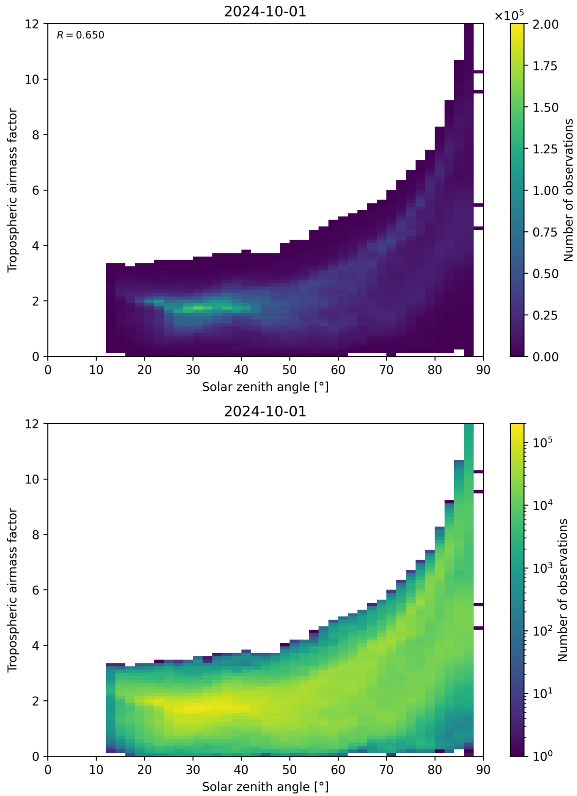
Figure 147: Scatter density plot of “Solar zenith angle” against “Tropospheric airmass factor” for 2024-09-30 to 2024-10-02.
