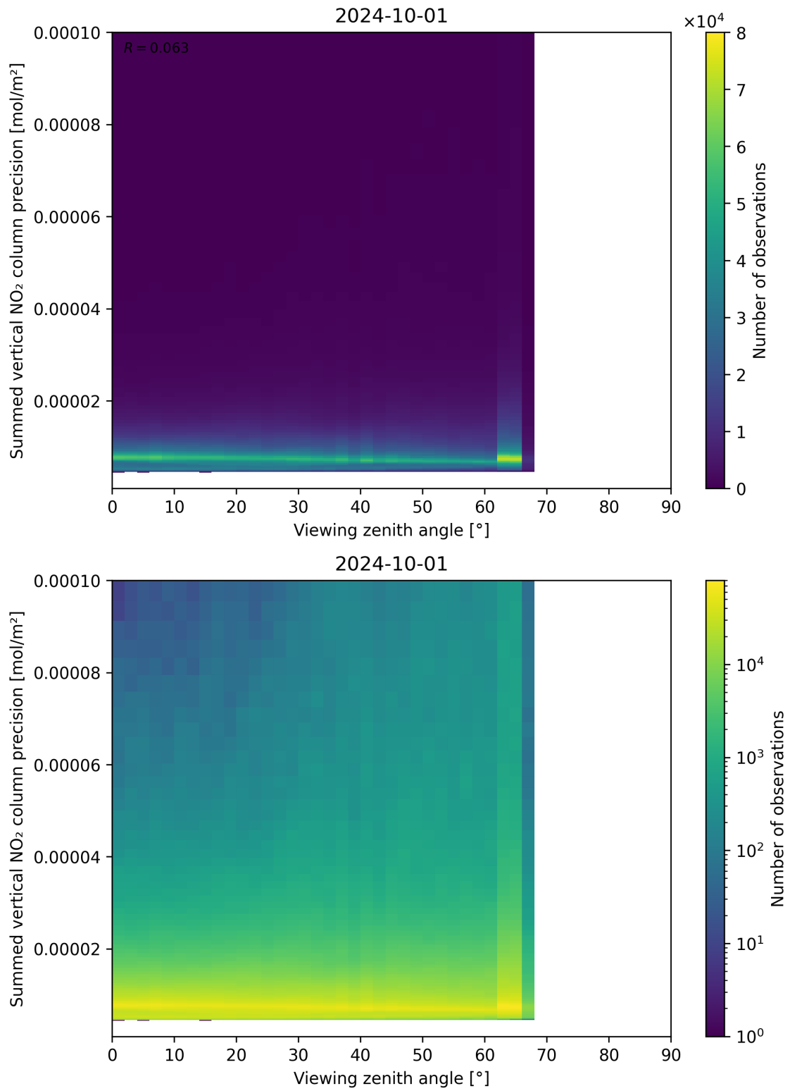
Figure 166: Scatter density plot of “Viewing zenith angle” against “Summed vertical NO 2 column precision” for 2024-09-30 to 2024-10-02.
