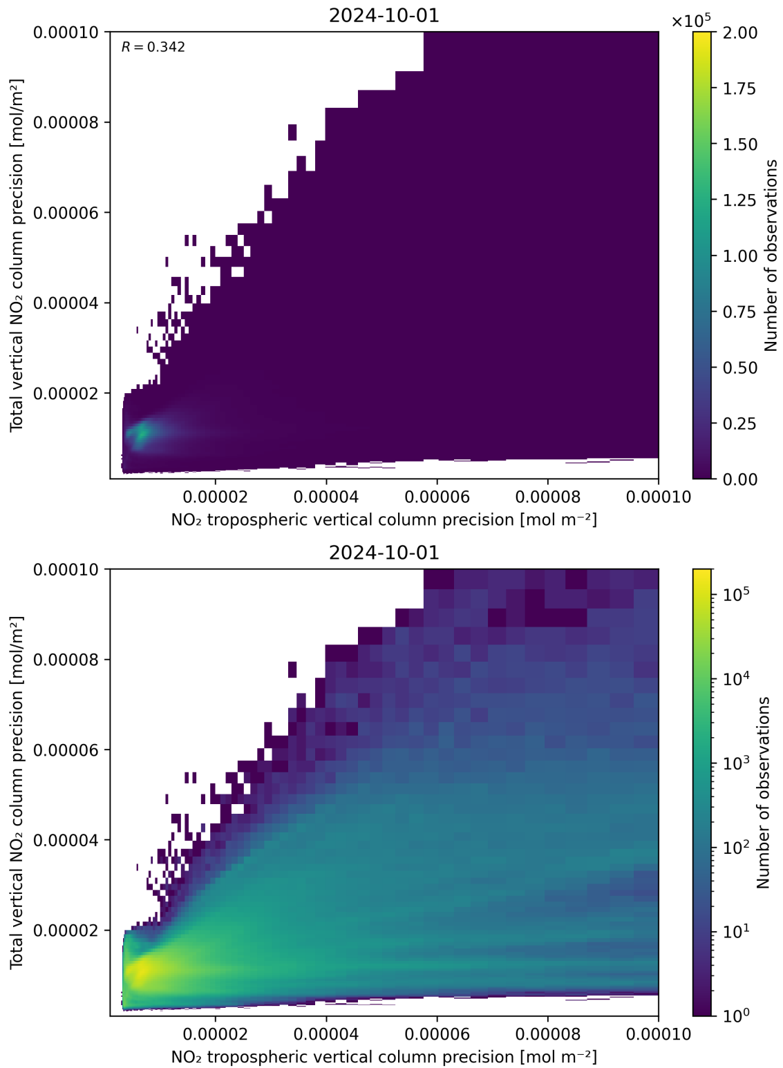
Figure 139: Scatter density plot of “NO 2 tropospheric vertical column precision” against “Total vertical NO 2 column precision” for 2024-09-30 to 2024-10-02.
