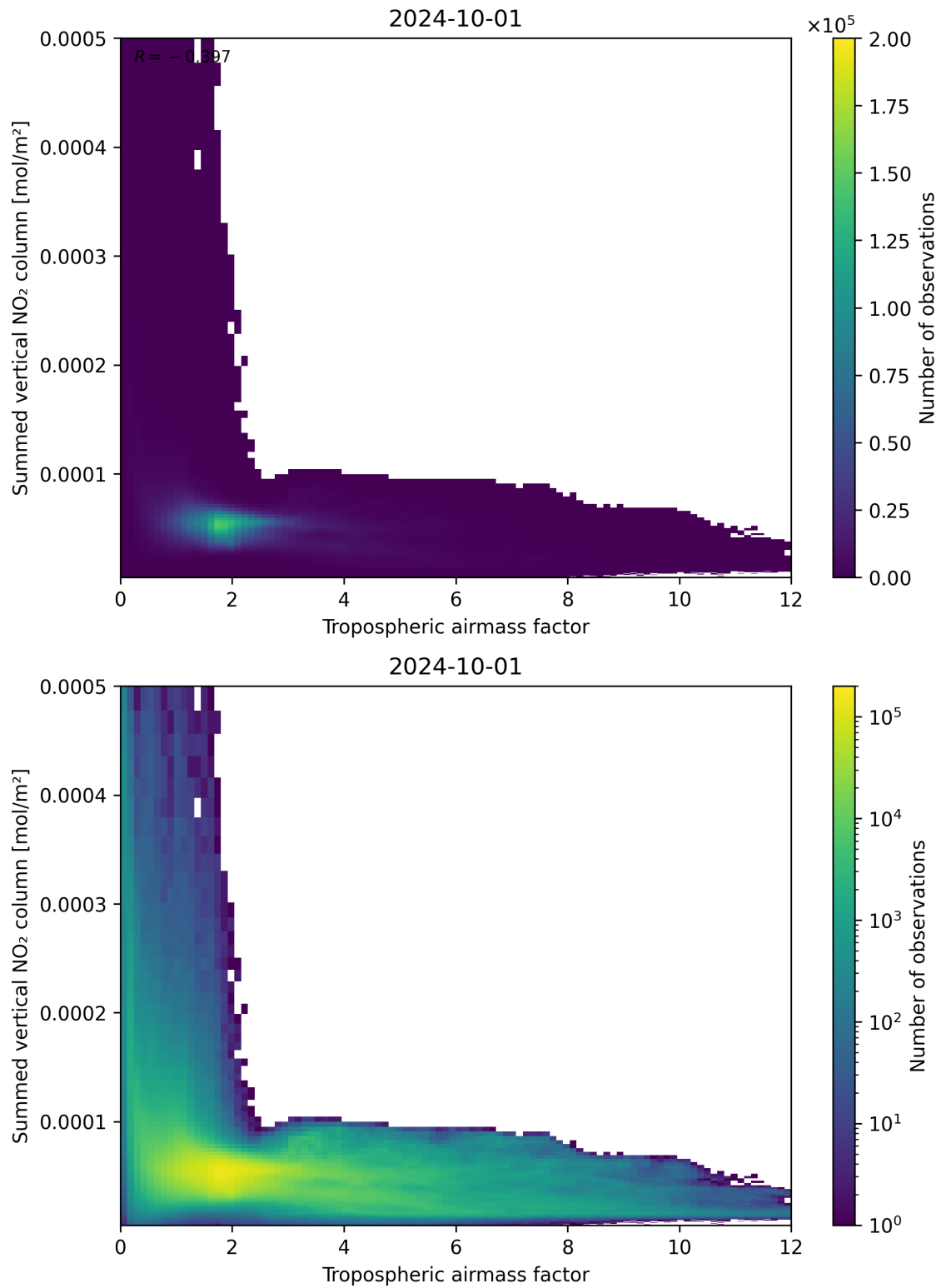
Figure 75: Scatter density plot of “Tropospheric airmass factor” against “Summed vertical NO 2 column” for 2024-09-30 to 2024-10-02.
