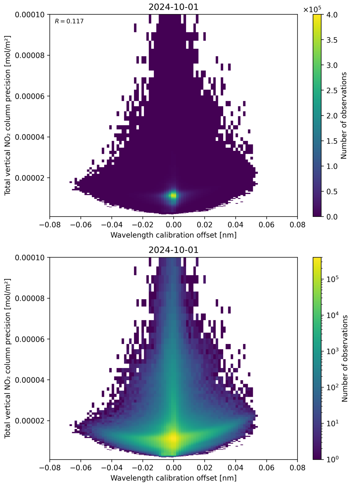
Figure 180: Scatter density plot of “Wavelength calibration offset” against “Total vertical NO 2 column precision” for 2024-09-30 to 2024-10-02.
