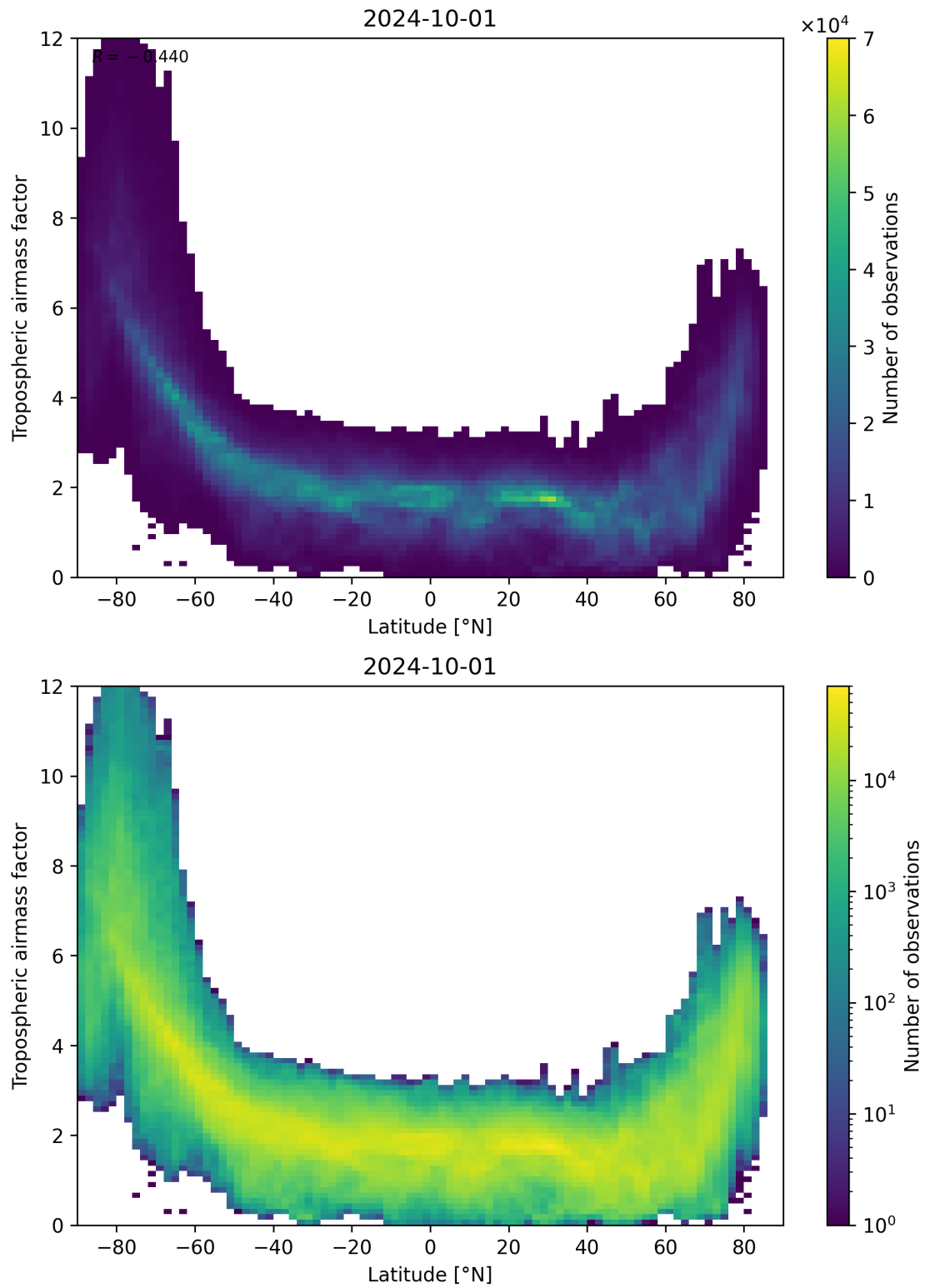
Figure 85: Scatter density plot of “Latitude” against “Tropospheric air mass factor” for 2024-09-30 to 2024-10-02.
