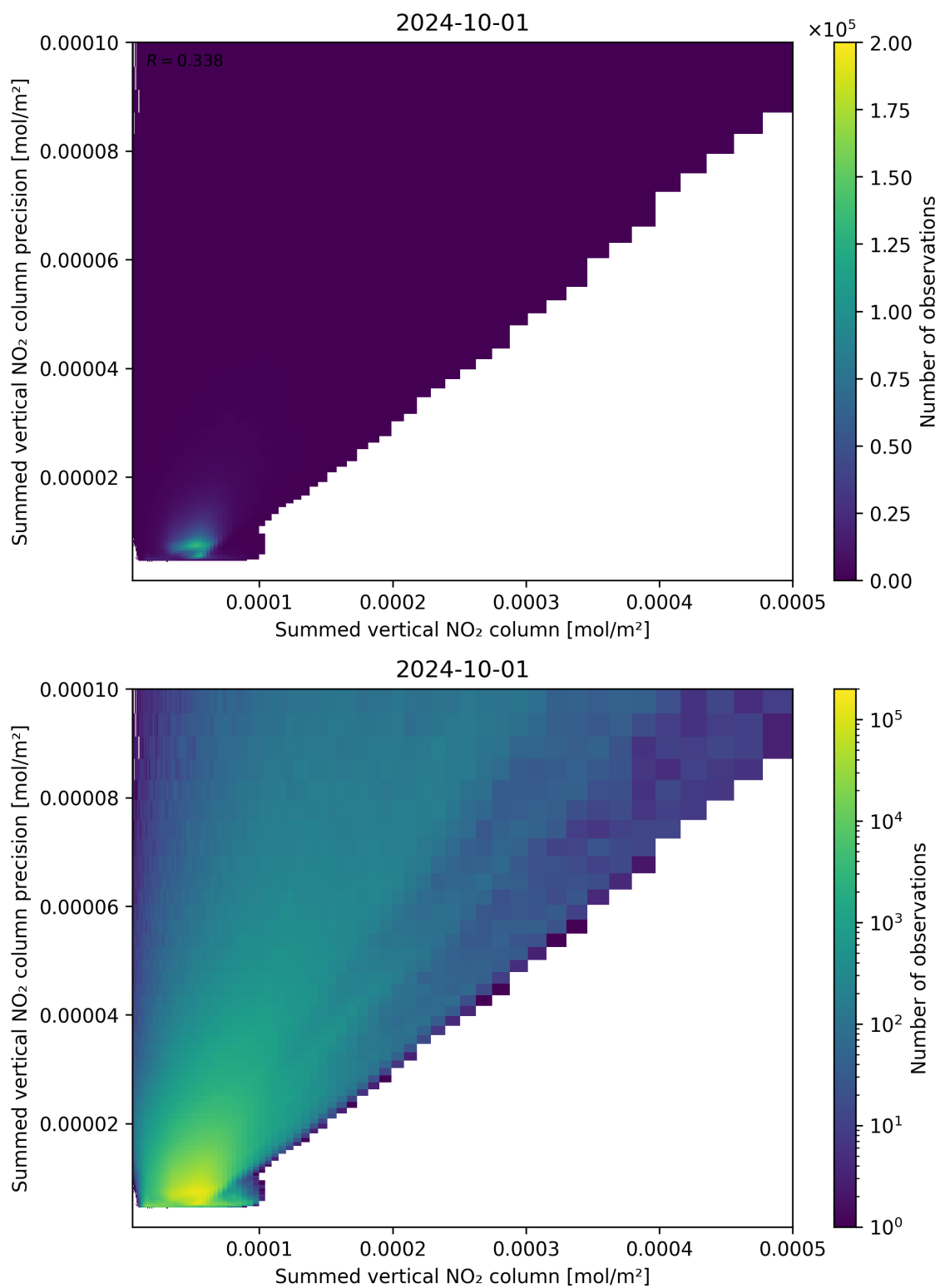
Figure 105: Scatter density plot of “Summed vertical NO 2 column” against “Summed vertical NO 2 column precision” for 2024-09-30 to 2024-10-02.
