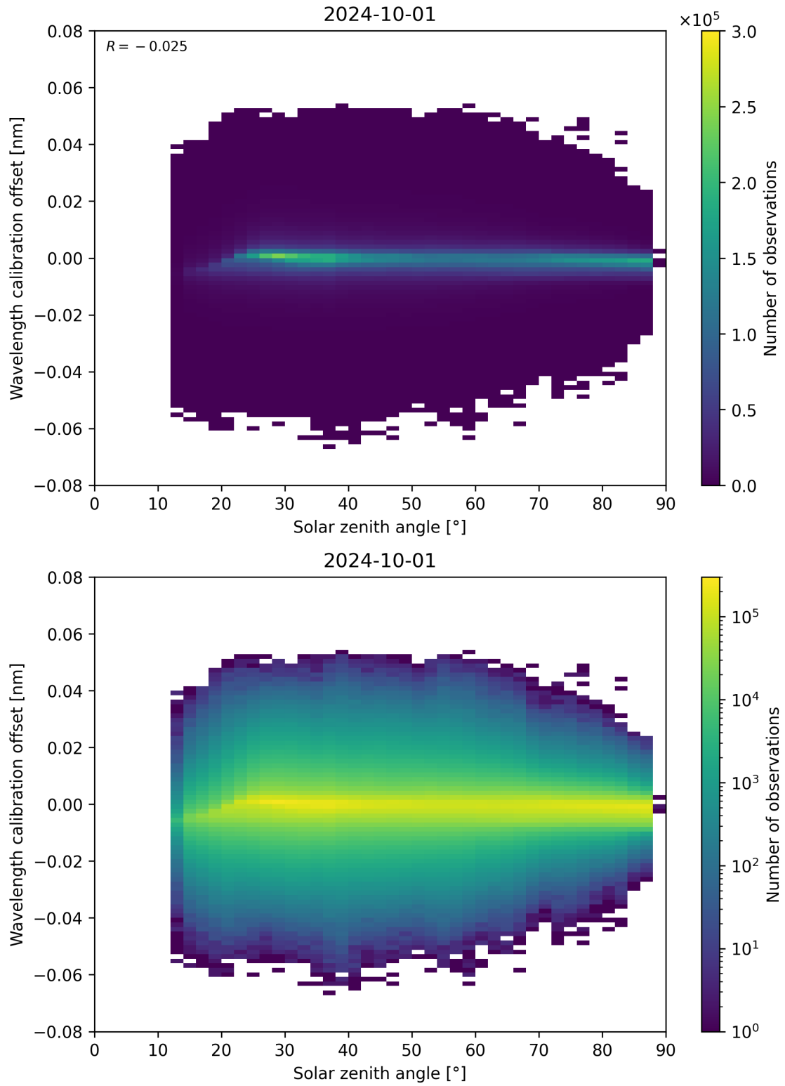
Figure 158: Scatter density plot of “Solar zenith angle” against “Wavelength calibration offset” for 2024-09-30 to 2024-10-02.
