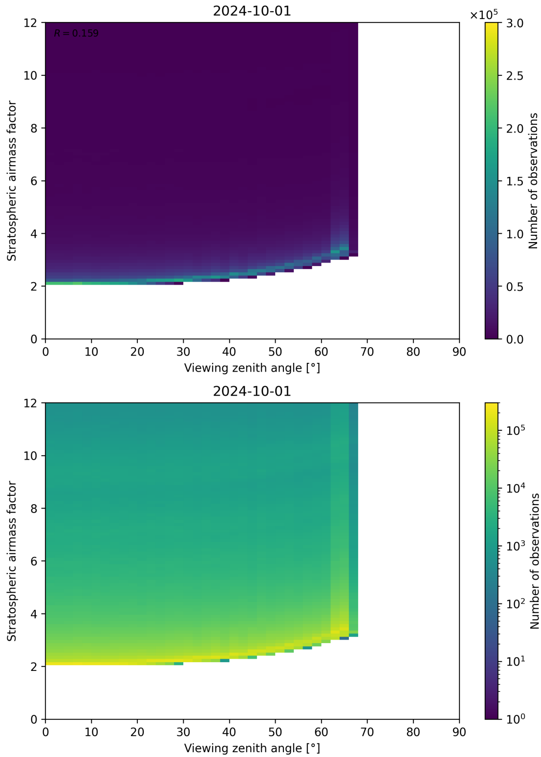
Figure 159: Scatter density plot of “Viewing zenith angle” against “Stratospheric airmass factor” for 2024-09-30 to 2024-10-02.
