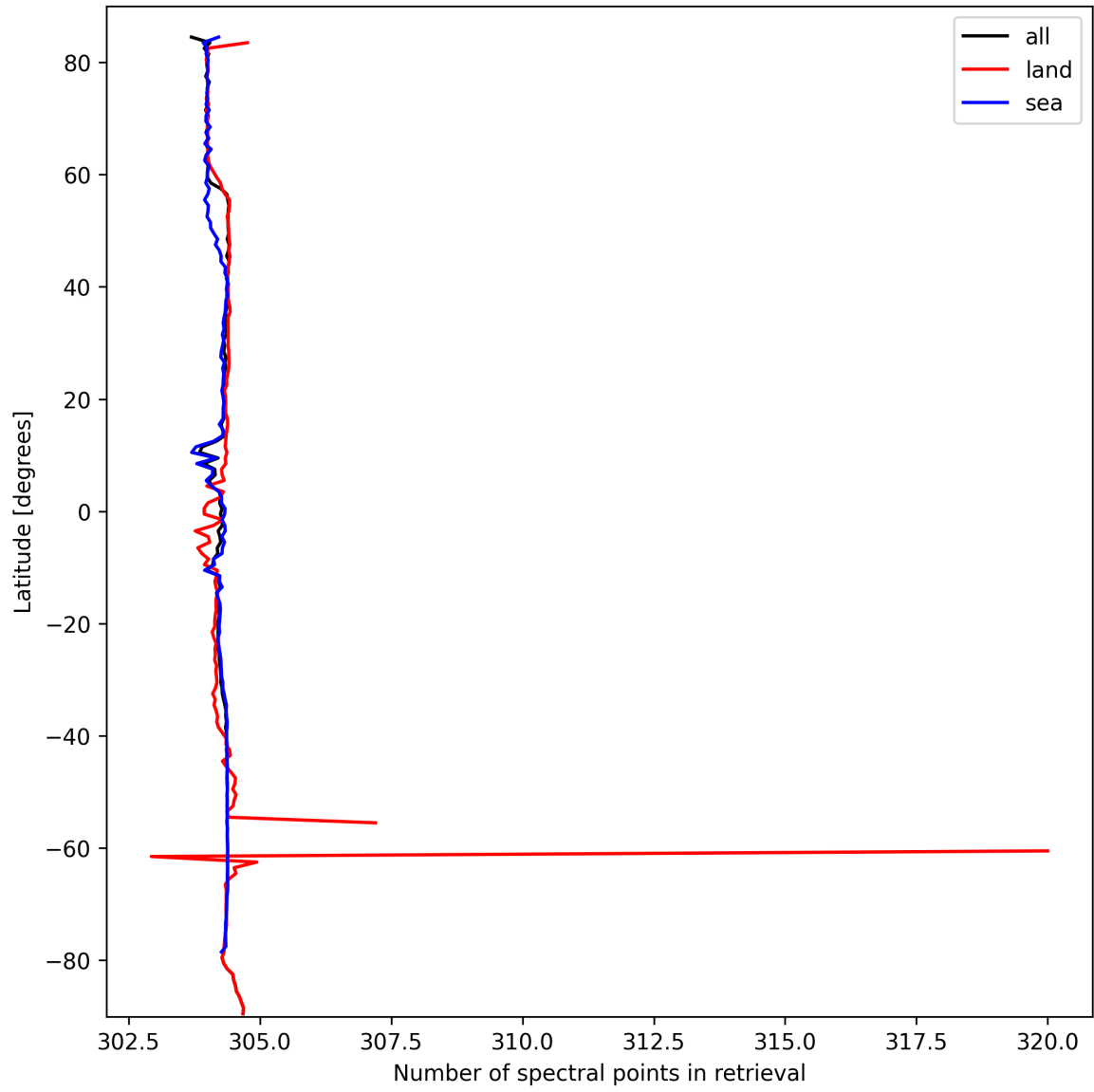
Figure 16: Zonal average of “Number of spectral points in retrieval” for 2024-09-30 to 2024-10-02.
