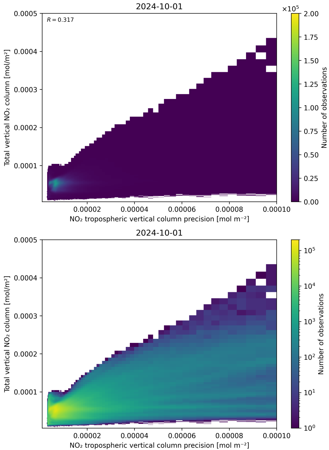
Figure 138: Scatter density plot of “NO 2 tropospheric vertical column precision” against “Total vertical NO 2 column” for 2024-09-30 to 2024-10-02.
