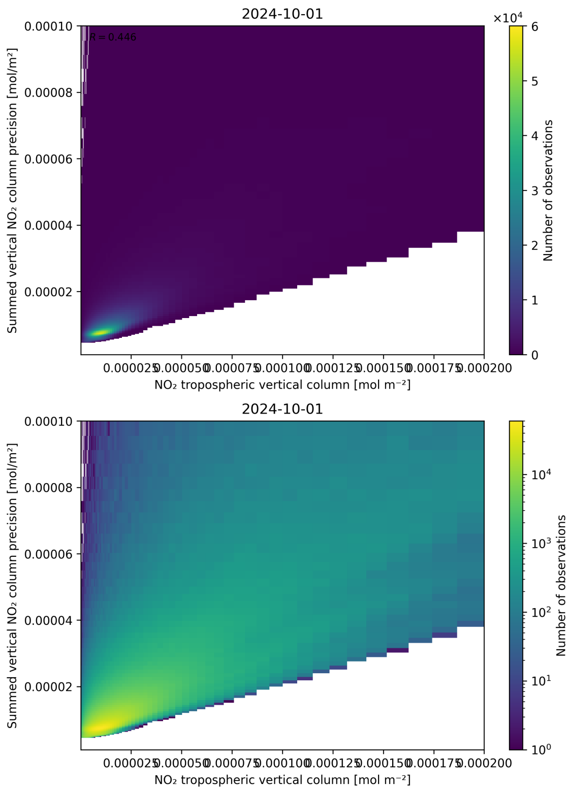
Figure 127: Scatter density plot of “NO 2 tropospheric vertical column” against “Summed vertical NO 2 column precision” for 2024-09-30 to 2024-10-02.
