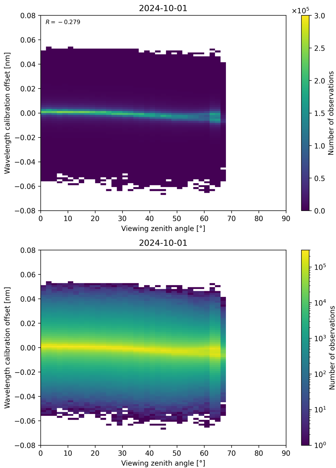
Figure 173: Scatter density plot of “Viewing zenith angle” against “Wavelength calibration offset” for 2024-09-30 to 2024-10-02.
