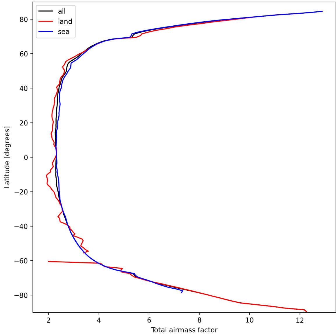
Figure 15: Zonal average of “Total airmass factor” for 2024-09-30 to 2024-10-02.
