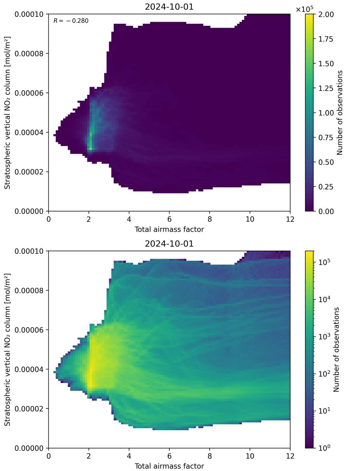
Figure 64: Scatter density plot of “Total airmass factor” against “Stratospheric vertical NO 2 column” for 2024-09-30 to 2024-10-02.
