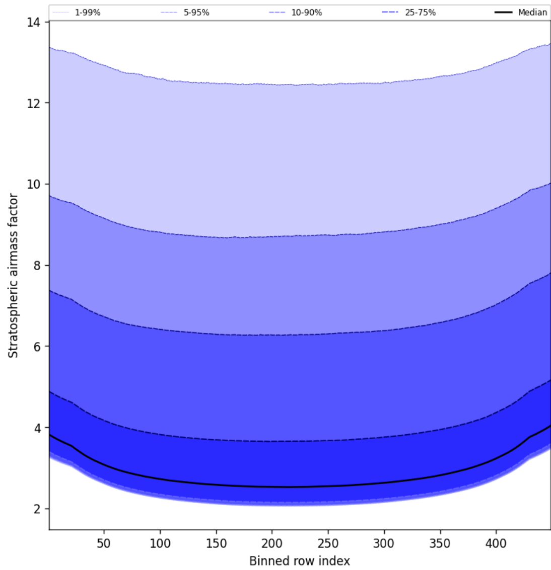
Figure 61: Along track statistics of “Stratospheric airmass factor” for 2024-09-30 to 2024-10-02
