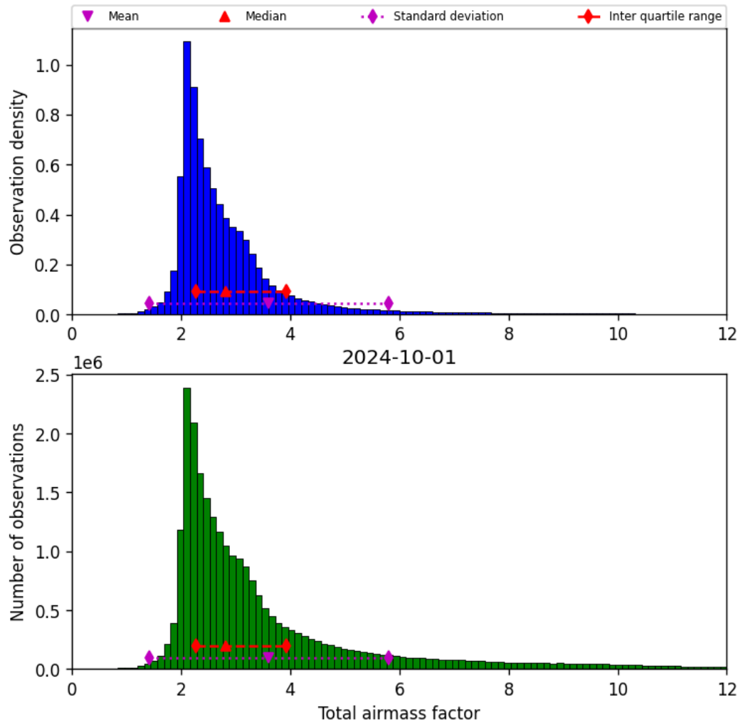
Figure 32: Histogram of “Total airmass factor” for 2024-09-30 to 2024-10-02
