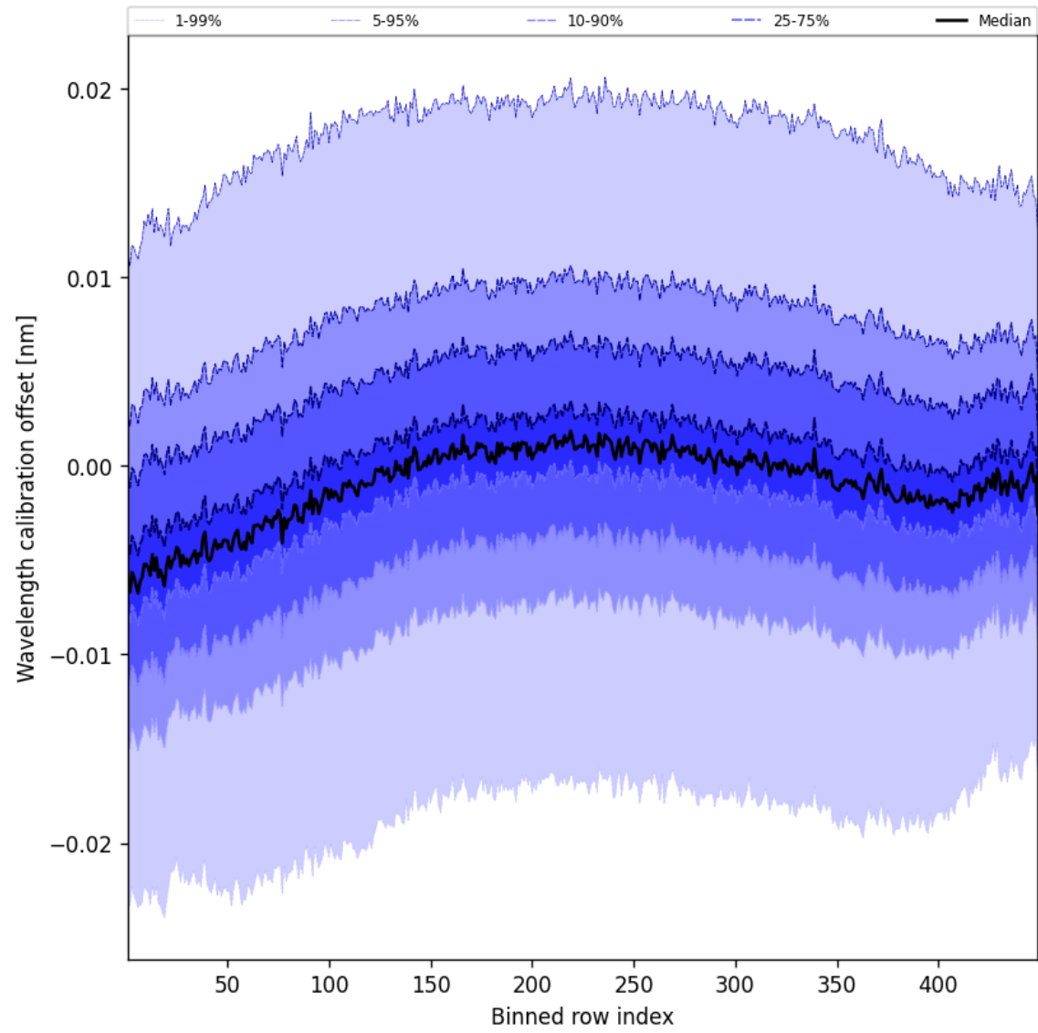
Figure 52: Along track statistics of “Wavelength calibration offset” for 2024-09-30 to 2024-10-02
