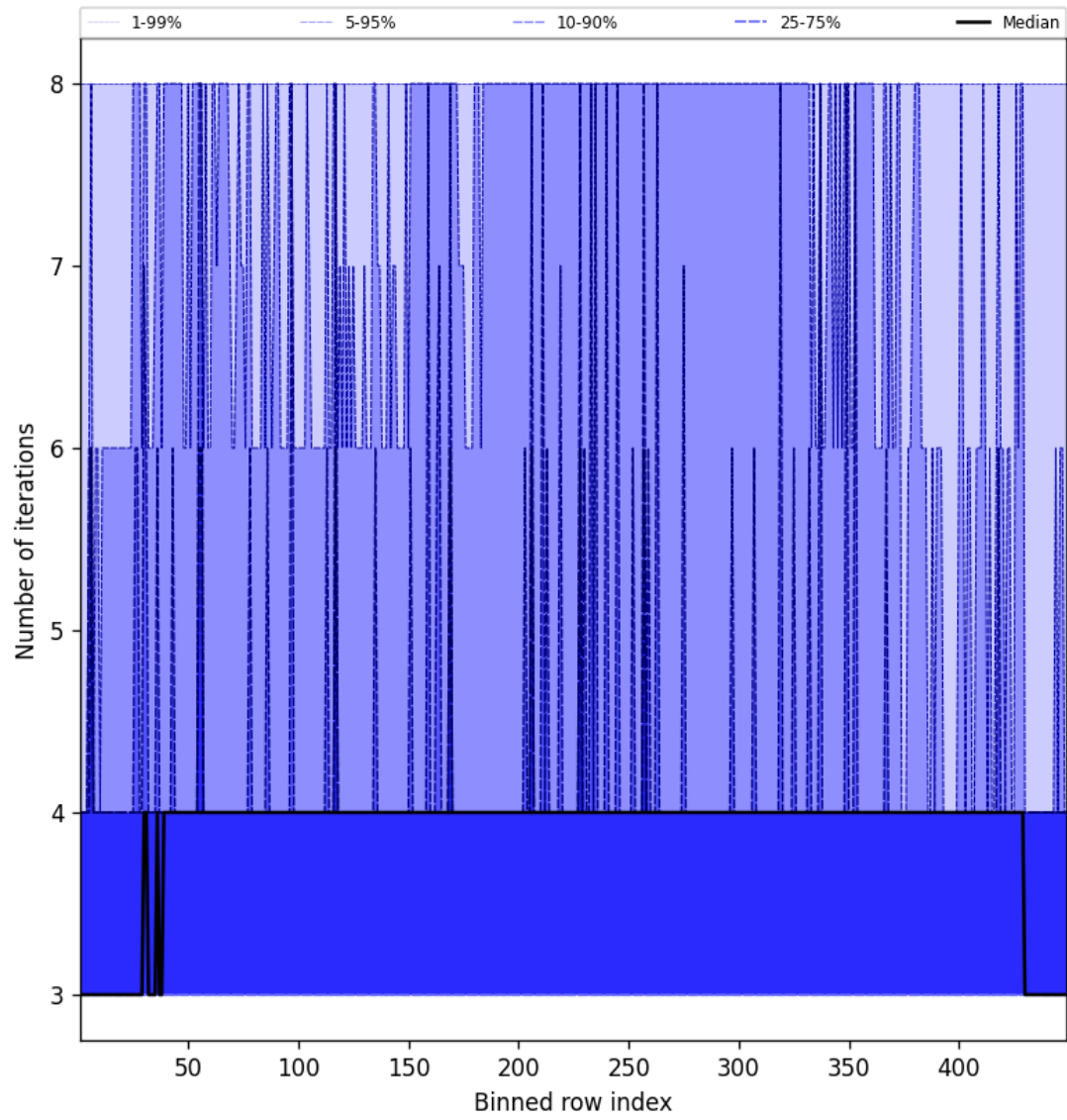
Figure 51: Along track statistics of “Number of iterations” for 2024-09-30 to 2024-10-02
