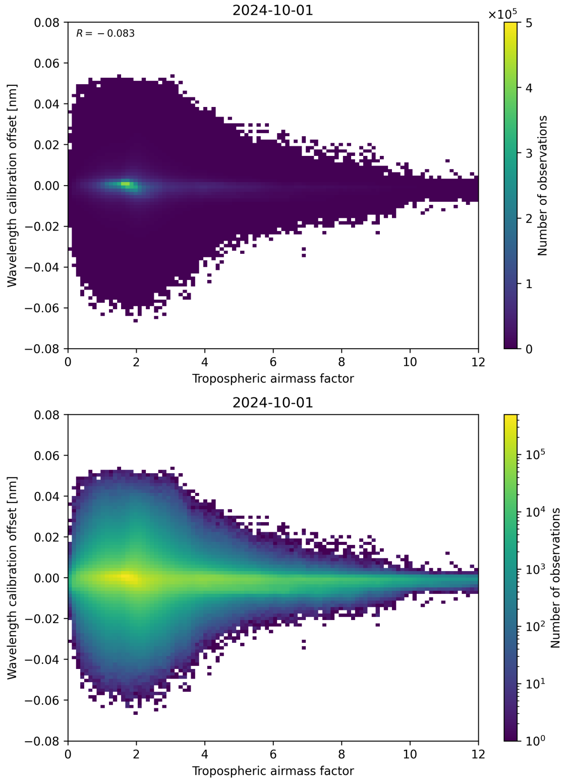
Figure 80: Scatter density plot of “Tropospheric airmass factor” against “Wavelength calibration offset” for 2024-09-30 to 2024-10-02.
