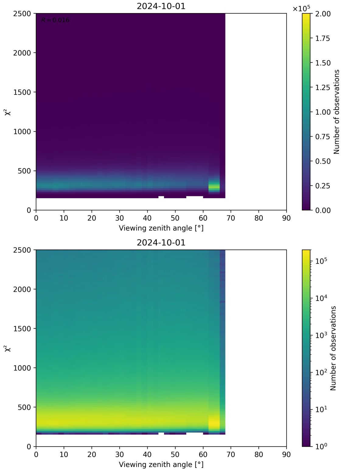
Figure 162: Scatter density plot of “Viewing zenith angle” against “ \chi^2 ” for 2024-09-30 to 2024-10-02.
