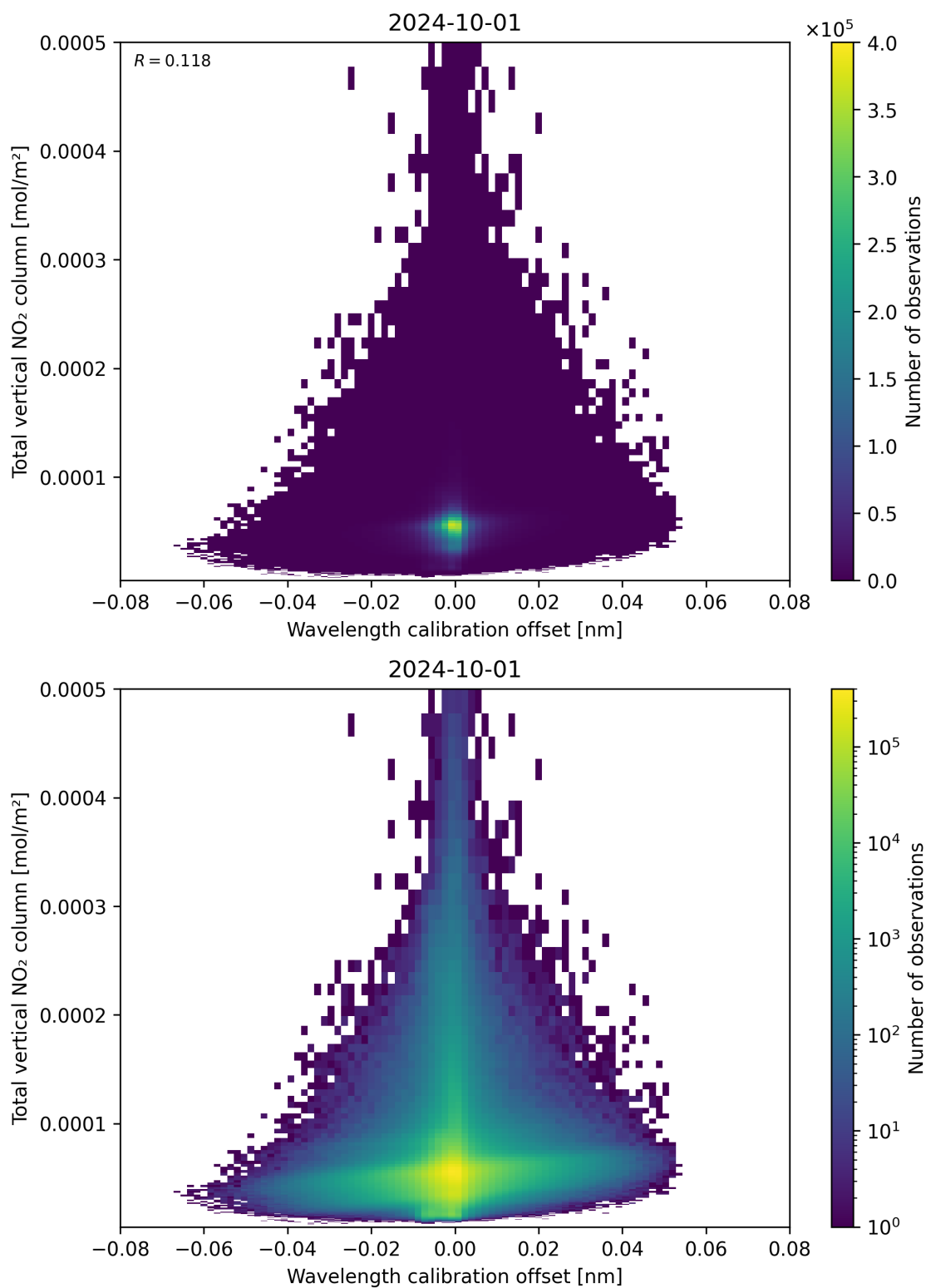
Figure 179: Scatter density plot of “Wavelength calibration offset” against “Total vertical NO 2 column” for 2024-09-30 to 2024-10-02.
