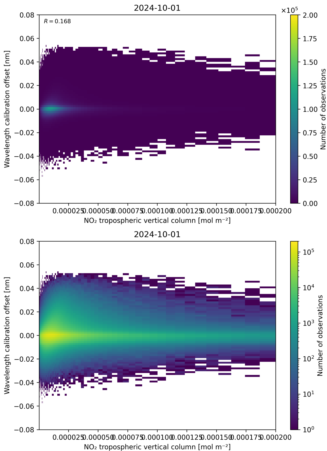
Figure 143: Scatter density plot of “NO 2 tropospheric vertical column” against “Wavelength calibration offset” for 2024-09-30 to 2024-10-02.
