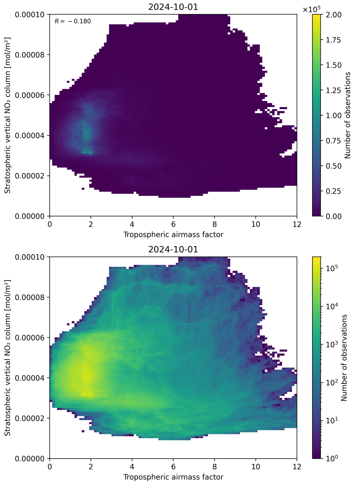
Figure 74: Scatter density plot of “Tropospheric airmass factor” against “Stratospheric vertical NO 2 column” for 2024-09-30 to 2024-10-02.
