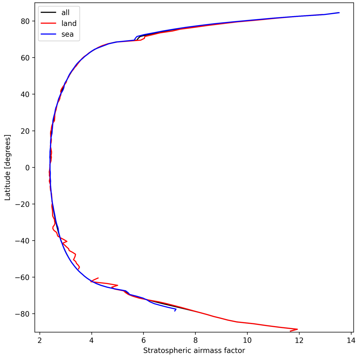
Figure 27: Zonal average of “Stratospheric airmass factor” for 2024-10-01 to 2024-10-03.
