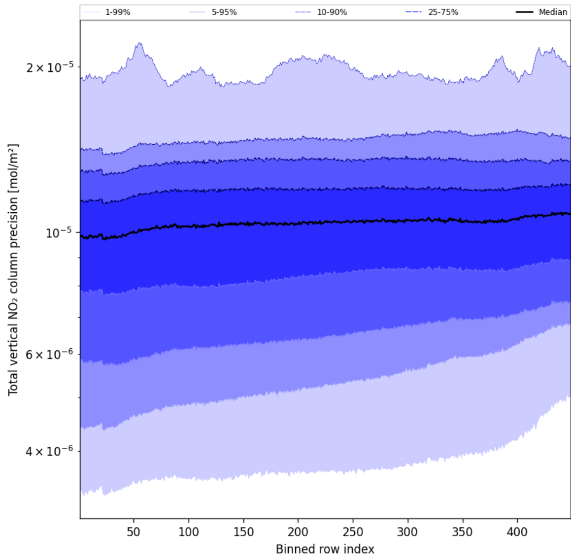
Figure 56: Along track statistics of “Total vertical NO 2 column precision” for 2024-10-01 to 2024-10-03
