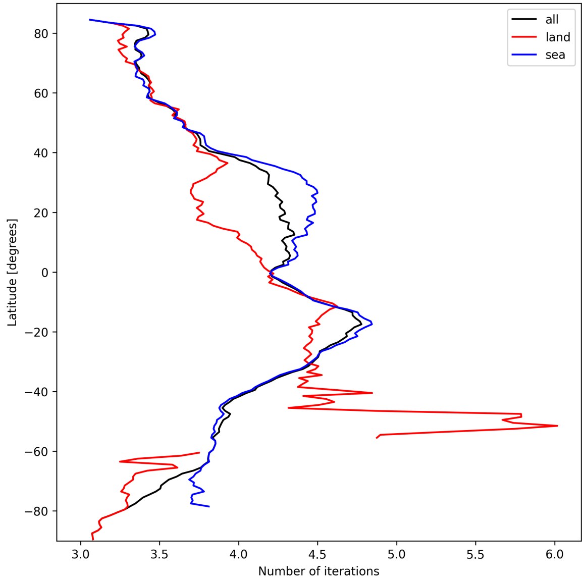
Figure 17: Zonal average of “Number of iterations” for 2024-10-01 to 2024-10-03.
