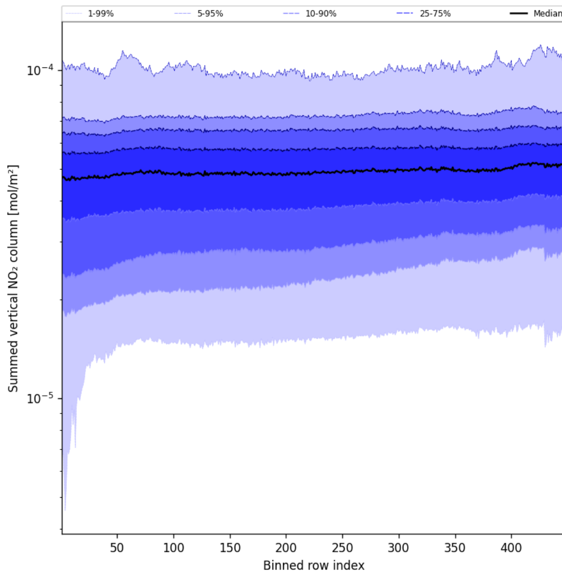
Figure 57: Along track statistics of “Summed vertical NO 2 column” for 2024-10-01 to 2024-10-03
