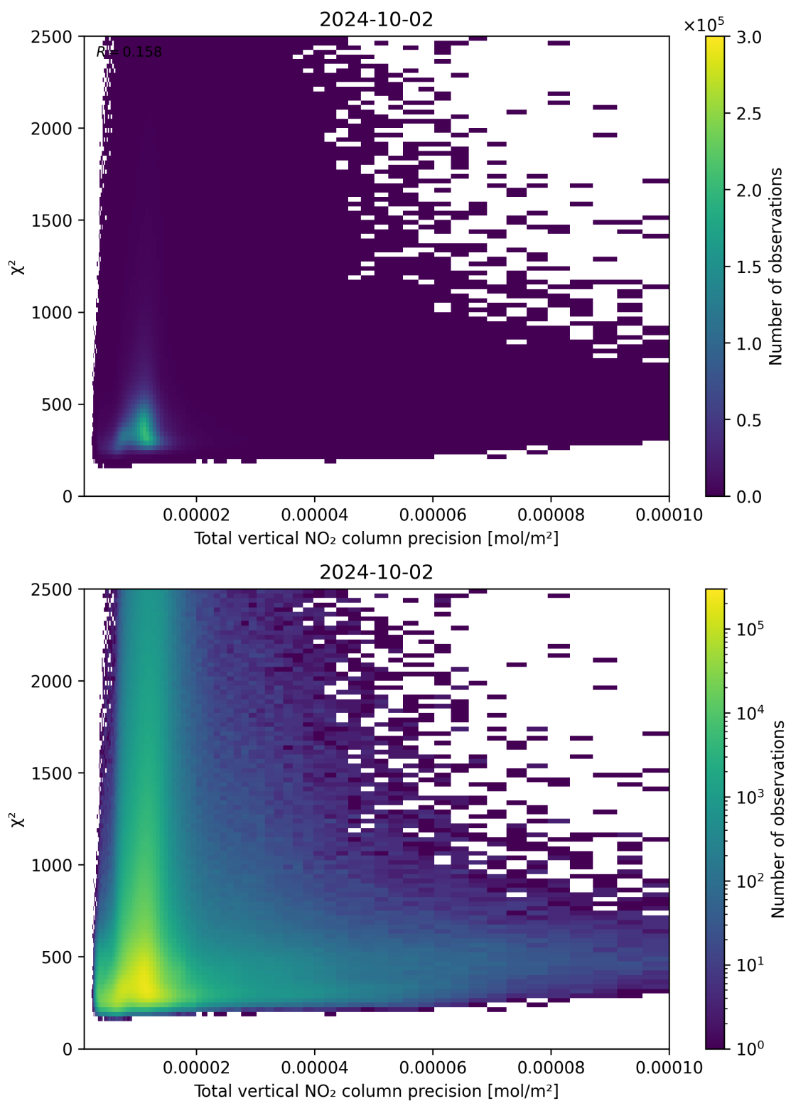
Figure 116: Scatter density plot of “Total vertical NO 2 column precision” against “ \chi^2 ” for 2024-10-01 to 2024-10-03.
