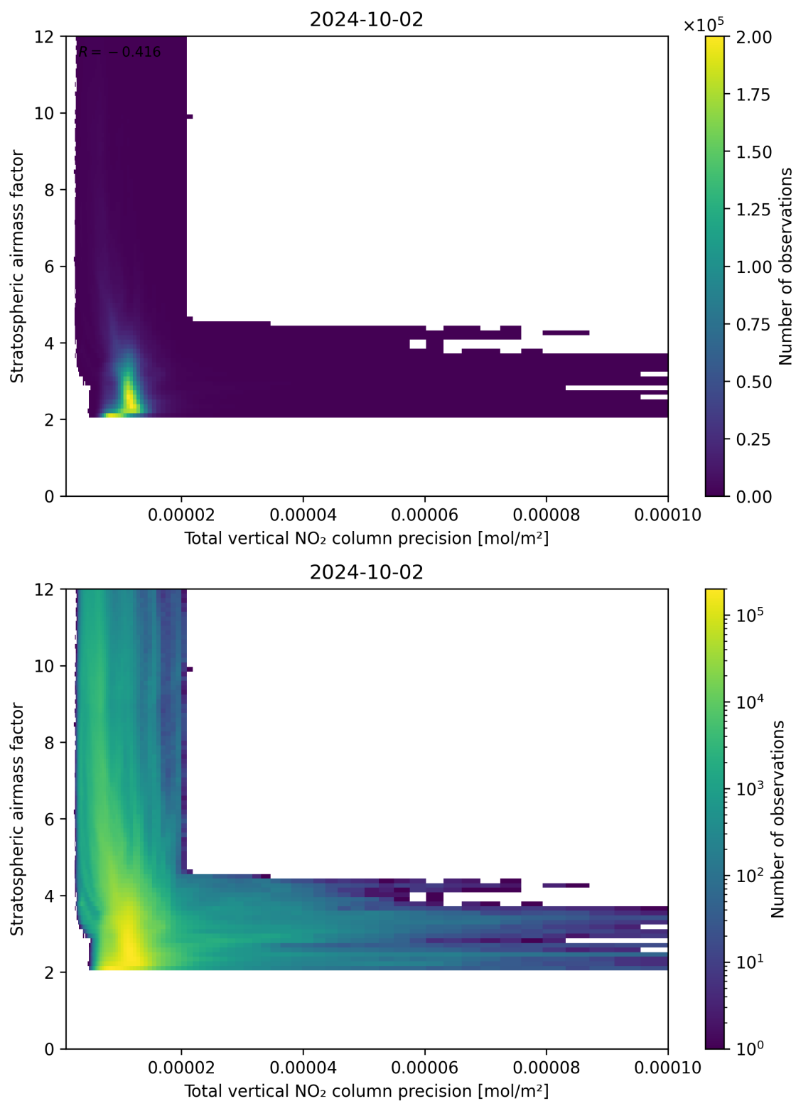
Figure 115: Scatter density plot of “Total vertical NO 2 column precision” against “Stratospheric air mass factor” for 2024-10-01 to 2024-10-03.
