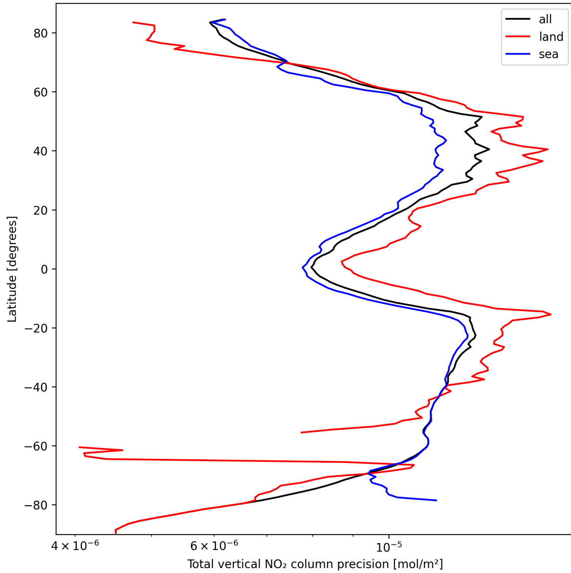
Figure 22: Zonal average of “Total vertical NO 2 column precision” for 2024-10-01 to 2024-10-03.
