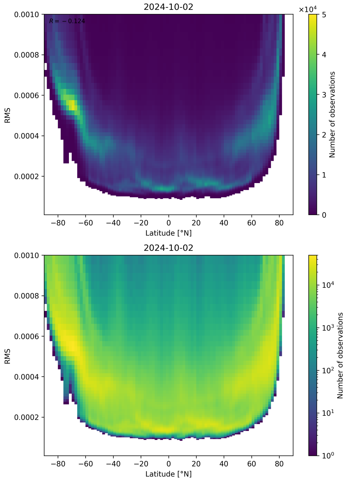
Figure 94: Scatter density plot of “Latitude” against “RMS” for 2024-10-01 to 2024-10-03.
