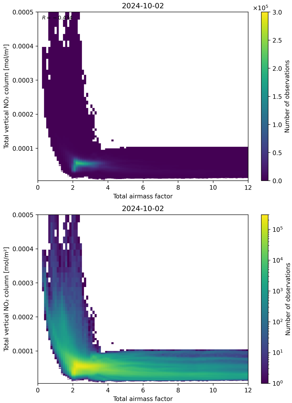
Figure 67: Scatter density plot of “Total air mass factor” against “Total vertical NO 2 column” for 2024-10-01 to 2024-10-03.
