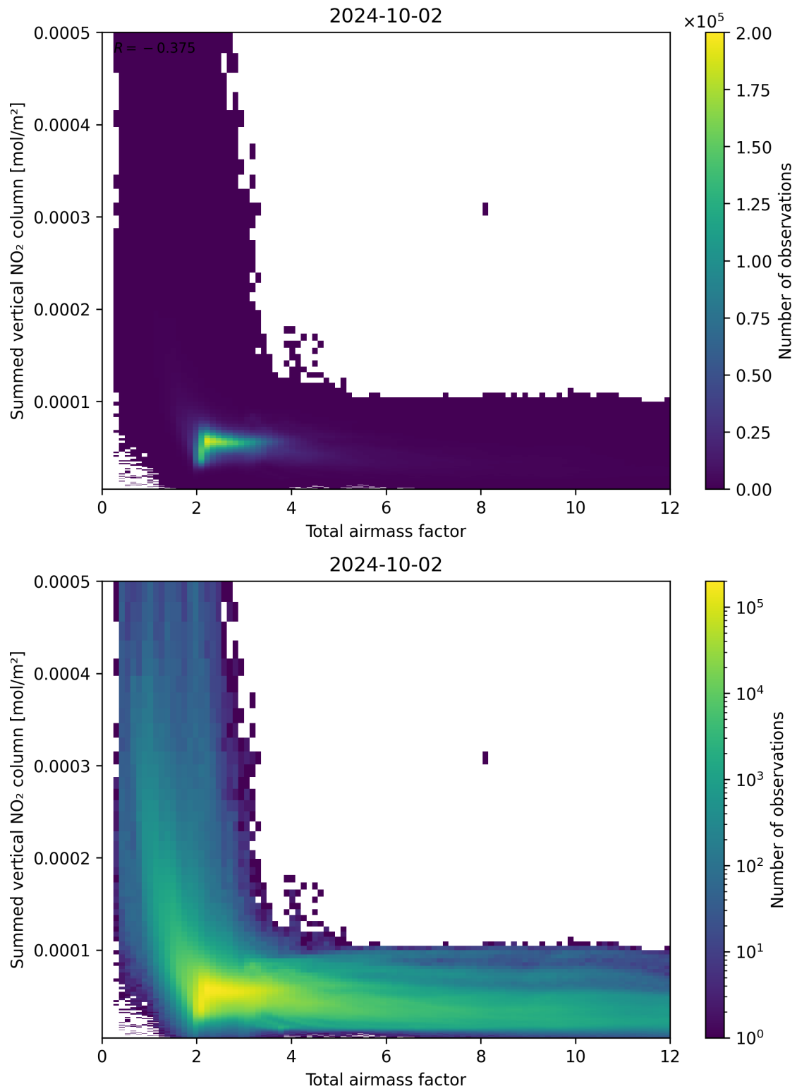
Figure 65: Scatter density plot of “Total airmass factor” against “Summed vertical NO 2 column” for 2024-10-01 to 2024-10-03.
