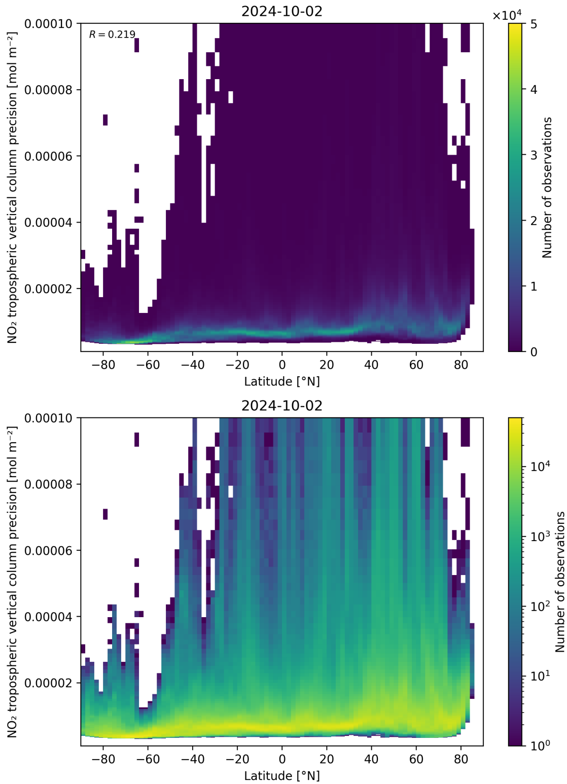
Figure 93: Scatter density plot of “Latitude” against “NO 2 tropospheric vertical column precision” for 2024-10-01 to 2024-10-03.
