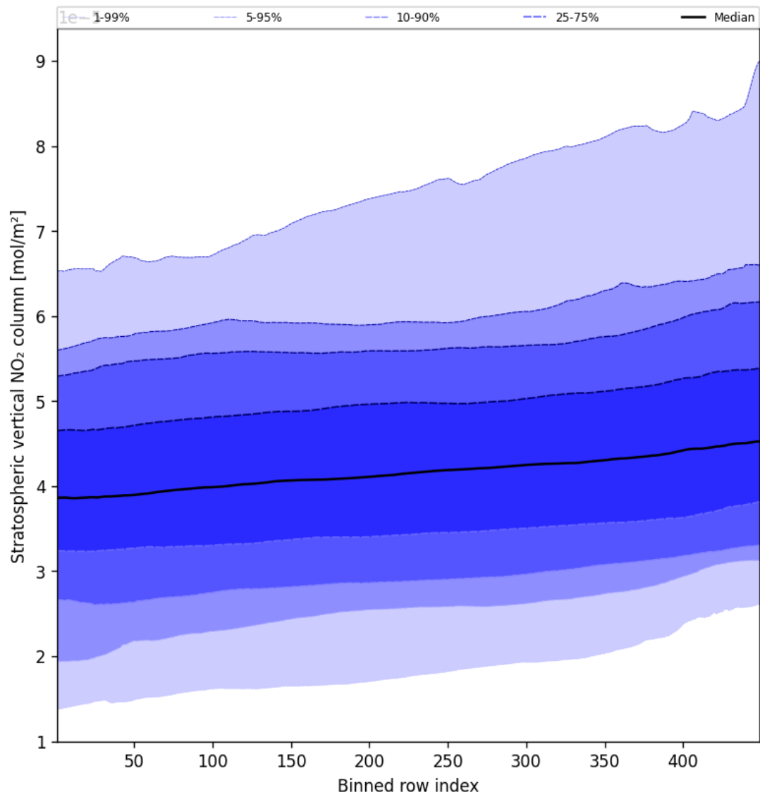
Figure 53: Along track statistics of “Stratospheric vertical NO 2 column” for 2024-10-01 to 2024-10-03
