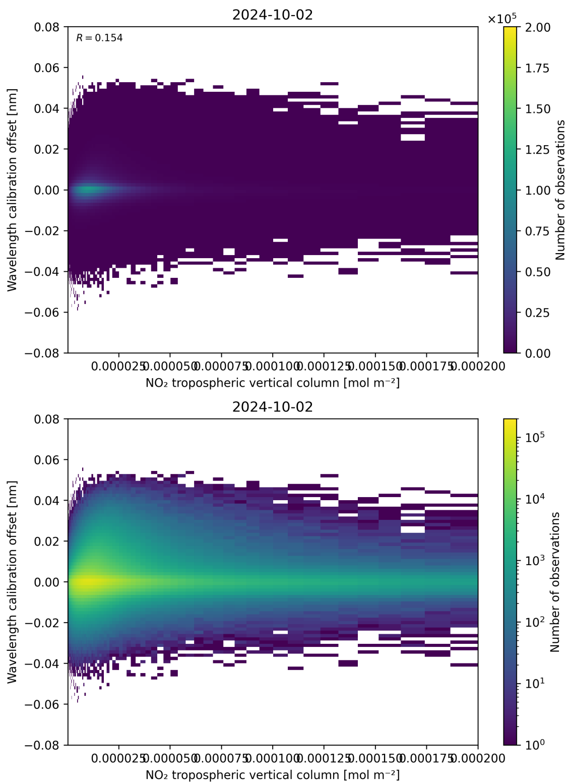
Figure 143: Scatter density plot of “NO 2 tropospheric vertical column” against “Wavelength calibration offset” for 2024-10-01 to 2024-10-03.
