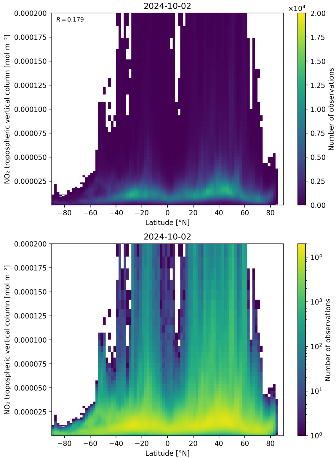
Figure 92: Scatter density plot of “Latitude” against “NO 2 tropospheric vertical column” for 2024-10-01 to 2024-10-03.
