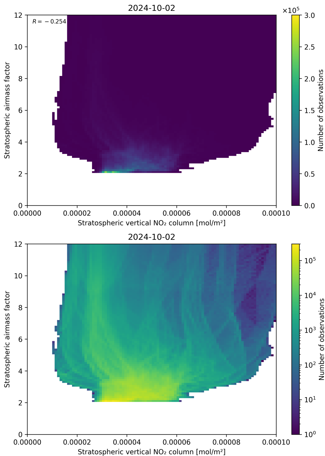
Figure 96: Scatter density plot of “Stratospheric vertical NO 2 column” against “Stratospheric airmass factor” for 2024-10-01 to 2024-10-03.
