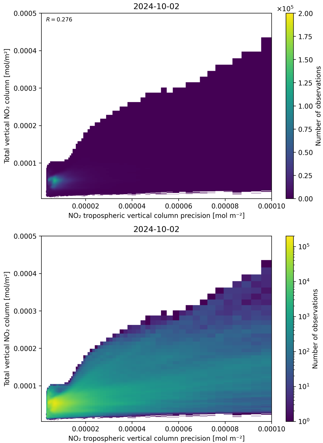
Figure 138: Scatter density plot of “NO 2 tropospheric vertical column precision” against “Total vertical NO 2 column” for 2024-10-01 to 2024-10-03.
