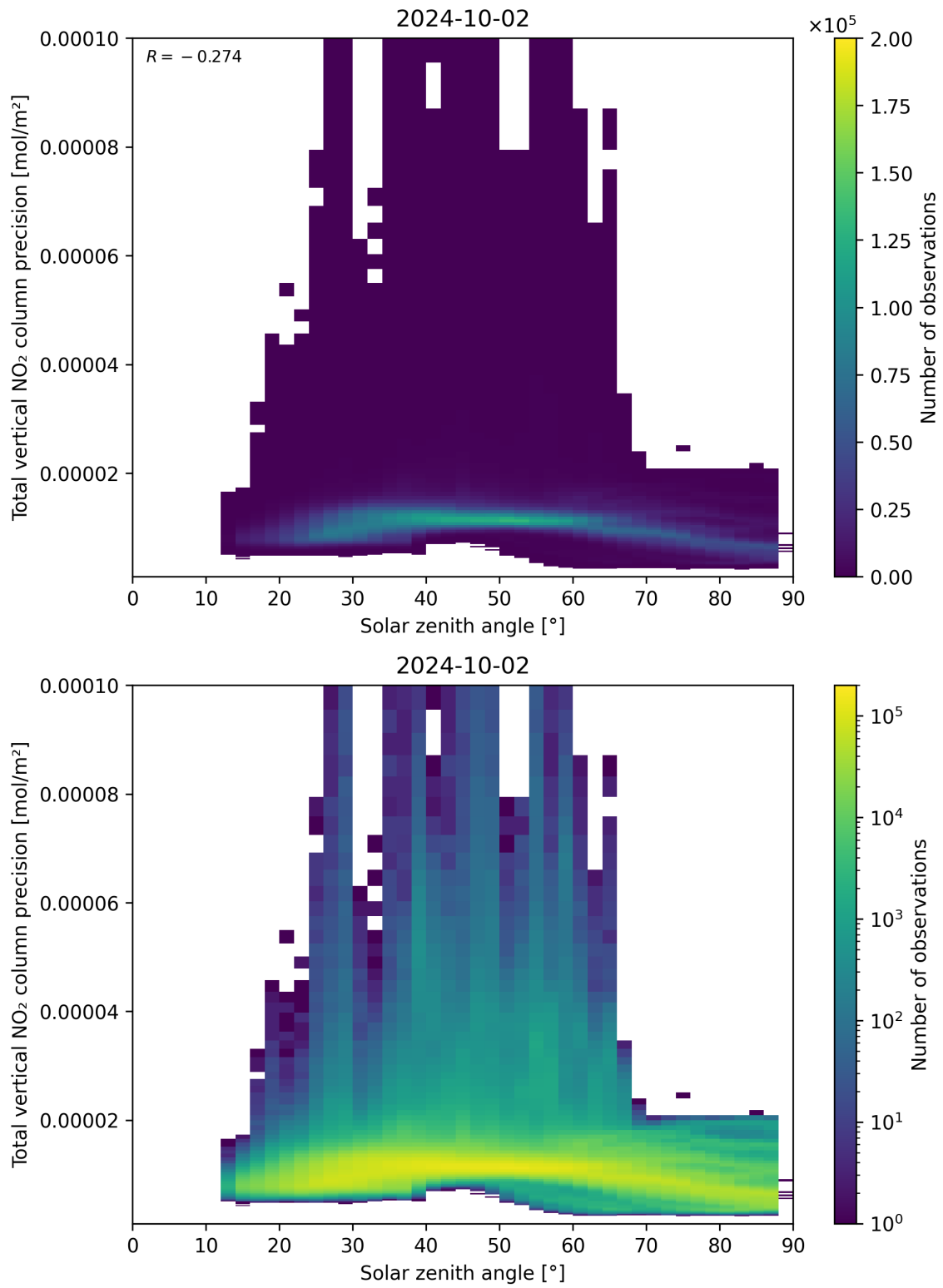
Figure 154: Scatter density plot of “Solar zenith angle” against “Total vertical NO 2 column precision” for 2024-10-01 to 2024-10-03.
