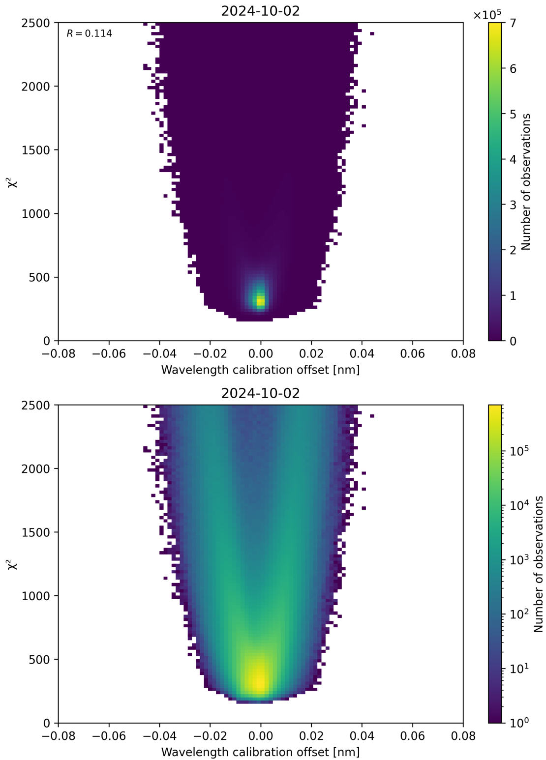
Figure 175: Scatter density plot of “Wavelength calibration offset” against “ \chi^2 ” for 2024-10-01 to 2024-10-03.
