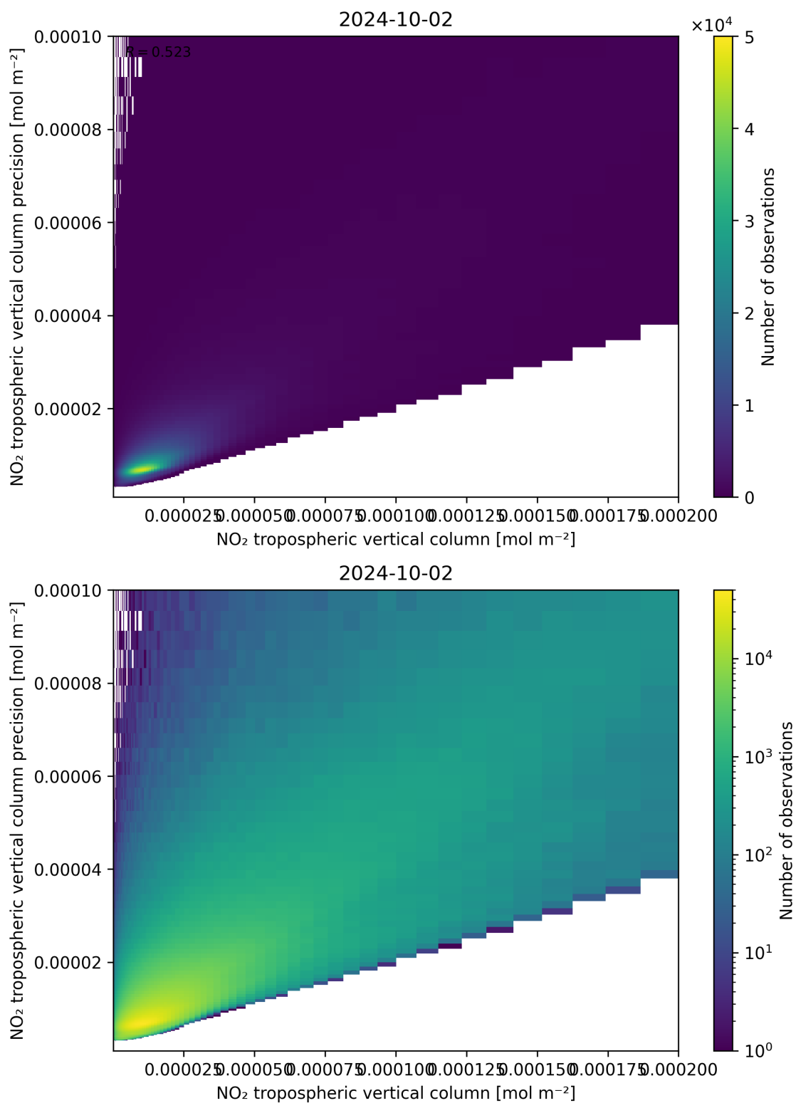
Figure 130: Scatter density plot of “NO 2 tropospheric vertical column” against “NO 2 tropospheric vertical column precision” for 2024-10-01 to 2024-10-03.
