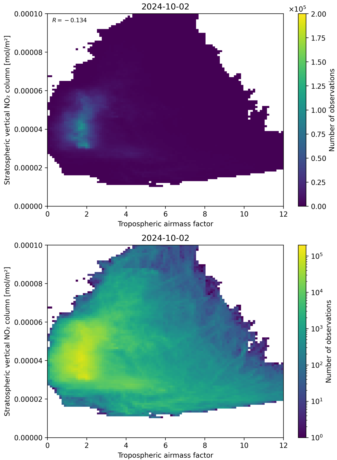
Figure 74: Scatter density plot of “Tropospheric airmass factor” against “Stratospheric vertical NO 2 column” for 2024-10-01 to 2024-10-03.
