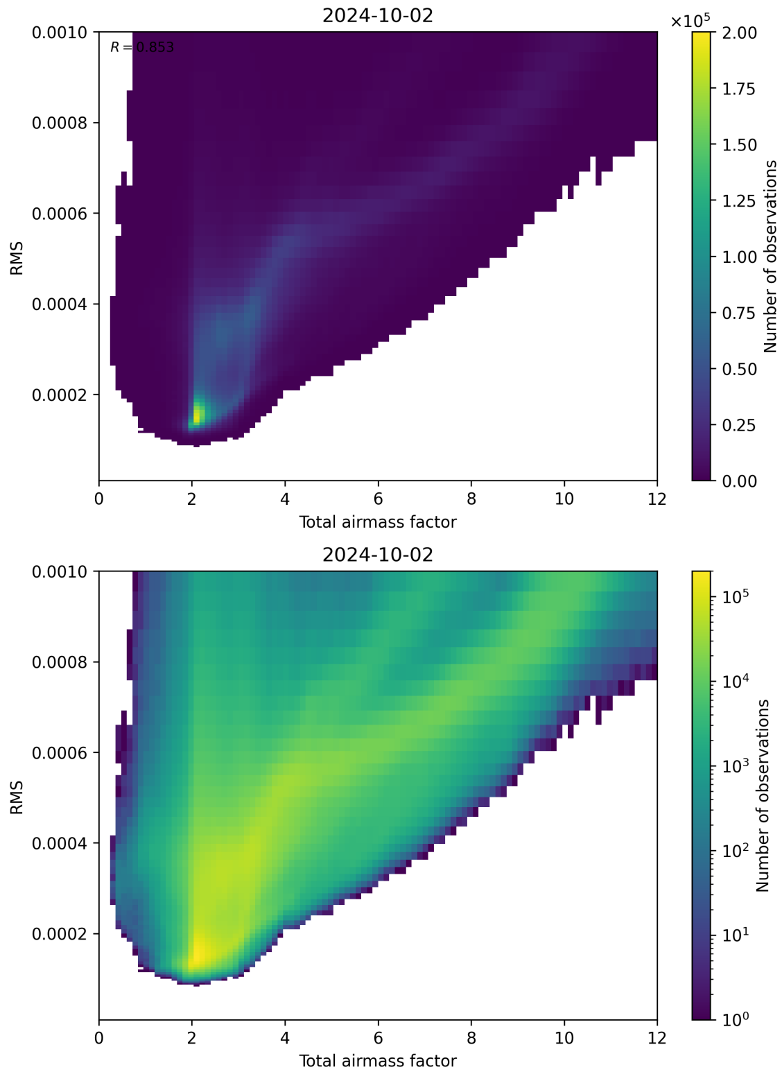
Figure 69: Scatter density plot of “Total airmass factor” against “RMS” for 2024-10-01 to 2024-10-03.
