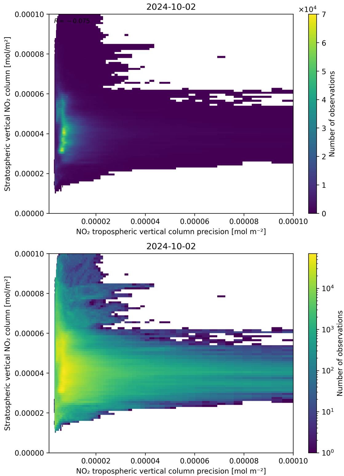
Figure 135: Scatter density plot of “NO 2 tropospheric vertical column precision” against “Stratospheric vertical NO 2 column” for 2024-10-01 to 2024-10-03.
