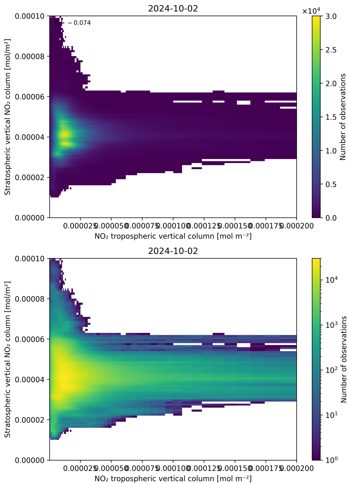
Figure 125: Scatter density plot of “NO 2 tropospheric vertical column” against “Stratospheric vertical NO 2 column” for 2024-10-01 to 2024-10-03.
