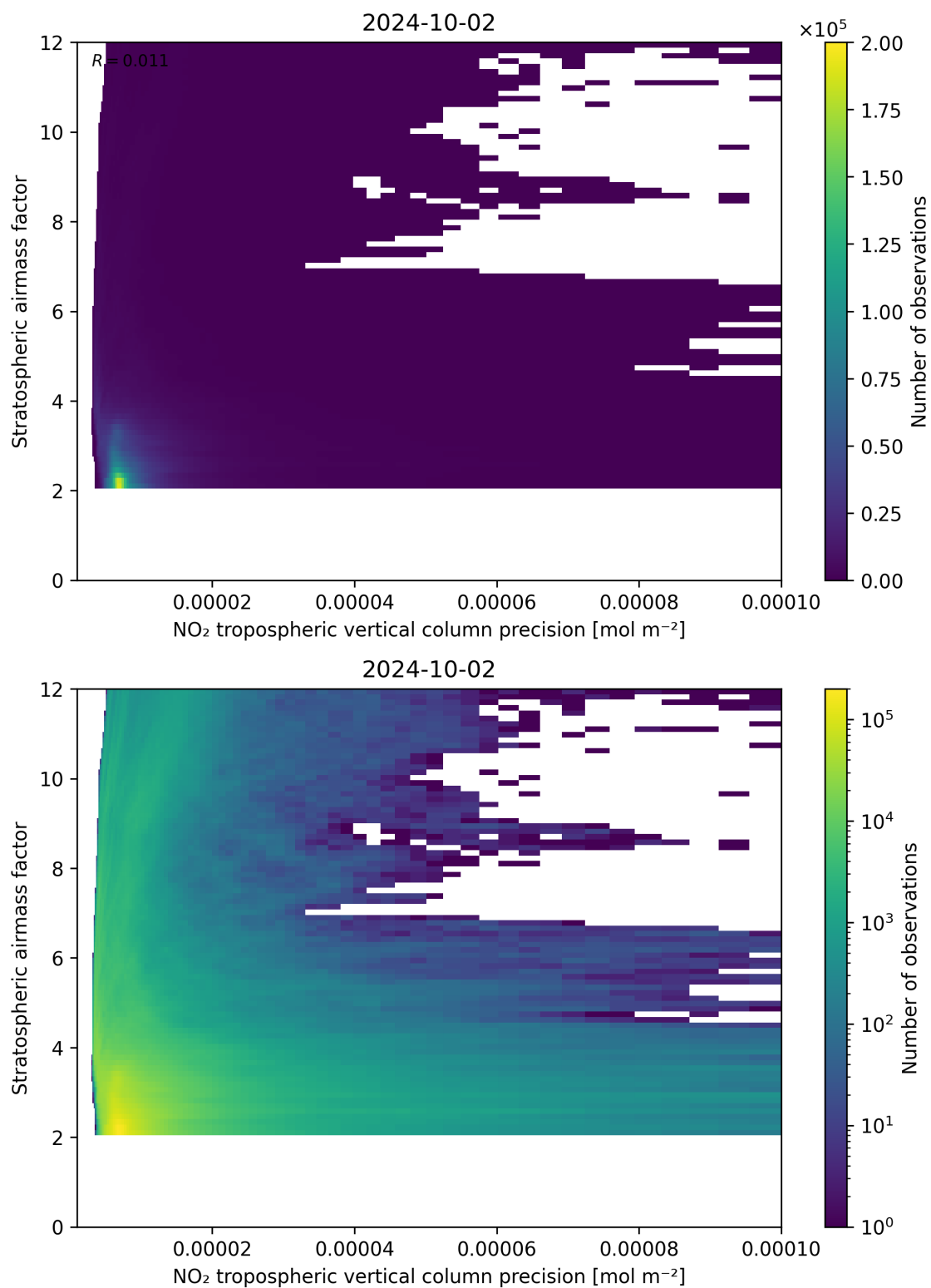
Figure 131: Scatter density plot of “NO 2 tropospheric vertical column precision” against “Stratospheric airmass factor” for 2024-10-01 to 2024-10-03.
