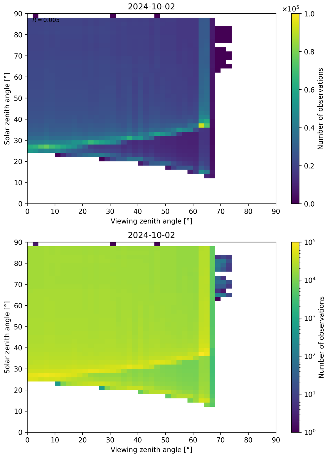
Figure 172: Scatter density plot of “Viewing zenith angle” against “Solar zenith angle” for 2024-10-01 to 2024-10-03.
