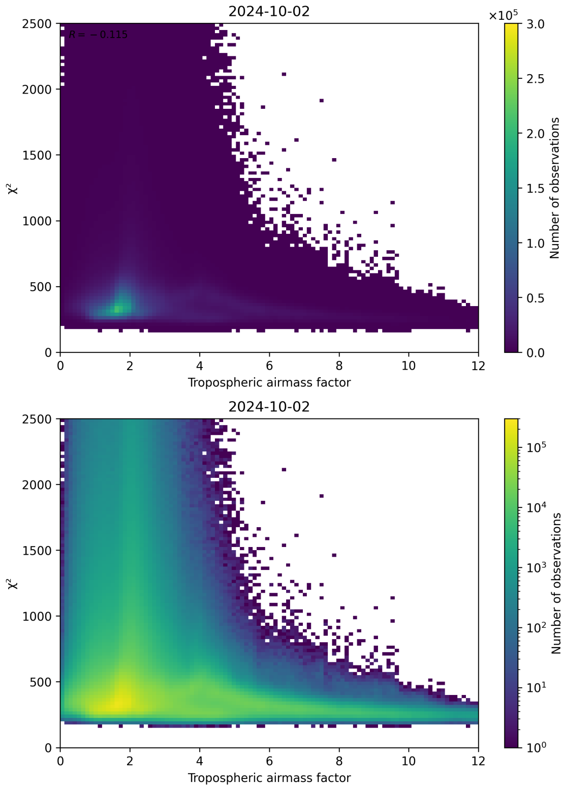
Figure 73: Scatter density plot of “Tropospheric airmass factor” against “ \chi^2 ” for 2024-10-01 to 2024-10-03.
