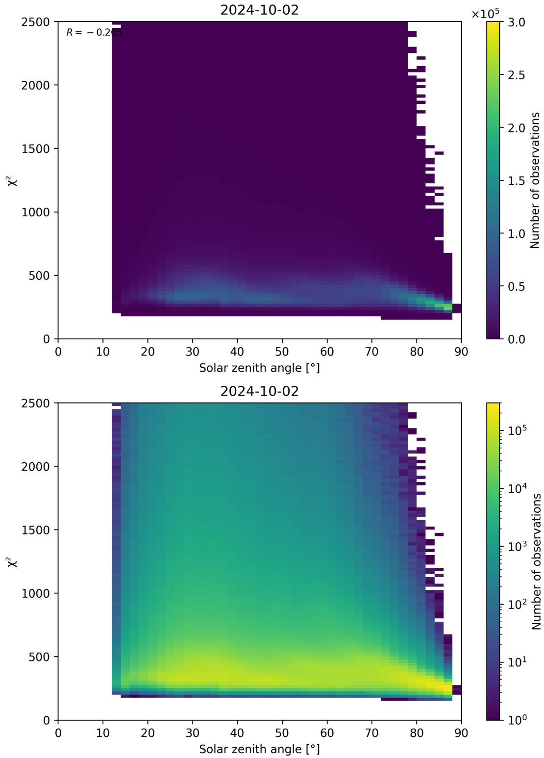
Figure 148: Scatter density plot of “Solar zenith angle” against “ \chi^2 ” for 2024-10-01 to 2024-10-03.
