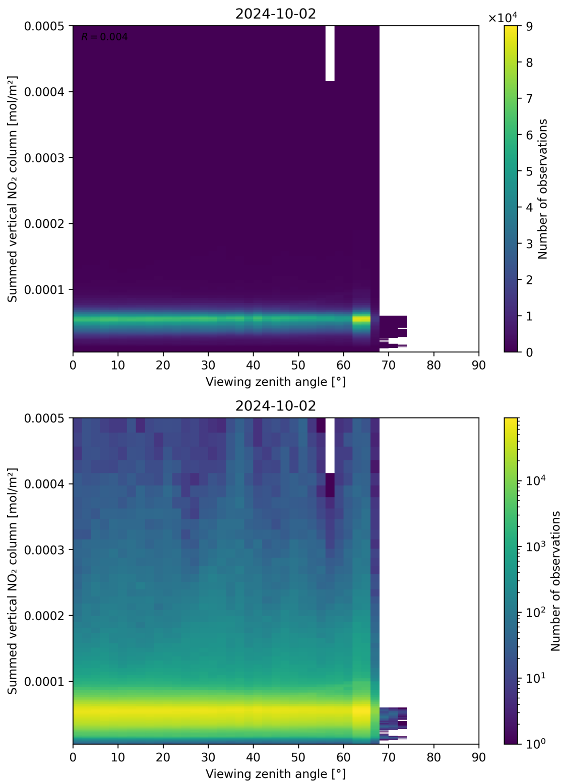
Figure 165: Scatter density plot of “Viewing zenith angle” against “Summed vertical NO 2 column” for 2024-10-01 to 2024-10-03.
