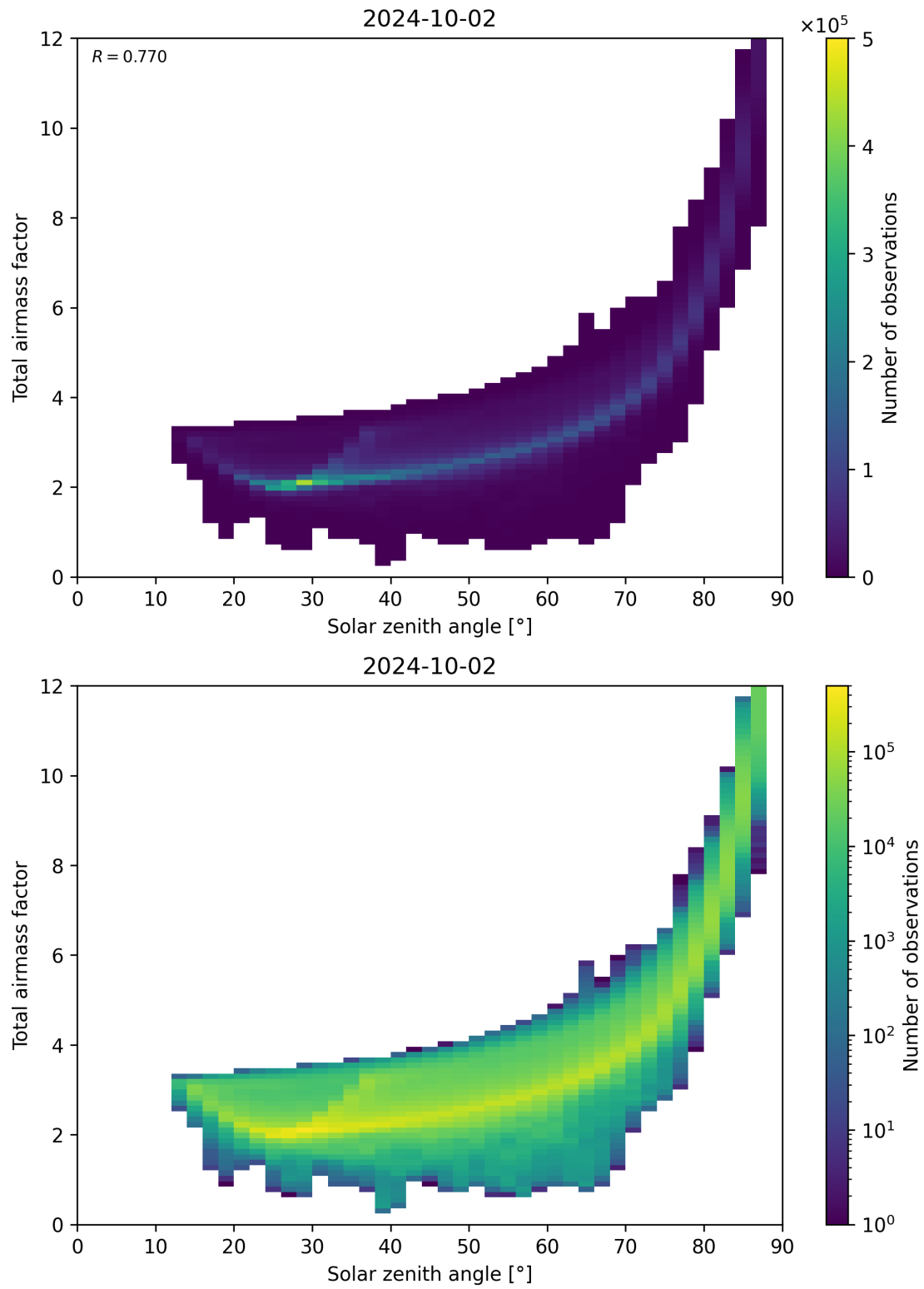
Figure 146: Scatter density plot of “Solar zenith angle” against “Total airmass factor” for 2024-10-01 to 2024-10-03.
