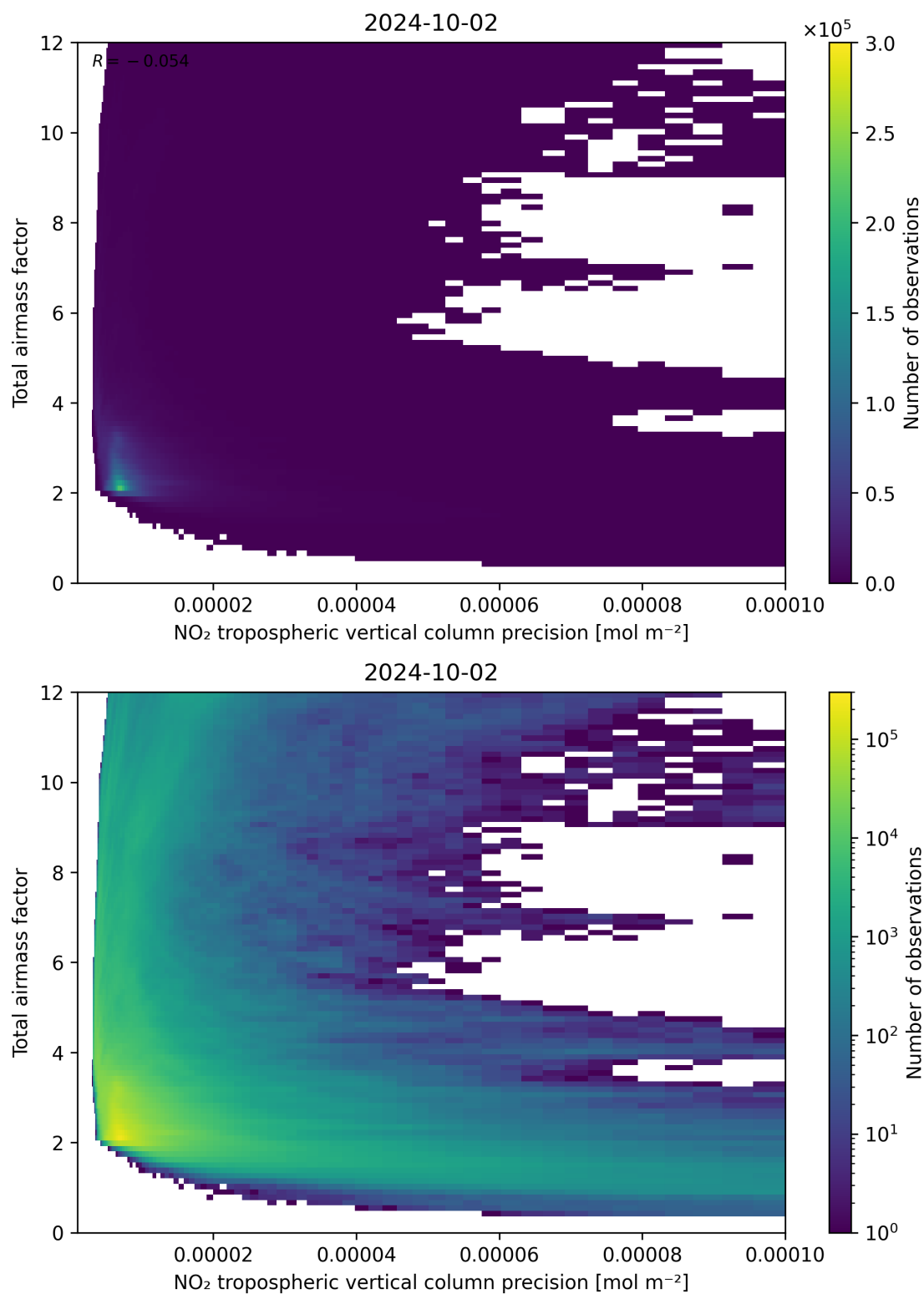
Figure 132: Scatter density plot of “NO 2 tropospheric vertical column precision” against “Total air mass factor” for 2024-10-01 to 2024-10-03.
