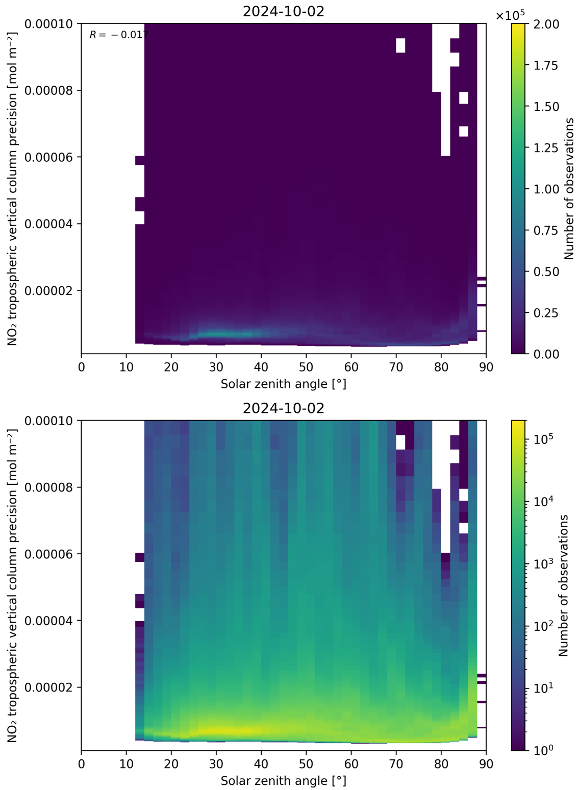
Figure 156: Scatter density plot of “Solar zenith angle” against “NO 2 tropospheric vertical column precision” for 2024-10-01 to 2024-10-03.
