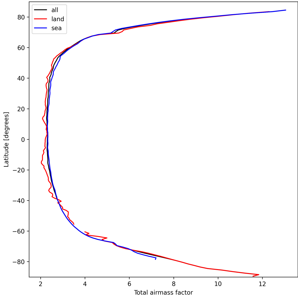
Figure 15: Zonal average of “Total airmass factor” for 2024-10-01 to 2024-10-03.
