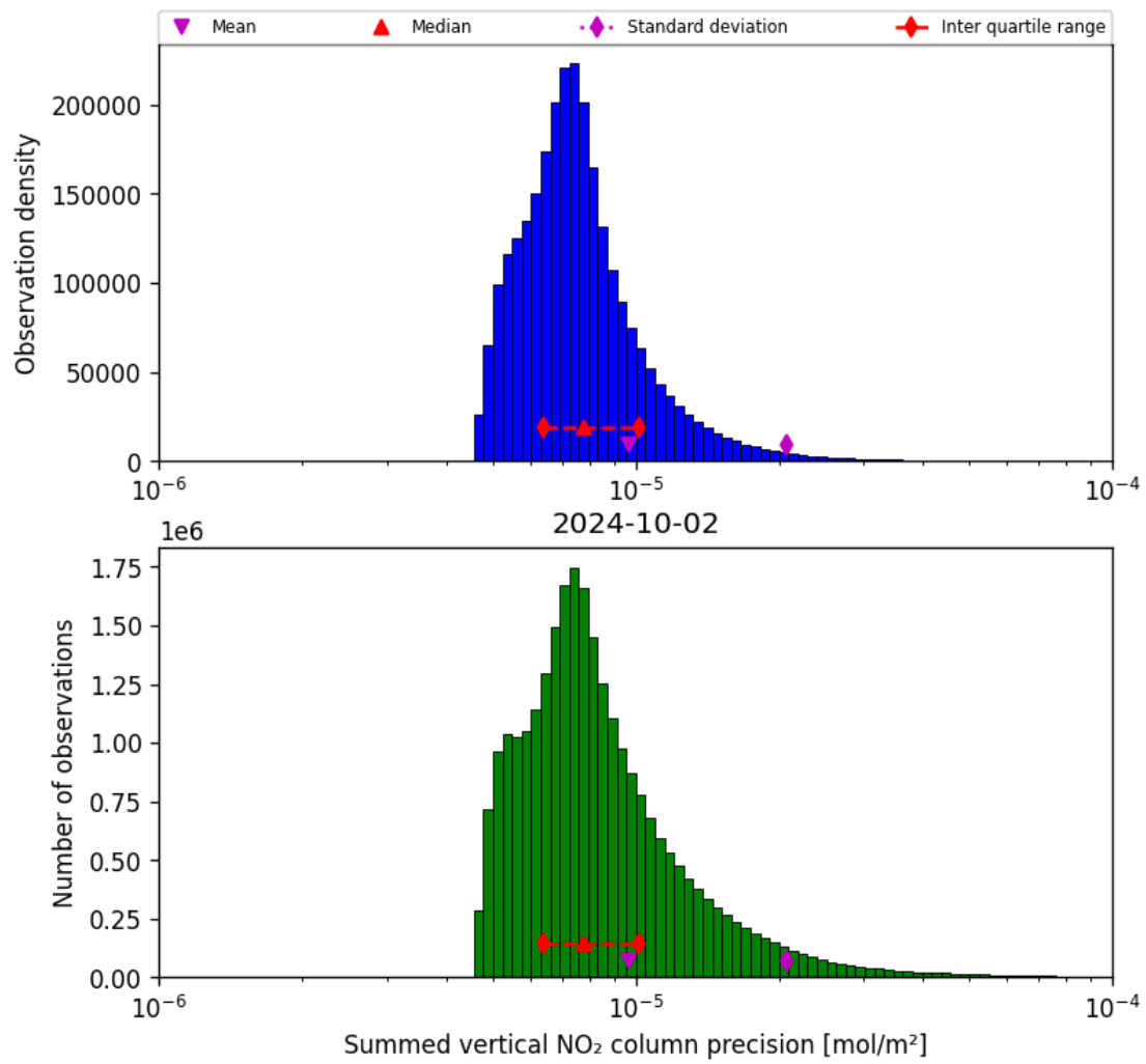
Figure 41: Histogram of “Summed vertical NO 2 column precision” for 2024-10-01 to 2024-10-03
