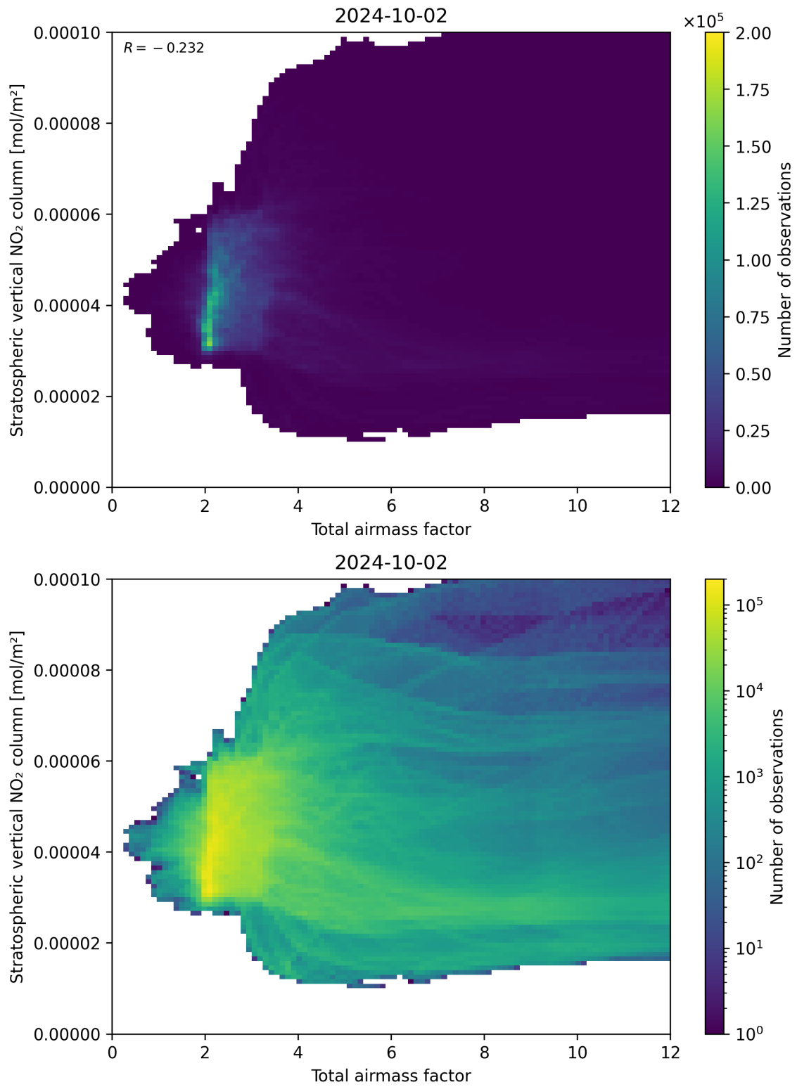
Figure 64: Scatter density plot of “Total airmass factor” against “Stratospheric vertical NO 2 column” for 2024-10-01 to 2024-10-03.
