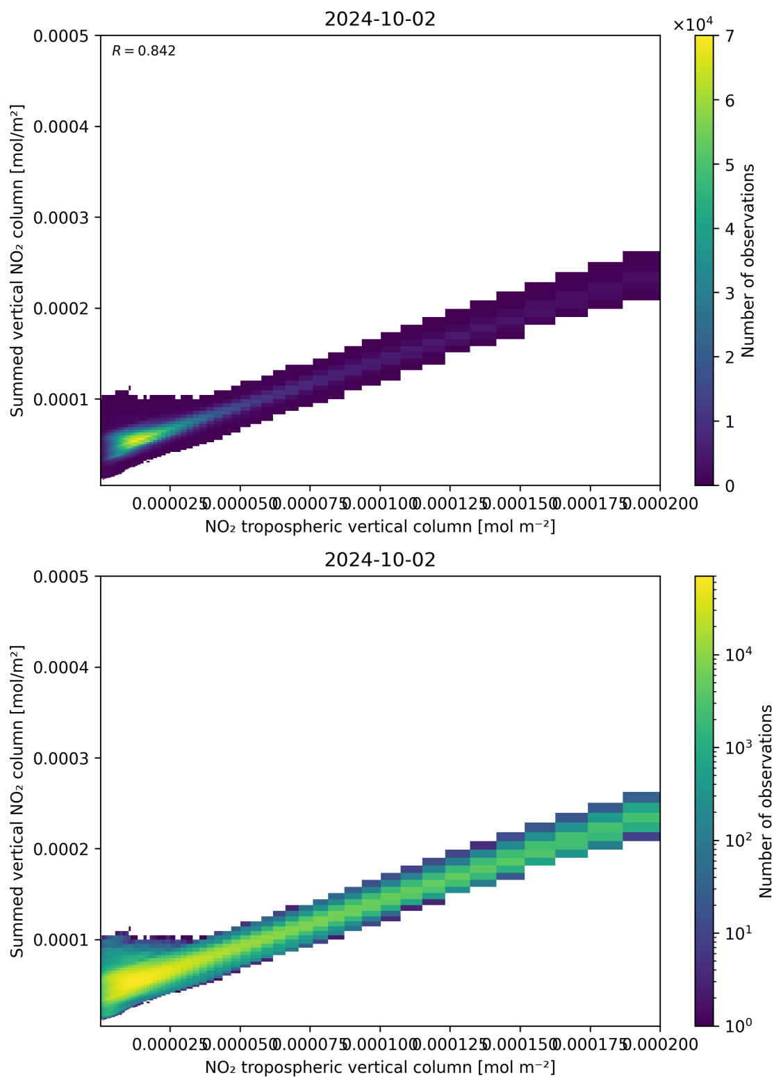
Figure 126: Scatter density plot of “NO 2 tropospheric vertical column” against “Summed vertical NO 2 column” for 2024-10-01 to 2024-10-03.
