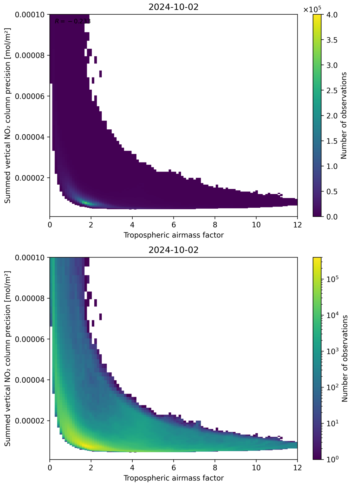
Figure 76: Scatter density plot of “Tropospheric airmass factor” against “Summed vertical NO 2 column precision” for 2024-10-01 to 2024-10-03.
