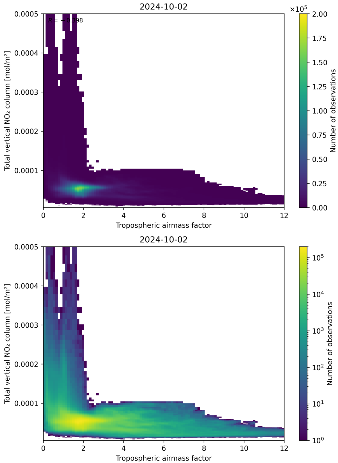
Figure 77: Scatter density plot of “Tropospheric airmass factor” against “Total vertical NO 2 column” for 2024-10-01 to 2024-10-03.
