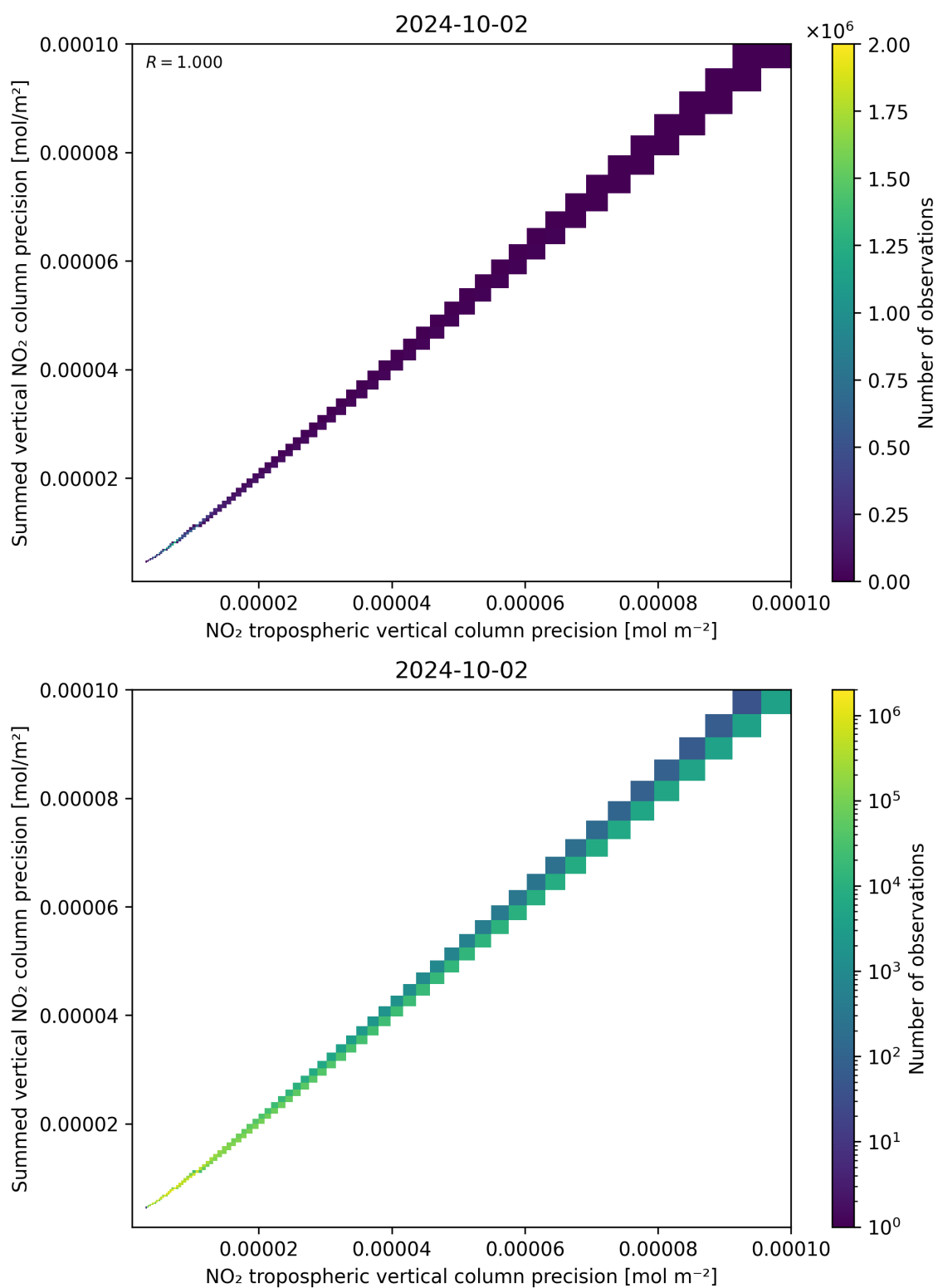
Figure 137: Scatter density plot of “NO 2 tropospheric vertical column precision” against “Summed vertical NO 2 column precision” for 2024-10-01 to 2024-10-03.
