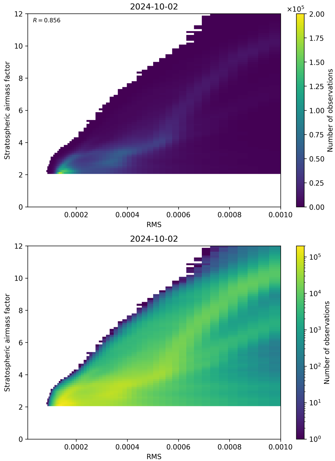
Figure 144: Scatter density plot of “RMS” against “Stratospheric airmass factor” for 2024-10-01 to 2024-10-03.
