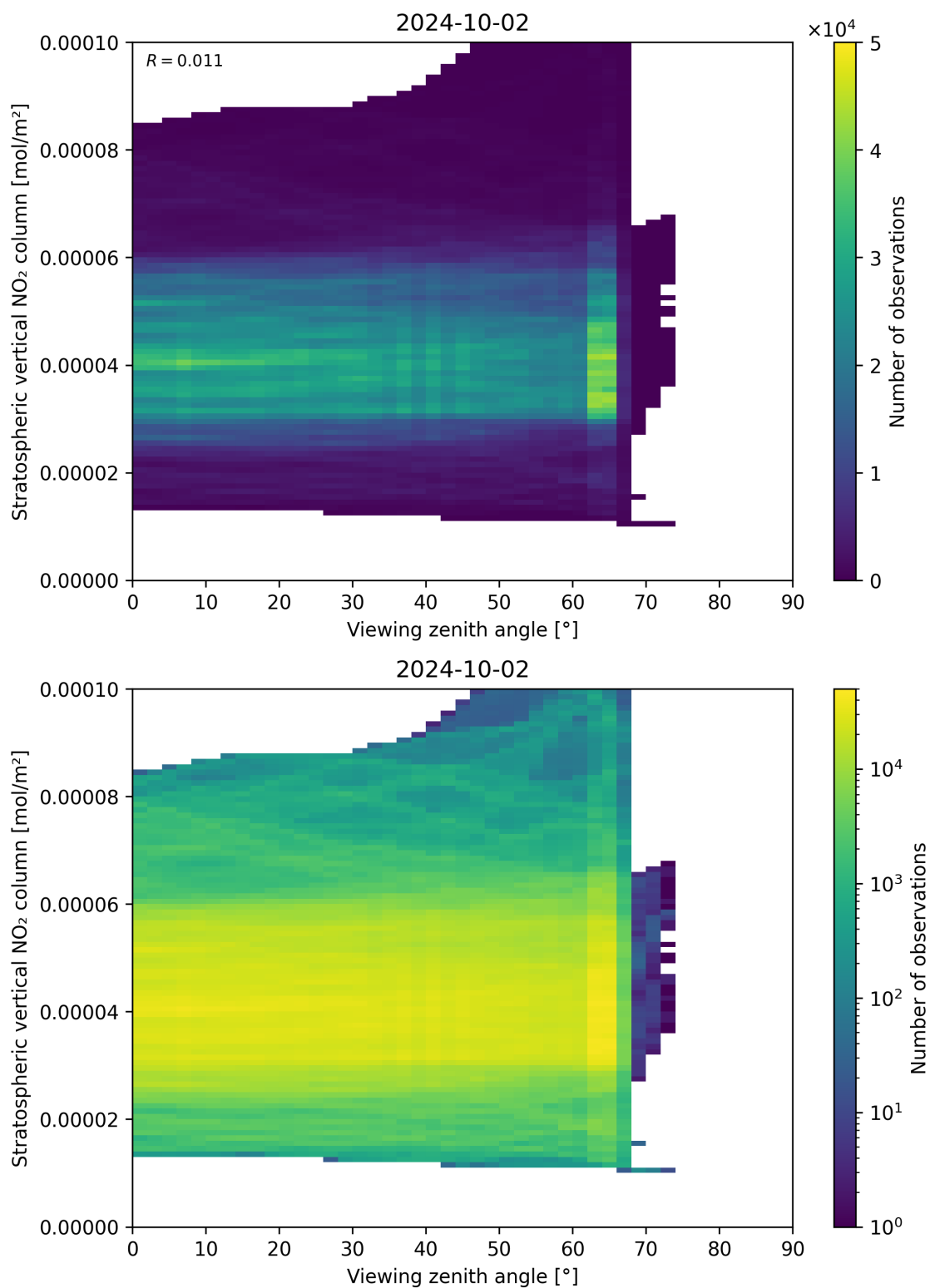
Figure 164: Scatter density plot of “Viewing zenith angle” against “Stratospheric vertical NO 2 column” for 2024-10-01 to 2024-10-03.
