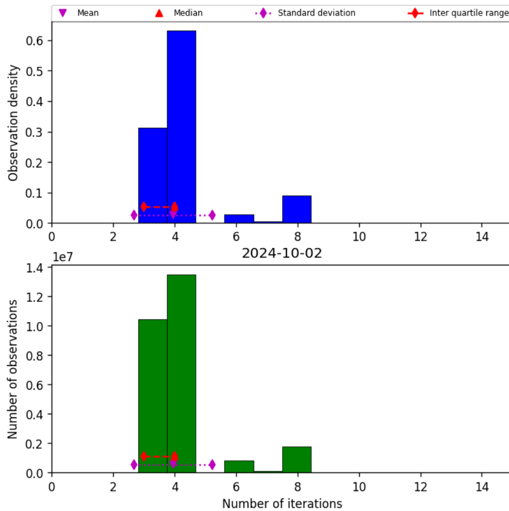
Figure 34: Histogram of “Number of iterations” for 2024-10-01 to 2024-10-03
