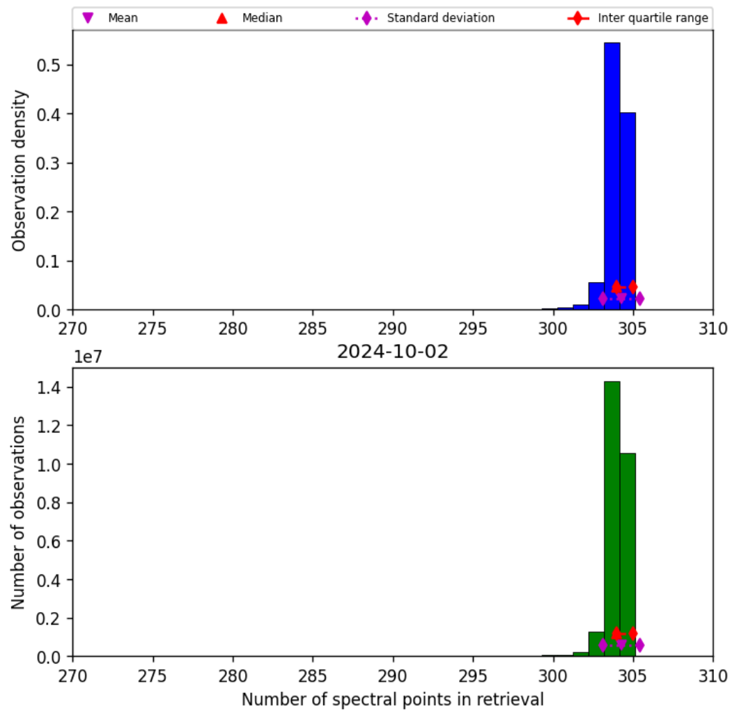
Figure 33: Histogram of “Number of spectral points in retrieval” for 2024-10-01 to 2024-10-03
