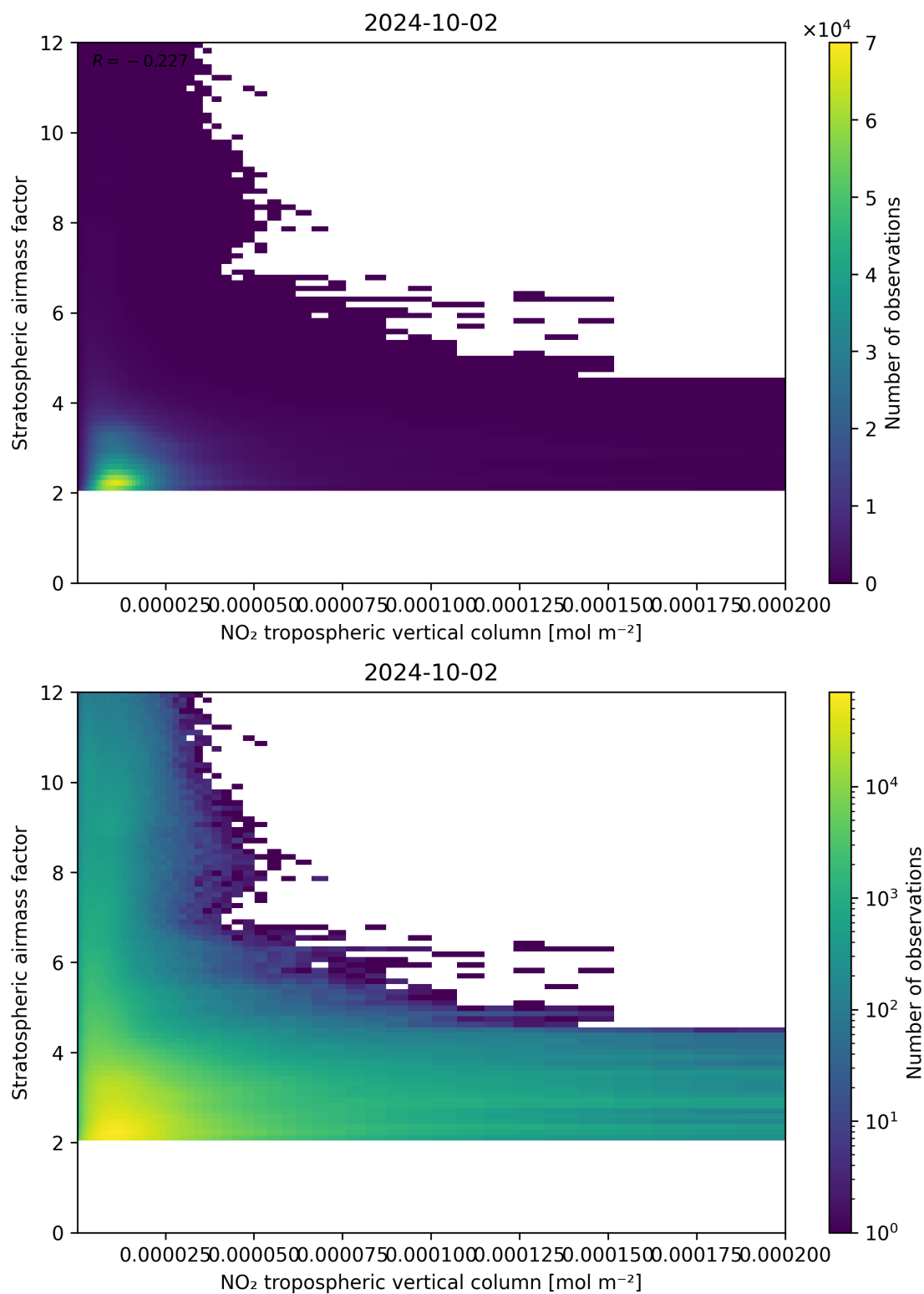
Figure 121: Scatter density plot of “NO 2 tropospheric vertical column” against “Stratospheric airmass factor” for 2024-10-01 to 2024-10-03.
