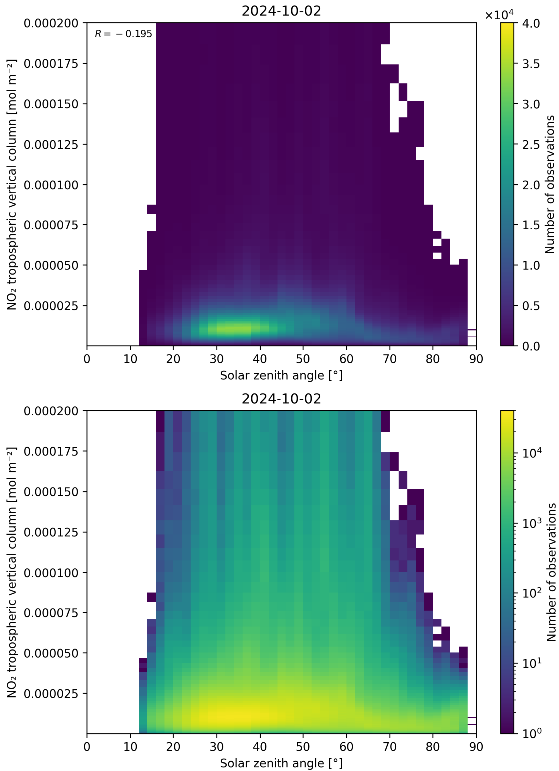
Figure 155: Scatter density plot of “Solar zenith angle” against “NO 2 tropospheric vertical column” for 2024-10-01 to 2024-10-03.
