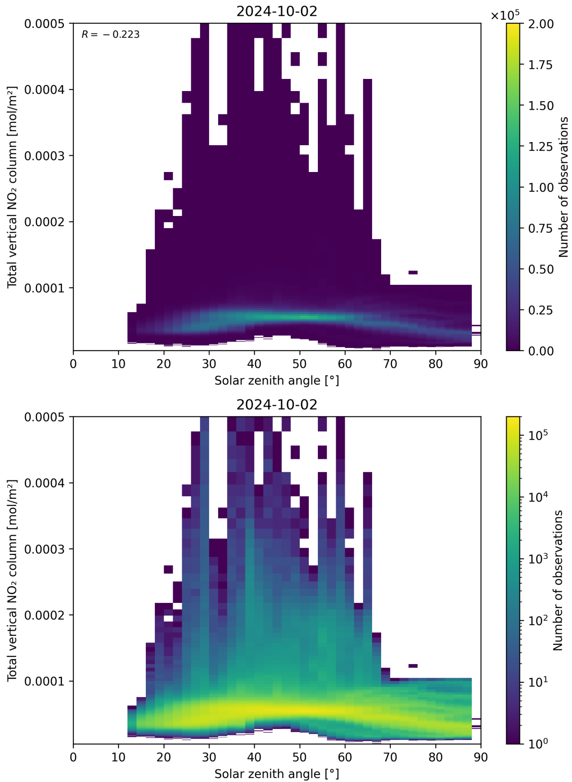
Figure 153: Scatter density plot of “Solar zenith angle” against “Total vertical NO 2 column” for 2024-10-01 to 2024-10-03.
