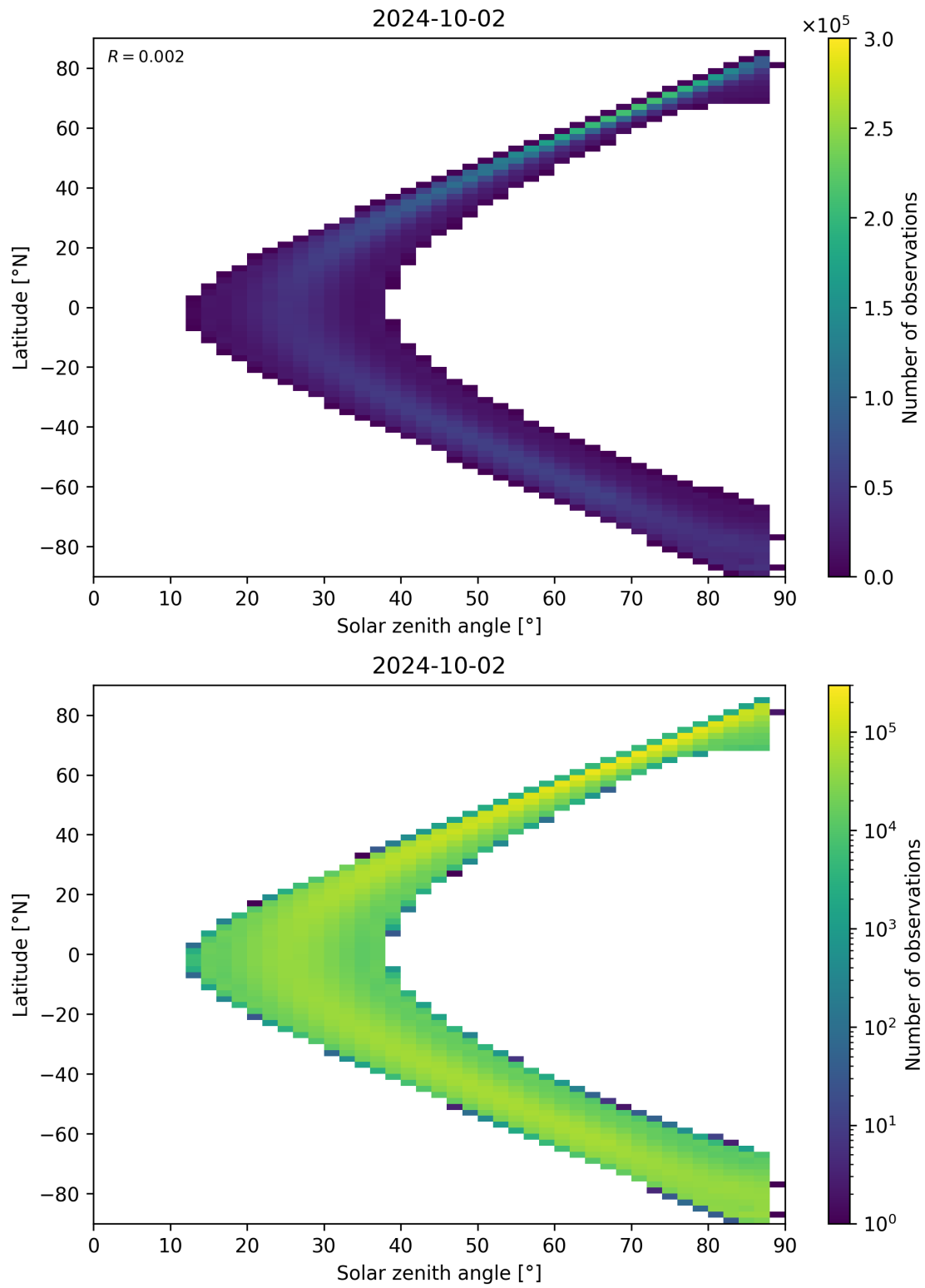
Figure 149: Scatter density plot of “Solar zenith angle” against “Latitude” for 2024-10-01 to 2024-10-03.
