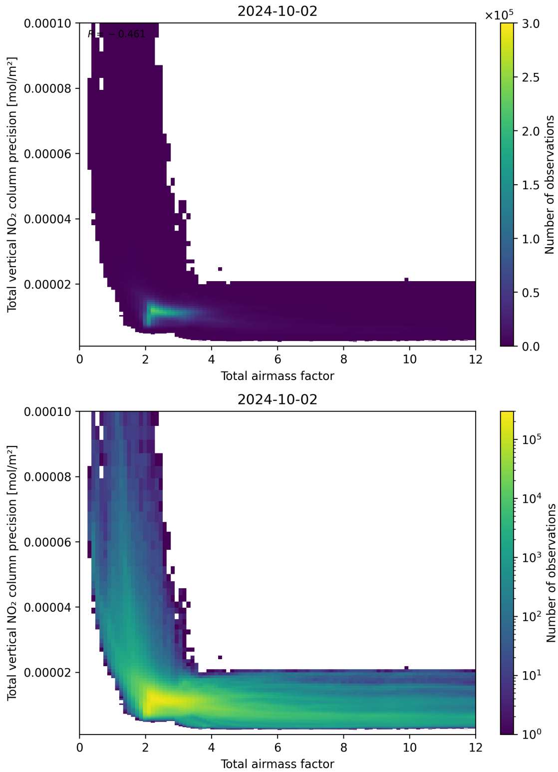
Figure 68: Scatter density plot of “Total airmass factor” against “Total vertical NO 2 column precision” for 2024-10-01 to 2024-10-03.
