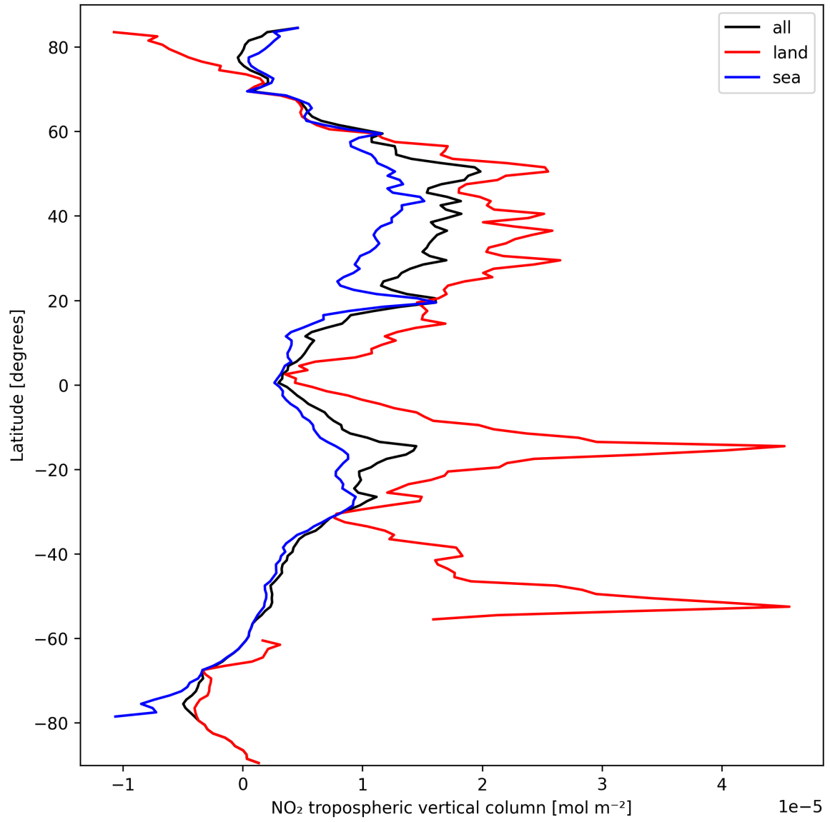
Figure 12: Zonal average of “NO 2 tropospheric vertical column” for 2024-10-01 to 2024-10-03.
