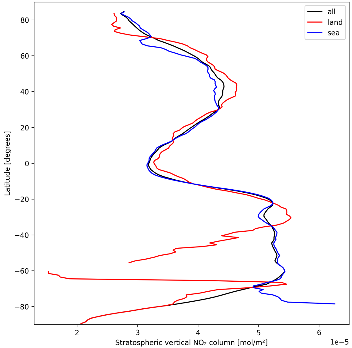
Figure 19: Zonal average of “Stratospheric vertical NO 2 column” for 2024-10-01 to 2024-10-03.
