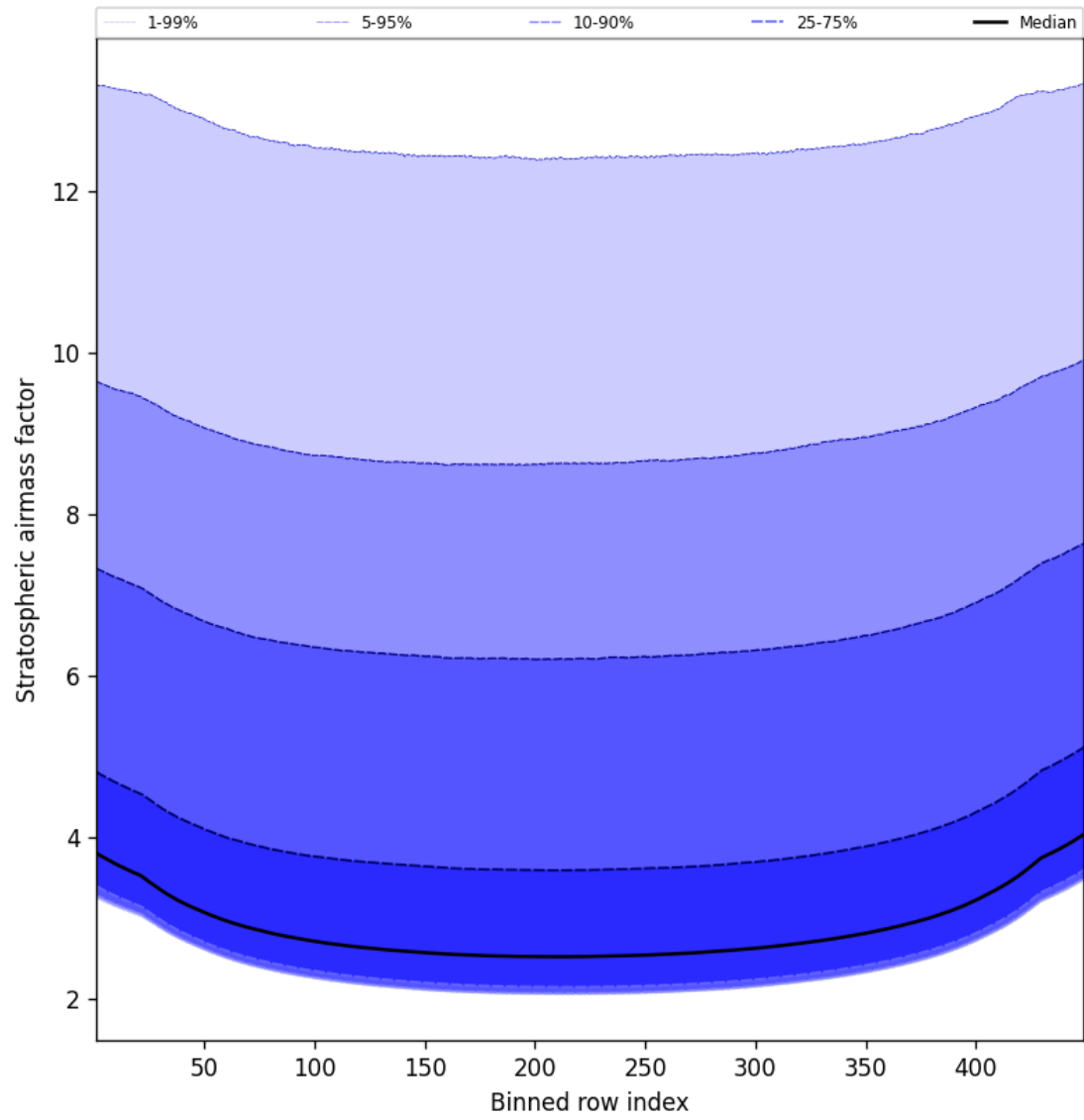
Figure 61: Along track statistics of “Stratospheric airmass factor” for 2024-10-01 to 2024-10-03
