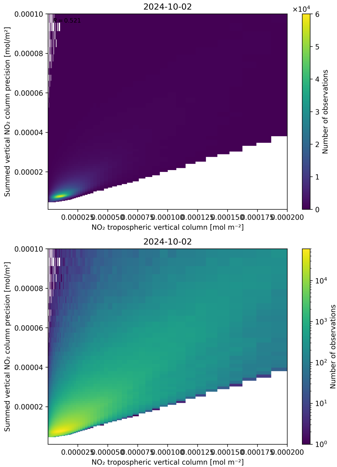
Figure 127: Scatter density plot of “NO 2 tropospheric vertical column” against “Summed vertical NO 2 column precision” for 2024-10-01 to 2024-10-03.
