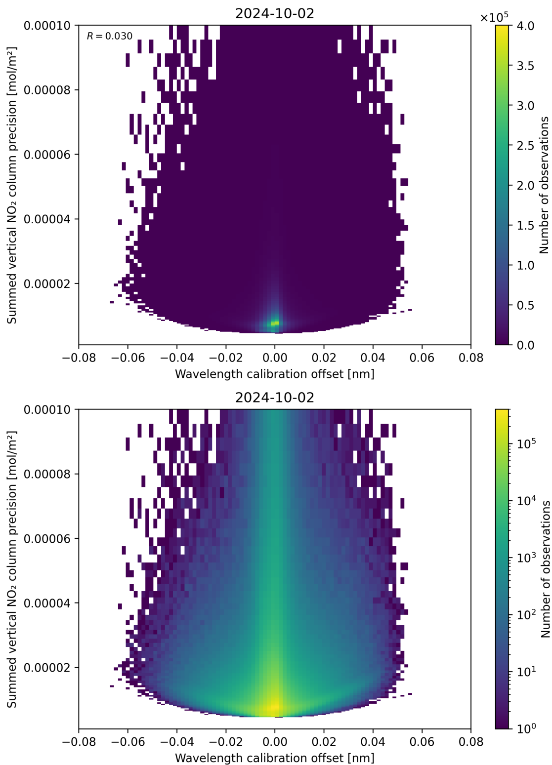
Figure 178: Scatter density plot of “Wavelength calibration offset” against “Summed vertical NO 2 column precision” for 2024-10-01 to 2024-10-03.
