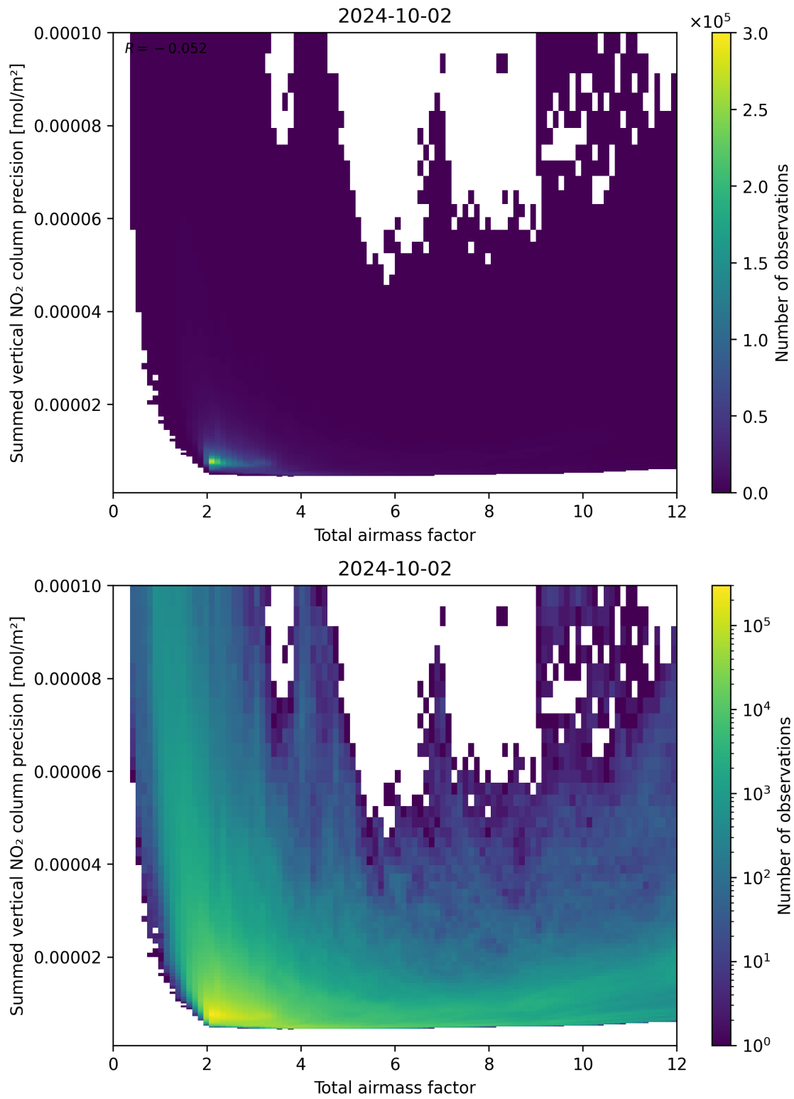
Figure 66: Scatter density plot of “Total airmass factor” against “Summed vertical NO 2 column precision” for 2024-10-01 to 2024-10-03.
