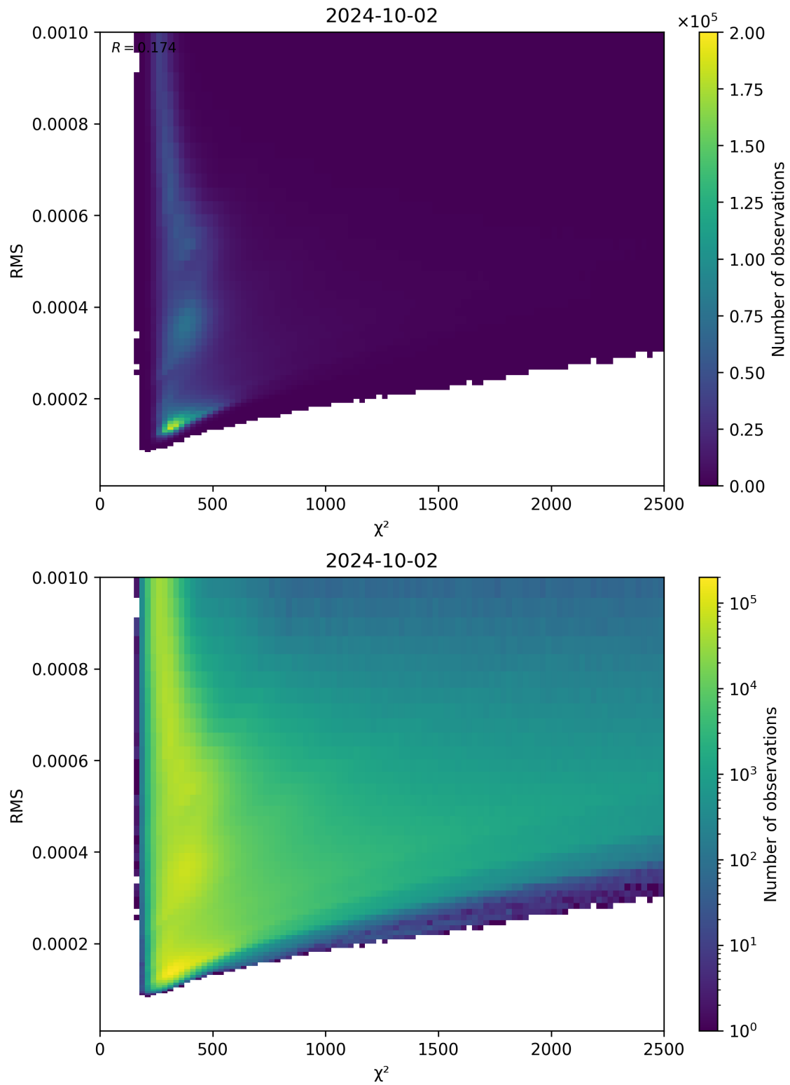
Figure 82: Scatter density plot of “ \chi^2 ” against “RMS” for 2024-10-01 to 2024-10-03.
