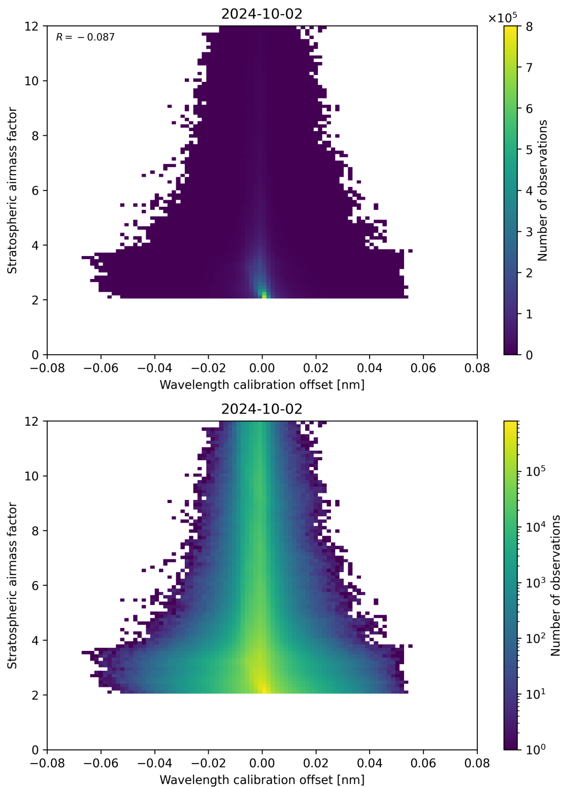
Figure 174: Scatter density plot of “Wavelength calibration offset” against “Stratospheric airmass factor” for 2024-10-01 to 2024-10-03.
