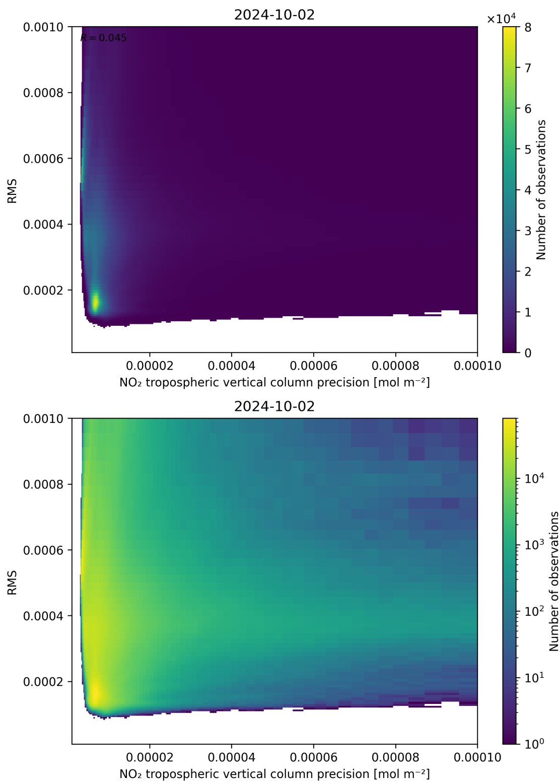
Figure 140: Scatter density plot of “NO 2 tropospheric vertical column precision” against “RMS” for 2024-10-01 to 2024-10-03.
