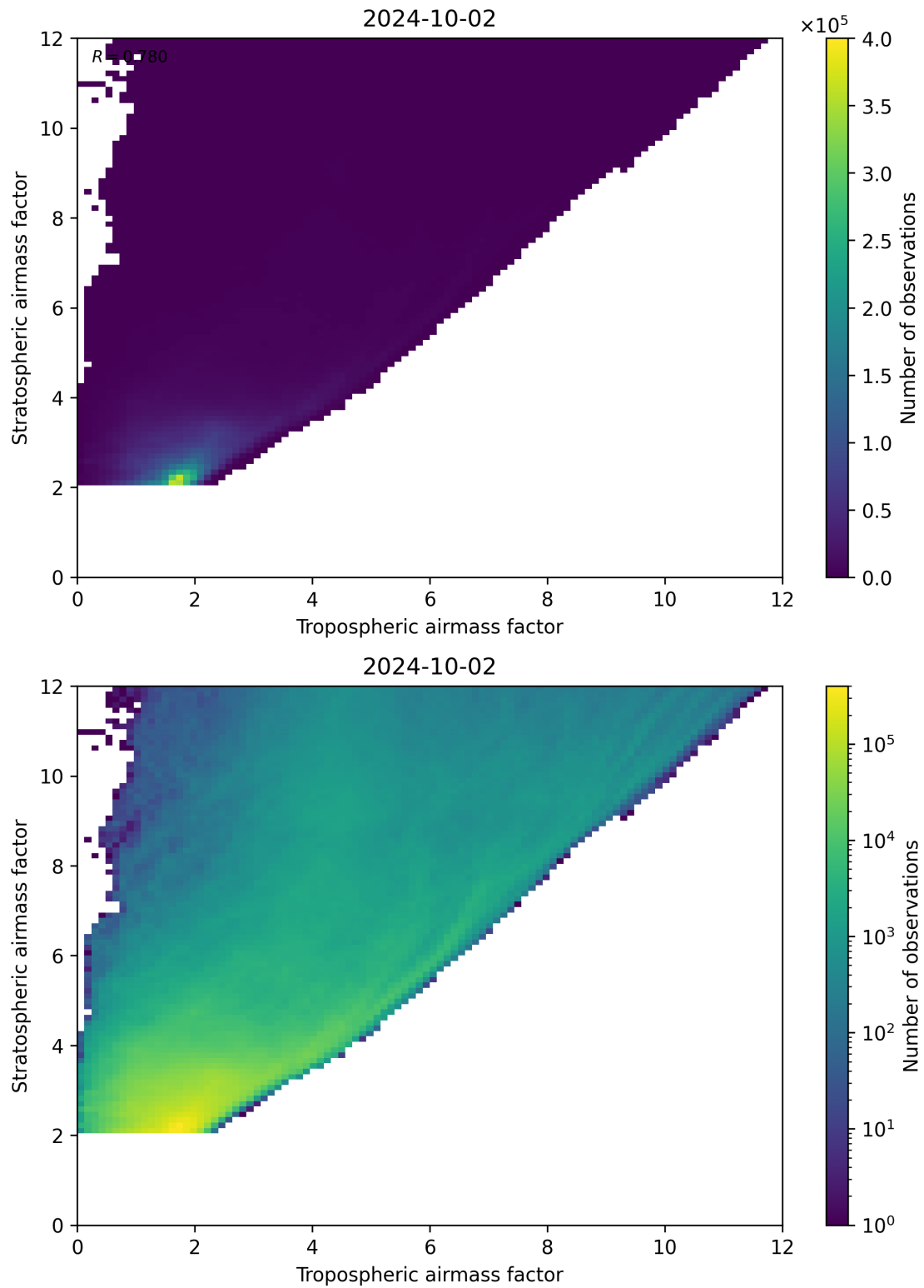
Figure 71: Scatter density plot of “Tropospheric airmass factor” against “Stratospheric airmass factor” for 2024-10-01 to 2024-10-03.
