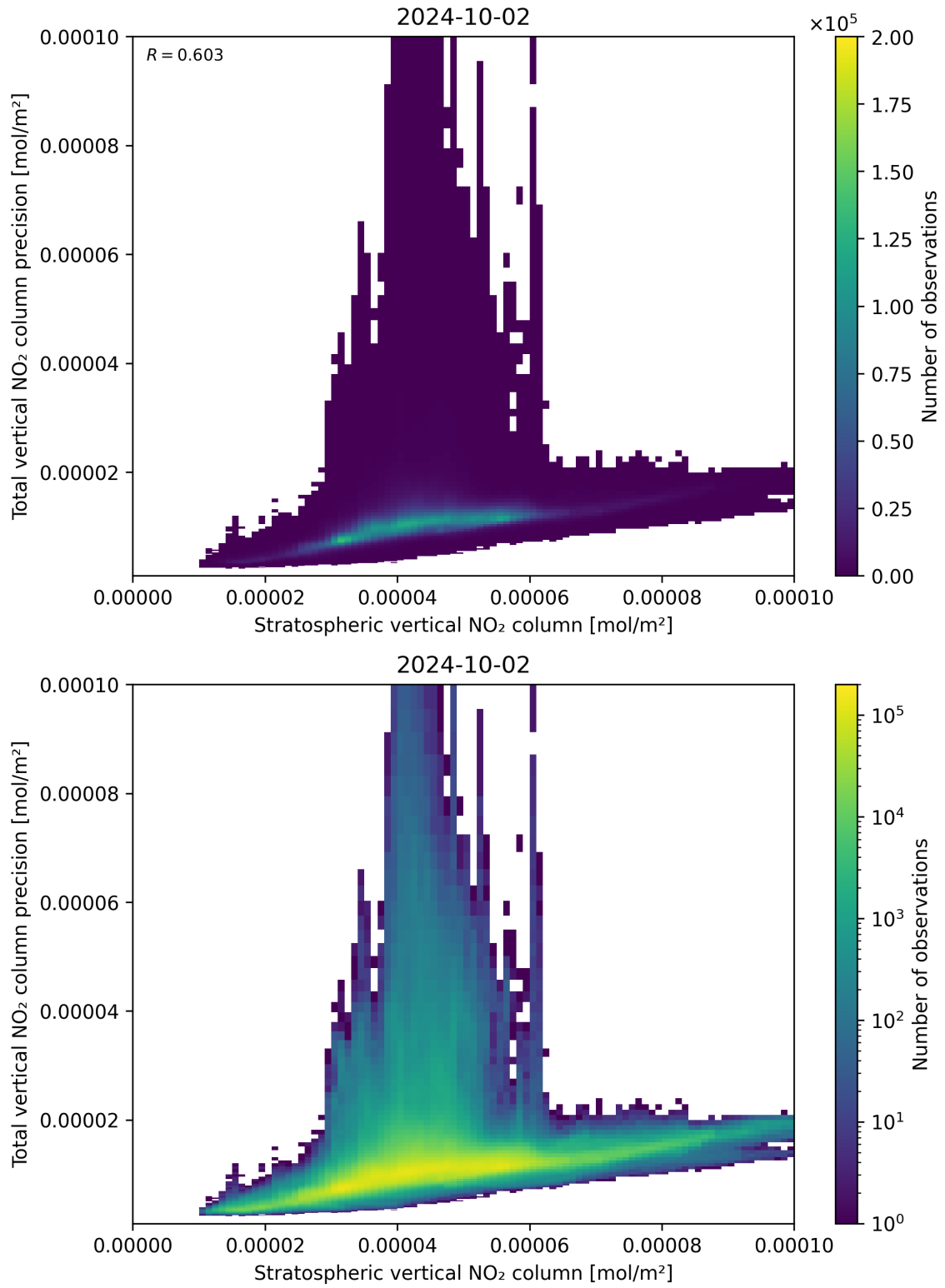
Figure 101: Scatter density plot of “Stratospheric vertical NO 2 column” against “Total vertical NO 2 column precision” for 2024-10-01 to 2024-10-03.
