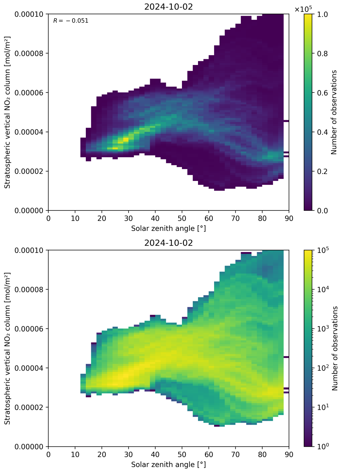
Figure 150: Scatter density plot of “Solar zenith angle” against “Stratospheric vertical NO 2 column” for 2024-10-01 to 2024-10-03.
