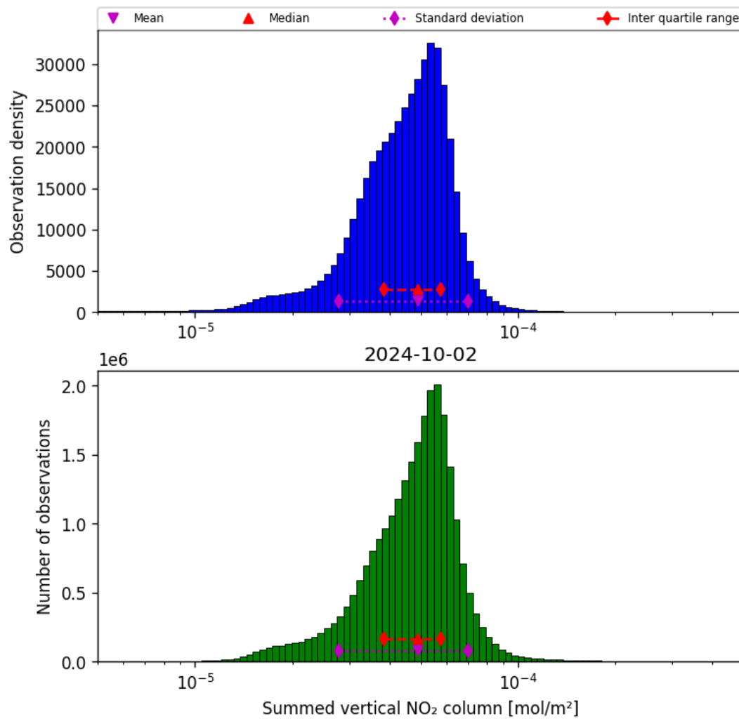
Figure 40: Histogram of “Summed vertical NO 2 column” for 2024-10-01 to 2024-10-03
