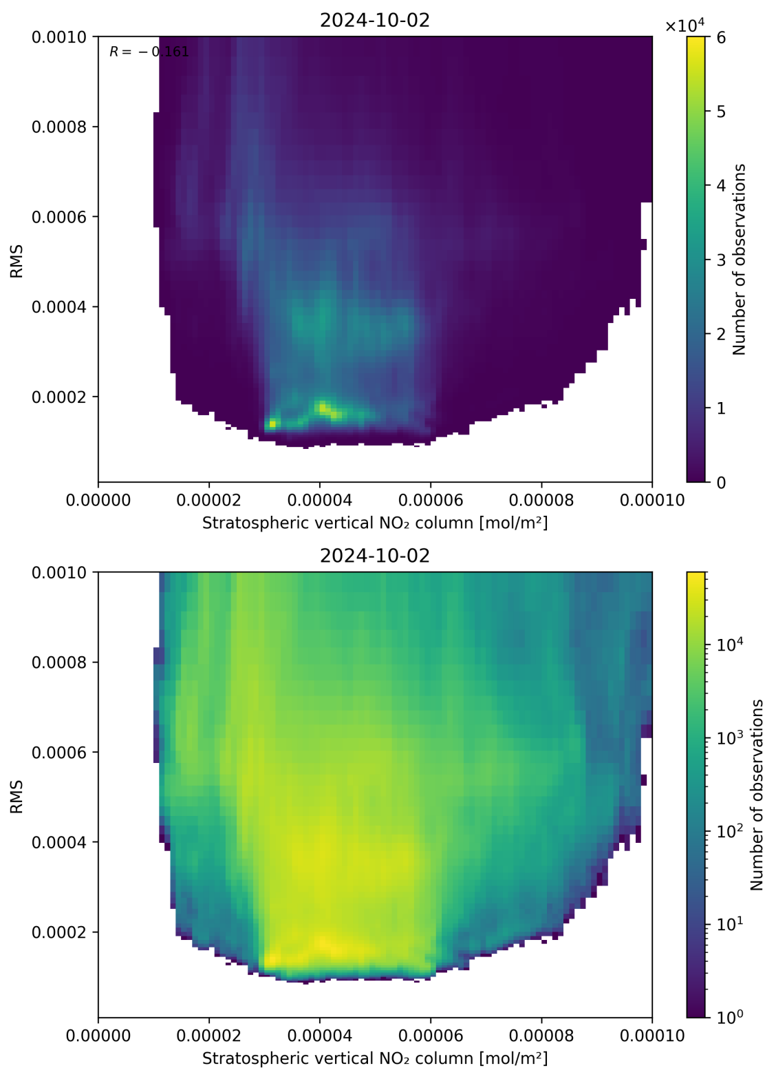
Figure 102: Scatter density plot of “Stratospheric vertical NO 2 column” against “RMS” for 2024-10-01 to 2024-10-03.
