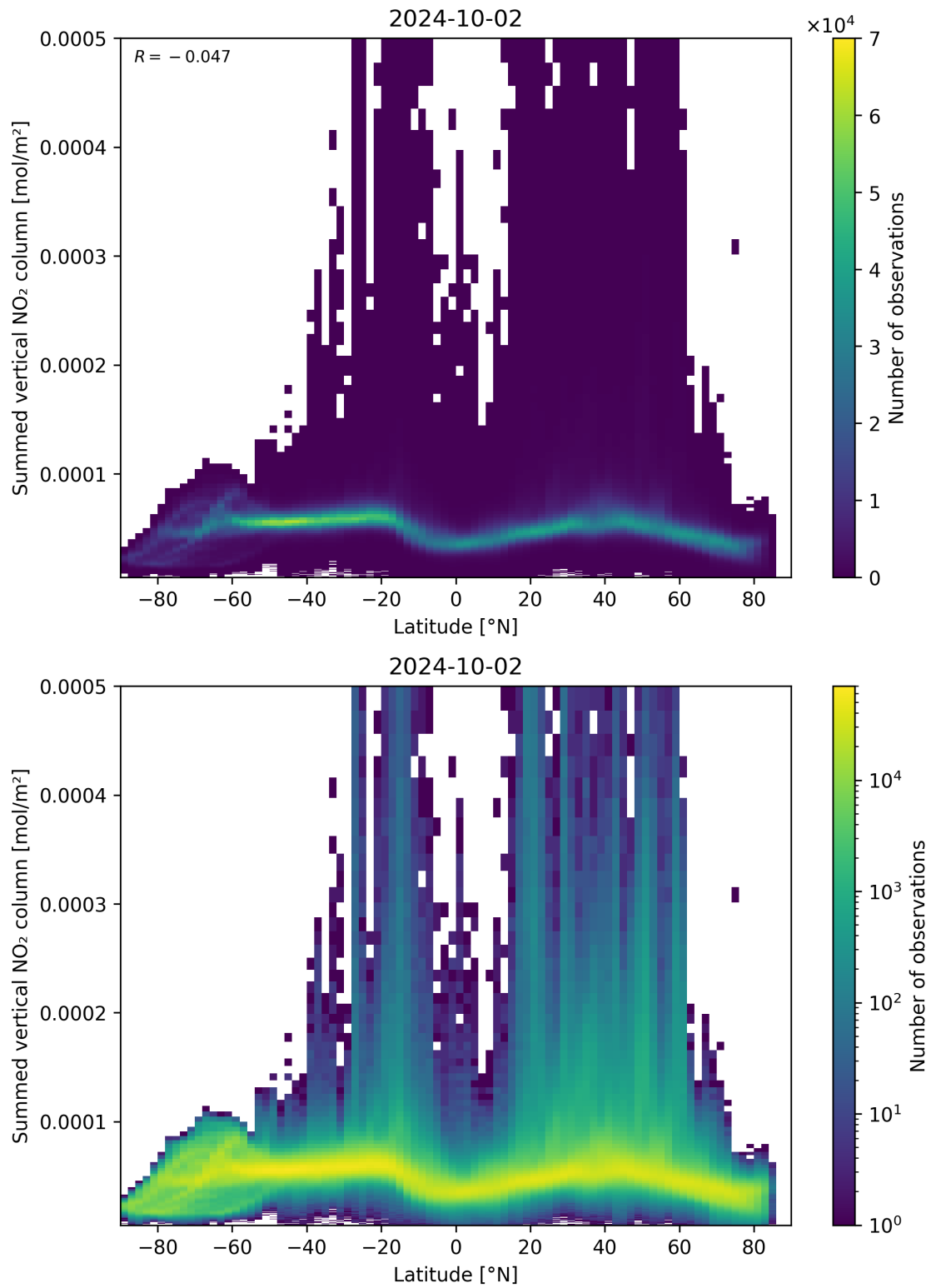
Figure 88: Scatter density plot of “Latitude” against “Summed vertical NO 2 column” for 2024-10-01 to 2024-10-03.
