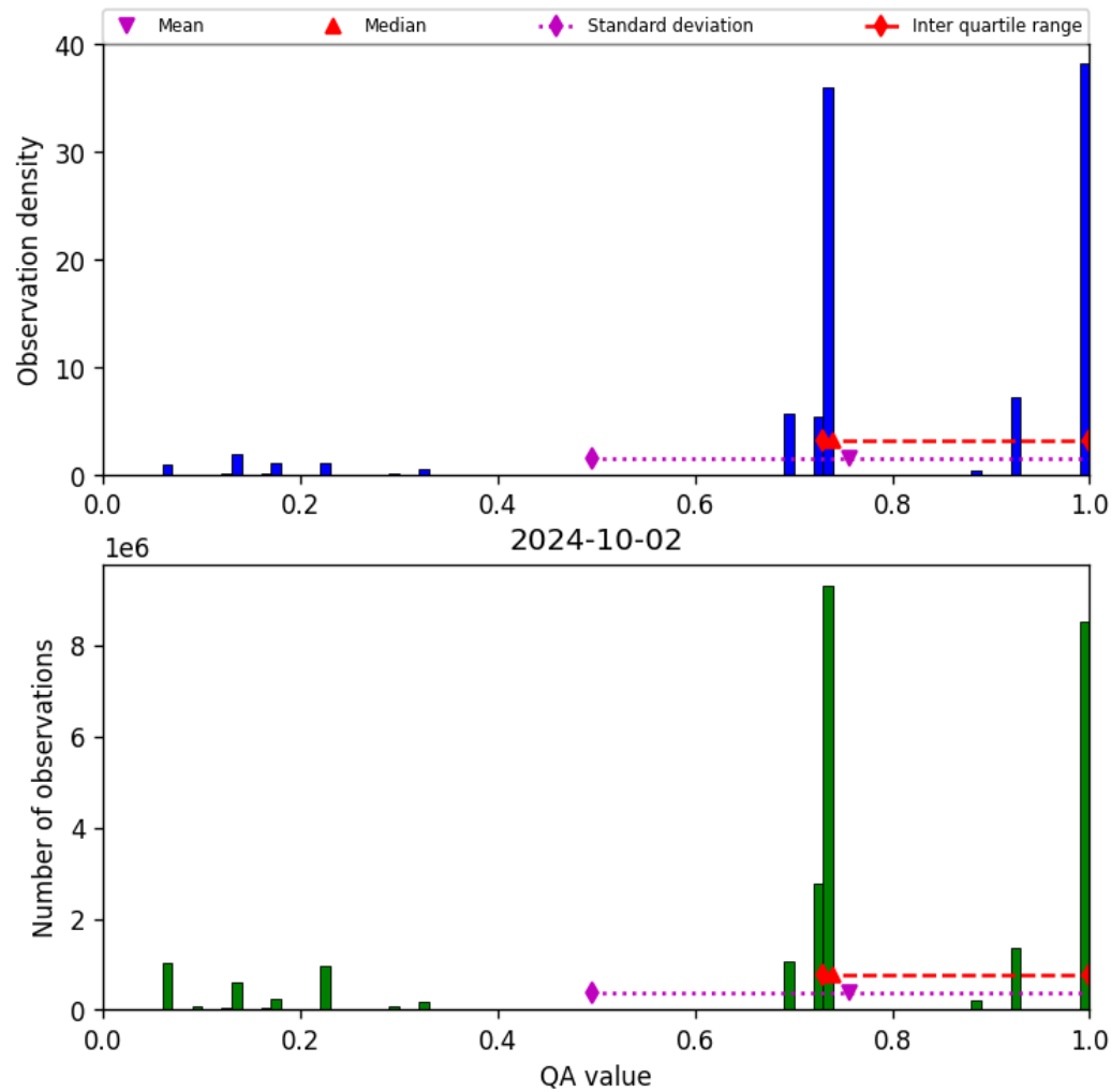
Figure 28: Histogram of “QA value” for 2024-10-01 to 2024-10-03
