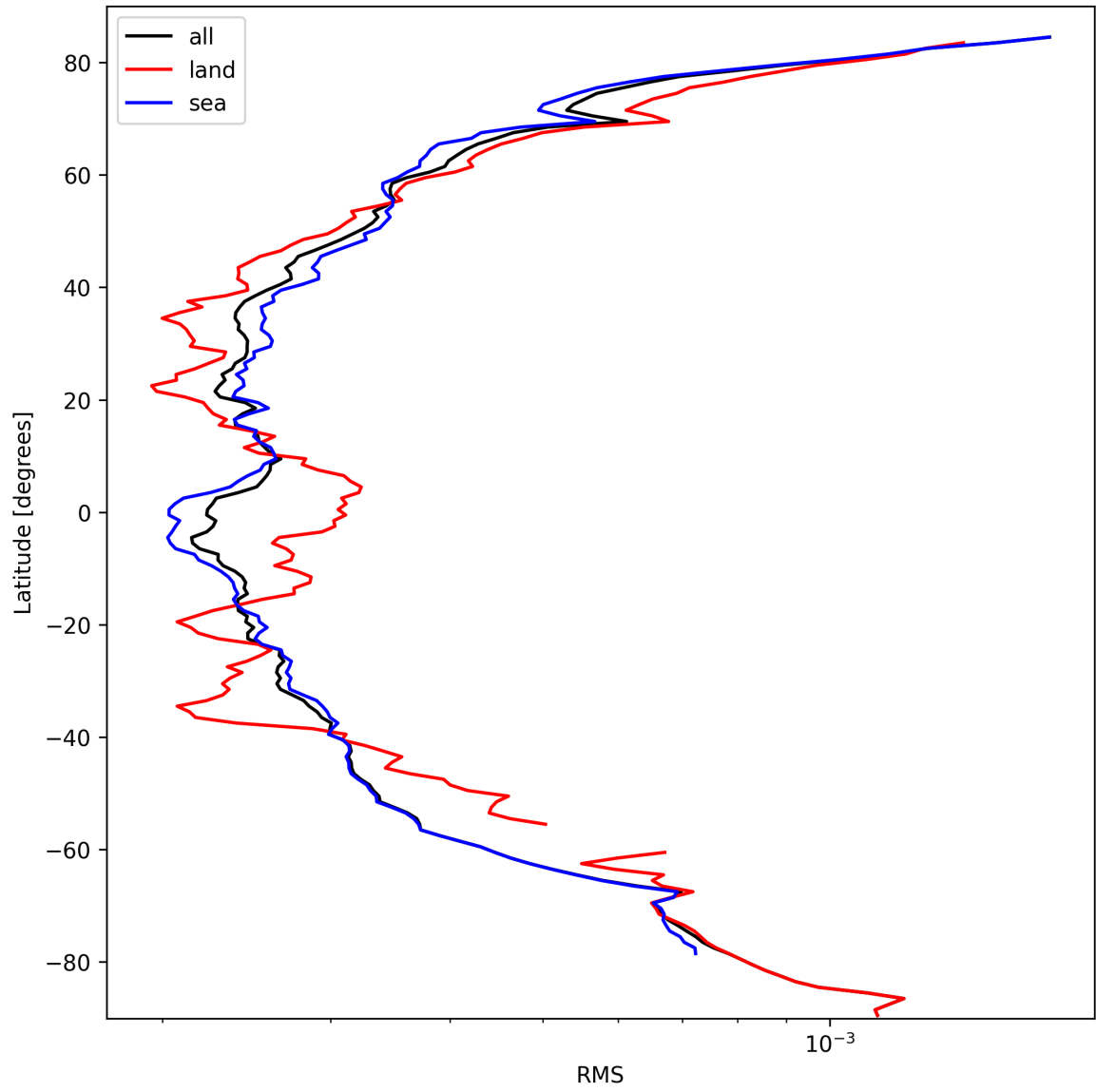
Figure 26: Zonal average of “RMS” for 2024-10-01 to 2024-10-03.
