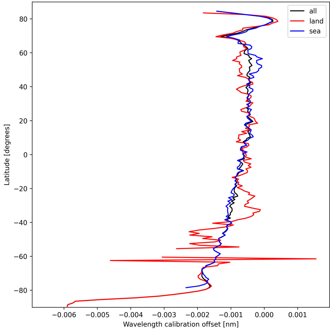
Figure 18: Zonal average of “Wavelength calibration offset” for 2024-10-01 to 2024-10-03.
