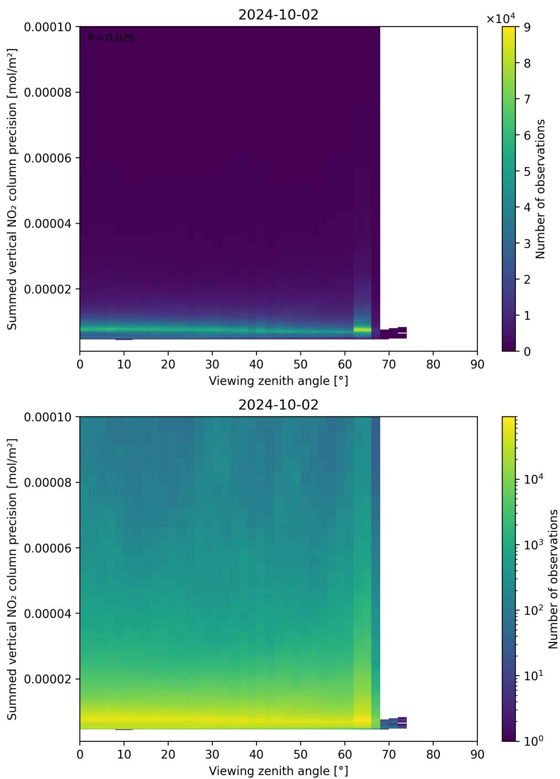
Figure 166: Scatter density plot of “Viewing zenith angle” against “Summed vertical NO 2 column precision” for 2024-10-01 to 2024-10-03.
