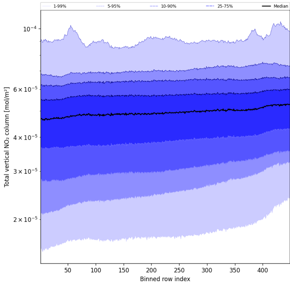
Figure 55: Along track statistics of “Total vertical NO 2 column” for 2024-10-01 to 2024-10-03
