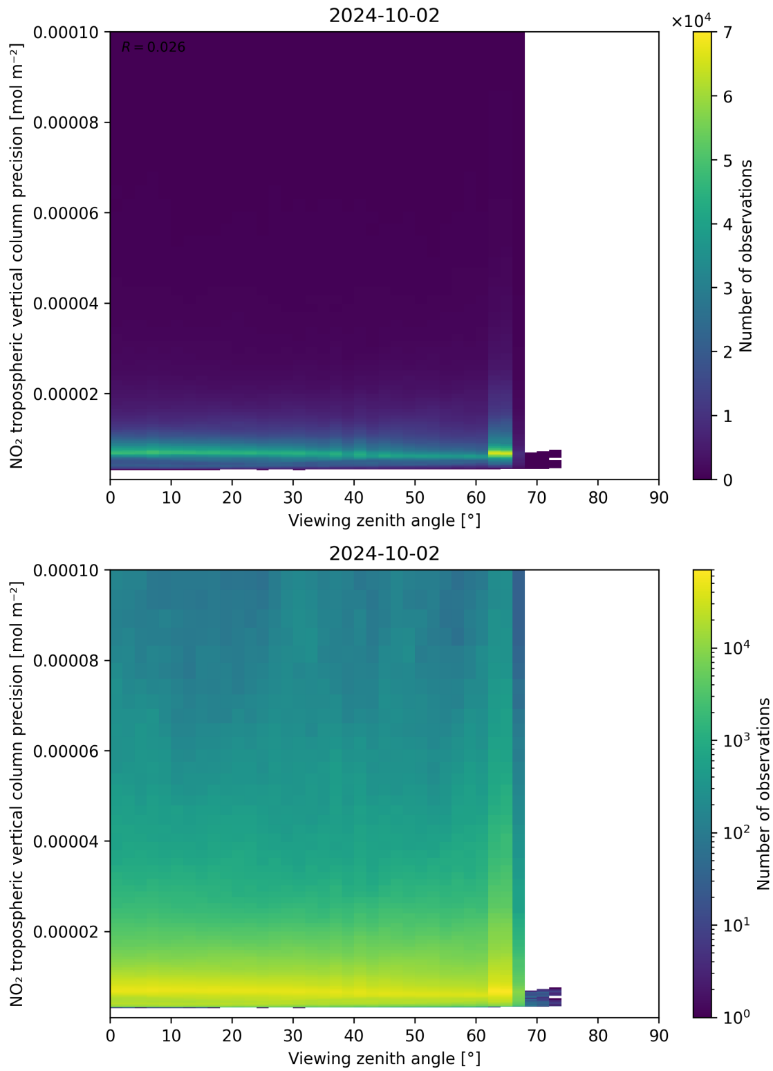
Figure 170: Scatter density plot of “Viewing zenith angle” against “NO 2 tropospheric vertical column precision” for 2024-10-01 to 2024-10-03.
