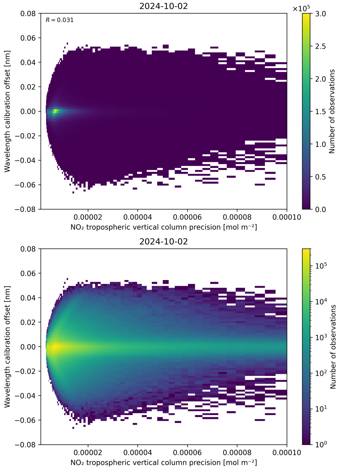
Figure 141: Scatter density plot of “NO 2 tropospheric vertical column precision” against “Wavelength calibration offset” for 2024-10-01 to 2024-10-03.
