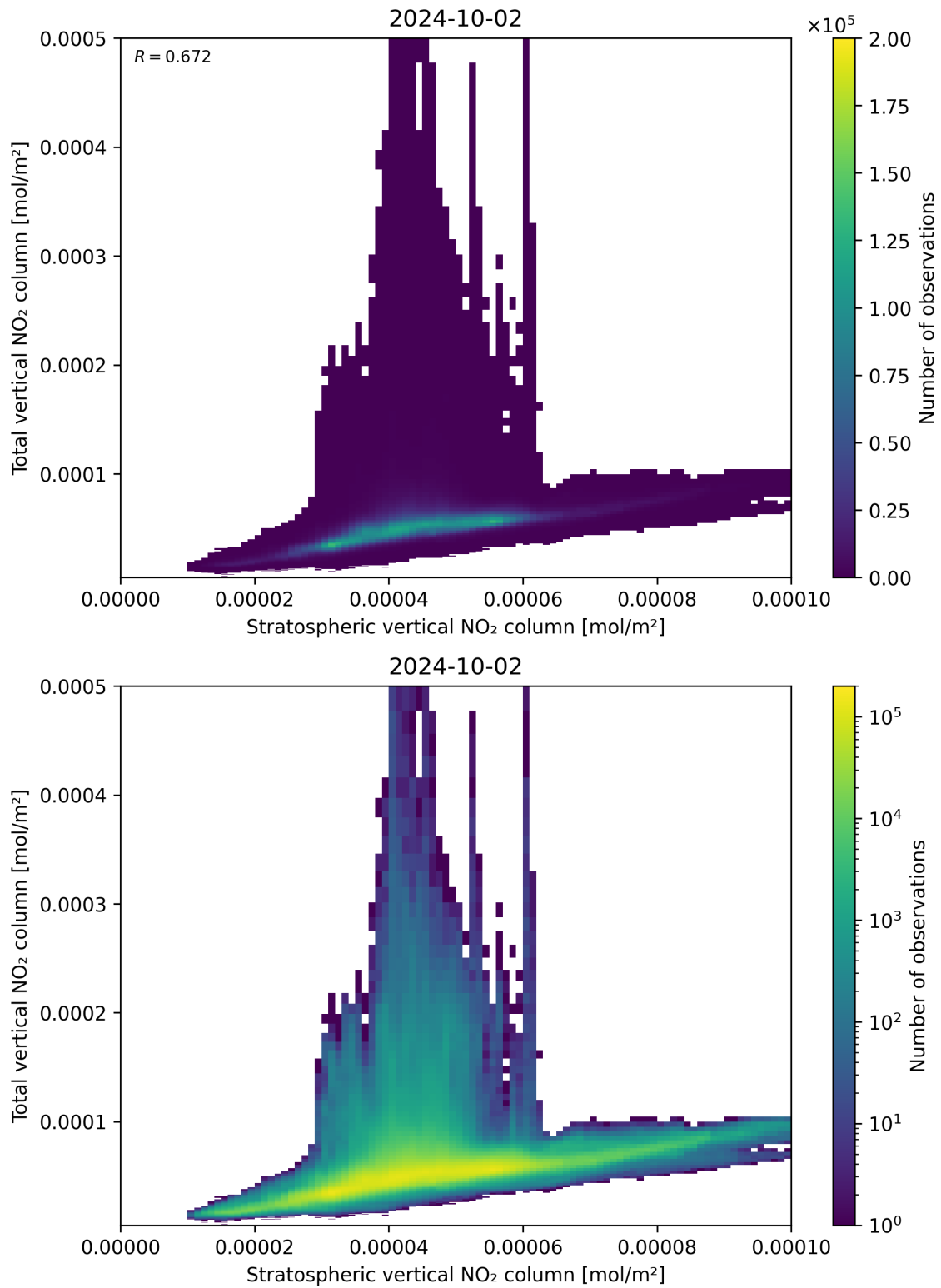
Figure 100: Scatter density plot of “Stratospheric vertical NO 2 column” against “Total vertical NO 2 column” for 2024-10-01 to 2024-10-03.
