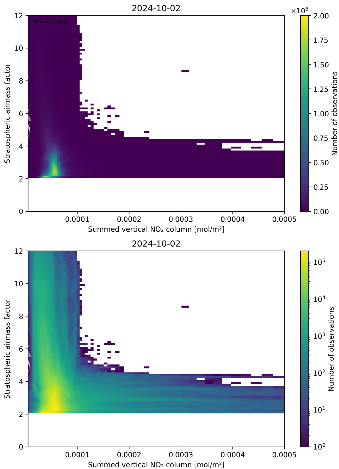
Figure 103: Scatter density plot of “Summed vertical NO 2 column” against “Stratospheric airmass factor” for 2024-10-01 to 2024-10-03.
