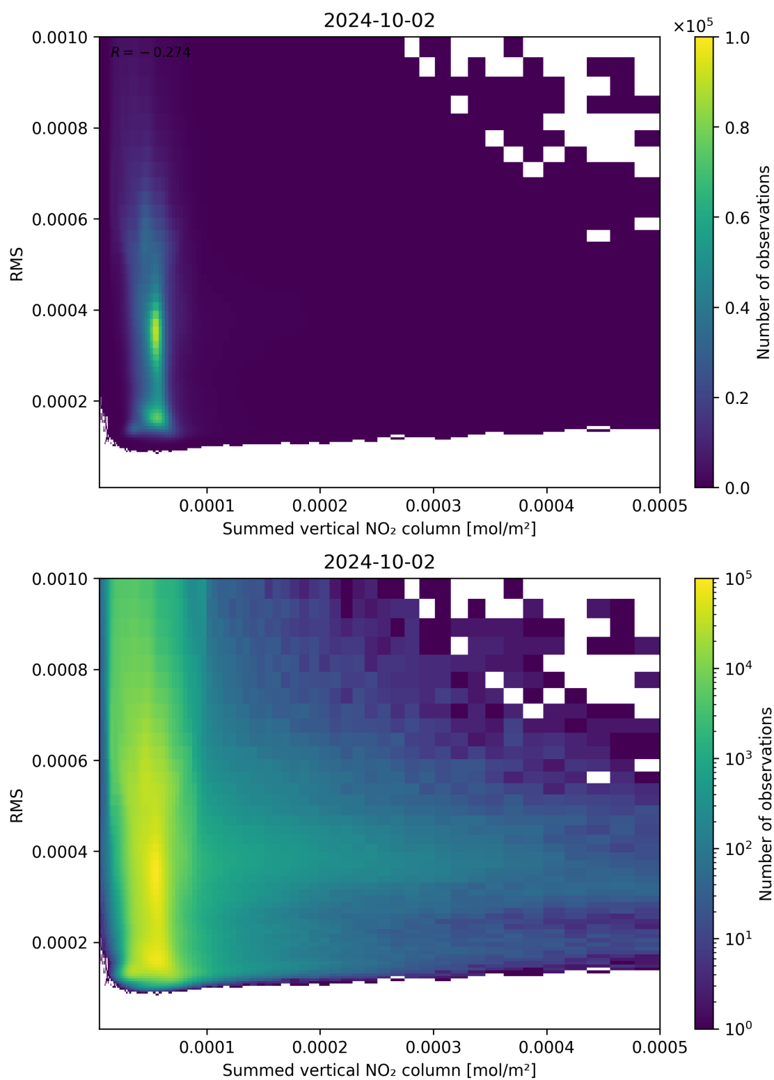
Figure 109: Scatter density plot of “Summed vertical NO 2 column” against “RMS” for 2024-10-01 to 2024-10-03.
