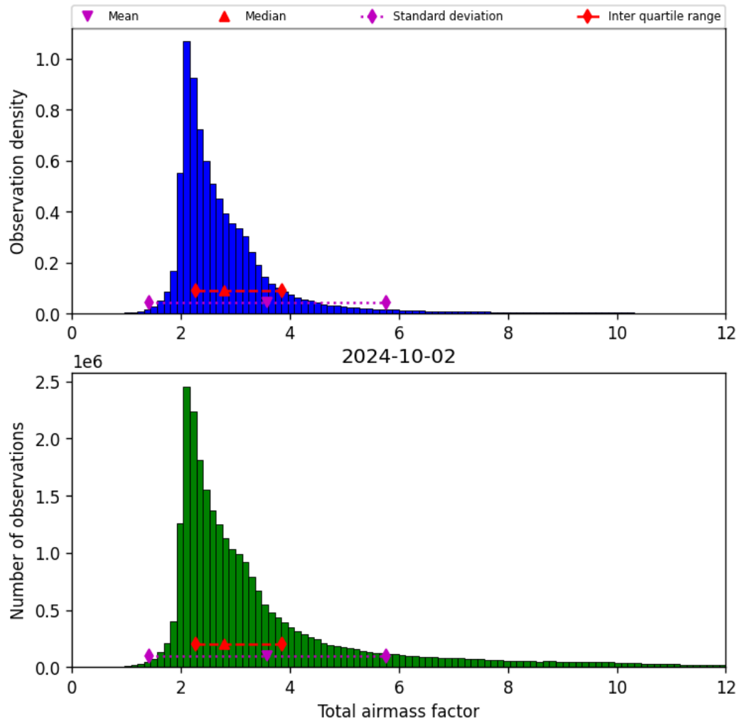
Figure 32: Histogram of “Total airmass factor” for 2024-10-01 to 2024-10-03
