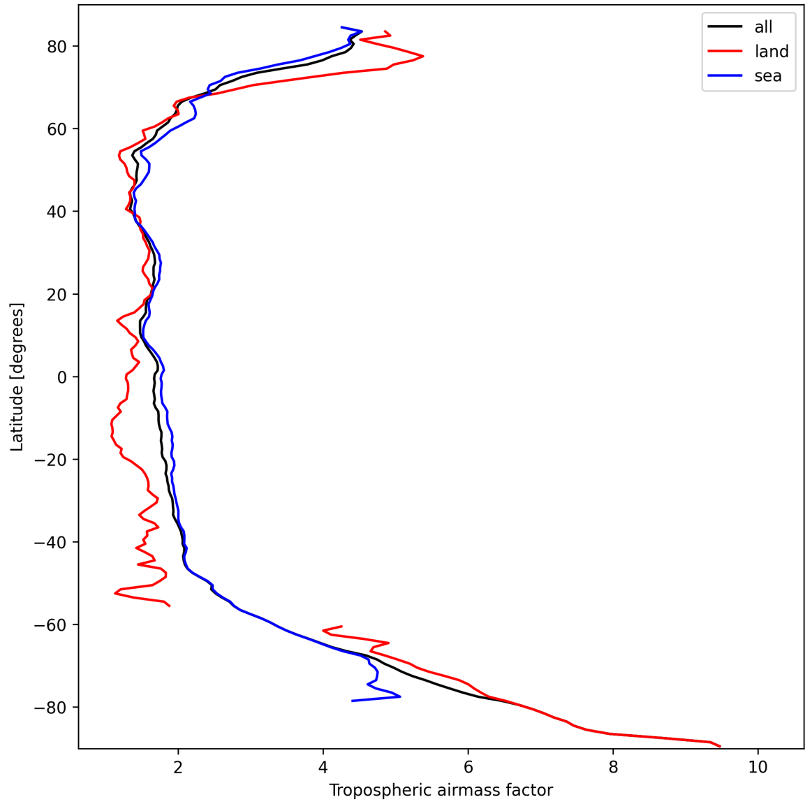
Figure 14: Zonal average of “Tropospheric air mass factor” for 2024-10-01 to 2024-10-03.
