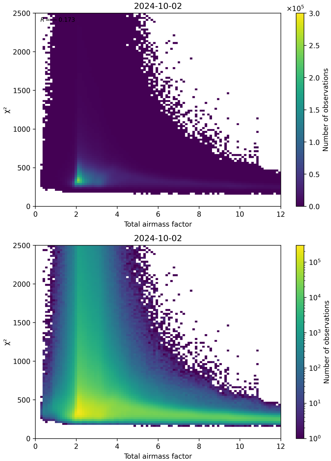
Figure 63: Scatter density plot of “Total airmass factor” against “ \chi^2 ” for 2024-10-01 to 2024-10-03.
