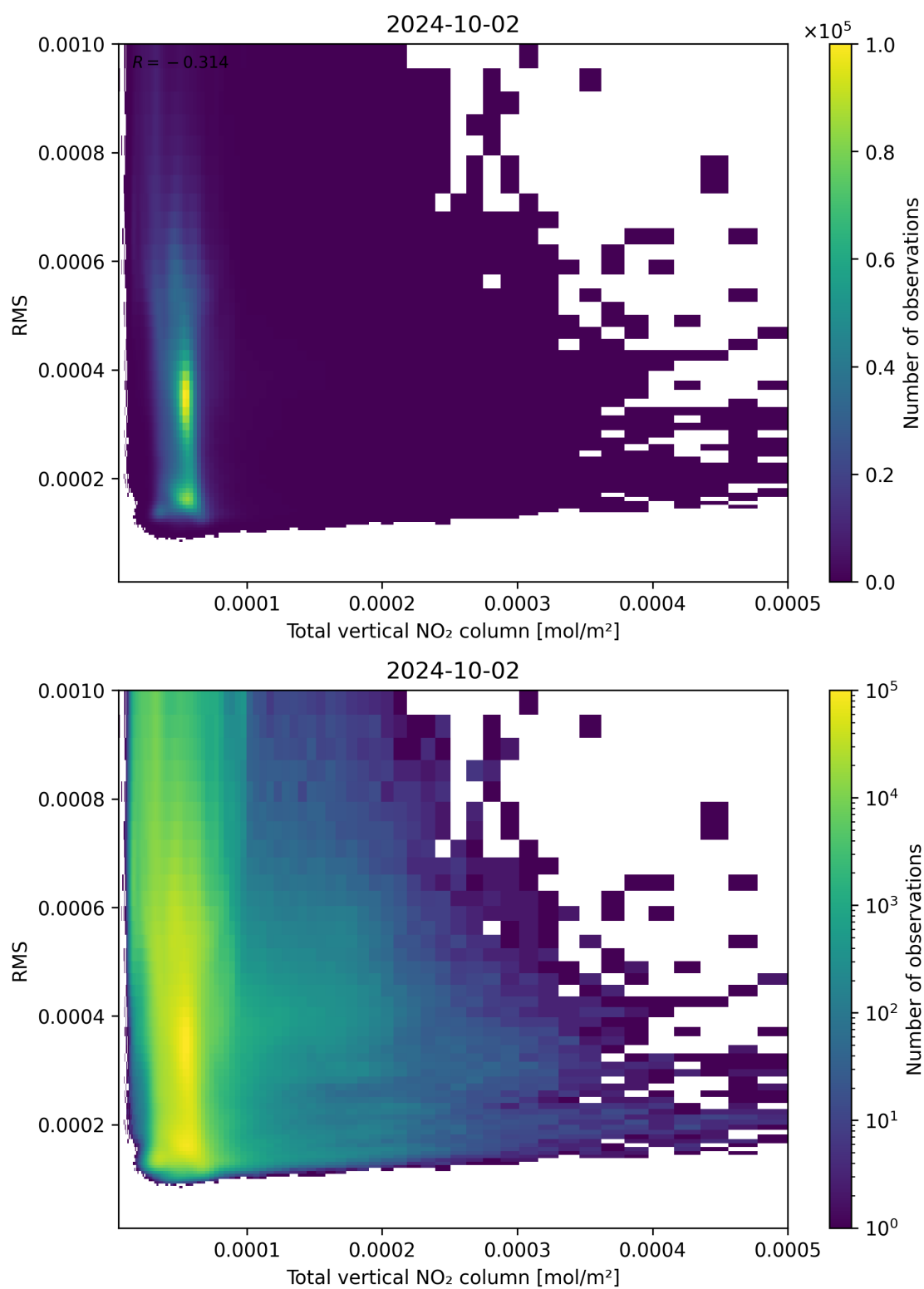
Figure 120: Scatter density plot of “Total vertical NO 2 column” against “RMS” for 2024-10-01 to 2024-10-03.
