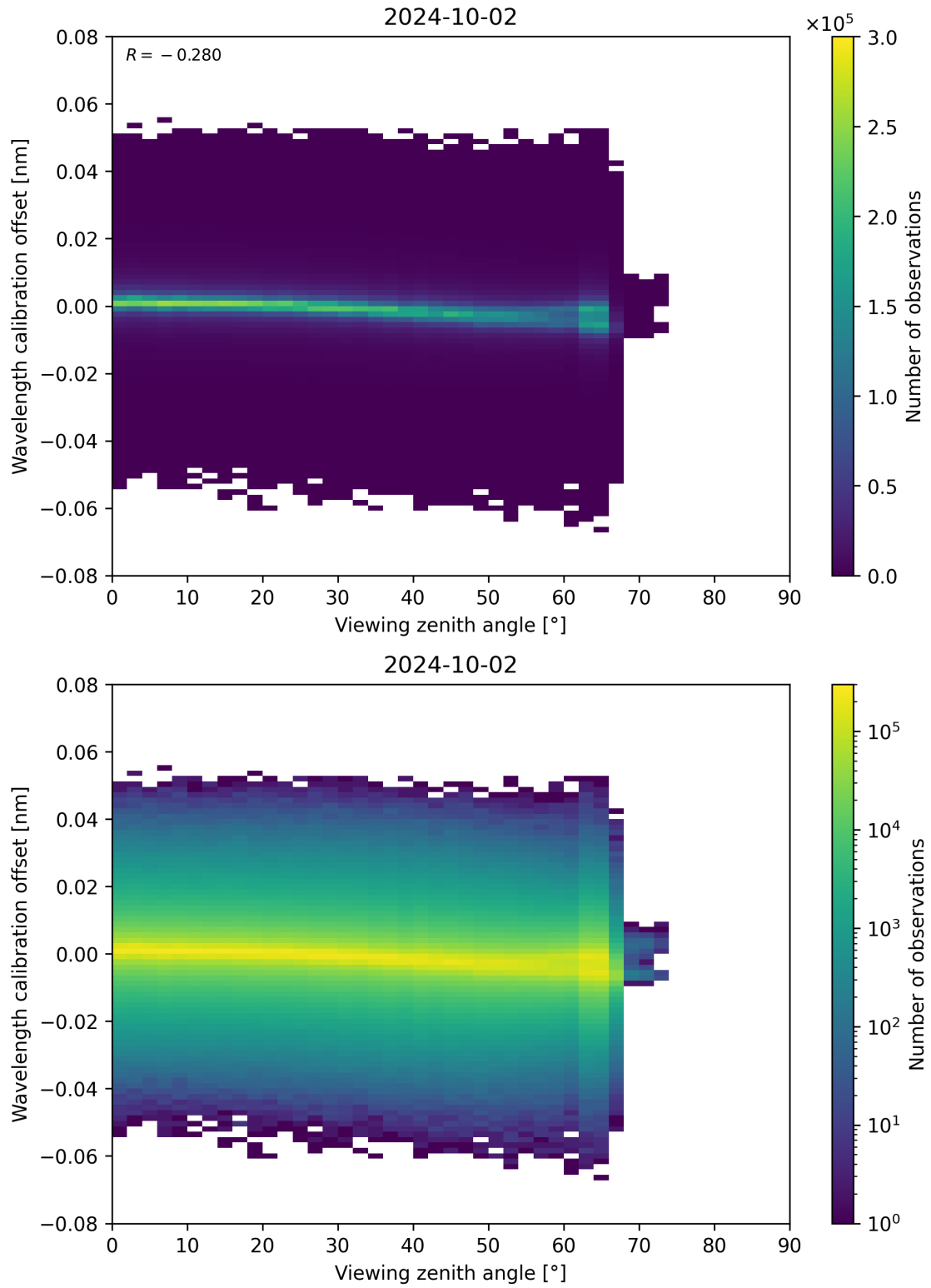
Figure 173: Scatter density plot of “Viewing zenith angle” against “Wavelength calibration offset” for 2024-10-01 to 2024-10-03.
