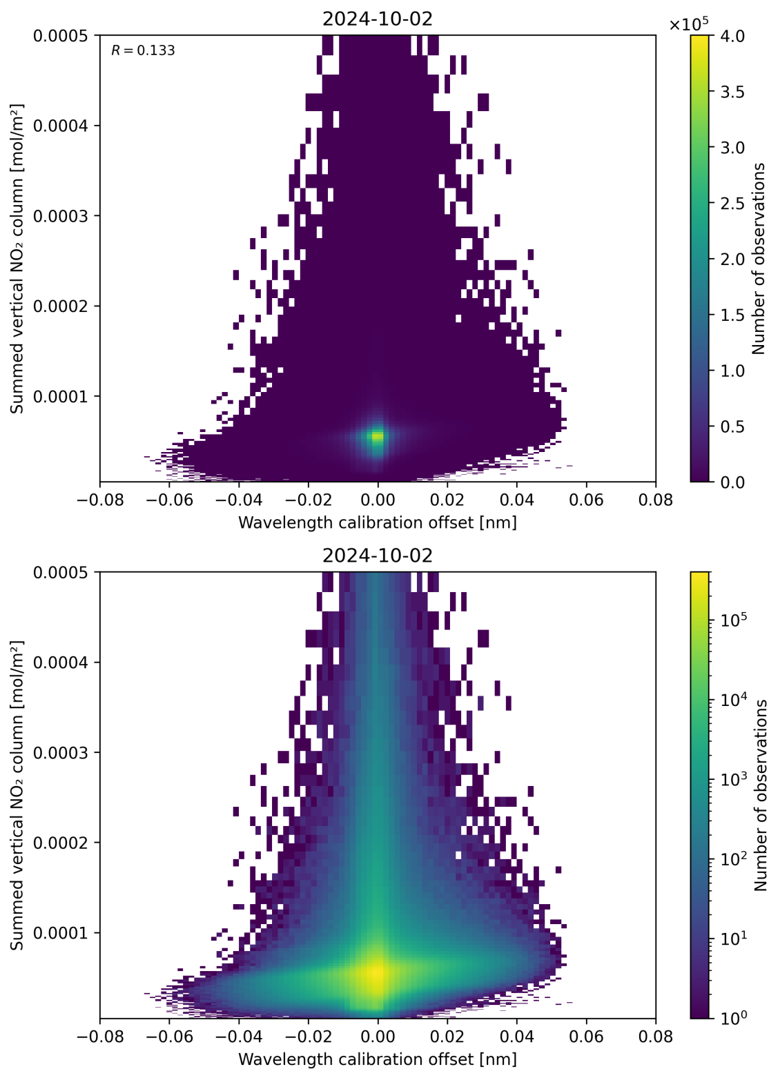
Figure 177: Scatter density plot of “Wavelength calibration offset” against “Summed vertical NO 2 column” for 2024-10-01 to 2024-10-03.
