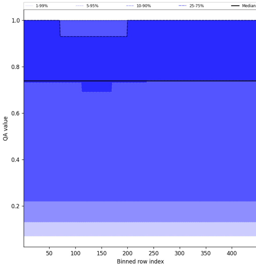
Figure 45: Along track statistics of “QA value” for 2024-10-01 to 2024-10-03
