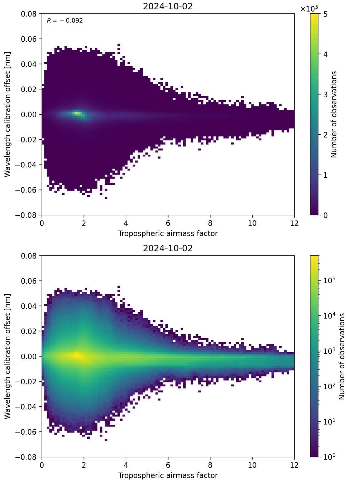
Figure 80: Scatter density plot of “Tropospheric airmass factor” against “Wavelength calibration offset” for 2024-10-01 to 2024-10-03.
