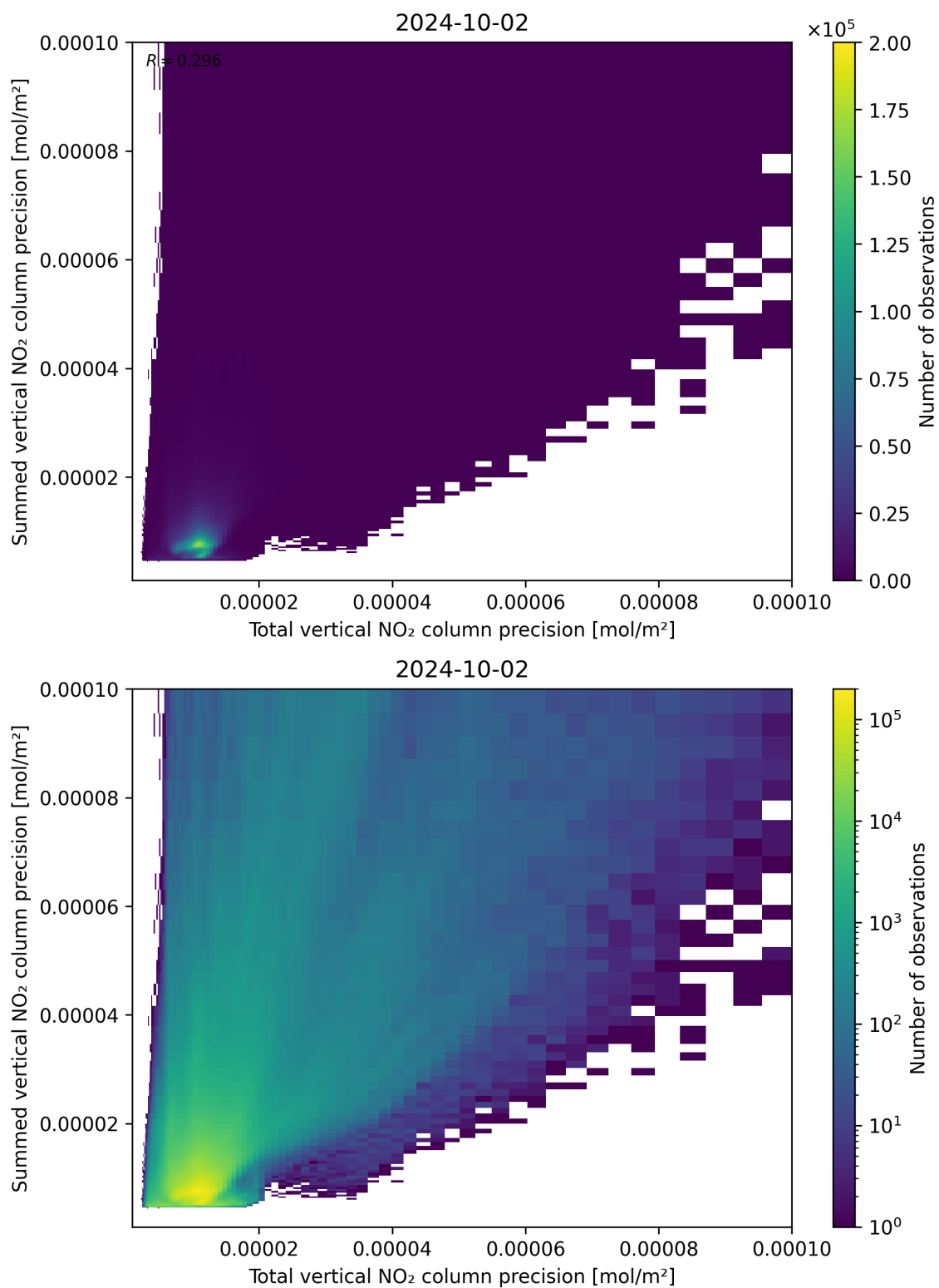
Figure 118: Scatter density plot of “Total vertical NO 2 column precision” against “Summed vertical NO 2 column precision” for 2024-10-01 to 2024-10-03.
