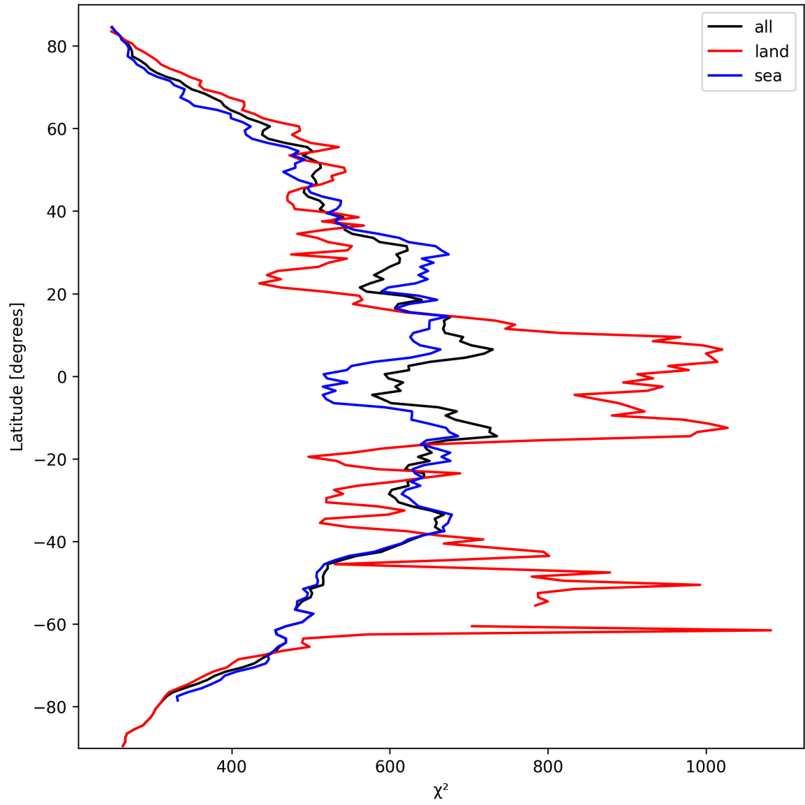
Figure 25: Zonal average of “ \chi^2 ” for 2024-10-01 to 2024-10-03.
