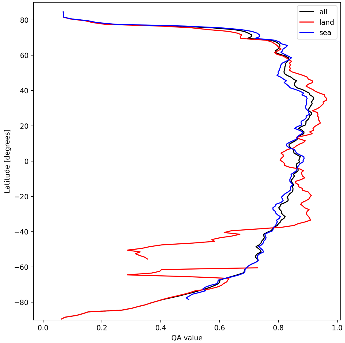
Figure 11: Zonal average of “QA value” for 2024-10-01 to 2024-10-03.
