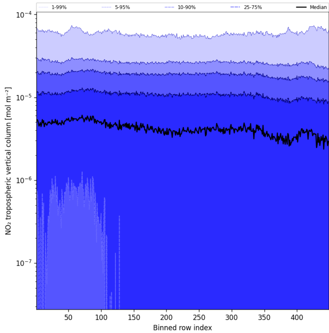
Figure 46: Along track statistics of “NO 2 tropospheric vertical column” for 2024-10-01 to 2024-10-03
