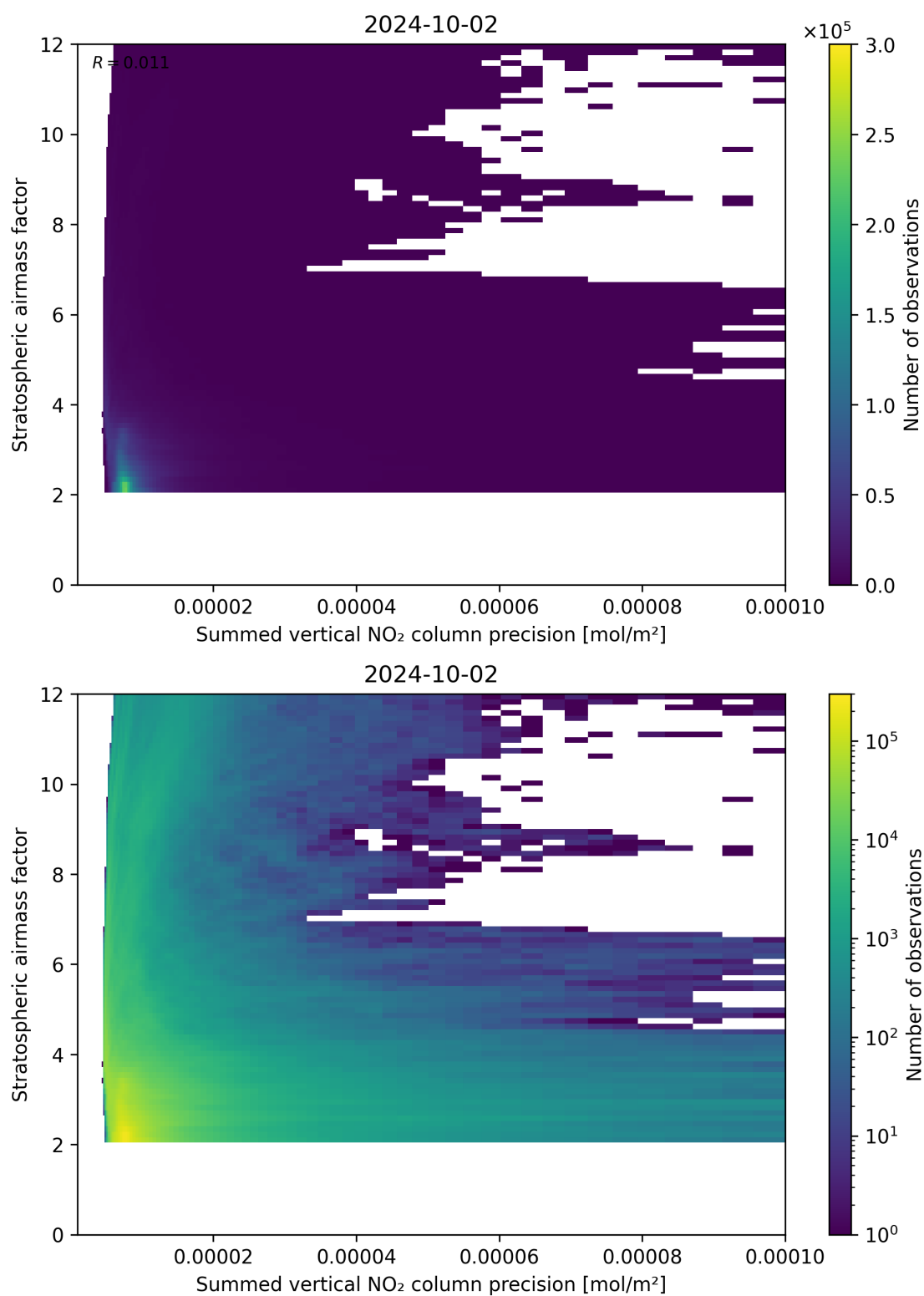
Figure 106: Scatter density plot of “Summed vertical NO 2 column precision” against “Stratospheric airmass factor” for 2024-10-01 to 2024-10-03.
