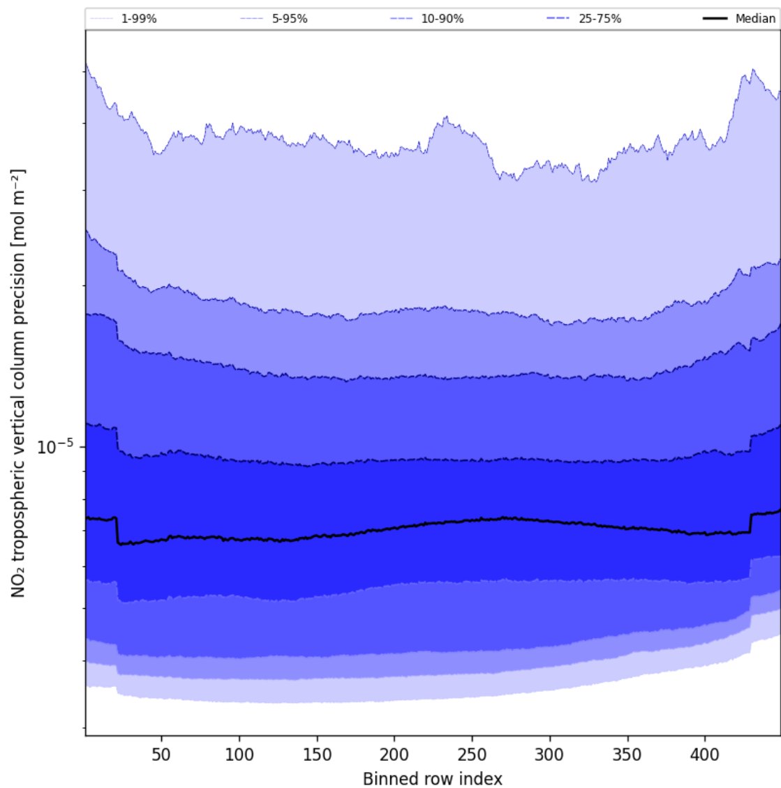
Figure 47: Along track statistics of “NO 2 tropospheric vertical column precision” for 2024-10-01 to 2024-10-03
