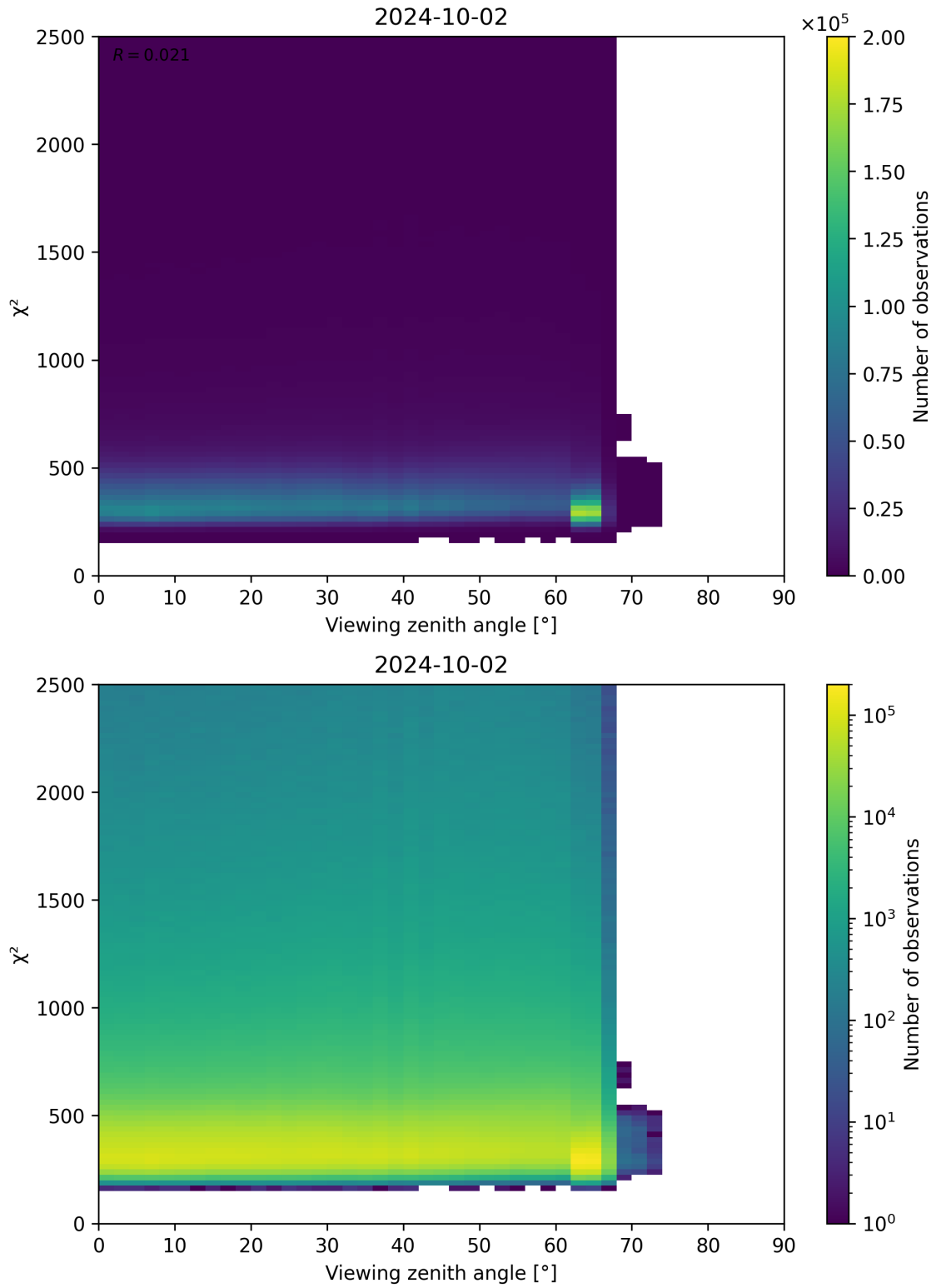
Figure 162: Scatter density plot of “Viewing zenith angle” against “ \chi^2 ” for 2024-10-01 to 2024-10-03.
