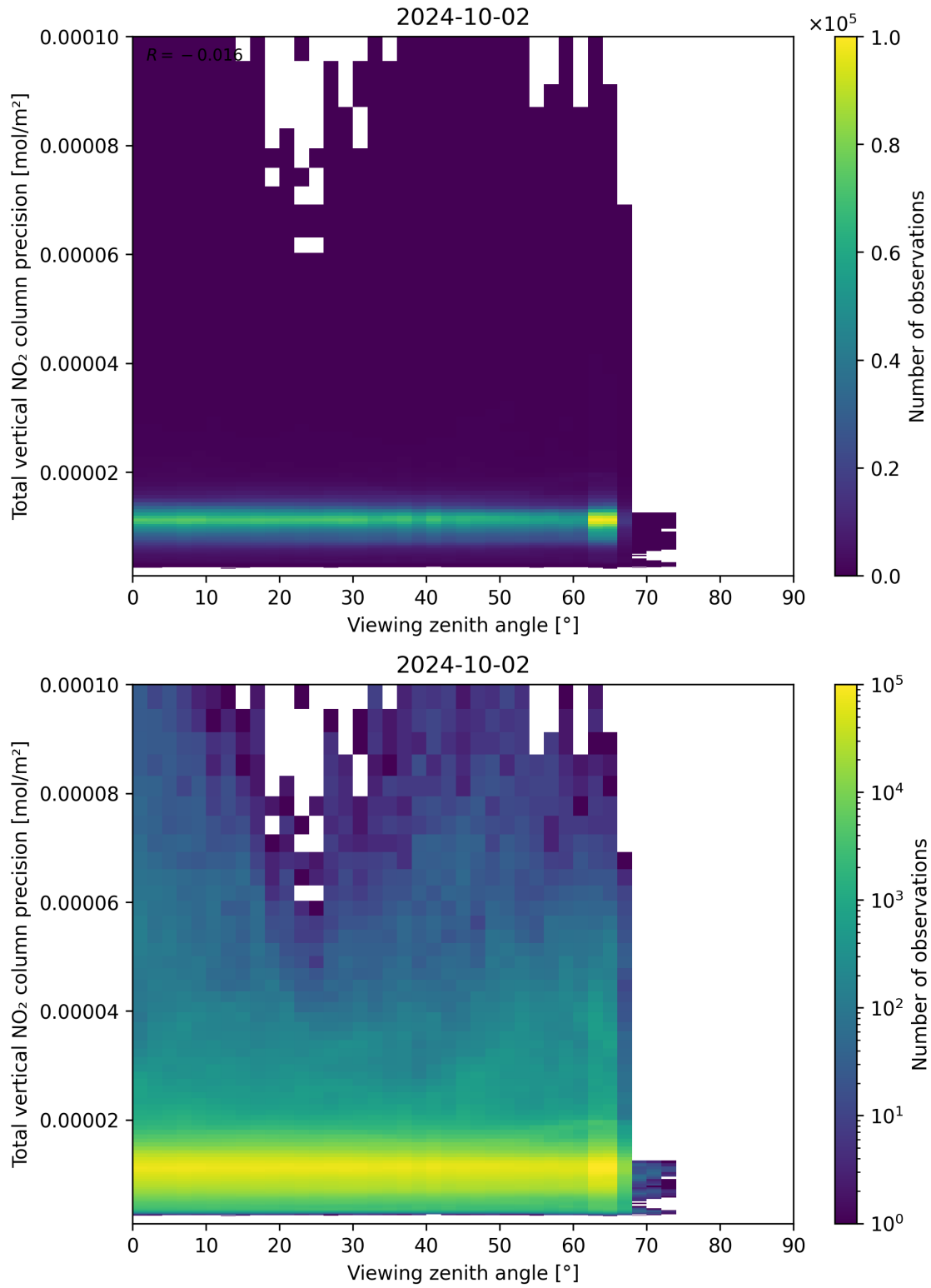
Figure 168: Scatter density plot of “Viewing zenith angle” against “Total vertical NO 2 column precision” for 2024-10-01 to 2024-10-03.
