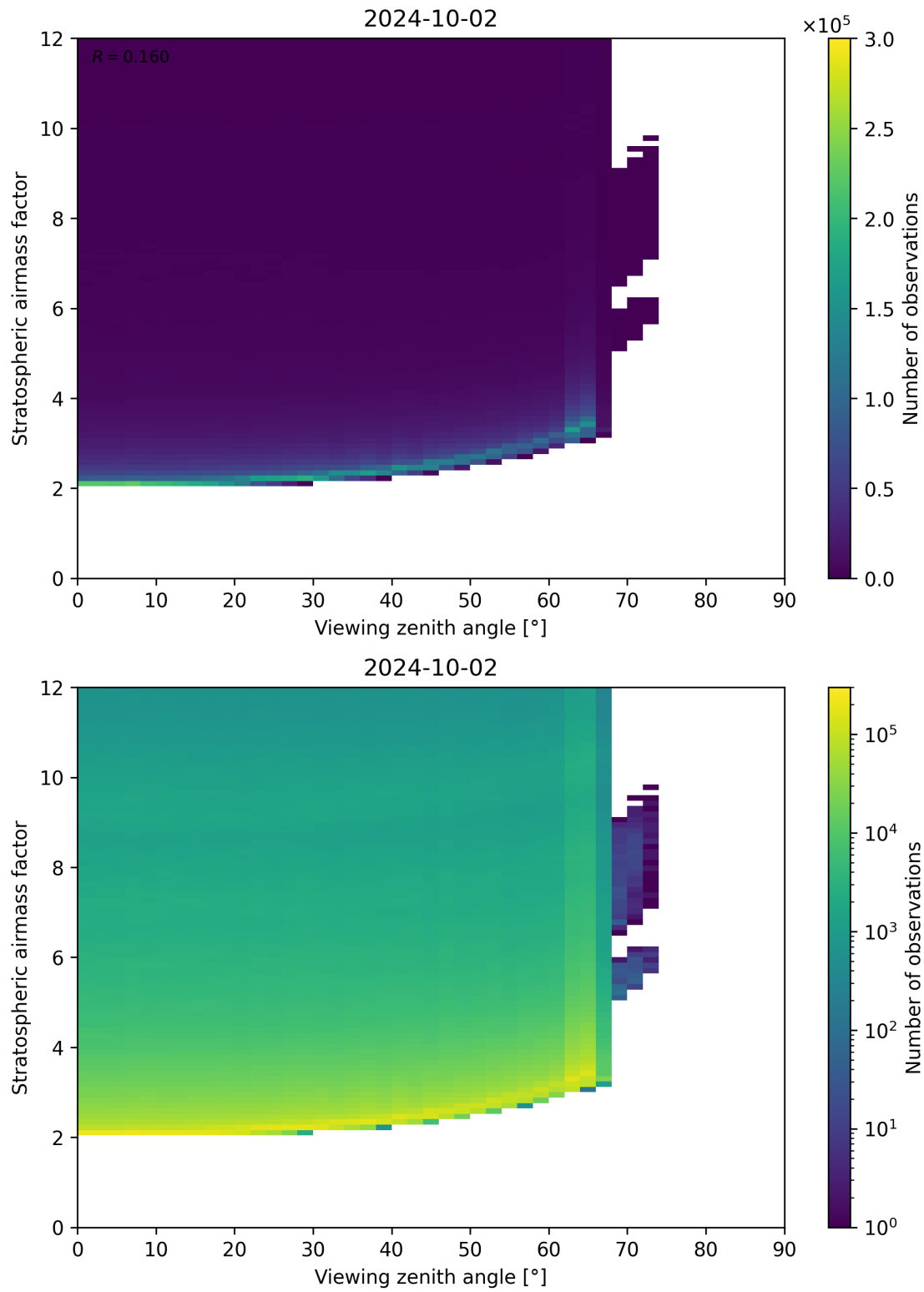
Figure 159: Scatter density plot of “Viewing zenith angle” against “Stratospheric airmass factor” for 2024-10-01 to 2024-10-03.
