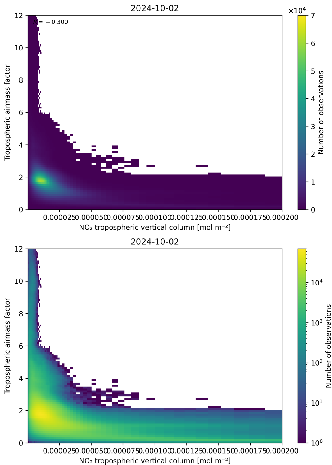
Figure 123: Scatter density plot of “NO 2 tropospheric vertical column” against “Tropospheric air mass factor” for 2024-10-01 to 2024-10-03.
