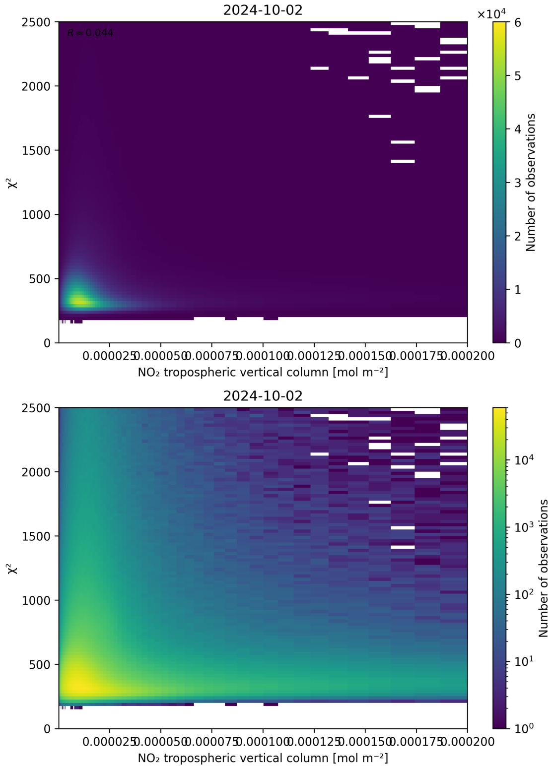
Figure 124: Scatter density plot of “NO 2 tropospheric vertical column” against “ \chi^2 ” for 2024-10-01 to 2024-10-03.
