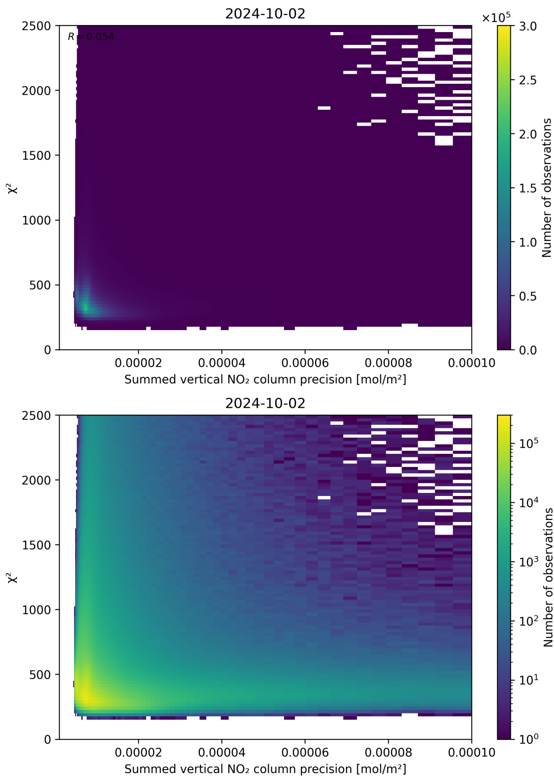
Figure 107: Scatter density plot of “Summed vertical NO 2 column precision” against “ \chi^2 ” for 2024-10-01 to 2024-10-03.
