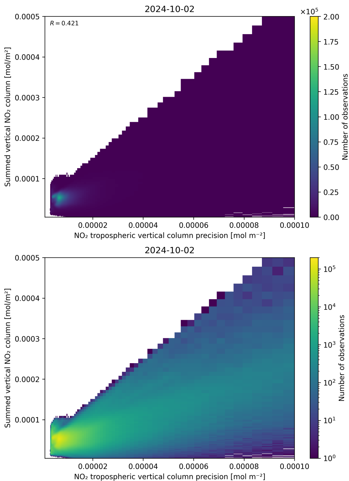
Figure 136: Scatter density plot of “NO 2 tropospheric vertical column precision” against “Summed vertical NO 2 column” for 2024-10-01 to 2024-10-03.
