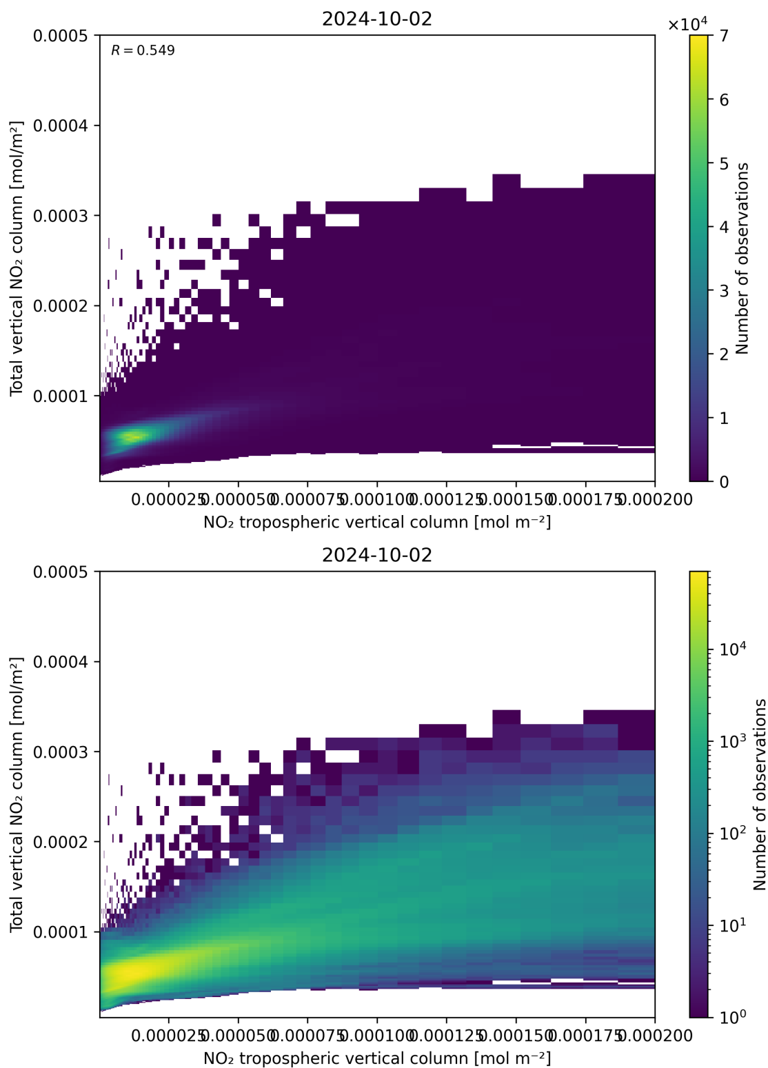
Figure 128: Scatter density plot of “NO 2 tropospheric vertical column” against “Total vertical NO 2 column” for 2024-10-01 to 2024-10-03.
