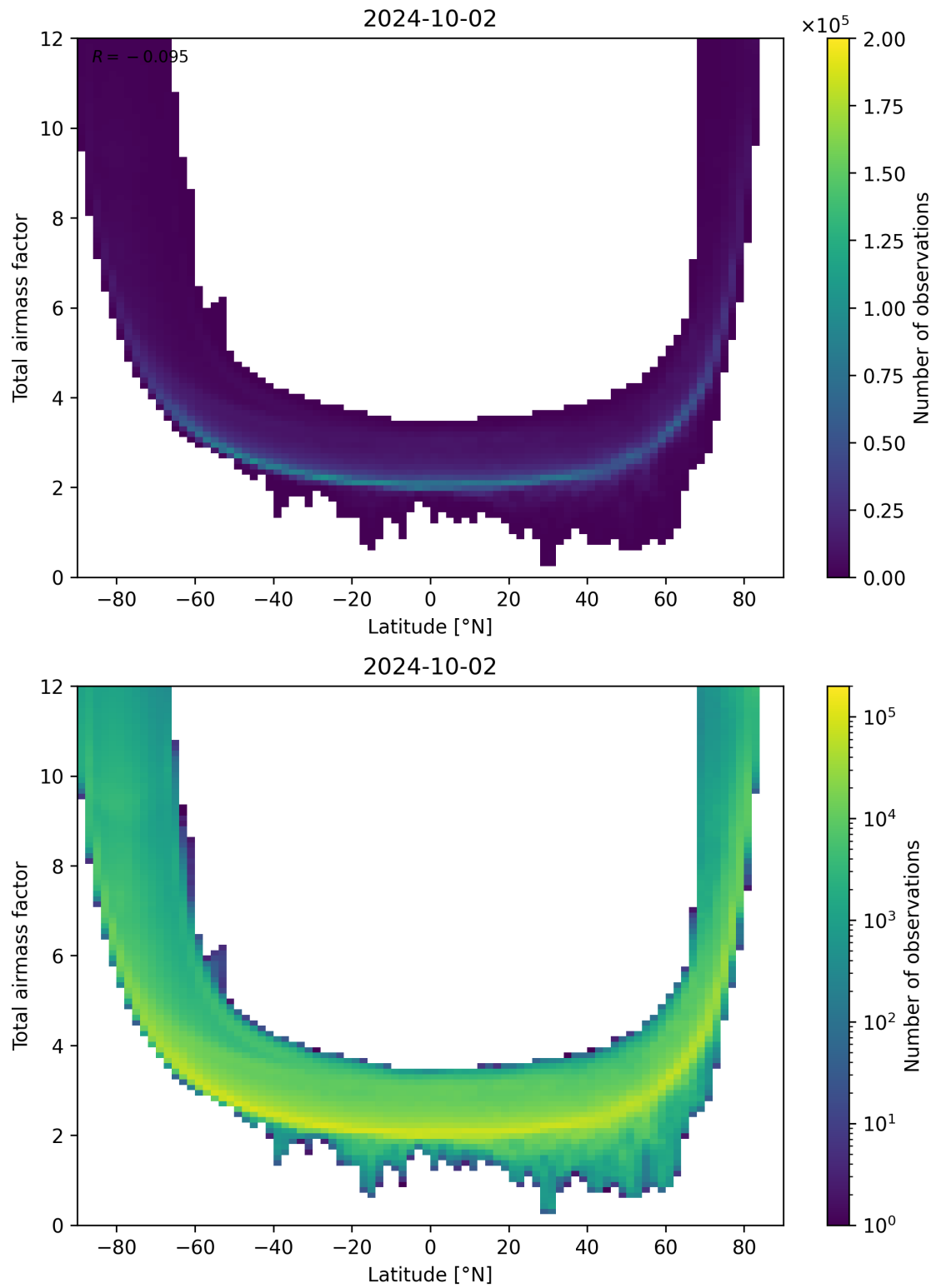
Figure 84: Scatter density plot of “Latitude” against “Total airmass factor” for 2024-10-01 to 2024-10-03.
