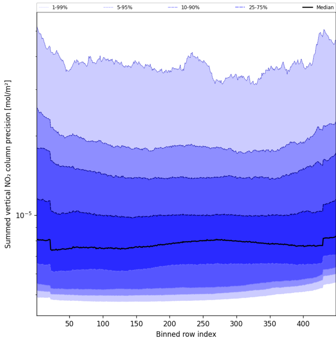
Figure 58: Along track statistics of “Summed vertical NO 2 column precision” for 2024-10-01 to 2024-10-03
