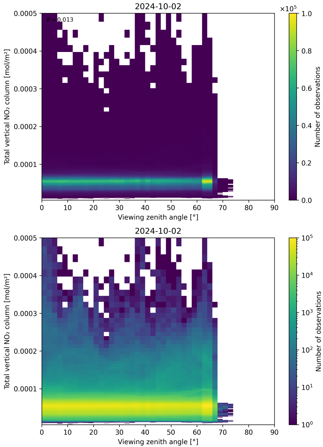
Figure 167: Scatter density plot of “Viewing zenith angle” against “Total vertical NO 2 column” for 2024-10-01 to 2024-10-03.
