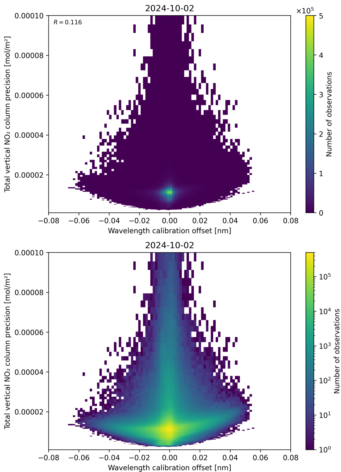
Figure 180: Scatter density plot of “Wavelength calibration offset” against “Total vertical NO 2 column precision” for 2024-10-01 to 2024-10-03.
