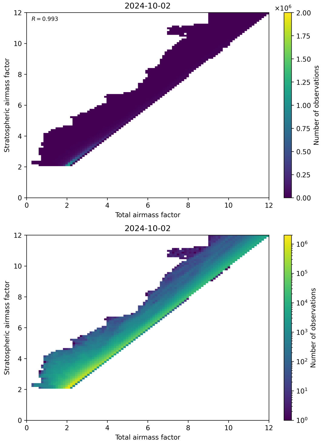
Figure 62: Scatter density plot of “Total airmass factor” against “Stratospheric airmass factor” for 2024-10-01 to 2024-10-03.
