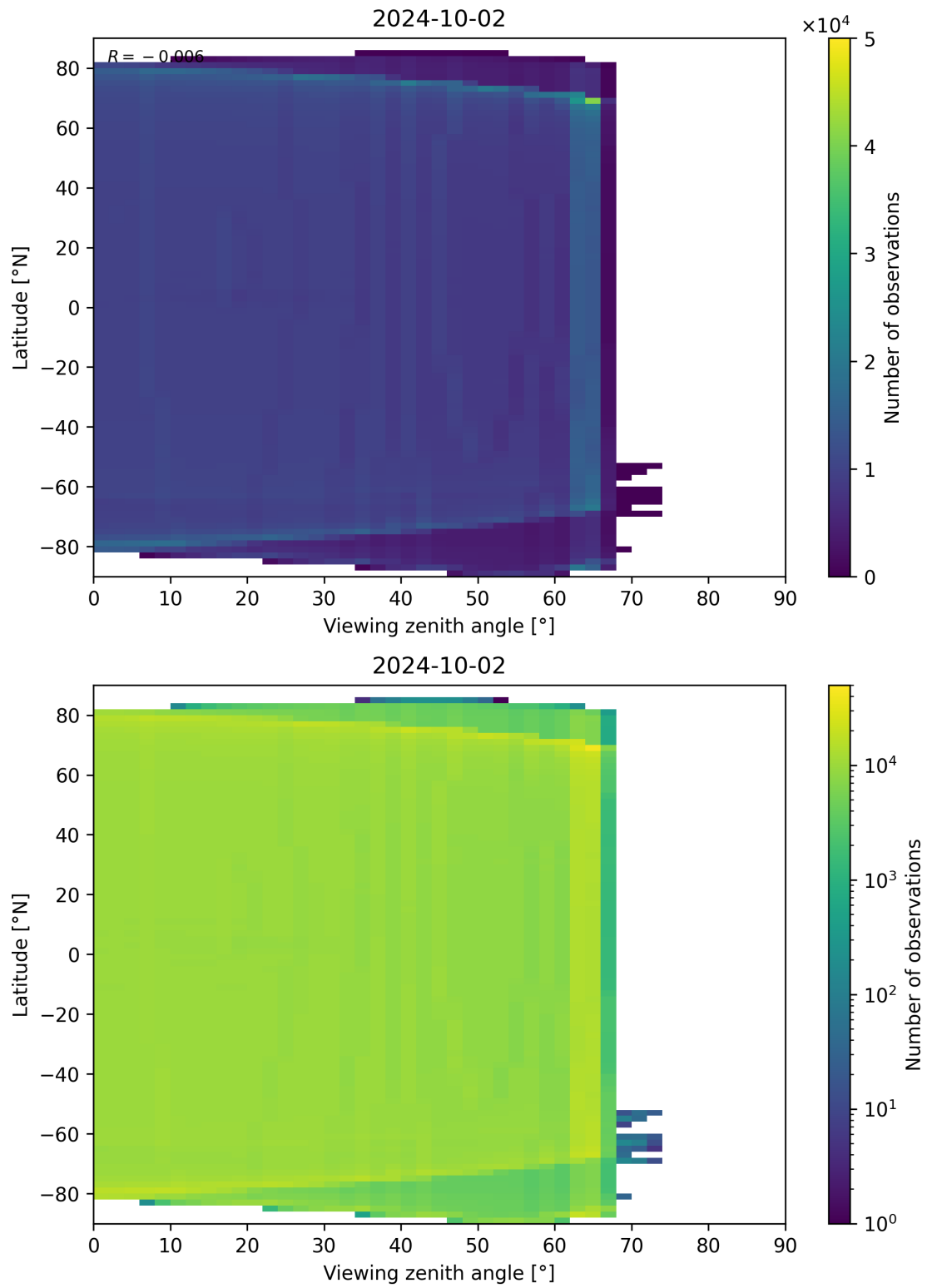
Figure 163: Scatter density plot of “Viewing zenith angle” against “Latitude” for 2024-10-01 to 2024-10-03.
