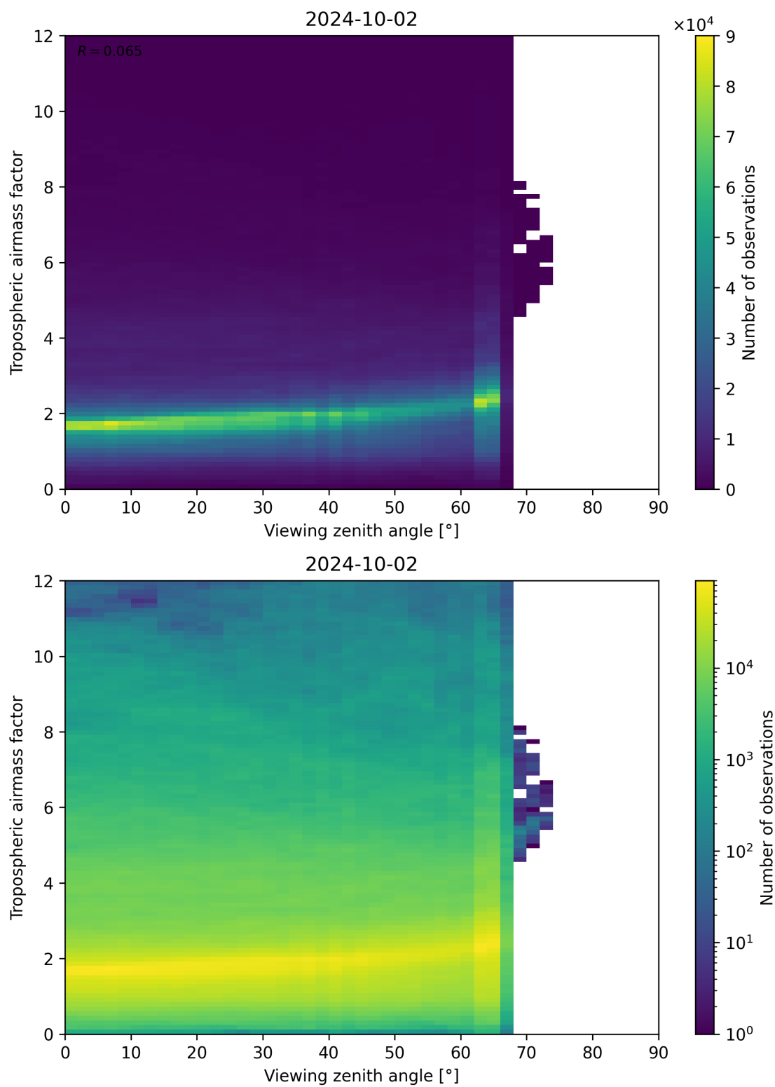
Figure 161: Scatter density plot of “Viewing zenith angle” against “Tropospheric air mass factor” for 2024-10-01 to 2024-10-03.
