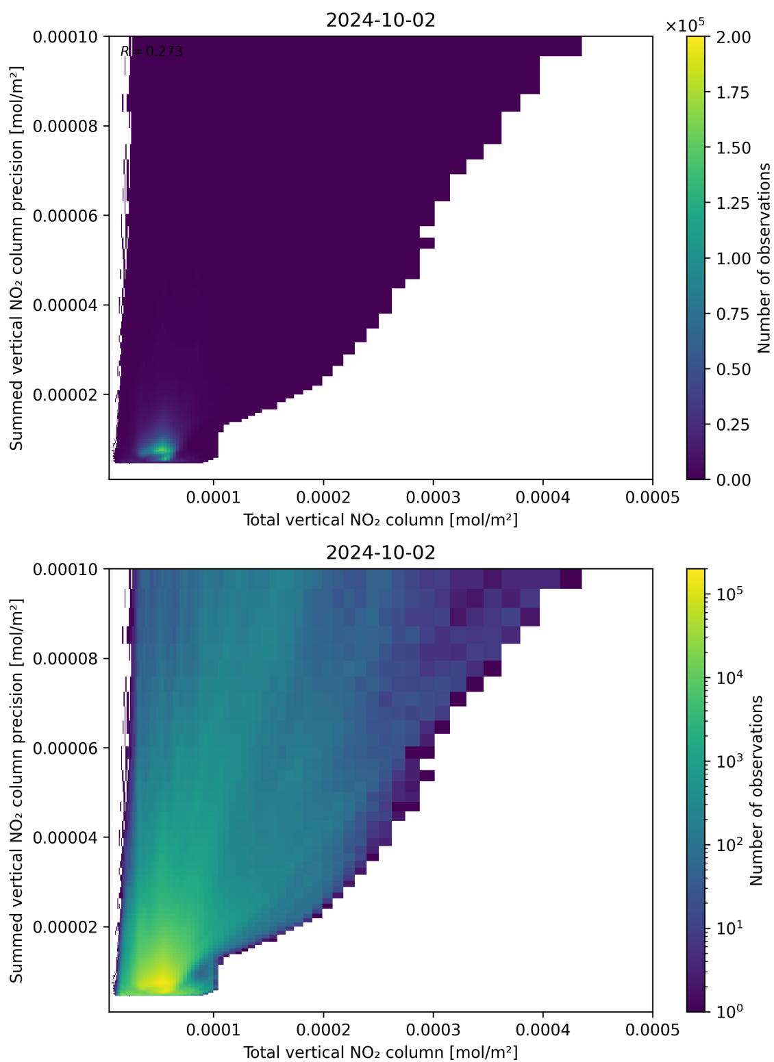
Figure 113: Scatter density plot of “Total vertical NO 2 column” against “Summed vertical NO 2 column precision” for 2024-10-01 to 2024-10-03.
