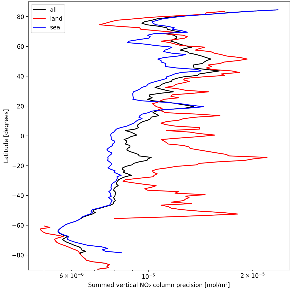
Figure 24: Zonal average of “Summed vertical NO 2 column precision” for 2024-10-01 to 2024-10-03.
