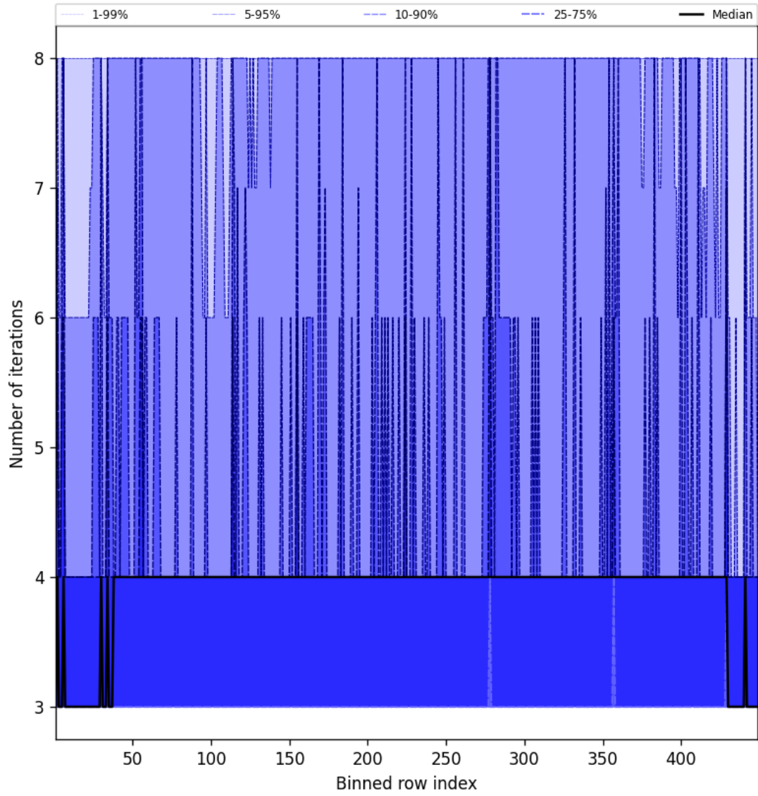
Figure 51: Along track statistics of “Number of iterations” for 2024-10-01 to 2024-10-03
