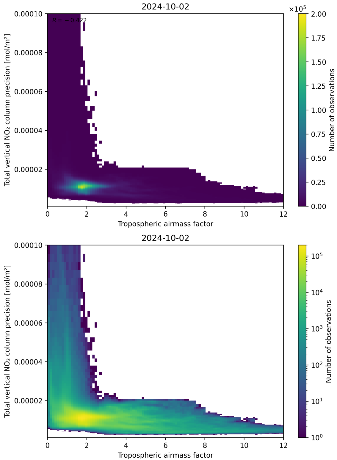
Figure 78: Scatter density plot of “Tropospheric air mass factor” against “Total vertical NO 2 column precision” for 2024-10-01 to 2024-10-03.
