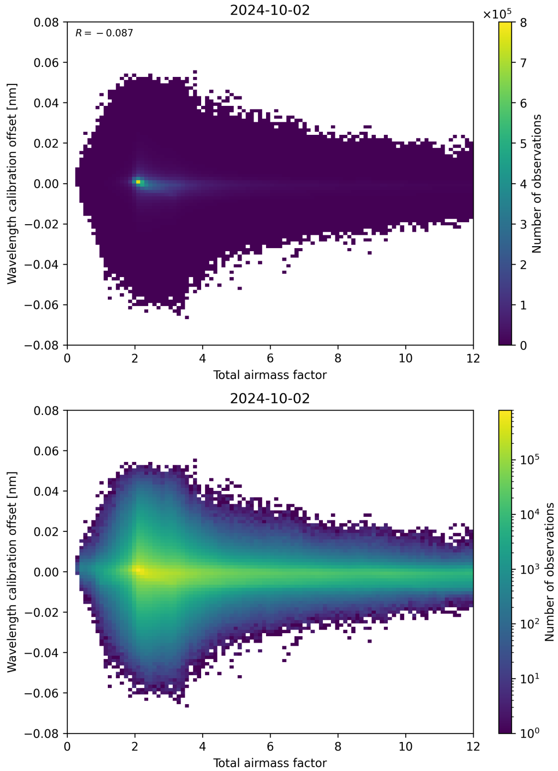
Figure 70: Scatter density plot of “Total airmass factor” against “Wavelength calibration offset” for 2024-10-01 to 2024-10-03.
