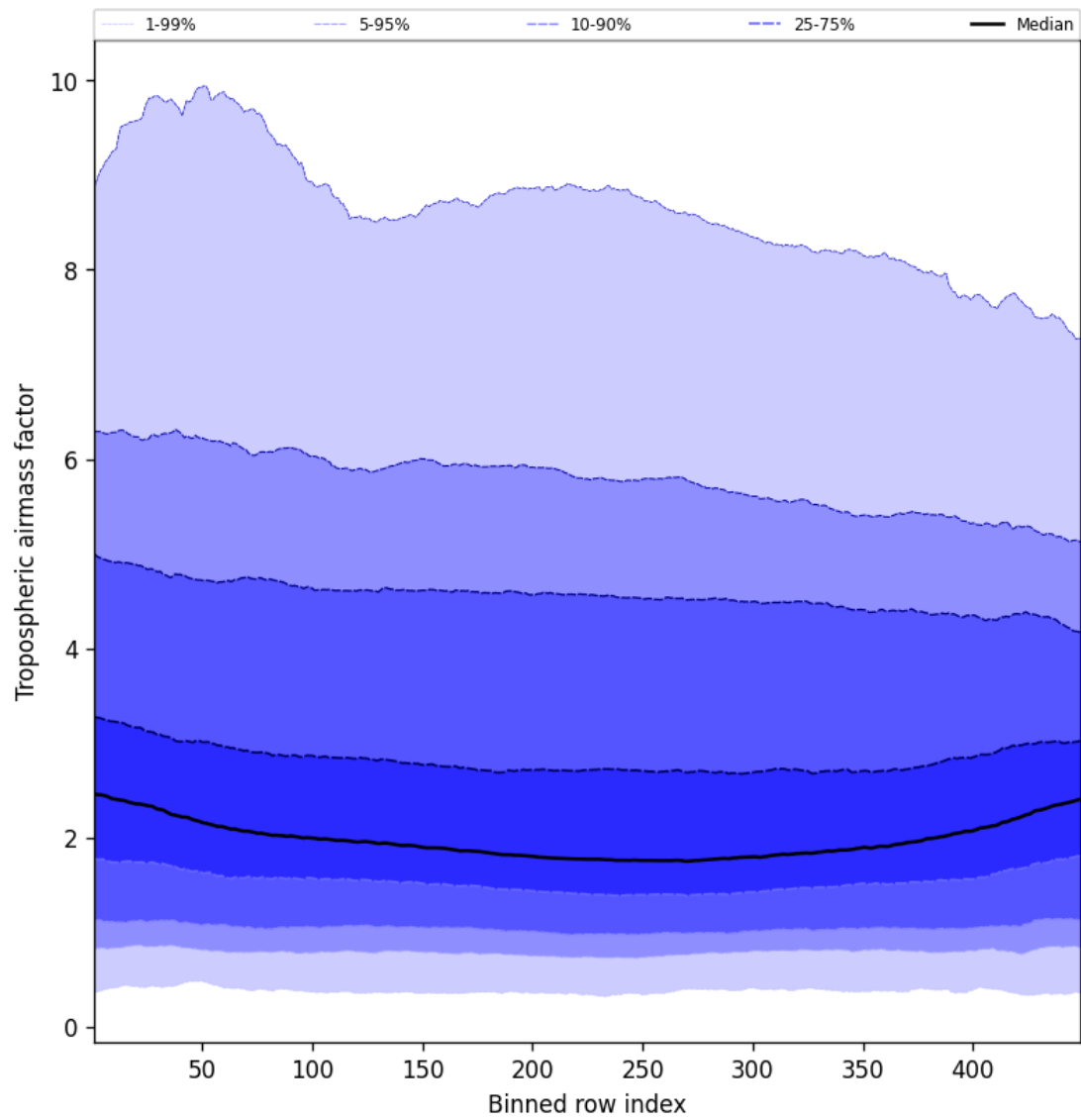
Figure 48: Along track statistics of “Tropospheric airmass factor” for 2024-10-01 to 2024-10-03
