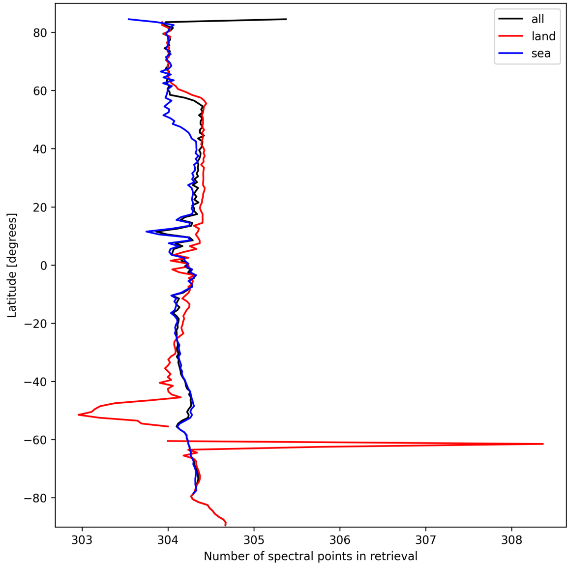
Figure 16: Zonal average of “Number of spectral points in retrieval” for 2024-10-01 to 2024-10-03.
