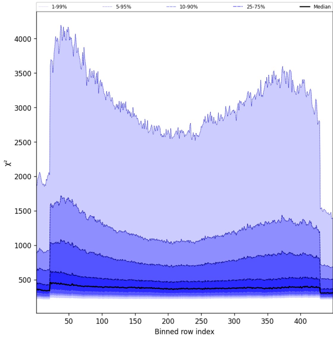
Figure 59: Along track statistics of “ \chi^2 ” for 2024-10-01 to 2024-10-03
