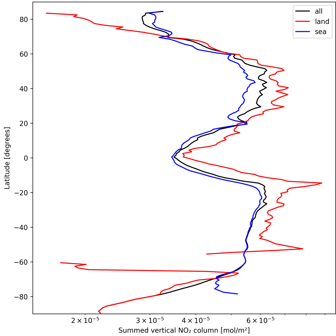
Figure 23: Zonal average of “Summed vertical NO 2 column” for 2024-10-01 to 2024-10-03.
