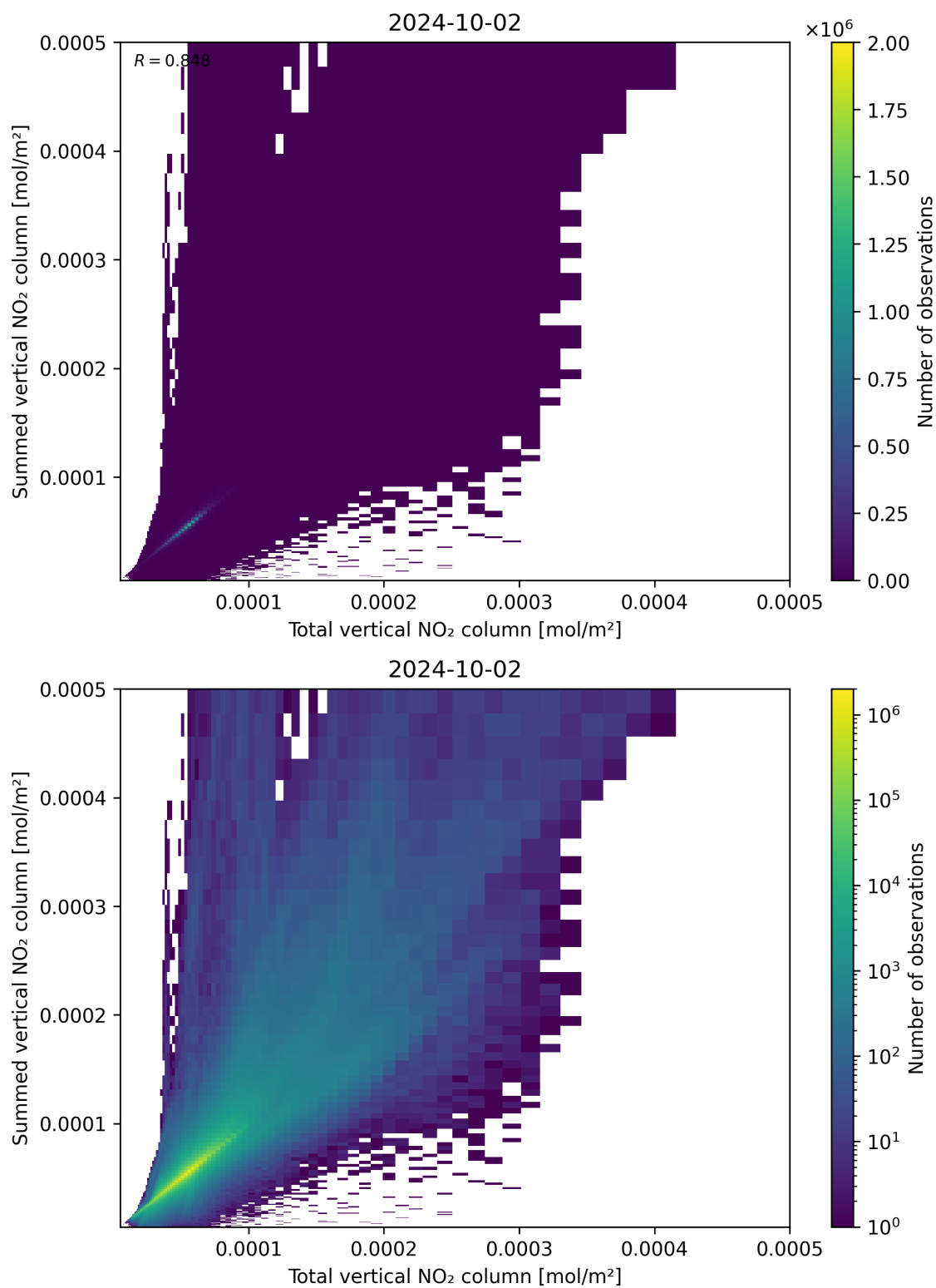
Figure 112: Scatter density plot of “Total vertical NO 2 column” against “Summed vertical NO 2 column” for 2024-10-01 to 2024-10-03.
