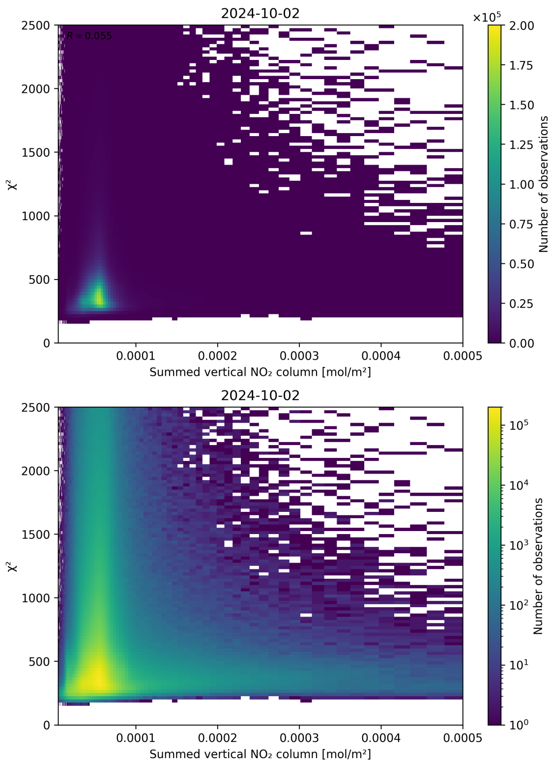
Figure 104: Scatter density plot of “Summed vertical NO 2 column” against “ \chi^2 ” for 2024-10-01 to 2024-10-03.
