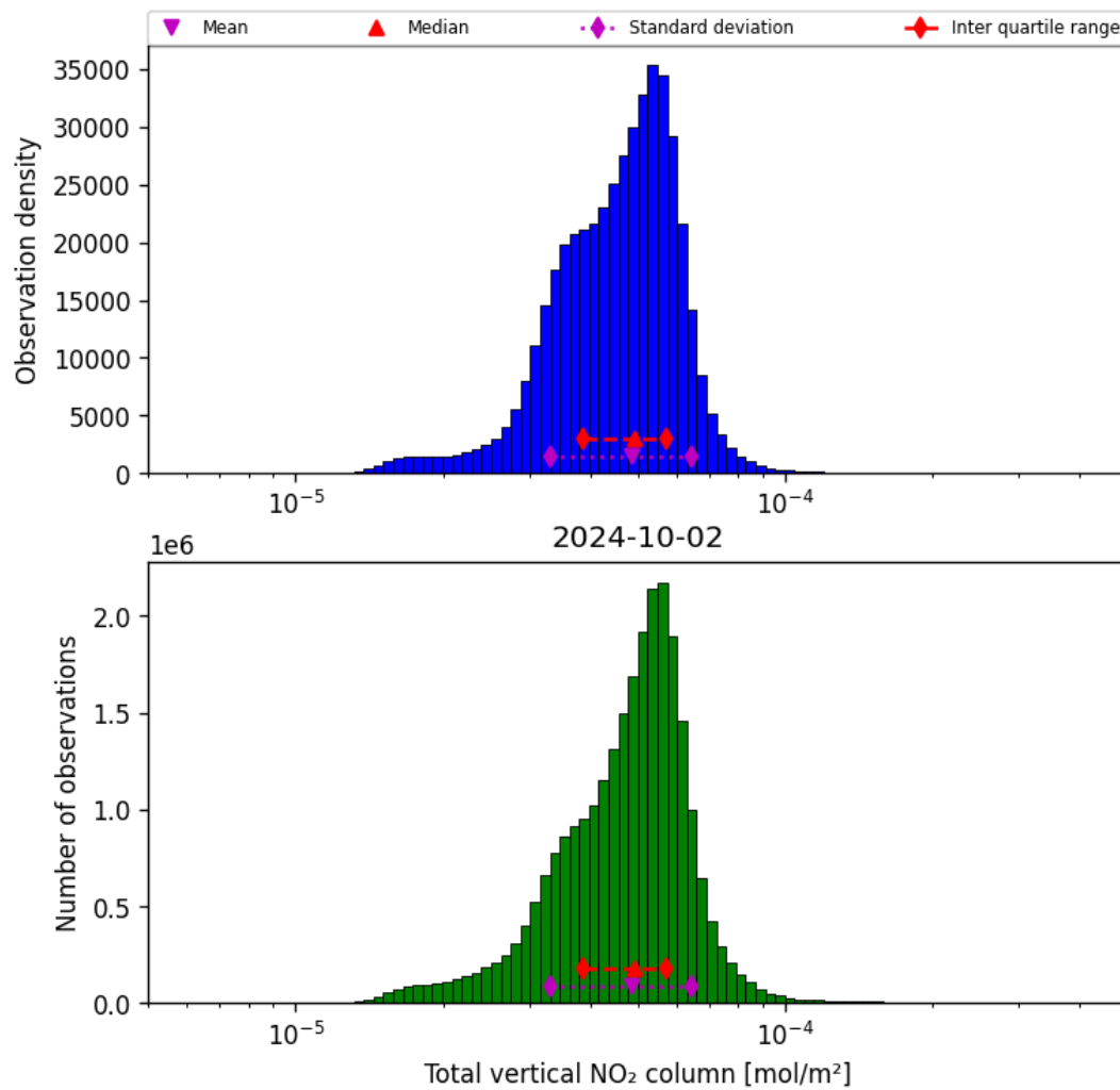
Figure 38: Histogram of “Total vertical NO 2 column” for 2024-10-01 to 2024-10-03
