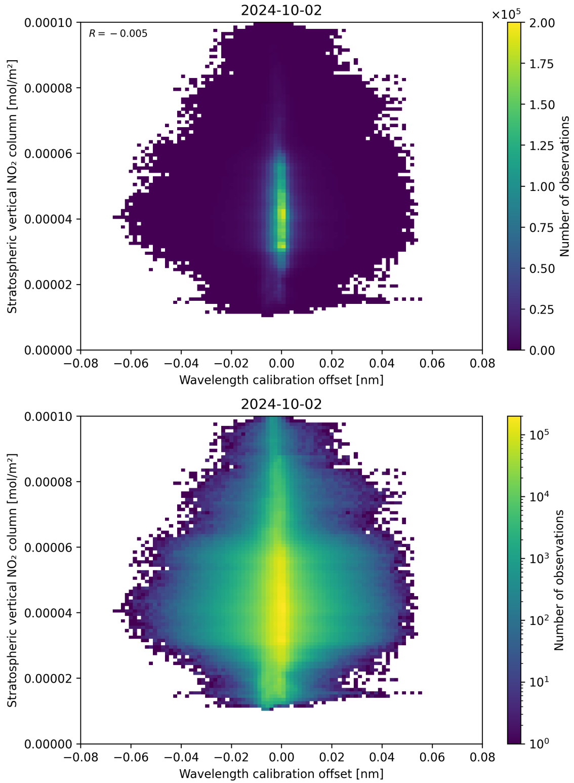
Figure 176: Scatter density plot of “Wavelength calibration offset” against “Stratospheric vertical NO 2 column” for 2024-10-01 to 2024-10-03.
