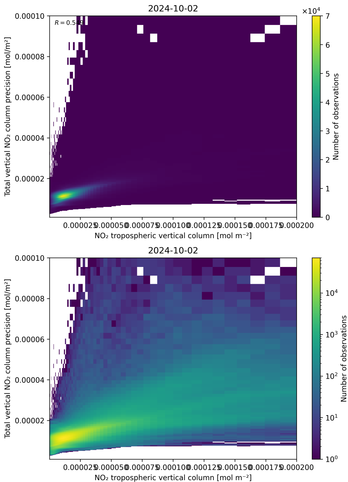
Figure 129: Scatter density plot of “NO 2 tropospheric vertical column” against “Total vertical NO 2 column precision” for 2024-10-01 to 2024-10-03.
