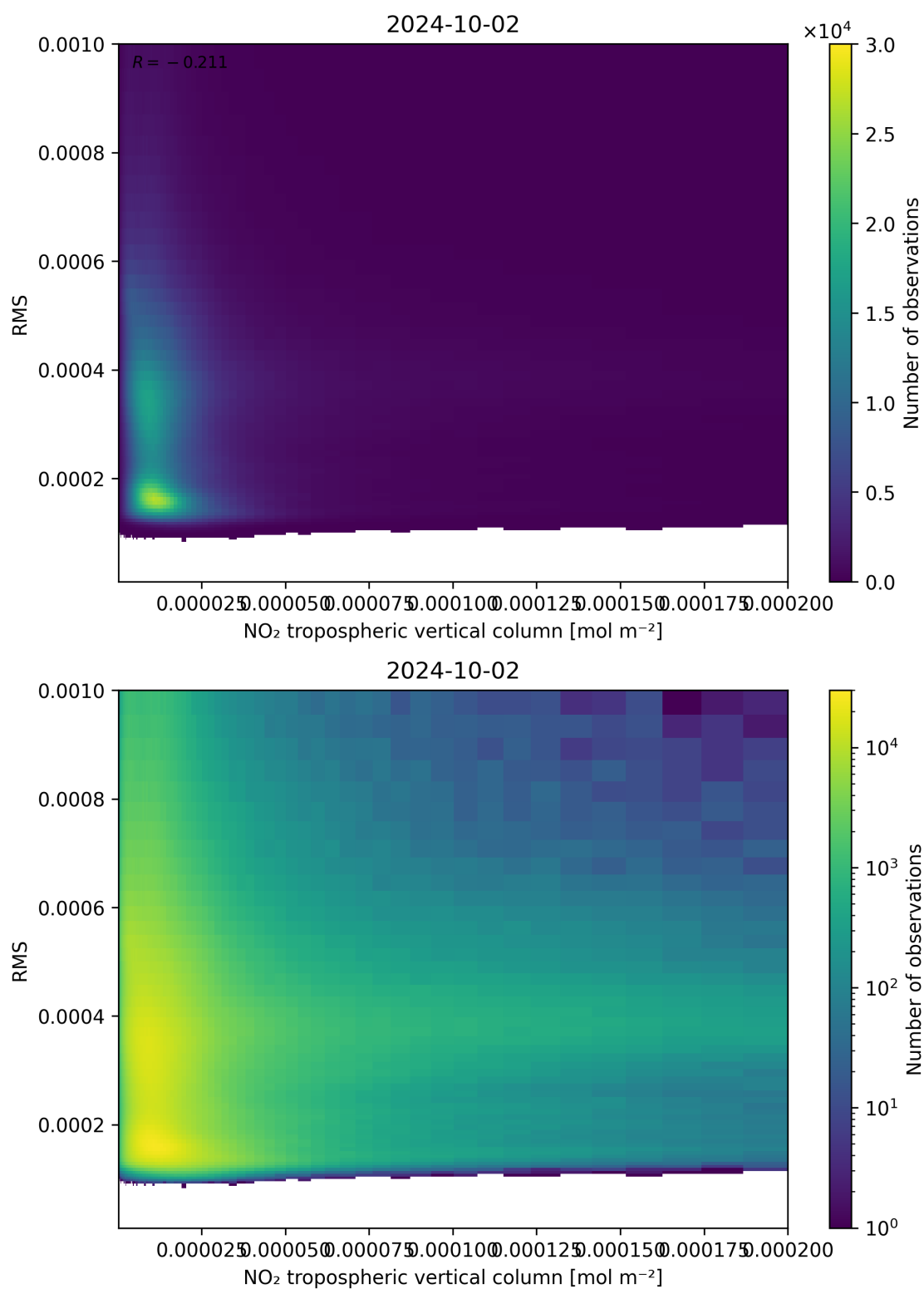
Figure 142: Scatter density plot of “NO 2 tropospheric vertical column” against “RMS” for 2024-10-01 to 2024-10-03.
