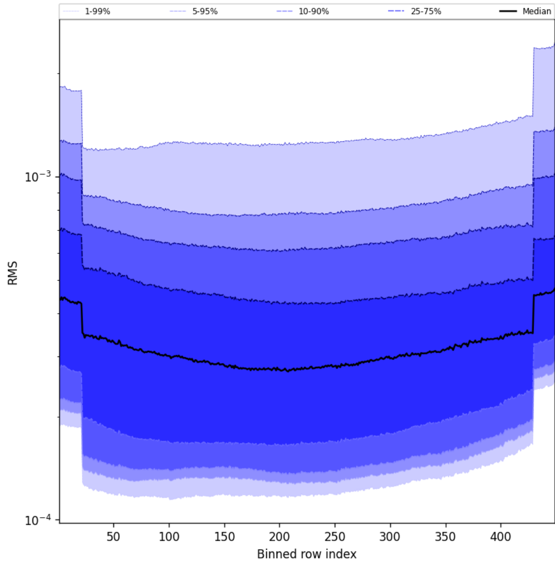
Figure 60: Along track statistics of “RMS” for 2024-10-01 to 2024-10-03
