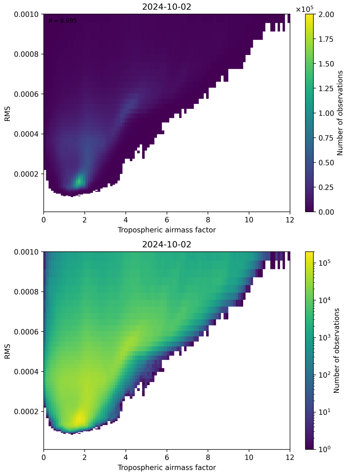
Figure 79: Scatter density plot of “Tropospheric airmass factor” against “RMS” for 2024-10-01 to 2024-10-03.
