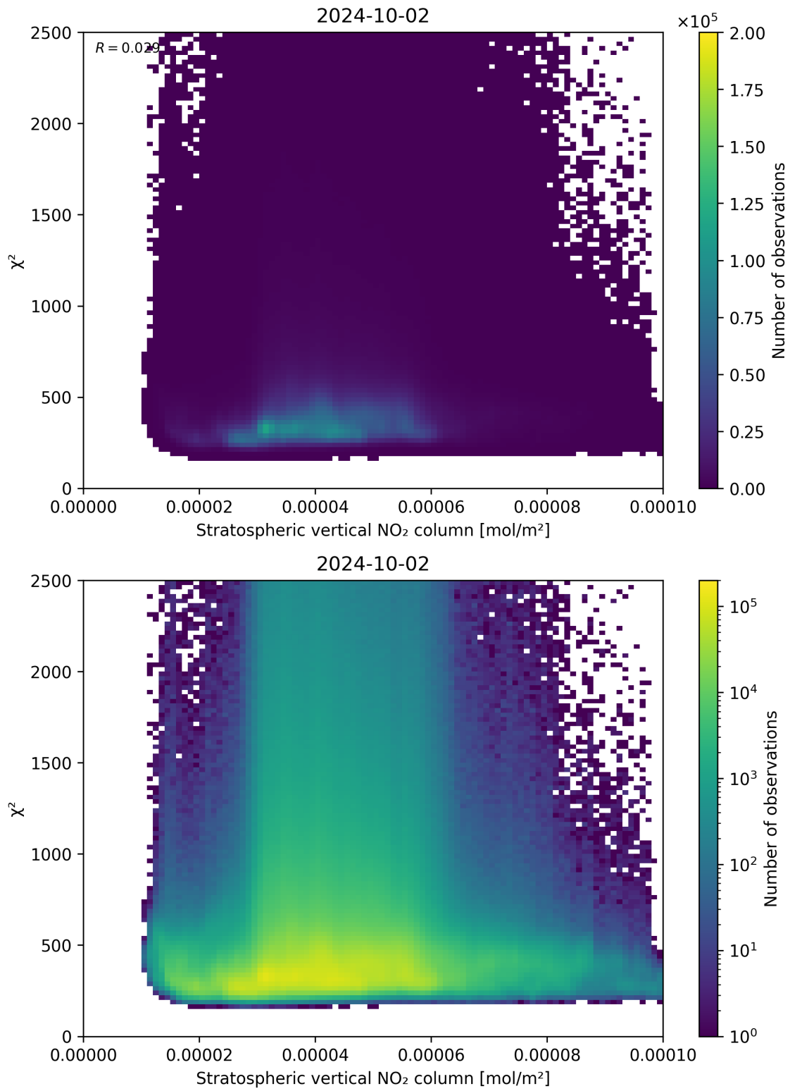
Figure 97: Scatter density plot of “Stratospheric vertical NO 2 column” against “ \chi^2 ” for 2024-10-01 to 2024-10-03.
