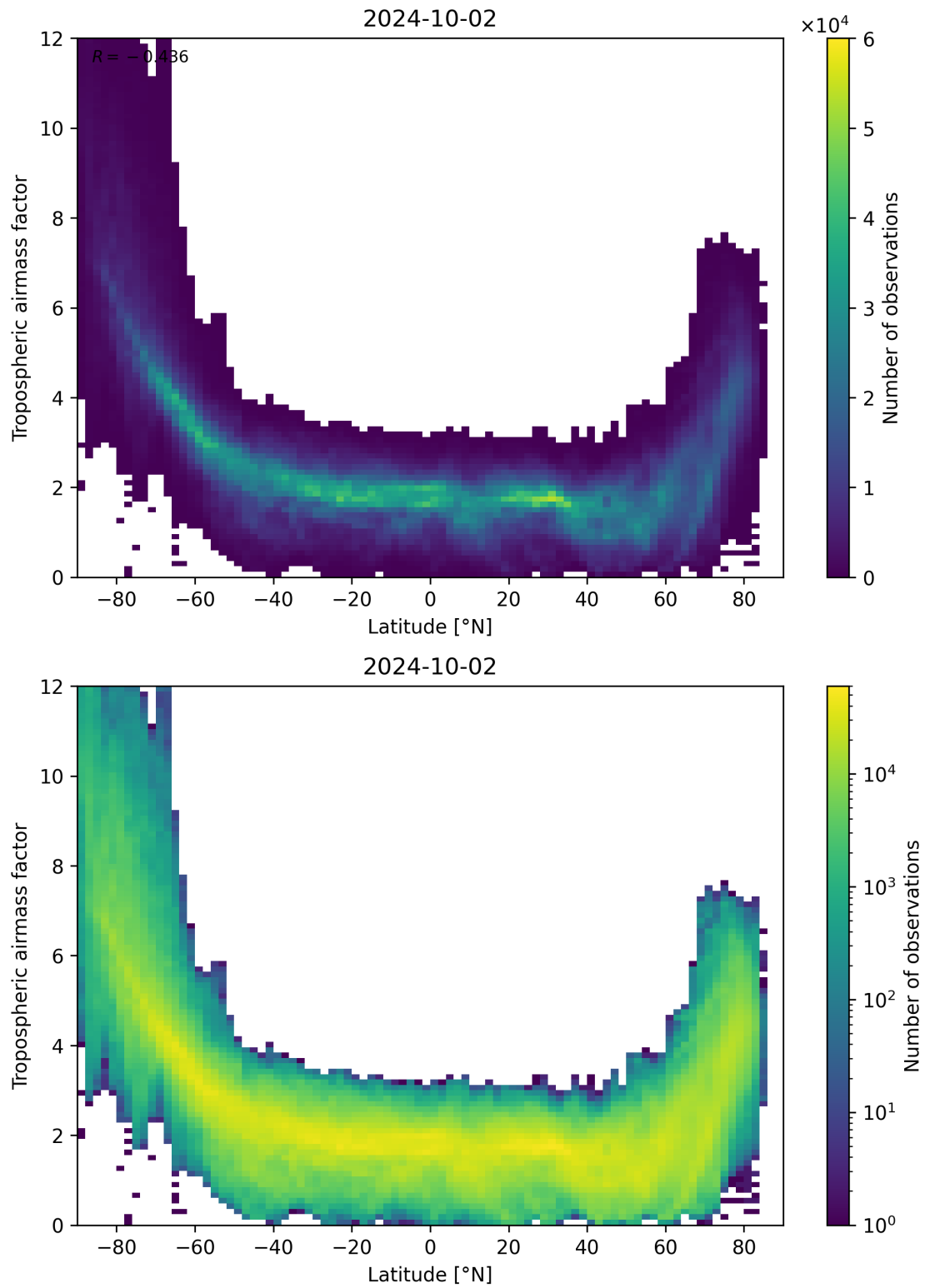
Figure 85: Scatter density plot of “Latitude” against “Tropospheric air mass factor” for 2024-10-01 to 2024-10-03.
