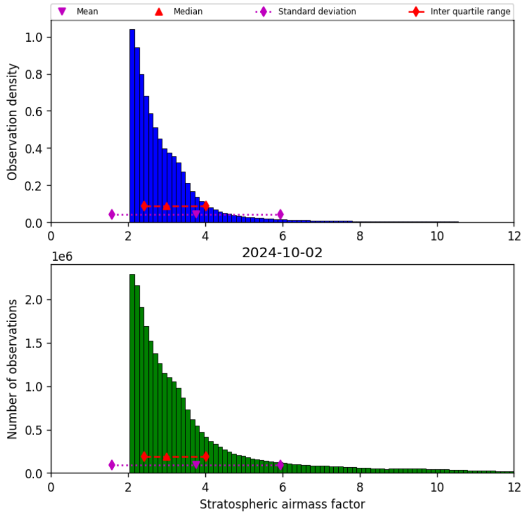
Figure 44: Histogram of “Stratospheric airmass factor” for 2024-10-01 to 2024-10-03
