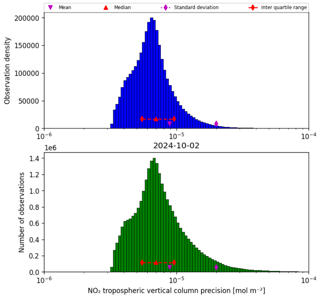
Figure 30: Histogram of “NO 2 tropospheric vertical column precision” for 2024-10-01 to 2024-10-03
