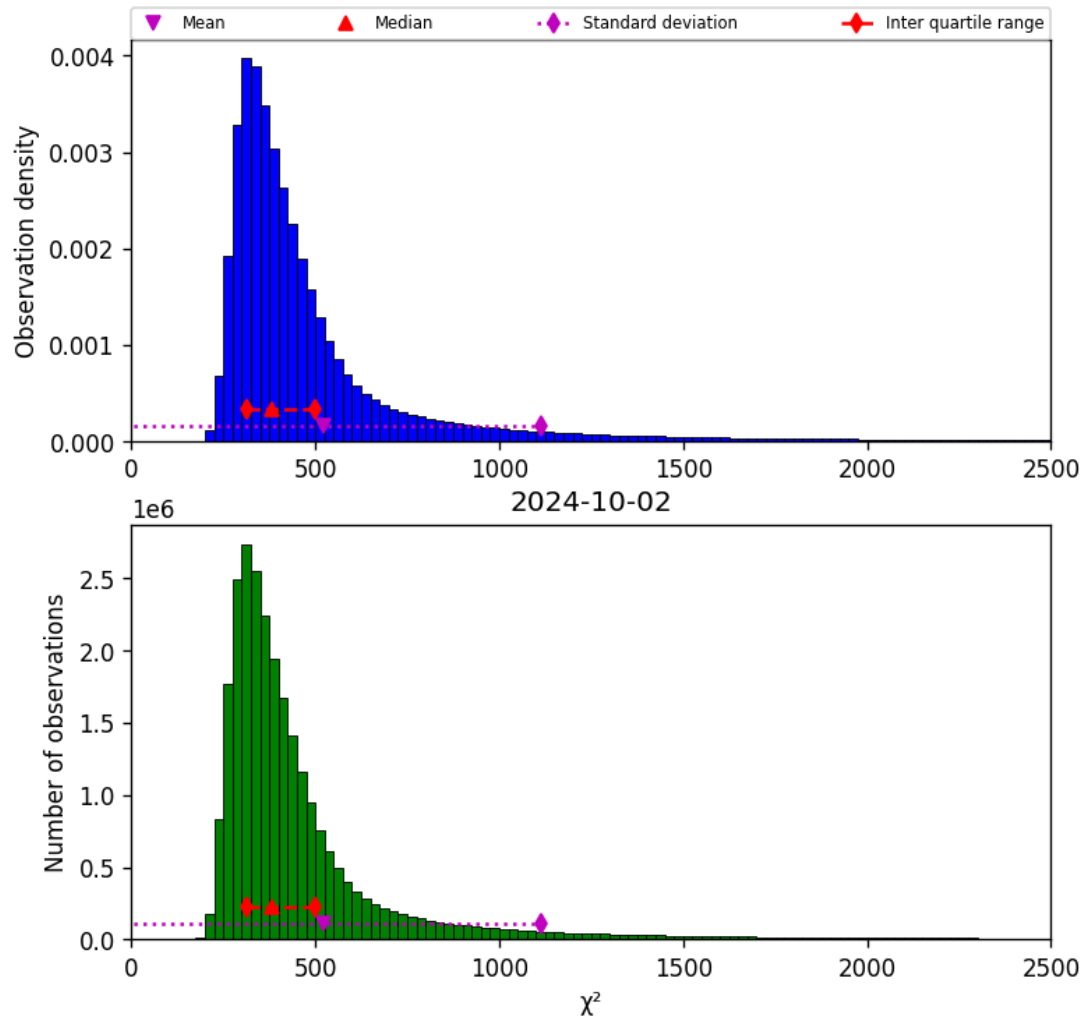
Figure 42: Histogram of “ \chi^2 ” for 2024-10-01 to 2024-10-03
