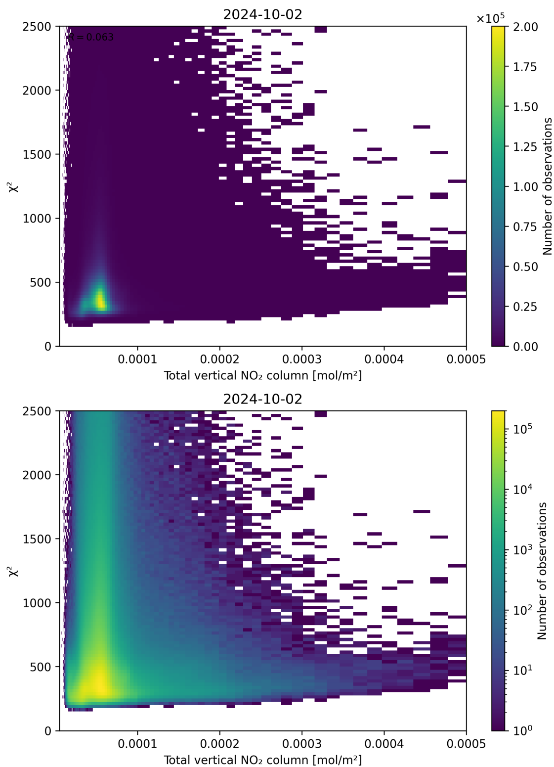
Figure 111: Scatter density plot of “Total vertical NO 2 column” against “ \chi^2 ” for 2024-10-01 to 2024-10-03.
