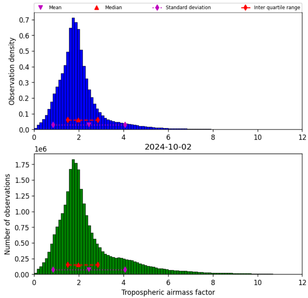
Figure 31: Histogram of “Tropospheric airmass factor” for 2024-10-01 to 2024-10-03
