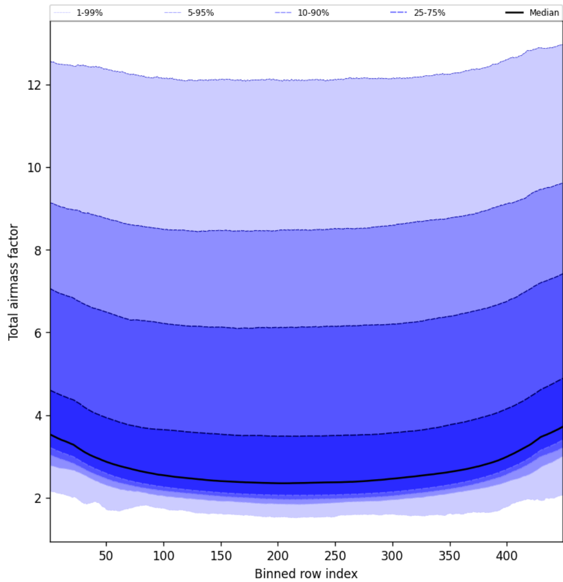
Figure 49: Along track statistics of “Total airmass factor” for 2024-10-01 to 2024-10-03
