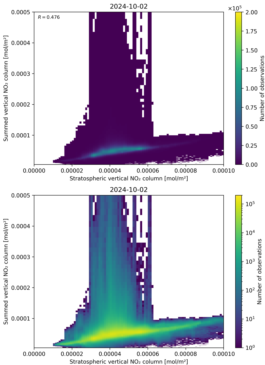
Figure 98: Scatter density plot of “Stratospheric vertical NO 2 column” against “Summed vertical NO 2 column” for 2024-10-01 to 2024-10-03.
