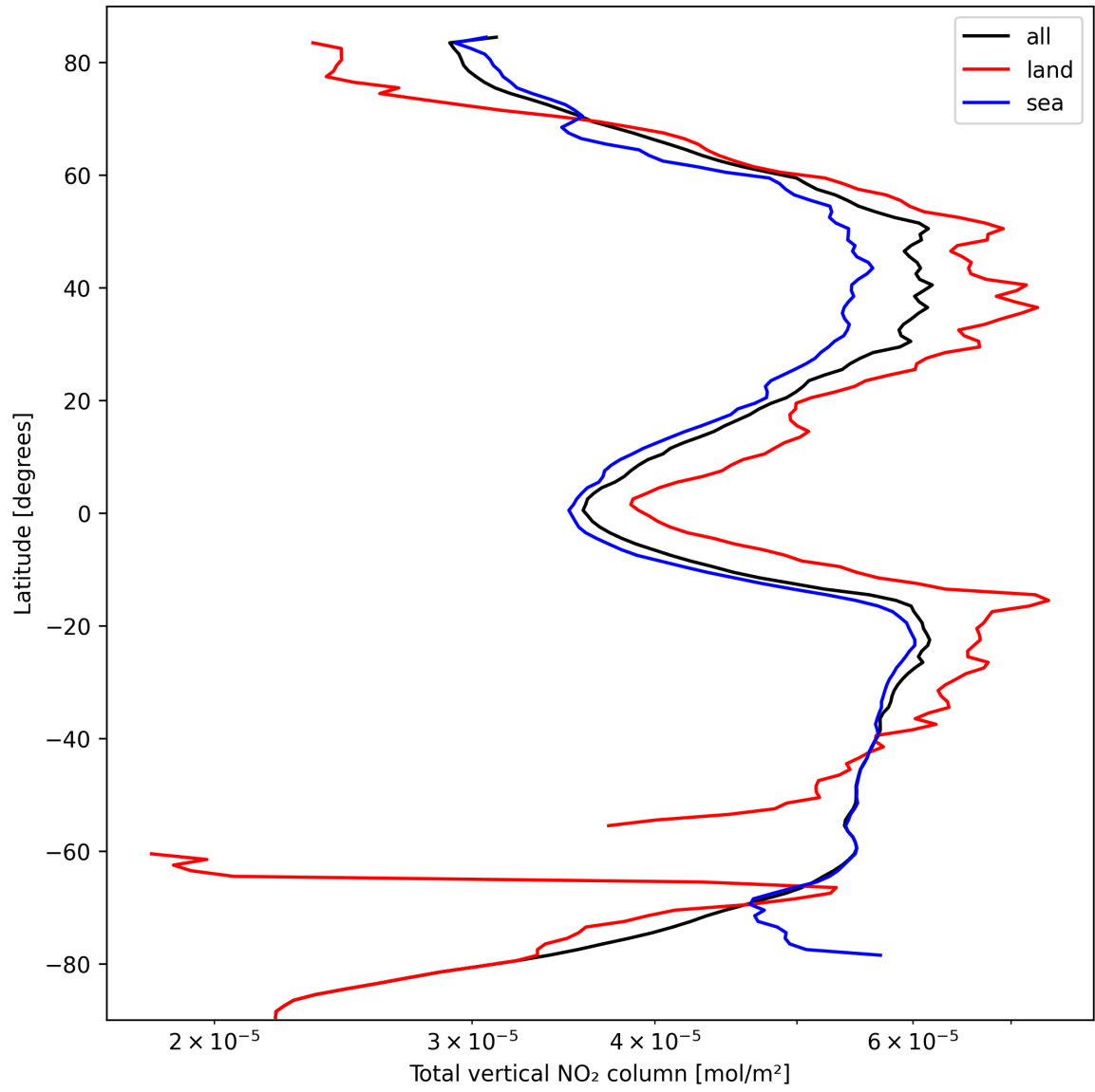
Figure 21: Zonal average of “Total vertical NO 2 column” for 2024-10-01 to 2024-10-03.
