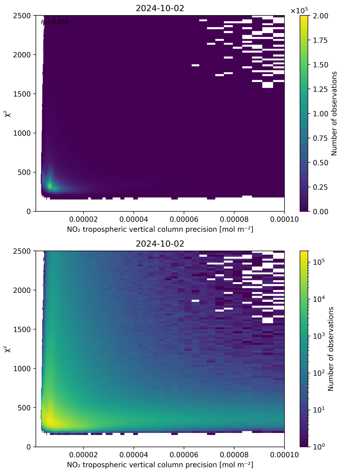
Figure 134: Scatter density plot of “NO 2 tropospheric vertical column precision” against “ \chi^2 ” for 2024-10-01 to 2024-10-03.
