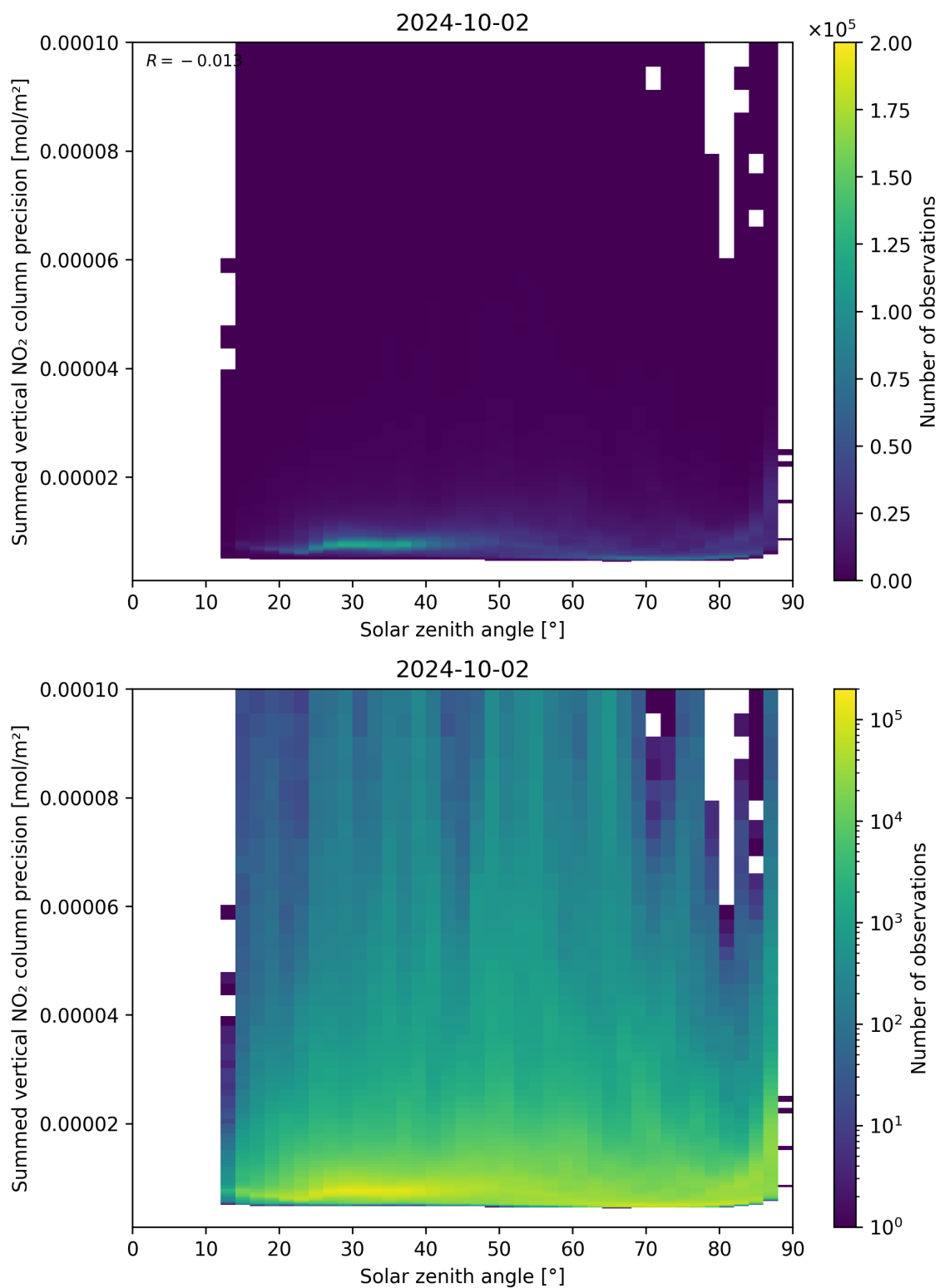
Figure 152: Scatter density plot of “Solar zenith angle” against “Summed vertical NO 2 column precision” for 2024-10-01 to 2024-10-03.
