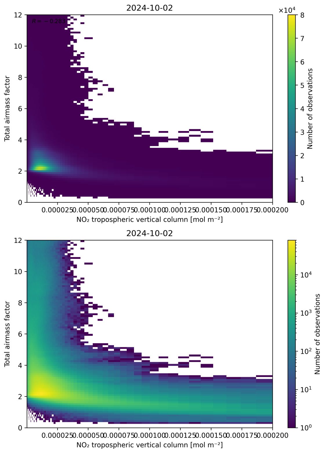
Figure 122: Scatter density plot of “NO 2 tropospheric vertical column” against “Total airmass factor” for 2024-10-01 to 2024-10-03.
