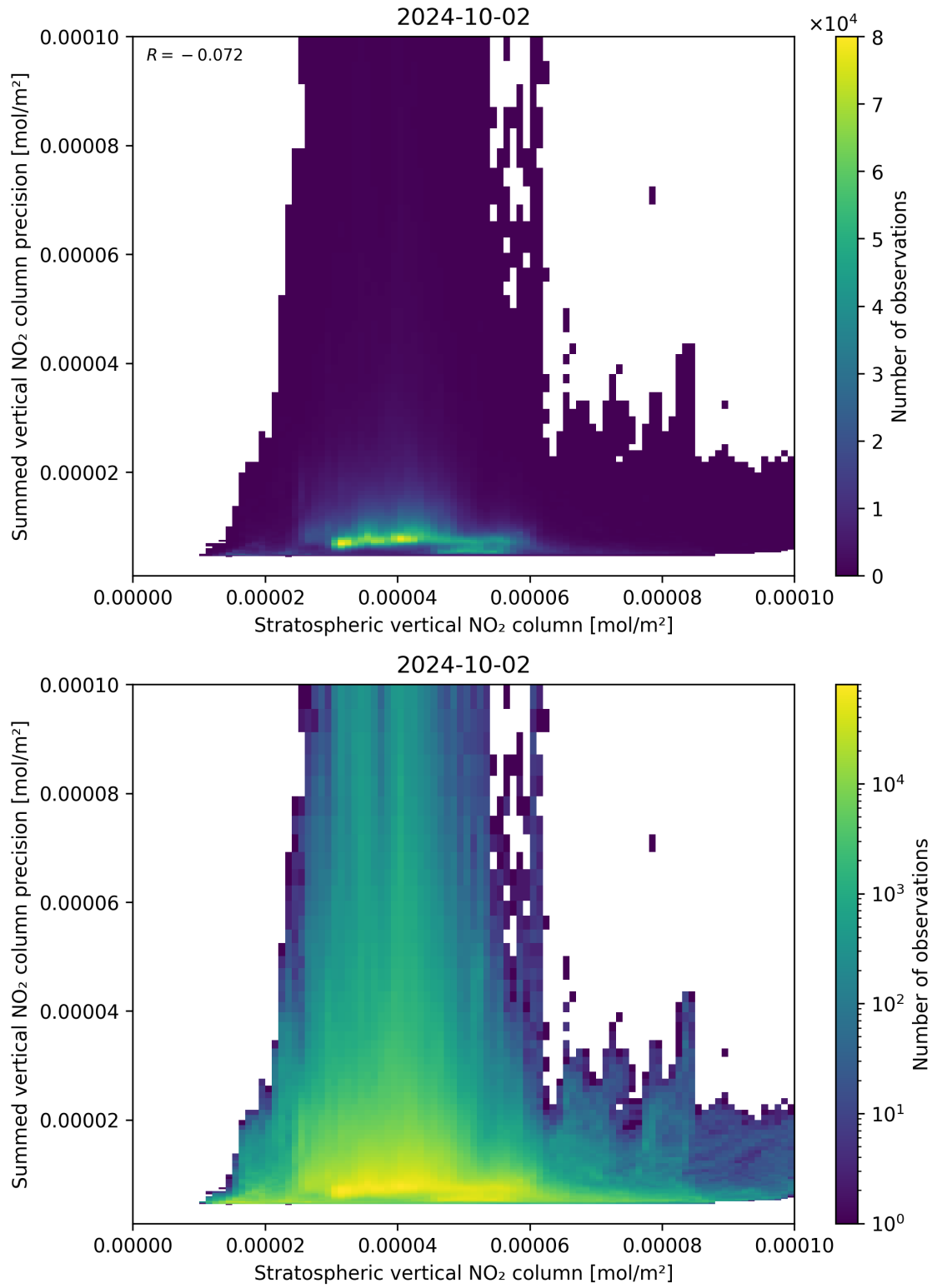
Figure 99: Scatter density plot of “Stratospheric vertical NO 2 column” against “Summed vertical NO 2 column precision” for 2024-10-01 to 2024-10-03.
