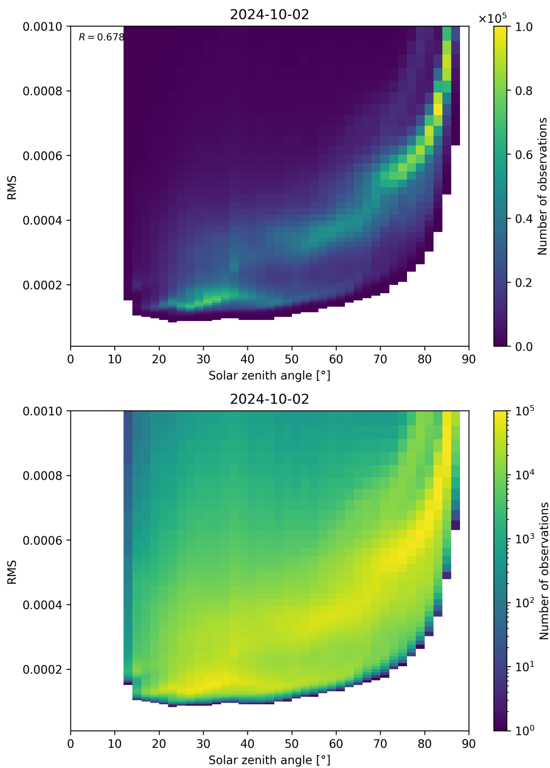
Figure 157: Scatter density plot of “Solar zenith angle” against “RMS” for 2024-10-01 to 2024-10-03.
