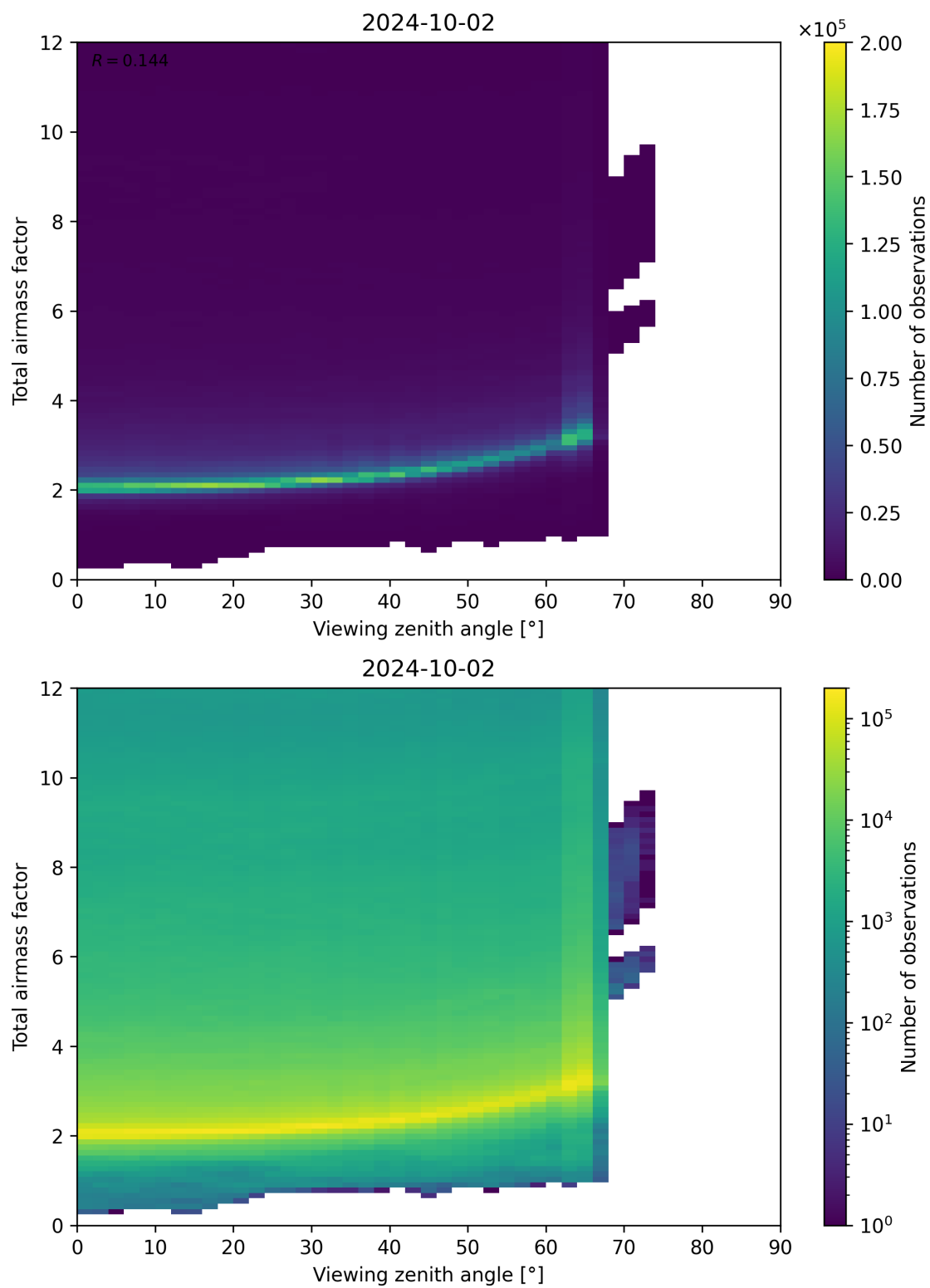
Figure 160: Scatter density plot of “Viewing zenith angle” against “Total airmass factor” for 2024-10-01 to 2024-10-03.
