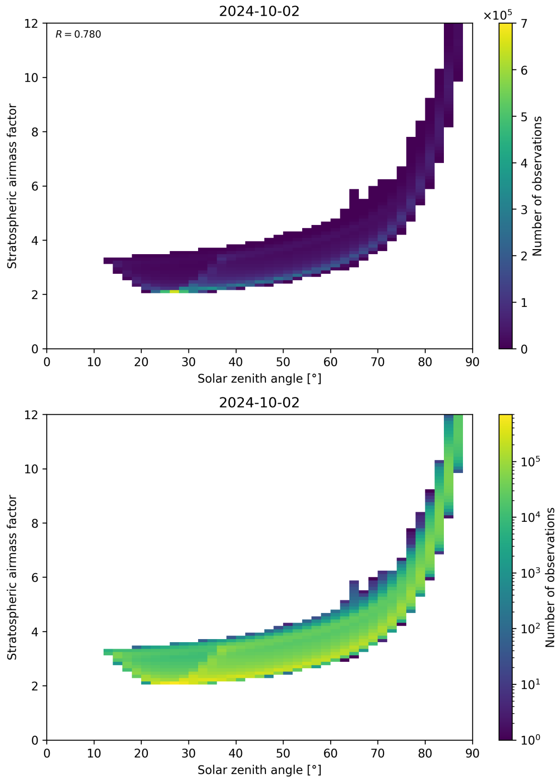
Figure 145: Scatter density plot of “Solar zenith angle” against “Stratospheric airmass factor” for 2024-10-01 to 2024-10-03.
