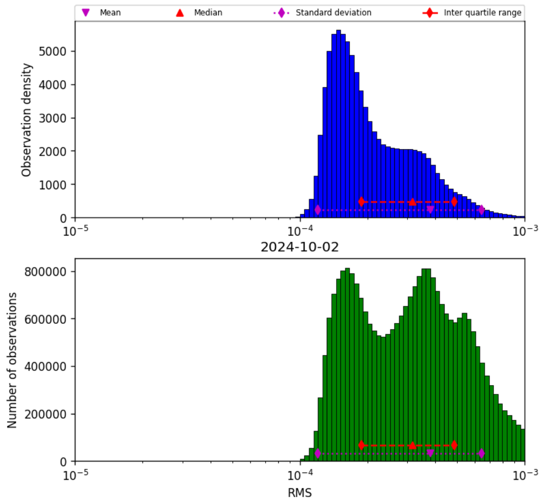
Figure 43: Histogram of “RMS” for 2024-10-01 to 2024-10-03
