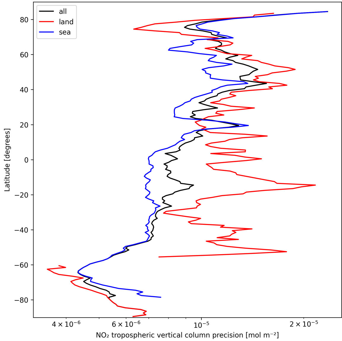
Figure 13: Zonal average of “NO 2 tropospheric vertical column precision” for 2024-10-01 to 2024-10-03.
