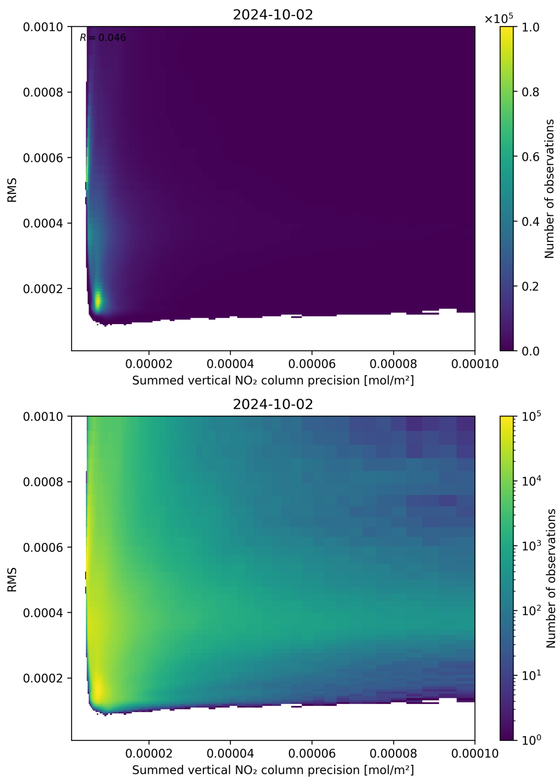
Figure 108: Scatter density plot of “Summed vertical NO 2 column precision” against “RMS” for 2024-10-01 to 2024-10-03.
