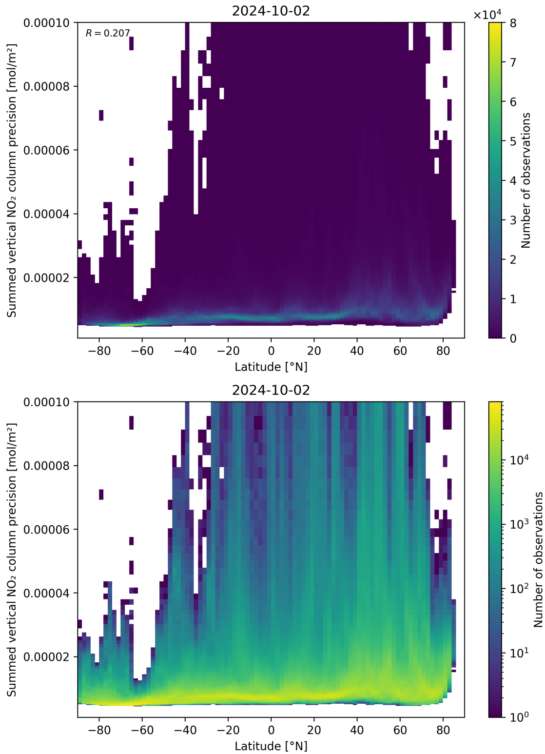
Figure 89: Scatter density plot of “Latitude” against “Summed vertical NO 2 column precision” for 2024-10-01 to 2024-10-03.
