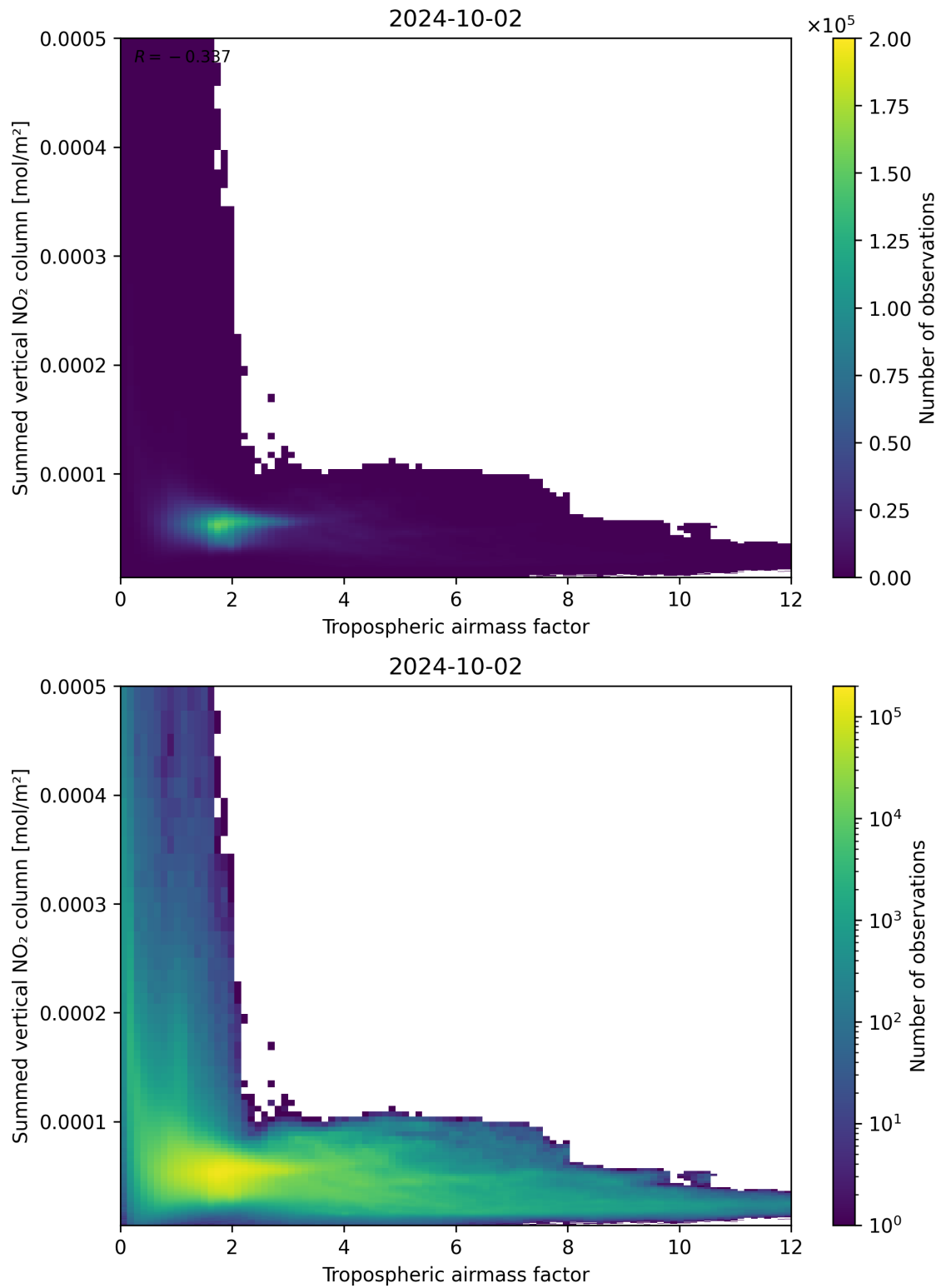
Figure 75: Scatter density plot of “Tropospheric air mass factor” against “Summed vertical NO 2 column” for 2024-10-01 to 2024-10-03.
