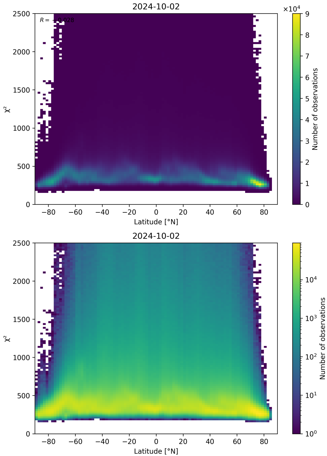
Figure 86: Scatter density plot of “Latitude” against “ \chi^2 ” for 2024-10-01 to 2024-10-03.
