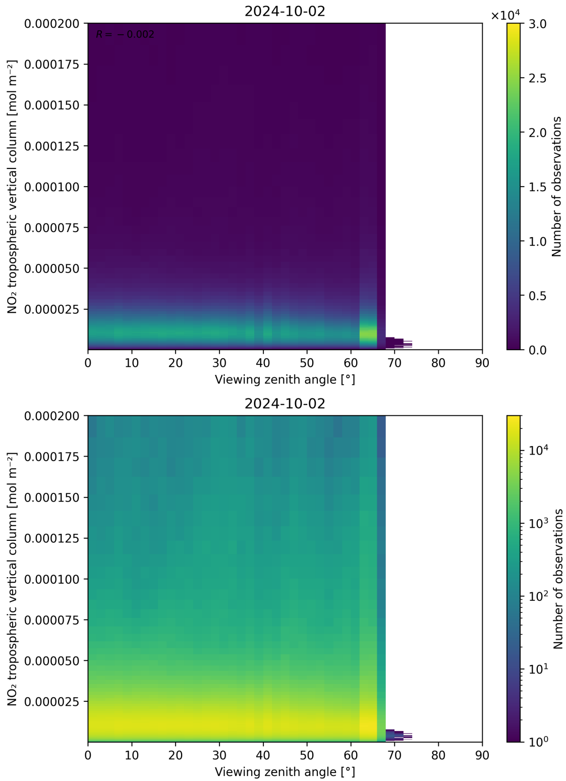
Figure 169: Scatter density plot of “Viewing zenith angle” against “NO 2 tropospheric vertical column” for 2024-10-01 to 2024-10-03.
