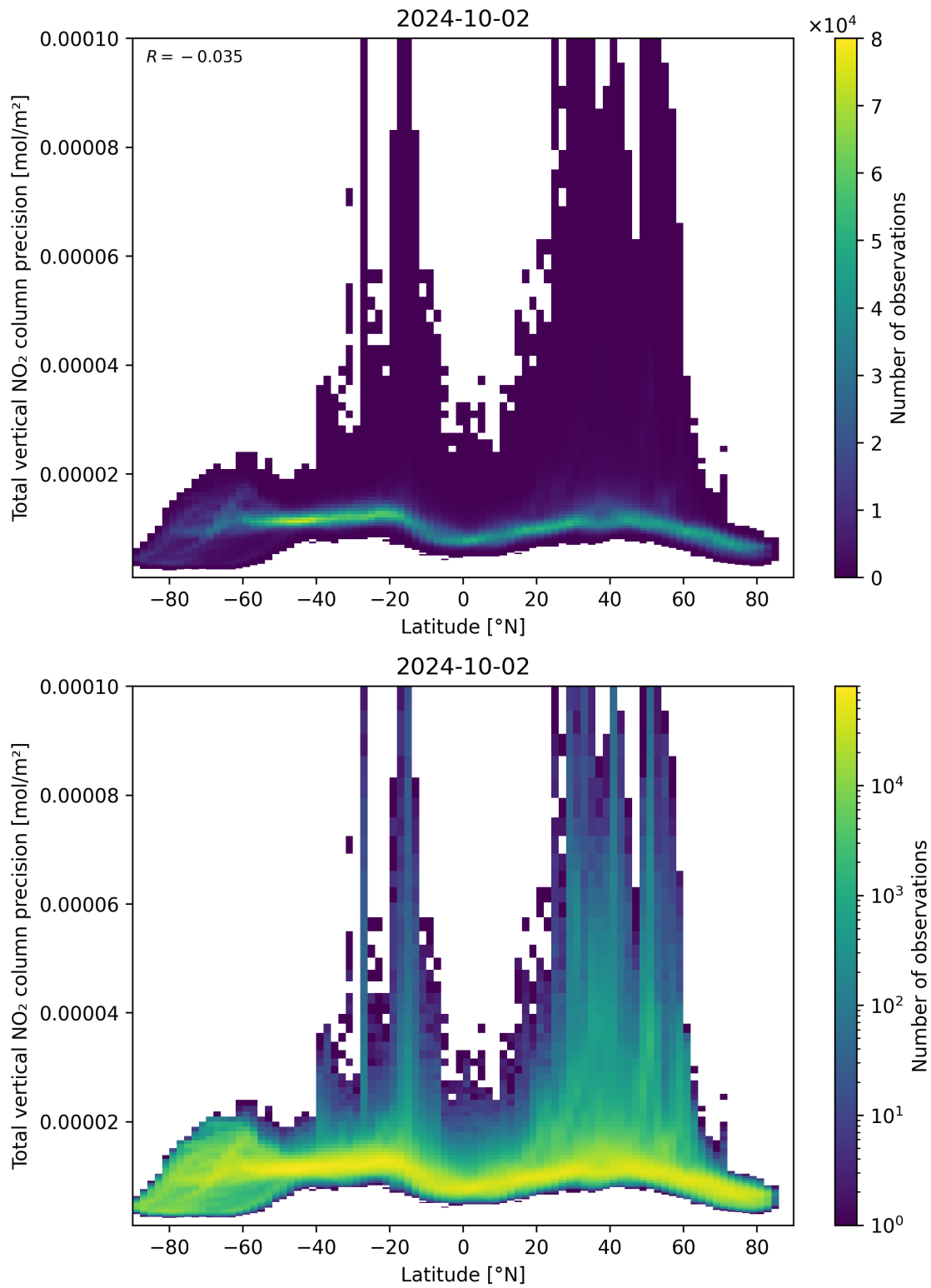
Figure 91: Scatter density plot of “Latitude” against “Total vertical NO 2 column precision” for 2024-10-01 to 2024-10-03.
