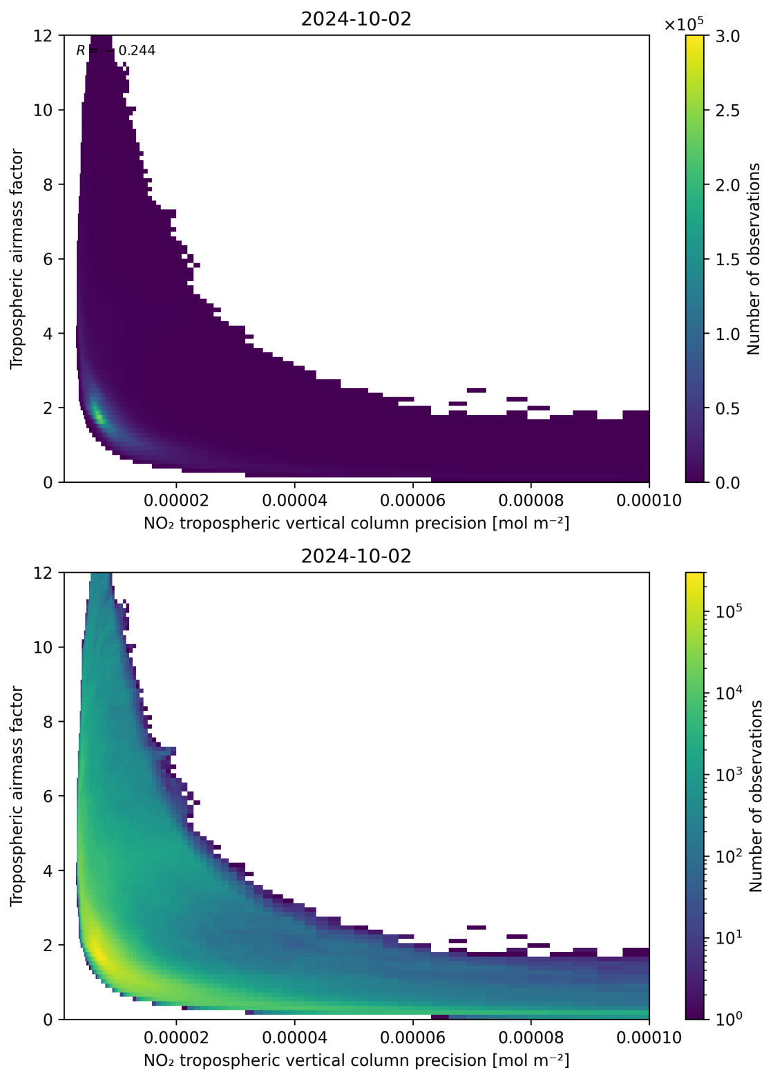
Figure 133: Scatter density plot of “NO 2 tropospheric vertical column precision” against “Tropospheric airmass factor” for 2024-10-01 to 2024-10-03.
