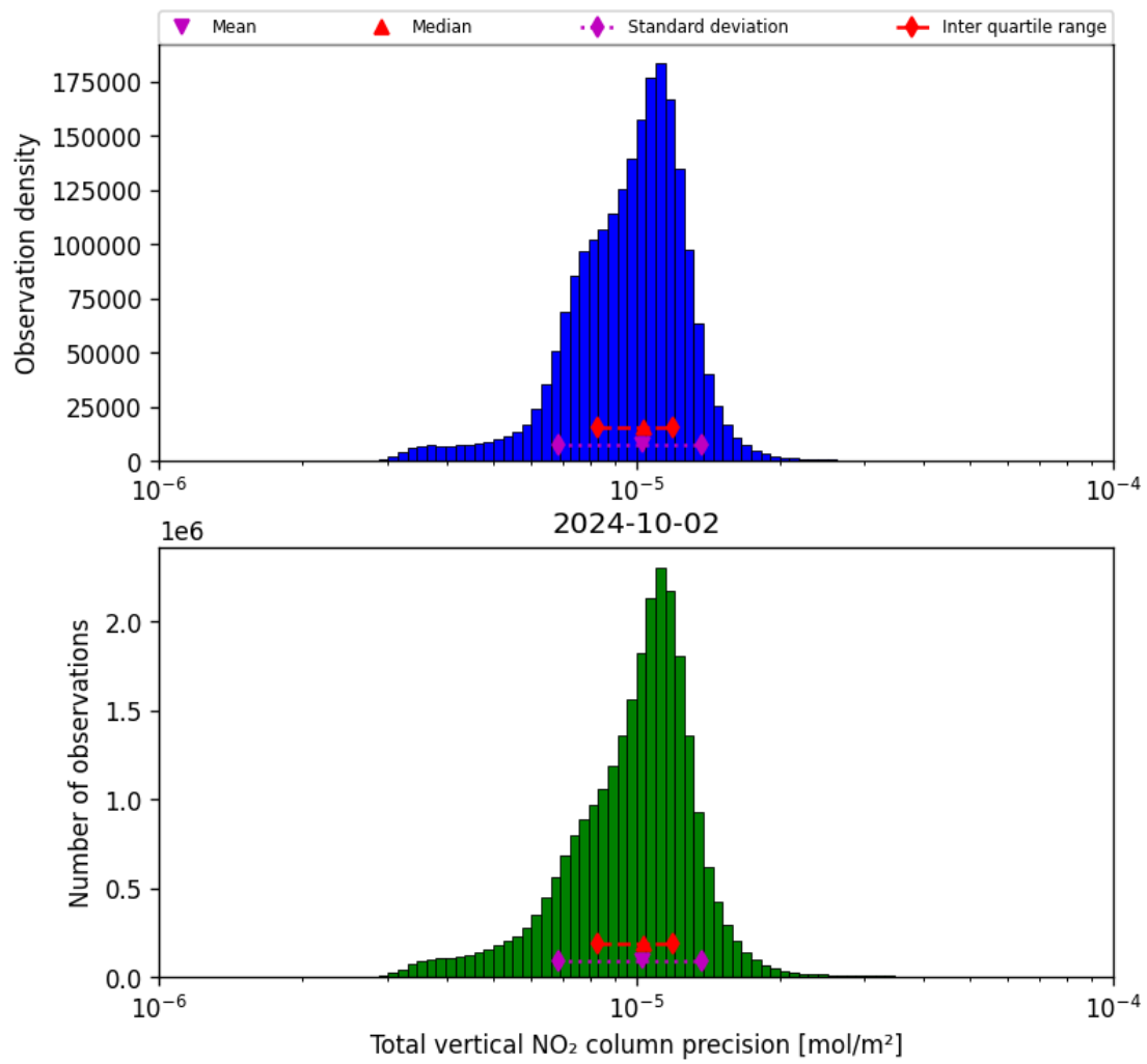
Figure 39: Histogram of "Total vertical NO 2 column precision" for 2024-10-01 to 2024-10-03
