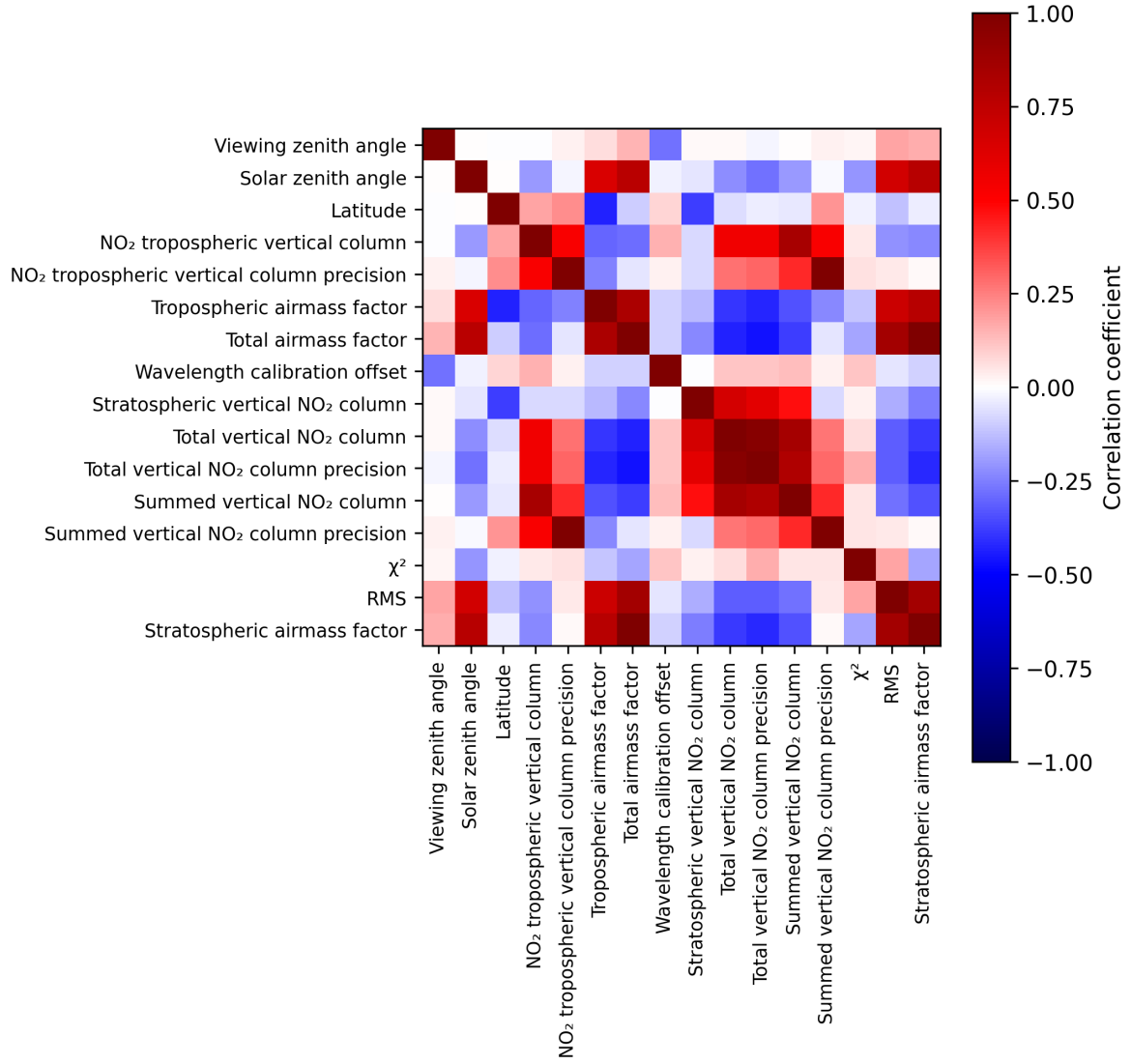
Figure 2: Map of correlation matrix for 2024-10-01 to 2024-10-03.
