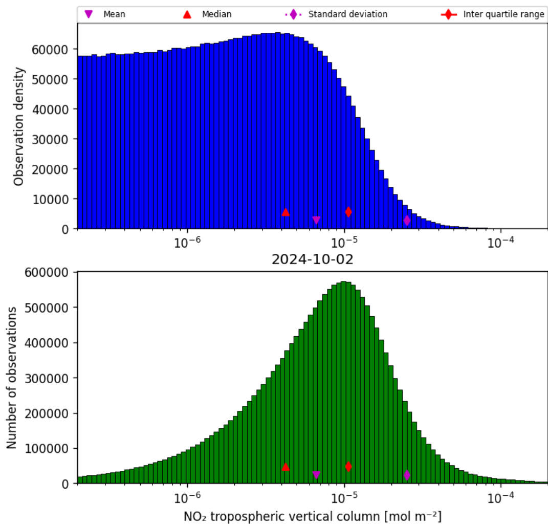
Figure 29: Histogram of “NO 2 tropospheric vertical column” for 2024-10-01 to 2024-10-03
