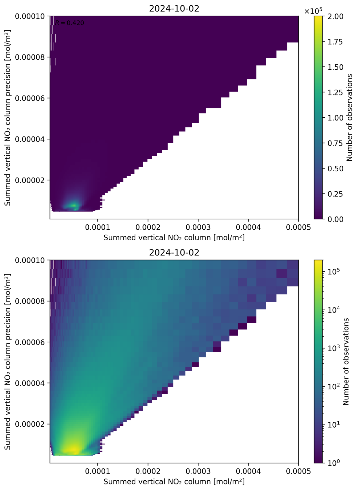
Figure 105: Scatter density plot of “Summed vertical NO 2 column” against “Summed vertical NO 2 column precision” for 2024-10-01 to 2024-10-03.
