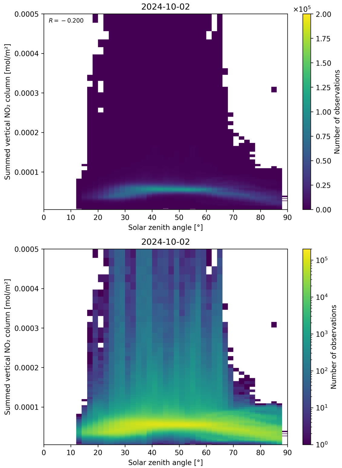
Figure 151: Scatter density plot of “Solar zenith angle” against “Summed vertical NO 2 column” for 2024-10-01 to 2024-10-03.
