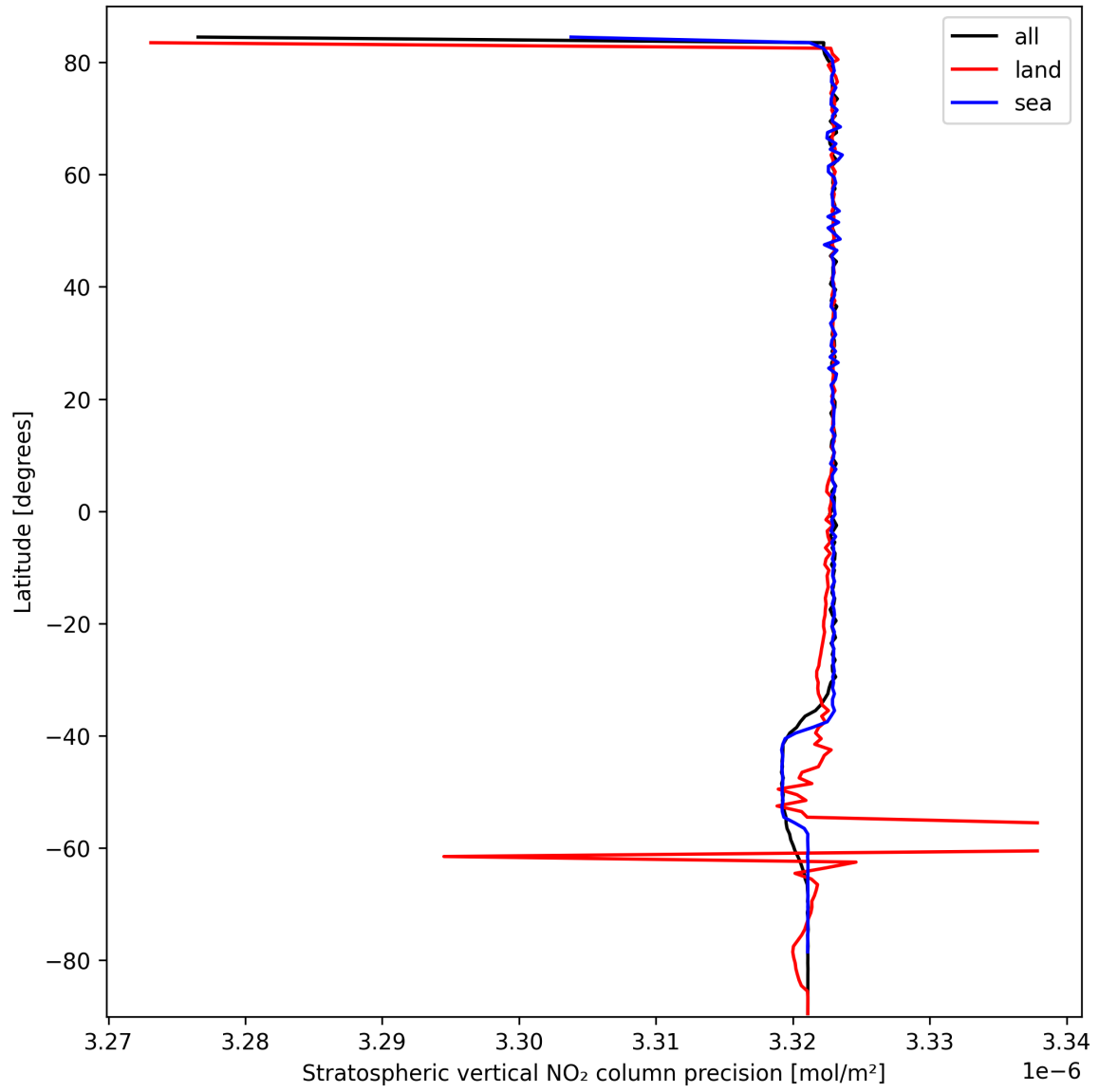
Figure 20: Zonal average of “Stratospheric vertical NO 2 column precision” for 2024-10-01 to 2024-10-03.
