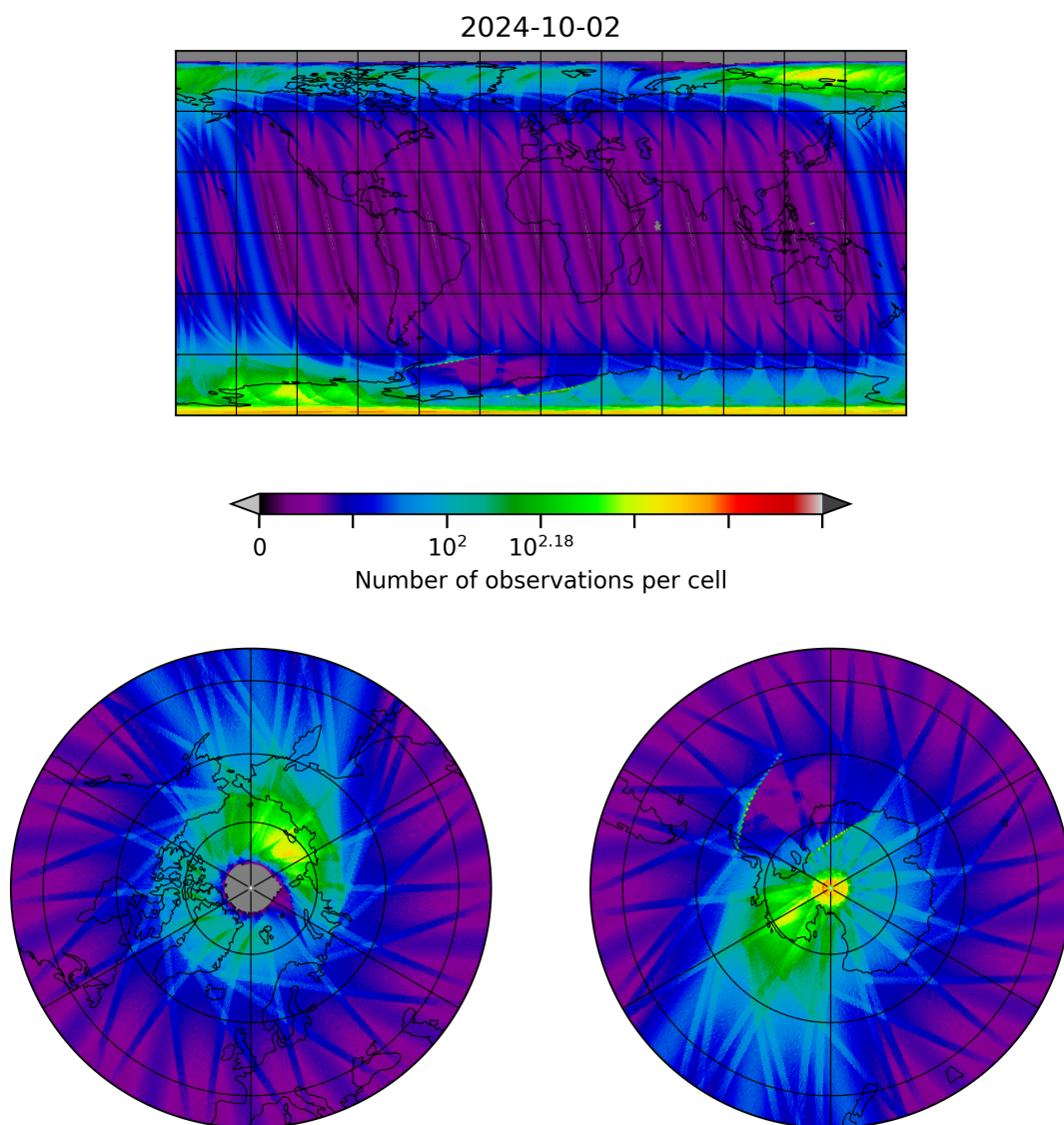
Figure 10: Map of the number of observations for 2024-10-01 to 2024-10-03
