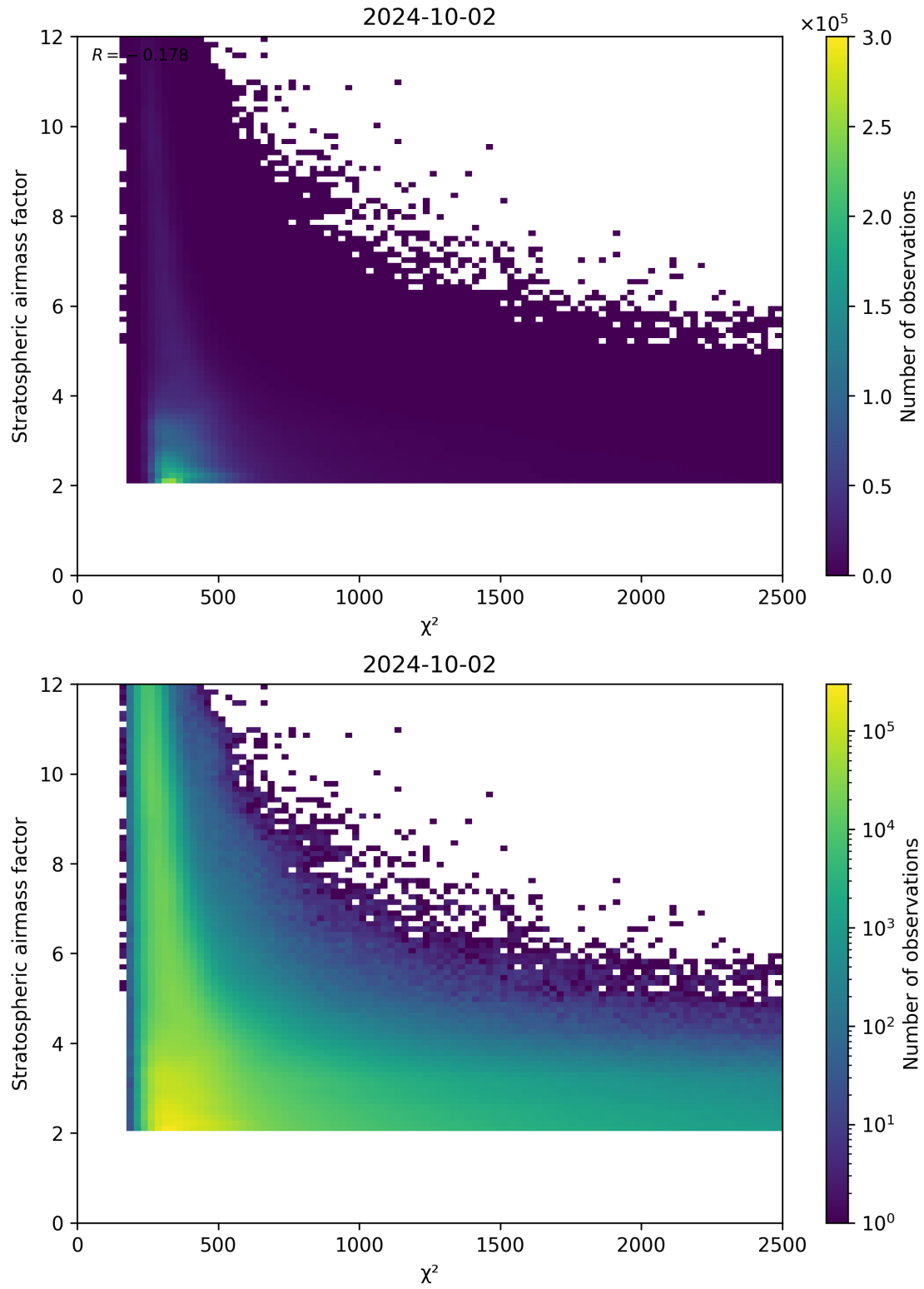
Figure 81: Scatter density plot of “ \chi^2 ” against “Stratospheric airmass factor” for 2024-10-01 to 2024-10-03.
