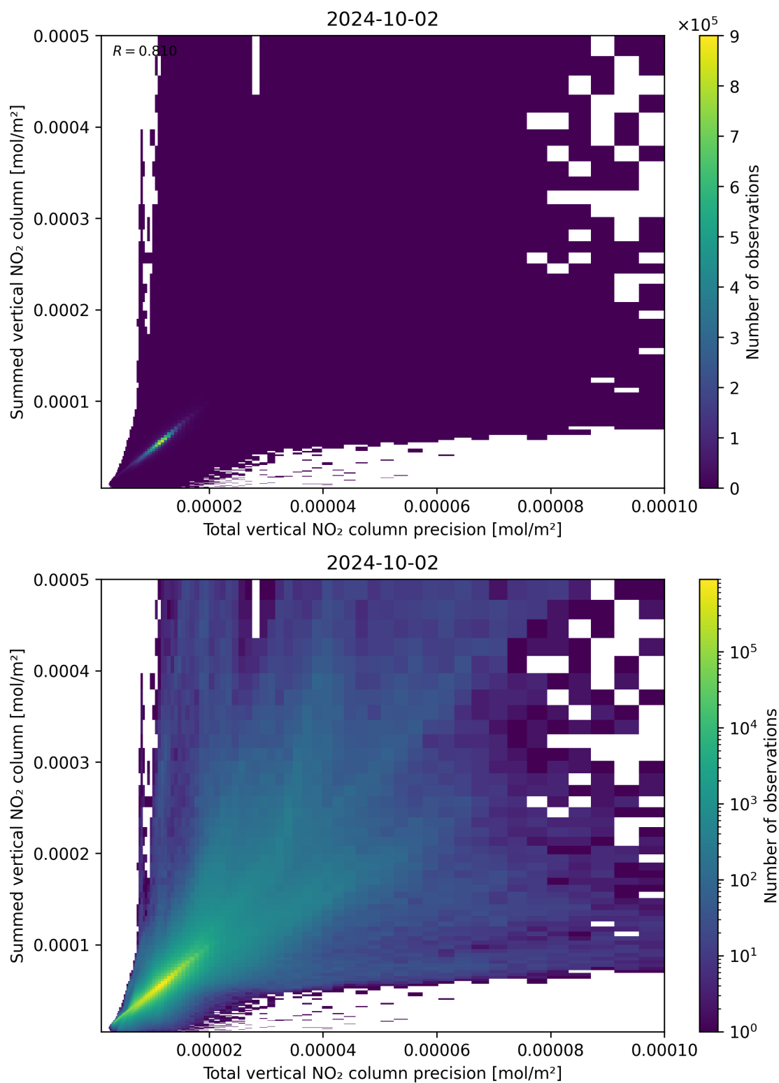
Figure 117: Scatter density plot of “Total vertical NO 2 column precision” against “Summed vertical NO 2 column” for 2024-10-01 to 2024-10-03.
