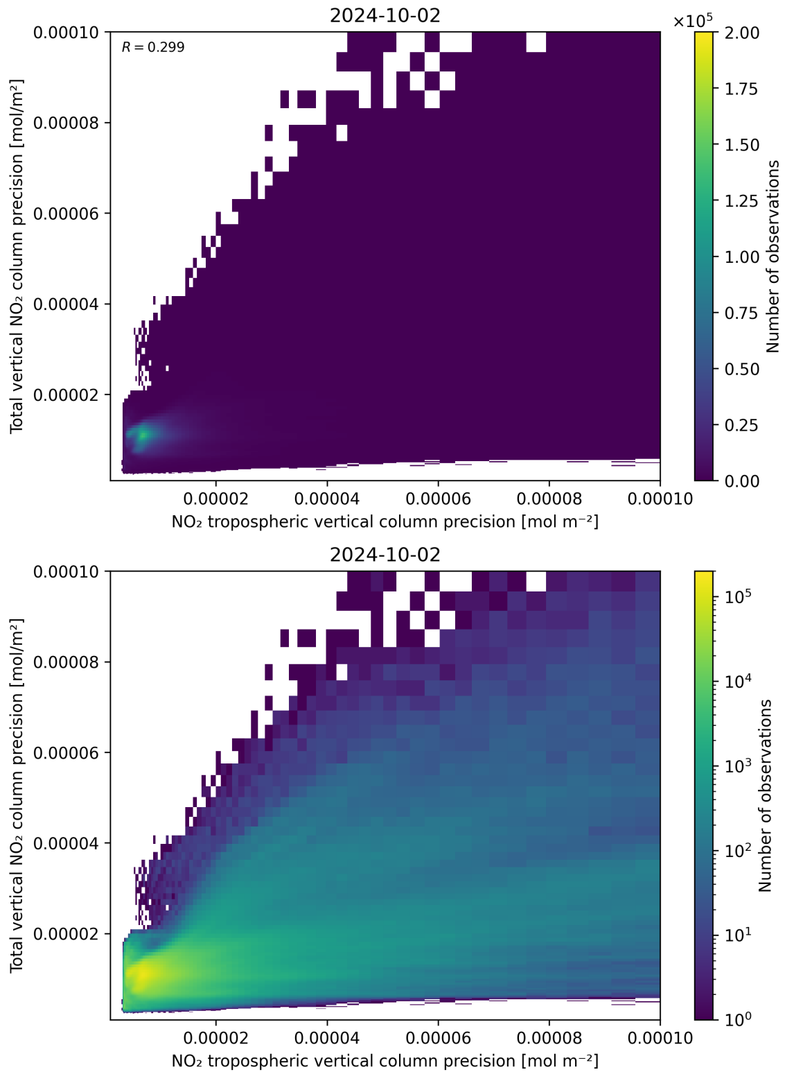
Figure 139: Scatter density plot of “NO 2 tropospheric vertical column precision” against “Total vertical NO 2 column precision” for 2024-10-01 to 2024-10-03.
