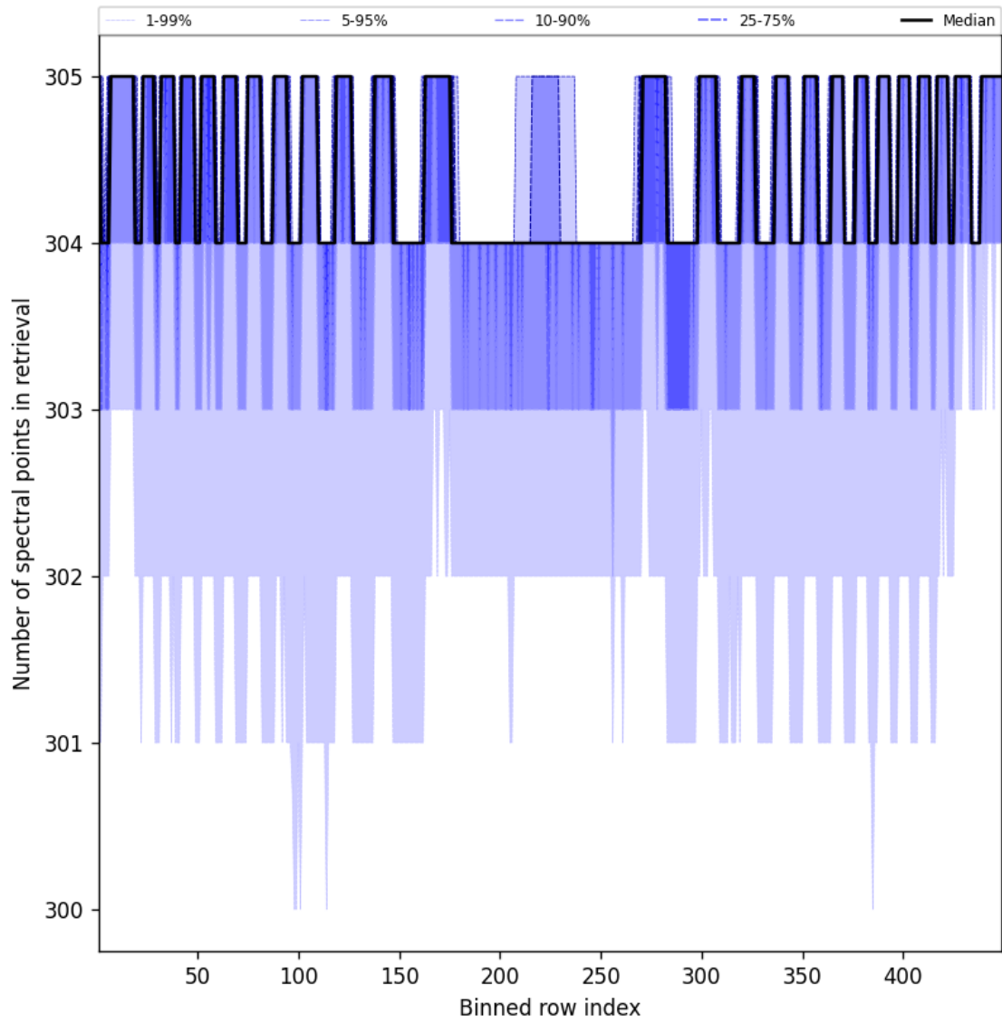
Figure 50: Along track statistics of “Number of spectral points in retrieval” for 2024-10-01 to 2024-10-03
