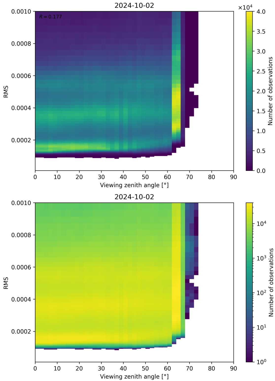
Figure 171: Scatter density plot of “Viewing zenith angle” against “RMS” for 2024-10-01 to 2024-10-03.
