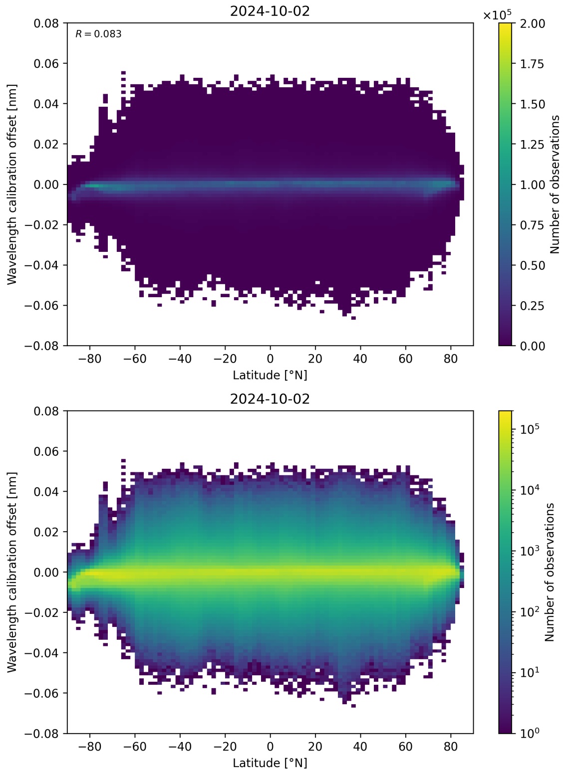
Figure 95: Scatter density plot of “Latitude” against “Wavelength calibration offset” for 2024-10-01 to 2024-10-03.
