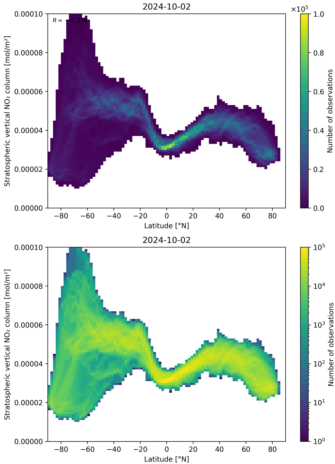
Figure 87: Scatter density plot of “Latitude” against “Stratospheric vertical NO 2 column” for 2024-10-01 to 2024-10-03.
