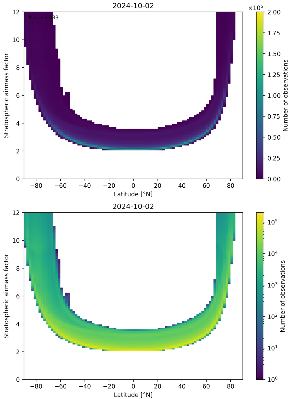
Figure 83: Scatter density plot of “Latitude” against “Stratospheric air mass factor” for 2024-10-01 to 2024-10-03.
