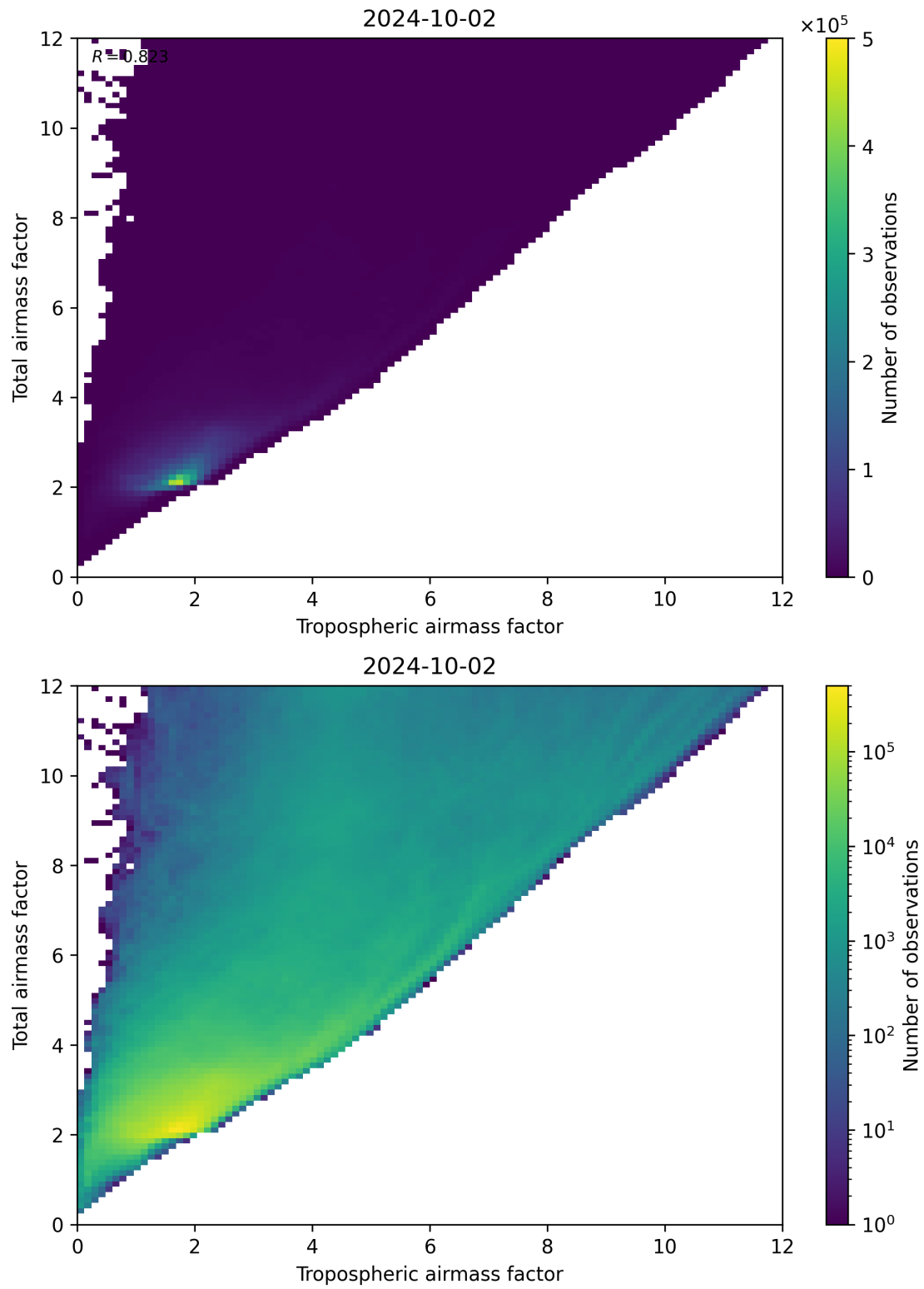
Figure 72: Scatter density plot of “Tropospheric airmass factor” against “Total airmass factor” for 2024-10-01 to 2024-10-03.
