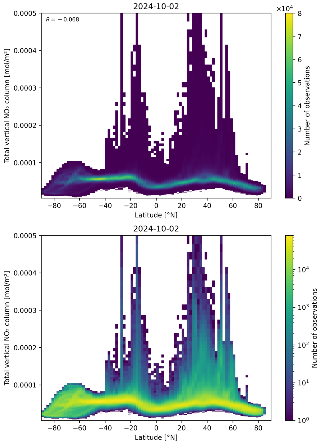
Figure 90: Scatter density plot of “Latitude” against “Total vertical NO 2 column” for 2024-10-01 to 2024-10-03.
