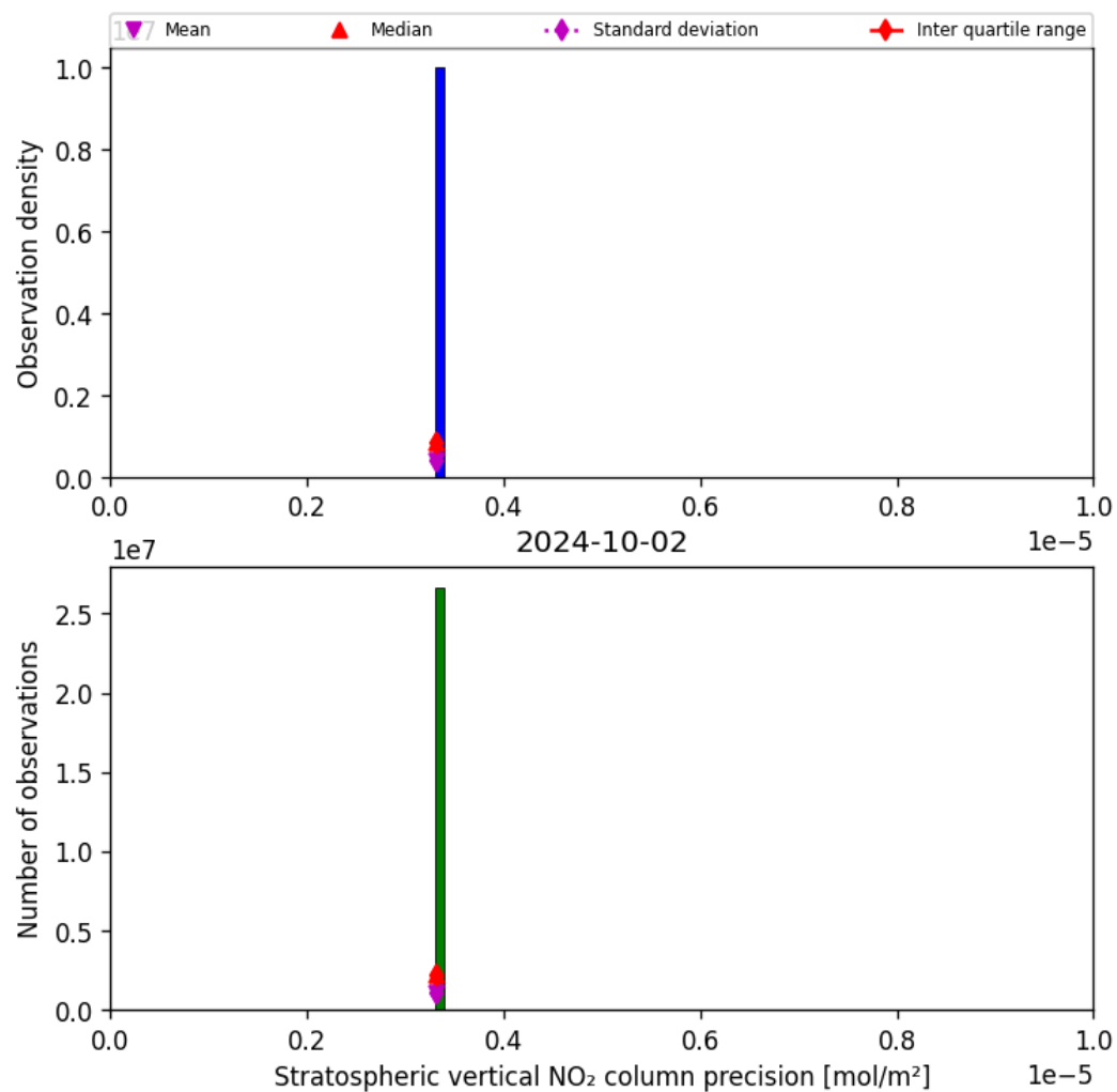
Figure 37: Histogram of “Stratospheric vertical NO 2 column precision” for 2024-10-01 to 2024-10-03
