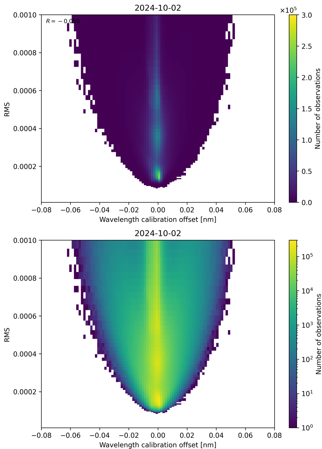
Figure 181: Scatter density plot of “Wavelength calibration offset” against “RMS” for 2024-10-01 to 2024-10-03.
