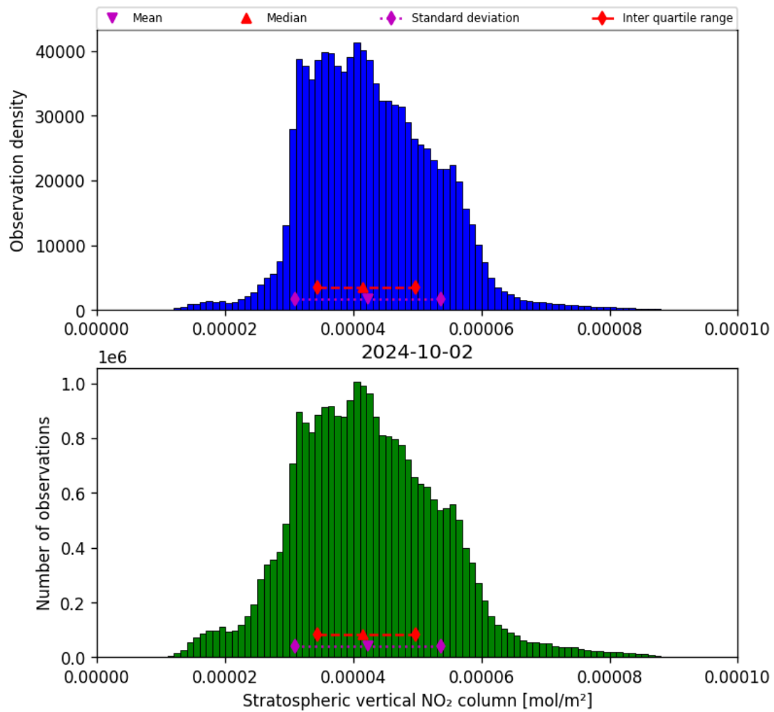
Figure 36: Histogram of “Stratospheric vertical NO 2 column” for 2024-10-01 to 2024-10-03
