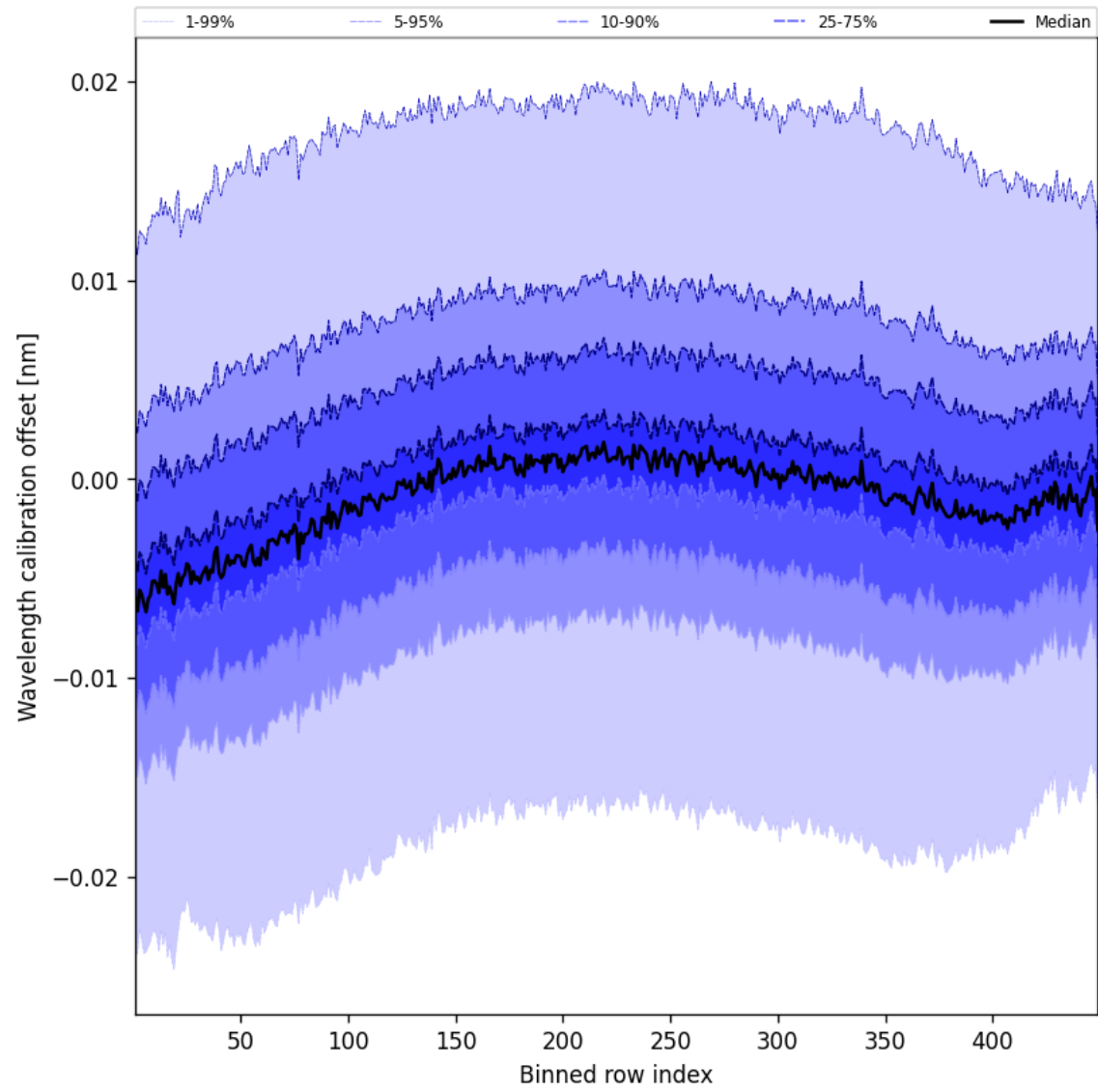
Figure 52: Along track statistics of “Wavelength calibration offset” for 2024-10-01 to 2024-10-03
