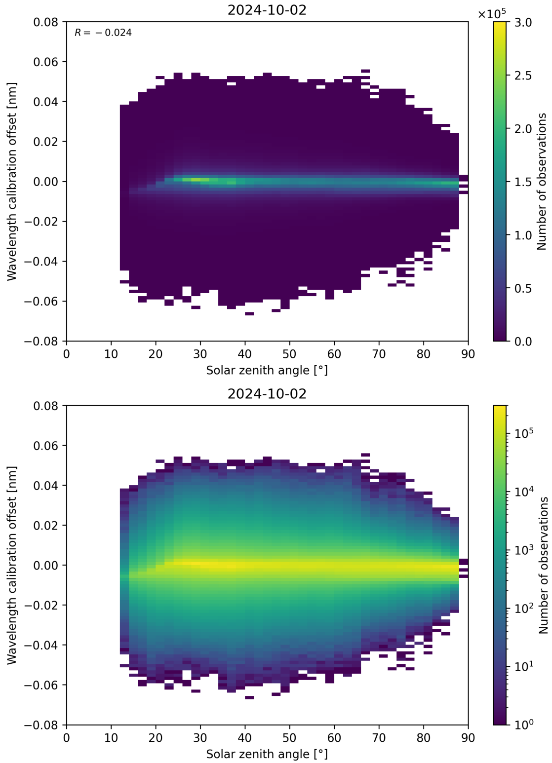
Figure 158: Scatter density plot of “Solar zenith angle” against “Wavelength calibration offset” for 2024-10-01 to 2024-10-03.
