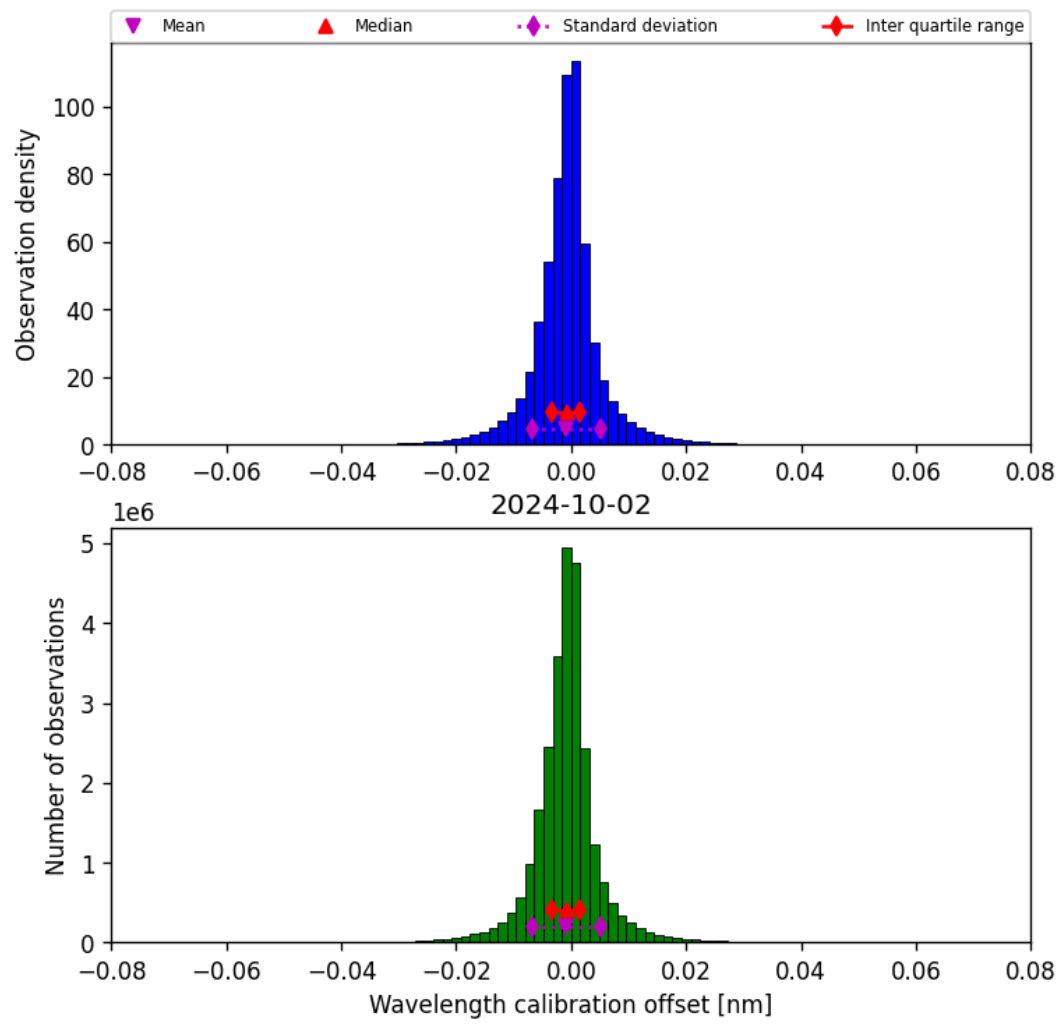
Figure 35: Histogram of “Wavelength calibration offset” for 2024-10-01 to 2024-10-03
