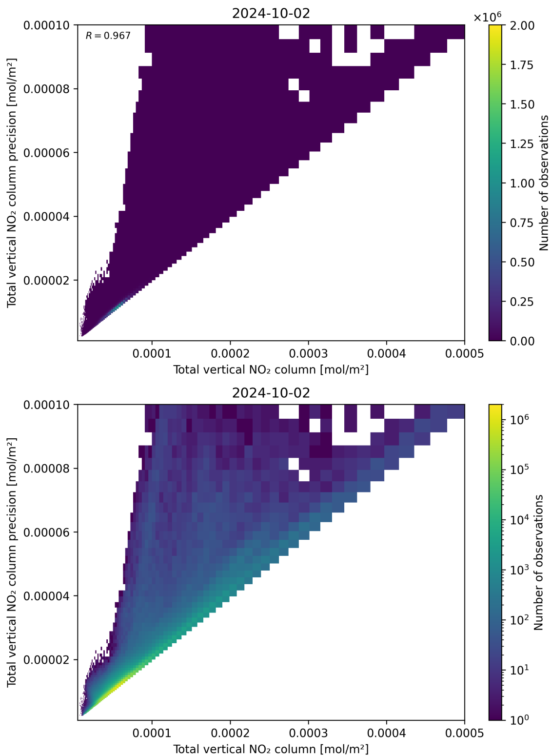
Figure 114: Scatter density plot of “Total vertical NO 2 column” against “Total vertical NO 2 column precision” for 2024-10-01 to 2024-10-03.
