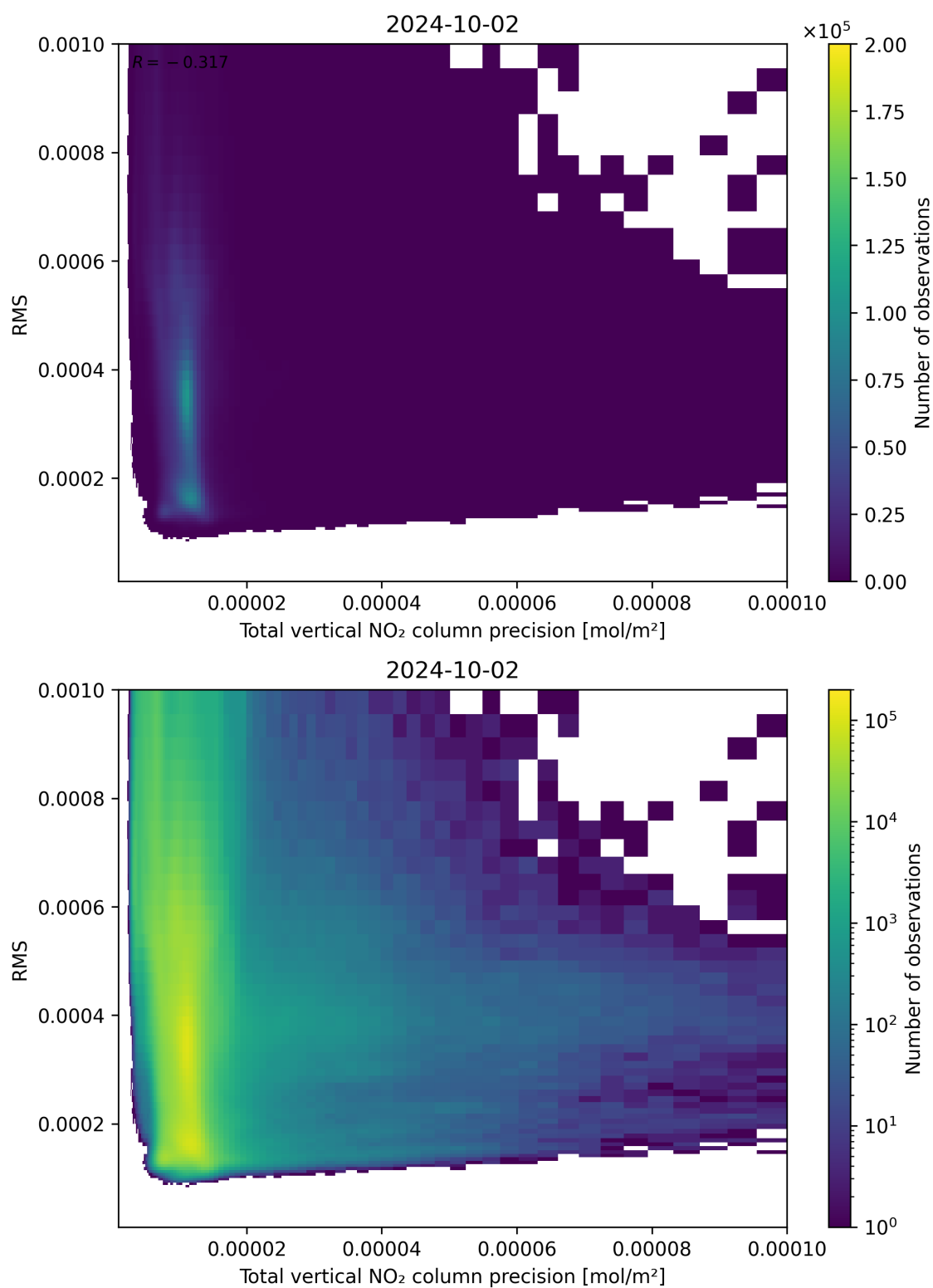
Figure 119: Scatter density plot of “Total vertical NO 2 column precision” against “RMS” for 2024-10-01 to 2024-10-03.
