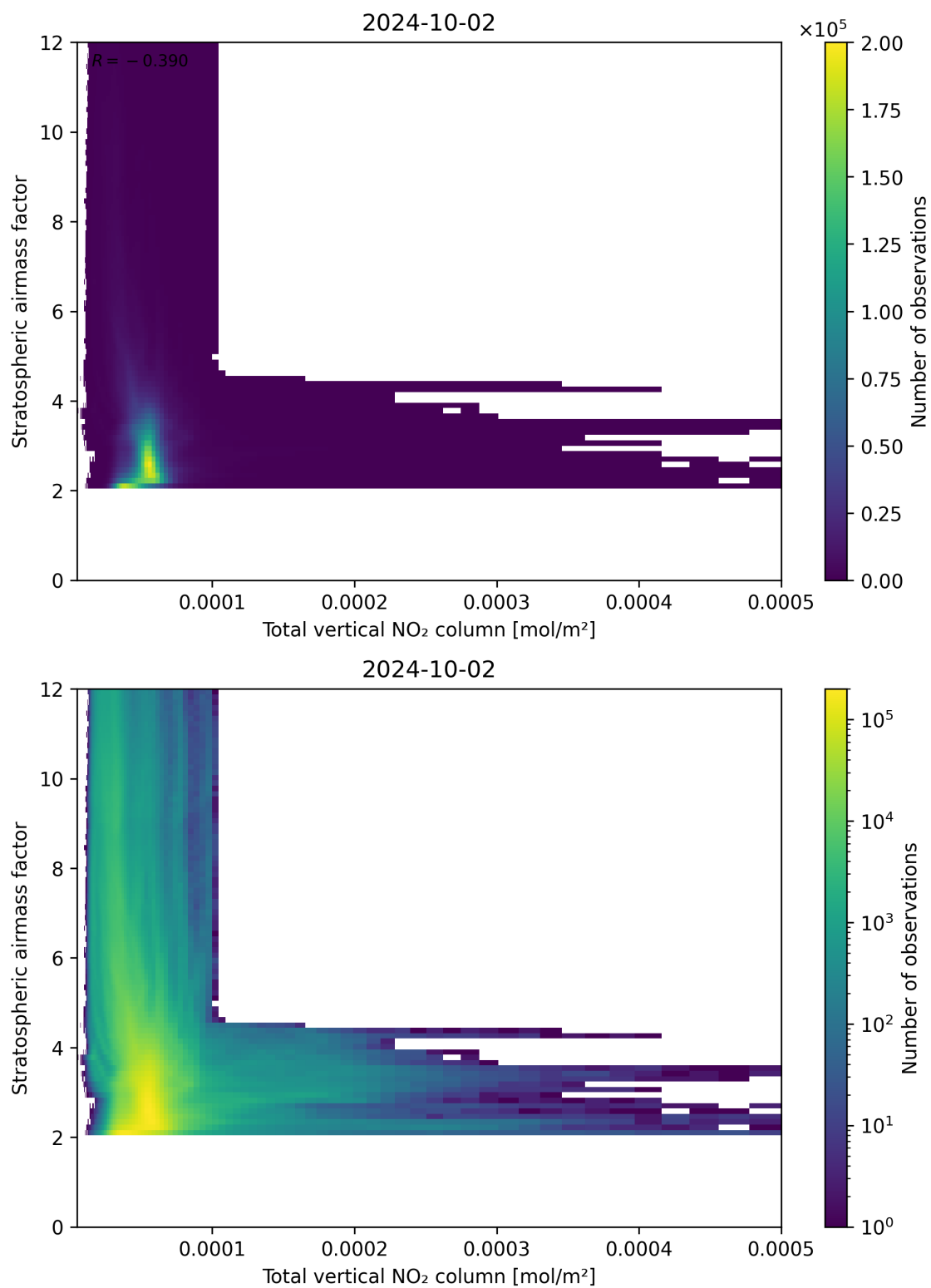
Figure 110: Scatter density plot of “Total vertical NO 2 column” against “Stratospheric airmass factor” for 2024-10-01 to 2024-10-03.
