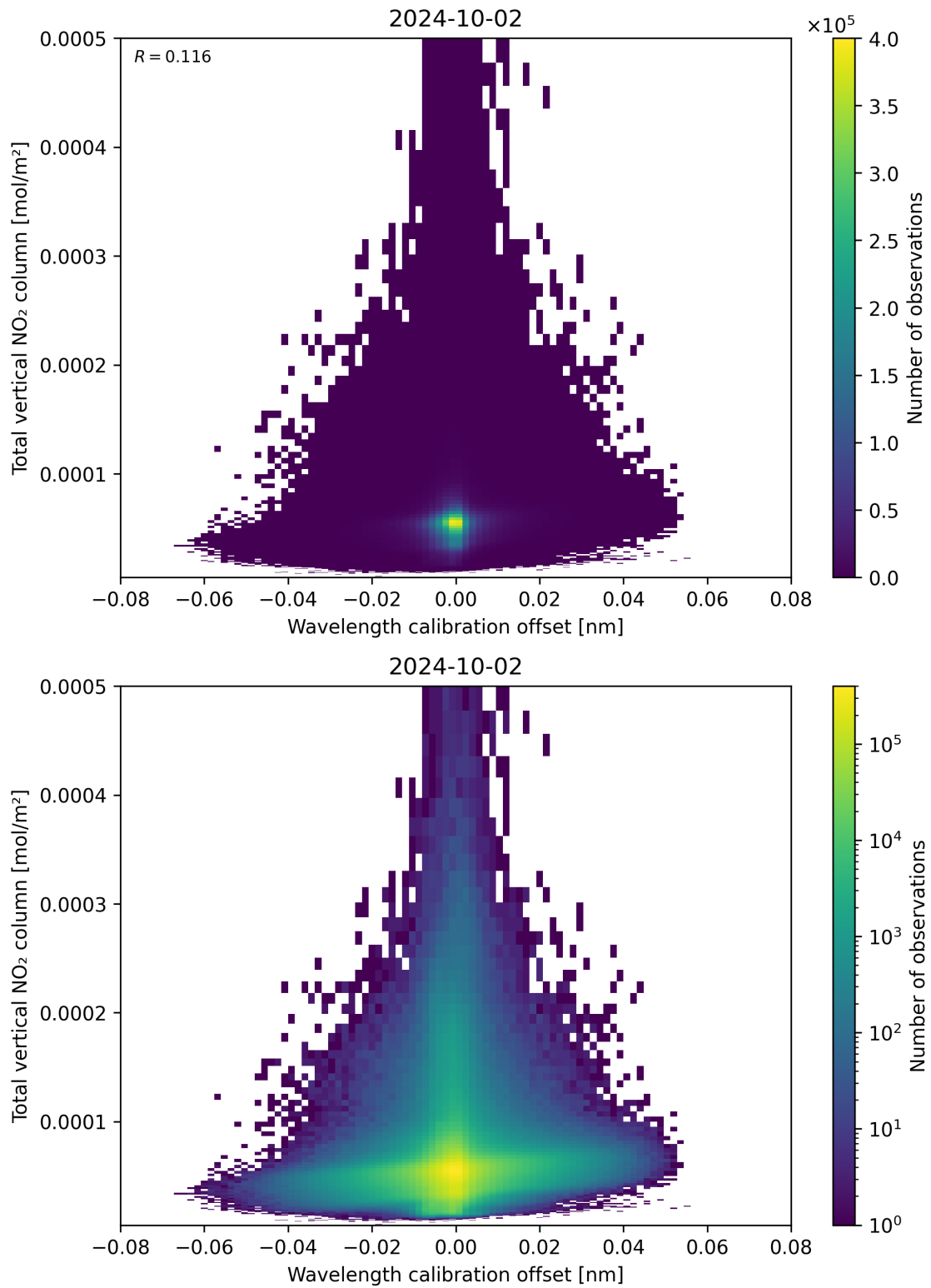
Figure 179: Scatter density plot of “Wavelength calibration offset” against “Total vertical NO 2 column” for 2024-10-01 to 2024-10-03.
