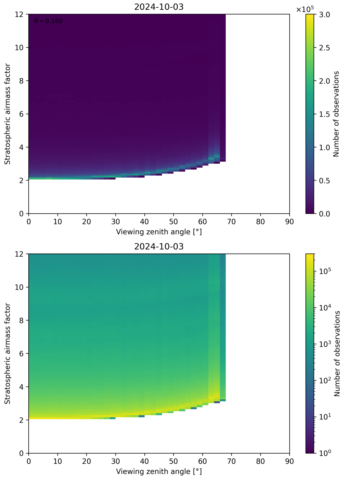
Figure 159: Scatter density plot of “Viewing zenith angle” against “Stratospheric airmass factor” for 2024-10-03 to 2024-10-04.
