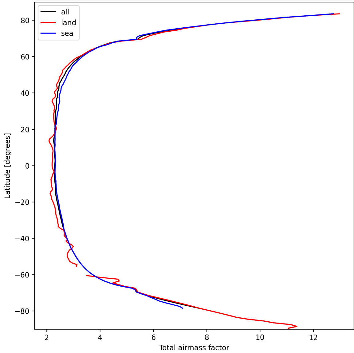
Figure 15: Zonal average of “Total airmass factor” for 2024-10-03 to 2024-10-04.
