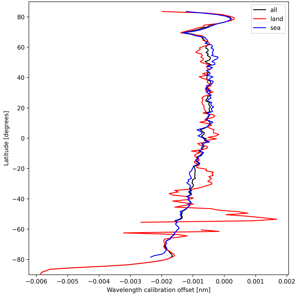
Figure 18: Zonal average of “Wavelength calibration offset” for 2024-10-03 to 2024-10-04.
