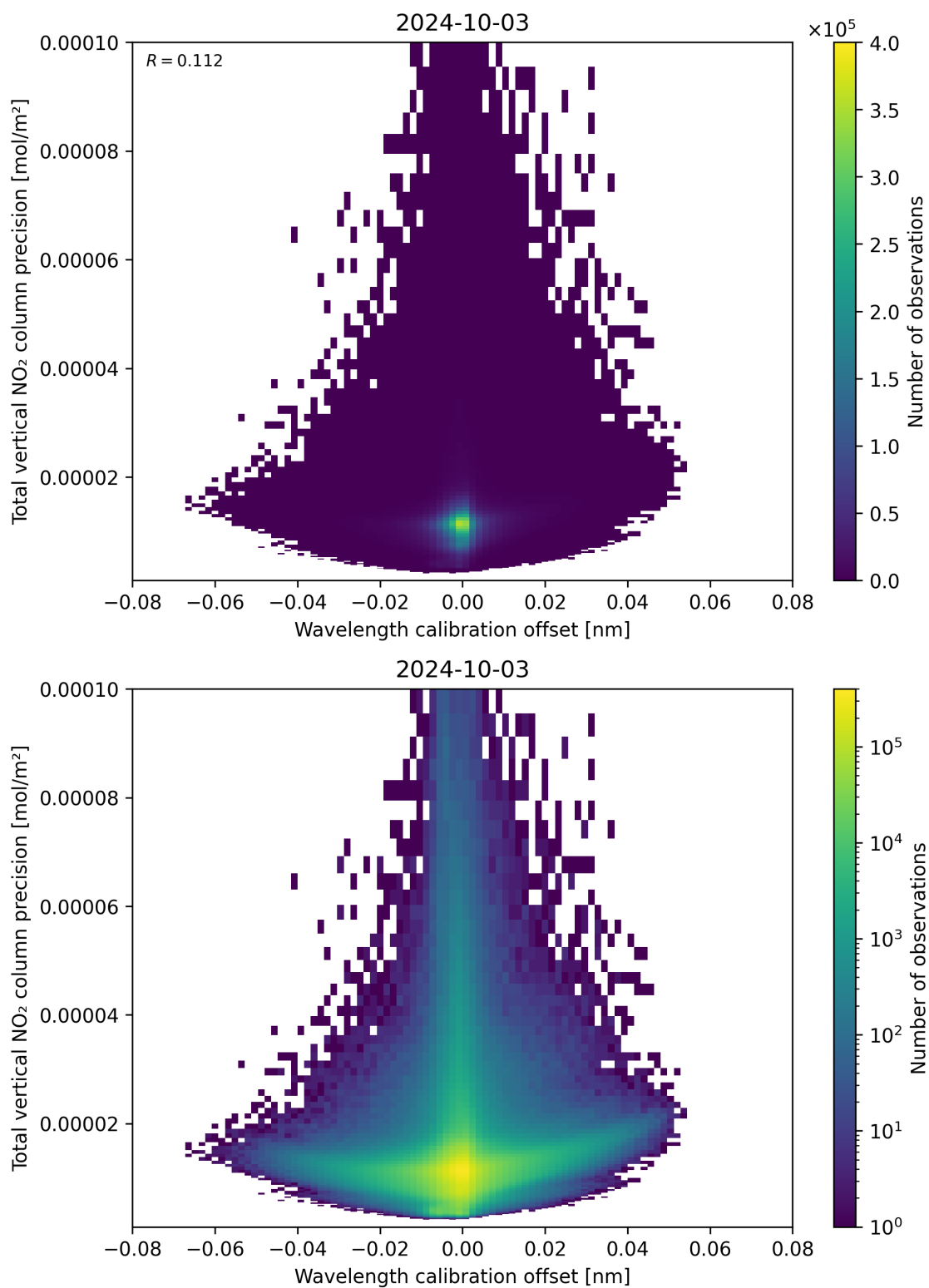
Figure 180: Scatter density plot of “Wavelength calibration offset” against “Total vertical NO 2 column precision” for 2024-10-03 to 2024-10-04.
