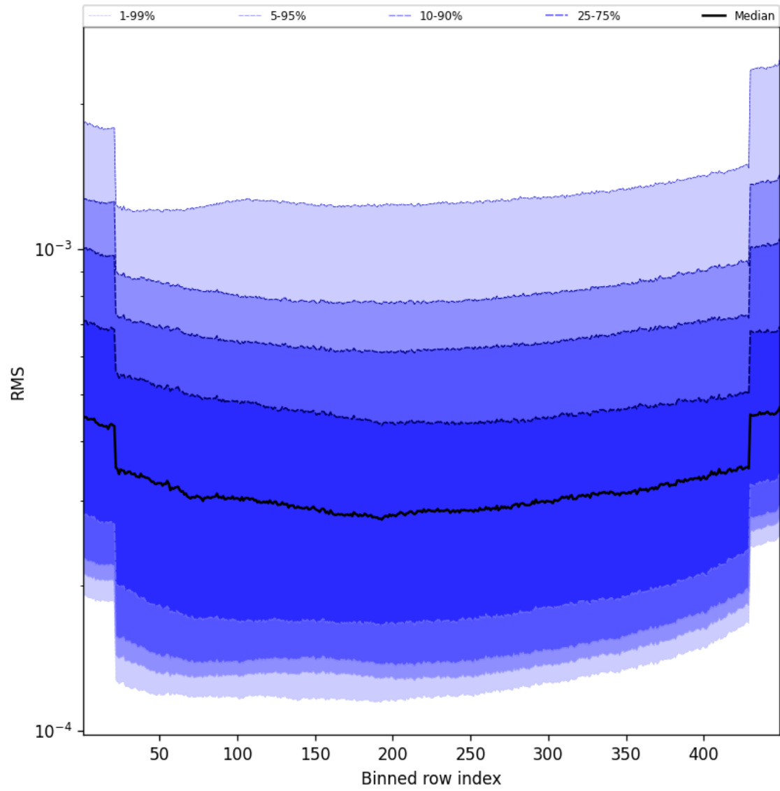
Figure 60: Along track statistics of “RMS” for 2024-10-03 to 2024-10-04
