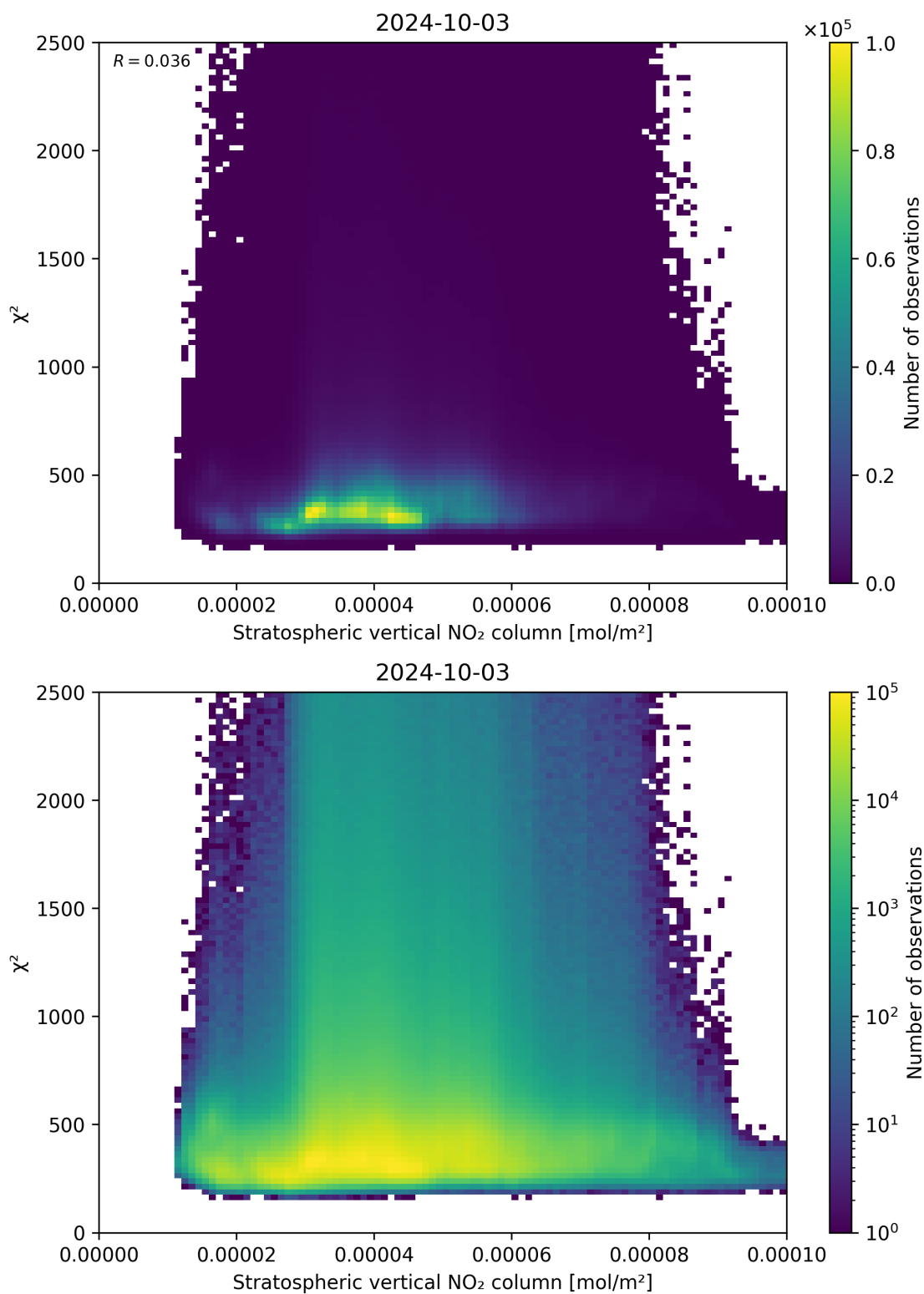
Figure 97: Scatter density plot of “Stratospheric vertical NO 2 column” against “ \chi^2 ” for 2024-10-03 to 2024-10-04.
