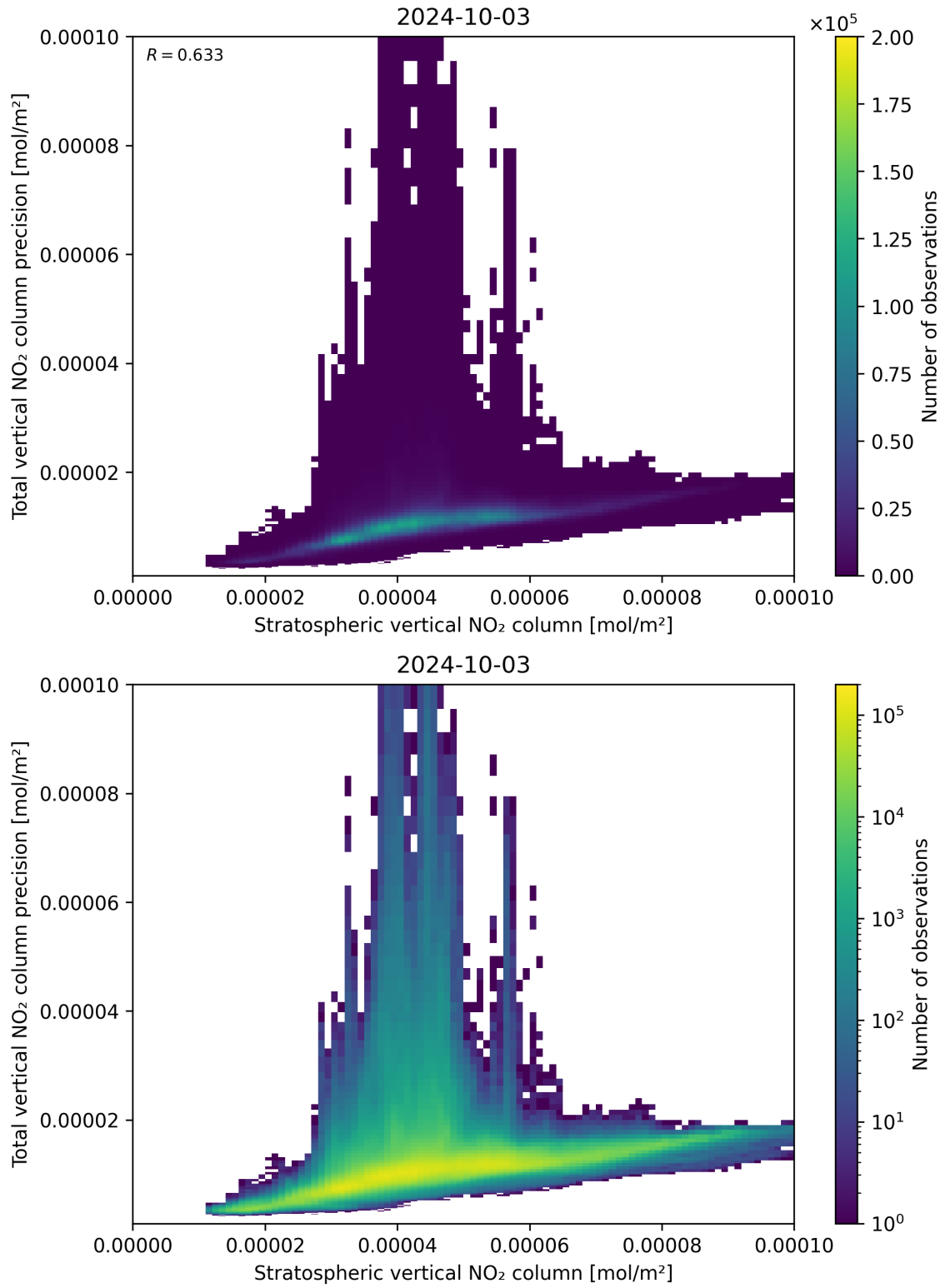
Figure 101: Scatter density plot of “Stratospheric vertical NO 2 column” against “Total vertical NO 2 column precision” for 2024-10-03 to 2024-10-04.
