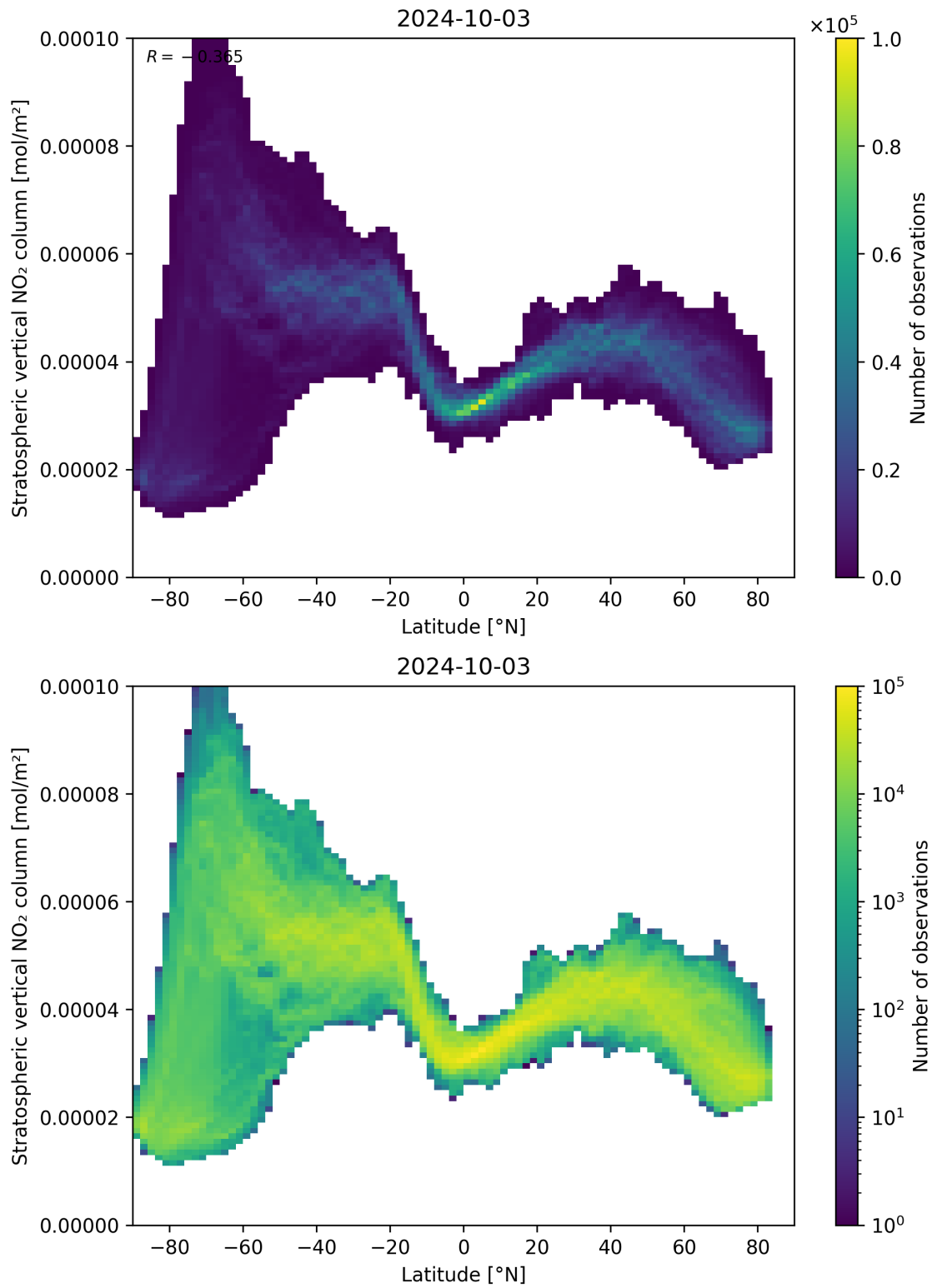
Figure 87: Scatter density plot of “Latitude” against “Stratospheric vertical NO 2 column” for 2024-10-03 to 2024-10-04.
