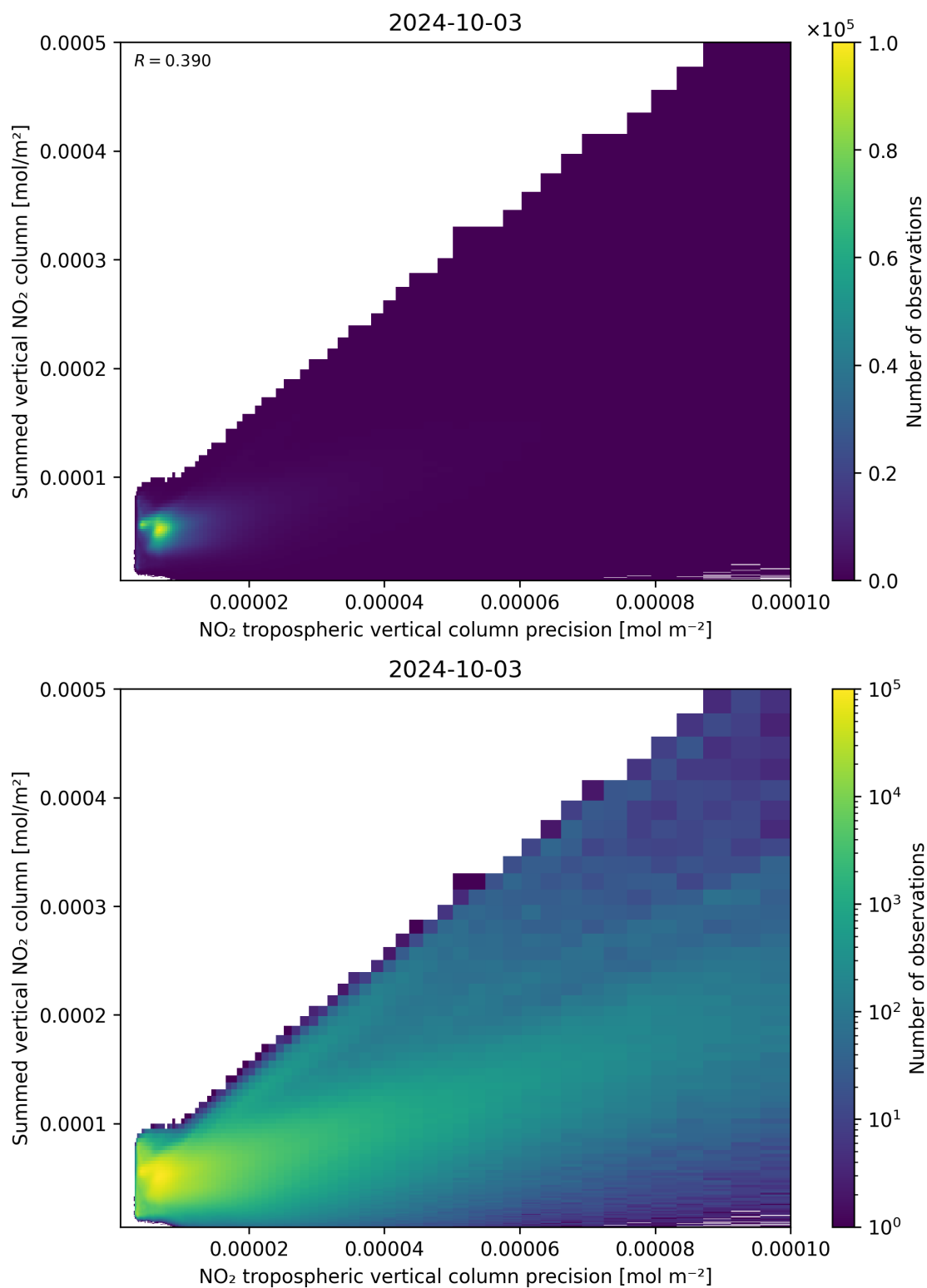
Figure 136: Scatter density plot of “NO 2 tropospheric vertical column precision” against “Summed vertical NO 2 column” for 2024-10-03 to 2024-10-04.
