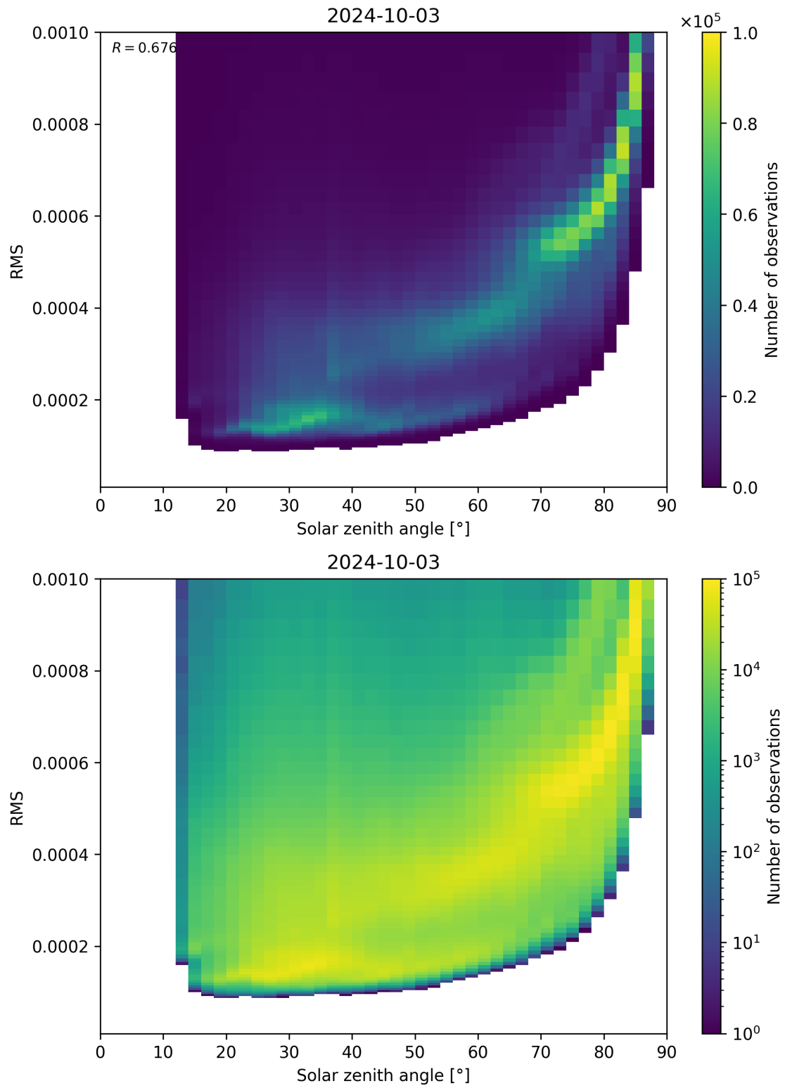
Figure 157: Scatter density plot of “Solar zenith angle” against “RMS” for 2024-10-03 to 2024-10-04.
