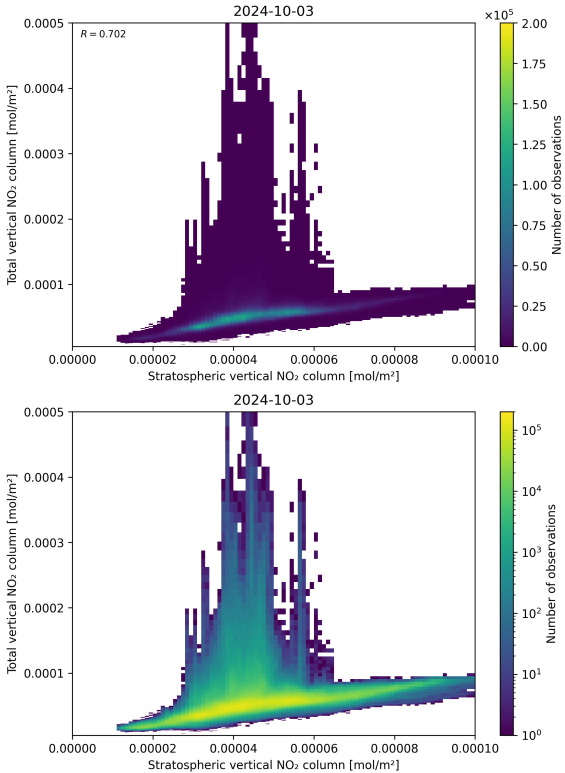
Figure 100: Scatter density plot of “Stratospheric vertical NO 2 column” against “Total vertical NO 2 column” for 2024-10-03 to 2024-10-04.
