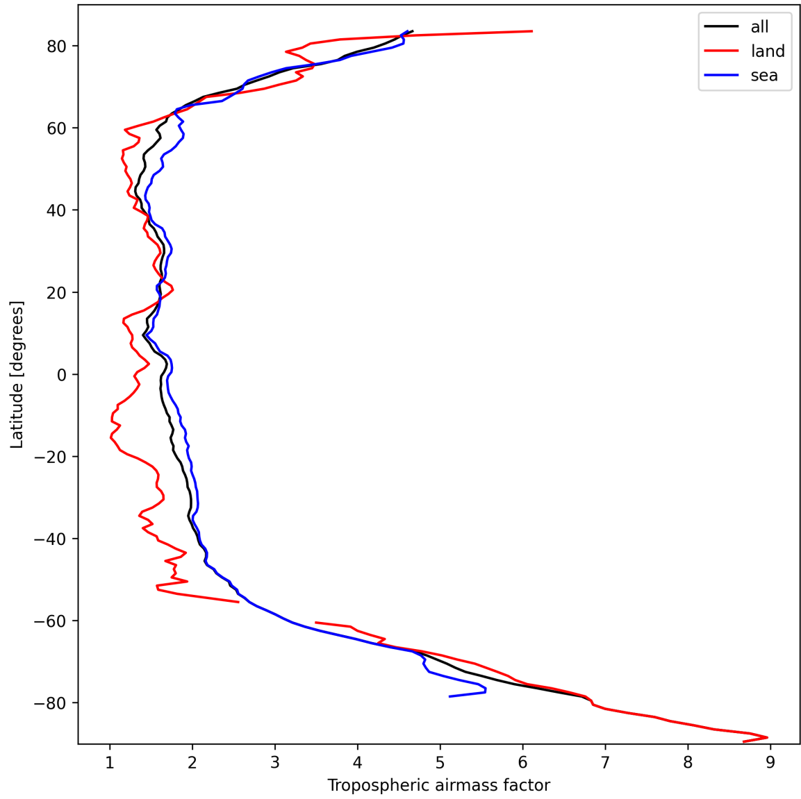
Figure 14: Zonal average of “Tropospheric air mass factor” for 2024-10-03 to 2024-10-04.
