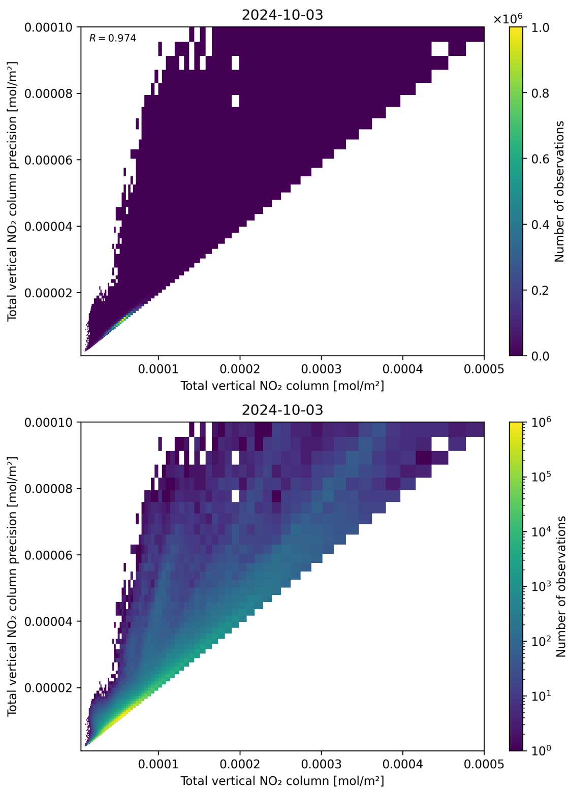
Figure 114: Scatter density plot of “Total vertical NO 2 column” against “Total vertical NO 2 column precision” for 2024-10-03 to 2024-10-04.
