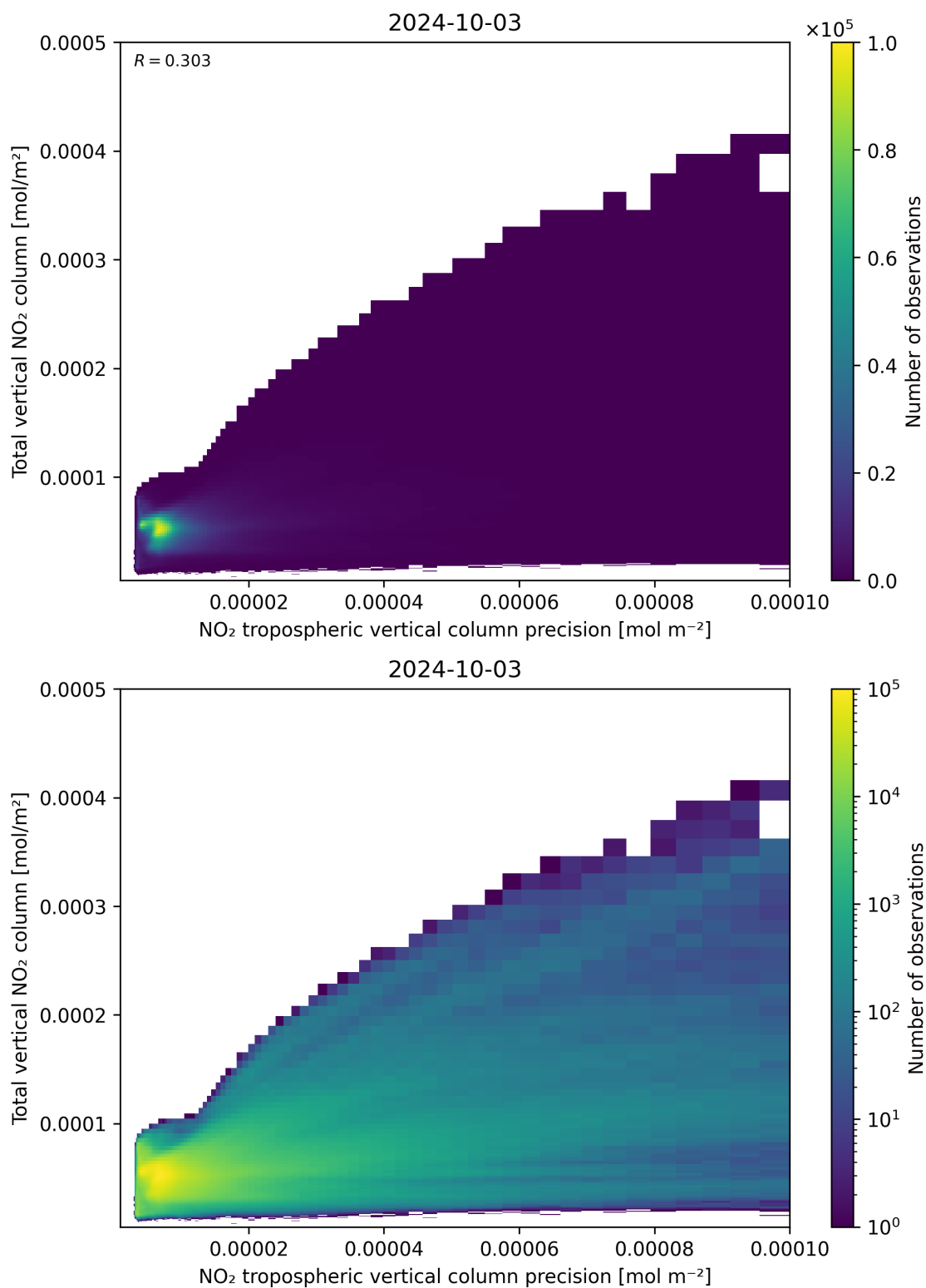
Figure 138: Scatter density plot of “NO 2 tropospheric vertical column precision” against “Total vertical NO 2 column” for 2024-10-03 to 2024-10-04.
