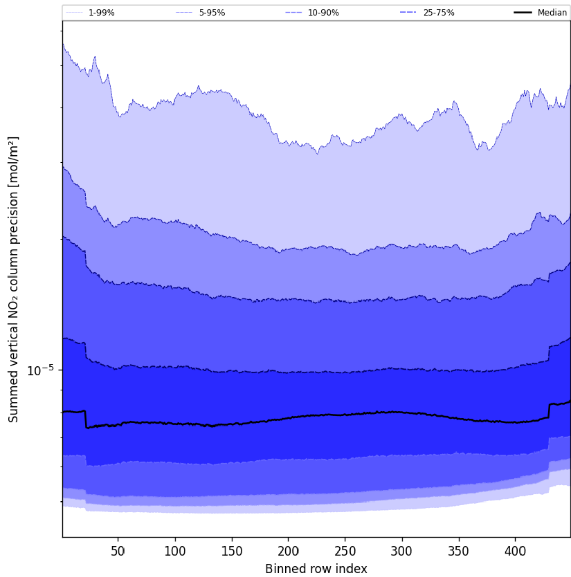
Figure 58: Along track statistics of “Summed vertical NO 2 column precision” for 2024-10-03 to 2024-10-04
