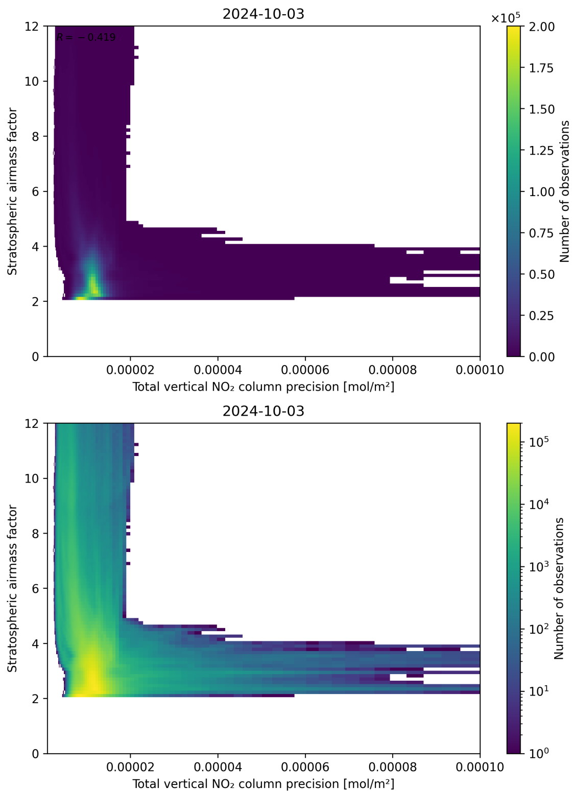
Figure 115: Scatter density plot of “Total vertical NO 2 column precision” against “Stratospheric air mass factor” for 2024-10-03 to 2024-10-04.
