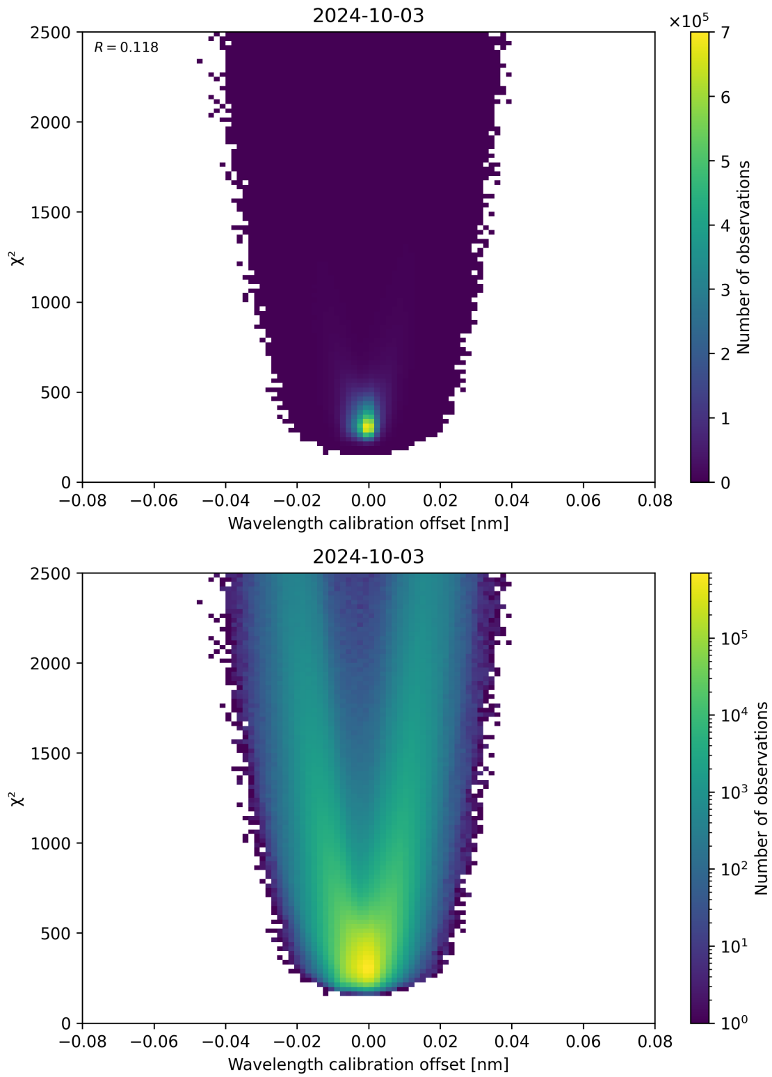
Figure 175: Scatter density plot of “Wavelength calibration offset” against “ \chi^2 ” for 2024-10-03 to 2024-10-04.
