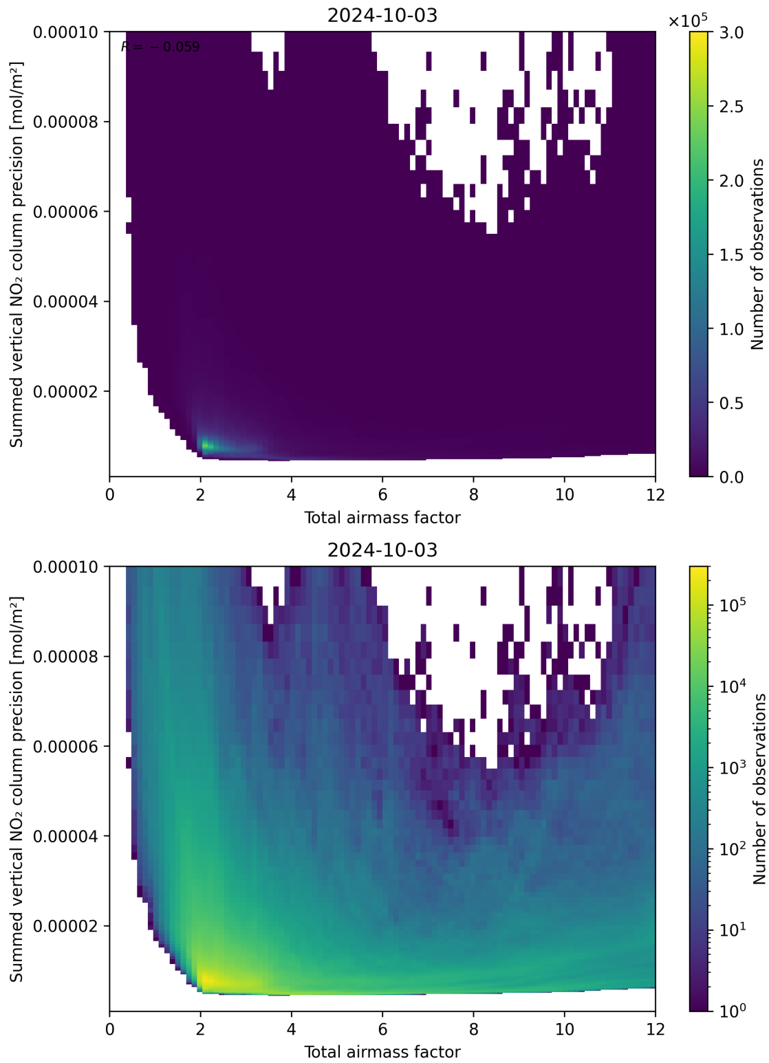
Figure 66: Scatter density plot of “Total airmass factor” against “Summed vertical NO 2 column precision” for 2024-10-03 to 2024-10-04.
