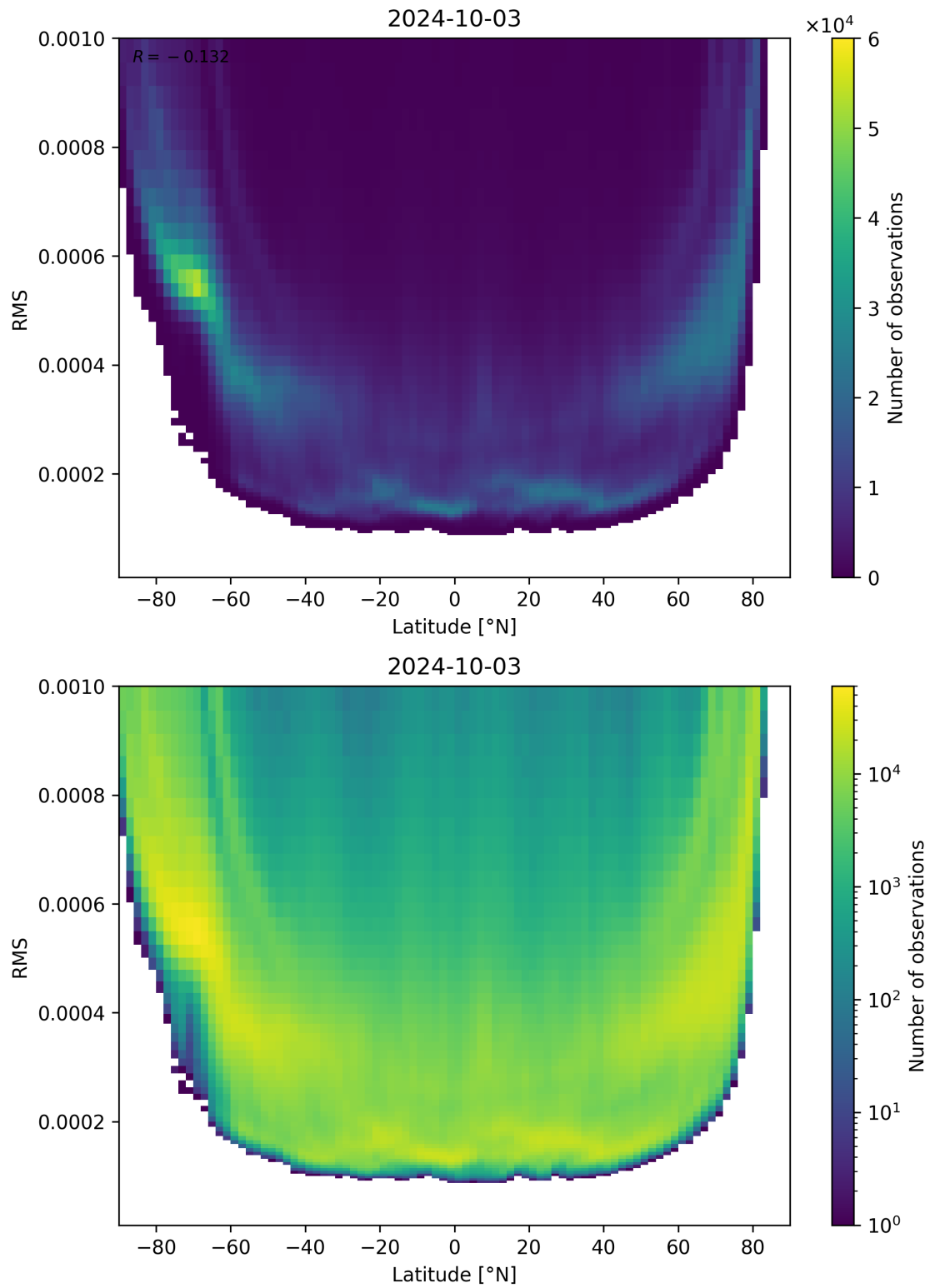
Figure 94: Scatter density plot of “Latitude” against “RMS” for 2024-10-03 to 2024-10-04.
