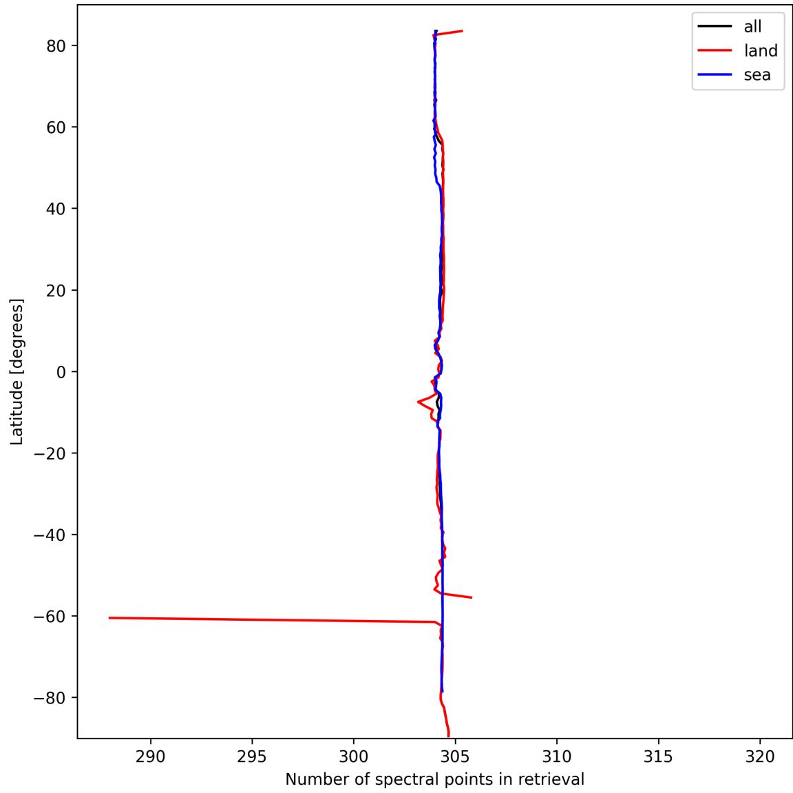
Figure 16: Zonal average of “Number of spectral points in retrieval” for 2024-10-03 to 2024-10-04.
