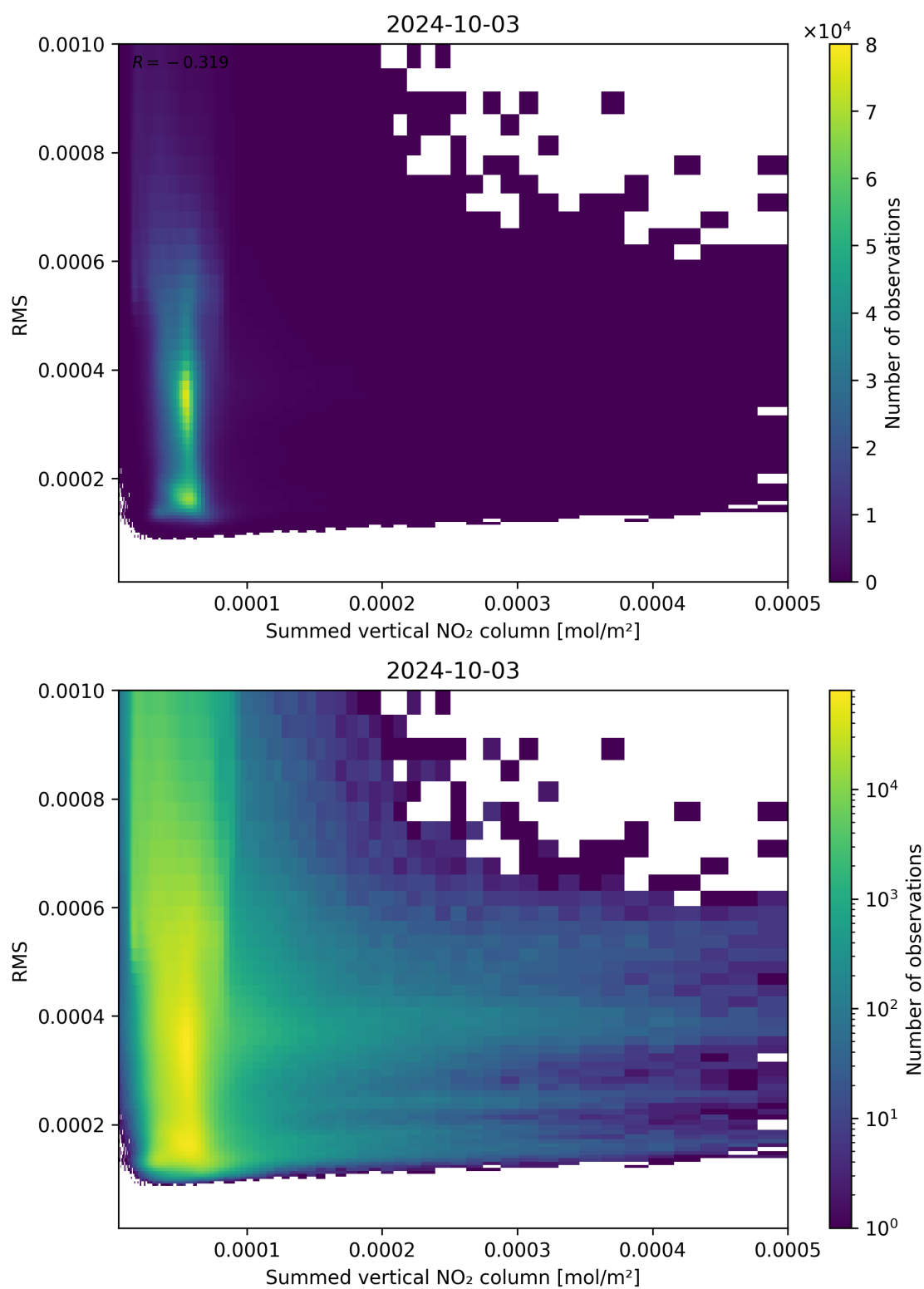
Figure 109: Scatter density plot of “Summed vertical NO 2 column” against “RMS” for 2024-10-03 to 2024-10-04.
