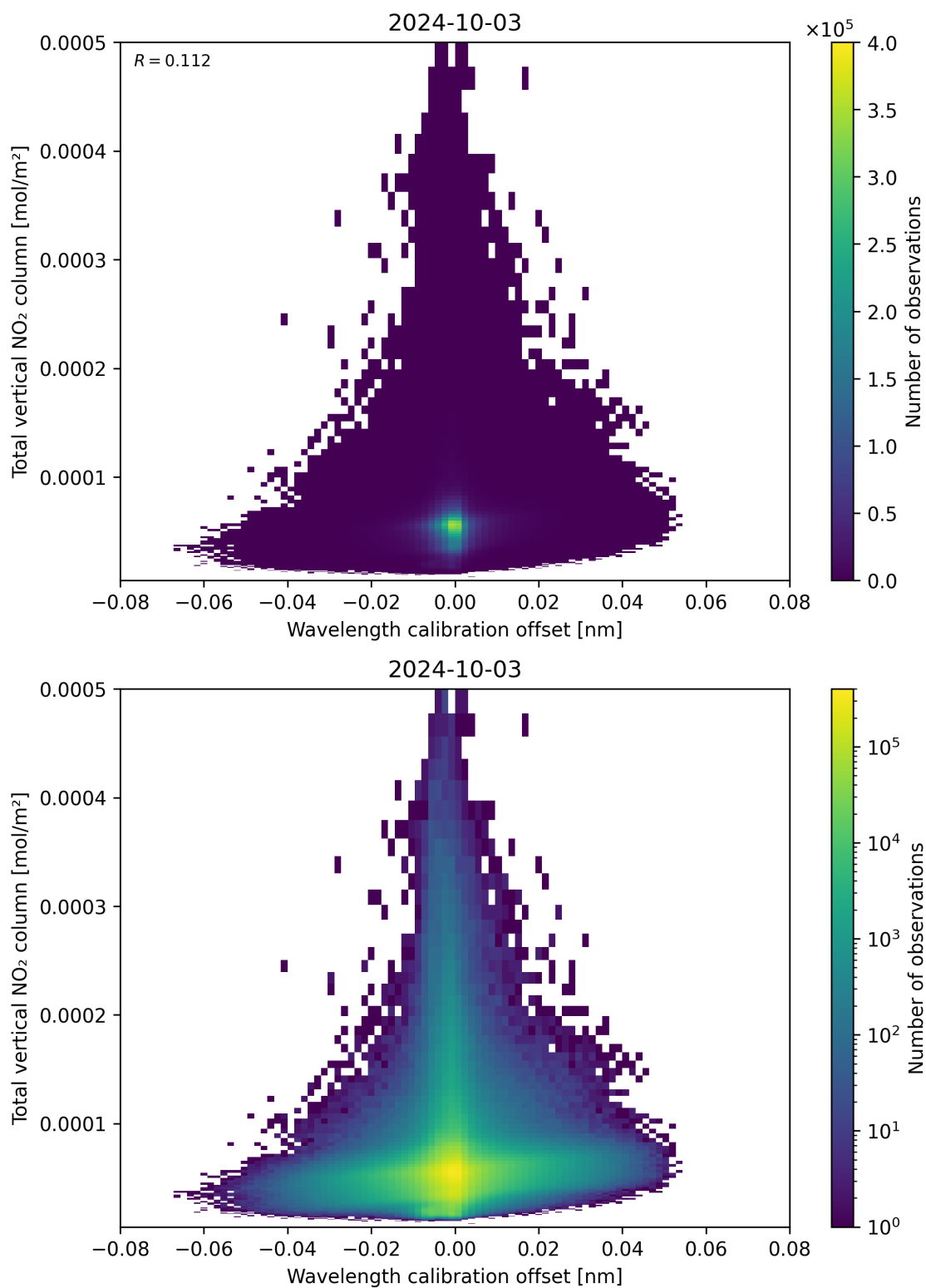
Figure 179: Scatter density plot of “Wavelength calibration offset” against “Total vertical NO 2 column” for 2024-10-03 to 2024-10-04.
