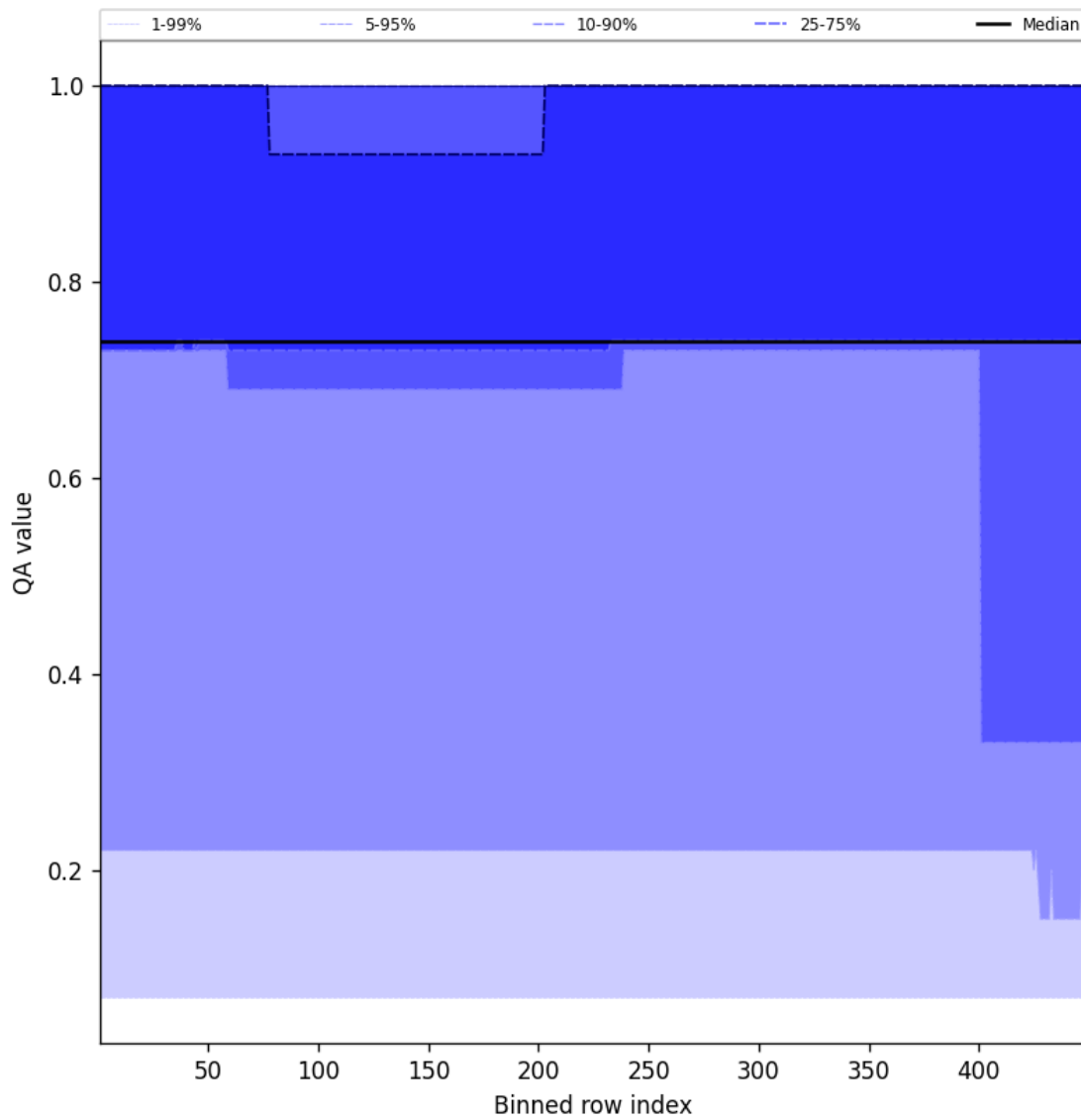
Figure 45: Along track statistics of “QA value” for 2024-10-03 to 2024-10-04
