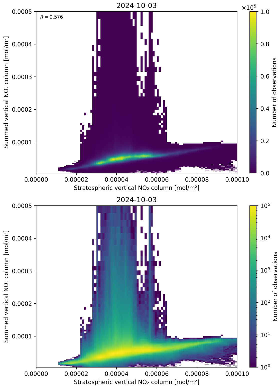
Figure 98: Scatter density plot of “Stratospheric vertical NO 2 column” against “Summed vertical NO 2 column” for 2024-10-03 to 2024-10-04.
