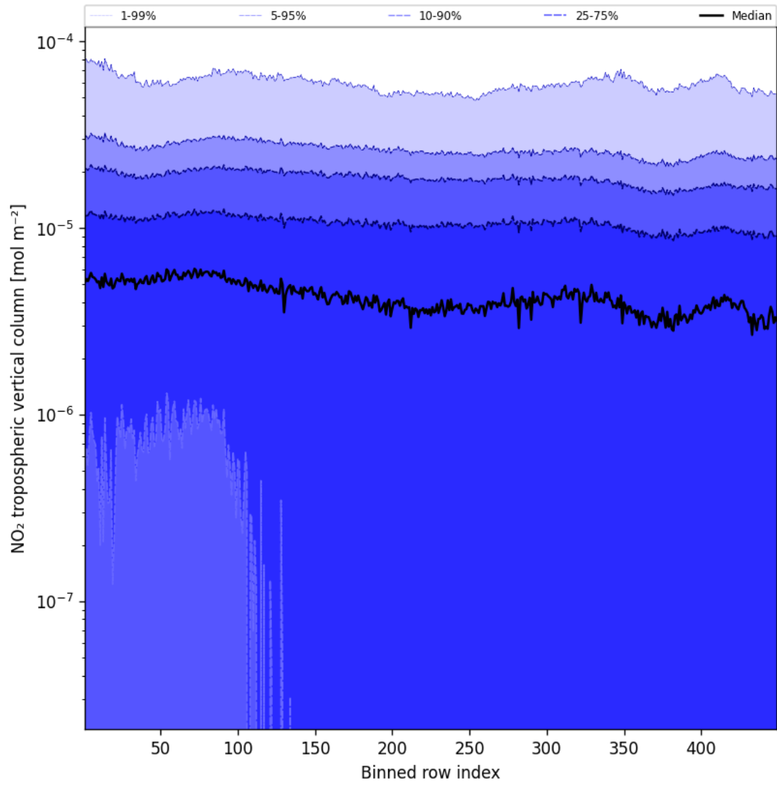
Figure 46: Along track statistics of “NO 2 tropospheric vertical column” for 2024-10-03 to 2024-10-04
