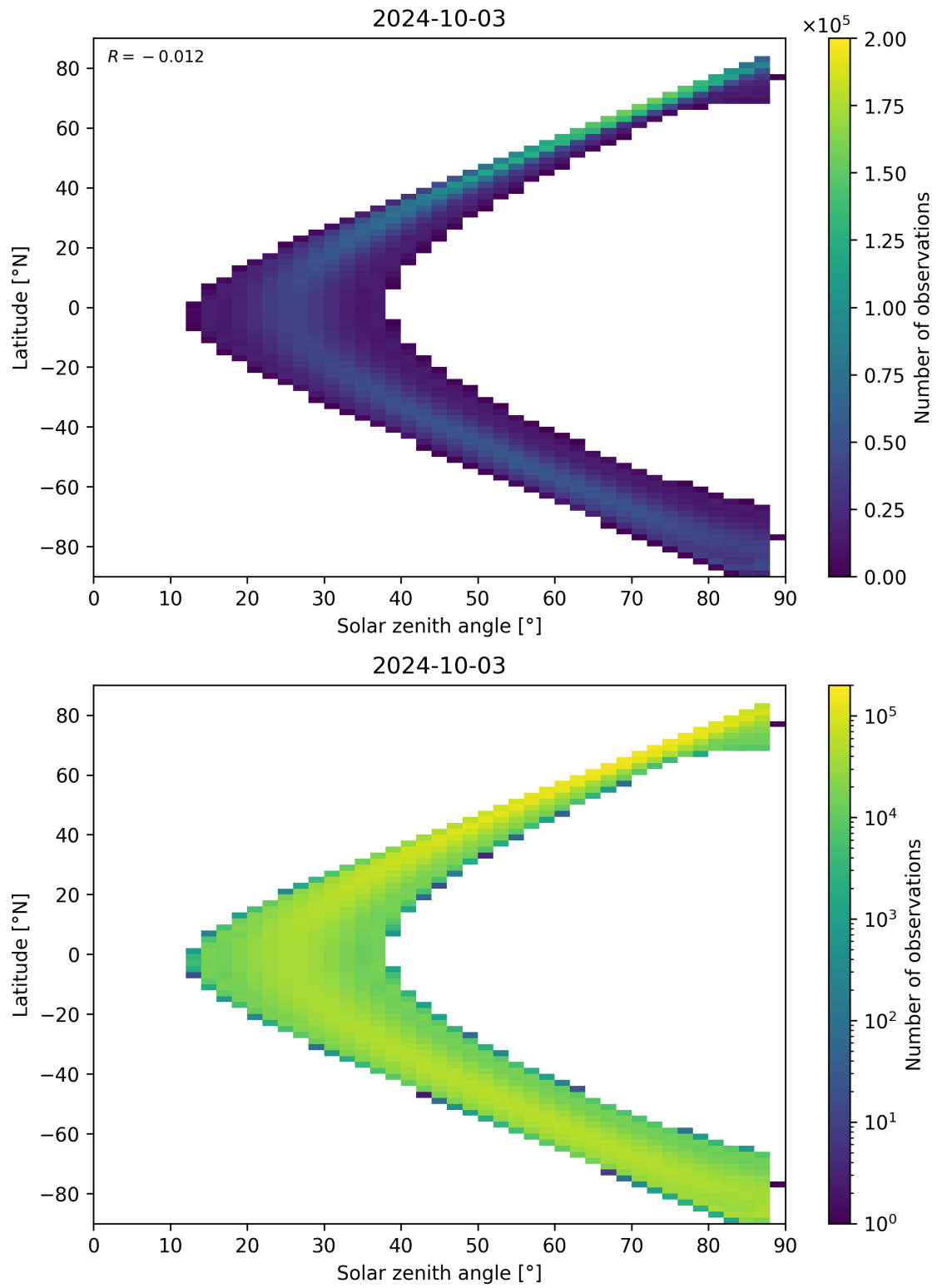
Figure 149: Scatter density plot of “Solar zenith angle” against “Latitude” for 2024-10-03 to 2024-10-04.
