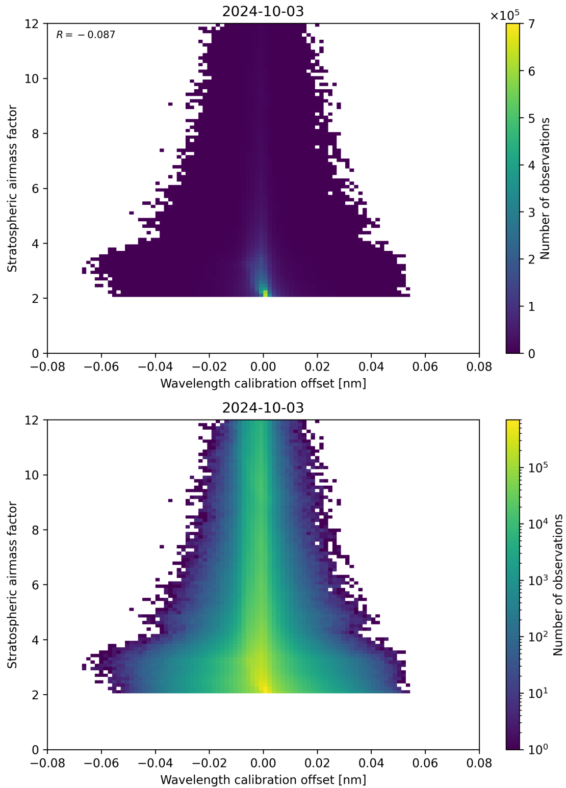
Figure 174: Scatter density plot of “Wavelength calibration offset” against “Stratospheric airmass factor” for 2024-10-03 to 2024-10-04.
