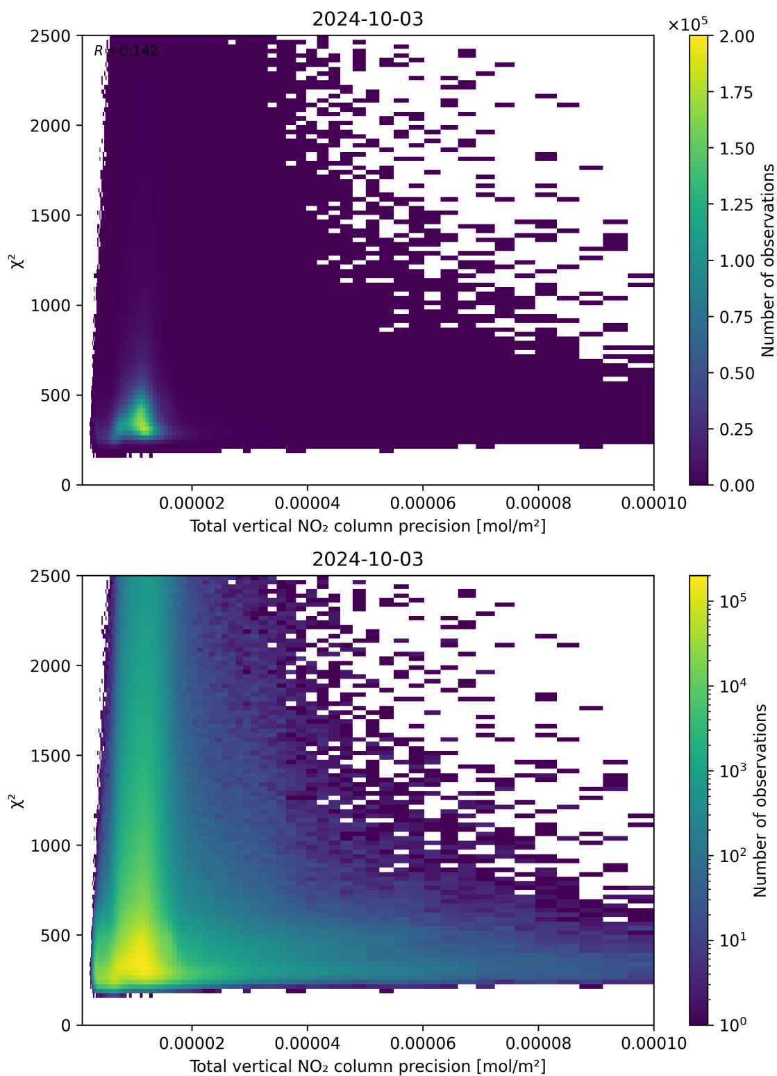
Figure 116: Scatter density plot of “Total vertical NO 2 column precision” against “ \chi^2 ” for 2024-10-03 to 2024-10-04.
