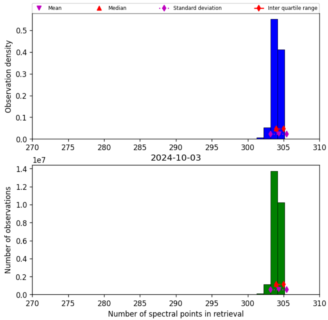
Figure 33: Histogram of “Number of spectral points in retrieval” for 2024-10-03 to 2024-10-04
