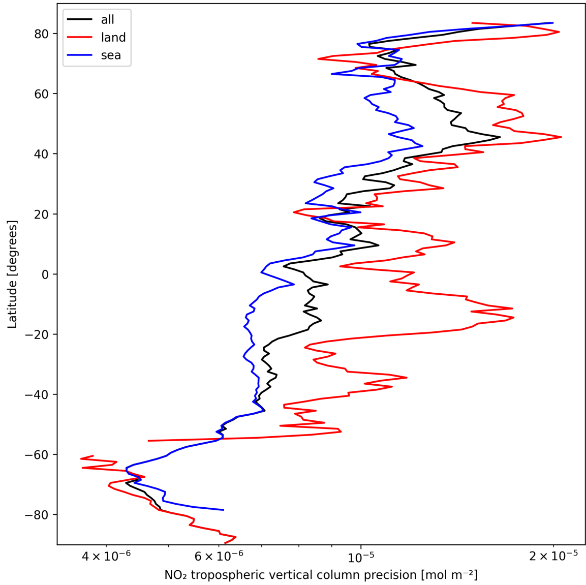
Figure 13: Zonal average of “NO 2 tropospheric vertical column precision” for 2024-10-03 to 2024-10-04.
