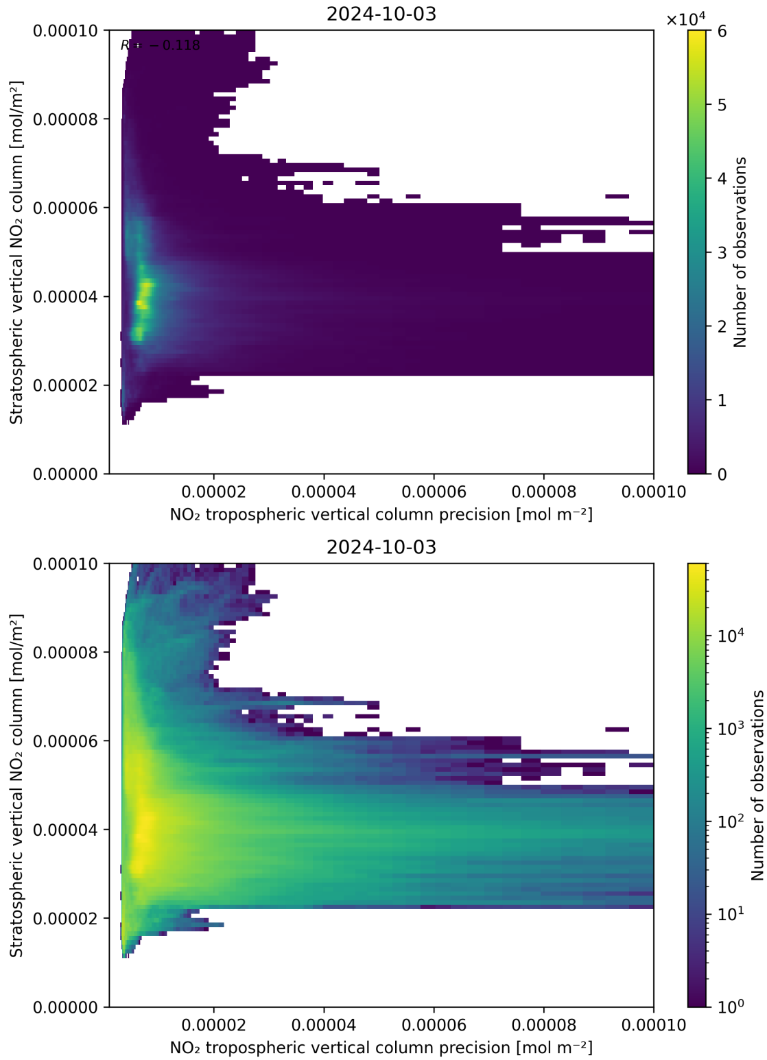
Figure 135: Scatter density plot of “NO 2 tropospheric vertical column precision” against “Stratospheric vertical NO 2 column” for 2024-10-03 to 2024-10-04.
