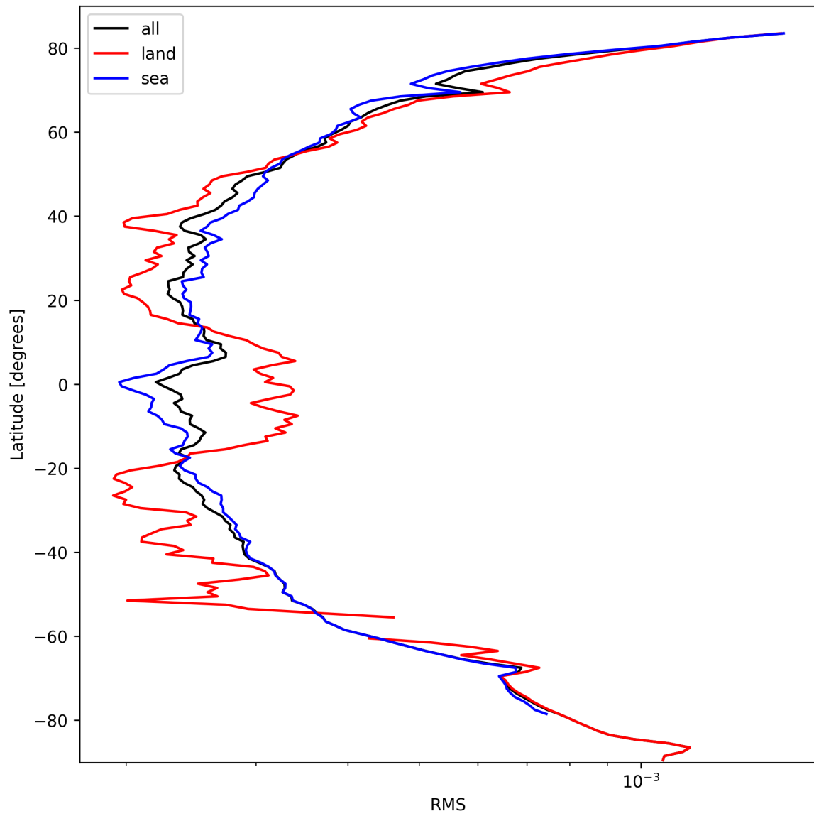
Figure 26: Zonal average of “RMS” for 2024-10-03 to 2024-10-04.
