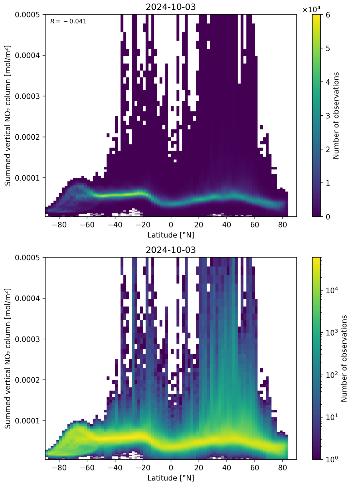
Figure 88: Scatter density plot of “Latitude” against “Summed vertical NO 2 column” for 2024-10-03 to 2024-10-04.
