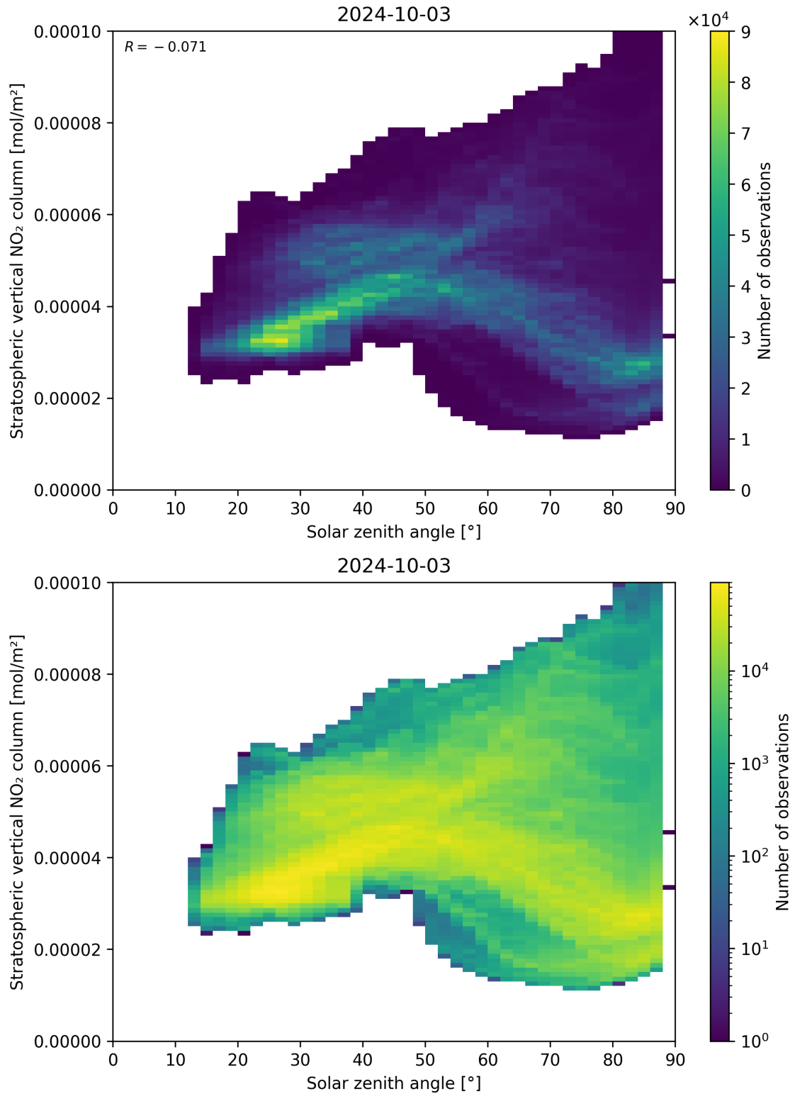
Figure 150: Scatter density plot of “Solar zenith angle” against “Stratospheric vertical NO 2 column” for 2024-10-03 to 2024-10-04.
