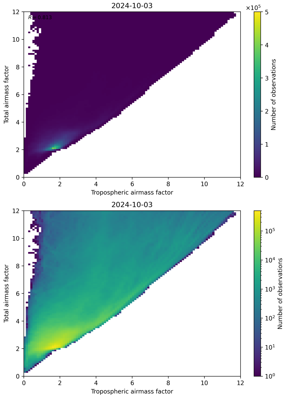
Figure 72: Scatter density plot of “Tropospheric airmass factor” against “Total airmass factor” for 2024-10-03 to 2024-10-04.
