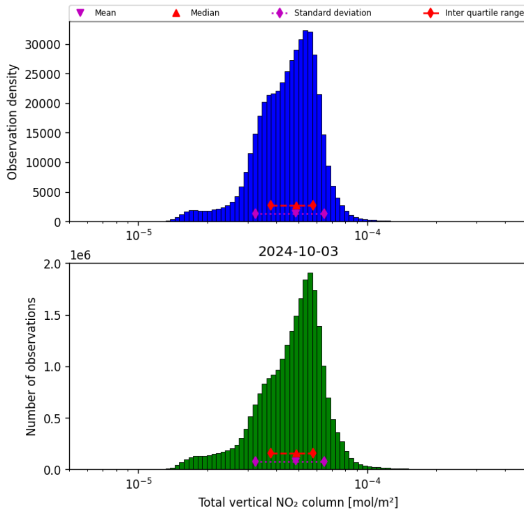
Figure 38: Histogram of “Total vertical NO 2 column” for 2024-10-03 to 2024-10-04
