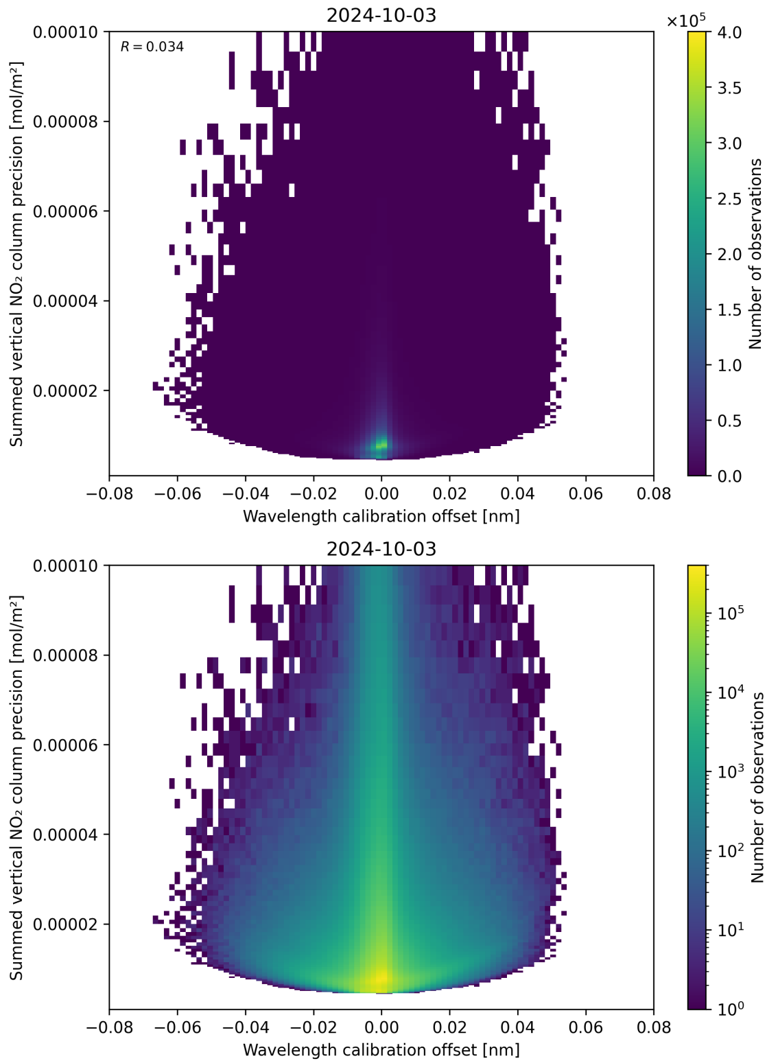
Figure 178: Scatter density plot of “Wavelength calibration offset” against “Summed vertical NO 2 column precision” for 2024-10-03 to 2024-10-04.
