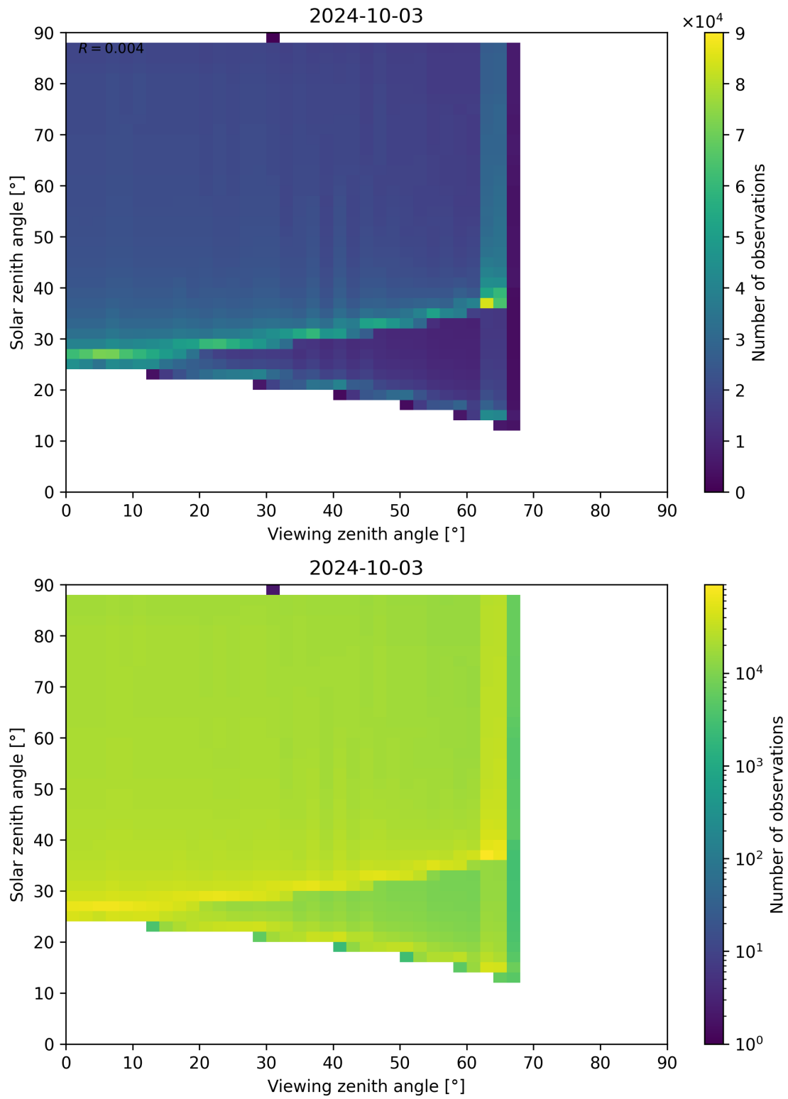
Figure 172: Scatter density plot of “Viewing zenith angle” against “Solar zenith angle” for 2024-10-03 to 2024-10-04.
