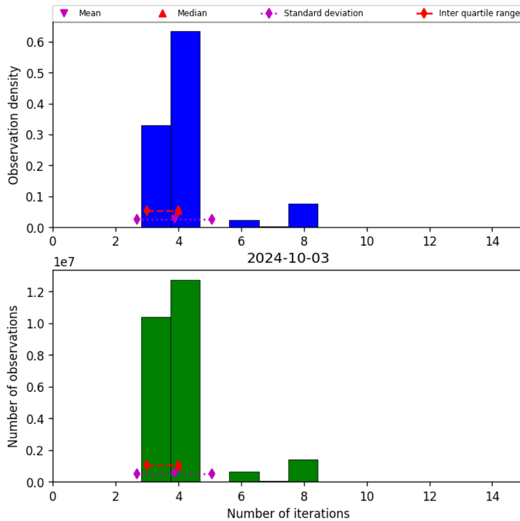
Figure 34: Histogram of “Number of iterations” for 2024-10-03 to 2024-10-04
