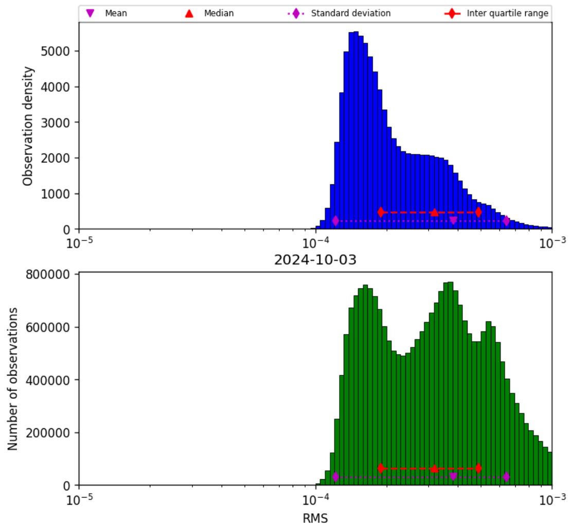
Figure 43: Histogram of “RMS” for 2024-10-03 to 2024-10-04
