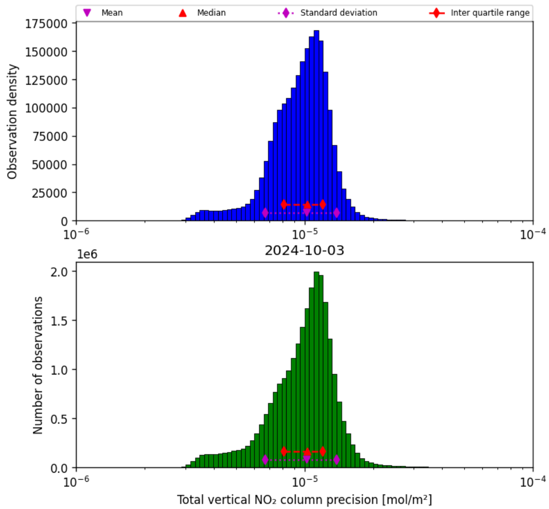
Figure 39: Histogram of “Total vertical NO 2 column precision” for 2024-10-03 to 2024-10-04
