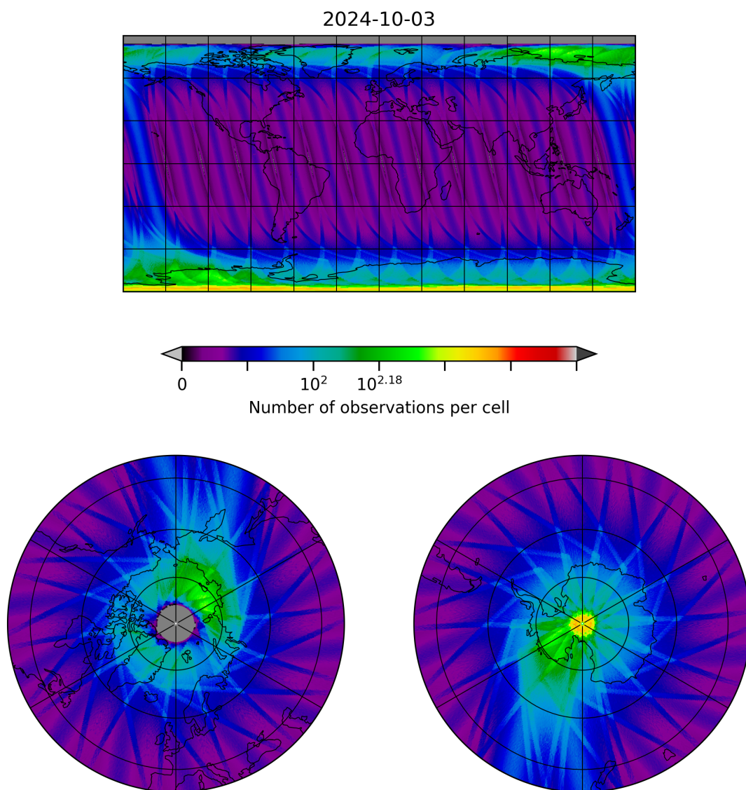
Figure 10: Map of the number of observations for 2024-10-03 to 2024-10-04
