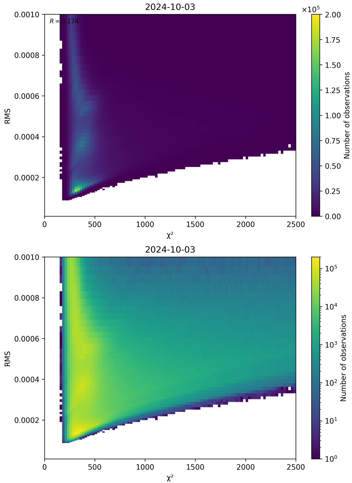
Figure 82: Scatter density plot of “ \chi^2 ” against “RMS” for 2024-10-03 to 2024-10-04.
