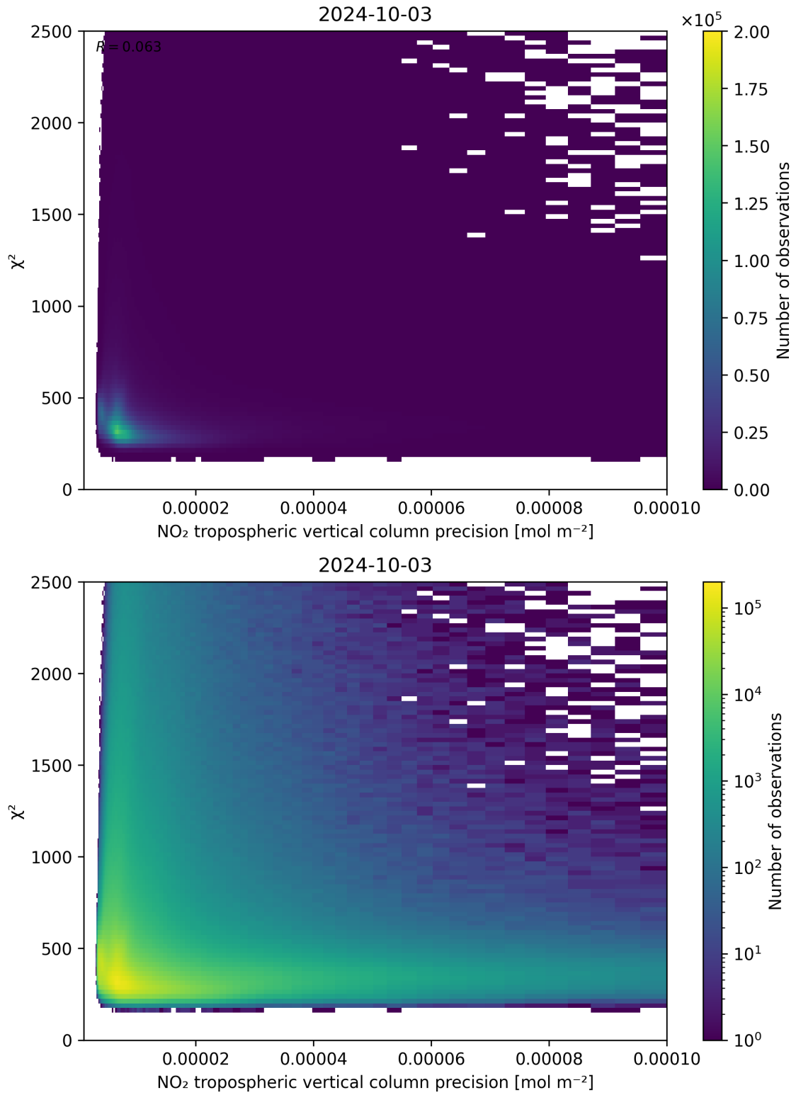
Figure 134: Scatter density plot of “NO 2 tropospheric vertical column precision” against “ \chi^2 ” for 2024-10-03 to 2024-10-04.
