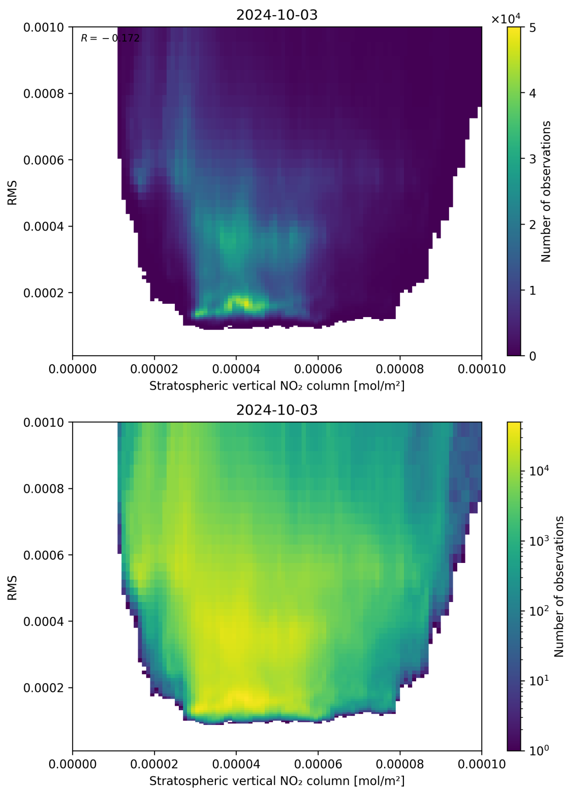
Figure 102: Scatter density plot of “Stratospheric vertical NO 2 column” against “RMS” for 2024-10-03 to 2024-10-04.
