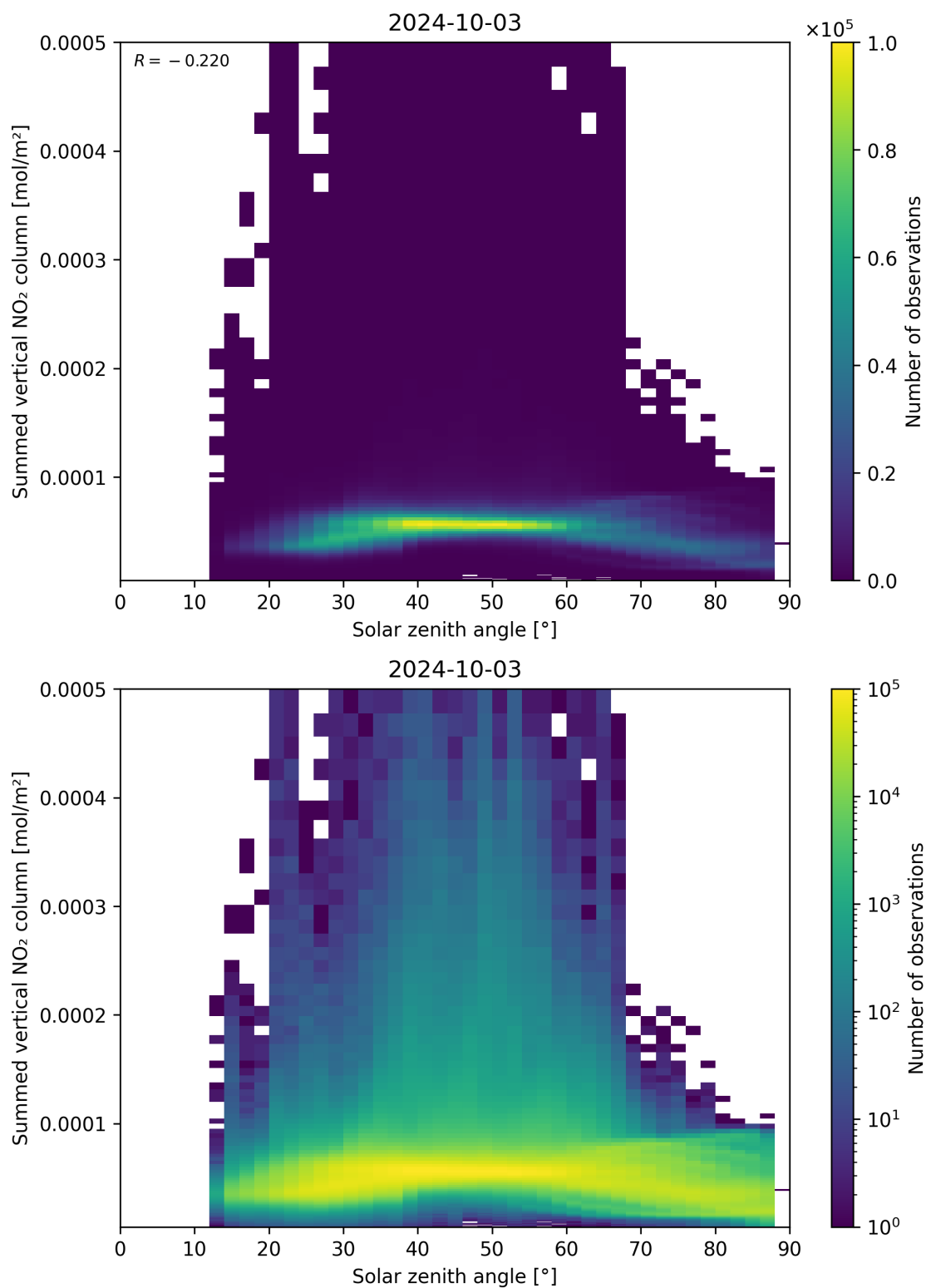
Figure 151: Scatter density plot of “Solar zenith angle” against “Summed vertical NO 2 column” for 2024-10-03 to 2024-10-04.
