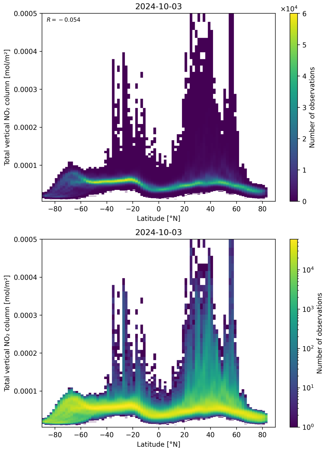
Figure 90: Scatter density plot of “Latitude” against “Total vertical NO 2 column” for 2024-10-03 to 2024-10-04.
