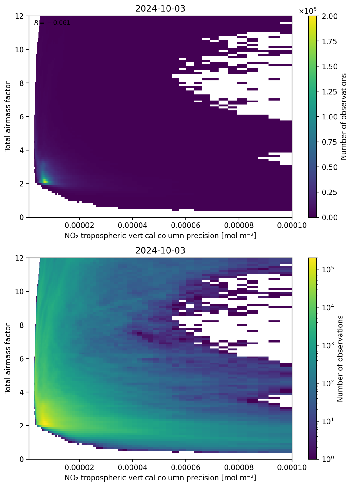
Figure 132: Scatter density plot of “NO 2 tropospheric vertical column precision” against “Total air mass factor” for 2024-10-03 to 2024-10-04.
