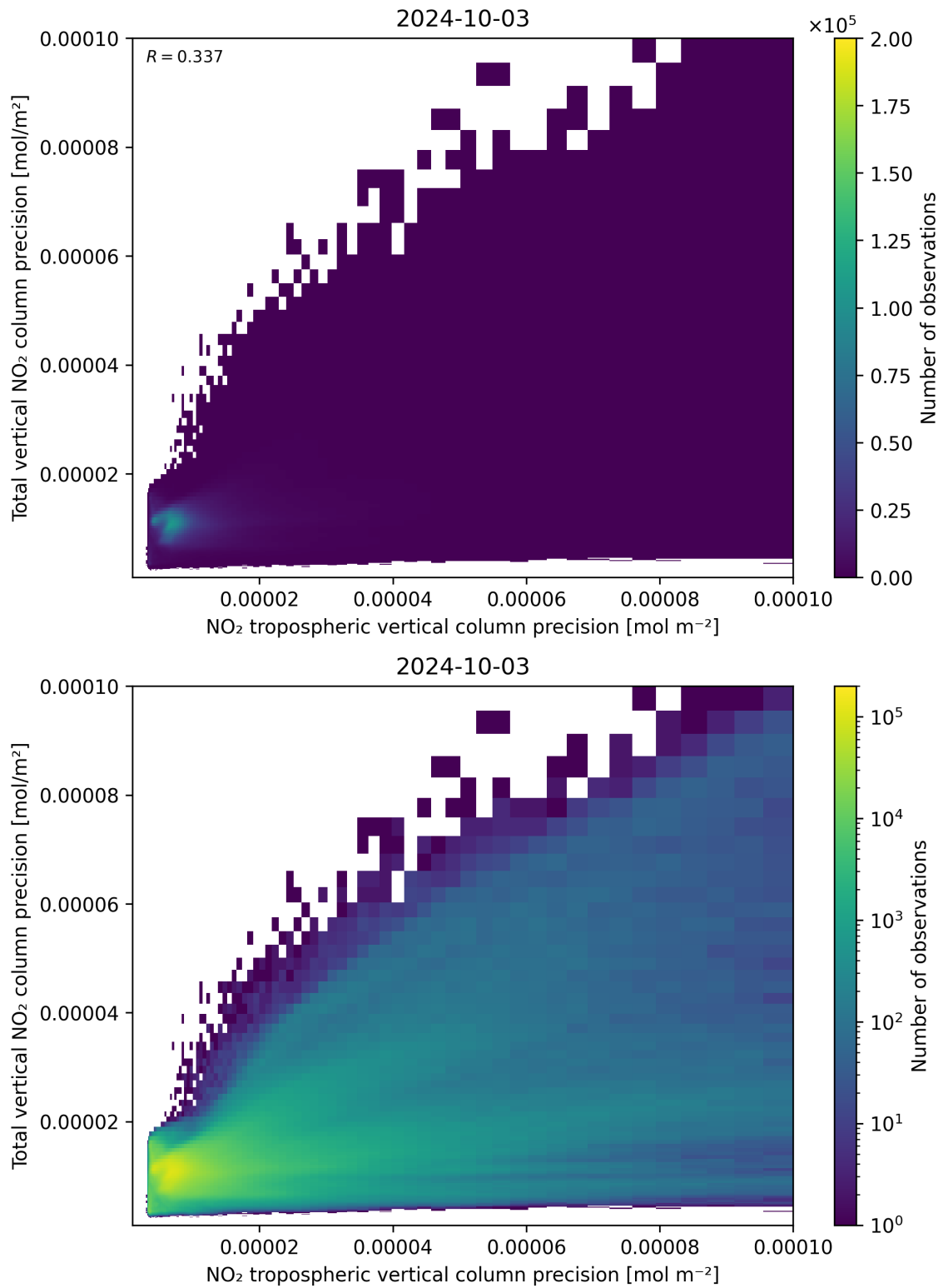
Figure 139: Scatter density plot of “NO 2 tropospheric vertical column precision” against “Total vertical NO 2 column precision” for 2024-10-03 to 2024-10-04.
