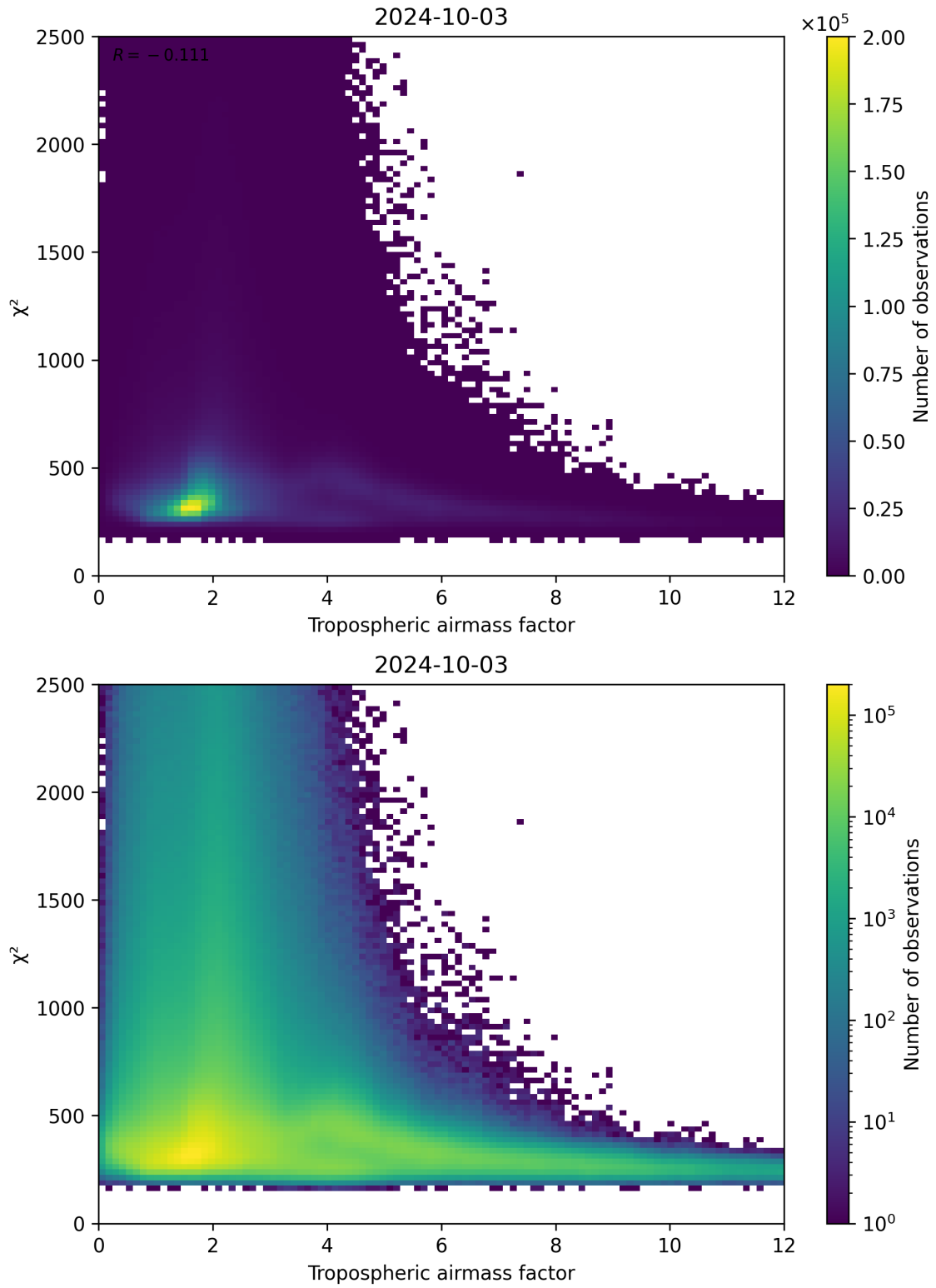
Figure 73: Scatter density plot of “Tropospheric airmass factor” against “ \chi^2 ” for 2024-10-03 to 2024-10-04.
