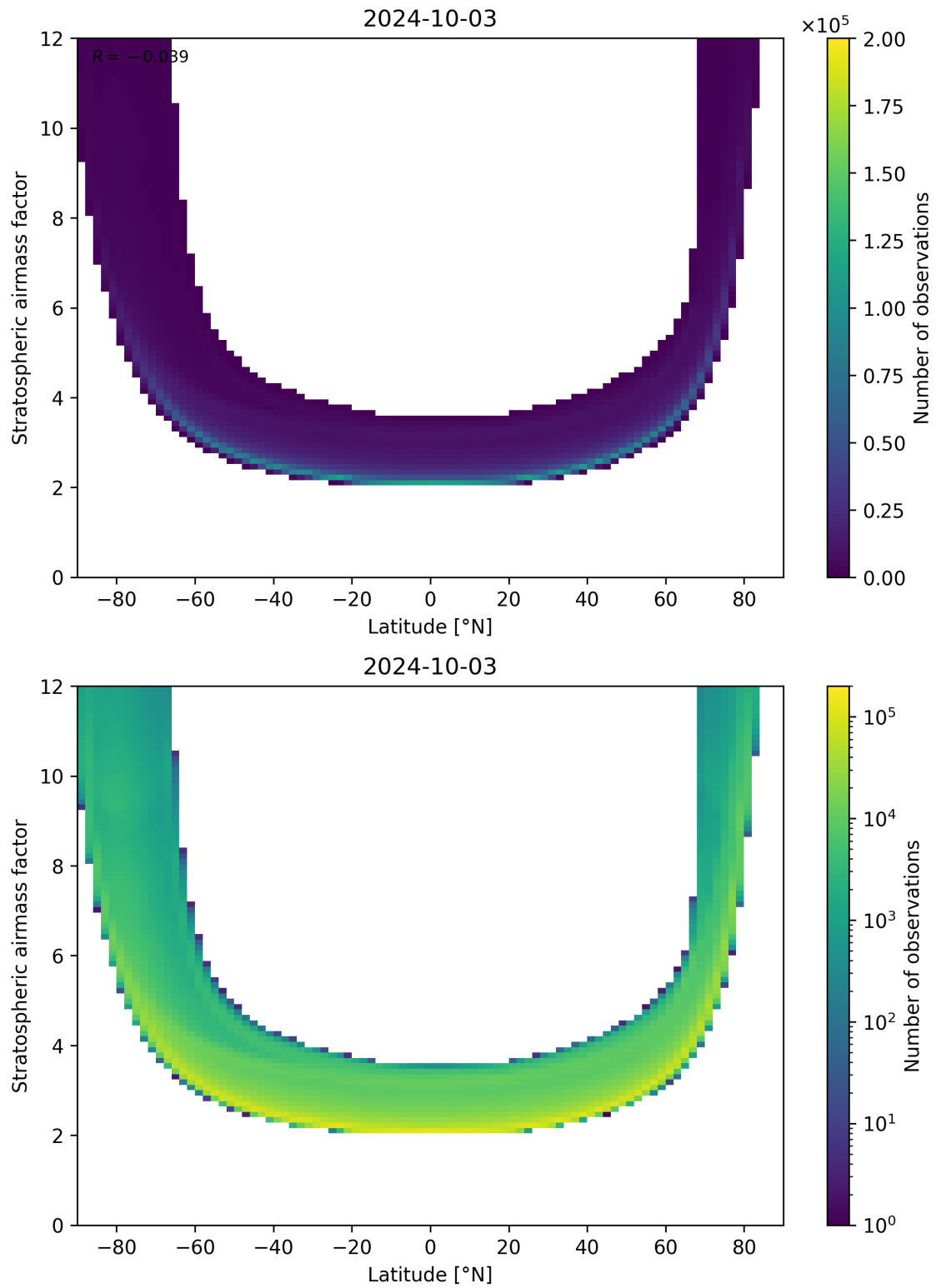
Figure 83: Scatter density plot of “Latitude” against “Stratospheric airmass factor” for 2024-10-03 to 2024-10-04.
