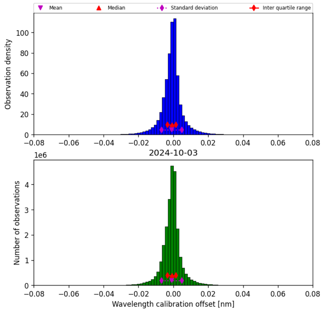
Figure 35: Histogram of “Wavelength calibration offset” for 2024-10-03 to 2024-10-04
