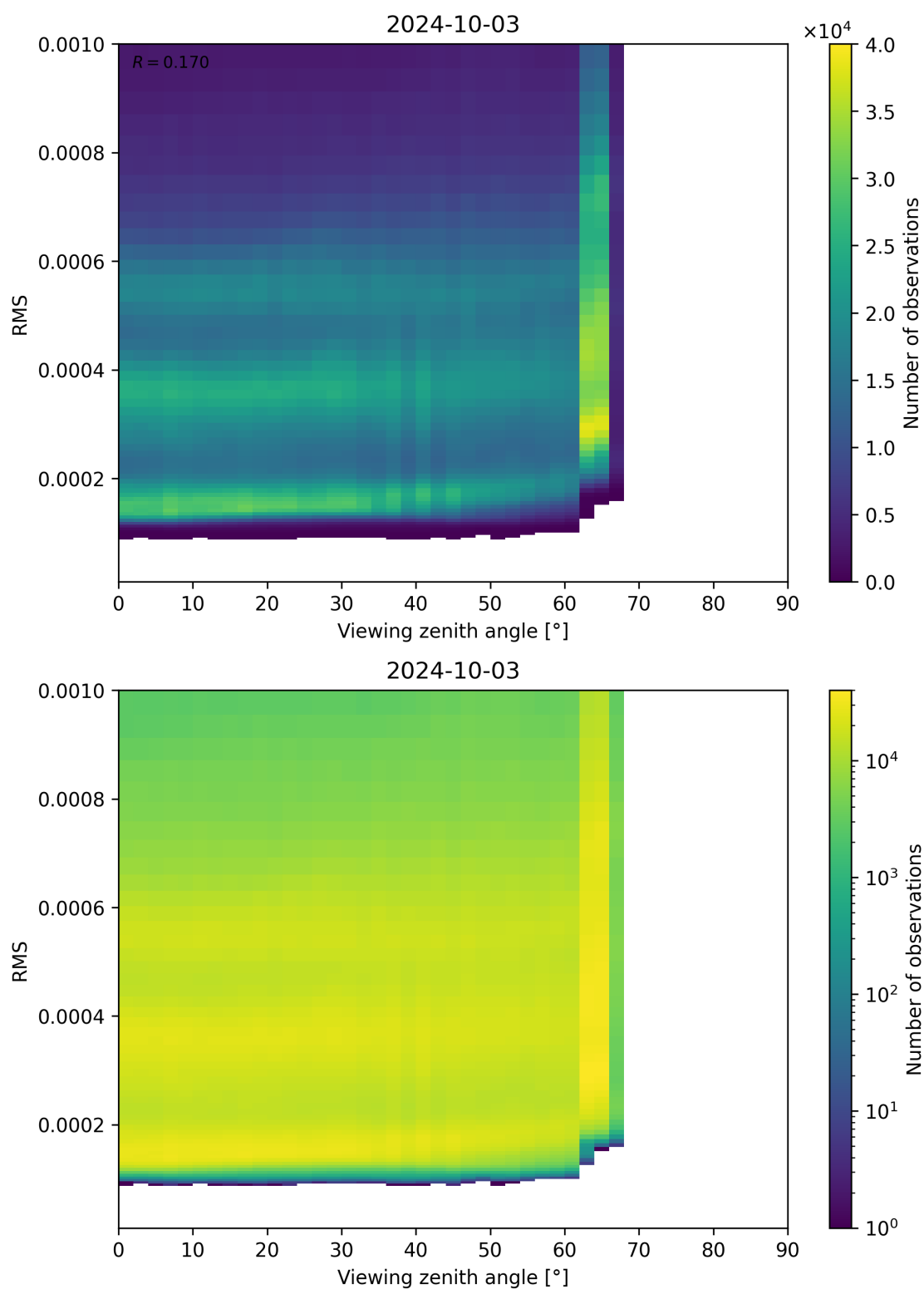
Figure 171: Scatter density plot of “Viewing zenith angle” against “RMS” for 2024-10-03 to 2024-10-04.
