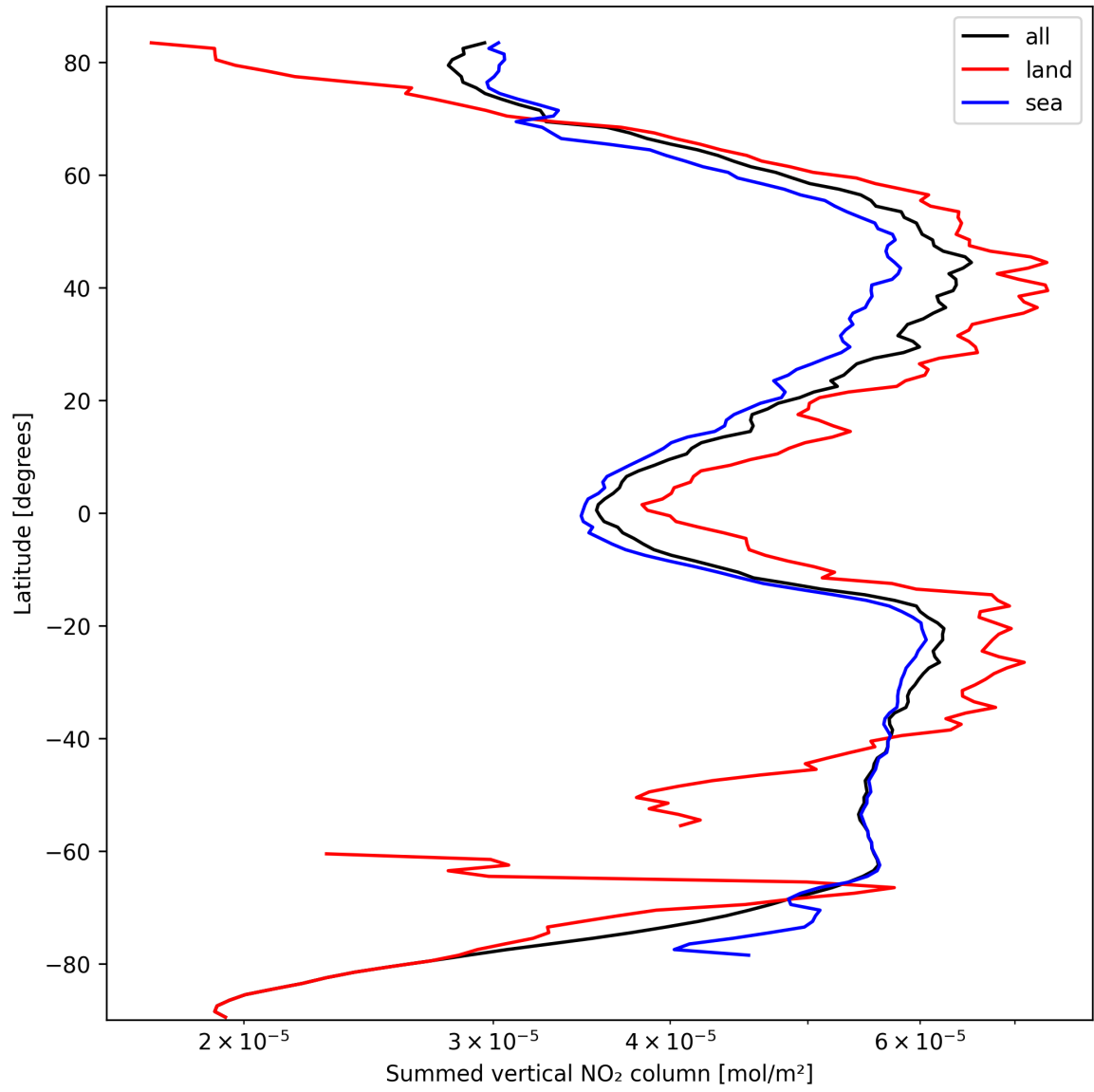
Figure 23: Zonal average of “Summed vertical NO 2 column” for 2024-10-03 to 2024-10-04.
