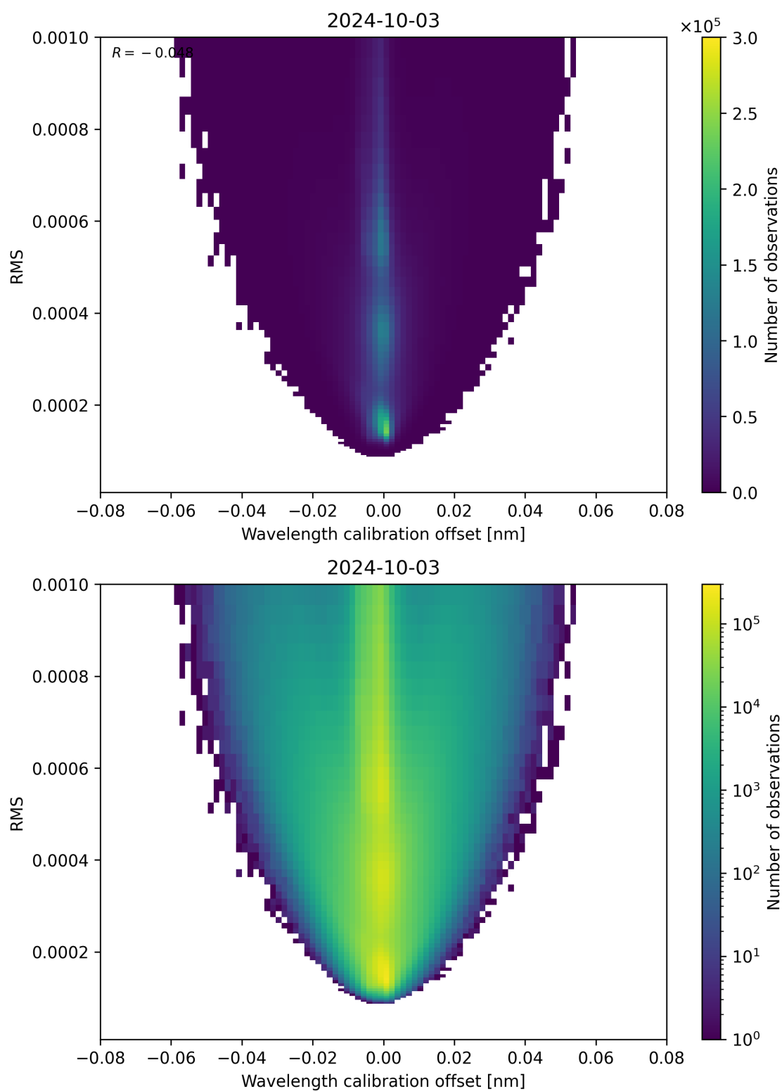
Figure 181: Scatter density plot of “Wavelength calibration offset” against “RMS” for 2024-10-03 to 2024-10-04.
