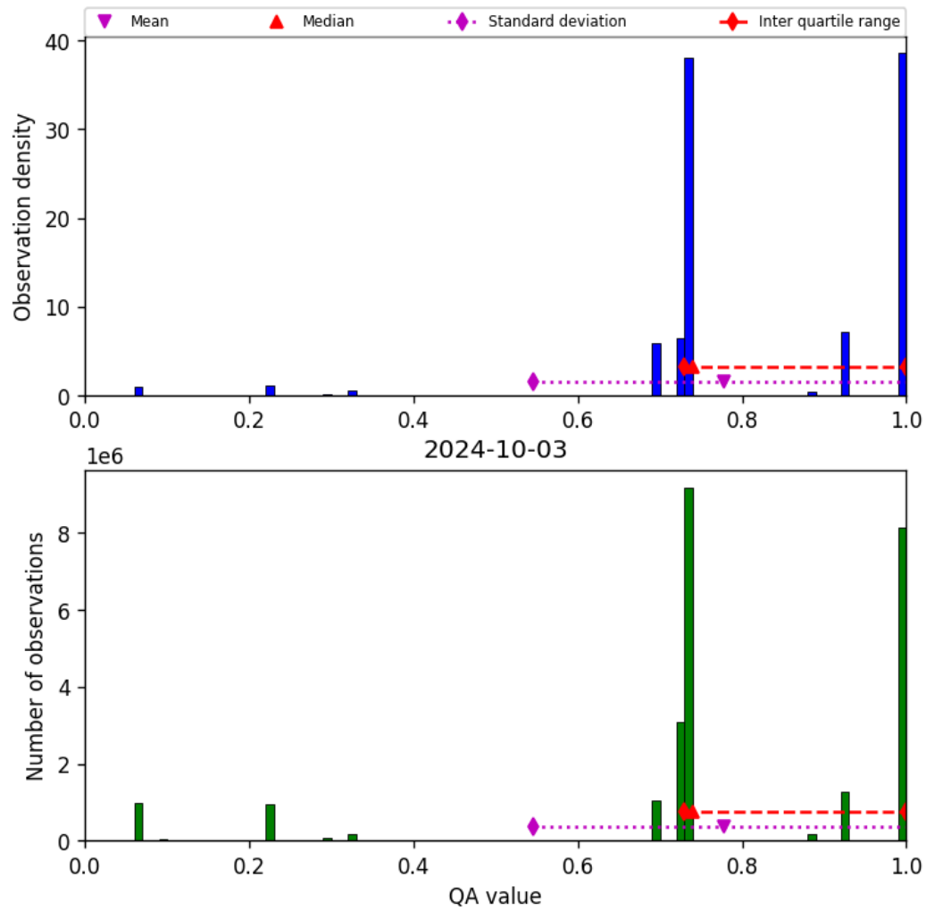
Figure 28: Histogram of “QA value” for 2024-10-03 to 2024-10-04
