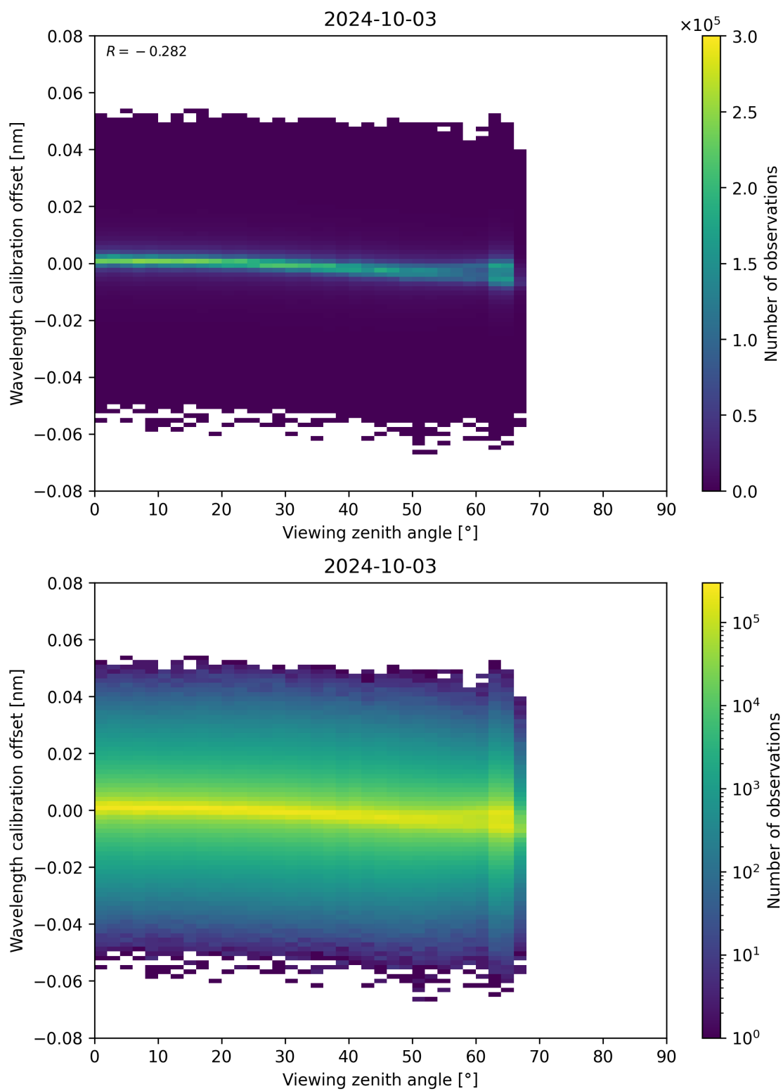
Figure 173: Scatter density plot of “Viewing zenith angle” against “Wavelength calibration offset” for 2024-10-03 to 2024-10-04.
