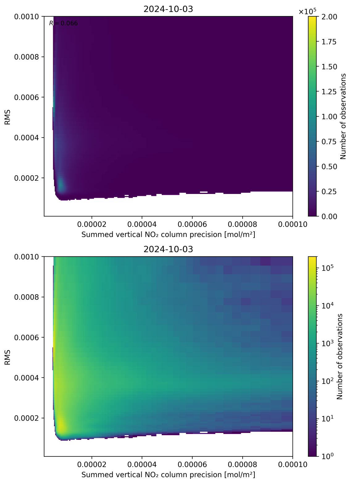
Figure 108: Scatter density plot of “Summed vertical NO 2 column precision” against “RMS” for 2024-10-03 to 2024-10-04.
