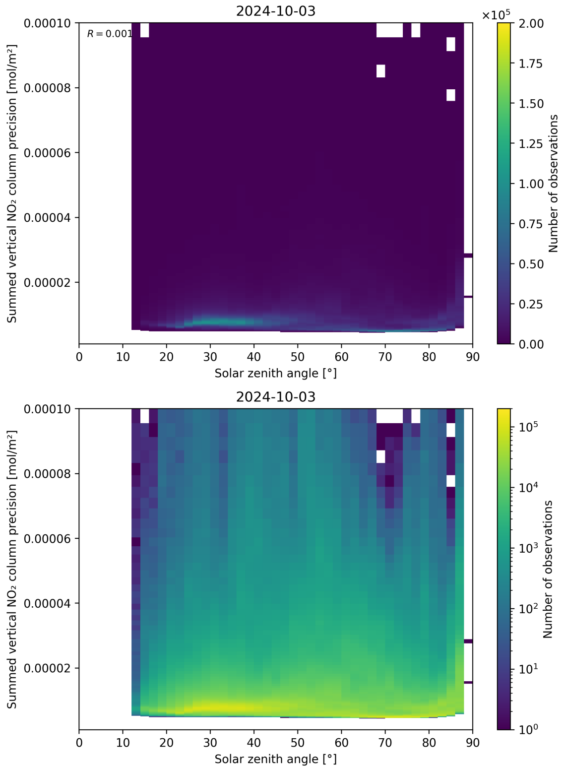
Figure 152: Scatter density plot of “Solar zenith angle” against “Summed vertical NO 2 column precision” for 2024-10-03 to 2024-10-04.
