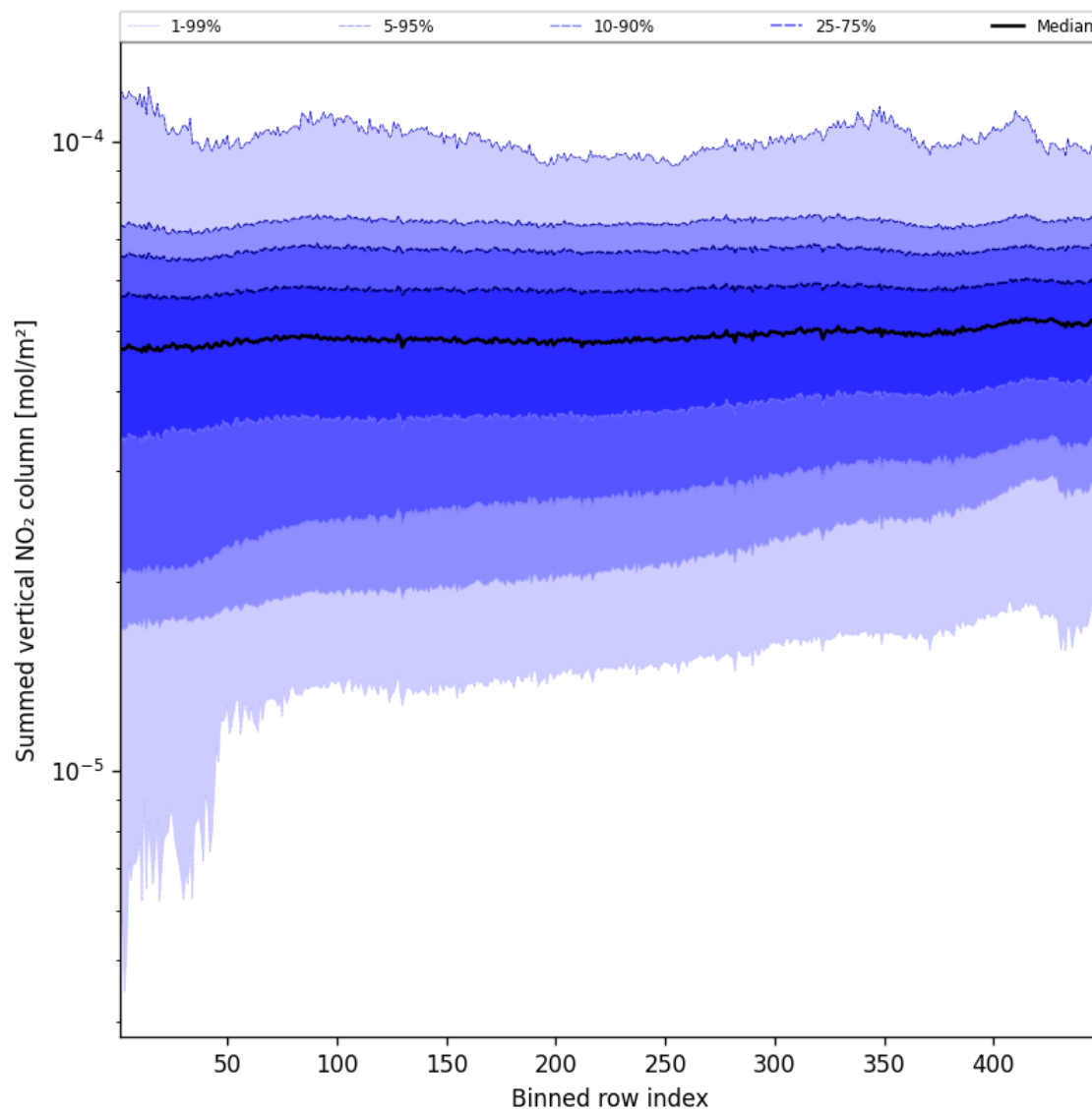
Figure 57: Along track statistics of “Summed vertical NO 2 column” for 2024-10-03 to 2024-10-04
