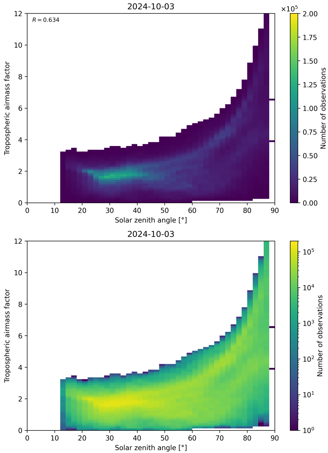
Figure 147: Scatter density plot of “Solar zenith angle” against “Tropospheric airmass factor” for 2024-10-03 to 2024-10-04.
