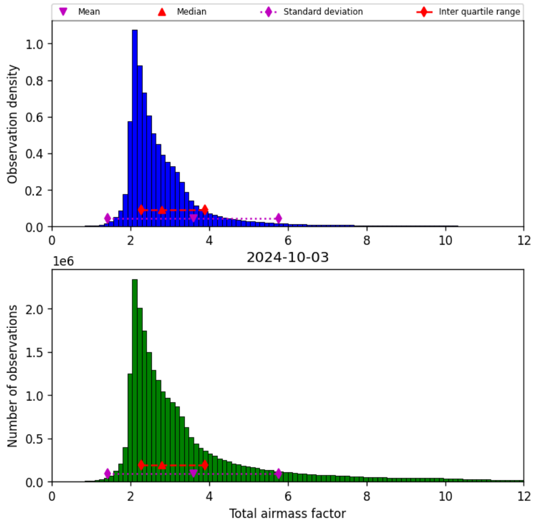
Figure 32: Histogram of “Total airmass factor” for 2024-10-03 to 2024-10-04
