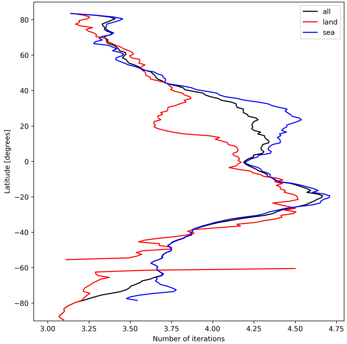
Figure 17: Zonal average of “Number of iterations” for 2024-10-03 to 2024-10-04.
