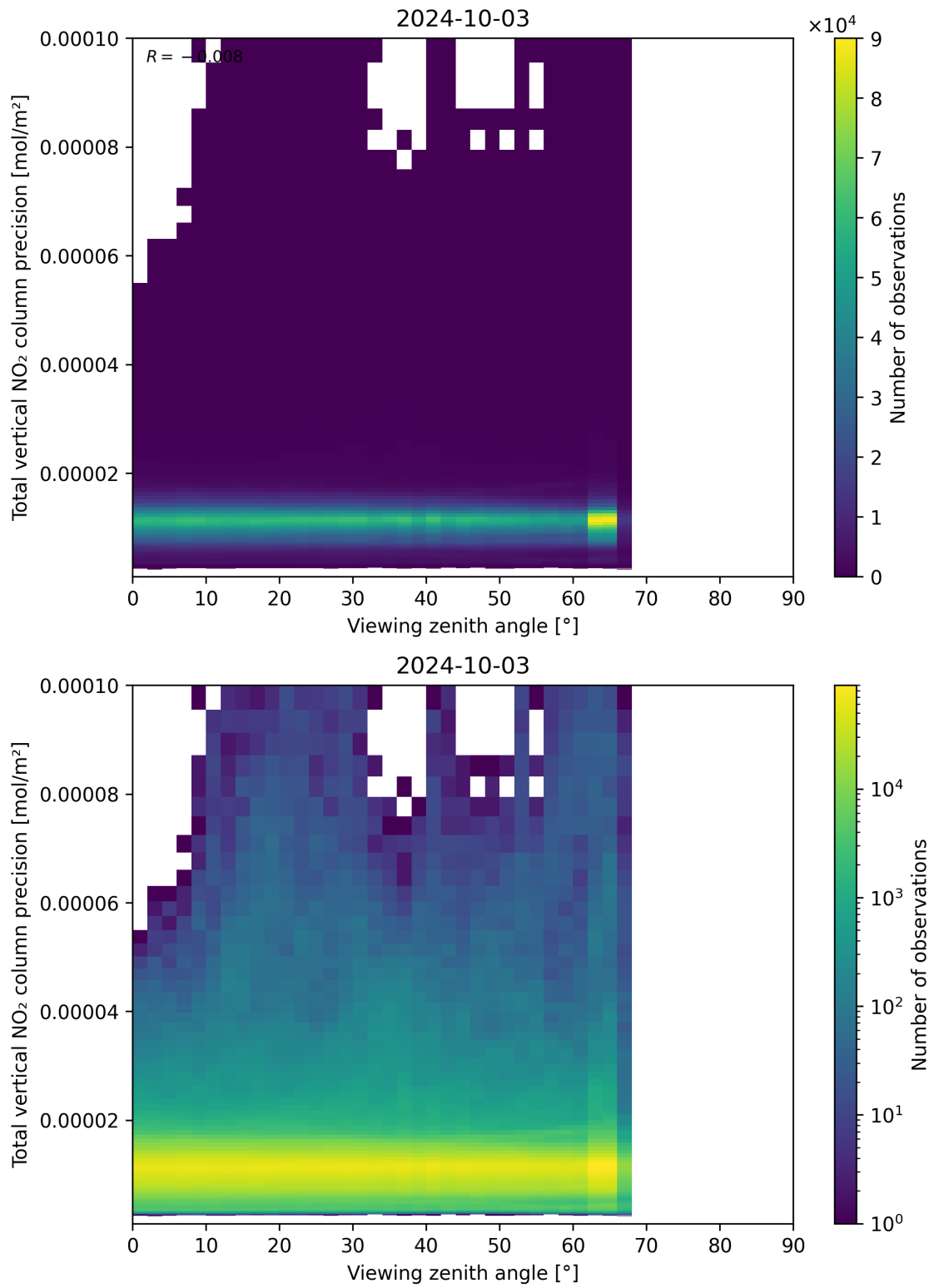
Figure 168: Scatter density plot of “Viewing zenith angle” against “Total vertical NO 2 column precision” for 2024-10-03 to 2024-10-04.
