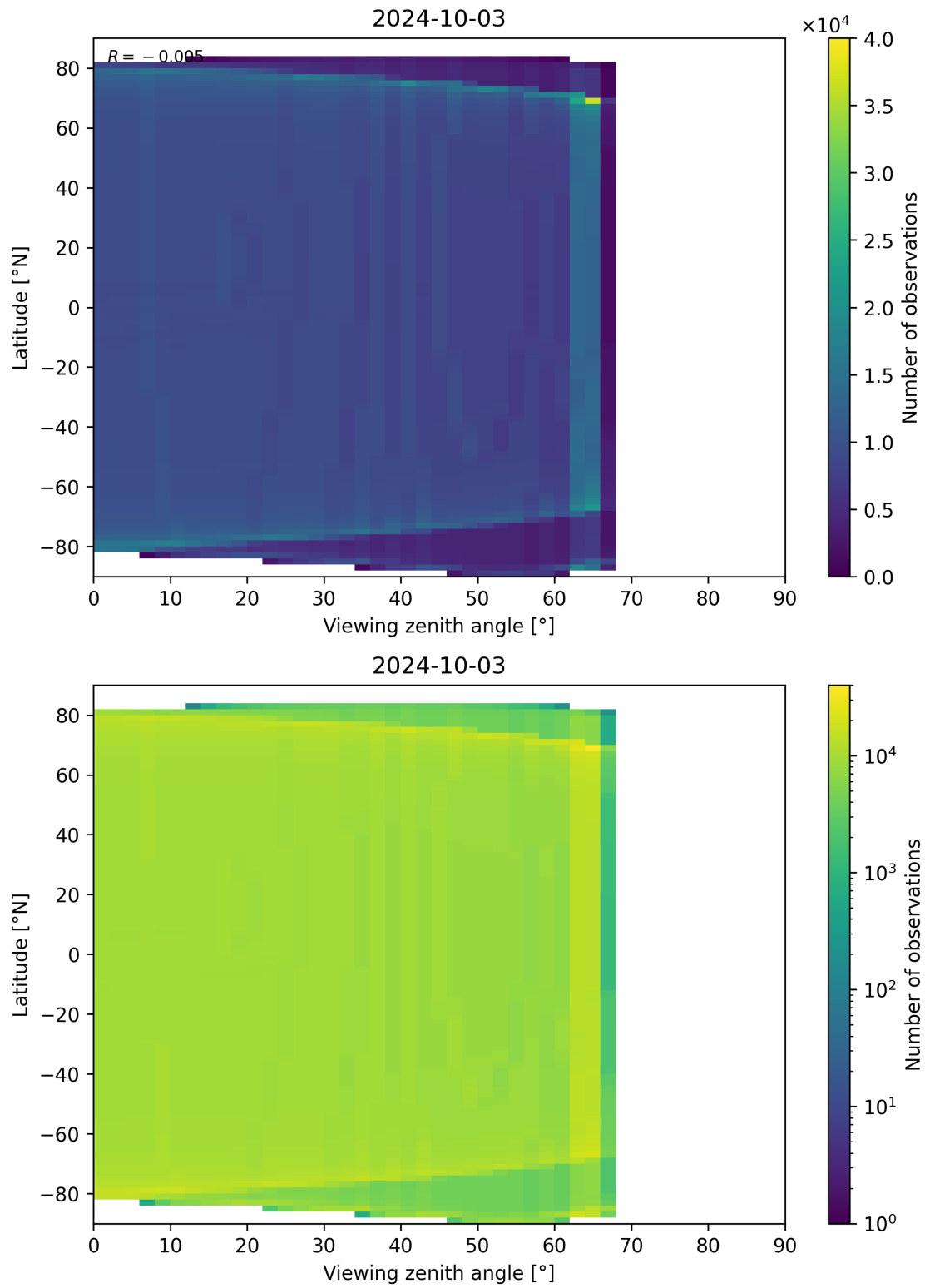
Figure 163: Scatter density plot of “Viewing zenith angle” against “Latitude” for 2024-10-03 to 2024-10-04.
