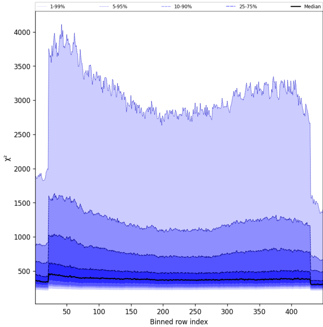
Figure 59: Along track statistics of “ \chi^2 ” for 2024-10-03 to 2024-10-04
