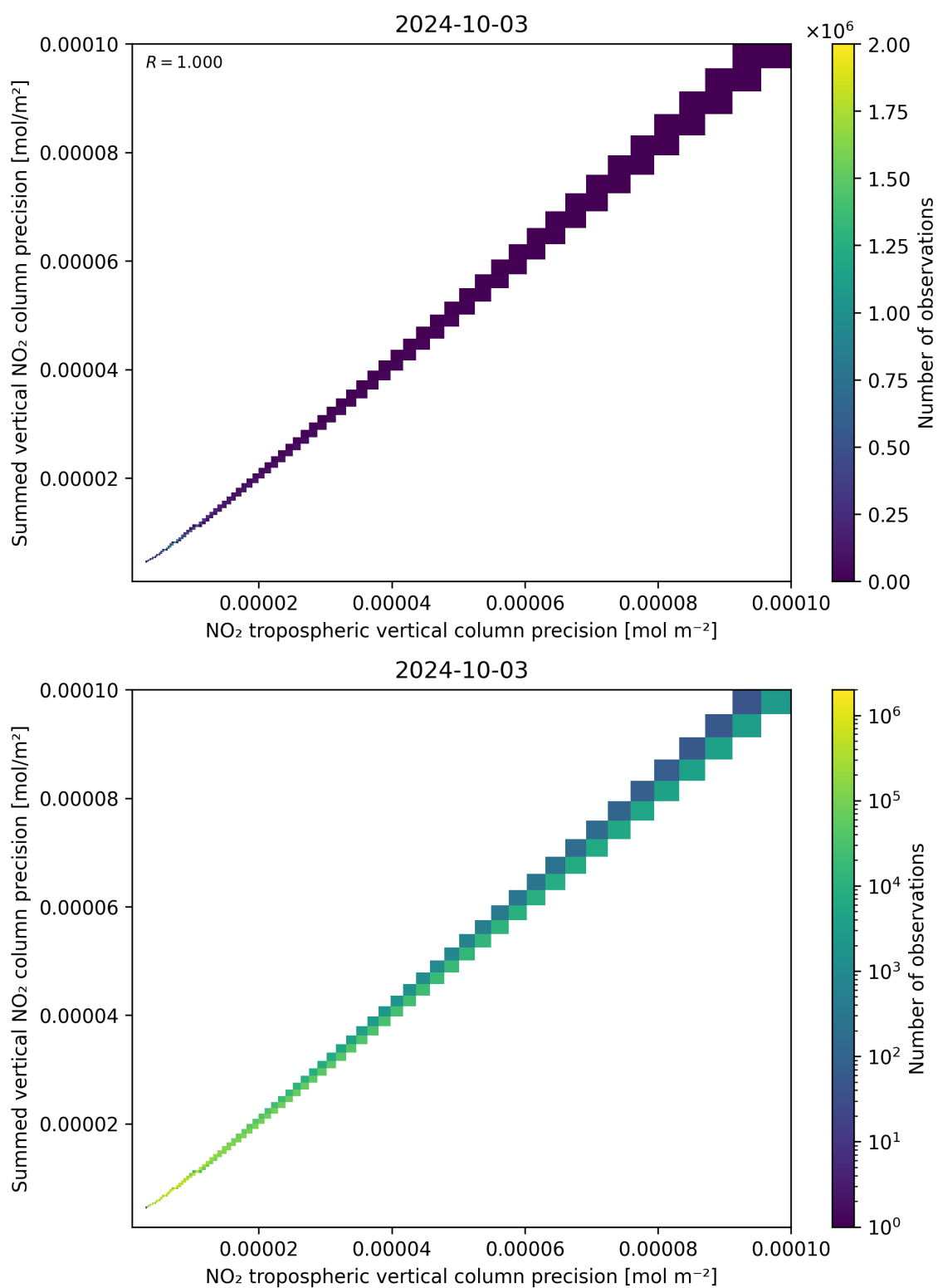
Figure 137: Scatter density plot of “NO 2 tropospheric vertical column precision” against “Summed vertical NO 2 column precision” for 2024-10-03 to 2024-10-04.
