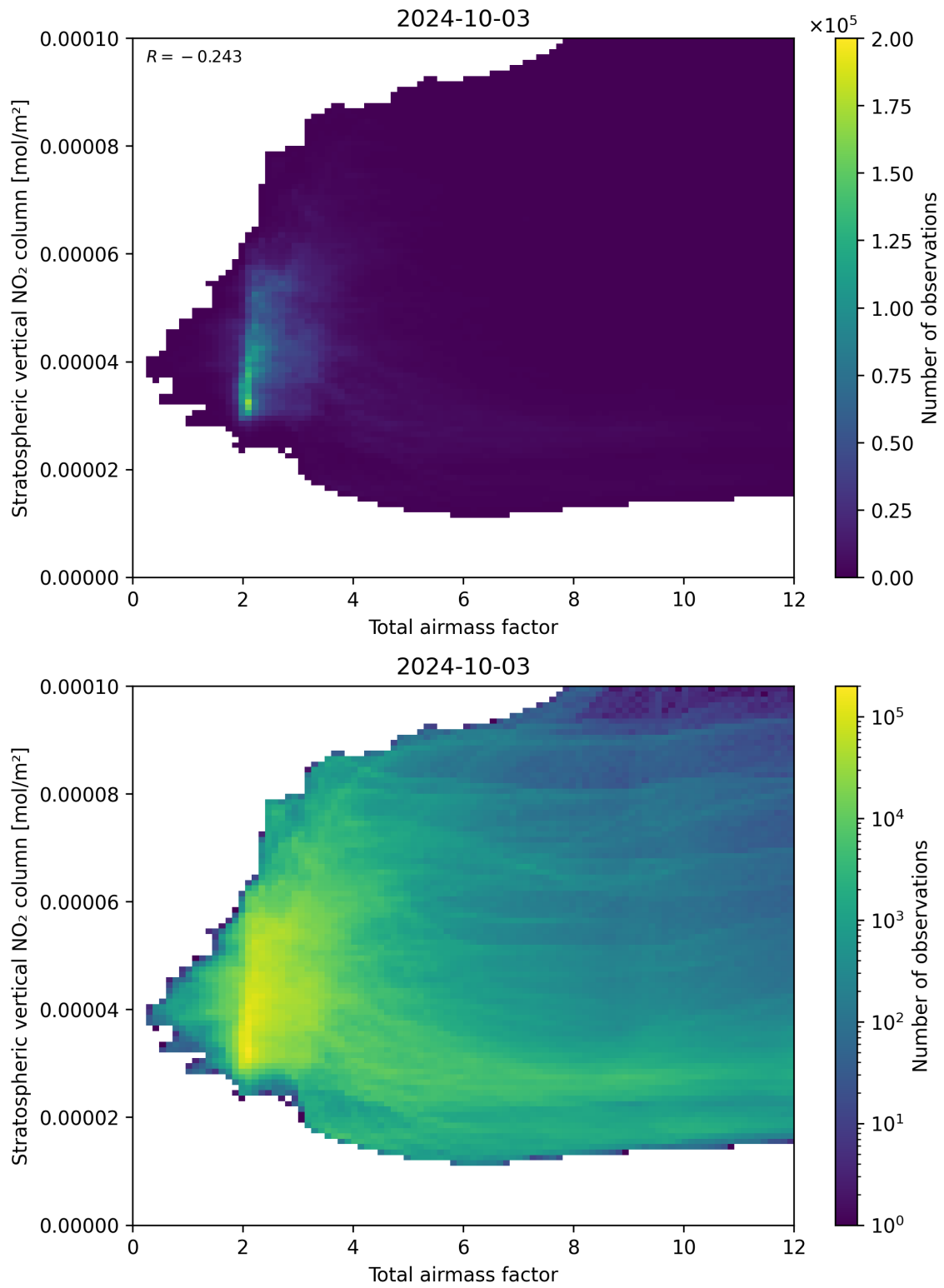
Figure 64: Scatter density plot of “Total airmass factor” against “Stratospheric vertical NO 2 column” for 2024-10-03 to 2024-10-04.
