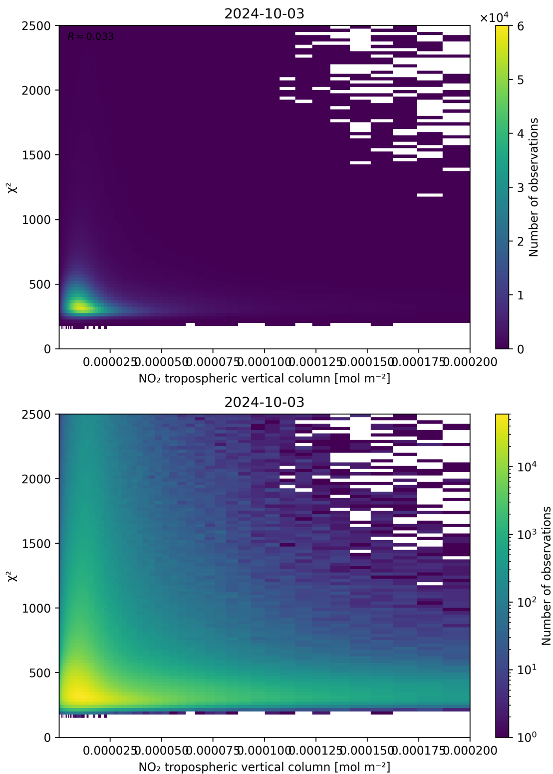
Figure 124: Scatter density plot of “NO 2 tropospheric vertical column” against “ \chi^2 ” for 2024-10-03 to 2024-10-04.
