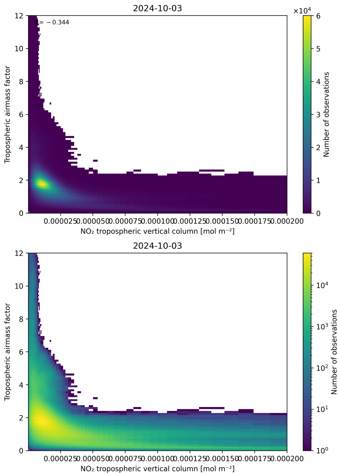
Figure 123: Scatter density plot of “NO 2 tropospheric vertical column” against “Tropospheric air mass factor” for 2024-10-03 to 2024-10-04.
