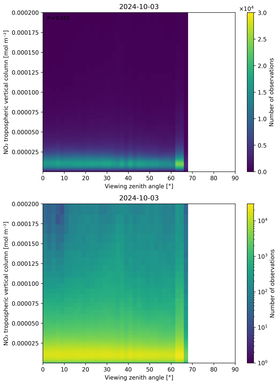
Figure 169: Scatter density plot of “Viewing zenith angle” against “NO 2 tropospheric vertical column” for 2024-10-03 to 2024-10-04.
