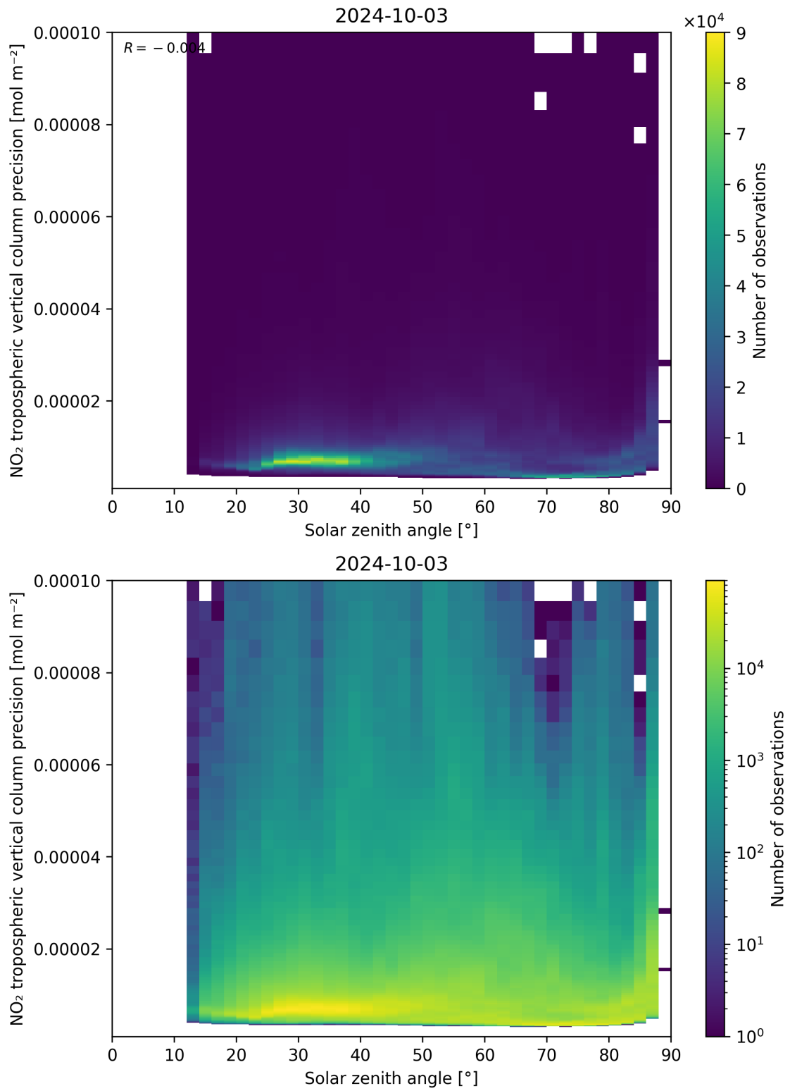
Figure 156: Scatter density plot of “Solar zenith angle” against “NO 2 tropospheric vertical column precision” for 2024-10-03 to 2024-10-04.
