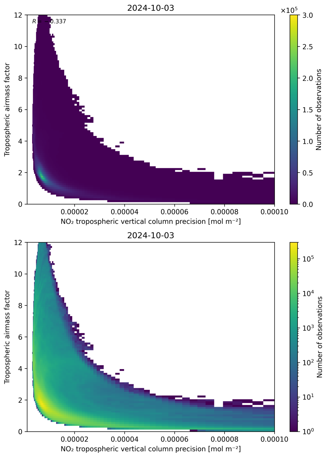
Figure 133: Scatter density plot of “NO 2 tropospheric vertical column precision” against “Tropospheric air mass factor” for 2024-10-03 to 2024-10-04.
