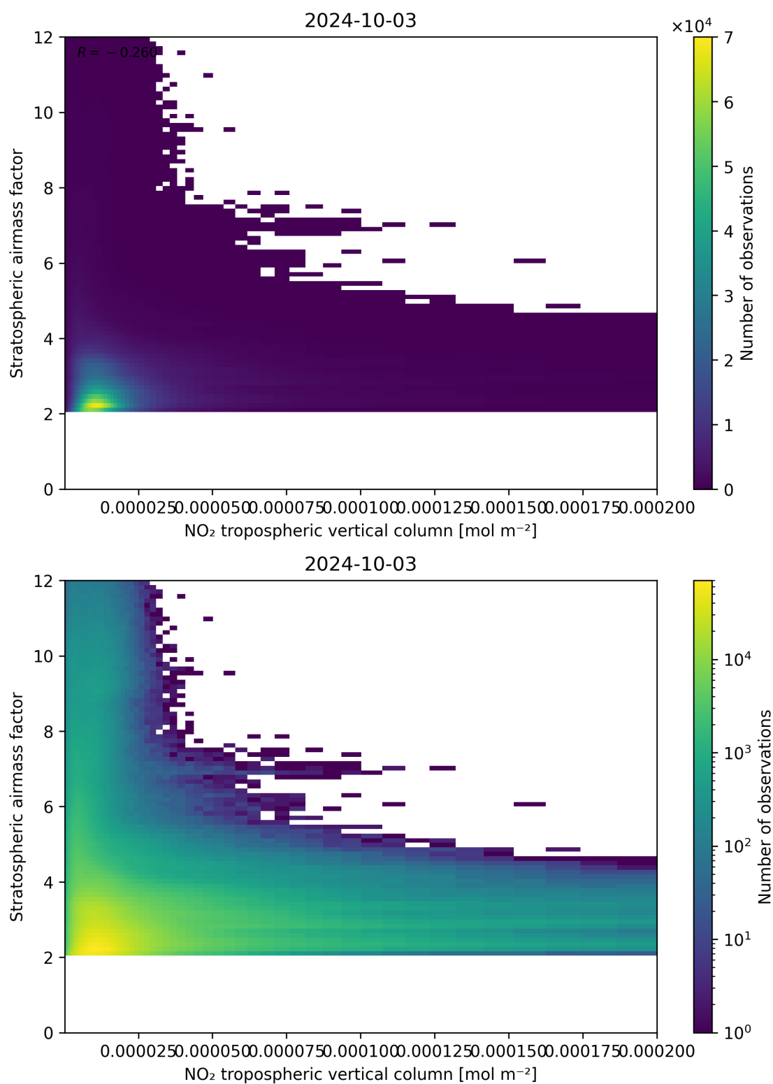
Figure 121: Scatter density plot of “NO 2 tropospheric vertical column” against “Stratospheric air mass factor” for 2024-10-03 to 2024-10-04.
