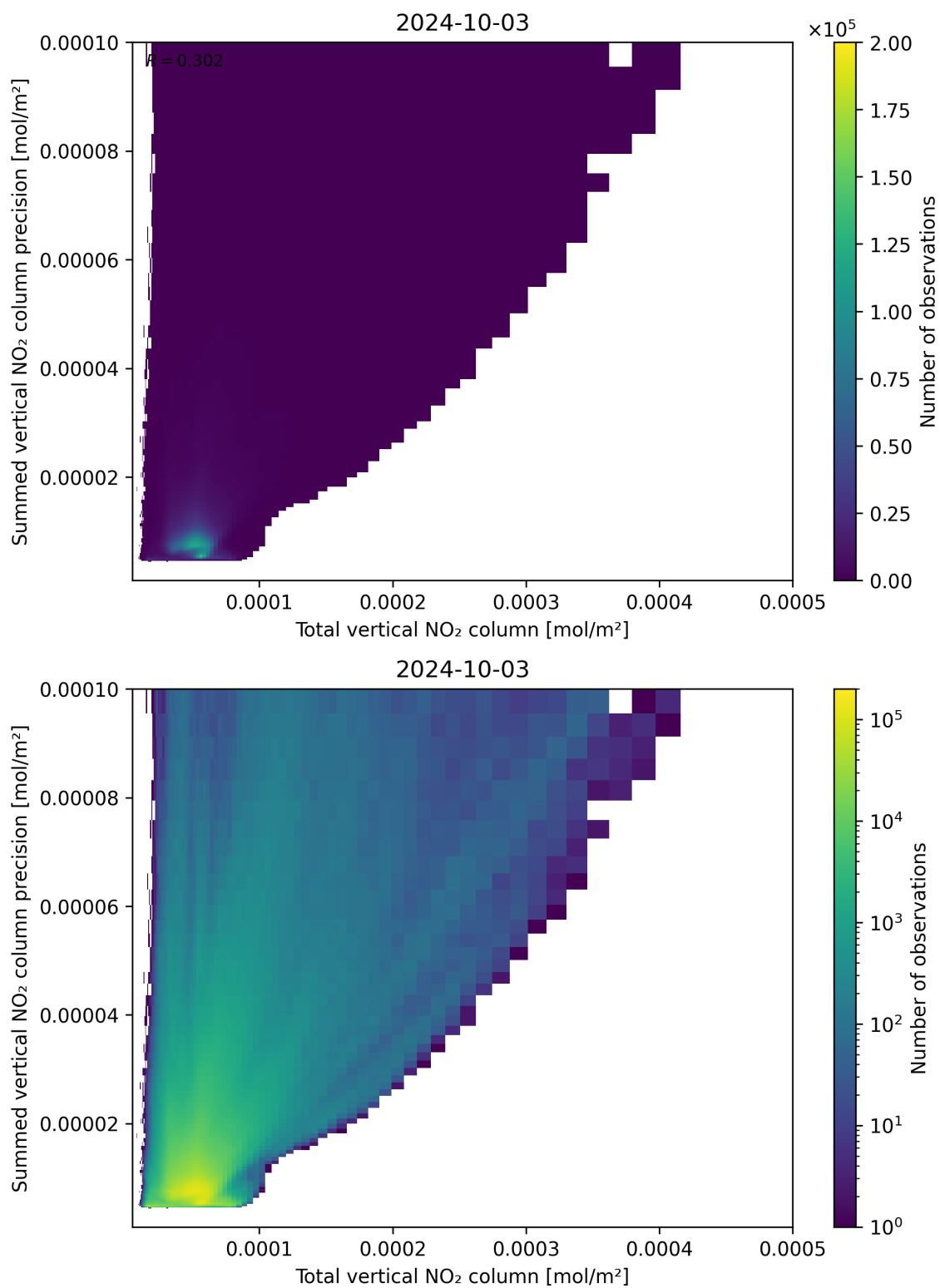
Figure 113: Scatter density plot of “Total vertical NO 2 column” against “Summed vertical NO 2 column precision” for 2024-10-03 to 2024-10-04.
