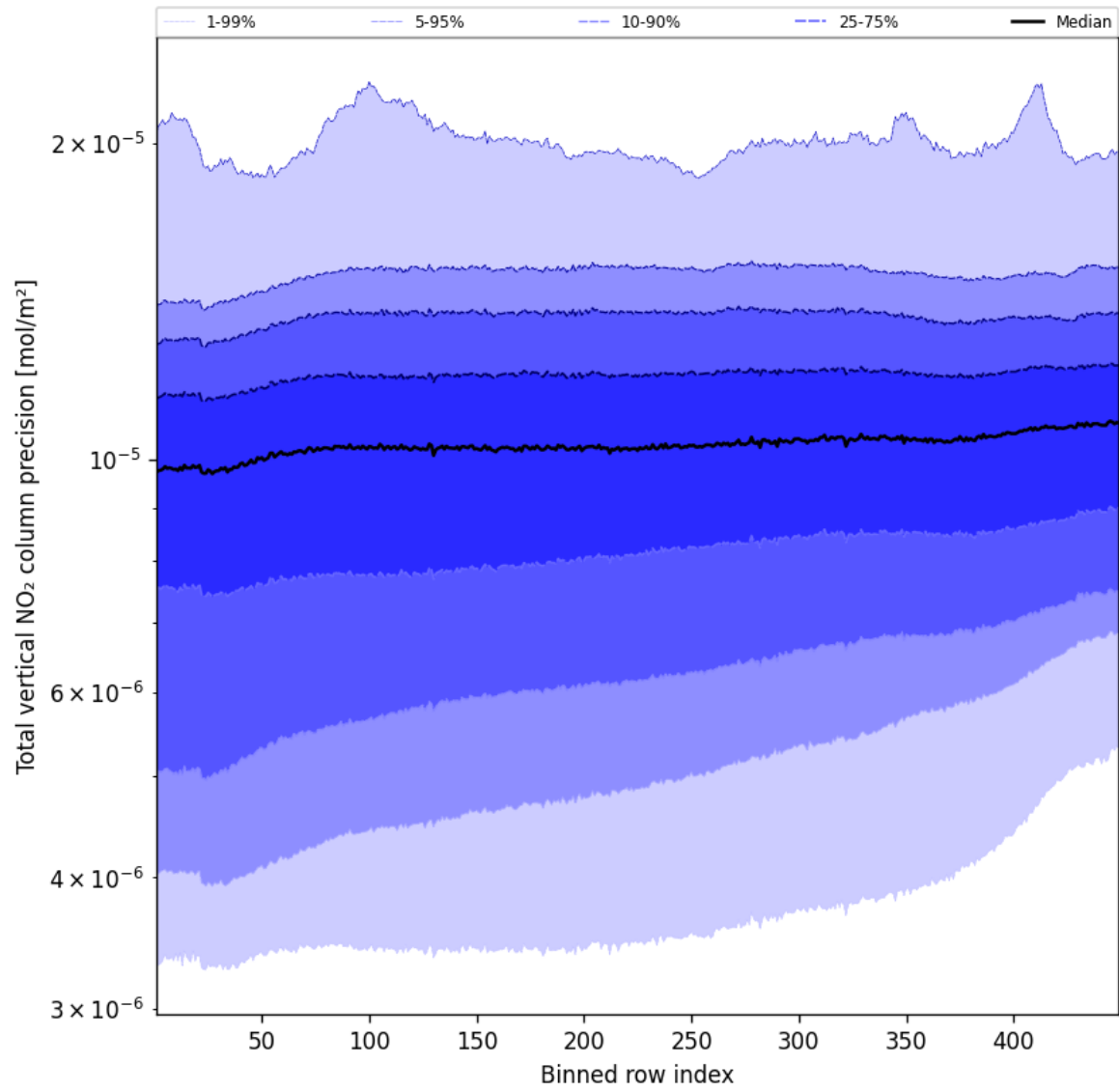
Figure 56: Along track statistics of “Total vertical NO 2 column precision” for 2024-10-03 to 2024-10-04
