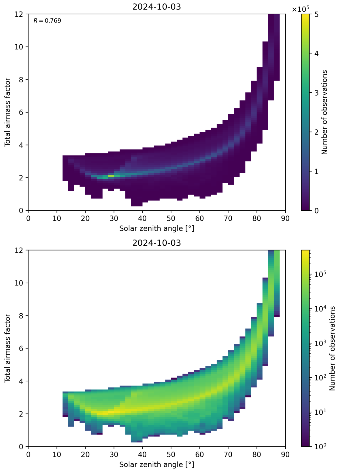
Figure 146: Scatter density plot of “Solar zenith angle” against “Total airmass factor” for 2024-10-03 to 2024-10-04.
