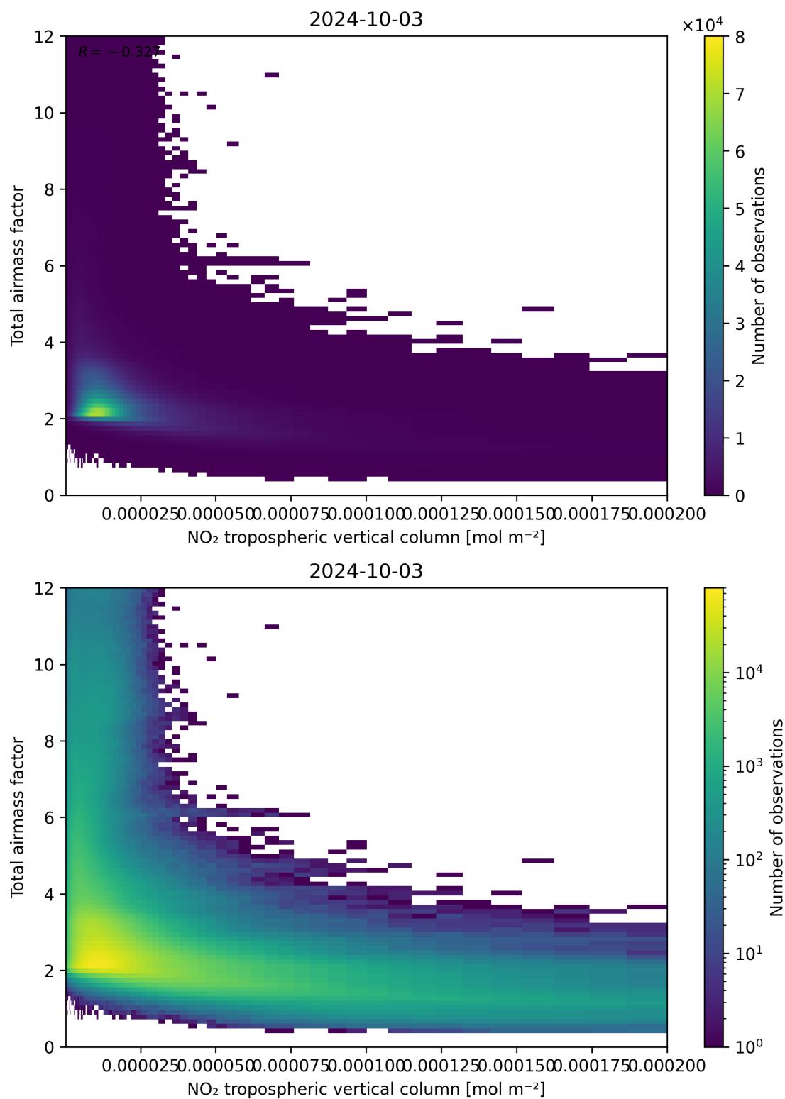
Figure 122: Scatter density plot of “NO 2 tropospheric vertical column” against “Total air mass factor” for 2024-10-03 to 2024-10-04.
