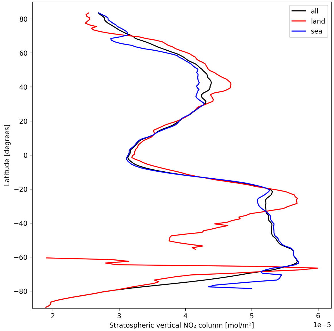
Figure 19: Zonal average of “Stratospheric vertical NO 2 column” for 2024-10-03 to 2024-10-04.
