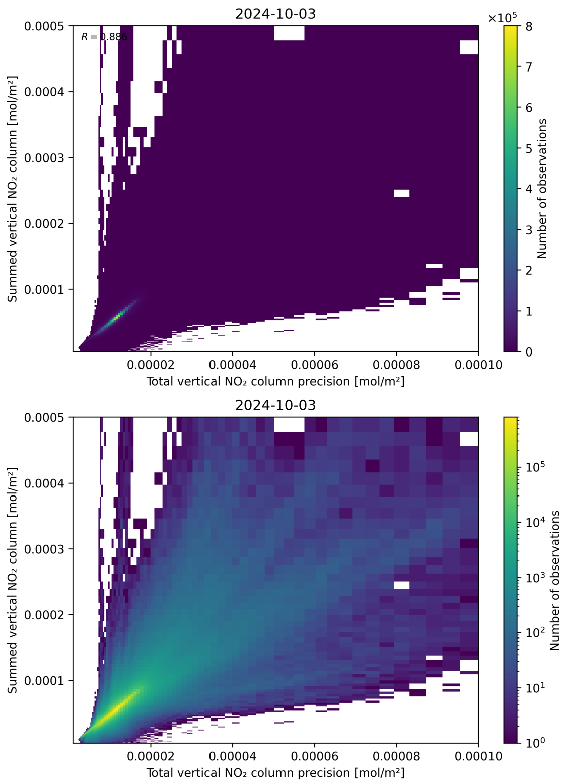
Figure 117: Scatter density plot of “Total vertical NO 2 column precision” against “Summed vertical NO 2 column” for 2024-10-03 to 2024-10-04.
