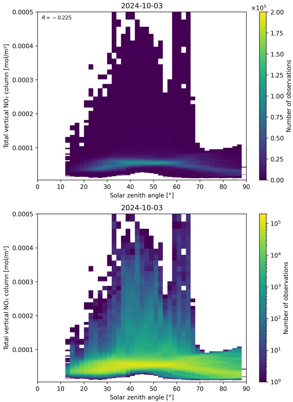
Figure 153: Scatter density plot of “Solar zenith angle” against “Total vertical NO 2 column” for 2024-10-03 to 2024-10-04.
