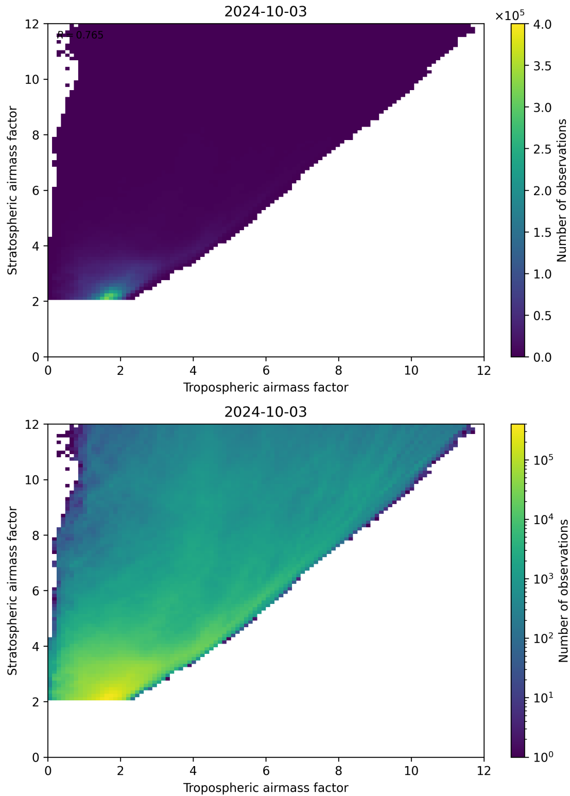
Figure 71: Scatter density plot of “Tropospheric airmass factor” against “Stratospheric airmass factor” for 2024-10-03 to 2024-10-04.
