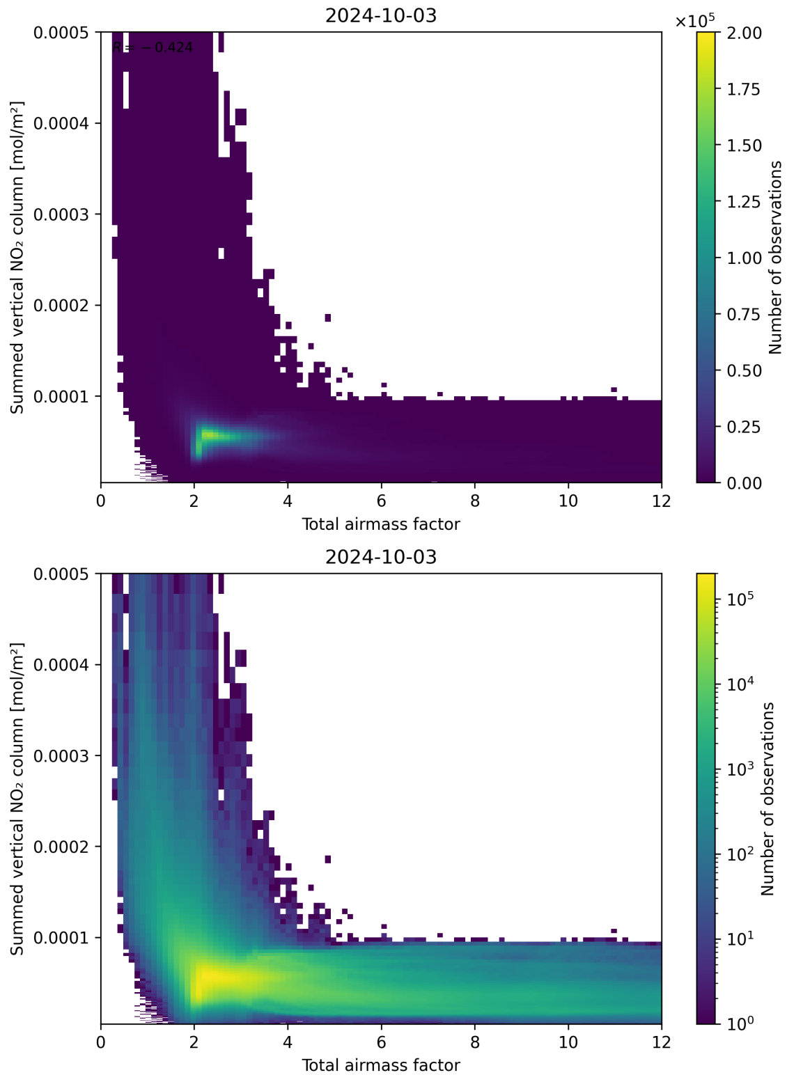
Figure 65: Scatter density plot of “Total airmass factor” against “Summed vertical NO 2 column” for 2024-10-03 to 2024-10-04.
