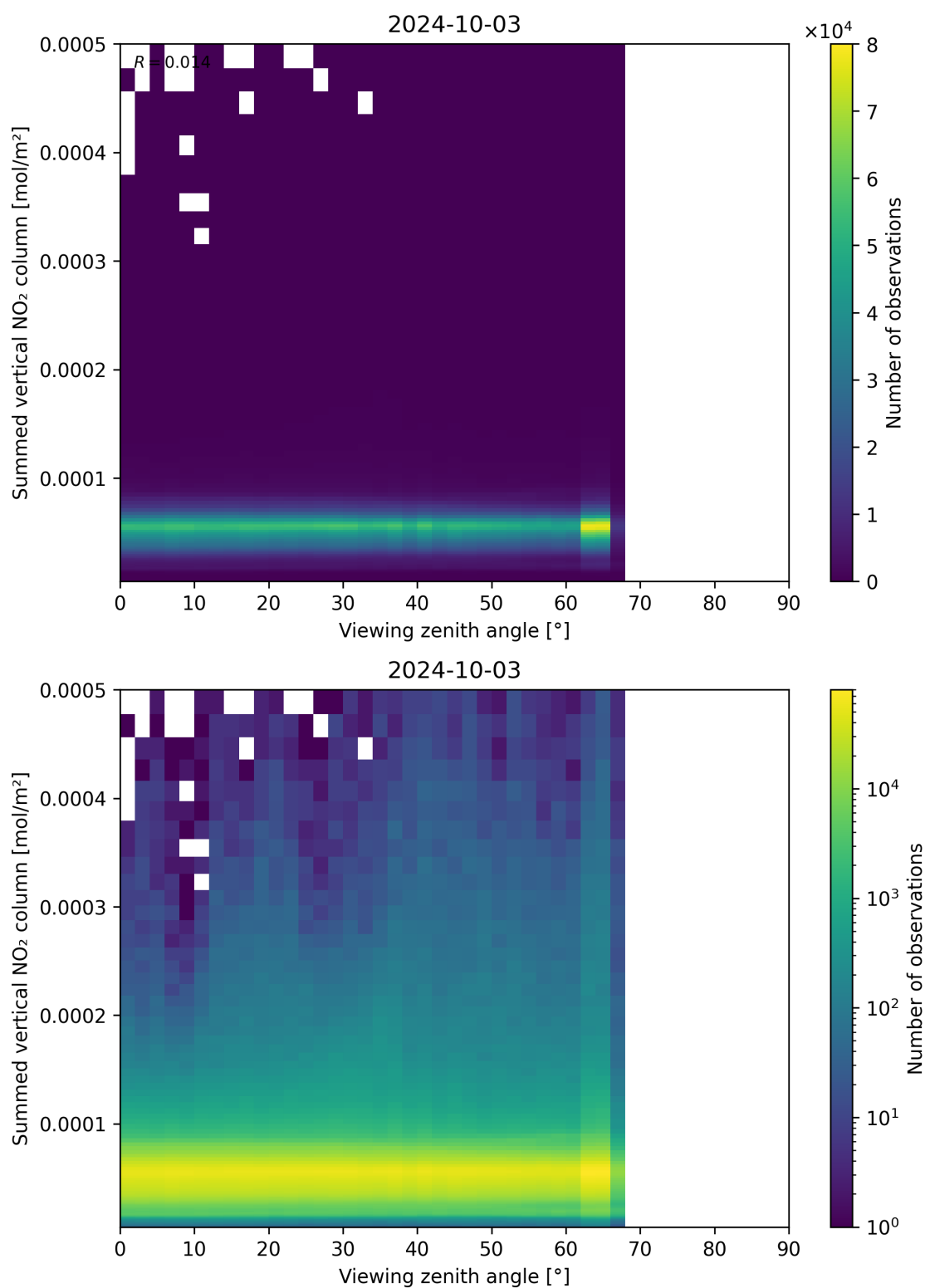
Figure 165: Scatter density plot of “Viewing zenith angle” against “Summed vertical NO 2 column” for 2024-10-03 to 2024-10-04.
