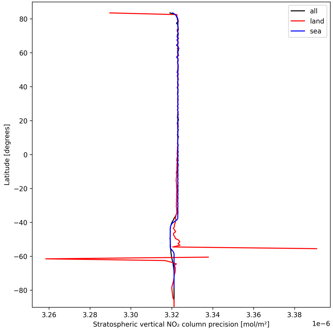
Figure 20: Zonal average of "Stratospheric vertical NO 2 column precision" for 2024-10-03 to 2024-10-04.
