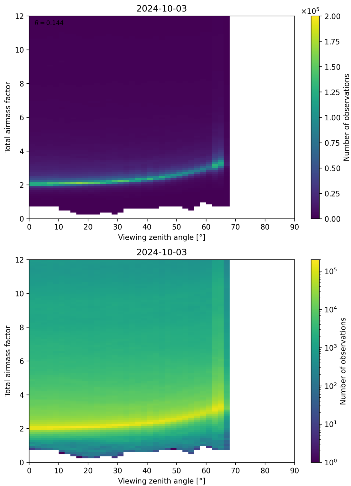
Figure 160: Scatter density plot of “Viewing zenith angle” against “Total airmass factor” for 2024-10-03 to 2024-10-04.
