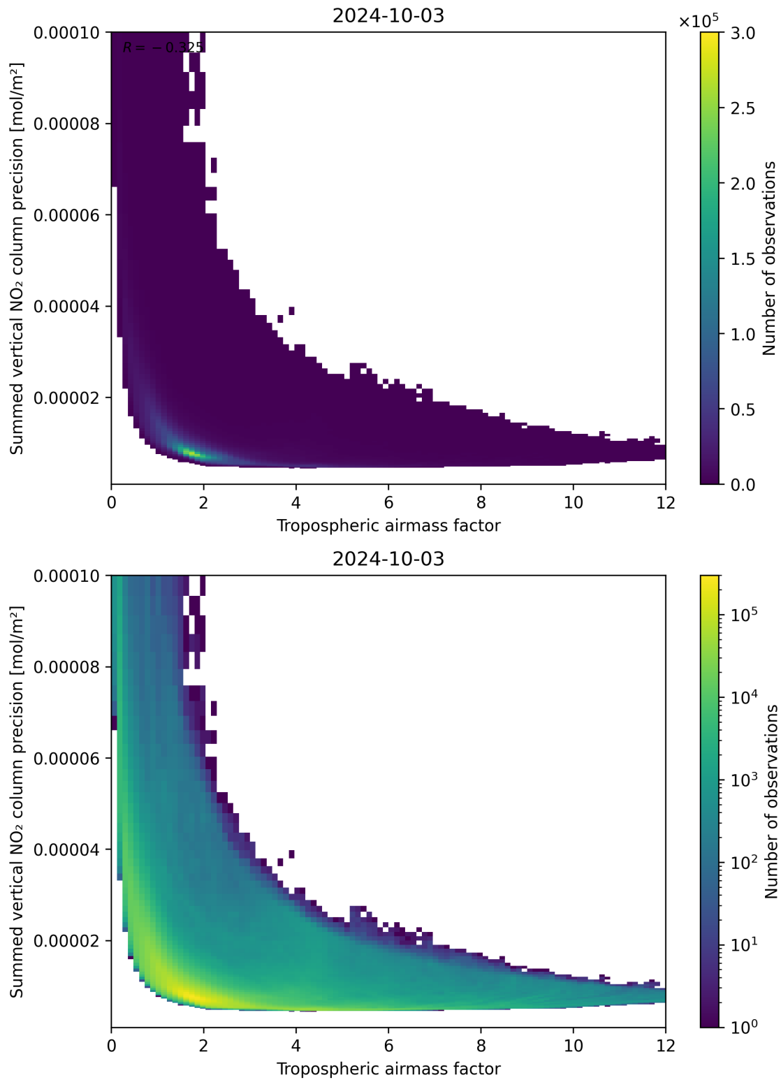
Figure 76: Scatter density plot of “Tropospheric air mass factor” against “Summed vertical NO 2 column precision” for 2024-10-03 to 2024-10-04.
