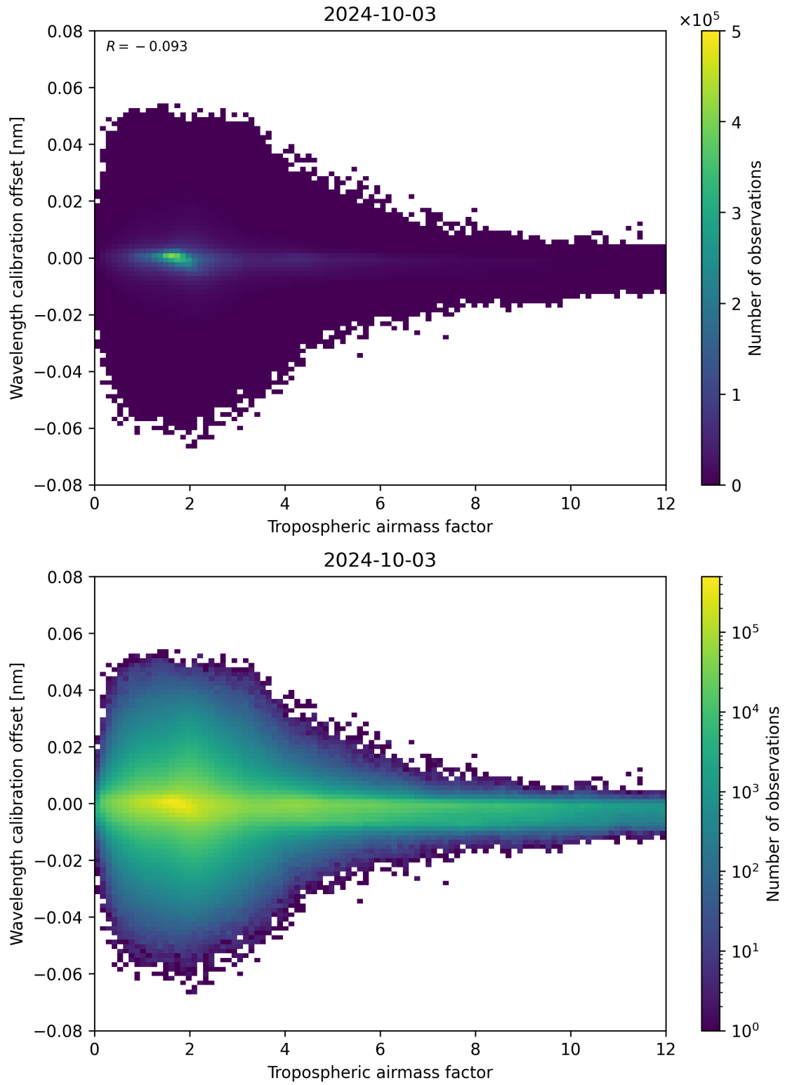
Figure 80: Scatter density plot of “Tropospheric airmass factor” against “Wavelength calibration offset” for 2024-10-03 to 2024-10-04.
