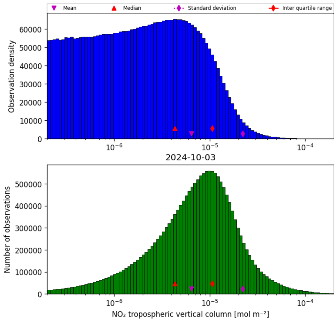
Figure 29: Histogram of “NO 2 tropospheric vertical column” for 2024-10-03 to 2024-10-04
