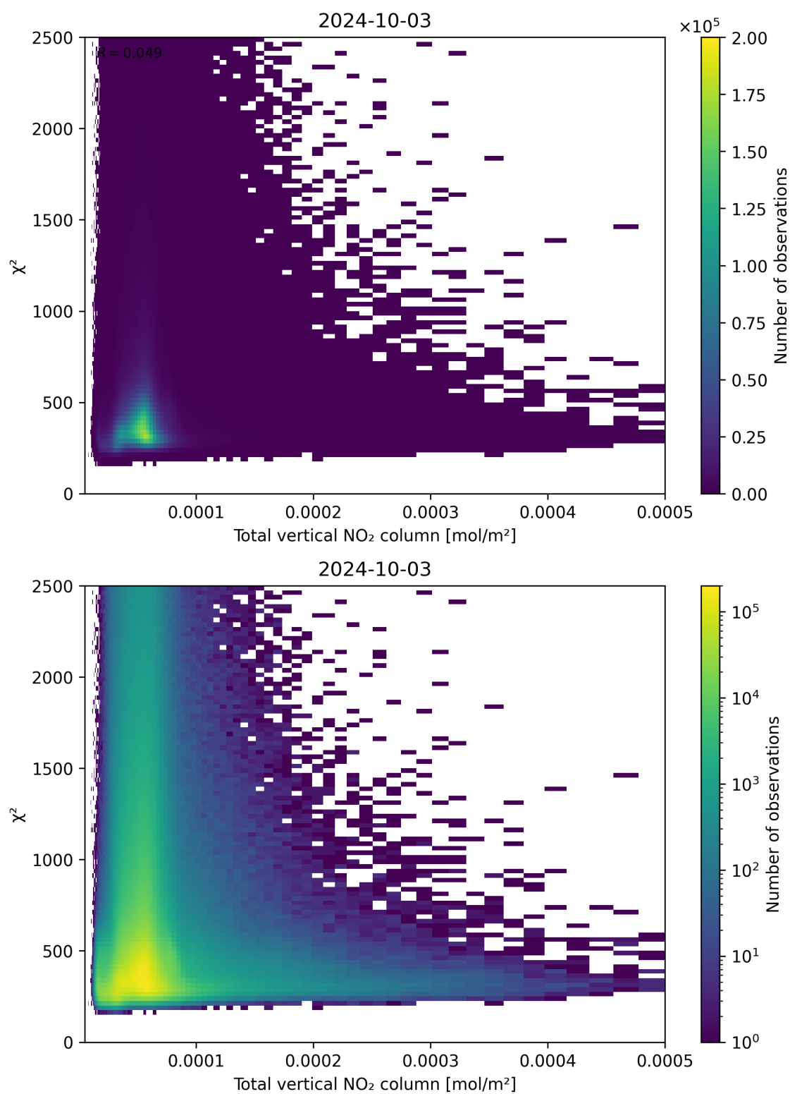
Figure 111: Scatter density plot of “Total vertical NO 2 column” against “ \chi^2 ” for 2024-10-03 to 2024-10-04.
