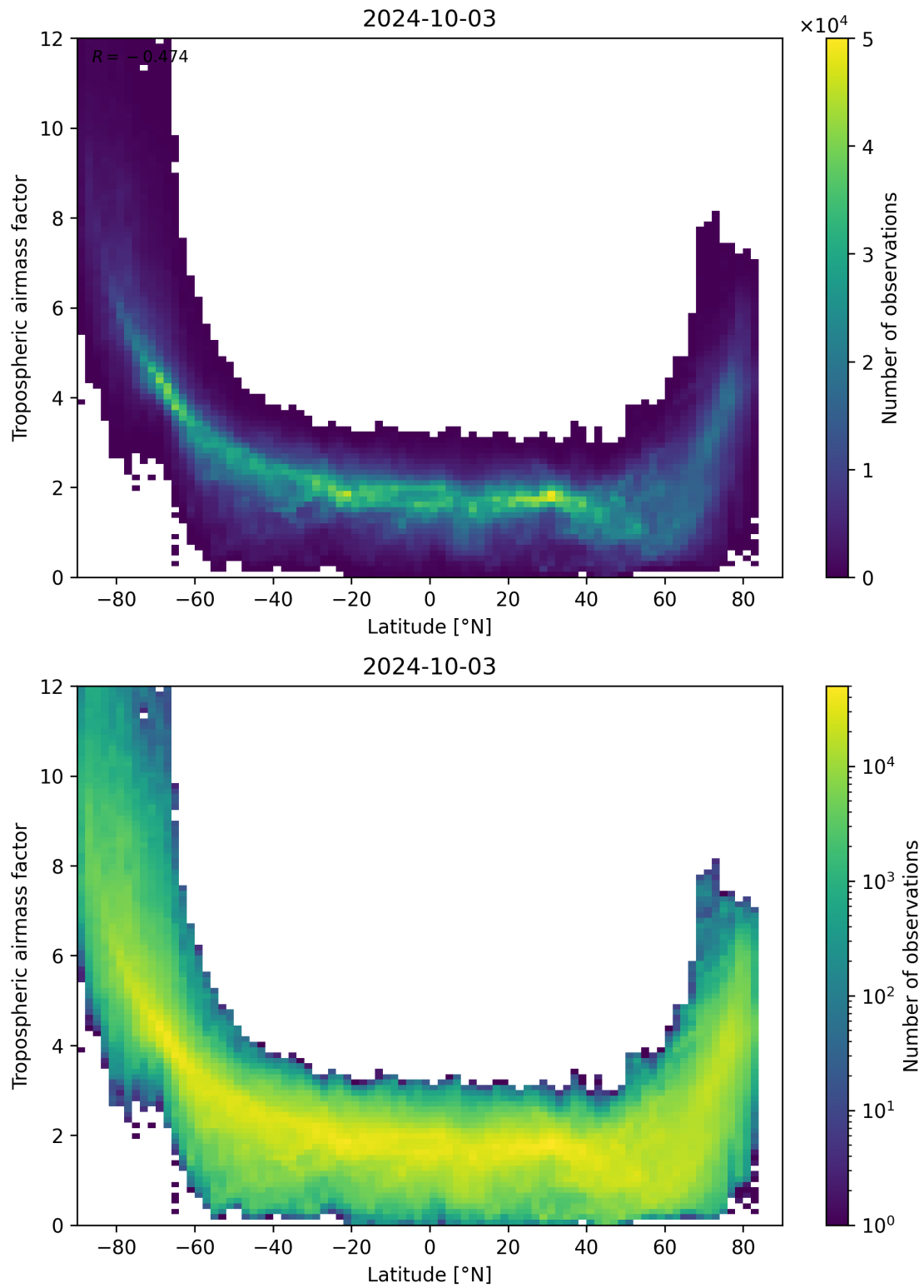
Figure 85: Scatter density plot of “Latitude” against “Tropospheric airmass factor” for 2024-10-03 to 2024-10-04.
