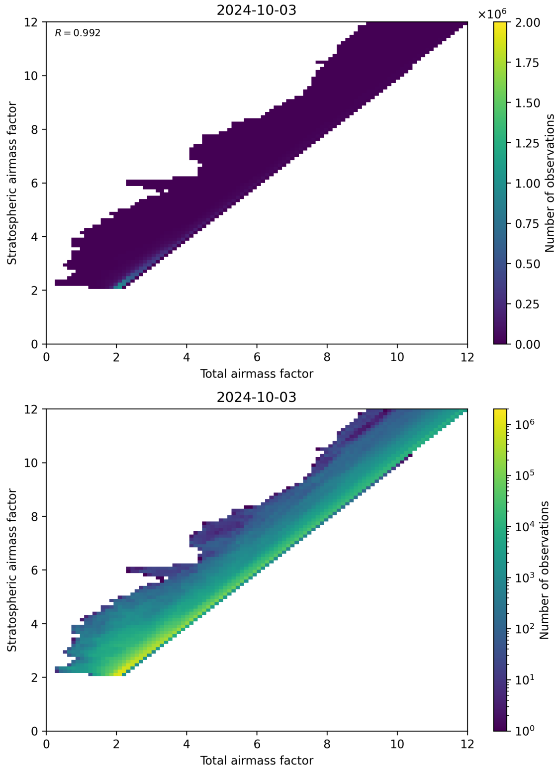
Figure 62: Scatter density plot of “Total airmass factor” against “Stratospheric airmass factor” for 2024-10-03 to 2024-10-04.
