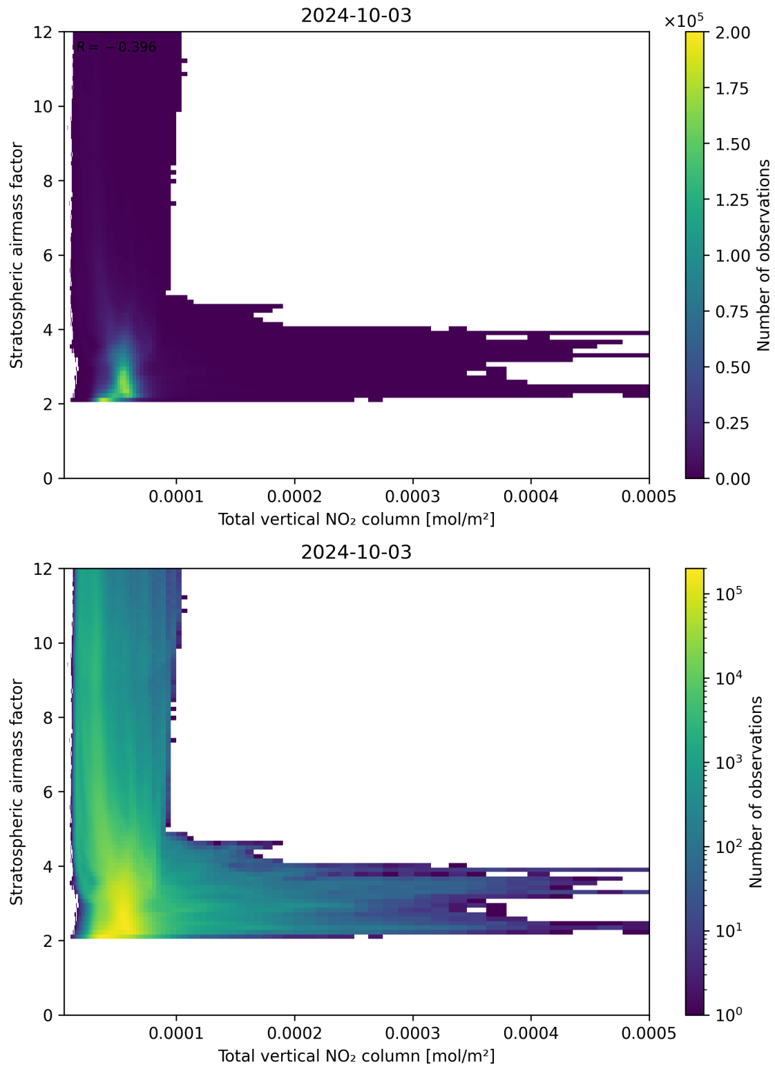
Figure 110: Scatter density plot of “Total vertical NO 2 column” against “Stratospheric airmass factor” for 2024-10-03 to 2024-10-04.
