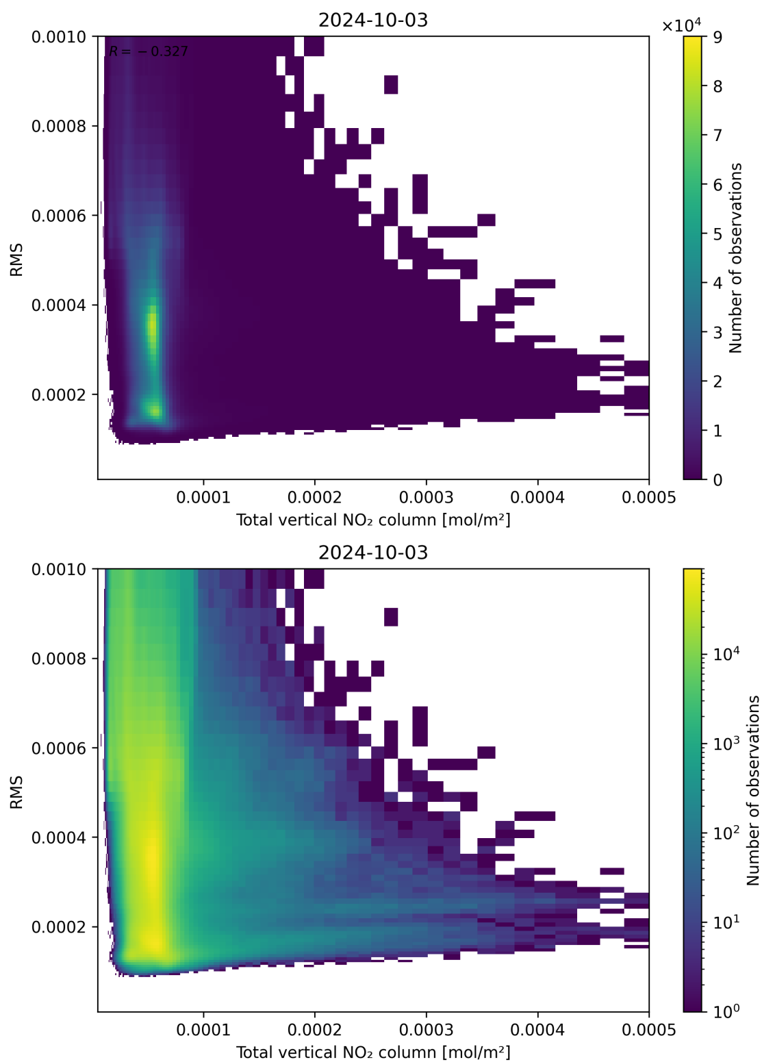
Figure 120: Scatter density plot of “Total vertical NO 2 column” against “RMS” for 2024-10-03 to 2024-10-04.
