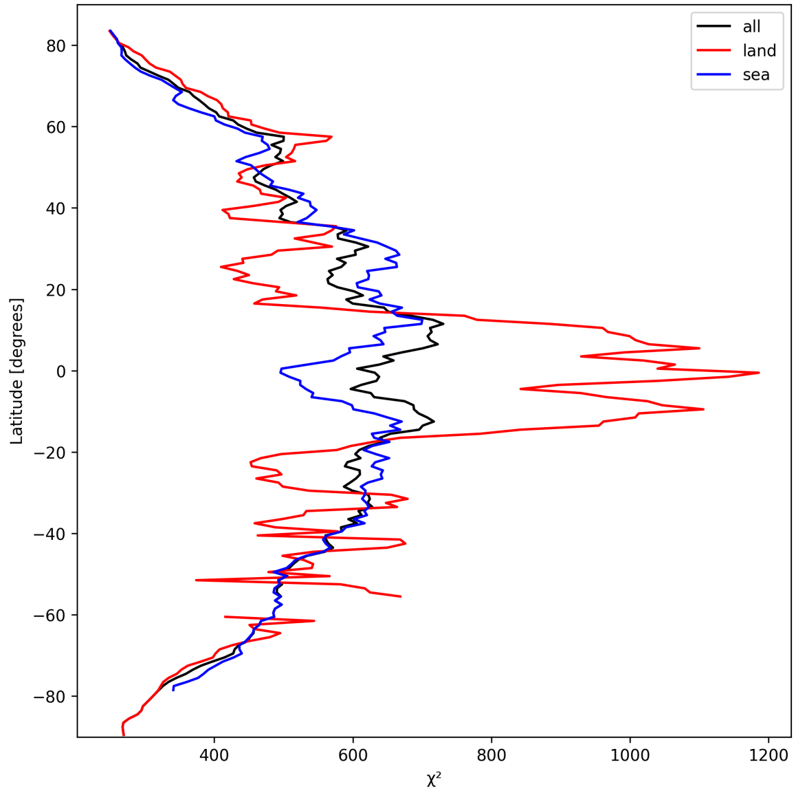
Figure 25: Zonal average of “ \chi^2 ” for 2024-10-03 to 2024-10-04.
