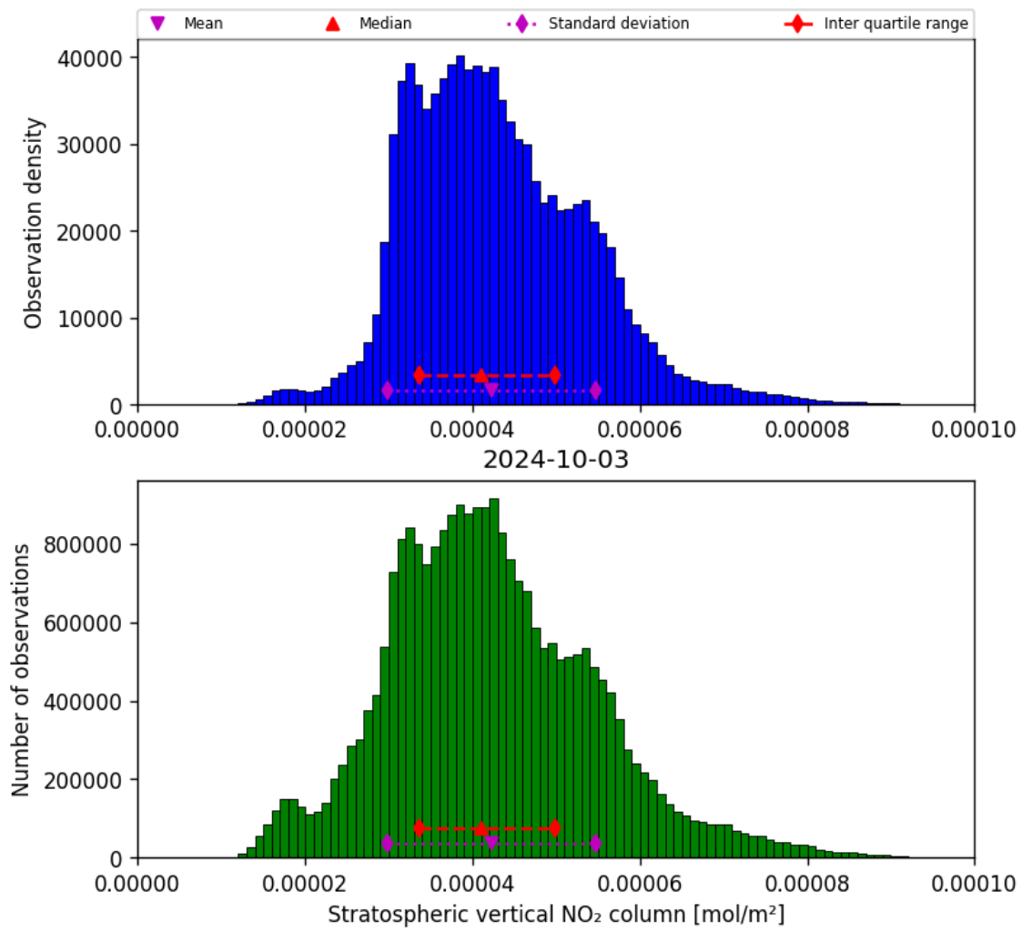
Figure 36: Histogram of “Stratospheric vertical NO 2 column” for 2024-10-03 to 2024-10-04
