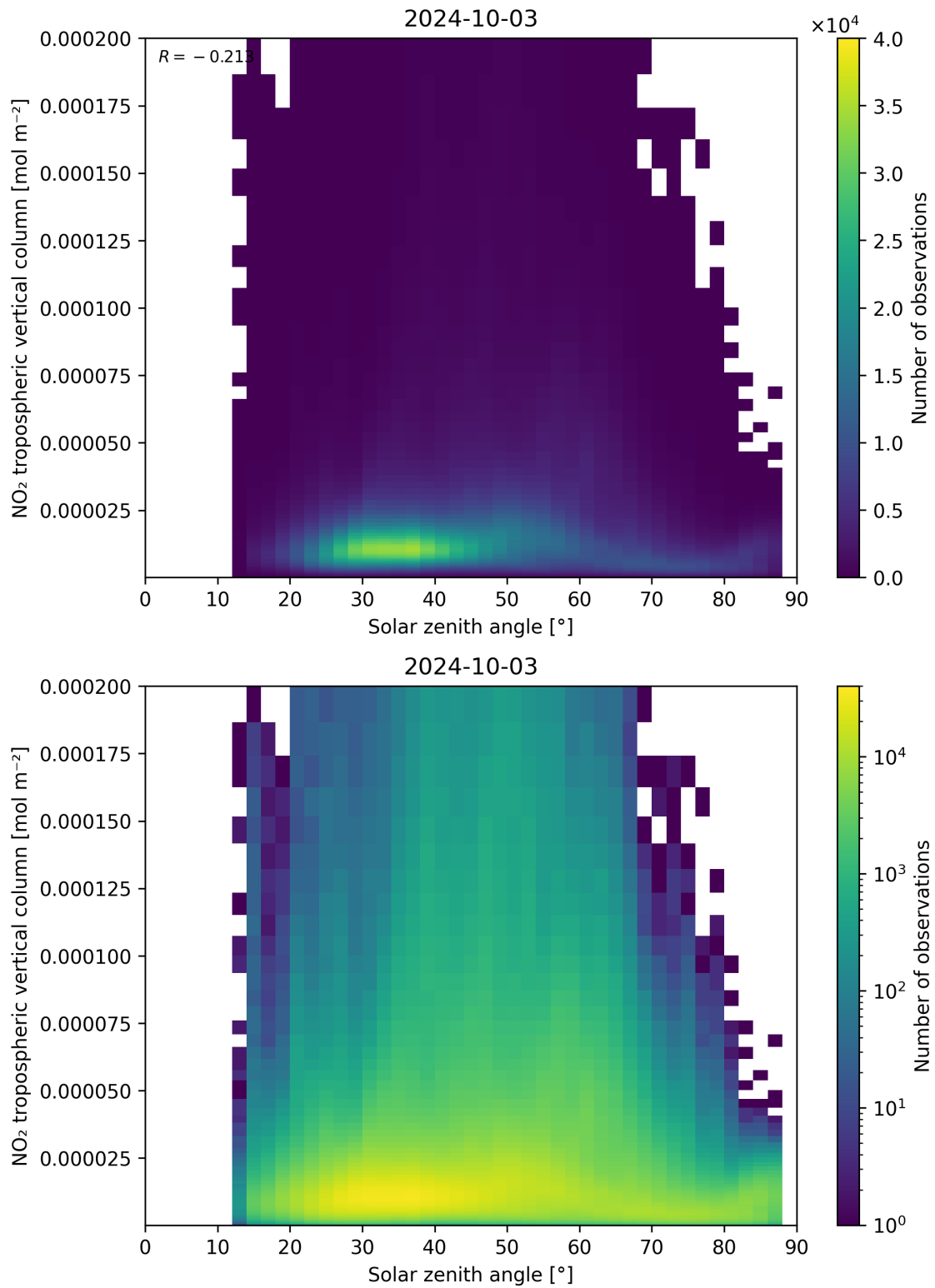
Figure 155: Scatter density plot of “Solar zenith angle” against “NO 2 tropospheric vertical column” for 2024-10-03 to 2024-10-04.
