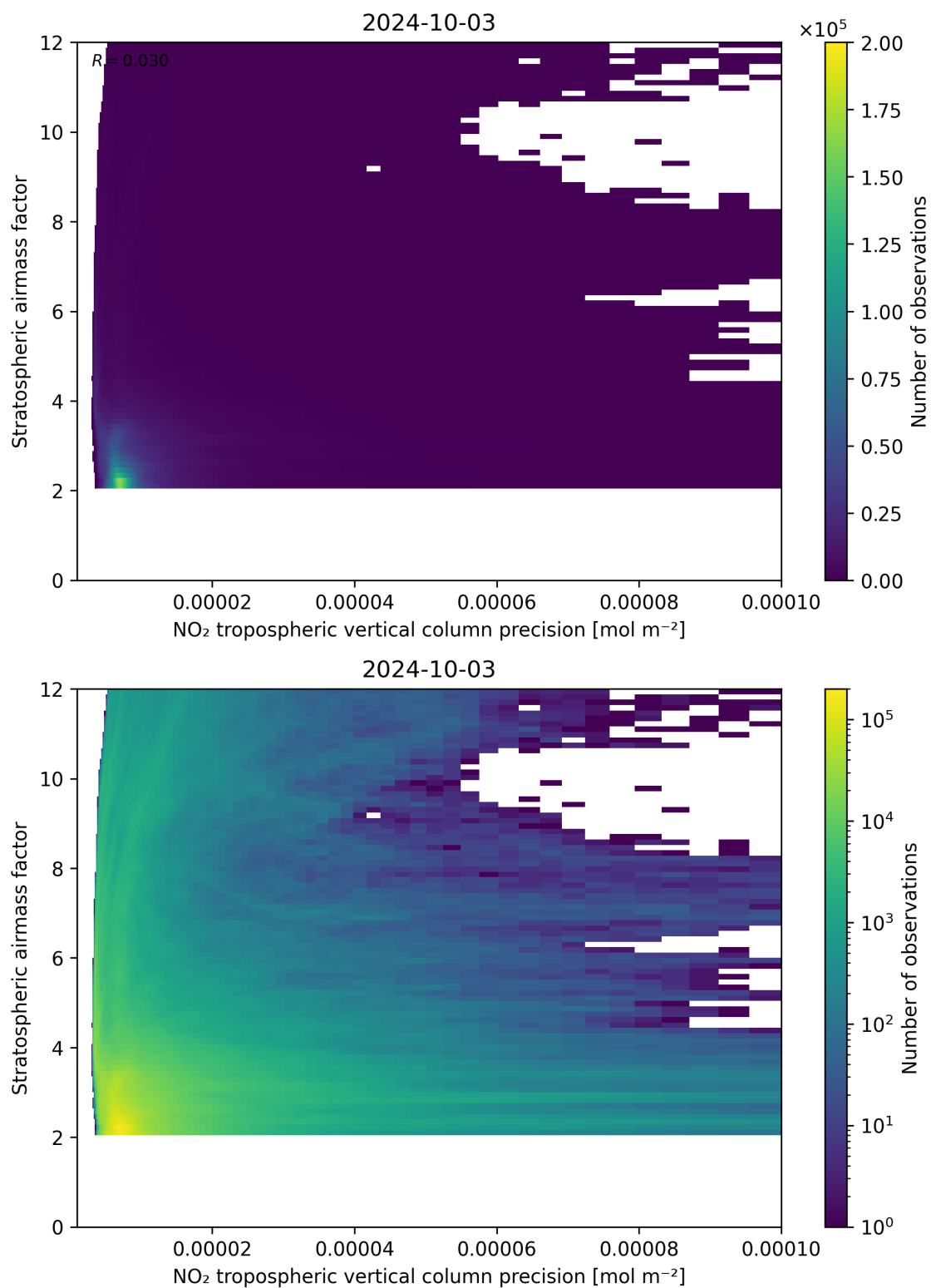
Figure 131: Scatter density plot of “NO 2 tropospheric vertical column precision” against “Stratospheric airmass factor” for 2024-10-03 to 2024-10-04.
