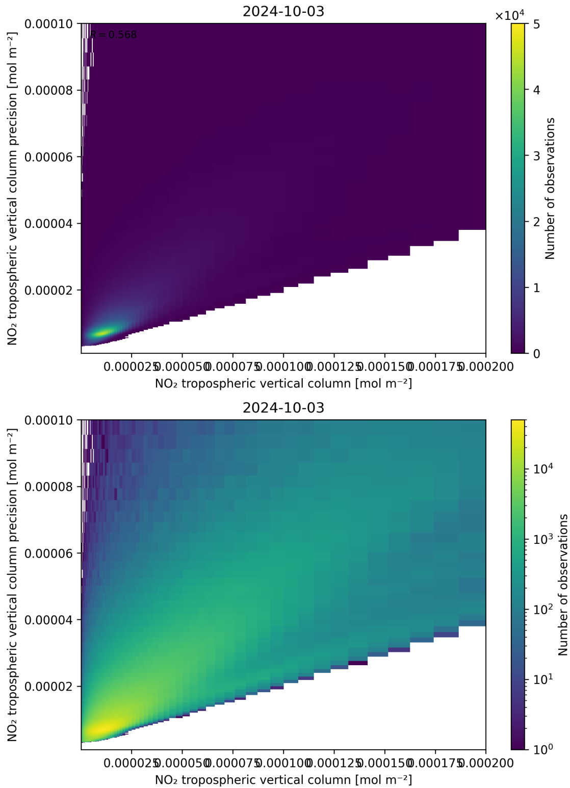
Figure 130: Scatter density plot of “NO 2 tropospheric vertical column” against “NO 2 tropospheric vertical column precision” for 2024-10-03 to 2024-10-04.
