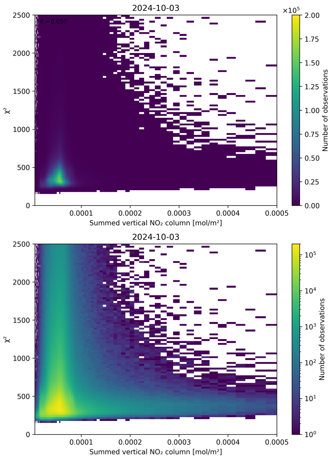
Figure 104: Scatter density plot of “Summed vertical NO 2 column” against “ \chi^2 ” for 2024-10-03 to 2024-10-04.
