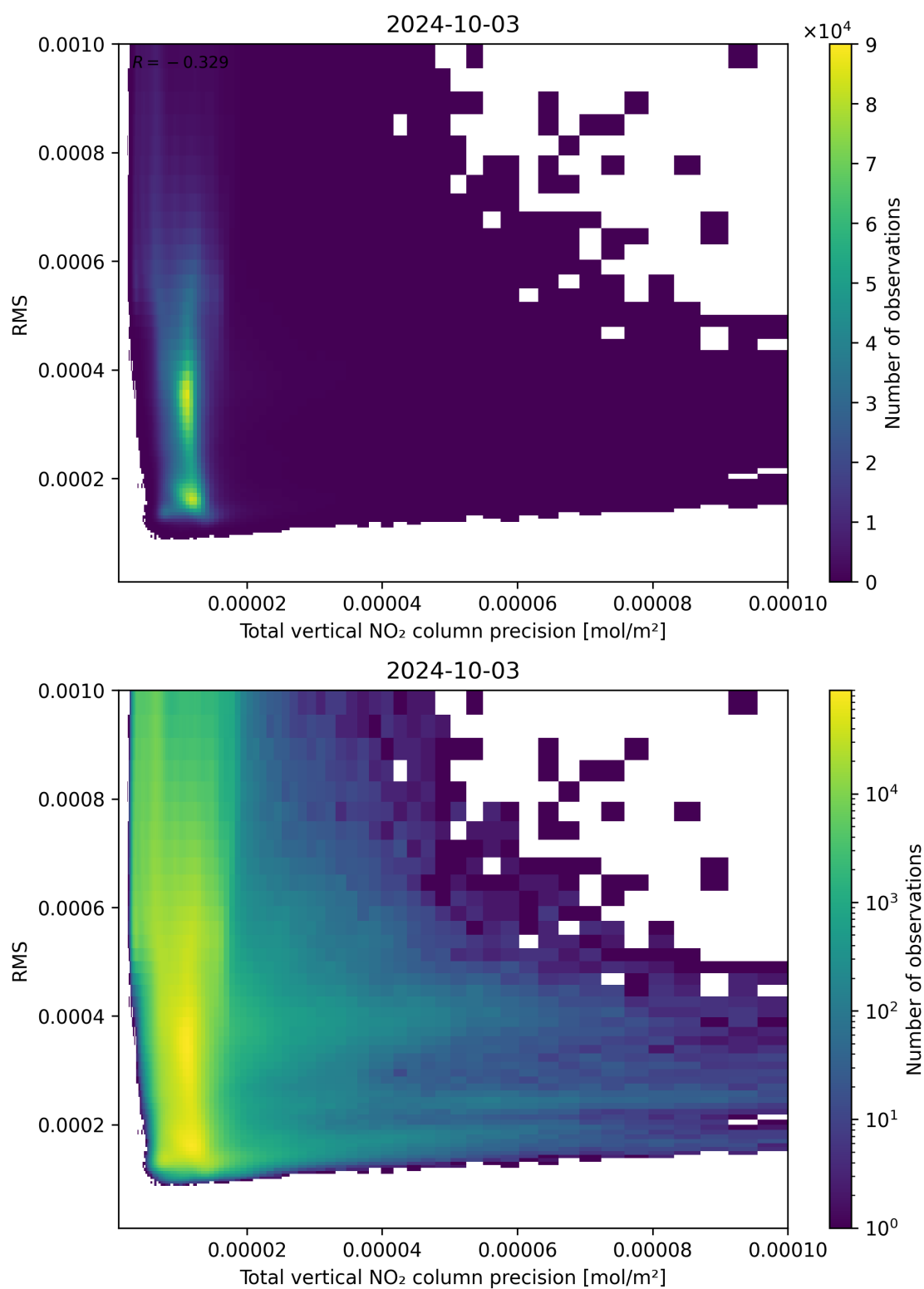
Figure 119: Scatter density plot of “Total vertical NO 2 column precision” against “RMS” for 2024-10-03 to 2024-10-04.
