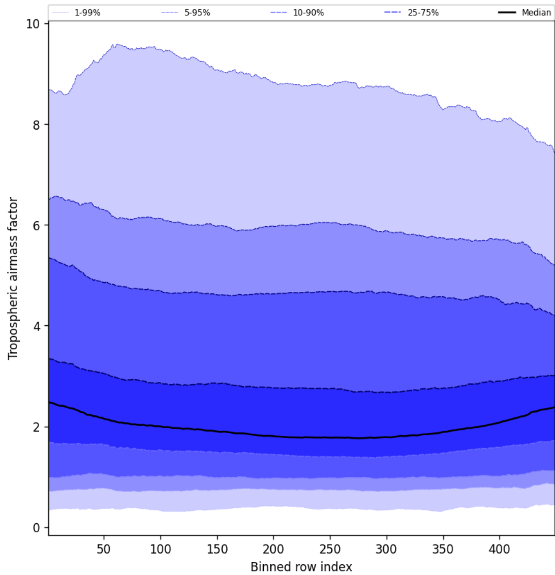
Figure 48: Along track statistics of “Tropospheric air mass factor” for 2024-10-03 to 2024-10-04
