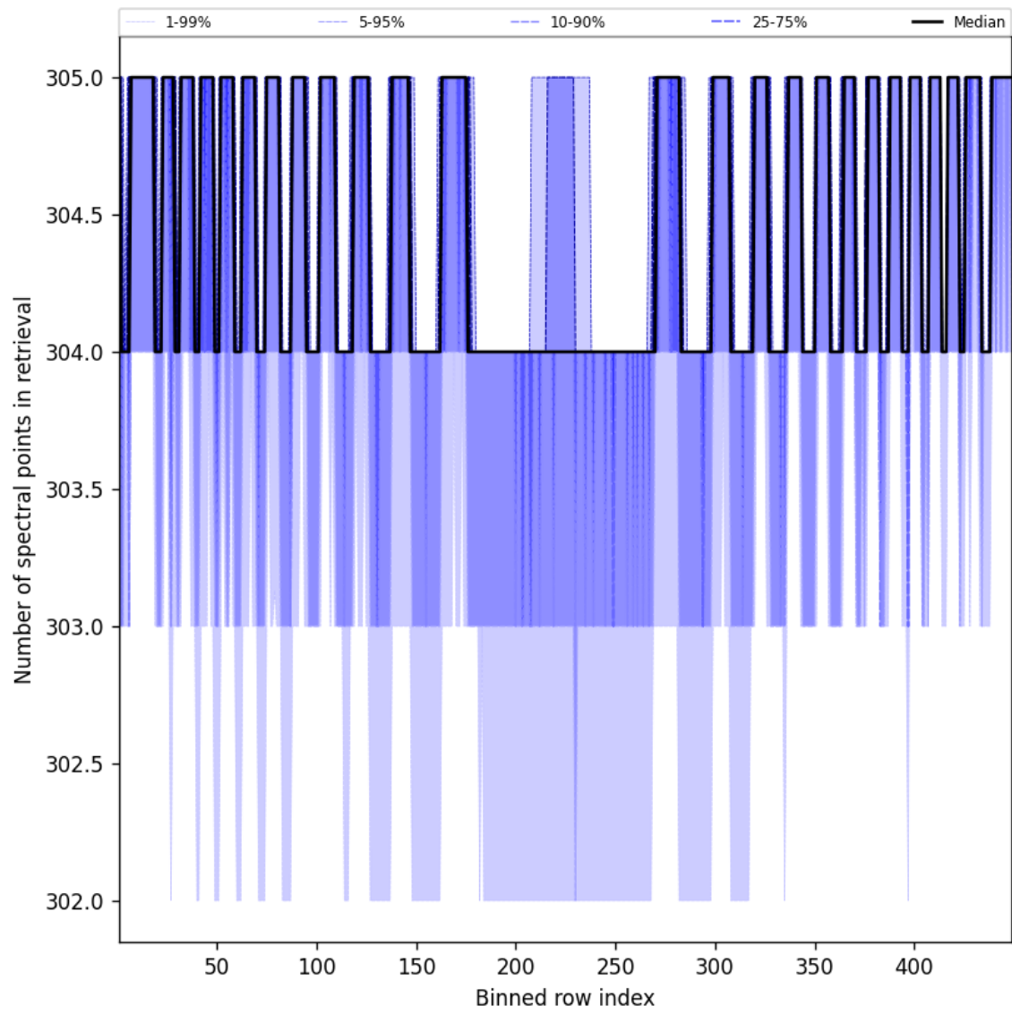
Figure 50: Along track statistics of “Number of spectral points in retrieval” for 2024-10-03 to 2024-10-04
