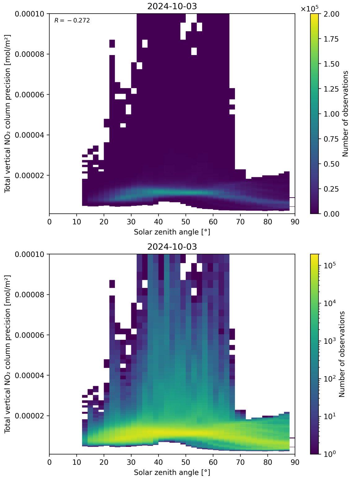
Figure 154: Scatter density plot of “Solar zenith angle” against “Total vertical NO 2 column precision” for 2024-10-03 to 2024-10-04.
