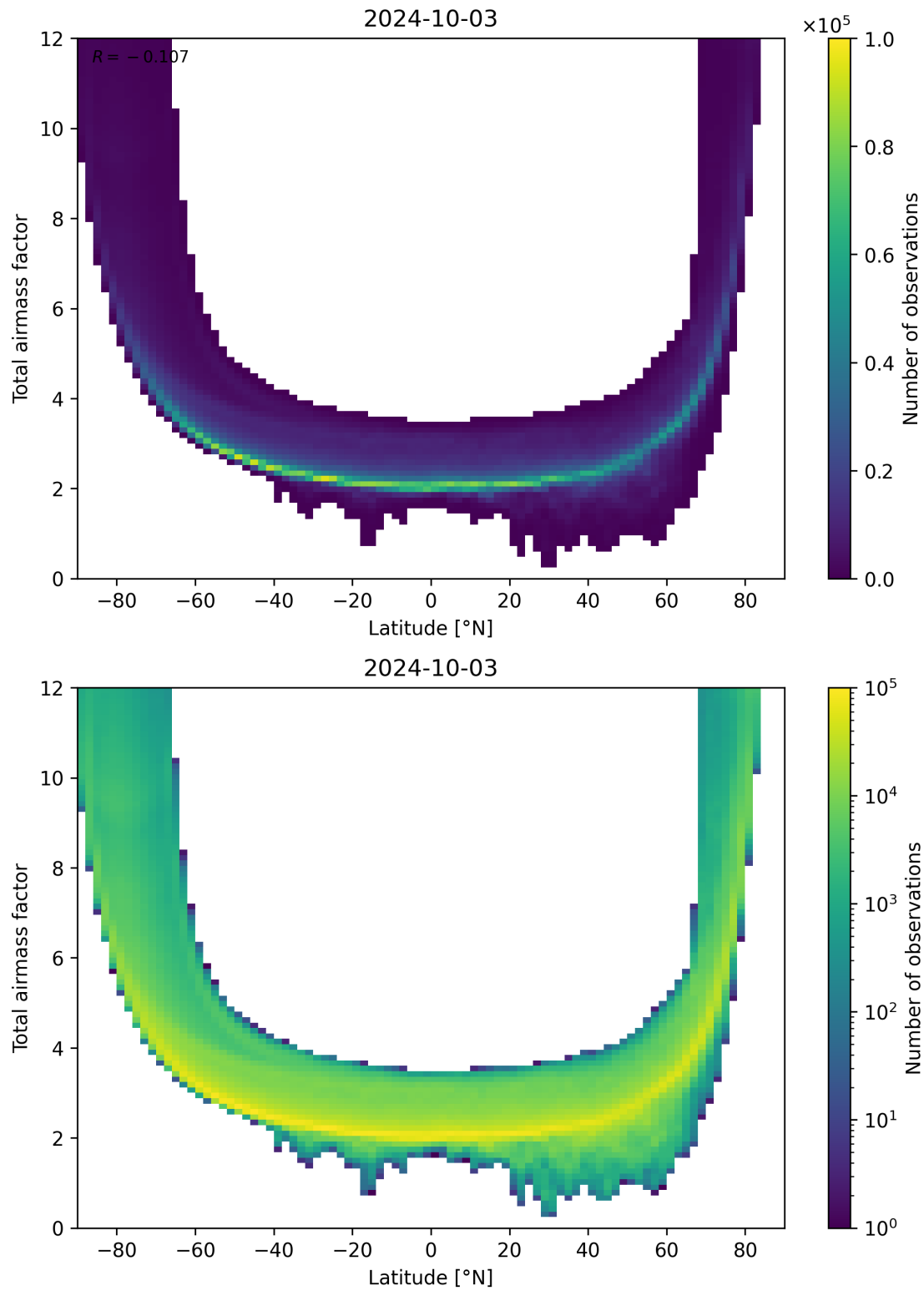
Figure 84: Scatter density plot of “Latitude” against “Total airmass factor” for 2024-10-03 to 2024-10-04.
