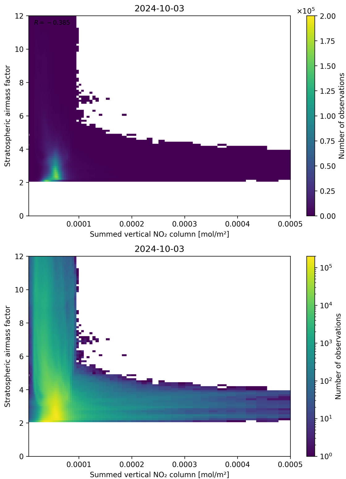
Figure 103: Scatter density plot of “Summed vertical NO 2 column” against “Stratospheric airmass factor” for 2024-10-03 to 2024-10-04.
