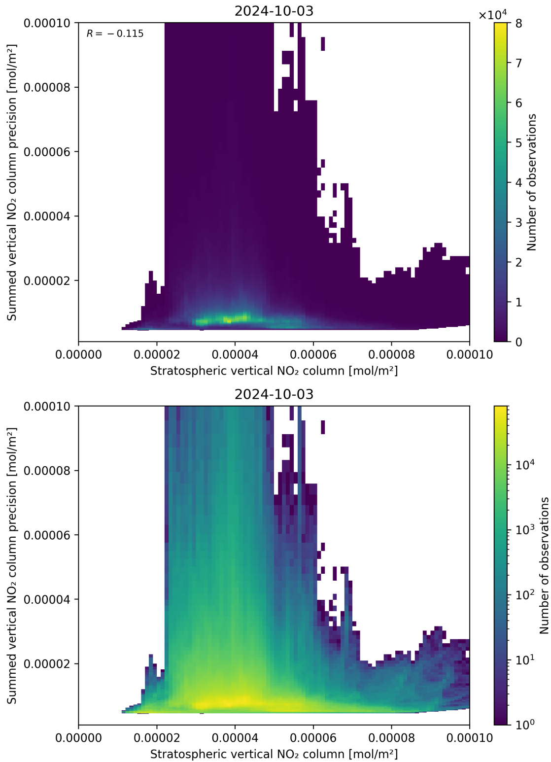
Figure 99: Scatter density plot of “Stratospheric vertical NO 2 column” against “Summed vertical NO 2 column precision” for 2024-10-03 to 2024-10-04.
