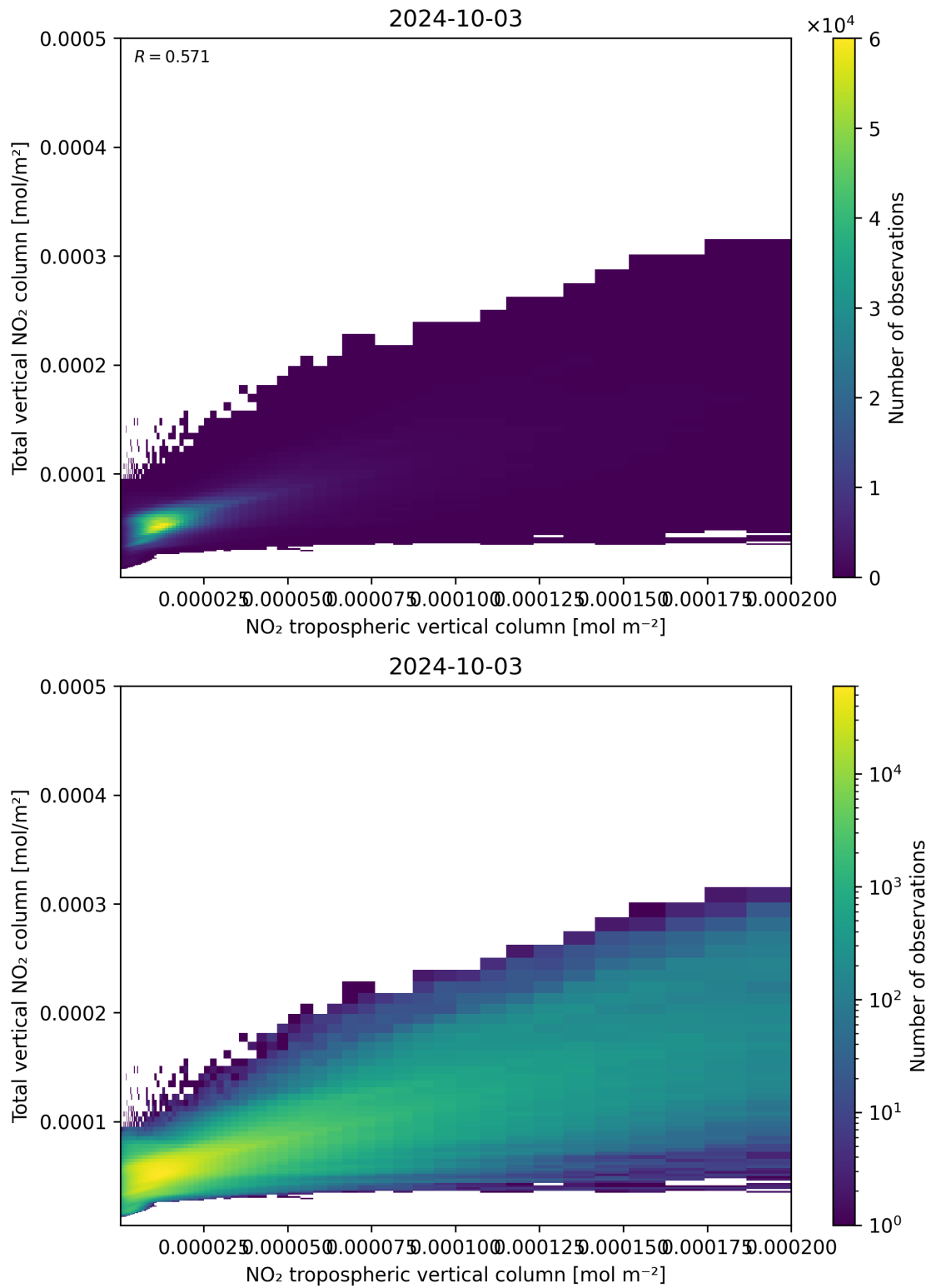
Figure 128: Scatter density plot of “NO 2 tropospheric vertical column” against “Total vertical NO 2 column” for 2024-10-03 to 2024-10-04.
