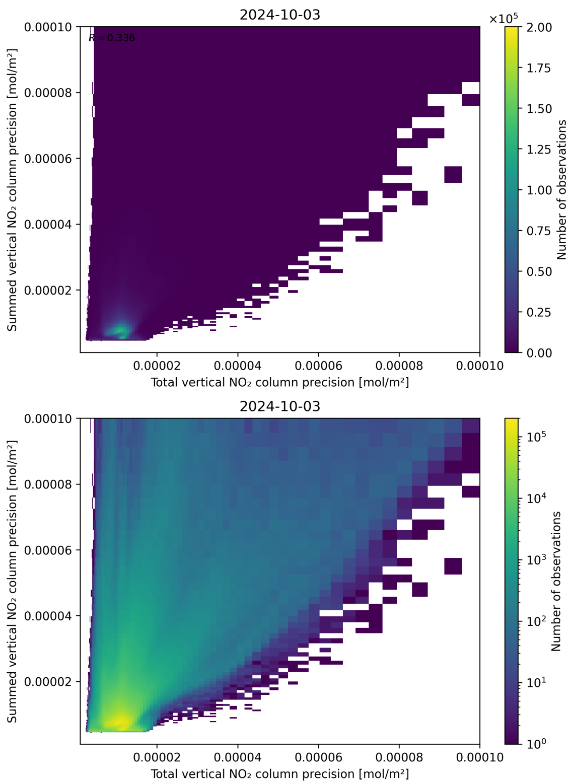
Figure 118: Scatter density plot of “Total vertical NO 2 column precision” against “Summed vertical NO 2 column precision” for 2024-10-03 to 2024-10-04.
