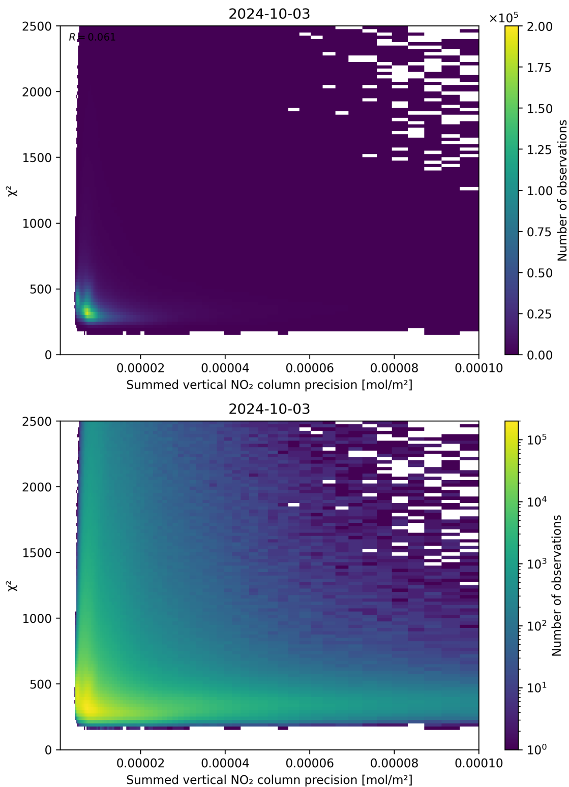
Figure 107: Scatter density plot of “Summed vertical NO 2 column precision” against “ \chi^2 ” for 2024-10-03 to 2024-10-04.
