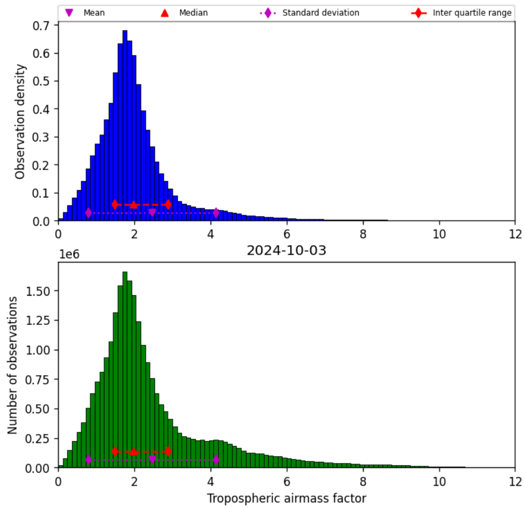
Figure 31: Histogram of “Tropospheric airmass factor” for 2024-10-03 to 2024-10-04
