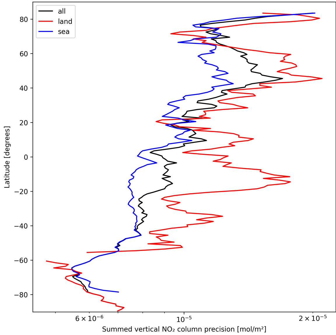
Figure 24: Zonal average of “Summed vertical NO 2 column precision” for 2024-10-03 to 2024-10-04.
