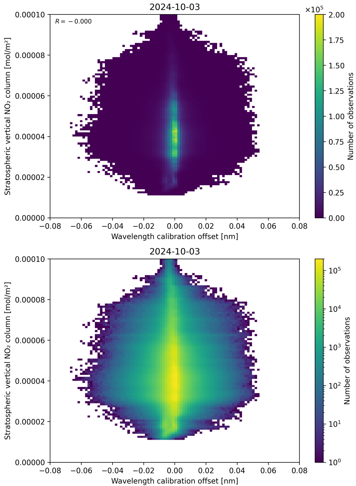
Figure 176: Scatter density plot of “Wavelength calibration offset” against “Stratospheric vertical NO 2 column” for 2024-10-03 to 2024-10-04.
