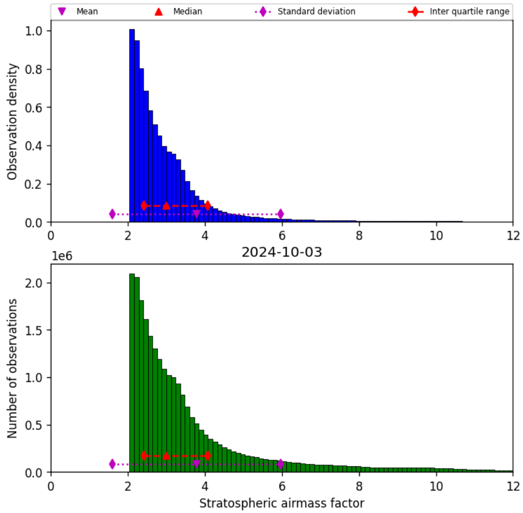
Figure 44: Histogram of “Stratospheric airmass factor” for 2024-10-03 to 2024-10-04
