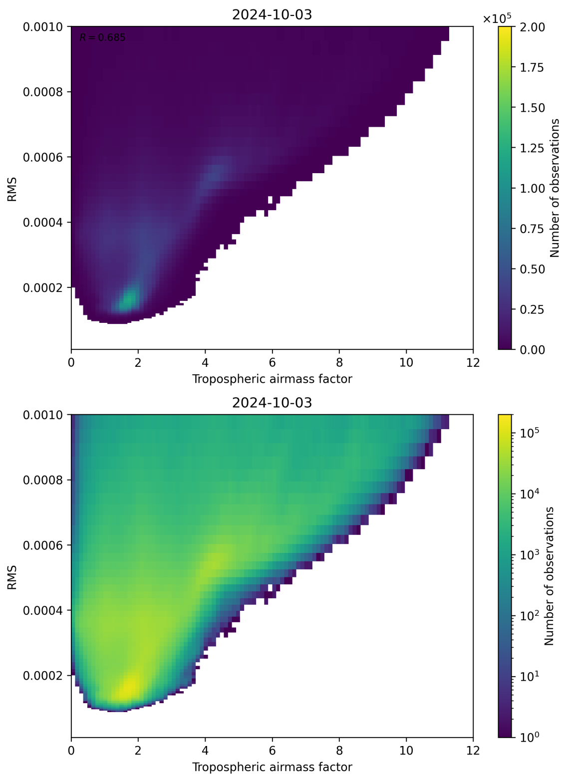
Figure 79: Scatter density plot of “Tropospheric airmass factor” against “RMS” for 2024-10-03 to 2024-10-04.
