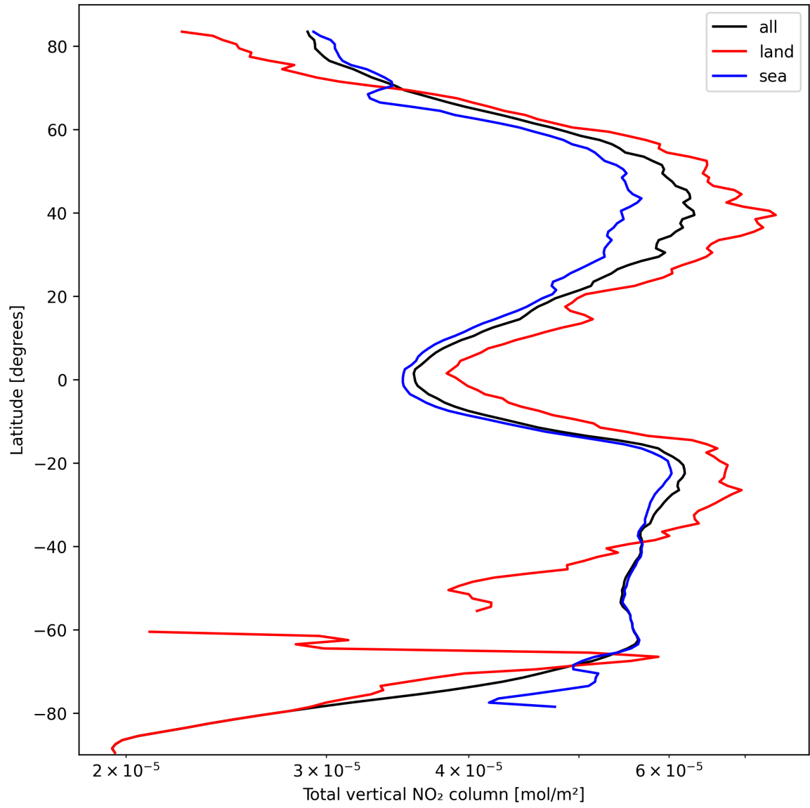
Figure 21: Zonal average of “Total vertical NO 2 column” for 2024-10-03 to 2024-10-04.
