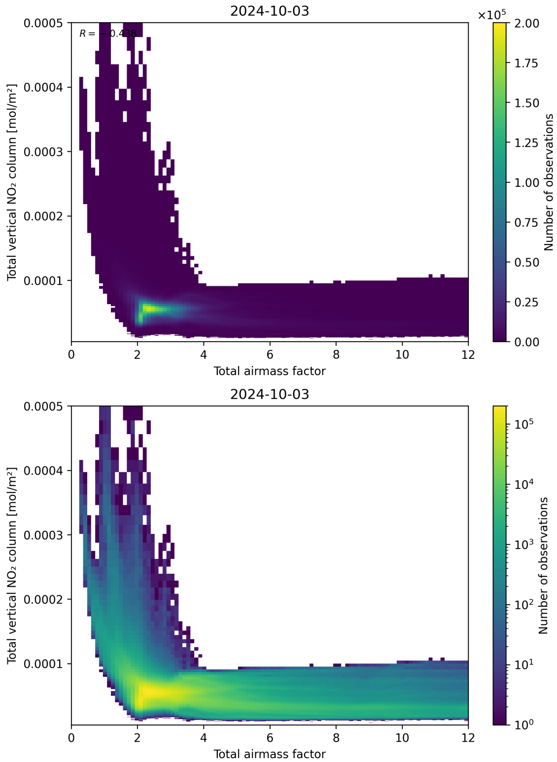
Figure 67: Scatter density plot of “Total airmass factor” against “Total vertical NO 2 column” for 2024-10-03 to 2024-10-04.
