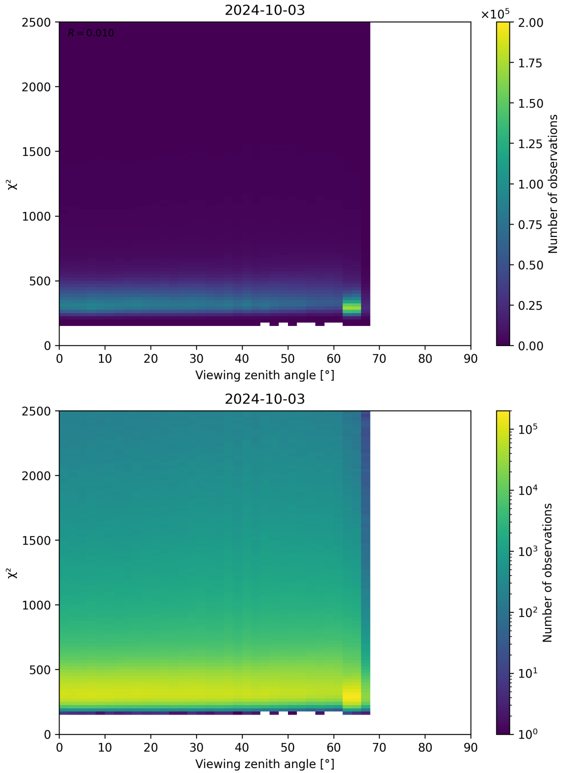
Figure 162: Scatter density plot of “Viewing zenith angle” against “ \chi^2 ” for 2024-10-03 to 2024-10-04.
