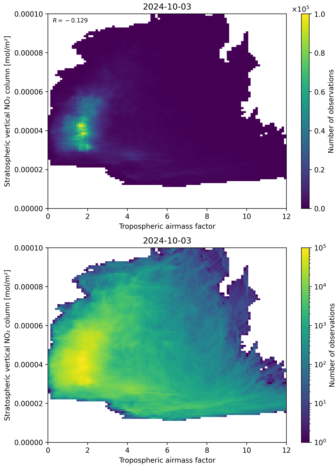
Figure 74: Scatter density plot of “Tropospheric airmass factor” against “Stratospheric vertical NO 2 column” for 2024-10-03 to 2024-10-04.
