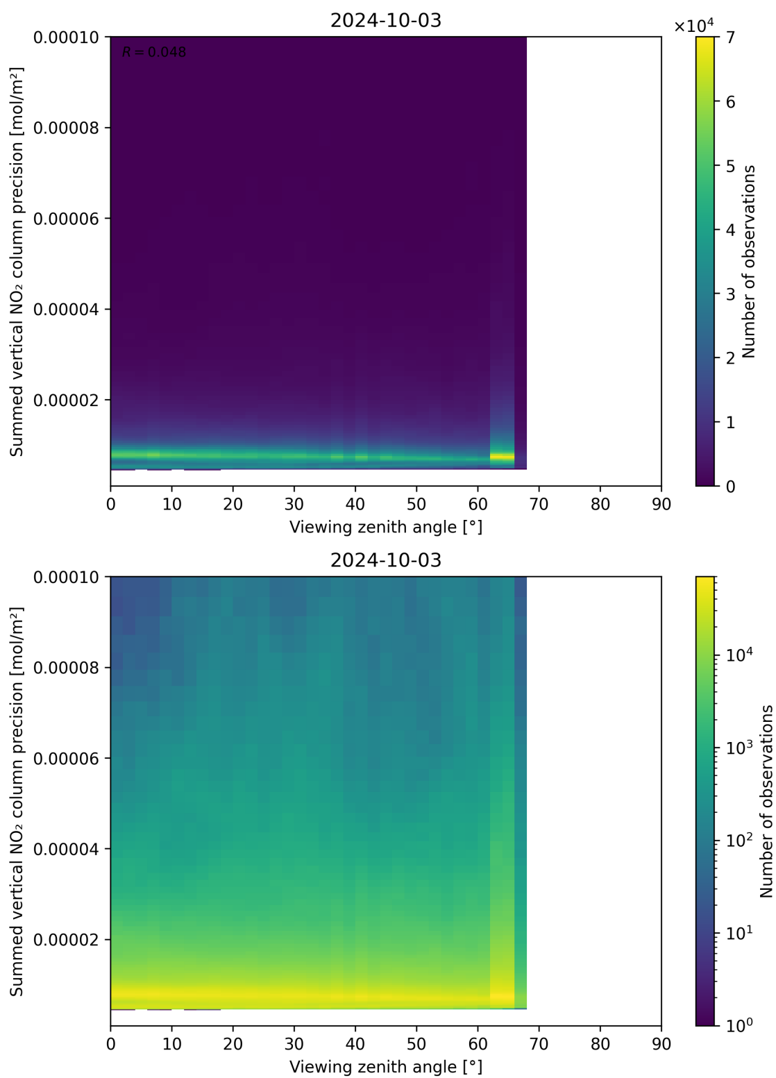
Figure 166: Scatter density plot of “Viewing zenith angle” against “Summed vertical NO 2 column precision” for 2024-10-03 to 2024-10-04.
