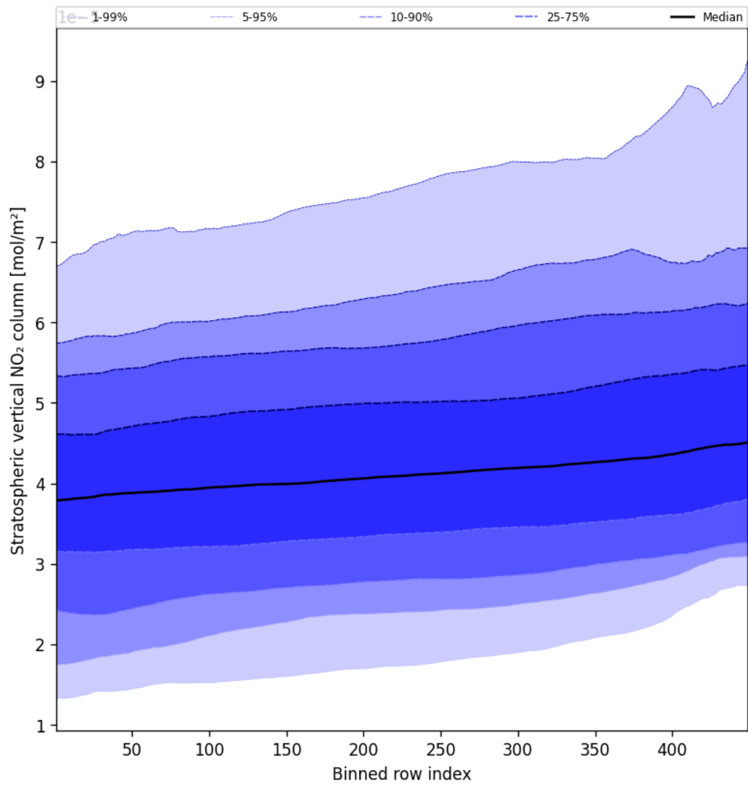
Figure 53: Along track statistics of “Stratospheric vertical NO 2 column” for 2024-10-03 to 2024-10-04
