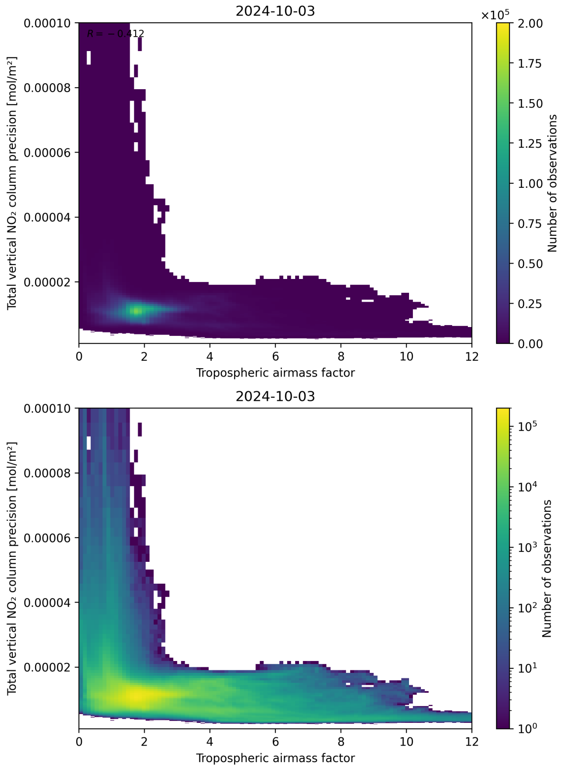
Figure 78: Scatter density plot of “Tropospheric airmass factor” against “Total vertical NO 2 column precision” for 2024-10-03 to 2024-10-04.
