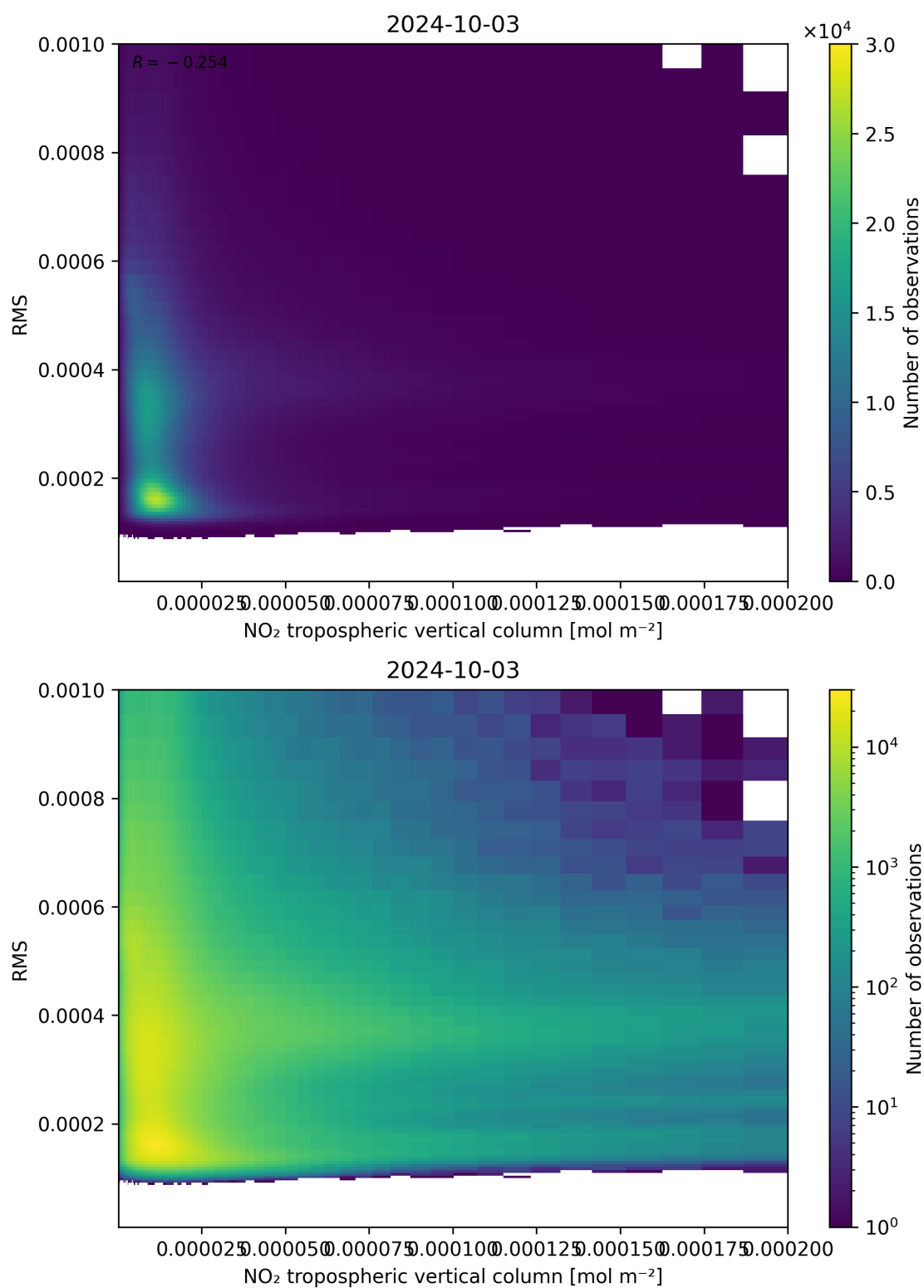
Figure 142: Scatter density plot of “NO 2 tropospheric vertical column” against “RMS” for 2024-10-03 to 2024-10-04.
