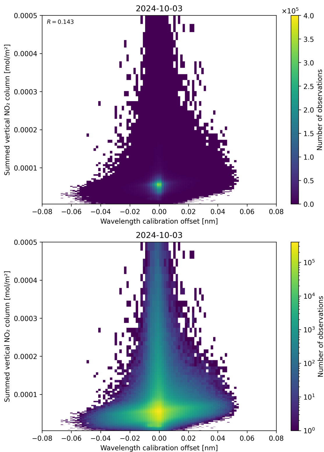
Figure 177: Scatter density plot of “Wavelength calibration offset” against “Summed vertical NO 2 column” for 2024-10-03 to 2024-10-04.
