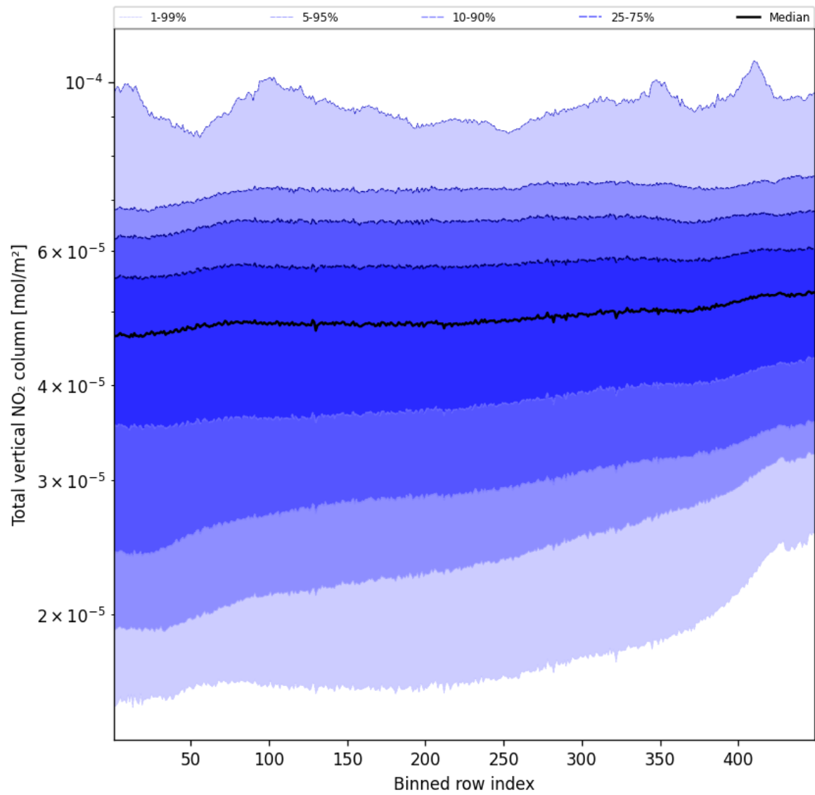
Figure 55: Along track statistics of “Total vertical NO 2 column” for 2024-10-03 to 2024-10-04
