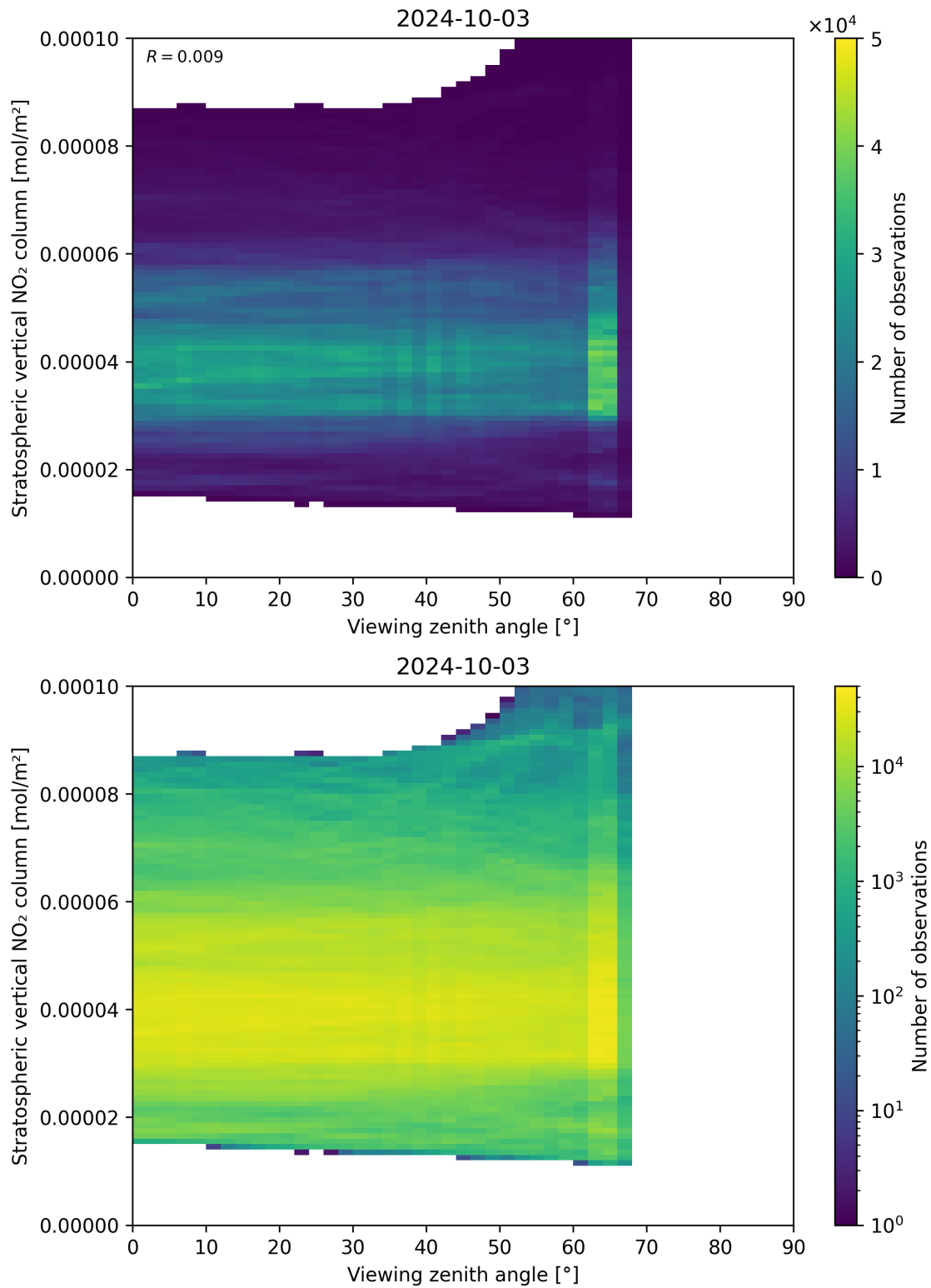
Figure 164: Scatter density plot of “Viewing zenith angle” against “Stratospheric vertical NO 2 column” for 2024-10-03 to 2024-10-04.
