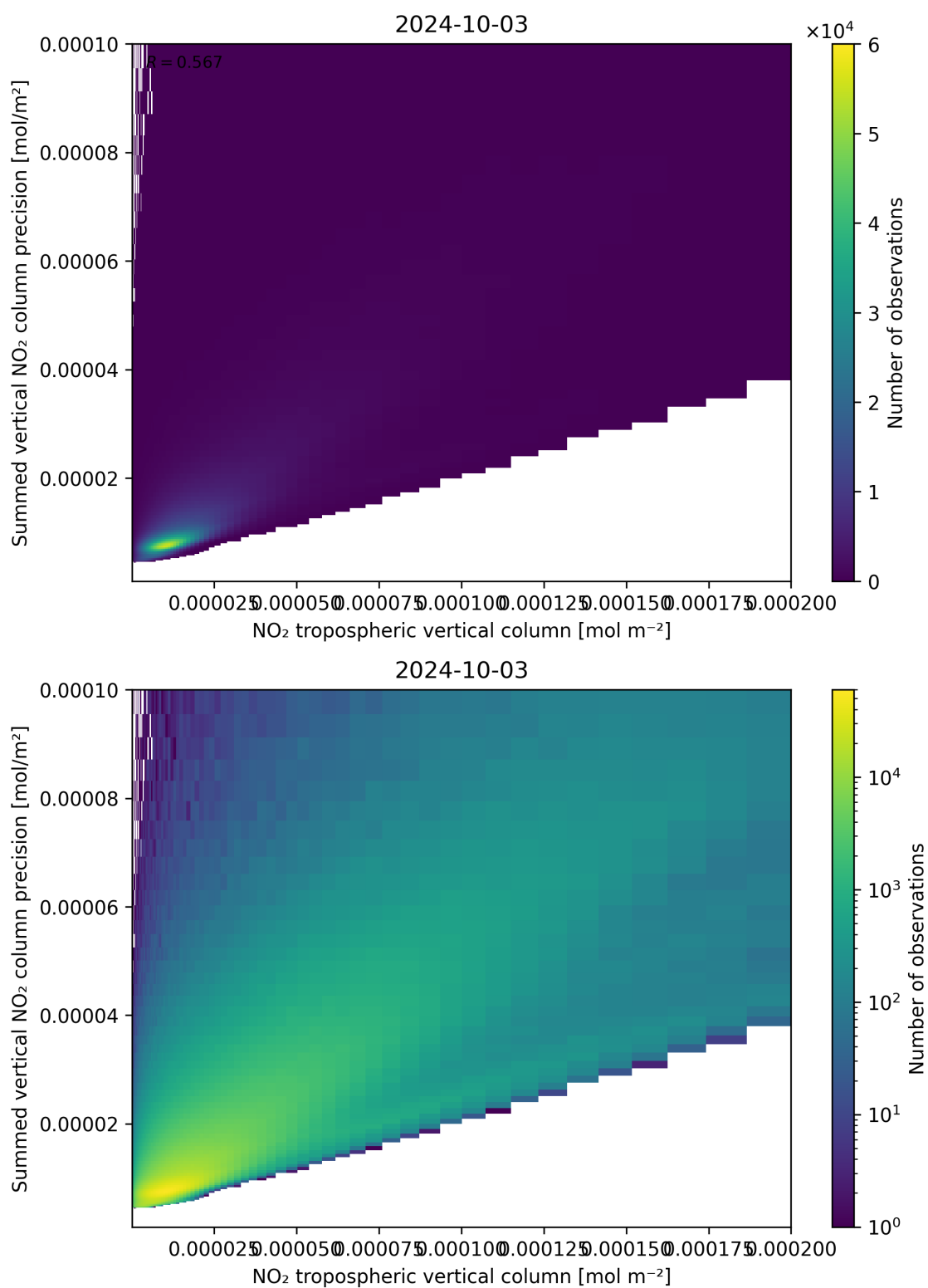
Figure 127: Scatter density plot of “NO 2 tropospheric vertical column” against “Summed vertical NO 2 column precision” for 2024-10-03 to 2024-10-04.
