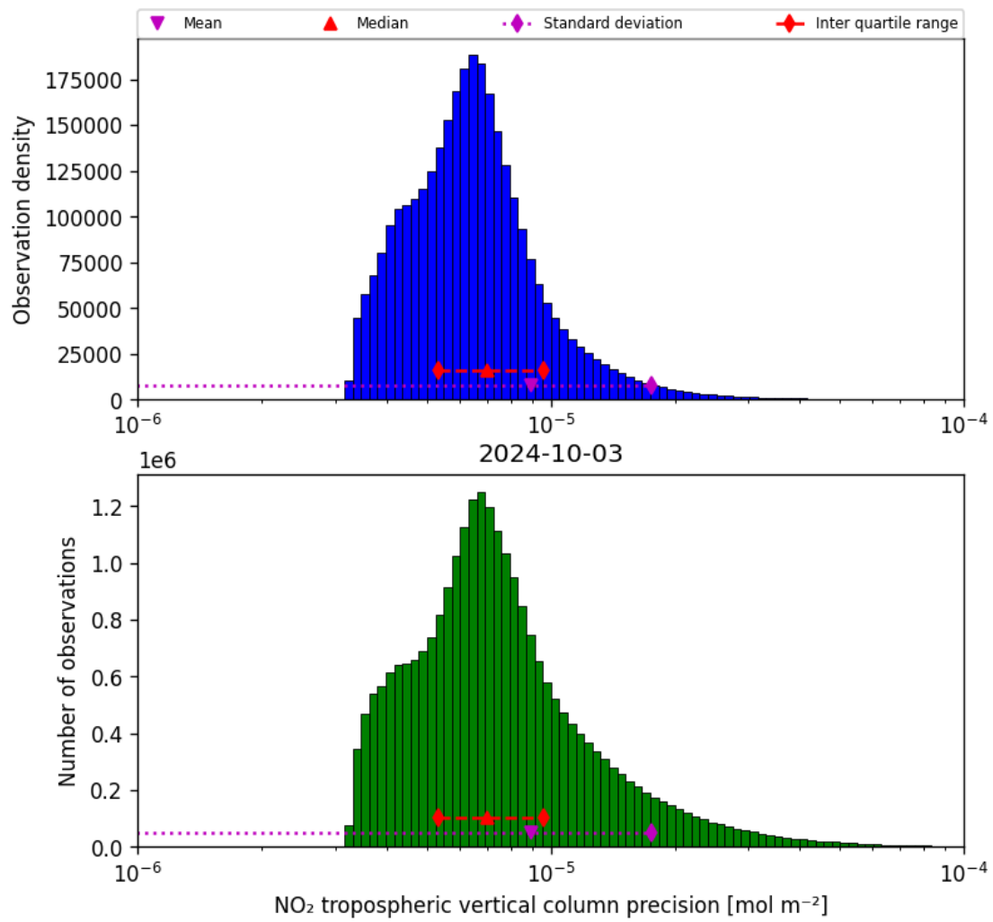
Figure 30: Histogram of “NO 2 tropospheric vertical column precision” for 2024-10-03 to 2024-10-04
