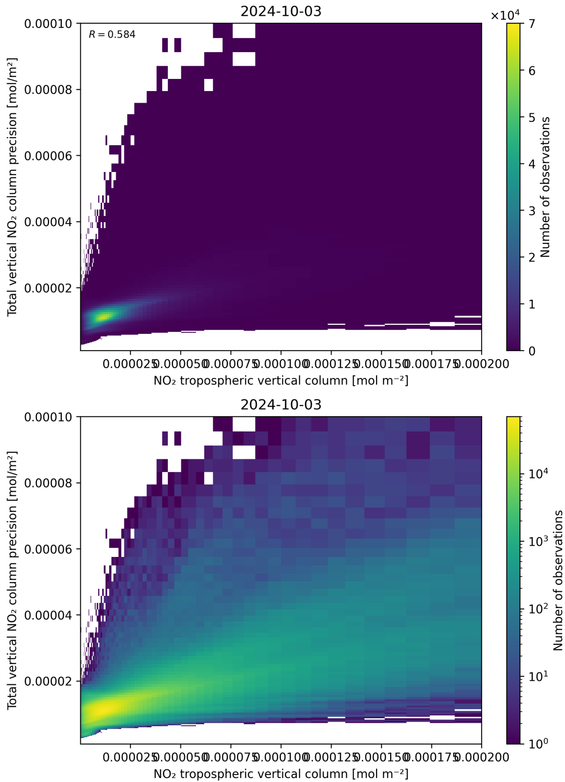
Figure 129: Scatter density plot of “NO 2 tropospheric vertical column” against “Total vertical NO 2 column precision” for 2024-10-03 to 2024-10-04.
