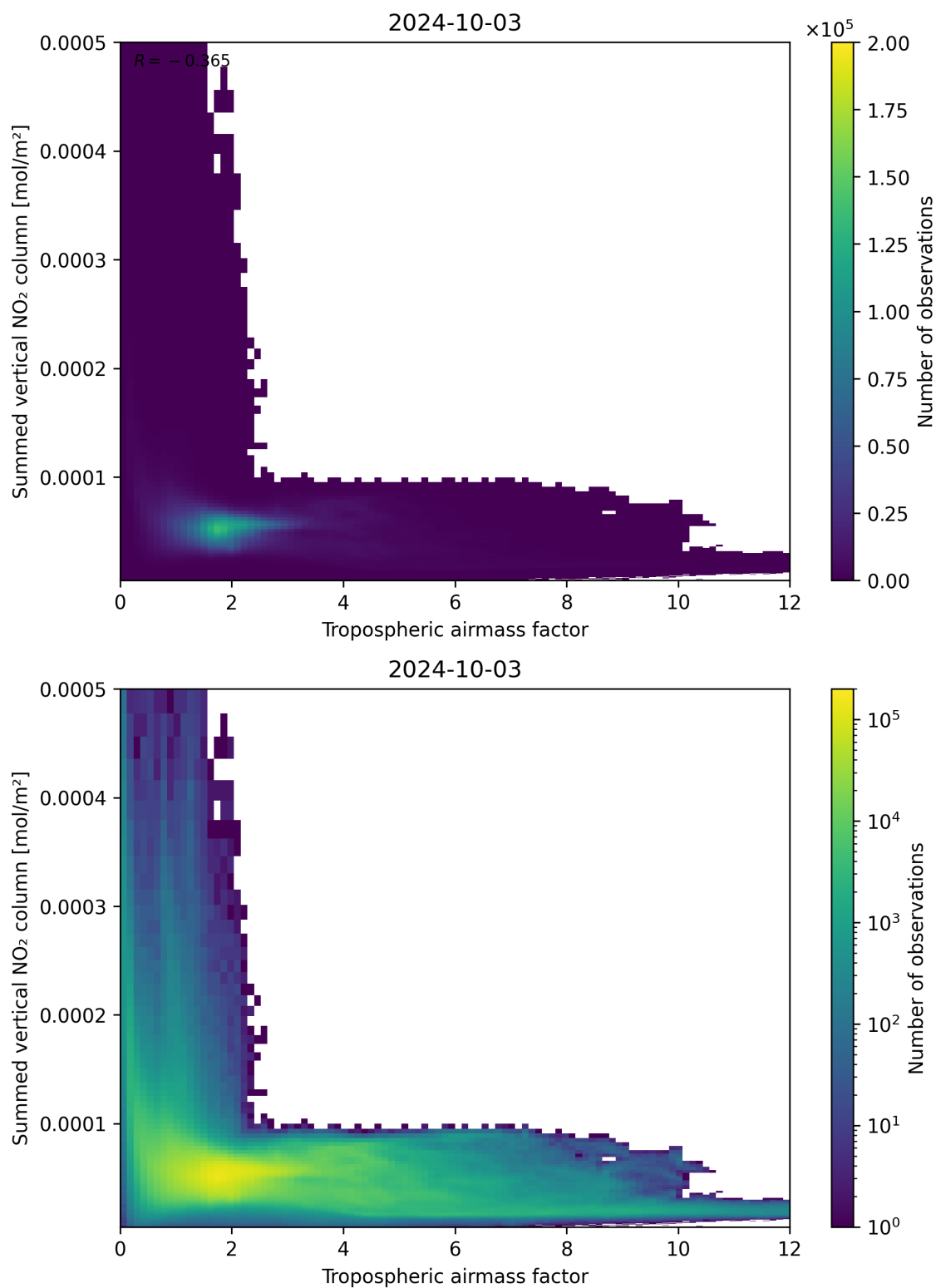
Figure 75: Scatter density plot of “Tropospheric air mass factor” against “Summed vertical NO 2 column” for 2024-10-03 to 2024-10-04.
