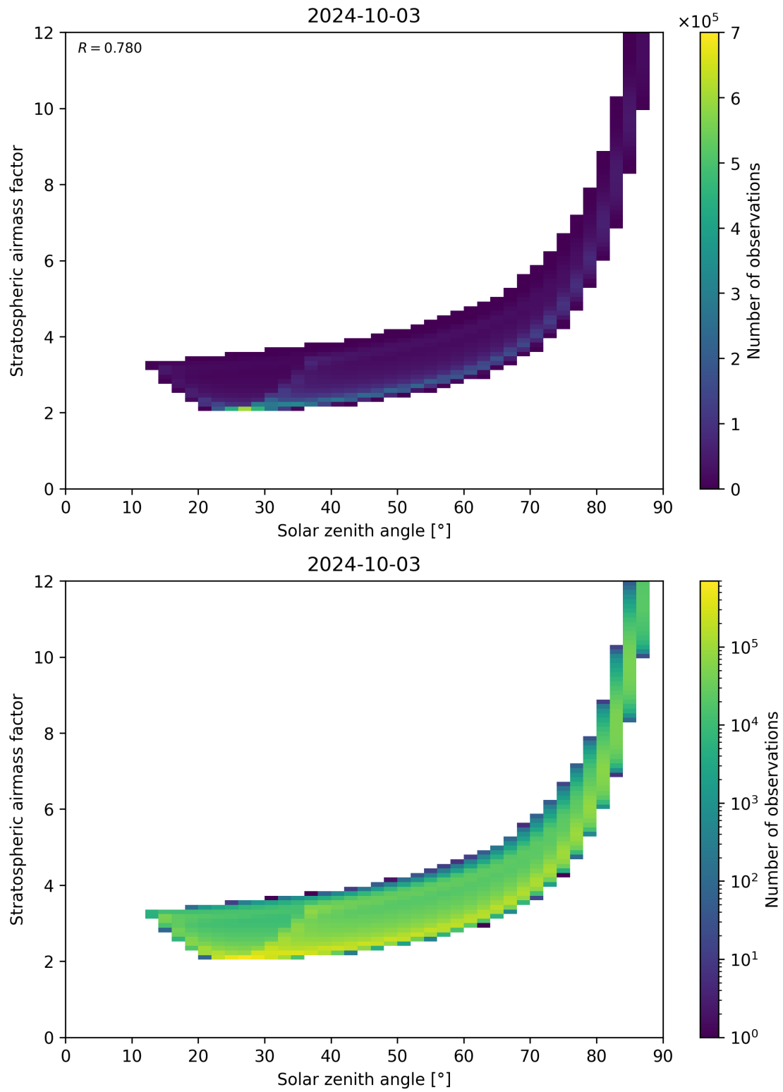
Figure 145: Scatter density plot of “Solar zenith angle” against “Stratospheric airmass factor” for 2024-10-03 to 2024-10-04.
