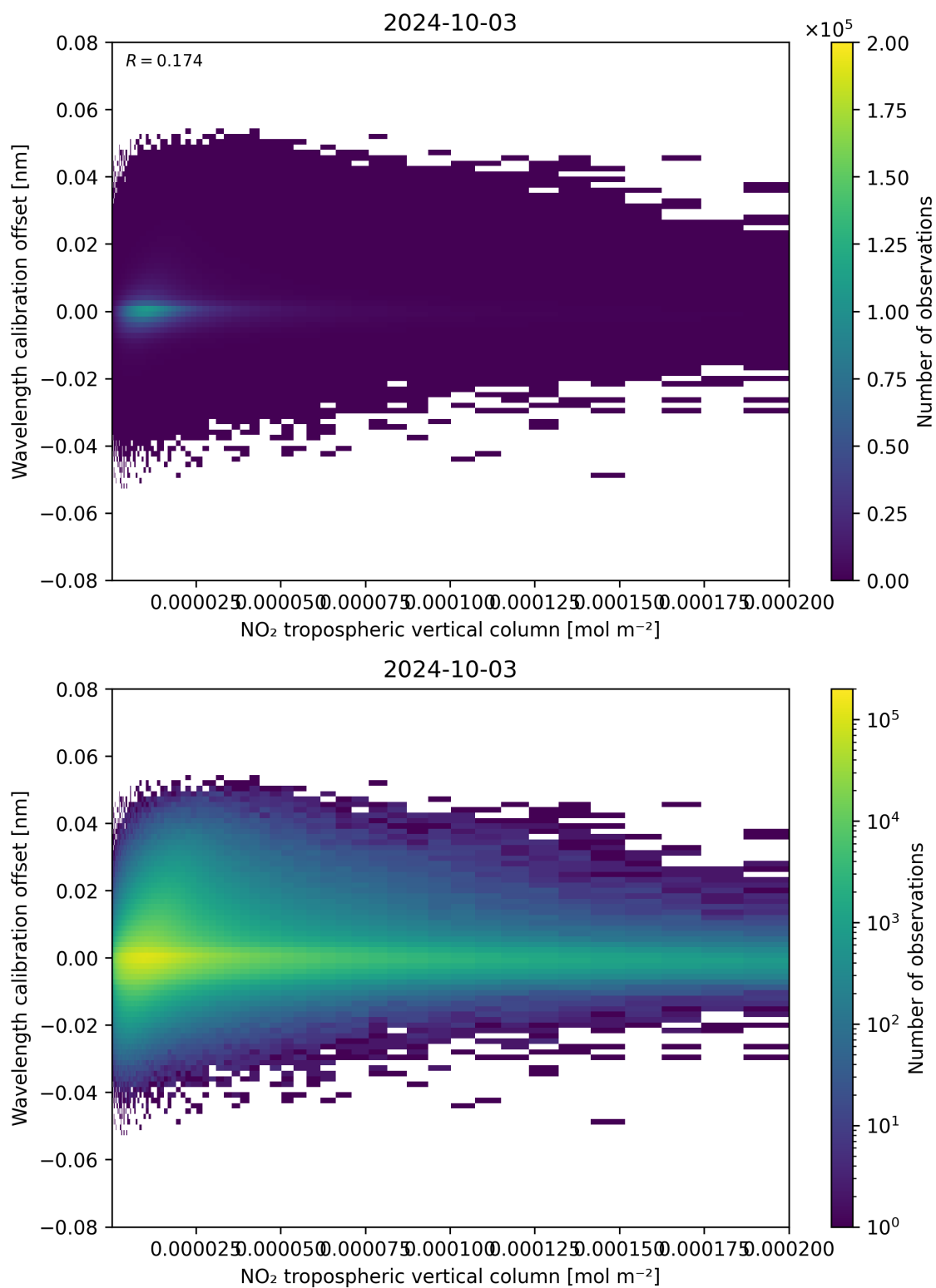
Figure 143: Scatter density plot of “NO 2 tropospheric vertical column” against “Wavelength calibration offset” for 2024-10-03 to 2024-10-04.
