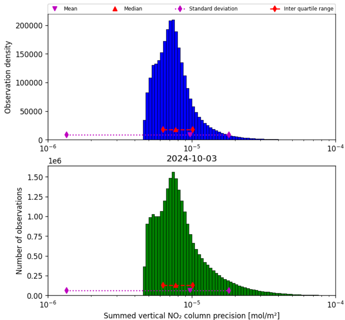
Figure 41: Histogram of “Summed vertical NO 2 column precision” for 2024-10-03 to 2024-10-04
