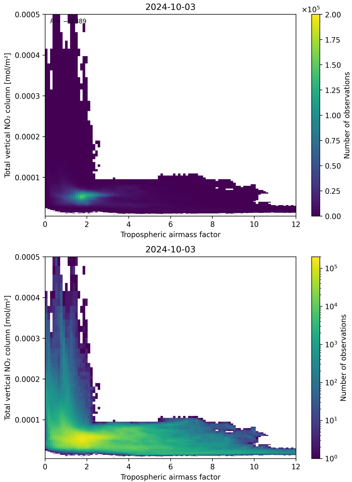
Figure 77: Scatter density plot of “Tropospheric airmass factor” against “Total vertical NO 2 column” for 2024-10-03 to 2024-10-04.
