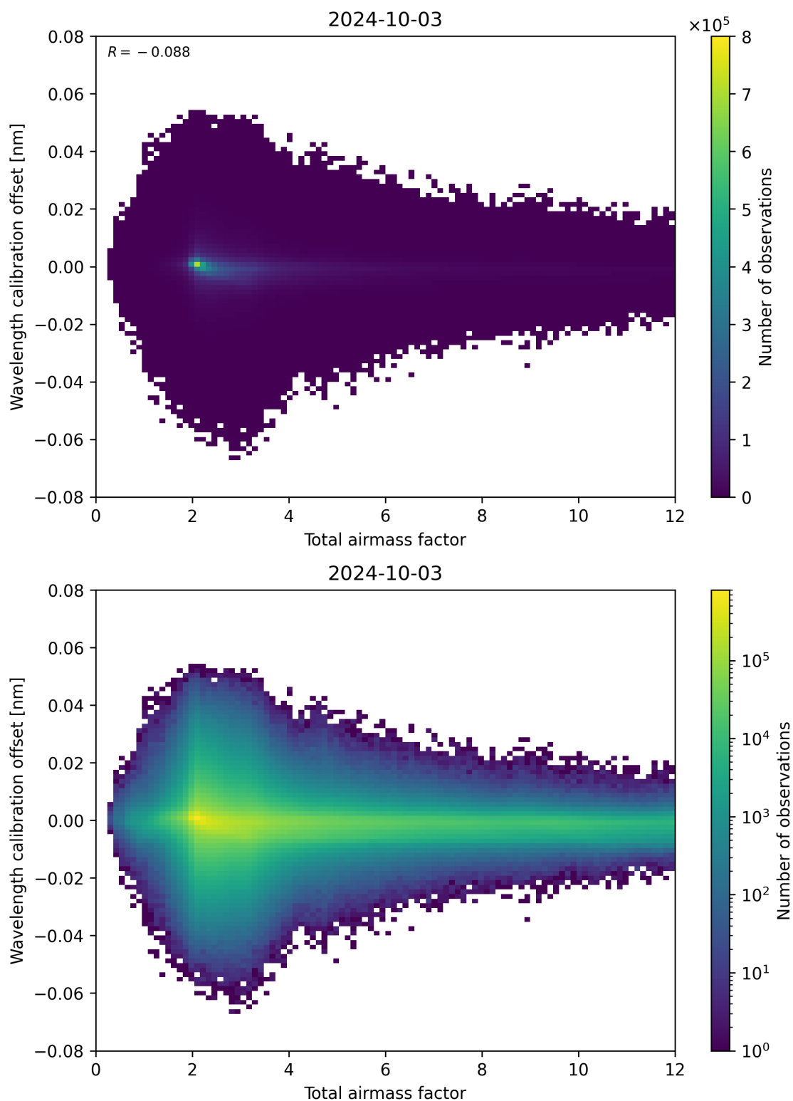
Figure 70: Scatter density plot of “Total airmass factor” against “Wavelength calibration offset” for 2024-10-03 to 2024-10-04.
