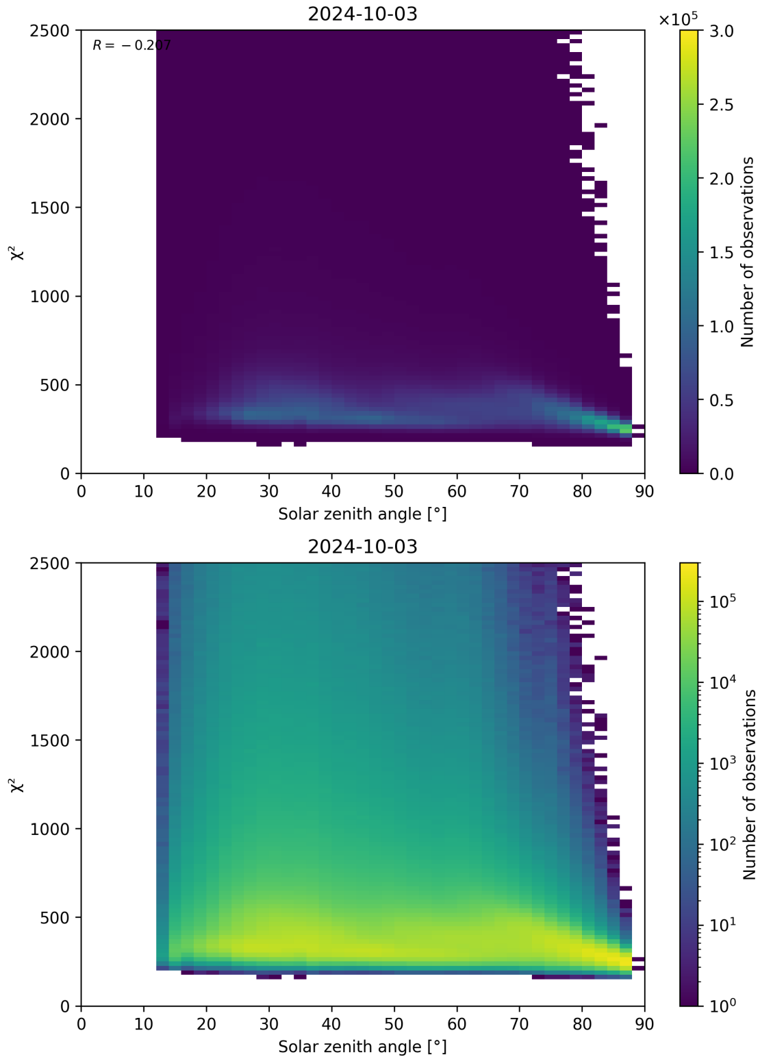
Figure 148: Scatter density plot of “Solar zenith angle” against “ \chi^2 ” for 2024-10-03 to 2024-10-04.
