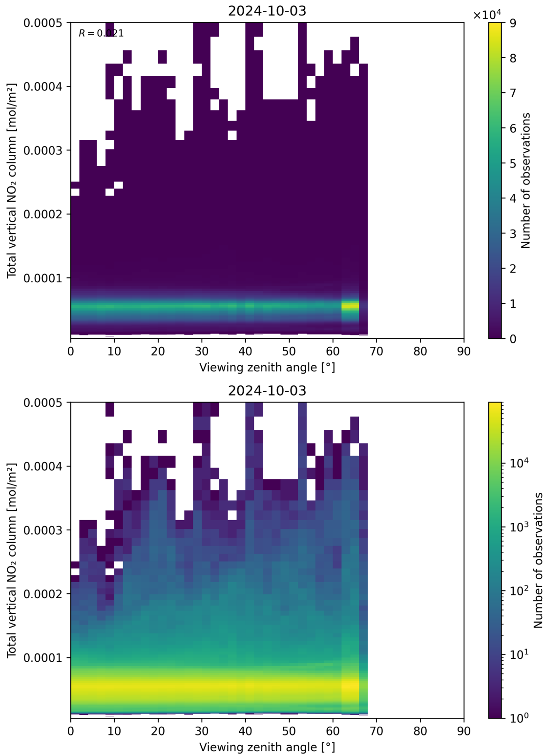
Figure 167: Scatter density plot of “Viewing zenith angle” against “Total vertical NO 2 column” for 2024-10-03 to 2024-10-04.
