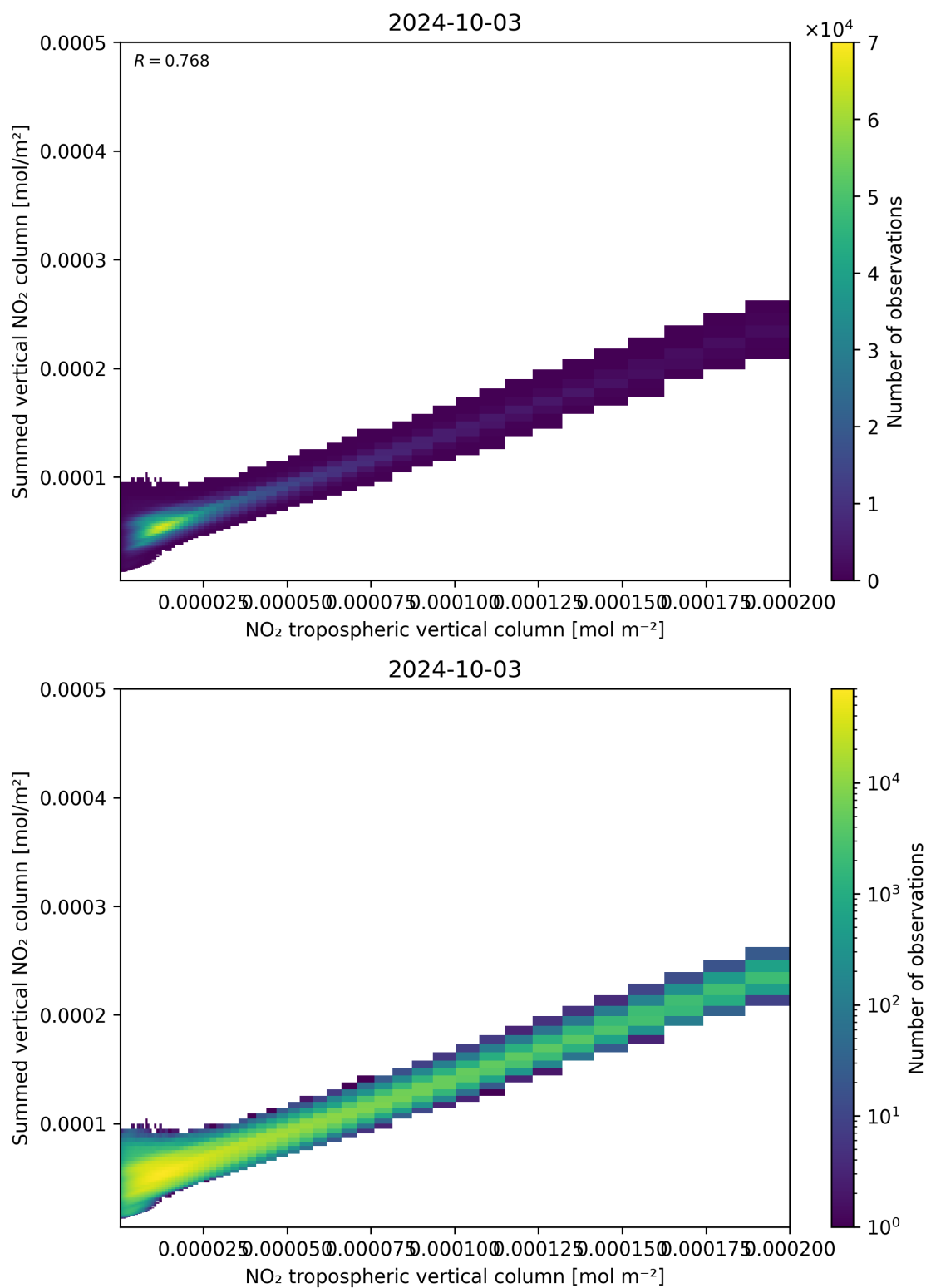
Figure 126: Scatter density plot of “NO 2 tropospheric vertical column” against “Summed vertical NO 2 column” for 2024-10-03 to 2024-10-04.
