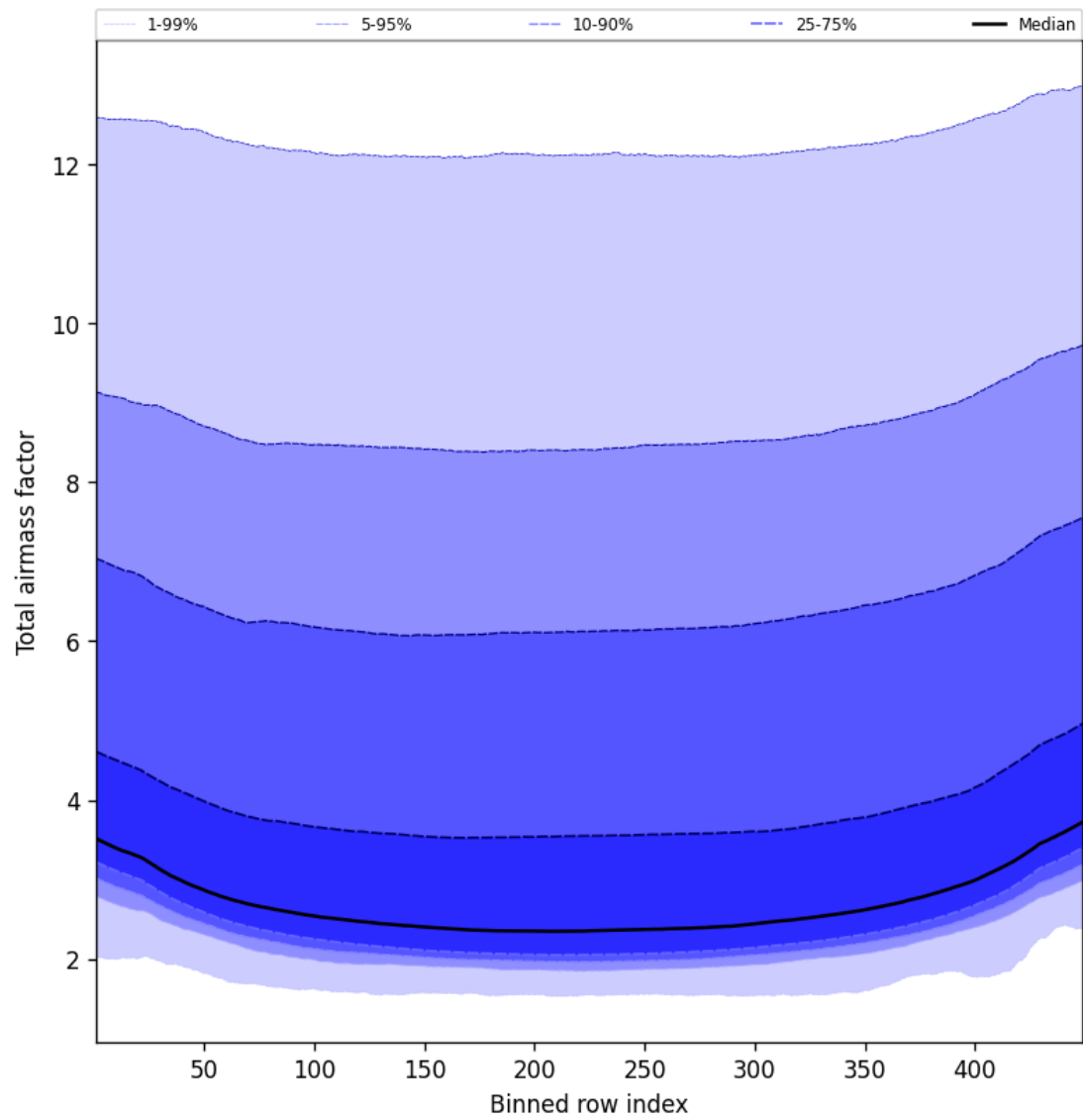
Figure 49: Along track statistics of “Total airmass factor” for 2024-10-03 to 2024-10-04
