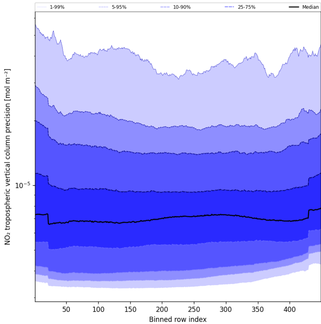
Figure 47: Along track statistics of “NO 2 tropospheric vertical column precision” for 2024-10-03 to 2024-10-04
