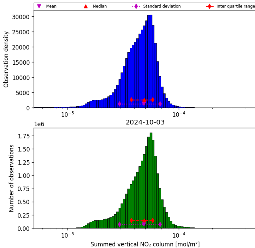
Figure 40: Histogram of “Summed vertical NO 2 column” for 2024-10-03 to 2024-10-04
