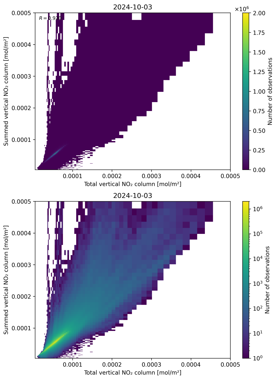
Figure 112: Scatter density plot of “Total vertical NO 2 column” against “Summed vertical NO 2 column” for 2024-10-03 to 2024-10-04.
