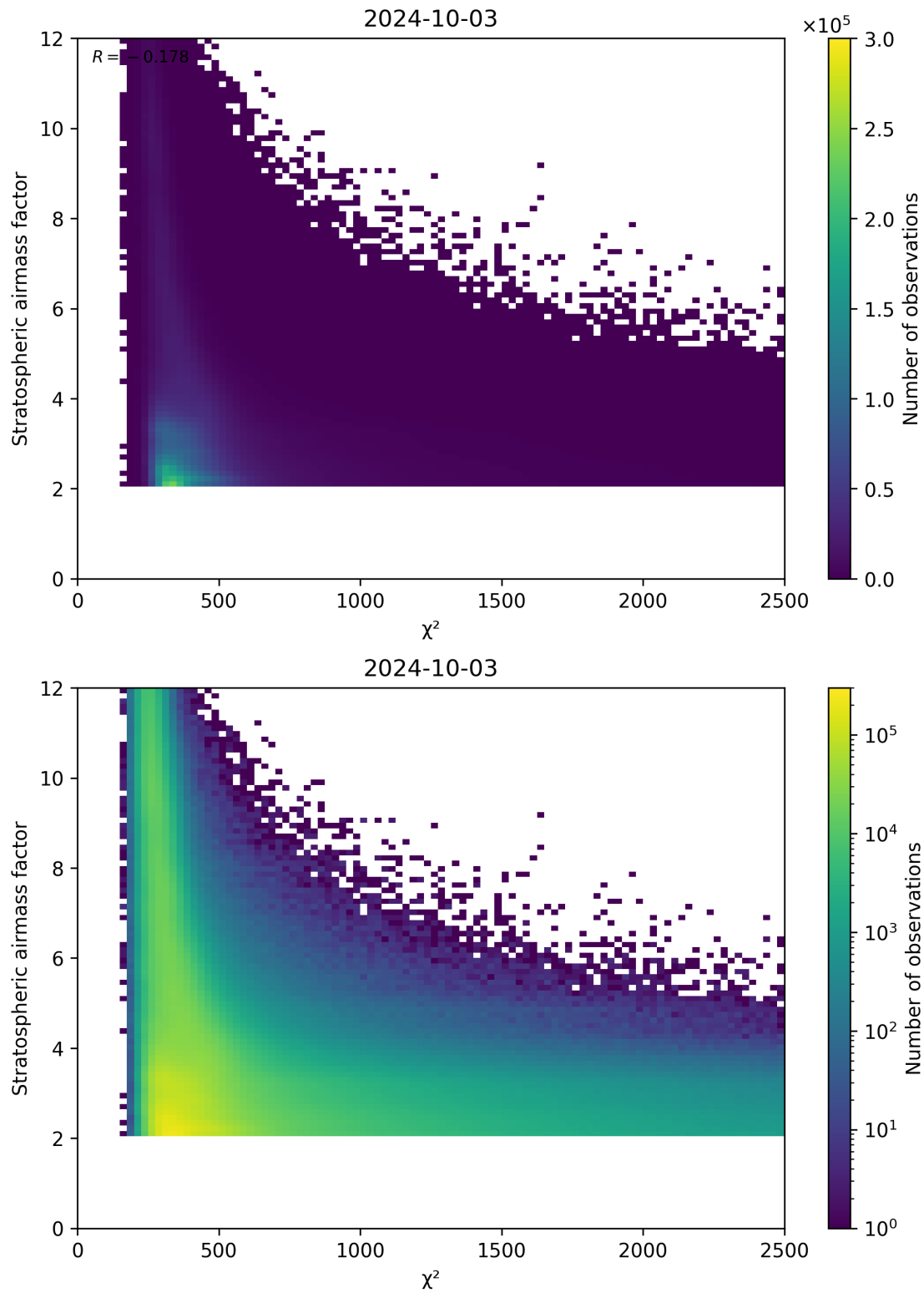
Figure 81: Scatter density plot of “ \chi^2 ” against “Stratospheric airmass factor” for 2024-10-03 to 2024-10-04.
