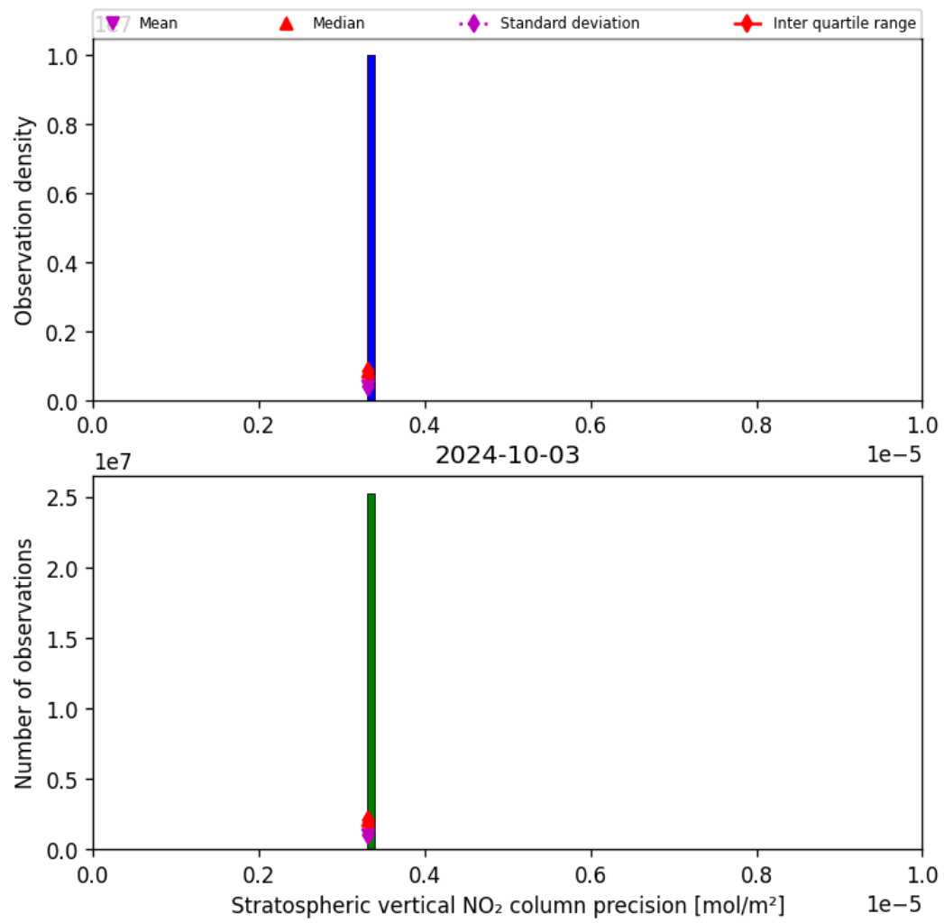
Figure 37: Histogram of “Stratospheric vertical NO 2 column precision” for 2024-10-03 to 2024-10-04
