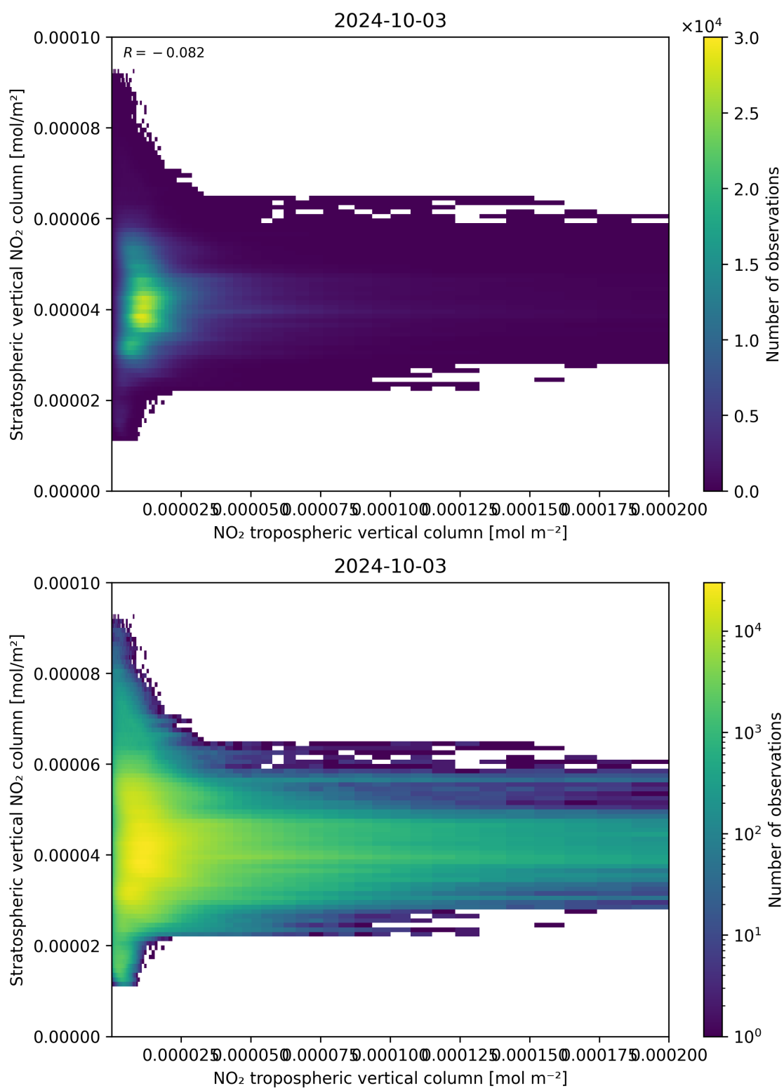
Figure 125: Scatter density plot of “NO 2 tropospheric vertical column” against “Stratospheric vertical NO 2 column” for 2024-10-03 to 2024-10-04.
