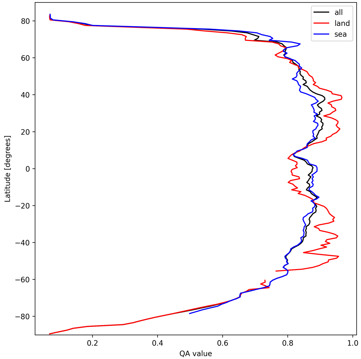
Figure 11: Zonal average of “QA value” for 2024-10-03 to 2024-10-04.
