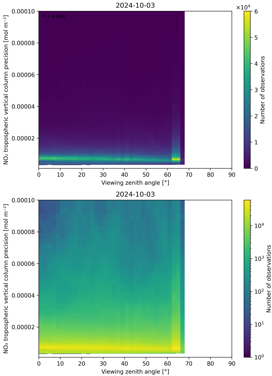
Figure 170: Scatter density plot of “Viewing zenith angle” against “NO 2 tropospheric vertical column precision” for 2024-10-03 to 2024-10-04.
