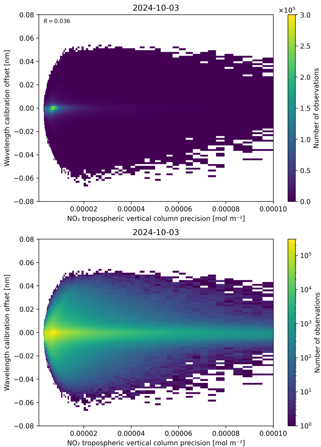
Figure 141: Scatter density plot of “NO 2 tropospheric vertical column precision” against “Wavelength calibration offset” for 2024-10-03 to 2024-10-04.
