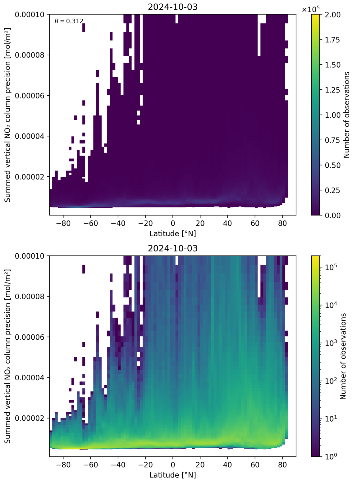
Figure 89: Scatter density plot of “Latitude” against “Summed vertical NO 2 column precision” for 2024-10-03 to 2024-10-04.
