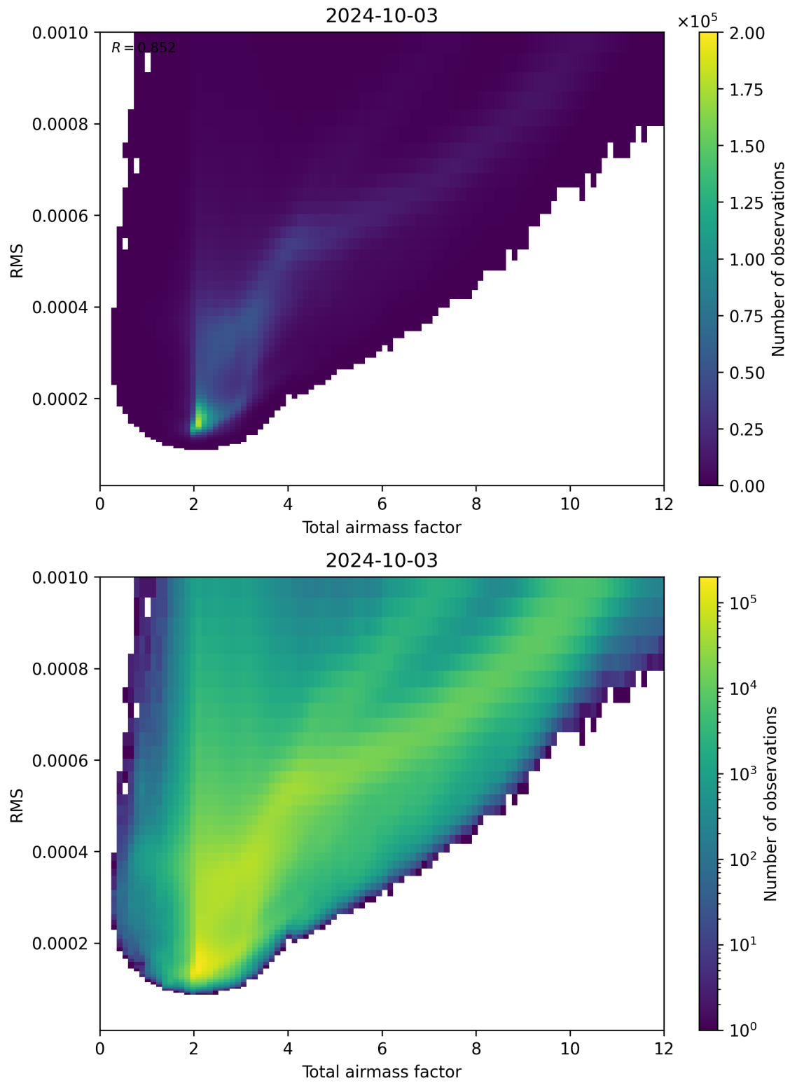
Figure 69: Scatter density plot of “Total airmass factor” against “RMS” for 2024-10-03 to 2024-10-04.
