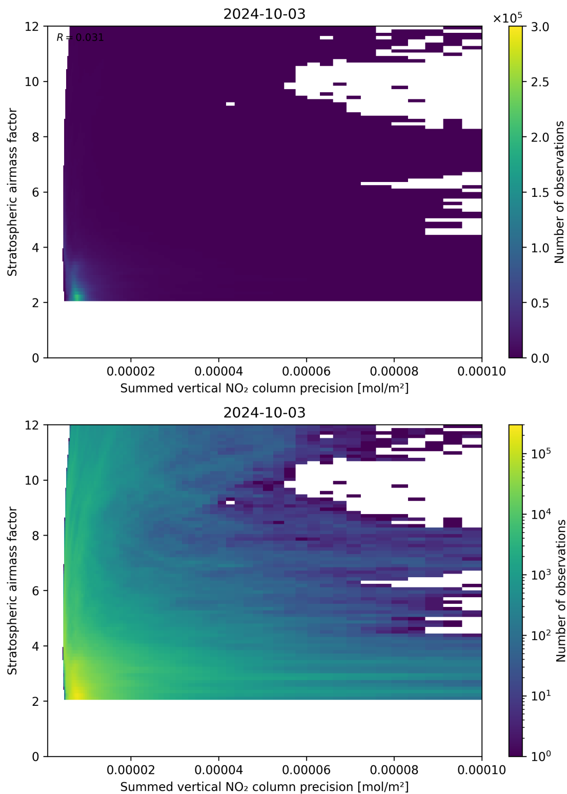
Figure 106: Scatter density plot of “Summed vertical NO 2 column precision” against “Stratospheric airmass factor” for 2024-10-03 to 2024-10-04.
