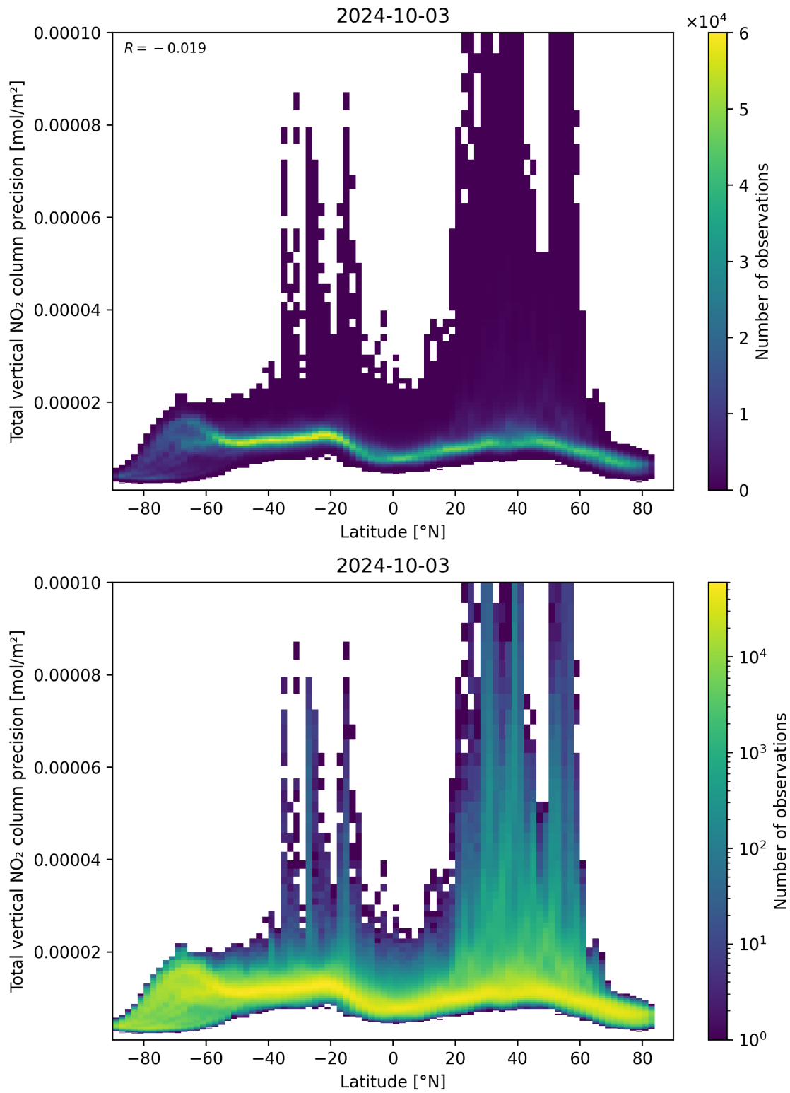
Figure 91: Scatter density plot of “Latitude” against “Total vertical NO 2 column precision” for 2024-10-03 to 2024-10-04.
