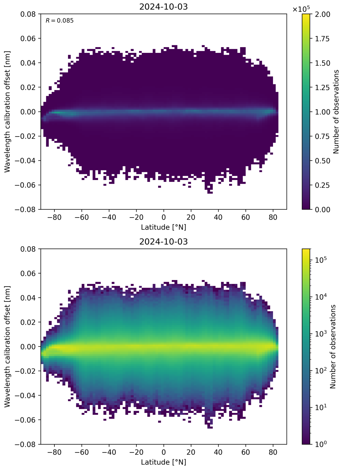
Figure 95: Scatter density plot of “Latitude” against “Wavelength calibration offset” for 2024-10-03 to 2024-10-04.
