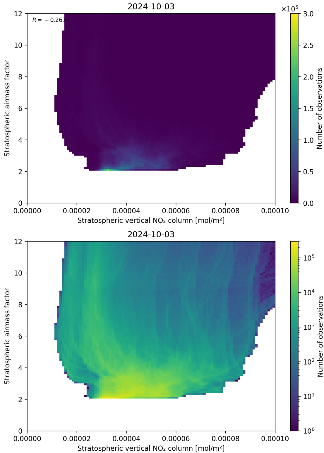
Figure 96: Scatter density plot of “Stratospheric vertical NO 2 column” against “Stratospheric airmass factor” for 2024-10-03 to 2024-10-04.
