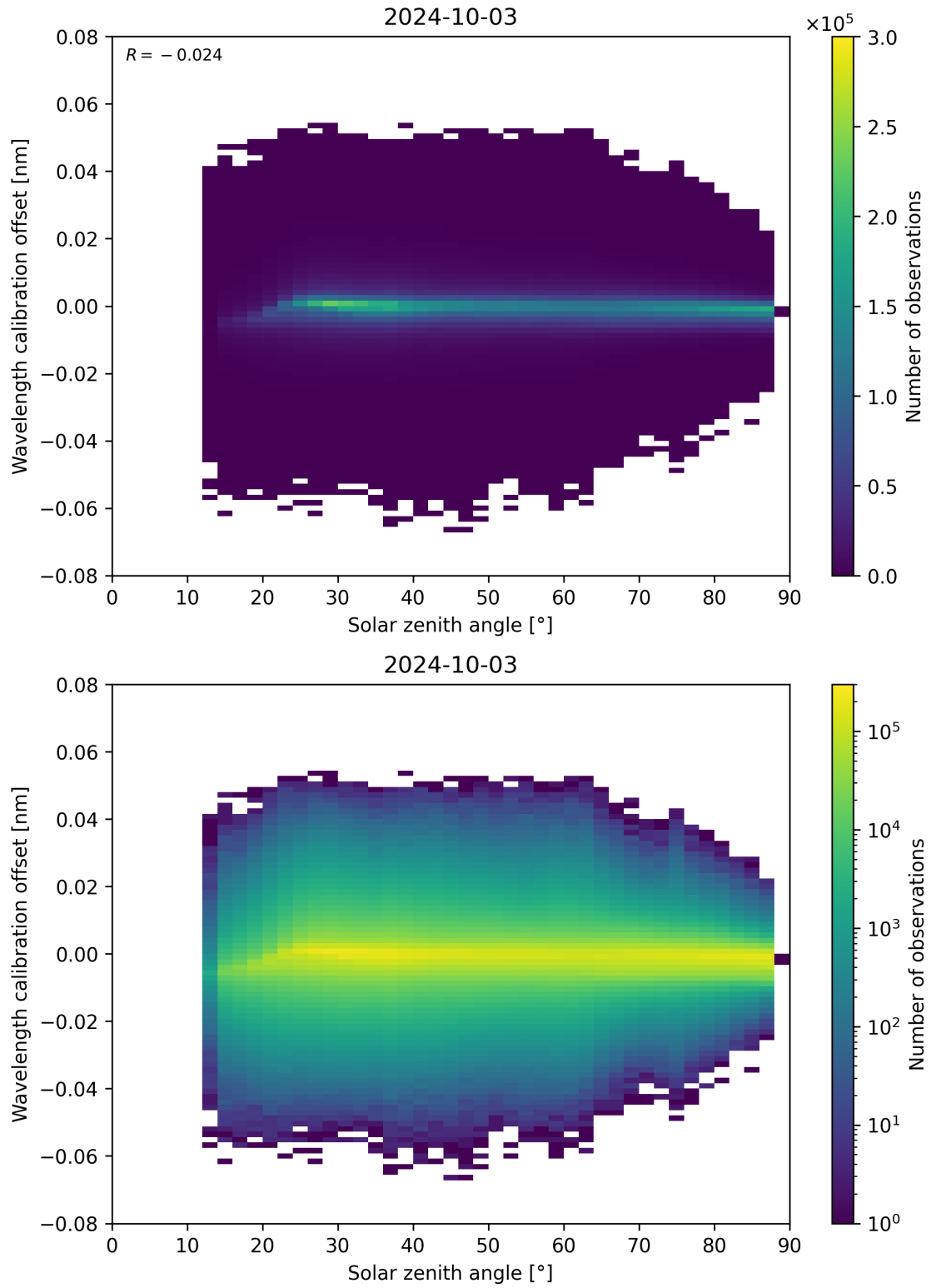
Figure 158: Scatter density plot of “Solar zenith angle” against “Wavelength calibration offset” for 2024-10-03 to 2024-10-04.
