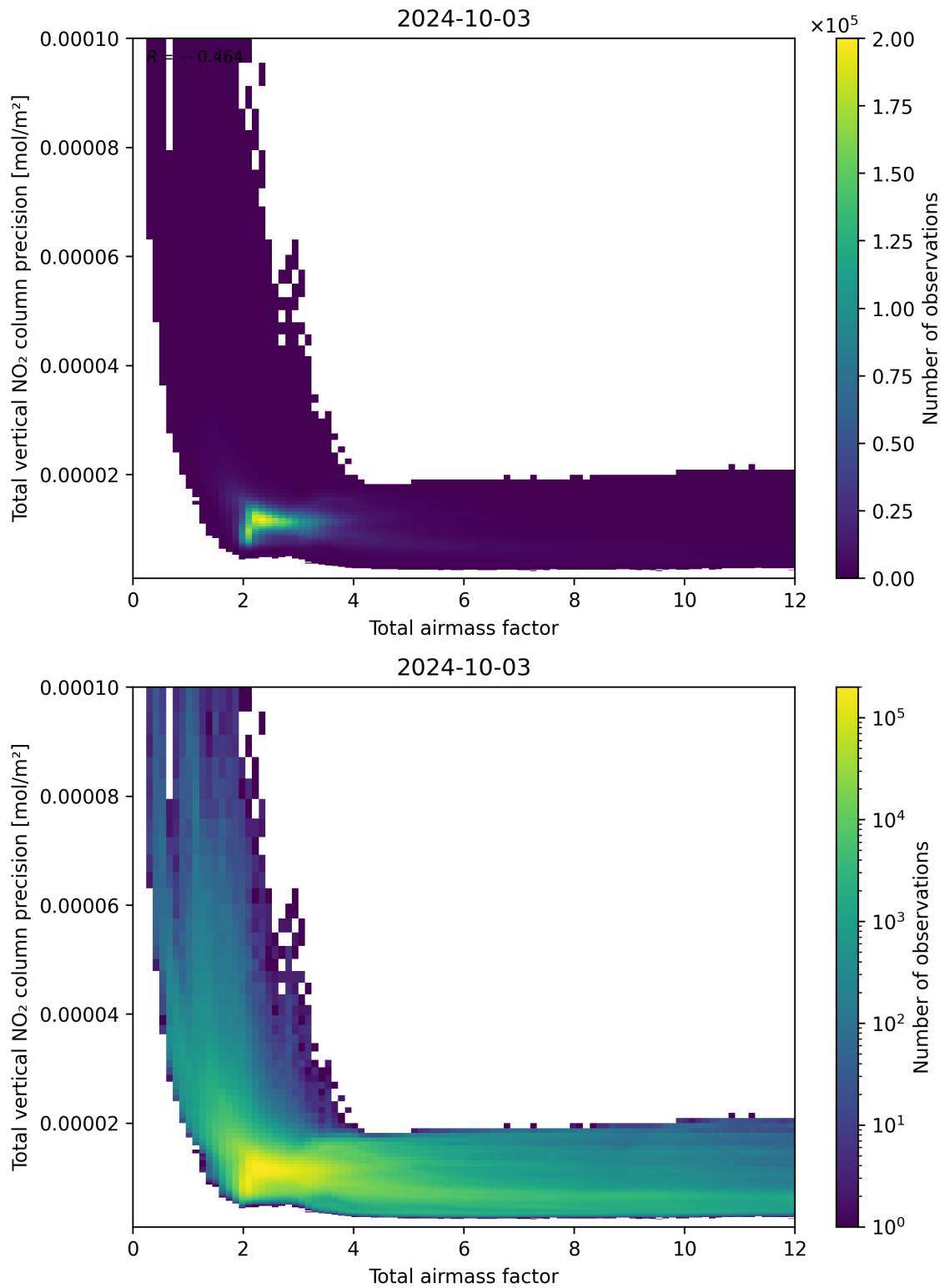
Figure 68: Scatter density plot of “Total airmass factor” against “Total vertical NO 2 column precision” for 2024-10-03 to 2024-10-04.
