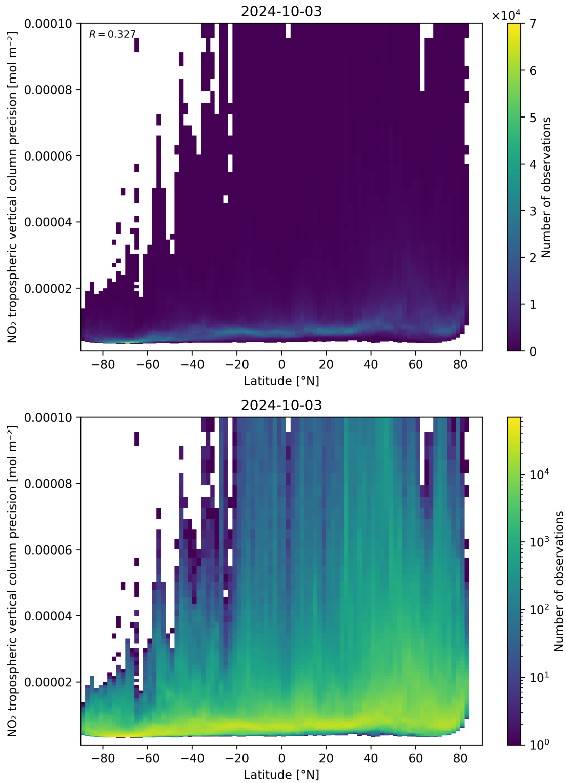
Figure 93: Scatter density plot of “Latitude” against “NO 2 tropospheric vertical column precision” for 2024-10-03 to 2024-10-04.
