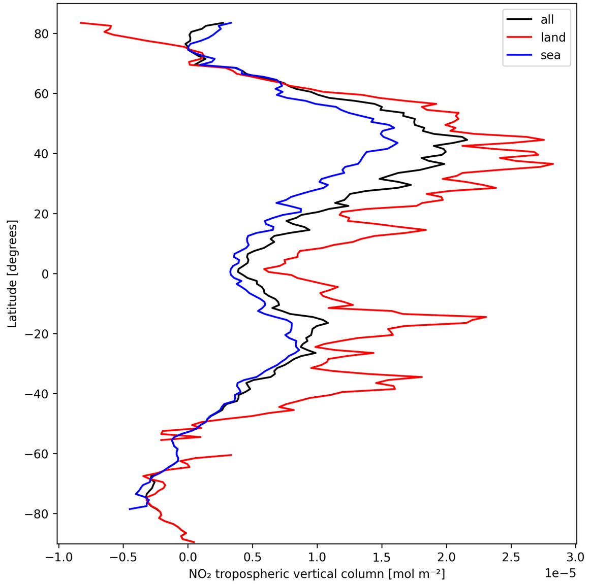
Figure 12: Zonal average of “NO 2 tropospheric vertical column” for 2024-10-03 to 2024-10-04.
