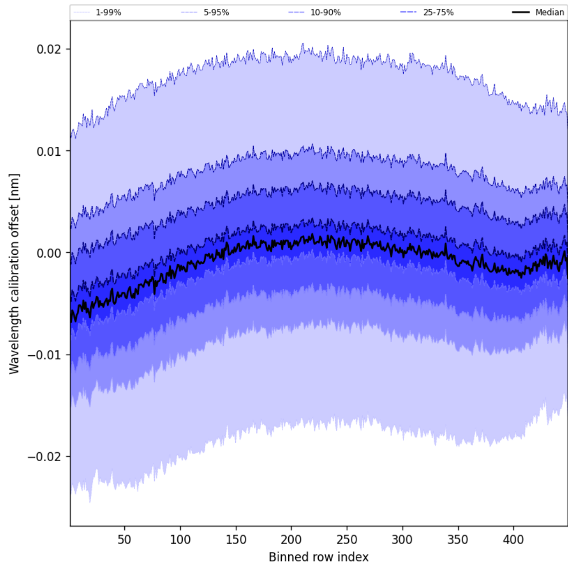
Figure 52: Along track statistics of “Wavelength calibration offset” for 2024-10-03 to 2024-10-04
