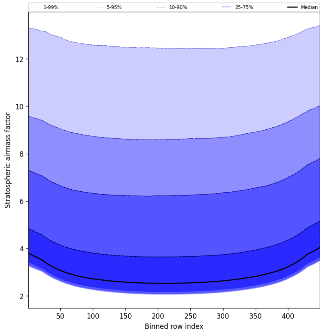
Figure 61: Along track statistics of “Stratospheric air mass factor” for 2024-10-03 to 2024-10-04
