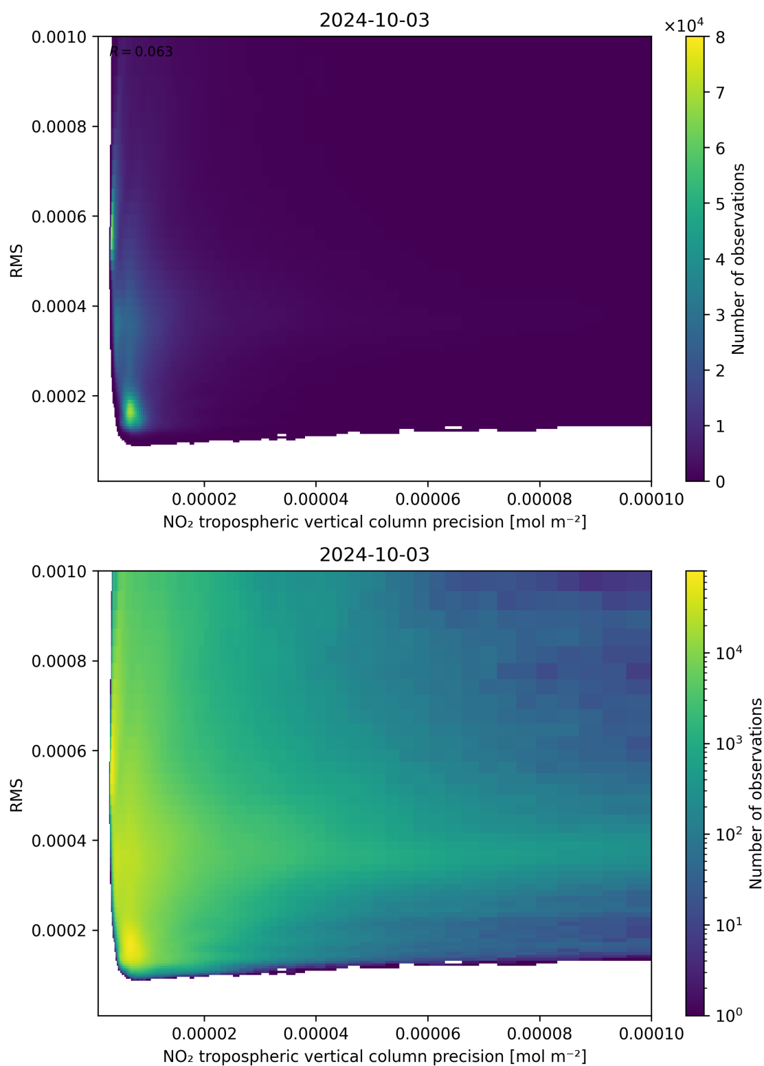
Figure 140: Scatter density plot of “NO 2 tropospheric vertical column precision” against “RMS” for 2024-10-03 to 2024-10-04.
