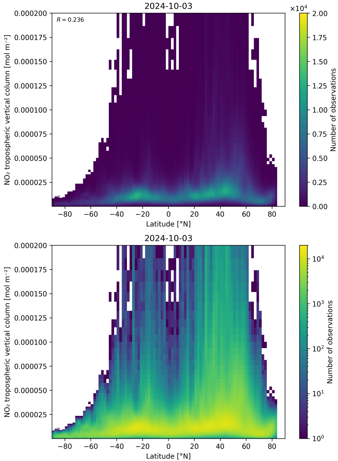
Figure 92: Scatter density plot of “Latitude” against “NO 2 tropospheric vertical column” for 2024-10-03 to 2024-10-04.
