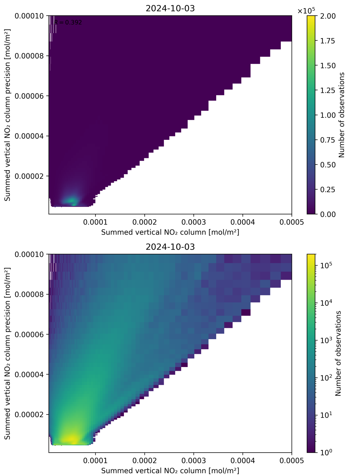
Figure 105: Scatter density plot of “Summed vertical NO 2 column” against “Summed vertical NO 2 column precision” for 2024-10-03 to 2024-10-04.
