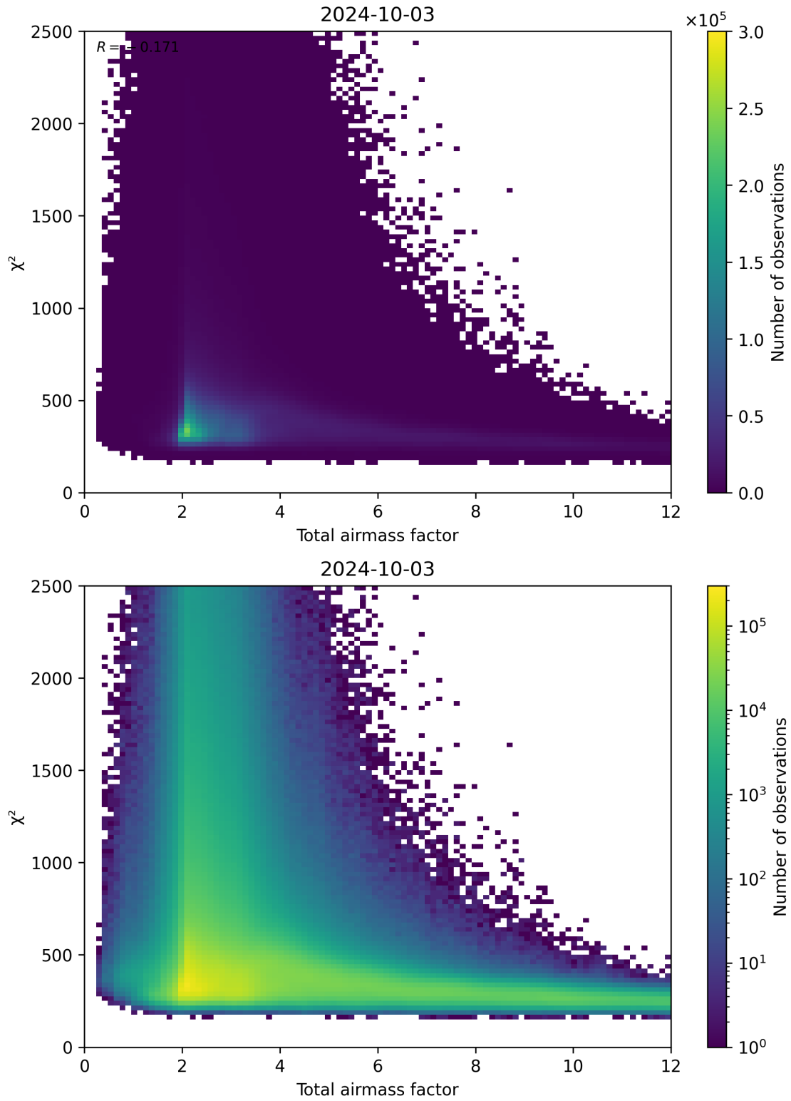
Figure 63: Scatter density plot of “Total airmass factor” against “ \chi^2 ” for 2024-10-03 to 2024-10-04.
