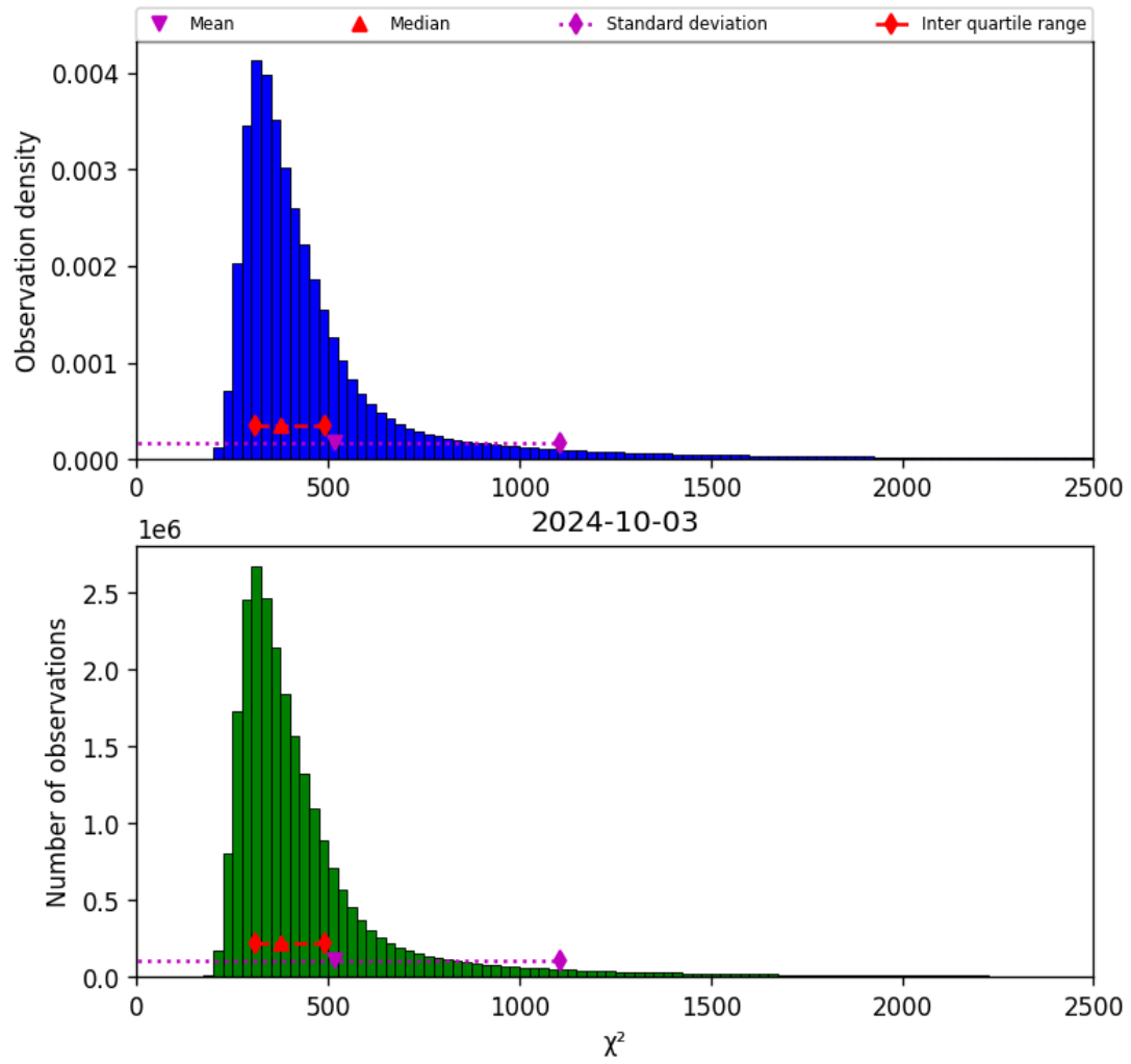
Figure 42: Histogram of “ \chi^2 ” for 2024-10-03 to 2024-10-04
