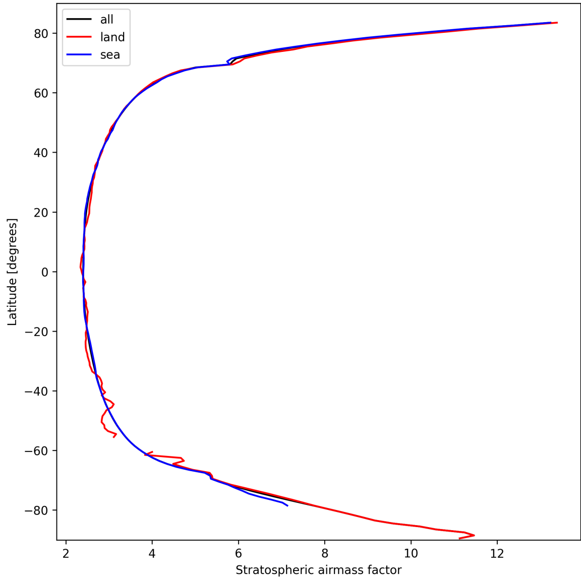
Figure 27: Zonal average of “Stratospheric air mass factor” for 2024-10-03 to 2024-10-04.
