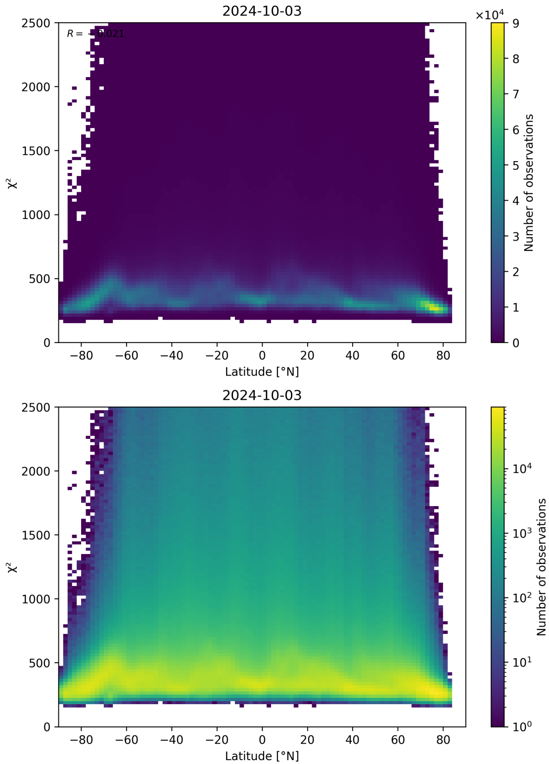
Figure 86: Scatter density plot of “Latitude” against “ \chi^2 ” for 2024-10-03 to 2024-10-04.
