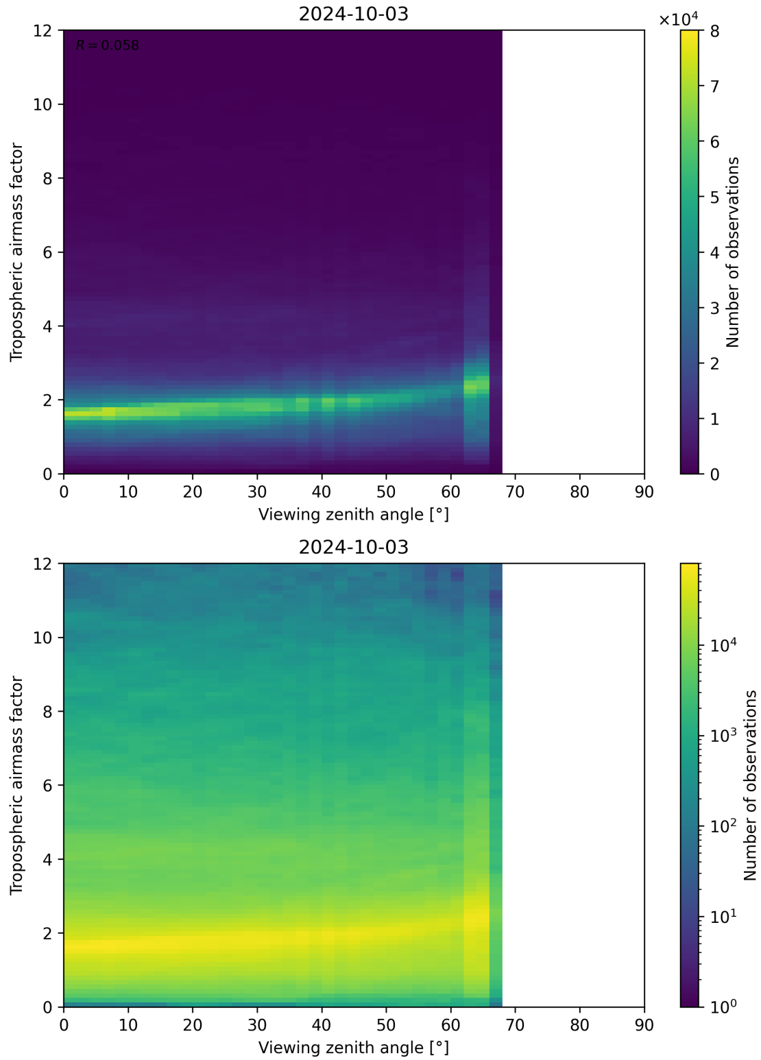
Figure 161: Scatter density plot of “Viewing zenith angle” against “Tropospheric air mass factor” for 2024-10-03 to 2024-10-04.
