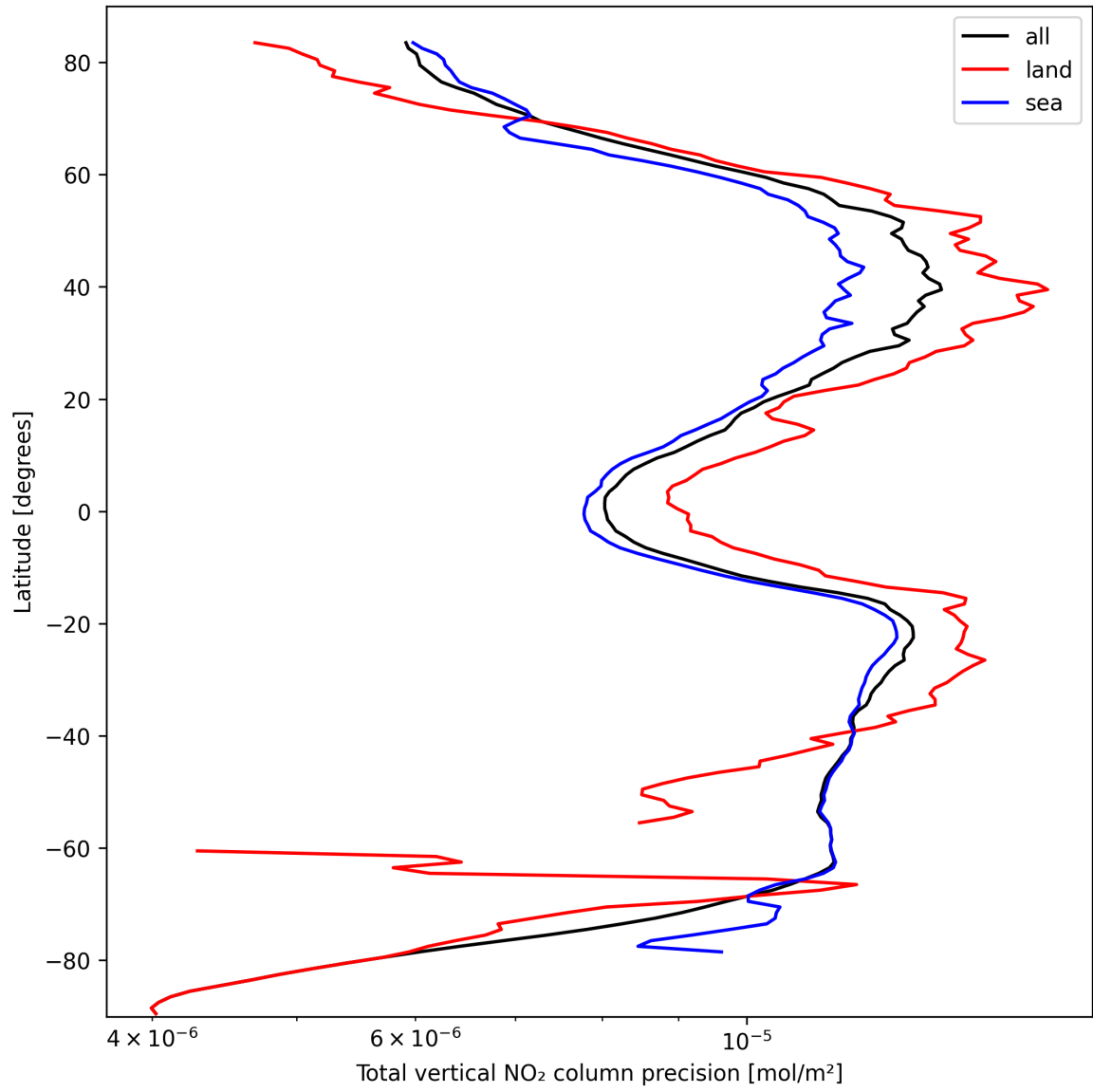
Figure 22: Zonal average of “Total vertical NO 2 column precision” for 2024-10-03 to 2024-10-04.
