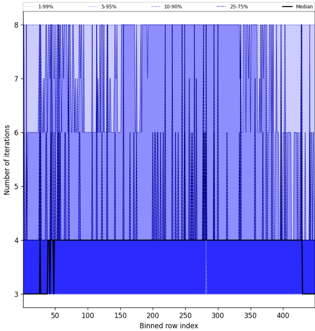
Figure 51: Along track statistics of “Number of iterations” for 2024-10-03 to 2024-10-04
