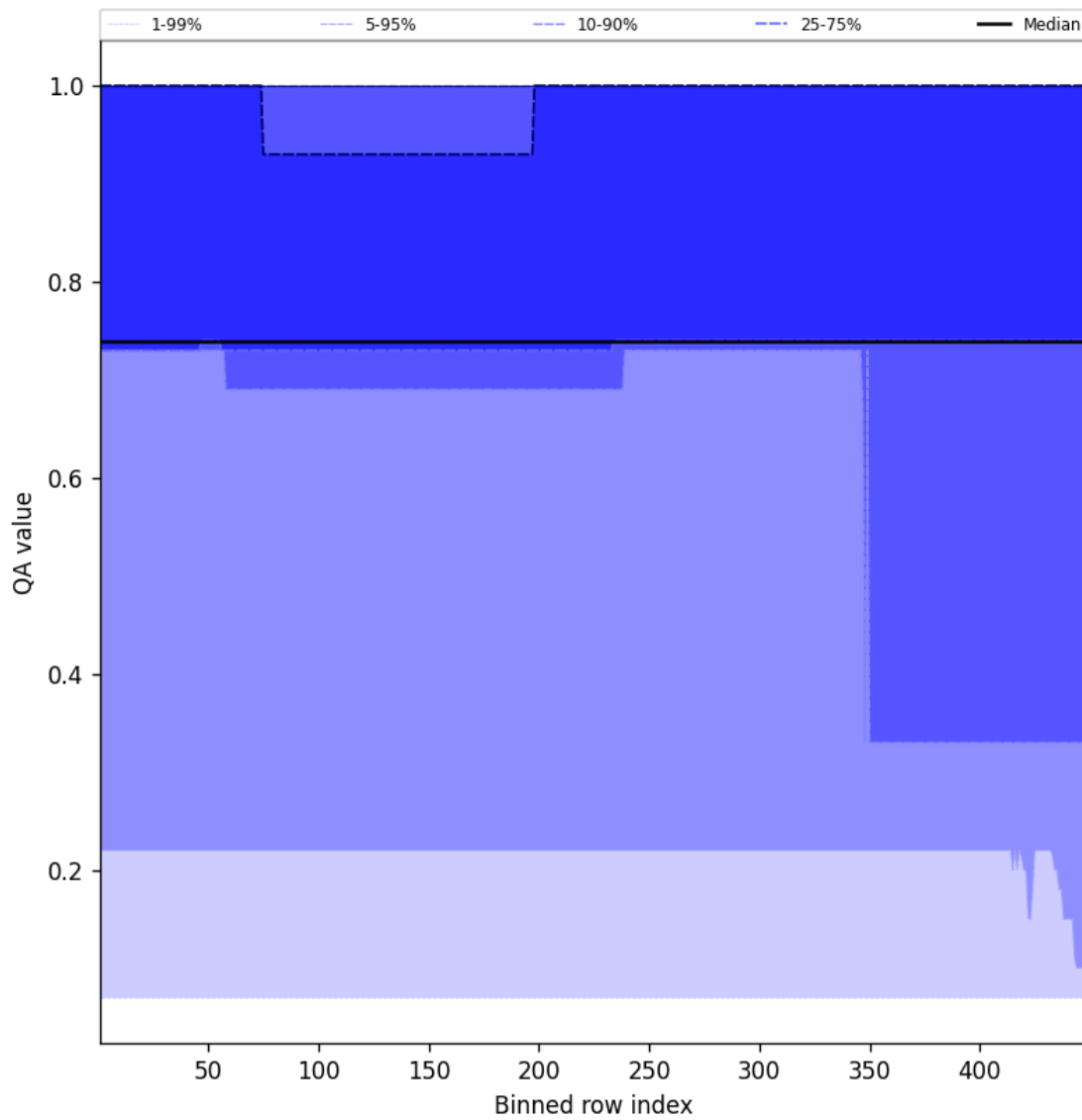
Figure 45: Along track statistics of “QA value” for 2024-10-03 to 2024-10-05
