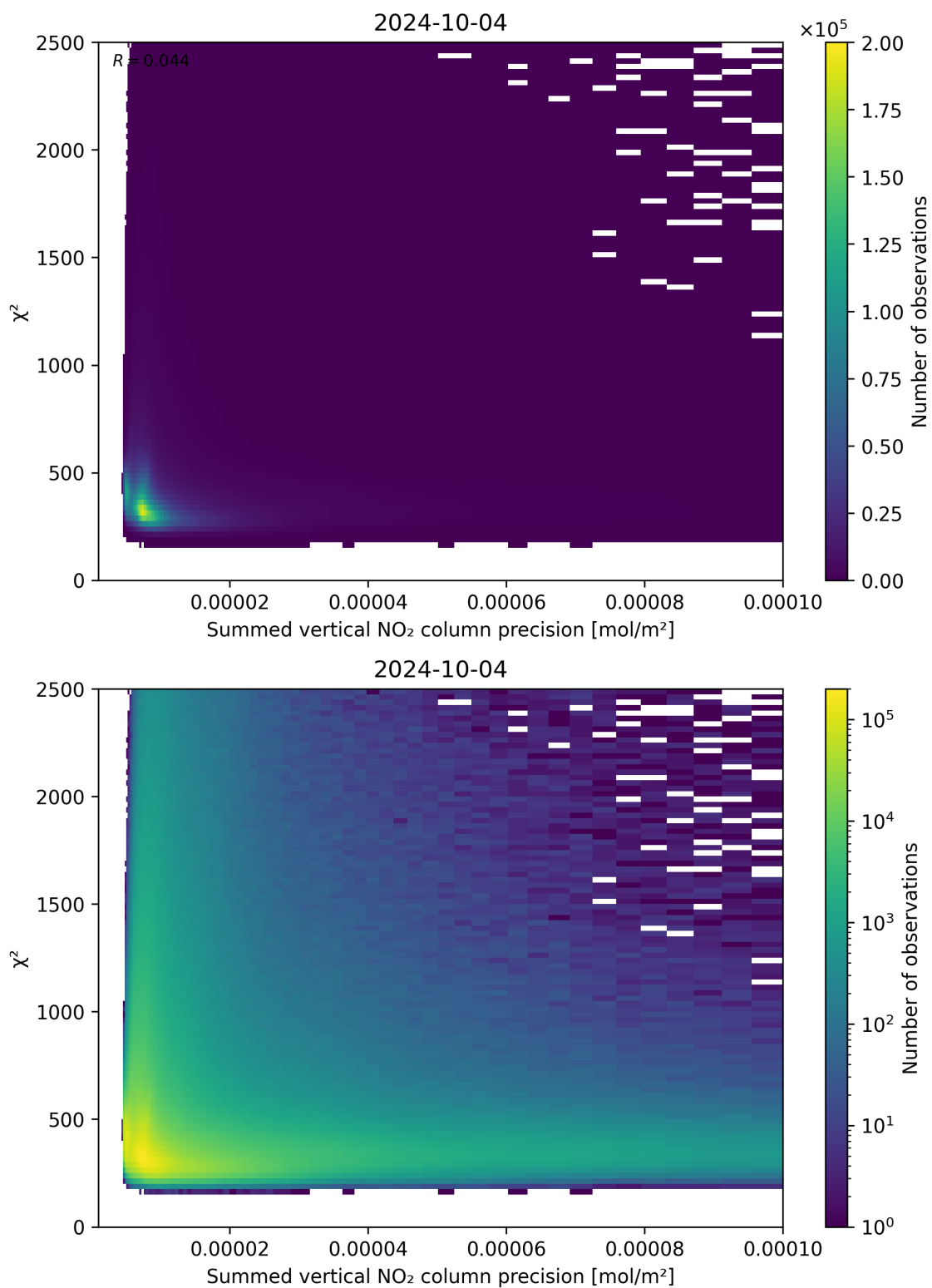
Figure 107: Scatter density plot of “Summed vertical NO 2 column precision” against “ \chi^2 ” for 2024-10-03 to 2024-10-05.
