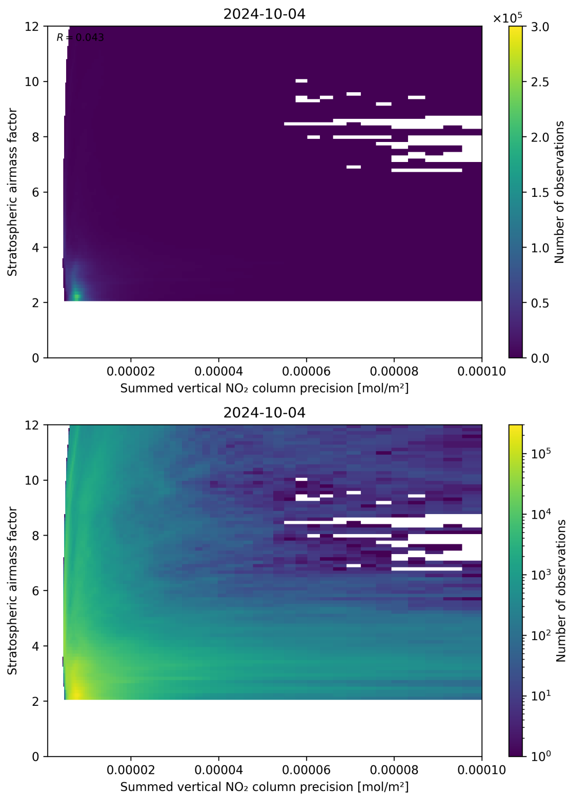
Figure 106: Scatter density plot of “Summed vertical NO 2 column precision” against “Stratospheric airmass factor” for 2024-10-03 to 2024-10-05.
