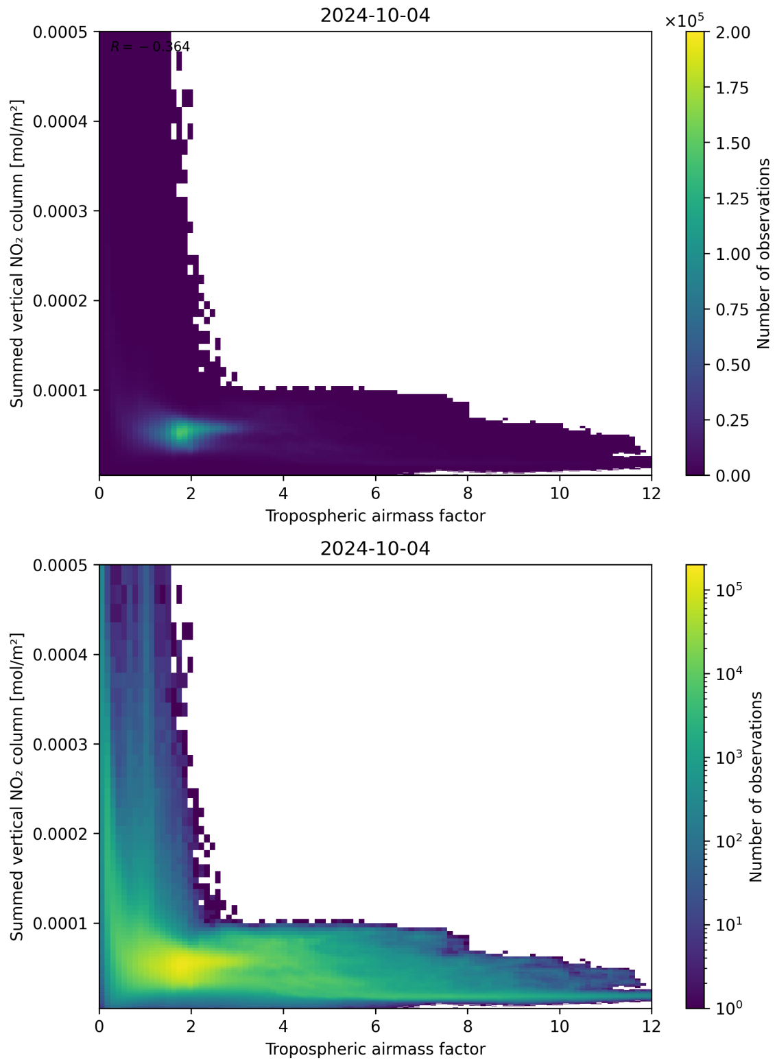
Figure 75: Scatter density plot of “Tropospheric airmass factor” against “Summed vertical NO 2 column” for 2024-10-03 to 2024-10-05.
