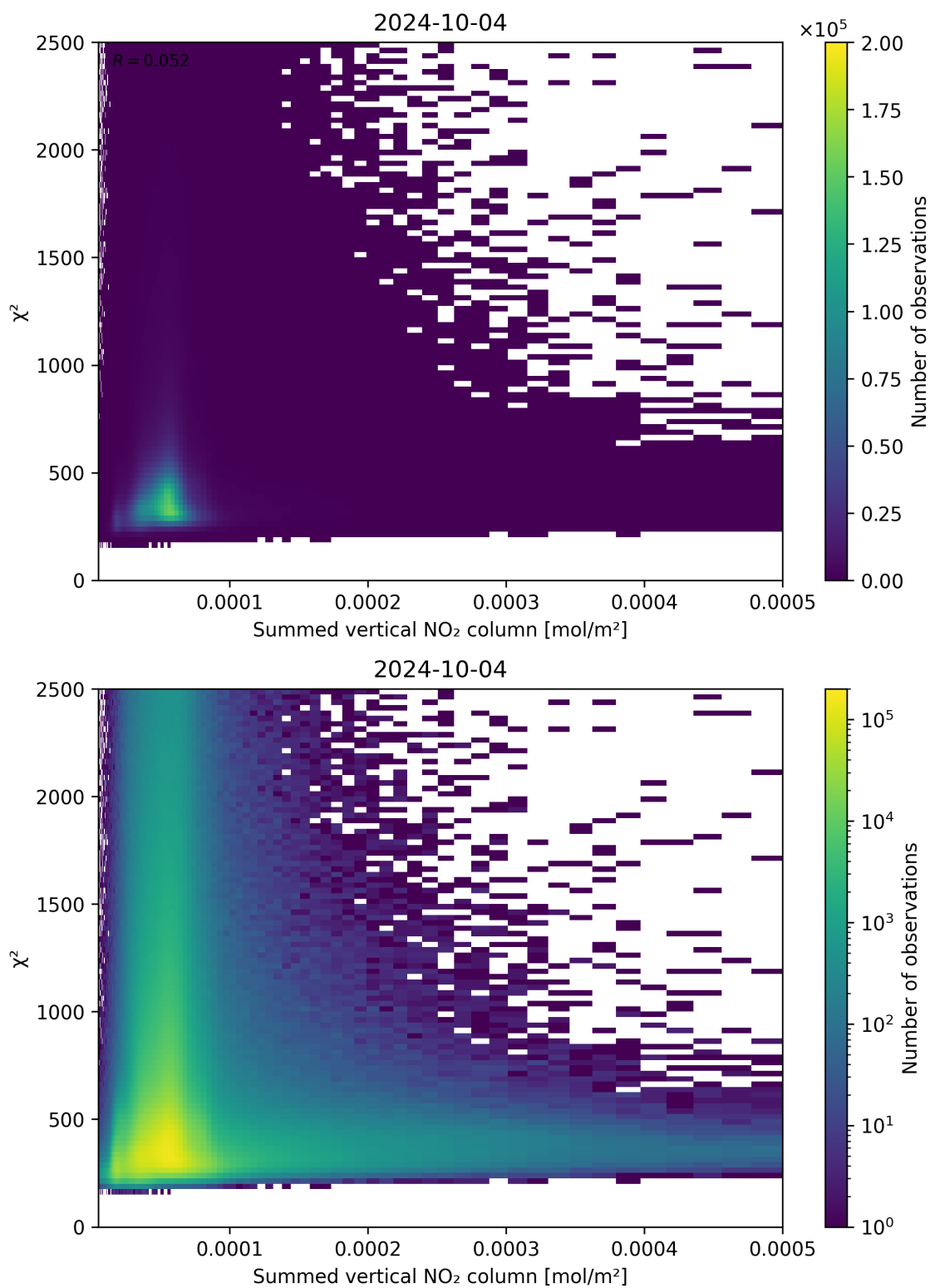
Figure 104: Scatter density plot of “Summed vertical NO 2 column” against “ \chi^2 ” for 2024-10-03 to 2024-10-05.
