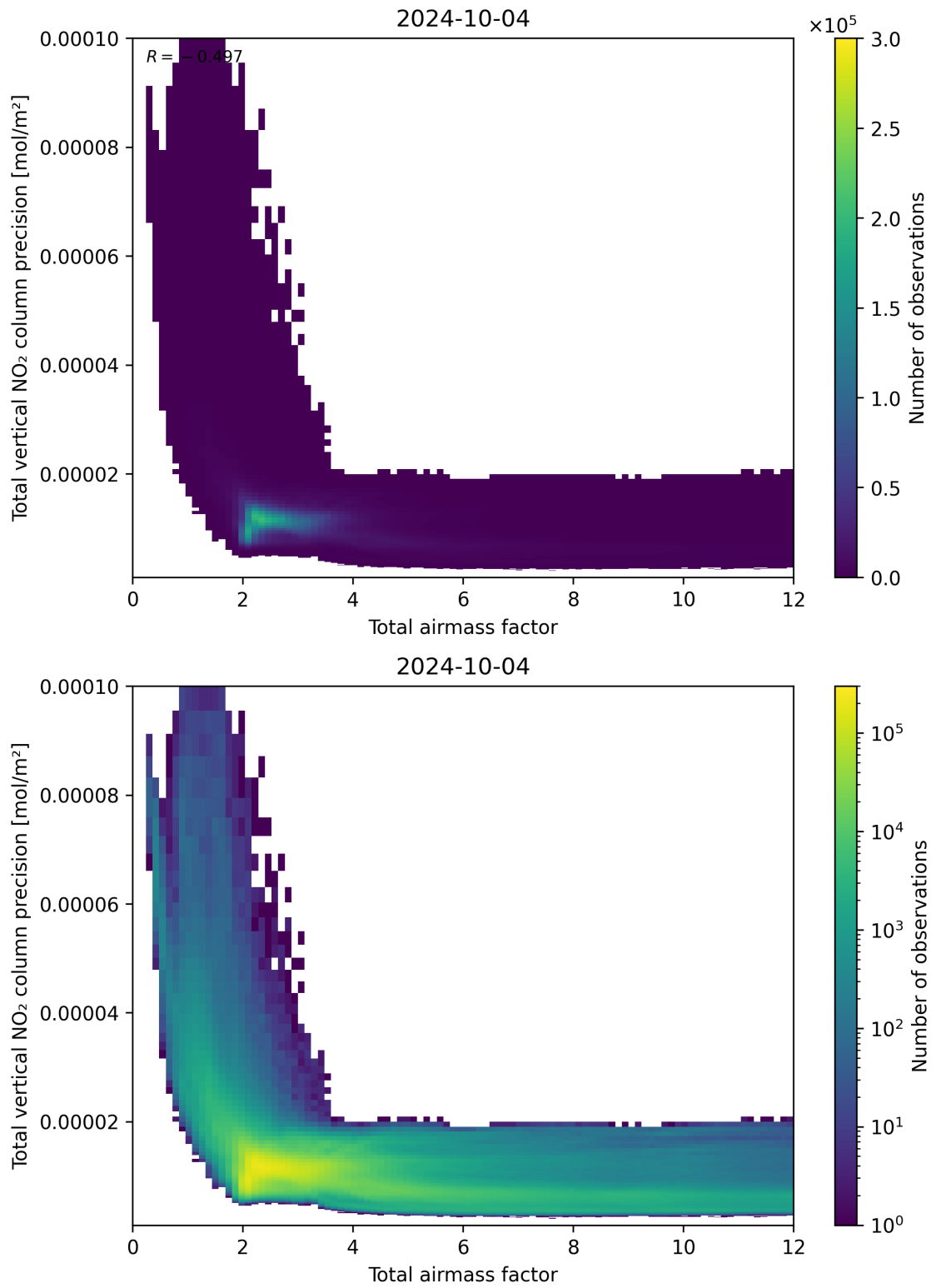
Figure 68: Scatter density plot of “Total airmass factor” against “Total vertical NO 2 column precision” for 2024-10-03 to 2024-10-05.
