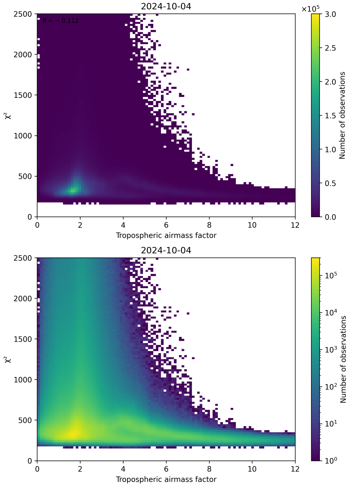
Figure 73: Scatter density plot of “Tropospheric airmass factor” against “ \chi^2 ” for 2024-10-03 to 2024-10-05.
