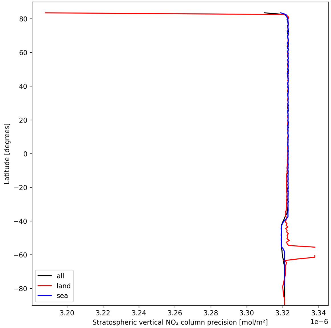
Figure 20: Zonal average of “Stratospheric vertical NO 2 column precision” for 2024-10-03 to 2024-10-05.
