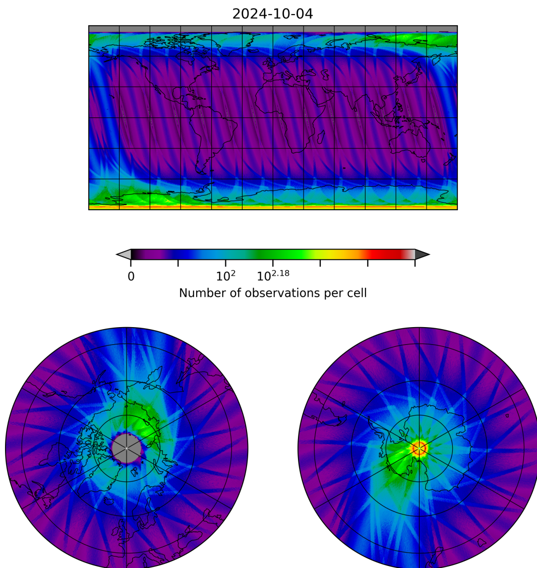
Figure 10: Map of the number of observations for 2024-10-03 to 2024-10-05
