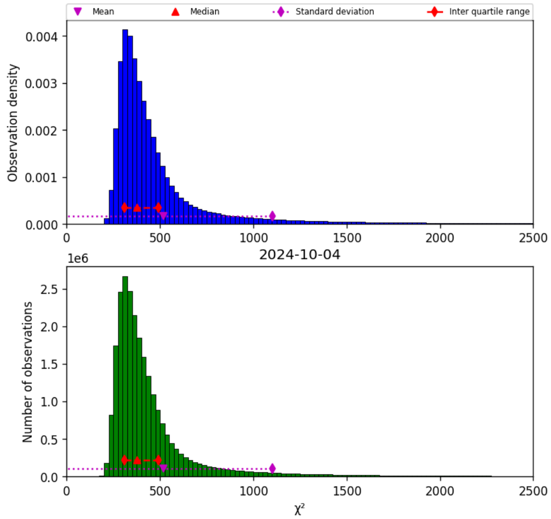
Figure 42: Histogram of " \chi^2 " for 2024-10-03 to 2024-10-05
