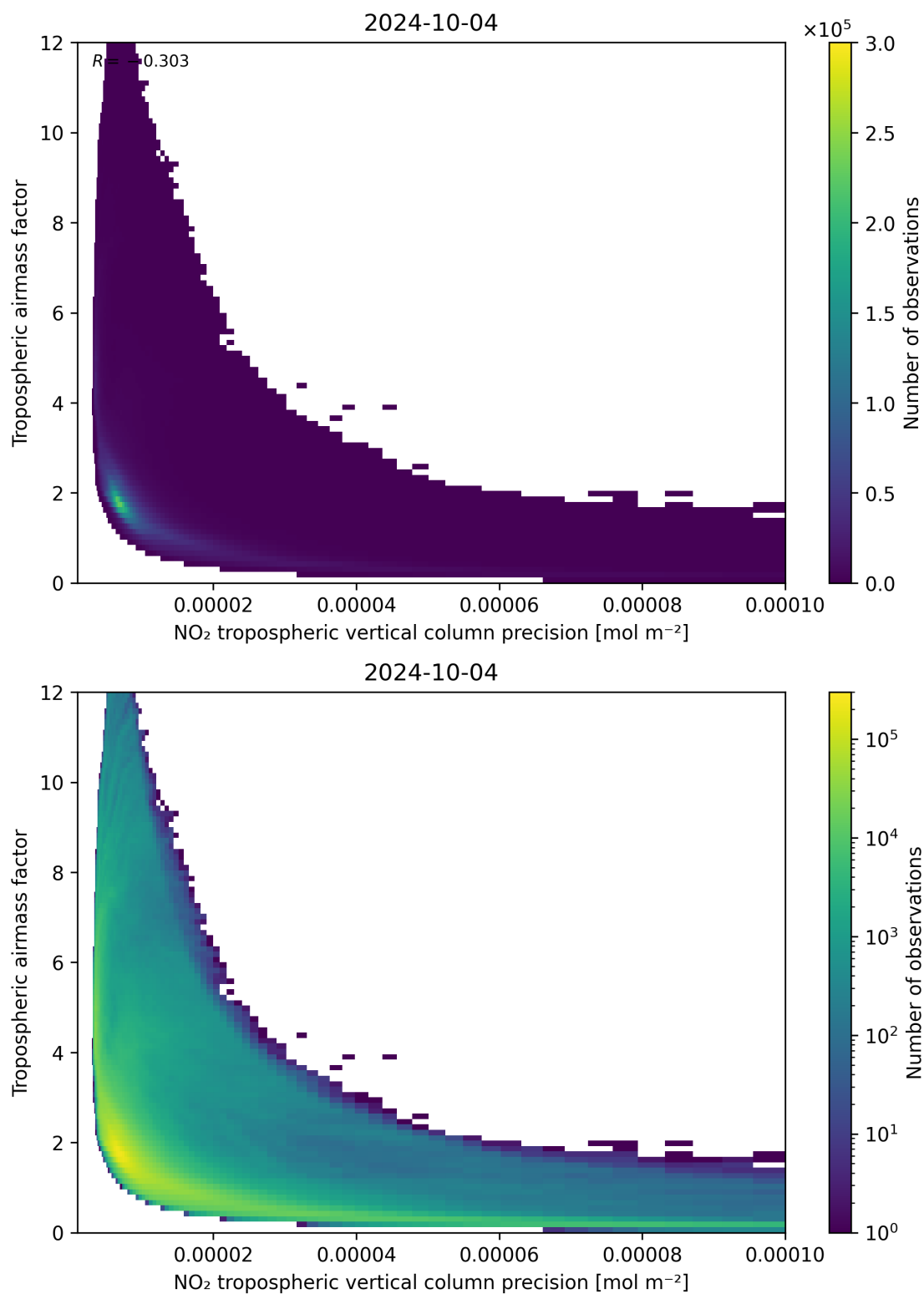
Figure 133: Scatter density plot of “NO 2 tropospheric vertical column precision” against “Tropospheric air mass factor” for 2024-10-03 to 2024-10-05.
