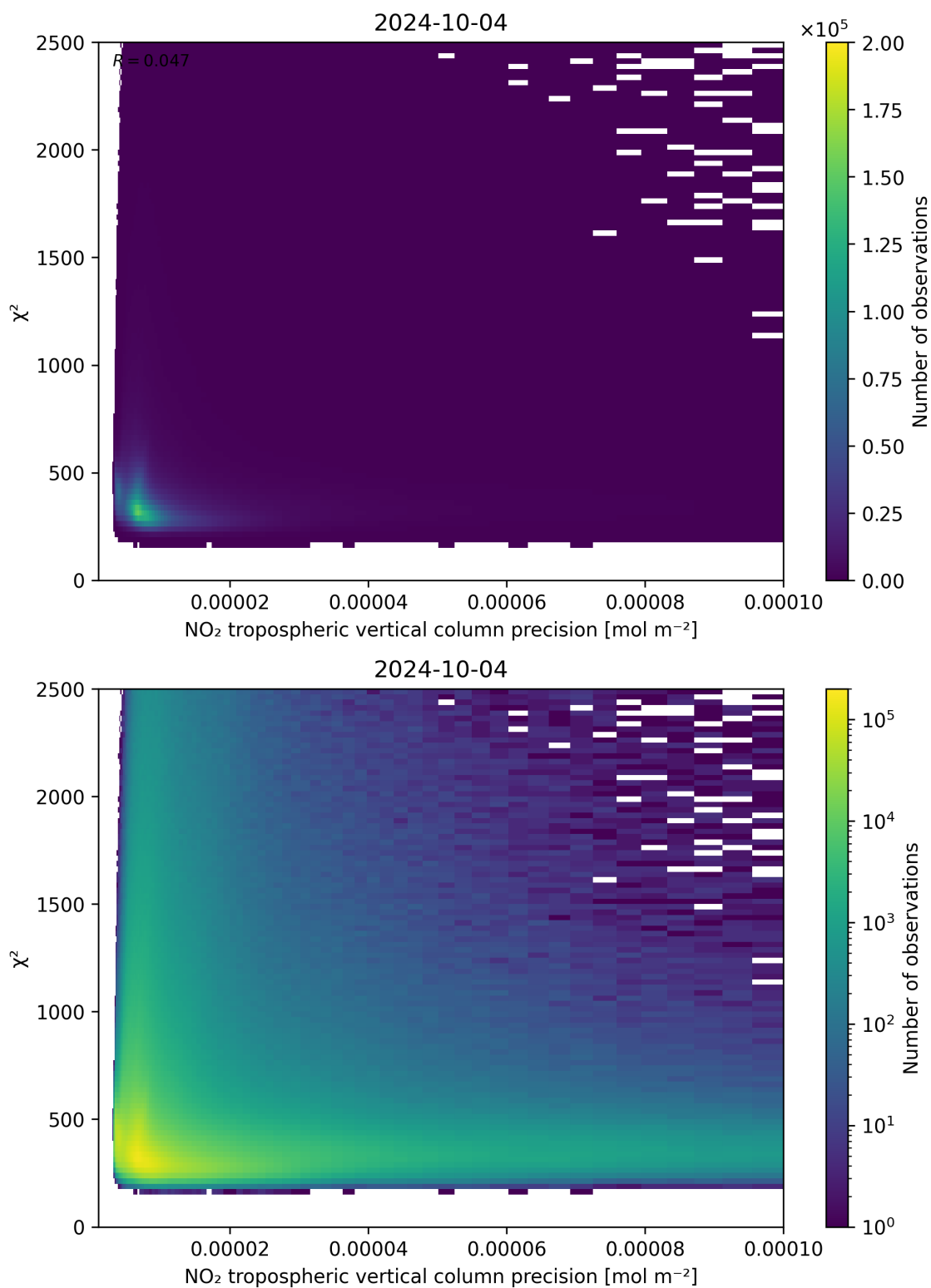
Figure 134: Scatter density plot of “NO 2 tropospheric vertical column precision” against “ \chi^2 ” for 2024-10-03 to 2024-10-05.
