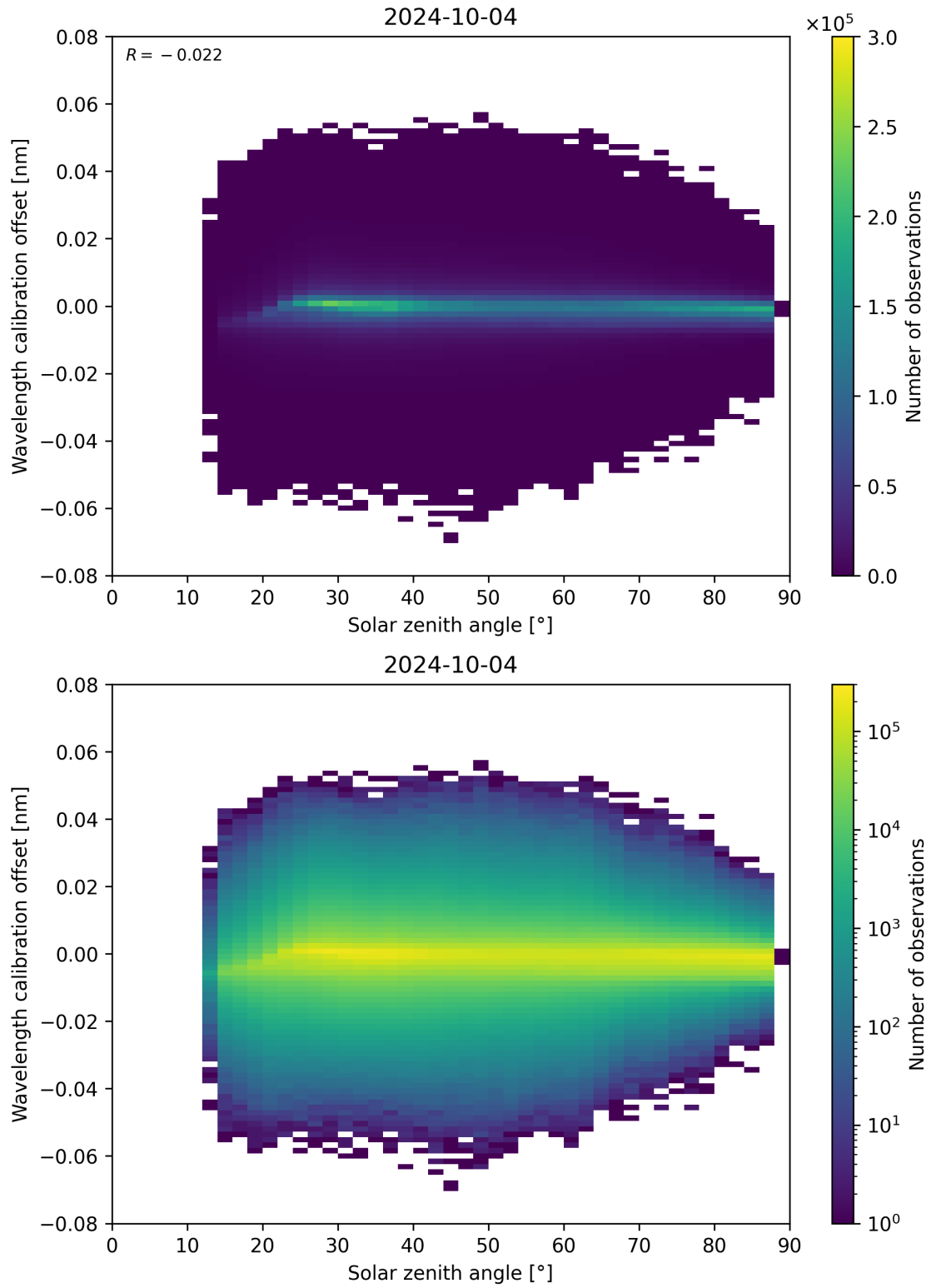
Figure 158: Scatter density plot of “Solar zenith angle” against “Wavelength calibration offset” for 2024-10-03 to 2024-10-05.
