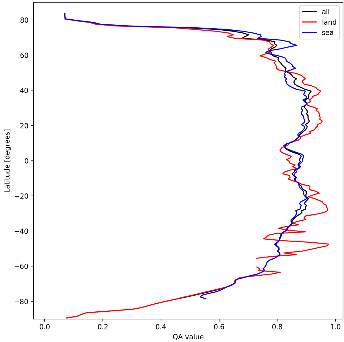
Figure 11: Zonal average of “QA value” for 2024-10-03 to 2024-10-05.
