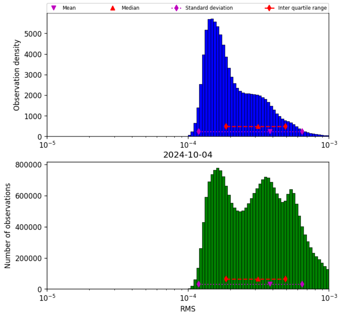
Figure 43: Histogram of “RMS” for 2024-10-03 to 2024-10-05
