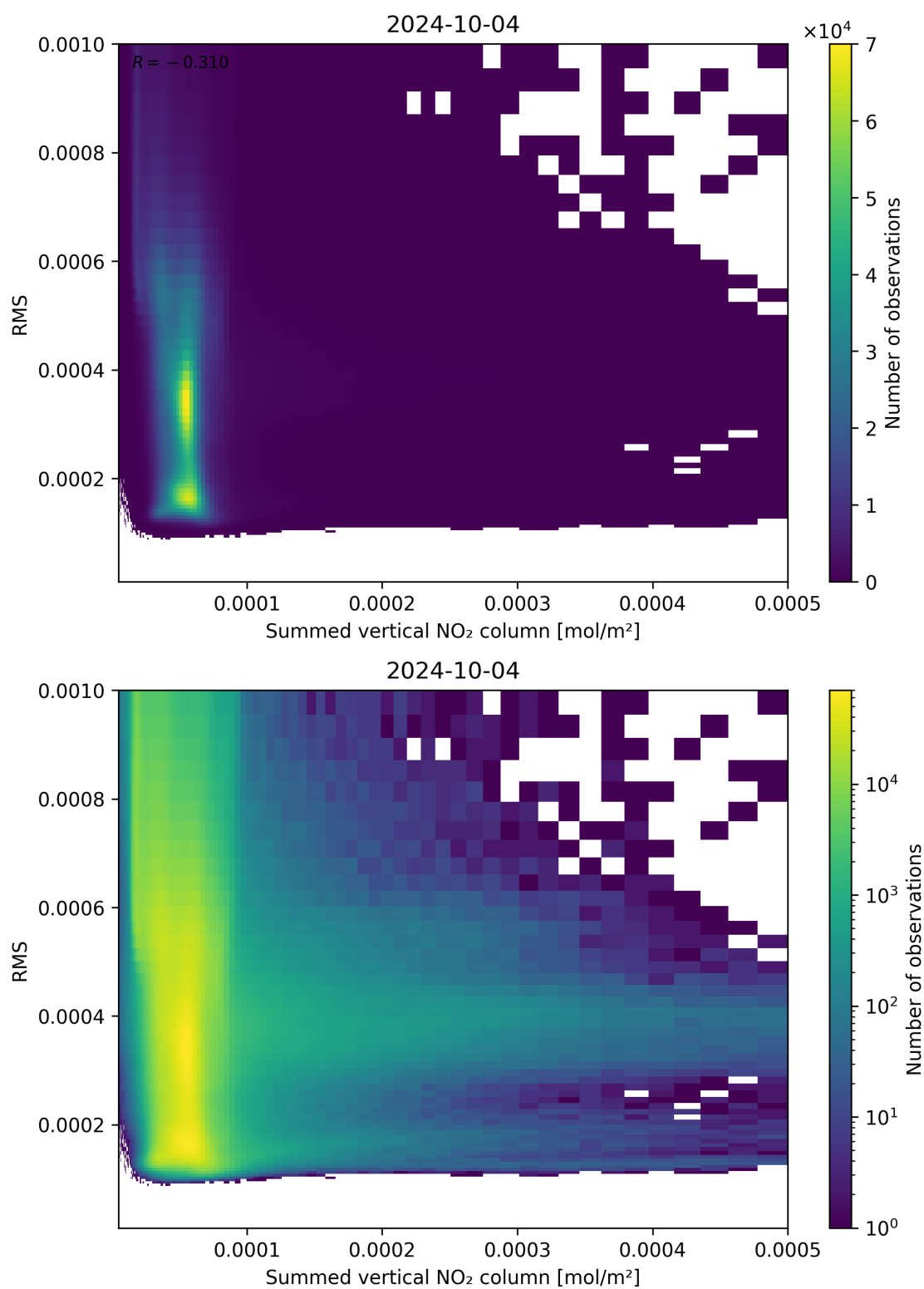
Figure 109: Scatter density plot of “Summed vertical NO 2 column” against “RMS” for 2024-10-03 to 2024-10-05.
