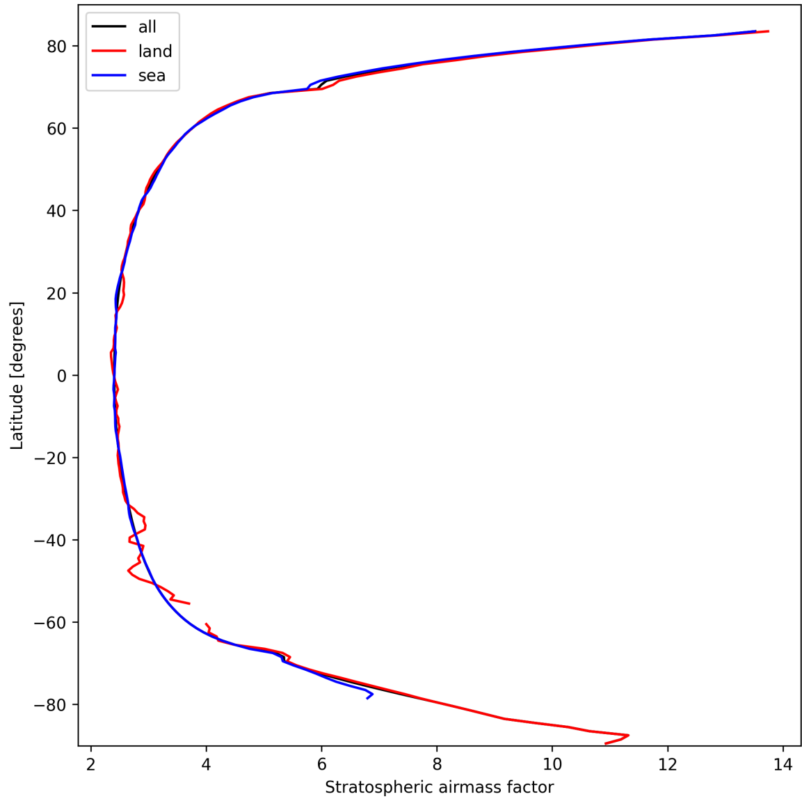
Figure 27: Zonal average of “Stratospheric air mass factor” for 2024-10-03 to 2024-10-05.
