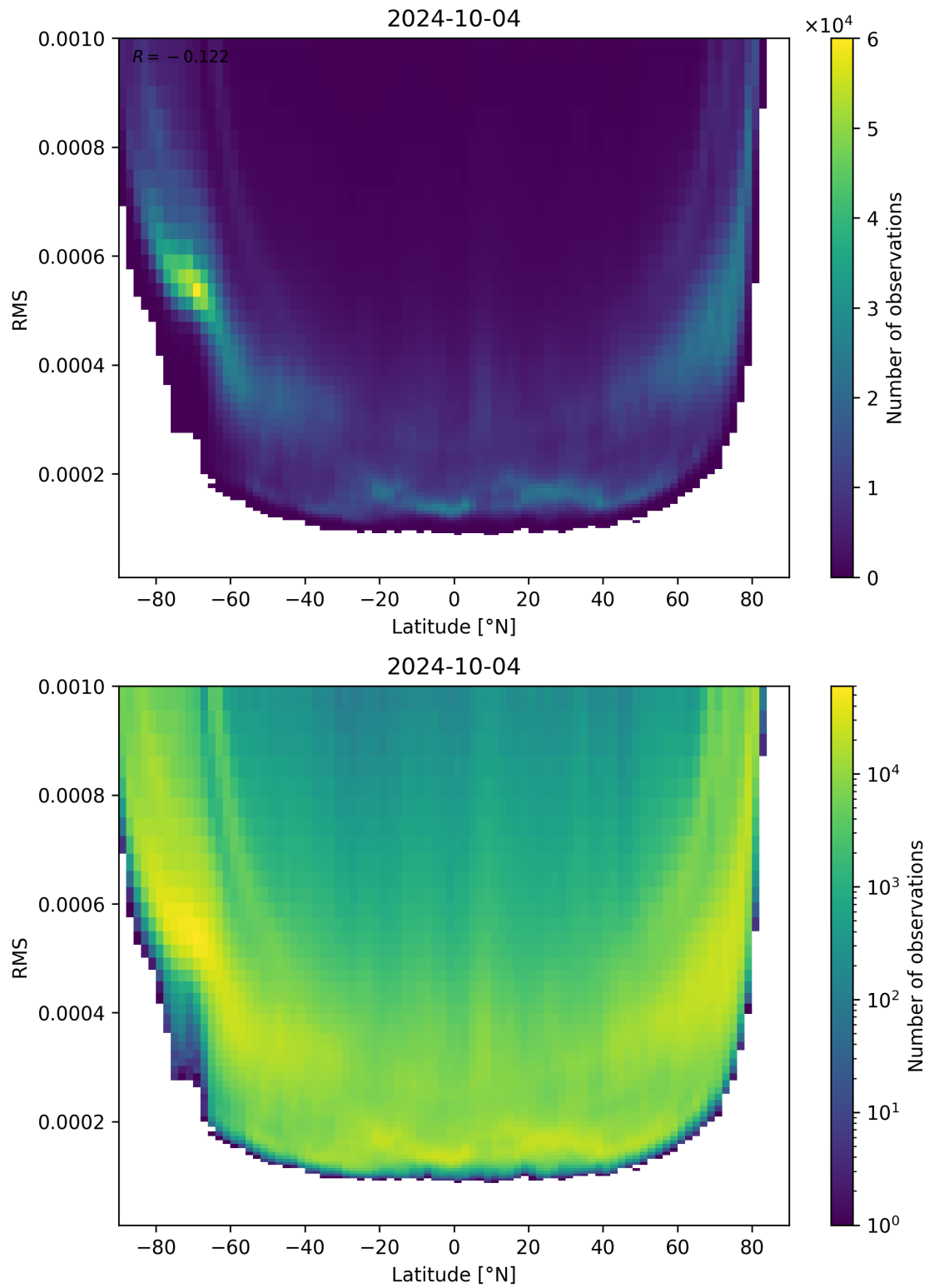
Figure 94: Scatter density plot of “Latitude” against “RMS” for 2024-10-03 to 2024-10-05.
