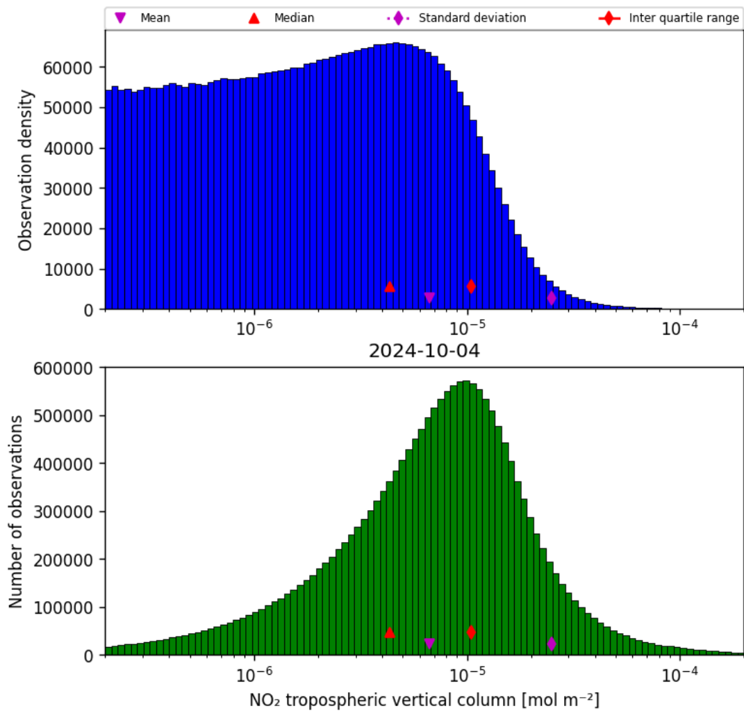
Figure 29: Histogram of “NO 2 tropospheric vertical column” for 2024-10-03 to 2024-10-05
