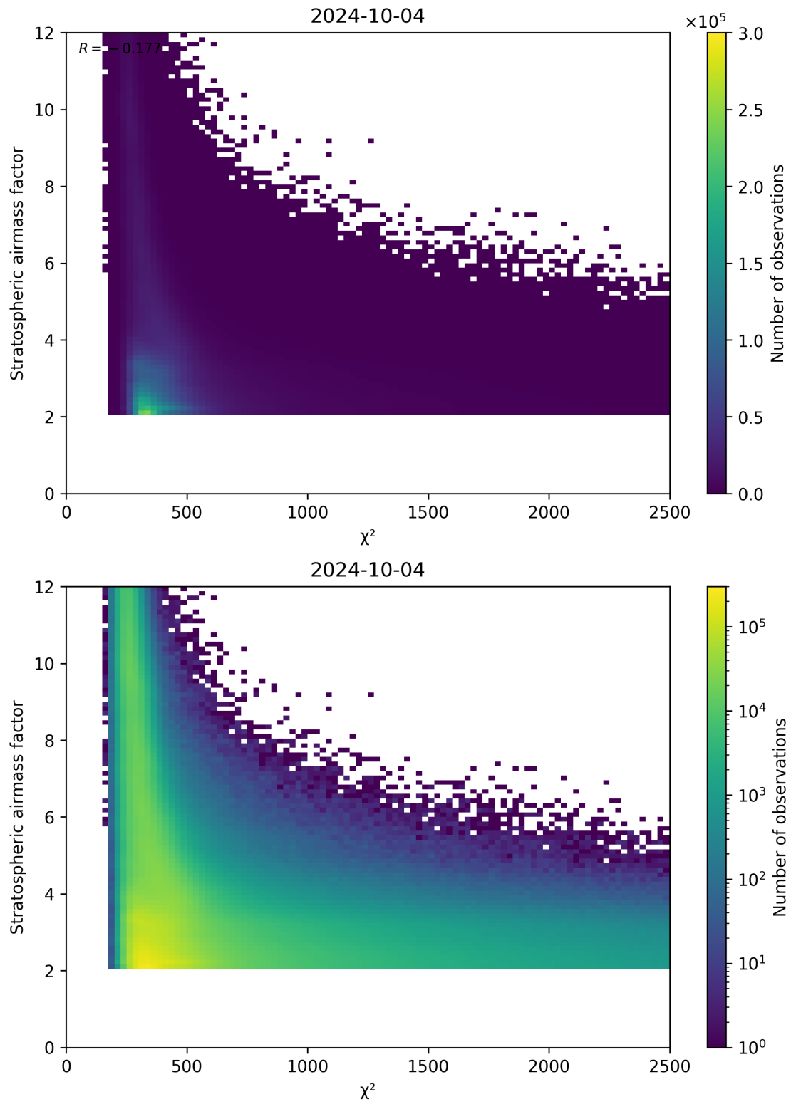
Figure 81: Scatter density plot of " \chi^2 " against "Stratospheric airmass factor" for 2024-10-03 to 2024-10-05.
