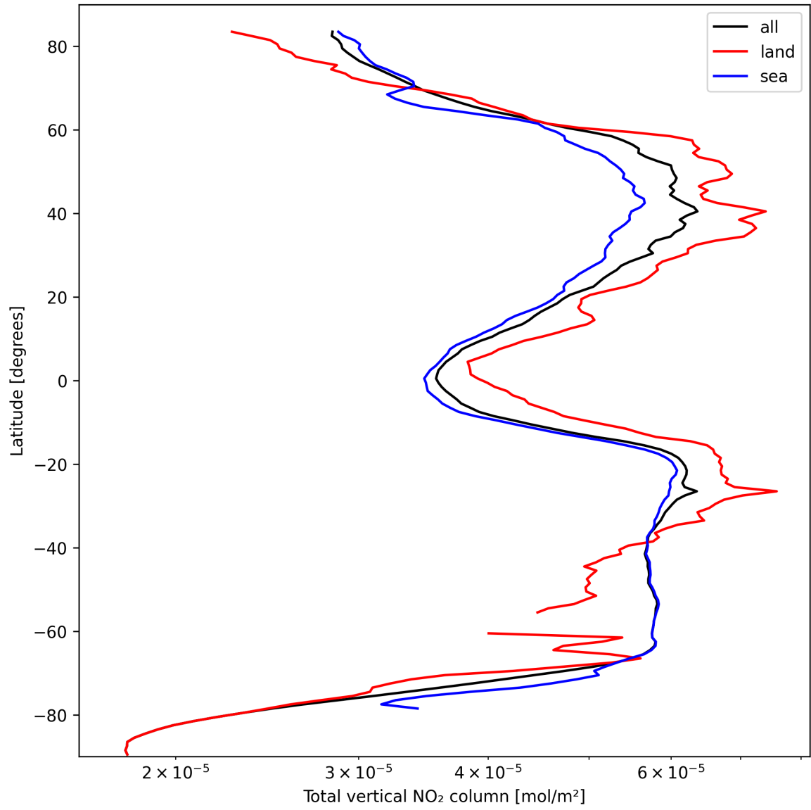
Figure 21: Zonal average of “Total vertical NO 2 column” for 2024-10-03 to 2024-10-05.
