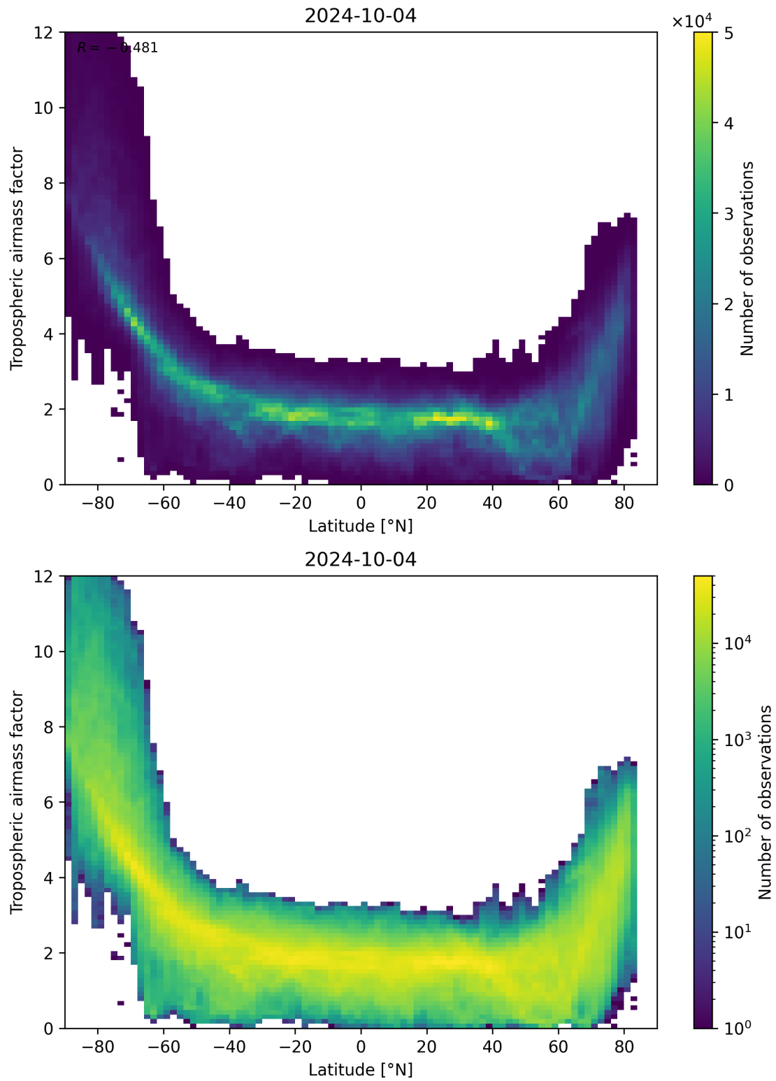
Figure 85: Scatter density plot of “Latitude” against “Tropospheric airmass factor” for 2024-10-03 to 2024-10-05.
