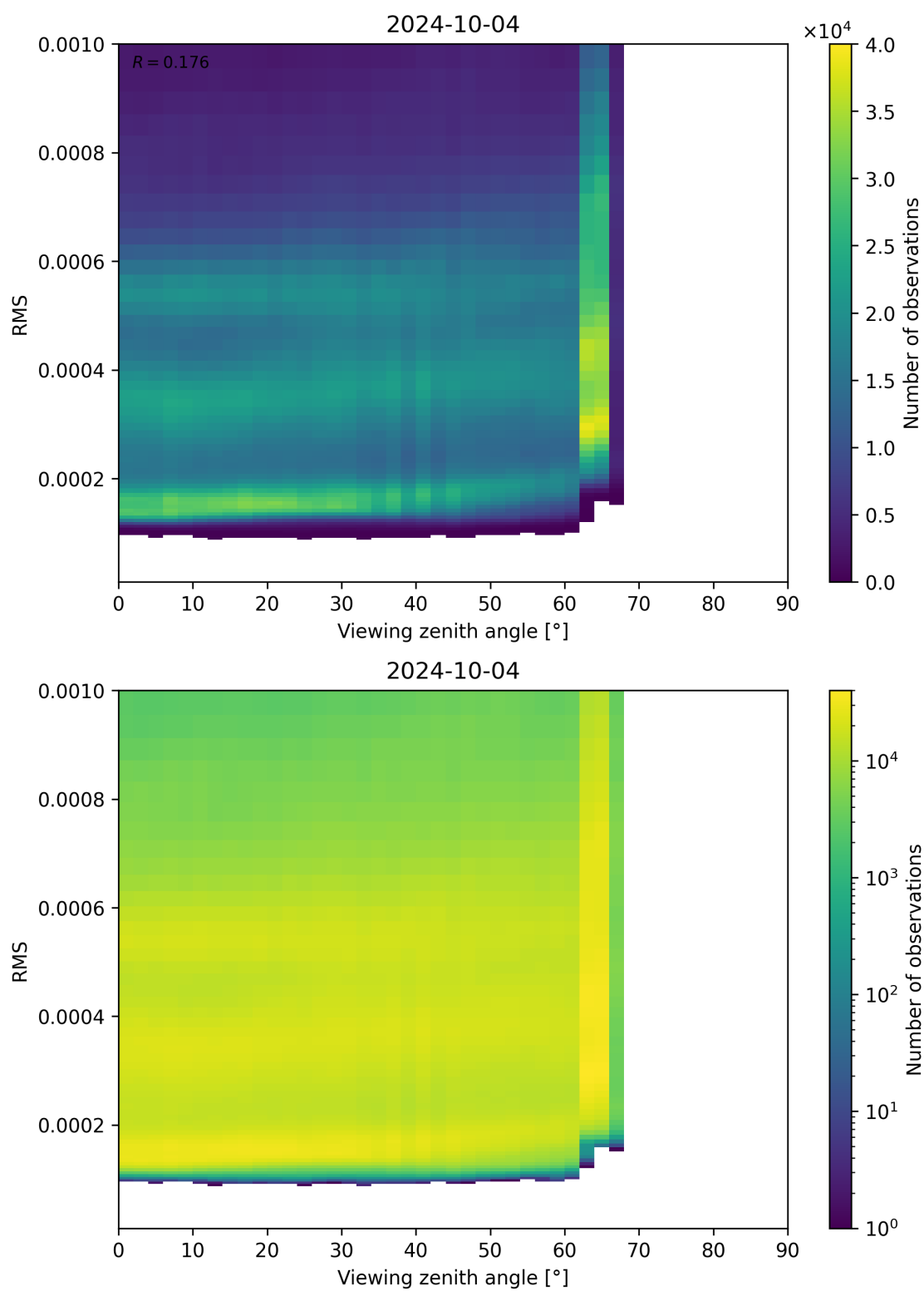
Figure 171: Scatter density plot of “Viewing zenith angle” against “RMS” for 2024-10-03 to 2024-10-05.
