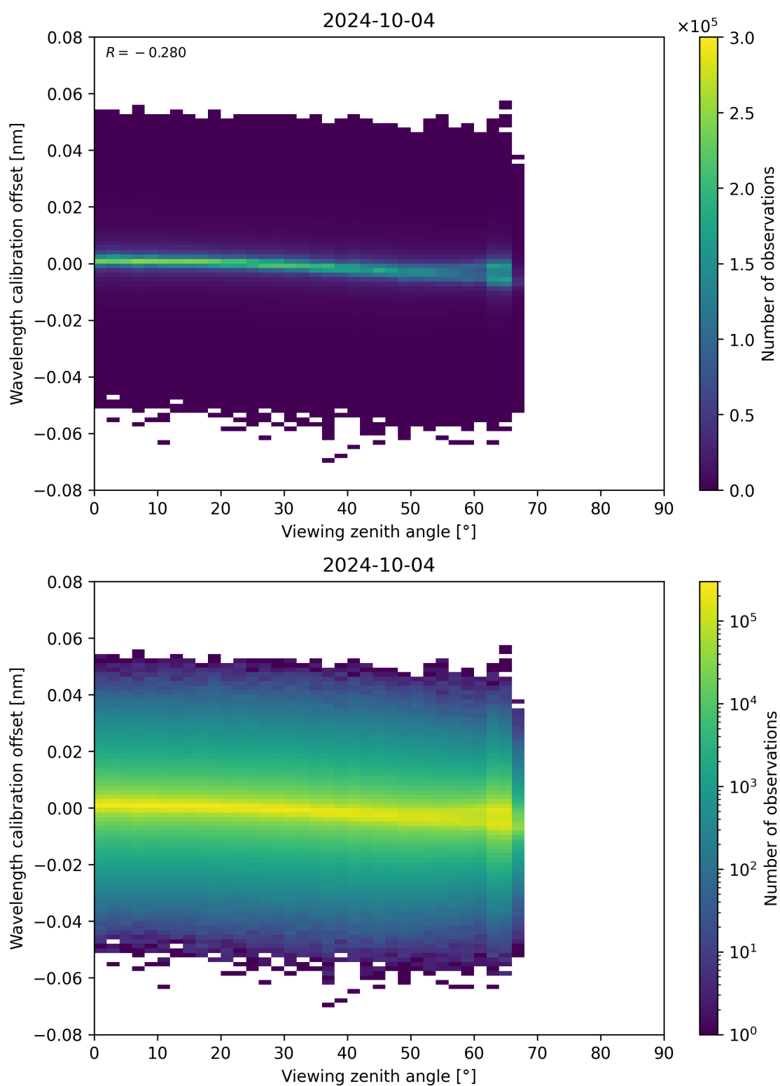
Figure 173: Scatter density plot of “Viewing zenith angle” against “Wavelength calibration offset” for 2024-10-03 to 2024-10-05.
