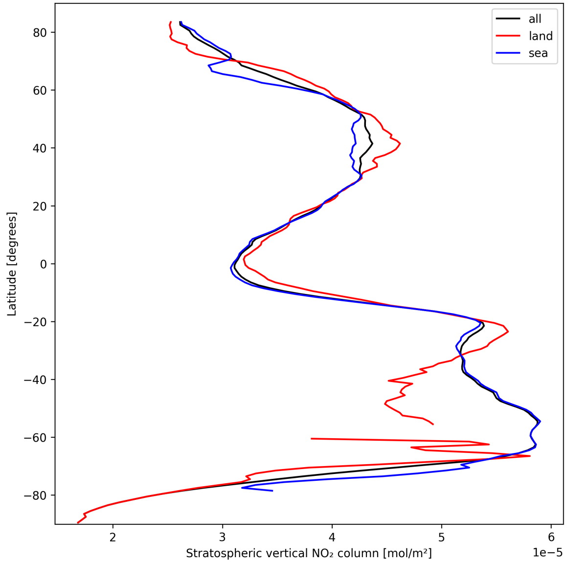
Figure 19: Zonal average of “Stratospheric vertical NO 2 column” for 2024-10-03 to 2024-10-05.
