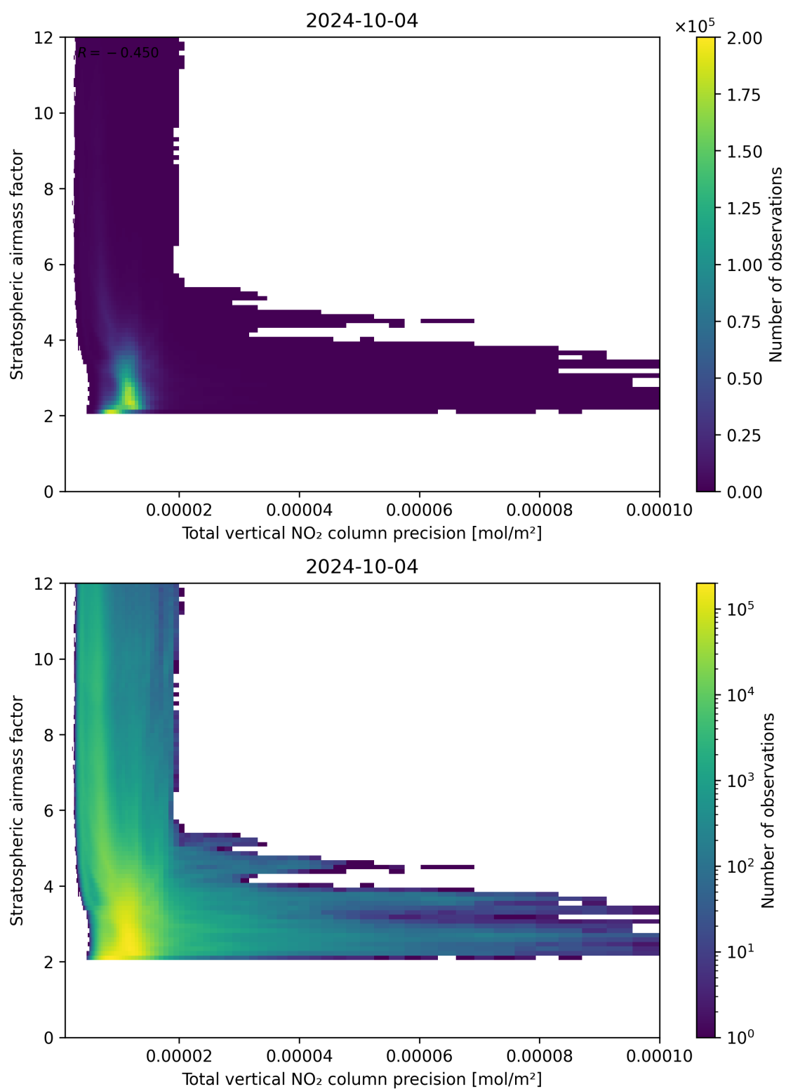
Figure 115: Scatter density plot of “Total vertical NO 2 column precision” against “Stratospheric airmass factor” for 2024-10-03 to 2024-10-05.
