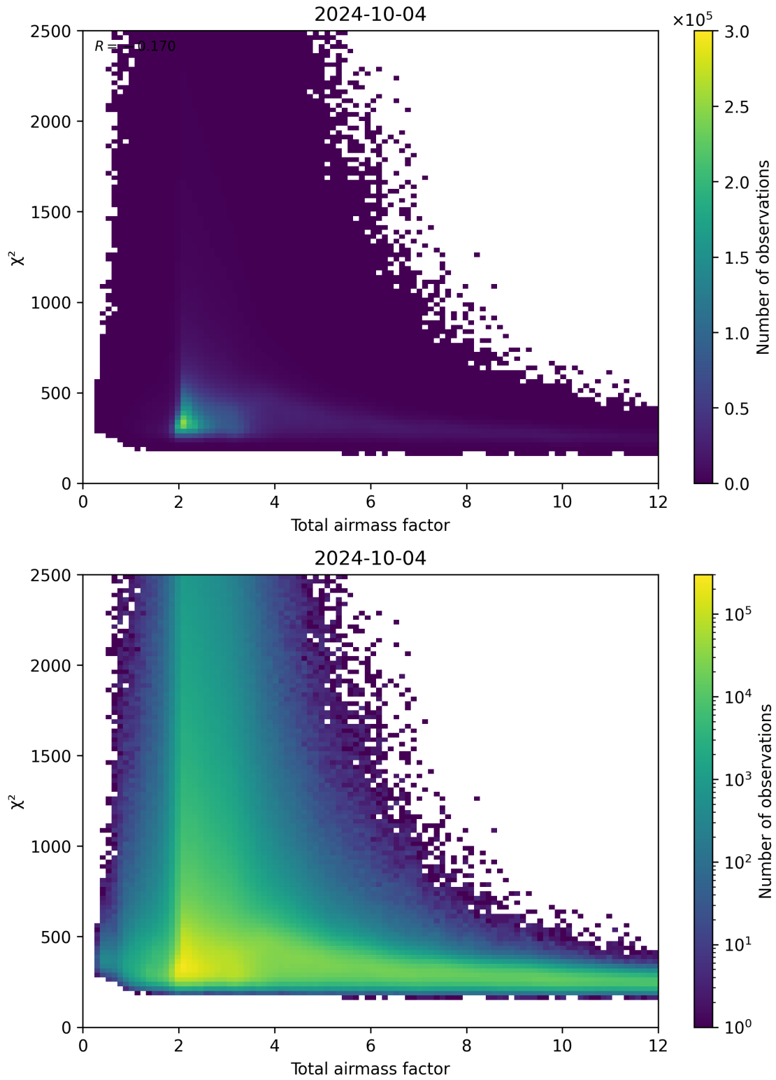
Figure 63: Scatter density plot of “Total airmass factor” against “ \chi^2 ” for 2024-10-03 to 2024-10-05.
