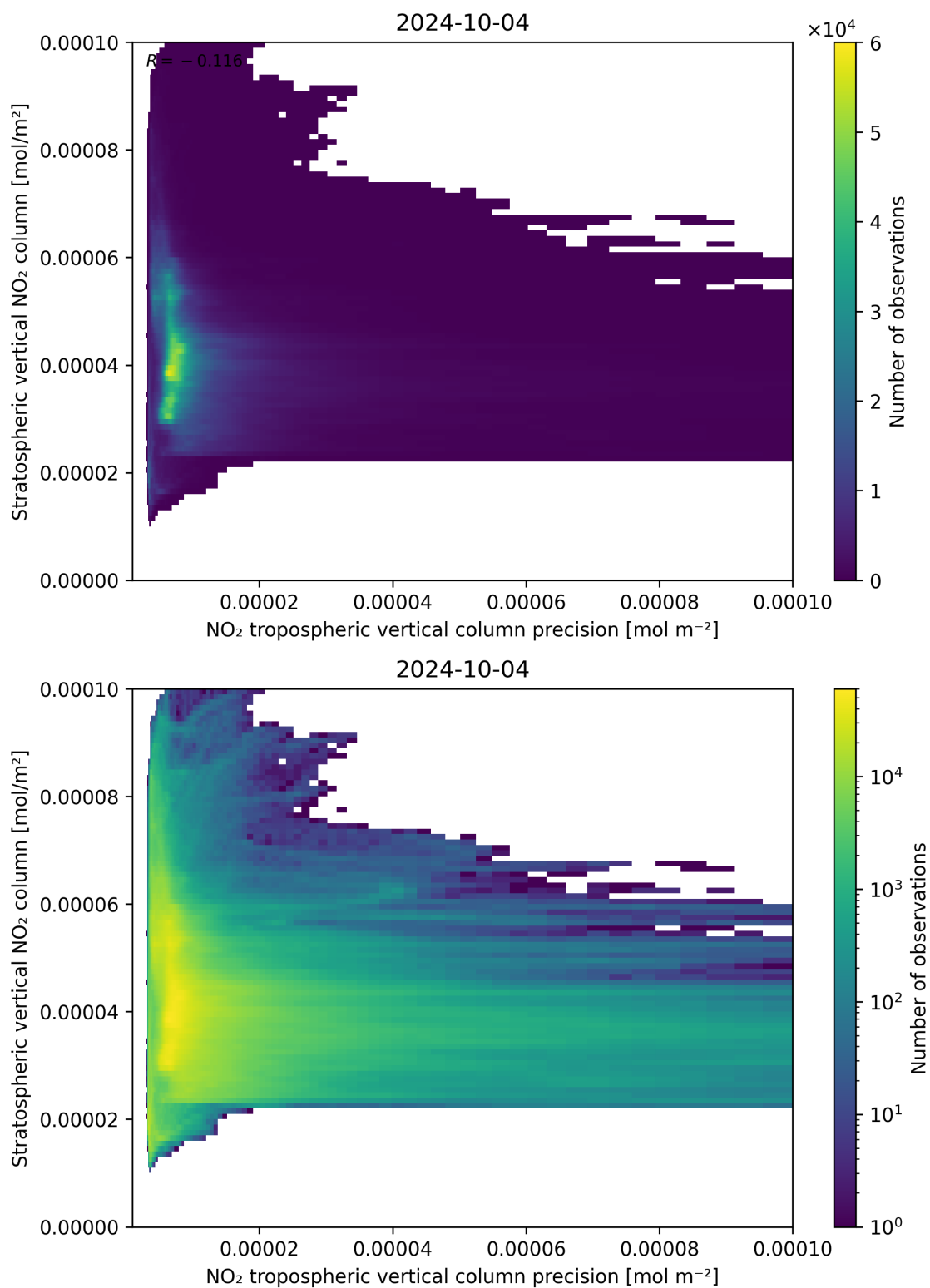
Figure 135: Scatter density plot of “NO 2 tropospheric vertical column precision” against “Stratospheric vertical NO 2 column” for 2024-10-03 to 2024-10-05.
