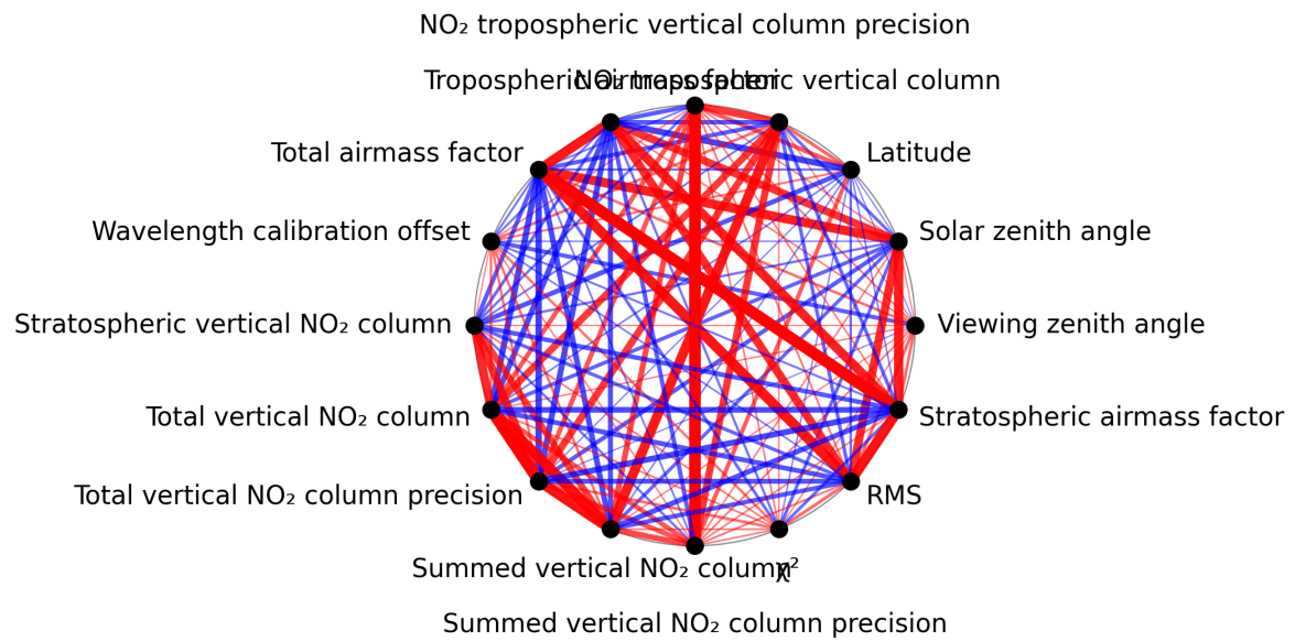
Figure 1: Map of correlation graph for 2024-10-03 to 2024-10-05.
