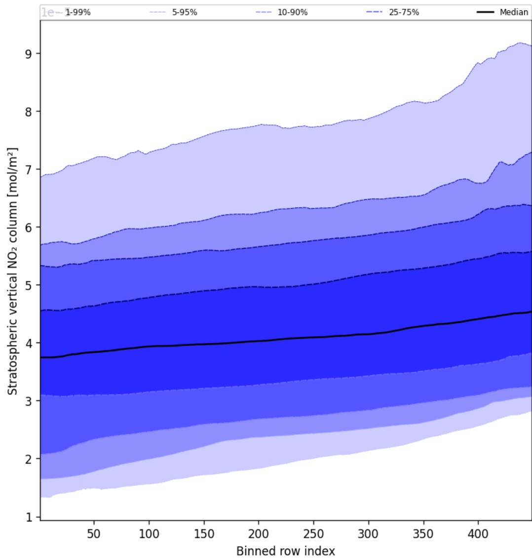
Figure 53: Along track statistics of “Stratospheric vertical NO 2 column” for 2024-10-03 to 2024-10-05
