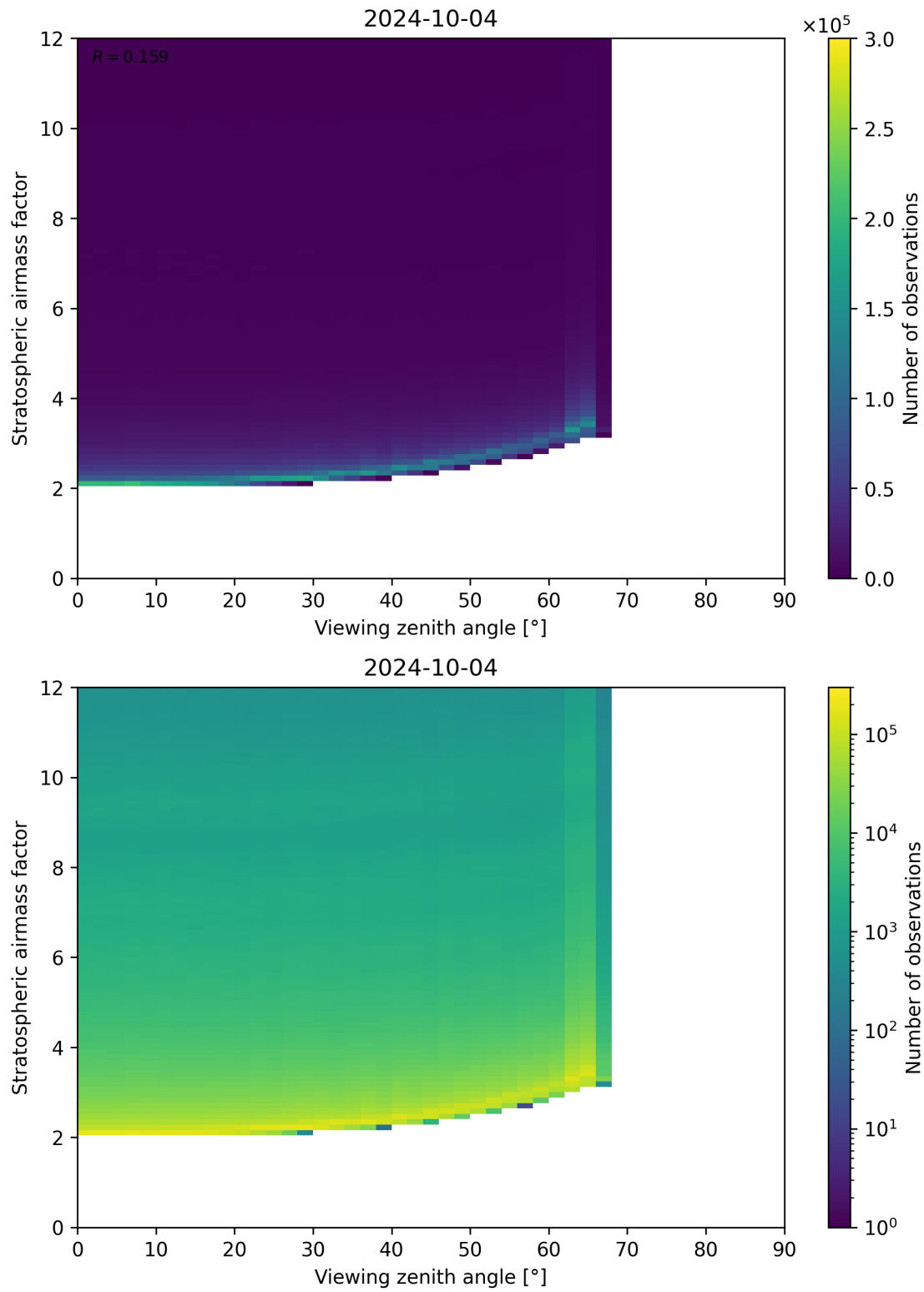
Figure 159: Scatter density plot of “Viewing zenith angle” against “Stratospheric airmass factor” for 2024-10-03 to 2024-10-05.
