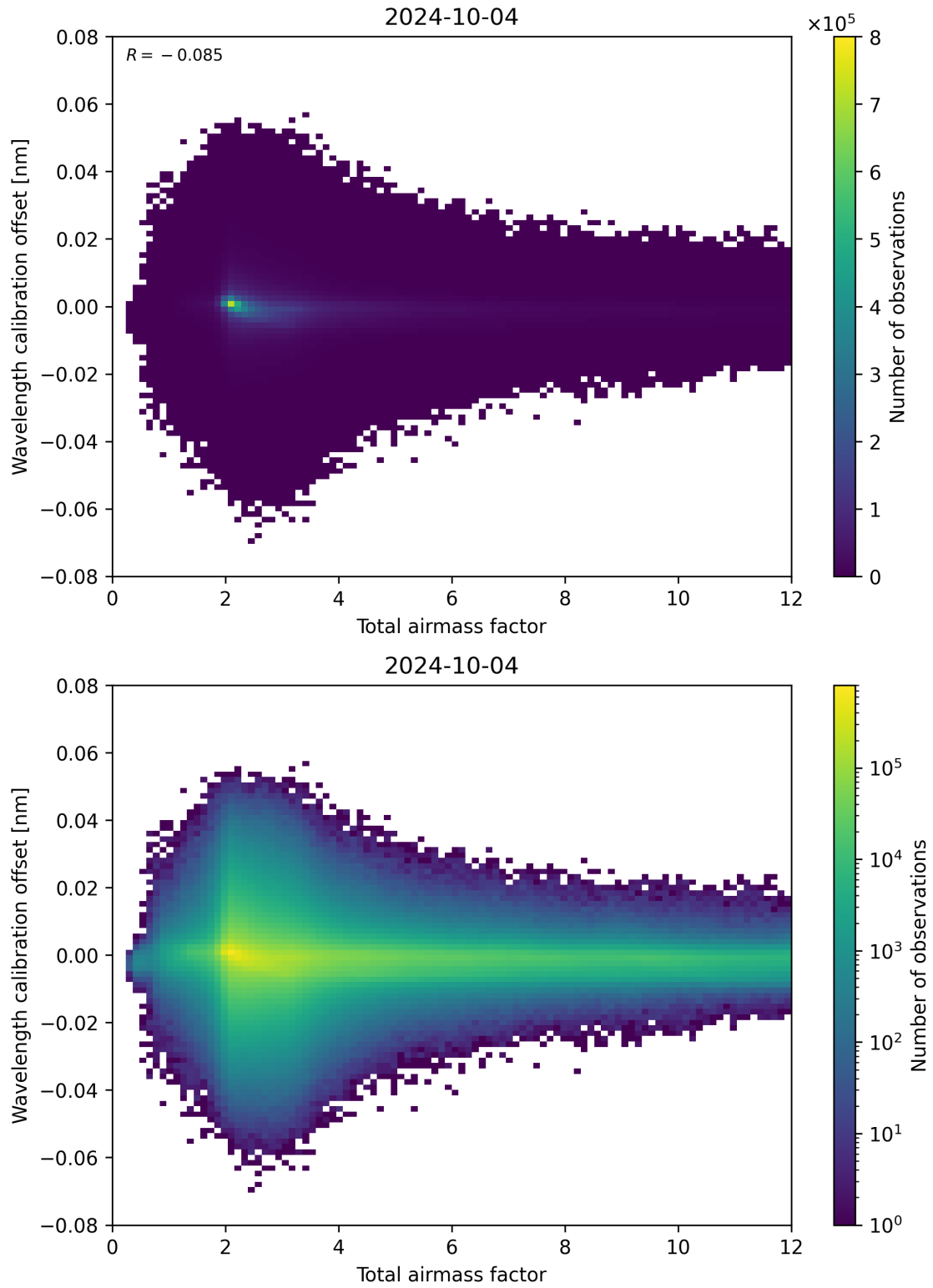
Figure 70: Scatter density plot of “Total airmass factor” against “Wavelength calibration offset” for 2024-10-03 to 2024-10-05.
