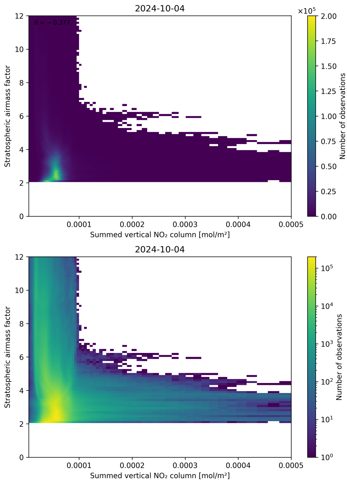
Figure 103: Scatter density plot of “Summed vertical NO 2 column” against “Stratospheric airmass factor” for 2024-10-03 to 2024-10-05.
