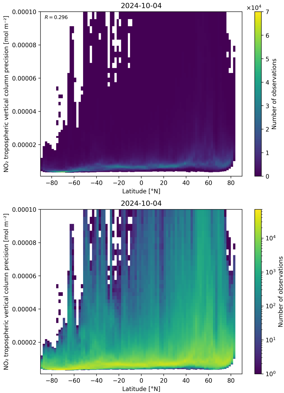
Figure 93: Scatter density plot of “Latitude” against “NO 2 tropospheric vertical column precision” for 2024-10-03 to 2024-10-05.
