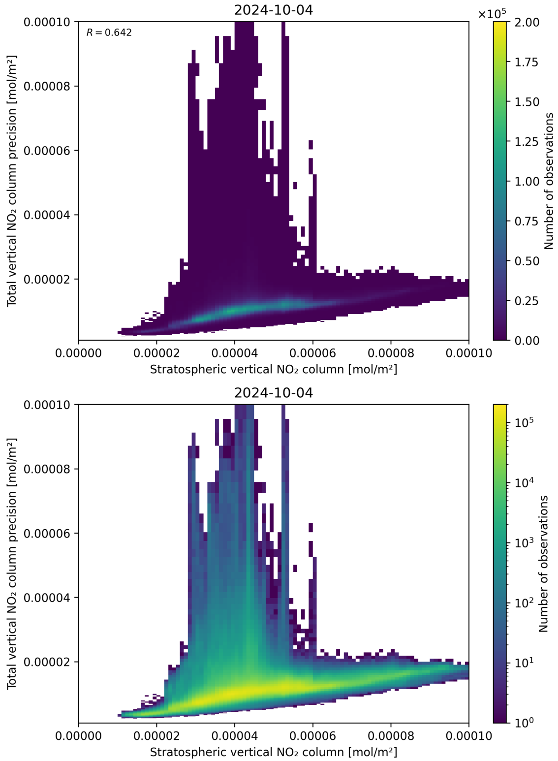
Figure 101: Scatter density plot of “Stratospheric vertical NO 2 column” against “Total vertical NO 2 column precision” for 2024-10-03 to 2024-10-05.
