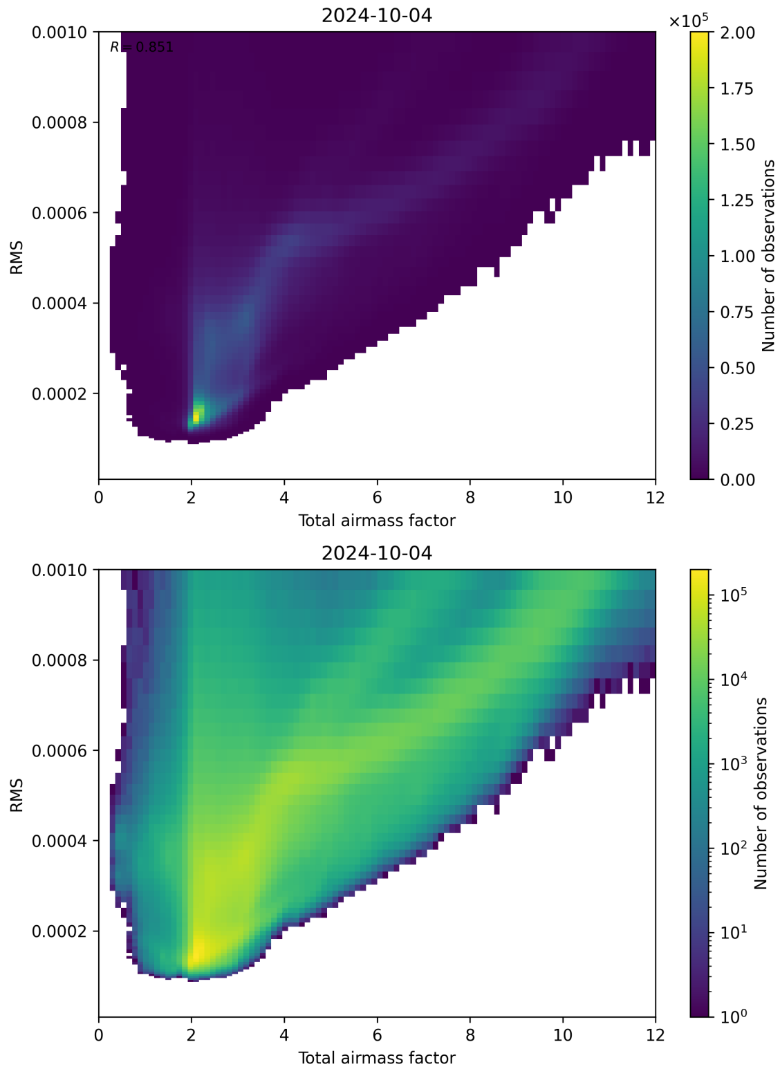
Figure 69: Scatter density plot of “Total airmass factor” against “RMS” for 2024-10-03 to 2024-10-05.
