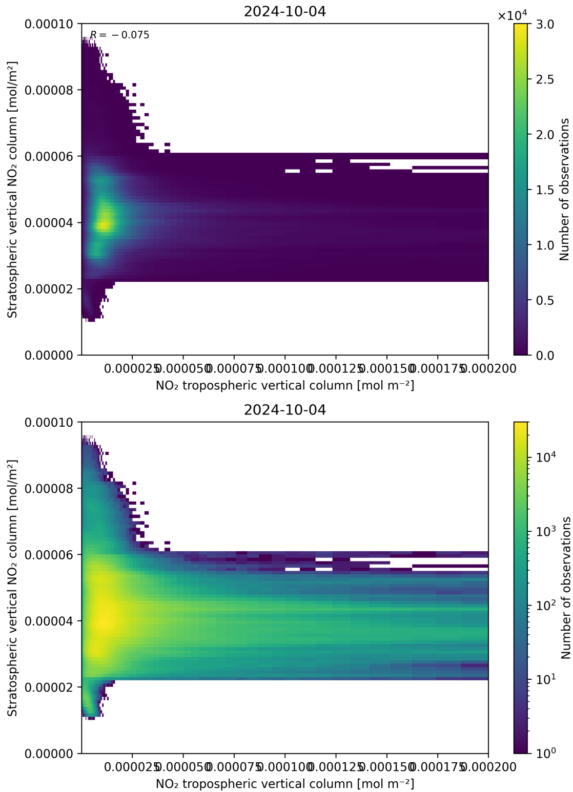
Figure 125: Scatter density plot of “NO 2 tropospheric vertical column” against “Stratospheric vertical NO 2 column” for 2024-10-03 to 2024-10-05.
