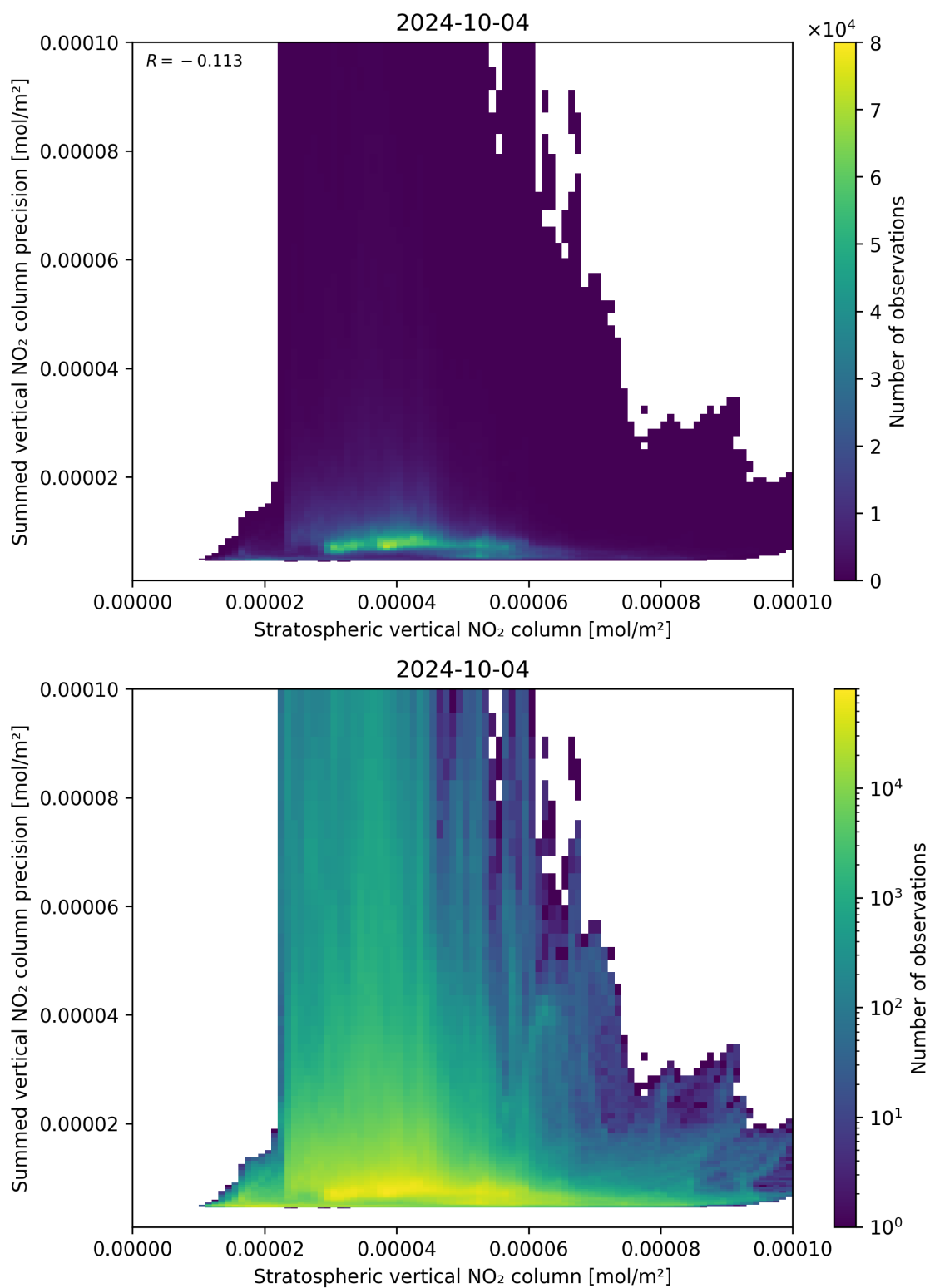
Figure 99: Scatter density plot of “Stratospheric vertical NO 2 column” against “Summed vertical NO 2 column precision” for 2024-10-03 to 2024-10-05.
