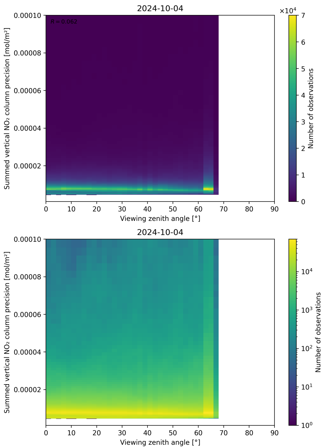
Figure 166: Scatter density plot of “Viewing zenith angle” against “Summed vertical NO 2 column precision” for 2024-10-03 to 2024-10-05.
