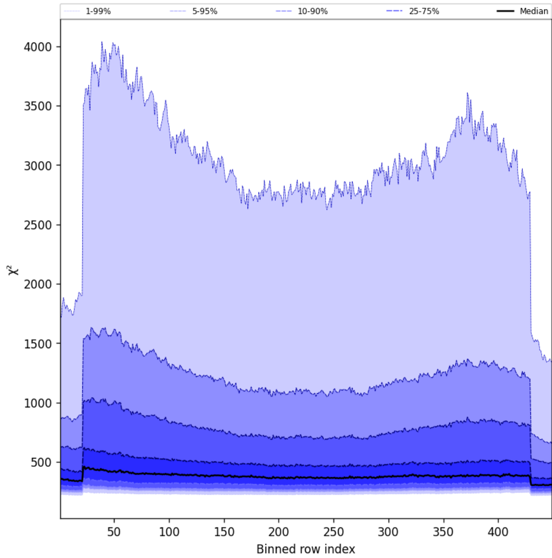
Figure 59: Along track statistics of “ \chi^2 ” for 2024-10-03 to 2024-10-05
