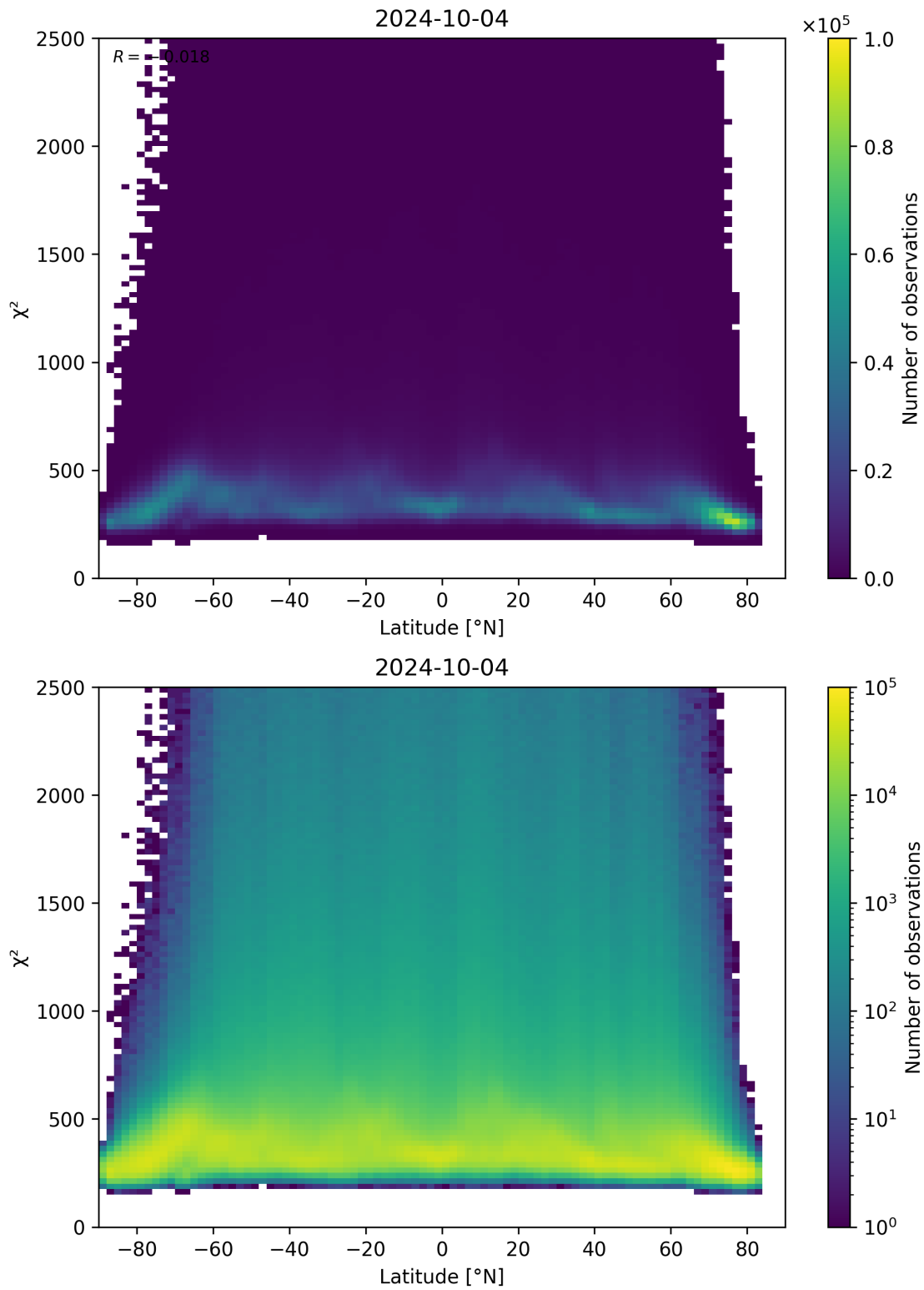
Figure 86: Scatter density plot of “Latitude” against “ \chi^2 ” for 2024-10-03 to 2024-10-05.
