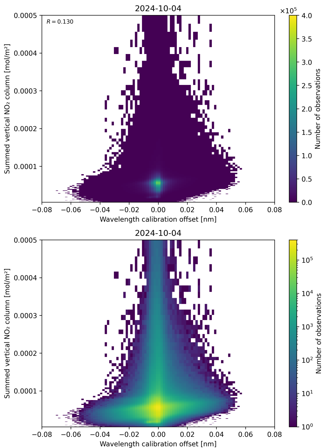
Figure 177: Scatter density plot of “Wavelength calibration offset” against “Summed vertical NO 2 column” for 2024-10-03 to 2024-10-05.
