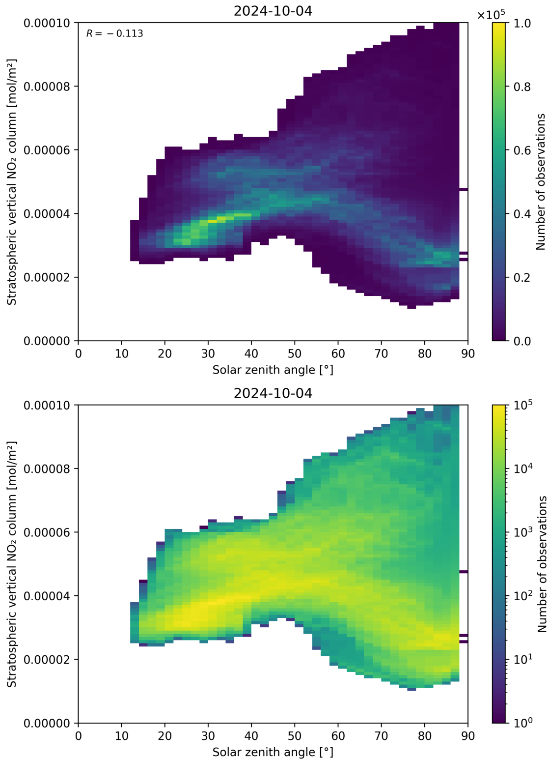
Figure 150: Scatter density plot of “Solar zenith angle” against “Stratospheric vertical NO 2 column” for 2024-10-03 to 2024-10-05.
