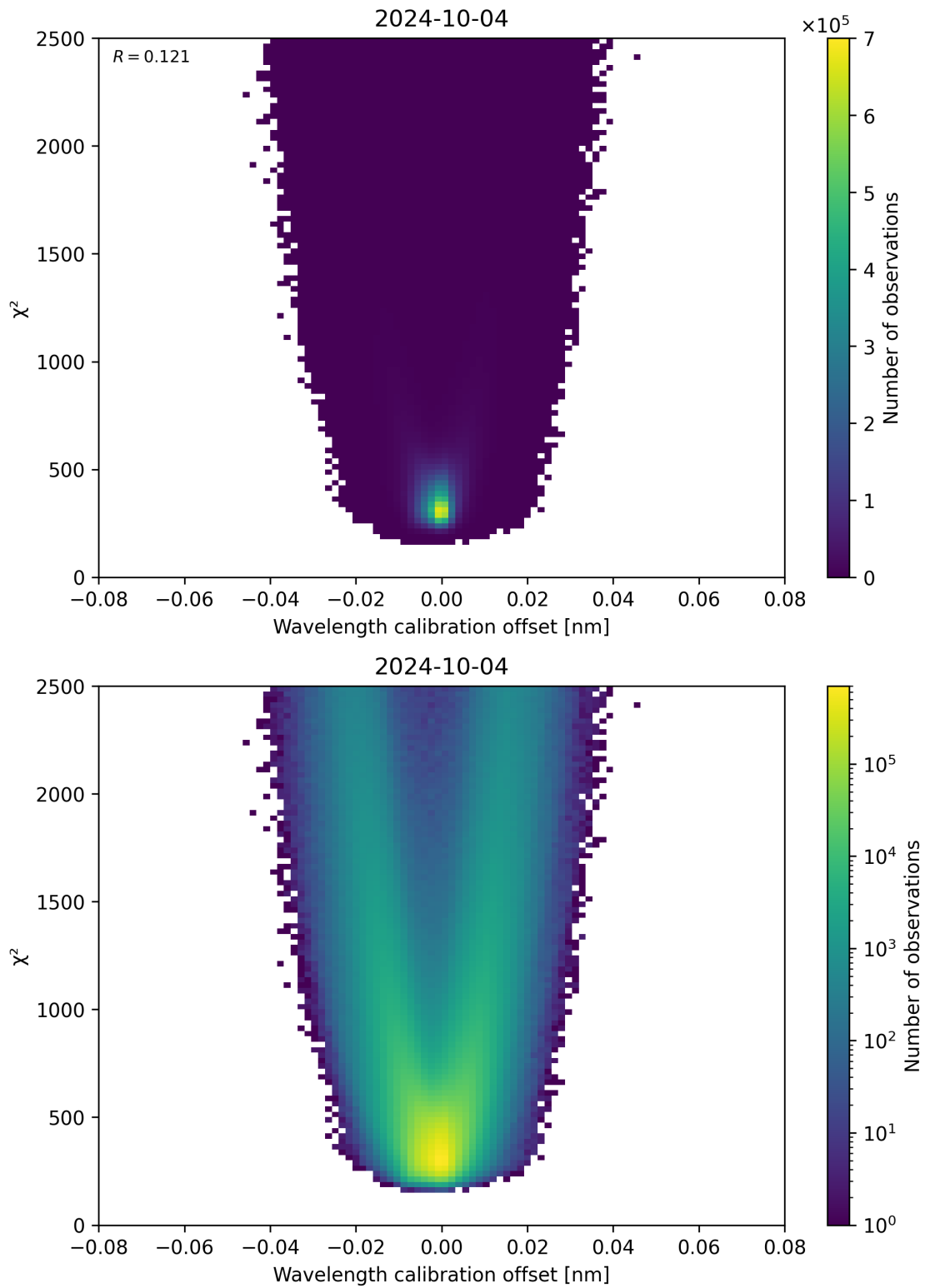
Figure 175: Scatter density plot of “Wavelength calibration offset” against “ \chi^2 ” for 2024-10-03 to 2024-10-05.
