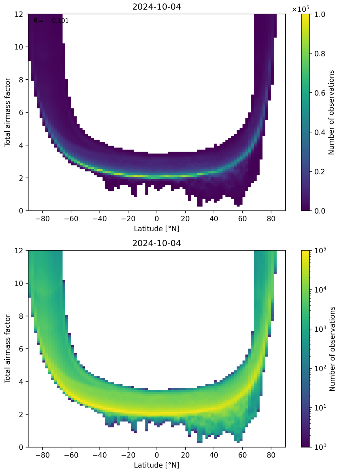
Figure 84: Scatter density plot of “Latitude” against “Total airmass factor” for 2024-10-03 to 2024-10-05.
