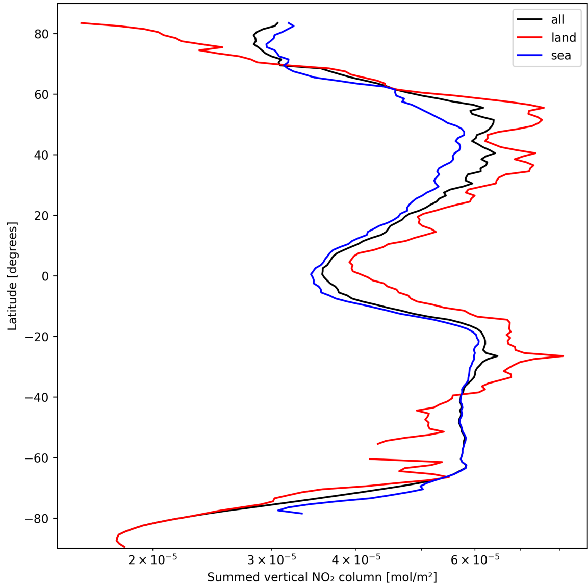
Figure 23: Zonal average of “Summed vertical NO 2 column” for 2024-10-03 to 2024-10-05.
