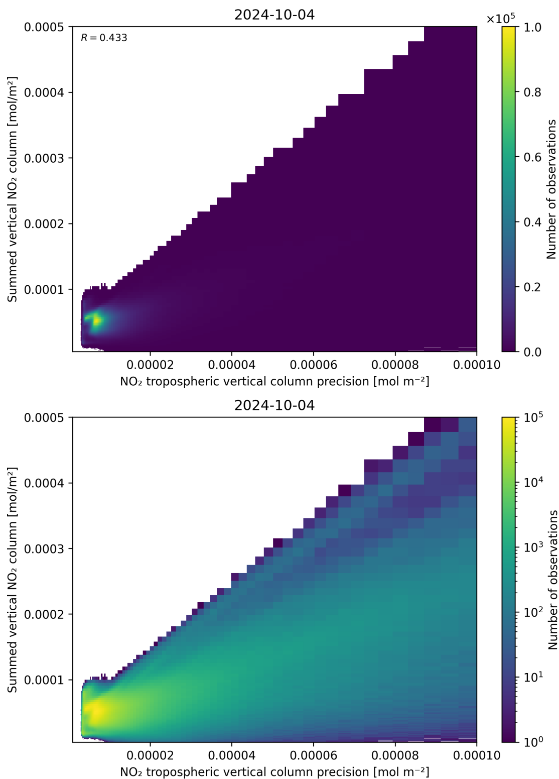
Figure 136: Scatter density plot of “NO 2 tropospheric vertical column precision” against “Summed vertical NO 2 column” for 2024-10-03 to 2024-10-05.
