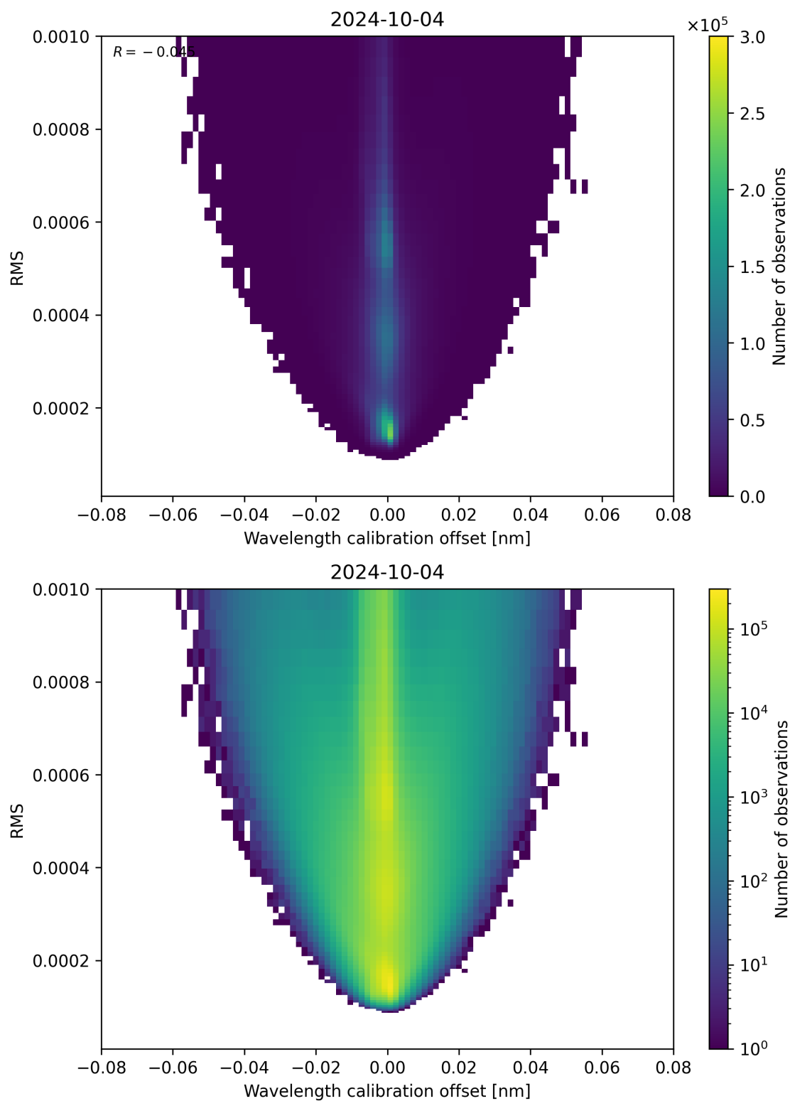
Figure 181: Scatter density plot of “Wavelength calibration offset” against “RMS” for 2024-10-03 to 2024-10-05.
