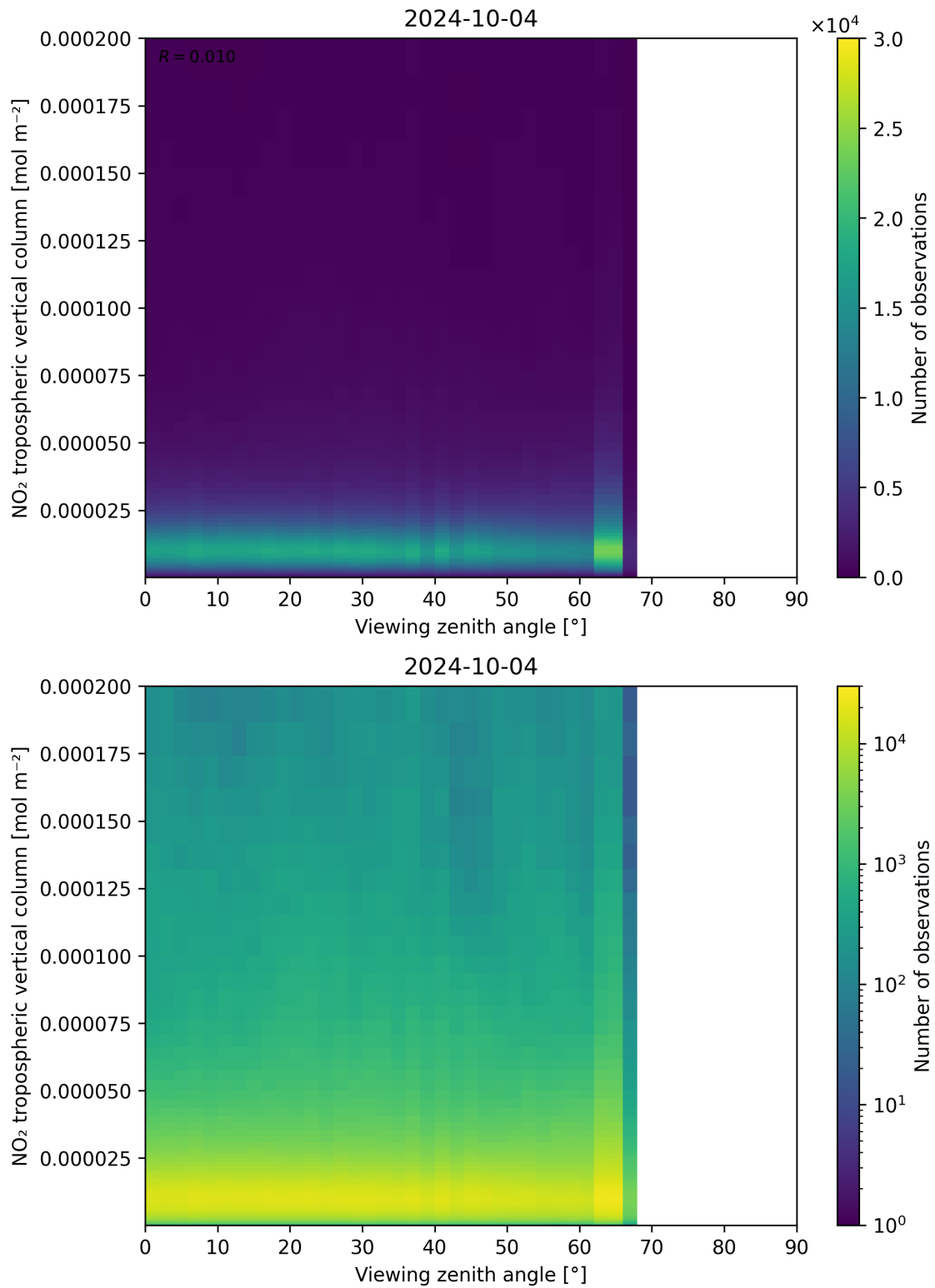
Figure 169: Scatter density plot of “Viewing zenith angle” against “NO 2 tropospheric vertical column” for 2024-10-03 to 2024-10-05.
