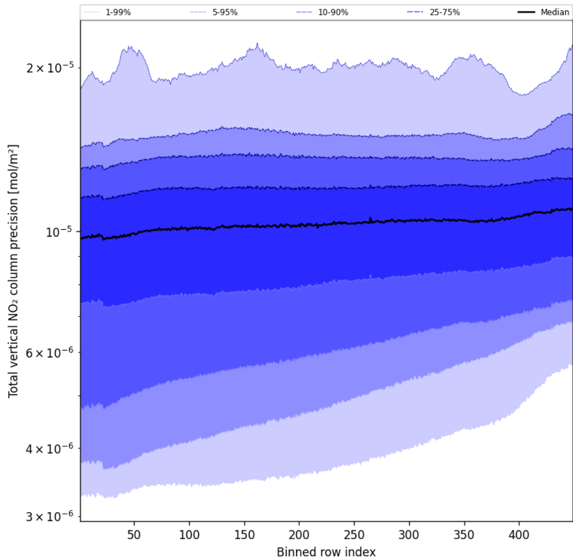
Figure 56: Along track statistics of “Total vertical NO 2 column precision” for 2024-10-03 to 2024-10-05
