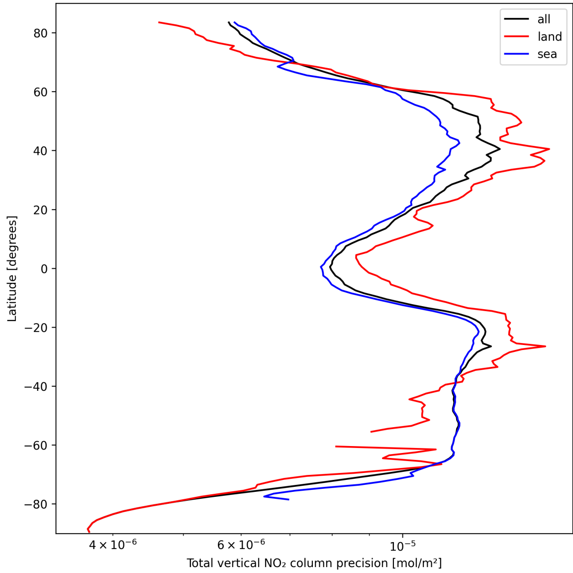
Figure 22: Zonal average of “Total vertical NO 2 column precision” for 2024-10-03 to 2024-10-05.
