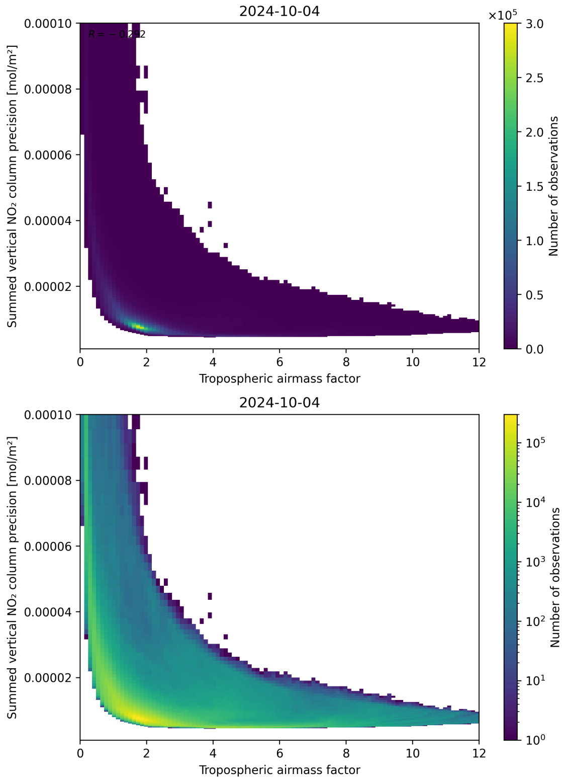
Figure 76: Scatter density plot of “Tropospheric airmass factor” against “Summed vertical NO 2 column precision” for 2024-10-03 to 2024-10-05.
