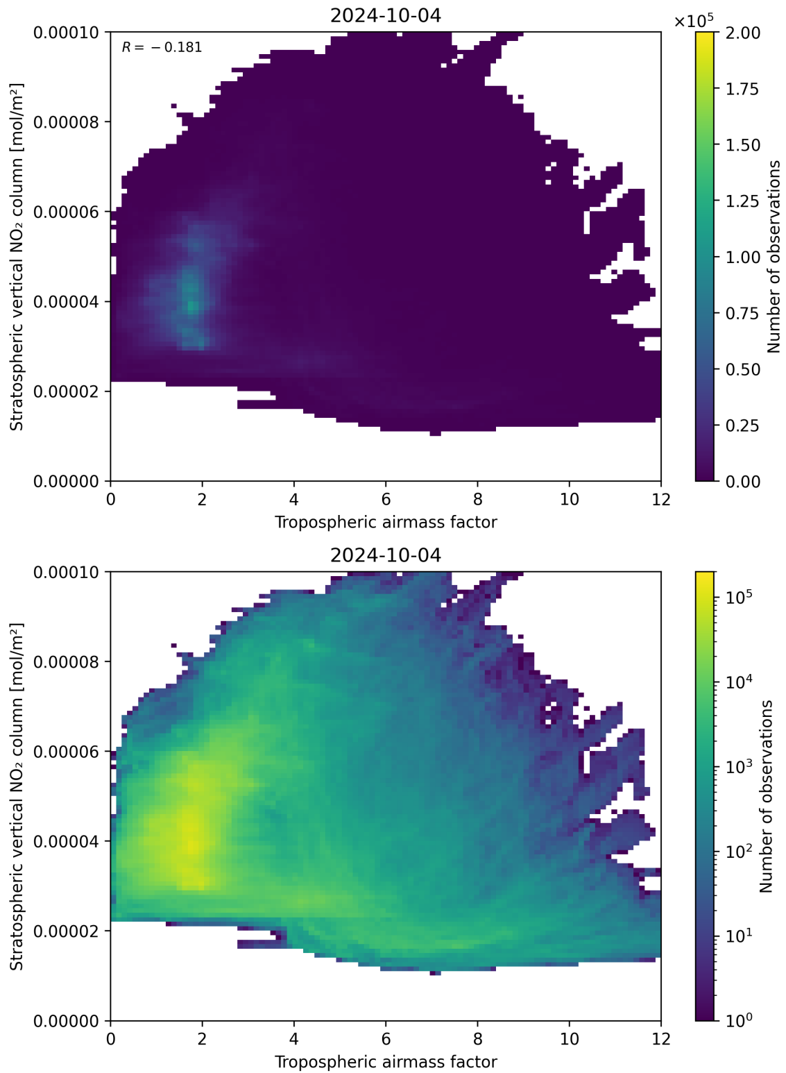
Figure 74: Scatter density plot of “Tropospheric air mass factor” against “Stratospheric vertical NO 2 column” for 2024-10-03 to 2024-10-05.
