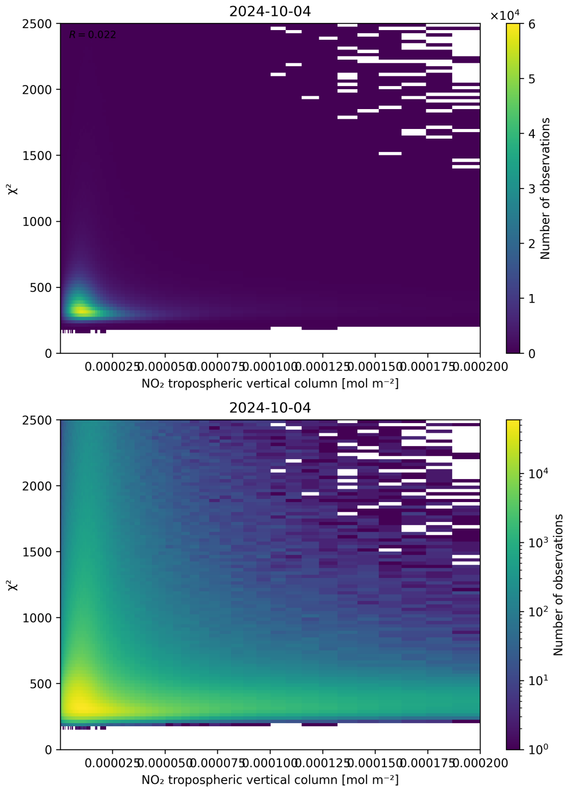
Figure 124: Scatter density plot of “NO 2 tropospheric vertical column” against “ \chi^2 ” for 2024-10-03 to 2024-10-05.
