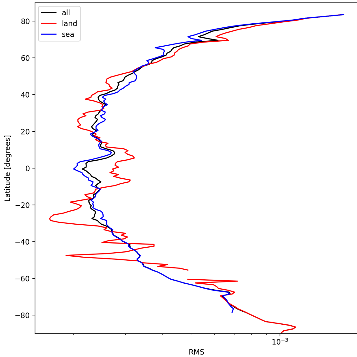
Figure 26: Zonal average of “RMS” for 2024-10-03 to 2024-10-05.
