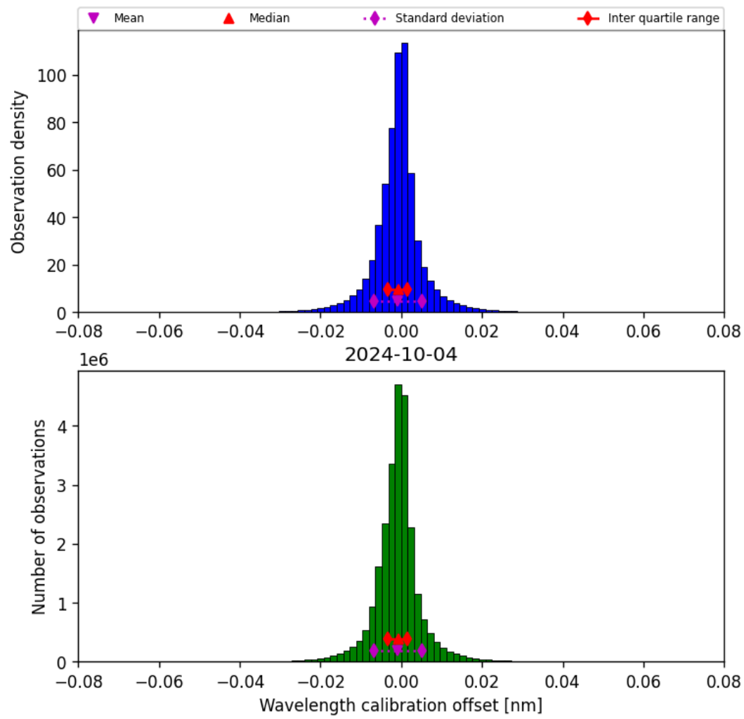
Figure 35: Histogram of "Wavelength calibration offset" for 2024-10-03 to 2024-10-05
