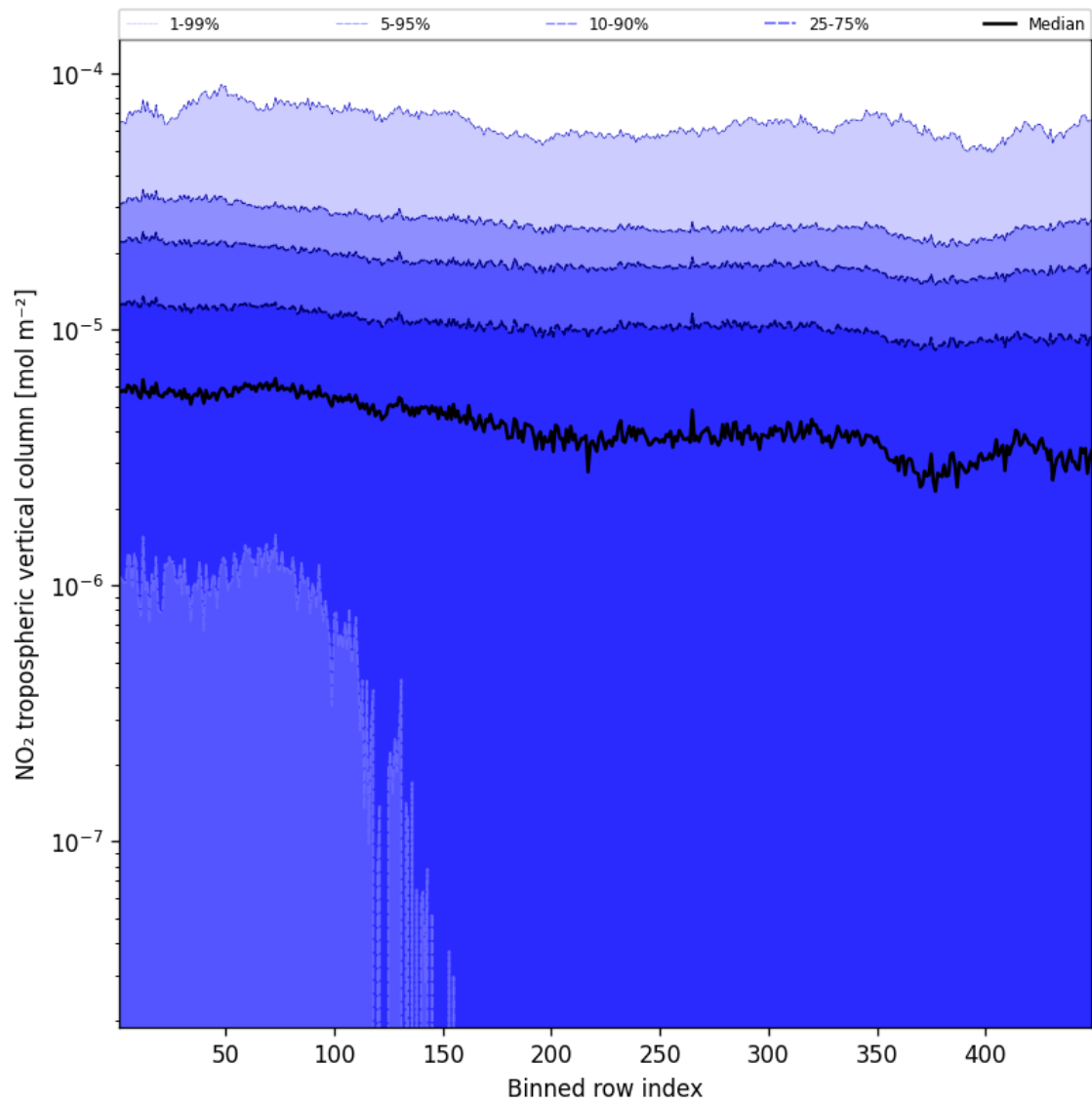
Figure 46: Along track statistics of “NO 2 tropospheric vertical column” for 2024-10-03 to 2024-10-05
