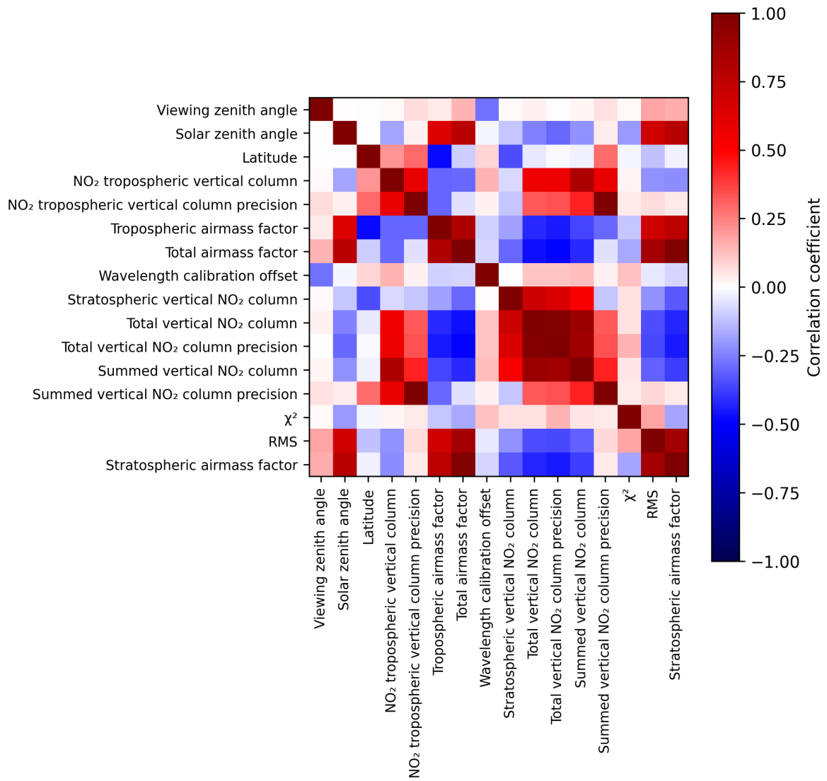
Figure 2: Map of correlation matrix for 2024-10-03 to 2024-10-05.
