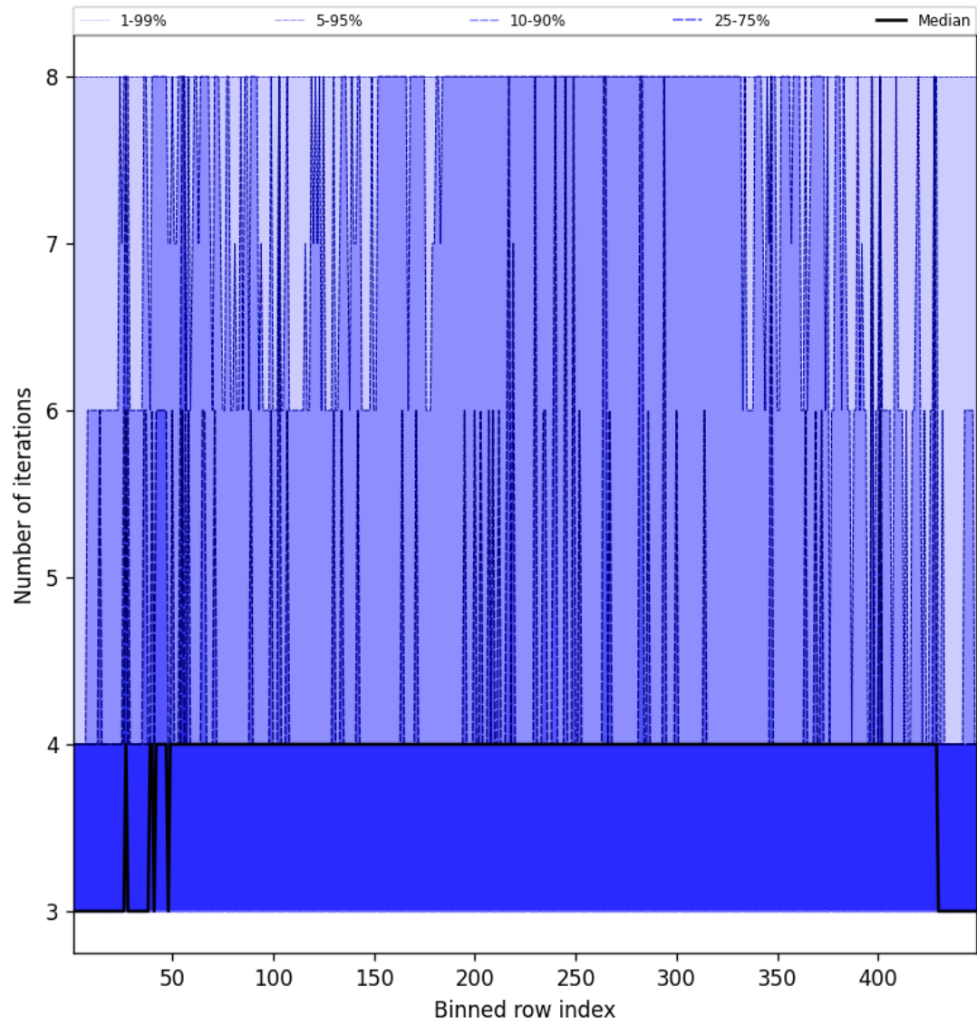
Figure 51: Along track statistics of “Number of iterations” for 2024-10-03 to 2024-10-05
