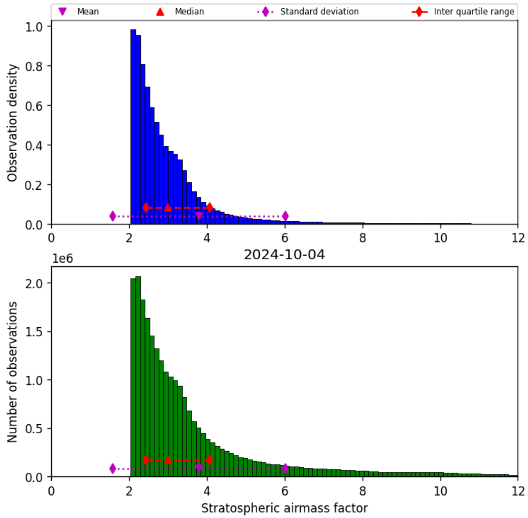
Figure 44: Histogram of “Stratospheric airmass factor” for 2024-10-03 to 2024-10-05
