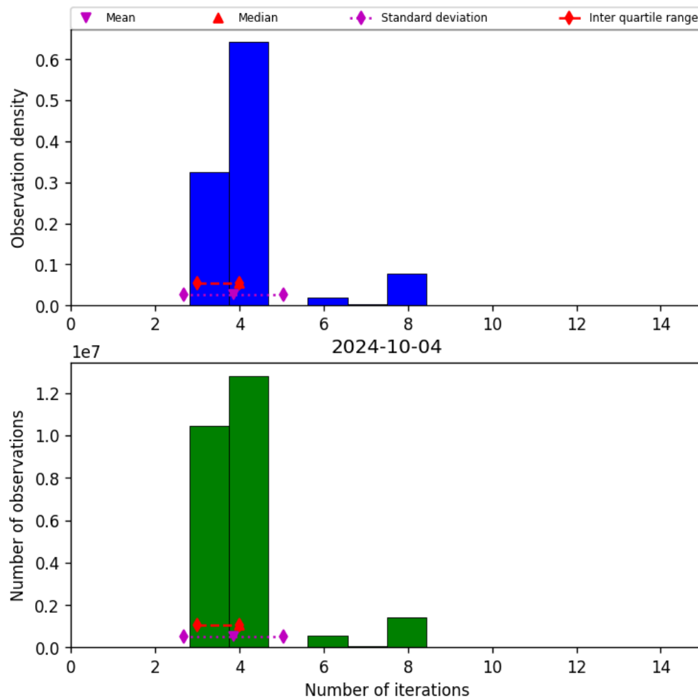
Figure 34: Histogram of “Number of iterations” for 2024-10-03 to 2024-10-05
