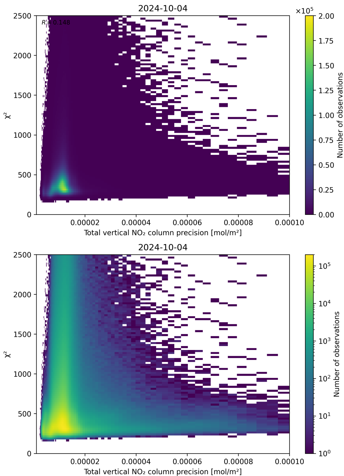
Figure 116: Scatter density plot of “Total vertical NO 2 column precision” against “ \chi^2 ” for 2024-10-03 to 2024-10-05.
