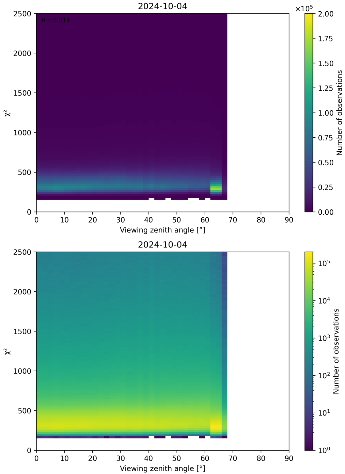
Figure 162: Scatter density plot of “Viewing zenith angle” against “ \chi^2 ” for 2024-10-03 to 2024-10-05.
