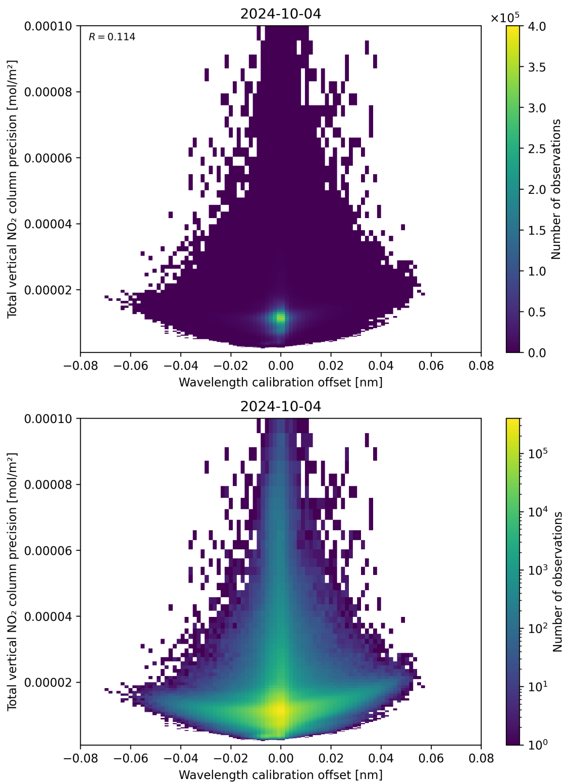
Figure 180: Scatter density plot of “Wavelength calibration offset” against “Total vertical NO 2 column precision” for 2024-10-03 to 2024-10-05.
