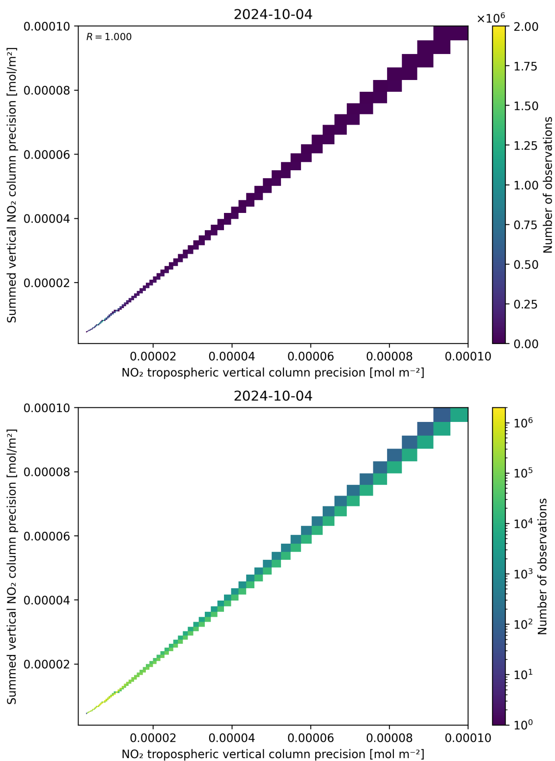
Figure 137: Scatter density plot of “NO 2 tropospheric vertical column precision” against “Summed vertical NO 2 column precision” for 2024-10-03 to 2024-10-05.
