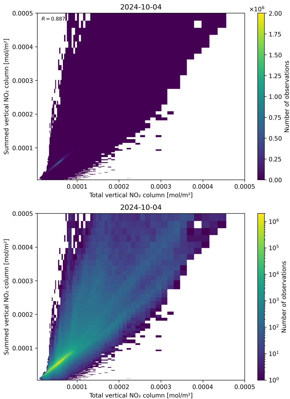
Figure 112: Scatter density plot of “Total vertical NO 2 column” against “Summed vertical NO 2 column” for 2024-10-03 to 2024-10-05.
