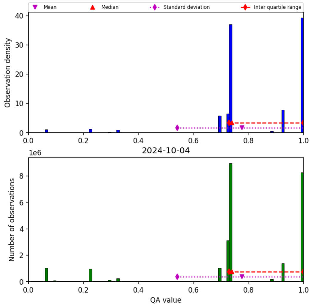
Figure 28: Histogram of “QA value” for 2024-10-03 to 2024-10-05
