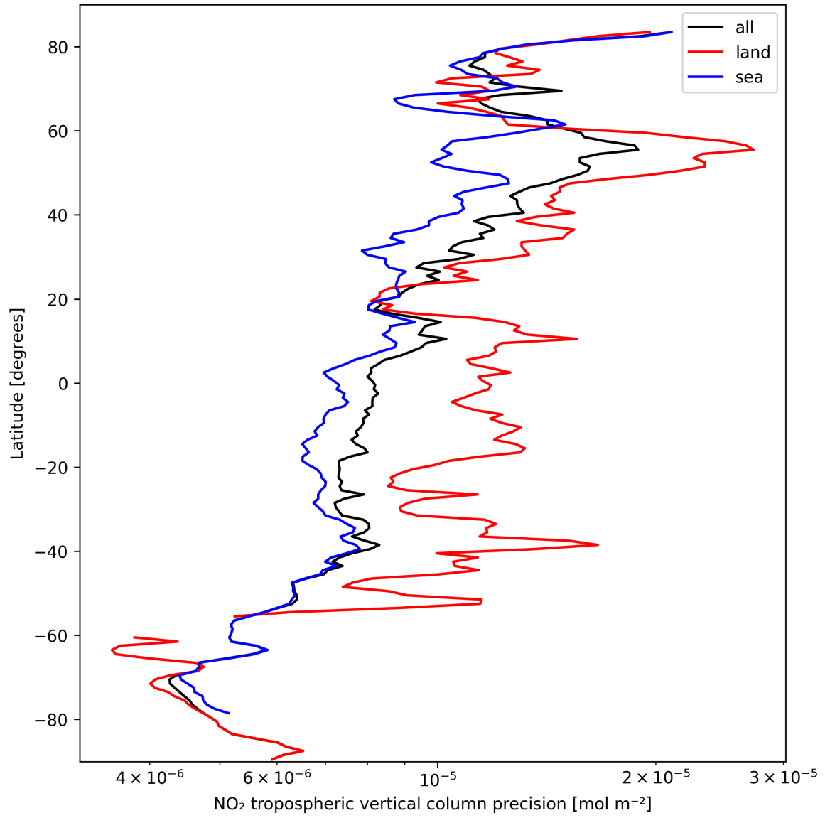
Figure 13: Zonal average of “NO 2 tropospheric vertical column precision” for 2024-10-03 to 2024-10-05.
