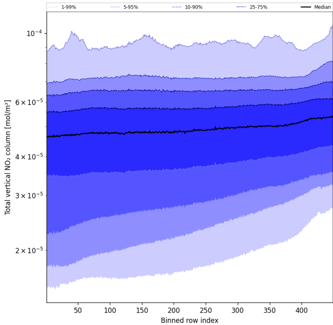
Figure 55: Along track statistics of “Total vertical NO 2 column” for 2024-10-03 to 2024-10-05
