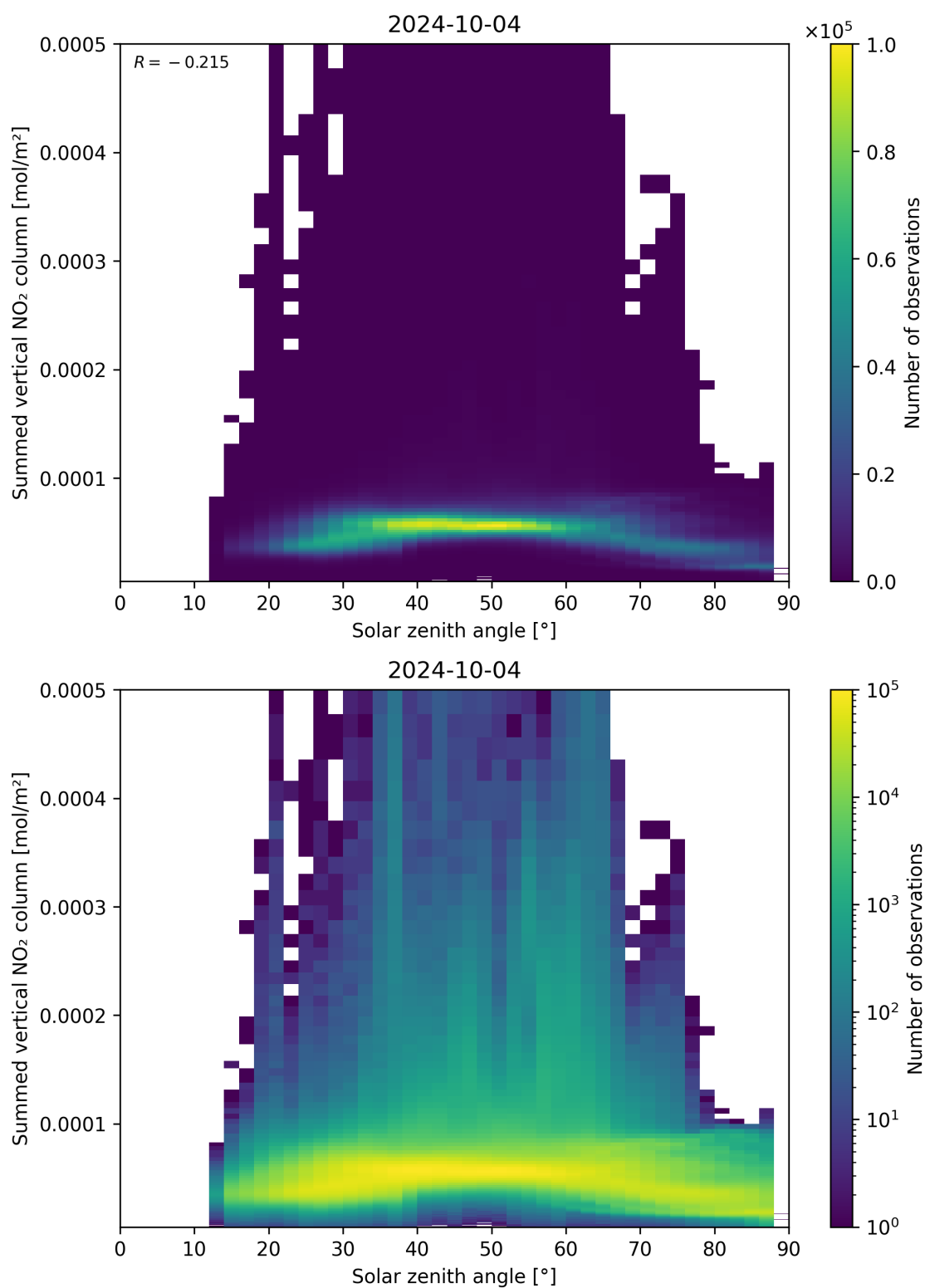
Figure 151: Scatter density plot of “Solar zenith angle” against “Summed vertical NO 2 column” for 2024-10-03 to 2024-10-05.
