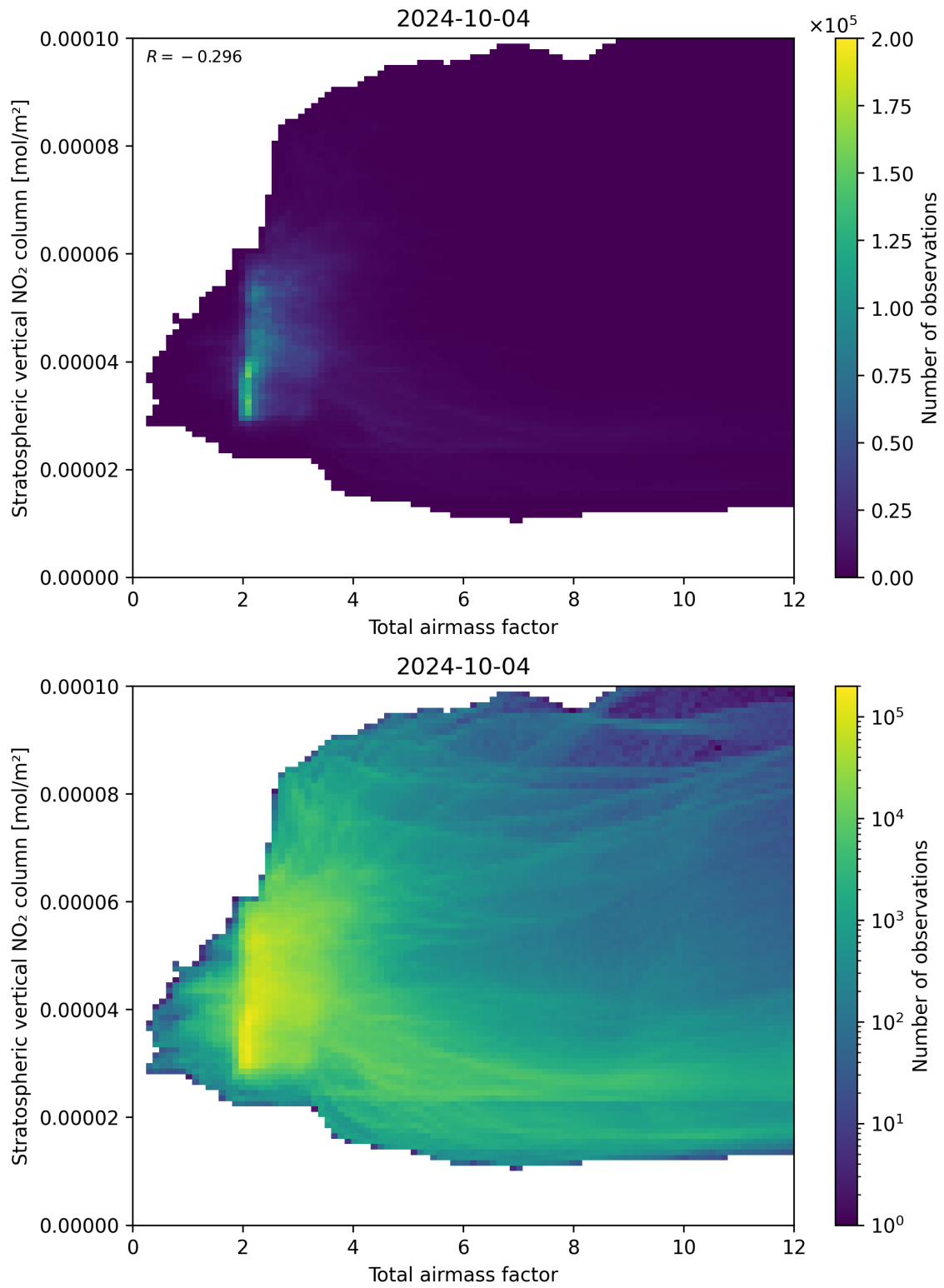
Figure 64: Scatter density plot of “Total airmass factor” against “Stratospheric vertical NO 2 column” for 2024-10-03 to 2024-10-05.
