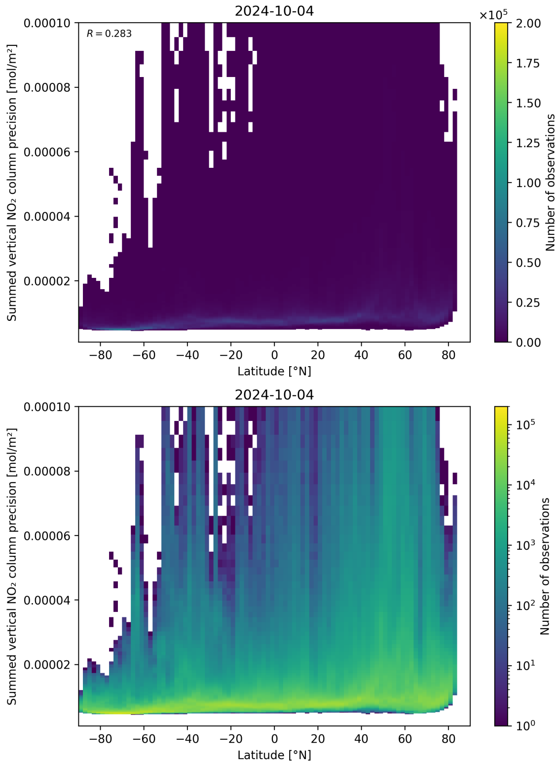
Figure 89: Scatter density plot of “Latitude” against “Summed vertical NO 2 column precision” for 2024-10-03 to 2024-10-05.
