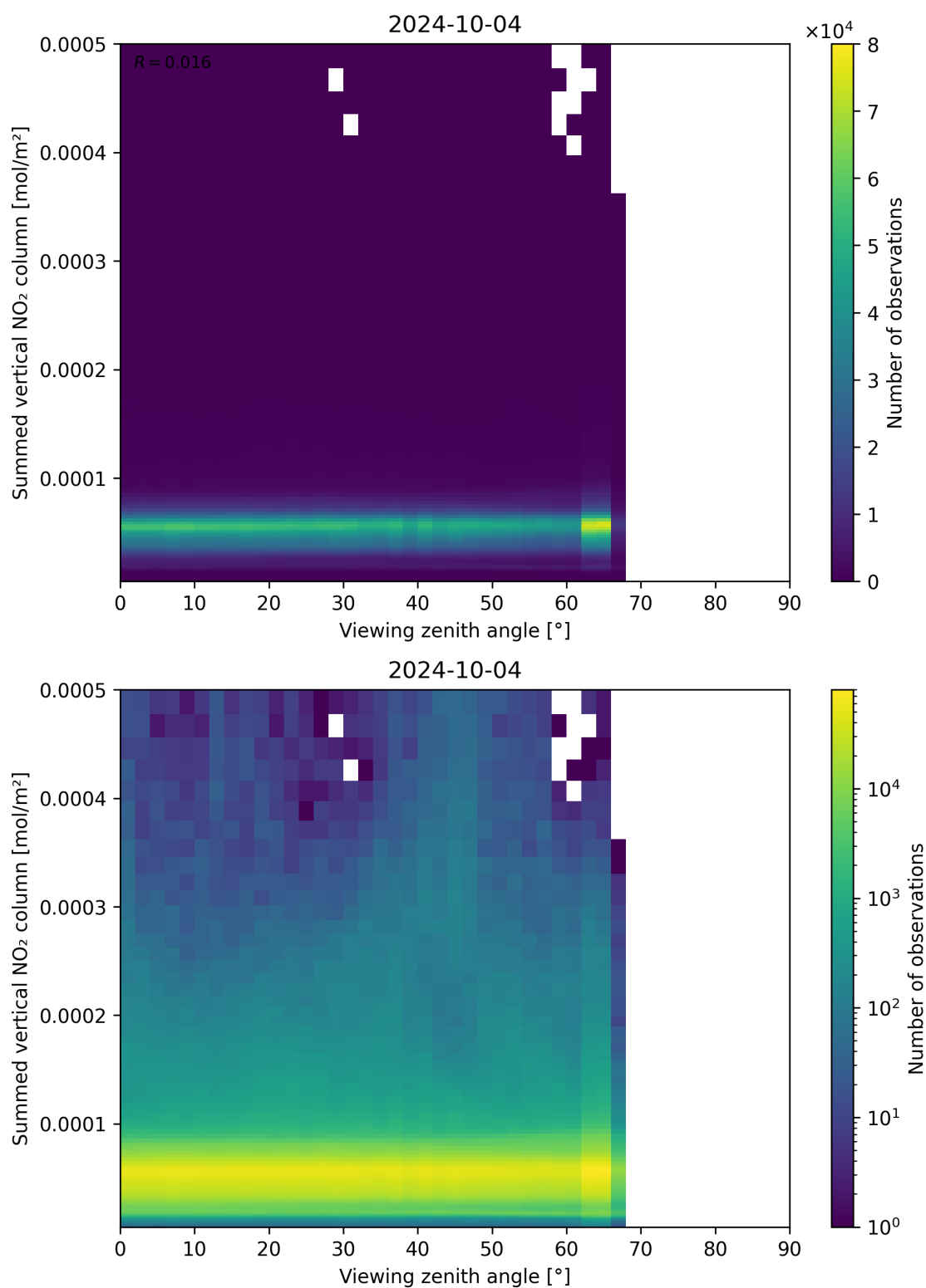
Figure 165: Scatter density plot of “Viewing zenith angle” against “Summed vertical NO 2 column” for 2024-10-03 to 2024-10-05.
