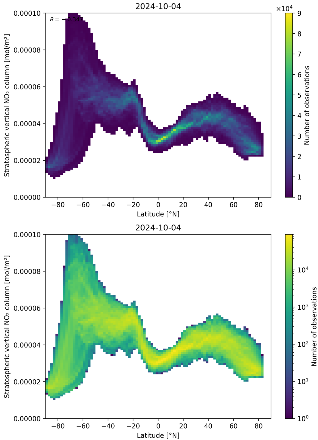
Figure 87: Scatter density plot of “Latitude” against “Stratospheric vertical NO 2 column” for 2024-10-03 to 2024-10-05.
