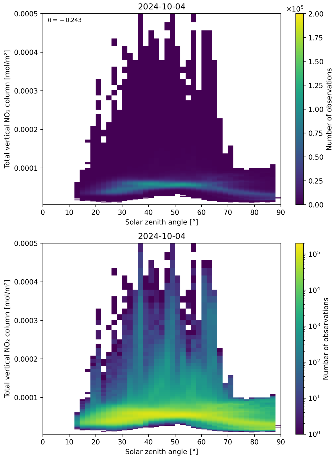
Figure 153: Scatter density plot of “Solar zenith angle” against “Total vertical NO 2 column” for 2024-10-03 to 2024-10-05.
