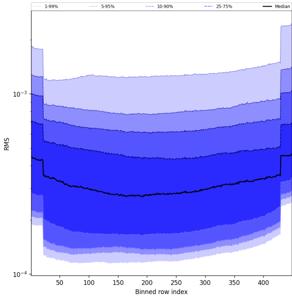
Figure 60: Along track statistics of “RMS” for 2024-10-03 to 2024-10-05
