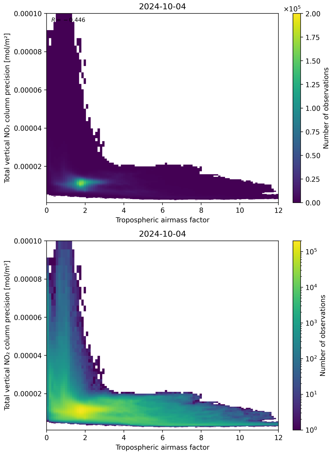
Figure 78: Scatter density plot of “Tropospheric air mass factor” against “Total vertical NO 2 column precision” for 2024-10-03 to 2024-10-05.
