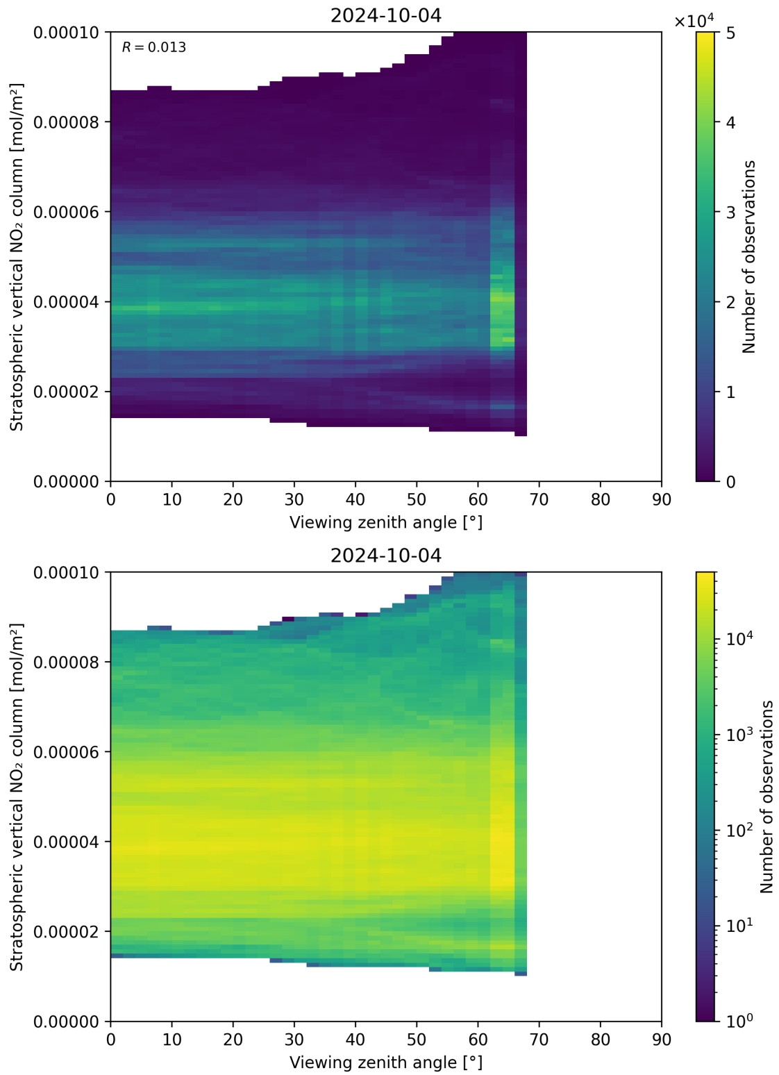
Figure 164: Scatter density plot of “Viewing zenith angle” against “Stratospheric vertical NO 2 column” for 2024-10-03 to 2024-10-05.
