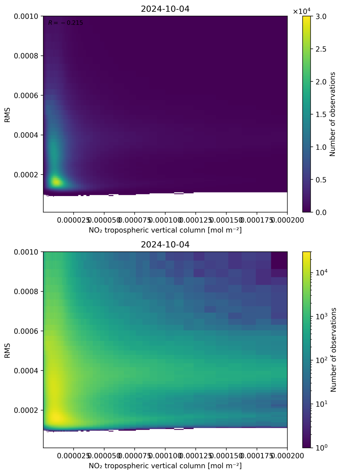
Figure 142: Scatter density plot of “NO 2 tropospheric vertical column” against “RMS” for 2024-10-03 to 2024-10-05.
