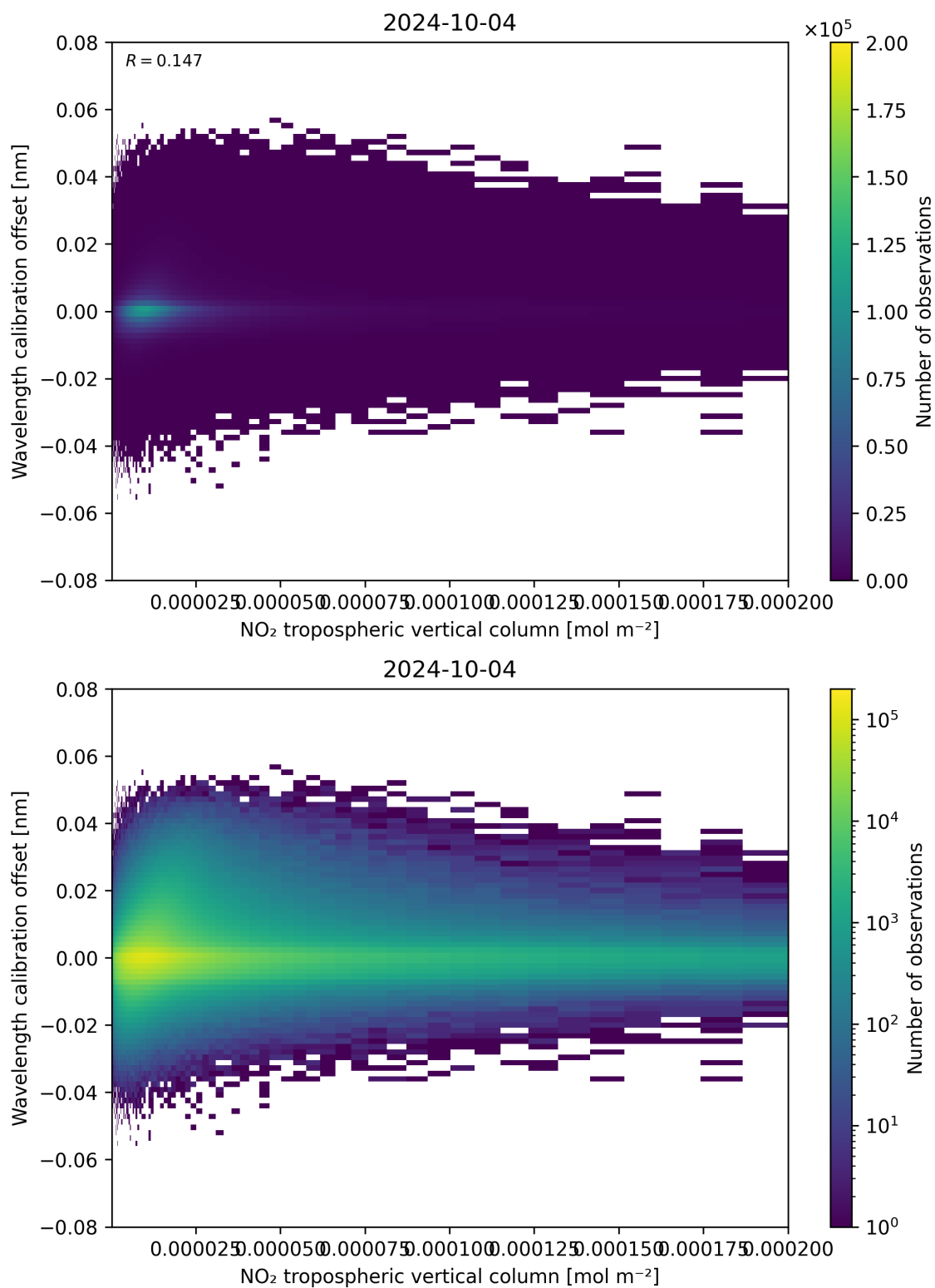
Figure 143: Scatter density plot of “NO 2 tropospheric vertical column” against “Wavelength calibration offset” for 2024-10-03 to 2024-10-05.
