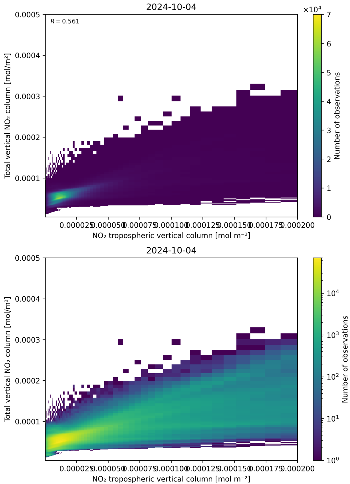
Figure 128: Scatter density plot of “NO 2 tropospheric vertical column” against “Total vertical NO 2 column” for 2024-10-03 to 2024-10-05.
