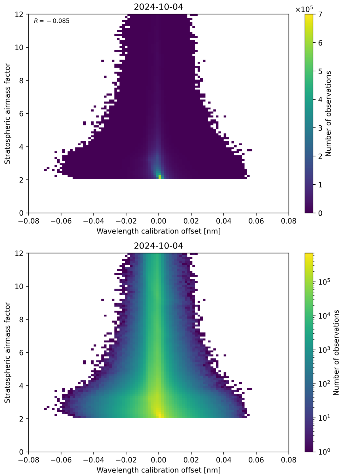
Figure 174: Scatter density plot of “Wavelength calibration offset” against “Stratospheric air mass factor” for 2024-10-03 to 2024-10-05.
