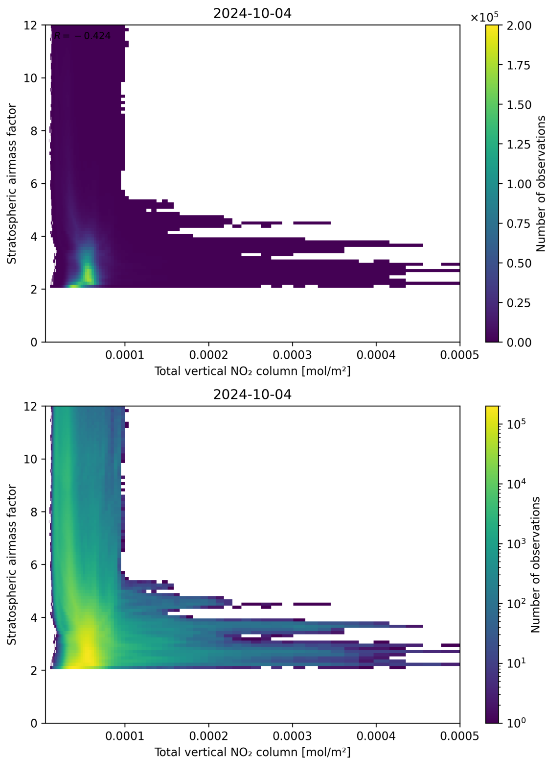
Figure 110: Scatter density plot of “Total vertical NO 2 column” against “Stratospheric airmass factor” for 2024-10-03 to 2024-10-05.
