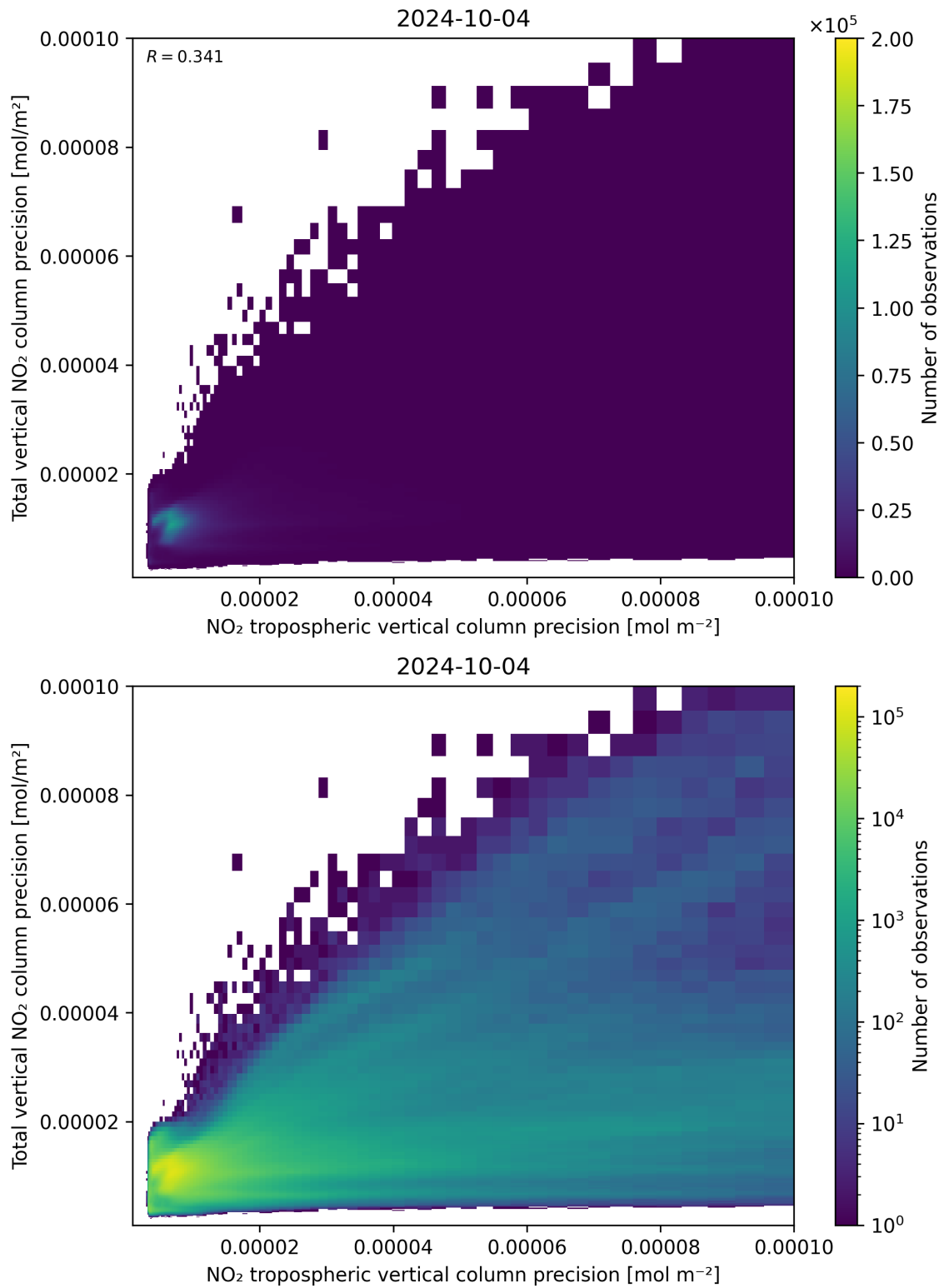
Figure 139: Scatter density plot of “NO 2 tropospheric vertical column precision” against “Total vertical NO 2 column precision” for 2024-10-03 to 2024-10-05.
