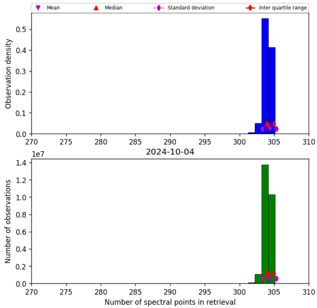
Figure 33: Histogram of “Number of spectral points in retrieval” for 2024-10-03 to 2024-10-05
