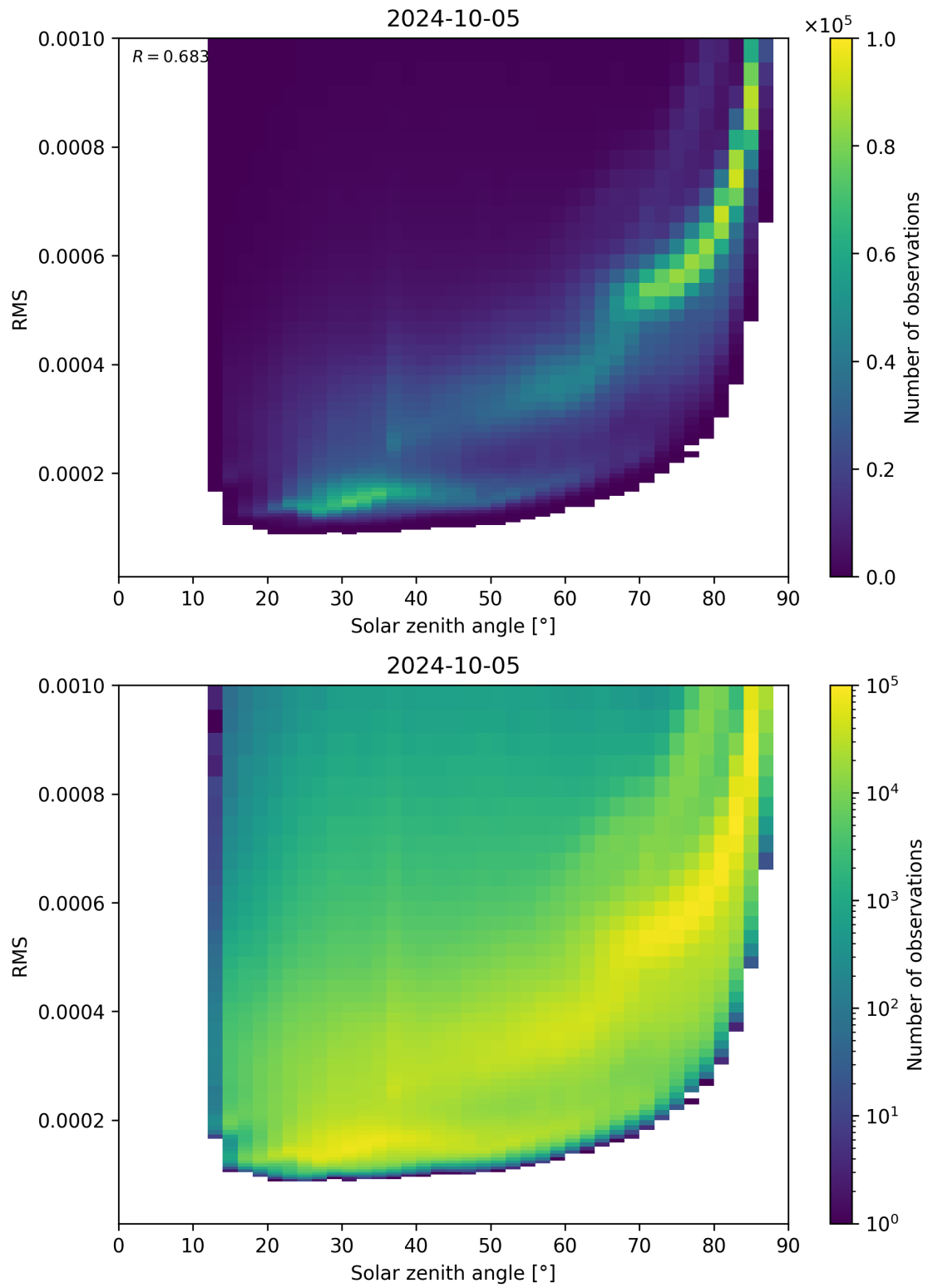
Figure 157: Scatter density plot of “Solar zenith angle” against “RMS” for 2024-10-04 to 2024-10-06.
