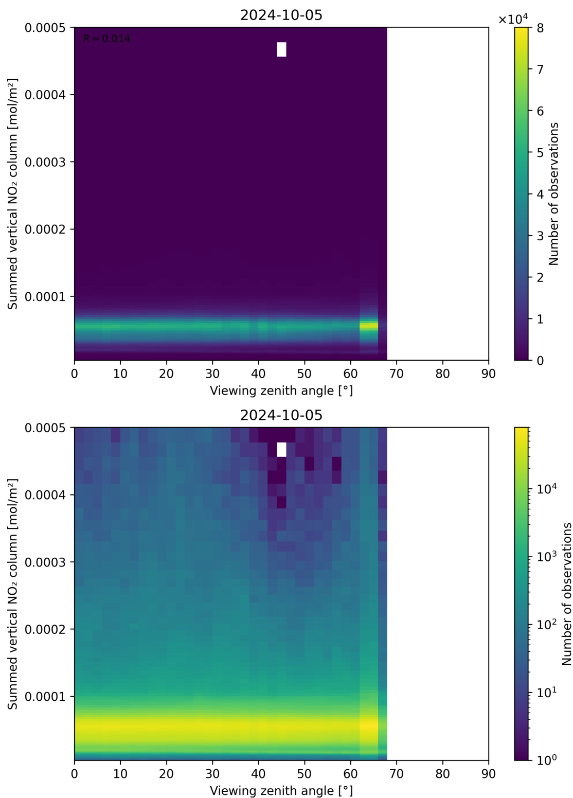
Figure 165: Scatter density plot of “Viewing zenith angle” against “Summed vertical NO 2 column” for 2024-10-04 to 2024-10-06.
