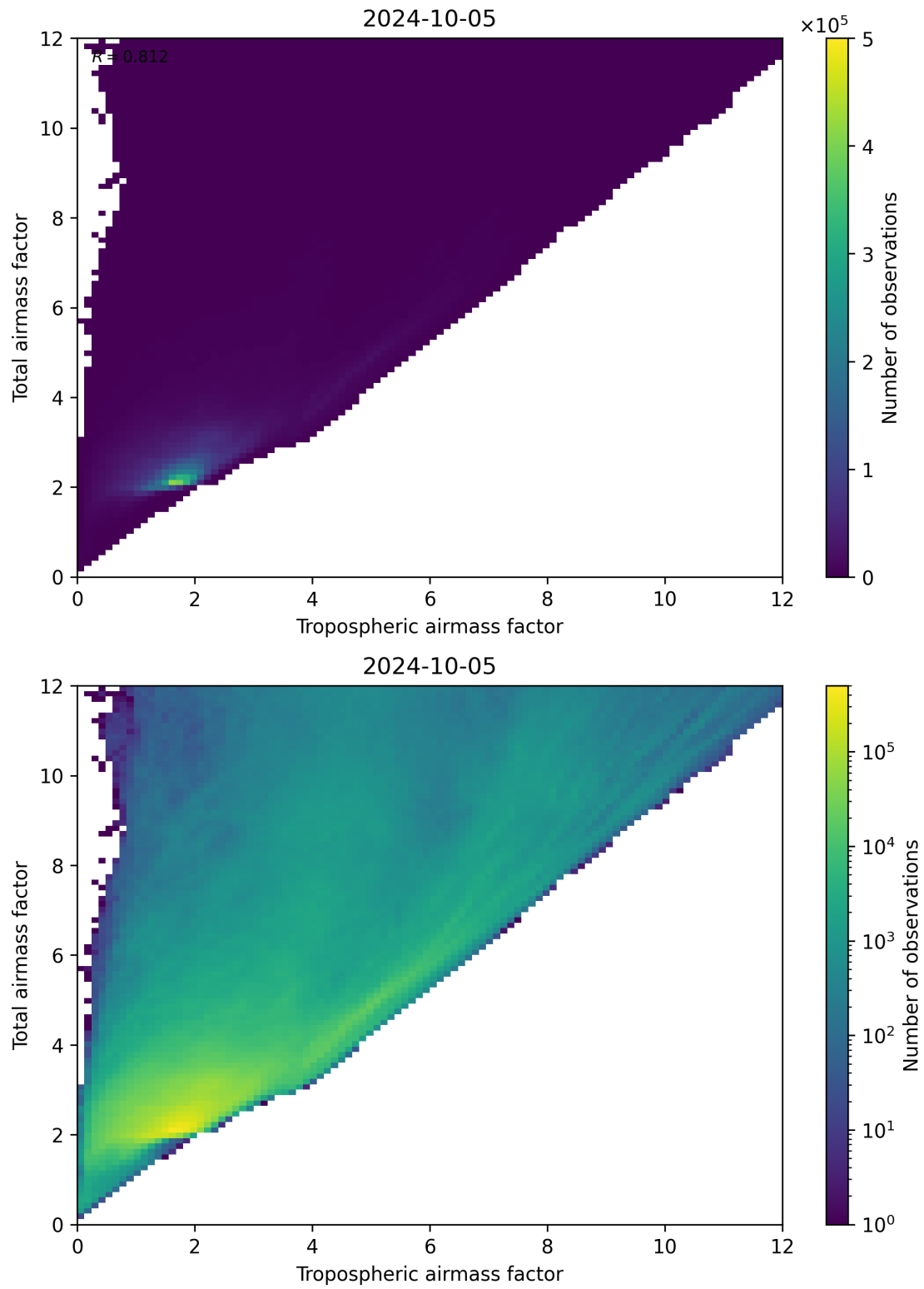
Figure 72: Scatter density plot of “Tropospheric airmass factor” against “Total airmass factor” for 2024-10-04 to 2024-10-06.
