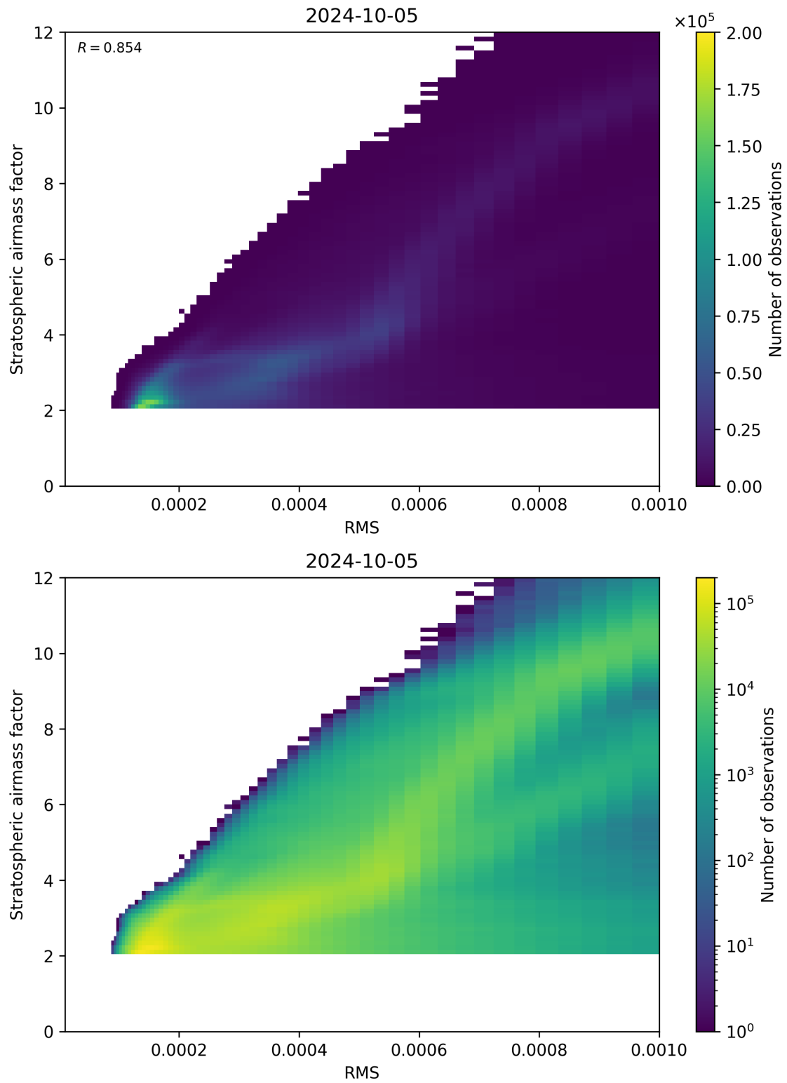
Figure 144: Scatter density plot of “RMS” against “Stratospheric airmass factor” for 2024-10-04 to 2024-10-06.
