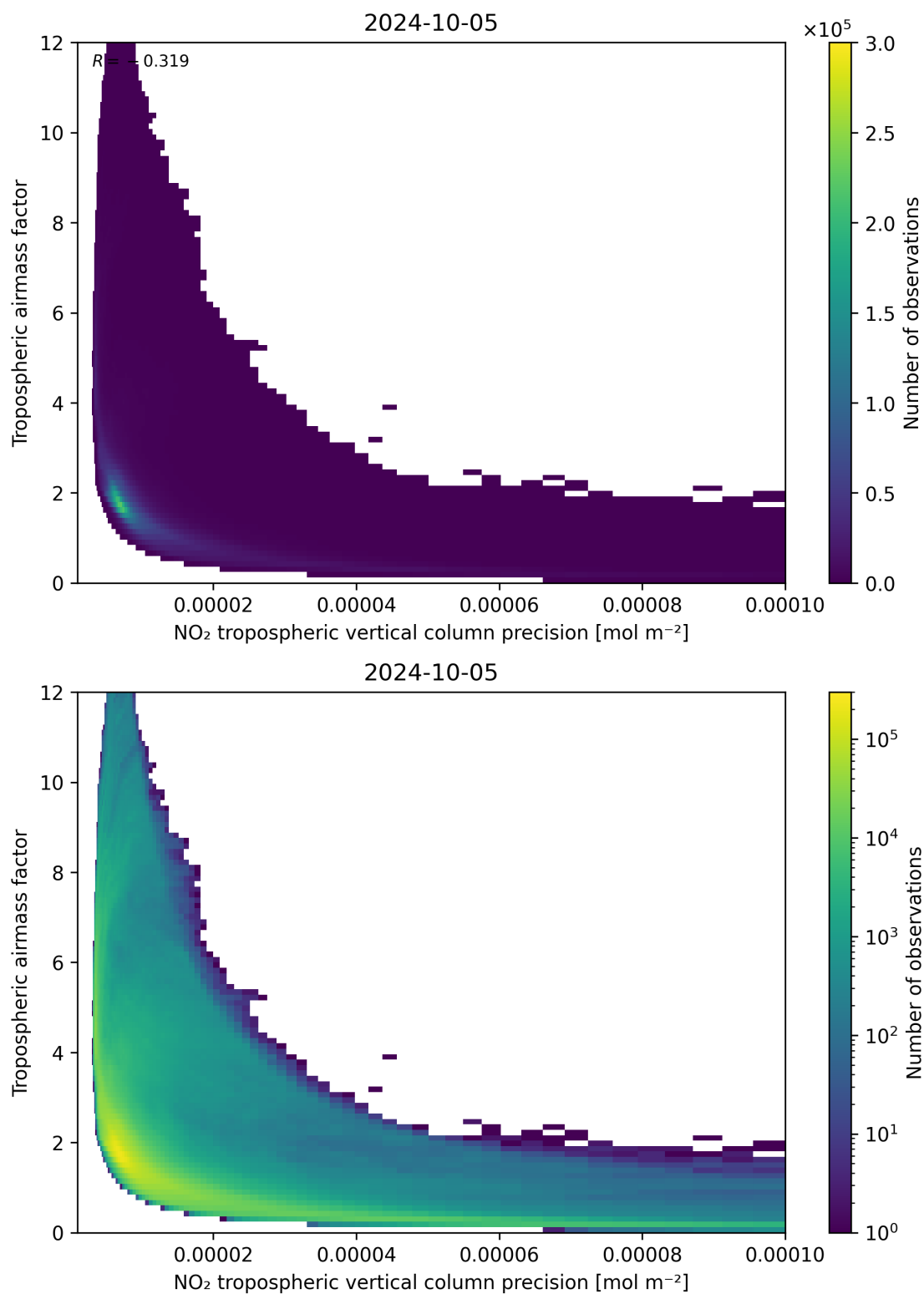
Figure 133: Scatter density plot of “NO 2 tropospheric vertical column precision” against “Tropospheric air mass factor” for 2024-10-04 to 2024-10-06.
