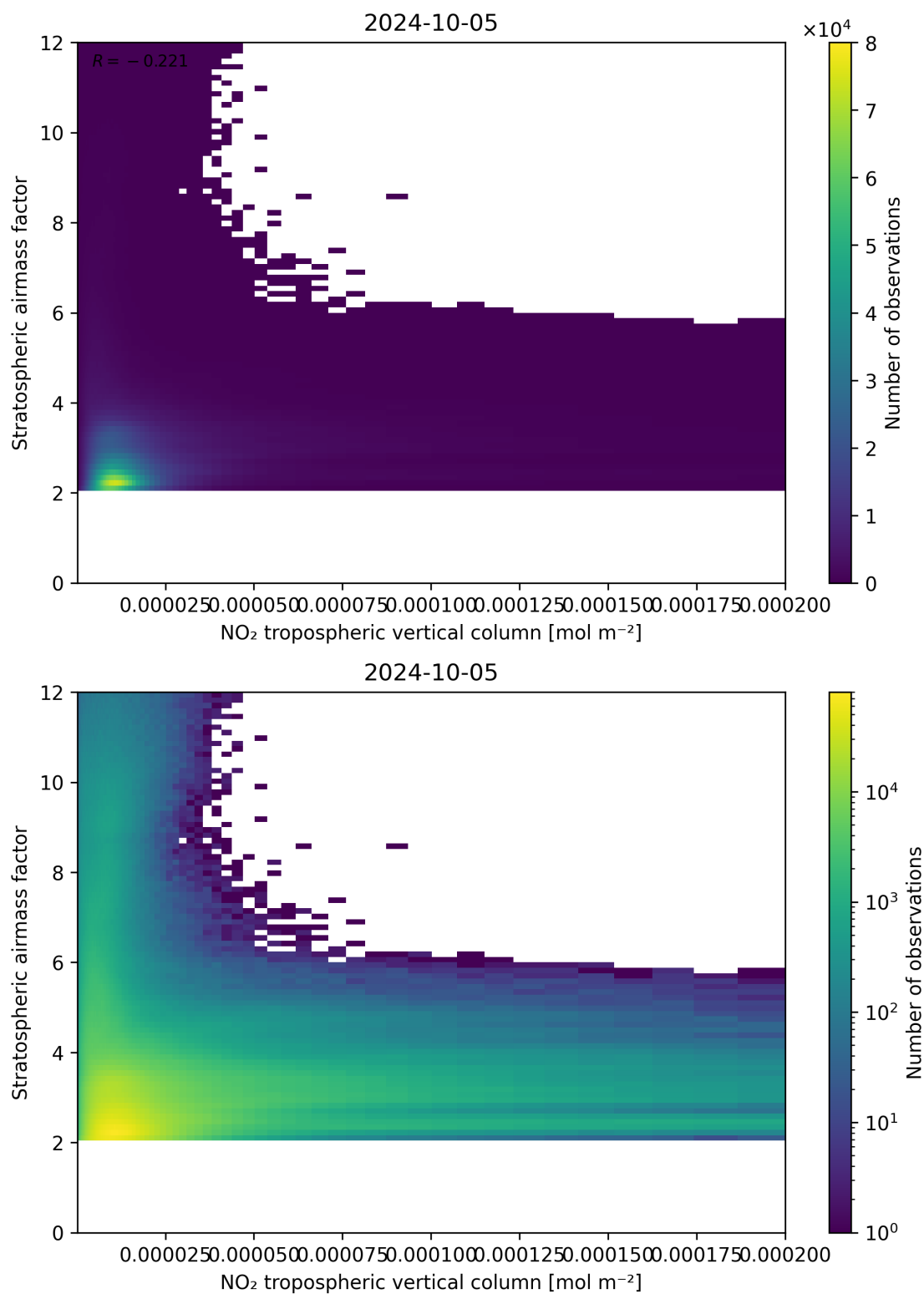
Figure 121: Scatter density plot of “NO 2 tropospheric vertical column” against “Stratospheric air mass factor” for 2024-10-04 to 2024-10-06.
