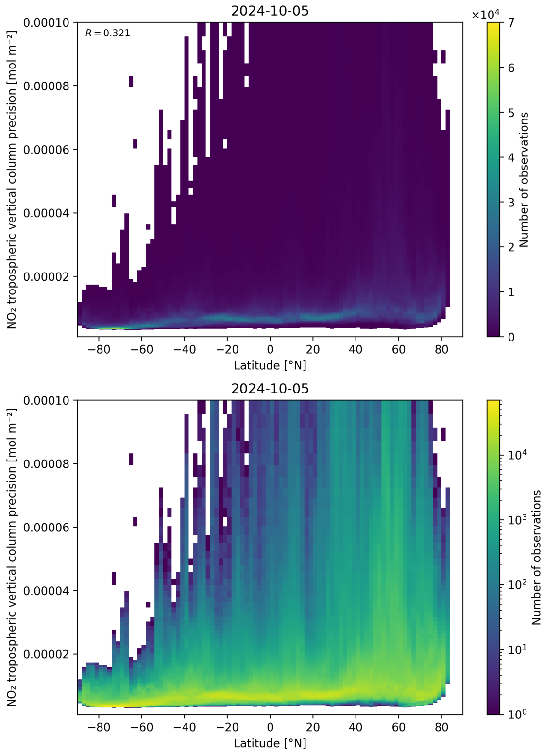
Figure 93: Scatter density plot of “Latitude” against “NO 2 tropospheric vertical column precision” for 2024-10-04 to 2024-10-06.
