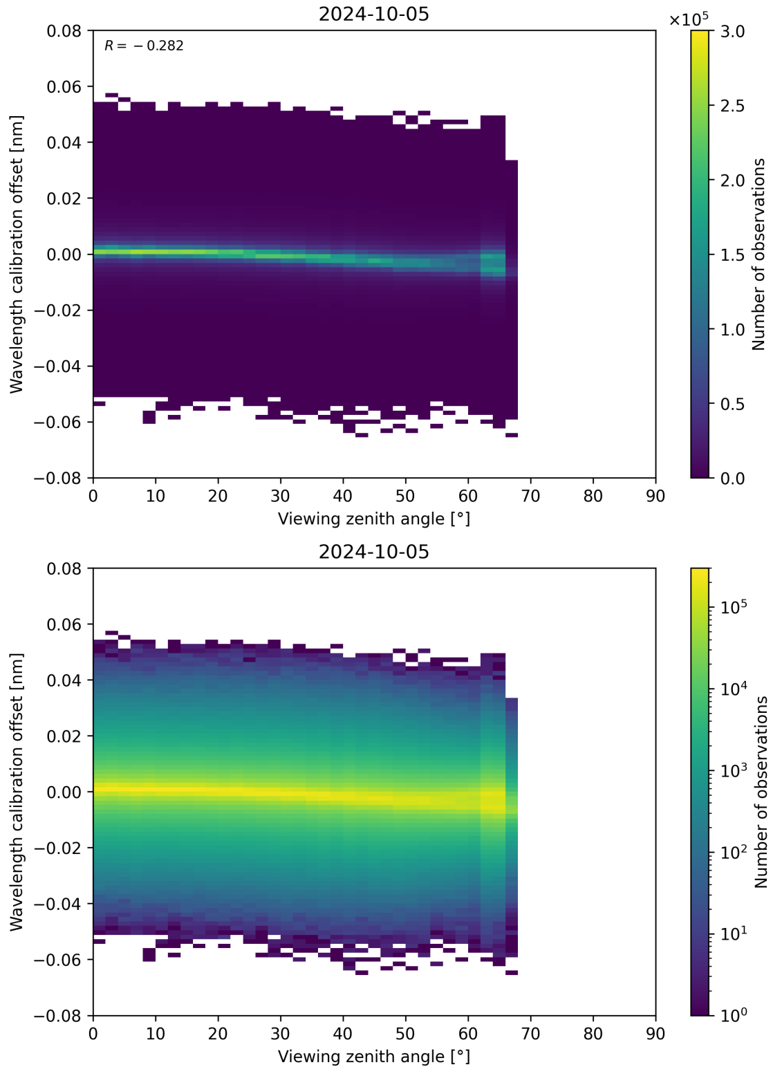
Figure 173: Scatter density plot of “Viewing zenith angle” against “Wavelength calibration offset” for 2024-10-04 to 2024-10-06.
