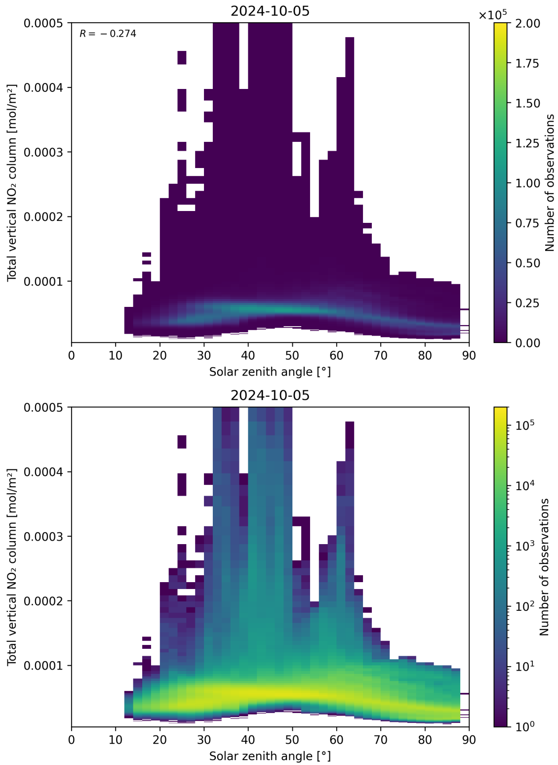
Figure 153: Scatter density plot of “Solar zenith angle” against “Total vertical NO 2 column” for 2024-10-04 to 2024-10-06.
