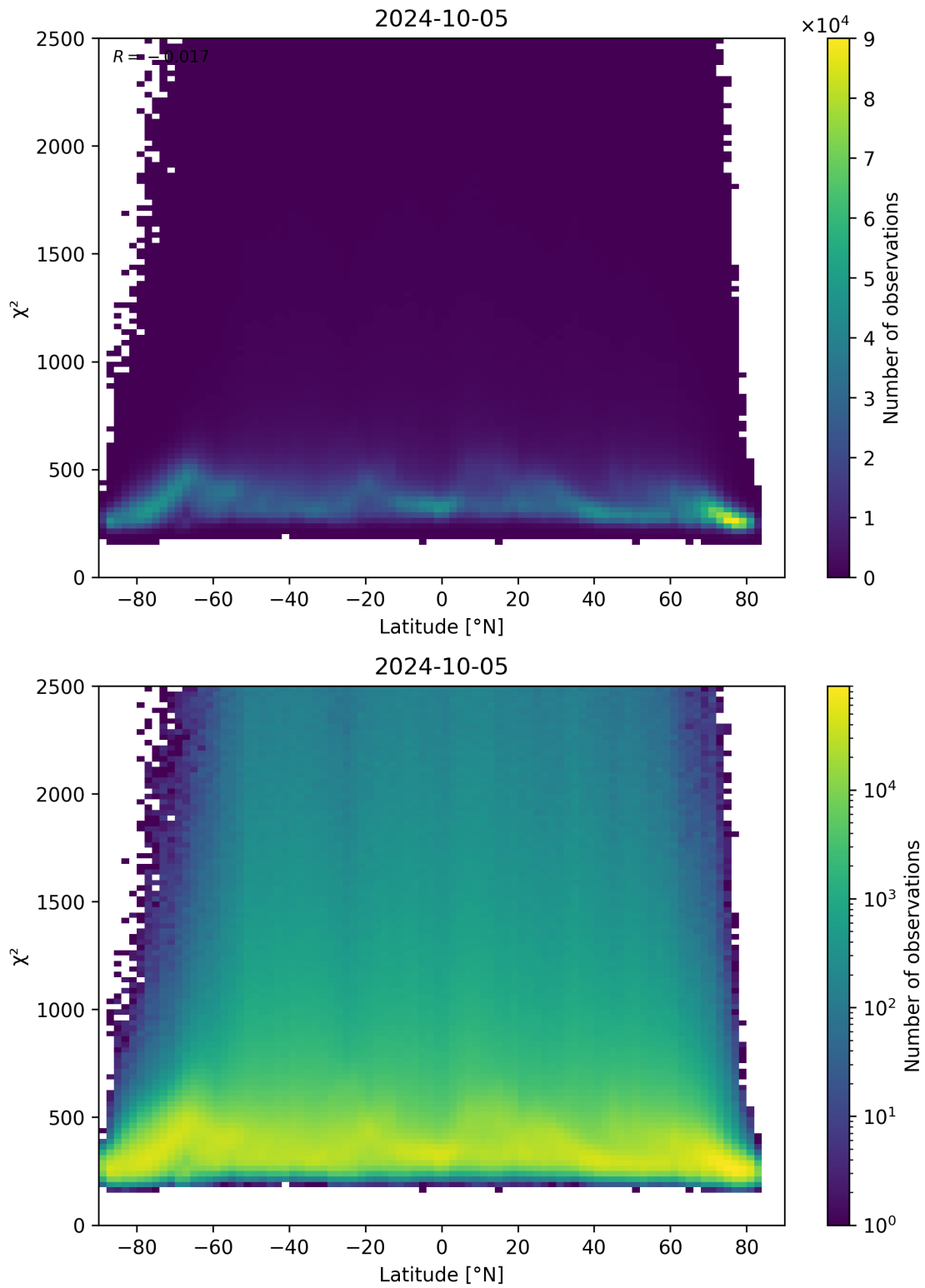
Figure 86: Scatter density plot of “Latitude” against “ \chi^2 ” for 2024-10-04 to 2024-10-06.
