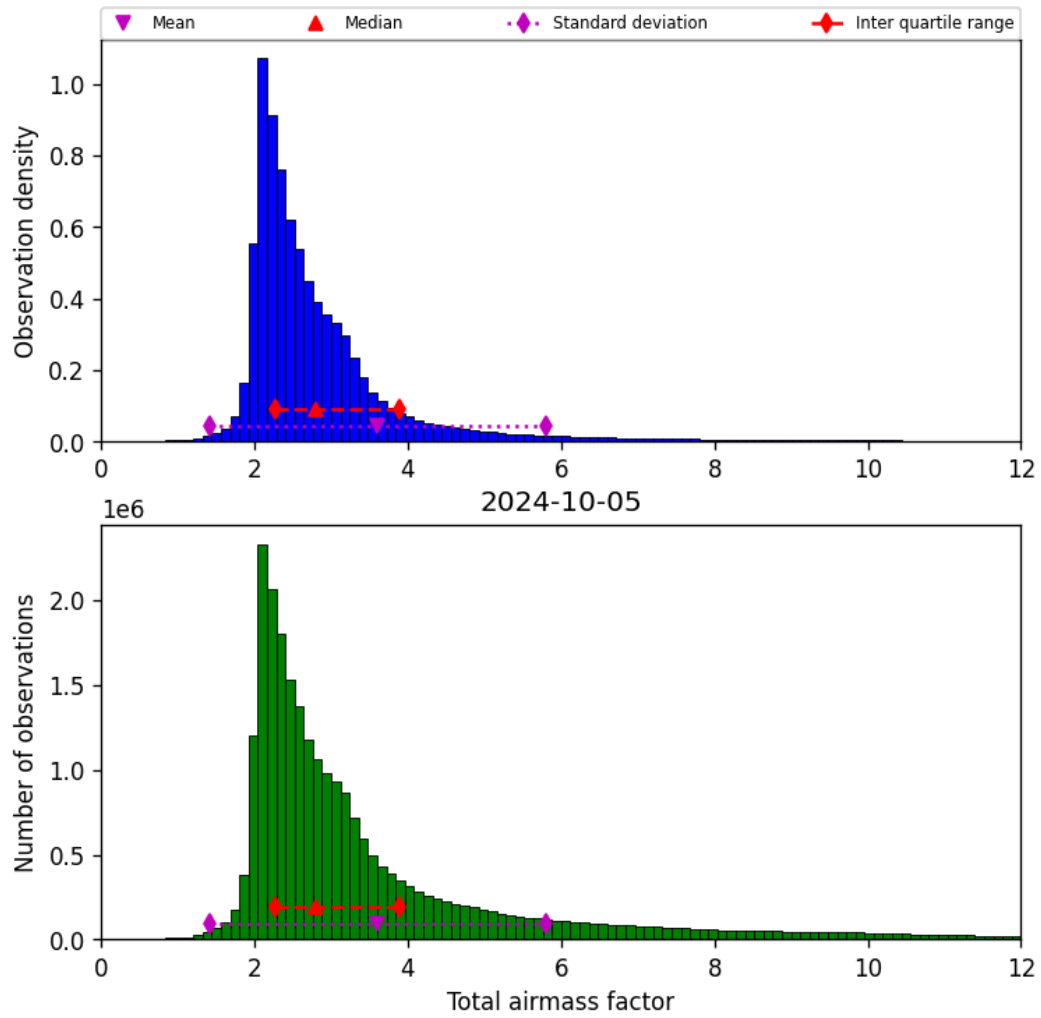
Figure 32: Histogram of “Total airmass factor” for 2024-10-04 to 2024-10-06
