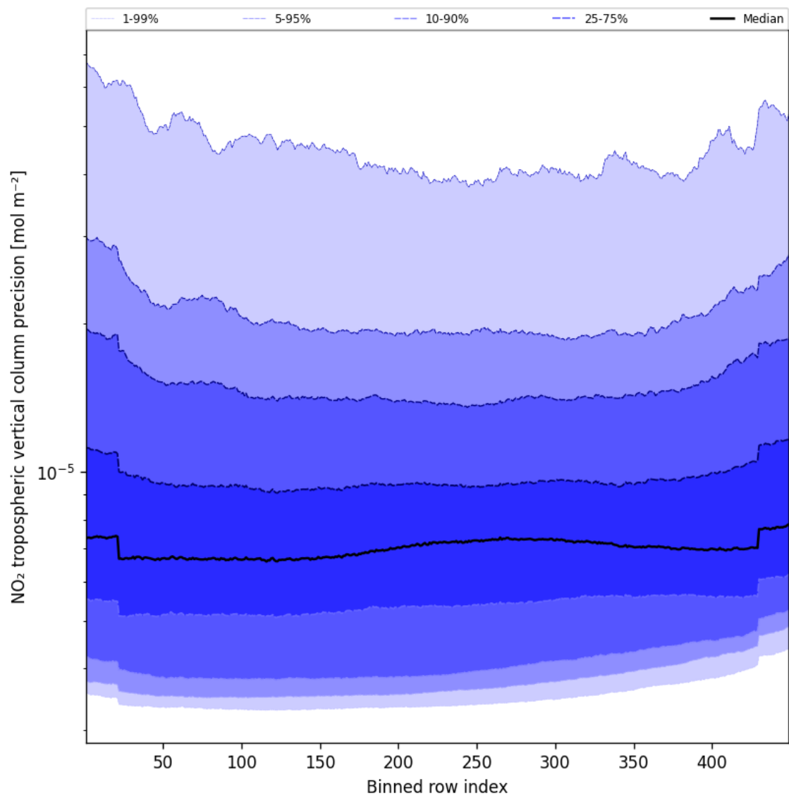
Figure 47: Along track statistics of “NO 2 tropospheric vertical column precision” for 2024-10-04 to 2024-10-06
