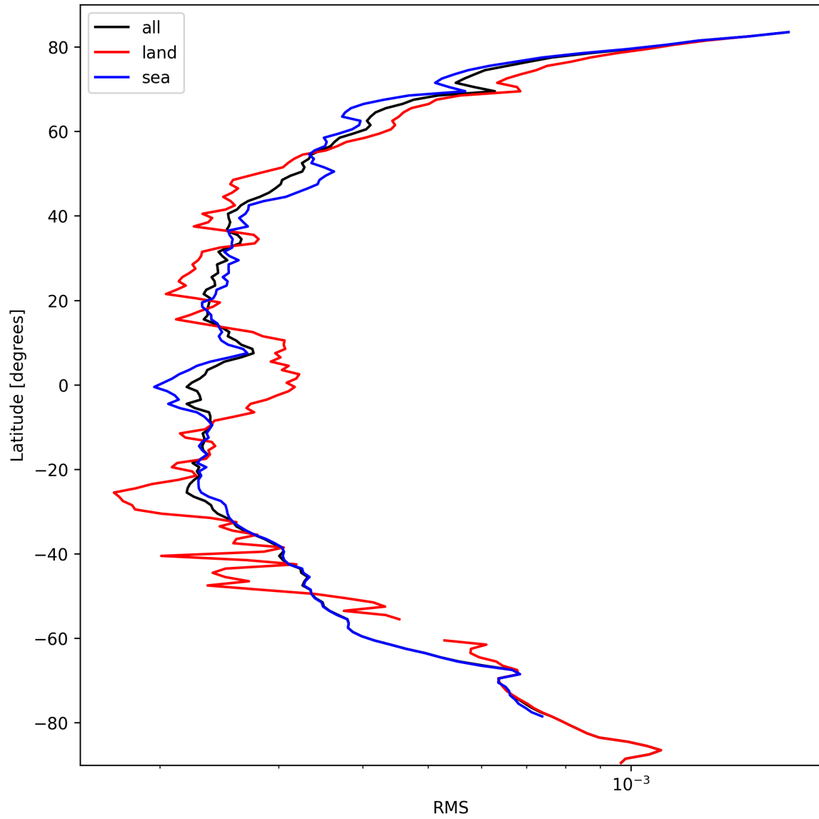
Figure 26: Zonal average of “RMS” for 2024-10-04 to 2024-10-06.
