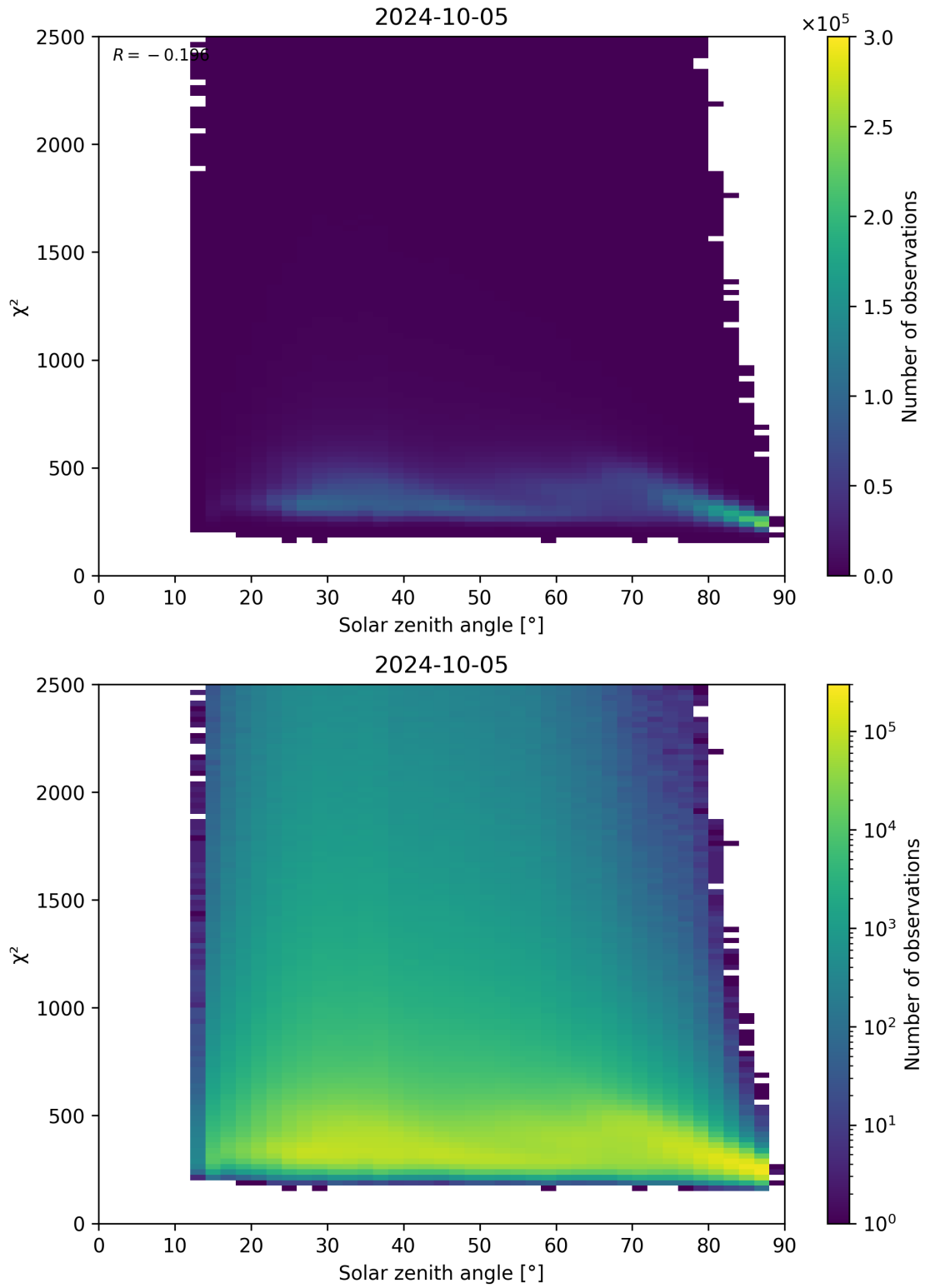
Figure 148: Scatter density plot of “Solar zenith angle” against “ \chi^2 ” for 2024-10-04 to 2024-10-06.
