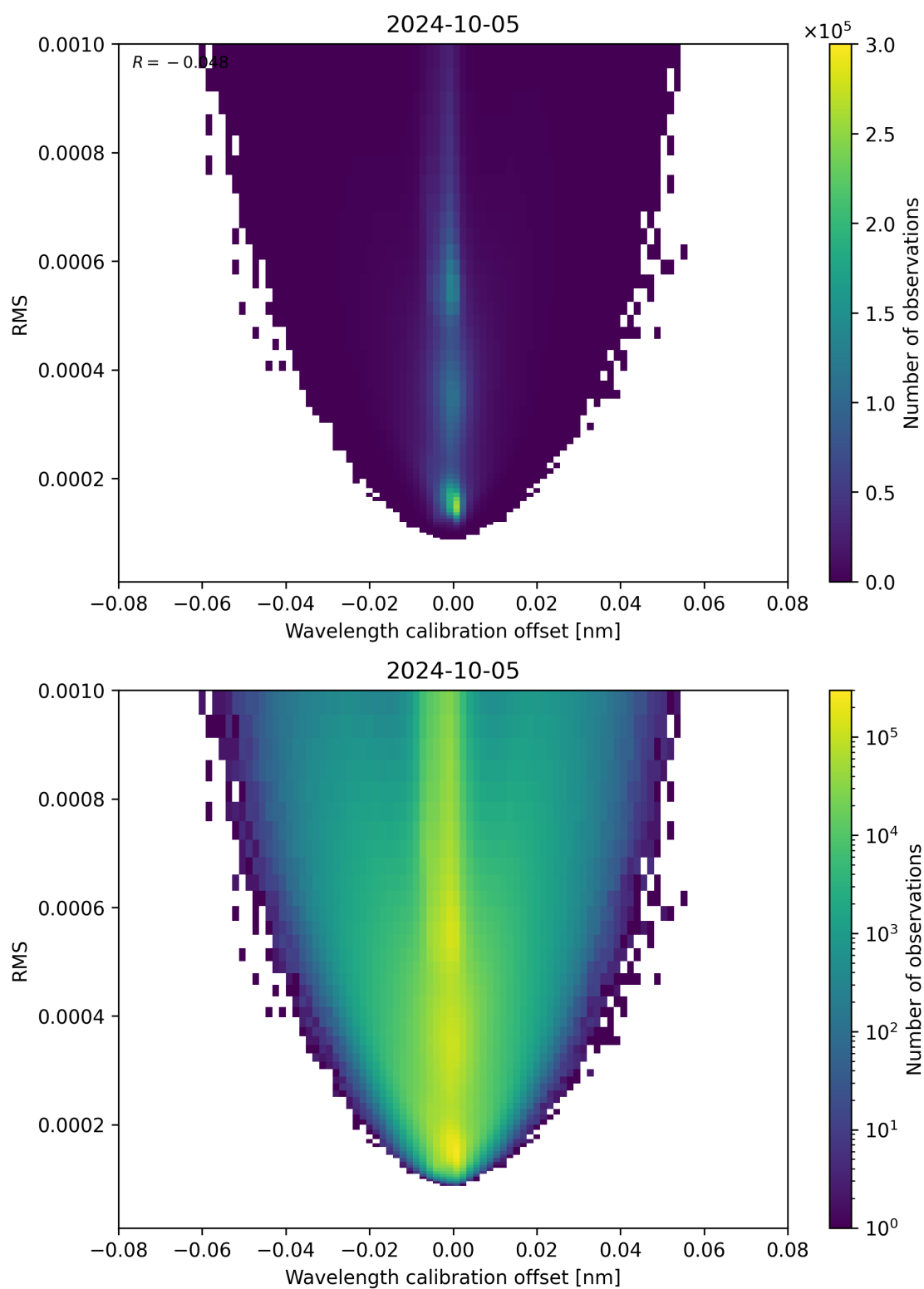
Figure 181: Scatter density plot of “Wavelength calibration offset” against “RMS” for 2024-10-04 to 2024-10-06.
