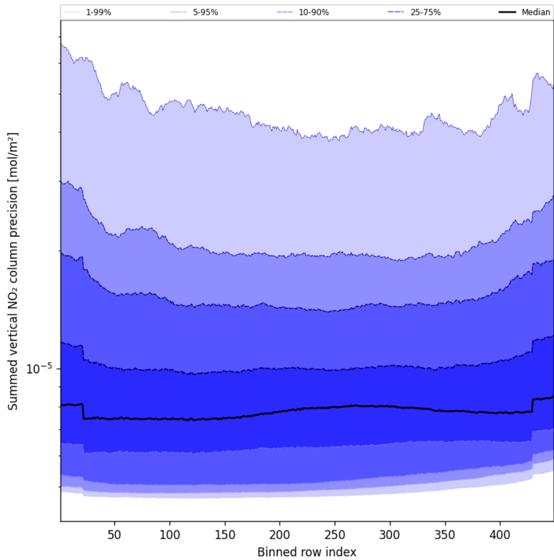
Figure 58: Along track statistics of “Summed vertical NO 2 column precision” for 2024-10-04 to 2024-10-06
