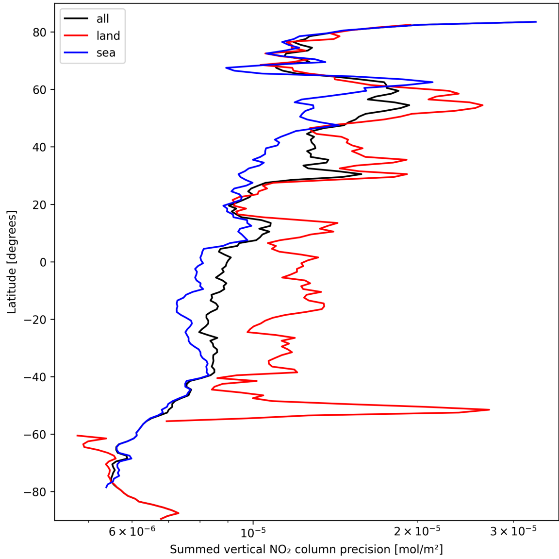
Figure 24: Zonal average of “Summed vertical NO 2 column precision” for 2024-10-04 to 2024-10-06.
