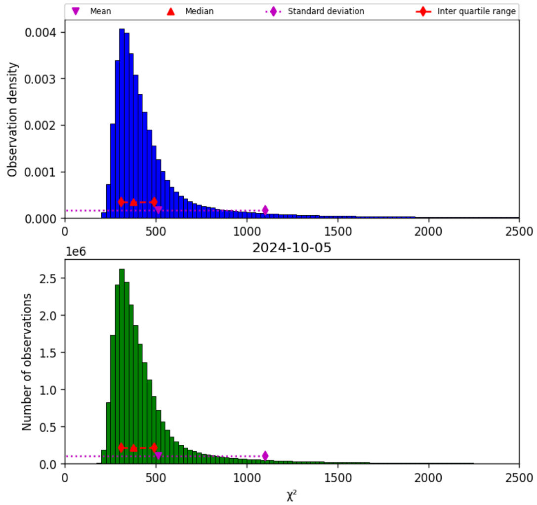
Figure 42: Histogram of “ \chi^2 ” for 2024-10-04 to 2024-10-06
