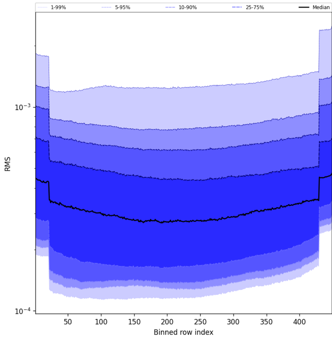
Figure 60: Along track statistics of “RMS” for 2024-10-04 to 2024-10-06
