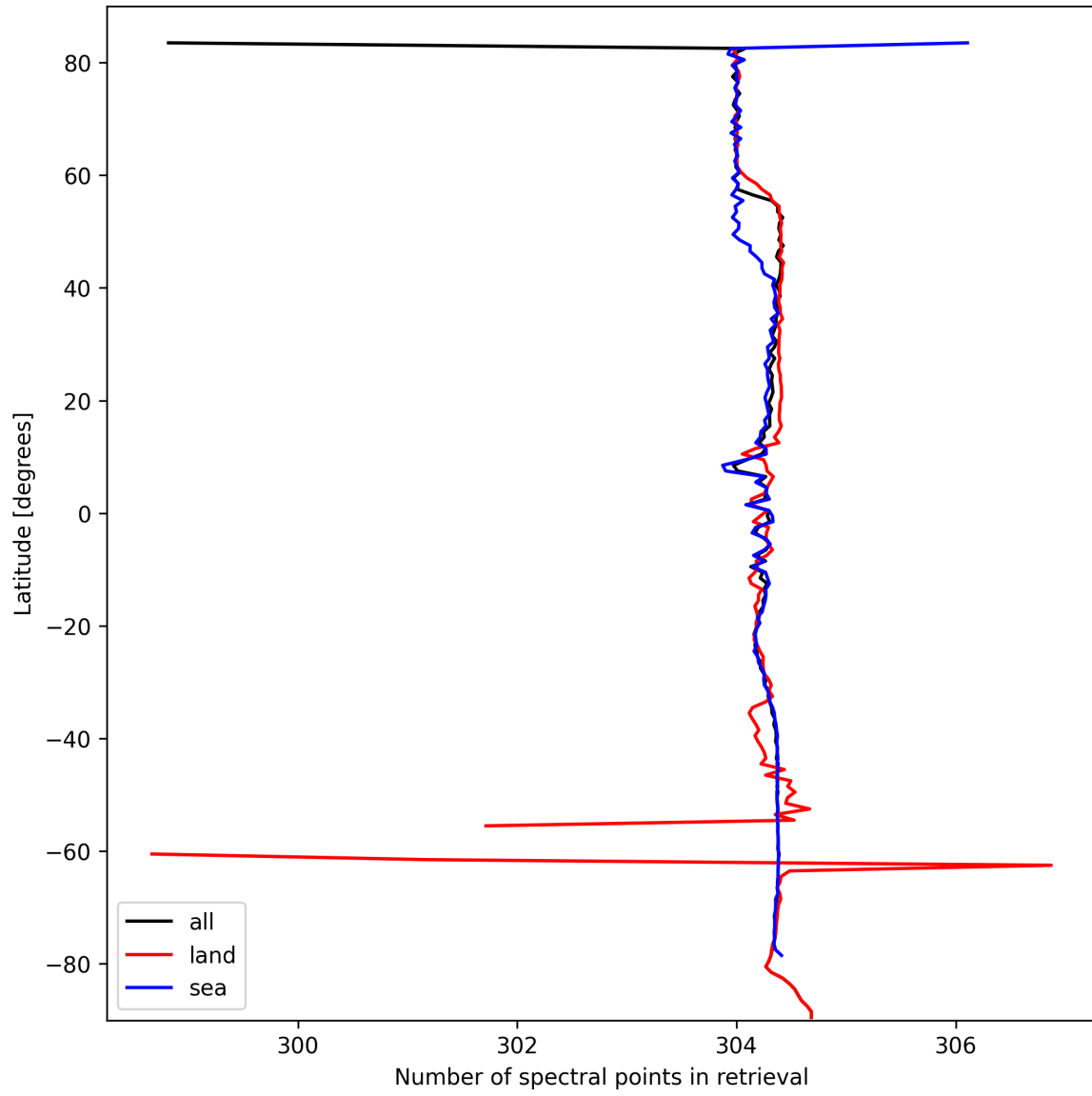
Figure 16: Zonal average of “Number of spectral points in retrieval” for 2024-10-04 to 2024-10-06.
