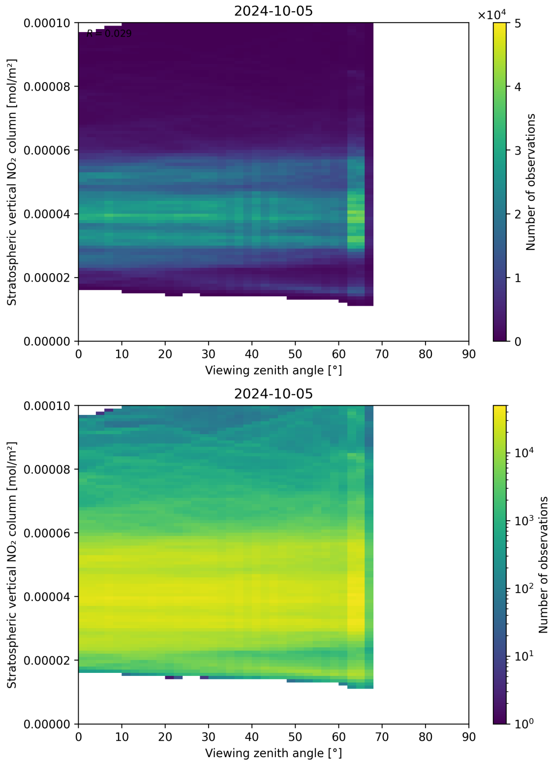
Figure 164: Scatter density plot of “Viewing zenith angle” against “Stratospheric vertical NO 2 column” for 2024-10-04 to 2024-10-06.
