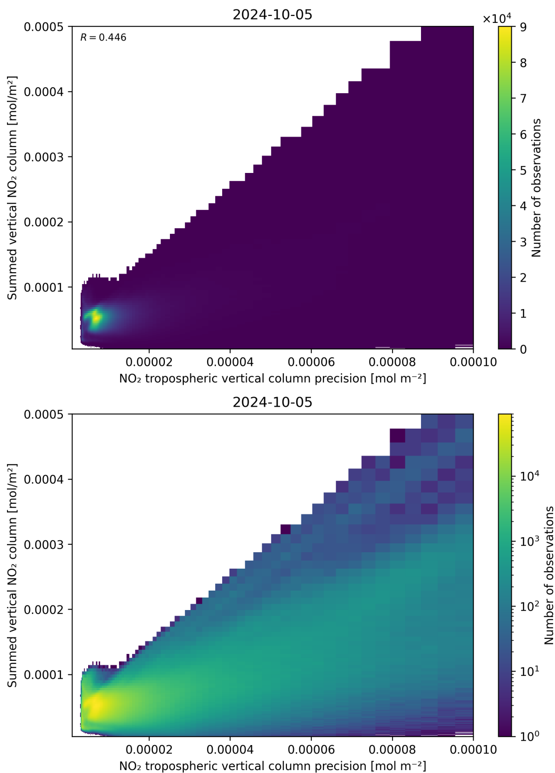
Figure 136: Scatter density plot of “NO 2 tropospheric vertical column precision” against “Summed vertical NO 2 column” for 2024-10-04 to 2024-10-06.
