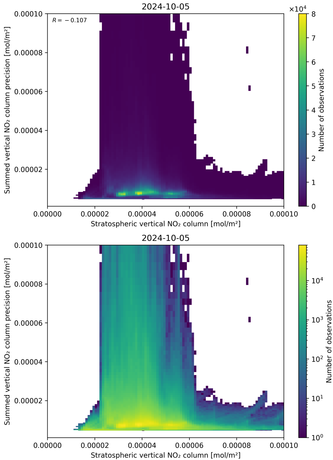
Figure 99: Scatter density plot of “Stratospheric vertical NO 2 column” against “Summed vertical NO 2 column precision” for 2024-10-04 to 2024-10-06.
