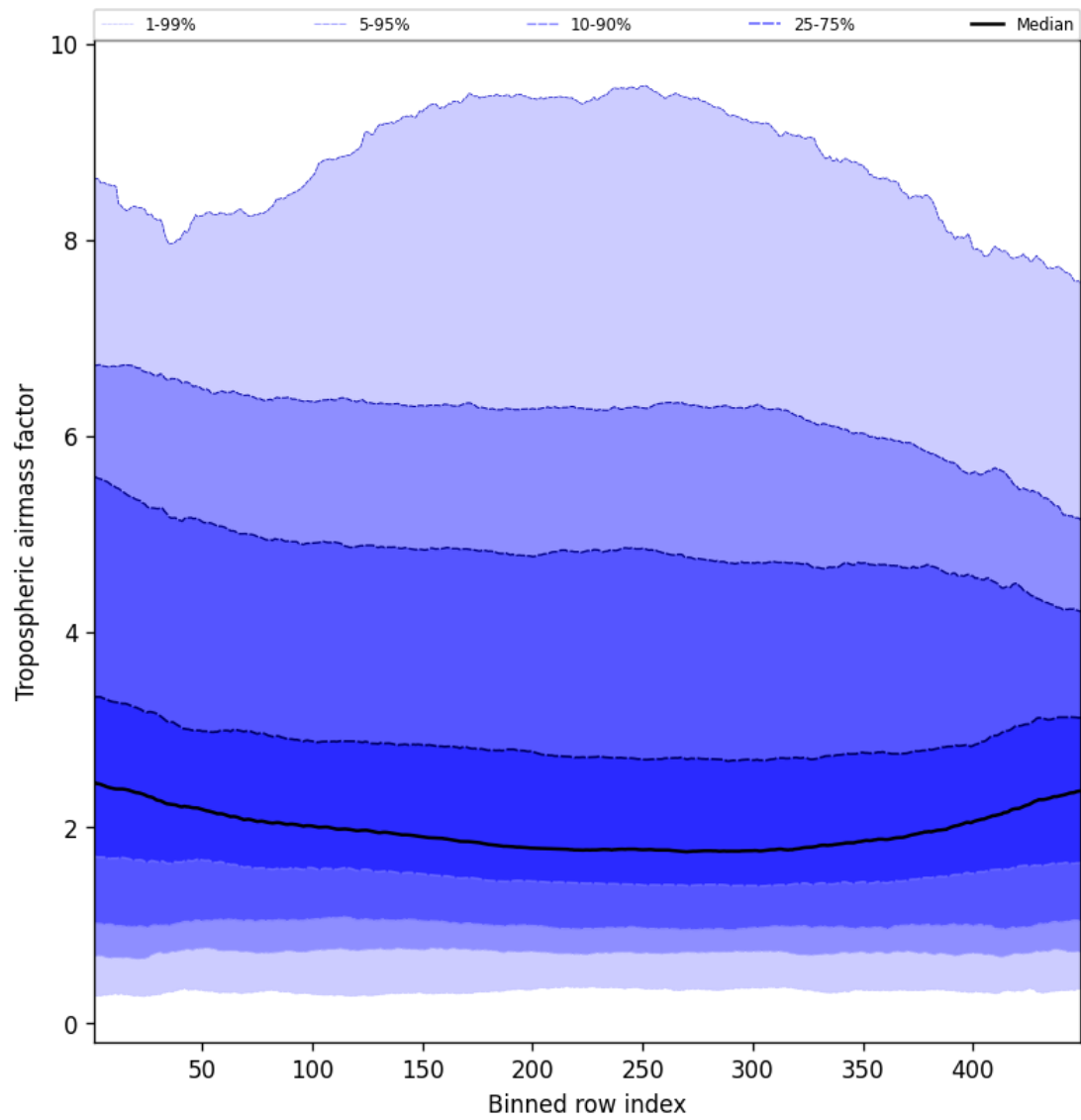
Figure 48: Along track statistics of “Tropospheric airmass factor” for 2024-10-04 to 2024-10-06
