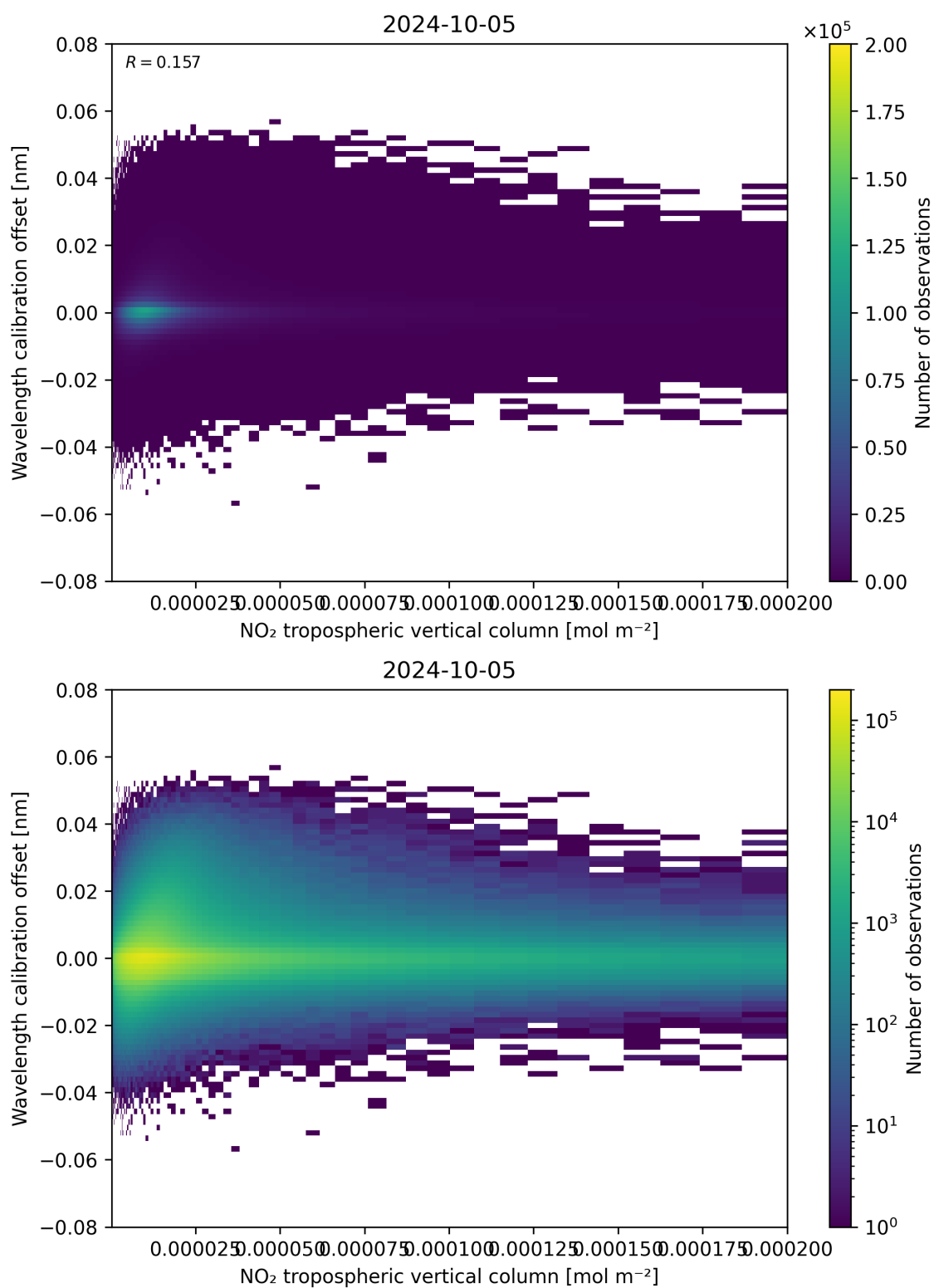
Figure 143: Scatter density plot of “NO 2 tropospheric vertical column” against “Wavelength calibration offset” for 2024-10-04 to 2024-10-06.
