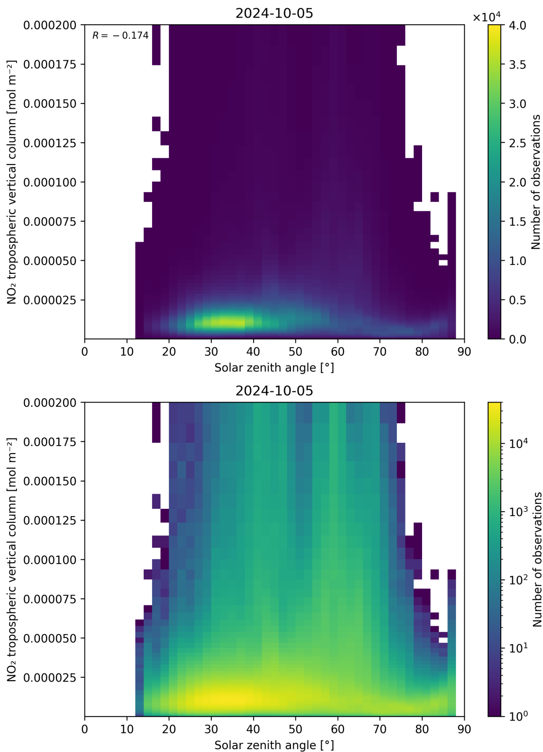
Figure 155: Scatter density plot of “Solar zenith angle” against “NO 2 tropospheric vertical column” for 2024-10-04 to 2024-10-06.
