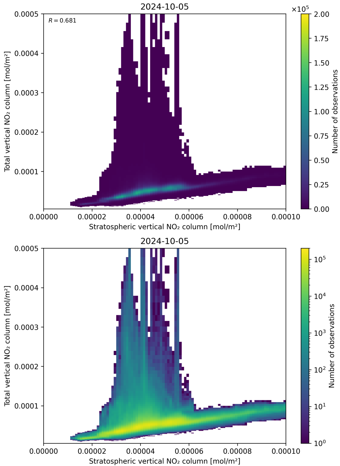
Figure 100: Scatter density plot of “Stratospheric vertical NO 2 column” against “Total vertical NO 2 column” for 2024-10-04 to 2024-10-06.
