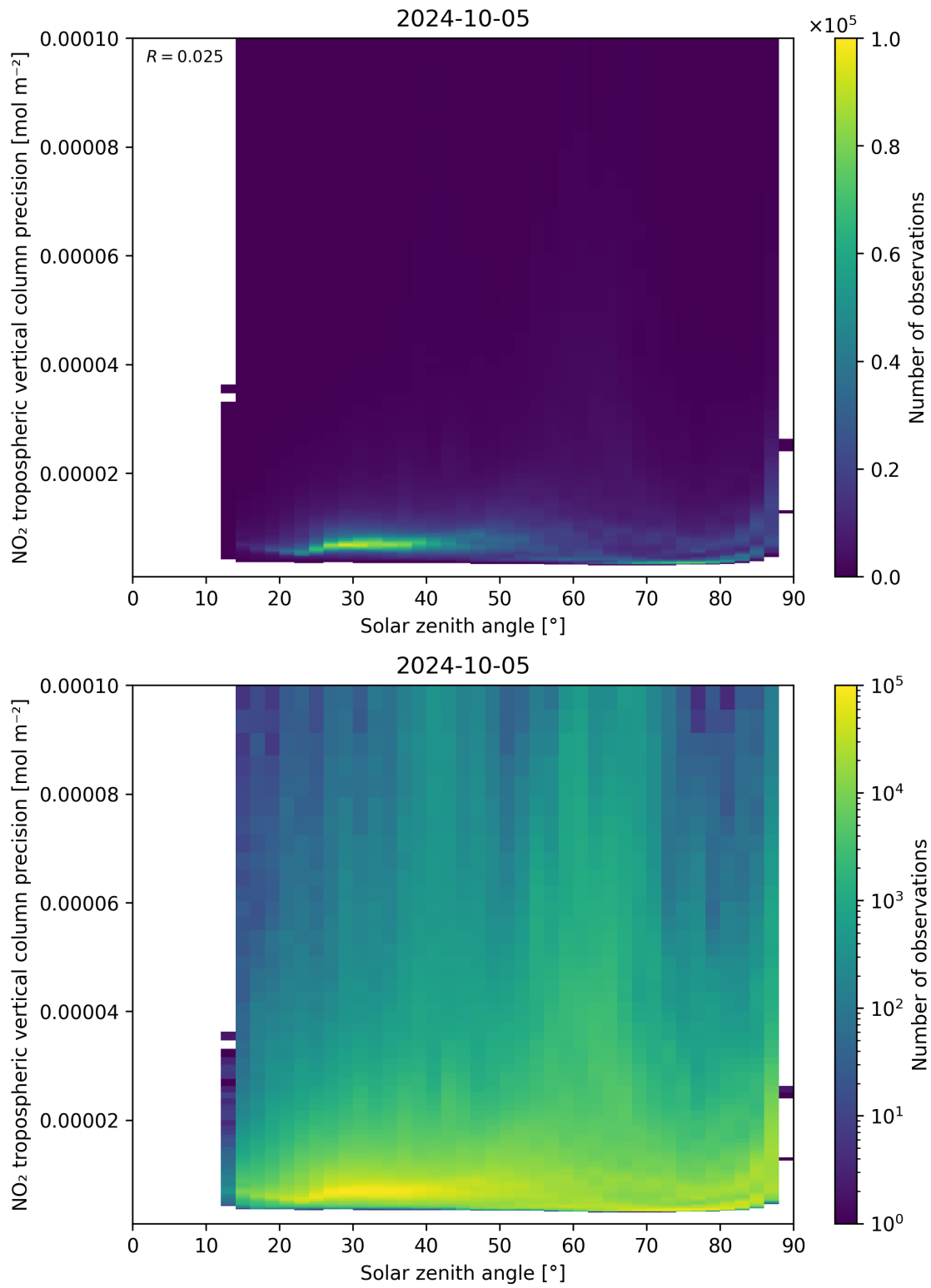
Figure 156: Scatter density plot of “Solar zenith angle” against “NO 2 tropospheric vertical column precision” for 2024-10-04 to 2024-10-06.
