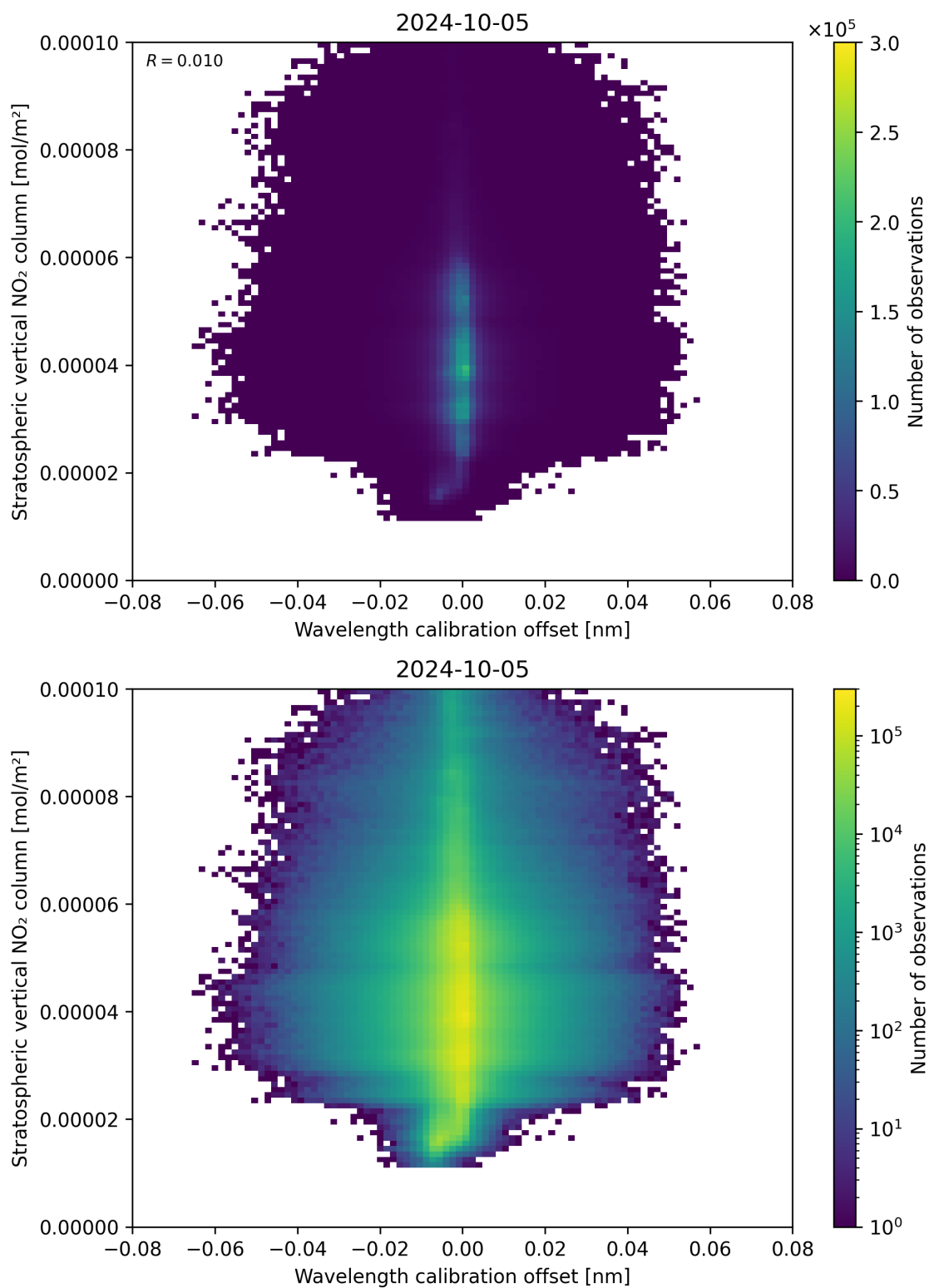
Figure 176: Scatter density plot of “Wavelength calibration offset” against “Stratospheric vertical NO 2 column” for 2024-10-04 to 2024-10-06.
