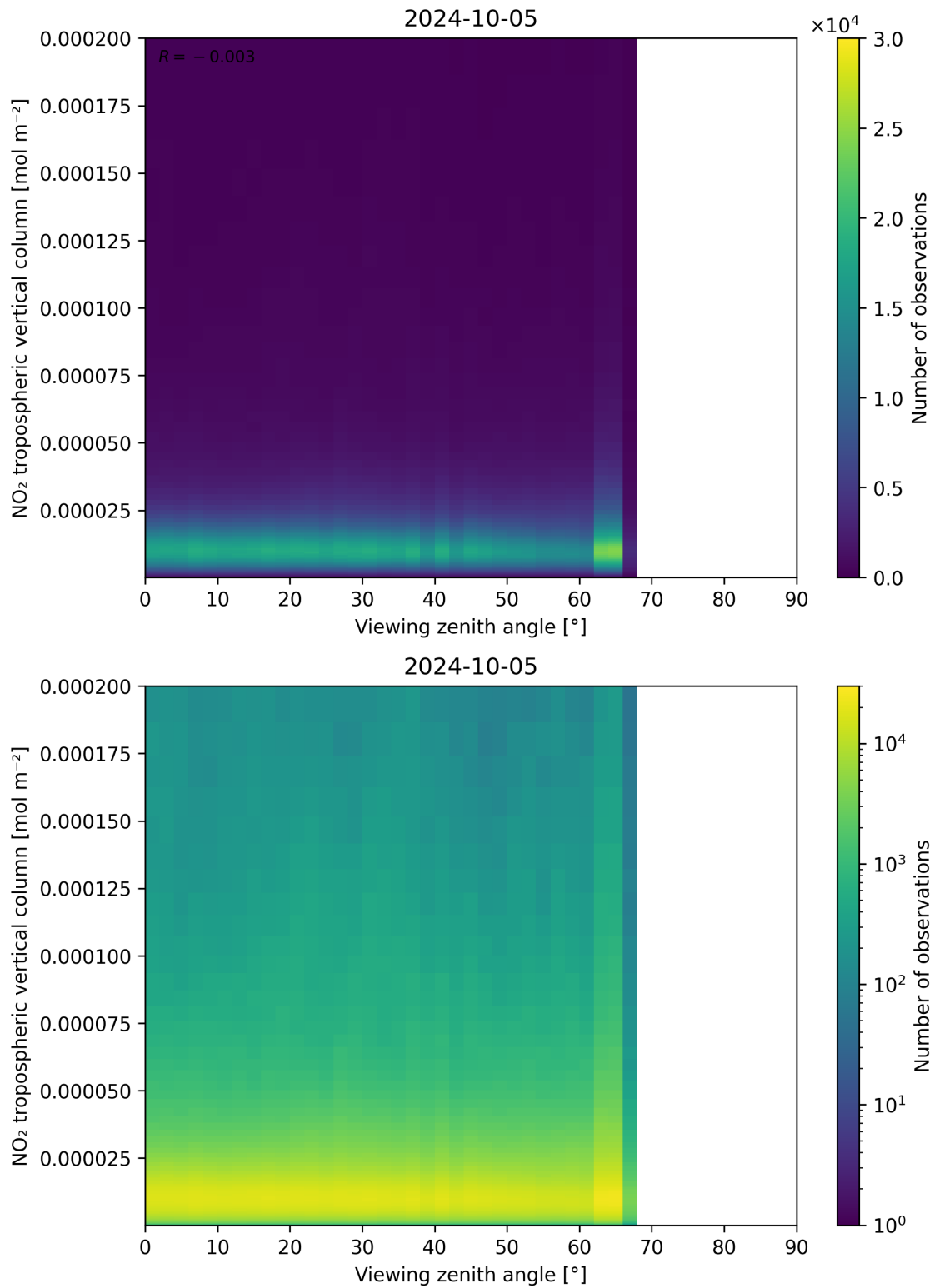
Figure 169: Scatter density plot of “Viewing zenith angle” against “NO 2 tropospheric vertical column” for 2024-10-04 to 2024-10-06.
