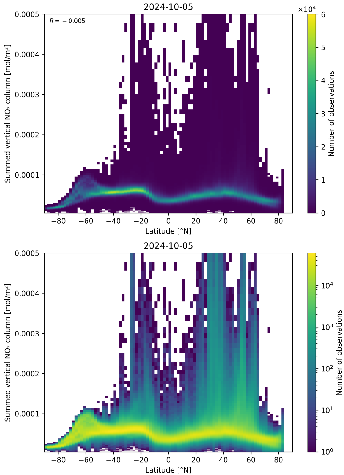
Figure 88: Scatter density plot of “Latitude” against “Summed vertical NO 2 column” for 2024-10-04 to 2024-10-06.
