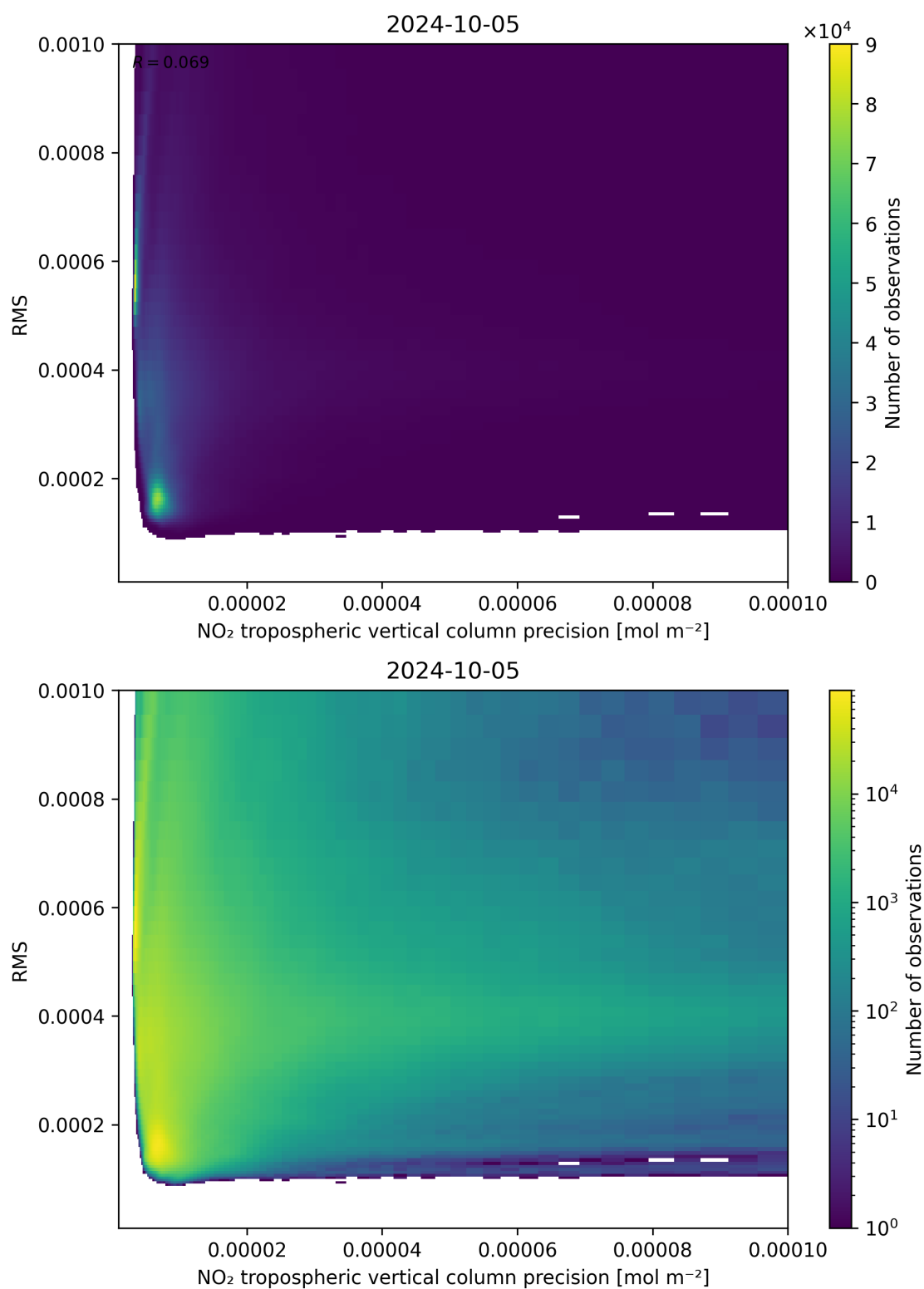
Figure 140: Scatter density plot of “NO 2 tropospheric vertical column precision” against “RMS” for 2024-10-04 to 2024-10-06.
