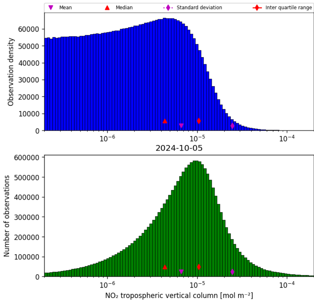
Figure 29: Histogram of “NO 2 tropospheric vertical column” for 2024-10-04 to 2024-10-06
