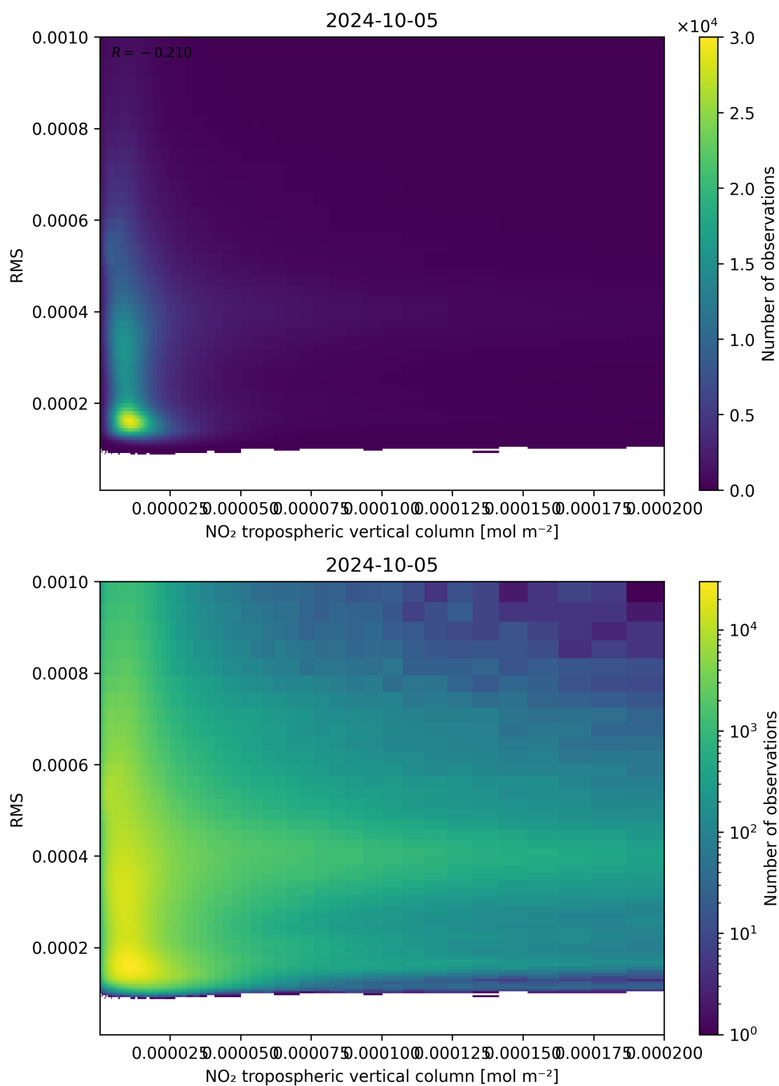
Figure 142: Scatter density plot of “NO 2 tropospheric vertical column” against “RMS” for 2024-10-04 to 2024-10-06.
