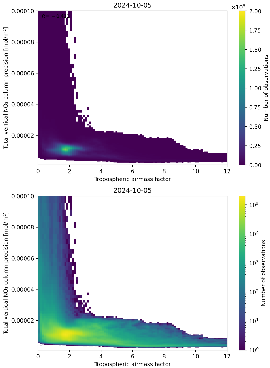
Figure 78: Scatter density plot of “Tropospheric air mass factor” against “Total vertical NO 2 column precision” for 2024-10-04 to 2024-10-06.
