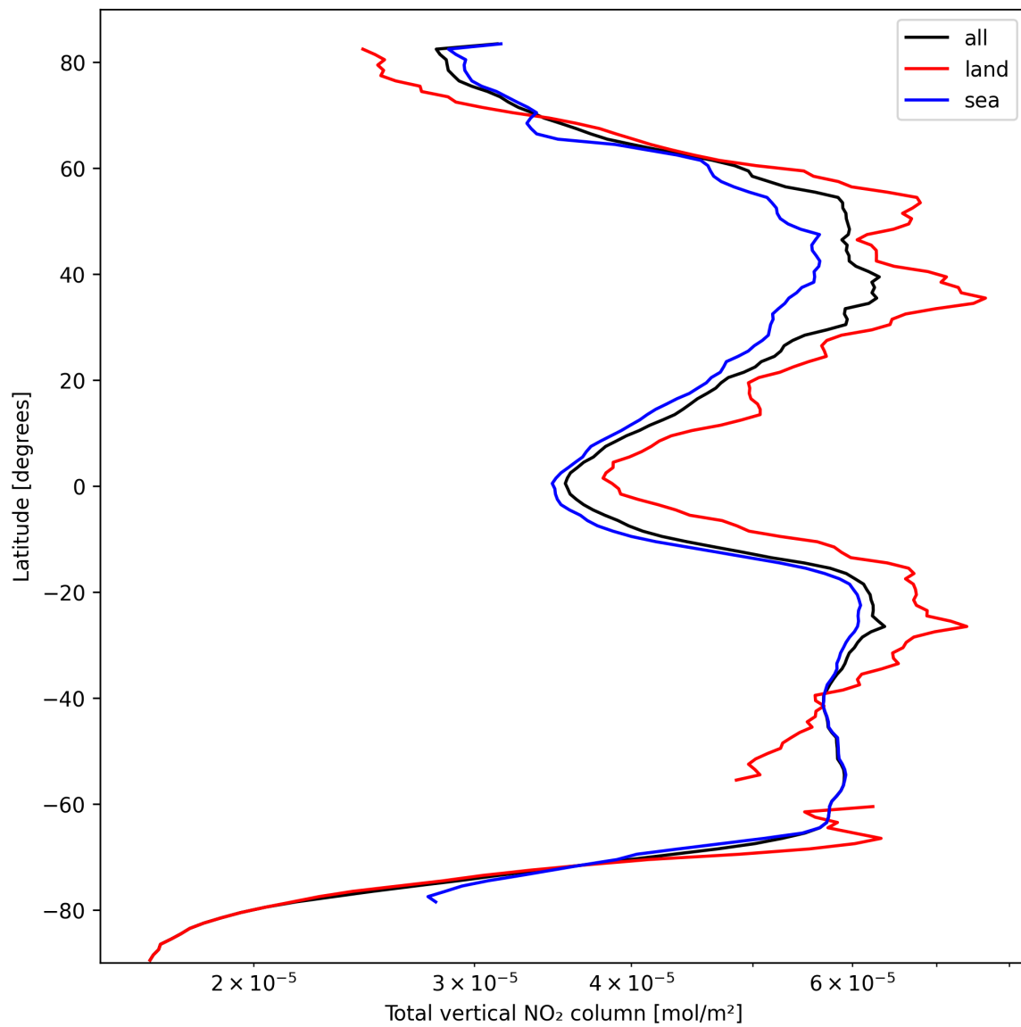
Figure 21: Zonal average of “Total vertical NO 2 column” for 2024-10-04 to 2024-10-06.
