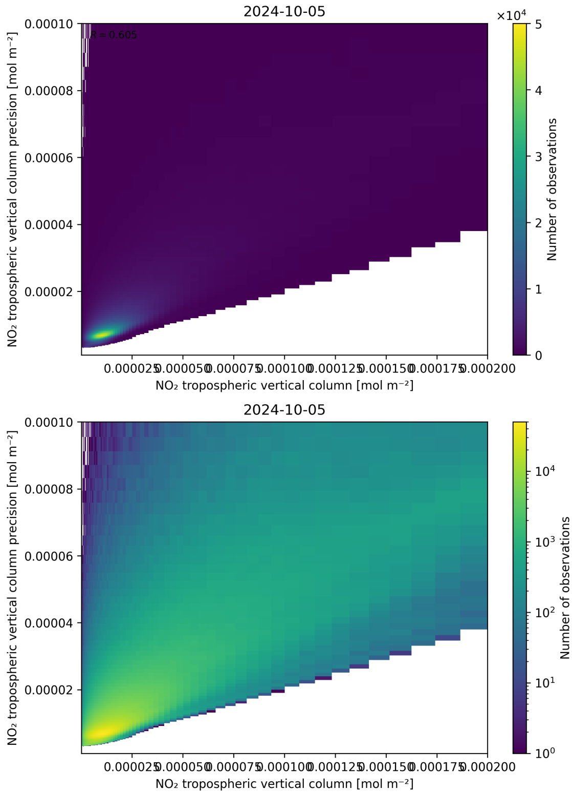
Figure 130: Scatter density plot of “NO 2 tropospheric vertical column” against “NO 2 tropospheric vertical column precision” for 2024-10-04 to 2024-10-06.
