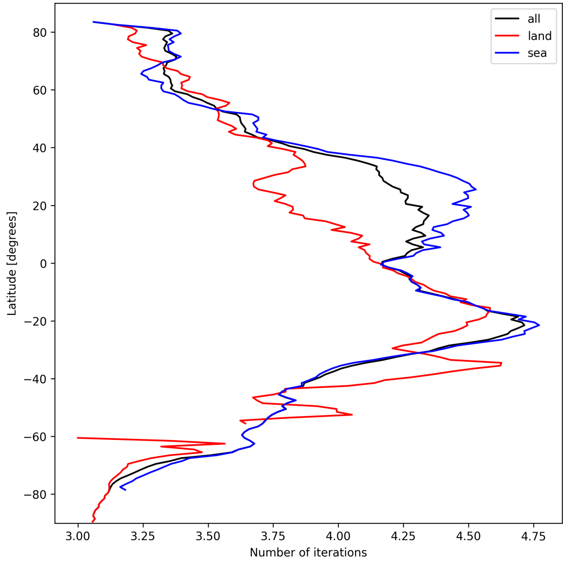
Figure 17: Zonal average of “Number of iterations” for 2024-10-04 to 2024-10-06.
