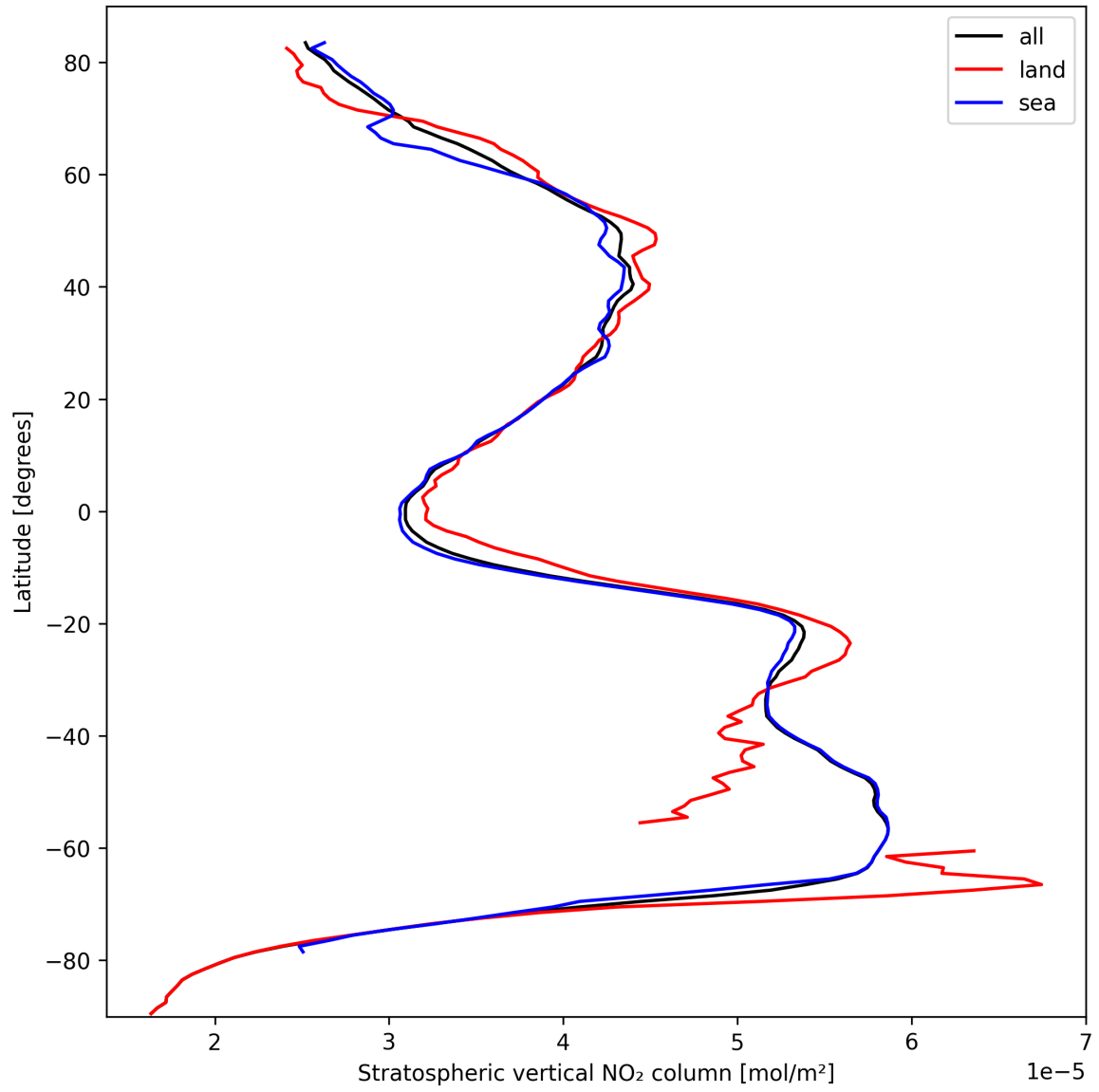
Figure 19: Zonal average of “Stratospheric vertical NO 2 column” for 2024-10-04 to 2024-10-06.
