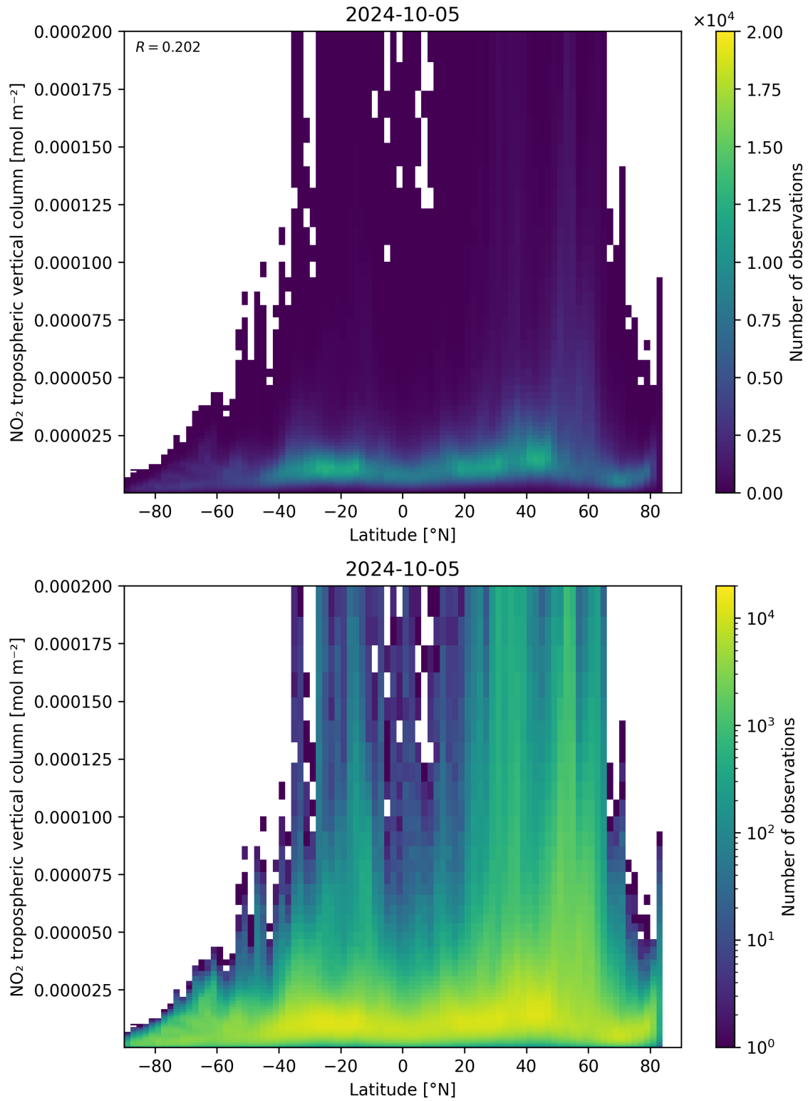
Figure 92: Scatter density plot of “Latitude” against “NO 2 tropospheric vertical column” for 2024-10-04 to 2024-10-06.
