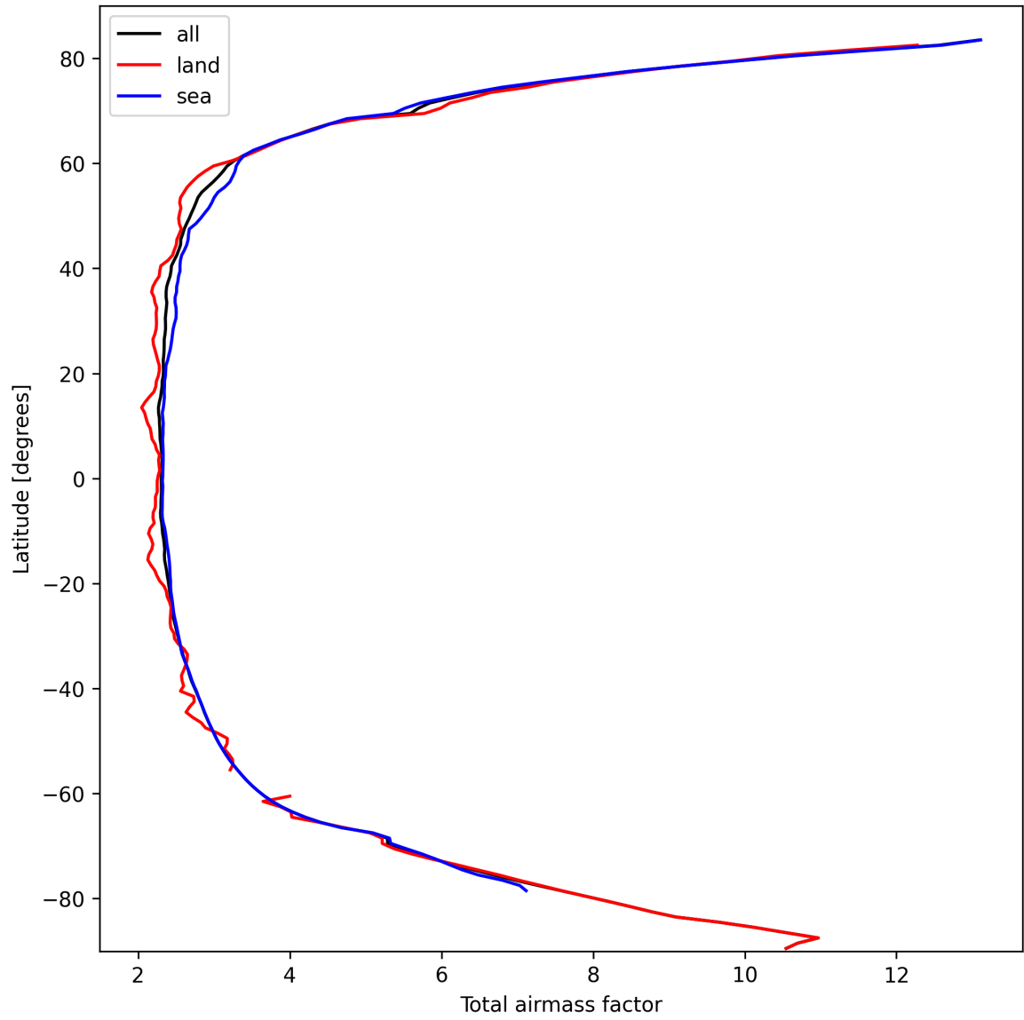
Figure 15: Zonal average of “Total airmass factor” for 2024-10-04 to 2024-10-06.
