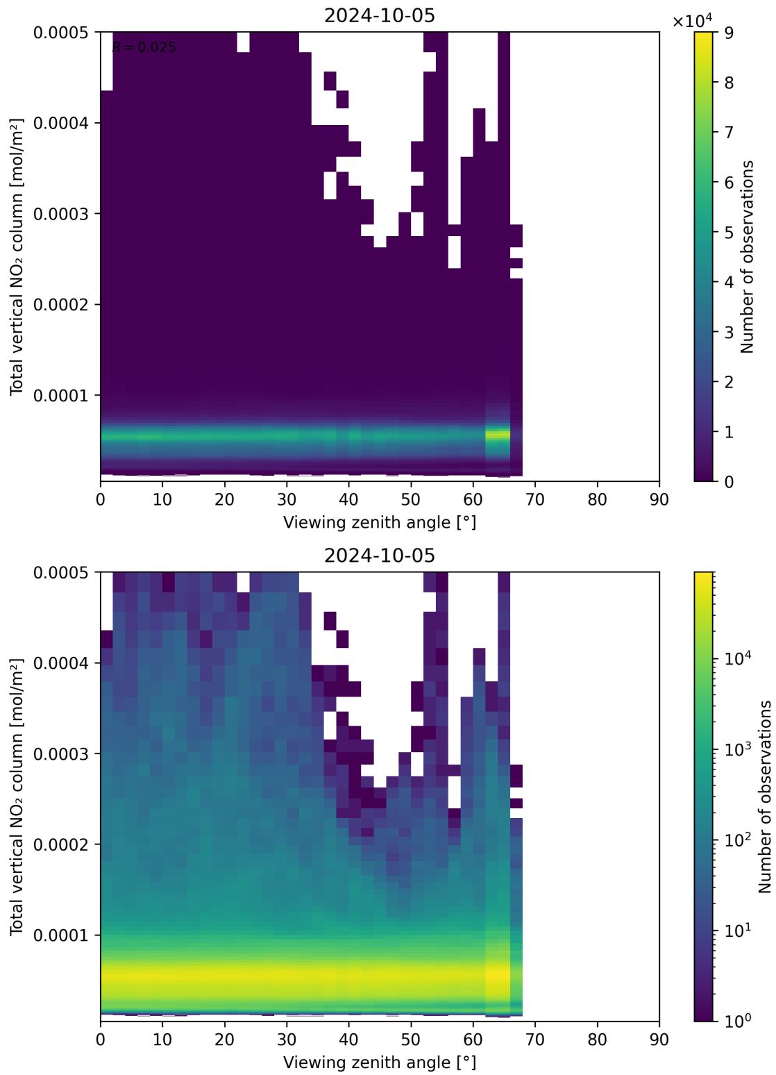
Figure 167: Scatter density plot of “Viewing zenith angle” against “Total vertical NO 2 column” for 2024-10-04 to 2024-10-06.
