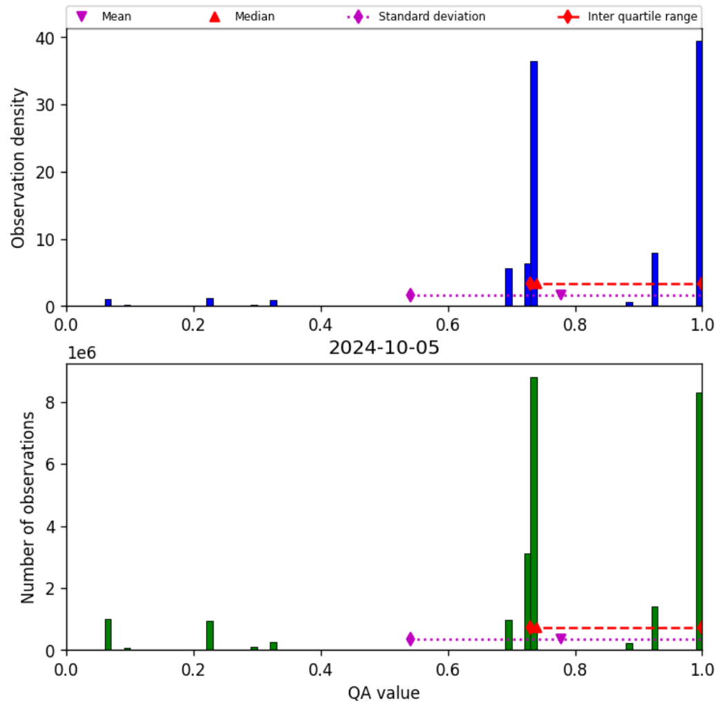
Figure 28: Histogram of “QA value” for 2024-10-04 to 2024-10-06
