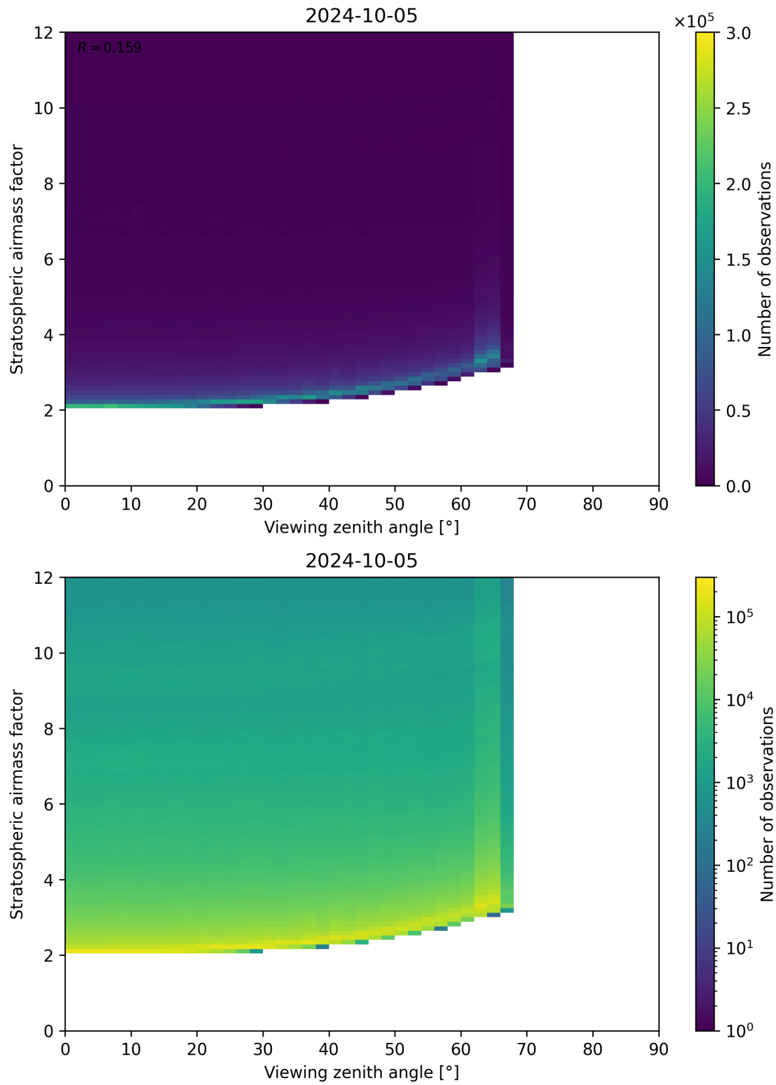
Figure 159: Scatter density plot of “Viewing zenith angle” against “Stratospheric airmass factor” for 2024-10-04 to 2024-10-06.
