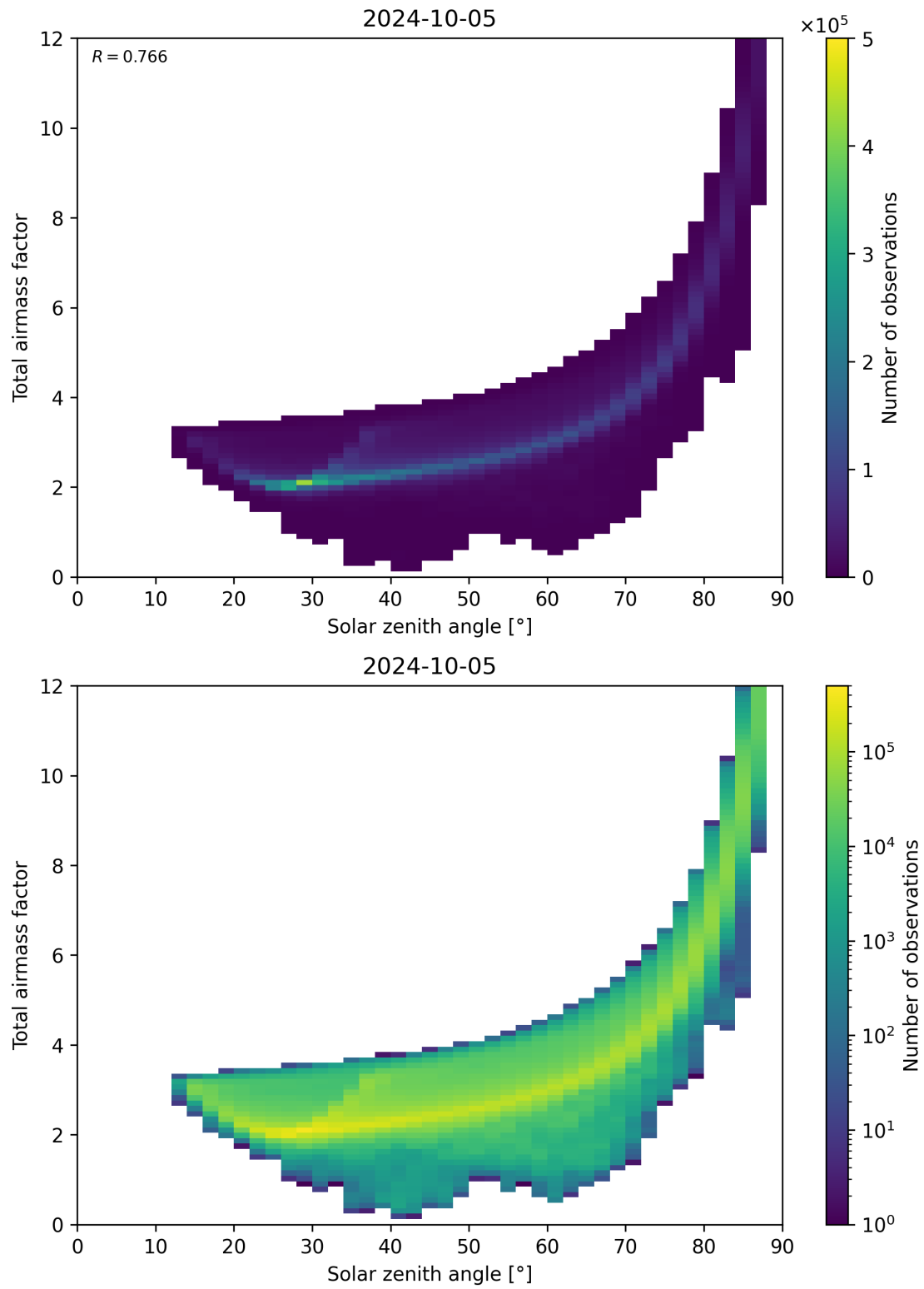
Figure 146: Scatter density plot of “Solar zenith angle” against “Total airmass factor” for 2024-10-04 to 2024-10-06.
