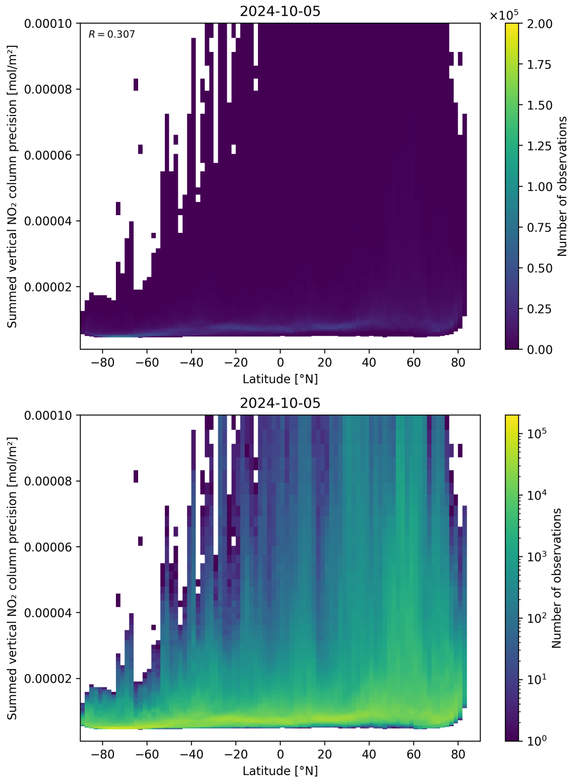
Figure 89: Scatter density plot of “Latitude” against “Summed vertical NO 2 column precision” for 2024-10-04 to 2024-10-06.
