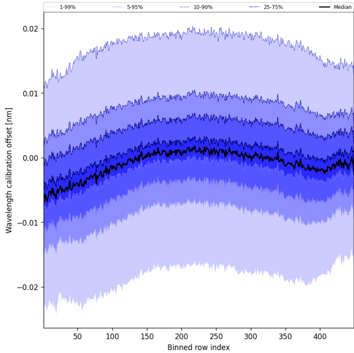
Figure 52: Along track statistics of “Wavelength calibration offset” for 2024-10-04 to 2024-10-06
