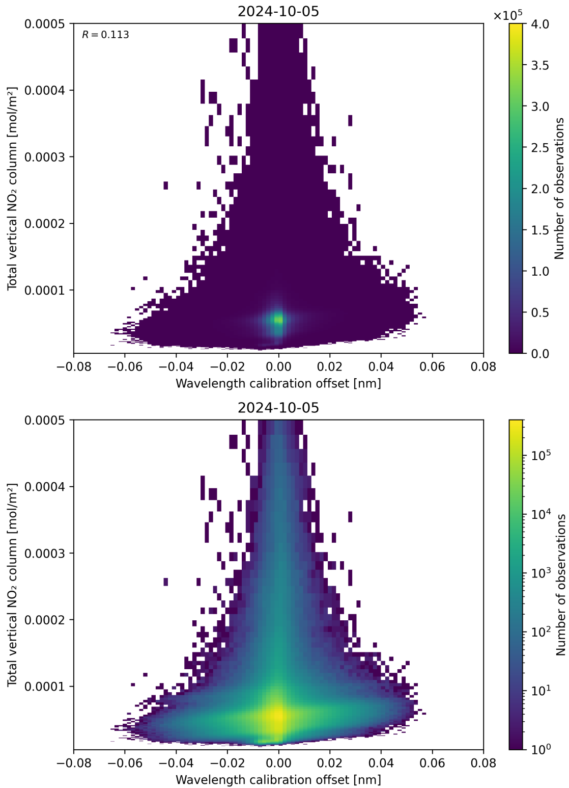
Figure 179: Scatter density plot of “Wavelength calibration offset” against “Total vertical NO 2 column” for 2024-10-04 to 2024-10-06.
