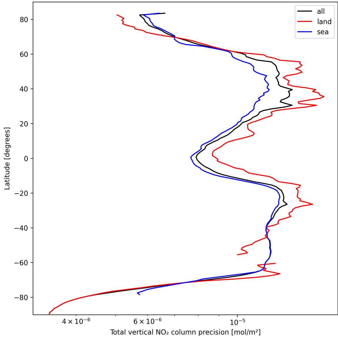
Figure 22: Zonal average of “Total vertical NO 2 column precision” for 2024-10-04 to 2024-10-06.
