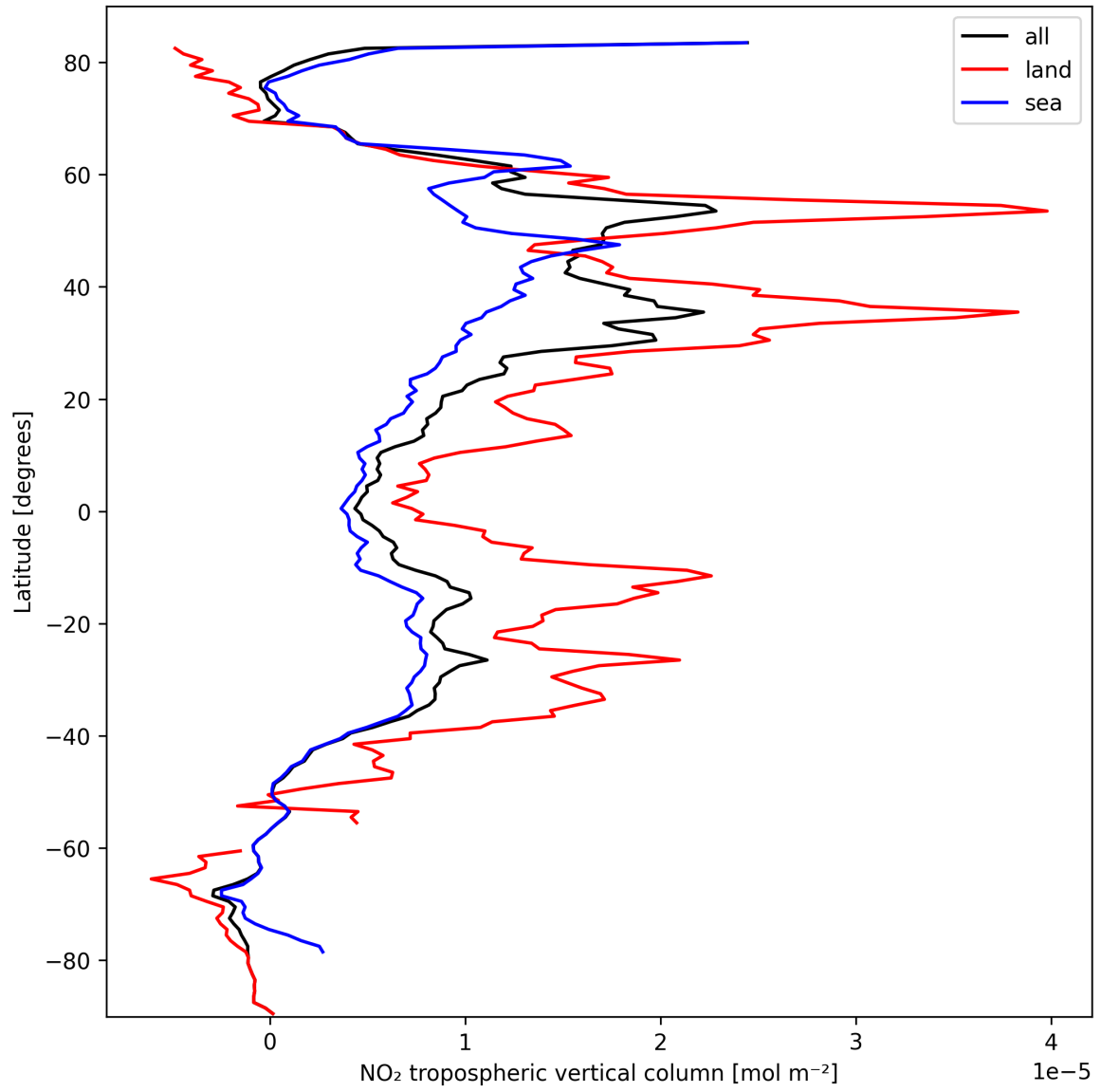
Figure 12: Zonal average of “NO 2 tropospheric vertical column” for 2024-10-04 to 2024-10-06.
