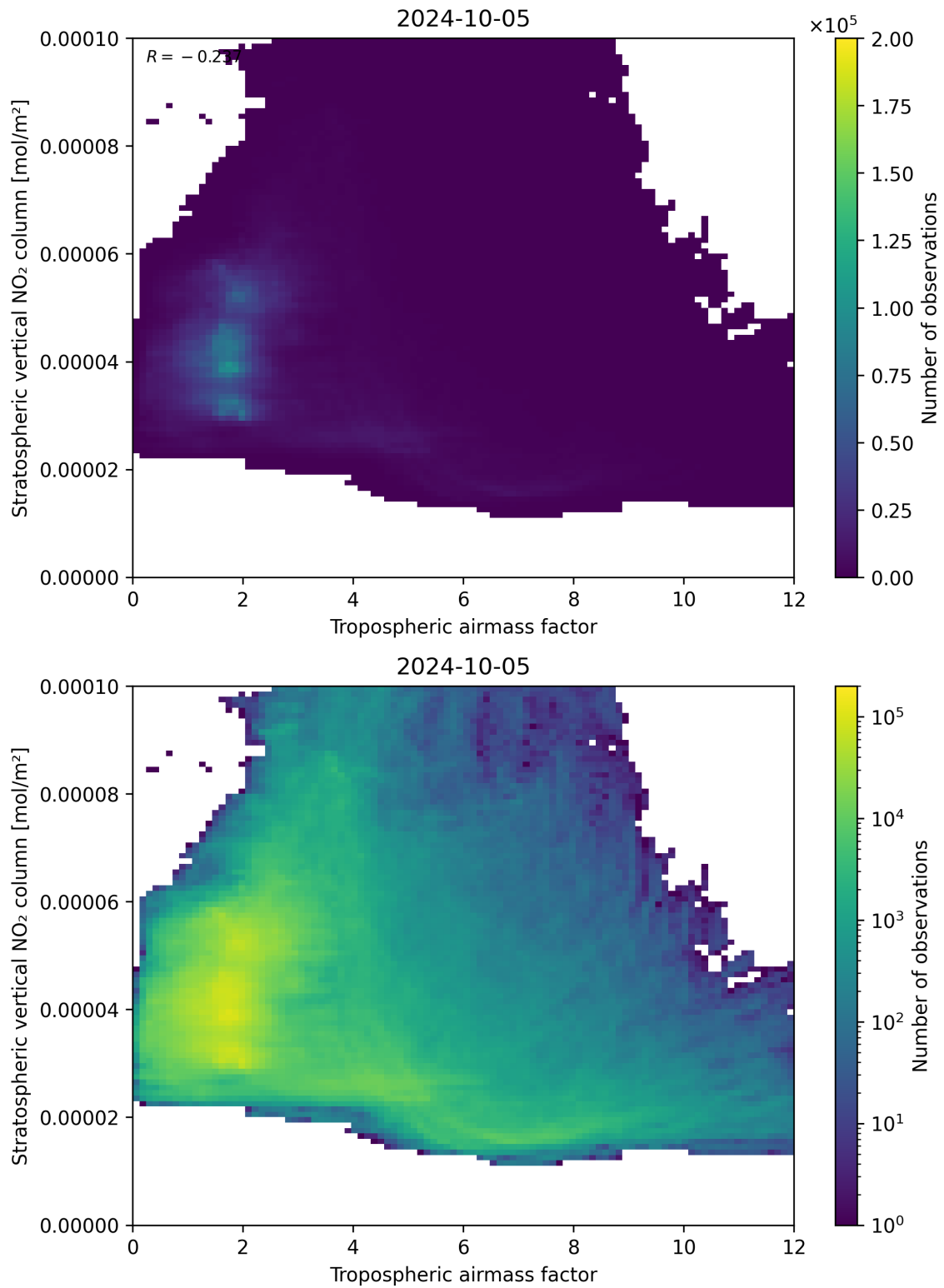
Figure 74: Scatter density plot of “Tropospheric air mass factor” against “Stratospheric vertical NO 2 column” for 2024-10-04 to 2024-10-06.
