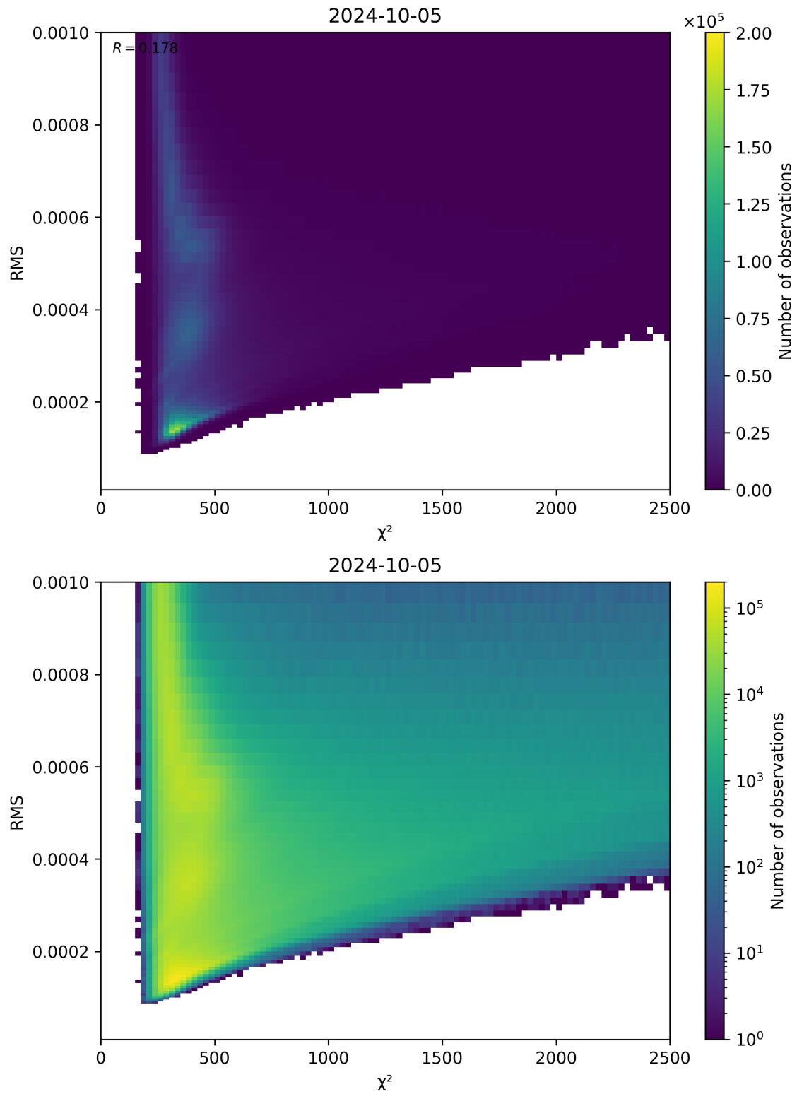
Figure 82: Scatter density plot of “ \chi^2 ” against “RMS” for 2024-10-04 to 2024-10-06.
