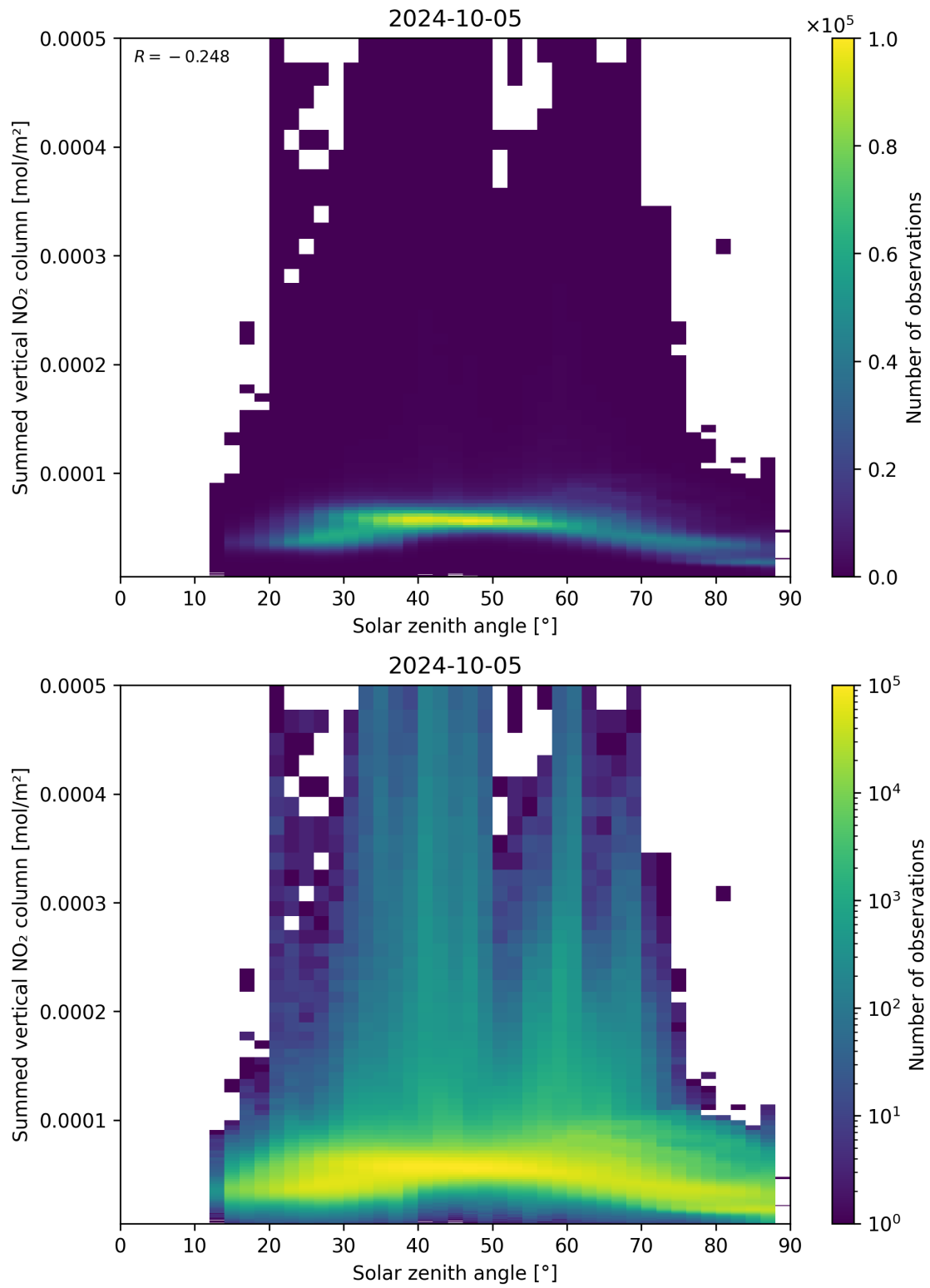
Figure 151: Scatter density plot of “Solar zenith angle” against “Summed vertical NO 2 column” for 2024-10-04 to 2024-10-06.
