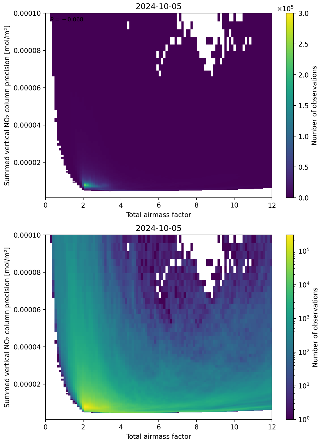
Figure 66: Scatter density plot of “Total airmass factor” against “Summed vertical NO 2 column precision” for 2024-10-04 to 2024-10-06.
