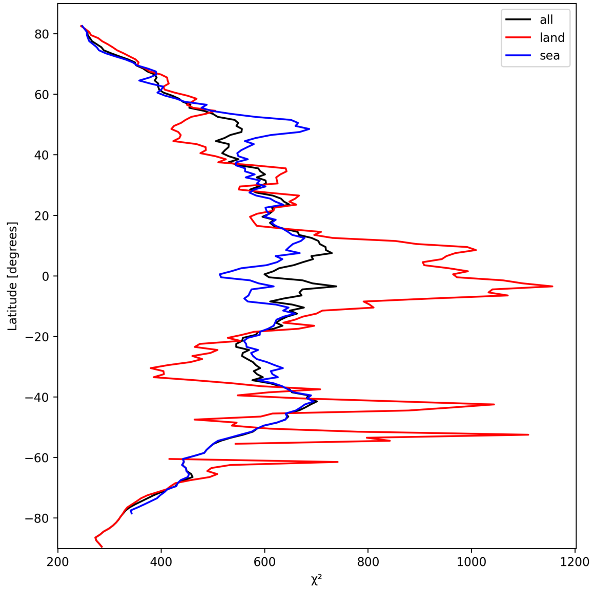
Figure 25: Zonal average of “ \chi^2 ” for 2024-10-05 to 2024-10-07.
