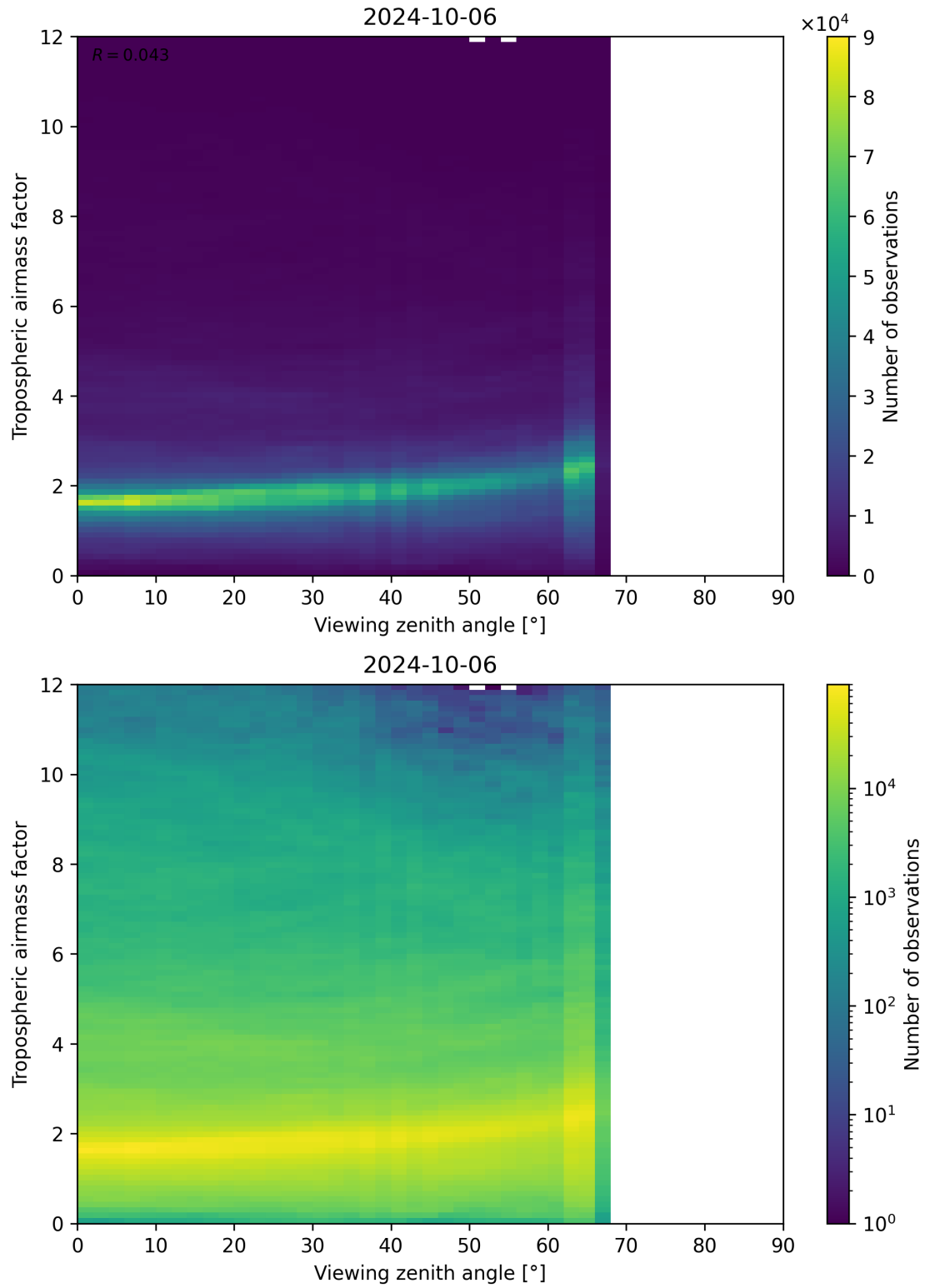
Figure 161: Scatter density plot of “Viewing zenith angle” against “Tropospheric airmass factor” for 2024-10-05 to 2024-10-07.
