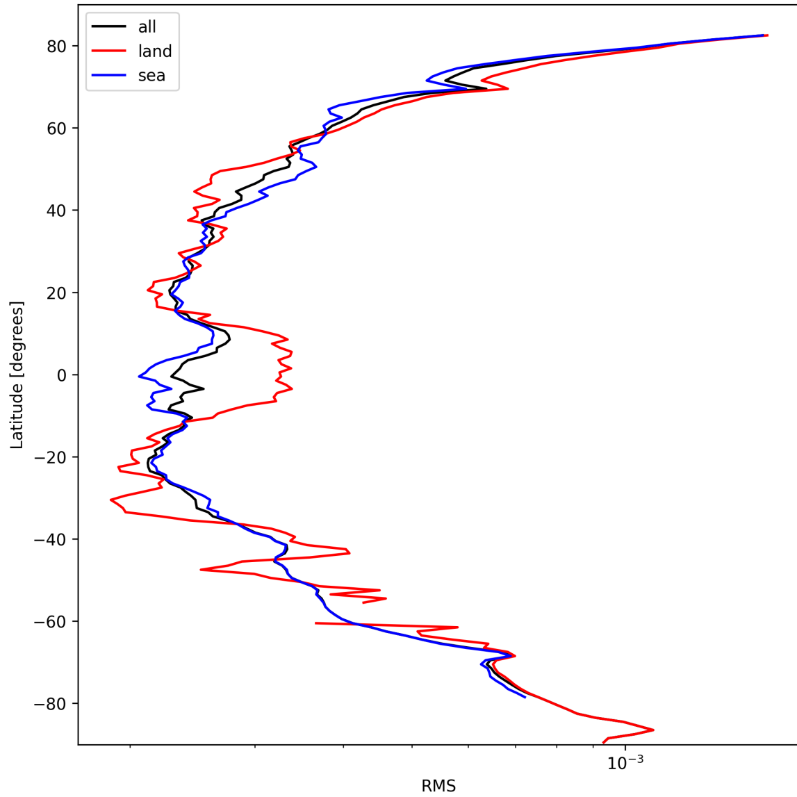
Figure 26: Zonal average of “RMS” for 2024-10-05 to 2024-10-07.
