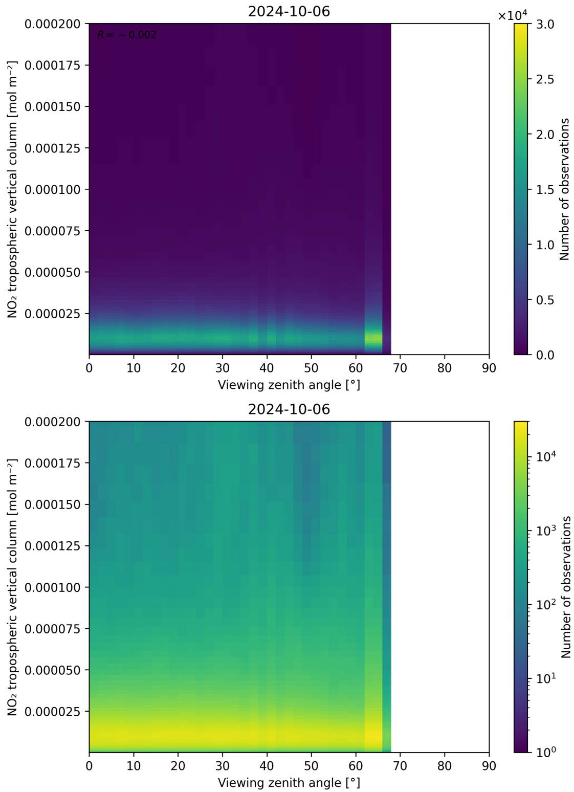
Figure 169: Scatter density plot of “Viewing zenith angle” against “NO 2 tropospheric vertical column” for 2024-10-05 to 2024-10-07.
