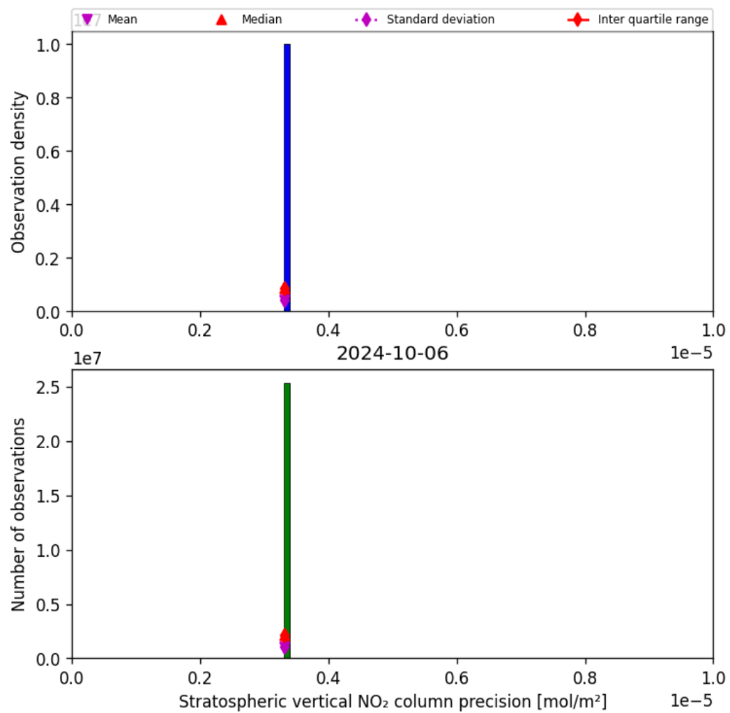
Figure 37: Histogram of “Stratospheric vertical NO 2 column precision” for 2024-10-05 to 2024-10-07
