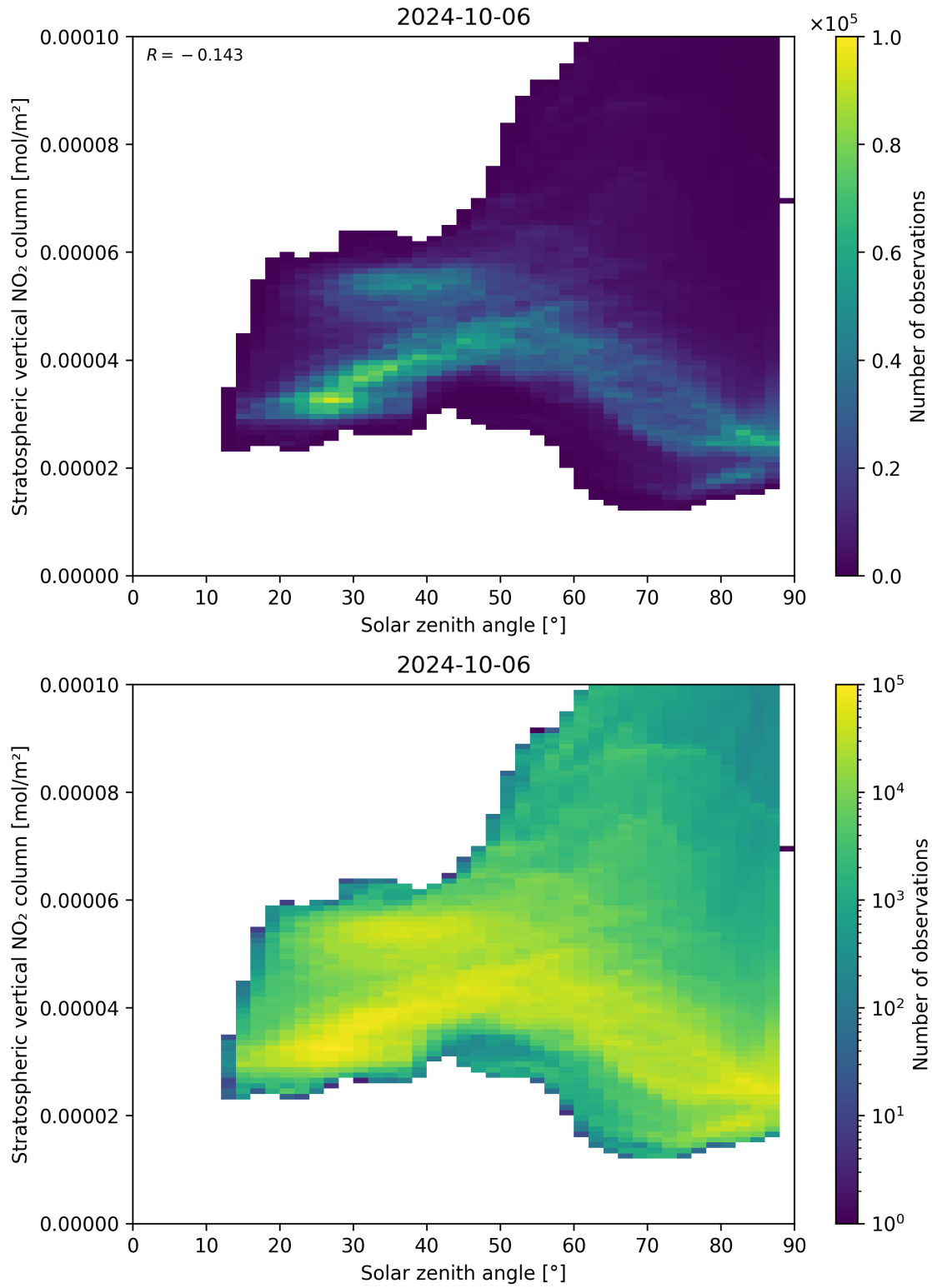
Figure 150: Scatter density plot of “Solar zenith angle” against “Stratospheric vertical NO 2 column” for 2024-10-05 to 2024-10-07.
