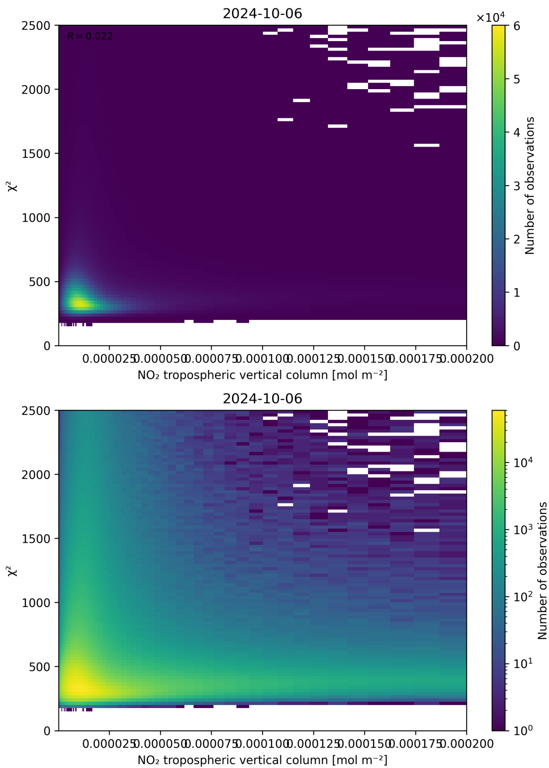
Figure 124: Scatter density plot of “NO 2 tropospheric vertical column” against “ \chi^2 ” for 2024-10-05 to 2024-10-07.
