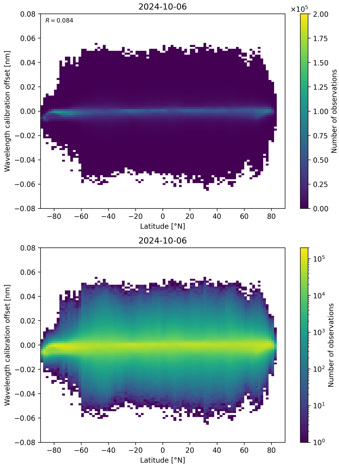
Figure 95: Scatter density plot of “Latitude” against “Wavelength calibration offset” for 2024-10-05 to 2024-10-07.
