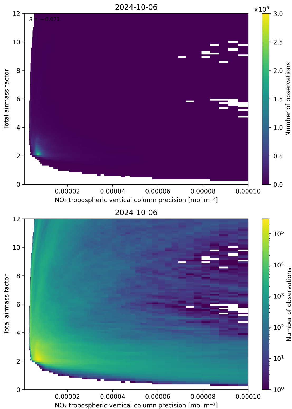
Figure 132: Scatter density plot of “NO 2 tropospheric vertical column precision” against “Total air mass factor” for 2024-10-05 to 2024-10-07.
