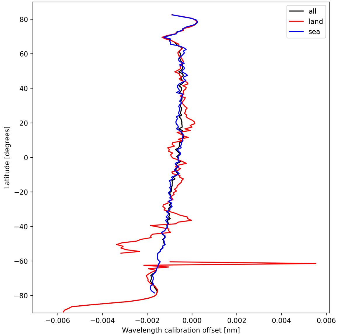
Figure 18: Zonal average of “Wavelength calibration offset” for 2024-10-05 to 2024-10-07.
