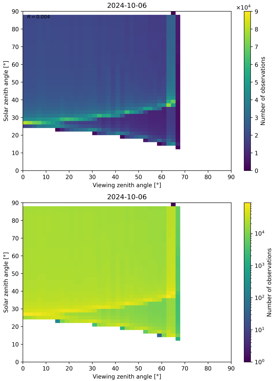
Figure 172: Scatter density plot of “Viewing zenith angle” against “Solar zenith angle” for 2024-10-05 to 2024-10-07.
