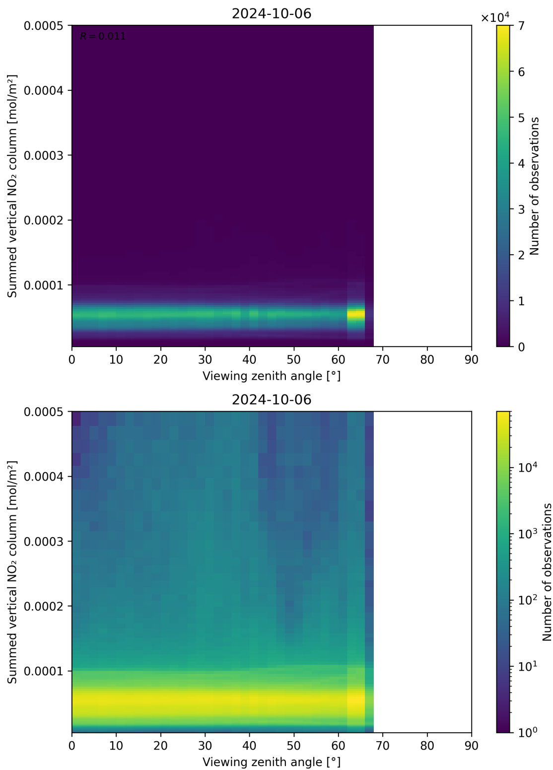
Figure 165: Scatter density plot of “Viewing zenith angle” against “Summed vertical NO 2 column” for 2024-10-05 to 2024-10-07.
