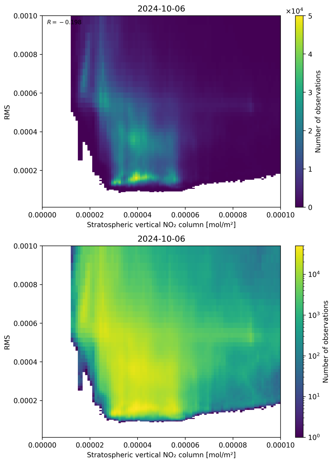
Figure 102: Scatter density plot of “Stratospheric vertical NO 2 column” against “RMS” for 2024-10-05 to 2024-10-07.
