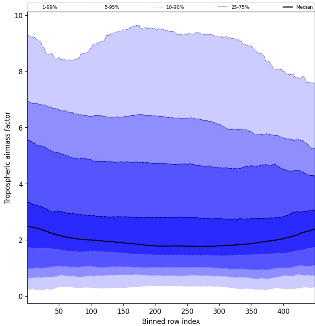
Figure 48: Along track statistics of “Tropospheric air mass factor” for 2024-10-05 to 2024-10-07
