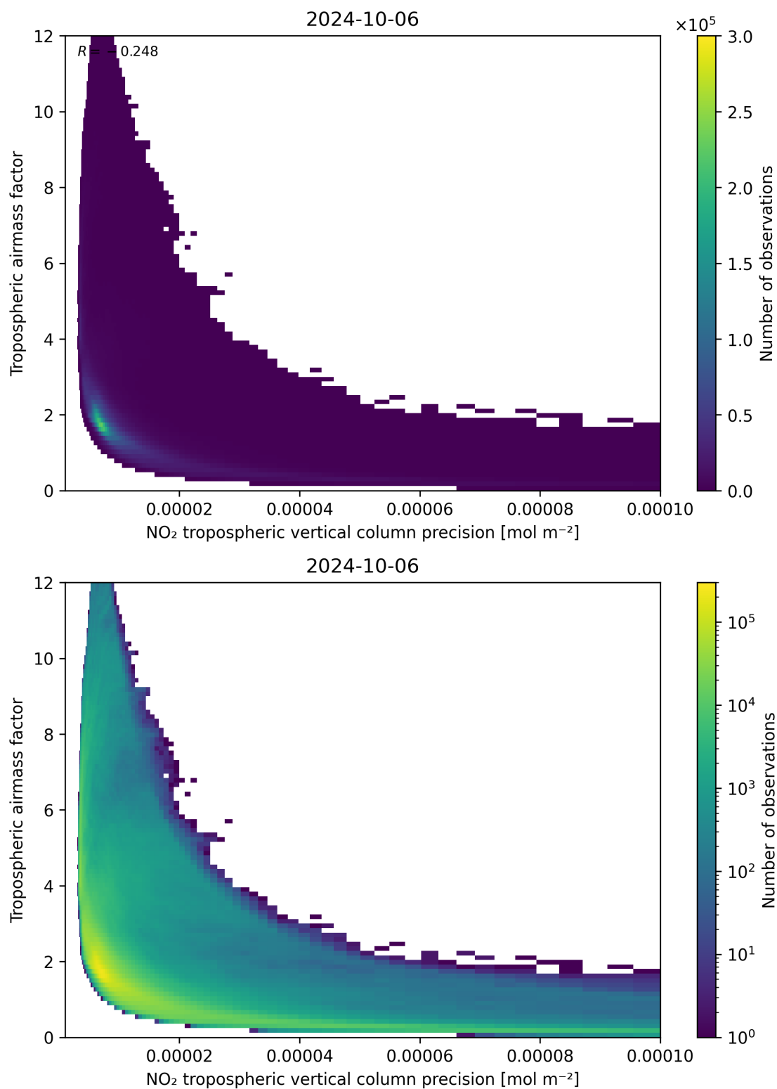
Figure 133: Scatter density plot of “NO 2 tropospheric vertical column precision” against “Tropospheric air mass factor” for 2024-10-05 to 2024-10-07.
