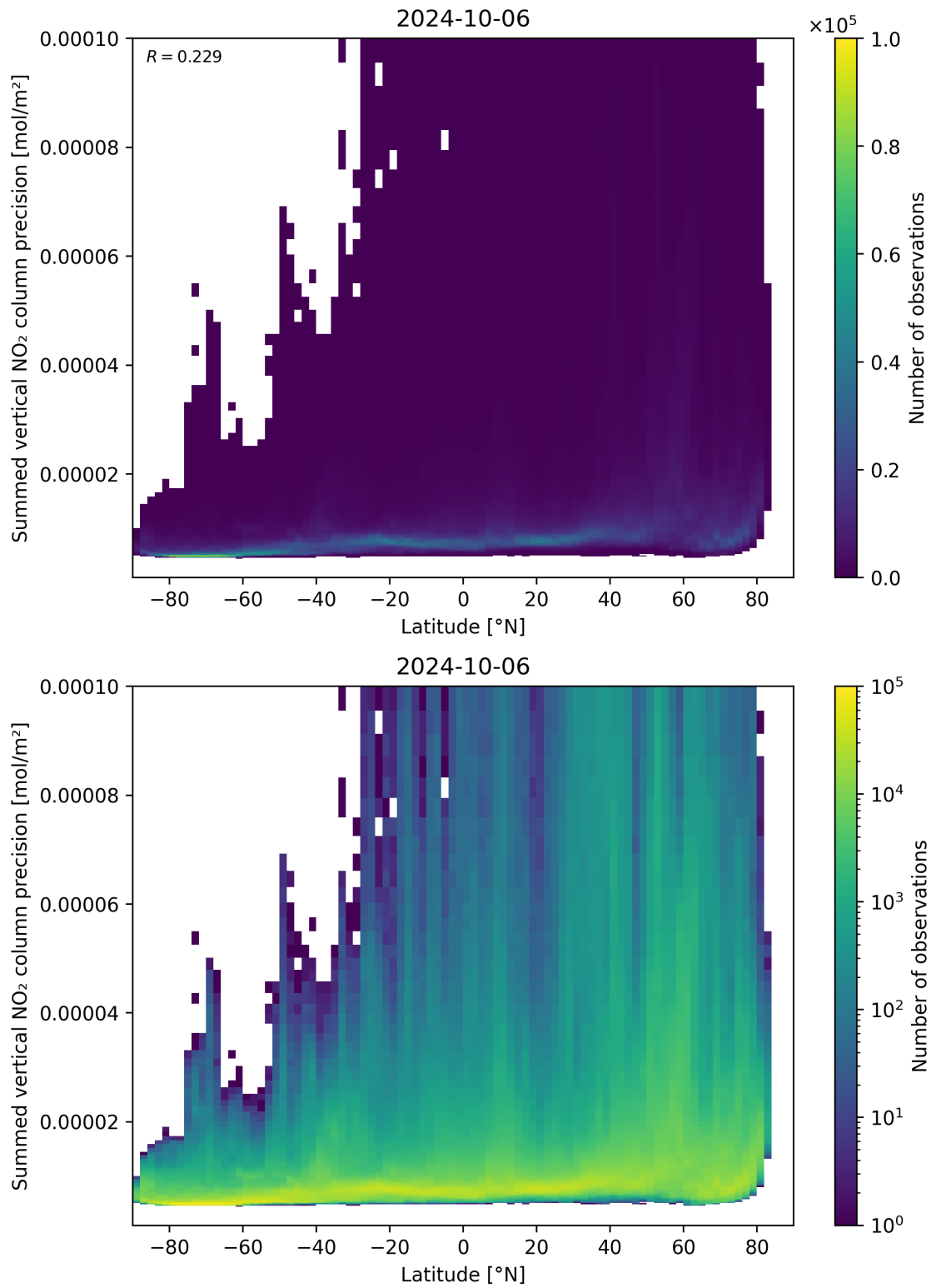
Figure 89: Scatter density plot of “Latitude” against “Summed vertical NO 2 column precision” for 2024-10-05 to 2024-10-07.
