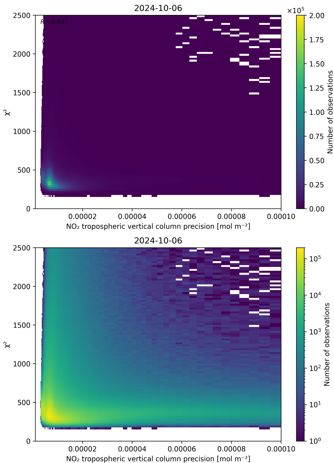
Figure 134: Scatter density plot of “NO 2 tropospheric vertical column precision” against “ \chi^2 ” for 2024-10-05 to 2024-10-07.
