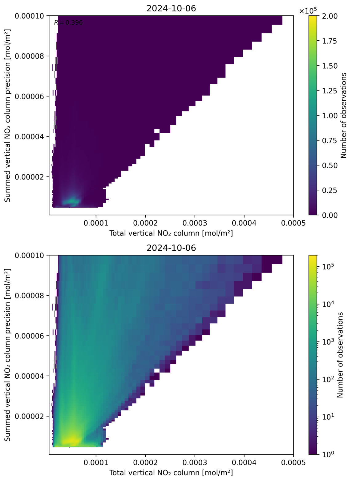
Figure 113: Scatter density plot of “Total vertical NO 2 column” against “Summed vertical NO 2 column precision” for 2024-10-05 to 2024-10-07.
