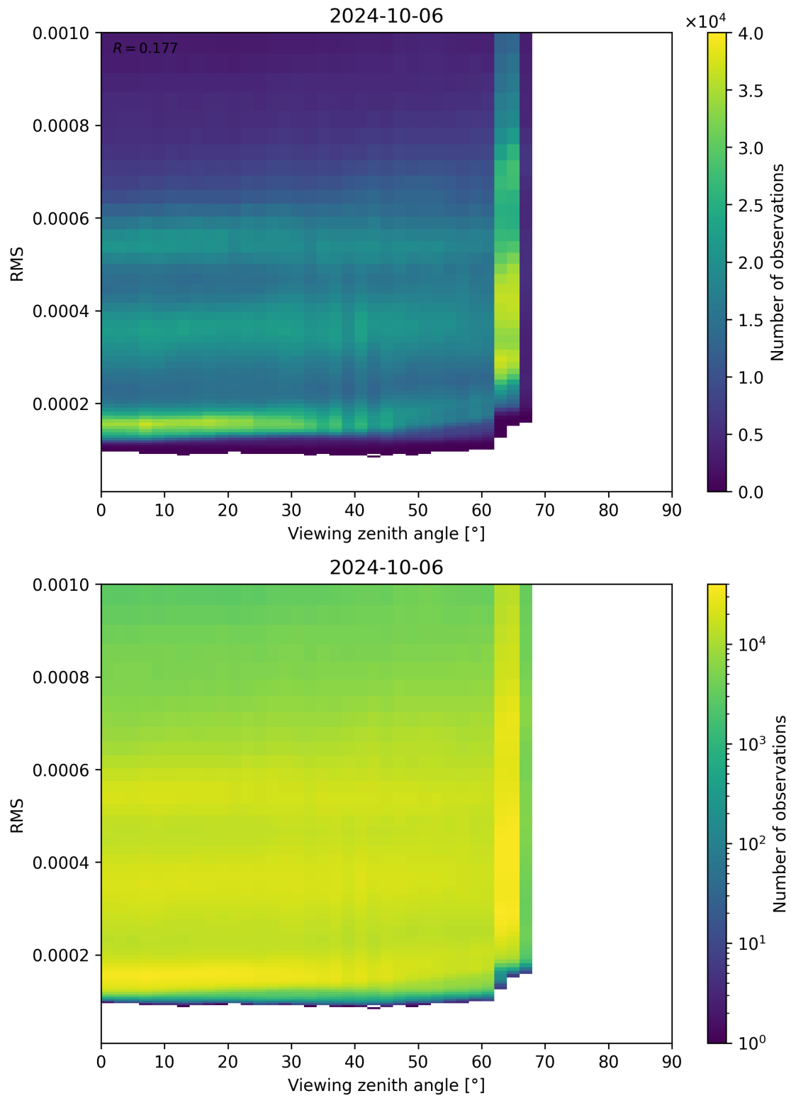
Figure 171: Scatter density plot of “Viewing zenith angle” against “RMS” for 2024-10-05 to 2024-10-07.
