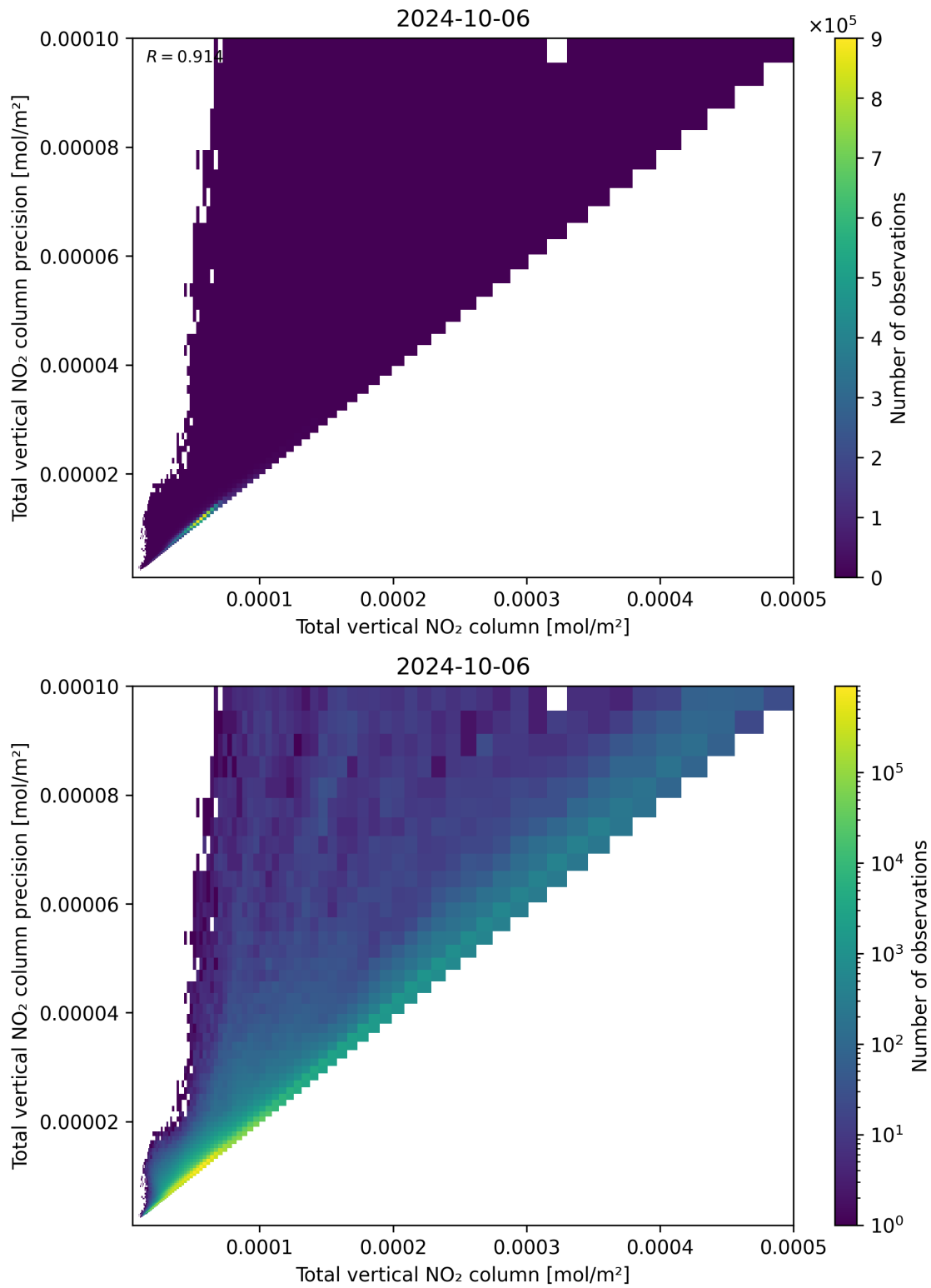
Figure 114: Scatter density plot of “Total vertical NO 2 column” against “Total vertical NO 2 column precision” for 2024-10-05 to 2024-10-07.
