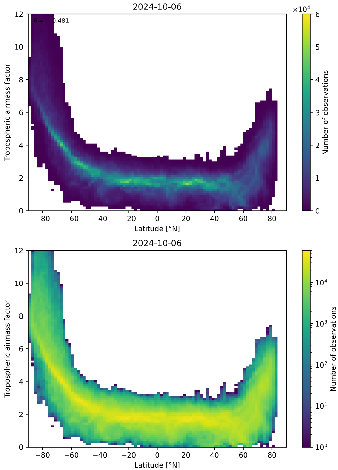
Figure 85: Scatter density plot of “Latitude” against “Tropospheric airmass factor” for 2024-10-05 to 2024-10-07.
