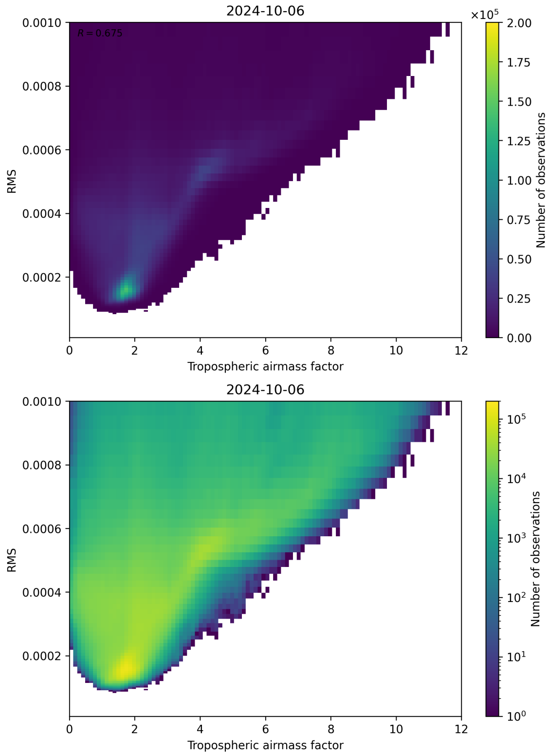
Figure 79: Scatter density plot of “Tropospheric airmass factor” against “RMS” for 2024-10-05 to 2024-10-07.
