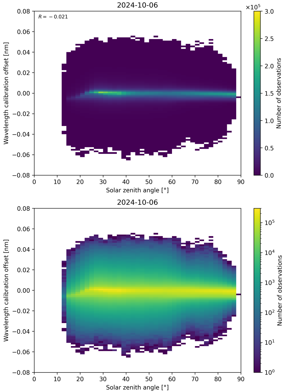
Figure 158: Scatter density plot of “Solar zenith angle” against “Wavelength calibration offset” for 2024-10-05 to 2024-10-07.
