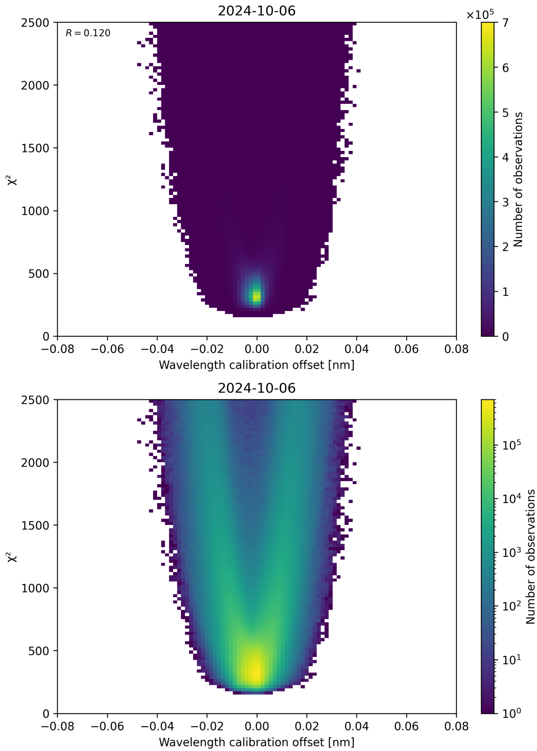
Figure 175: Scatter density plot of “Wavelength calibration offset” against “ \chi^2 ” for 2024-10-05 to 2024-10-07.
