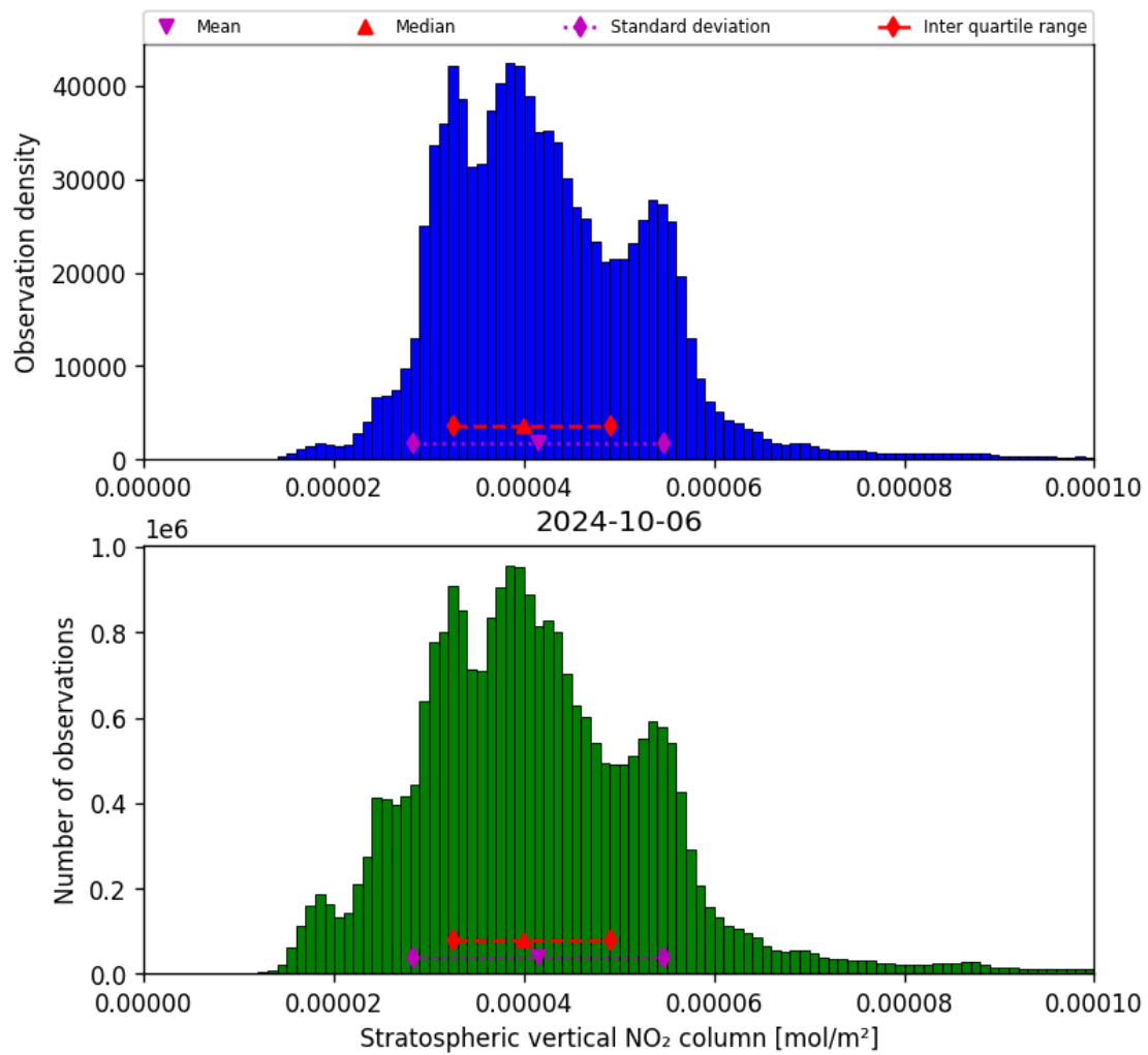
Figure 36: Histogram of “Stratospheric vertical NO 2 column” for 2024-10-05 to 2024-10-07
