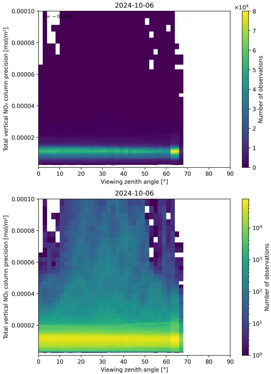
Figure 168: Scatter density plot of “Viewing zenith angle” against “Total vertical NO 2 column precision” for 2024-10-05 to 2024-10-07.
