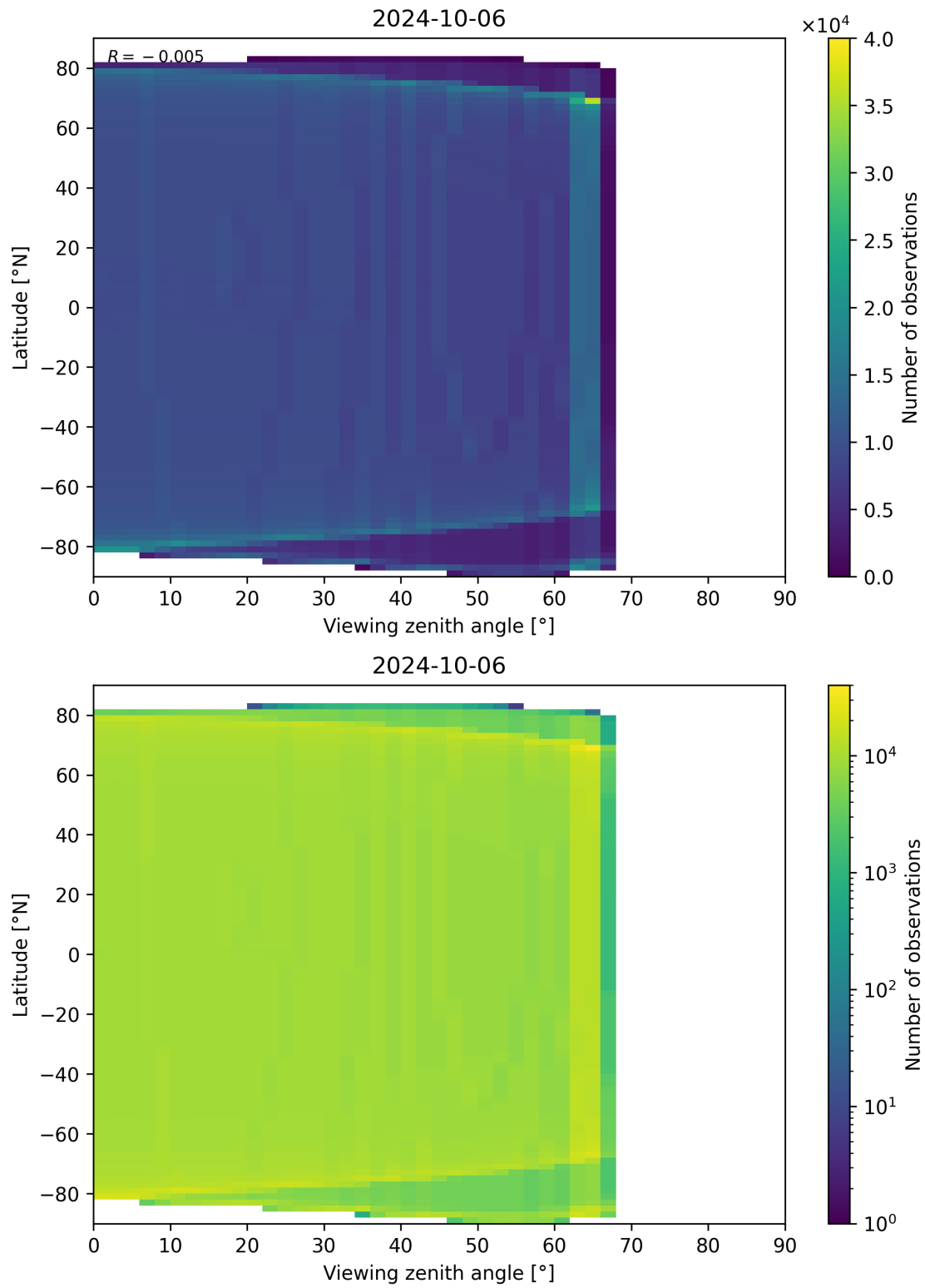
Figure 163: Scatter density plot of “Viewing zenith angle” against “Latitude” for 2024-10-05 to 2024-10-07.
