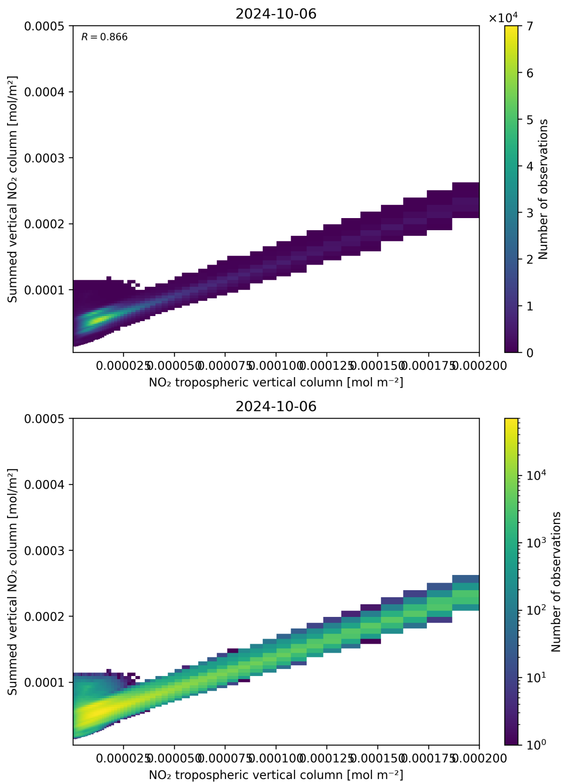
Figure 126: Scatter density plot of “NO 2 tropospheric vertical column” against “Summed vertical NO 2 column” for 2024-10-05 to 2024-10-07.
