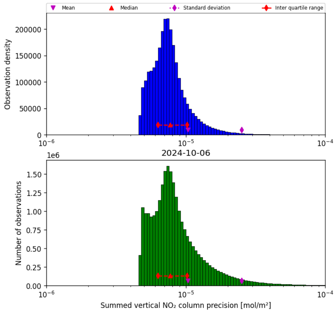
Figure 41: Histogram of "Summed vertical NO 2 column precision" for 2024-10-05 to 2024-10-07
