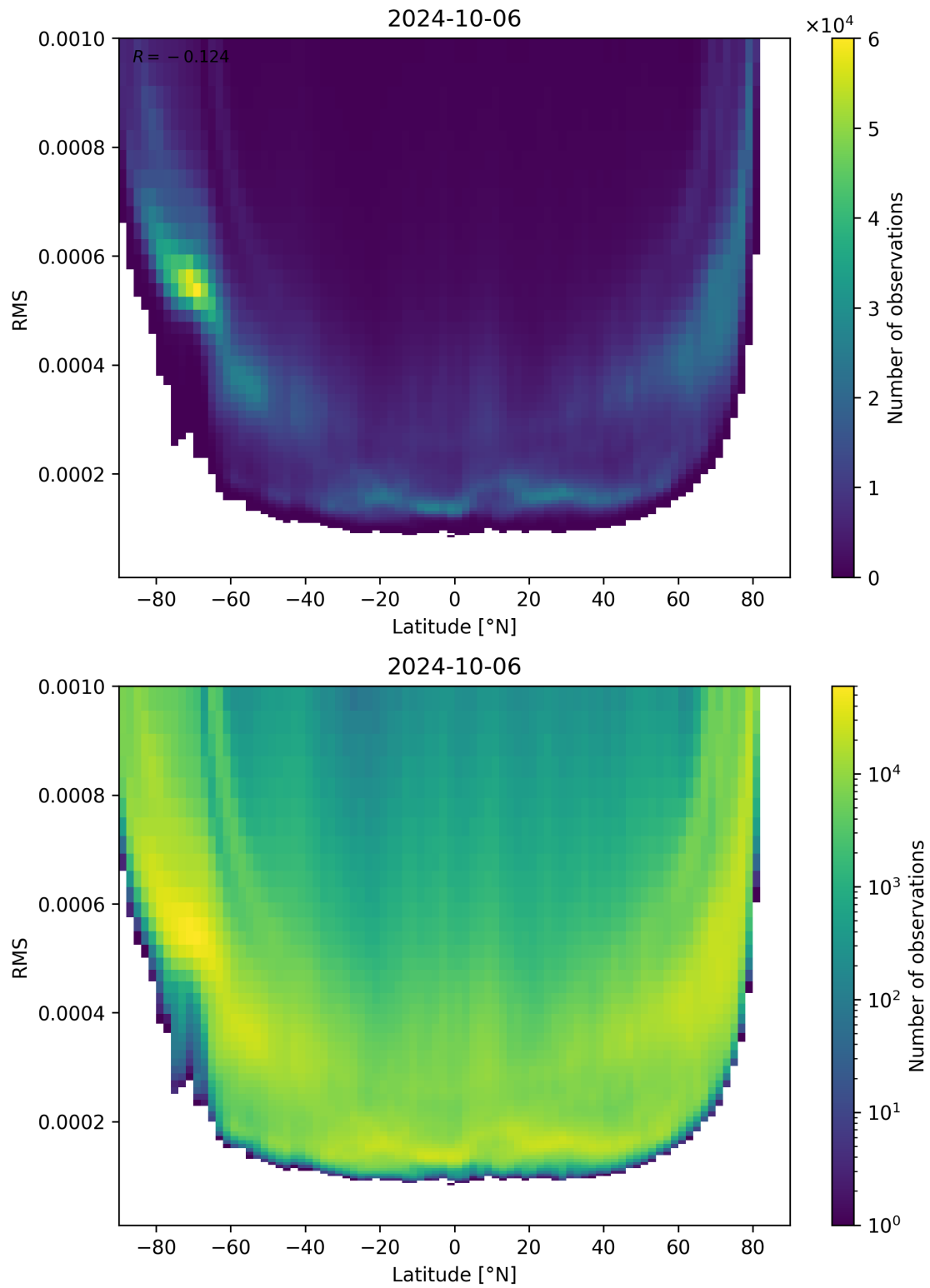
Figure 94: Scatter density plot of “Latitude” against “RMS” for 2024-10-05 to 2024-10-07.
