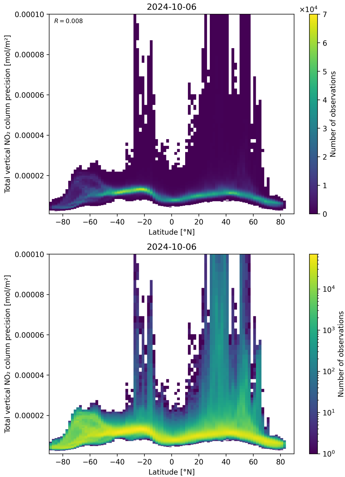
Figure 91: Scatter density plot of “Latitude” against “Total vertical NO 2 column precision” for 2024-10-05 to 2024-10-07.
