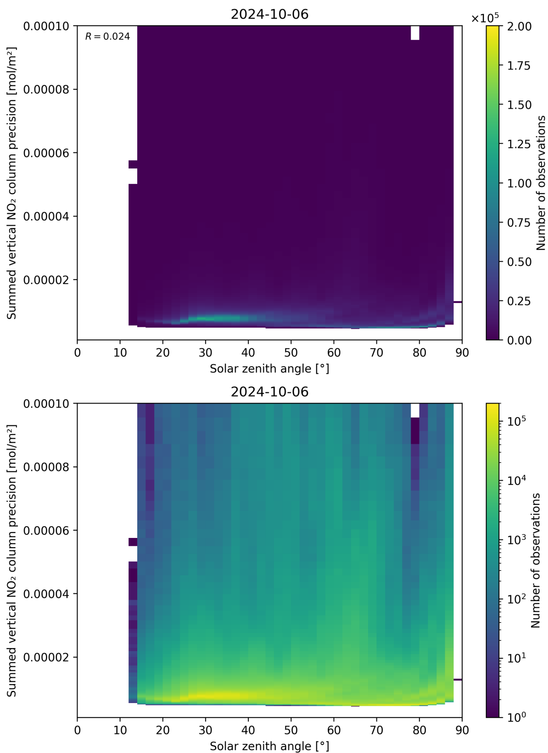
Figure 152: Scatter density plot of “Solar zenith angle” against “Summed vertical NO 2 column precision” for 2024-10-05 to 2024-10-07.
