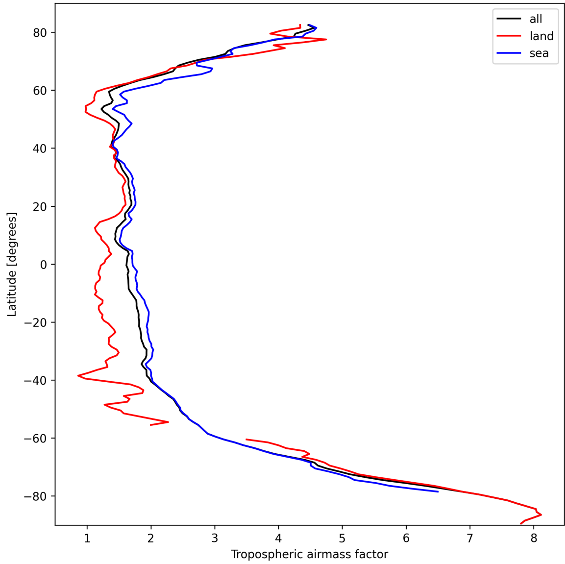
Figure 14: Zonal average of “Tropospheric air mass factor” for 2024-10-05 to 2024-10-07.
