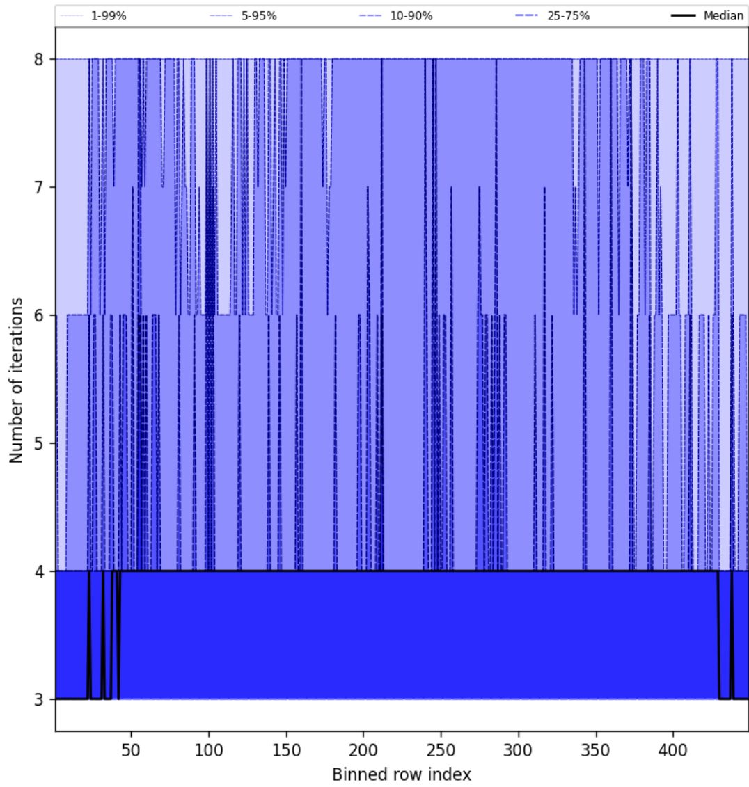
Figure 51: Along track statistics of “Number of iterations” for 2024-10-05 to 2024-10-07
