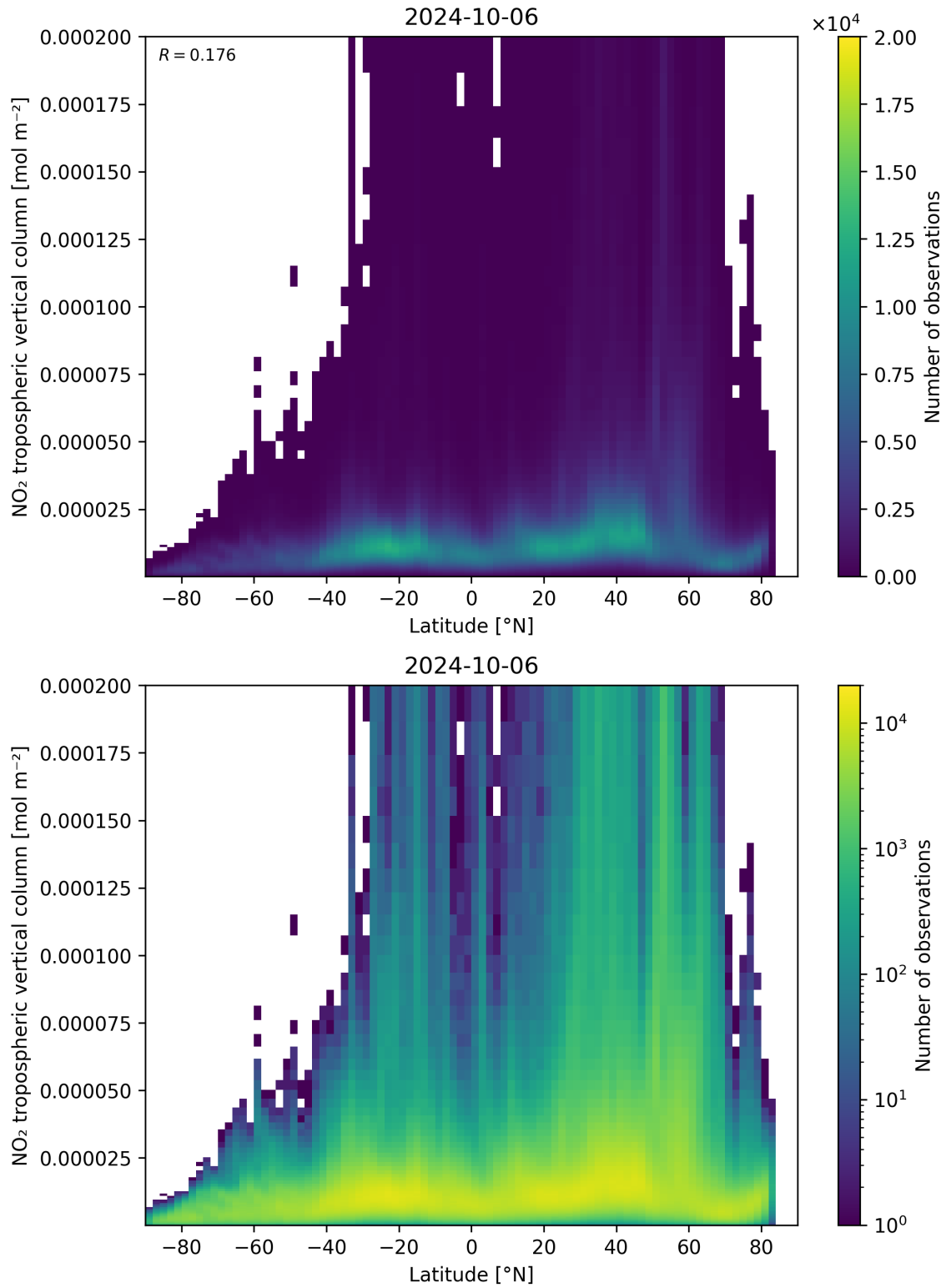
Figure 92: Scatter density plot of “Latitude” against “NO 2 tropospheric vertical column” for 2024-10-05 to 2024-10-07.
