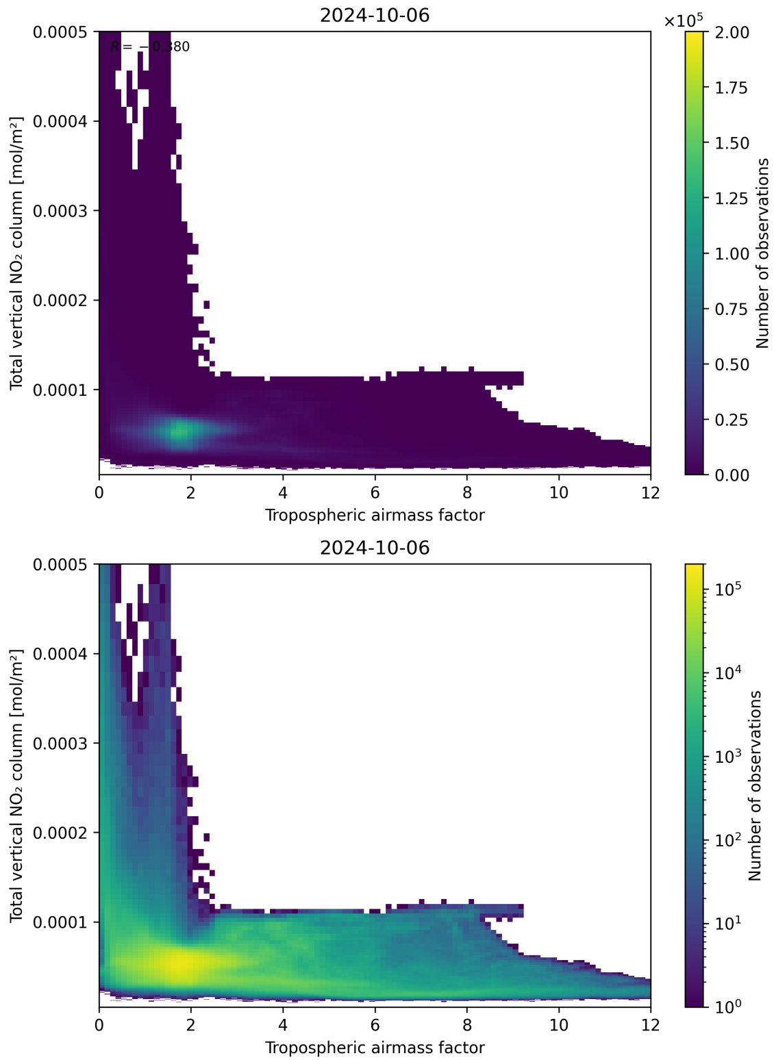
Figure 77: Scatter density plot of “Tropospheric airmass factor” against “Total vertical NO 2 column” for 2024-10-05 to 2024-10-07.
