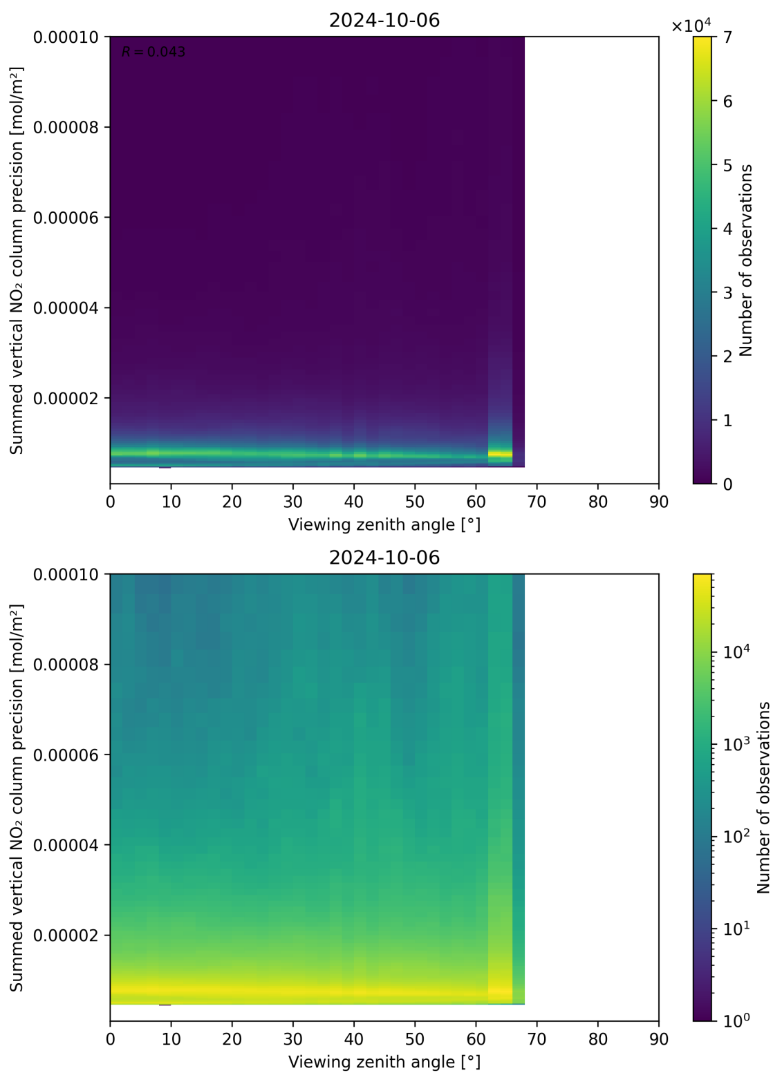
Figure 166: Scatter density plot of “Viewing zenith angle” against “Summed vertical NO 2 column precision” for 2024-10-05 to 2024-10-07.
