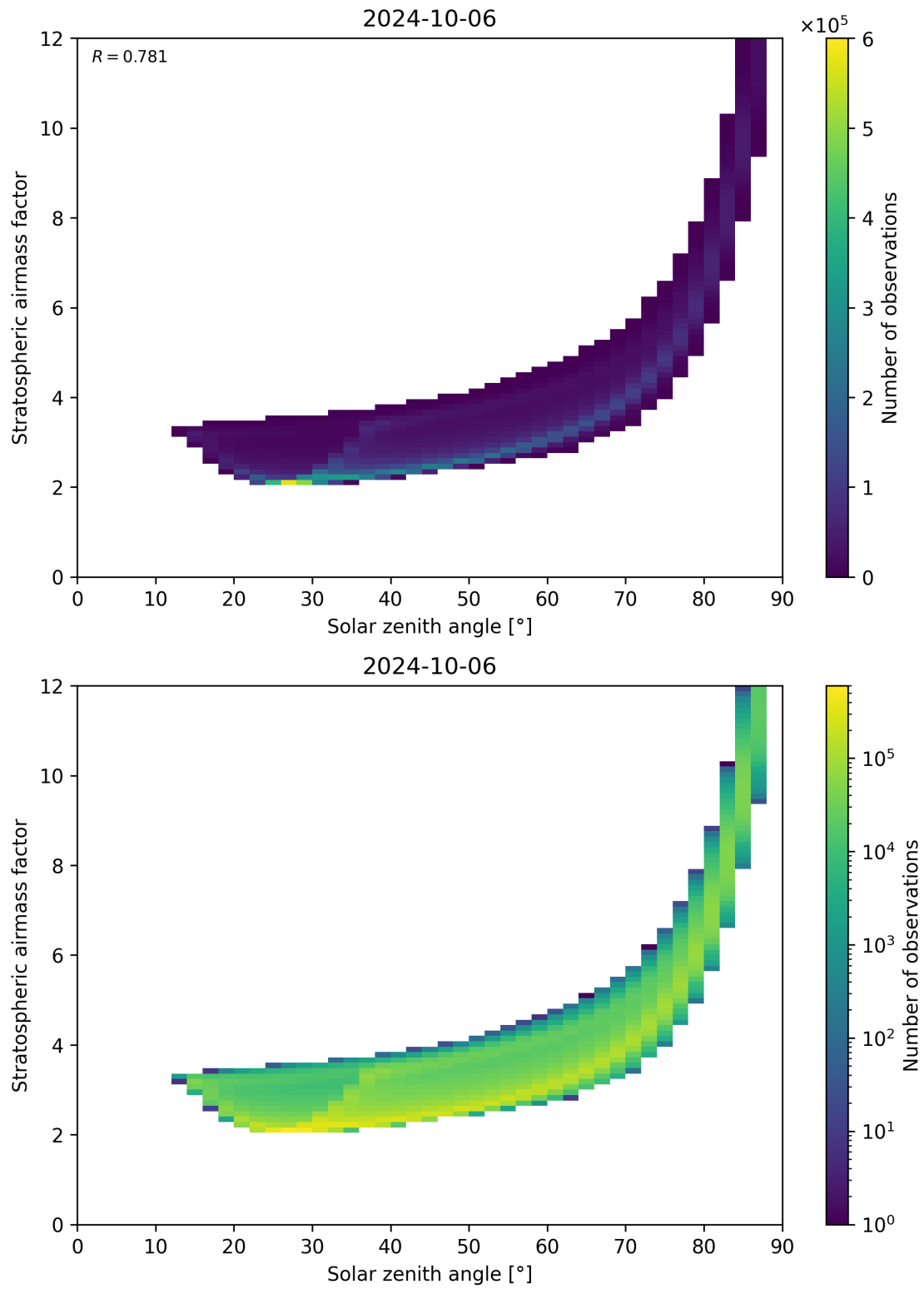
Figure 145: Scatter density plot of “Solar zenith angle” against “Stratospheric airmass factor” for 2024-10-05 to 2024-10-07.
