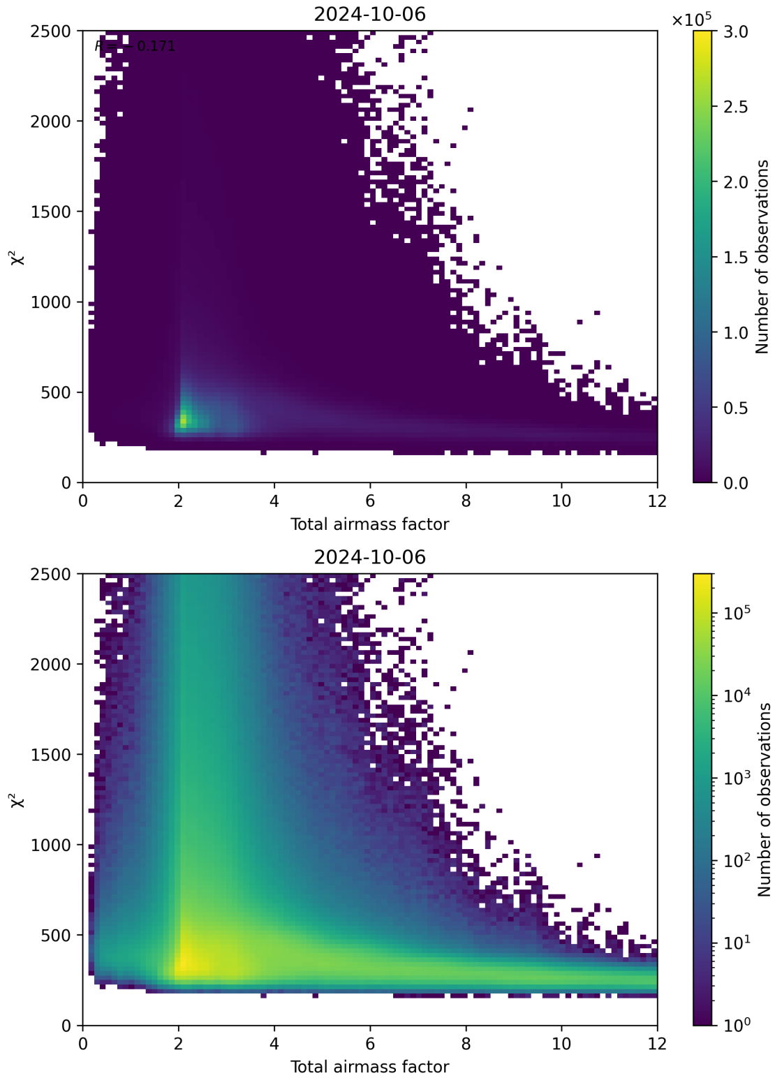
Figure 63: Scatter density plot of “Total airmass factor” against “ \chi^2 ” for 2024-10-05 to 2024-10-07.
