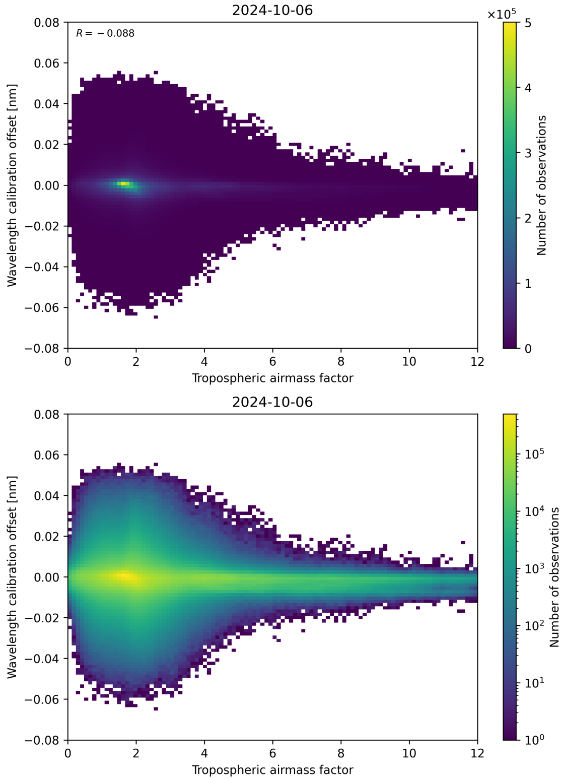
Figure 80: Scatter density plot of “Tropospheric airmass factor” against “Wavelength calibration offset” for 2024-10-05 to 2024-10-07.
