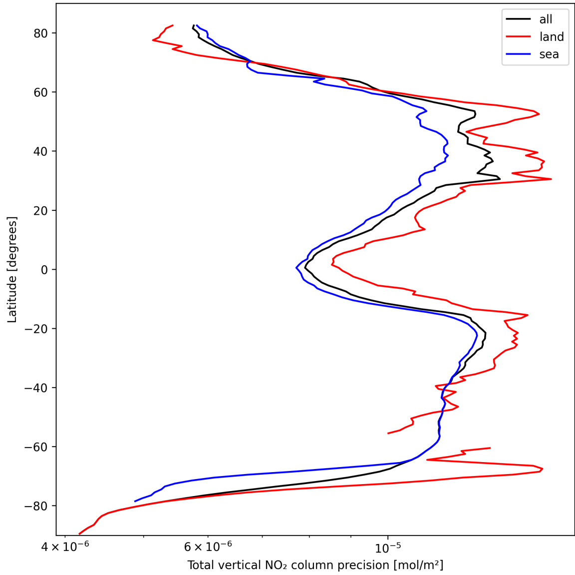
Figure 22: Zonal average of “Total vertical NO 2 column precision” for 2024-10-05 to 2024-10-07.
