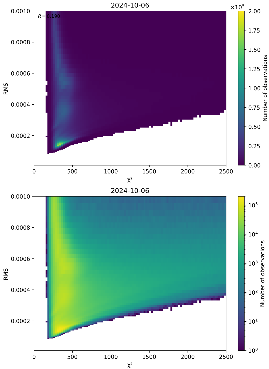
Figure 82: Scatter density plot of “ \chi^2 ” against “RMS” for 2024-10-05 to 2024-10-07.
