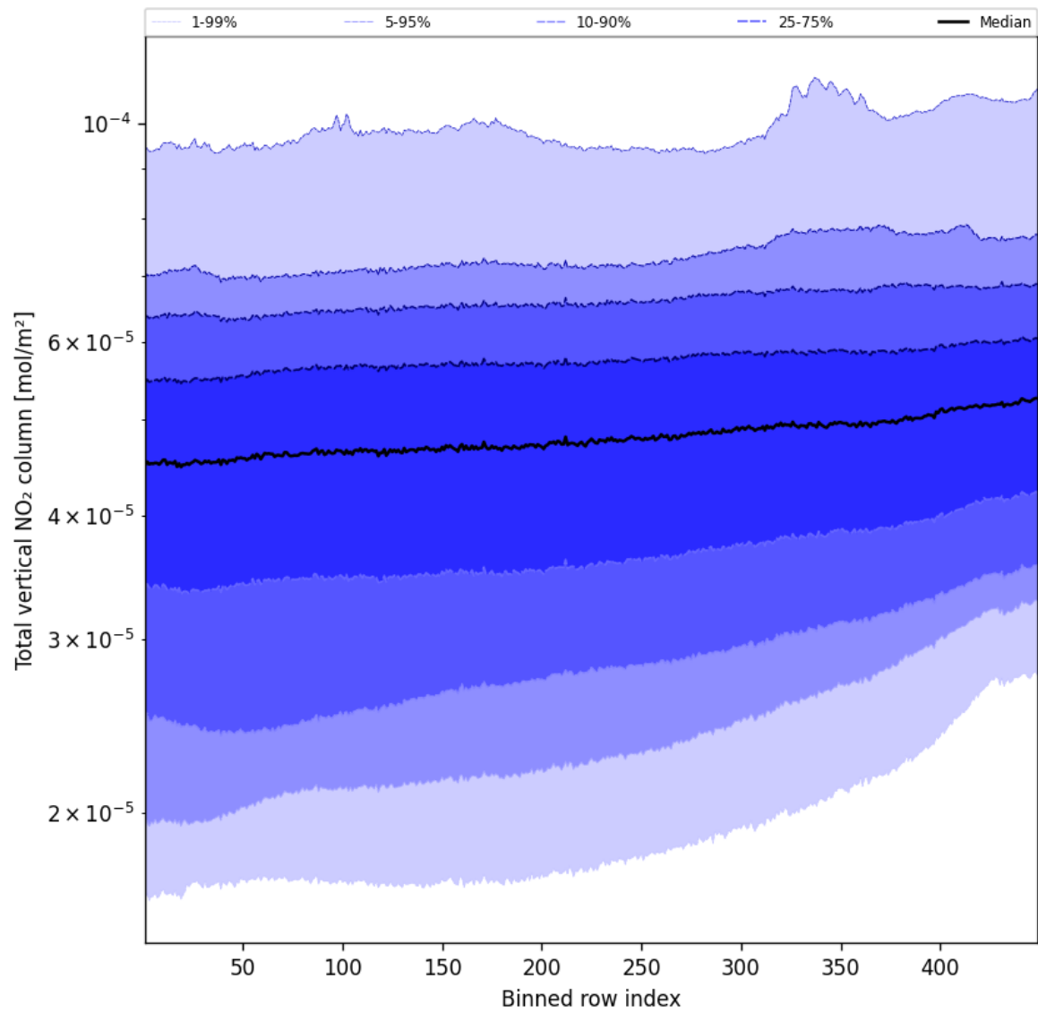
Figure 55: Along track statistics of “Total vertical NO 2 column” for 2024-10-05 to 2024-10-07
