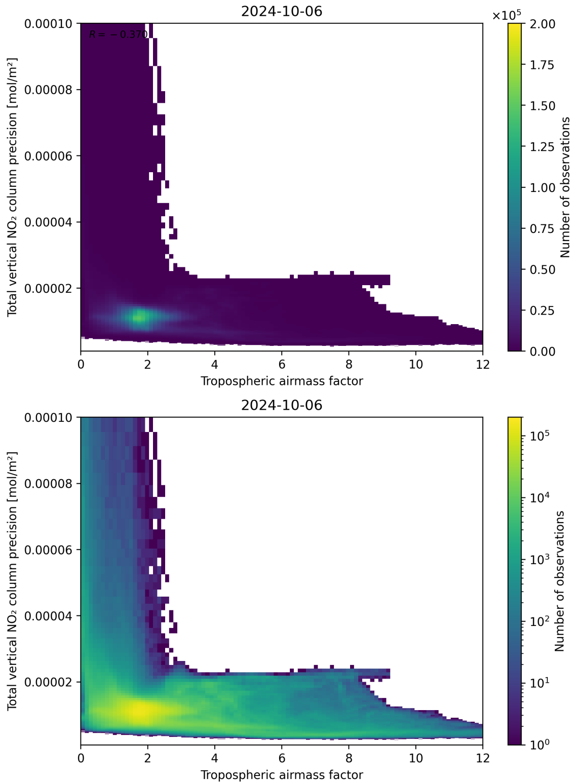
Figure 78: Scatter density plot of “Tropospheric air mass factor” against “Total vertical NO 2 column precision” for 2024-10-05 to 2024-10-07.
