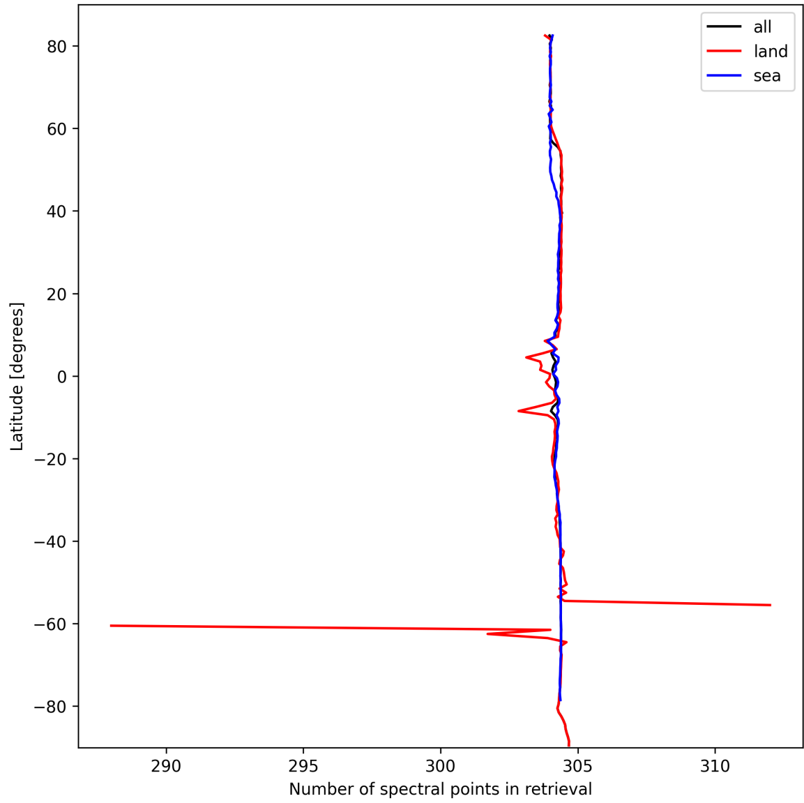
Figure 16: Zonal average of “Number of spectral points in retrieval” for 2024-10-05 to 2024-10-07.
