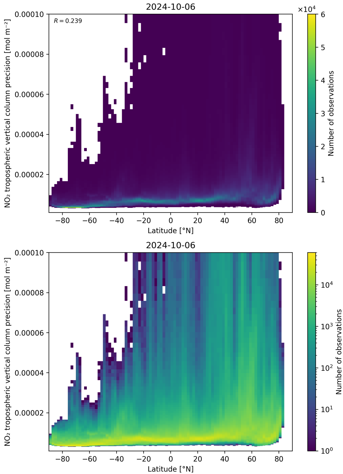
Figure 93: Scatter density plot of “Latitude” against “NO 2 tropospheric vertical column precision” for 2024-10-05 to 2024-10-07.
