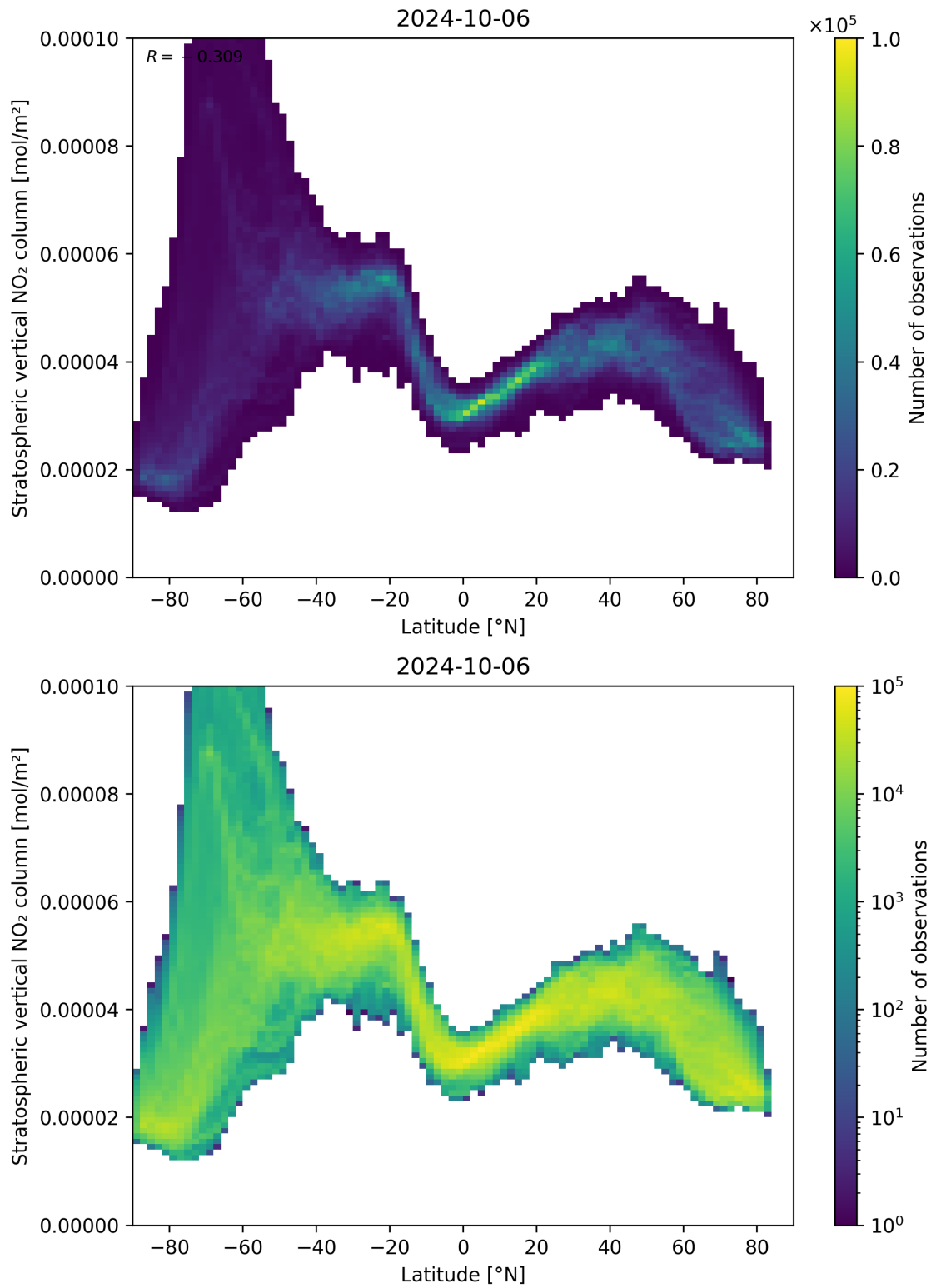
Figure 87: Scatter density plot of “Latitude” against “Stratospheric vertical NO 2 column” for 2024-10-05 to 2024-10-07.
