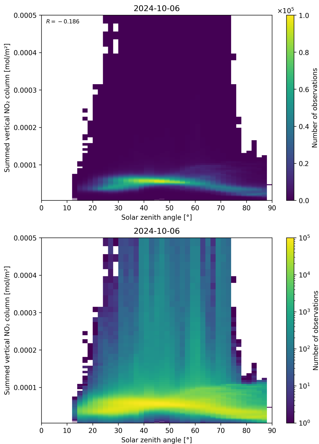
Figure 151: Scatter density plot of “Solar zenith angle” against “Summed vertical NO 2 column” for 2024-10-05 to 2024-10-07.
