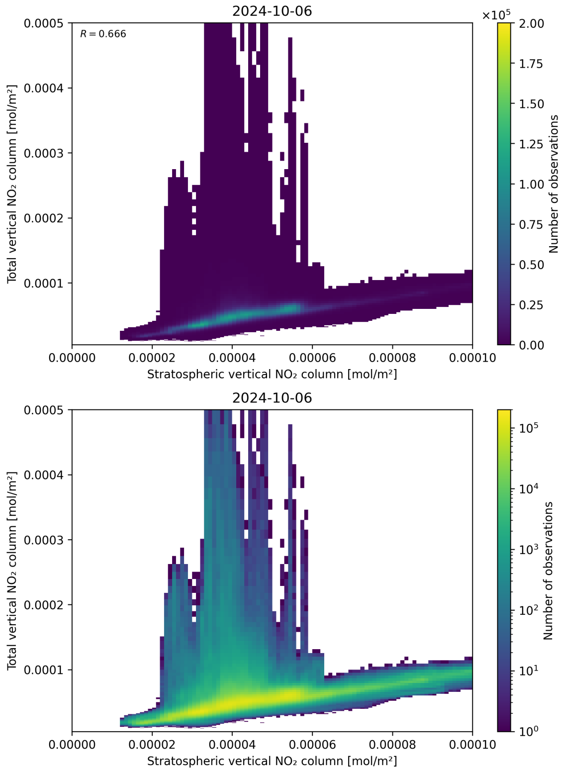
Figure 100: Scatter density plot of “Stratospheric vertical NO 2 column” against “Total vertical NO 2 column” for 2024-10-05 to 2024-10-07.
