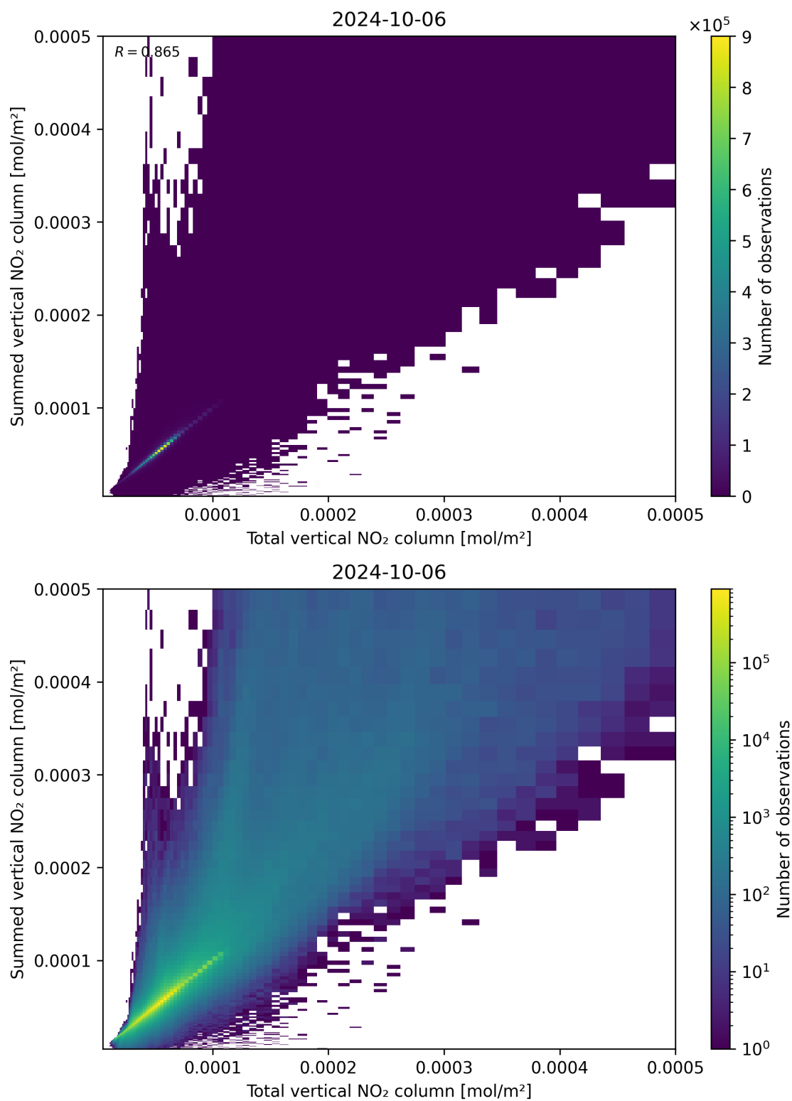
Figure 112: Scatter density plot of “Total vertical NO 2 column” against “Summed vertical NO 2 column” for 2024-10-05 to 2024-10-07.
