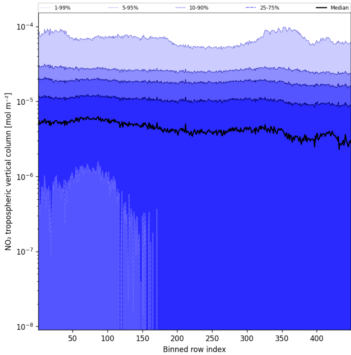
Figure 46: Along track statistics of “NO 2 tropospheric vertical column” for 2024-10-05 to 2024-10-07
