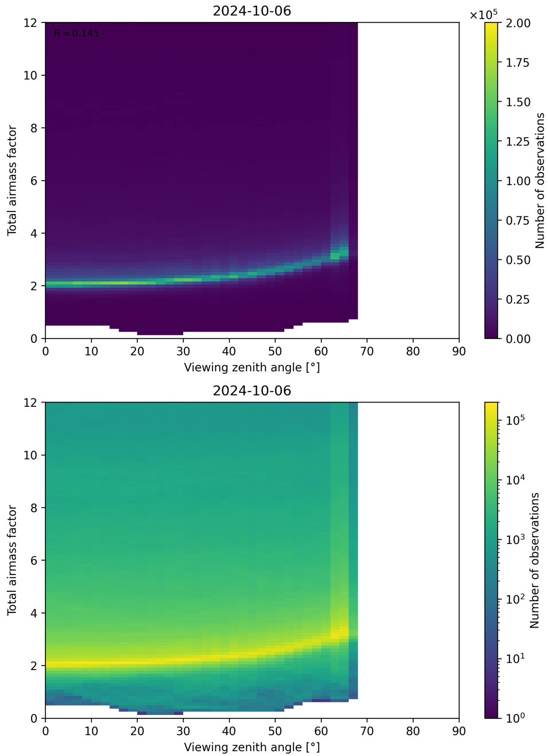
Figure 160: Scatter density plot of “Viewing zenith angle” against “Total airmass factor” for 2024-10-05 to 2024-10-07.
