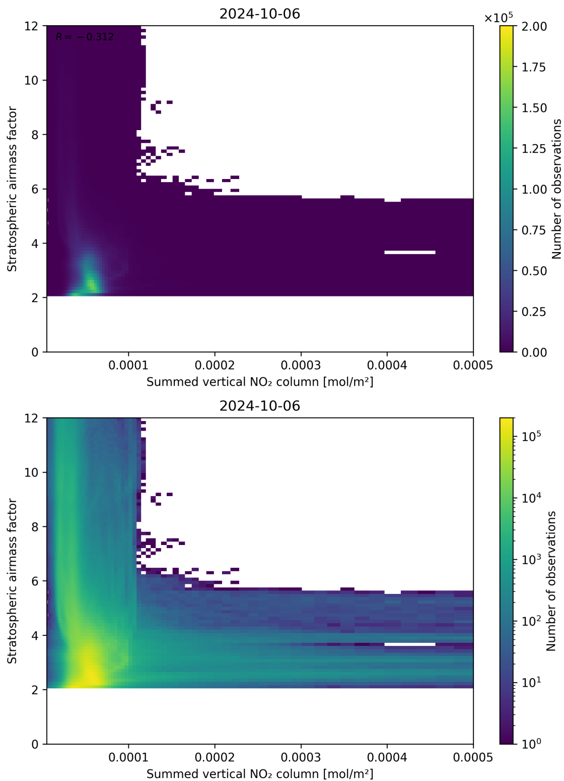
Figure 103: Scatter density plot of “Summed vertical NO 2 column” against “Stratospheric airmass factor” for 2024-10-05 to 2024-10-07.
