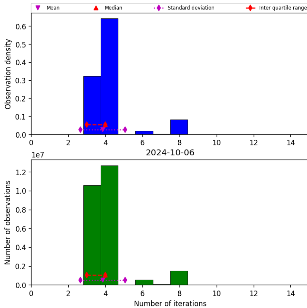
Figure 34: Histogram of “Number of iterations” for 2024-10-05 to 2024-10-07
