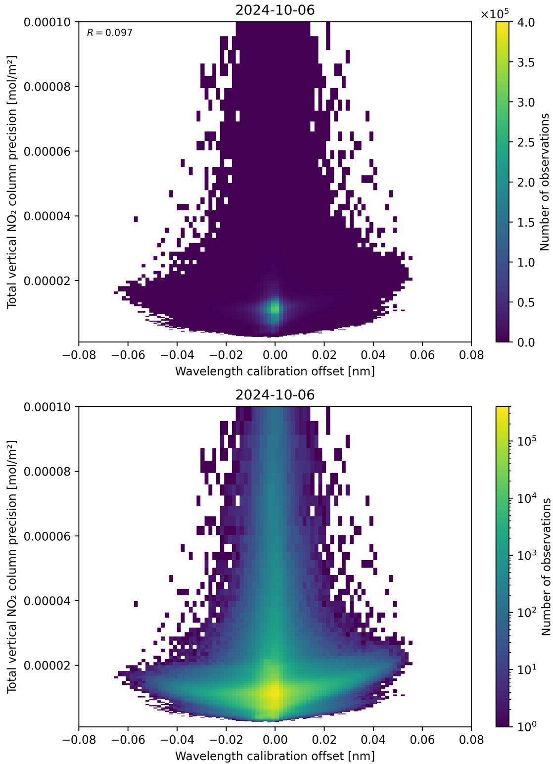
Figure 180: Scatter density plot of “Wavelength calibration offset” against “Total vertical NO 2 column precision” for 2024-10-05 to 2024-10-07.
