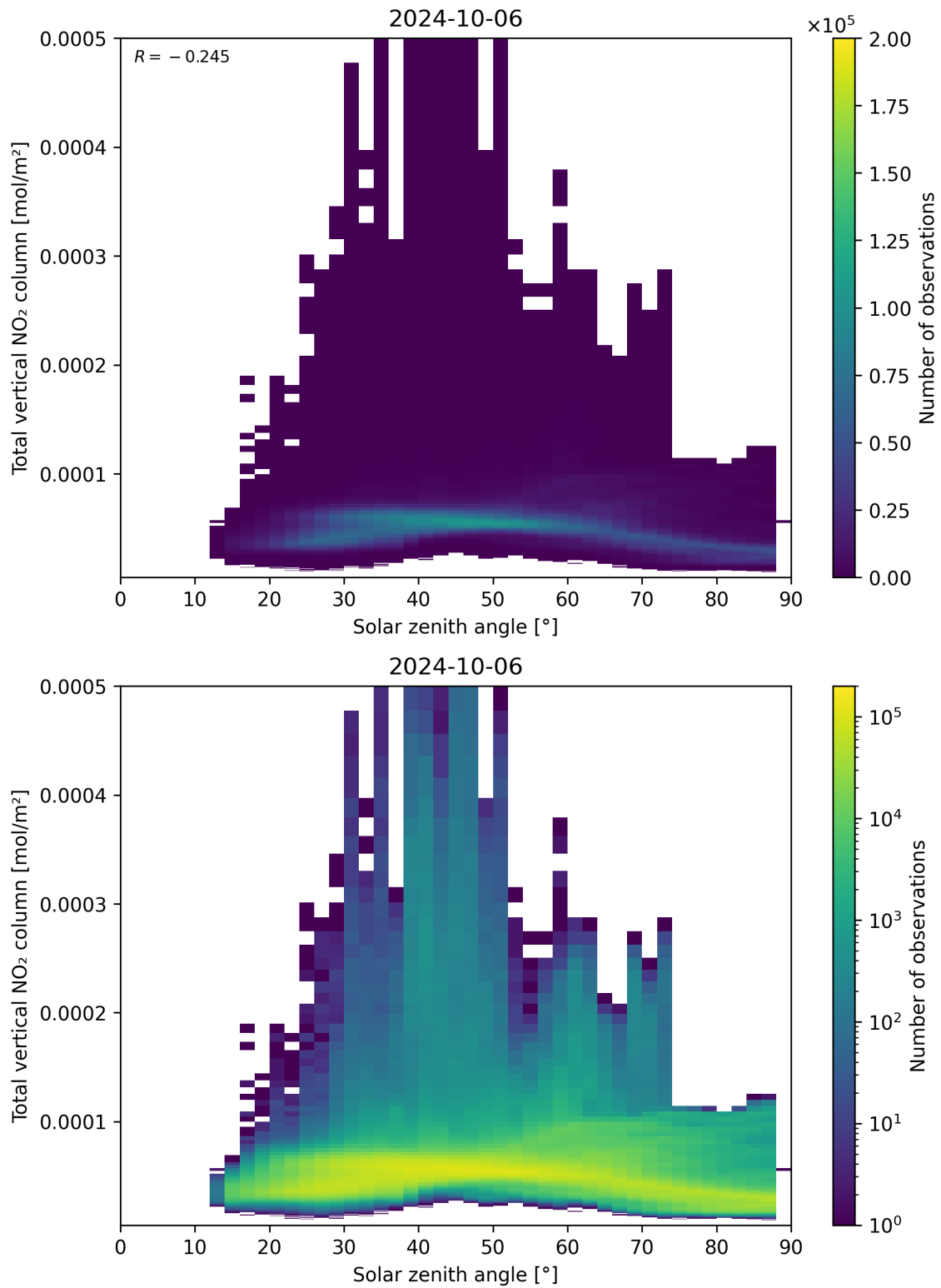
Figure 153: Scatter density plot of “Solar zenith angle” against “Total vertical NO 2 column” for 2024-10-05 to 2024-10-07.
