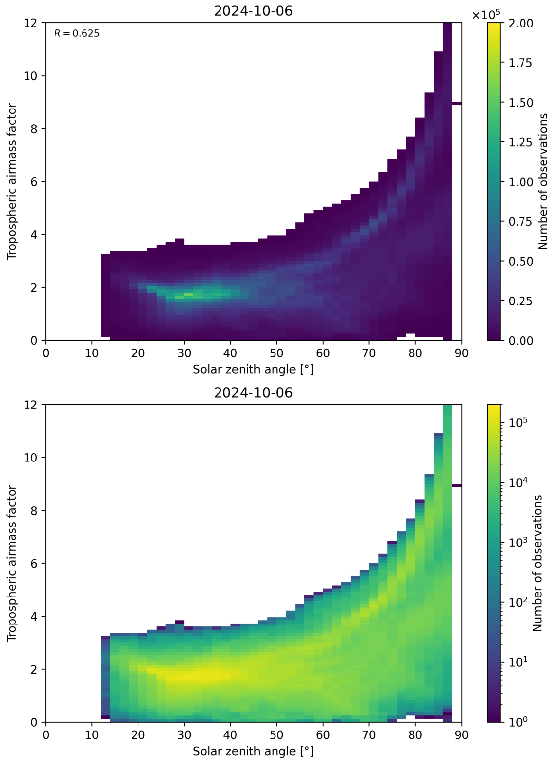
Figure 147: Scatter density plot of “Solar zenith angle” against “Tropospheric airmass factor” for 2024-10-05 to 2024-10-07.
