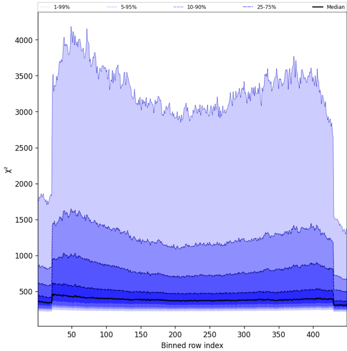
Figure 59: Along track statistics of “ \chi^2 ” for 2024-10-05 to 2024-10-07
