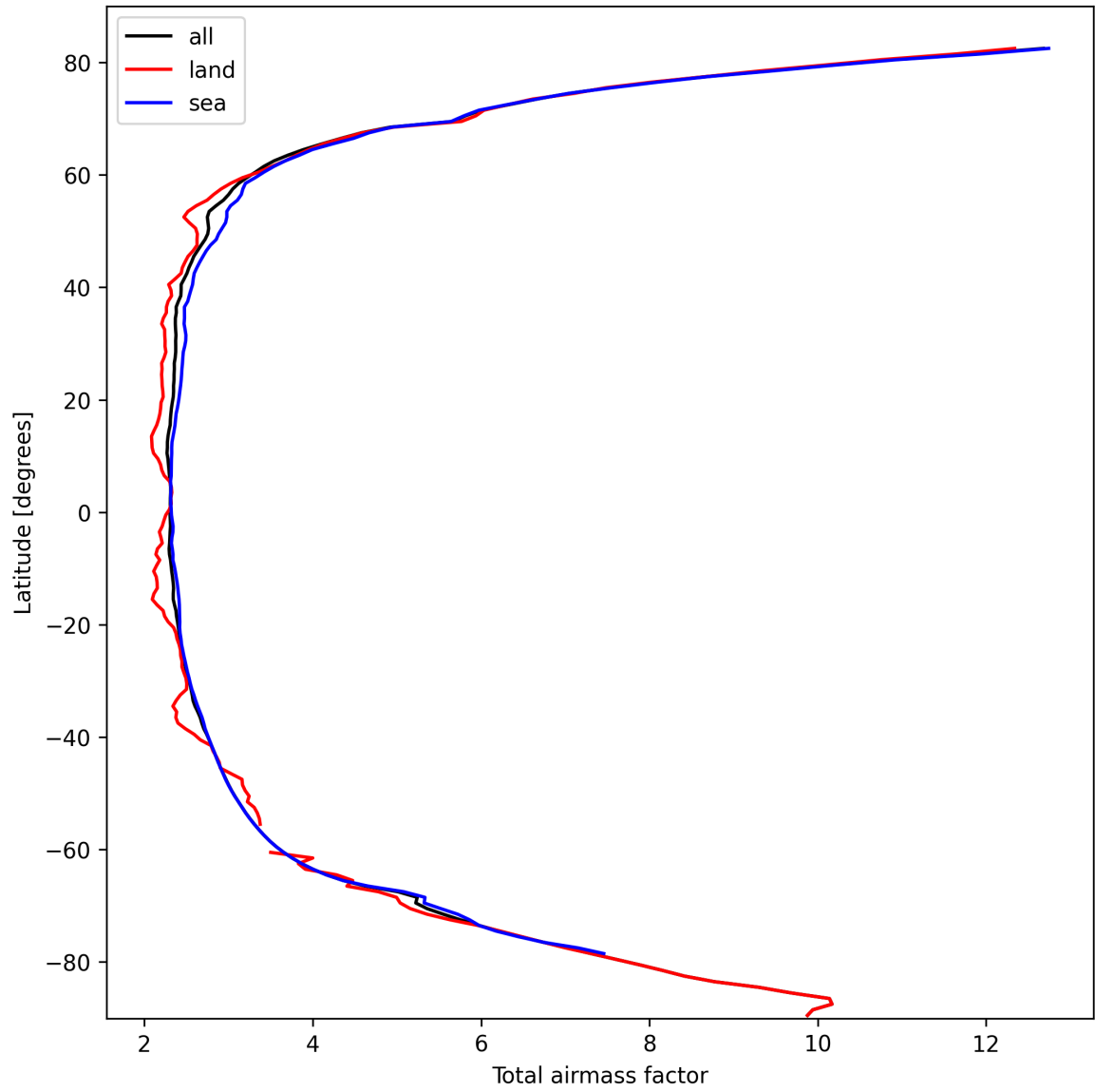
Figure 15: Zonal average of “Total airmass factor” for 2024-10-05 to 2024-10-07.
