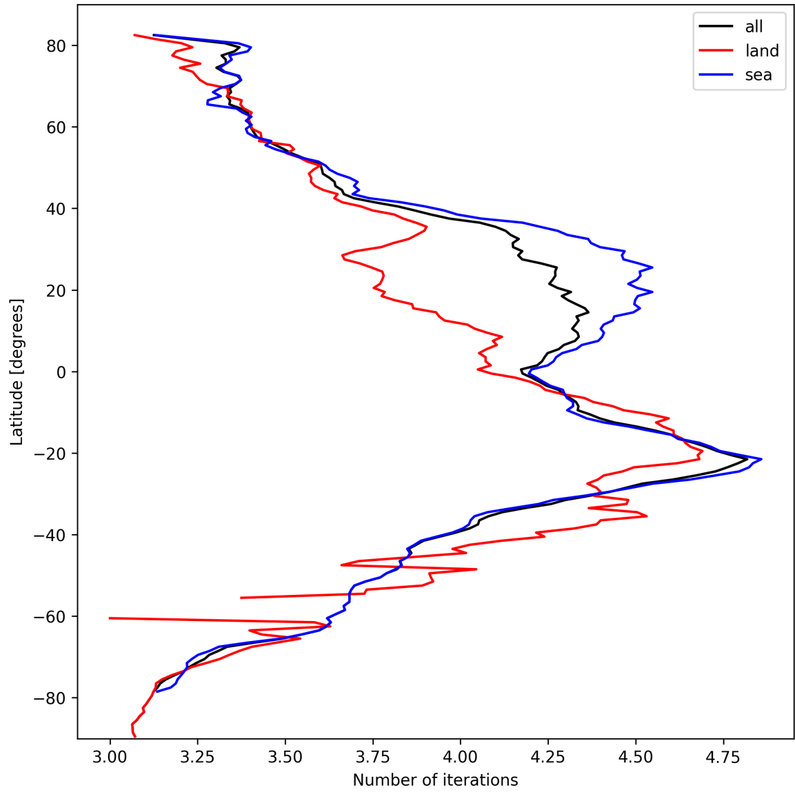
Figure 17: Zonal average of “Number of iterations” for 2024-10-05 to 2024-10-07.
