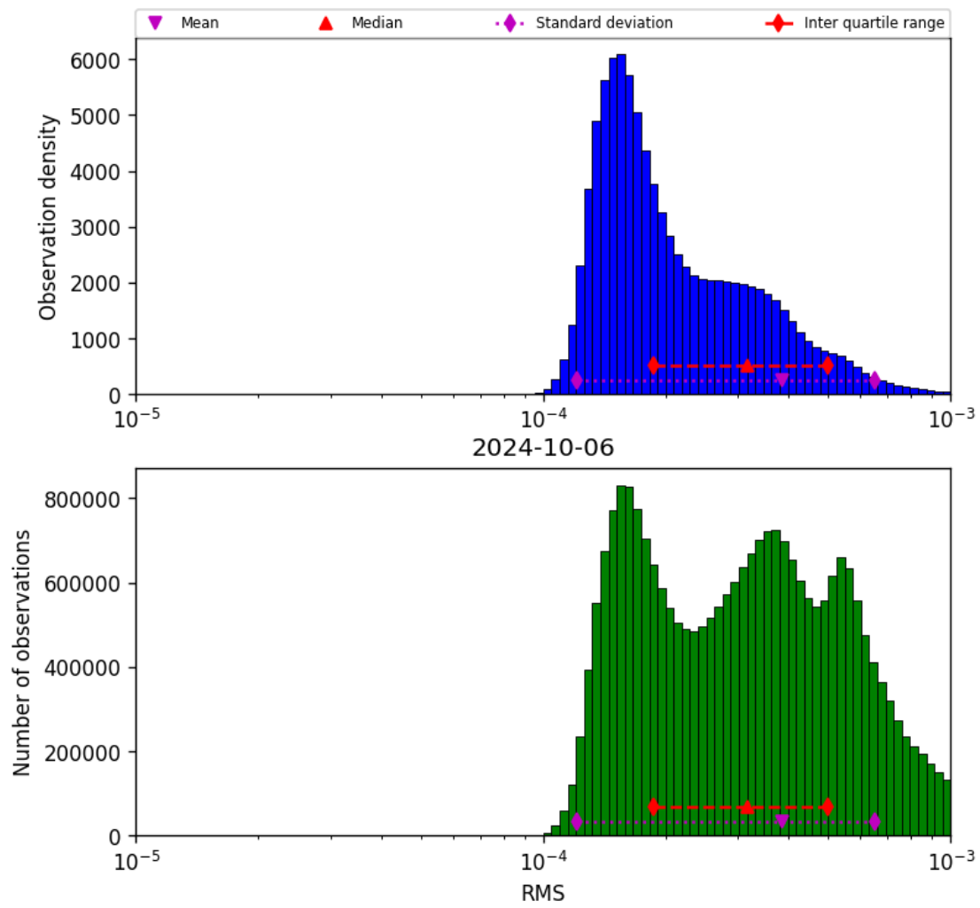
Figure 43: Histogram of “RMS” for 2024-10-05 to 2024-10-07
