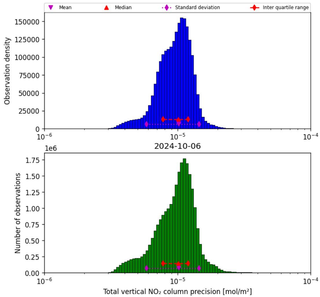
Figure 39: Histogram of “Total vertical NO 2 column precision” for 2024-10-05 to 2024-10-07
