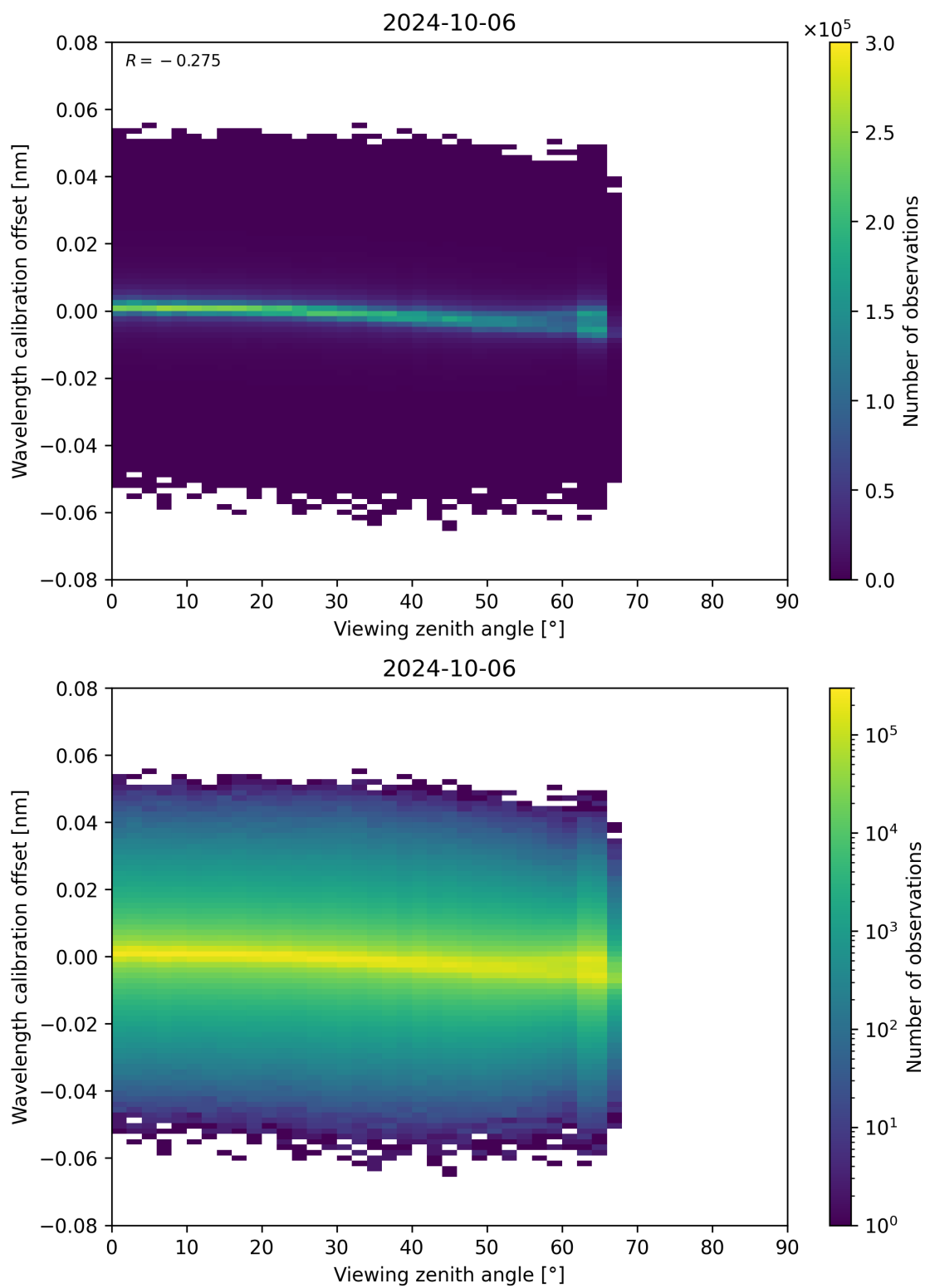
Figure 173: Scatter density plot of “Viewing zenith angle” against “Wavelength calibration offset” for 2024-10-05 to 2024-10-07.
