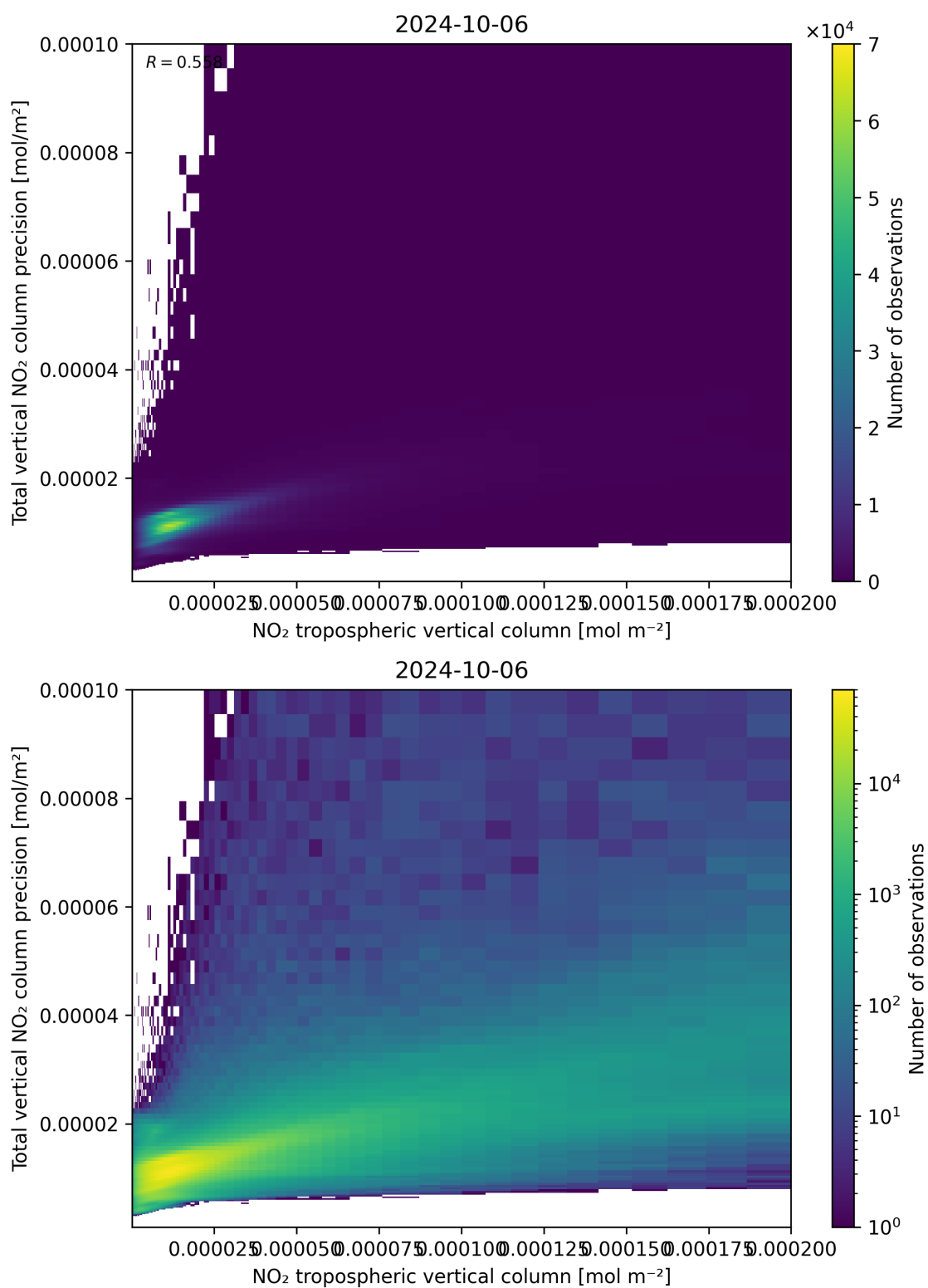
Figure 129: Scatter density plot of “NO 2 tropospheric vertical column” against “Total vertical NO 2 column precision” for 2024-10-05 to 2024-10-07.
