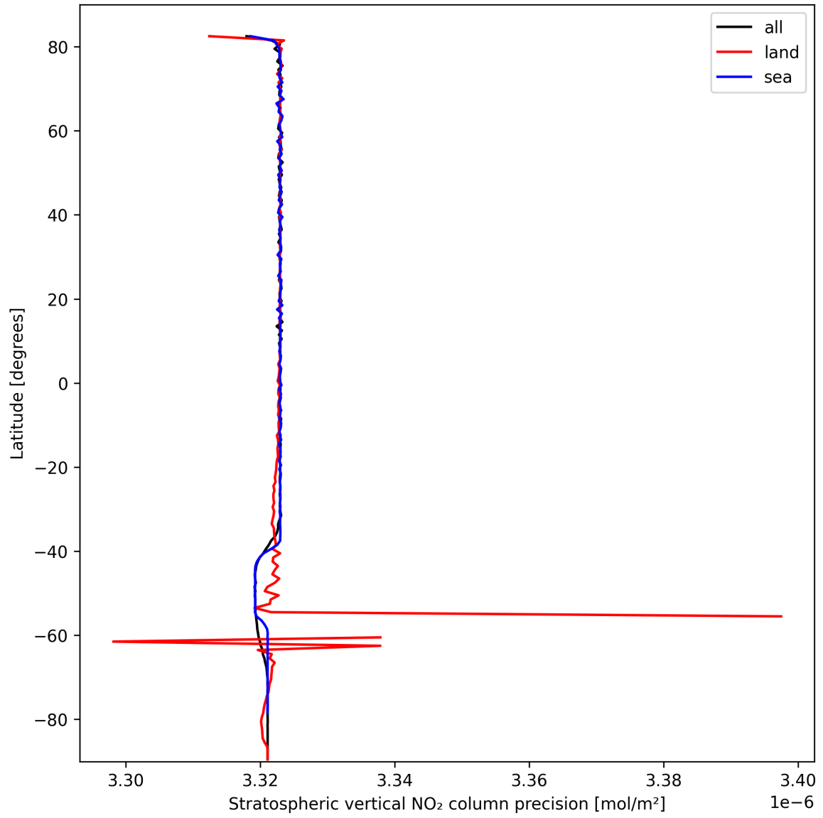
Figure 20: Zonal average of “Stratospheric vertical NO 2 column precision” for 2024-10-05 to 2024-10-07.
