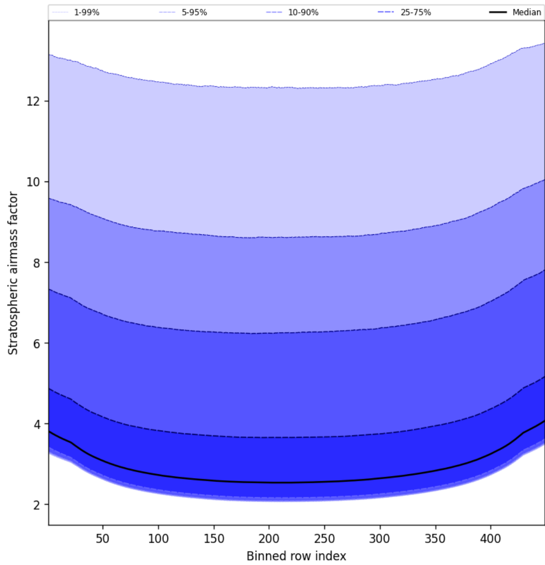
Figure 61: Along track statistics of “Stratospheric airmass factor” for 2024-10-05 to 2024-10-07
