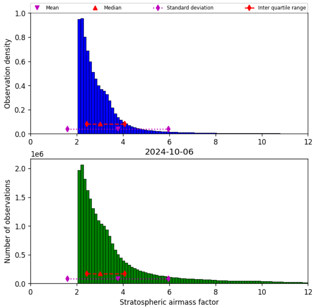
Figure 44: Histogram of “Stratospheric airmass factor” for 2024-10-05 to 2024-10-07
