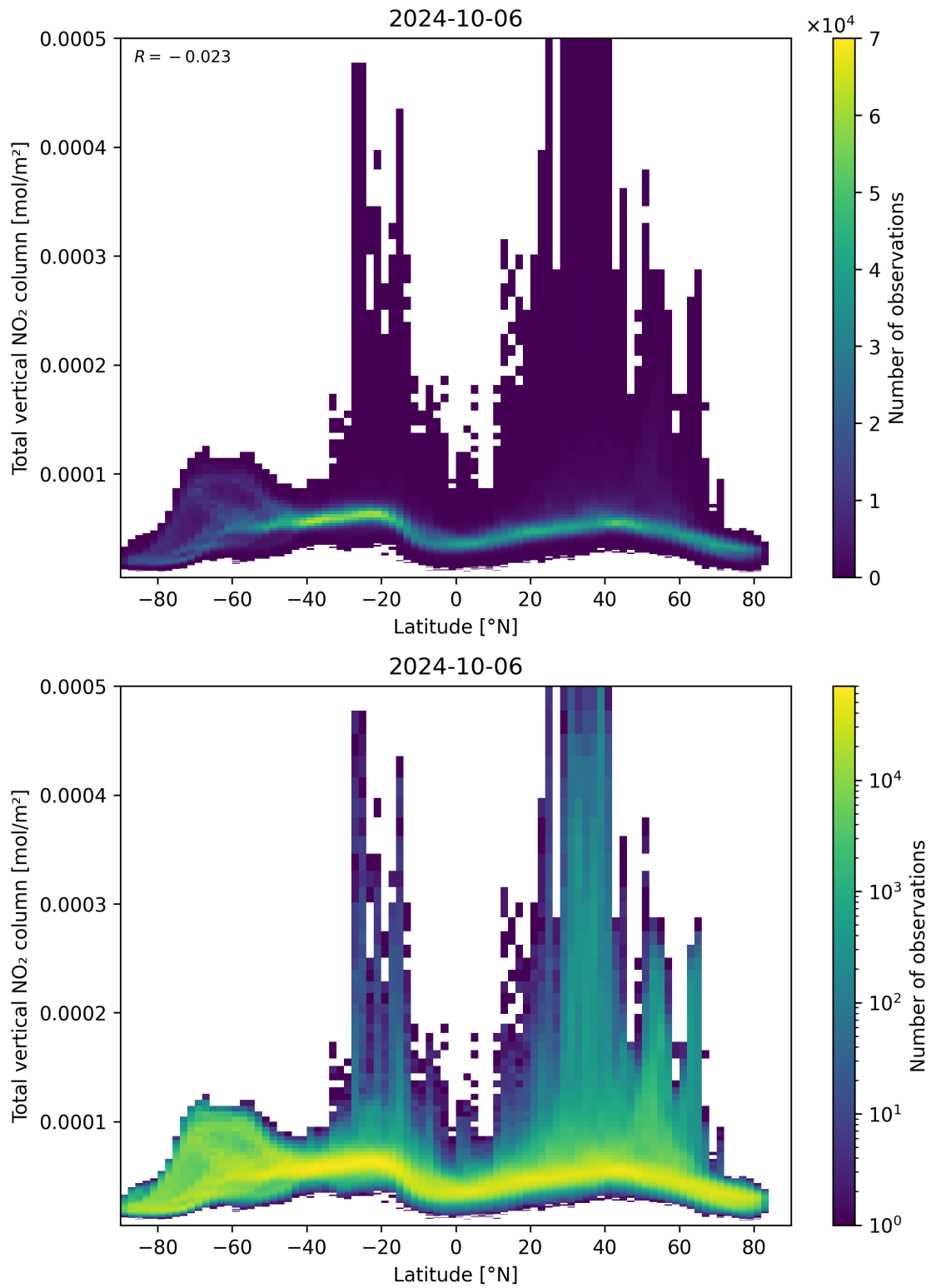
Figure 90: Scatter density plot of “Latitude” against “Total vertical NO 2 column” for 2024-10-05 to 2024-10-07.
