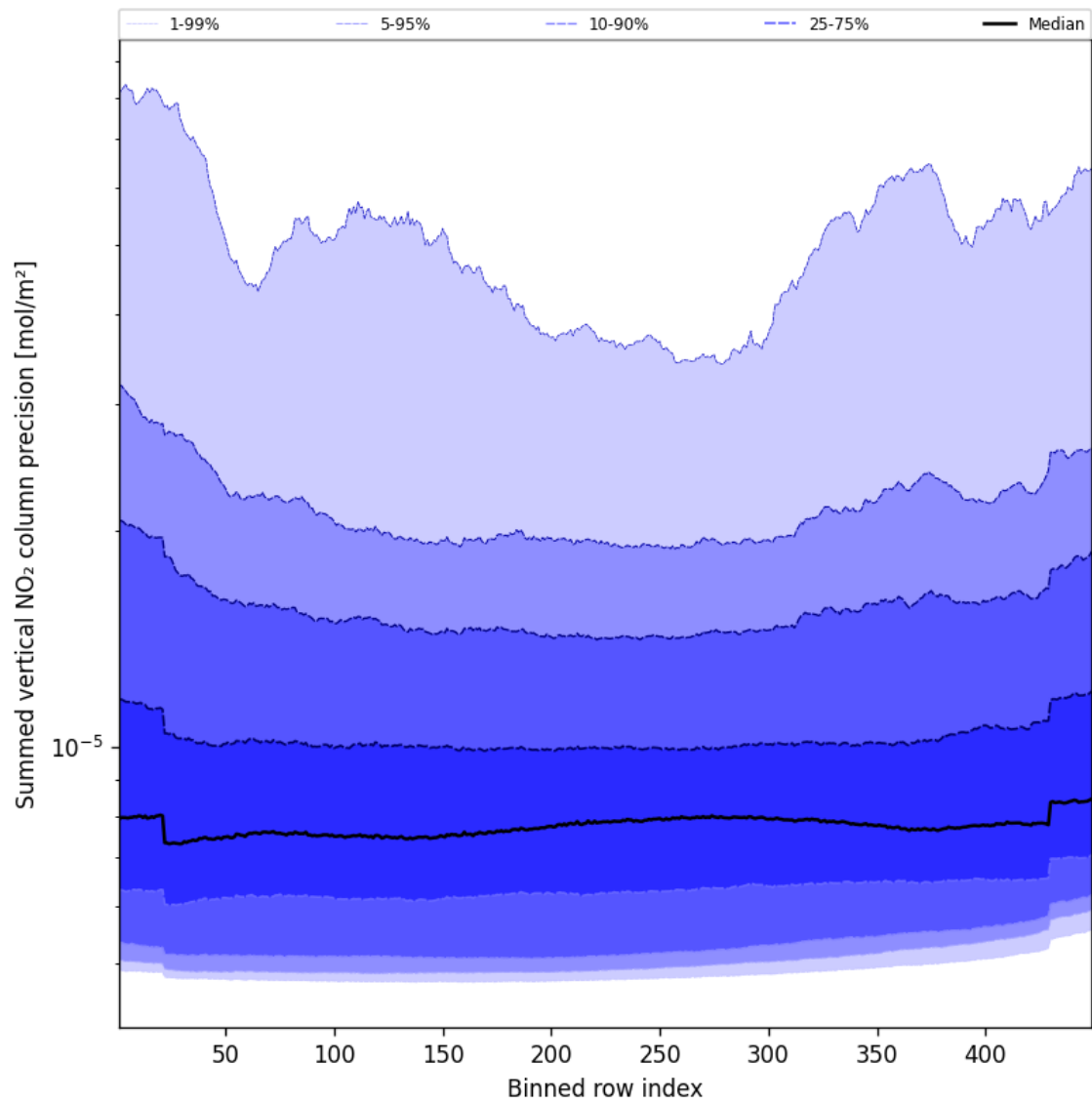
Figure 58: Along track statistics of “Summed vertical NO 2 column precision” for 2024-10-05 to 2024-10-07
