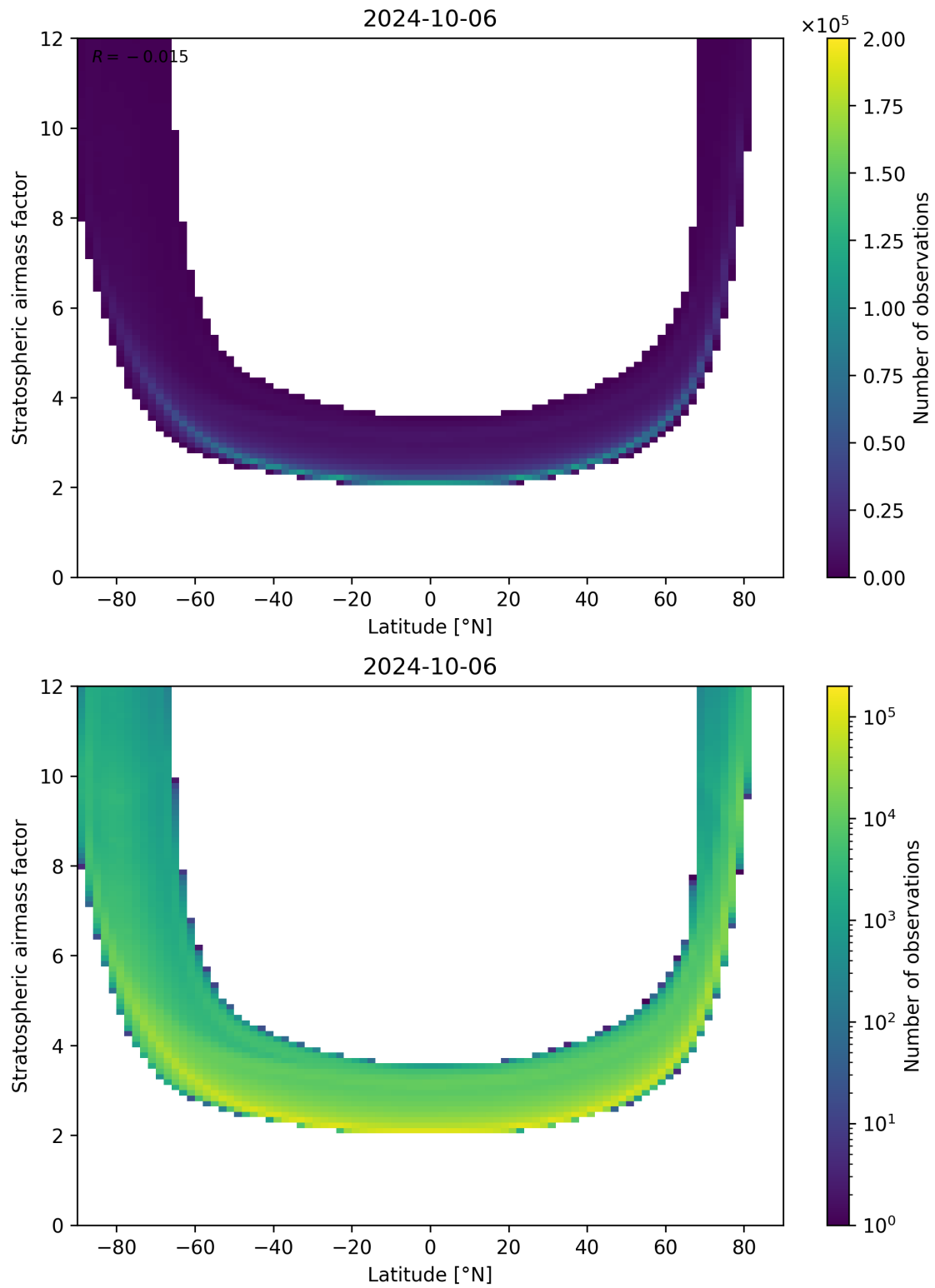
Figure 83: Scatter density plot of “Latitude” against “Stratospheric airmass factor” for 2024-10-05 to 2024-10-07.
