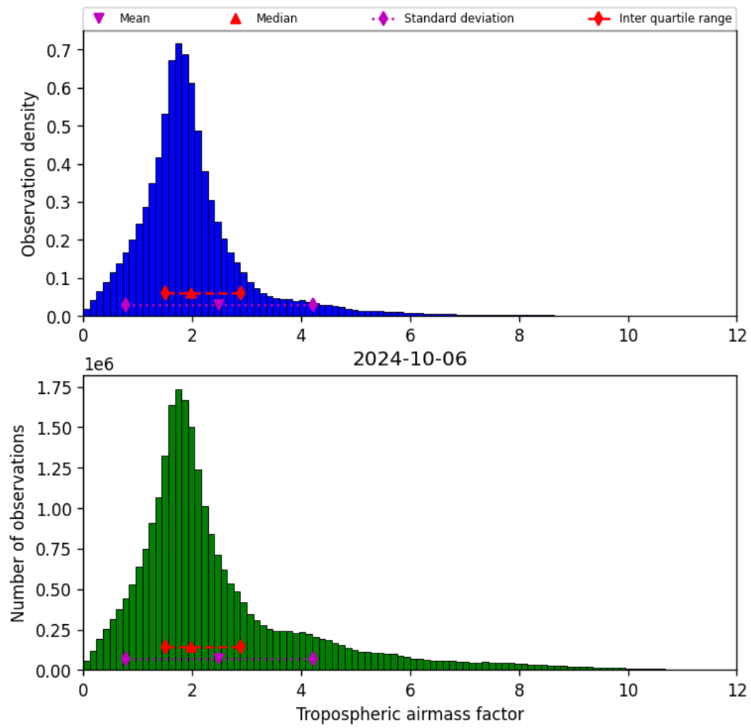
Figure 31: Histogram of “Tropospheric airmass factor” for 2024-10-05 to 2024-10-07
