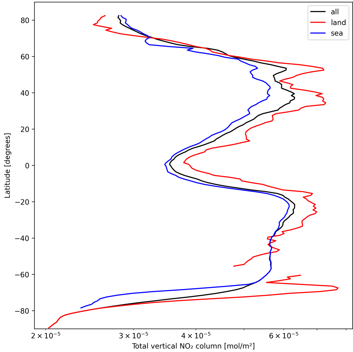
Figure 21: Zonal average of “Total vertical NO 2 column” for 2024-10-05 to 2024-10-07.
