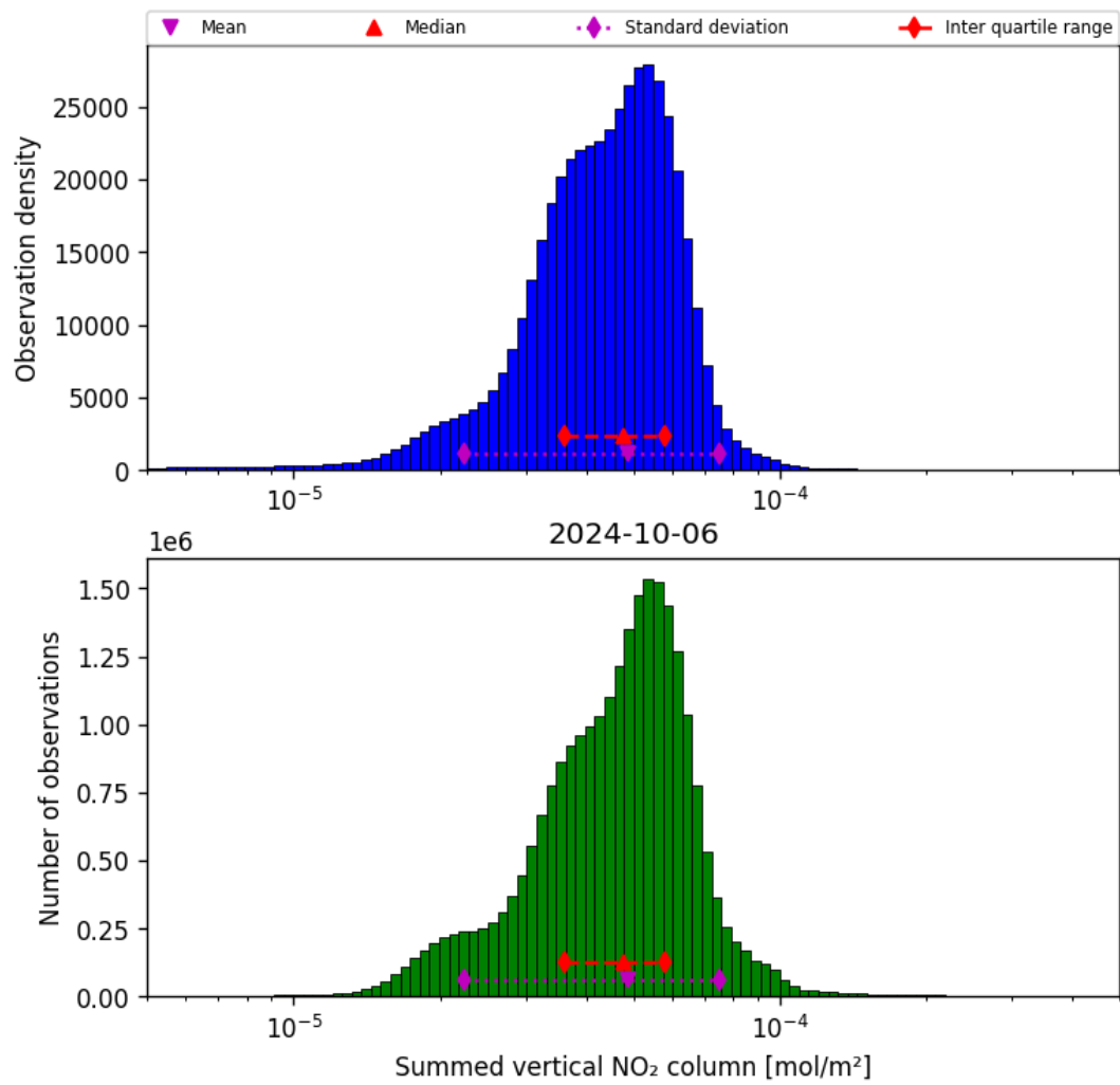
Figure 40: Histogram of “Summed vertical NO 2 column” for 2024-10-05 to 2024-10-07
