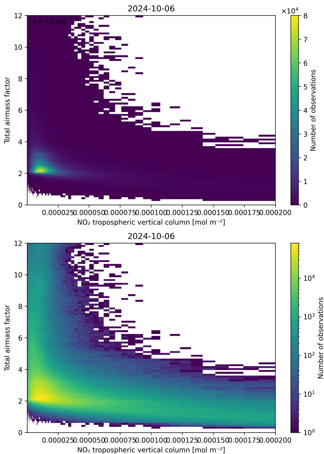
Figure 122: Scatter density plot of “NO 2 tropospheric vertical column” against “Total air mass factor” for 2024-10-05 to 2024-10-07.
