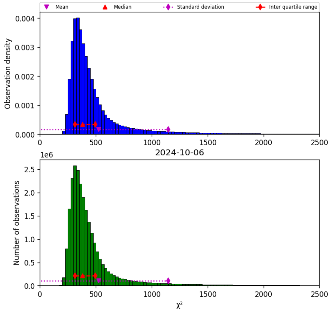
Figure 42: Histogram of “ \chi^2 ” for 2024-10-05 to 2024-10-07
