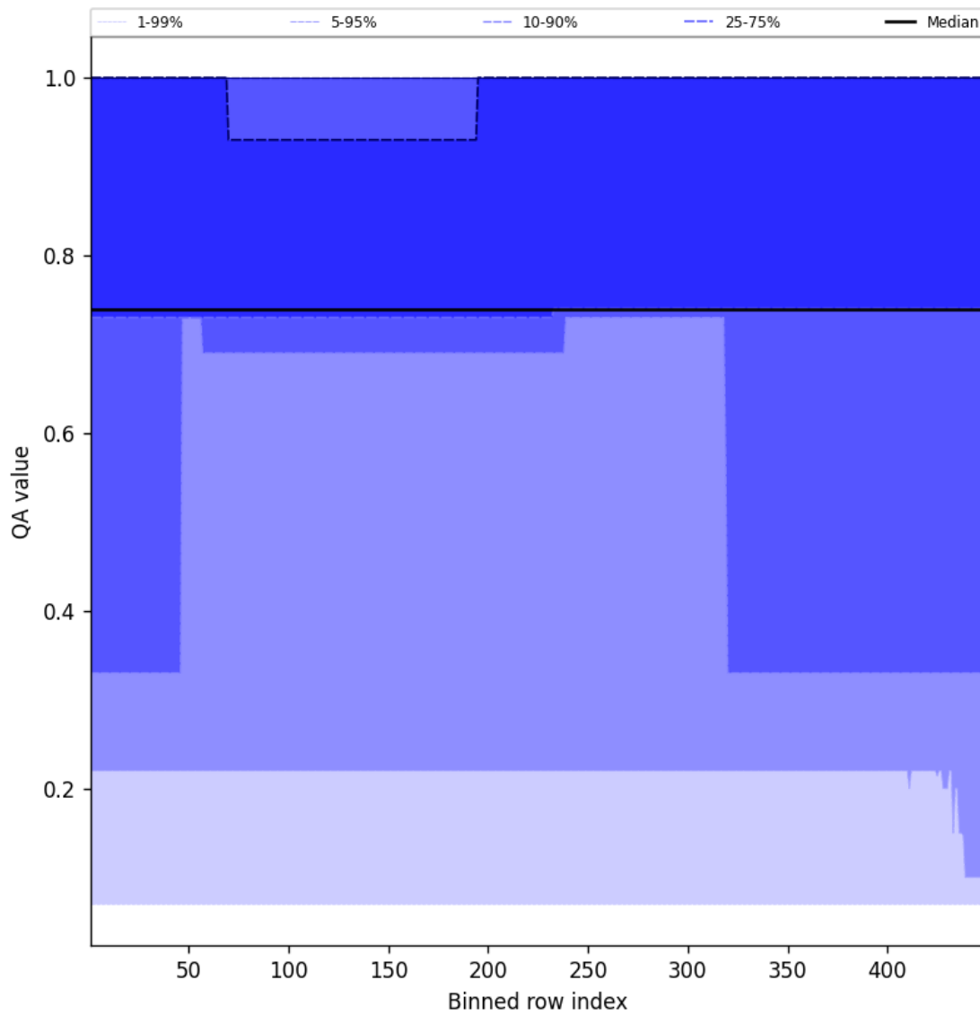
Figure 45: Along track statistics of “QA value” for 2024-10-05 to 2024-10-07
