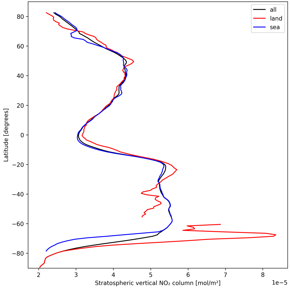
Figure 19: Zonal average of “Stratospheric vertical NO 2 column” for 2024-10-05 to 2024-10-07.
