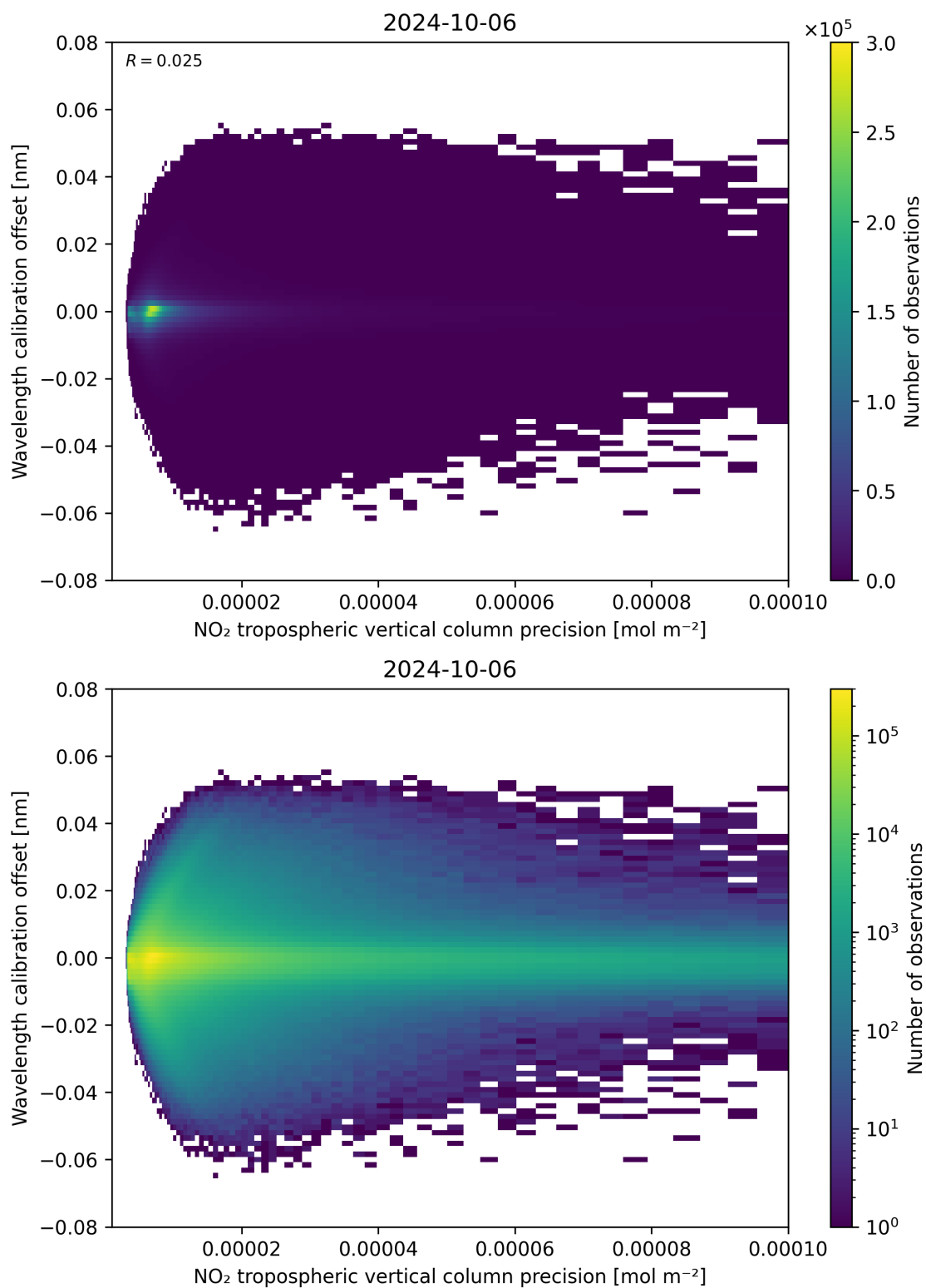
Figure 141: Scatter density plot of “NO 2 tropospheric vertical column precision” against “Wavelength calibration offset” for 2024-10-05 to 2024-10-07.
