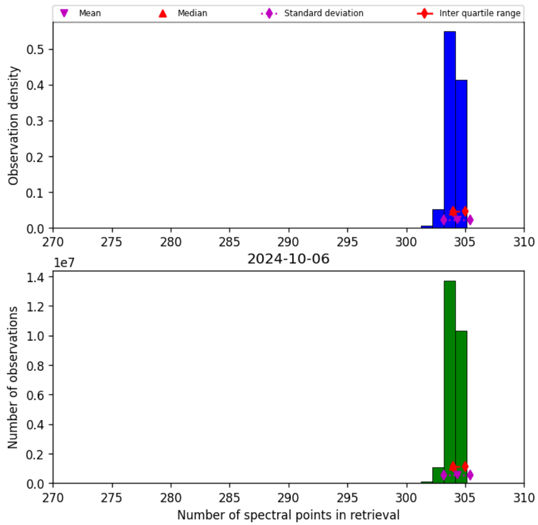
Figure 33: Histogram of “Number of spectral points in retrieval” for 2024-10-05 to 2024-10-07
