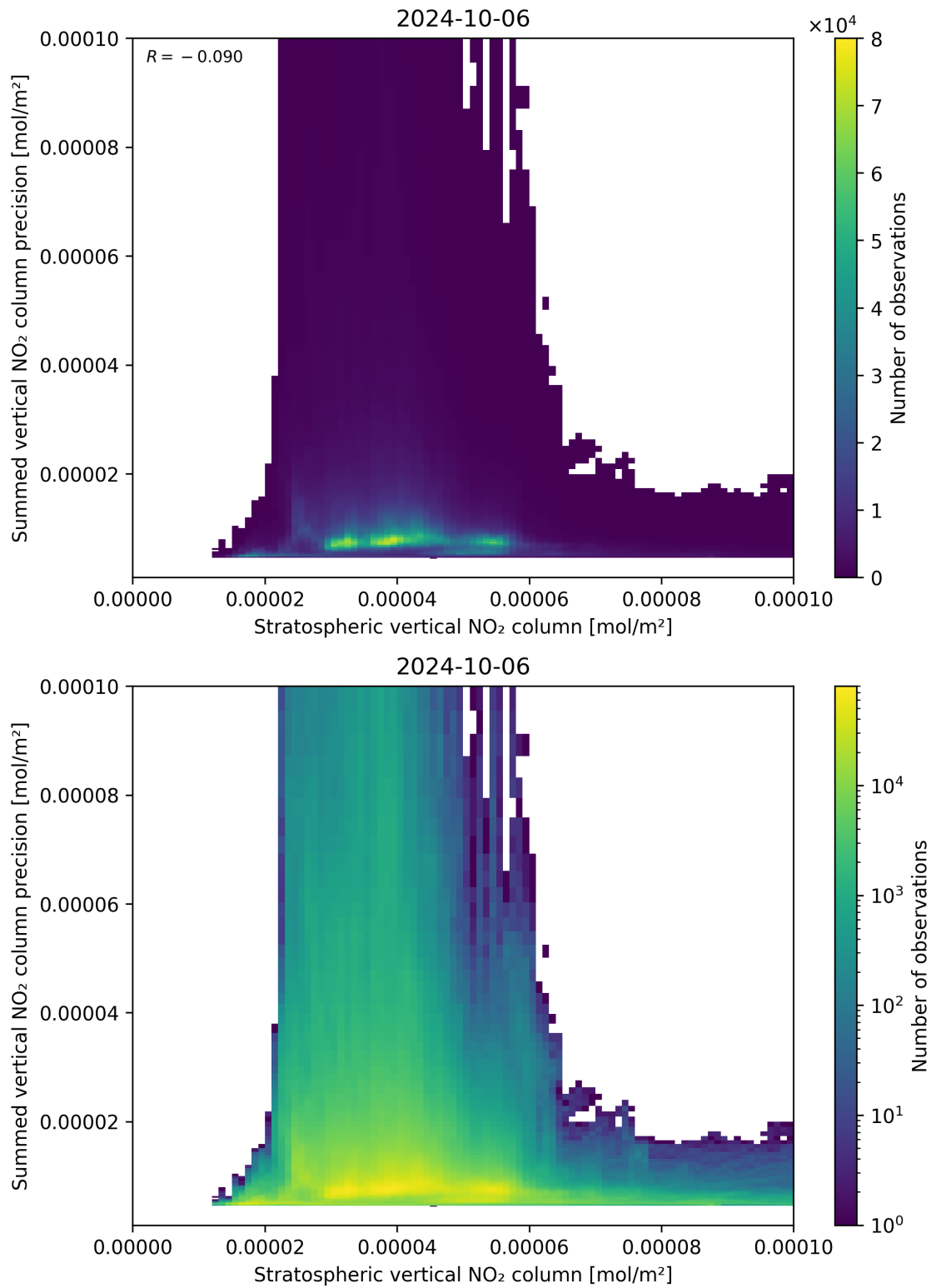
Figure 99: Scatter density plot of “Stratospheric vertical NO 2 column” against “Summed vertical NO 2 column precision” for 2024-10-05 to 2024-10-07.
