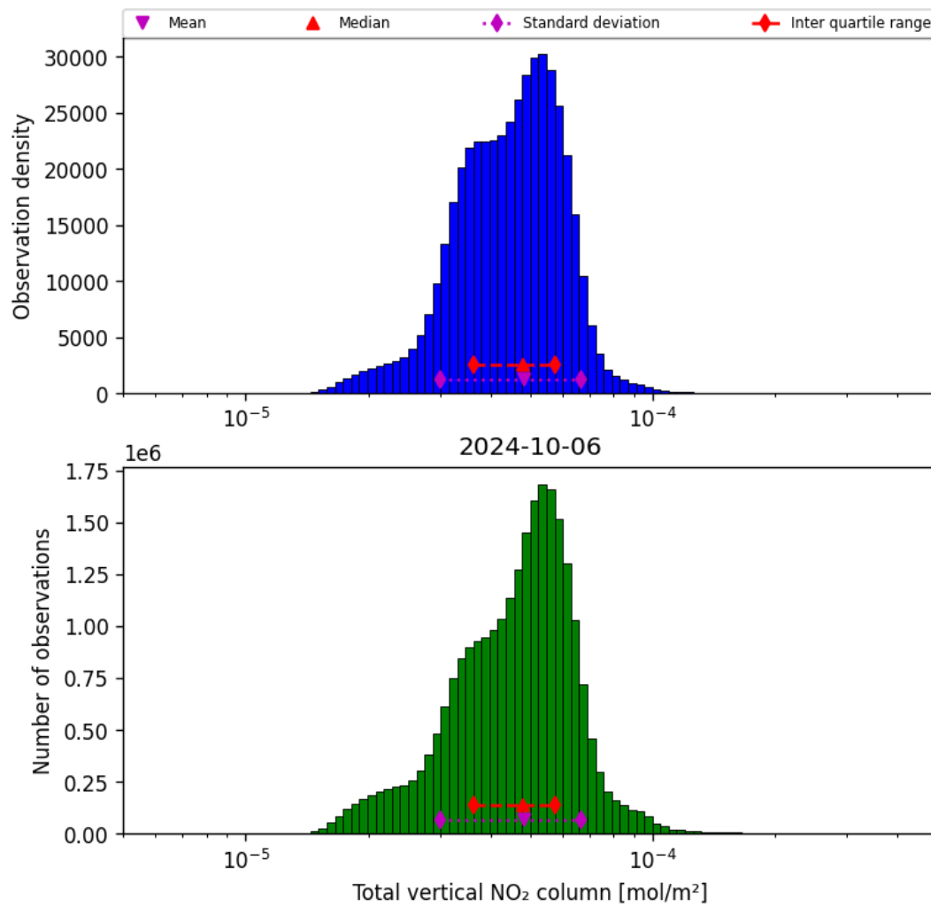
Figure 38: Histogram of “Total vertical NO 2 column” for 2024-10-05 to 2024-10-07
