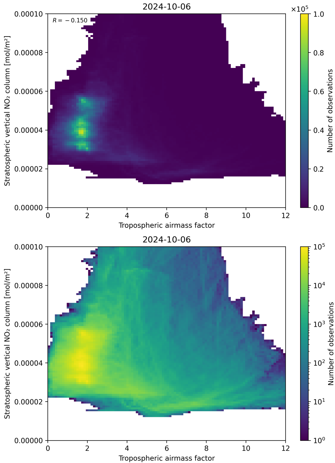
Figure 74: Scatter density plot of “Tropospheric air mass factor” against “Stratospheric vertical NO 2 column” for 2024-10-05 to 2024-10-07.
