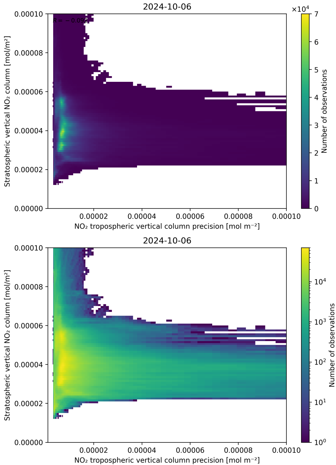
Figure 135: Scatter density plot of “NO 2 tropospheric vertical column precision” against “Stratospheric vertical NO 2 column” for 2024-10-05 to 2024-10-07.
