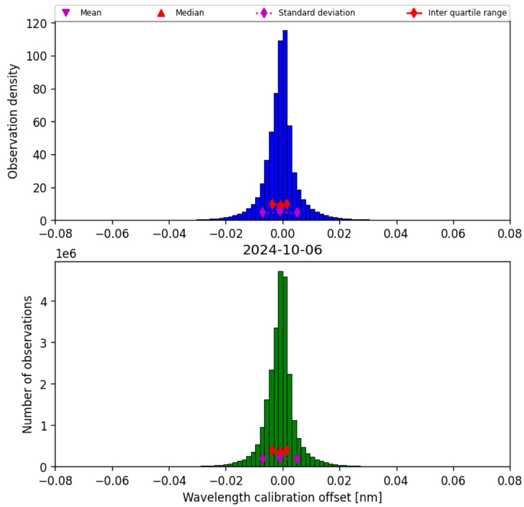
Figure 35: Histogram of “Wavelength calibration offset” for 2024-10-05 to 2024-10-07
