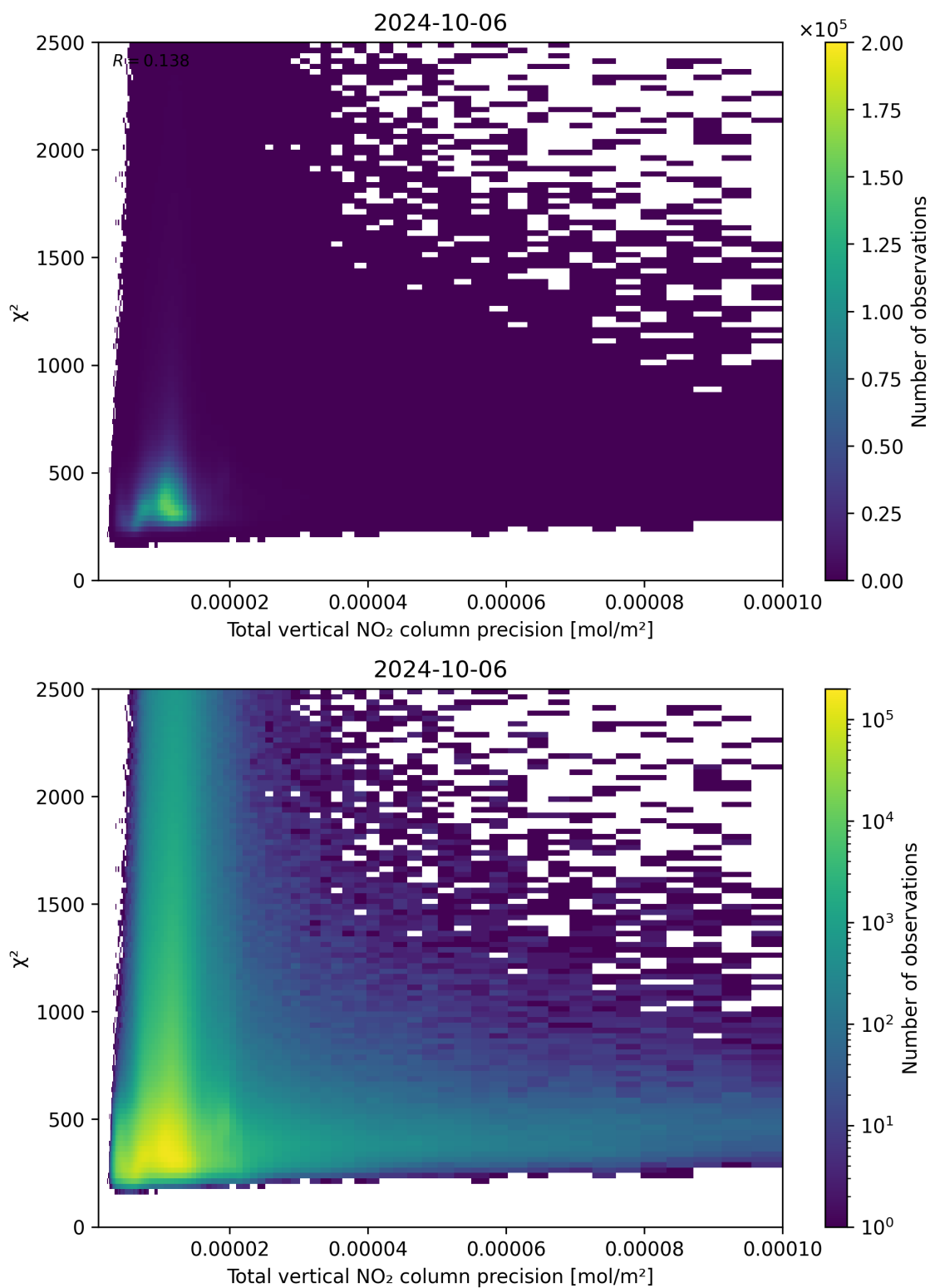
Figure 116: Scatter density plot of “Total vertical NO 2 column precision” against “ \chi^2 ” for 2024-10-05 to 2024-10-07.
