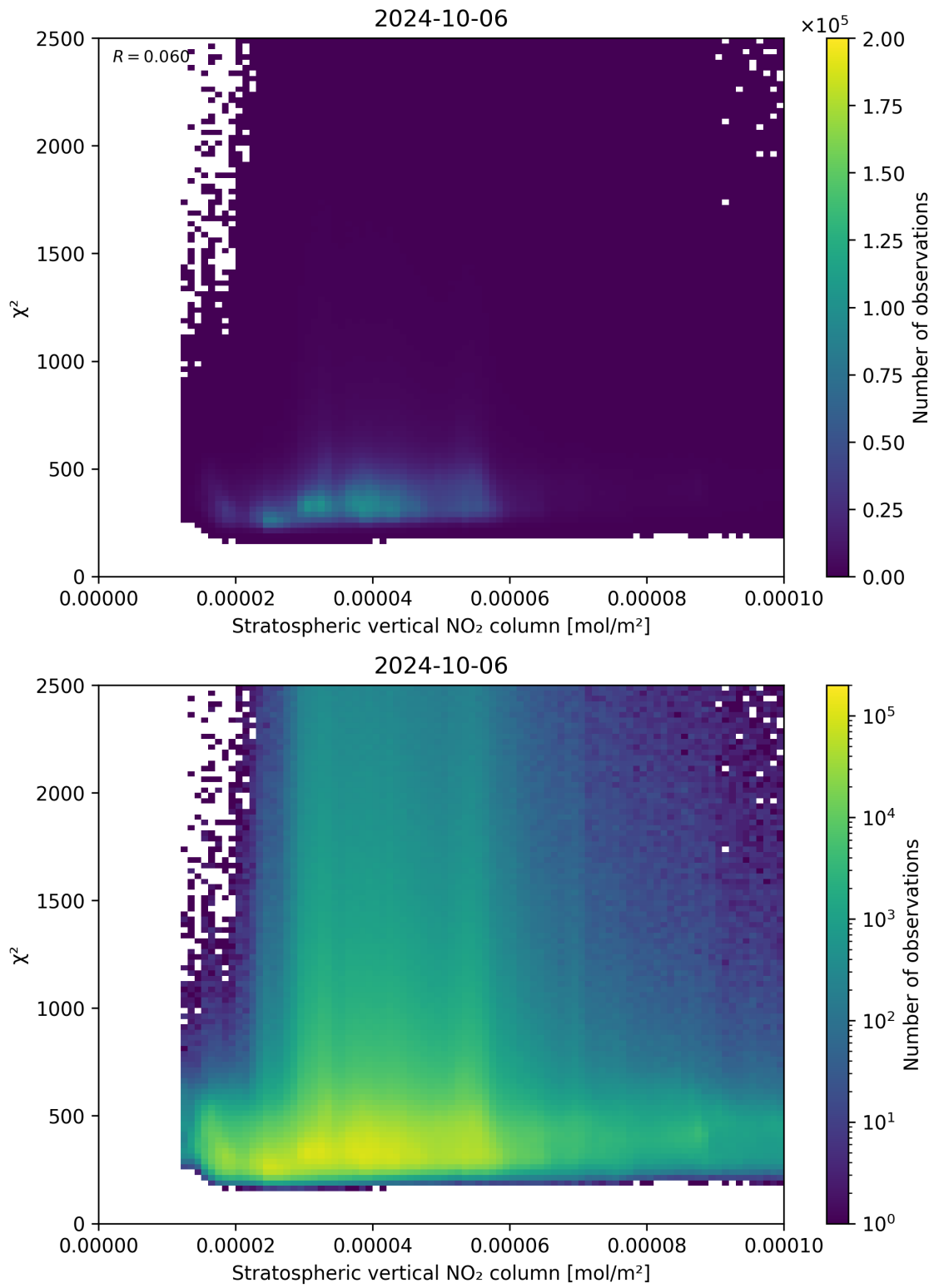
Figure 97: Scatter density plot of “Stratospheric vertical NO 2 column” against “ \chi^2 ” for 2024-10-05 to 2024-10-07.
