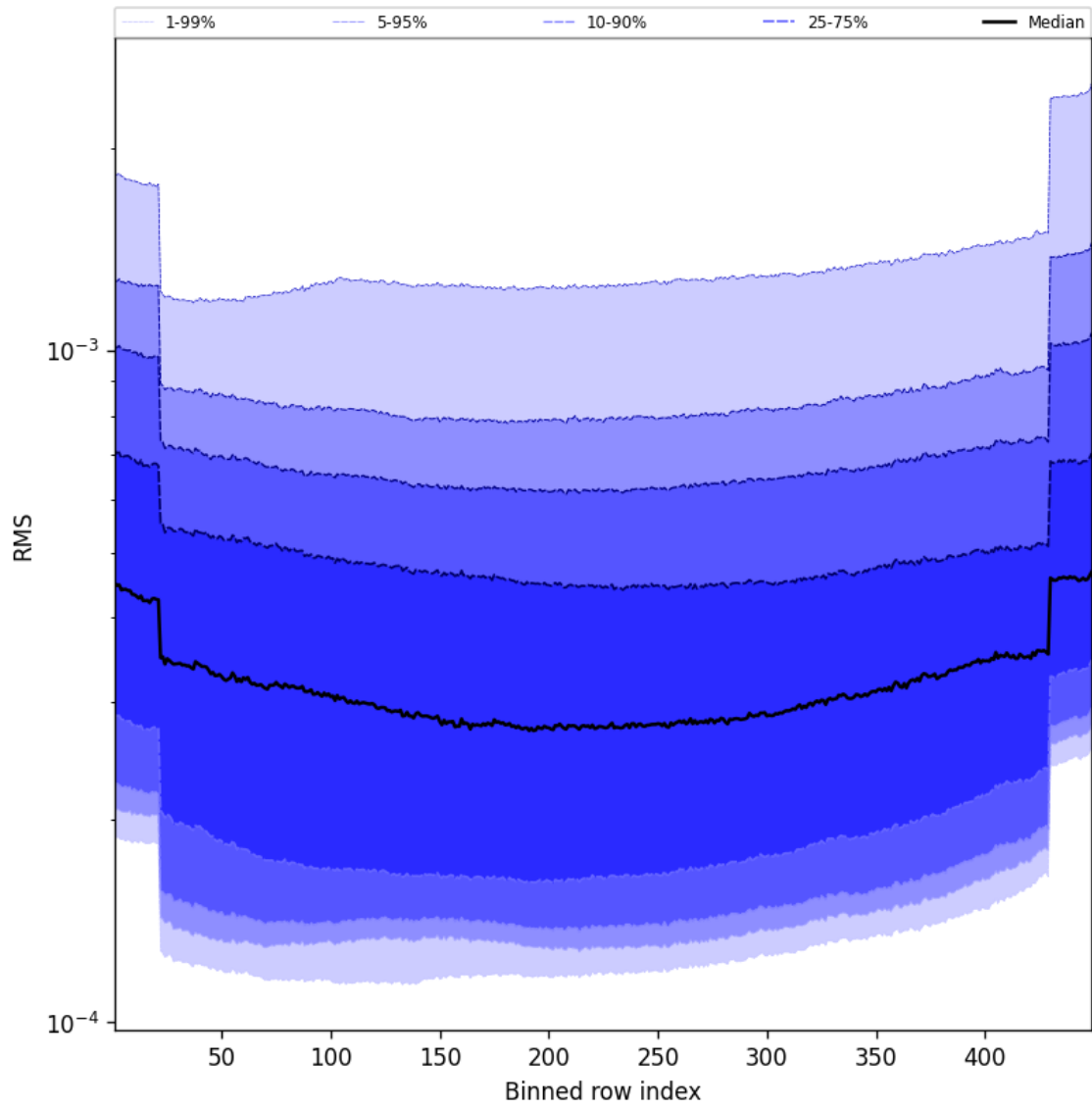
Figure 60: Along track statistics of “RMS” for 2024-10-05 to 2024-10-07
