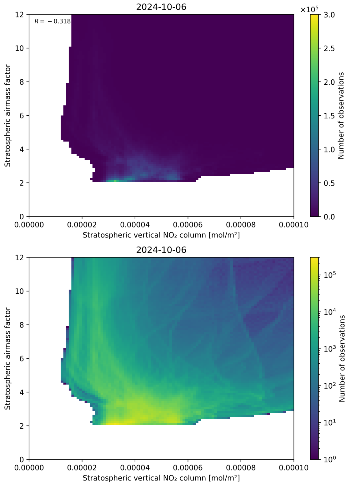
Figure 96: Scatter density plot of “Stratospheric vertical NO 2 column” against “Stratospheric airmass factor” for 2024-10-05 to 2024-10-07.
