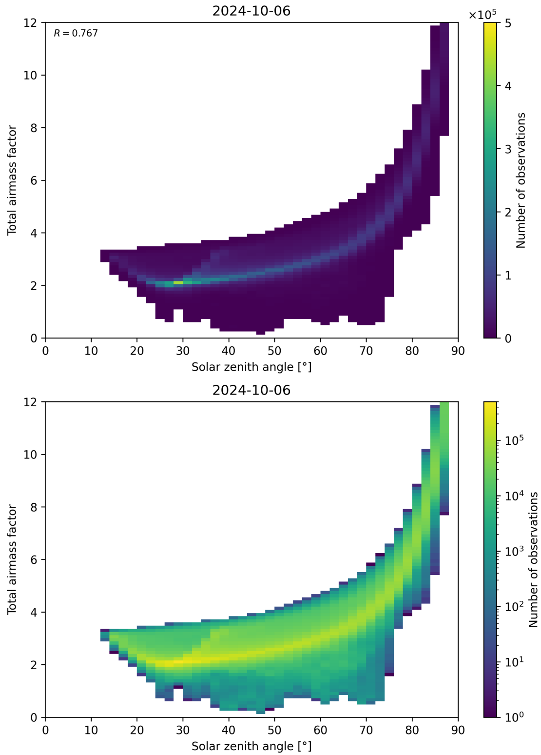
Figure 146: Scatter density plot of “Solar zenith angle” against “Total airmass factor” for 2024-10-05 to 2024-10-07.
