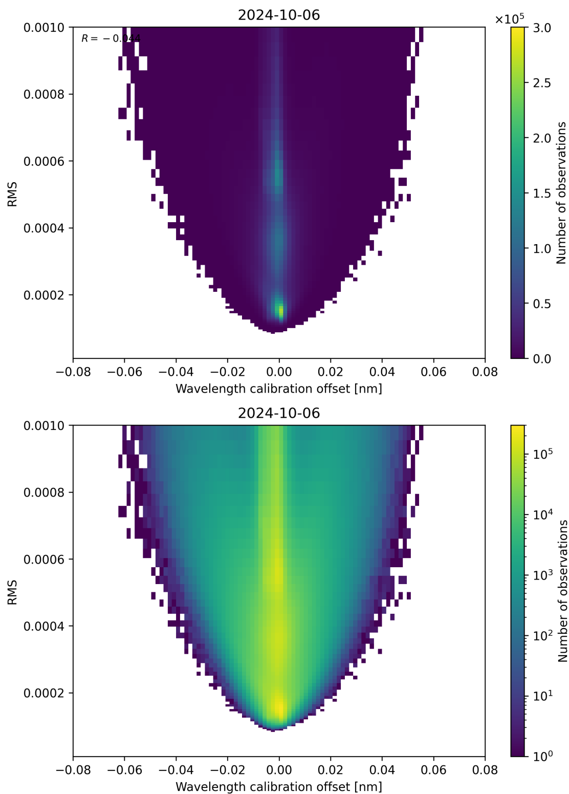
Figure 181: Scatter density plot of “Wavelength calibration offset” against “RMS” for 2024-10-05 to 2024-10-07.
