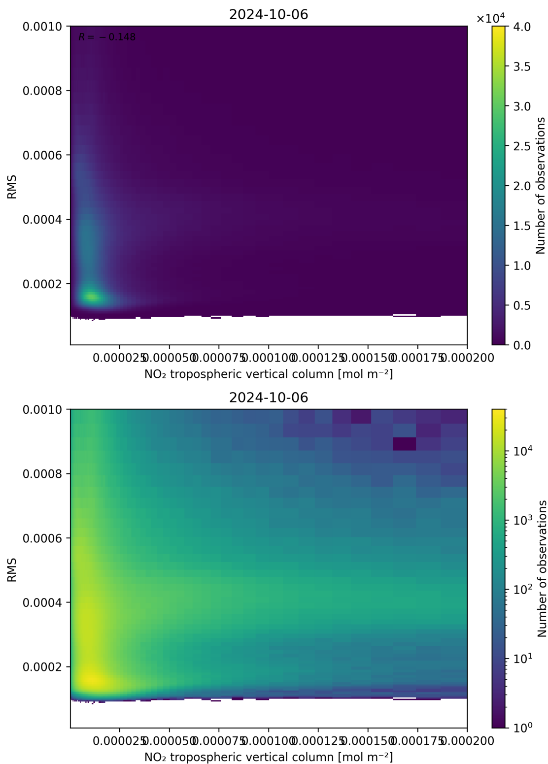
Figure 142: Scatter density plot of “NO 2 tropospheric vertical column” against “RMS” for 2024-10-05 to 2024-10-07.
