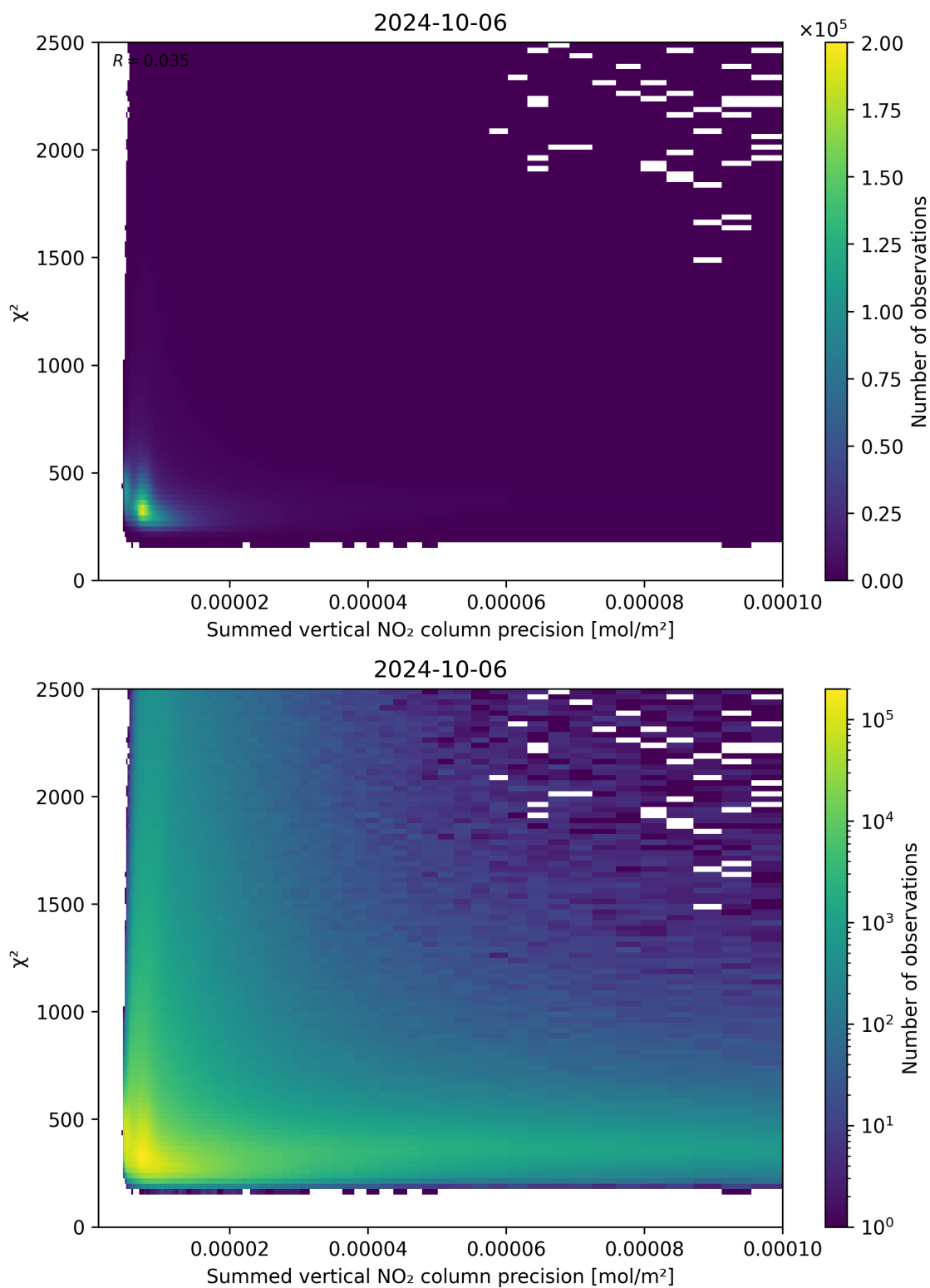
Figure 107: Scatter density plot of “Summed vertical NO 2 column precision” against “ \chi^2 ” for 2024-10-05 to 2024-10-07.
