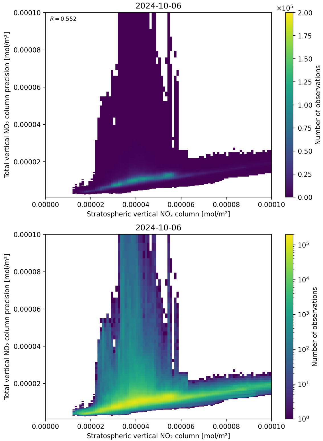
Figure 101: Scatter density plot of “Stratospheric vertical NO 2 column” against “Total vertical NO 2 column precision” for 2024-10-05 to 2024-10-07.
