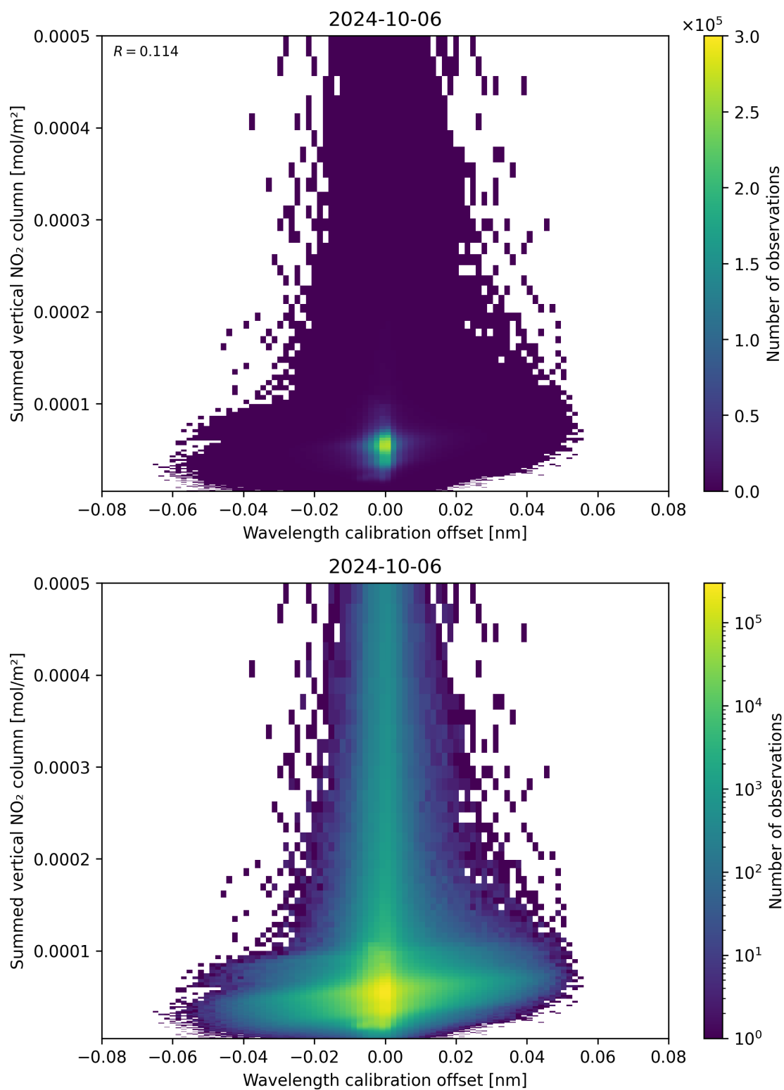
Figure 177: Scatter density plot of “Wavelength calibration offset” against “Summed vertical NO 2 column” for 2024-10-05 to 2024-10-07.
