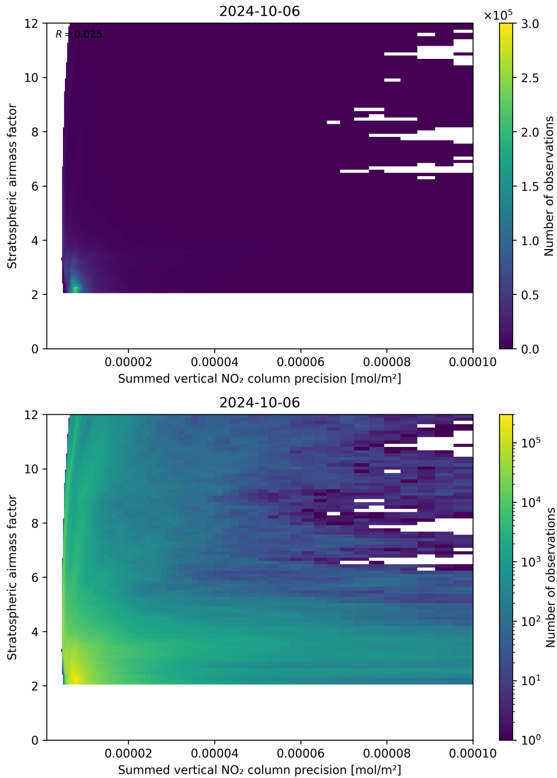
Figure 106: Scatter density plot of “Summed vertical NO 2 column precision” against “Stratospheric airmass factor” for 2024-10-05 to 2024-10-07.
