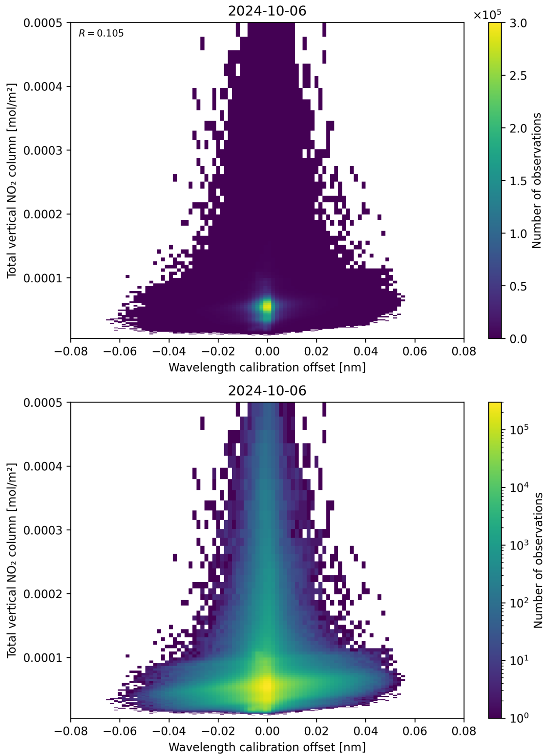
Figure 179: Scatter density plot of “Wavelength calibration offset” against “Total vertical NO 2 column” for 2024-10-05 to 2024-10-07.
