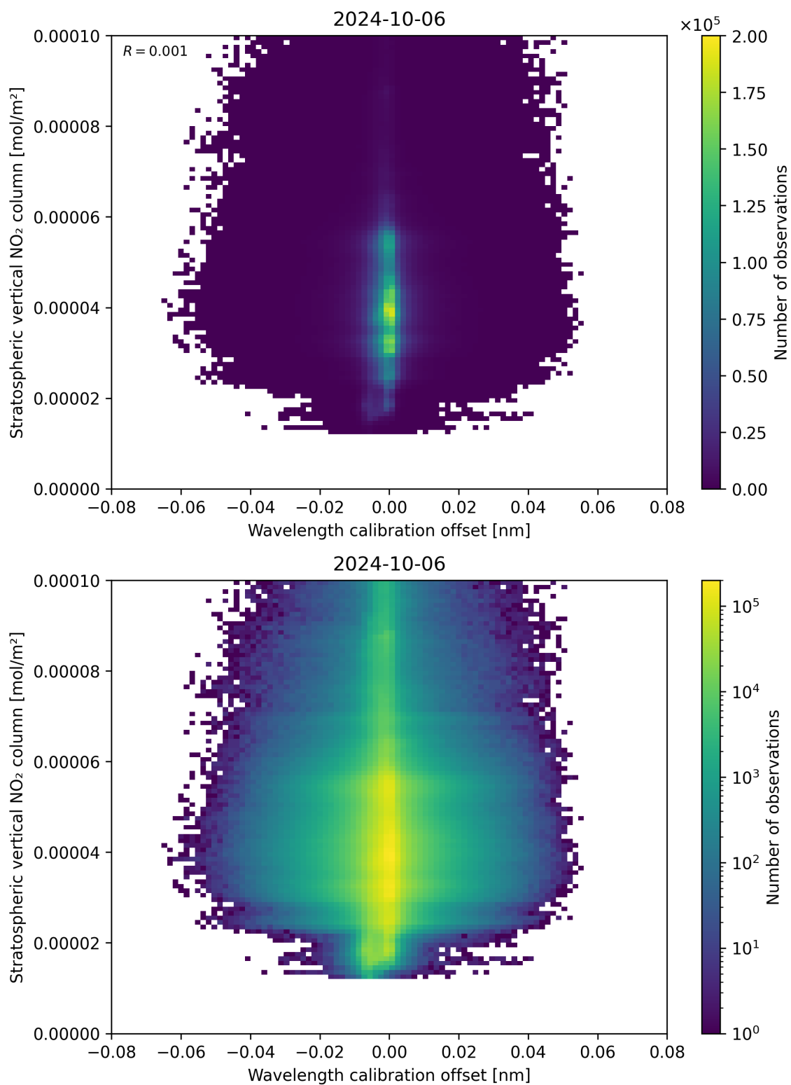
Figure 176: Scatter density plot of “Wavelength calibration offset” against “Stratospheric vertical NO 2 column” for 2024-10-05 to 2024-10-07.
