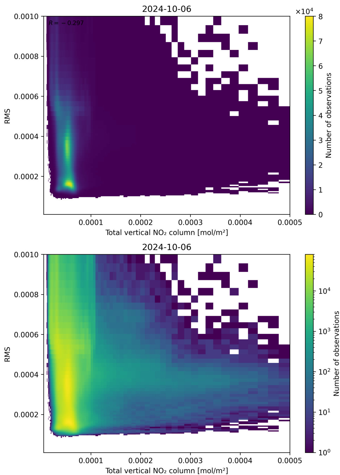
Figure 120: Scatter density plot of “Total vertical NO 2 column” against “RMS” for 2024-10-05 to 2024-10-07.
