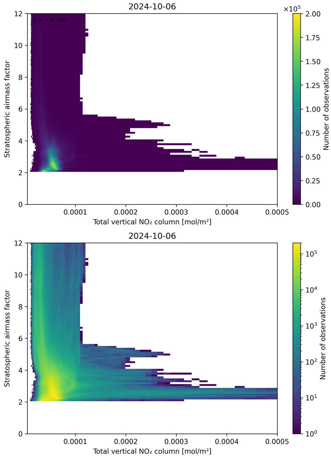
Figure 110: Scatter density plot of “Total vertical NO 2 column” against “Stratospheric airmass factor” for 2024-10-05 to 2024-10-07.
