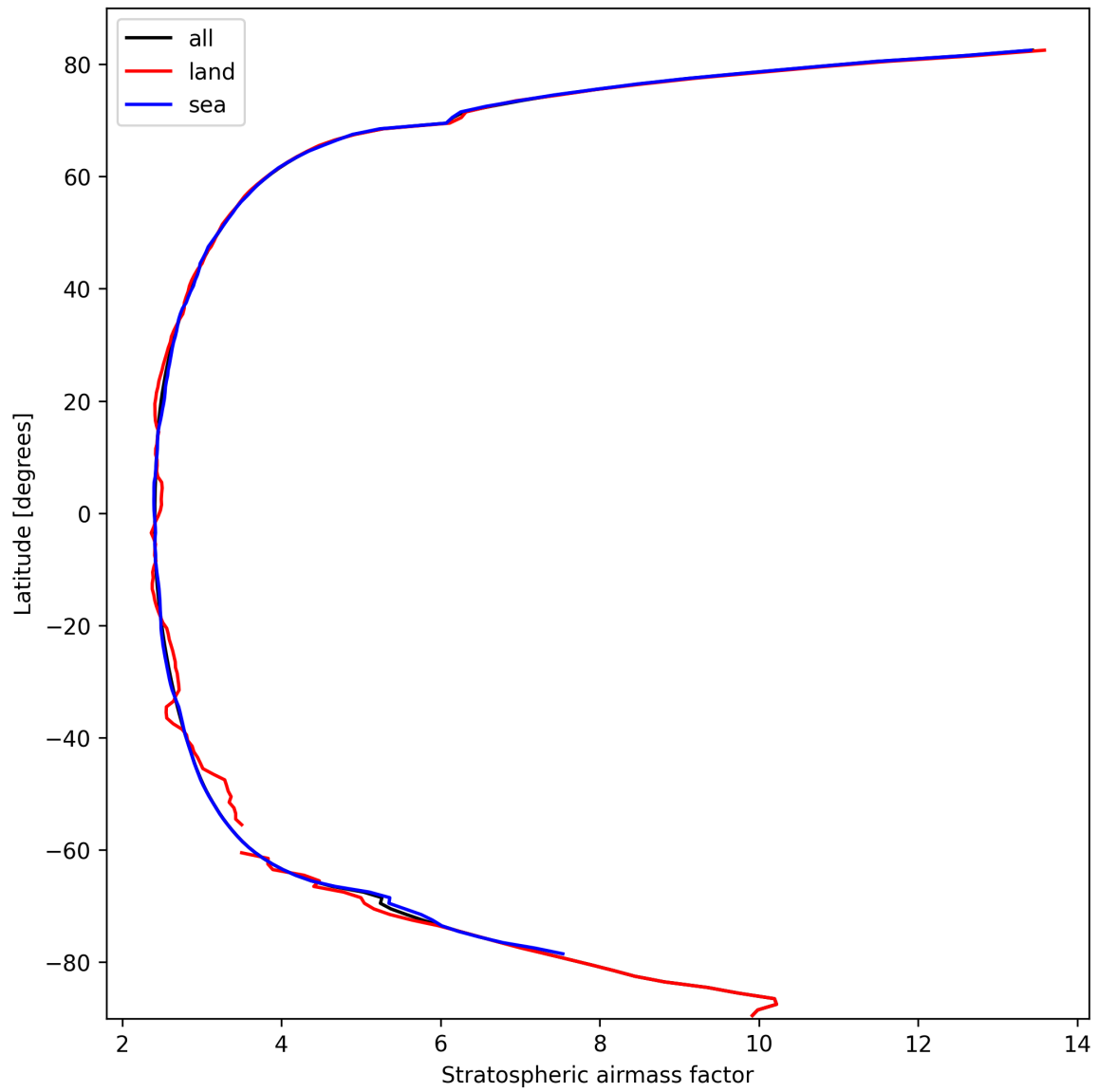
Figure 27: Zonal average of “Stratospheric airmass factor” for 2024-10-05 to 2024-10-07.
