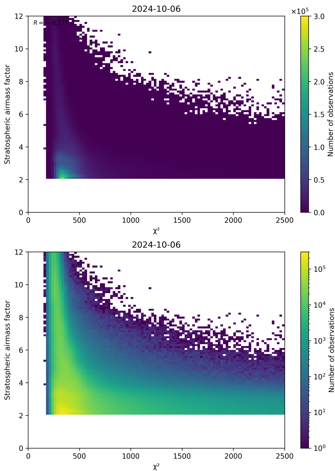
Figure 81: Scatter density plot of “ \chi^2 ” against “Stratospheric airmass factor” for 2024-10-05 to 2024-10-07.
