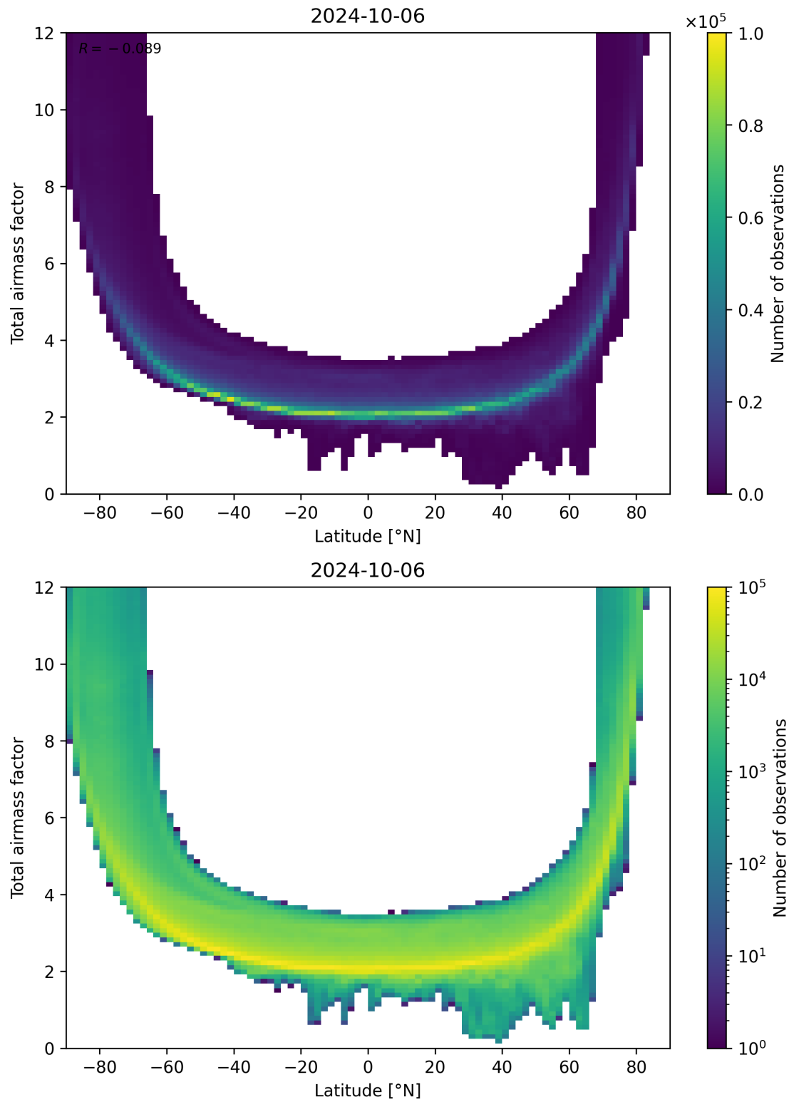
Figure 84: Scatter density plot of “Latitude” against “Total airmass factor” for 2024-10-05 to 2024-10-07.
