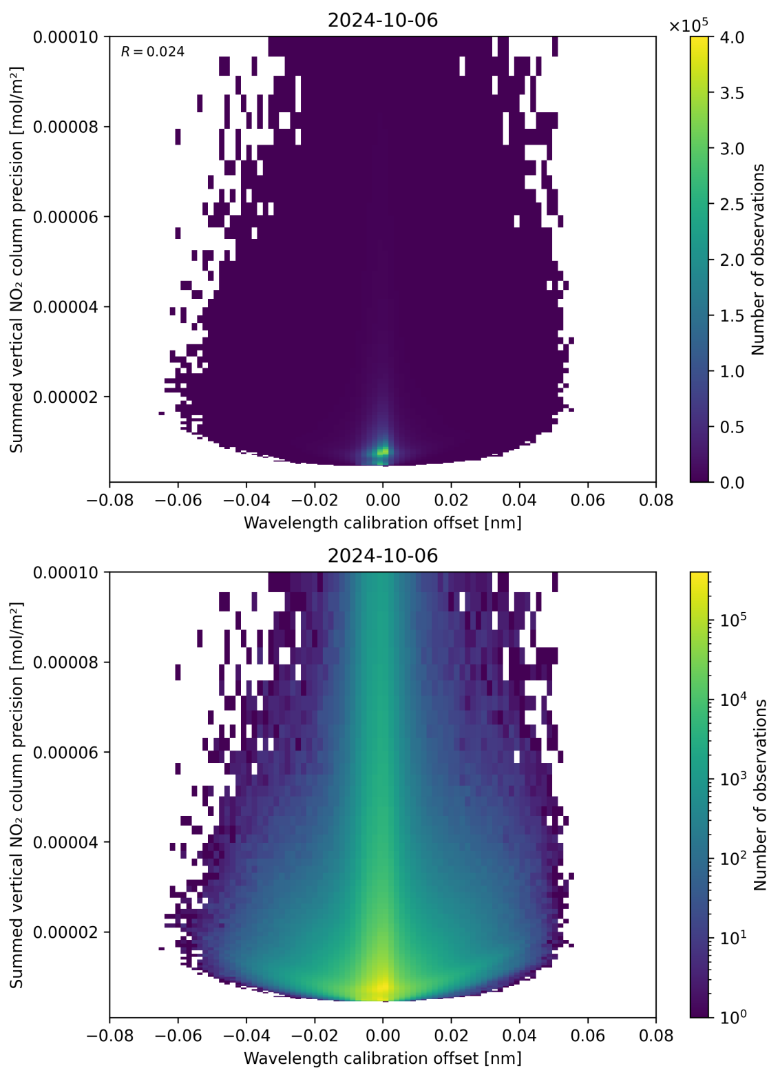
Figure 178: Scatter density plot of “Wavelength calibration offset” against “Summed vertical NO 2 column precision” for 2024-10-05 to 2024-10-07.
