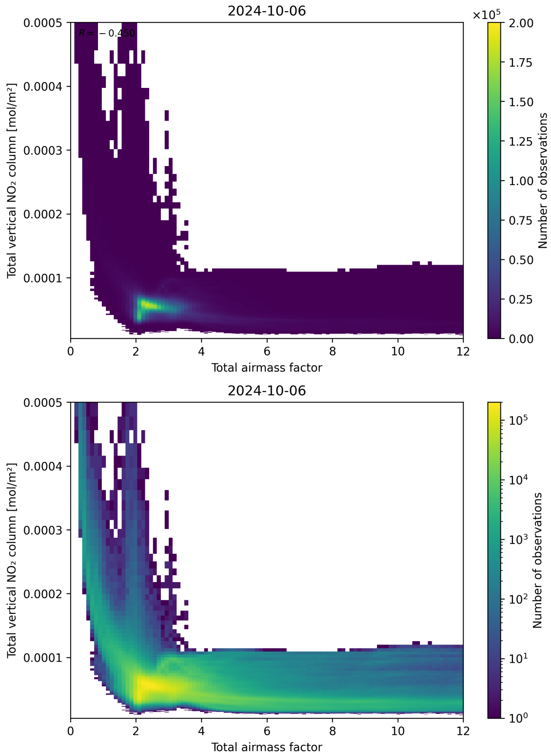
Figure 67: Scatter density plot of “Total air mass factor” against “Total vertical NO 2 column” for 2024-10-05 to 2024-10-07.
