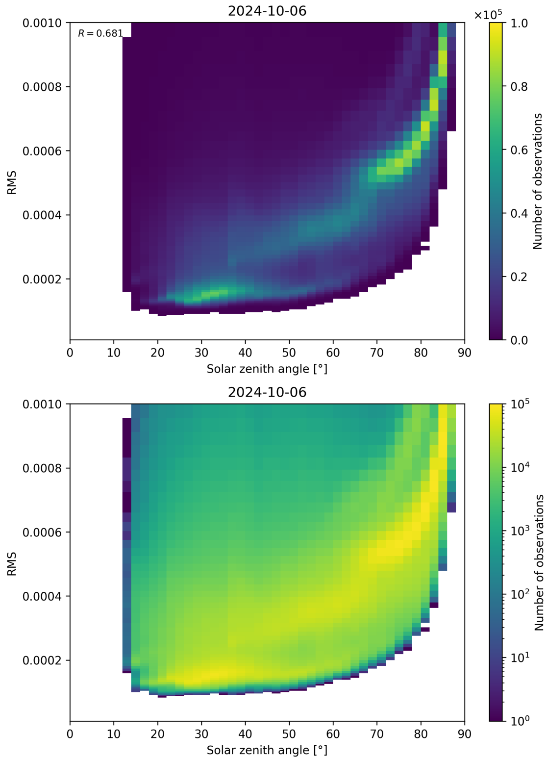
Figure 157: Scatter density plot of “Solar zenith angle” against “RMS” for 2024-10-05 to 2024-10-07.
