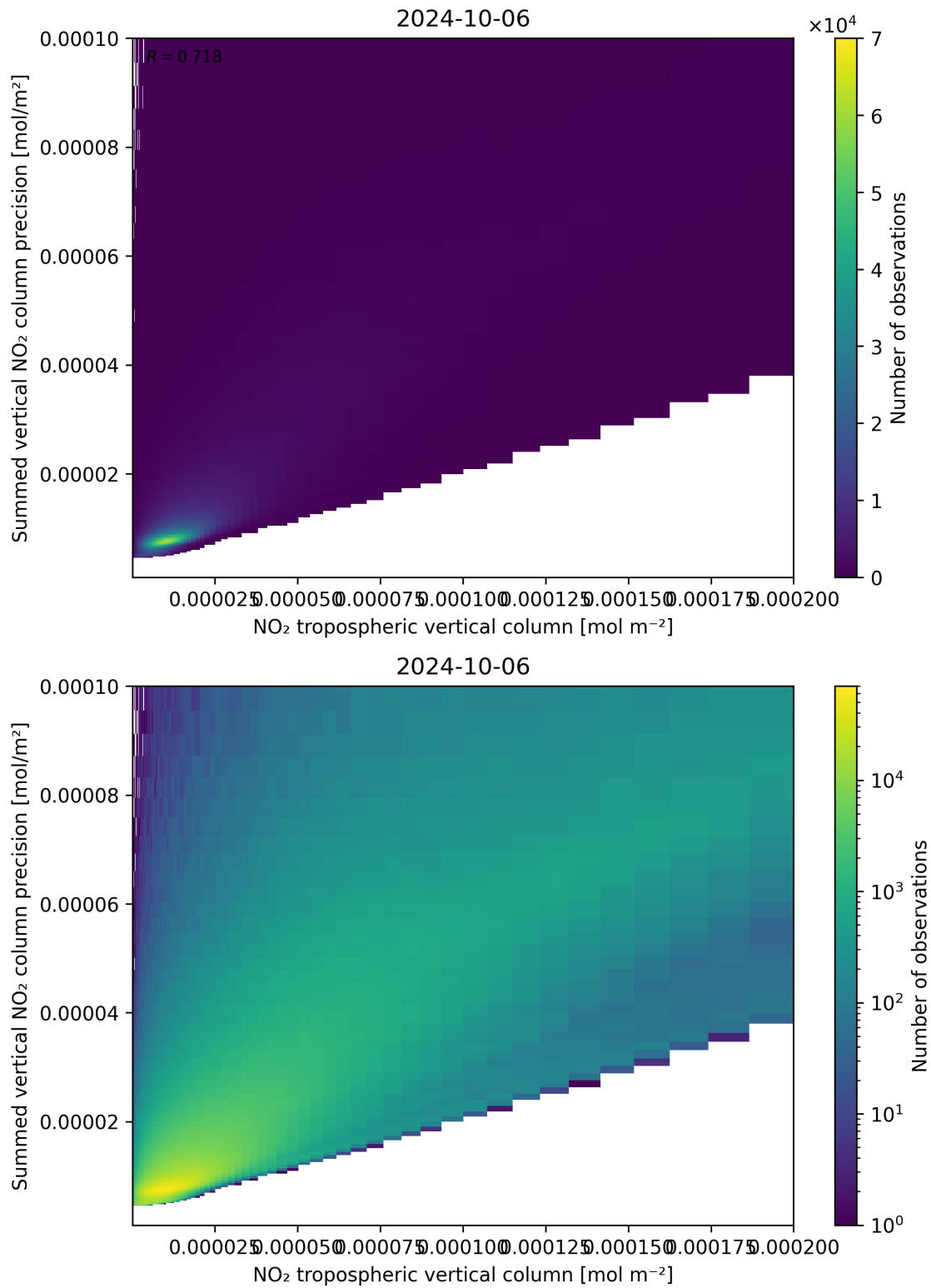
Figure 127: Scatter density plot of “NO 2 tropospheric vertical column” against “Summed vertical NO 2 column precision” for 2024-10-05 to 2024-10-07.
