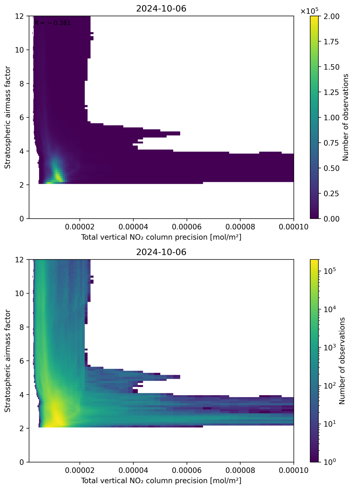
Figure 115: Scatter density plot of “Total vertical NO 2 column precision” against “Stratospheric air mass factor” for 2024-10-05 to 2024-10-07.
