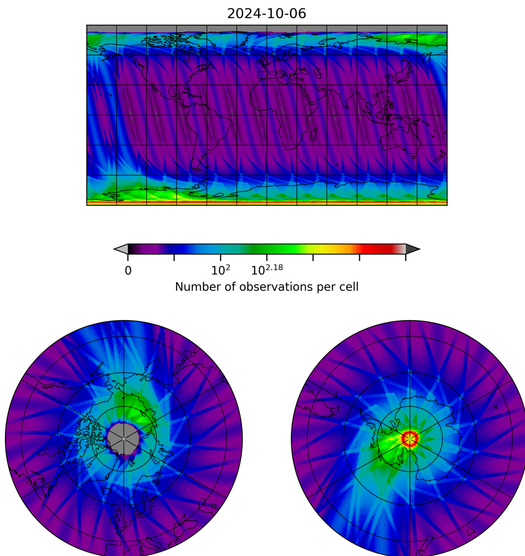
Figure 10: Map of the number of observations for 2024-10-05 to 2024-10-07
