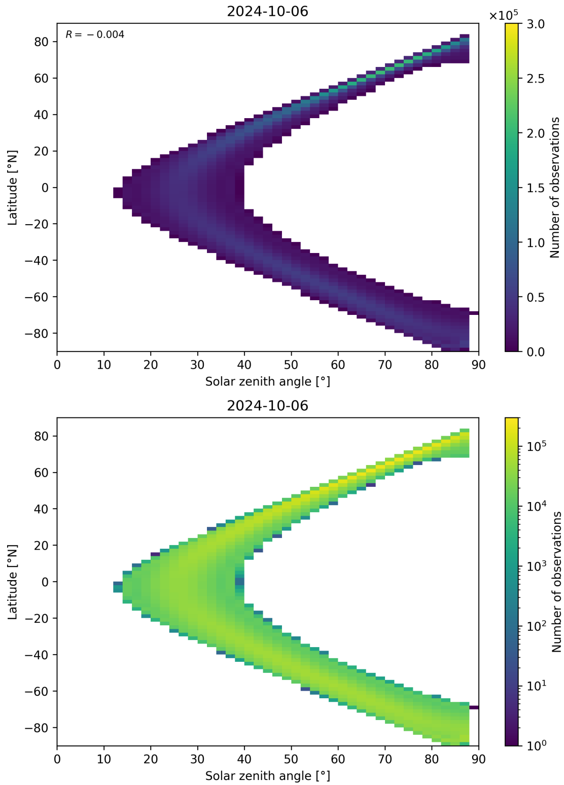
Figure 149: Scatter density plot of “Solar zenith angle” against “Latitude” for 2024-10-05 to 2024-10-07.
