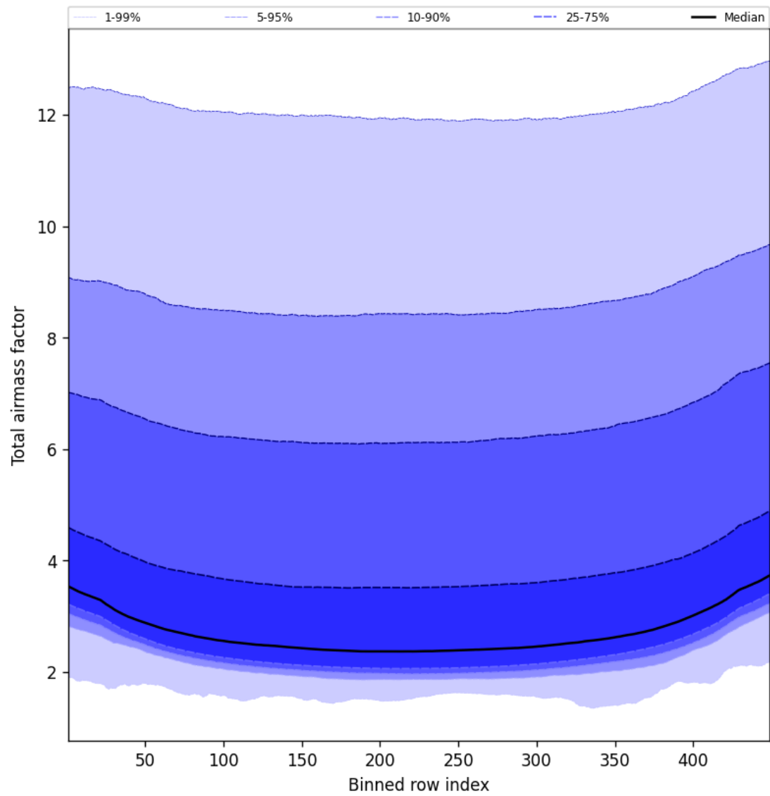
Figure 49: Along track statistics of “Total airmass factor” for 2024-10-05 to 2024-10-07
