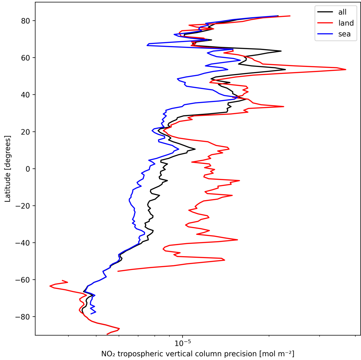
Figure 13: Zonal average of “NO 2 tropospheric vertical column precision” for 2024-10-05 to 2024-10-07.
