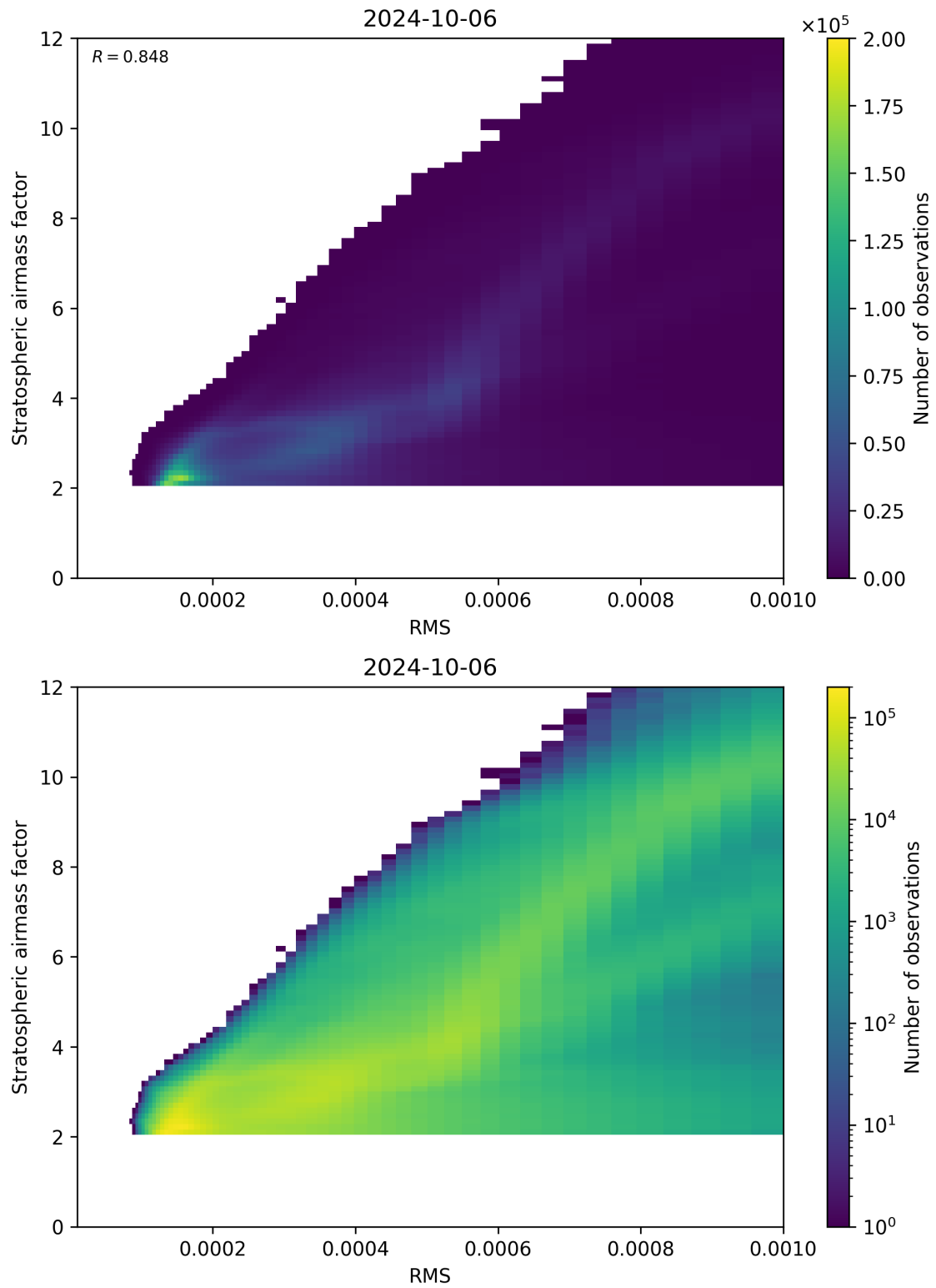
Figure 144: Scatter density plot of “RMS” against “Stratospheric airmass factor” for 2024-10-05 to 2024-10-07.
