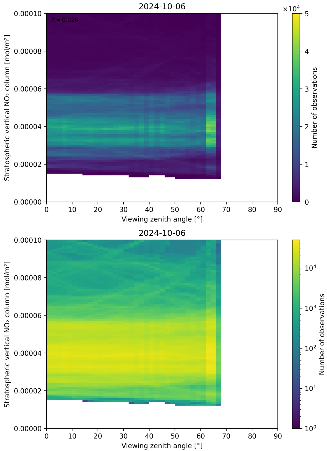
Figure 164: Scatter density plot of “Viewing zenith angle” against “Stratospheric vertical NO 2 column” for 2024-10-05 to 2024-10-07.
