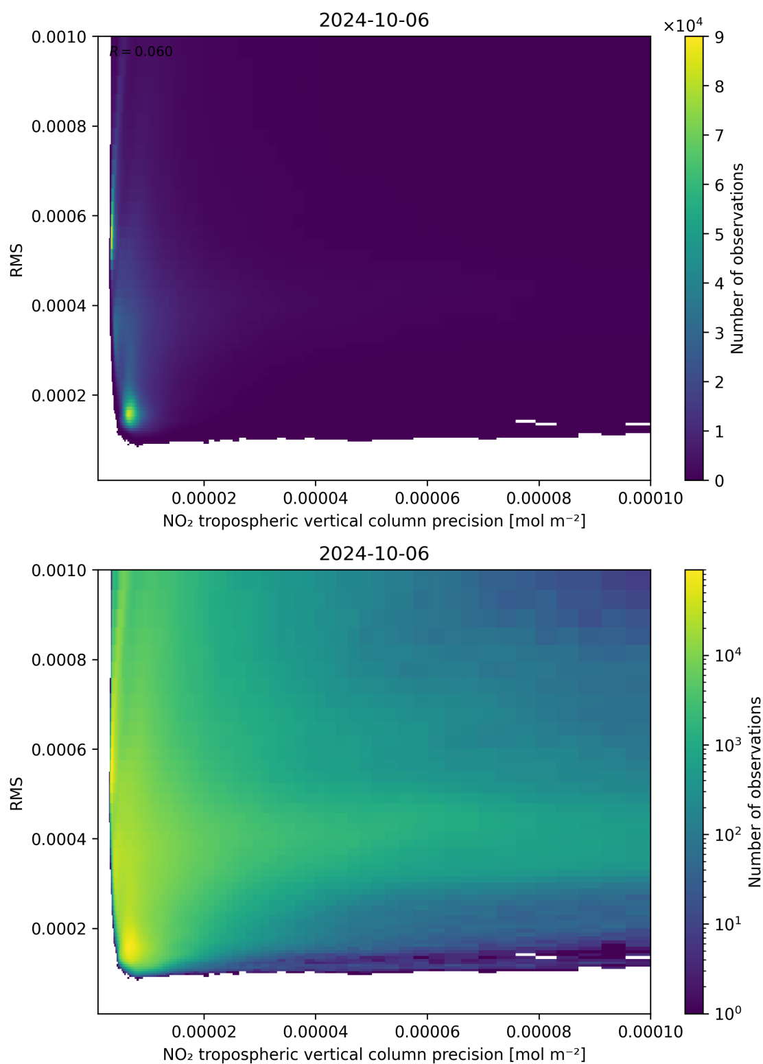
Figure 140: Scatter density plot of “NO 2 tropospheric vertical column precision” against “RMS” for 2024-10-05 to 2024-10-07.
