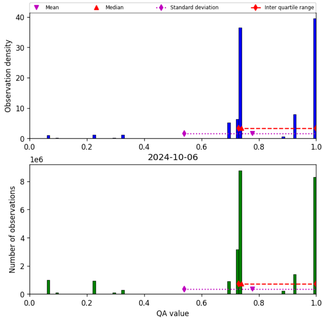
Figure 28: Histogram of “QA value” for 2024-10-05 to 2024-10-07
