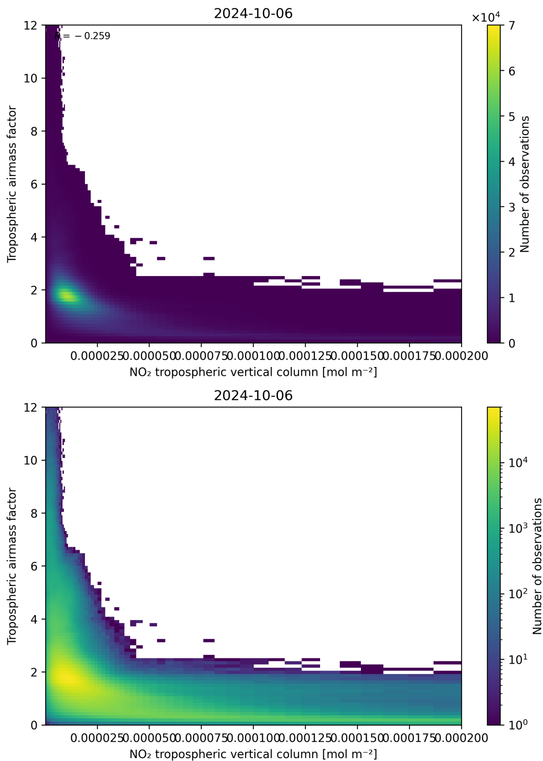
Figure 123: Scatter density plot of “NO 2 tropospheric vertical column” against “Tropospheric air mass factor” for 2024-10-05 to 2024-10-07.
