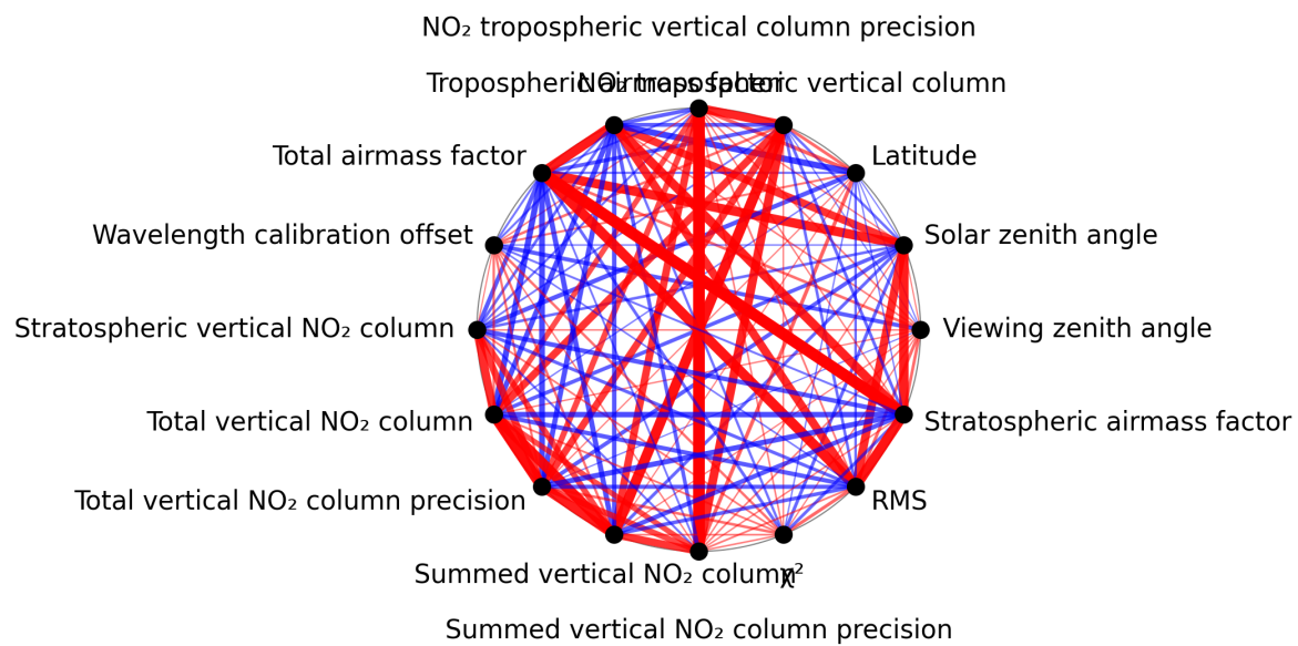
Figure 1: Map of correlation graph for 2024-10-05 to 2024-10-07.
