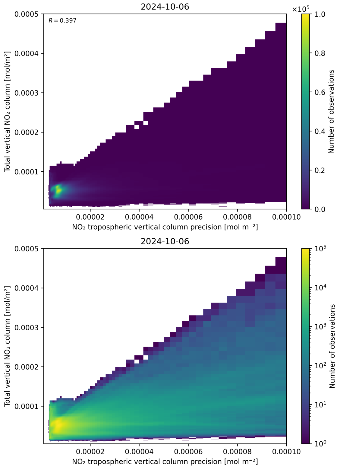
Figure 138: Scatter density plot of “NO 2 tropospheric vertical column precision” against “Total vertical NO 2 column” for 2024-10-05 to 2024-10-07.
