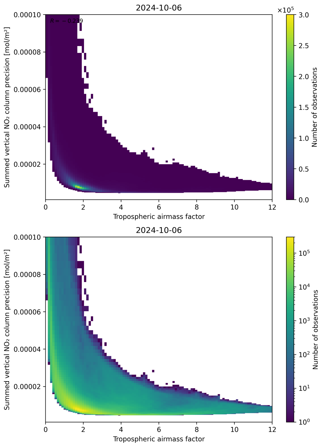
Figure 76: Scatter density plot of “Tropospheric air mass factor” against “Summed vertical NO 2 column precision” for 2024-10-05 to 2024-10-07.
