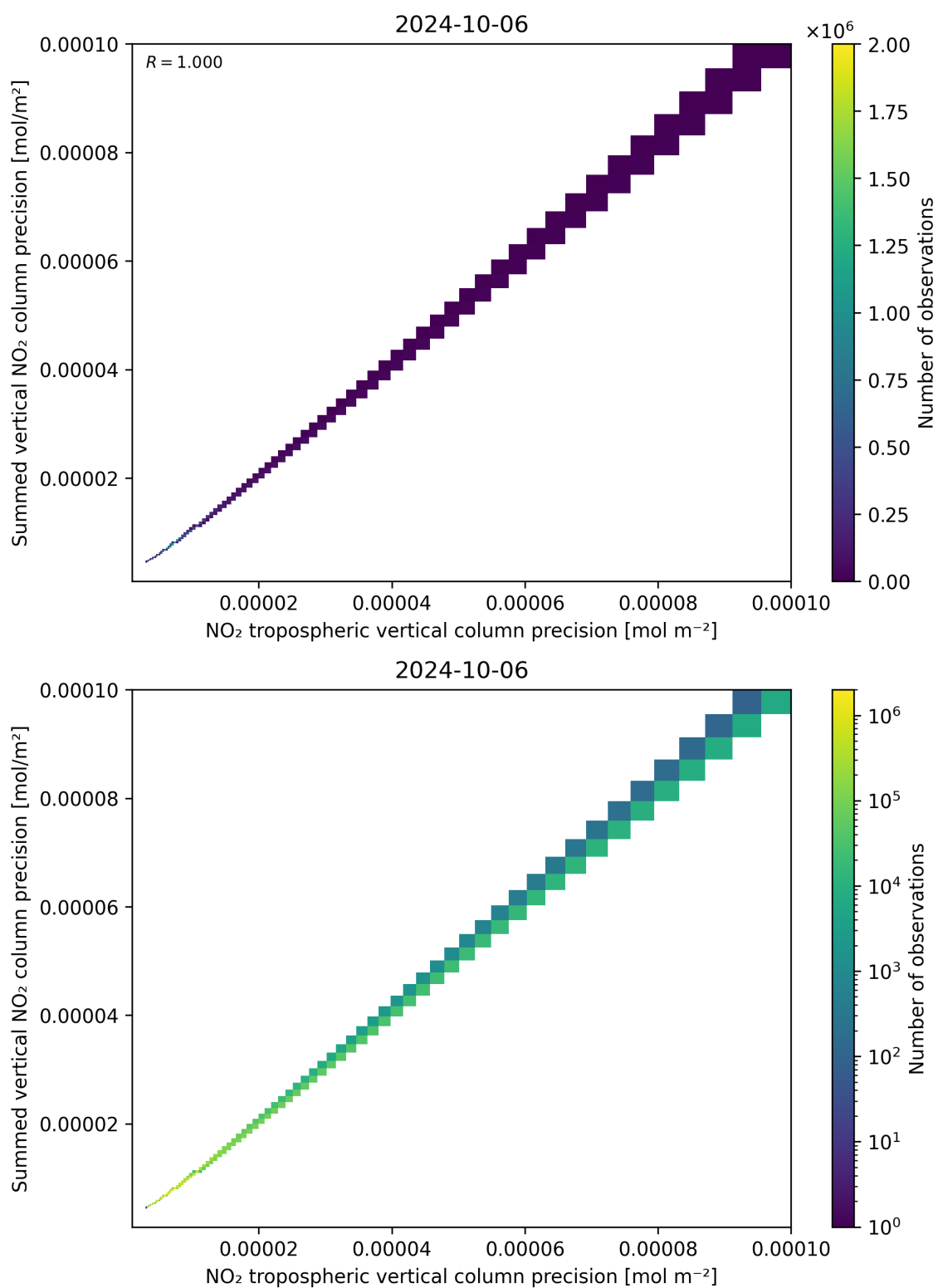
Figure 137: Scatter density plot of “NO 2 tropospheric vertical column precision” against “Summed vertical NO 2 column precision” for 2024-10-05 to 2024-10-07.
