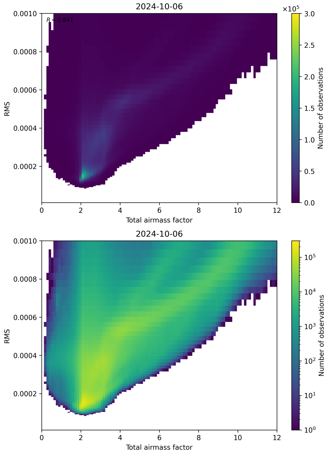
Figure 69: Scatter density plot of “Total airmass factor” against “RMS” for 2024-10-05 to 2024-10-07.
