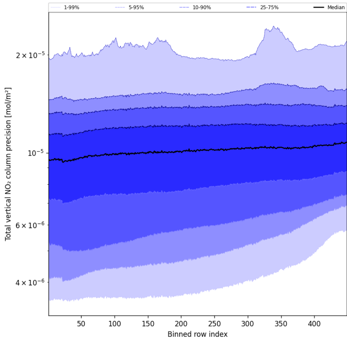
Figure 56: Along track statistics of “Total vertical NO 2 column precision” for 2024-10-05 to 2024-10-07
