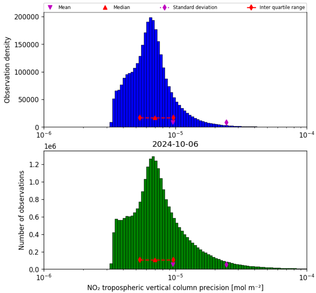
Figure 30: Histogram of “NO 2 tropospheric vertical column precision” for 2024-10-05 to 2024-10-07
