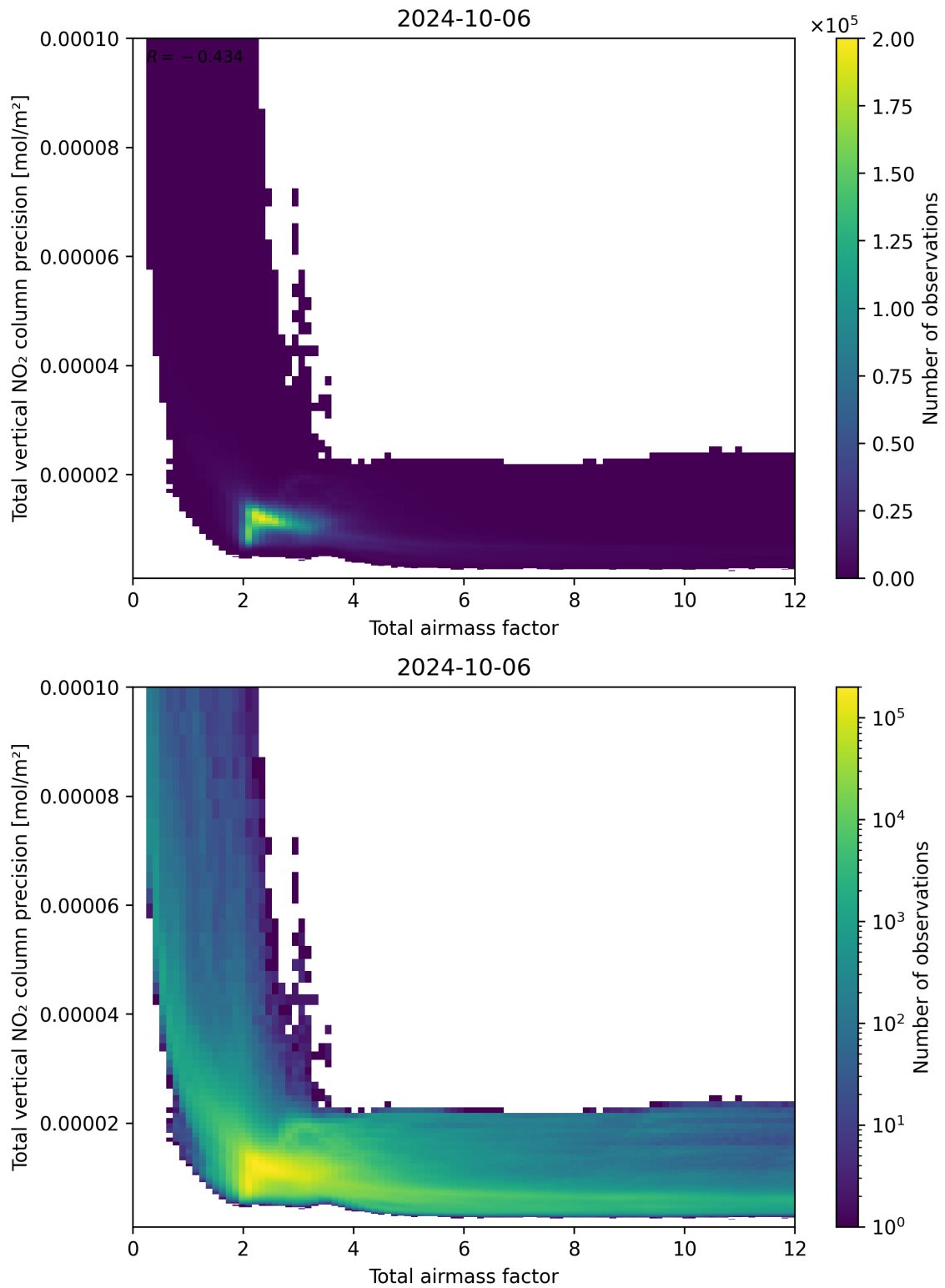
Figure 68: Scatter density plot of “Total airmass factor” against “Total vertical NO 2 column precision” for 2024-10-05 to 2024-10-07.
