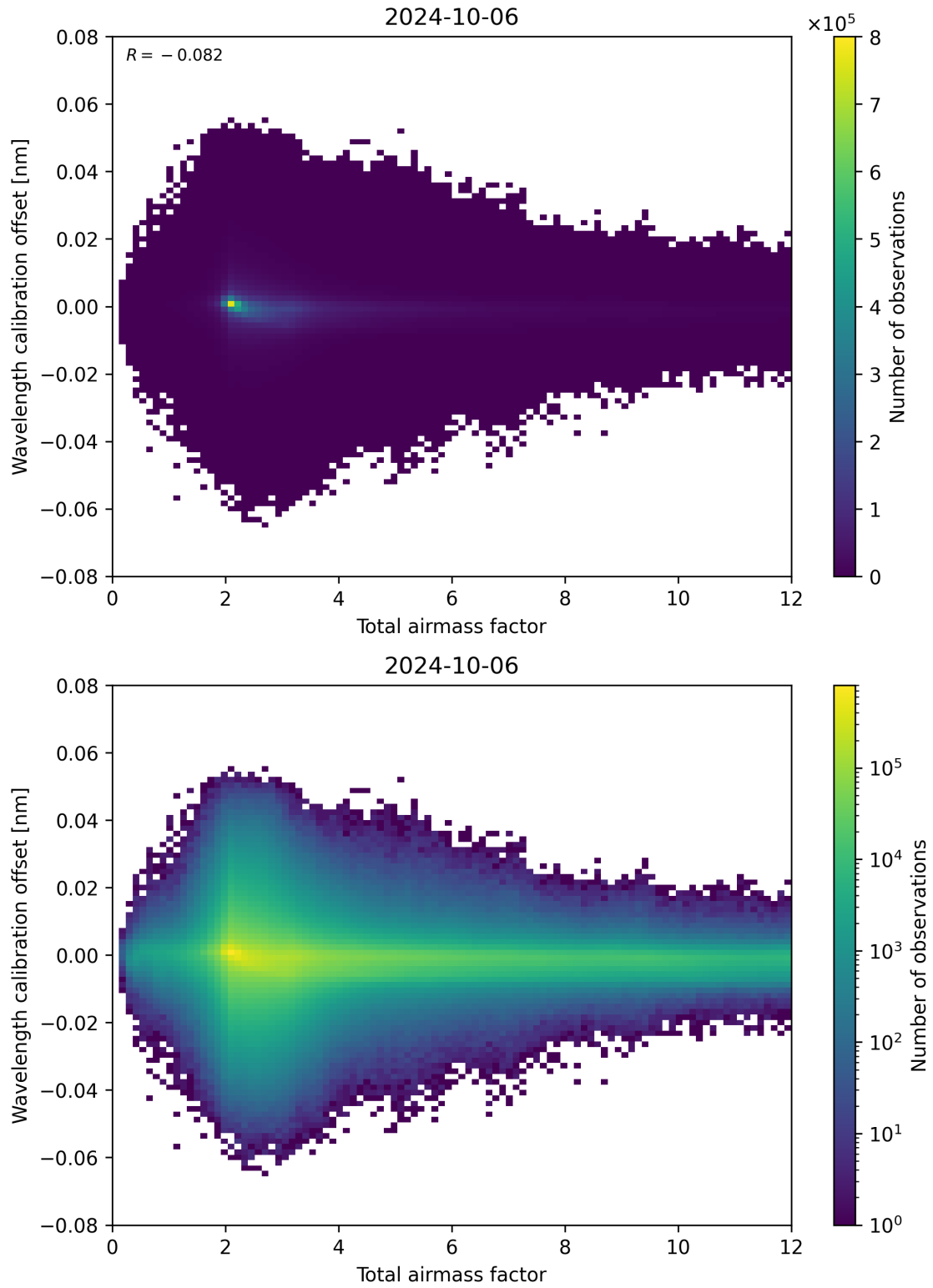
Figure 70: Scatter density plot of “Total airmass factor” against “Wavelength calibration offset” for 2024-10-05 to 2024-10-07.
