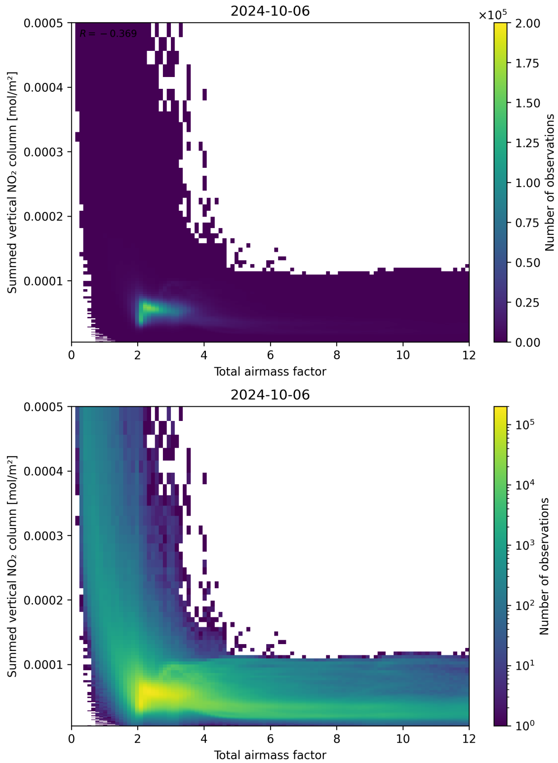
Figure 65: Scatter density plot of “Total airmass factor” against “Summed vertical NO 2 column” for 2024-10-05 to 2024-10-07.
