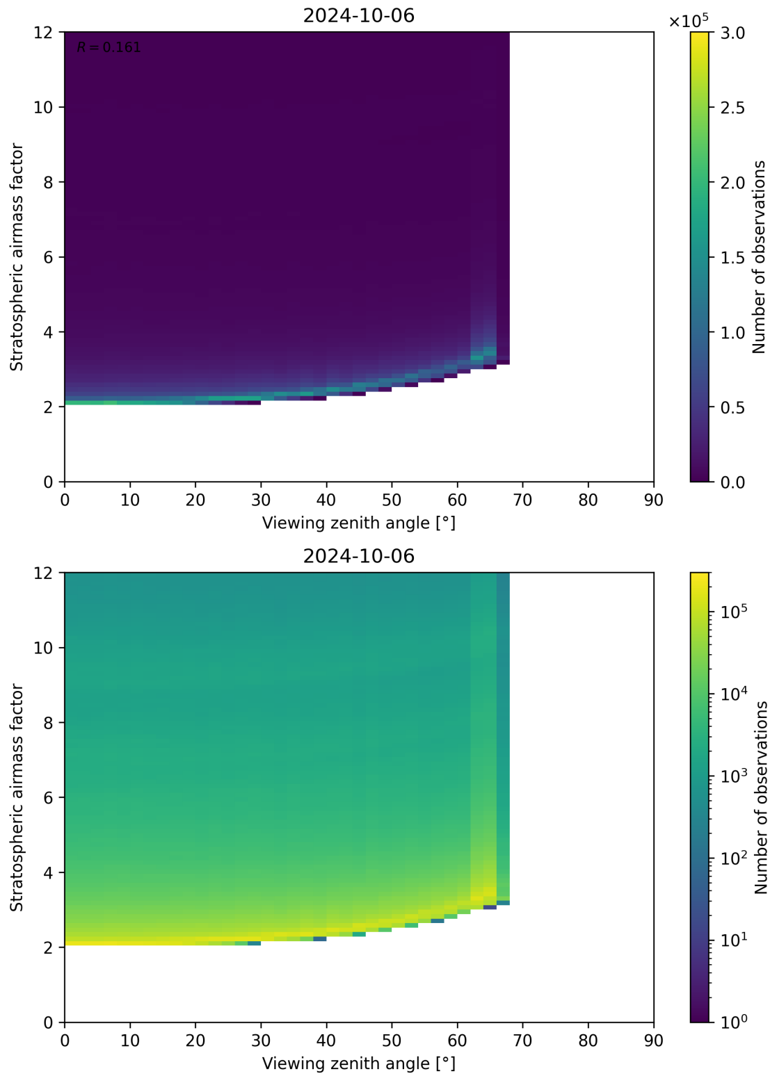
Figure 159: Scatter density plot of “Viewing zenith angle” against “Stratospheric airmass factor” for 2024-10-05 to 2024-10-07.
