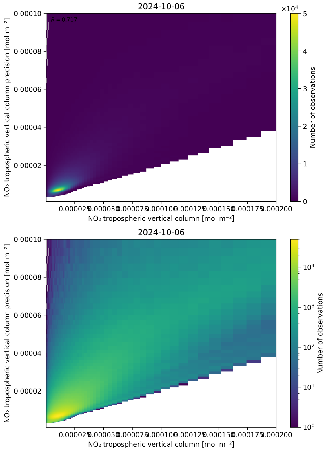
Figure 130: Scatter density plot of “NO 2 tropospheric vertical column” against “NO 2 tropospheric vertical column precision” for 2024-10-05 to 2024-10-07.
