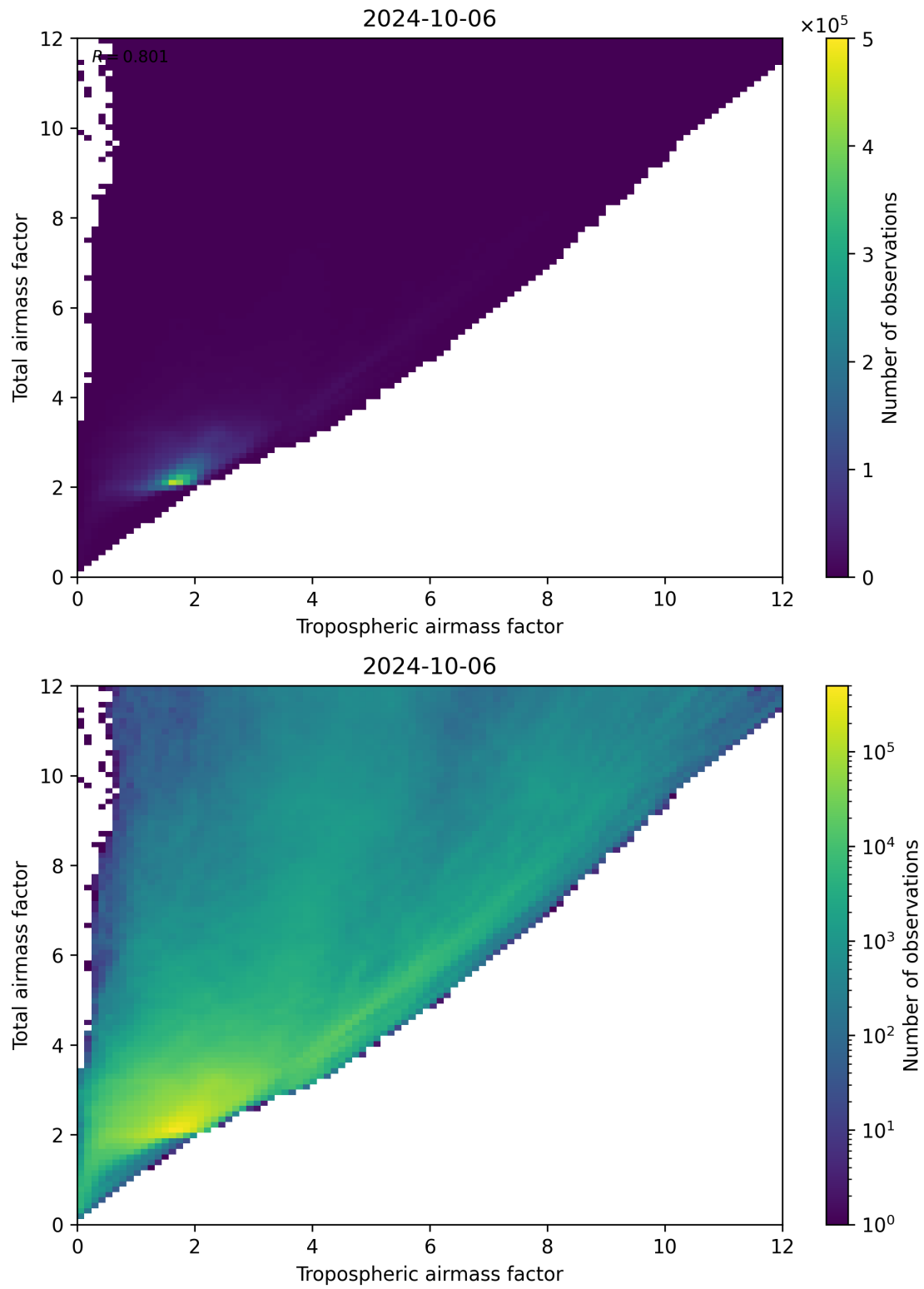
Figure 72: Scatter density plot of “Tropospheric airmass factor” against “Total airmass factor” for 2024-10-05 to 2024-10-07.
