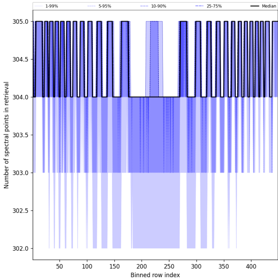
Figure 50: Along track statistics of “Number of spectral points in retrieval” for 2024-10-05 to 2024-10-07
