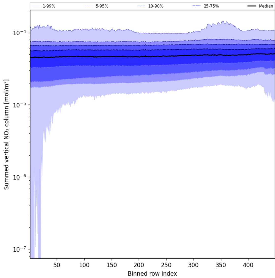
Figure 57: Along track statistics of “Summed vertical NO 2 column” for 2024-10-05 to 2024-10-07
