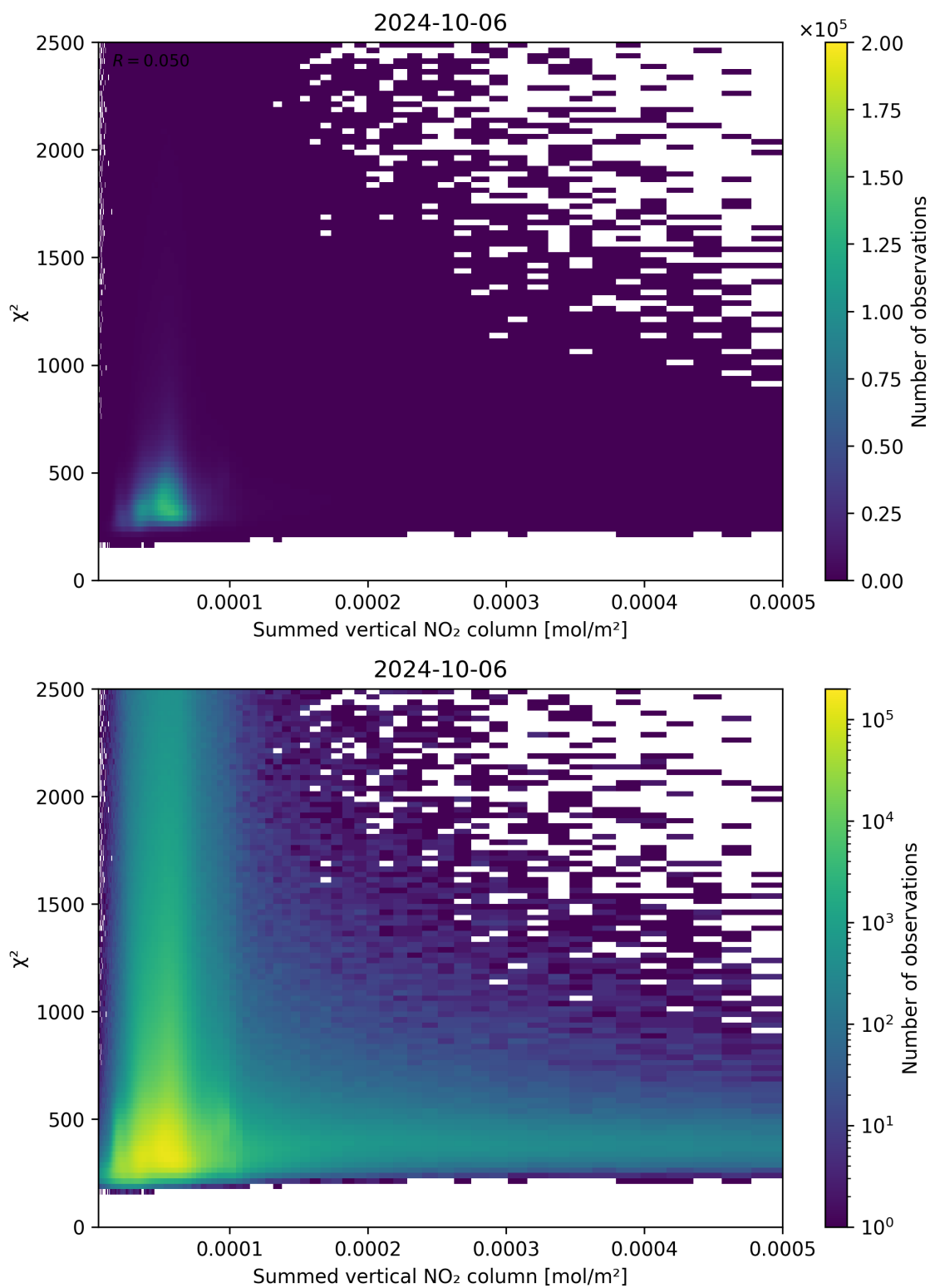
Figure 104: Scatter density plot of “Summed vertical NO 2 column” against “ \chi^2 ” for 2024-10-05 to 2024-10-07.
