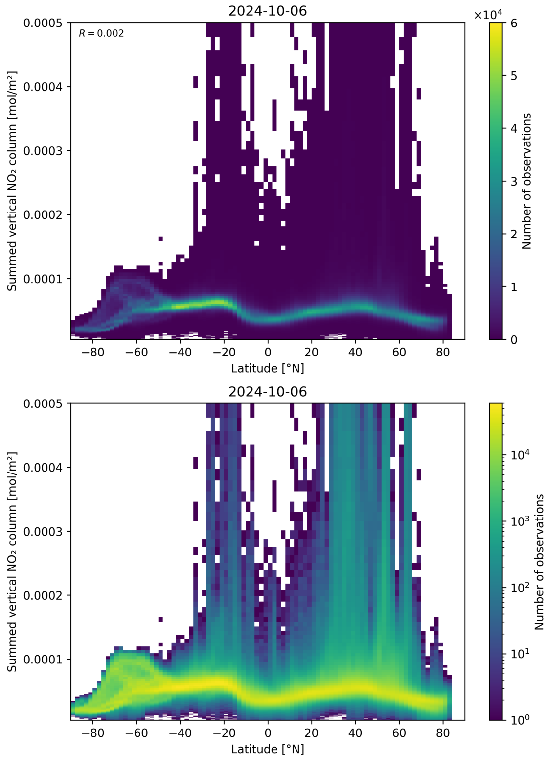
Figure 88: Scatter density plot of “Latitude” against “Summed vertical NO 2 column” for 2024-10-05 to 2024-10-07.
