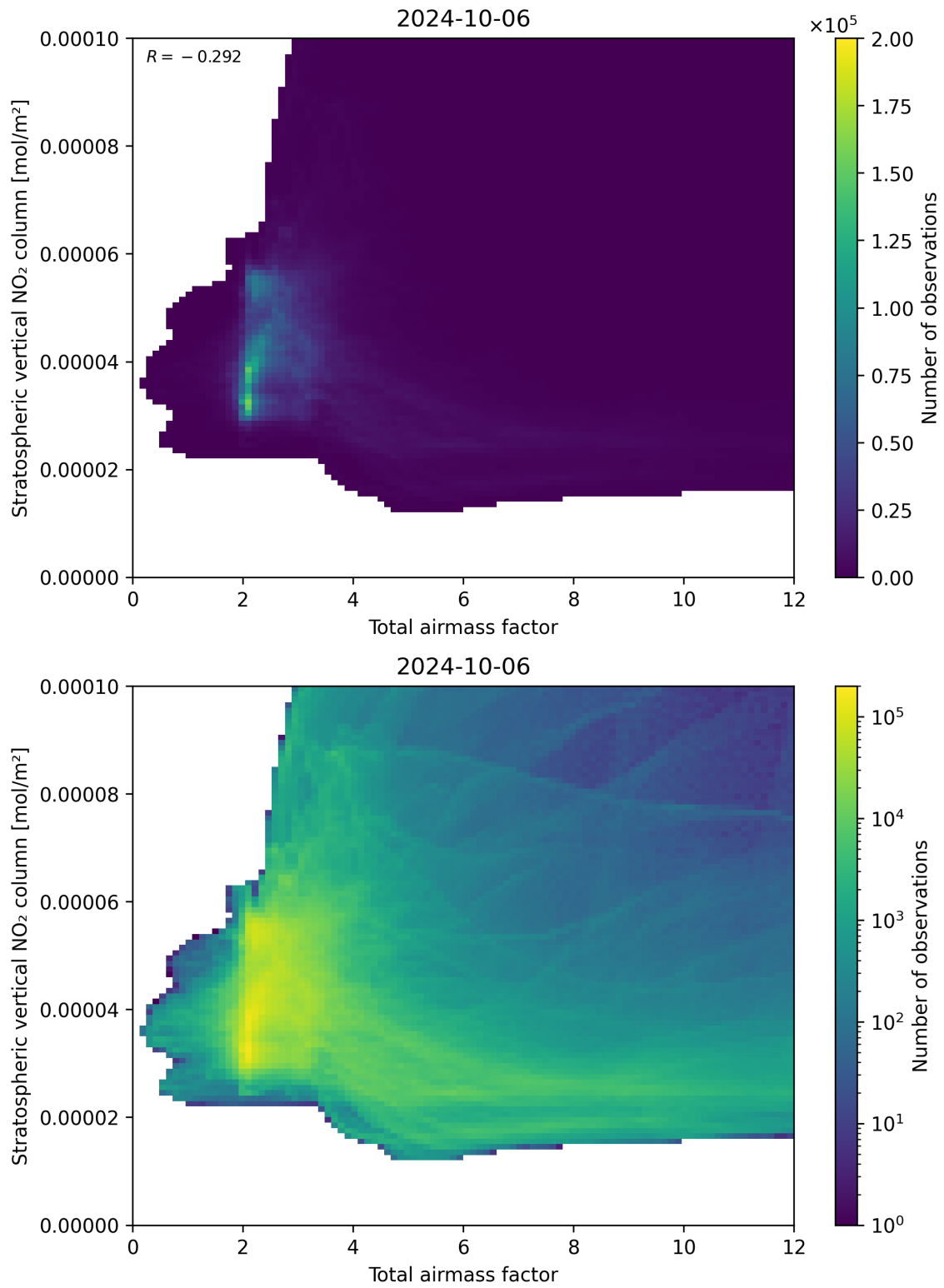
Figure 64: Scatter density plot of “Total airmass factor” against “Stratospheric vertical NO 2 column” for 2024-10-05 to 2024-10-07.
