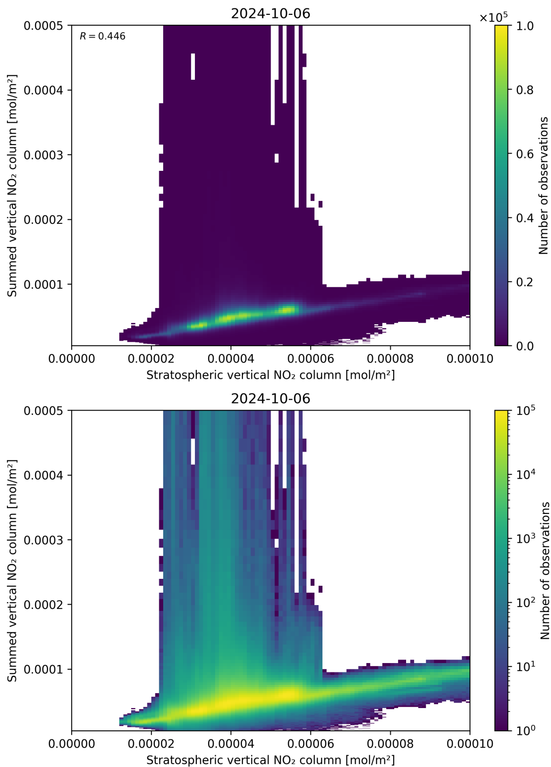
Figure 98: Scatter density plot of “Stratospheric vertical NO 2 column” against “Summed vertical NO 2 column” for 2024-10-05 to 2024-10-07.
