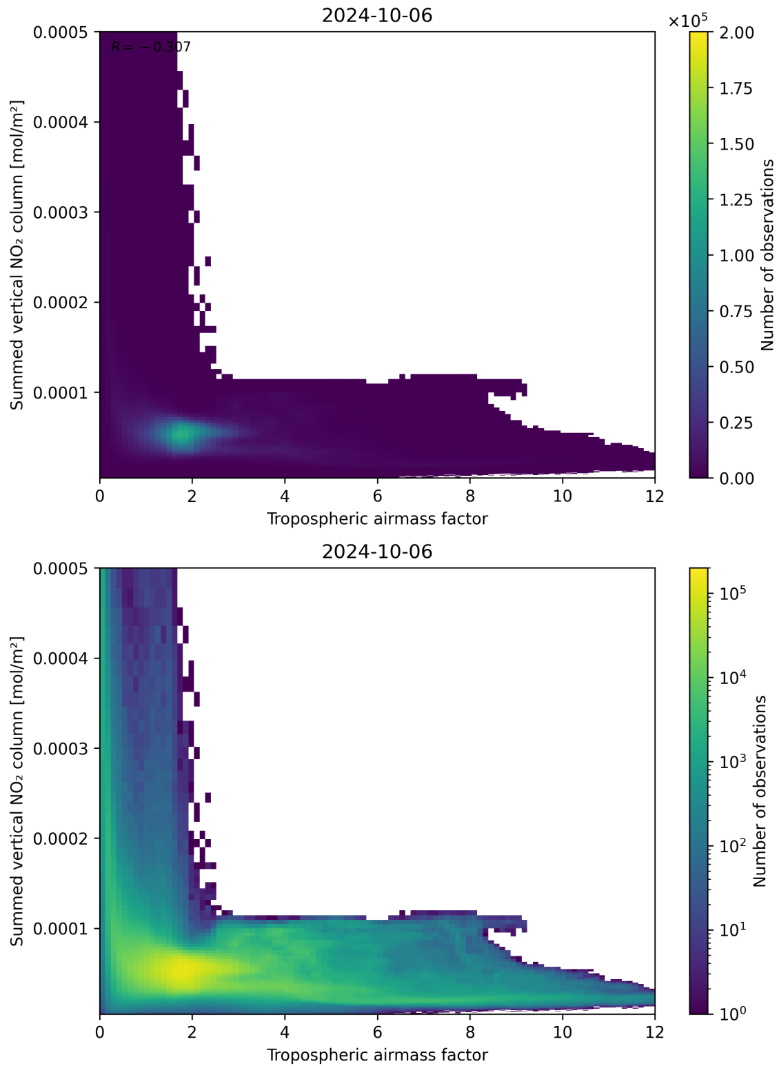
Figure 75: Scatter density plot of “Tropospheric air mass factor” against “Summed vertical NO 2 column” for 2024-10-05 to 2024-10-07.
