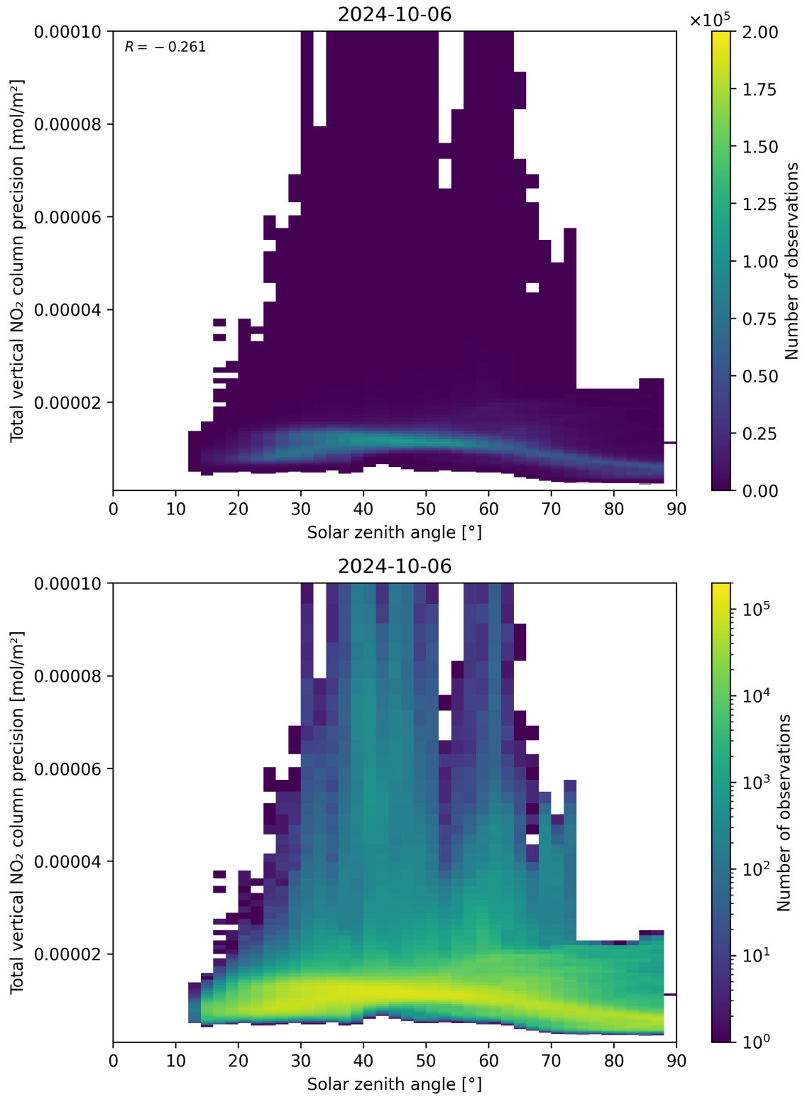
Figure 154: Scatter density plot of “Solar zenith angle” against “Total vertical NO 2 column precision” for 2024-10-05 to 2024-10-07.
