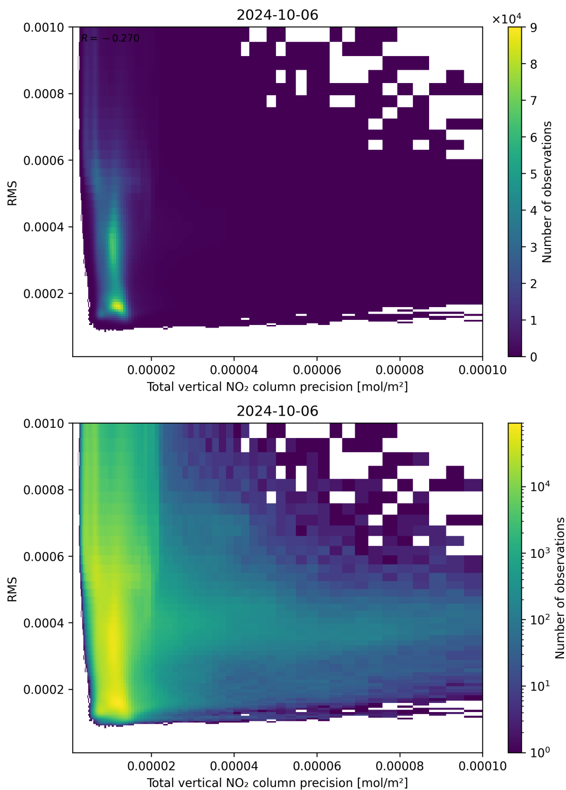
Figure 119: Scatter density plot of “Total vertical NO 2 column precision” against “RMS” for 2024-10-05 to 2024-10-07.
