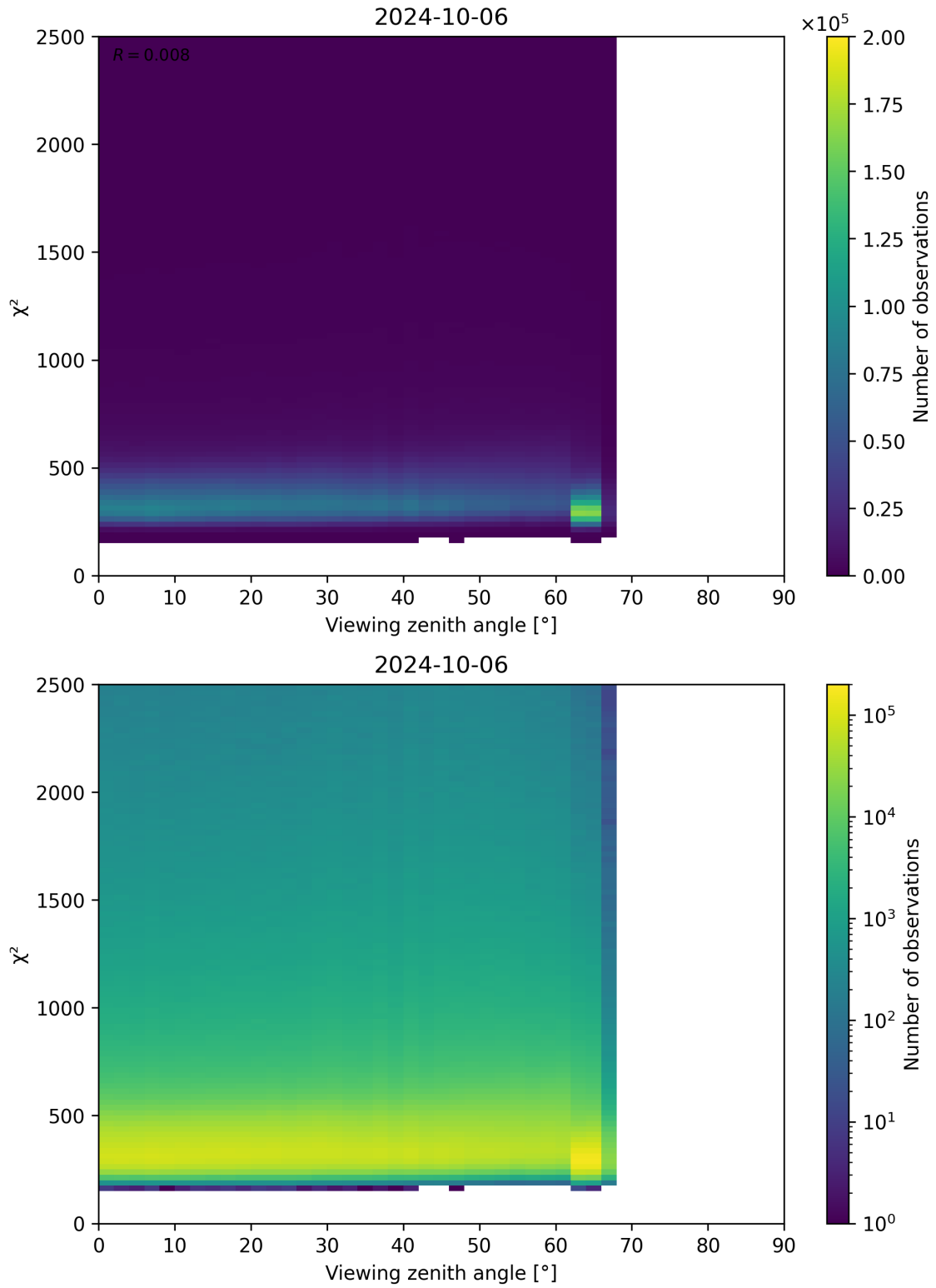
Figure 162: Scatter density plot of “Viewing zenith angle” against “ \chi^2 ” for 2024-10-05 to 2024-10-07.
