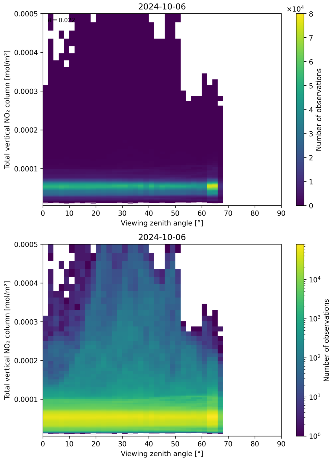
Figure 167: Scatter density plot of “Viewing zenith angle” against “Total vertical NO 2 column” for 2024-10-05 to 2024-10-07.
