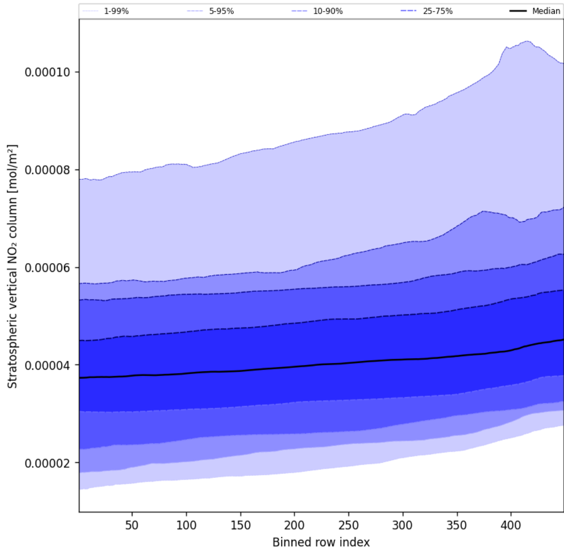
Figure 53: Along track statistics of “Stratospheric vertical NO 2 column” for 2024-10-05 to 2024-10-07
