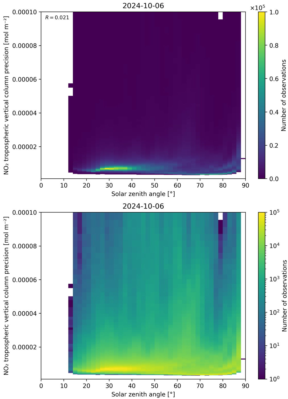
Figure 156: Scatter density plot of “Solar zenith angle” against “NO 2 tropospheric vertical column precision” for 2024-10-05 to 2024-10-07.
