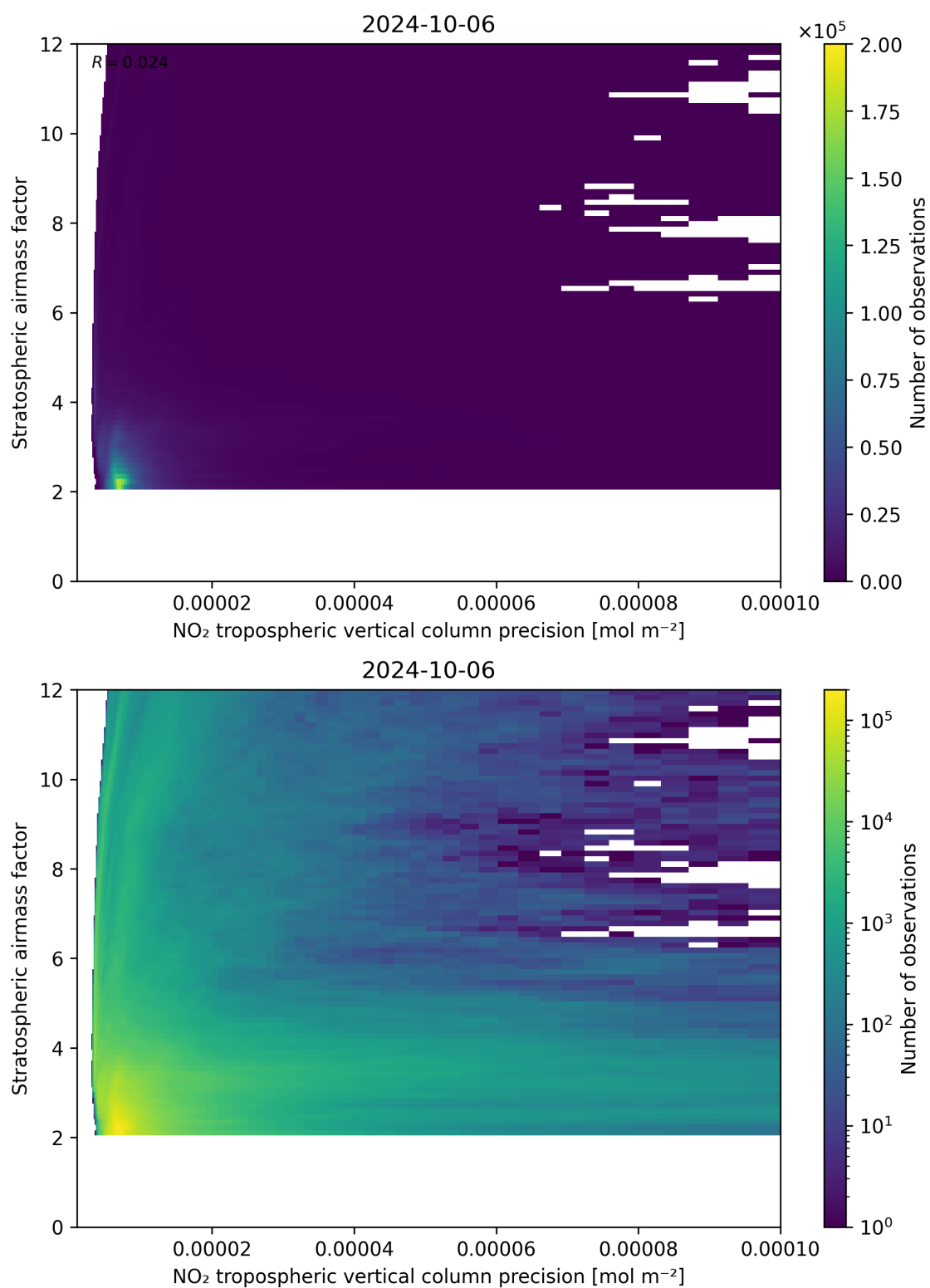
Figure 131: Scatter density plot of “NO 2 tropospheric vertical column precision” against “Stratospheric airmass factor” for 2024-10-05 to 2024-10-07.
