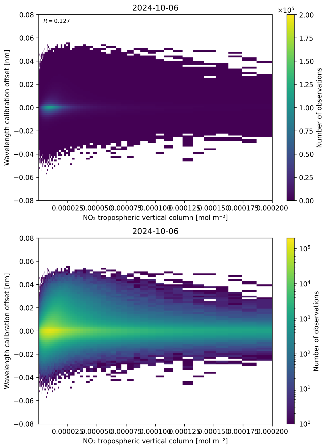
Figure 143: Scatter density plot of “NO 2 tropospheric vertical column” against “Wavelength calibration offset” for 2024-10-05 to 2024-10-07.
