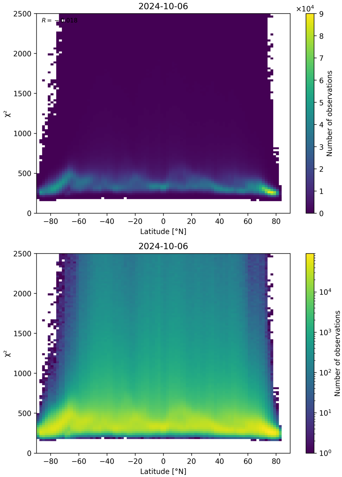
Figure 86: Scatter density plot of “Latitude” against “ \chi^2 ” for 2024-10-05 to 2024-10-07.
