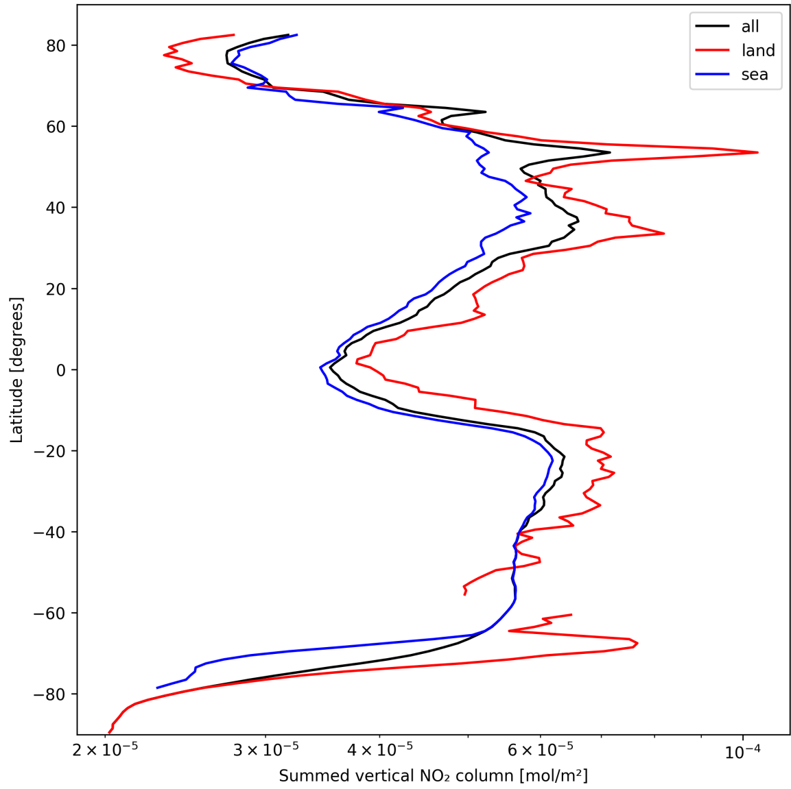
Figure 23: Zonal average of “Summed vertical NO 2 column” for 2024-10-05 to 2024-10-07.
