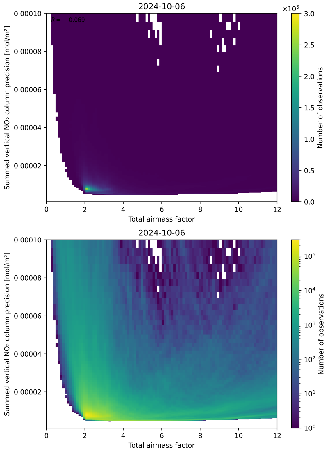
Figure 66: Scatter density plot of “Total airmass factor” against “Summed vertical NO 2 column precision” for 2024-10-05 to 2024-10-07.
