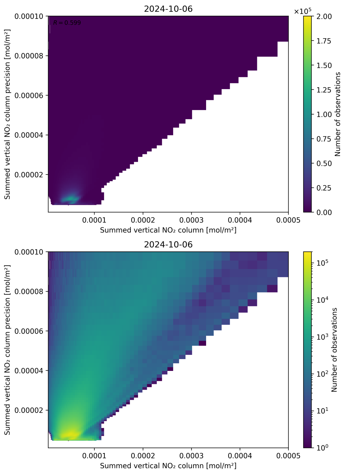
Figure 105: Scatter density plot of “Summed vertical NO 2 column” against “Summed vertical NO 2 column precision” for 2024-10-05 to 2024-10-07.
