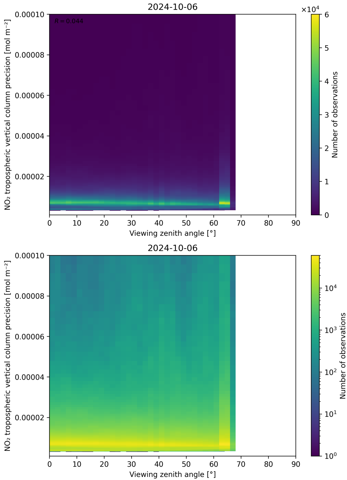
Figure 170: Scatter density plot of “Viewing zenith angle” against “NO 2 tropospheric vertical column precision” for 2024-10-05 to 2024-10-07.
