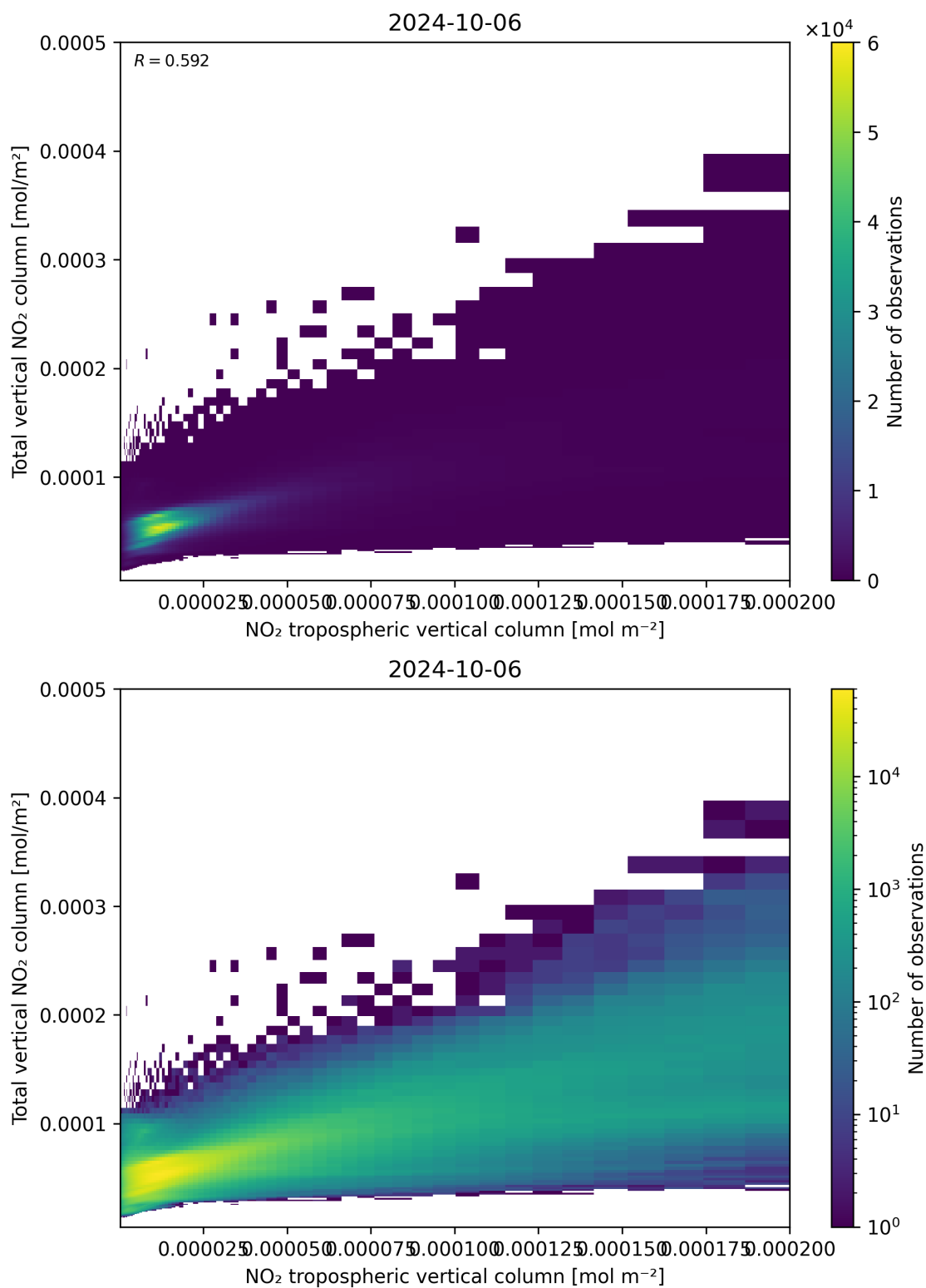
Figure 128: Scatter density plot of “NO 2 tropospheric vertical column” against “Total vertical NO 2 column” for 2024-10-05 to 2024-10-07.
