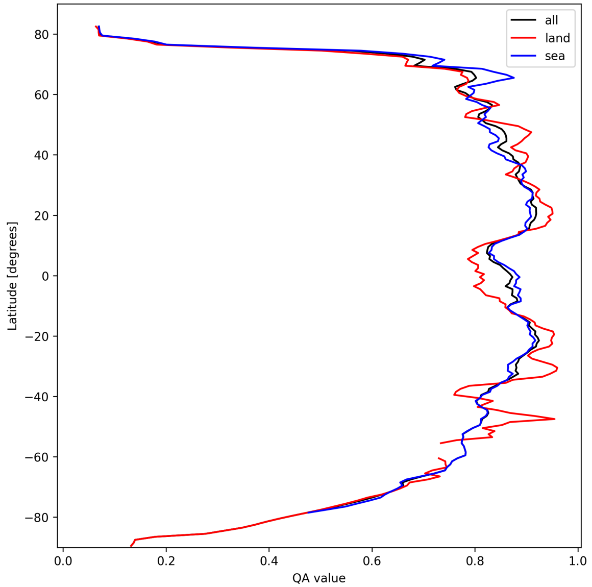
Figure 11: Zonal average of “QA value” for 2024-10-05 to 2024-10-07.
