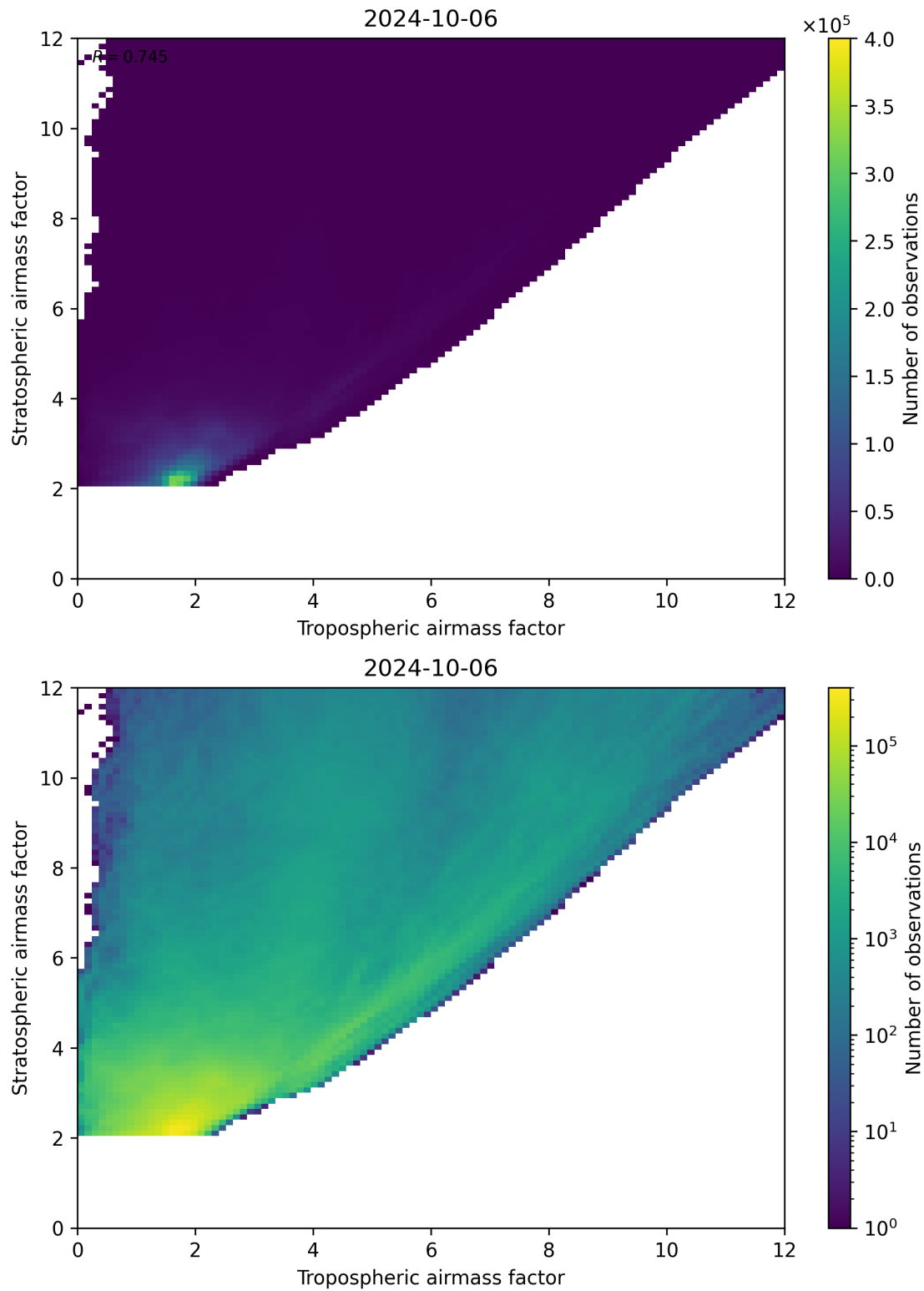
Figure 71: Scatter density plot of “Tropospheric airmass factor” against “Stratospheric airmass factor” for 2024-10-05 to 2024-10-07.
