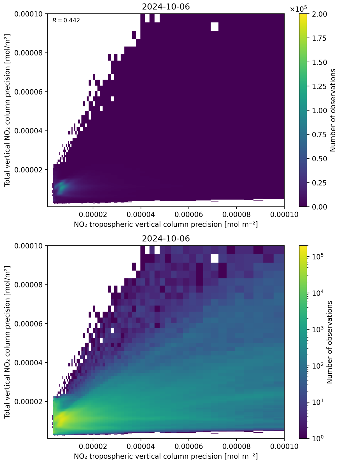
Figure 139: Scatter density plot of “NO 2 tropospheric vertical column precision” against “Total vertical NO 2 column precision” for 2024-10-05 to 2024-10-07.
