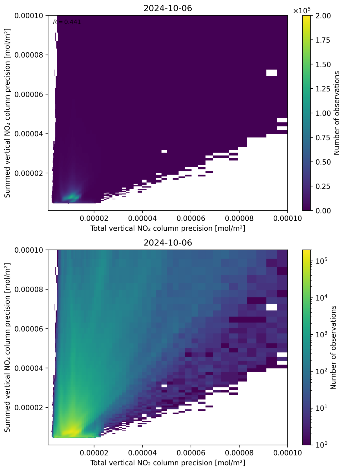
Figure 118: Scatter density plot of “Total vertical NO 2 column precision” against “Summed vertical NO 2 column precision” for 2024-10-05 to 2024-10-07.
