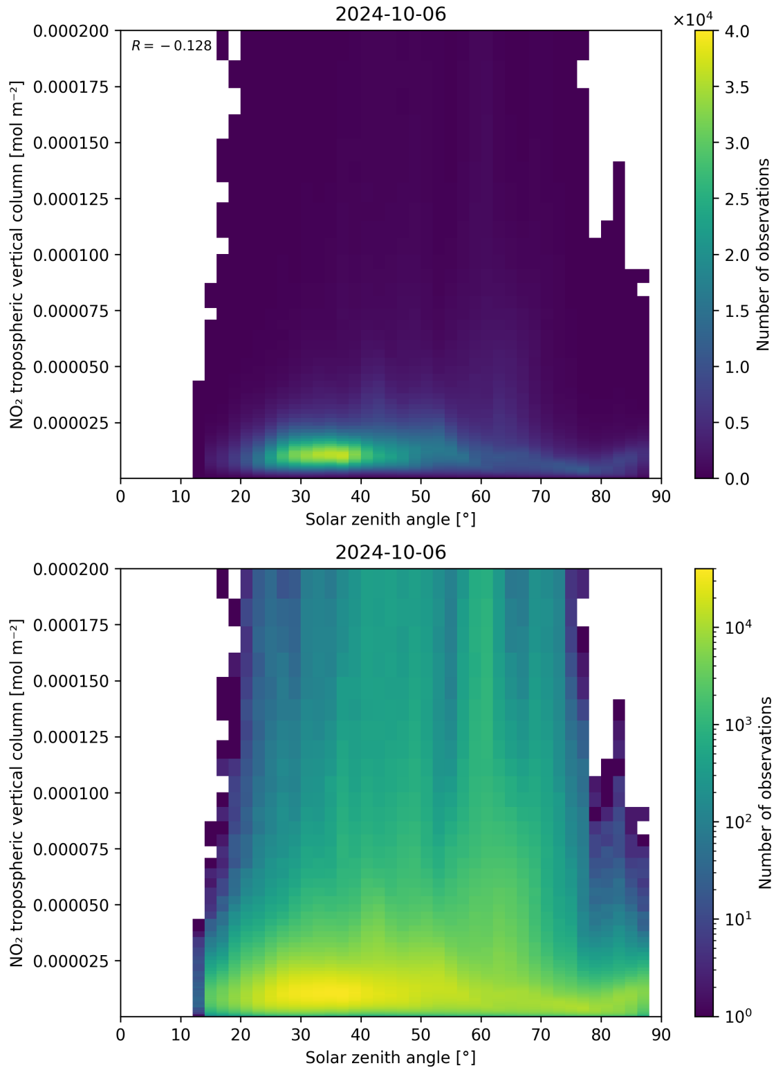
Figure 155: Scatter density plot of “Solar zenith angle” against “NO 2 tropospheric vertical column” for 2024-10-05 to 2024-10-07.
