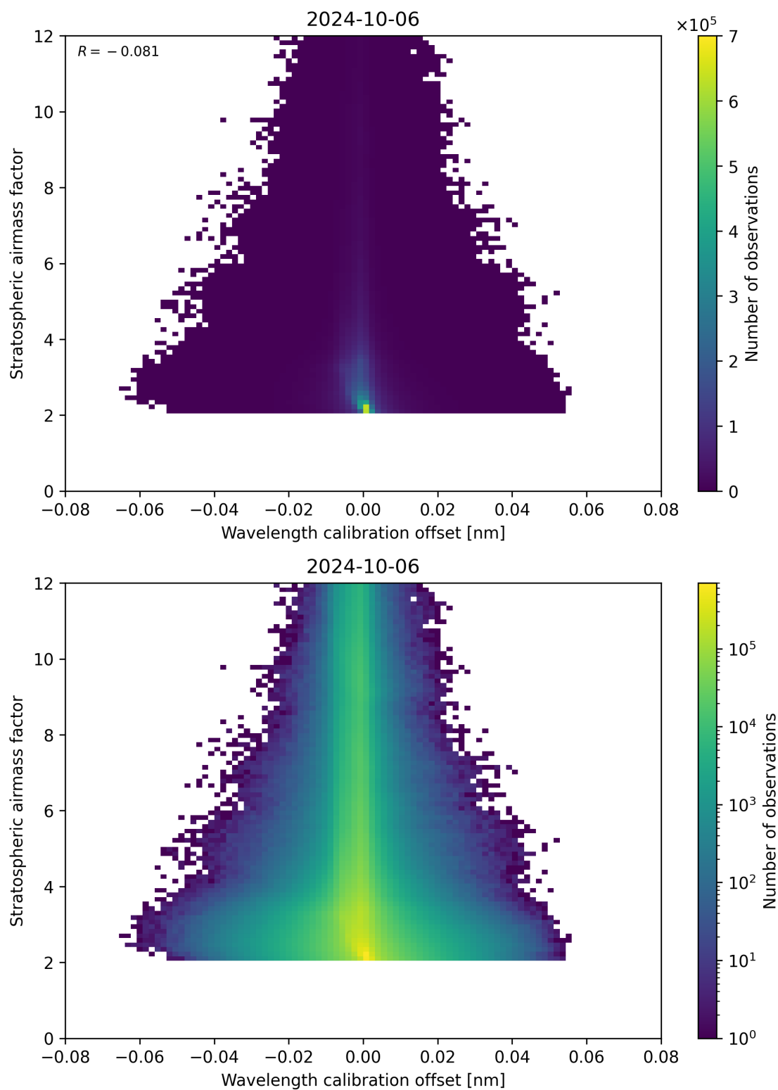
Figure 174: Scatter density plot of “Wavelength calibration offset” against “Stratospheric airmass factor” for 2024-10-05 to 2024-10-07.
