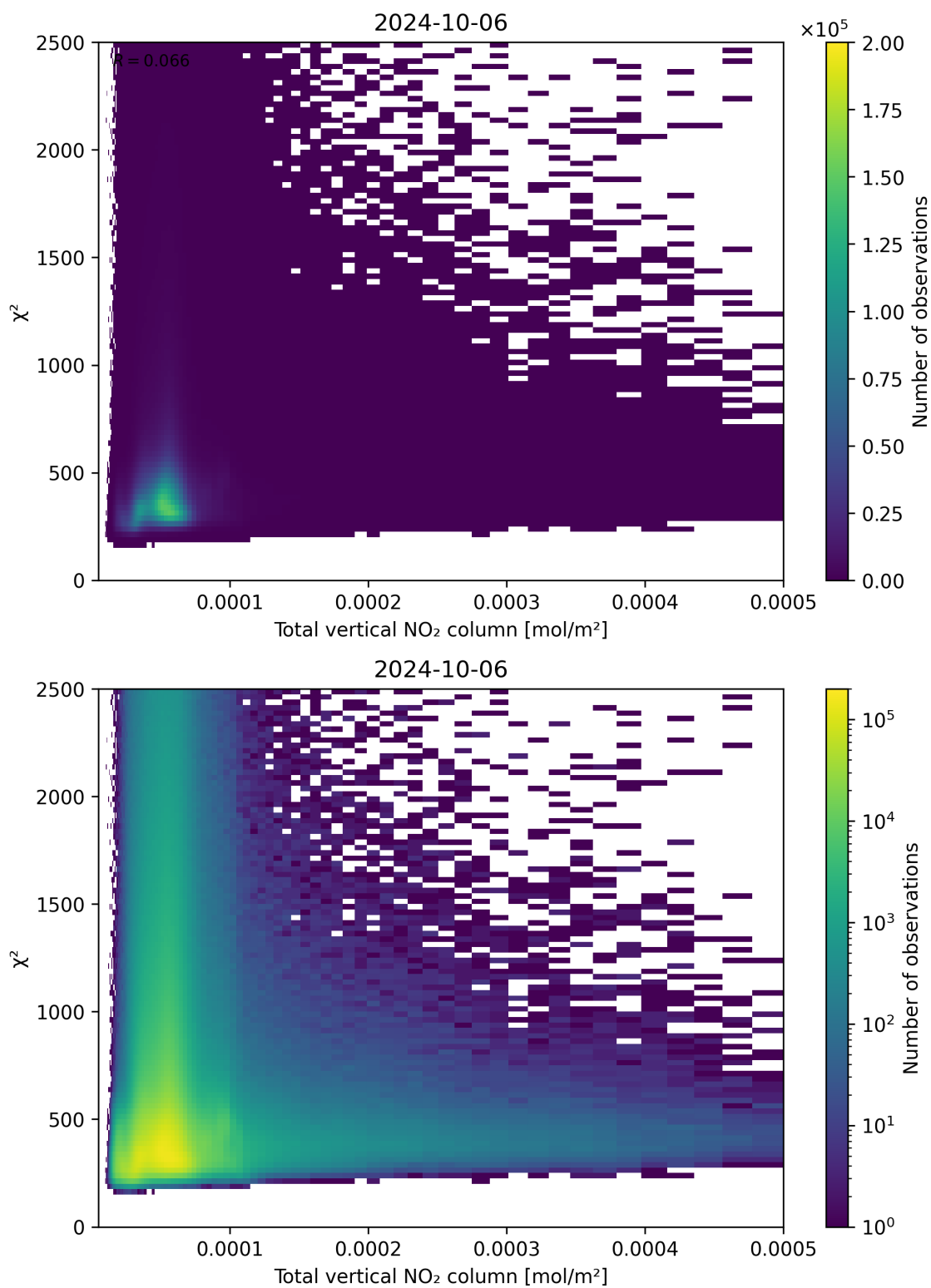
Figure 111: Scatter density plot of “Total vertical NO 2 column” against “ \chi^2 ” for 2024-10-05 to 2024-10-07.
