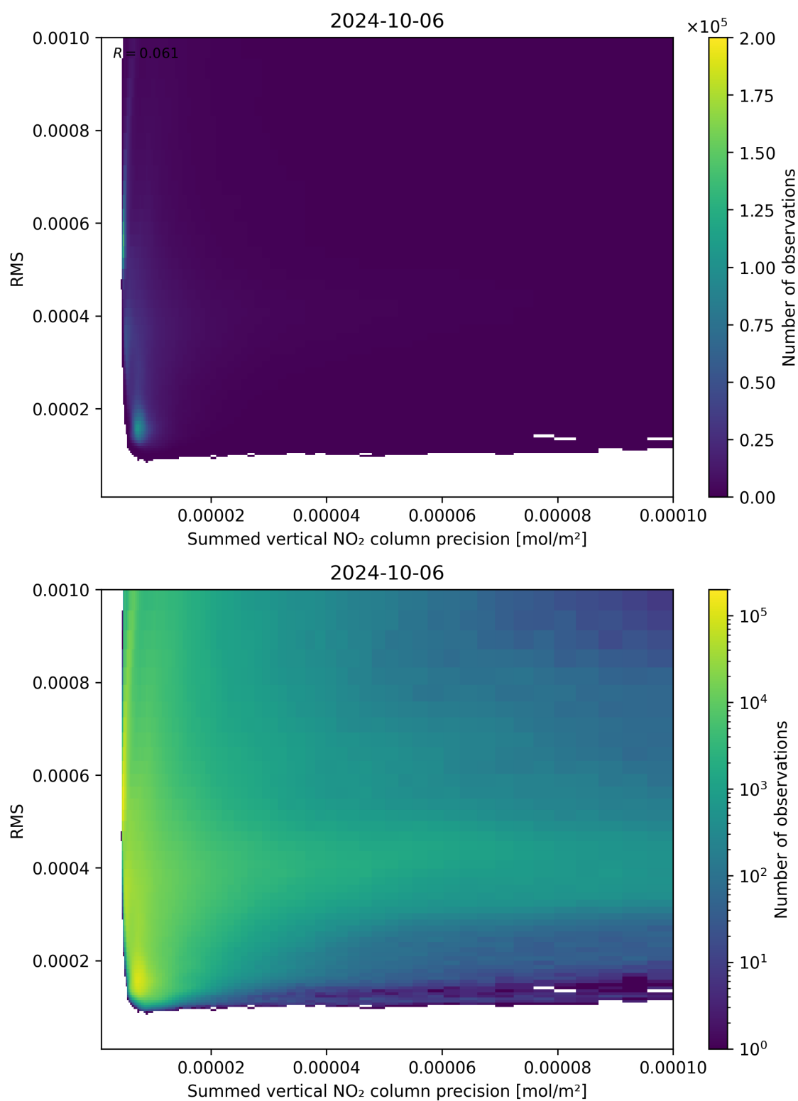
Figure 108: Scatter density plot of “Summed vertical NO 2 column precision” against “RMS” for 2024-10-05 to 2024-10-07.
