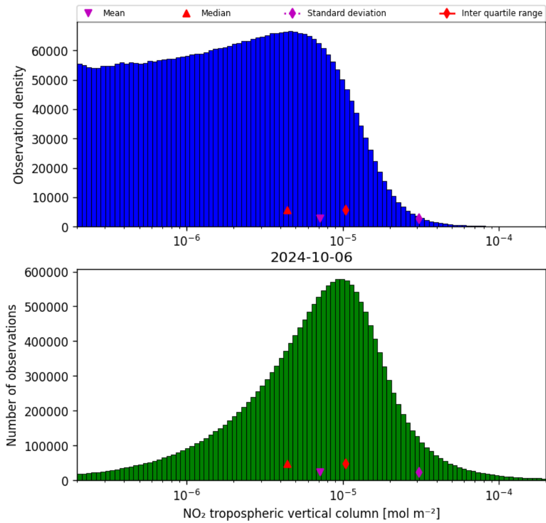
Figure 29: Histogram of “ \text{NO}_2 tropospheric vertical column” for 2024-10-05 to 2024-10-07
