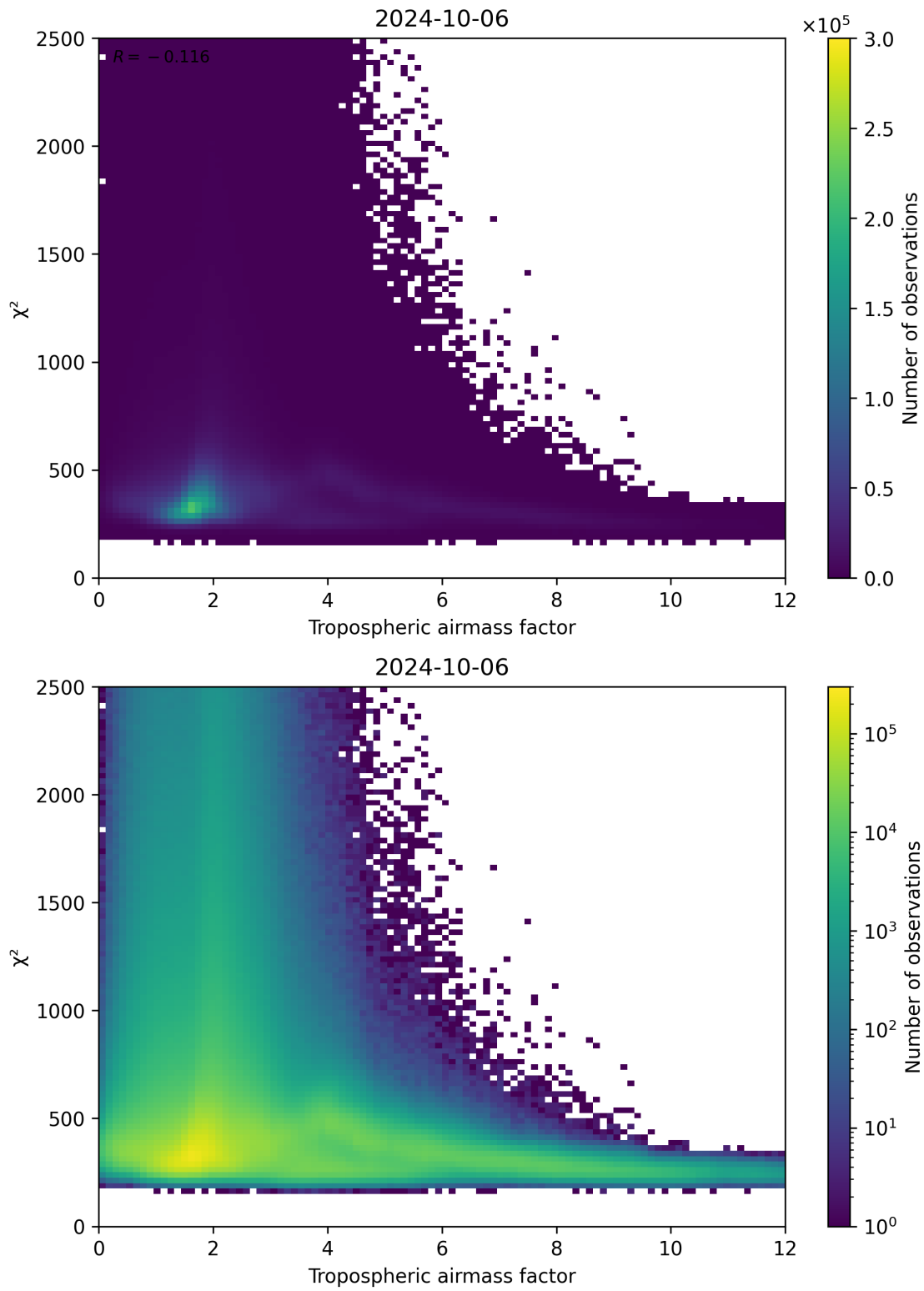
Figure 73: Scatter density plot of “Tropospheric airmass factor” against “ \chi^2 ” for 2024-10-05 to 2024-10-07.
