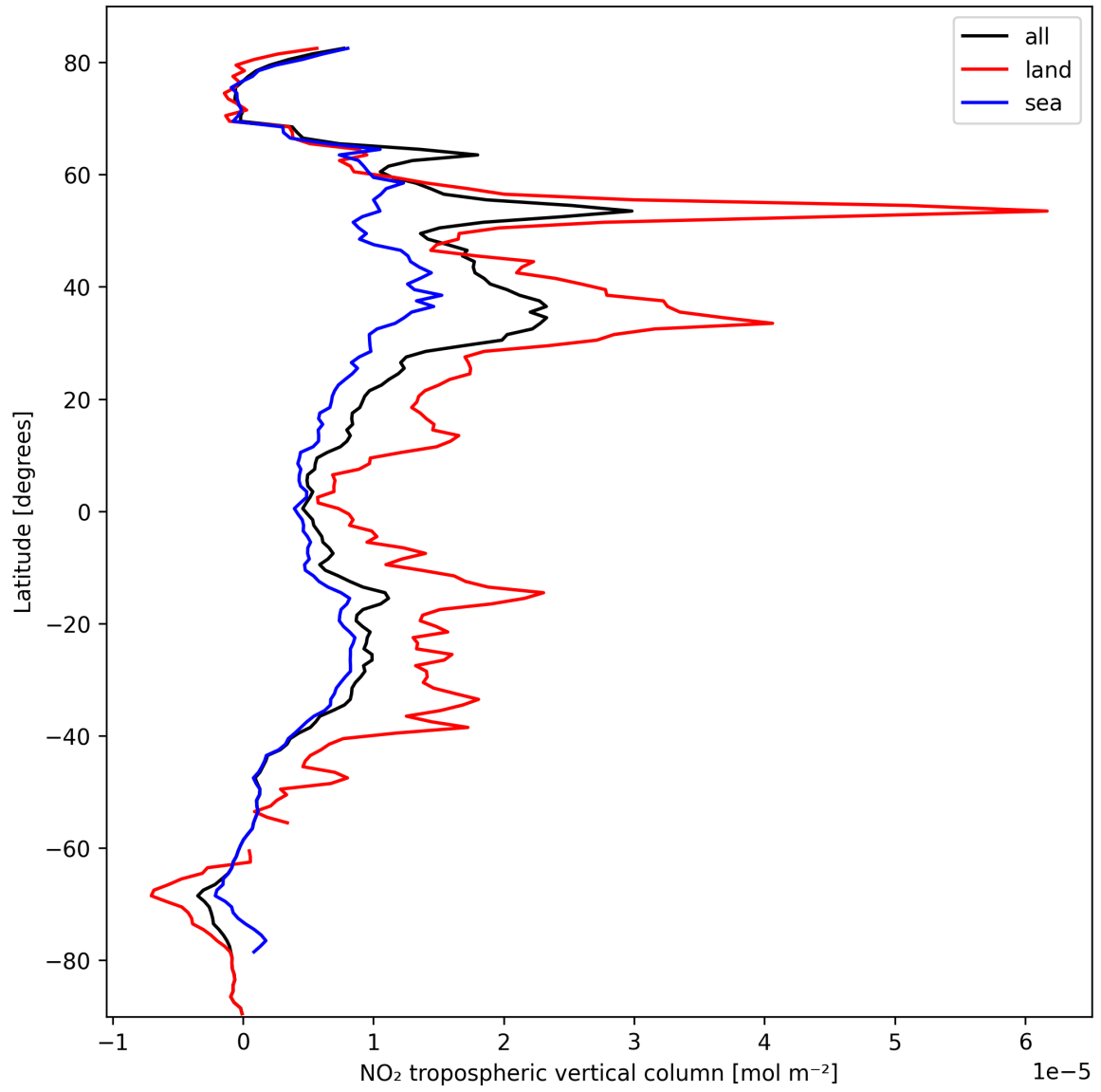
Figure 12: Zonal average of “NO 2 tropospheric vertical column” for 2024-10-05 to 2024-10-07.
