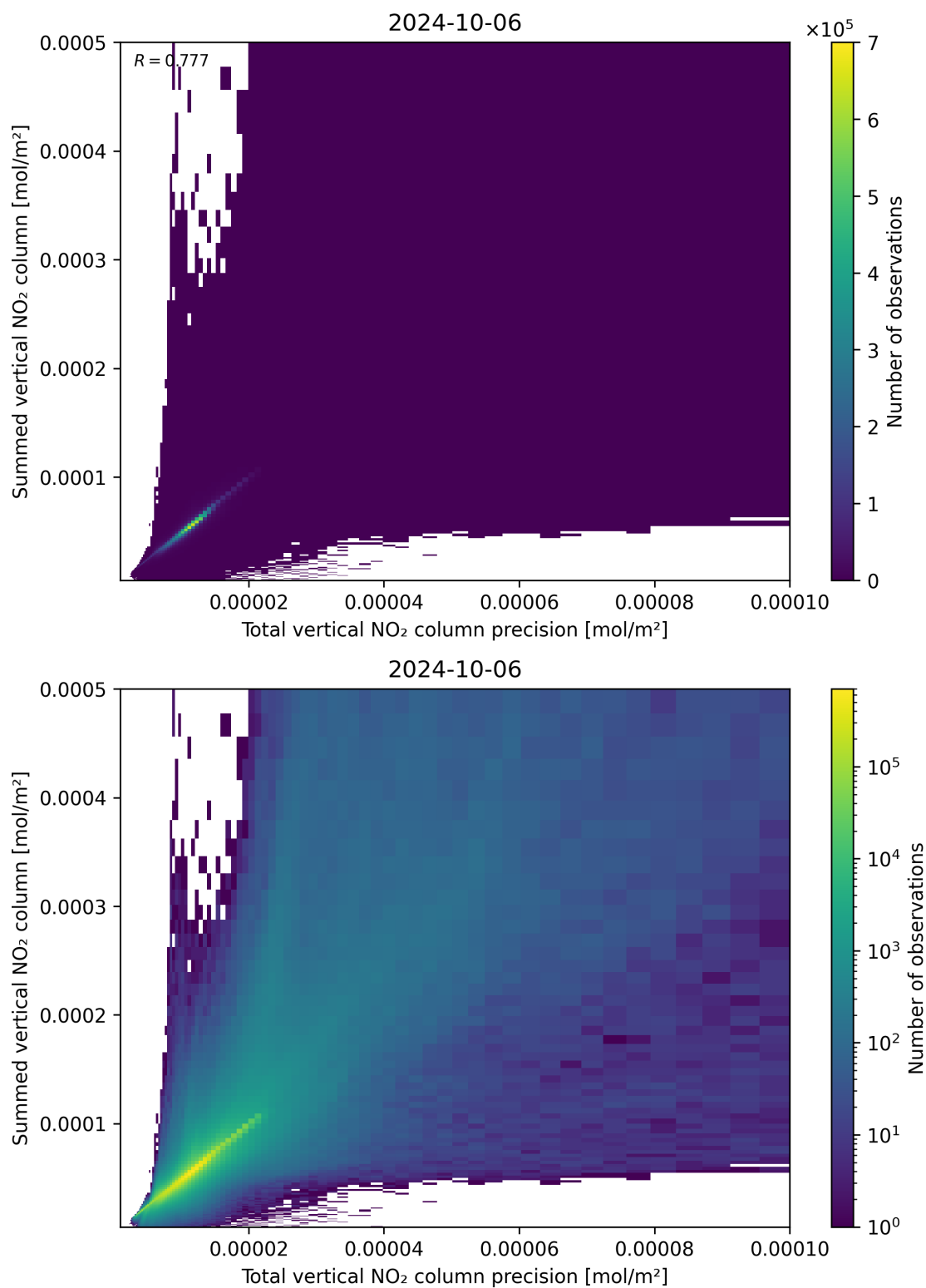
Figure 117: Scatter density plot of “Total vertical NO 2 column precision” against “Summed vertical NO 2 column” for 2024-10-05 to 2024-10-07.
