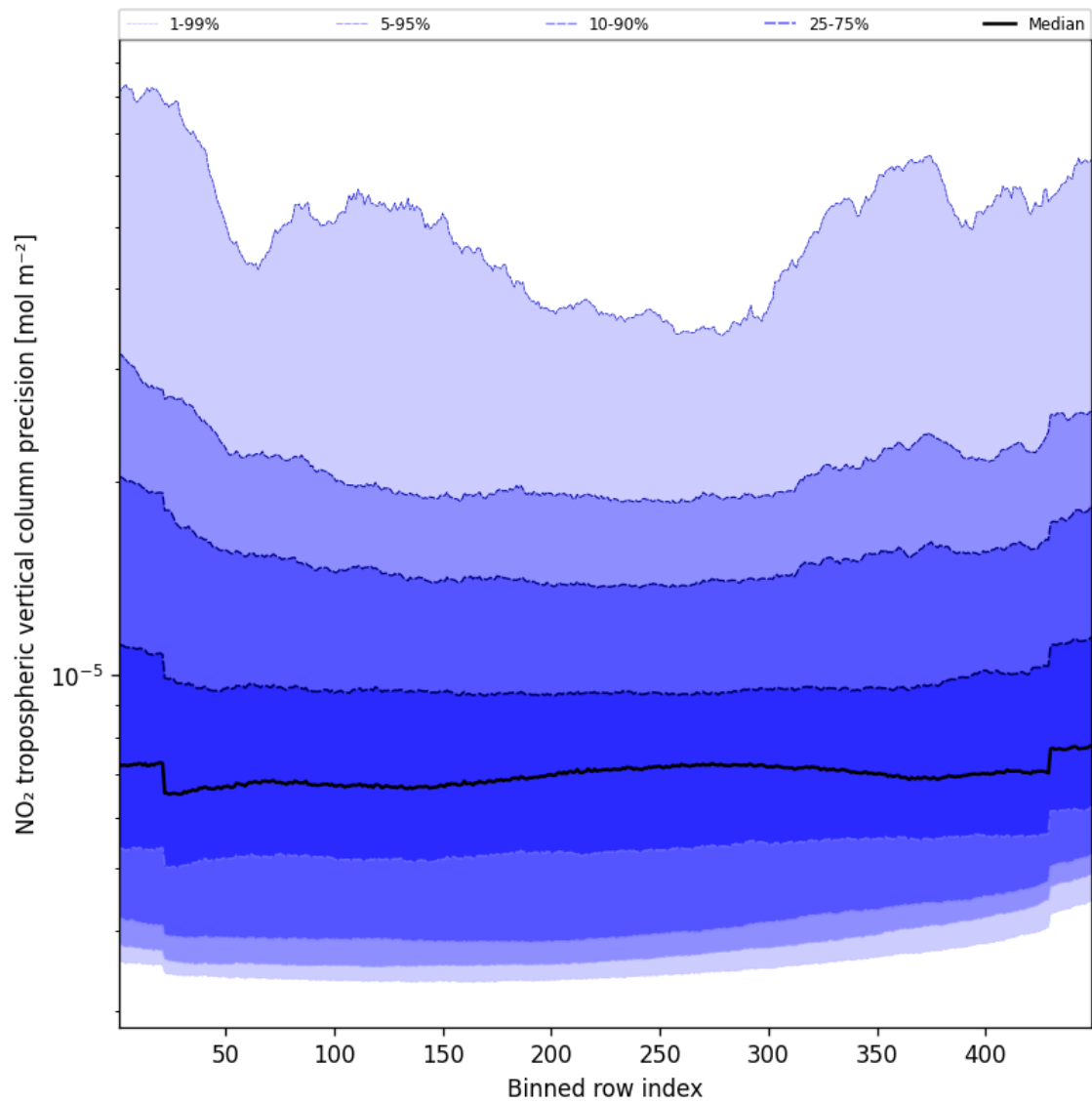
Figure 47: Along track statistics of “NO 2 tropospheric vertical column precision” for 2024-10-05 to 2024-10-07
