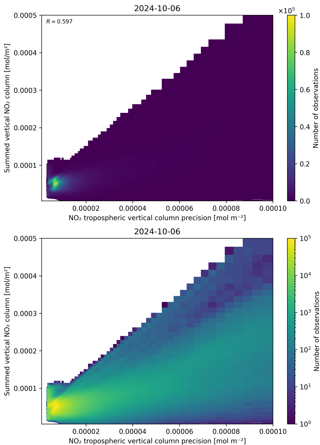
Figure 136: Scatter density plot of “NO 2 tropospheric vertical column precision” against “Summed vertical NO 2 column” for 2024-10-05 to 2024-10-07.
