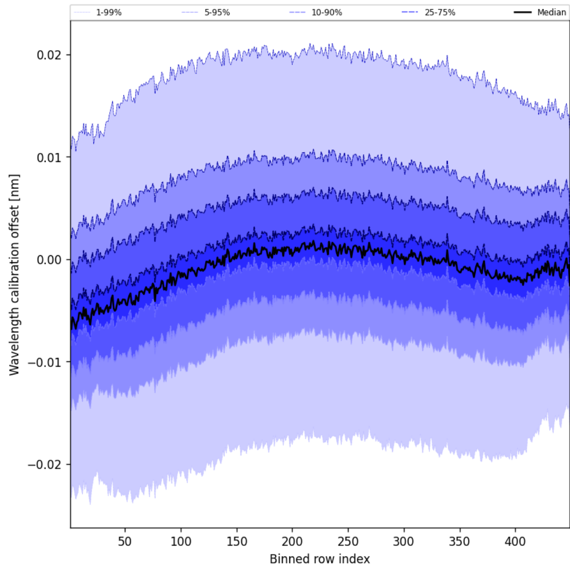
Figure 52: Along track statistics of “Wavelength calibration offset” for 2024-10-05 to 2024-10-07
