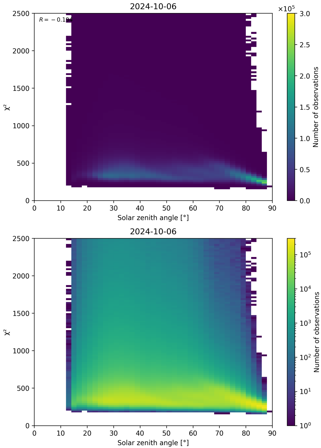
Figure 148: Scatter density plot of “Solar zenith angle” against “ \chi^2 ” for 2024-10-05 to 2024-10-07.
