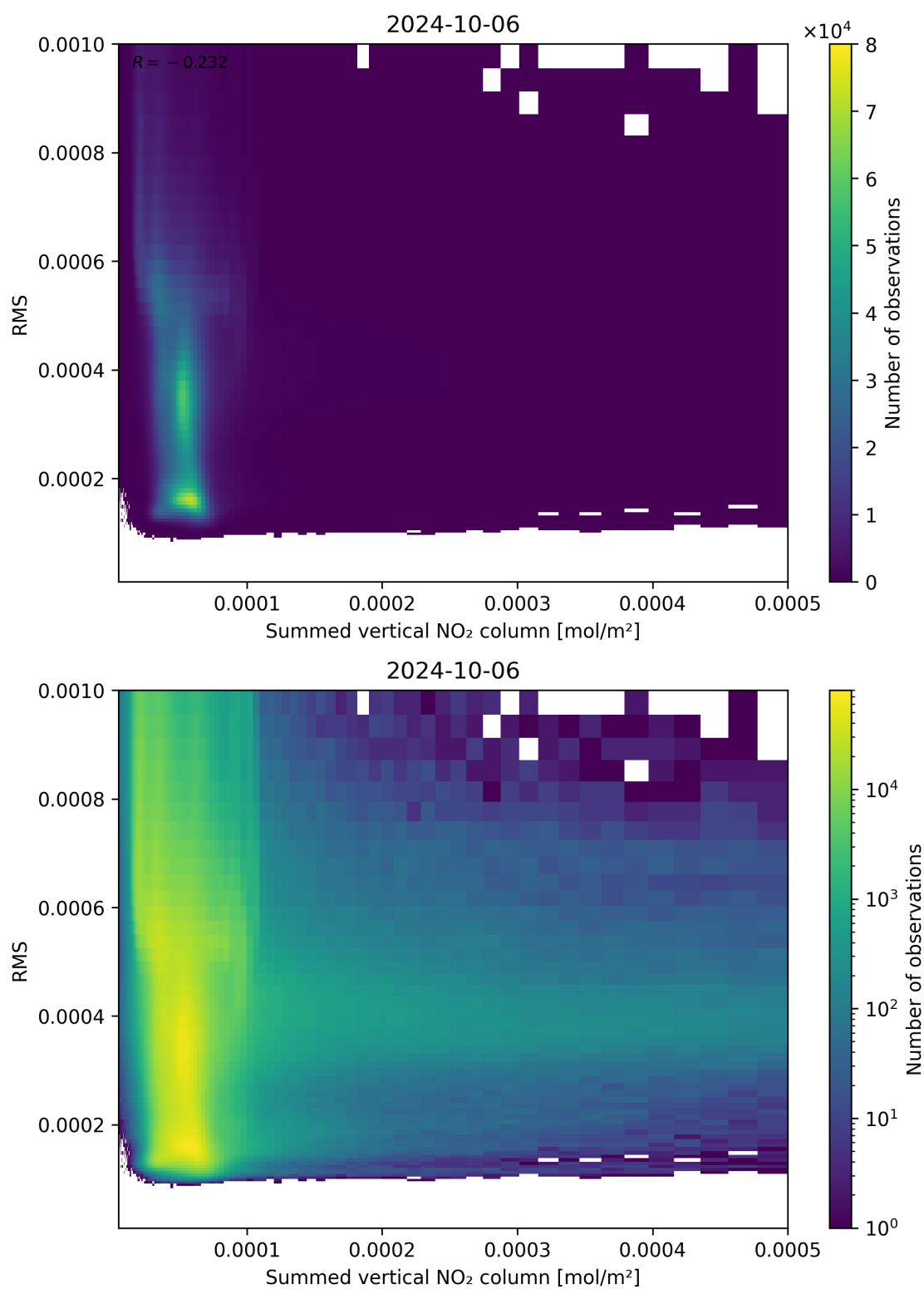
Figure 109: Scatter density plot of “Summed vertical NO 2 column” against “RMS” for 2024-10-05 to 2024-10-07.
