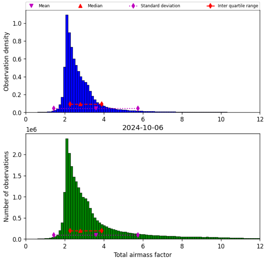
Figure 32: Histogram of “Total airmass factor” for 2024-10-05 to 2024-10-07
