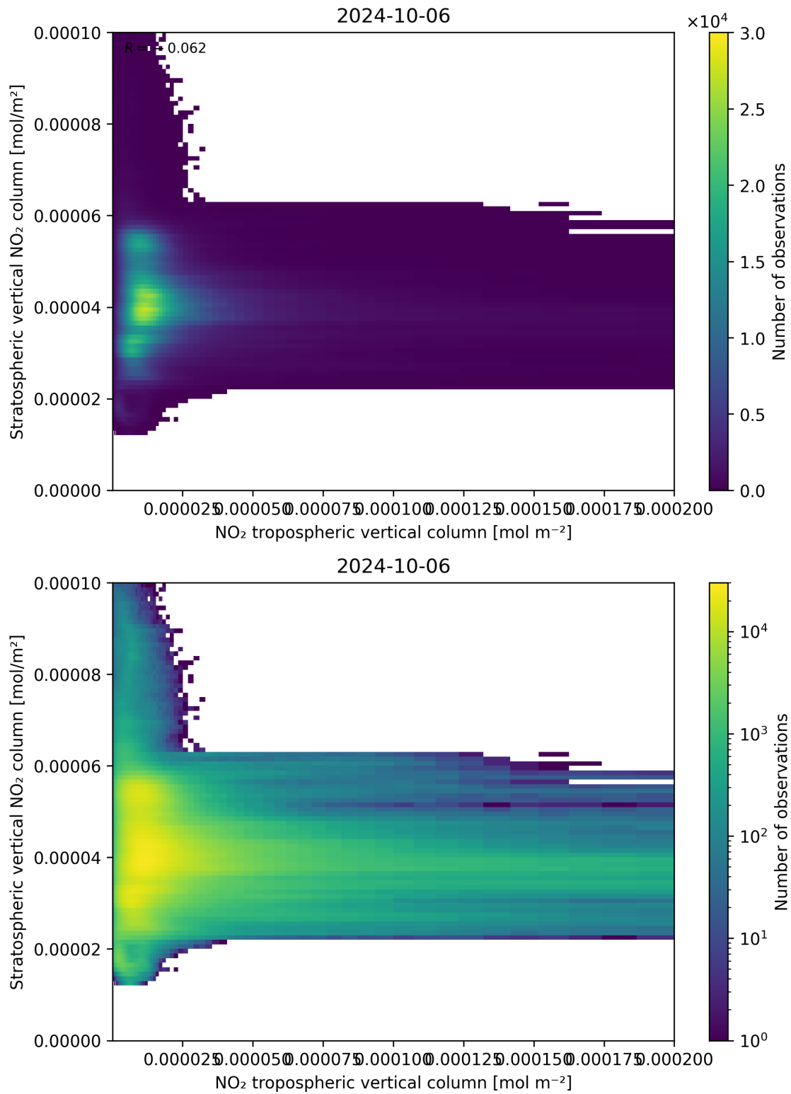
Figure 125: Scatter density plot of “NO 2 tropospheric vertical column” against “Stratospheric vertical NO 2 column” for 2024-10-05 to 2024-10-07.
