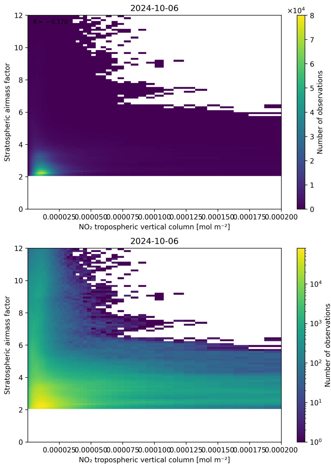
Figure 121: Scatter density plot of “NO 2 tropospheric vertical column” against “Stratospheric air mass factor” for 2024-10-05 to 2024-10-07.
