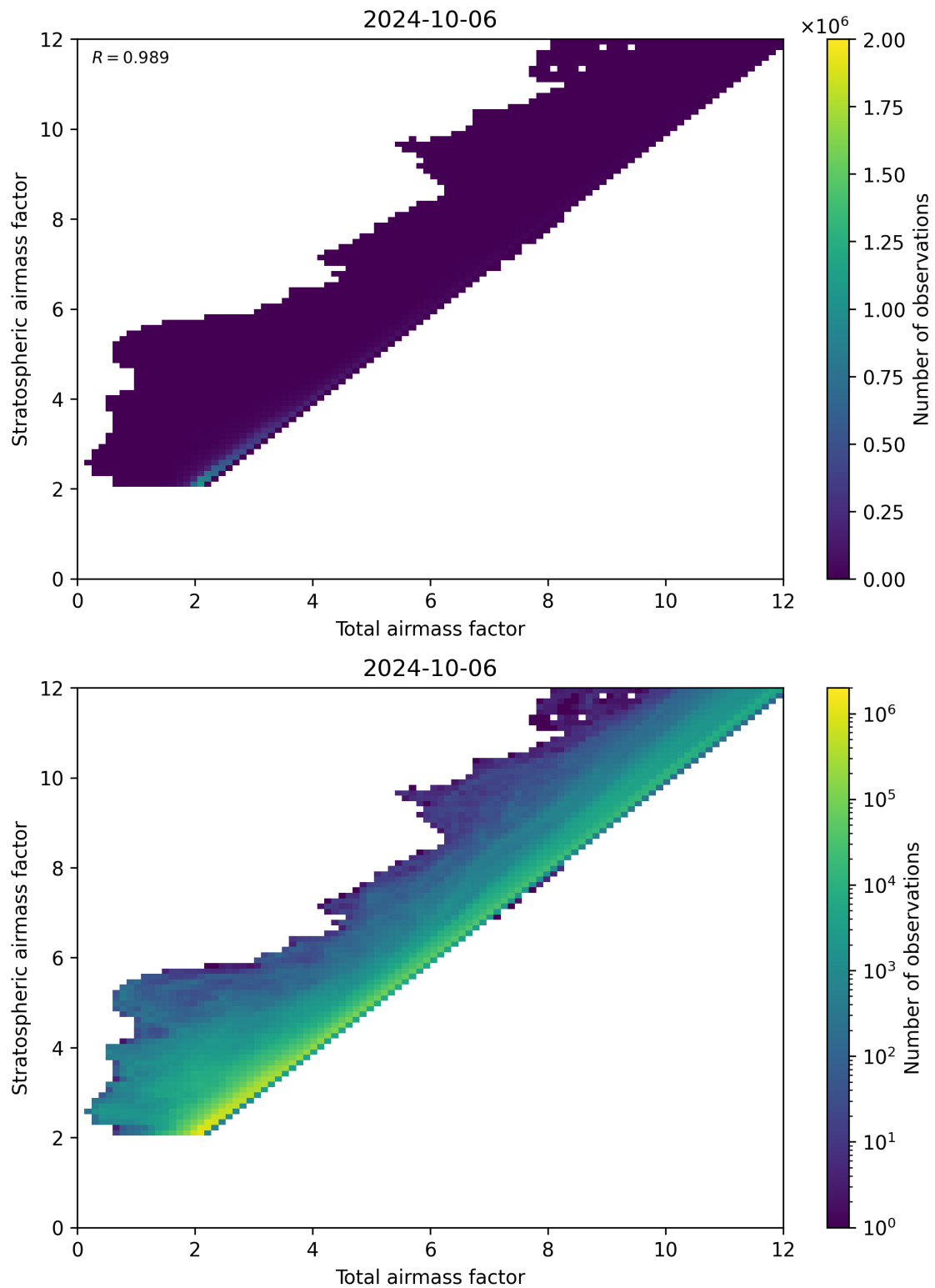
Figure 62: Scatter density plot of “Total airmass factor” against “Stratospheric airmass factor” for 2024-10-05 to 2024-10-07.
