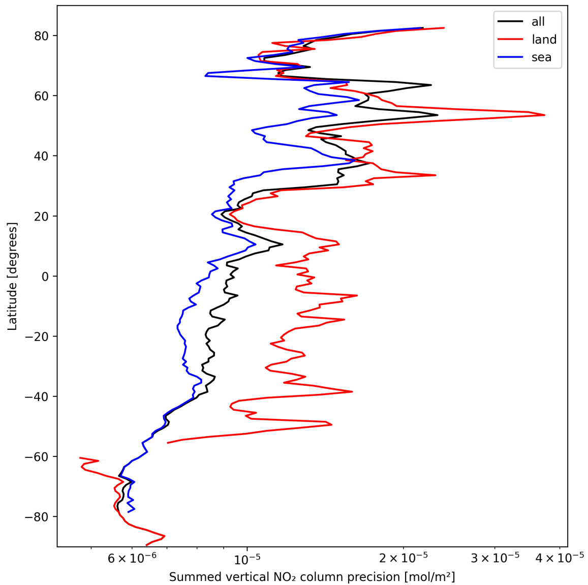
Figure 24: Zonal average of “Summed vertical NO 2 column precision” for 2024-10-05 to 2024-10-07.
