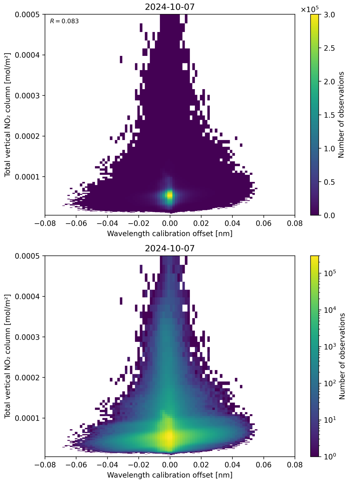
Figure 179: Scatter density plot of “Wavelength calibration offset” against “Total vertical NO 2 column” for 2024-10-06 to 2024-10-08.
