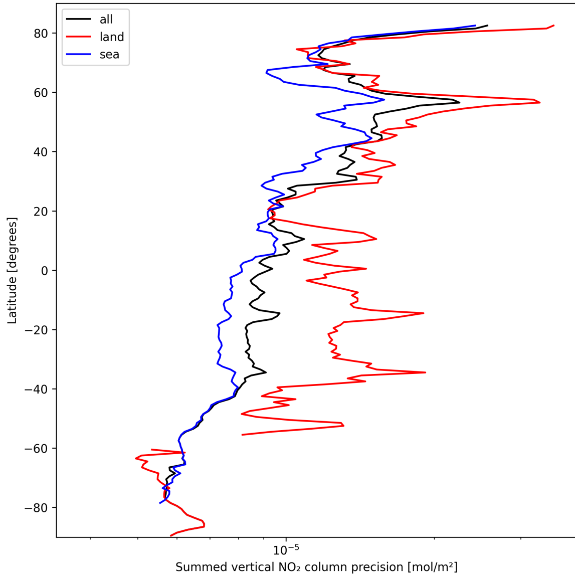
Figure 24: Zonal average of “Summed vertical NO 2 column precision” for 2024-10-06 to 2024-10-08.
