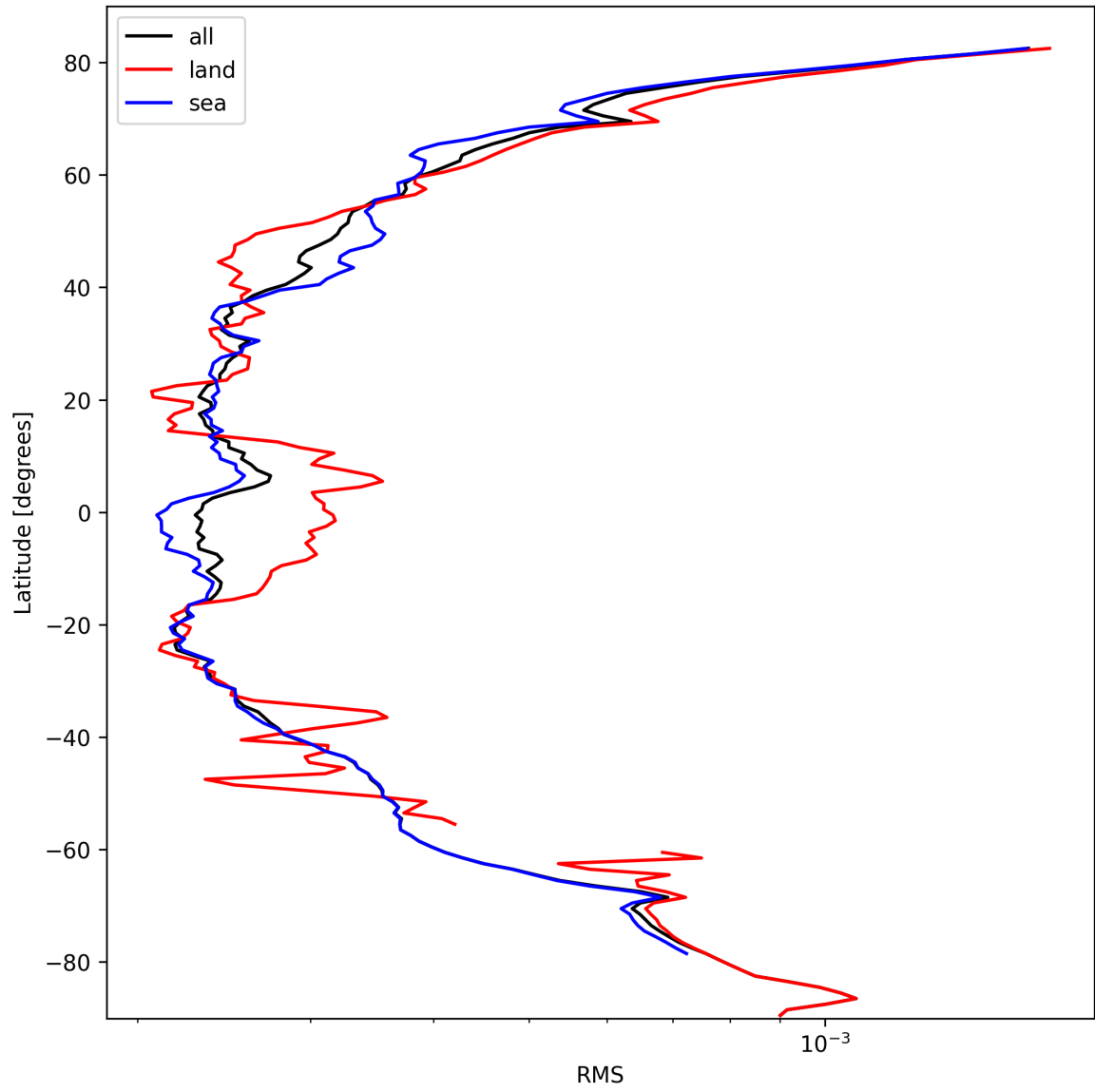
Figure 26: Zonal average of “RMS” for 2024-10-06 to 2024-10-08.
