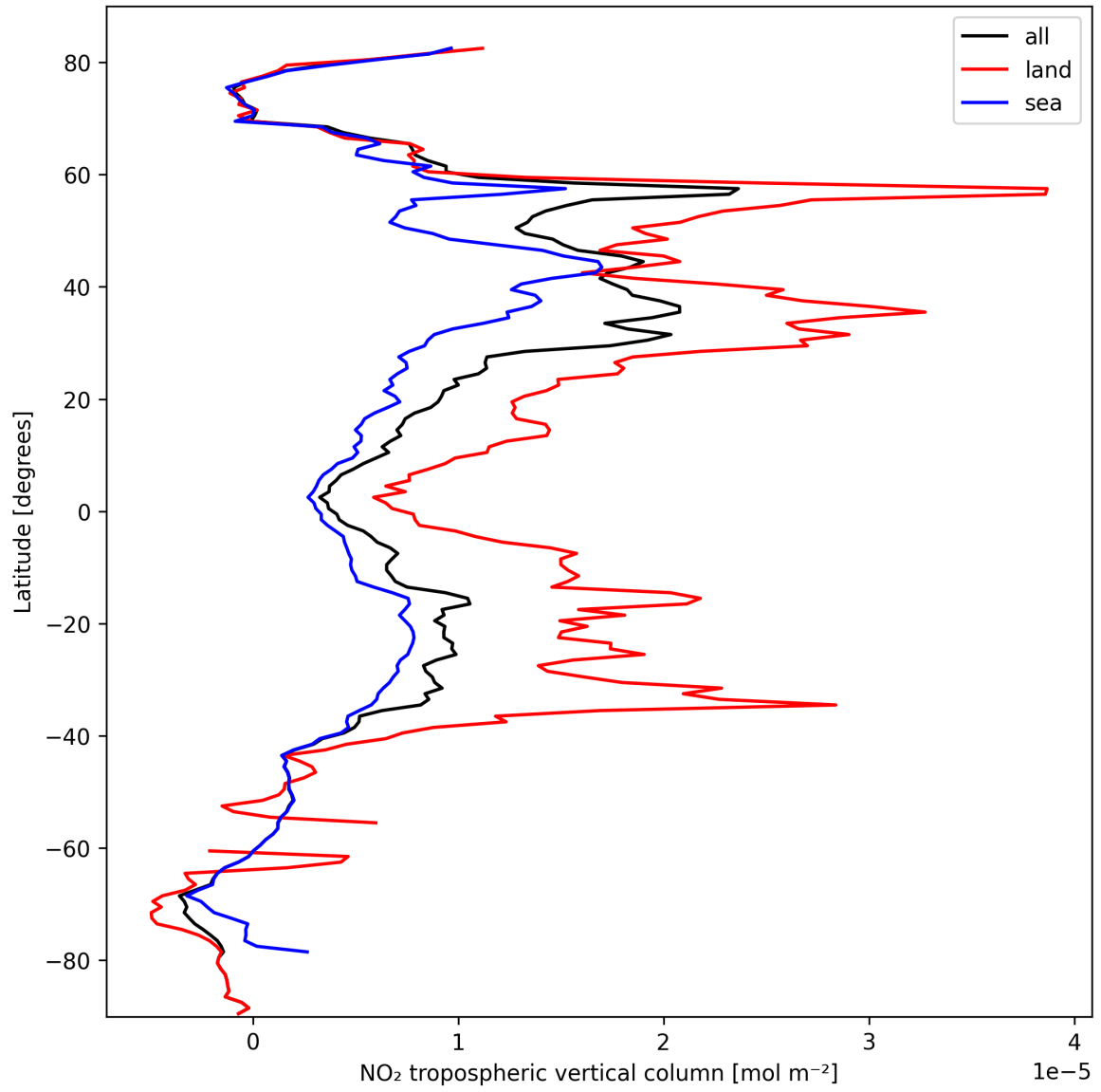
Figure 12: Zonal average of “NO 2 tropospheric vertical column” for 2024-10-06 to 2024-10-08.
