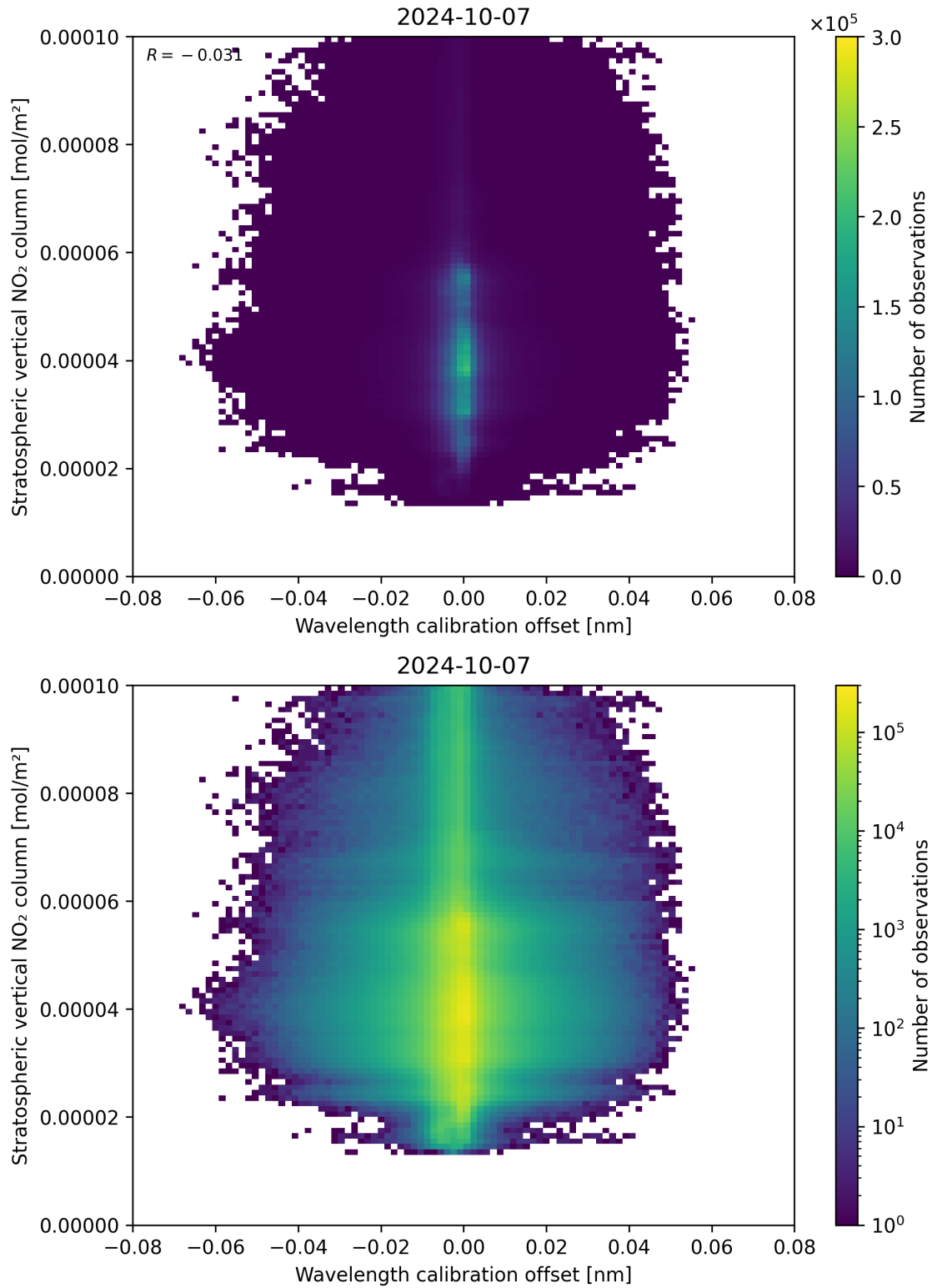
Figure 176: Scatter density plot of “Wavelength calibration offset” against “Stratospheric vertical NO 2 column” for 2024-10-06 to 2024-10-08.
