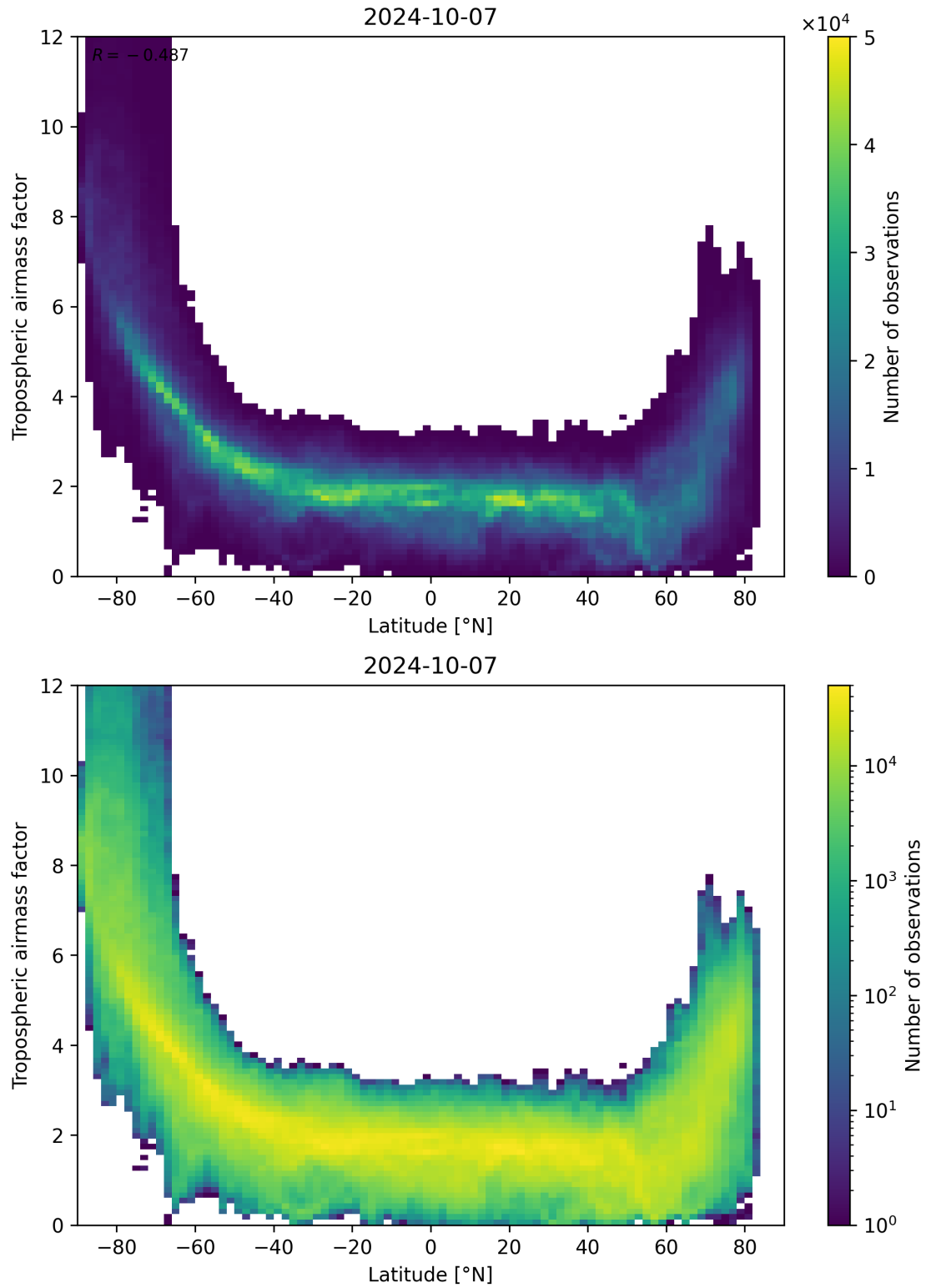
Figure 85: Scatter density plot of “Latitude” against “Tropospheric airmass factor” for 2024-10-06 to 2024-10-08.
