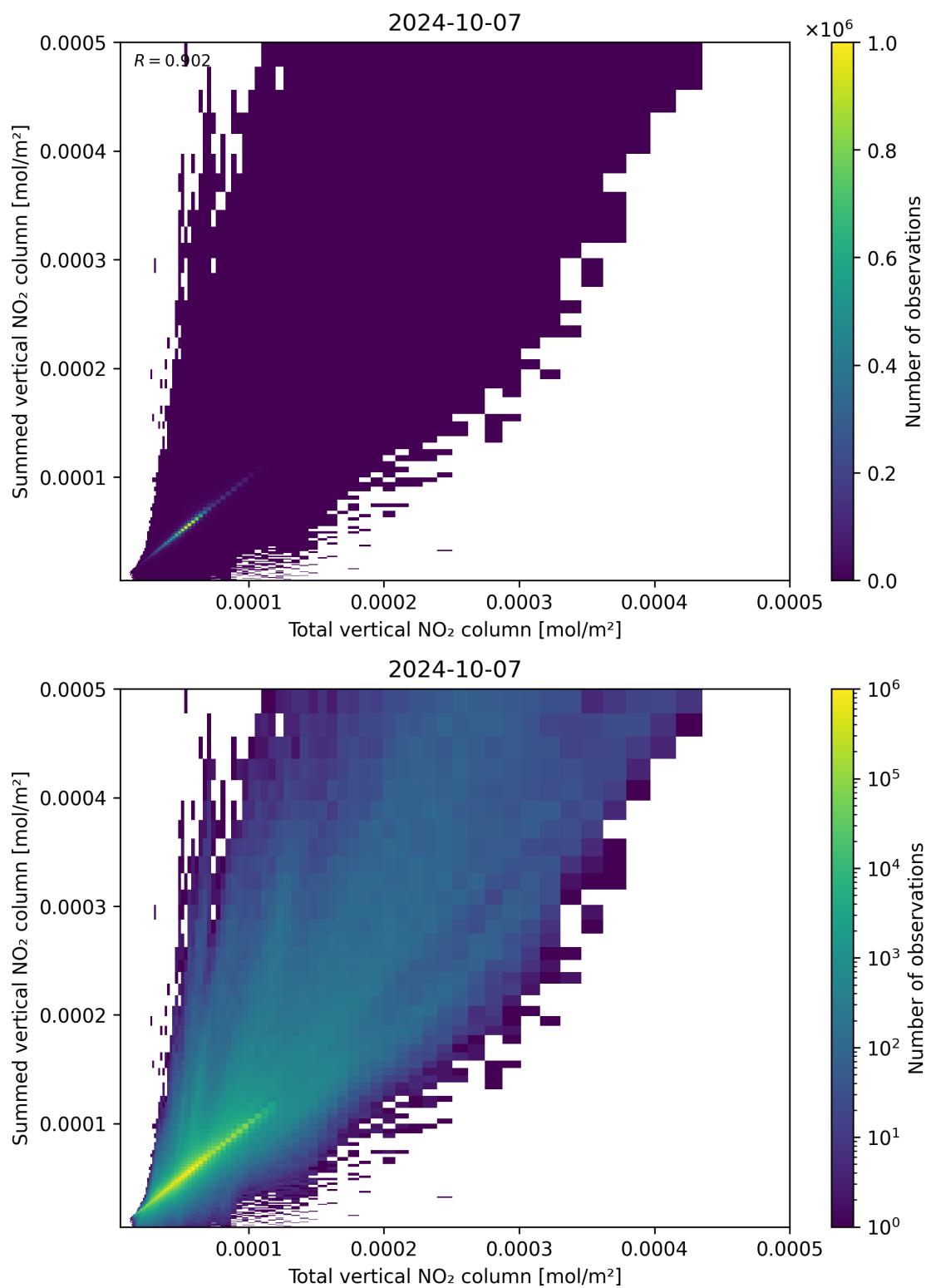
Figure 112: Scatter density plot of “Total vertical NO 2 column” against “Summed vertical NO 2 column” for 2024-10-06 to 2024-10-08.
