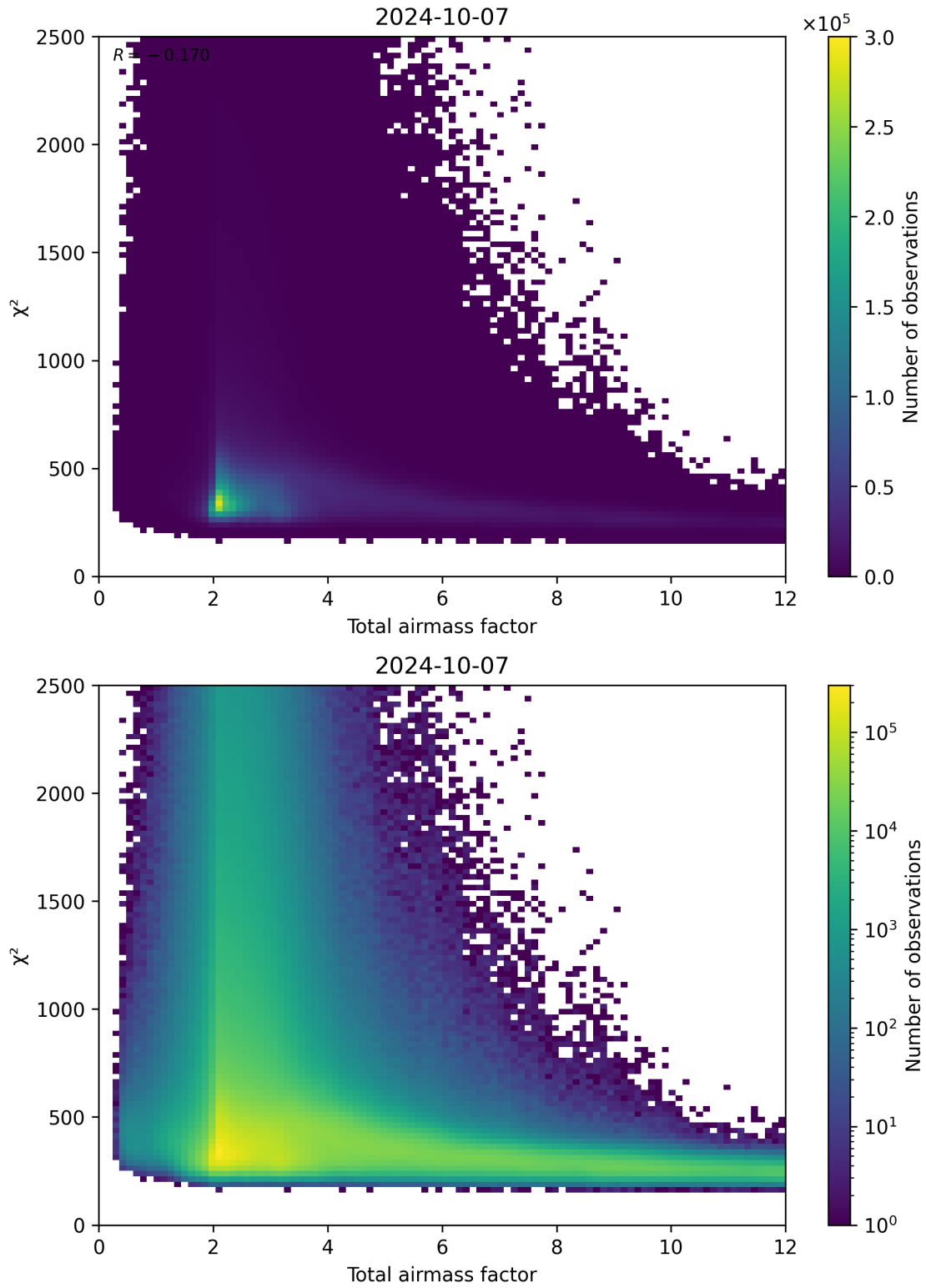
Figure 63: Scatter density plot of “Total airmass factor” against “ \chi^2 ” for 2024-10-06 to 2024-10-08.
