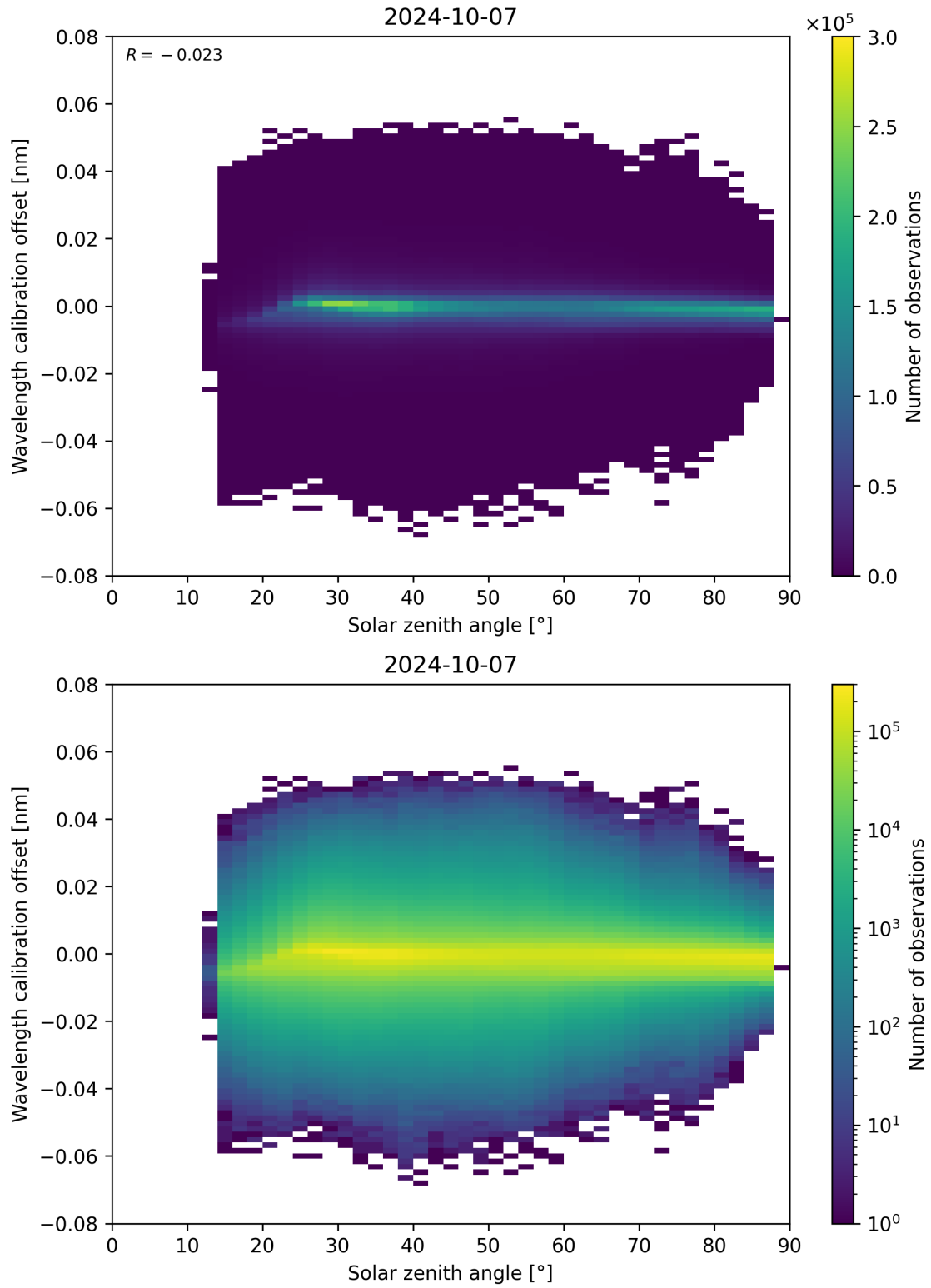
Figure 158: Scatter density plot of “Solar zenith angle” against “Wavelength calibration offset” for 2024-10-06 to 2024-10-08.
