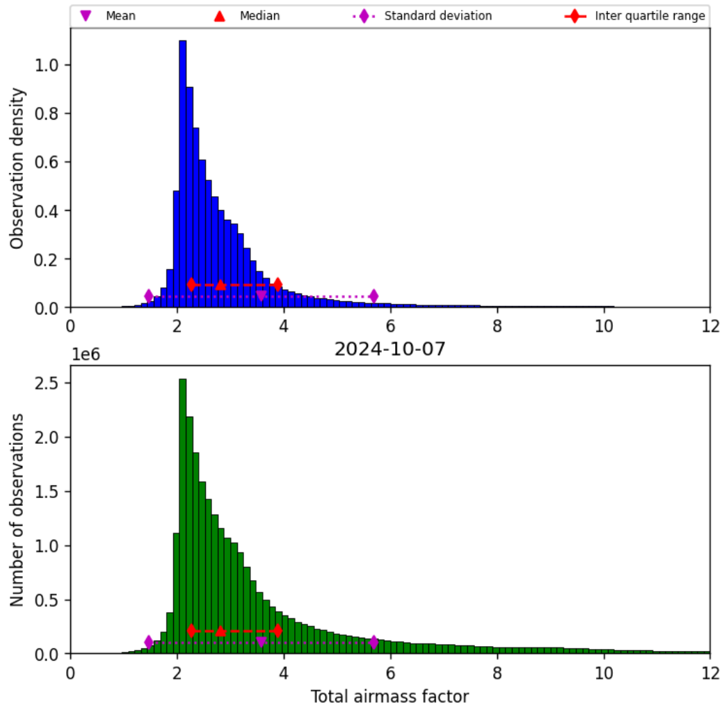
Figure 32: Histogram of “Total airmass factor” for 2024-10-06 to 2024-10-08
