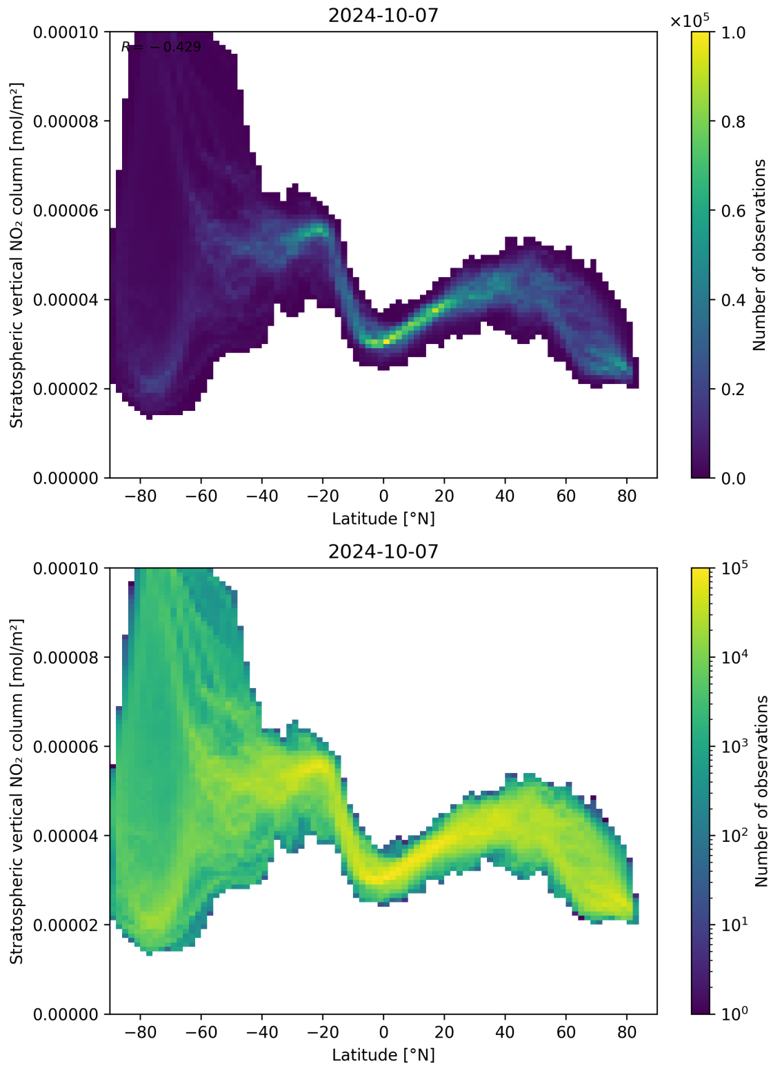
Figure 87: Scatter density plot of “Latitude” against “Stratospheric vertical NO 2 column” for 2024-10-06 to 2024-10-08.
