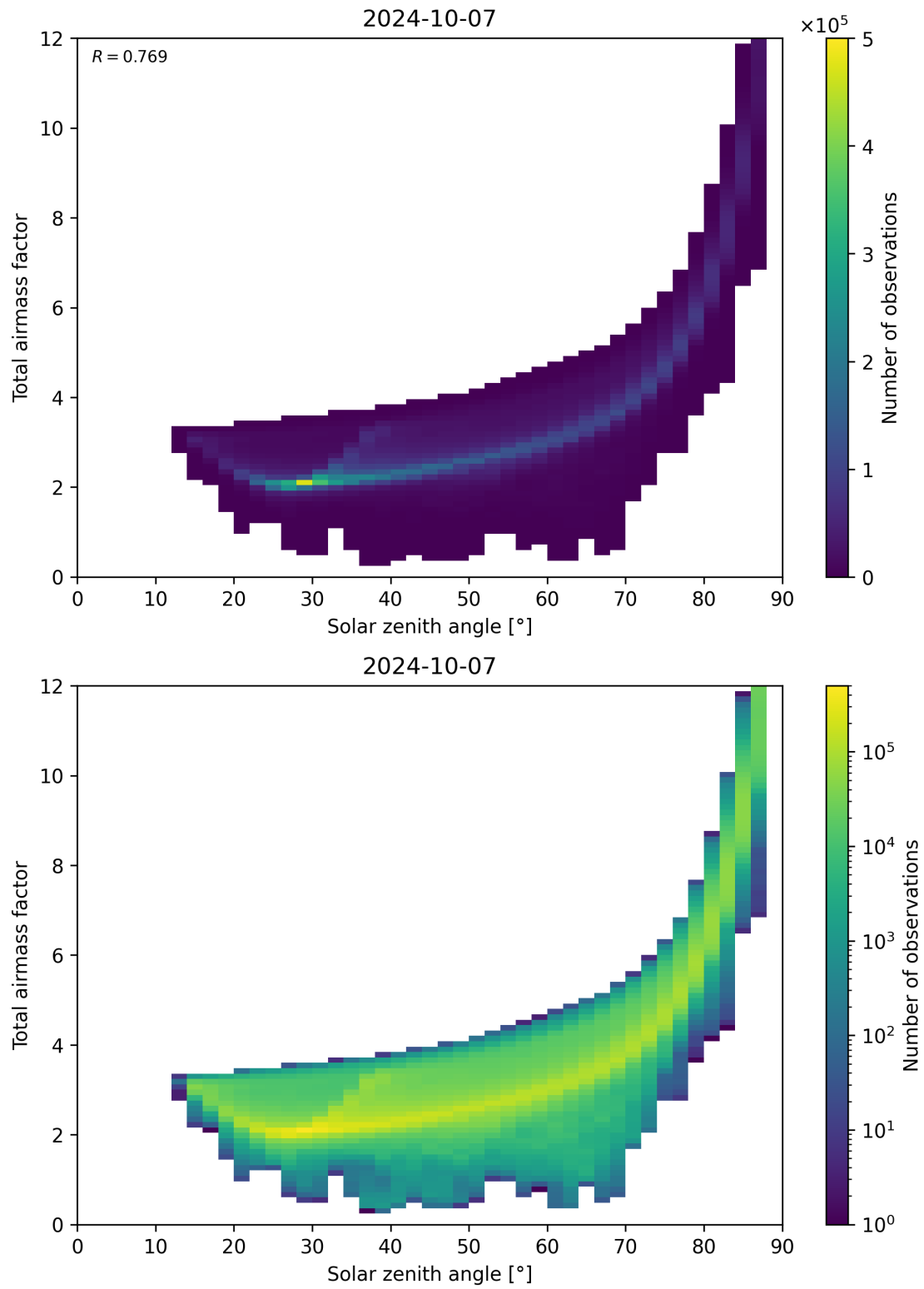
Figure 146: Scatter density plot of “Solar zenith angle” against “Total air mass factor” for 2024-10-06 to 2024-10-08.
