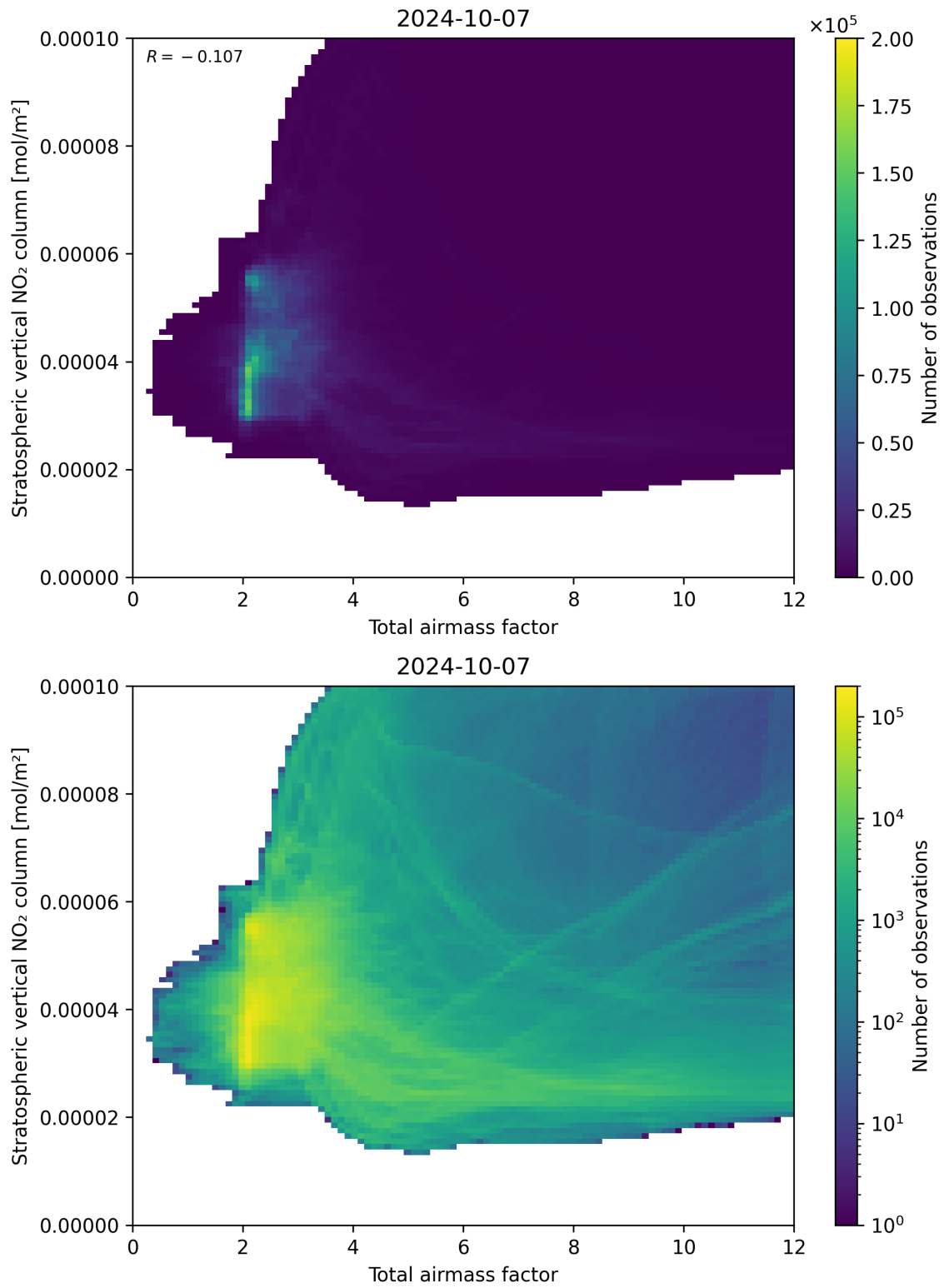
Figure 64: Scatter density plot of “Total airmass factor” against “Stratospheric vertical NO 2 column” for 2024-10-06 to 2024-10-08.
