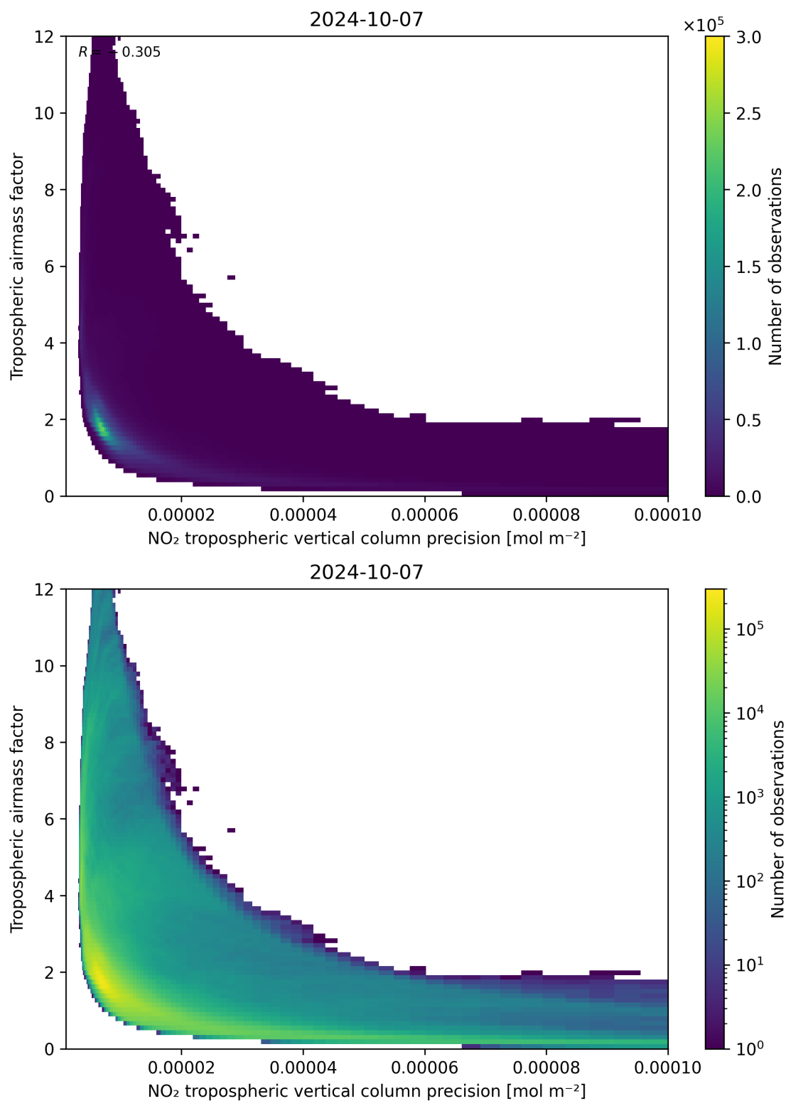
Figure 133: Scatter density plot of “NO 2 tropospheric vertical column precision” against “Tropospheric airmass factor” for 2024-10-06 to 2024-10-08.
