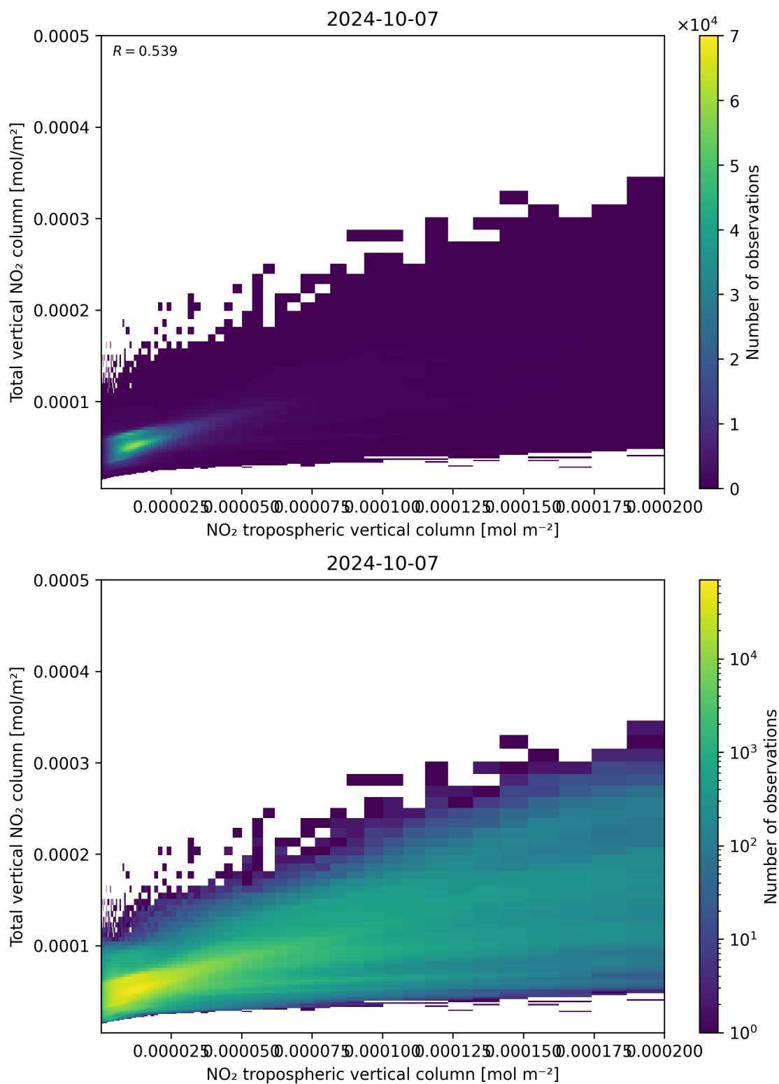
Figure 128: Scatter density plot of “NO 2 tropospheric vertical column” against “Total vertical NO 2 column” for 2024-10-06 to 2024-10-08.
