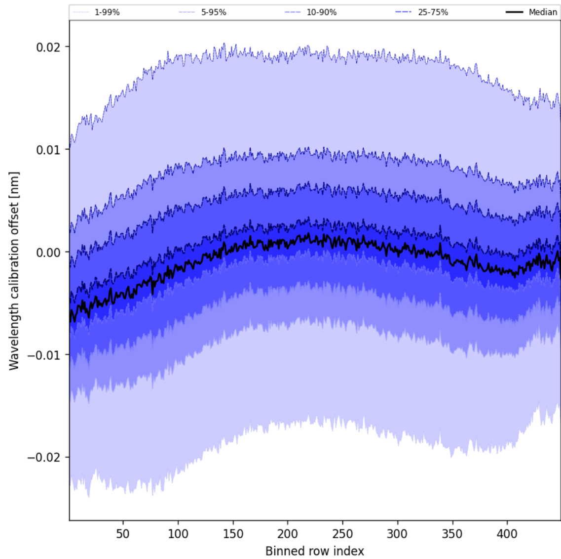
Figure 52: Along track statistics of “Wavelength calibration offset” for 2024-10-06 to 2024-10-08
