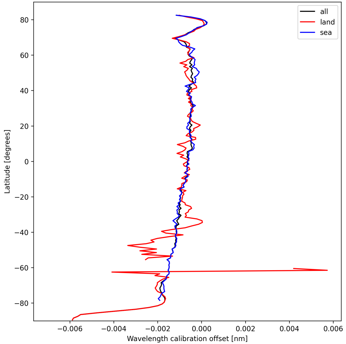
Figure 18: Zonal average of “Wavelength calibration offset” for 2024-10-06 to 2024-10-08.
