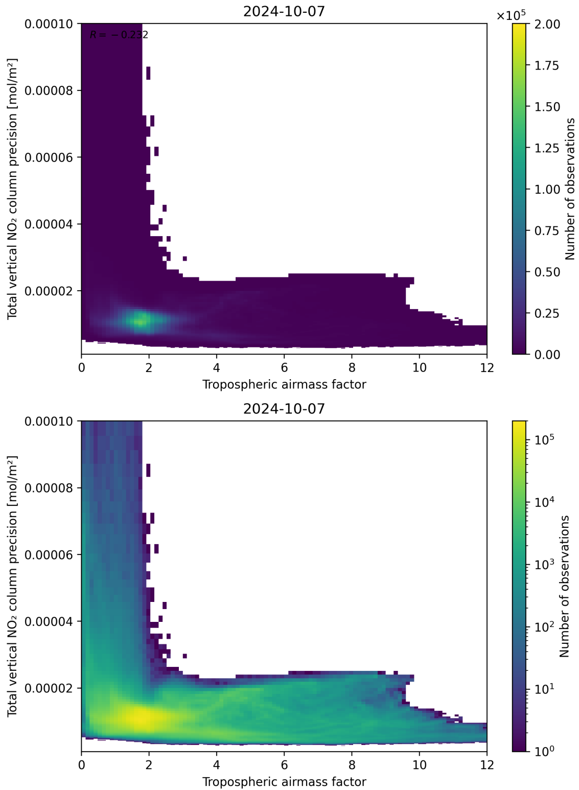
Figure 78: Scatter density plot of “Tropospheric air mass factor” against “Total vertical NO 2 column precision” for 2024-10-06 to 2024-10-08.
