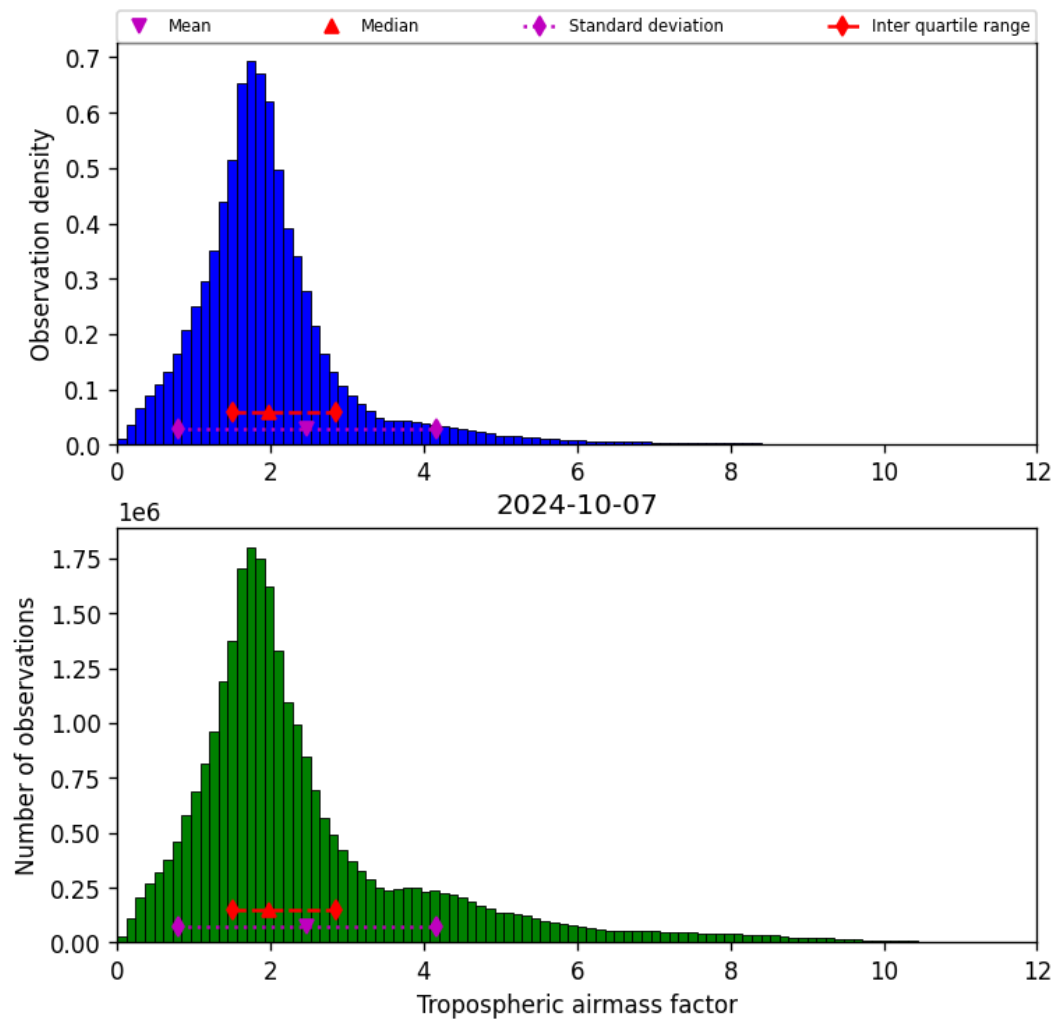
Figure 31: Histogram of “Tropospheric airmass factor” for 2024-10-06 to 2024-10-08
