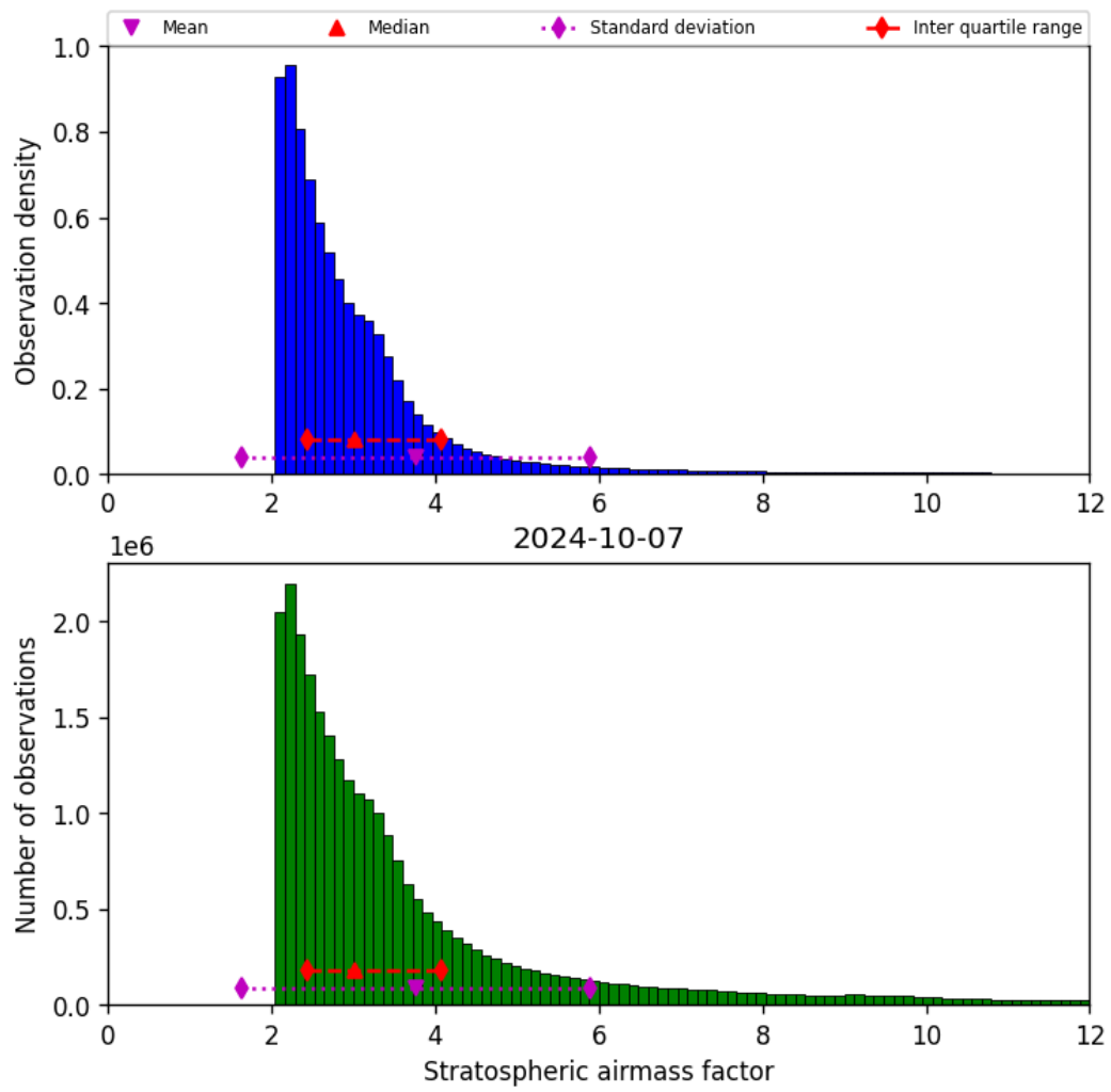
Figure 44: Histogram of “Stratospheric airmass factor” for 2024-10-06 to 2024-10-08
