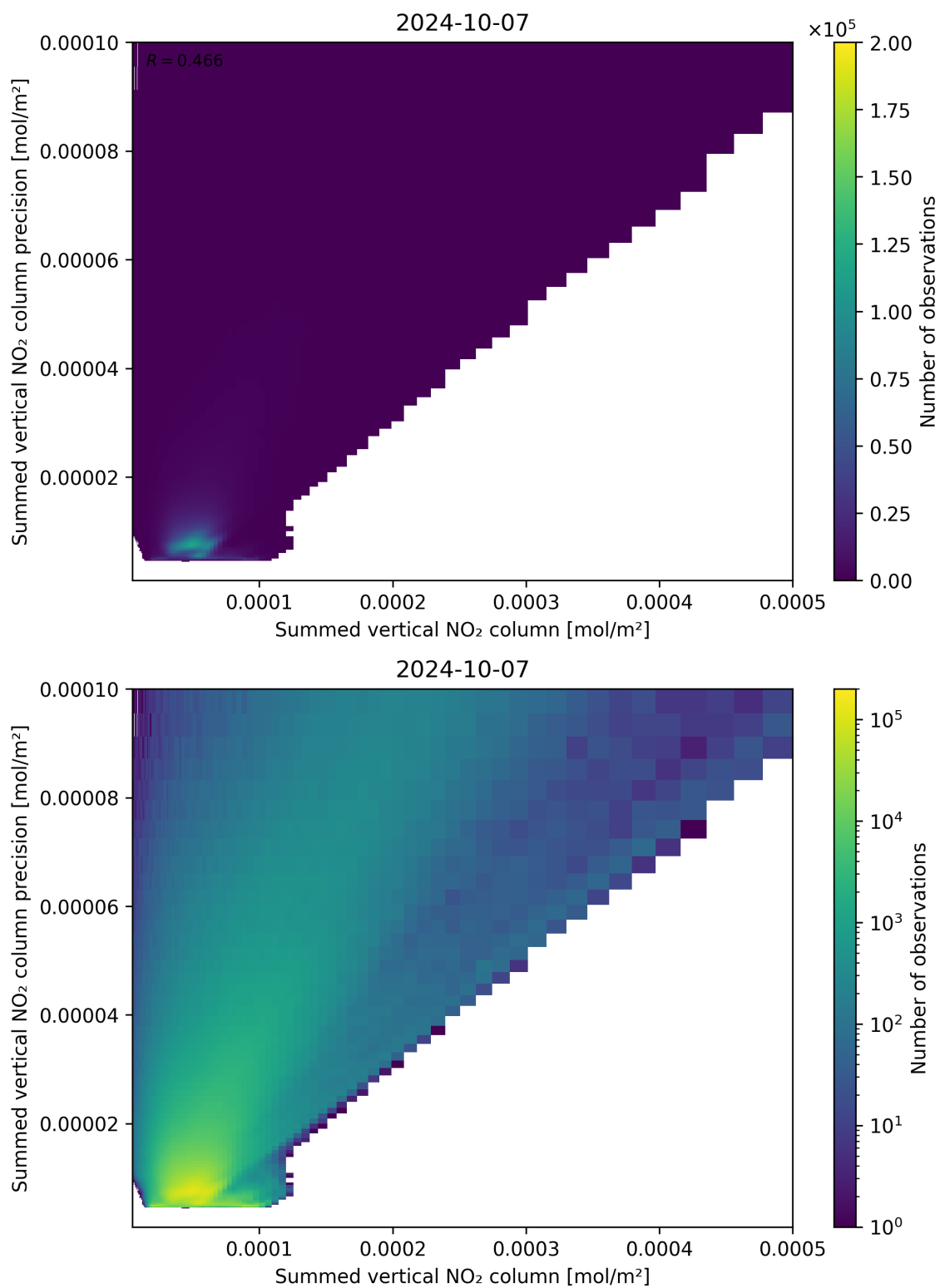
Figure 105: Scatter density plot of “Summed vertical NO 2 column” against “Summed vertical NO 2 column precision” for 2024-10-06 to 2024-10-08.
