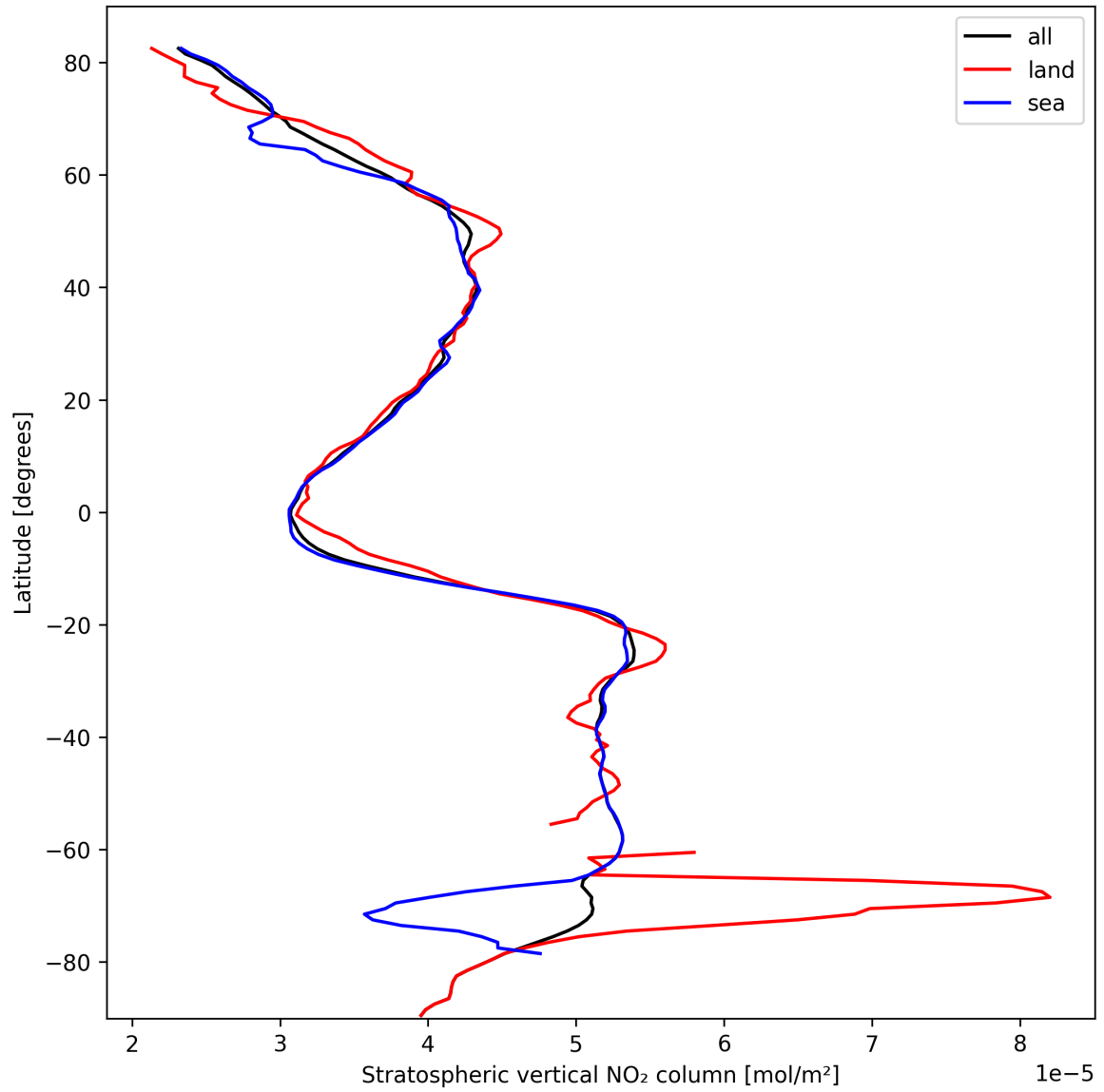
Figure 19: Zonal average of “Stratospheric vertical NO 2 column” for 2024-10-06 to 2024-10-08.
