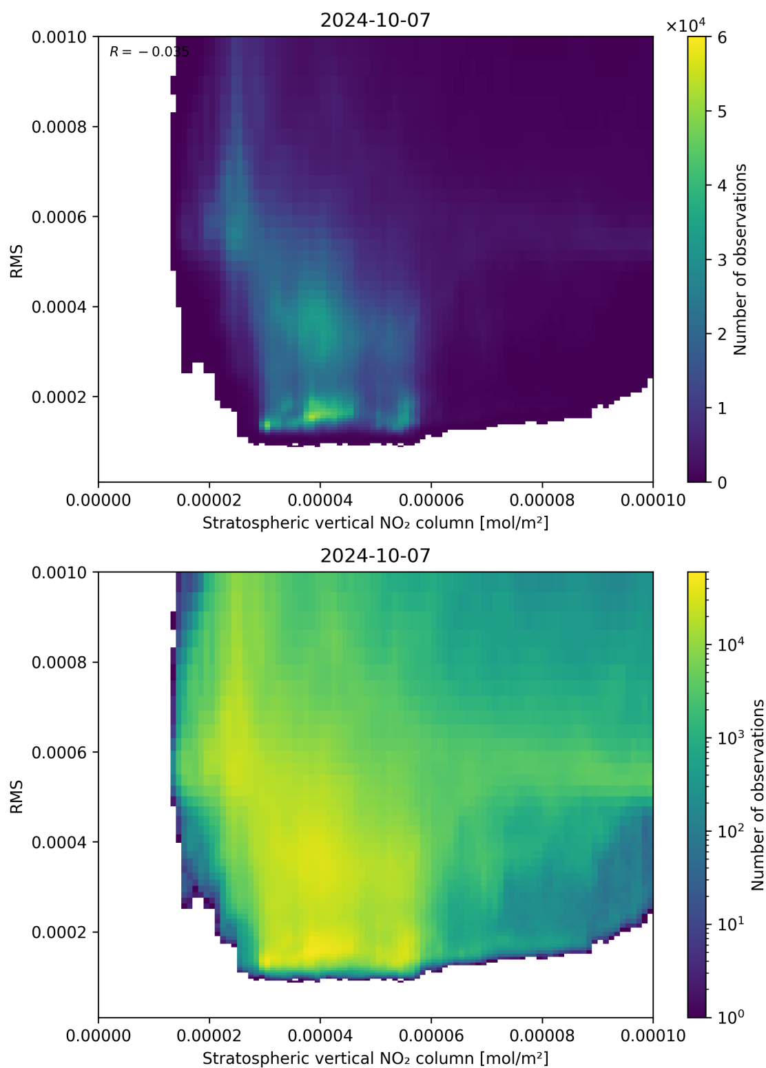
Figure 102: Scatter density plot of “Stratospheric vertical NO 2 column” against “RMS” for 2024-10-06 to 2024-10-08.
