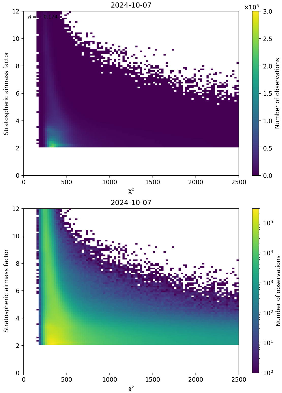
Figure 81: Scatter density plot of “ \chi^2 ” against “Stratospheric airmass factor” for 2024-10-06 to 2024-10-08.
