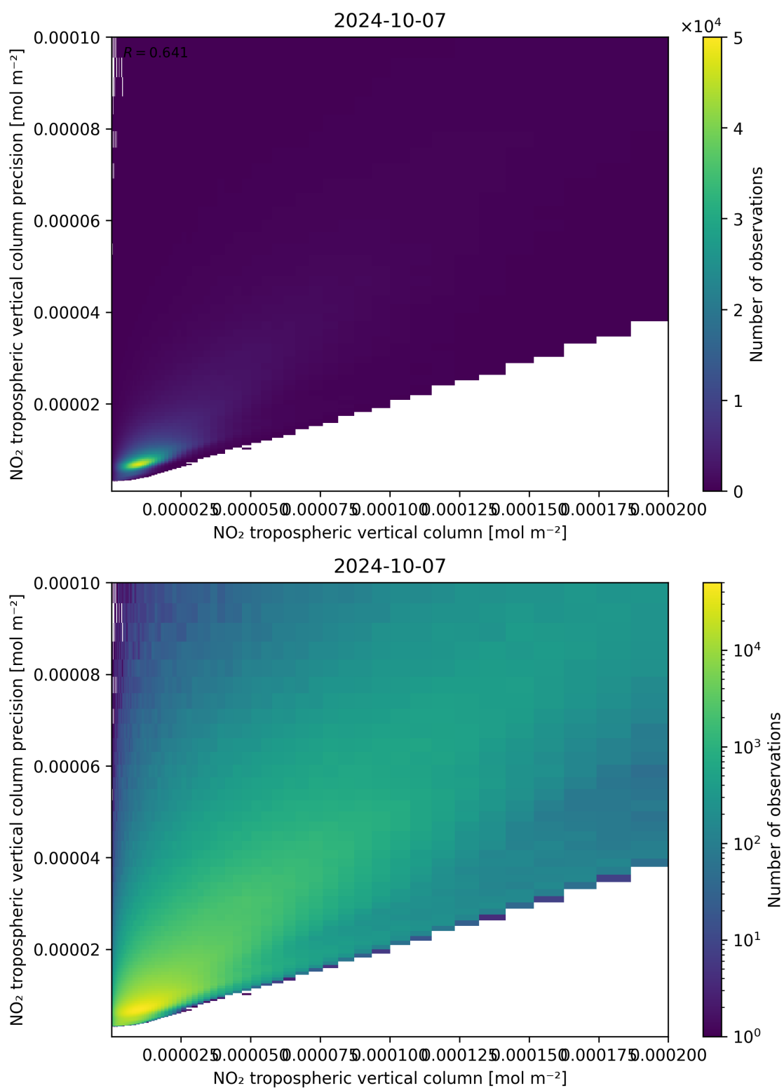
Figure 130: Scatter density plot of “NO 2 tropospheric vertical column” against “NO 2 tropospheric vertical column precision” for 2024-10-06 to 2024-10-08.
