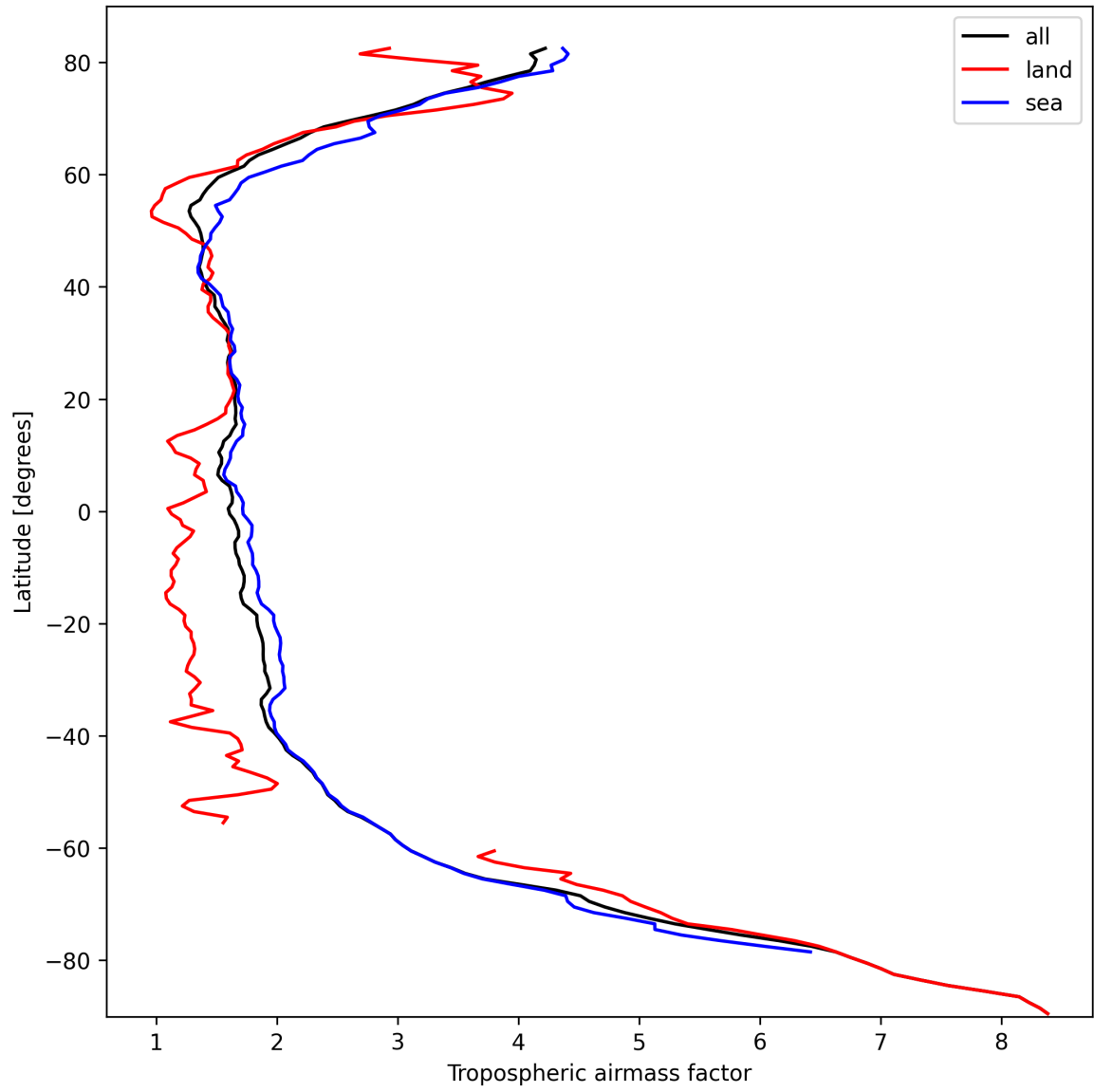
Figure 14: Zonal average of “Tropospheric airmass factor” for 2024-10-06 to 2024-10-08.
