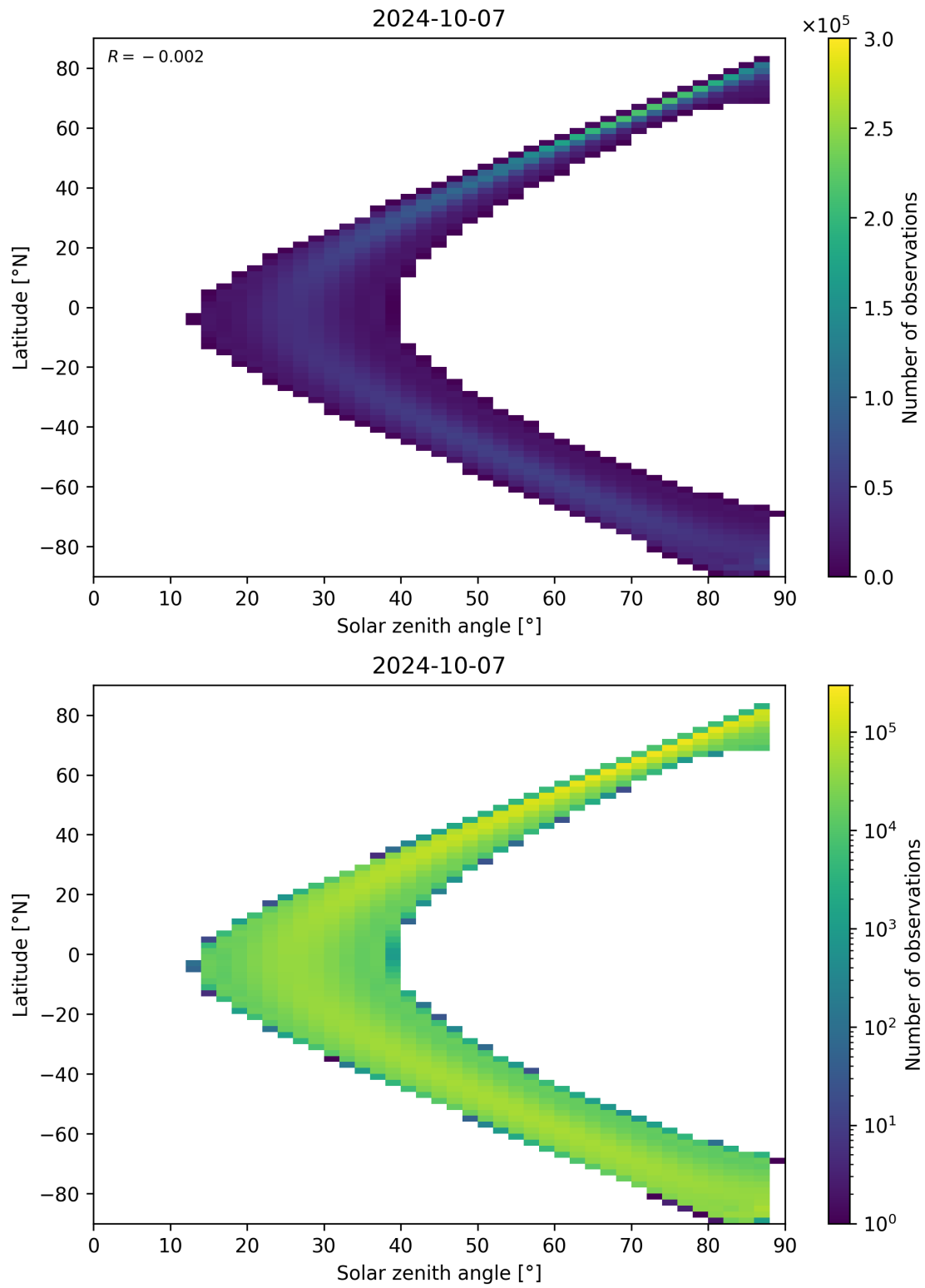
Figure 149: Scatter density plot of “Solar zenith angle” against “Latitude” for 2024-10-06 to 2024-10-08.
