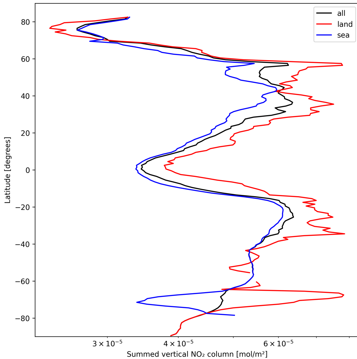
Figure 23: Zonal average of “Summed vertical NO 2 column” for 2024-10-06 to 2024-10-08.
