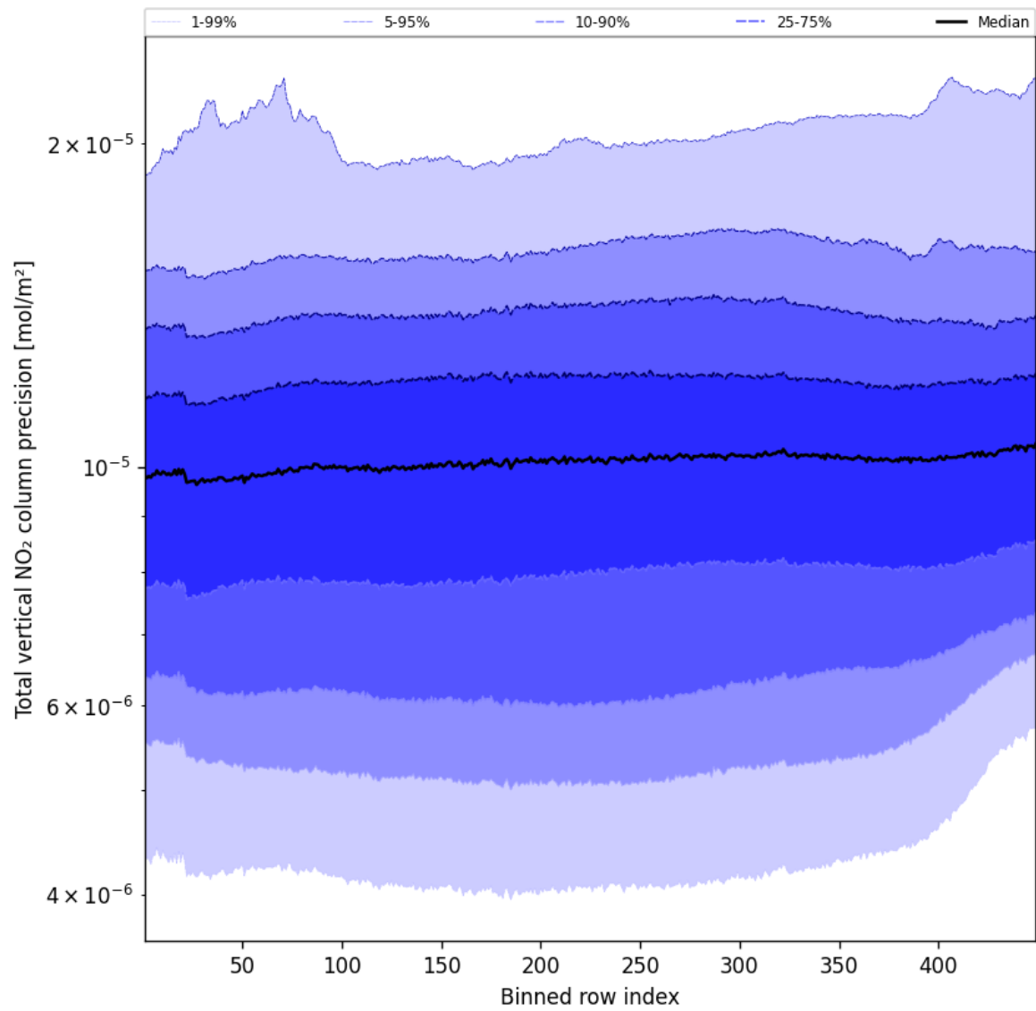
Figure 56: Along track statistics of “Total vertical NO 2 column precision” for 2024-10-06 to 2024-10-08
