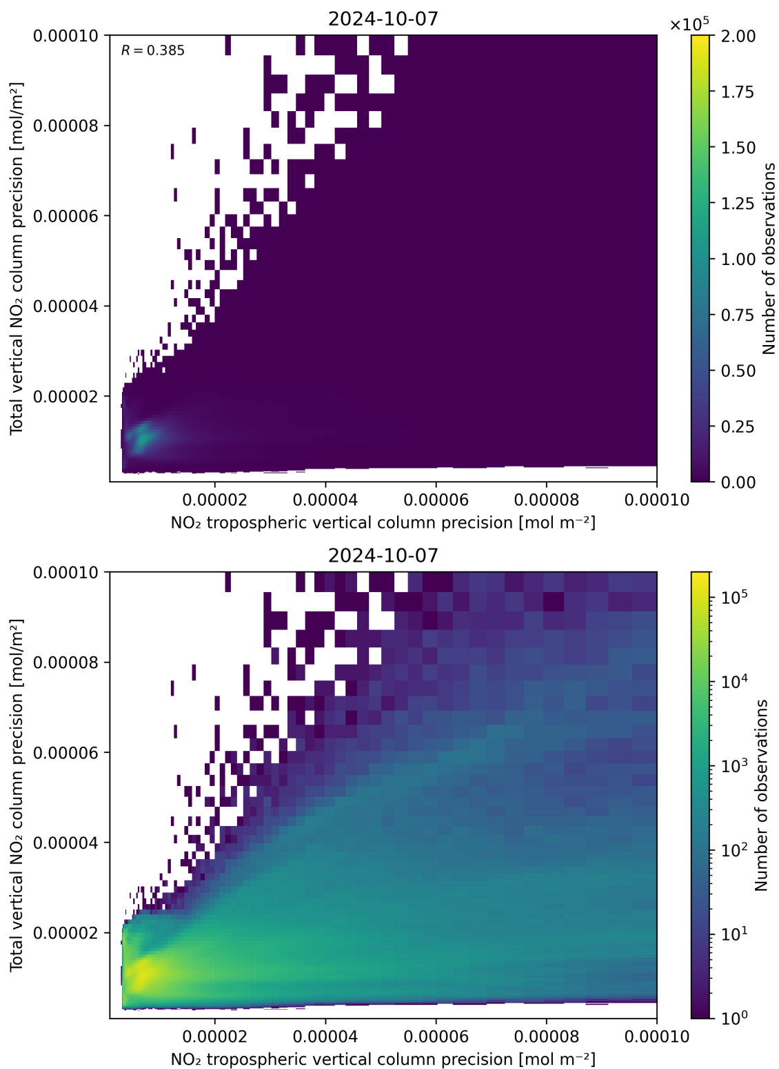
Figure 139: Scatter density plot of “NO 2 tropospheric vertical column precision” against “Total vertical NO 2 column precision” for 2024-10-06 to 2024-10-08.
