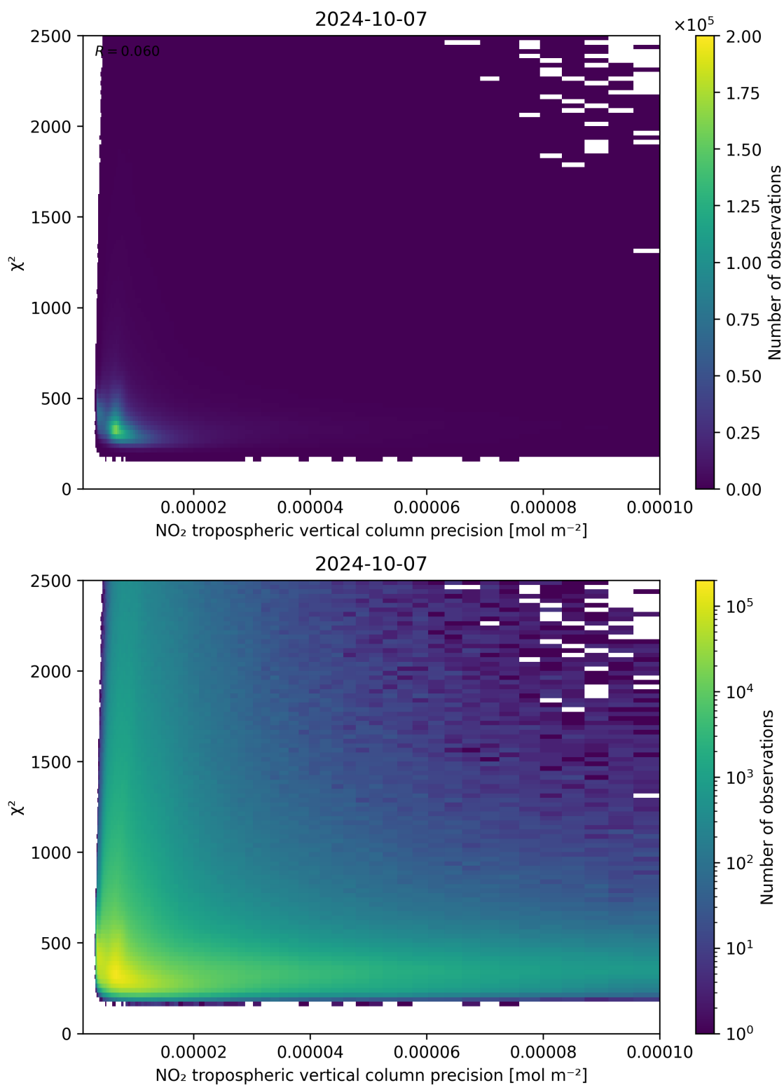
Figure 134: Scatter density plot of “NO 2 tropospheric vertical column precision” against “ \chi^2 ” for 2024-10-06 to 2024-10-08.
