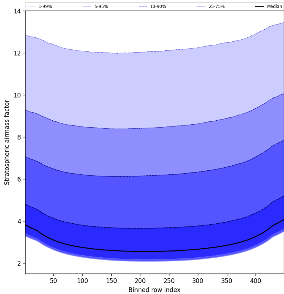
Figure 61: Along track statistics of “Stratospheric airmass factor” for 2024-10-06 to 2024-10-08
