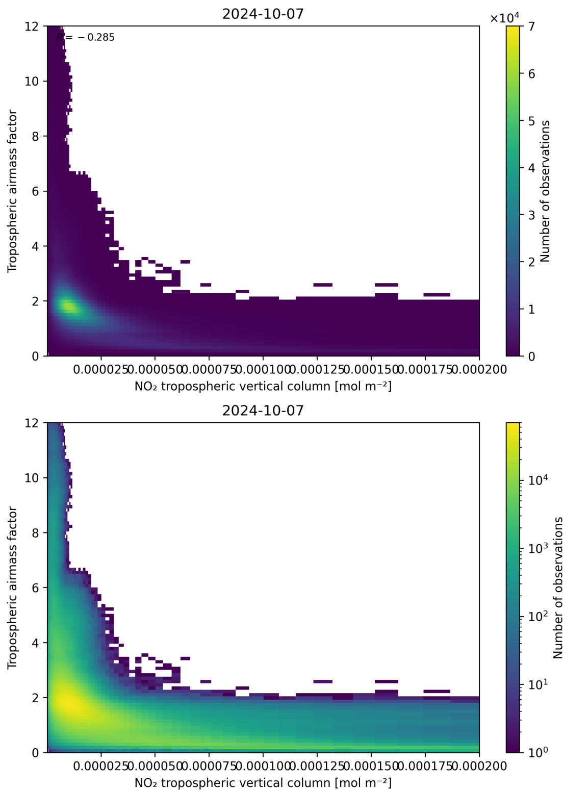
Figure 123: Scatter density plot of “NO 2 tropospheric vertical column” against “Tropospheric air mass factor” for 2024-10-06 to 2024-10-08.
