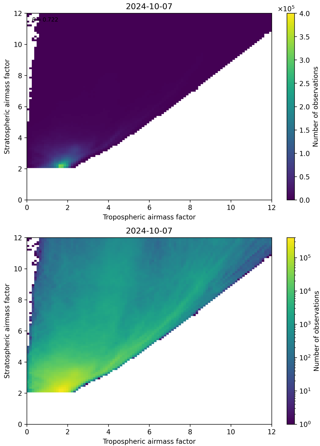
Figure 71: Scatter density plot of “Tropospheric airmass factor” against “Stratospheric airmass factor” for 2024-10-06 to 2024-10-08.
