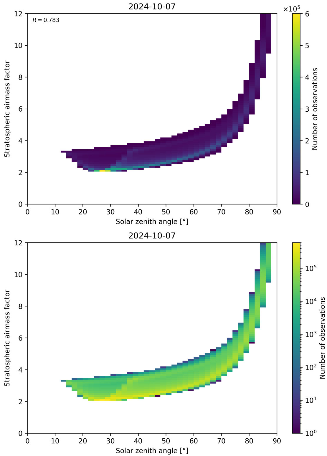
Figure 145: Scatter density plot of “Solar zenith angle” against “Stratospheric airmass factor” for 2024-10-06 to 2024-10-08.
