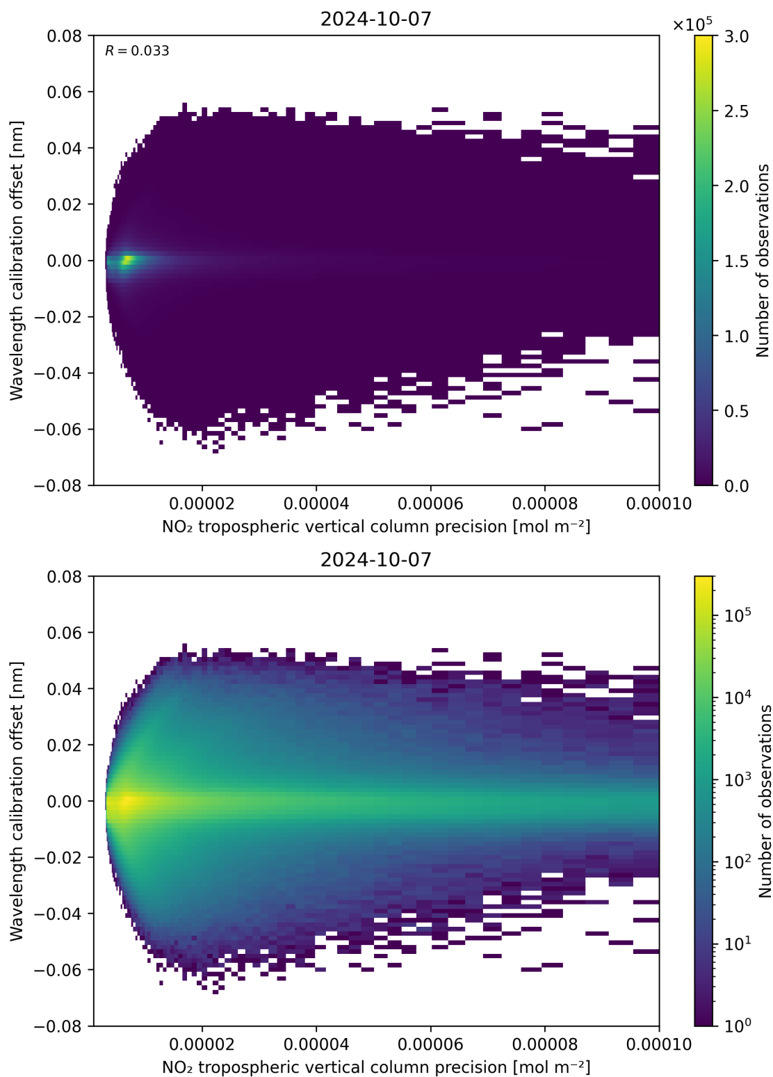
Figure 141: Scatter density plot of “NO 2 tropospheric vertical column precision” against “Wavelength calibration offset” for 2024-10-06 to 2024-10-08.
