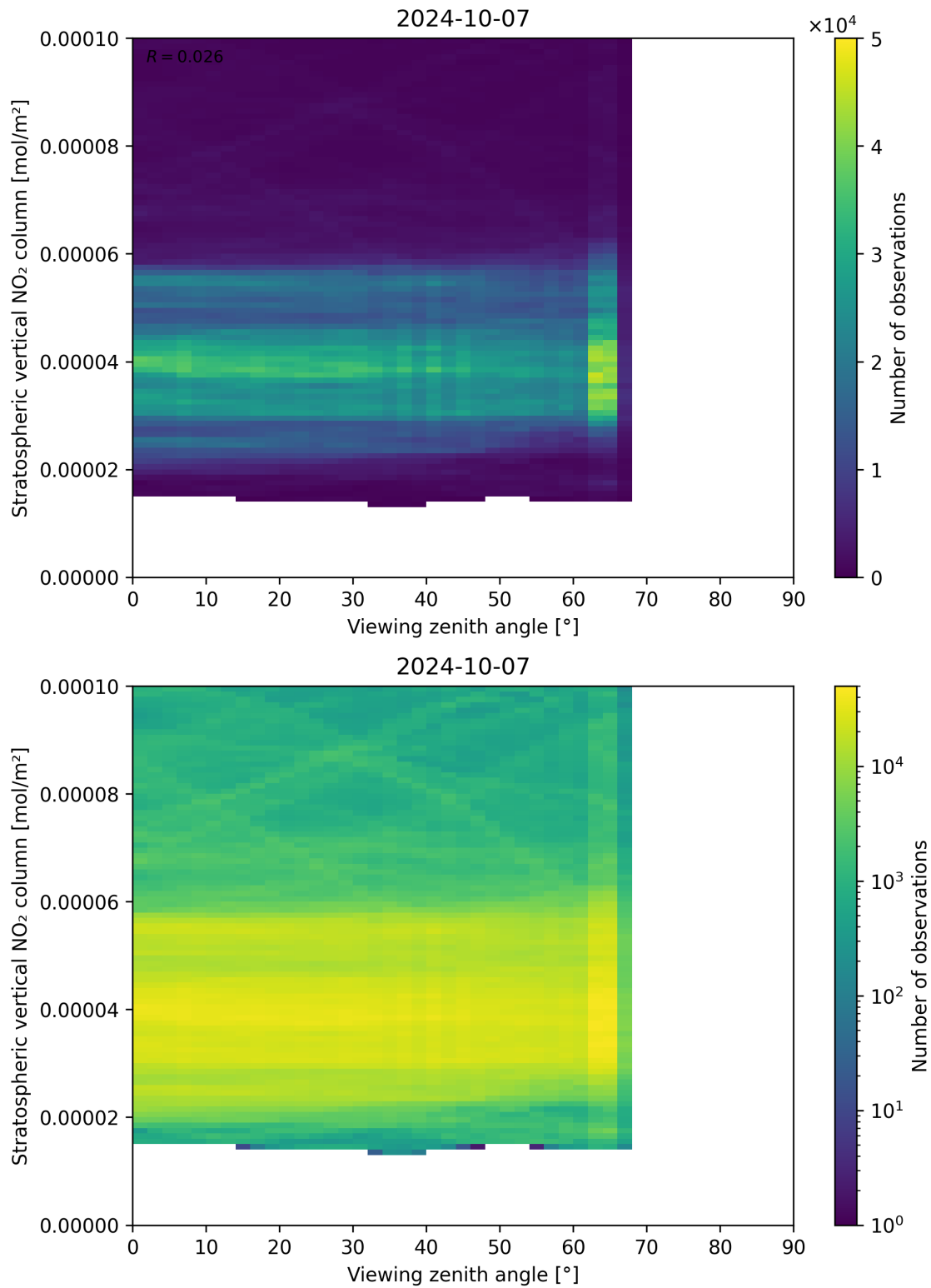
Figure 164: Scatter density plot of “Viewing zenith angle” against “Stratospheric vertical NO 2 column” for 2024-10-06 to 2024-10-08.
