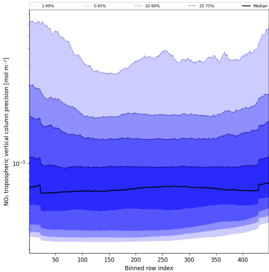
Figure 47: Along track statistics of “NO 2 tropospheric vertical column precision” for 2024-10-06 to 2024-10-08
