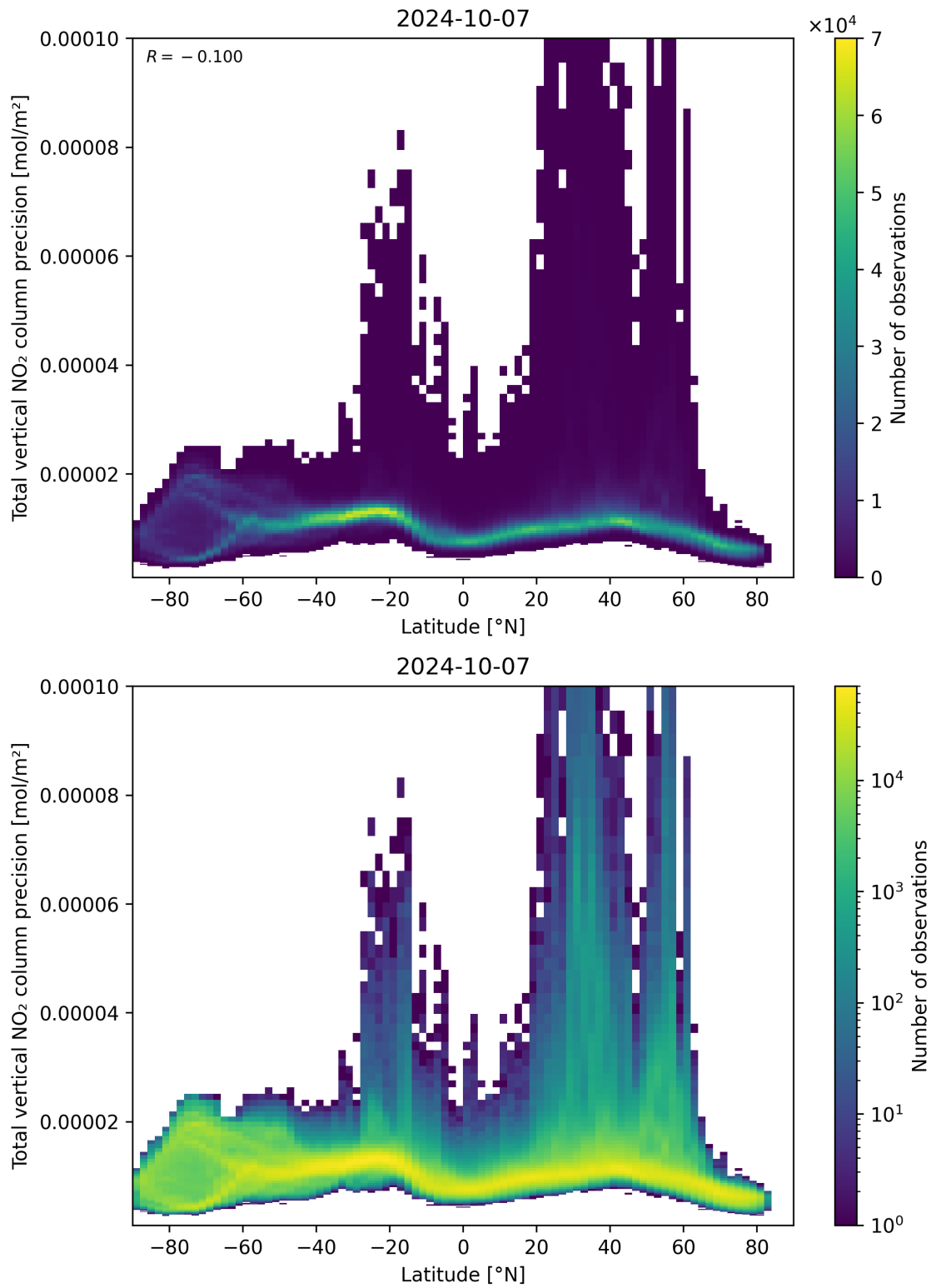
Figure 91: Scatter density plot of “Latitude” against “Total vertical NO 2 column precision” for 2024-10-06 to 2024-10-08.
