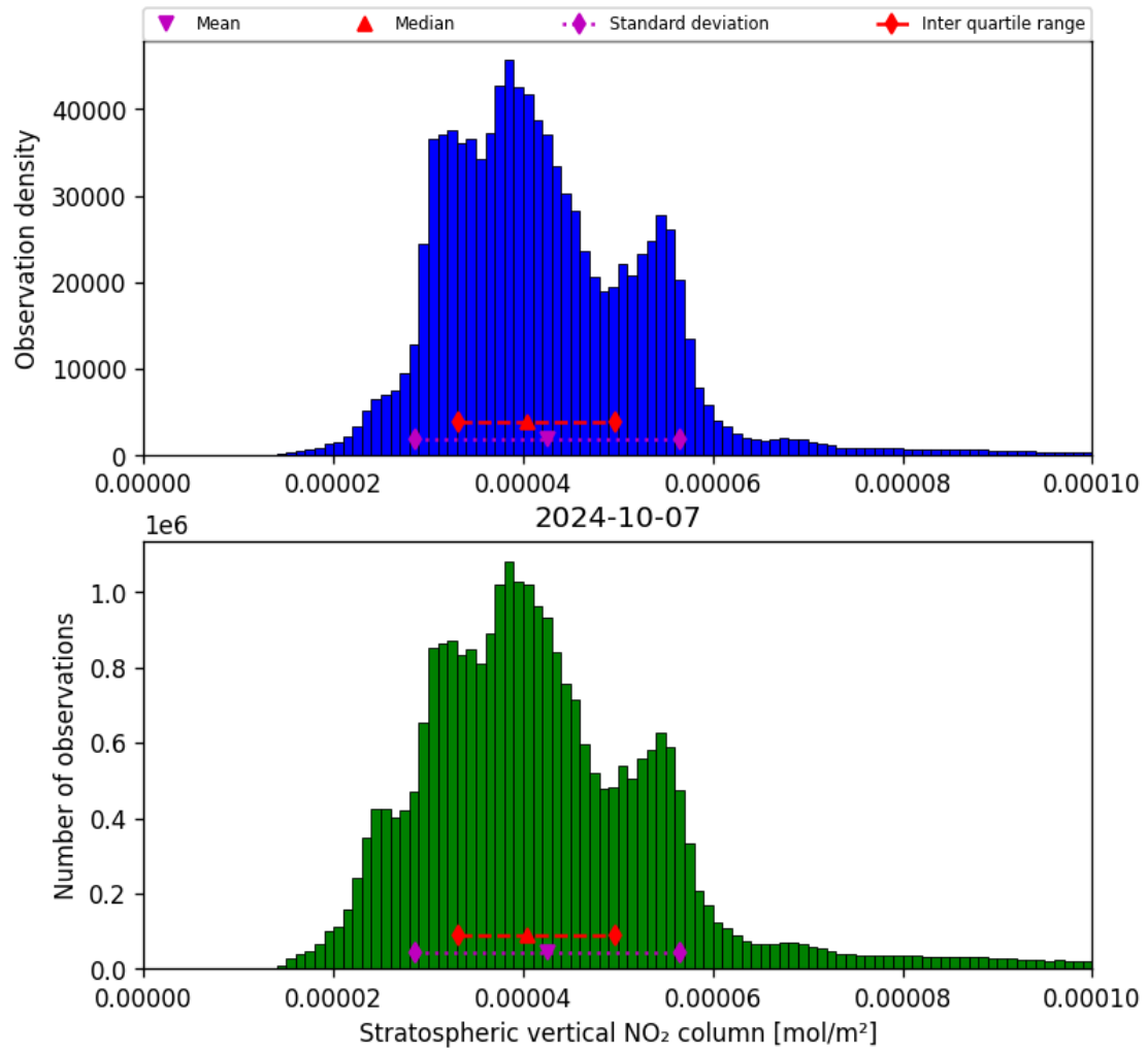
Figure 36: Histogram of “Stratospheric vertical NO 2 column” for 2024-10-06 to 2024-10-08
