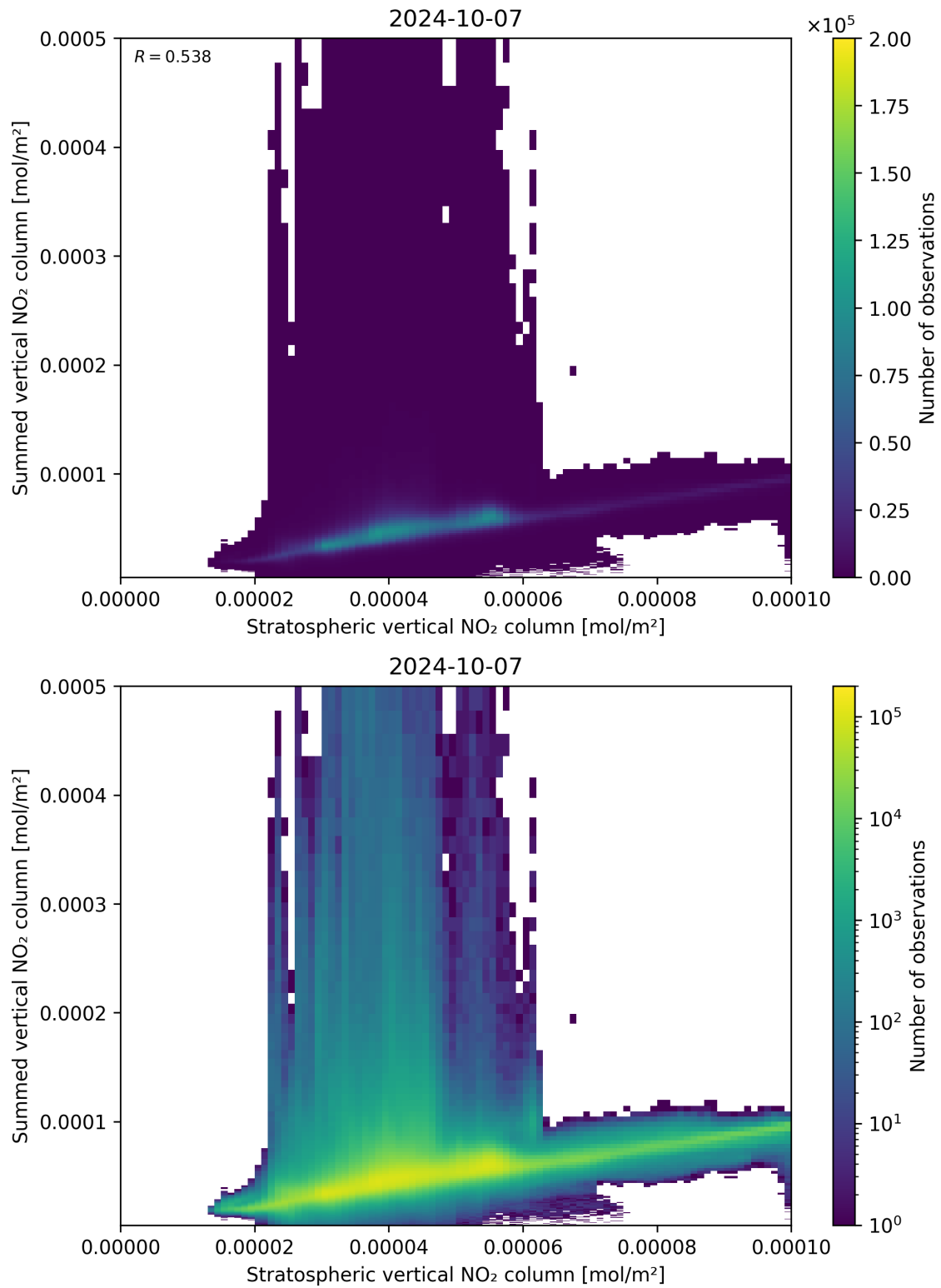
Figure 98: Scatter density plot of “Stratospheric vertical NO 2 column” against “Summed vertical NO 2 column” for 2024-10-06 to 2024-10-08.
