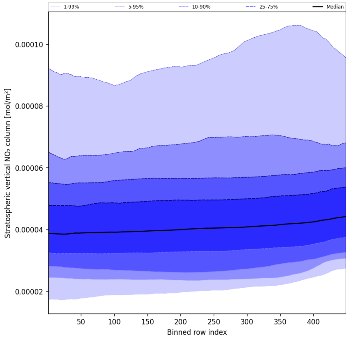
Figure 53: Along track statistics of “Stratospheric vertical NO 2 column” for 2024-10-06 to 2024-10-08
