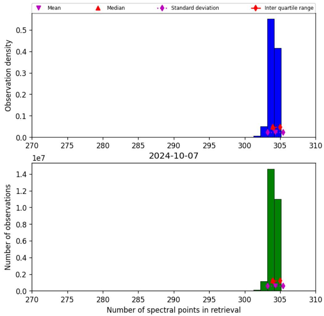
Figure 33: Histogram of “Number of spectral points in retrieval” for 2024-10-06 to 2024-10-08
