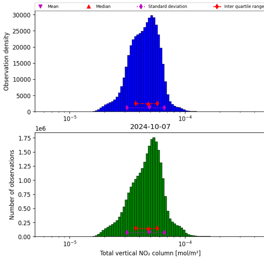
Figure 38: Histogram of “Total vertical NO 2 column” for 2024-10-06 to 2024-10-08
