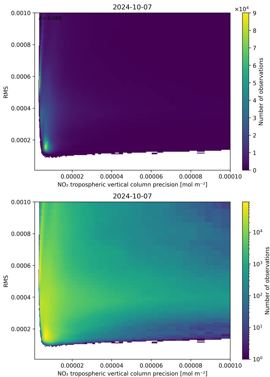
Figure 140: Scatter density plot of “NO 2 tropospheric vertical column precision” against “RMS” for 2024-10-06 to 2024-10-08.
