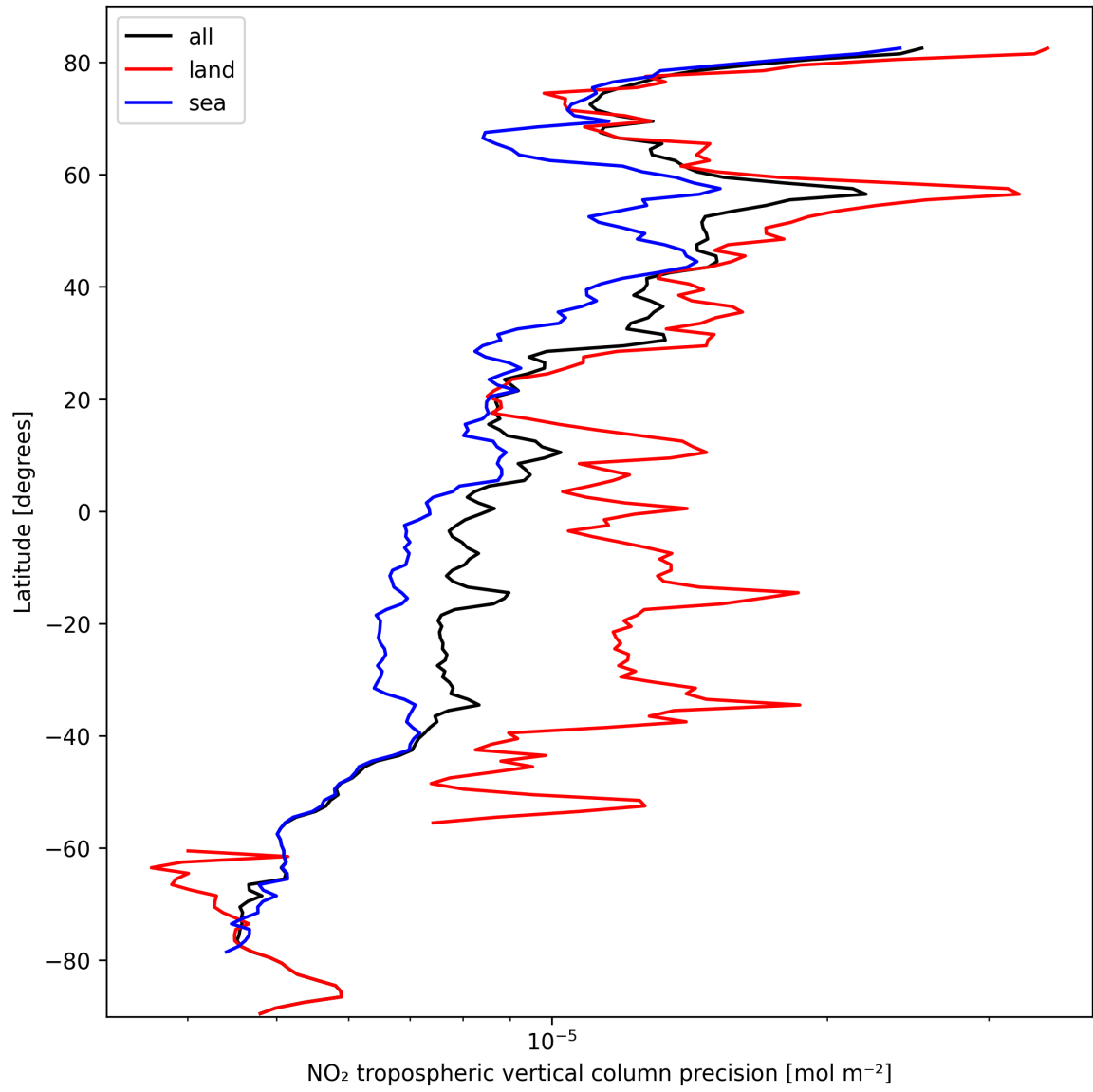
Figure 13: Zonal average of “NO 2 tropospheric vertical column precision” for 2024-10-06 to 2024-10-08.
