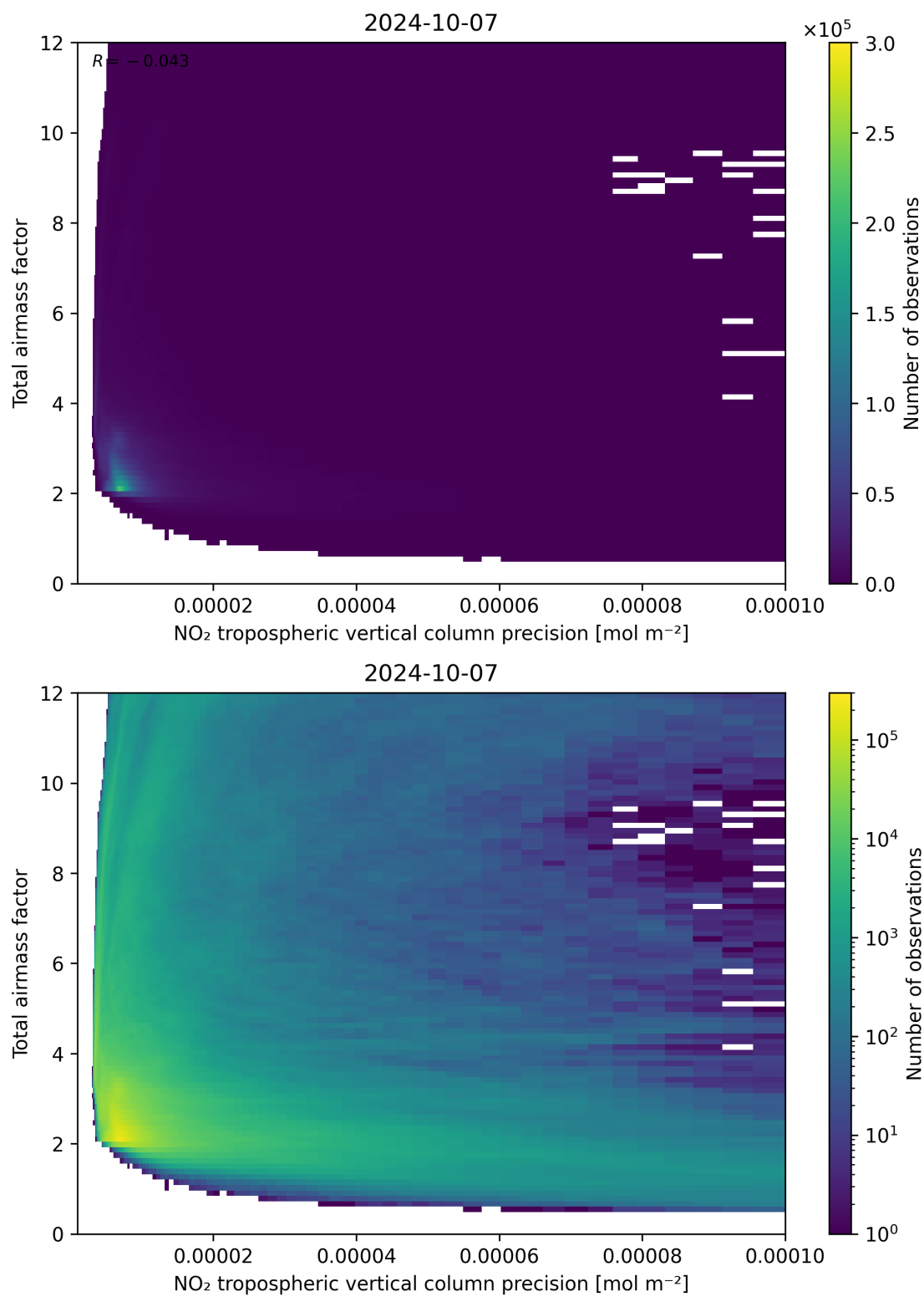
Figure 132: Scatter density plot of “NO 2 tropospheric vertical column precision” against “Total air mass factor” for 2024-10-06 to 2024-10-08.
