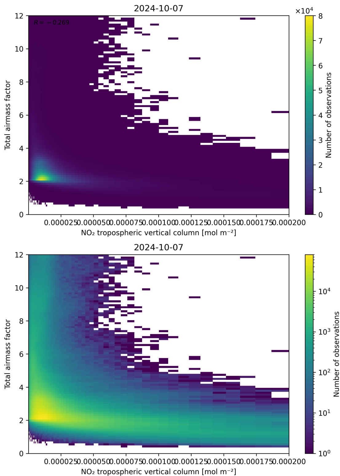
Figure 122: Scatter density plot of “NO 2 tropospheric vertical column” against “Total air mass factor” for 2024-10-06 to 2024-10-08.
