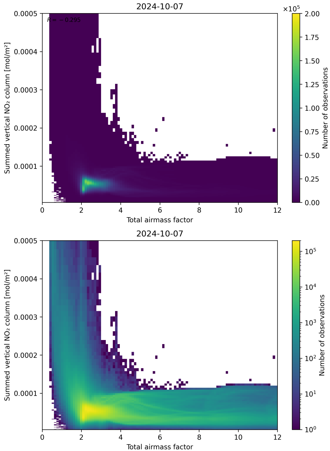
Figure 65: Scatter density plot of “Total airmass factor” against “Summed vertical NO 2 column” for 2024-10-06 to 2024-10-08.
