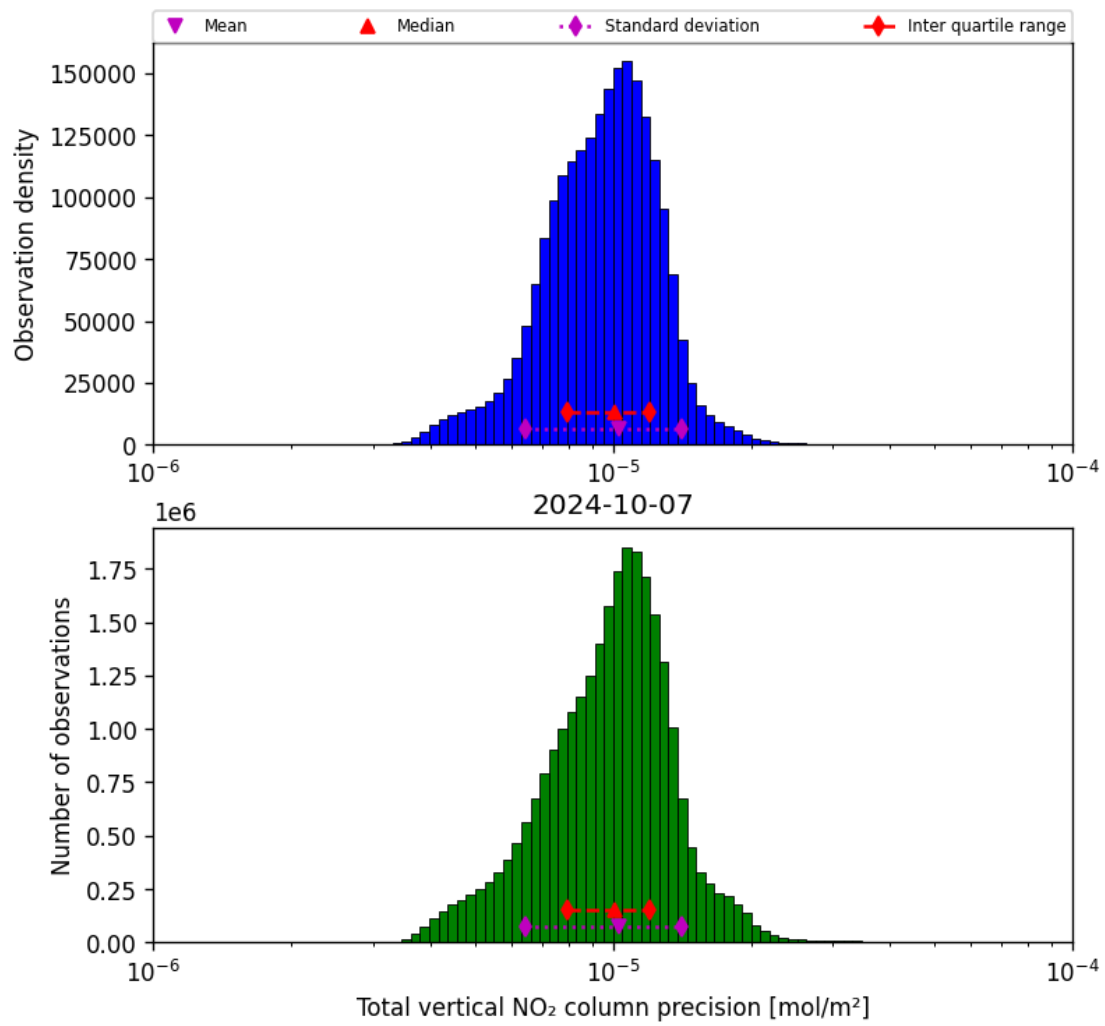
Figure 39: Histogram of "Total vertical NO 2 column precision" for 2024-10-06 to 2024-10-08
