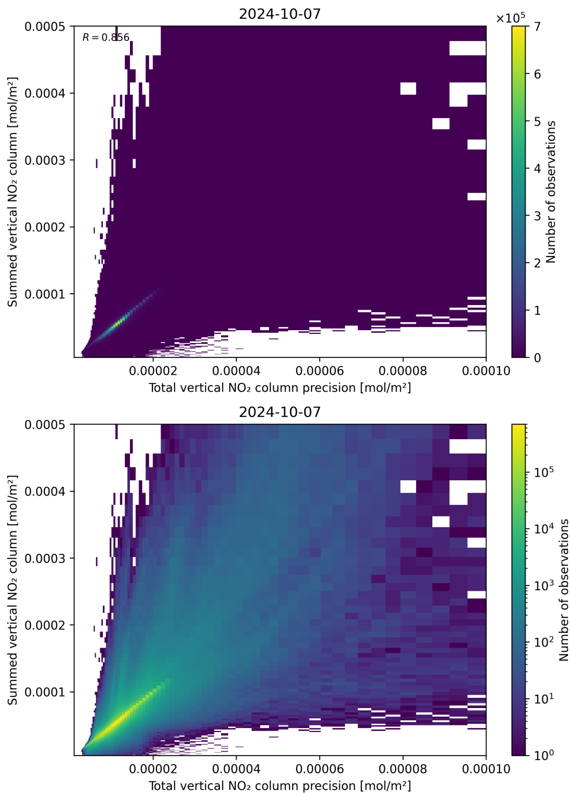
Figure 117: Scatter density plot of “Total vertical NO 2 column precision” against “Summed vertical NO 2 column” for 2024-10-06 to 2024-10-08.
