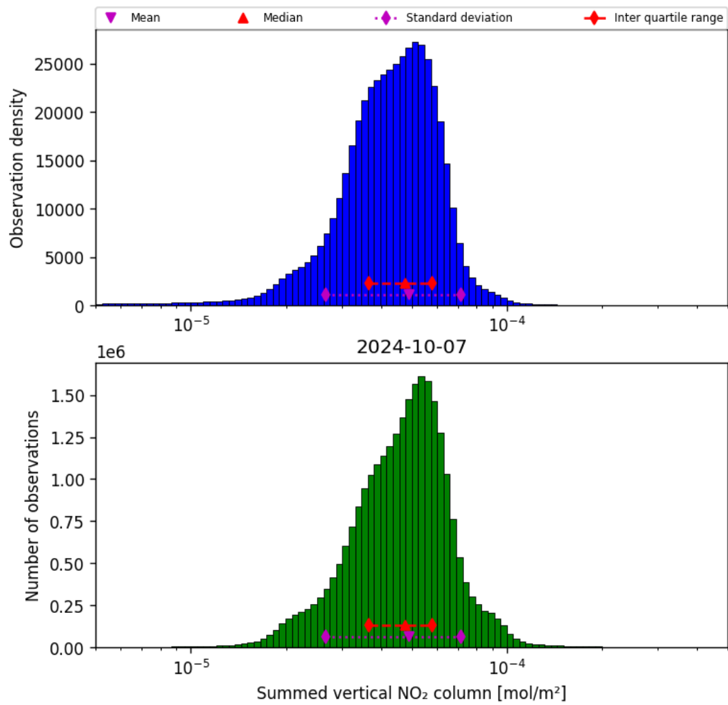
Figure 40: Histogram of “Summed vertical NO 2 column” for 2024-10-06 to 2024-10-08
