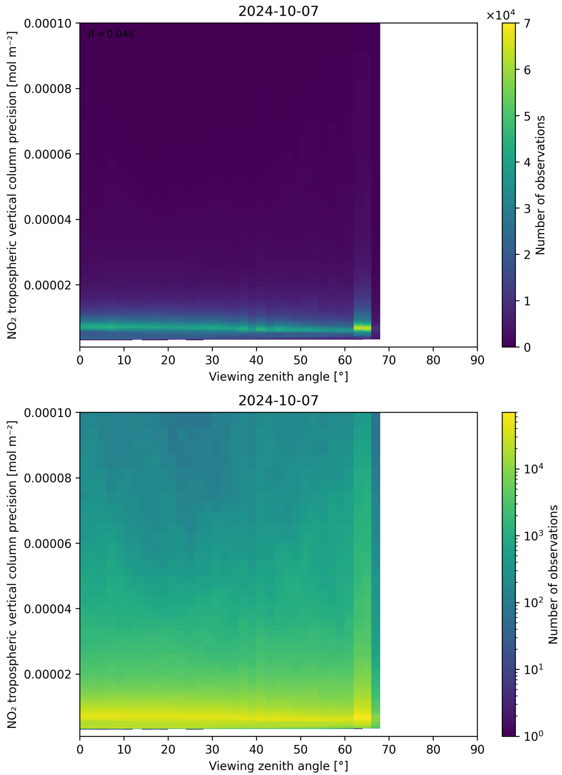
Figure 170: Scatter density plot of “Viewing zenith angle” against “NO 2 tropospheric vertical column precision” for 2024-10-06 to 2024-10-08.
