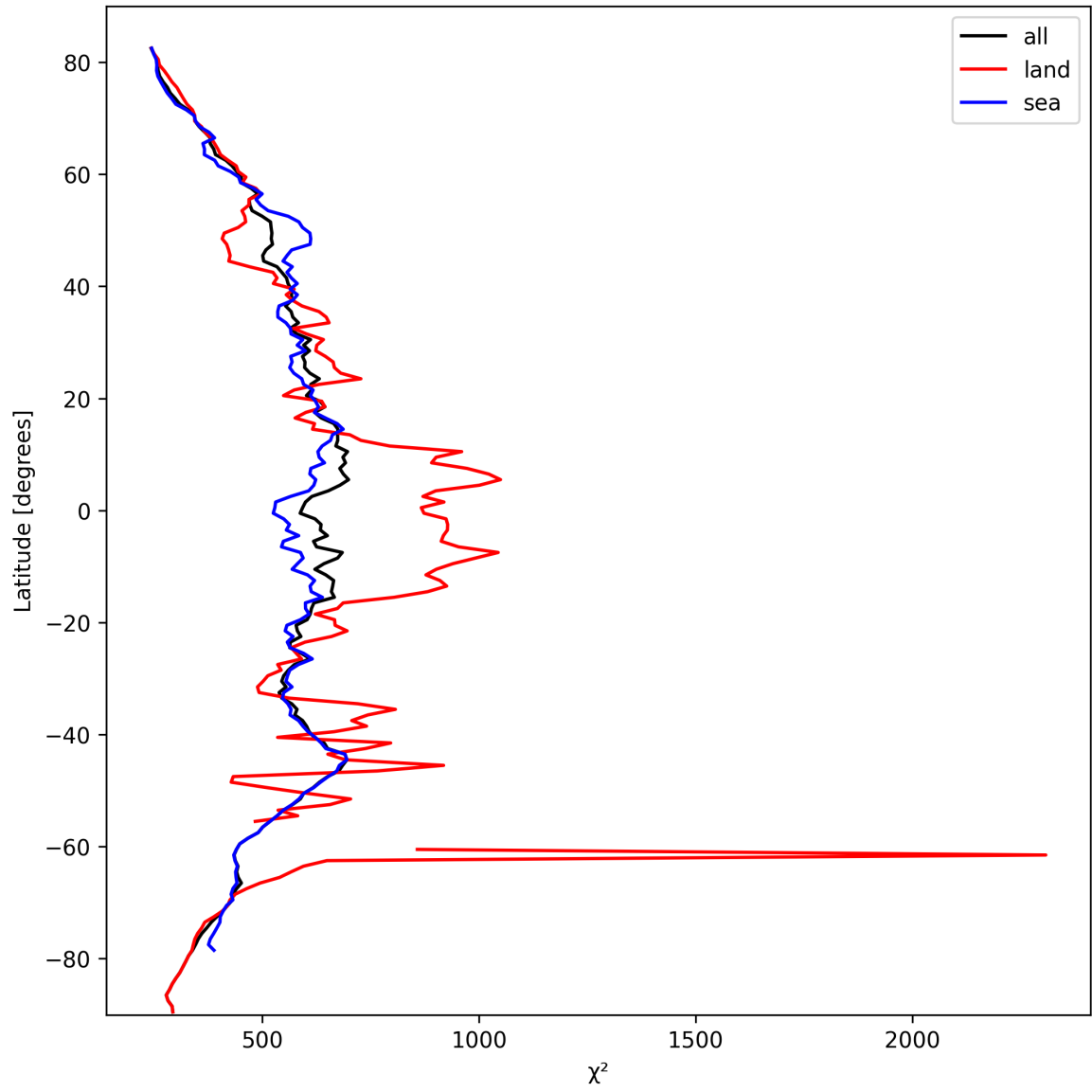
Figure 25: Zonal average of “ \chi^2 ” for 2024-10-06 to 2024-10-08.
