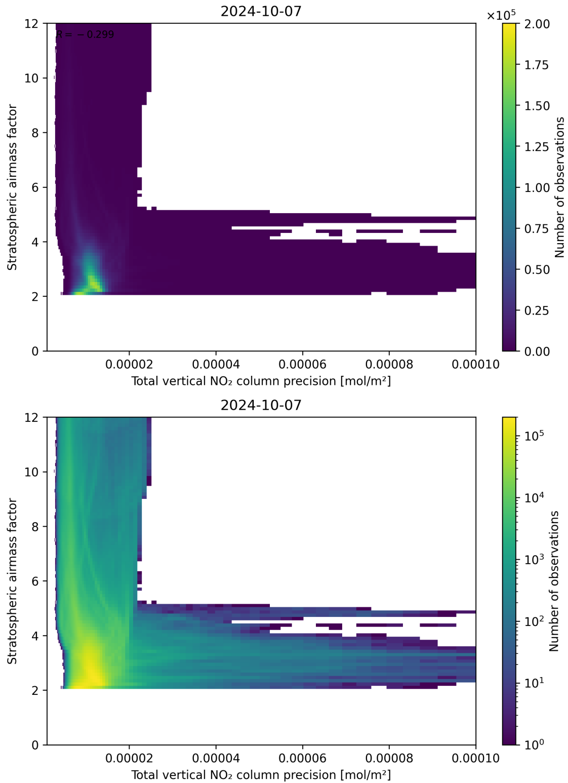
Figure 115: Scatter density plot of “Total vertical NO 2 column precision” against “Stratospheric air mass factor” for 2024-10-06 to 2024-10-08.
