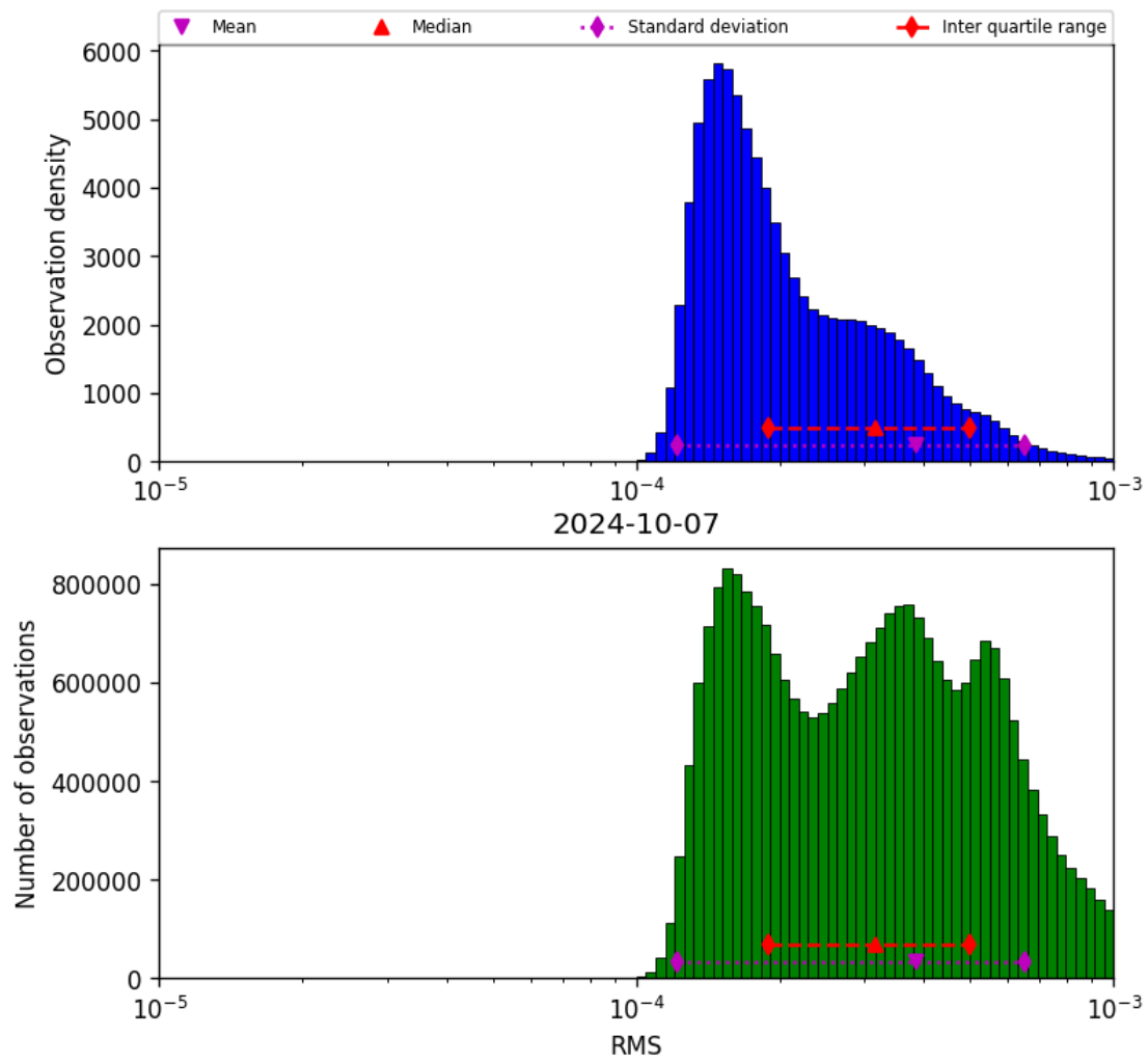
Figure 43: Histogram of “RMS” for 2024-10-06 to 2024-10-08
