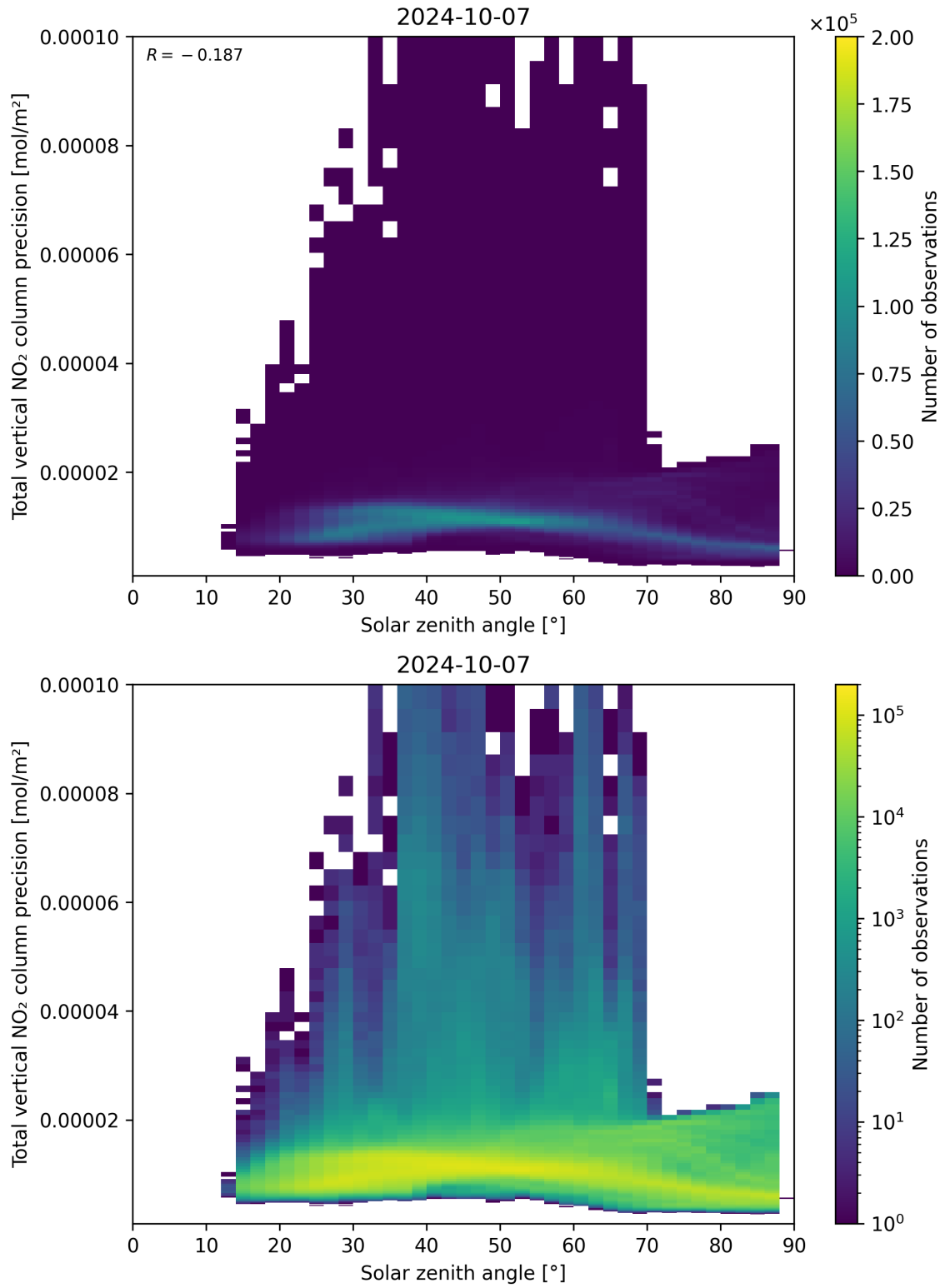
Figure 154: Scatter density plot of “Solar zenith angle” against “Total vertical NO 2 column precision” for 2024-10-06 to 2024-10-08.
