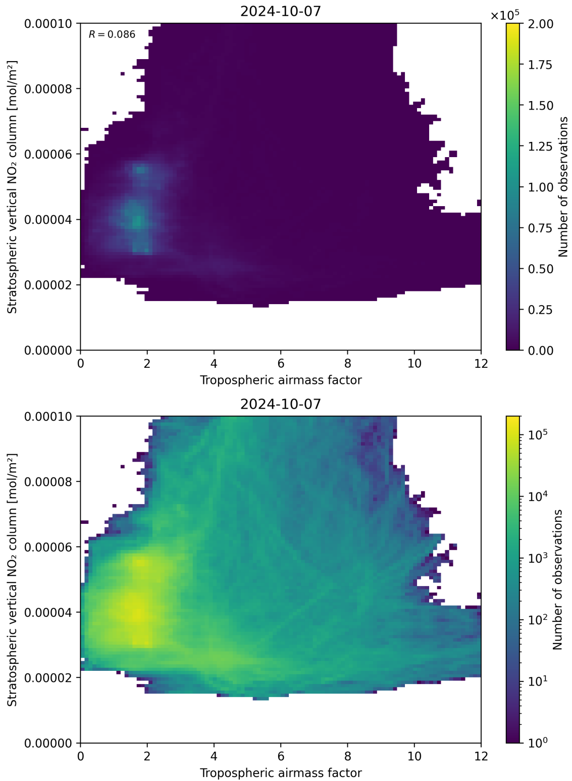
Figure 74: Scatter density plot of “Tropospheric air mass factor” against “Stratospheric vertical NO 2 column” for 2024-10-06 to 2024-10-08.
