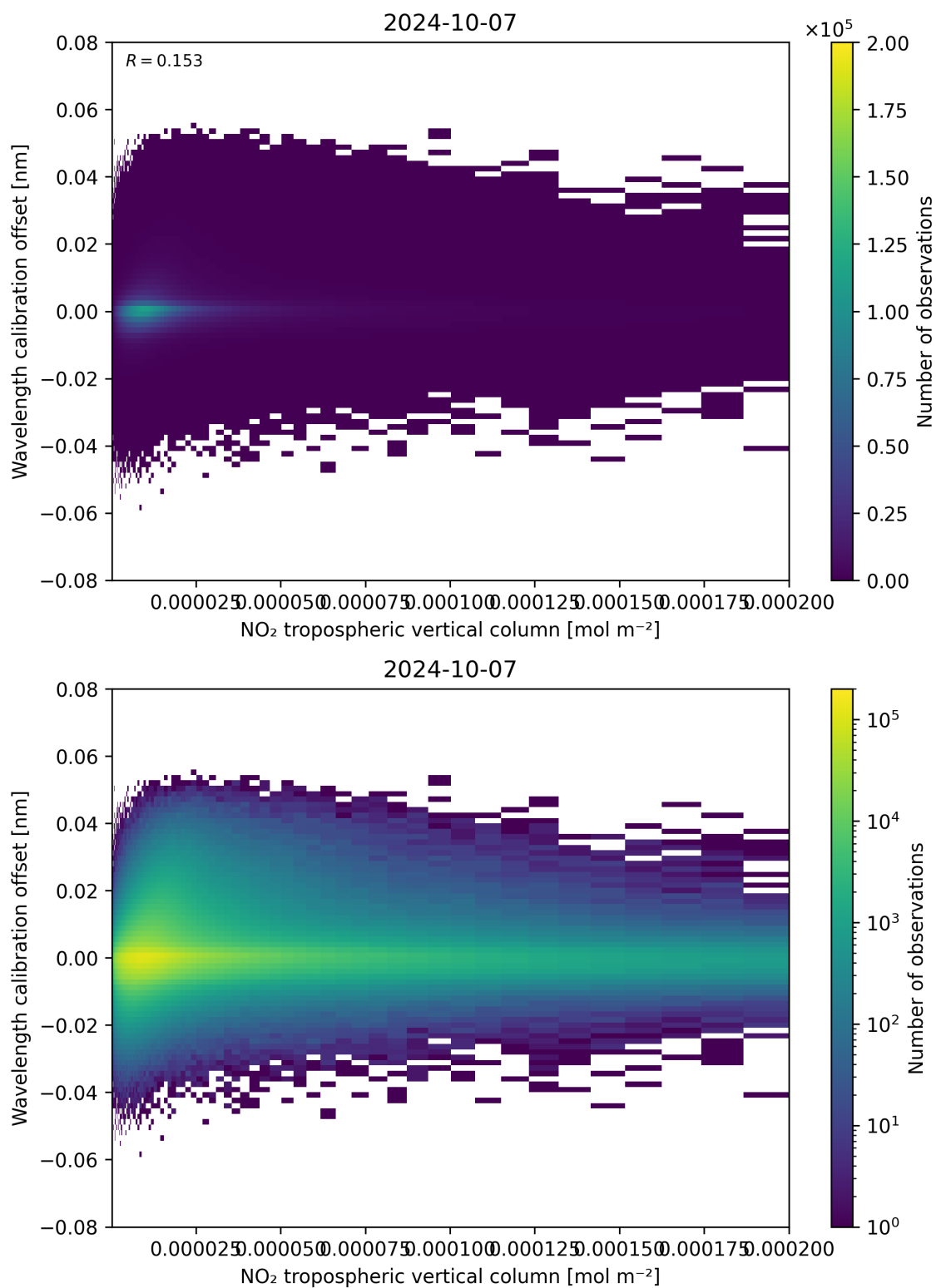
Figure 143: Scatter density plot of “NO 2 tropospheric vertical column” against “Wavelength calibration offset” for 2024-10-06 to 2024-10-08.
