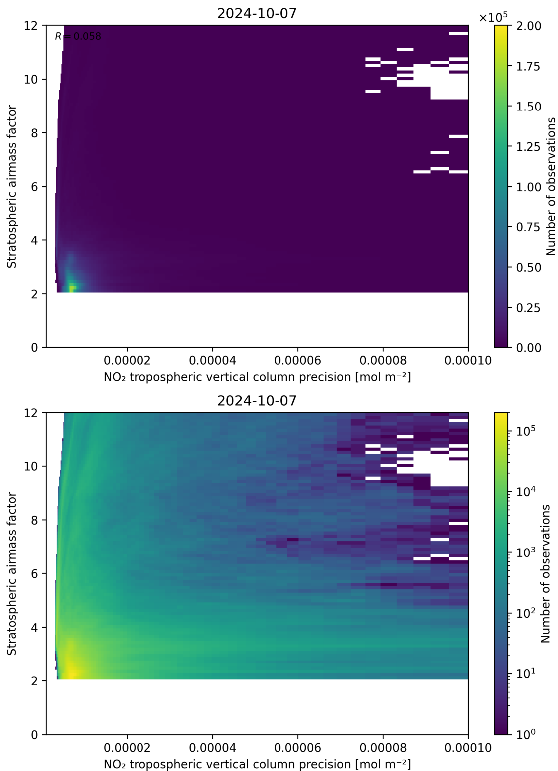
Figure 131: Scatter density plot of “NO 2 tropospheric vertical column precision” against “Stratospheric airmass factor” for 2024-10-06 to 2024-10-08.
