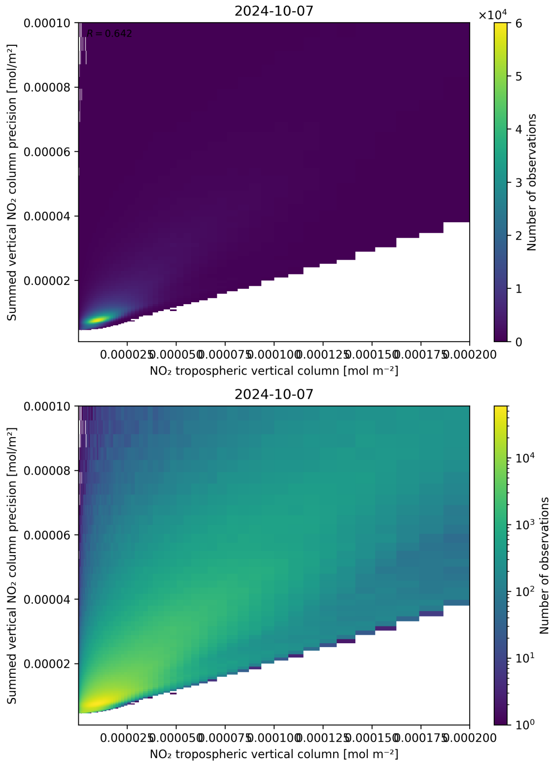
Figure 127: Scatter density plot of “NO 2 tropospheric vertical column” against “Summed vertical NO 2 column precision” for 2024-10-06 to 2024-10-08.
