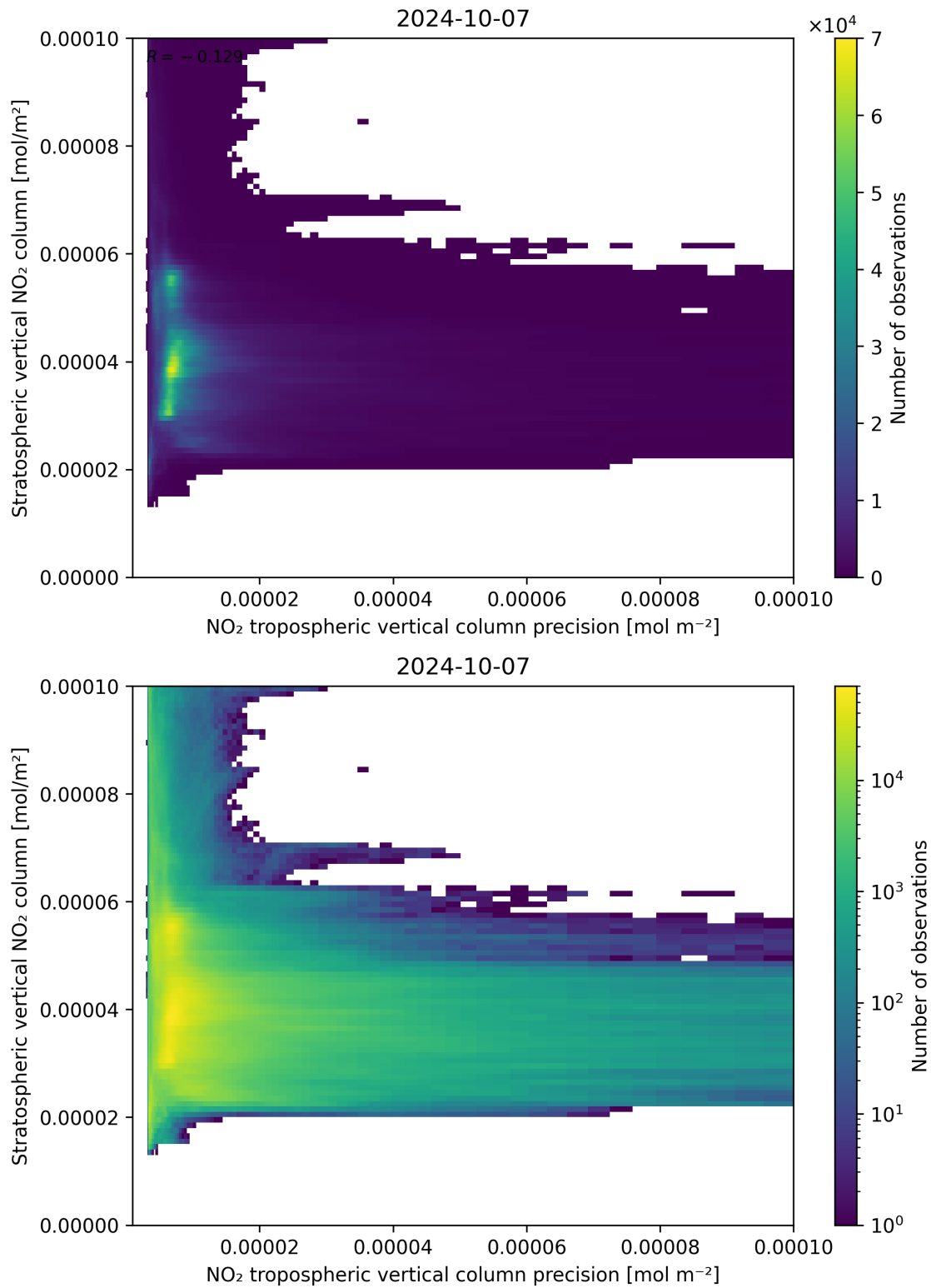
Figure 135: Scatter density plot of “NO 2 tropospheric vertical column precision” against “Stratospheric vertical NO 2 column” for 2024-10-06 to 2024-10-08.
