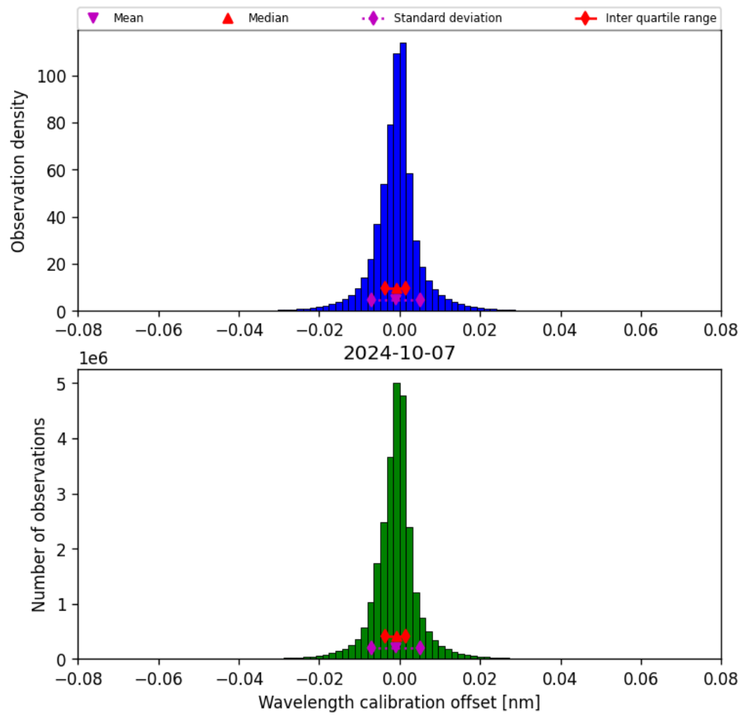
Figure 35: Histogram of “Wavelength calibration offset” for 2024-10-06 to 2024-10-08
