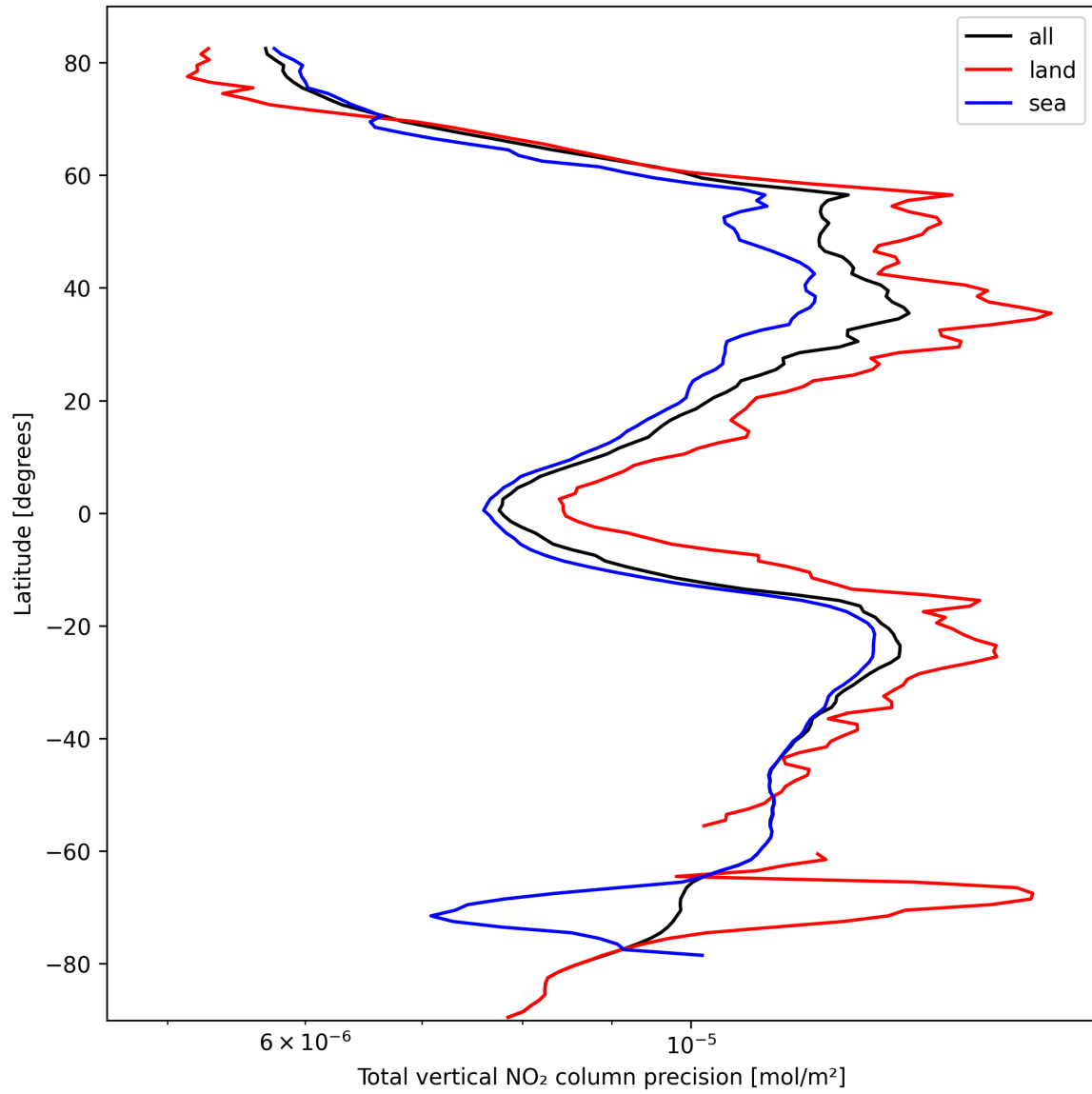
Figure 22: Zonal average of "Total vertical NO 2 column precision" for 2024-10-06 to 2024-10-08.
