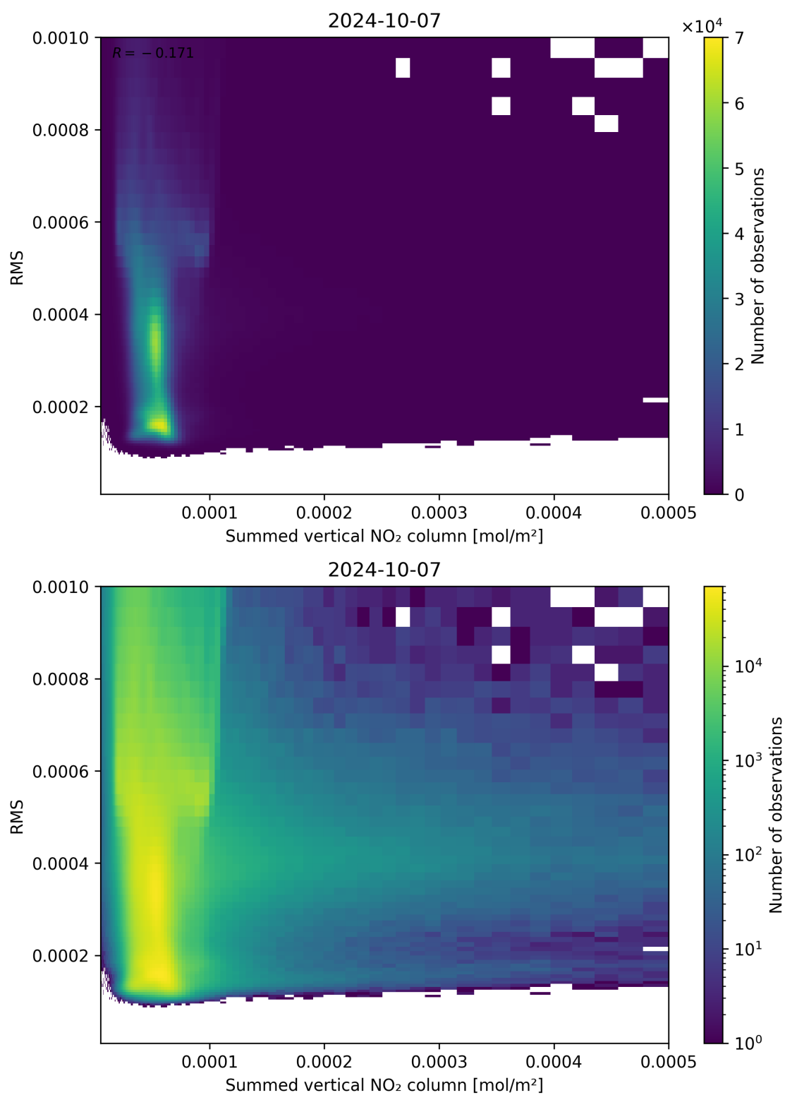
Figure 109: Scatter density plot of “Summed vertical NO 2 column” against “RMS” for 2024-10-06 to 2024-10-08.
