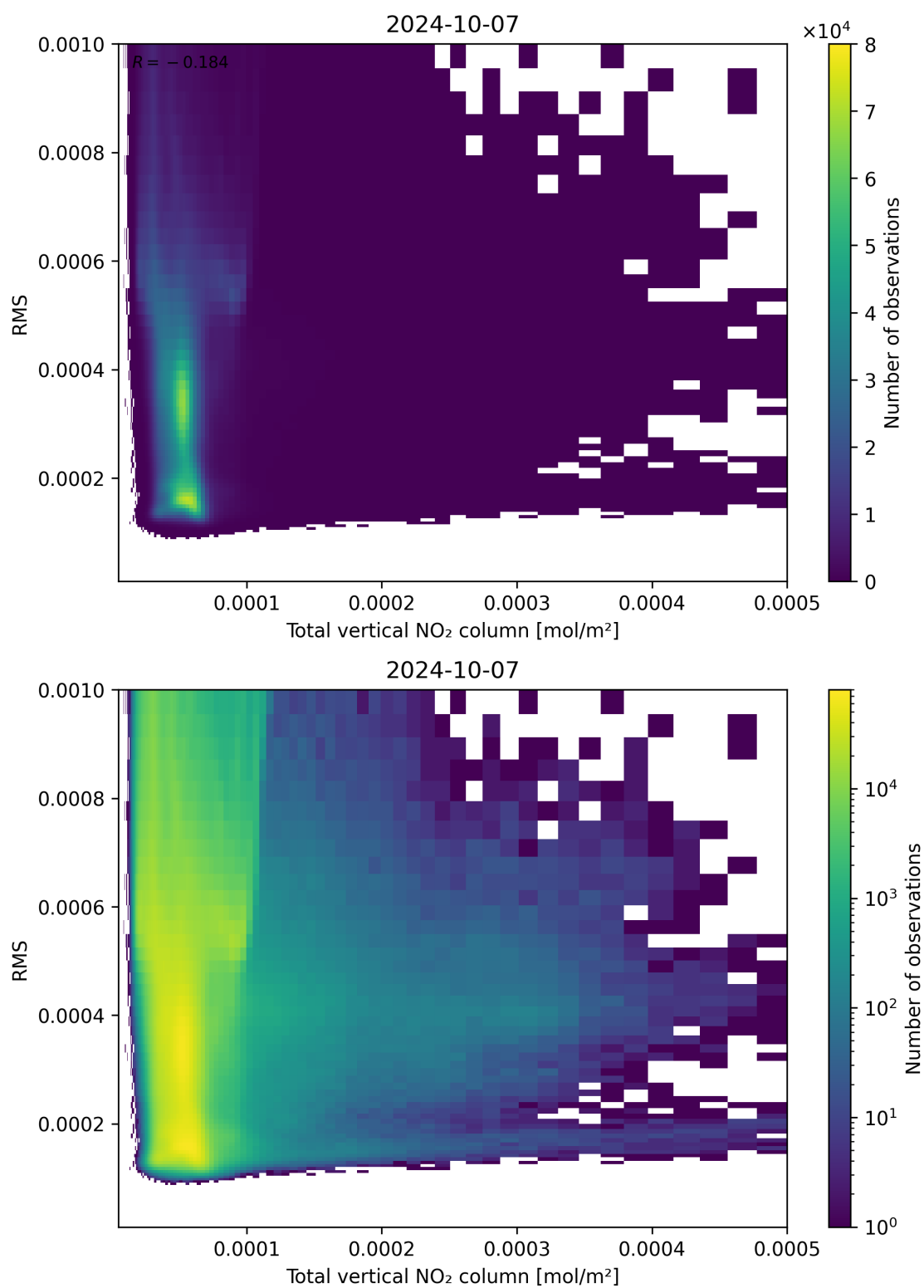
Figure 120: Scatter density plot of “Total vertical NO 2 column” against “RMS” for 2024-10-06 to 2024-10-08.
