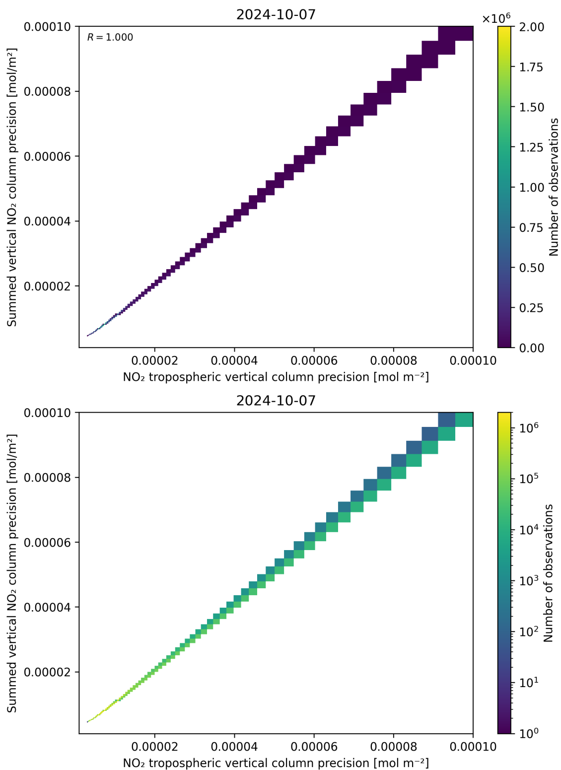
Figure 137: Scatter density plot of “NO 2 tropospheric vertical column precision” against “Summed vertical NO 2 column precision” for 2024-10-06 to 2024-10-08.
