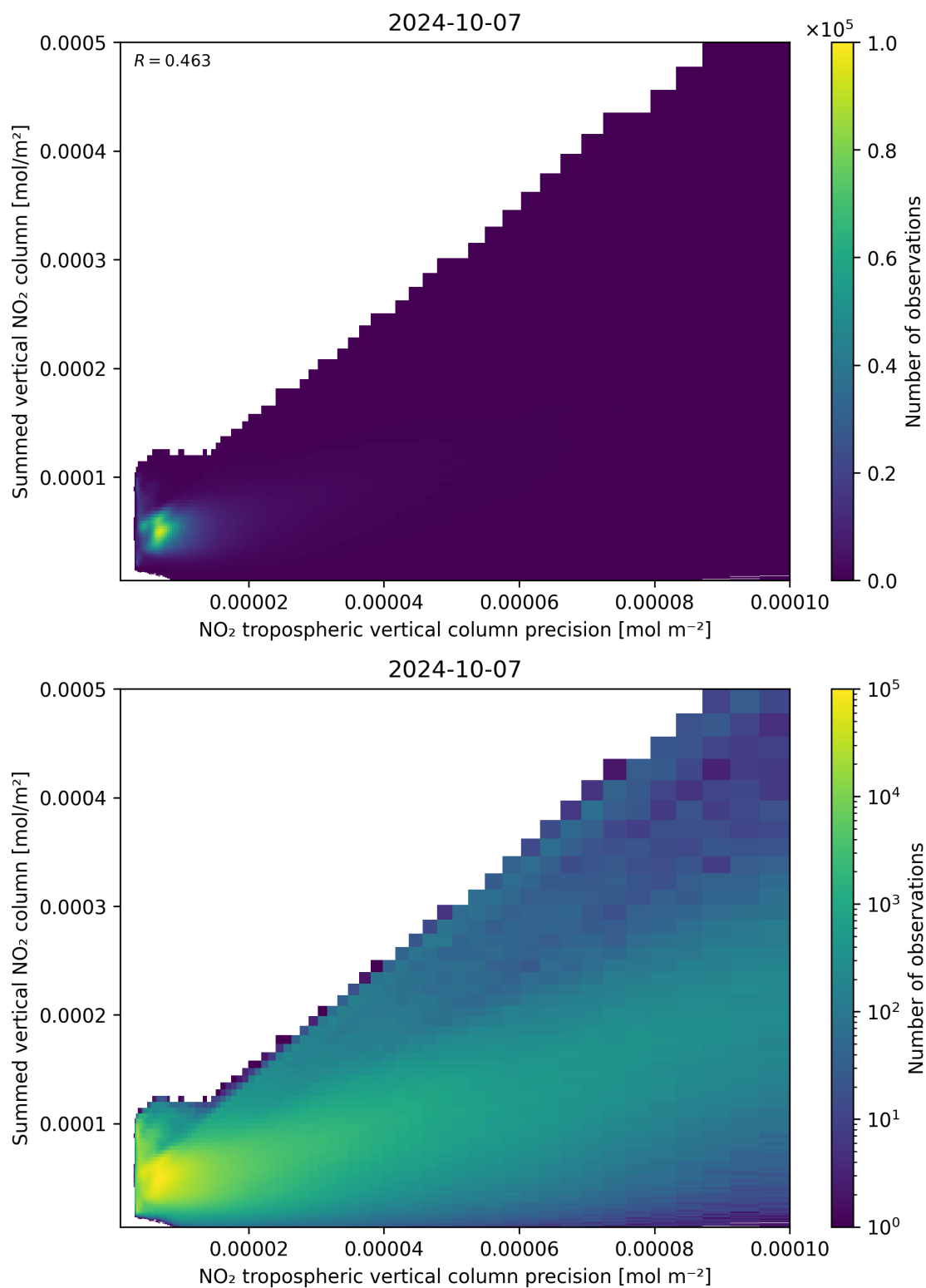
Figure 136: Scatter density plot of “NO 2 tropospheric vertical column precision” against “Summed vertical NO 2 column” for 2024-10-06 to 2024-10-08.
