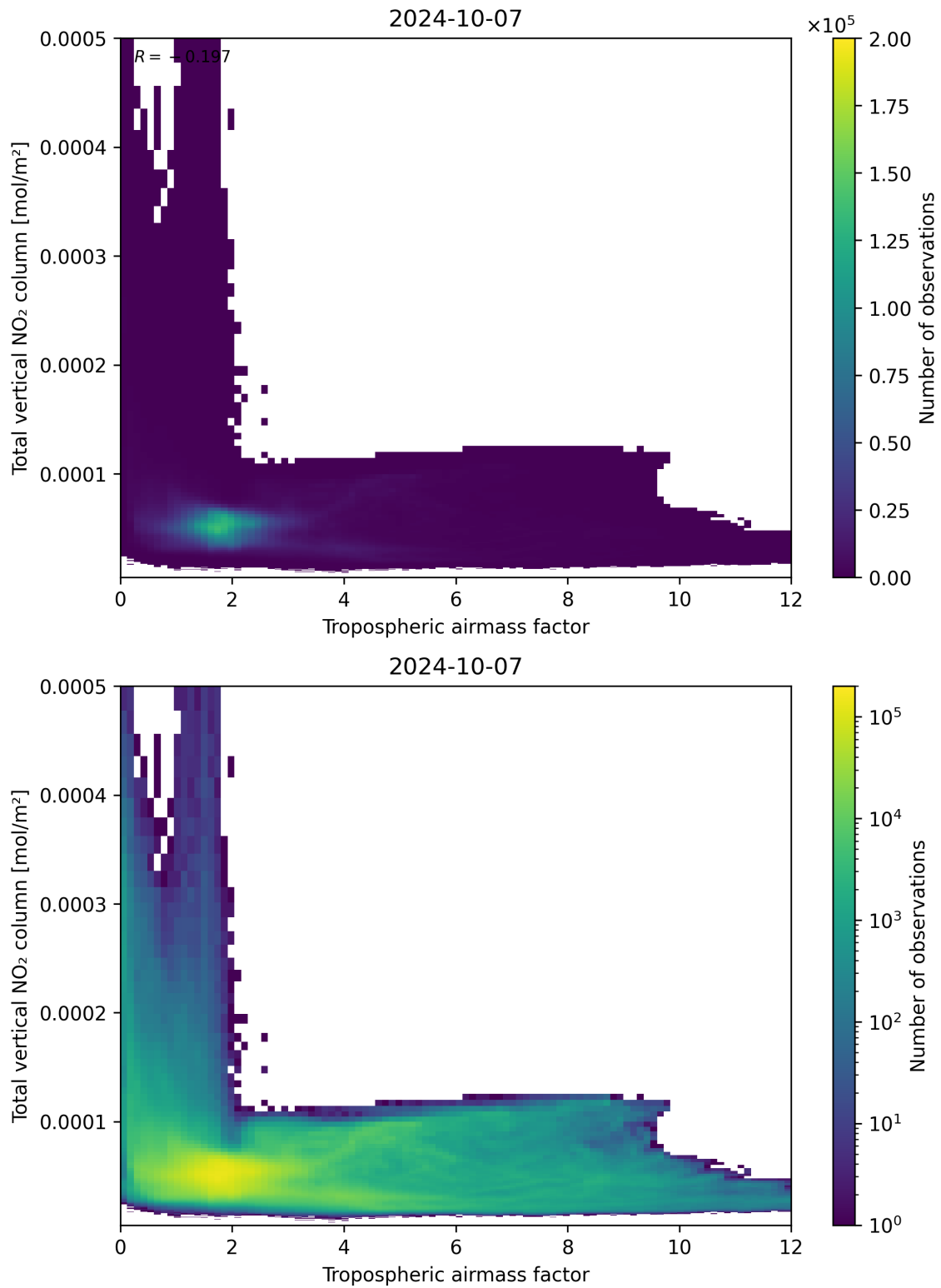
Figure 77: Scatter density plot of “Tropospheric airmass factor” against “Total vertical NO 2 column” for 2024-10-06 to 2024-10-08.
