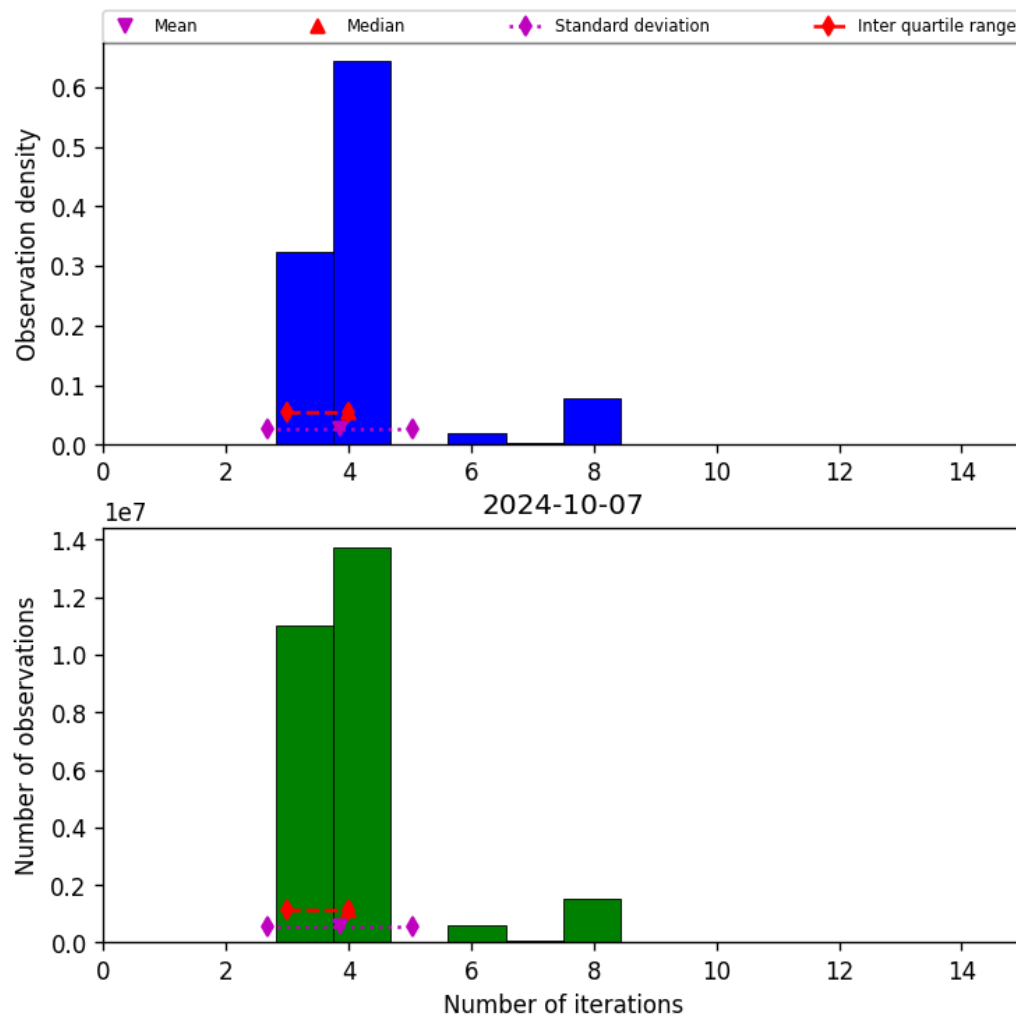
Figure 34: Histogram of “Number of iterations” for 2024-10-06 to 2024-10-08
