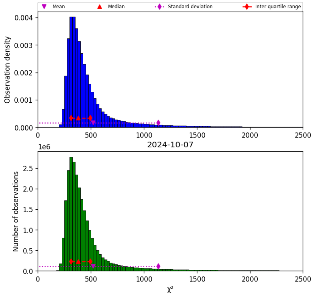
Figure 42: Histogram of “ \chi^2 ” for 2024-10-06 to 2024-10-08
