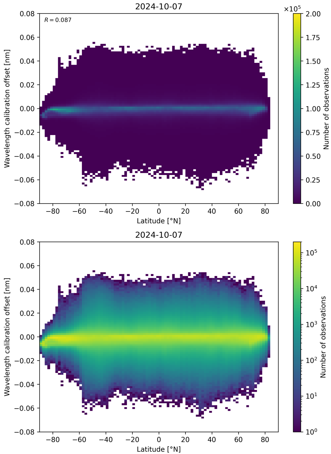
Figure 95: Scatter density plot of “Latitude” against “Wavelength calibration offset” for 2024-10-06 to 2024-10-08.
