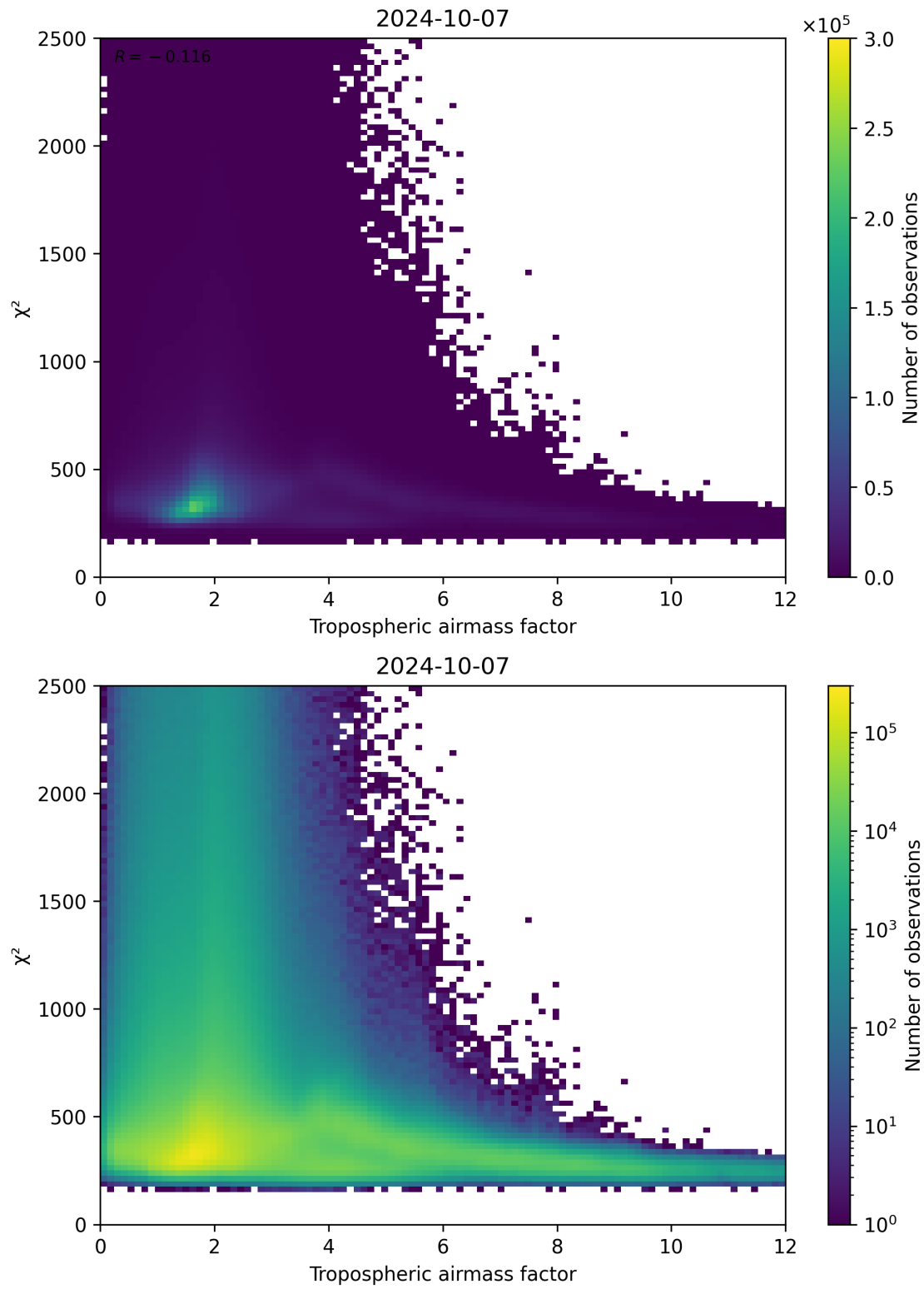
Figure 73: Scatter density plot of “Tropospheric airmass factor” against “ \chi^2 ” for 2024-10-06 to 2024-10-08.
