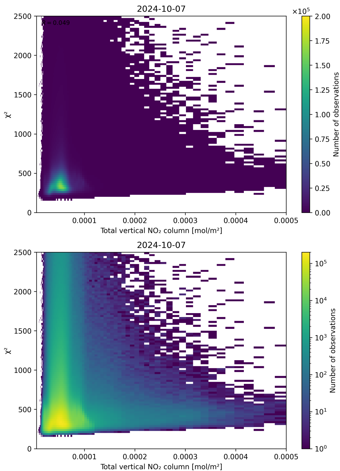
Figure 111: Scatter density plot of “Total vertical NO 2 column” against “ \chi^2 ” for 2024-10-06 to 2024-10-08.
