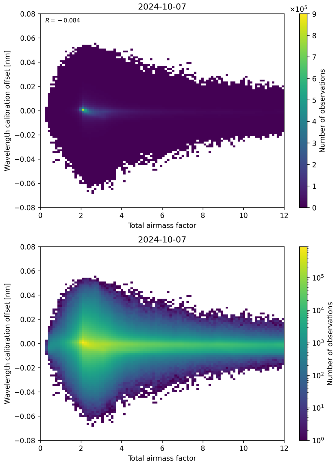
Figure 70: Scatter density plot of “Total airmass factor” against “Wavelength calibration offset” for 2024-10-06 to 2024-10-08.
