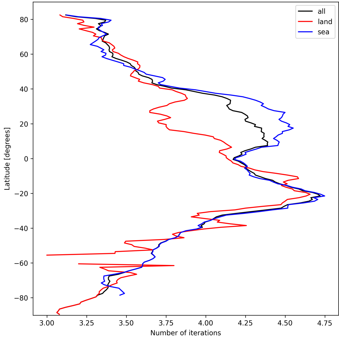
Figure 17: Zonal average of “Number of iterations” for 2024-10-06 to 2024-10-08.
