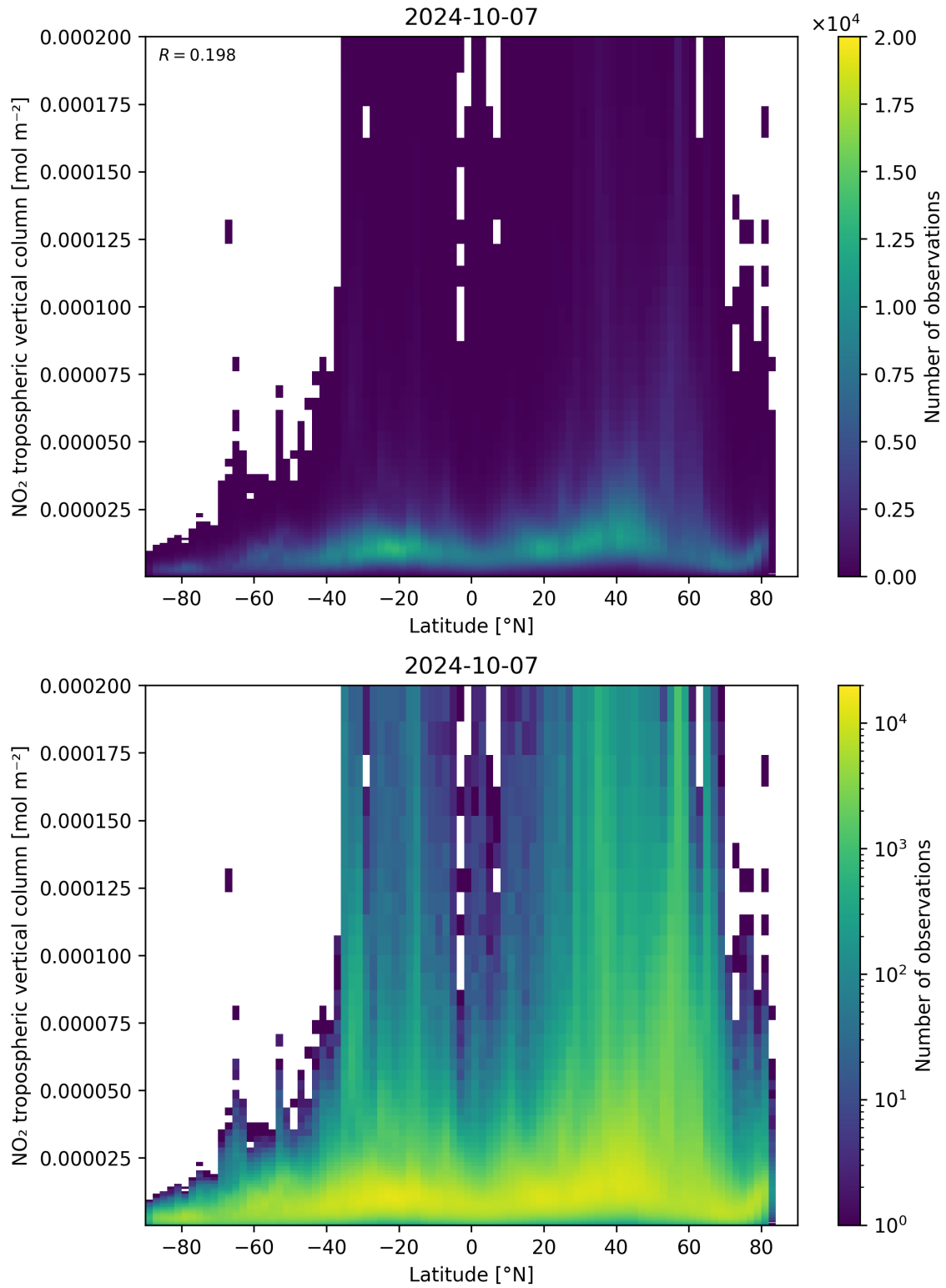
Figure 92: Scatter density plot of “Latitude” against “NO 2 tropospheric vertical column” for 2024-10-06 to 2024-10-08.
