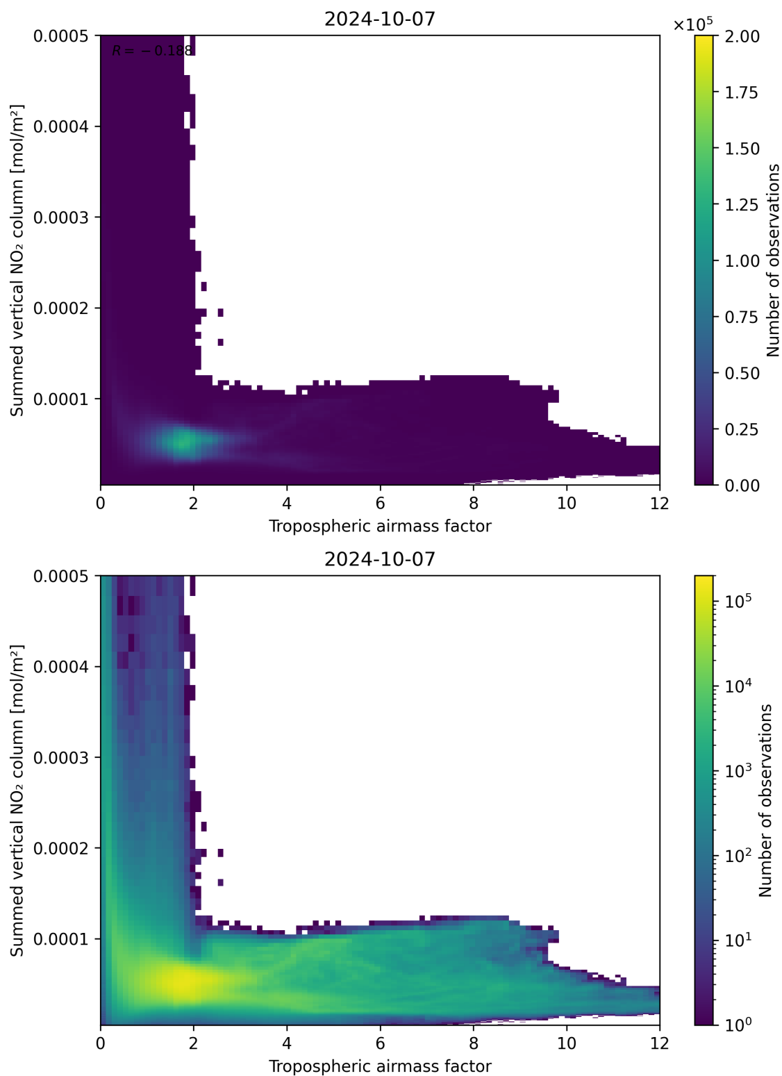
Figure 75: Scatter density plot of “Tropospheric air mass factor” against “Summed vertical NO 2 column” for 2024-10-06 to 2024-10-08.
