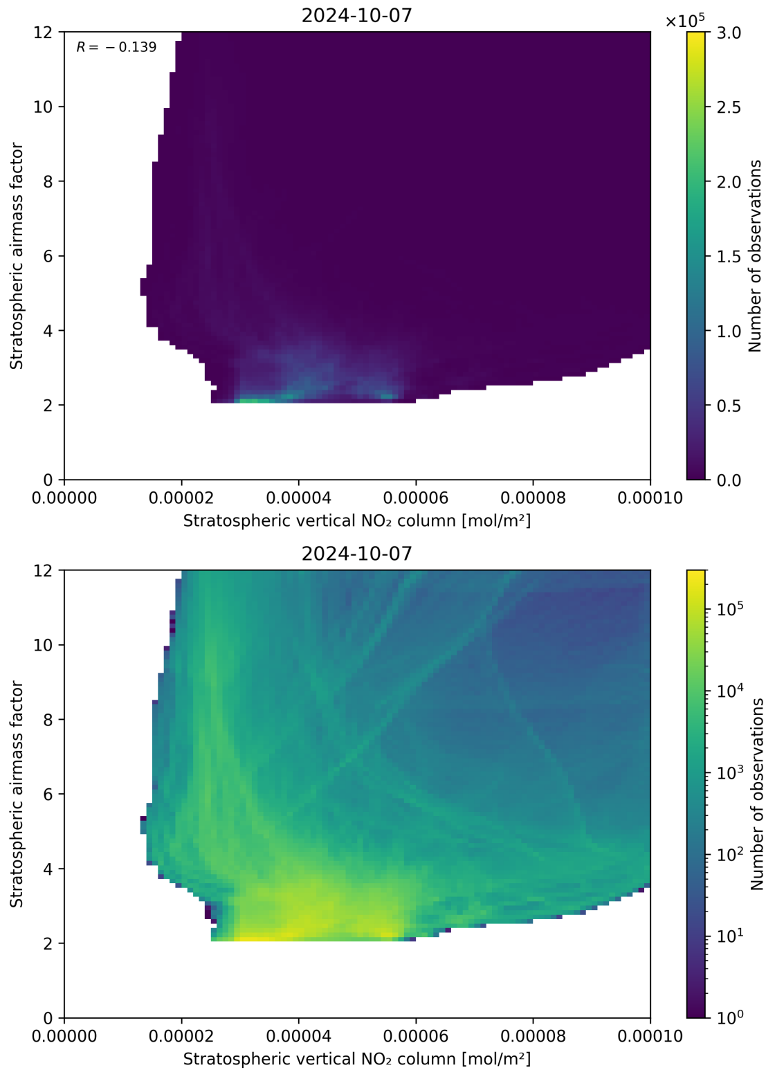
Figure 96: Scatter density plot of “Stratospheric vertical NO 2 column” against “Stratospheric airmass factor” for 2024-10-06 to 2024-10-08.
