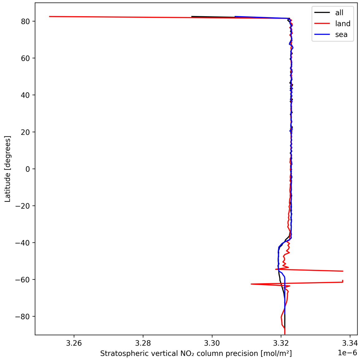
Figure 20: Zonal average of “Stratospheric vertical NO 2 column precision” for 2024-10-06 to 2024-10-08.
