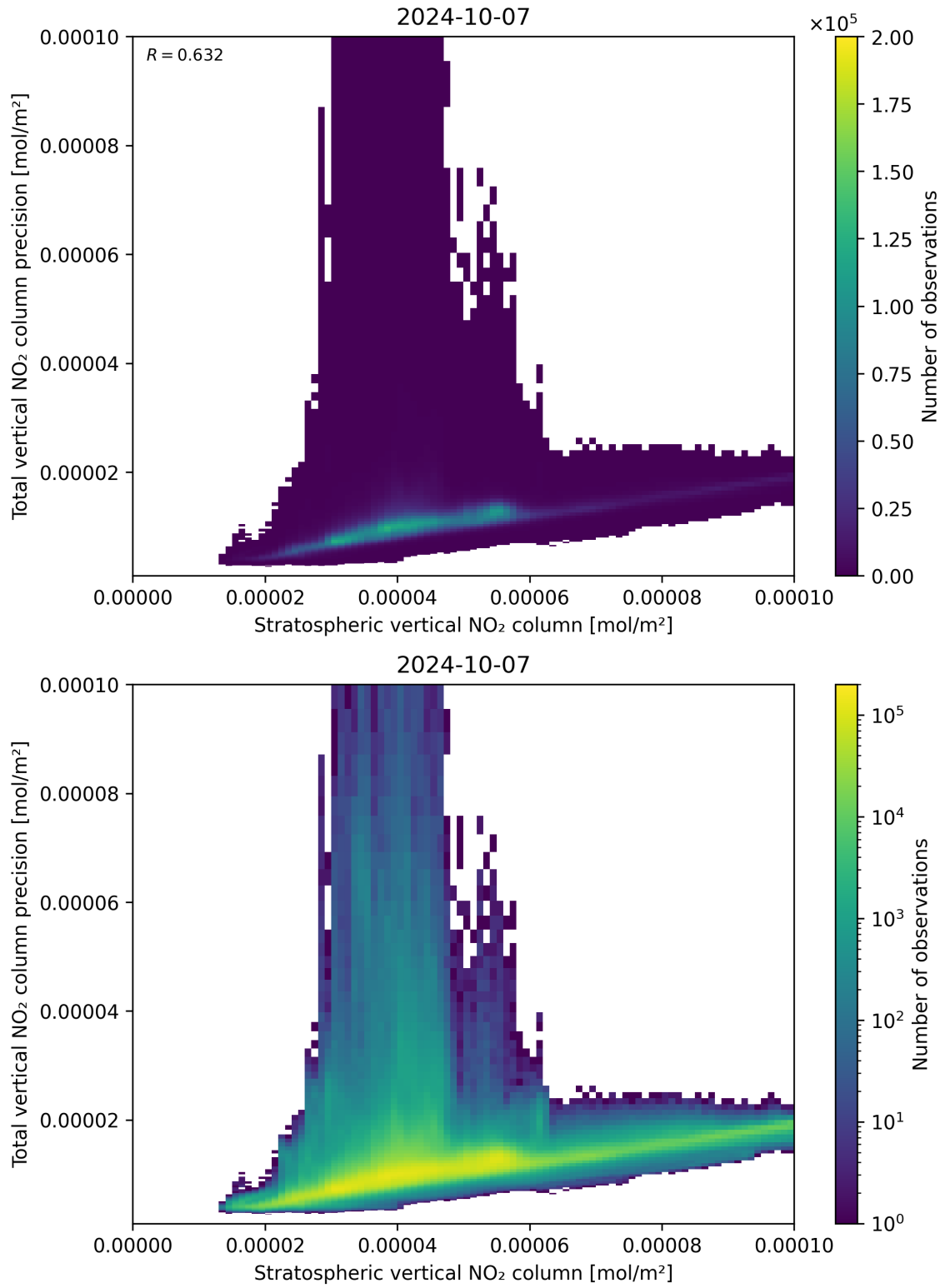
Figure 101: Scatter density plot of “Stratospheric vertical NO 2 column” against “Total vertical NO 2 column precision” for 2024-10-06 to 2024-10-08.
