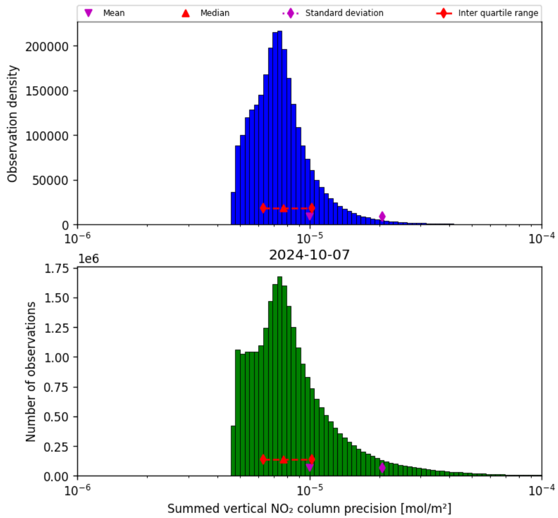
Figure 41: Histogram of "Summed vertical NO 2 column precision" for 2024-10-06 to 2024-10-08
