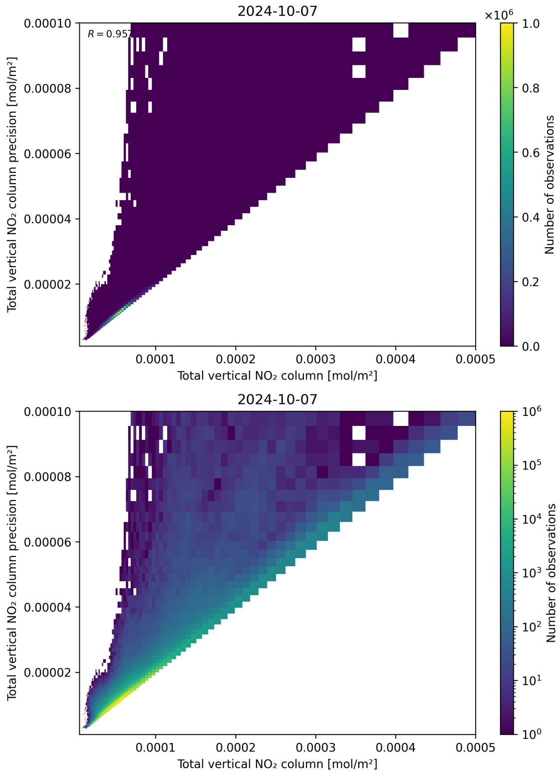
Figure 114: Scatter density plot of “Total vertical NO 2 column” against “Total vertical NO 2 column precision” for 2024-10-06 to 2024-10-08.
