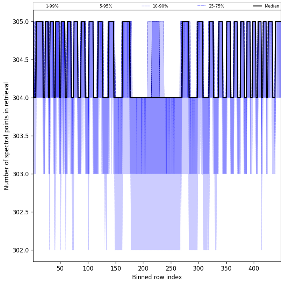
Figure 50: Along track statistics of “Number of spectral points in retrieval” for 2024-10-06 to 2024-10-08
