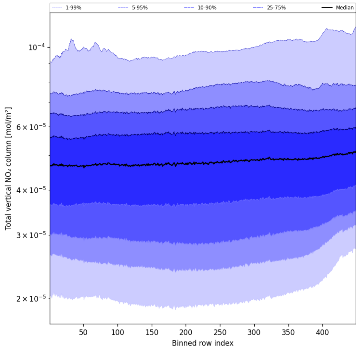
Figure 55: Along track statistics of “Total vertical NO 2 column” for 2024-10-06 to 2024-10-08
