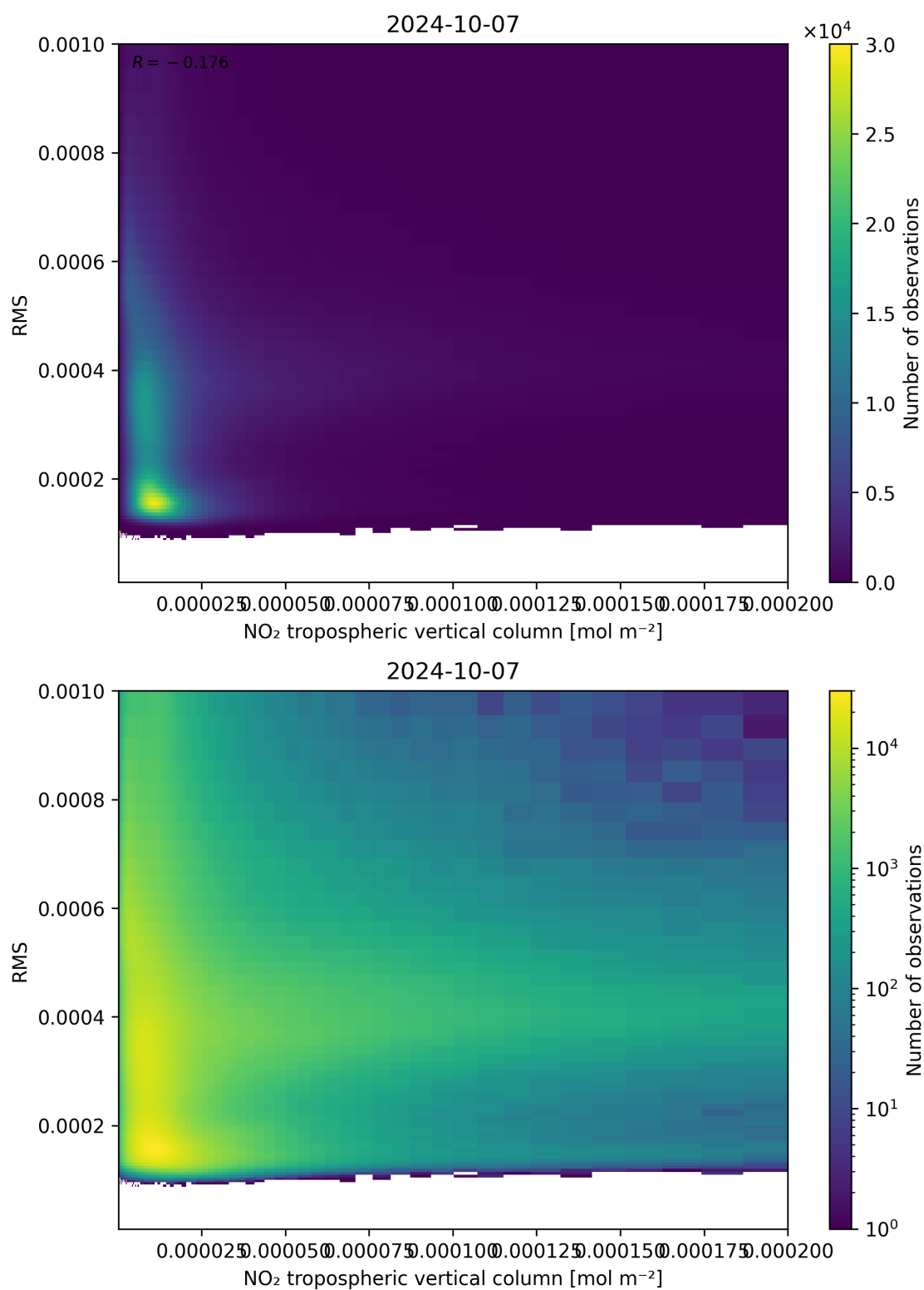
Figure 142: Scatter density plot of “NO 2 tropospheric vertical column” against “RMS” for 2024-10-06 to 2024-10-08.
