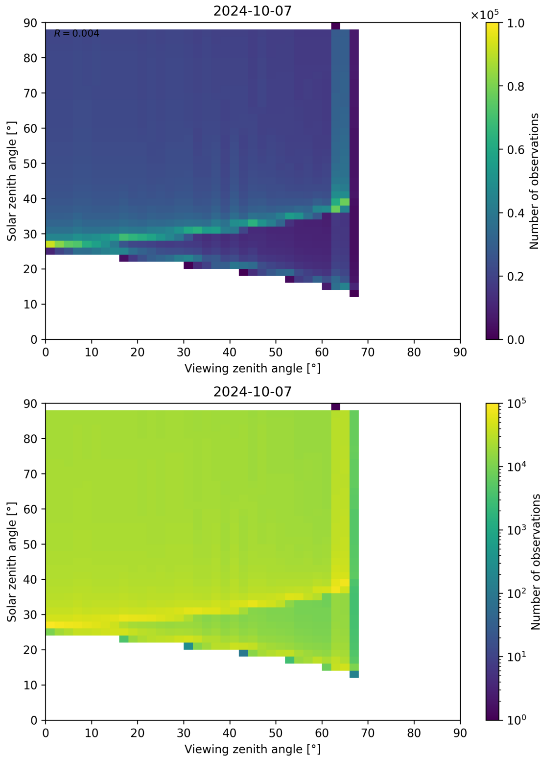
Figure 172: Scatter density plot of “Viewing zenith angle” against “Solar zenith angle” for 2024-10-06 to 2024-10-08.
