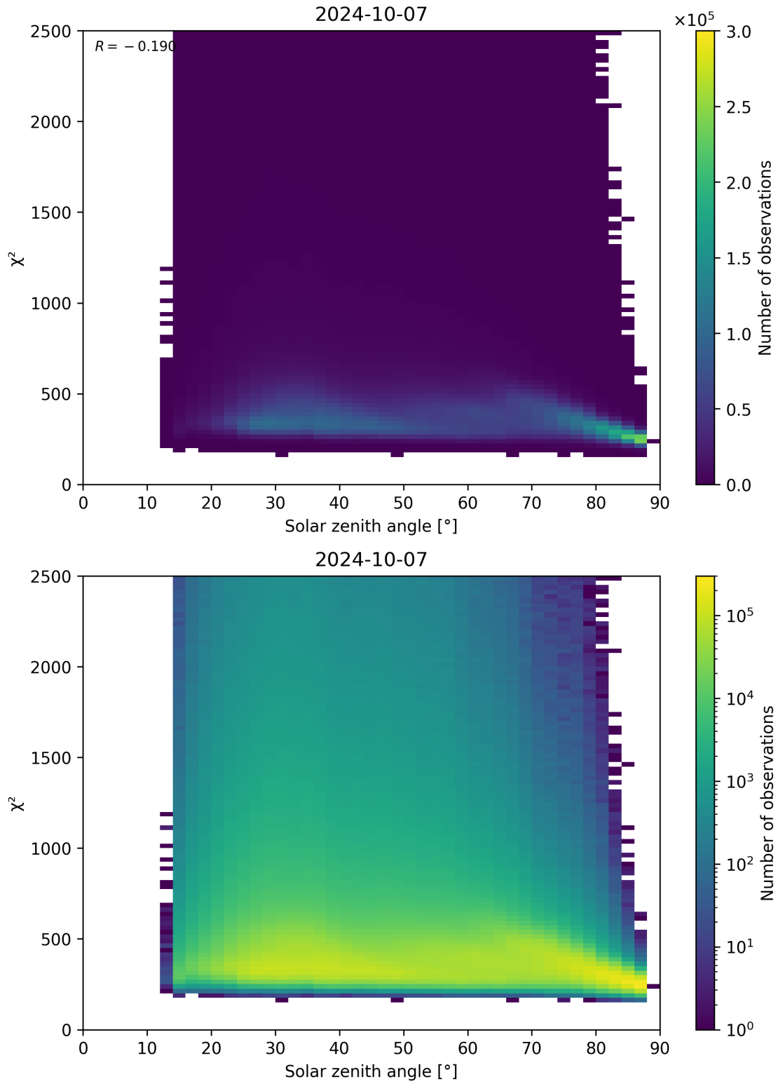
Figure 148: Scatter density plot of “Solar zenith angle” against “ \chi^2 ” for 2024-10-06 to 2024-10-08.
