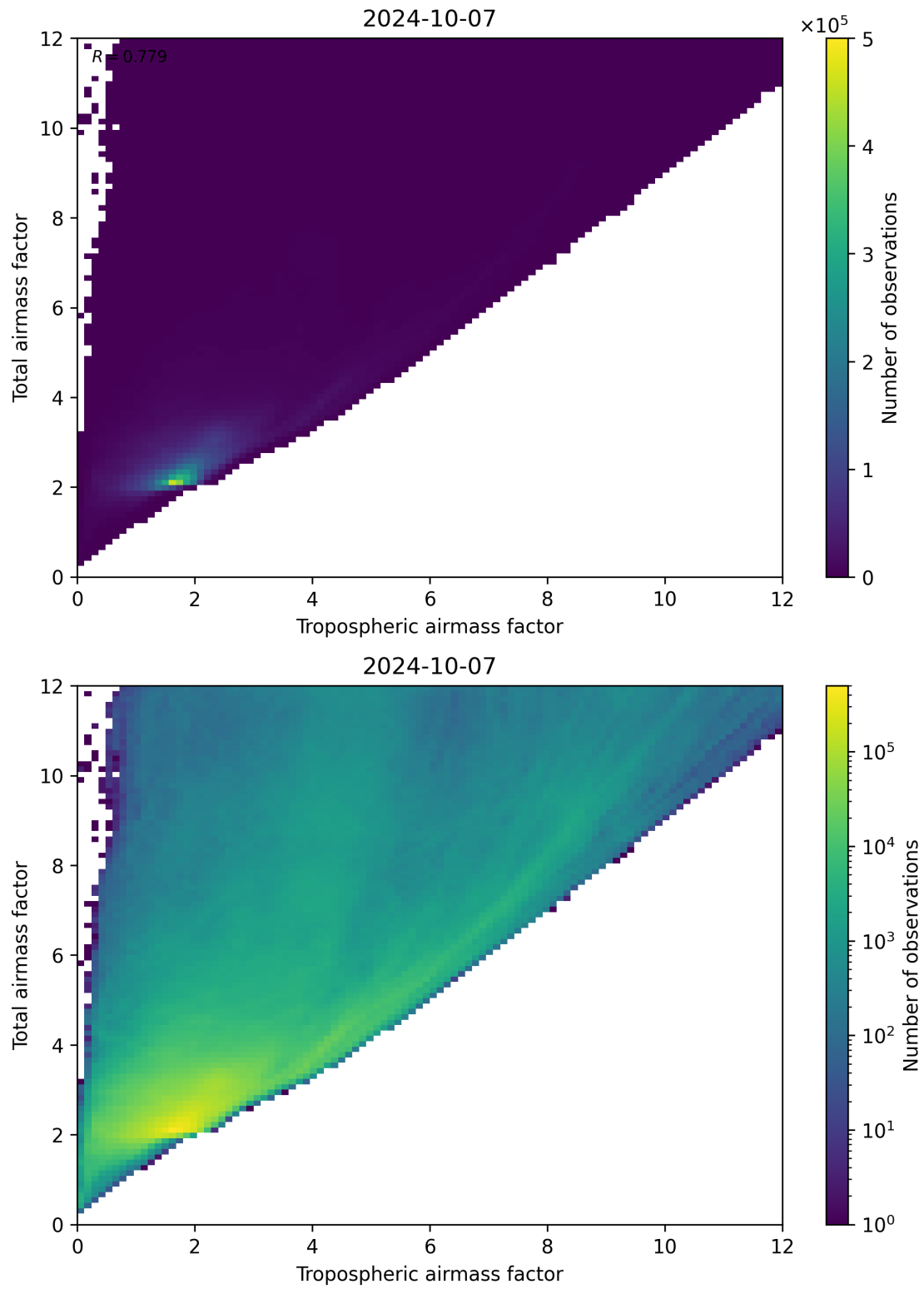
Figure 72: Scatter density plot of “Tropospheric airmass factor” against “Total airmass factor” for 2024-10-06 to 2024-10-08.
