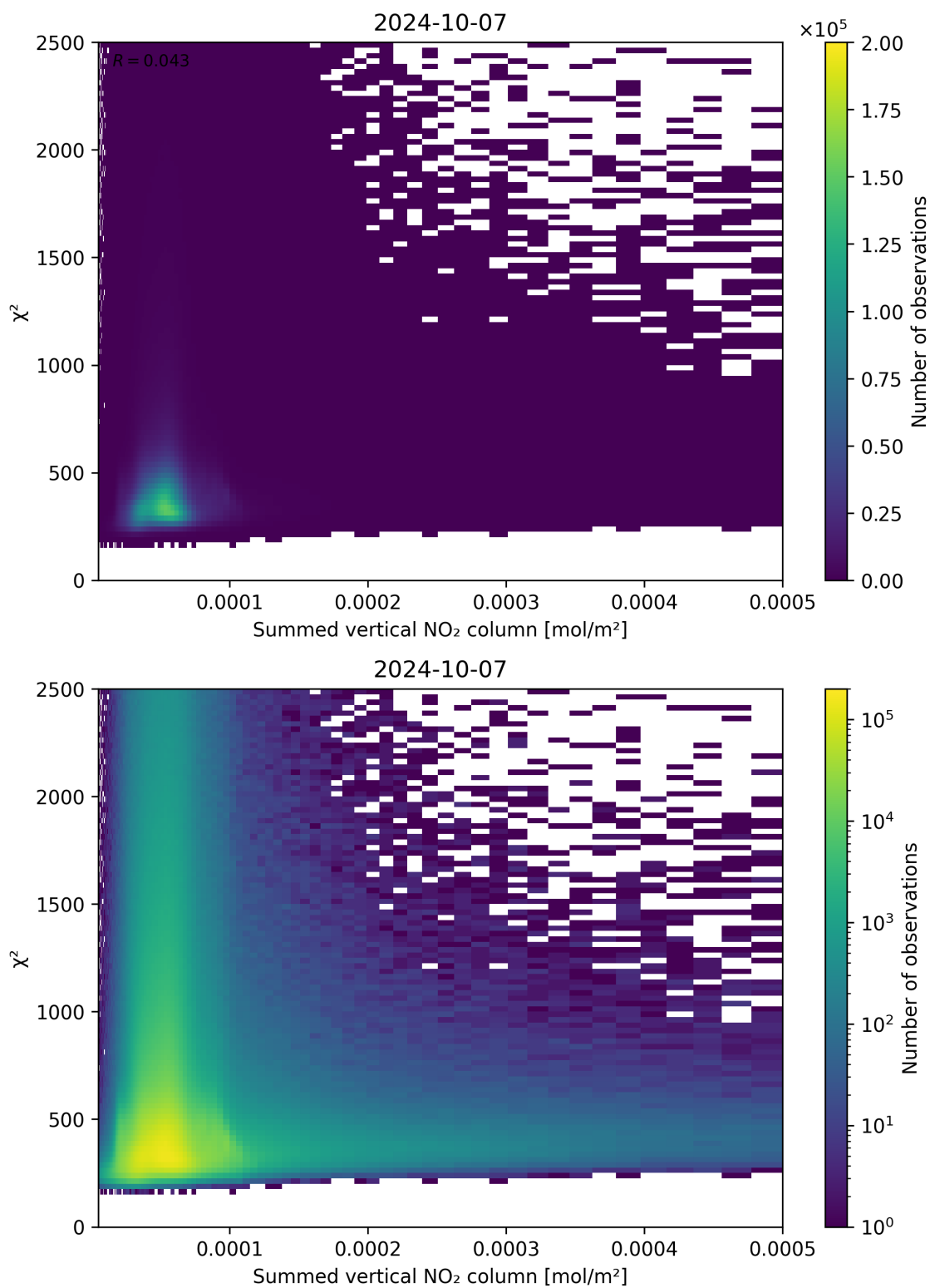
Figure 104: Scatter density plot of “Summed vertical NO 2 column” against “ \chi^2 ” for 2024-10-06 to 2024-10-08.
