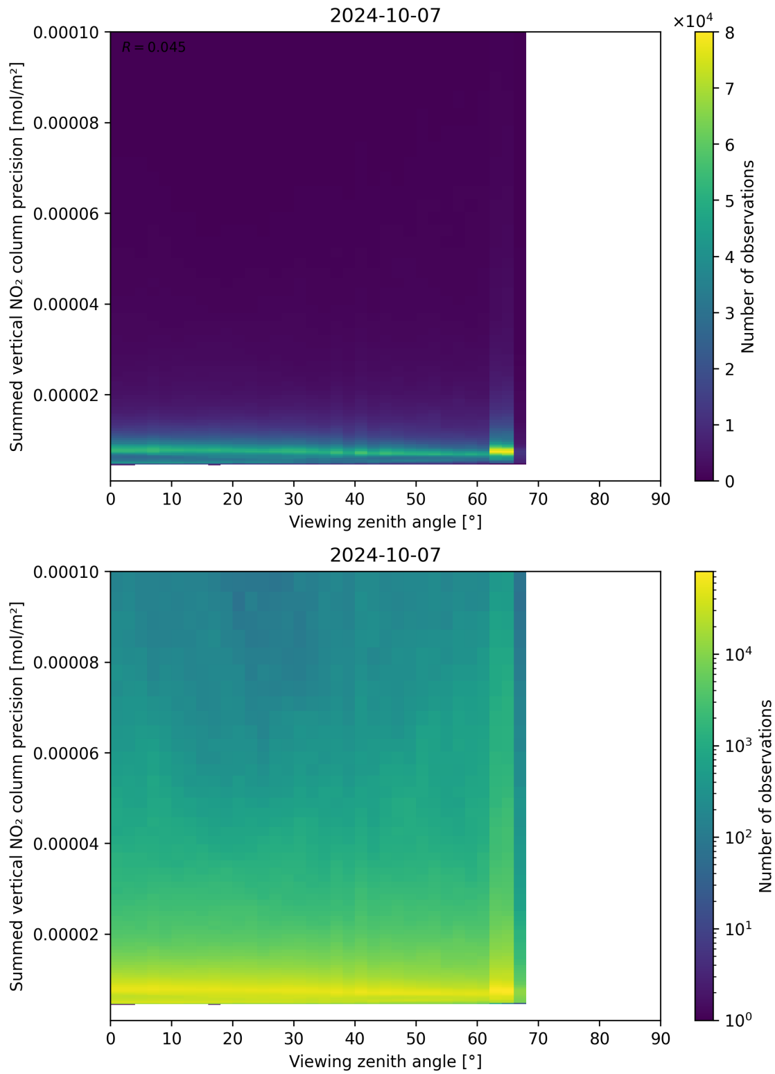
Figure 166: Scatter density plot of “Viewing zenith angle” against “Summed vertical NO 2 column precision” for 2024-10-06 to 2024-10-08.
