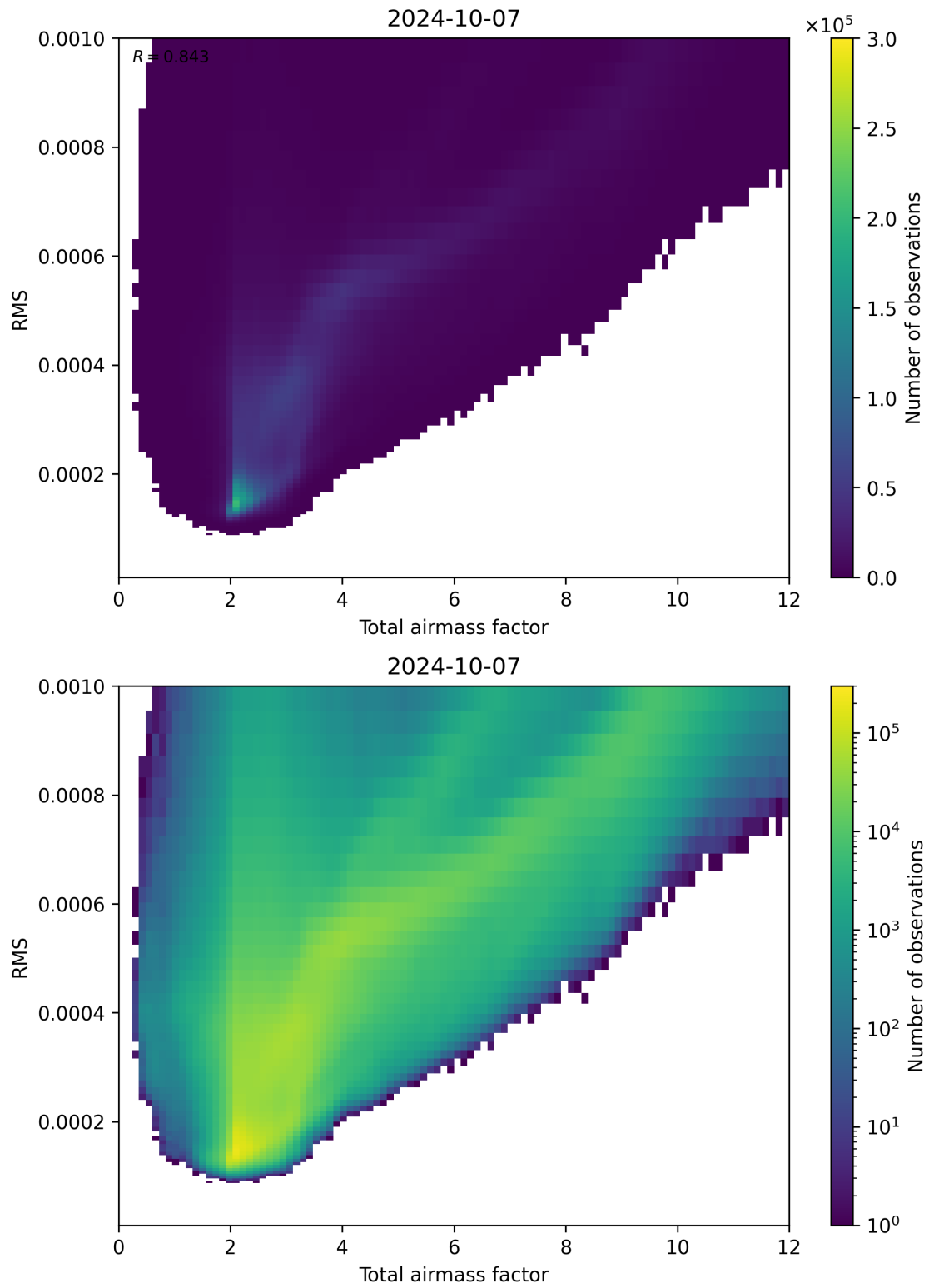
Figure 69: Scatter density plot of “Total airmass factor” against “RMS” for 2024-10-06 to 2024-10-08.
