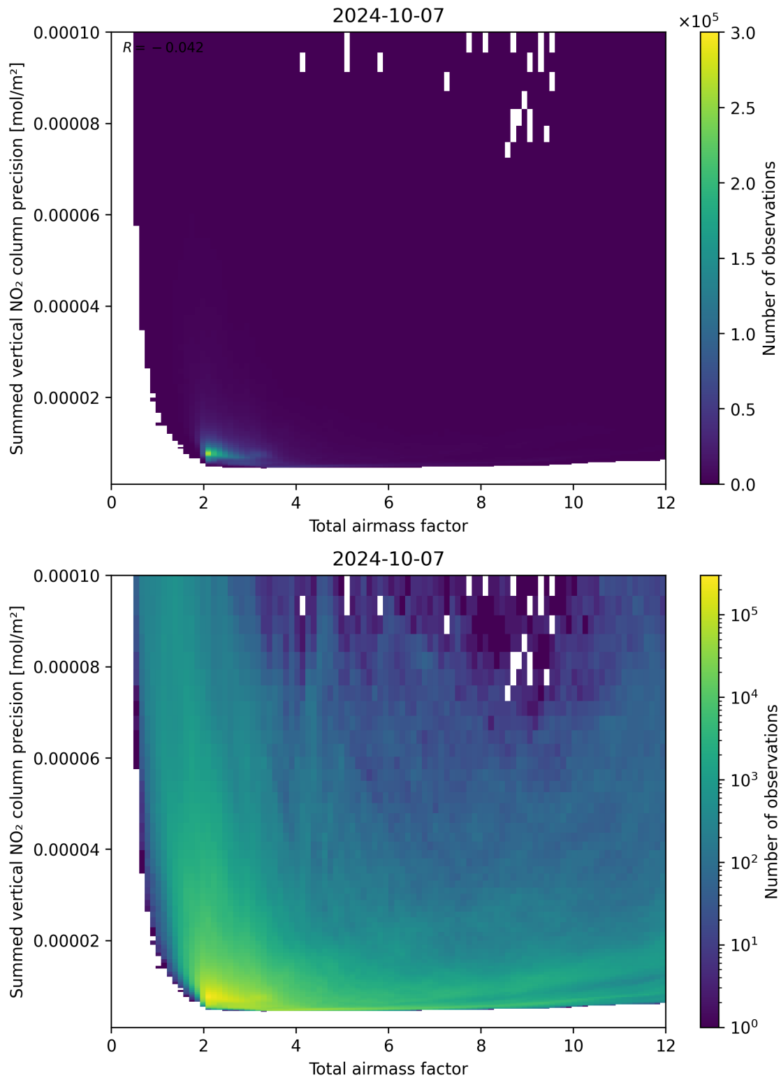
Figure 66: Scatter density plot of “Total airmass factor” against “Summed vertical NO 2 column precision” for 2024-10-06 to 2024-10-08.
