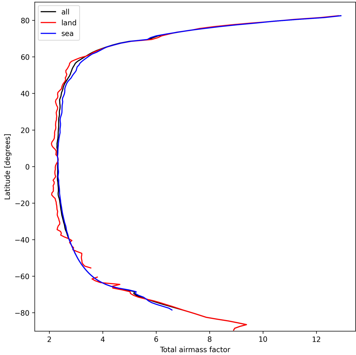
Figure 15: Zonal average of “Total airmass factor” for 2024-10-06 to 2024-10-08.
