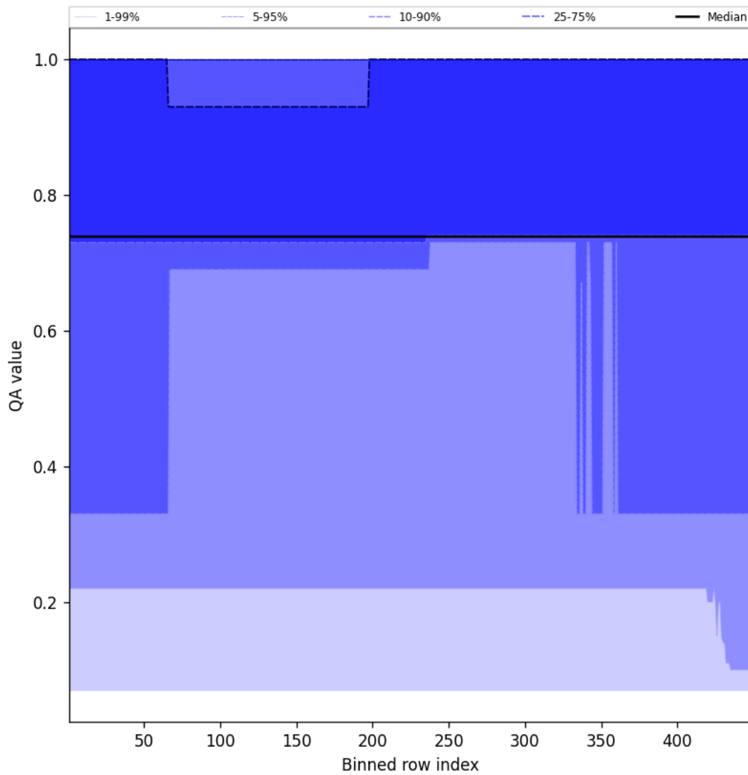
Figure 45: Along track statistics of “QA value” for 2024-10-06 to 2024-10-08
