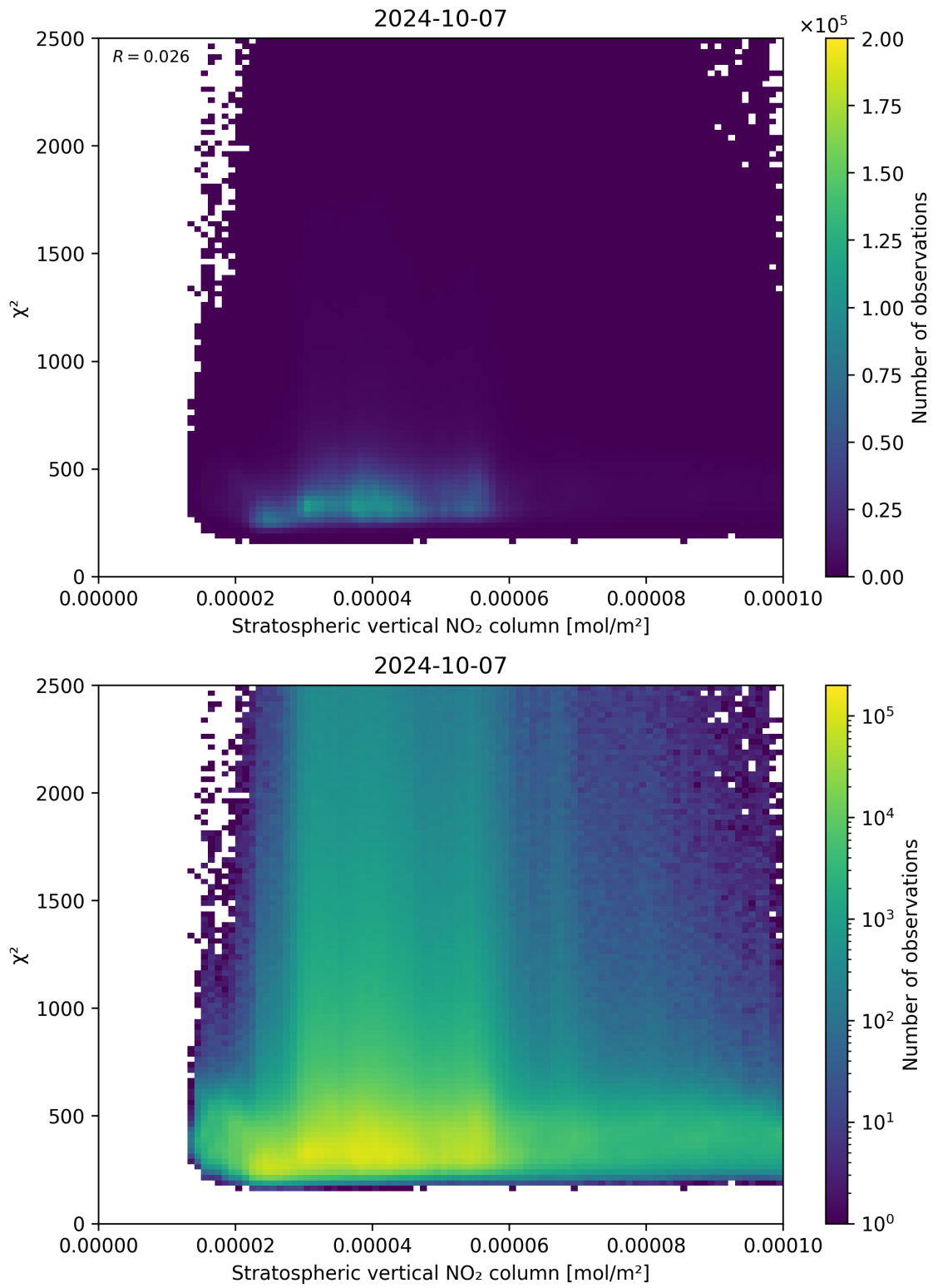
Figure 97: Scatter density plot of “Stratospheric vertical NO 2 column” against “ \chi^2 ” for 2024-10-06 to 2024-10-08.
