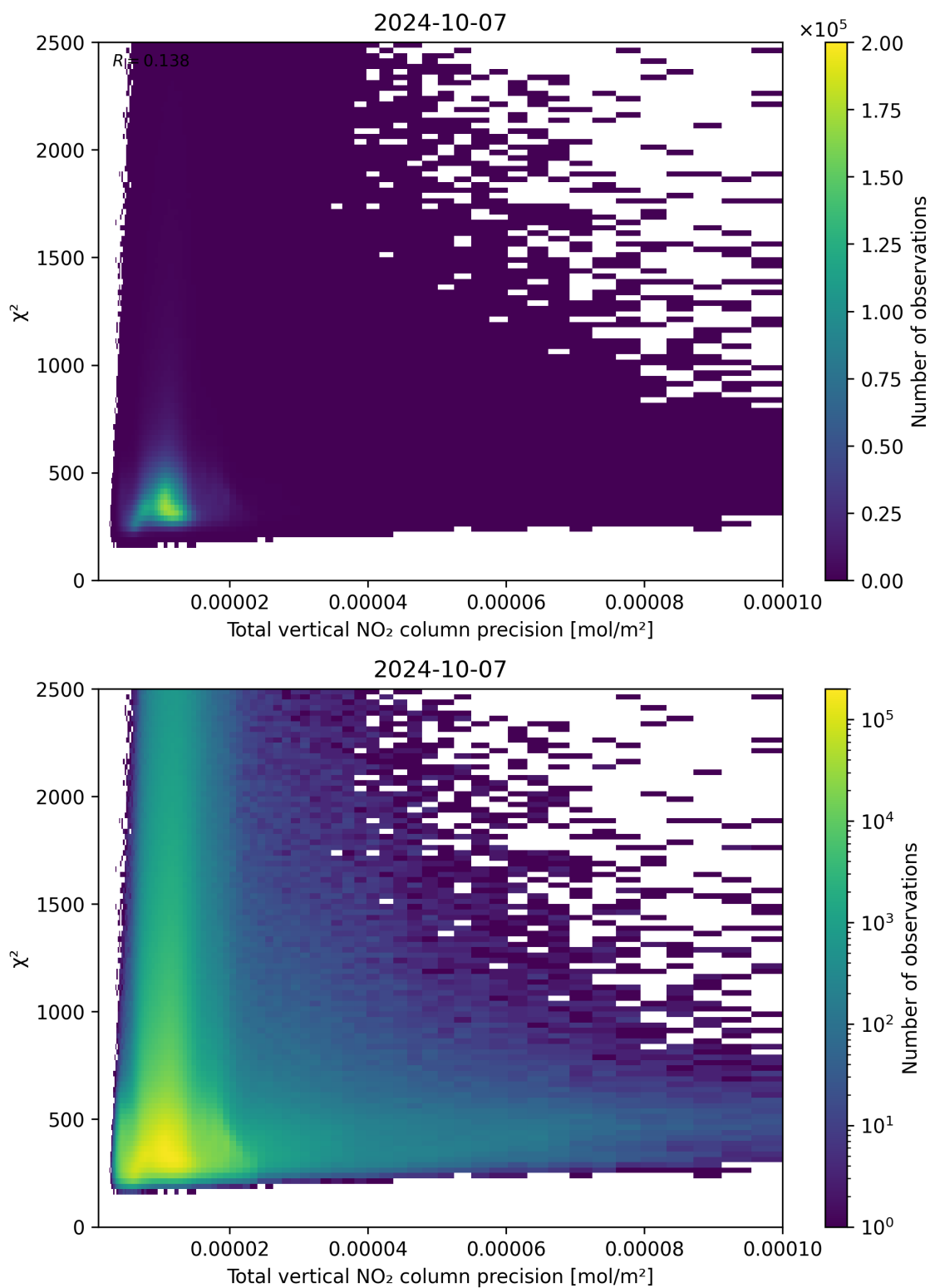
Figure 116: Scatter density plot of “Total vertical NO 2 column precision” against “ \chi^2 ” for 2024-10-06 to 2024-10-08.
