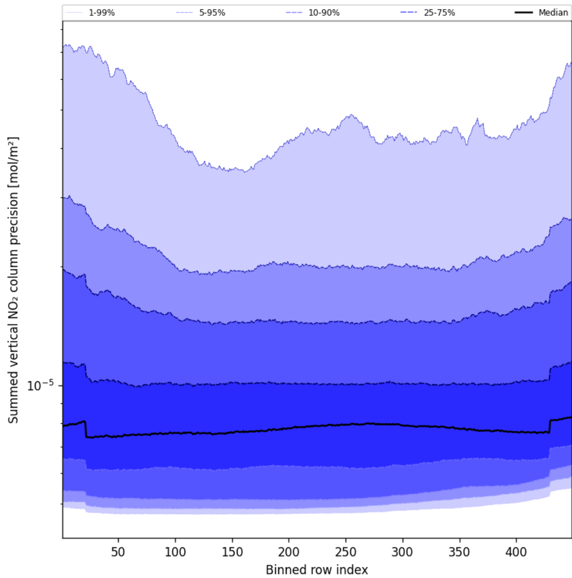
Figure 58: Along track statistics of “Summed vertical NO 2 column precision” for 2024-10-06 to 2024-10-08
