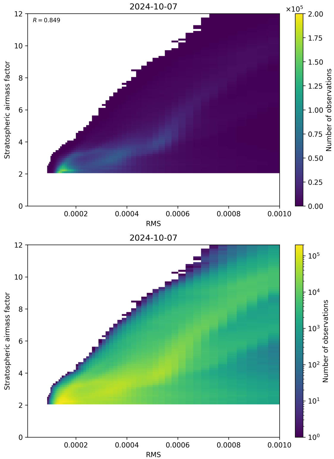
Figure 144: Scatter density plot of “RMS” against “Stratospheric airmass factor” for 2024-10-06 to 2024-10-08.
