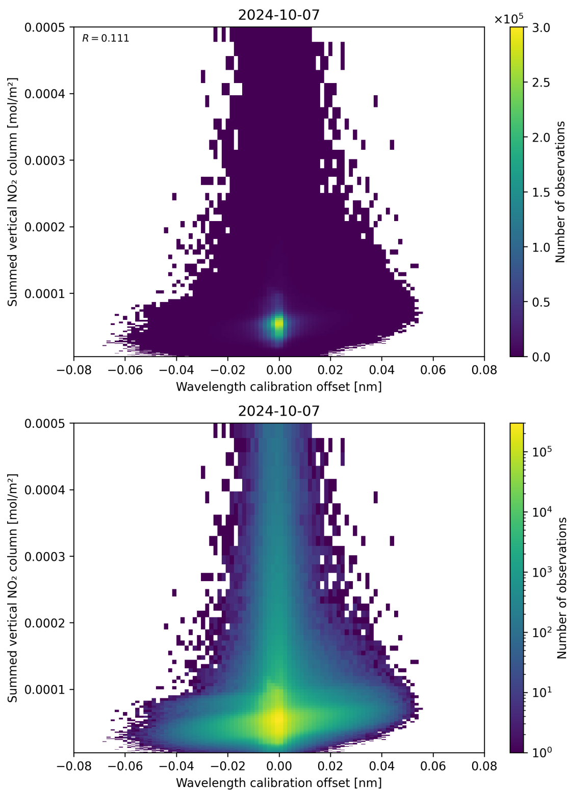
Figure 177: Scatter density plot of “Wavelength calibration offset” against “Summed vertical NO 2 column” for 2024-10-06 to 2024-10-08.
