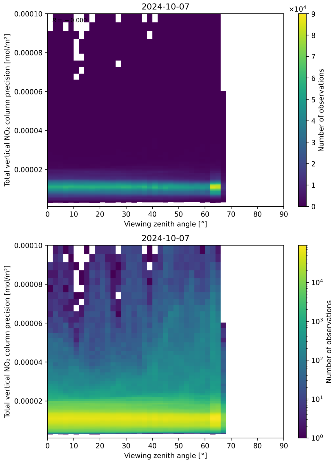
Figure 168: Scatter density plot of “Viewing zenith angle” against “Total vertical NO 2 column precision” for 2024-10-06 to 2024-10-08.
