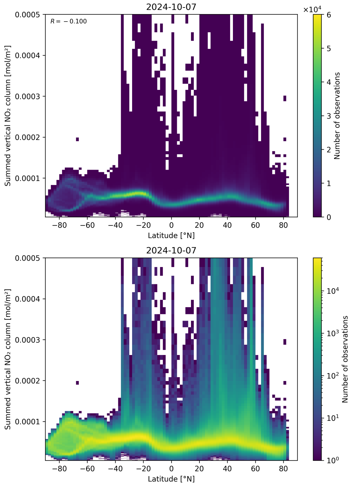
Figure 88: Scatter density plot of “Latitude” against “Summed vertical NO 2 column” for 2024-10-06 to 2024-10-08.
