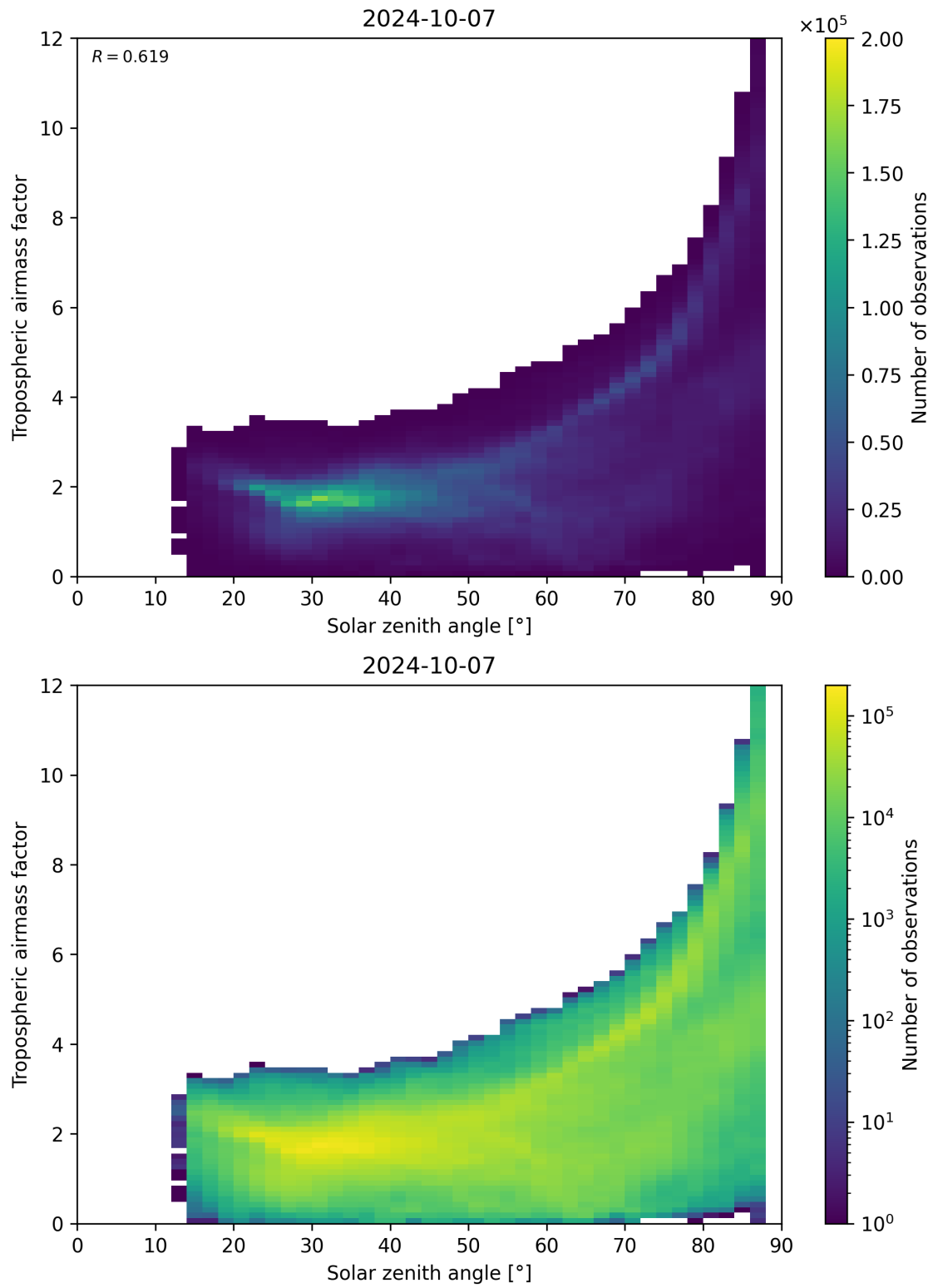
Figure 147: Scatter density plot of “Solar zenith angle” against “Tropospheric airmass factor” for 2024-10-06 to 2024-10-08.
