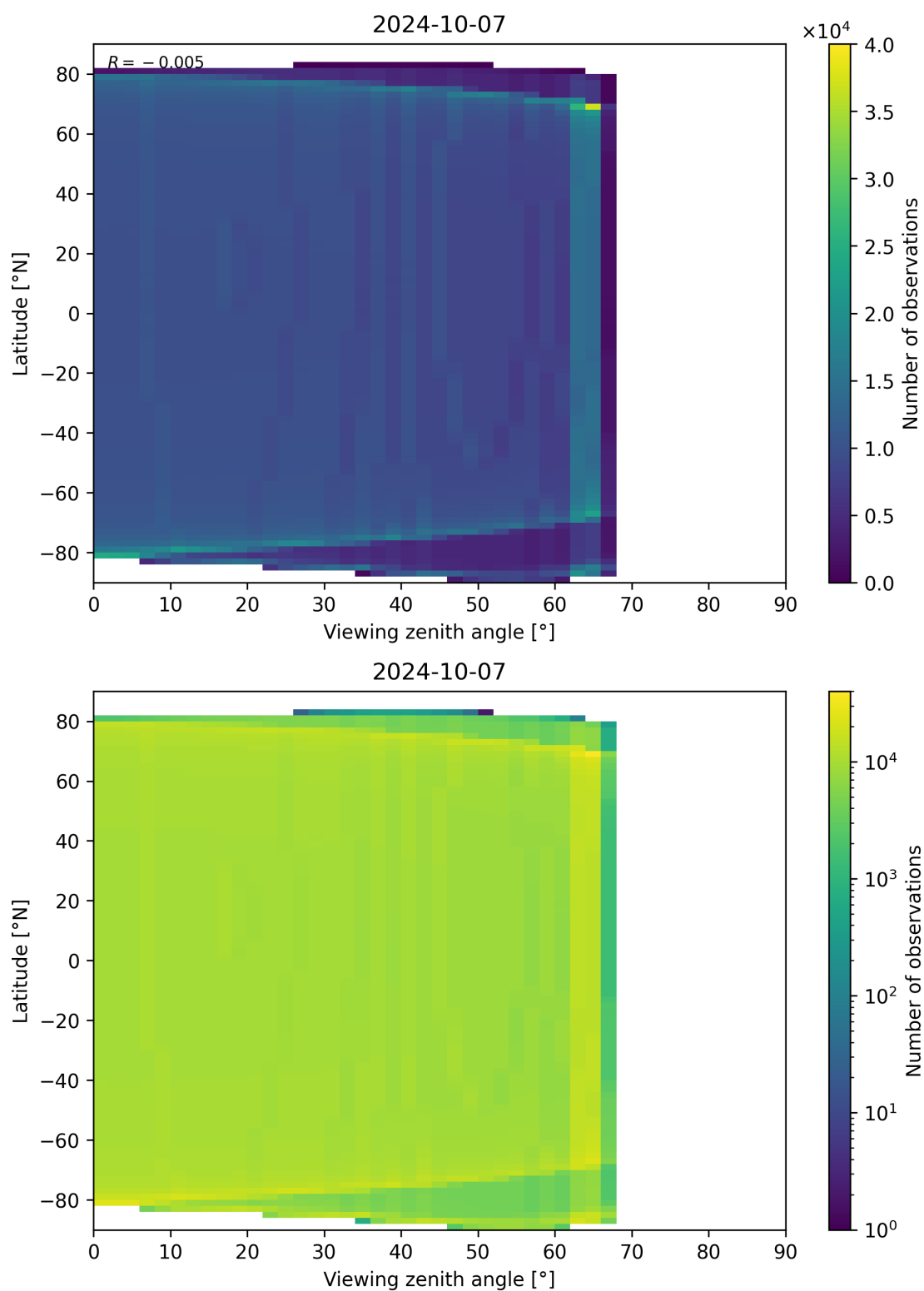
Figure 163: Scatter density plot of “Viewing zenith angle” against “Latitude” for 2024-10-06 to 2024-10-08.
