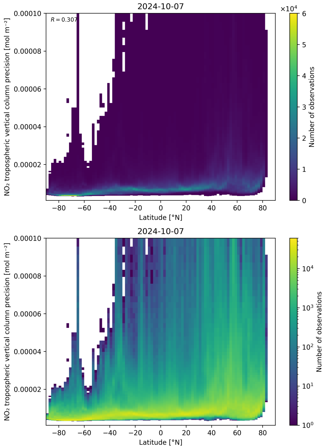
Figure 93: Scatter density plot of “Latitude” against “NO 2 tropospheric vertical column precision” for 2024-10-06 to 2024-10-08.
