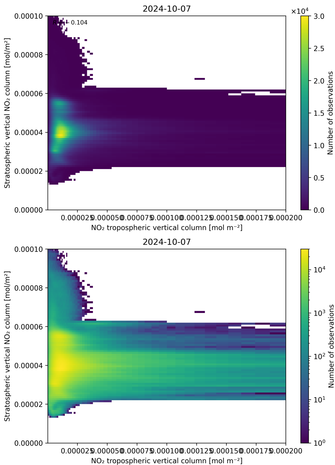
Figure 125: Scatter density plot of “NO 2 tropospheric vertical column” against “Stratospheric vertical NO 2 column” for 2024-10-06 to 2024-10-08.
