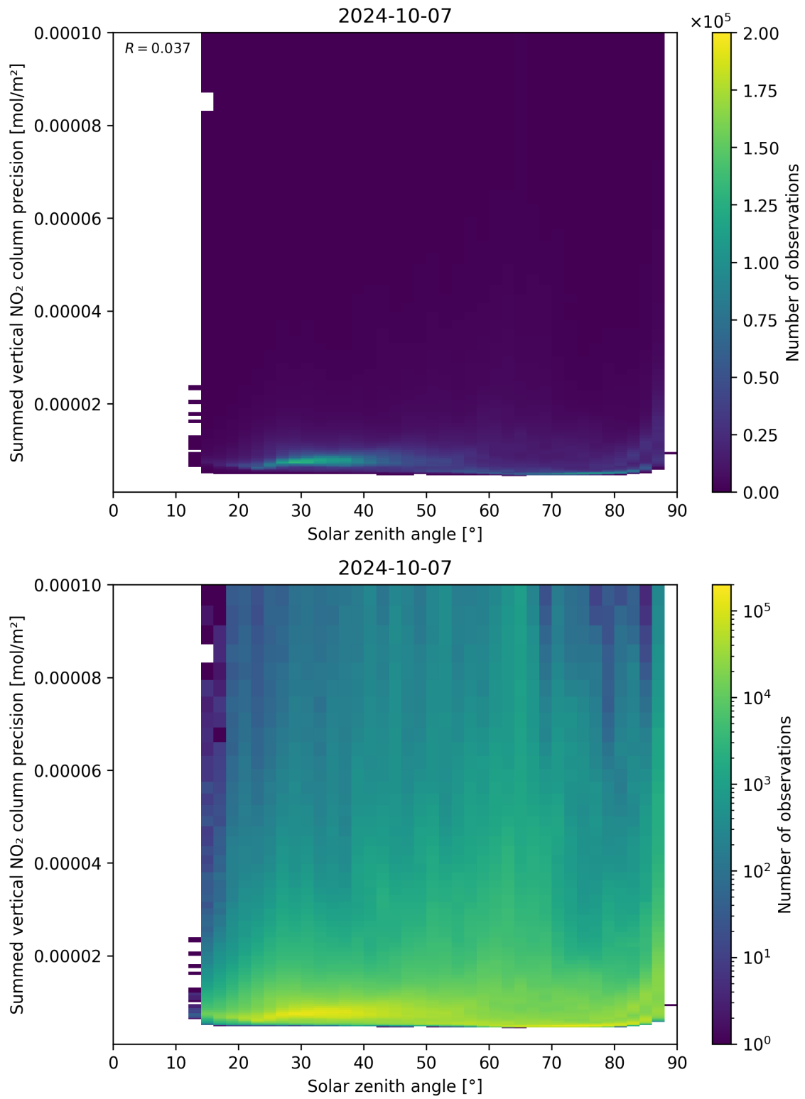
Figure 152: Scatter density plot of “Solar zenith angle” against “Summed vertical NO 2 column precision” for 2024-10-06 to 2024-10-08.
