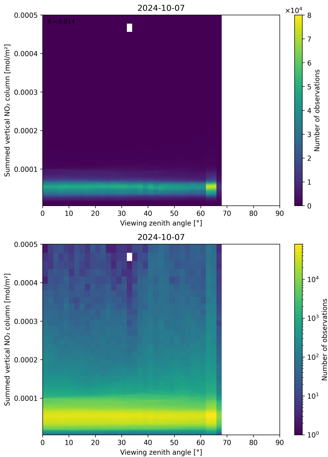
Figure 165: Scatter density plot of “Viewing zenith angle” against “Summed vertical NO 2 column” for 2024-10-06 to 2024-10-08.
