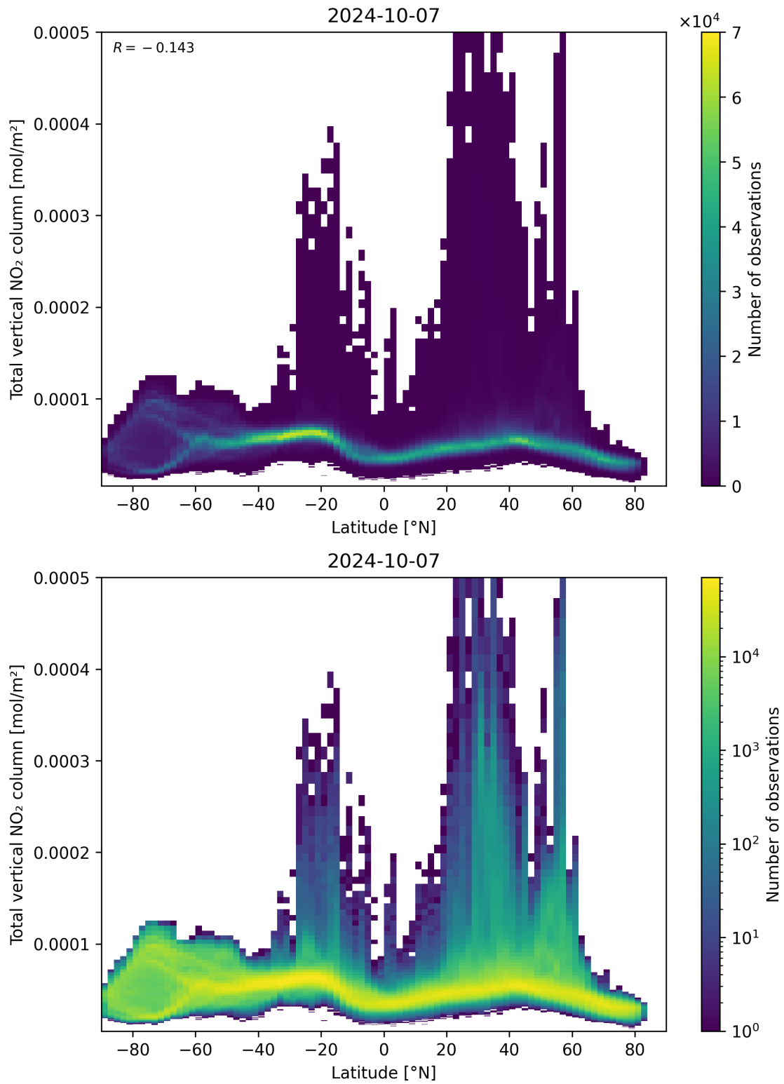
Figure 90: Scatter density plot of “Latitude” against “Total vertical NO 2 column” for 2024-10-06 to 2024-10-08.
