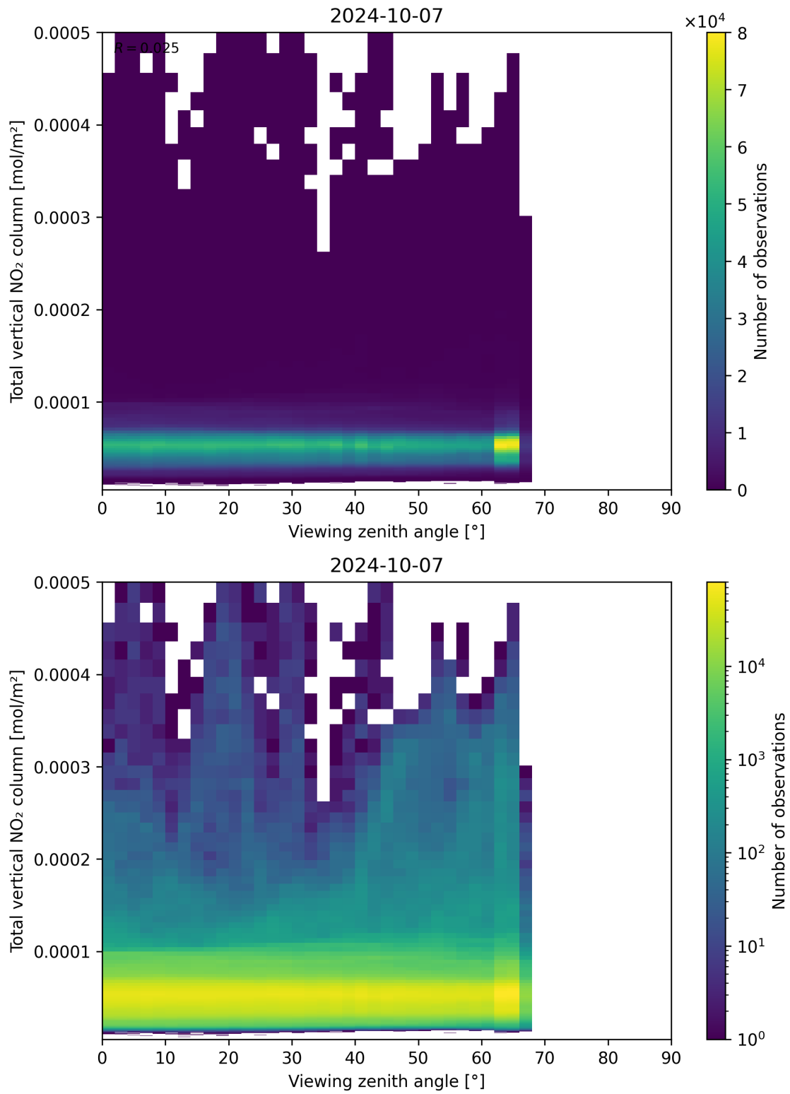
Figure 167: Scatter density plot of “Viewing zenith angle” against “Total vertical NO 2 column” for 2024-10-06 to 2024-10-08.
