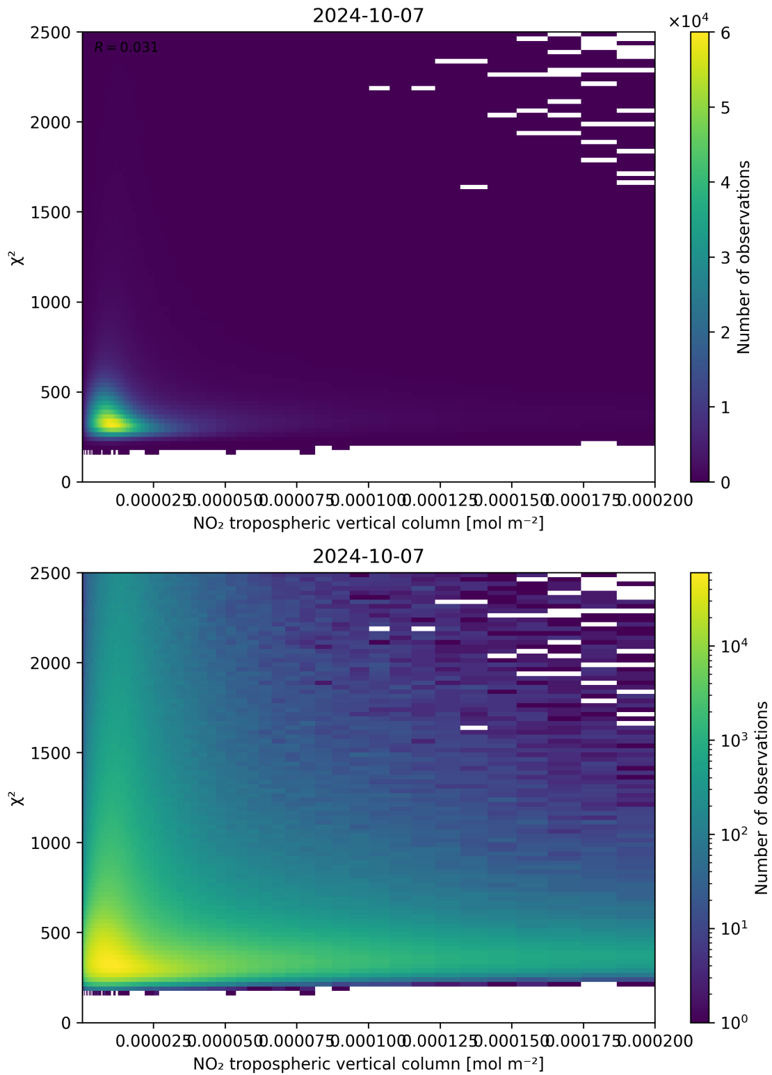
Figure 124: Scatter density plot of “NO 2 tropospheric vertical column” against “ \chi^2 ” for 2024-10-06 to 2024-10-08.
