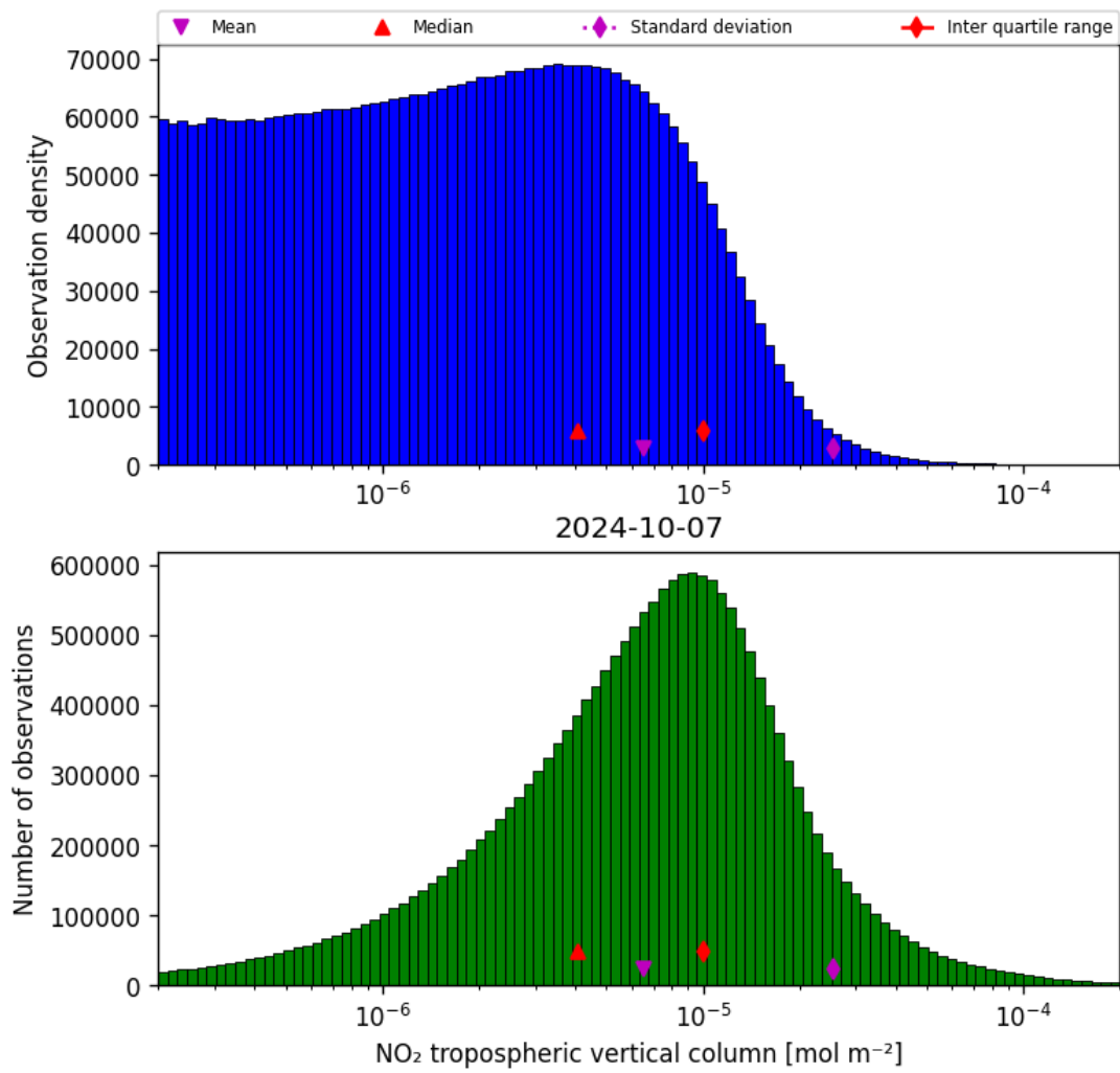
Figure 29: Histogram of “NO 2 tropospheric vertical column” for 2024-10-06 to 2024-10-08
