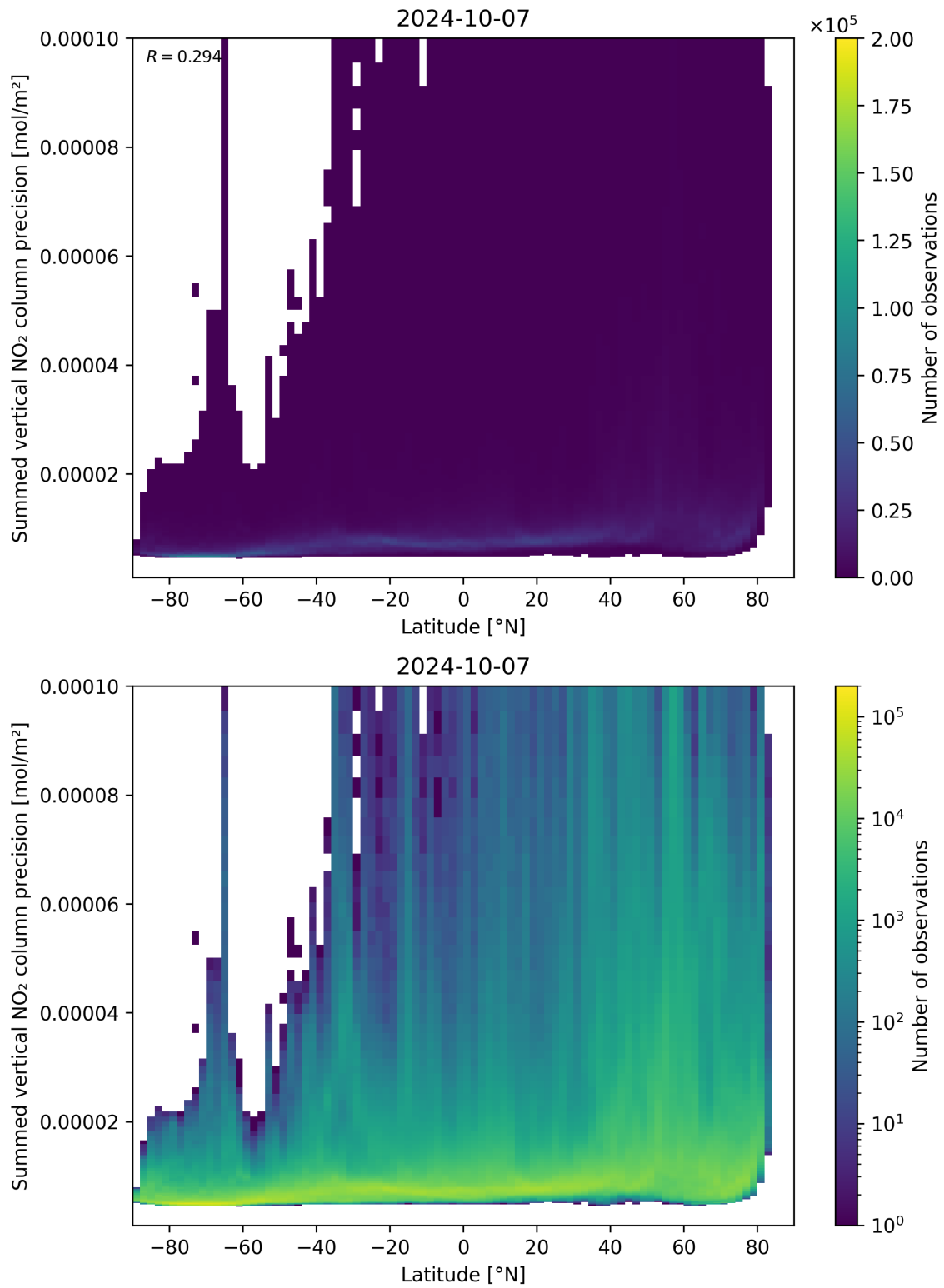
Figure 89: Scatter density plot of “Latitude” against “Summed vertical NO 2 column precision” for 2024-10-06 to 2024-10-08.
