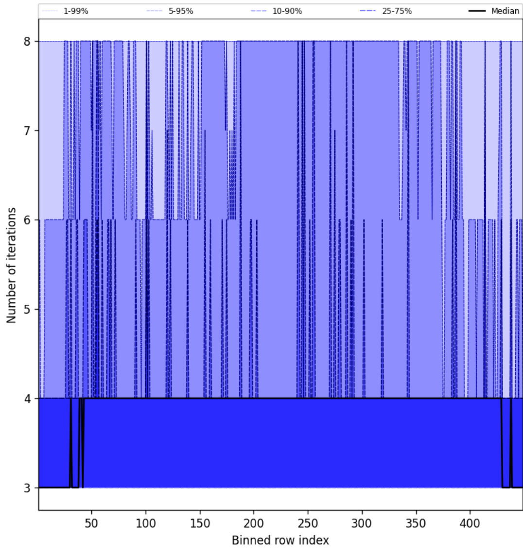
Figure 51: Along track statistics of “Number of iterations” for 2024-10-06 to 2024-10-08
