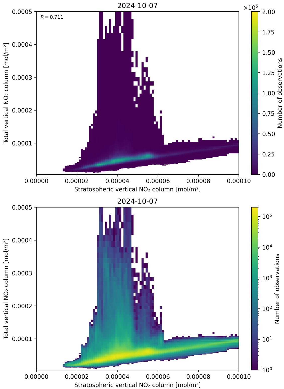
Figure 100: Scatter density plot of “Stratospheric vertical NO 2 column” against “Total vertical NO 2 column” for 2024-10-06 to 2024-10-08.
