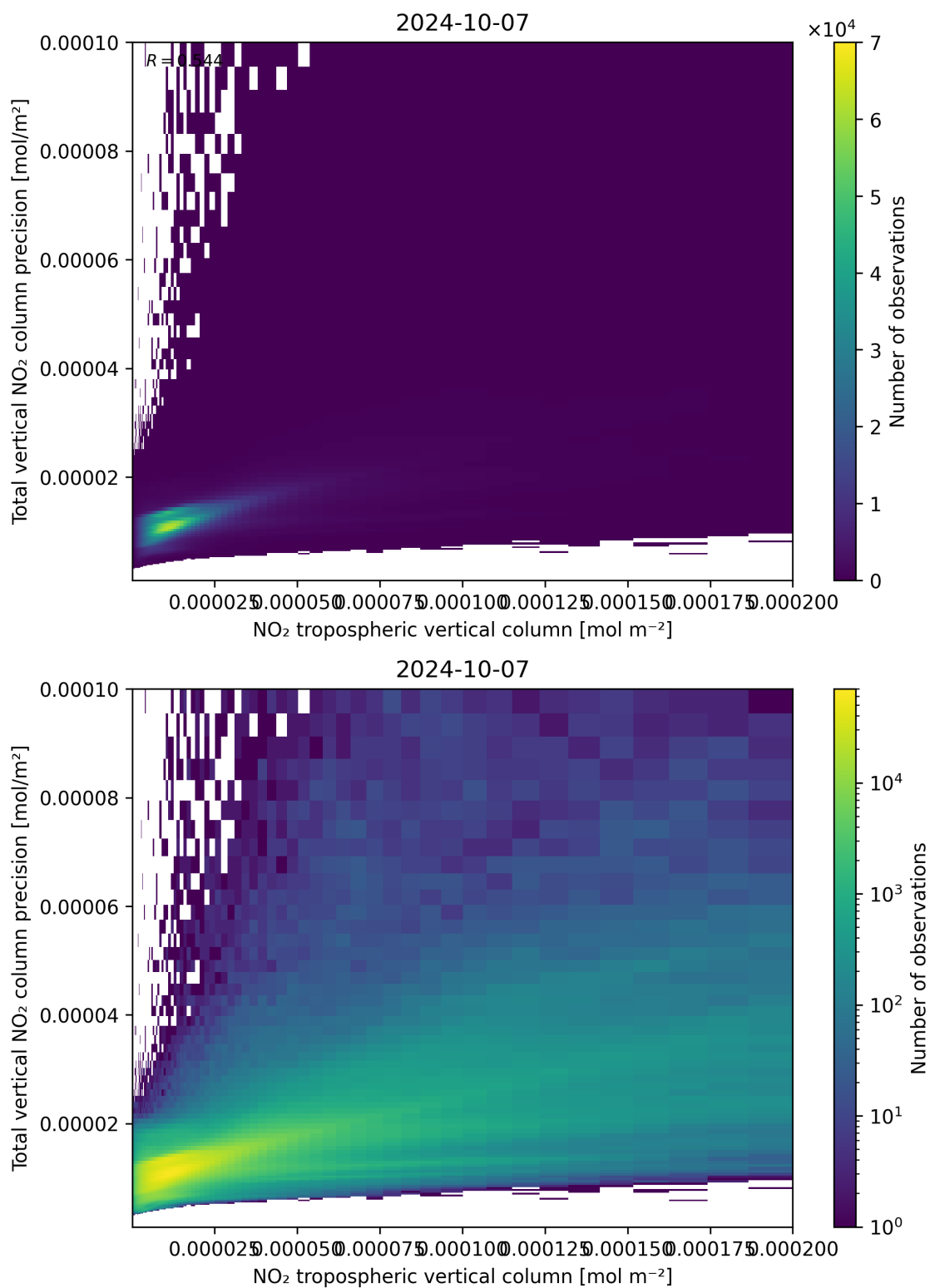
Figure 129: Scatter density plot of “NO 2 tropospheric vertical column” against “Total vertical NO 2 column precision” for 2024-10-06 to 2024-10-08.
