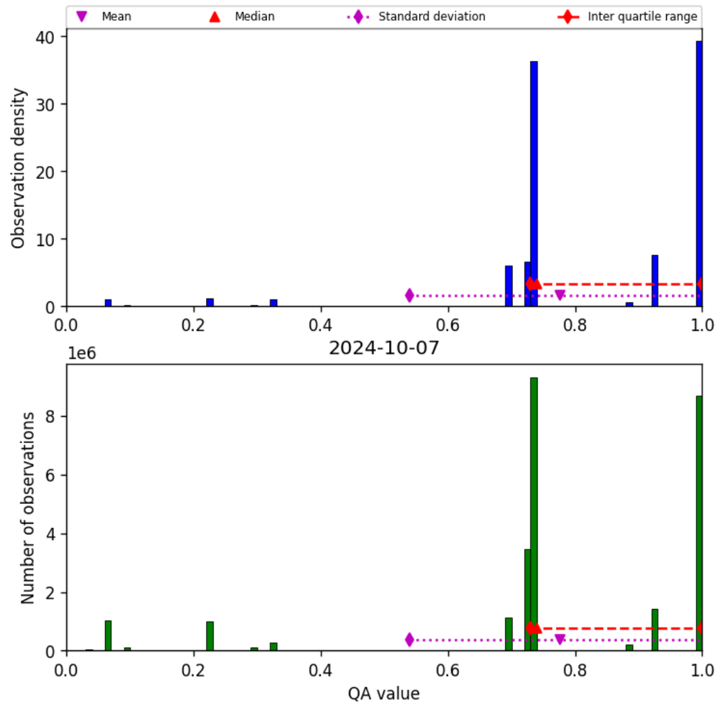
Figure 28: Histogram of “QA value” for 2024-10-06 to 2024-10-08
