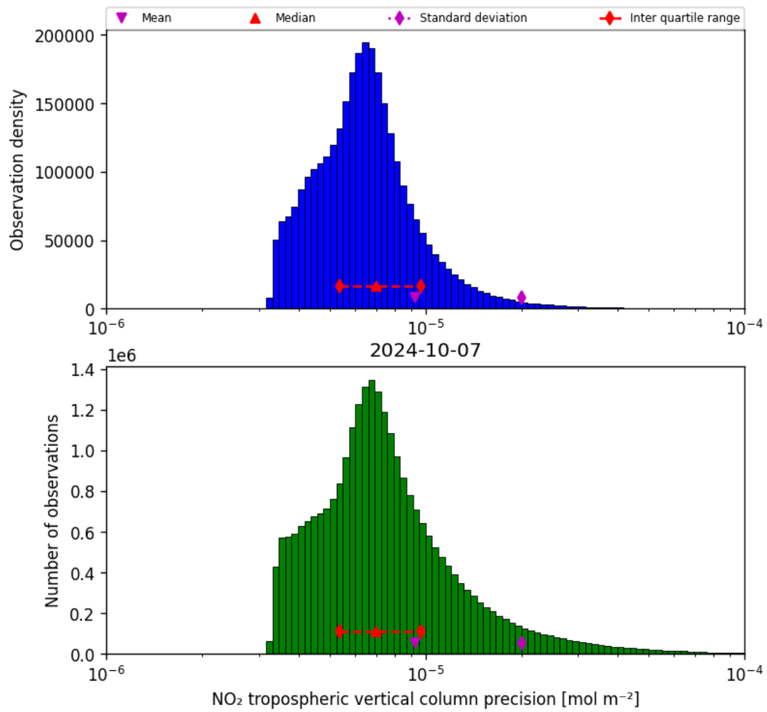
Figure 30: Histogram of “NO 2 tropospheric vertical column precision” for 2024-10-06 to 2024-10-08
