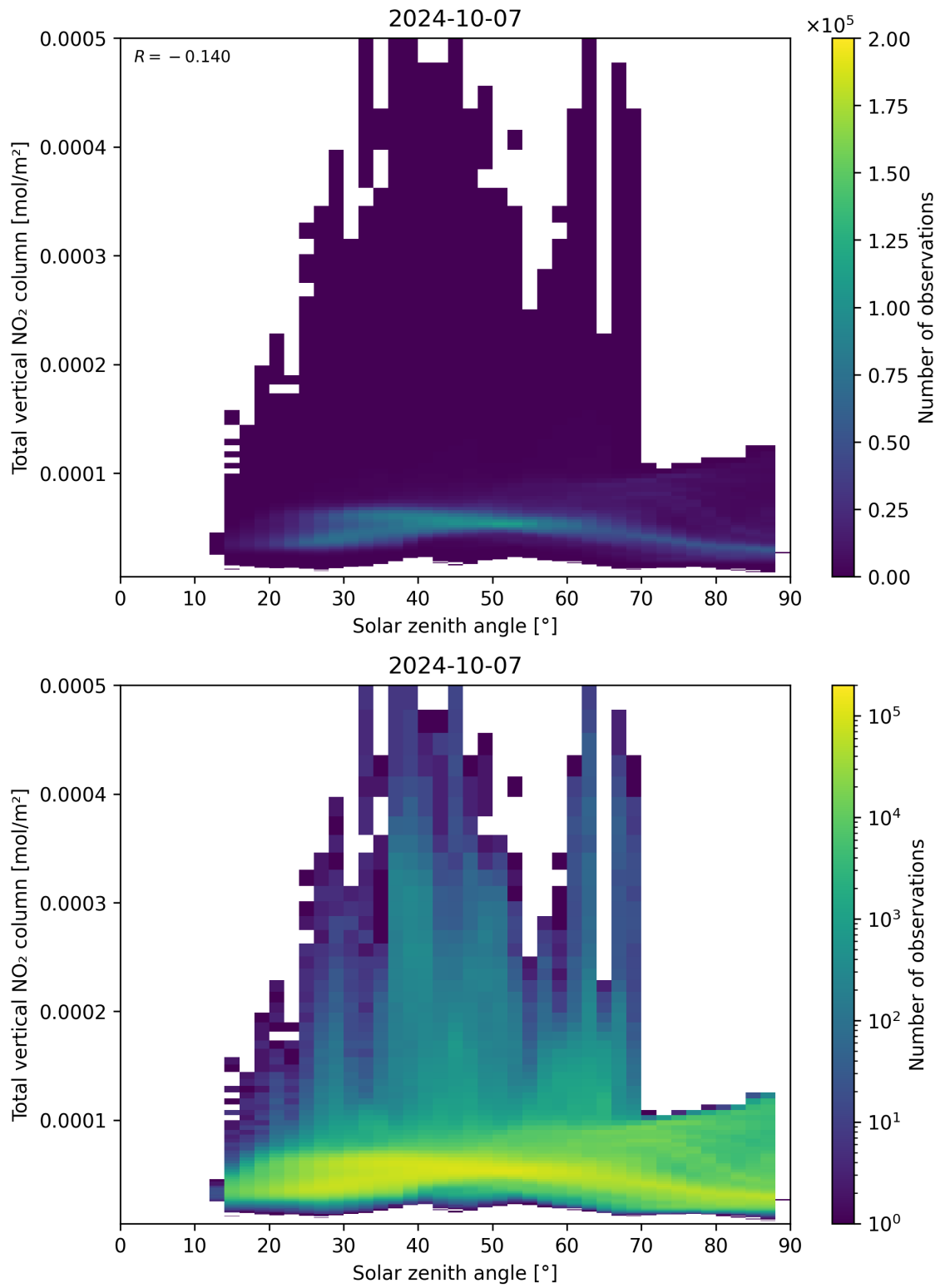
Figure 153: Scatter density plot of “Solar zenith angle” against “Total vertical NO 2 column” for 2024-10-06 to 2024-10-08.
