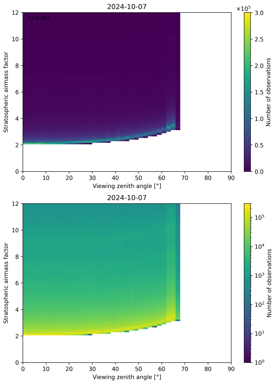
Figure 159: Scatter density plot of “Viewing zenith angle” against “Stratospheric airmass factor” for 2024-10-06 to 2024-10-08.
