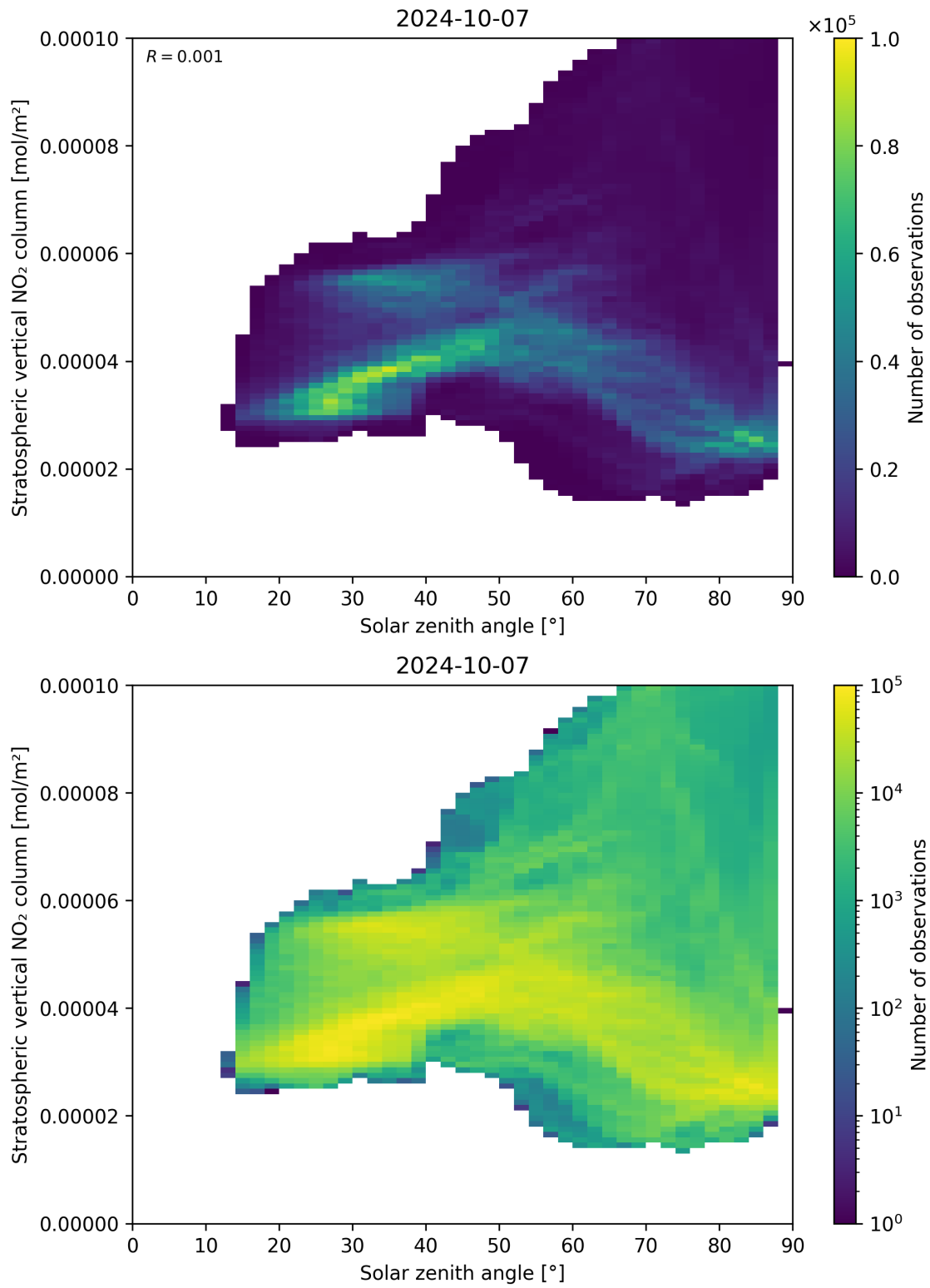
Figure 150: Scatter density plot of “Solar zenith angle” against “Stratospheric vertical NO 2 column” for 2024-10-06 to 2024-10-08.
