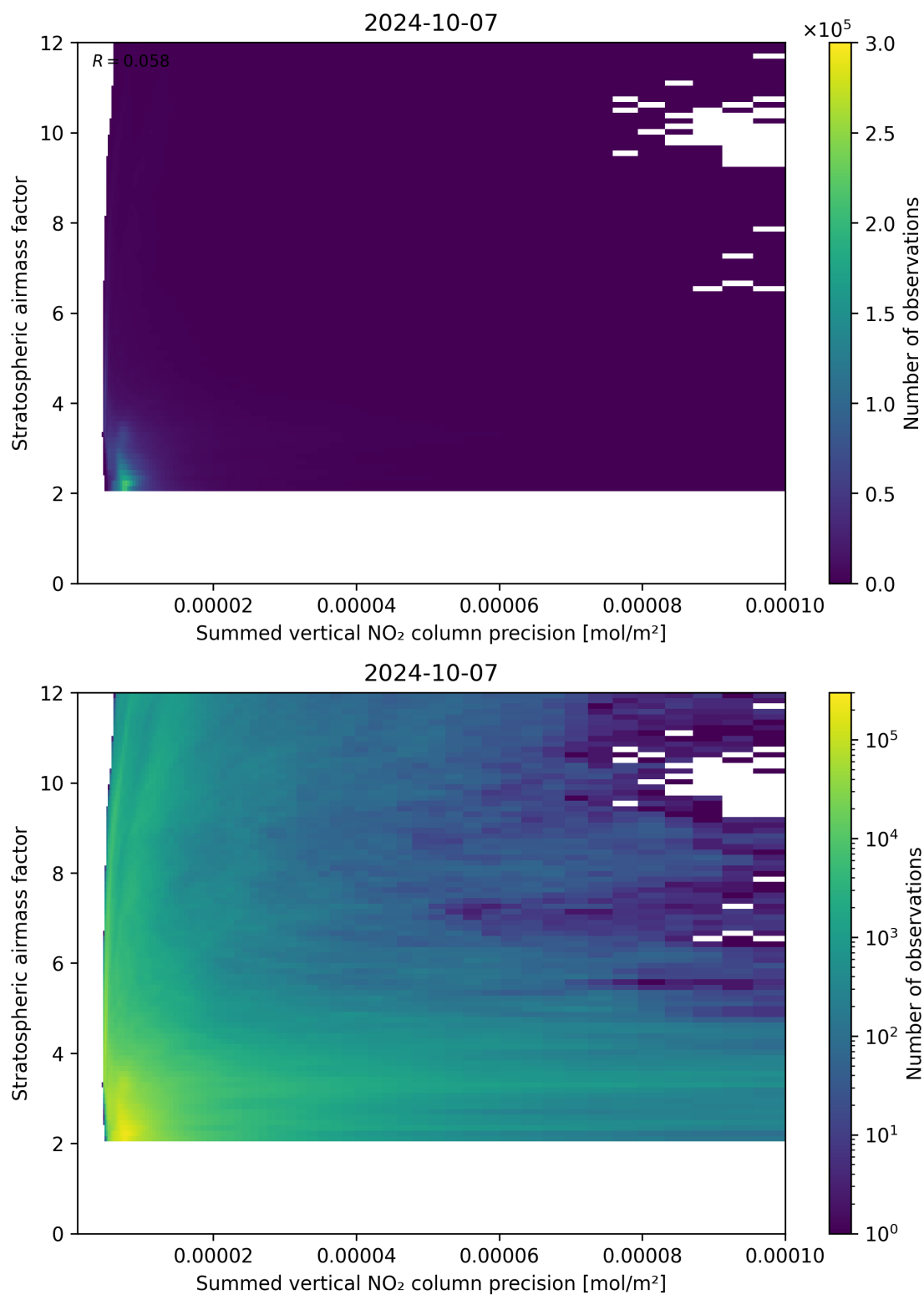
Figure 106: Scatter density plot of “Summed vertical NO 2 column precision” against “Stratospheric airmass factor” for 2024-10-06 to 2024-10-08.
