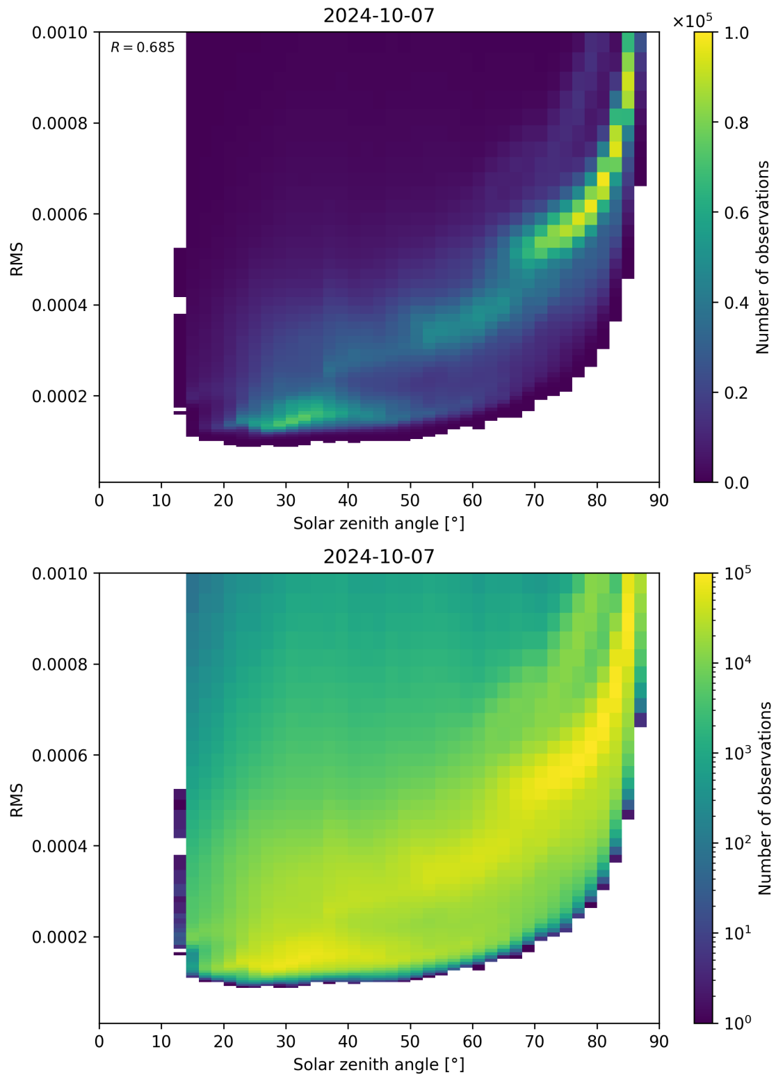
Figure 157: Scatter density plot of “Solar zenith angle” against “RMS” for 2024-10-06 to 2024-10-08.
