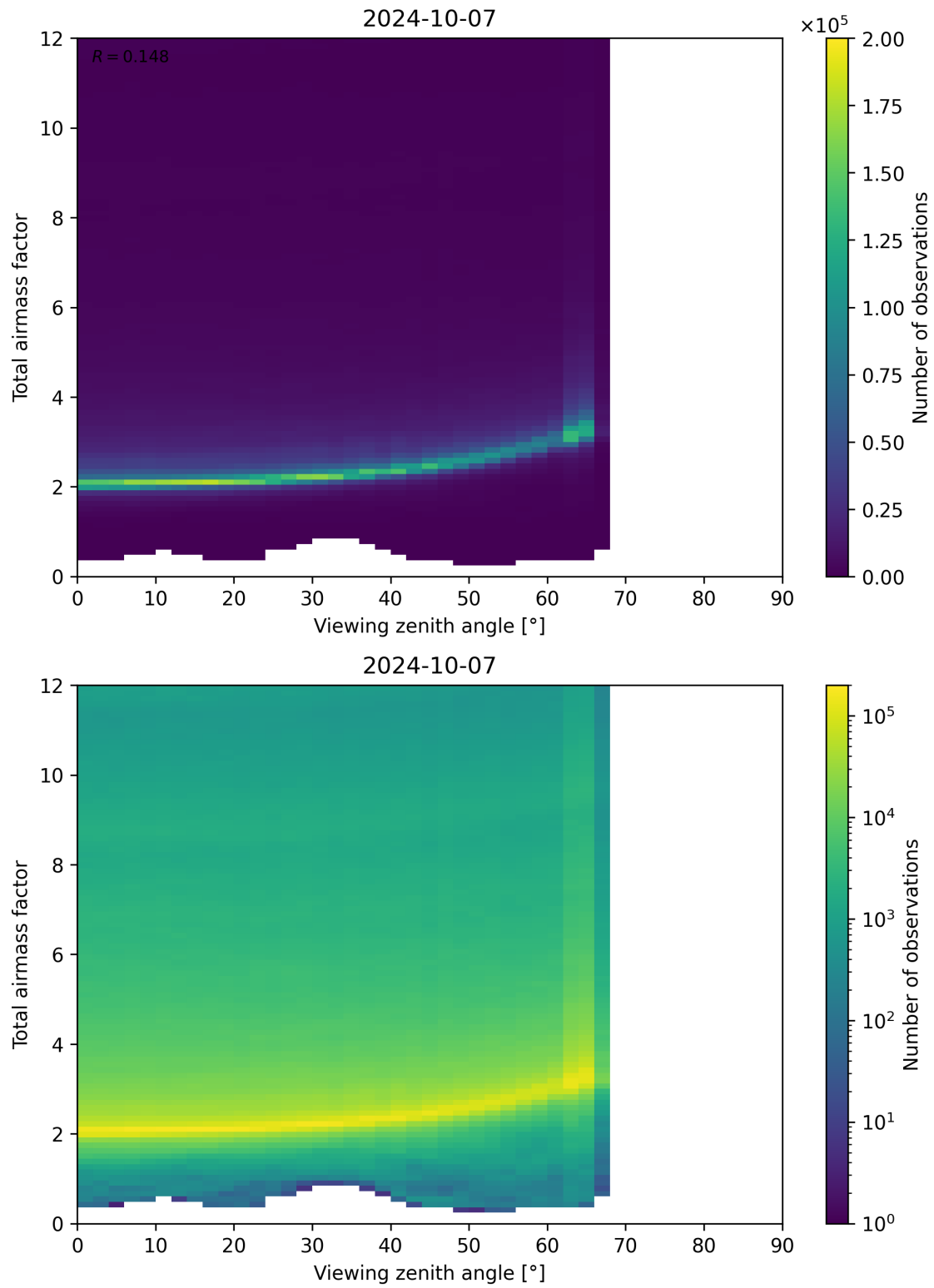
Figure 160: Scatter density plot of “Viewing zenith angle” against “Total airmass factor” for 2024-10-06 to 2024-10-08.
