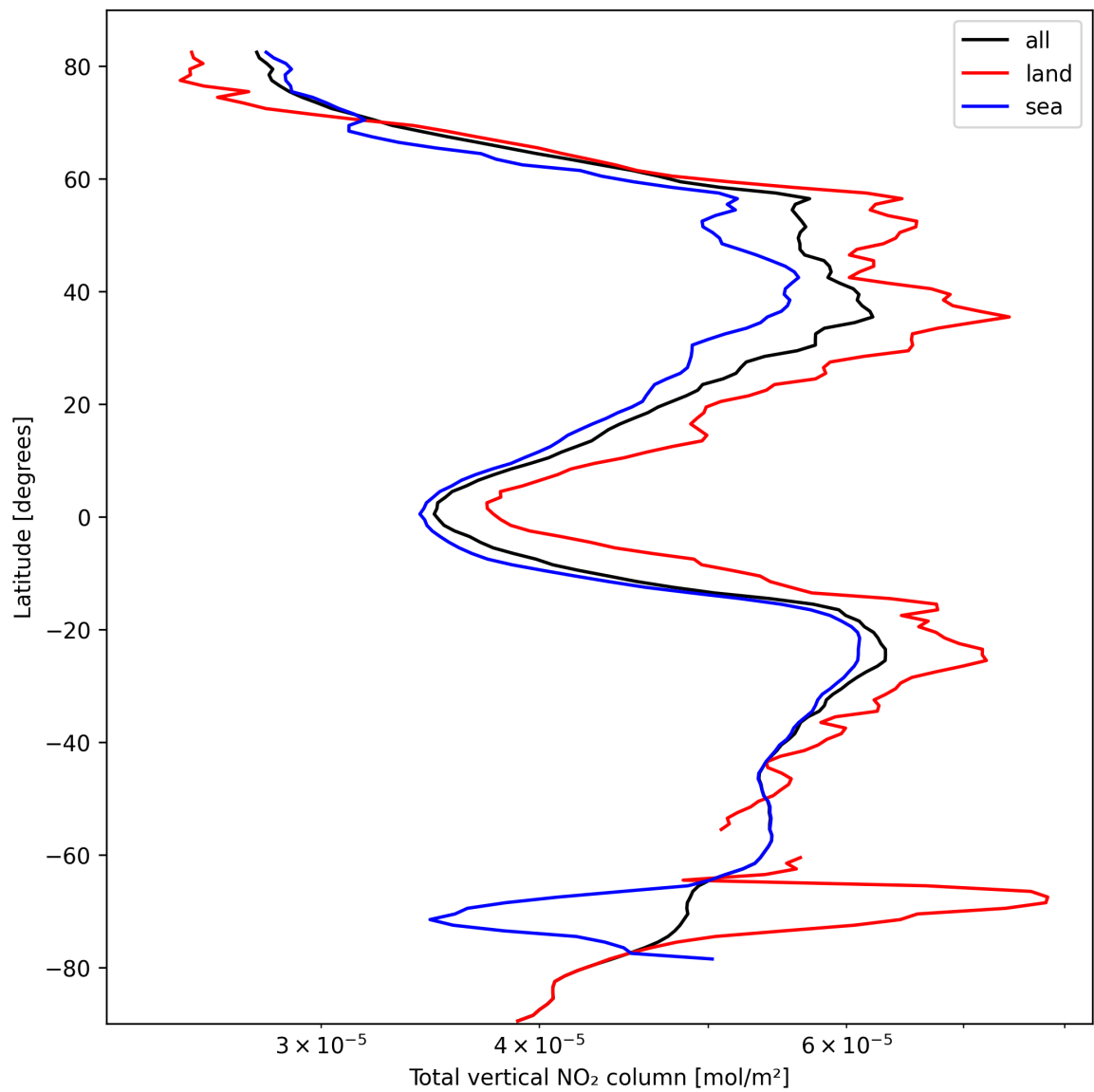
Figure 21: Zonal average of “Total vertical NO 2 column” for 2024-10-06 to 2024-10-08.
