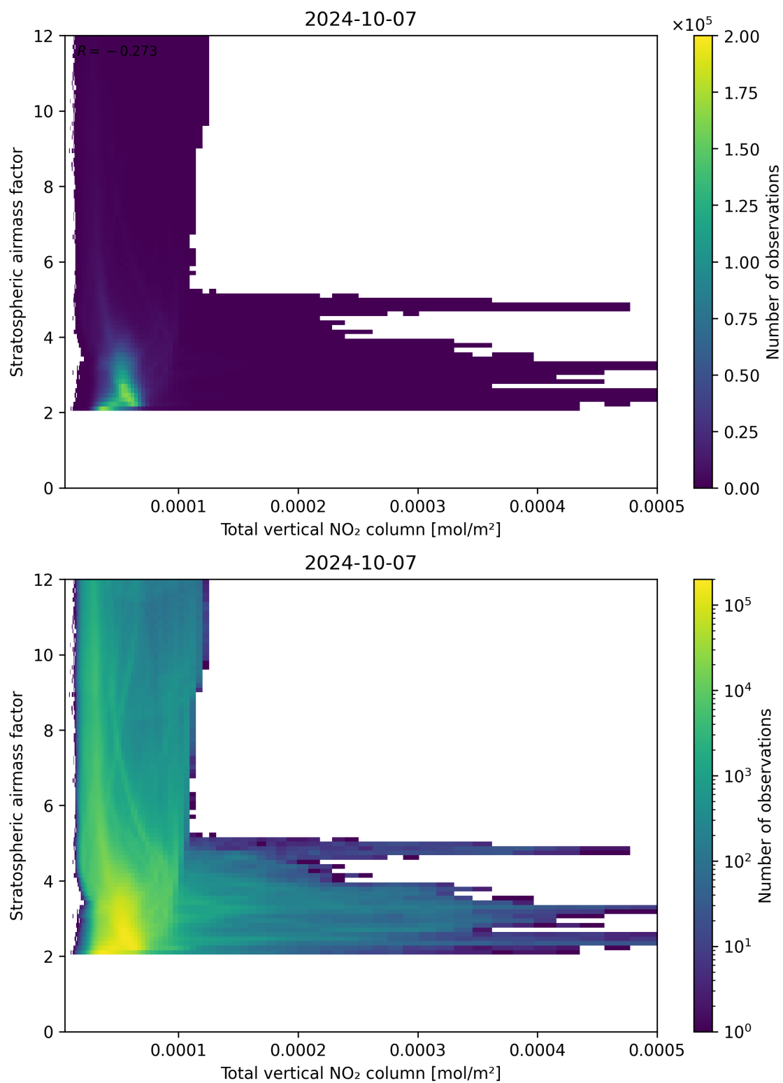
Figure 110: Scatter density plot of “Total vertical NO 2 column” against “Stratospheric airmass factor” for 2024-10-06 to 2024-10-08.
