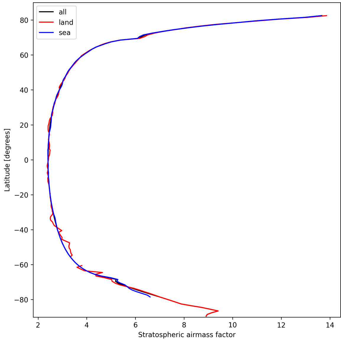
Figure 27: Zonal average of “Stratospheric airmass factor” for 2024-10-06 to 2024-10-08.
