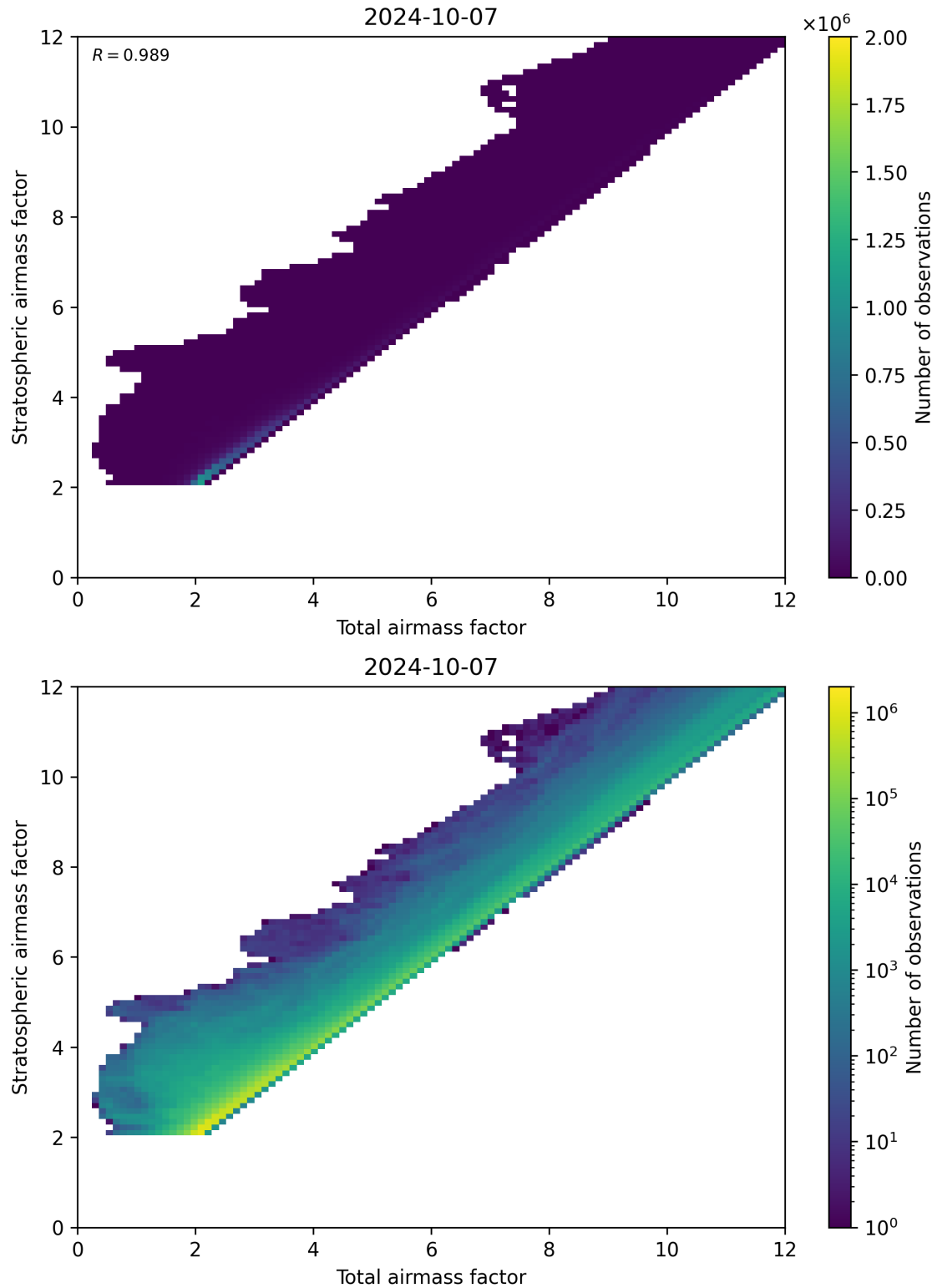
Figure 62: Scatter density plot of “Total airmass factor” against “Stratospheric airmass factor” for 2024-10-06 to 2024-10-08.
