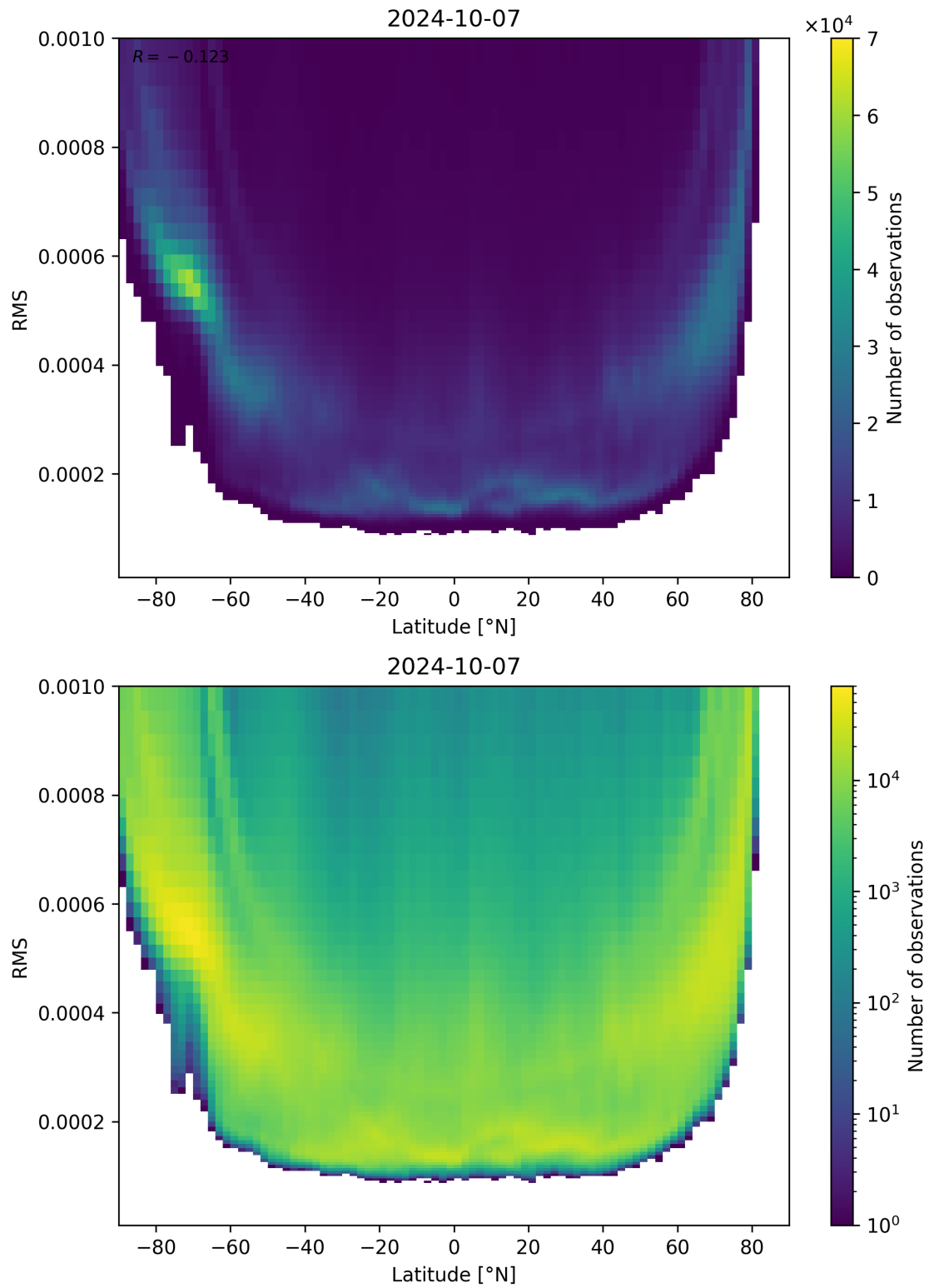
Figure 94: Scatter density plot of “Latitude” against “RMS” for 2024-10-06 to 2024-10-08.
