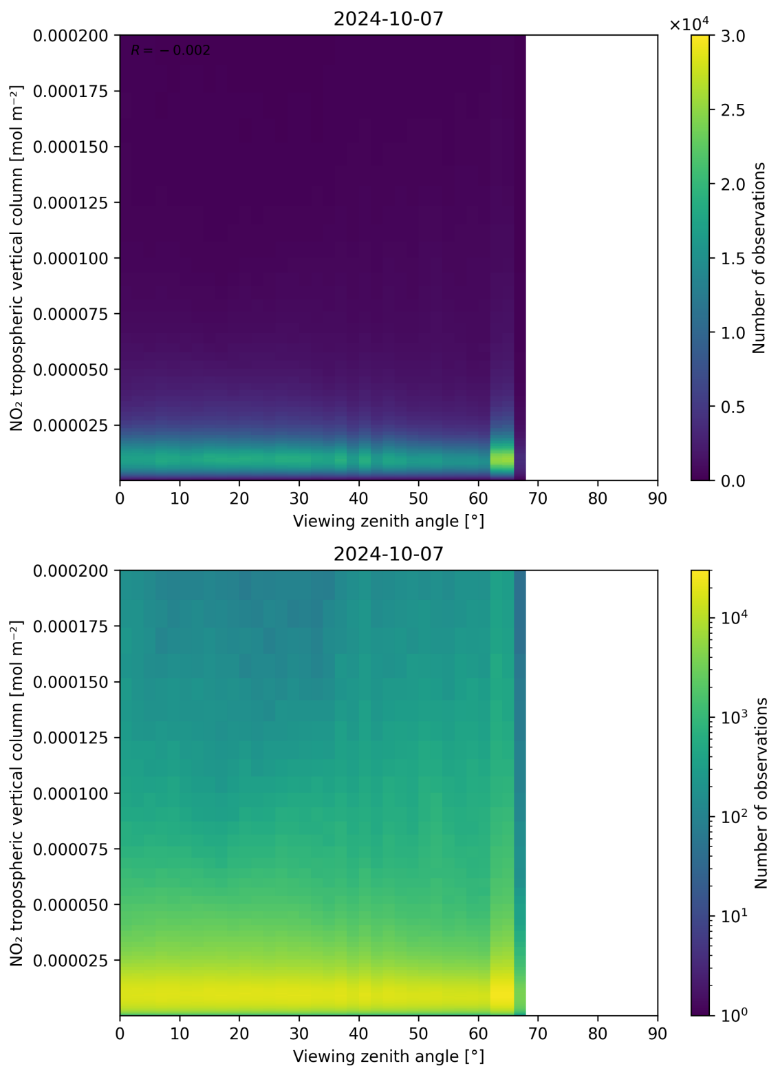
Figure 169: Scatter density plot of “Viewing zenith angle” against “NO 2 tropospheric vertical column” for 2024-10-06 to 2024-10-08.
