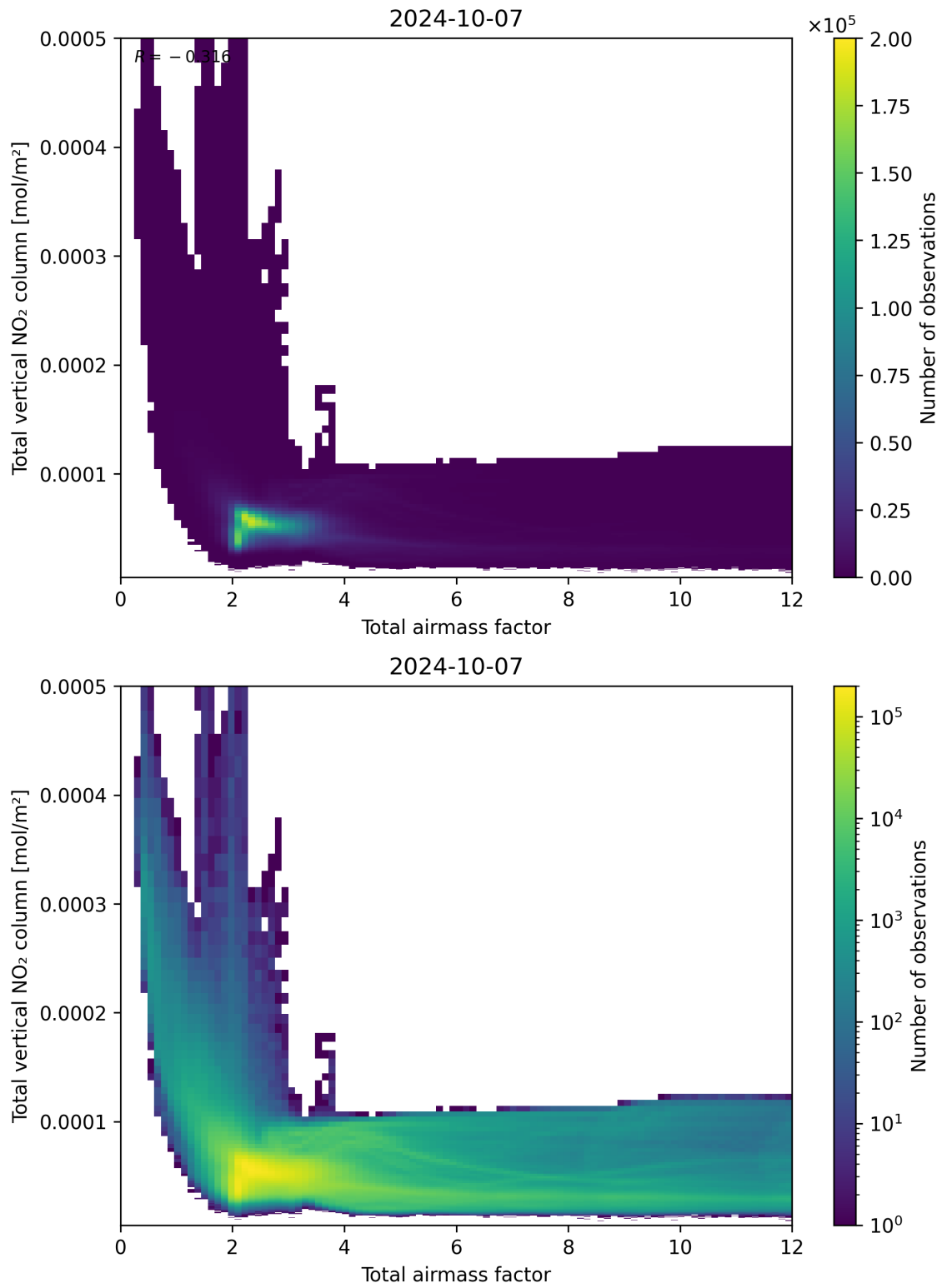
Figure 67: Scatter density plot of “Total airmass factor” against “Total vertical NO 2 column” for 2024-10-06 to 2024-10-08.
