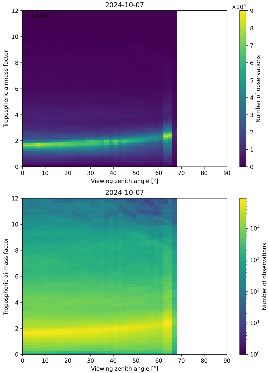
Figure 161: Scatter density plot of “Viewing zenith angle” against “Tropospheric air mass factor” for 2024-10-06 to 2024-10-08.
