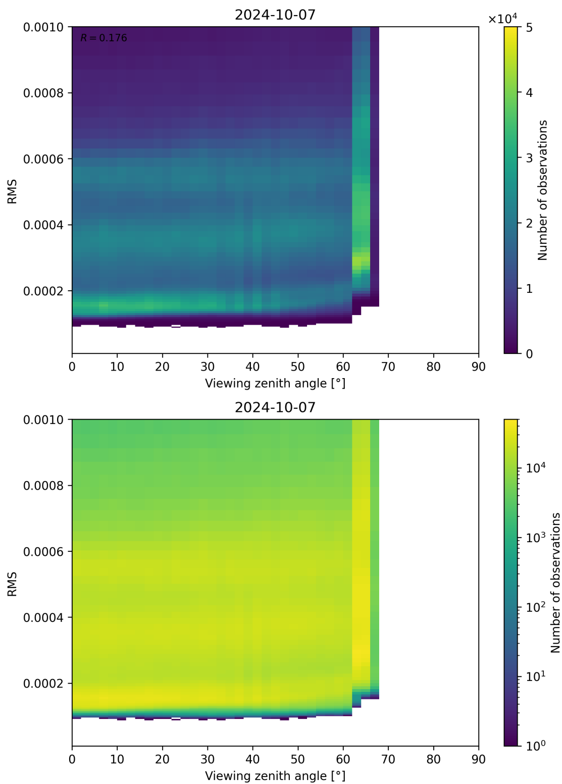
Figure 171: Scatter density plot of “Viewing zenith angle” against “RMS” for 2024-10-06 to 2024-10-08.
