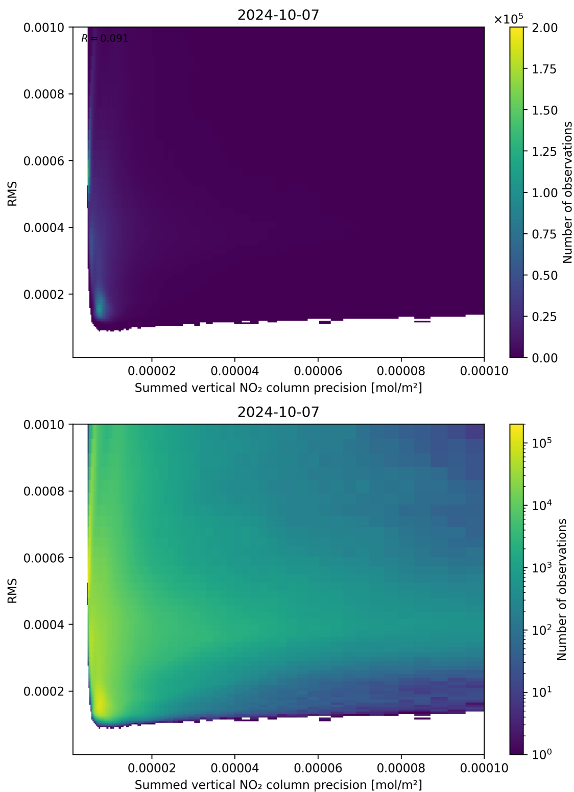
Figure 108: Scatter density plot of “Summed vertical NO 2 column precision” against “RMS” for 2024-10-06 to 2024-10-08.
