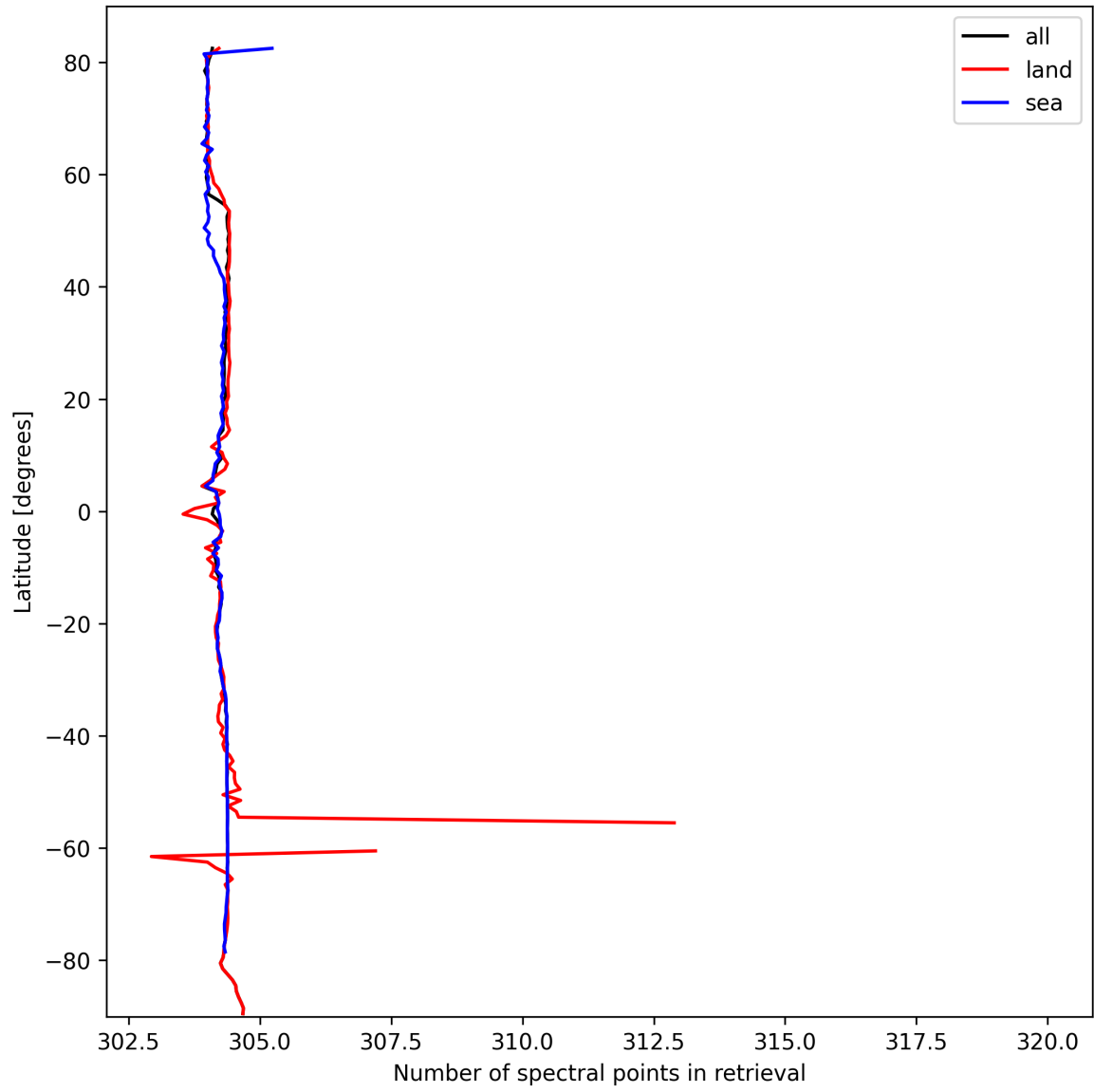
Figure 16: Zonal average of “Number of spectral points in retrieval” for 2024-10-06 to 2024-10-08.
