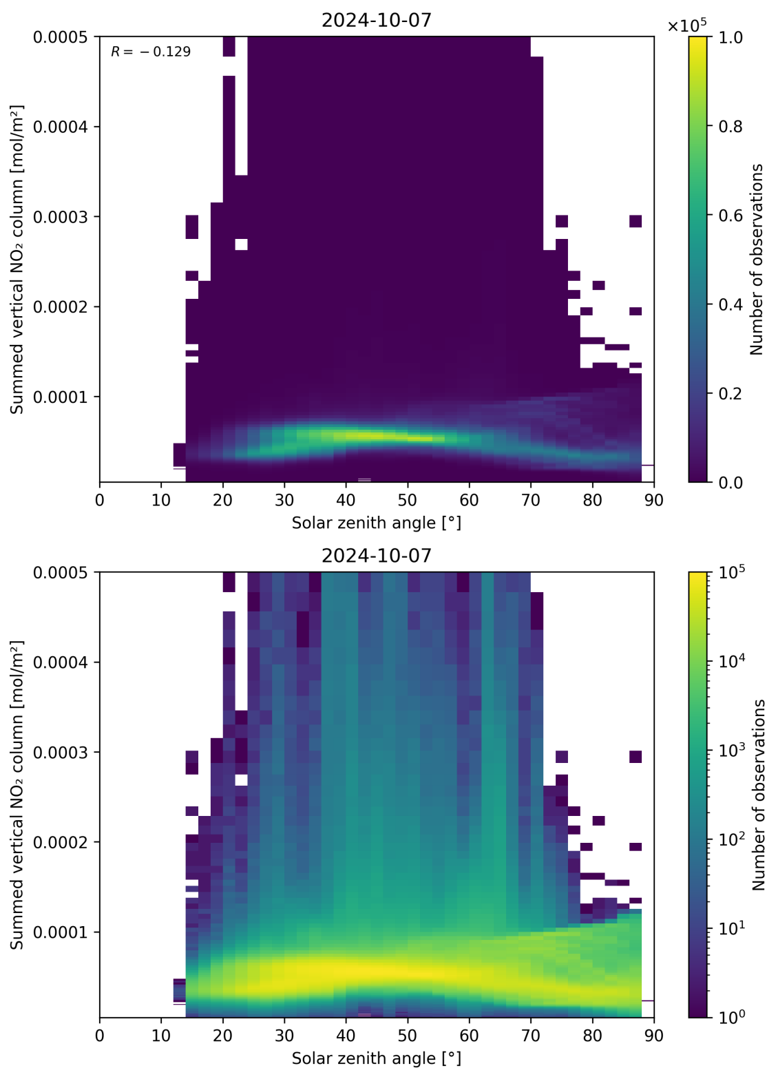
Figure 151: Scatter density plot of “Solar zenith angle” against “Summed vertical NO 2 column” for 2024-10-06 to 2024-10-08.
