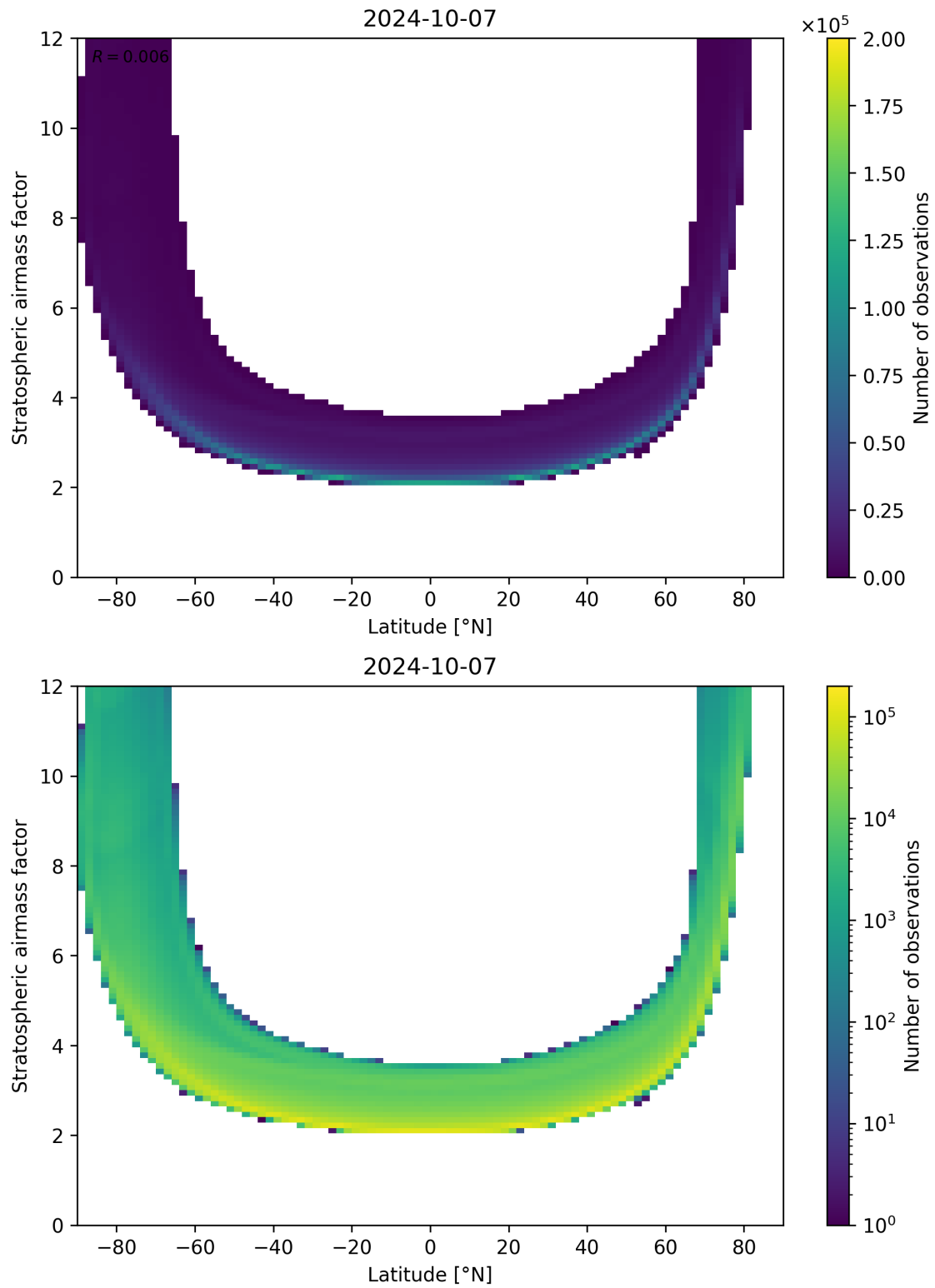
Figure 83: Scatter density plot of “Latitude” against “Stratospheric airmass factor” for 2024-10-06 to 2024-10-08.
