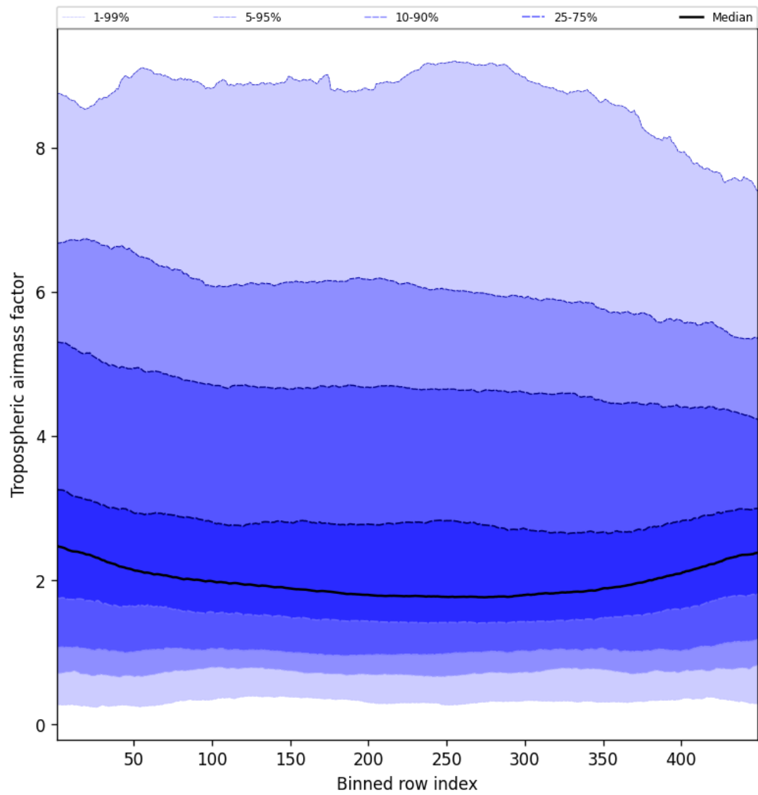
Figure 48: Along track statistics of “Tropospheric air mass factor” for 2024-10-06 to 2024-10-08
