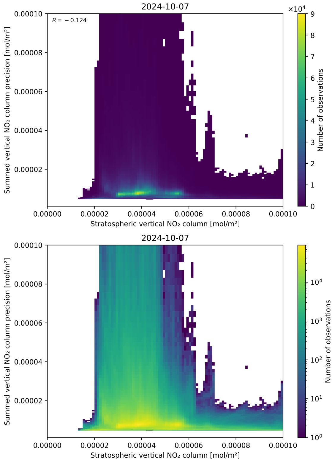
Figure 99: Scatter density plot of “Stratospheric vertical NO 2 column” against “Summed vertical NO 2 column precision” for 2024-10-06 to 2024-10-08.
