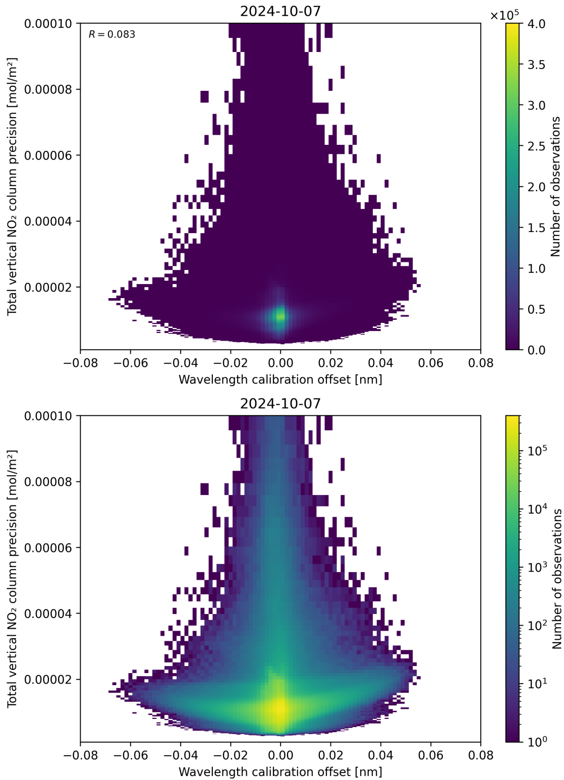
Figure 180: Scatter density plot of “Wavelength calibration offset” against “Total vertical NO 2 column precision” for 2024-10-06 to 2024-10-08.
