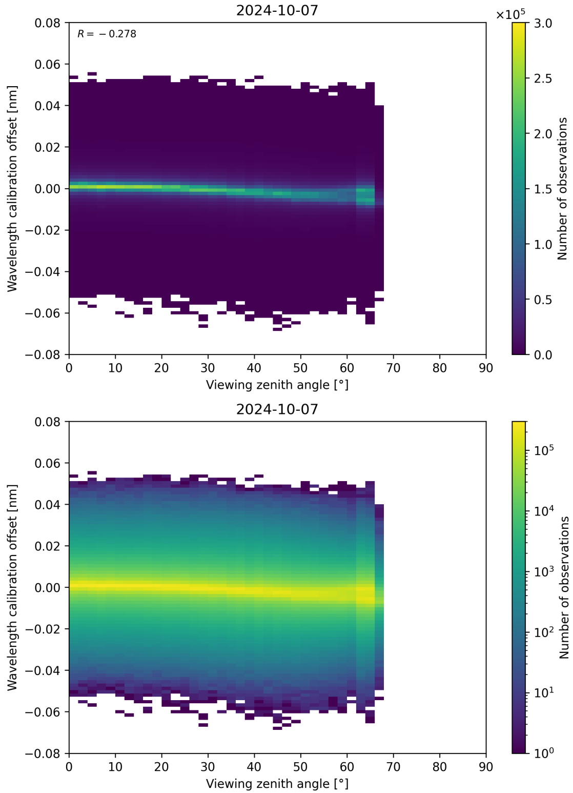
Figure 173: Scatter density plot of “Viewing zenith angle” against “Wavelength calibration offset” for 2024-10-06 to 2024-10-08.
