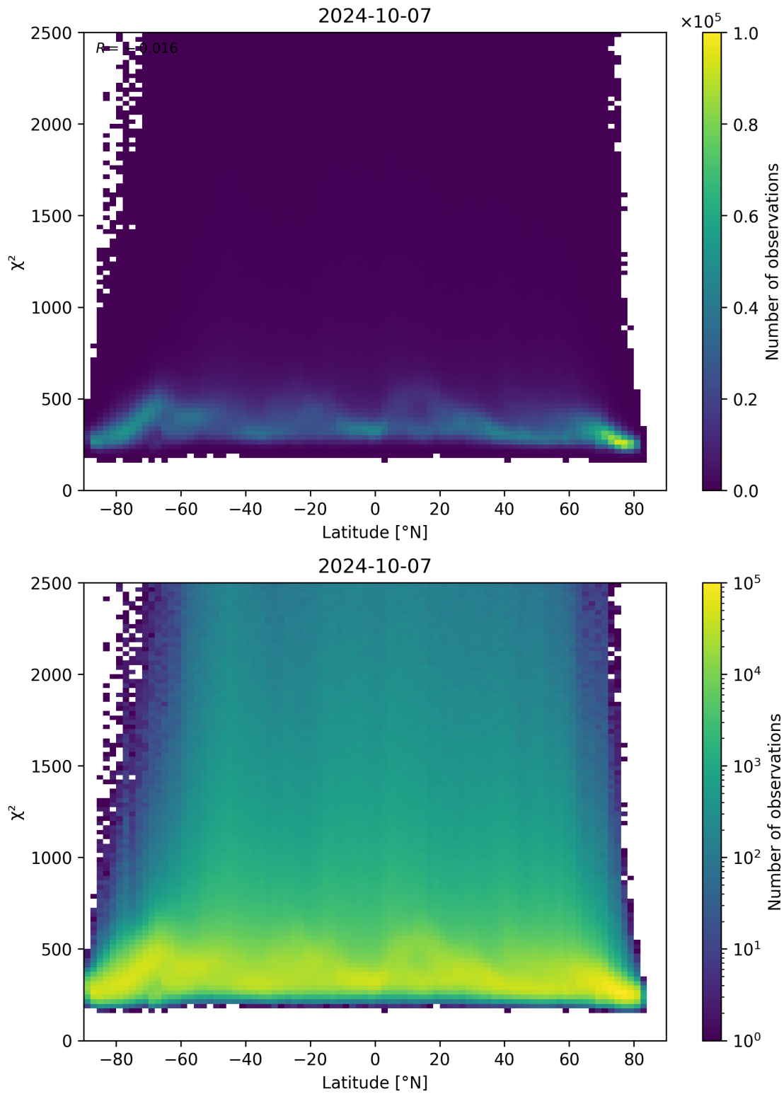
Figure 86: Scatter density plot of “Latitude” against “ \chi^2 ” for 2024-10-06 to 2024-10-08.
