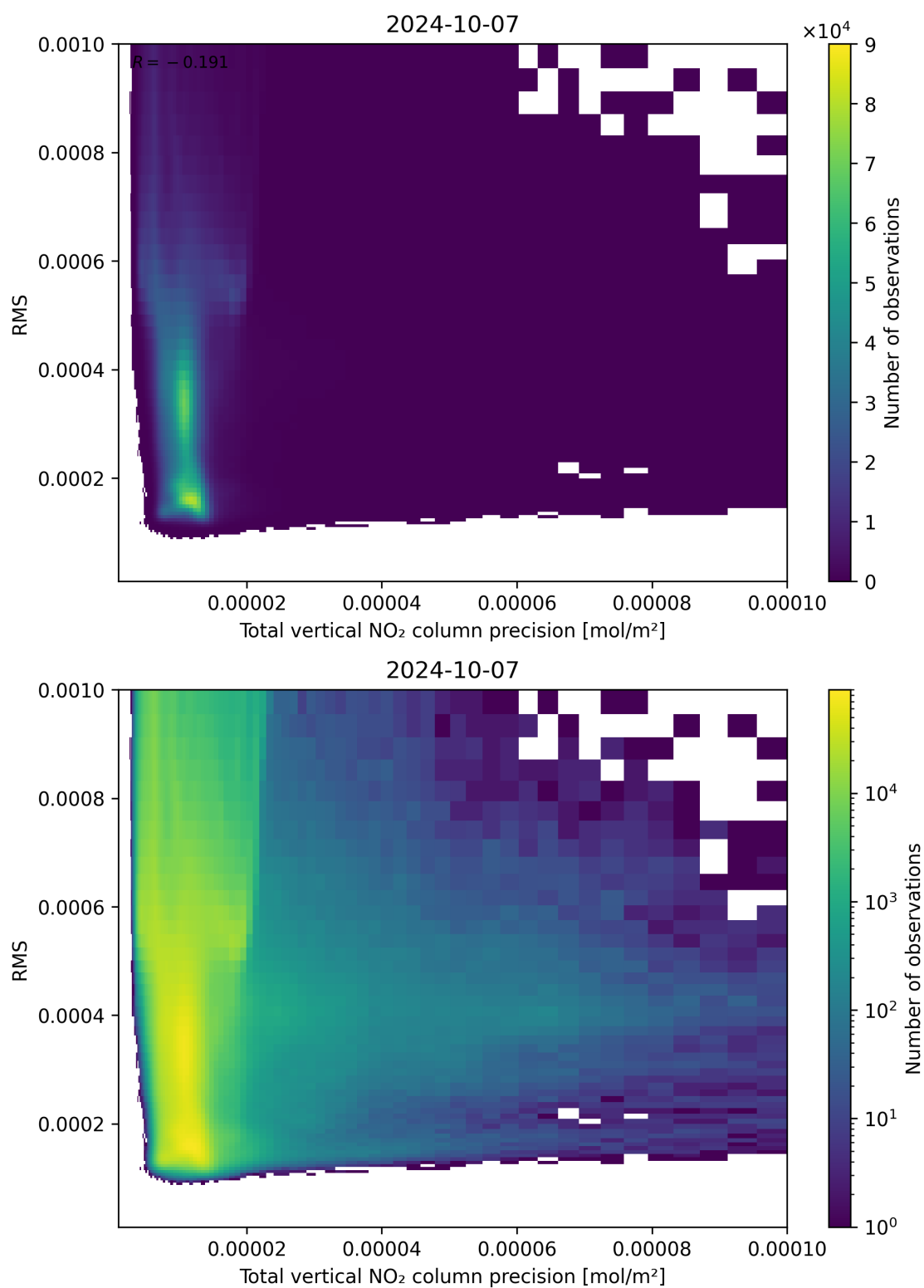
Figure 119: Scatter density plot of “Total vertical NO 2 column precision” against “RMS” for 2024-10-06 to 2024-10-08.
