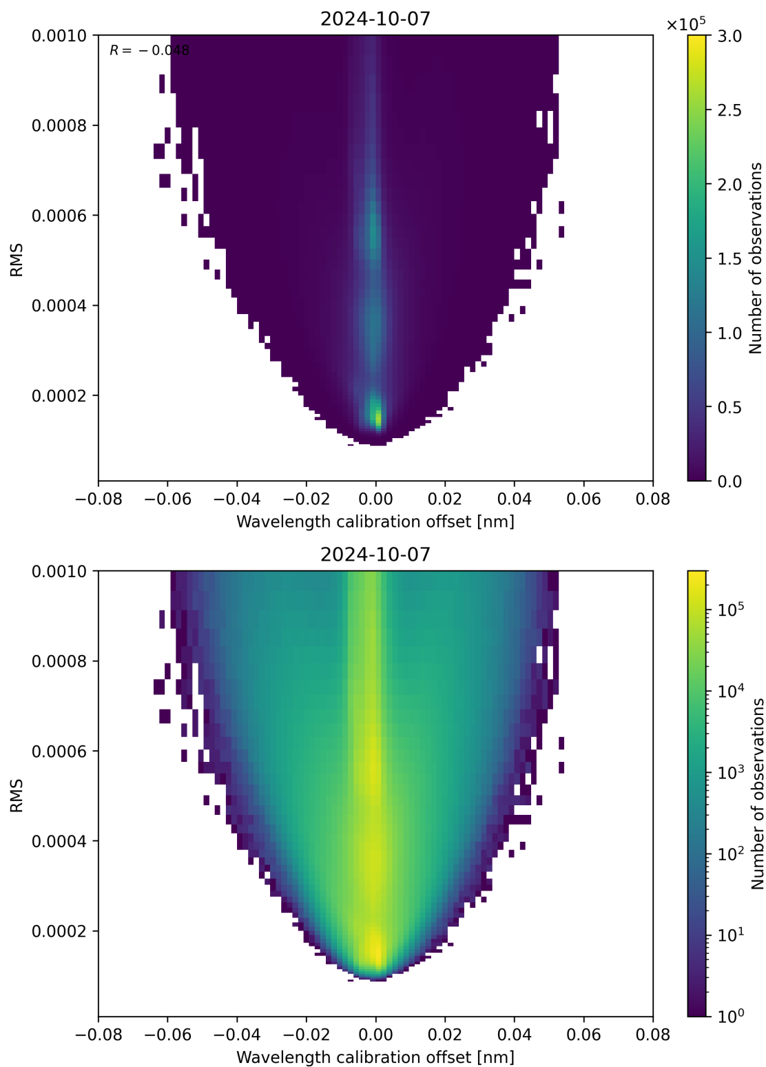
Figure 181: Scatter density plot of “Wavelength calibration offset” against “RMS” for 2024-10-06 to 2024-10-08.
