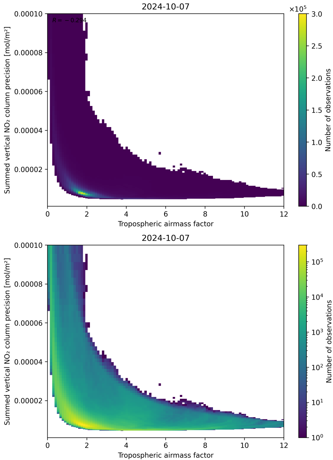
Figure 76: Scatter density plot of “Tropospheric air mass factor” against “Summed vertical NO 2 column precision” for 2024-10-06 to 2024-10-08.
