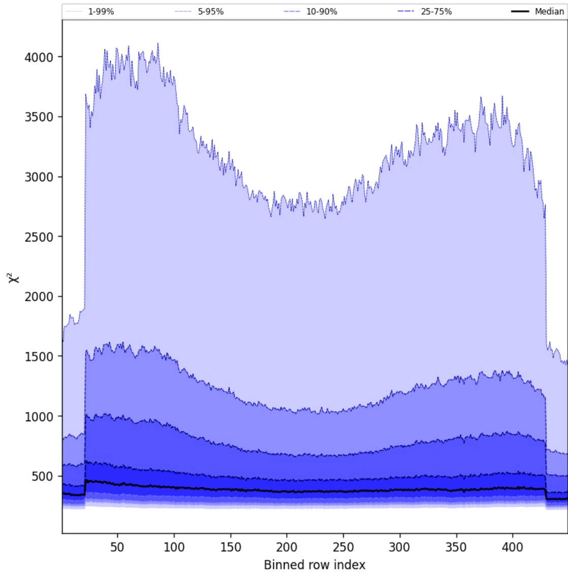
Figure 59: Along track statistics of “ \chi^2 ” for 2024-10-06 to 2024-10-08
