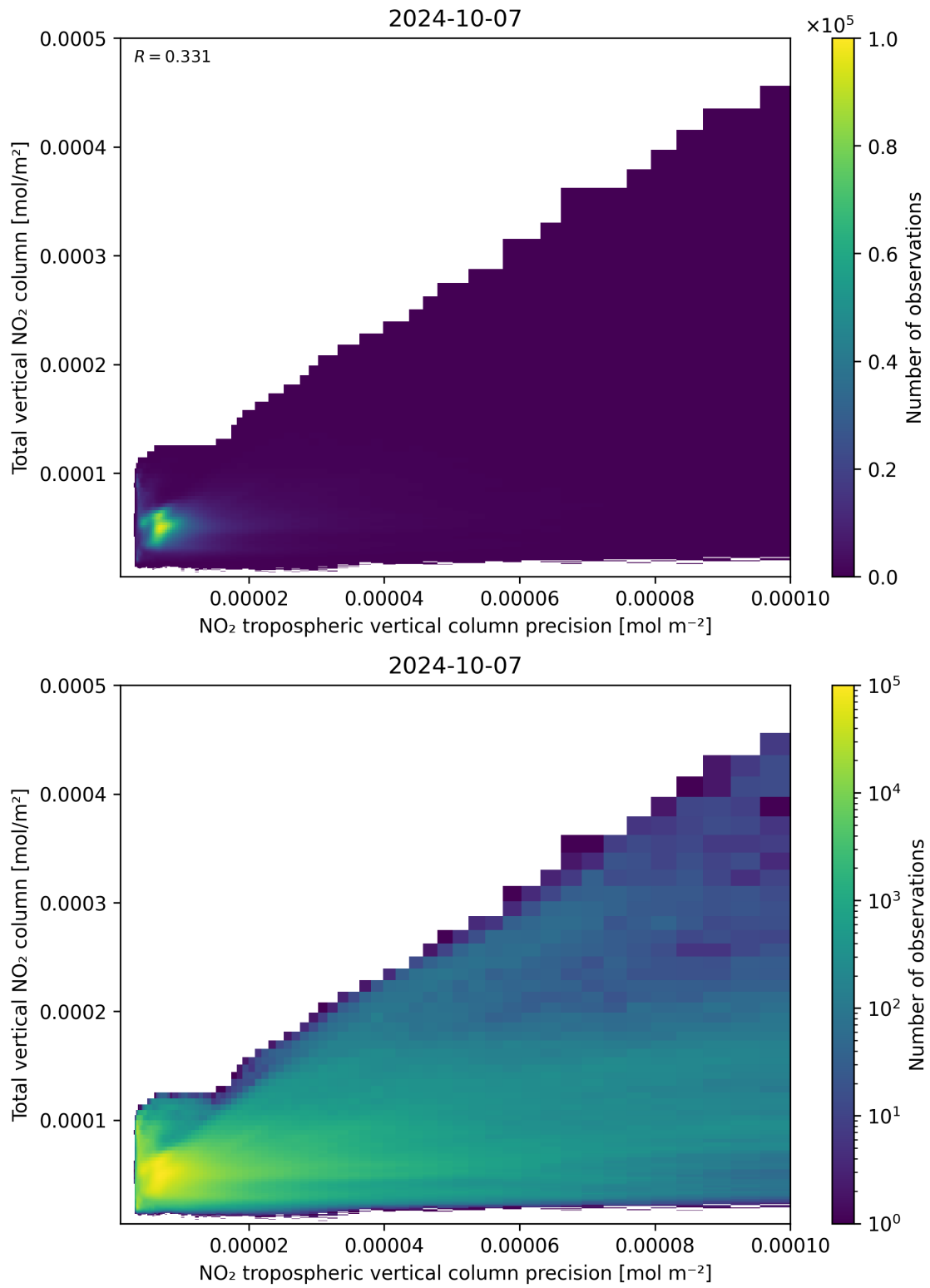
Figure 138: Scatter density plot of “NO 2 tropospheric vertical column precision” against “Total vertical NO 2 column” for 2024-10-06 to 2024-10-08.
