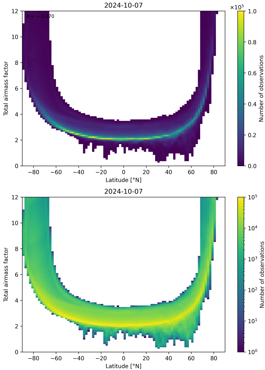
Figure 84: Scatter density plot of “Latitude” against “Total airmass factor” for 2024-10-06 to 2024-10-08.
