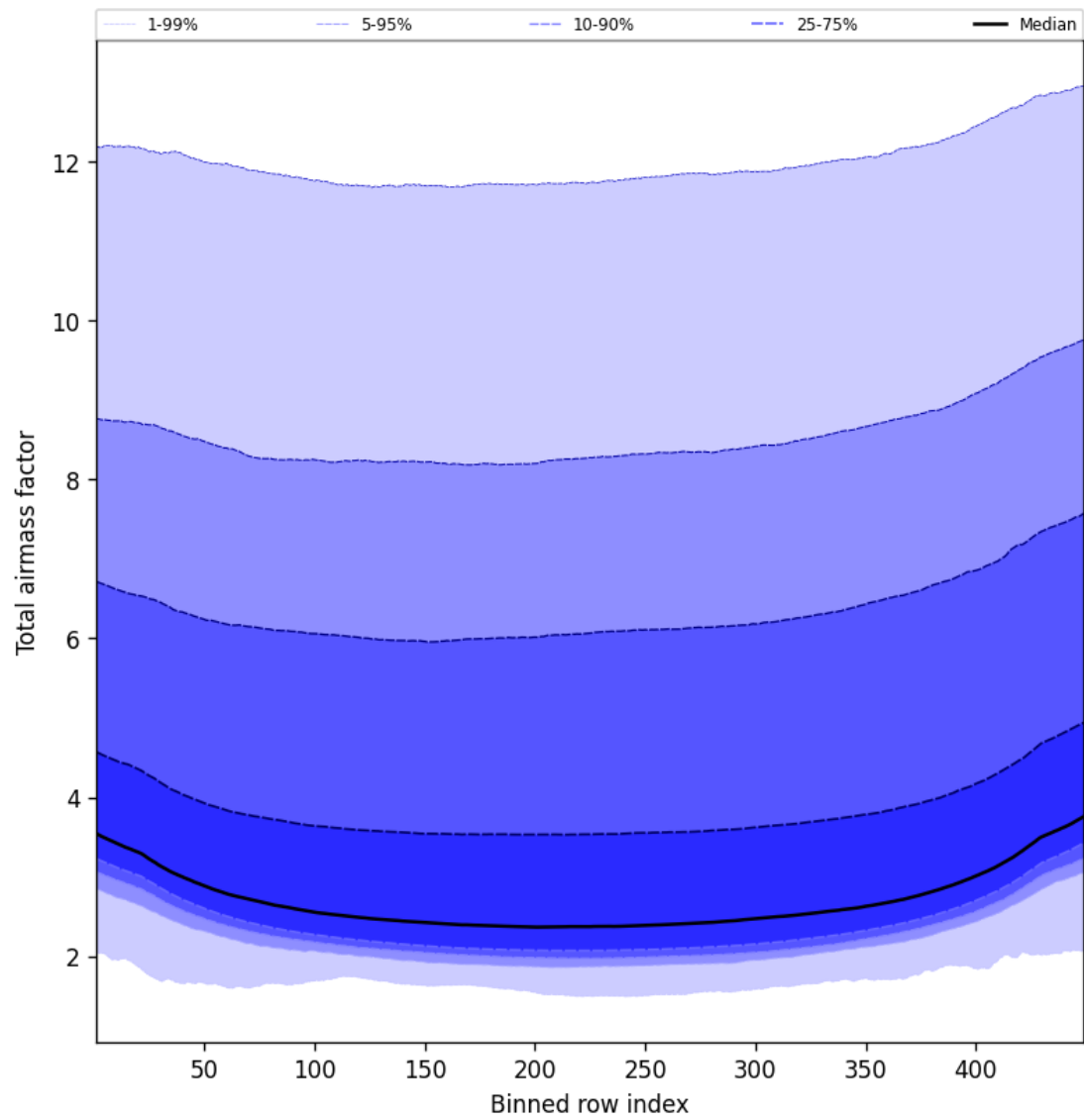
Figure 49: Along track statistics of “Total airmass factor” for 2024-10-06 to 2024-10-08
