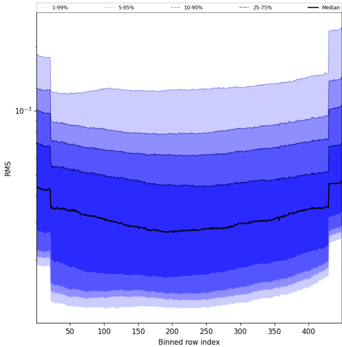
Figure 60: Along track statistics of “RMS” for 2024-10-06 to 2024-10-08
