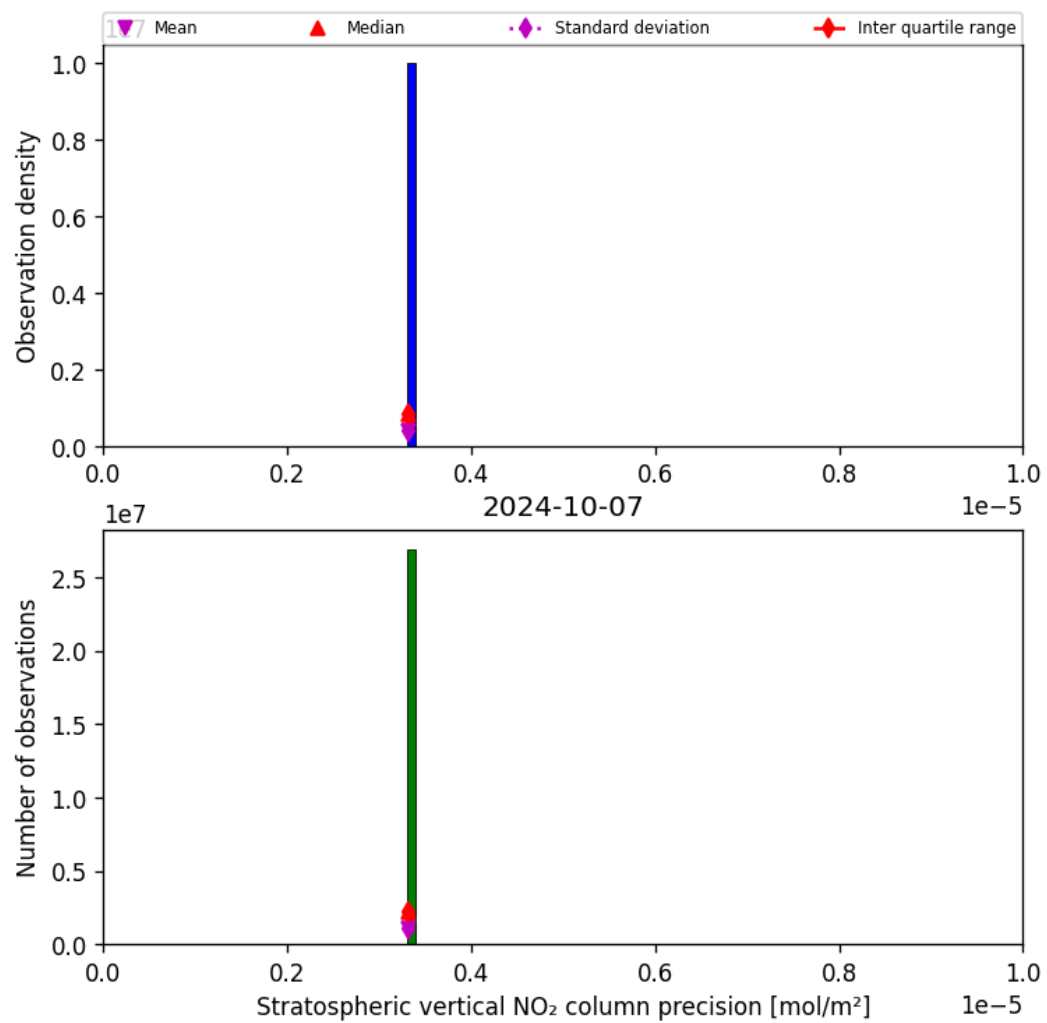
Figure 37: Histogram of “Stratospheric vertical NO 2 column precision” for 2024-10-06 to 2024-10-08
