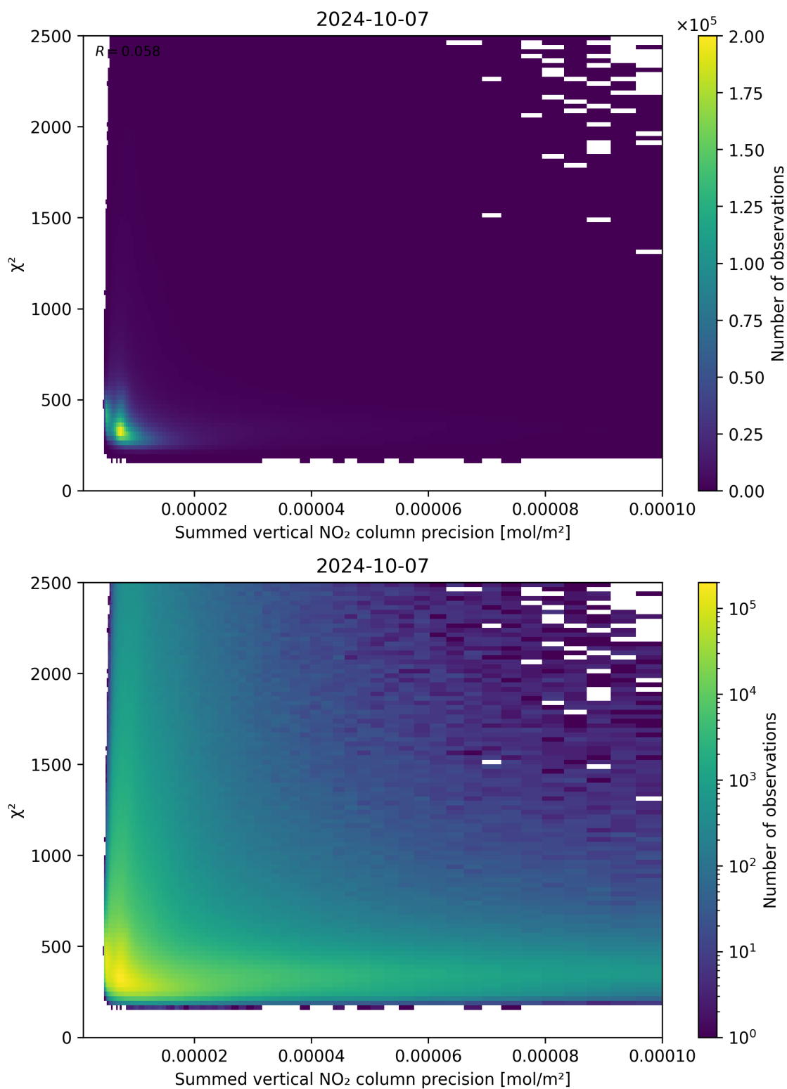
Figure 107: Scatter density plot of “Summed vertical NO 2 column precision” against “ \chi^2 ” for 2024-10-06 to 2024-10-08.
