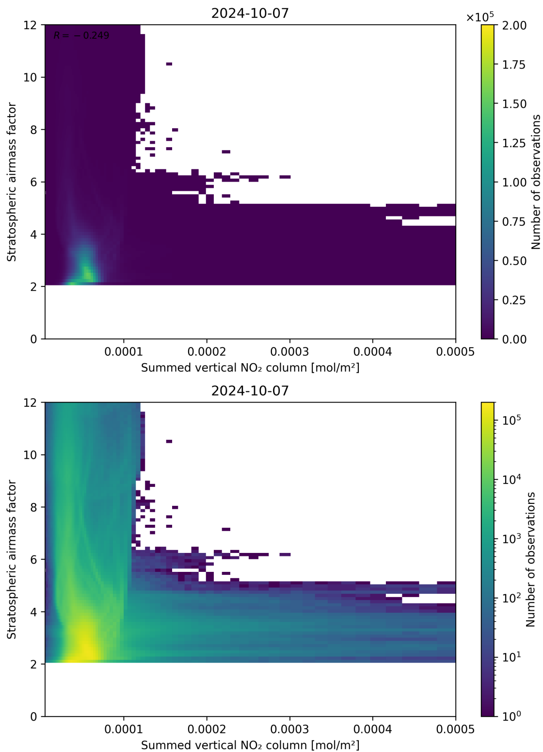
Figure 103: Scatter density plot of “Summed vertical NO 2 column” against “Stratospheric airmass factor” for 2024-10-06 to 2024-10-08.
