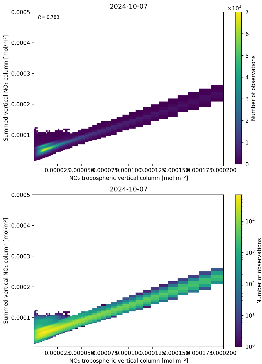
Figure 126: Scatter density plot of “NO 2 tropospheric vertical column” against “Summed vertical NO 2 column” for 2024-10-06 to 2024-10-08.
