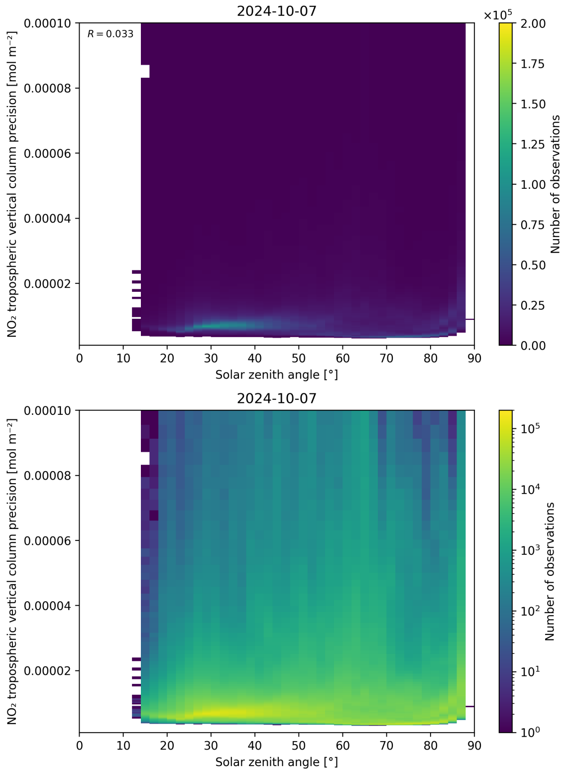
Figure 156: Scatter density plot of “Solar zenith angle” against “NO 2 tropospheric vertical column precision” for 2024-10-06 to 2024-10-08.
