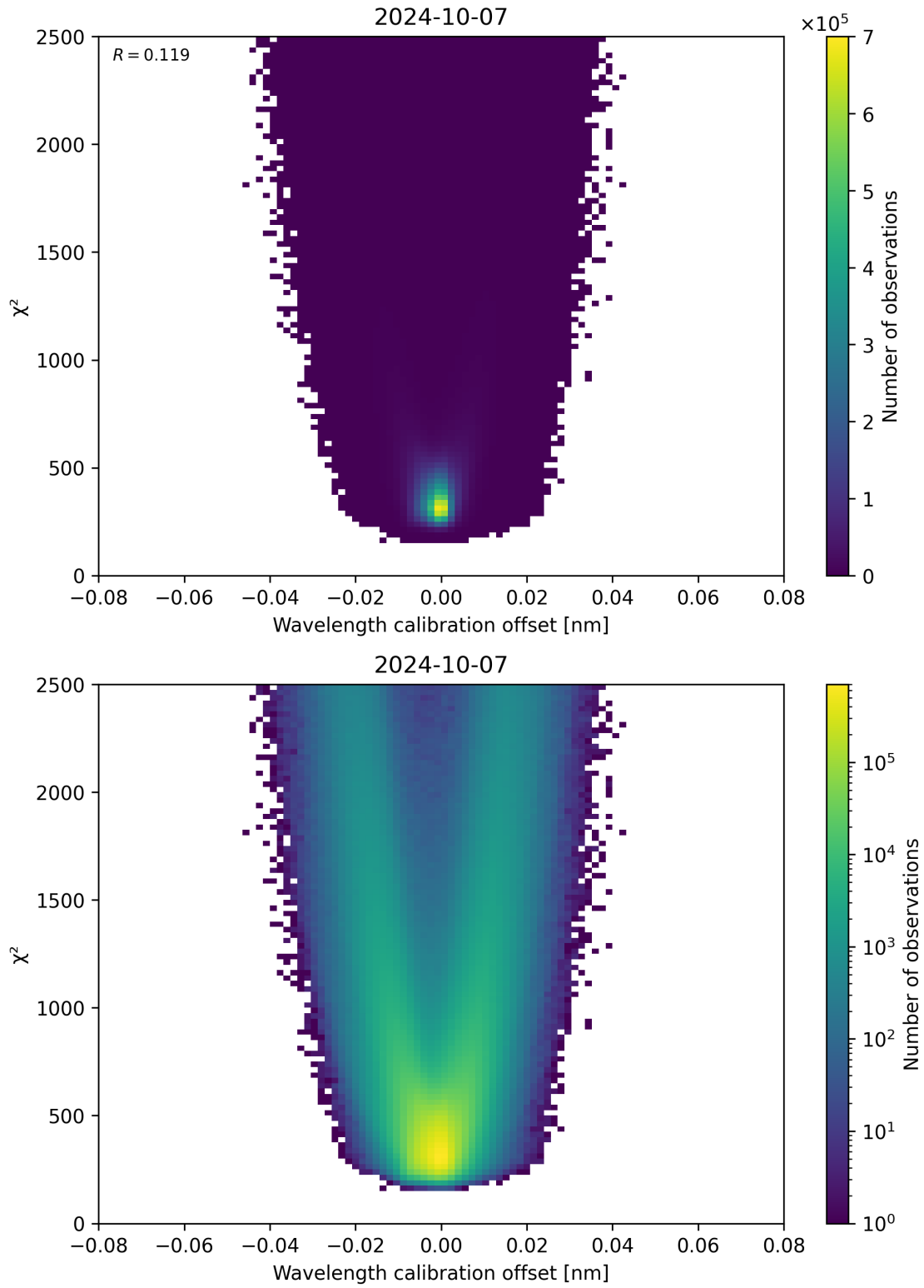
Figure 175: Scatter density plot of “Wavelength calibration offset” against “ \chi^2 ” for 2024-10-06 to 2024-10-08.
