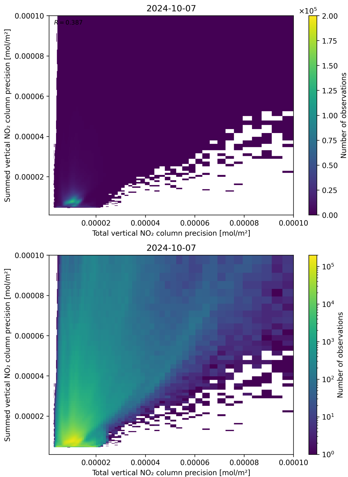
Figure 118: Scatter density plot of “Total vertical NO 2 column precision” against “Summed vertical NO 2 column precision” for 2024-10-06 to 2024-10-08.
