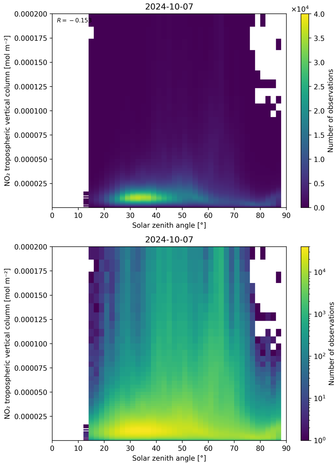
Figure 155: Scatter density plot of “Solar zenith angle” against “NO 2 tropospheric vertical column” for 2024-10-06 to 2024-10-08.
