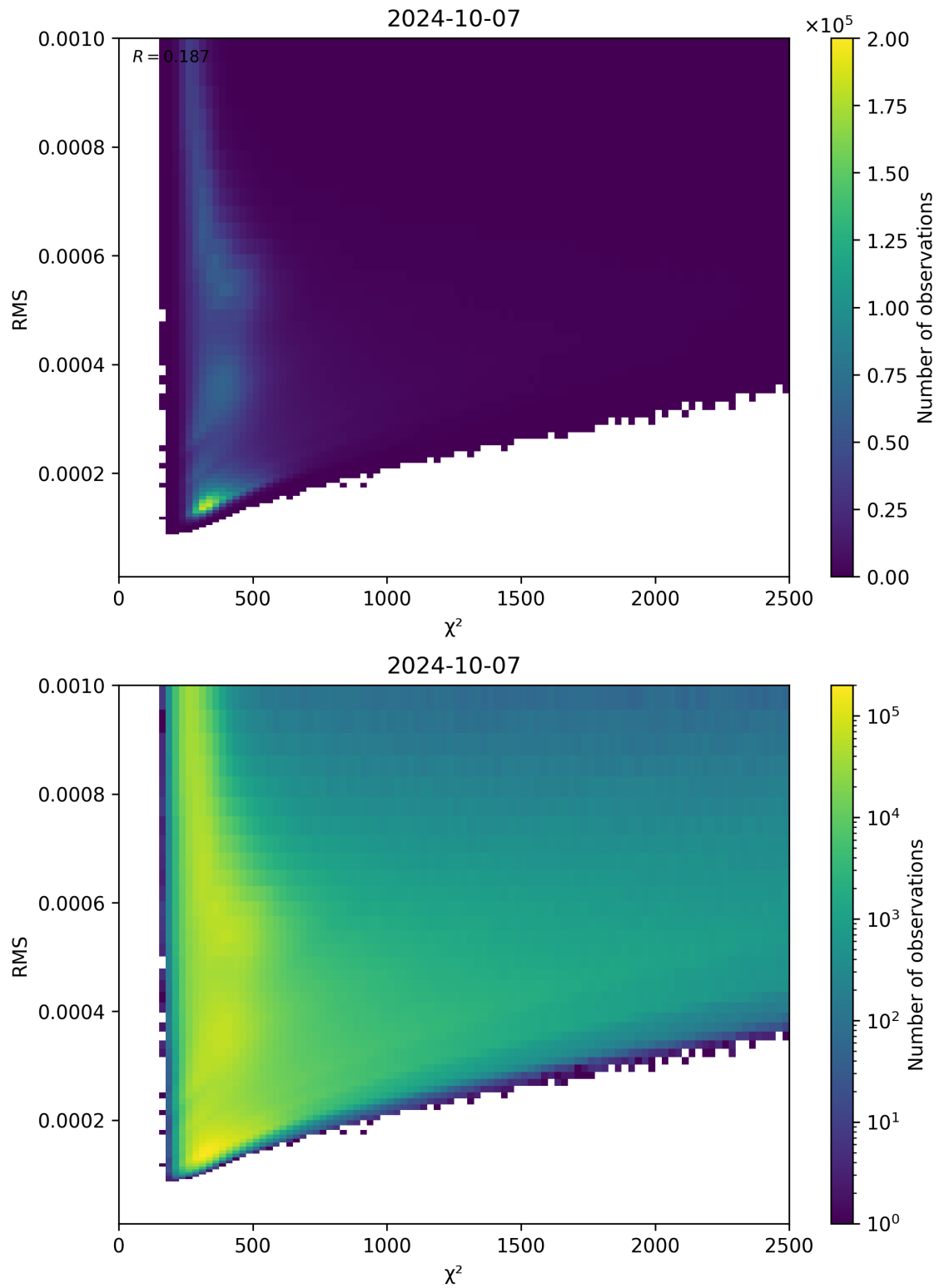
Figure 82: Scatter density plot of “ \chi^2 ” against “RMS” for 2024-10-06 to 2024-10-08.
