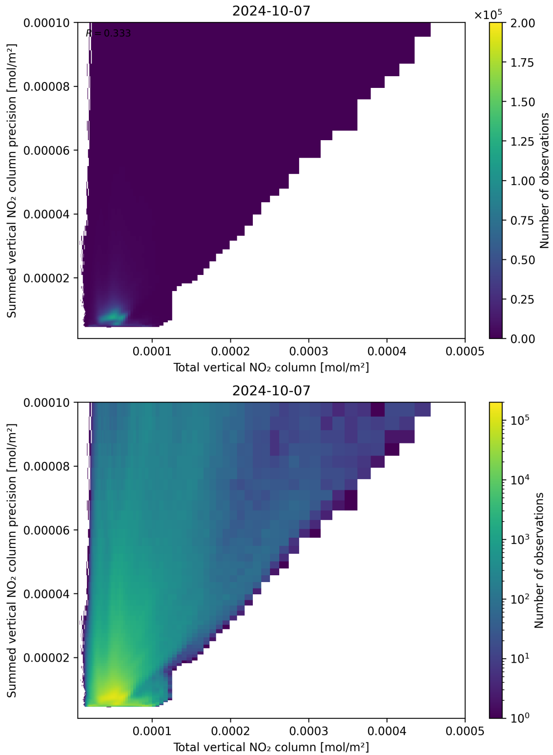
Figure 113: Scatter density plot of “Total vertical NO 2 column” against “Summed vertical NO 2 column precision” for 2024-10-06 to 2024-10-08.
