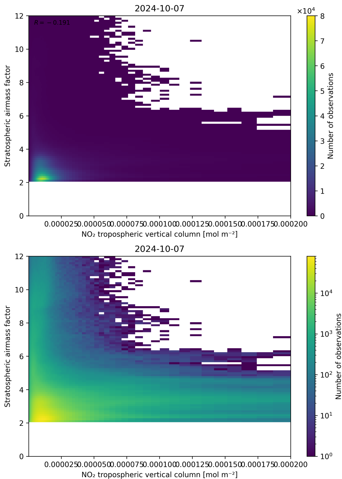
Figure 121: Scatter density plot of “NO 2 tropospheric vertical column” against “Stratospheric air mass factor” for 2024-10-06 to 2024-10-08.
