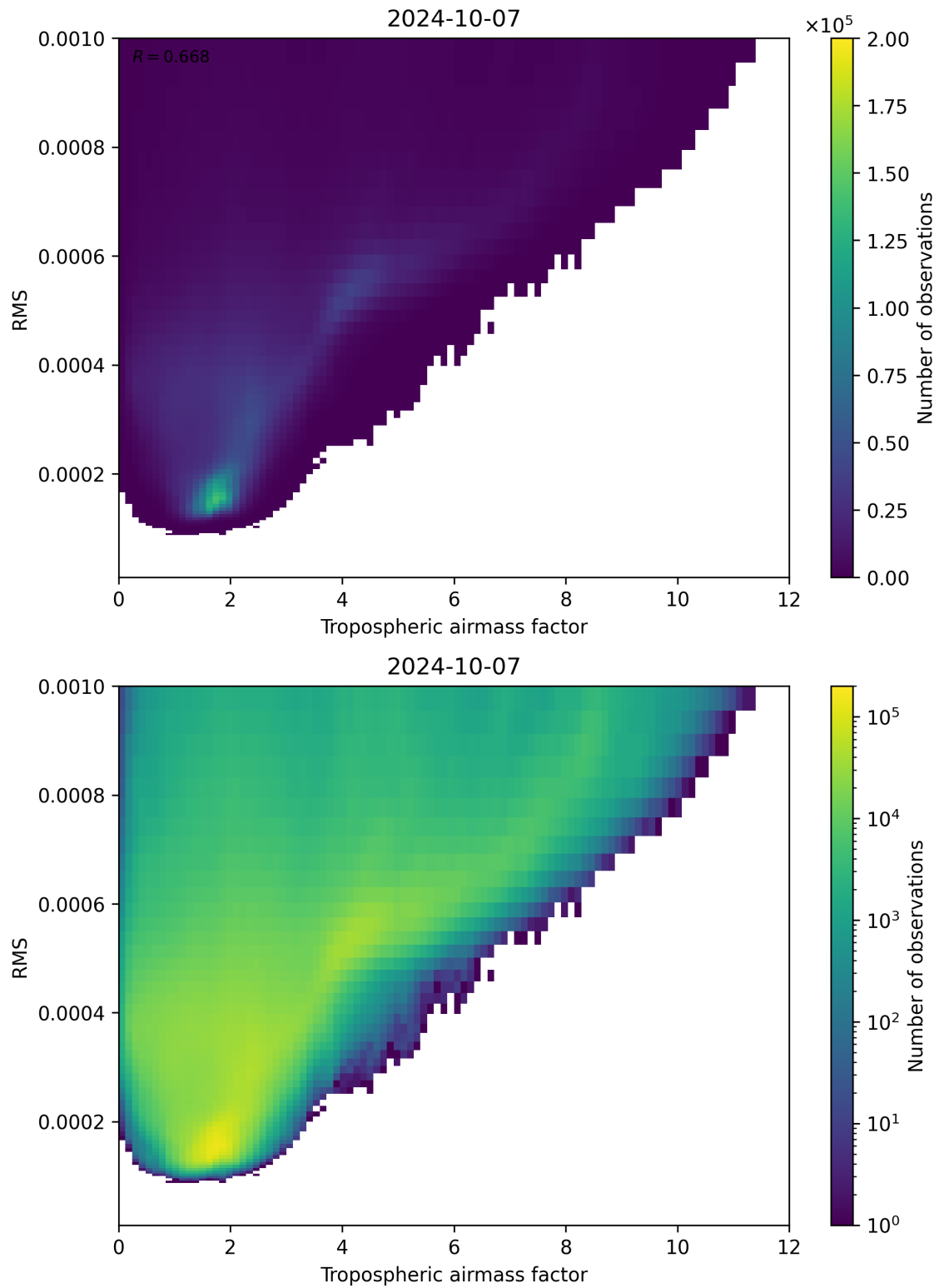
Figure 79: Scatter density plot of “Tropospheric airmass factor” against “RMS” for 2024-10-06 to 2024-10-08.
