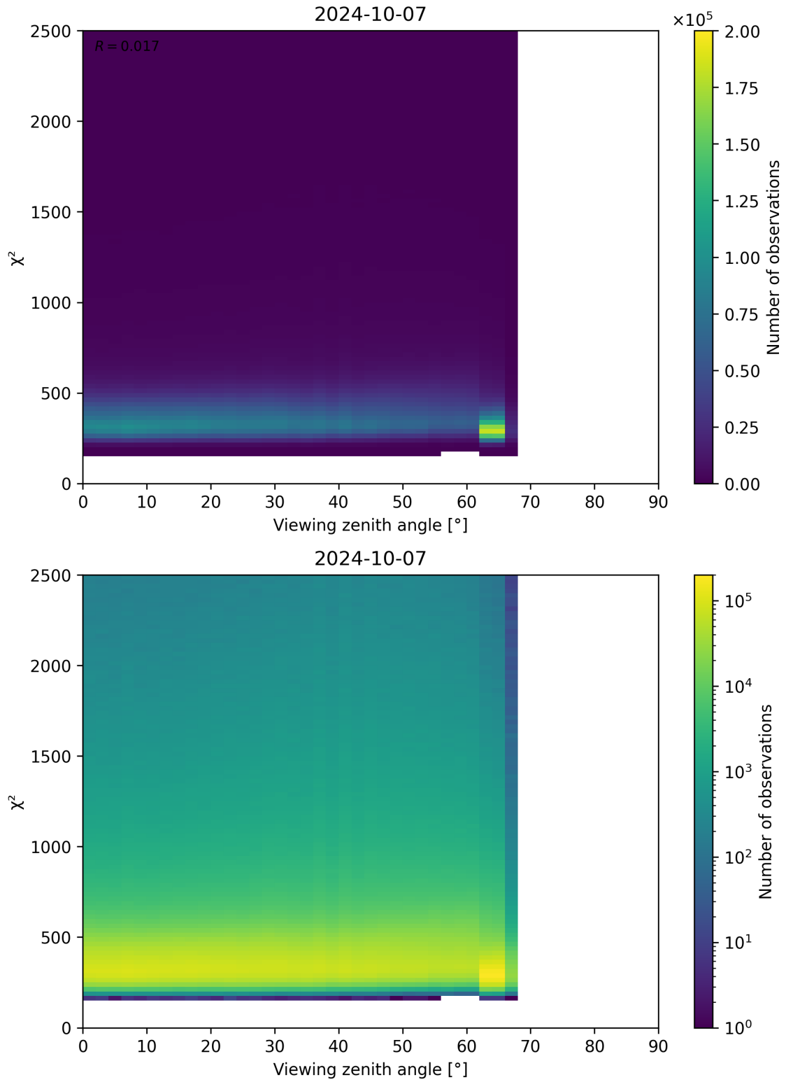
Figure 162: Scatter density plot of “Viewing zenith angle” against “ \chi^2 ” for 2024-10-06 to 2024-10-08.
