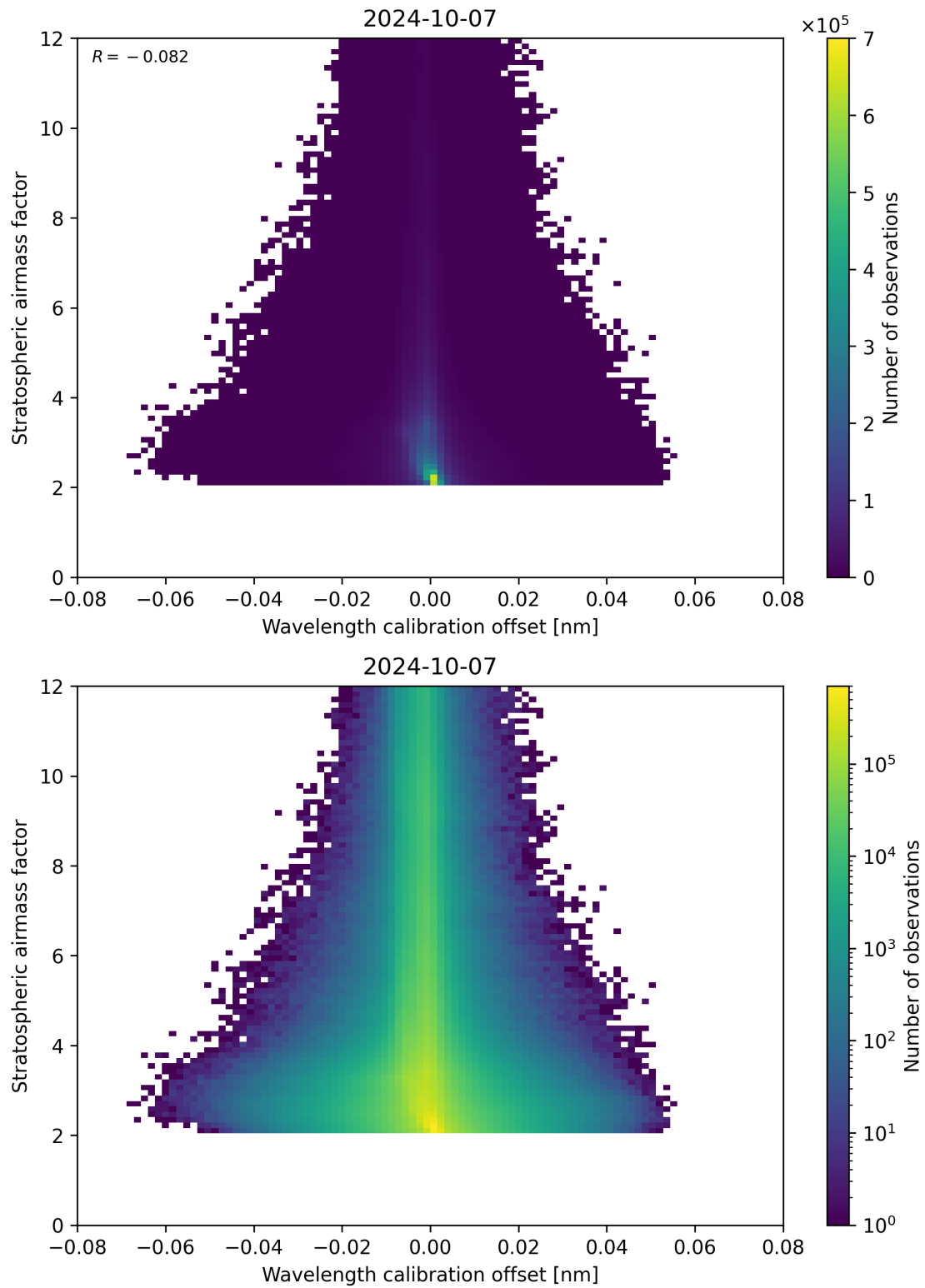
Figure 174: Scatter density plot of “Wavelength calibration offset” against “Stratospheric airmass factor” for 2024-10-06 to 2024-10-08.
