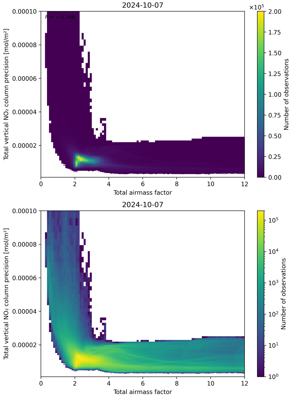
Figure 68: Scatter density plot of “Total airmass factor” against “Total vertical NO 2 column precision” for 2024-10-06 to 2024-10-08.
