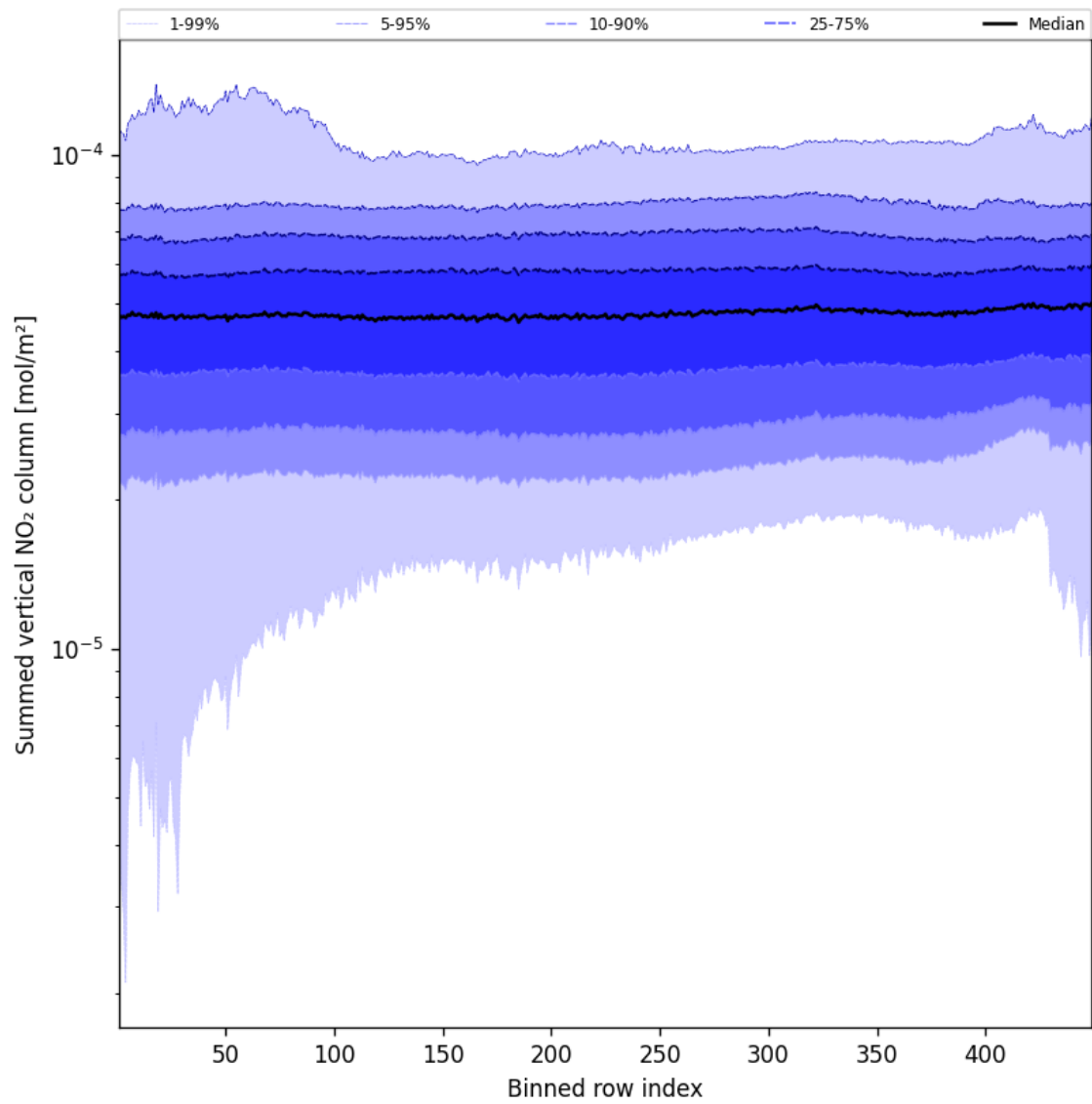
Figure 57: Along track statistics of “Summed vertical NO 2 column” for 2024-10-06 to 2024-10-08
