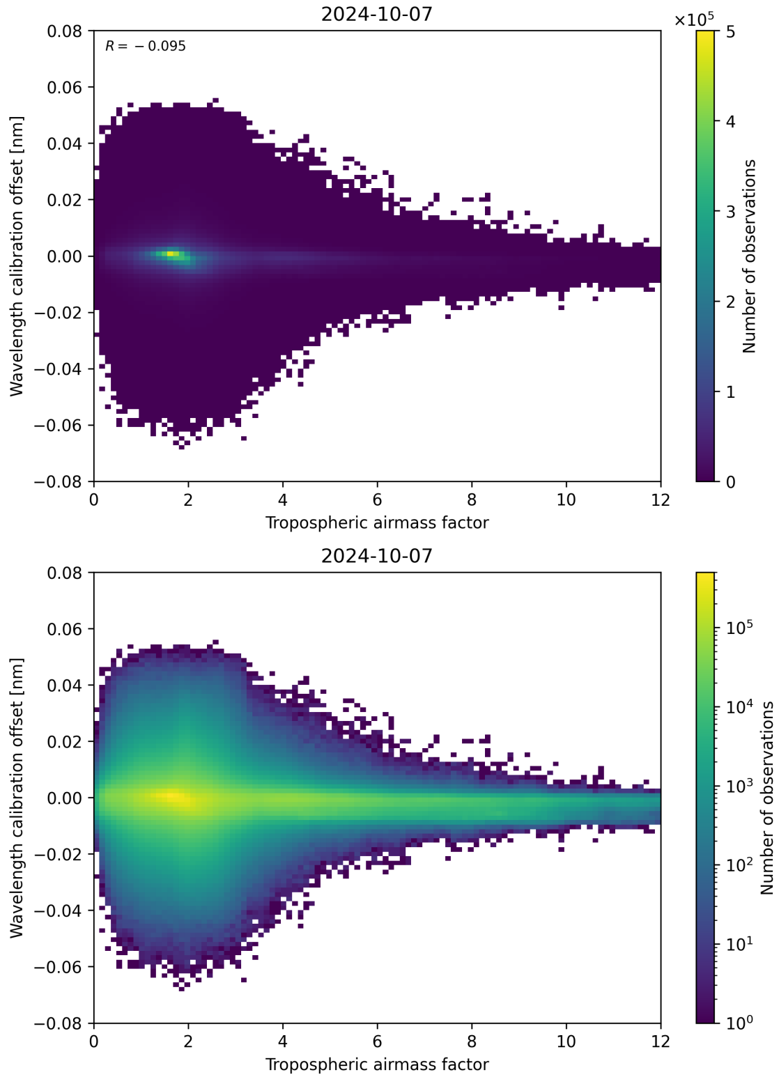
Figure 80: Scatter density plot of “Tropospheric airmass factor” against “Wavelength calibration offset” for 2024-10-06 to 2024-10-08.
