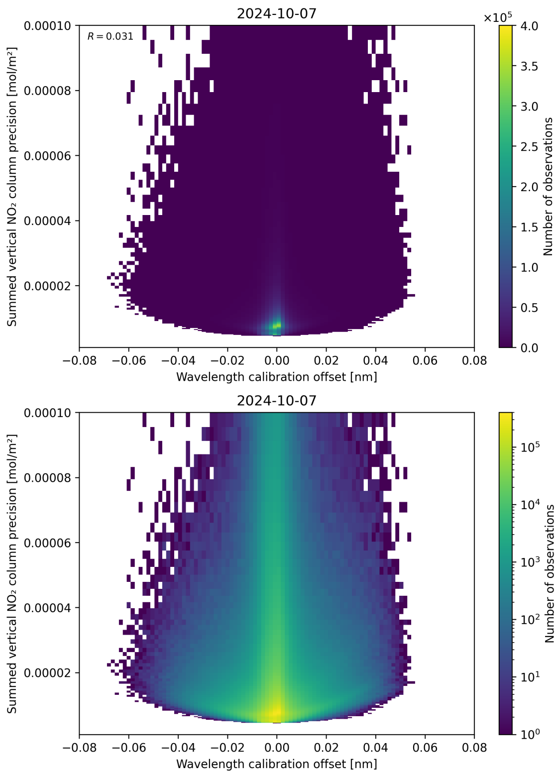
Figure 178: Scatter density plot of “Wavelength calibration offset” against “Summed vertical NO 2 column precision” for 2024-10-06 to 2024-10-08.
