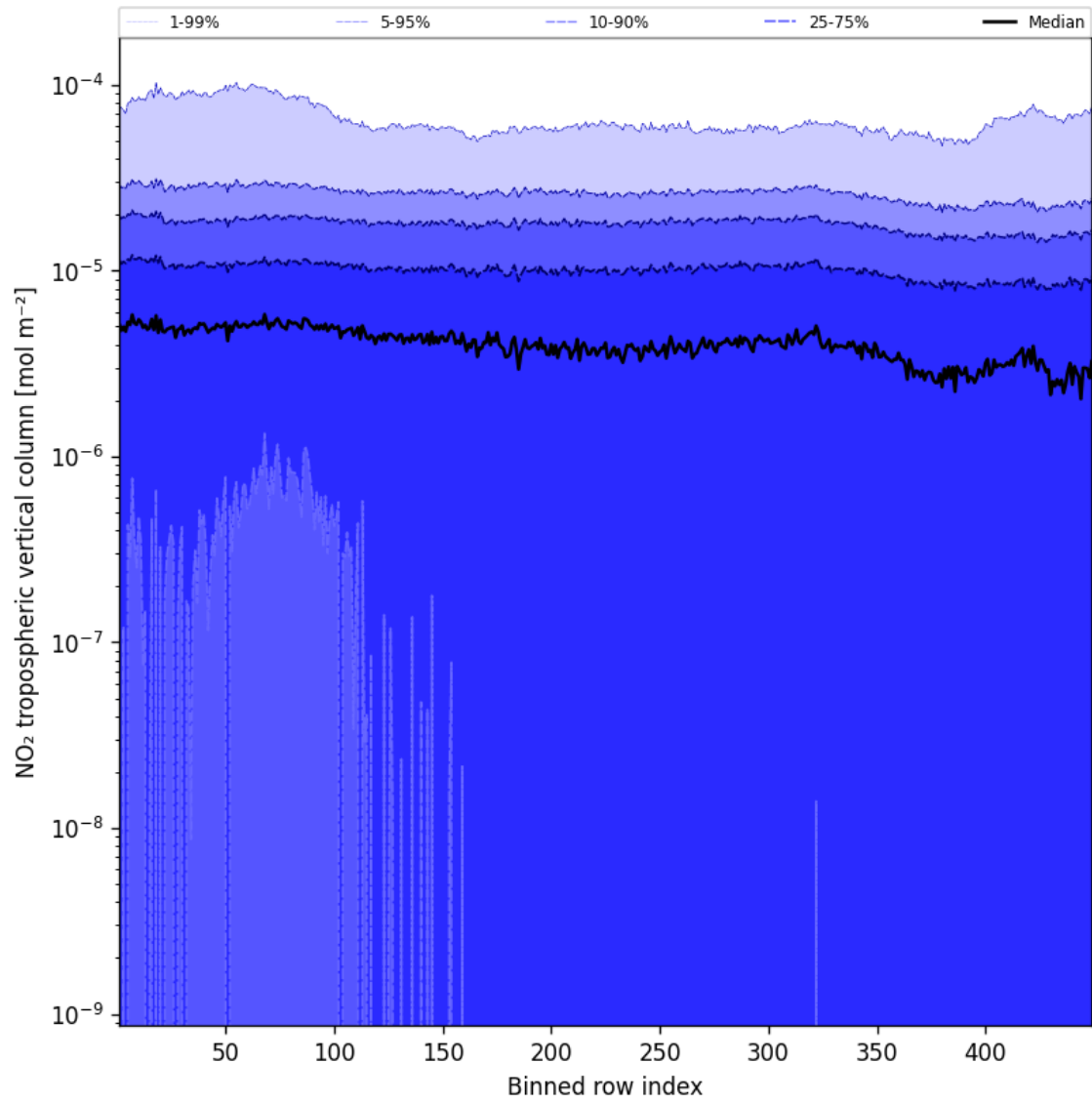
Figure 46: Along track statistics of “NO 2 tropospheric vertical column” for 2024-10-06 to 2024-10-08
