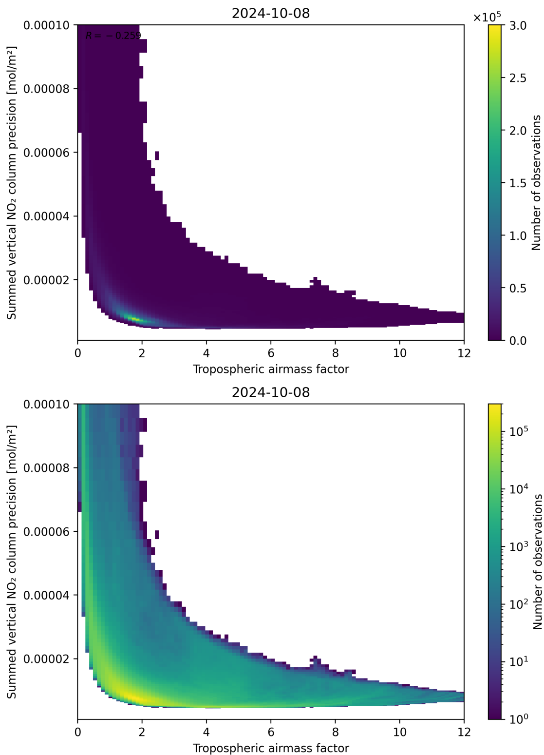
Figure 76: Scatter density plot of “Tropospheric airmass factor” against “Summed vertical NO 2 column precision” for 2024-10-08 to 2024-10-09.
