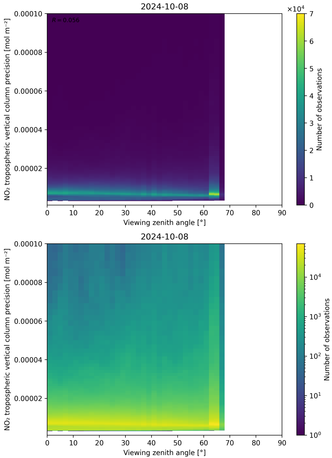
Figure 170: Scatter density plot of “Viewing zenith angle” against “NO 2 tropospheric vertical column precision” for 2024-10-08 to 2024-10-09.
