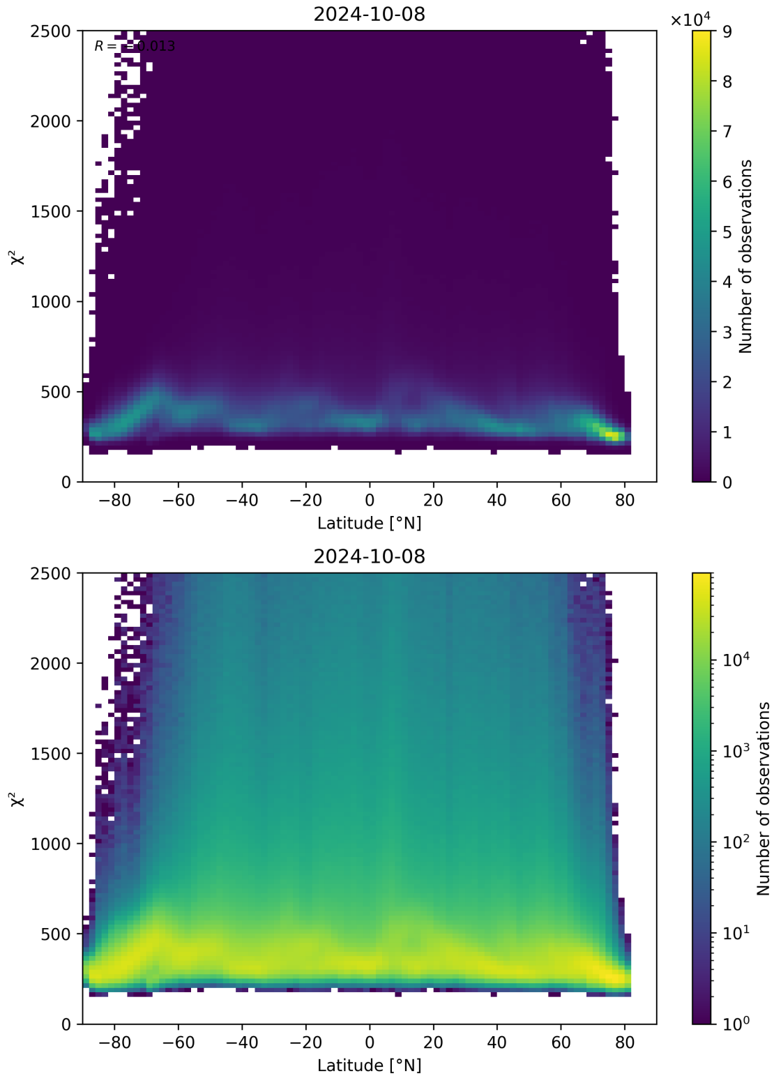
Figure 86: Scatter density plot of “Latitude” against “ \chi^2 ” for 2024-10-08 to 2024-10-09.
