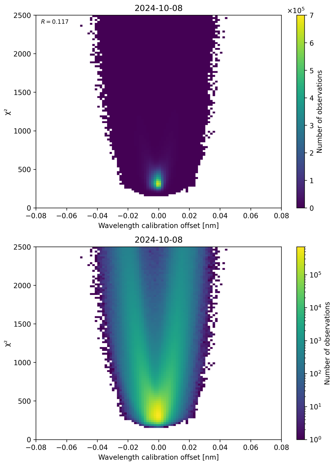
Figure 175: Scatter density plot of “Wavelength calibration offset” against “ \chi^2 ” for 2024-10-08 to 2024-10-09.
