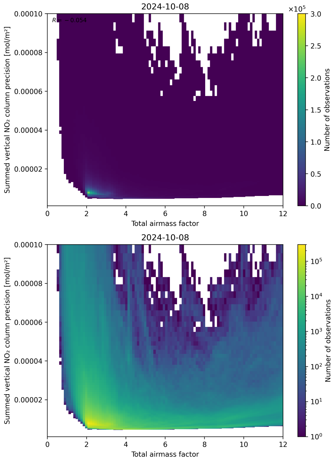
Figure 66: Scatter density plot of “Total airmass factor” against “Summed vertical NO 2 column precision” for 2024-10-08 to 2024-10-09.
