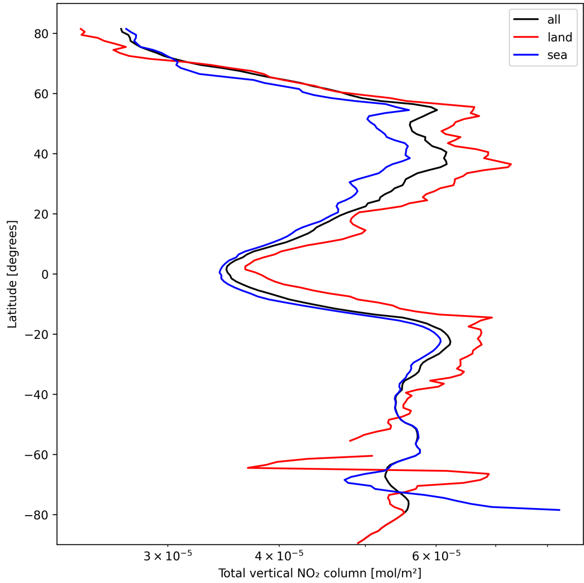
Figure 21: Zonal average of “Total vertical NO 2 column” for 2024-10-08 to 2024-10-09.
