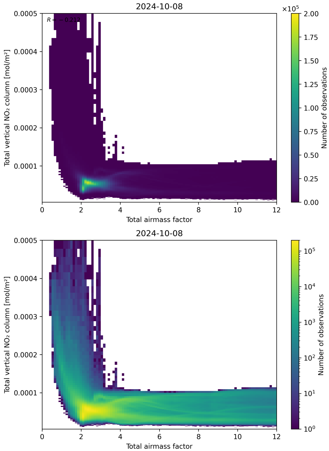
Figure 67: Scatter density plot of “Total airmass factor” against “Total vertical NO 2 column” for 2024-10-08 to 2024-10-09.
