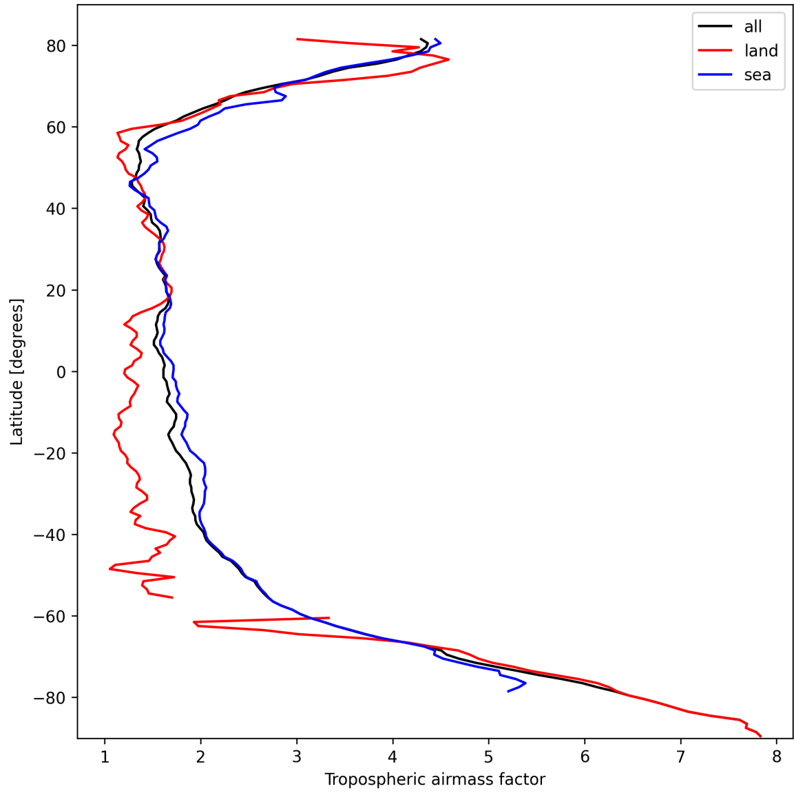
Figure 14: Zonal average of “Tropospheric airmass factor” for 2024-10-08 to 2024-10-09.
