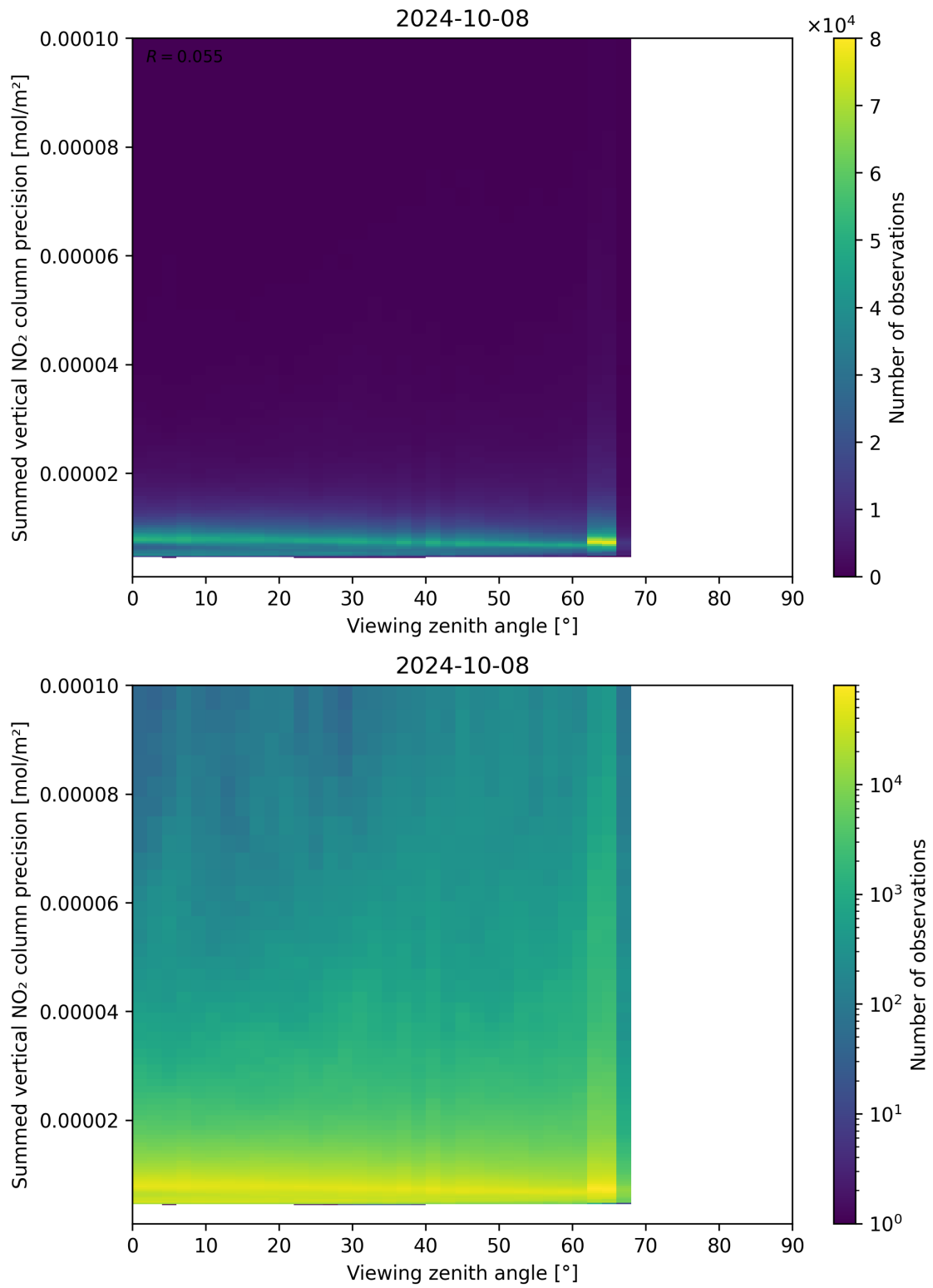
Figure 166: Scatter density plot of “Viewing zenith angle” against “Summed vertical NO 2 column precision” for 2024-10-08 to 2024-10-09.
