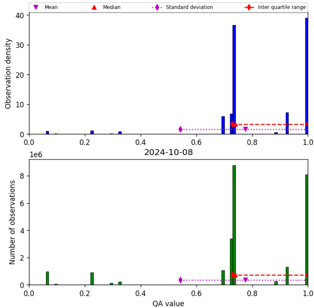
Figure 28: Histogram of “QA value” for 2024-10-08 to 2024-10-09
