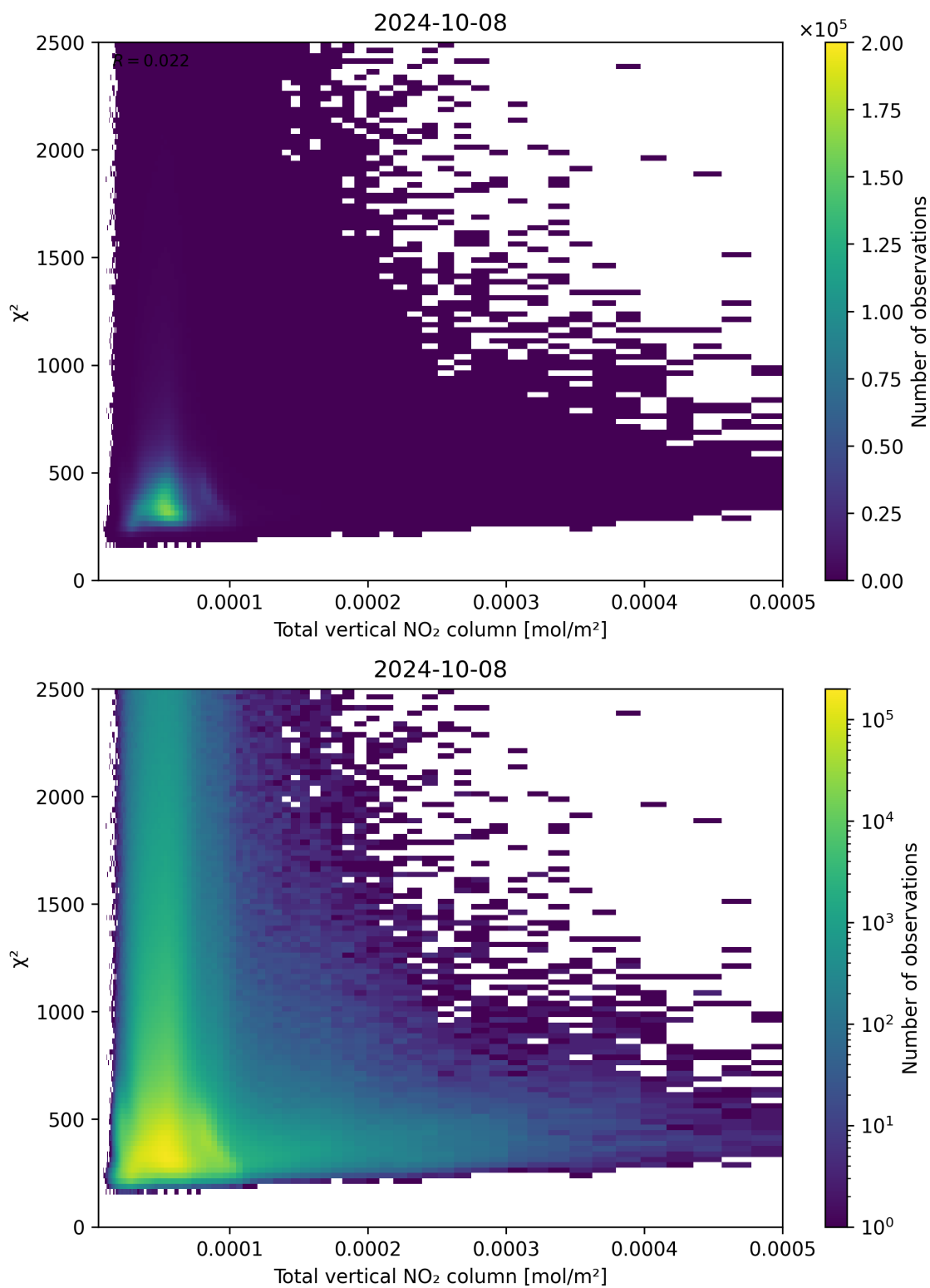
Figure 111: Scatter density plot of “Total vertical NO 2 column” against “ \chi^2 ” for 2024-10-08 to 2024-10-09.
