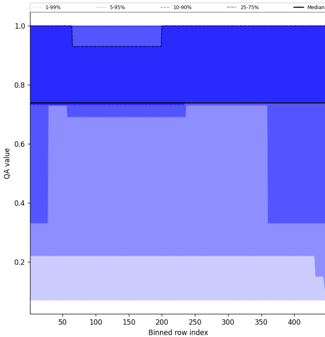
Figure 45: Along track statistics of “QA value” for 2024-10-08 to 2024-10-09
