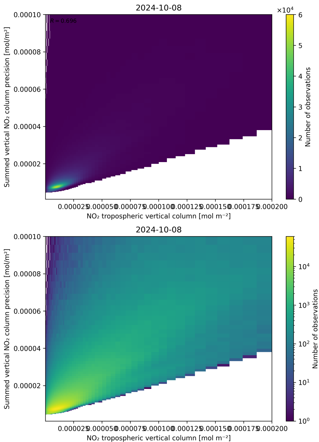
Figure 127: Scatter density plot of “NO 2 tropospheric vertical column” against “Summed vertical NO 2 column precision” for 2024-10-08 to 2024-10-09.
