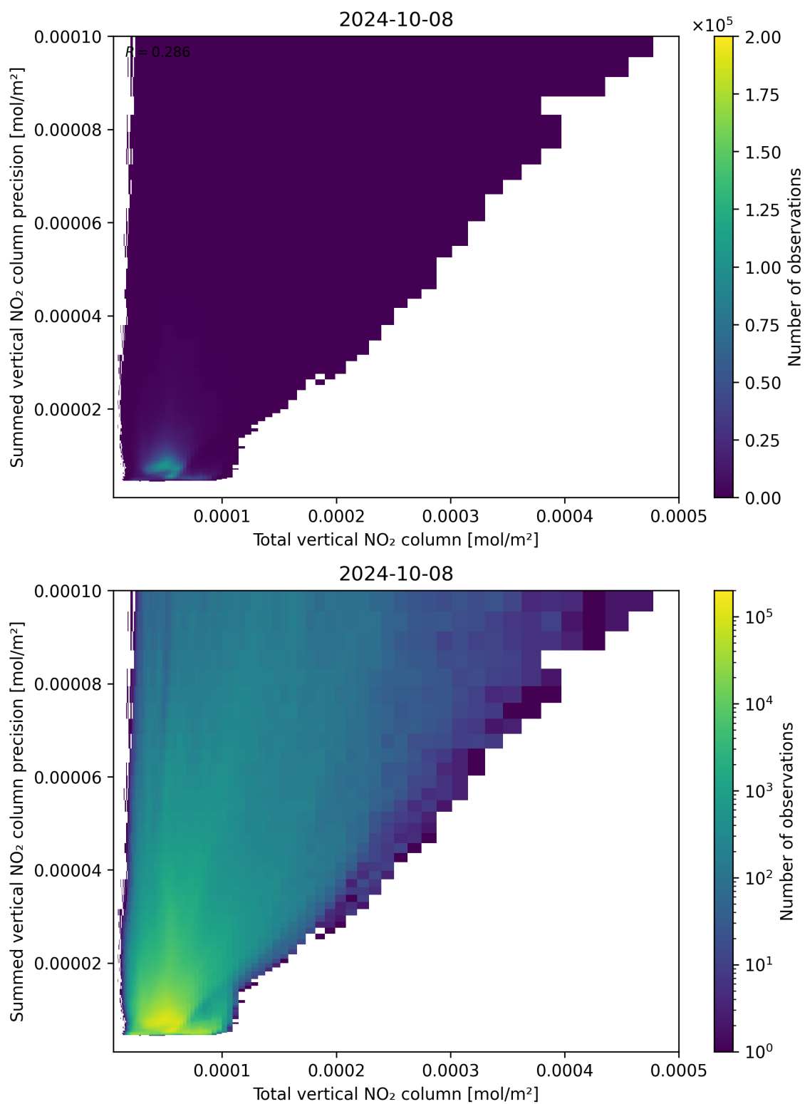
Figure 113: Scatter density plot of “Total vertical NO 2 column” against “Summed vertical NO 2 column precision” for 2024-10-08 to 2024-10-09.
