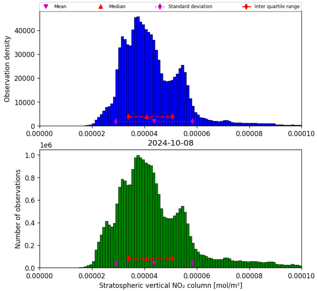
Figure 36: Histogram of “Stratospheric vertical NO 2 column” for 2024-10-08 to 2024-10-09
