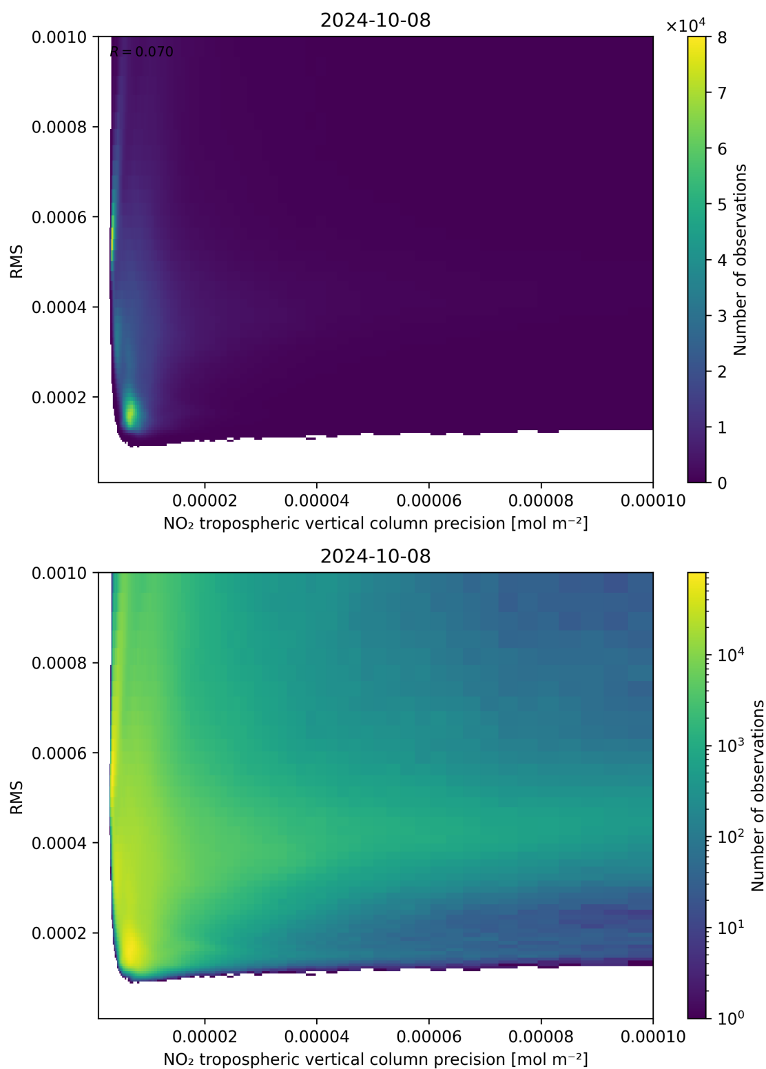
Figure 140: Scatter density plot of “NO 2 tropospheric vertical column precision” against “RMS” for 2024-10-08 to 2024-10-09.
