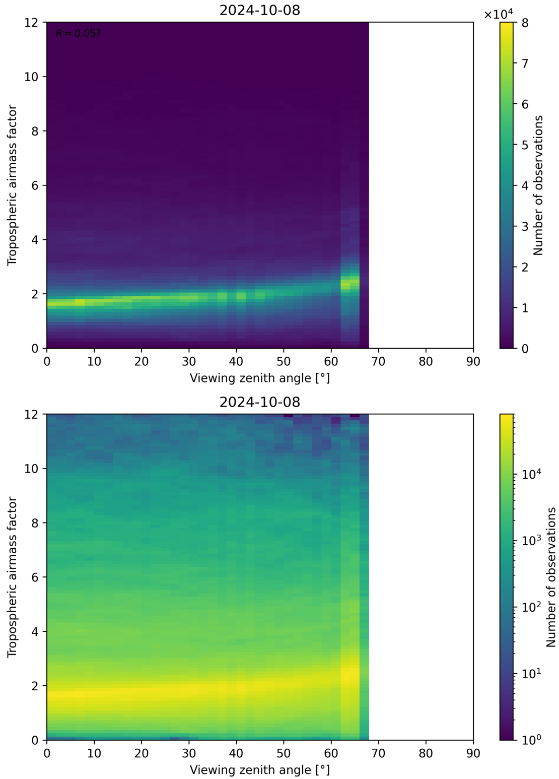
Figure 161: Scatter density plot of “Viewing zenith angle” against “Tropospheric airmass factor” for 2024-10-08 to 2024-10-09.
