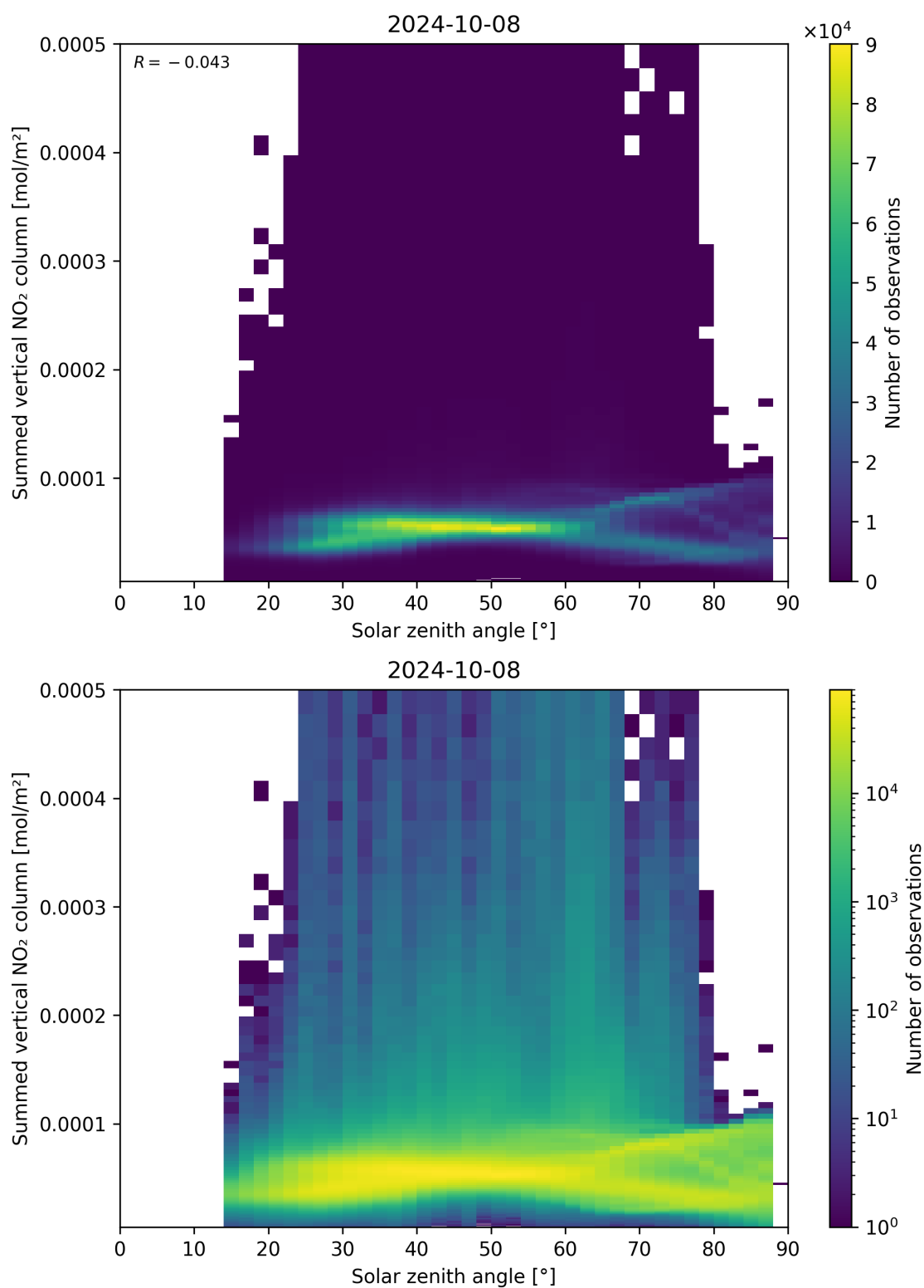
Figure 151: Scatter density plot of “Solar zenith angle” against “Summed vertical NO 2 column” for 2024-10-08 to 2024-10-09.
