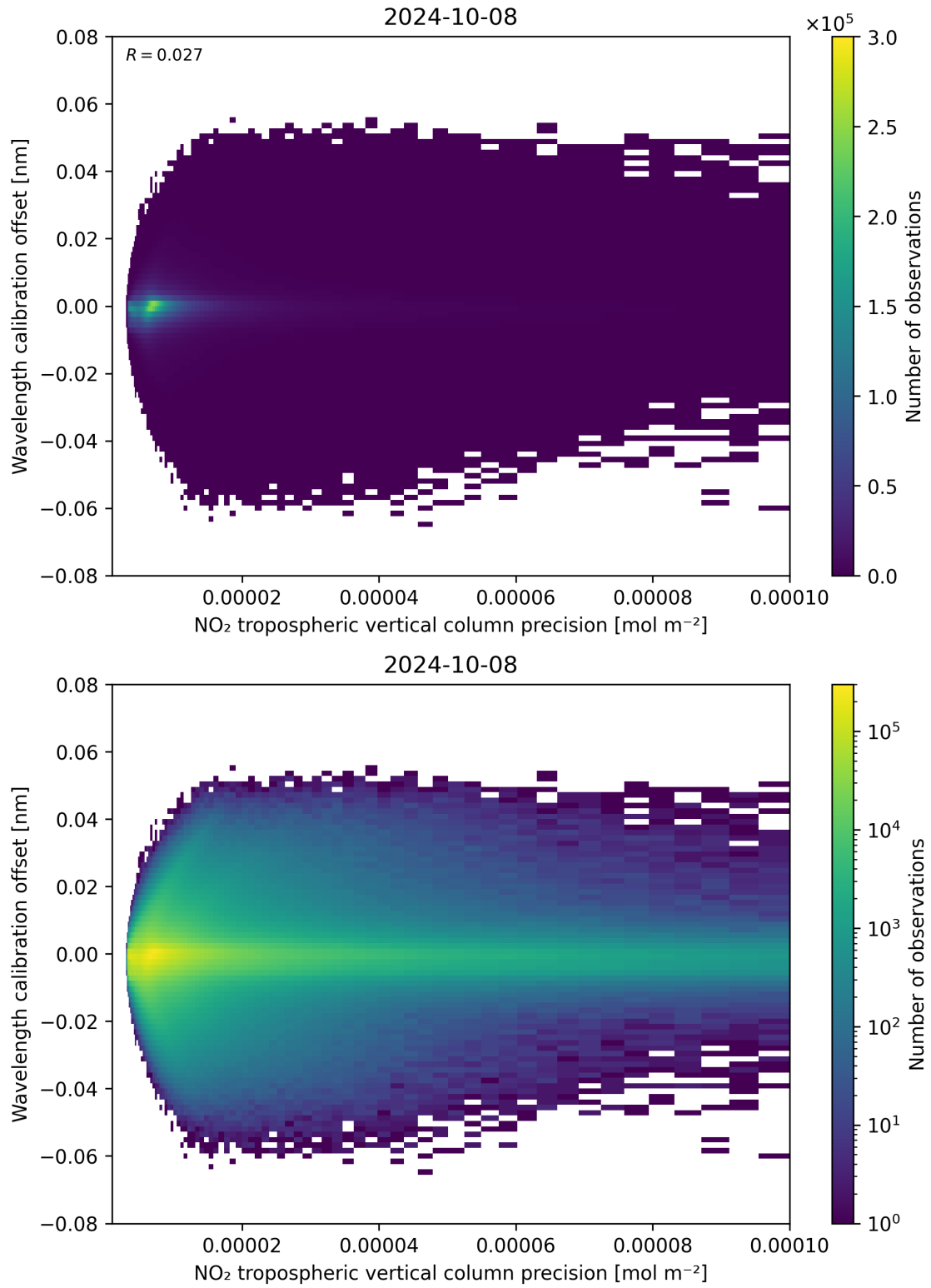
Figure 141: Scatter density plot of “NO 2 tropospheric vertical column precision” against “Wavelength calibration offset” for 2024-10-08 to 2024-10-09.
