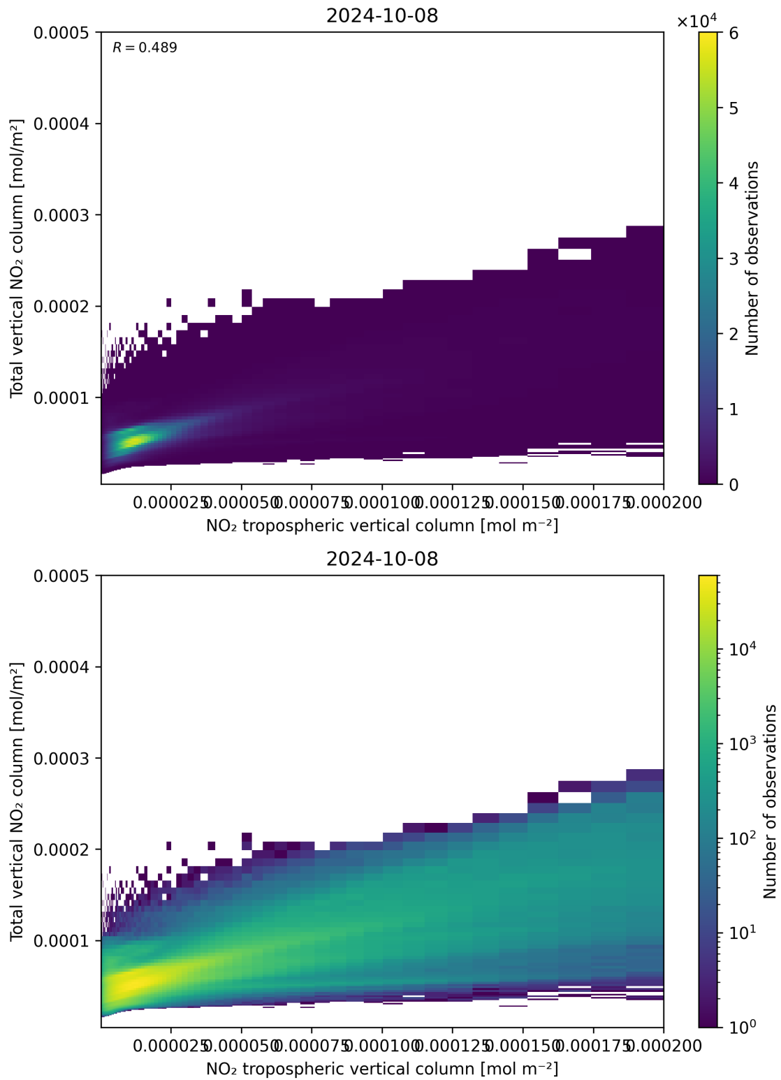
Figure 128: Scatter density plot of “NO 2 tropospheric vertical column” against “Total vertical NO 2 column” for 2024-10-08 to 2024-10-09.
