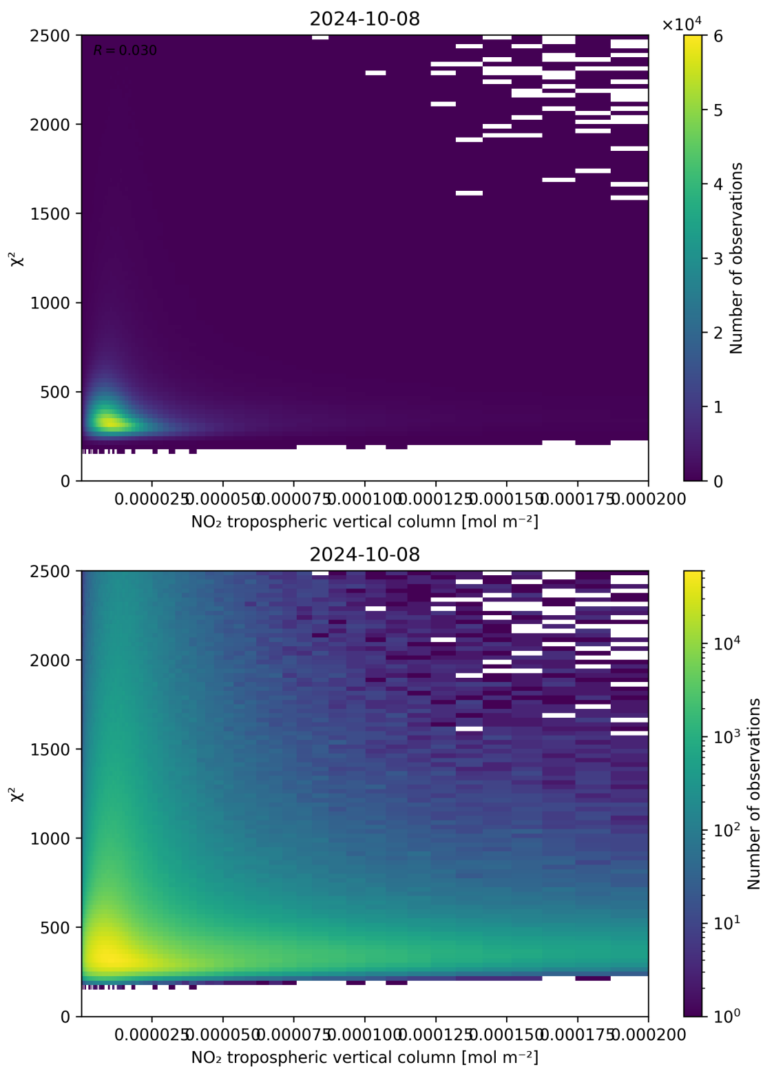
Figure 124: Scatter density plot of “NO 2 tropospheric vertical column” against “ \chi^2 ” for 2024-10-08 to 2024-10-09.
