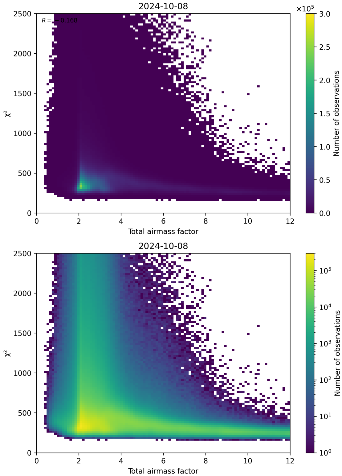
Figure 63: Scatter density plot of “Total airmass factor” against “ \chi^2 ” for 2024-10-08 to 2024-10-09.
