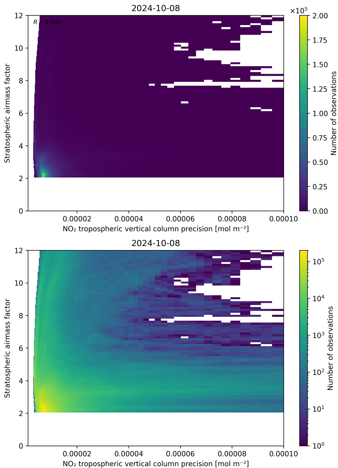
Figure 131: Scatter density plot of “NO 2 tropospheric vertical column precision” against “Stratospheric airmass factor” for 2024-10-08 to 2024-10-09.
