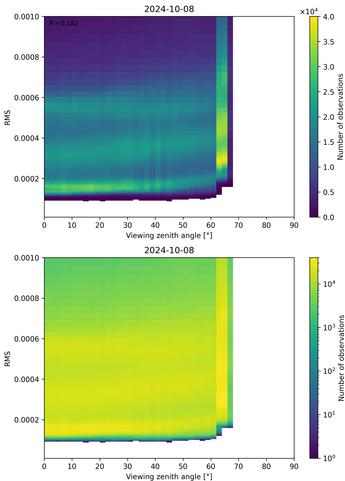
Figure 171: Scatter density plot of “Viewing zenith angle” against “RMS” for 2024-10-08 to 2024-10-09.
