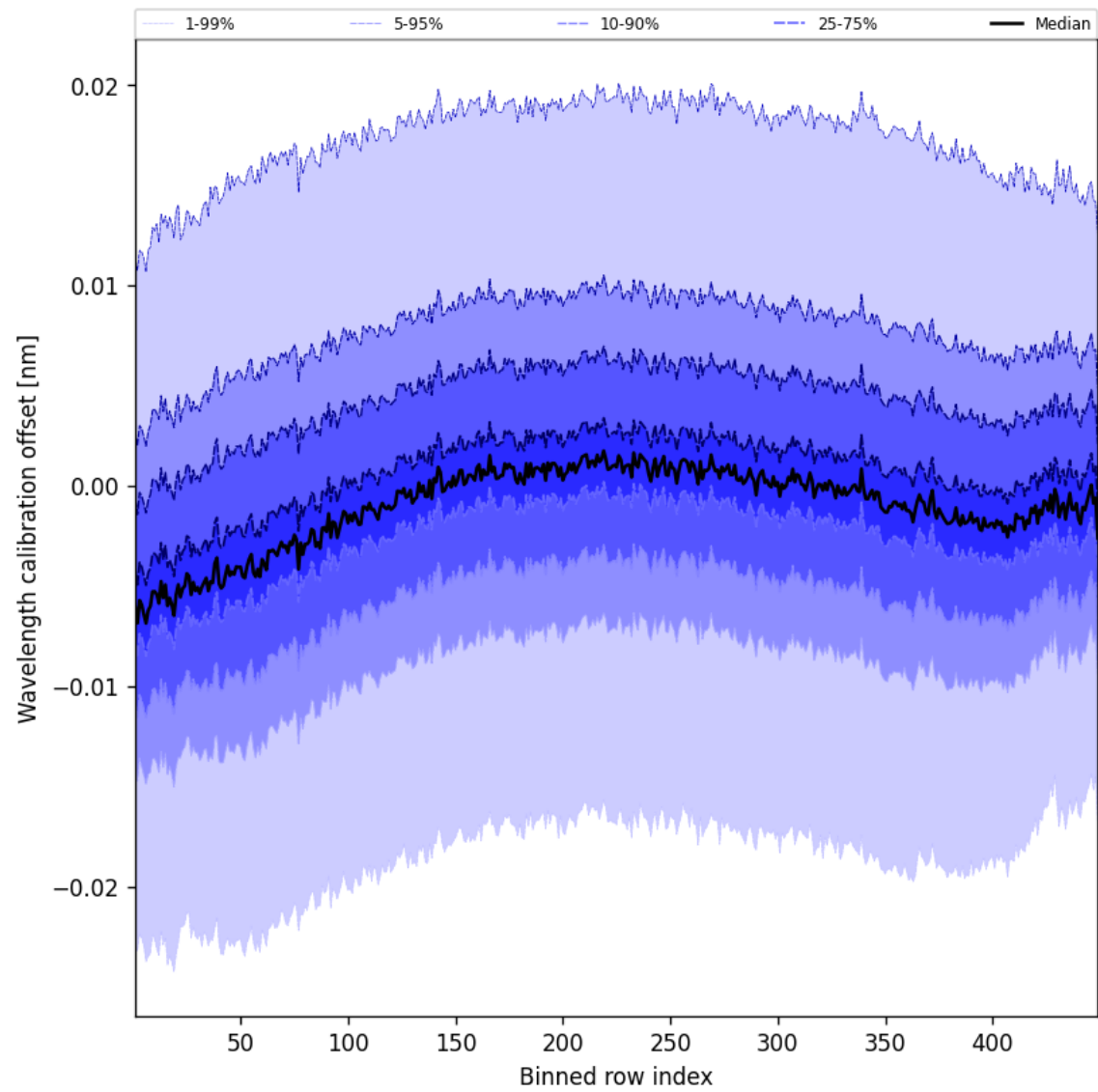
Figure 52: Along track statistics of “Wavelength calibration offset” for 2024-10-08 to 2024-10-09
