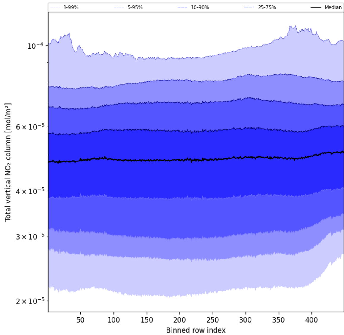
Figure 55: Along track statistics of “Total vertical NO 2 column” for 2024-10-08 to 2024-10-09
