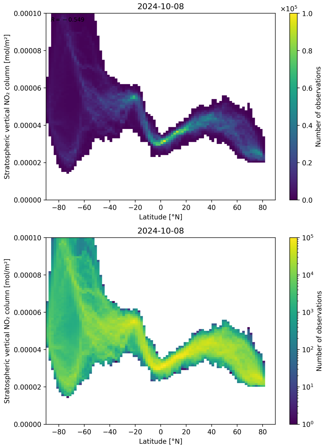
Figure 87: Scatter density plot of “Latitude” against “Stratospheric vertical NO 2 column” for 2024-10-08 to 2024-10-09.
