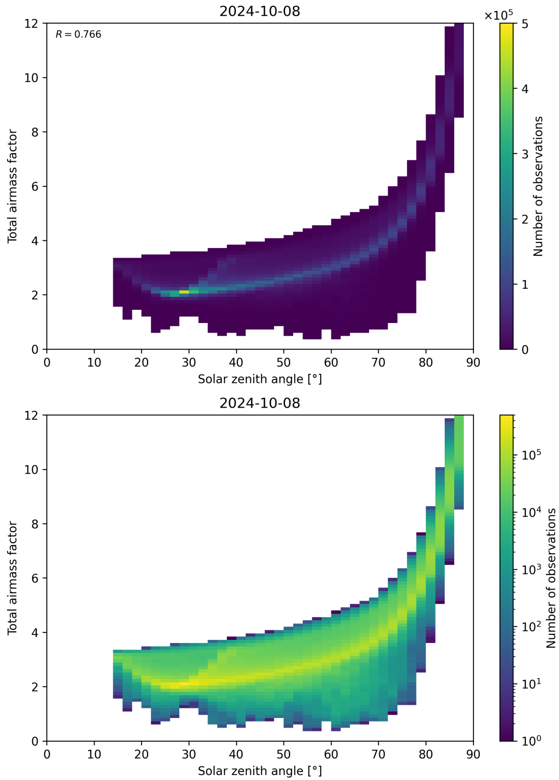
Figure 146: Scatter density plot of “Solar zenith angle” against “Total airmass factor” for 2024-10-08 to 2024-10-09.
