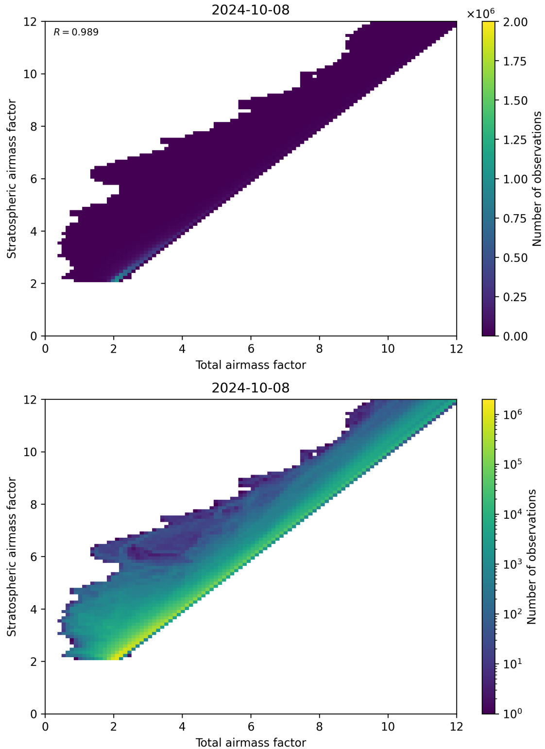
Figure 62: Scatter density plot of “Total airmass factor” against “Stratospheric airmass factor” for 2024-10-08 to 2024-10-09.
