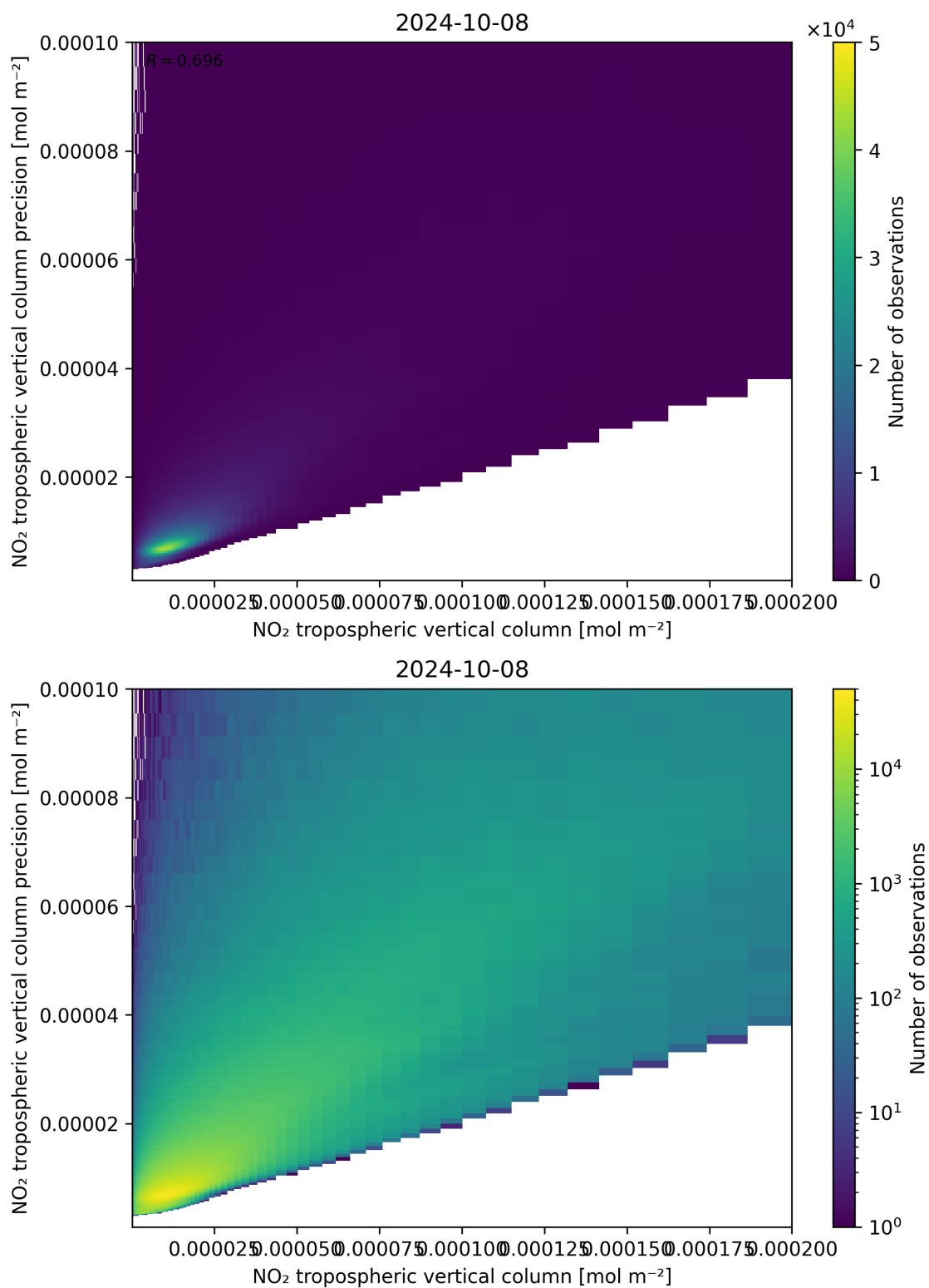
Figure 130: Scatter density plot of “NO 2 tropospheric vertical column” against “NO 2 tropospheric vertical column precision” for 2024-10-08 to 2024-10-09.
