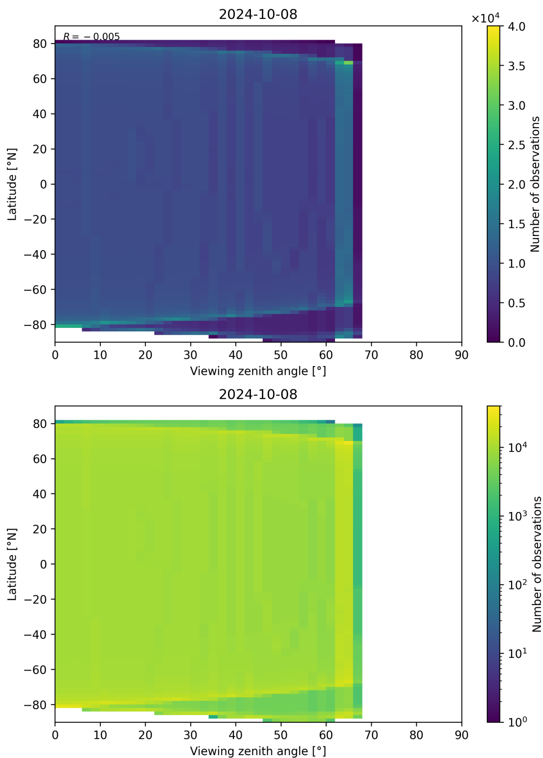
Figure 163: Scatter density plot of “Viewing zenith angle” against “Latitude” for 2024-10-08 to 2024-10-09.
