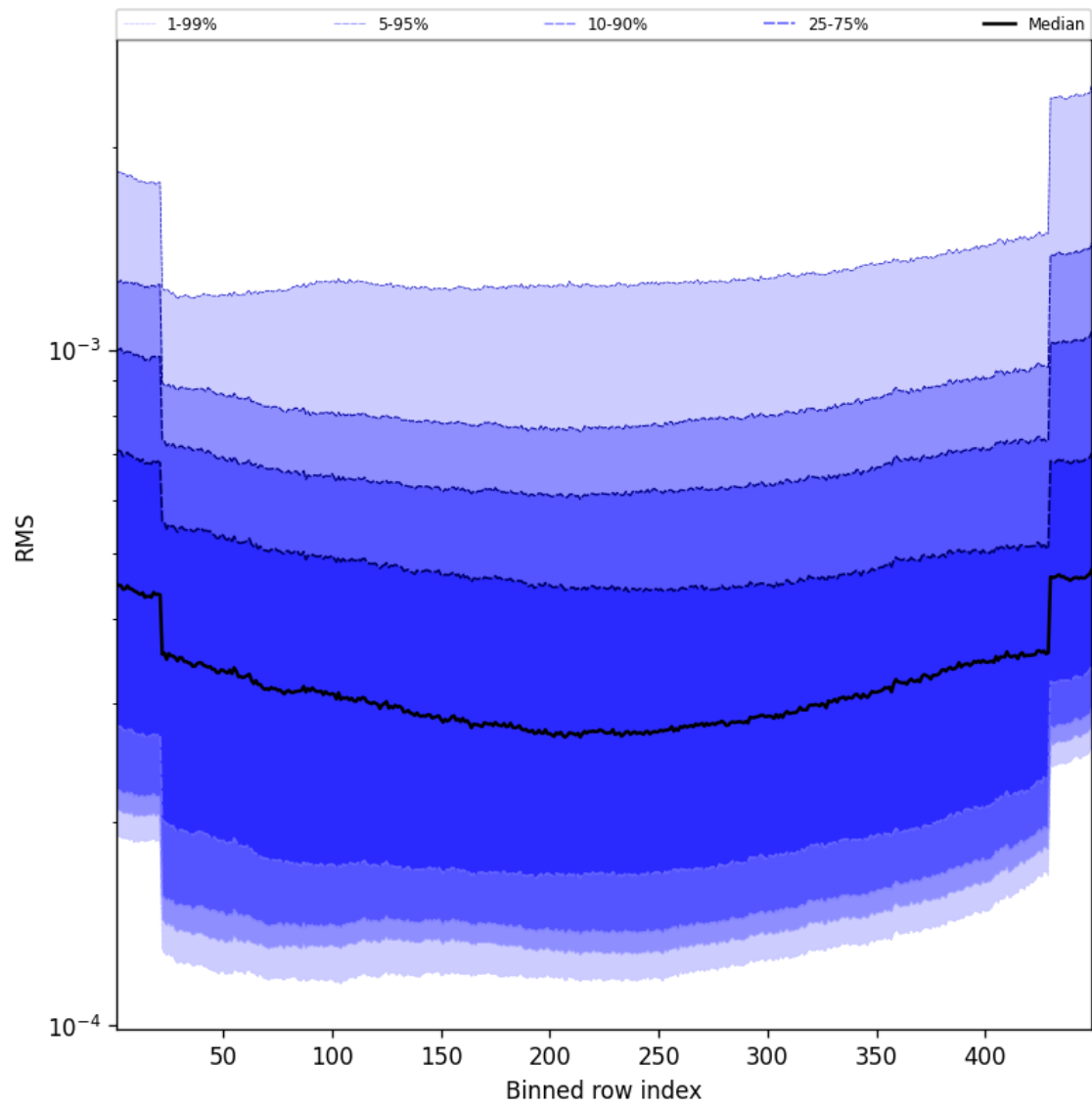
Figure 60: Along track statistics of “RMS” for 2024-10-08 to 2024-10-09
