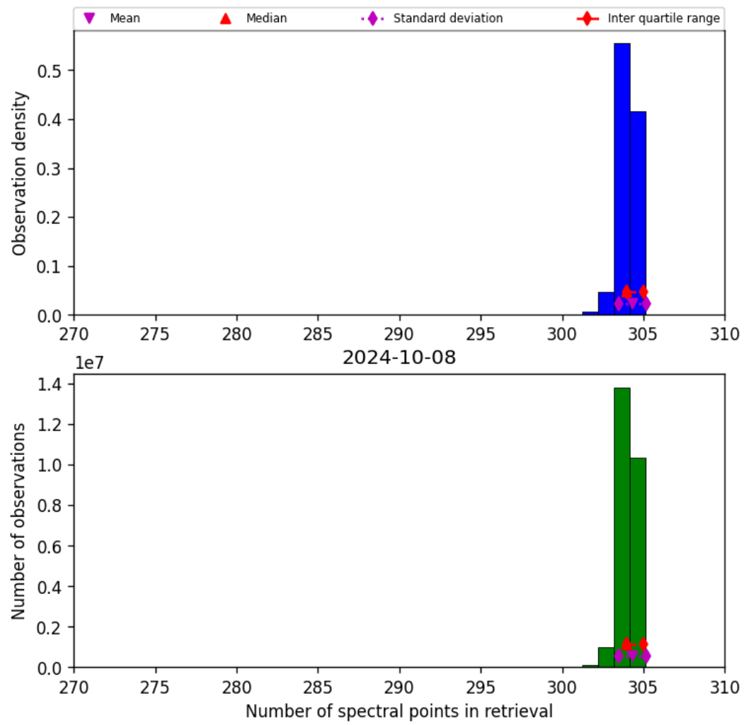
Figure 33: Histogram of “Number of spectral points in retrieval” for 2024-10-08 to 2024-10-09
