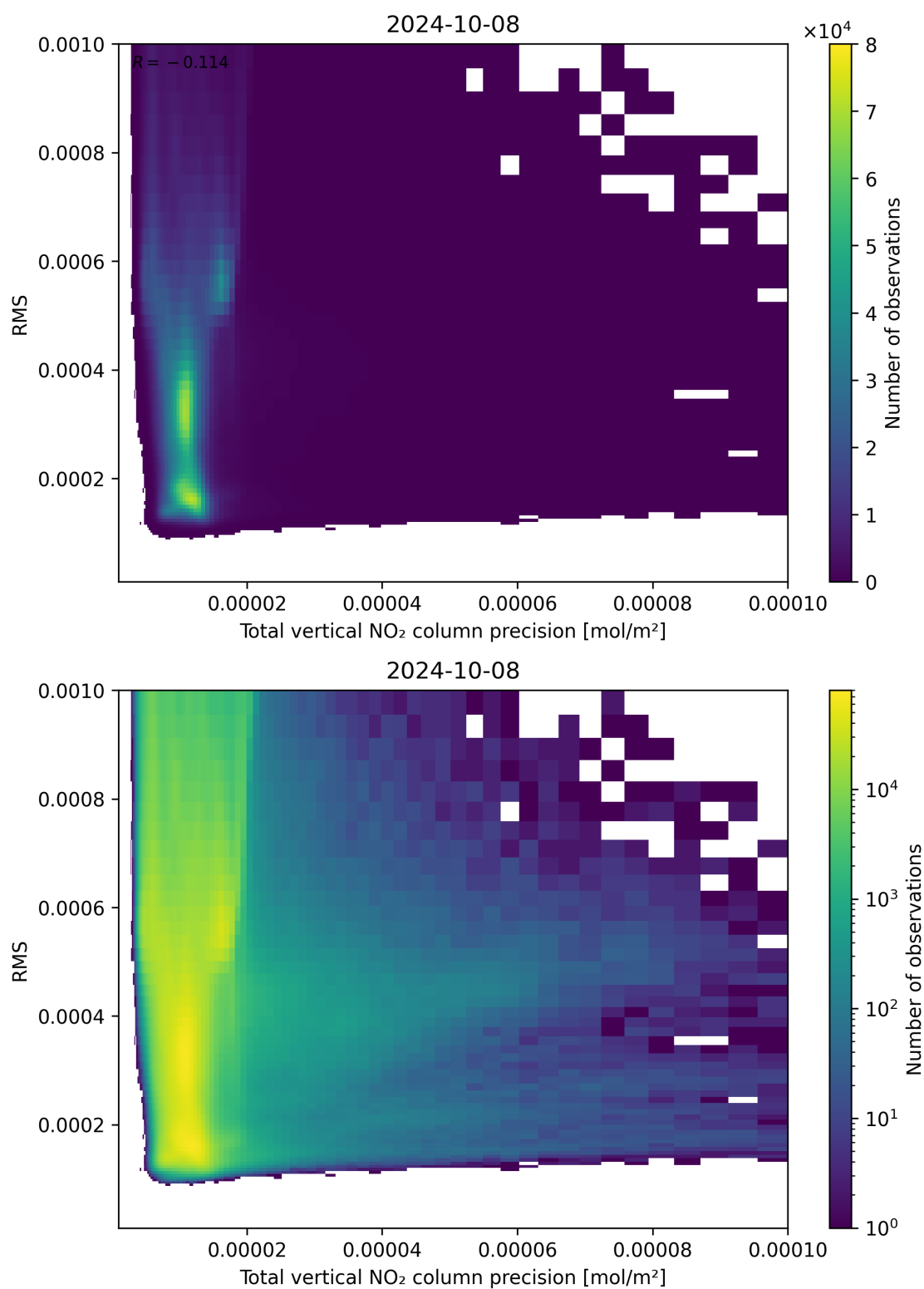
Figure 119: Scatter density plot of “Total vertical NO 2 column precision” against “RMS” for 2024-10-08 to 2024-10-09.
