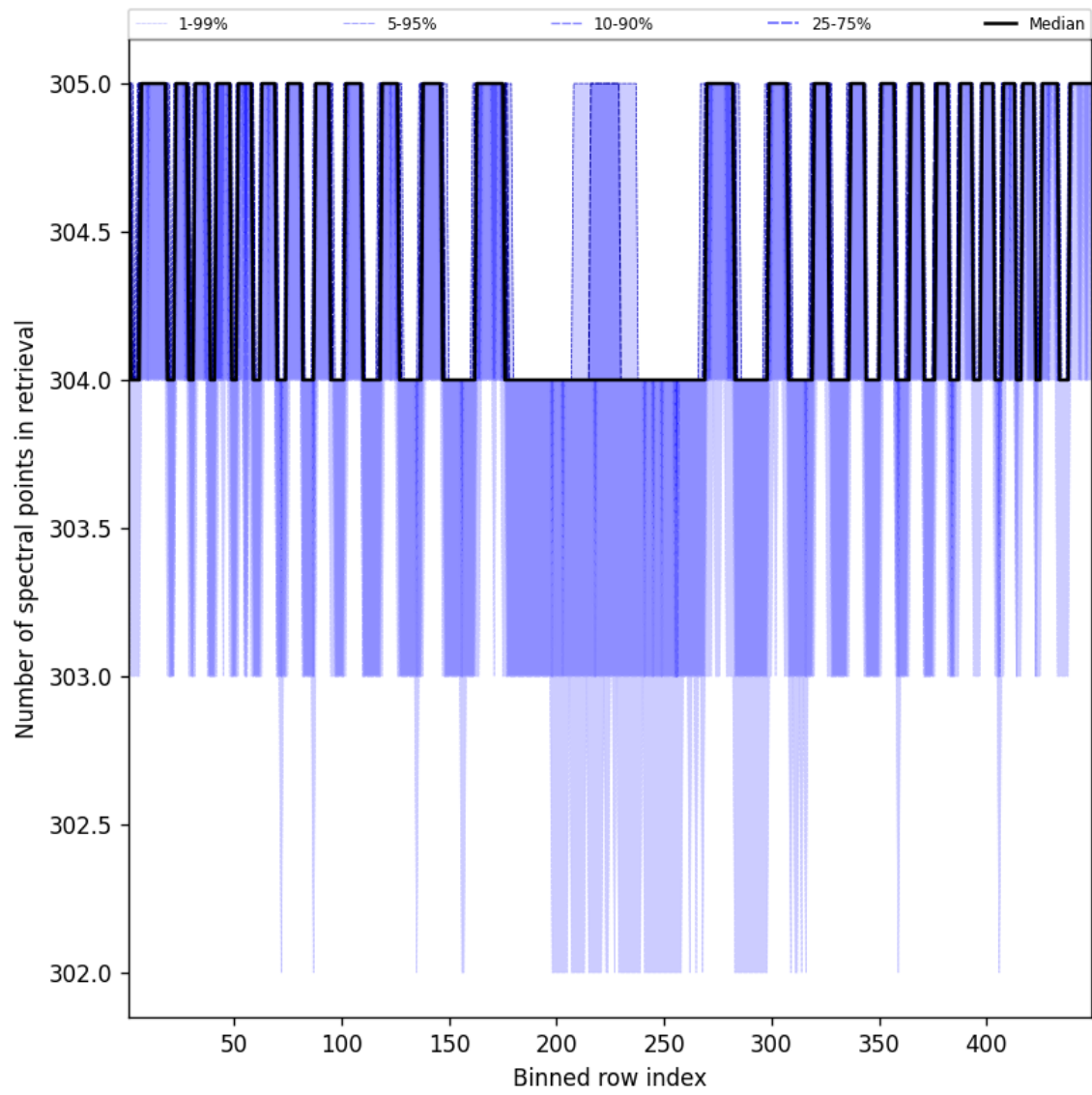
Figure 50: Along track statistics of “Number of spectral points in retrieval” for 2024-10-08 to 2024-10-09
