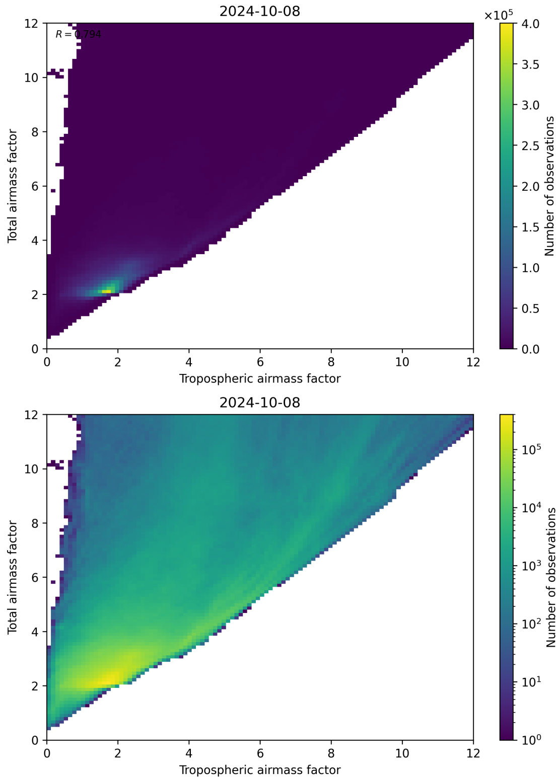
Figure 72: Scatter density plot of “Tropospheric airmass factor” against “Total airmass factor” for 2024-10-08 to 2024-10-09.
