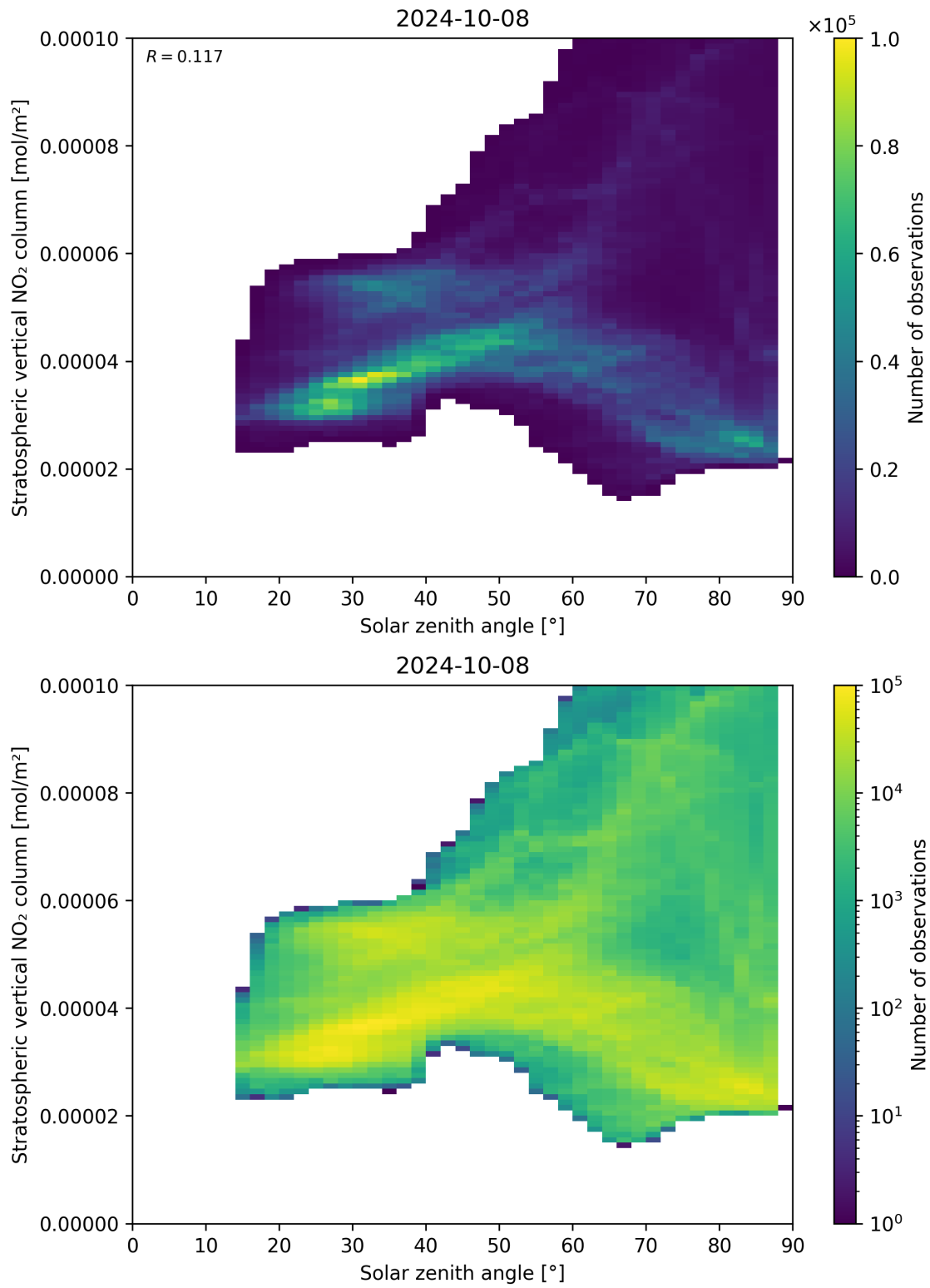
Figure 150: Scatter density plot of “Solar zenith angle” against “Stratospheric vertical NO 2 column” for 2024-10-08 to 2024-10-09.
