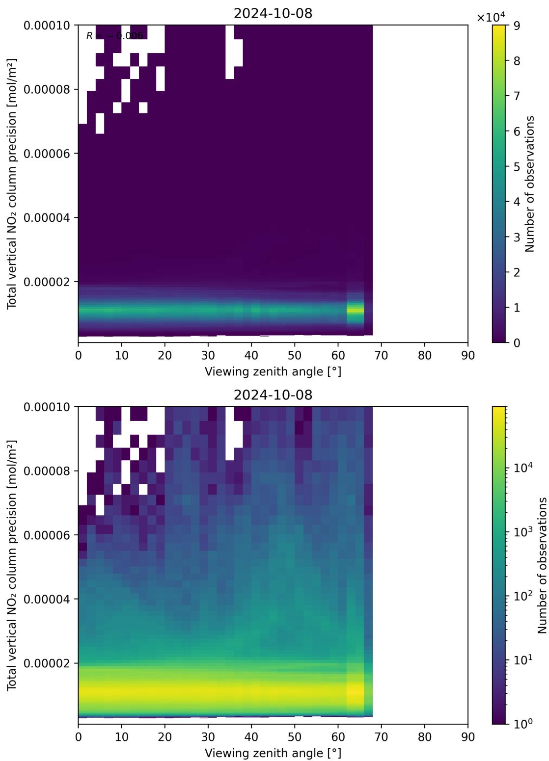
Figure 168: Scatter density plot of “Viewing zenith angle” against “Total vertical NO 2 column precision” for 2024-10-08 to 2024-10-09.
