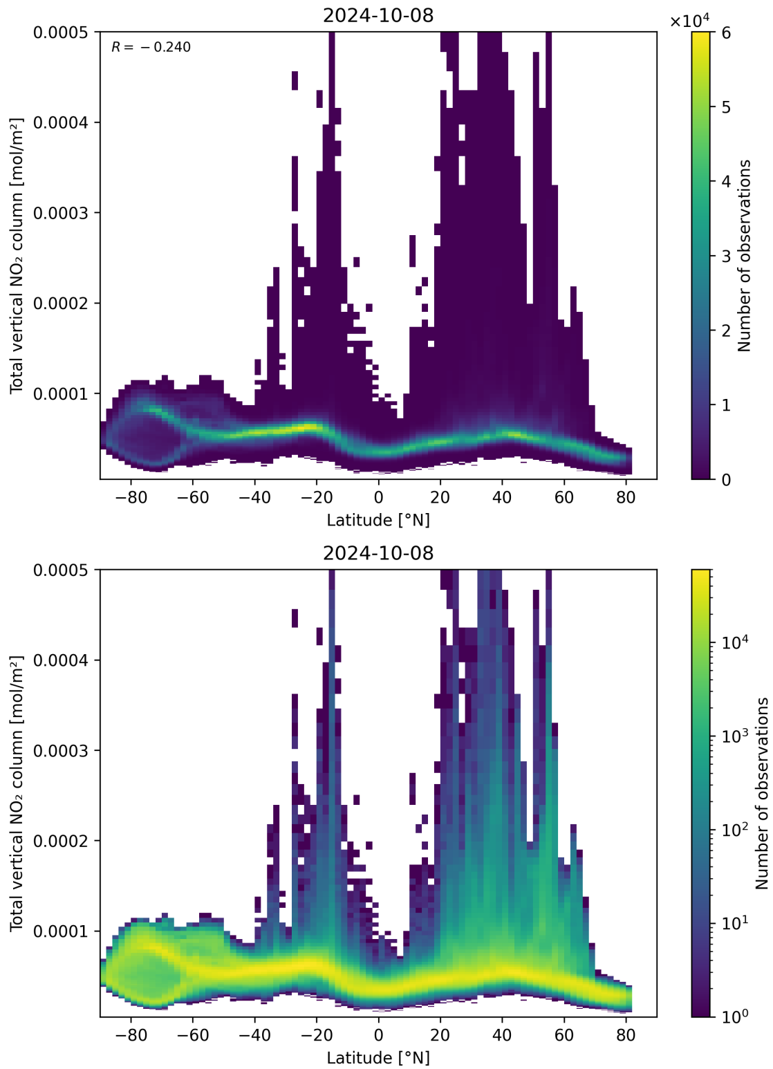
Figure 90: Scatter density plot of “Latitude” against “Total vertical NO 2 column” for 2024-10-08 to 2024-10-09.
