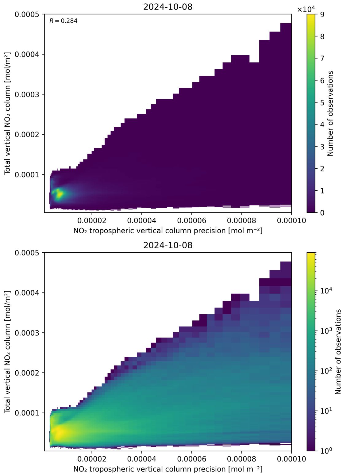
Figure 138: Scatter density plot of “NO 2 tropospheric vertical column precision” against “Total vertical NO 2 column” for 2024-10-08 to 2024-10-09.
