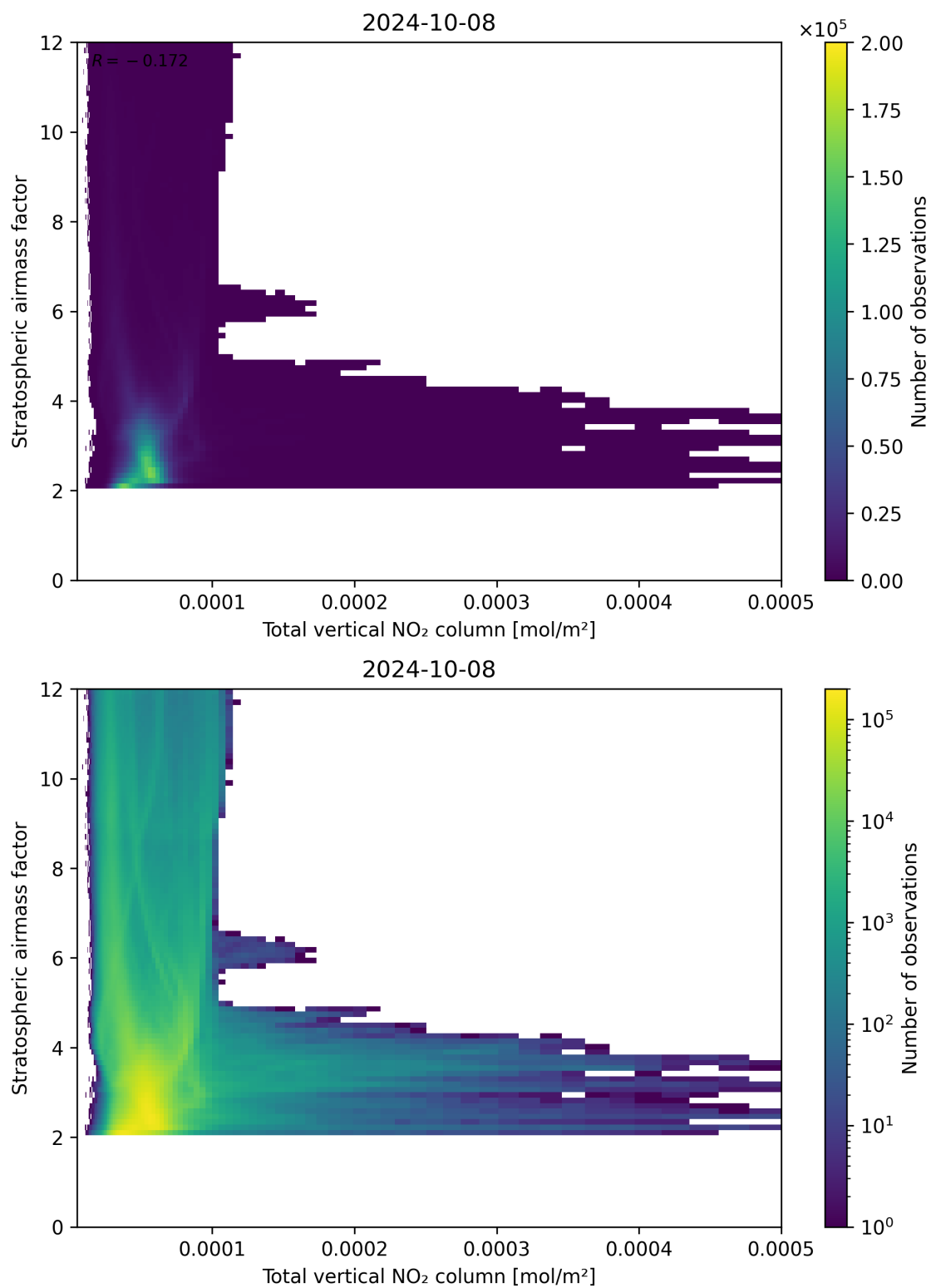
Figure 110: Scatter density plot of “Total vertical NO 2 column” against “Stratospheric airmass factor” for 2024-10-08 to 2024-10-09.
