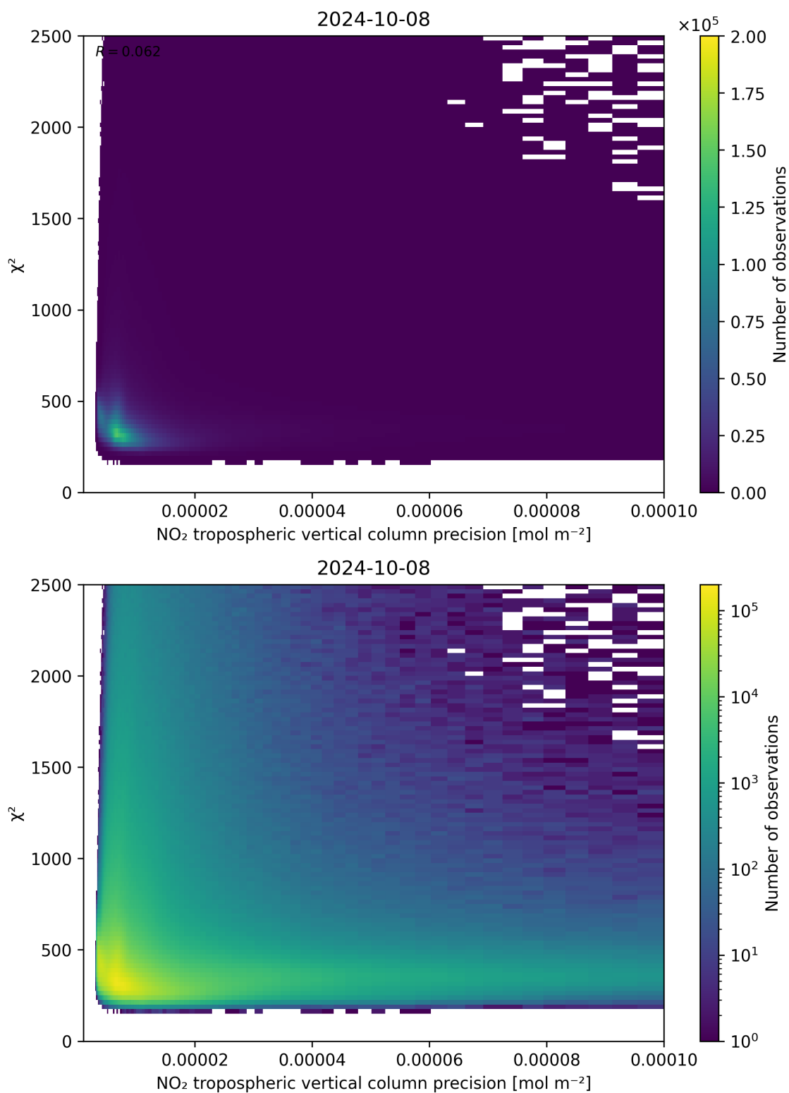
Figure 134: Scatter density plot of “NO 2 tropospheric vertical column precision” against “ \chi^2 ” for 2024-10-08 to 2024-10-09.
