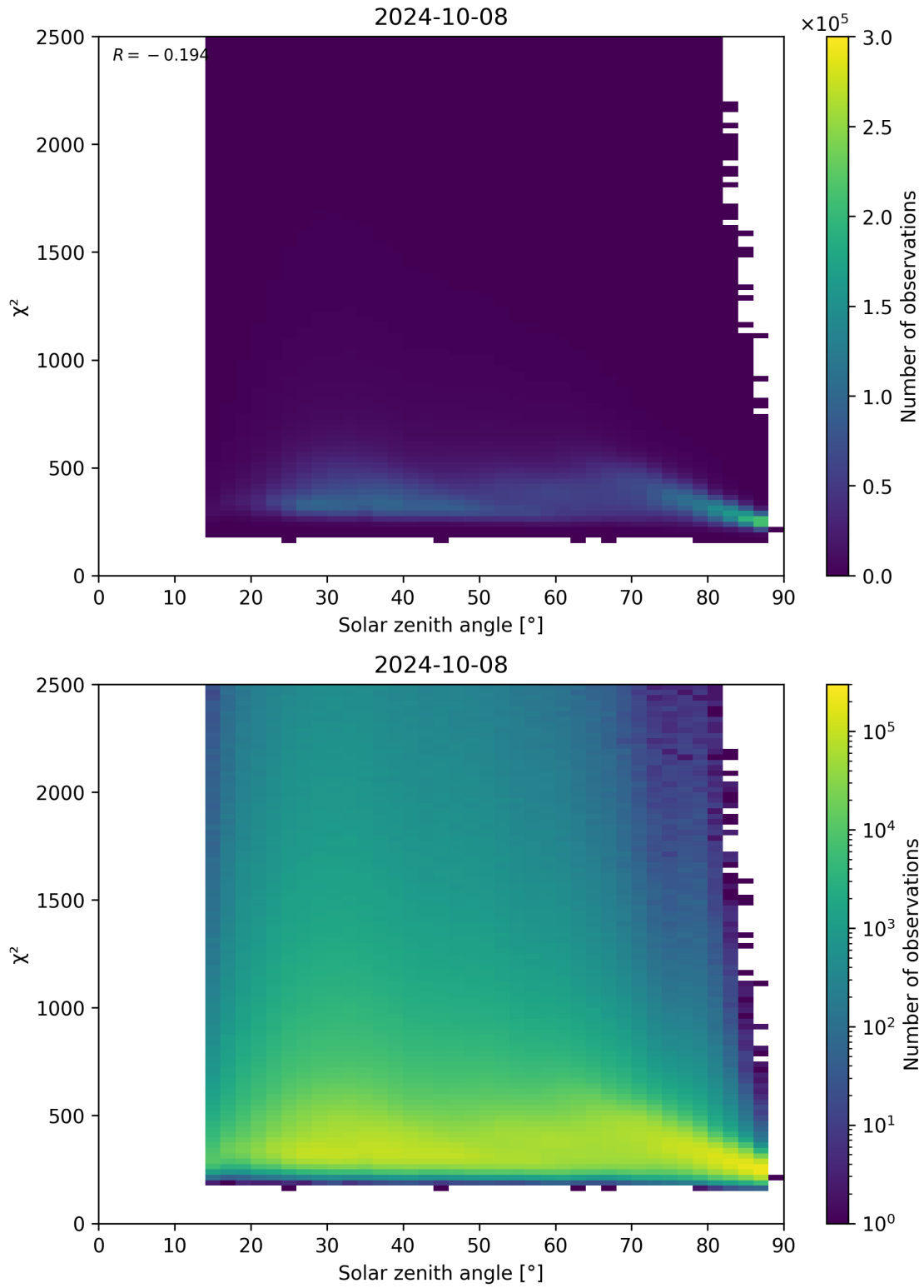
Figure 148: Scatter density plot of “Solar zenith angle” against “ \chi^2 ” for 2024-10-08 to 2024-10-09.
