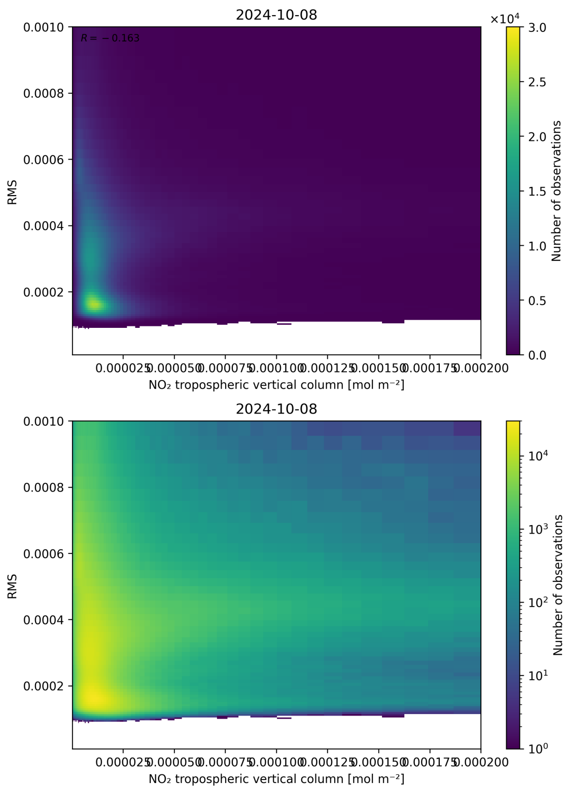
Figure 142: Scatter density plot of “NO 2 tropospheric vertical column” against “RMS” for 2024-10-08 to 2024-10-09.
