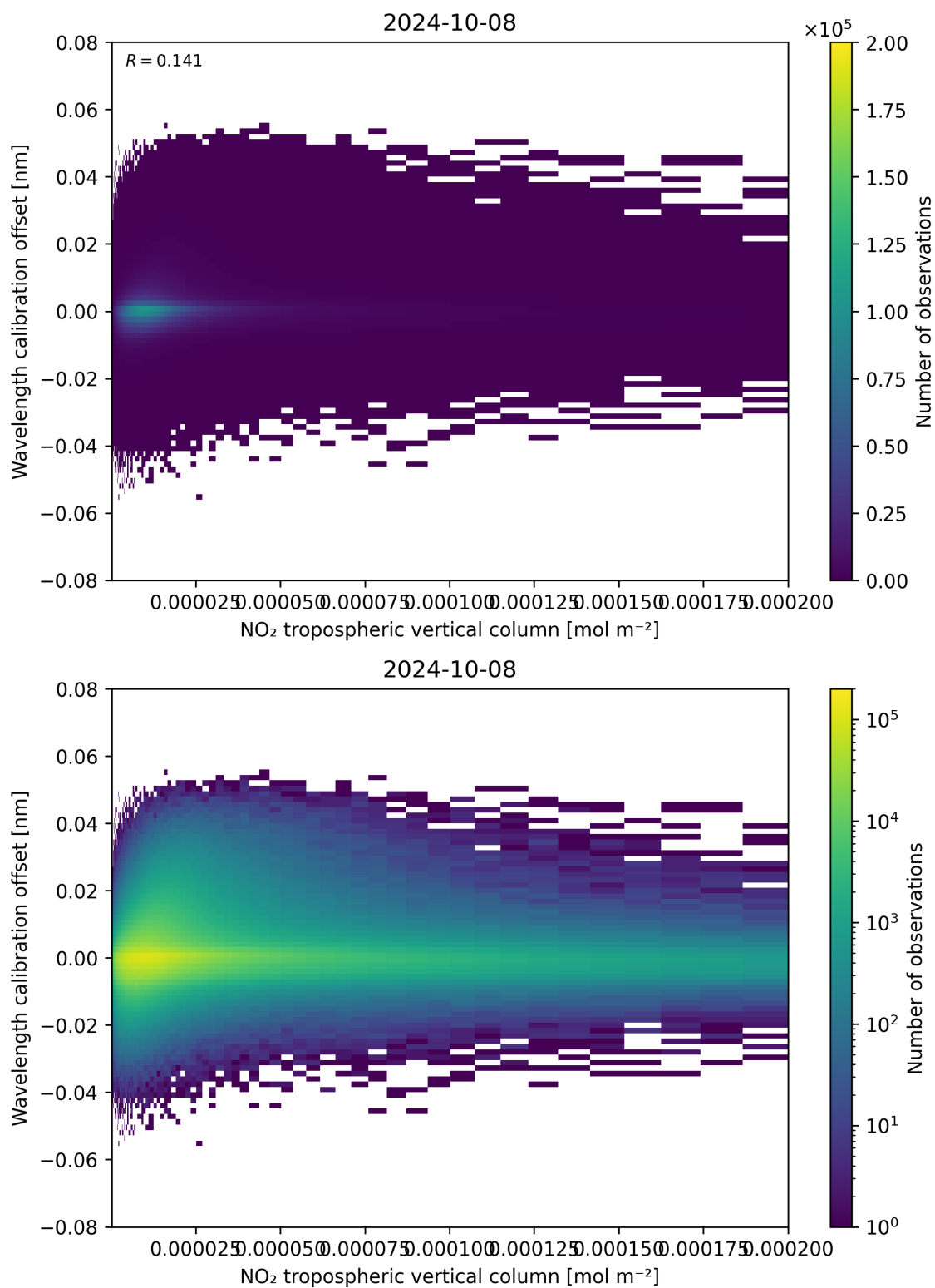
Figure 143: Scatter density plot of “NO 2 tropospheric vertical column” against “Wavelength calibration offset” for 2024-10-08 to 2024-10-09.
