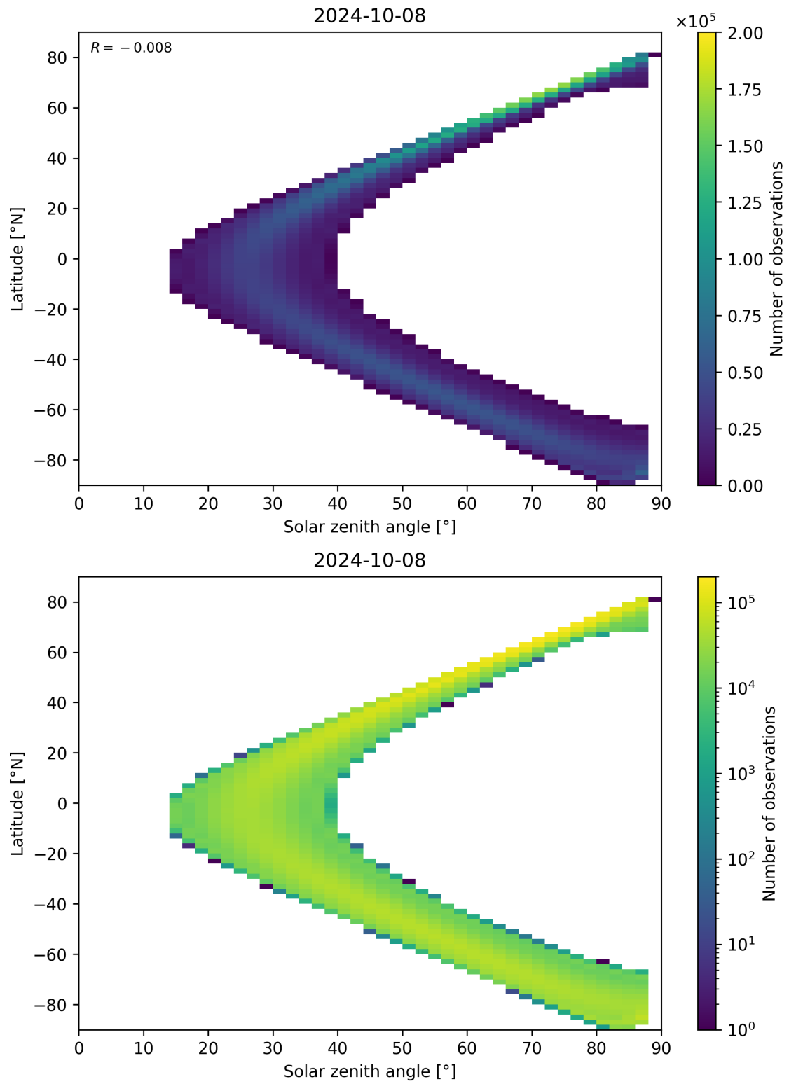
Figure 149: Scatter density plot of “Solar zenith angle” against “Latitude” for 2024-10-08 to 2024-10-09.
