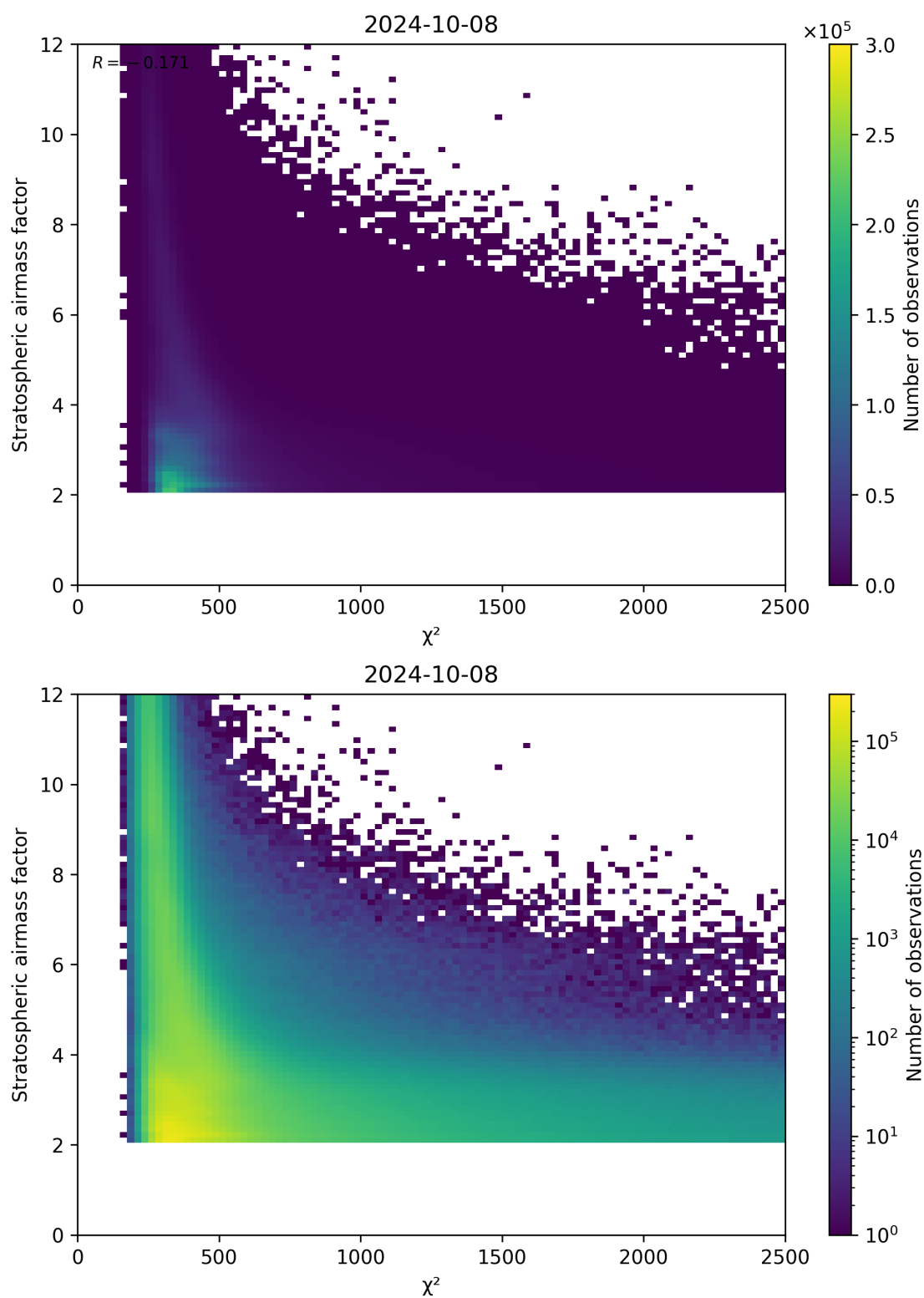
Figure 81: Scatter density plot of “ \chi^2 ” against “Stratospheric airmass factor” for 2024-10-08 to 2024-10-09.
