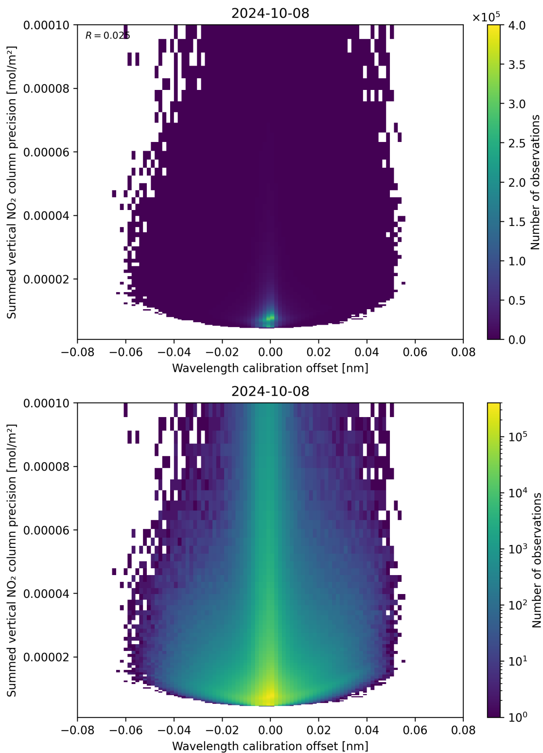
Figure 178: Scatter density plot of “Wavelength calibration offset” against “Summed vertical NO 2 column precision” for 2024-10-08 to 2024-10-09.
