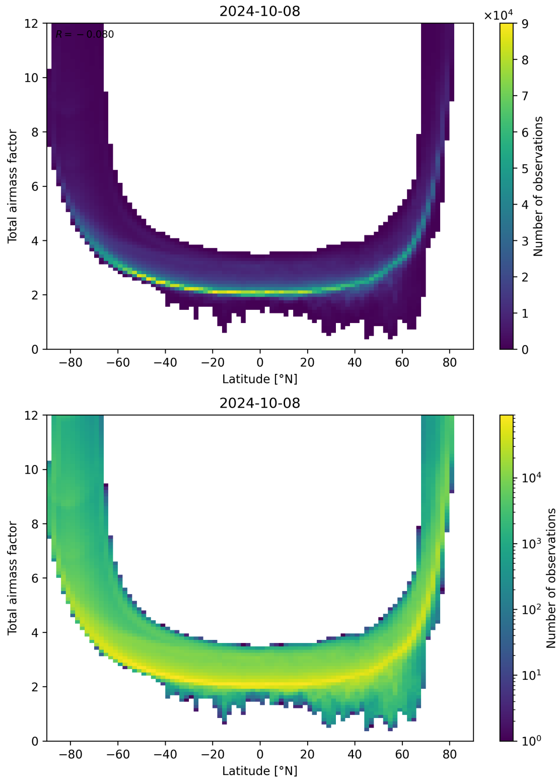
Figure 84: Scatter density plot of “Latitude” against “Total airmass factor” for 2024-10-08 to 2024-10-09.
