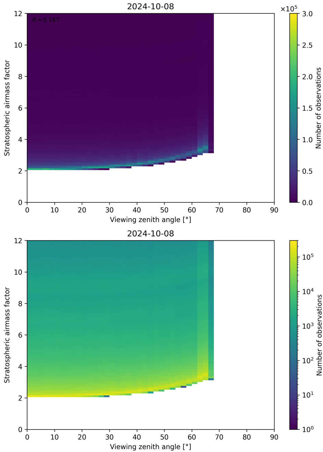
Figure 159: Scatter density plot of “Viewing zenith angle” against “Stratospheric airmass factor” for 2024-10-08 to 2024-10-09.
