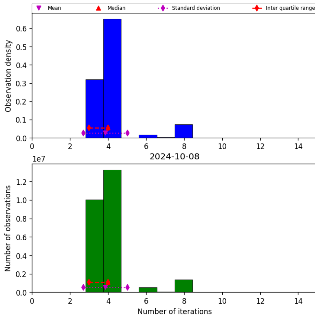
Figure 34: Histogram of “Number of iterations” for 2024-10-08 to 2024-10-09
