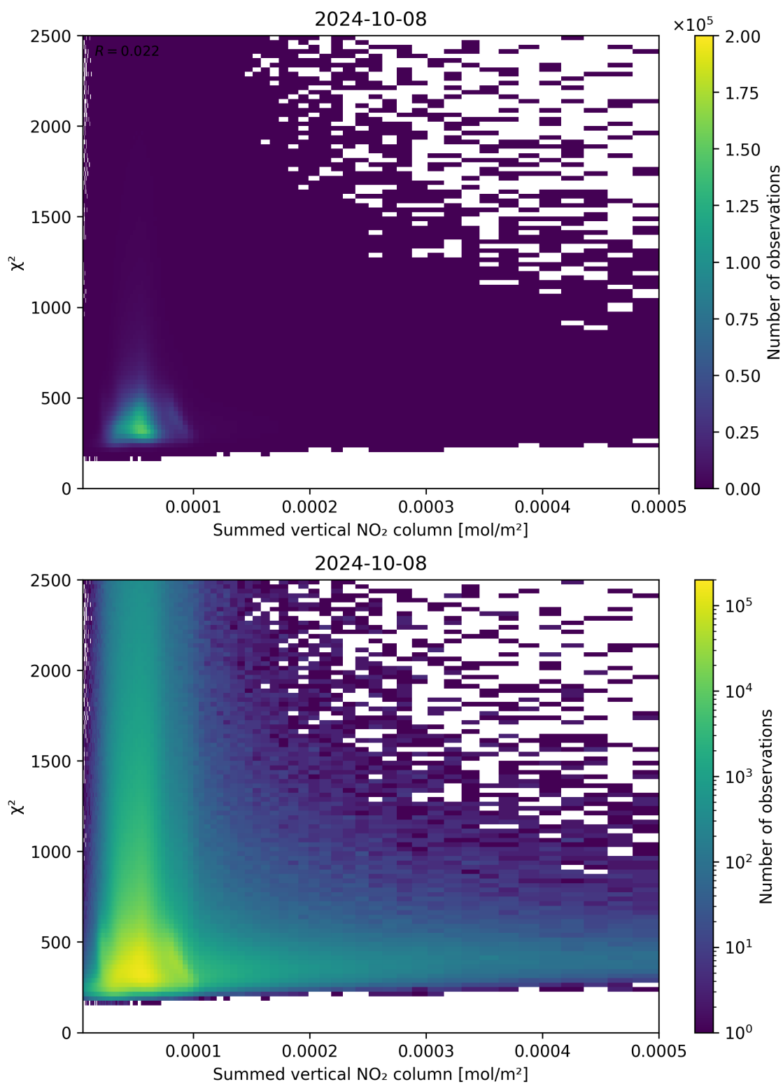
Figure 104: Scatter density plot of “Summed vertical NO 2 column” against “ \chi^2 ” for 2024-10-08 to 2024-10-09.
