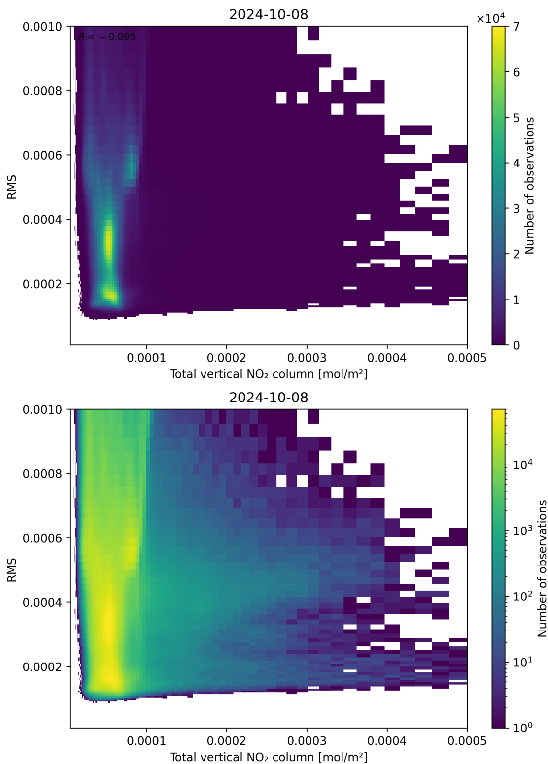
Figure 120: Scatter density plot of “Total vertical NO 2 column” against “RMS” for 2024-10-08 to 2024-10-09.
