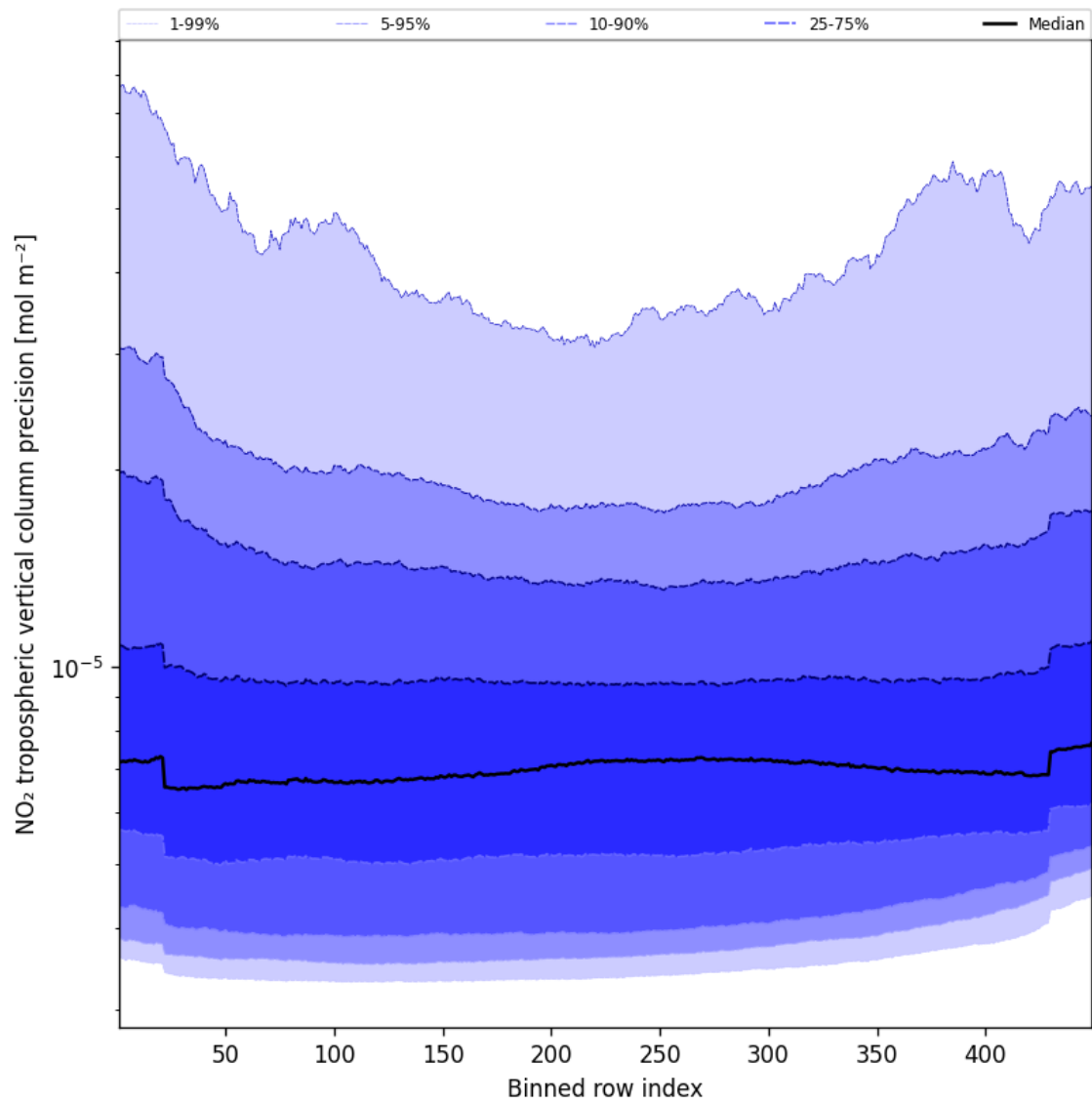
Figure 47: Along track statistics of “NO 2 tropospheric vertical column precision” for 2024-10-08 to 2024-10-09
