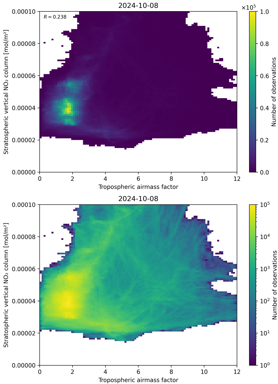
Figure 74: Scatter density plot of “Tropospheric air mass factor” against “Stratospheric vertical NO 2 column” for 2024-10-08 to 2024-10-09.
