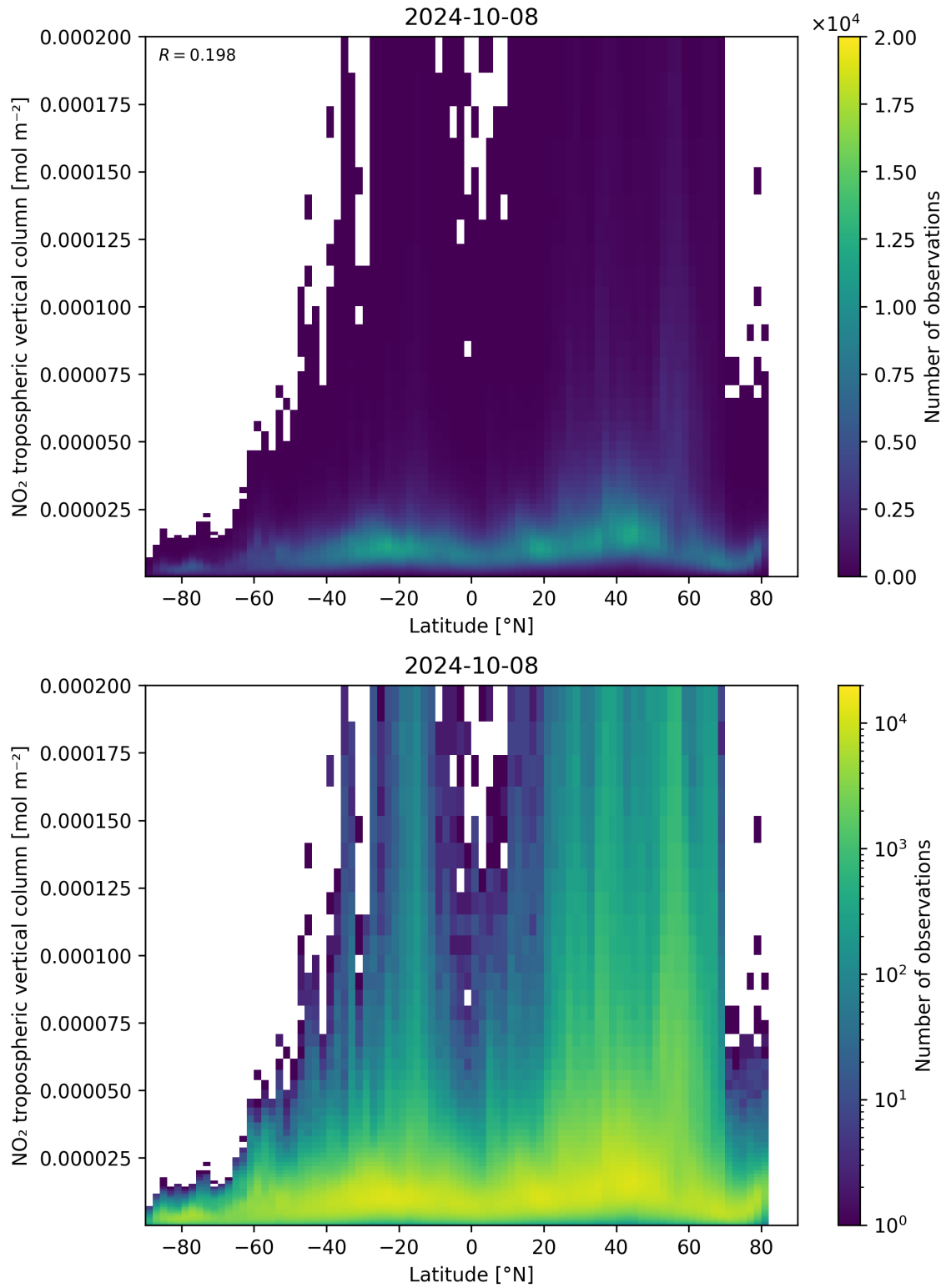
Figure 92: Scatter density plot of “Latitude” against “NO 2 tropospheric vertical column” for 2024-10-08 to 2024-10-09.
