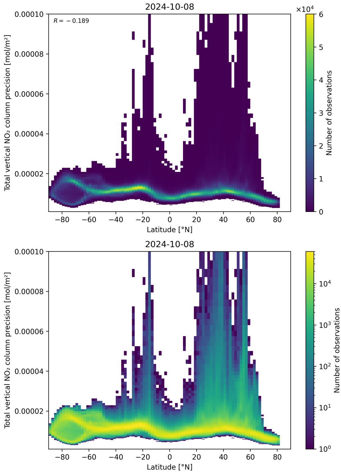
Figure 91: Scatter density plot of “Latitude” against “Total vertical NO 2 column precision” for 2024-10-08 to 2024-10-09.
