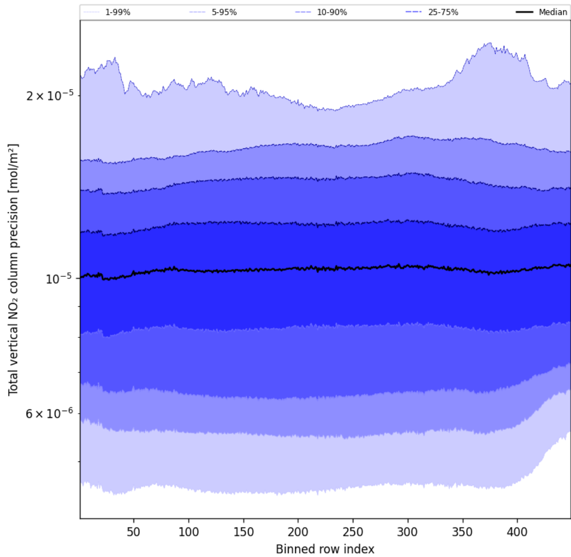
Figure 56: Along track statistics of “Total vertical NO 2 column precision” for 2024-10-08 to 2024-10-09
