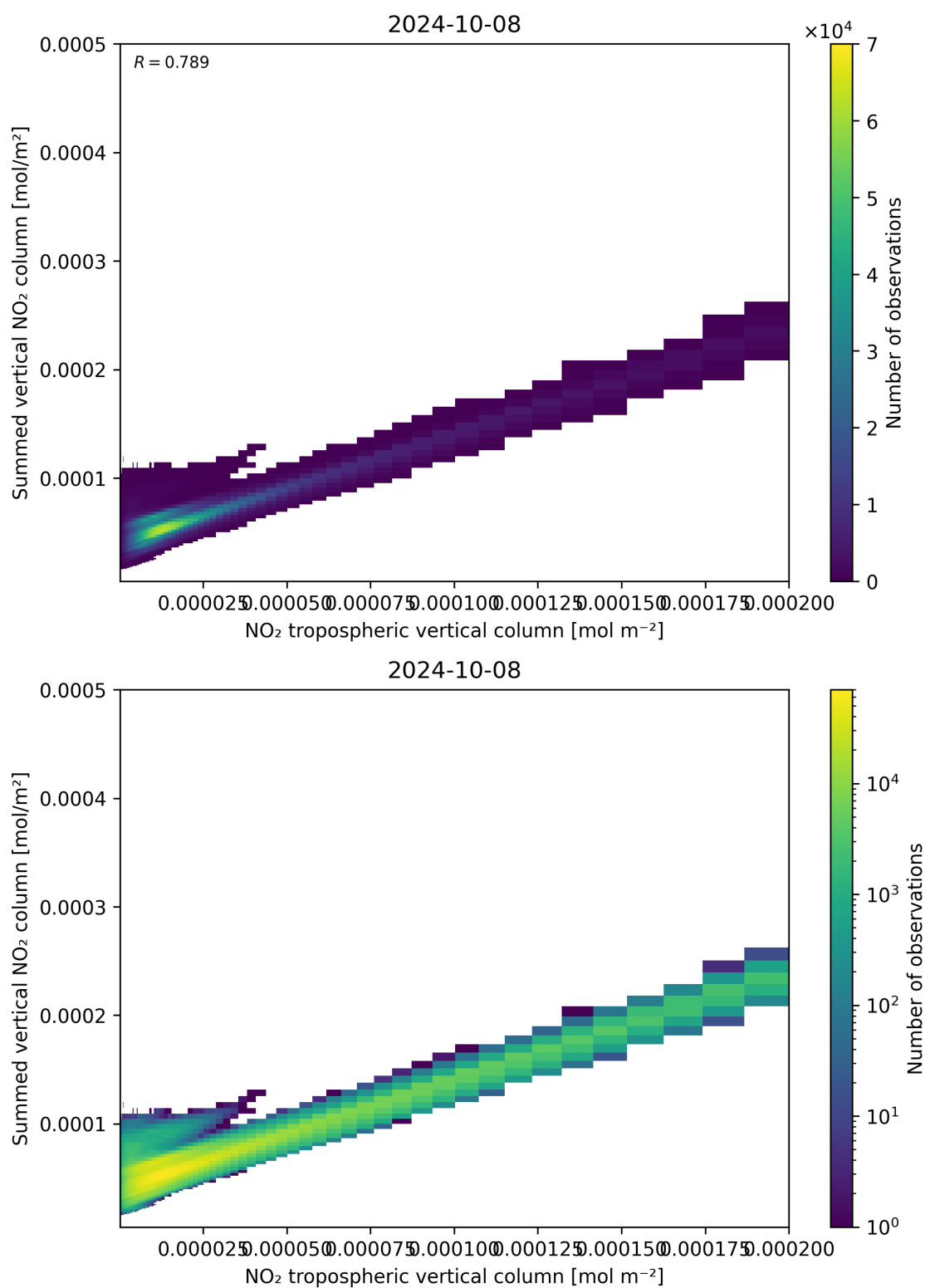
Figure 126: Scatter density plot of “NO 2 tropospheric vertical column” against “Summed vertical NO 2 column” for 2024-10-08 to 2024-10-09.
