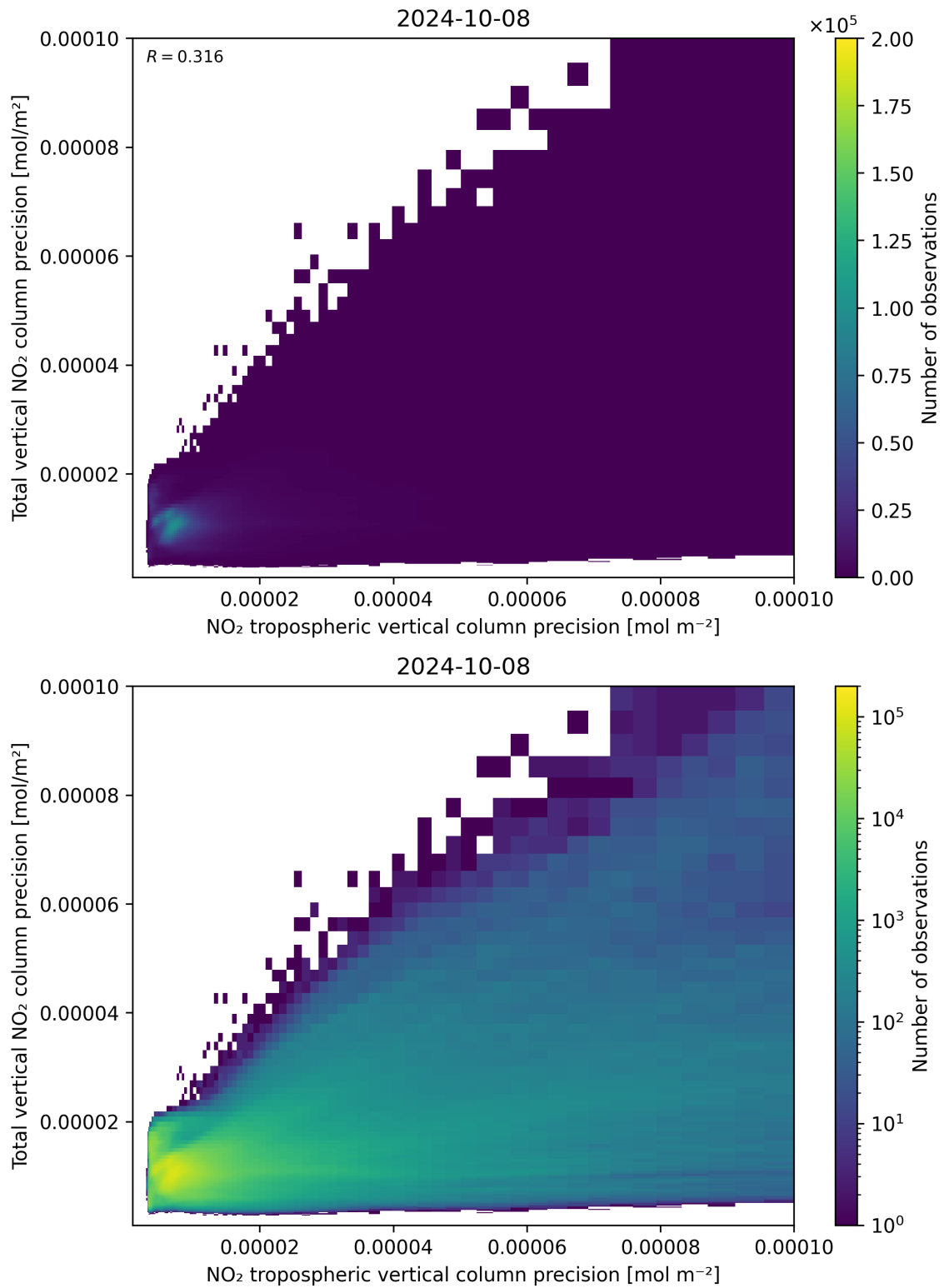
Figure 139: Scatter density plot of “NO 2 tropospheric vertical column precision” against “Total vertical NO 2 column precision” for 2024-10-08 to 2024-10-09.
