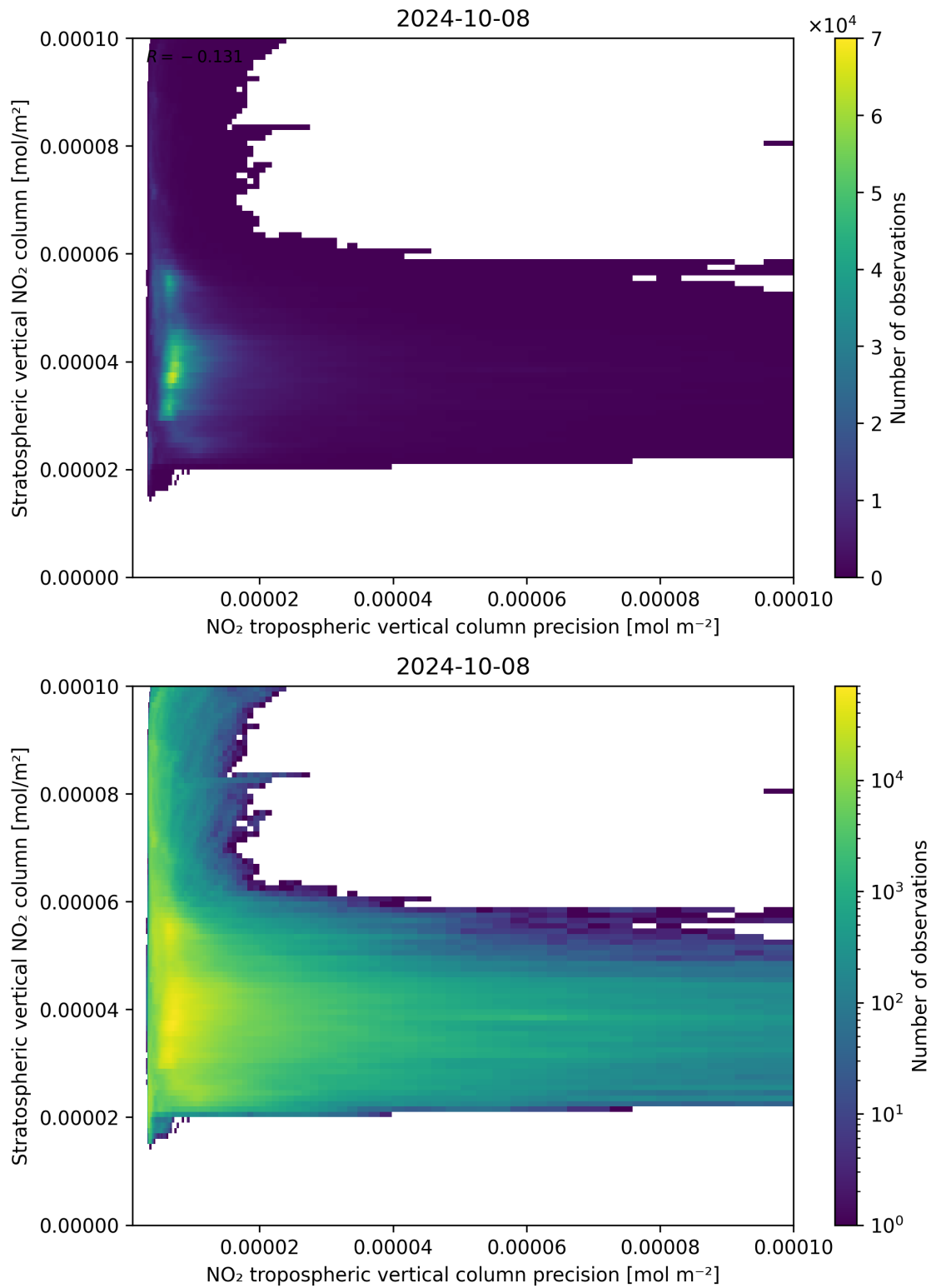
Figure 135: Scatter density plot of “NO 2 tropospheric vertical column precision” against “Stratospheric vertical NO 2 column” for 2024-10-08 to 2024-10-09.
