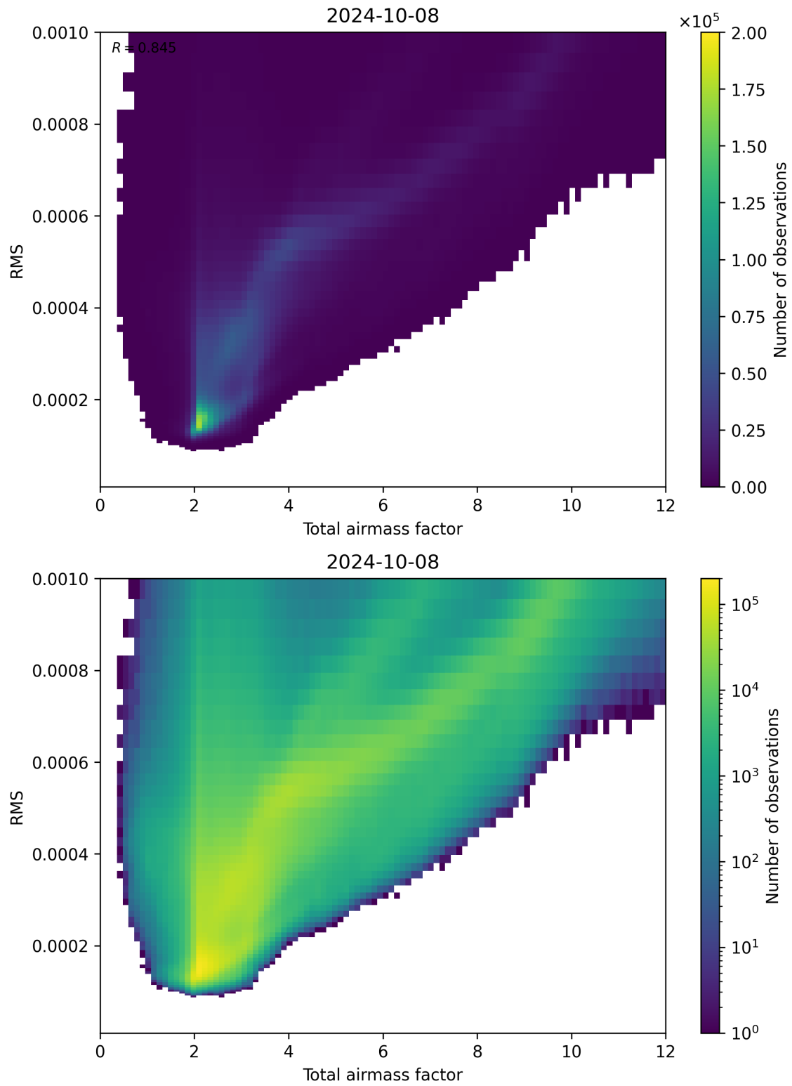
Figure 69: Scatter density plot of “Total airmass factor” against “RMS” for 2024-10-08 to 2024-10-09.
