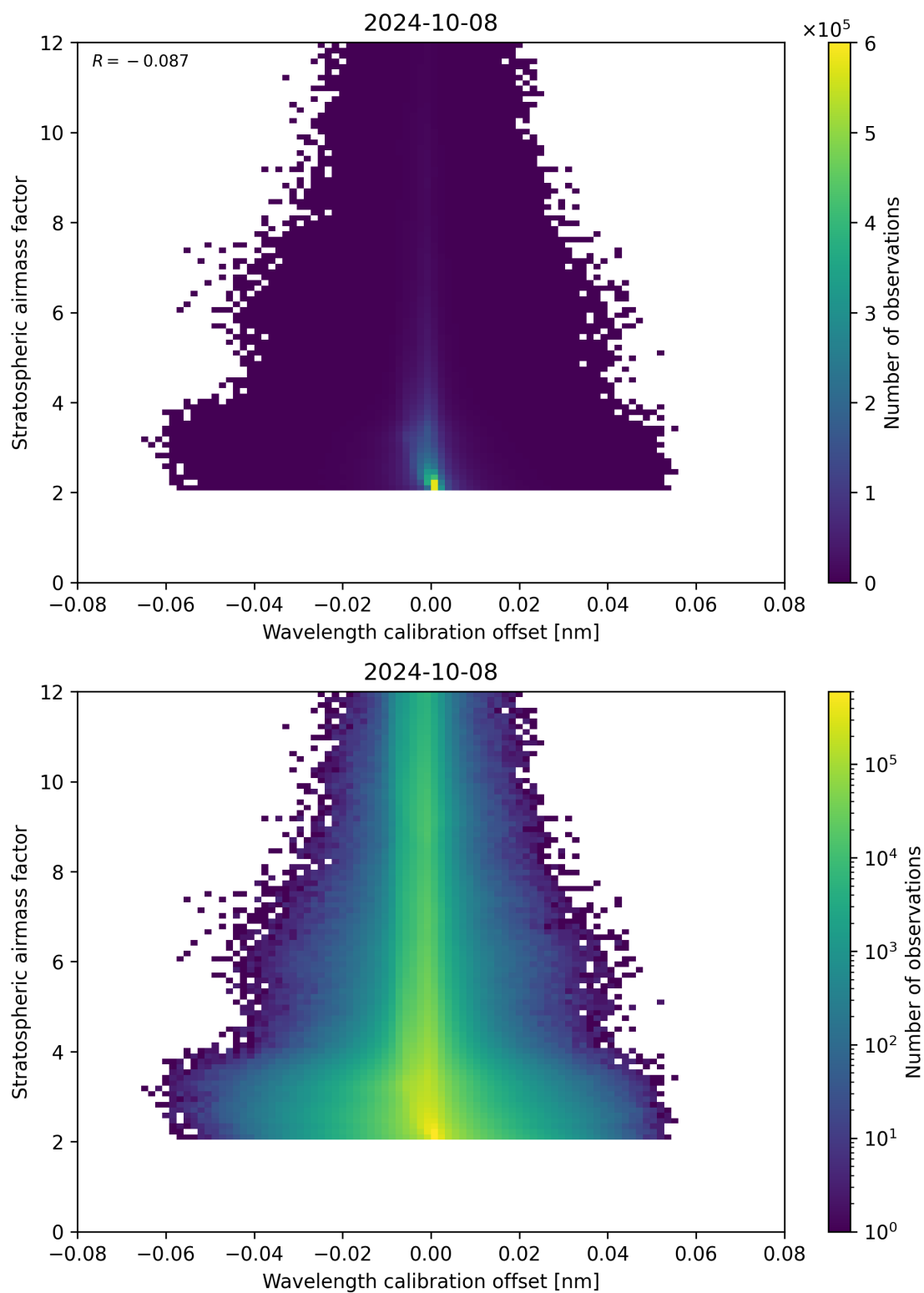
Figure 174: Scatter density plot of “Wavelength calibration offset” against “Stratospheric air mass factor” for 2024-10-08 to 2024-10-09.
