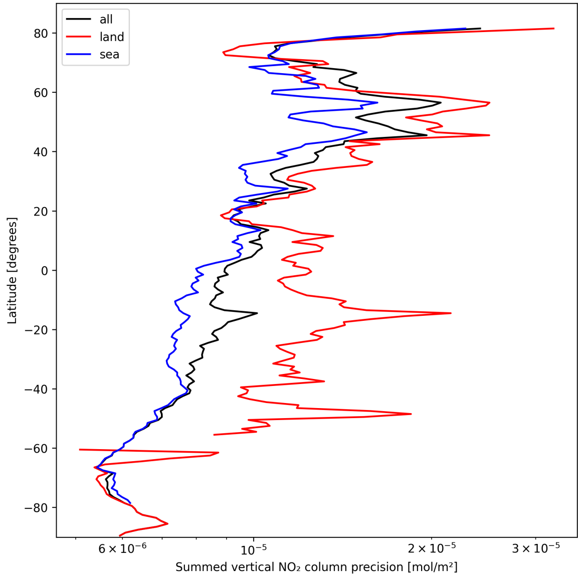
Figure 24: Zonal average of “Summed vertical NO 2 column precision” for 2024-10-08 to 2024-10-09.
