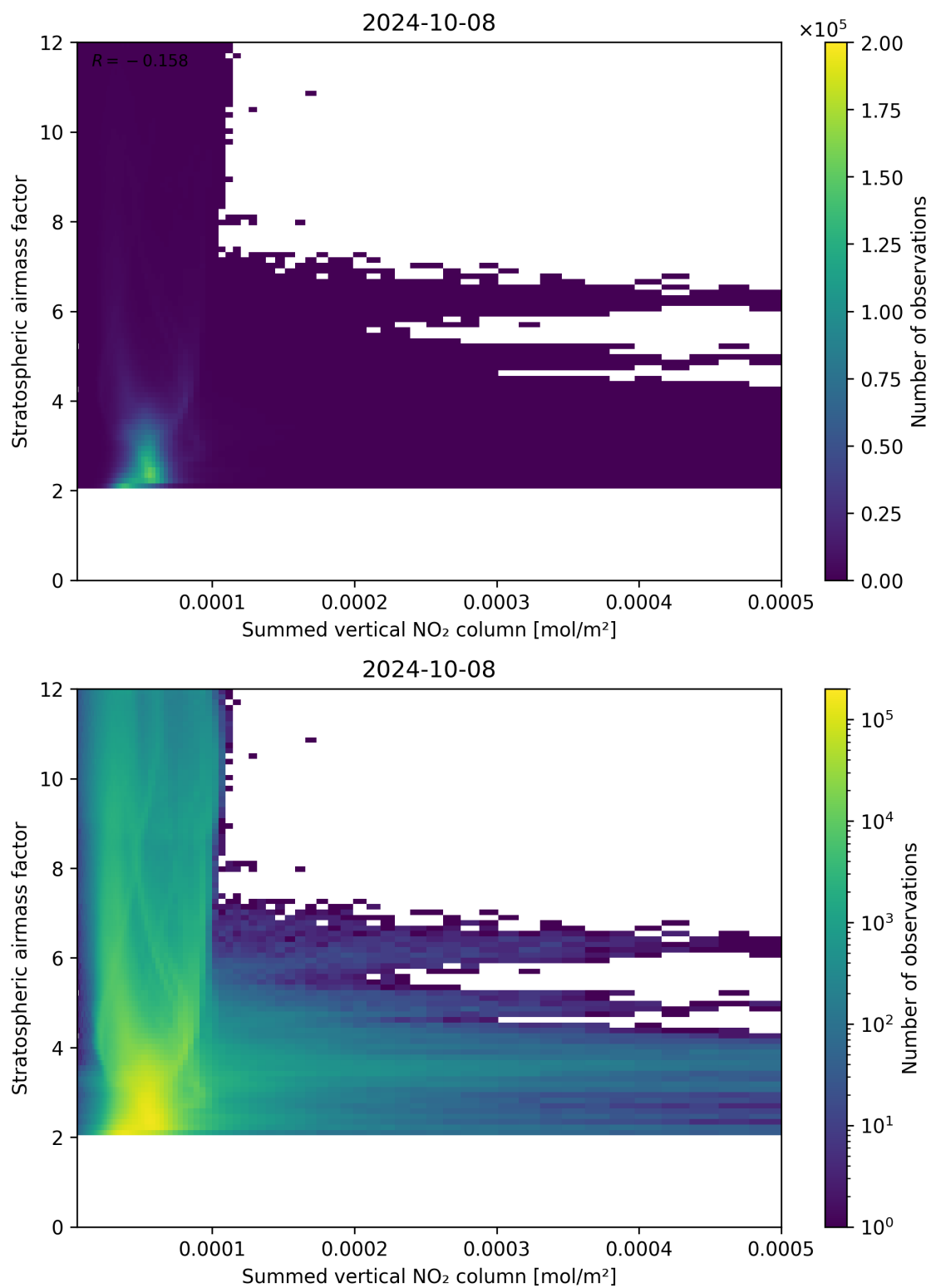
Figure 103: Scatter density plot of “Summed vertical NO 2 column” against “Stratospheric airmass factor” for 2024-10-08 to 2024-10-09.
