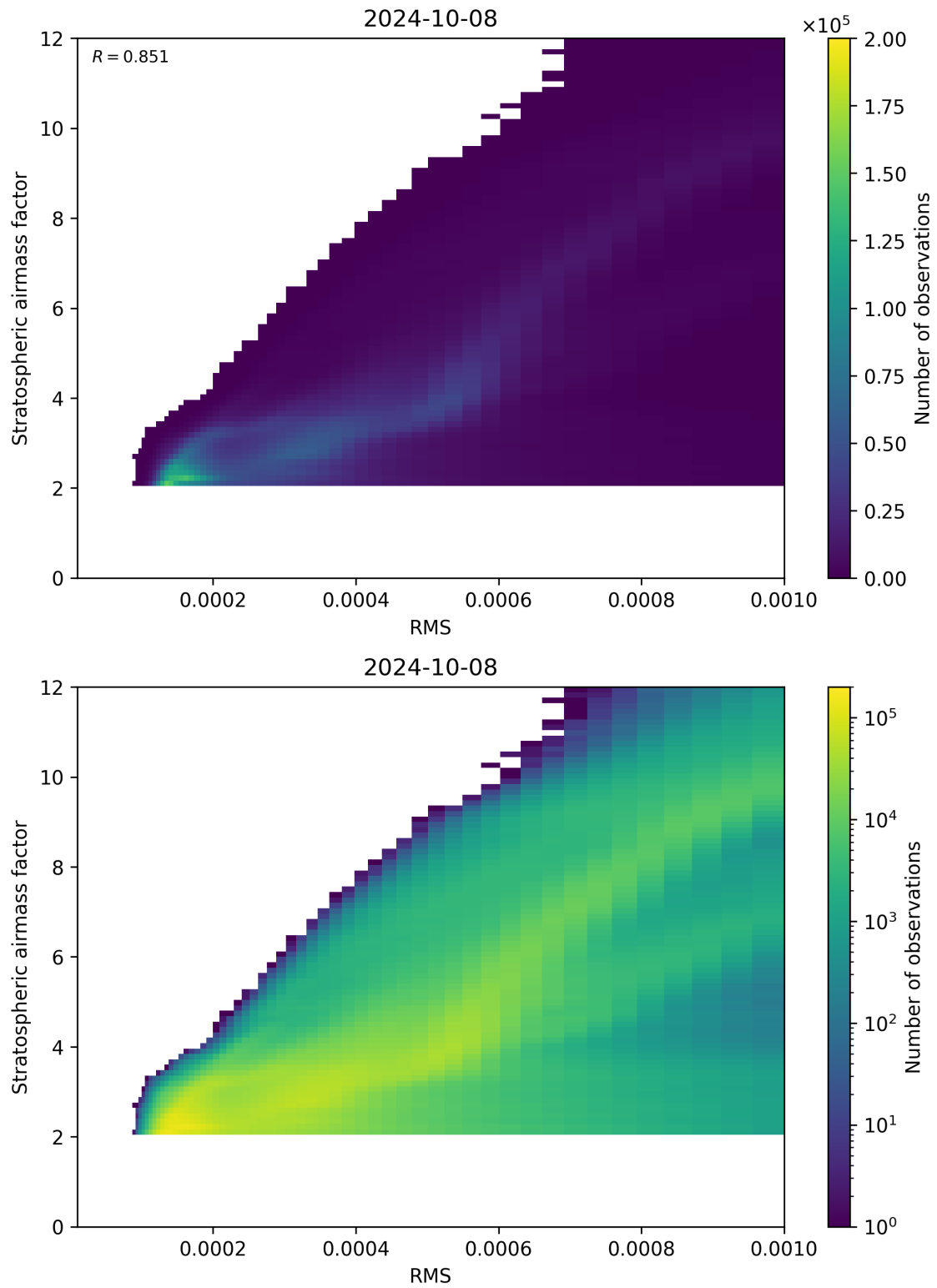
Figure 144: Scatter density plot of “RMS” against “Stratospheric airmass factor” for 2024-10-08 to 2024-10-09.
