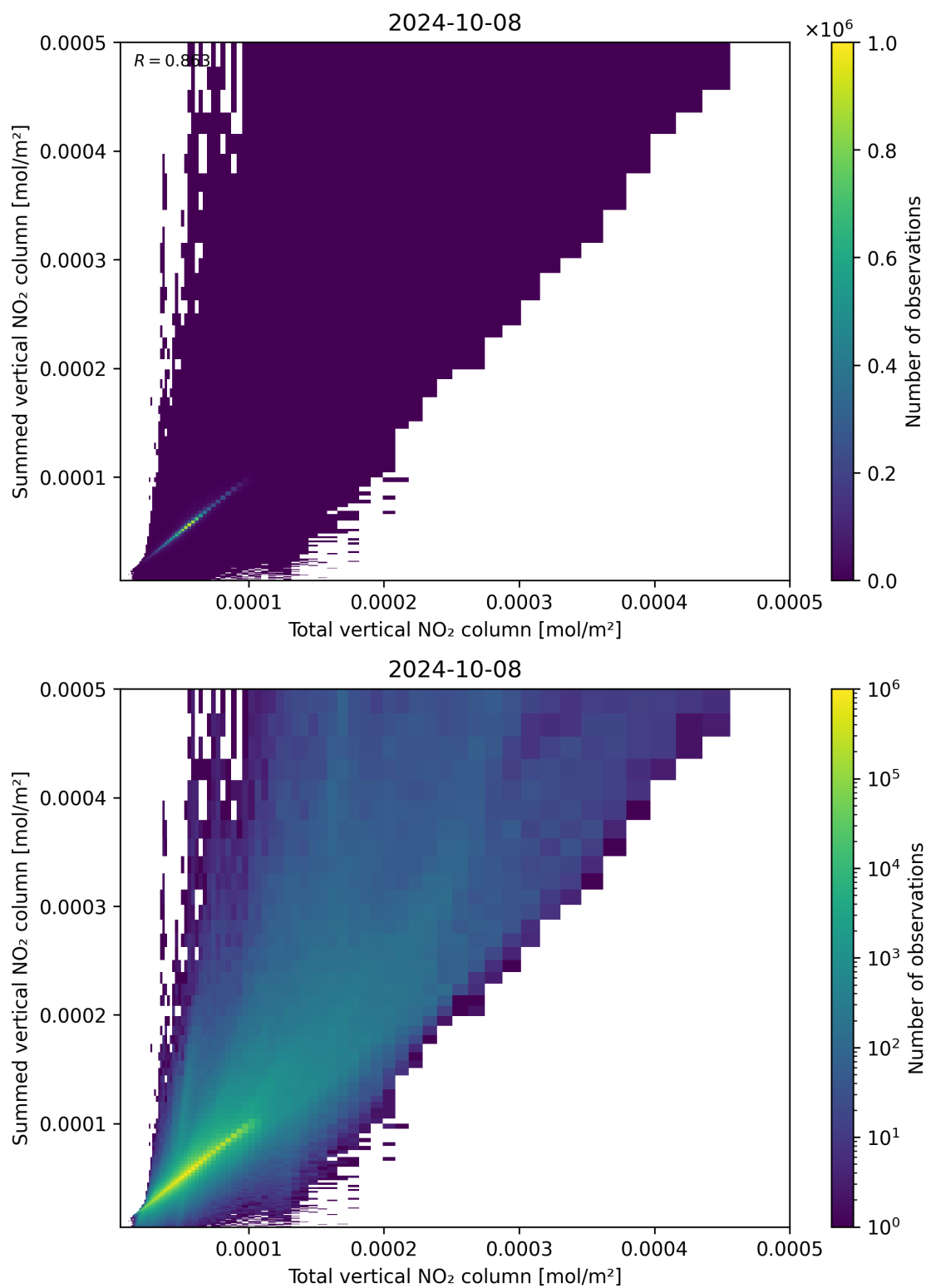
Figure 112: Scatter density plot of “Total vertical NO 2 column” against “Summed vertical NO 2 column” for 2024-10-08 to 2024-10-09.
