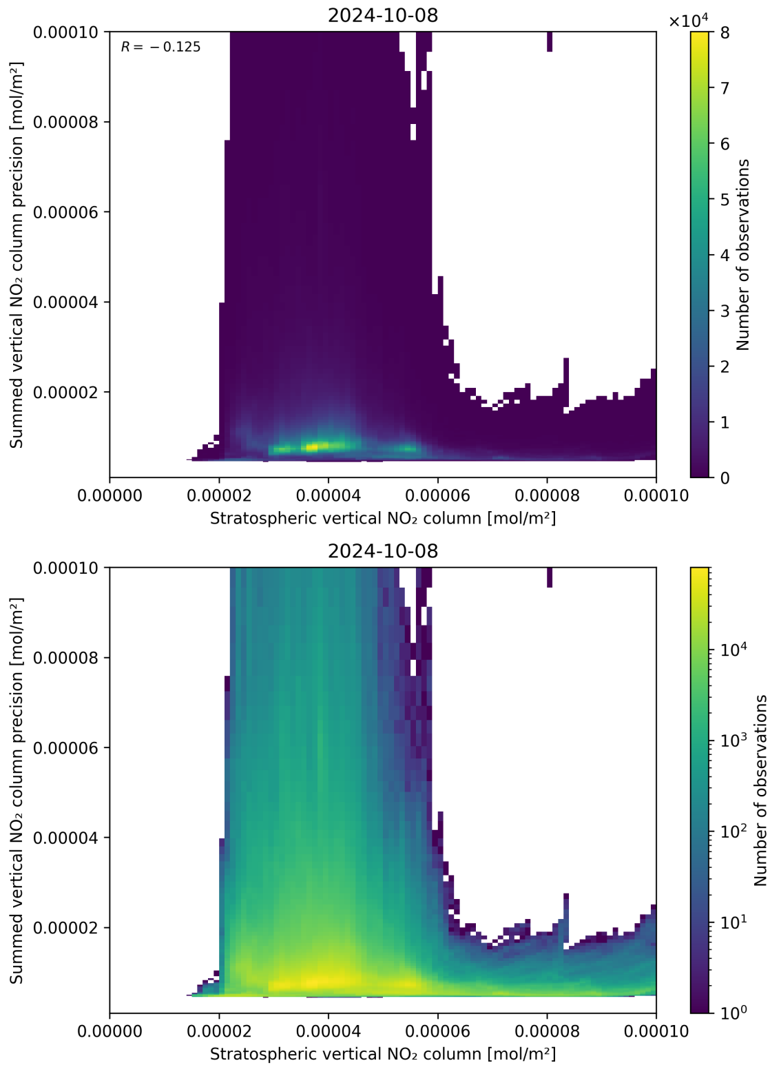
Figure 99: Scatter density plot of “Stratospheric vertical NO 2 column” against “Summed vertical NO 2 column precision” for 2024-10-08 to 2024-10-09.
