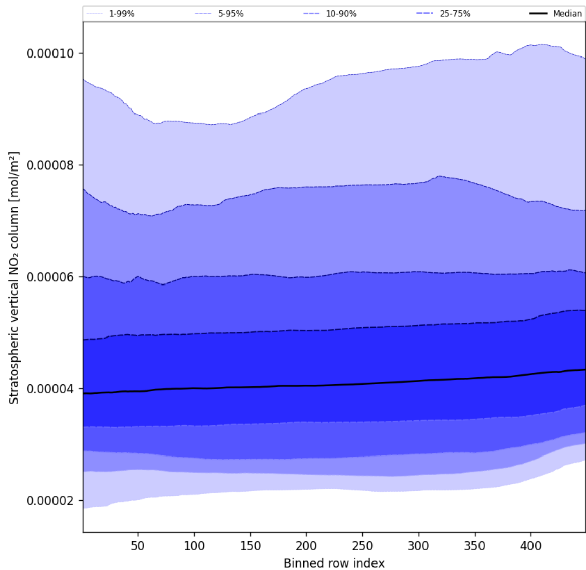
Figure 53: Along track statistics of “Stratospheric vertical NO 2 column” for 2024-10-08 to 2024-10-09
