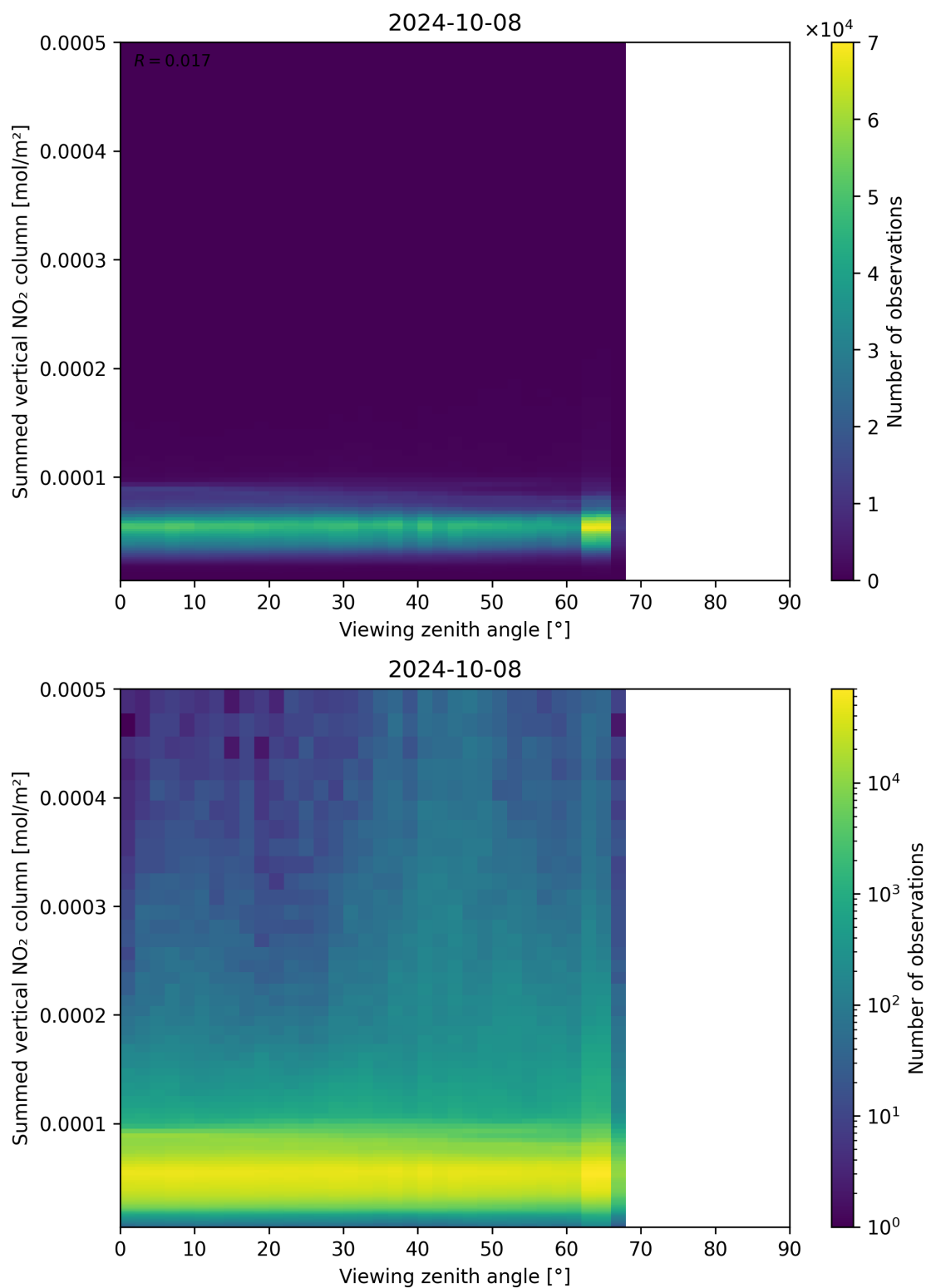
Figure 165: Scatter density plot of “Viewing zenith angle” against “Summed vertical NO 2 column” for 2024-10-08 to 2024-10-09.
