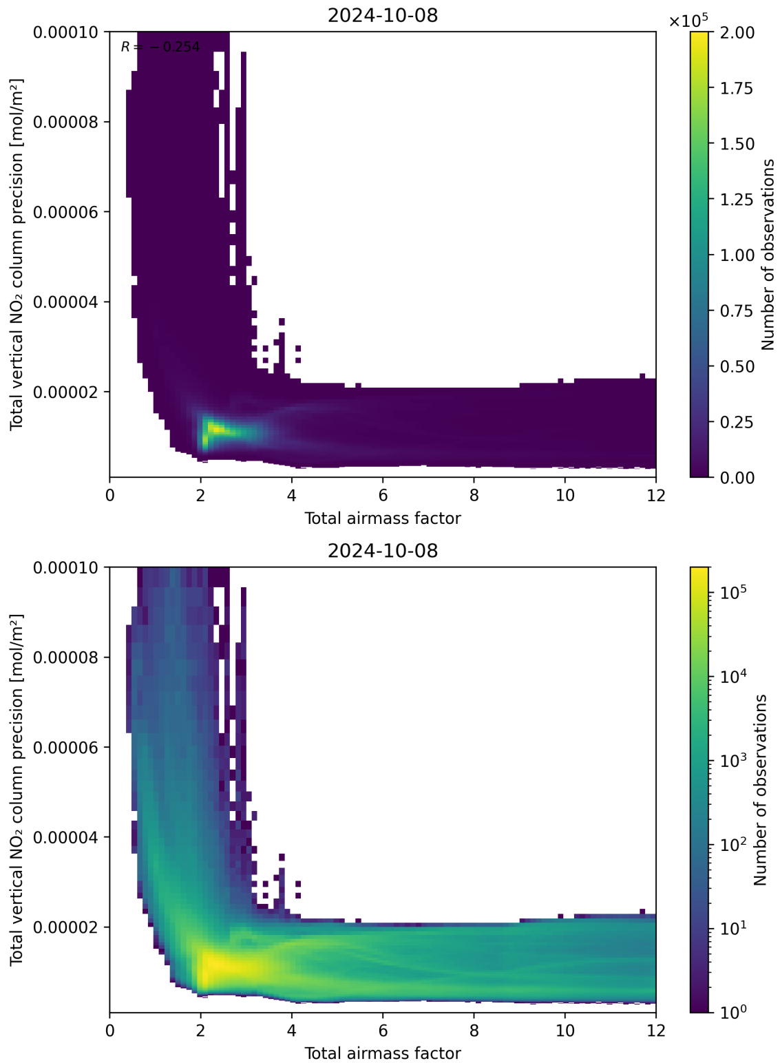
Figure 68: Scatter density plot of “Total airmass factor” against “Total vertical NO 2 column precision” for 2024-10-08 to 2024-10-09.
