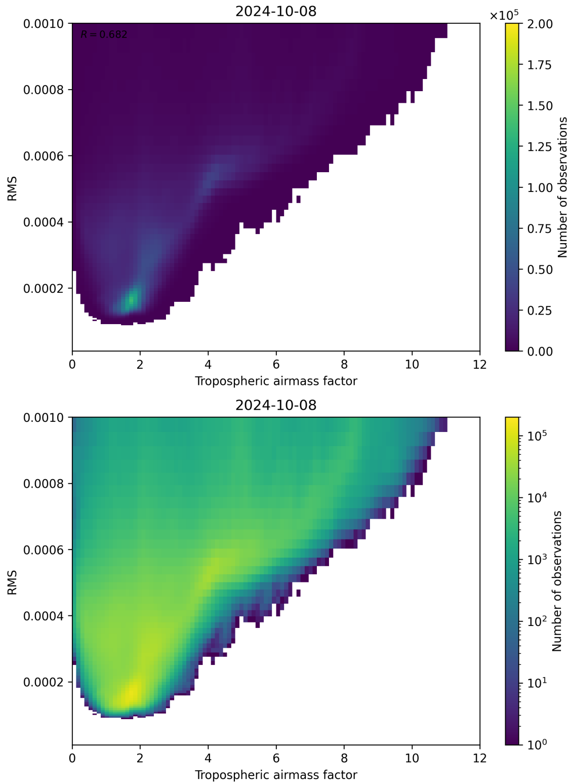
Figure 79: Scatter density plot of “Tropospheric airmass factor” against “RMS” for 2024-10-08 to 2024-10-09.
