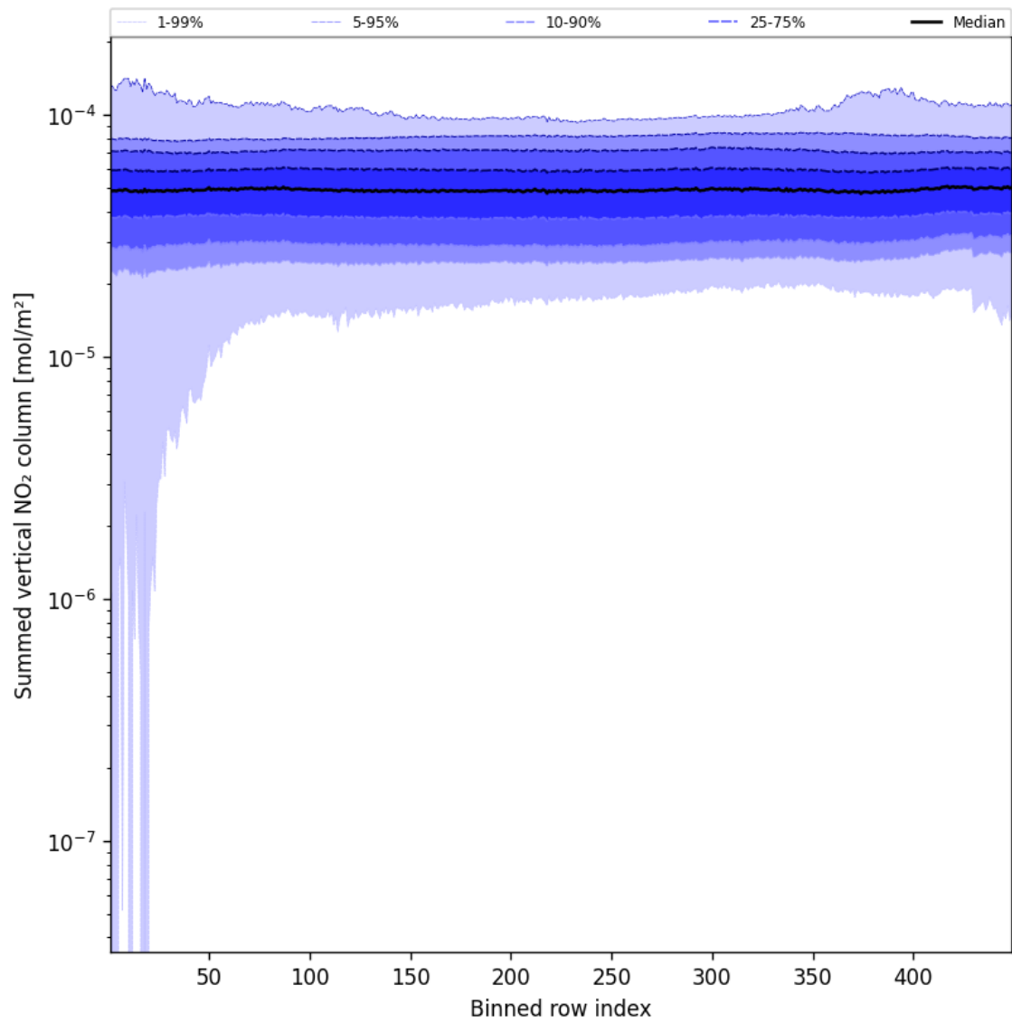
Figure 57: Along track statistics of “Summed vertical NO 2 column” for 2024-10-08 to 2024-10-09
