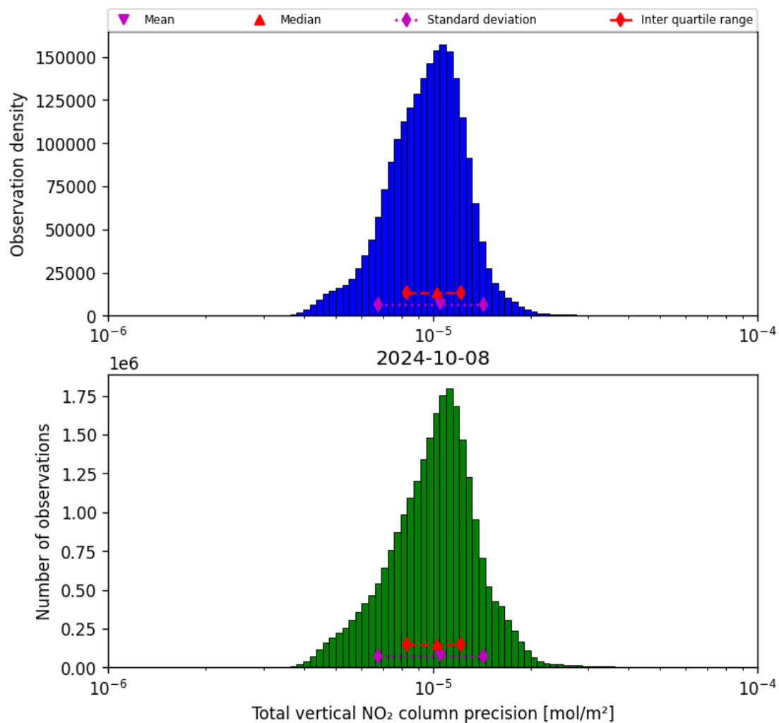
Figure 39: Histogram of “Total vertical NO 2 column precision” for 2024-10-08 to 2024-10-09
