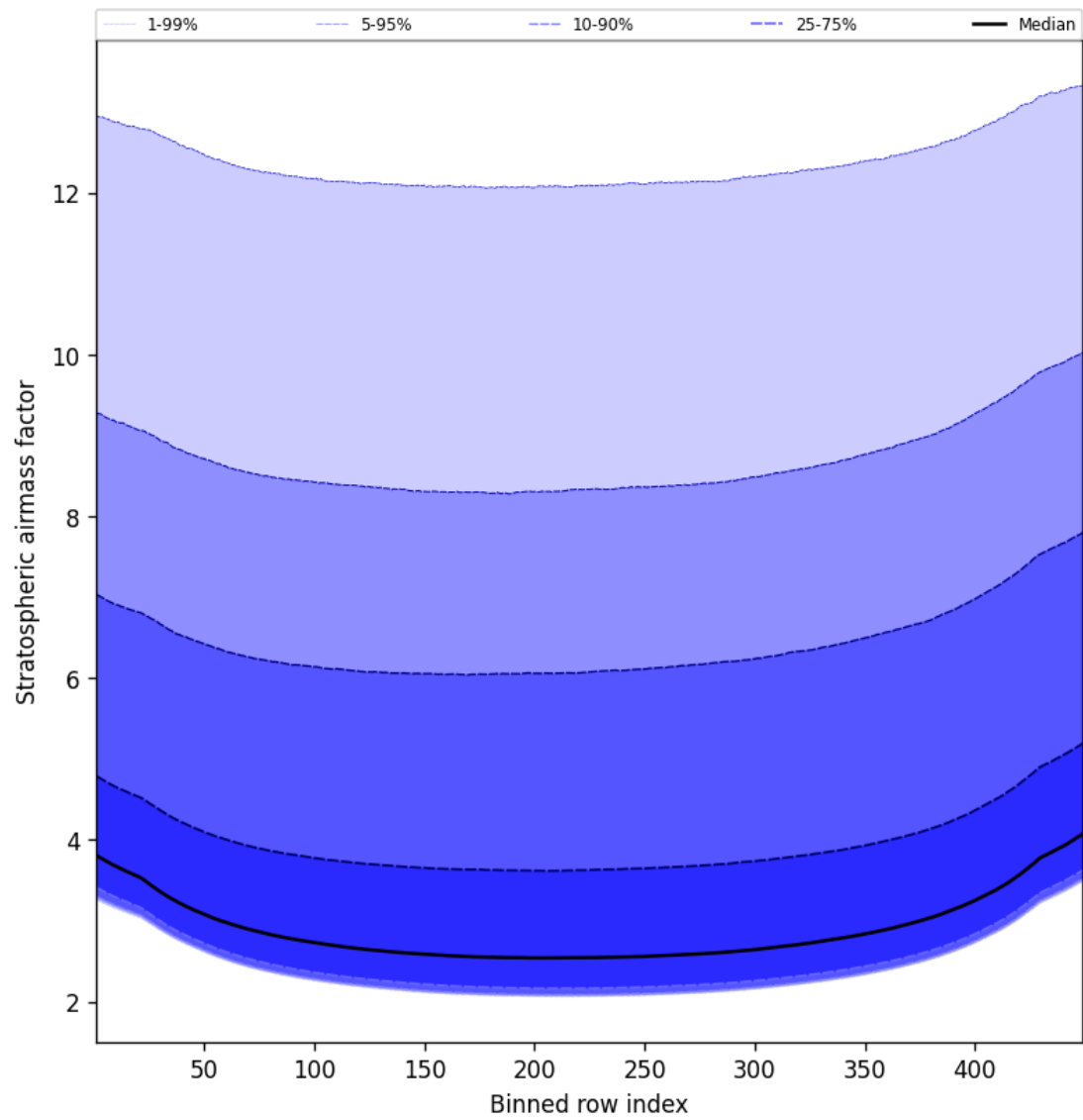
Figure 61: Along track statistics of “Stratospheric airmass factor” for 2024-10-08 to 2024-10-09
