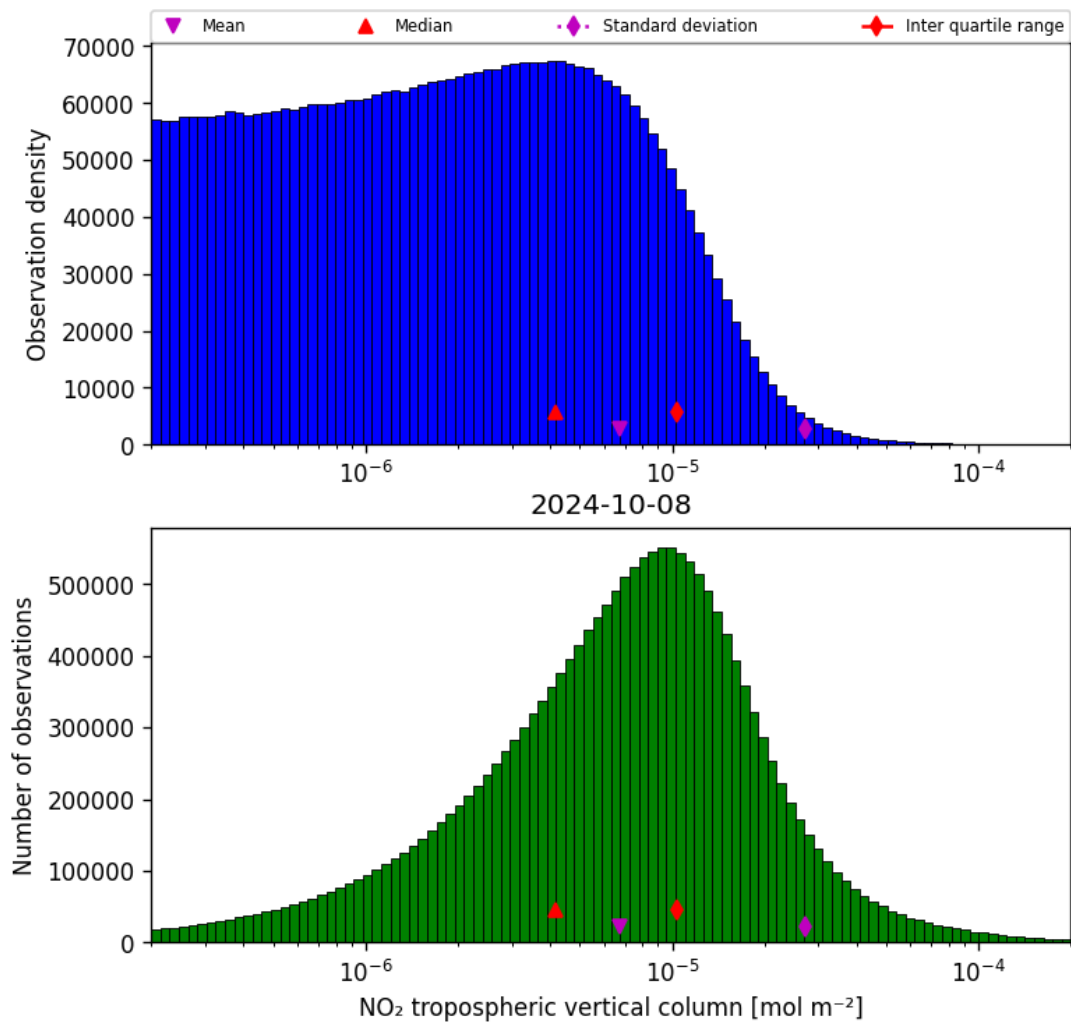
Figure 29: Histogram of “NO 2 tropospheric vertical column” for 2024-10-08 to 2024-10-09
