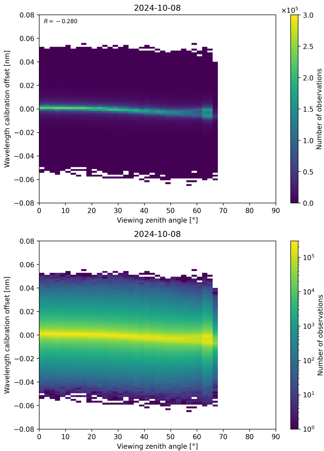
Figure 173: Scatter density plot of “Viewing zenith angle” against “Wavelength calibration offset” for 2024-10-08 to 2024-10-09.
