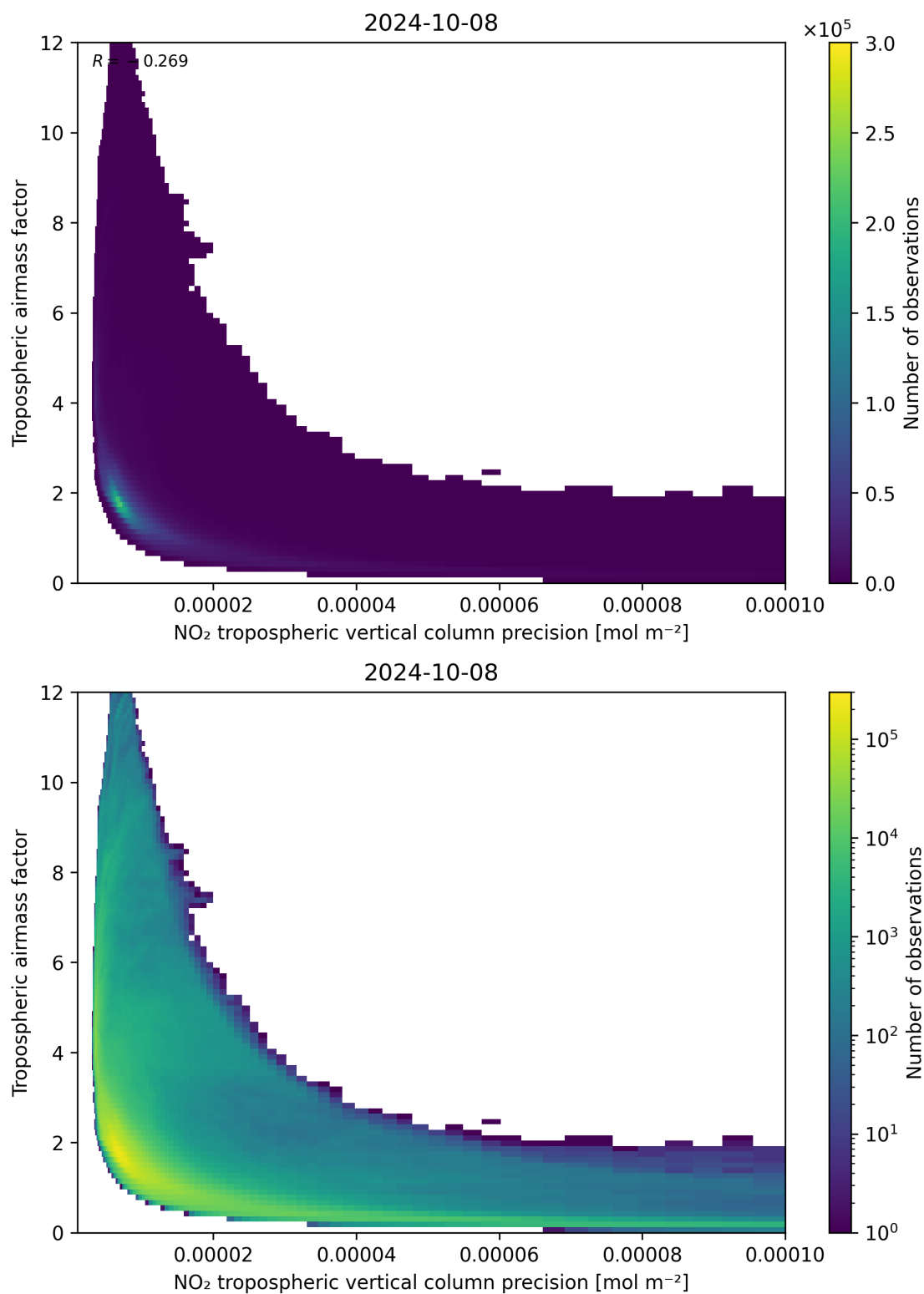
Figure 133: Scatter density plot of “NO 2 tropospheric vertical column precision” against “Tropospheric airmass factor” for 2024-10-08 to 2024-10-09.
