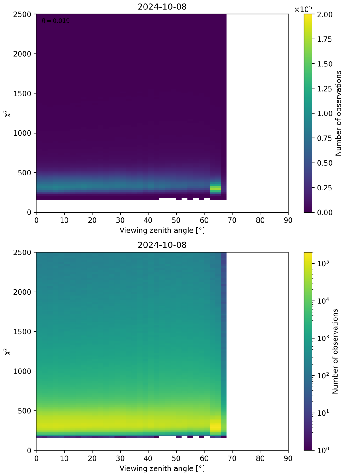
Figure 162: Scatter density plot of “Viewing zenith angle” against “ \chi^2 ” for 2024-10-08 to 2024-10-09.
