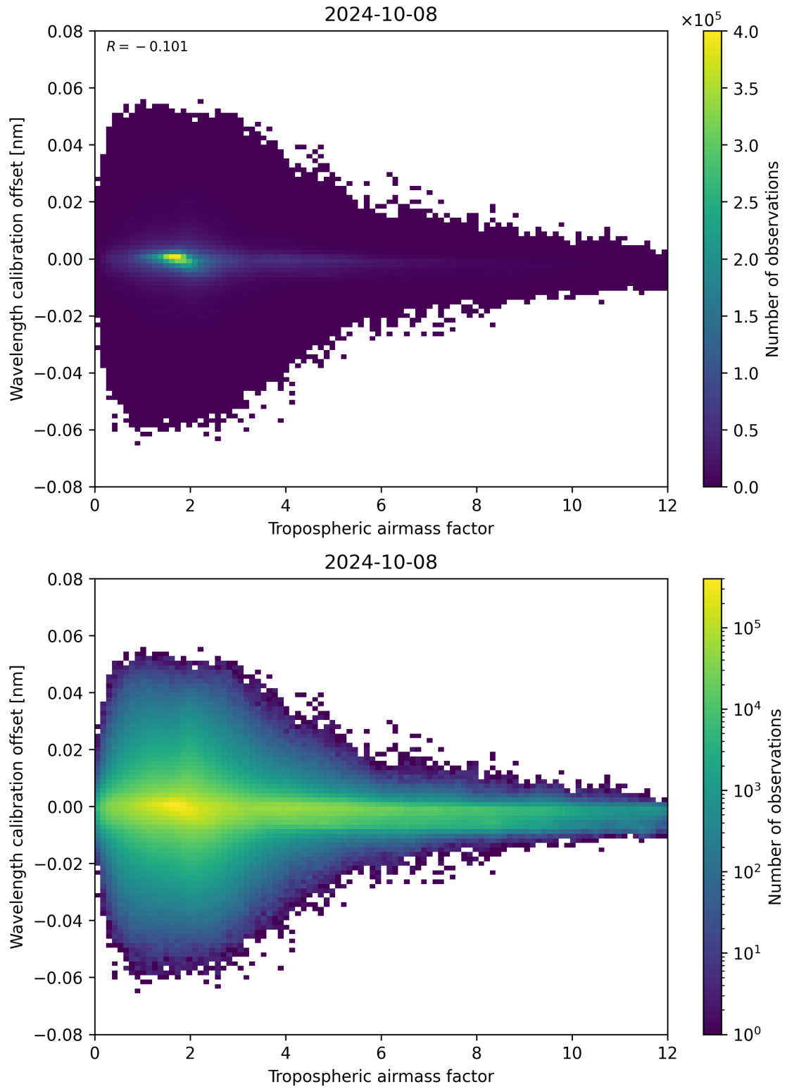
Figure 80: Scatter density plot of “Tropospheric airmass factor” against “Wavelength calibration offset” for 2024-10-08 to 2024-10-09.
