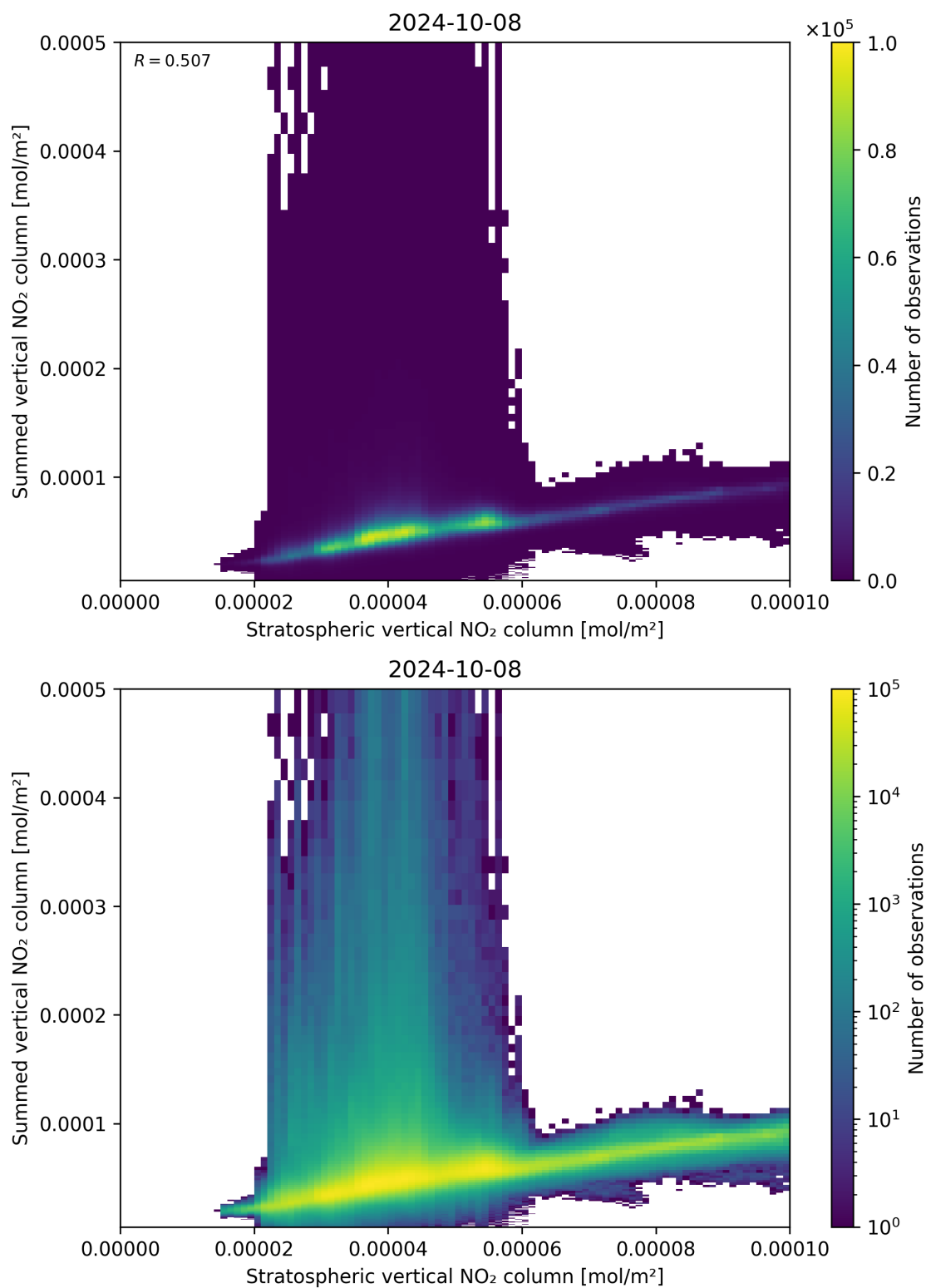
Figure 98: Scatter density plot of “Stratospheric vertical NO 2 column” against “Summed vertical NO 2 column” for 2024-10-08 to 2024-10-09.
