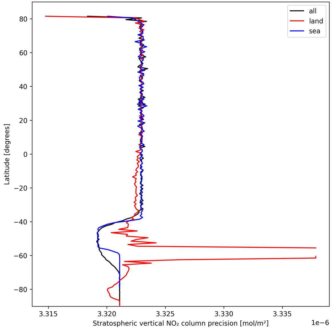
Figure 20: Zonal average of “Stratospheric vertical NO 2 column precision” for 2024-10-08 to 2024-10-09.
