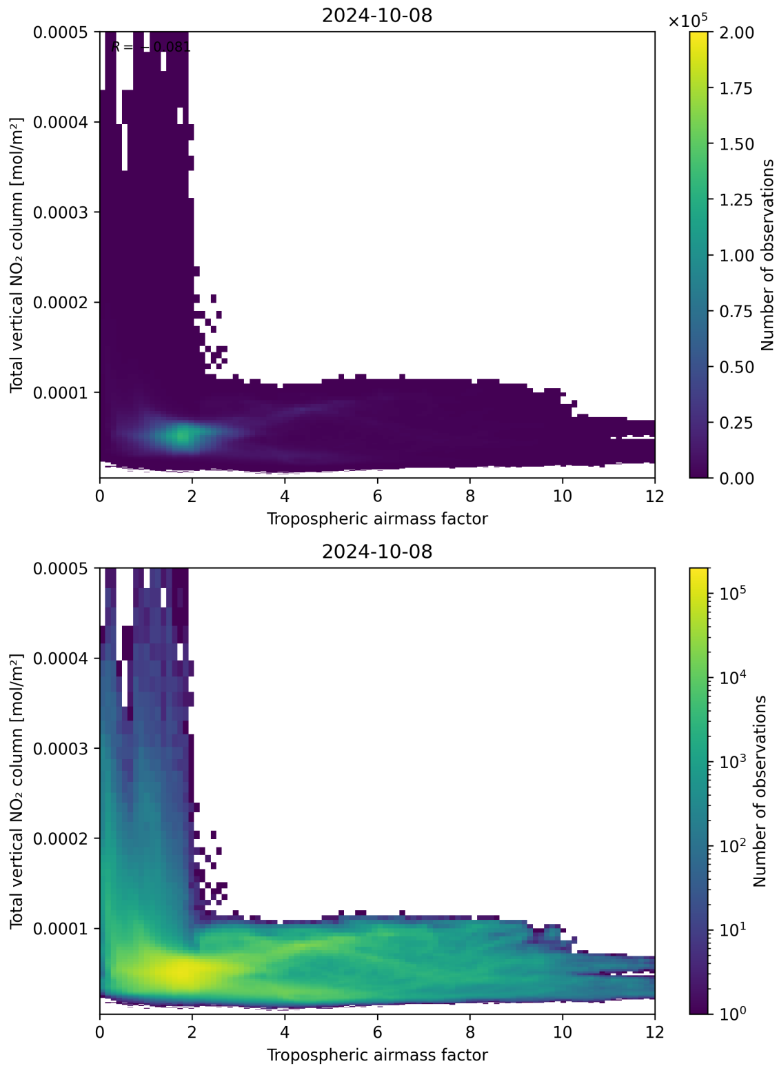
Figure 77: Scatter density plot of “Tropospheric airmass factor” against “Total vertical NO 2 column” for 2024-10-08 to 2024-10-09.
