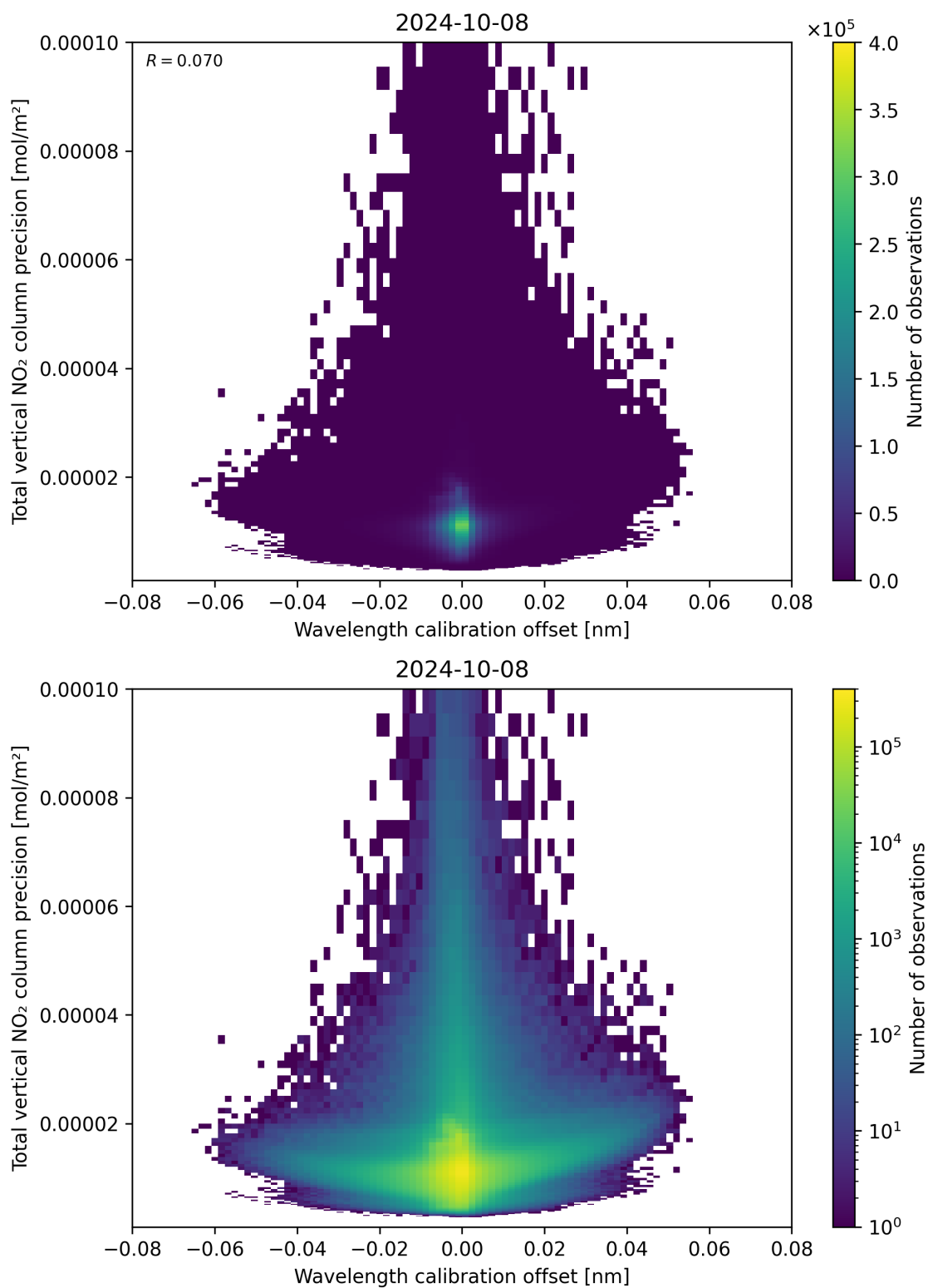
Figure 180: Scatter density plot of “Wavelength calibration offset” against “Total vertical NO 2 column precision” for 2024-10-08 to 2024-10-09.
