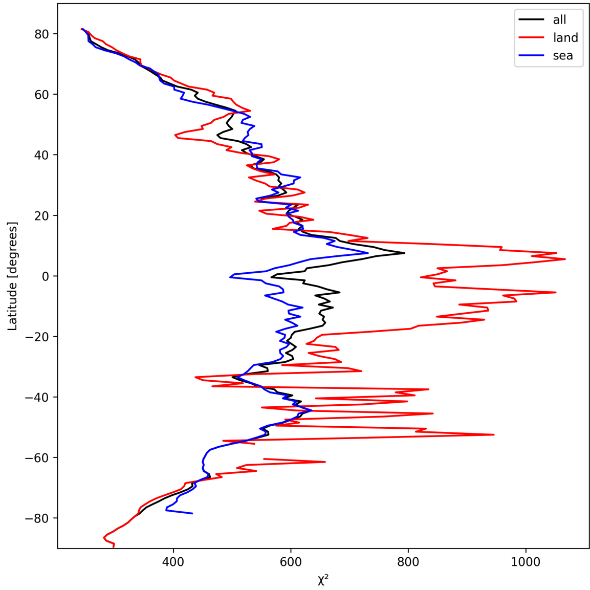
Figure 25: Zonal average of “ \chi^2 ” for 2024-10-08 to 2024-10-09.
