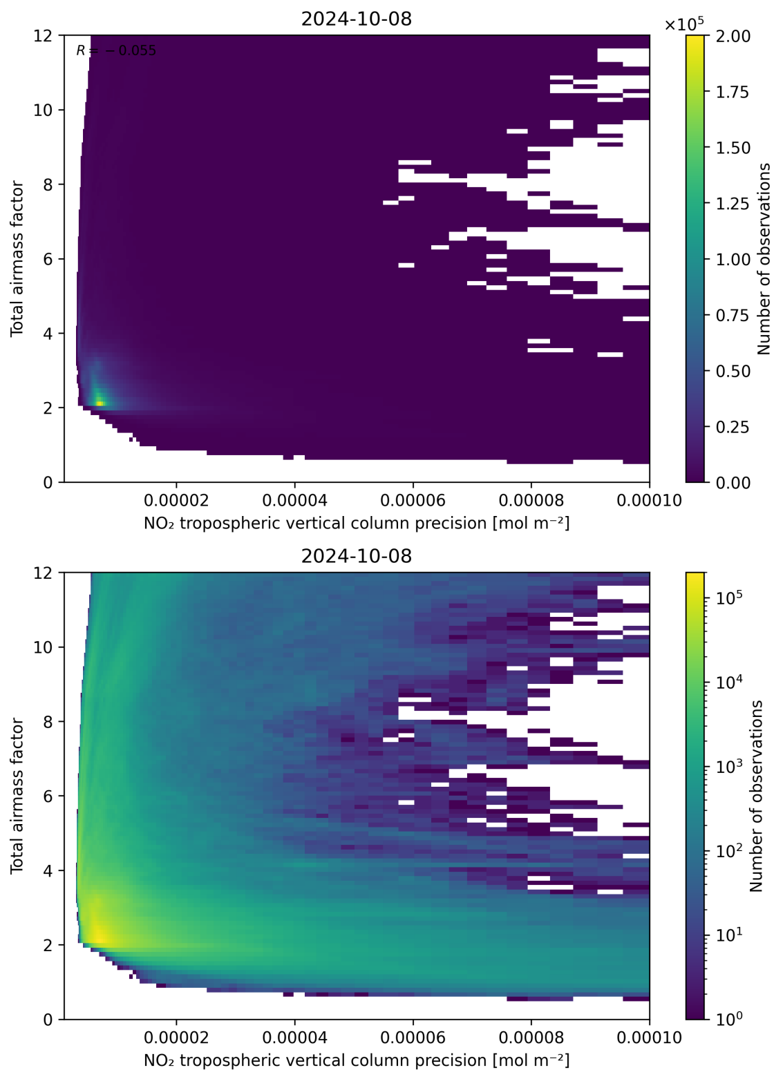
Figure 132: Scatter density plot of “NO 2 tropospheric vertical column precision” against “Total air mass factor” for 2024-10-08 to 2024-10-09.
