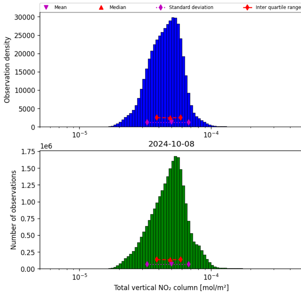
Figure 38: Histogram of “Total vertical NO 2 column” for 2024-10-08 to 2024-10-09
