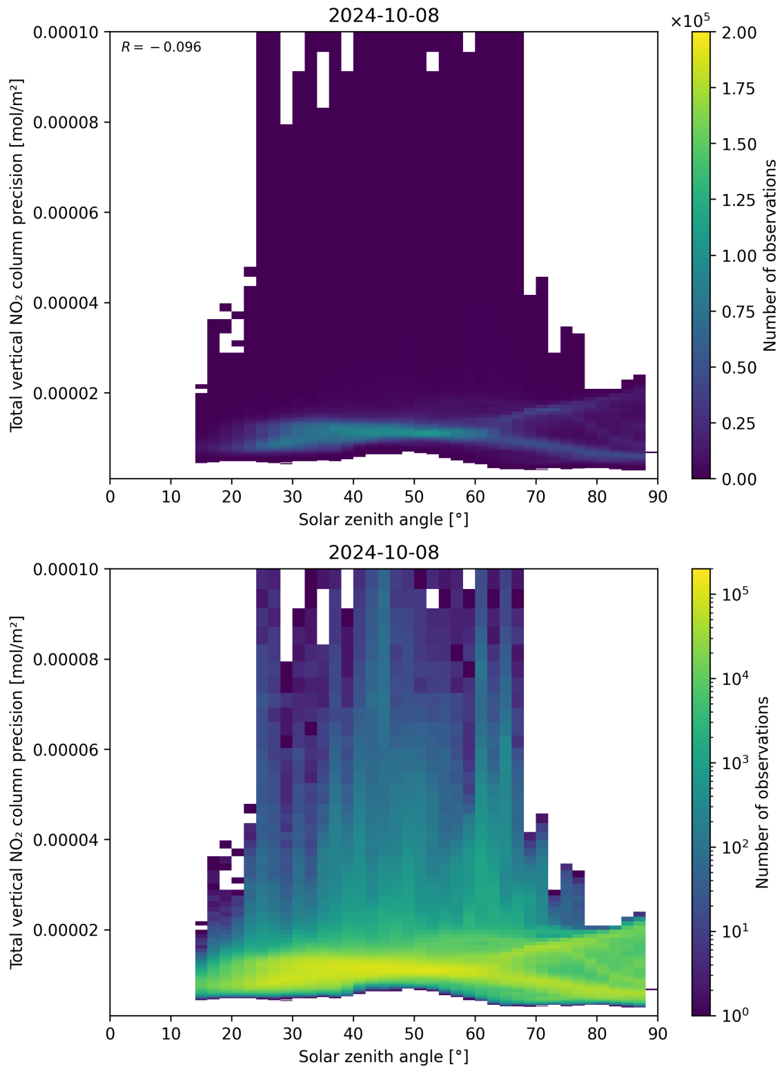
Figure 154: Scatter density plot of “Solar zenith angle” against “Total vertical NO 2 column precision” for 2024-10-08 to 2024-10-09.
