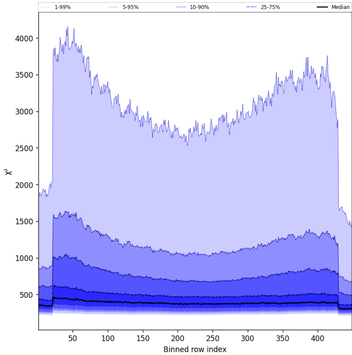
Figure 59: Along track statistics of “ \chi^2 ” for 2024-10-08 to 2024-10-09
