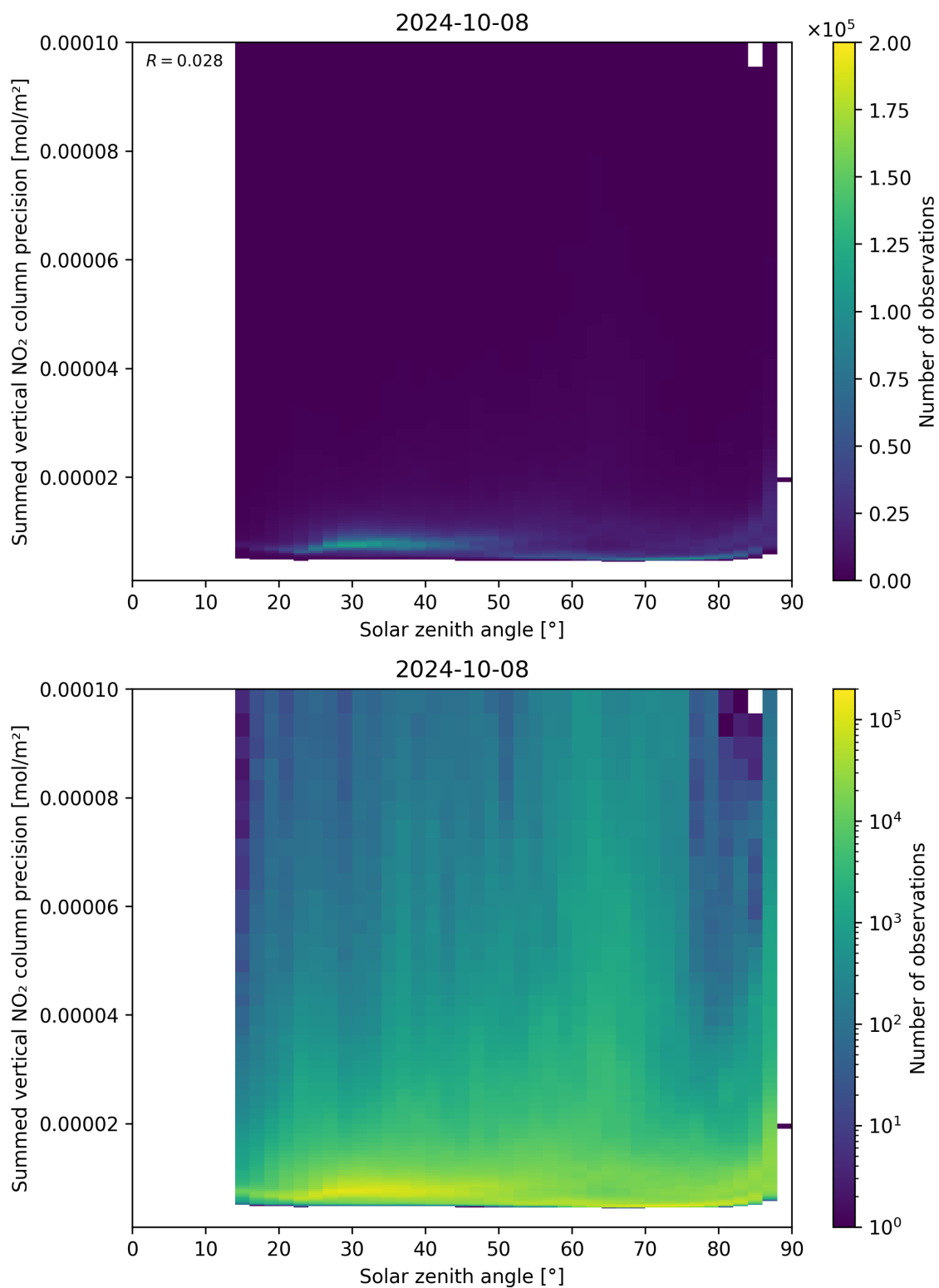
Figure 152: Scatter density plot of “Solar zenith angle” against “Summed vertical NO 2 column precision” for 2024-10-08 to 2024-10-09.
