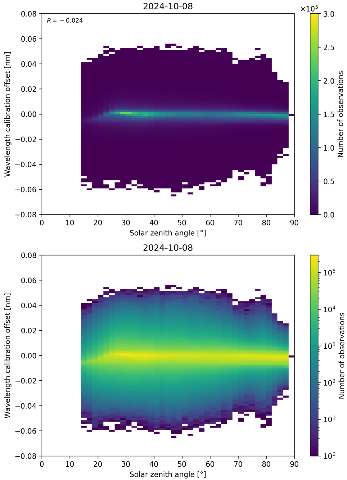
Figure 158: Scatter density plot of “Solar zenith angle” against “Wavelength calibration offset” for 2024-10-08 to 2024-10-09.
