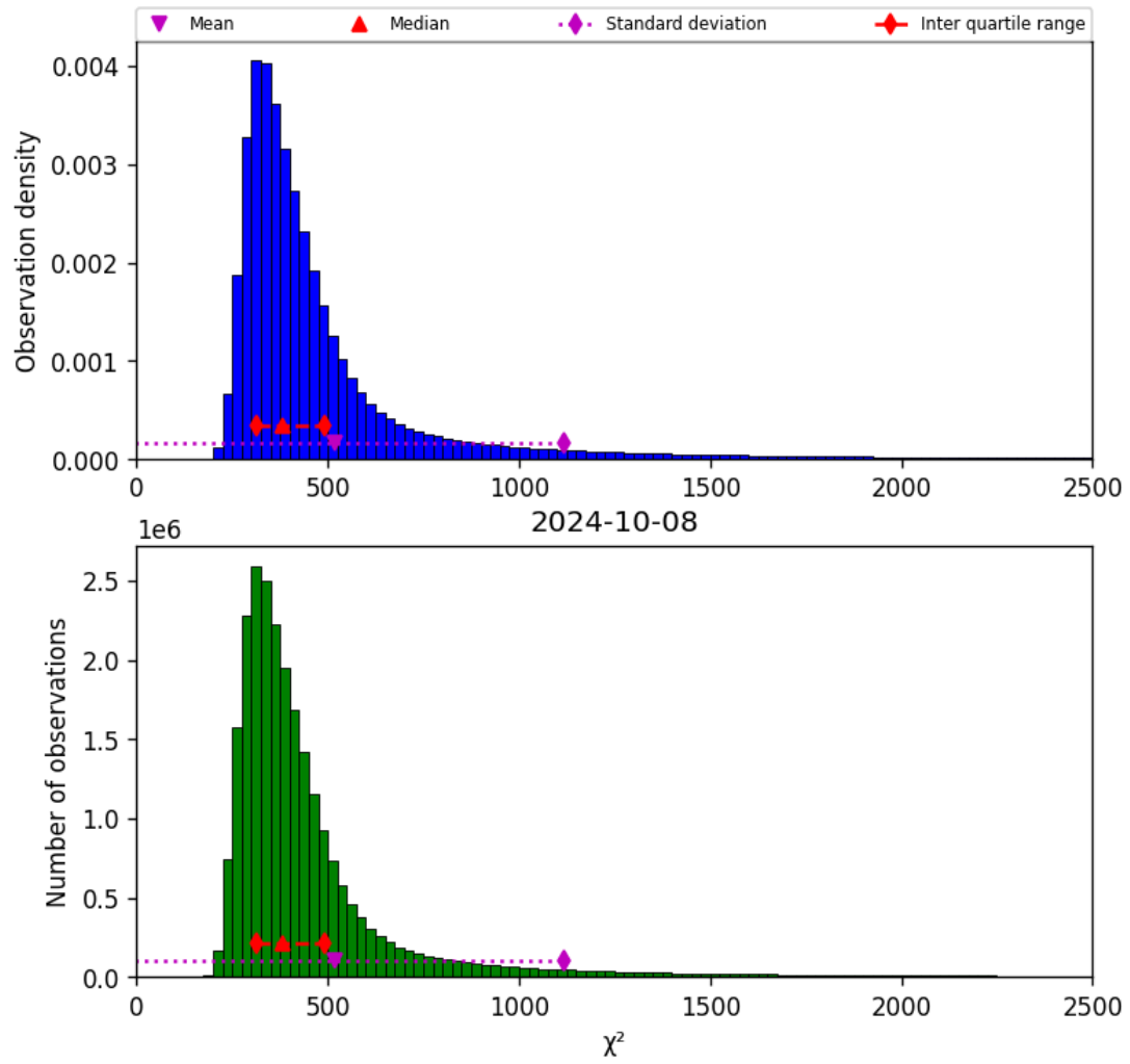
Figure 42: Histogram of “ \chi^2 ” for 2024-10-08 to 2024-10-09
