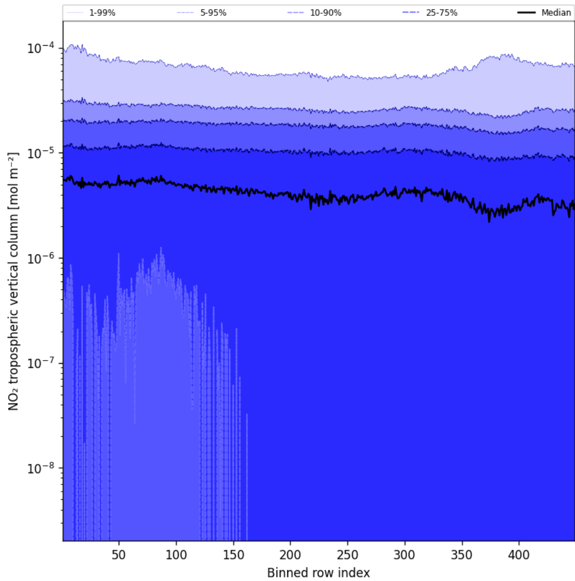
Figure 46: Along track statistics of “NO 2 tropospheric vertical column” for 2024-10-08 to 2024-10-09
