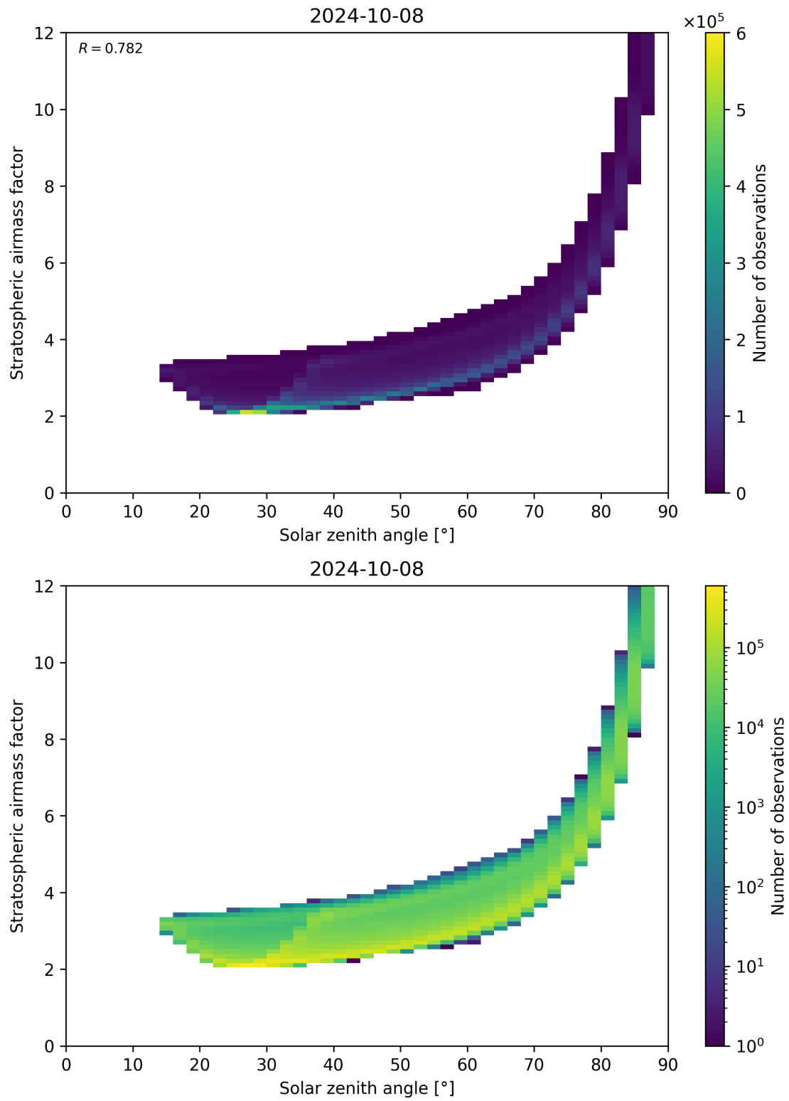
Figure 145: Scatter density plot of “Solar zenith angle” against “Stratospheric airmass factor” for 2024-10-08 to 2024-10-09.
