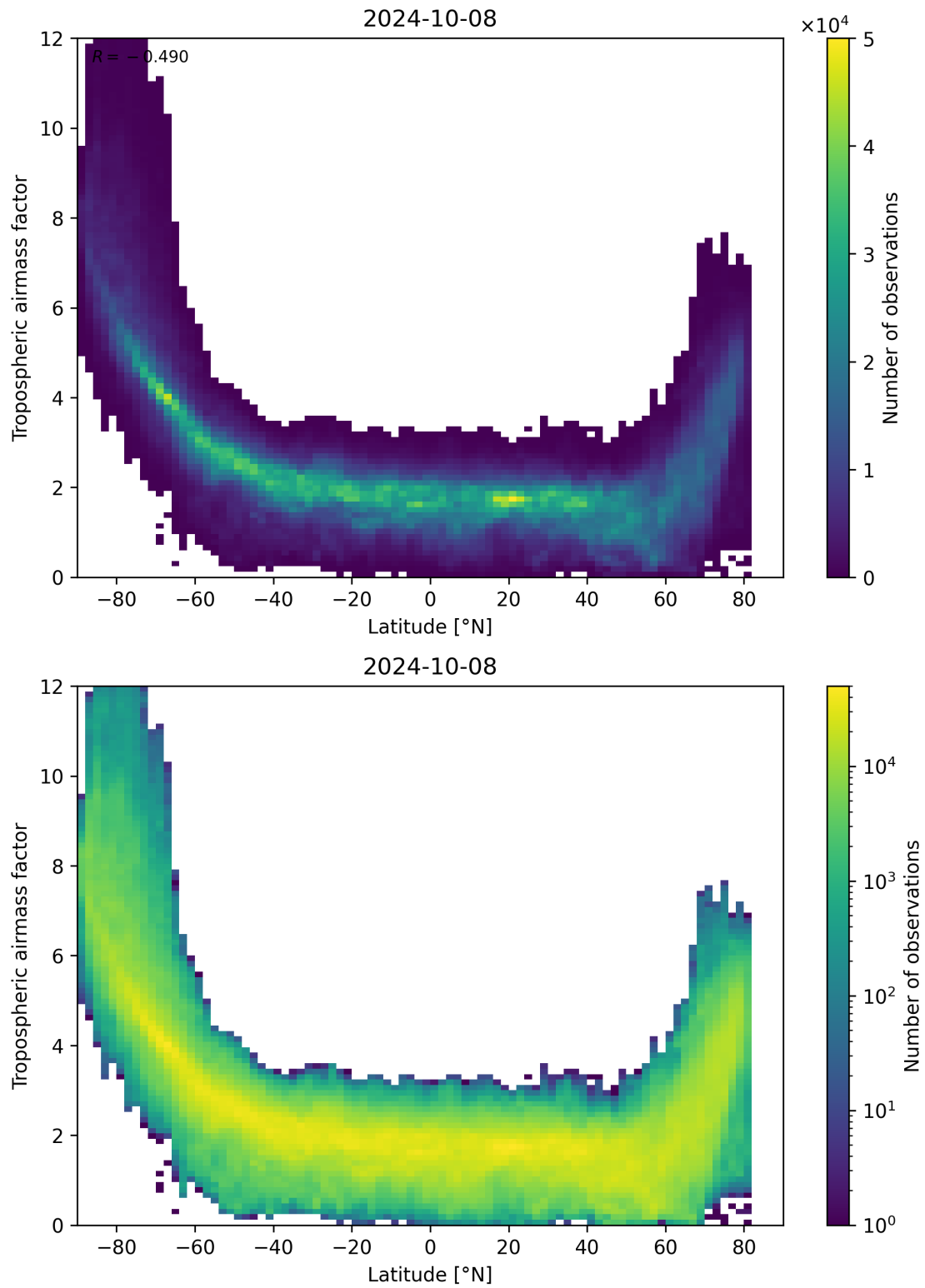
Figure 85: Scatter density plot of “Latitude” against “Tropospheric air mass factor” for 2024-10-08 to 2024-10-09.
