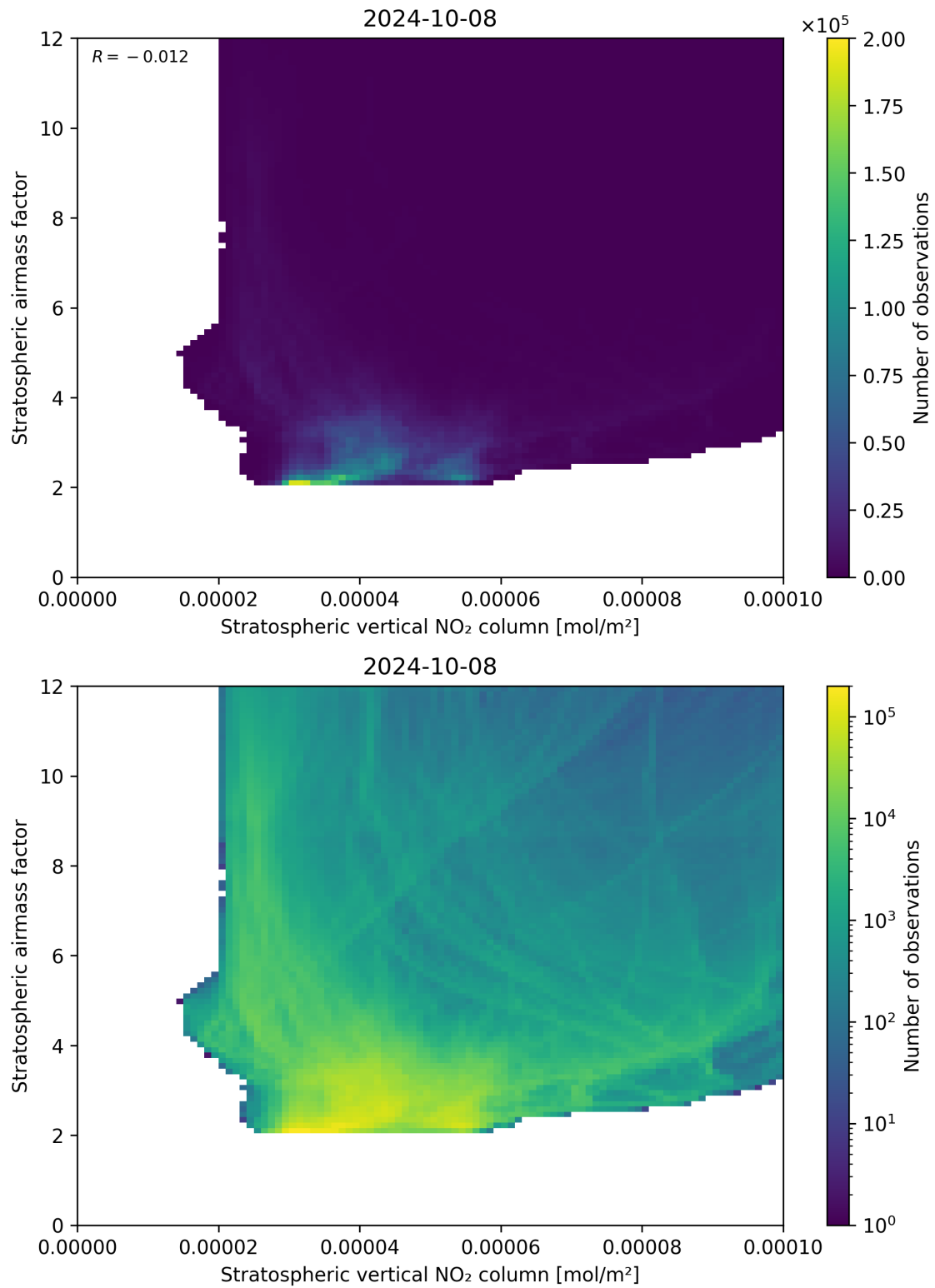
Figure 96: Scatter density plot of “Stratospheric vertical NO 2 column” against “Stratospheric airmass factor” for 2024-10-08 to 2024-10-09.
