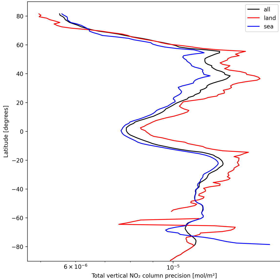
Figure 22: Zonal average of “Total vertical NO 2 column precision” for 2024-10-08 to 2024-10-09.
