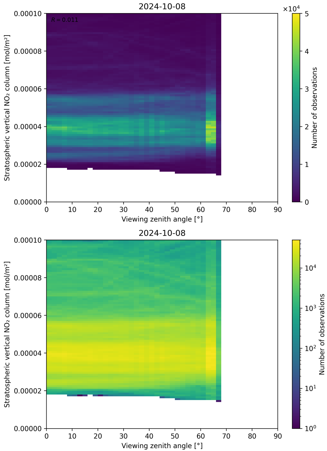
Figure 164: Scatter density plot of “Viewing zenith angle” against “Stratospheric vertical NO 2 column” for 2024-10-08 to 2024-10-09.
