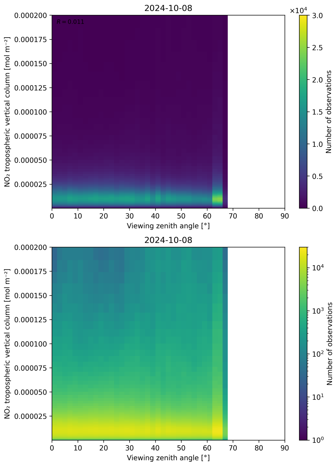
Figure 169: Scatter density plot of “Viewing zenith angle” against “NO 2 tropospheric vertical column” for 2024-10-08 to 2024-10-09.
