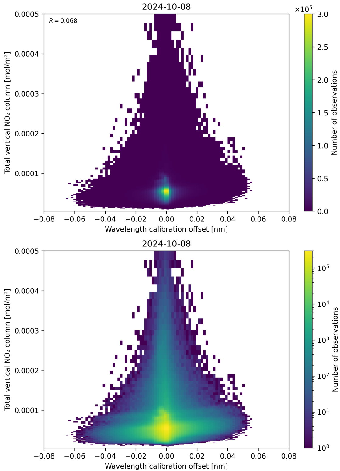
Figure 179: Scatter density plot of “Wavelength calibration offset” against “Total vertical NO 2 column” for 2024-10-08 to 2024-10-09.
