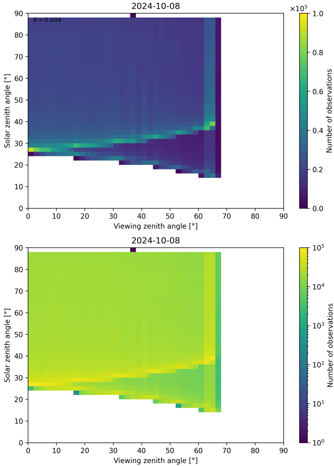
Figure 172: Scatter density plot of “Viewing zenith angle” against “Solar zenith angle” for 2024-10-08 to 2024-10-09.
