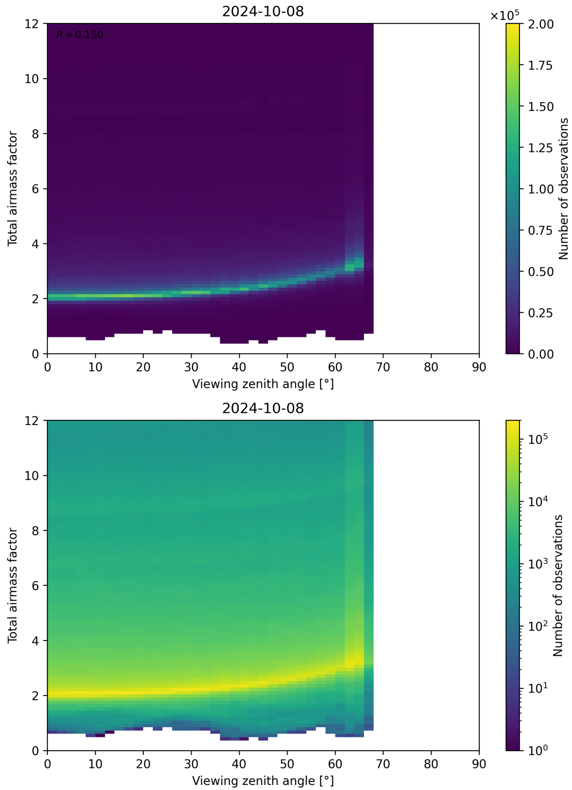
Figure 160: Scatter density plot of “Viewing zenith angle” against “Total airmass factor” for 2024-10-08 to 2024-10-09.
