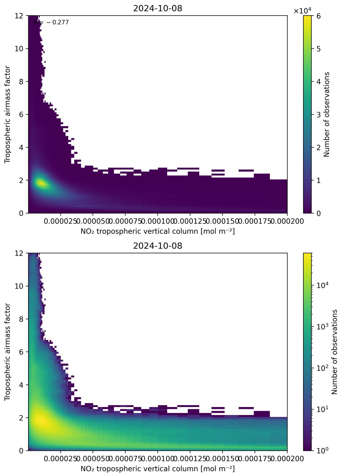
Figure 123: Scatter density plot of “NO 2 tropospheric vertical column” against “Tropospheric air mass factor” for 2024-10-08 to 2024-10-09.
