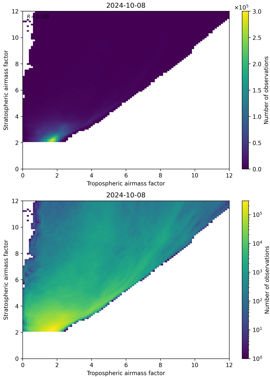
Figure 71: Scatter density plot of “Tropospheric airmass factor” against “Stratospheric airmass factor” for 2024-10-08 to 2024-10-09.
