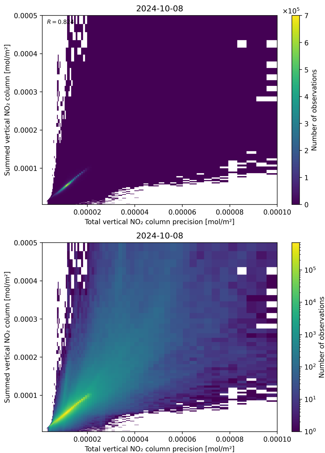
Figure 117: Scatter density plot of “Total vertical NO 2 column precision” against “Summed vertical NO 2 column” for 2024-10-08 to 2024-10-09.
