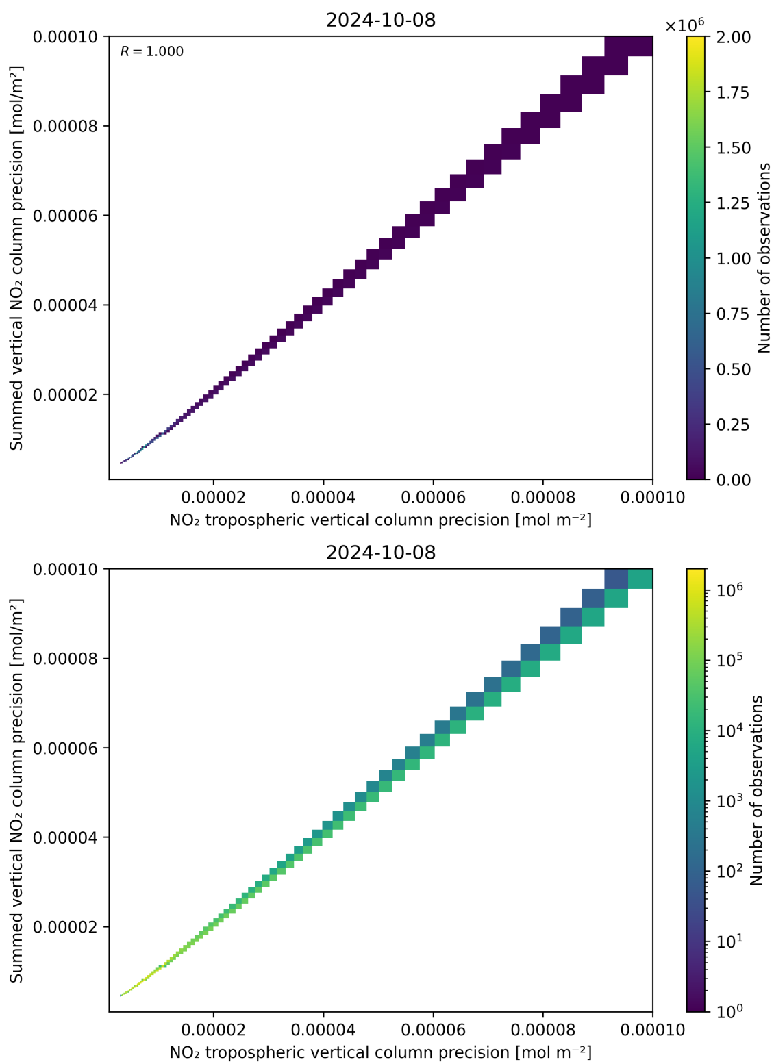
Figure 137: Scatter density plot of “NO 2 tropospheric vertical column precision” against “Summed vertical NO 2 column precision” for 2024-10-08 to 2024-10-09.
