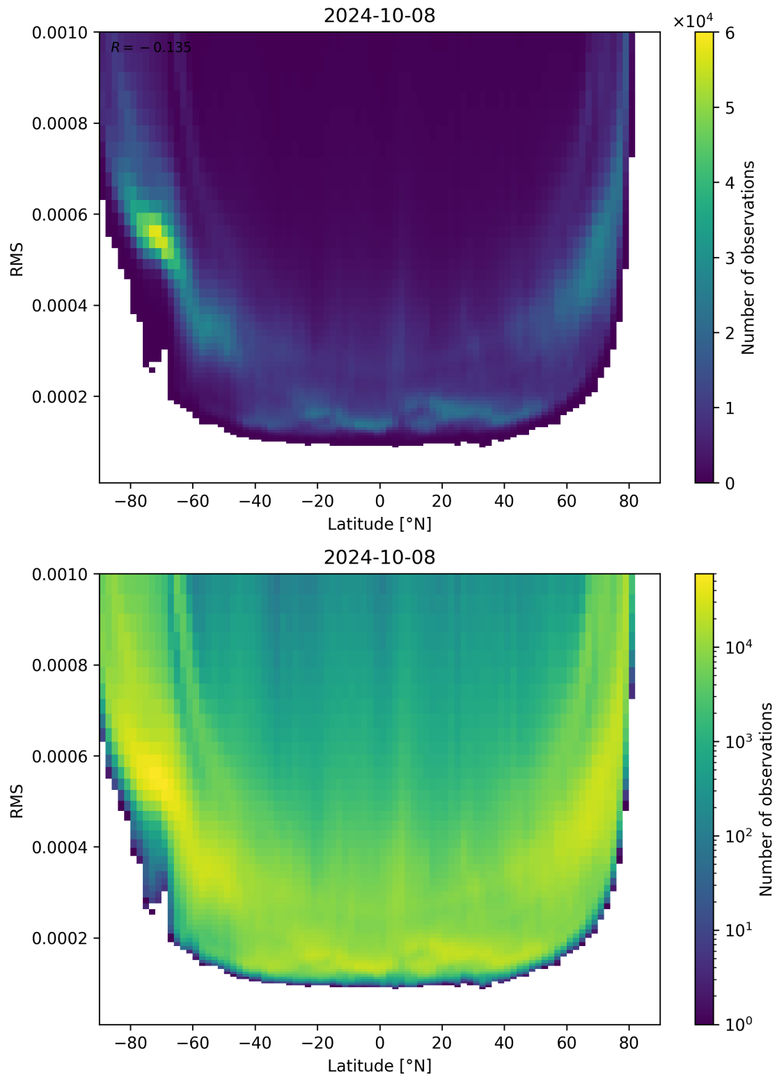
Figure 94: Scatter density plot of “Latitude” against “RMS” for 2024-10-08 to 2024-10-09.
