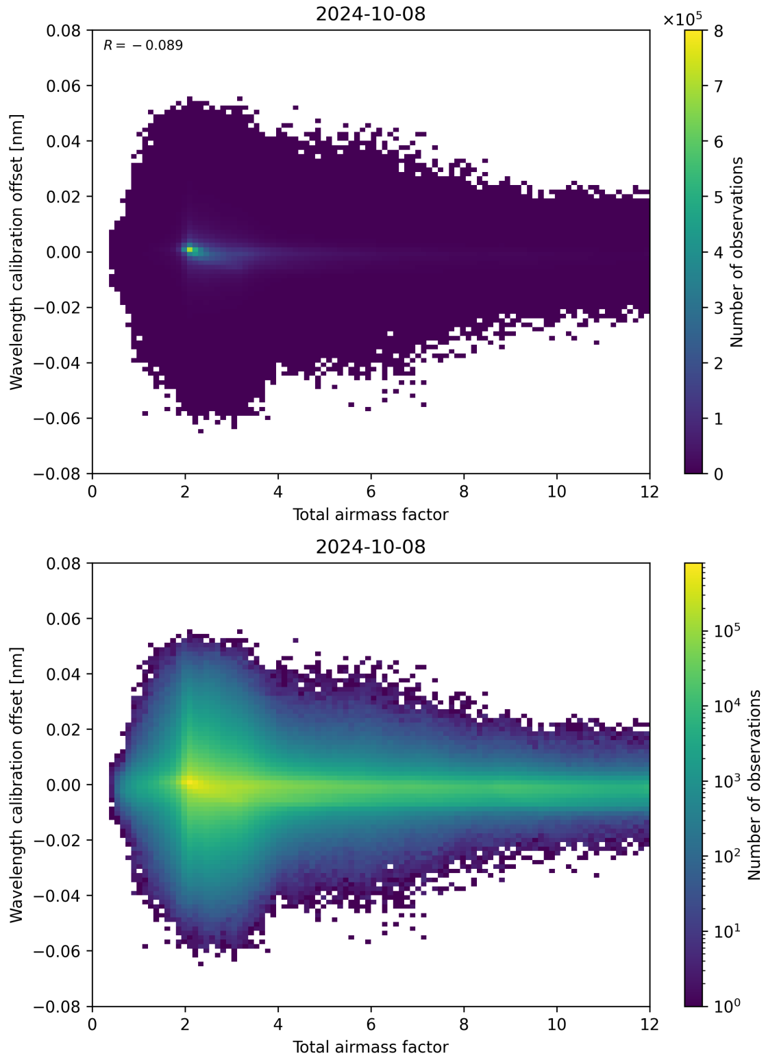
Figure 70: Scatter density plot of “Total airmass factor” against “Wavelength calibration offset” for 2024-10-08 to 2024-10-09.
