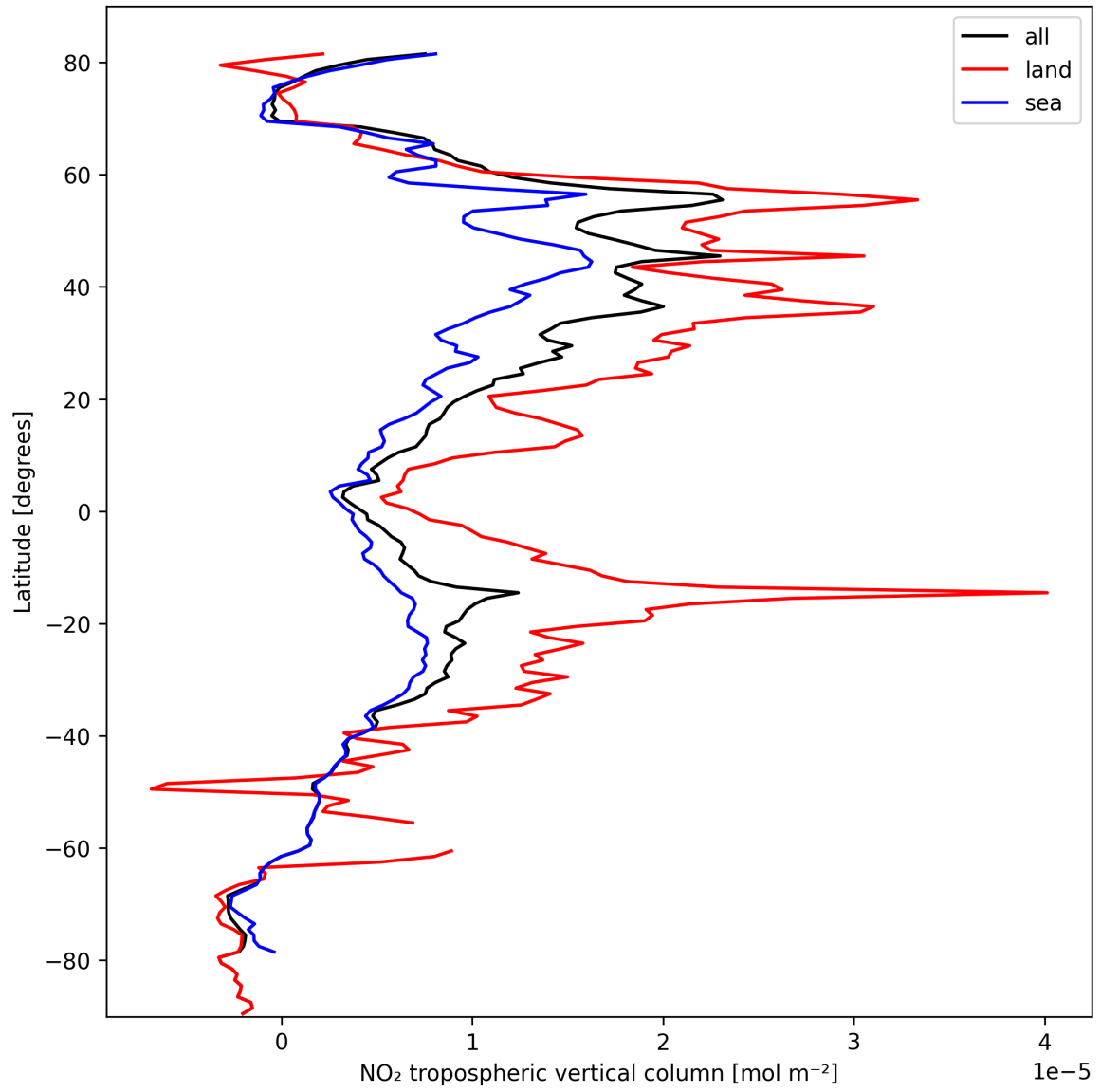
Figure 12: Zonal average of “NO 2 tropospheric vertical column” for 2024-10-08 to 2024-10-09.
