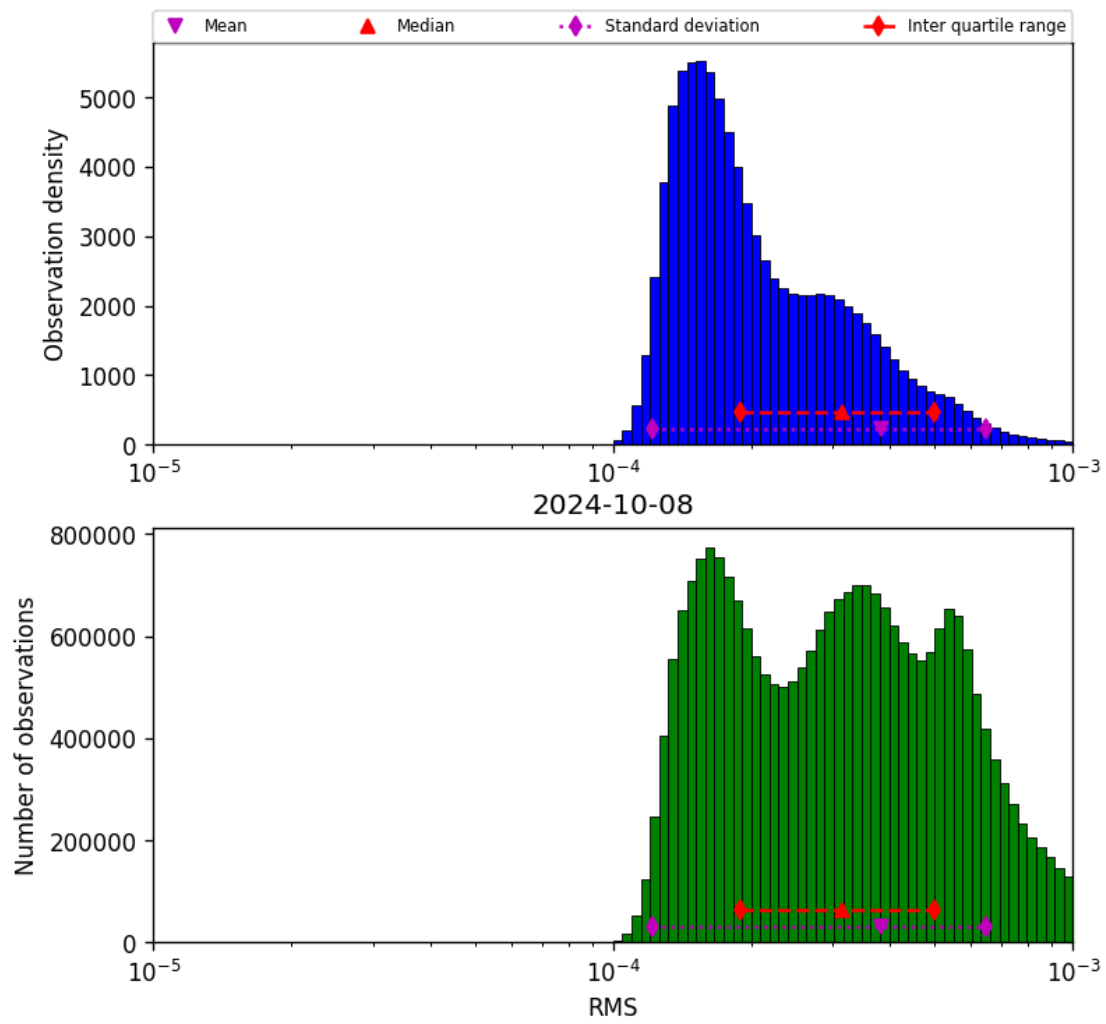
Figure 43: Histogram of “RMS” for 2024-10-08 to 2024-10-09
