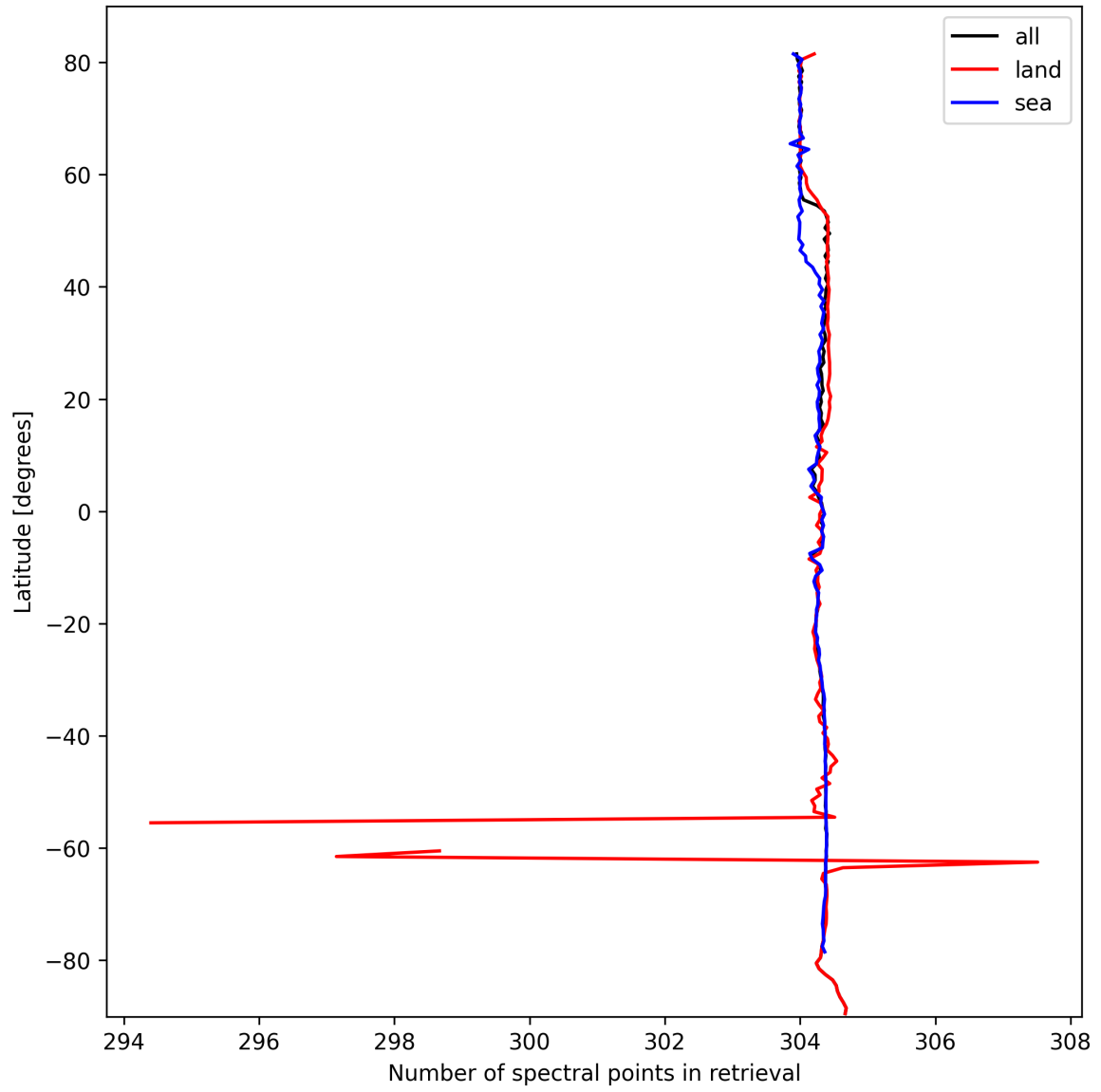
Figure 16: Zonal average of “Number of spectral points in retrieval” for 2024-10-08 to 2024-10-09.
