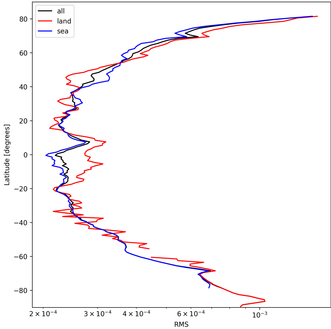
Figure 26: Zonal average of “RMS” for 2024-10-08 to 2024-10-09.
