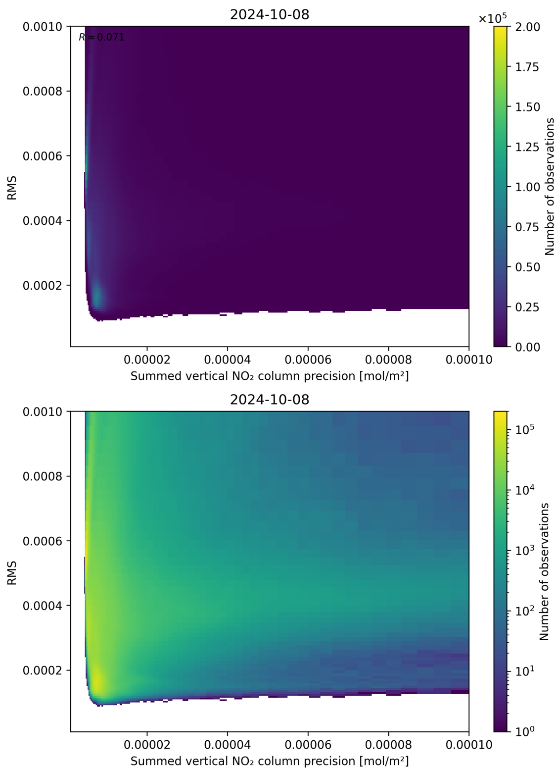
Figure 108: Scatter density plot of “Summed vertical NO 2 column precision” against “RMS” for 2024-10-08 to 2024-10-09.
