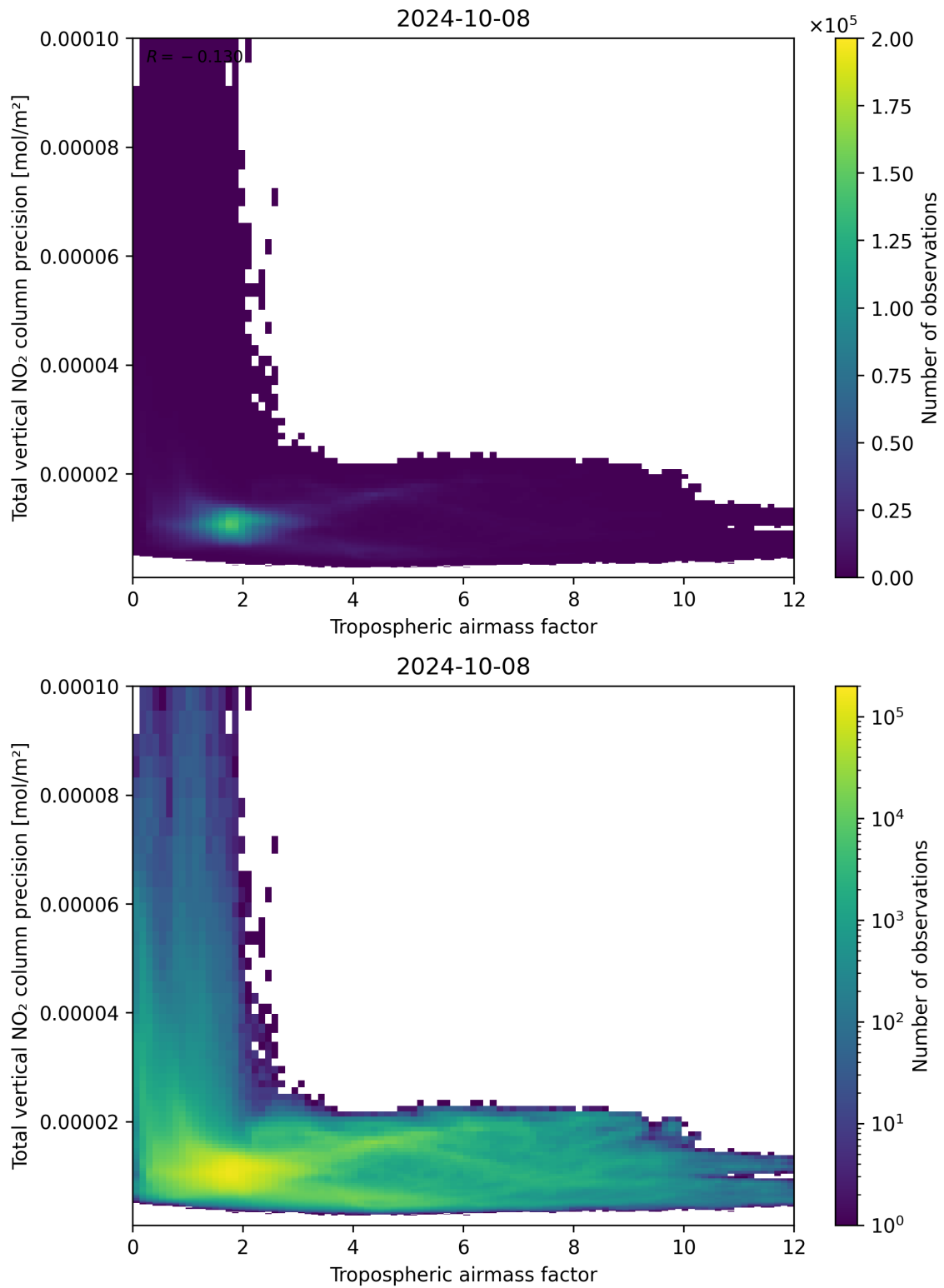
Figure 78: Scatter density plot of “Tropospheric airmass factor” against “Total vertical NO 2 column precision” for 2024-10-08 to 2024-10-09.
