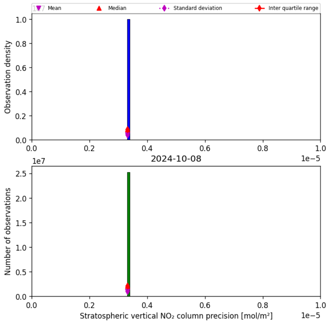
Figure 37: Histogram of “Stratospheric vertical NO 2 column precision” for 2024-10-08 to 2024-10-09
