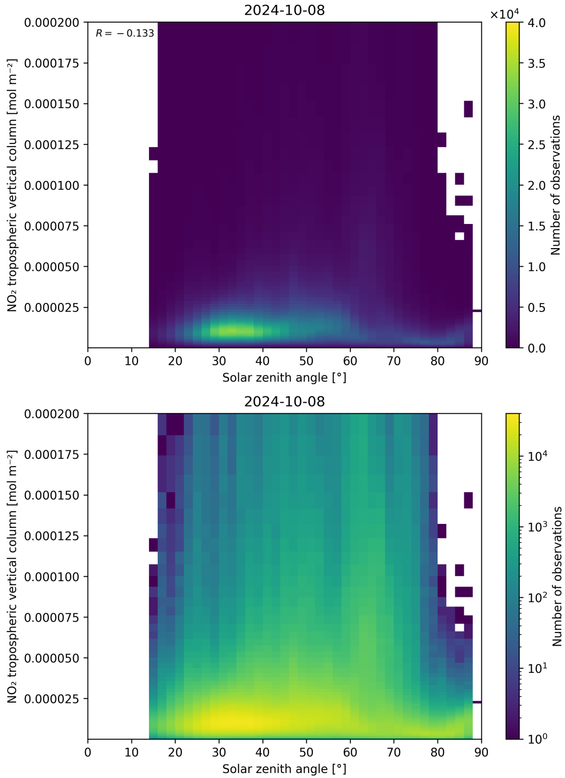
Figure 155: Scatter density plot of “Solar zenith angle” against “NO 2 tropospheric vertical column” for 2024-10-08 to 2024-10-09.
