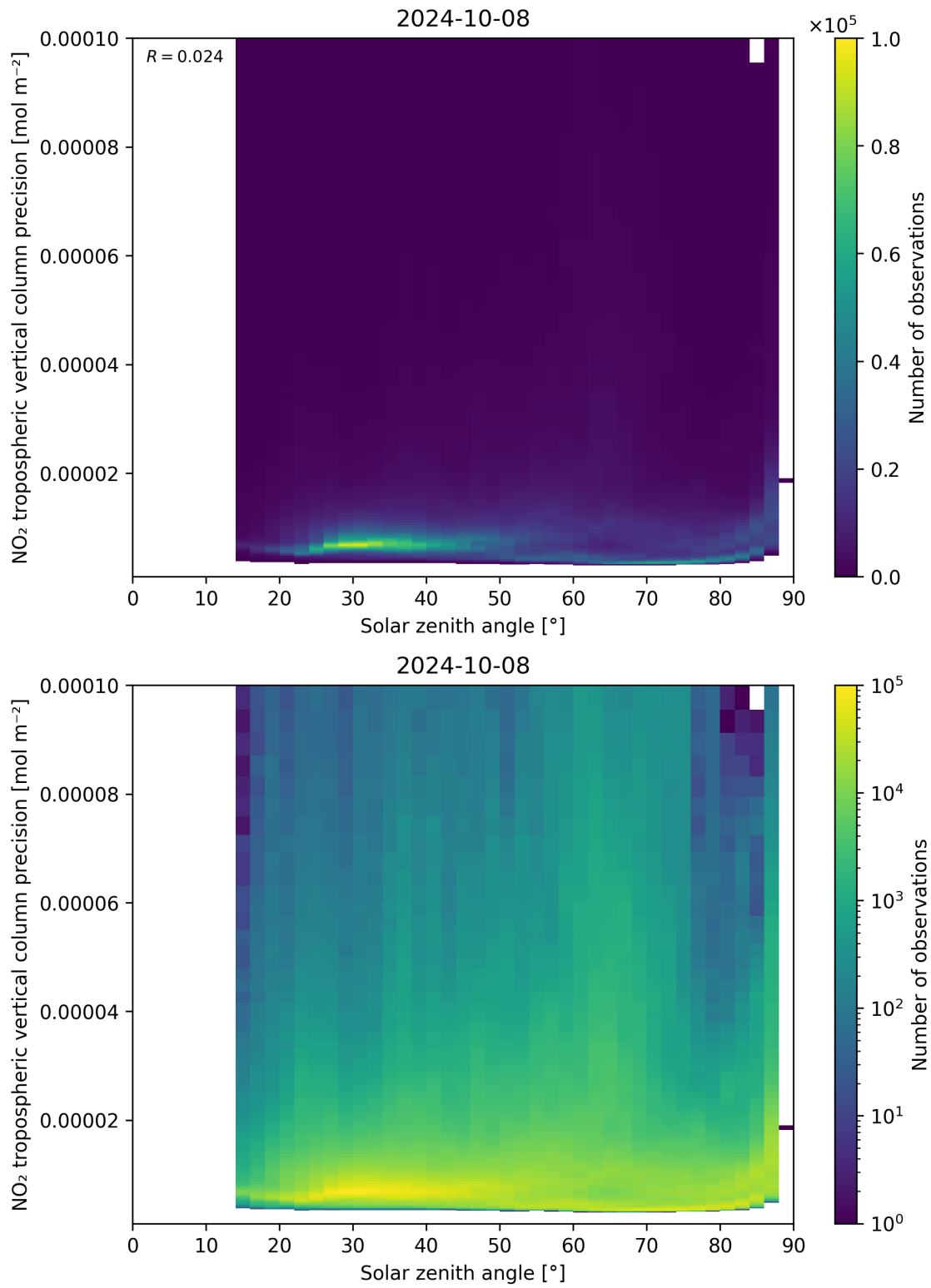
Figure 156: Scatter density plot of “Solar zenith angle” against “NO 2 tropospheric vertical column precision” for 2024-10-08 to 2024-10-09.
