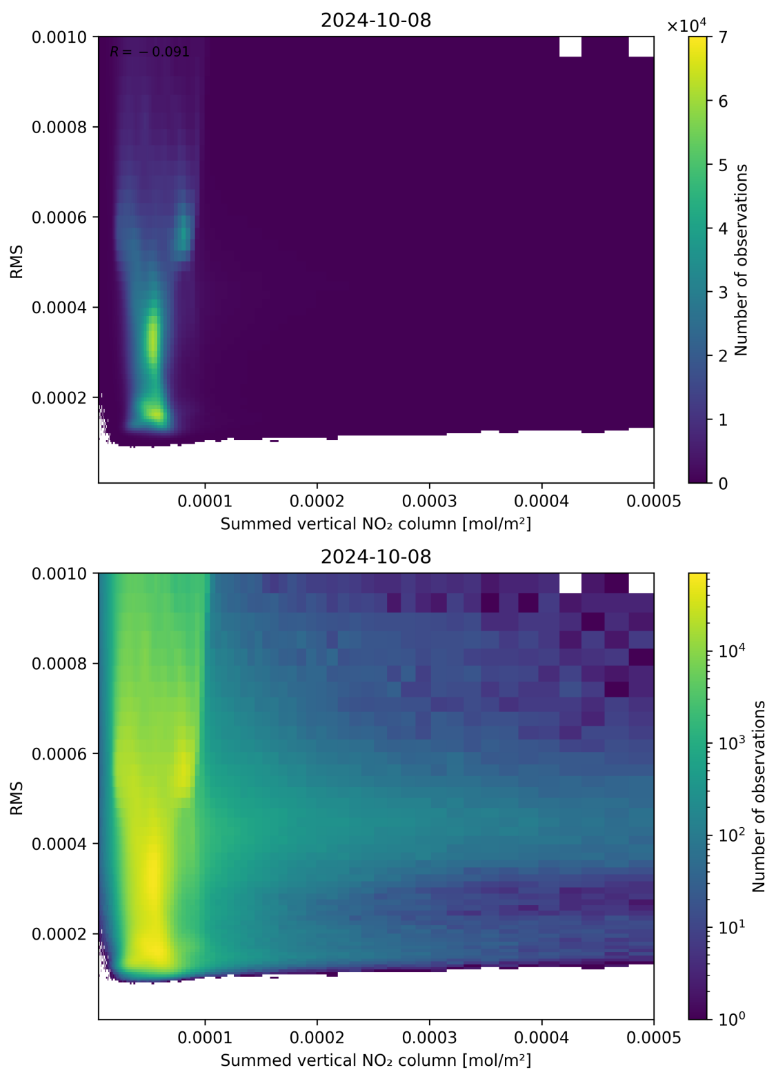
Figure 109: Scatter density plot of “Summed vertical NO 2 column” against “RMS” for 2024-10-08 to 2024-10-09.
