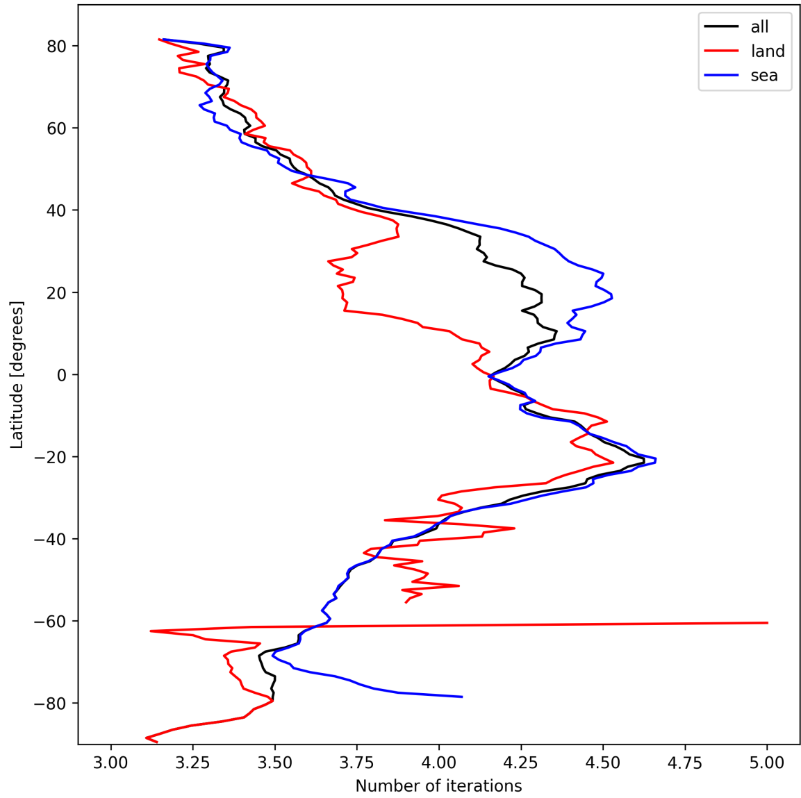
Figure 17: Zonal average of “Number of iterations” for 2024-10-08 to 2024-10-09.
