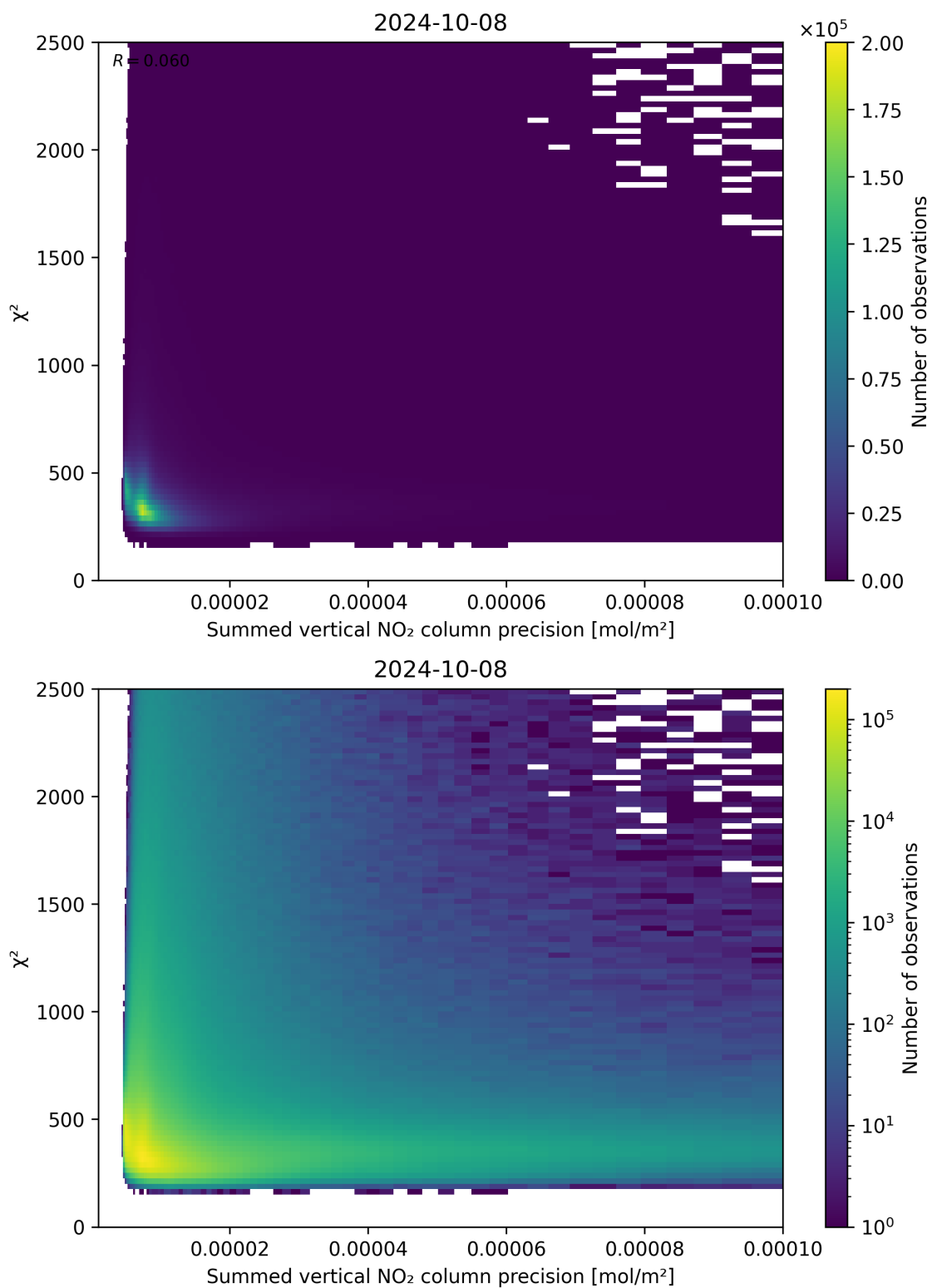
Figure 107: Scatter density plot of “Summed vertical NO 2 column precision” against “ \chi^2 ” for 2024-10-08 to 2024-10-09.
