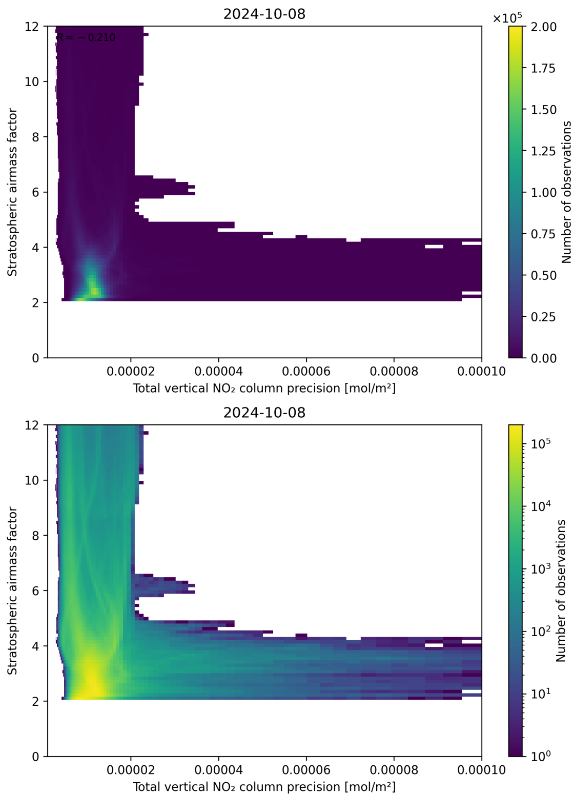
Figure 115: Scatter density plot of “Total vertical NO 2 column precision” against “Stratospheric air mass factor” for 2024-10-08 to 2024-10-09.
