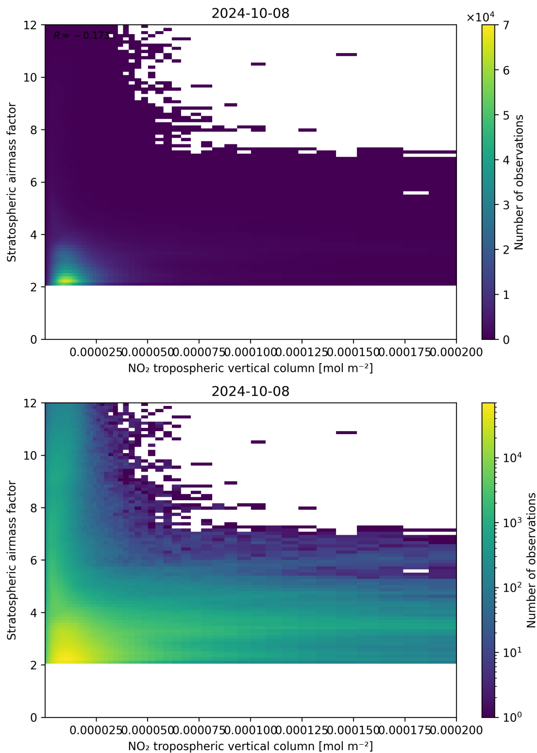
Figure 121: Scatter density plot of “NO 2 tropospheric vertical column” against “Stratospheric air mass factor” for 2024-10-08 to 2024-10-09.
