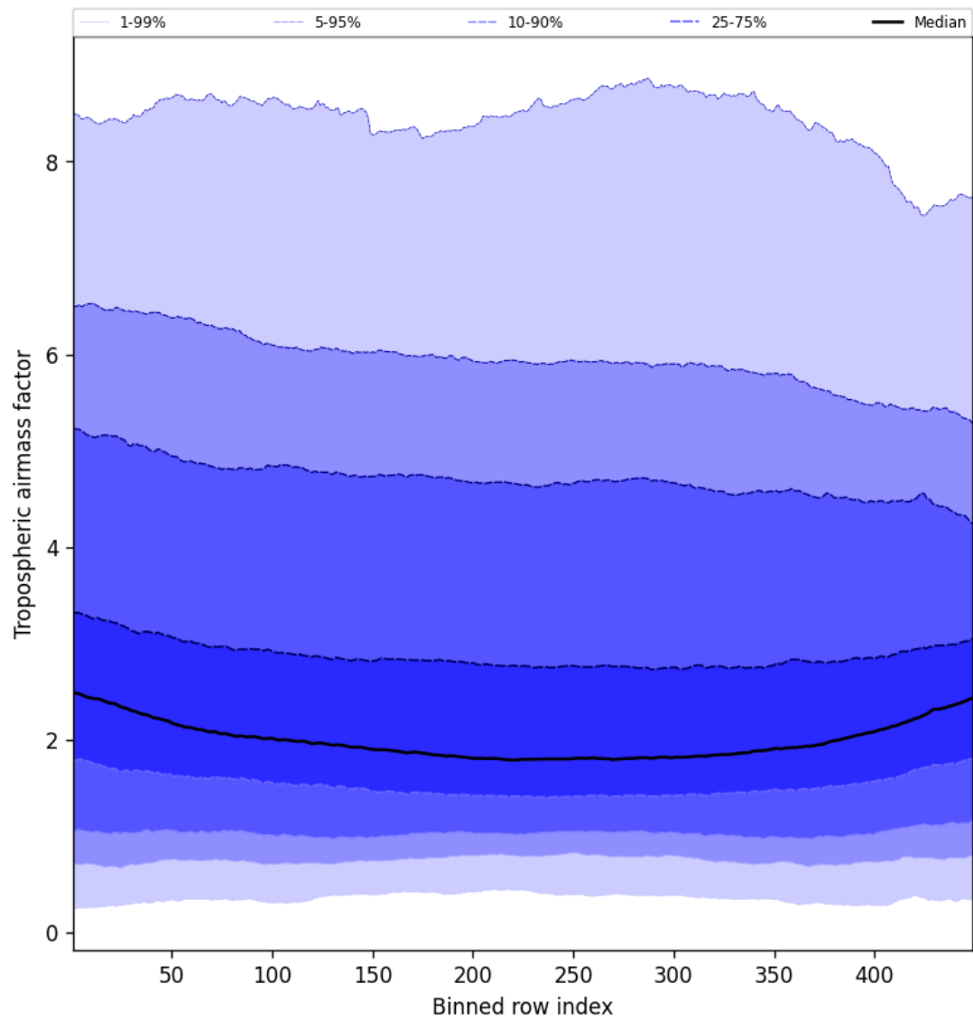
Figure 48: Along track statistics of “Tropospheric air mass factor” for 2024-10-08 to 2024-10-09
