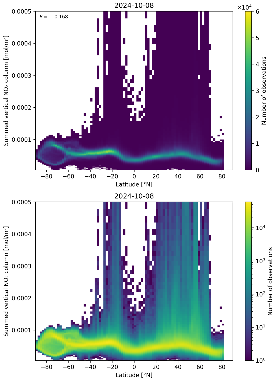
Figure 88: Scatter density plot of “Latitude” against “Summed vertical NO 2 column” for 2024-10-08 to 2024-10-09.
