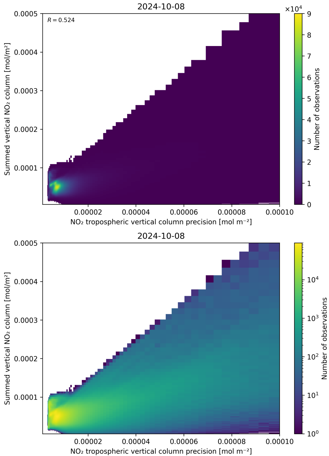
Figure 136: Scatter density plot of “NO 2 tropospheric vertical column precision” against “Summed vertical NO 2 column” for 2024-10-08 to 2024-10-09.
