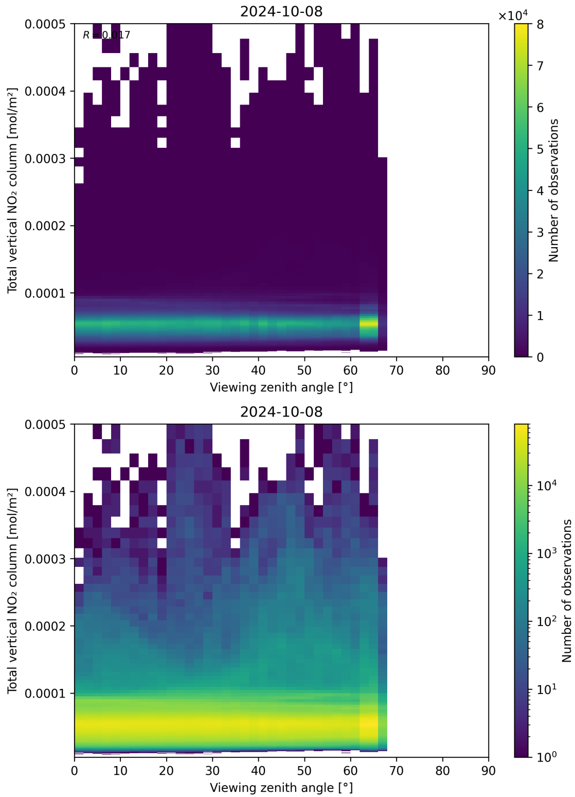
Figure 167: Scatter density plot of “Viewing zenith angle” against “Total vertical NO 2 column” for 2024-10-08 to 2024-10-09.
