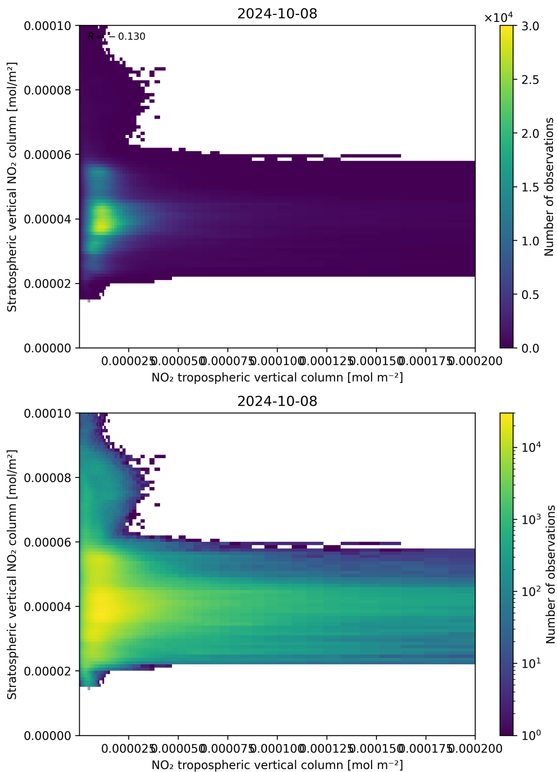
Figure 125: Scatter density plot of “NO 2 tropospheric vertical column” against “Stratospheric vertical NO 2 column” for 2024-10-08 to 2024-10-09.
