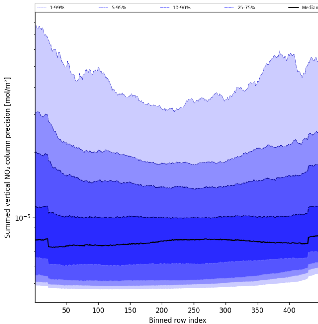
Figure 58: Along track statistics of “Summed vertical NO 2 column precision” for 2024-10-08 to 2024-10-09
