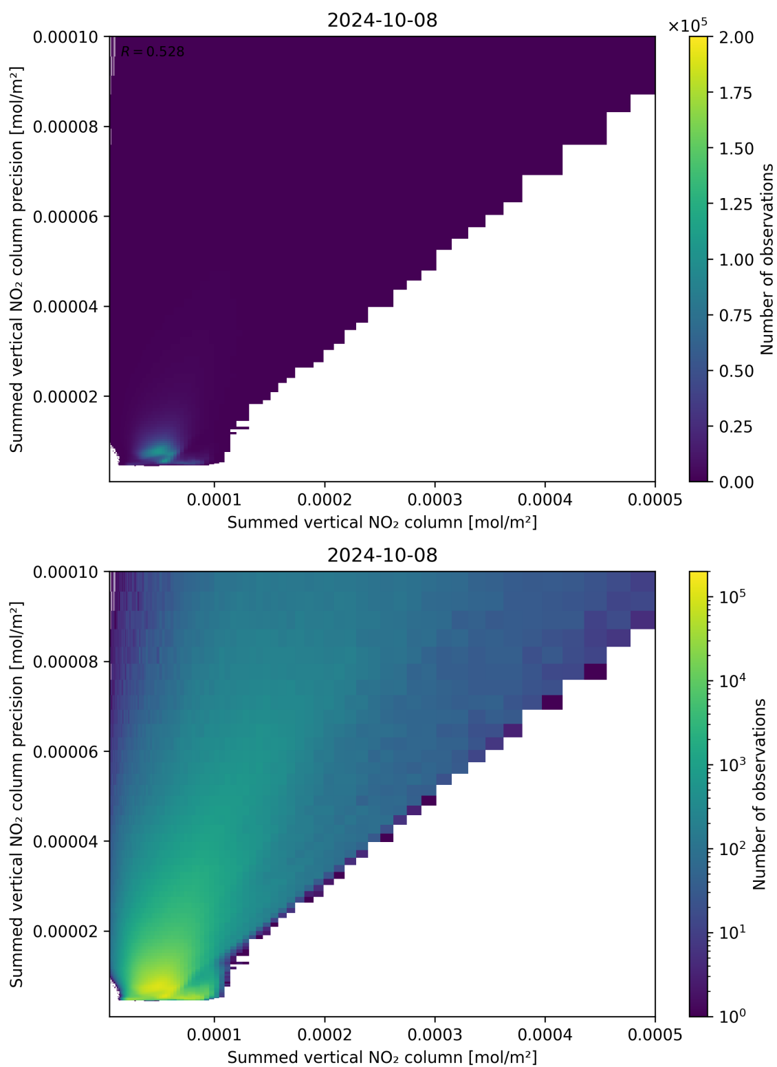
Figure 105: Scatter density plot of “Summed vertical NO 2 column” against “Summed vertical NO 2 column precision” for 2024-10-08 to 2024-10-09.
