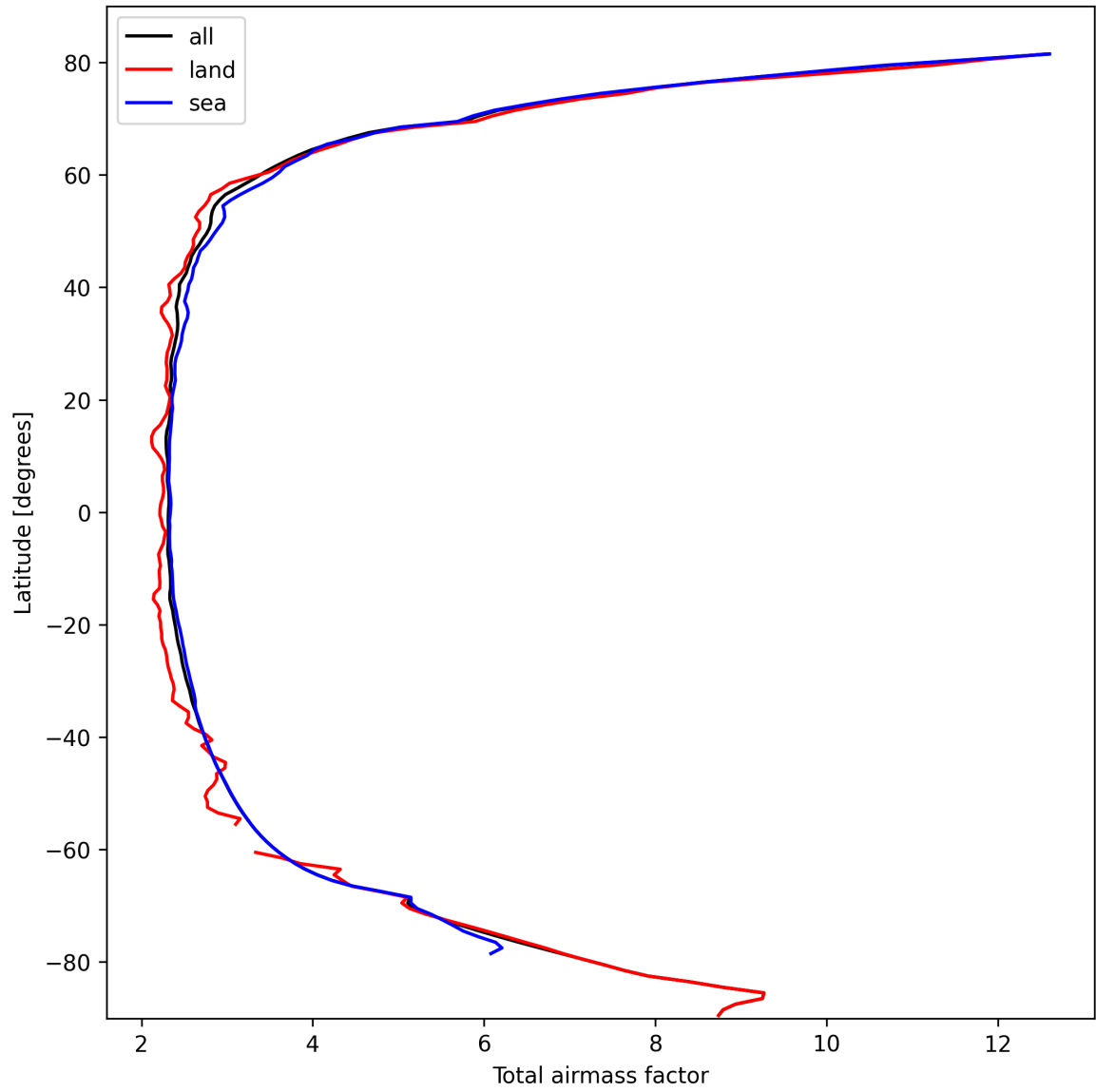
Figure 15: Zonal average of “Total airmass factor” for 2024-10-08 to 2024-10-09.
