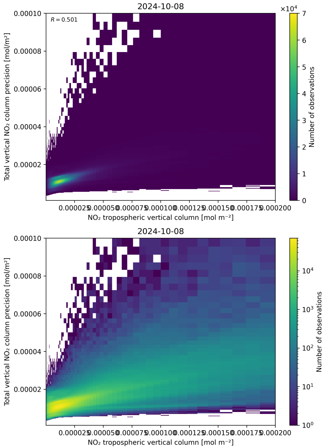
Figure 129: Scatter density plot of “NO 2 tropospheric vertical column” against “Total vertical NO 2 column precision” for 2024-10-08 to 2024-10-09.
