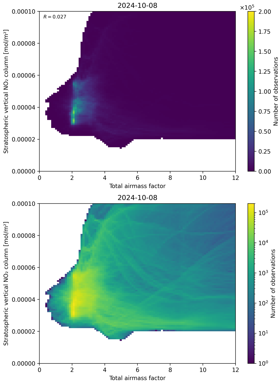
Figure 64: Scatter density plot of “Total airmass factor” against “Stratospheric vertical NO 2 column” for 2024-10-08 to 2024-10-09.
