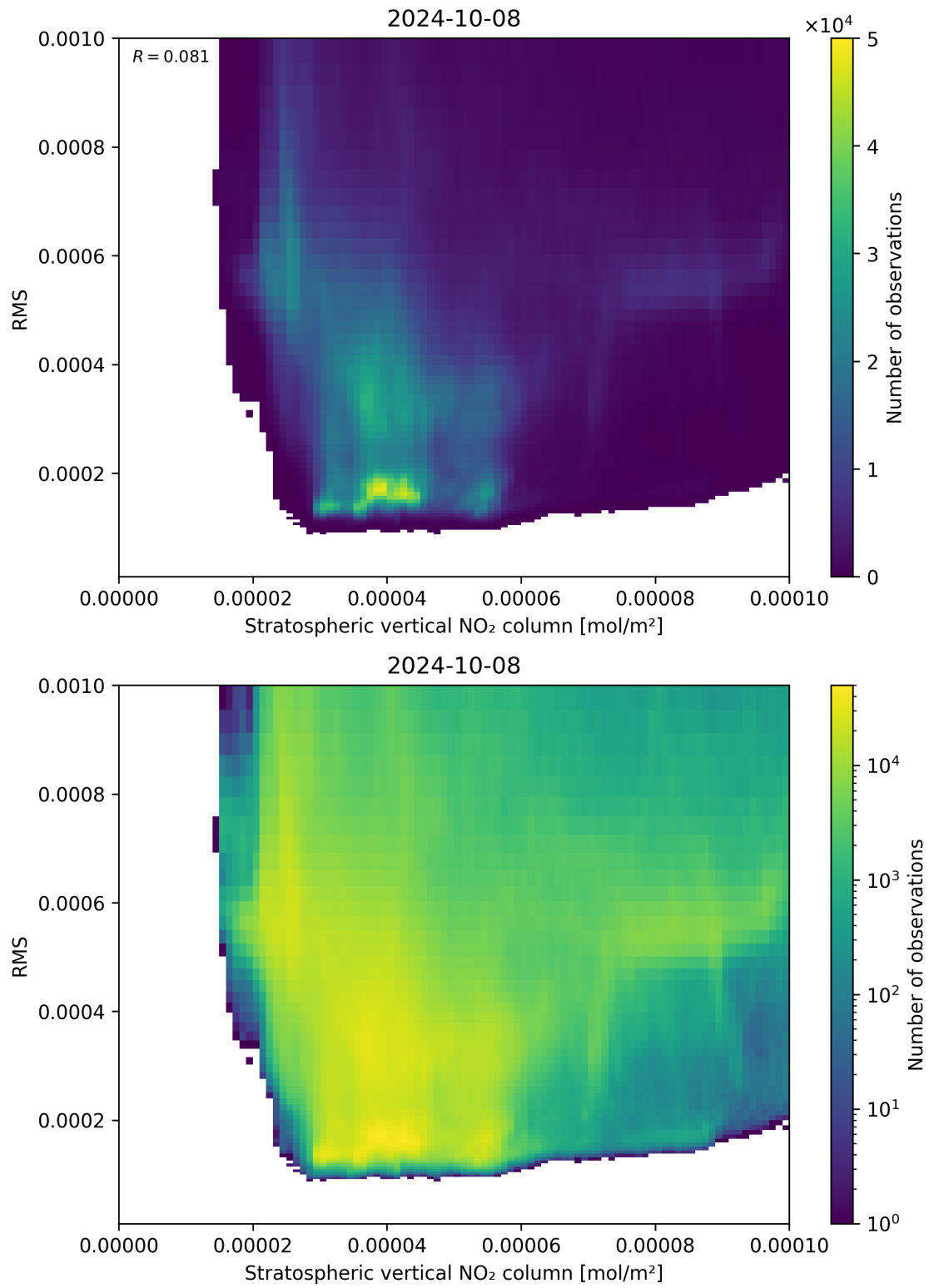
Figure 102: Scatter density plot of “Stratospheric vertical NO 2 column” against “RMS” for 2024-10-08 to 2024-10-09.
