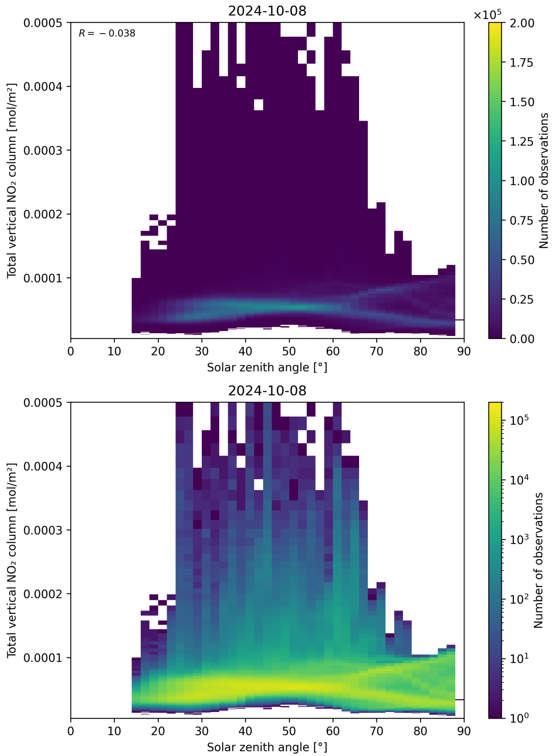
Figure 153: Scatter density plot of “Solar zenith angle” against “Total vertical NO 2 column” for 2024-10-08 to 2024-10-09.
