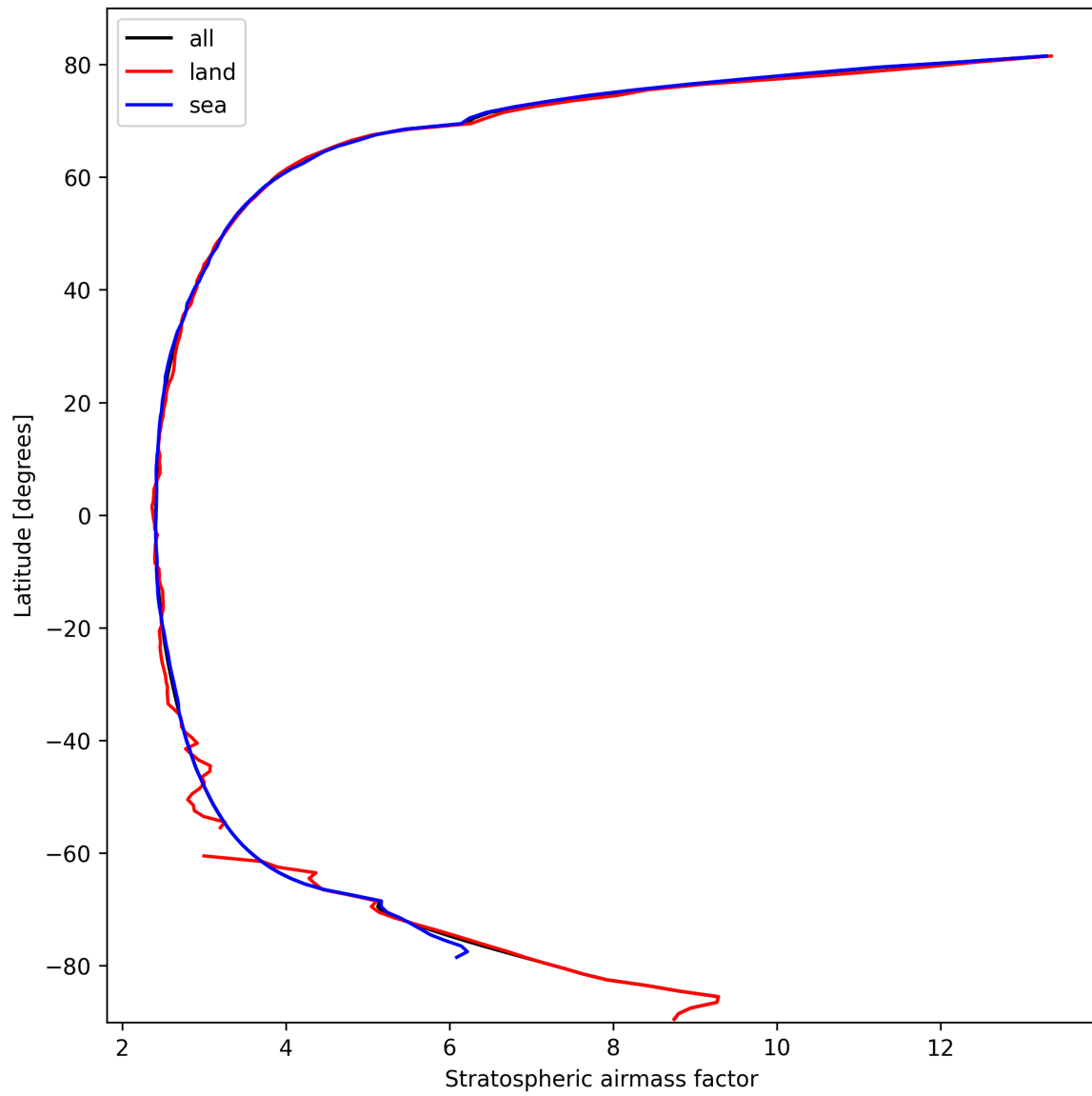
Figure 27: Zonal average of “Stratospheric air mass factor” for 2024-10-08 to 2024-10-09.
