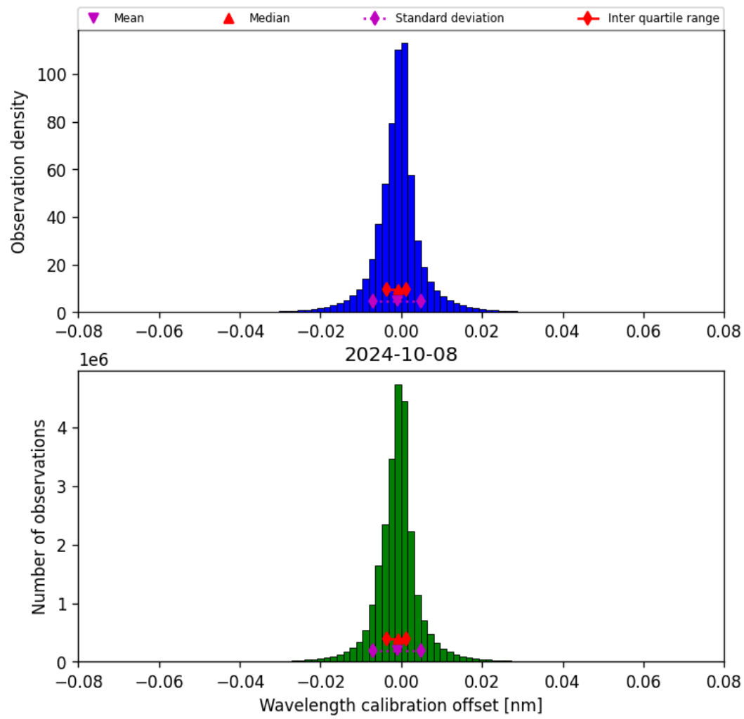
Figure 35: Histogram of “Wavelength calibration offset” for 2024-10-08 to 2024-10-09
