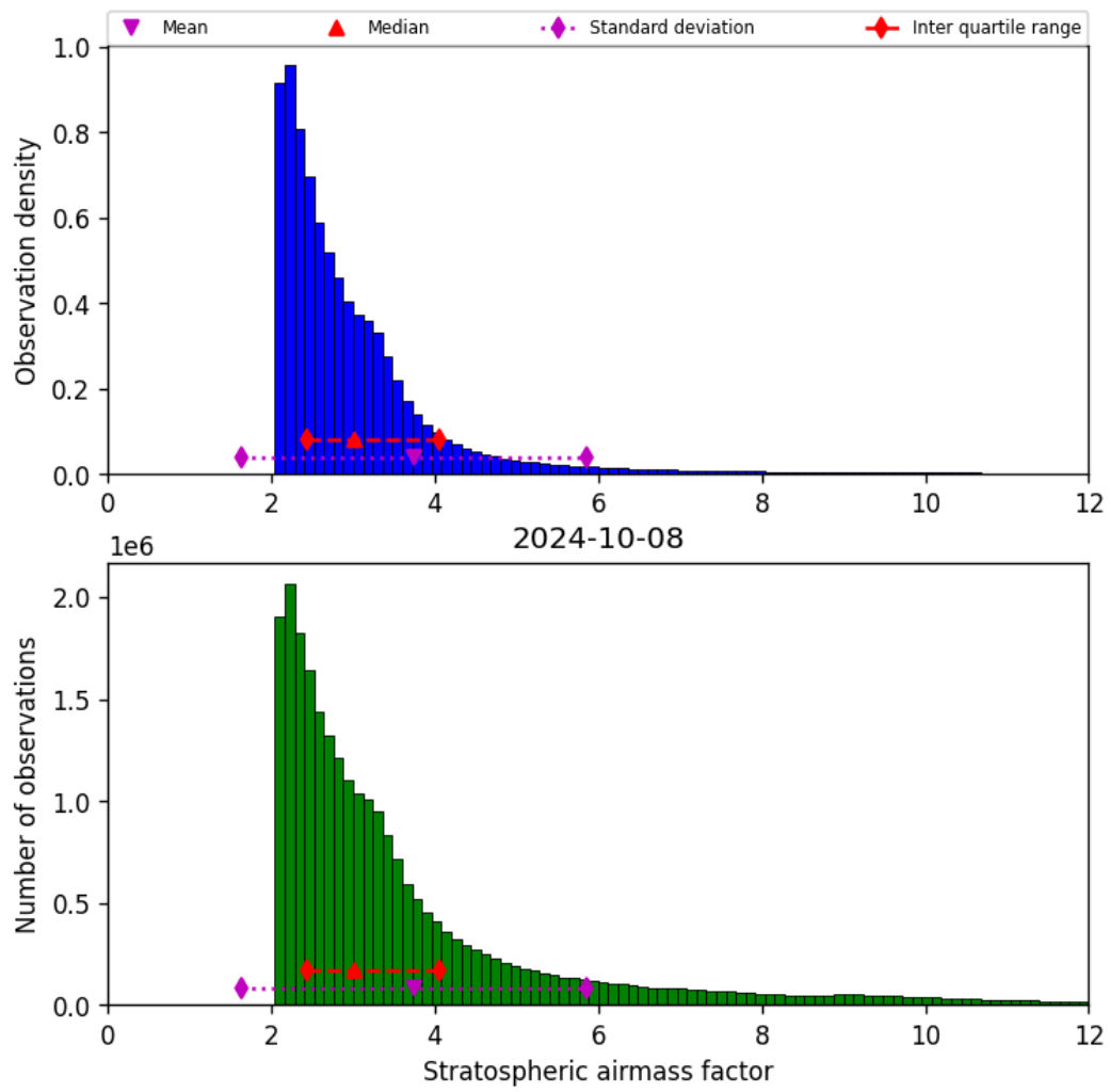
Figure 44: Histogram of “Stratospheric airmass factor” for 2024-10-08 to 2024-10-09
