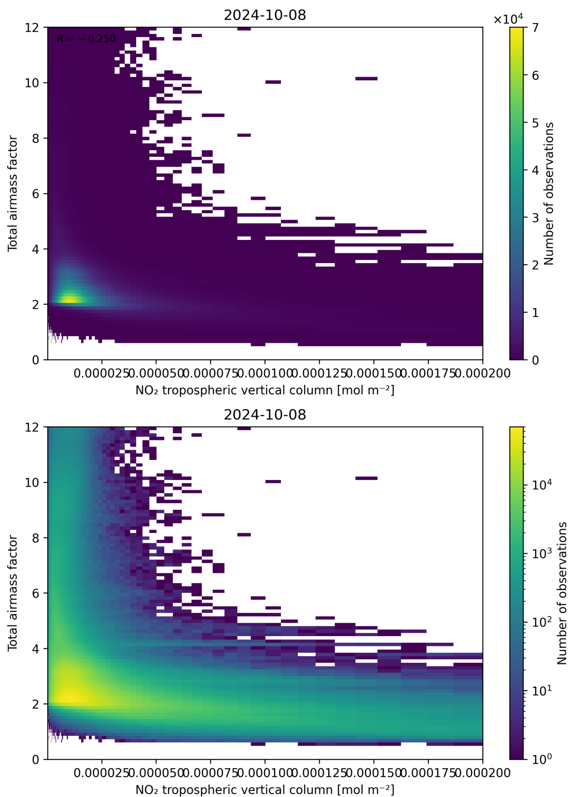
Figure 122: Scatter density plot of “NO 2 tropospheric vertical column” against “Total air mass factor” for 2024-10-08 to 2024-10-09.
