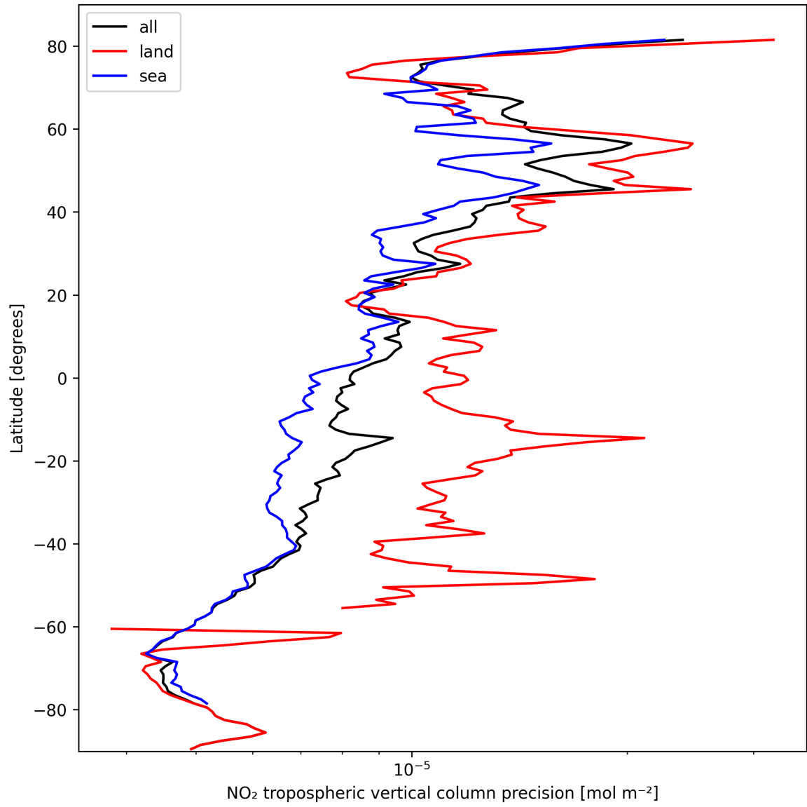
Figure 13: Zonal average of “NO 2 tropospheric vertical column precision” for 2024-10-08 to 2024-10-09.
