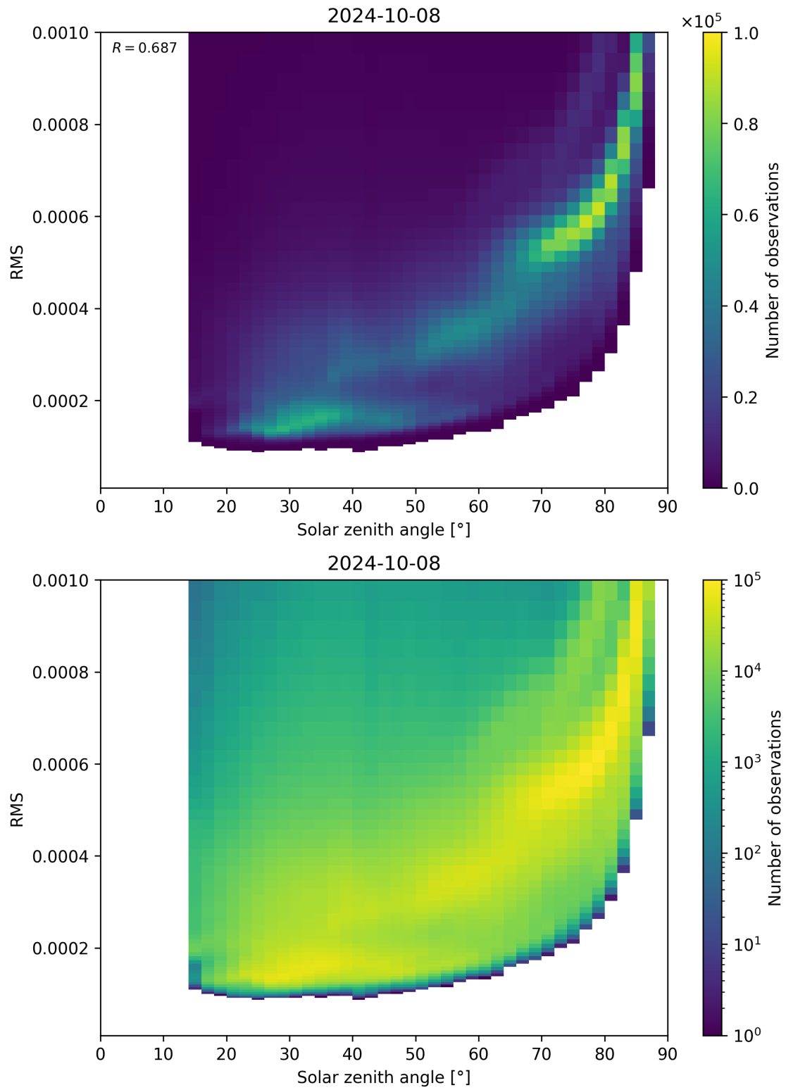
Figure 157: Scatter density plot of “Solar zenith angle” against “RMS” for 2024-10-08 to 2024-10-09.
