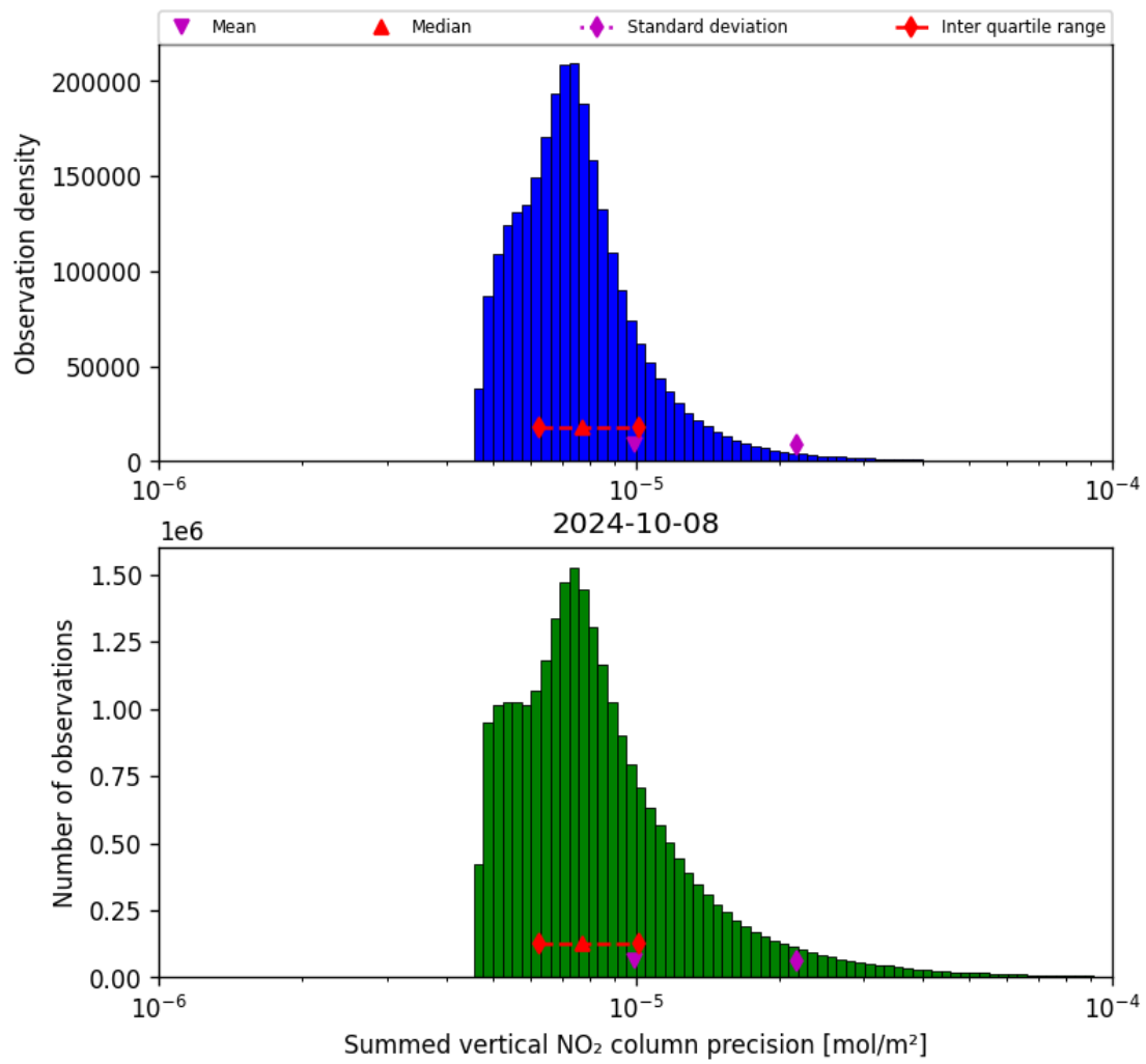
Figure 41: Histogram of "Summed vertical NO 2 column precision" for 2024-10-08 to 2024-10-09
