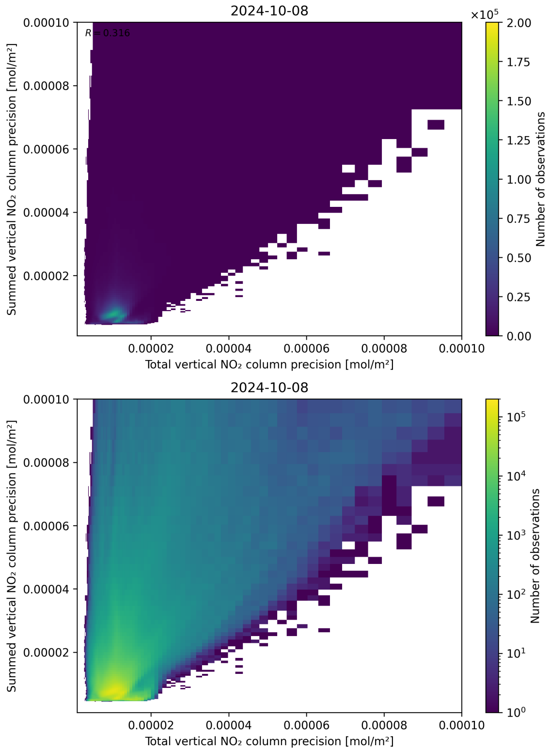
Figure 118: Scatter density plot of “Total vertical NO 2 column precision” against “Summed vertical NO 2 column precision” for 2024-10-08 to 2024-10-09.
