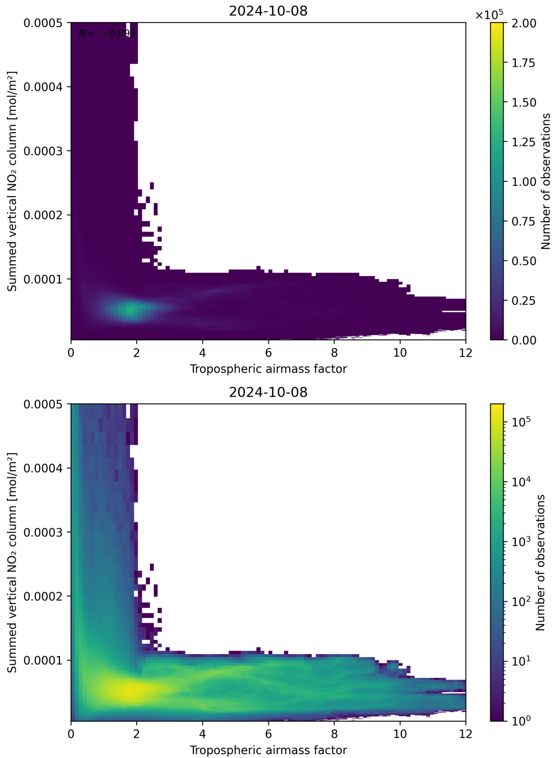
Figure 75: Scatter density plot of “Tropospheric air mass factor” against “Summed vertical NO 2 column” for 2024-10-08 to 2024-10-09.
