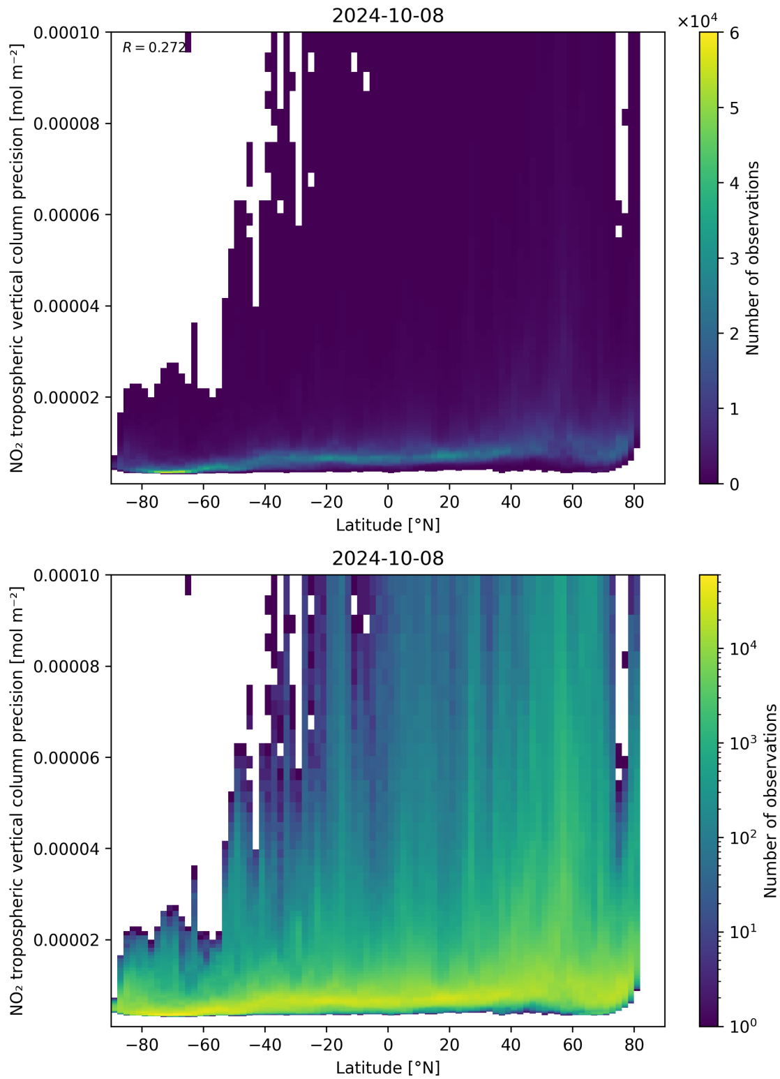
Figure 93: Scatter density plot of “Latitude” against “NO 2 tropospheric vertical column precision” for 2024-10-08 to 2024-10-09.
