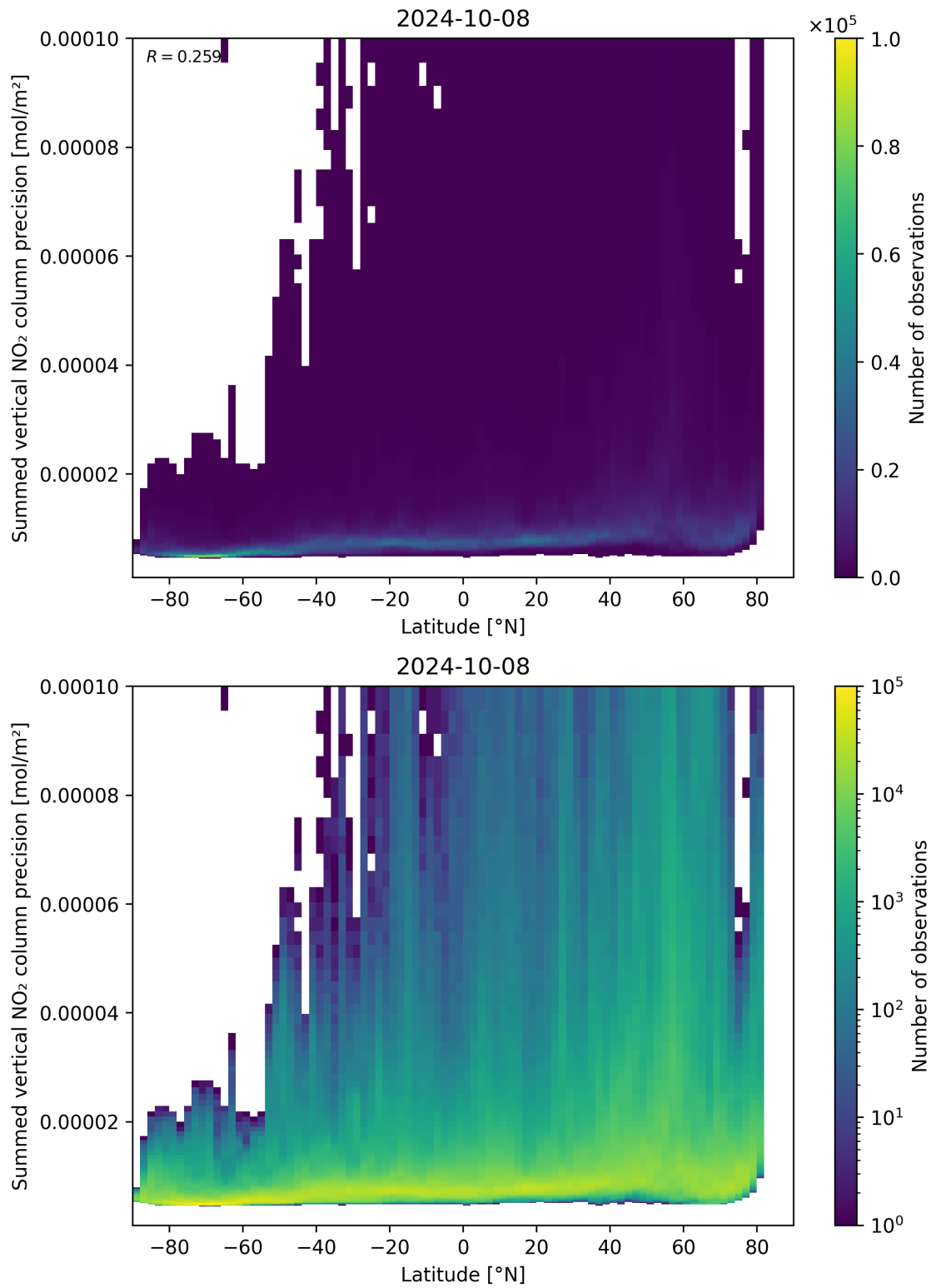
Figure 89: Scatter density plot of “Latitude” against “Summed vertical NO 2 column precision” for 2024-10-08 to 2024-10-09.
