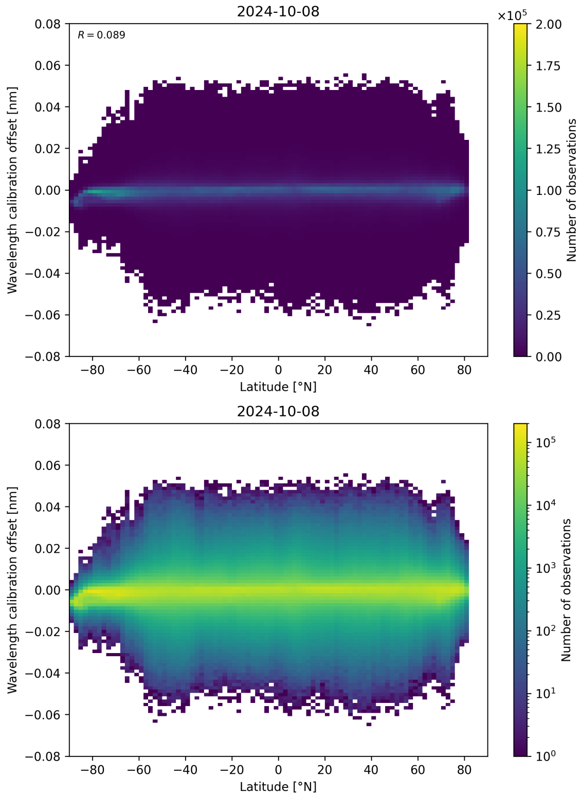
Figure 95: Scatter density plot of “Latitude” against “Wavelength calibration offset” for 2024-10-08 to 2024-10-09.
