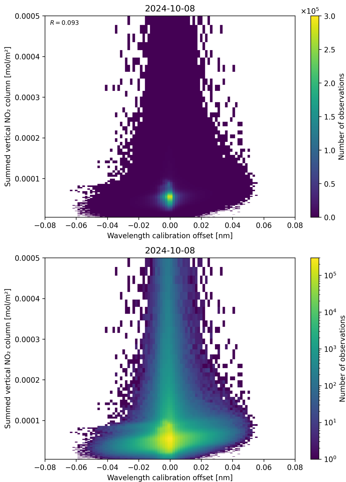
Figure 177: Scatter density plot of “Wavelength calibration offset” against “Summed vertical NO 2 column” for 2024-10-08 to 2024-10-09.
