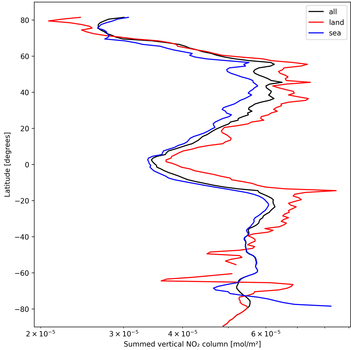
Figure 23: Zonal average of “Summed vertical NO 2 column” for 2024-10-08 to 2024-10-09.
