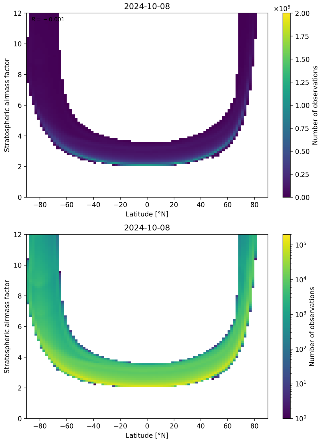
Figure 83: Scatter density plot of “Latitude” against “Stratospheric airmass factor” for 2024-10-08 to 2024-10-09.
