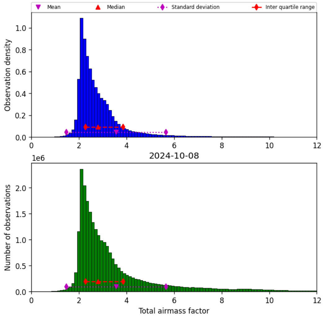
Figure 32: Histogram of “Total airmass factor” for 2024-10-08 to 2024-10-09
