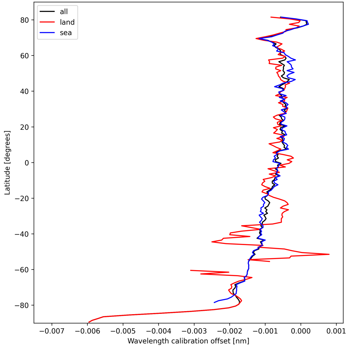
Figure 18: Zonal average of “Wavelength calibration offset” for 2024-10-08 to 2024-10-09.
