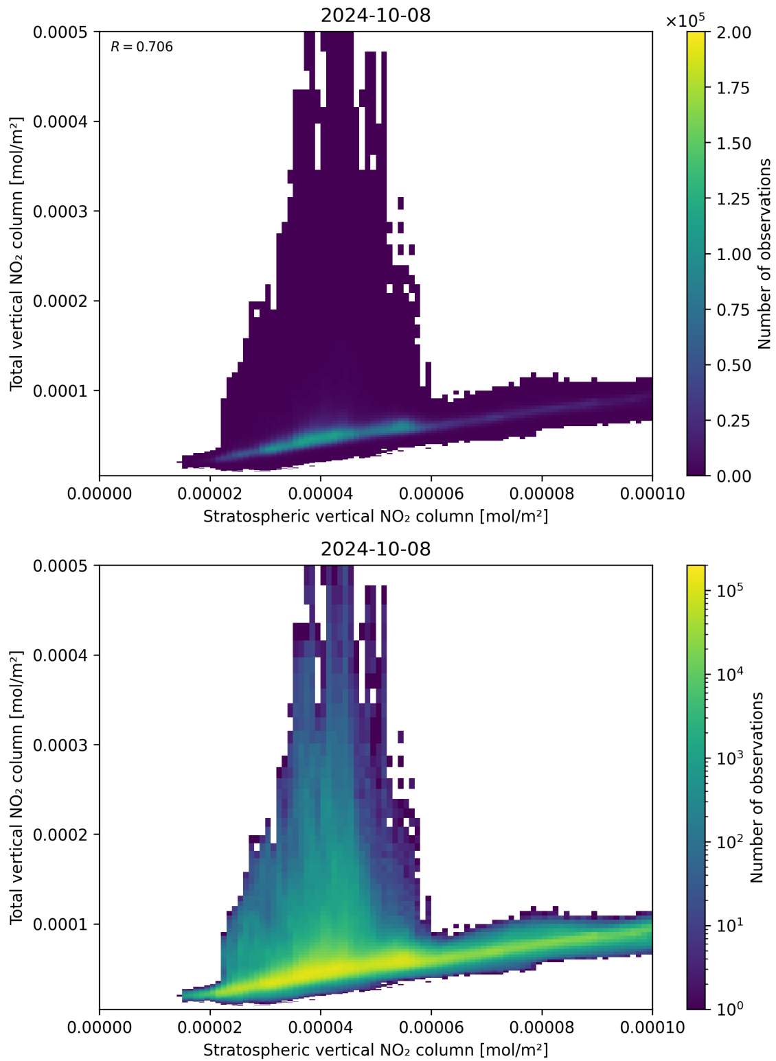
Figure 100: Scatter density plot of “Stratospheric vertical NO 2 column” against “Total vertical NO 2 column” for 2024-10-08 to 2024-10-09.
