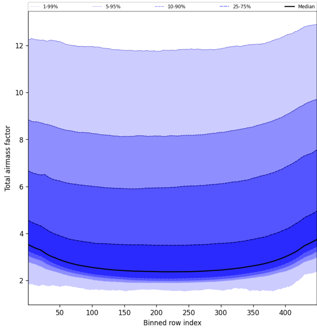
Figure 49: Along track statistics of “Total airmass factor” for 2024-10-08 to 2024-10-09
