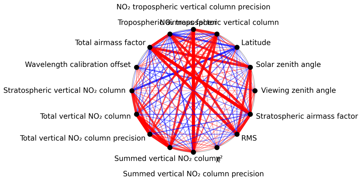
Figure 1: Map of correlation graph for 2024-10-08 to 2024-10-09.
