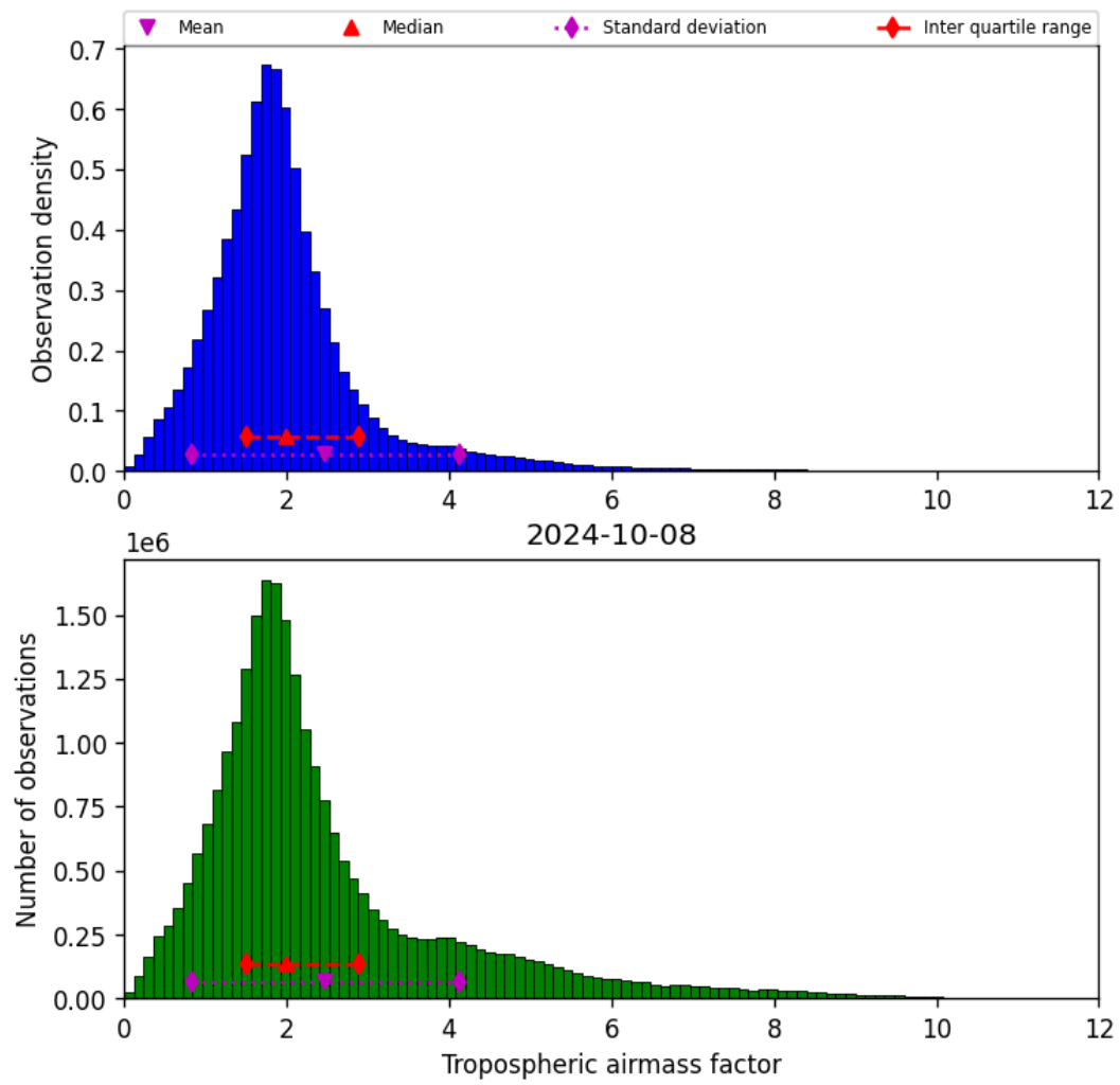
Figure 31: Histogram of “Tropospheric airmass factor” for 2024-10-08 to 2024-10-09
