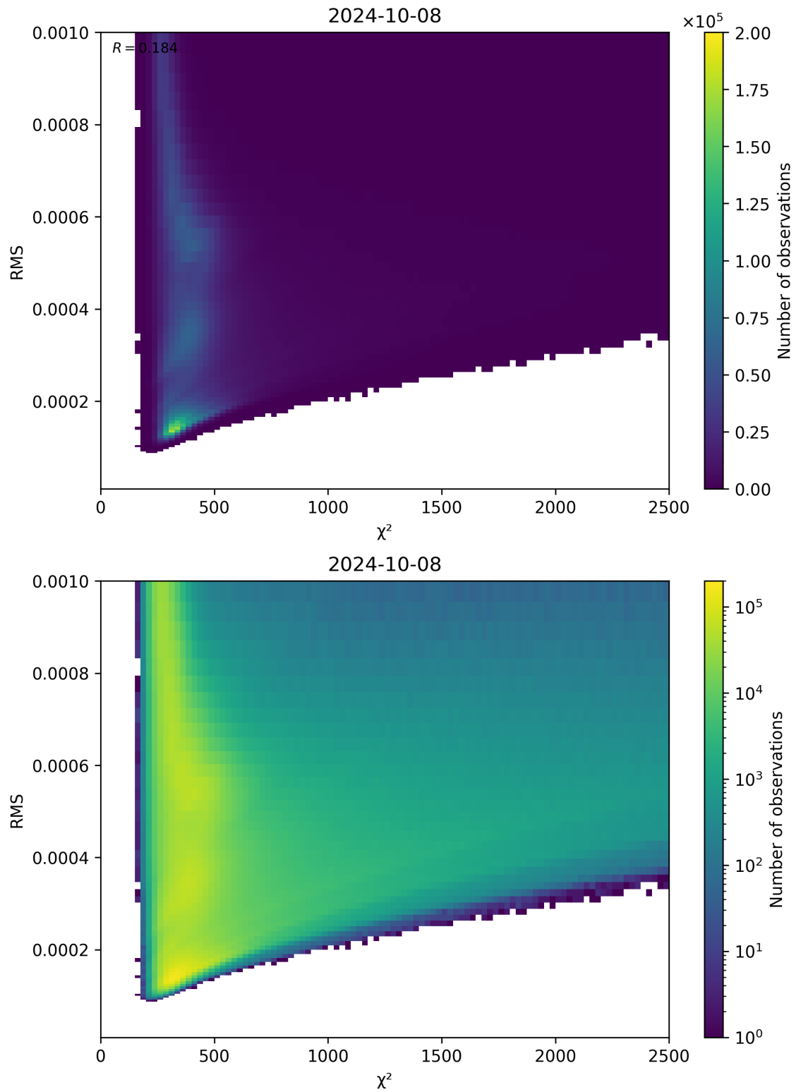
Figure 82: Scatter density plot of “ \chi^2 ” against “RMS” for 2024-10-08 to 2024-10-09.
