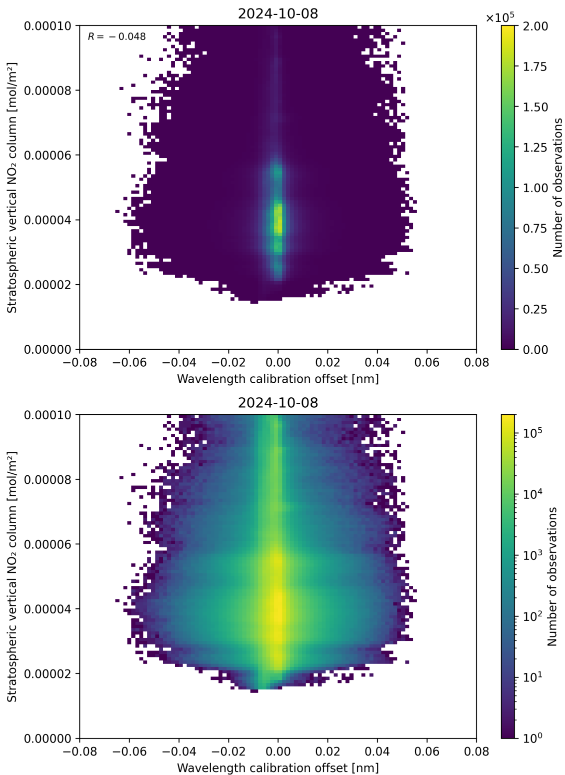
Figure 176: Scatter density plot of “Wavelength calibration offset” against “Stratospheric vertical NO 2 column” for 2024-10-08 to 2024-10-09.
