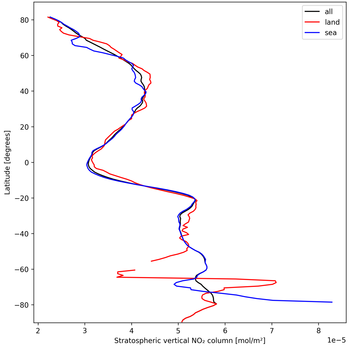
Figure 19: Zonal average of “Stratospheric vertical NO 2 column” for 2024-10-08 to 2024-10-09.
