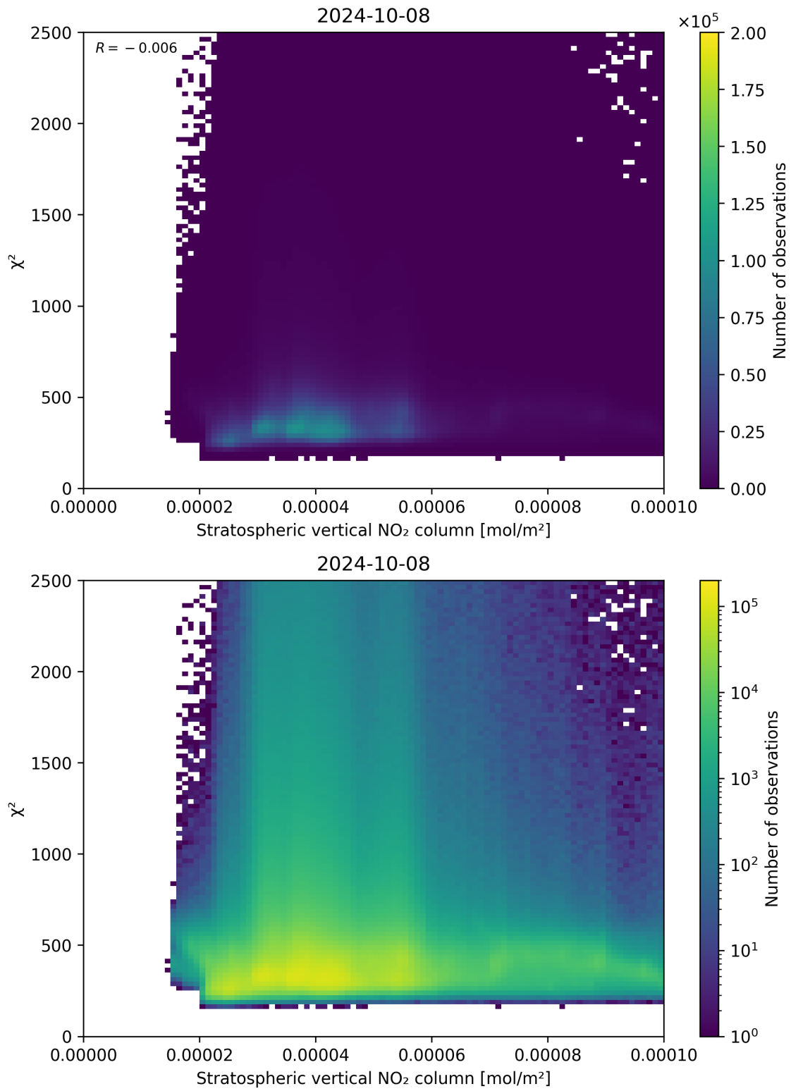
Figure 97: Scatter density plot of “Stratospheric vertical NO 2 column” against “ \chi^2 ” for 2024-10-08 to 2024-10-09.
