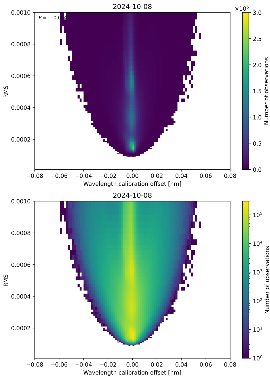
Figure 181: Scatter density plot of “Wavelength calibration offset” against “RMS” for 2024-10-08 to 2024-10-09.
