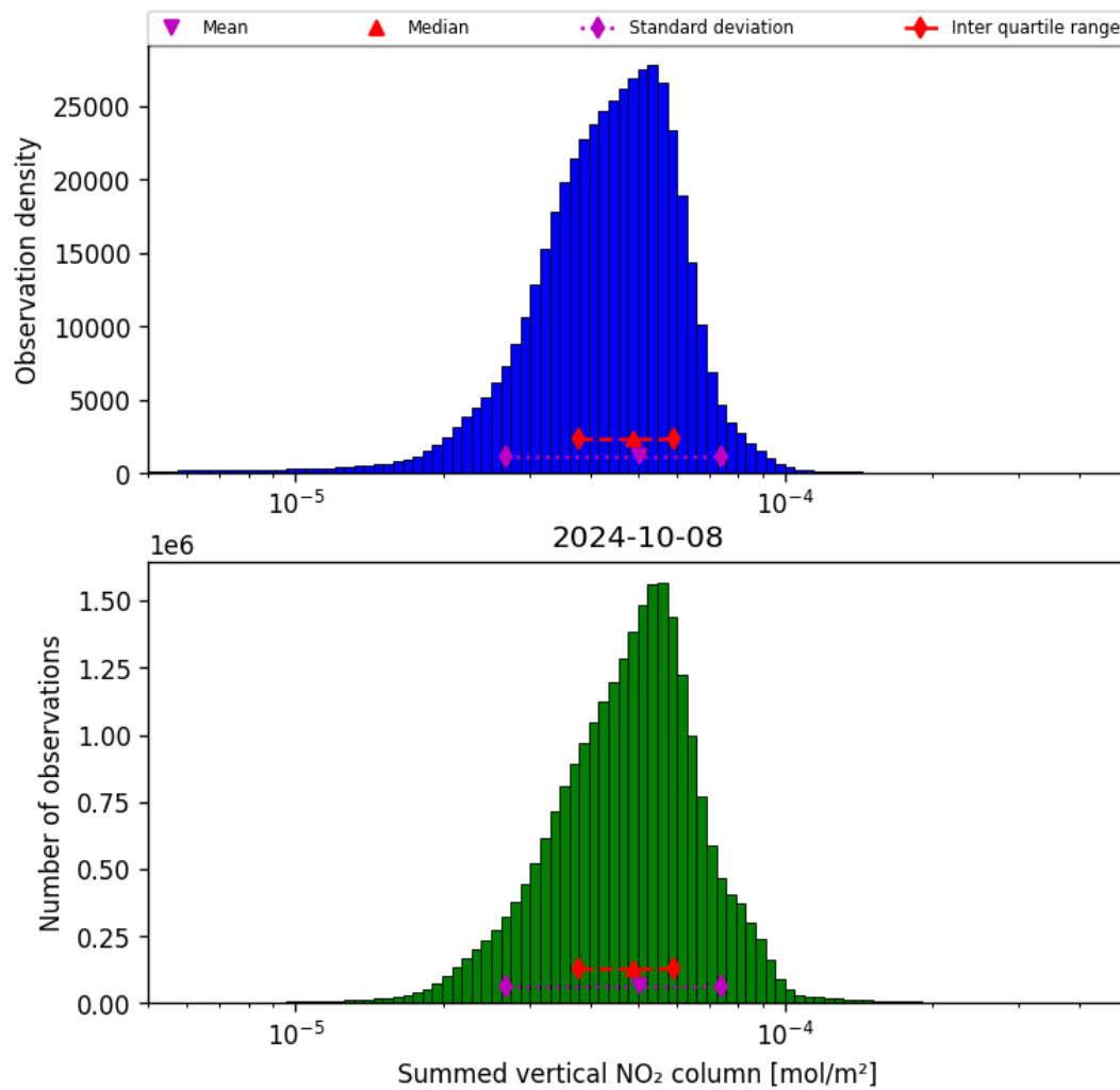
Figure 40: Histogram of “Summed vertical NO 2 column” for 2024-10-08 to 2024-10-09
