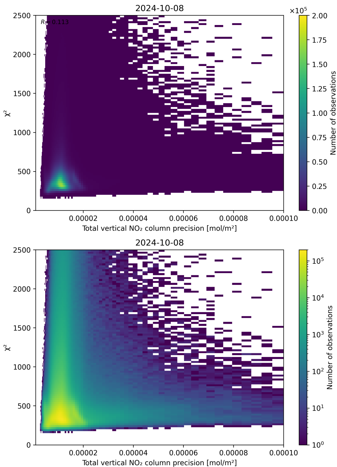
Figure 116: Scatter density plot of “Total vertical NO 2 column precision” against “ \chi^2 ” for 2024-10-08 to 2024-10-09.
