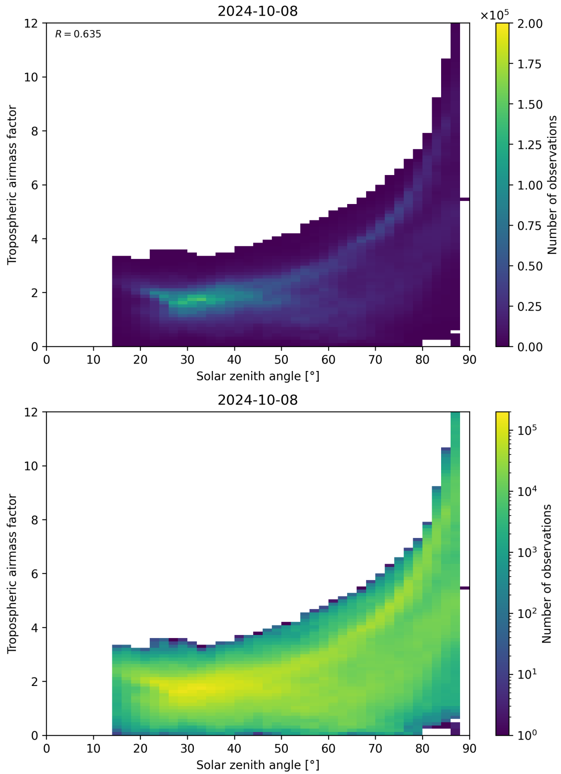
Figure 147: Scatter density plot of “Solar zenith angle” against “Tropospheric airmass factor” for 2024-10-08 to 2024-10-09.
