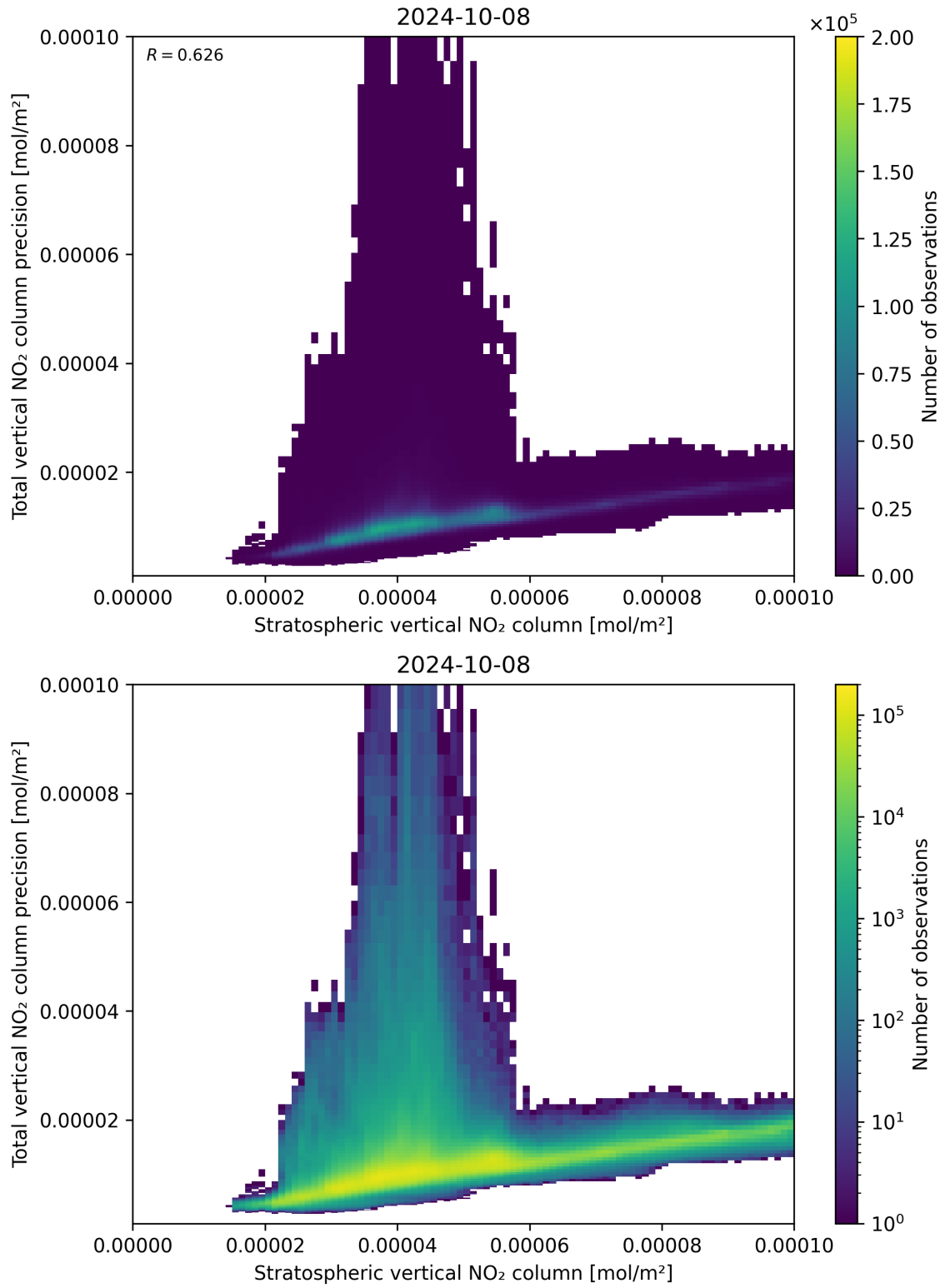
Figure 101: Scatter density plot of “Stratospheric vertical NO 2 column” against “Total vertical NO 2 column precision” for 2024-10-08 to 2024-10-09.
