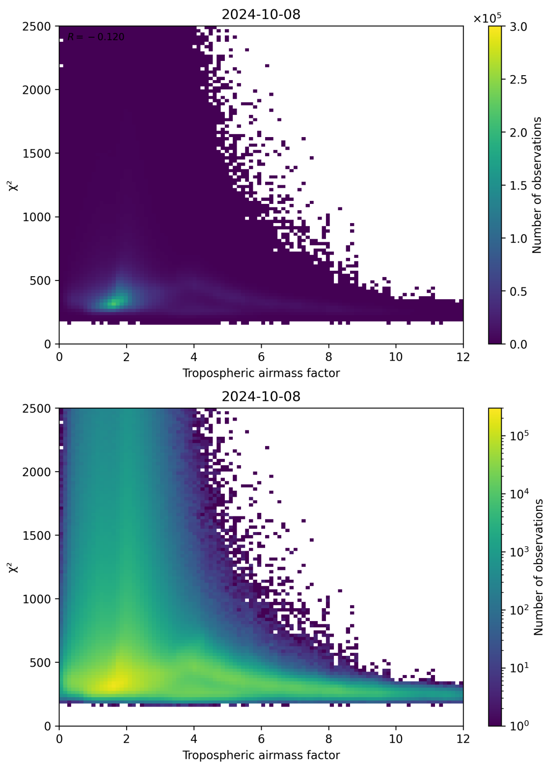
Figure 73: Scatter density plot of “Tropospheric airmass factor” against “ \chi^2 ” for 2024-10-08 to 2024-10-09.
