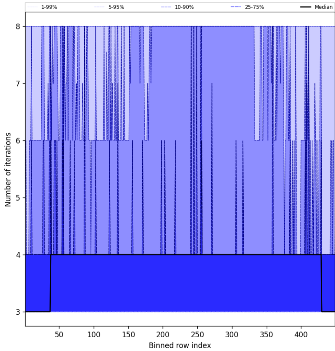
Figure 51: Along track statistics of “Number of iterations” for 2024-10-08 to 2024-10-09
