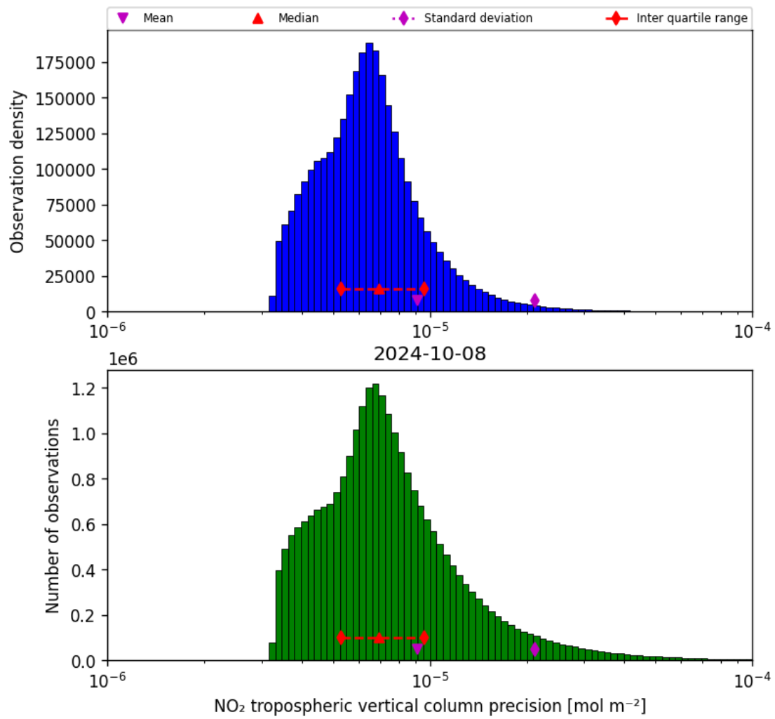
Figure 30: Histogram of “NO 2 tropospheric vertical column precision” for 2024-10-08 to 2024-10-09
