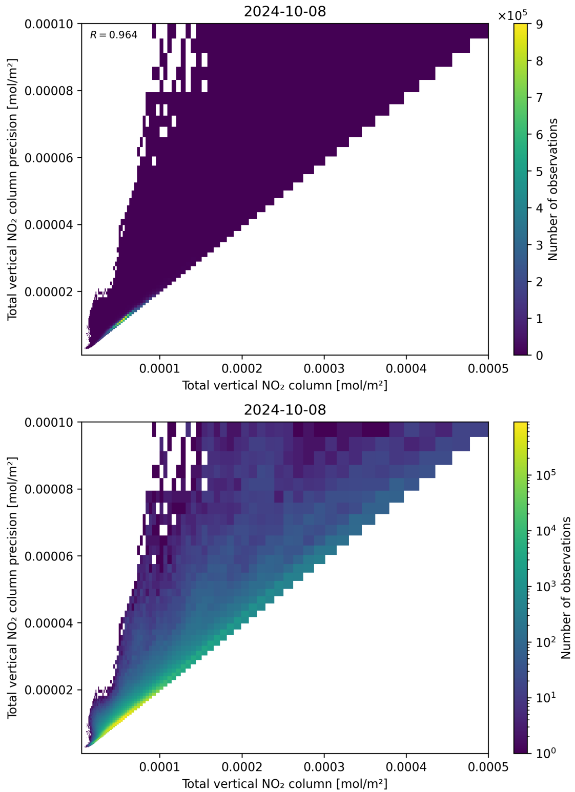
Figure 114: Scatter density plot of “Total vertical NO 2 column” against “Total vertical NO 2 column precision” for 2024-10-08 to 2024-10-09.
