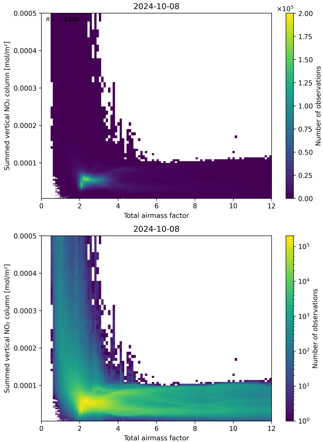
Figure 65: Scatter density plot of “Total airmass factor” against “Summed vertical NO 2 column” for 2024-10-08 to 2024-10-09.
