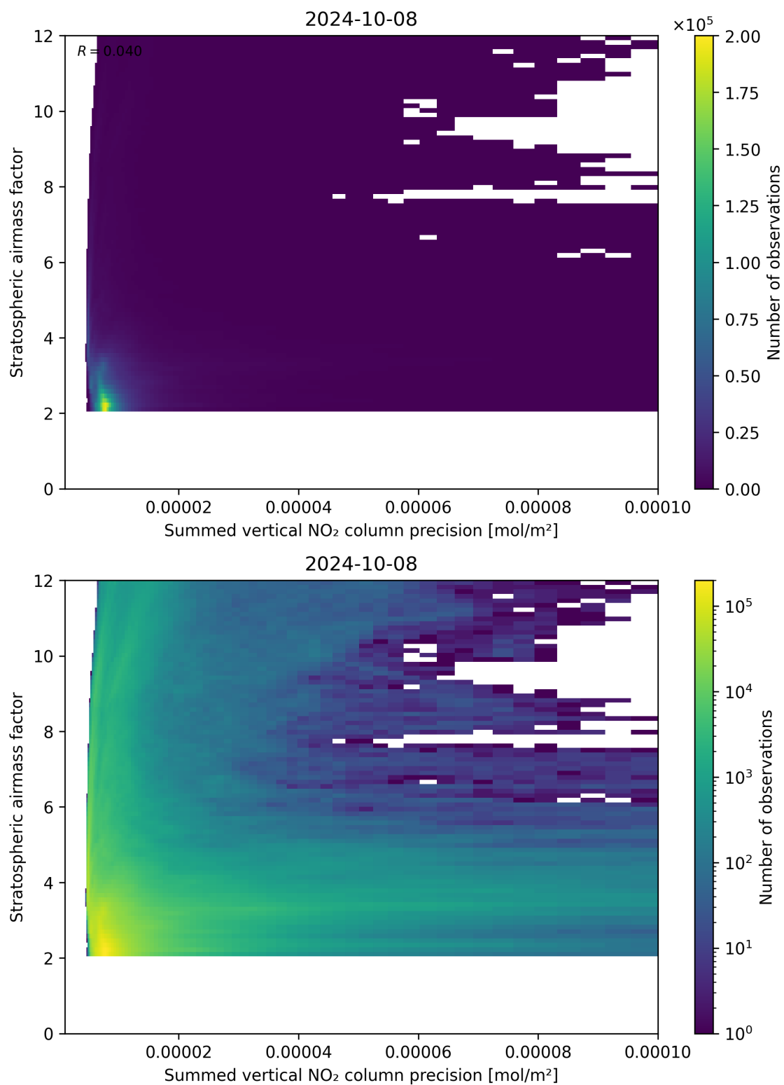
Figure 106: Scatter density plot of “Summed vertical NO 2 column precision” against “Stratospheric airmass factor” for 2024-10-08 to 2024-10-09.
