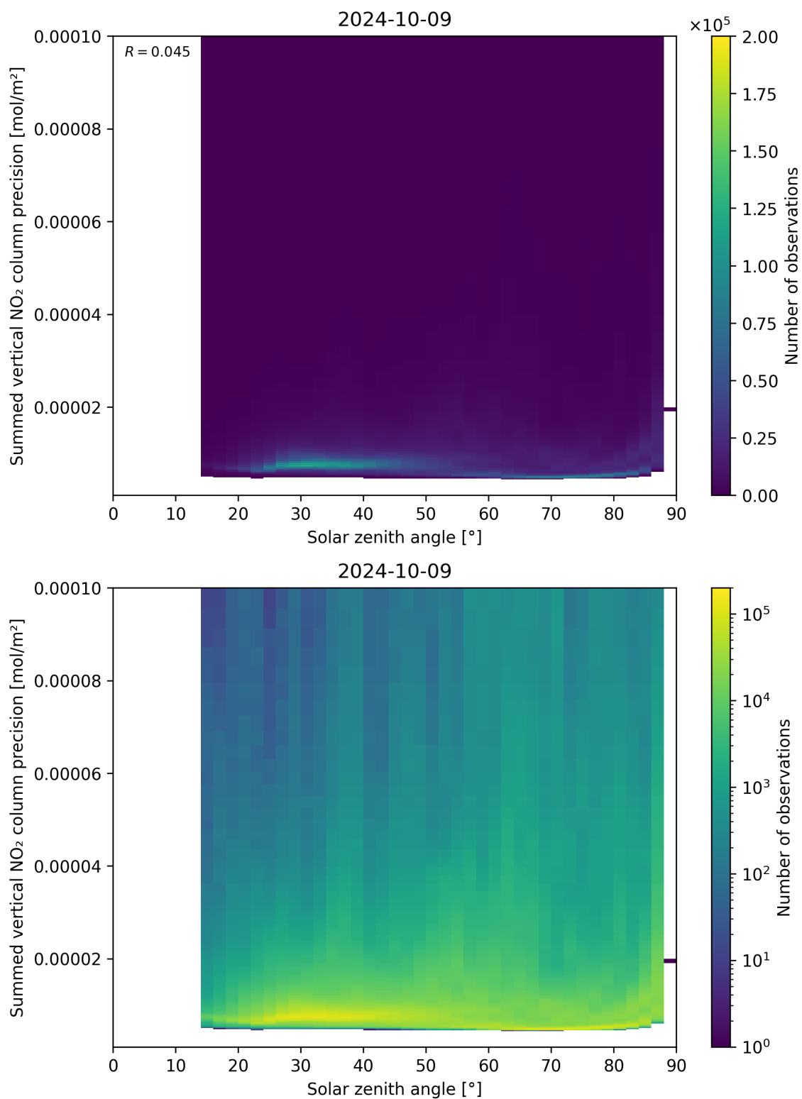
Figure 152: Scatter density plot of “Solar zenith angle” against “Summed vertical NO 2 column precision” for 2024-10-08 to 2024-10-10.
