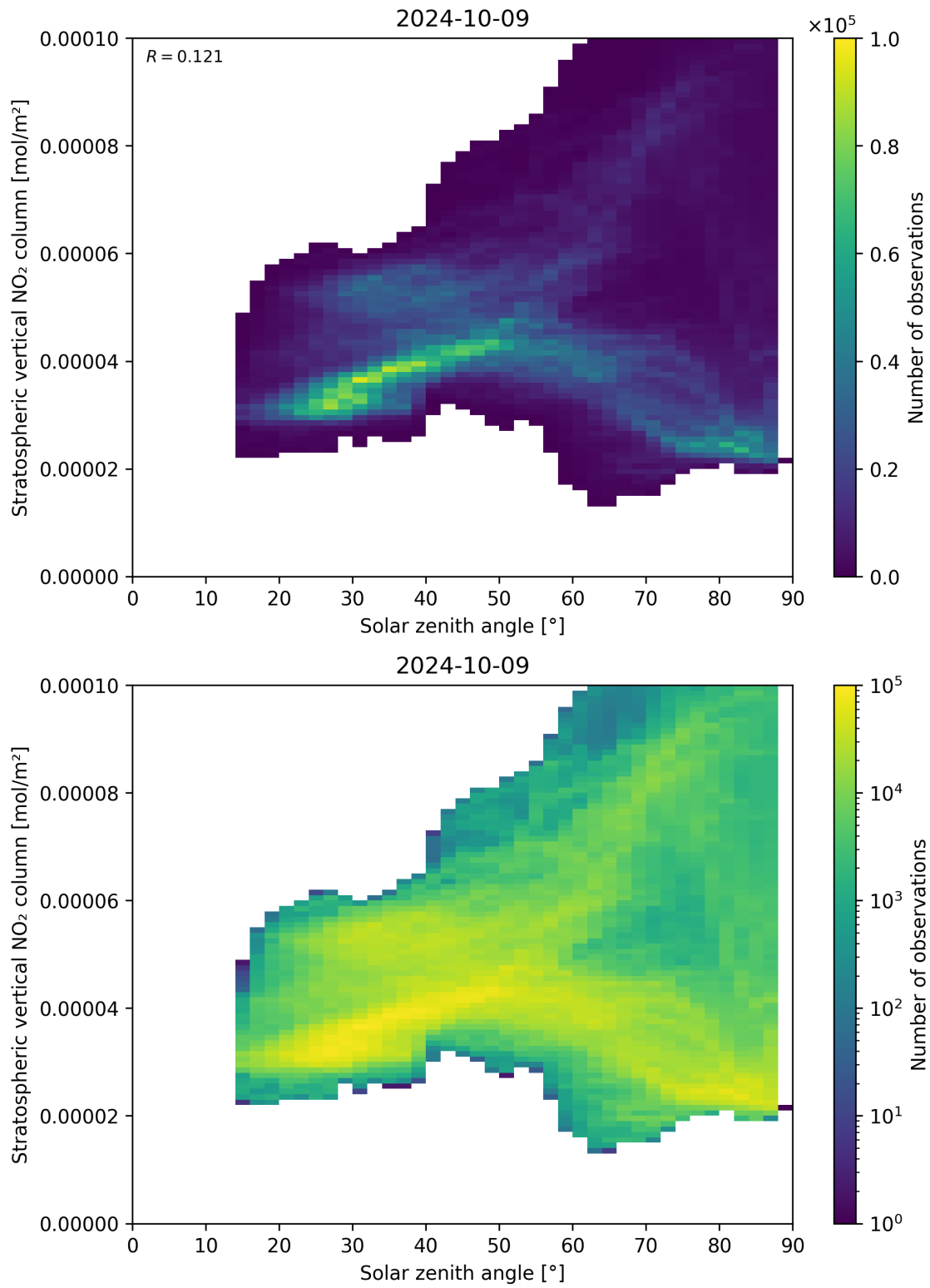
Figure 150: Scatter density plot of “Solar zenith angle” against “Stratospheric vertical NO 2 column” for 2024-10-08 to 2024-10-10.
