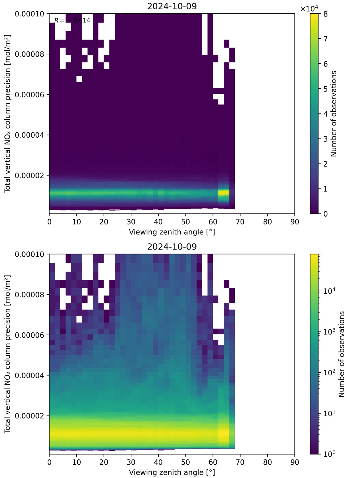
Figure 168: Scatter density plot of “Viewing zenith angle” against “Total vertical NO 2 column precision” for 2024-10-08 to 2024-10-10.
