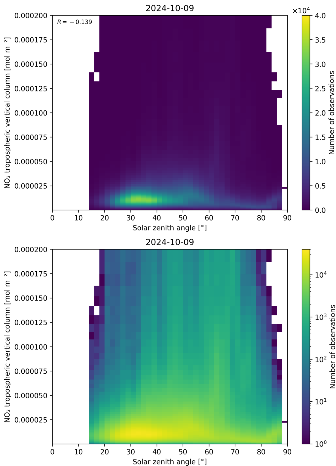
Figure 155: Scatter density plot of “Solar zenith angle” against “NO 2 tropospheric vertical column” for 2024-10-08 to 2024-10-10.
