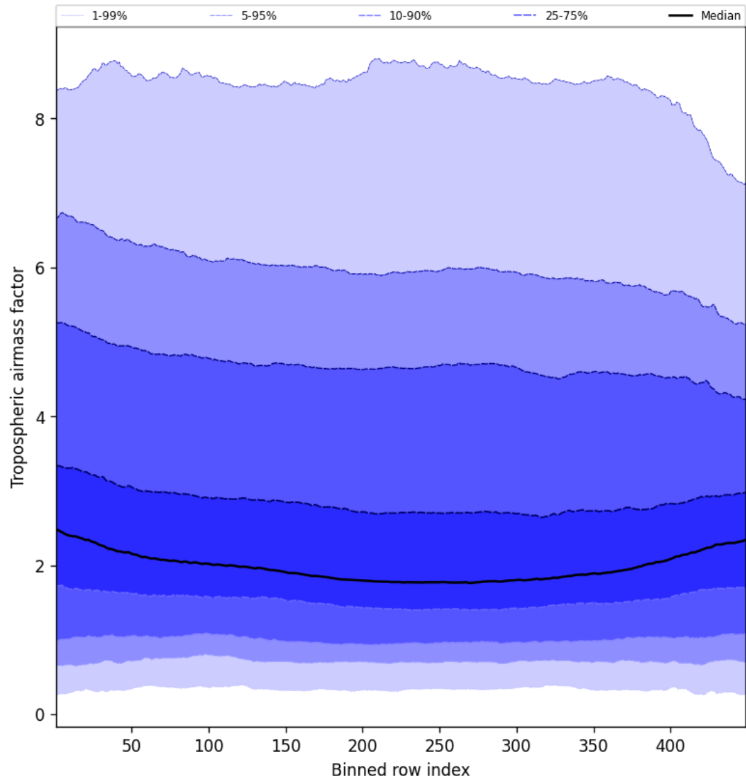
Figure 48: Along track statistics of “Tropospheric air mass factor” for 2024-10-08 to 2024-10-10
