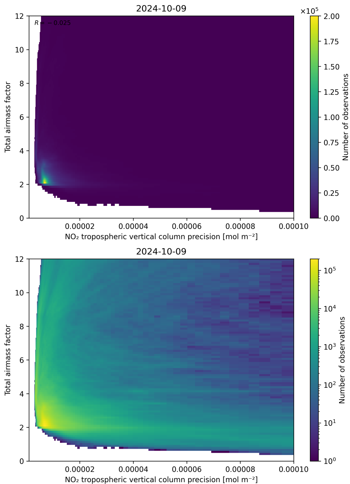
Figure 132: Scatter density plot of “NO 2 tropospheric vertical column precision” against “Total air mass factor” for 2024-10-08 to 2024-10-10.
