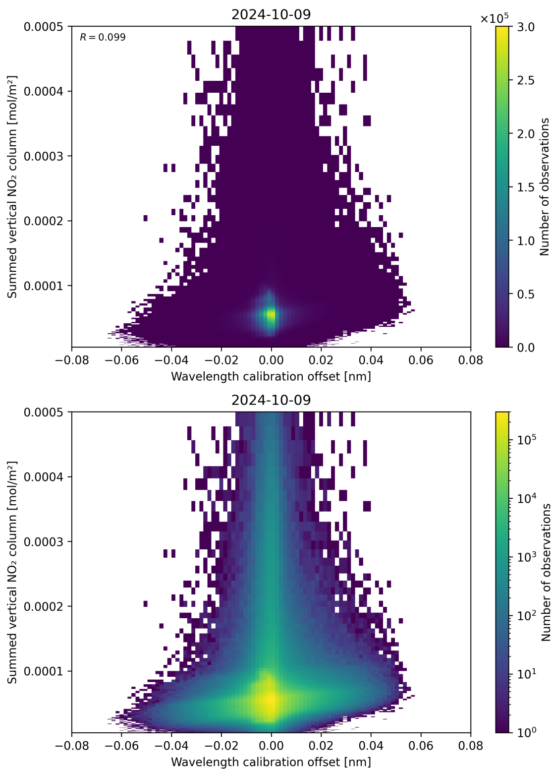
Figure 177: Scatter density plot of “Wavelength calibration offset” against “Summed vertical NO 2 column” for 2024-10-08 to 2024-10-10.
