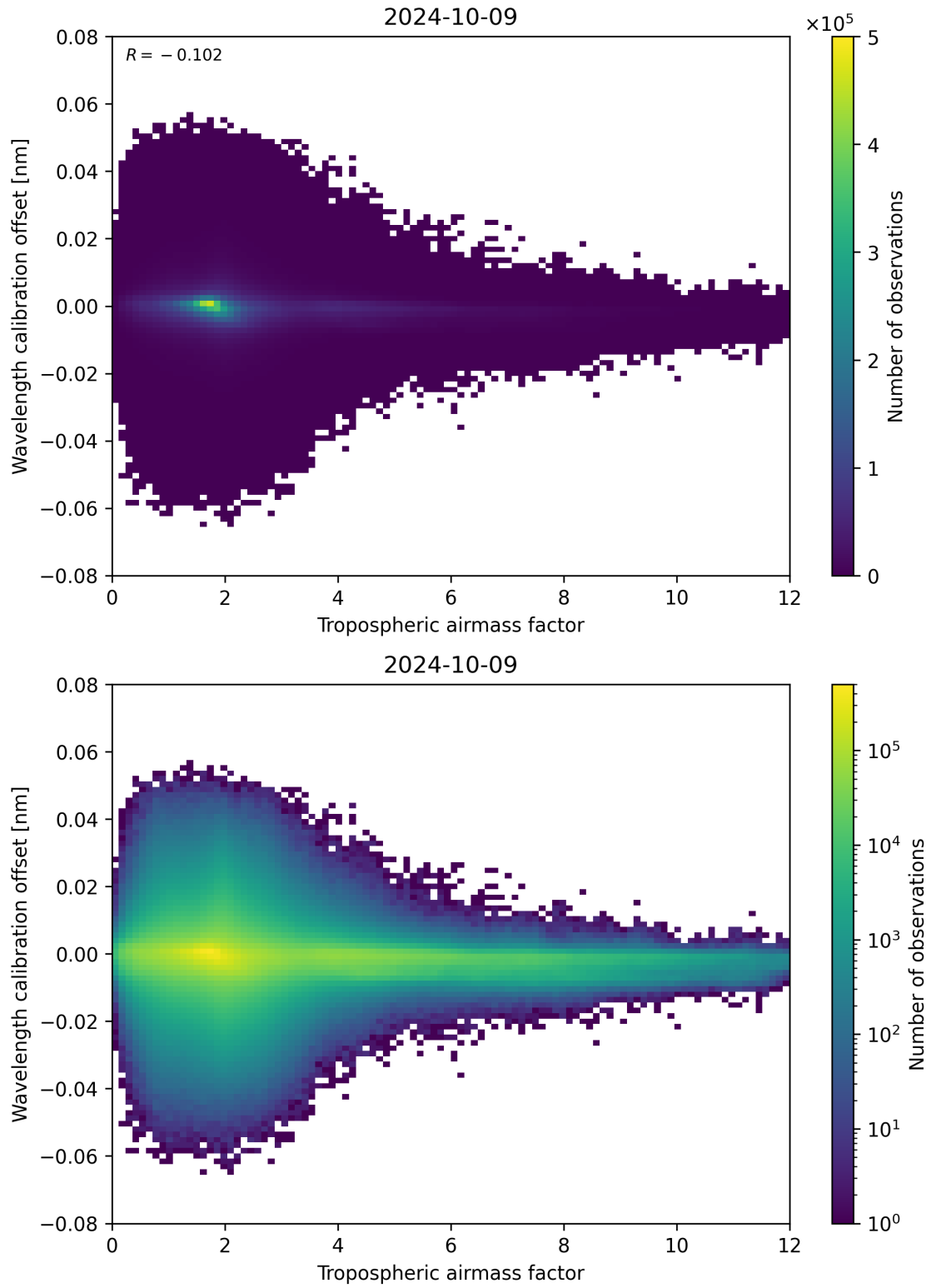
Figure 80: Scatter density plot of “Tropospheric airmass factor” against “Wavelength calibration offset” for 2024-10-08 to 2024-10-10.
