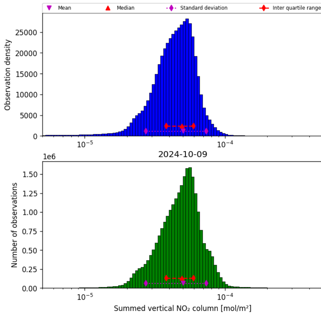
Figure 40: Histogram of “Summed vertical NO 2 column” for 2024-10-08 to 2024-10-10
