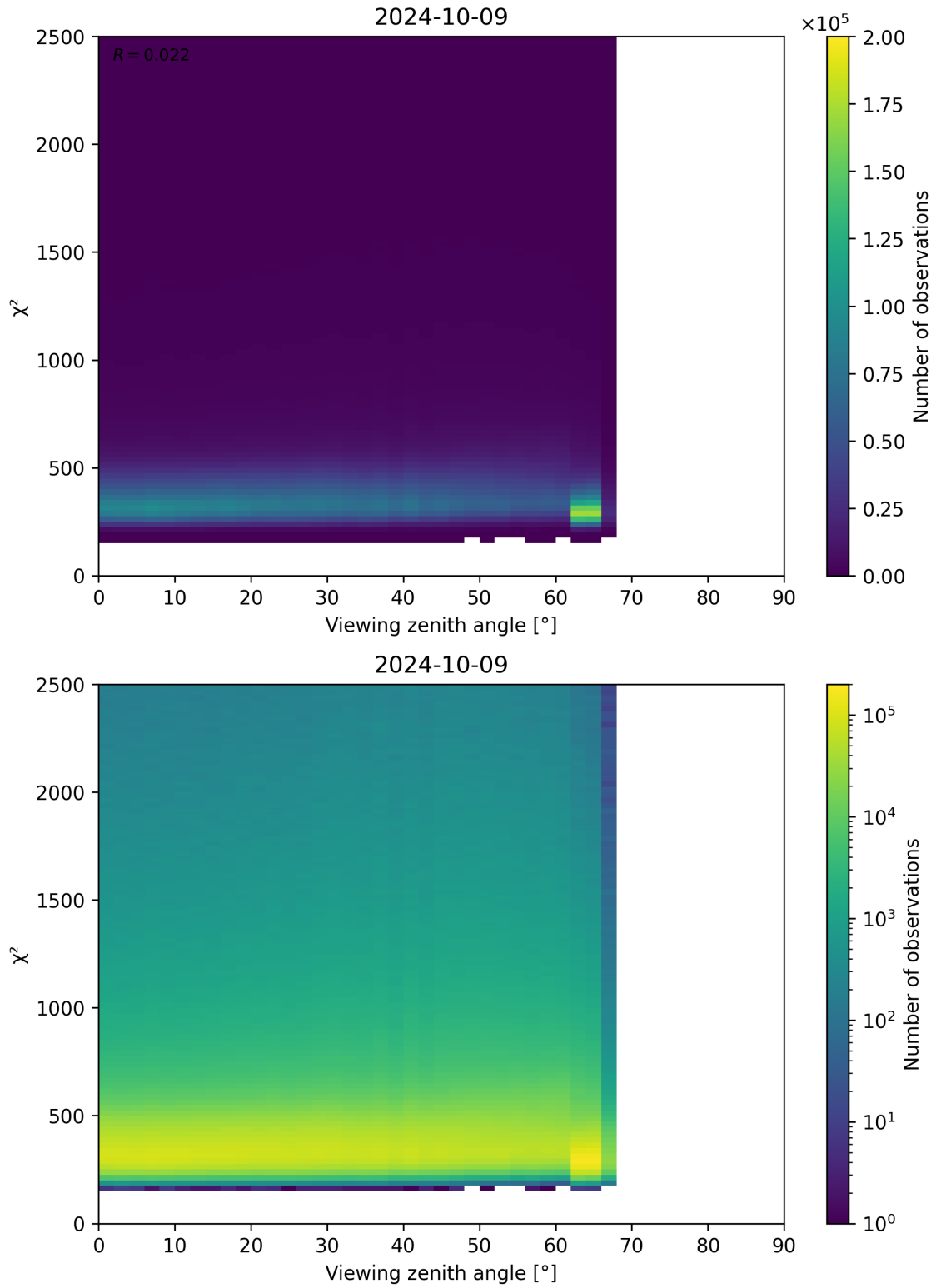
Figure 162: Scatter density plot of “Viewing zenith angle” against “ \chi^2 ” for 2024-10-08 to 2024-10-10.
