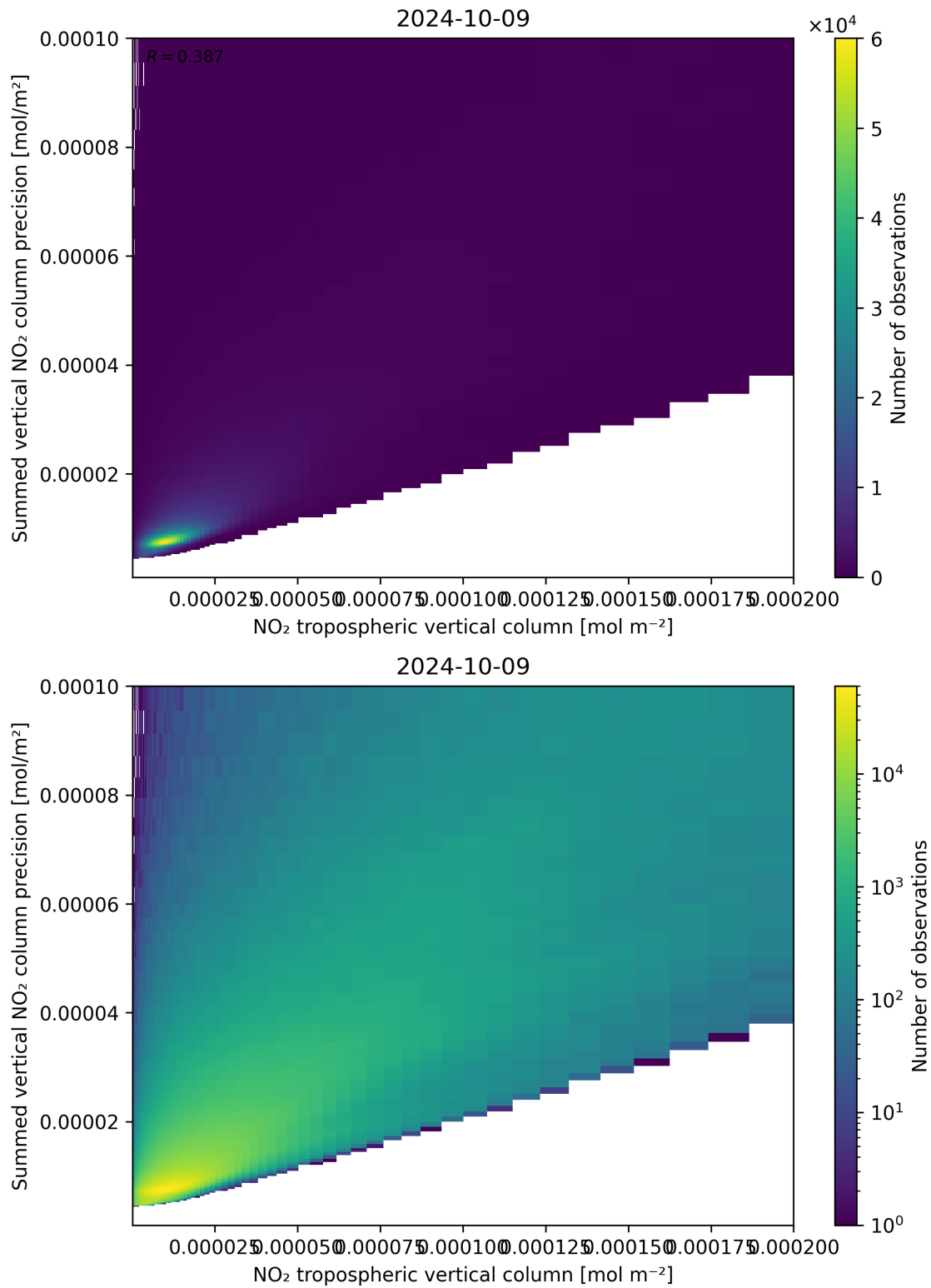
Figure 127: Scatter density plot of “NO 2 tropospheric vertical column” against “Summed vertical NO 2 column precision” for 2024-10-08 to 2024-10-10.
