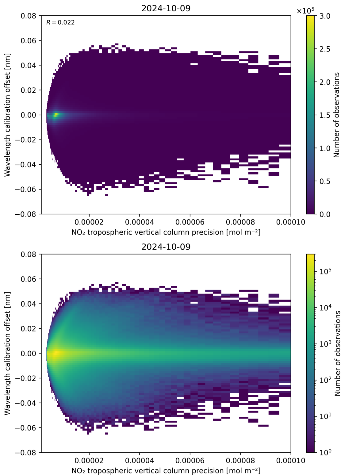
Figure 141: Scatter density plot of “NO 2 tropospheric vertical column precision” against “Wavelength calibration offset” for 2024-10-08 to 2024-10-10.
