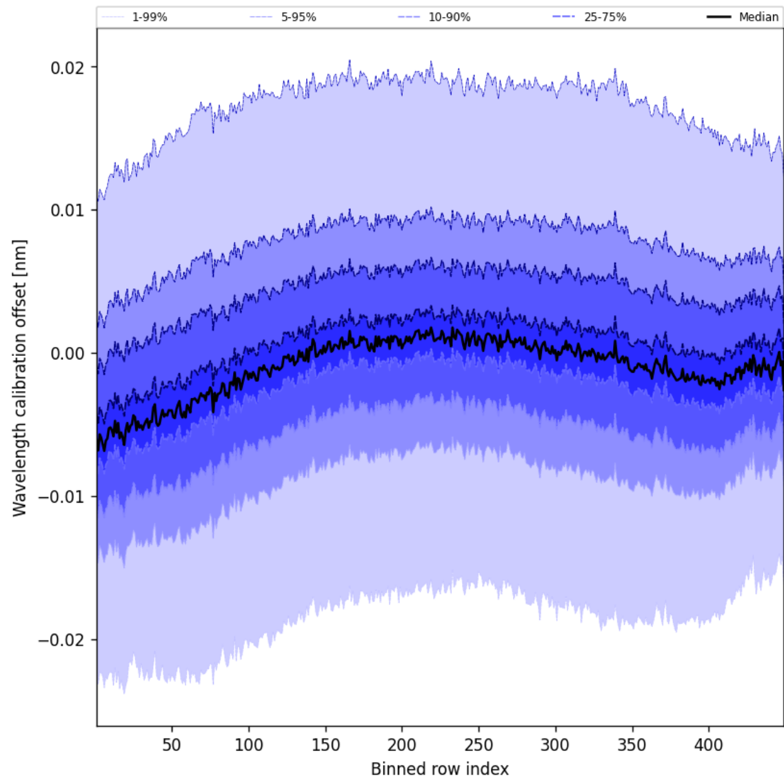
Figure 52: Along track statistics of “Wavelength calibration offset” for 2024-10-08 to 2024-10-10
