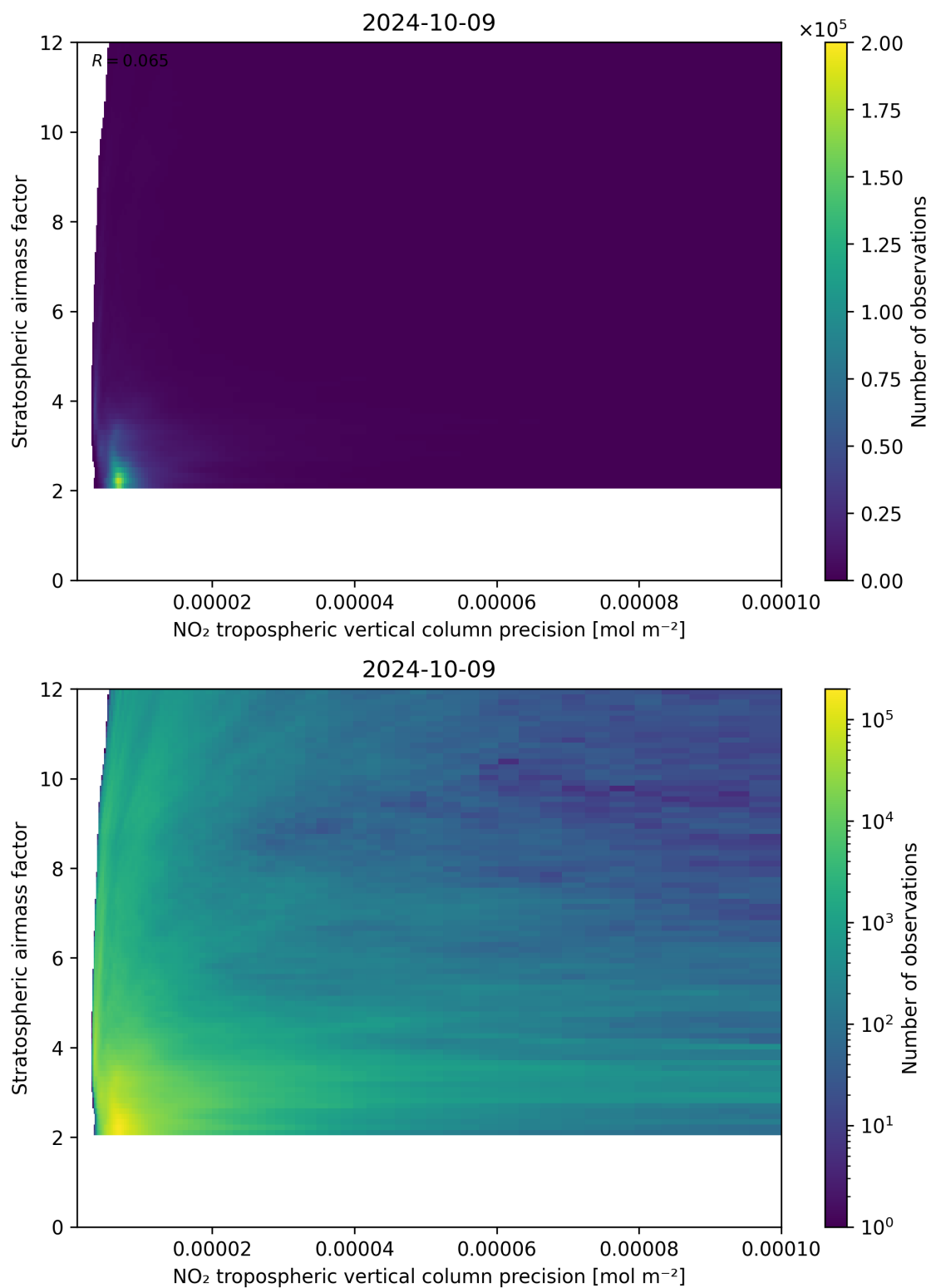
Figure 131: Scatter density plot of “NO 2 tropospheric vertical column precision” against “Stratospheric airmass factor” for 2024-10-08 to 2024-10-10.
