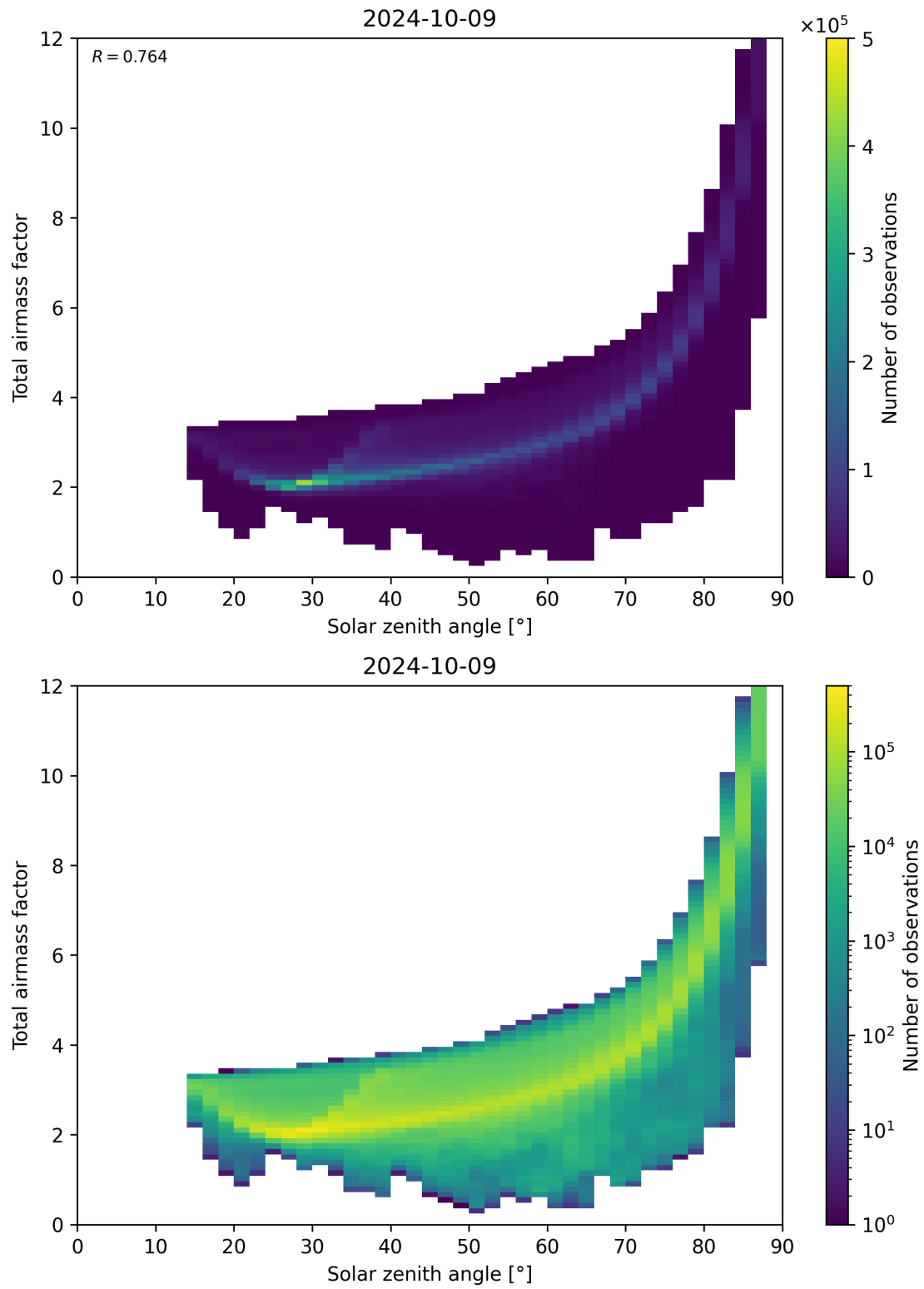
Figure 146: Scatter density plot of “Solar zenith angle” against “Total air mass factor” for 2024-10-08 to 2024-10-10.
