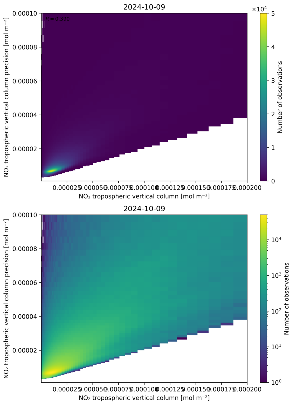
Figure 130: Scatter density plot of “NO 2 tropospheric vertical column” against “NO 2 tropospheric vertical column precision” for 2024-10-08 to 2024-10-10.
