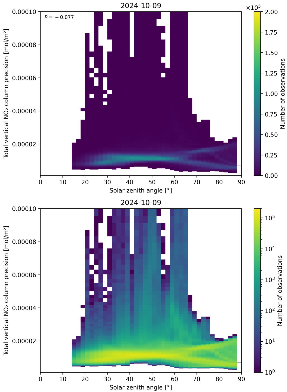
Figure 154: Scatter density plot of “Solar zenith angle” against “Total vertical NO 2 column precision” for 2024-10-08 to 2024-10-10.
