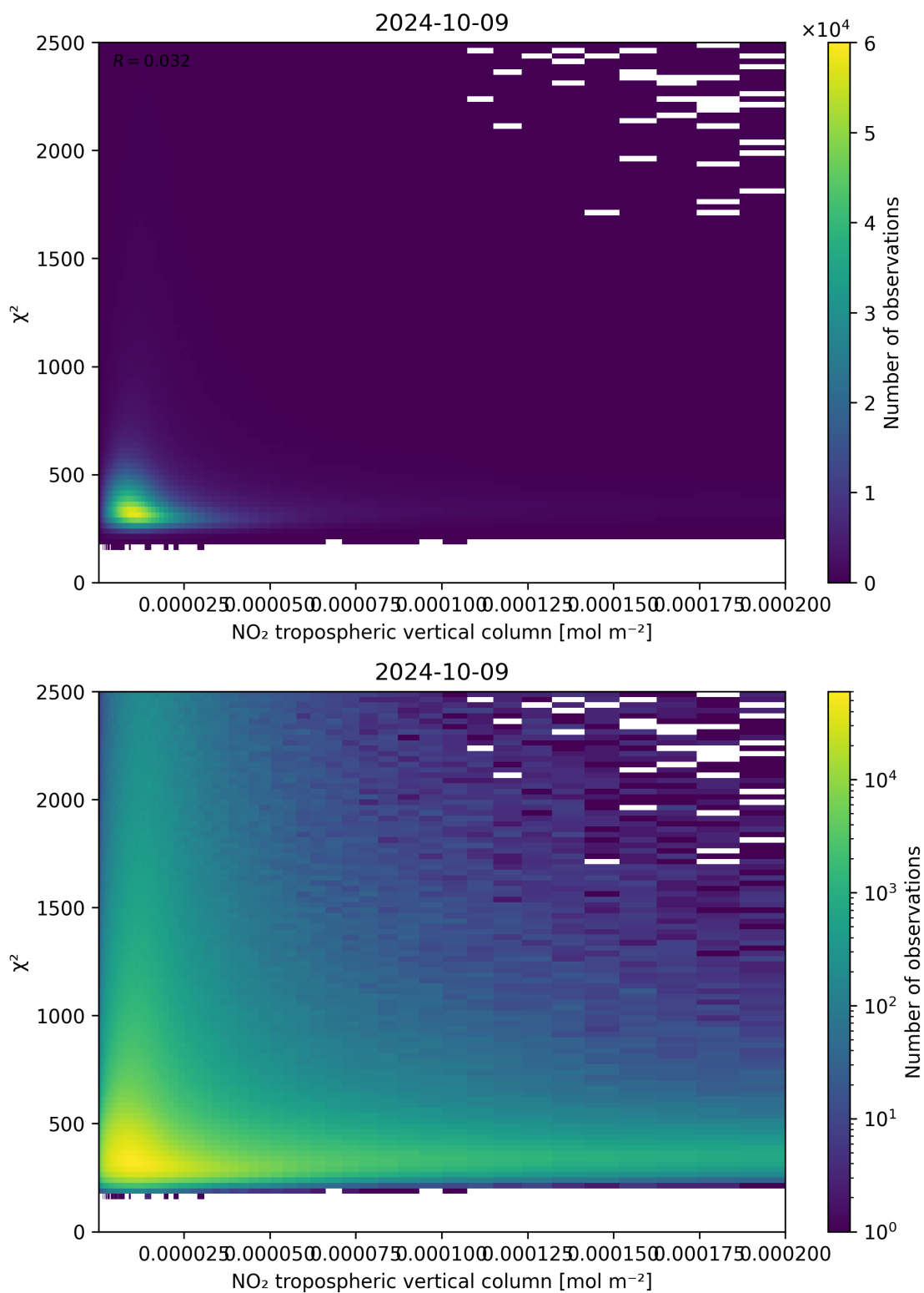
Figure 124: Scatter density plot of “NO 2 tropospheric vertical column” against “ \chi^2 ” for 2024-10-08 to 2024-10-10.
