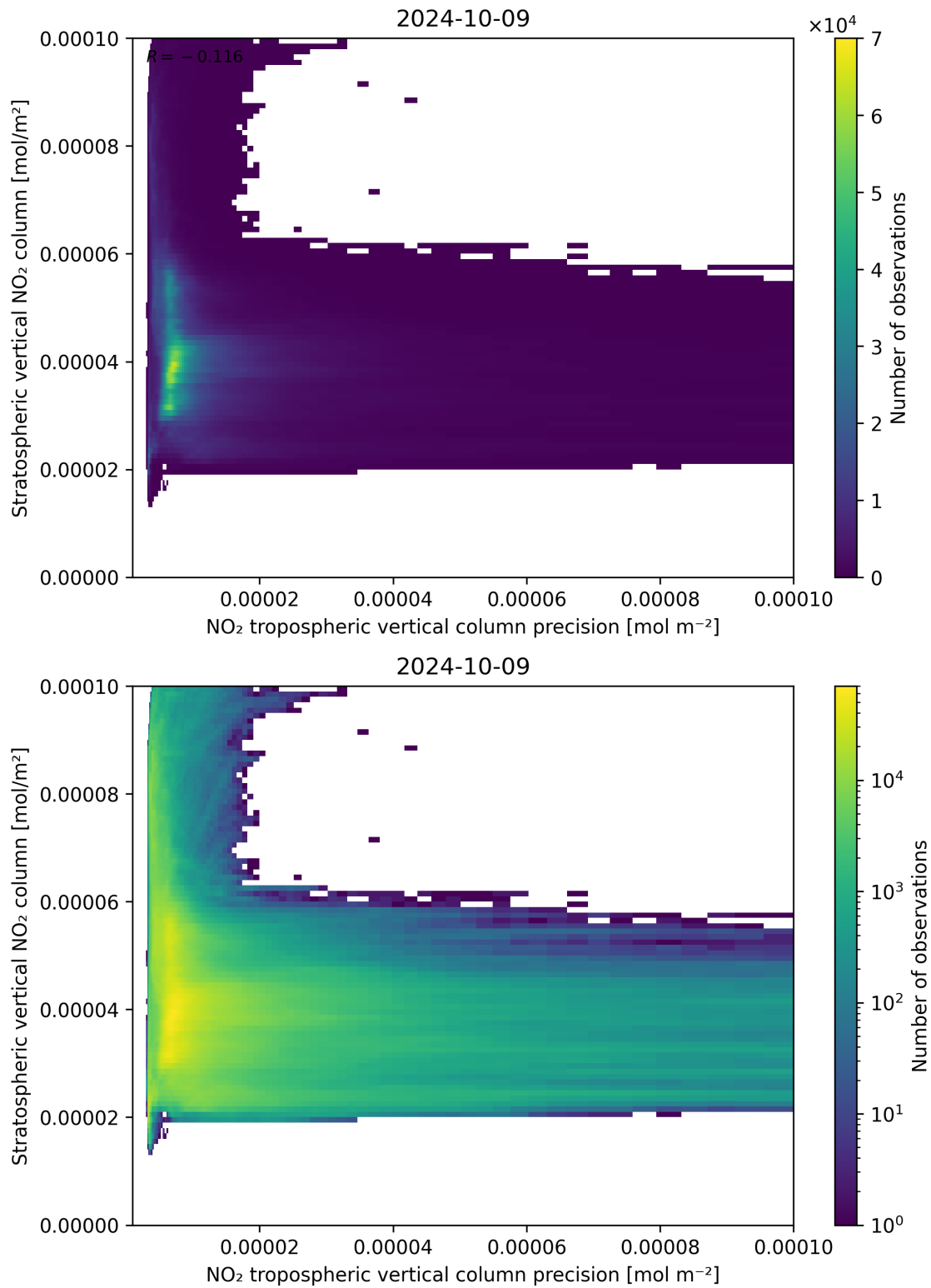
Figure 135: Scatter density plot of “NO 2 tropospheric vertical column precision” against “Stratospheric vertical NO 2 column” for 2024-10-08 to 2024-10-10.
