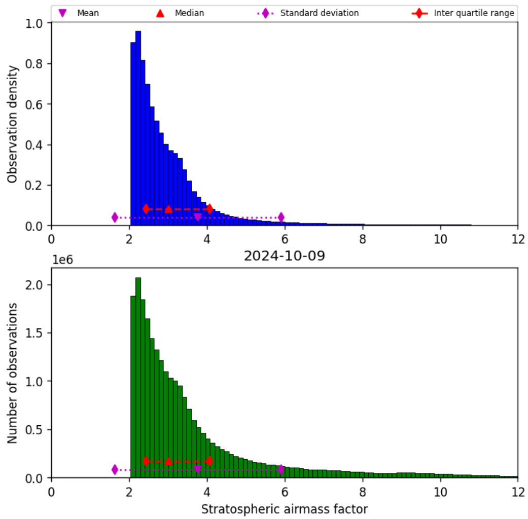
Figure 44: Histogram of “Stratospheric airmass factor” for 2024-10-08 to 2024-10-10
