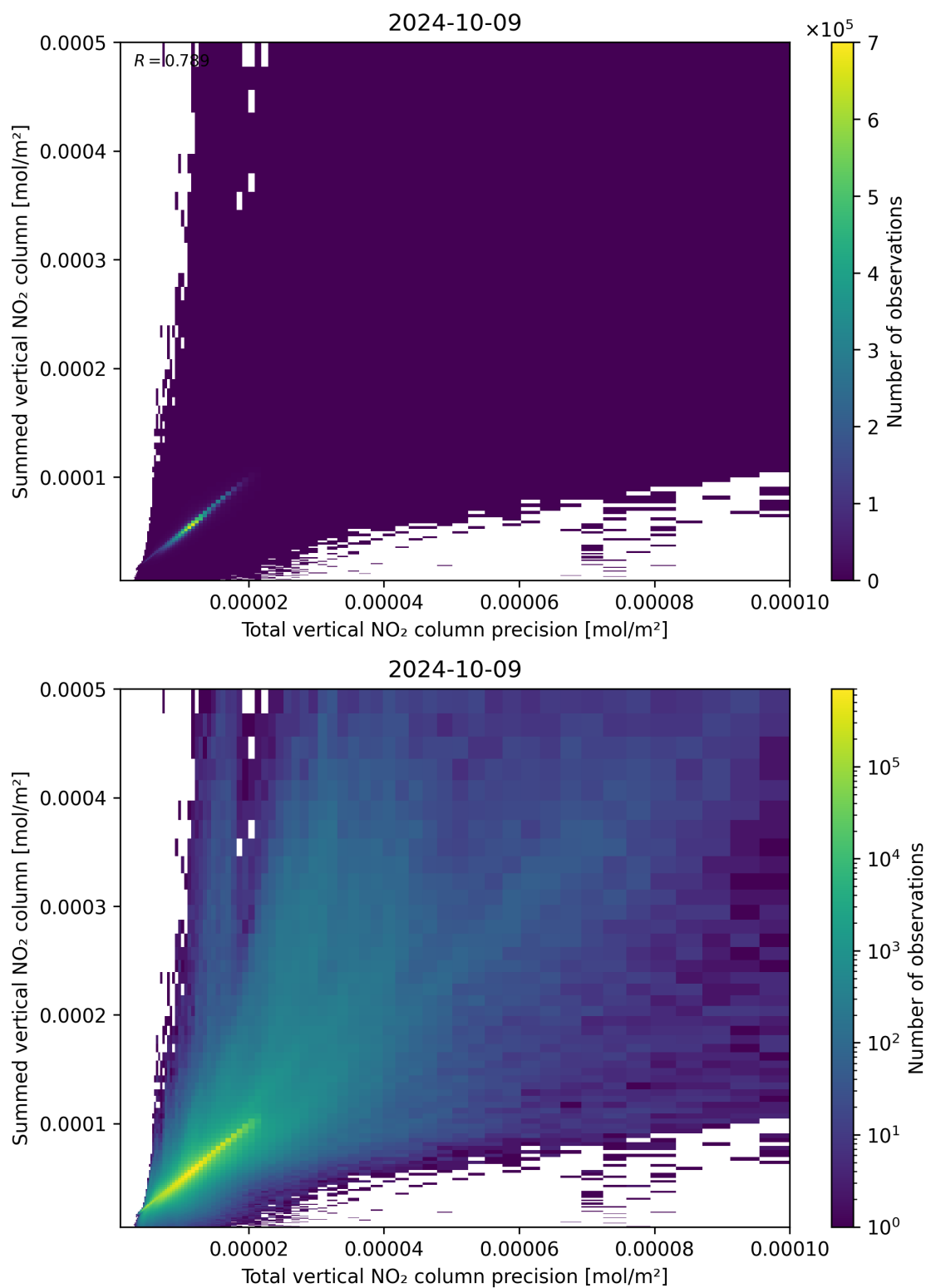
Figure 117: Scatter density plot of “Total vertical NO 2 column precision” against “Summed vertical NO 2 column” for 2024-10-08 to 2024-10-10.
