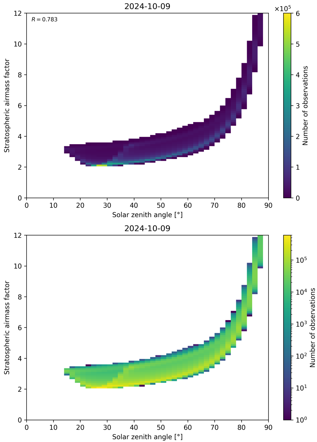
Figure 145: Scatter density plot of “Solar zenith angle” against “Stratospheric airmass factor” for 2024-10-08 to 2024-10-10.
