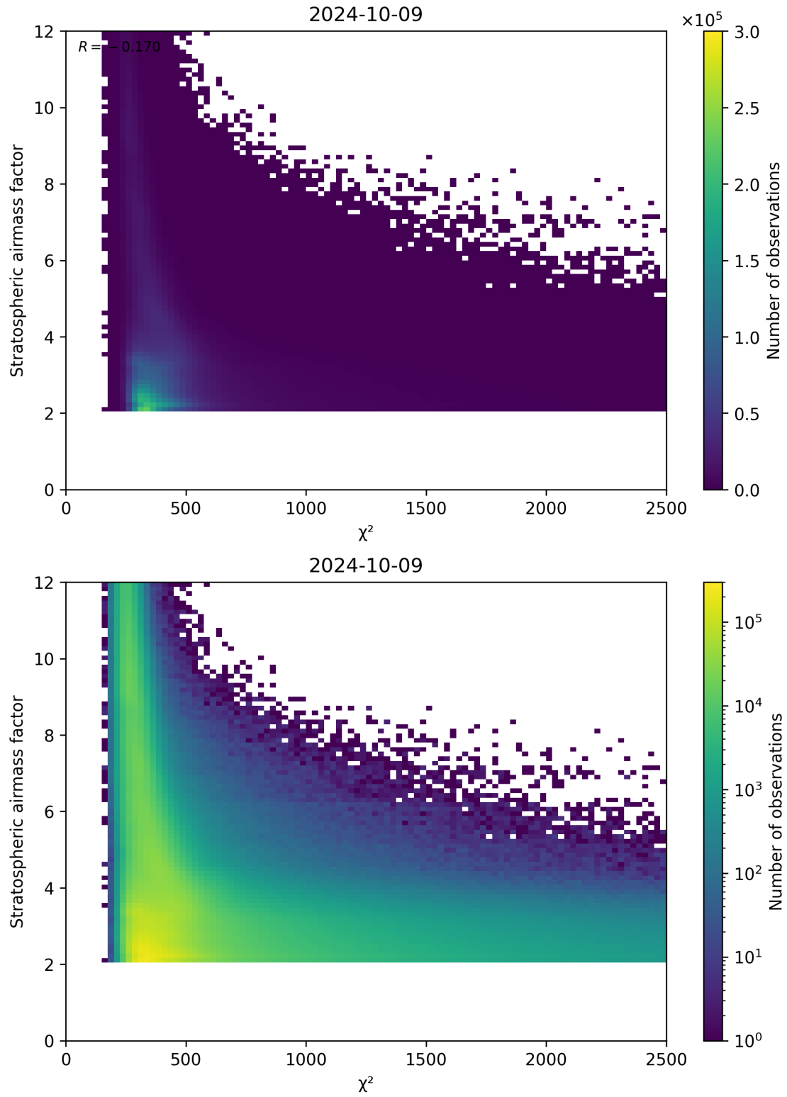
Figure 81: Scatter density plot of “ \chi^2 ” against “Stratospheric airmass factor” for 2024-10-08 to 2024-10-10.
