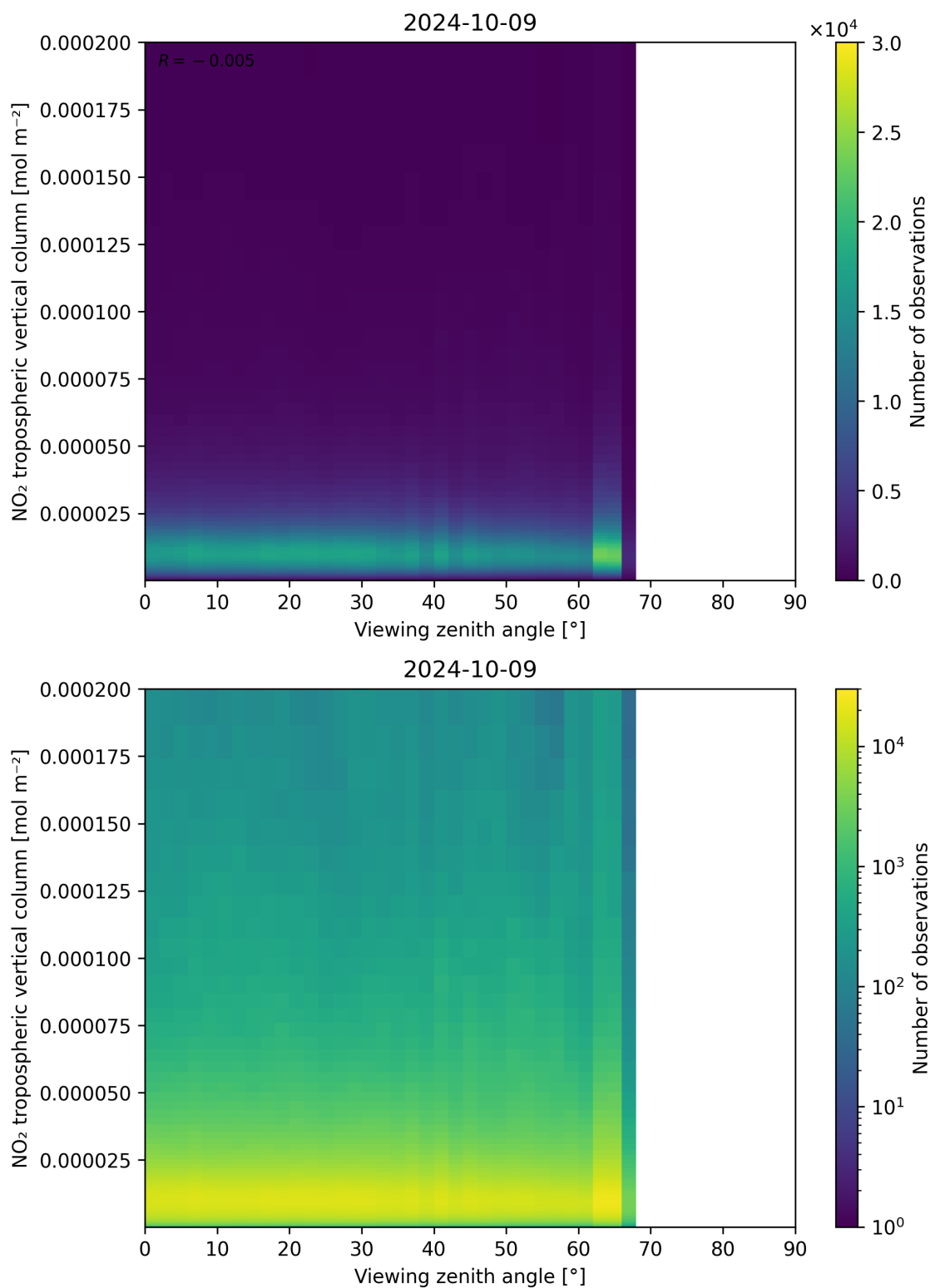
Figure 169: Scatter density plot of “Viewing zenith angle” against “NO 2 tropospheric vertical column” for 2024-10-08 to 2024-10-10.
