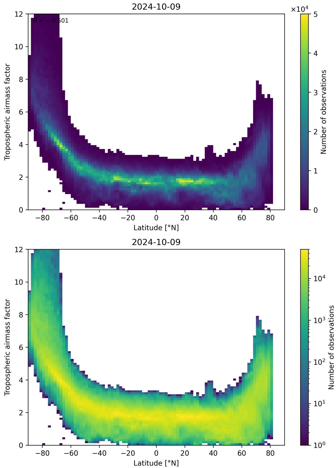
Figure 85: Scatter density plot of “Latitude” against “Tropospheric airmass factor” for 2024-10-08 to 2024-10-10.
