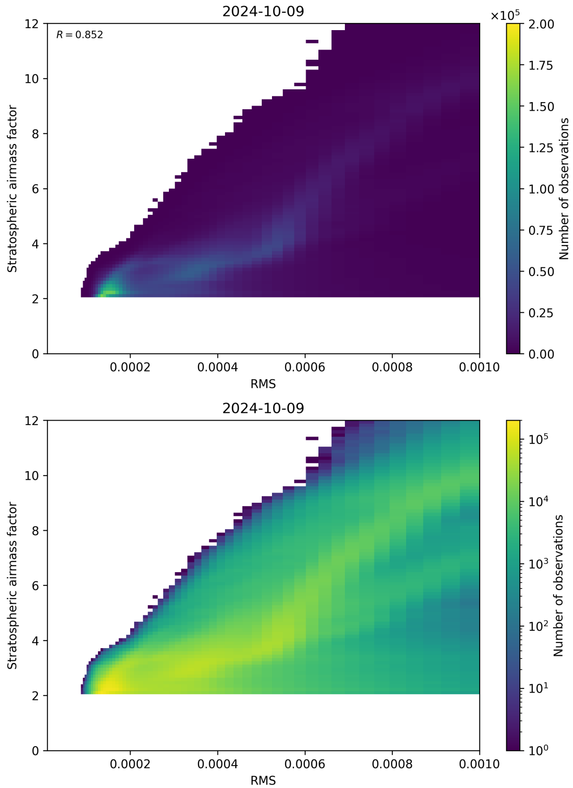
Figure 144: Scatter density plot of “RMS” against “Stratospheric airmass factor” for 2024-10-08 to 2024-10-10.
