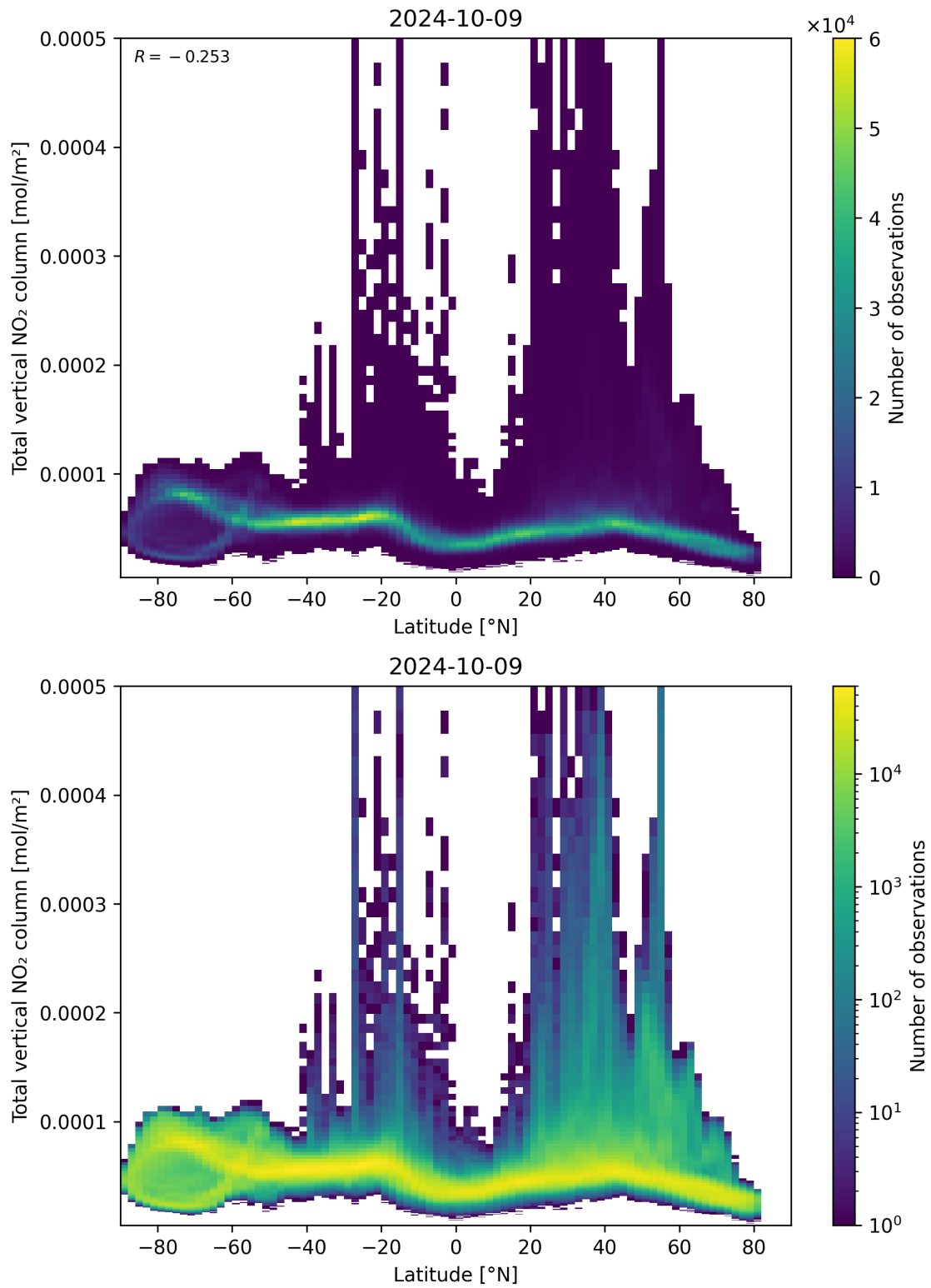
Figure 90: Scatter density plot of “Latitude” against “Total vertical NO 2 column” for 2024-10-08 to 2024-10-10.
