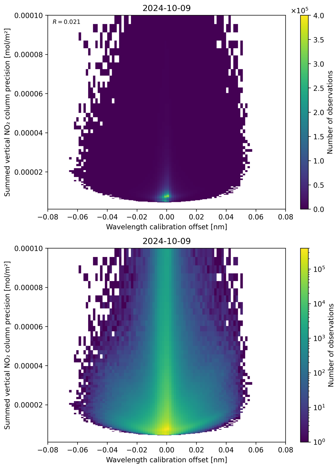
Figure 178: Scatter density plot of “Wavelength calibration offset” against “Summed vertical NO 2 column precision” for 2024-10-08 to 2024-10-10.
