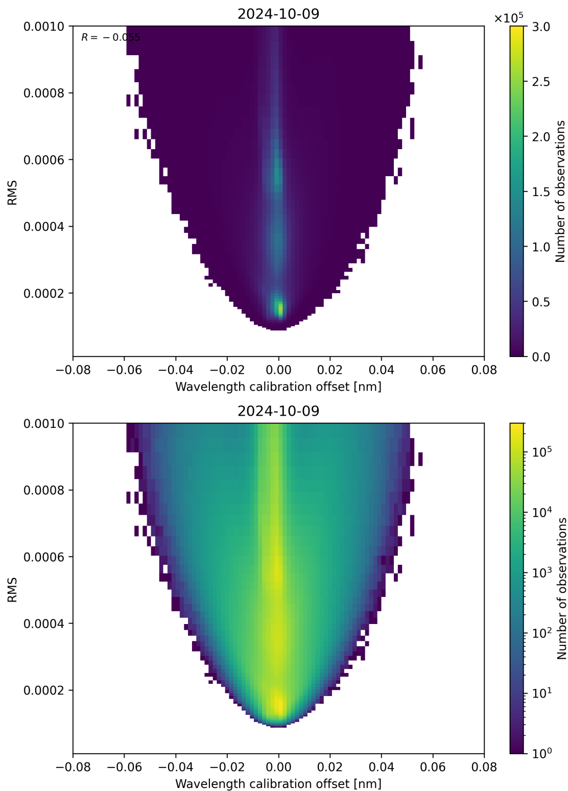
Figure 181: Scatter density plot of “Wavelength calibration offset” against “RMS” for 2024-10-08 to 2024-10-10.
