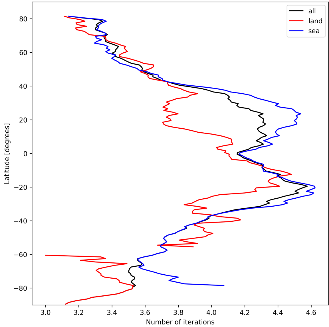
Figure 17: Zonal average of “Number of iterations” for 2024-10-08 to 2024-10-10.
