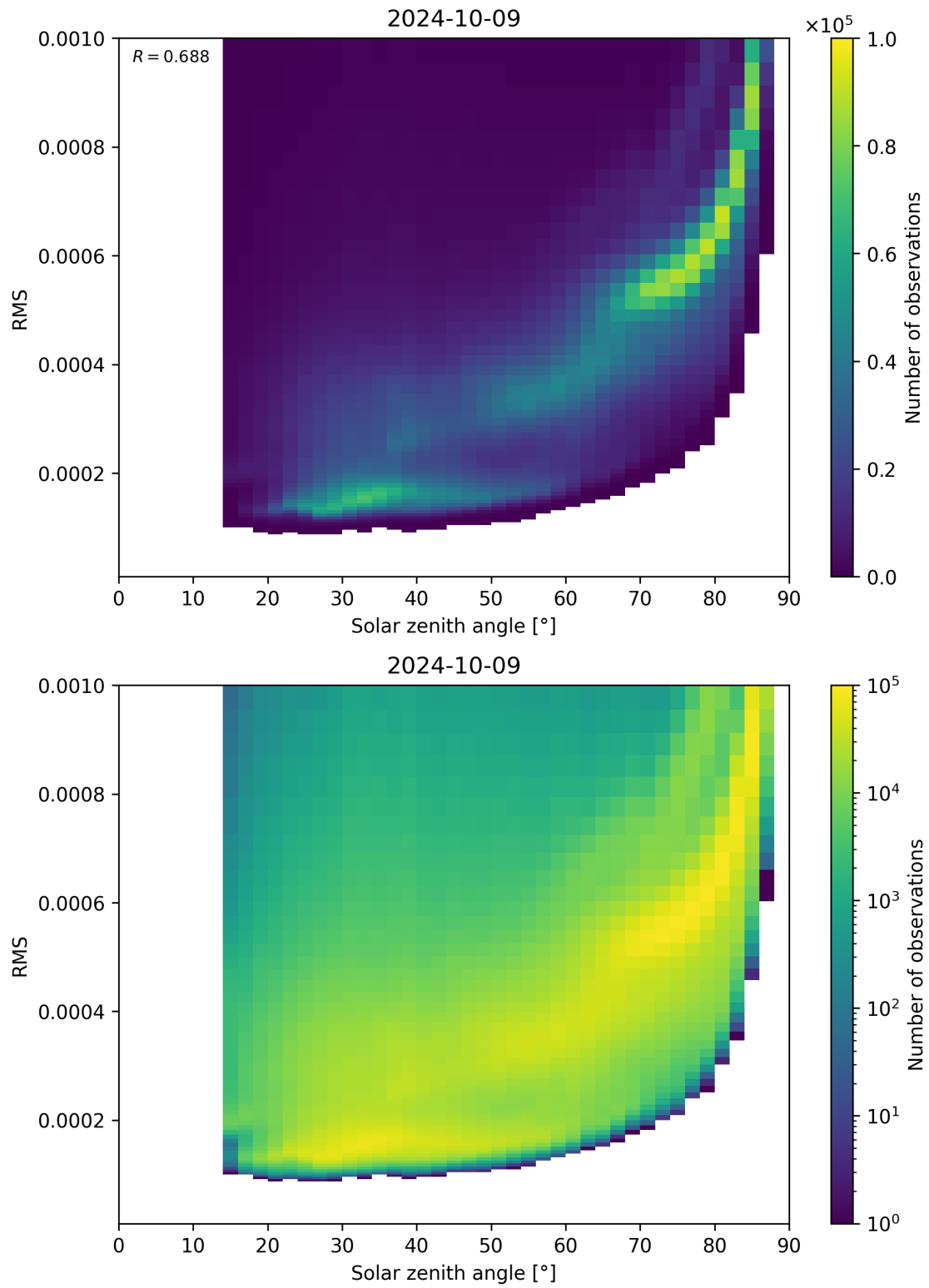
Figure 157: Scatter density plot of “Solar zenith angle” against “RMS” for 2024-10-08 to 2024-10-10.
