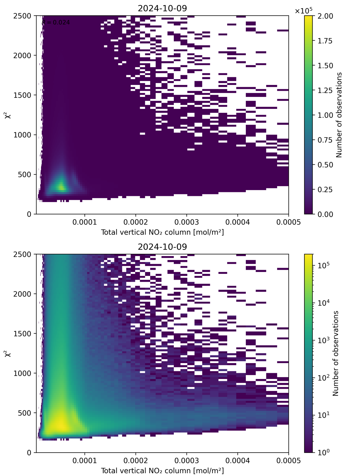
Figure 111: Scatter density plot of “Total vertical NO 2 column” against “ \chi^2 ” for 2024-10-08 to 2024-10-10.
