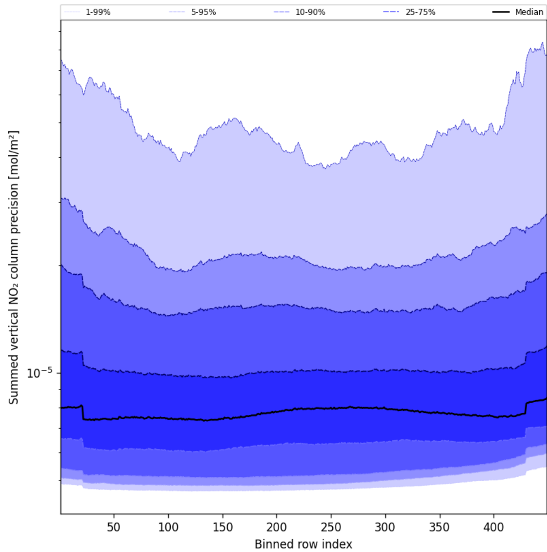
Figure 58: Along track statistics of “Summed vertical NO 2 column precision” for 2024-10-08 to 2024-10-10
