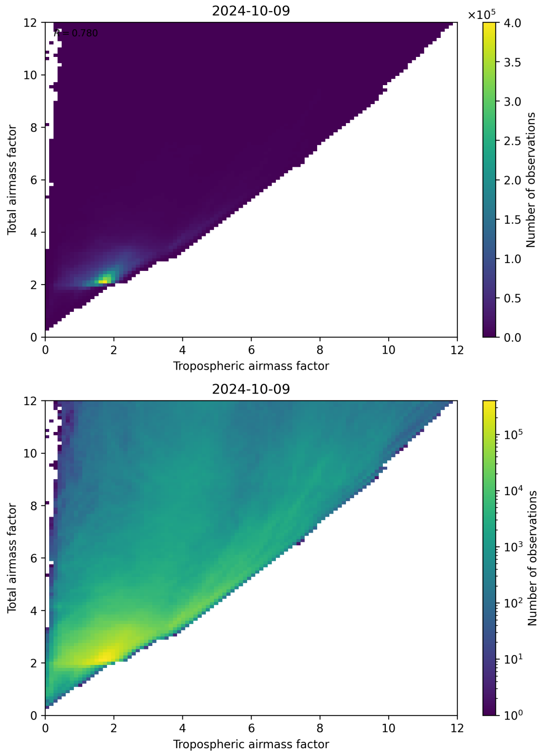
Figure 72: Scatter density plot of “Tropospheric airmass factor” against “Total airmass factor” for 2024-10-08 to 2024-10-10.
