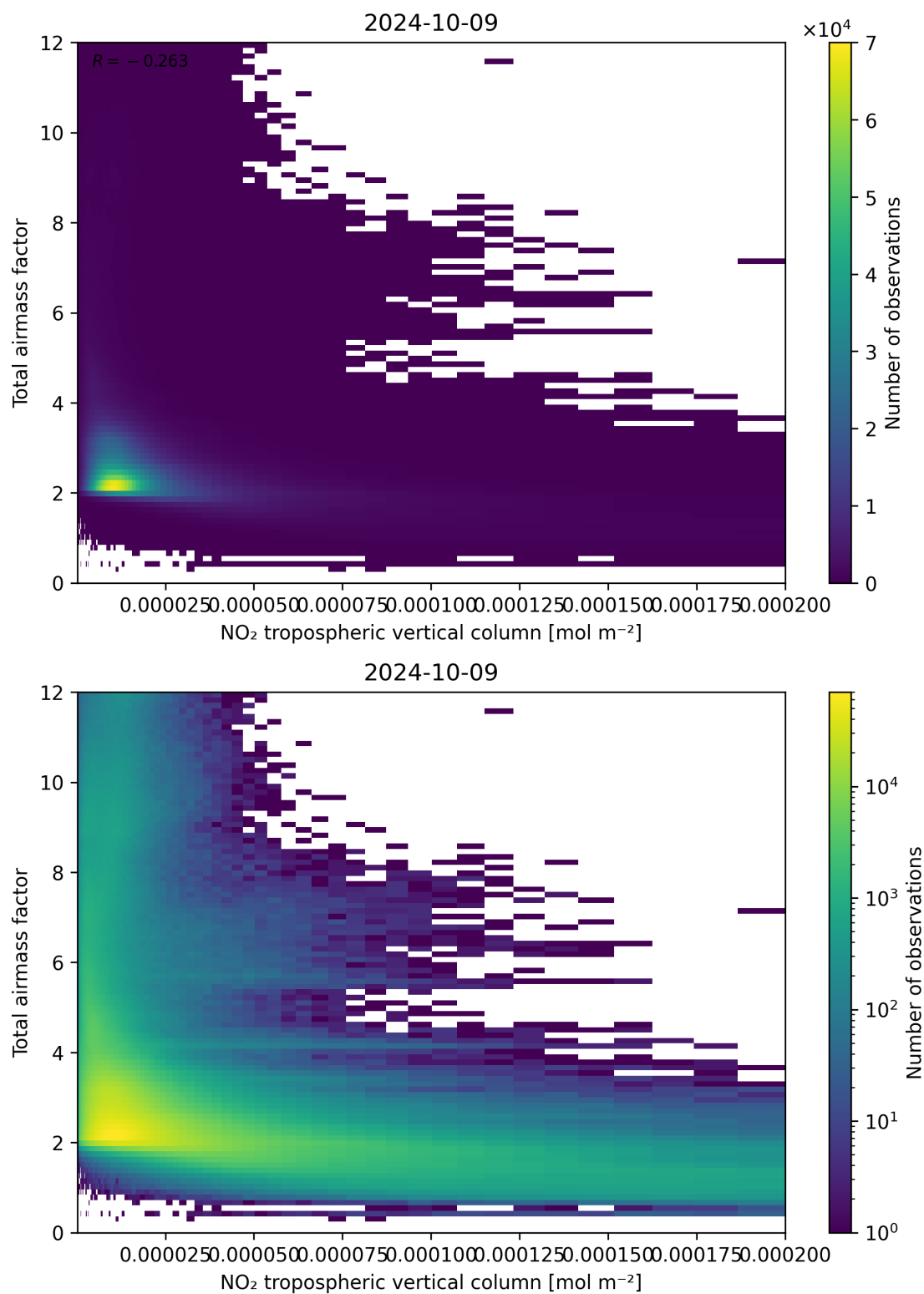
Figure 122: Scatter density plot of “NO 2 tropospheric vertical column” against “Total air mass factor” for 2024-10-08 to 2024-10-10.
