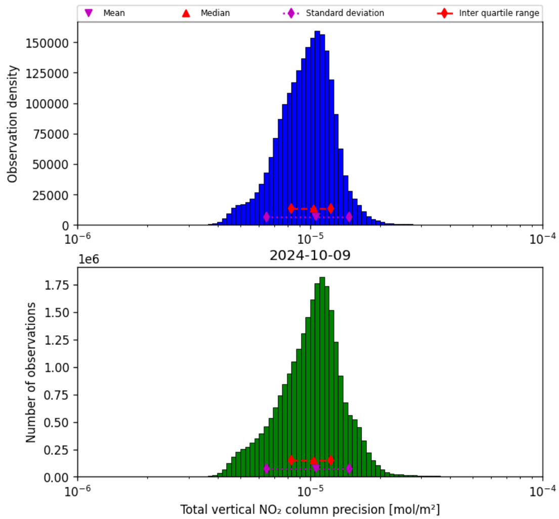
Figure 39: Histogram of “Total vertical NO 2 column precision” for 2024-10-08 to 2024-10-10
