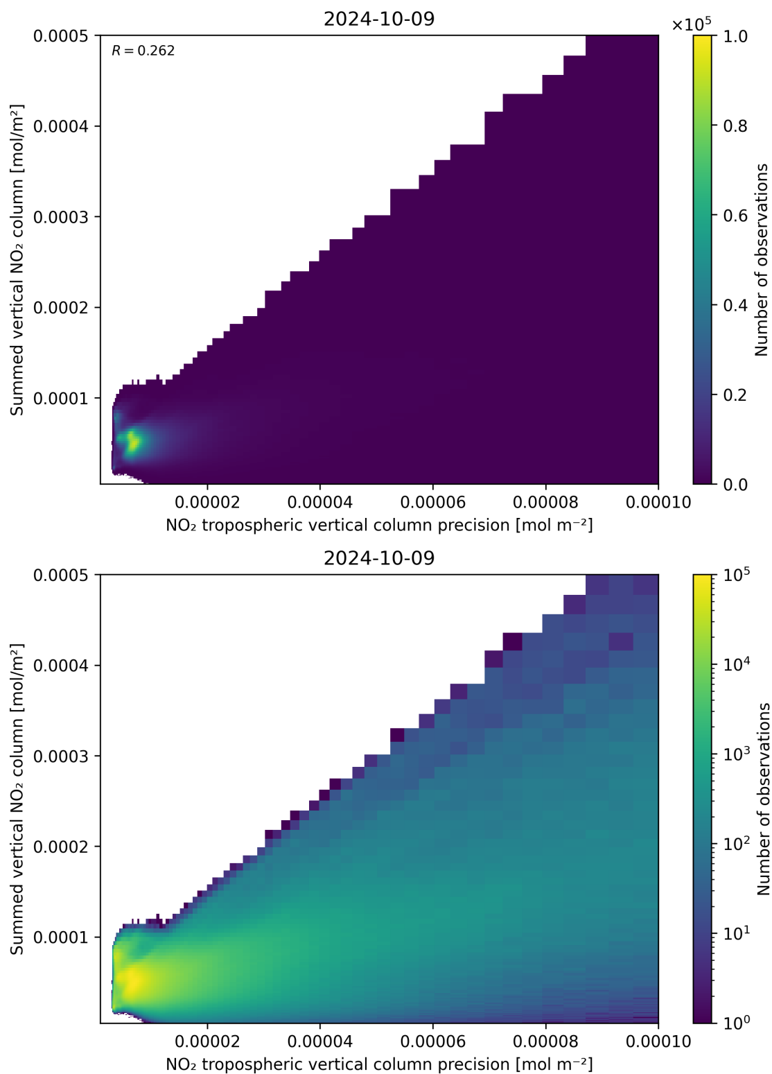
Figure 136: Scatter density plot of “NO 2 tropospheric vertical column precision” against “Summed vertical NO 2 column” for 2024-10-08 to 2024-10-10.
