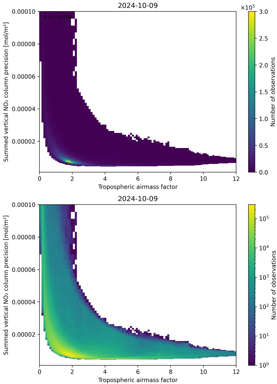
Figure 76: Scatter density plot of “Tropospheric air mass factor” against “Summed vertical NO 2 column precision” for 2024-10-08 to 2024-10-10.
