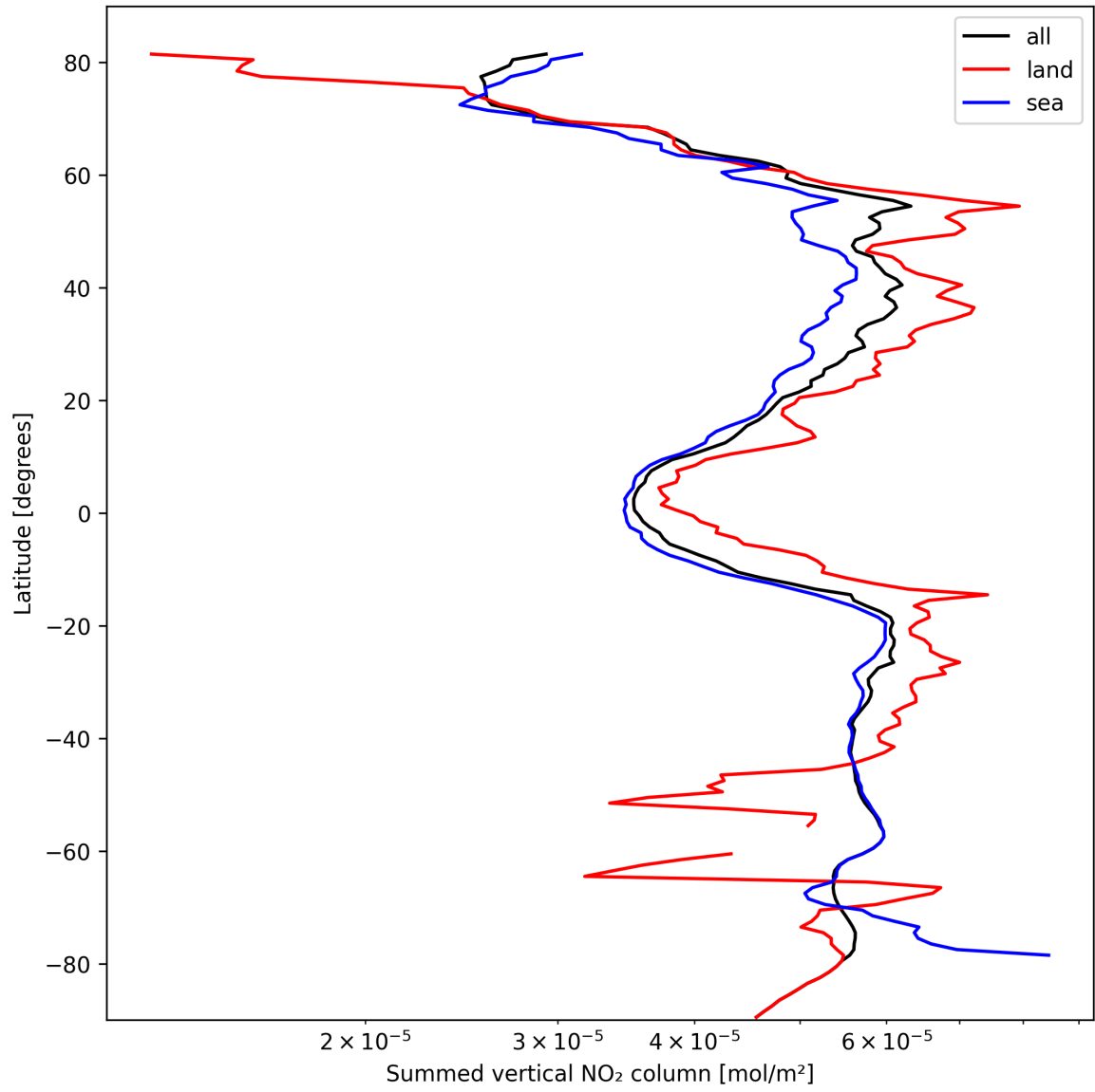
Figure 23: Zonal average of “Summed vertical NO 2 column” for 2024-10-08 to 2024-10-10.
