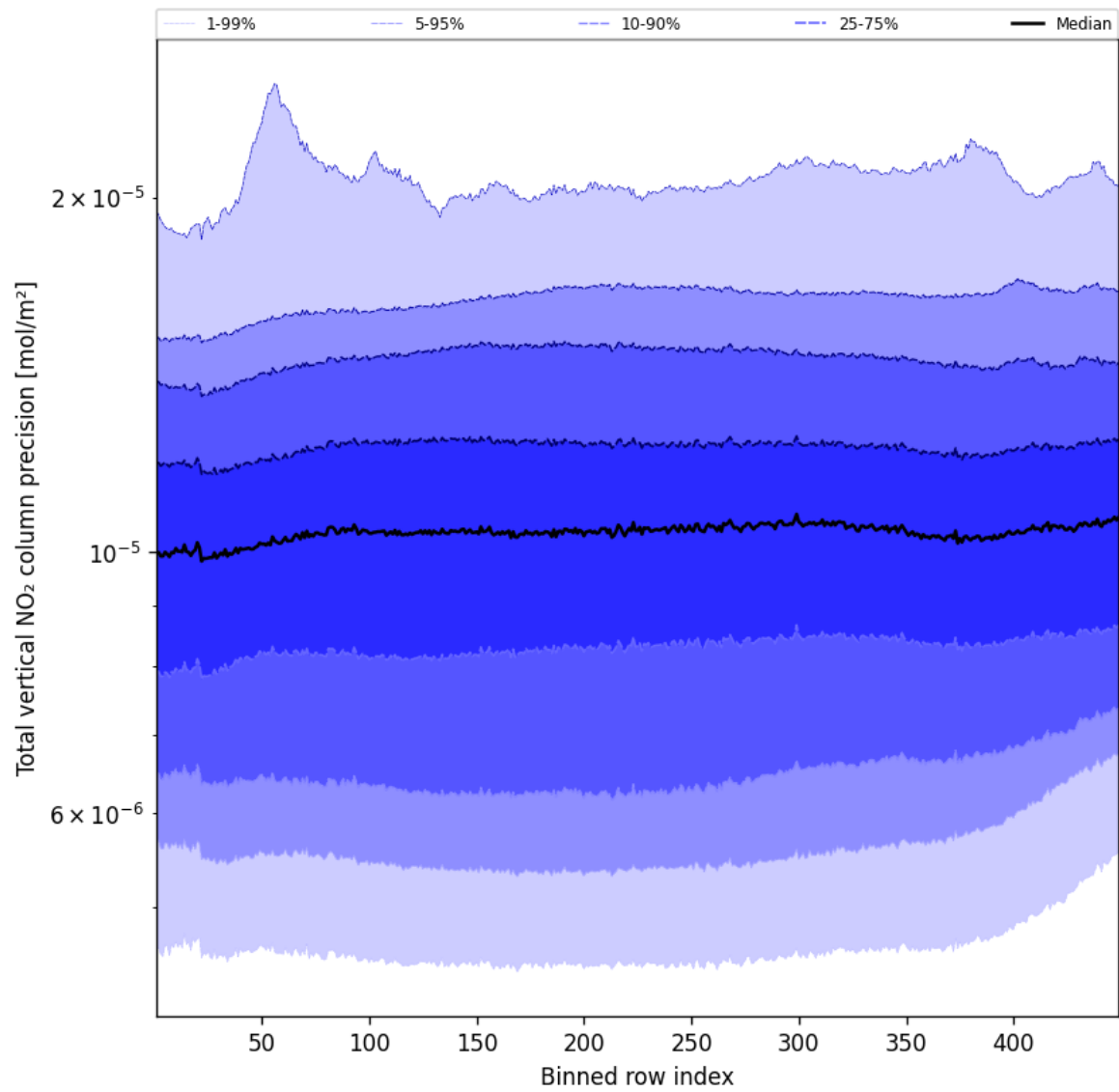
Figure 56: Along track statistics of “Total vertical NO 2 column precision” for 2024-10-08 to 2024-10-10
