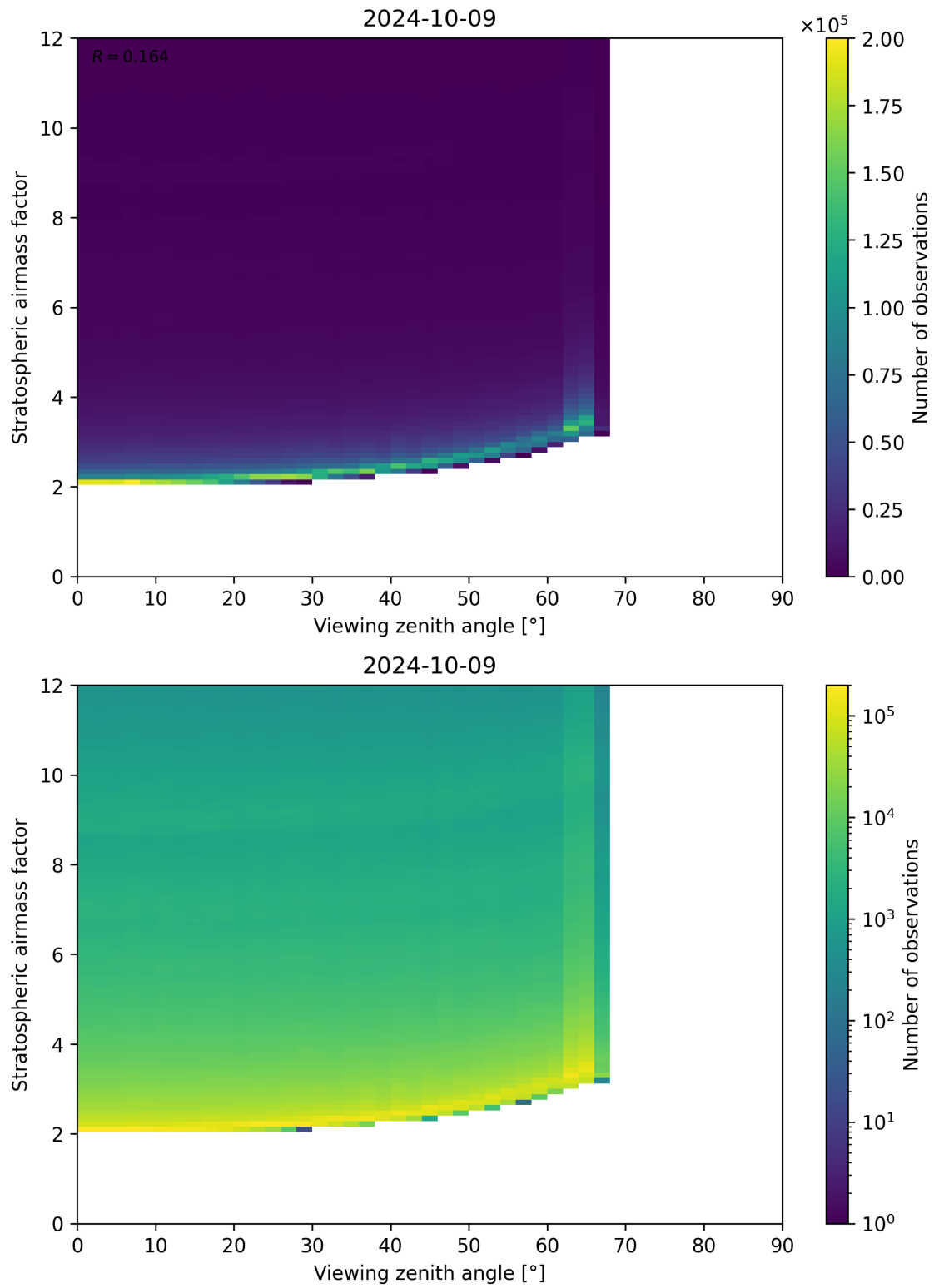
Figure 159: Scatter density plot of “Viewing zenith angle” against “Stratospheric airmass factor” for 2024-10-08 to 2024-10-10.
