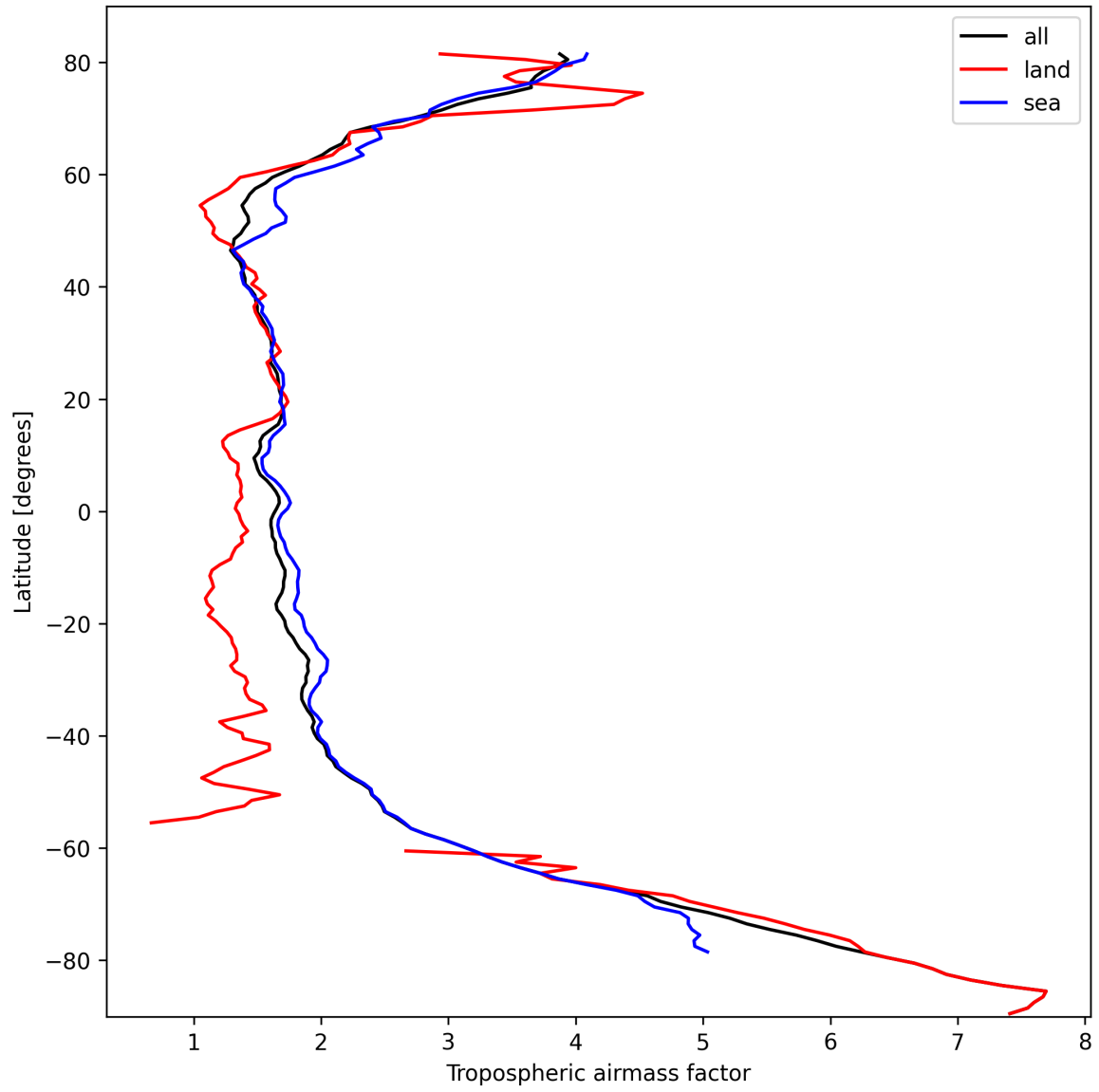
Figure 14: Zonal average of “Tropospheric airmass factor” for 2024-10-08 to 2024-10-10.
