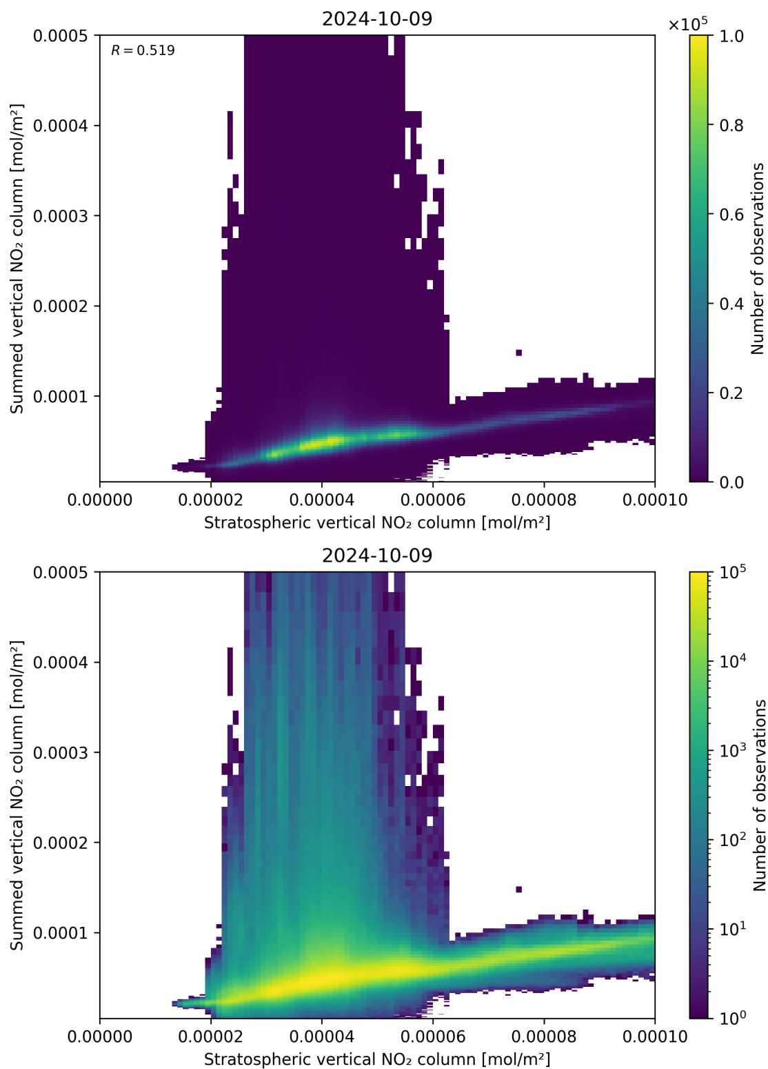
Figure 98: Scatter density plot of “Stratospheric vertical NO 2 column” against “Summed vertical NO 2 column” for 2024-10-08 to 2024-10-10.
