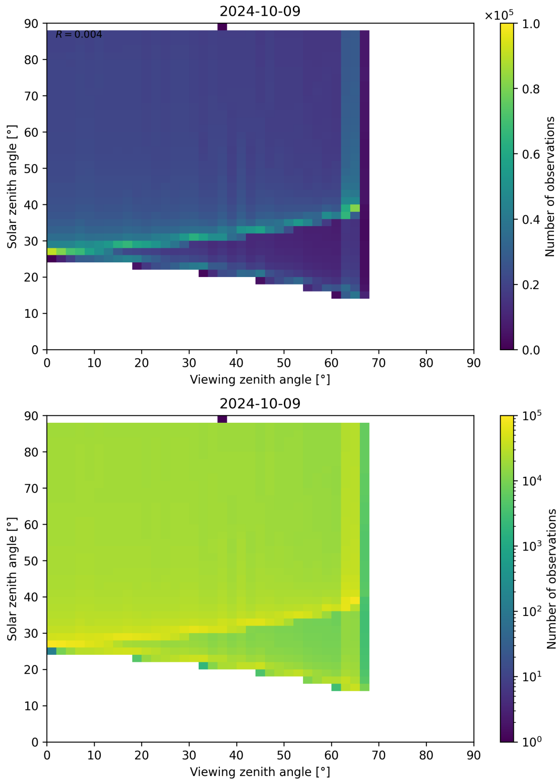
Figure 172: Scatter density plot of “Viewing zenith angle” against “Solar zenith angle” for 2024-10-08 to 2024-10-10.
