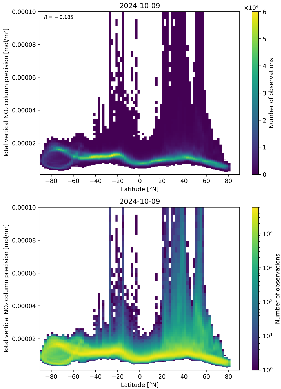
Figure 91: Scatter density plot of “Latitude” against “Total vertical NO 2 column precision” for 2024-10-08 to 2024-10-10.
