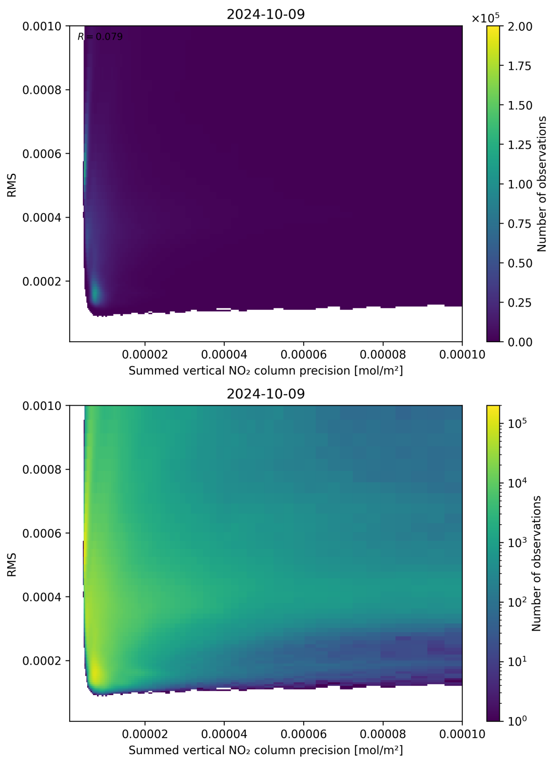
Figure 108: Scatter density plot of “Summed vertical NO 2 column precision” against “RMS” for 2024-10-08 to 2024-10-10.
