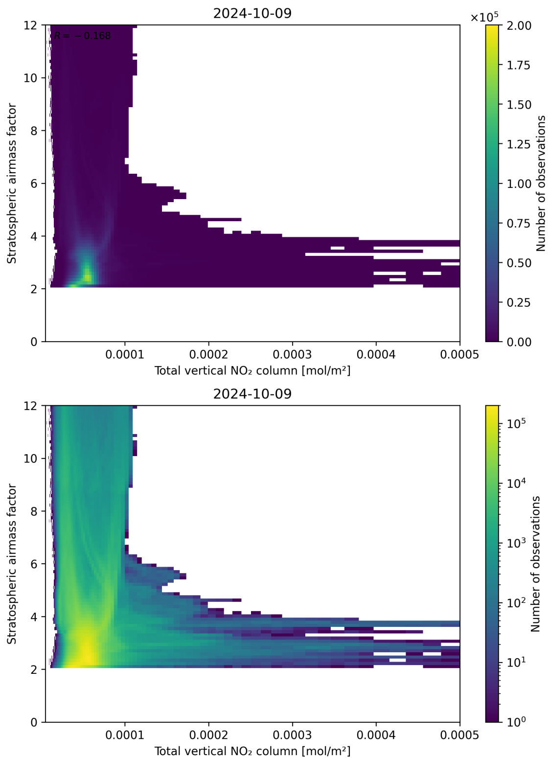
Figure 110: Scatter density plot of “Total vertical NO 2 column” against “Stratospheric airmass factor” for 2024-10-08 to 2024-10-10.
