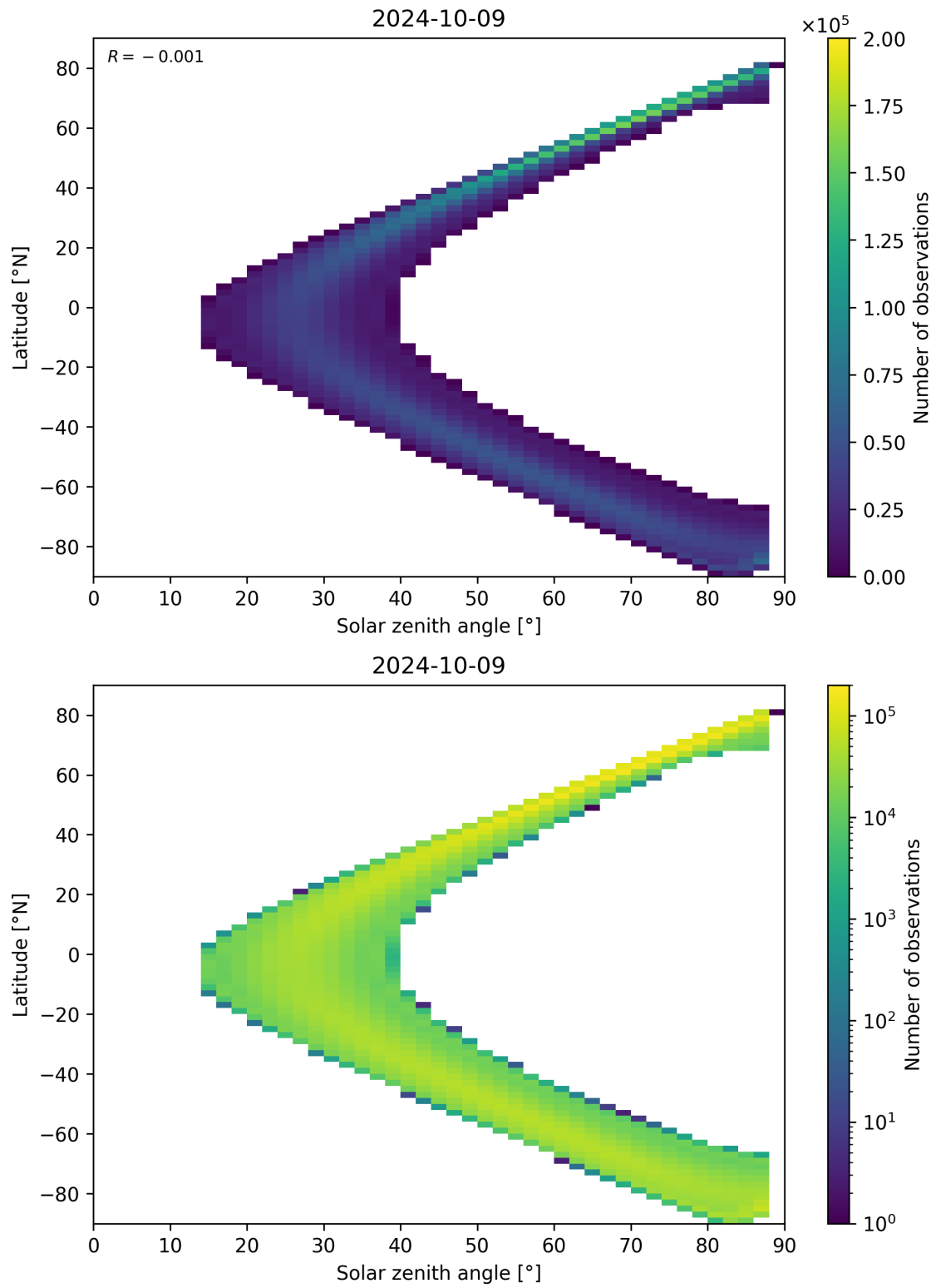
Figure 149: Scatter density plot of “Solar zenith angle” against “Latitude” for 2024-10-08 to 2024-10-10.
