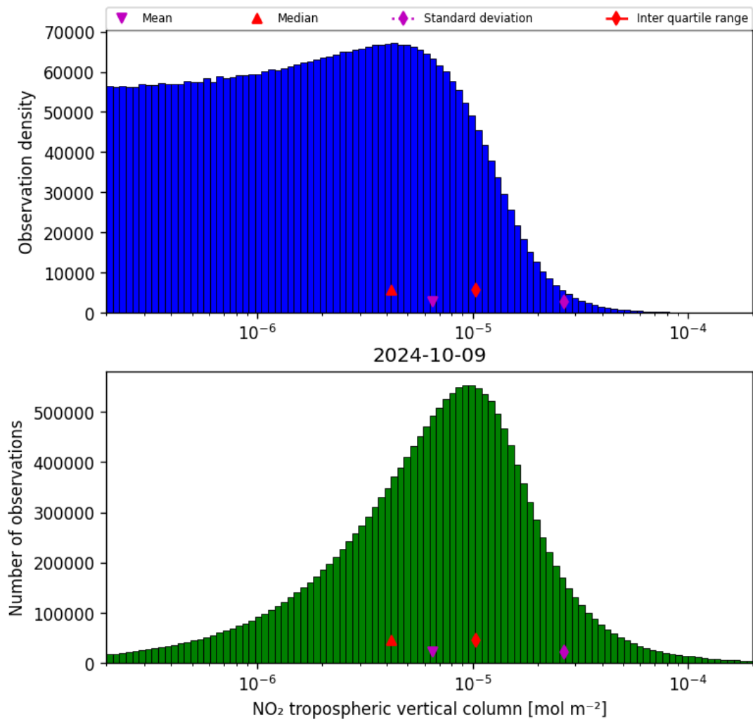
Figure 29: Histogram of “NO 2 tropospheric vertical column” for 2024-10-08 to 2024-10-10
