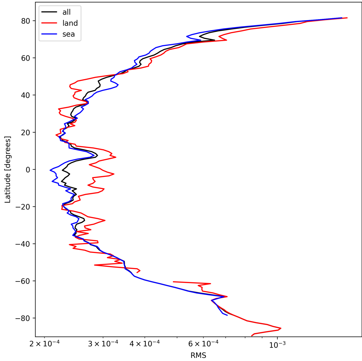
Figure 26: Zonal average of “RMS” for 2024-10-08 to 2024-10-10.
