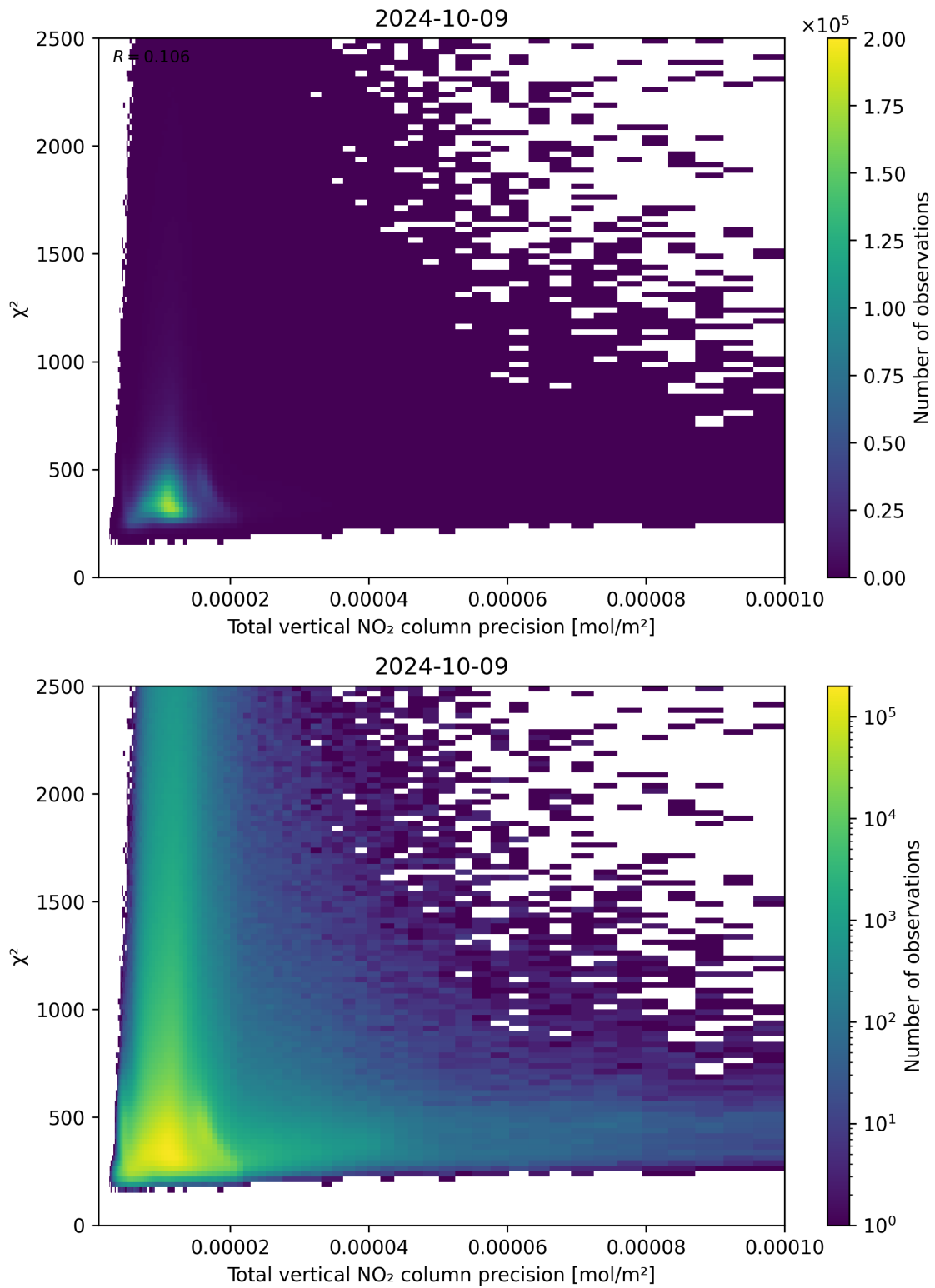
Figure 116: Scatter density plot of “Total vertical NO 2 column precision” against “ \chi^2 ” for 2024-10-08 to 2024-10-10.
