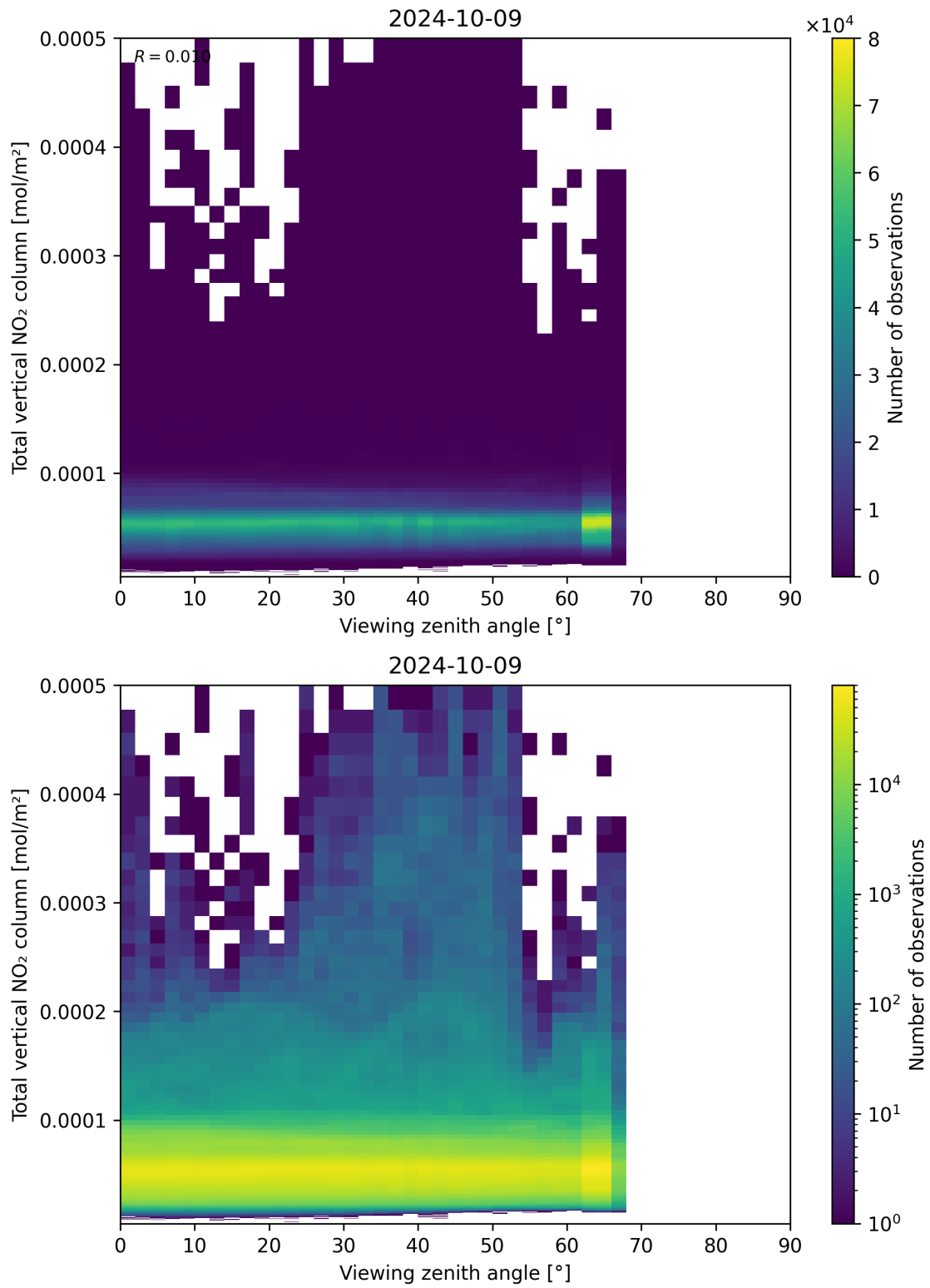
Figure 167: Scatter density plot of “Viewing zenith angle” against “Total vertical NO 2 column” for 2024-10-08 to 2024-10-10.
