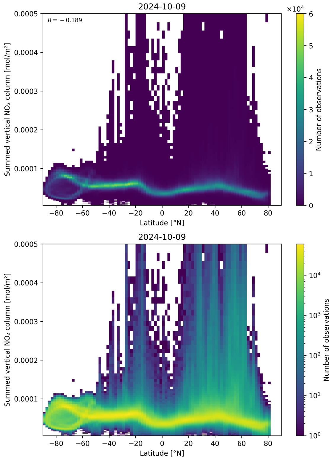
Figure 88: Scatter density plot of “Latitude” against “Summed vertical NO 2 column” for 2024-10-08 to 2024-10-10.
