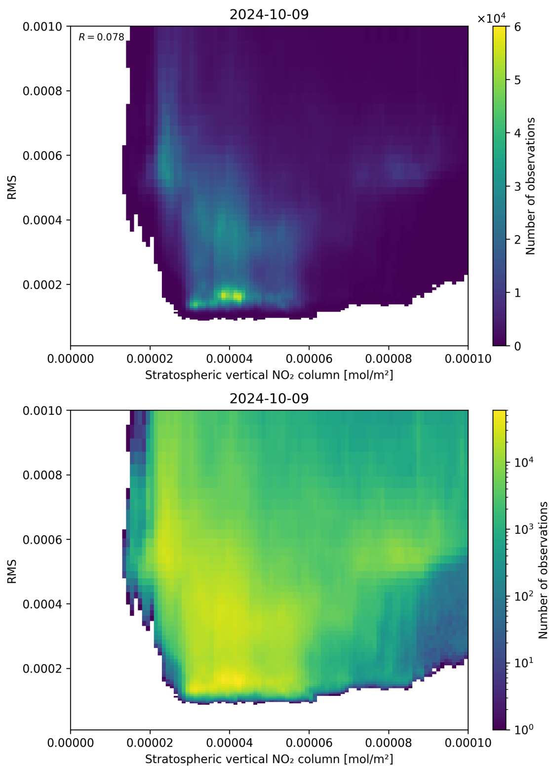
Figure 102: Scatter density plot of “Stratospheric vertical NO 2 column” against “RMS” for 2024-10-08 to 2024-10-10.
