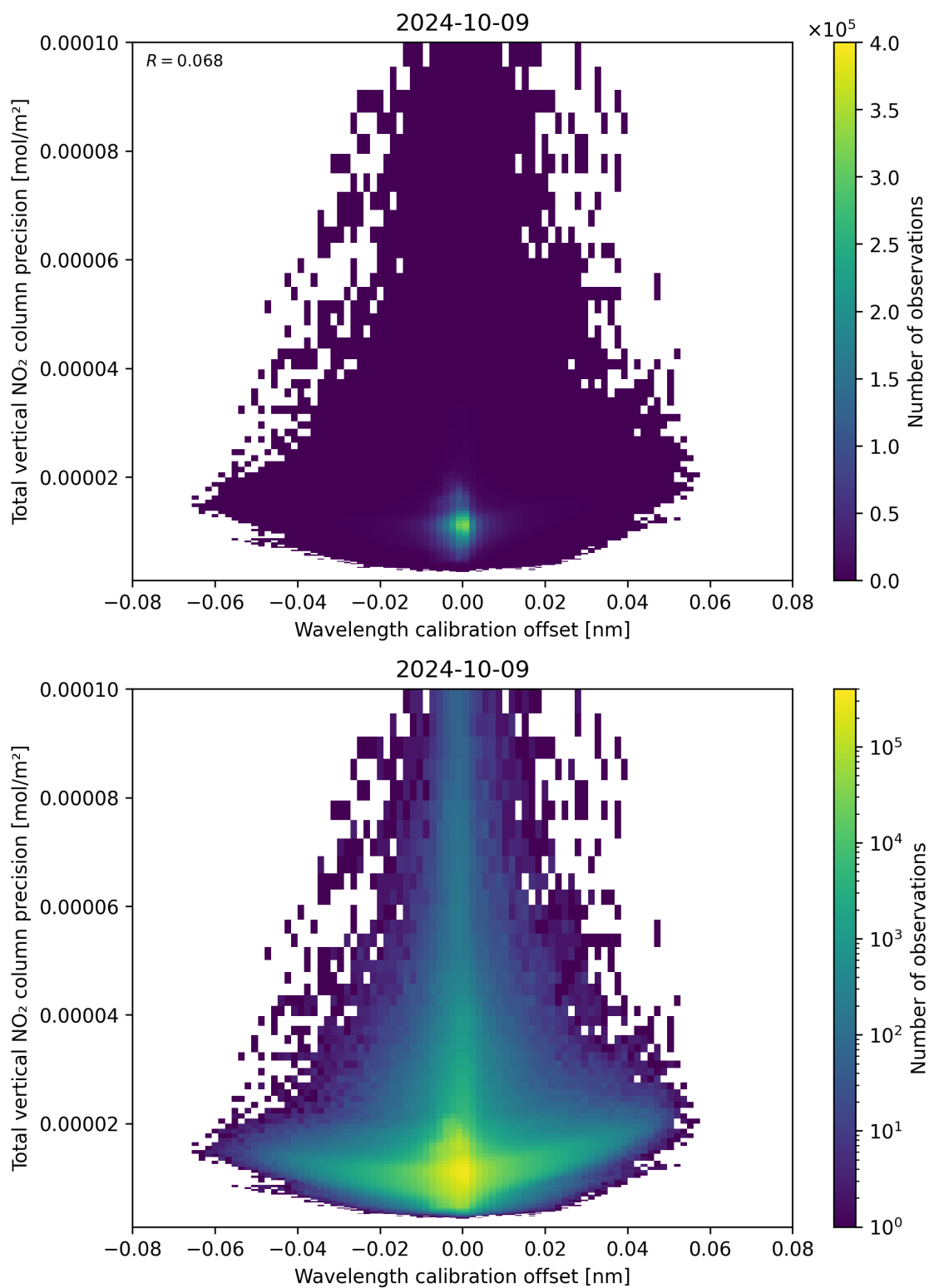
Figure 180: Scatter density plot of “Wavelength calibration offset” against “Total vertical NO 2 column precision” for 2024-10-08 to 2024-10-10.
