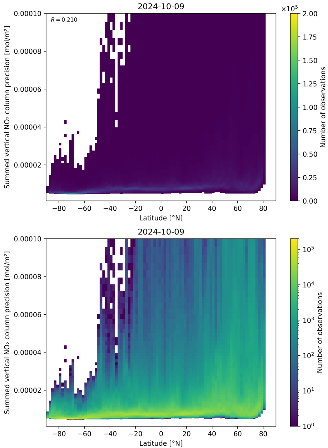
Figure 89: Scatter density plot of “Latitude” against “Summed vertical NO 2 column precision” for 2024-10-08 to 2024-10-10.
