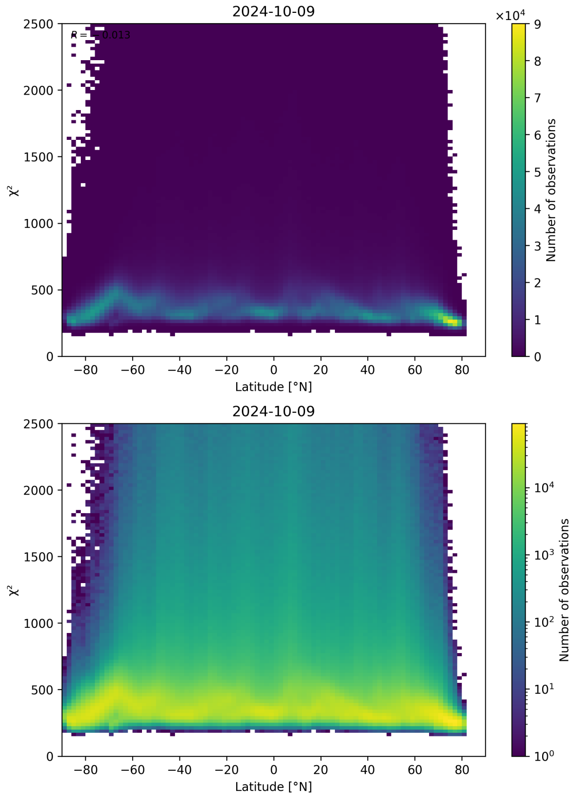
Figure 86: Scatter density plot of “Latitude” against “ \chi^2 ” for 2024-10-08 to 2024-10-10.
