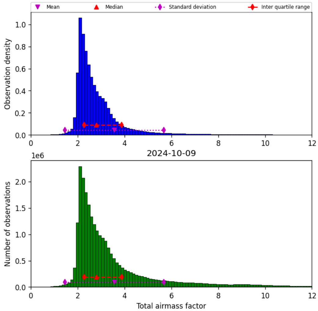
Figure 32: Histogram of “Total airmass factor” for 2024-10-08 to 2024-10-10
