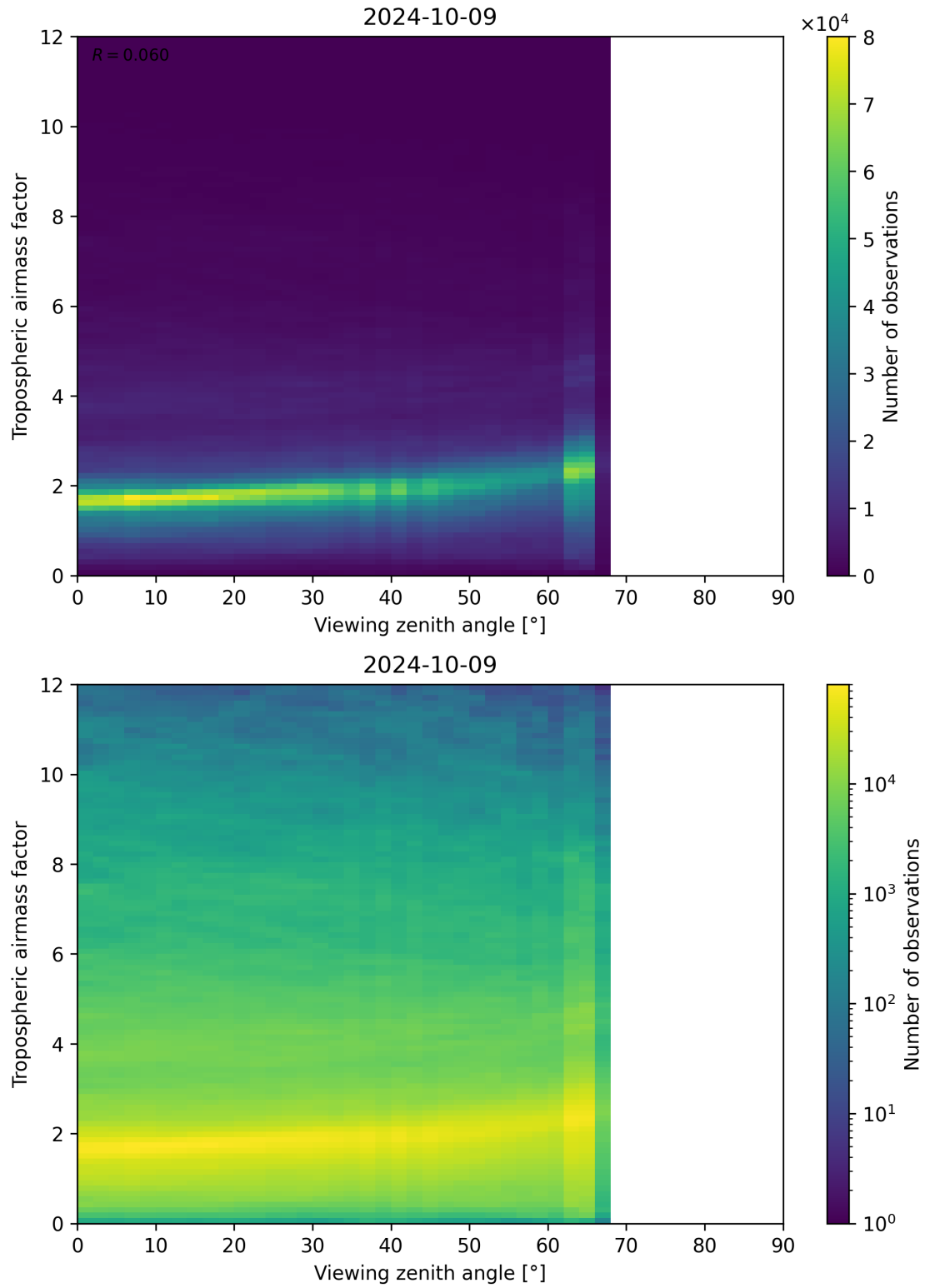
Figure 161: Scatter density plot of “Viewing zenith angle” against “Tropospheric airmass factor” for 2024-10-08 to 2024-10-10.
