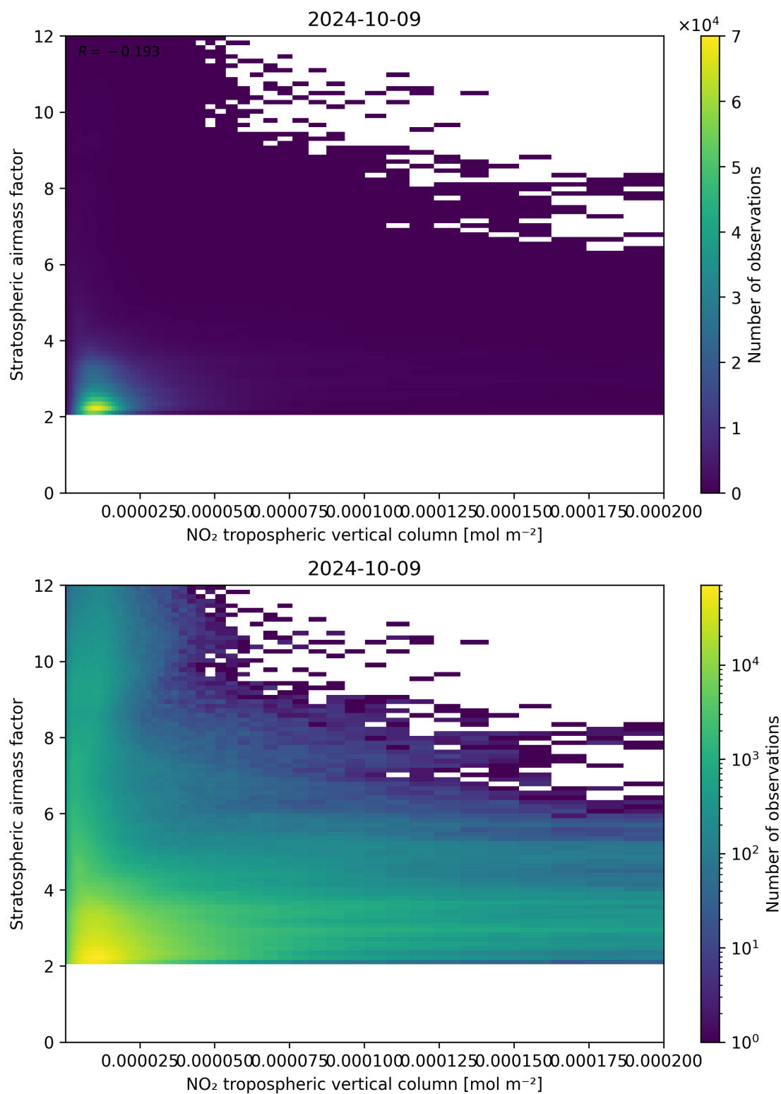
Figure 121: Scatter density plot of “NO 2 tropospheric vertical column” against “Stratospheric airmass factor” for 2024-10-08 to 2024-10-10.
