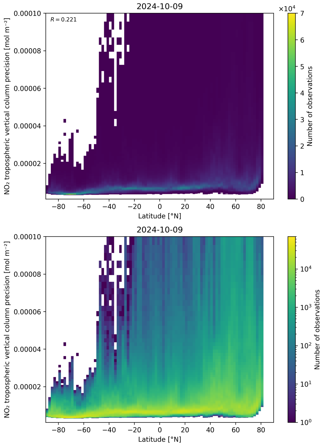
Figure 93: Scatter density plot of “Latitude” against “NO 2 tropospheric vertical column precision” for 2024-10-08 to 2024-10-10.
