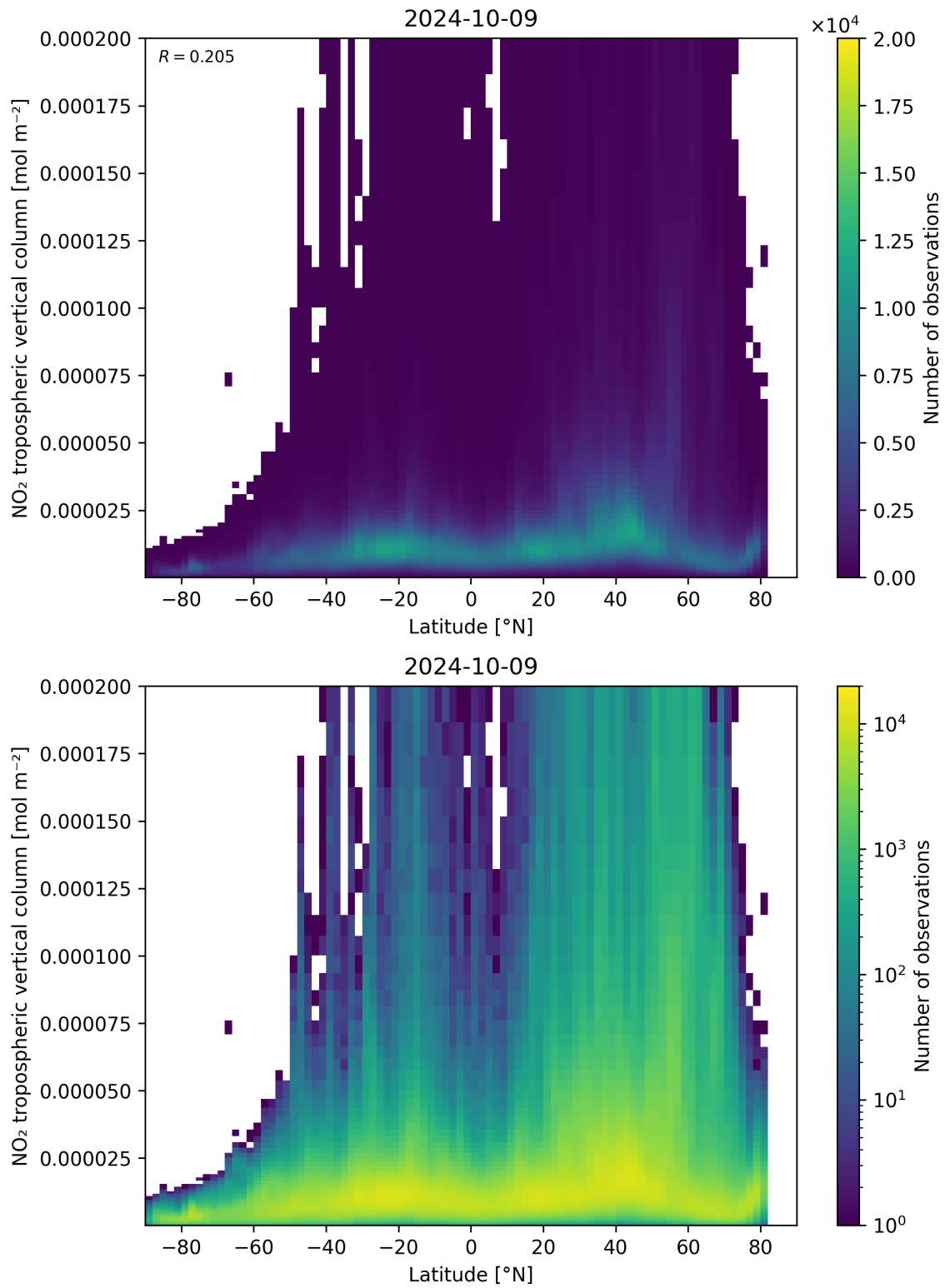
Figure 92: Scatter density plot of “Latitude” against “NO 2 tropospheric vertical column” for 2024-10-08 to 2024-10-10.
