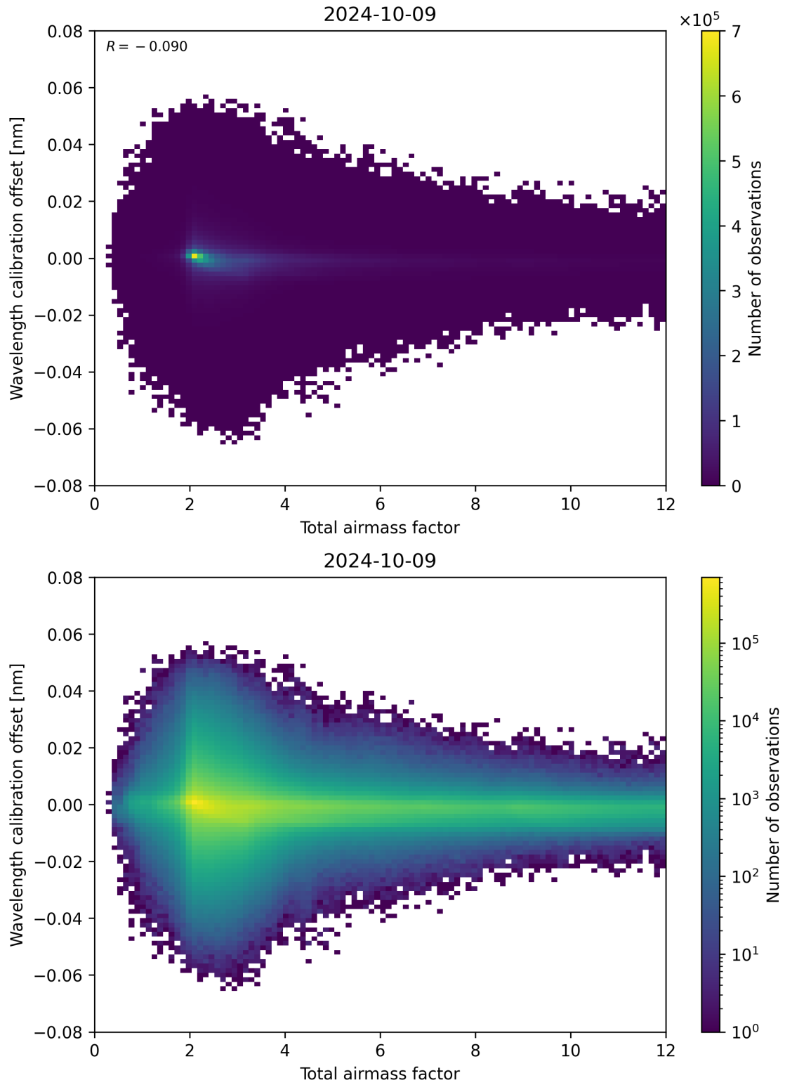
Figure 70: Scatter density plot of “Total airmass factor” against “Wavelength calibration offset” for 2024-10-08 to 2024-10-10.
