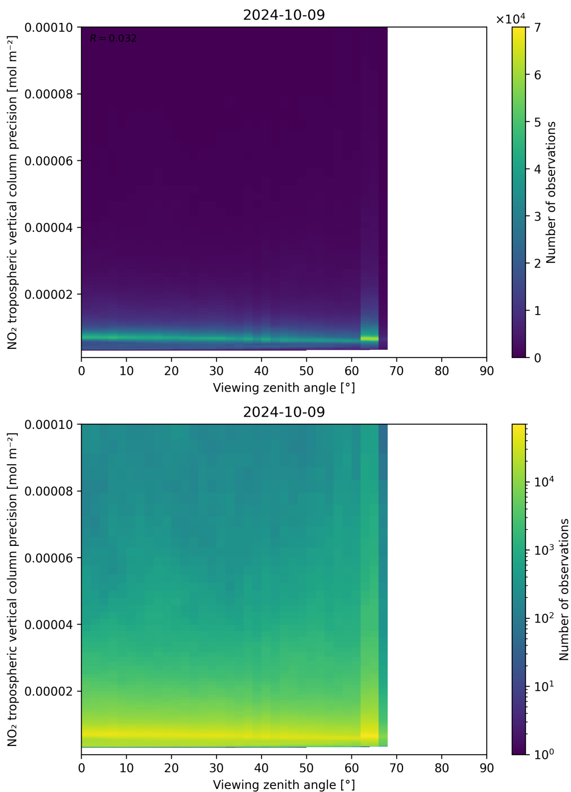
Figure 170: Scatter density plot of “Viewing zenith angle” against “NO 2 tropospheric vertical column precision” for 2024-10-08 to 2024-10-10.
