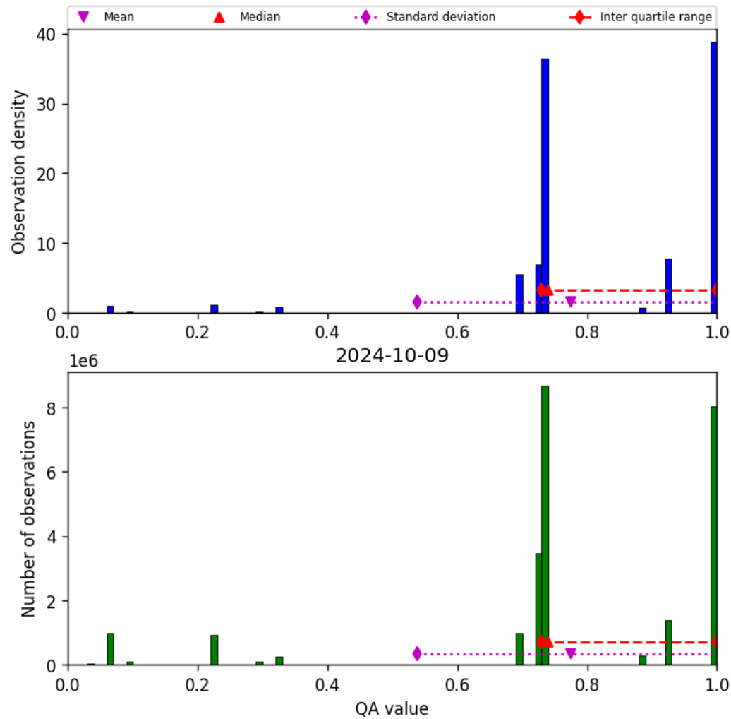
Figure 28: Histogram of “QA value” for 2024-10-08 to 2024-10-10
