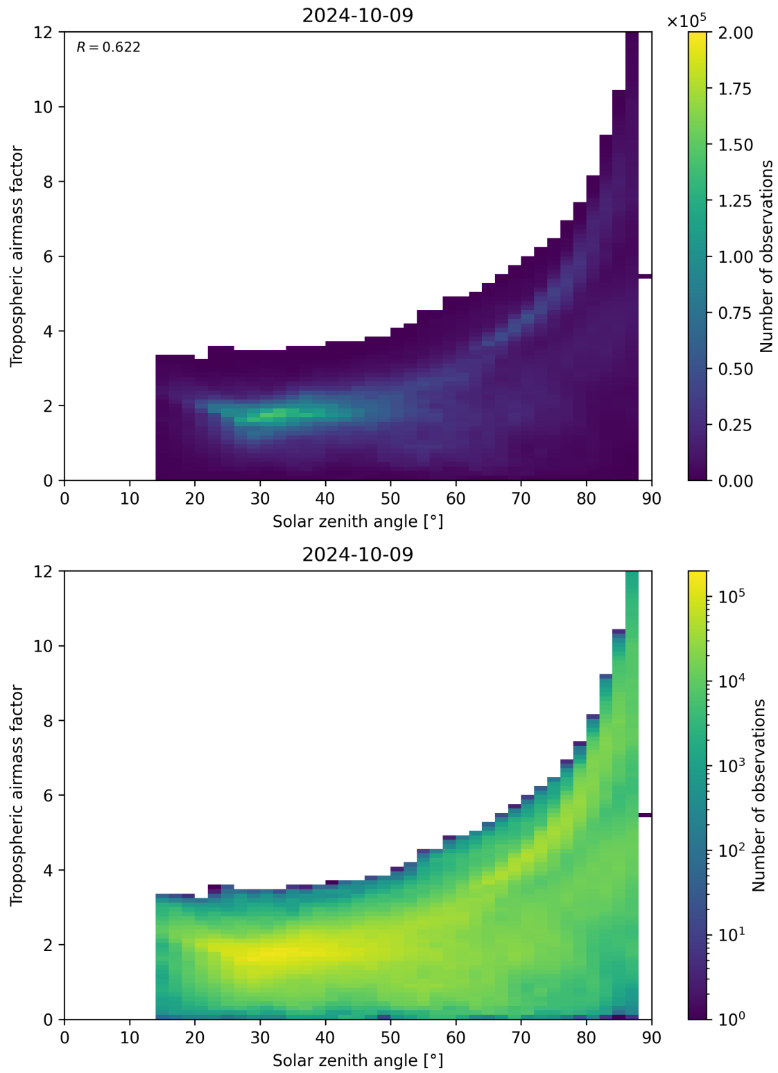
Figure 147: Scatter density plot of “Solar zenith angle” against “Tropospheric airmass factor” for 2024-10-08 to 2024-10-10.
