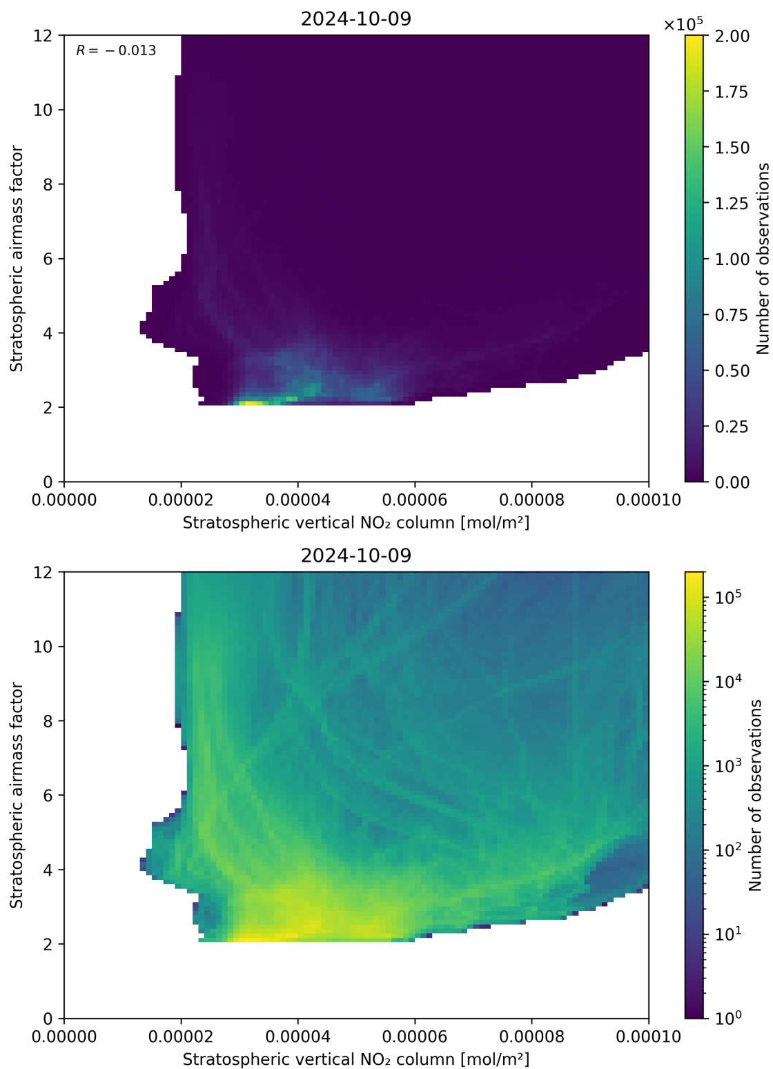
Figure 96: Scatter density plot of “Stratospheric vertical NO 2 column” against “Stratospheric airmass factor” for 2024-10-08 to 2024-10-10.
