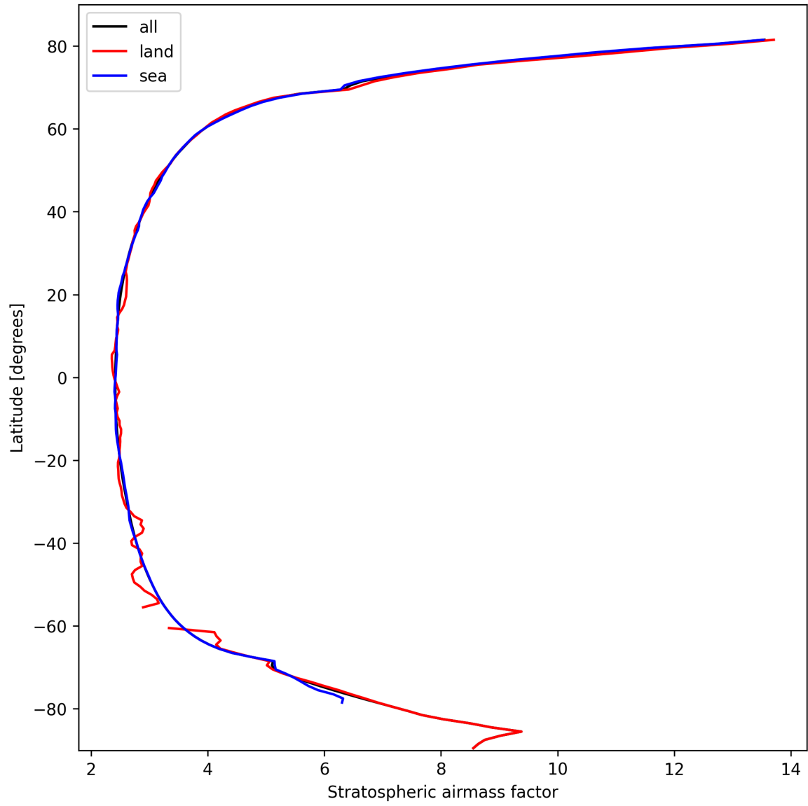
Figure 27: Zonal average of “Stratospheric air mass factor” for 2024-10-08 to 2024-10-10.
