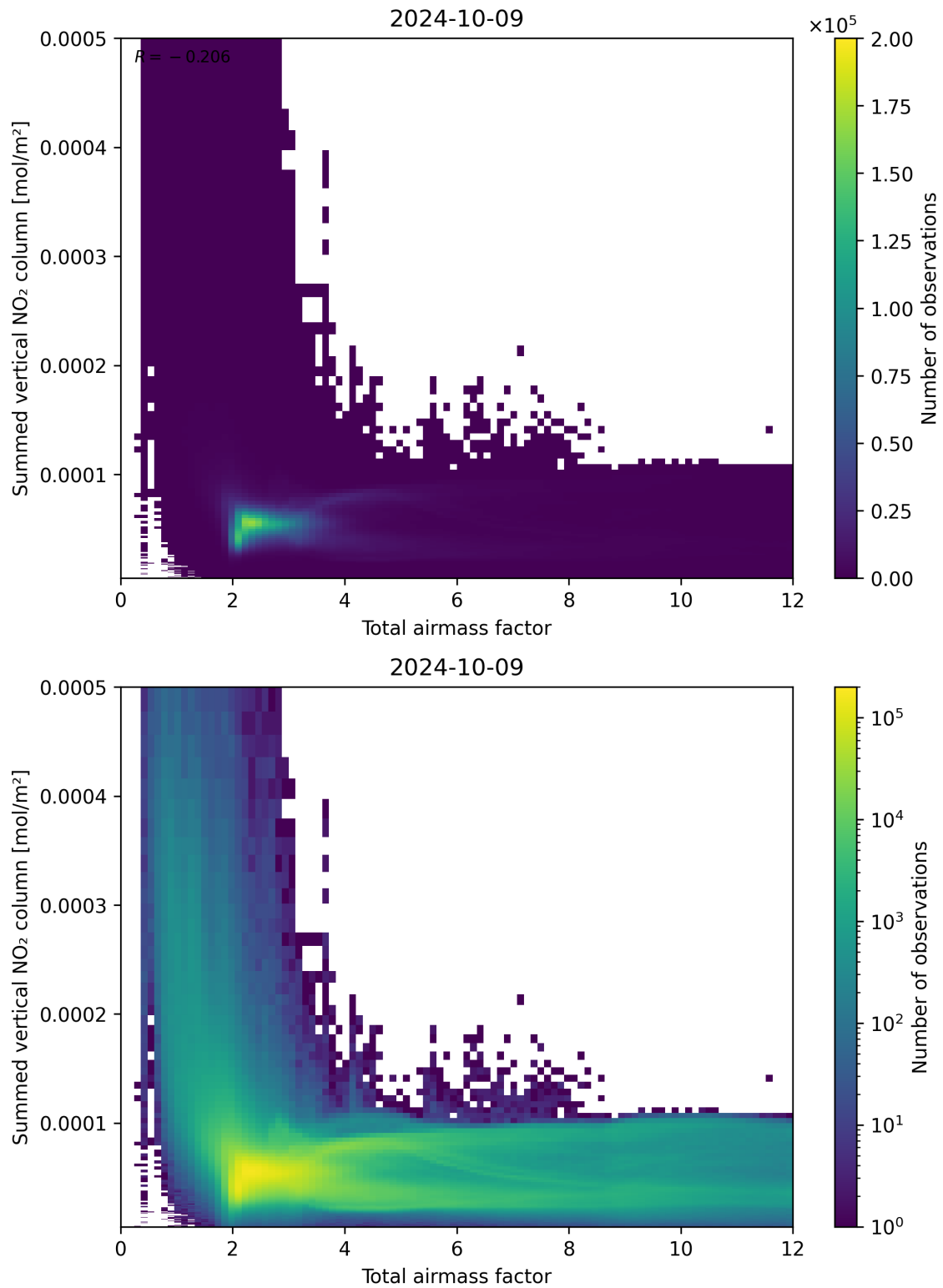
Figure 65: Scatter density plot of “Total airmass factor” against “Summed vertical NO 2 column” for 2024-10-08 to 2024-10-10.
