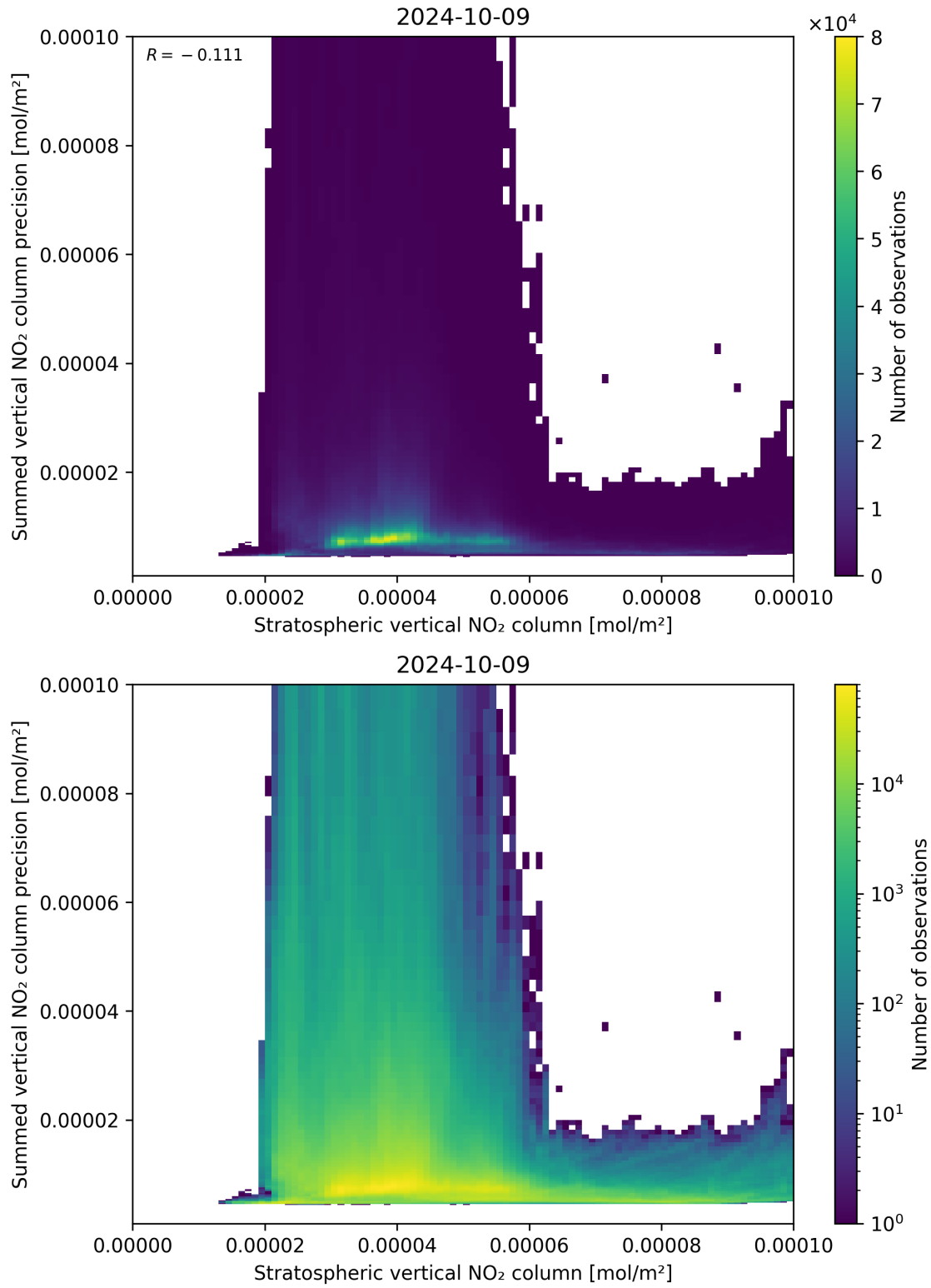
Figure 99: Scatter density plot of “Stratospheric vertical NO 2 column” against “Summed vertical NO 2 column precision” for 2024-10-08 to 2024-10-10.
