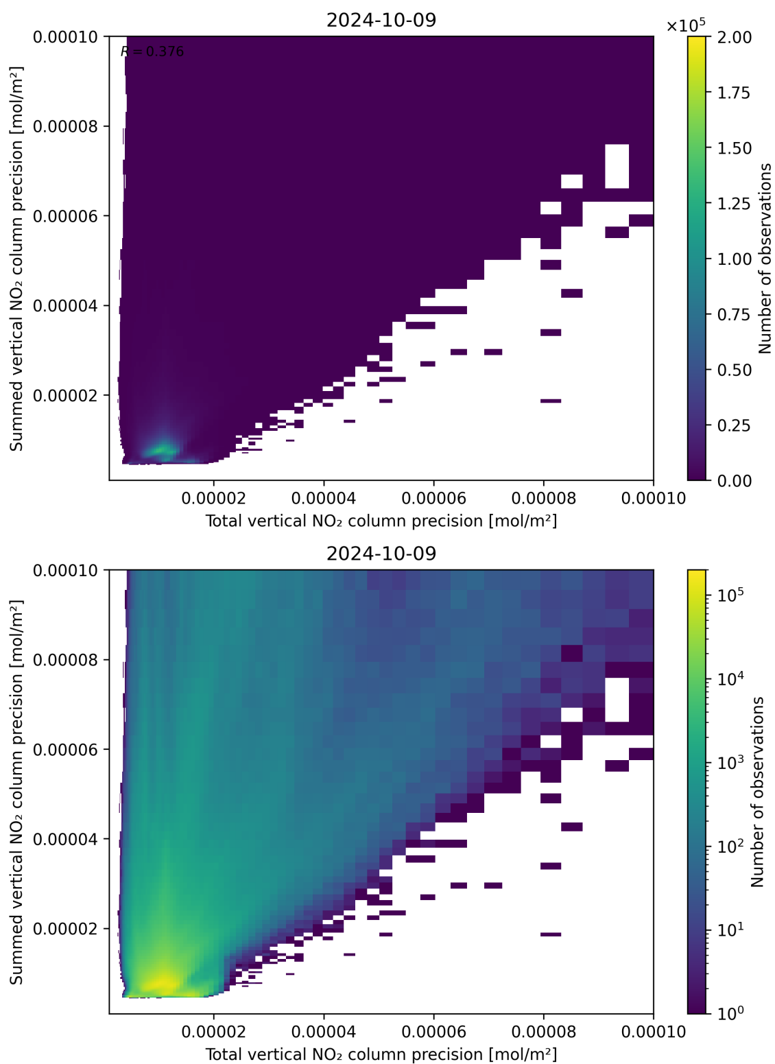
Figure 118: Scatter density plot of “Total vertical NO 2 column precision” against “Summed vertical NO 2 column precision” for 2024-10-08 to 2024-10-10.
