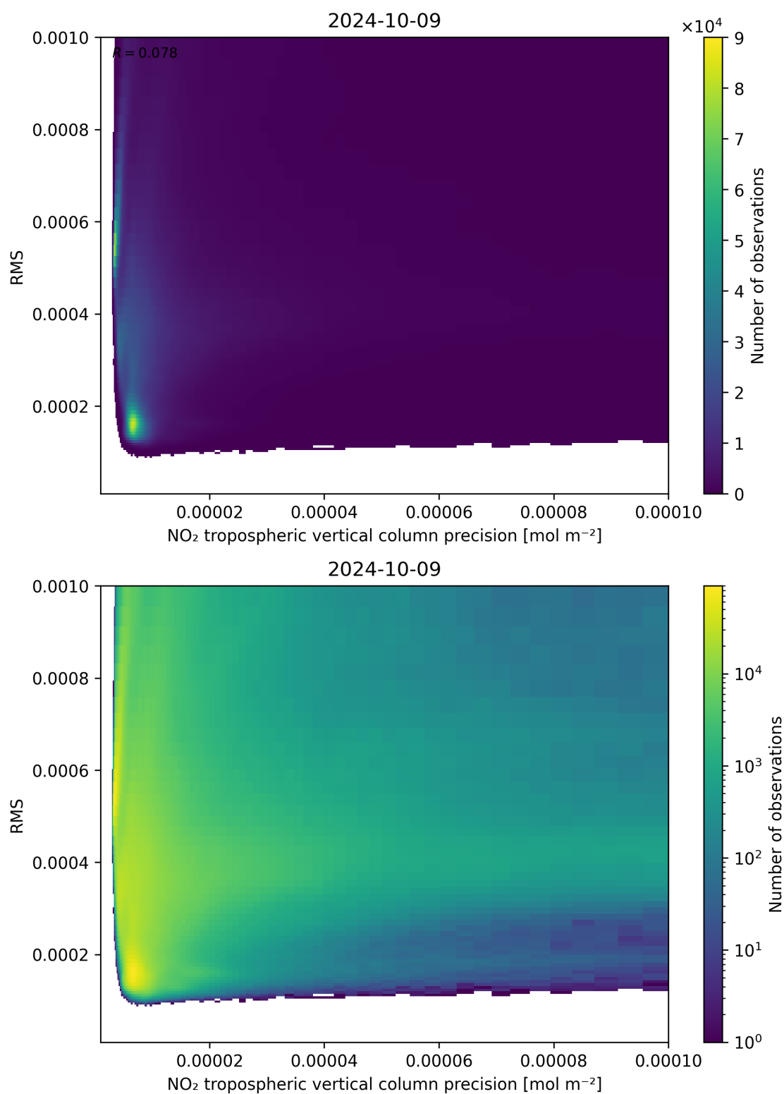
Figure 140: Scatter density plot of “NO 2 tropospheric vertical column precision” against “RMS” for 2024-10-08 to 2024-10-10.
