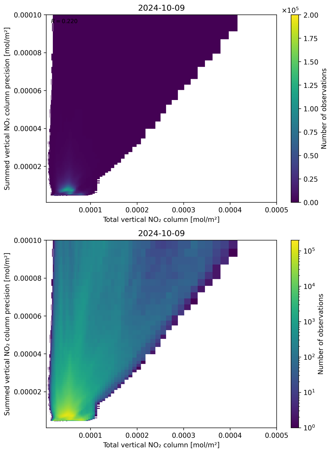
Figure 113: Scatter density plot of “Total vertical NO 2 column” against “Summed vertical NO 2 column precision” for 2024-10-08 to 2024-10-10.
