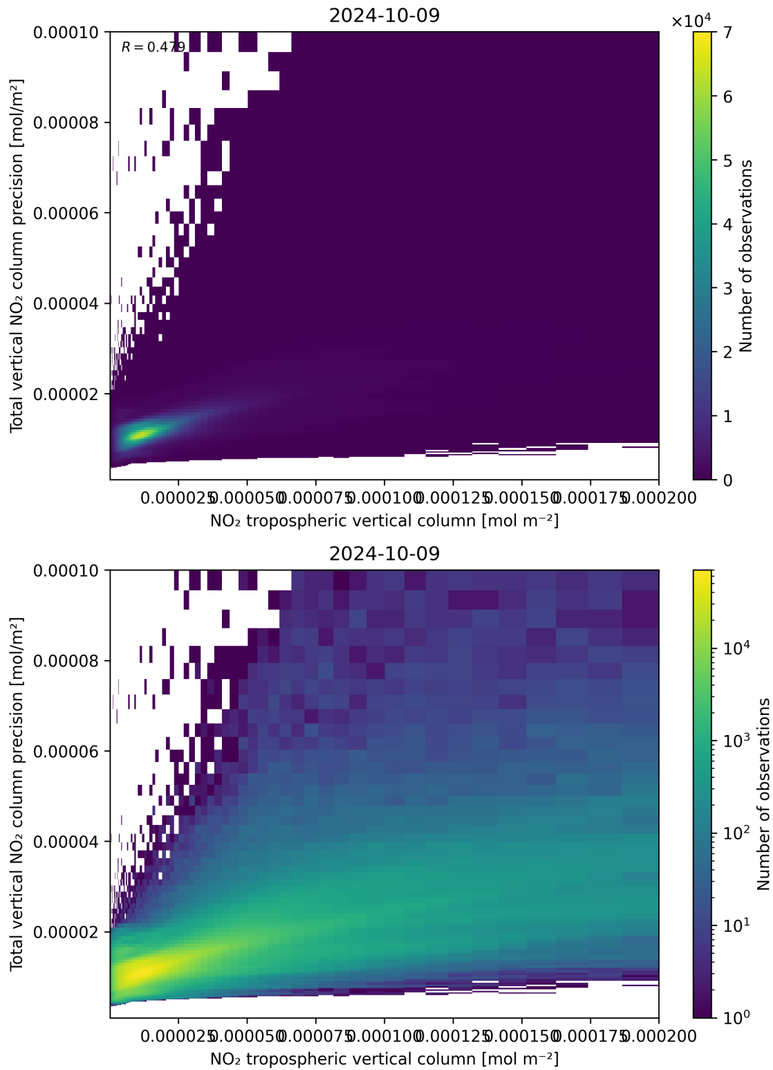
Figure 129: Scatter density plot of “NO 2 tropospheric vertical column” against “Total vertical NO 2 column precision” for 2024-10-08 to 2024-10-10.
