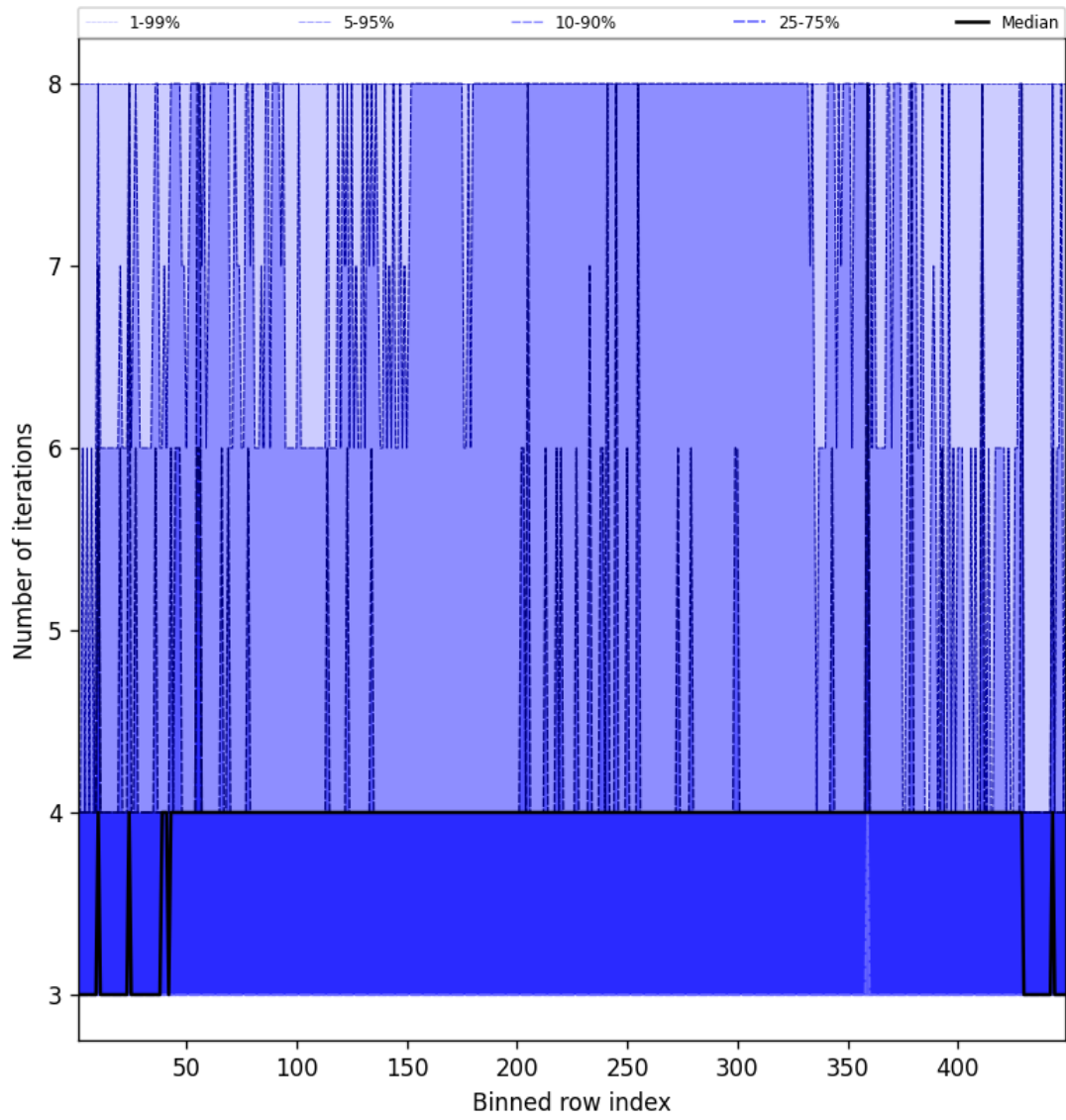
Figure 51: Along track statistics of “Number of iterations” for 2024-10-08 to 2024-10-10
