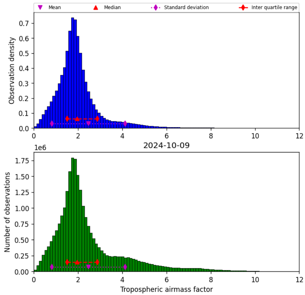
Figure 31: Histogram of “Tropospheric airmass factor” for 2024-10-08 to 2024-10-10
