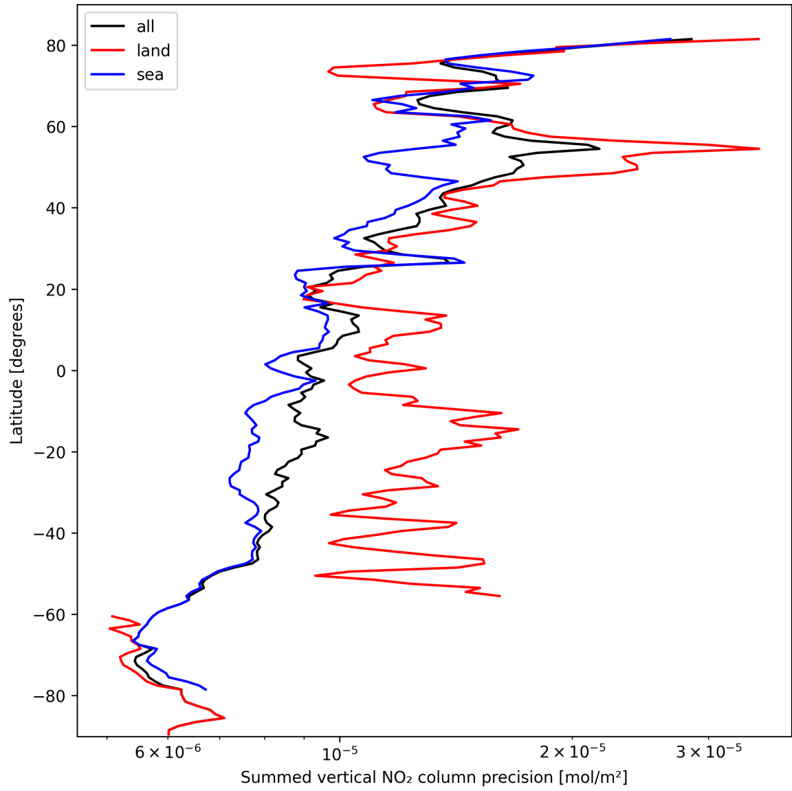
Figure 24: Zonal average of “Summed vertical NO 2 column precision” for 2024-10-08 to 2024-10-10.
