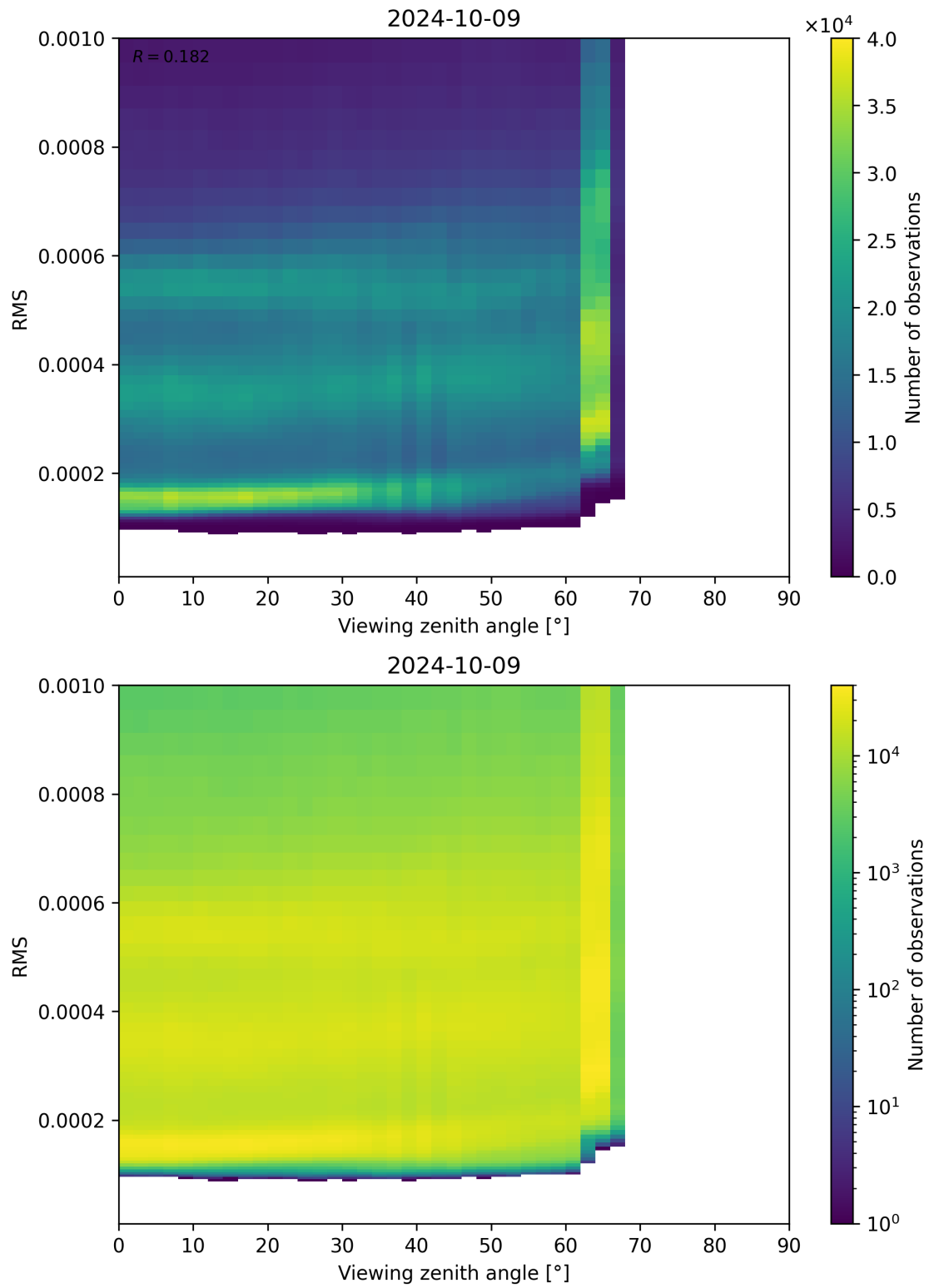
Figure 171: Scatter density plot of “Viewing zenith angle” against “RMS” for 2024-10-08 to 2024-10-10.
