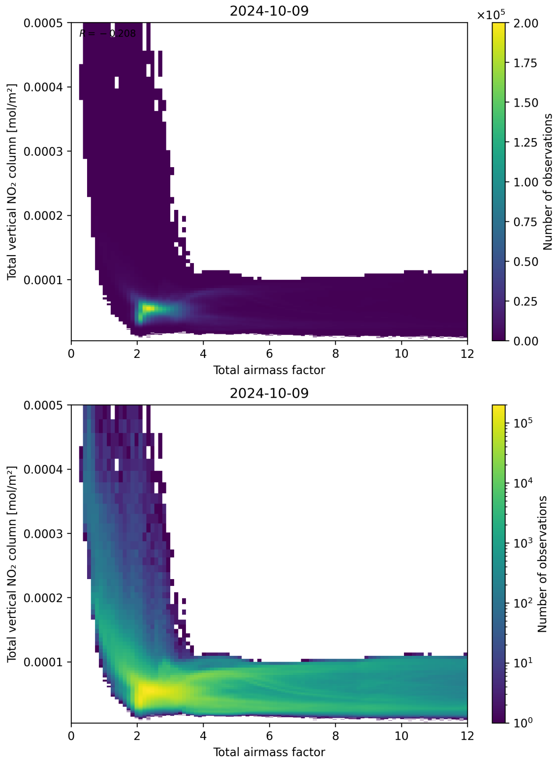
Figure 67: Scatter density plot of “Total airmass factor” against “Total vertical NO 2 column” for 2024-10-08 to 2024-10-10.
