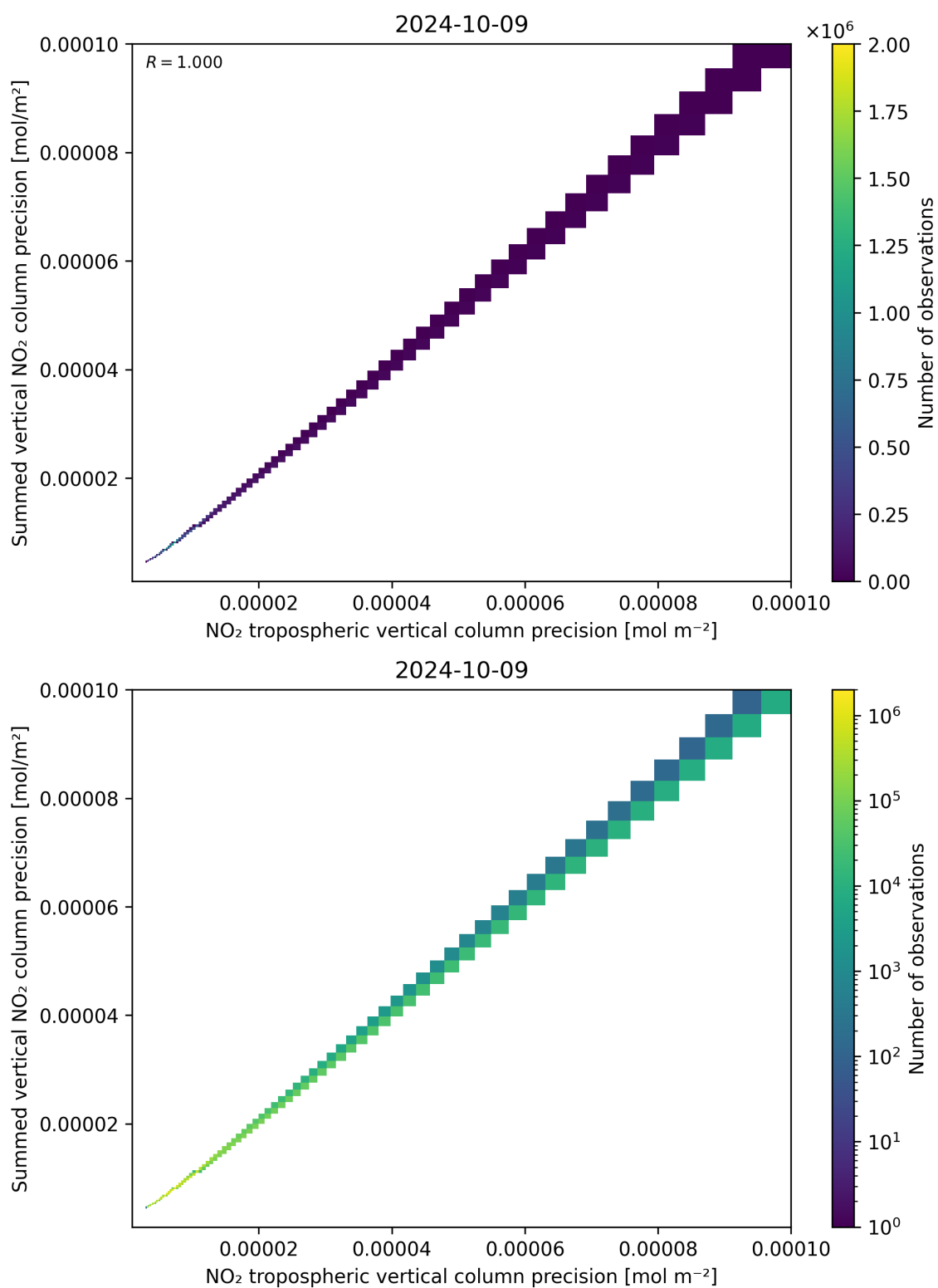
Figure 137: Scatter density plot of “NO 2 tropospheric vertical column precision” against “Summed vertical NO 2 column precision” for 2024-10-08 to 2024-10-10.
