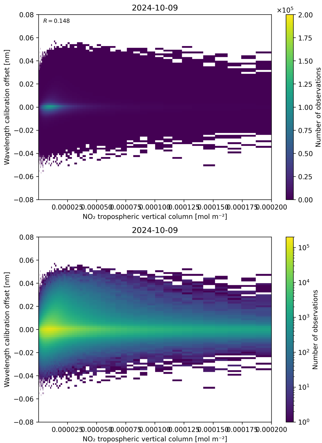
Figure 143: Scatter density plot of “NO 2 tropospheric vertical column” against “Wavelength calibration offset” for 2024-10-08 to 2024-10-10.
