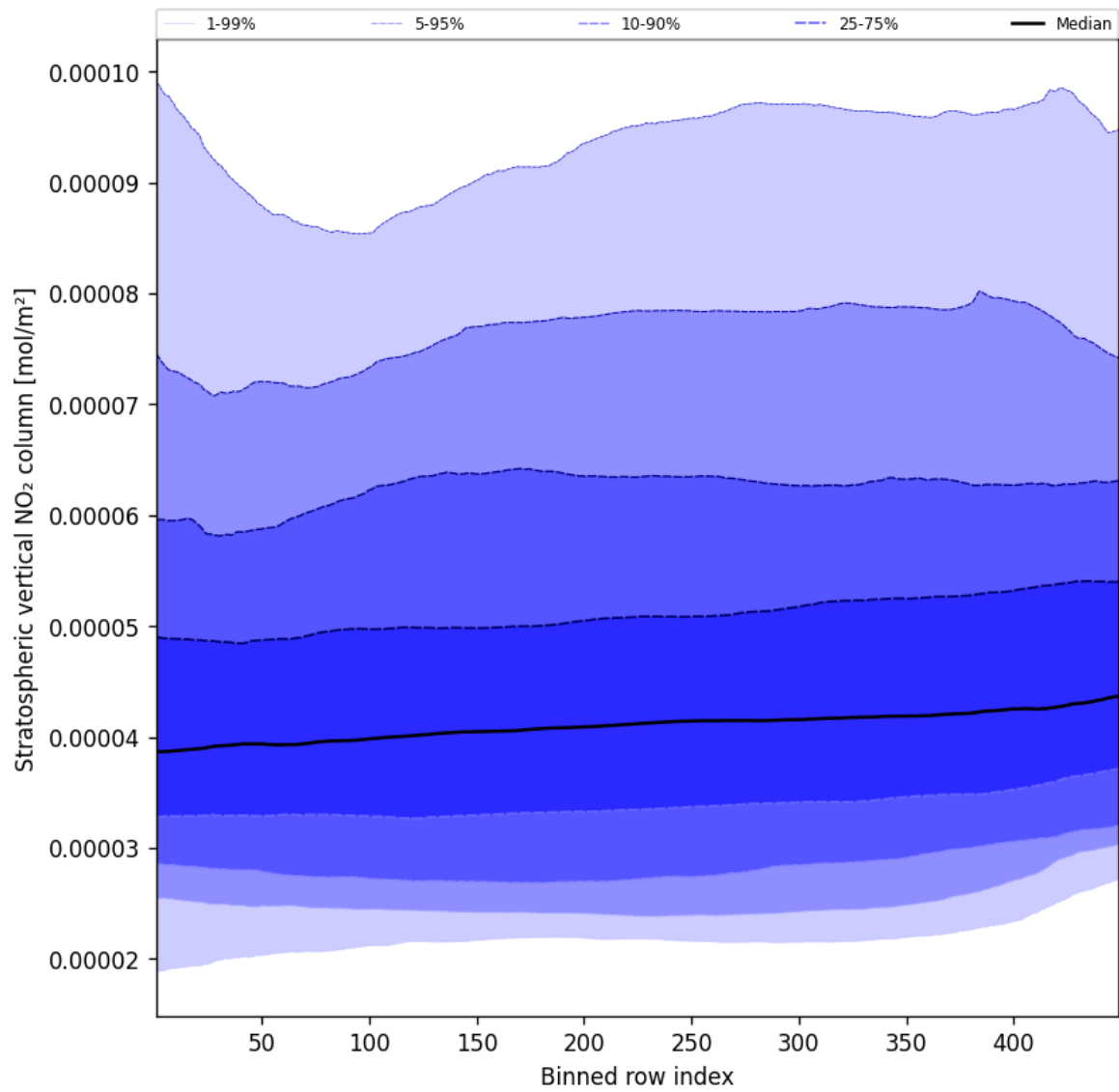
Figure 53: Along track statistics of “Stratospheric vertical NO 2 column” for 2024-10-08 to 2024-10-10
