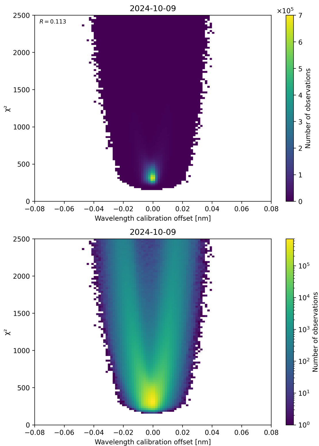
Figure 175: Scatter density plot of “Wavelength calibration offset” against “ \chi^2 ” for 2024-10-08 to 2024-10-10.
