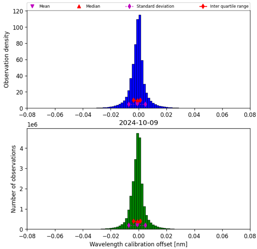
Figure 35: Histogram of “Wavelength calibration offset” for 2024-10-08 to 2024-10-10
