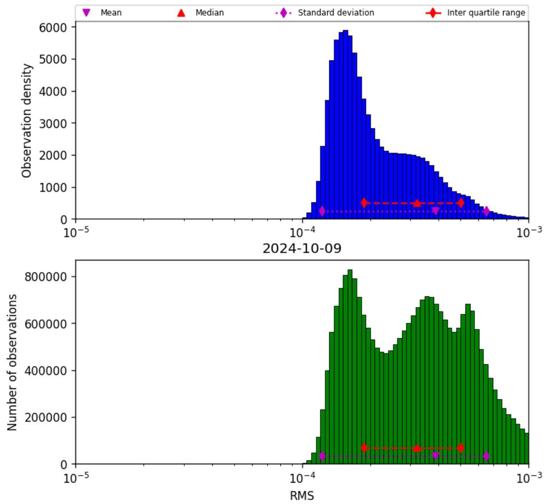
Figure 43: Histogram of “RMS” for 2024-10-08 to 2024-10-10
