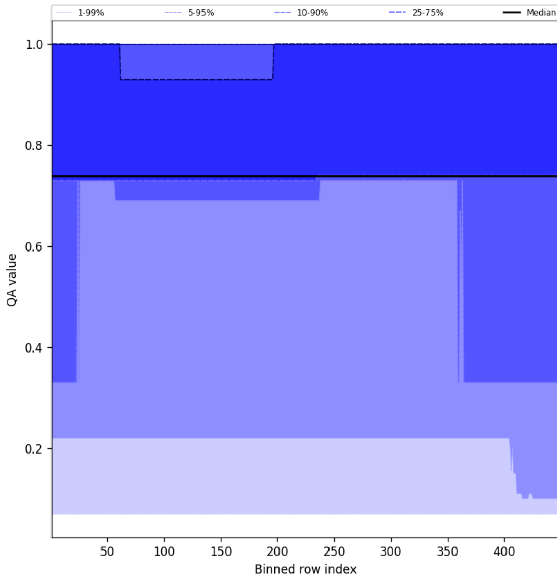
Figure 45: Along track statistics of “QA value” for 2024-10-08 to 2024-10-10
