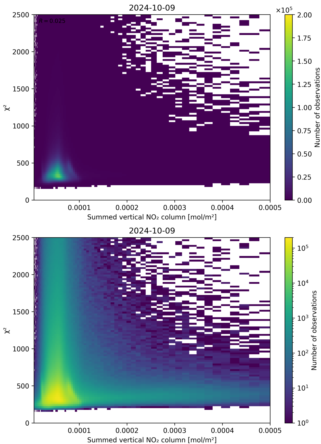
Figure 104: Scatter density plot of “Summed vertical NO 2 column” against “ \chi^2 ” for 2024-10-08 to 2024-10-10.
