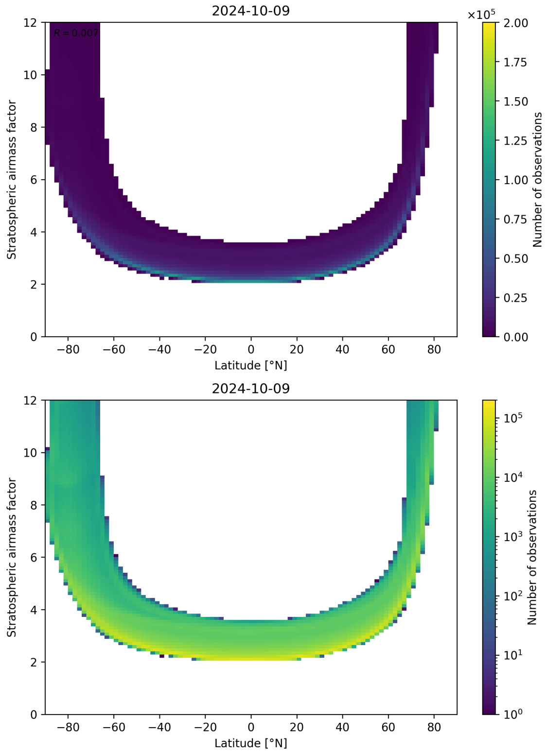
Figure 83: Scatter density plot of “Latitude” against “Stratospheric airmass factor” for 2024-10-08 to 2024-10-10.
