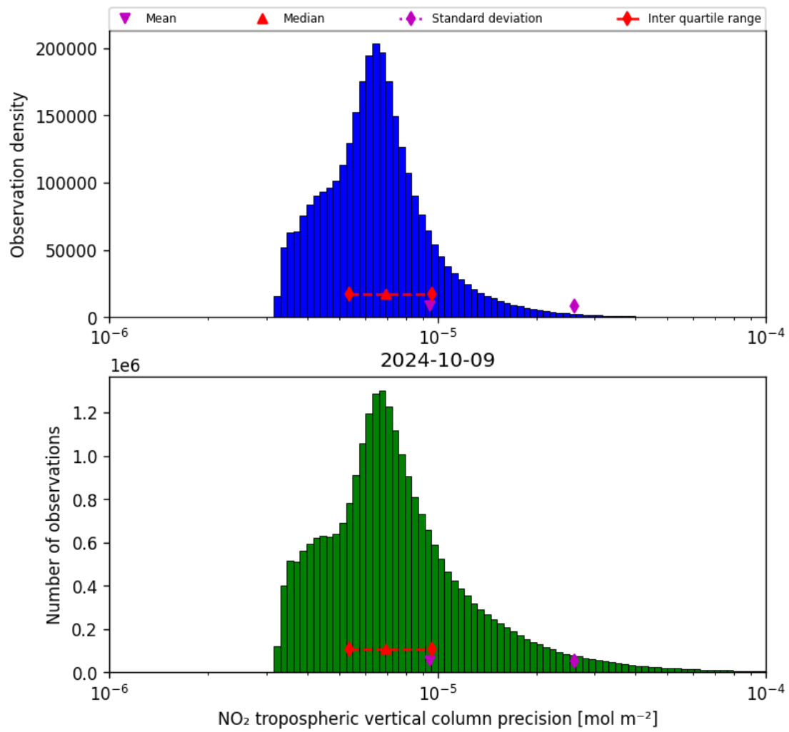
Figure 30: Histogram of “NO 2 tropospheric vertical column precision” for 2024-10-08 to 2024-10-10
