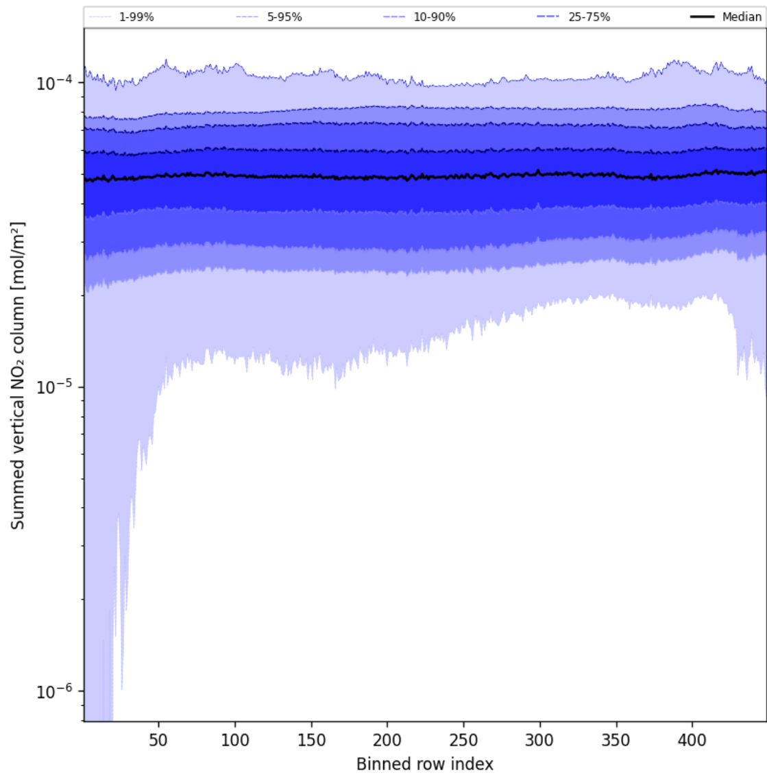
Figure 57: Along track statistics of “Summed vertical NO 2 column” for 2024-10-08 to 2024-10-10
