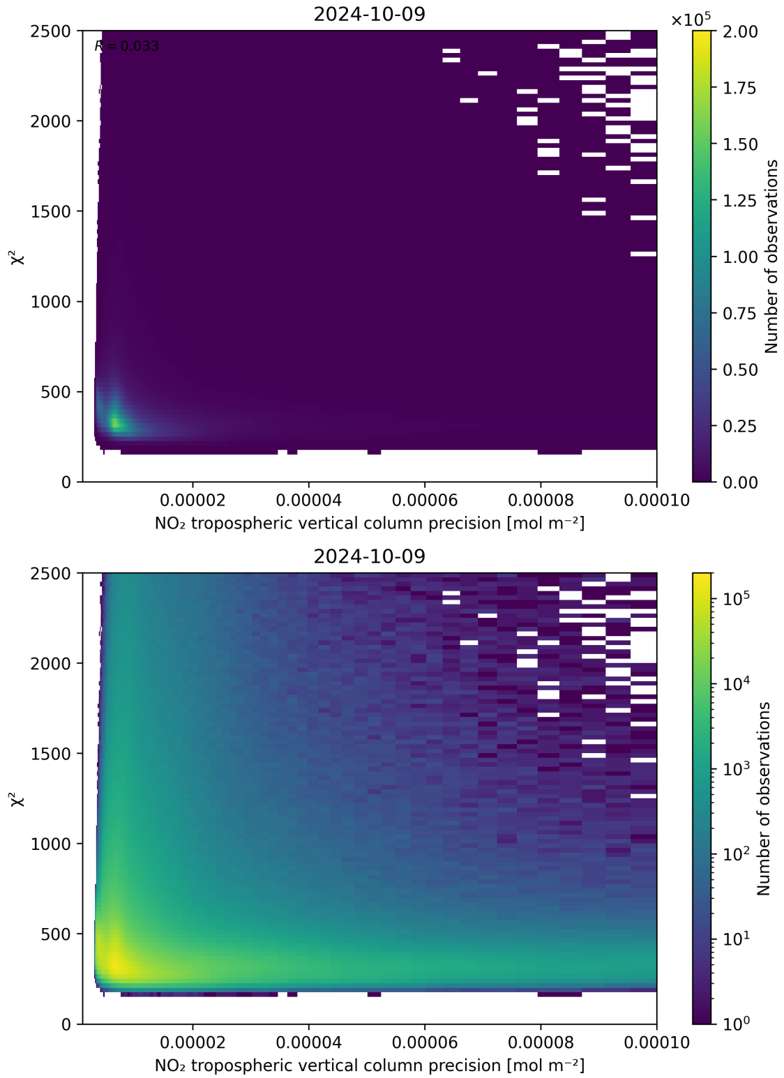
Figure 134: Scatter density plot of “NO 2 tropospheric vertical column precision” against “ \chi^2 ” for 2024-10-08 to 2024-10-10.
