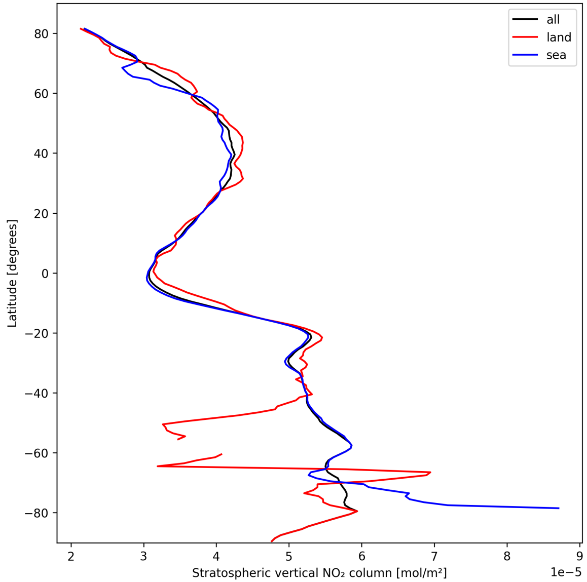
Figure 19: Zonal average of “Stratospheric vertical NO 2 column” for 2024-10-08 to 2024-10-10.
