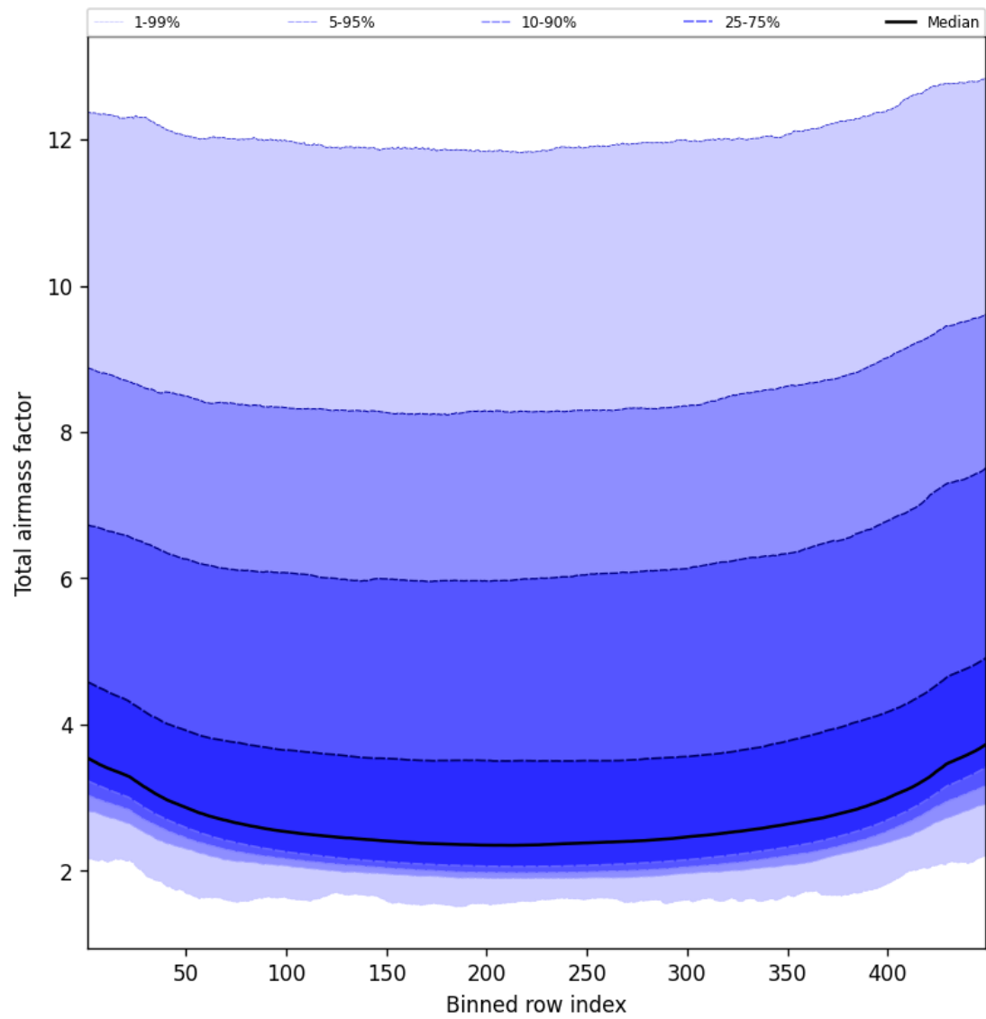
Figure 49: Along track statistics of “Total airmass factor” for 2024-10-08 to 2024-10-10
