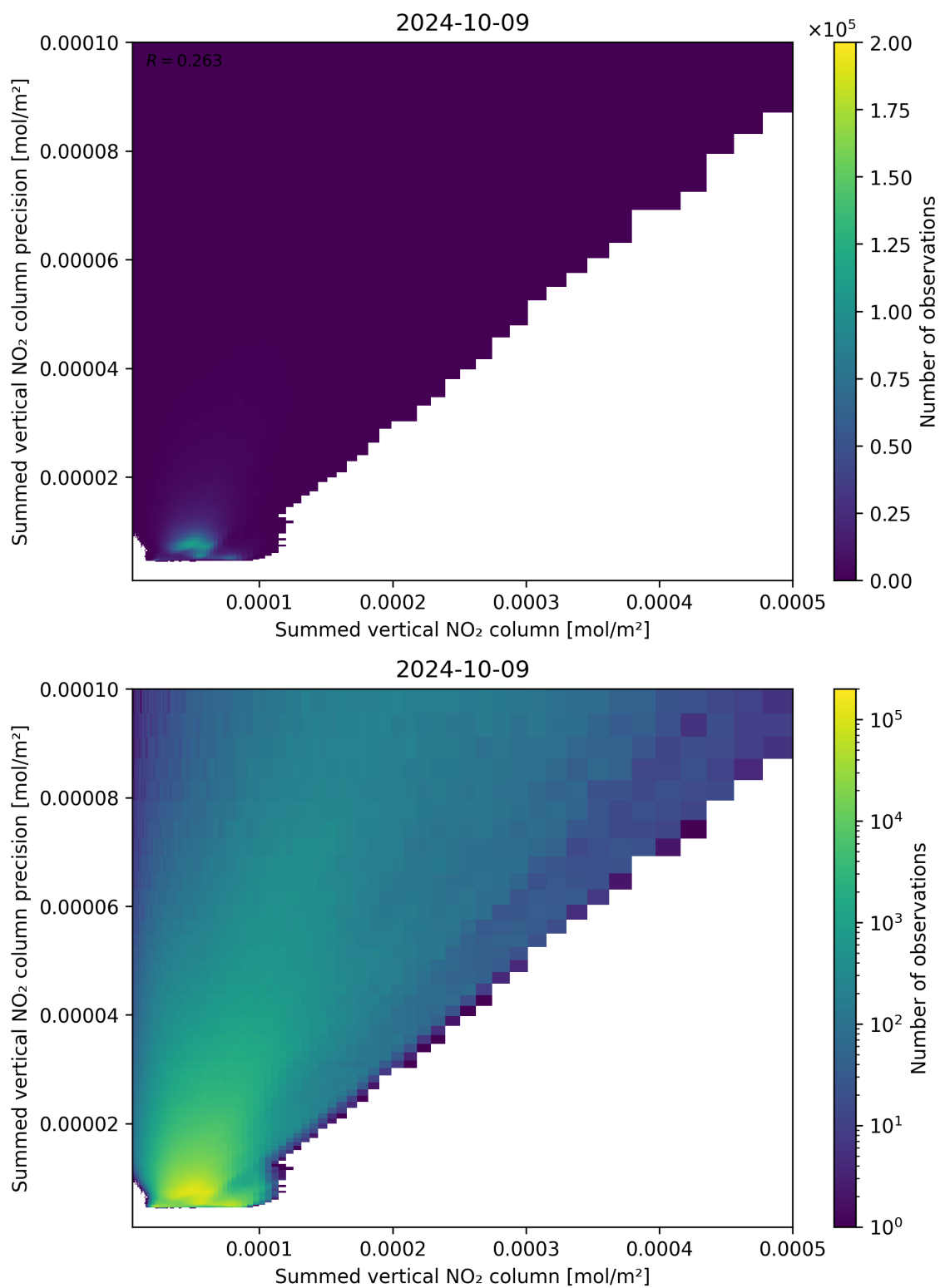
Figure 105: Scatter density plot of “Summed vertical NO 2 column” against “Summed vertical NO 2 column precision” for 2024-10-08 to 2024-10-10.
