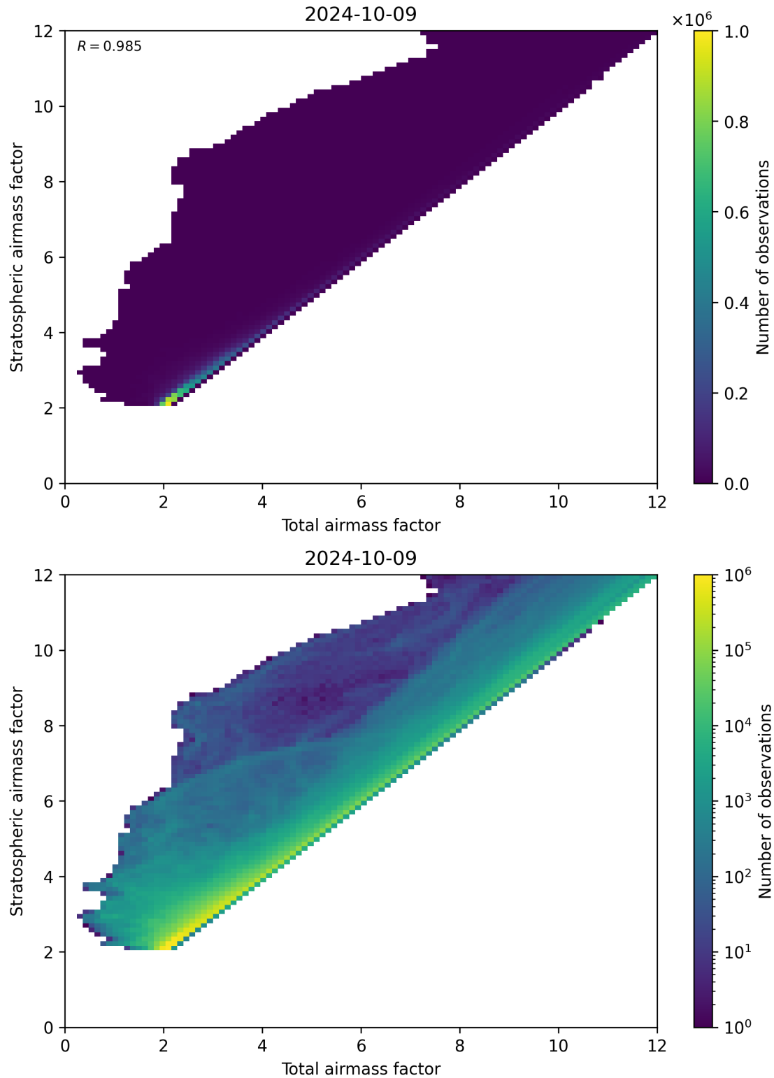
Figure 62: Scatter density plot of “Total air mass factor” against “Stratospheric air mass factor” for 2024-10-08 to 2024-10-10.
