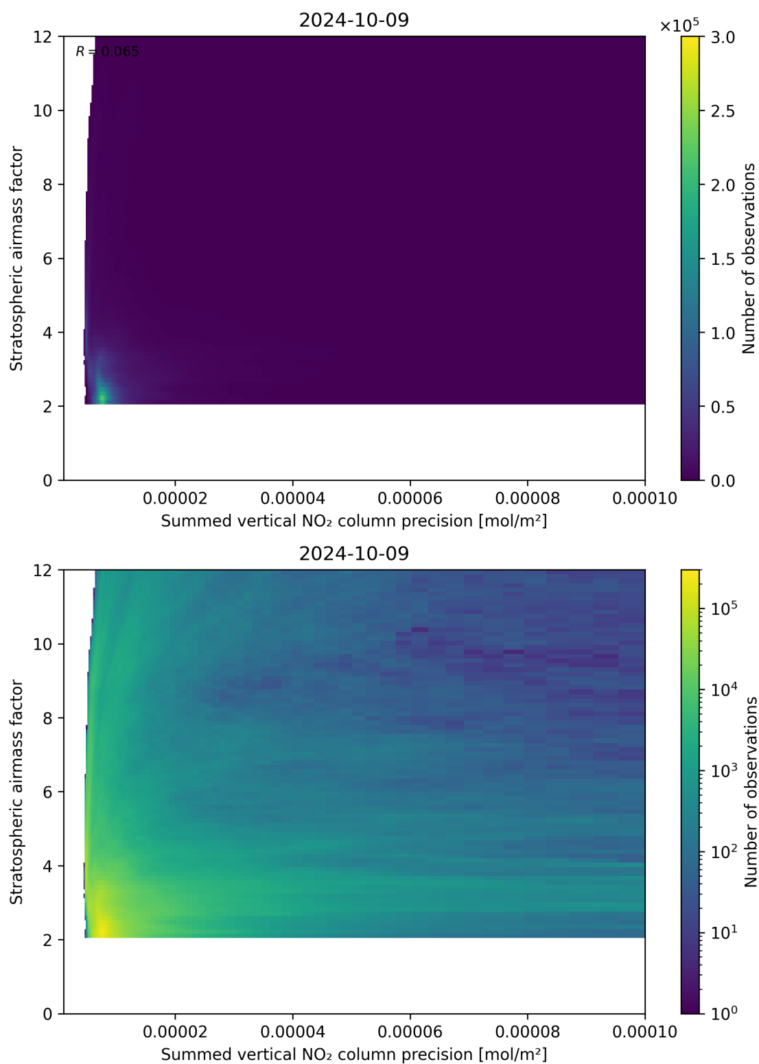
Figure 106: Scatter density plot of “Summed vertical NO 2 column precision” against “Stratospheric airmass factor” for 2024-10-08 to 2024-10-10.
