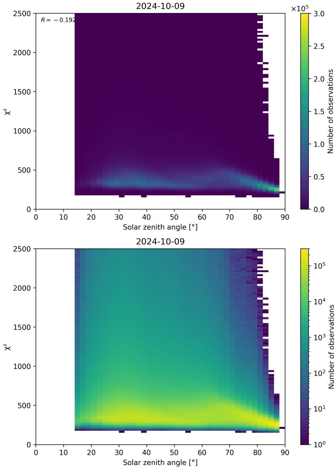
Figure 148: Scatter density plot of “Solar zenith angle” against “ \chi^2 ” for 2024-10-08 to 2024-10-10.
