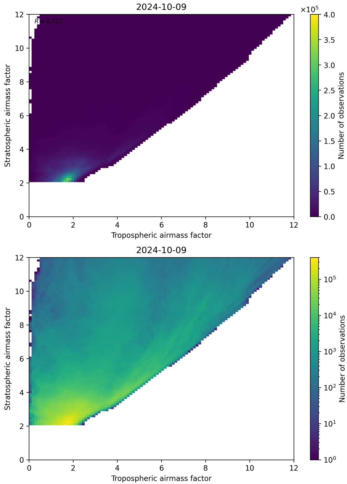
Figure 71: Scatter density plot of “Tropospheric airmass factor” against “Stratospheric airmass factor” for 2024-10-08 to 2024-10-10.
