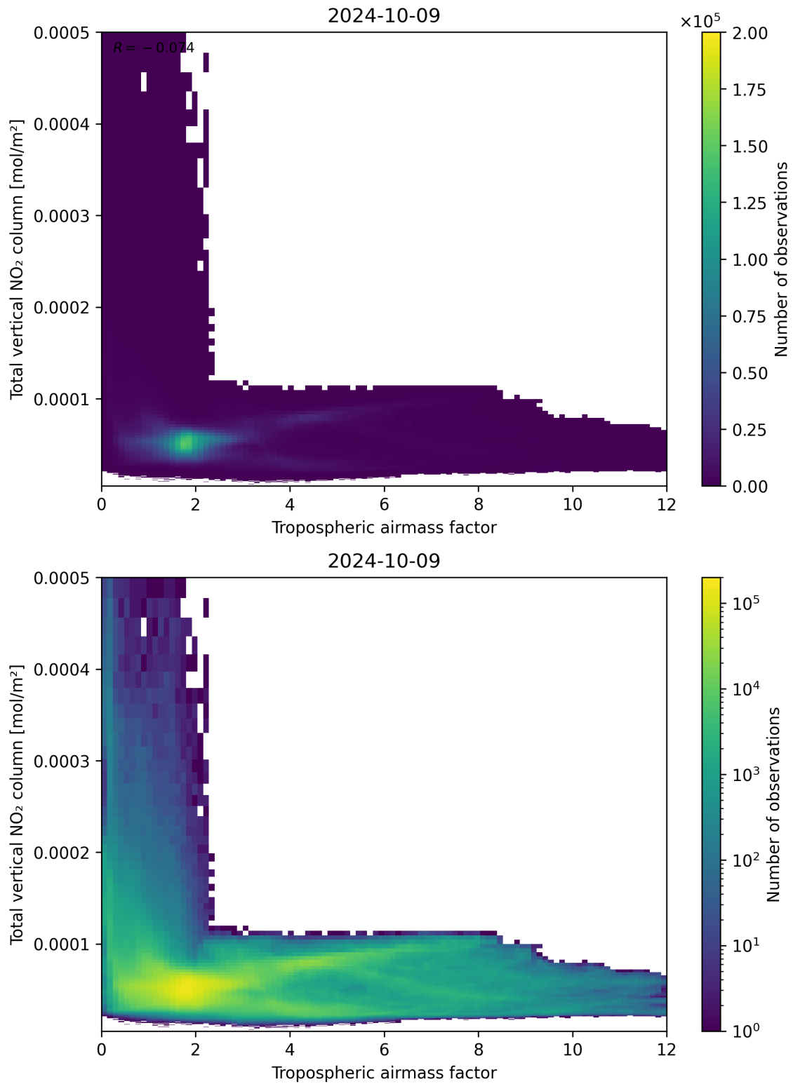
Figure 77: Scatter density plot of “Tropospheric airmass factor” against “Total vertical NO 2 column” for 2024-10-08 to 2024-10-10.
