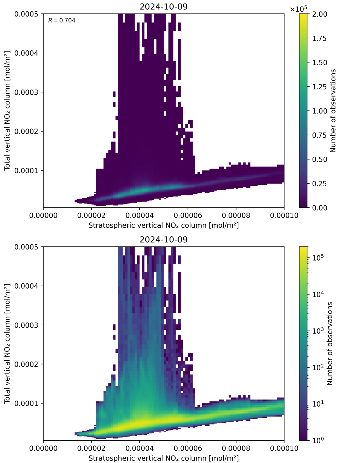
Figure 100: Scatter density plot of “Stratospheric vertical NO 2 column” against “Total vertical NO 2 column” for 2024-10-08 to 2024-10-10.
