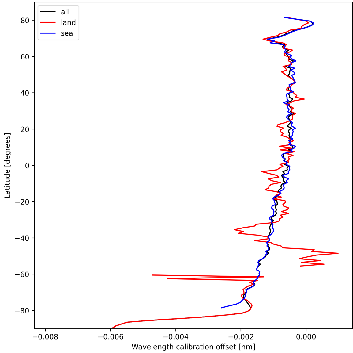
Figure 18: Zonal average of “Wavelength calibration offset” for 2024-10-08 to 2024-10-10.
