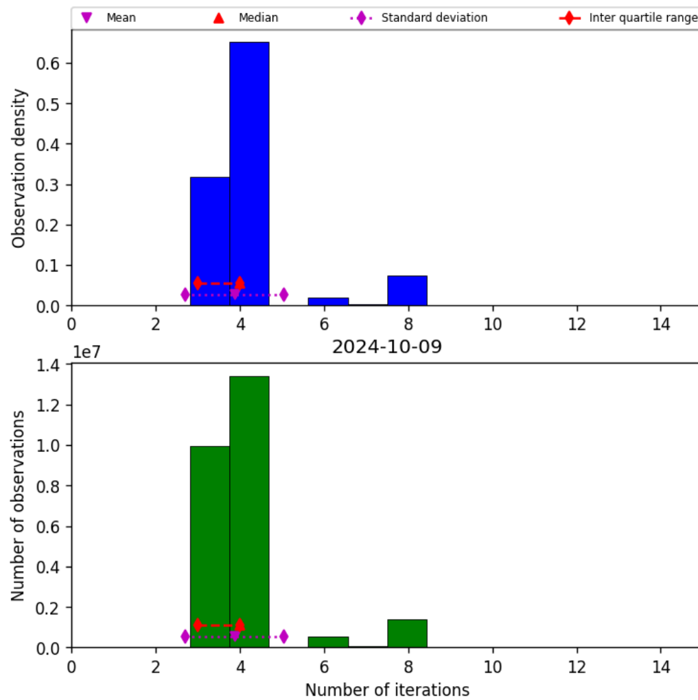
Figure 34: Histogram of “Number of iterations” for 2024-10-08 to 2024-10-10
