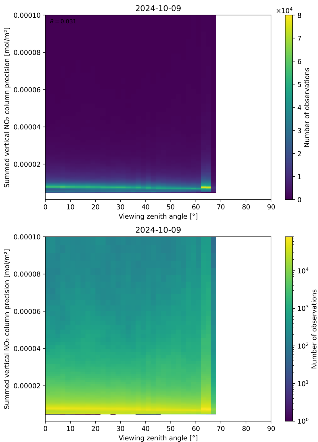
Figure 166: Scatter density plot of “Viewing zenith angle” against “Summed vertical NO 2 column precision” for 2024-10-08 to 2024-10-10.
