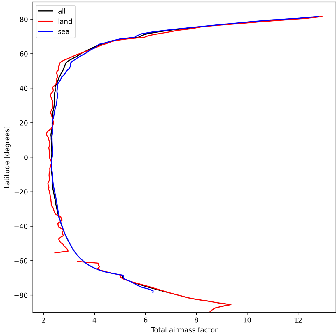
Figure 15: Zonal average of “Total airmass factor” for 2024-10-08 to 2024-10-10.
