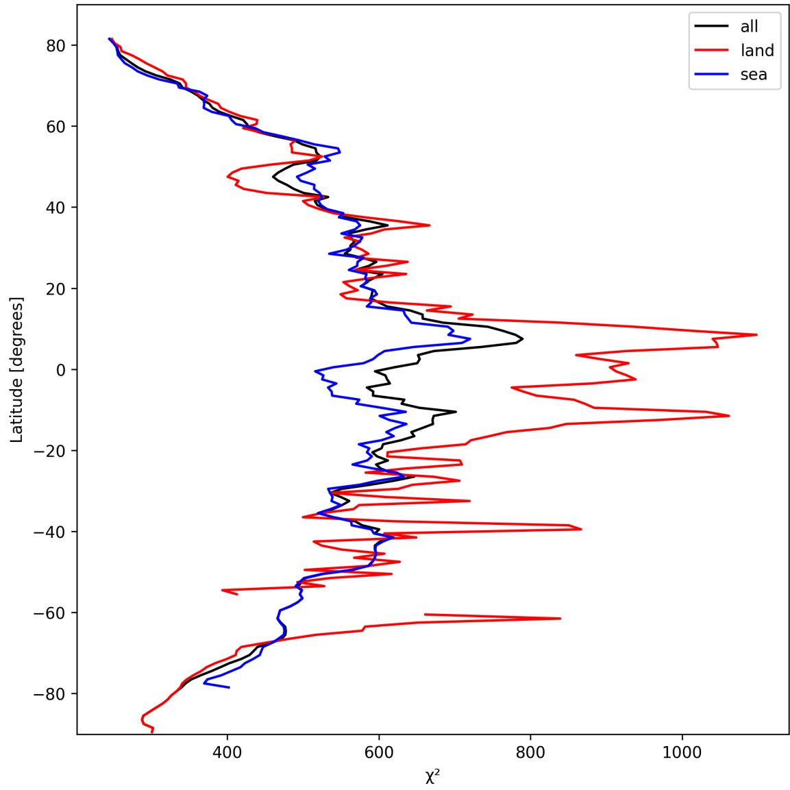
Figure 25: Zonal average of “ \chi^2 ” for 2024-10-08 to 2024-10-10.
