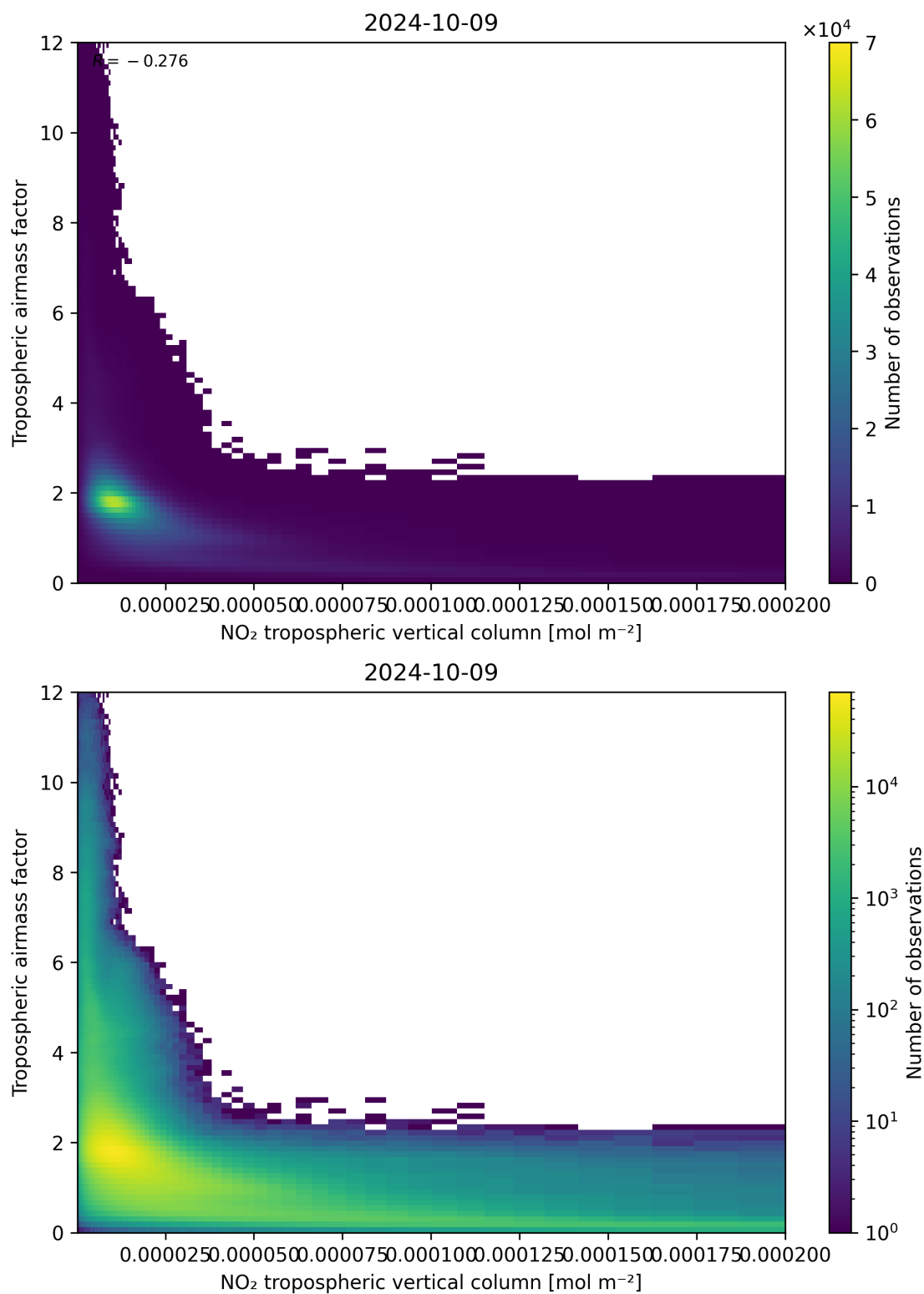
Figure 123: Scatter density plot of “NO 2 tropospheric vertical column” against “Tropospheric air mass factor” for 2024-10-08 to 2024-10-10.
