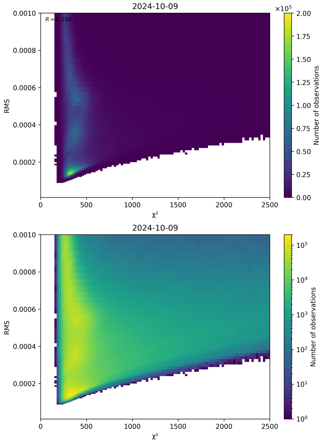
Figure 82: Scatter density plot of “ \chi^2 ” against “RMS” for 2024-10-08 to 2024-10-10.
