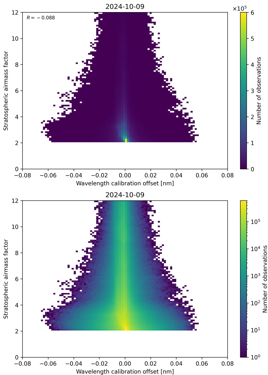
Figure 174: Scatter density plot of “Wavelength calibration offset” against “Stratospheric airmass factor” for 2024-10-08 to 2024-10-10.
