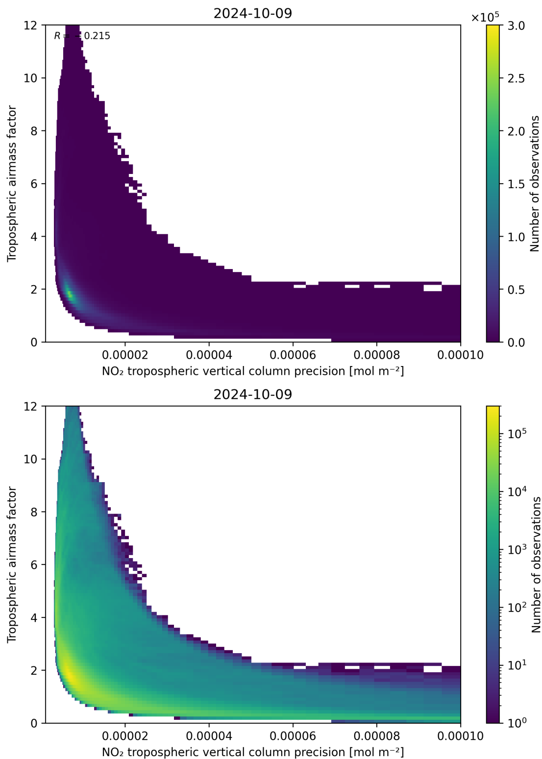
Figure 133: Scatter density plot of “NO 2 tropospheric vertical column precision” against “Tropospheric air mass factor” for 2024-10-08 to 2024-10-10.
