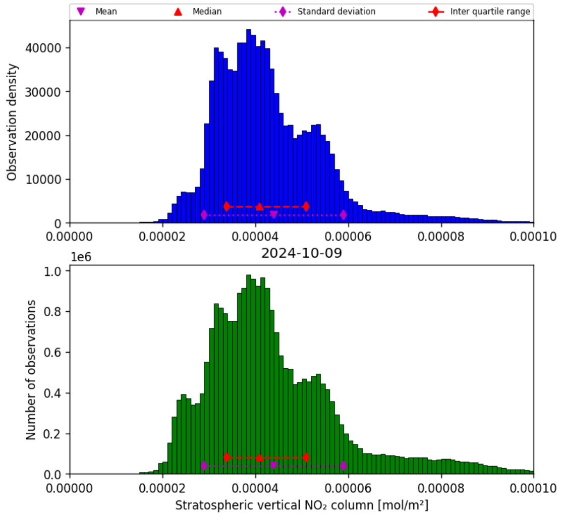
Figure 36: Histogram of “Stratospheric vertical NO 2 column” for 2024-10-08 to 2024-10-10
