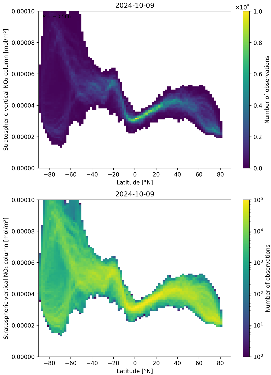
Figure 87: Scatter density plot of “Latitude” against “Stratospheric vertical NO 2 column” for 2024-10-08 to 2024-10-10.
