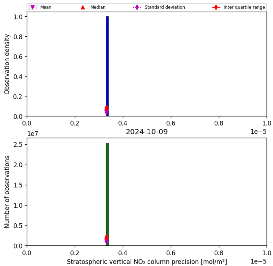
Figure 37: Histogram of “Stratospheric vertical NO 2 column precision” for 2024-10-08 to 2024-10-10
