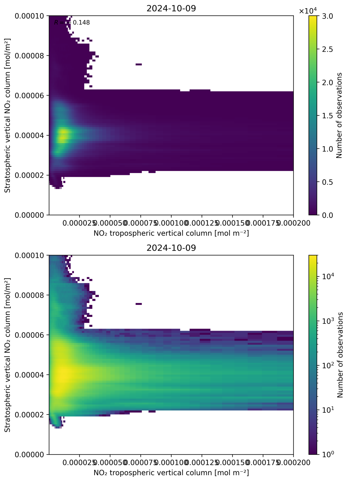
Figure 125: Scatter density plot of “NO 2 tropospheric vertical column” against “Stratospheric vertical NO 2 column” for 2024-10-08 to 2024-10-10.
