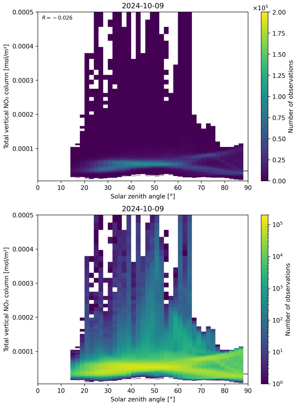
Figure 153: Scatter density plot of “Solar zenith angle” against “Total vertical NO 2 column” for 2024-10-08 to 2024-10-10.
