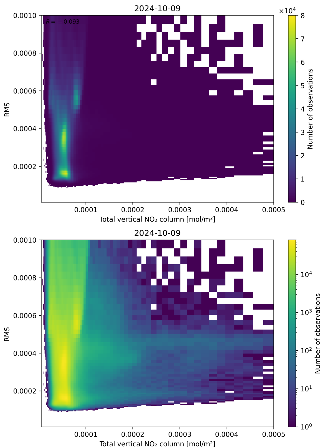
Figure 120: Scatter density plot of “Total vertical NO 2 column” against “RMS” for 2024-10-08 to 2024-10-10.
