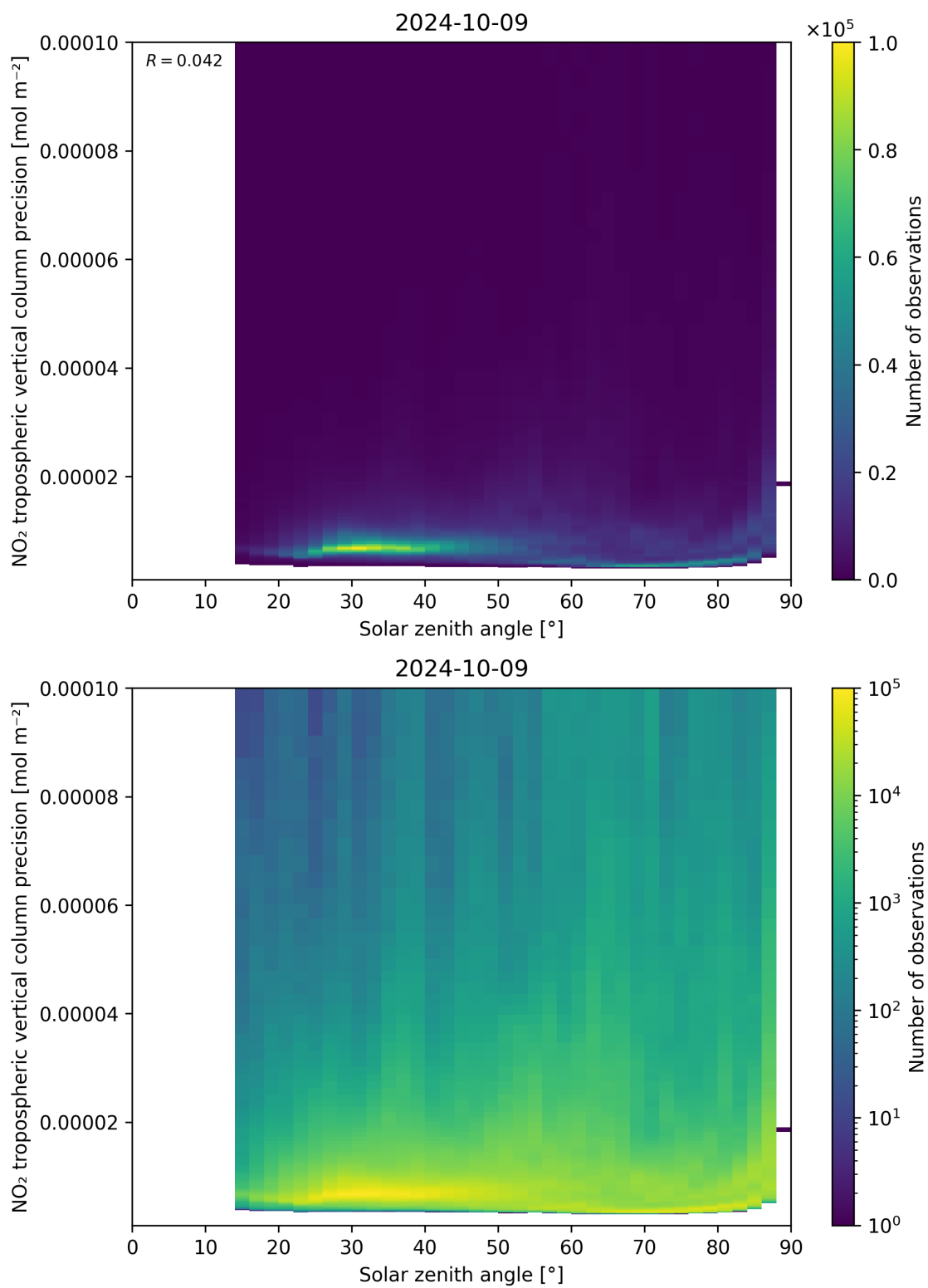
Figure 156: Scatter density plot of “Solar zenith angle” against “NO 2 tropospheric vertical column precision” for 2024-10-08 to 2024-10-10.
