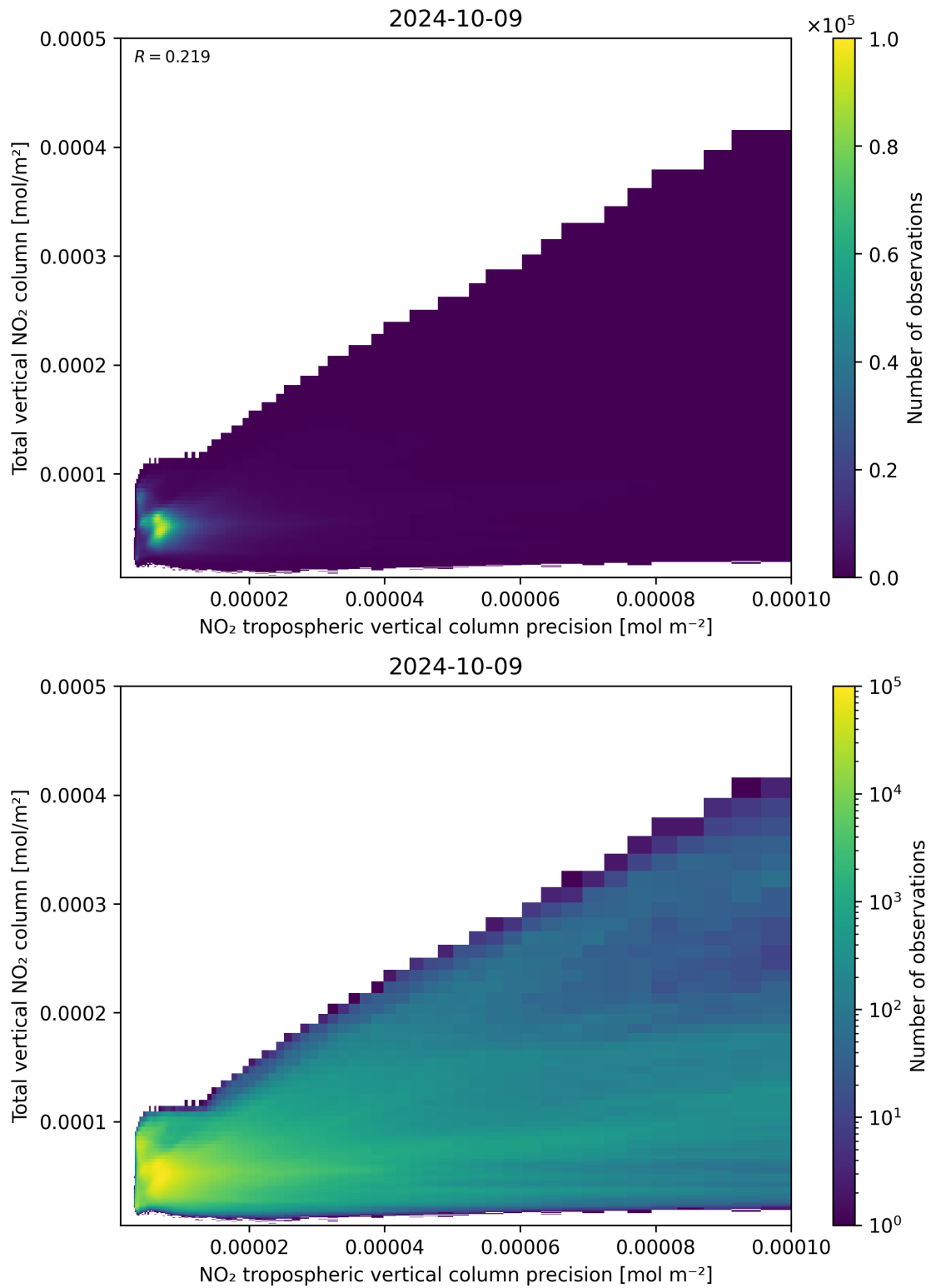
Figure 138: Scatter density plot of “NO 2 tropospheric vertical column precision” against “Total vertical NO 2 column” for 2024-10-08 to 2024-10-10.
