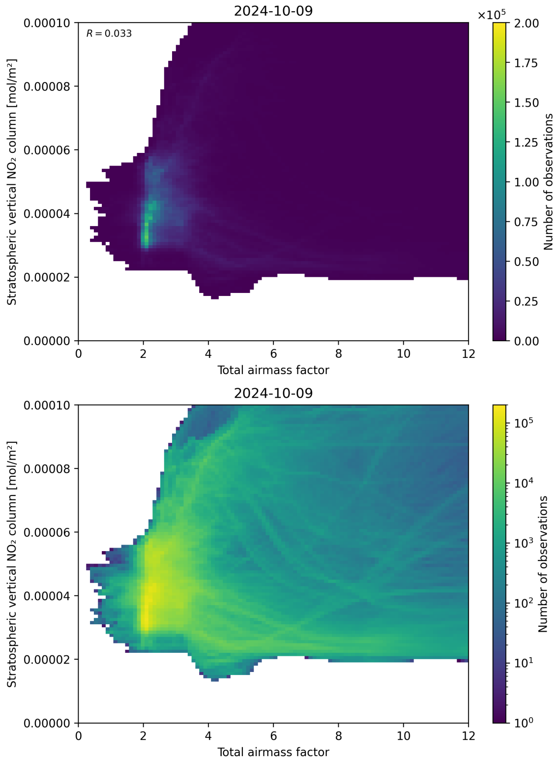
Figure 64: Scatter density plot of “Total airmass factor” against “Stratospheric vertical NO 2 column” for 2024-10-08 to 2024-10-10.
