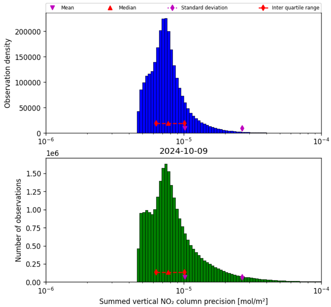
Figure 41: Histogram of “Summed vertical NO 2 column precision” for 2024-10-08 to 2024-10-10
