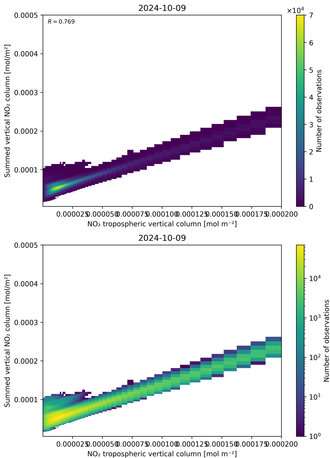
Figure 126: Scatter density plot of “NO 2 tropospheric vertical column” against “Summed vertical NO 2 column” for 2024-10-08 to 2024-10-10.
