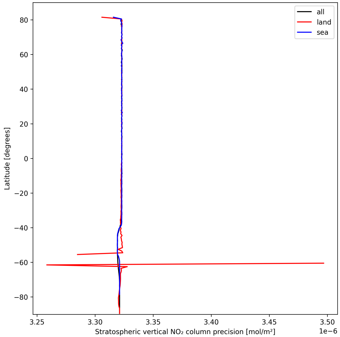
Figure 20: Zonal average of “Stratospheric vertical NO 2 column precision” for 2024-10-08 to 2024-10-10.
