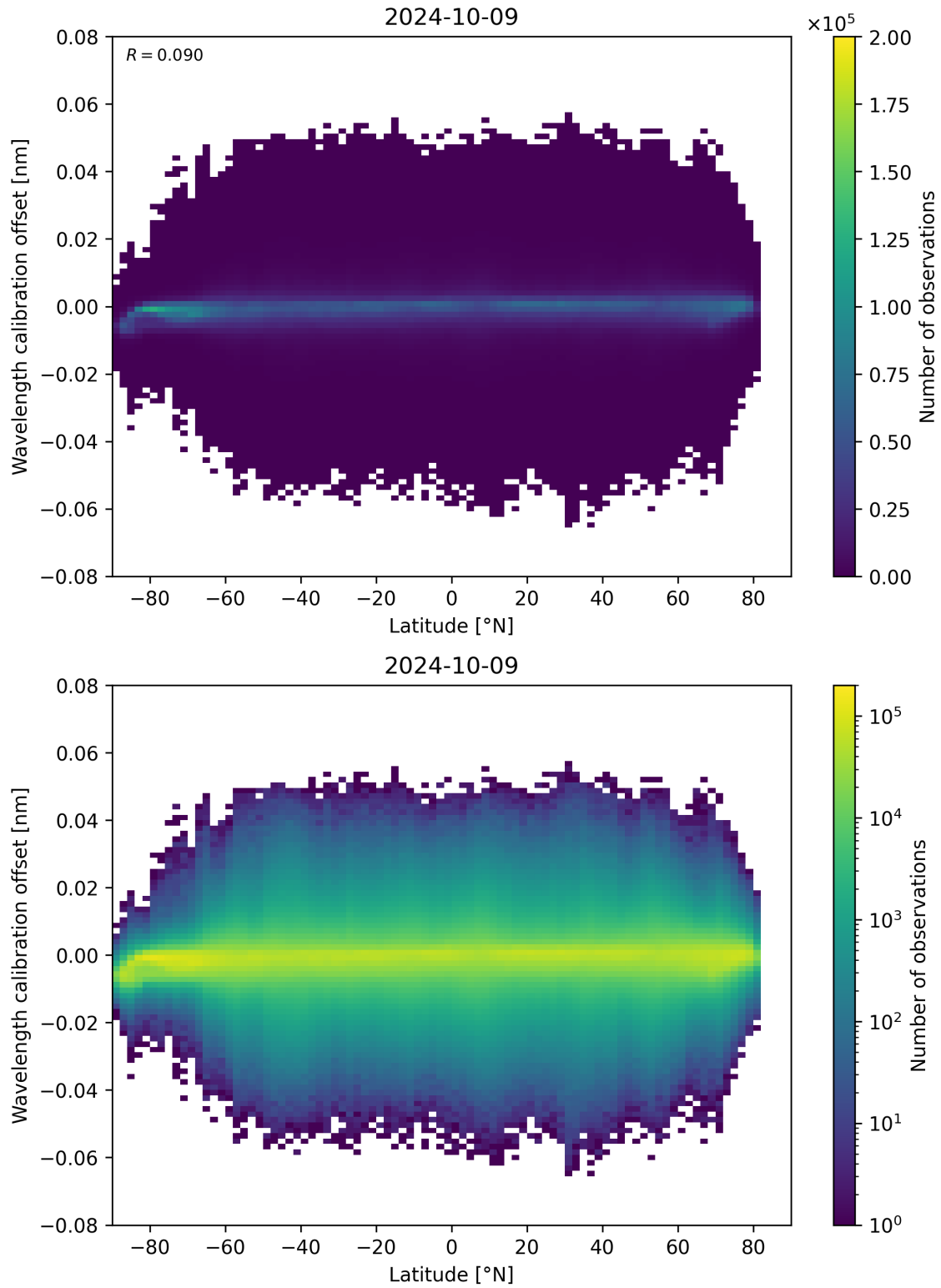
Figure 95: Scatter density plot of “Latitude” against “Wavelength calibration offset” for 2024-10-08 to 2024-10-10.
