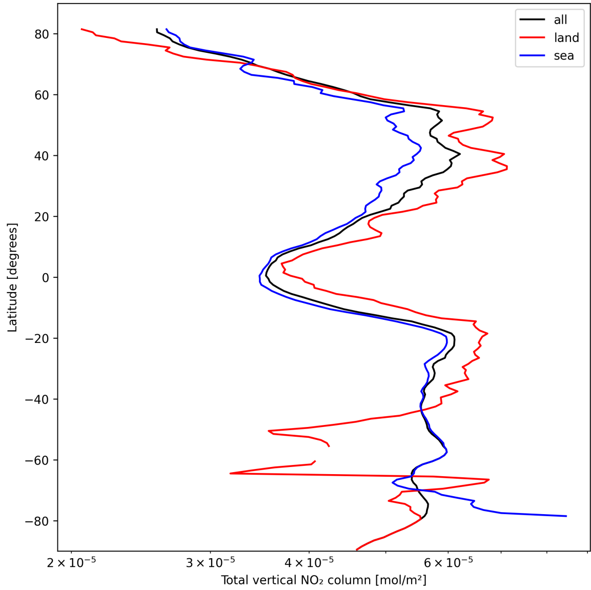
Figure 21: Zonal average of “Total vertical NO 2 column” for 2024-10-08 to 2024-10-10.
