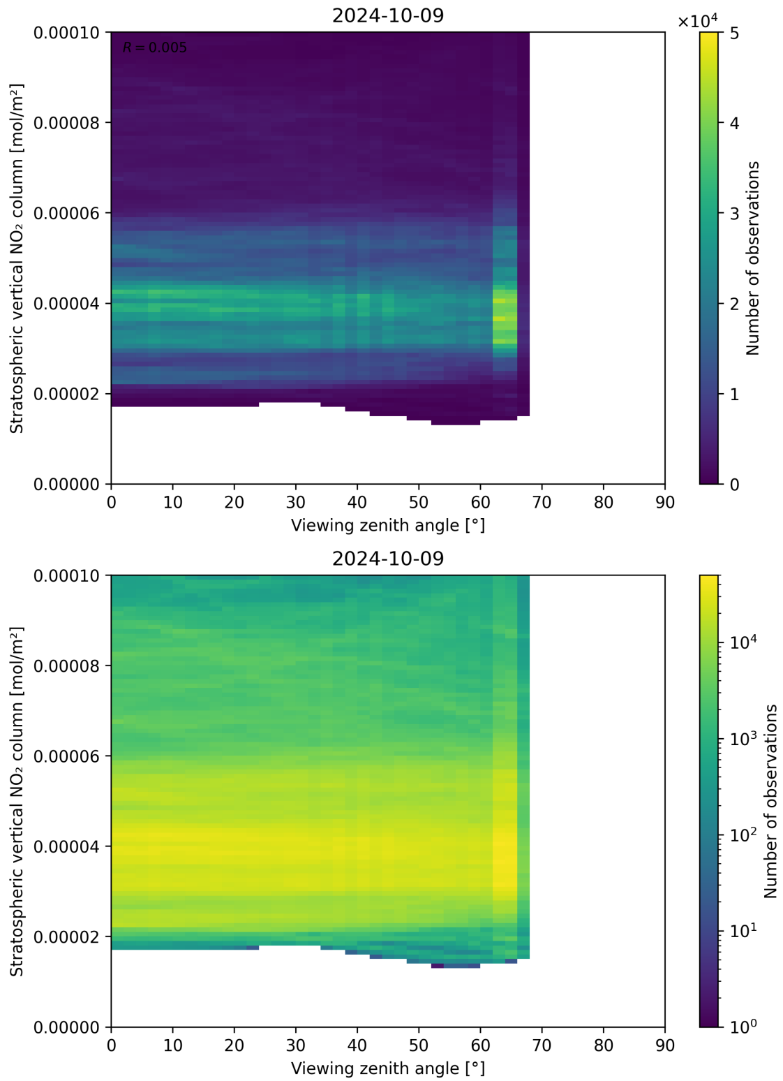
Figure 164: Scatter density plot of “Viewing zenith angle” against “Stratospheric vertical NO 2 column” for 2024-10-08 to 2024-10-10.
