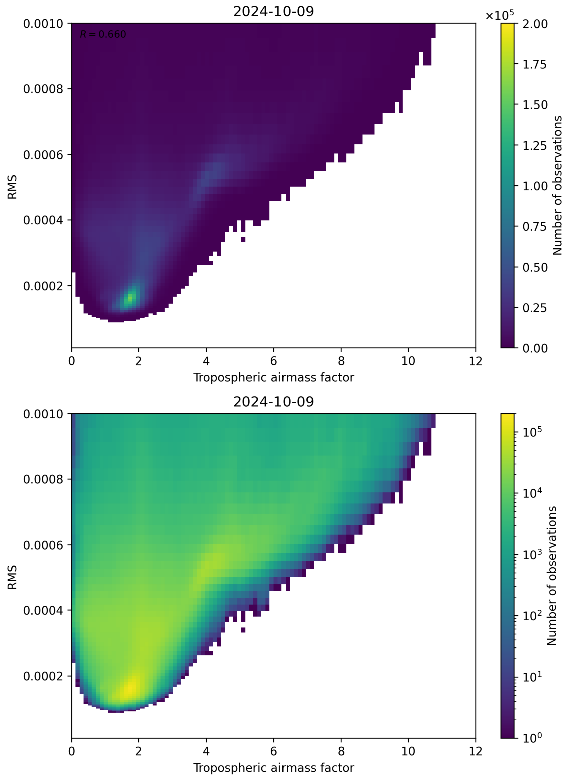
Figure 79: Scatter density plot of “Tropospheric airmass factor” against “RMS” for 2024-10-08 to 2024-10-10.
