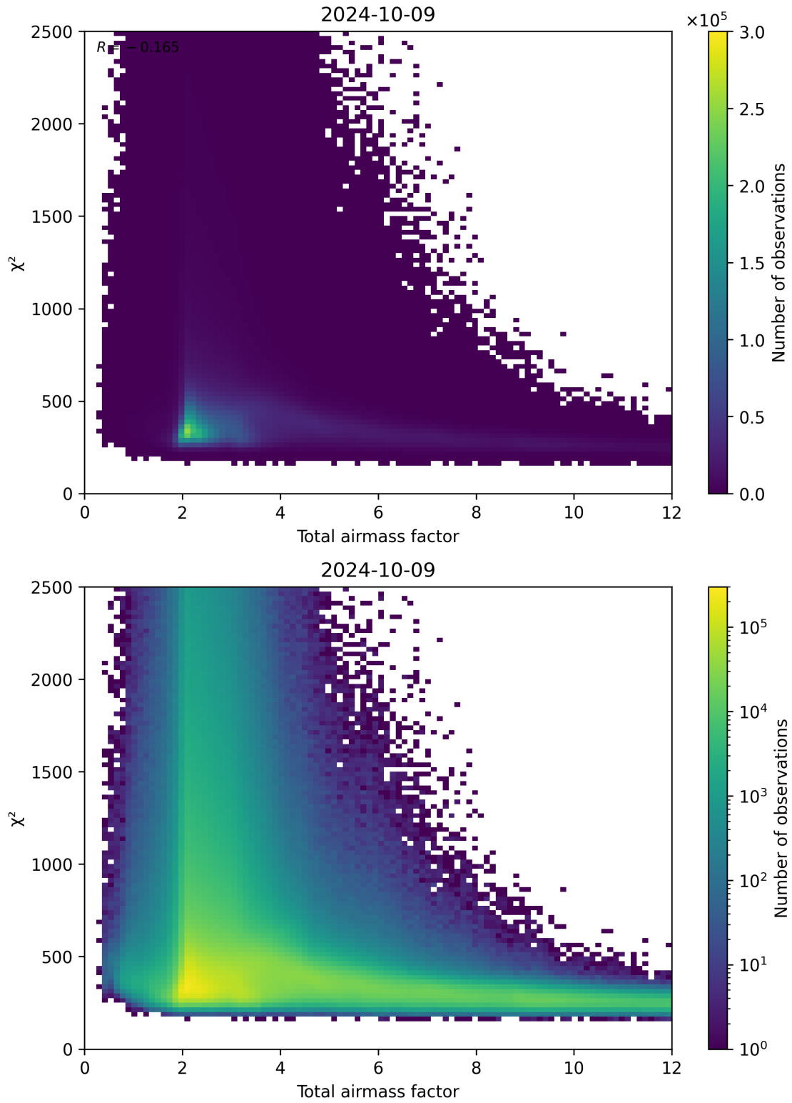
Figure 63: Scatter density plot of “Total airmass factor” against “ \chi^2 ” for 2024-10-08 to 2024-10-10.
