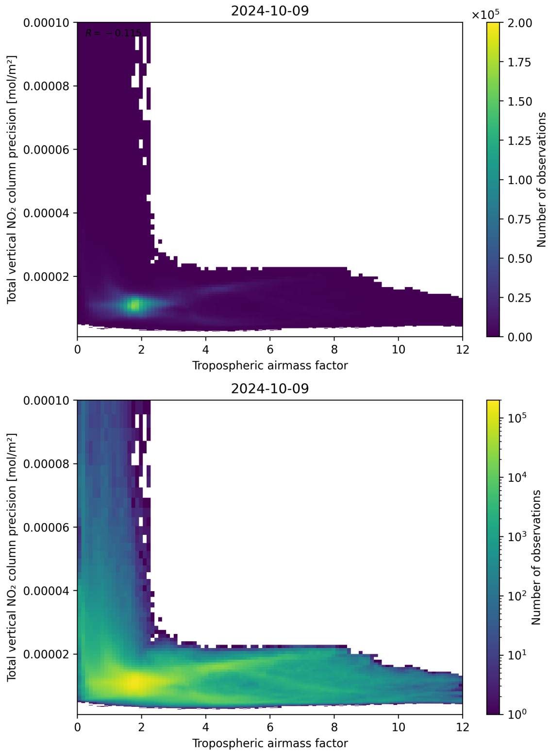
Figure 78: Scatter density plot of “Tropospheric air mass factor” against “Total vertical NO 2 column precision” for 2024-10-08 to 2024-10-10.
