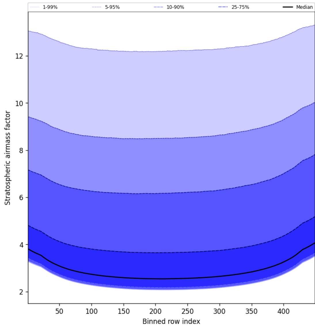
Figure 61: Along track statistics of “Stratospheric airmass factor” for 2024-10-08 to 2024-10-10
