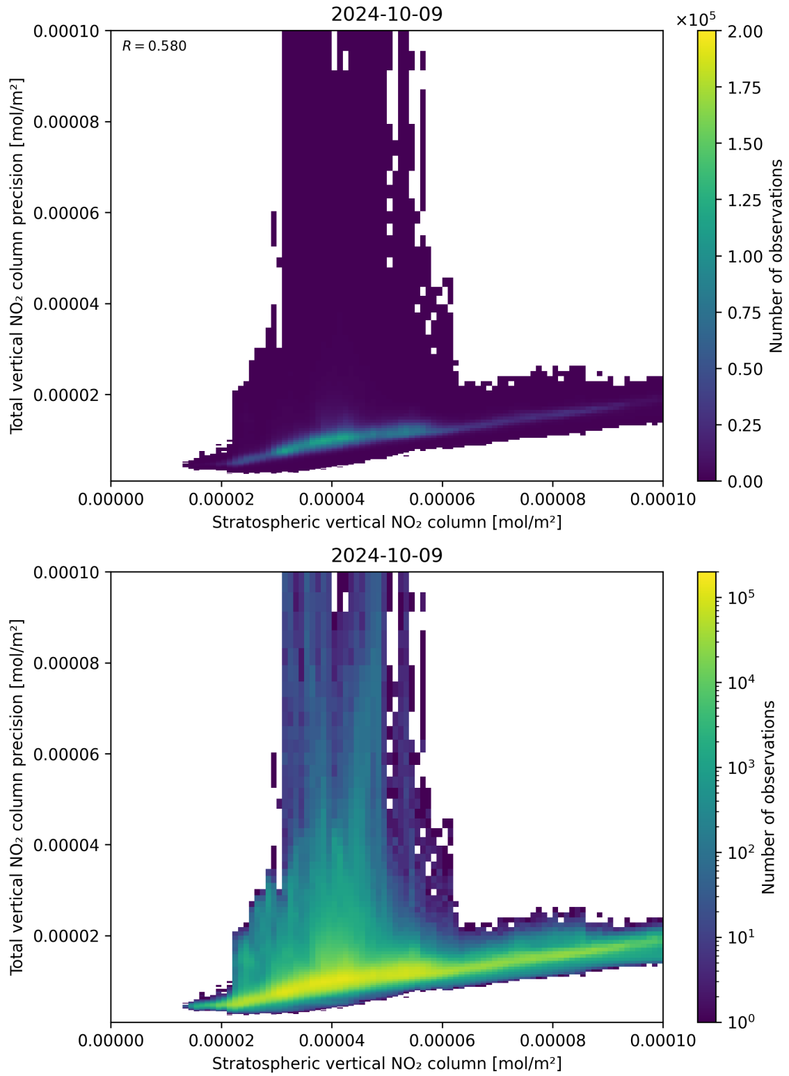
Figure 101: Scatter density plot of “Stratospheric vertical NO 2 column” against “Total vertical NO 2 column precision” for 2024-10-08 to 2024-10-10.
