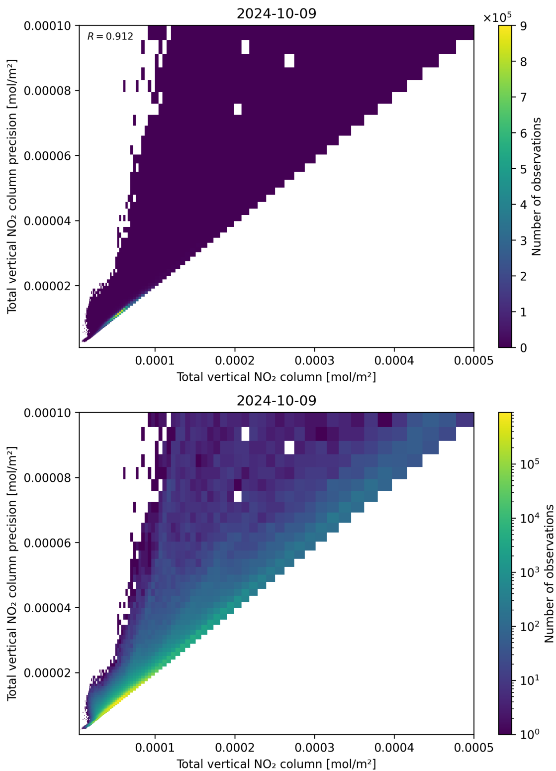
Figure 114: Scatter density plot of “Total vertical NO 2 column” against “Total vertical NO 2 column precision” for 2024-10-08 to 2024-10-10.
