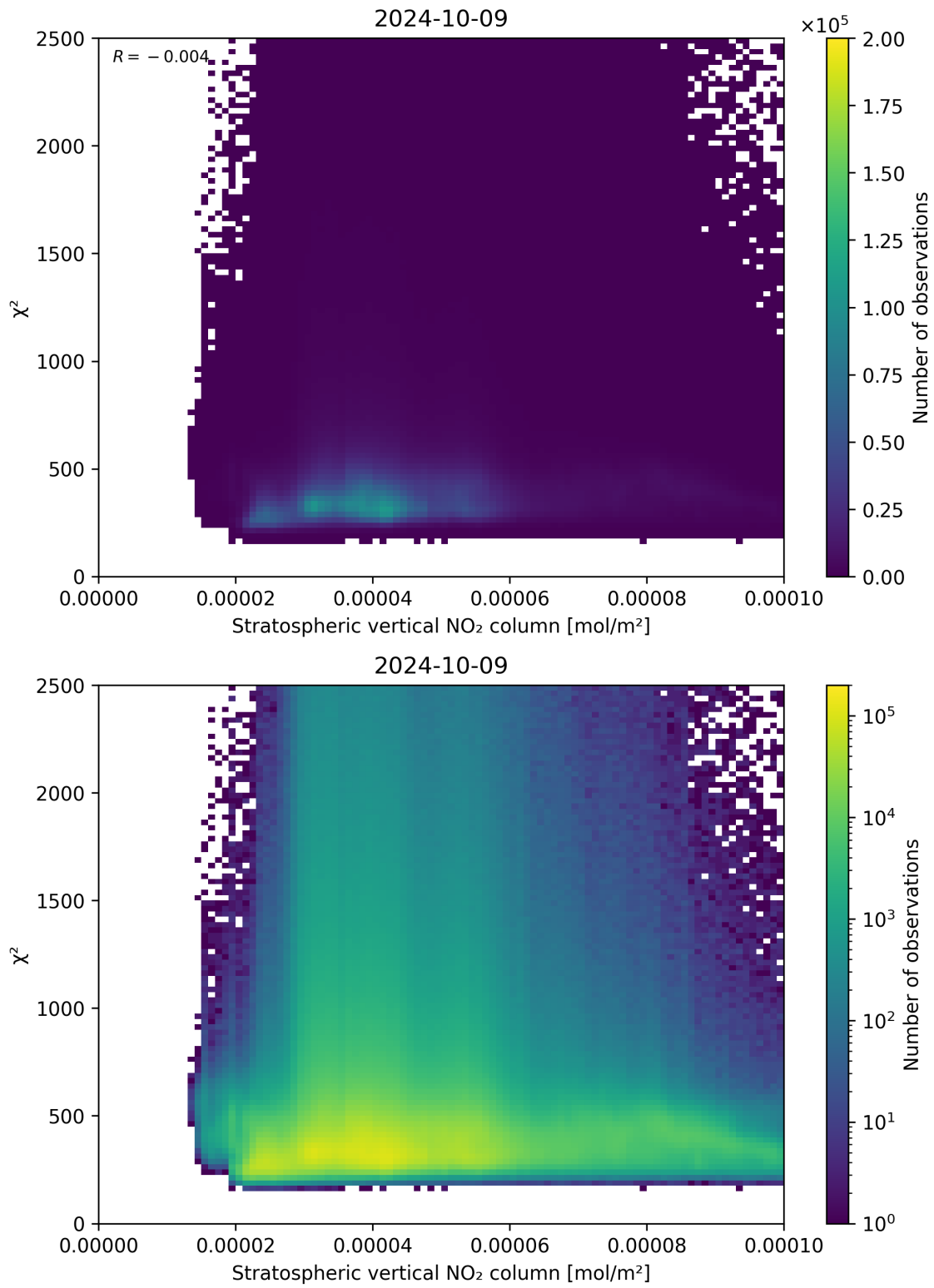
Figure 97: Scatter density plot of “Stratospheric vertical NO 2 column” against “ \chi^2 ” for 2024-10-08 to 2024-10-10.
