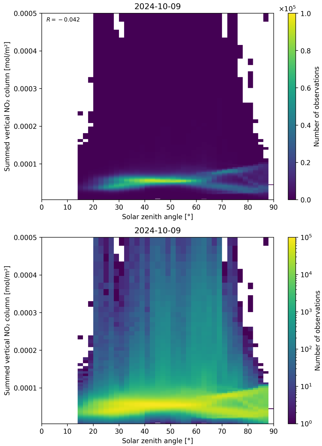
Figure 151: Scatter density plot of “Solar zenith angle” against “Summed vertical NO 2 column” for 2024-10-08 to 2024-10-10.
