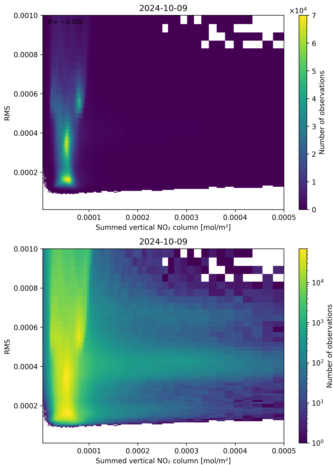
Figure 109: Scatter density plot of “Summed vertical NO 2 column” against “RMS” for 2024-10-08 to 2024-10-10.
