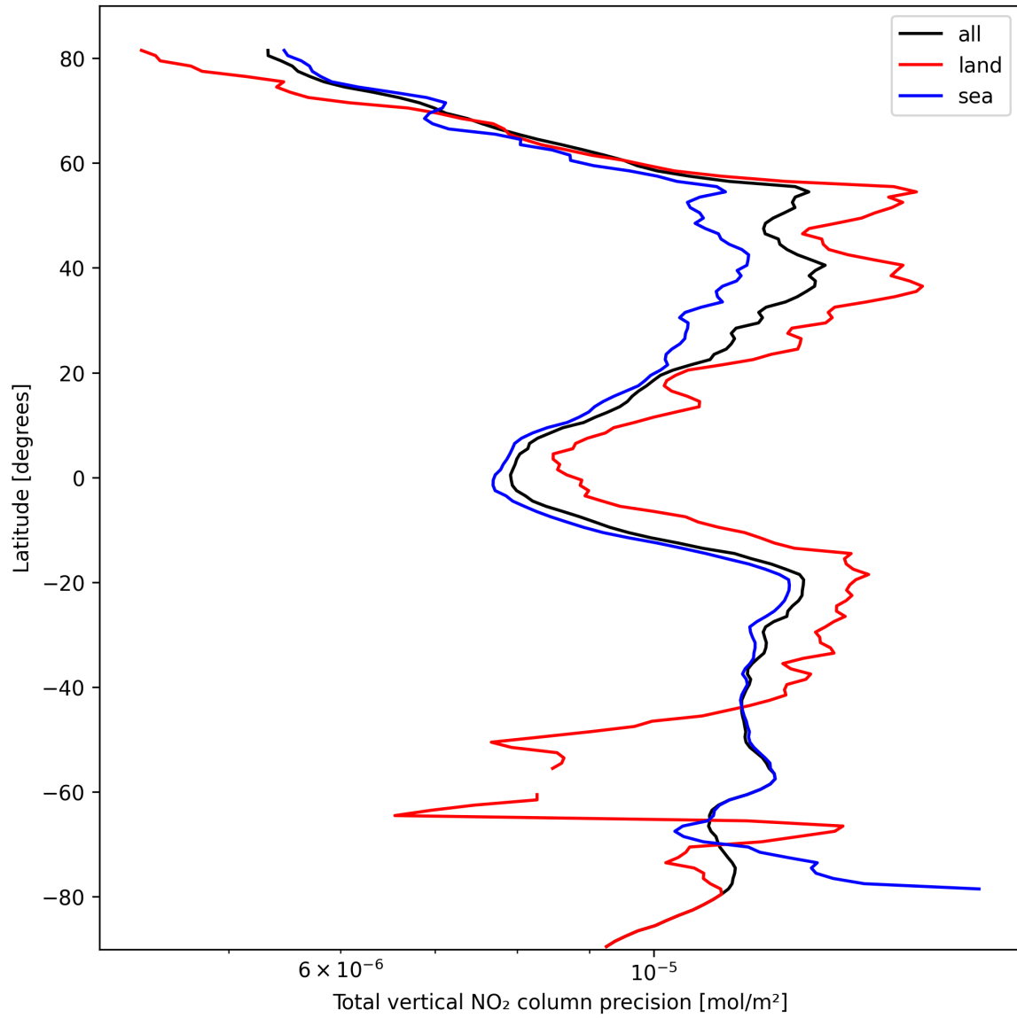
Figure 22: Zonal average of “Total vertical NO 2 column precision” for 2024-10-08 to 2024-10-10.
