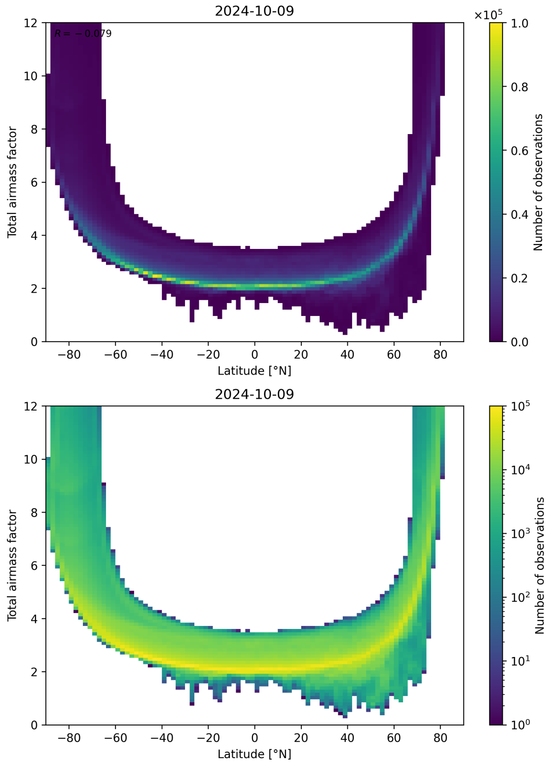
Figure 84: Scatter density plot of “Latitude” against “Total airmass factor” for 2024-10-08 to 2024-10-10.
