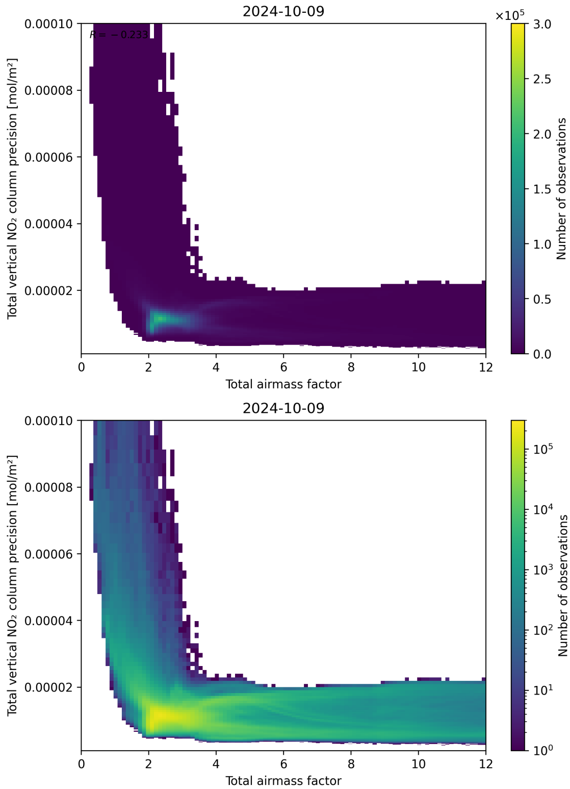
Figure 68: Scatter density plot of “Total airmass factor” against “Total vertical NO 2 column precision” for 2024-10-08 to 2024-10-10.
