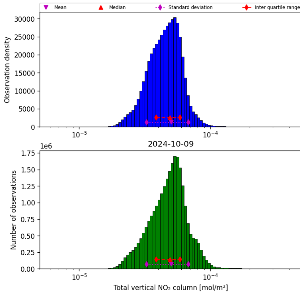
Figure 38: Histogram of “Total vertical NO 2 column” for 2024-10-08 to 2024-10-10
