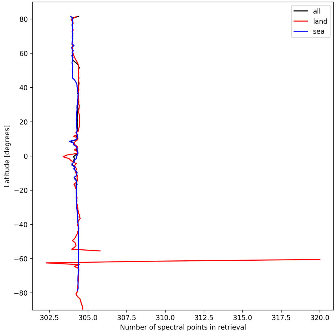
Figure 16: Zonal average of “Number of spectral points in retrieval” for 2024-10-08 to 2024-10-10.
