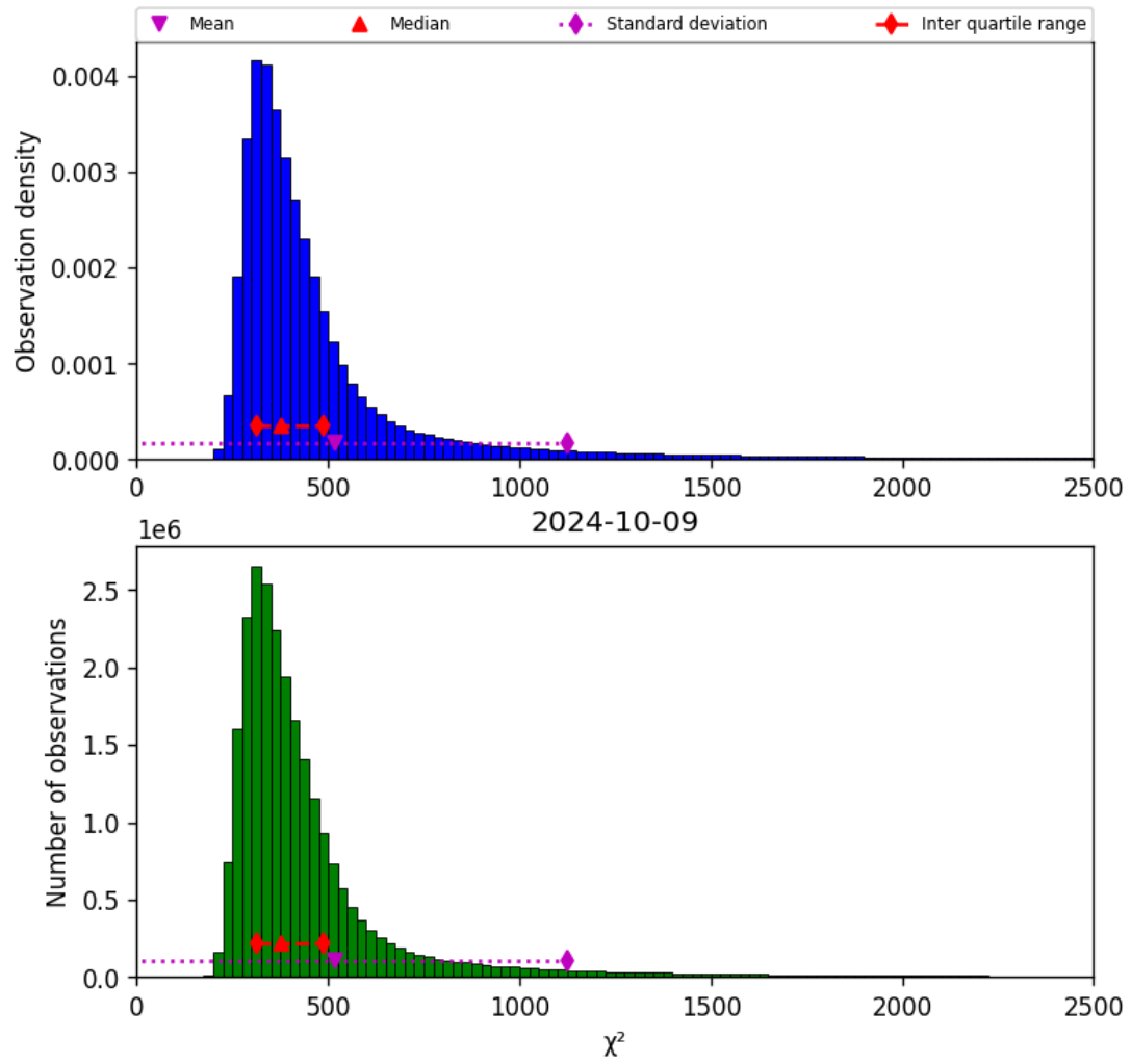
Figure 42: Histogram of “ \chi^2 ” for 2024-10-08 to 2024-10-10
