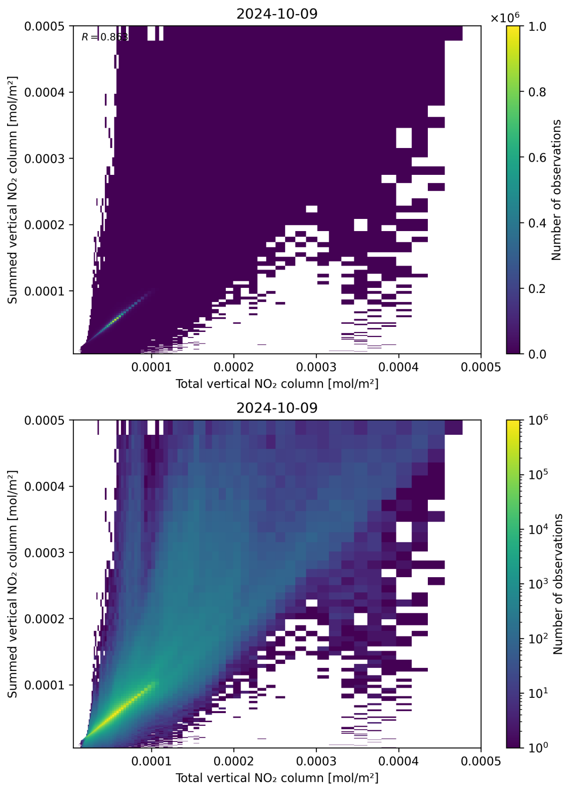
Figure 112: Scatter density plot of “Total vertical NO 2 column” against “Summed vertical NO 2 column” for 2024-10-08 to 2024-10-10.
