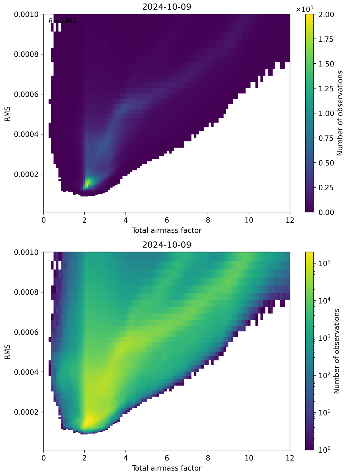
Figure 69: Scatter density plot of “Total airmass factor” against “RMS” for 2024-10-08 to 2024-10-10.
