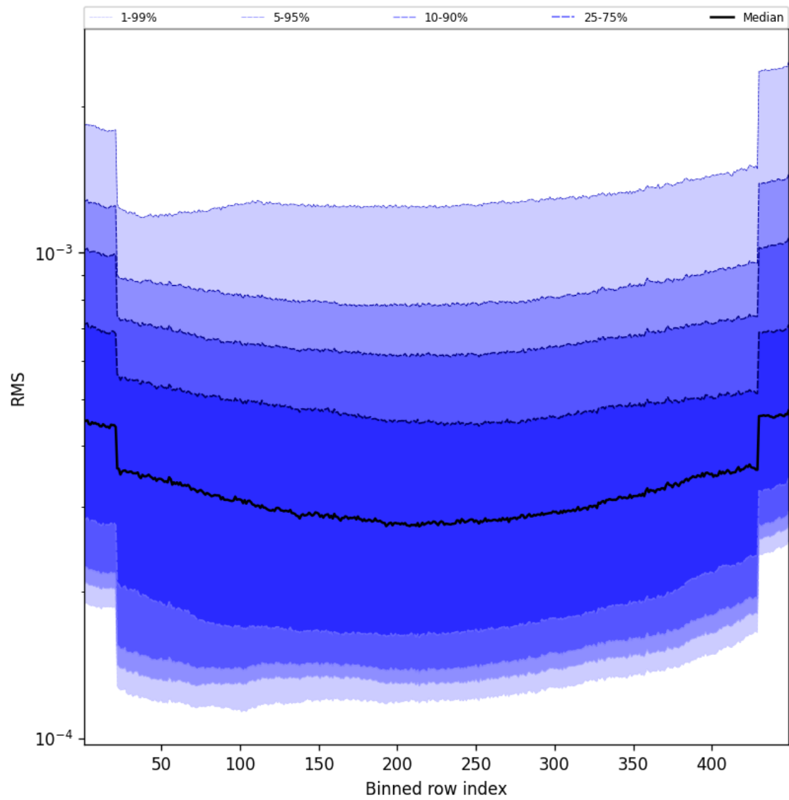
Figure 60: Along track statistics of “RMS” for 2024-10-08 to 2024-10-10
