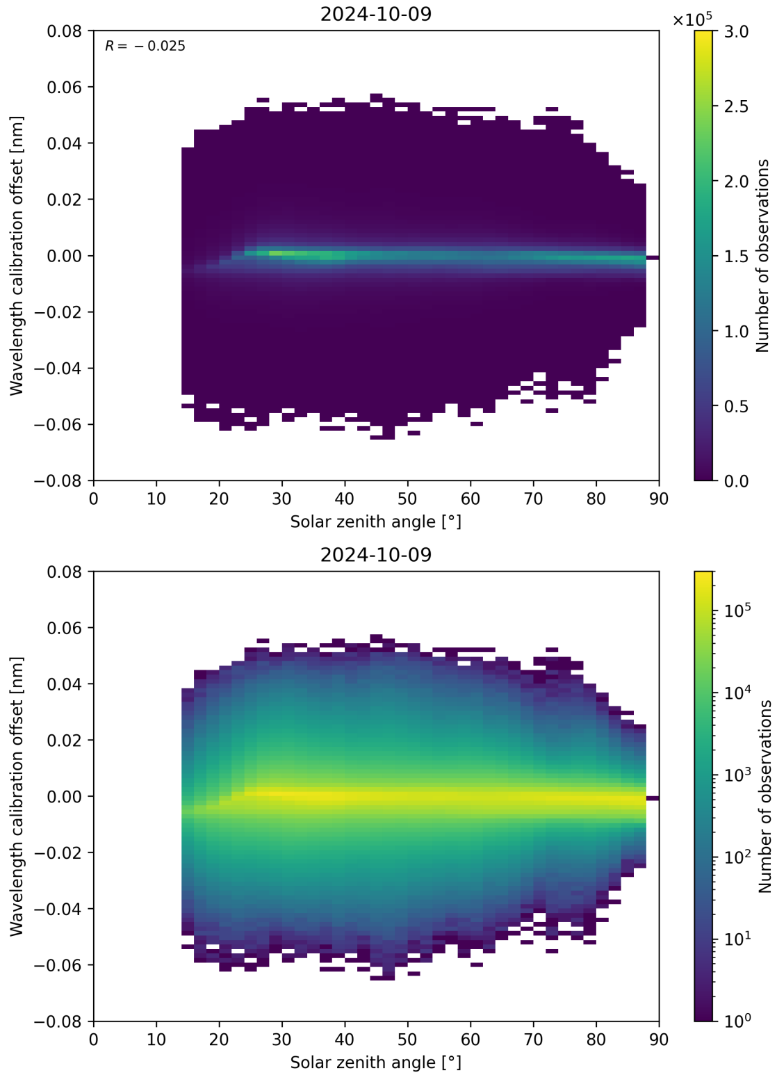
Figure 158: Scatter density plot of “Solar zenith angle” against “Wavelength calibration offset” for 2024-10-08 to 2024-10-10.
