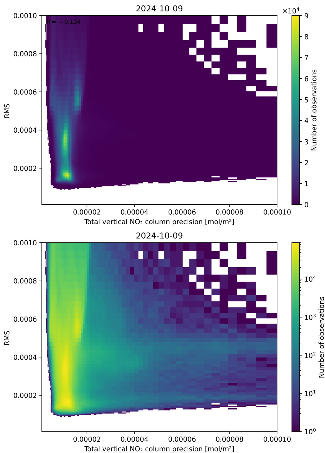
Figure 119: Scatter density plot of “Total vertical NO 2 column precision” against “RMS” for 2024-10-08 to 2024-10-10.
