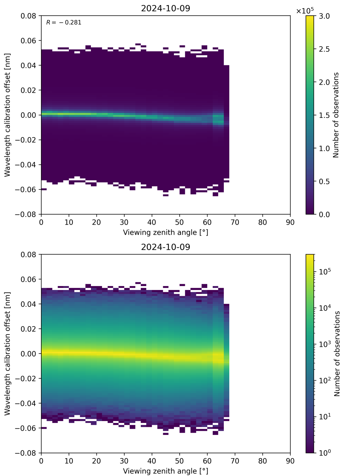
Figure 173: Scatter density plot of “Viewing zenith angle” against “Wavelength calibration offset” for 2024-10-08 to 2024-10-10.
