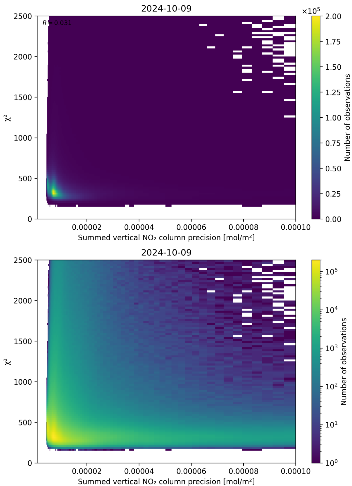
Figure 107: Scatter density plot of “Summed vertical NO 2 column precision” against “ \chi^2 ” for 2024-10-08 to 2024-10-10.
