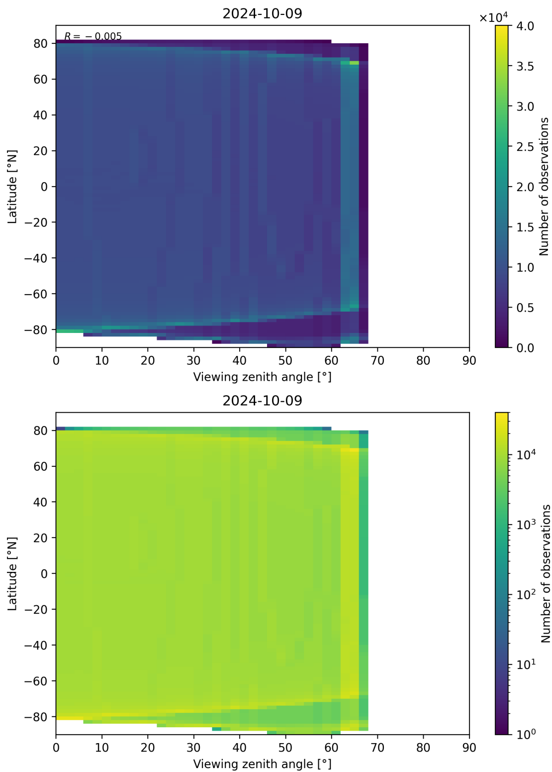
Figure 163: Scatter density plot of “Viewing zenith angle” against “Latitude” for 2024-10-08 to 2024-10-10.
