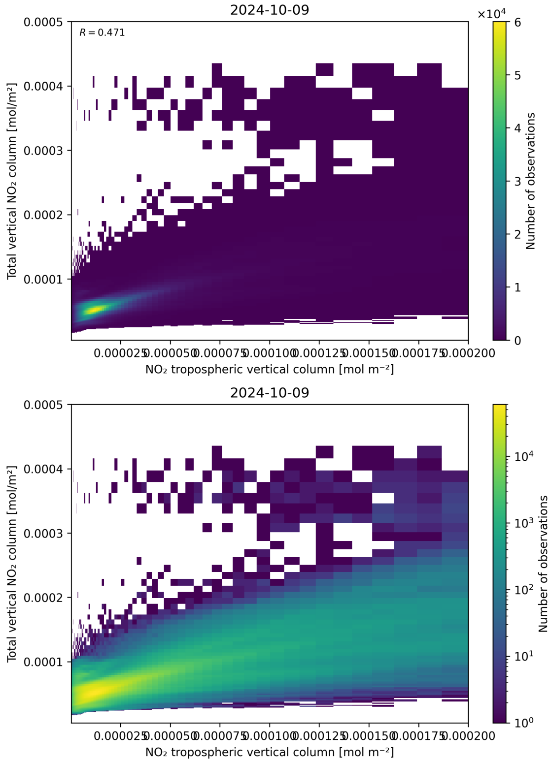
Figure 128: Scatter density plot of “NO 2 tropospheric vertical column” against “Total vertical NO 2 column” for 2024-10-08 to 2024-10-10.
