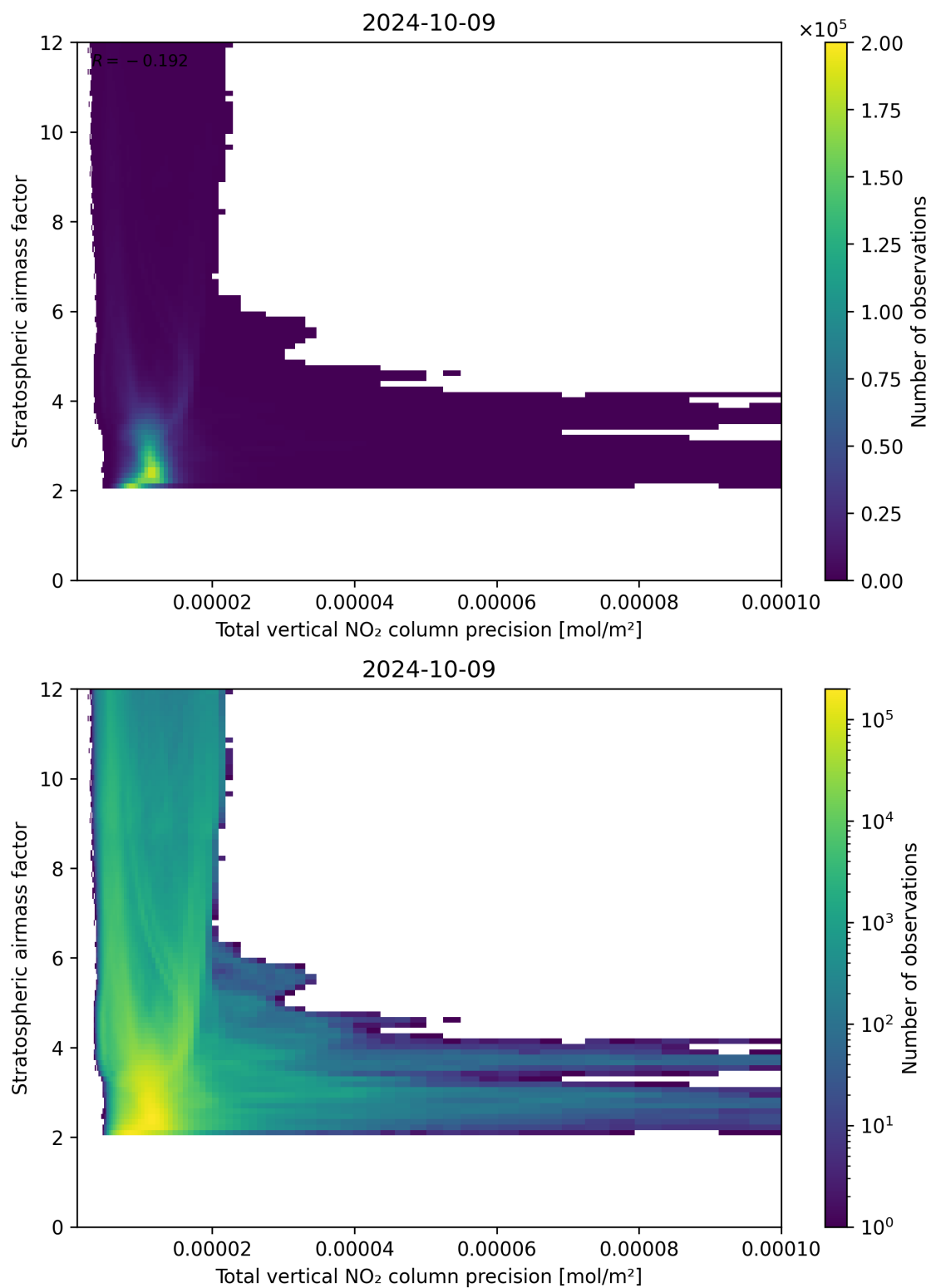
Figure 115: Scatter density plot of “Total vertical NO 2 column precision” against “Stratospheric airmass factor” for 2024-10-08 to 2024-10-10.
