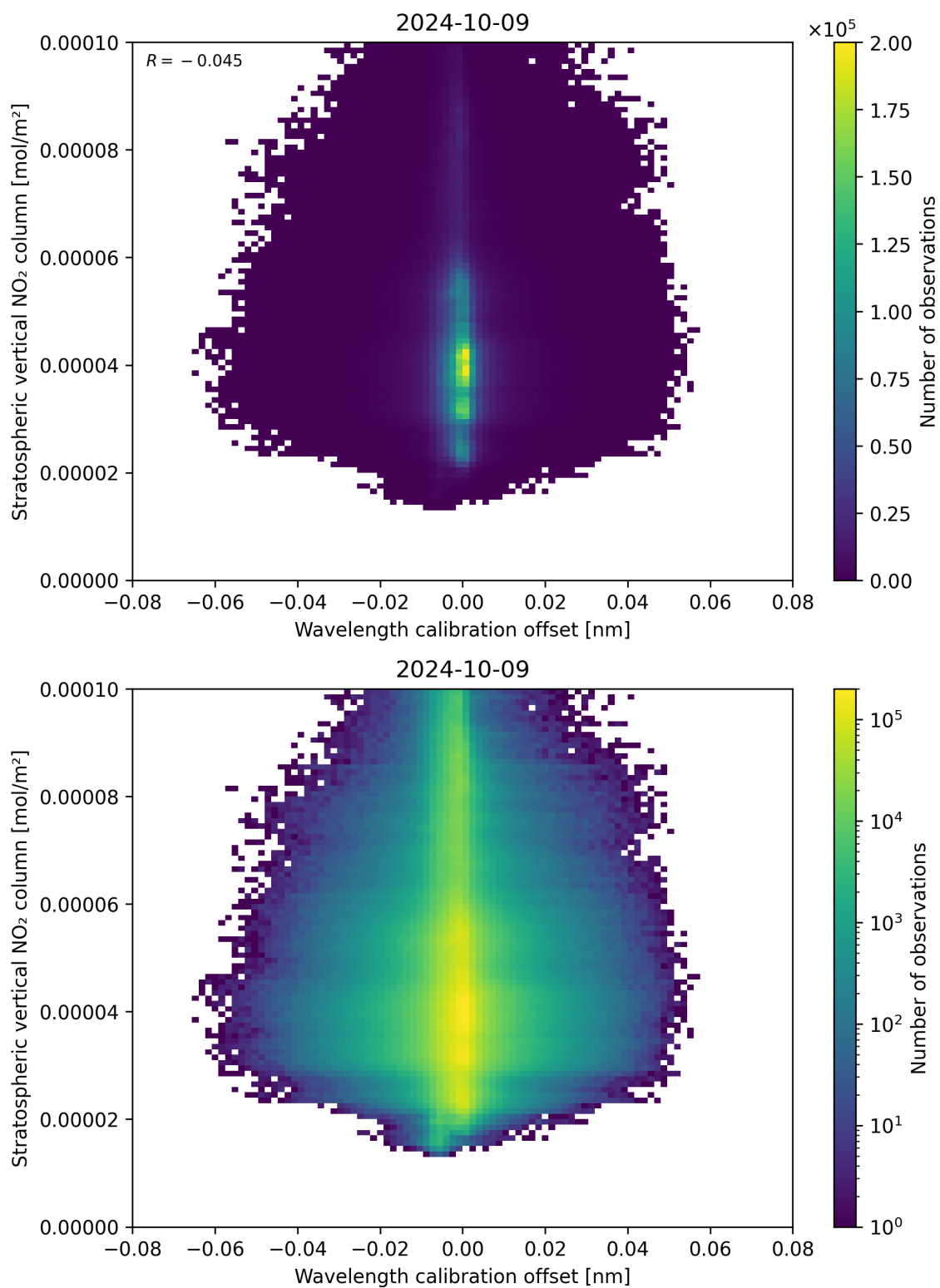
Figure 176: Scatter density plot of “Wavelength calibration offset” against “Stratospheric vertical NO 2 column” for 2024-10-08 to 2024-10-10.
