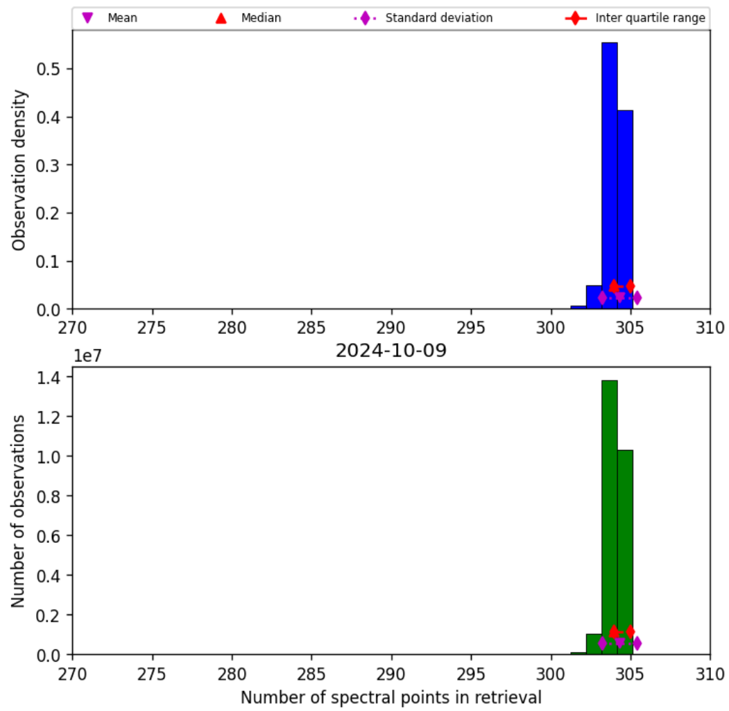
Figure 33: Histogram of “Number of spectral points in retrieval” for 2024-10-08 to 2024-10-10
