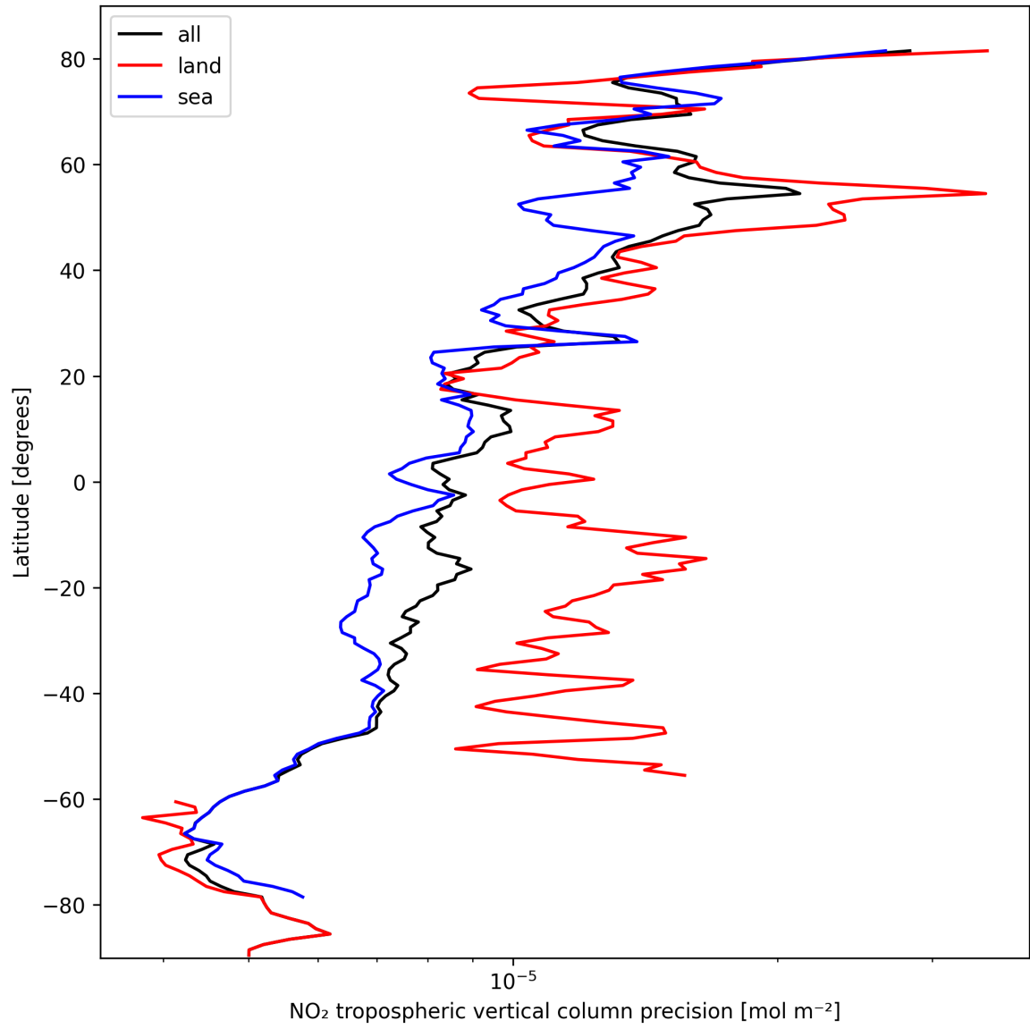
Figure 13: Zonal average of “NO 2 tropospheric vertical column precision” for 2024-10-08 to 2024-10-10.
