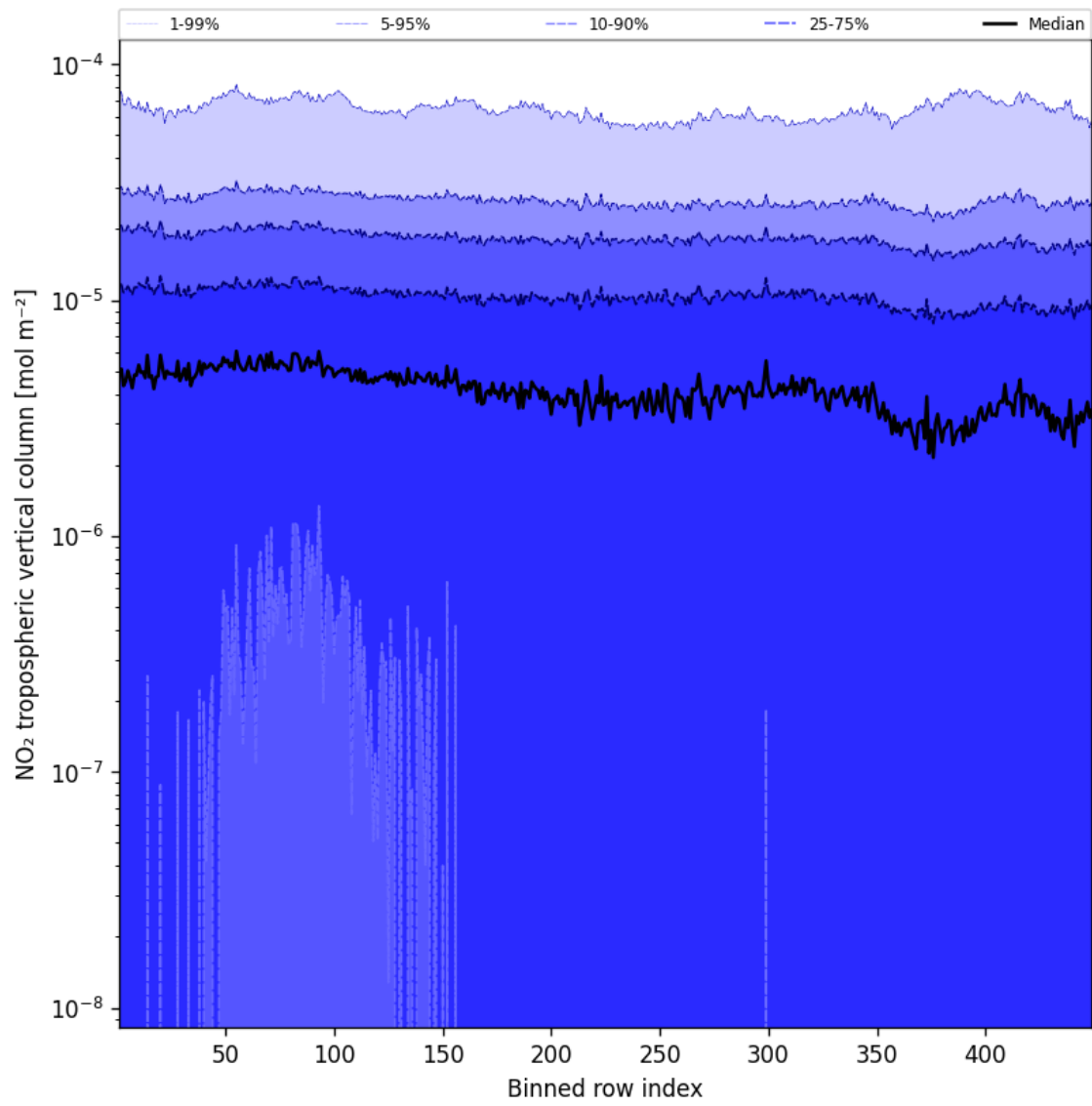
Figure 46: Along track statistics of “NO 2 tropospheric vertical column” for 2024-10-08 to 2024-10-10
