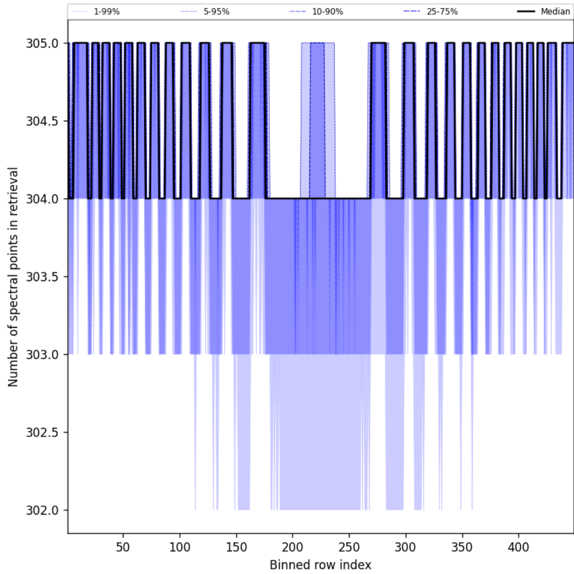
Figure 50: Along track statistics of “Number of spectral points in retrieval” for 2024-10-08 to 2024-10-10
