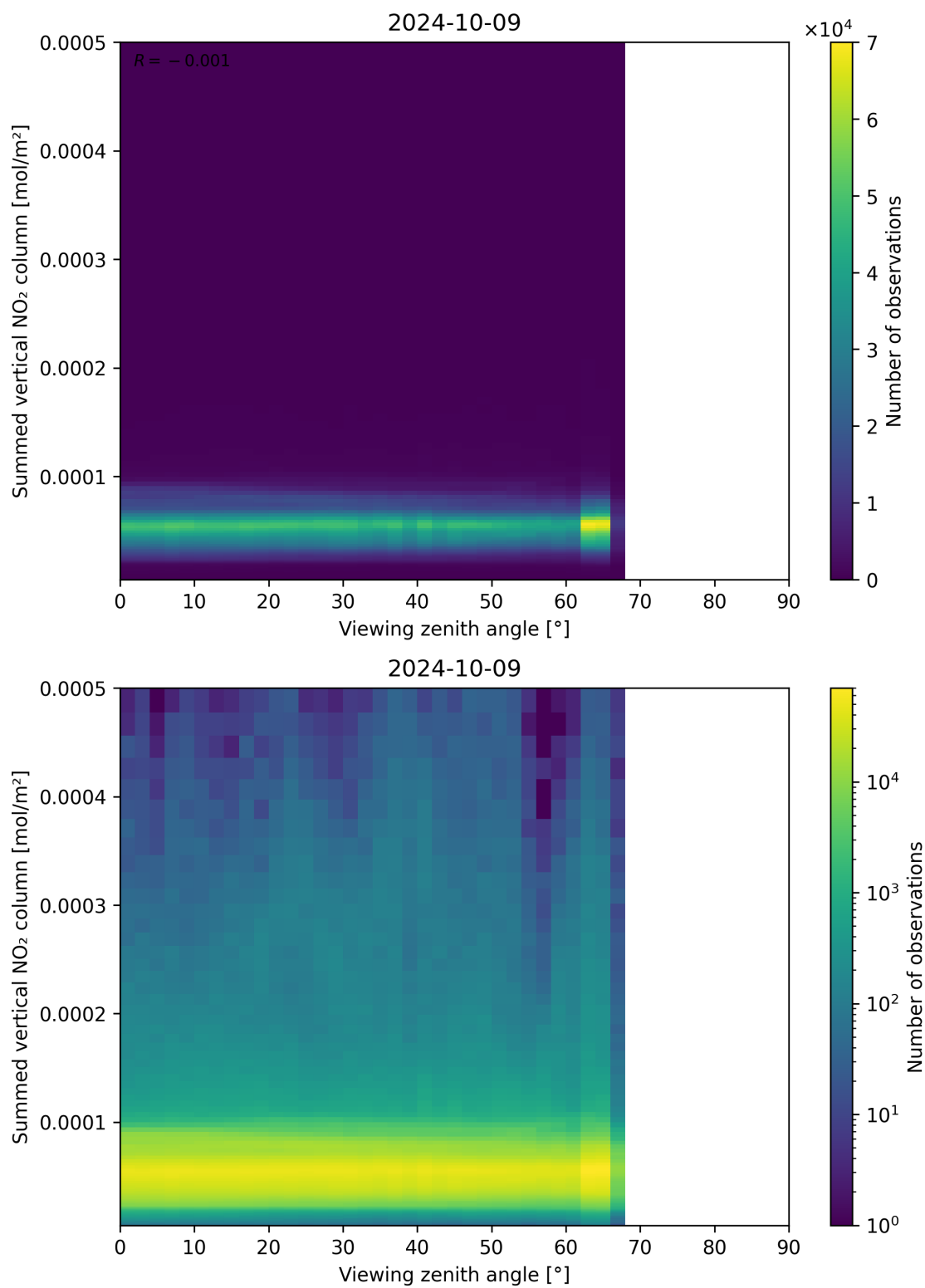
Figure 165: Scatter density plot of “Viewing zenith angle” against “Summed vertical NO 2 column” for 2024-10-08 to 2024-10-10.
