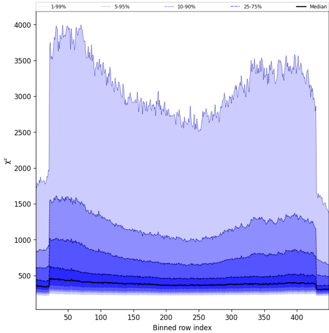
Figure 59: Along track statistics of “ \chi^2 ” for 2024-10-08 to 2024-10-10
