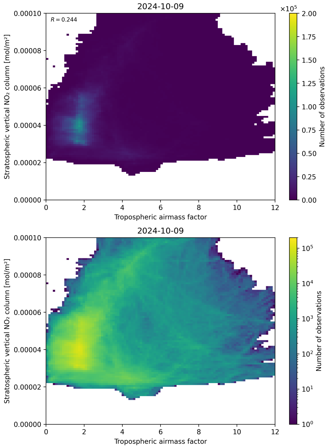
Figure 74: Scatter density plot of “Tropospheric air mass factor” against “Stratospheric vertical NO 2 column” for 2024-10-08 to 2024-10-10.
