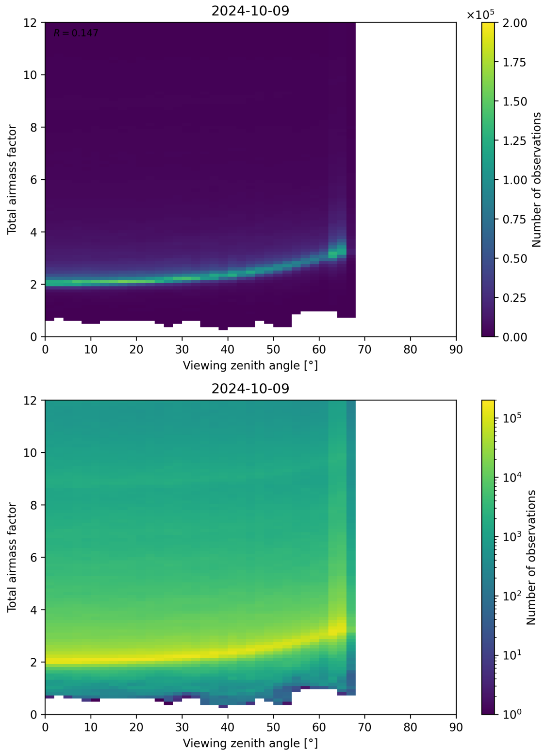
Figure 160: Scatter density plot of “Viewing zenith angle” against “Total airmass factor” for 2024-10-08 to 2024-10-10.
