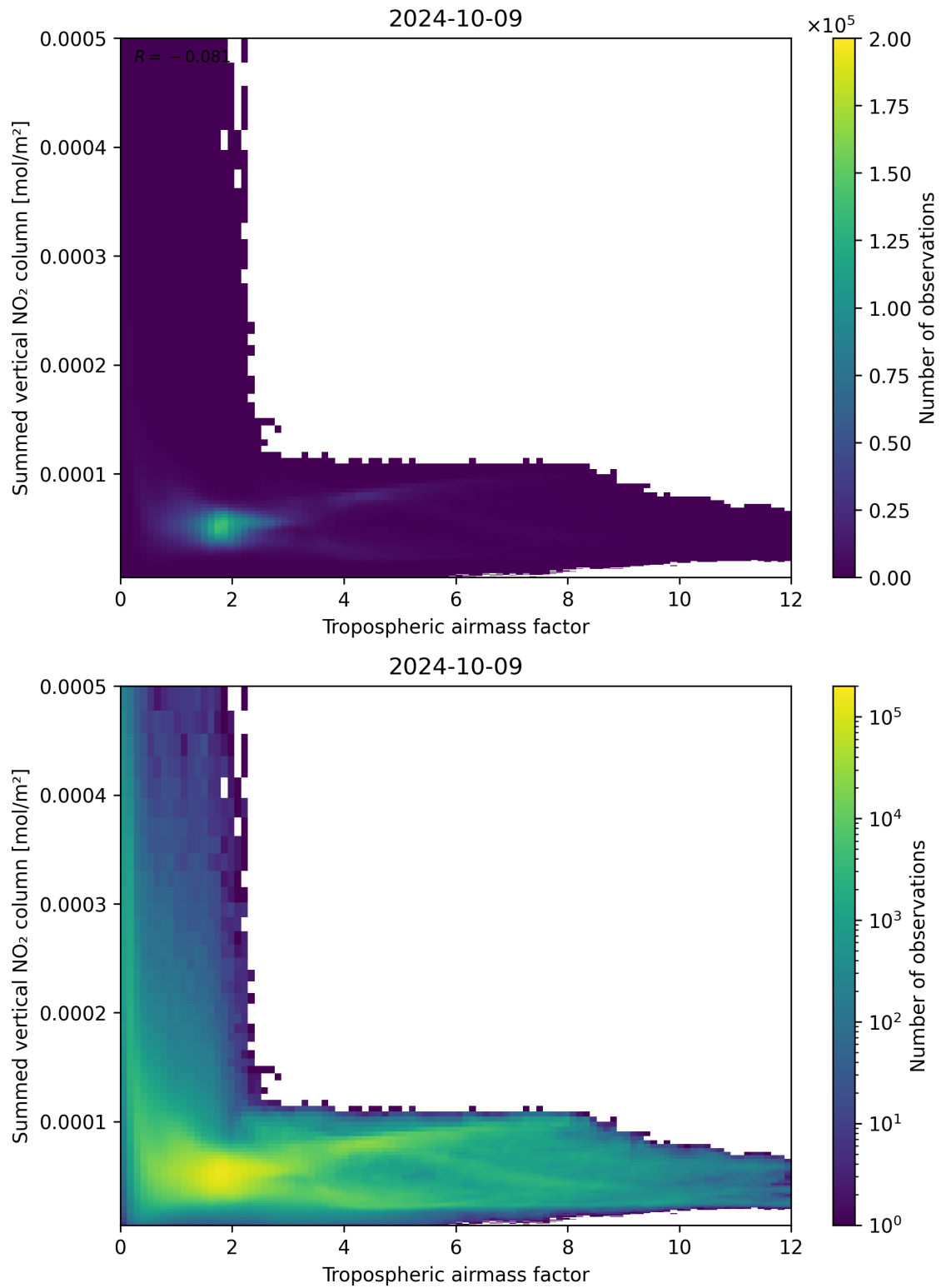
Figure 75: Scatter density plot of “Tropospheric air mass factor” against “Summed vertical NO 2 column” for 2024-10-08 to 2024-10-10.
