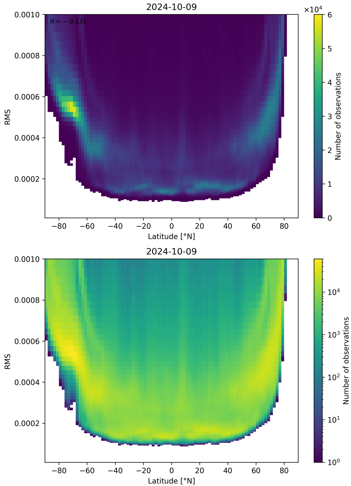
Figure 94: Scatter density plot of “Latitude” against “RMS” for 2024-10-08 to 2024-10-10.
