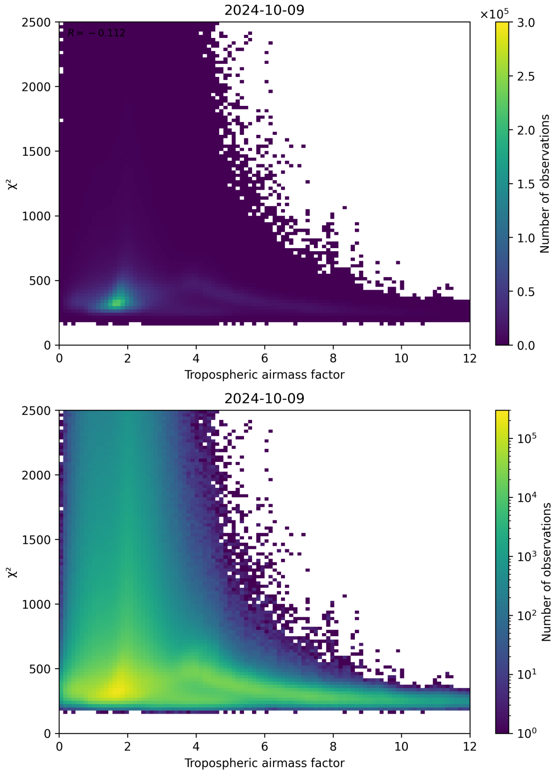
Figure 73: Scatter density plot of “Tropospheric airmass factor” against “ \chi^2 ” for 2024-10-08 to 2024-10-10.
