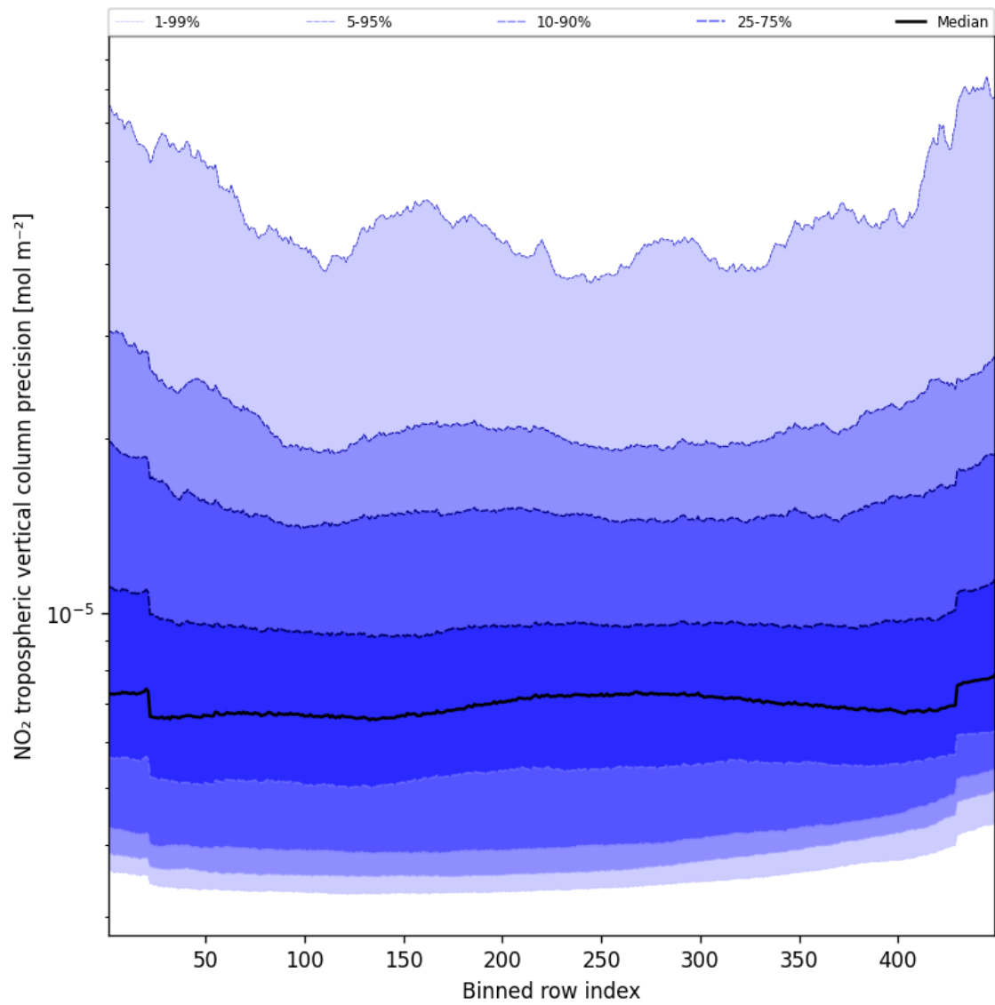
Figure 47: Along track statistics of “NO 2 tropospheric vertical column precision” for 2024-10-08 to 2024-10-10
