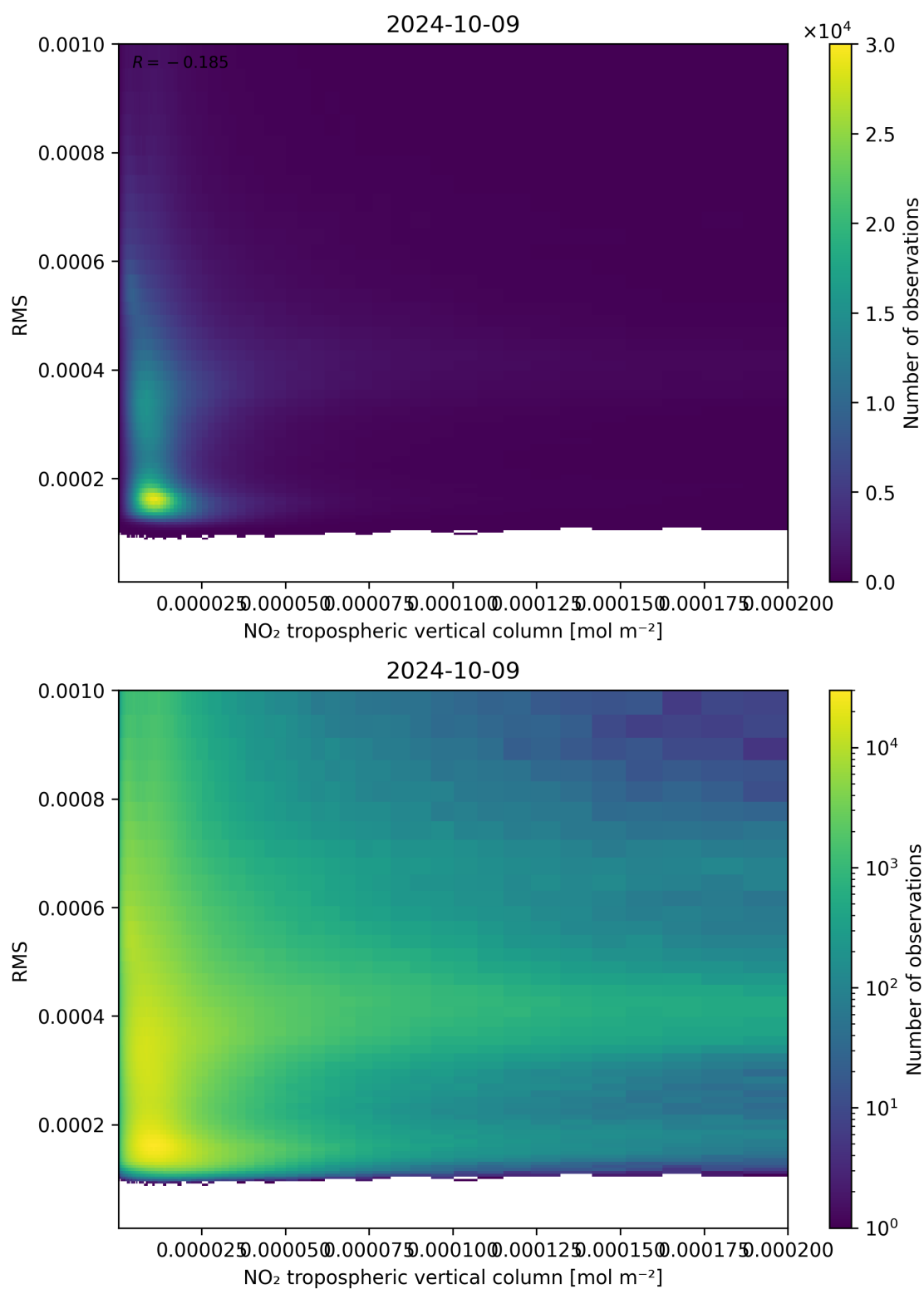
Figure 142: Scatter density plot of “NO 2 tropospheric vertical column” against “RMS” for 2024-10-08 to 2024-10-10.
