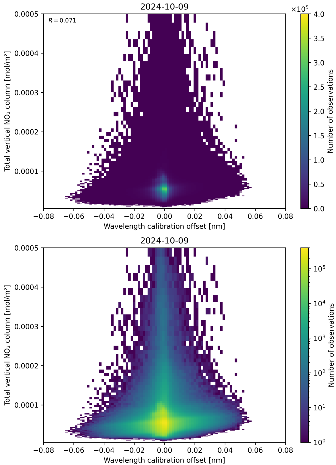
Figure 179: Scatter density plot of “Wavelength calibration offset” against “Total vertical NO 2 column” for 2024-10-08 to 2024-10-10.
