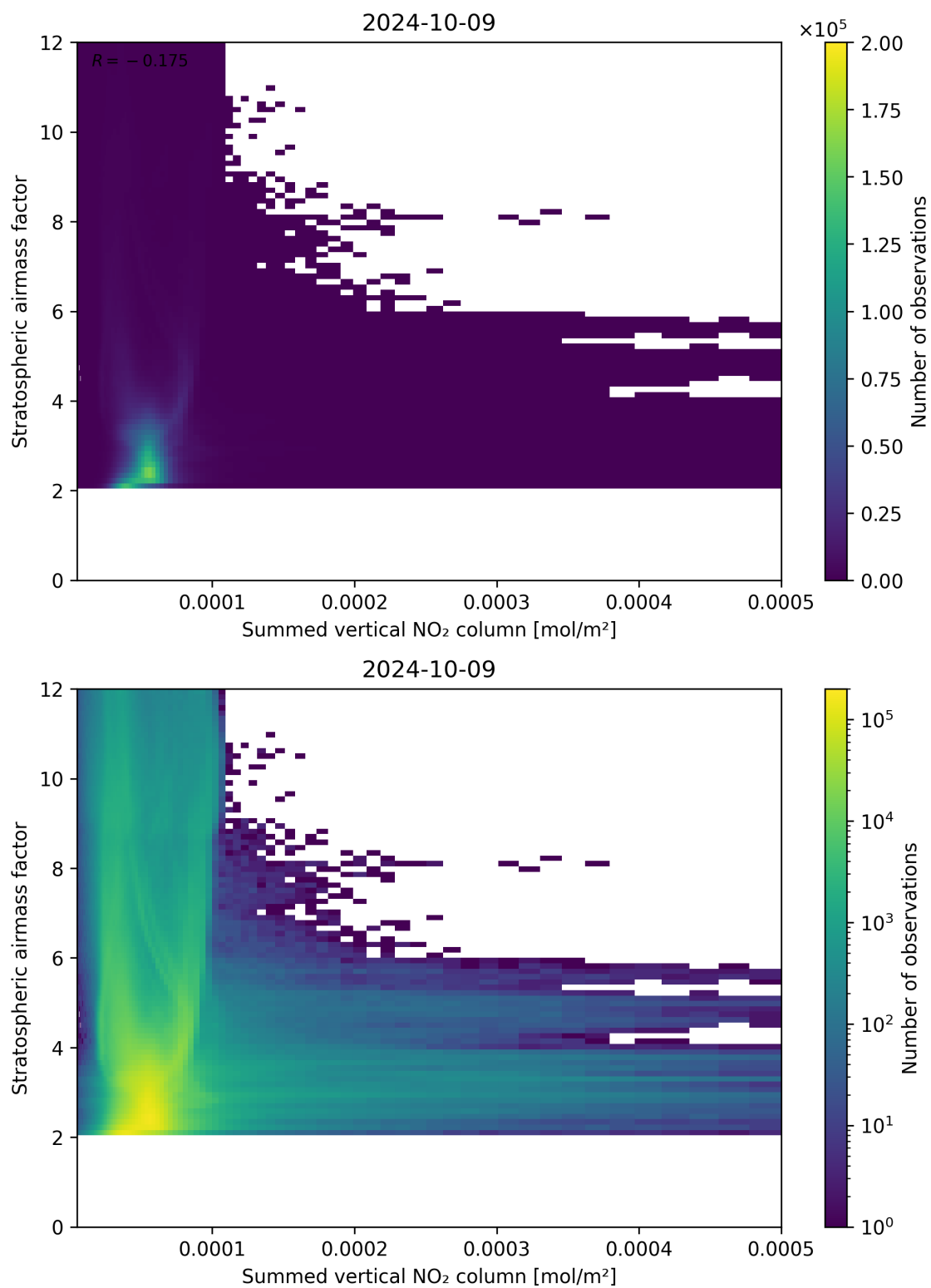
Figure 103: Scatter density plot of “Summed vertical NO 2 column” against “Stratospheric airmass factor” for 2024-10-08 to 2024-10-10.
