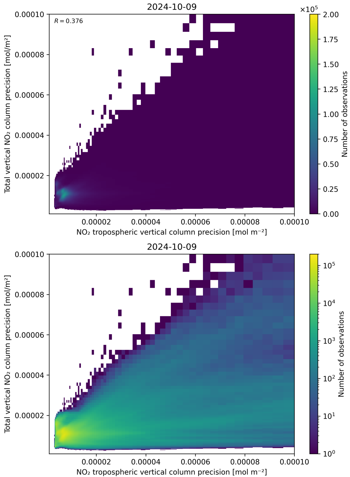
Figure 139: Scatter density plot of “NO 2 tropospheric vertical column precision” against “Total vertical NO 2 column precision” for 2024-10-08 to 2024-10-10.
