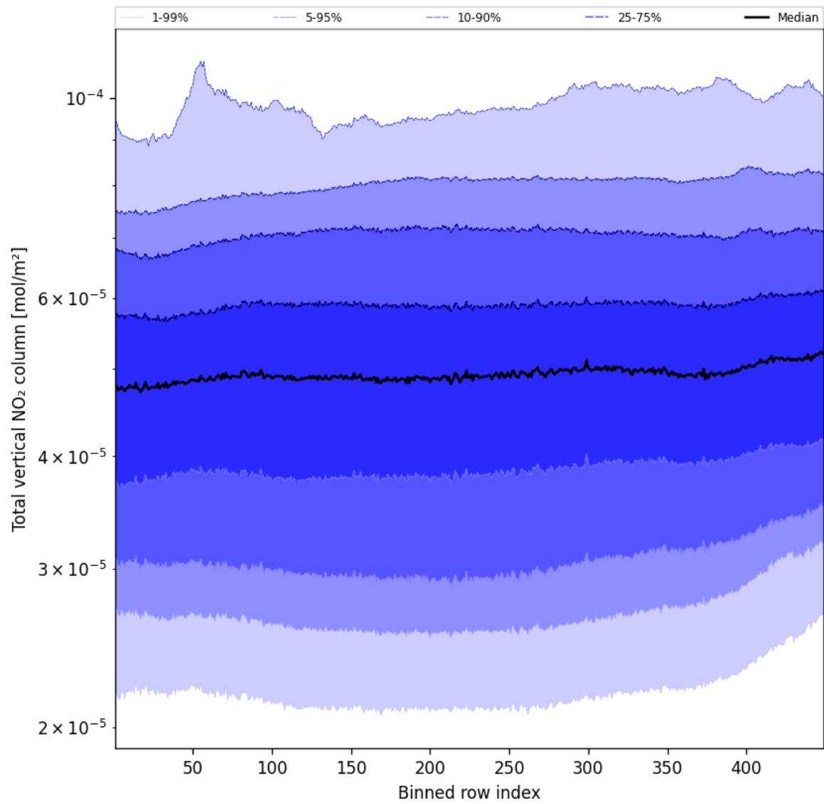
Figure 55: Along track statistics of “Total vertical NO 2 column” for 2024-10-08 to 2024-10-10
