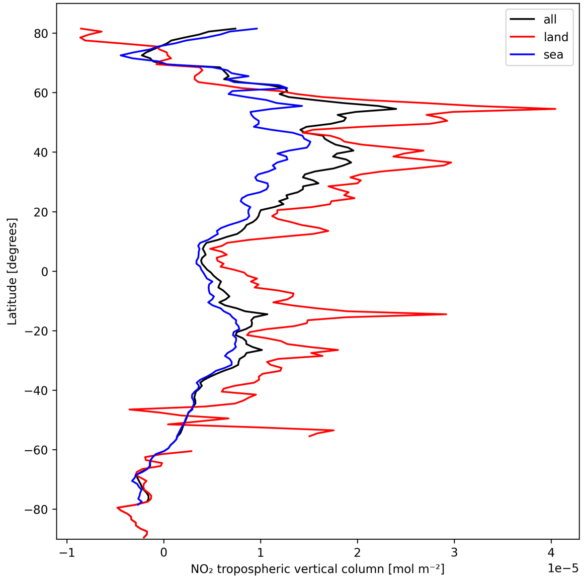
Figure 12: Zonal average of “NO 2 tropospheric vertical column” for 2024-10-08 to 2024-10-10.
