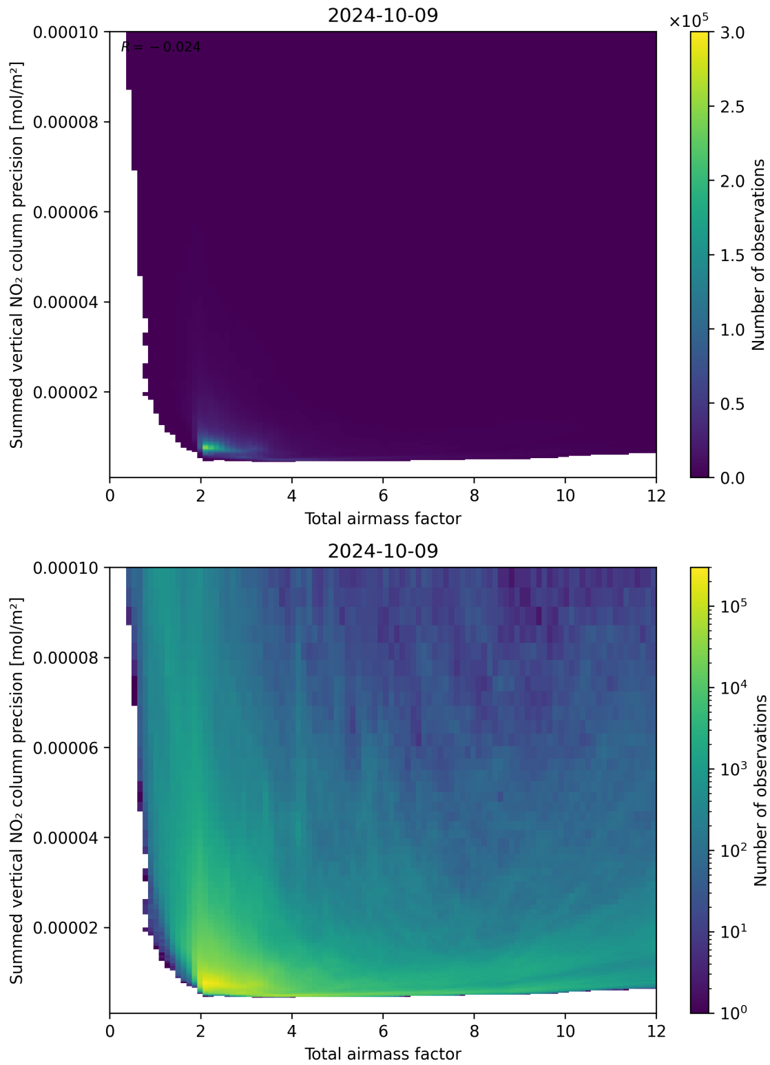
Figure 66: Scatter density plot of “Total airmass factor” against “Summed vertical NO 2 column precision” for 2024-10-08 to 2024-10-10.
