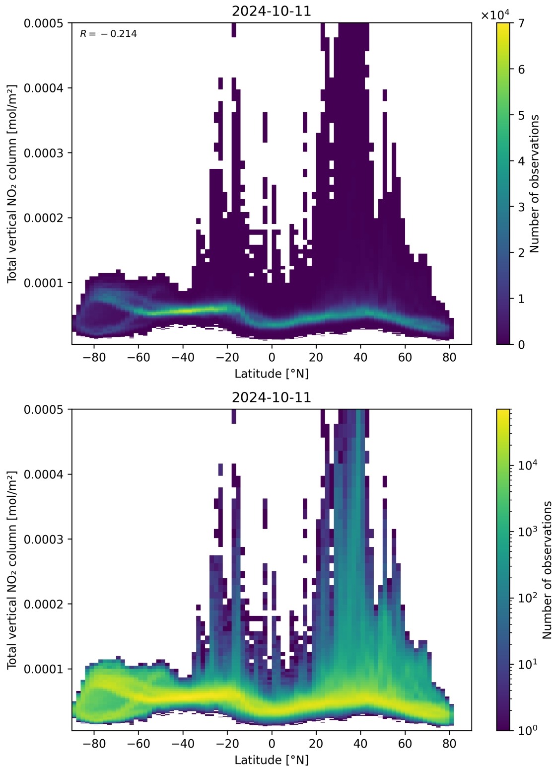
Figure 90: Scatter density plot of “Latitude” against “Total vertical NO 2 column” for 2024-10-10 to 2024-10-12.
