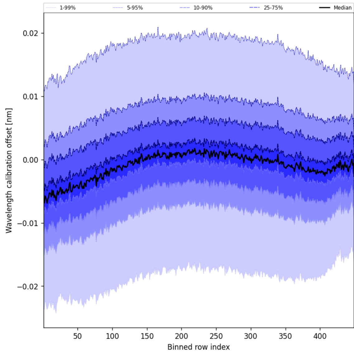
Figure 52: Along track statistics of “Wavelength calibration offset” for 2024-10-10 to 2024-10-12
