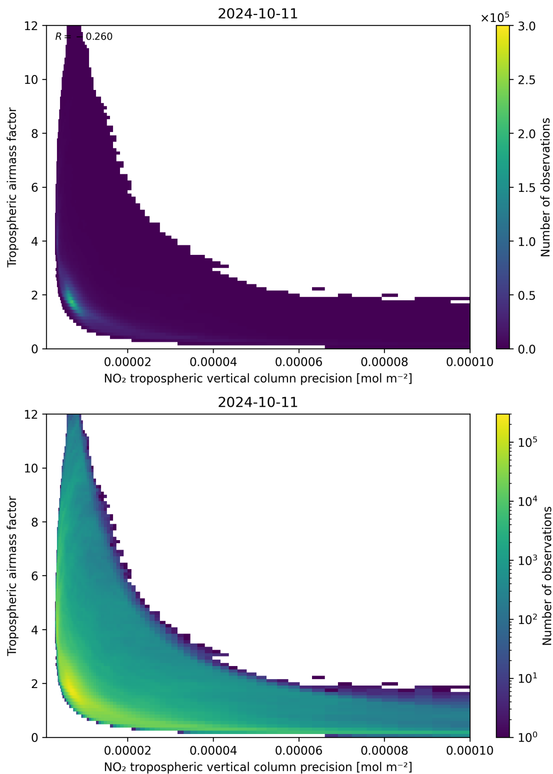
Figure 133: Scatter density plot of “NO 2 tropospheric vertical column precision” against “Tropospheric air mass factor” for 2024-10-10 to 2024-10-12.
