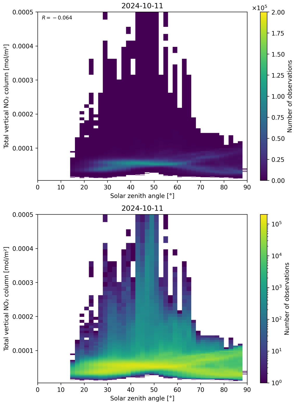
Figure 153: Scatter density plot of “Solar zenith angle” against “Total vertical NO 2 column” for 2024-10-10 to 2024-10-12.
