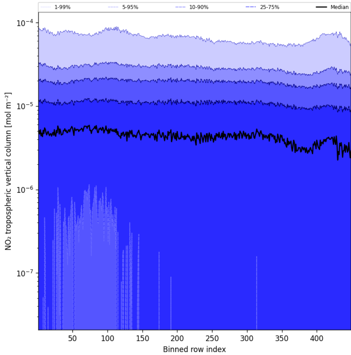
Figure 46: Along track statistics of “NO 2 tropospheric vertical column” for 2024-10-10 to 2024-10-12
