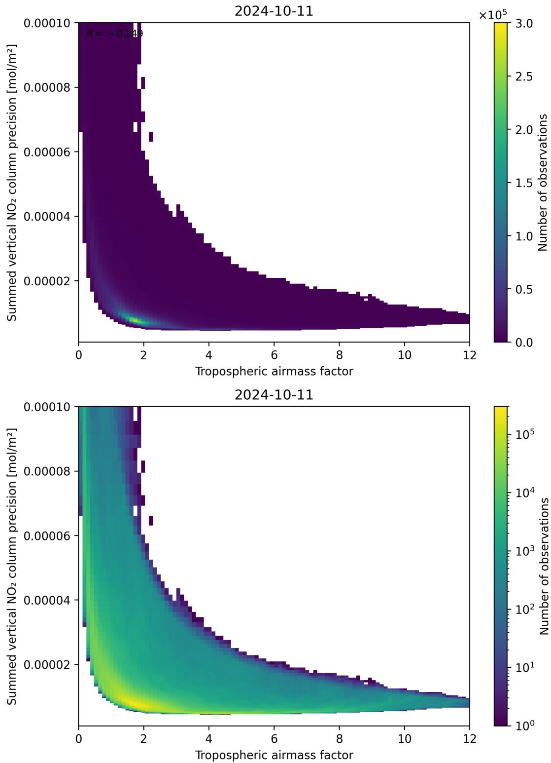
Figure 76: Scatter density plot of “Tropospheric airmass factor” against “Summed vertical NO 2 column precision” for 2024-10-10 to 2024-10-12.
