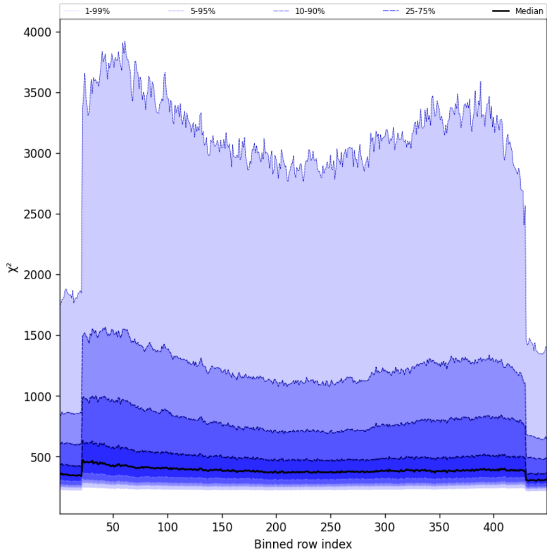
Figure 59: Along track statistics of “ \chi^2 ” for 2024-10-10 to 2024-10-12
