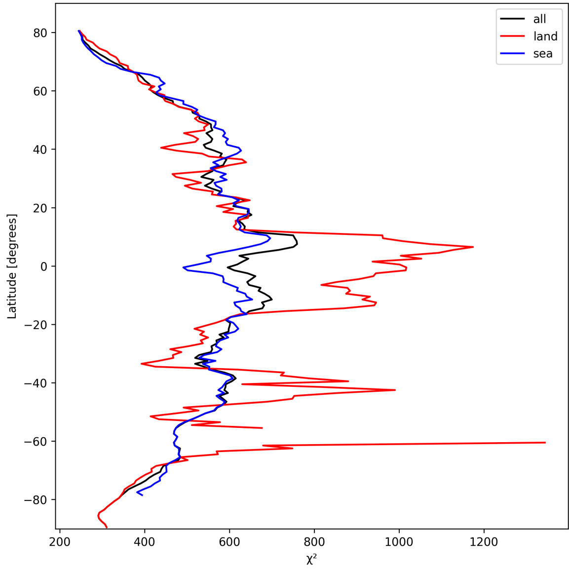
Figure 25: Zonal average of “ \chi^2 ” for 2024-10-10 to 2024-10-12.
