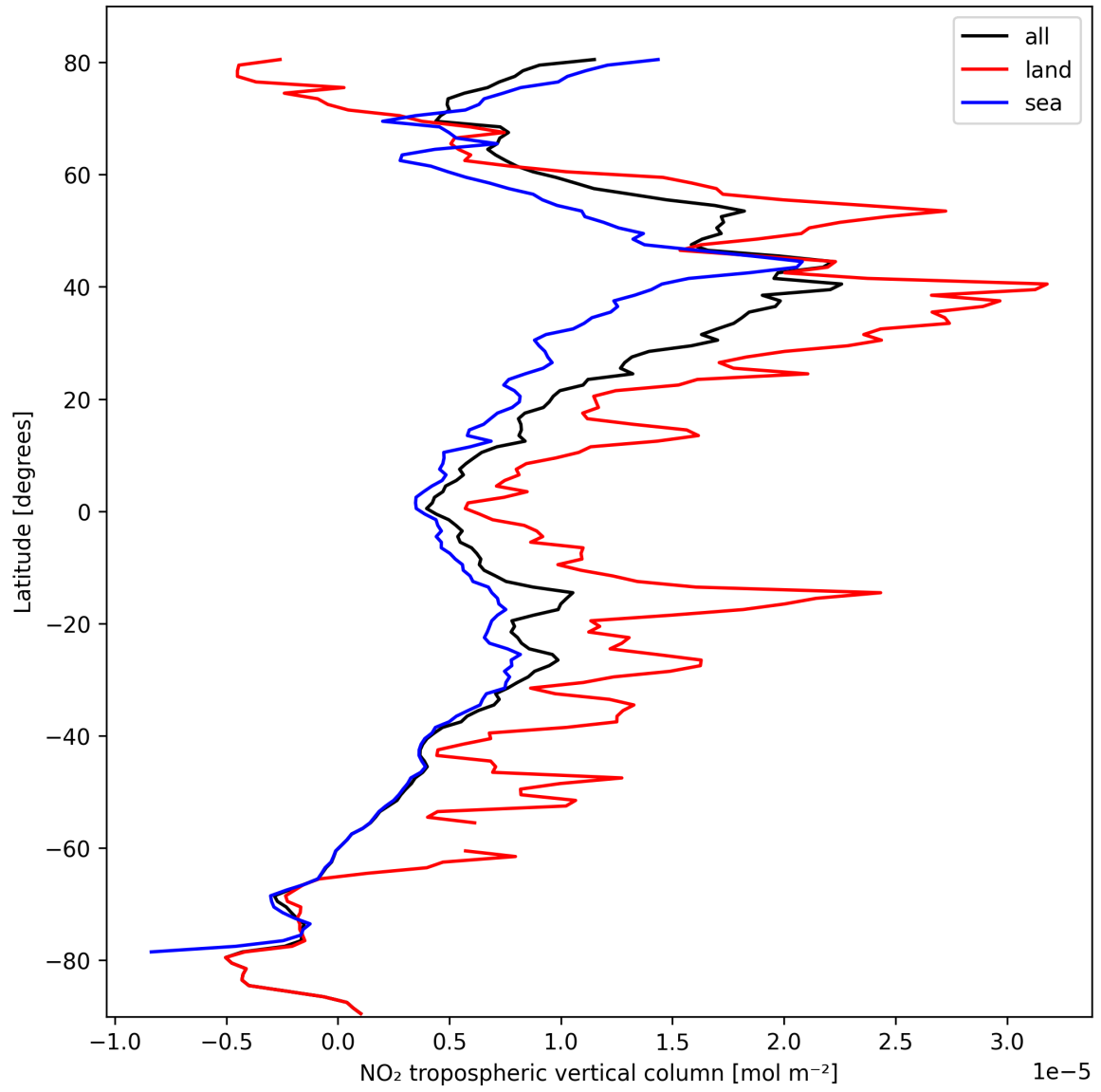
Figure 12: Zonal average of “NO 2 tropospheric vertical column” for 2024-10-10 to 2024-10-12.
