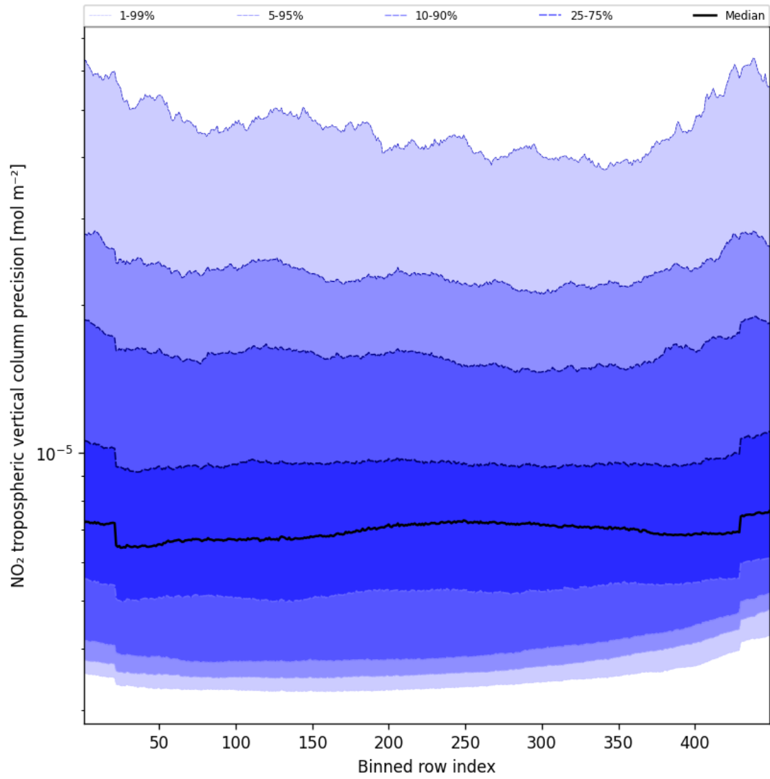
Figure 47: Along track statistics of “NO 2 tropospheric vertical column precision” for 2024-10-10 to 2024-10-12
