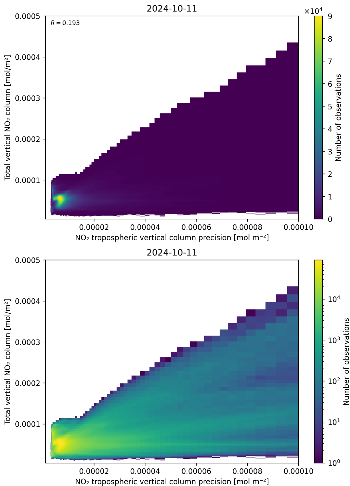
Figure 138: Scatter density plot of “NO 2 tropospheric vertical column precision” against “Total vertical NO 2 column” for 2024-10-10 to 2024-10-12.
