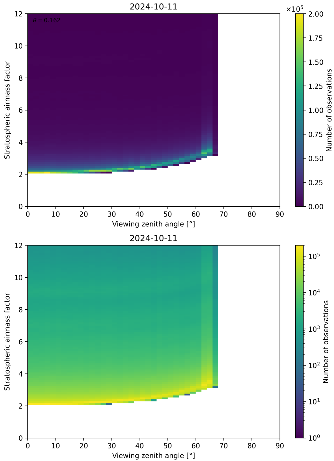
Figure 159: Scatter density plot of “Viewing zenith angle” against “Stratospheric airmass factor” for 2024-10-10 to 2024-10-12.
