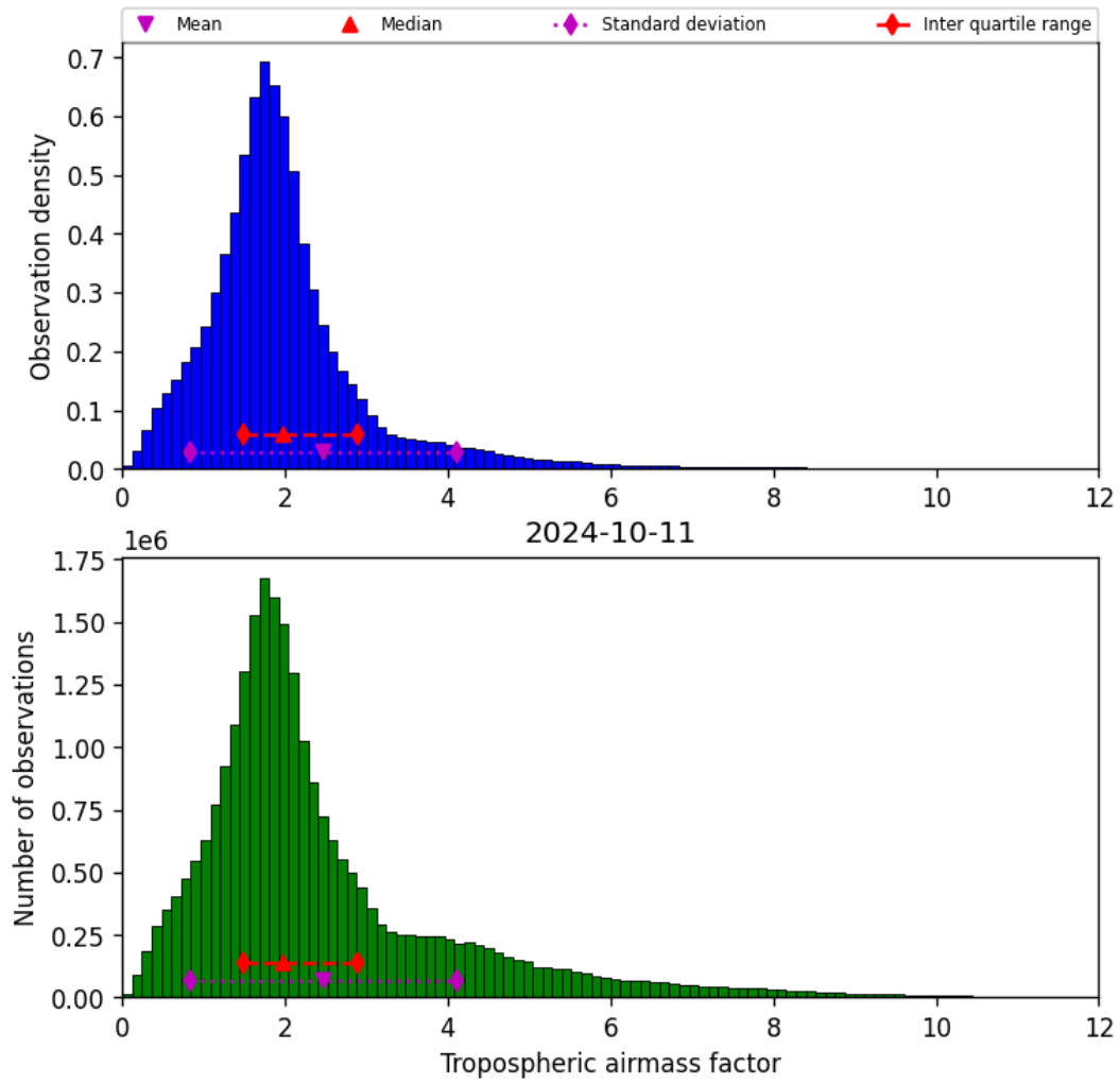
Figure 31: Histogram of “Tropospheric airmass factor” for 2024-10-10 to 2024-10-12
