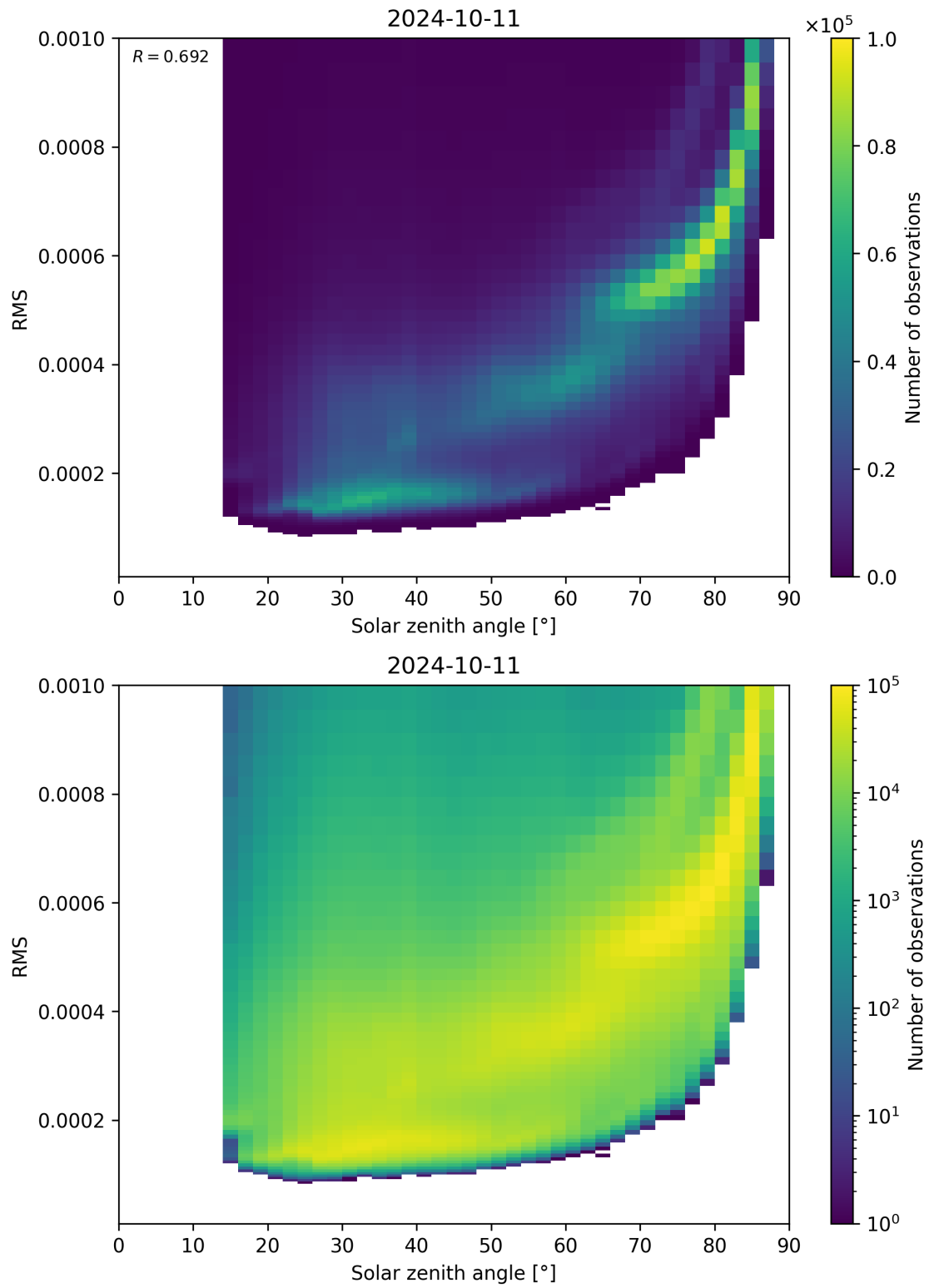
Figure 157: Scatter density plot of “Solar zenith angle” against “RMS” for 2024-10-10 to 2024-10-12.
