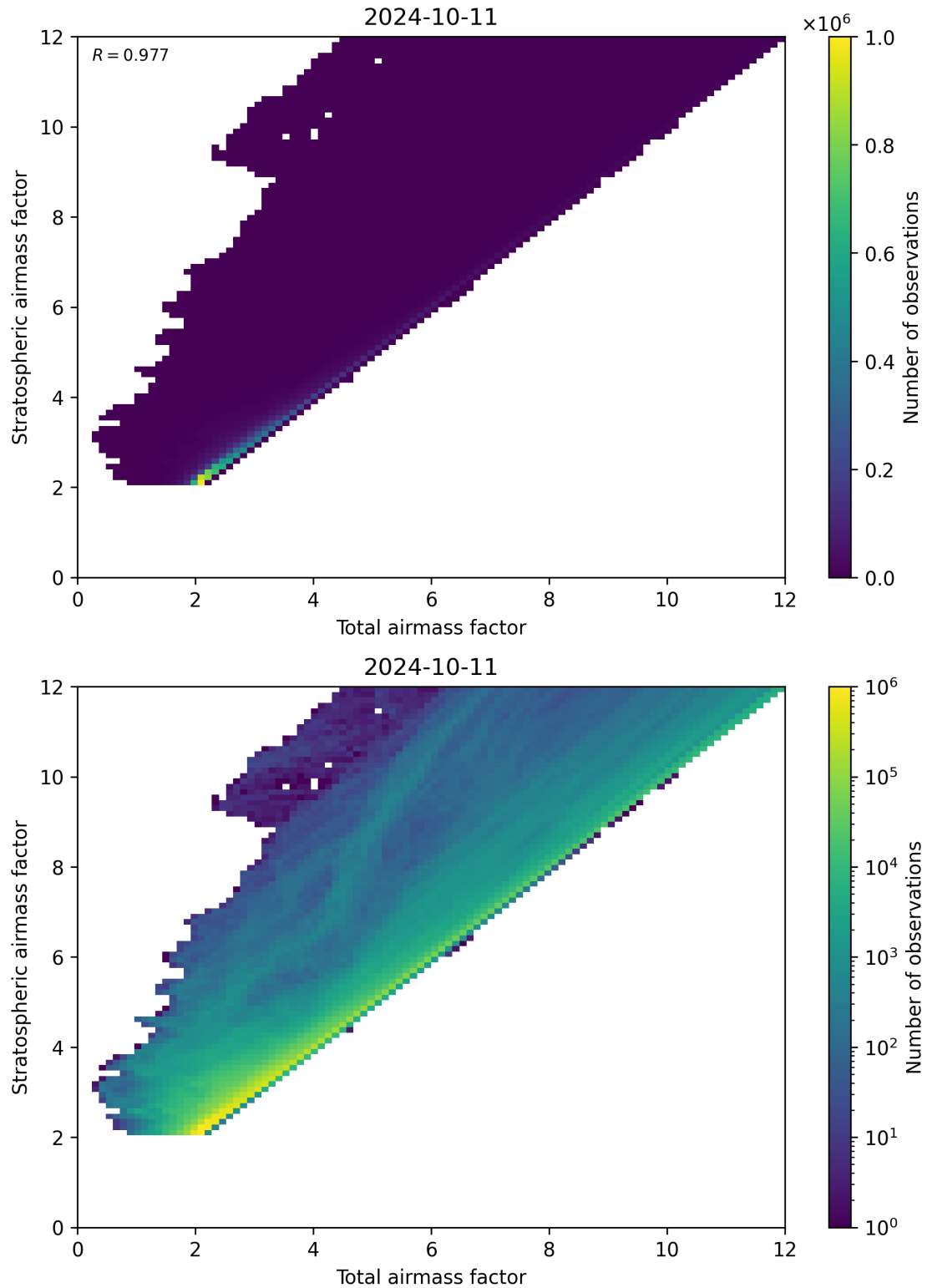
Figure 62: Scatter density plot of “Total airmass factor” against “Stratospheric airmass factor” for 2024-10-10 to 2024-10-12.
