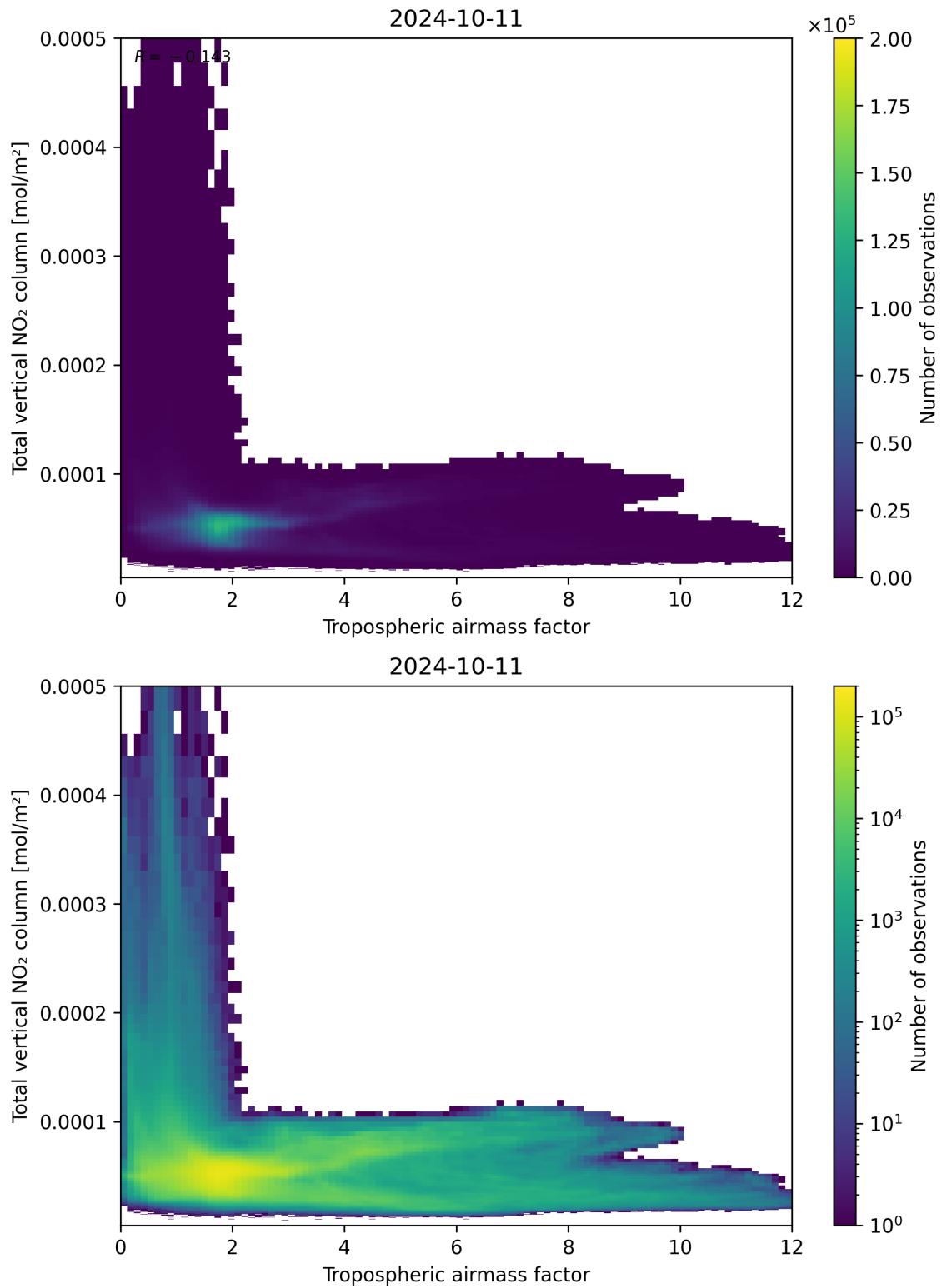
Figure 77: Scatter density plot of “Tropospheric airmass factor” against “Total vertical NO 2 column” for 2024-10-10 to 2024-10-12.
