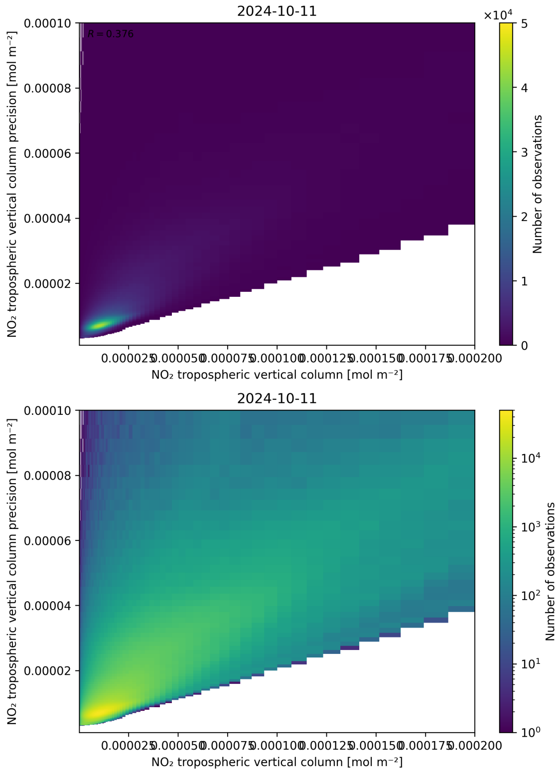
Figure 130: Scatter density plot of “NO 2 tropospheric vertical column” against “NO 2 tropospheric vertical column precision” for 2024-10-10 to 2024-10-12.
