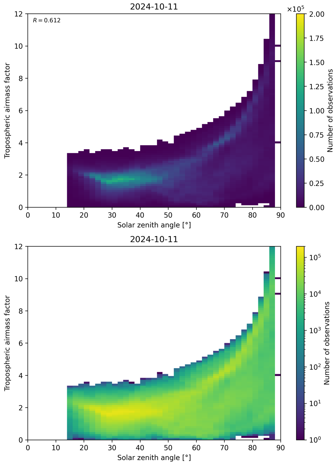
Figure 147: Scatter density plot of “Solar zenith angle” against “Tropospheric airmass factor” for 2024-10-10 to 2024-10-12.
