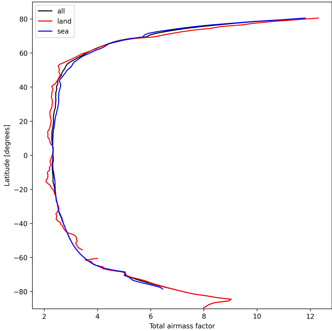
Figure 15: Zonal average of “Total airmass factor” for 2024-10-10 to 2024-10-12.
