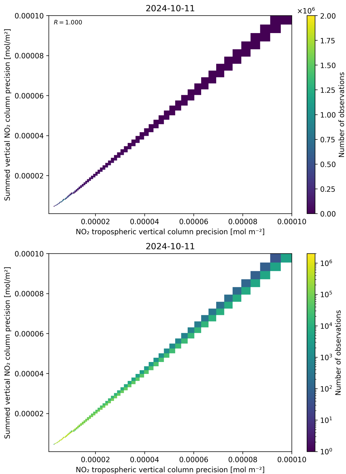
Figure 137: Scatter density plot of “NO 2 tropospheric vertical column precision” against “Summed vertical NO 2 column precision” for 2024-10-10 to 2024-10-12.
