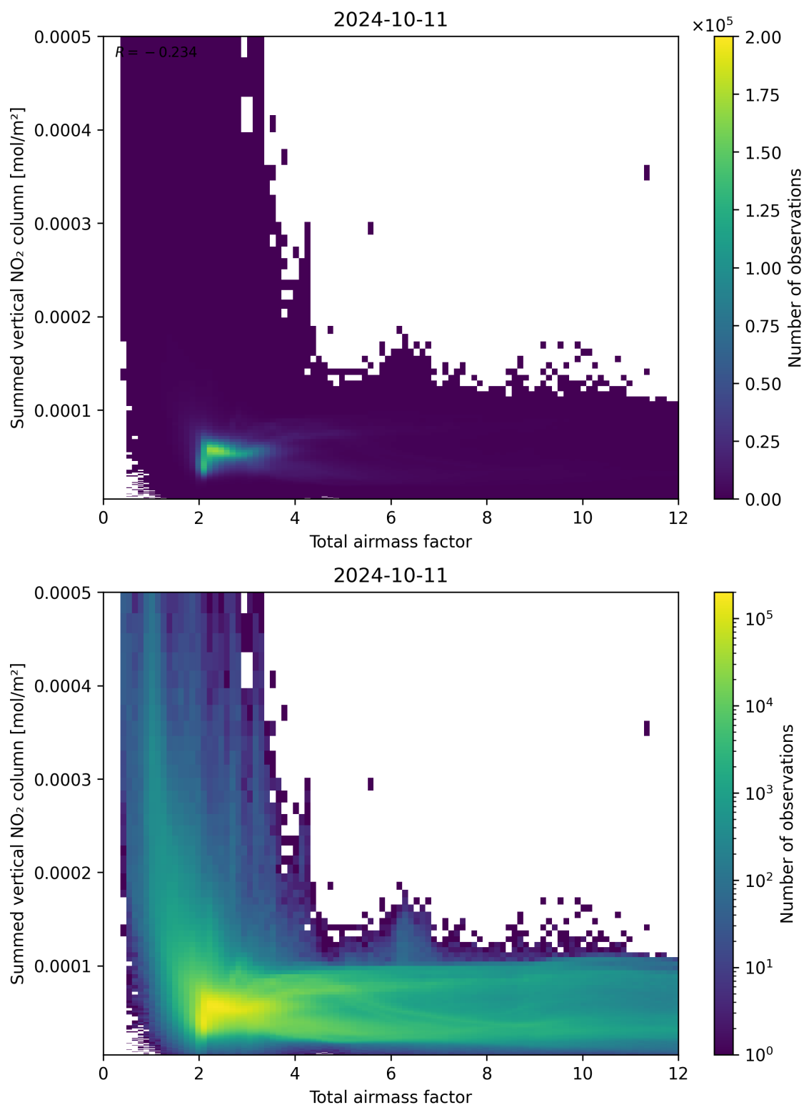
Figure 65: Scatter density plot of “Total airmass factor” against “Summed vertical NO 2 column” for 2024-10-10 to 2024-10-12.
