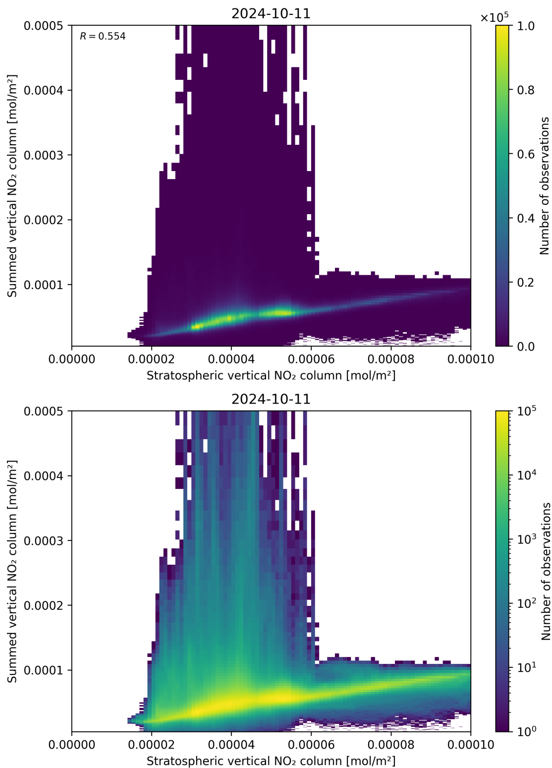
Figure 98: Scatter density plot of “Stratospheric vertical NO 2 column” against “Summed vertical NO 2 column” for 2024-10-10 to 2024-10-12.
