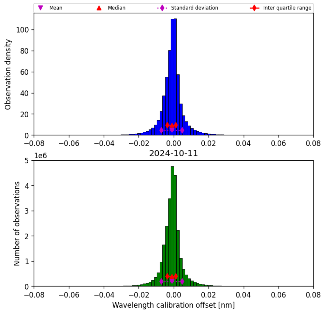
Figure 35: Histogram of “Wavelength calibration offset” for 2024-10-10 to 2024-10-12
