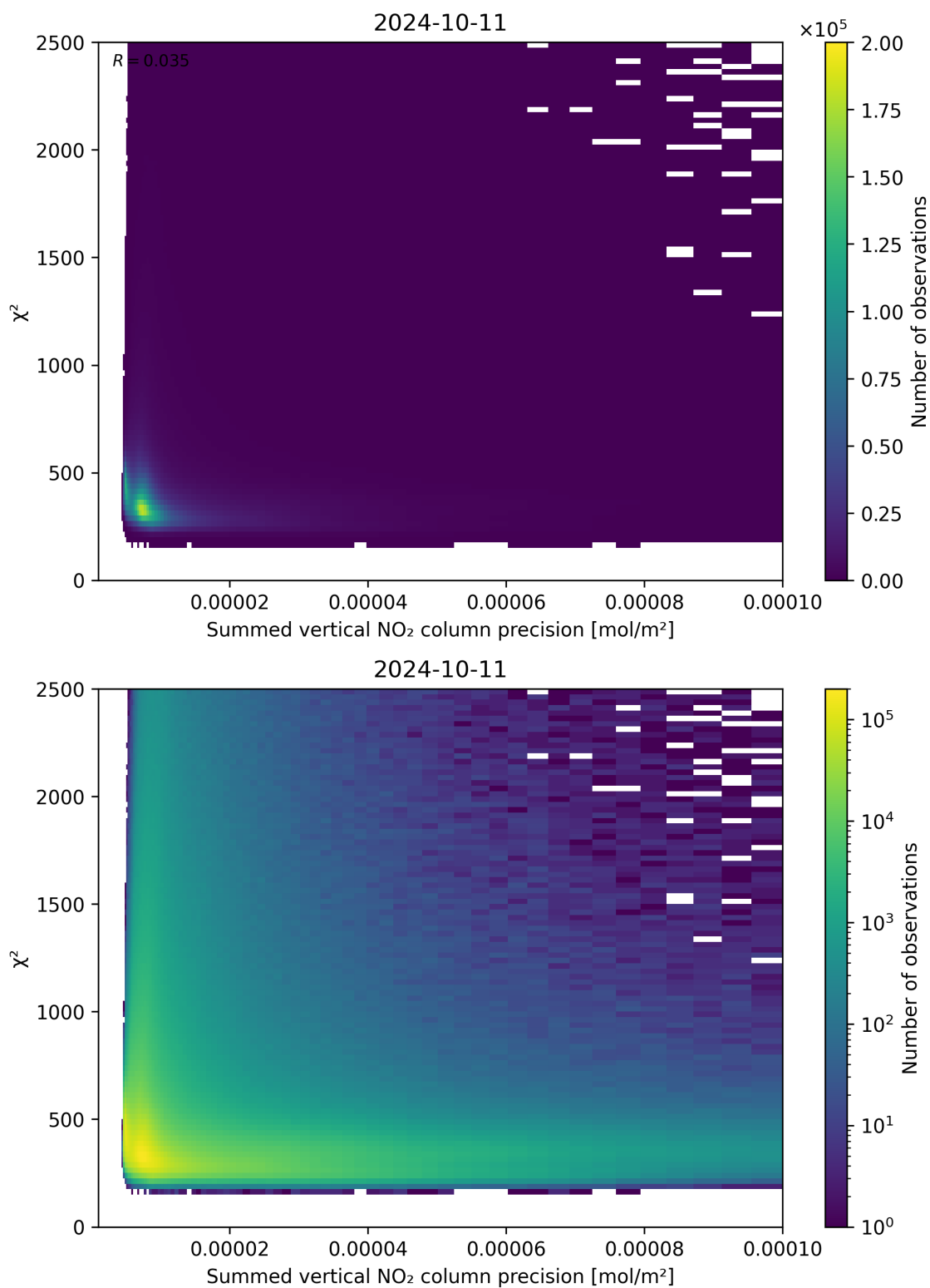
Figure 107: Scatter density plot of “Summed vertical NO 2 column precision” against “ \chi^2 ” for 2024-10-10 to 2024-10-12.
