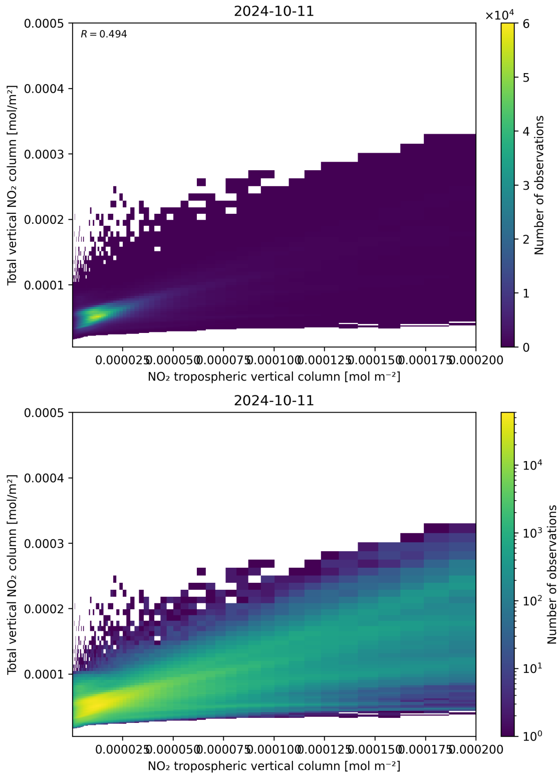
Figure 128: Scatter density plot of “NO 2 tropospheric vertical column” against “Total vertical NO 2 column” for 2024-10-10 to 2024-10-12.
