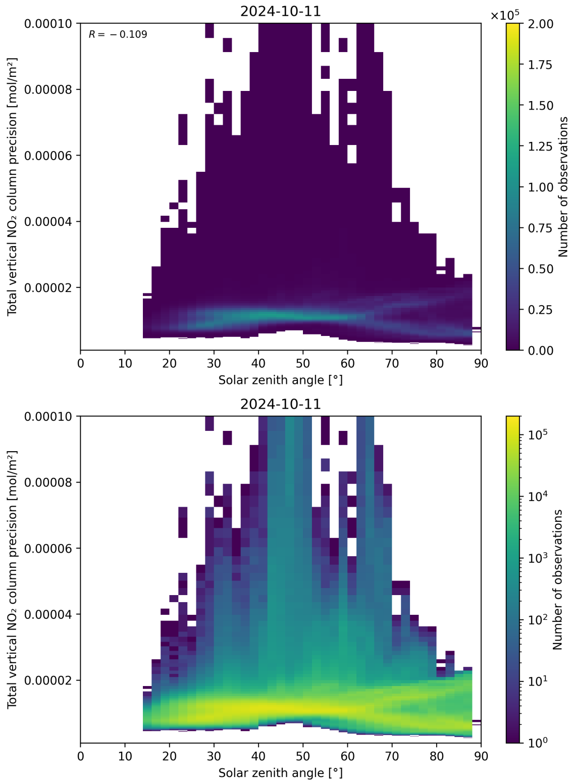
Figure 154: Scatter density plot of “Solar zenith angle” against “Total vertical NO 2 column precision” for 2024-10-10 to 2024-10-12.
