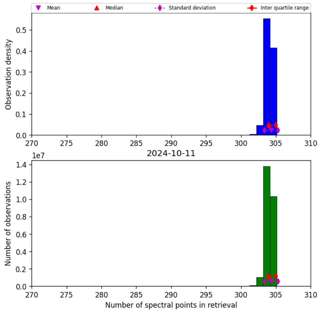
Figure 33: Histogram of “Number of spectral points in retrieval” for 2024-10-10 to 2024-10-12
