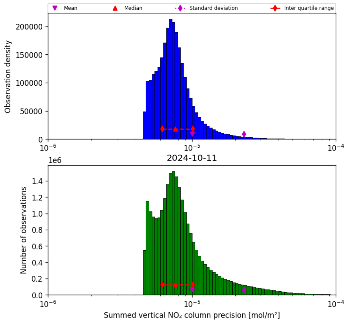
Figure 41: Histogram of "Summed vertical NO 2 column precision" for 2024-10-10 to 2024-10-12
