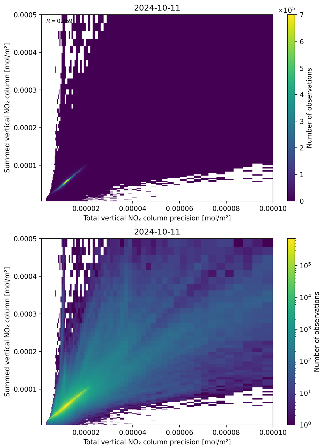
Figure 117: Scatter density plot of “Total vertical NO 2 column precision” against “Summed vertical NO 2 column” for 2024-10-10 to 2024-10-12.
