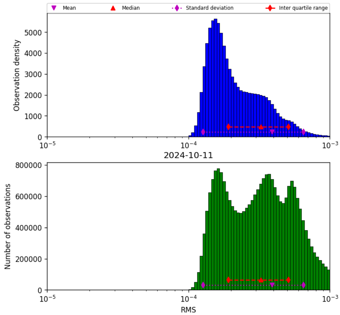
Figure 43: Histogram of “RMS” for 2024-10-10 to 2024-10-12
