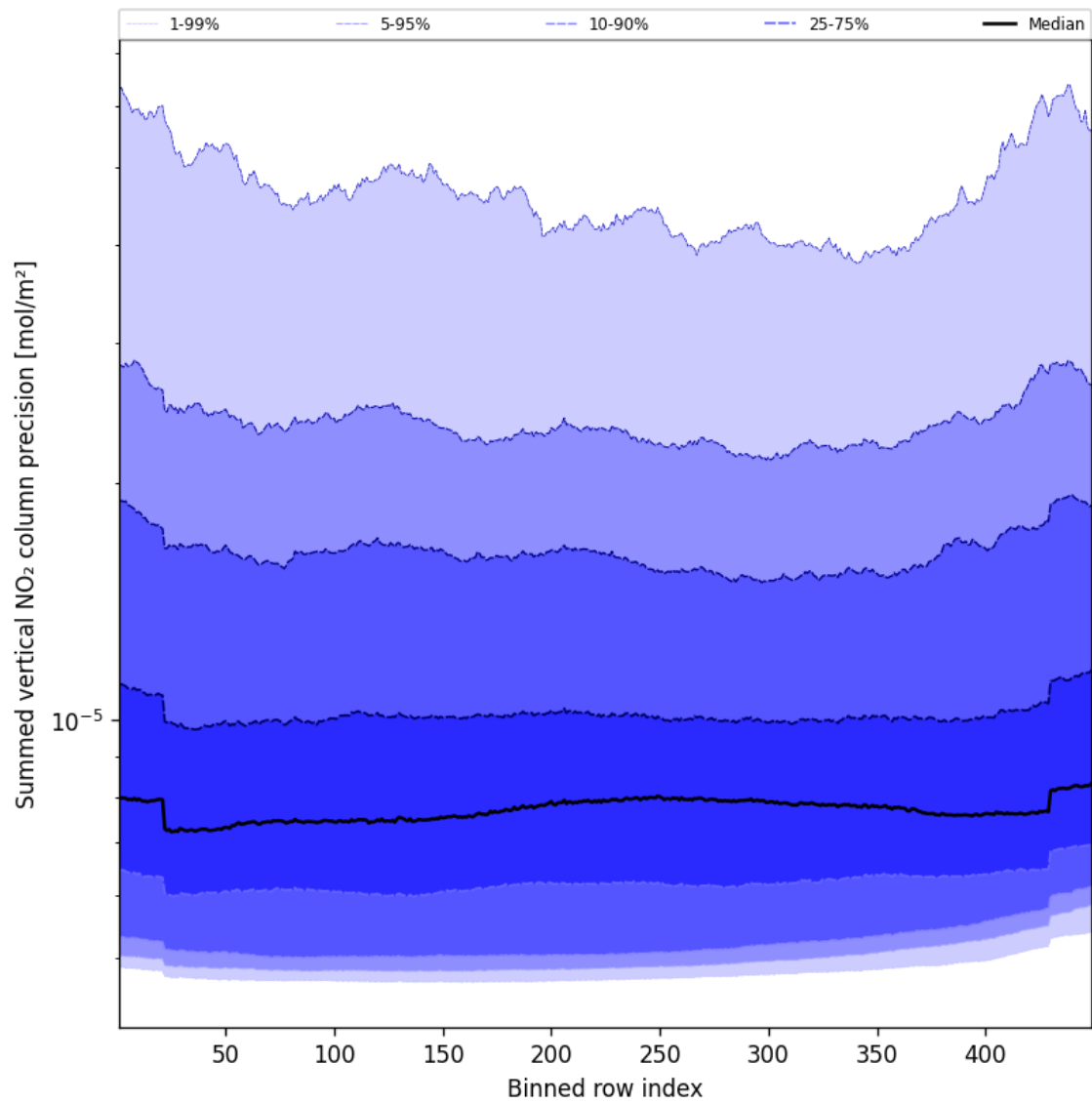
Figure 58: Along track statistics of “Summed vertical NO 2 column precision” for 2024-10-10 to 2024-10-12
