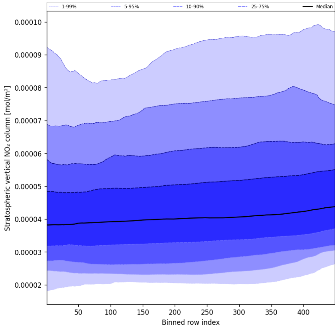
Figure 53: Along track statistics of “Stratospheric vertical NO 2 column” for 2024-10-10 to 2024-10-12
