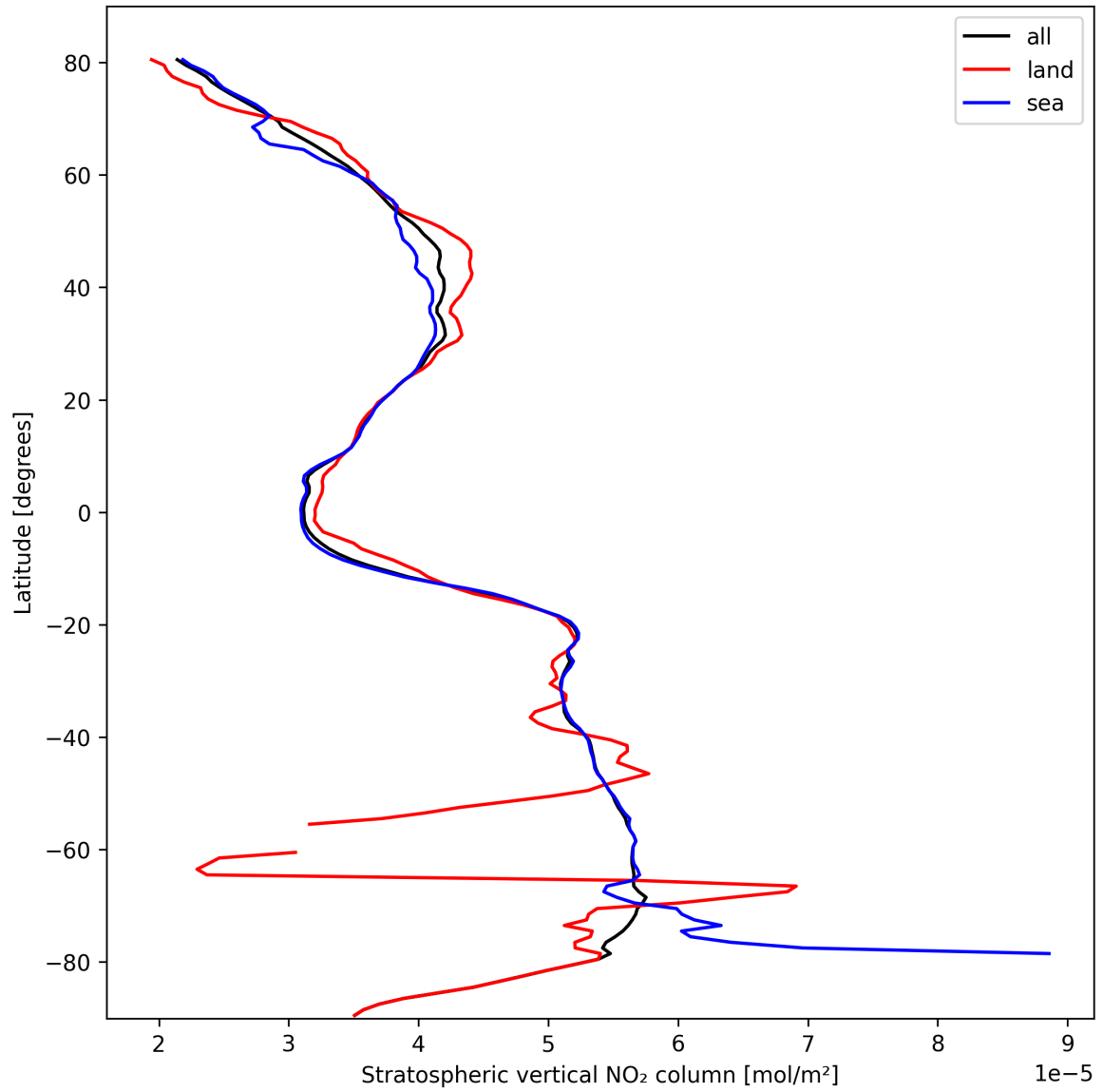
Figure 19: Zonal average of “Stratospheric vertical NO 2 column” for 2024-10-10 to 2024-10-12.
