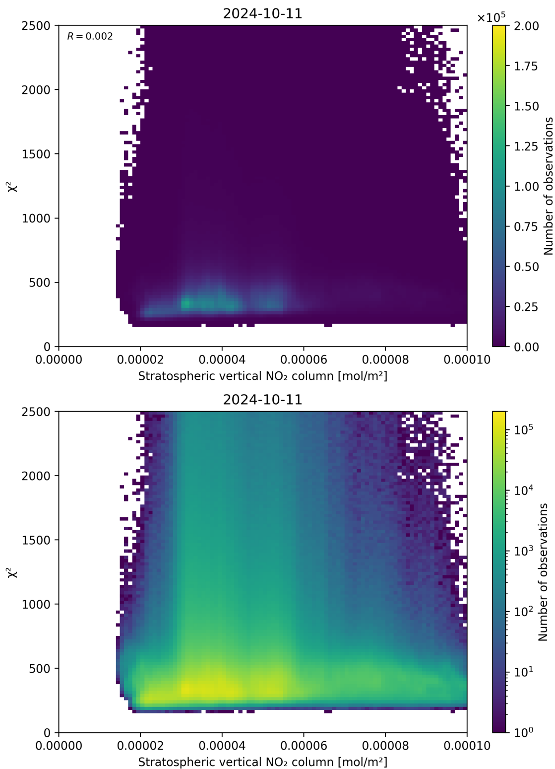
Figure 97: Scatter density plot of “Stratospheric vertical NO 2 column” against “ \chi^2 ” for 2024-10-10 to 2024-10-12.
