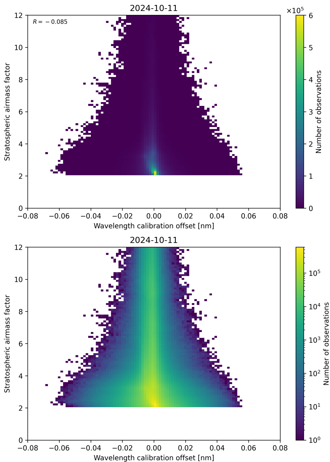
Figure 174: Scatter density plot of “Wavelength calibration offset” against “Stratospheric airmass factor” for 2024-10-10 to 2024-10-12.
