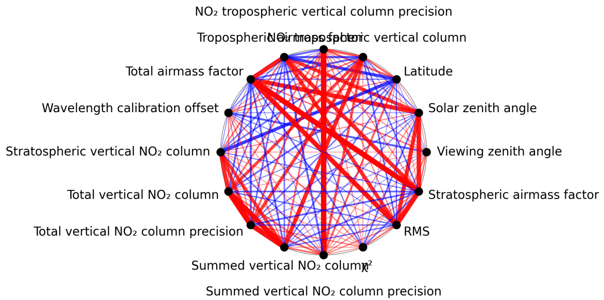
Figure 1: Map of correlation graph for 2024-10-10 to 2024-10-12.
