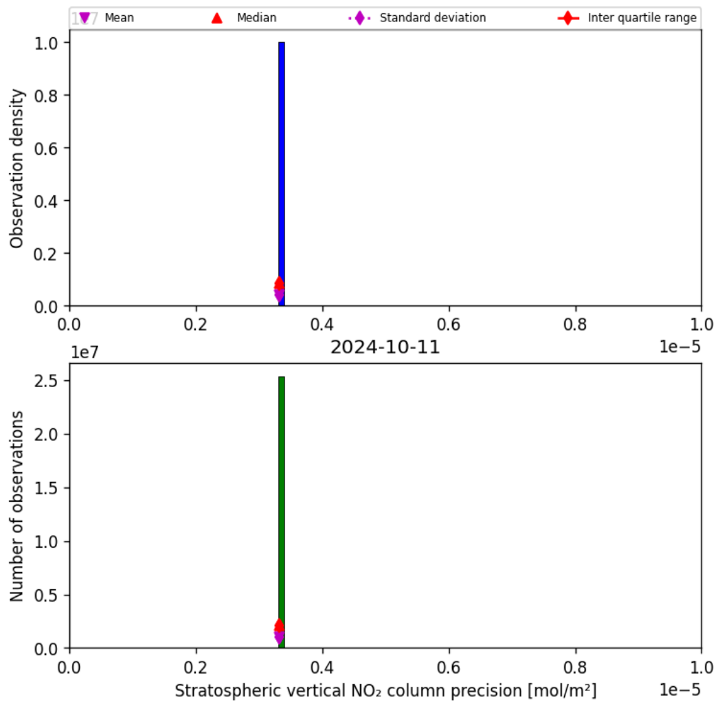
Figure 37: Histogram of “Stratospheric vertical NO 2 column precision” for 2024-10-10 to 2024-10-12
