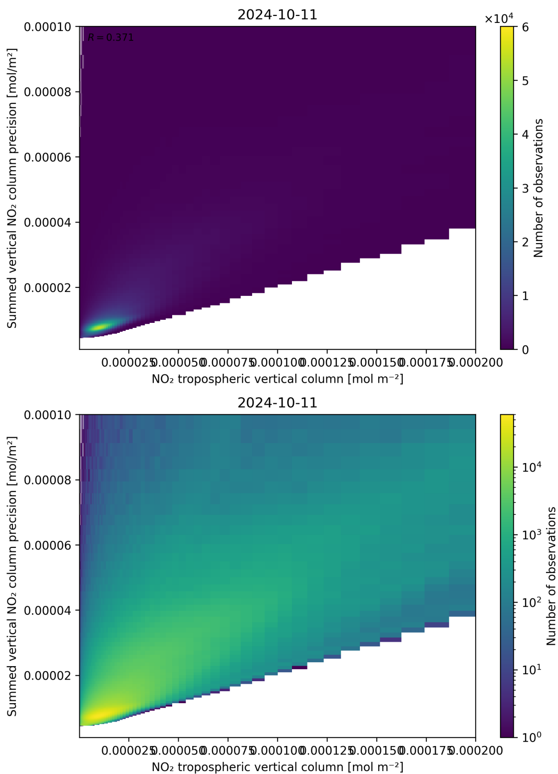
Figure 127: Scatter density plot of “NO 2 tropospheric vertical column” against “Summed vertical NO 2 column precision” for 2024-10-10 to 2024-10-12.
