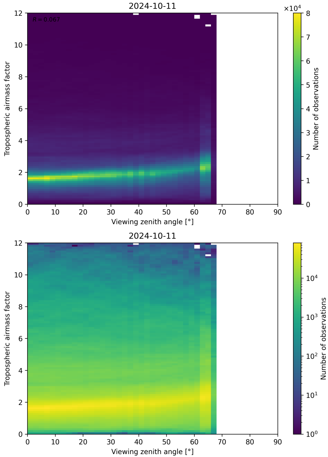
Figure 161: Scatter density plot of “Viewing zenith angle” against “Tropospheric airmass factor” for 2024-10-10 to 2024-10-12.
