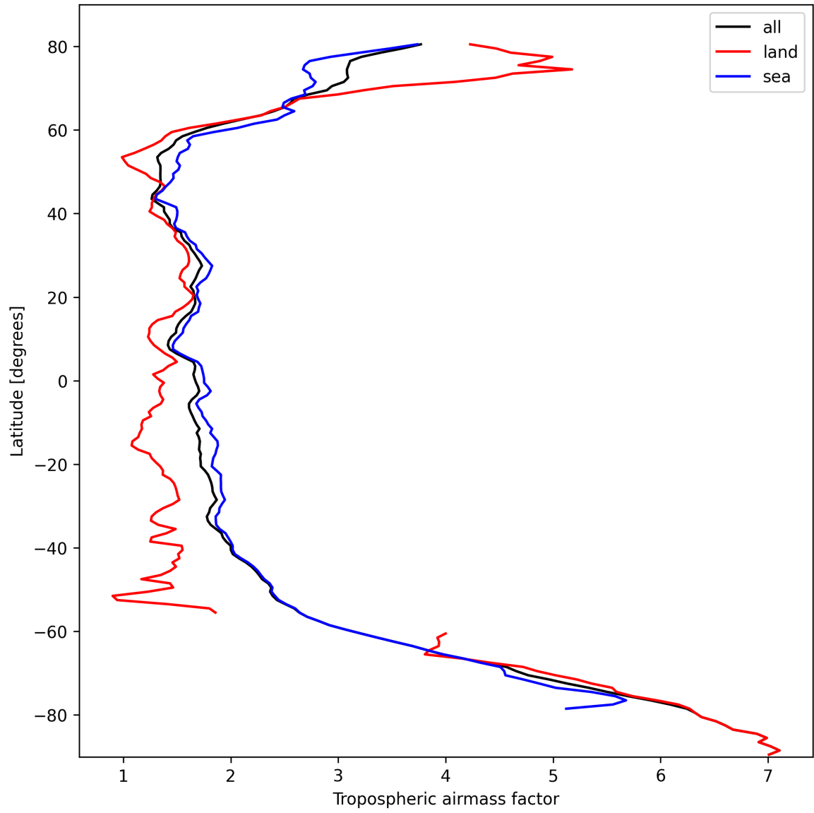
Figure 14: Zonal average of “Tropospheric air mass factor” for 2024-10-10 to 2024-10-12.
