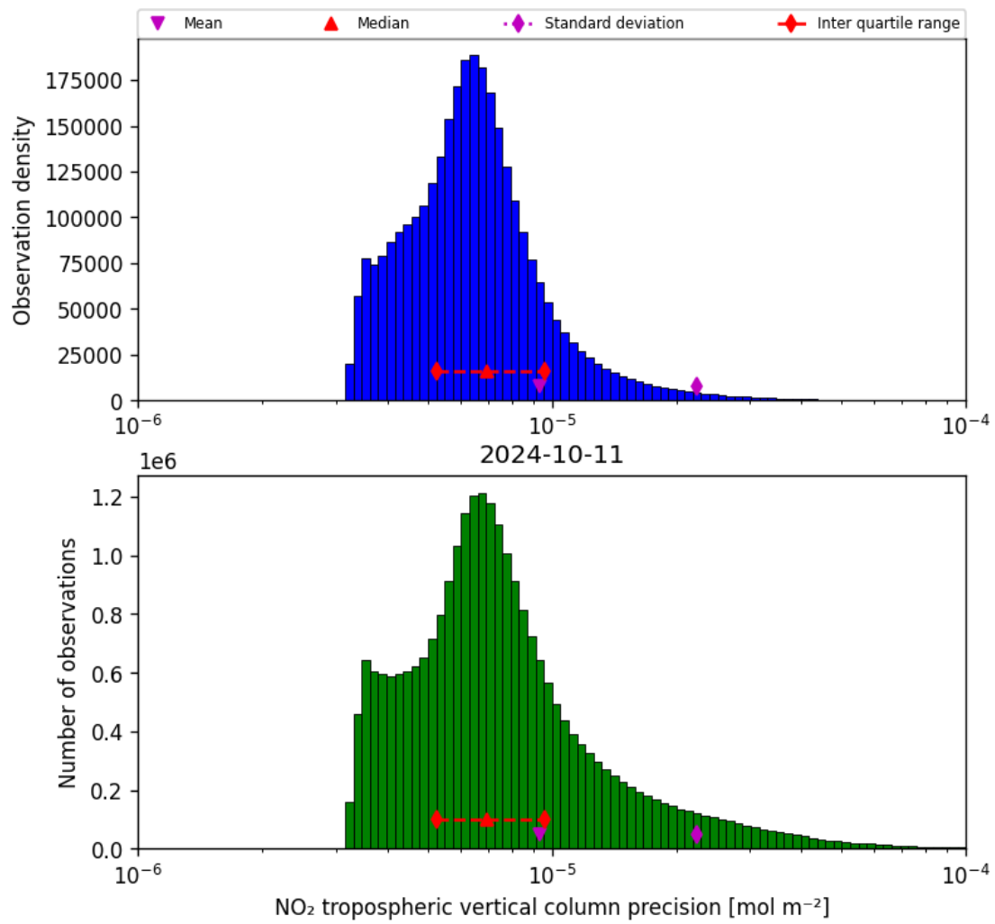
Figure 30: Histogram of “NO 2 tropospheric vertical column precision” for 2024-10-10 to 2024-10-12
