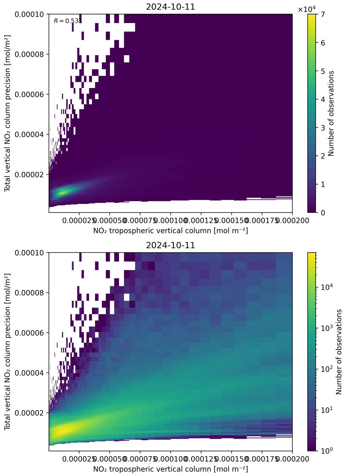
Figure 129: Scatter density plot of “NO 2 tropospheric vertical column” against “Total vertical NO 2 column precision” for 2024-10-10 to 2024-10-12.
