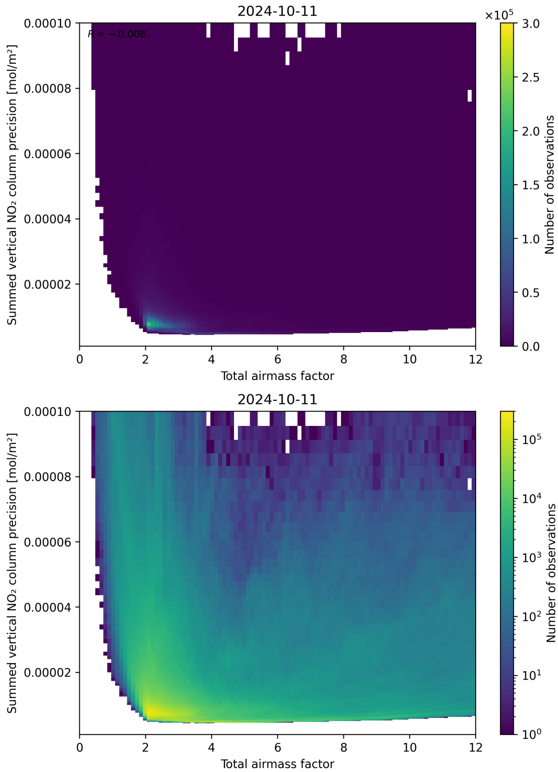
Figure 66: Scatter density plot of “Total airmass factor” against “Summed vertical NO 2 column precision” for 2024-10-10 to 2024-10-12.
