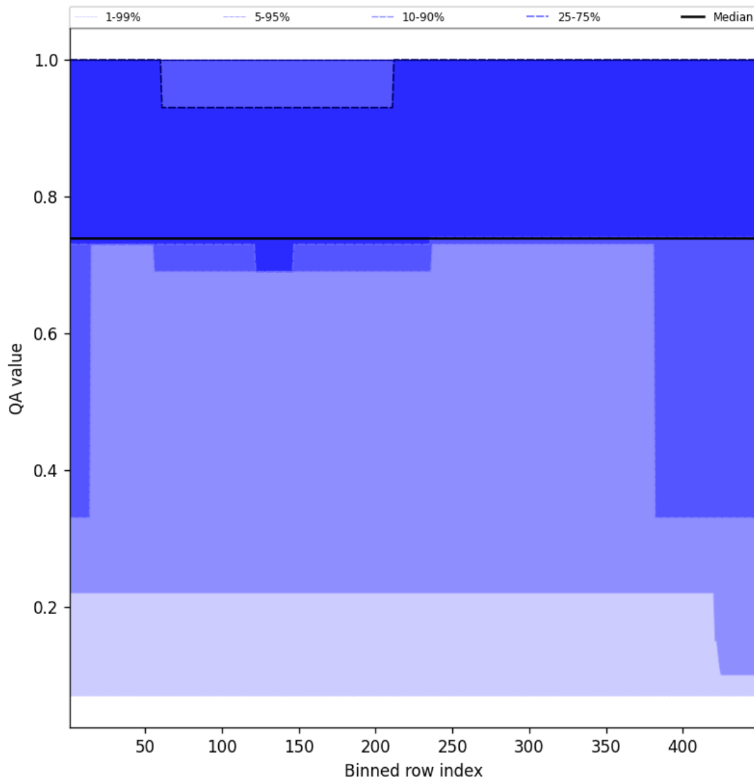
Figure 45: Along track statistics of “QA value” for 2024-10-10 to 2024-10-12
