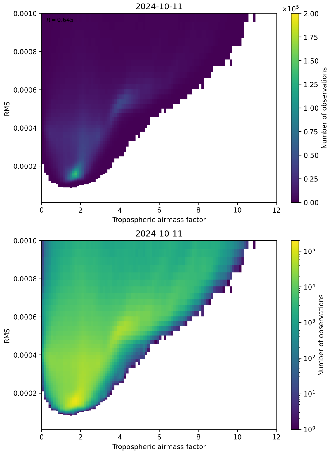
Figure 79: Scatter density plot of “Tropospheric airmass factor” against “RMS” for 2024-10-10 to 2024-10-12.
