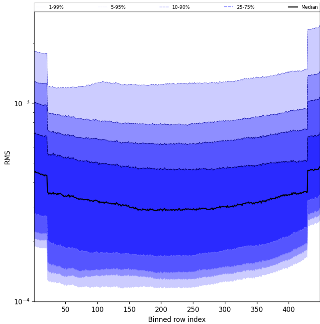
Figure 60: Along track statistics of “RMS” for 2024-10-10 to 2024-10-12
