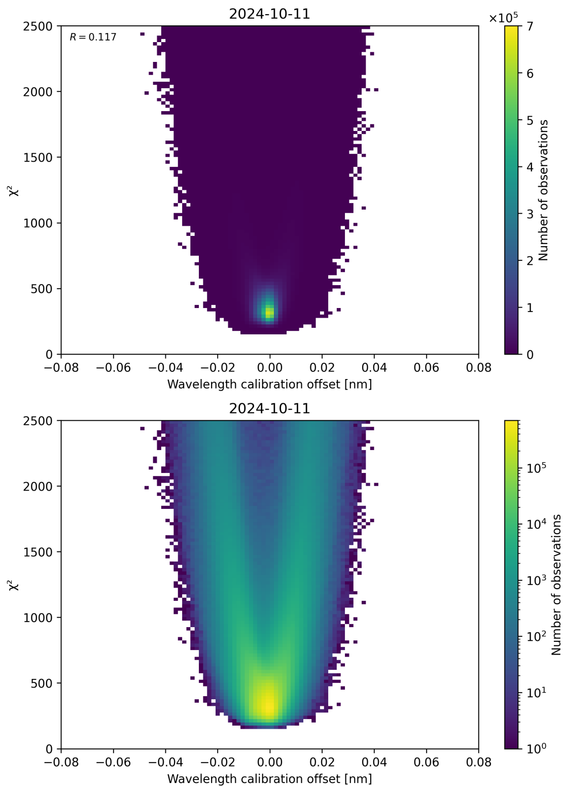
Figure 175: Scatter density plot of “Wavelength calibration offset” against “ \chi^2 ” for 2024-10-10 to 2024-10-12.
