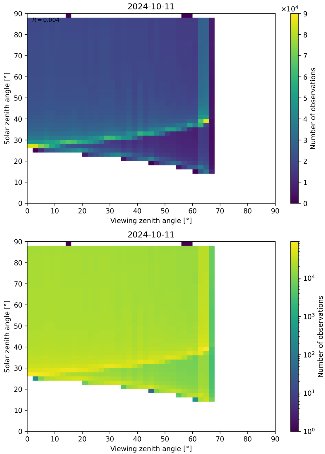
Figure 172: Scatter density plot of “Viewing zenith angle” against “Solar zenith angle” for 2024-10-10 to 2024-10-12.
