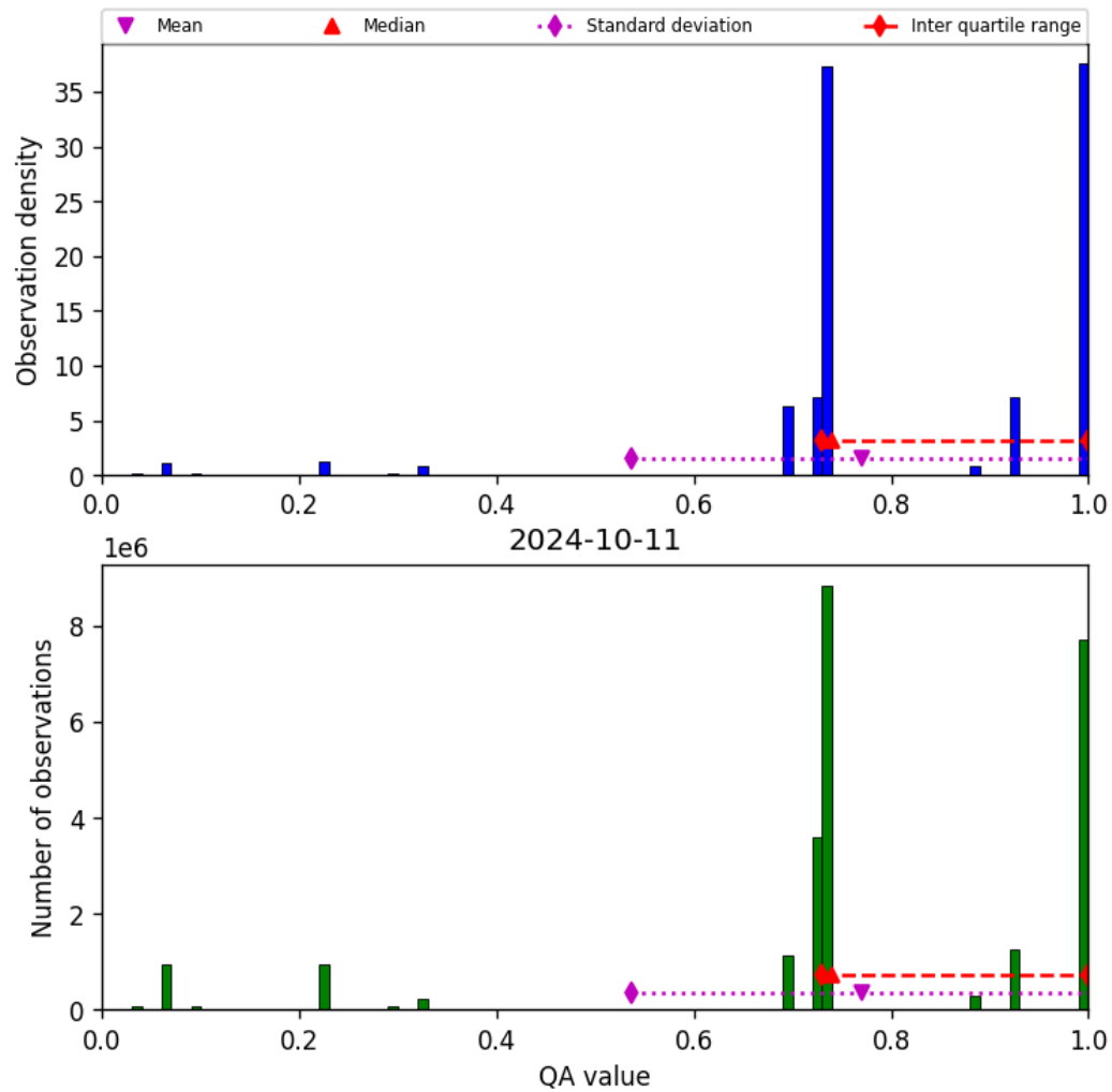
Figure 28: Histogram of “QA value” for 2024-10-10 to 2024-10-12
