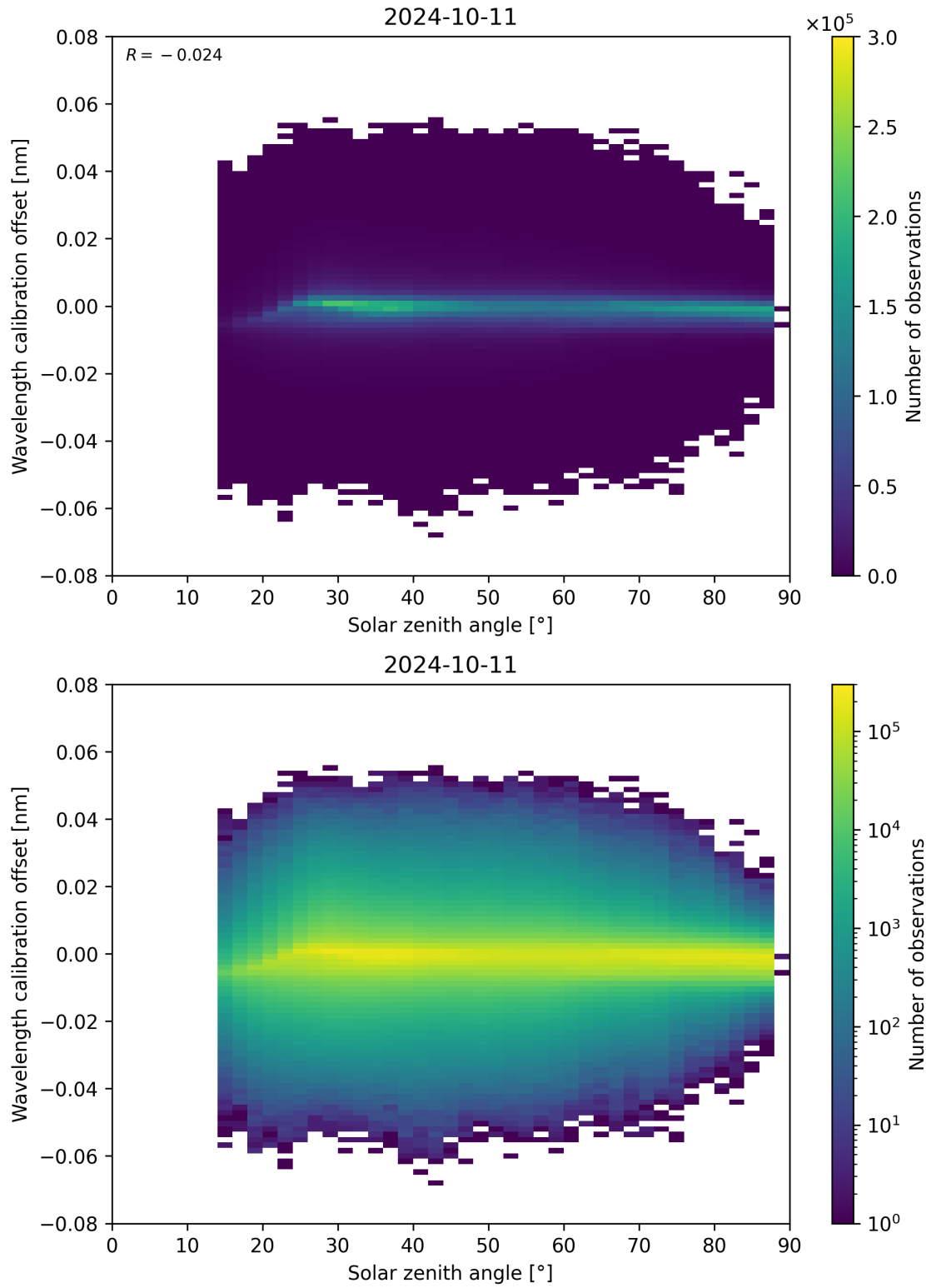
Figure 158: Scatter density plot of “Solar zenith angle” against “Wavelength calibration offset” for 2024-10-10 to 2024-10-12.
