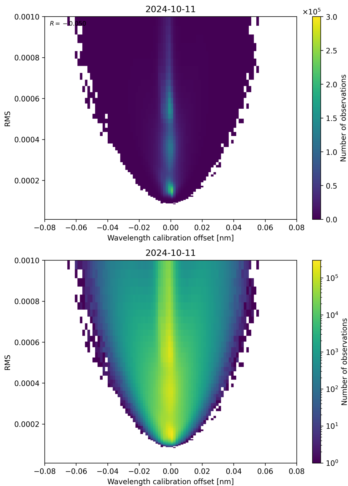
Figure 181: Scatter density plot of “Wavelength calibration offset” against “RMS” for 2024-10-10 to 2024-10-12.
