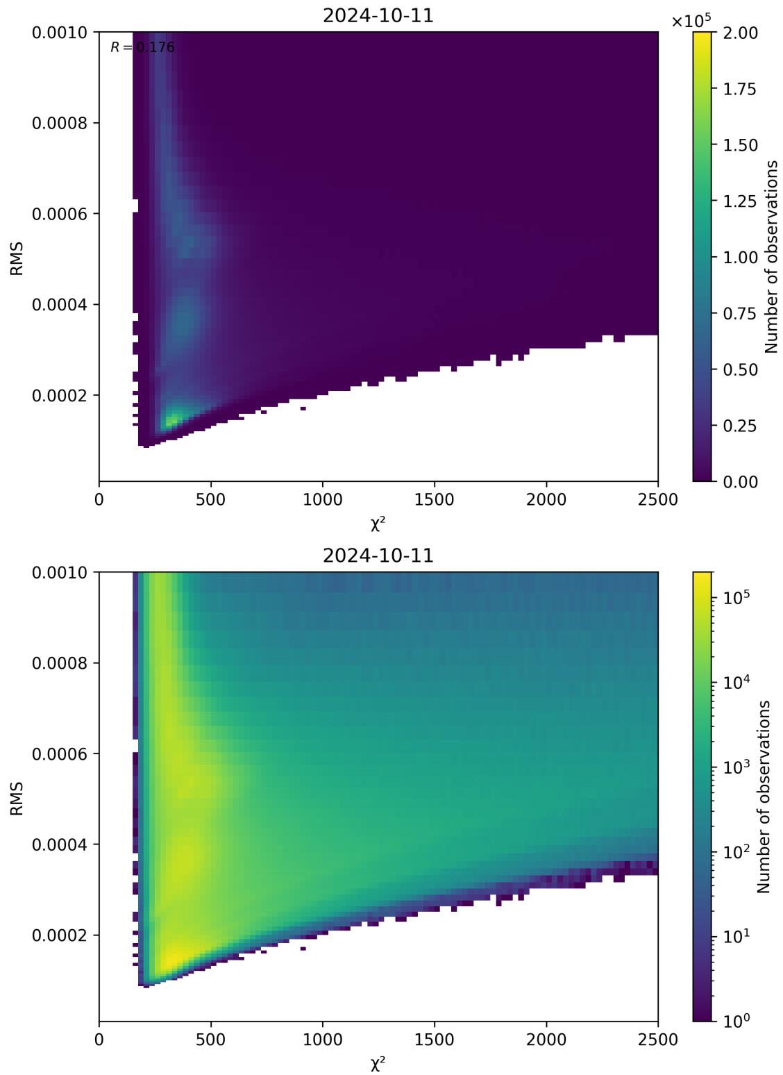
Figure 82: Scatter density plot of “ \chi^2 ” against “RMS” for 2024-10-10 to 2024-10-12.
