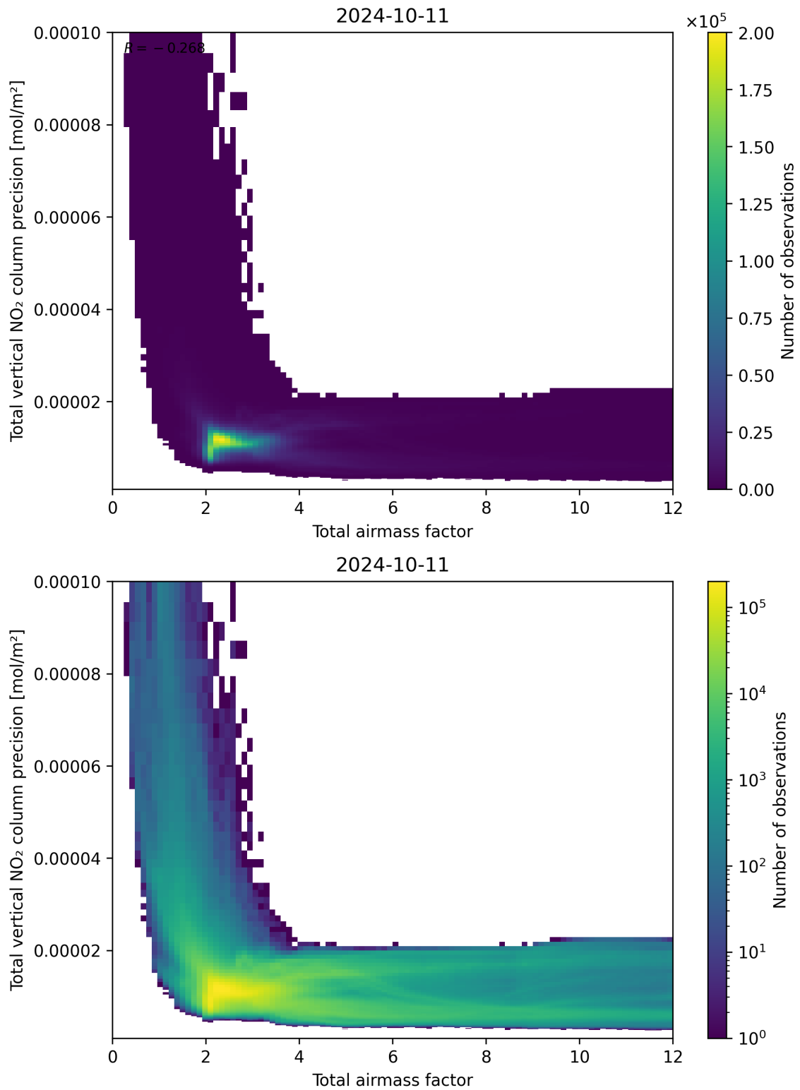
Figure 68: Scatter density plot of “Total airmass factor” against “Total vertical NO 2 column precision” for 2024-10-10 to 2024-10-12.
