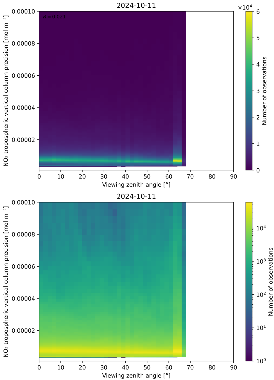
Figure 170: Scatter density plot of “Viewing zenith angle” against “NO 2 tropospheric vertical column precision” for 2024-10-10 to 2024-10-12.
