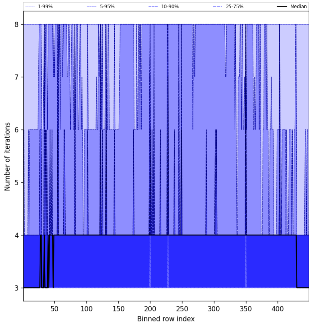
Figure 51: Along track statistics of “Number of iterations” for 2024-10-10 to 2024-10-12
