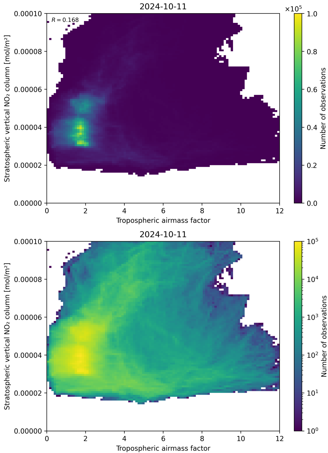
Figure 74: Scatter density plot of “Tropospheric air mass factor” against “Stratospheric vertical NO 2 column” for 2024-10-10 to 2024-10-12.
