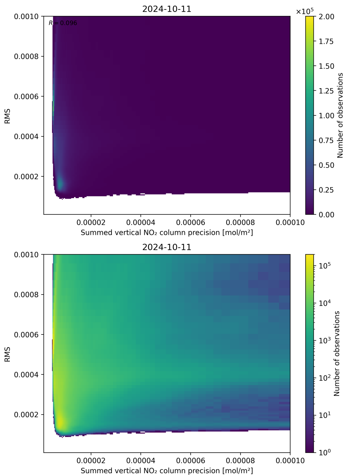
Figure 108: Scatter density plot of “Summed vertical NO 2 column precision” against “RMS” for 2024-10-10 to 2024-10-12.
