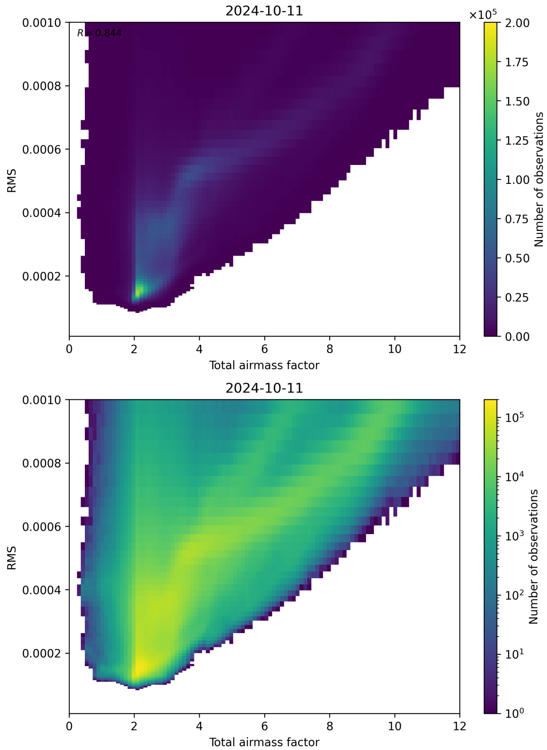
Figure 69: Scatter density plot of “Total airmass factor” against “RMS” for 2024-10-10 to 2024-10-12.
