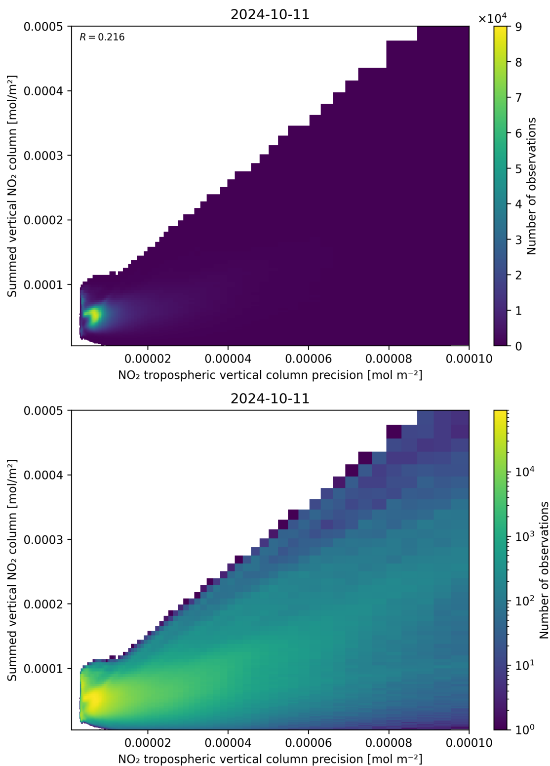
Figure 136: Scatter density plot of “NO 2 tropospheric vertical column precision” against “Summed vertical NO 2 column” for 2024-10-10 to 2024-10-12.
