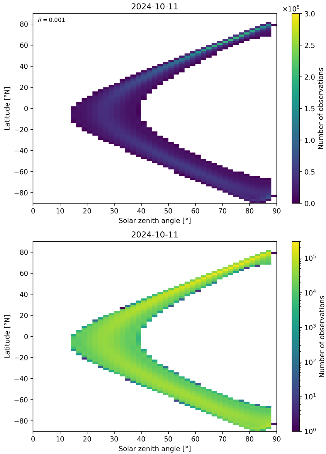
Figure 149: Scatter density plot of “Solar zenith angle” against “Latitude” for 2024-10-10 to 2024-10-12.
