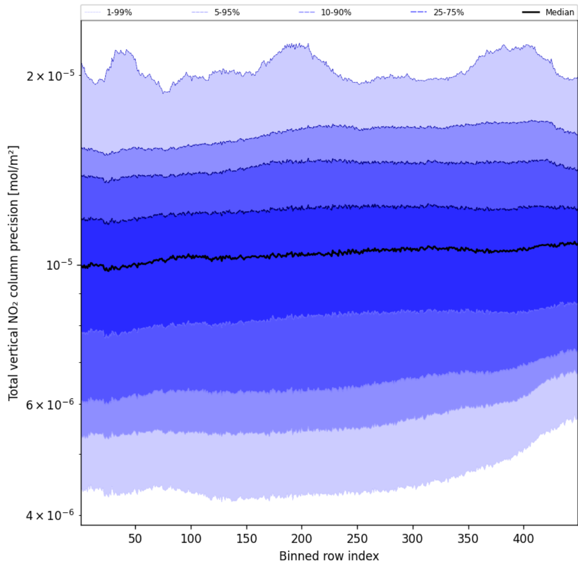
Figure 56: Along track statistics of “Total vertical NO 2 column precision” for 2024-10-10 to 2024-10-12
