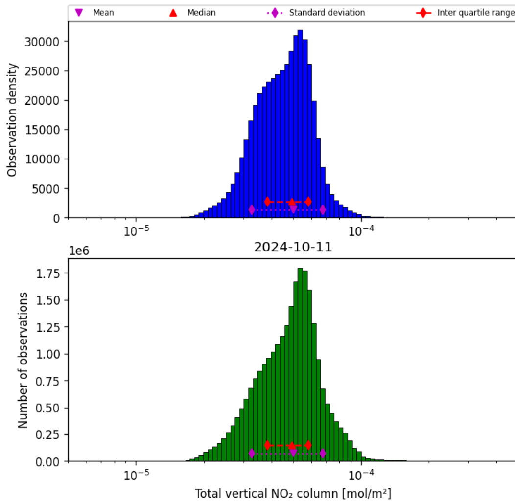
Figure 38: Histogram of “Total vertical NO 2 column” for 2024-10-10 to 2024-10-12
