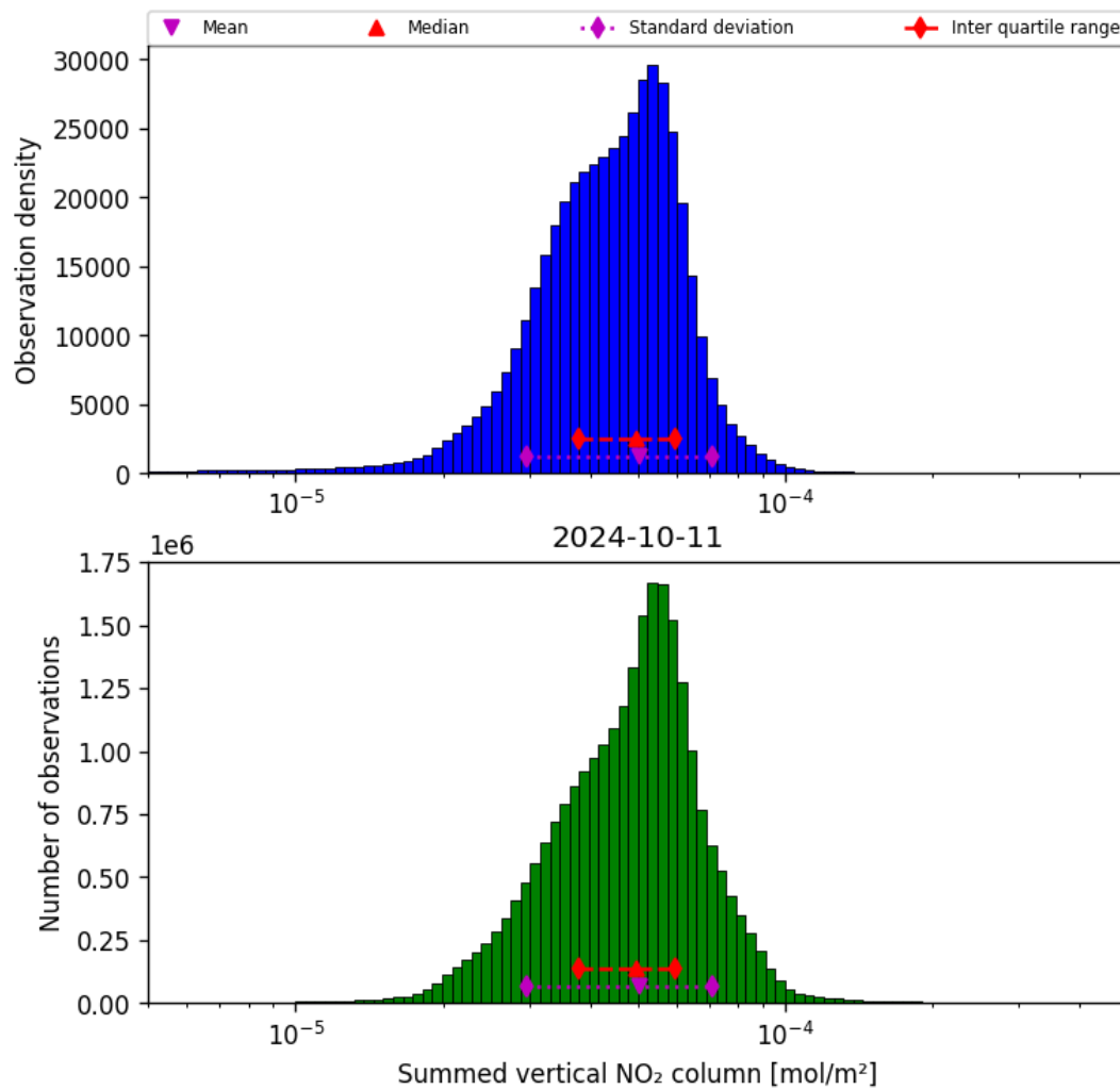
Figure 40: Histogram of “Summed vertical NO 2 column” for 2024-10-10 to 2024-10-12
