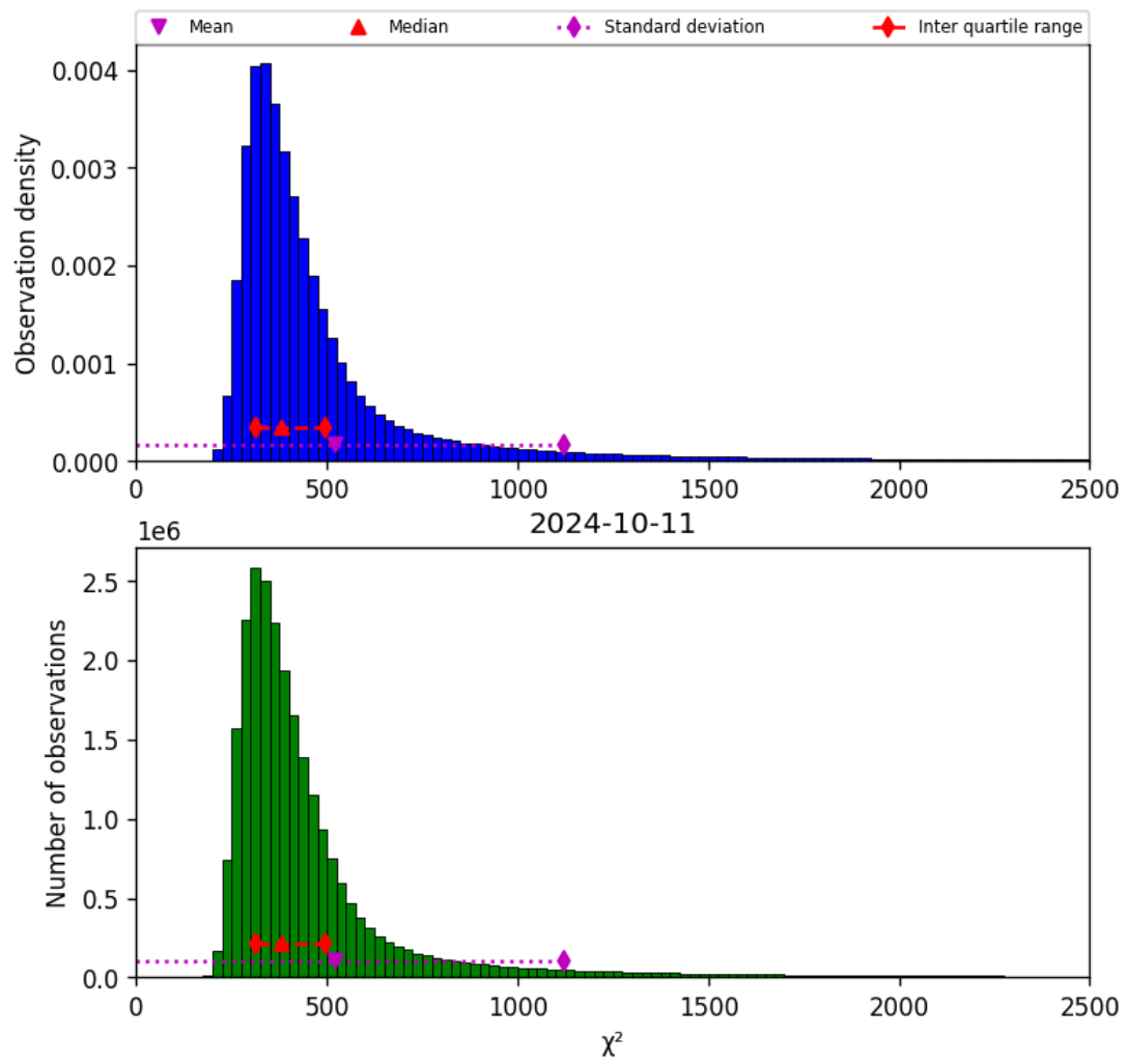
Figure 42: Histogram of “ \chi^2 ” for 2024-10-10 to 2024-10-12
