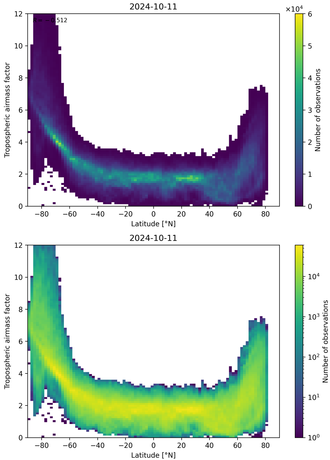
Figure 85: Scatter density plot of “Latitude” against “Tropospheric air mass factor” for 2024-10-10 to 2024-10-12.
