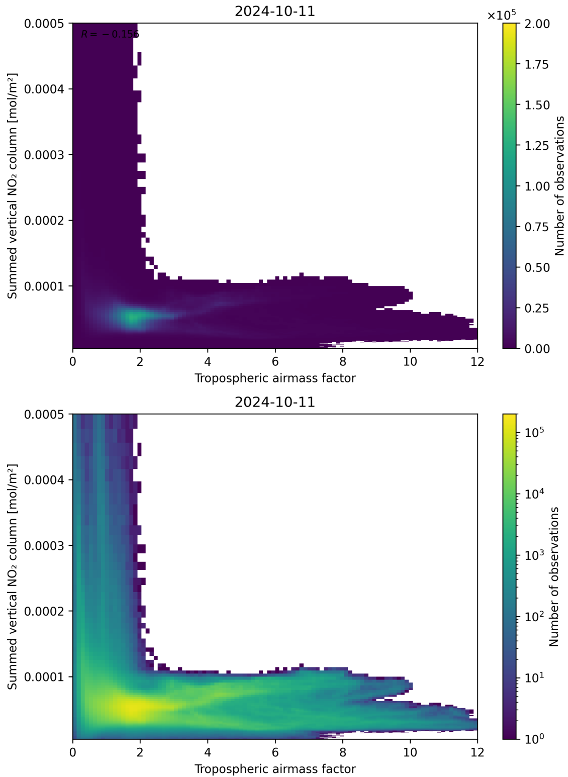
Figure 75: Scatter density plot of “Tropospheric air mass factor” against “Summed vertical NO 2 column” for 2024-10-10 to 2024-10-12.
