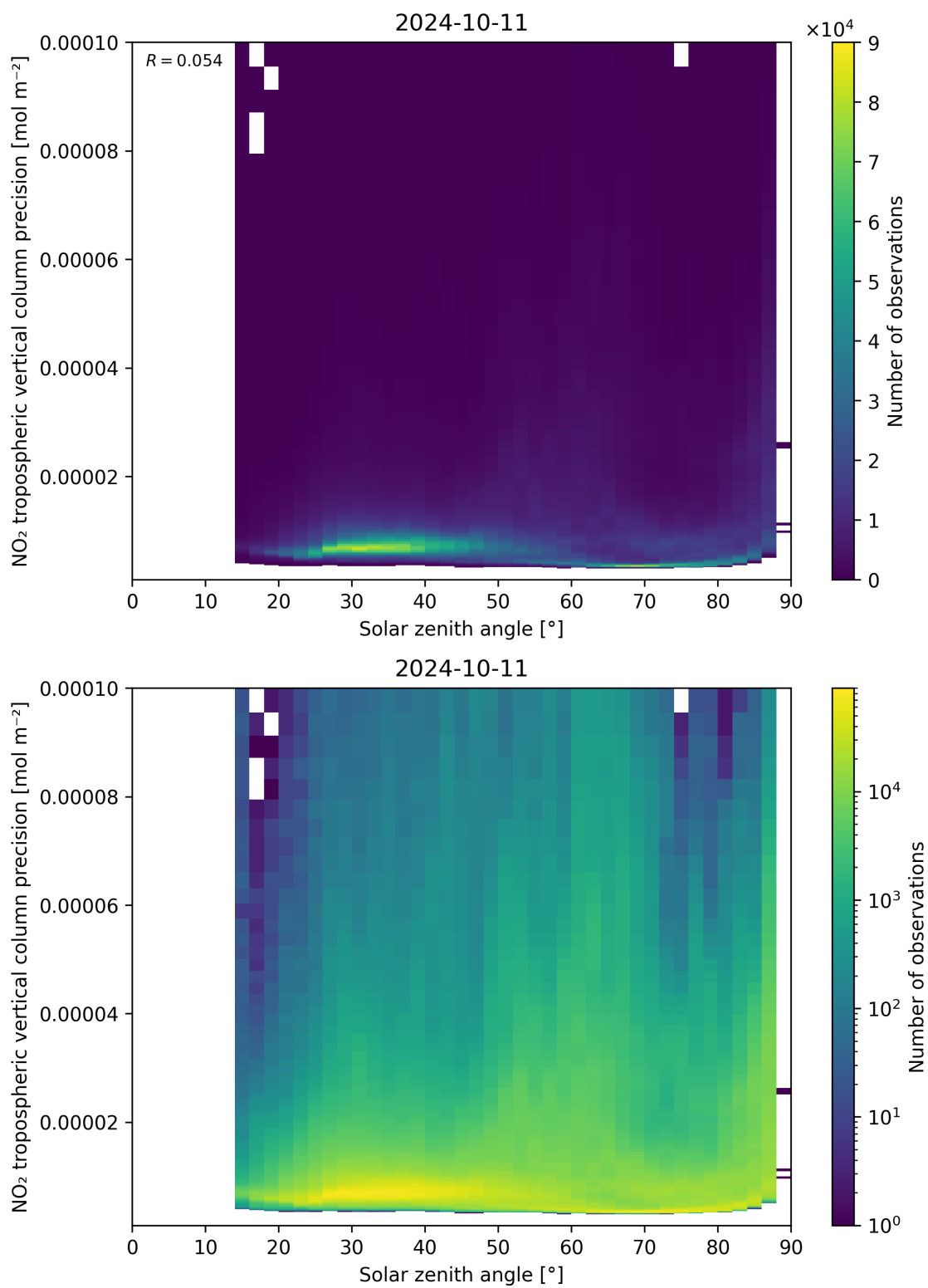
Figure 156: Scatter density plot of “Solar zenith angle” against “NO 2 tropospheric vertical column precision” for 2024-10-10 to 2024-10-12.
