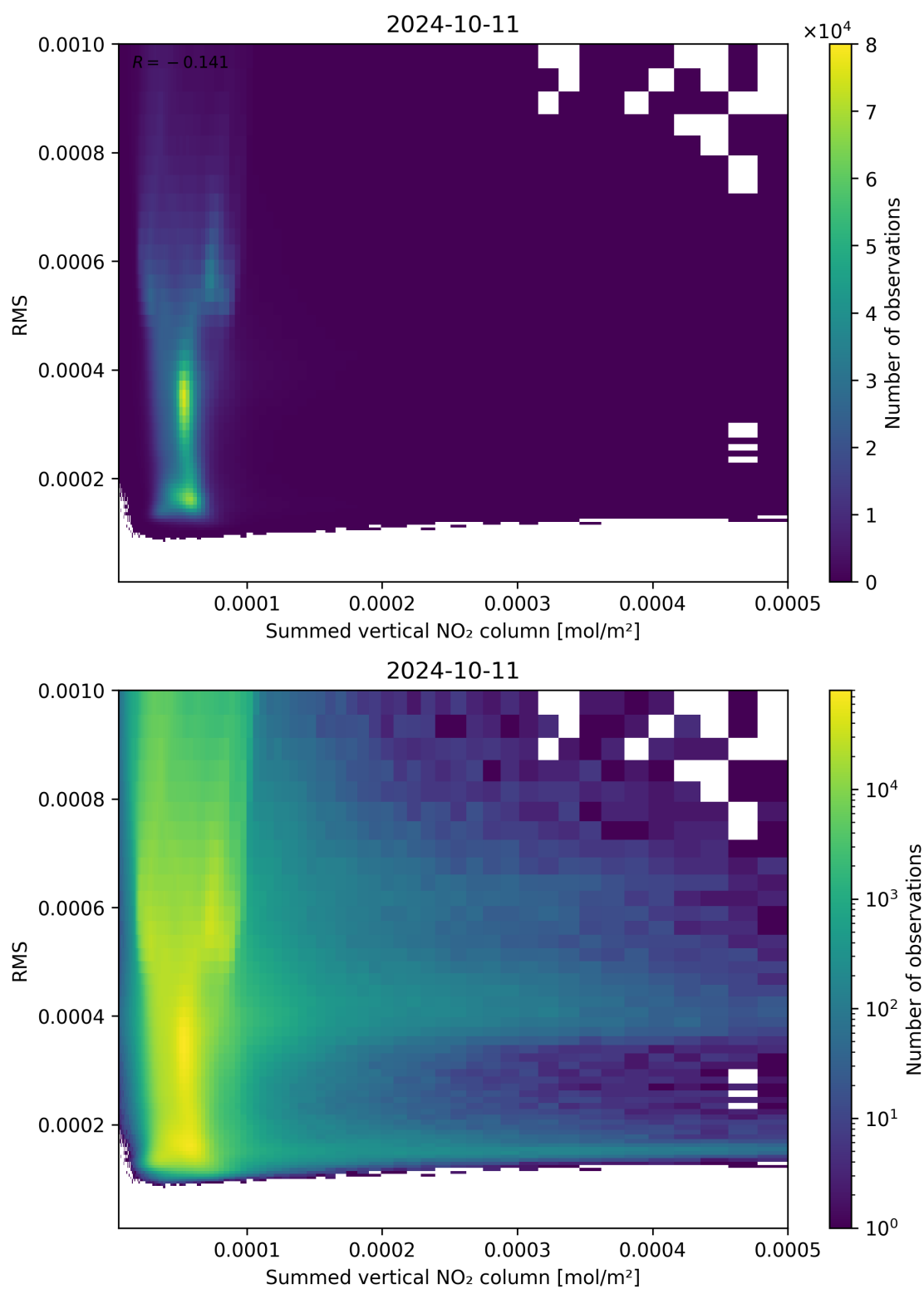
Figure 109: Scatter density plot of “Summed vertical NO 2 column” against “RMS” for 2024-10-10 to 2024-10-12.
