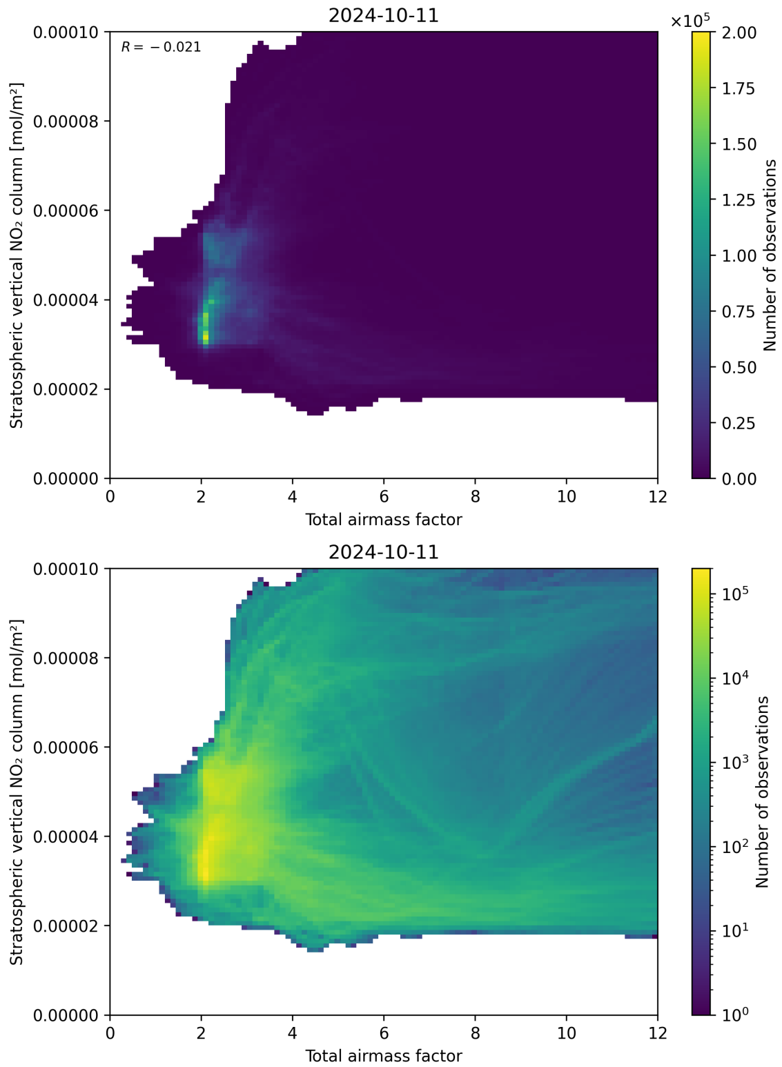
Figure 64: Scatter density plot of “Total airmass factor” against “Stratospheric vertical NO 2 column” for 2024-10-10 to 2024-10-12.
