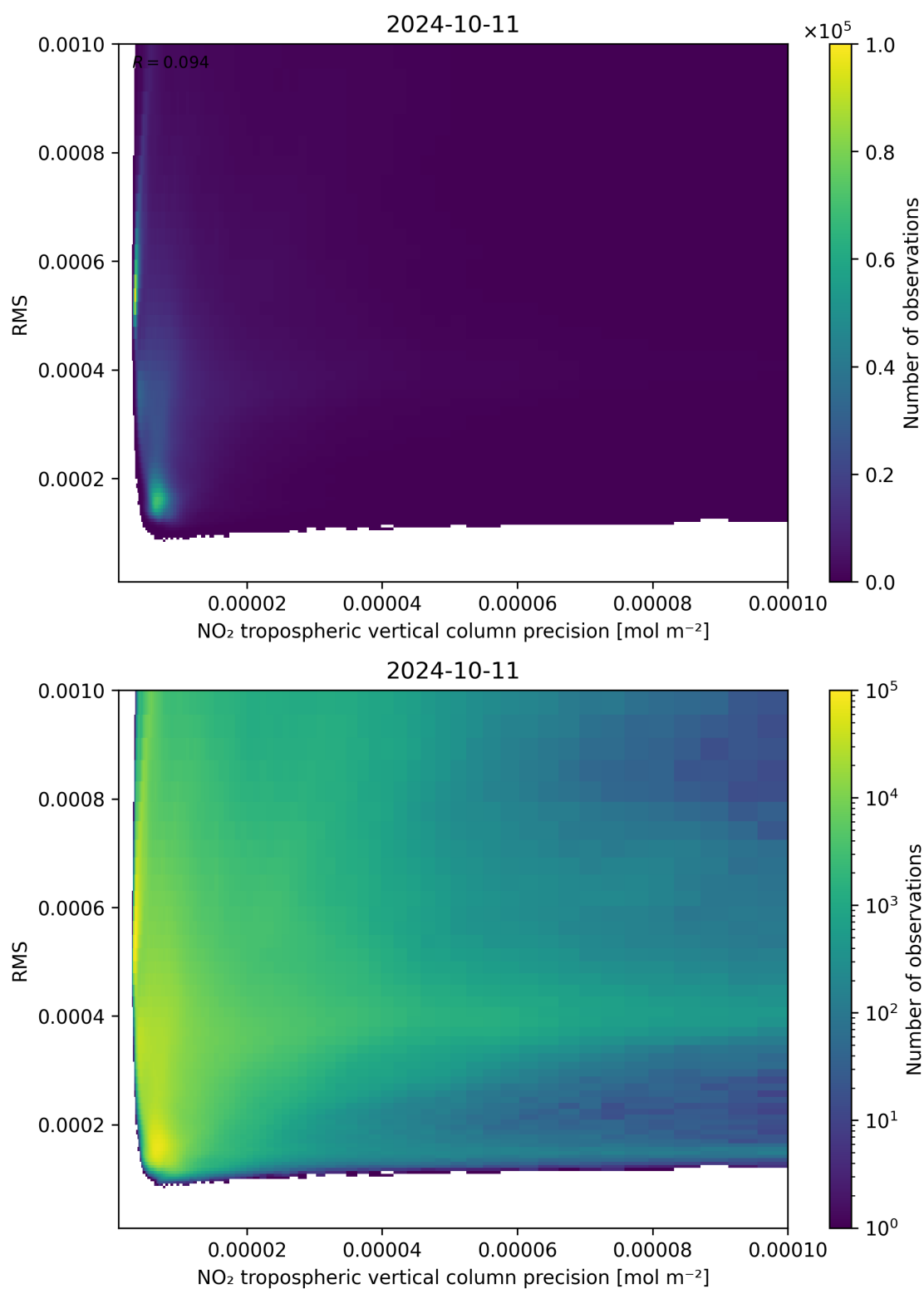
Figure 140: Scatter density plot of “NO 2 tropospheric vertical column precision” against “RMS” for 2024-10-10 to 2024-10-12.
