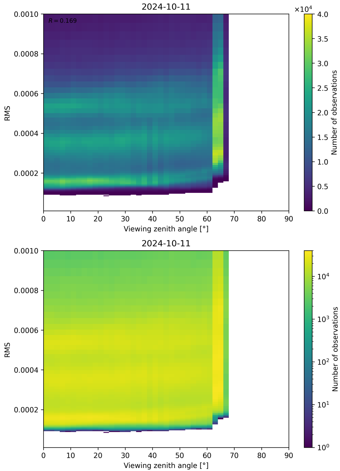
Figure 171: Scatter density plot of “Viewing zenith angle” against “RMS” for 2024-10-10 to 2024-10-12.
