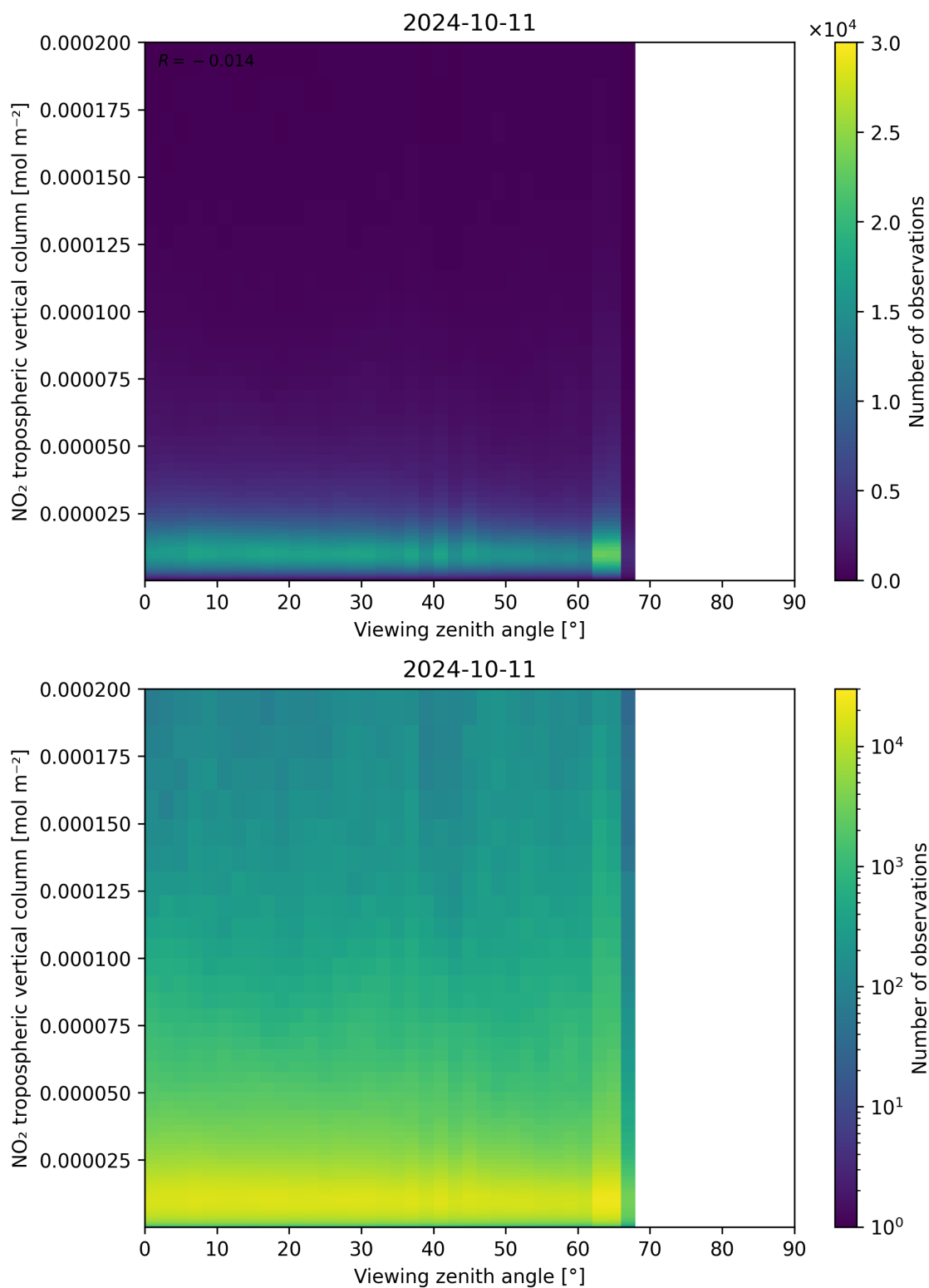
Figure 169: Scatter density plot of “Viewing zenith angle” against “NO 2 tropospheric vertical column” for 2024-10-10 to 2024-10-12.
