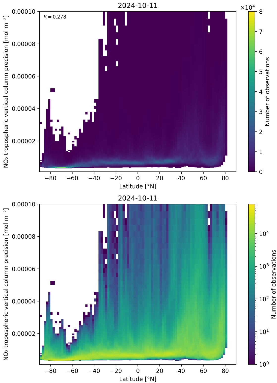
Figure 93: Scatter density plot of “Latitude” against “NO 2 tropospheric vertical column precision” for 2024-10-10 to 2024-10-12.
