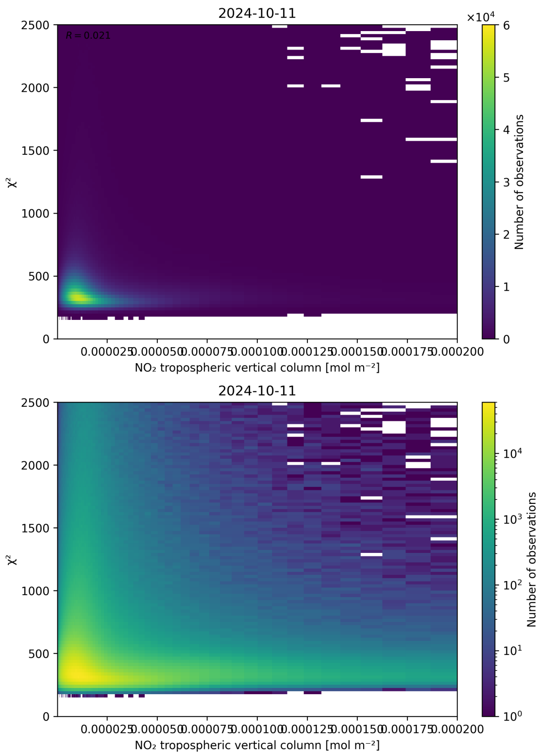
Figure 124: Scatter density plot of “NO 2 tropospheric vertical column” against “ \chi^2 ” for 2024-10-10 to 2024-10-12.
