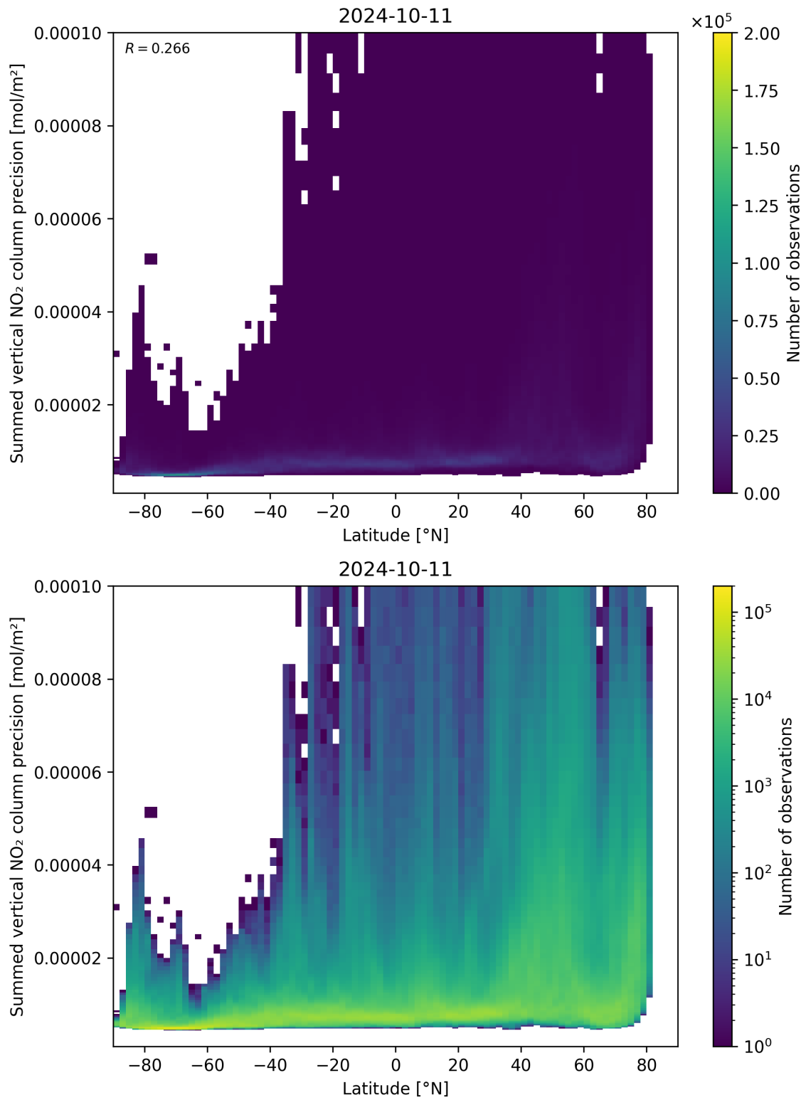
Figure 89: Scatter density plot of “Latitude” against “Summed vertical NO 2 column precision” for 2024-10-10 to 2024-10-12.
