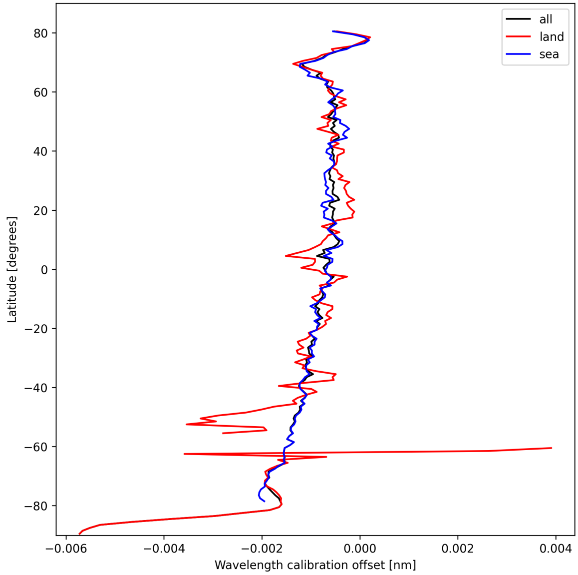
Figure 18: Zonal average of “Wavelength calibration offset” for 2024-10-10 to 2024-10-12.
