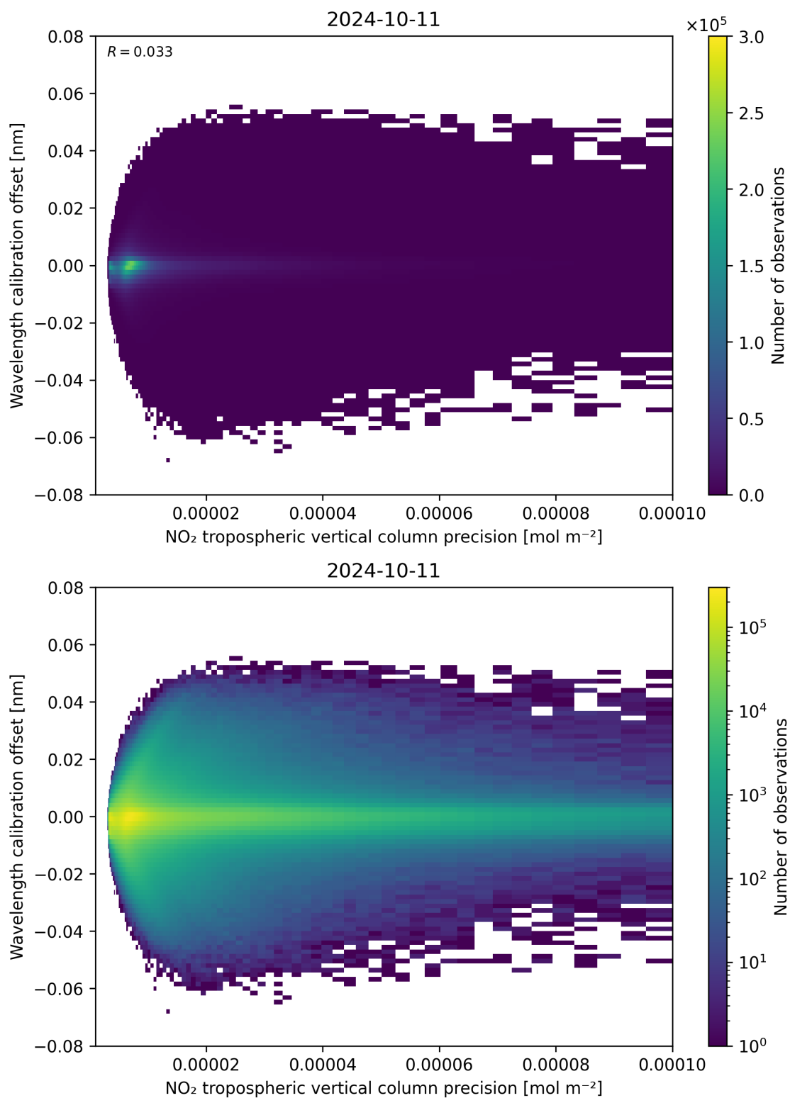
Figure 141: Scatter density plot of “NO 2 tropospheric vertical column precision” against “Wavelength calibration offset” for 2024-10-10 to 2024-10-12.
