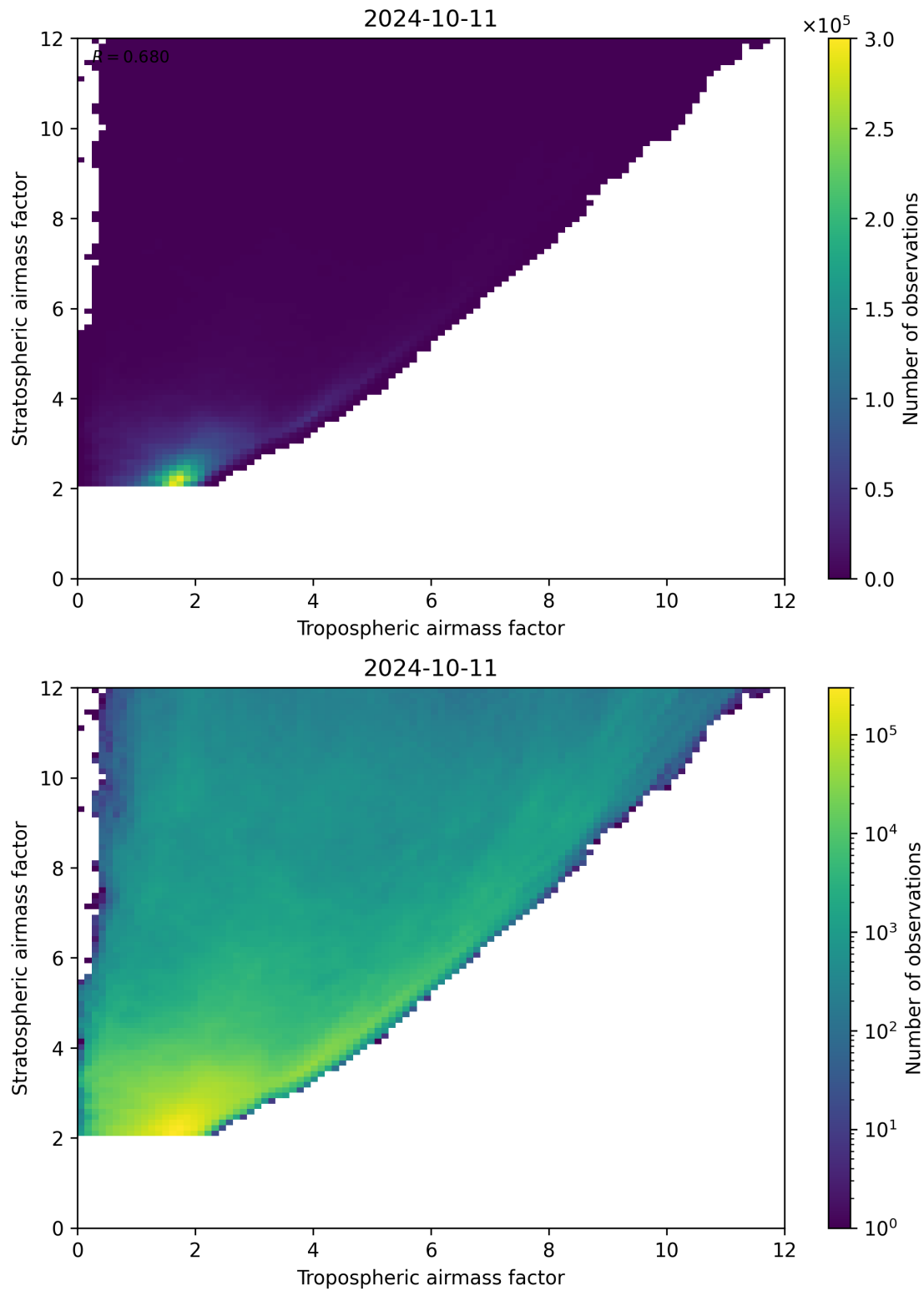
Figure 71: Scatter density plot of “Tropospheric airmass factor” against “Stratospheric airmass factor” for 2024-10-10 to 2024-10-12.
