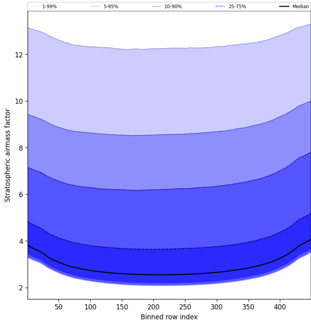
Figure 61: Along track statistics of “Stratospheric airmass factor” for 2024-10-10 to 2024-10-12
