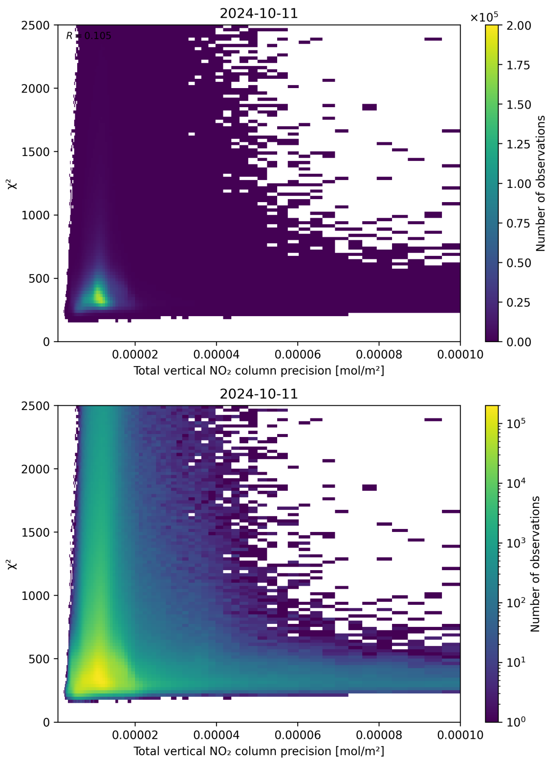
Figure 116: Scatter density plot of “Total vertical NO 2 column precision” against “ \chi^2 ” for 2024-10-10 to 2024-10-12.
