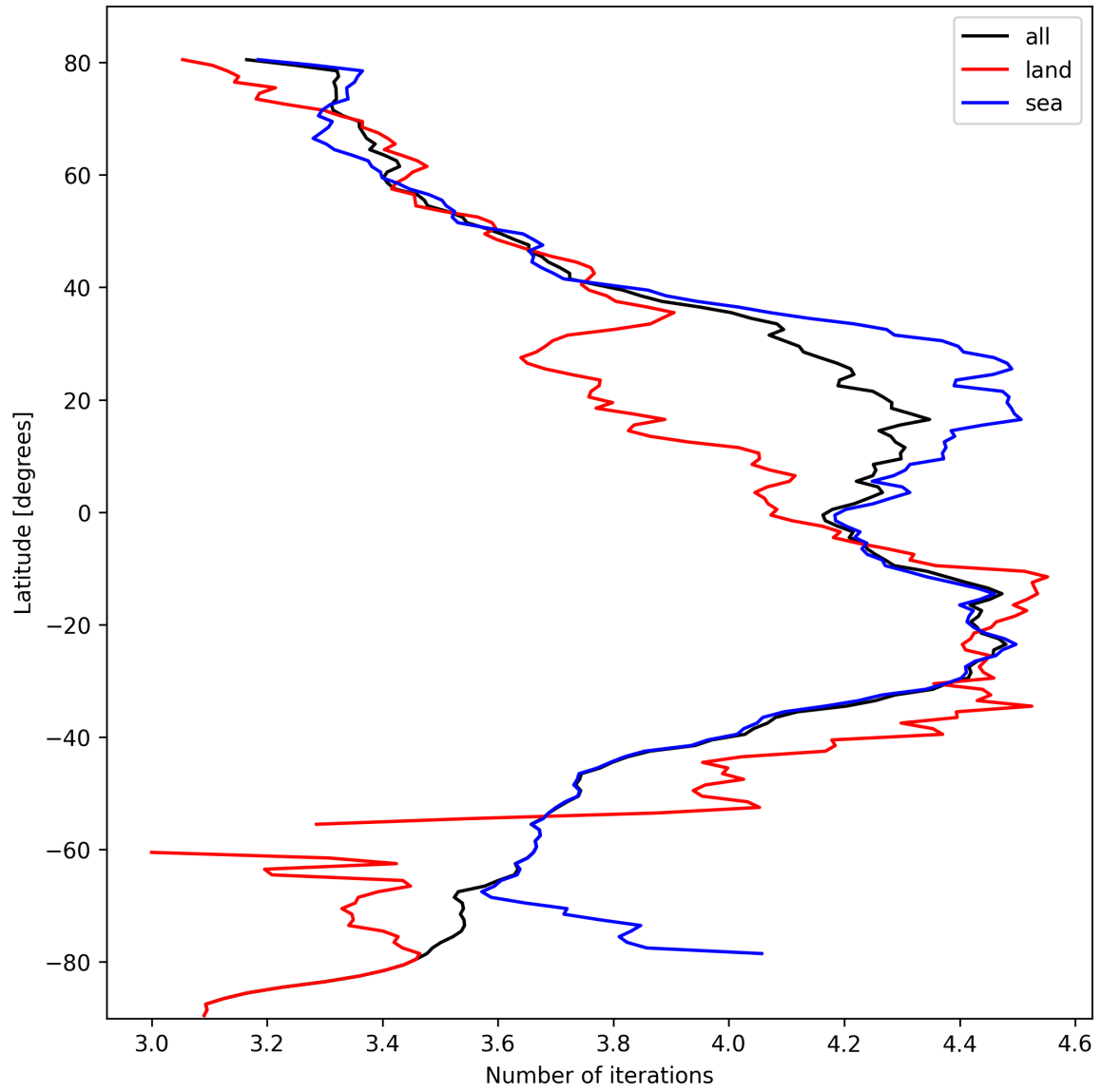
Figure 17: Zonal average of “Number of iterations” for 2024-10-10 to 2024-10-12.
