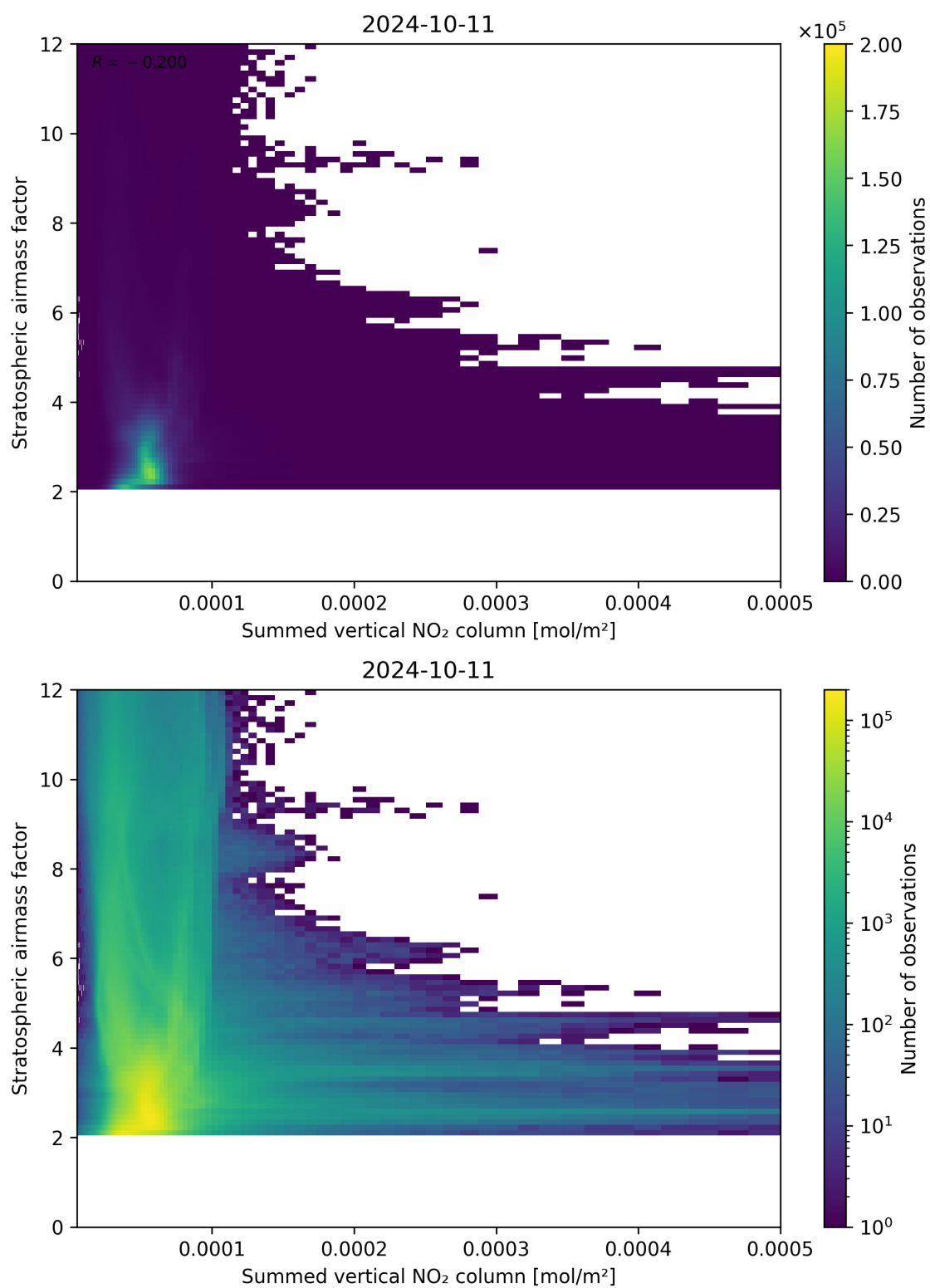
Figure 103: Scatter density plot of “Summed vertical NO 2 column” against “Stratospheric airmass factor” for 2024-10-10 to 2024-10-12.
