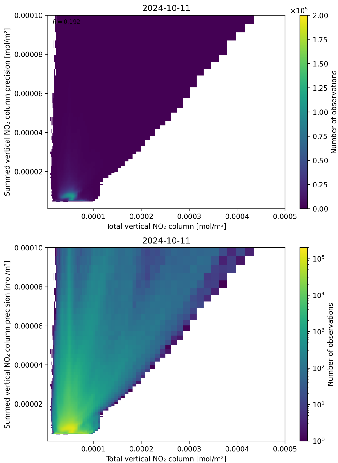
Figure 113: Scatter density plot of “Total vertical NO 2 column” against “Summed vertical NO 2 column precision” for 2024-10-10 to 2024-10-12.
