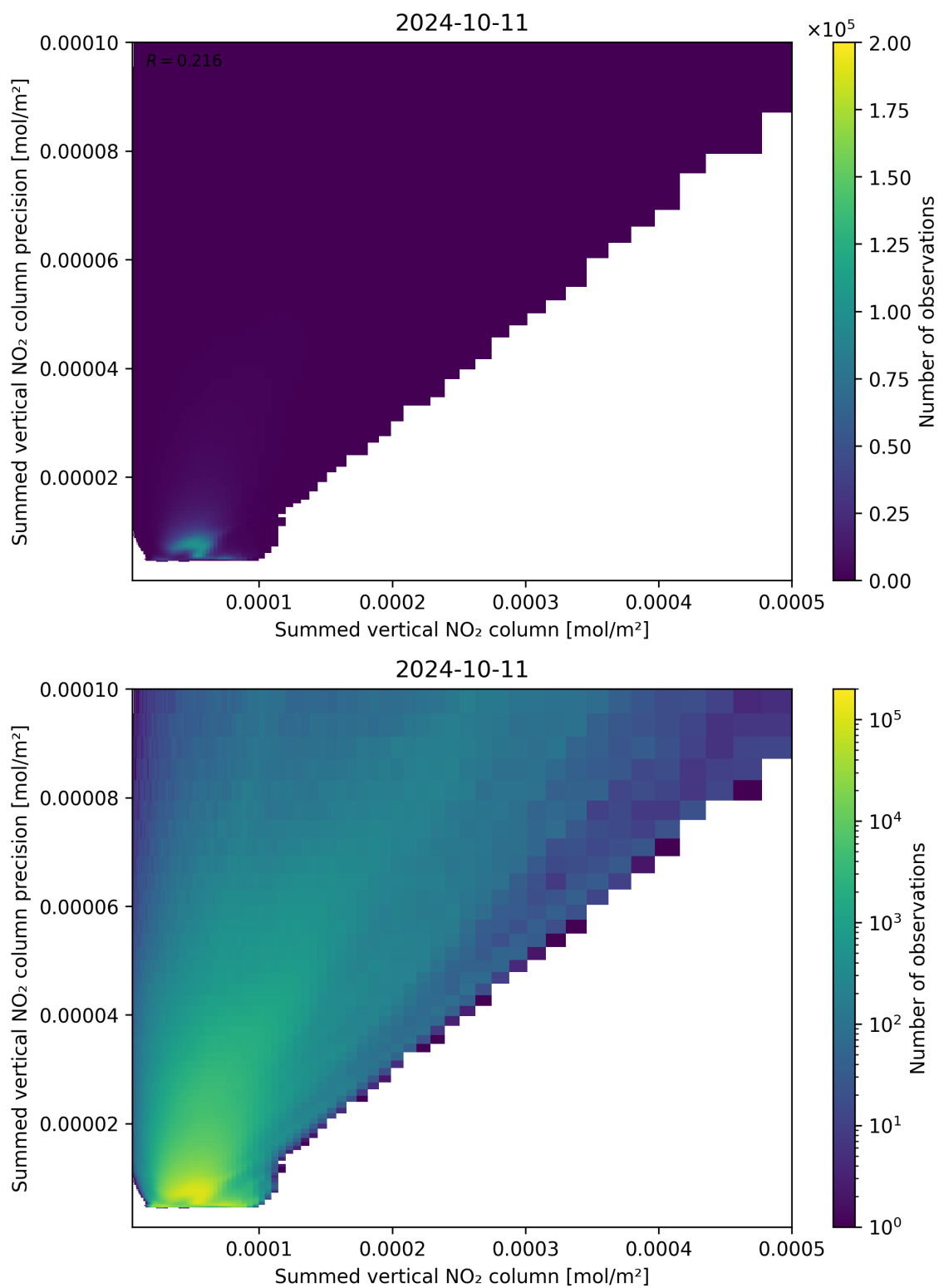
Figure 105: Scatter density plot of “Summed vertical NO 2 column” against “Summed vertical NO 2 column precision” for 2024-10-10 to 2024-10-12.
