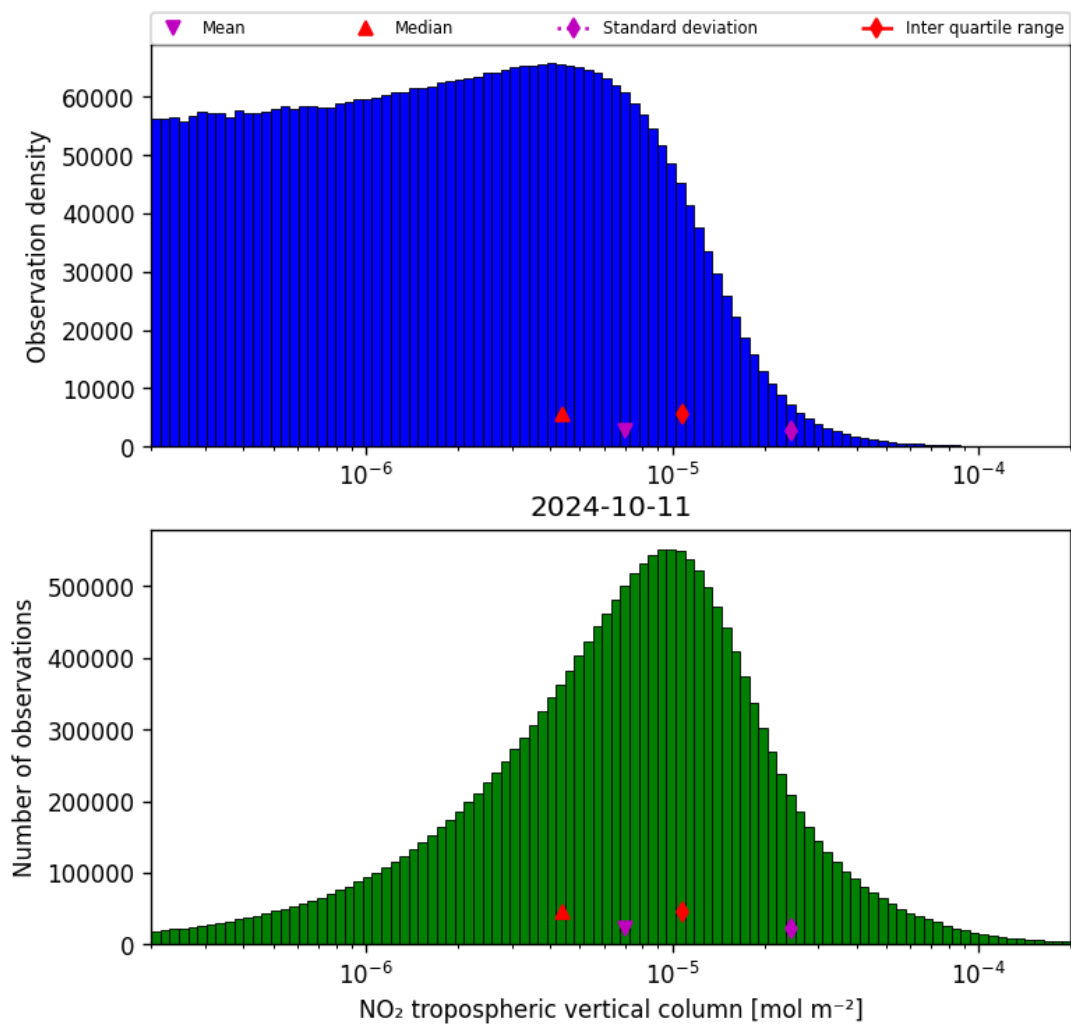
Figure 29: Histogram of “NO 2 tropospheric vertical column” for 2024-10-10 to 2024-10-12
