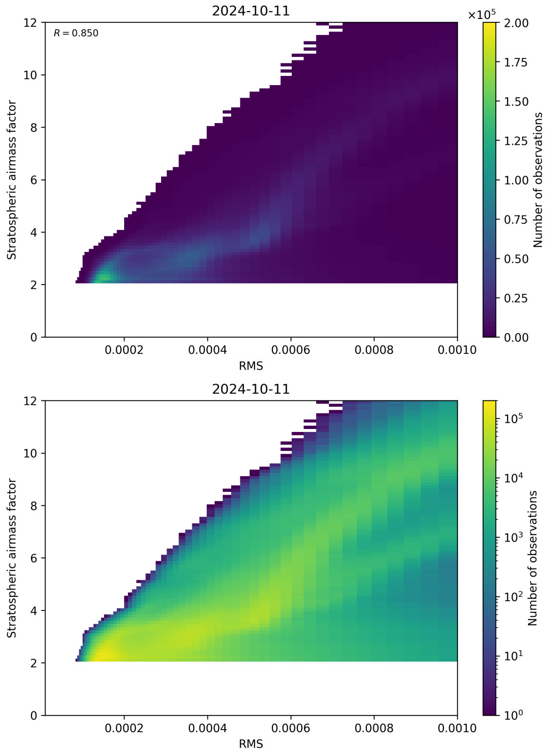
Figure 144: Scatter density plot of “RMS” against “Stratospheric airmass factor” for 2024-10-10 to 2024-10-12.
