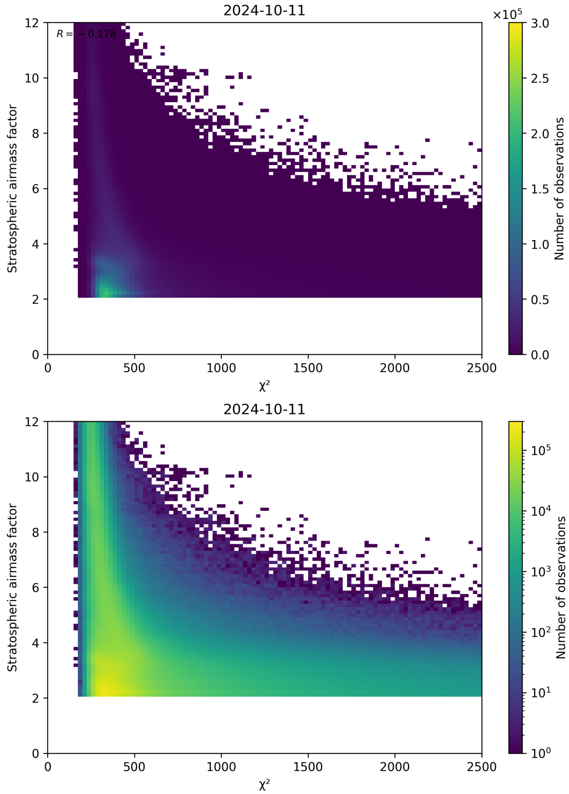
Figure 81: Scatter density plot of “ \chi^2 ” against “Stratospheric airmass factor” for 2024-10-10 to 2024-10-12.
