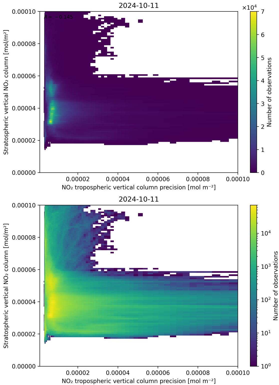
Figure 135: Scatter density plot of “NO 2 tropospheric vertical column precision” against “Stratospheric vertical NO 2 column” for 2024-10-10 to 2024-10-12.
