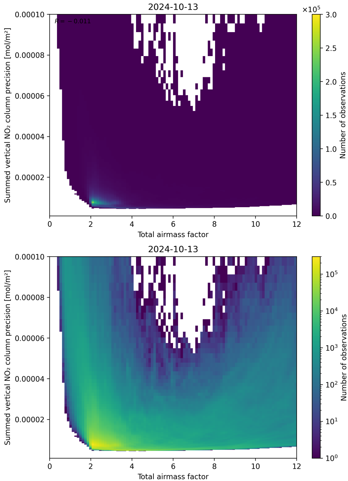
Figure 66: Scatter density plot of “Total airmass factor” against “Summed vertical NO 2 column precision” for 2024-10-12 to 2024-10-14.
