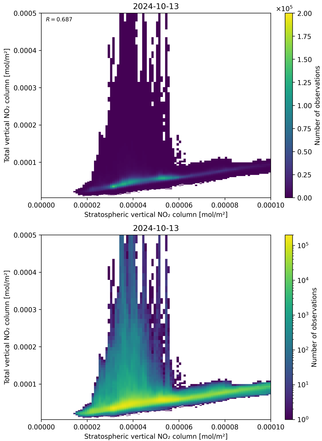
Figure 100: Scatter density plot of “Stratospheric vertical NO 2 column” against “Total vertical NO 2 column” for 2024-10-12 to 2024-10-14.
