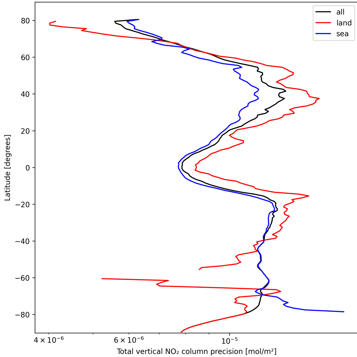
Figure 22: Zonal average of “Total vertical NO 2 column precision” for 2024-10-12 to 2024-10-14.
