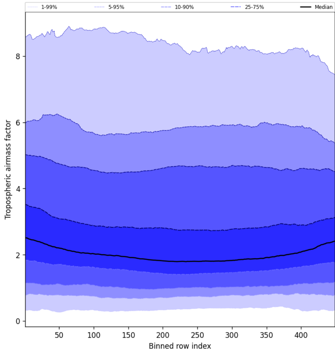
Figure 48: Along track statistics of “Tropospheric airmass factor” for 2024-10-12 to 2024-10-14
