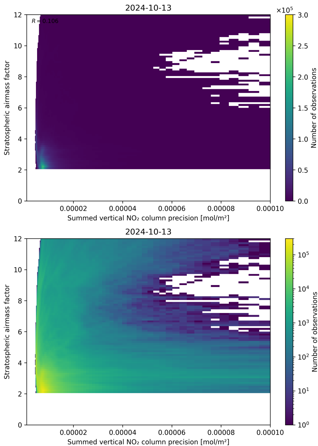
Figure 106: Scatter density plot of “Summed vertical NO 2 column precision” against “Stratospheric airmass factor” for 2024-10-12 to 2024-10-14.
