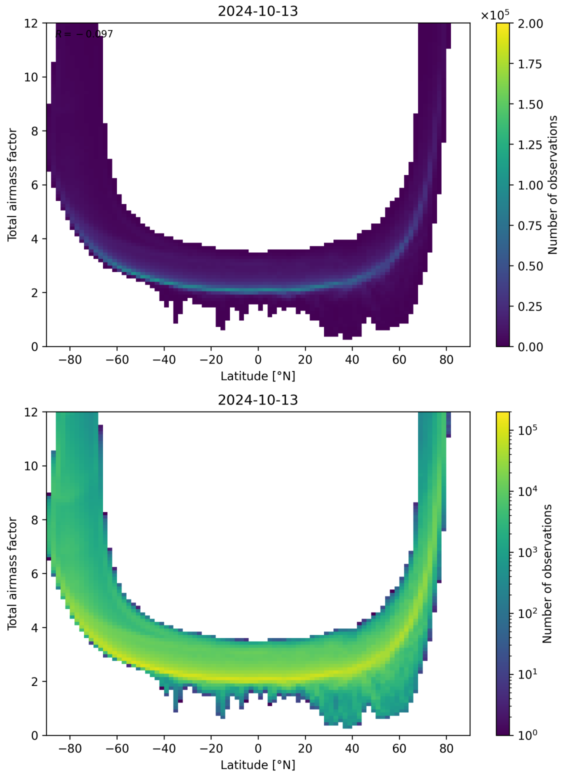
Figure 84: Scatter density plot of “Latitude” against “Total airmass factor” for 2024-10-12 to 2024-10-14.
