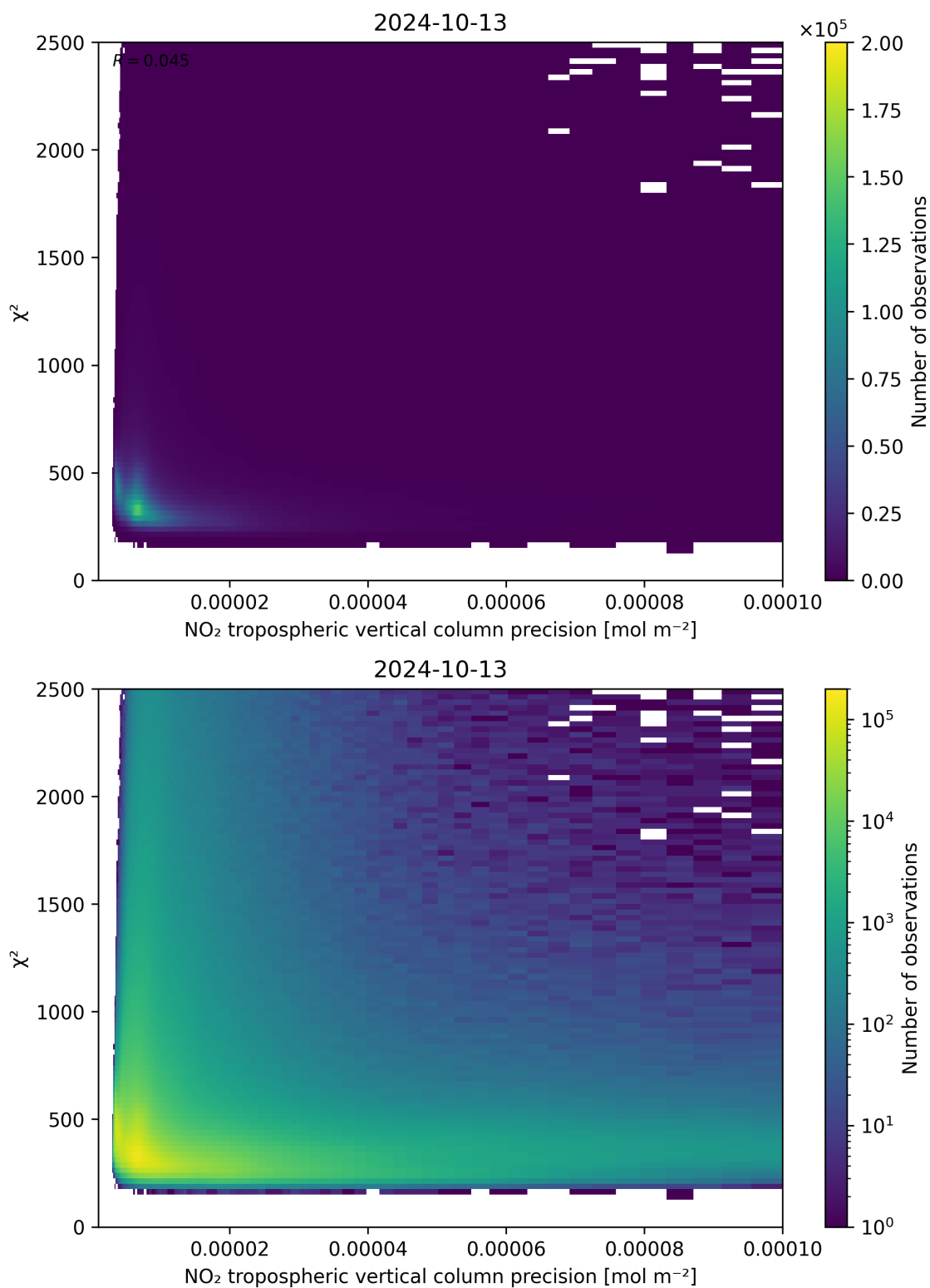
Figure 134: Scatter density plot of “NO 2 tropospheric vertical column precision” against “ \chi^2 ” for 2024-10-12 to 2024-10-14.
