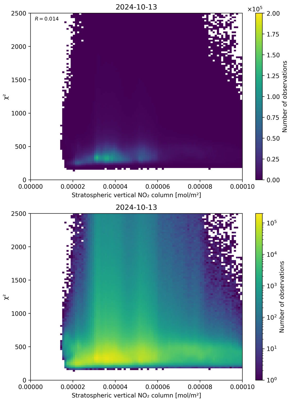
Figure 97: Scatter density plot of “Stratospheric vertical NO 2 column” against “ \chi^2 ” for 2024-10-12 to 2024-10-14.
