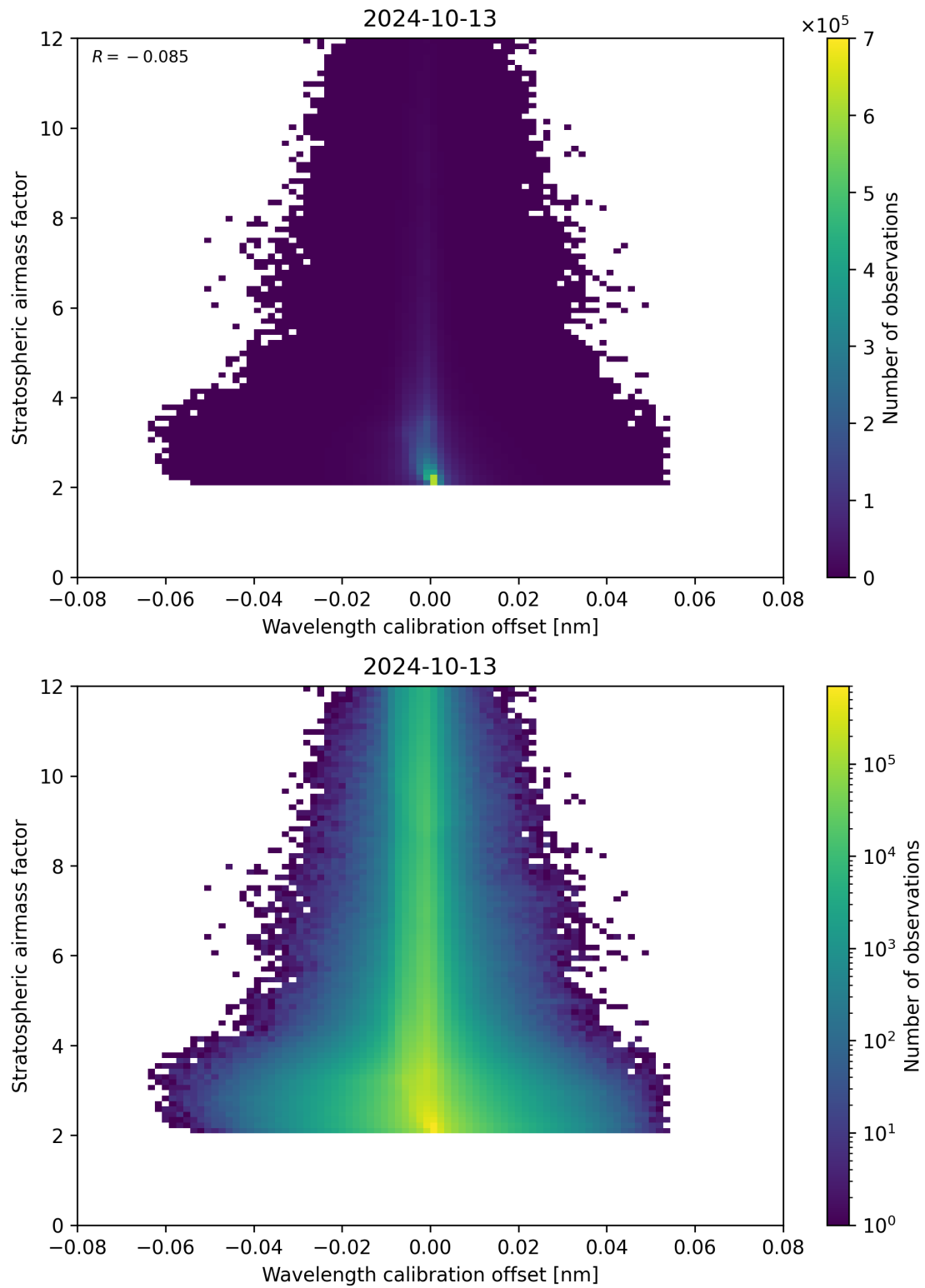
Figure 174: Scatter density plot of “Wavelength calibration offset” against “Stratospheric airmass factor” for 2024-10-12 to 2024-10-14.
