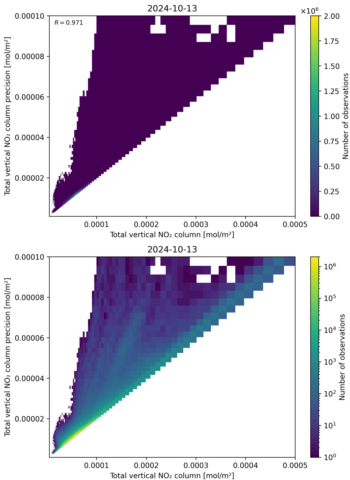
Figure 114: Scatter density plot of “Total vertical NO 2 column” against “Total vertical NO 2 column precision” for 2024-10-12 to 2024-10-14.
