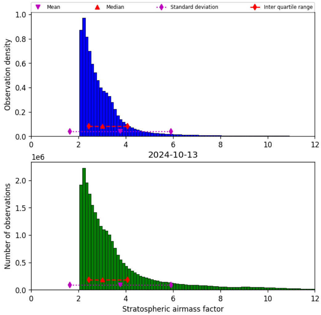
Figure 44: Histogram of “Stratospheric airmass factor” for 2024-10-12 to 2024-10-14
