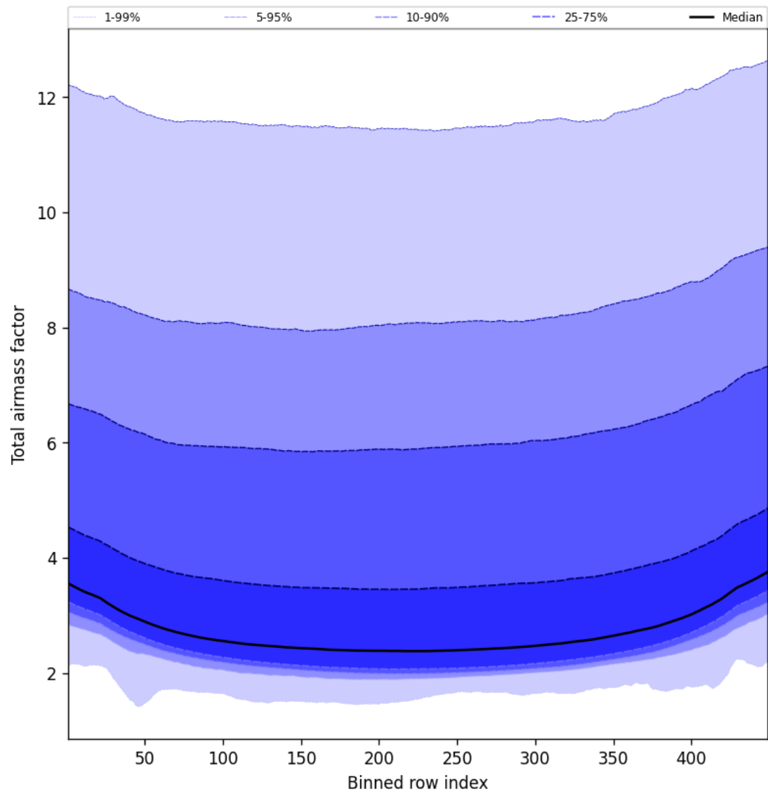
Figure 49: Along track statistics of “Total airmass factor” for 2024-10-12 to 2024-10-14
