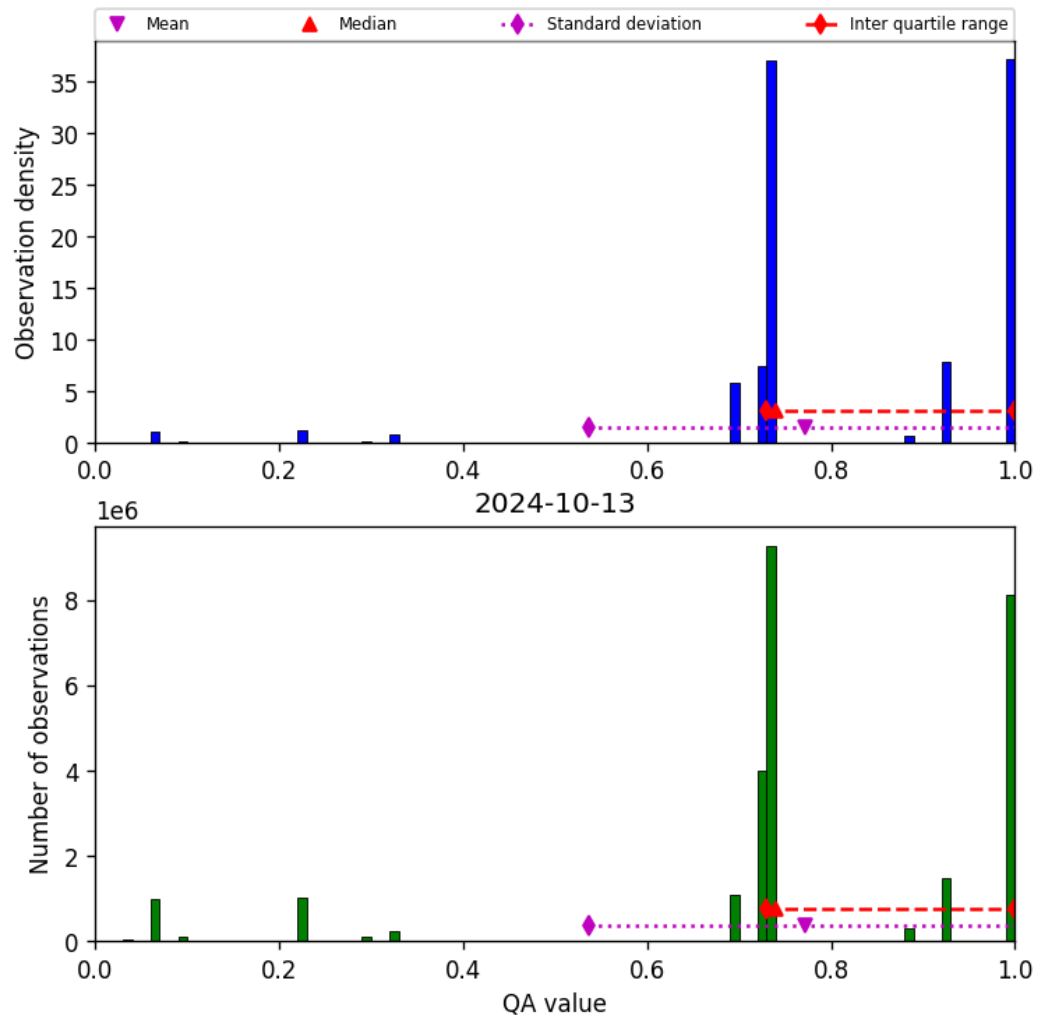
Figure 28: Histogram of “QA value” for 2024-10-12 to 2024-10-14
