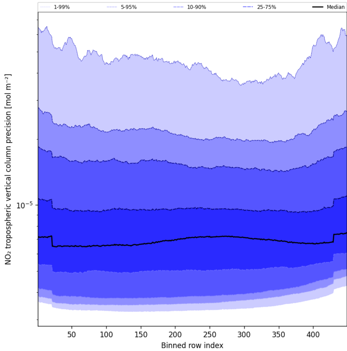
Figure 47: Along track statistics of “NO 2 tropospheric vertical column precision” for 2024-10-12 to 2024-10-14
