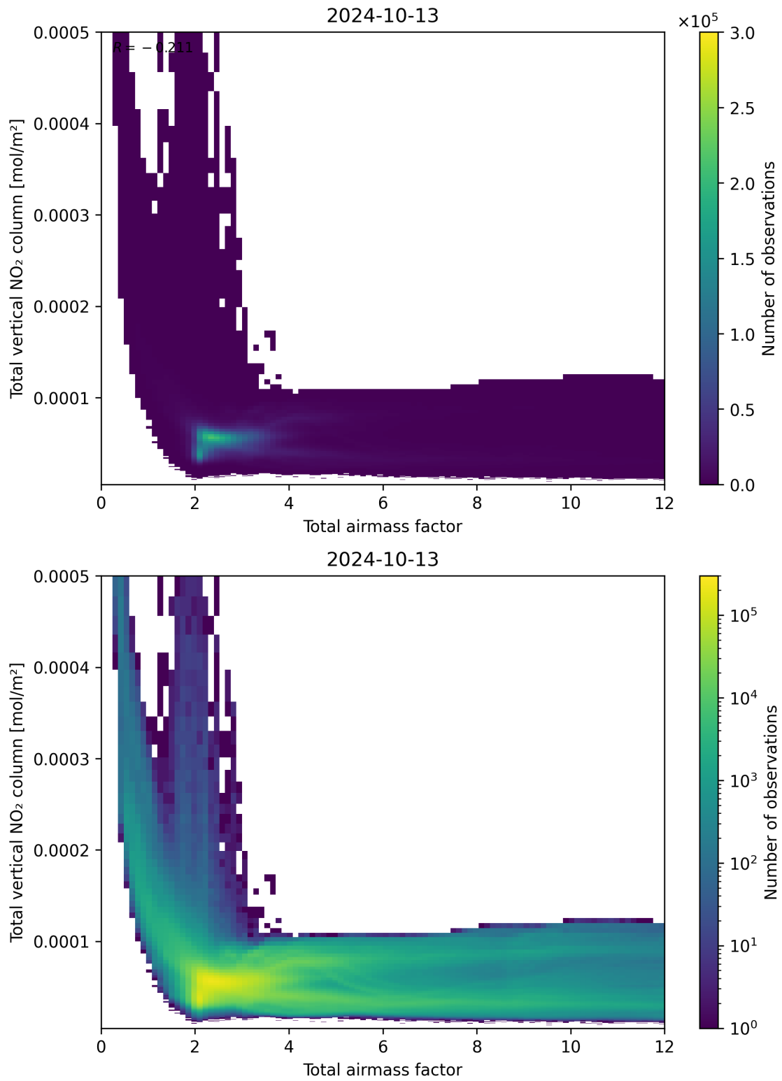
Figure 67: Scatter density plot of “Total airmass factor” against “Total vertical NO 2 column” for 2024-10-12 to 2024-10-14.
