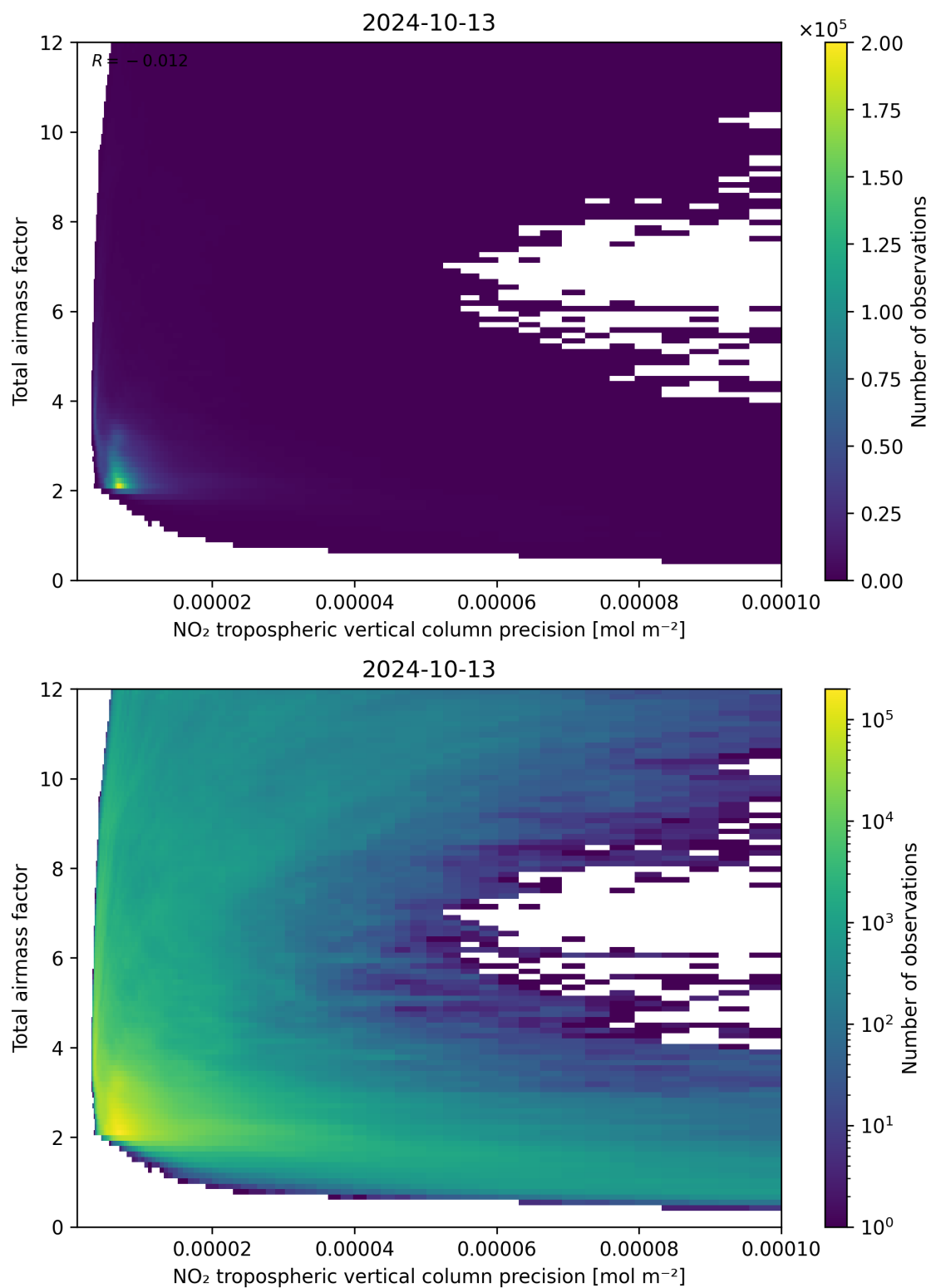
Figure 132: Scatter density plot of “NO 2 tropospheric vertical column precision” against “Total air mass factor” for 2024-10-12 to 2024-10-14.
