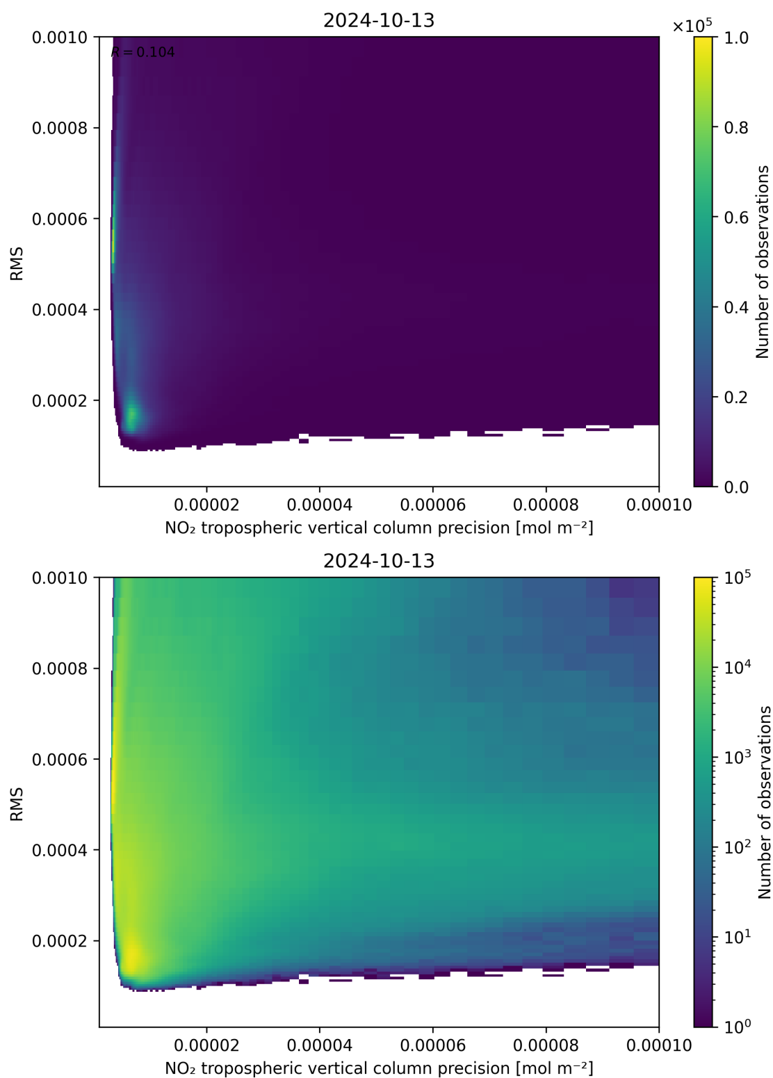
Figure 140: Scatter density plot of “NO 2 tropospheric vertical column precision” against “RMS” for 2024-10-12 to 2024-10-14.
