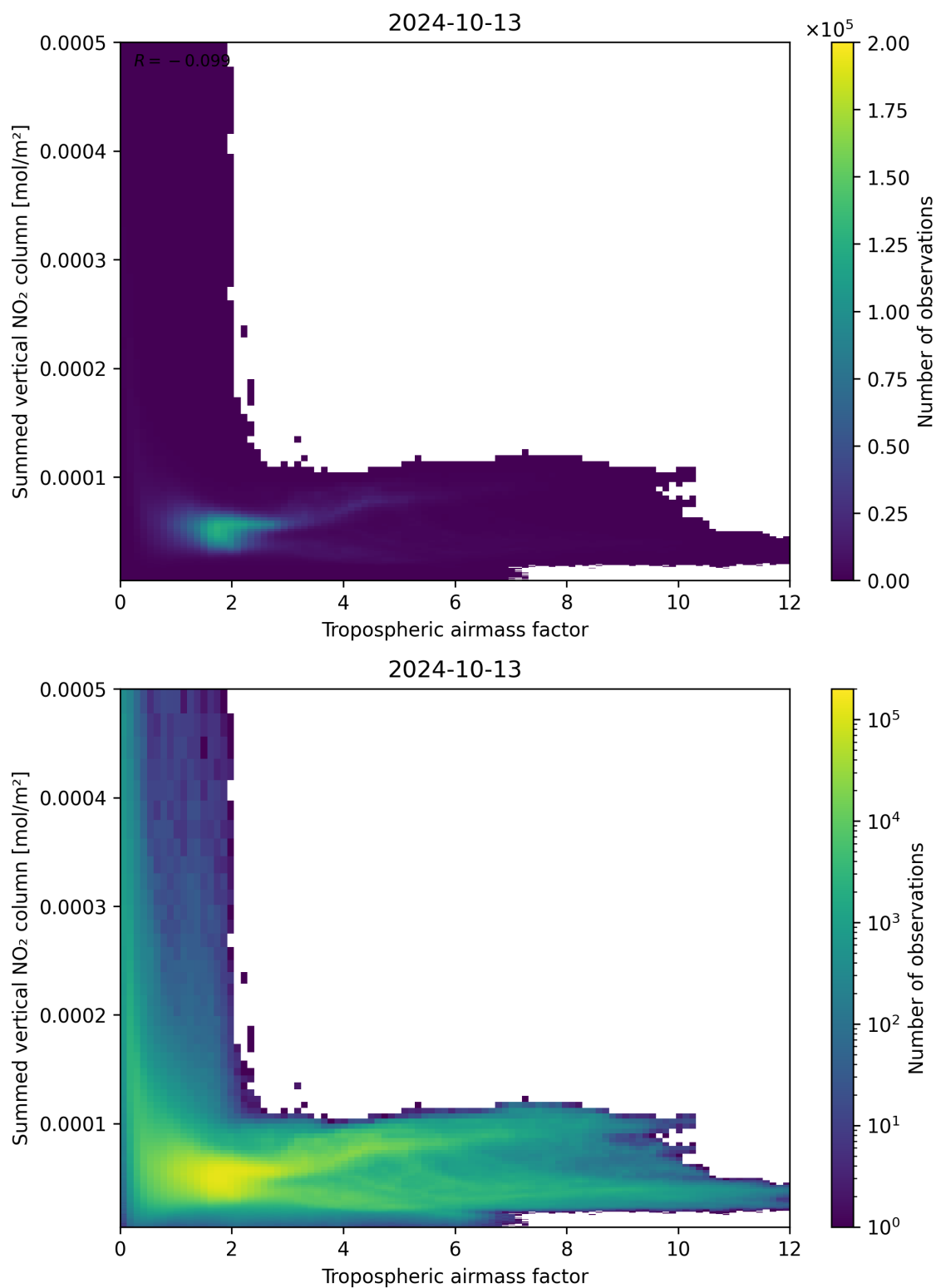
Figure 75: Scatter density plot of “Tropospheric air mass factor” against “Summed vertical NO 2 column” for 2024-10-12 to 2024-10-14.
