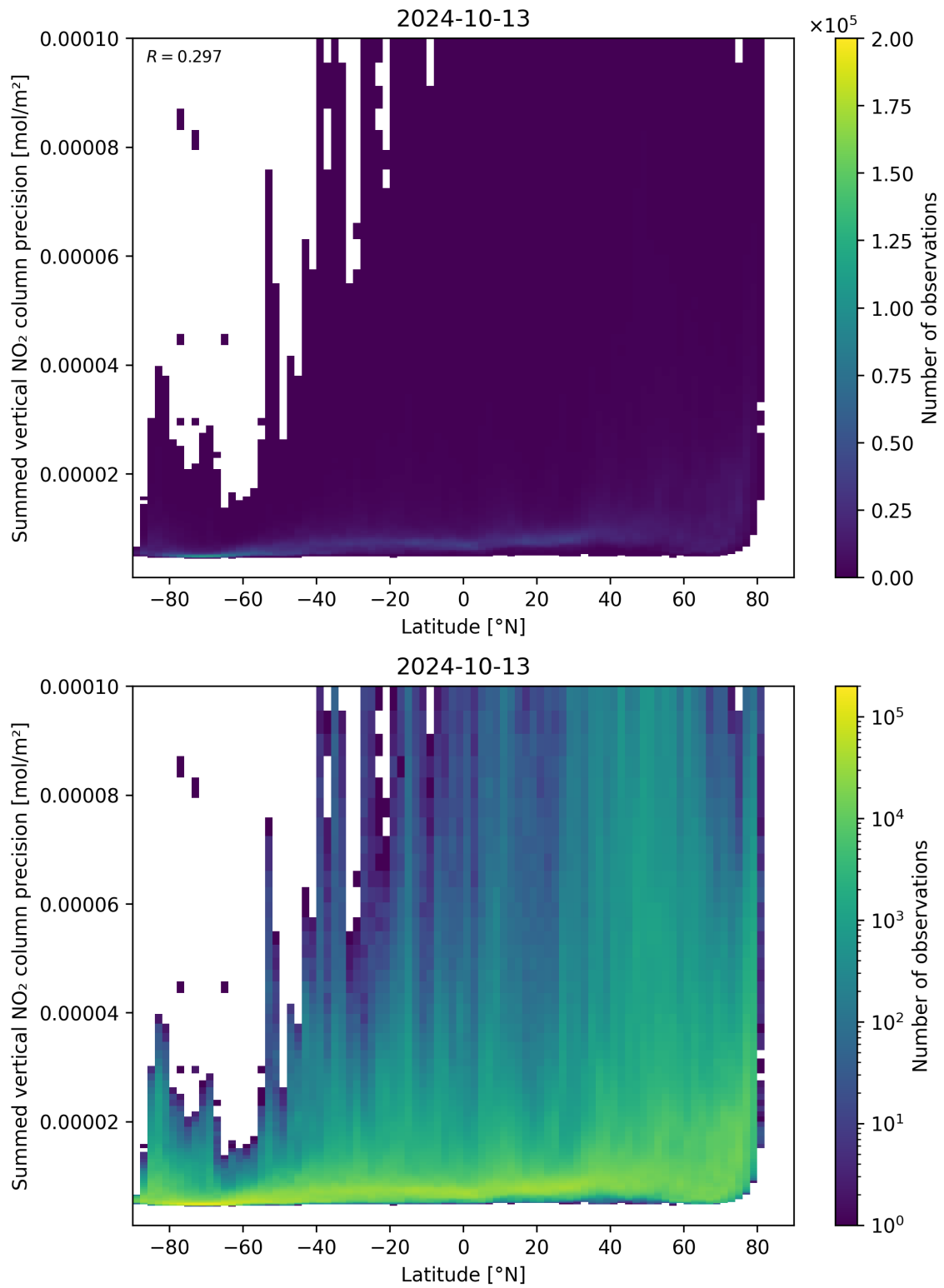
Figure 89: Scatter density plot of “Latitude” against “Summed vertical NO 2 column precision” for 2024-10-12 to 2024-10-14.
