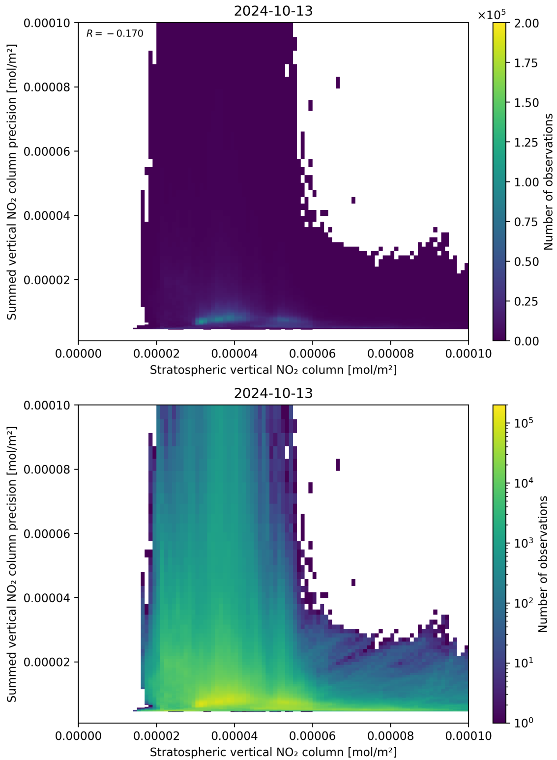
Figure 99: Scatter density plot of “Stratospheric vertical NO 2 column” against “Summed vertical NO 2 column precision” for 2024-10-12 to 2024-10-14.
