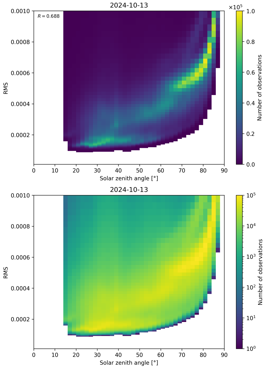
Figure 157: Scatter density plot of “Solar zenith angle” against “RMS” for 2024-10-12 to 2024-10-14.
