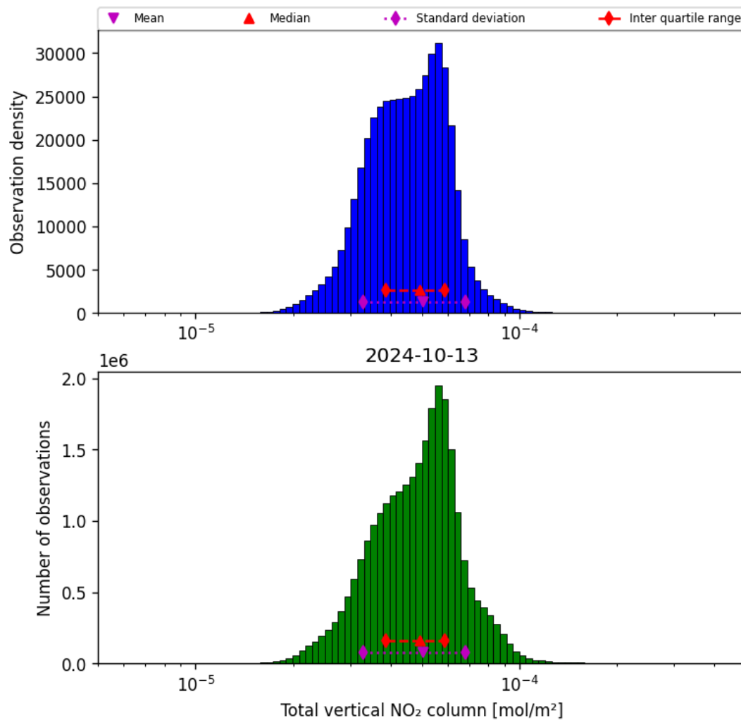
Figure 38: Histogram of “Total vertical NO 2 column” for 2024-10-12 to 2024-10-14
