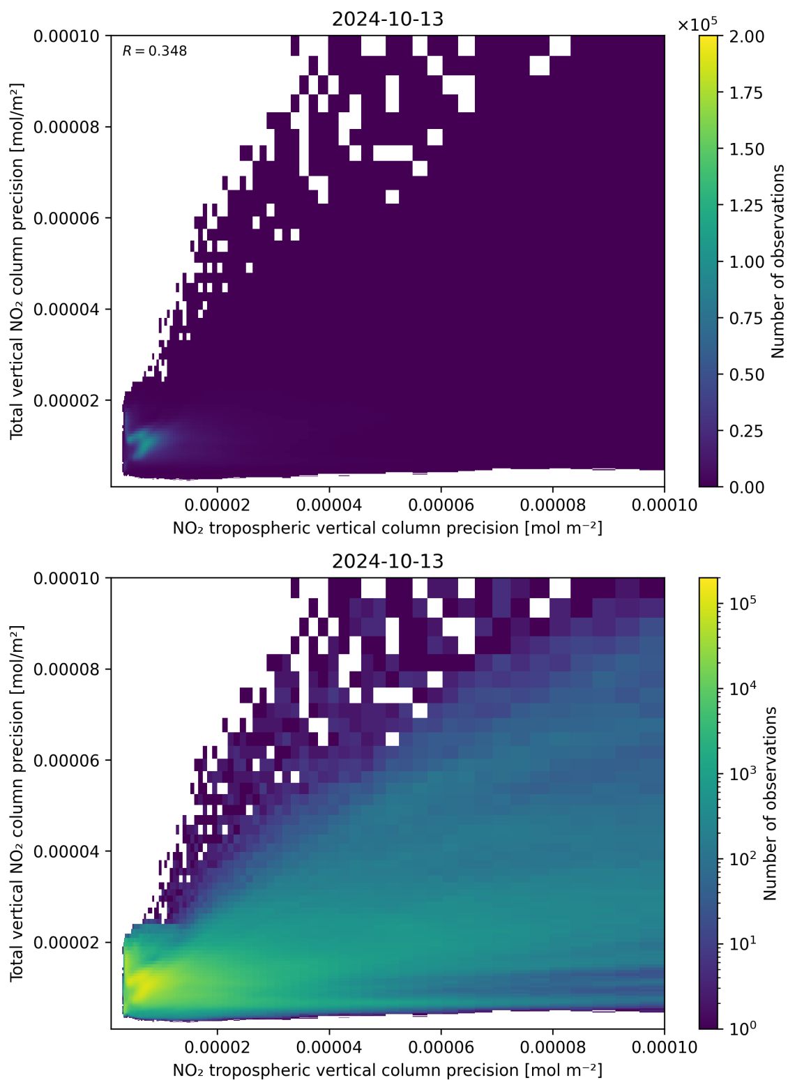
Figure 139: Scatter density plot of “NO 2 tropospheric vertical column precision” against “Total vertical NO 2 column precision” for 2024-10-12 to 2024-10-14.
