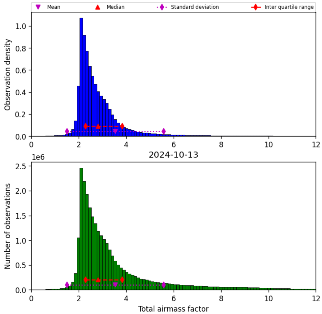
Figure 32: Histogram of “Total airmass factor” for 2024-10-12 to 2024-10-14
