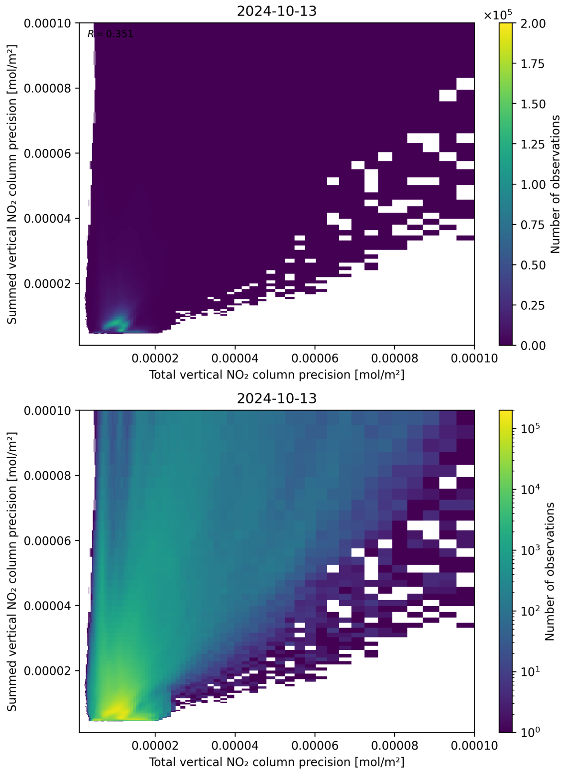
Figure 118: Scatter density plot of “Total vertical NO 2 column precision” against “Summed vertical NO 2 column precision” for 2024-10-12 to 2024-10-14.
