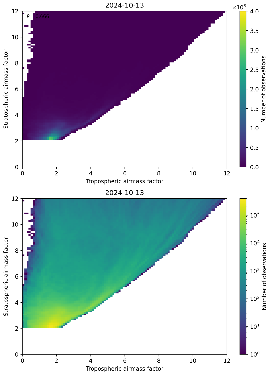
Figure 71: Scatter density plot of “Tropospheric airmass factor” against “Stratospheric airmass factor” for 2024-10-12 to 2024-10-14.
