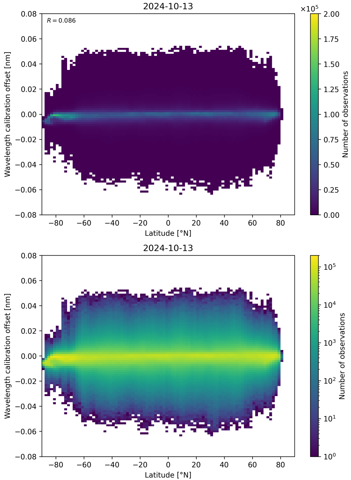
Figure 95: Scatter density plot of “Latitude” against “Wavelength calibration offset” for 2024-10-12 to 2024-10-14.
