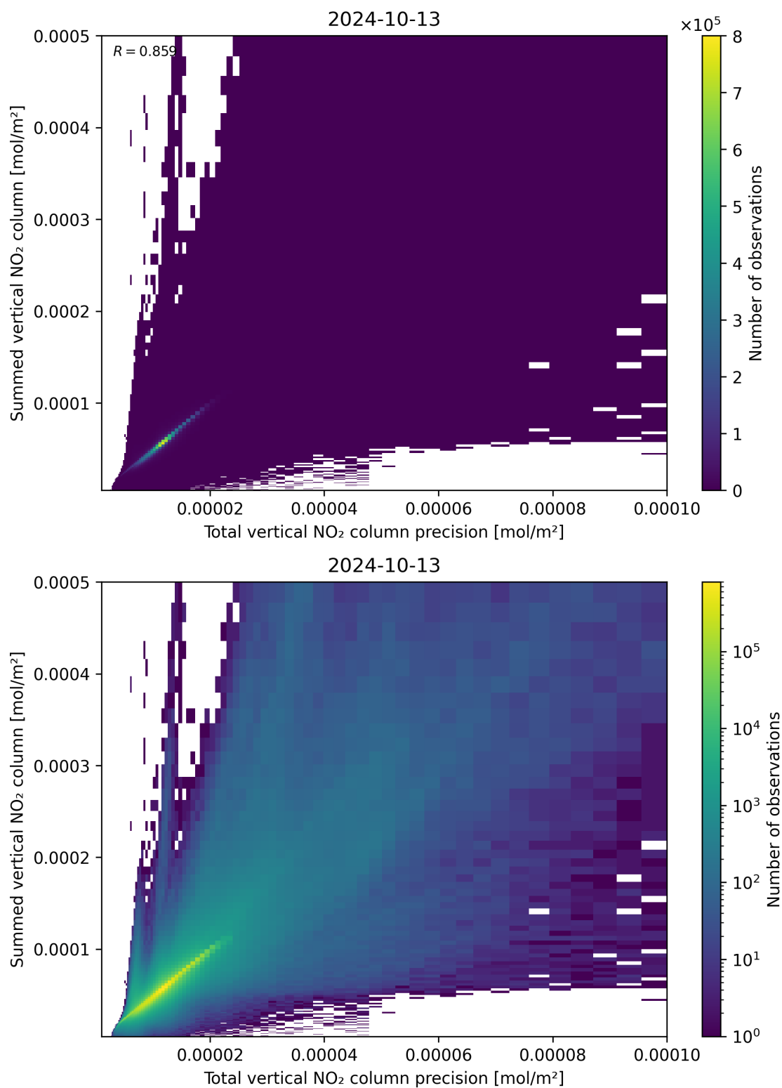
Figure 117: Scatter density plot of “Total vertical NO 2 column precision” against “Summed vertical NO 2 column” for 2024-10-12 to 2024-10-14.
