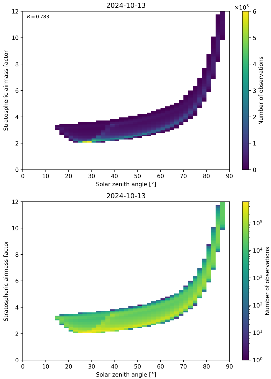
Figure 145: Scatter density plot of “Solar zenith angle” against “Stratospheric airmass factor” for 2024-10-12 to 2024-10-14.
