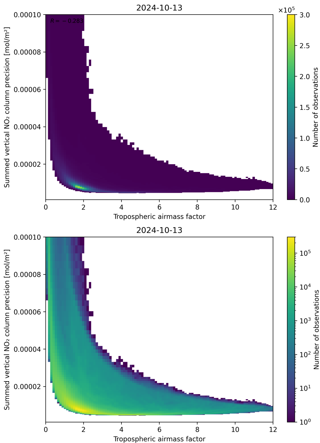
Figure 76: Scatter density plot of “Tropospheric air mass factor” against “Summed vertical NO 2 column precision” for 2024-10-12 to 2024-10-14.
