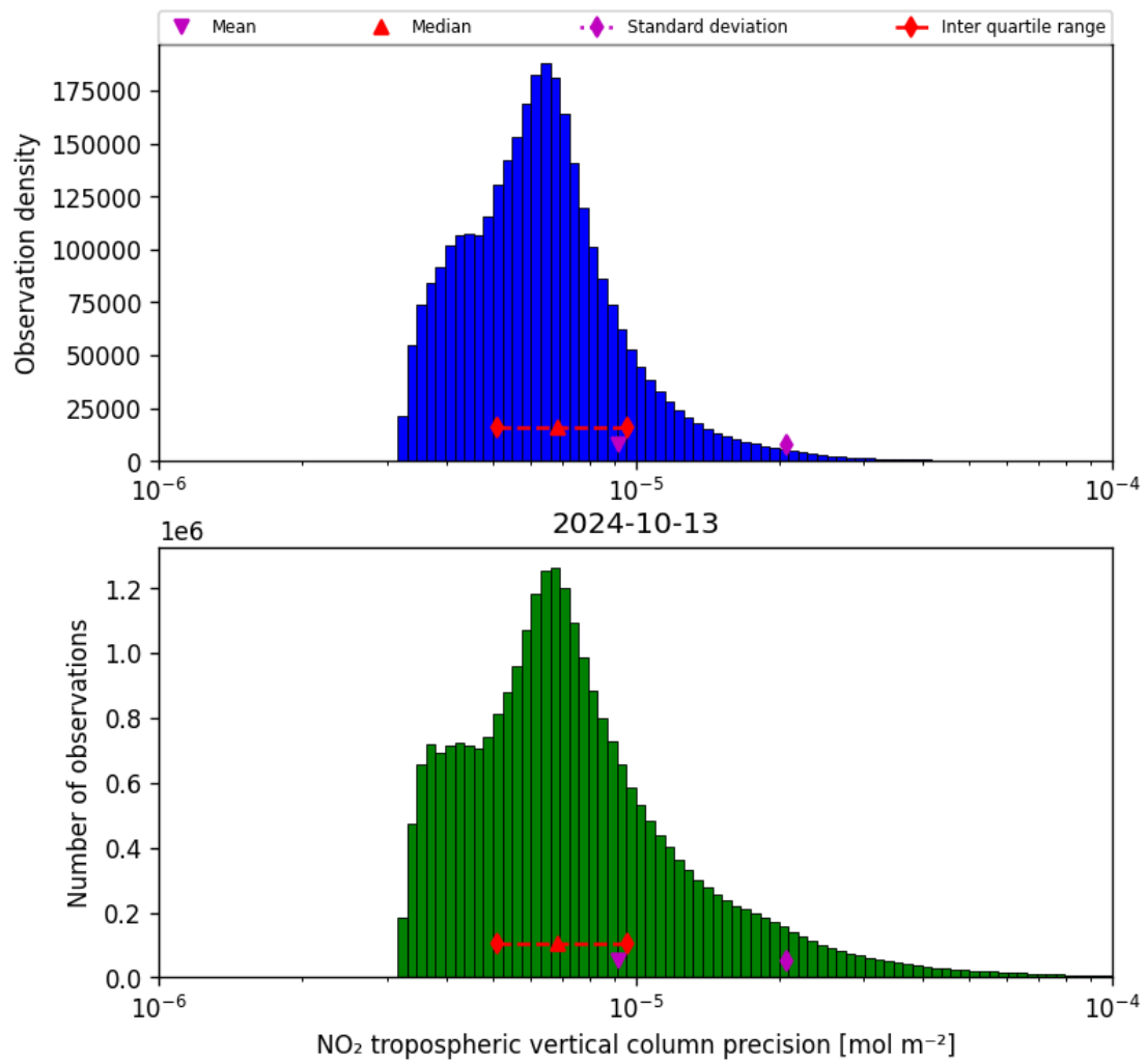
Figure 30: Histogram of “NO 2 tropospheric vertical column precision” for 2024-10-12 to 2024-10-14
