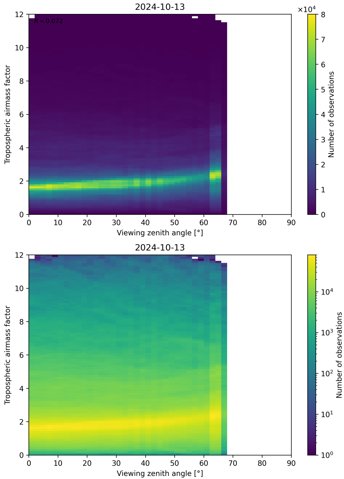
Figure 161: Scatter density plot of “Viewing zenith angle” against “Tropospheric airmass factor” for 2024-10-12 to 2024-10-14.
