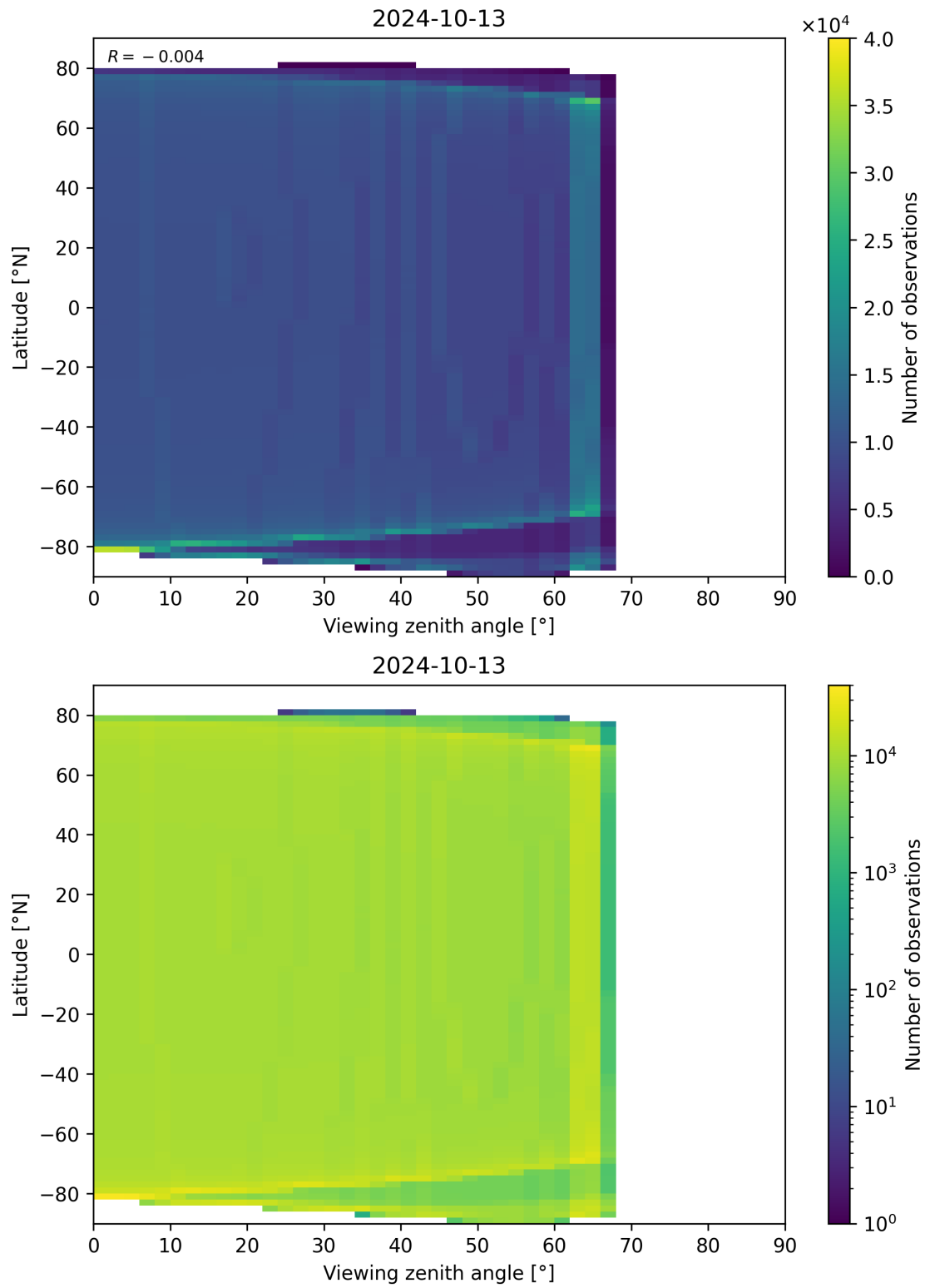
Figure 163: Scatter density plot of “Viewing zenith angle” against “Latitude” for 2024-10-12 to 2024-10-14.
