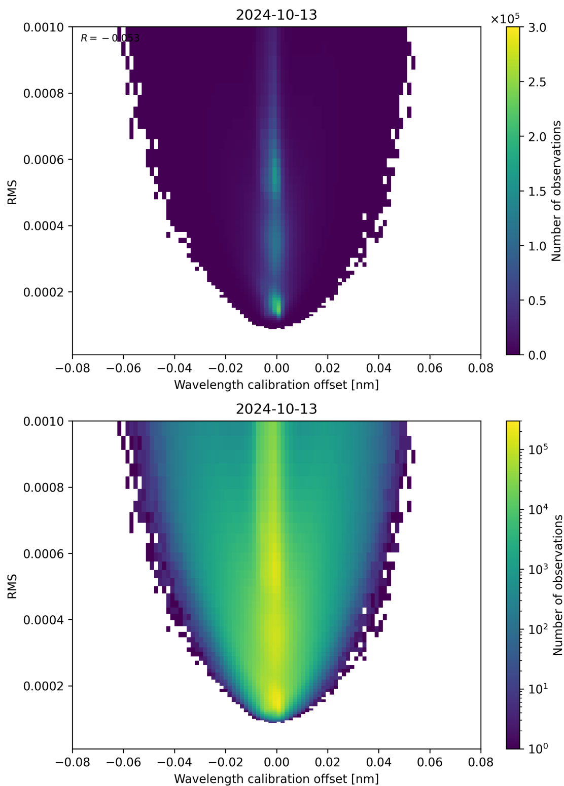
Figure 181: Scatter density plot of “Wavelength calibration offset” against “RMS” for 2024-10-12 to 2024-10-14.
