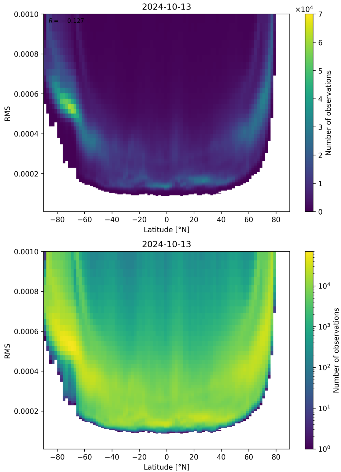
Figure 94: Scatter density plot of “Latitude” against “RMS” for 2024-10-12 to 2024-10-14.
