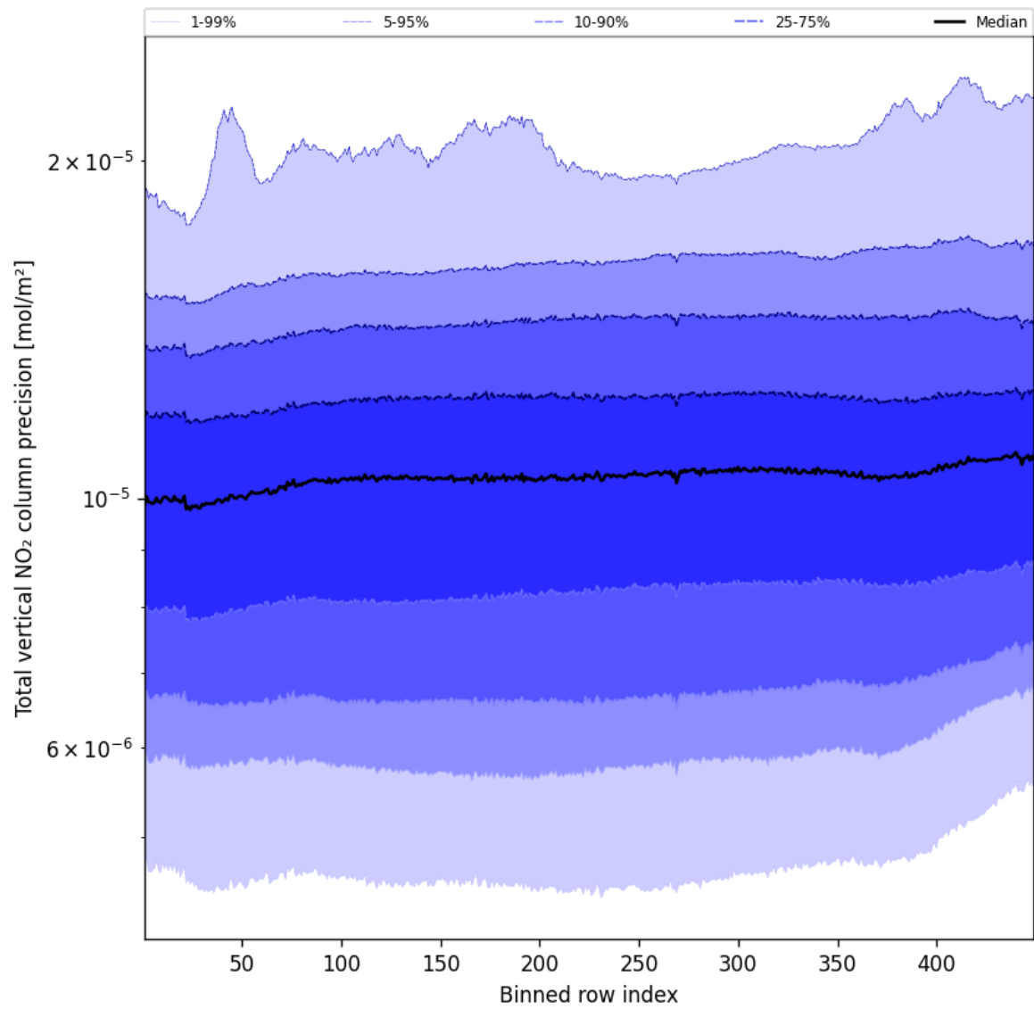
Figure 56: Along track statistics of "Total vertical NO 2 column precision" for 2024-10-12 to 2024-10-14
