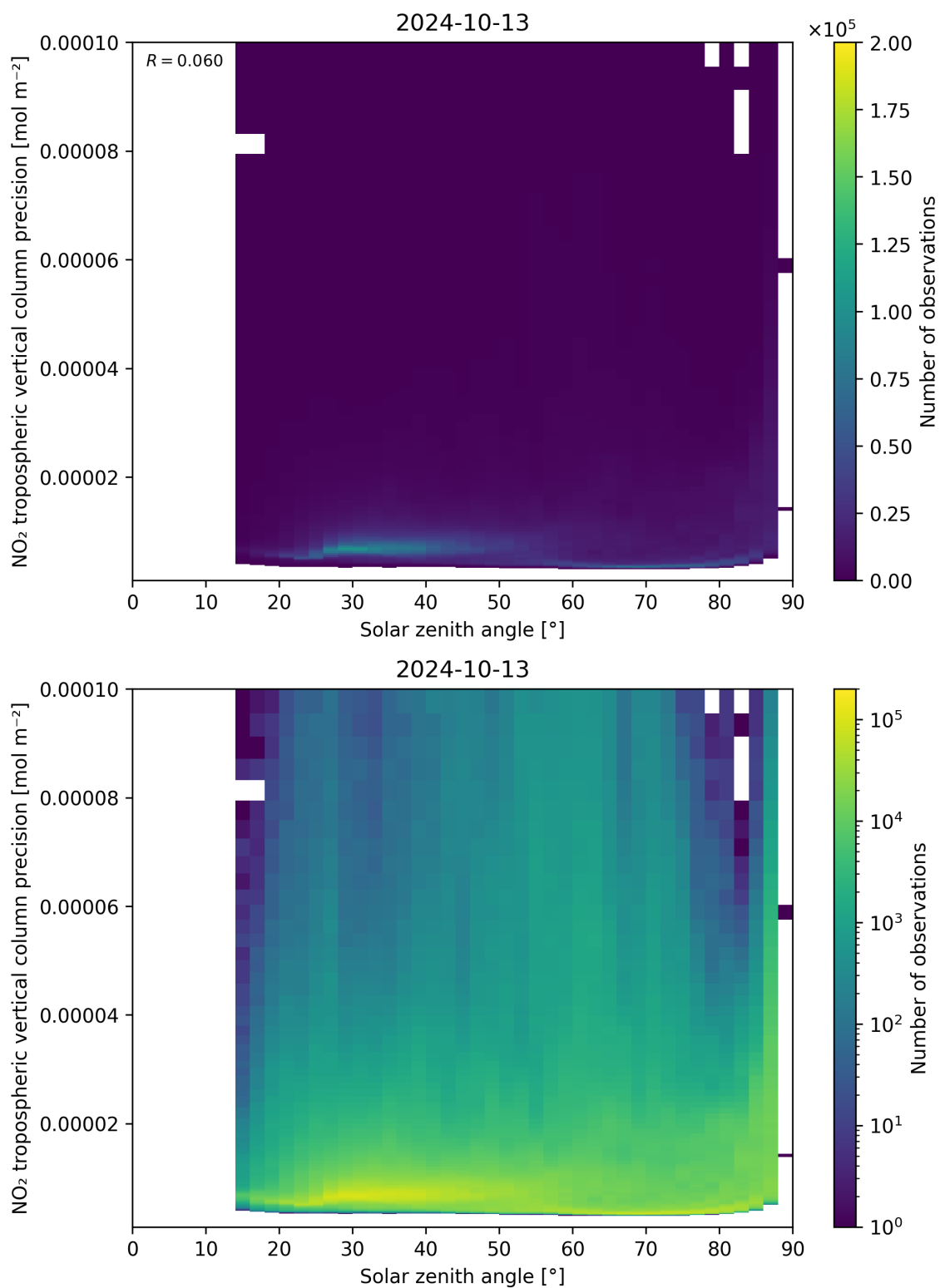
Figure 156: Scatter density plot of “Solar zenith angle” against “NO 2 tropospheric vertical column precision” for 2024-10-12 to 2024-10-14.
