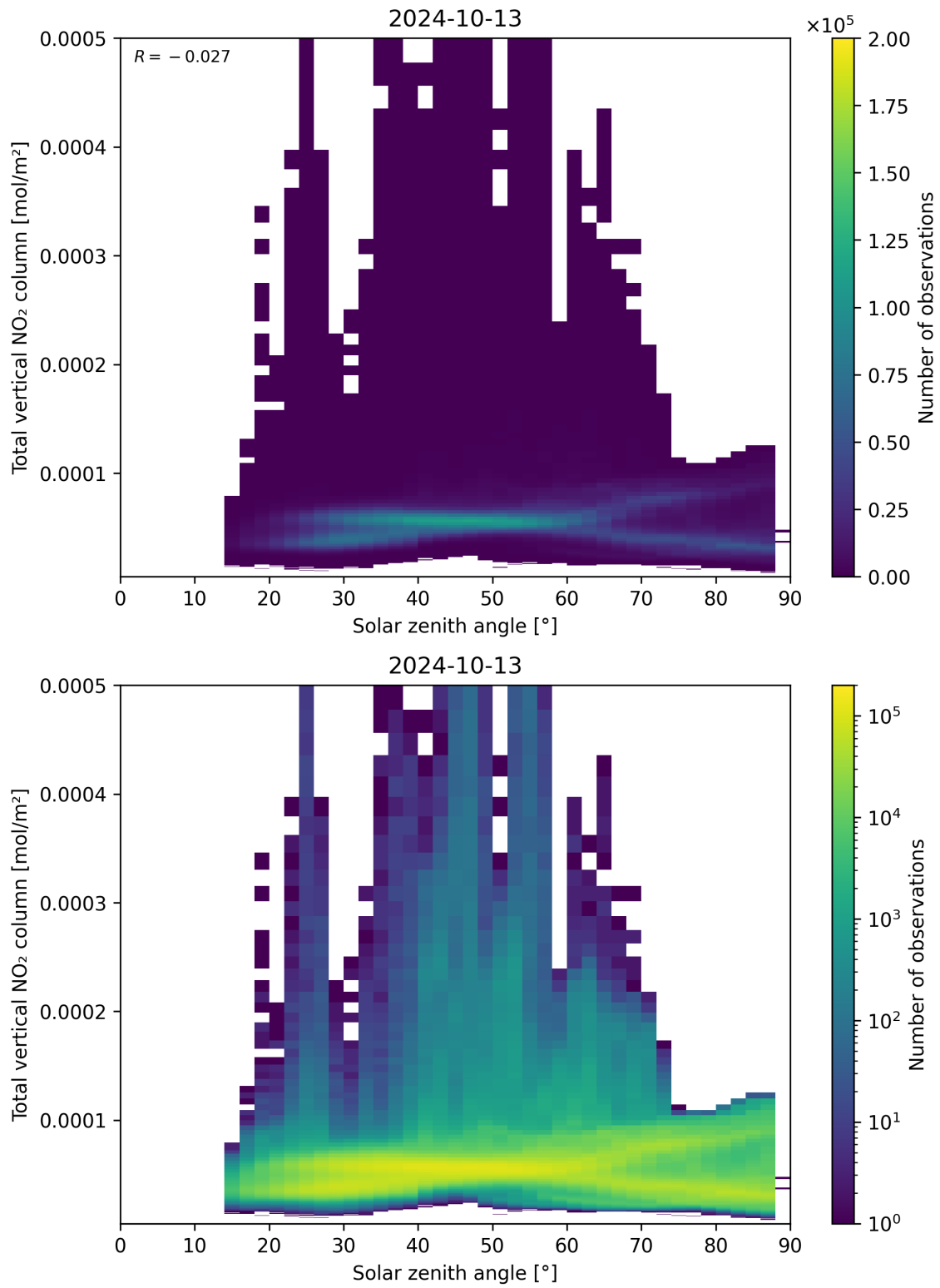
Figure 153: Scatter density plot of “Solar zenith angle” against “Total vertical NO 2 column” for 2024-10-12 to 2024-10-14.
