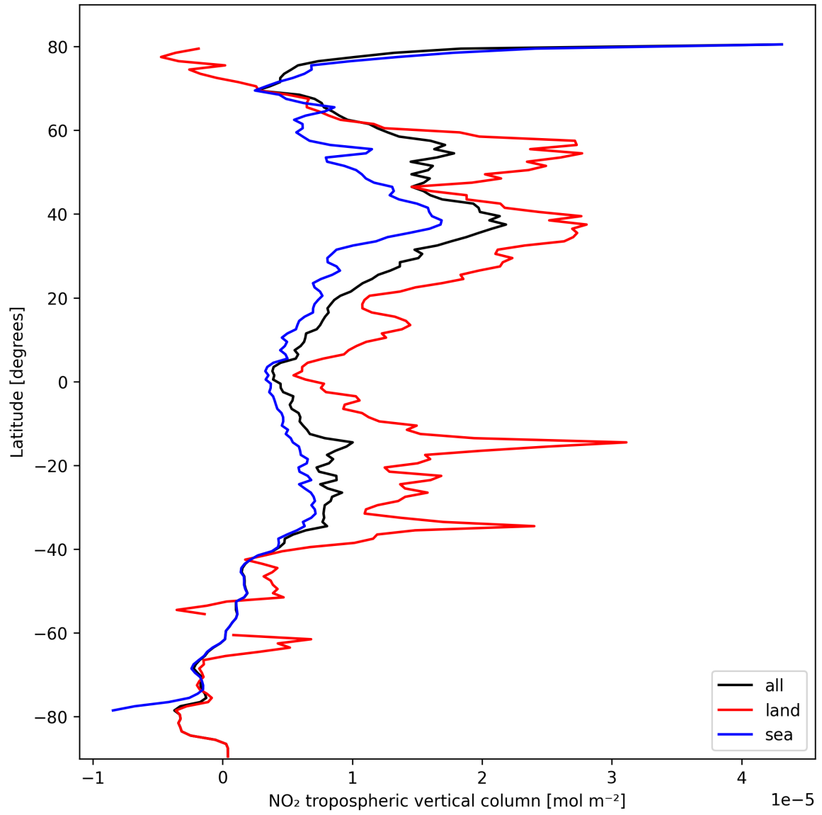
Figure 12: Zonal average of “NO 2 tropospheric vertical column” for 2024-10-12 to 2024-10-14.
