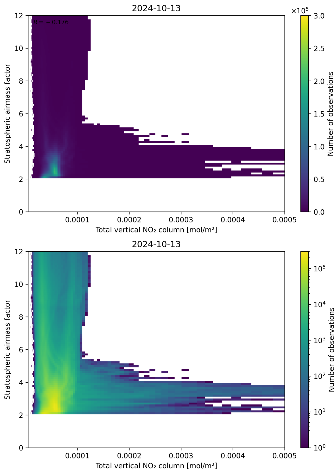
Figure 110: Scatter density plot of “Total vertical NO 2 column” against “Stratospheric airmass factor” for 2024-10-12 to 2024-10-14.
