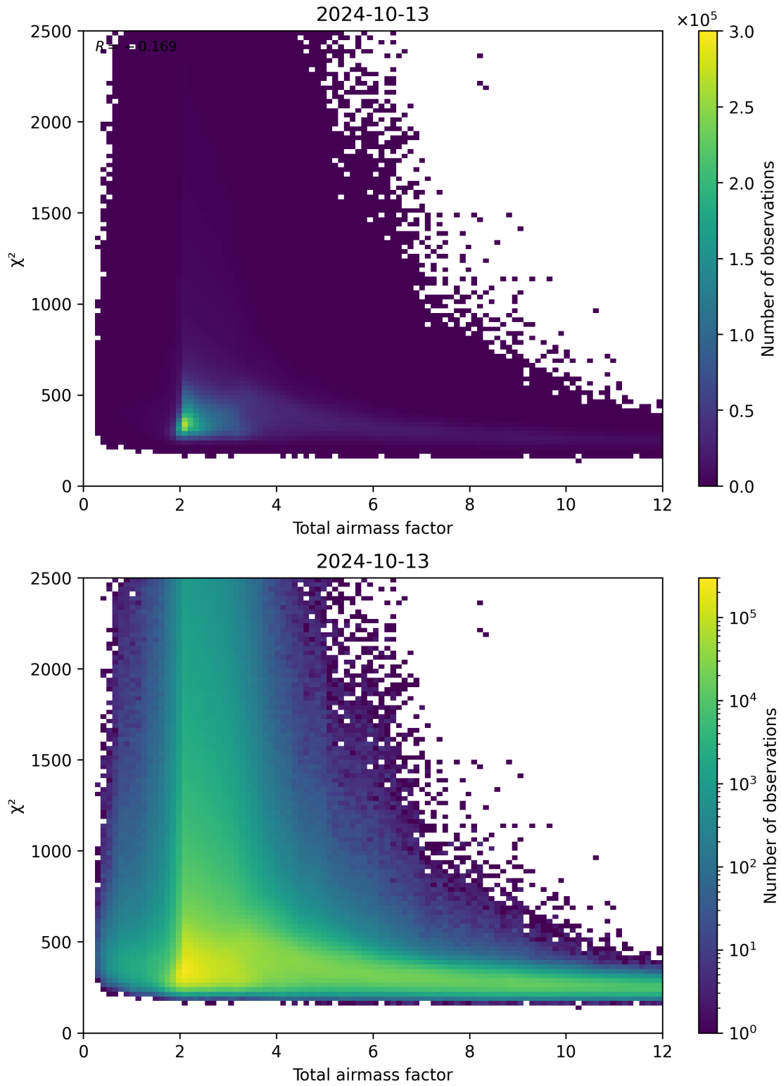
Figure 63: Scatter density plot of “Total airmass factor” against “ \chi^2 ” for 2024-10-12 to 2024-10-14.
