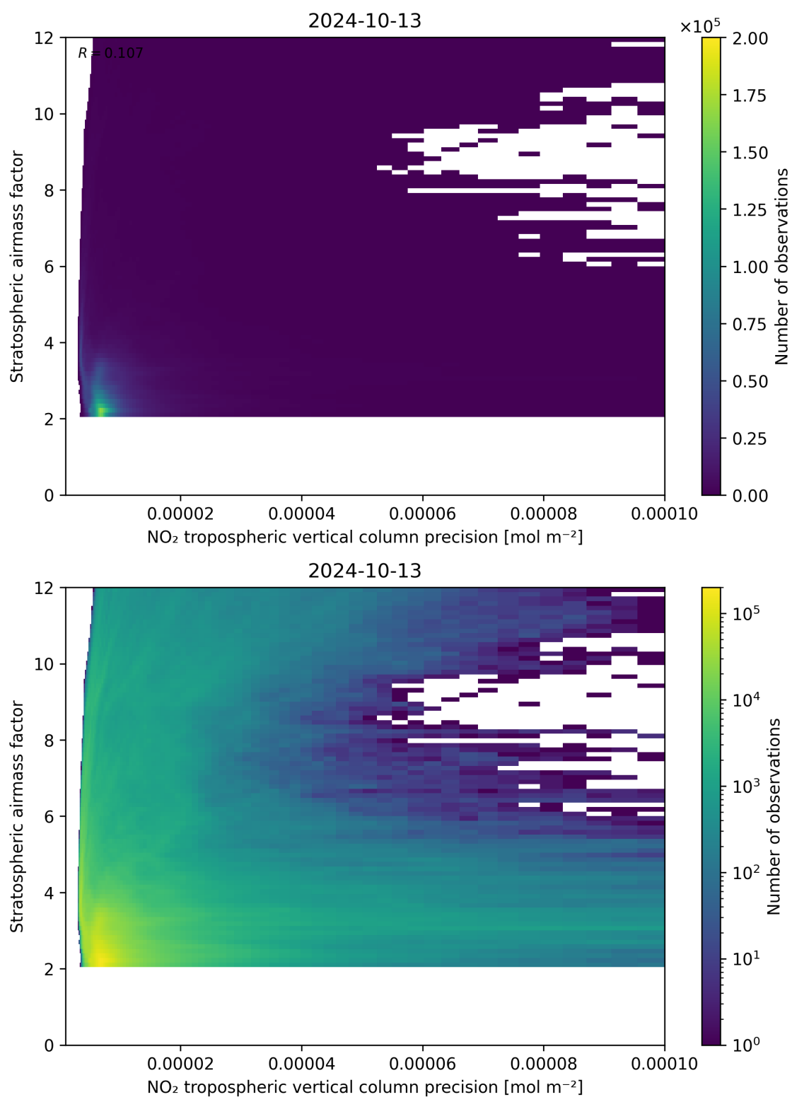
Figure 131: Scatter density plot of “NO 2 tropospheric vertical column precision” against “Stratospheric airmass factor” for 2024-10-12 to 2024-10-14.
