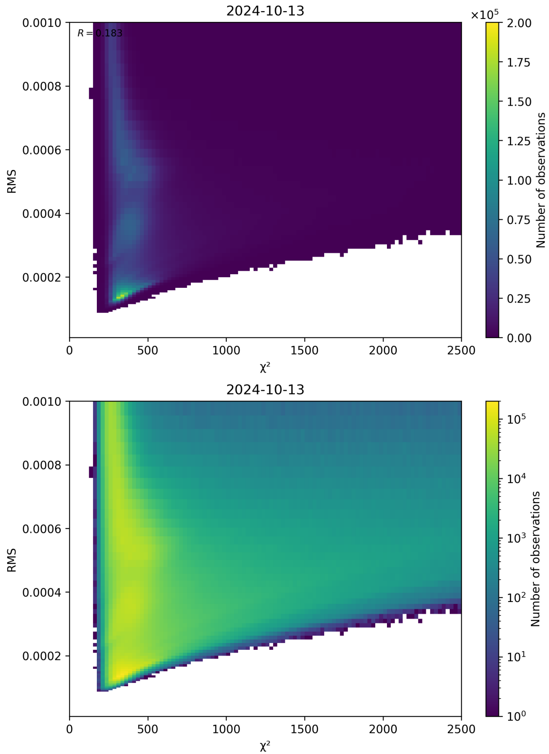
Figure 82: Scatter density plot of “ \chi^2 ” against “RMS” for 2024-10-12 to 2024-10-14.
