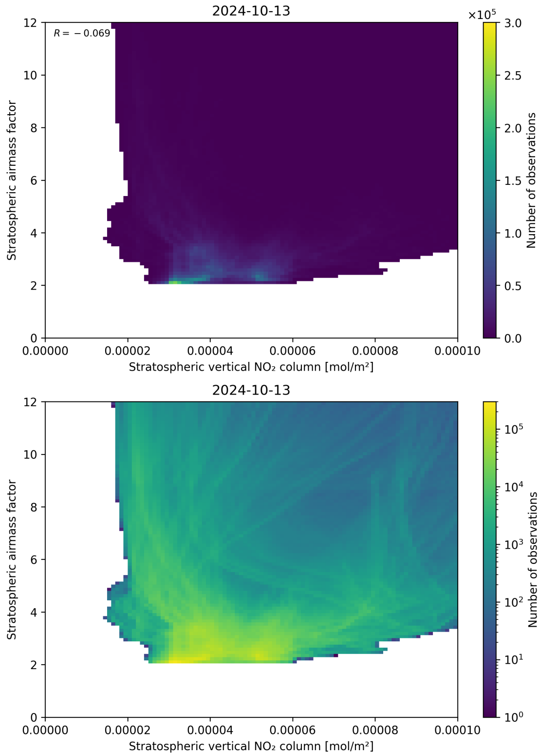
Figure 96: Scatter density plot of “Stratospheric vertical NO 2 column” against “Stratospheric airmass factor” for 2024-10-12 to 2024-10-14.
