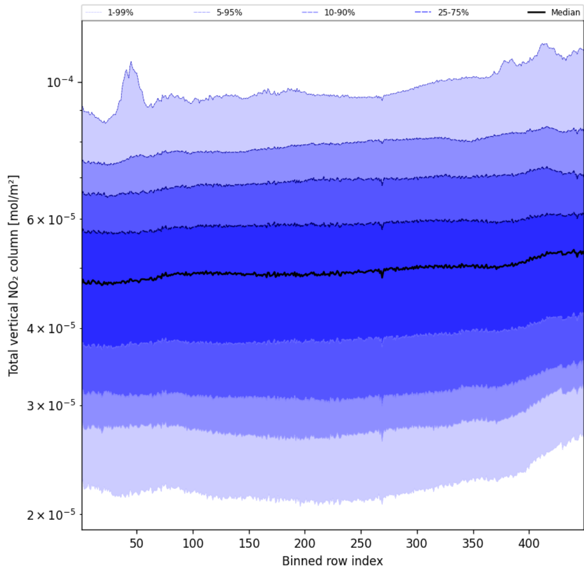
Figure 55: Along track statistics of “Total vertical NO 2 column” for 2024-10-12 to 2024-10-14
