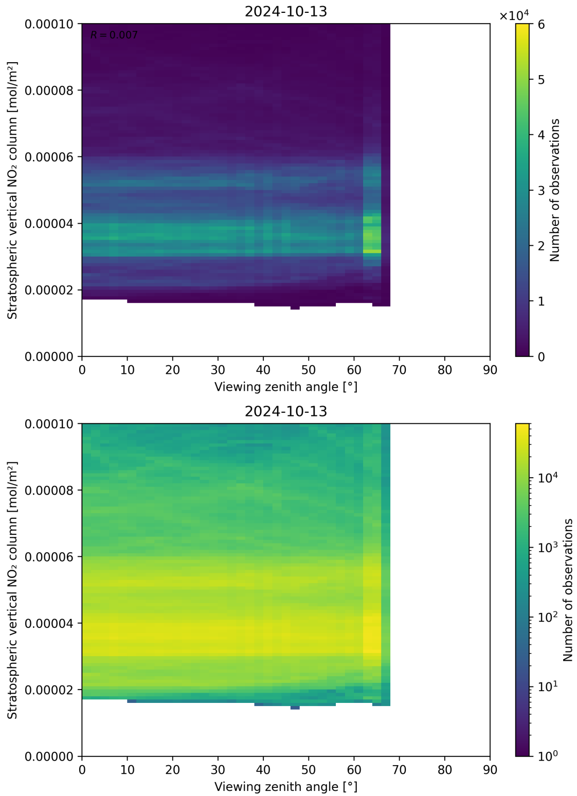
Figure 164: Scatter density plot of “Viewing zenith angle” against “Stratospheric vertical NO 2 column” for 2024-10-12 to 2024-10-14.
