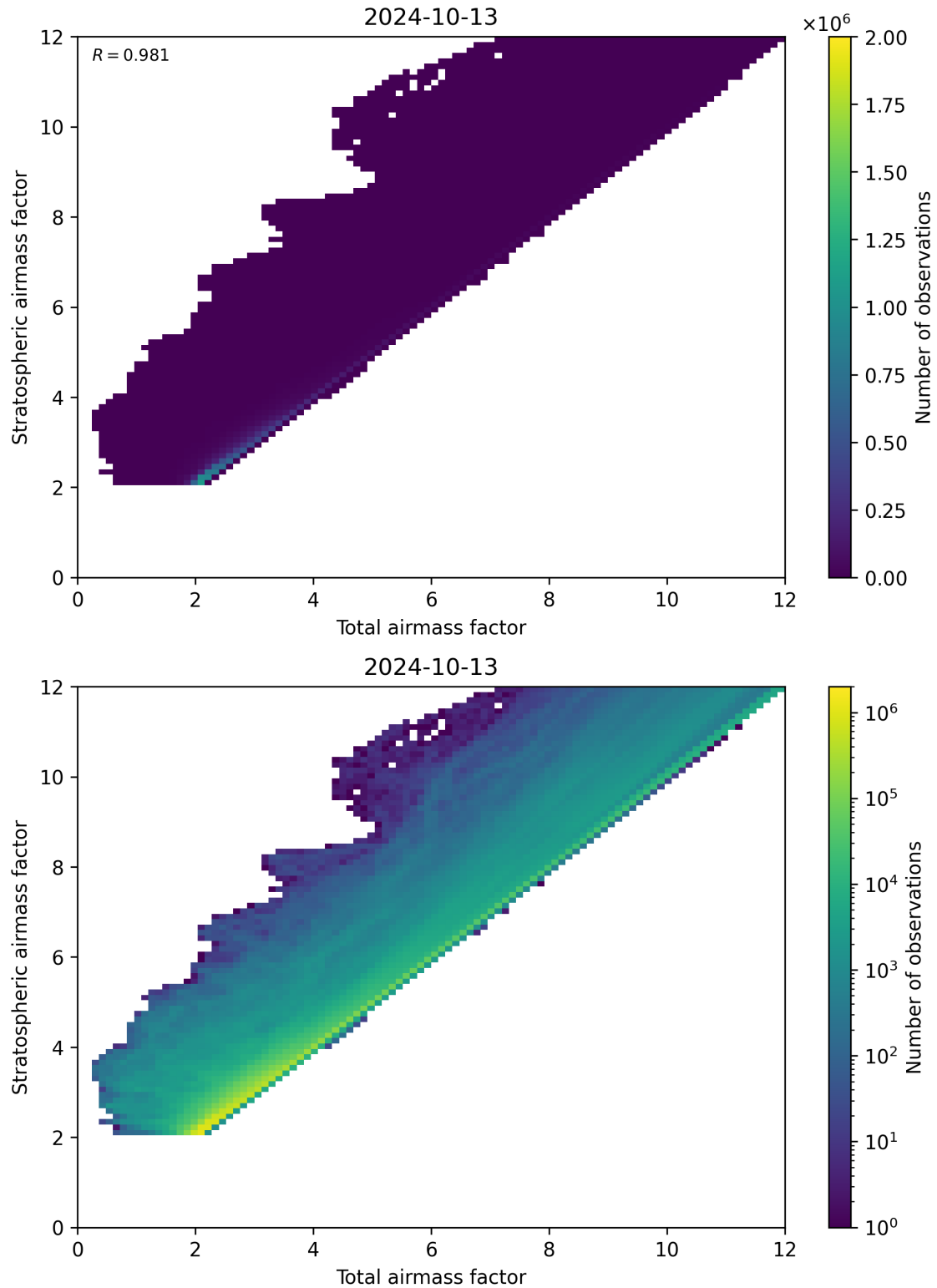
Figure 62: Scatter density plot of “Total airmass factor” against “Stratospheric airmass factor” for 2024-10-12 to 2024-10-14.
