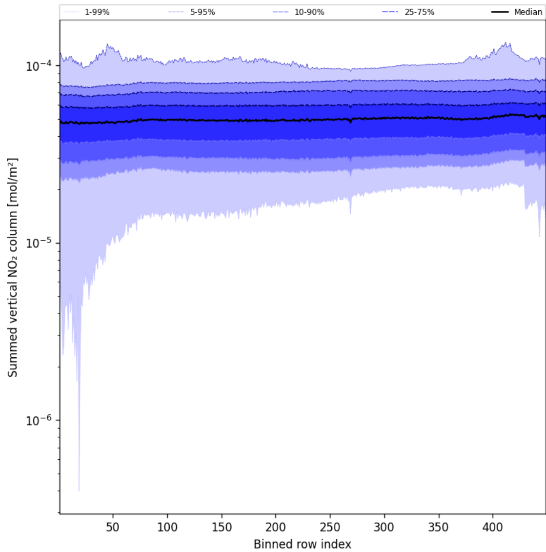
Figure 57: Along track statistics of “Summed vertical NO 2 column” for 2024-10-12 to 2024-10-14
