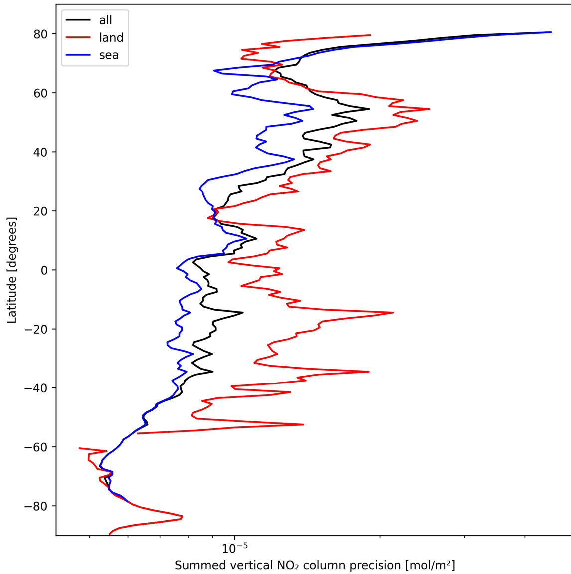
Figure 24: Zonal average of “Summed vertical NO 2 column precision” for 2024-10-12 to 2024-10-14.
