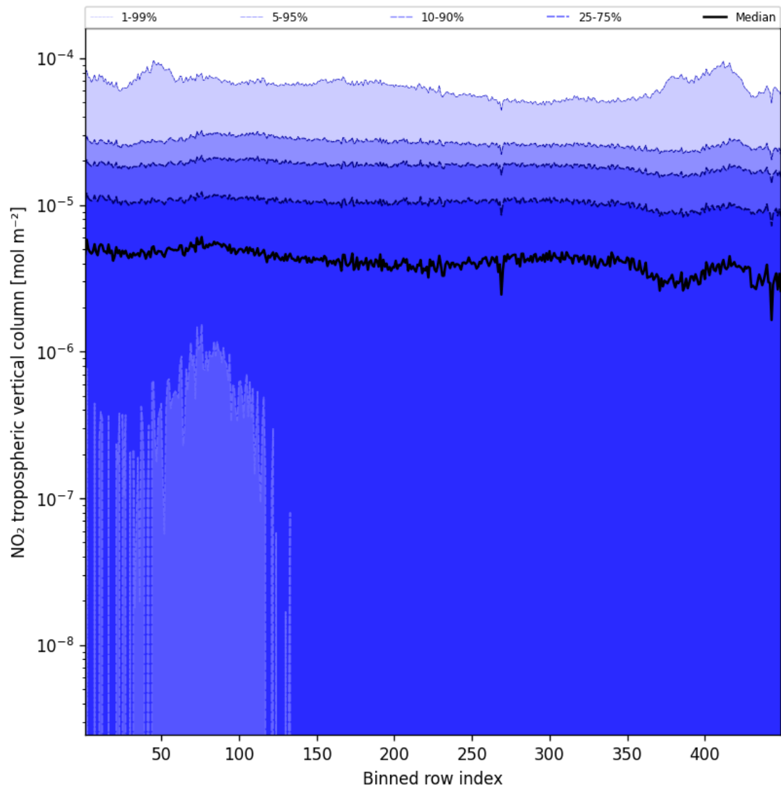
Figure 46: Along track statistics of “NO 2 tropospheric vertical column” for 2024-10-12 to 2024-10-14
