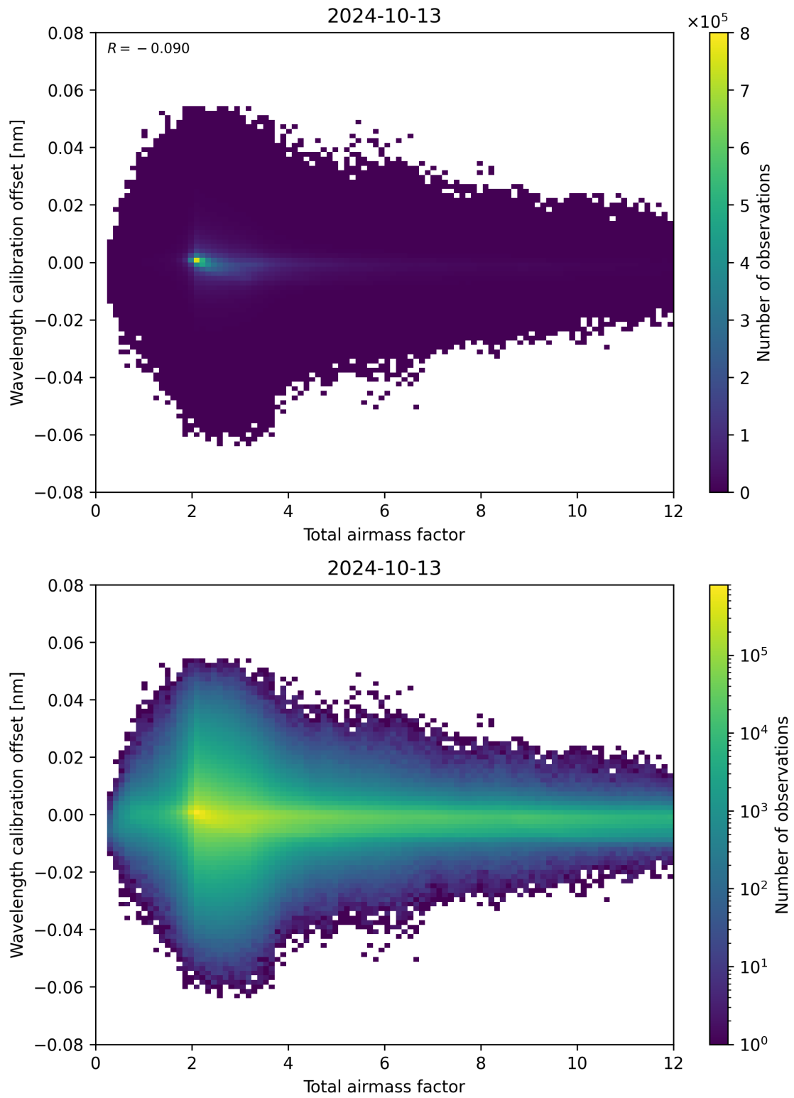
Figure 70: Scatter density plot of “Total airmass factor” against “Wavelength calibration offset” for 2024-10-12 to 2024-10-14.
