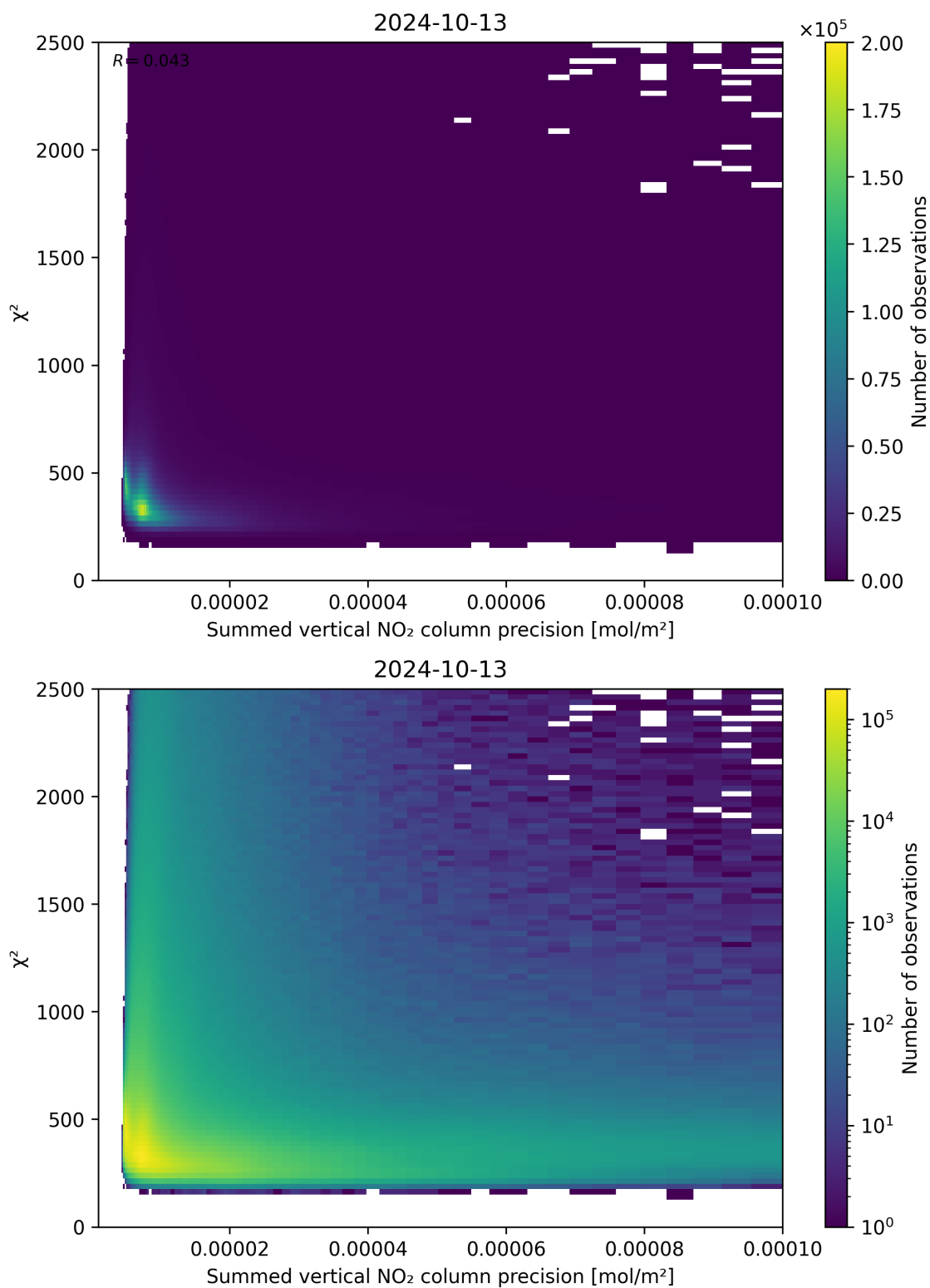
Figure 107: Scatter density plot of “Summed vertical NO 2 column precision” against “ \chi^2 ” for 2024-10-12 to 2024-10-14.
