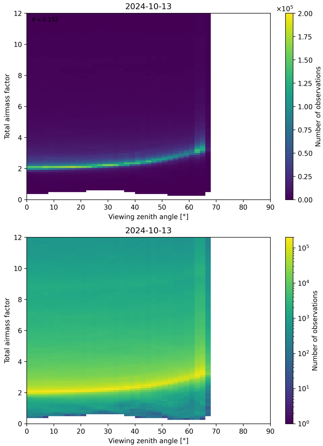
Figure 160: Scatter density plot of “Viewing zenith angle” against “Total airmass factor” for 2024-10-12 to 2024-10-14.
