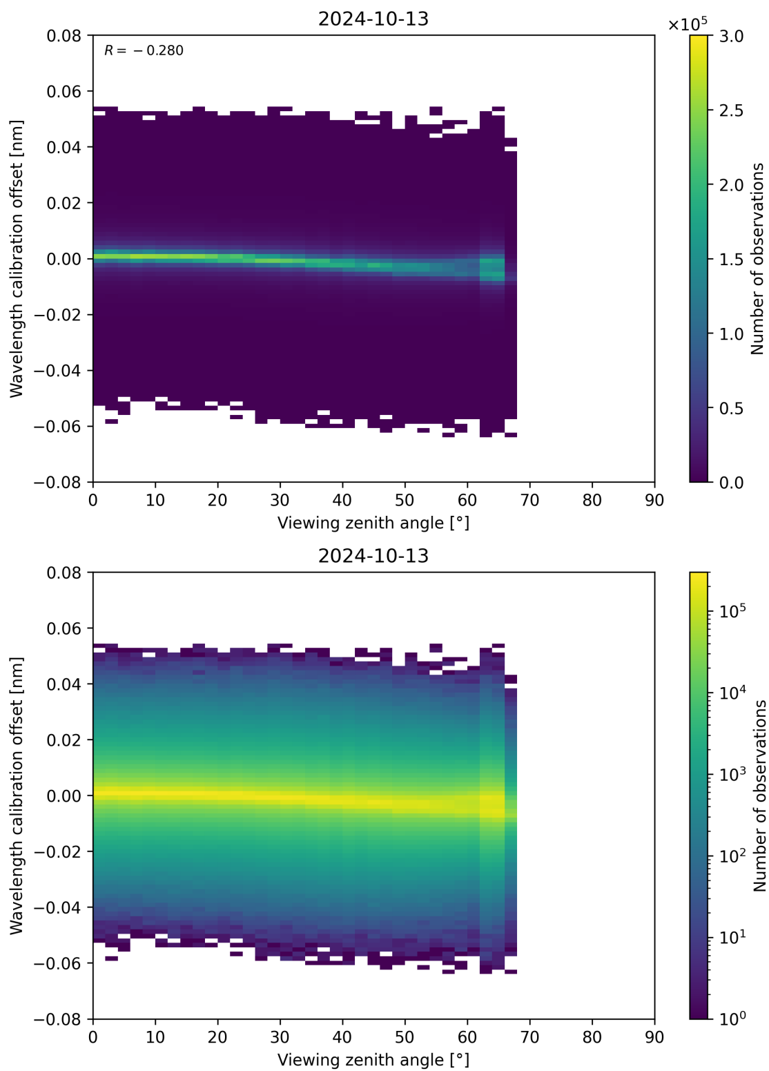
Figure 173: Scatter density plot of “Viewing zenith angle” against “Wavelength calibration offset” for 2024-10-12 to 2024-10-14.
