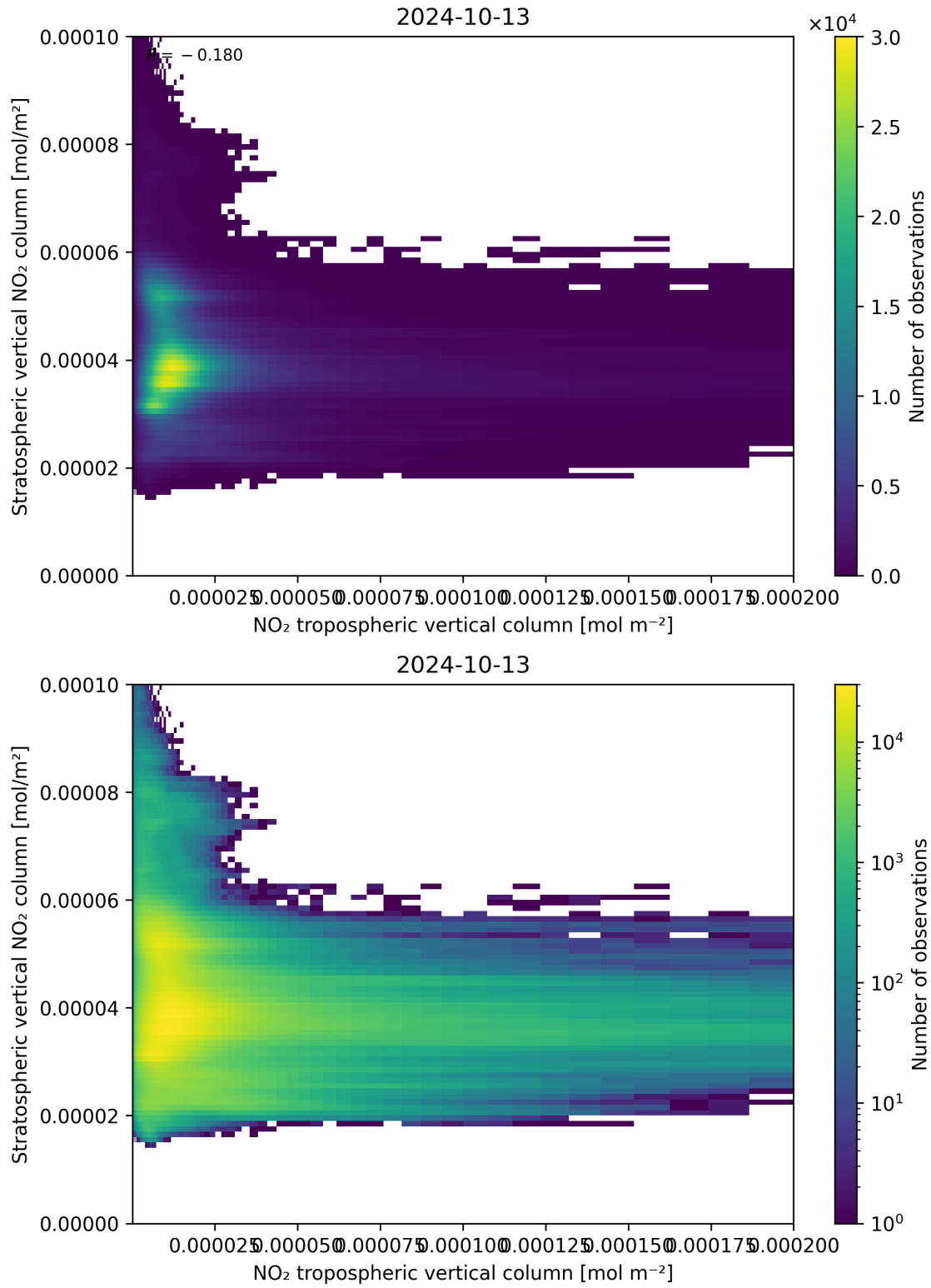
Figure 125: Scatter density plot of “NO 2 tropospheric vertical column” against “Stratospheric vertical NO 2 column” for 2024-10-12 to 2024-10-14.
