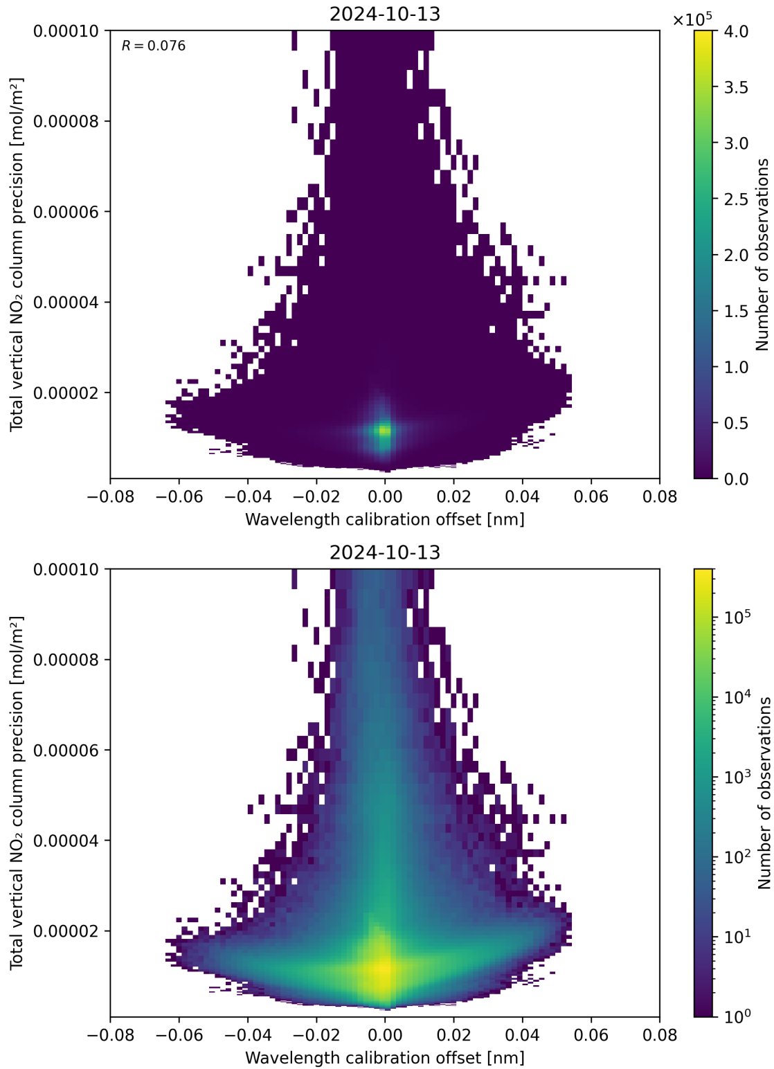
Figure 180: Scatter density plot of “Wavelength calibration offset” against “Total vertical NO 2 column precision” for 2024-10-12 to 2024-10-14.
