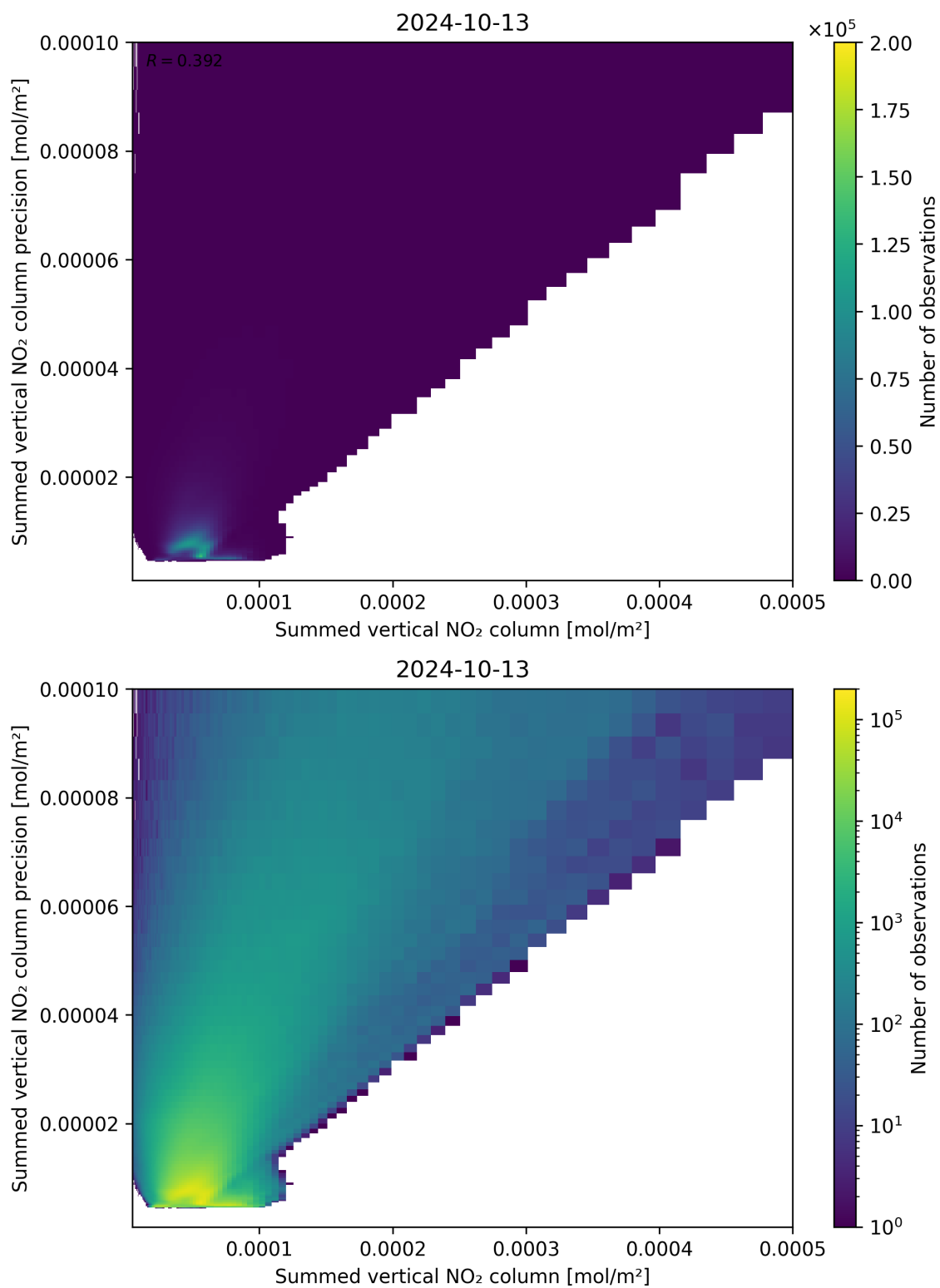
Figure 105: Scatter density plot of “Summed vertical NO 2 column” against “Summed vertical NO 2 column precision” for 2024-10-12 to 2024-10-14.
