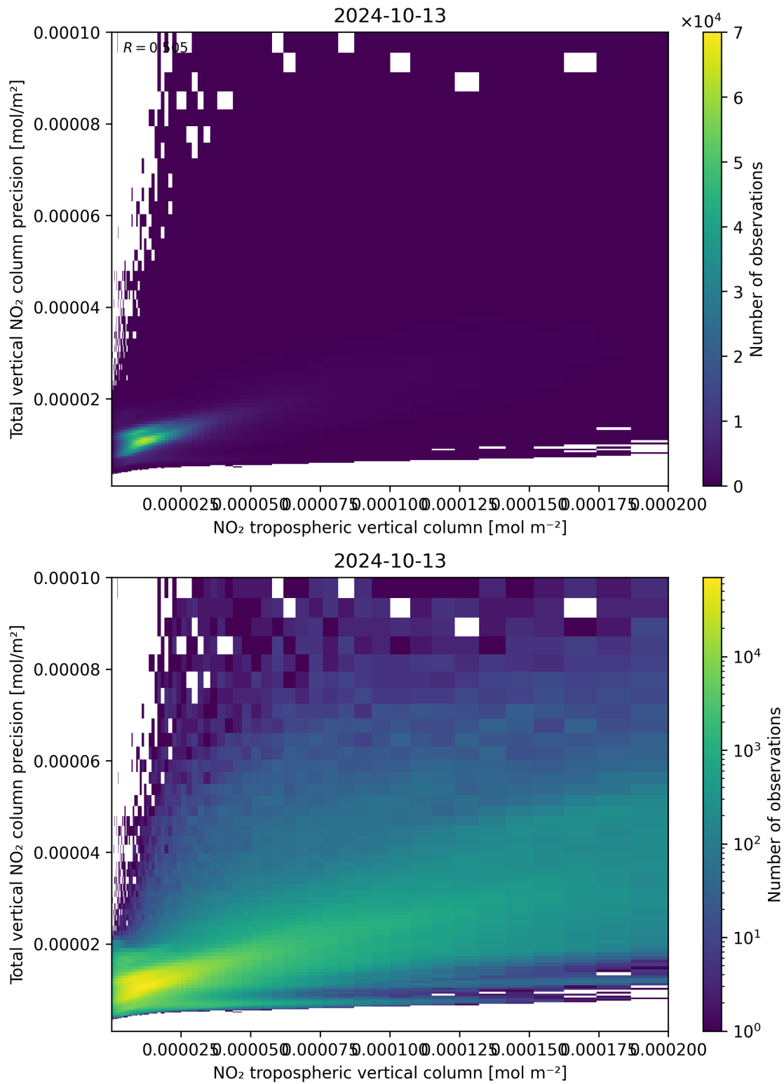
Figure 129: Scatter density plot of “NO 2 tropospheric vertical column” against “Total vertical NO 2 column precision” for 2024-10-12 to 2024-10-14.
