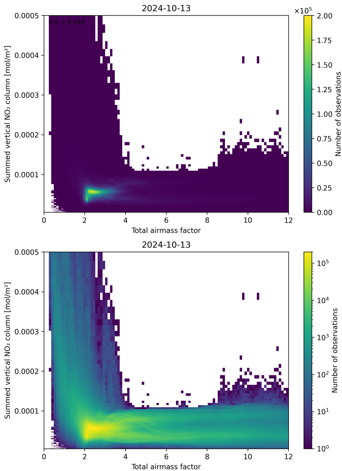
Figure 65: Scatter density plot of “Total airmass factor” against “Summed vertical NO 2 column” for 2024-10-12 to 2024-10-14.
