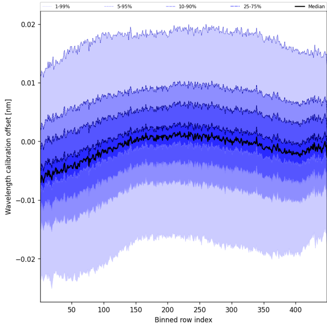
Figure 52: Along track statistics of “Wavelength calibration offset” for 2024-10-12 to 2024-10-14
