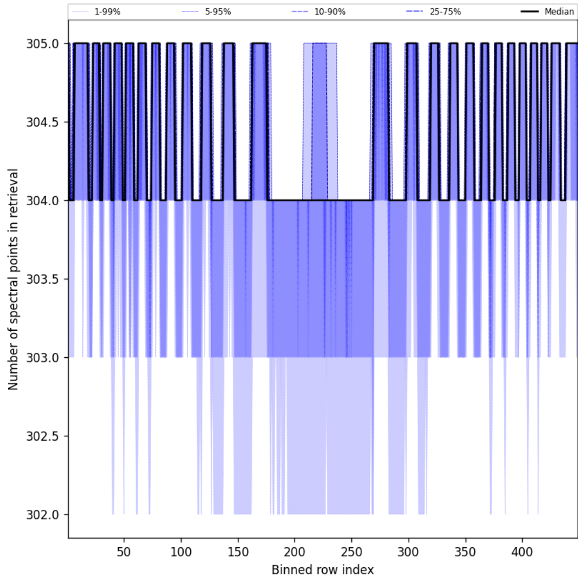
Figure 50: Along track statistics of “Number of spectral points in retrieval” for 2024-10-12 to 2024-10-14
