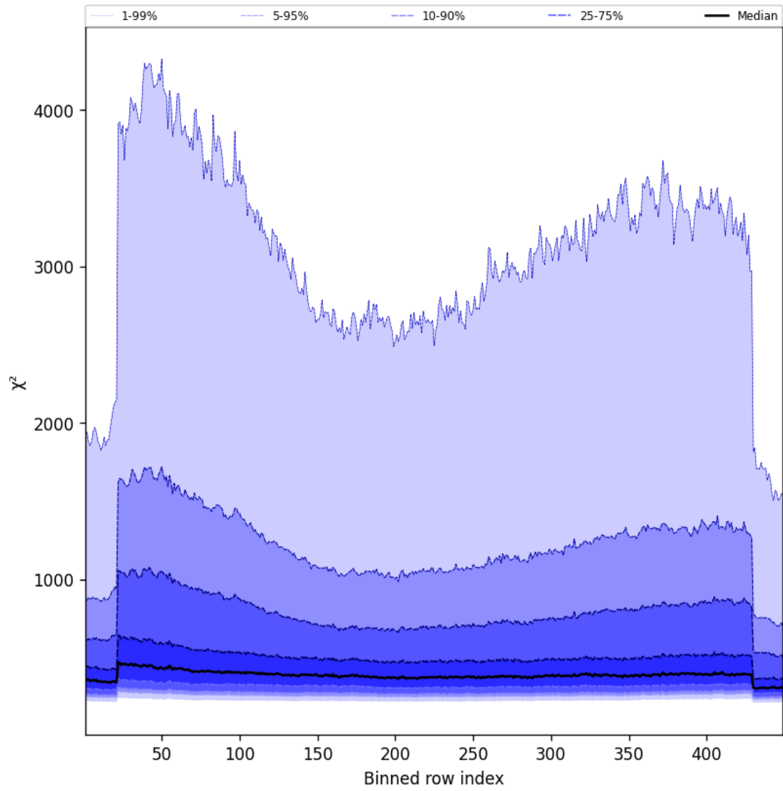
Figure 59: Along track statistics of “ \chi^2 ” for 2024-10-12 to 2024-10-14
