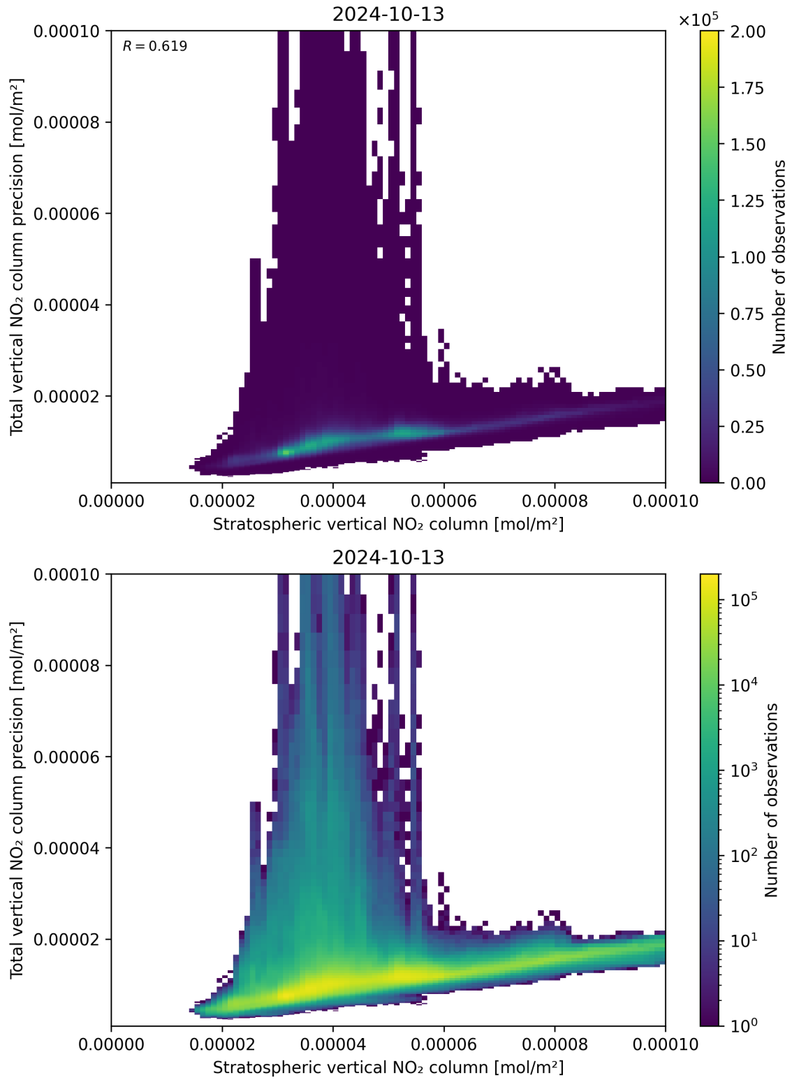
Figure 101: Scatter density plot of “Stratospheric vertical NO 2 column” against “Total vertical NO 2 column precision” for 2024-10-12 to 2024-10-14.
