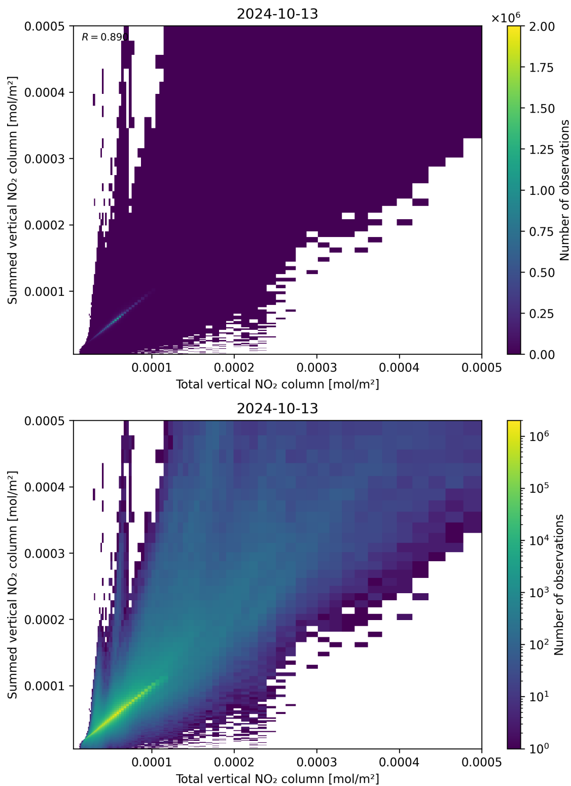
Figure 112: Scatter density plot of “Total vertical NO 2 column” against “Summed vertical NO 2 column” for 2024-10-12 to 2024-10-14.
