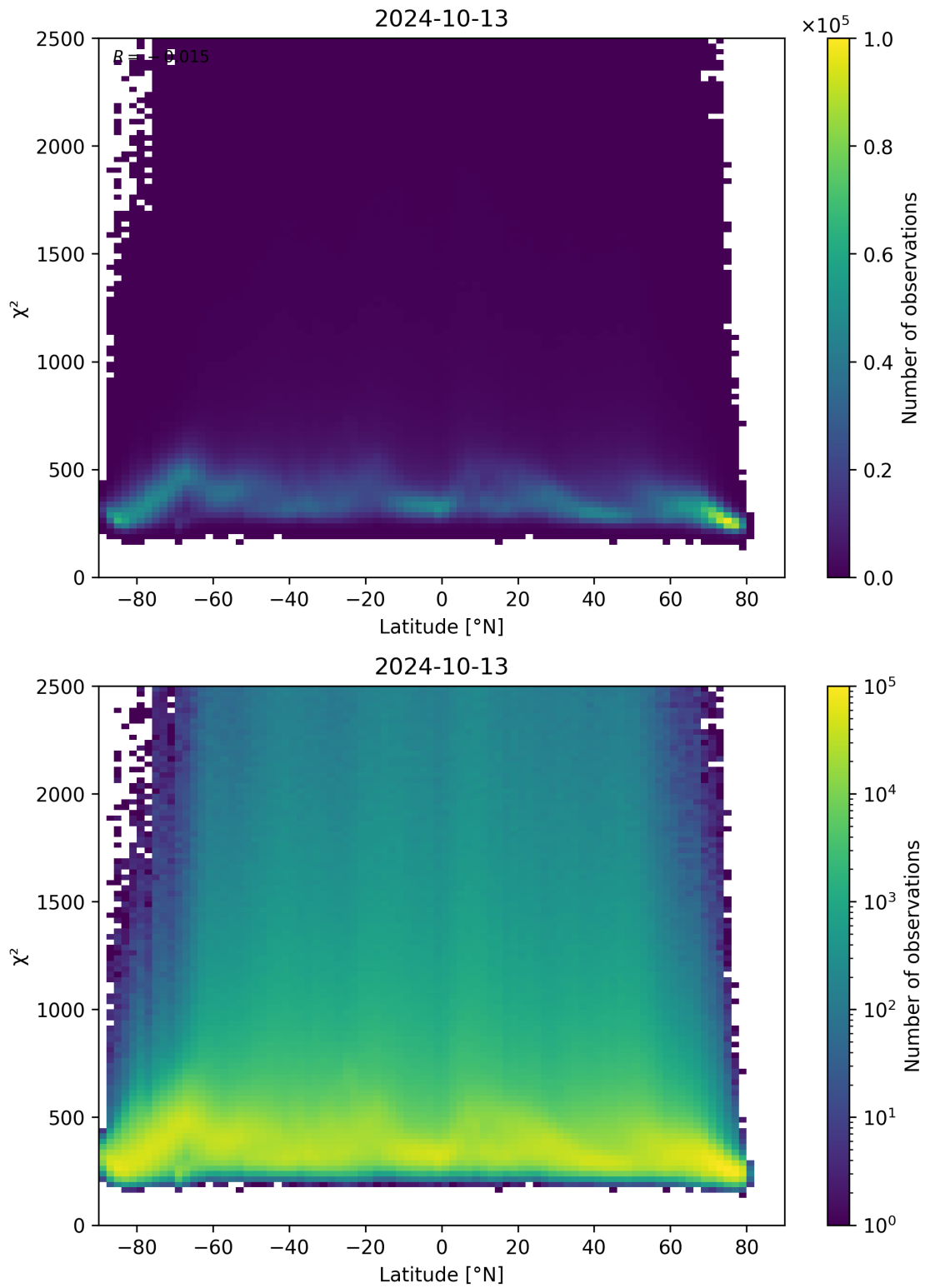
Figure 86: Scatter density plot of “Latitude” against “ \chi^2 ” for 2024-10-12 to 2024-10-14.
