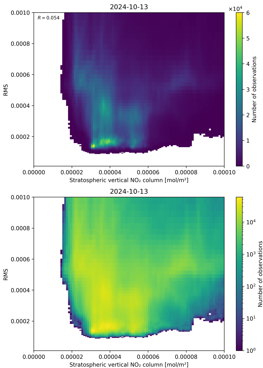
Figure 102: Scatter density plot of “Stratospheric vertical NO 2 column” against “RMS” for 2024-10-12 to 2024-10-14.
