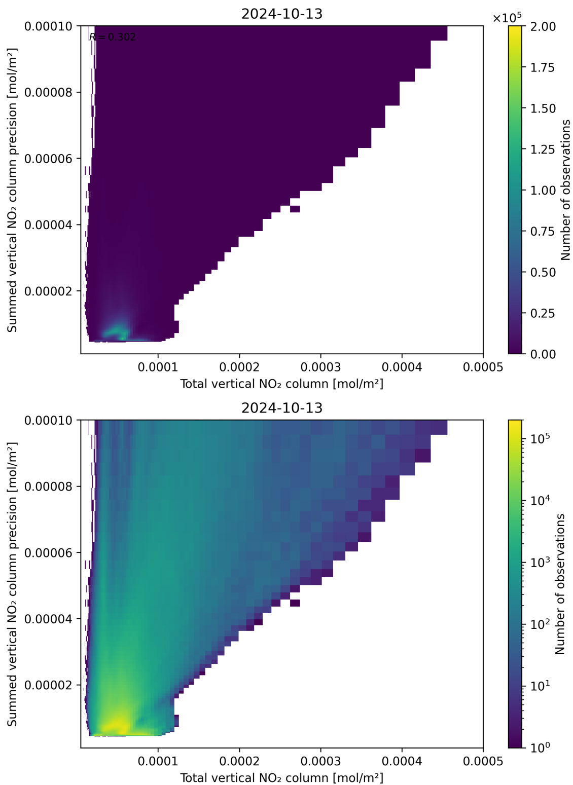
Figure 113: Scatter density plot of “Total vertical NO 2 column” against “Summed vertical NO 2 column precision” for 2024-10-12 to 2024-10-14.
