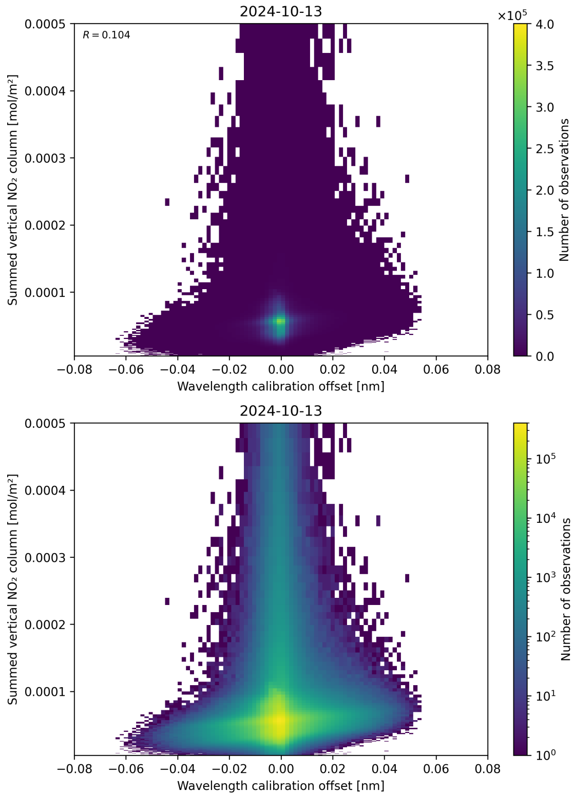
Figure 177: Scatter density plot of “Wavelength calibration offset” against “Summed vertical NO 2 column” for 2024-10-12 to 2024-10-14.
