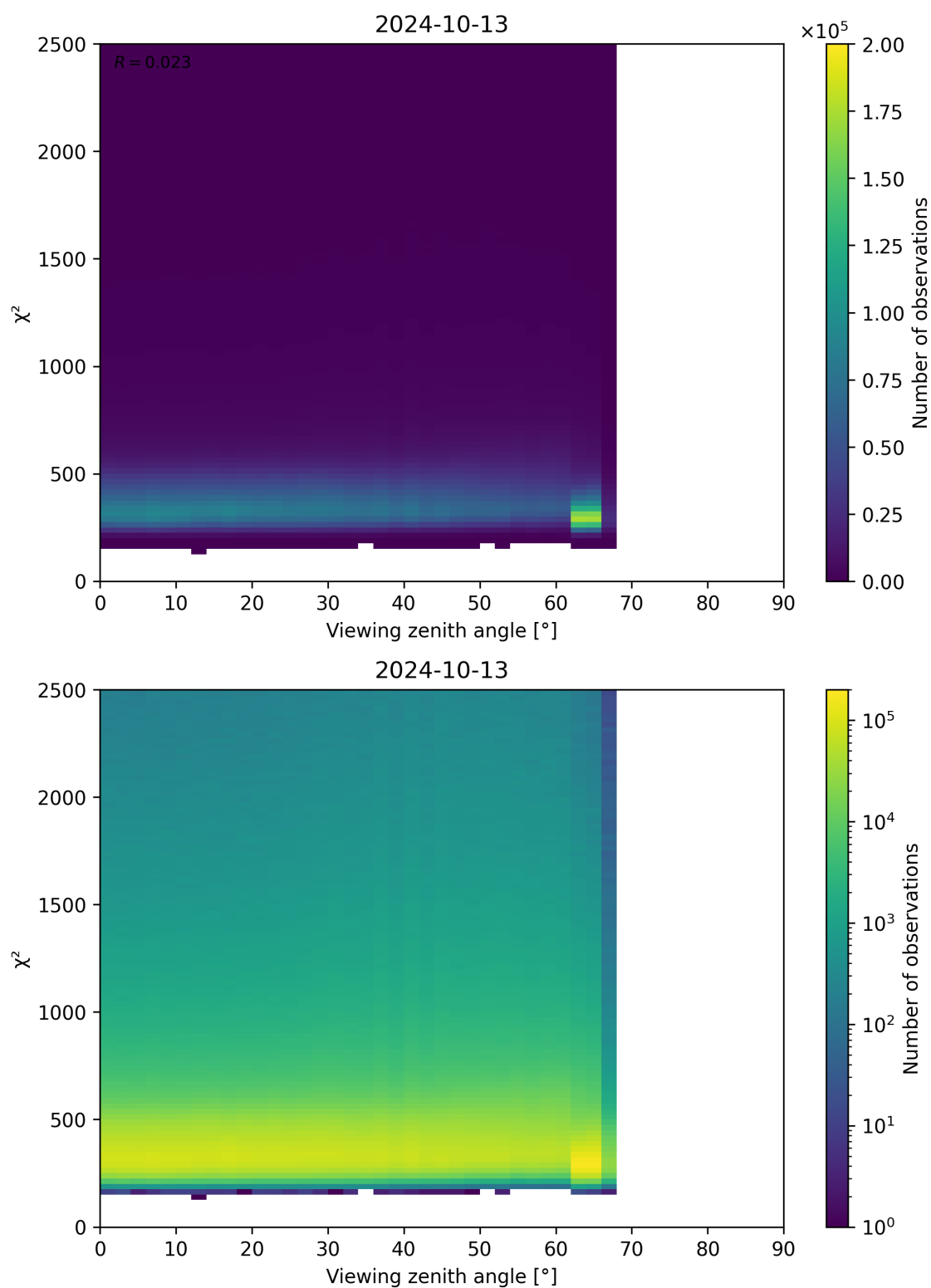
Figure 162: Scatter density plot of “Viewing zenith angle” against “ \chi^2 ” for 2024-10-12 to 2024-10-14.
