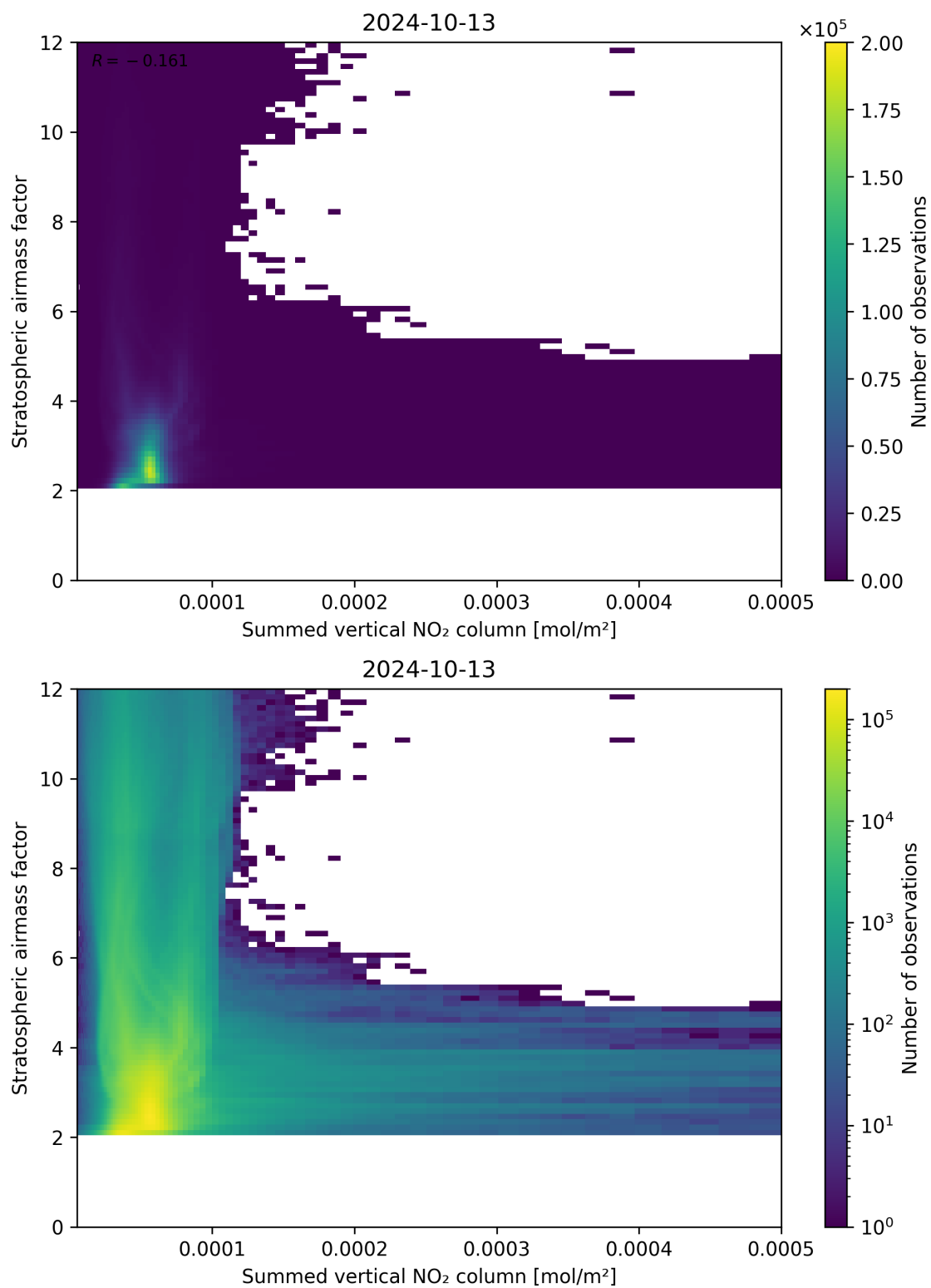
Figure 103: Scatter density plot of “Summed vertical NO 2 column” against “Stratospheric airmass factor” for 2024-10-12 to 2024-10-14.
