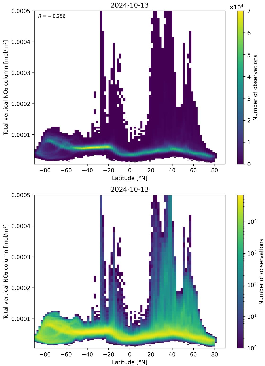
Figure 90: Scatter density plot of “Latitude” against “Total vertical NO 2 column” for 2024-10-12 to 2024-10-14.
