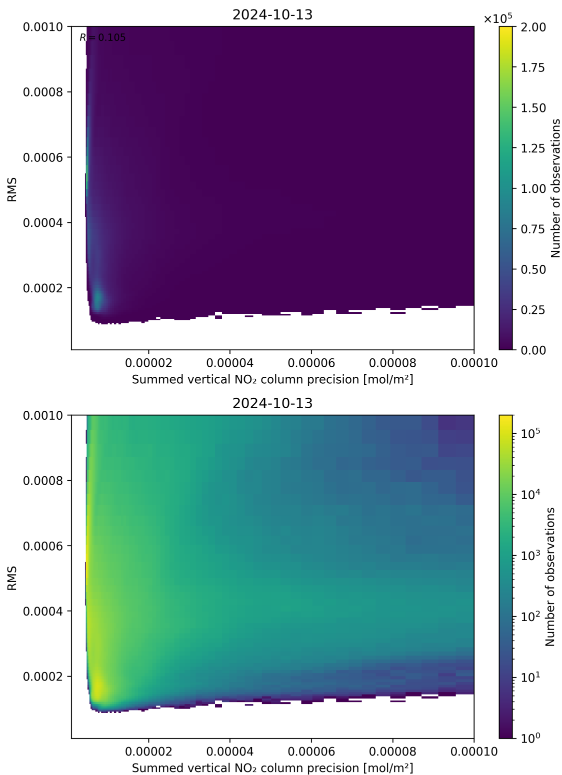
Figure 108: Scatter density plot of “Summed vertical NO 2 column precision” against “RMS” for 2024-10-12 to 2024-10-14.
