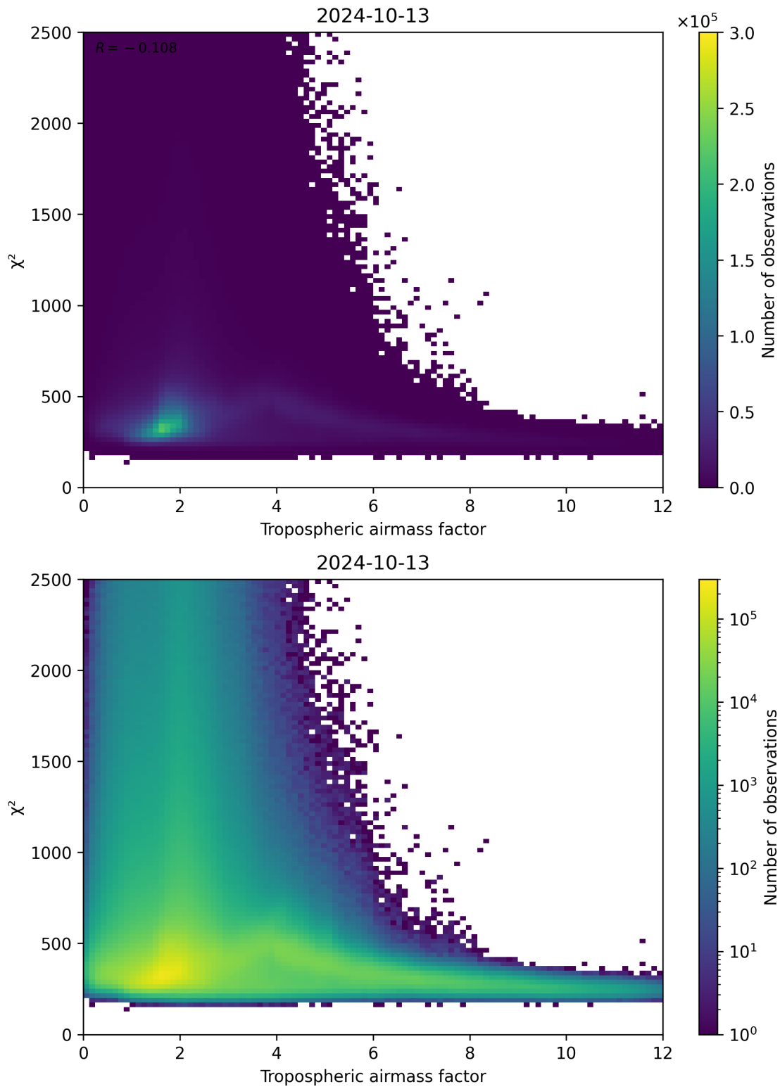
Figure 73: Scatter density plot of “Tropospheric airmass factor” against “ \chi^2 ” for 2024-10-12 to 2024-10-14.
