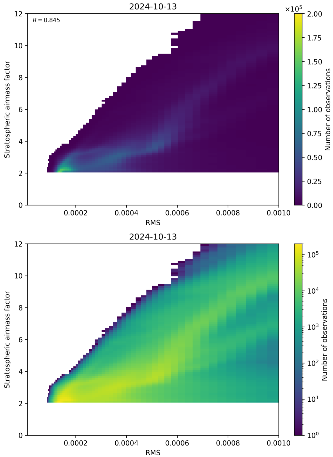
Figure 144: Scatter density plot of “RMS” against “Stratospheric airmass factor” for 2024-10-12 to 2024-10-14.
