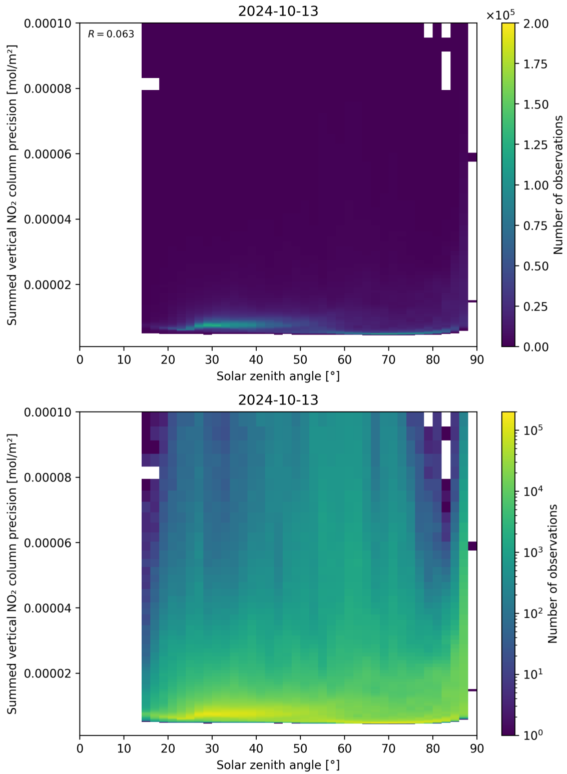
Figure 152: Scatter density plot of “Solar zenith angle” against “Summed vertical NO 2 column precision” for 2024-10-12 to 2024-10-14.
