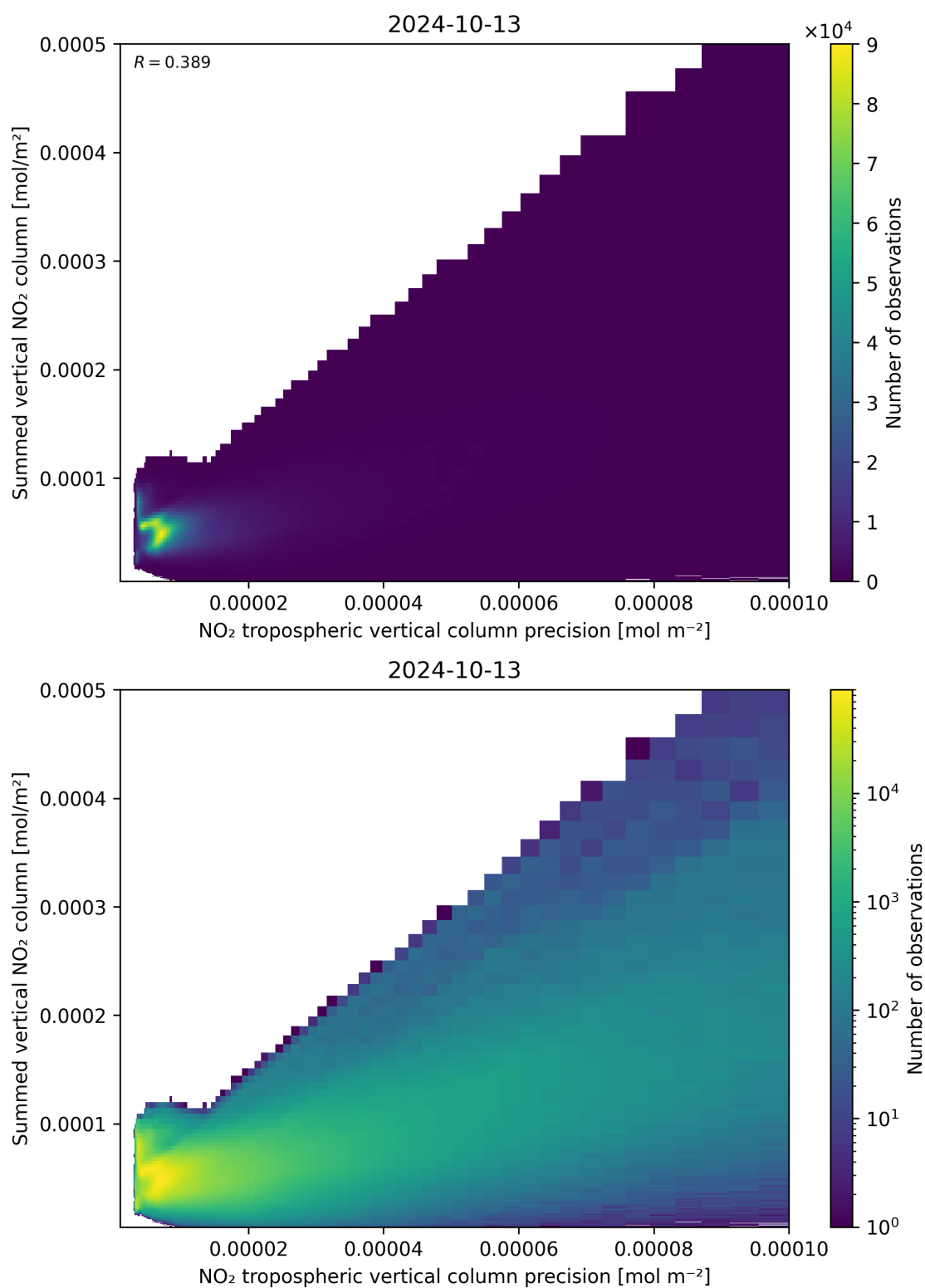
Figure 136: Scatter density plot of “NO 2 tropospheric vertical column precision” against “Summed vertical NO 2 column” for 2024-10-12 to 2024-10-14.
