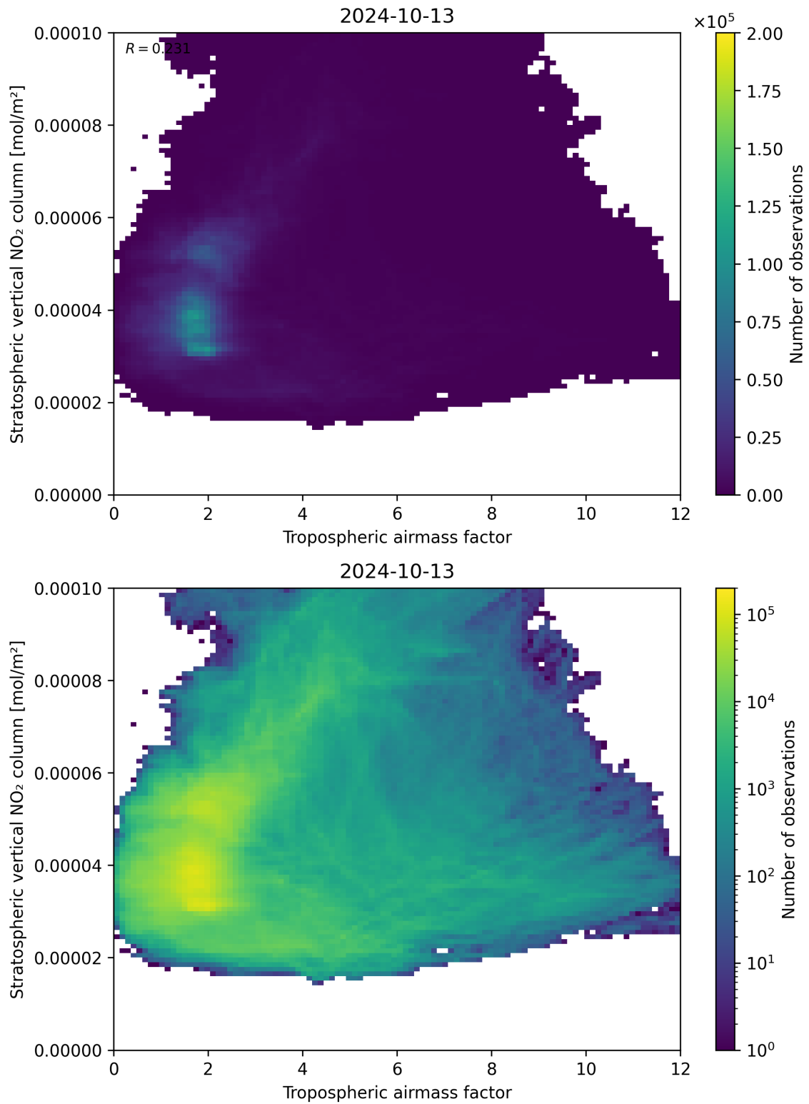
Figure 74: Scatter density plot of “Tropospheric airmass factor” against “Stratospheric vertical NO 2 column” for 2024-10-12 to 2024-10-14.
