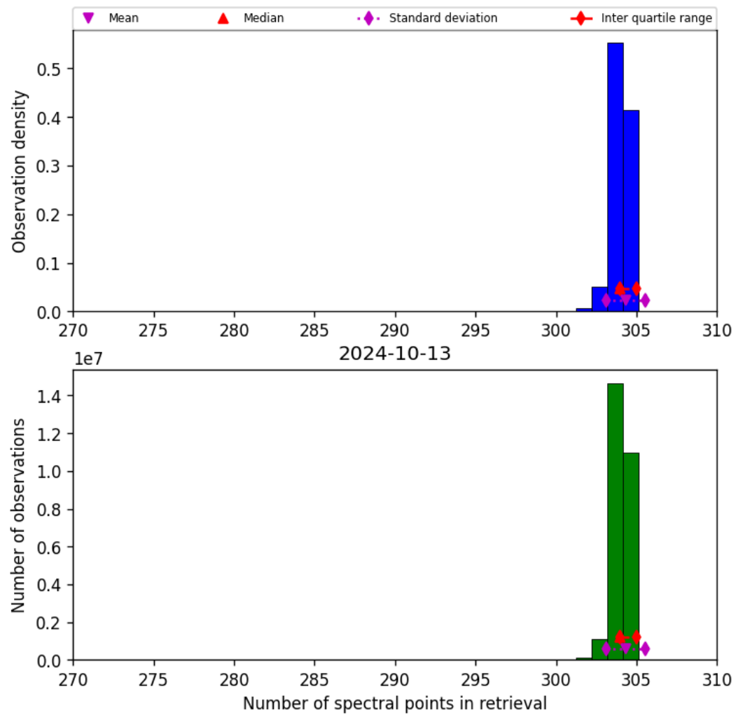
Figure 33: Histogram of “Number of spectral points in retrieval” for 2024-10-12 to 2024-10-14
