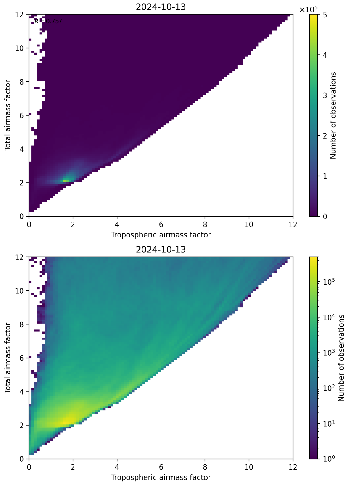
Figure 72: Scatter density plot of “Tropospheric airmass factor” against “Total airmass factor” for 2024-10-12 to 2024-10-14.
