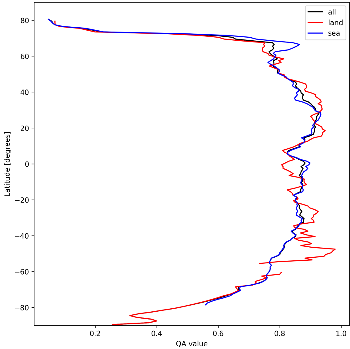
Figure 11: Zonal average of “QA value” for 2024-10-12 to 2024-10-14.
