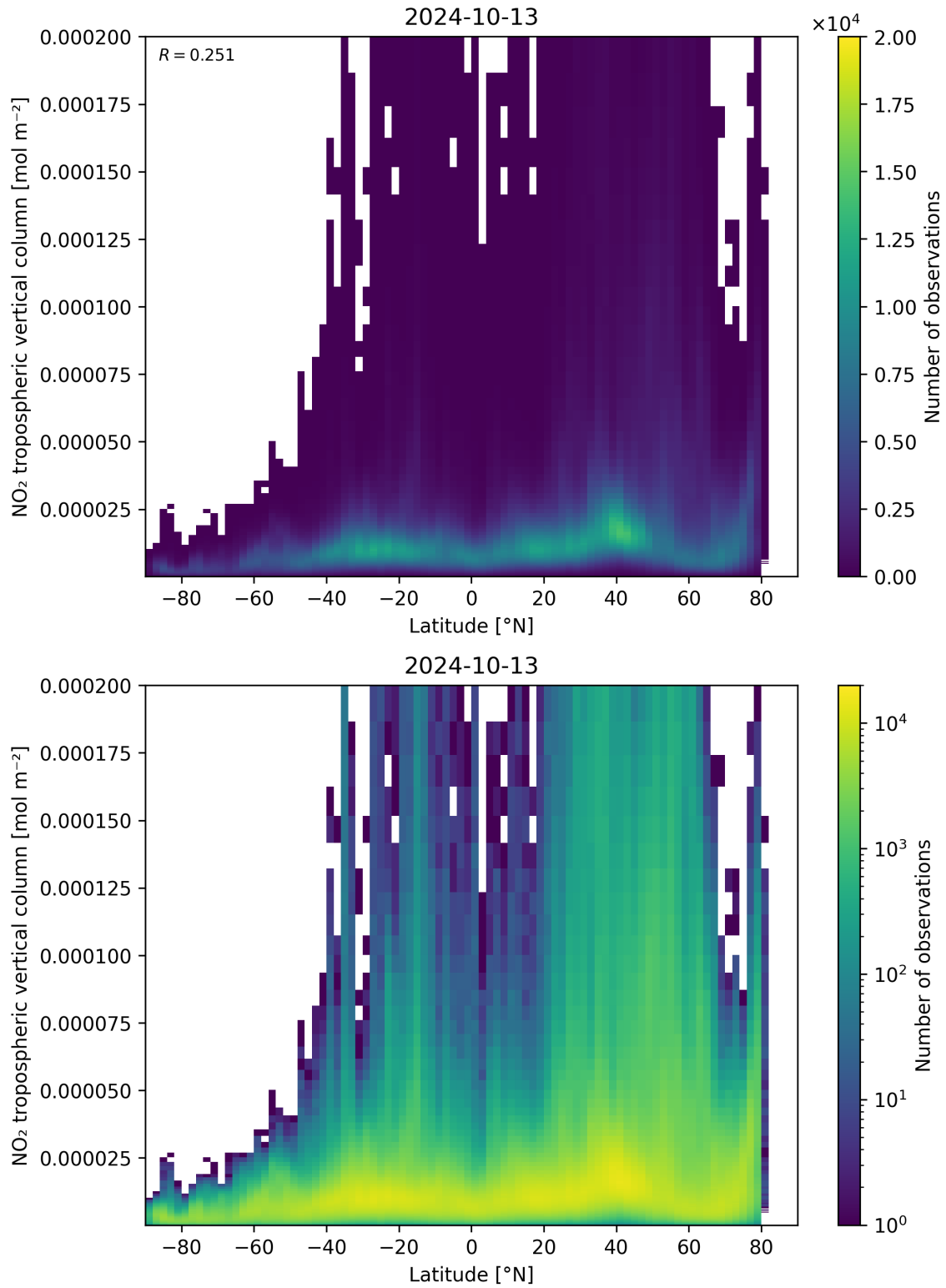
Figure 92: Scatter density plot of “Latitude” against “NO 2 tropospheric vertical column” for 2024-10-12 to 2024-10-14.
