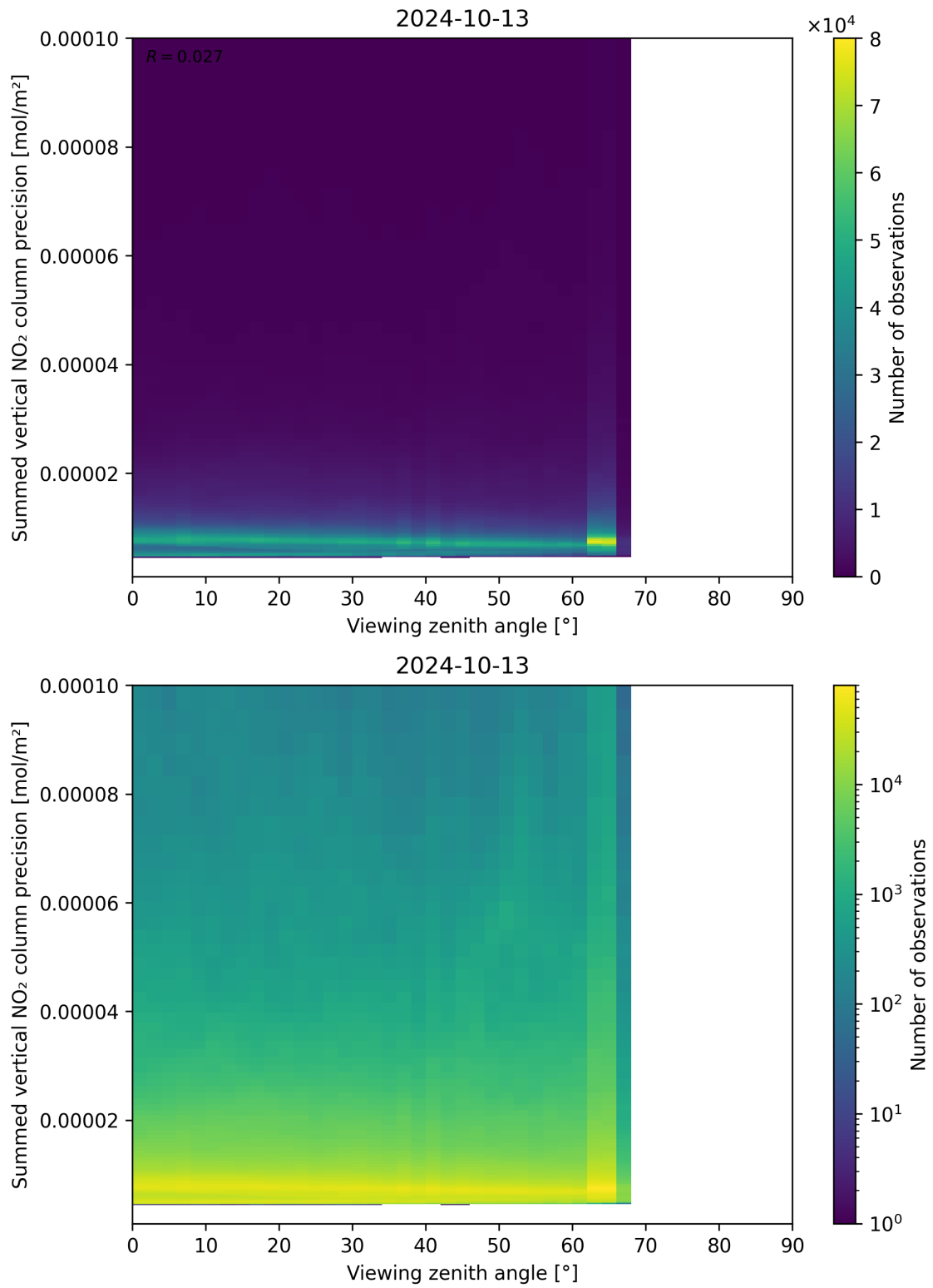
Figure 166: Scatter density plot of “Viewing zenith angle” against “Summed vertical NO 2 column precision” for 2024-10-12 to 2024-10-14.
