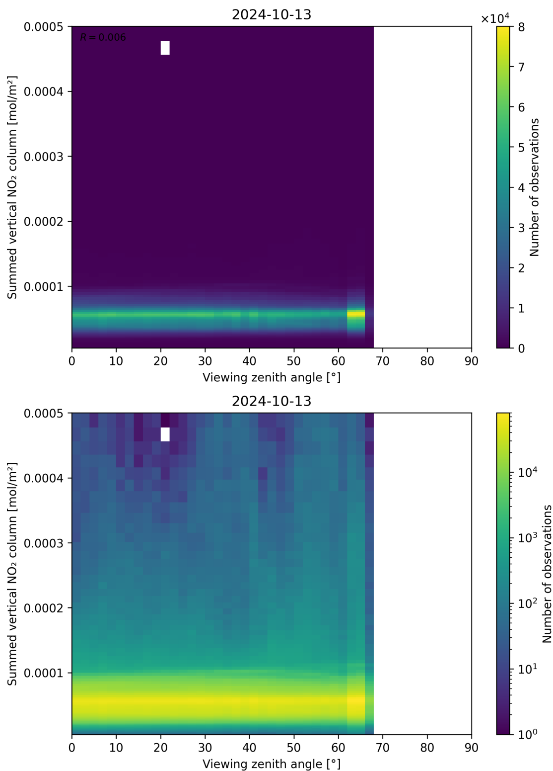
Figure 165: Scatter density plot of “Viewing zenith angle” against “Summed vertical NO 2 column” for 2024-10-12 to 2024-10-14.
