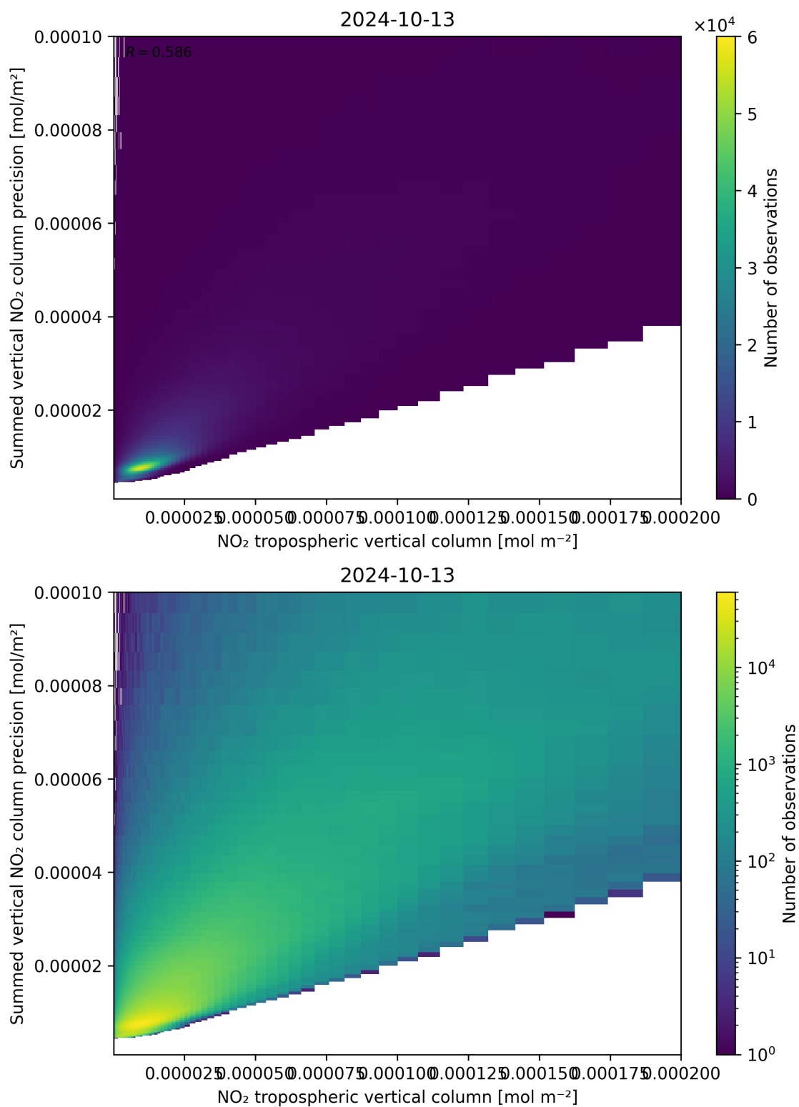
Figure 127: Scatter density plot of “NO 2 tropospheric vertical column” against “Summed vertical NO 2 column precision” for 2024-10-12 to 2024-10-14.
