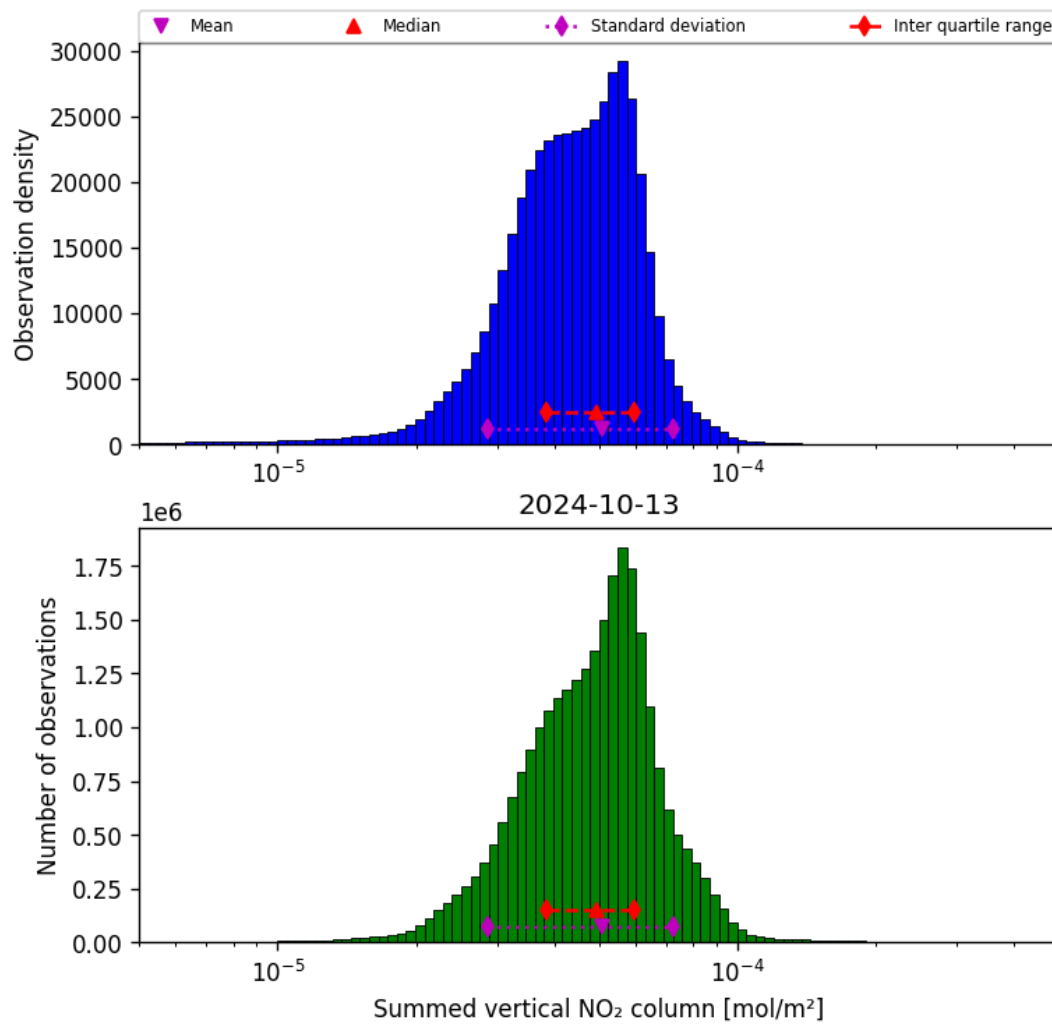
Figure 40: Histogram of “Summed vertical NO 2 column” for 2024-10-12 to 2024-10-14
