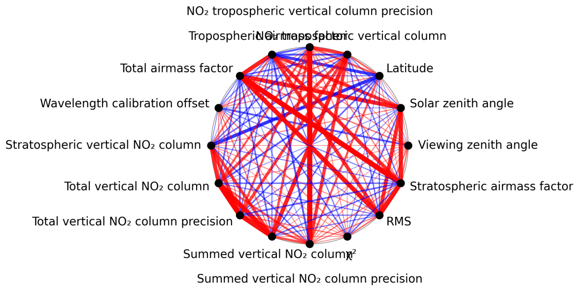
Figure 1: Map of correlation graph for 2024-10-12 to 2024-10-14.
