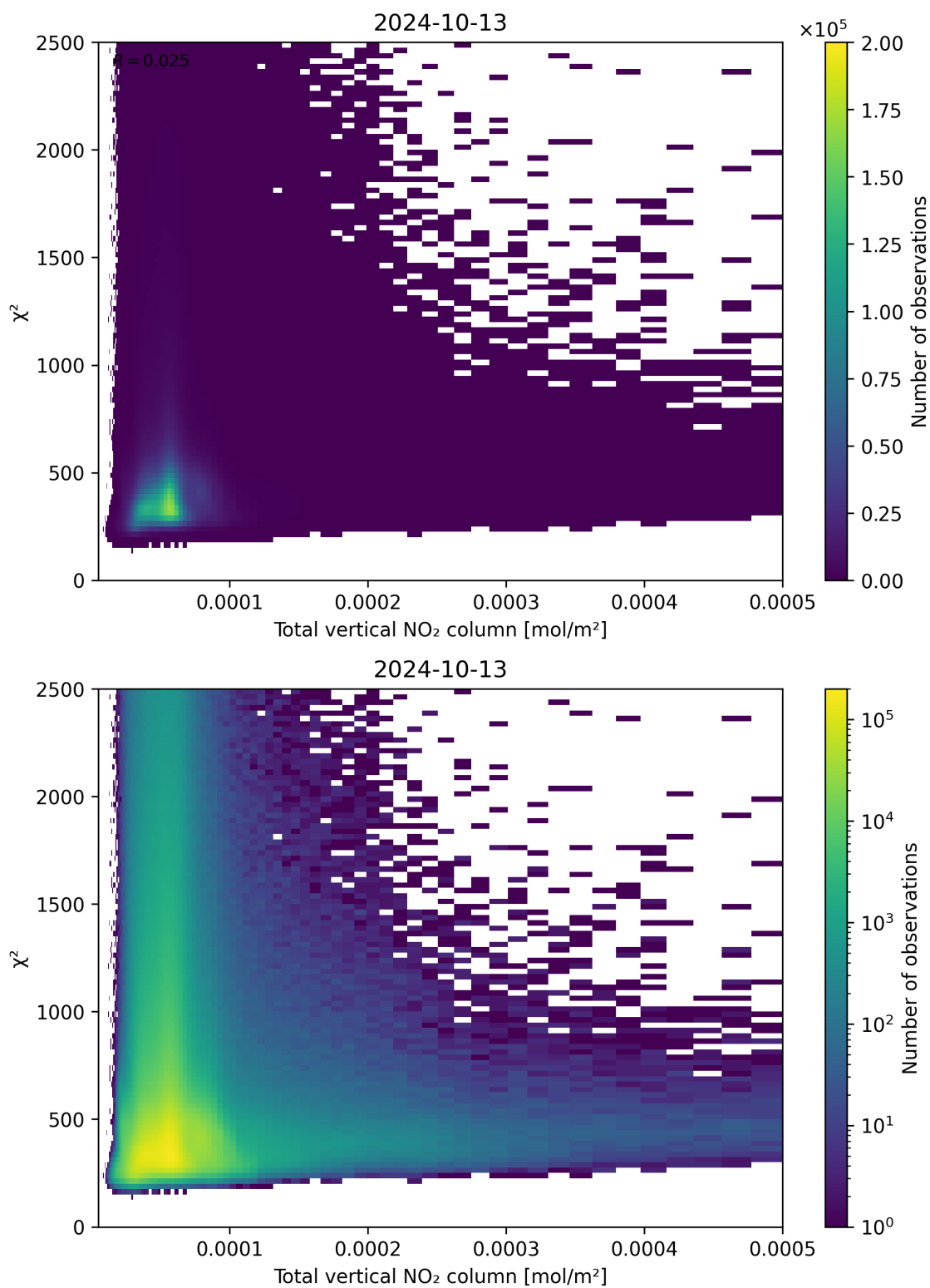
Figure 111: Scatter density plot of “Total vertical NO 2 column” against “ \chi^2 ” for 2024-10-12 to 2024-10-14.
