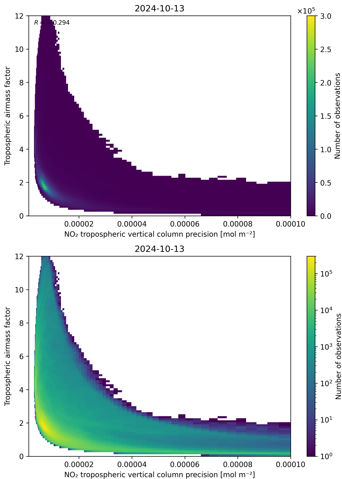
Figure 133: Scatter density plot of “NO 2 tropospheric vertical column precision” against “Tropospheric airmass factor” for 2024-10-12 to 2024-10-14.
