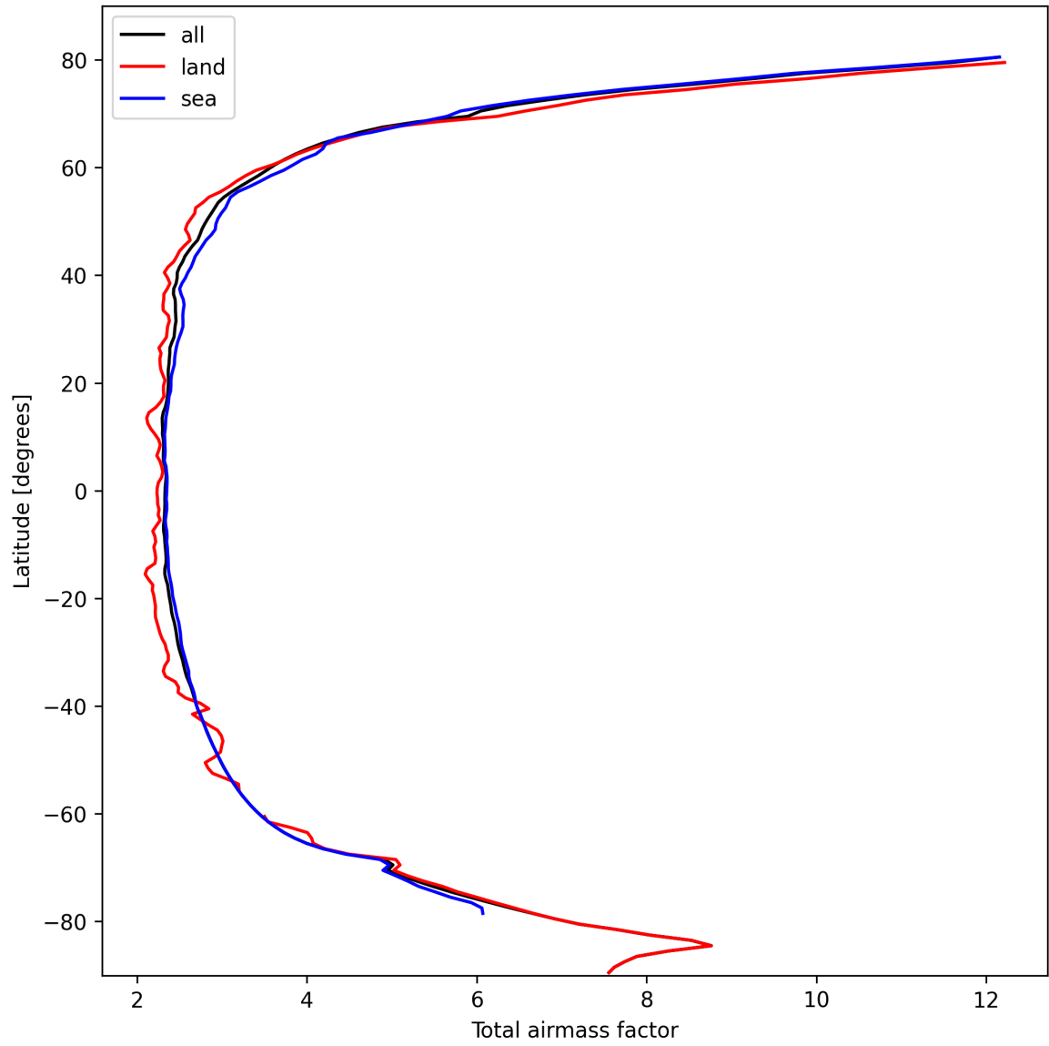
Figure 15: Zonal average of “Total airmass factor” for 2024-10-12 to 2024-10-14.
