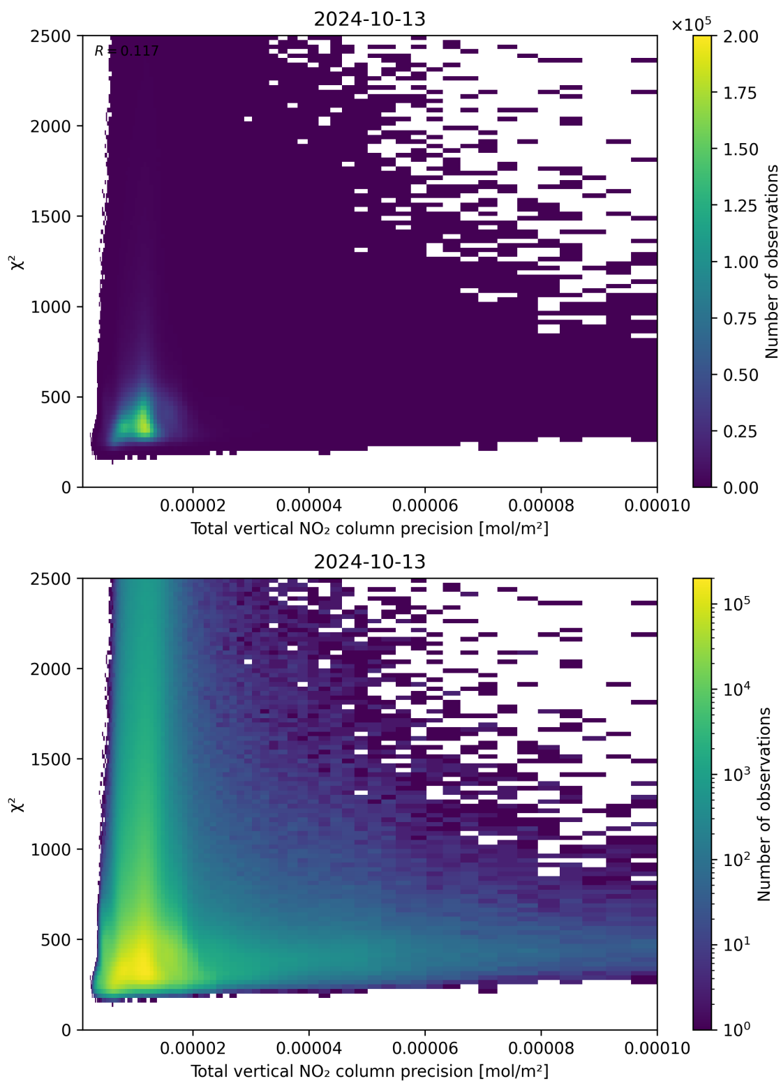
Figure 116: Scatter density plot of “Total vertical NO 2 column precision” against “ \chi^2 ” for 2024-10-12 to 2024-10-14.
