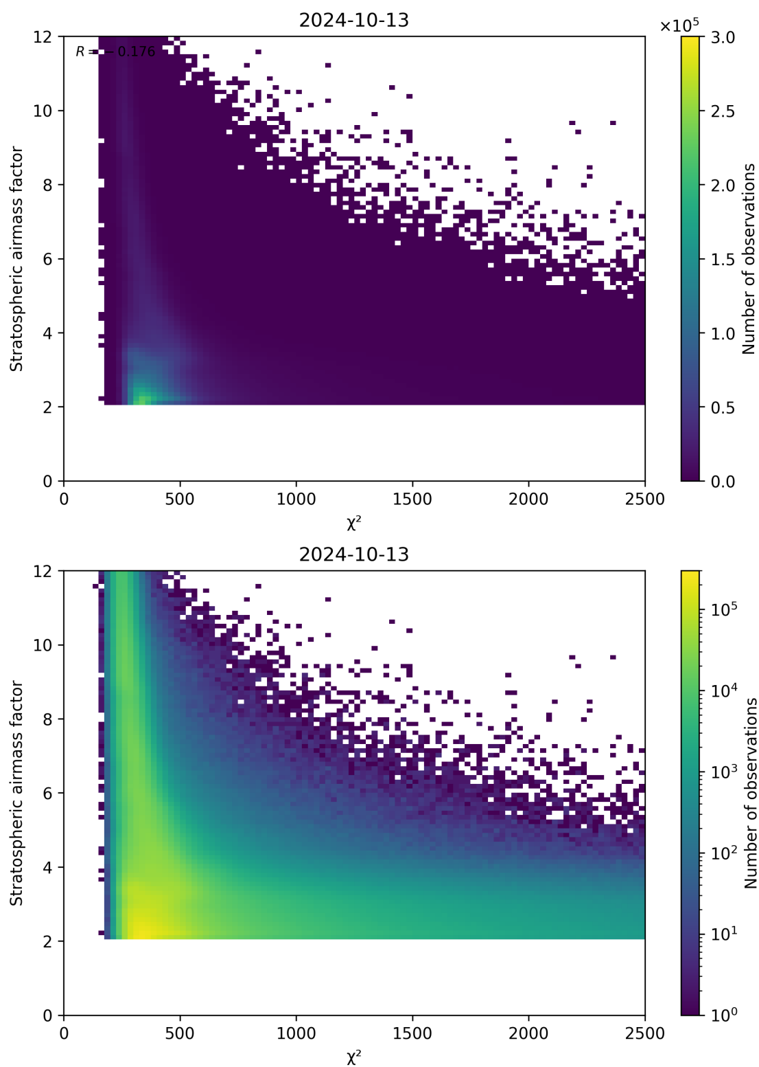
Figure 81: Scatter density plot of “ \chi^2 ” against “Stratospheric airmass factor” for 2024-10-12 to 2024-10-14.
