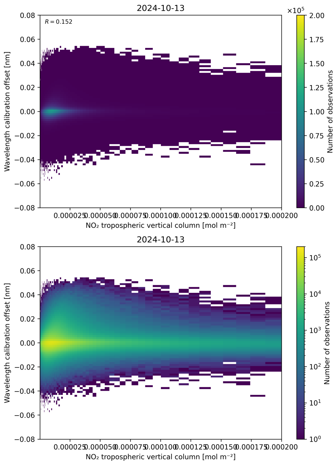
Figure 143: Scatter density plot of “NO 2 tropospheric vertical column” against “Wavelength calibration offset” for 2024-10-12 to 2024-10-14.
