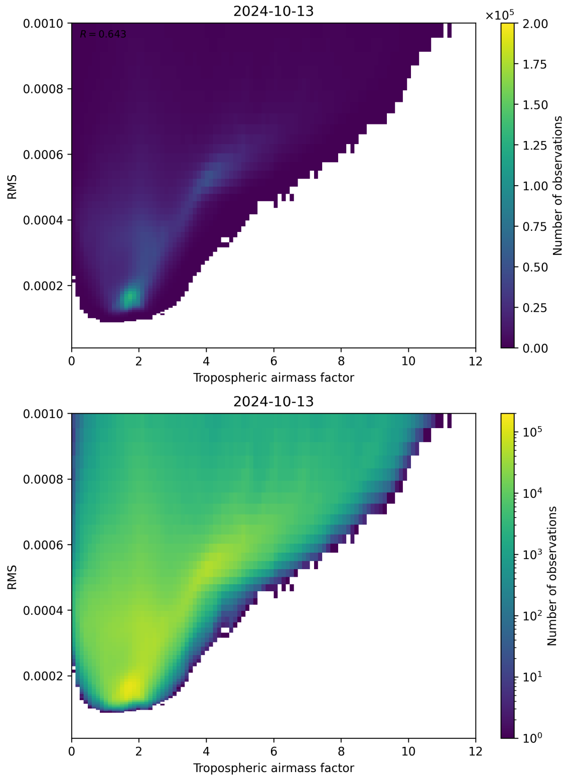
Figure 79: Scatter density plot of “Tropospheric airmass factor” against “RMS” for 2024-10-12 to 2024-10-14.
