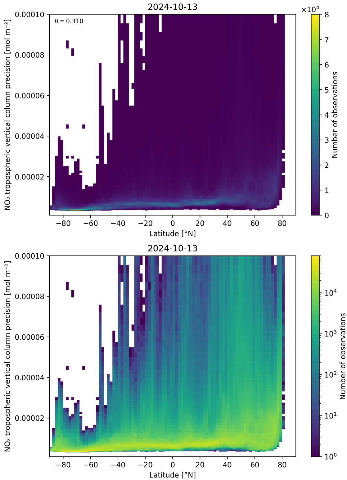
Figure 93: Scatter density plot of “Latitude” against “NO 2 tropospheric vertical column precision” for 2024-10-12 to 2024-10-14.
