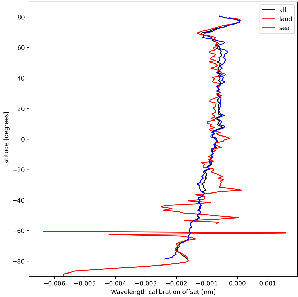
Figure 18: Zonal average of “Wavelength calibration offset” for 2024-10-12 to 2024-10-14.
