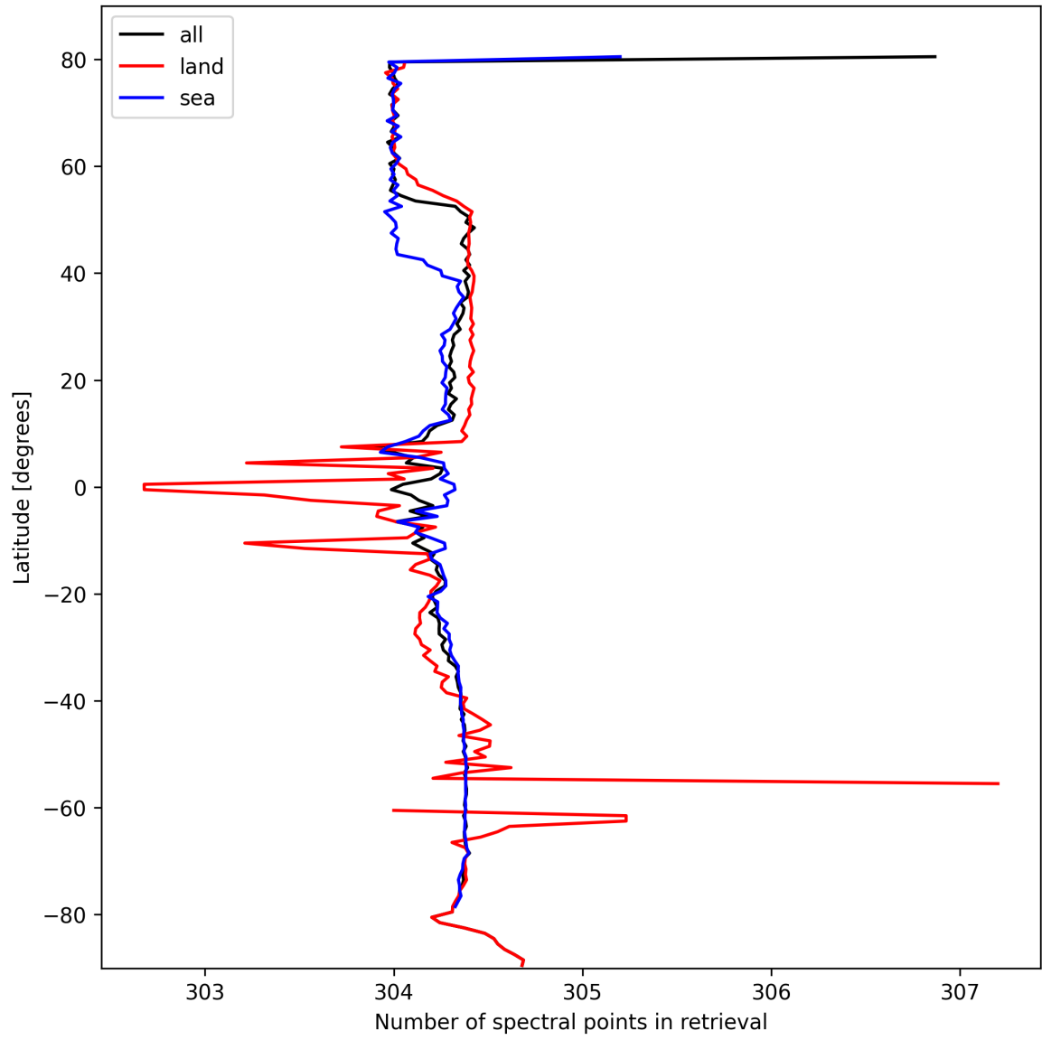
Figure 16: Zonal average of “Number of spectral points in retrieval” for 2024-10-12 to 2024-10-14.
