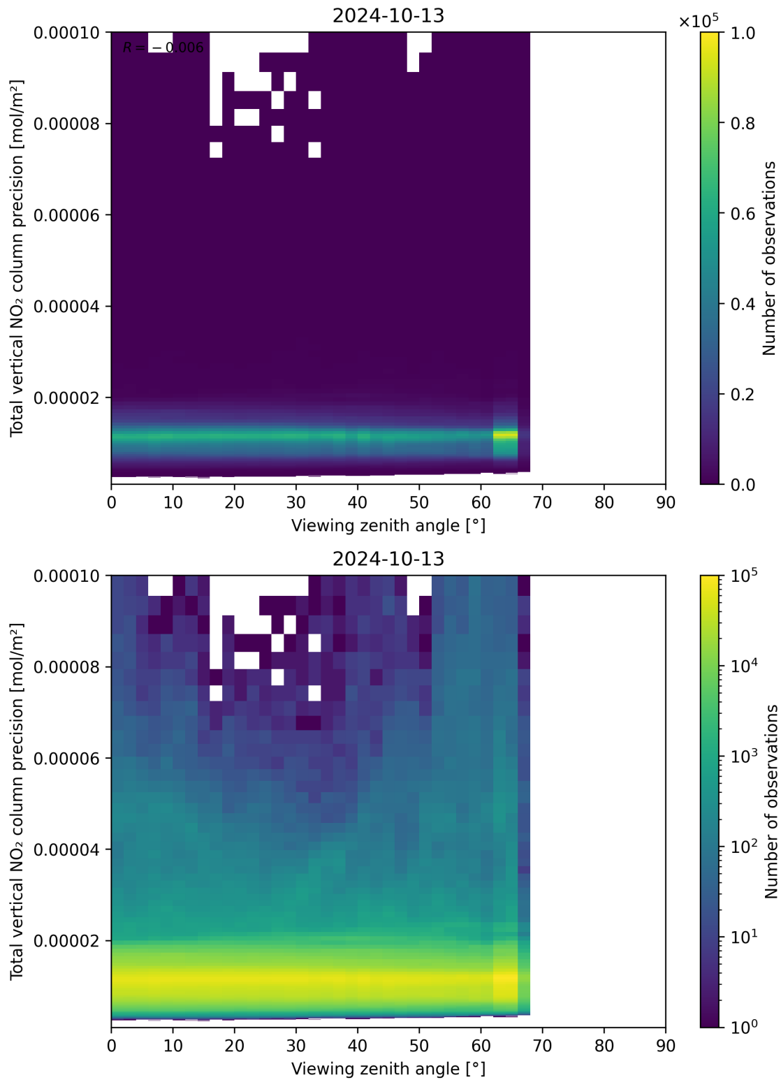
Figure 168: Scatter density plot of “Viewing zenith angle” against “Total vertical NO 2 column precision” for 2024-10-12 to 2024-10-14.
