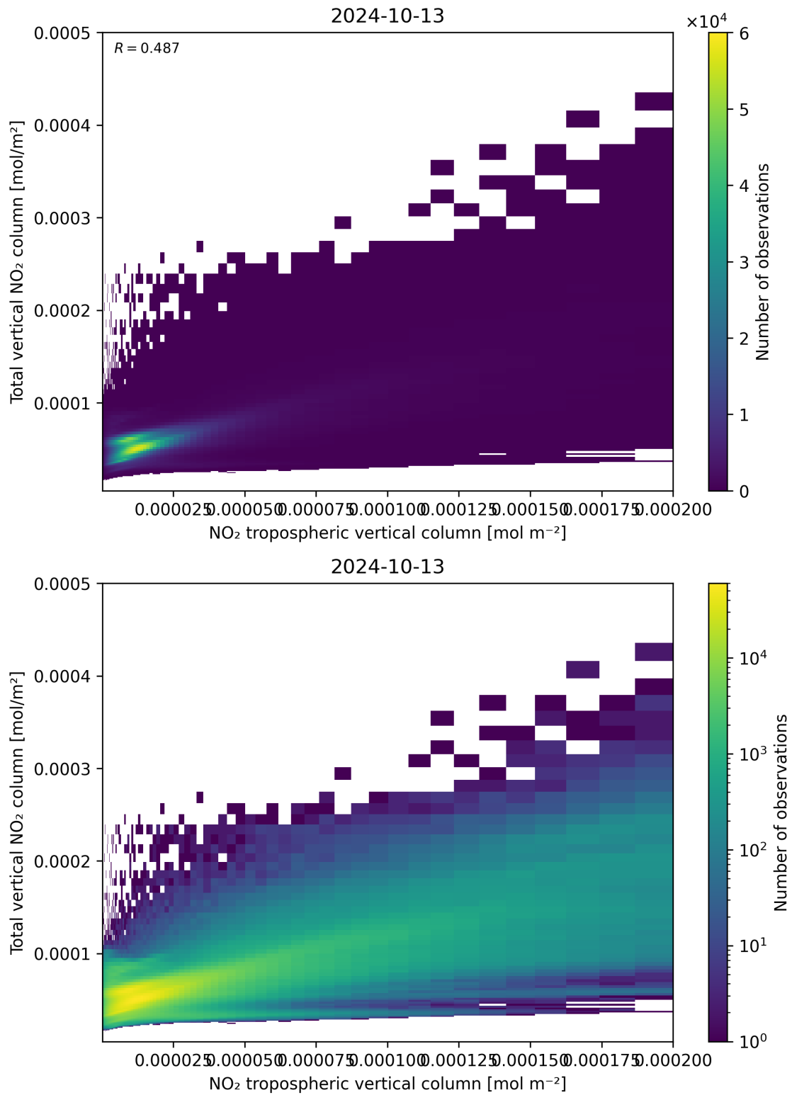
Figure 128: Scatter density plot of “NO 2 tropospheric vertical column” against “Total vertical NO 2 column” for 2024-10-12 to 2024-10-14.
