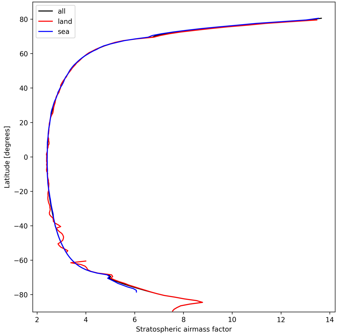
Figure 27: Zonal average of “Stratospheric air mass factor” for 2024-10-12 to 2024-10-14.
