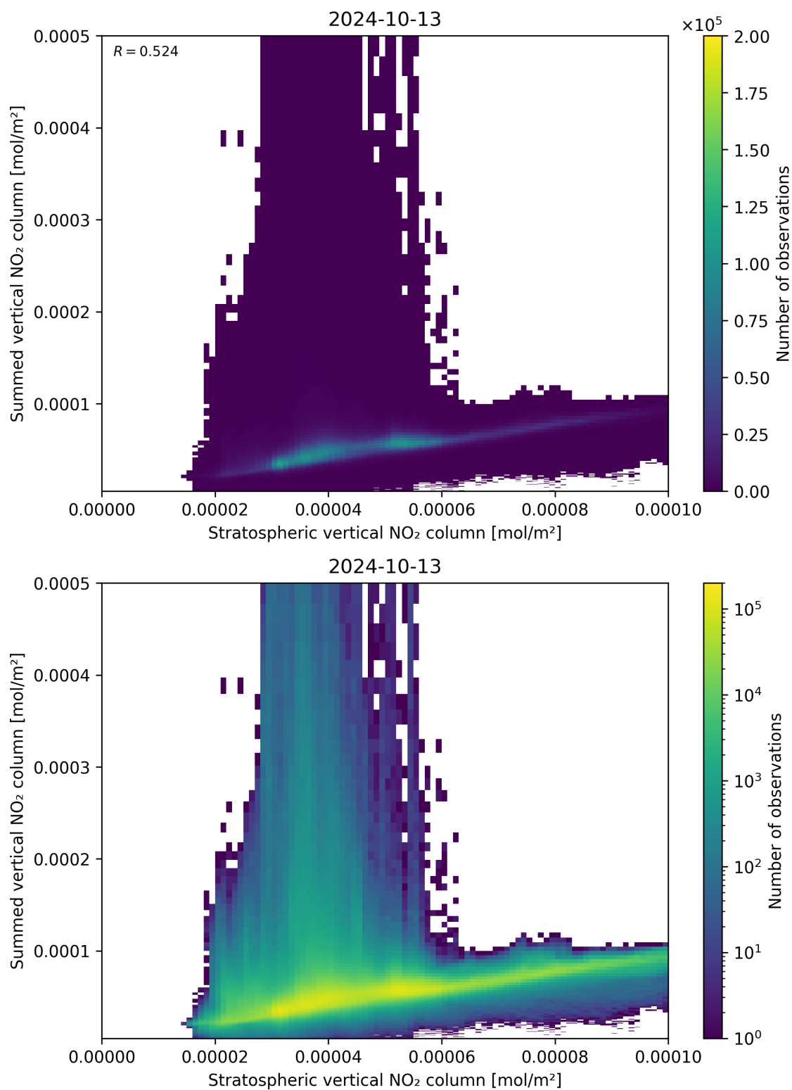
Figure 98: Scatter density plot of “Stratospheric vertical NO 2 column” against “Summed vertical NO 2 column” for 2024-10-12 to 2024-10-14.
