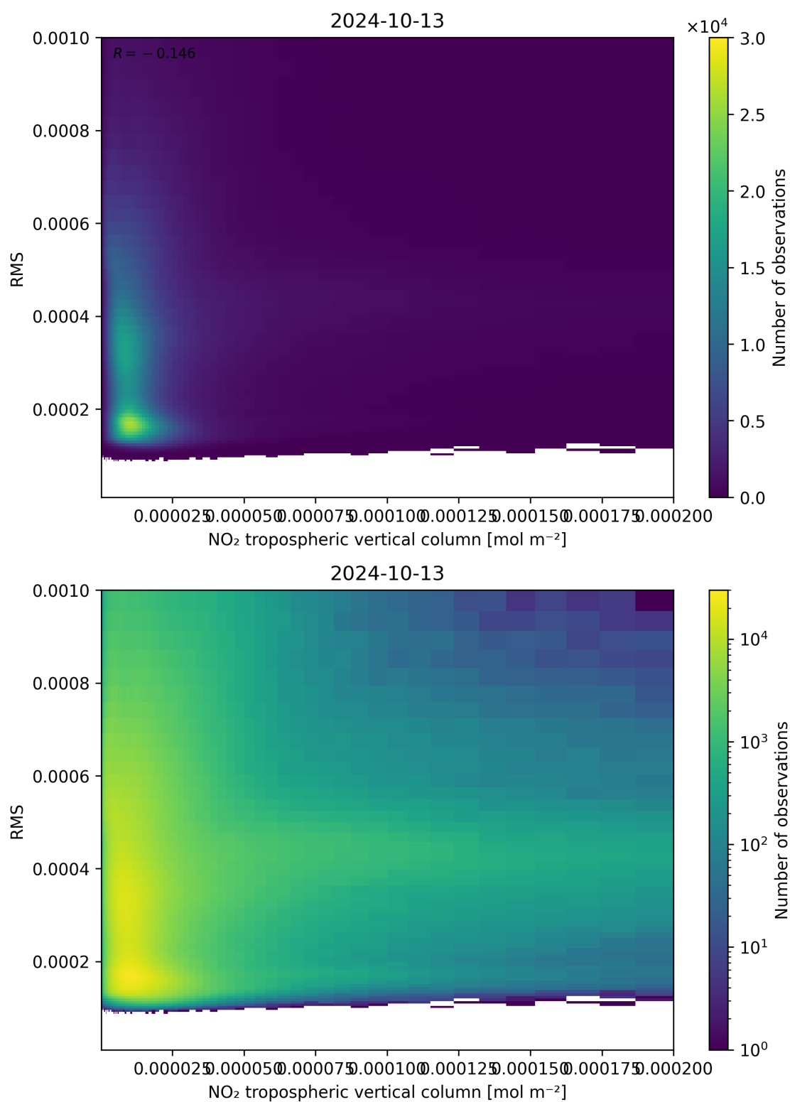
Figure 142: Scatter density plot of “NO 2 tropospheric vertical column” against “RMS” for 2024-10-12 to 2024-10-14.
