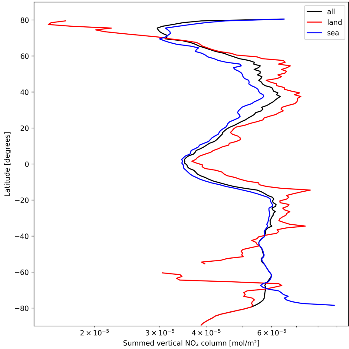
Figure 23: Zonal average of “Summed vertical NO 2 column” for 2024-10-12 to 2024-10-14.
