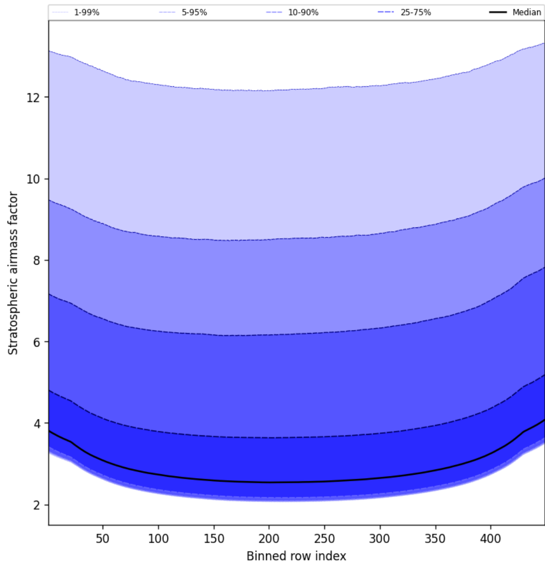
Figure 61: Along track statistics of “Stratospheric airmass factor” for 2024-10-12 to 2024-10-14
