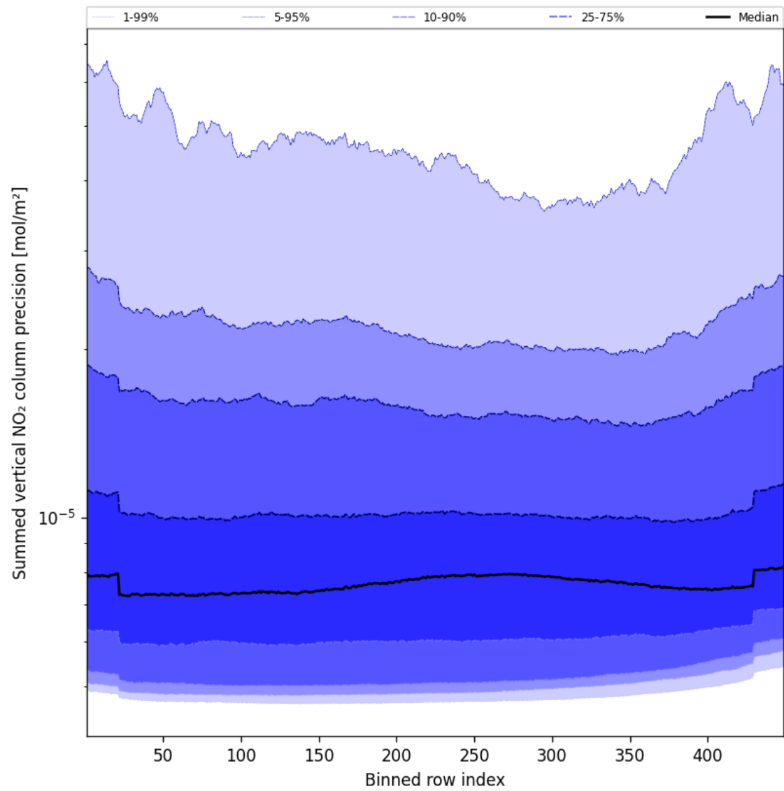
Figure 58: Along track statistics of “Summed vertical NO 2 column precision” for 2024-10-12 to 2024-10-14
