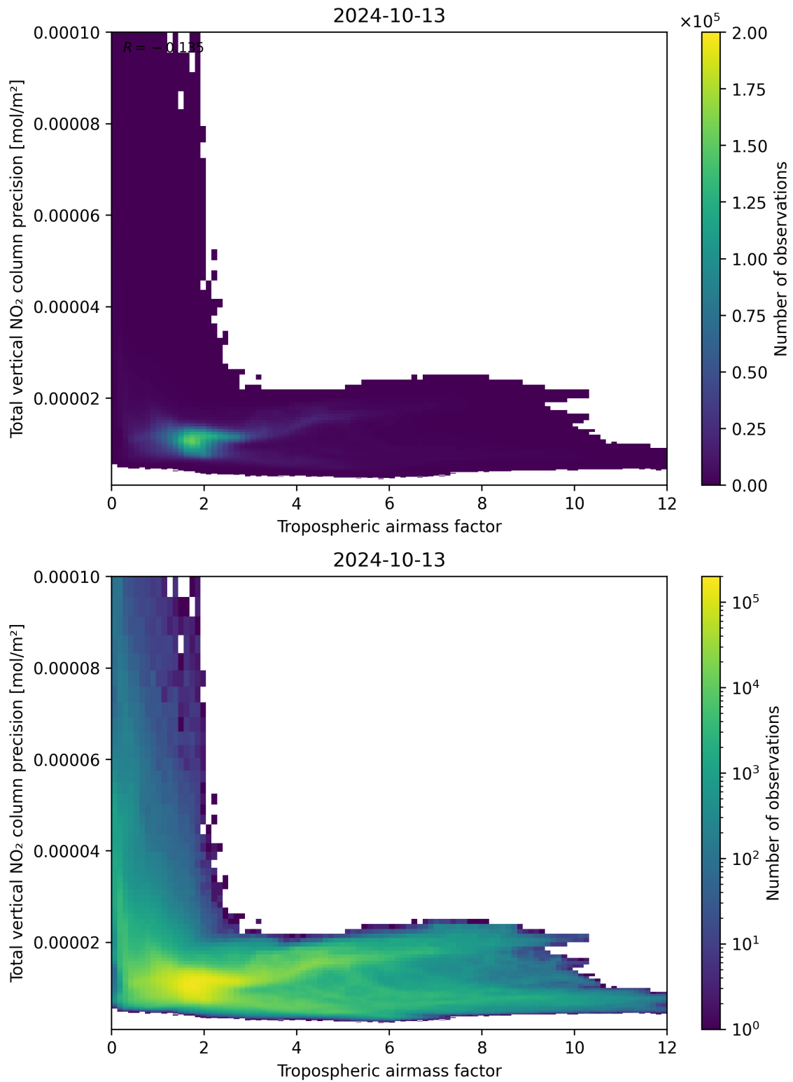
Figure 78: Scatter density plot of “Tropospheric airmass factor” against “Total vertical NO 2 column precision” for 2024-10-12 to 2024-10-14.
