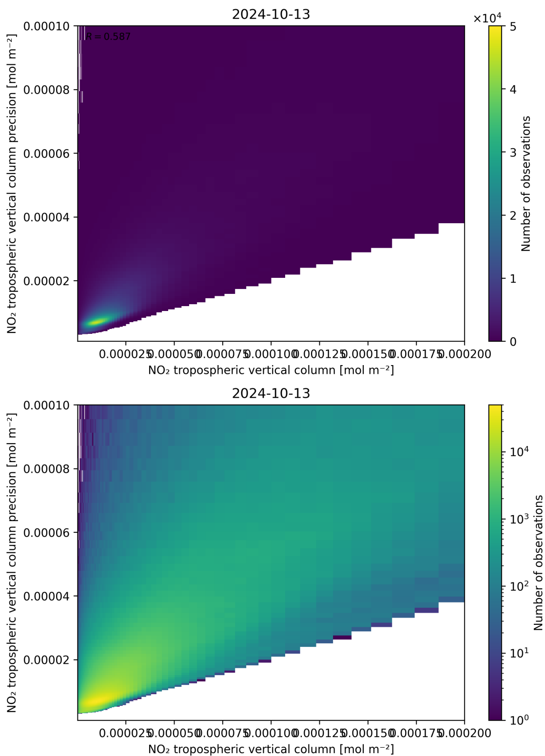
Figure 130: Scatter density plot of “NO 2 tropospheric vertical column” against “NO 2 tropospheric vertical column precision” for 2024-10-12 to 2024-10-14.
