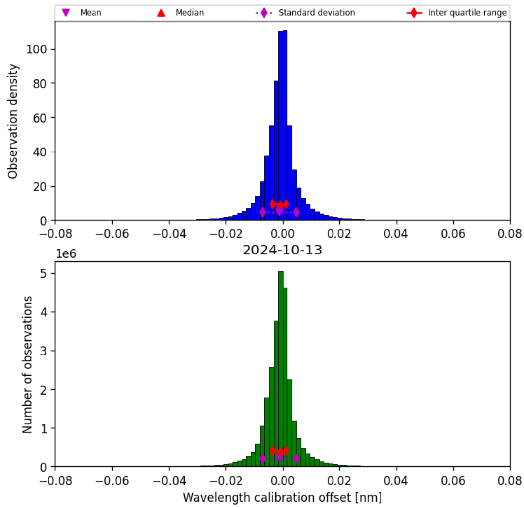
Figure 35: Histogram of “Wavelength calibration offset” for 2024-10-12 to 2024-10-14
