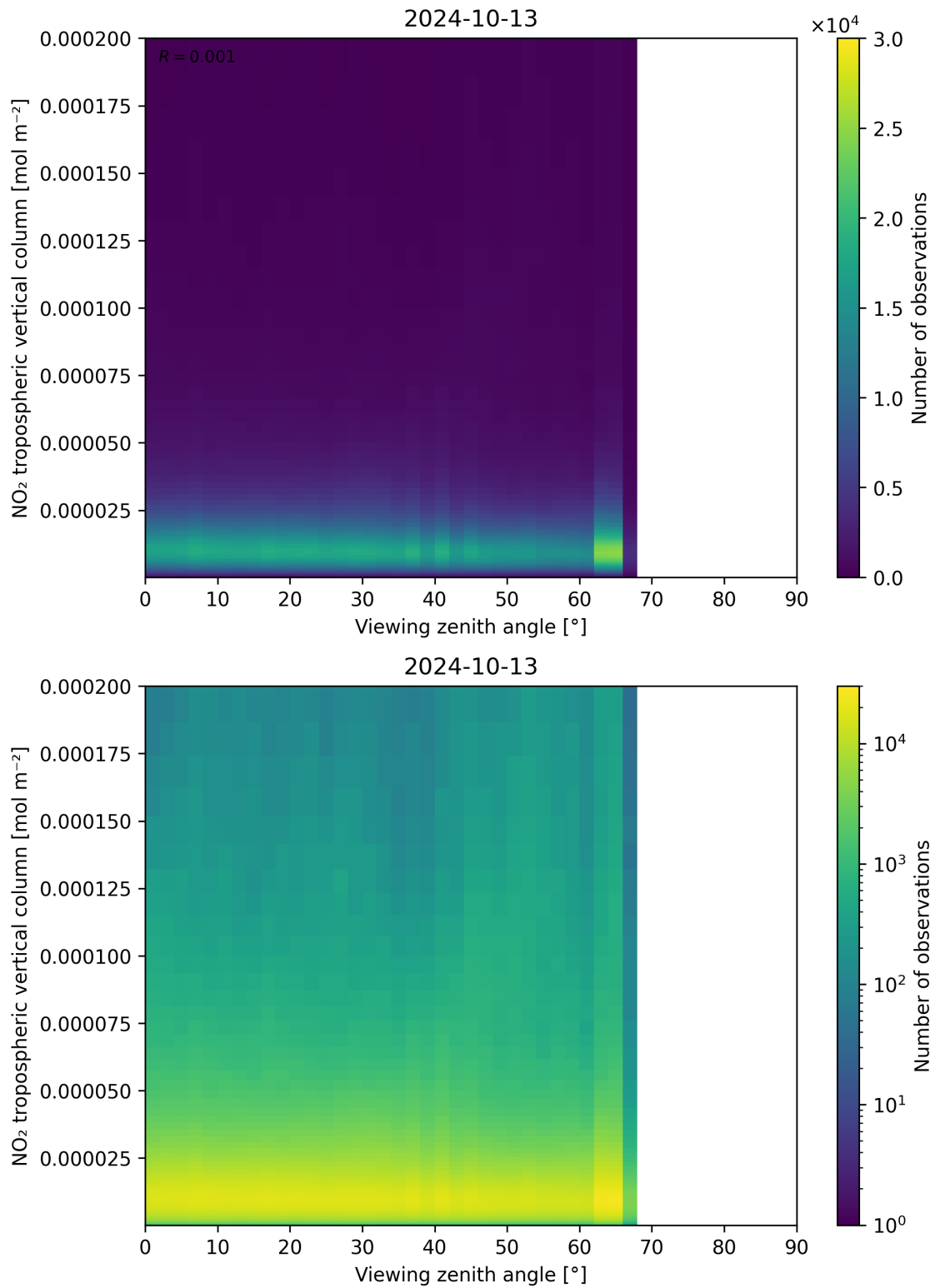
Figure 169: Scatter density plot of “Viewing zenith angle” against “NO 2 tropospheric vertical column” for 2024-10-12 to 2024-10-14.
