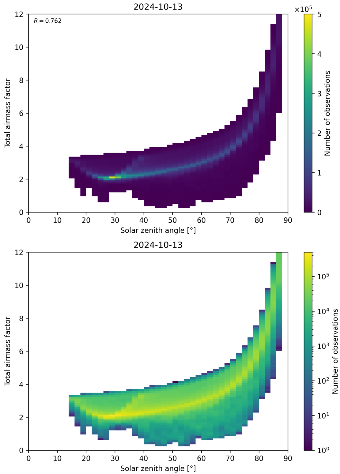
Figure 146: Scatter density plot of “Solar zenith angle” against “Total air mass factor” for 2024-10-12 to 2024-10-14.
