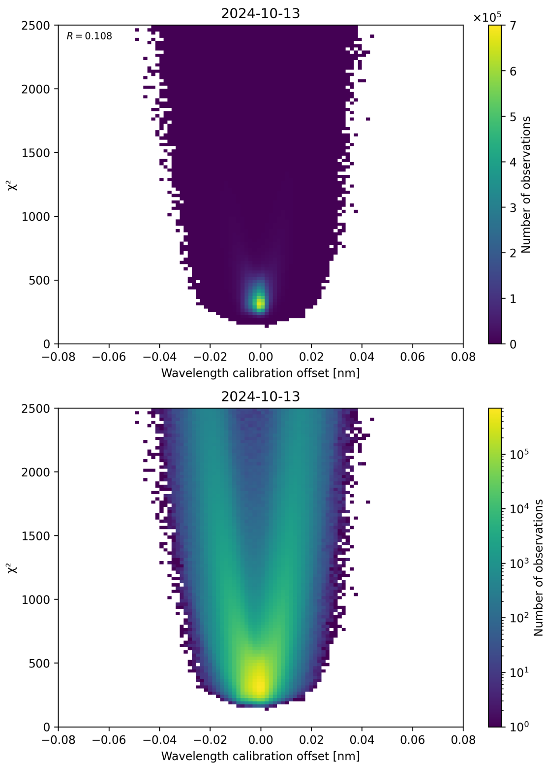
Figure 175: Scatter density plot of “Wavelength calibration offset” against “ \chi^2 ” for 2024-10-12 to 2024-10-14.
