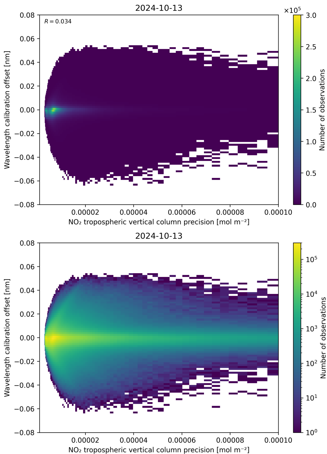
Figure 141: Scatter density plot of “NO 2 tropospheric vertical column precision” against “Wavelength calibration offset” for 2024-10-12 to 2024-10-14.
