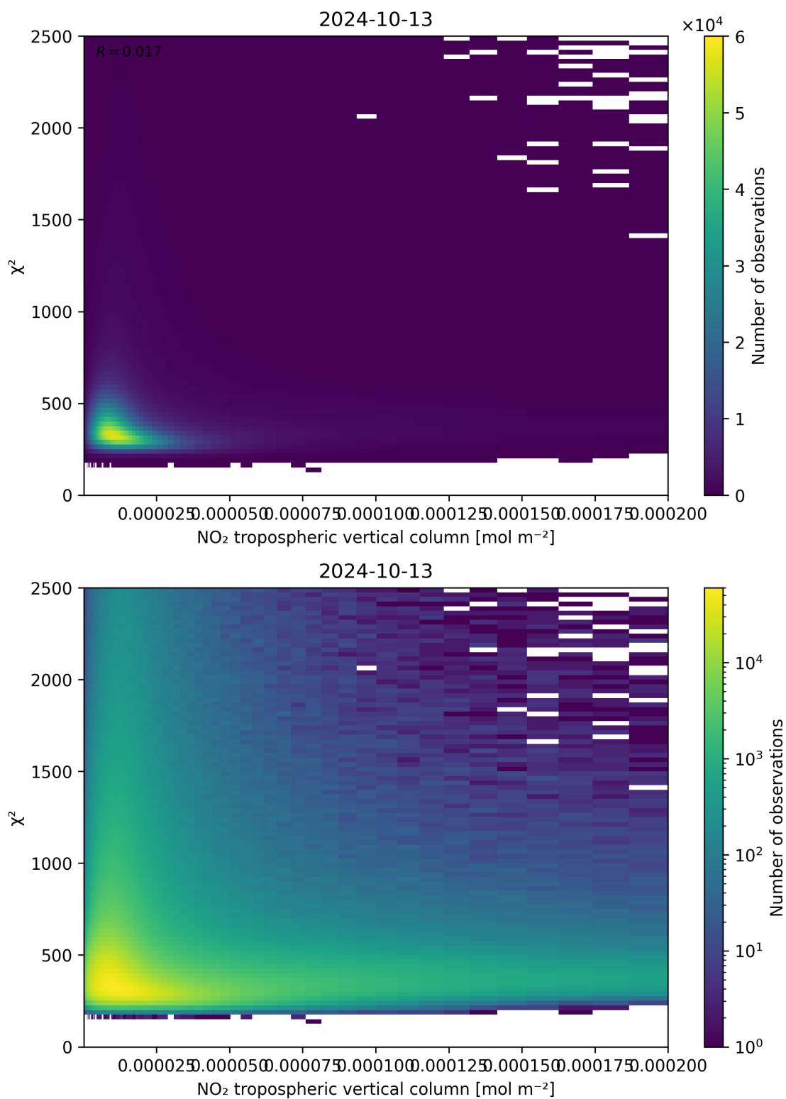
Figure 124: Scatter density plot of “NO 2 tropospheric vertical column” against “ \chi^2 ” for 2024-10-12 to 2024-10-14.
