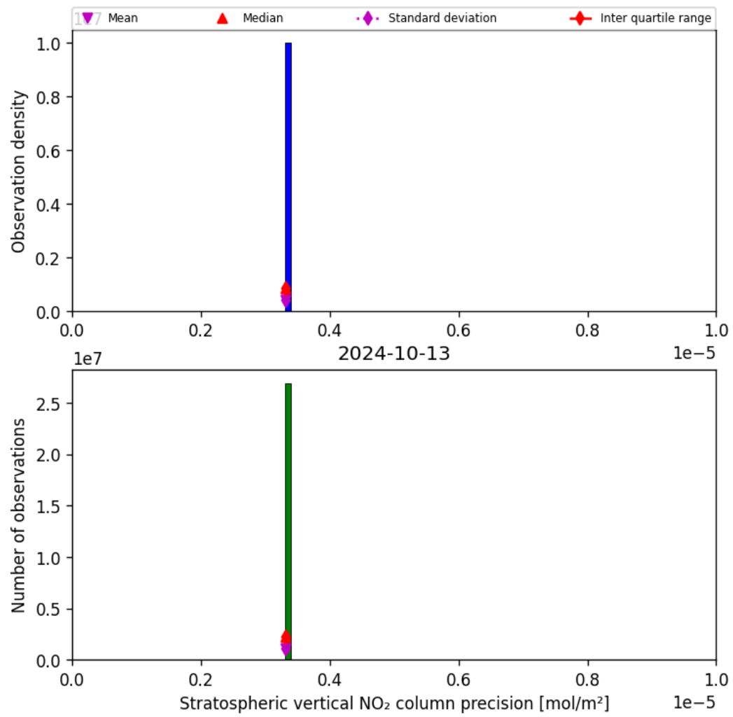
Figure 37: Histogram of “Stratospheric vertical NO 2 column precision” for 2024-10-12 to 2024-10-14
