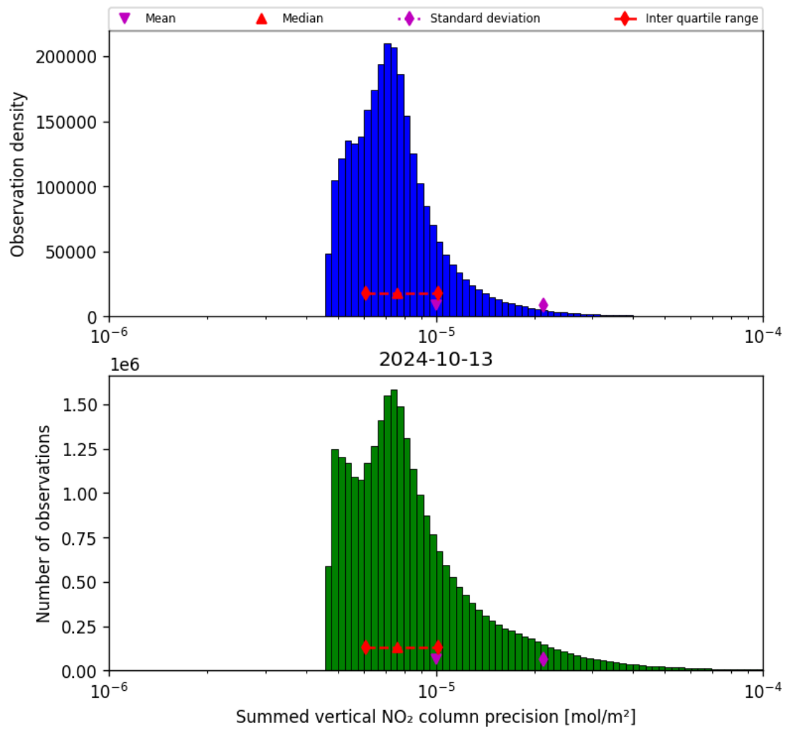
Figure 41: Histogram of "Summed vertical NO 2 column precision" for 2024-10-12 to 2024-10-14
