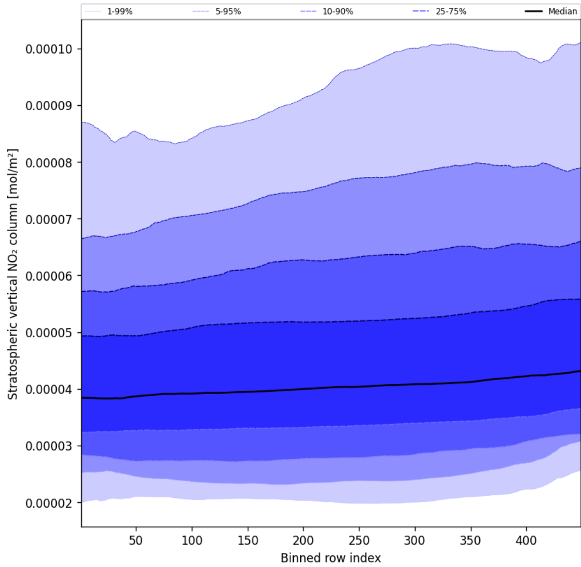
Figure 53: Along track statistics of “Stratospheric vertical NO 2 column” for 2024-10-12 to 2024-10-14
