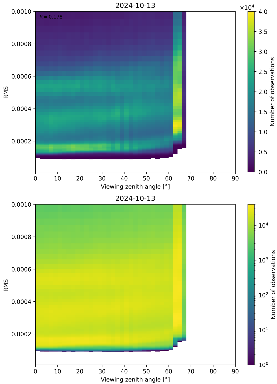
Figure 171: Scatter density plot of “Viewing zenith angle” against “RMS” for 2024-10-12 to 2024-10-14.
