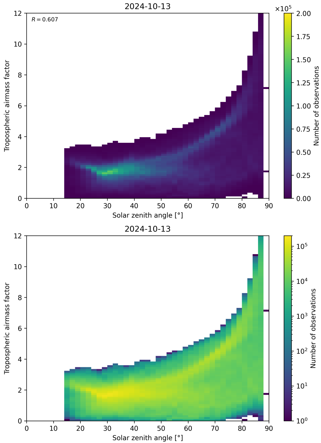
Figure 147: Scatter density plot of “Solar zenith angle” against “Tropospheric airmass factor” for 2024-10-12 to 2024-10-14.
