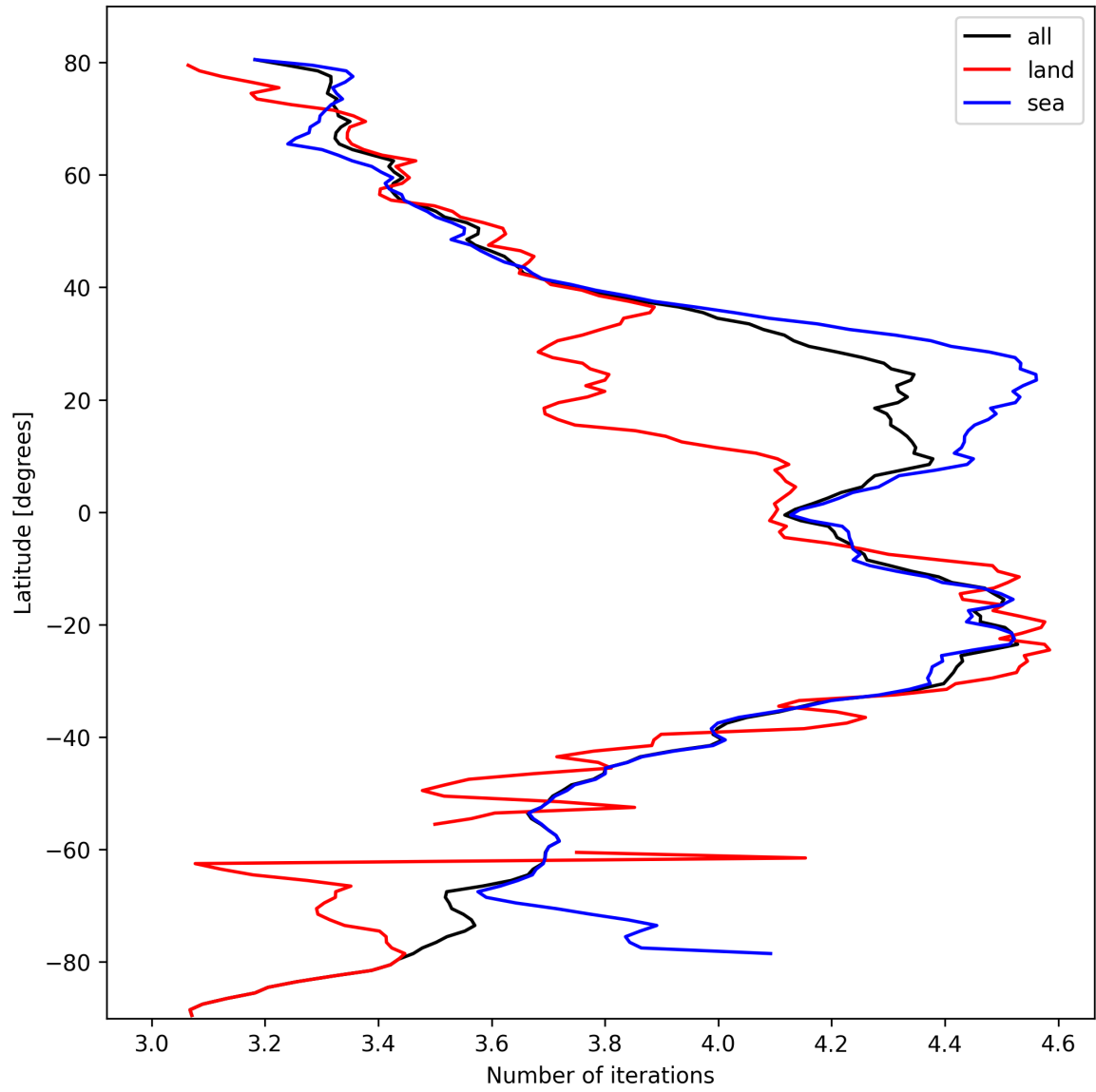
Figure 17: Zonal average of “Number of iterations” for 2024-10-12 to 2024-10-14.
