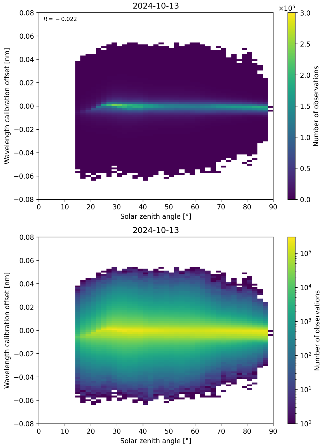
Figure 158: Scatter density plot of “Solar zenith angle” against “Wavelength calibration offset” for 2024-10-12 to 2024-10-14.
