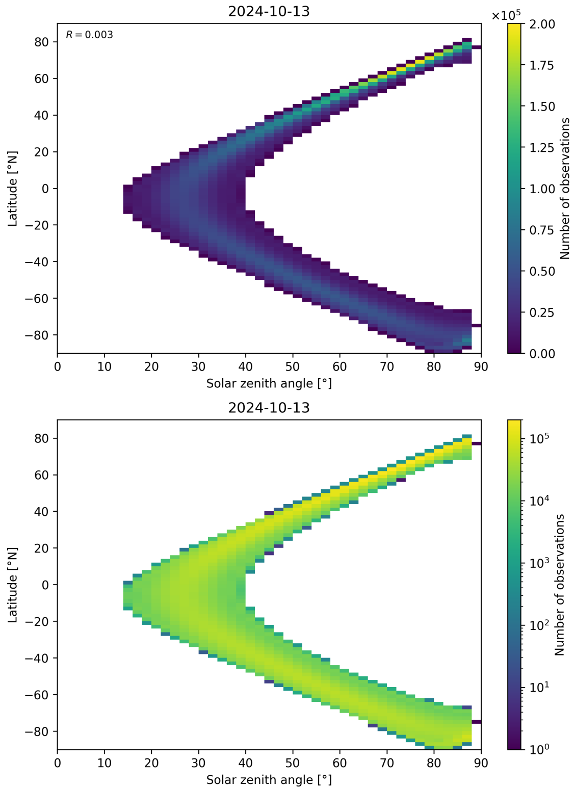
Figure 149: Scatter density plot of “Solar zenith angle” against “Latitude” for 2024-10-12 to 2024-10-14.
