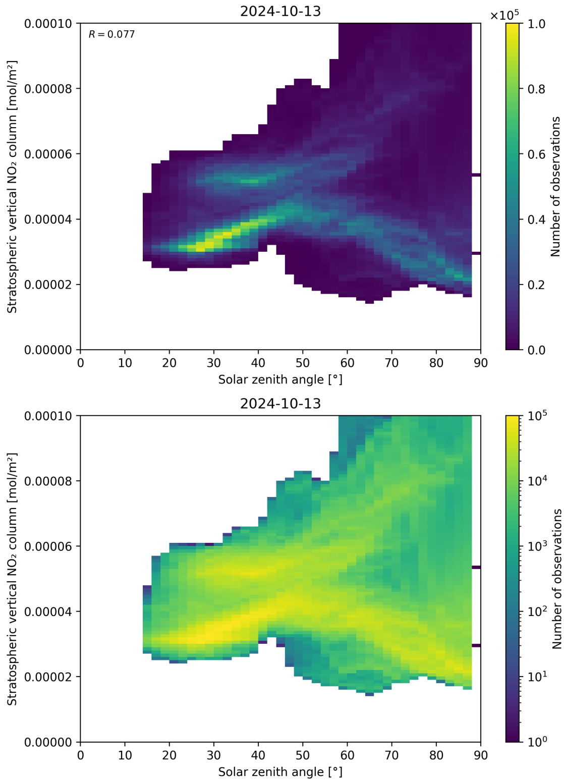
Figure 150: Scatter density plot of “Solar zenith angle” against “Stratospheric vertical NO 2 column” for 2024-10-12 to 2024-10-14.
