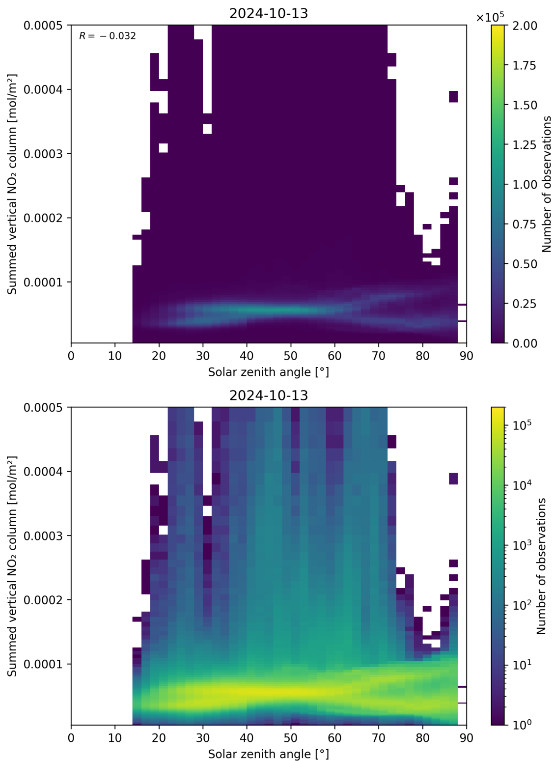
Figure 151: Scatter density plot of “Solar zenith angle” against “Summed vertical NO 2 column” for 2024-10-12 to 2024-10-14.
