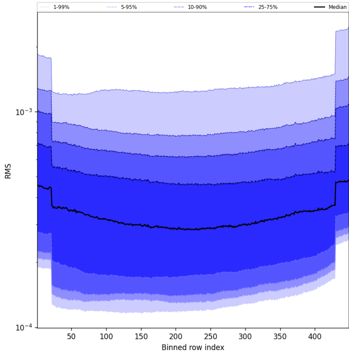
Figure 60: Along track statistics of “RMS” for 2024-10-12 to 2024-10-14
