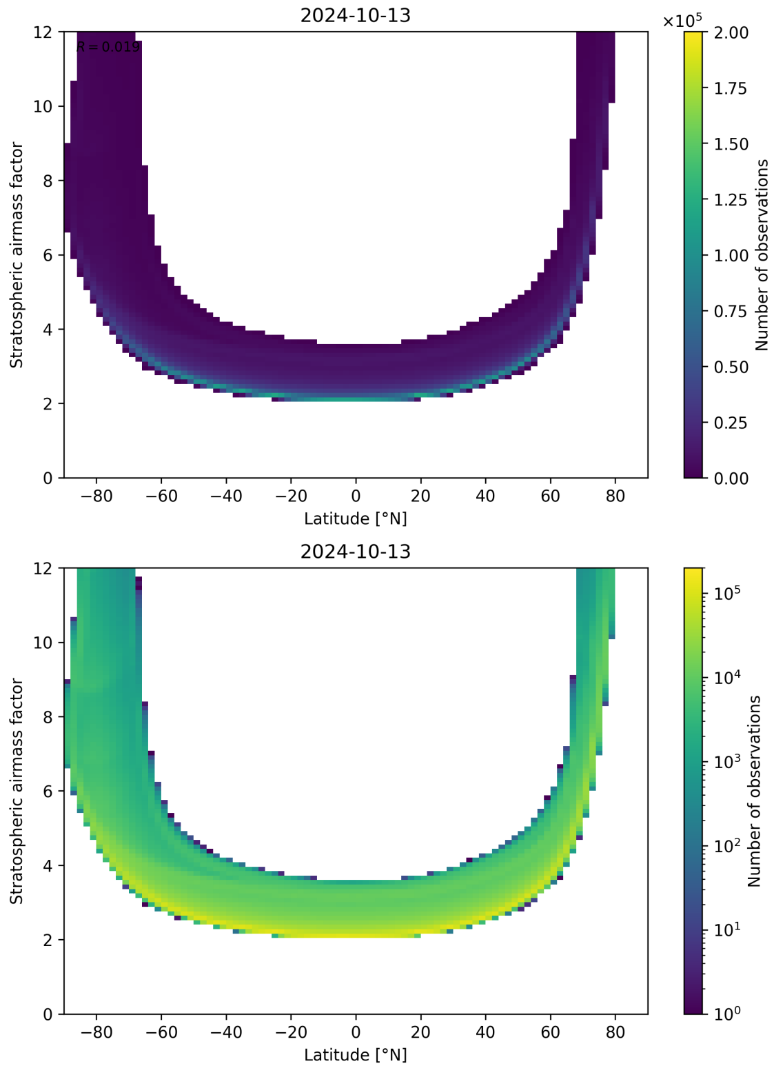
Figure 83: Scatter density plot of “Latitude” against “Stratospheric airmass factor” for 2024-10-12 to 2024-10-14.
