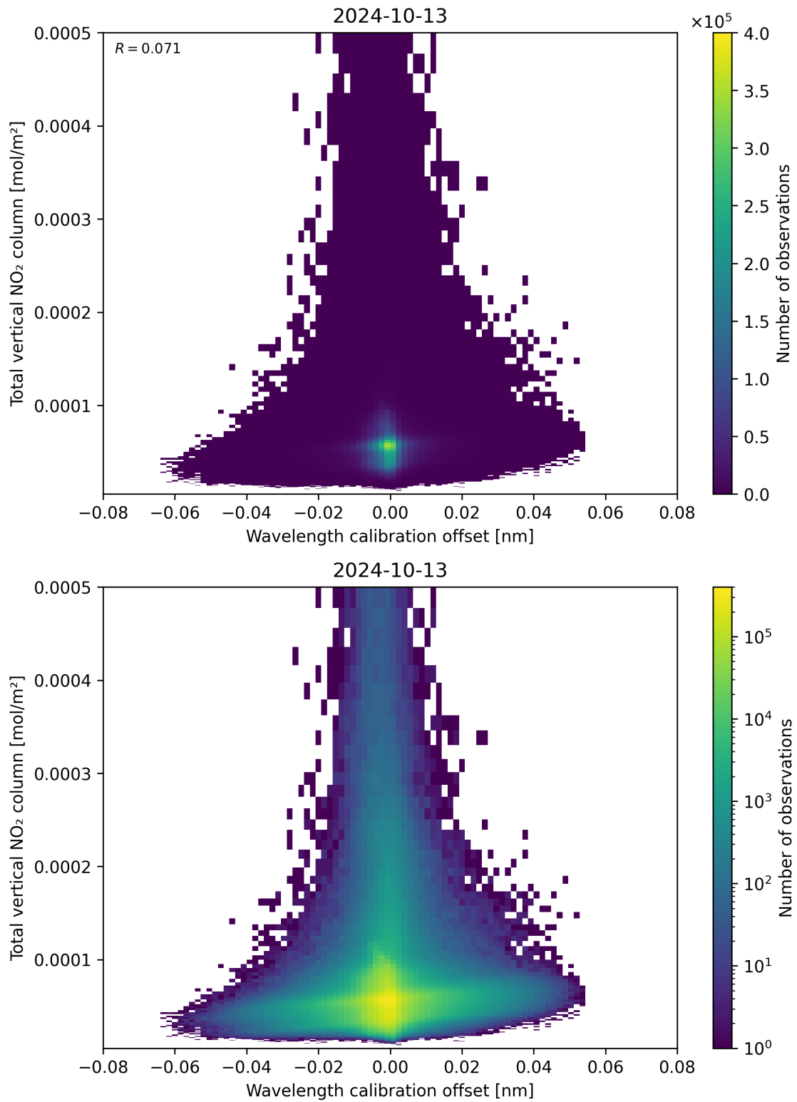
Figure 179: Scatter density plot of “Wavelength calibration offset” against “Total vertical NO 2 column” for 2024-10-12 to 2024-10-14.
