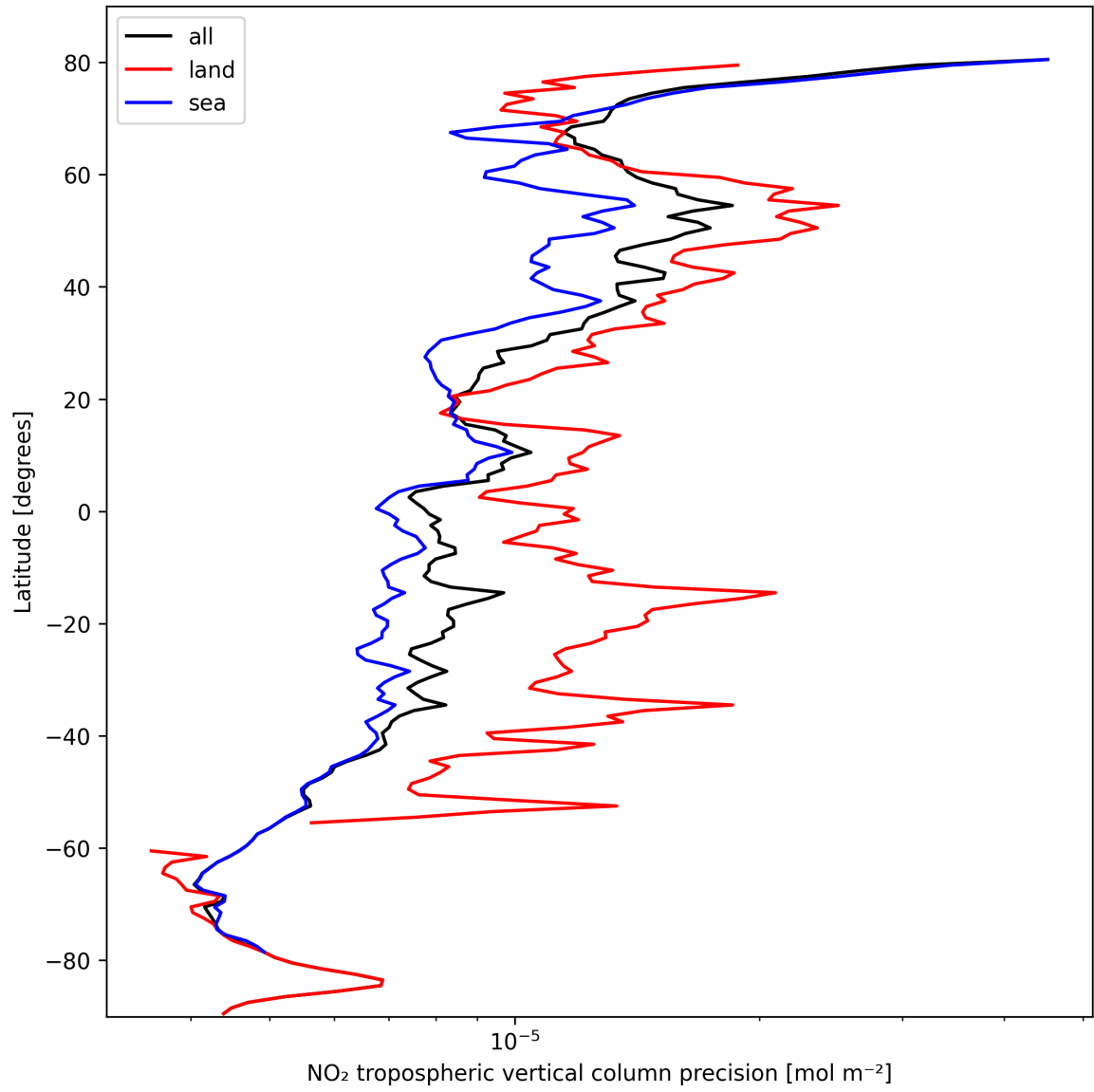
Figure 13: Zonal average of “NO 2 tropospheric vertical column precision” for 2024-10-12 to 2024-10-14.
