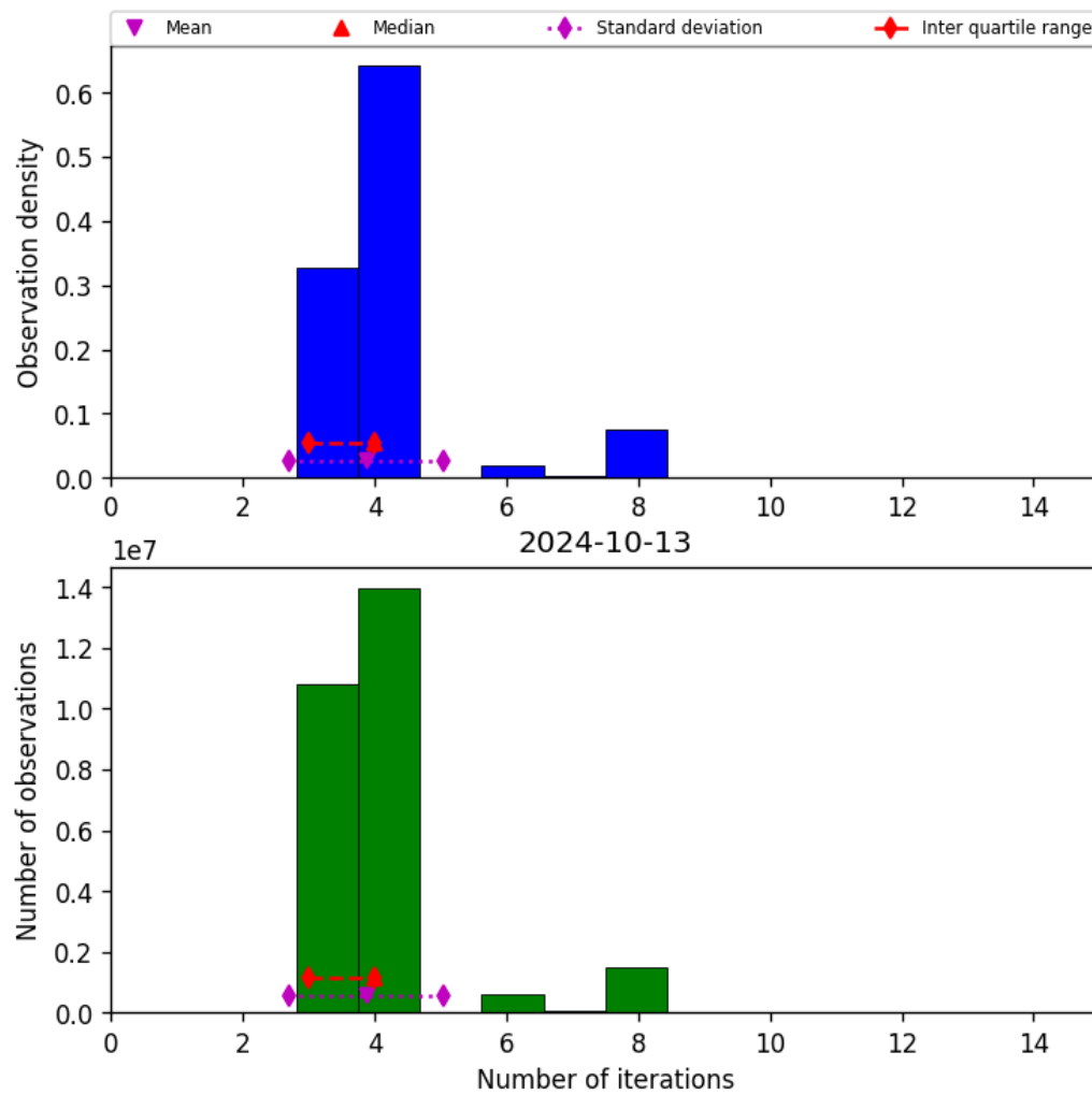
Figure 34: Histogram of “Number of iterations” for 2024-10-12 to 2024-10-14
