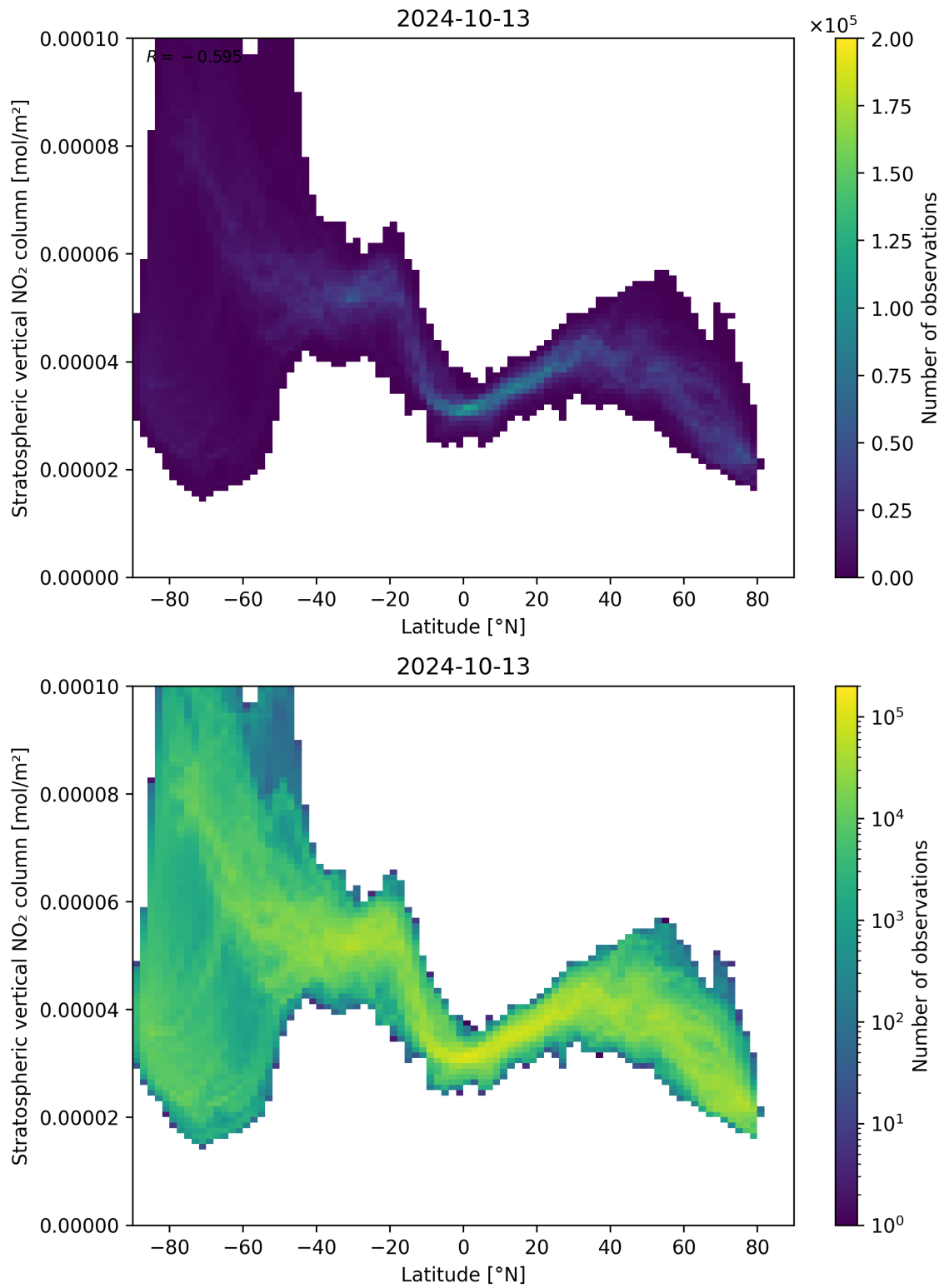
Figure 87: Scatter density plot of “Latitude” against “Stratospheric vertical NO 2 column” for 2024-10-12 to 2024-10-14.
