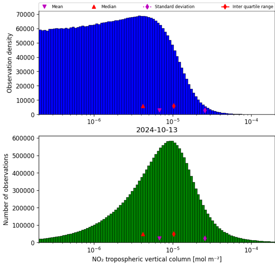
Figure 29: Histogram of “NO 2 tropospheric vertical column” for 2024-10-12 to 2024-10-14
