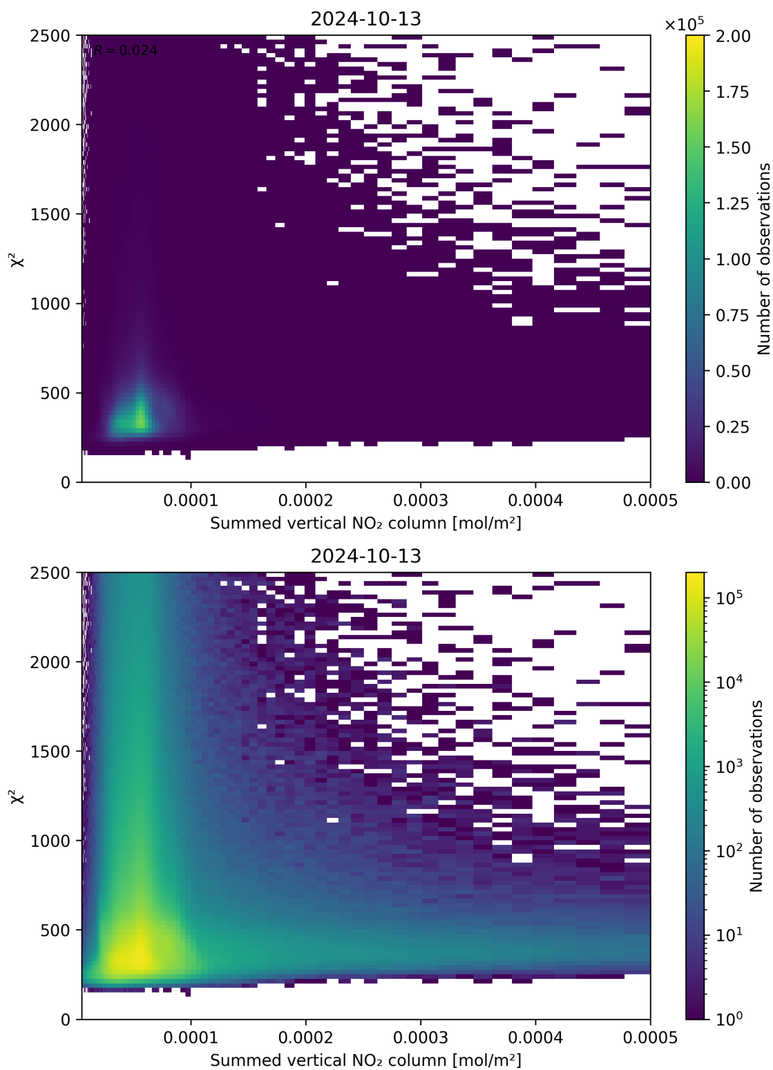
Figure 104: Scatter density plot of “Summed vertical NO 2 column” against “ \chi^2 ” for 2024-10-12 to 2024-10-14.
