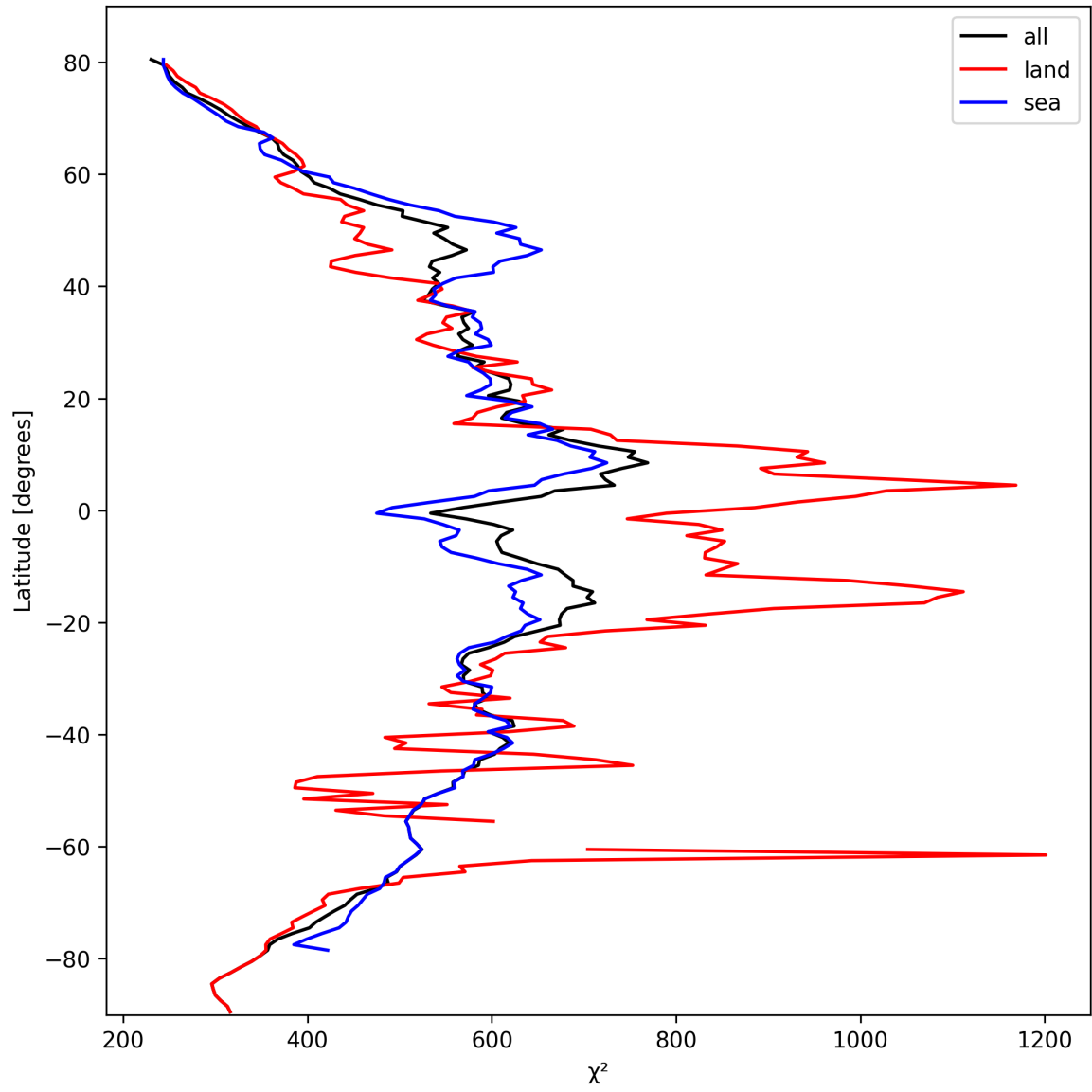
Figure 25: Zonal average of “ \chi^2 ” for 2024-10-12 to 2024-10-14.
