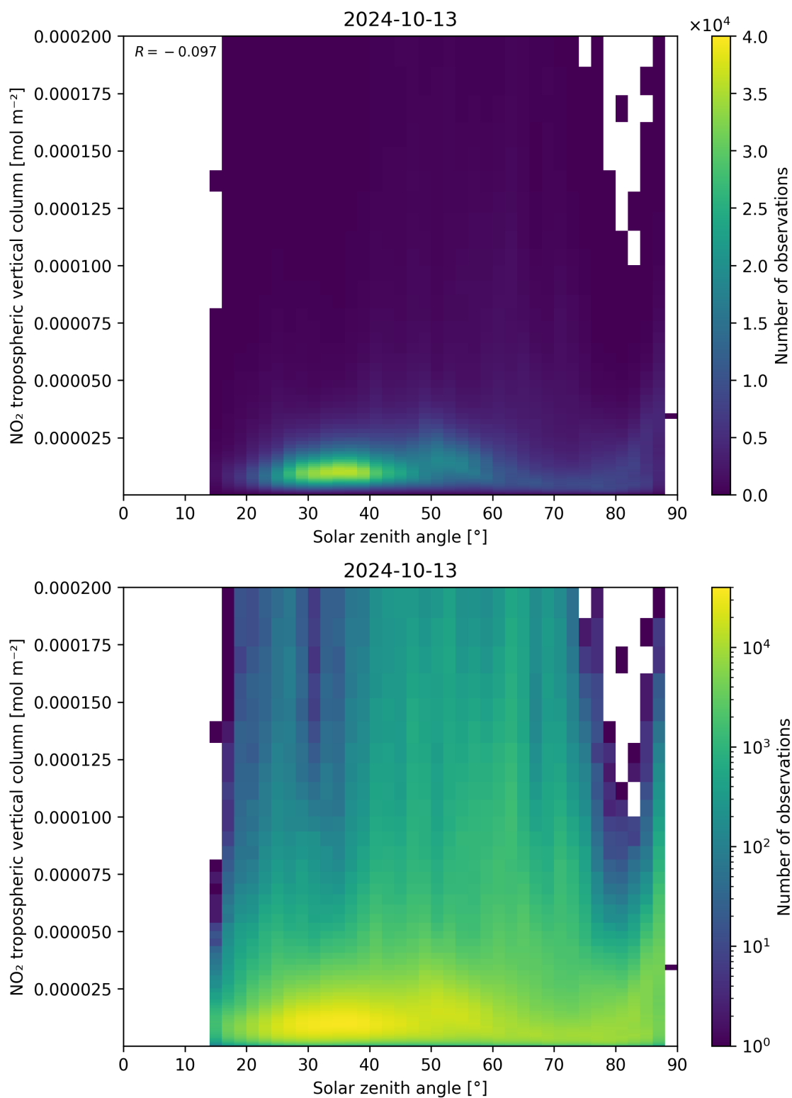
Figure 155: Scatter density plot of “Solar zenith angle” against “NO 2 tropospheric vertical column” for 2024-10-12 to 2024-10-14.
