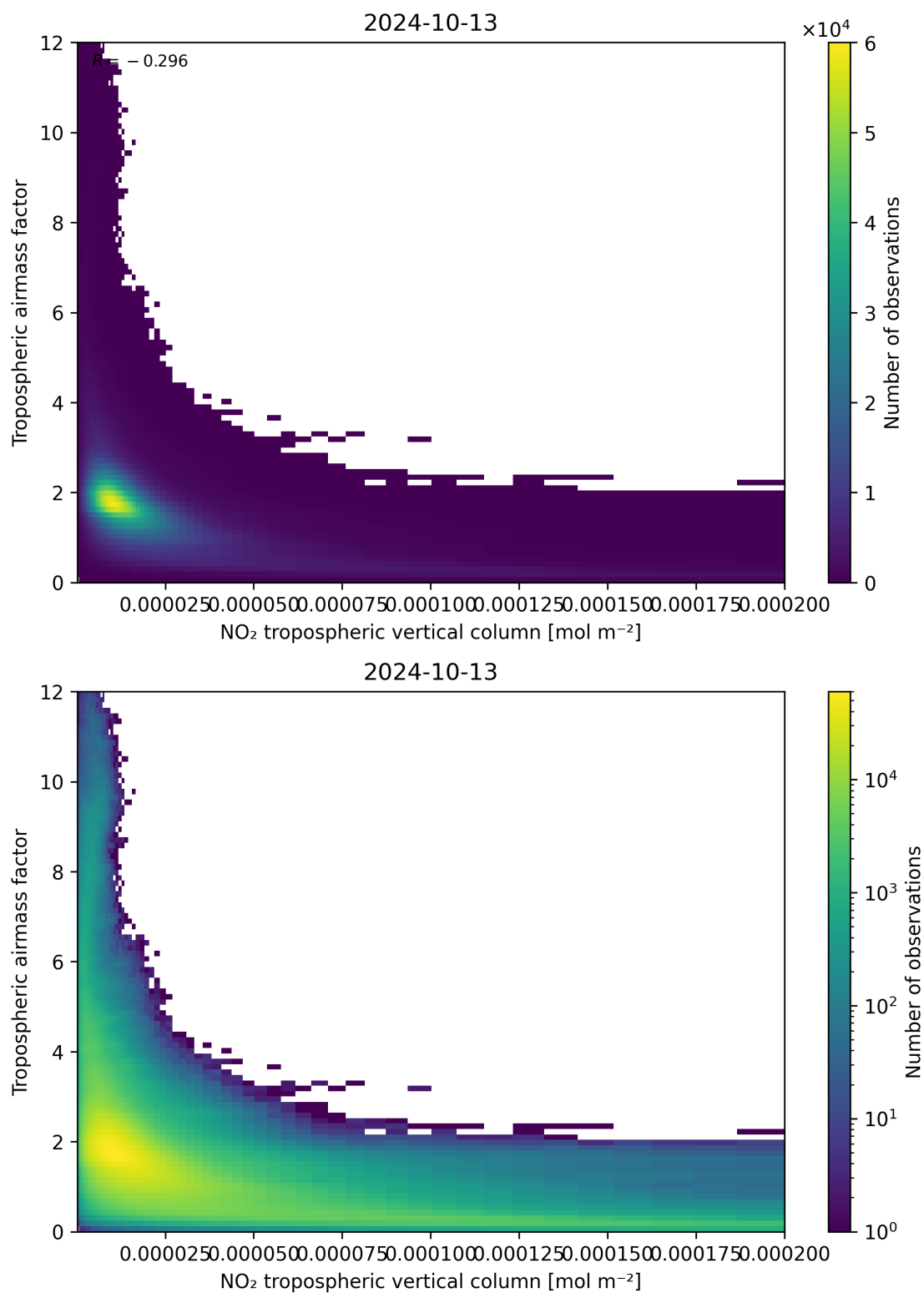
Figure 123: Scatter density plot of “NO 2 tropospheric vertical column” against “Tropospheric air mass factor” for 2024-10-12 to 2024-10-14.
