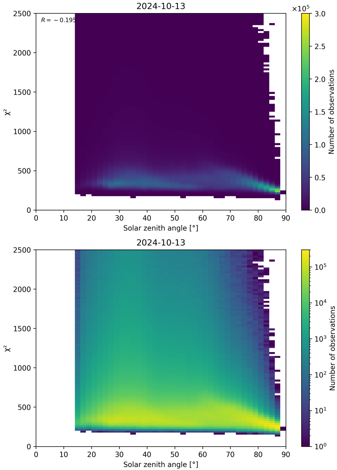
Figure 148: Scatter density plot of “Solar zenith angle” against “ \chi^2 ” for 2024-10-12 to 2024-10-14.
