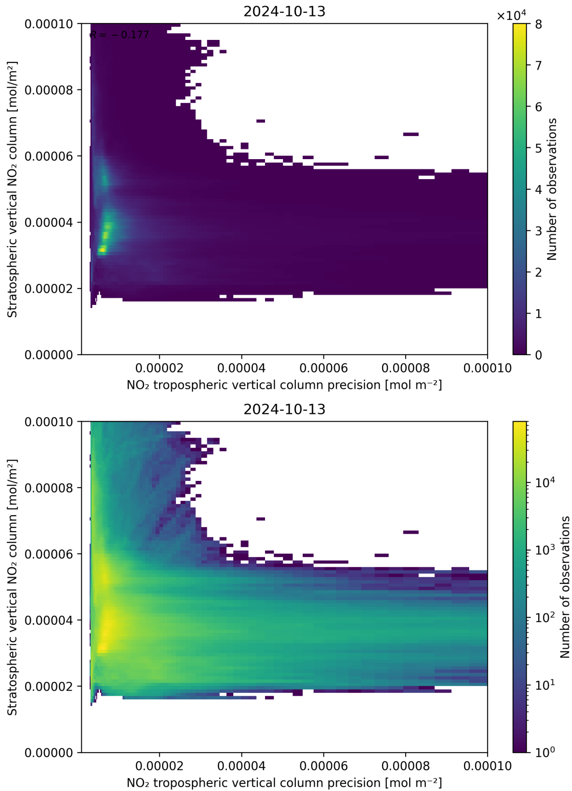
Figure 135: Scatter density plot of “NO 2 tropospheric vertical column precision” against “Stratospheric vertical NO 2 column” for 2024-10-12 to 2024-10-14.
