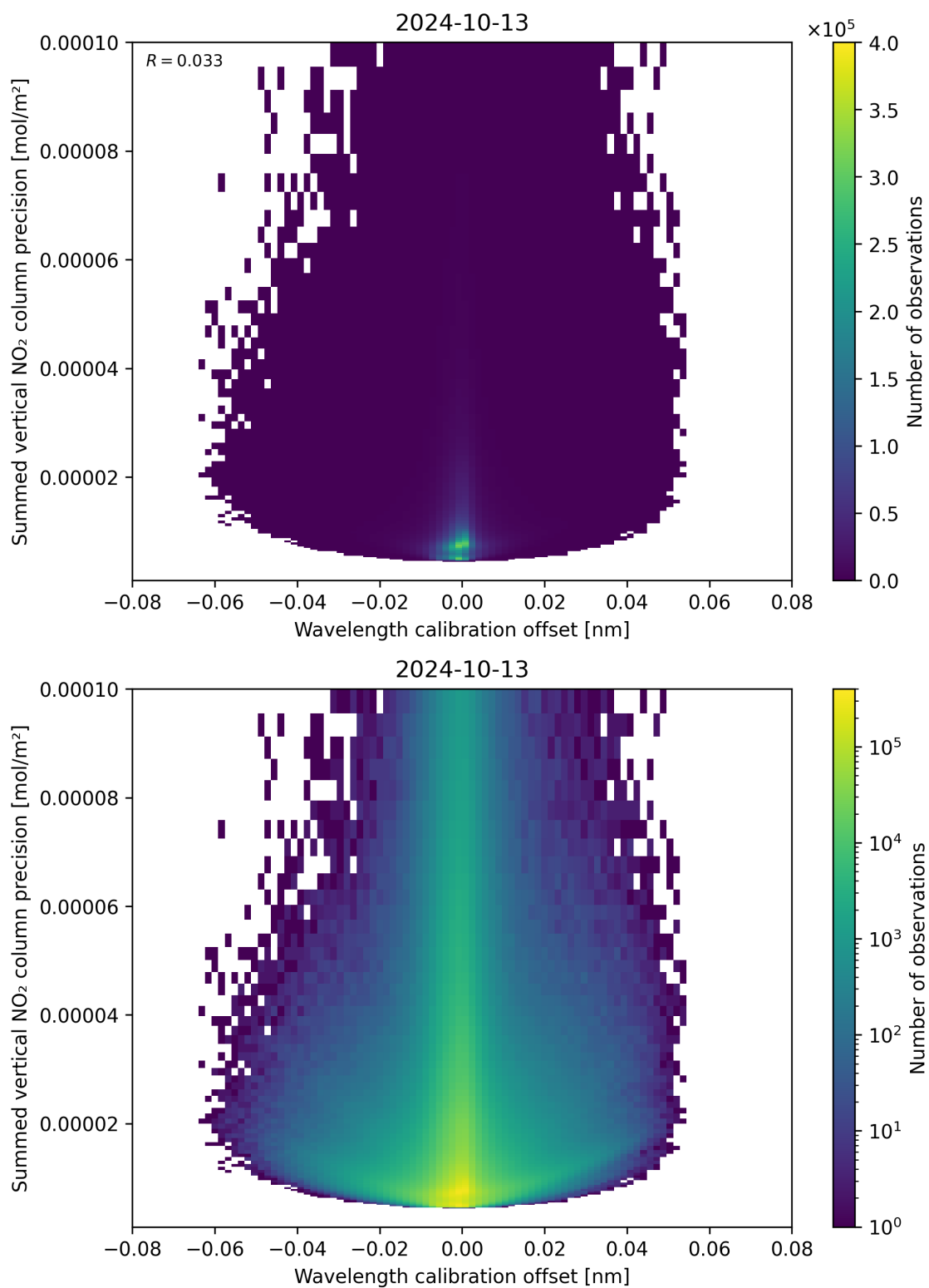
Figure 178: Scatter density plot of “Wavelength calibration offset” against “Summed vertical NO 2 column precision” for 2024-10-12 to 2024-10-14.
