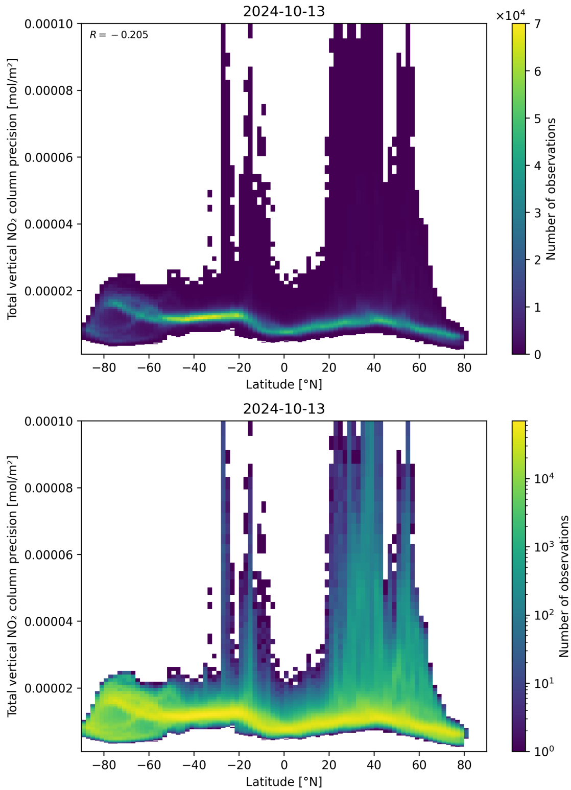
Figure 91: Scatter density plot of “Latitude” against “Total vertical NO 2 column precision” for 2024-10-12 to 2024-10-14.
