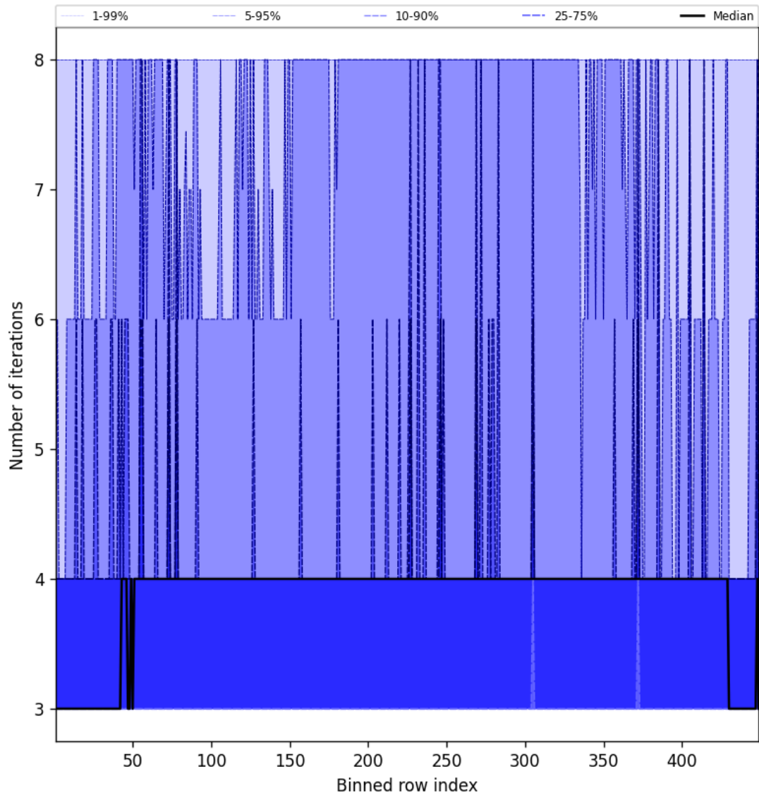
Figure 51: Along track statistics of “Number of iterations” for 2024-10-12 to 2024-10-14
