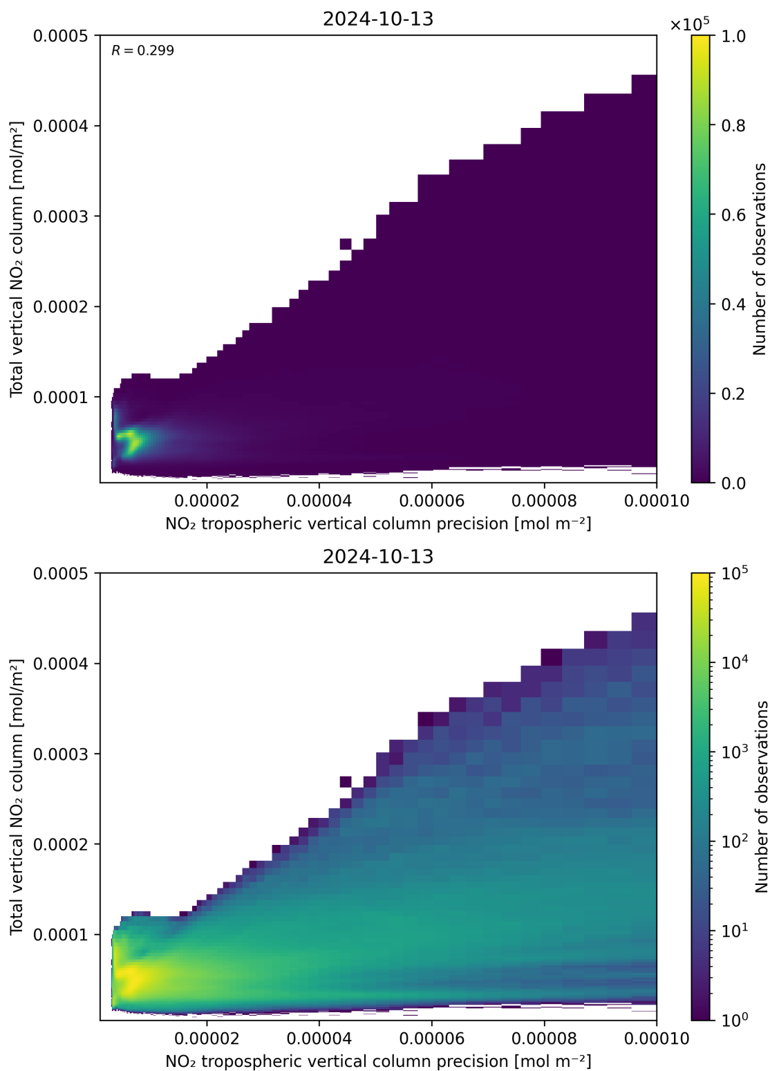
Figure 138: Scatter density plot of “NO 2 tropospheric vertical column precision” against “Total vertical NO 2 column” for 2024-10-12 to 2024-10-14.
