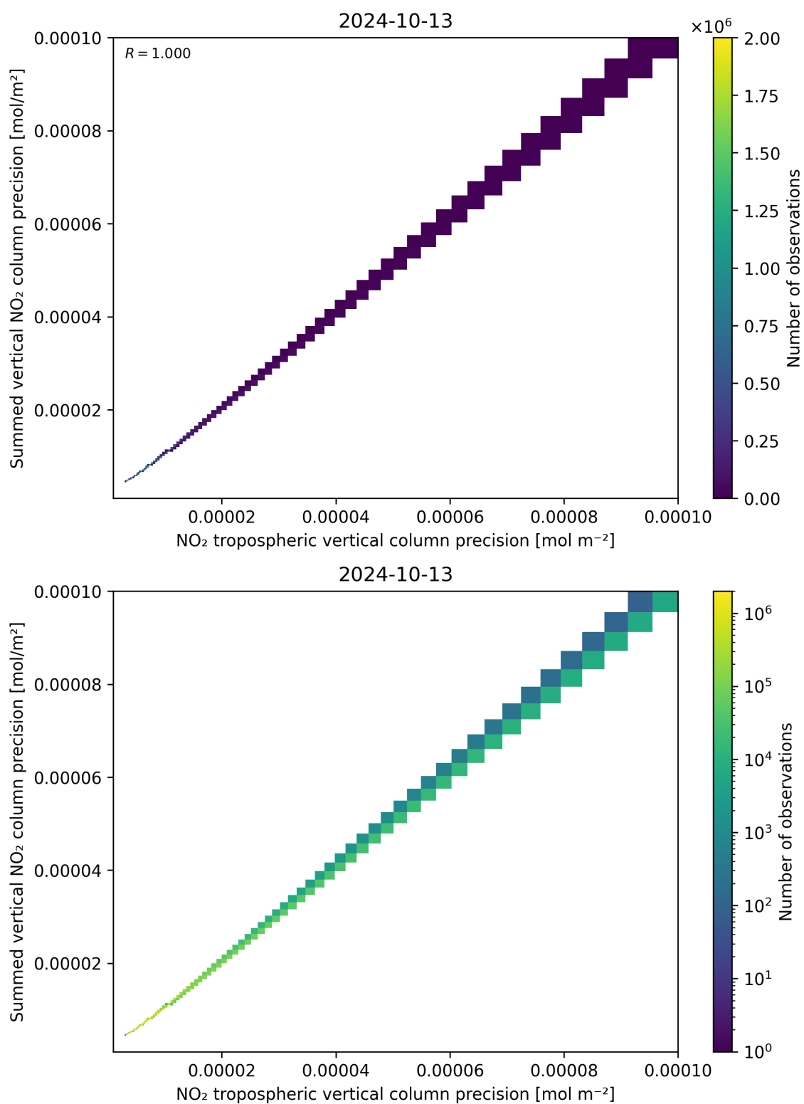
Figure 137: Scatter density plot of “NO 2 tropospheric vertical column precision” against “Summed vertical NO 2 column precision” for 2024-10-12 to 2024-10-14.
