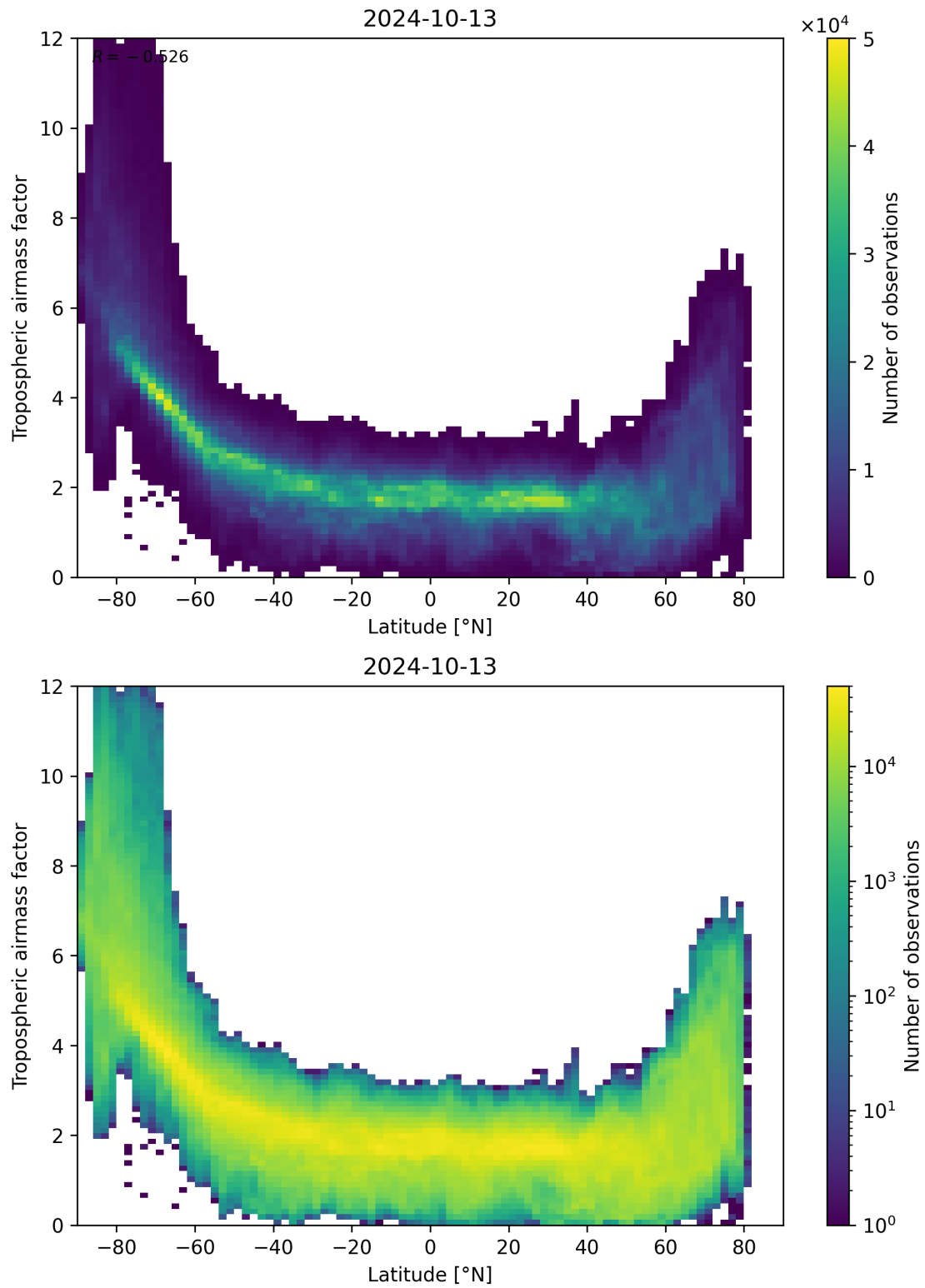
Figure 85: Scatter density plot of “Latitude” against “Tropospheric airmass factor” for 2024-10-12 to 2024-10-14.
