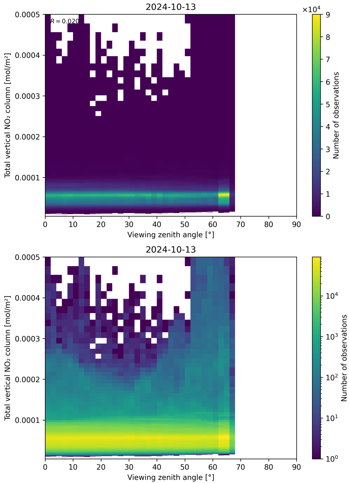
Figure 167: Scatter density plot of “Viewing zenith angle” against “Total vertical NO 2 column” for 2024-10-12 to 2024-10-14.
