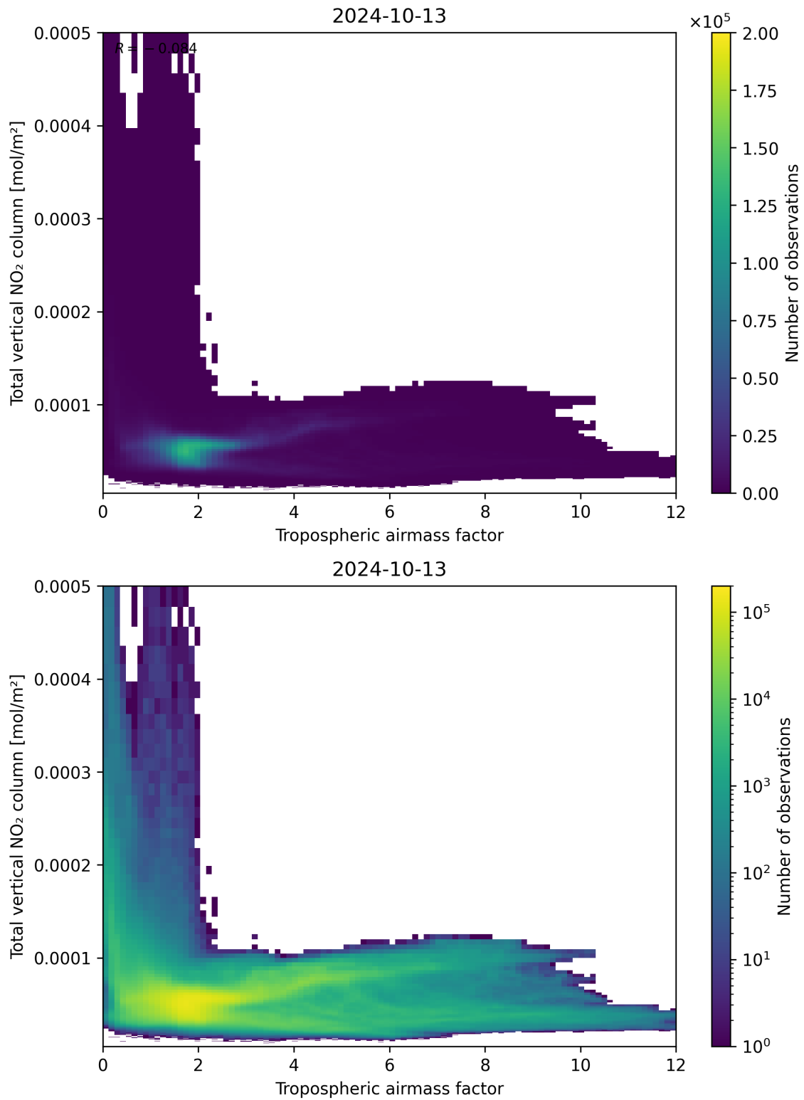
Figure 77: Scatter density plot of “Tropospheric airmass factor” against “Total vertical NO 2 column” for 2024-10-12 to 2024-10-14.
