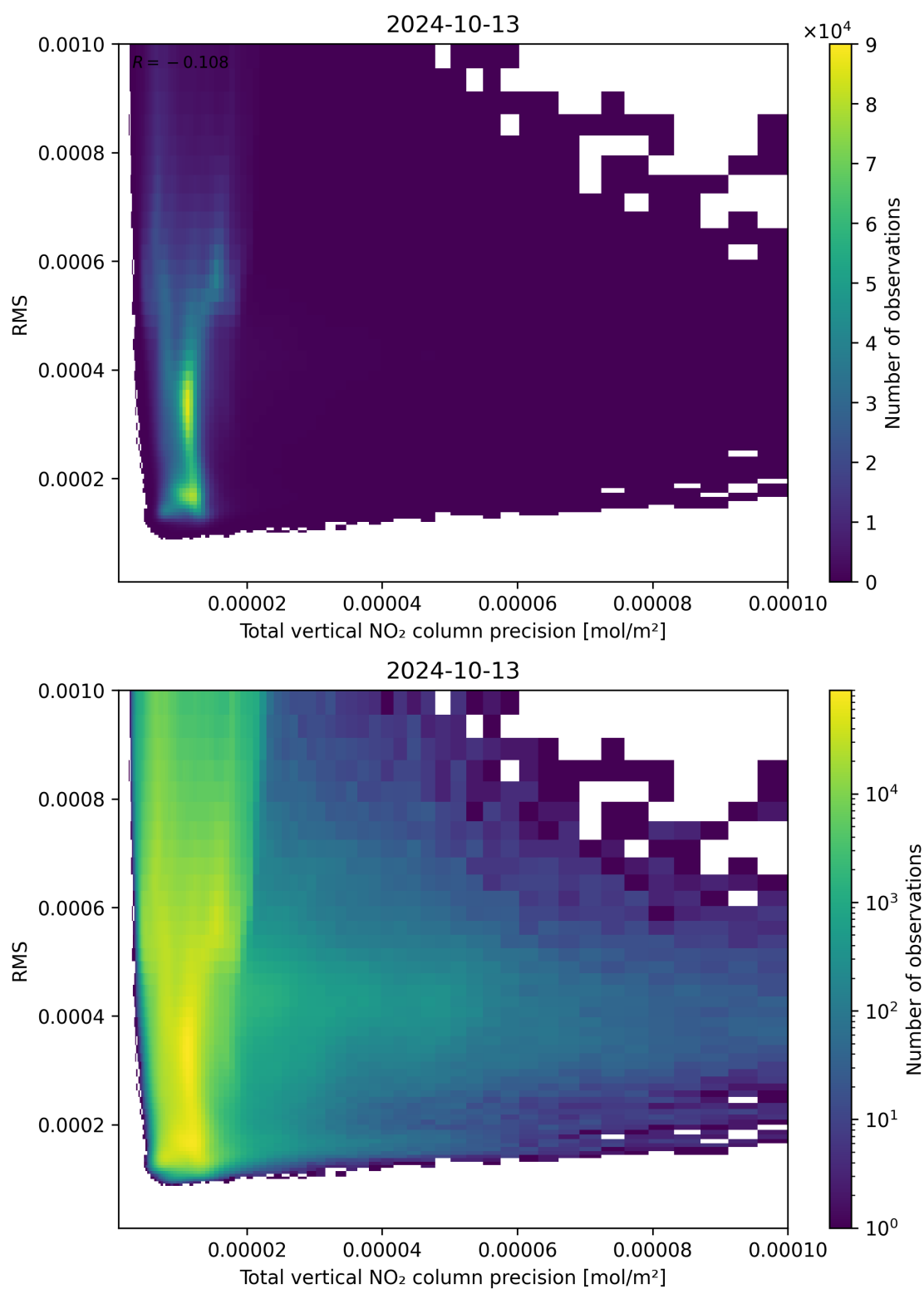
Figure 119: Scatter density plot of “Total vertical NO 2 column precision” against “RMS” for 2024-10-12 to 2024-10-14.
