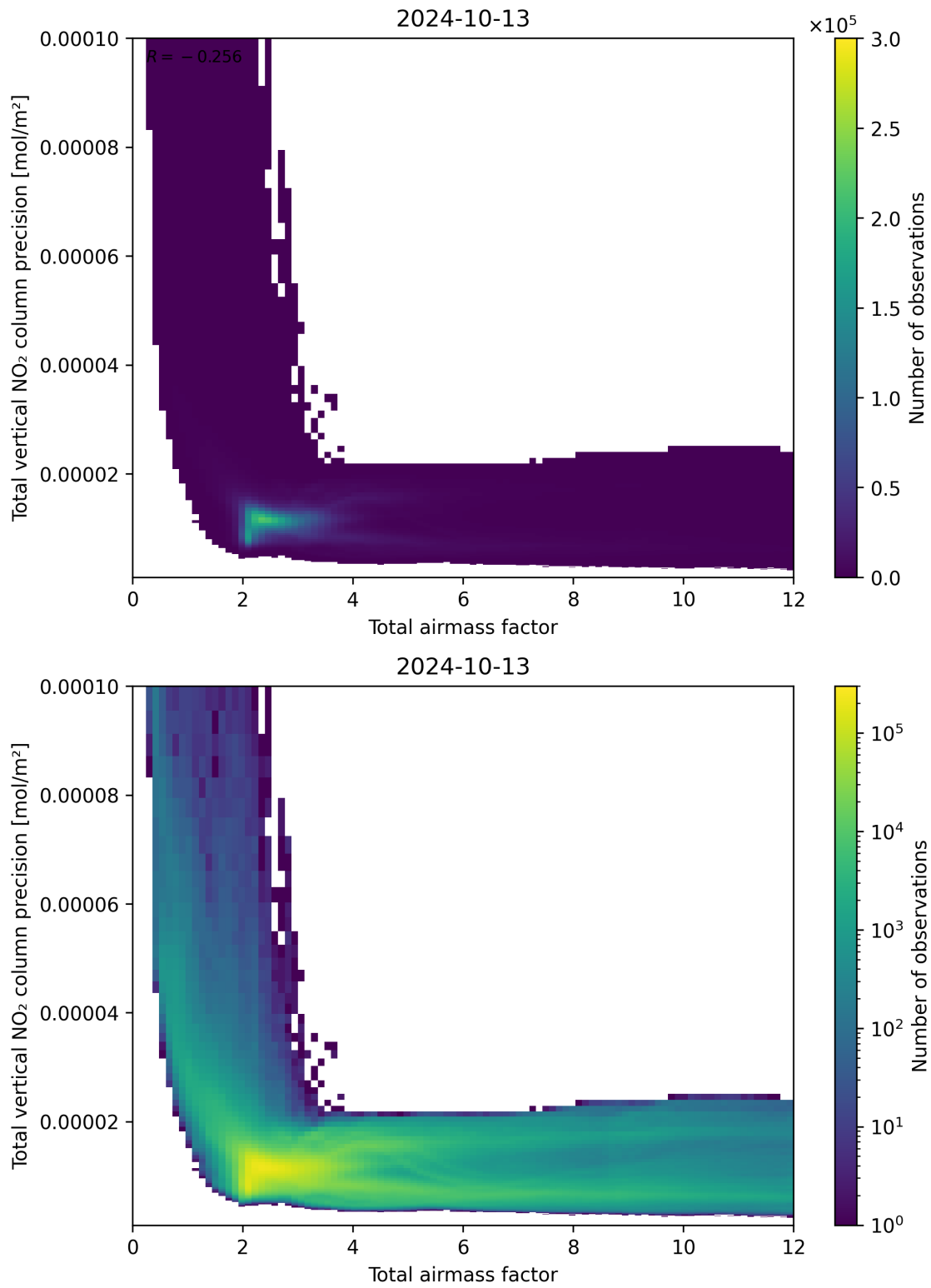
Figure 68: Scatter density plot of “Total airmass factor” against “Total vertical NO 2 column precision” for 2024-10-12 to 2024-10-14.
