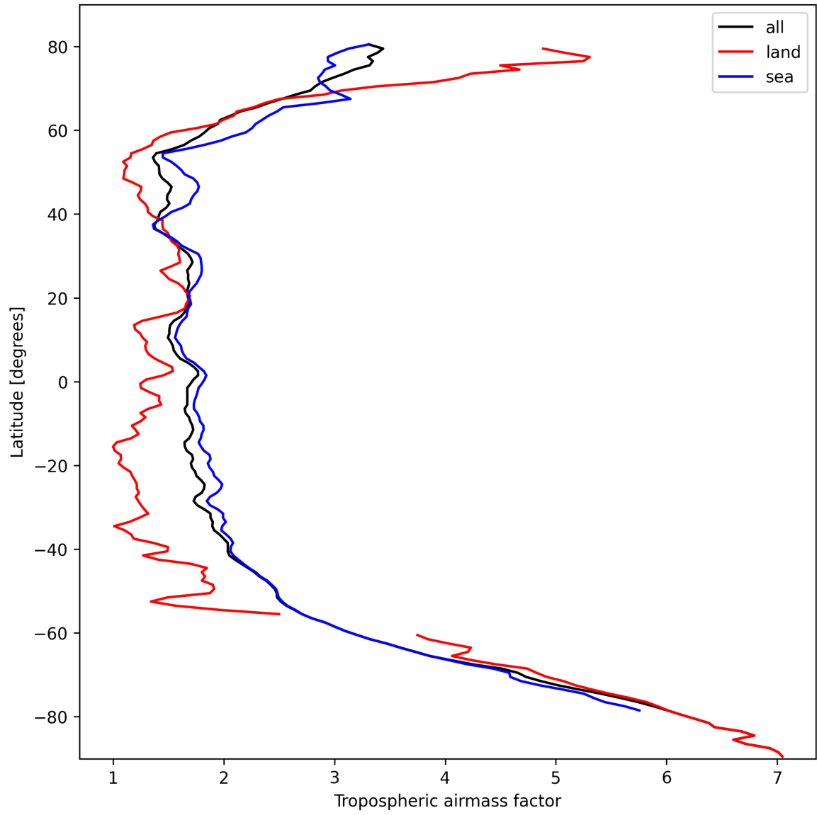
Figure 14: Zonal average of “Tropospheric airmass factor” for 2024-10-12 to 2024-10-14.
