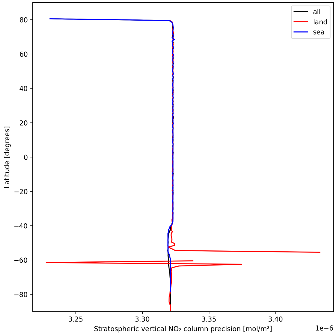
Figure 20: Zonal average of “Stratospheric vertical NO 2 column precision” for 2024-10-12 to 2024-10-14.
