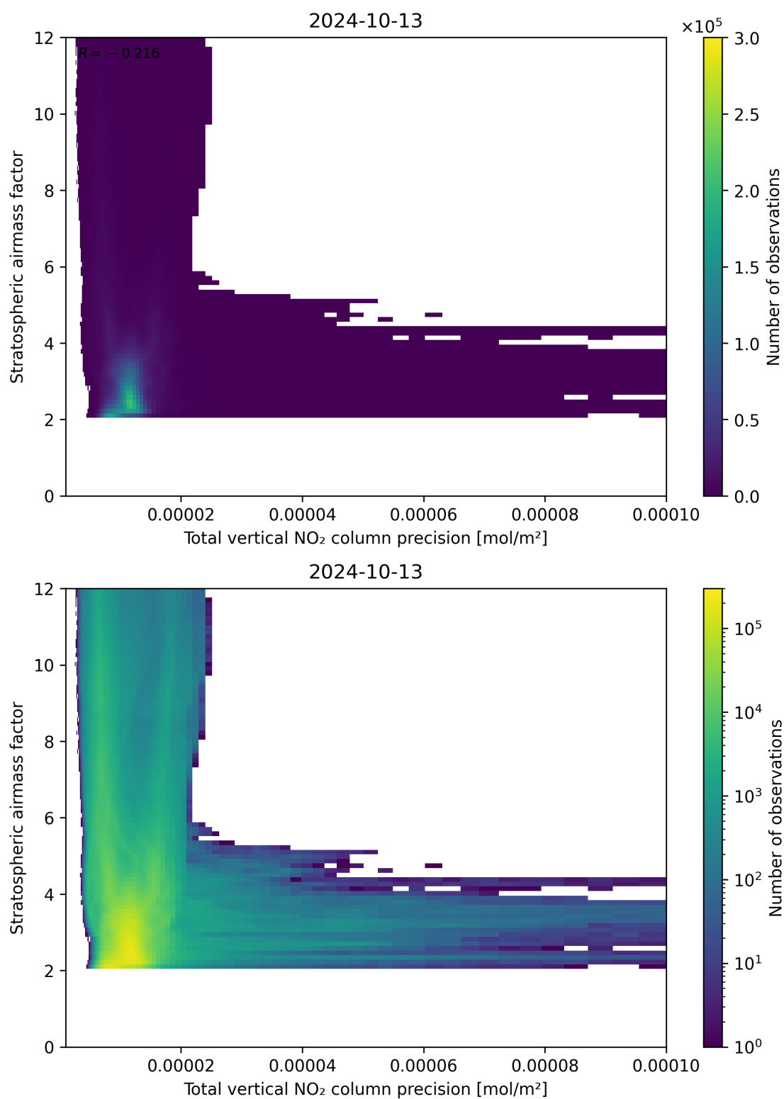
Figure 115: Scatter density plot of “Total vertical NO 2 column precision” against “Stratospheric air mass factor” for 2024-10-12 to 2024-10-14.
