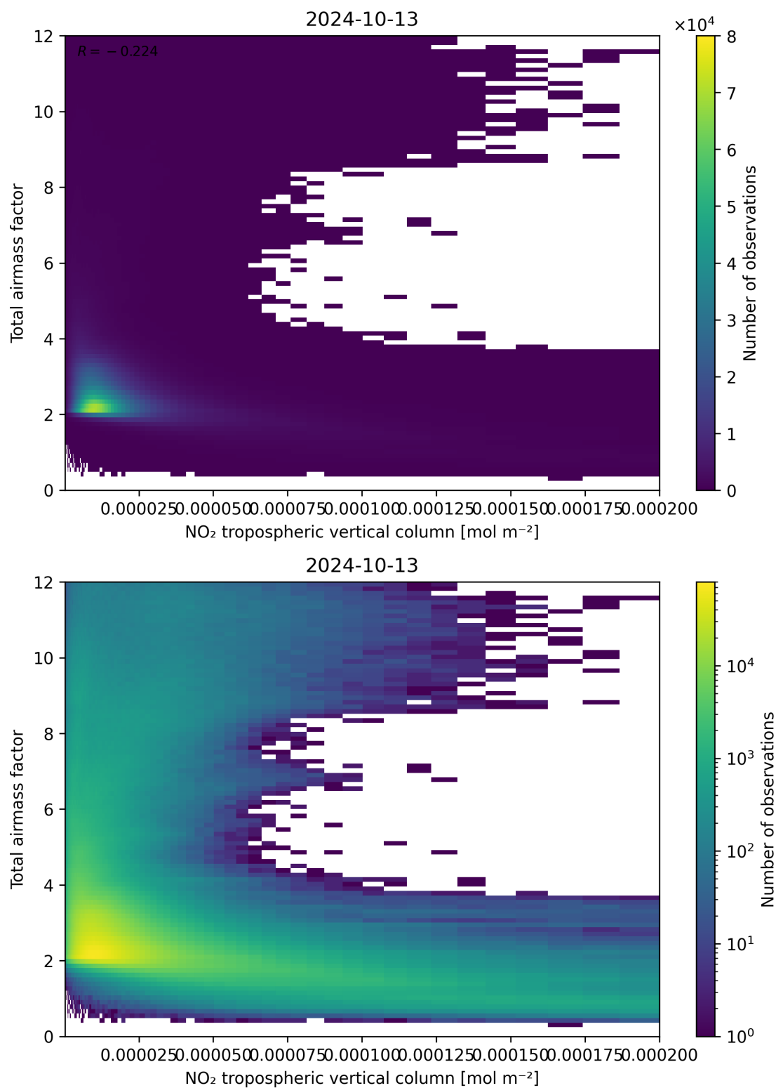
Figure 122: Scatter density plot of “NO 2 tropospheric vertical column” against “Total air mass factor” for 2024-10-12 to 2024-10-14.
