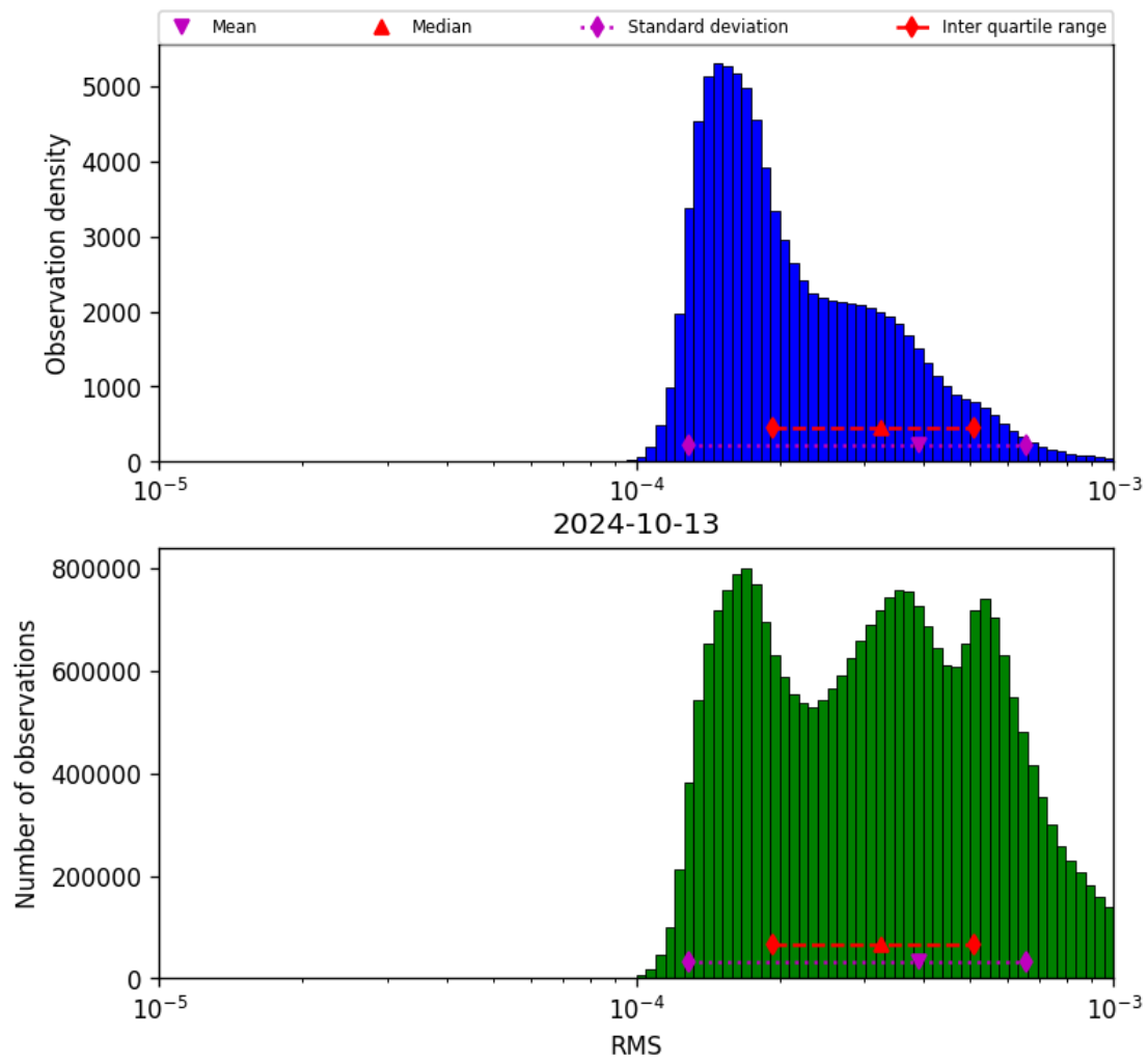
Figure 43: Histogram of “RMS” for 2024-10-12 to 2024-10-14
