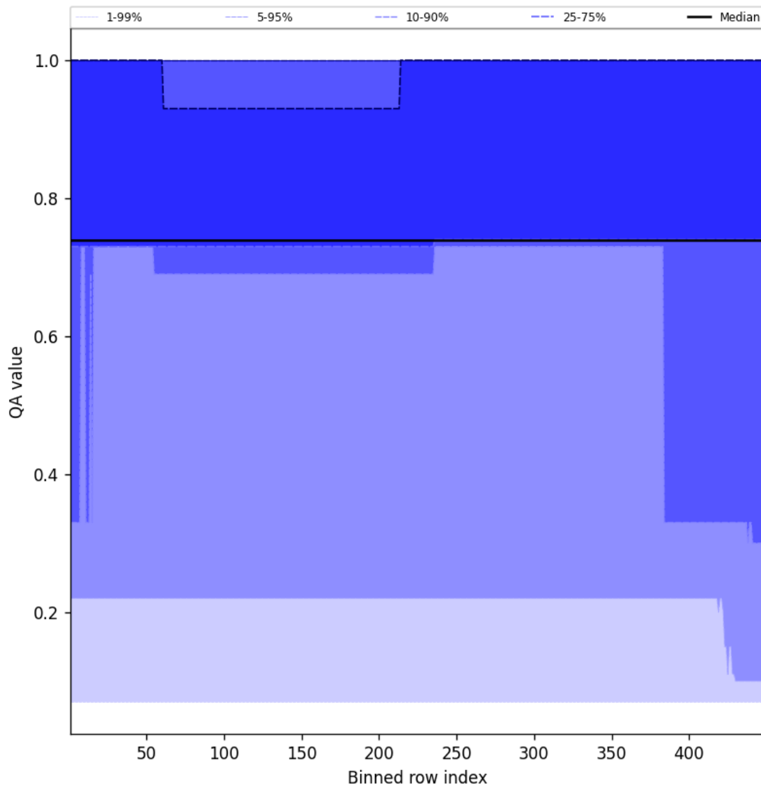
Figure 45: Along track statistics of “QA value” for 2024-10-12 to 2024-10-14
