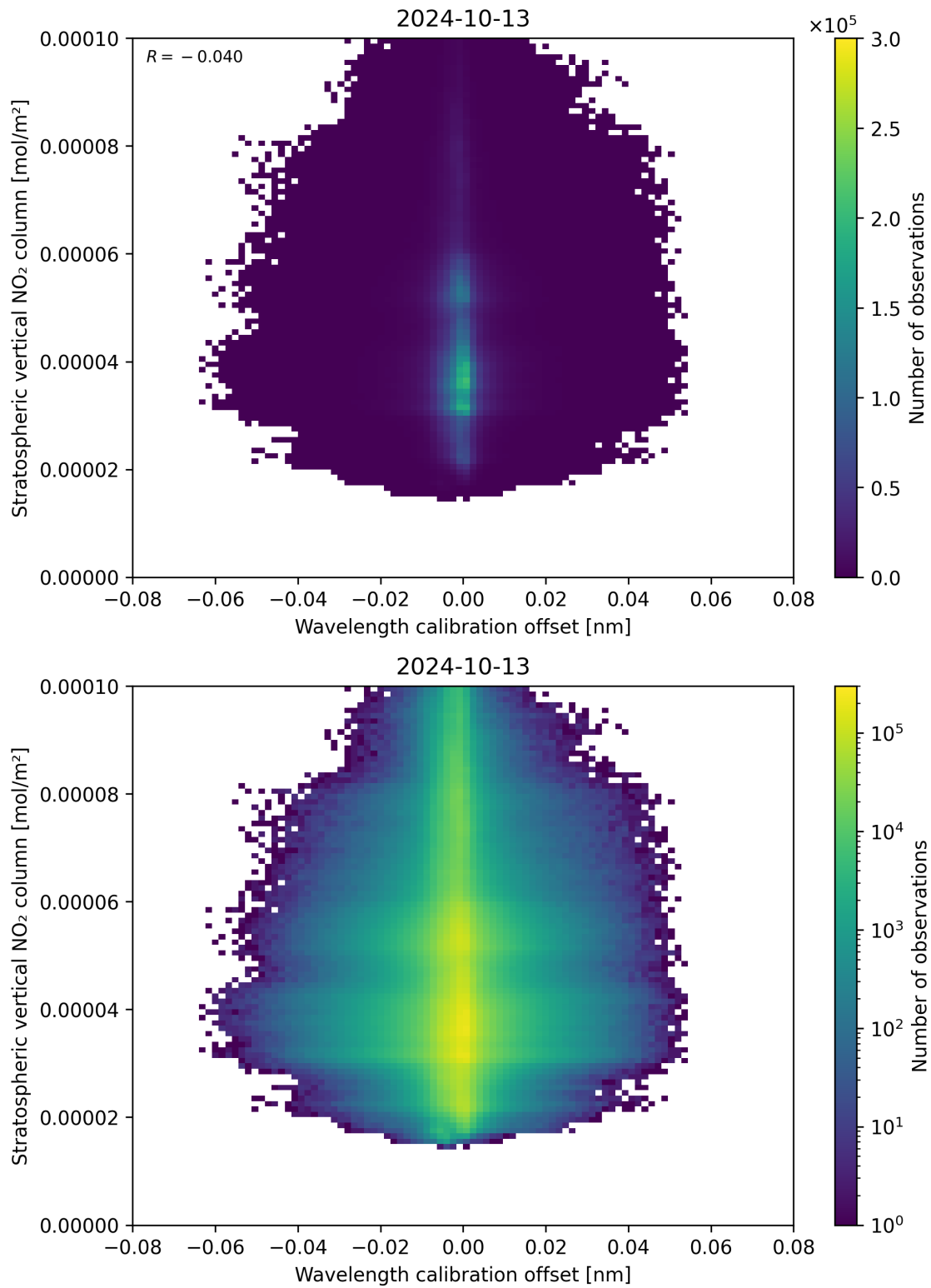
Figure 176: Scatter density plot of “Wavelength calibration offset” against “Stratospheric vertical NO 2 column” for 2024-10-12 to 2024-10-14.
