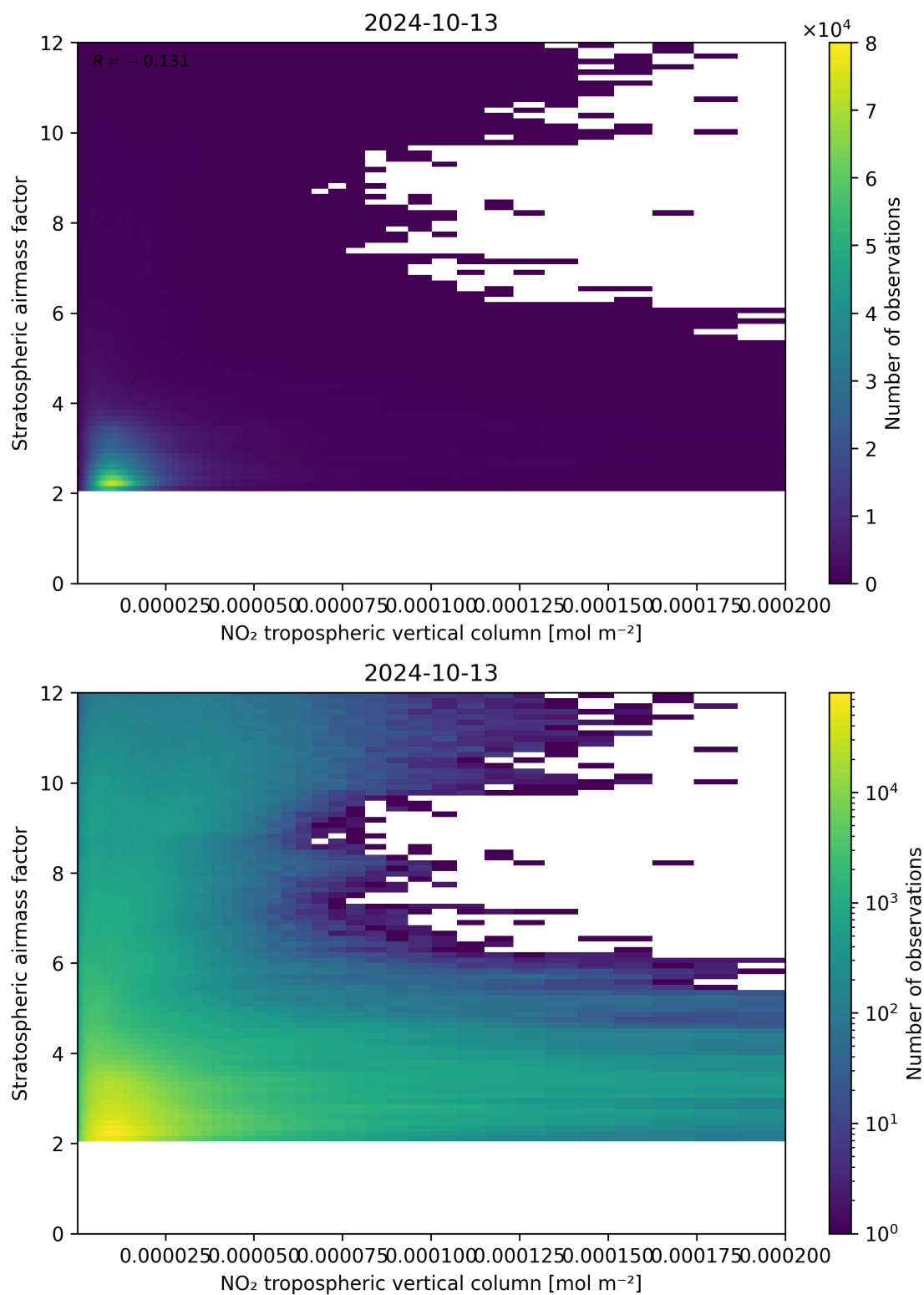
Figure 121: Scatter density plot of “NO 2 tropospheric vertical column” against “Stratospheric air mass factor” for 2024-10-12 to 2024-10-14.
