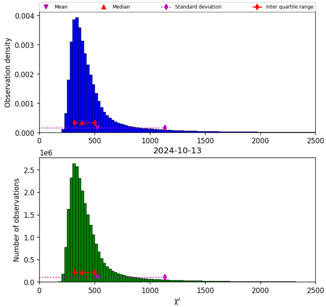
Figure 42: Histogram of “ \chi^2 ” for 2024-10-12 to 2024-10-14
