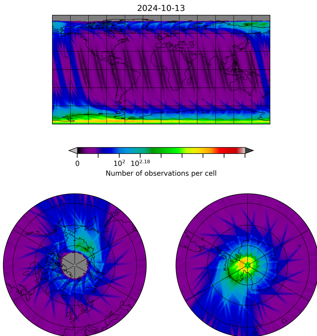
Figure 10: Map of the number of observations for 2024-10-12 to 2024-10-14
