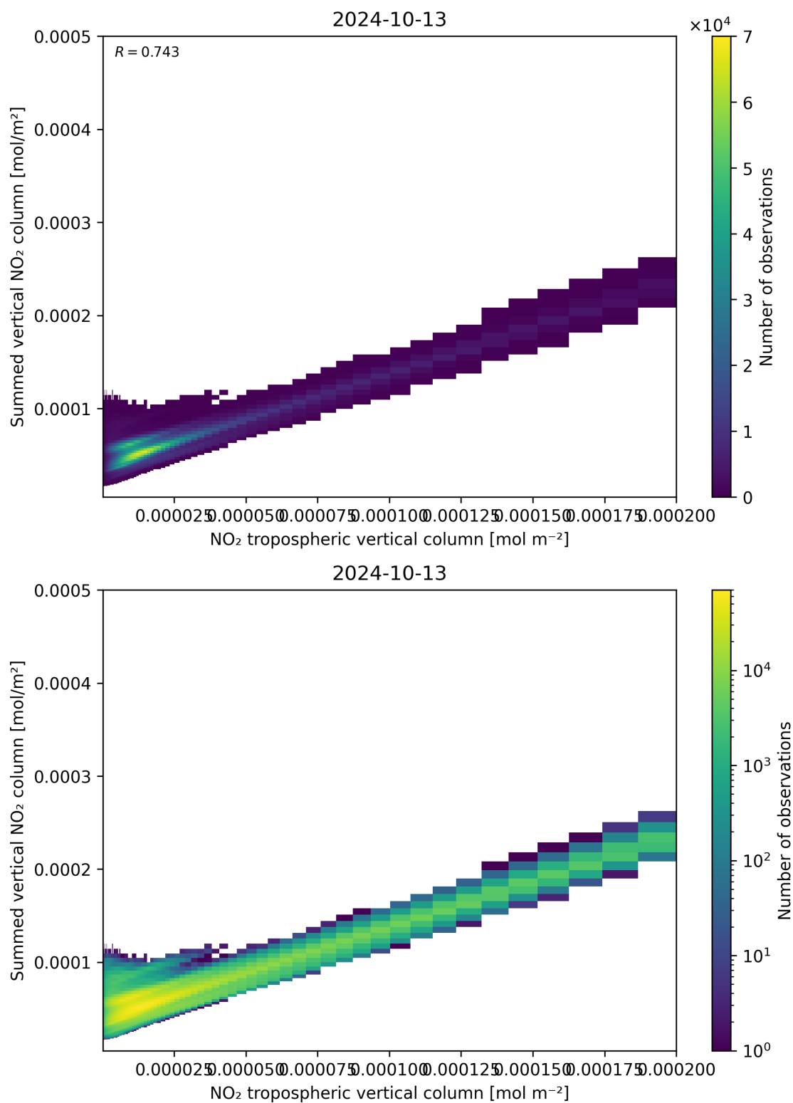
Figure 126: Scatter density plot of “NO 2 tropospheric vertical column” against “Summed vertical NO 2 column” for 2024-10-12 to 2024-10-14.
