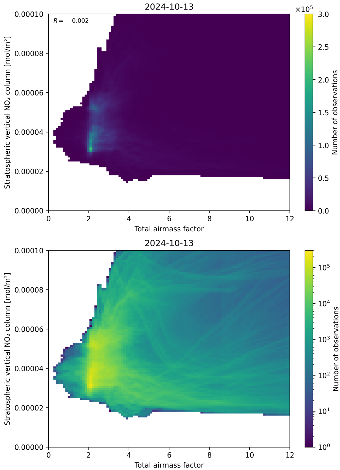
Figure 64: Scatter density plot of “Total airmass factor” against “Stratospheric vertical NO 2 column” for 2024-10-12 to 2024-10-14.
