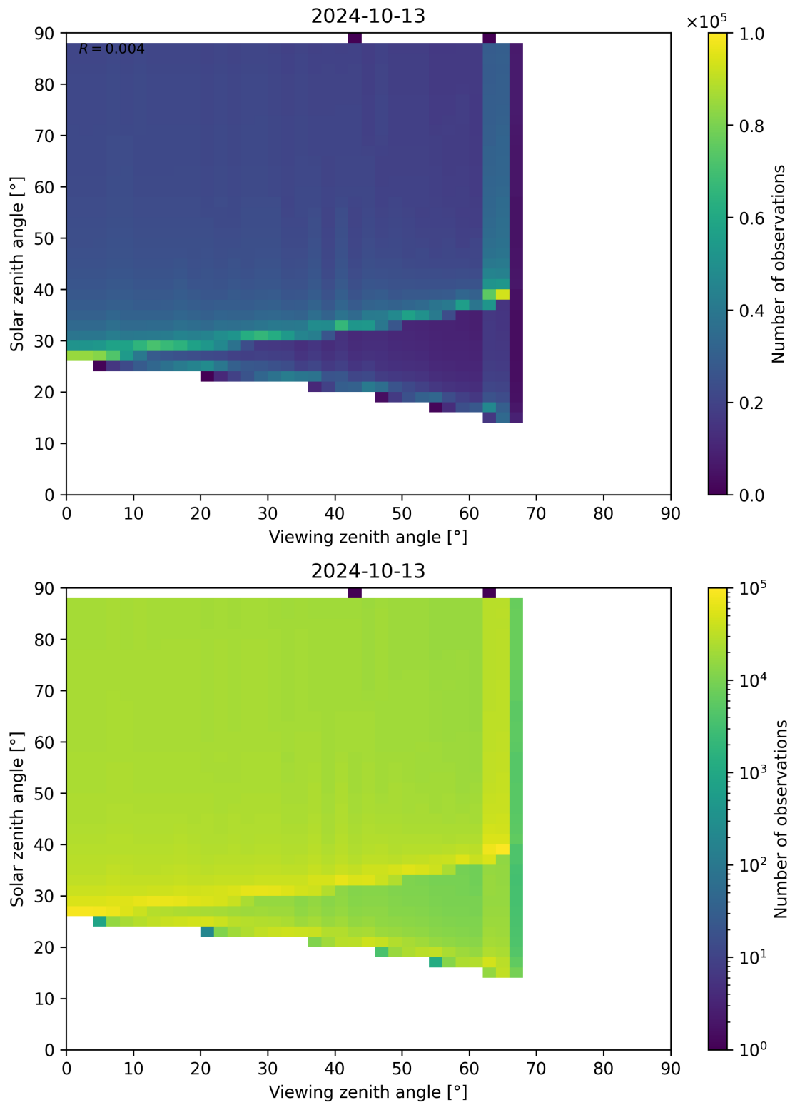
Figure 172: Scatter density plot of “Viewing zenith angle” against “Solar zenith angle” for 2024-10-12 to 2024-10-14.
