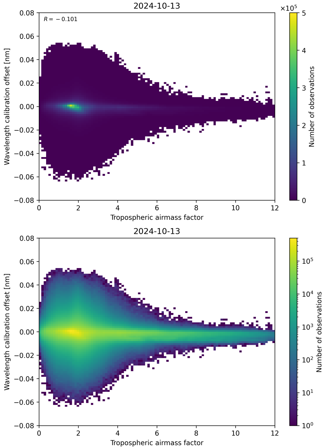
Figure 80: Scatter density plot of “Tropospheric airmass factor” against “Wavelength calibration offset” for 2024-10-12 to 2024-10-14.
