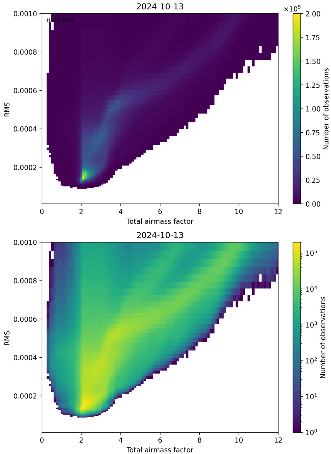
Figure 69: Scatter density plot of “Total airmass factor” against “RMS” for 2024-10-12 to 2024-10-14.
