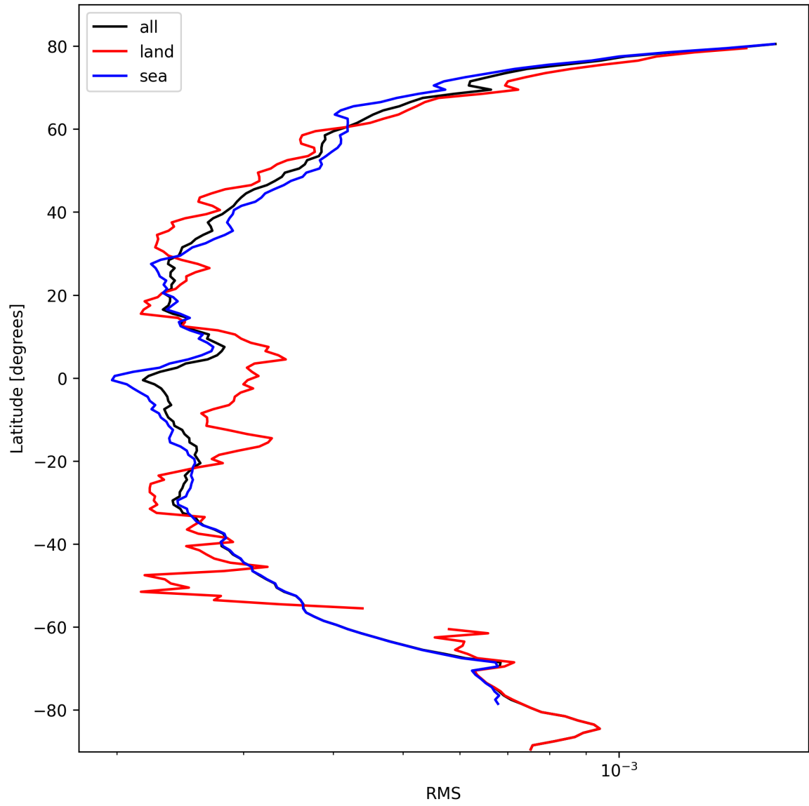
Figure 26: Zonal average of “RMS” for 2024-10-12 to 2024-10-14.
