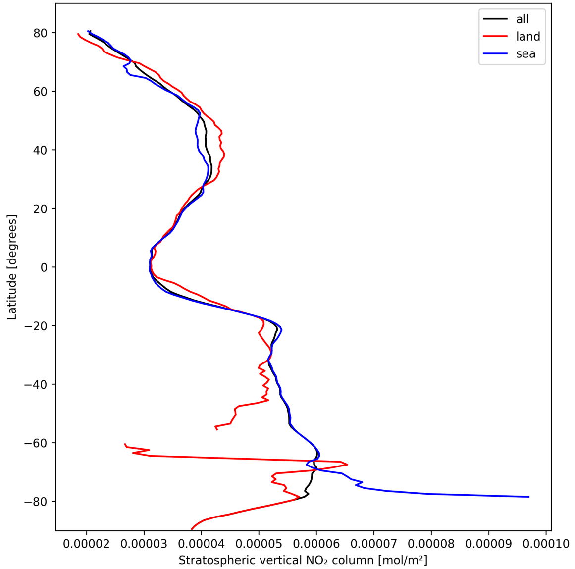
Figure 19: Zonal average of “Stratospheric vertical NO 2 column” for 2024-10-12 to 2024-10-14.
