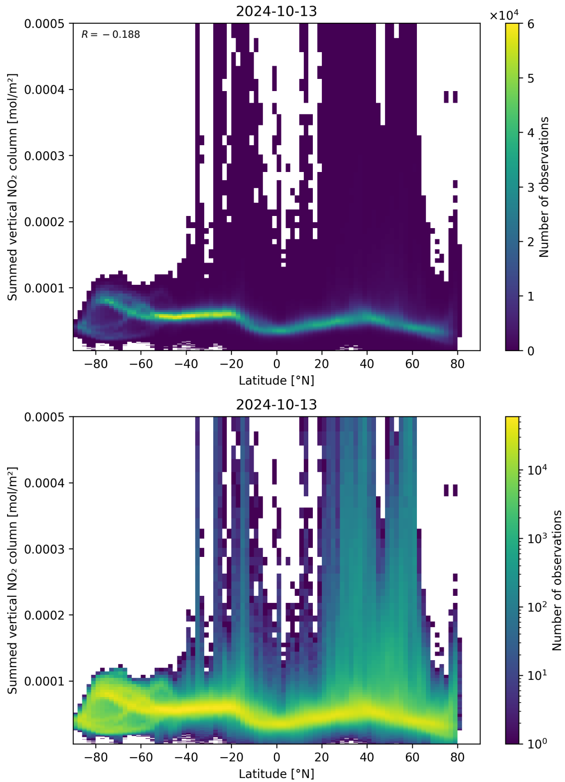
Figure 88: Scatter density plot of “Latitude” against “Summed vertical NO 2 column” for 2024-10-12 to 2024-10-14.
