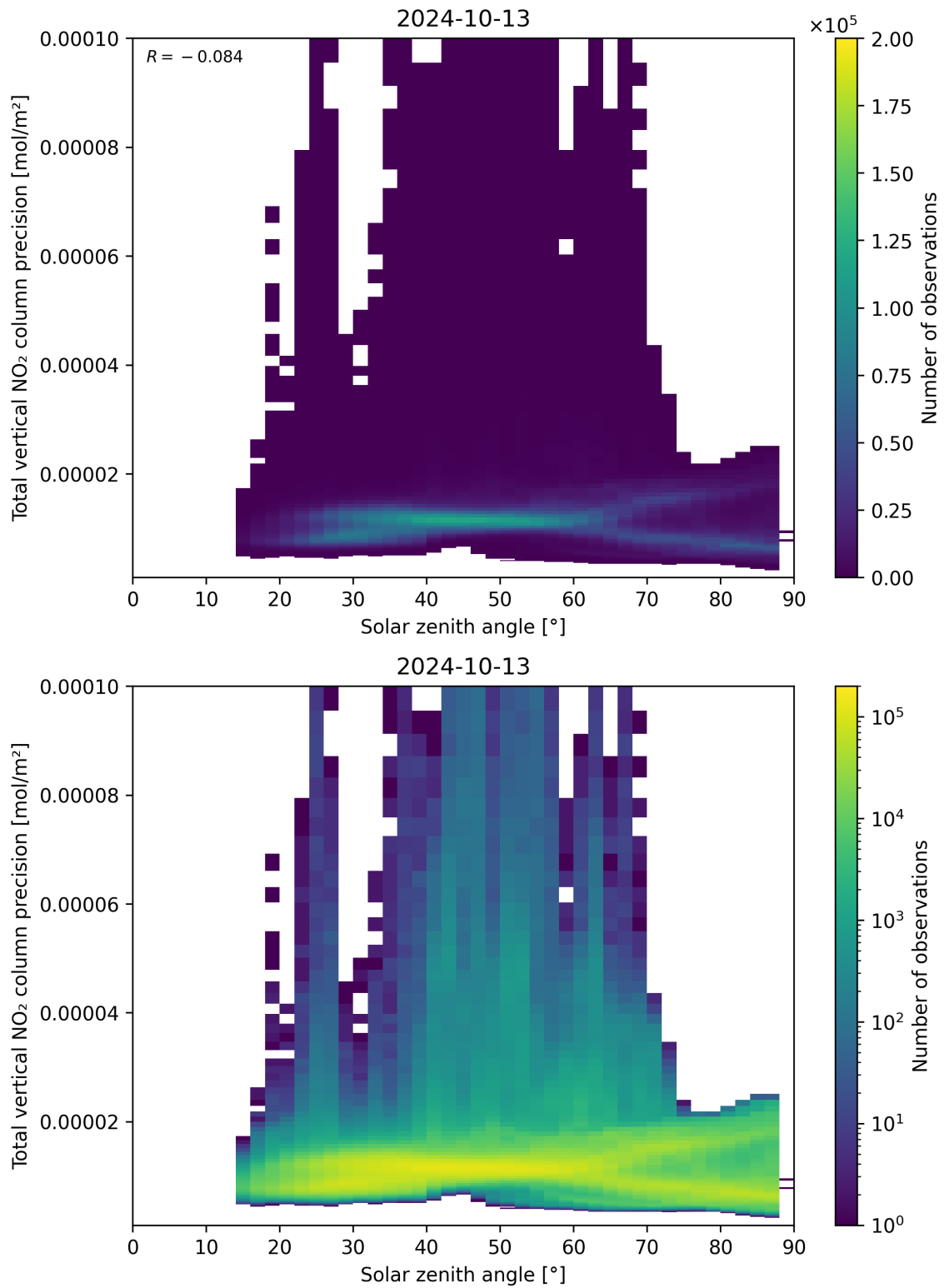
Figure 154: Scatter density plot of “Solar zenith angle” against “Total vertical NO 2 column precision” for 2024-10-12 to 2024-10-14.
