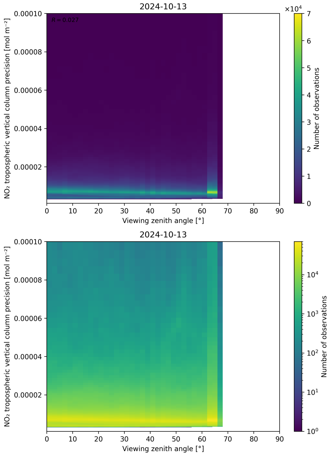
Figure 170: Scatter density plot of “Viewing zenith angle” against “NO 2 tropospheric vertical column precision” for 2024-10-12 to 2024-10-14.
