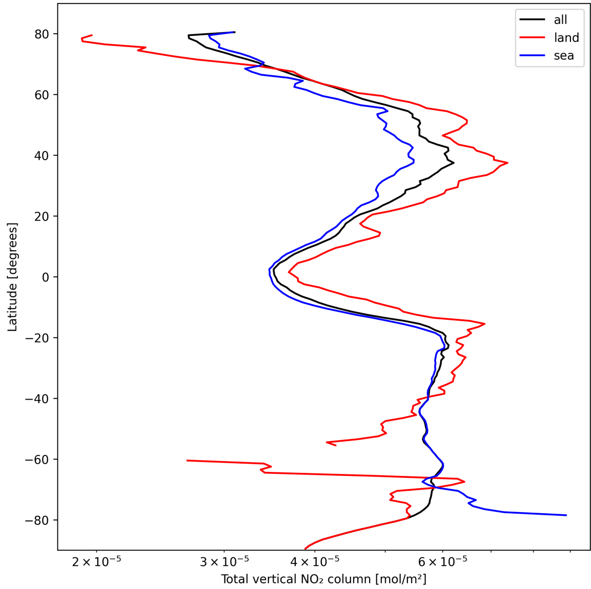
Figure 21: Zonal average of “Total vertical NO 2 column” for 2024-10-12 to 2024-10-14.
