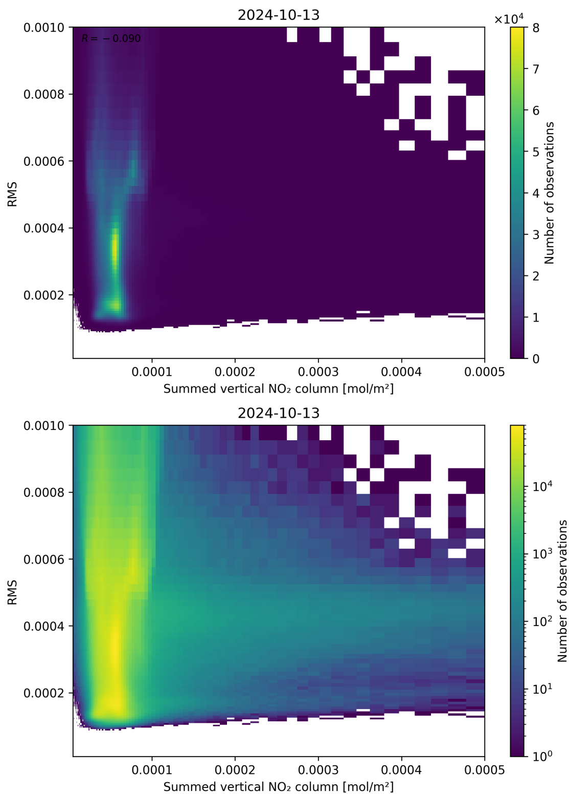
Figure 109: Scatter density plot of “Summed vertical NO 2 column” against “RMS” for 2024-10-12 to 2024-10-14.
