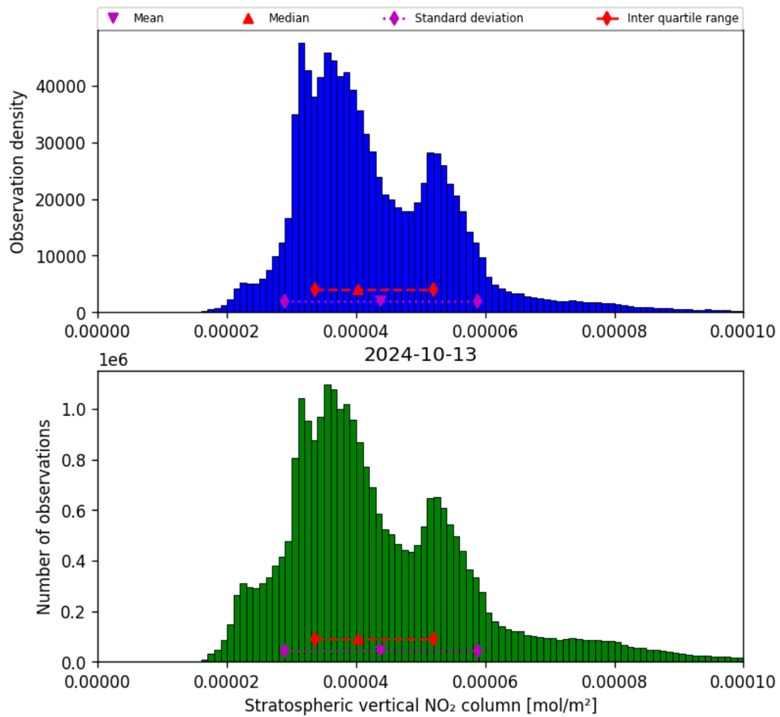
Figure 36: Histogram of “Stratospheric vertical NO 2 column” for 2024-10-12 to 2024-10-14
