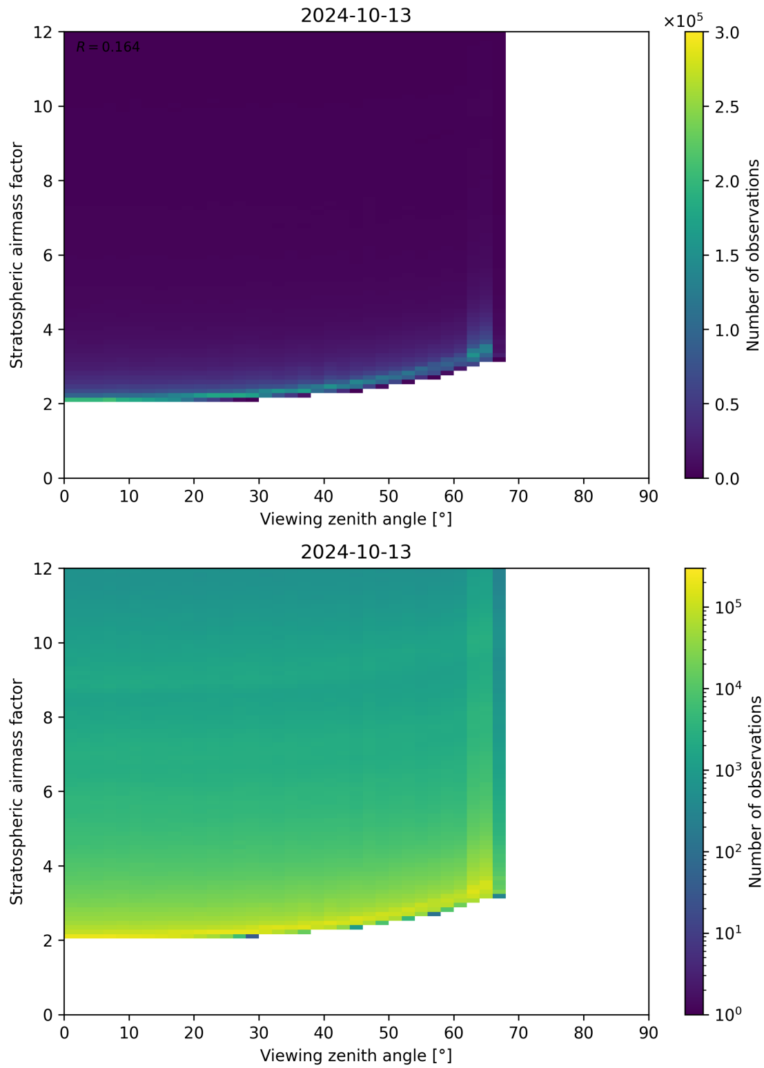
Figure 159: Scatter density plot of “Viewing zenith angle” against “Stratospheric airmass factor” for 2024-10-12 to 2024-10-14.
