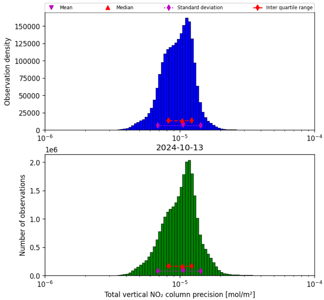
Figure 39: Histogram of “Total vertical NO 2 column precision” for 2024-10-12 to 2024-10-14
