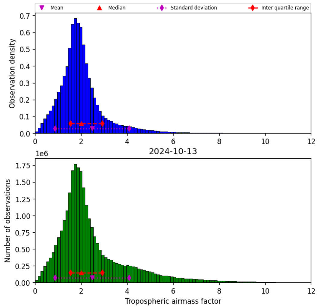
Figure 31: Histogram of “Tropospheric airmass factor” for 2024-10-12 to 2024-10-14
