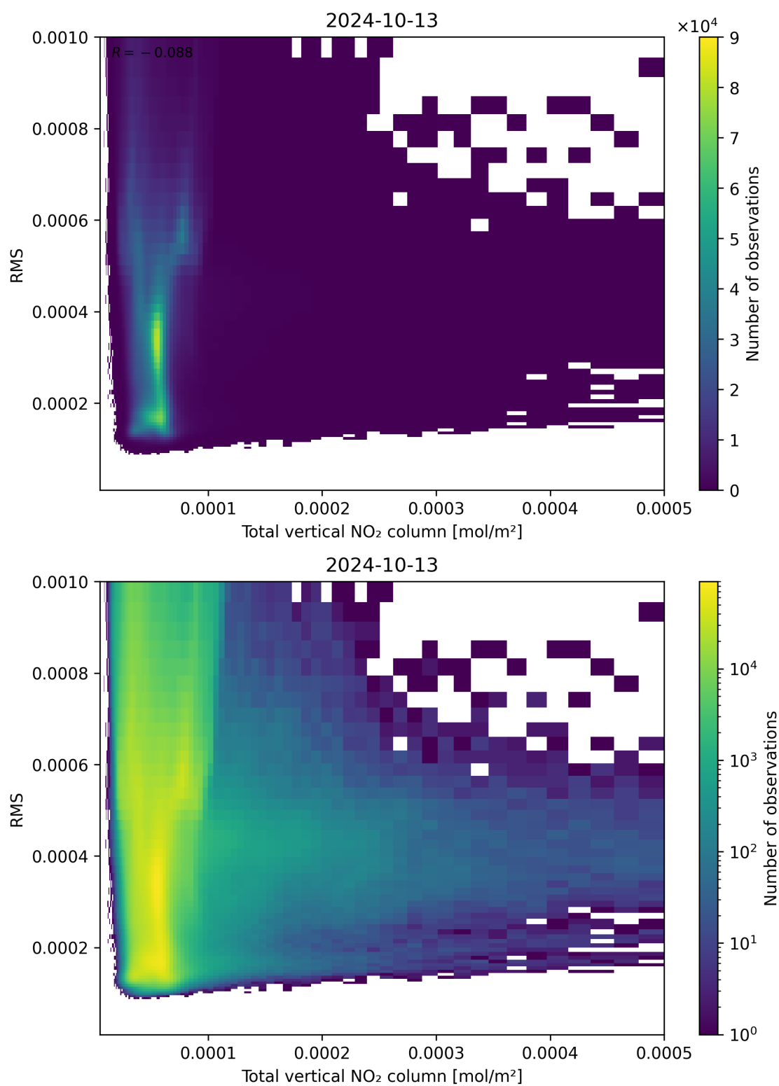
Figure 120: Scatter density plot of “Total vertical NO 2 column” against “RMS” for 2024-10-12 to 2024-10-14.
