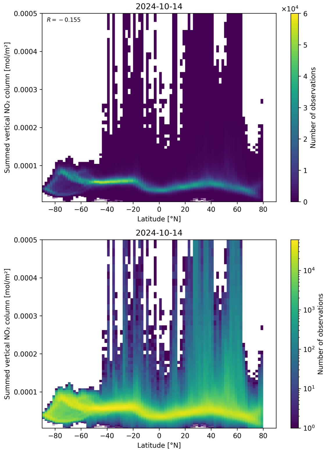
Figure 88: Scatter density plot of “Latitude” against “Summed vertical NO 2 column” for 2024-10-14 to 2024-10-15.
