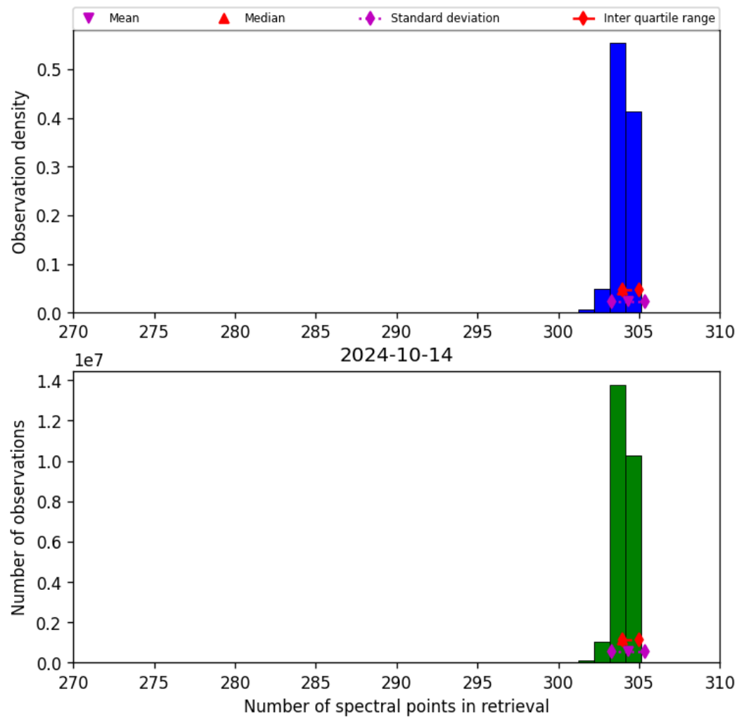
Figure 33: Histogram of “Number of spectral points in retrieval” for 2024-10-14 to 2024-10-15
