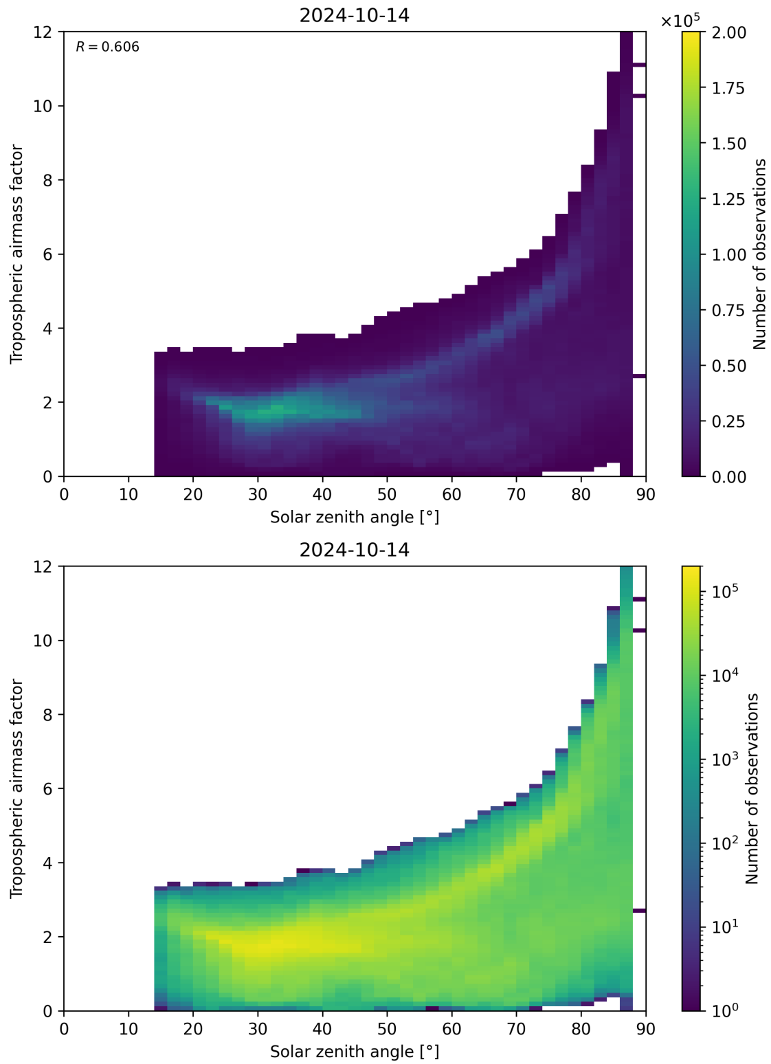
Figure 147: Scatter density plot of “Solar zenith angle” against “Tropospheric airmass factor” for 2024-10-14 to 2024-10-15.
