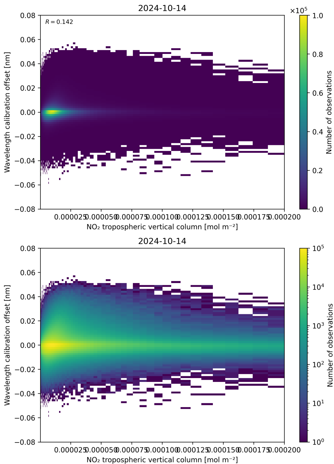
Figure 143: Scatter density plot of “NO 2 tropospheric vertical column” against “Wavelength calibration offset” for 2024-10-14 to 2024-10-15.
