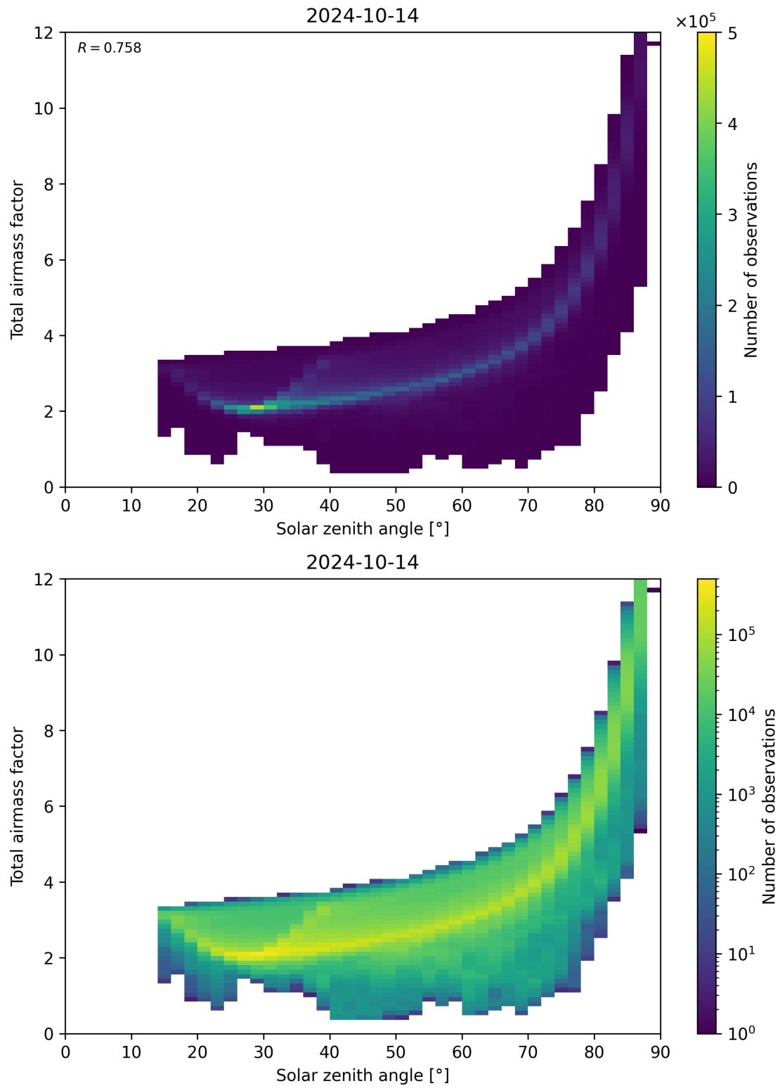
Figure 146: Scatter density plot of “Solar zenith angle” against “Total airmass factor” for 2024-10-14 to 2024-10-15.
