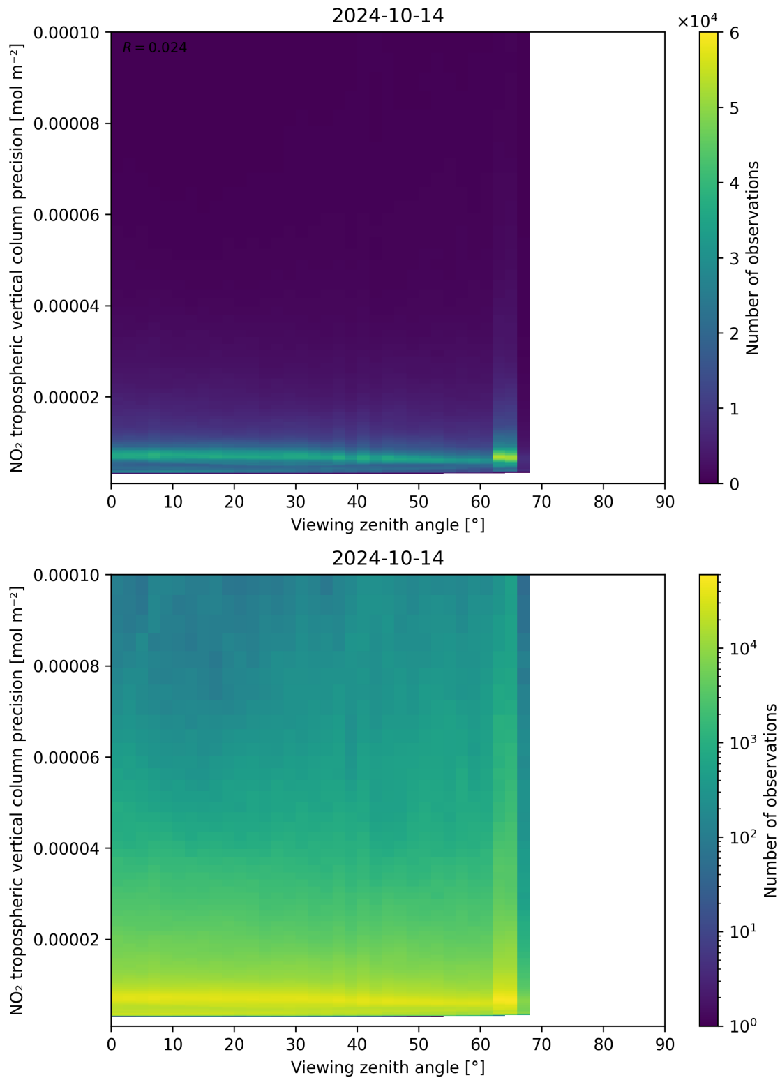
Figure 170: Scatter density plot of “Viewing zenith angle” against “NO 2 tropospheric vertical column precision” for 2024-10-14 to 2024-10-15.
