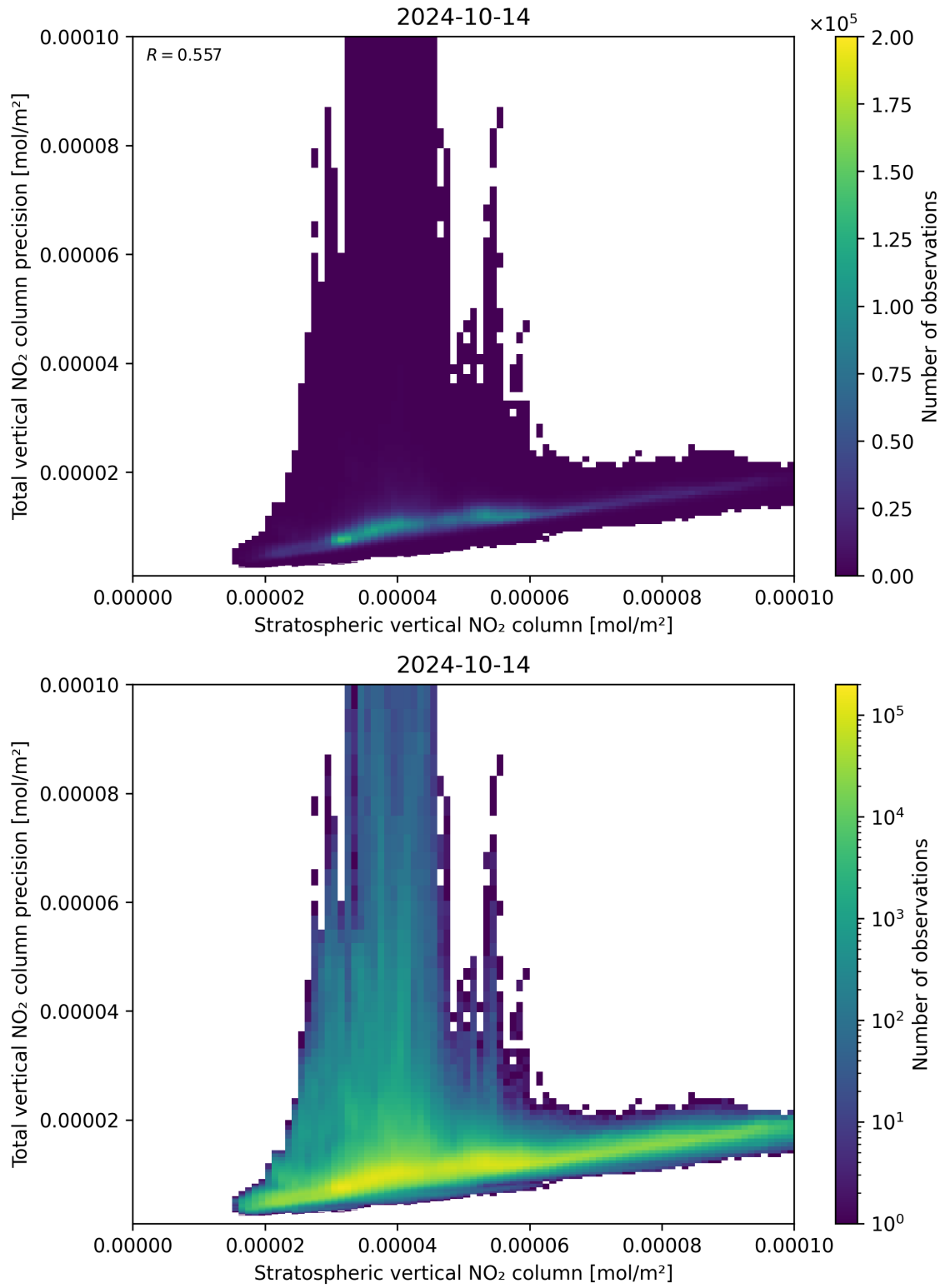
Figure 101: Scatter density plot of “Stratospheric vertical NO 2 column” against “Total vertical NO 2 column precision” for 2024-10-14 to 2024-10-15.
