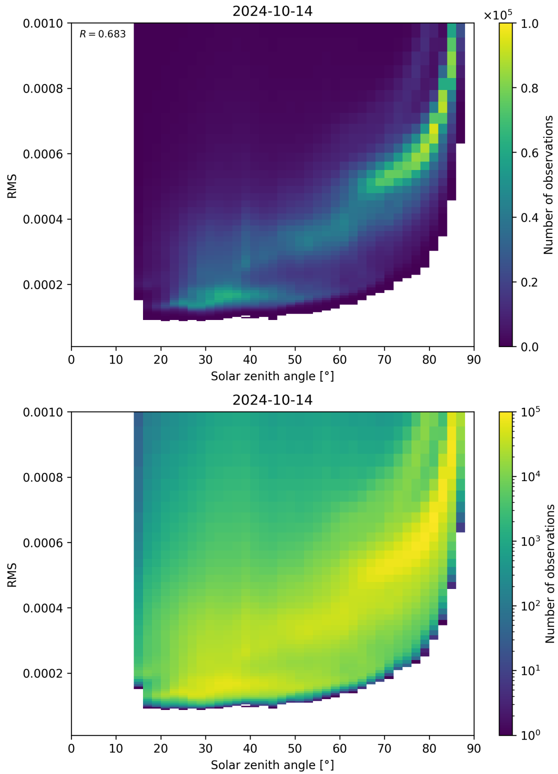
Figure 157: Scatter density plot of “Solar zenith angle” against “RMS” for 2024-10-14 to 2024-10-15.
