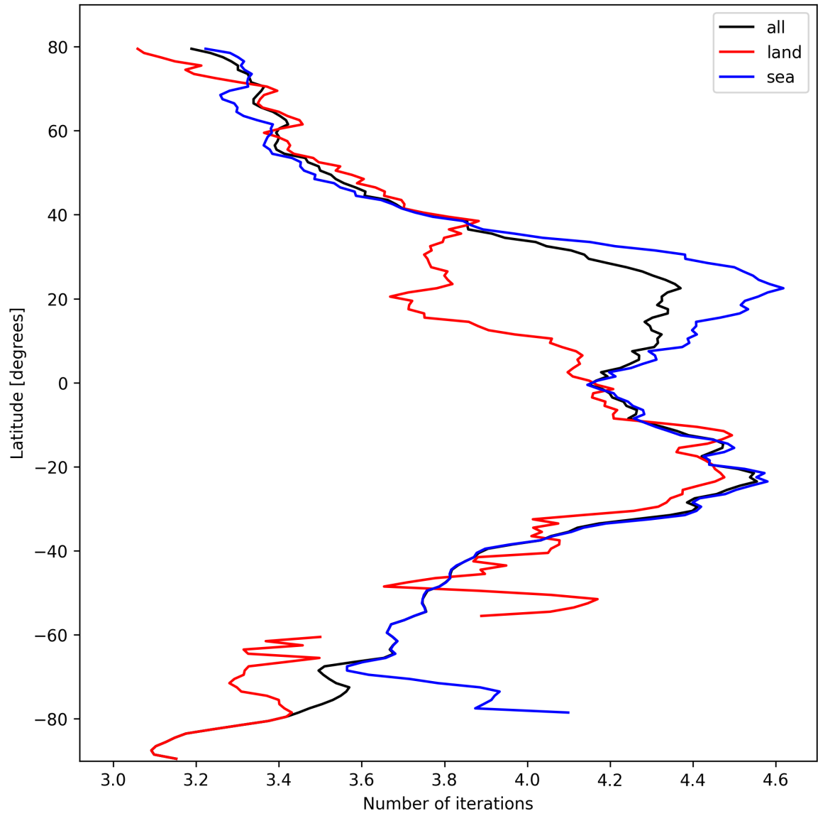
Figure 17: Zonal average of “Number of iterations” for 2024-10-14 to 2024-10-15.
