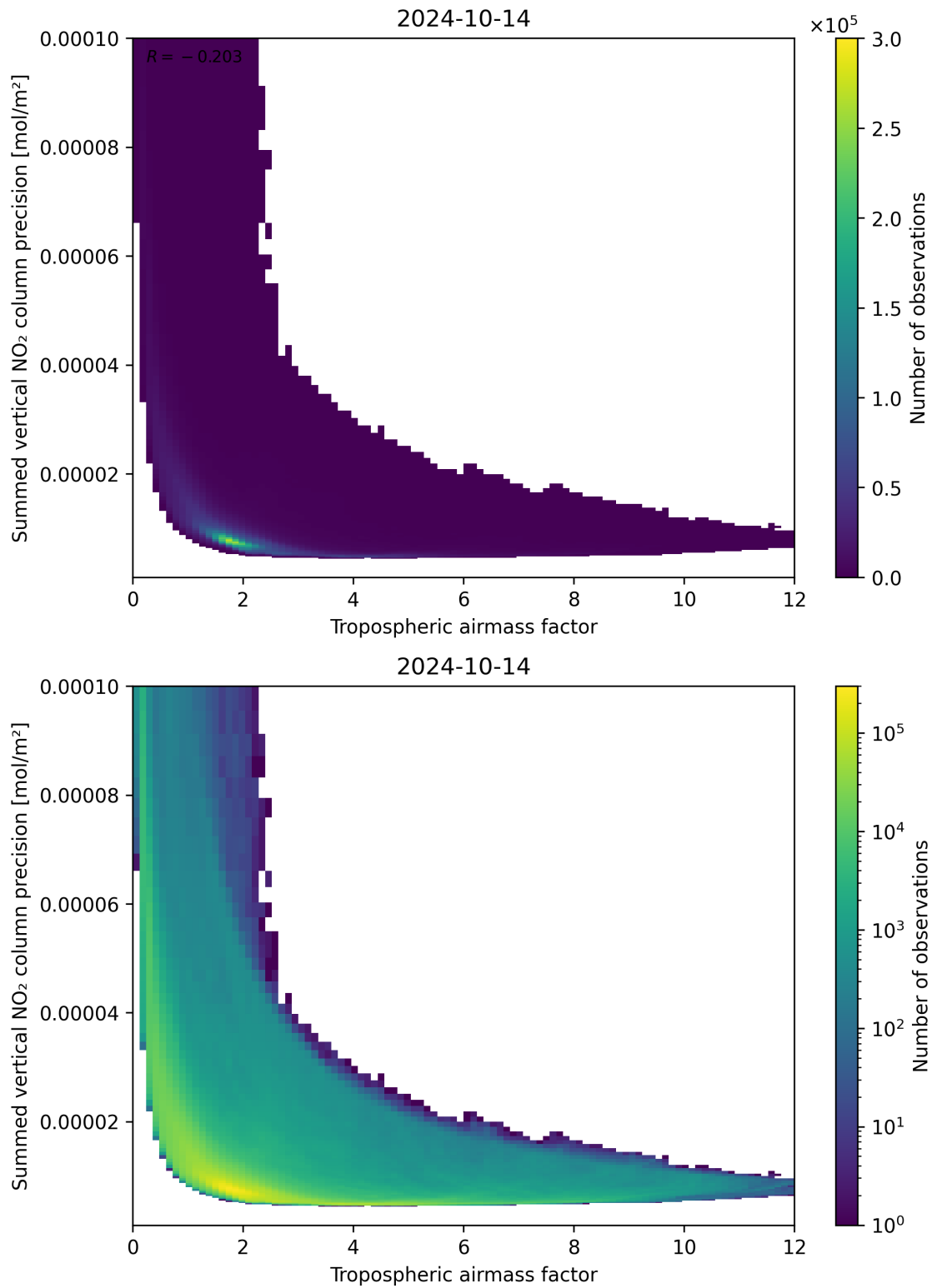
Figure 76: Scatter density plot of “Tropospheric air mass factor” against “Summed vertical NO 2 column precision” for 2024-10-14 to 2024-10-15.
