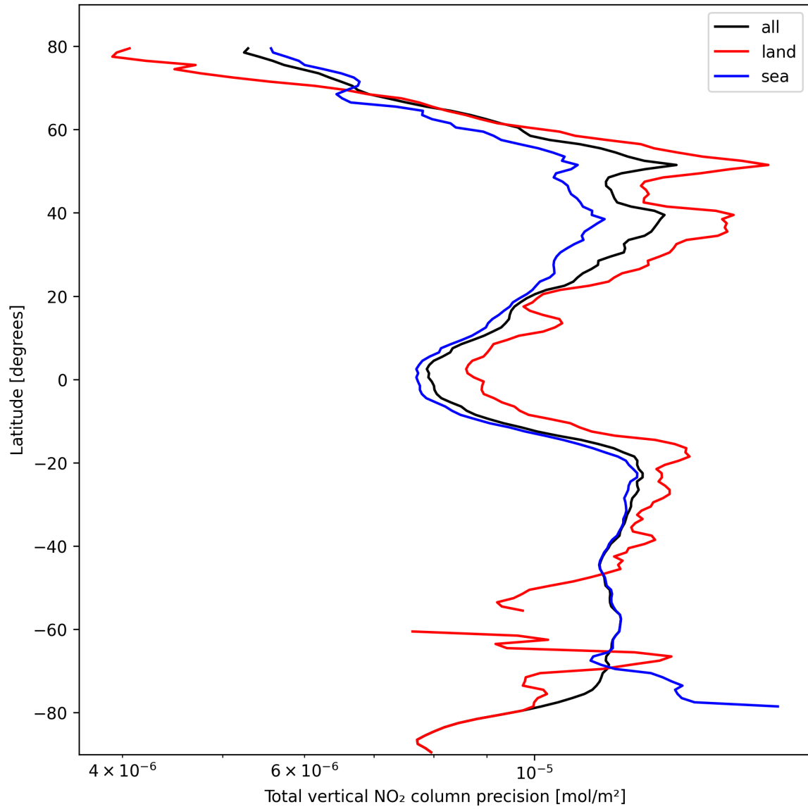
Figure 22: Zonal average of “Total vertical NO 2 column precision” for 2024-10-14 to 2024-10-15.
