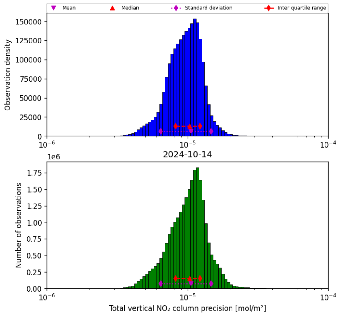
Figure 39: Histogram of “Total vertical NO 2 column precision” for 2024-10-14 to 2024-10-15
