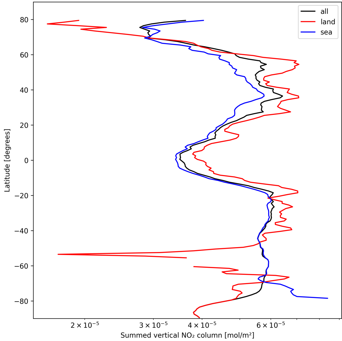
Figure 23: Zonal average of “Summed vertical NO 2 column” for 2024-10-14 to 2024-10-15.
