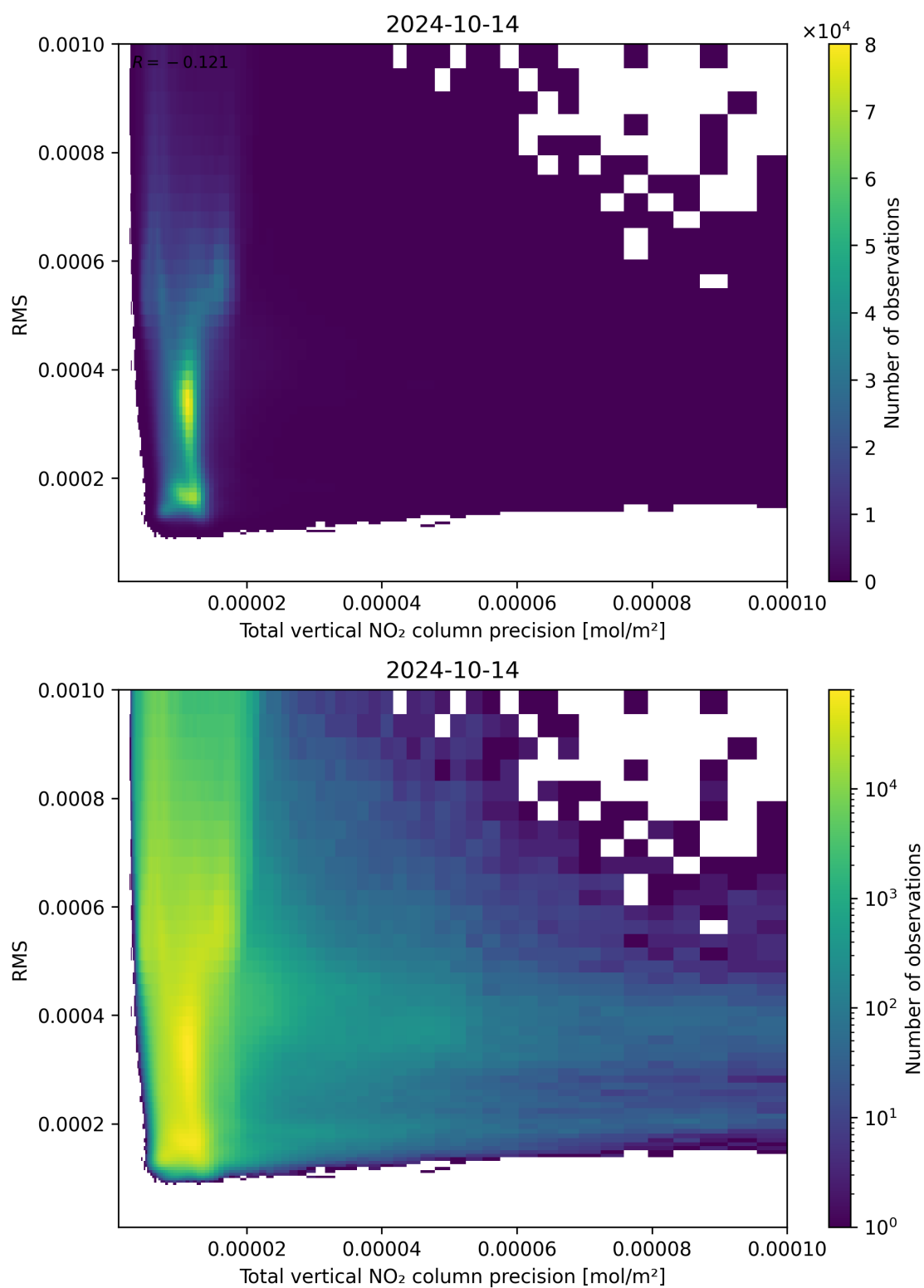
Figure 119: Scatter density plot of “Total vertical NO 2 column precision” against “RMS” for 2024-10-14 to 2024-10-15.
