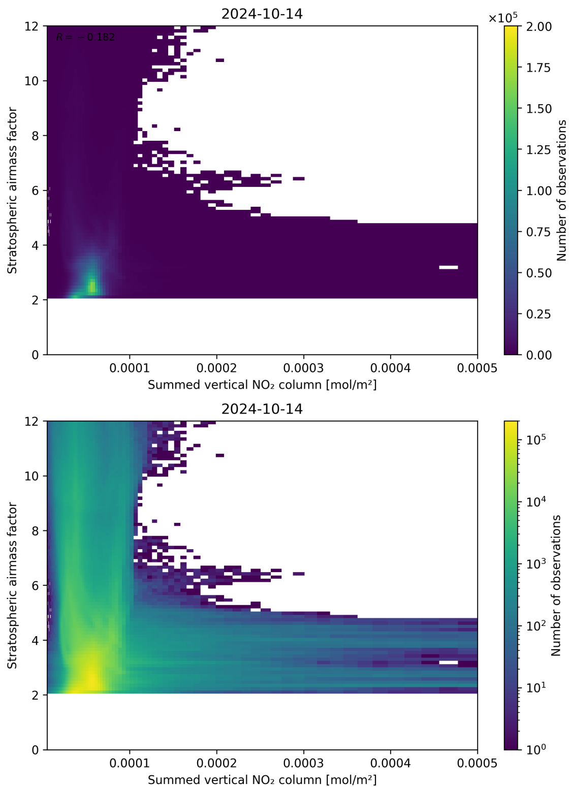
Figure 103: Scatter density plot of “Summed vertical NO 2 column” against “Stratospheric air mass factor” for 2024-10-14 to 2024-10-15.
