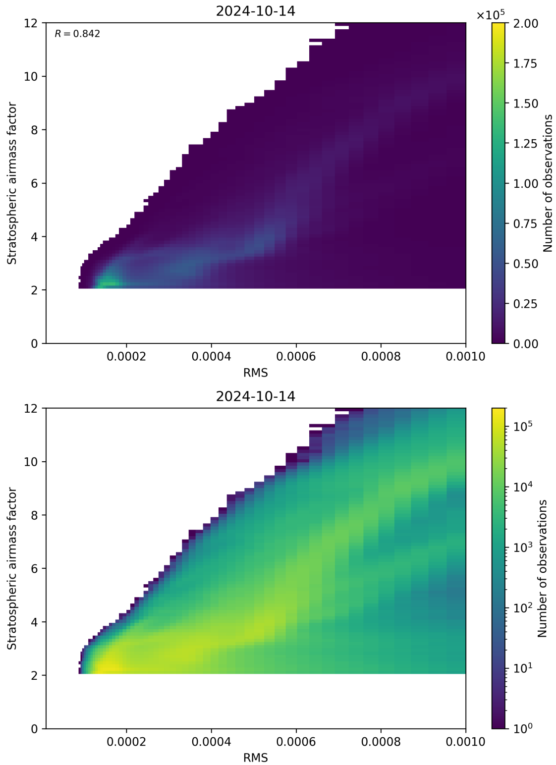
Figure 144: Scatter density plot of “RMS” against “Stratospheric airmass factor” for 2024-10-14 to 2024-10-15.
