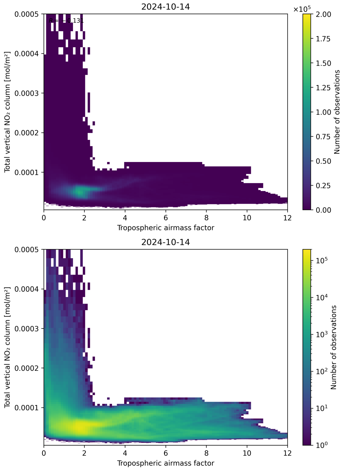
Figure 77: Scatter density plot of “Tropospheric airmass factor” against “Total vertical NO 2 column” for 2024-10-14 to 2024-10-15.
