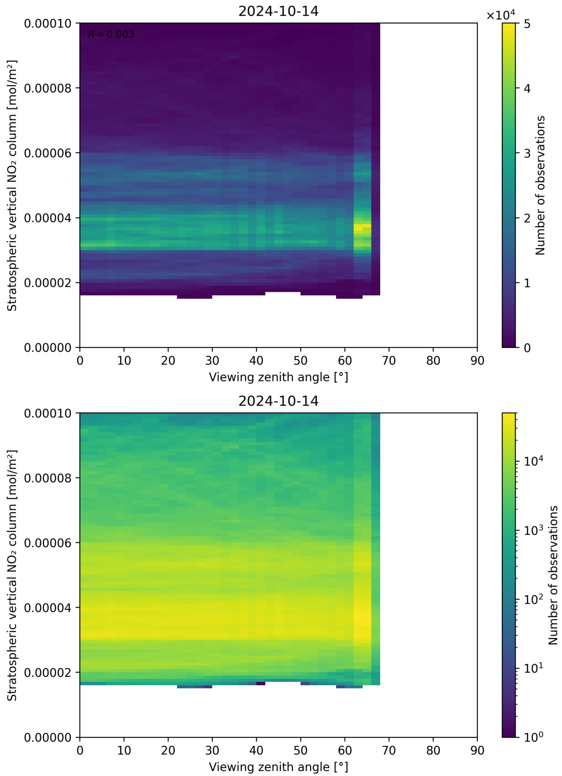
Figure 164: Scatter density plot of “Viewing zenith angle” against “Stratospheric vertical NO 2 column” for 2024-10-14 to 2024-10-15.
