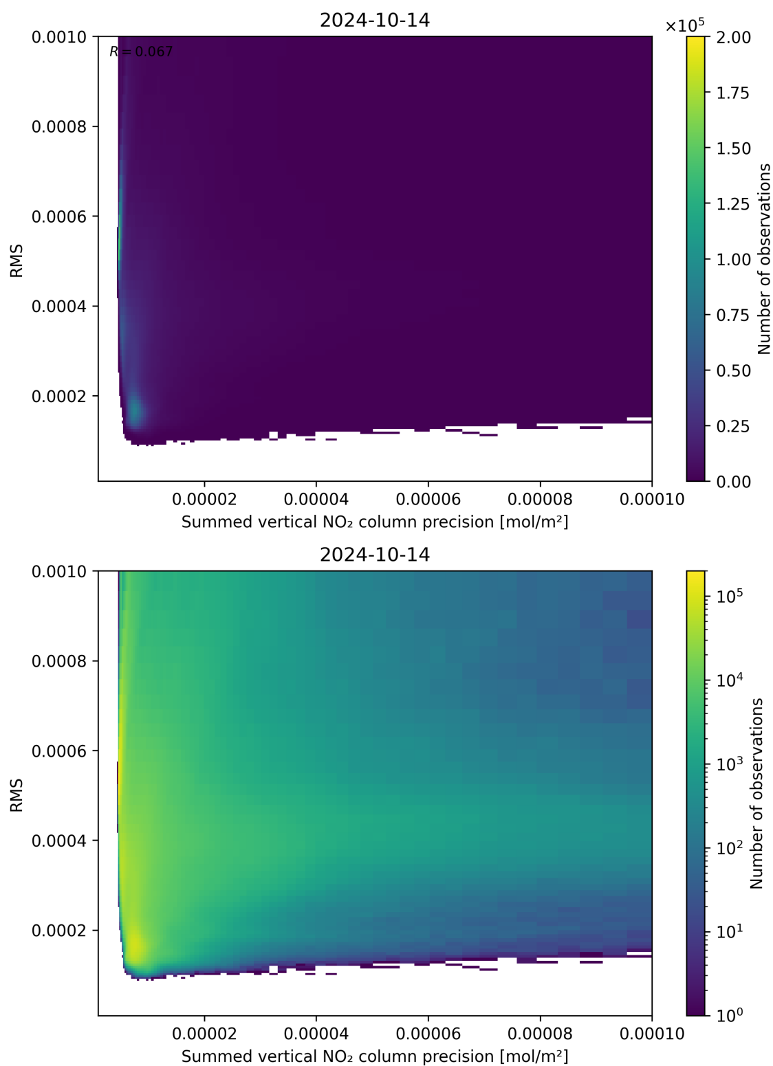
Figure 108: Scatter density plot of “Summed vertical NO 2 column precision” against “RMS” for 2024-10-14 to 2024-10-15.
