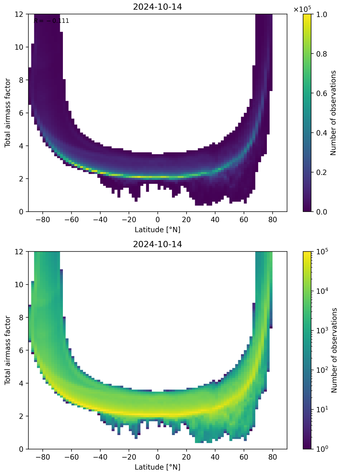
Figure 84: Scatter density plot of “Latitude” against “Total airmass factor” for 2024-10-14 to 2024-10-15.
