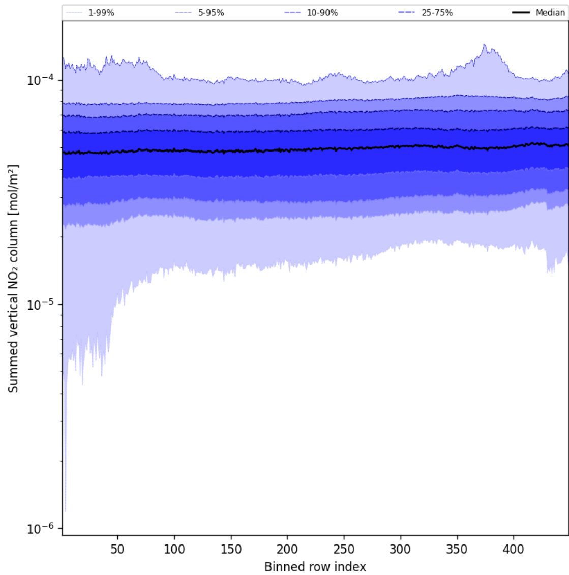
Figure 57: Along track statistics of “Summed vertical NO 2 column” for 2024-10-14 to 2024-10-15
