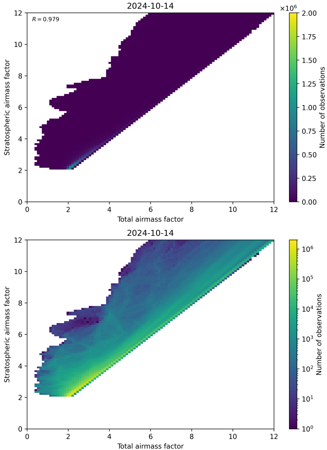
Figure 62: Scatter density plot of “Total airmass factor” against “Stratospheric airmass factor” for 2024-10-14 to 2024-10-15.
