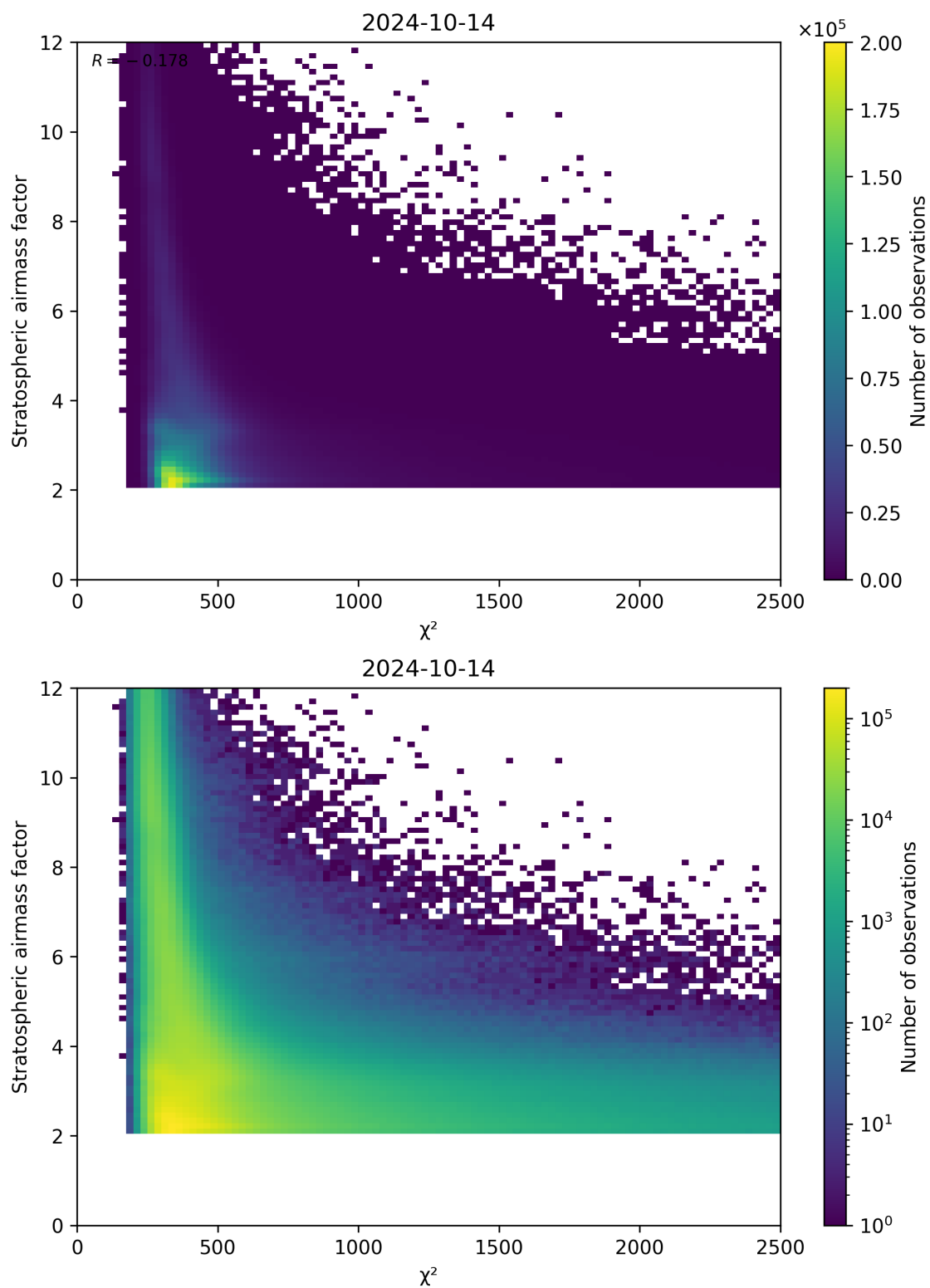
Figure 81: Scatter density plot of “ \chi^2 ” against “Stratospheric airmass factor” for 2024-10-14 to 2024-10-15.
