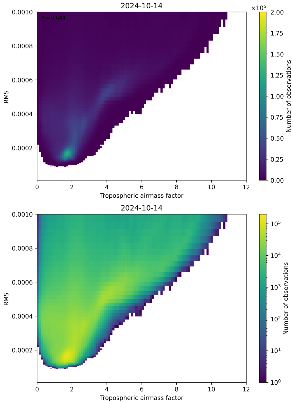
Figure 79: Scatter density plot of “Tropospheric airmass factor” against “RMS” for 2024-10-14 to 2024-10-15.
