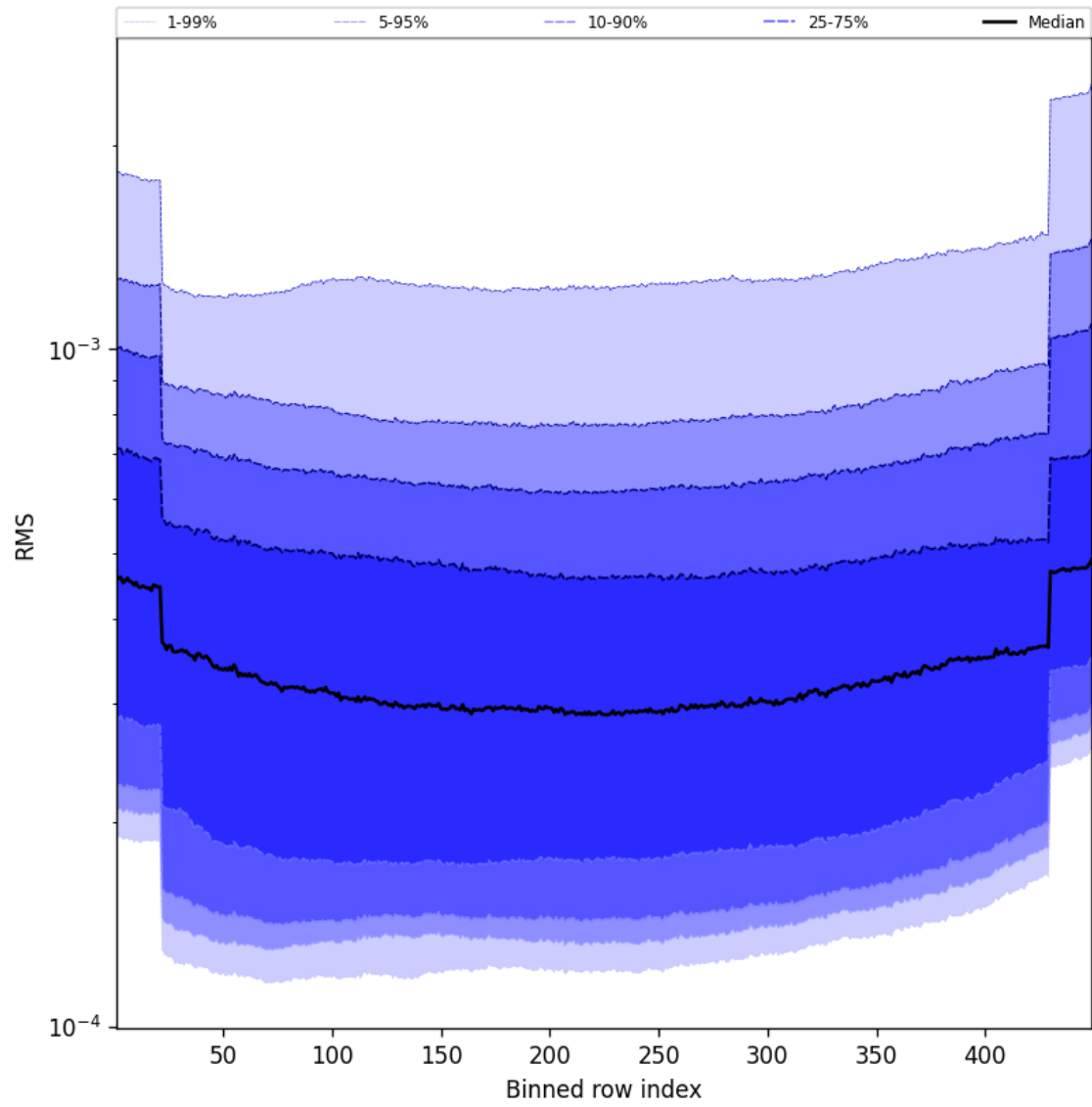
Figure 60: Along track statistics of “RMS” for 2024-10-14 to 2024-10-15
