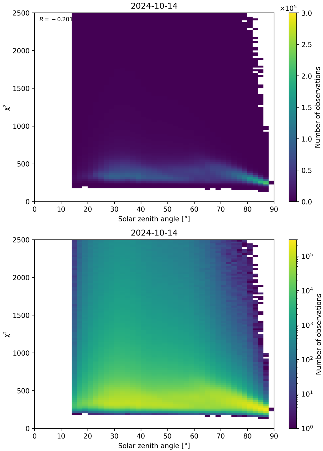
Figure 148: Scatter density plot of “Solar zenith angle” against “ \chi^2 ” for 2024-10-14 to 2024-10-15.
