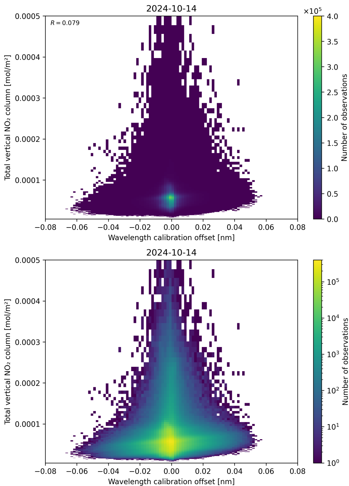
Figure 179: Scatter density plot of “Wavelength calibration offset” against “Total vertical NO 2 column” for 2024-10-14 to 2024-10-15.
