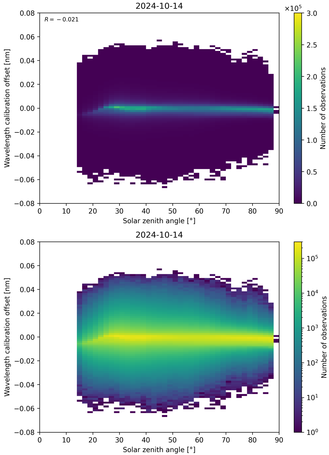
Figure 158: Scatter density plot of “Solar zenith angle” against “Wavelength calibration offset” for 2024-10-14 to 2024-10-15.
