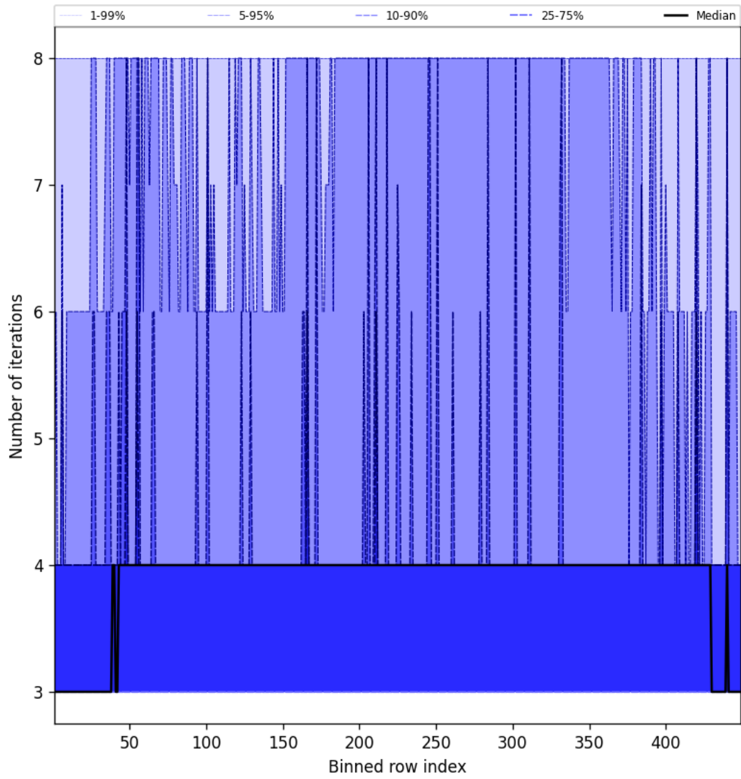
Figure 51: Along track statistics of “Number of iterations” for 2024-10-14 to 2024-10-15
