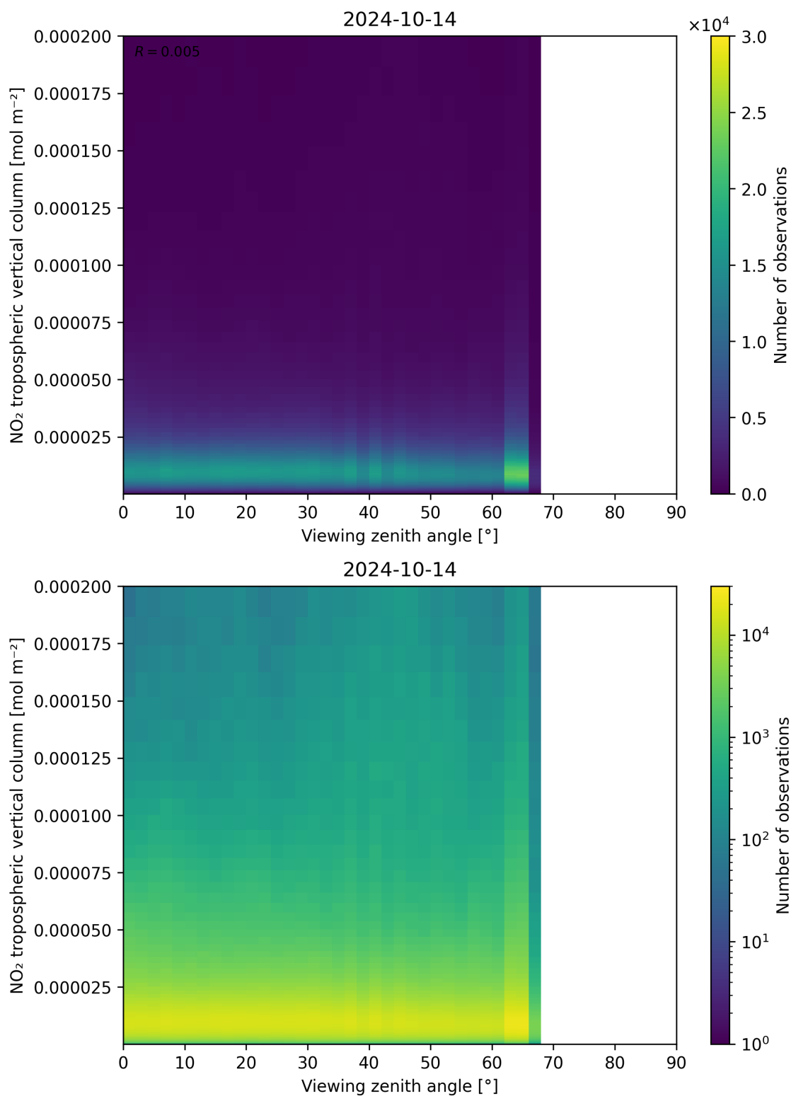
Figure 169: Scatter density plot of “Viewing zenith angle” against “NO 2 tropospheric vertical column” for 2024-10-14 to 2024-10-15.
