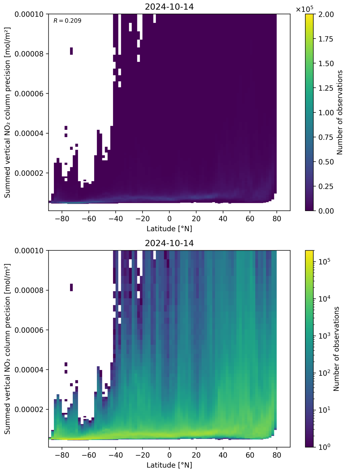
Figure 89: Scatter density plot of “Latitude” against “Summed vertical NO 2 column precision” for 2024-10-14 to 2024-10-15.
