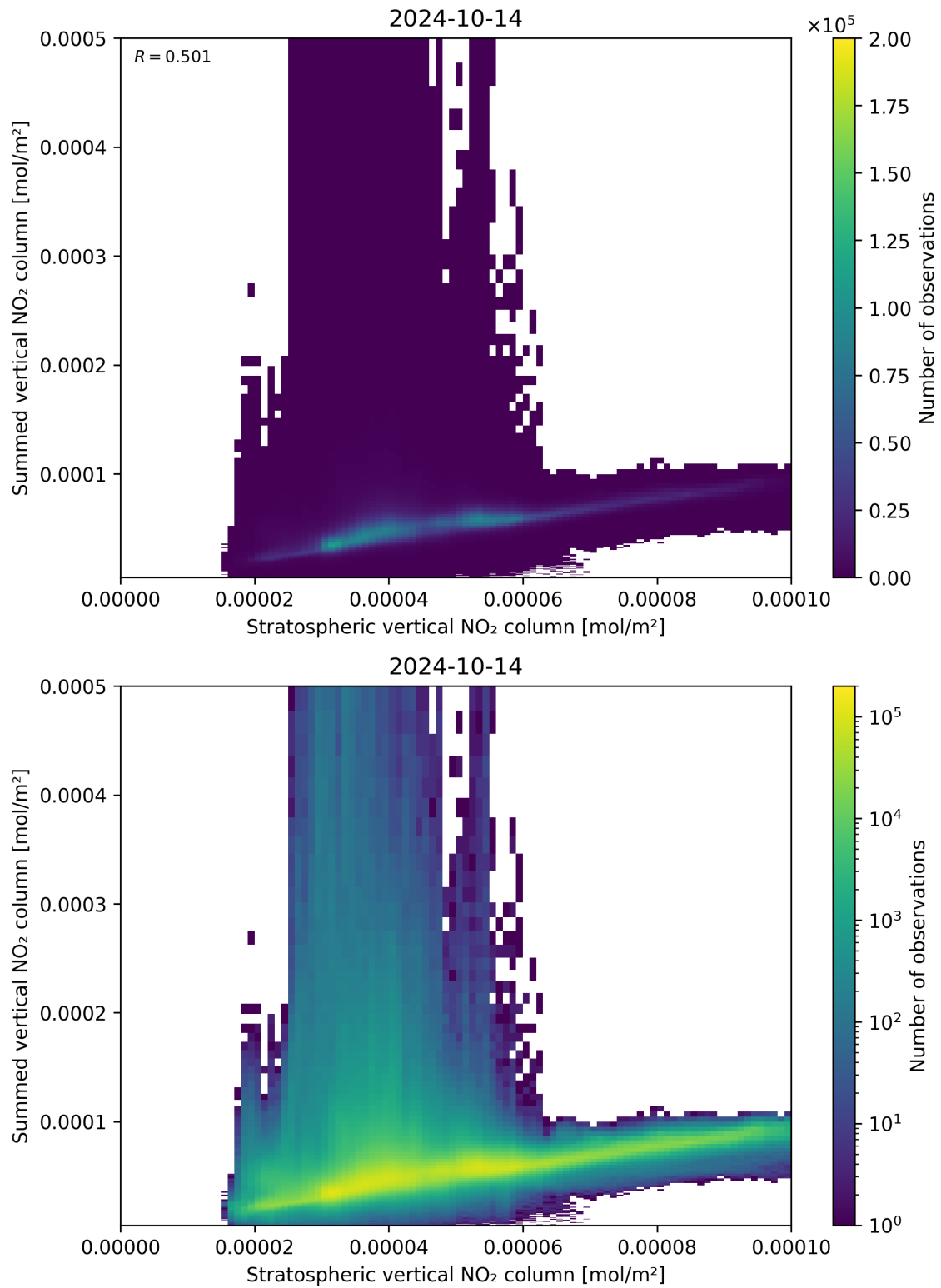
Figure 98: Scatter density plot of “Stratospheric vertical NO 2 column” against “Summed vertical NO 2 column” for 2024-10-14 to 2024-10-15.
