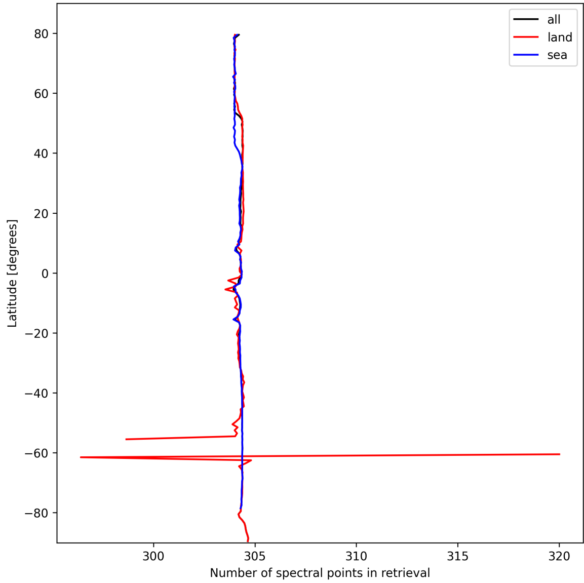
Figure 16: Zonal average of “Number of spectral points in retrieval” for 2024-10-14 to 2024-10-15.
