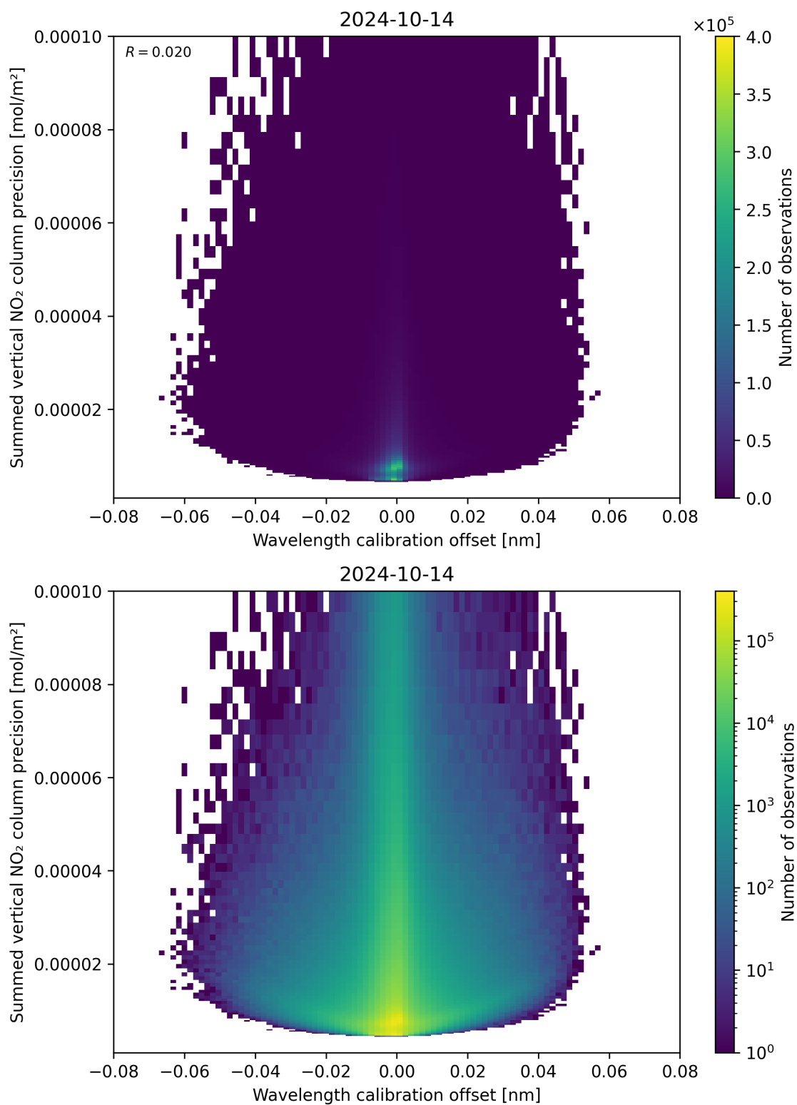
Figure 178: Scatter density plot of “Wavelength calibration offset” against “Summed vertical NO 2 column precision” for 2024-10-14 to 2024-10-15.
