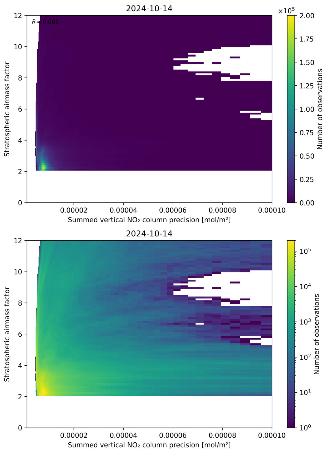
Figure 106: Scatter density plot of “Summed vertical NO 2 column precision” against “Stratospheric airmass factor” for 2024-10-14 to 2024-10-15.
