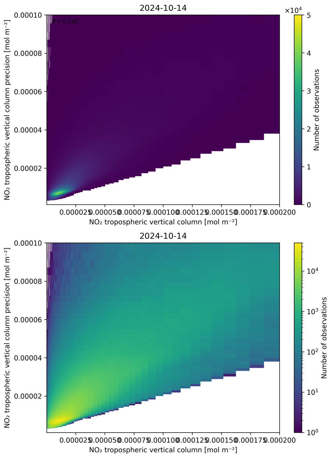
Figure 130: Scatter density plot of “NO 2 tropospheric vertical column” against “NO 2 tropospheric vertical column precision” for 2024-10-14 to 2024-10-15.
