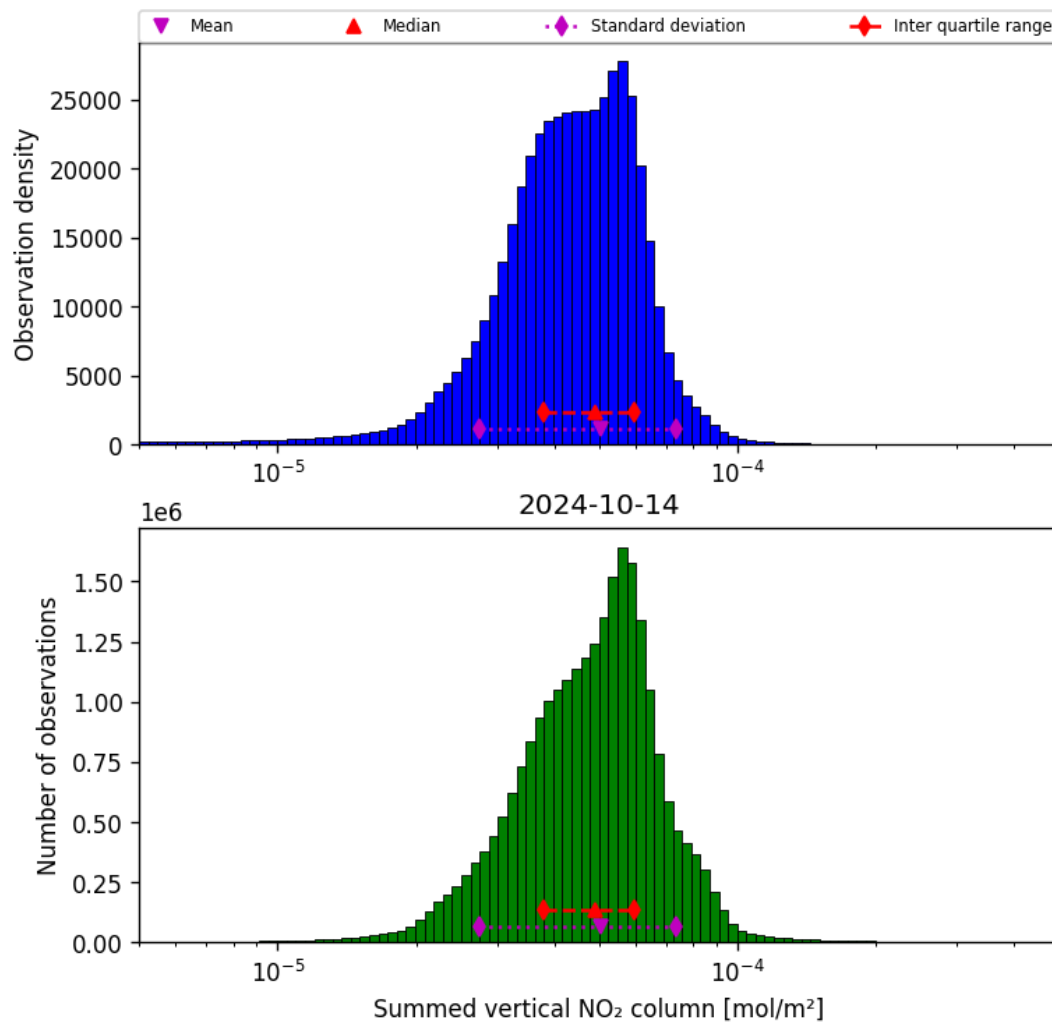
Figure 40: Histogram of “Summed vertical NO 2 column” for 2024-10-14 to 2024-10-15
