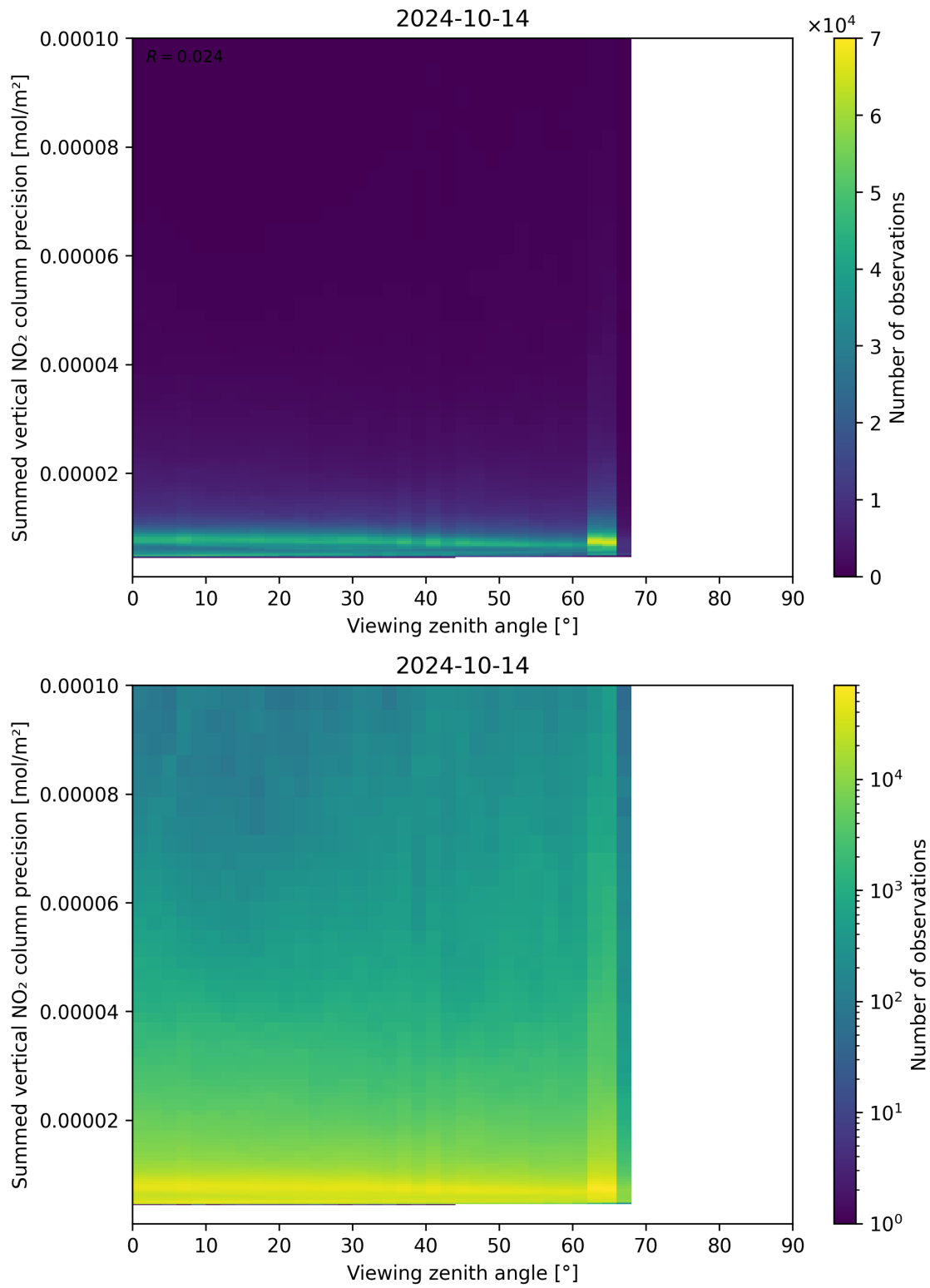
Figure 166: Scatter density plot of “Viewing zenith angle” against “Summed vertical NO 2 column precision” for 2024-10-14 to 2024-10-15.
