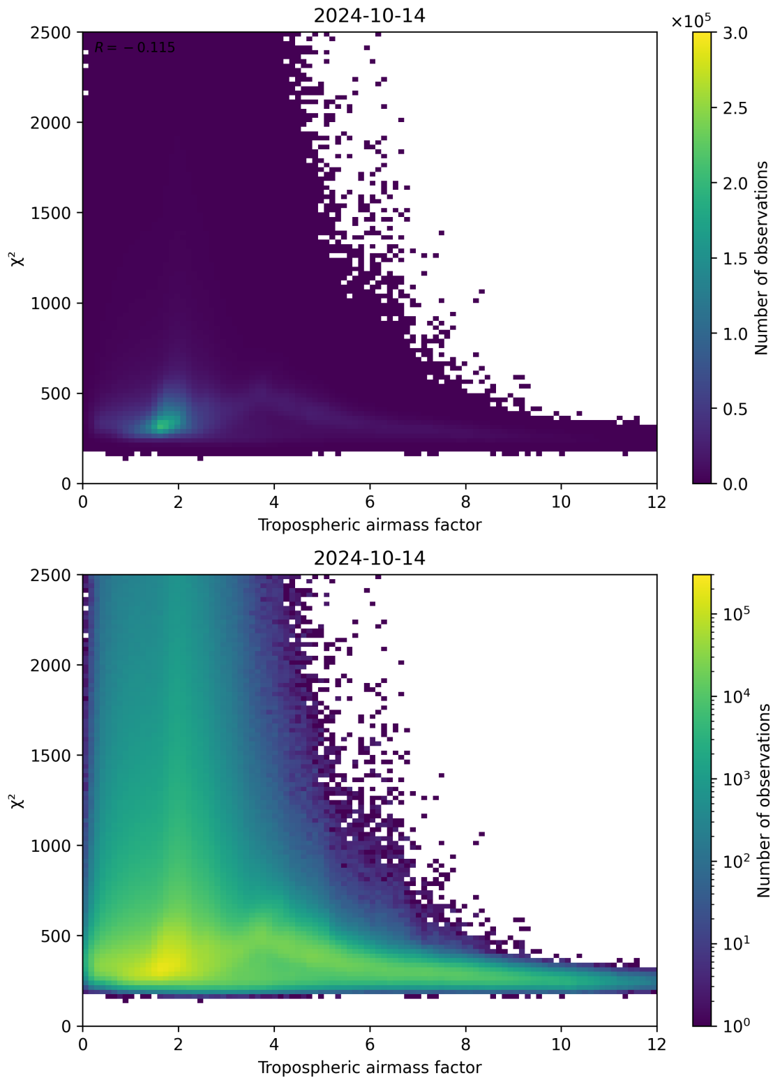
Figure 73: Scatter density plot of “Tropospheric airmass factor” against “ \chi^2 ” for 2024-10-14 to 2024-10-15.
