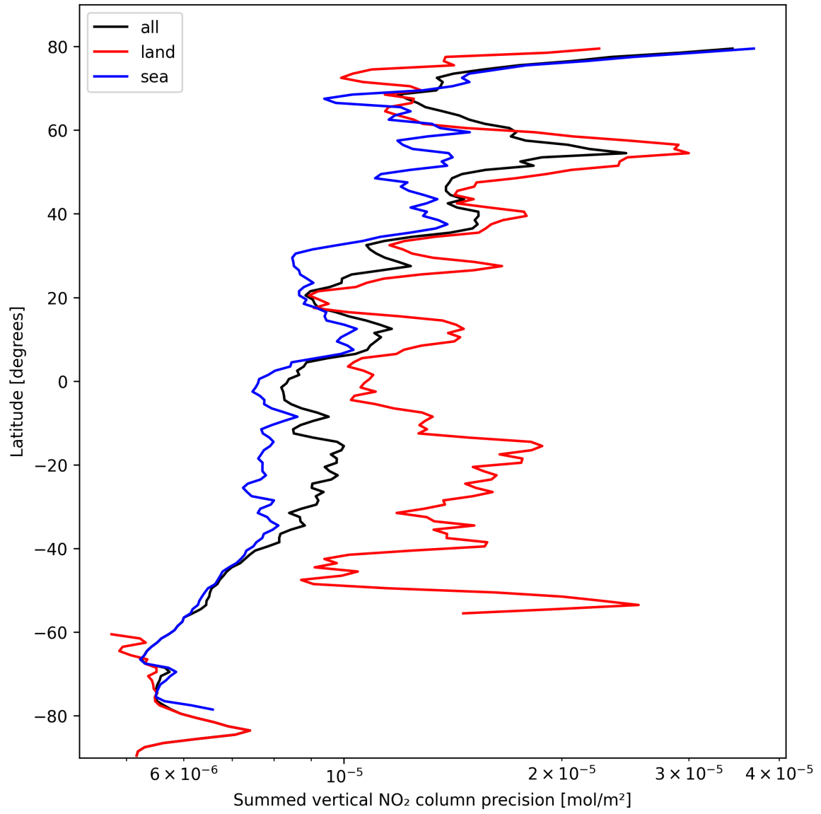
Figure 24: Zonal average of “Summed vertical NO 2 column precision” for 2024-10-14 to 2024-10-15.
