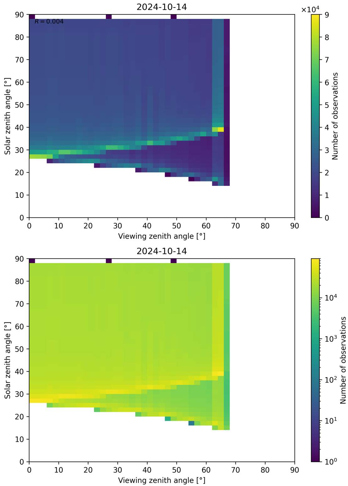
Figure 172: Scatter density plot of “Viewing zenith angle” against “Solar zenith angle” for 2024-10-14 to 2024-10-15.
