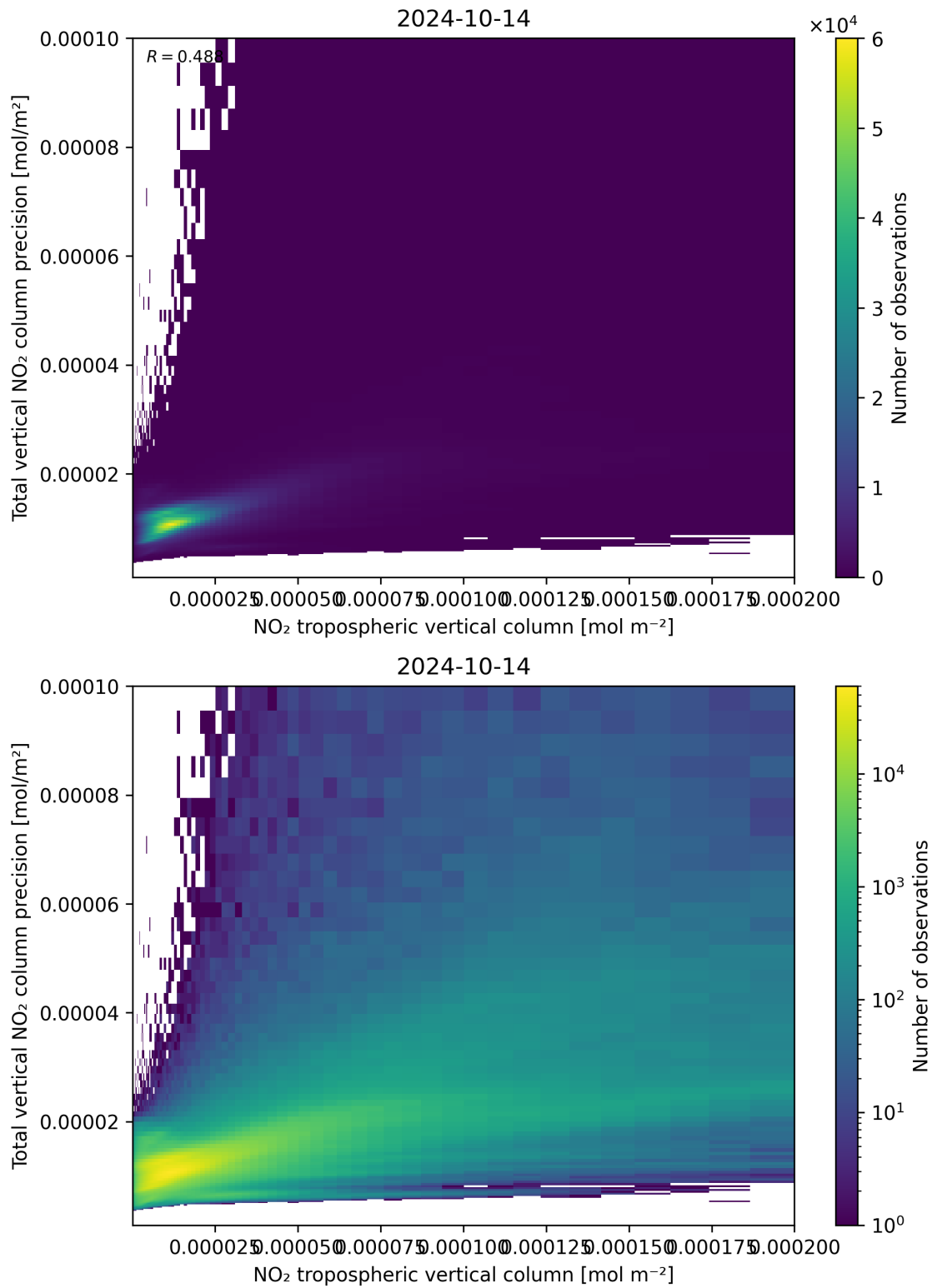
Figure 129: Scatter density plot of “NO 2 tropospheric vertical column” against “Total vertical NO 2 column precision” for 2024-10-14 to 2024-10-15.
