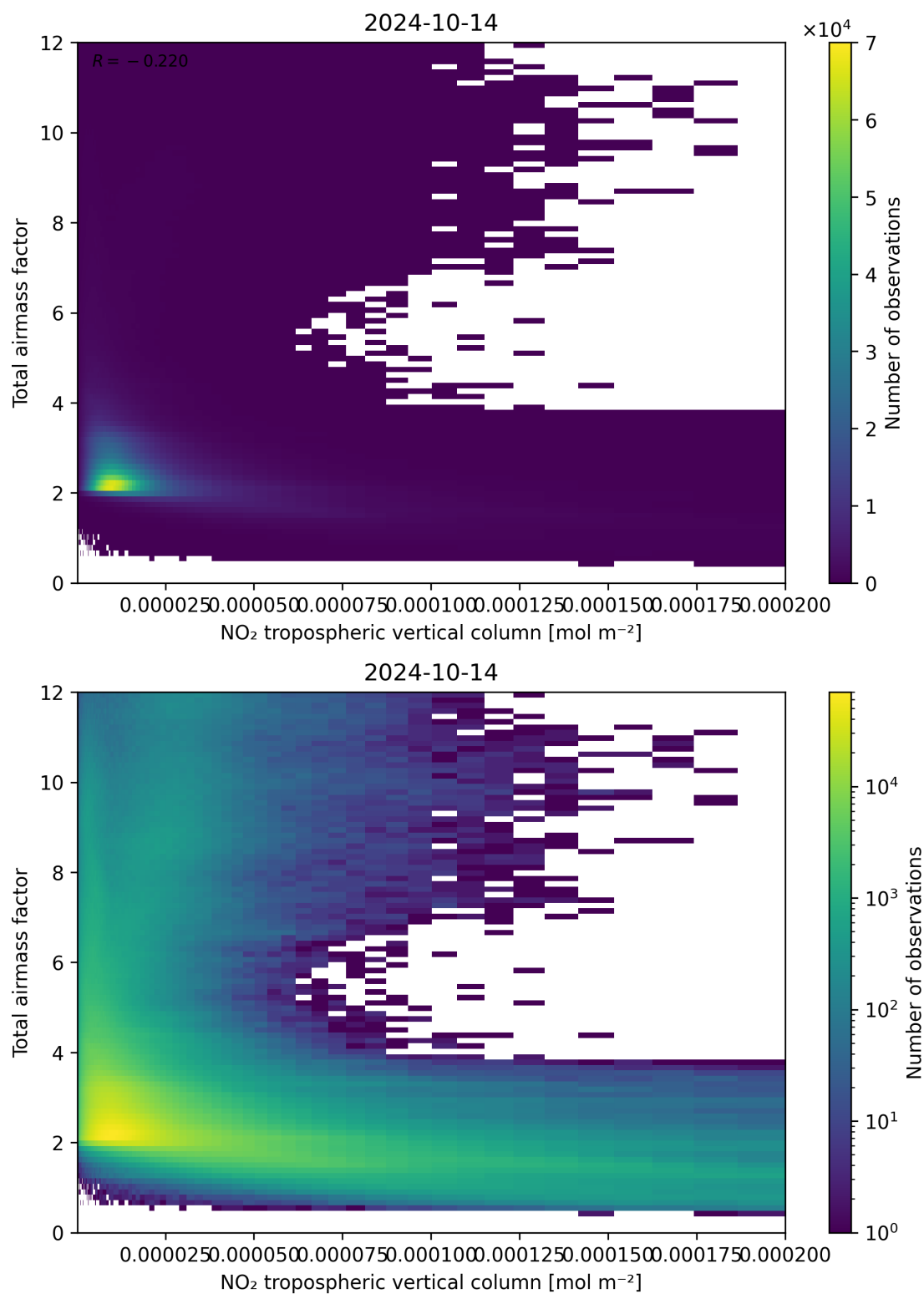
Figure 122: Scatter density plot of “NO 2 tropospheric vertical column” against “Total airmass factor” for 2024-10-14 to 2024-10-15.
