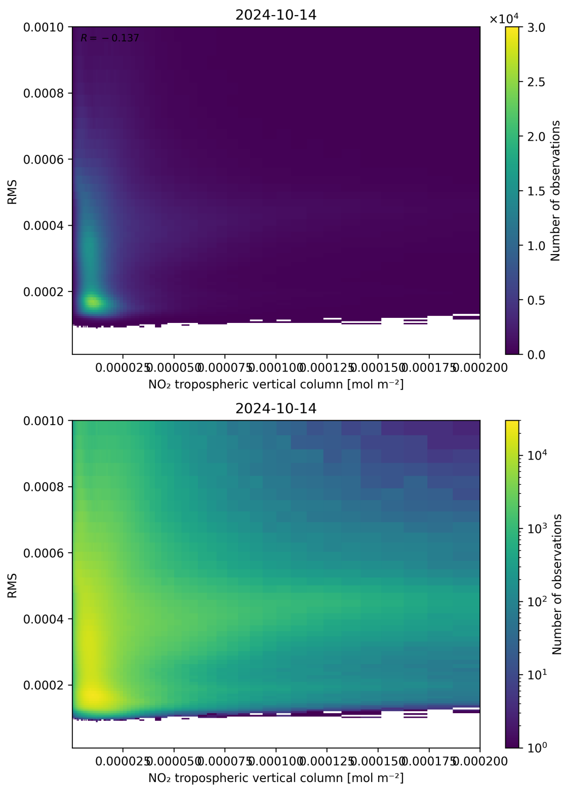
Figure 142: Scatter density plot of “NO 2 tropospheric vertical column” against “RMS” for 2024-10-14 to 2024-10-15.
