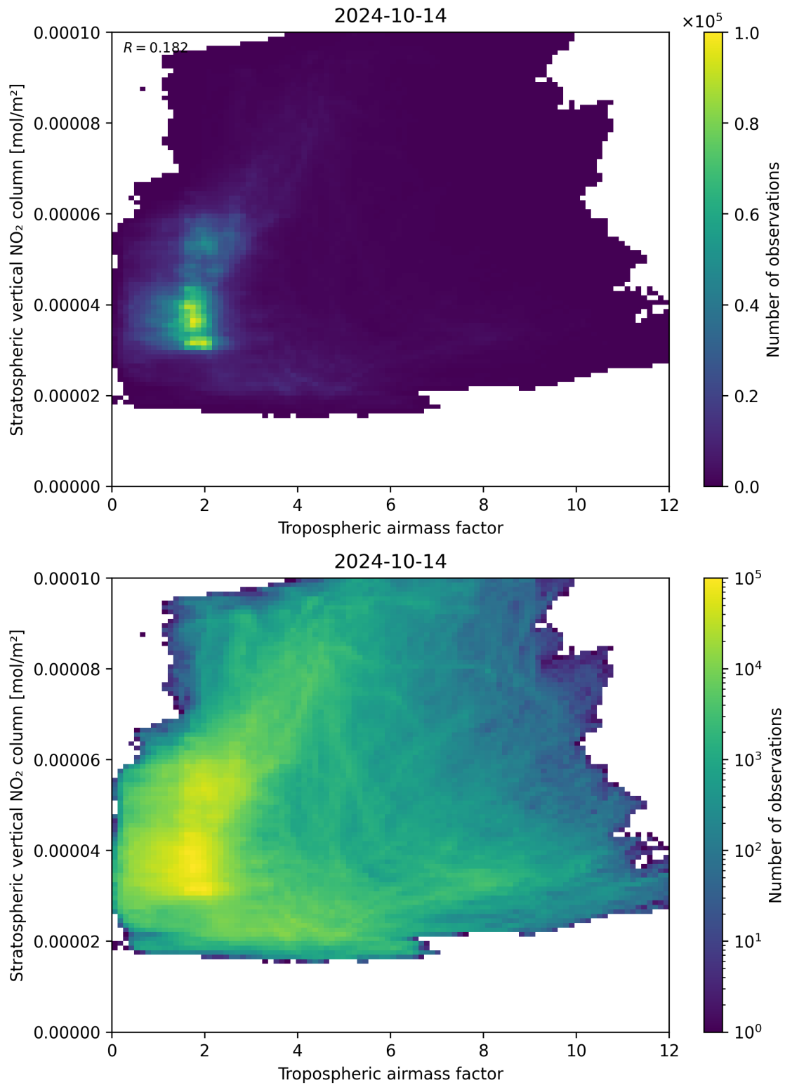
Figure 74: Scatter density plot of “Tropospheric air mass factor” against “Stratospheric vertical NO 2 column” for 2024-10-14 to 2024-10-15.
