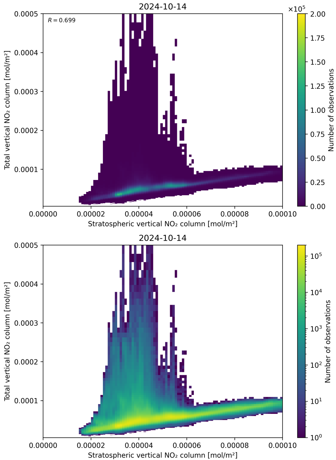
Figure 100: Scatter density plot of “Stratospheric vertical NO 2 column” against “Total vertical NO 2 column” for 2024-10-14 to 2024-10-15.
