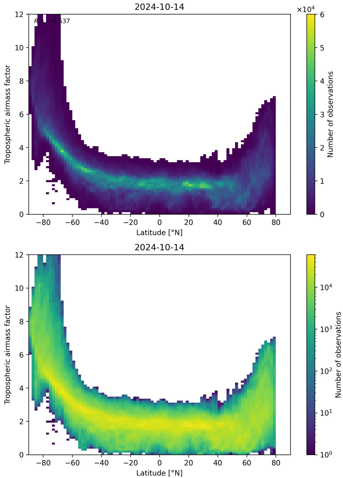
Figure 85: Scatter density plot of “Latitude” against “Tropospheric air mass factor” for 2024-10-14 to 2024-10-15.
