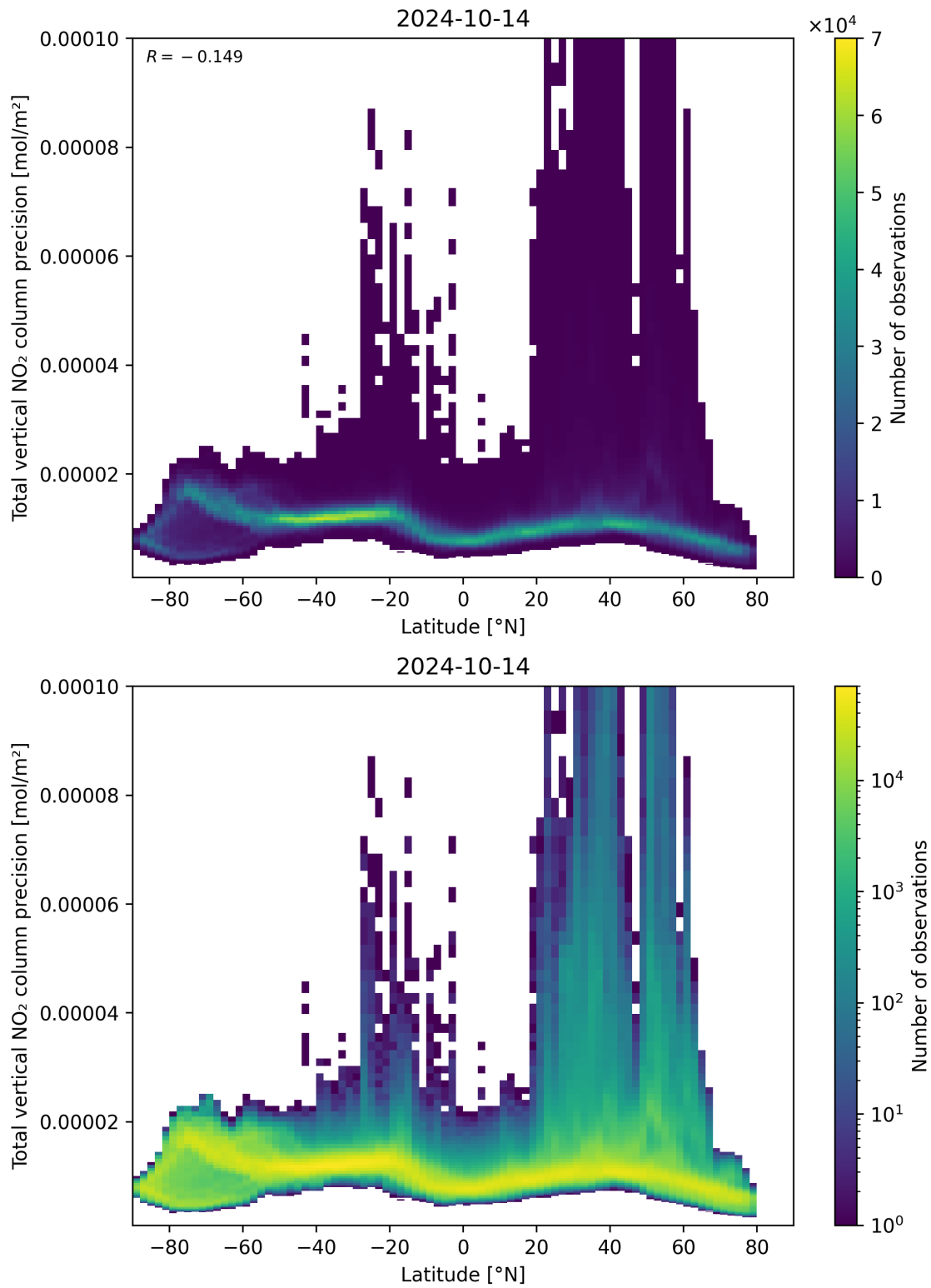
Figure 91: Scatter density plot of “Latitude” against “Total vertical NO 2 column precision” for 2024-10-14 to 2024-10-15.
