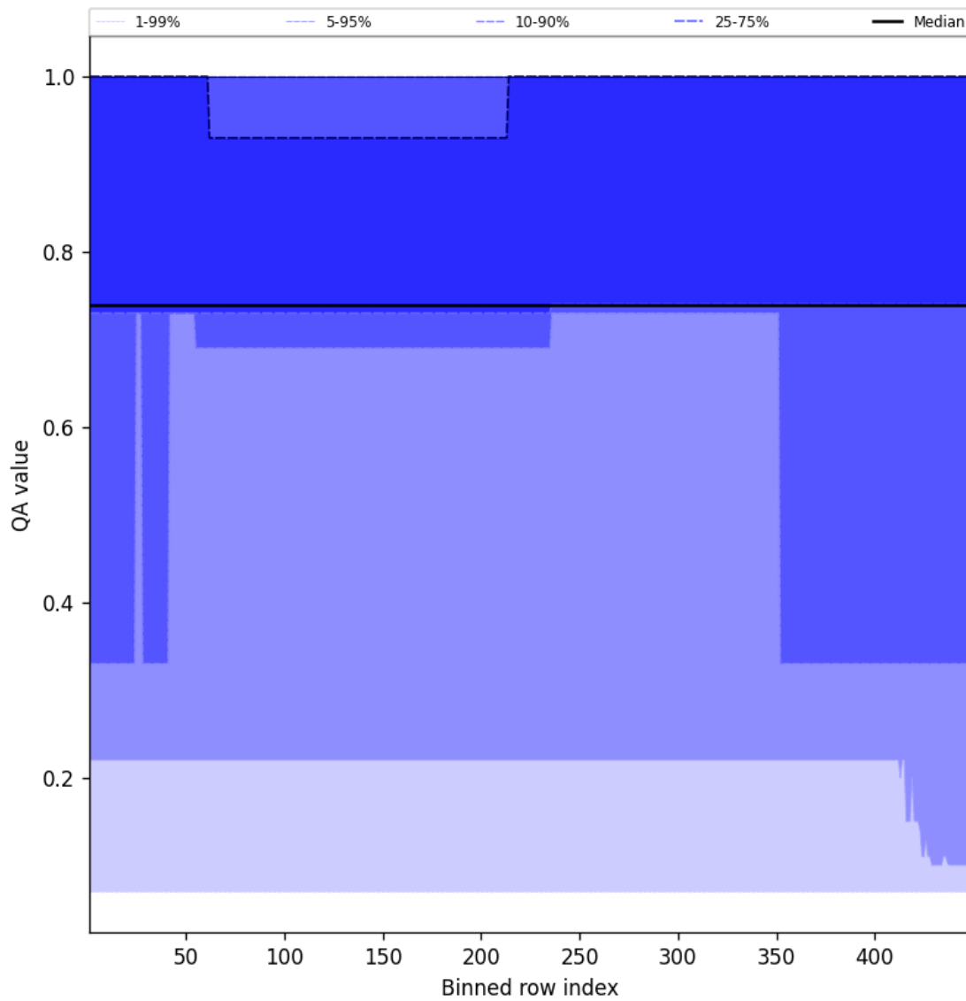
Figure 45: Along track statistics of “QA value” for 2024-10-14 to 2024-10-15
