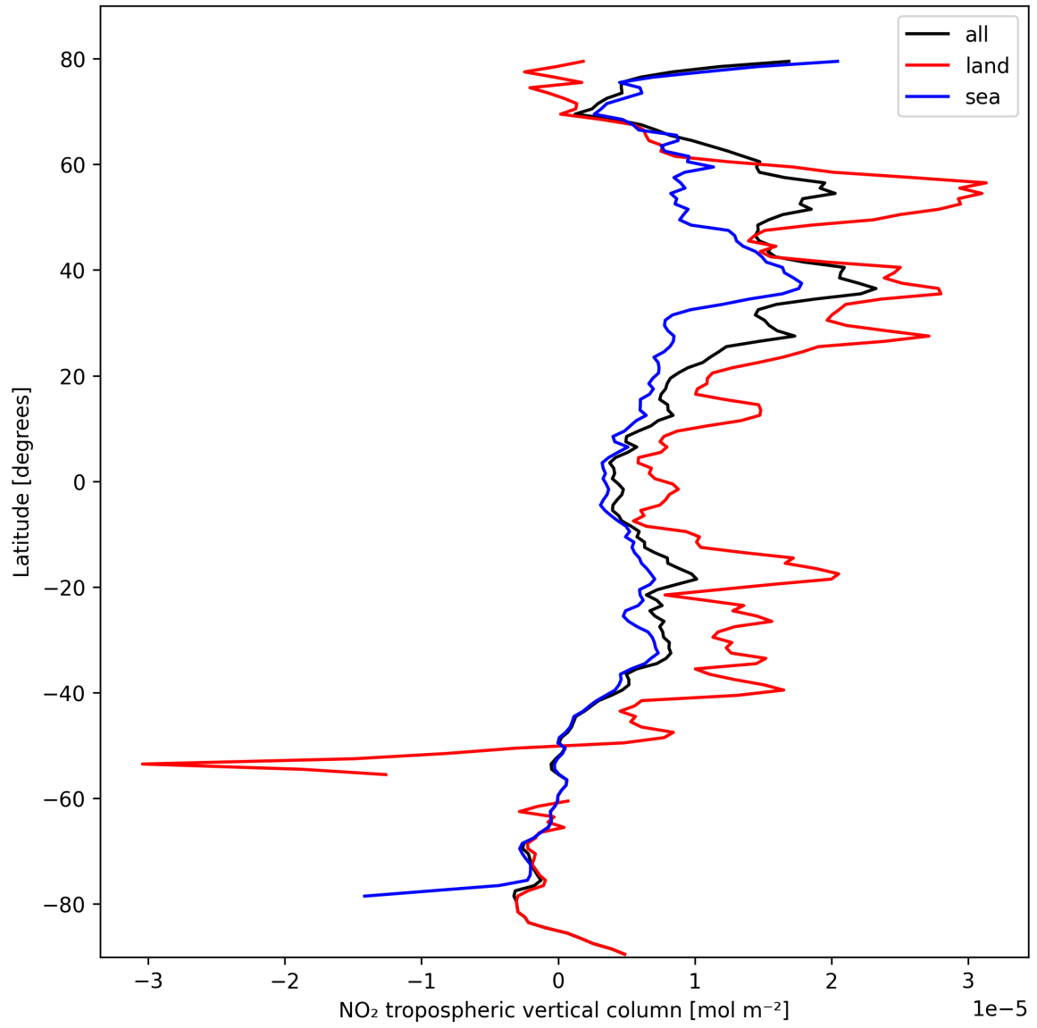
Figure 12: Zonal average of “NO 2 tropospheric vertical column” for 2024-10-14 to 2024-10-15.
