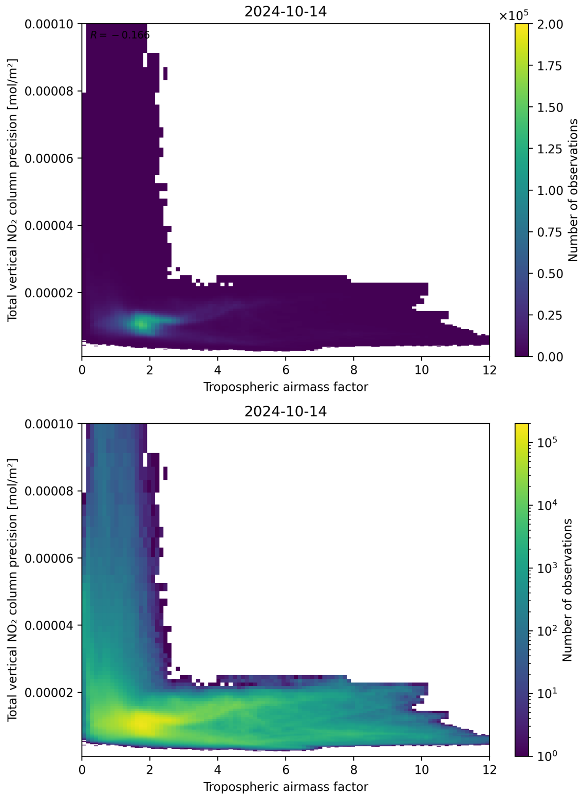
Figure 78: Scatter density plot of “Tropospheric air mass factor” against “Total vertical NO 2 column precision” for 2024-10-14 to 2024-10-15.
