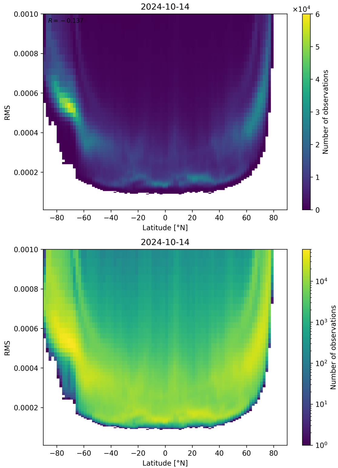
Figure 94: Scatter density plot of “Latitude” against “RMS” for 2024-10-14 to 2024-10-15.
