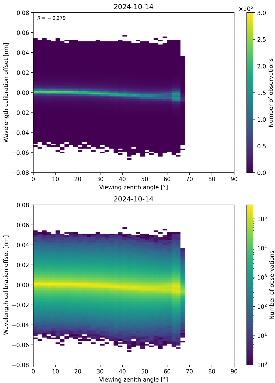
Figure 173: Scatter density plot of “Viewing zenith angle” against “Wavelength calibration offset” for 2024-10-14 to 2024-10-15.
