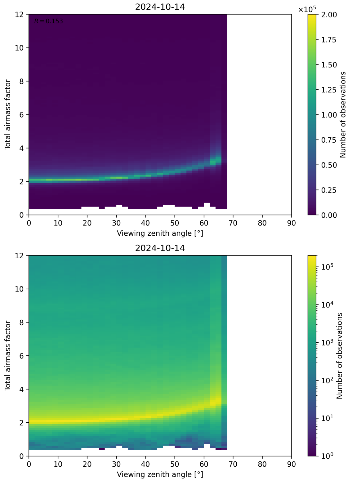
Figure 160: Scatter density plot of “Viewing zenith angle” against “Total airmass factor” for 2024-10-14 to 2024-10-15.
