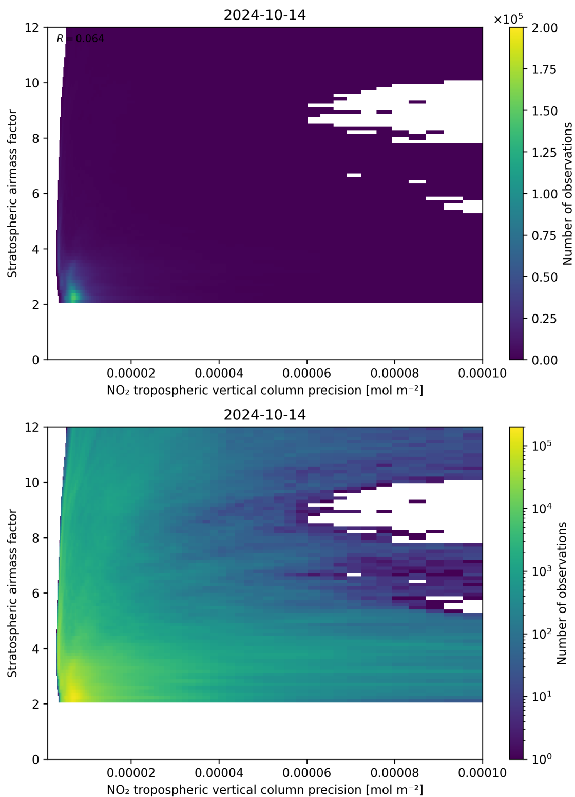
Figure 131: Scatter density plot of “NO 2 tropospheric vertical column precision” against “Stratospheric airmass factor” for 2024-10-14 to 2024-10-15.
