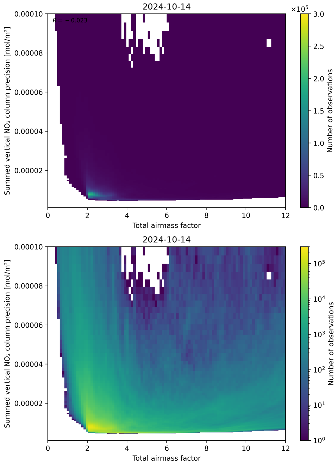
Figure 66: Scatter density plot of “Total airmass factor” against “Summed vertical NO 2 column precision” for 2024-10-14 to 2024-10-15.
