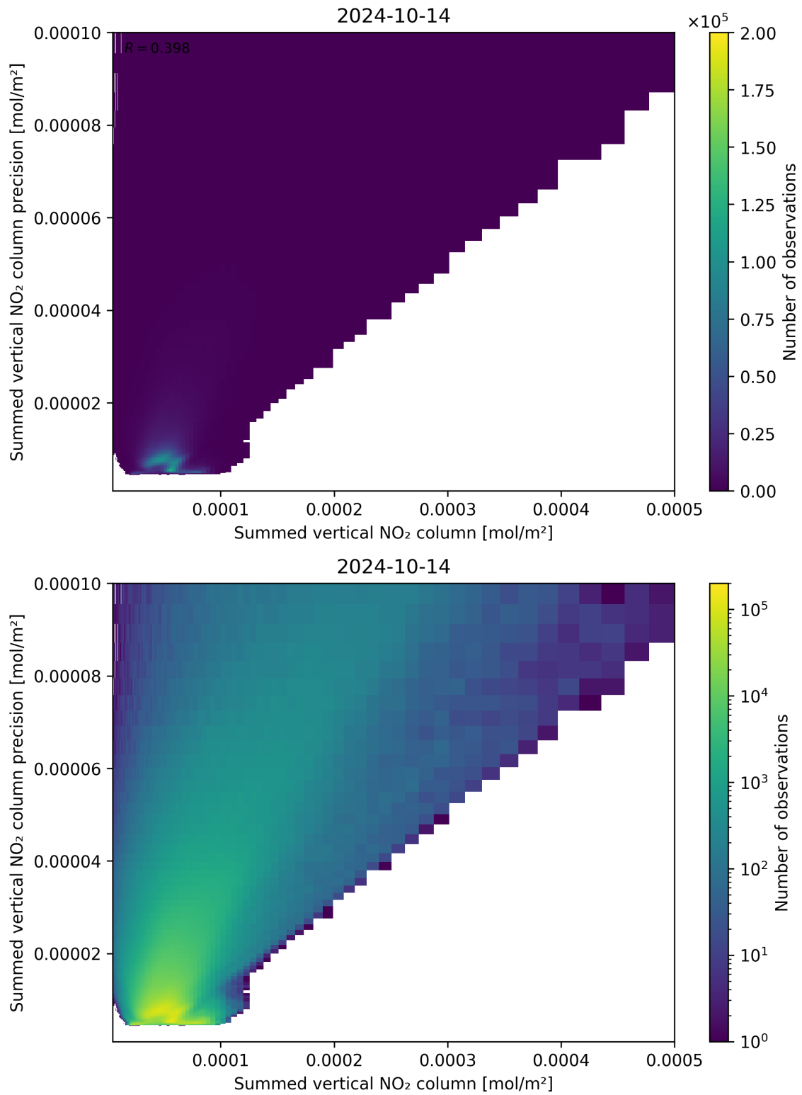
Figure 105: Scatter density plot of “Summed vertical NO 2 column” against “Summed vertical NO 2 column precision” for 2024-10-14 to 2024-10-15.
