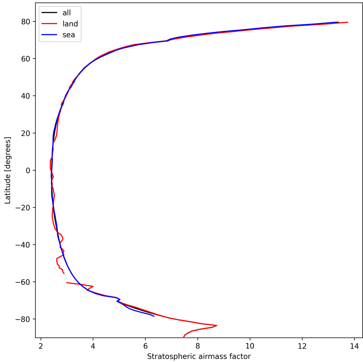
Figure 27: Zonal average of “Stratospheric air mass factor” for 2024-10-14 to 2024-10-15.
