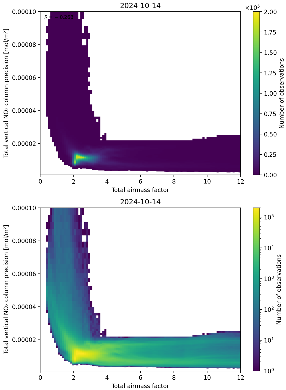
Figure 68: Scatter density plot of “Total airmass factor” against “Total vertical NO 2 column precision” for 2024-10-14 to 2024-10-15.
