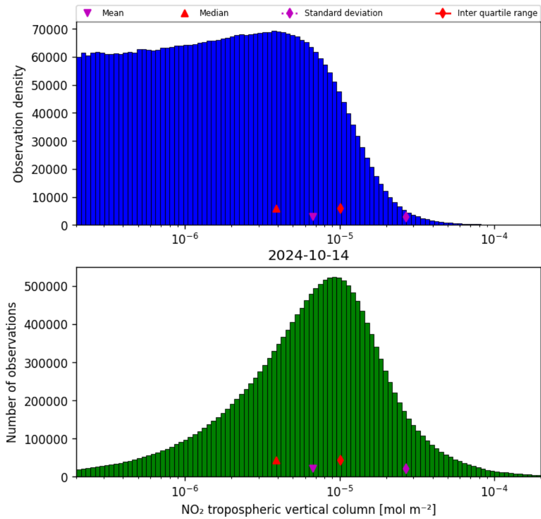
Figure 29: Histogram of “NO 2 tropospheric vertical column” for 2024-10-14 to 2024-10-15
