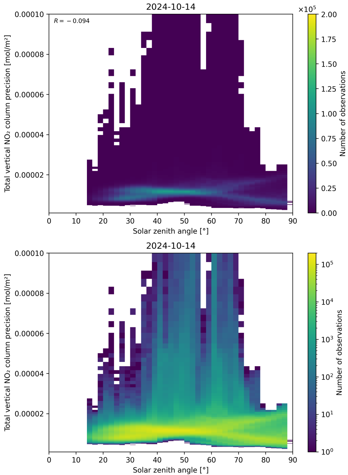
Figure 154: Scatter density plot of “Solar zenith angle” against “Total vertical NO 2 column precision” for 2024-10-14 to 2024-10-15.
