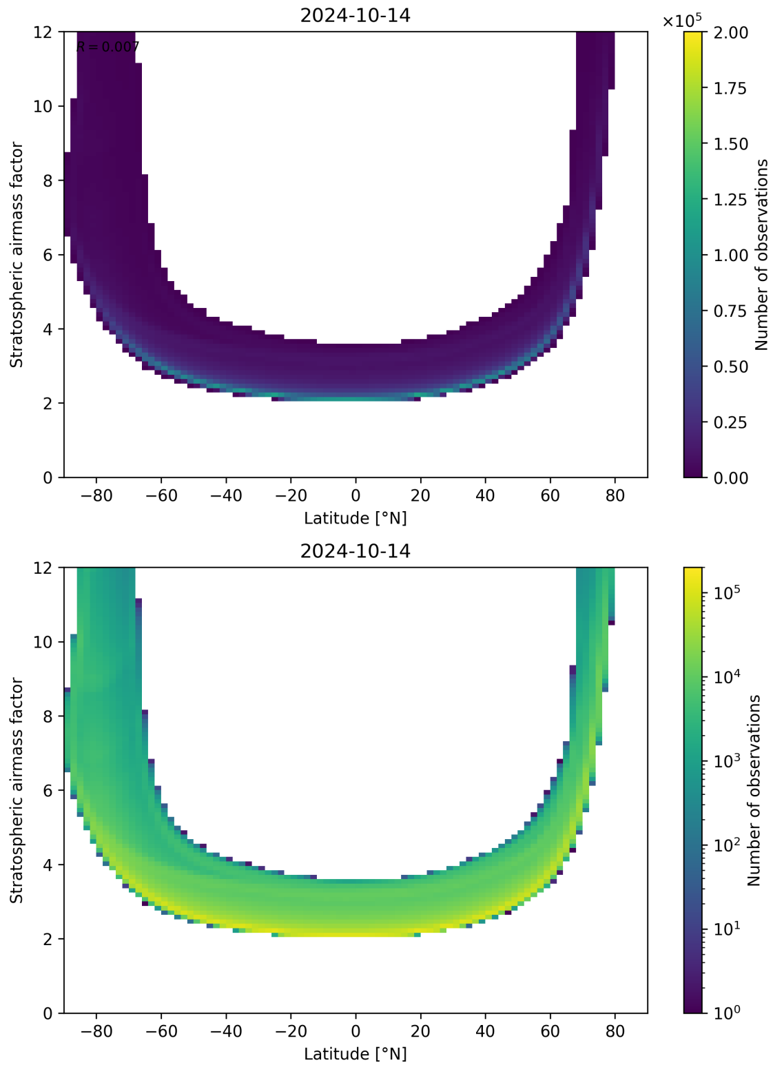
Figure 83: Scatter density plot of “Latitude” against “Stratospheric air mass factor” for 2024-10-14 to 2024-10-15.
