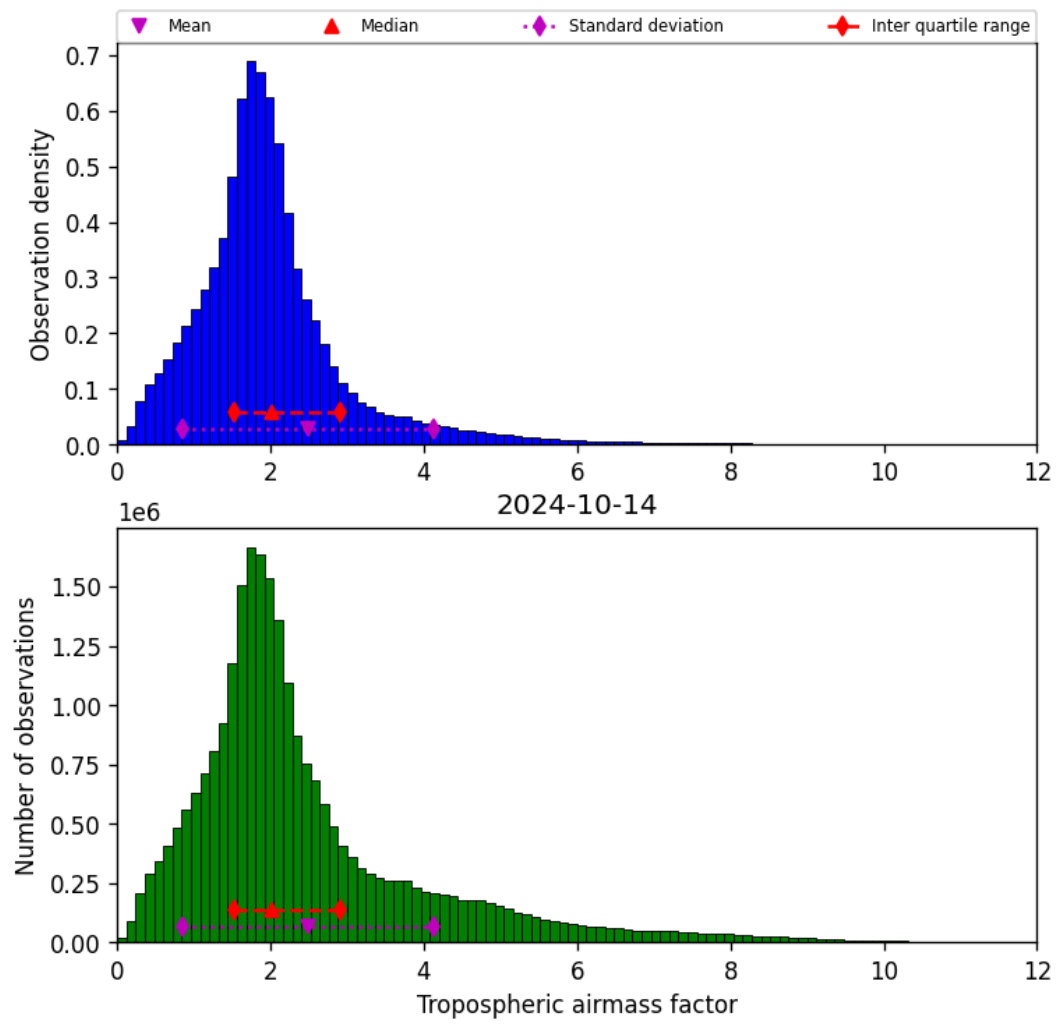
Figure 31: Histogram of “Tropospheric airmass factor” for 2024-10-14 to 2024-10-15
