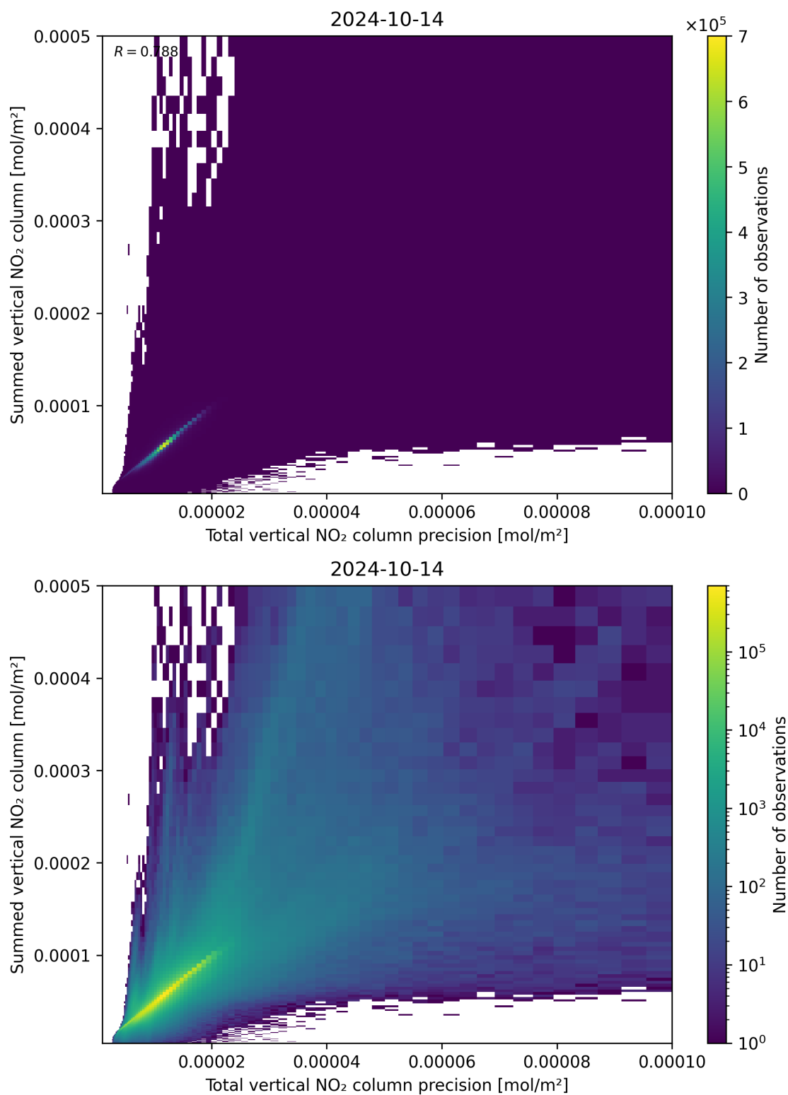
Figure 117: Scatter density plot of “Total vertical NO 2 column precision” against “Summed vertical NO 2 column” for 2024-10-14 to 2024-10-15.
