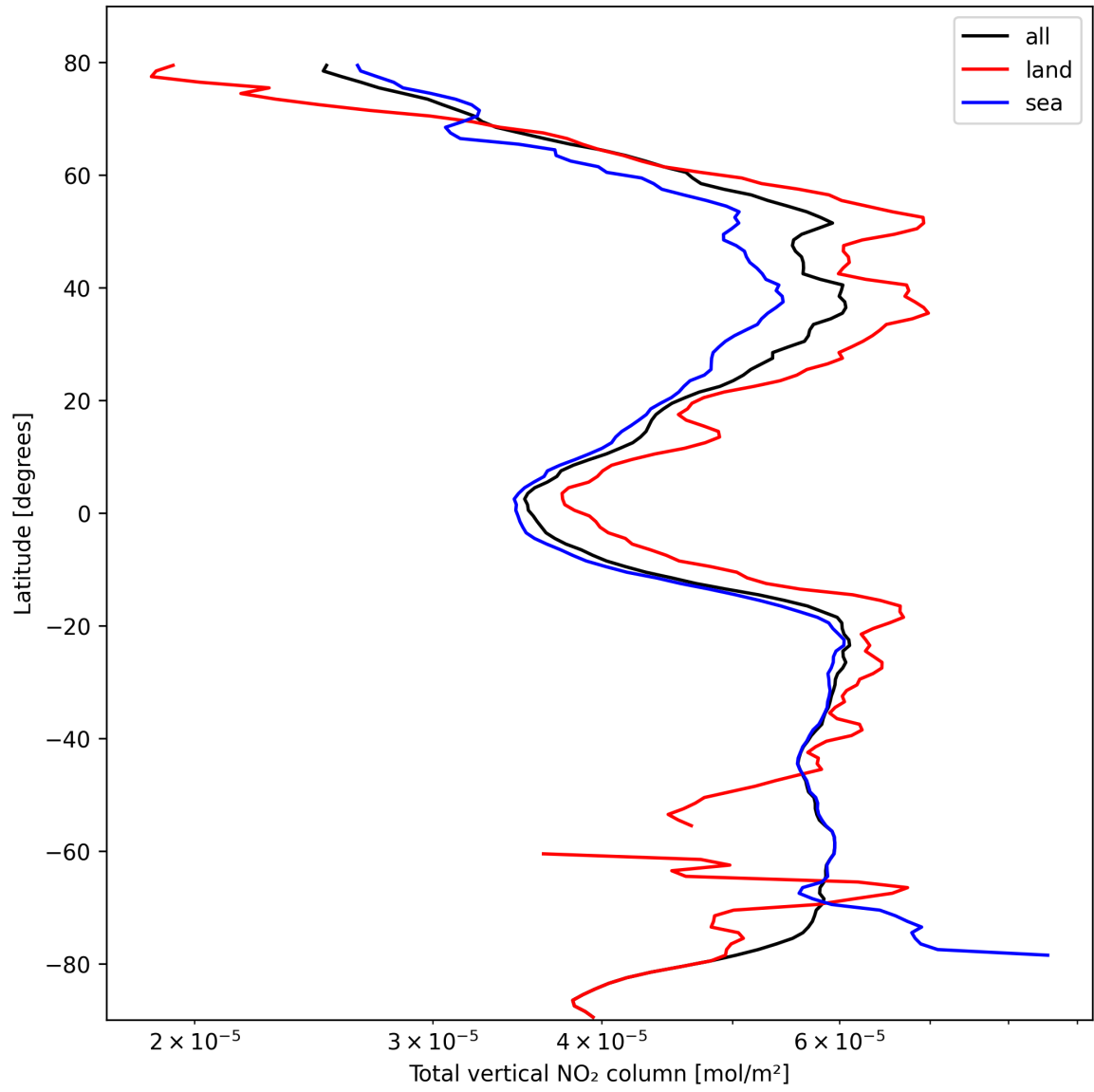
Figure 21: Zonal average of “Total vertical NO 2 column” for 2024-10-14 to 2024-10-15.
