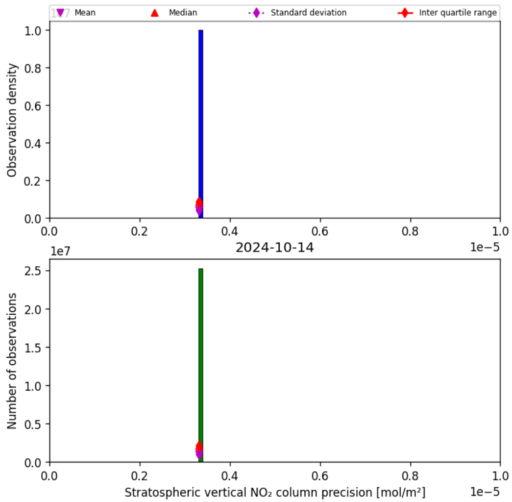
Figure 37: Histogram of “Stratospheric vertical NO 2 column precision” for 2024-10-14 to 2024-10-15
