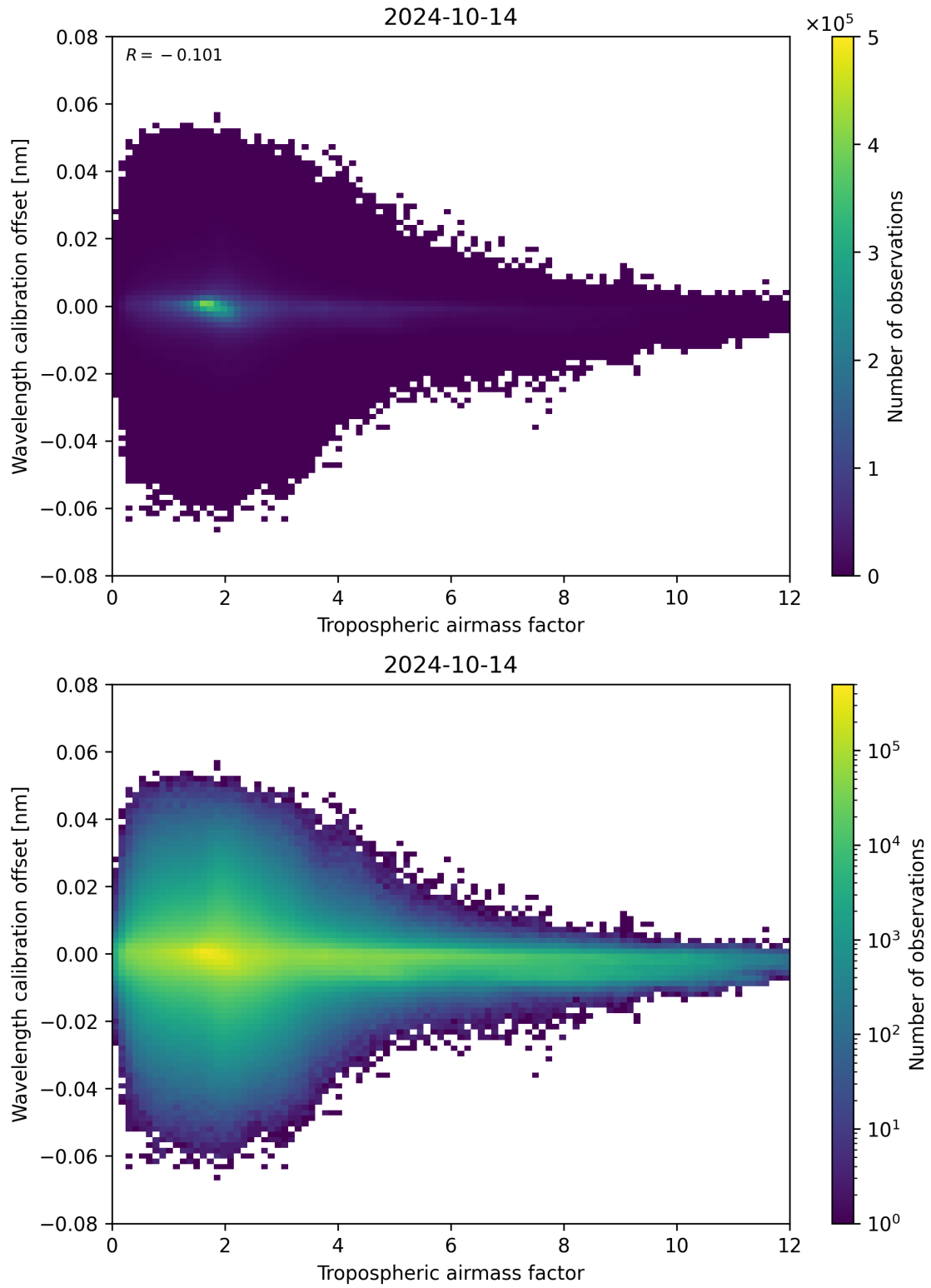
Figure 80: Scatter density plot of “Tropospheric airmass factor” against “Wavelength calibration offset” for 2024-10-14 to 2024-10-15.
