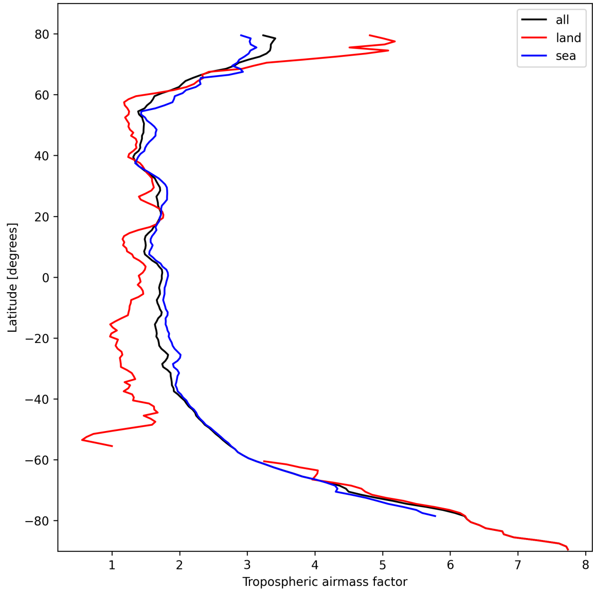
Figure 14: Zonal average of “Tropospheric airmass factor” for 2024-10-14 to 2024-10-15.
