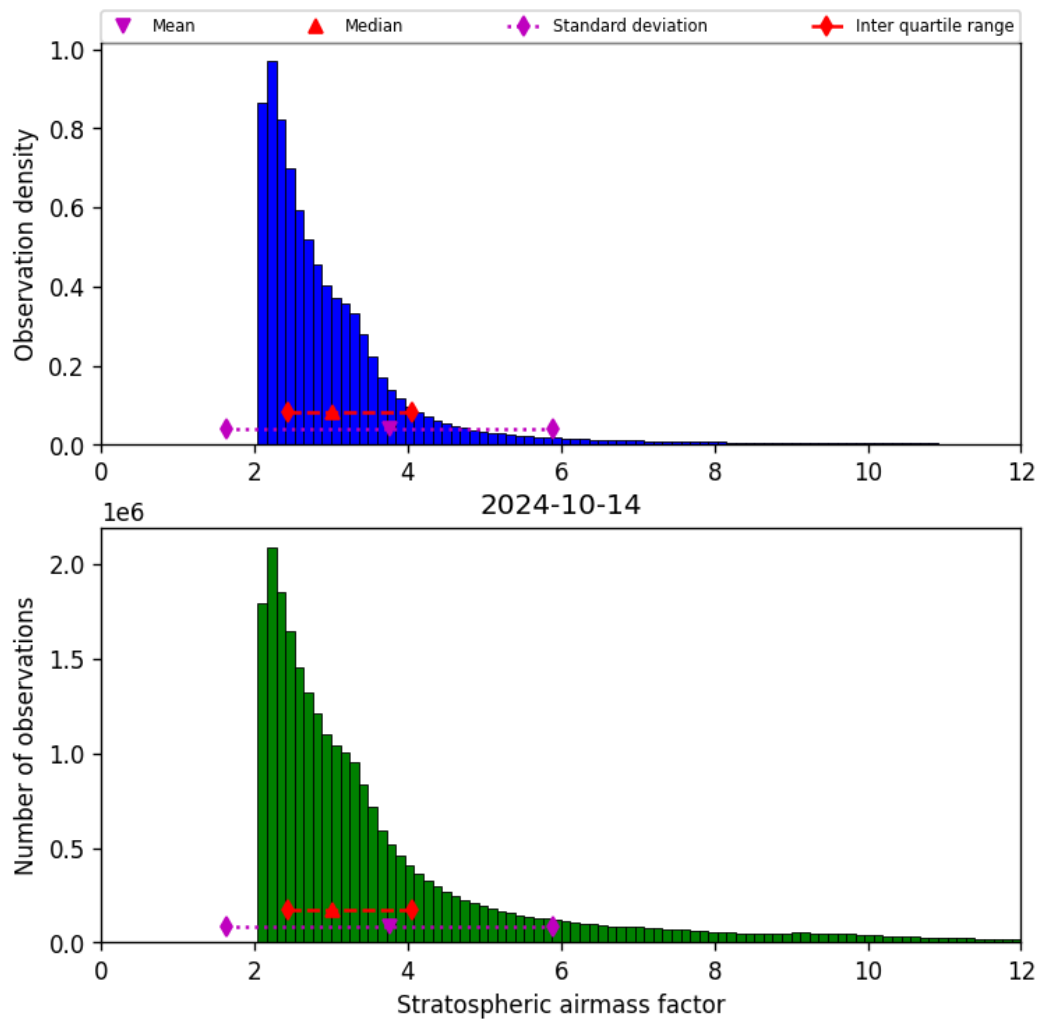
Figure 44: Histogram of “Stratospheric airmass factor” for 2024-10-14 to 2024-10-15
