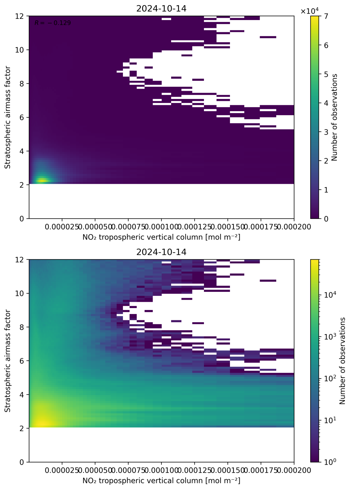
Figure 121: Scatter density plot of “NO 2 tropospheric vertical column” against “Stratospheric airmass factor” for 2024-10-14 to 2024-10-15.
