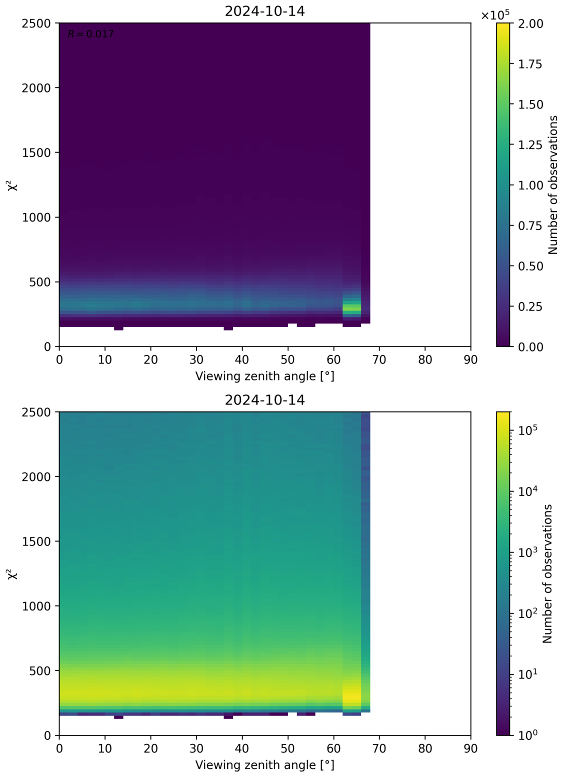
Figure 162: Scatter density plot of “Viewing zenith angle” against “ \chi^2 ” for 2024-10-14 to 2024-10-15.
