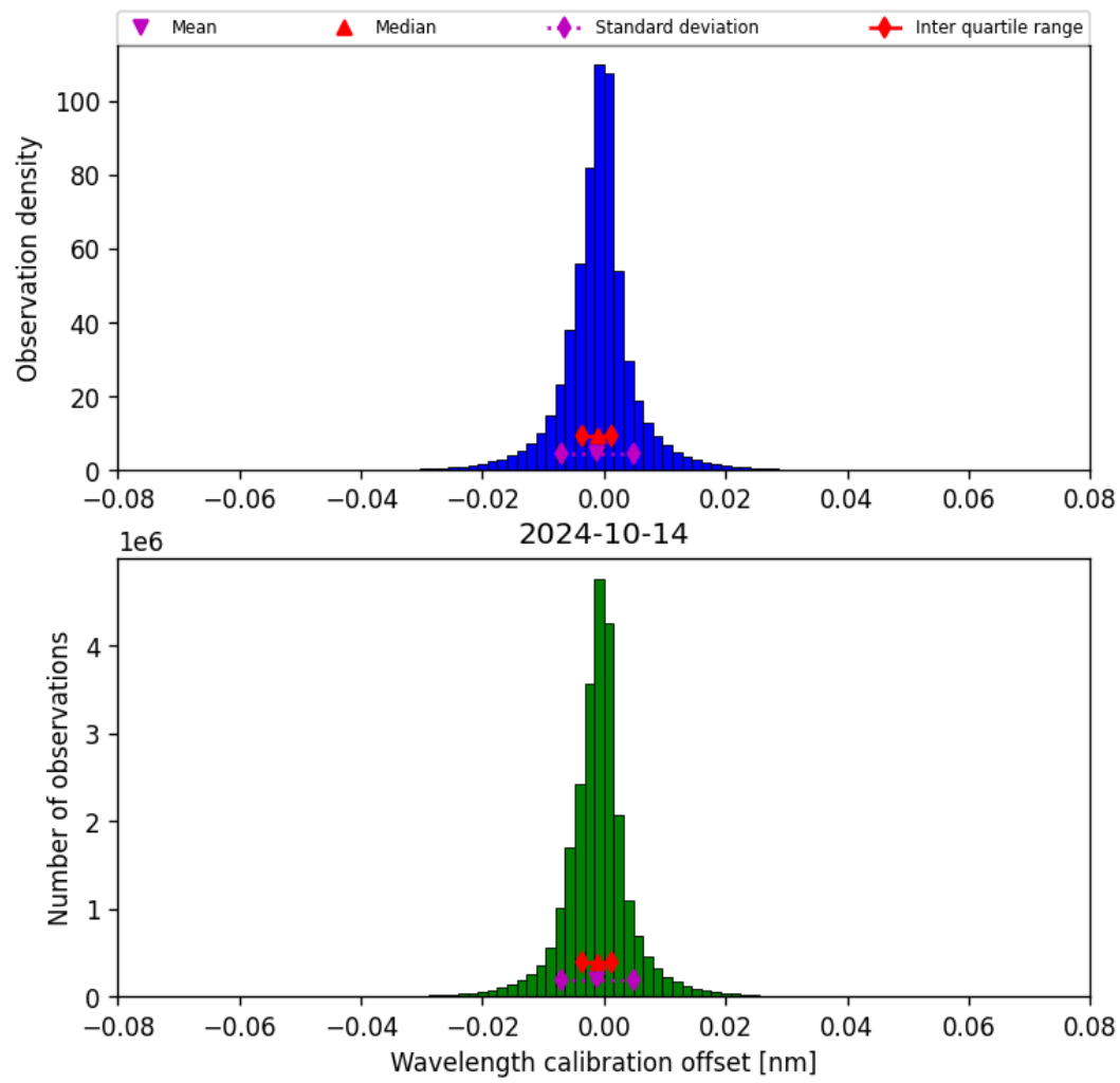
Figure 35: Histogram of “Wavelength calibration offset” for 2024-10-14 to 2024-10-15
