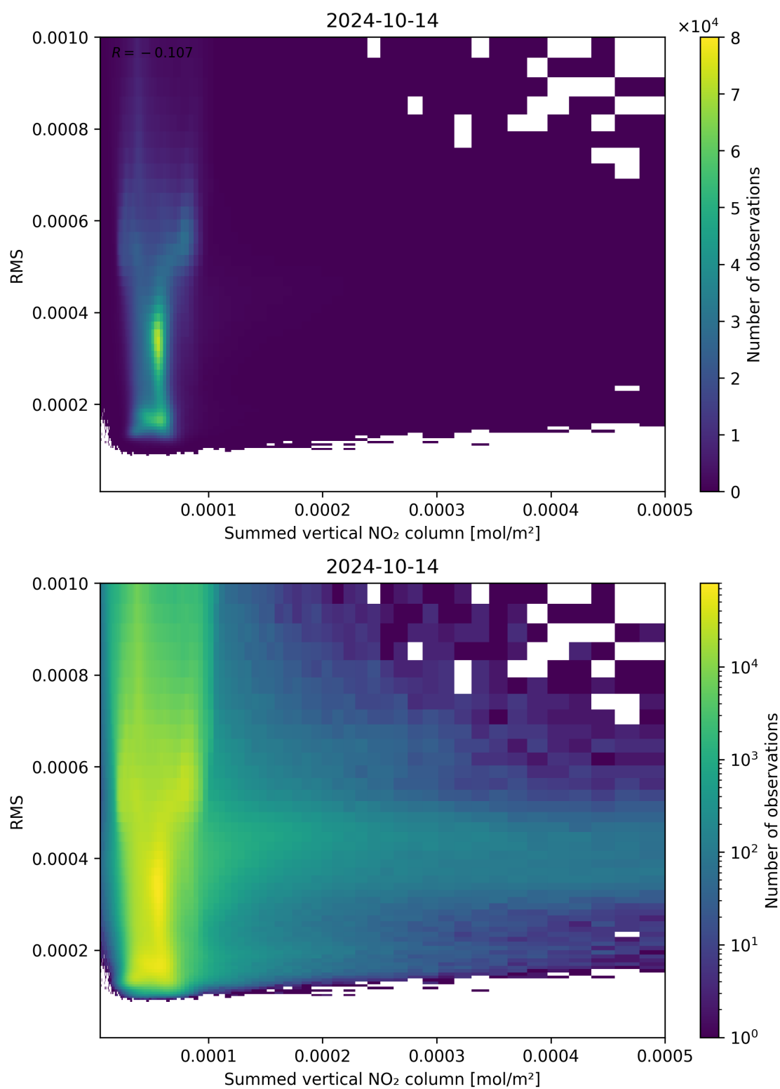
Figure 109: Scatter density plot of “Summed vertical NO 2 column” against “RMS” for 2024-10-14 to 2024-10-15.
