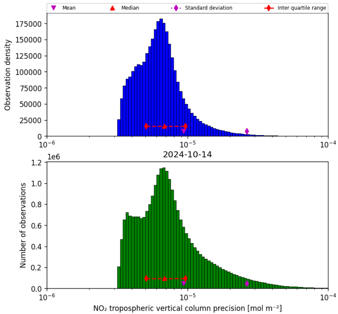
Figure 30: Histogram of “NO 2 tropospheric vertical column precision” for 2024-10-14 to 2024-10-15
