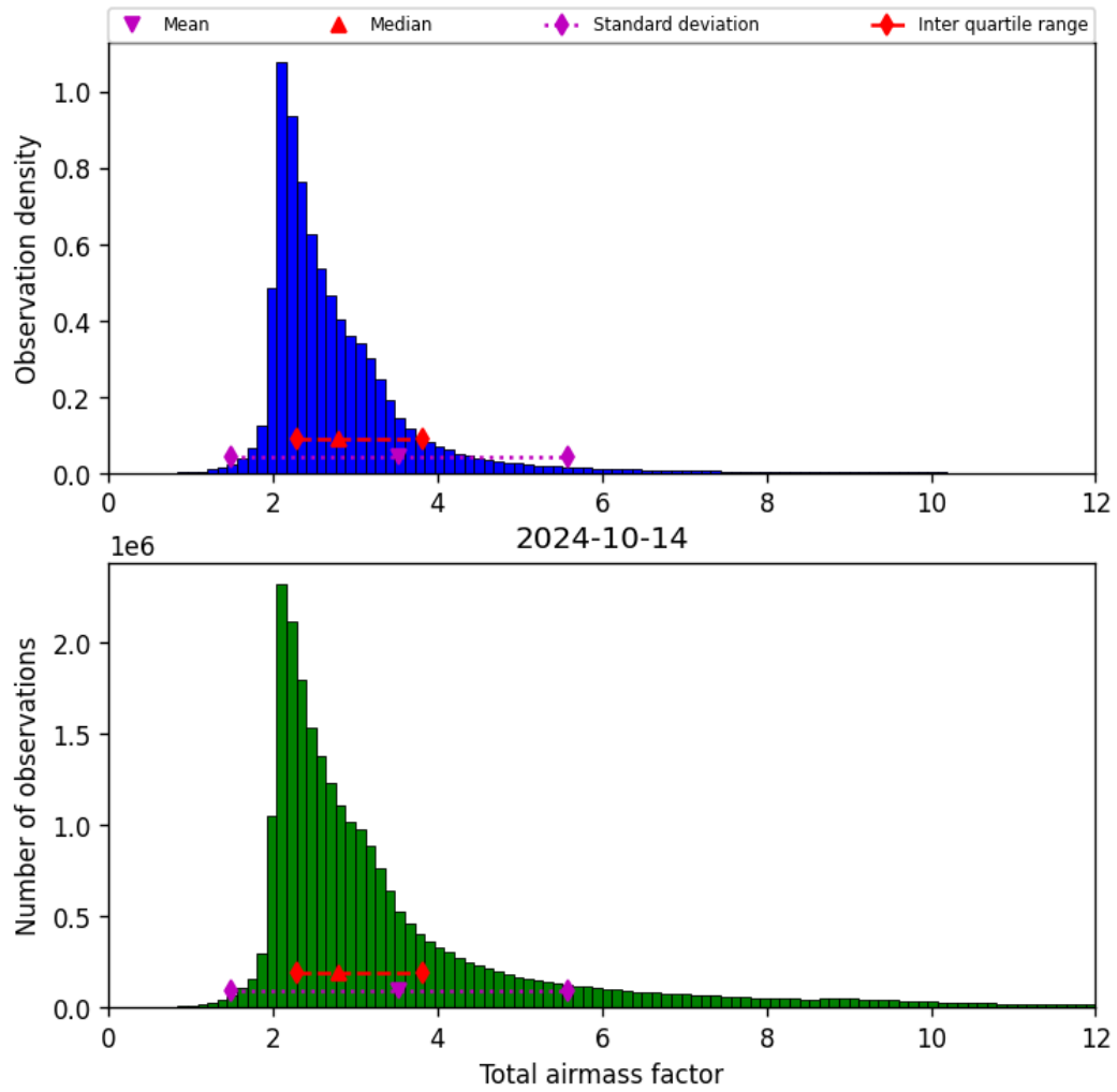
Figure 32: Histogram of “Total airmass factor” for 2024-10-14 to 2024-10-15
