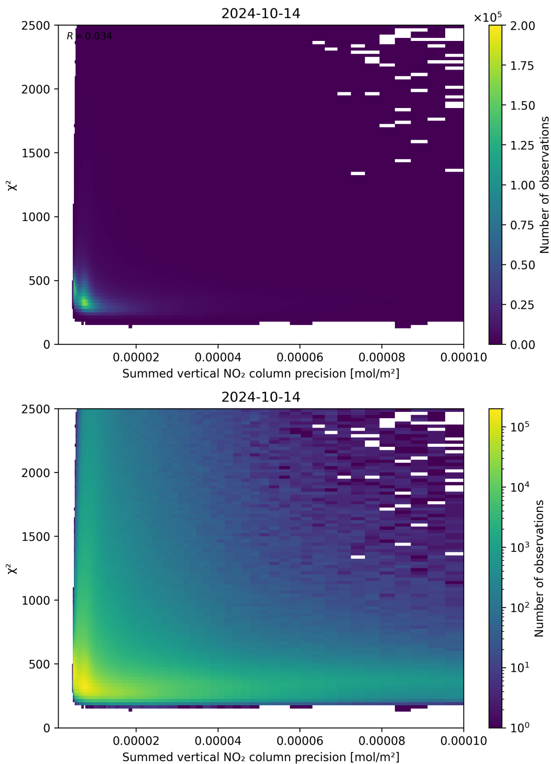
Figure 107: Scatter density plot of “Summed vertical NO 2 column precision” against “ \chi^2 ” for 2024-10-14 to 2024-10-15.
