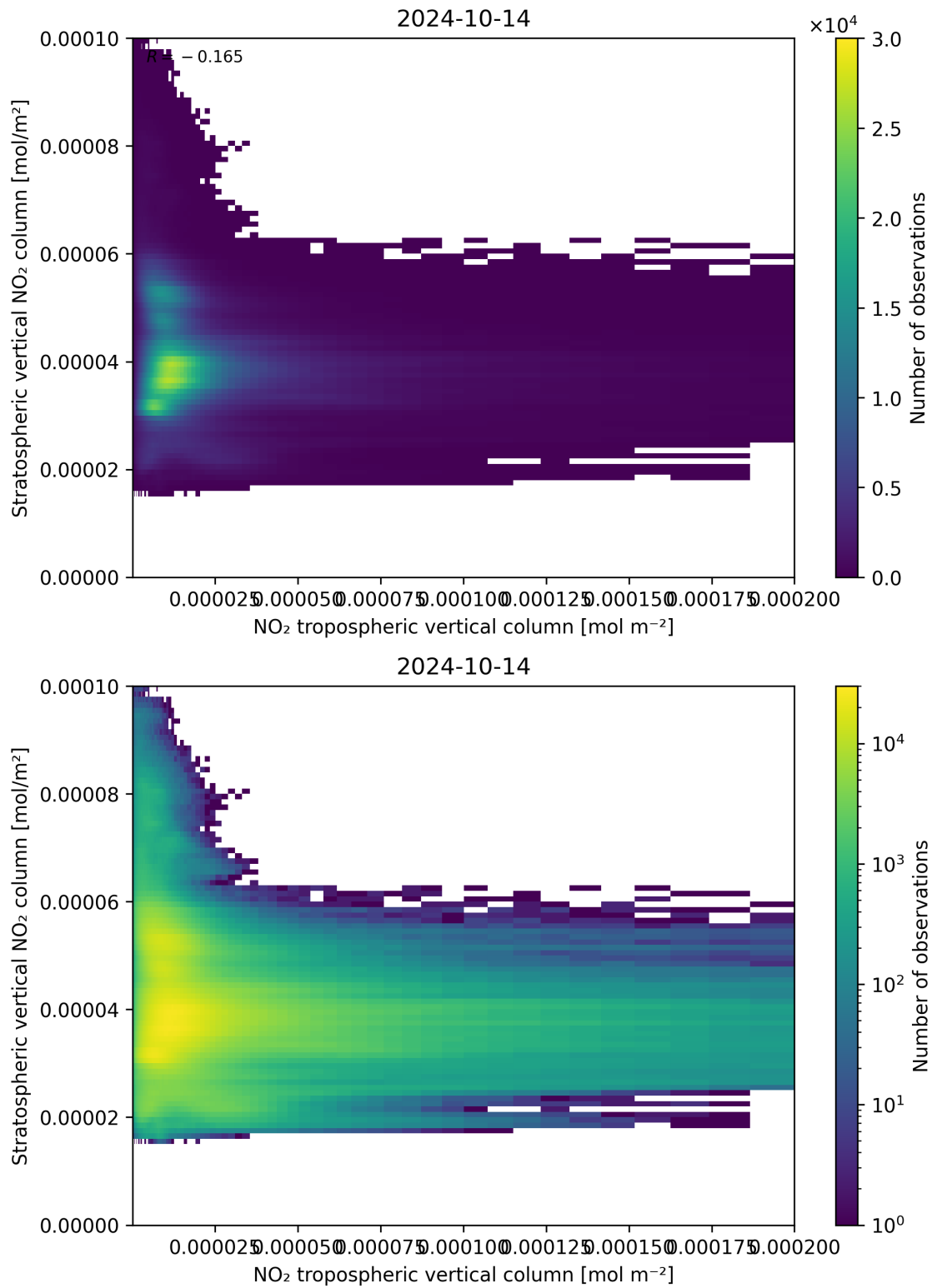
Figure 125: Scatter density plot of “NO 2 tropospheric vertical column” against “Stratospheric vertical NO 2 column” for 2024-10-14 to 2024-10-15.
