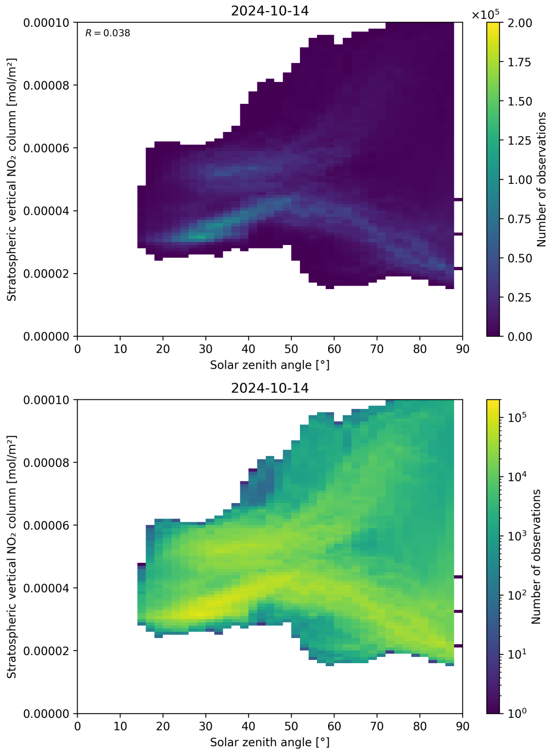
Figure 150: Scatter density plot of “Solar zenith angle” against “Stratospheric vertical NO 2 column” for 2024-10-14 to 2024-10-15.
