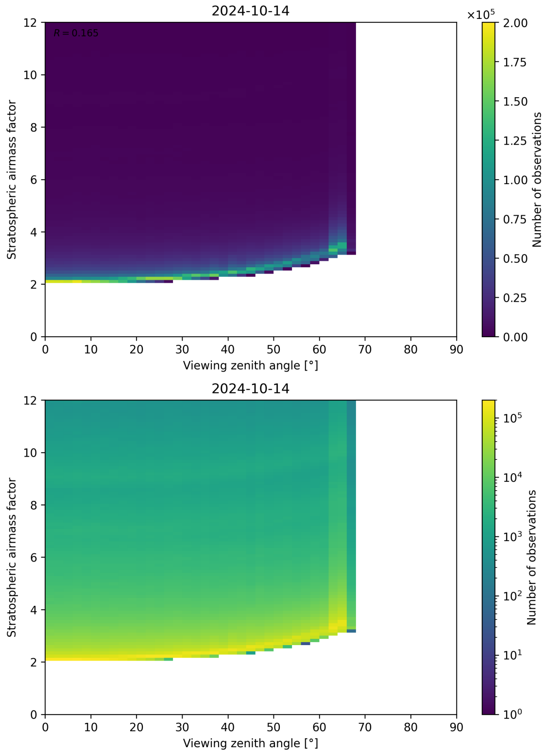
Figure 159: Scatter density plot of “Viewing zenith angle” against “Stratospheric airmass factor” for 2024-10-14 to 2024-10-15.
