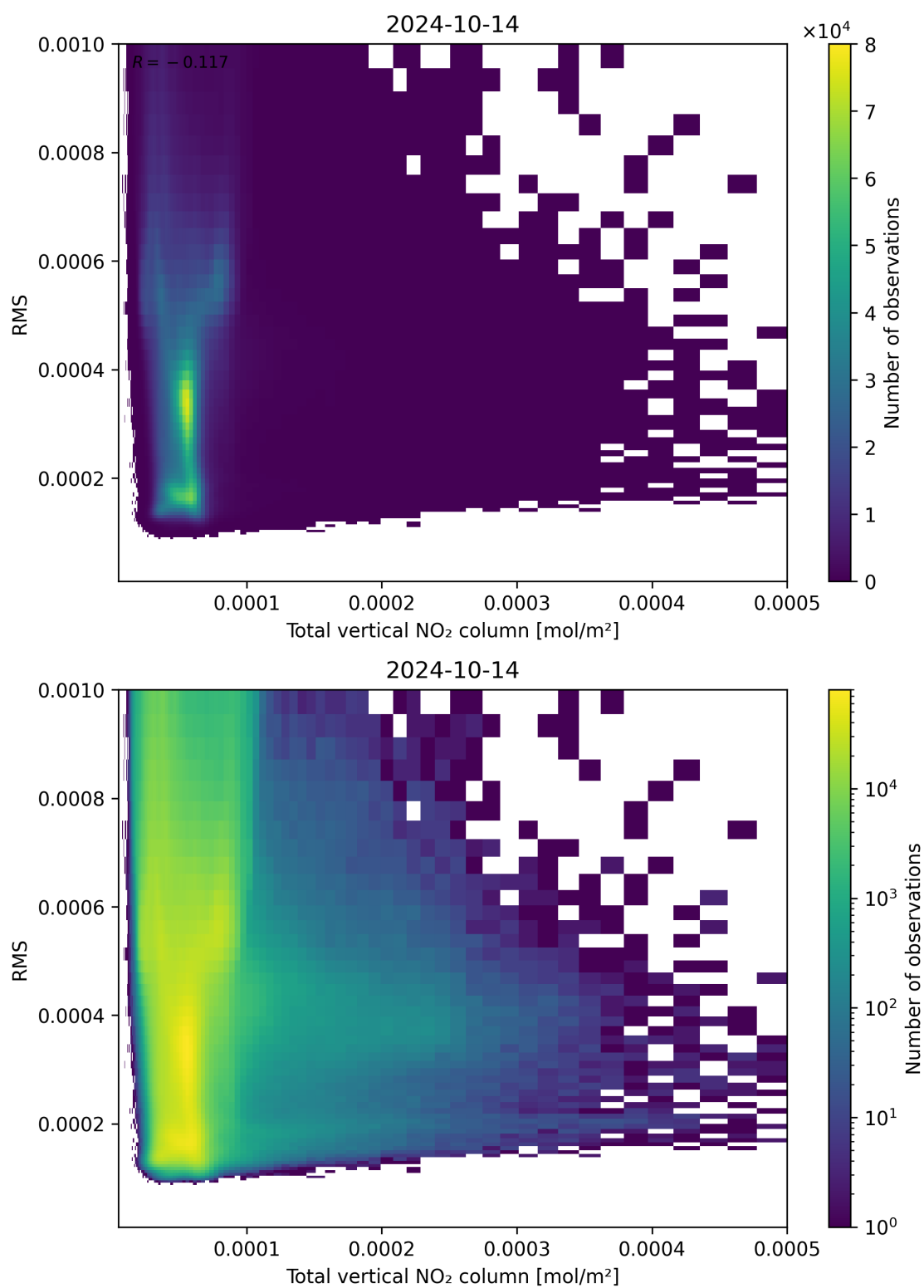
Figure 120: Scatter density plot of “Total vertical NO 2 column” against “RMS” for 2024-10-14 to 2024-10-15.
