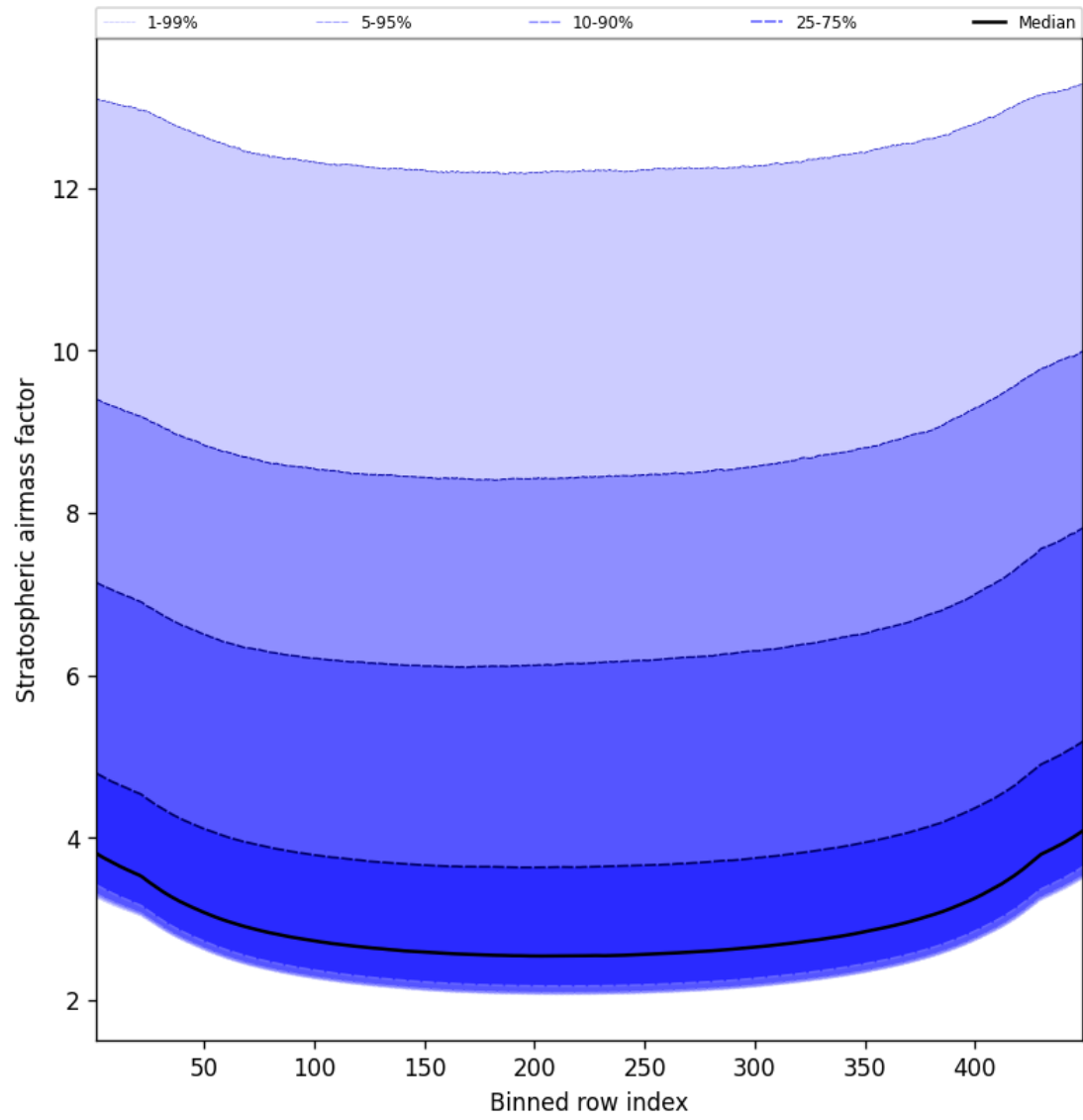
Figure 61: Along track statistics of “Stratospheric airmass factor” for 2024-10-14 to 2024-10-15
