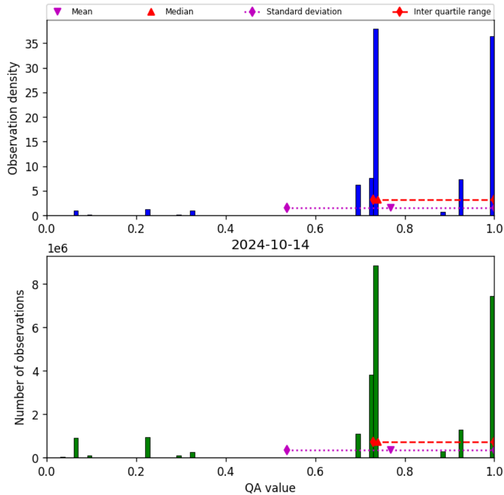
Figure 28: Histogram of “QA value” for 2024-10-14 to 2024-10-15
