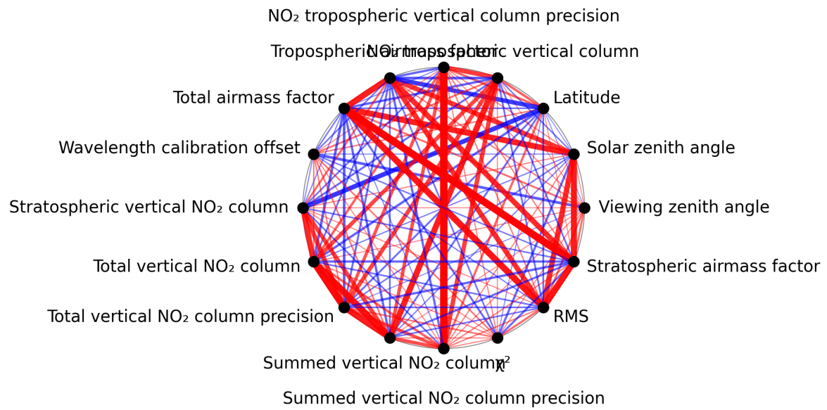
Figure 1: Map of correlation graph for 2024-10-14 to 2024-10-15.
