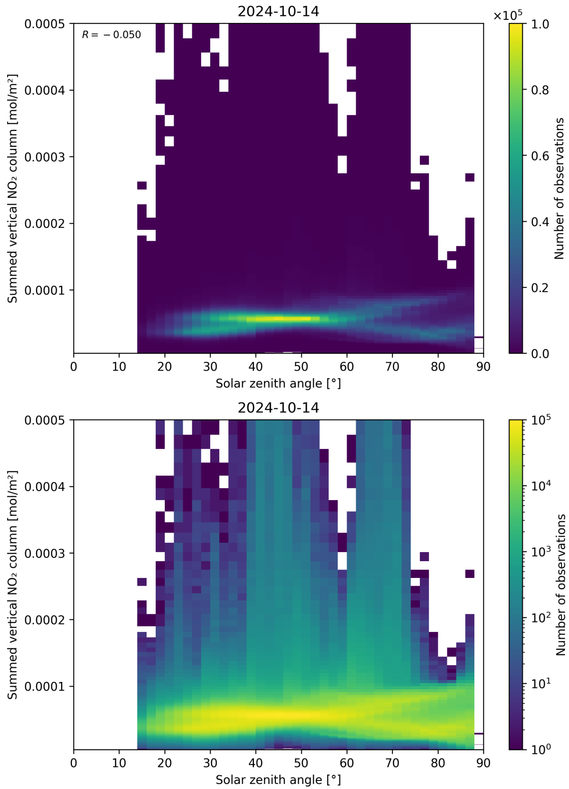
Figure 151: Scatter density plot of “Solar zenith angle” against “Summed vertical NO 2 column” for 2024-10-14 to 2024-10-15.
