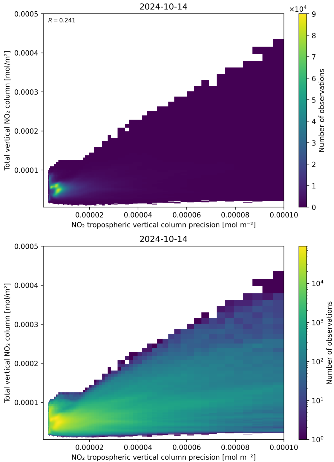
Figure 138: Scatter density plot of “NO 2 tropospheric vertical column precision” against “Total vertical NO 2 column” for 2024-10-14 to 2024-10-15.
