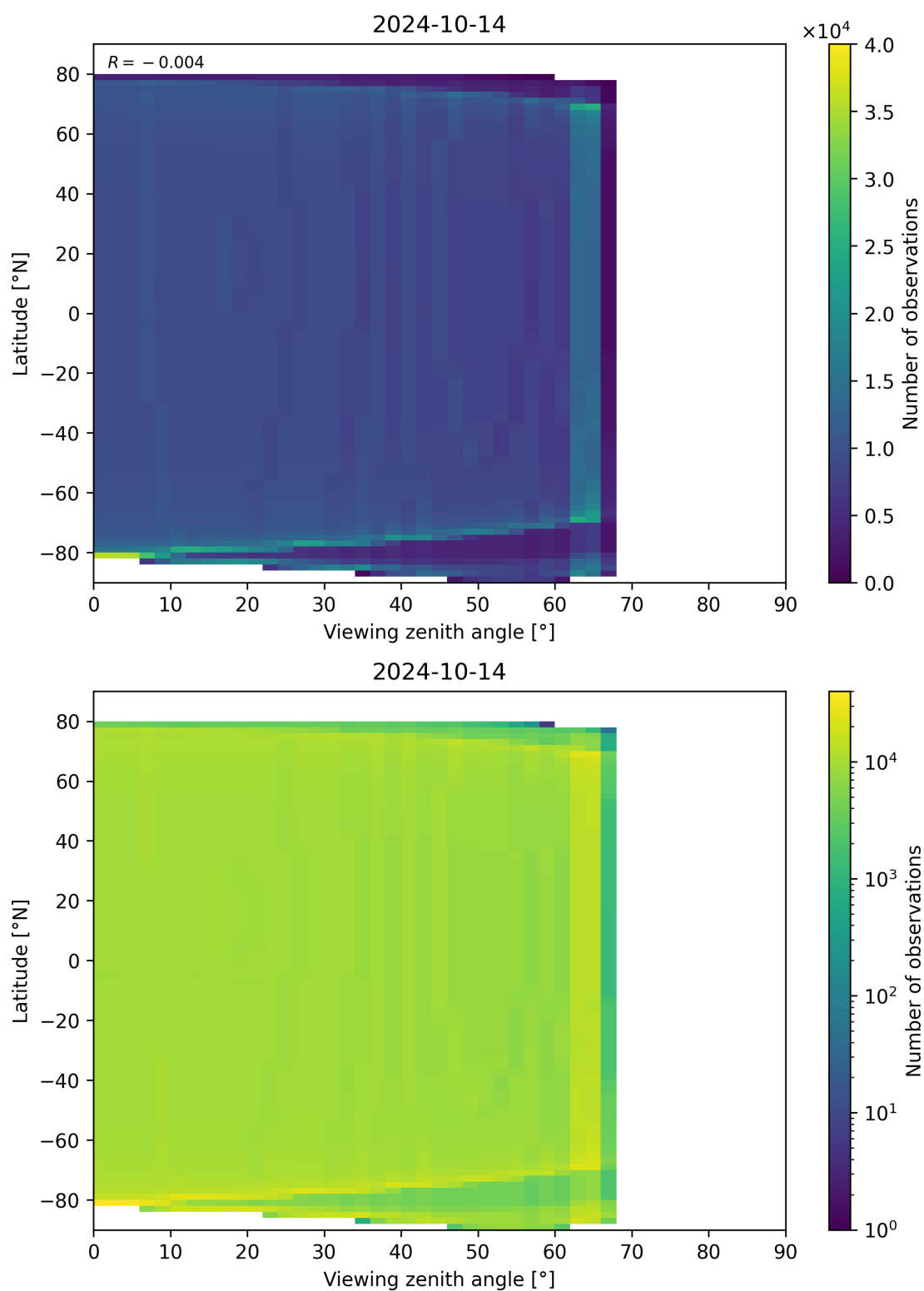
Figure 163: Scatter density plot of “Viewing zenith angle” against “Latitude” for 2024-10-14 to 2024-10-15.
