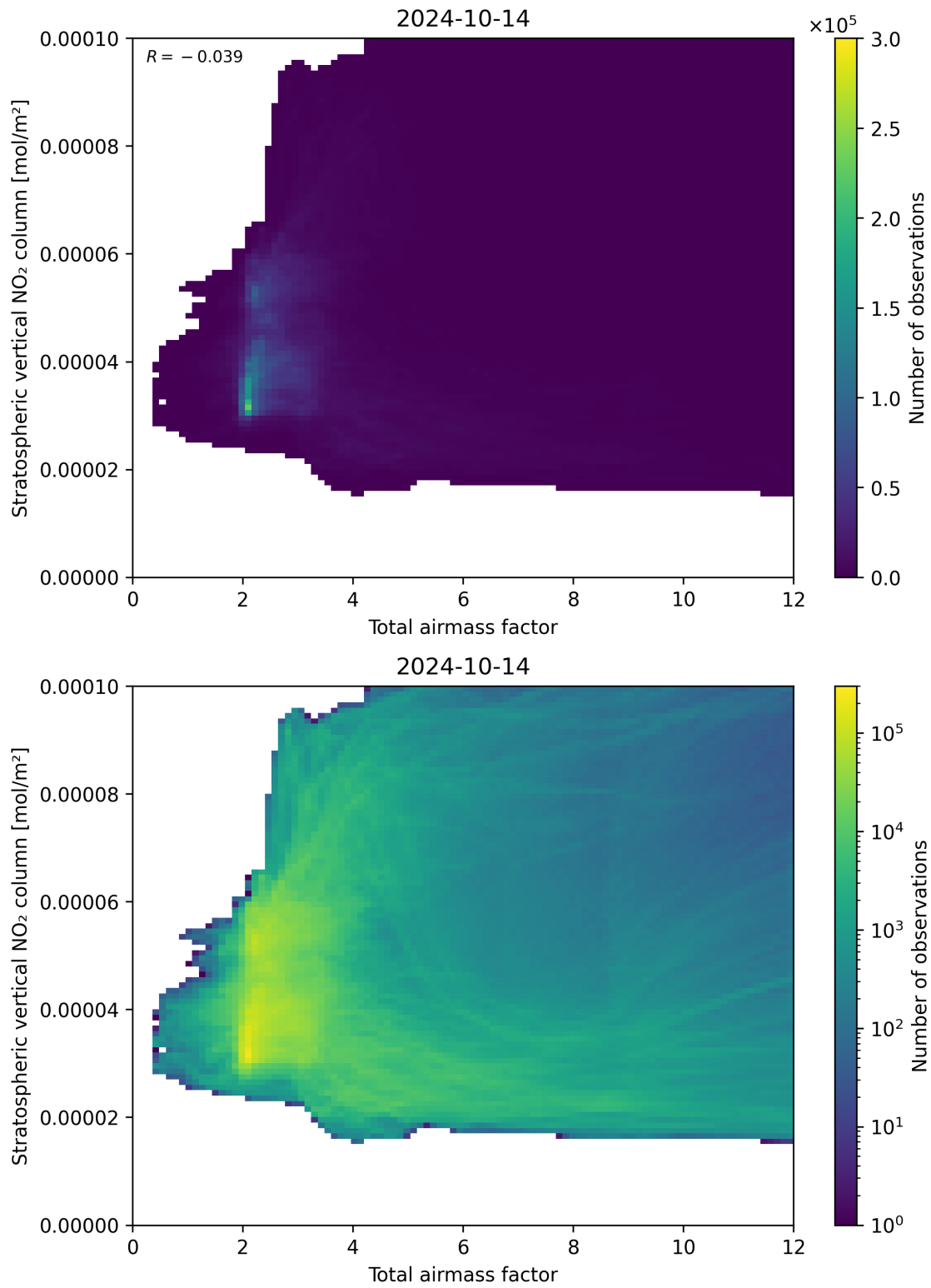
Figure 64: Scatter density plot of “Total airmass factor” against “Stratospheric vertical NO 2 column” for 2024-10-14 to 2024-10-15.
