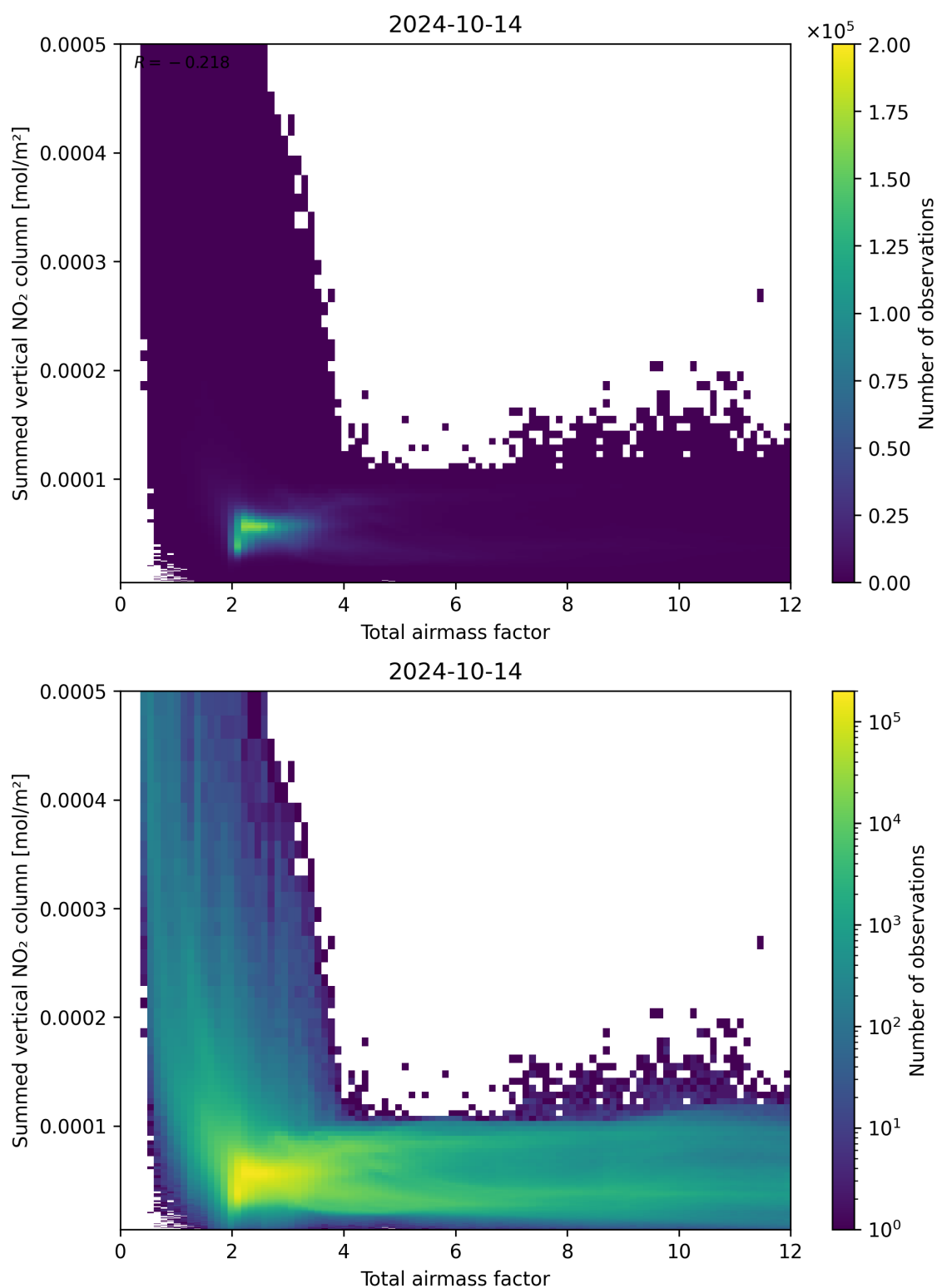
Figure 65: Scatter density plot of “Total airmass factor” against “Summed vertical NO 2 column” for 2024-10-14 to 2024-10-15.
