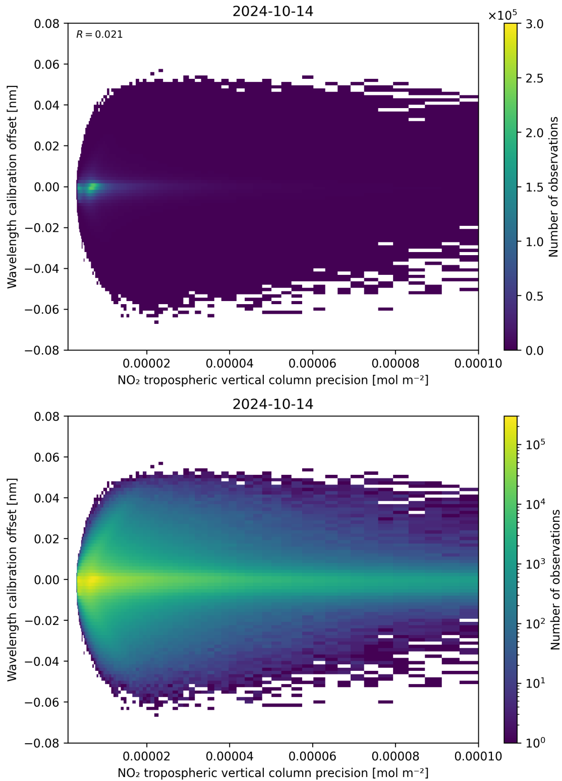
Figure 141: Scatter density plot of “NO 2 tropospheric vertical column precision” against “Wavelength calibration offset” for 2024-10-14 to 2024-10-15.
