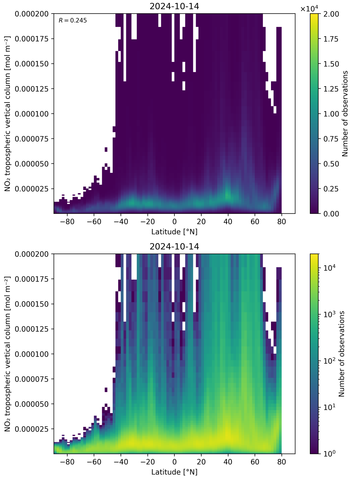
Figure 92: Scatter density plot of “Latitude” against “NO 2 tropospheric vertical column” for 2024-10-14 to 2024-10-15.
