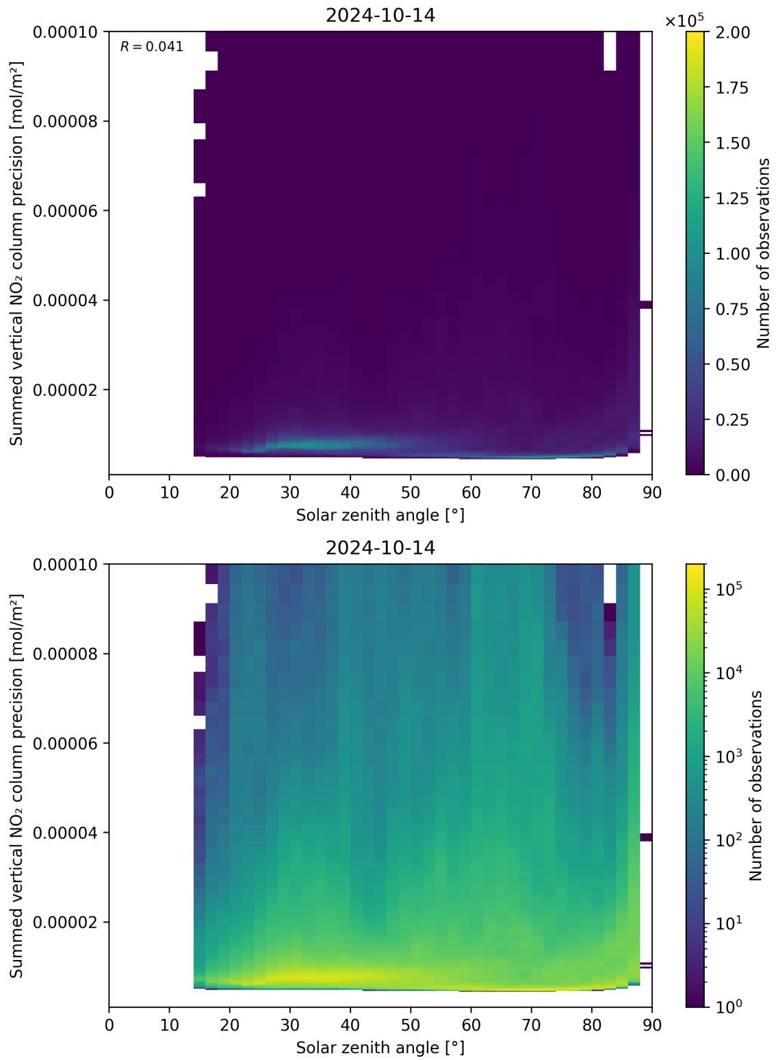
Figure 152: Scatter density plot of “Solar zenith angle” against “Summed vertical NO 2 column precision” for 2024-10-14 to 2024-10-15.
