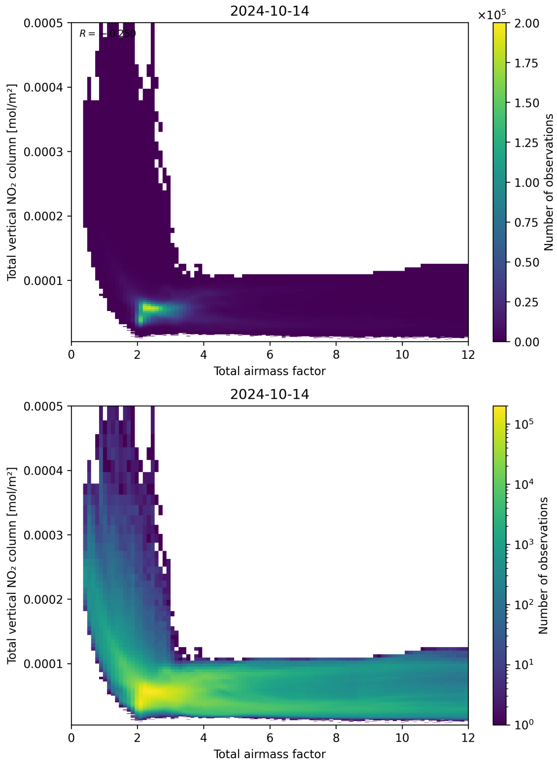
Figure 67: Scatter density plot of “Total airmass factor” against “Total vertical NO 2 column” for 2024-10-14 to 2024-10-15.
