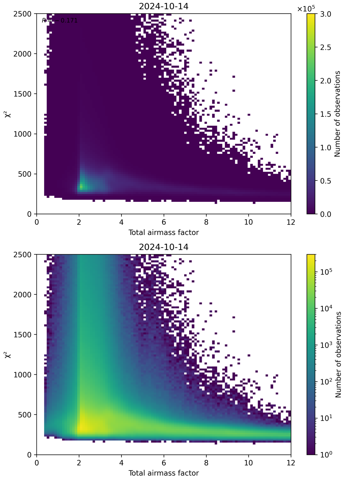
Figure 63: Scatter density plot of “Total airmass factor” against “ \chi^2 ” for 2024-10-14 to 2024-10-15.
