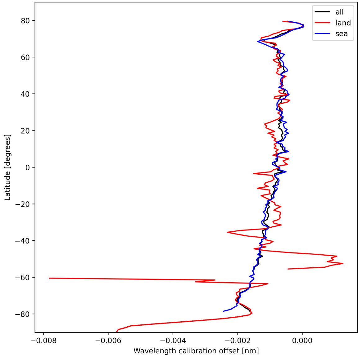
Figure 18: Zonal average of “Wavelength calibration offset” for 2024-10-14 to 2024-10-15.
