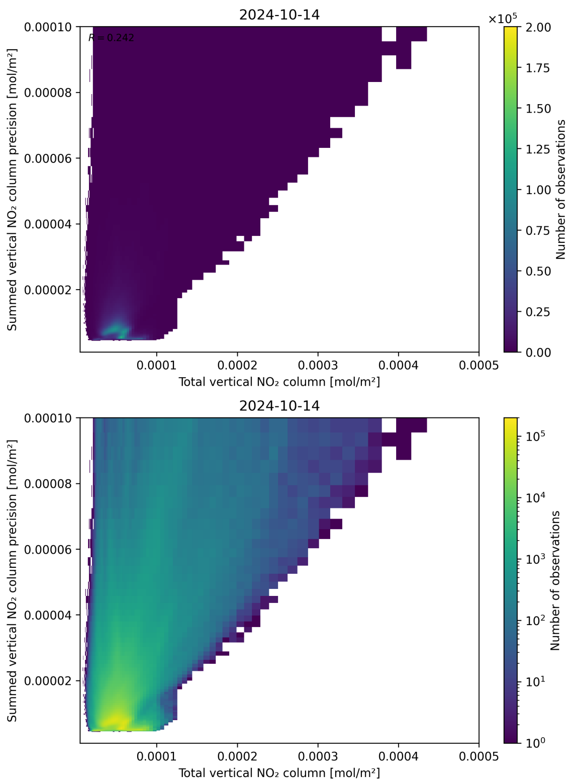
Figure 113: Scatter density plot of “Total vertical NO 2 column” against “Summed vertical NO 2 column precision” for 2024-10-14 to 2024-10-15.
