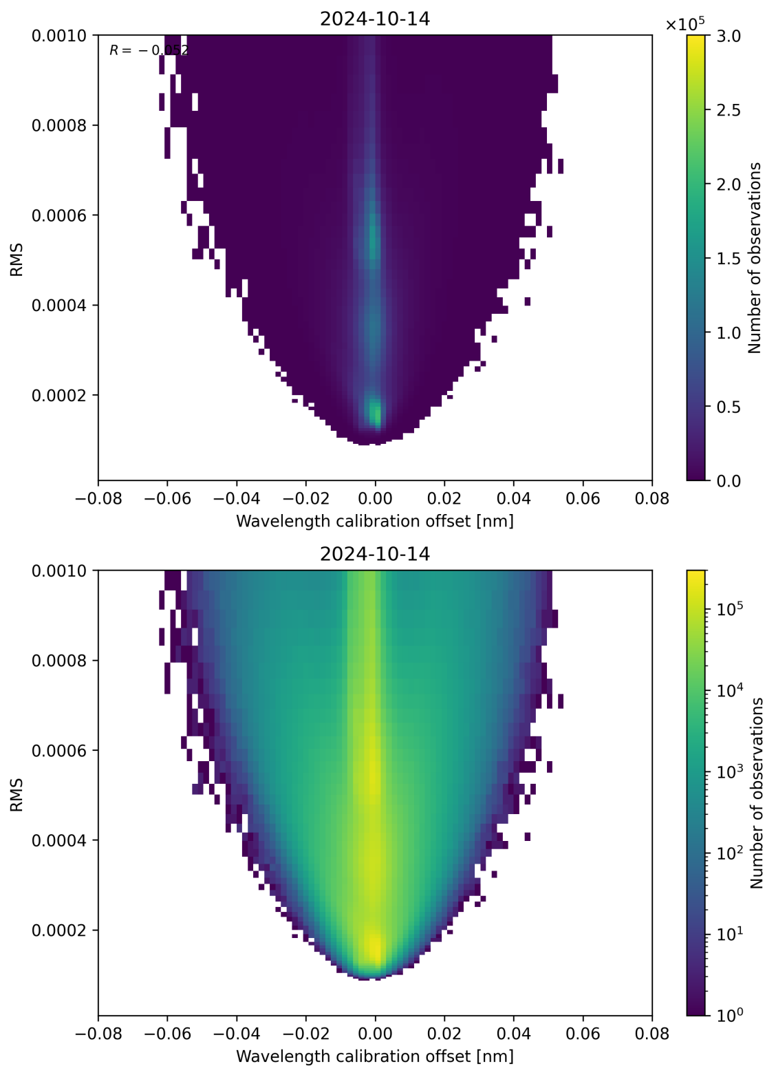
Figure 181: Scatter density plot of “Wavelength calibration offset” against “RMS” for 2024-10-14 to 2024-10-15.
