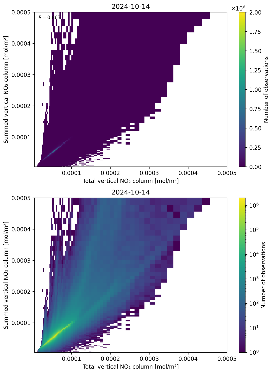
Figure 112: Scatter density plot of “Total vertical NO 2 column” against “Summed vertical NO 2 column” for 2024-10-14 to 2024-10-15.
