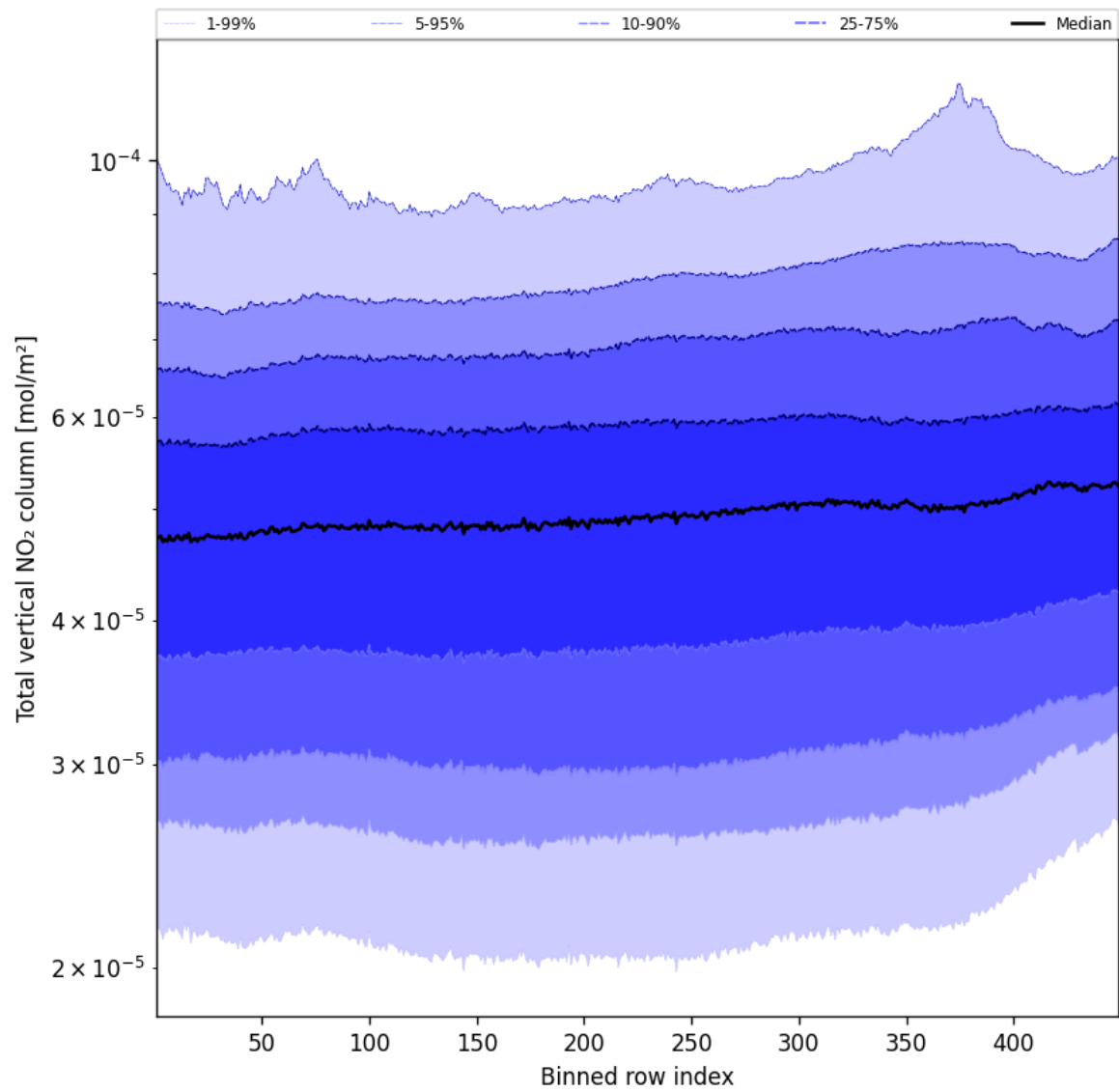
Figure 55: Along track statistics of “Total vertical NO 2 column” for 2024-10-14 to 2024-10-15
