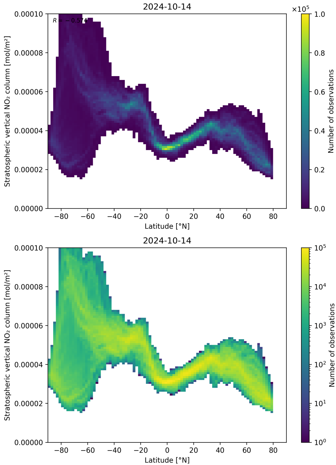
Figure 87: Scatter density plot of “Latitude” against “Stratospheric vertical NO 2 column” for 2024-10-14 to 2024-10-15.
