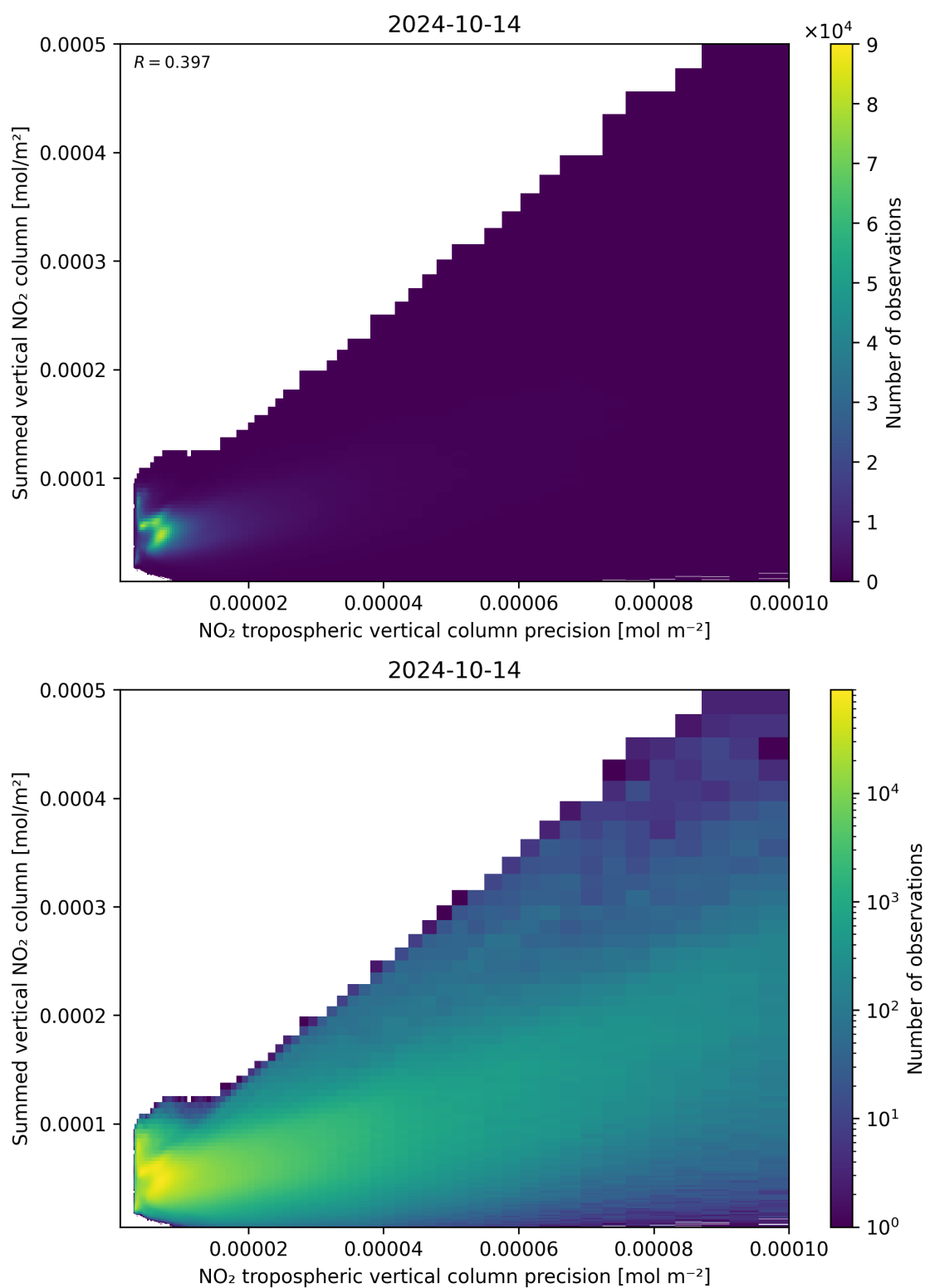
Figure 136: Scatter density plot of “NO 2 tropospheric vertical column precision” against “Summed vertical NO 2 column” for 2024-10-14 to 2024-10-15.
