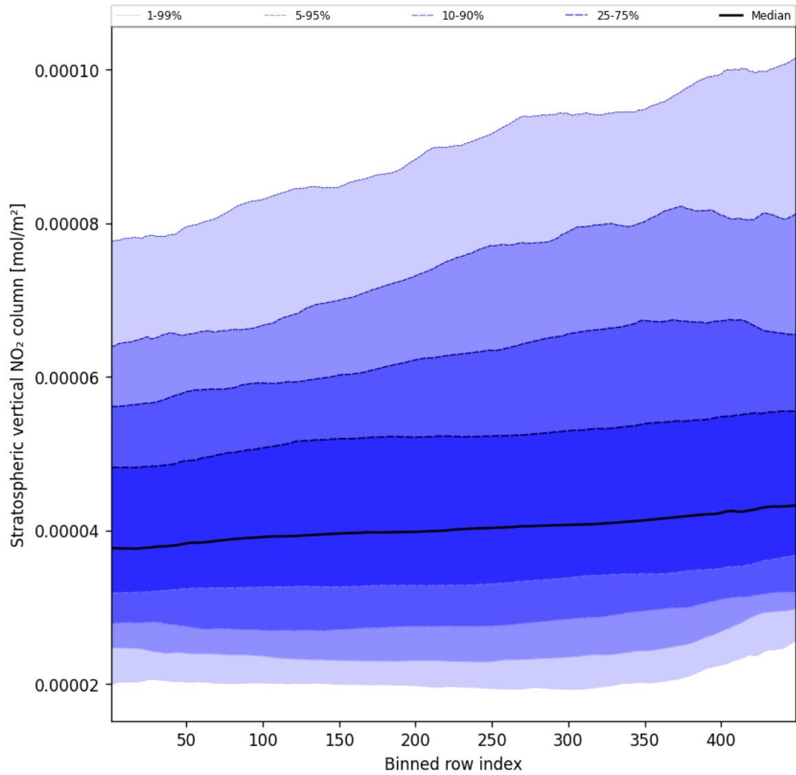
Figure 53: Along track statistics of “Stratospheric vertical NO 2 column” for 2024-10-14 to 2024-10-15
