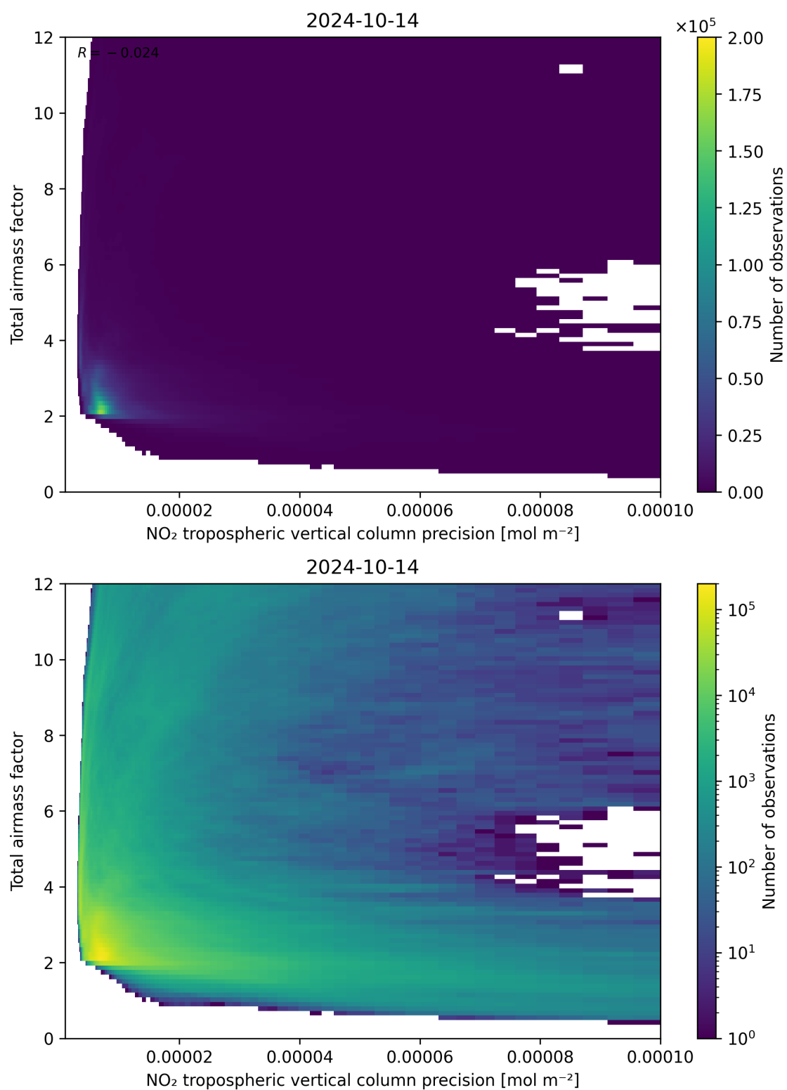
Figure 132: Scatter density plot of “NO 2 tropospheric vertical column precision” against “Total air mass factor” for 2024-10-14 to 2024-10-15.
