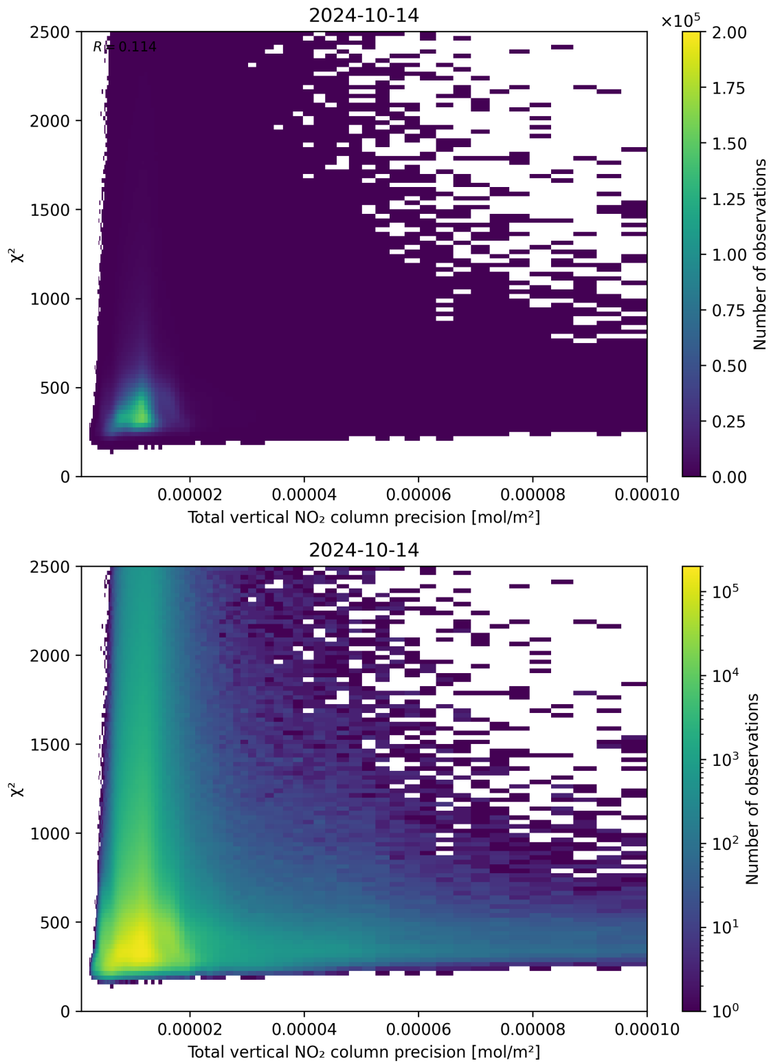
Figure 116: Scatter density plot of “Total vertical NO 2 column precision” against “ \chi^2 ” for 2024-10-14 to 2024-10-15.
