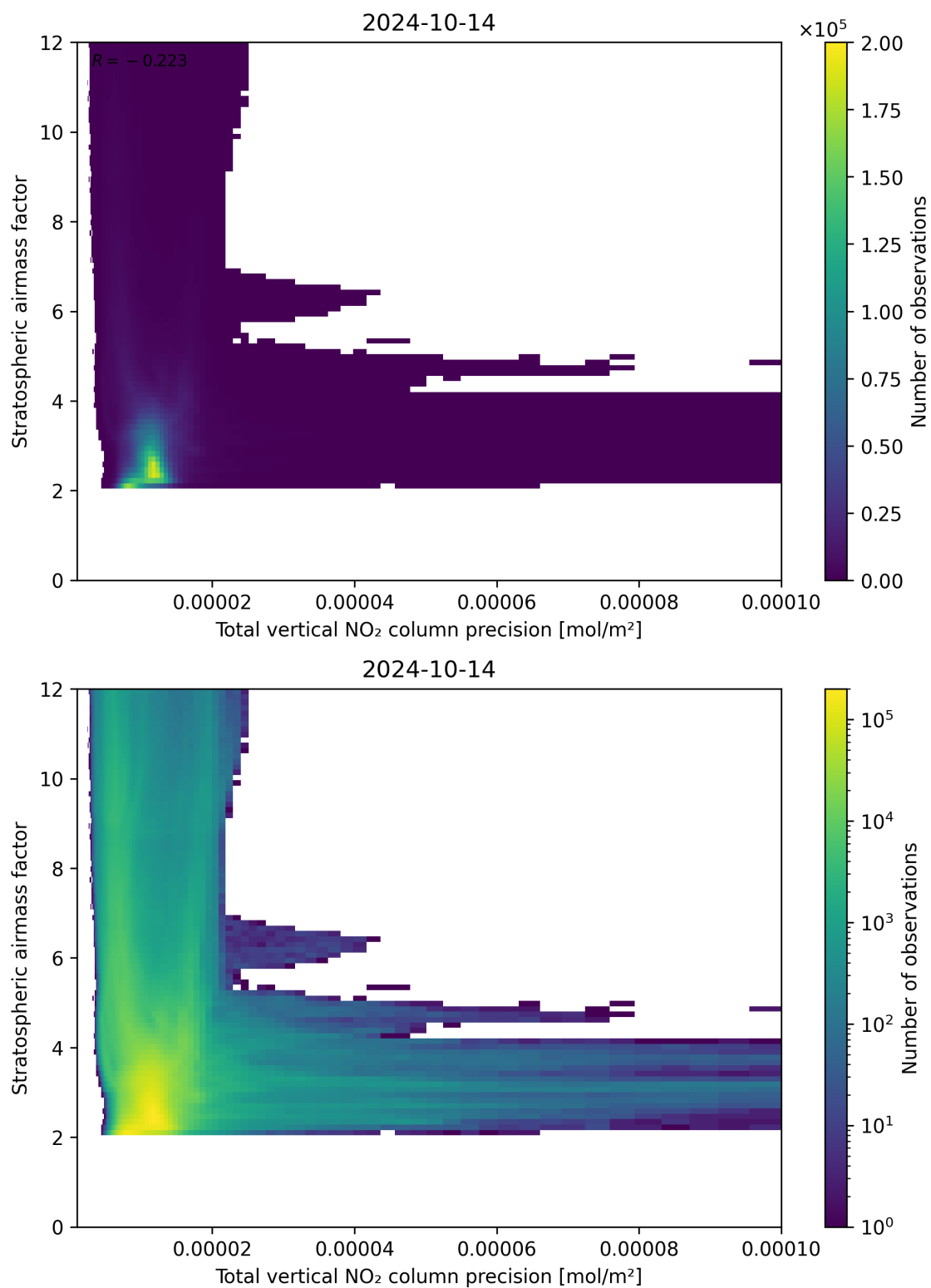
Figure 115: Scatter density plot of “Total vertical NO 2 column precision” against “Stratospheric air mass factor” for 2024-10-14 to 2024-10-15.
