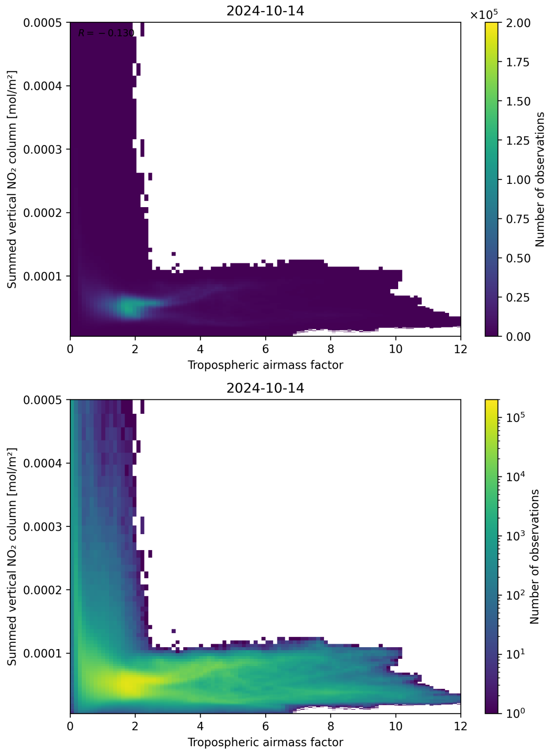
Figure 75: Scatter density plot of “Tropospheric air mass factor” against “Summed vertical NO 2 column” for 2024-10-14 to 2024-10-15.
