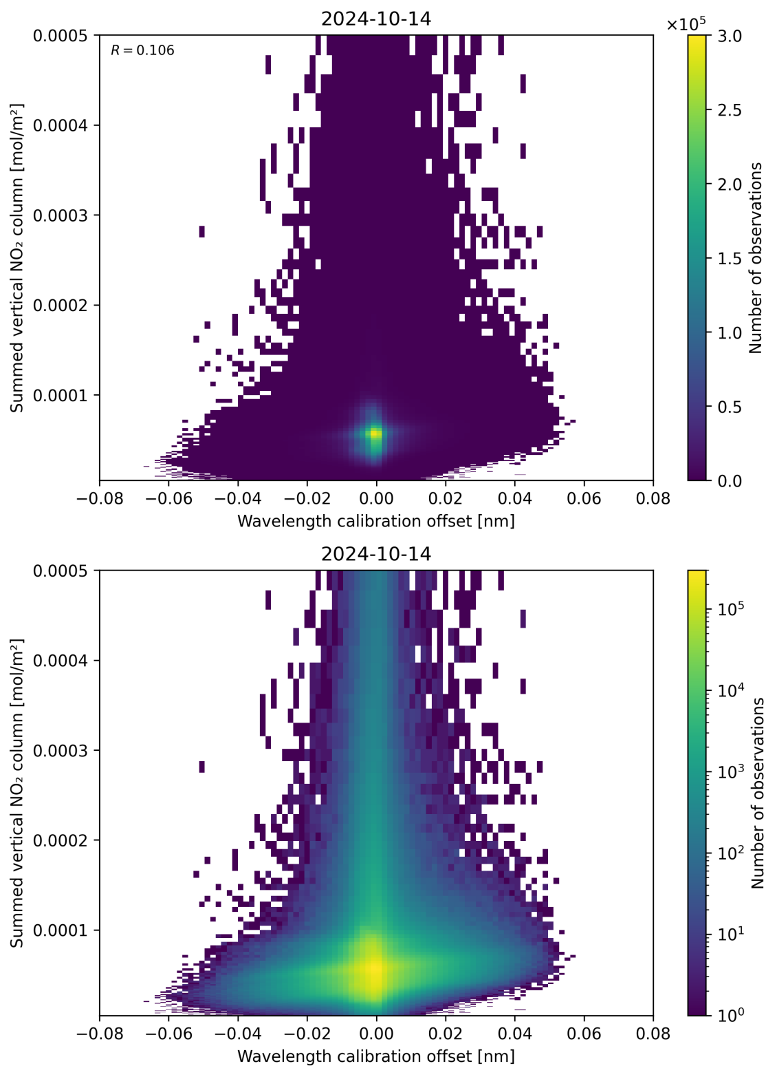
Figure 177: Scatter density plot of “Wavelength calibration offset” against “Summed vertical NO 2 column” for 2024-10-14 to 2024-10-15.
