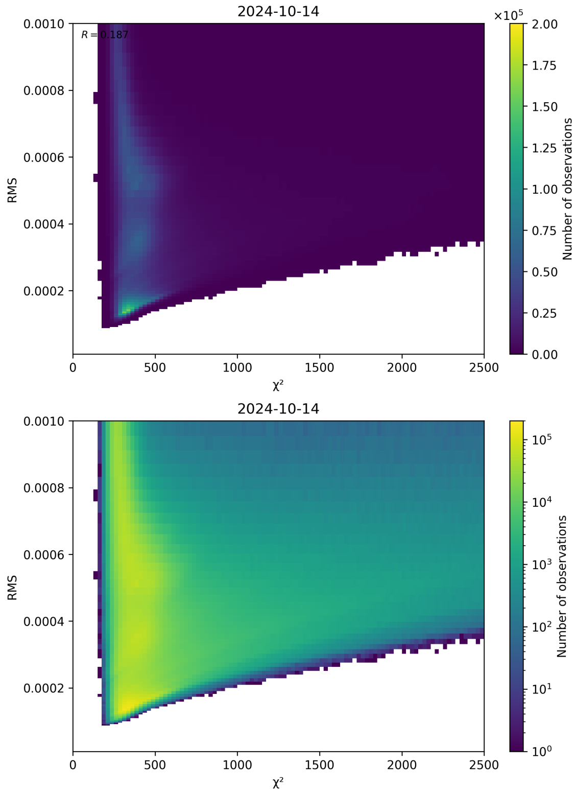
Figure 82: Scatter density plot of “ \chi^2 ” against “RMS” for 2024-10-14 to 2024-10-15.
