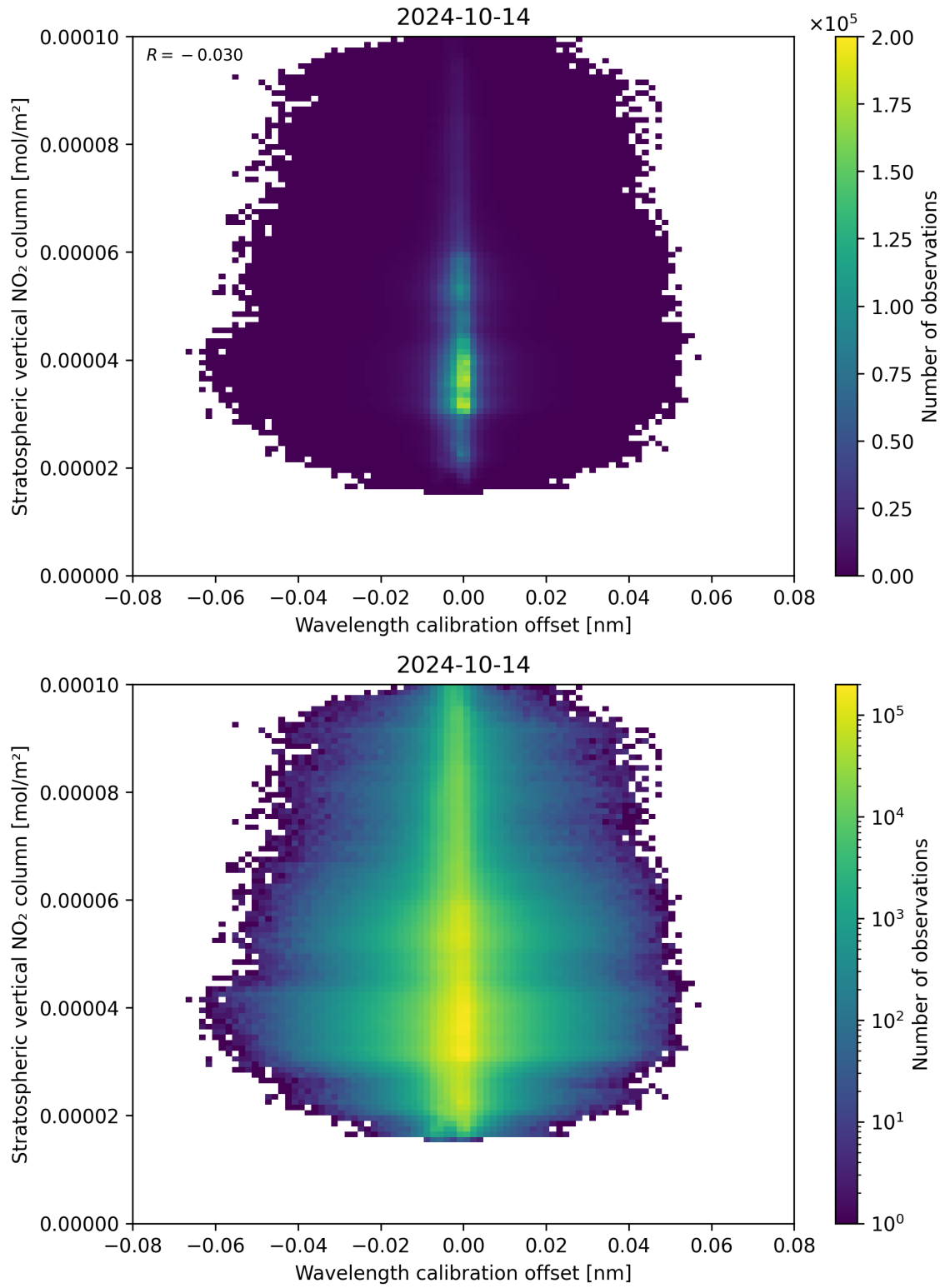
Figure 176: Scatter density plot of “Wavelength calibration offset” against “Stratospheric vertical NO 2 column” for 2024-10-14 to 2024-10-15.
