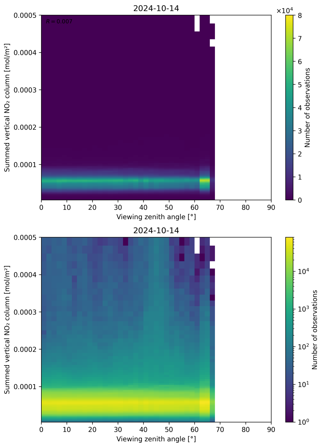
Figure 165: Scatter density plot of “Viewing zenith angle” against “Summed vertical NO 2 column” for 2024-10-14 to 2024-10-15.
