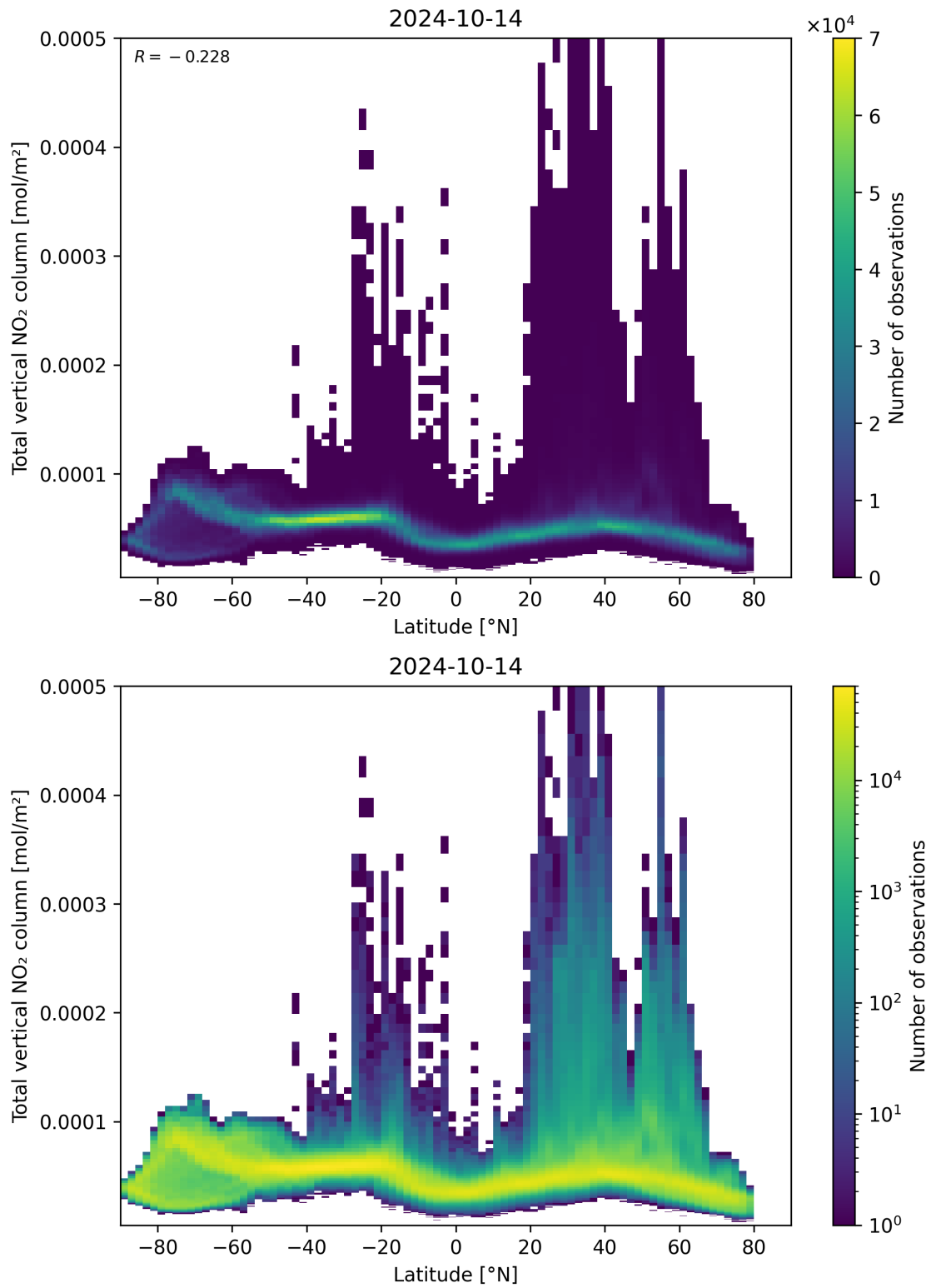
Figure 90: Scatter density plot of “Latitude” against “Total vertical NO 2 column” for 2024-10-14 to 2024-10-15.
