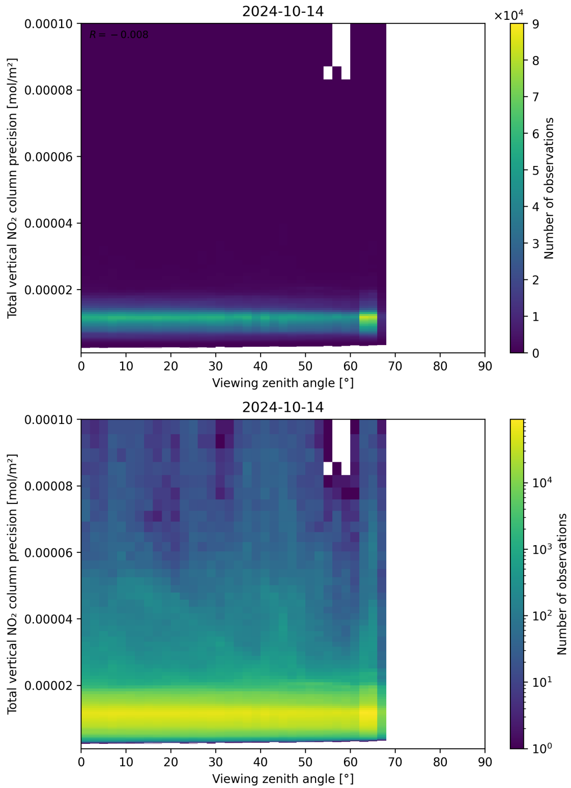
Figure 168: Scatter density plot of “Viewing zenith angle” against “Total vertical NO 2 column precision” for 2024-10-14 to 2024-10-15.
