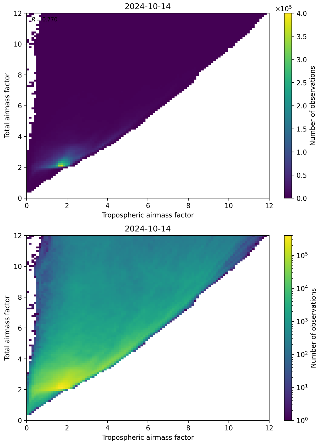
Figure 72: Scatter density plot of “Tropospheric airmass factor” against “Total airmass factor” for 2024-10-14 to 2024-10-15.
