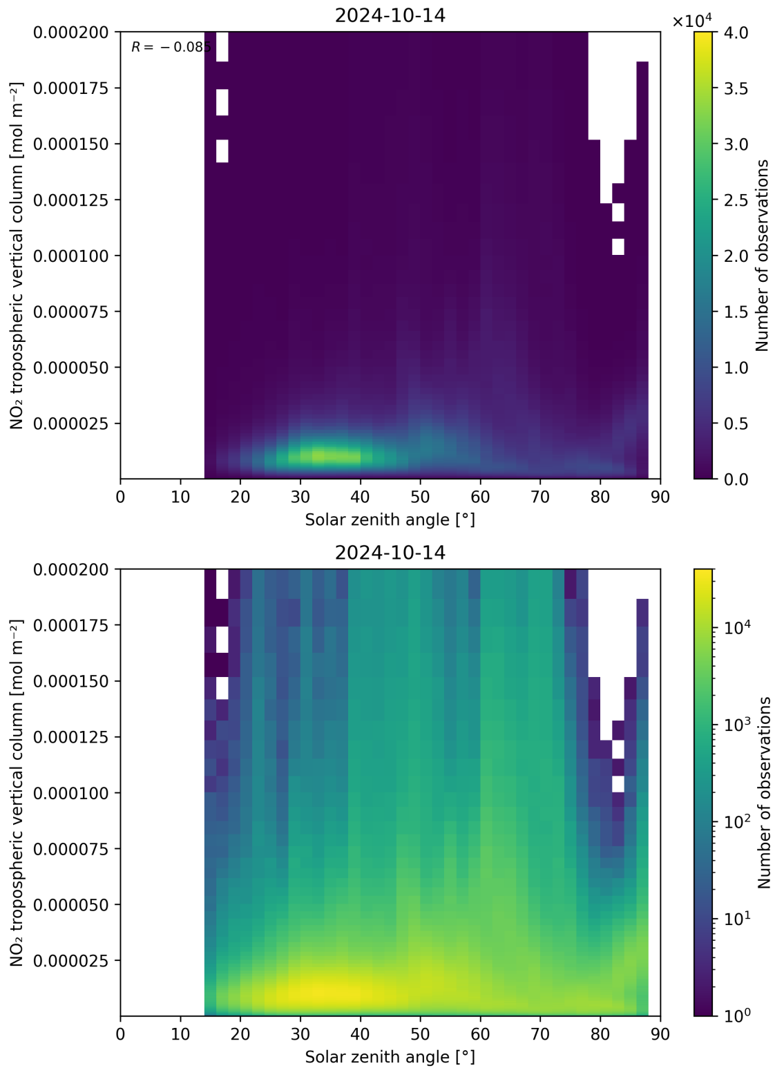
Figure 155: Scatter density plot of “Solar zenith angle” against “NO 2 tropospheric vertical column” for 2024-10-14 to 2024-10-15.
