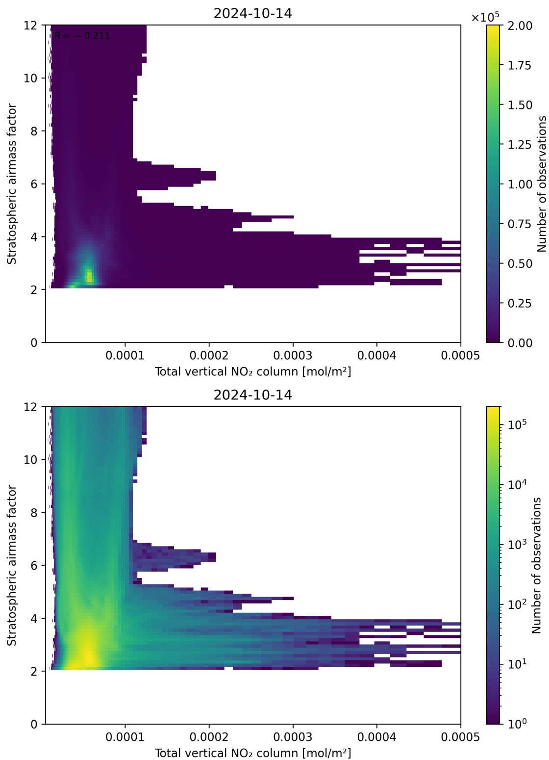
Figure 110: Scatter density plot of “Total vertical NO 2 column” against “Stratospheric airmass factor” for 2024-10-14 to 2024-10-15.
