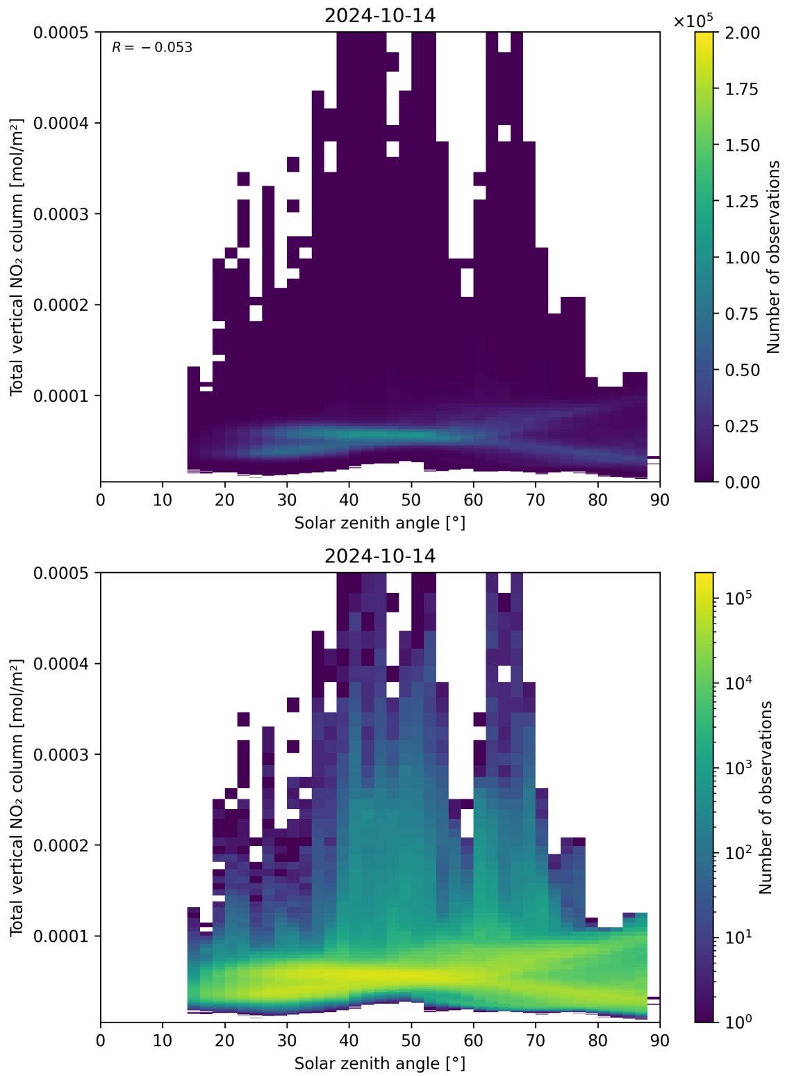
Figure 153: Scatter density plot of “Solar zenith angle” against “Total vertical NO 2 column” for 2024-10-14 to 2024-10-15.
