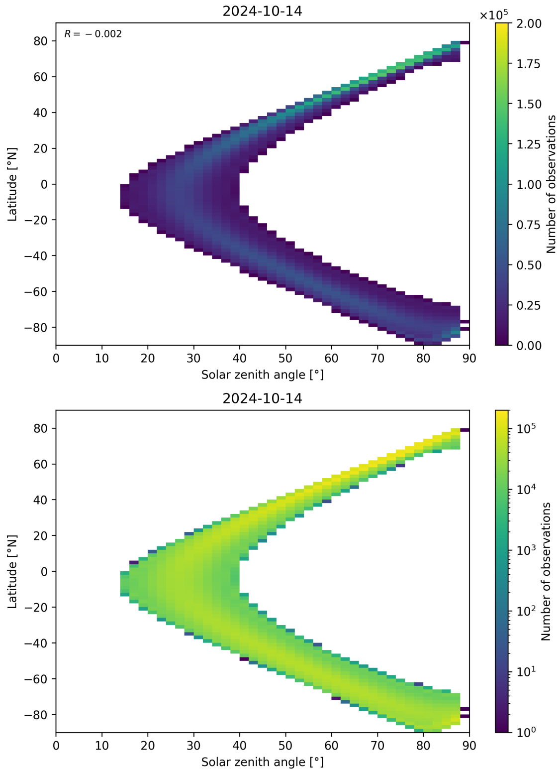
Figure 149: Scatter density plot of “Solar zenith angle” against “Latitude” for 2024-10-14 to 2024-10-15.
