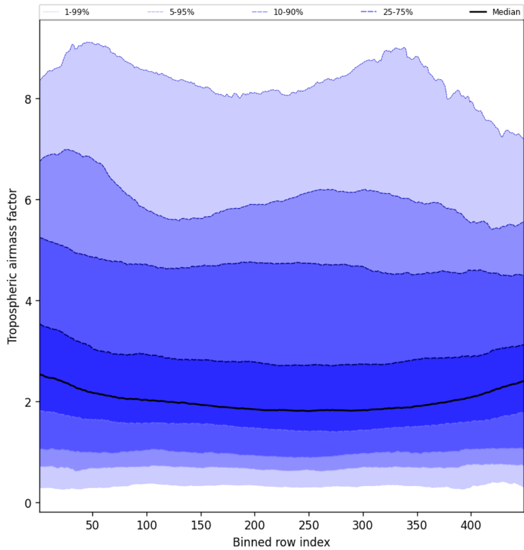
Figure 48: Along track statistics of “Tropospheric air mass factor” for 2024-10-14 to 2024-10-15
