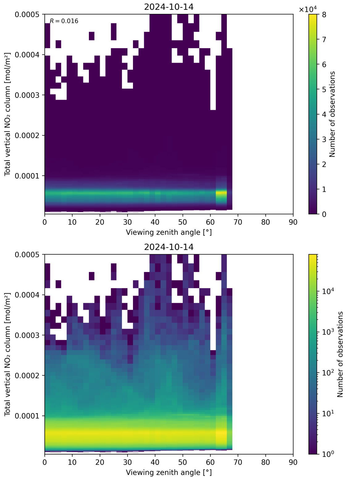
Figure 167: Scatter density plot of “Viewing zenith angle” against “Total vertical NO 2 column” for 2024-10-14 to 2024-10-15.
