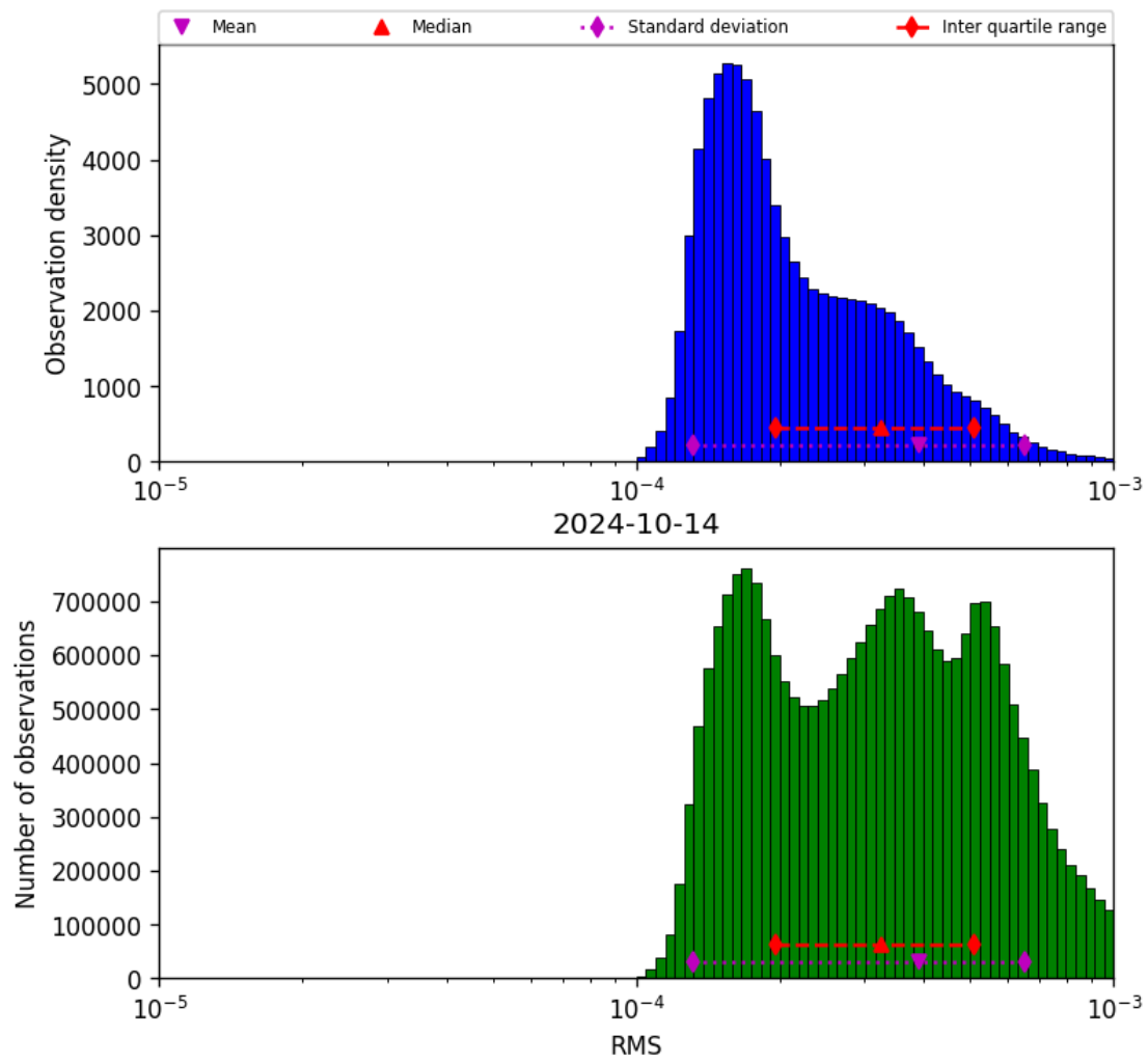
Figure 43: Histogram of “RMS” for 2024-10-14 to 2024-10-15
