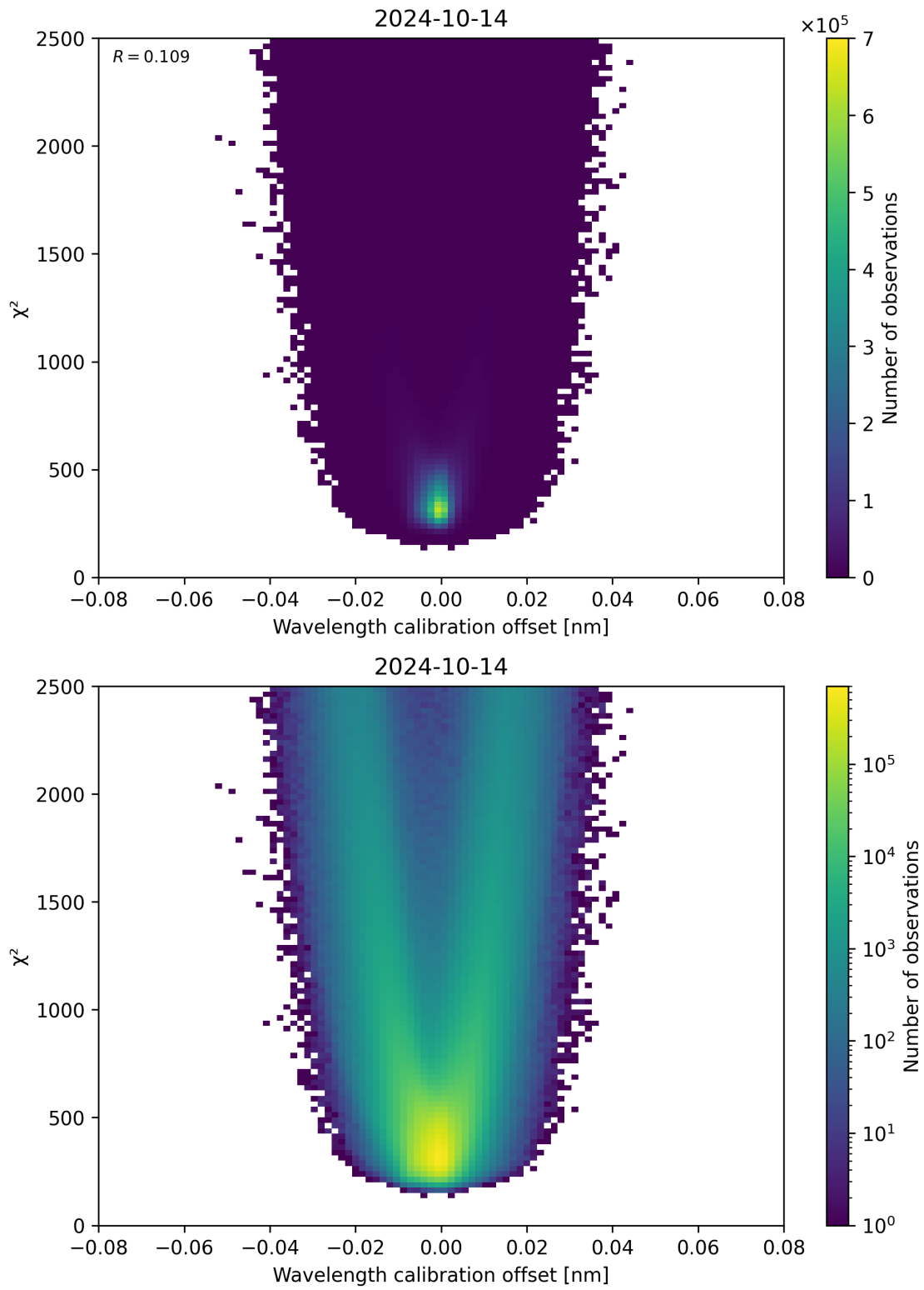
Figure 175: Scatter density plot of “Wavelength calibration offset” against “ \chi^2 ” for 2024-10-14 to 2024-10-15.
