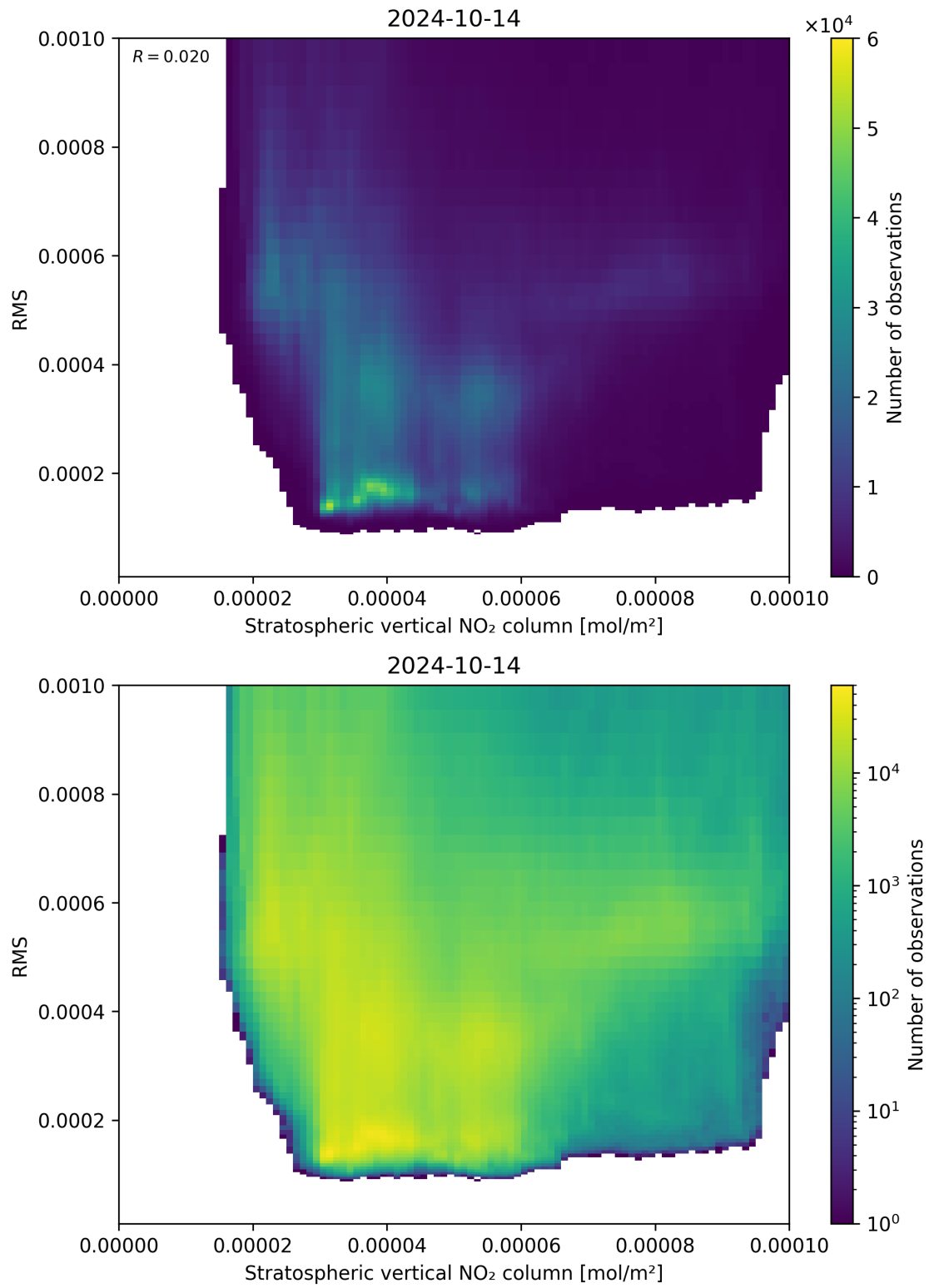
Figure 102: Scatter density plot of “Stratospheric vertical NO 2 column” against “RMS” for 2024-10-14 to 2024-10-15.
