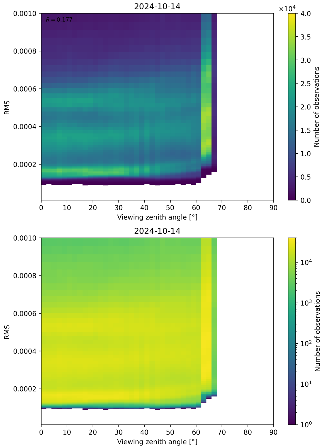
Figure 171: Scatter density plot of “Viewing zenith angle” against “RMS” for 2024-10-14 to 2024-10-15.
