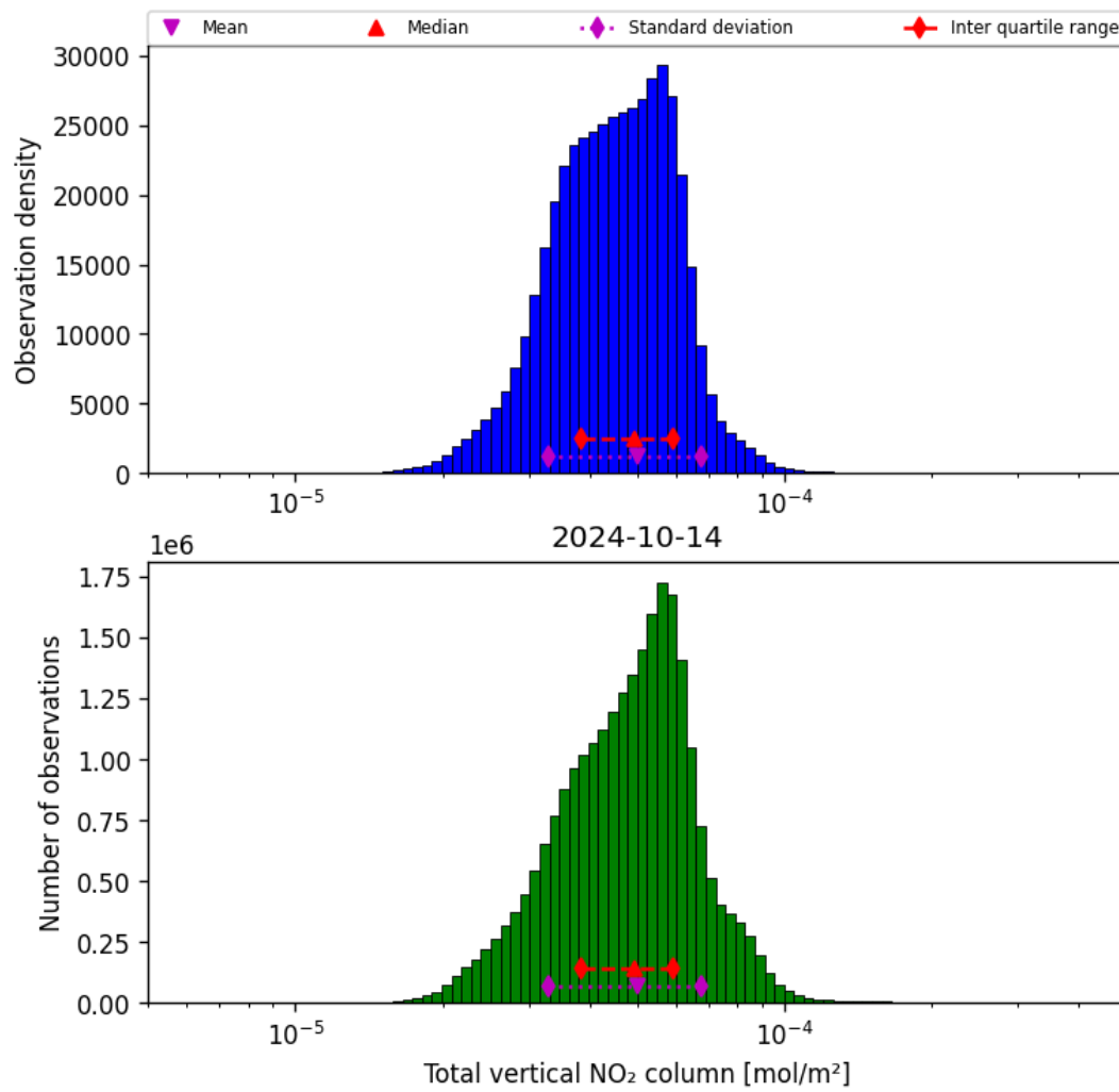
Figure 38: Histogram of “Total vertical NO 2 column” for 2024-10-14 to 2024-10-15
