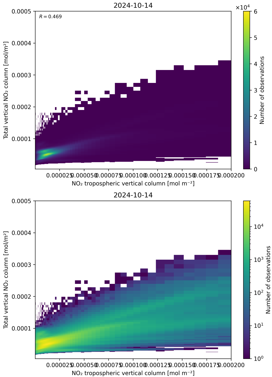
Figure 128: Scatter density plot of “NO 2 tropospheric vertical column” against “Total vertical NO 2 column” for 2024-10-14 to 2024-10-15.
