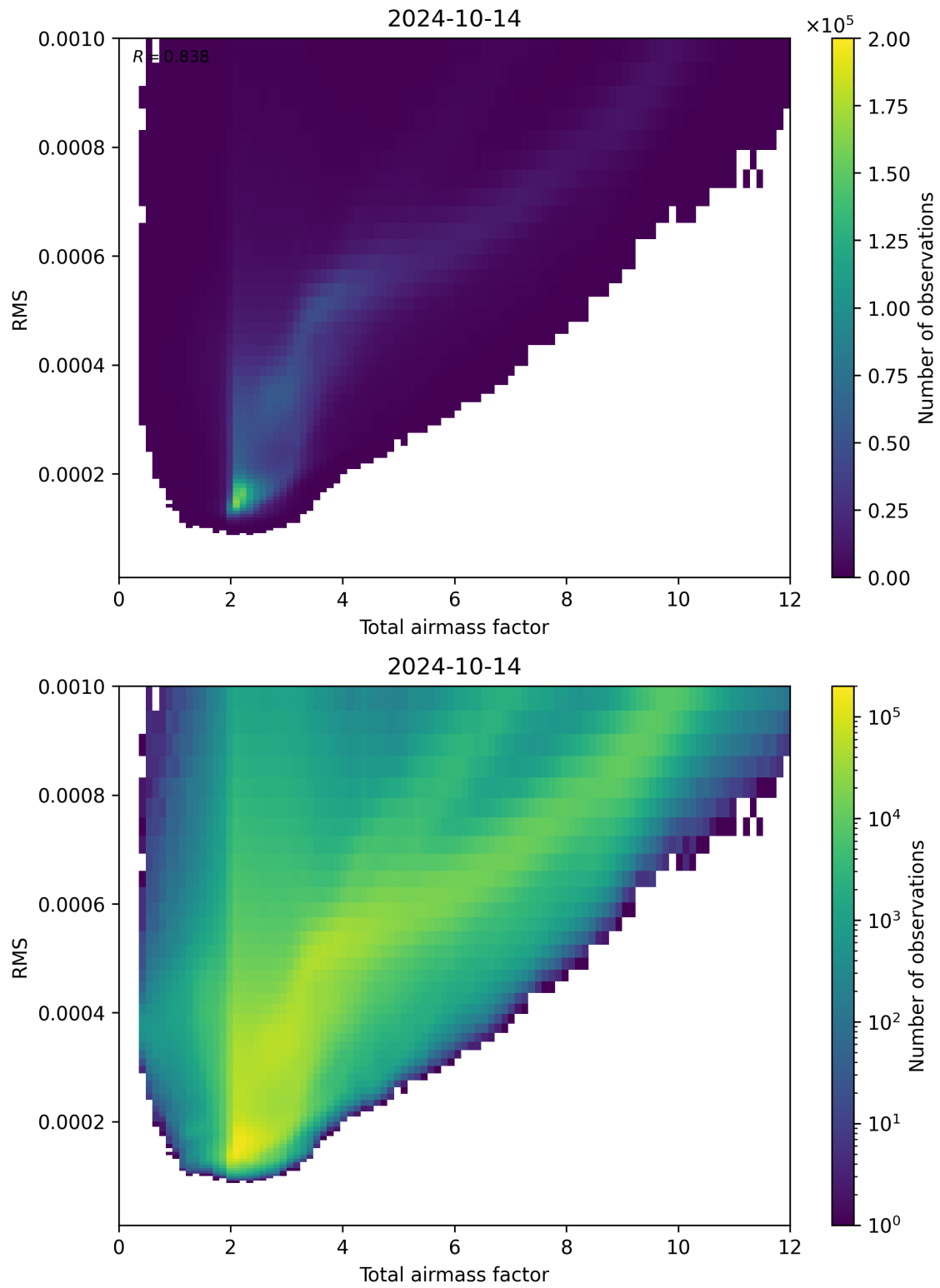
Figure 69: Scatter density plot of “Total airmass factor” against “RMS” for 2024-10-14 to 2024-10-15.
