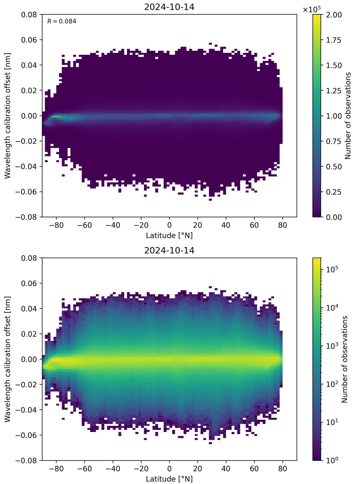
Figure 95: Scatter density plot of “Latitude” against “Wavelength calibration offset” for 2024-10-14 to 2024-10-15.
