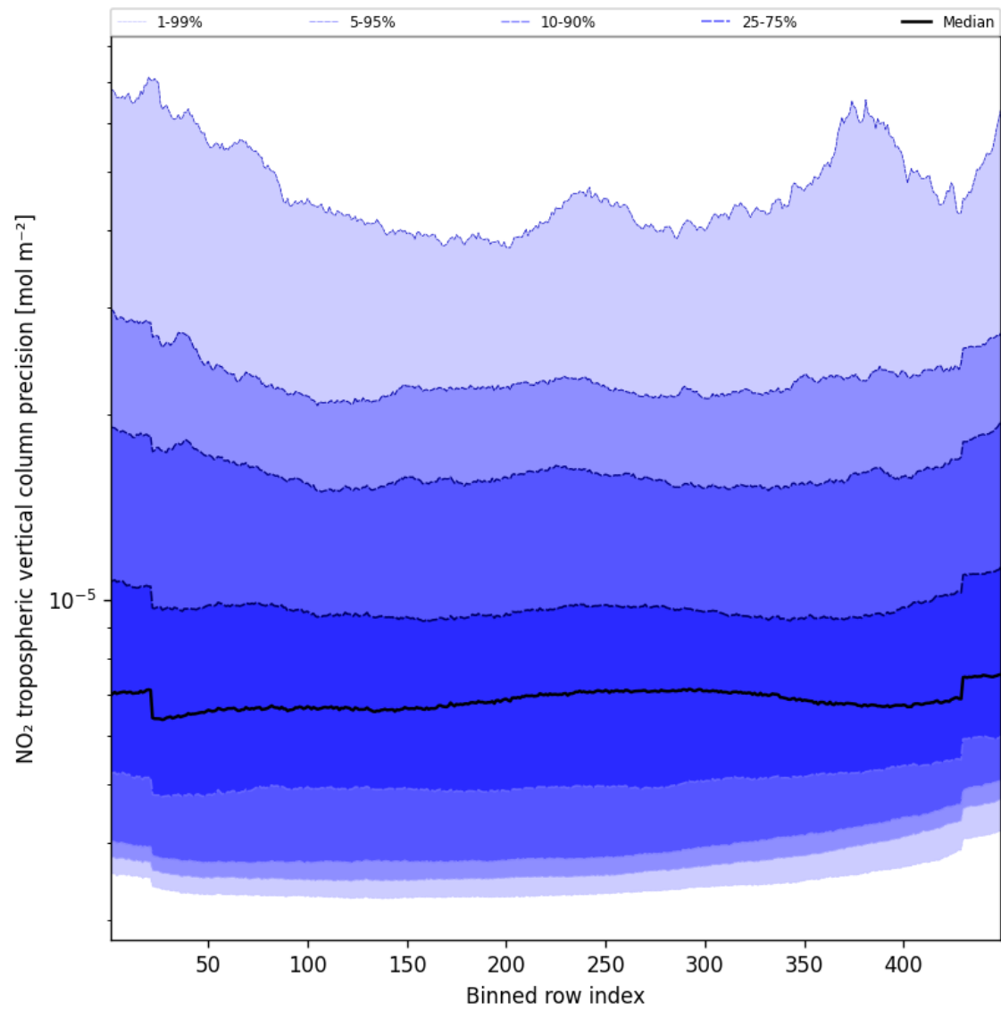
Figure 47: Along track statistics of “NO 2 tropospheric vertical column precision” for 2024-10-14 to 2024-10-15
