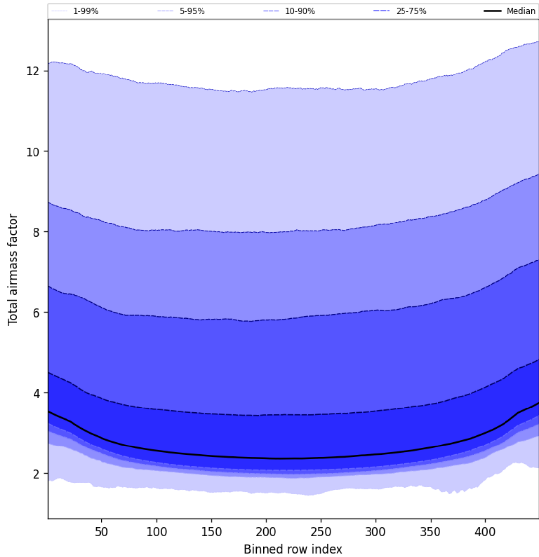
Figure 49: Along track statistics of “Total airmass factor” for 2024-10-14 to 2024-10-15
