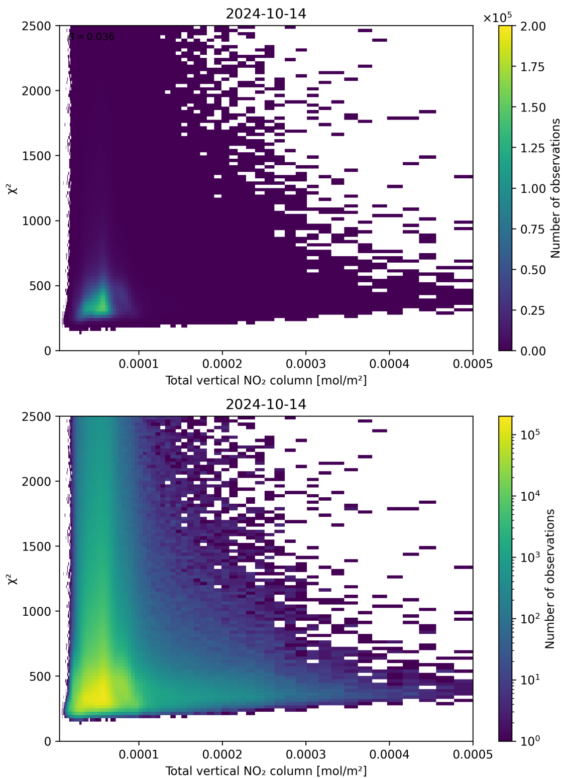
Figure 111: Scatter density plot of “Total vertical NO 2 column” against “ \chi^2 ” for 2024-10-14 to 2024-10-15.
