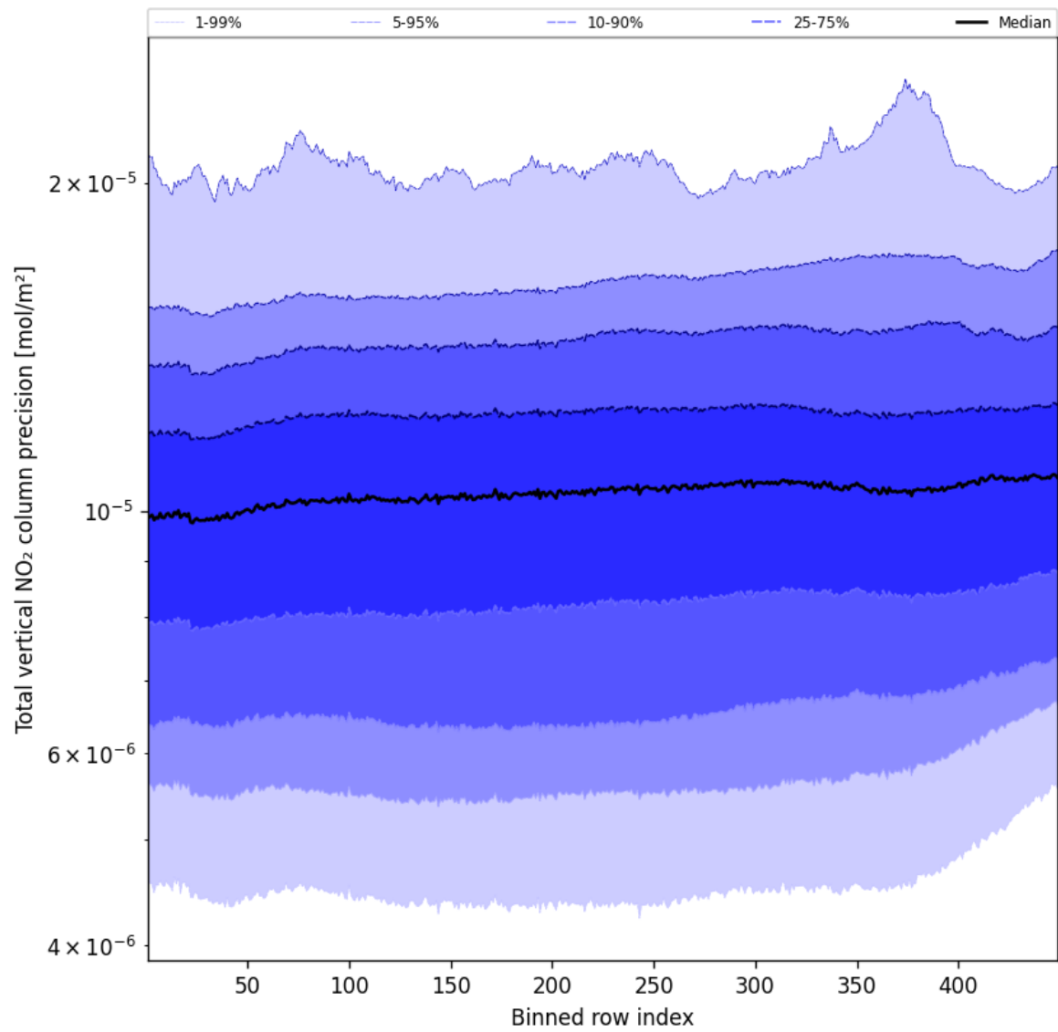
Figure 56: Along track statistics of “Total vertical NO 2 column precision” for 2024-10-14 to 2024-10-15
