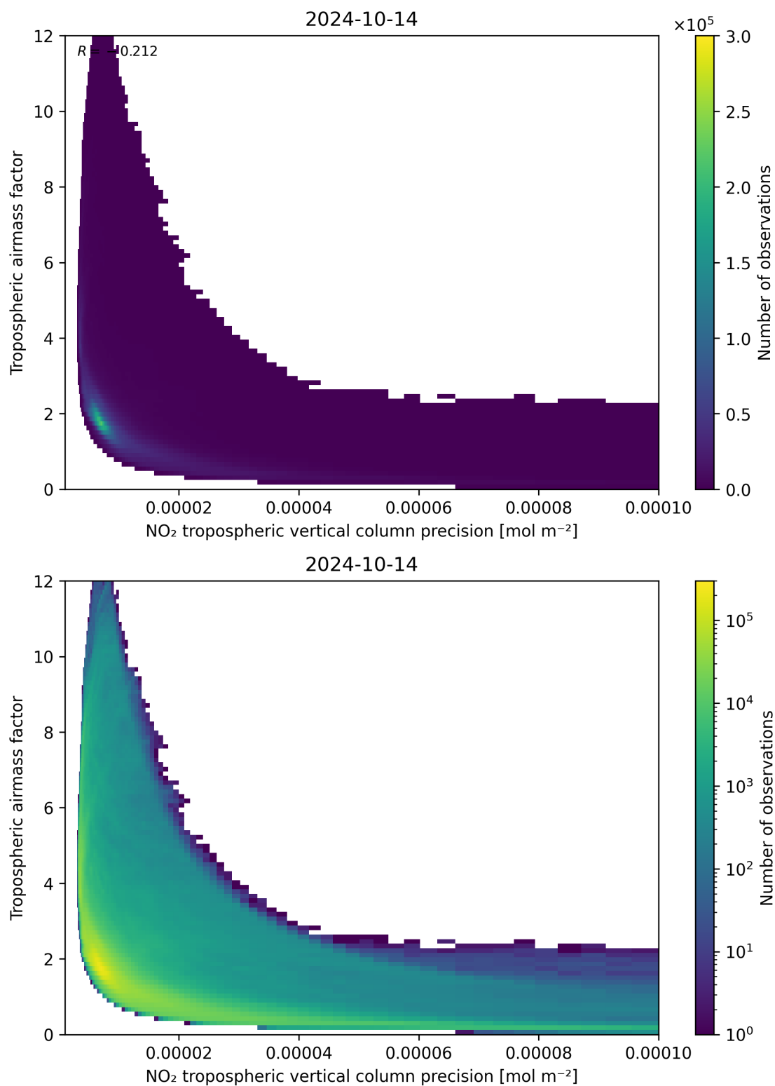
Figure 133: Scatter density plot of “NO 2 tropospheric vertical column precision” against “Tropospheric airmass factor” for 2024-10-14 to 2024-10-15.
