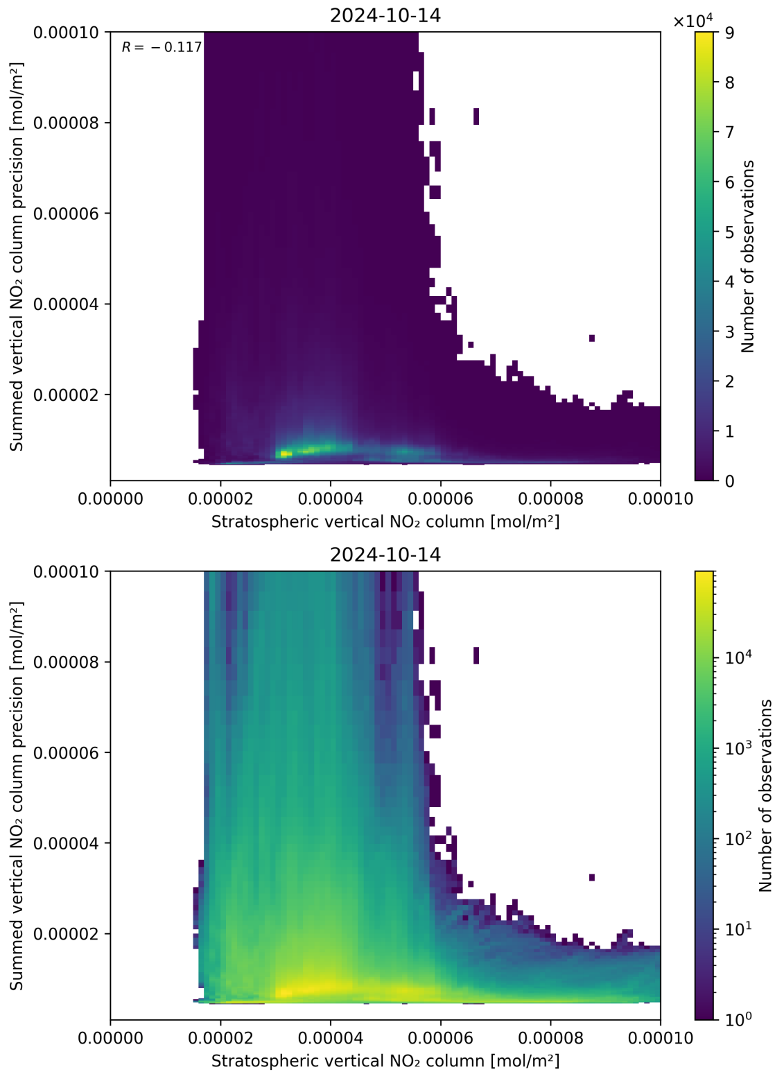
Figure 99: Scatter density plot of “Stratospheric vertical NO 2 column” against “Summed vertical NO 2 column precision” for 2024-10-14 to 2024-10-15.
