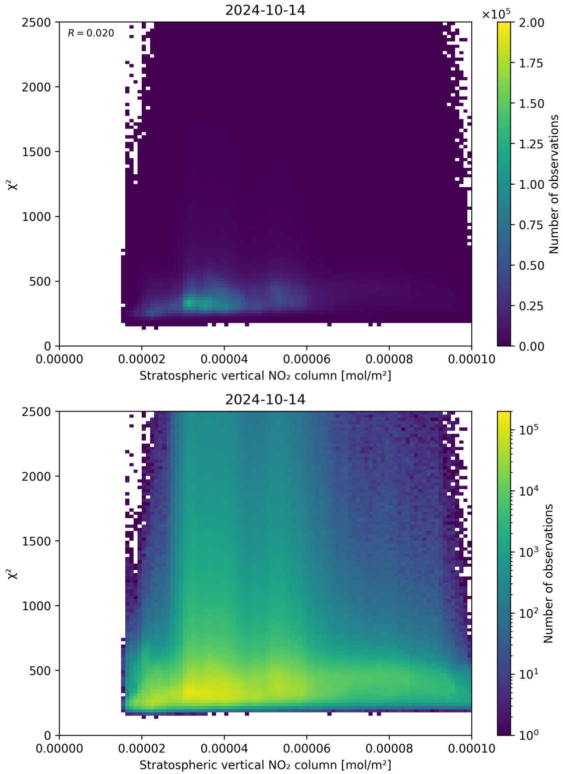
Figure 97: Scatter density plot of “Stratospheric vertical NO 2 column” against “ \chi^2 ” for 2024-10-14 to 2024-10-15.
