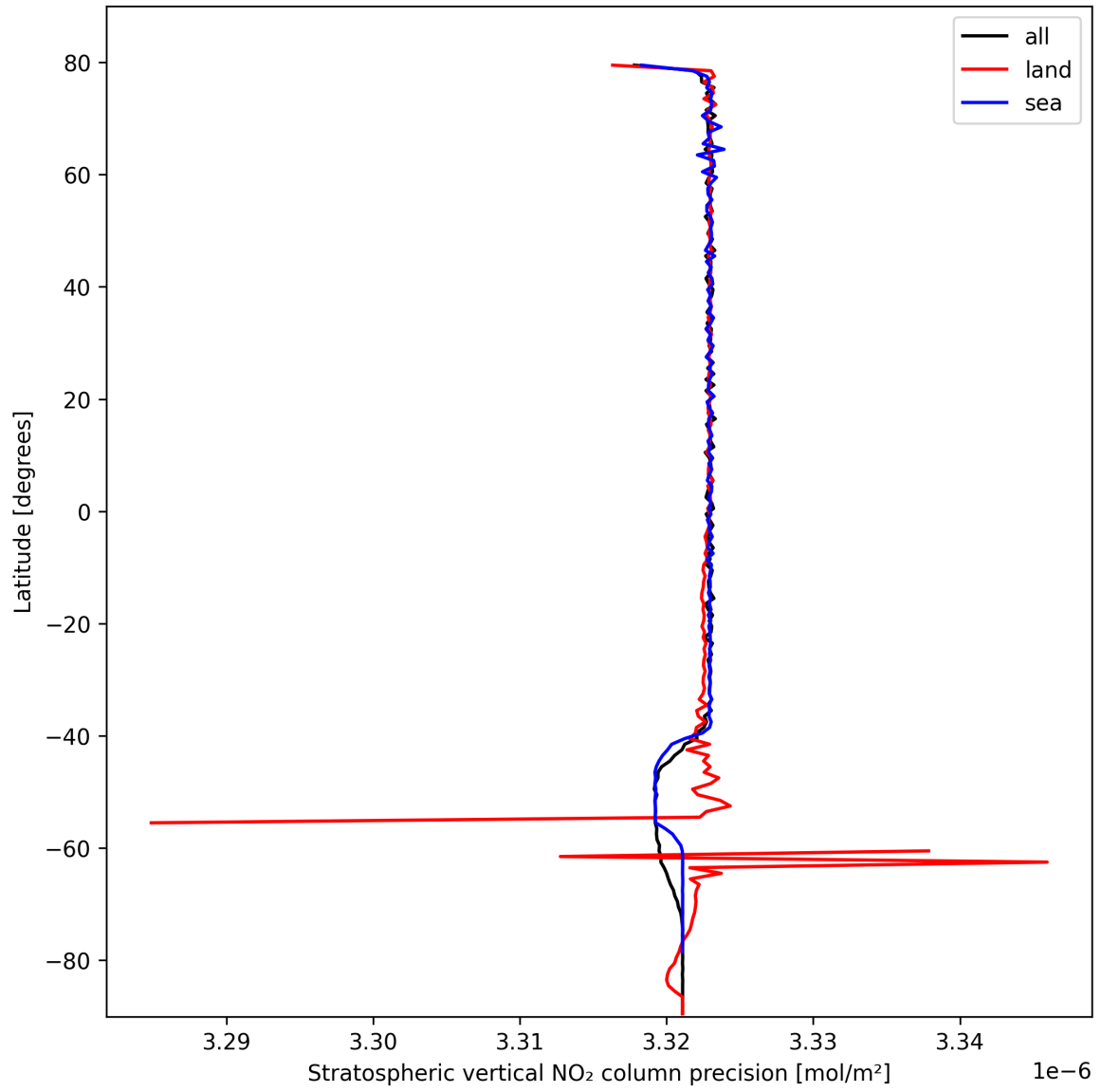
Figure 20: Zonal average of “Stratospheric vertical NO 2 column precision” for 2024-10-14 to 2024-10-15.
