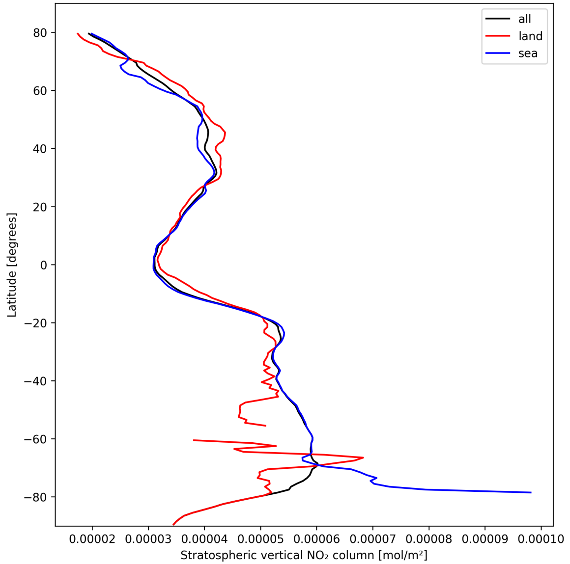
Figure 19: Zonal average of “Stratospheric vertical NO 2 column” for 2024-10-14 to 2024-10-15.
