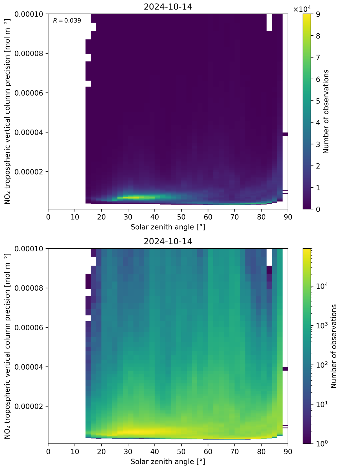
Figure 156: Scatter density plot of “Solar zenith angle” against “NO 2 tropospheric vertical column precision” for 2024-10-14 to 2024-10-15.
