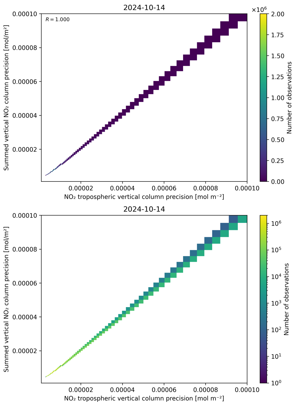
Figure 137: Scatter density plot of “NO 2 tropospheric vertical column precision” against “Summed vertical NO 2 column precision” for 2024-10-14 to 2024-10-15.
