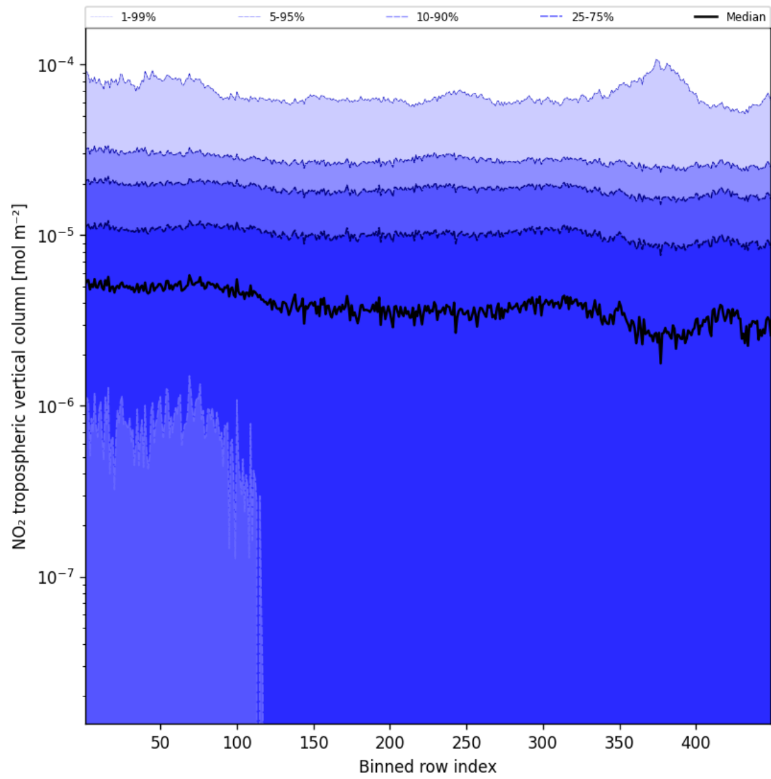
Figure 46: Along track statistics of "NO 2 tropospheric vertical column" for 2024-10-14 to 2024-10-15
