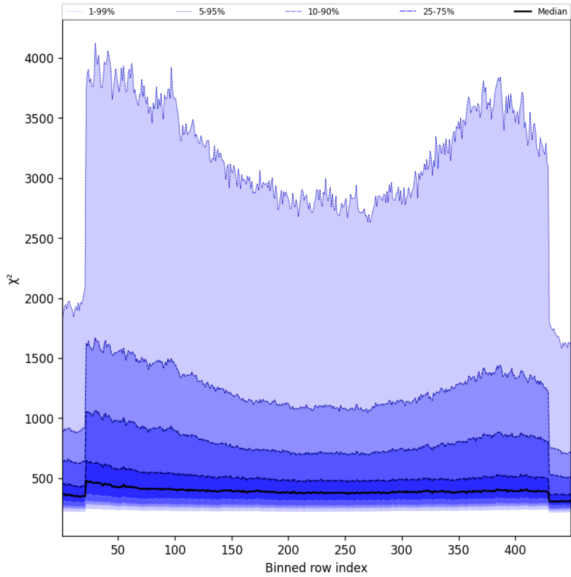
Figure 59: Along track statistics of “ \chi^2 ” for 2024-10-14 to 2024-10-15
