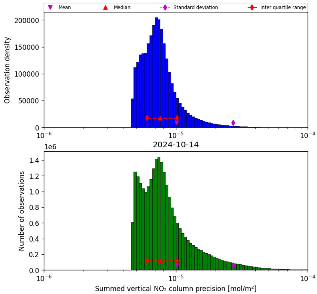
Figure 41: Histogram of “Summed vertical NO 2 column precision” for 2024-10-14 to 2024-10-15
