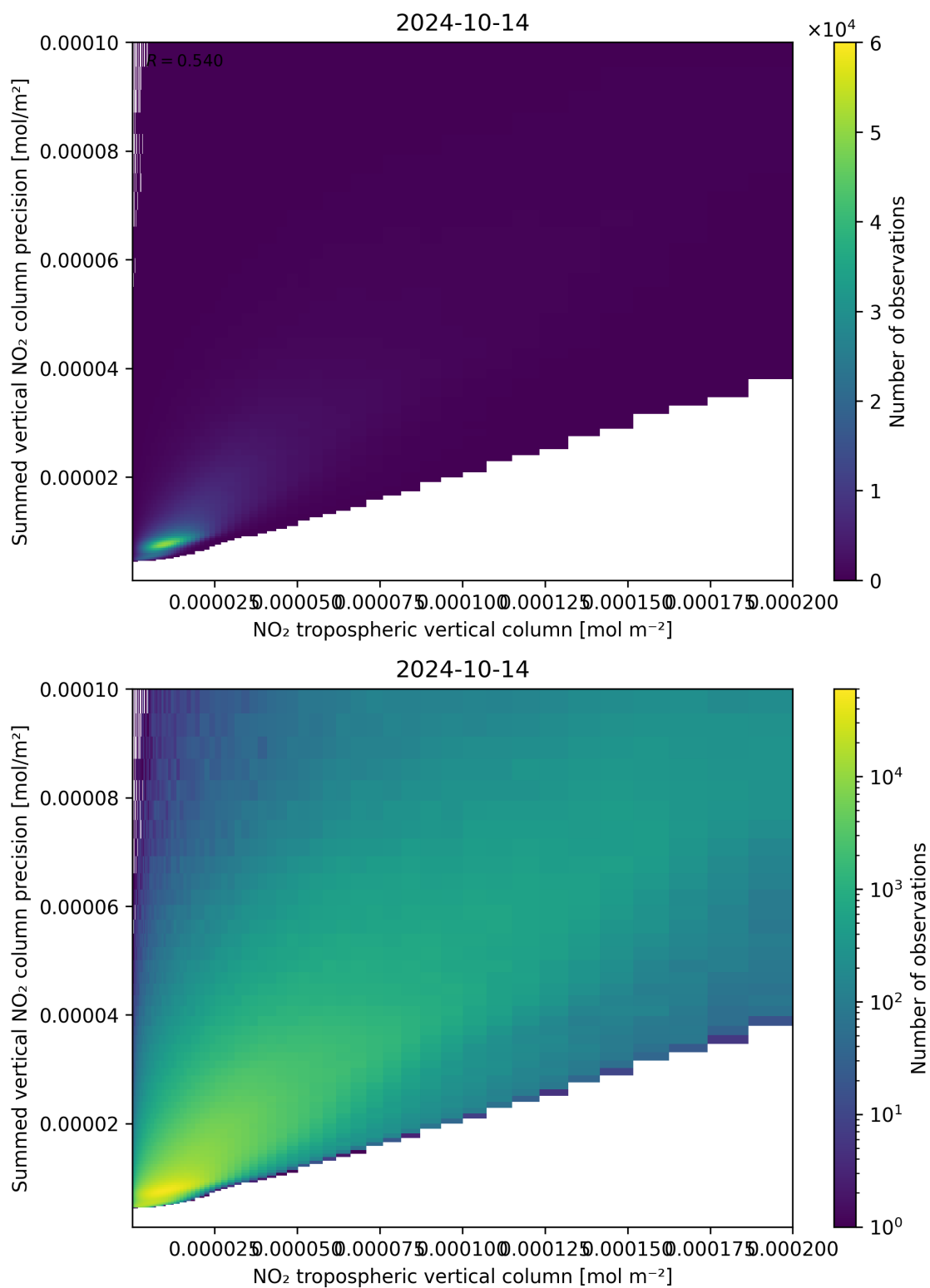
Figure 127: Scatter density plot of “NO 2 tropospheric vertical column” against “Summed vertical NO 2 column precision” for 2024-10-14 to 2024-10-15.
