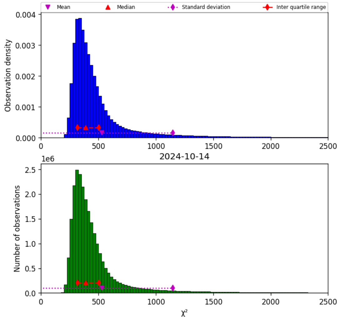
Figure 42: Histogram of " \chi^2 " for 2024-10-14 to 2024-10-15
