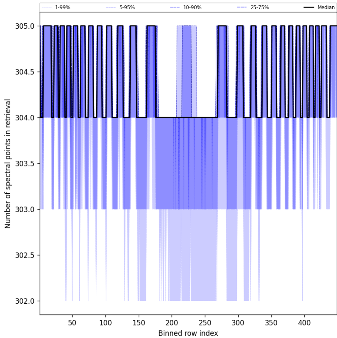
Figure 50: Along track statistics of “Number of spectral points in retrieval” for 2024-10-14 to 2024-10-15
