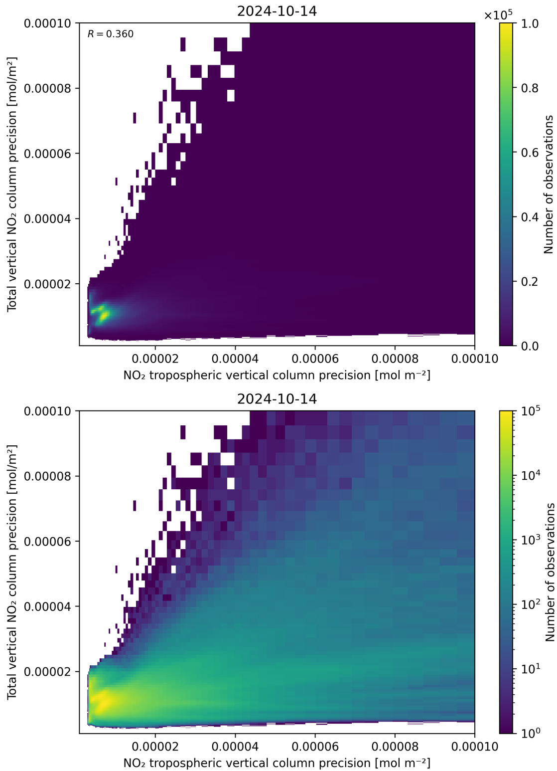
Figure 139: Scatter density plot of “NO 2 tropospheric vertical column precision” against “Total vertical NO 2 column precision” for 2024-10-14 to 2024-10-15.
