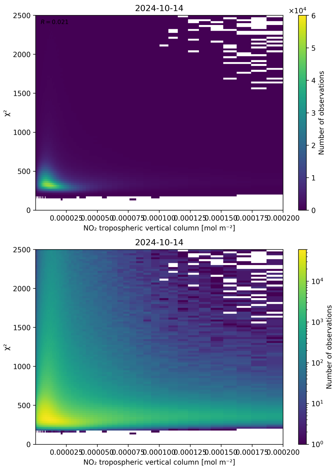
Figure 124: Scatter density plot of “NO 2 tropospheric vertical column” against “ \chi^2 ” for 2024-10-14 to 2024-10-15.
