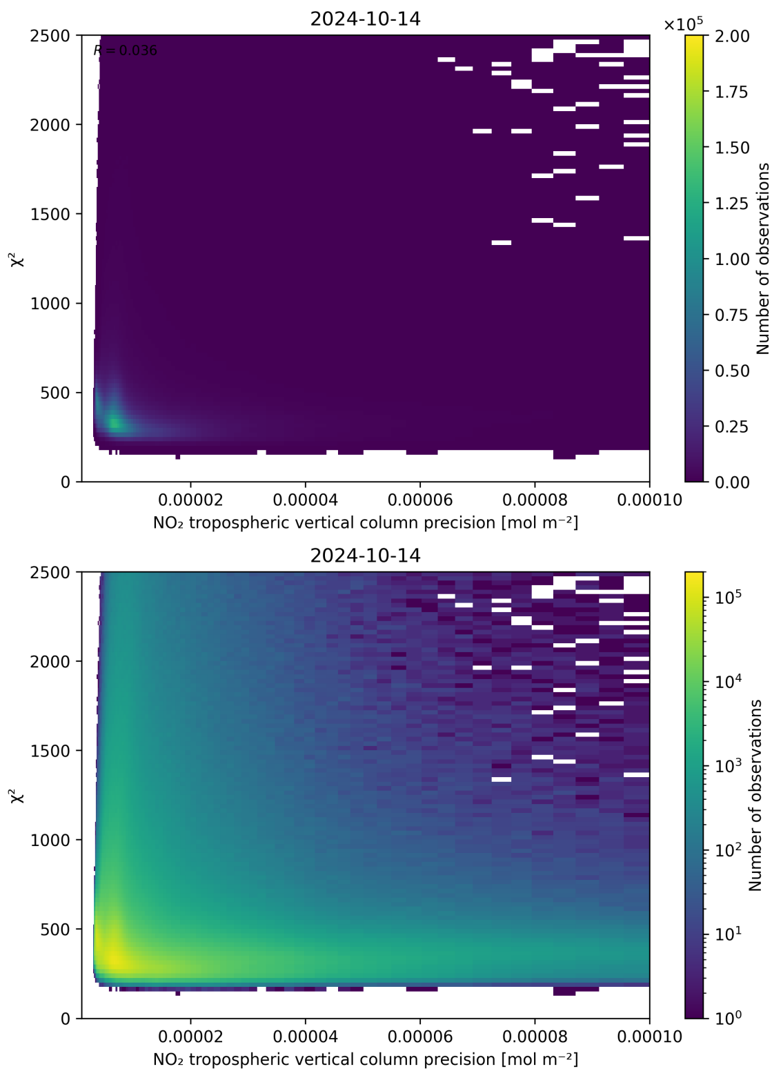
Figure 134: Scatter density plot of “NO 2 tropospheric vertical column precision” against “ \chi^2 ” for 2024-10-14 to 2024-10-15.
