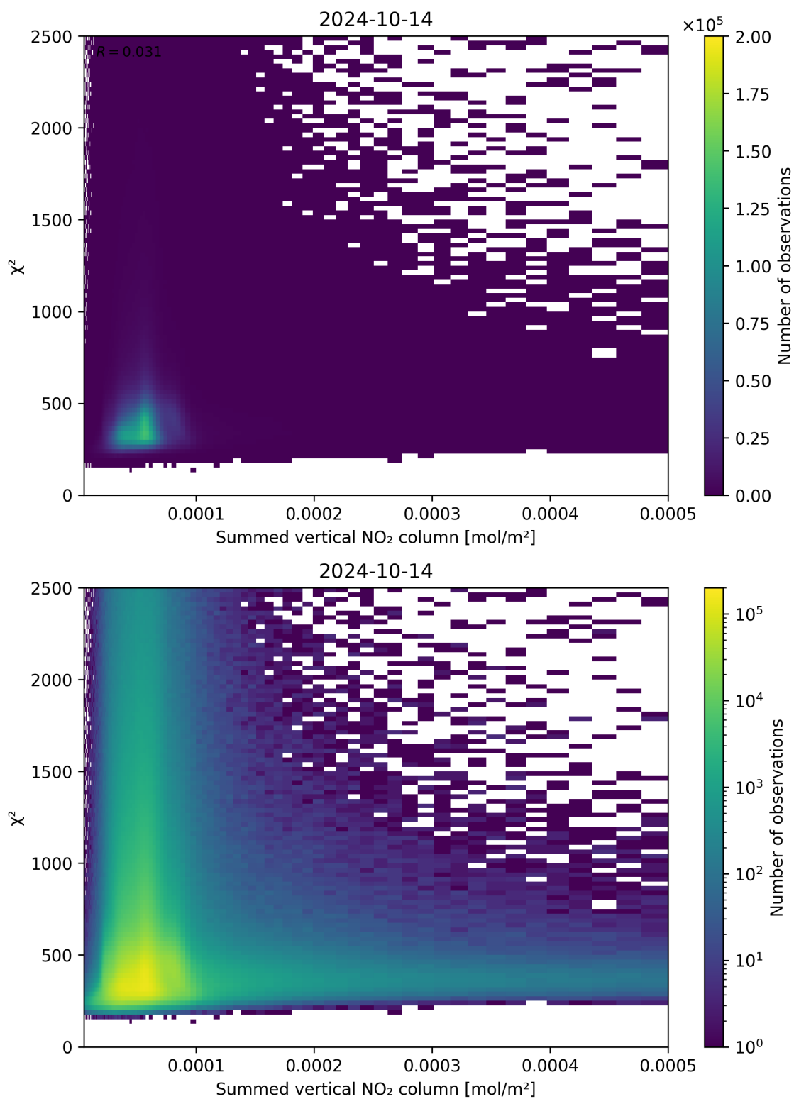
Figure 104: Scatter density plot of “Summed vertical NO 2 column” against “ \chi^2 ” for 2024-10-14 to 2024-10-15.
