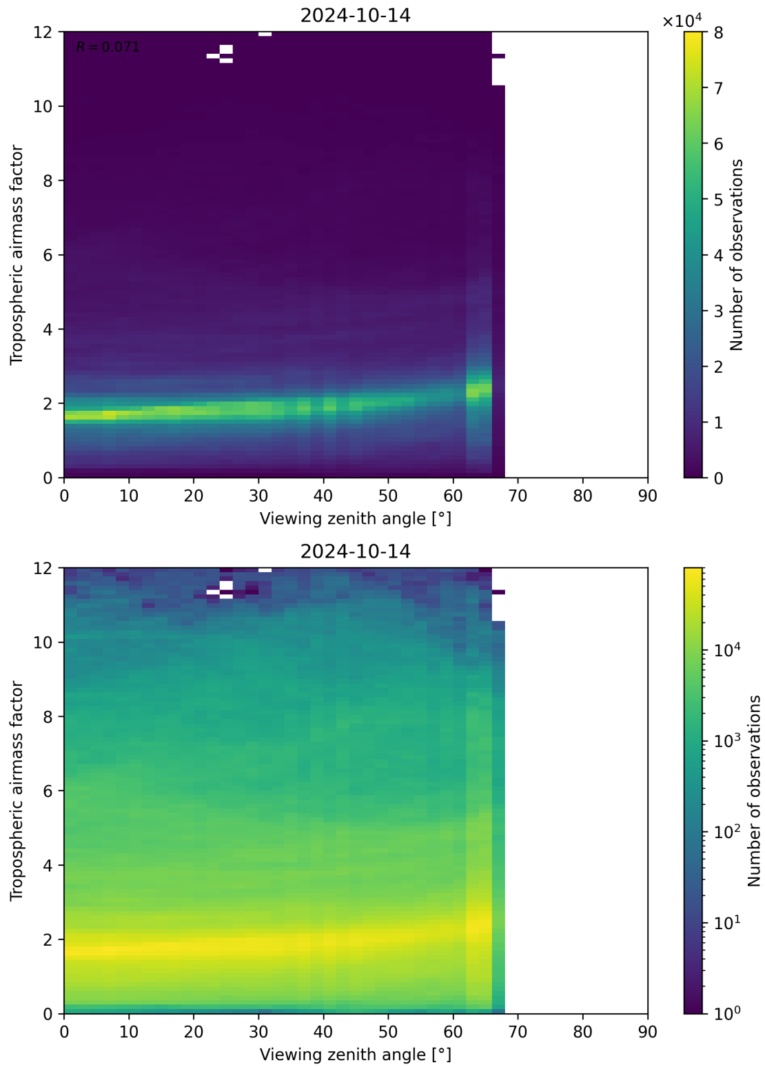
Figure 161: Scatter density plot of “Viewing zenith angle” against “Tropospheric airmass factor” for 2024-10-14 to 2024-10-15.
