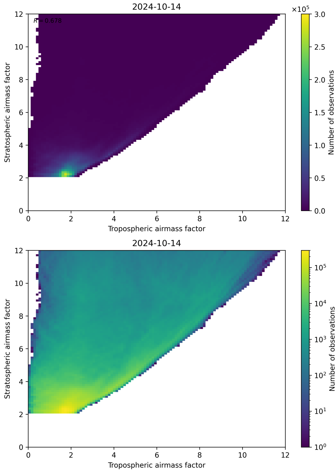
Figure 71: Scatter density plot of “Tropospheric airmass factor” against “Stratospheric airmass factor” for 2024-10-14 to 2024-10-15.
