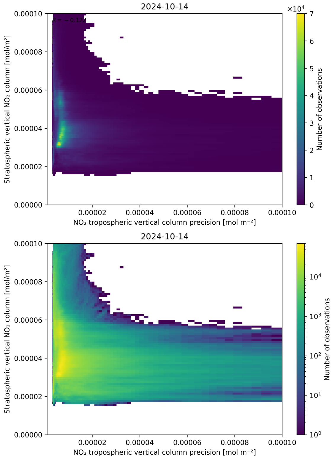
Figure 135: Scatter density plot of “NO 2 tropospheric vertical column precision” against “Stratospheric vertical NO 2 column” for 2024-10-14 to 2024-10-15.
