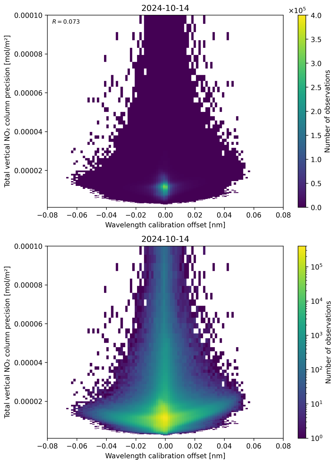
Figure 180: Scatter density plot of “Wavelength calibration offset” against “Total vertical NO 2 column precision” for 2024-10-14 to 2024-10-15.
