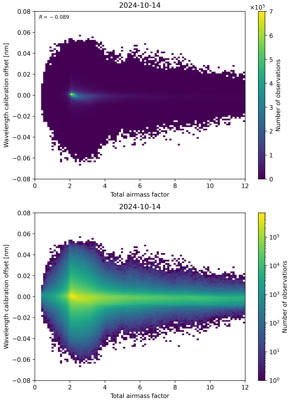
Figure 70: Scatter density plot of “Total airmass factor” against “Wavelength calibration offset” for 2024-10-14 to 2024-10-15.
