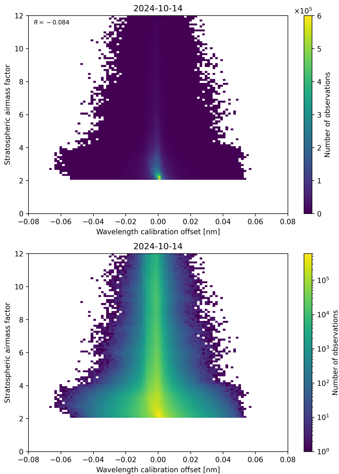
Figure 174: Scatter density plot of “Wavelength calibration offset” against “Stratospheric air mass factor” for 2024-10-14 to 2024-10-15.
