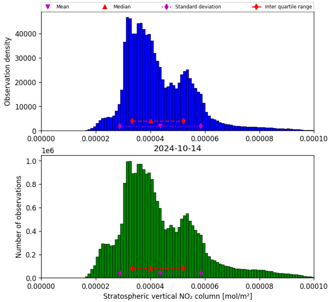
Figure 36: Histogram of “Stratospheric vertical NO 2 column” for 2024-10-14 to 2024-10-15
