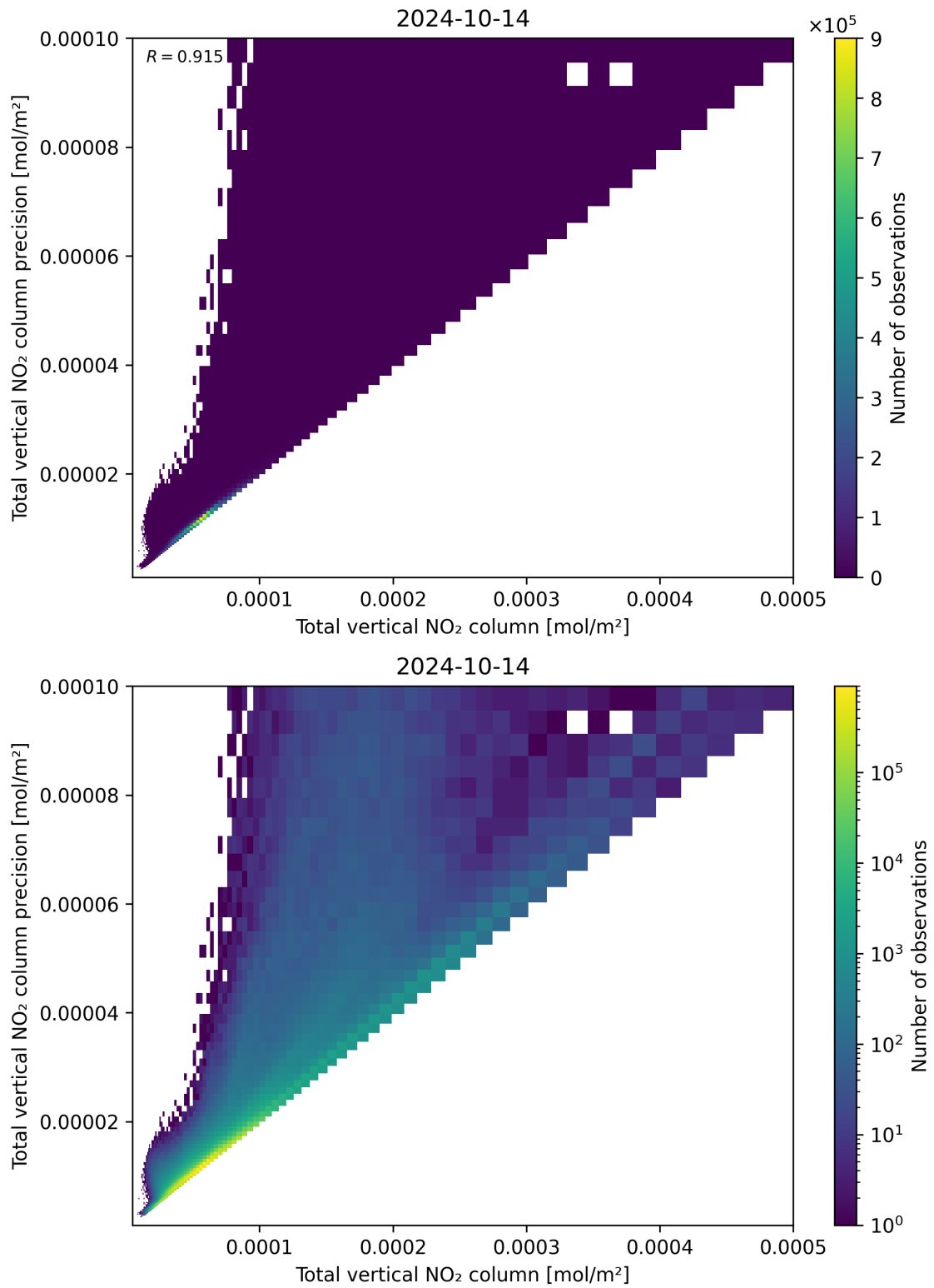
Figure 114: Scatter density plot of “Total vertical NO 2 column” against “Total vertical NO 2 column precision” for 2024-10-14 to 2024-10-15.
