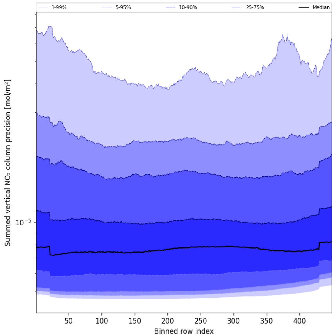
Figure 58: Along track statistics of “Summed vertical NO 2 column precision” for 2024-10-14 to 2024-10-15
