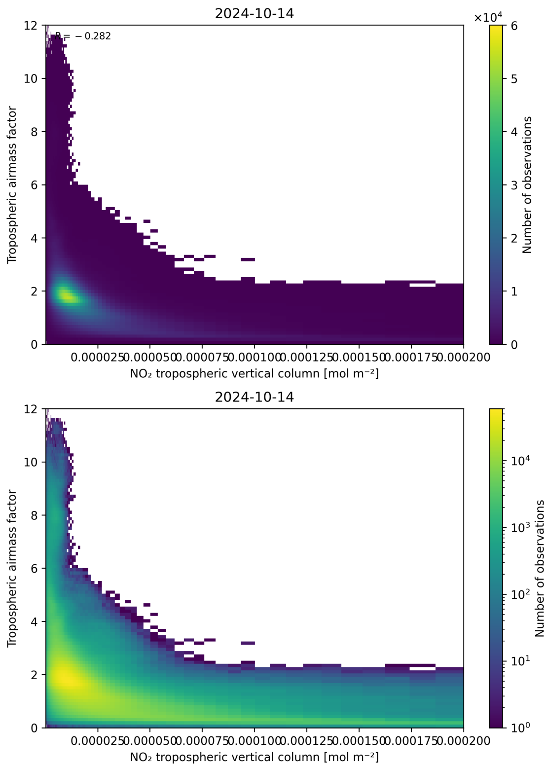
Figure 123: Scatter density plot of “NO 2 tropospheric vertical column” against “Tropospheric air mass factor” for 2024-10-14 to 2024-10-15.
