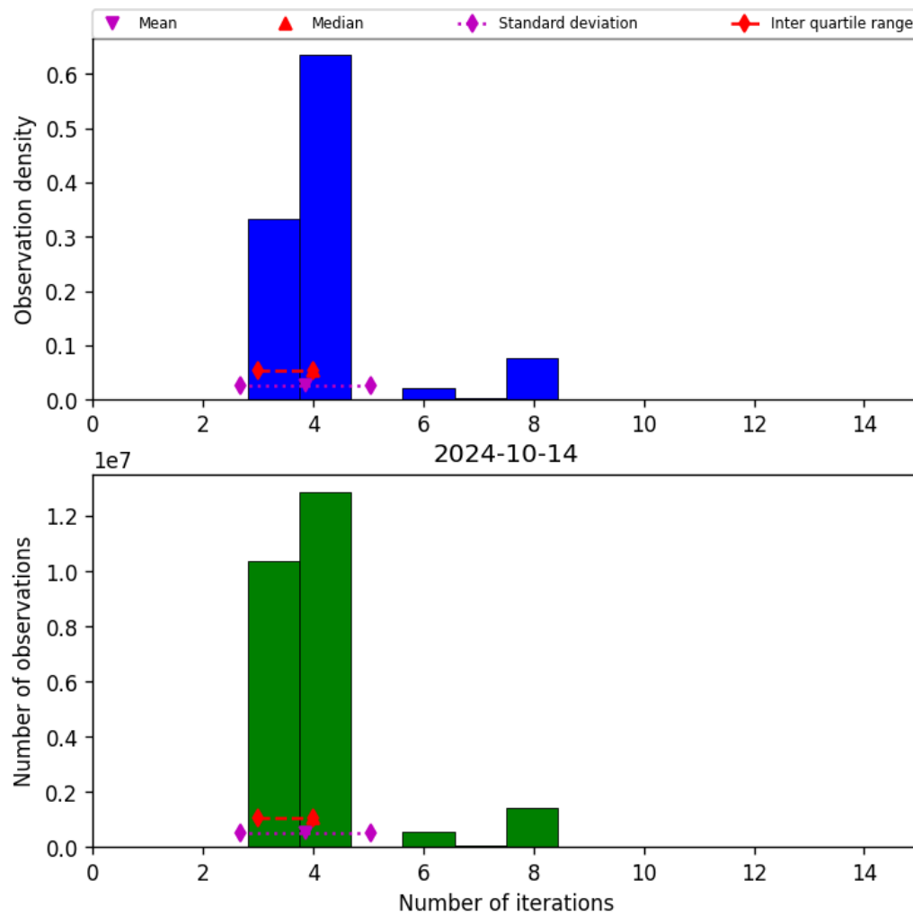
Figure 34: Histogram of “Number of iterations” for 2024-10-14 to 2024-10-15
