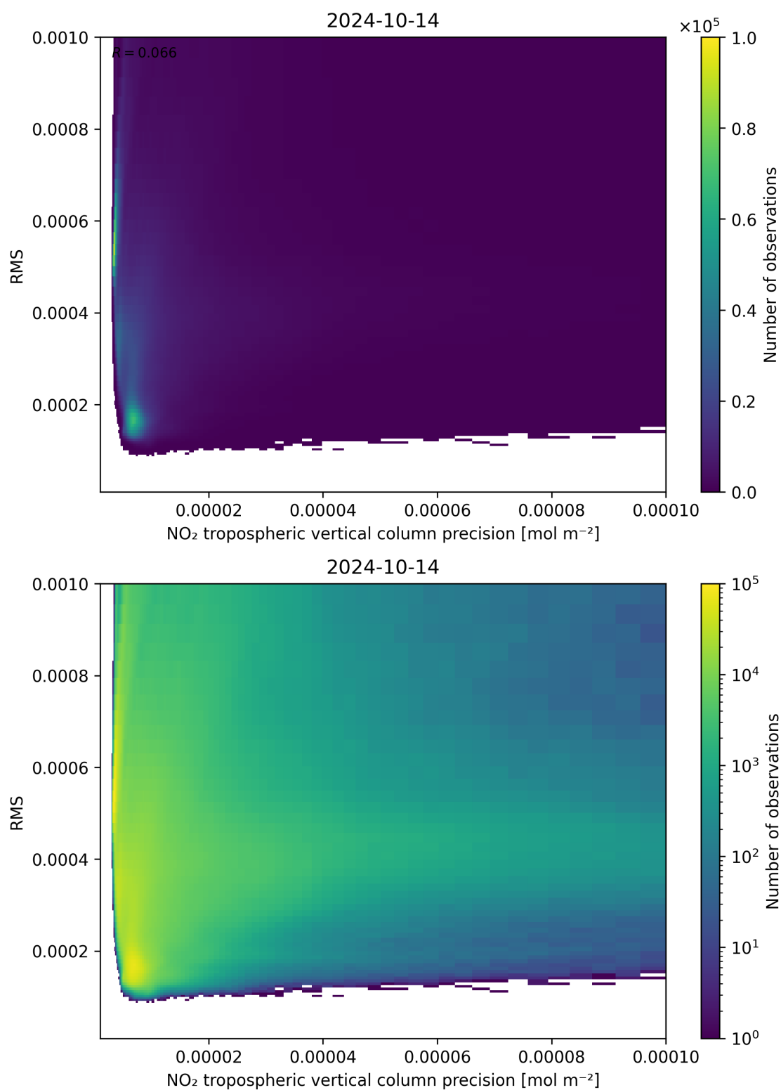
Figure 140: Scatter density plot of “NO 2 tropospheric vertical column precision” against “RMS” for 2024-10-14 to 2024-10-15.
