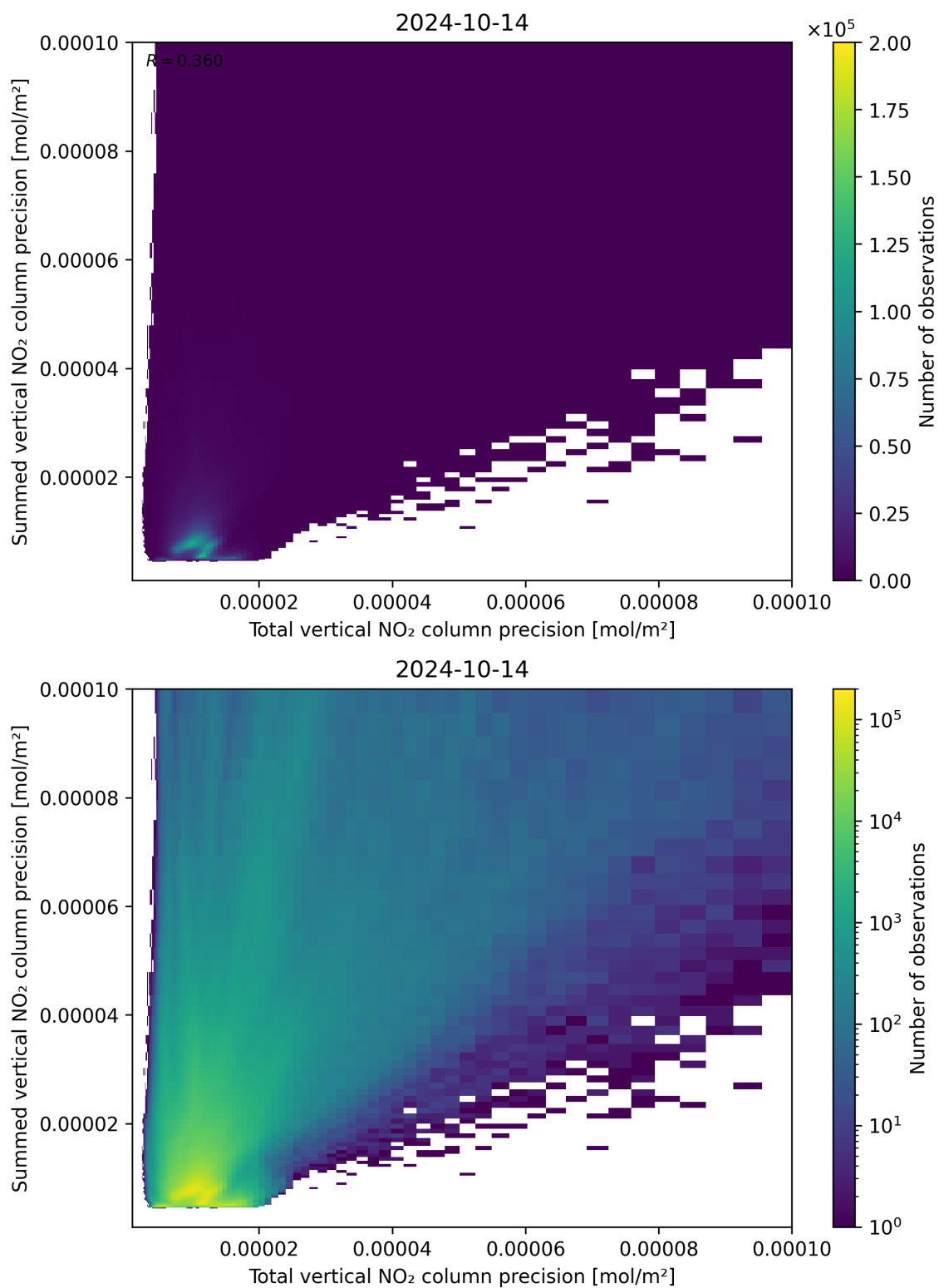
Figure 118: Scatter density plot of “Total vertical NO 2 column precision” against “Summed vertical NO 2 column precision” for 2024-10-14 to 2024-10-15.
