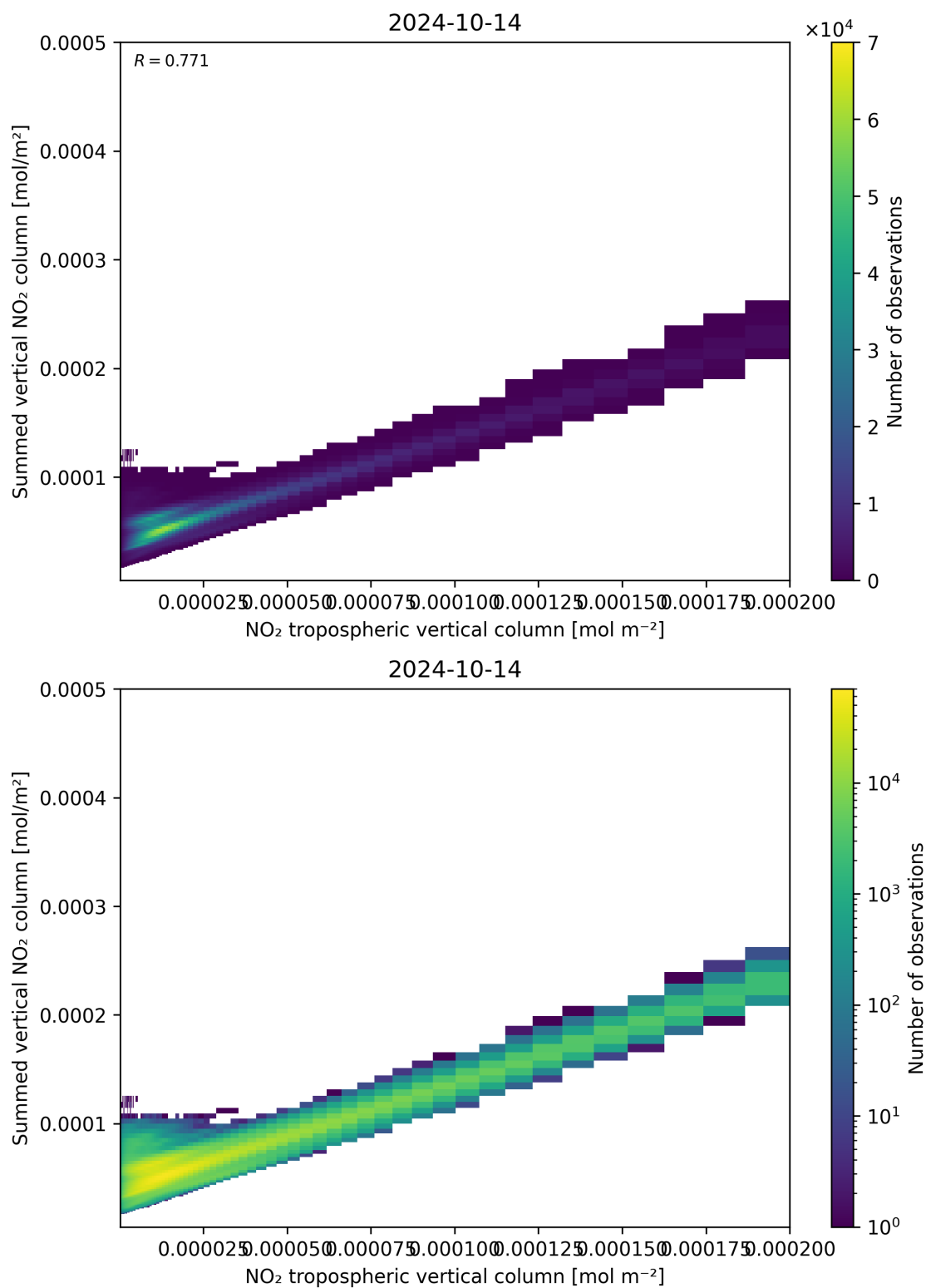
Figure 126: Scatter density plot of “NO 2 tropospheric vertical column” against “Summed vertical NO 2 column” for 2024-10-14 to 2024-10-15.
