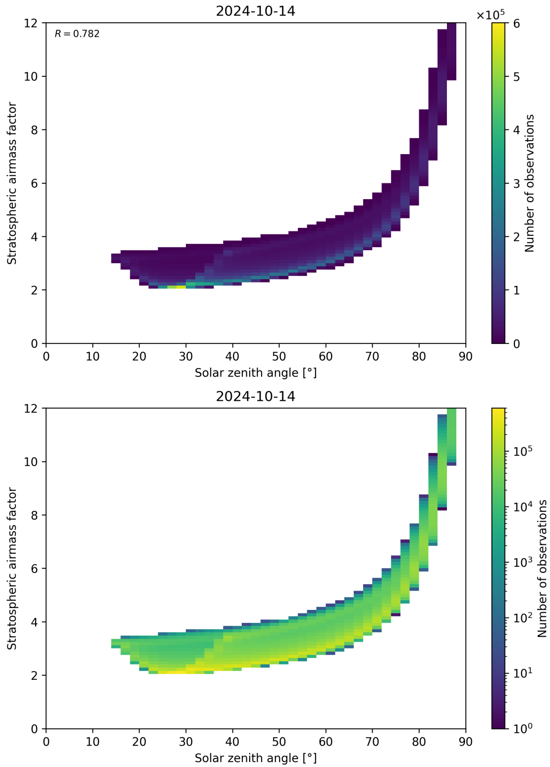
Figure 145: Scatter density plot of “Solar zenith angle” against “Stratospheric airmass factor” for 2024-10-14 to 2024-10-15.
