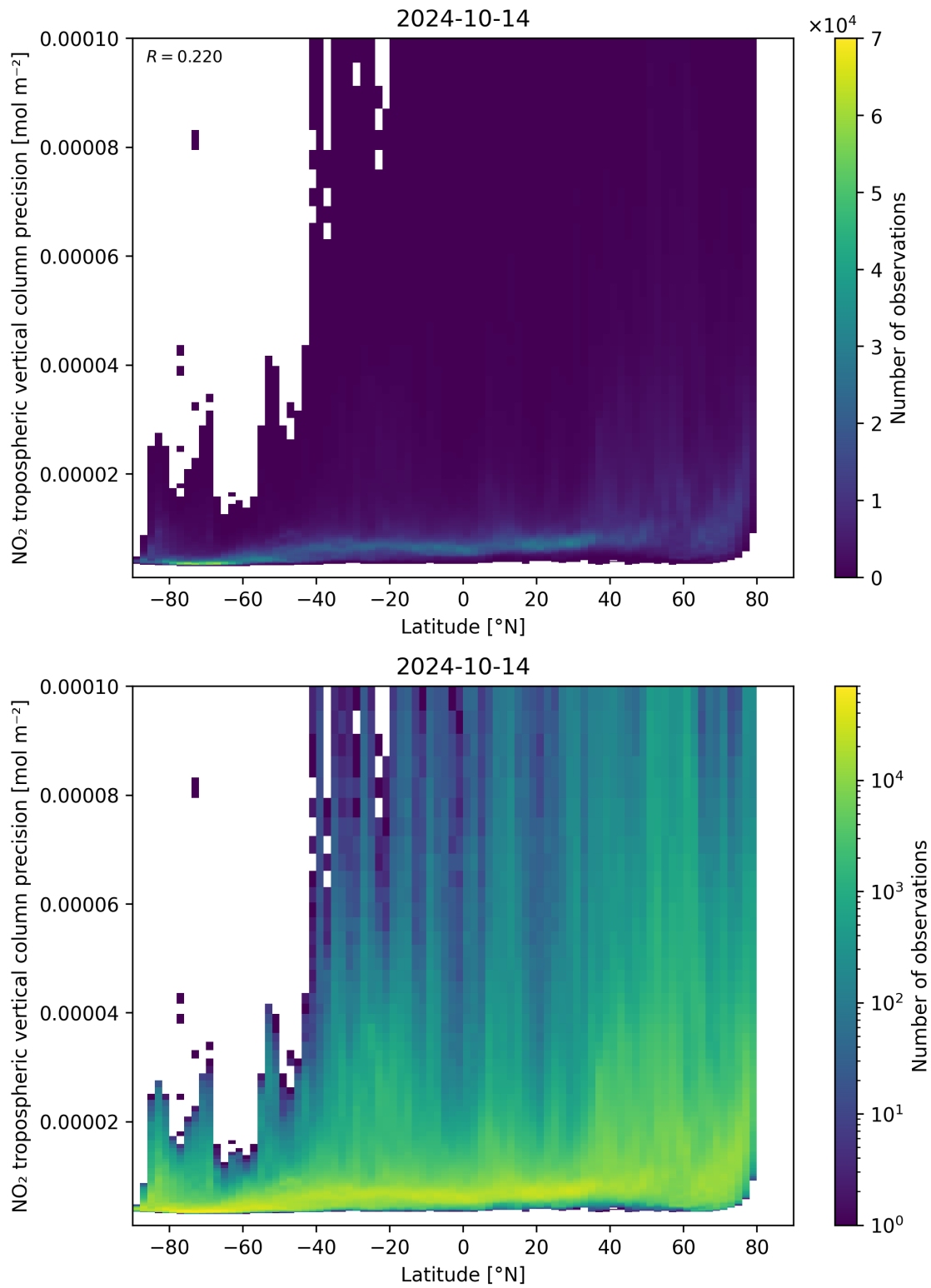
Figure 93: Scatter density plot of “Latitude” against “NO 2 tropospheric vertical column precision” for 2024-10-14 to 2024-10-15.
