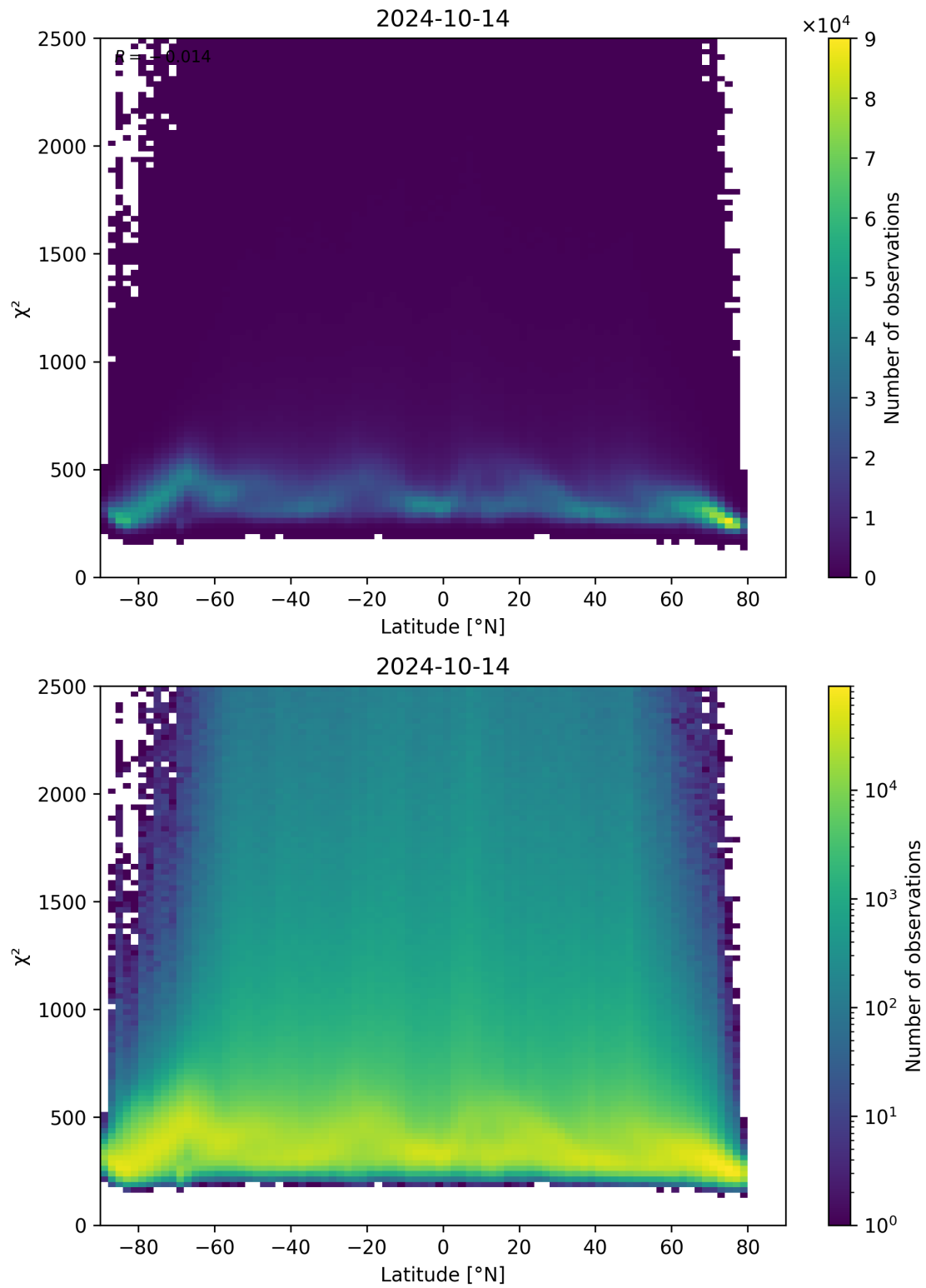
Figure 86: Scatter density plot of “Latitude” against “ \chi^2 ” for 2024-10-14 to 2024-10-15.
