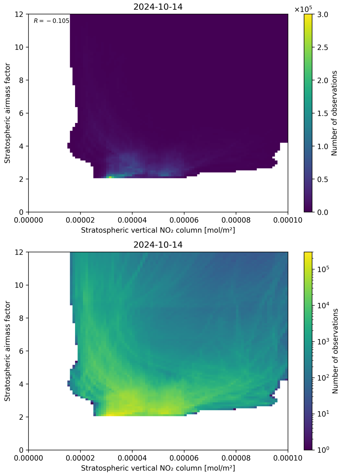
Figure 96: Scatter density plot of “Stratospheric vertical NO 2 column” against “Stratospheric airmass factor” for 2024-10-14 to 2024-10-15.
