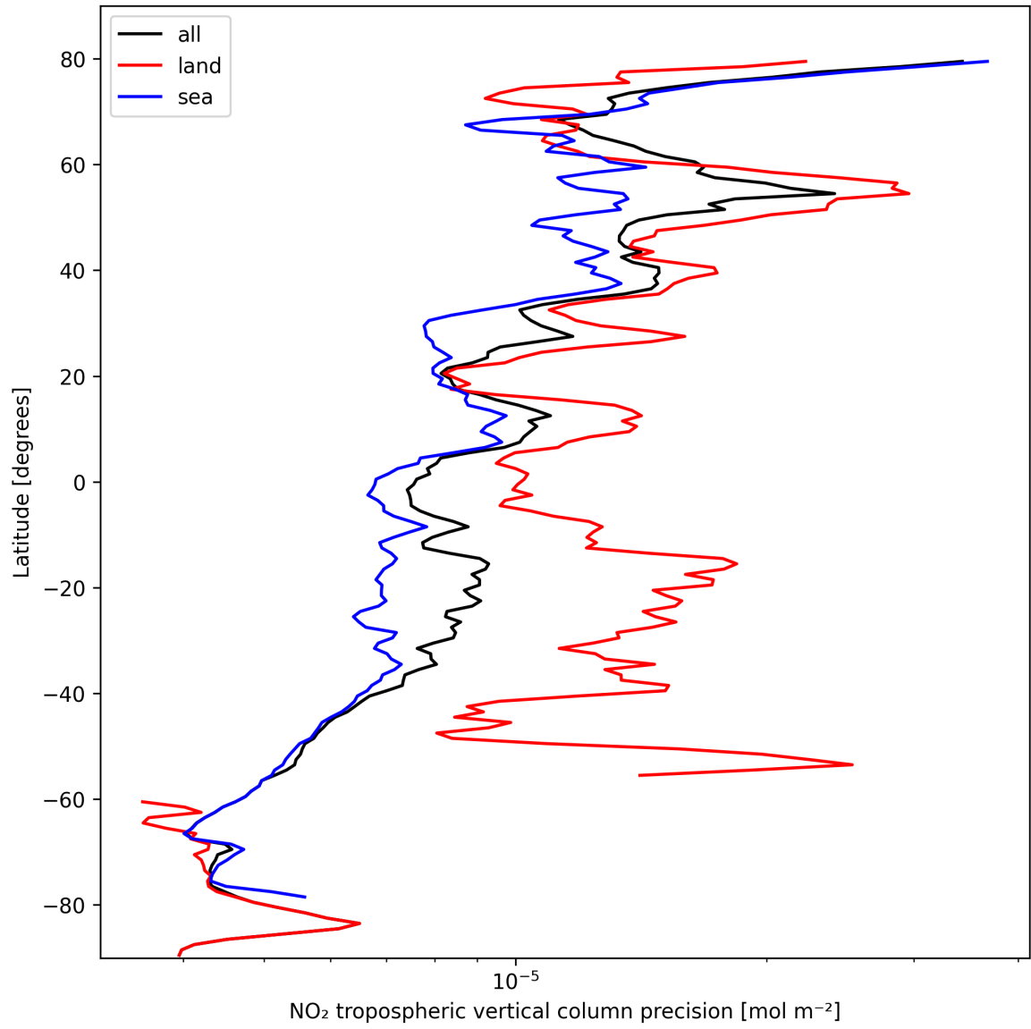
Figure 13: Zonal average of “NO 2 tropospheric vertical column precision” for 2024-10-14 to 2024-10-15.
