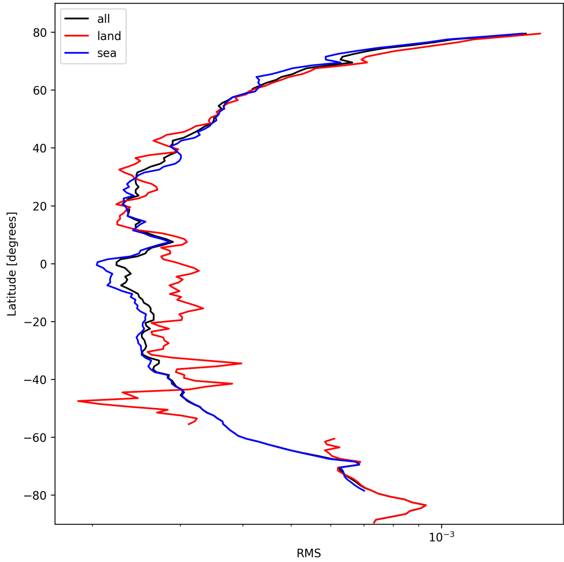
Figure 26: Zonal average of “RMS” for 2024-10-14 to 2024-10-15.
