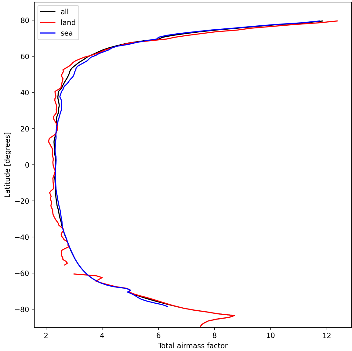
Figure 15: Zonal average of “Total airmass factor” for 2024-10-14 to 2024-10-15.
