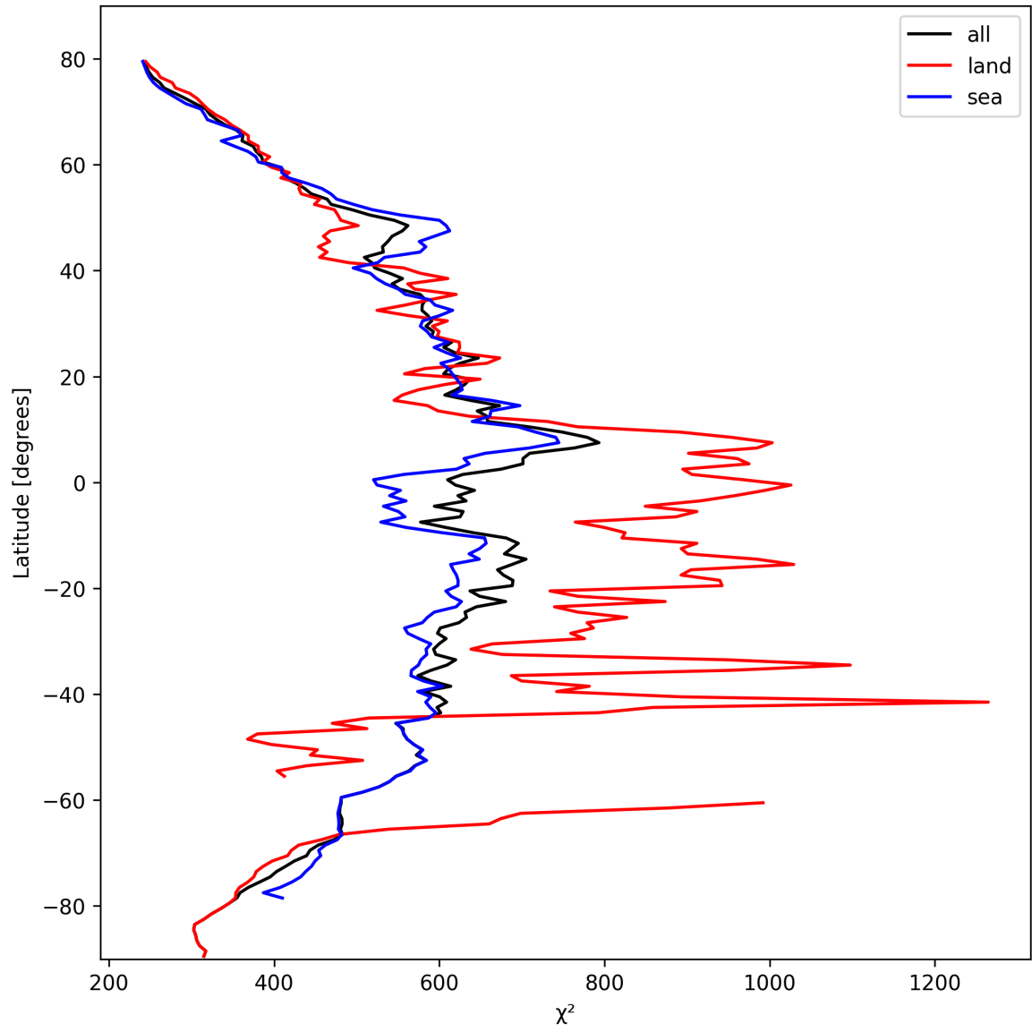
Figure 25: Zonal average of “ \chi^2 ” for 2024-10-14 to 2024-10-15.
