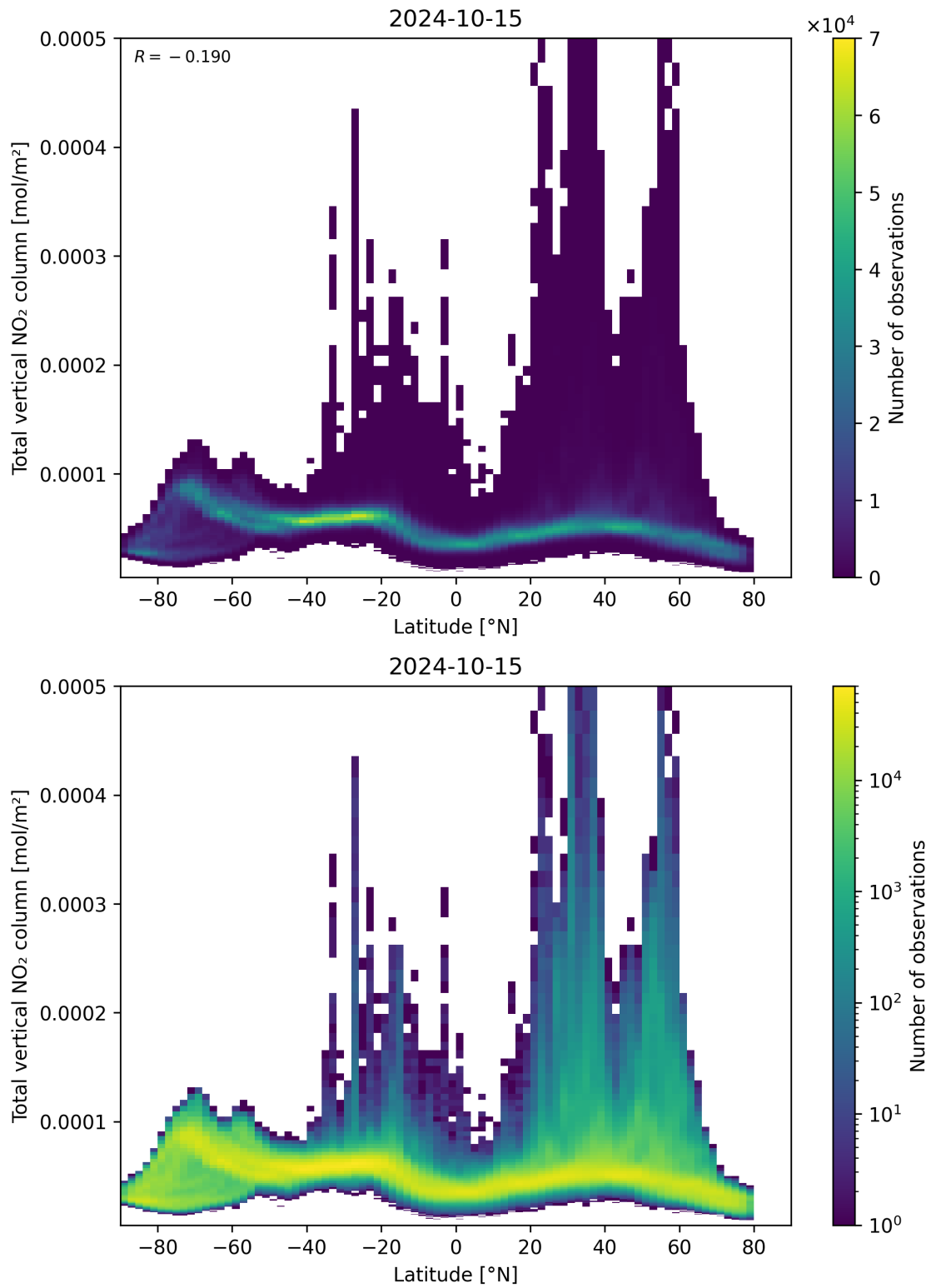
Figure 90: Scatter density plot of “Latitude” against “Total vertical NO 2 column” for 2024-10-14 to 2024-10-16.
