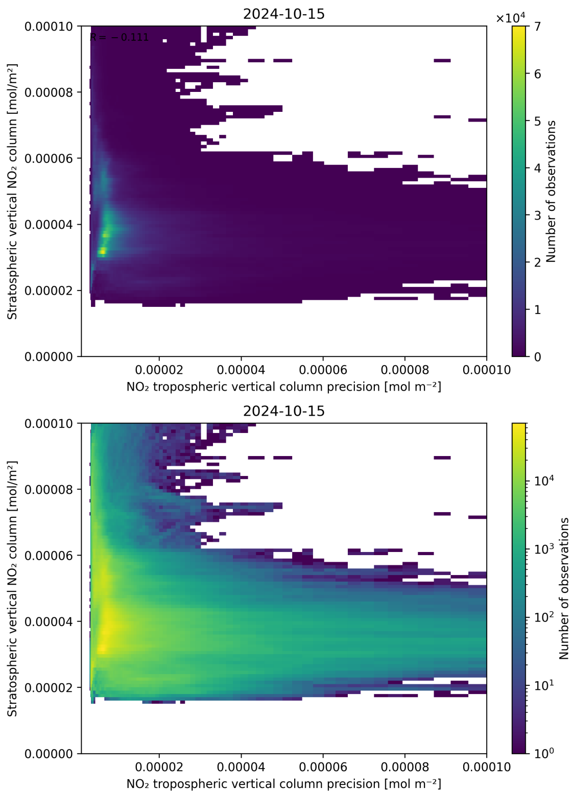
Figure 135: Scatter density plot of “NO 2 tropospheric vertical column precision” against “Stratospheric vertical NO 2 column” for 2024-10-14 to 2024-10-16.
