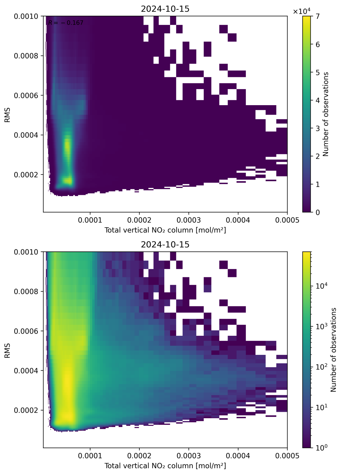
Figure 120: Scatter density plot of “Total vertical NO 2 column” against “RMS” for 2024-10-14 to 2024-10-16.
