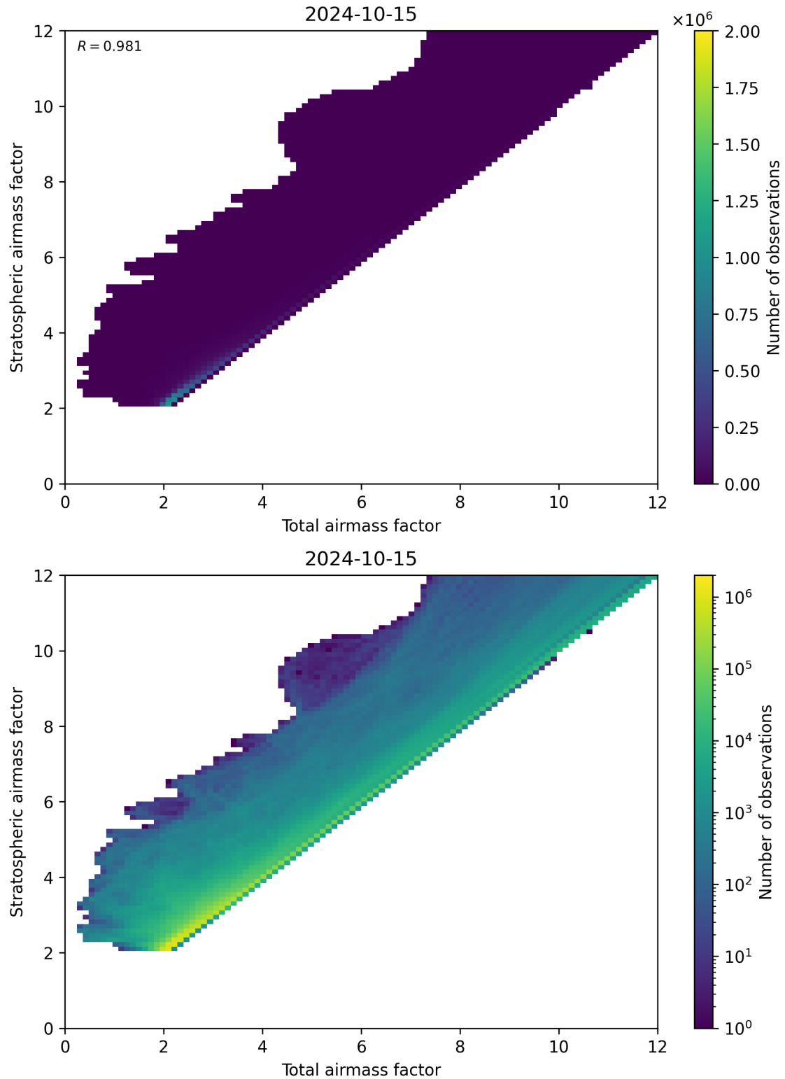
Figure 62: Scatter density plot of “Total airmass factor” against “Stratospheric airmass factor” for 2024-10-14 to 2024-10-16.
