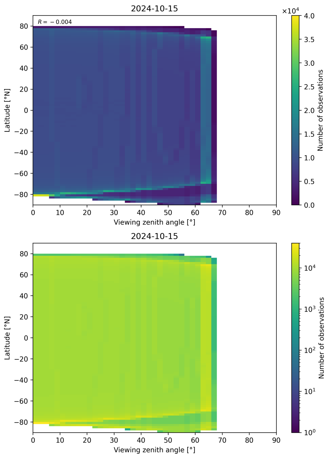
Figure 163: Scatter density plot of “Viewing zenith angle” against “Latitude” for 2024-10-14 to 2024-10-16.
