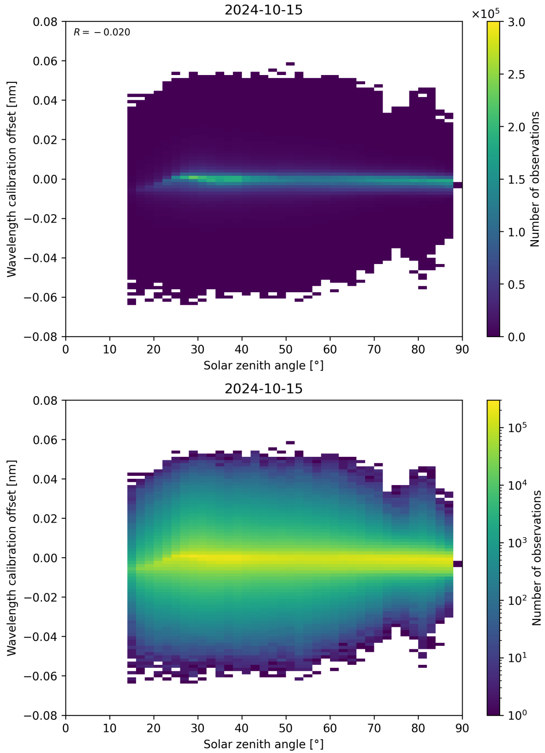
Figure 158: Scatter density plot of “Solar zenith angle” against “Wavelength calibration offset” for 2024-10-14 to 2024-10-16.
