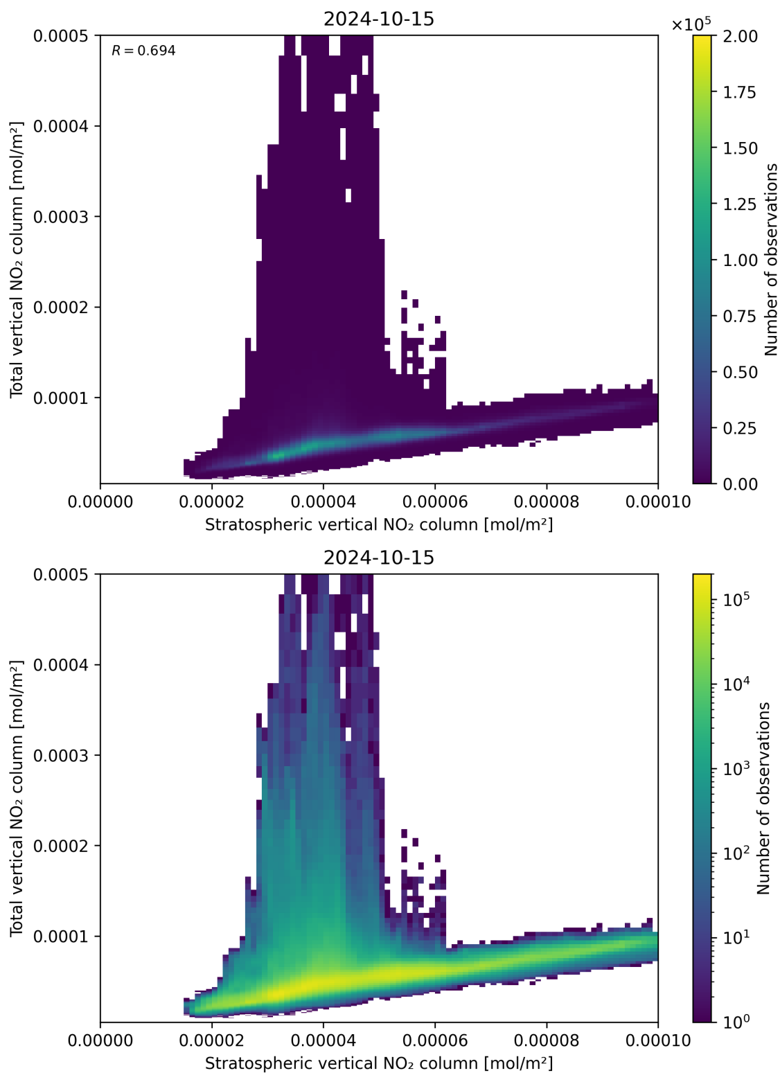
Figure 100: Scatter density plot of “Stratospheric vertical NO 2 column” against “Total vertical NO 2 column” for 2024-10-14 to 2024-10-16.
