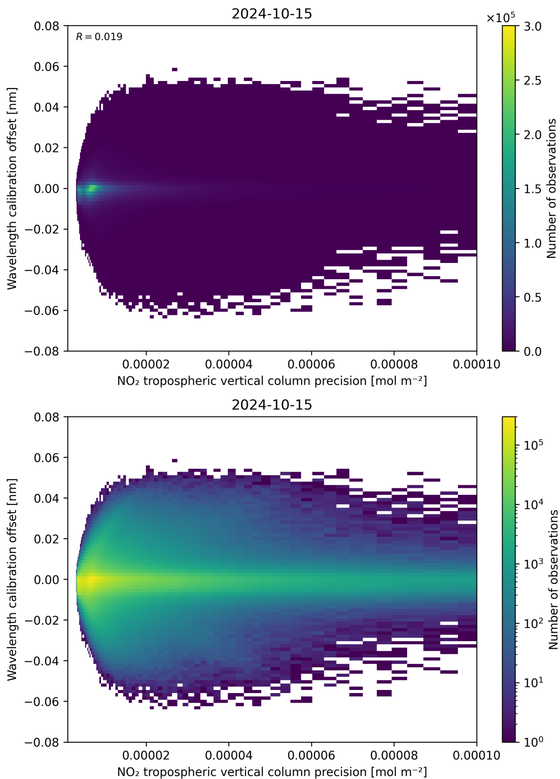
Figure 141: Scatter density plot of “NO 2 tropospheric vertical column precision” against “Wavelength calibration offset” for 2024-10-14 to 2024-10-16.
