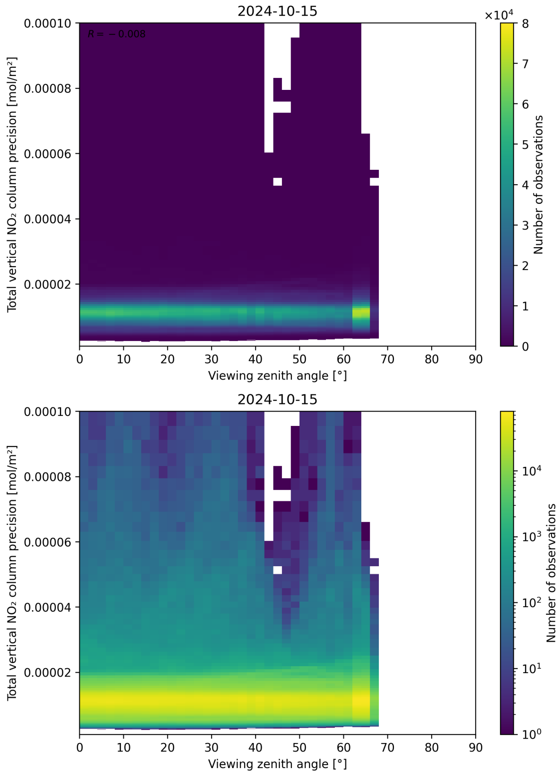
Figure 168: Scatter density plot of “Viewing zenith angle” against “Total vertical NO 2 column precision” for 2024-10-14 to 2024-10-16.
