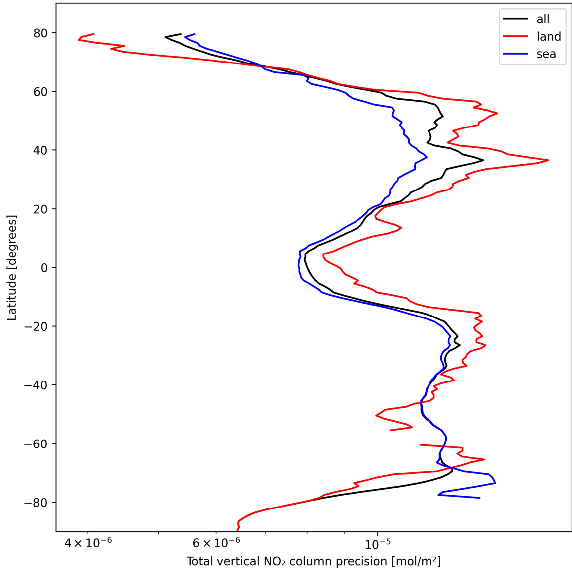
Figure 22: Zonal average of “Total vertical NO 2 column precision” for 2024-10-14 to 2024-10-16.
