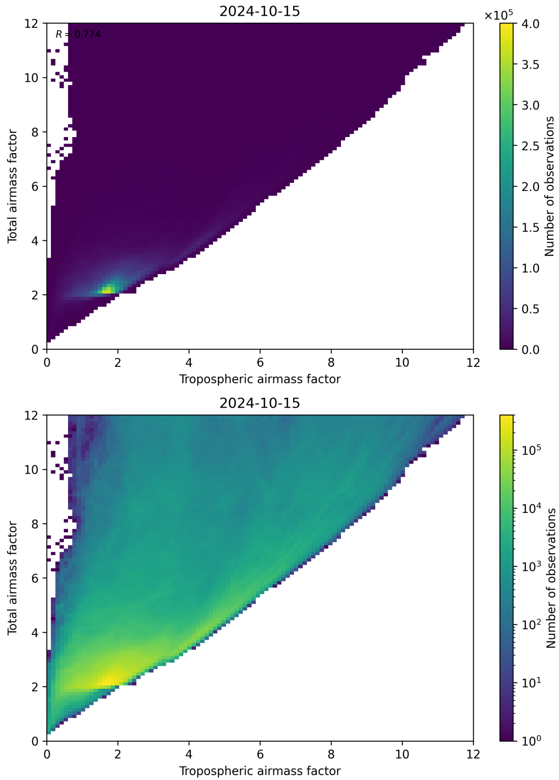
Figure 72: Scatter density plot of “Tropospheric airmass factor” against “Total airmass factor” for 2024-10-14 to 2024-10-16.
