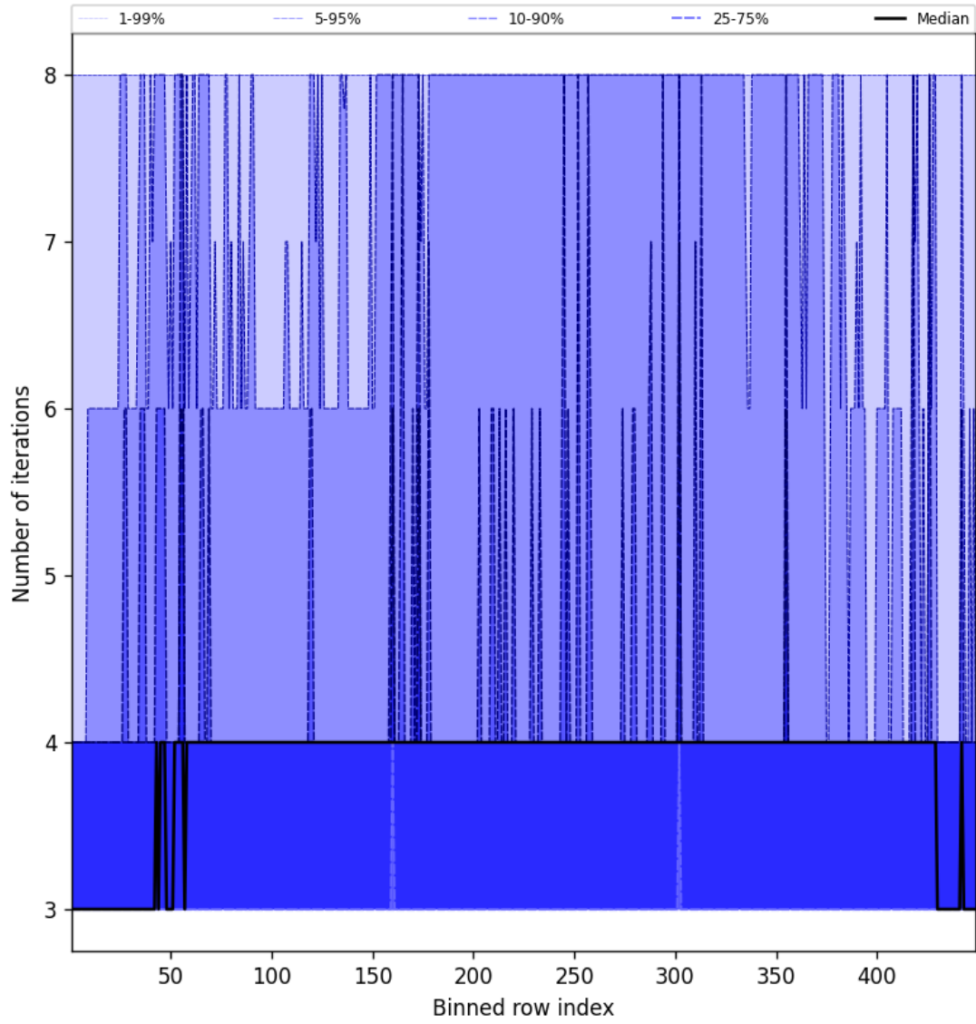
Figure 51: Along track statistics of “Number of iterations” for 2024-10-14 to 2024-10-16
