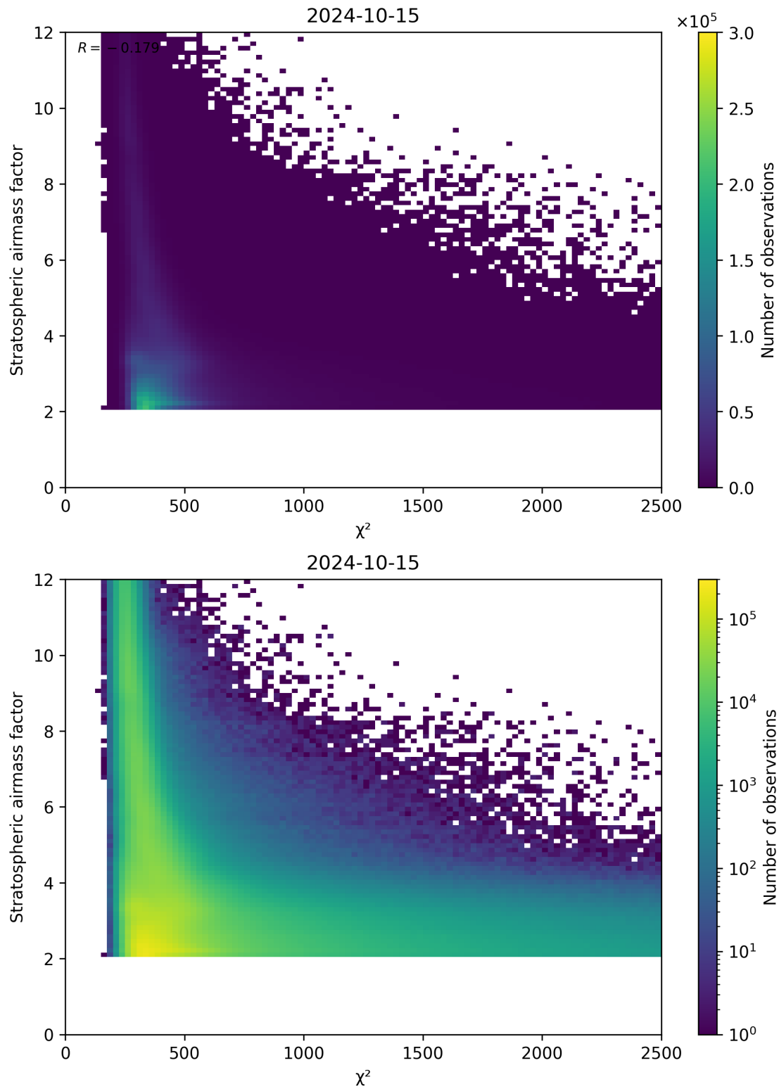
Figure 81: Scatter density plot of “ \chi^2 ” against “Stratospheric airmass factor” for 2024-10-14 to 2024-10-16.
