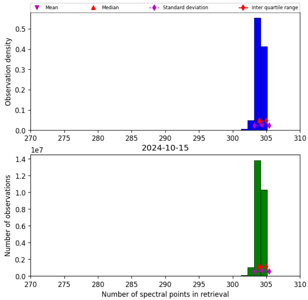
Figure 33: Histogram of “Number of spectral points in retrieval” for 2024-10-14 to 2024-10-16
