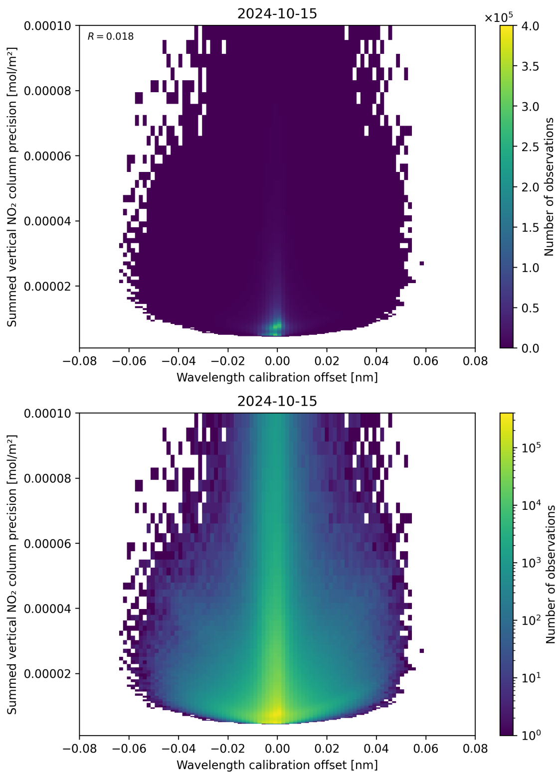
Figure 178: Scatter density plot of “Wavelength calibration offset” against “Summed vertical NO 2 column precision” for 2024-10-14 to 2024-10-16.
