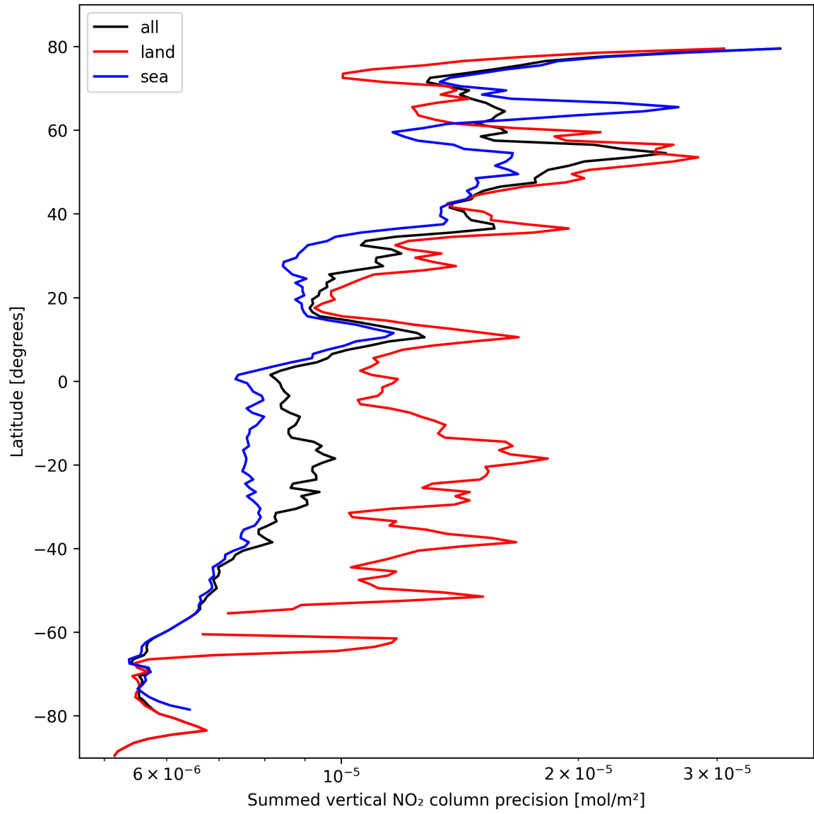
Figure 24: Zonal average of “Summed vertical NO 2 column precision” for 2024-10-14 to 2024-10-16.
