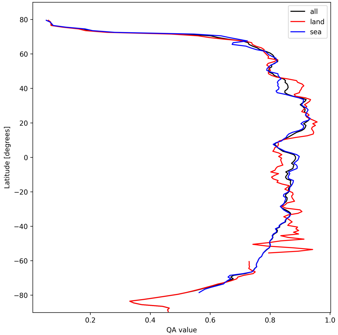
Figure 11: Zonal average of “QA value” for 2024-10-14 to 2024-10-16.
