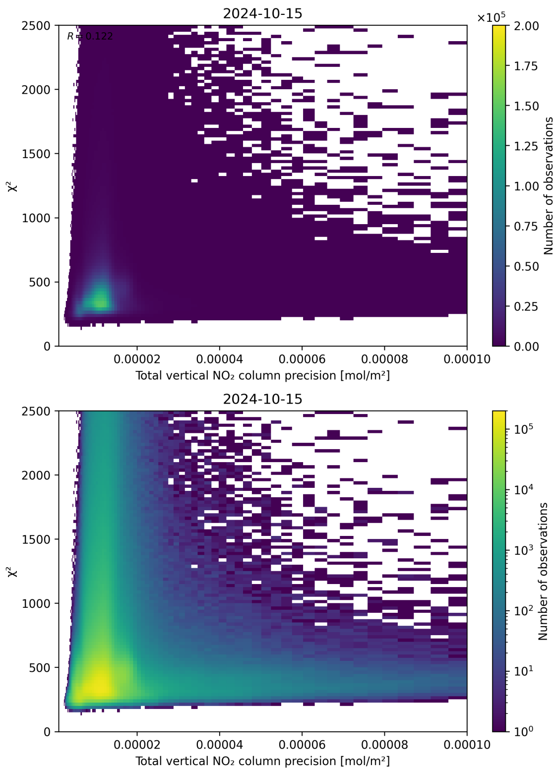
Figure 116: Scatter density plot of “Total vertical NO 2 column precision” against “ \chi^2 ” for 2024-10-14 to 2024-10-16.
