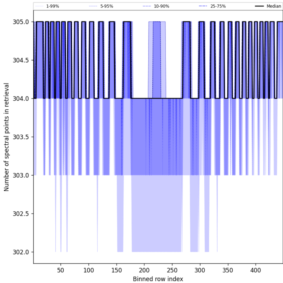
Figure 50: Along track statistics of “Number of spectral points in retrieval” for 2024-10-14 to 2024-10-16
