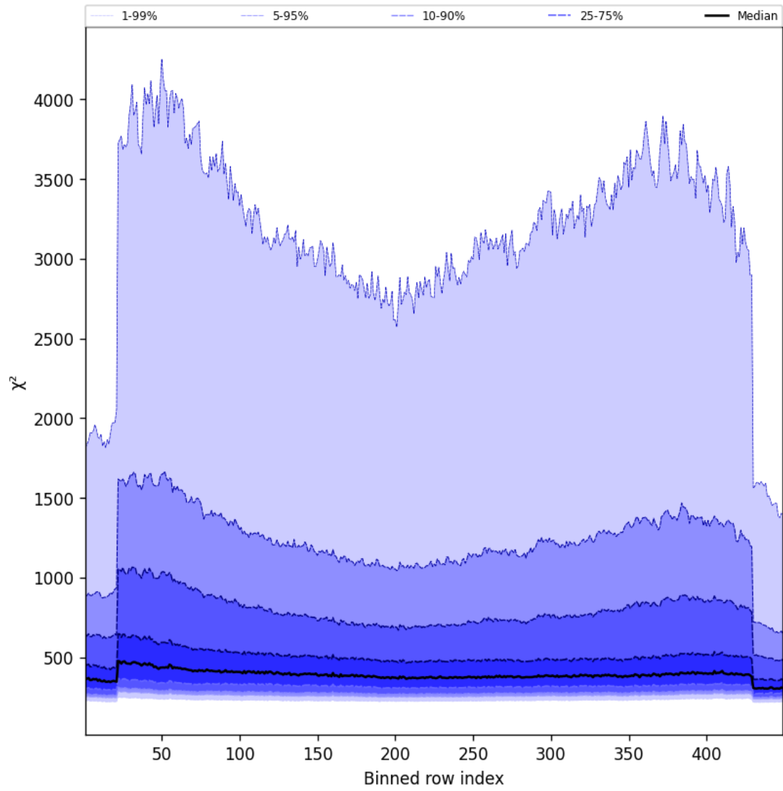
Figure 59: Along track statistics of “ \chi^2 ” for 2024-10-14 to 2024-10-16
