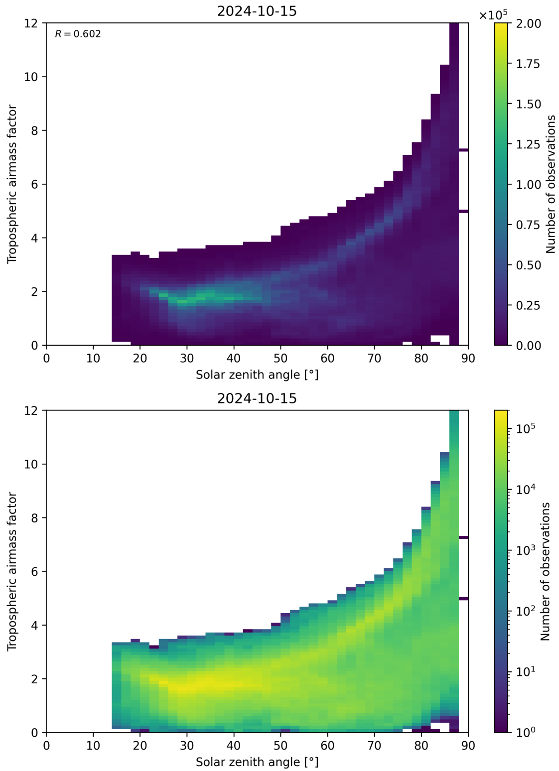
Figure 147: Scatter density plot of “Solar zenith angle” against “Tropospheric airmass factor” for 2024-10-14 to 2024-10-16.
