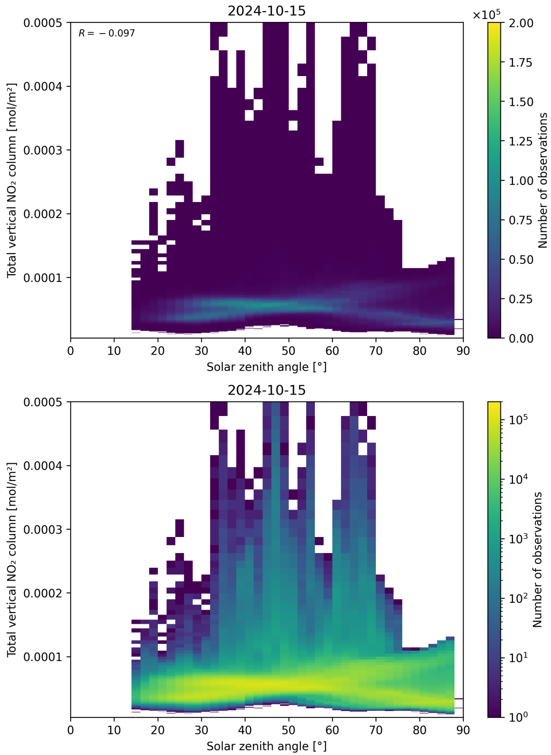
Figure 153: Scatter density plot of “Solar zenith angle” against “Total vertical NO 2 column” for 2024-10-14 to 2024-10-16.
