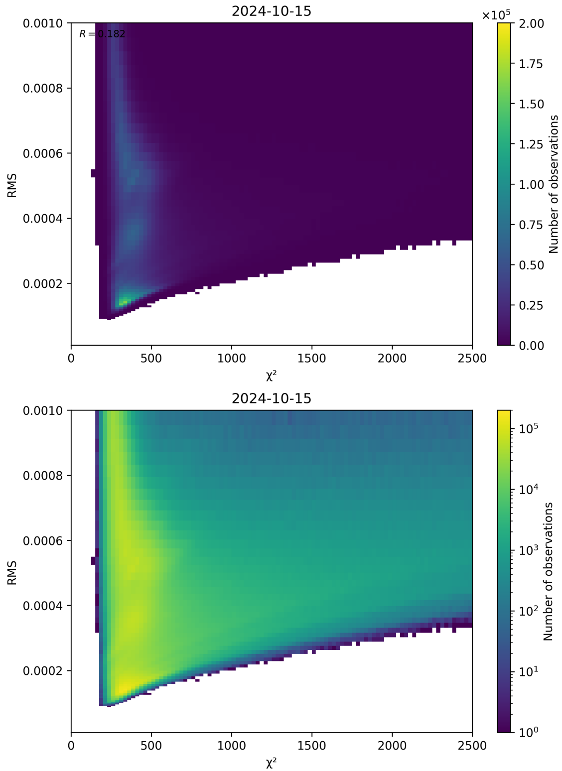
Figure 82: Scatter density plot of “ \chi^2 ” against “RMS” for 2024-10-14 to 2024-10-16.
