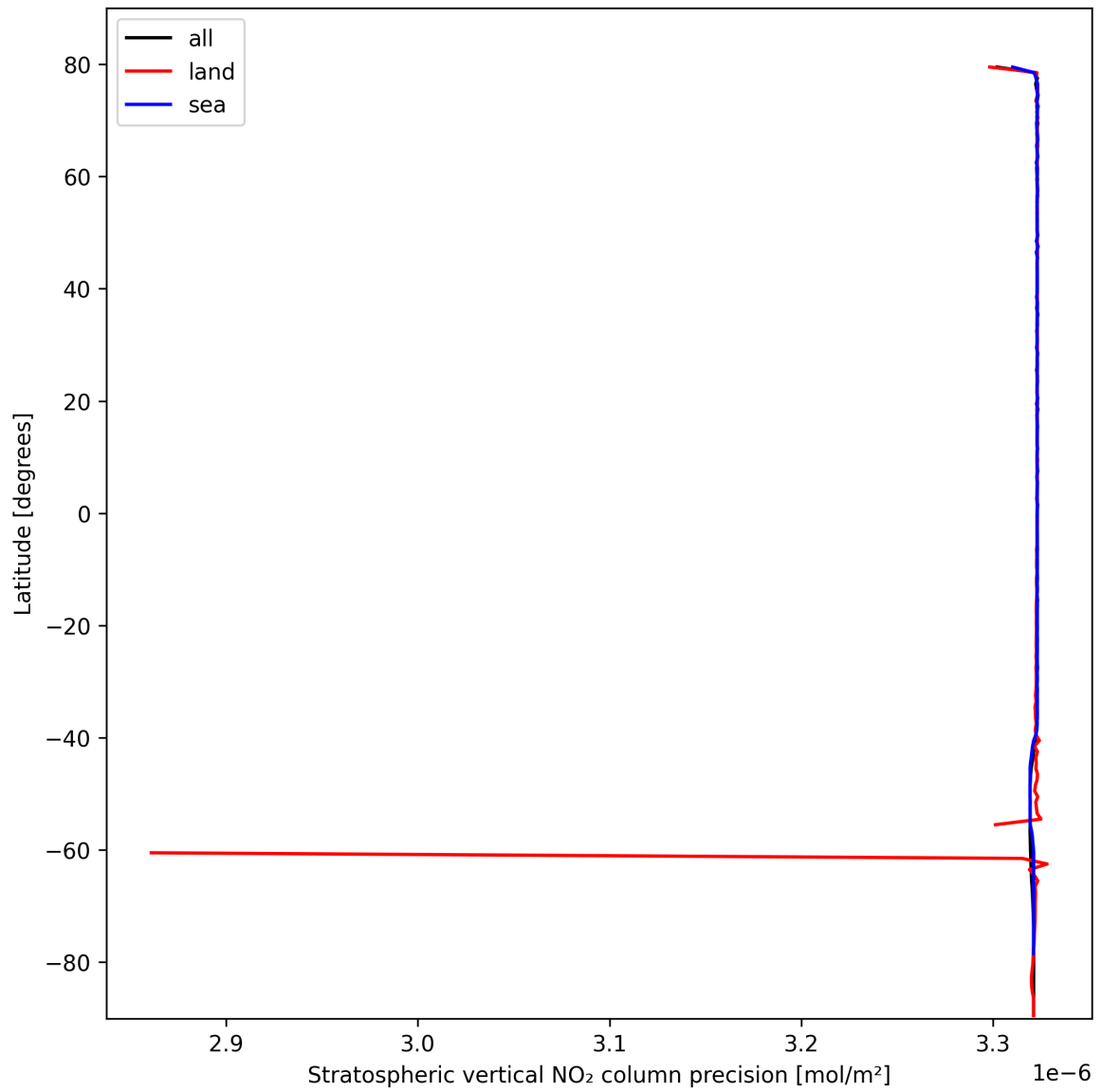
Figure 20: Zonal average of “Stratospheric vertical NO 2 column precision” for 2024-10-14 to 2024-10-16.
