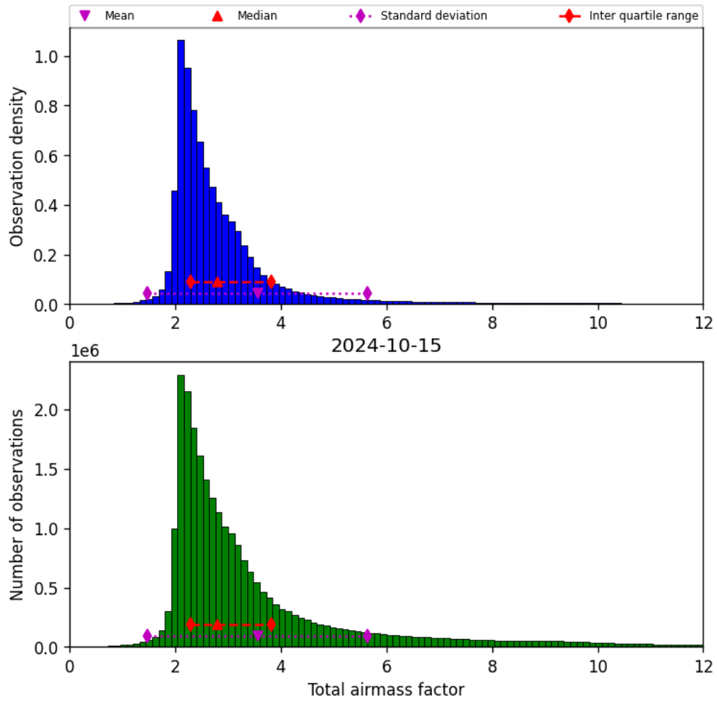
Figure 32: Histogram of “Total airmass factor” for 2024-10-14 to 2024-10-16
