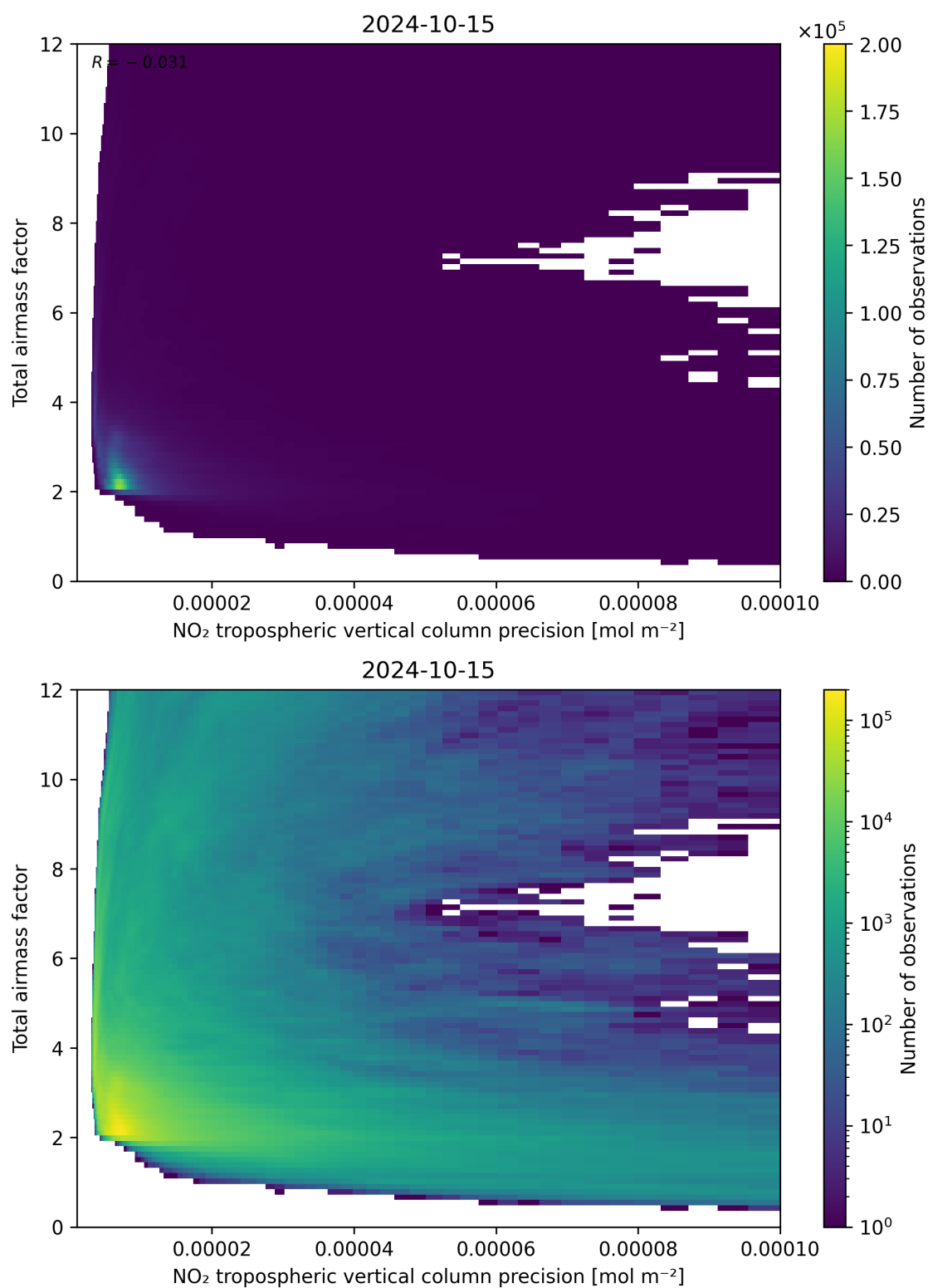
Figure 132: Scatter density plot of “NO 2 tropospheric vertical column precision” against “Total air mass factor” for 2024-10-14 to 2024-10-16.
