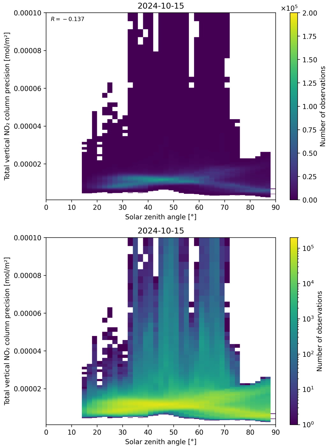
Figure 154: Scatter density plot of “Solar zenith angle” against “Total vertical NO 2 column precision” for 2024-10-14 to 2024-10-16.
