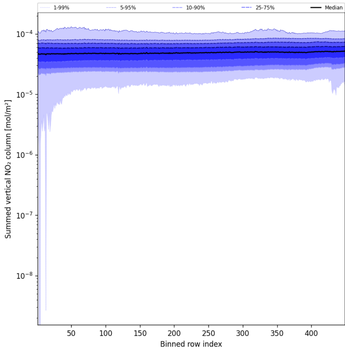
Figure 57: Along track statistics of “Summed vertical NO 2 column” for 2024-10-14 to 2024-10-16
