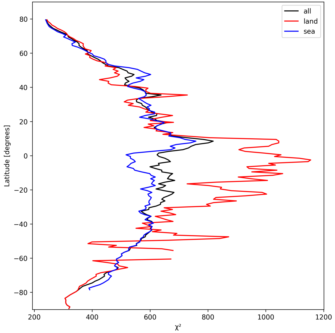
Figure 25: Zonal average of “ \chi^2 ” for 2024-10-14 to 2024-10-16.
