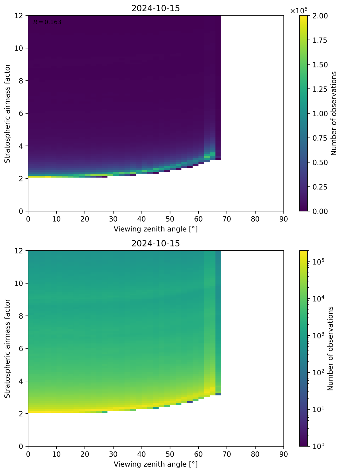
Figure 159: Scatter density plot of “Viewing zenith angle” against “Stratospheric airmass factor” for 2024-10-14 to 2024-10-16.
