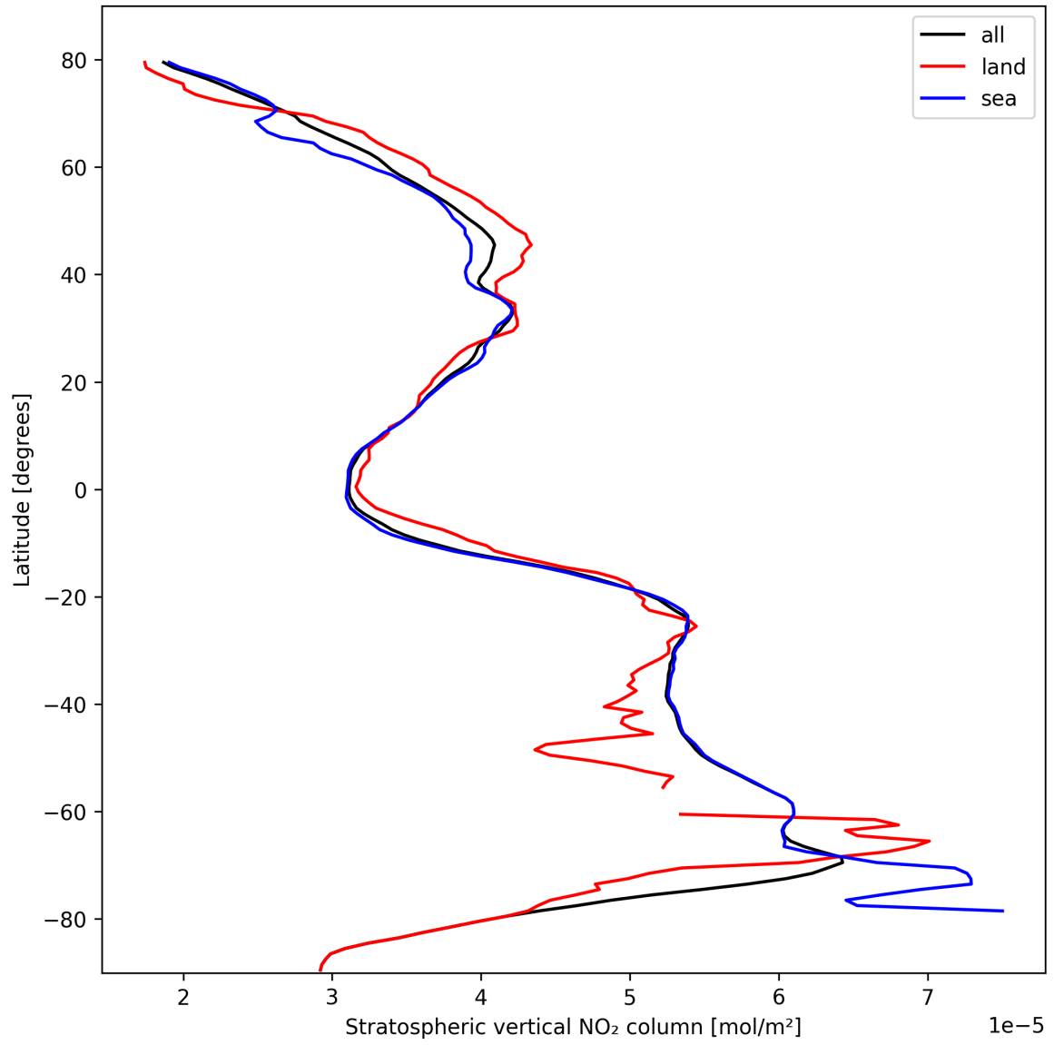
Figure 19: Zonal average of “Stratospheric vertical NO 2 column” for 2024-10-14 to 2024-10-16.
