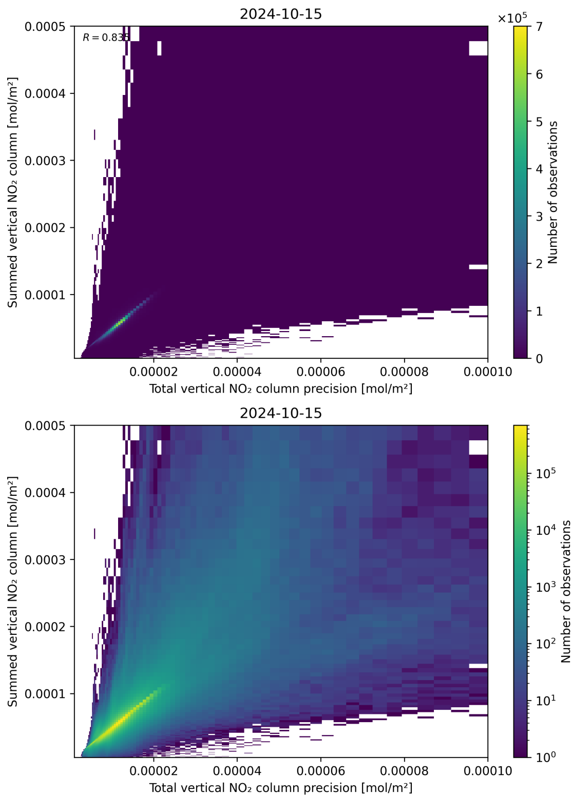
Figure 117: Scatter density plot of “Total vertical NO 2 column precision” against “Summed vertical NO 2 column” for 2024-10-14 to 2024-10-16.
