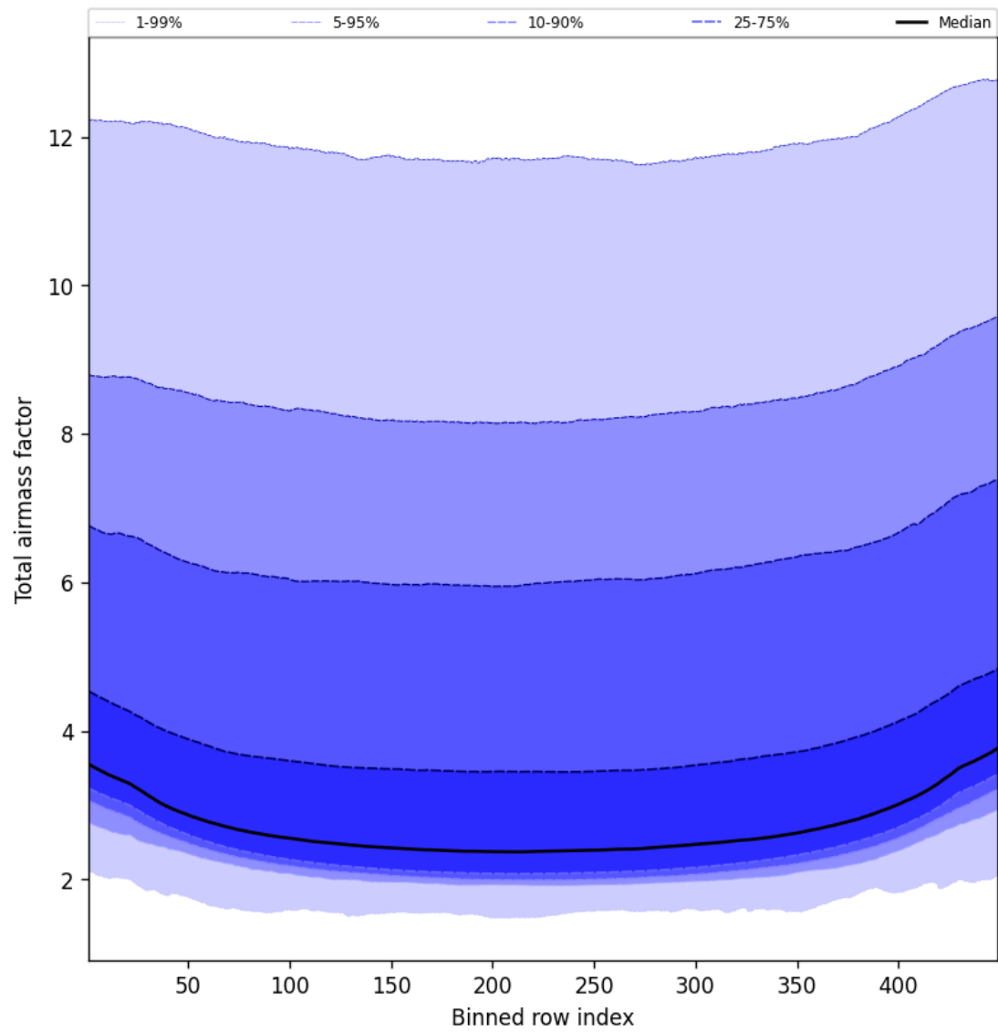
Figure 49: Along track statistics of “Total airmass factor” for 2024-10-14 to 2024-10-16
