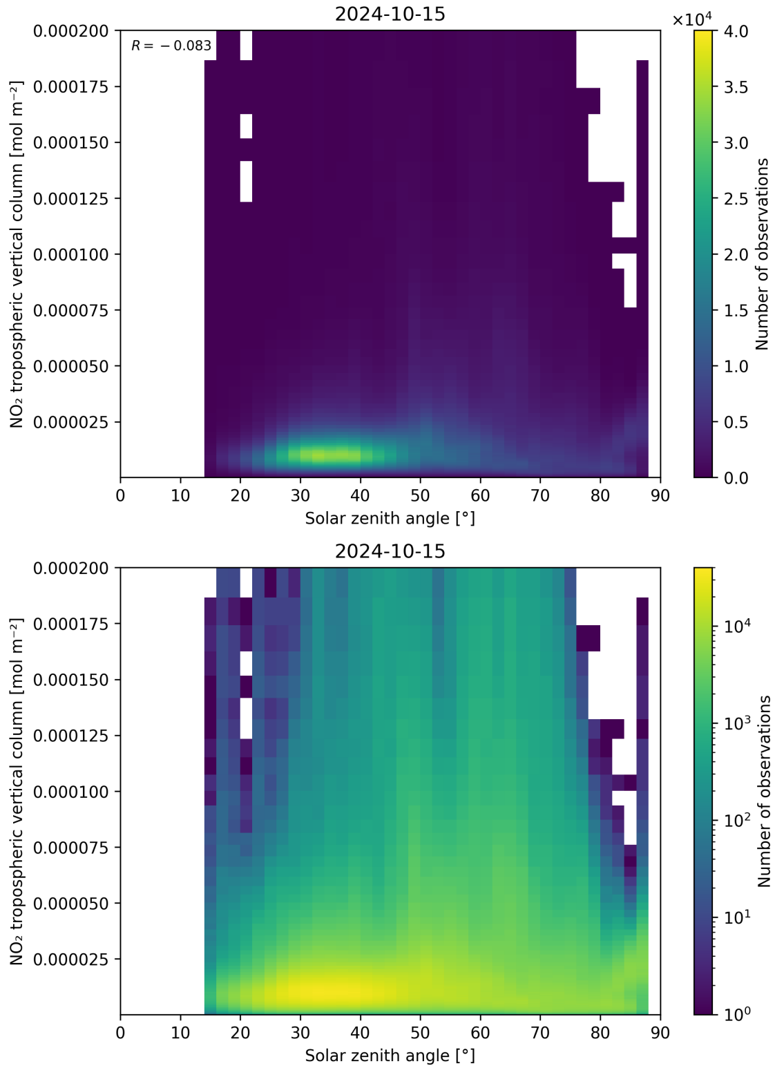
Figure 155: Scatter density plot of “Solar zenith angle” against “NO 2 tropospheric vertical column” for 2024-10-14 to 2024-10-16.
