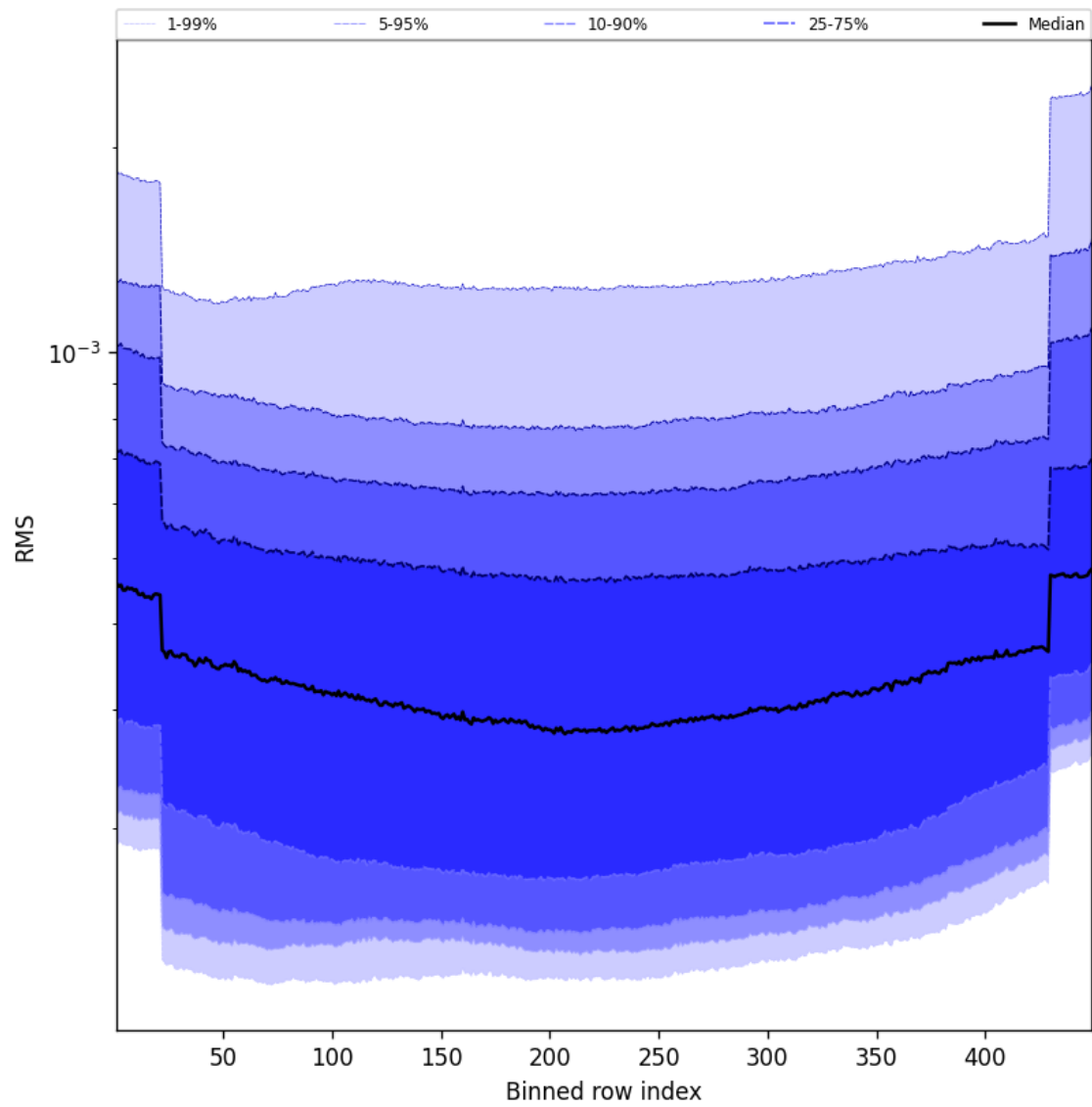
Figure 60: Along track statistics of “RMS” for 2024-10-14 to 2024-10-16
