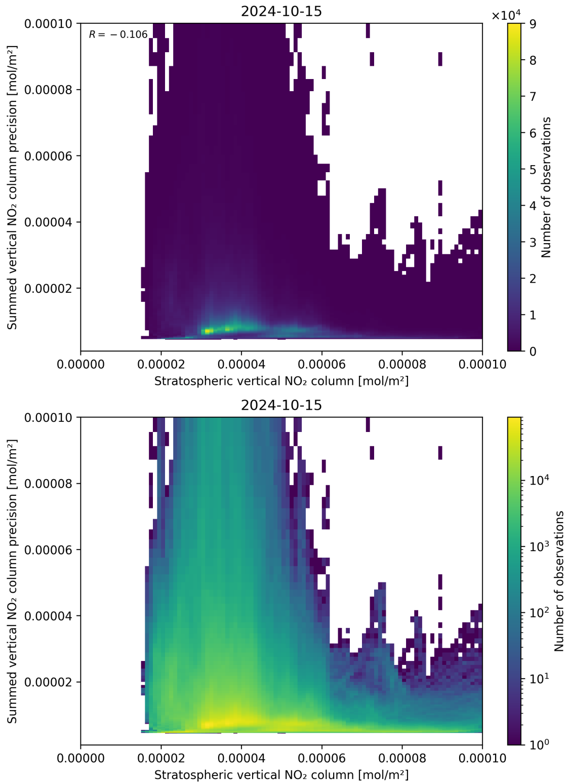
Figure 99: Scatter density plot of “Stratospheric vertical NO 2 column” against “Summed vertical NO 2 column precision” for 2024-10-14 to 2024-10-16.
