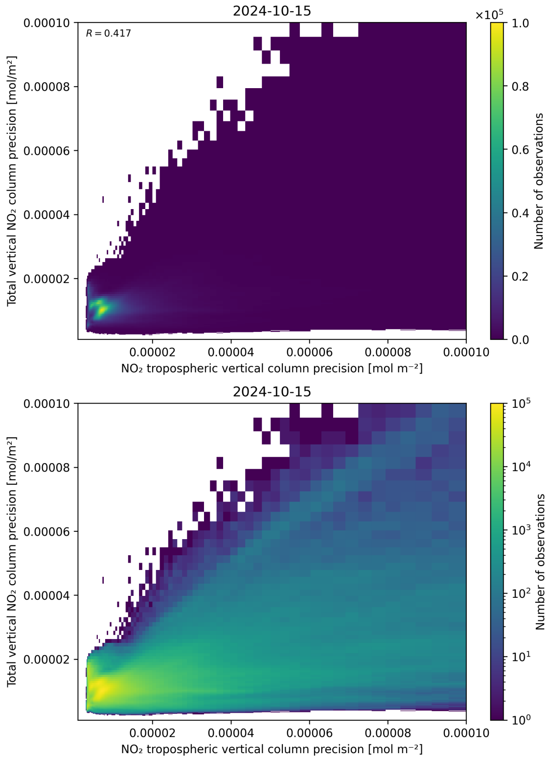
Figure 139: Scatter density plot of “NO 2 tropospheric vertical column precision” against “Total vertical NO 2 column precision” for 2024-10-14 to 2024-10-16.
