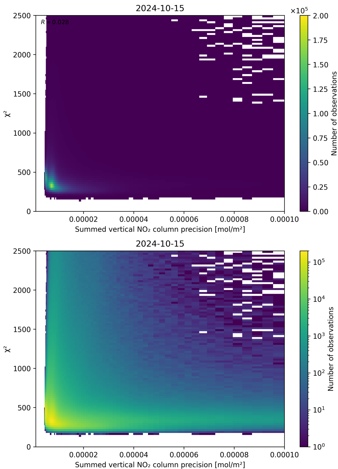
Figure 107: Scatter density plot of “Summed vertical NO 2 column precision” against “ \chi^2 ” for 2024-10-14 to 2024-10-16.
