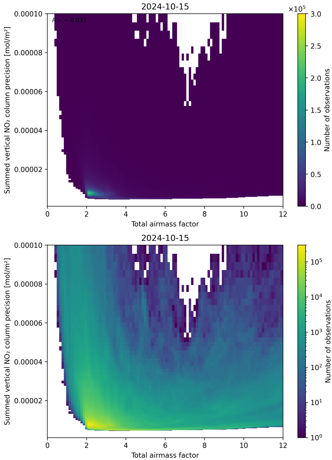
Figure 66: Scatter density plot of “Total airmass factor” against “Summed vertical NO 2 column precision” for 2024-10-14 to 2024-10-16.
