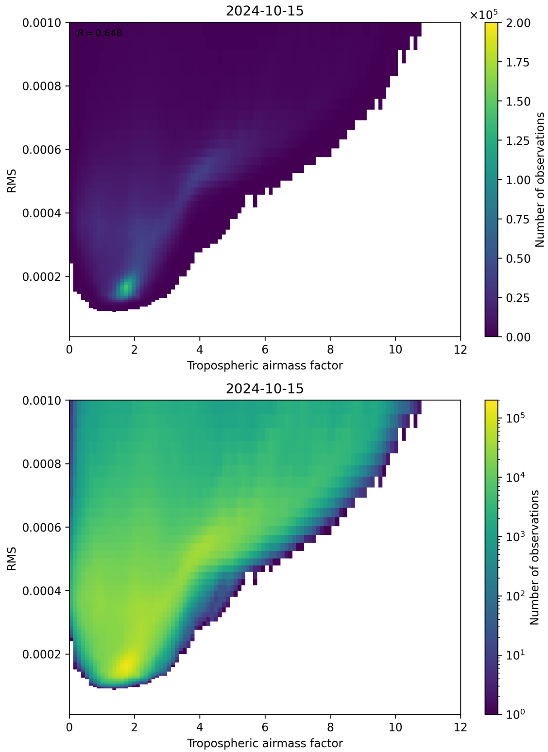
Figure 79: Scatter density plot of “Tropospheric airmass factor” against “RMS” for 2024-10-14 to 2024-10-16.
