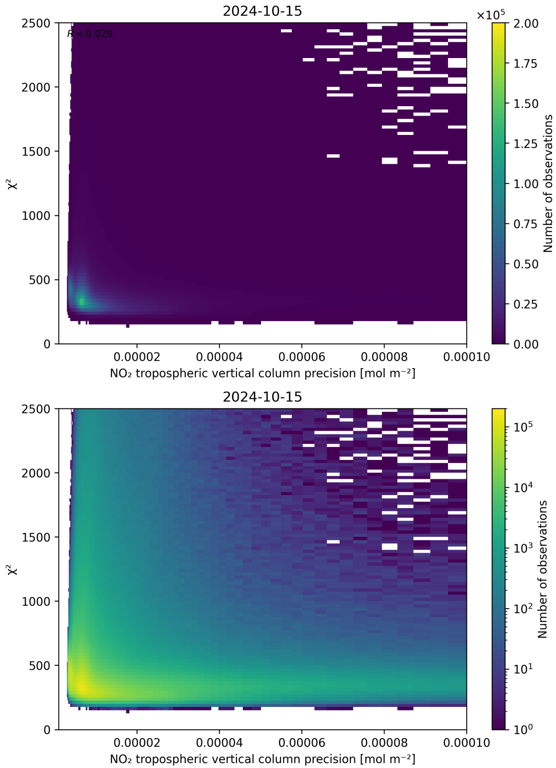
Figure 134: Scatter density plot of “NO 2 tropospheric vertical column precision” against “ \chi^2 ” for 2024-10-14 to 2024-10-16.
