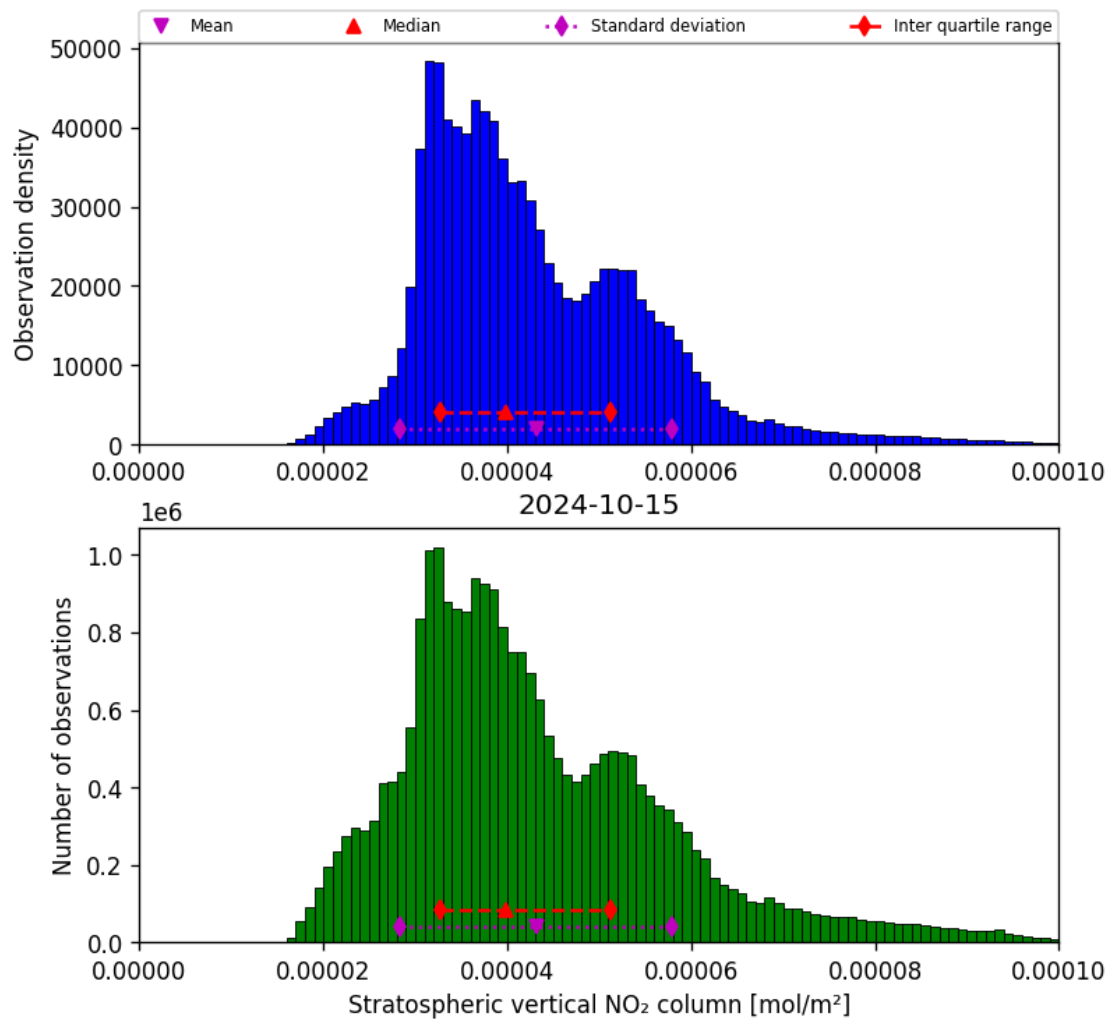
Figure 36: Histogram of “Stratospheric vertical NO 2 column” for 2024-10-14 to 2024-10-16
