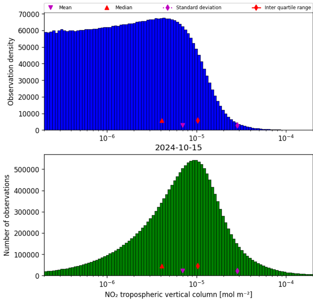
Figure 29: Histogram of “NO 2 tropospheric vertical column” for 2024-10-14 to 2024-10-16
