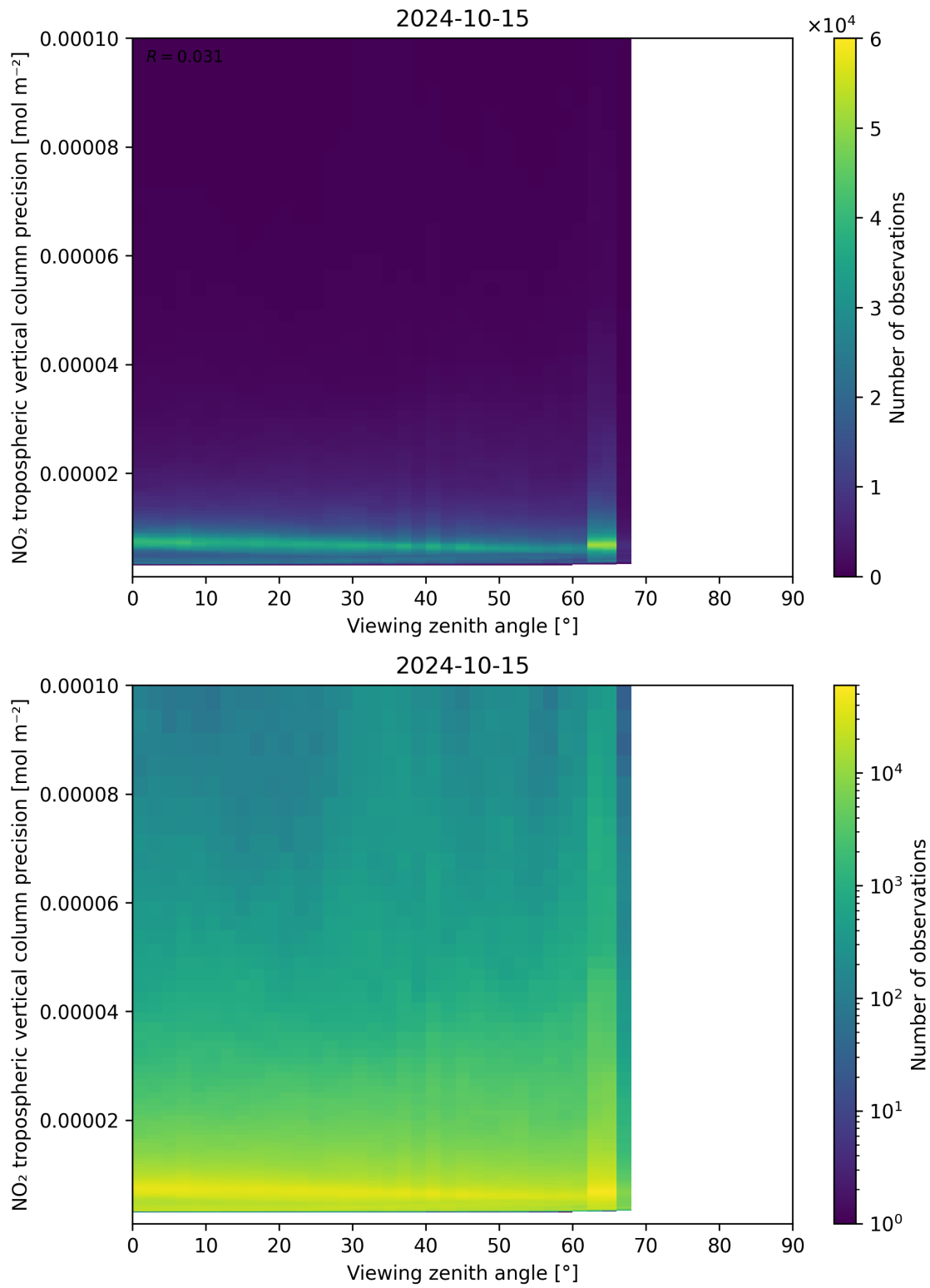
Figure 170: Scatter density plot of “Viewing zenith angle” against “NO 2 tropospheric vertical column precision” for 2024-10-14 to 2024-10-16.
