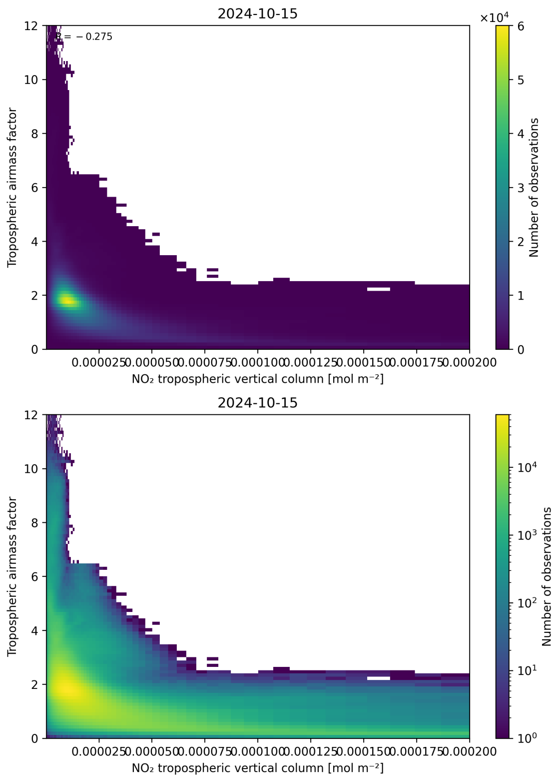
Figure 123: Scatter density plot of “NO 2 tropospheric vertical column” against “Tropospheric air mass factor” for 2024-10-14 to 2024-10-16.
