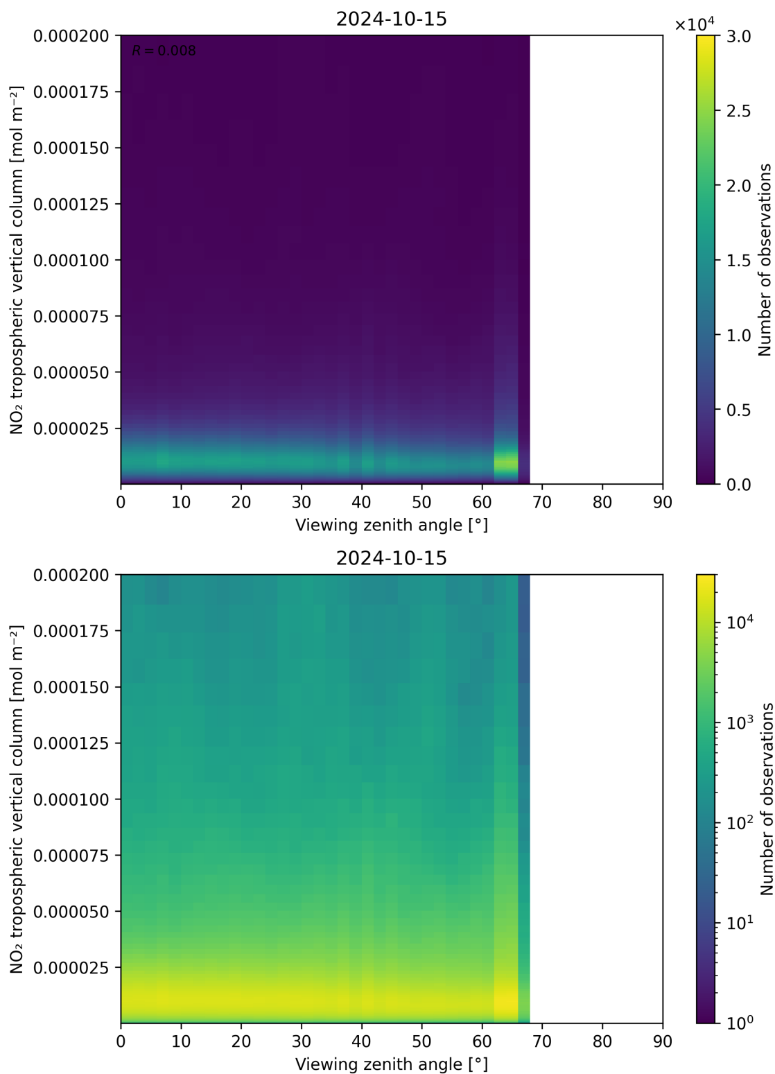
Figure 169: Scatter density plot of “Viewing zenith angle” against “NO 2 tropospheric vertical column” for 2024-10-14 to 2024-10-16.
