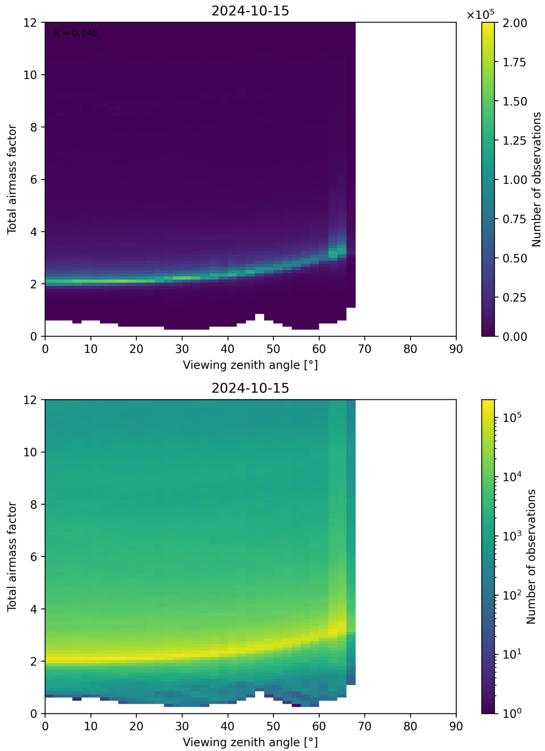
Figure 160: Scatter density plot of “Viewing zenith angle” against “Total airmass factor” for 2024-10-14 to 2024-10-16.
