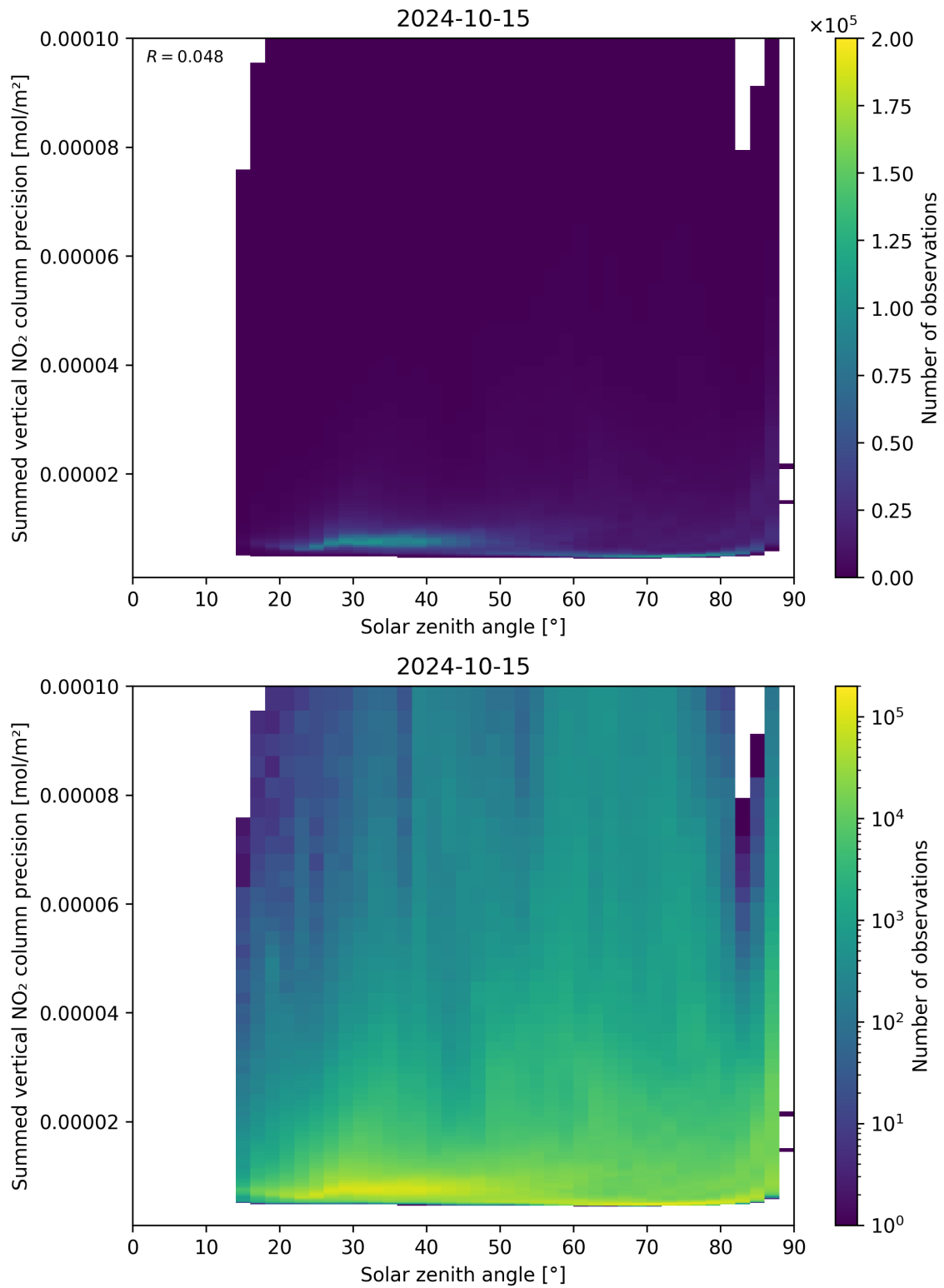
Figure 152: Scatter density plot of “Solar zenith angle” against “Summed vertical NO 2 column precision” for 2024-10-14 to 2024-10-16.
