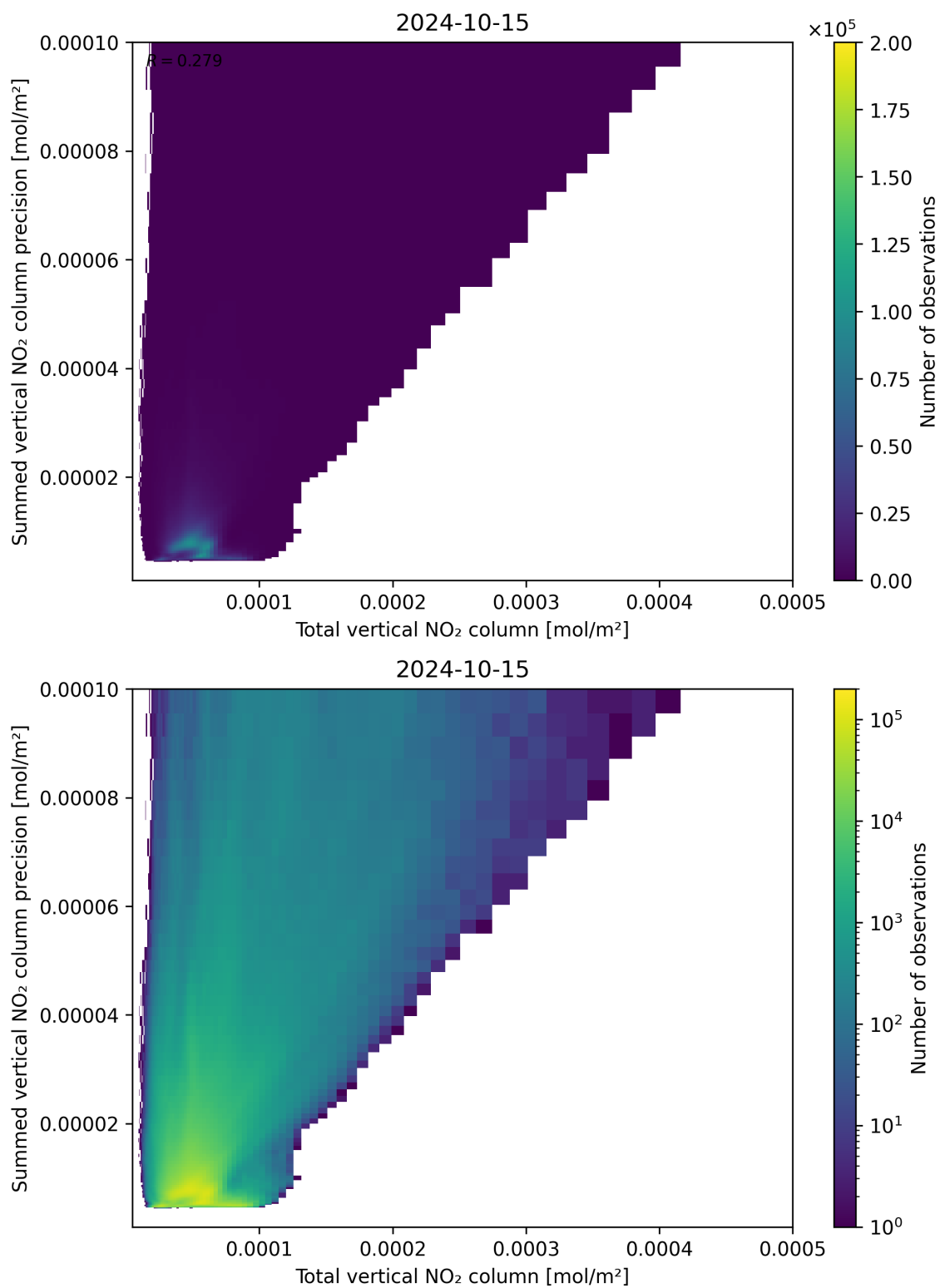
Figure 113: Scatter density plot of “Total vertical NO 2 column” against “Summed vertical NO 2 column precision” for 2024-10-14 to 2024-10-16.
