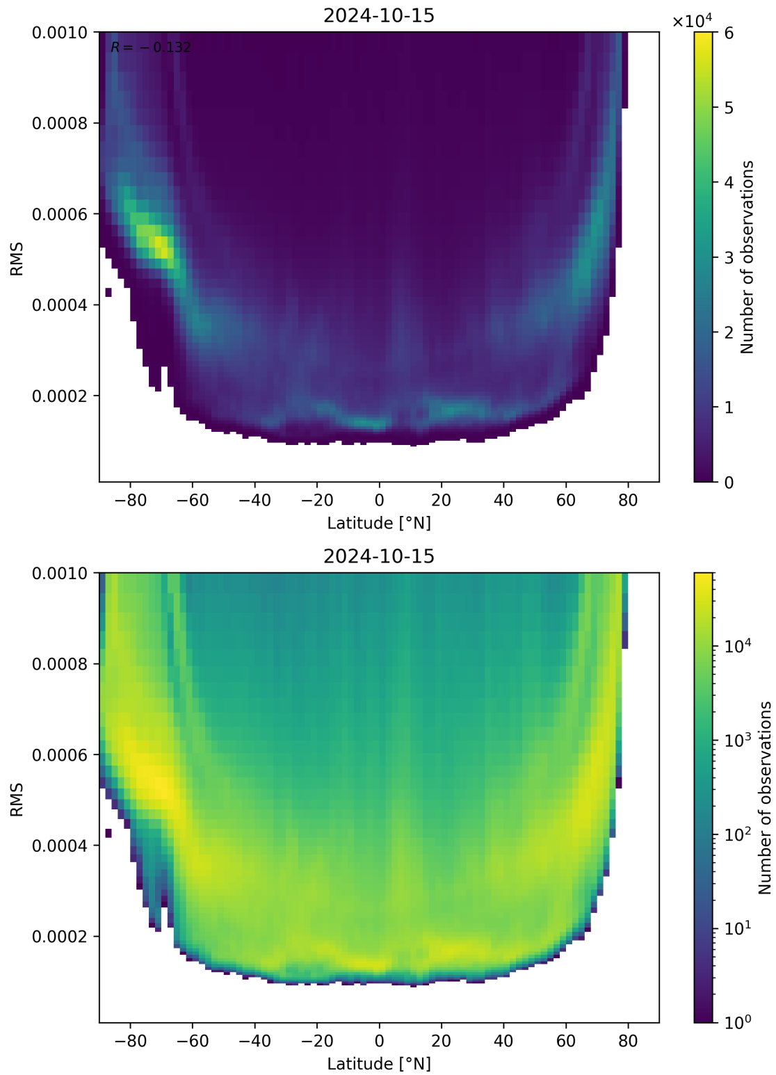
Figure 94: Scatter density plot of “Latitude” against “RMS” for 2024-10-14 to 2024-10-16.
