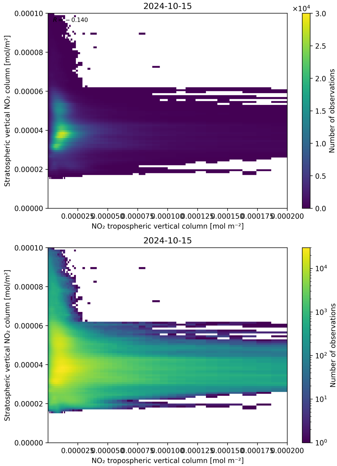
Figure 125: Scatter density plot of “NO 2 tropospheric vertical column” against “Stratospheric vertical NO 2 column” for 2024-10-14 to 2024-10-16.
