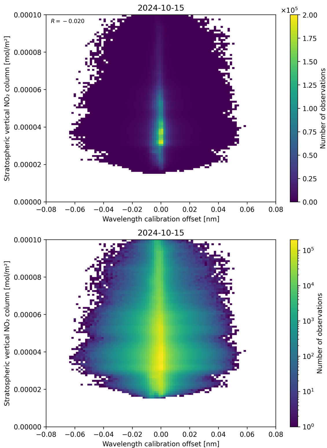
Figure 176: Scatter density plot of “Wavelength calibration offset” against “Stratospheric vertical NO 2 column” for 2024-10-14 to 2024-10-16.
