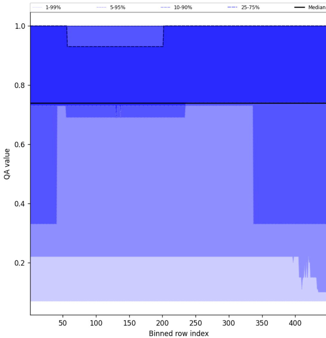
Figure 45: Along track statistics of “QA value” for 2024-10-14 to 2024-10-16
