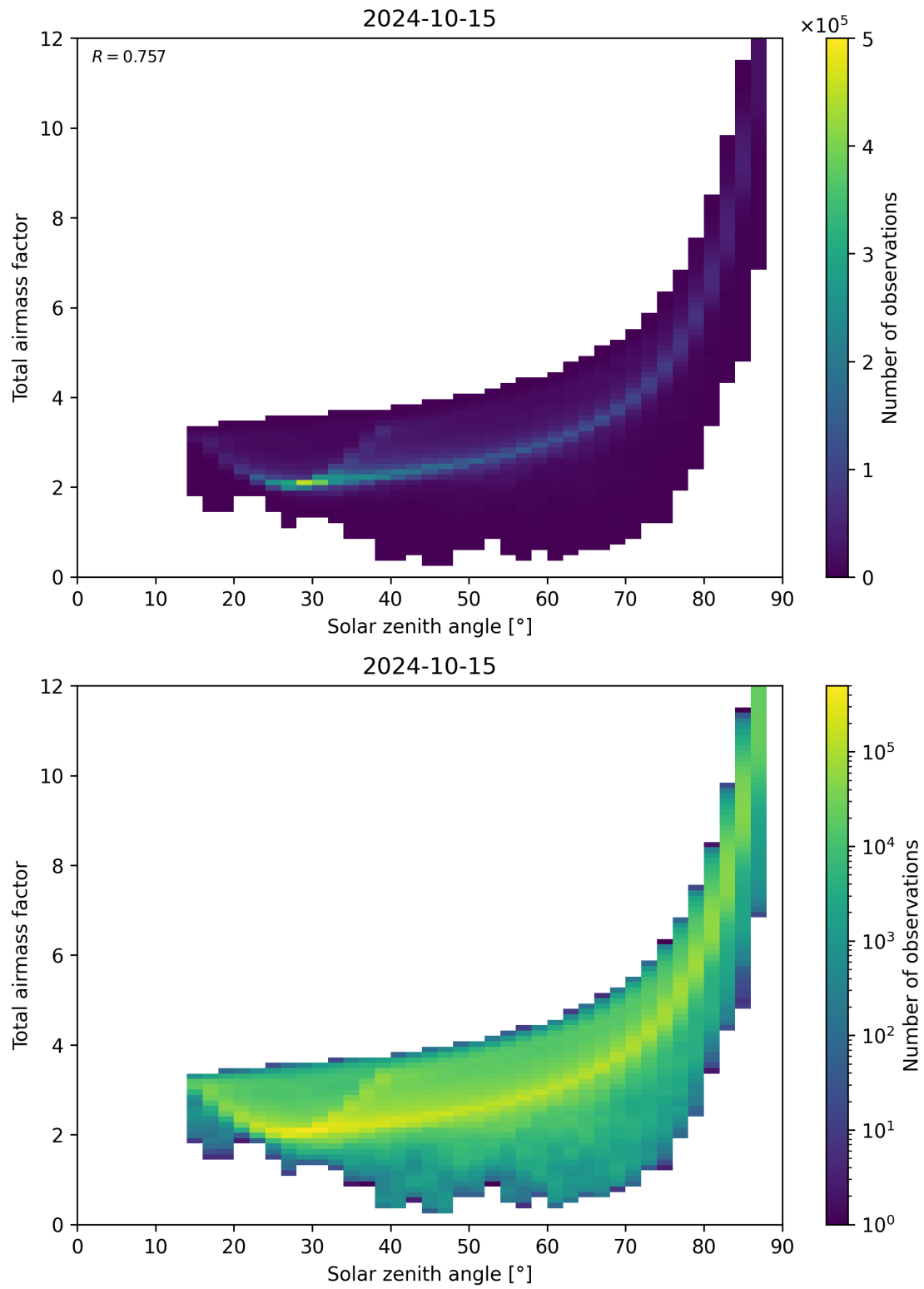
Figure 146: Scatter density plot of “Solar zenith angle” against “Total air mass factor” for 2024-10-14 to 2024-10-16.
