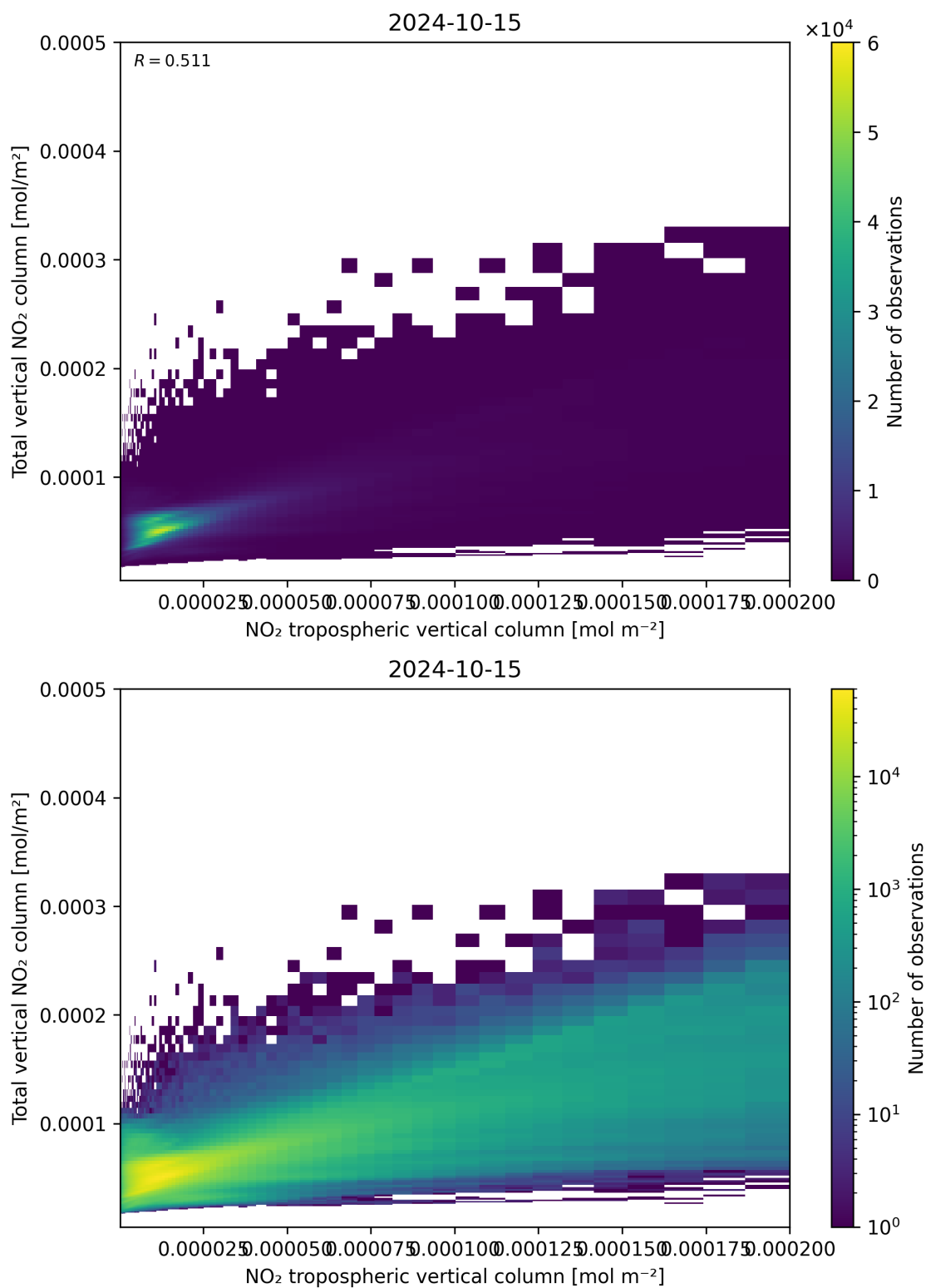
Figure 128: Scatter density plot of “NO 2 tropospheric vertical column” against “Total vertical NO 2 column” for 2024-10-14 to 2024-10-16.
