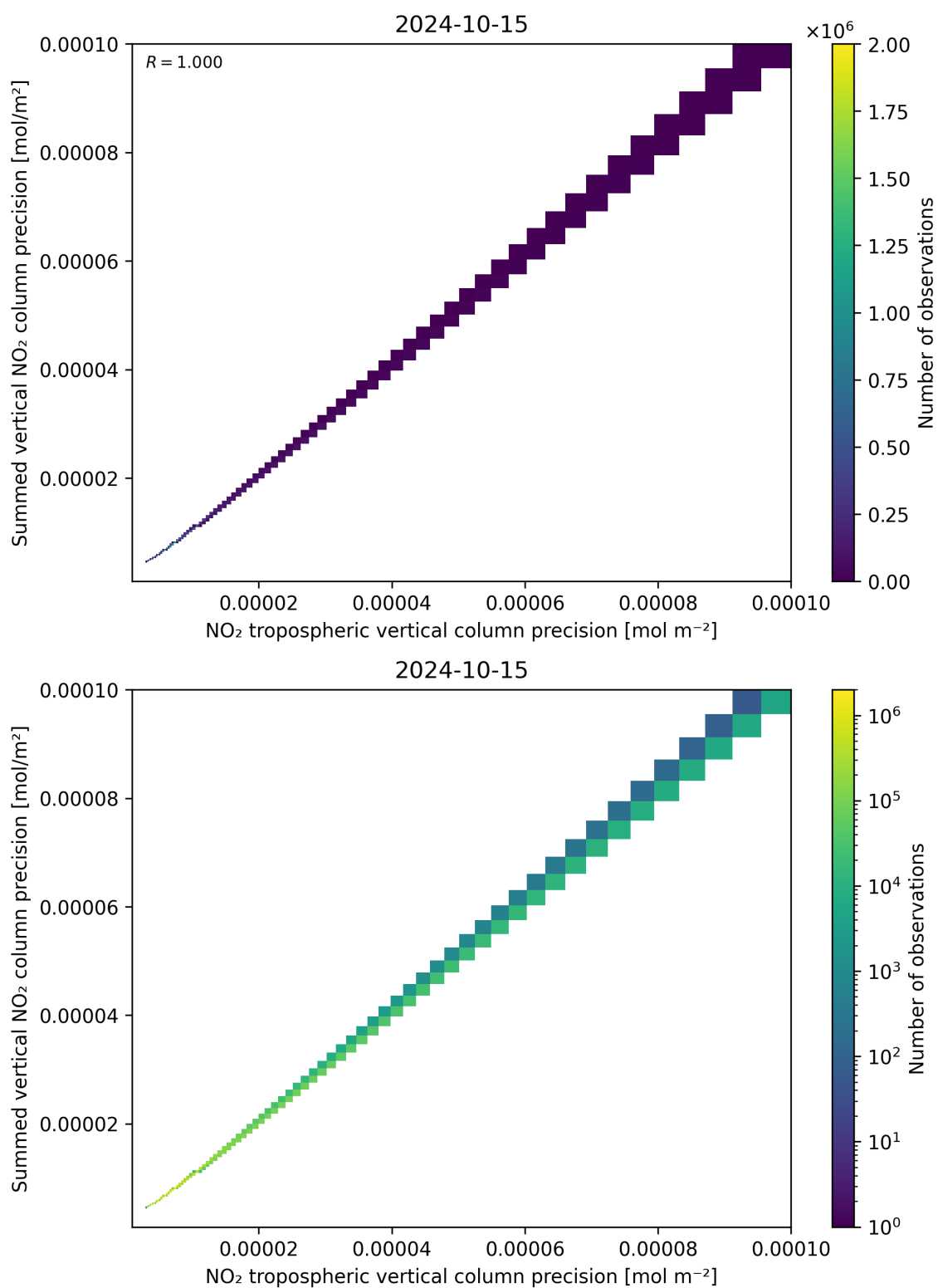
Figure 137: Scatter density plot of “NO 2 tropospheric vertical column precision” against “Summed vertical NO 2 column precision” for 2024-10-14 to 2024-10-16.
