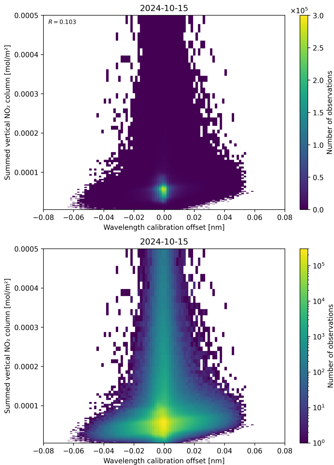
Figure 177: Scatter density plot of “Wavelength calibration offset” against “Summed vertical NO 2 column” for 2024-10-14 to 2024-10-16.
