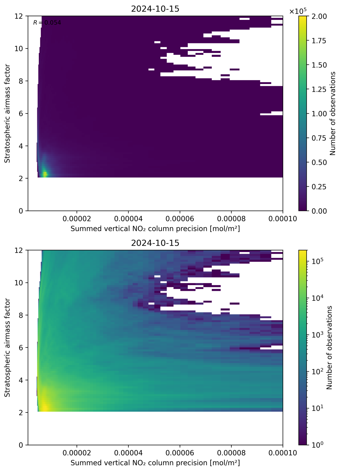
Figure 106: Scatter density plot of “Summed vertical NO 2 column precision” against “Stratospheric airmass factor” for 2024-10-14 to 2024-10-16.
