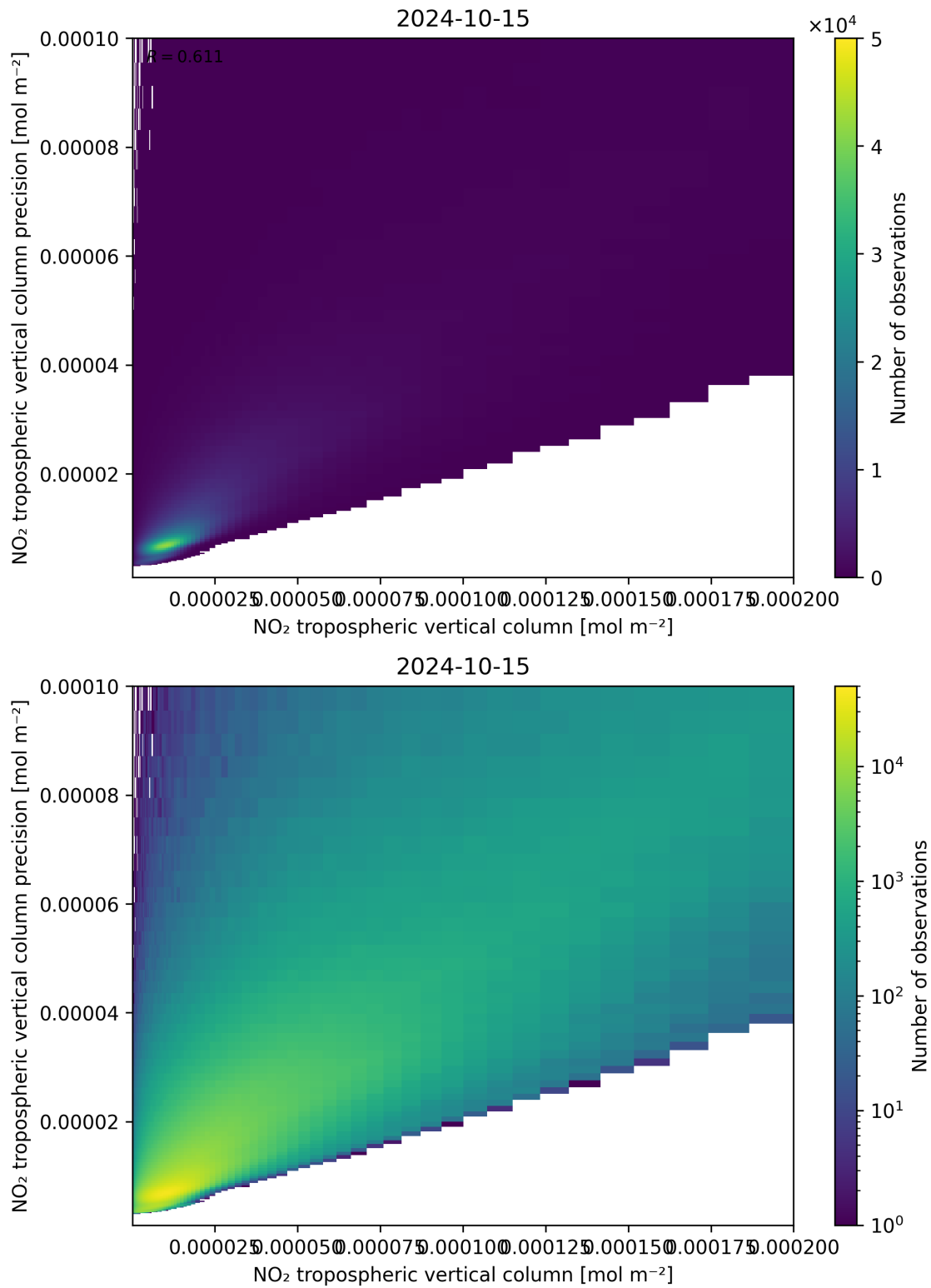
Figure 130: Scatter density plot of “NO 2 tropospheric vertical column” against “NO 2 tropospheric vertical column precision” for 2024-10-14 to 2024-10-16.
