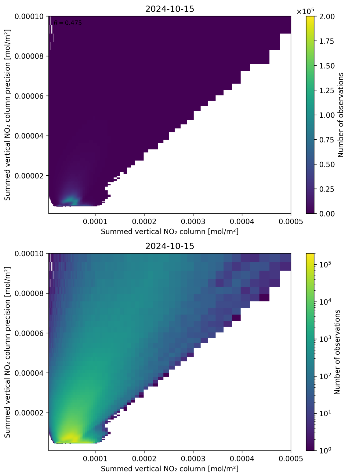
Figure 105: Scatter density plot of “Summed vertical NO 2 column” against “Summed vertical NO 2 column precision” for 2024-10-14 to 2024-10-16.
