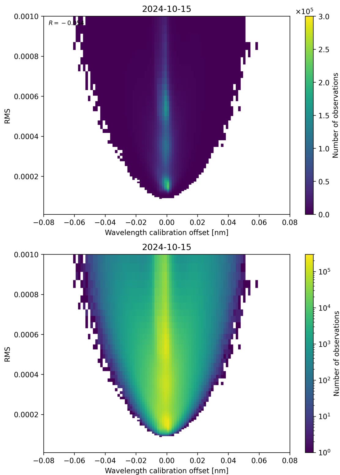
Figure 181: Scatter density plot of “Wavelength calibration offset” against “RMS” for 2024-10-14 to 2024-10-16.
