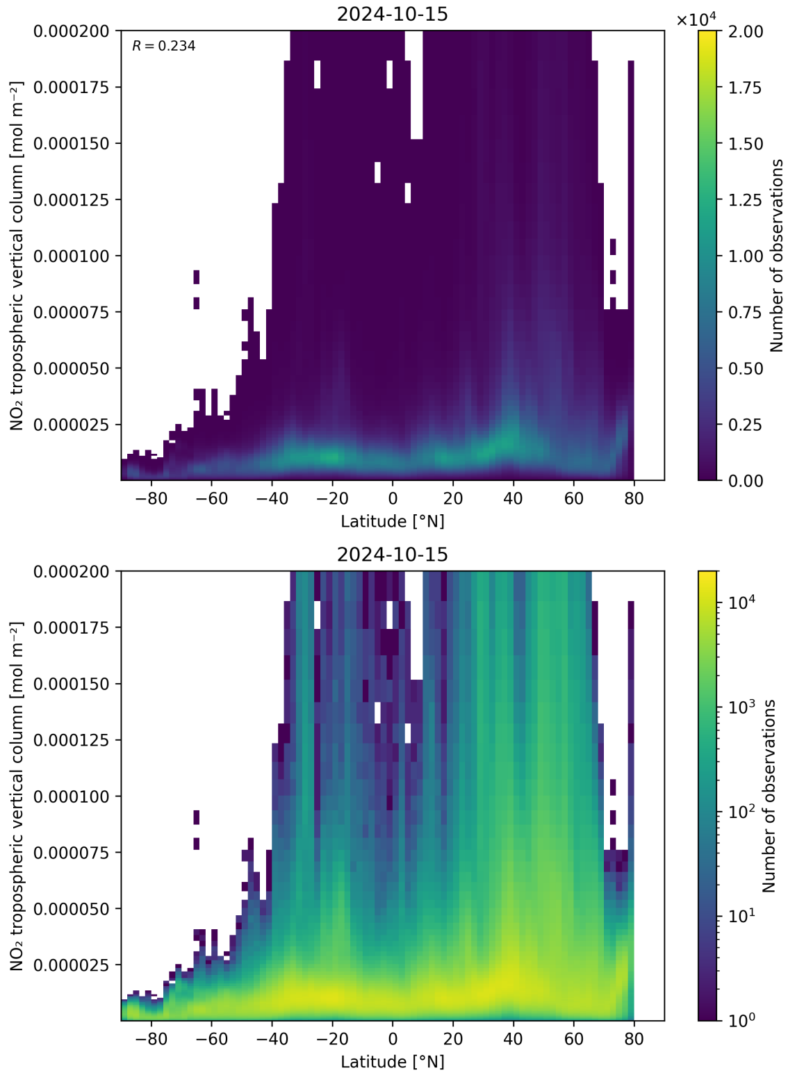
Figure 92: Scatter density plot of “Latitude” against “NO 2 tropospheric vertical column” for 2024-10-14 to 2024-10-16.
