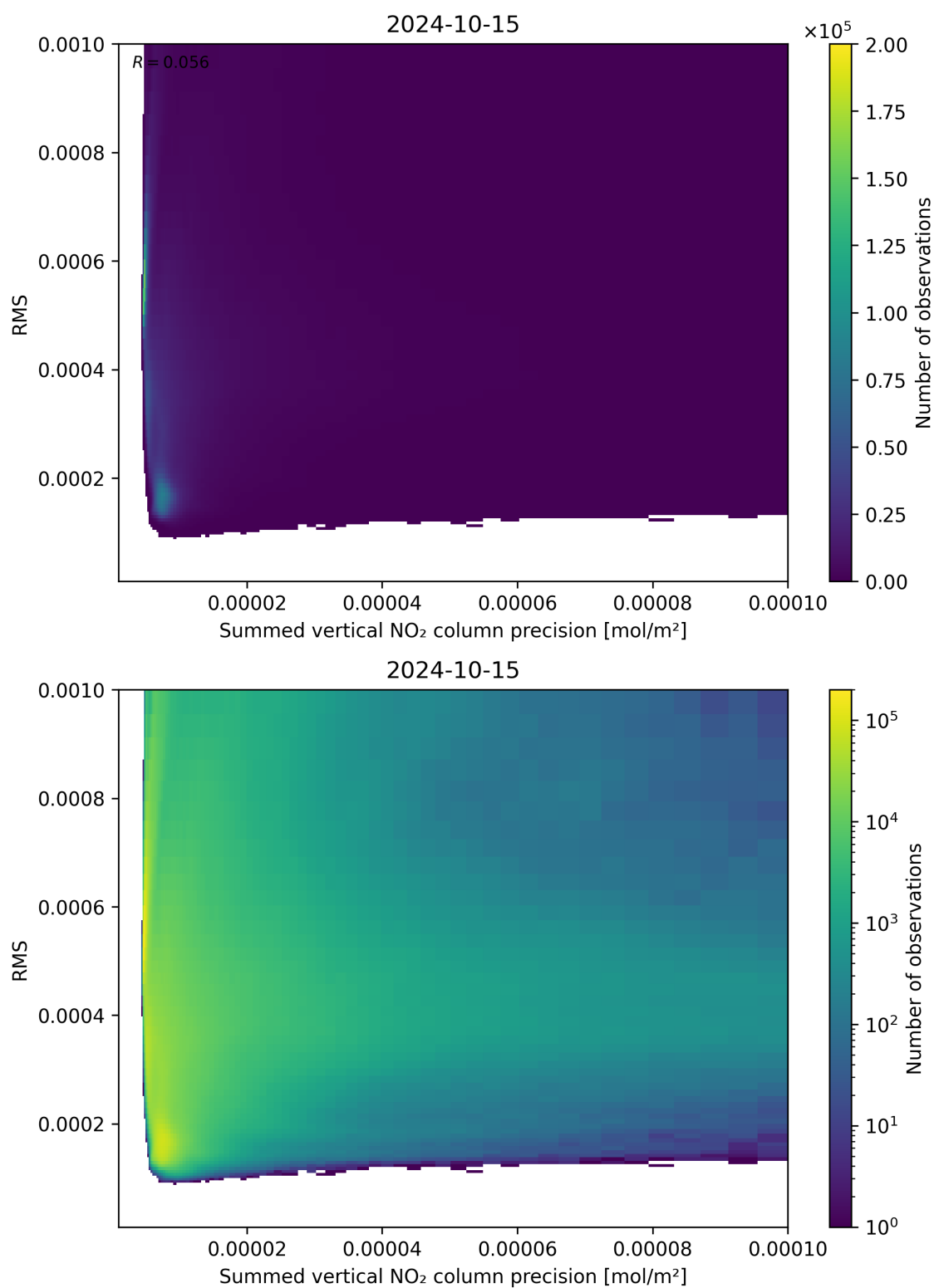
Figure 108: Scatter density plot of “Summed vertical NO 2 column precision” against “RMS” for 2024-10-14 to 2024-10-16.
