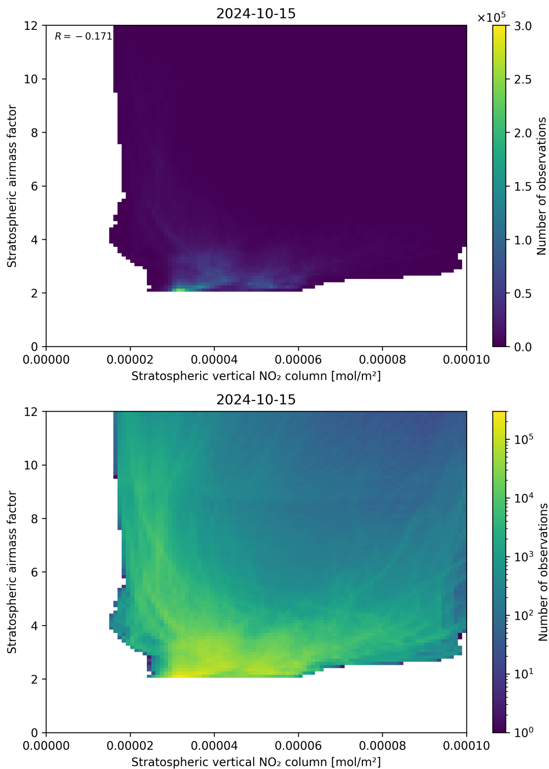
Figure 96: Scatter density plot of “Stratospheric vertical NO 2 column” against “Stratospheric airmass factor” for 2024-10-14 to 2024-10-16.
