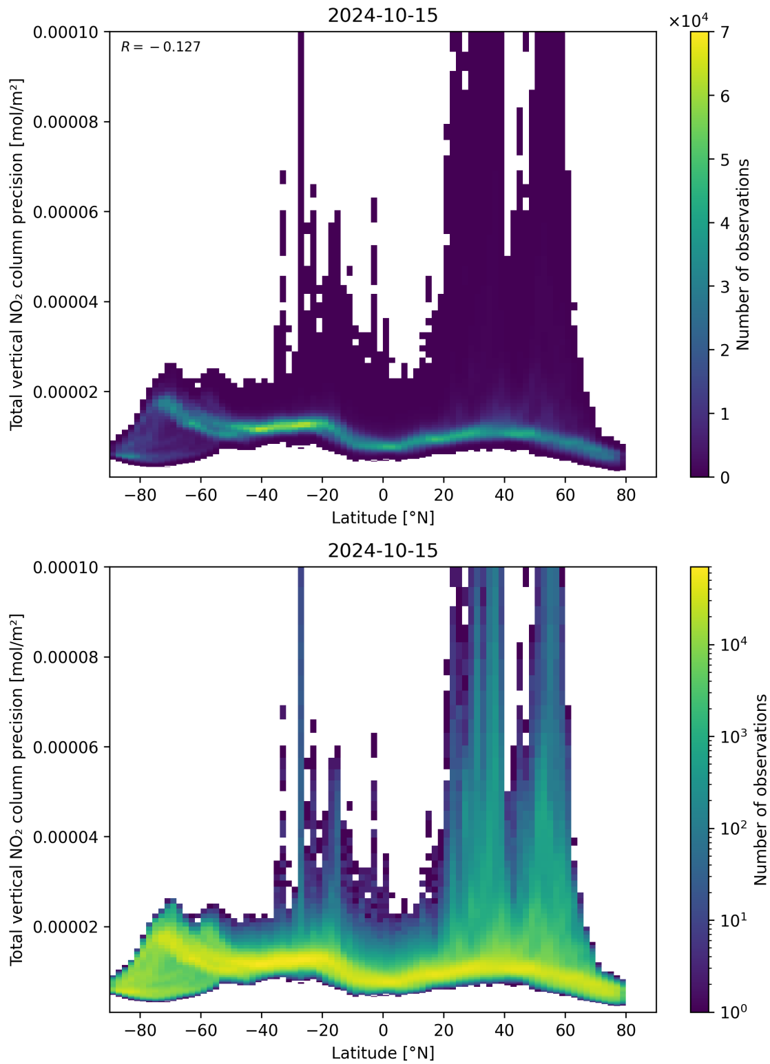
Figure 91: Scatter density plot of “Latitude” against “Total vertical NO 2 column precision” for 2024-10-14 to 2024-10-16.
