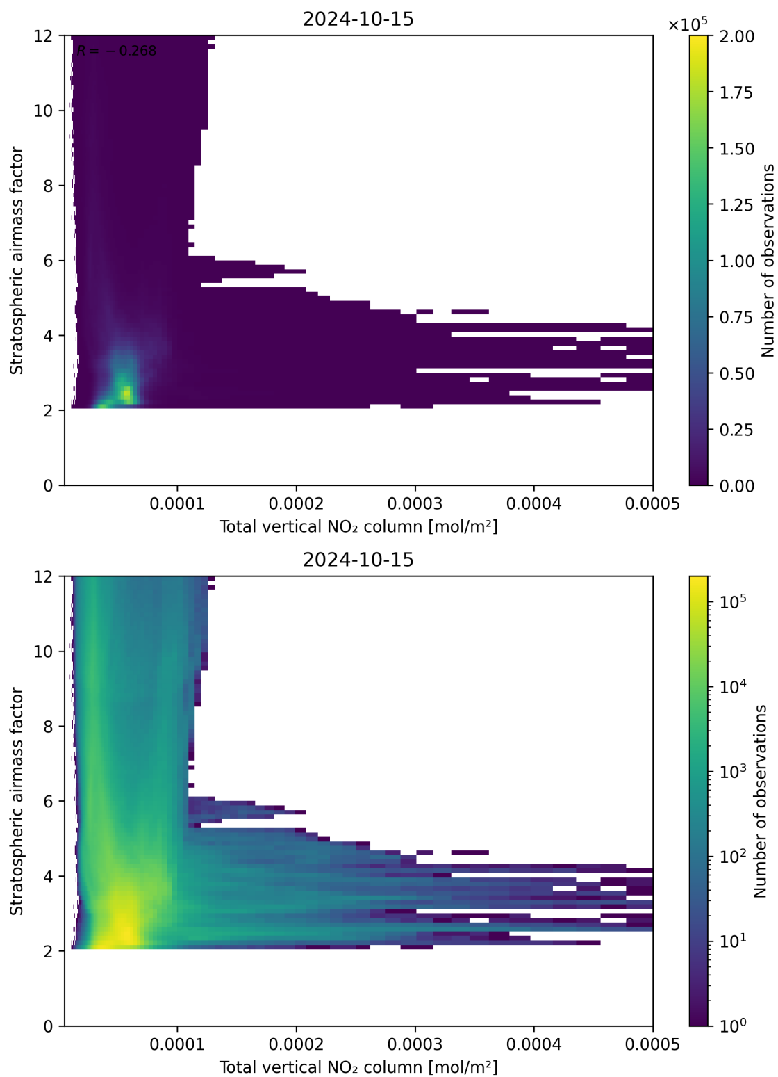
Figure 110: Scatter density plot of “Total vertical NO 2 column” against “Stratospheric airmass factor” for 2024-10-14 to 2024-10-16.
