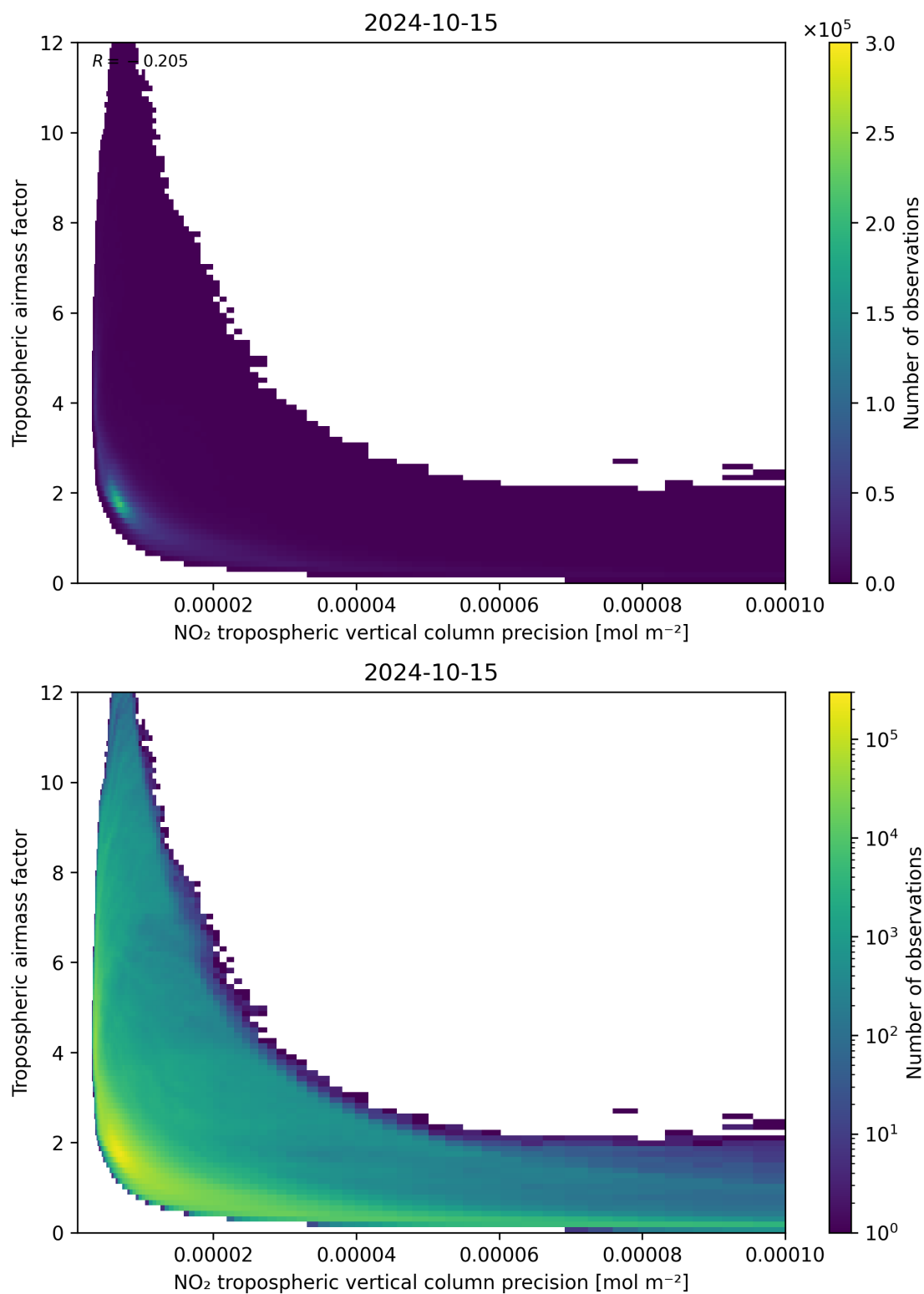
Figure 133: Scatter density plot of “NO 2 tropospheric vertical column precision” against “Tropospheric airmass factor” for 2024-10-14 to 2024-10-16.
