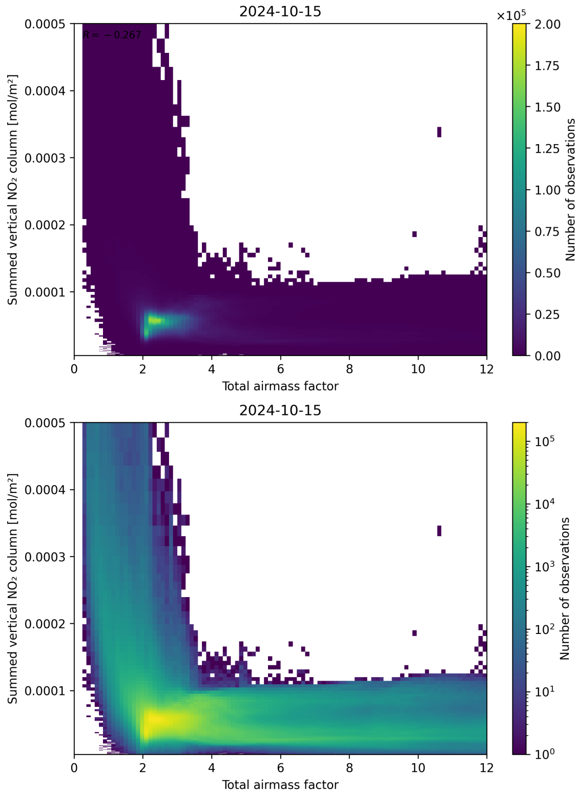
Figure 65: Scatter density plot of “Total airmass factor” against “Summed vertical NO 2 column” for 2024-10-14 to 2024-10-16.
