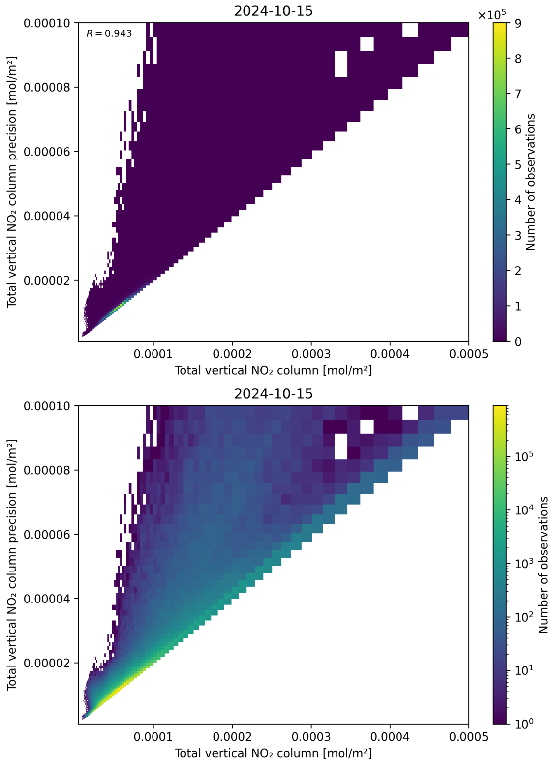
Figure 114: Scatter density plot of “Total vertical NO 2 column” against “Total vertical NO 2 column precision” for 2024-10-14 to 2024-10-16.
