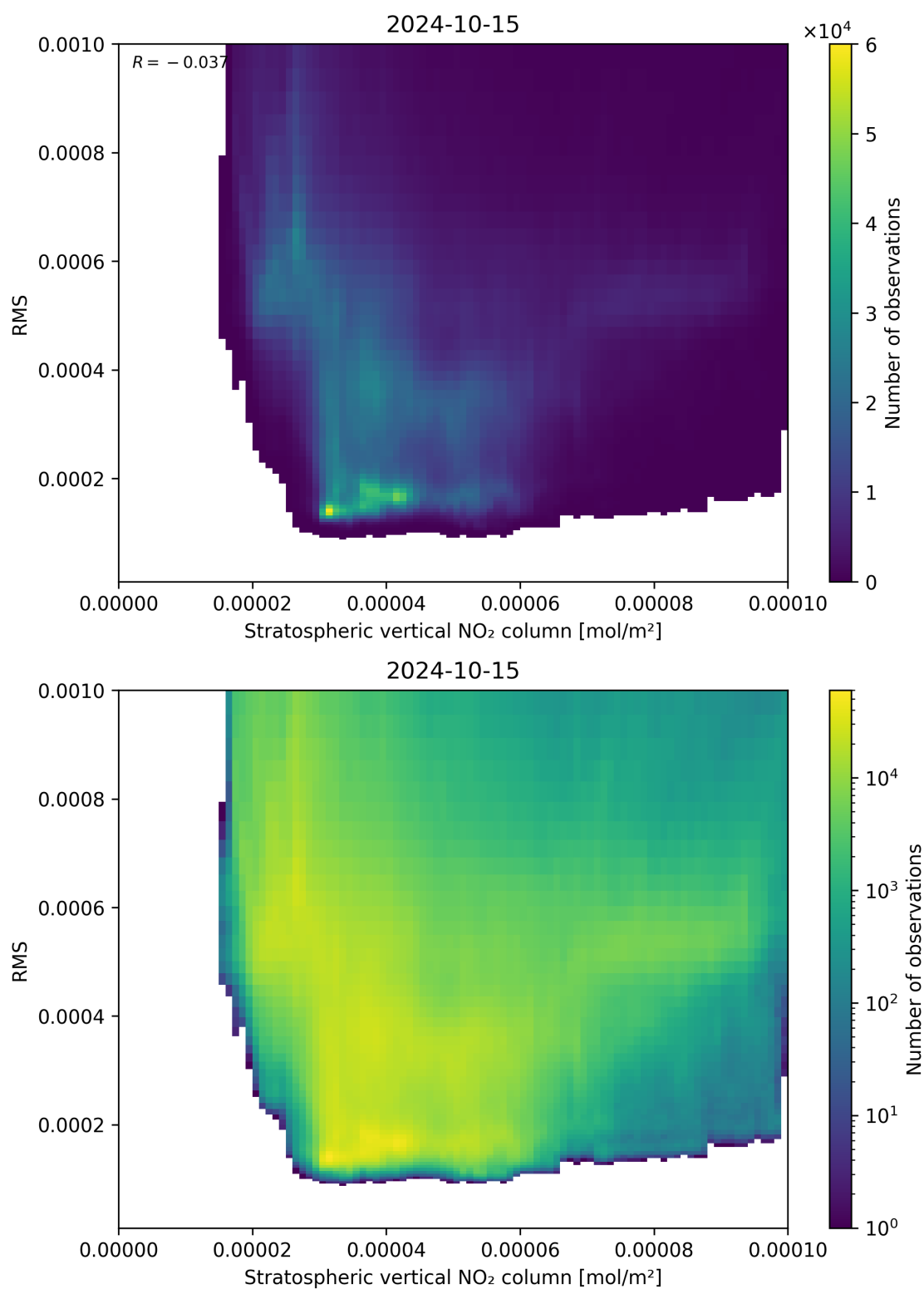
Figure 102: Scatter density plot of “Stratospheric vertical NO 2 column” against “RMS” for 2024-10-14 to 2024-10-16.
