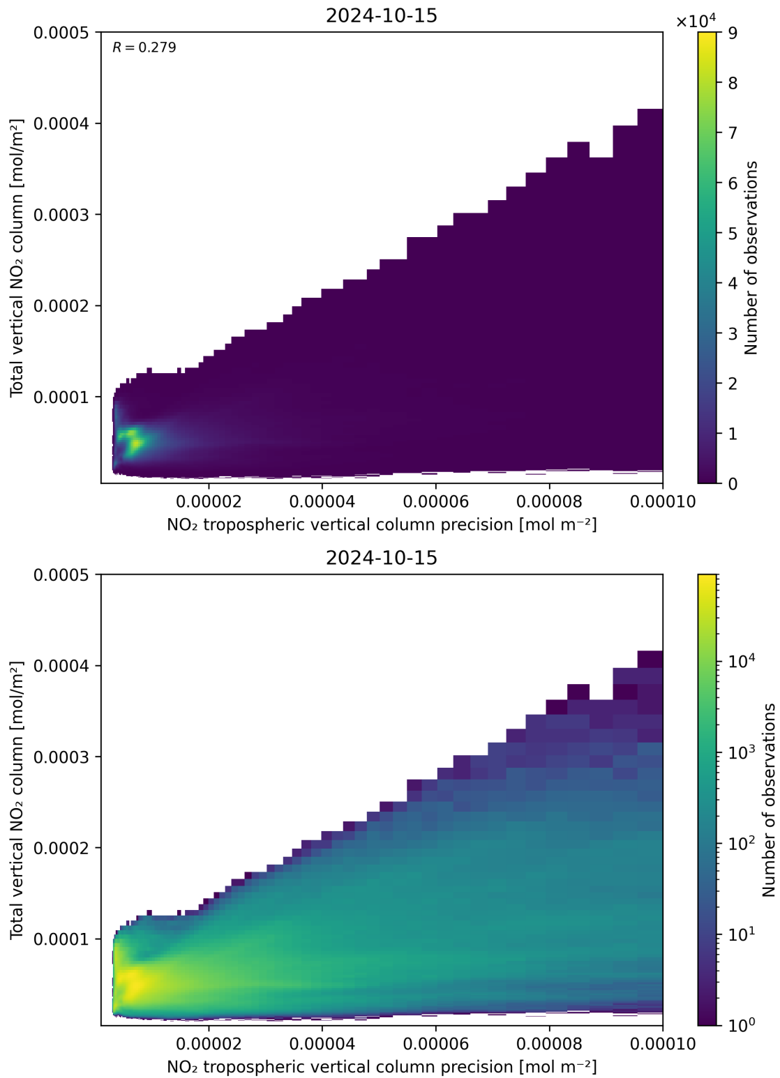
Figure 138: Scatter density plot of “NO 2 tropospheric vertical column precision” against “Total vertical NO 2 column” for 2024-10-14 to 2024-10-16.
