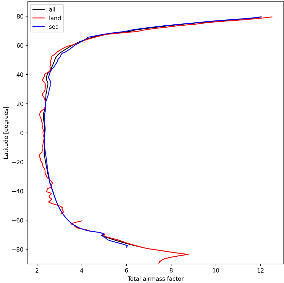
Figure 15: Zonal average of “Total airmass factor” for 2024-10-14 to 2024-10-16.
