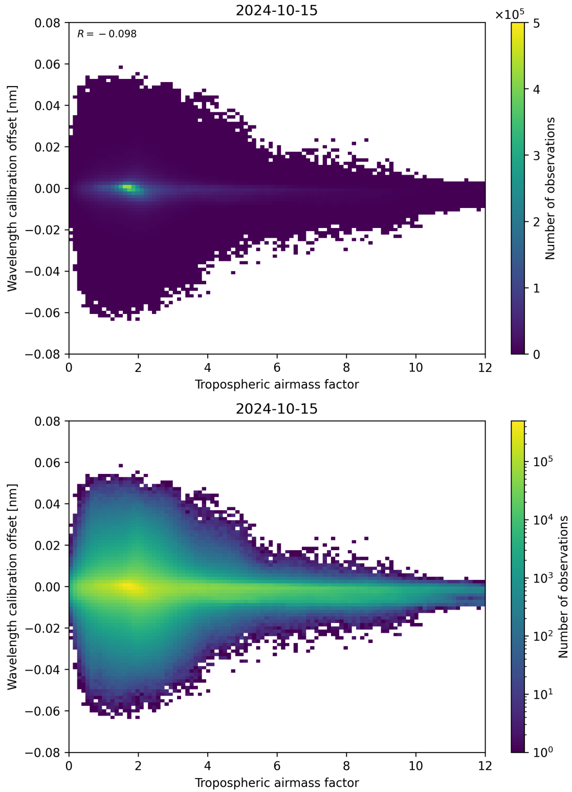
Figure 80: Scatter density plot of “Tropospheric airmass factor” against “Wavelength calibration offset” for 2024-10-14 to 2024-10-16.
