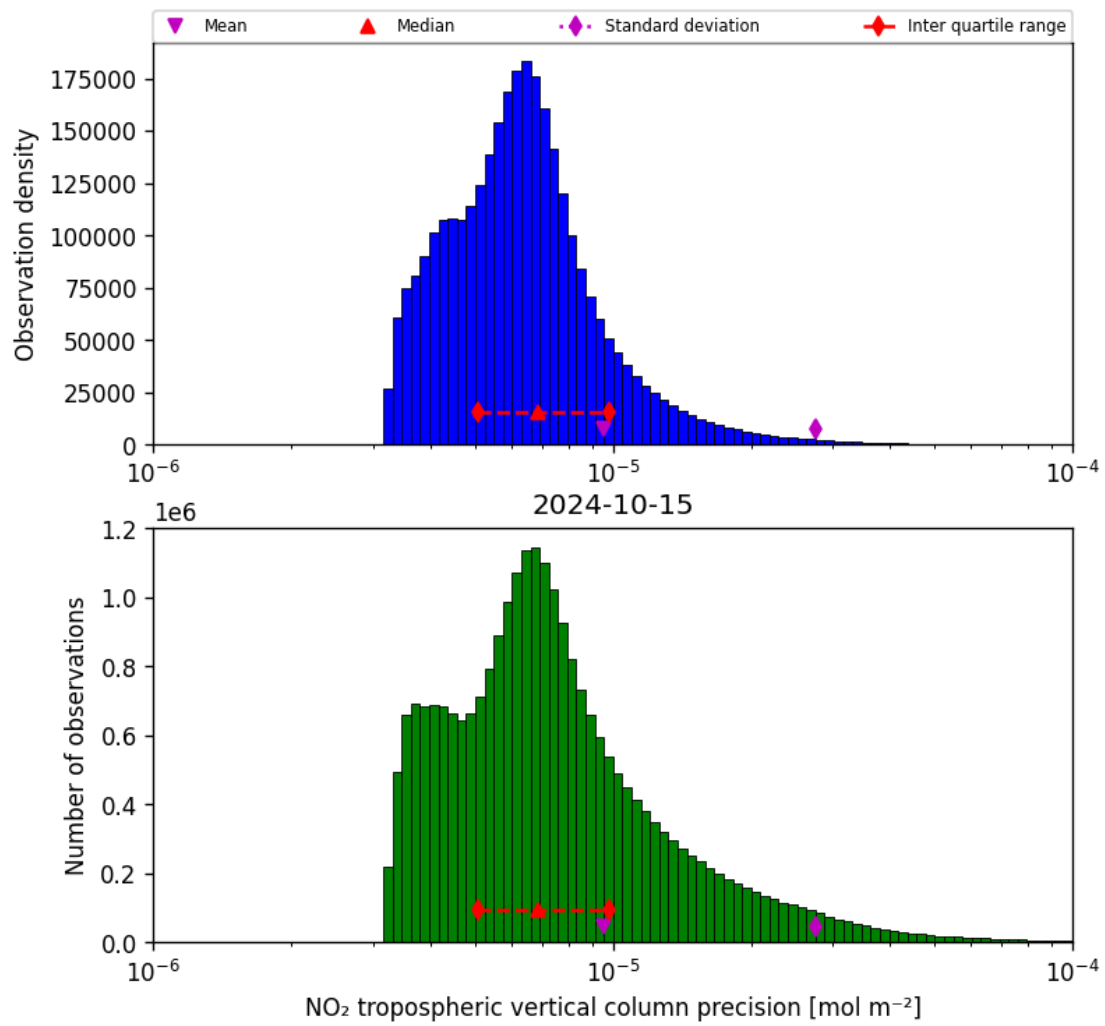
Figure 30: Histogram of “NO 2 tropospheric vertical column precision” for 2024-10-14 to 2024-10-16
