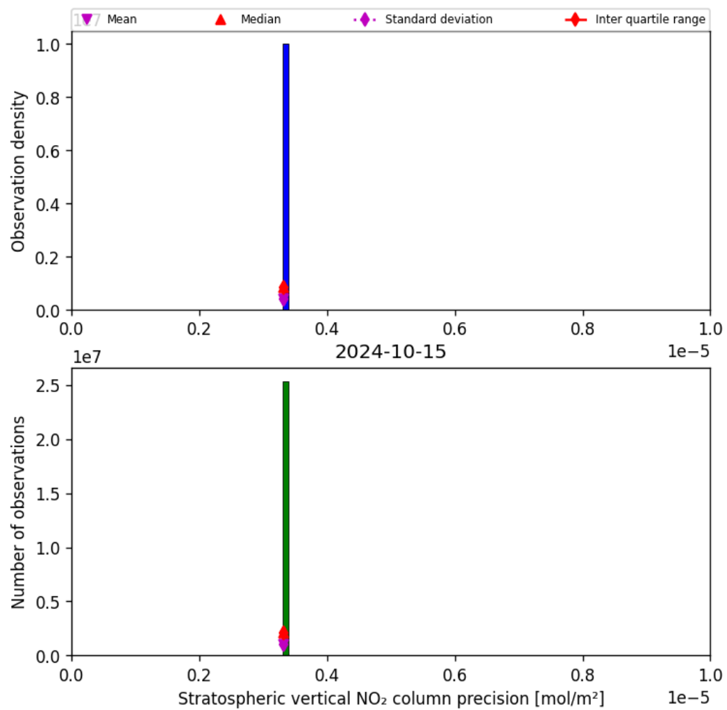
Figure 37: Histogram of “Stratospheric vertical NO 2 column precision” for 2024-10-14 to 2024-10-16
