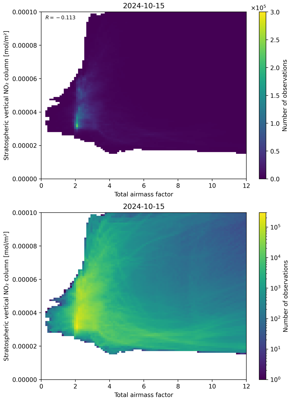
Figure 64: Scatter density plot of “Total airmass factor” against “Stratospheric vertical \text{NO}_2 column” for 2024-10-14 to 2024-10-16.
