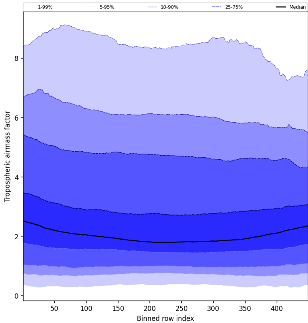
Figure 48: Along track statistics of “Tropospheric airmass factor” for 2024-10-14 to 2024-10-16
