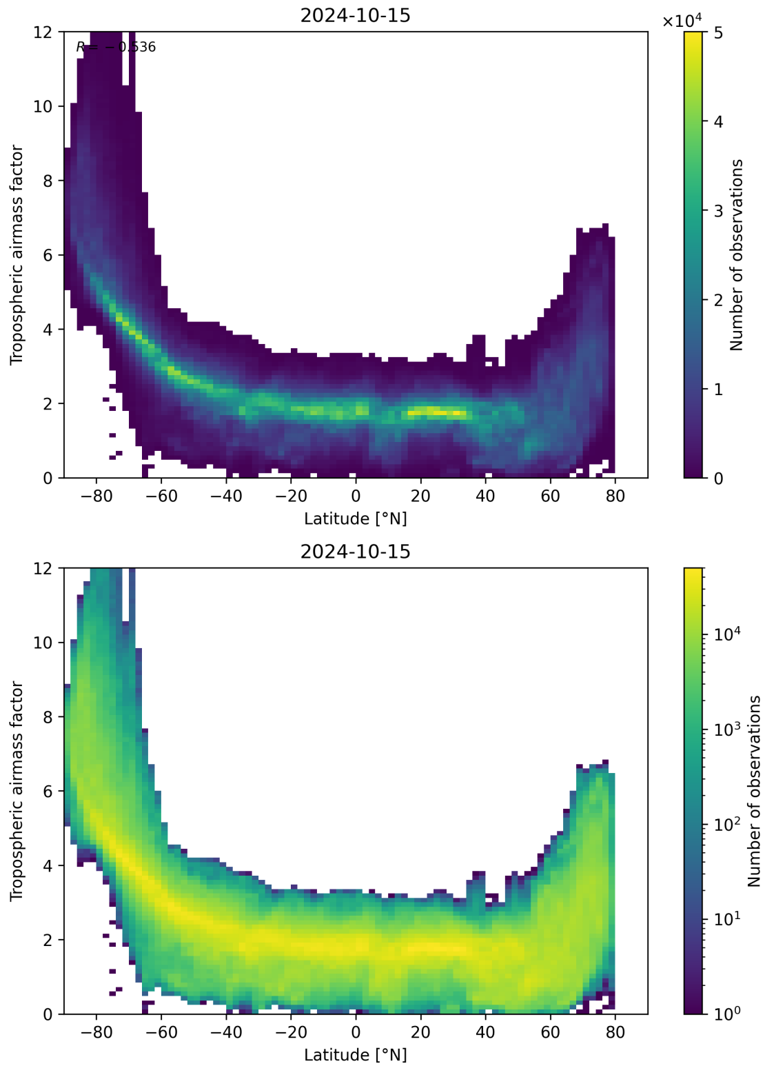
Figure 85: Scatter density plot of “Latitude” against “Tropospheric airmass factor” for 2024-10-14 to 2024-10-16.
