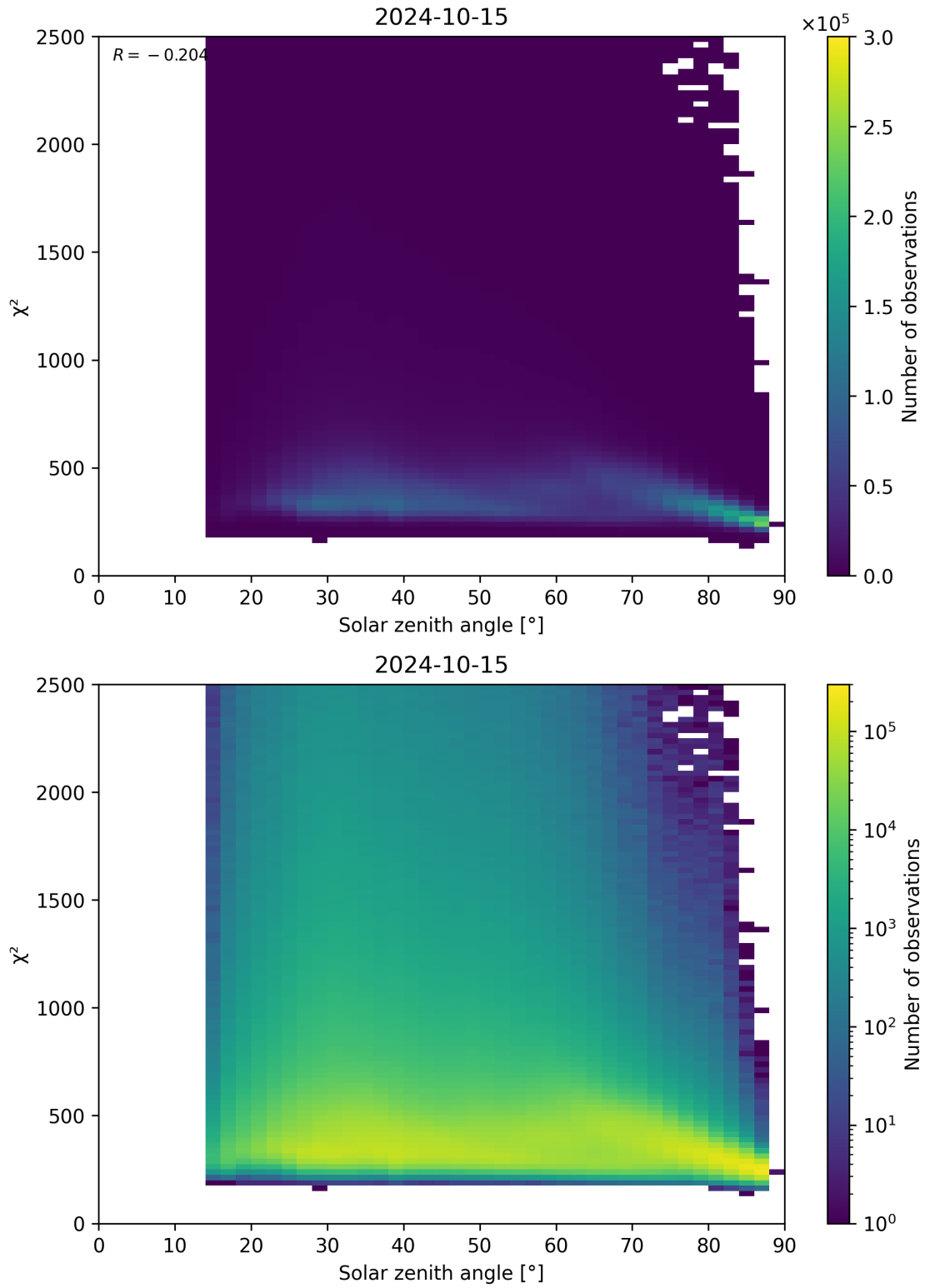
Figure 148: Scatter density plot of “Solar zenith angle” against “ \chi^2 ” for 2024-10-14 to 2024-10-16.
