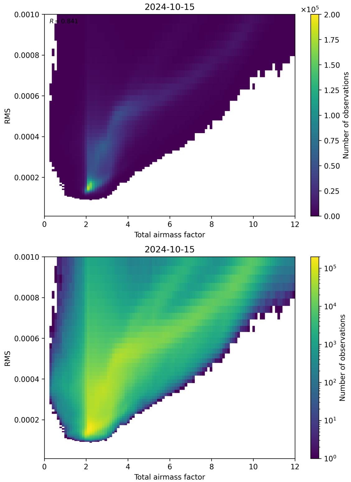
Figure 69: Scatter density plot of “Total airmass factor” against “RMS” for 2024-10-14 to 2024-10-16.
