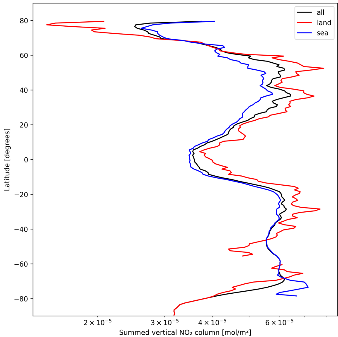
Figure 23: Zonal average of “Summed vertical NO 2 column” for 2024-10-14 to 2024-10-16.
