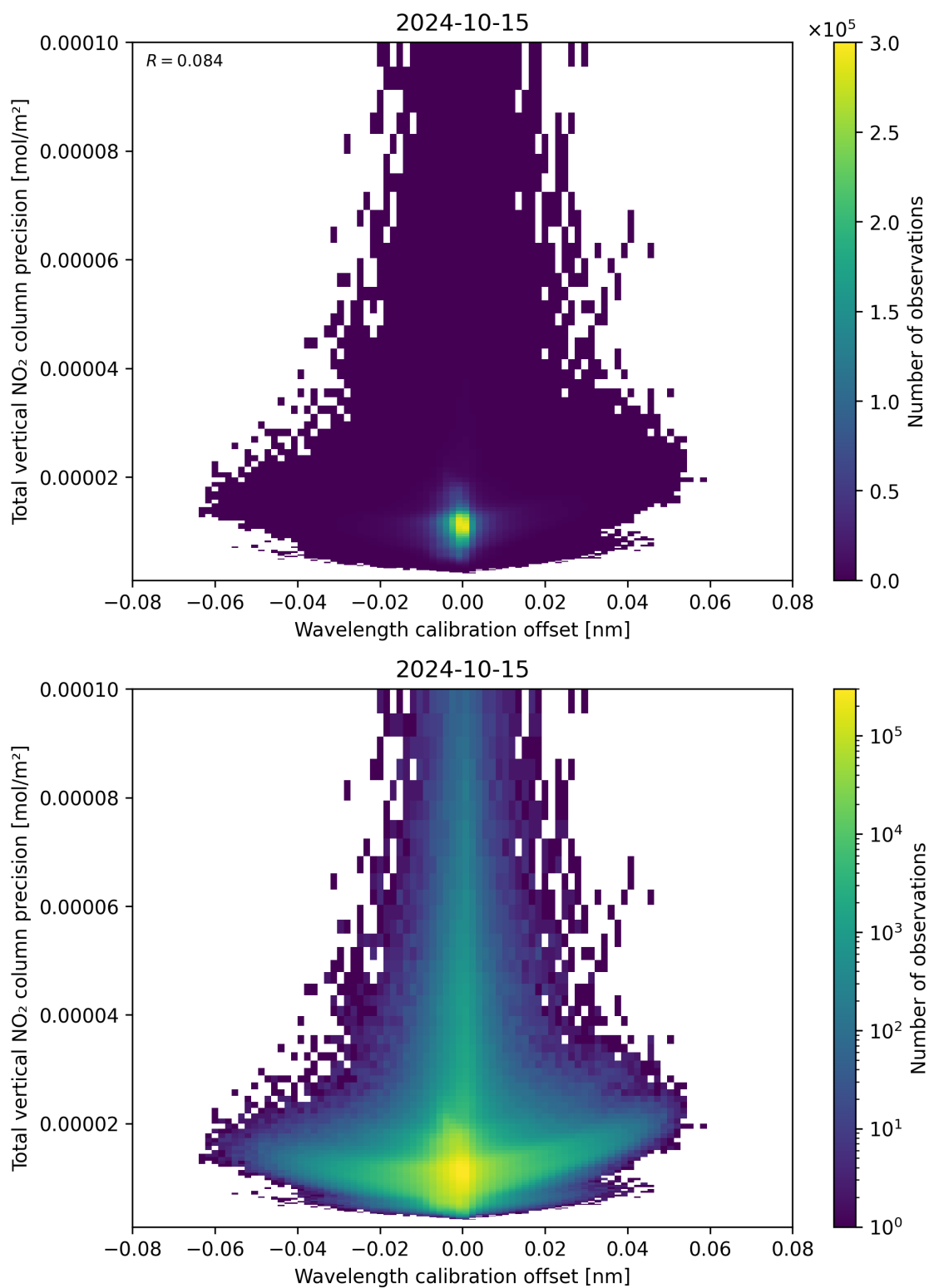
Figure 180: Scatter density plot of “Wavelength calibration offset” against “Total vertical NO 2 column precision” for 2024-10-14 to 2024-10-16.
