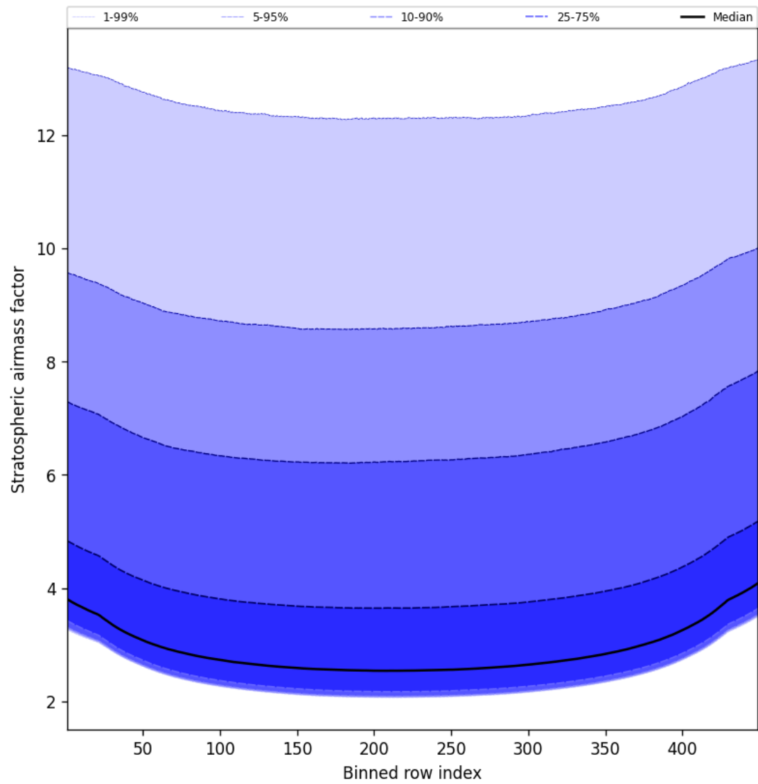
Figure 61: Along track statistics of “Stratospheric air mass factor” for 2024-10-14 to 2024-10-16
