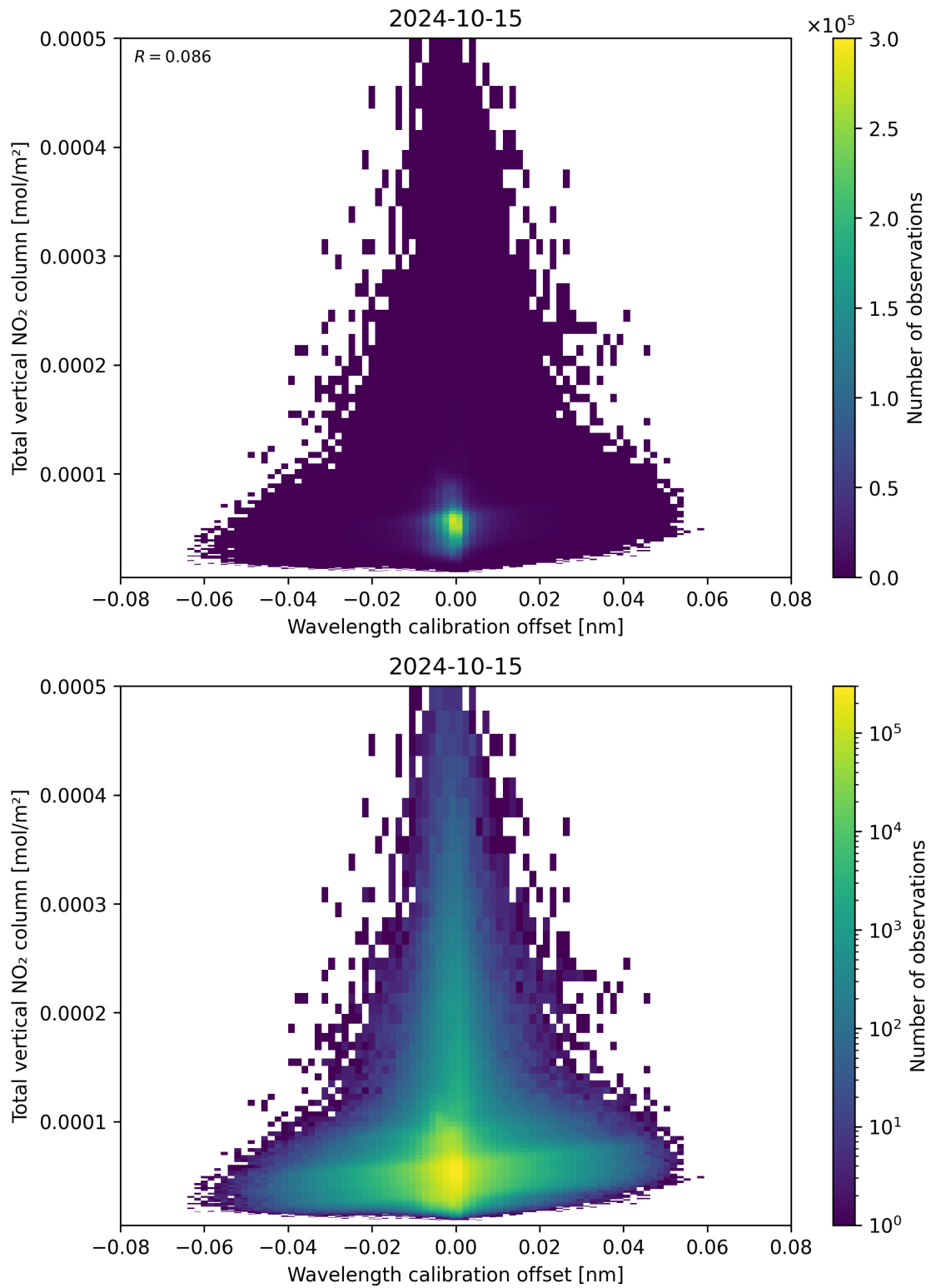
Figure 179: Scatter density plot of “Wavelength calibration offset” against “Total vertical NO 2 column” for 2024-10-14 to 2024-10-16.
