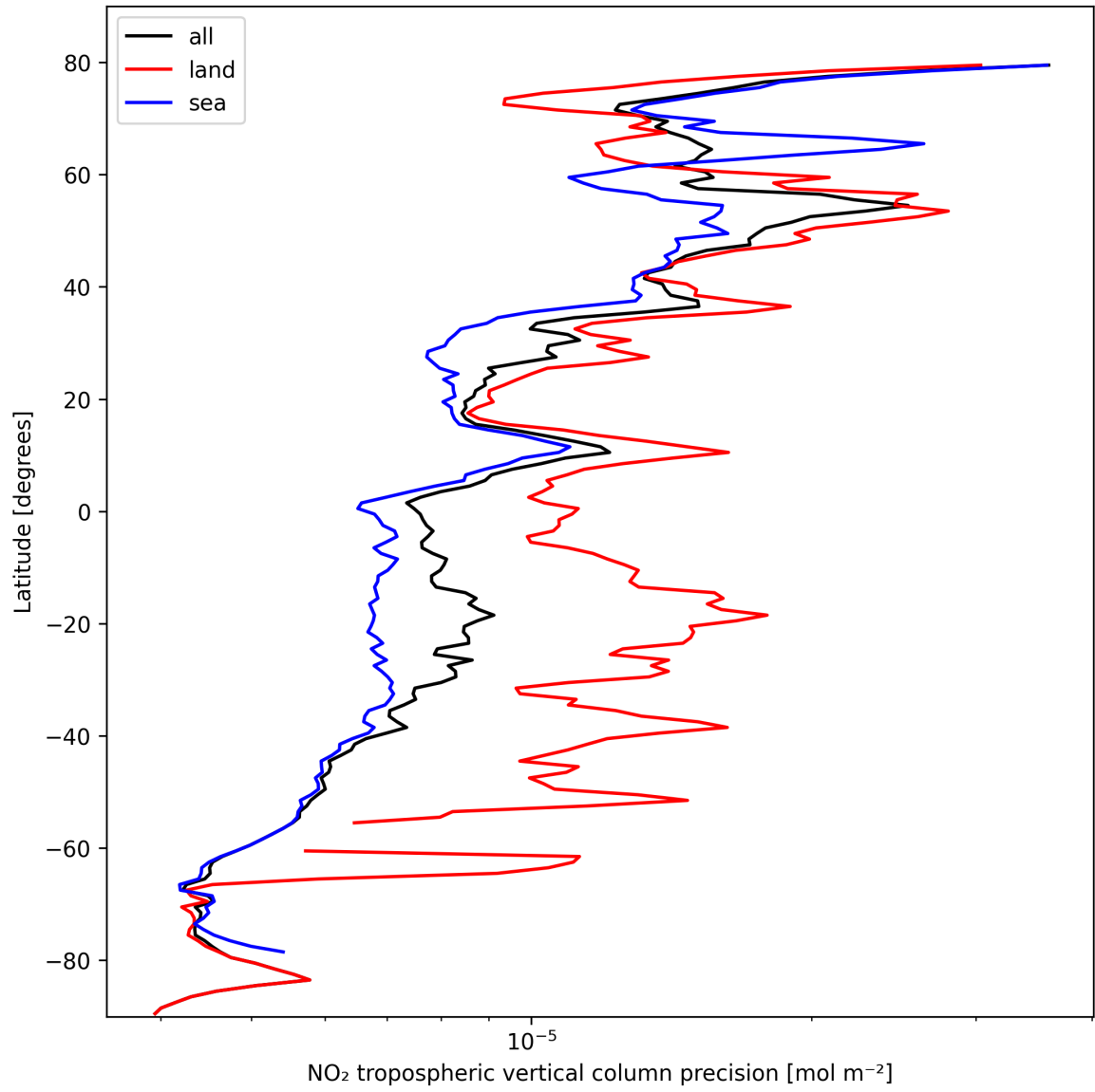
Figure 13: Zonal average of “NO 2 tropospheric vertical column precision” for 2024-10-14 to 2024-10-16.
