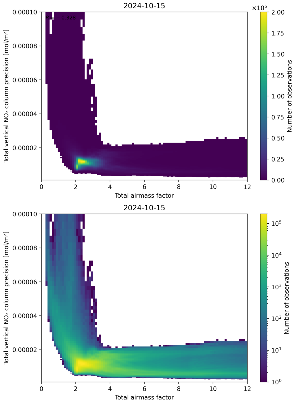
Figure 68: Scatter density plot of “Total airmass factor” against “Total vertical NO 2 column precision” for 2024-10-14 to 2024-10-16.
