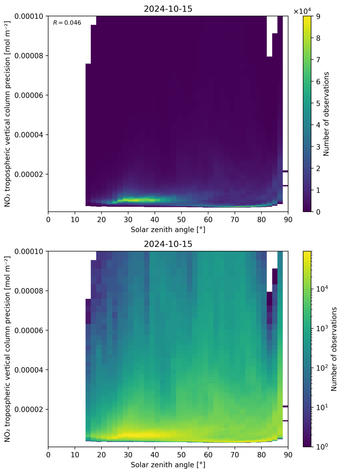
Figure 156: Scatter density plot of “Solar zenith angle” against “NO 2 tropospheric vertical column precision” for 2024-10-14 to 2024-10-16.
