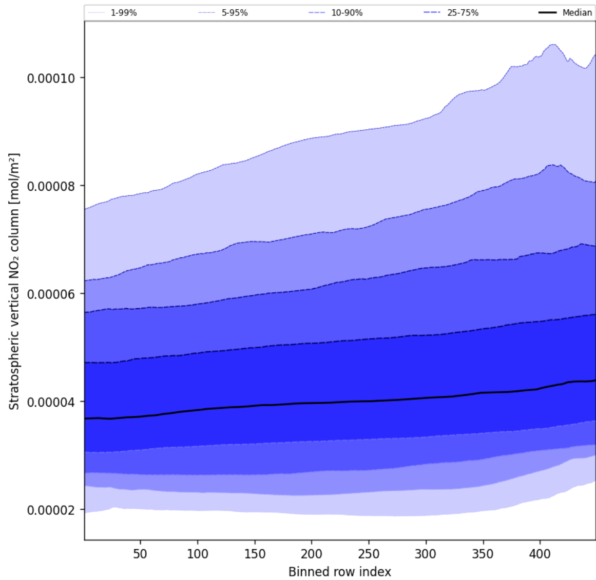
Figure 53: Along track statistics of “Stratospheric vertical NO 2 column” for 2024-10-14 to 2024-10-16
