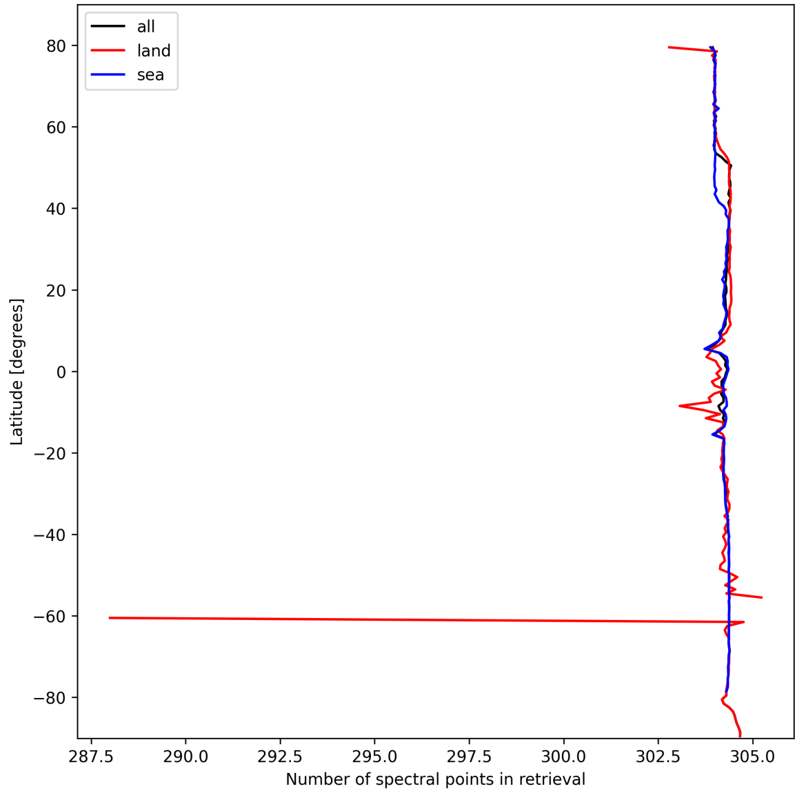
Figure 16: Zonal average of “Number of spectral points in retrieval” for 2024-10-14 to 2024-10-16.
