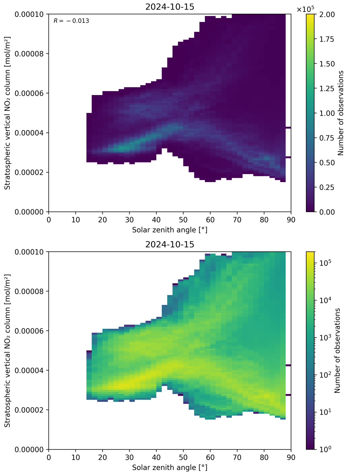
Figure 150: Scatter density plot of “Solar zenith angle” against “Stratospheric vertical NO 2 column” for 2024-10-14 to 2024-10-16.
