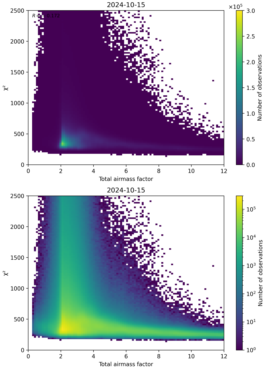
Figure 63: Scatter density plot of “Total airmass factor” against “ \chi^2 ” for 2024-10-14 to 2024-10-16.
