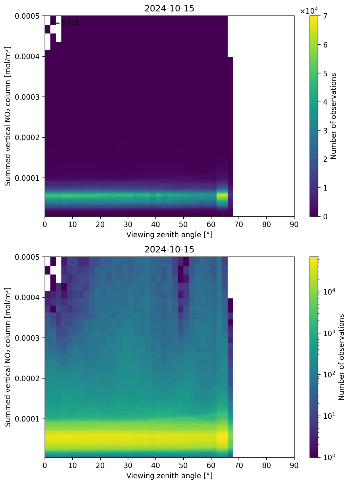
Figure 165: Scatter density plot of “Viewing zenith angle” against “Summed vertical NO 2 column” for 2024-10-14 to 2024-10-16.
