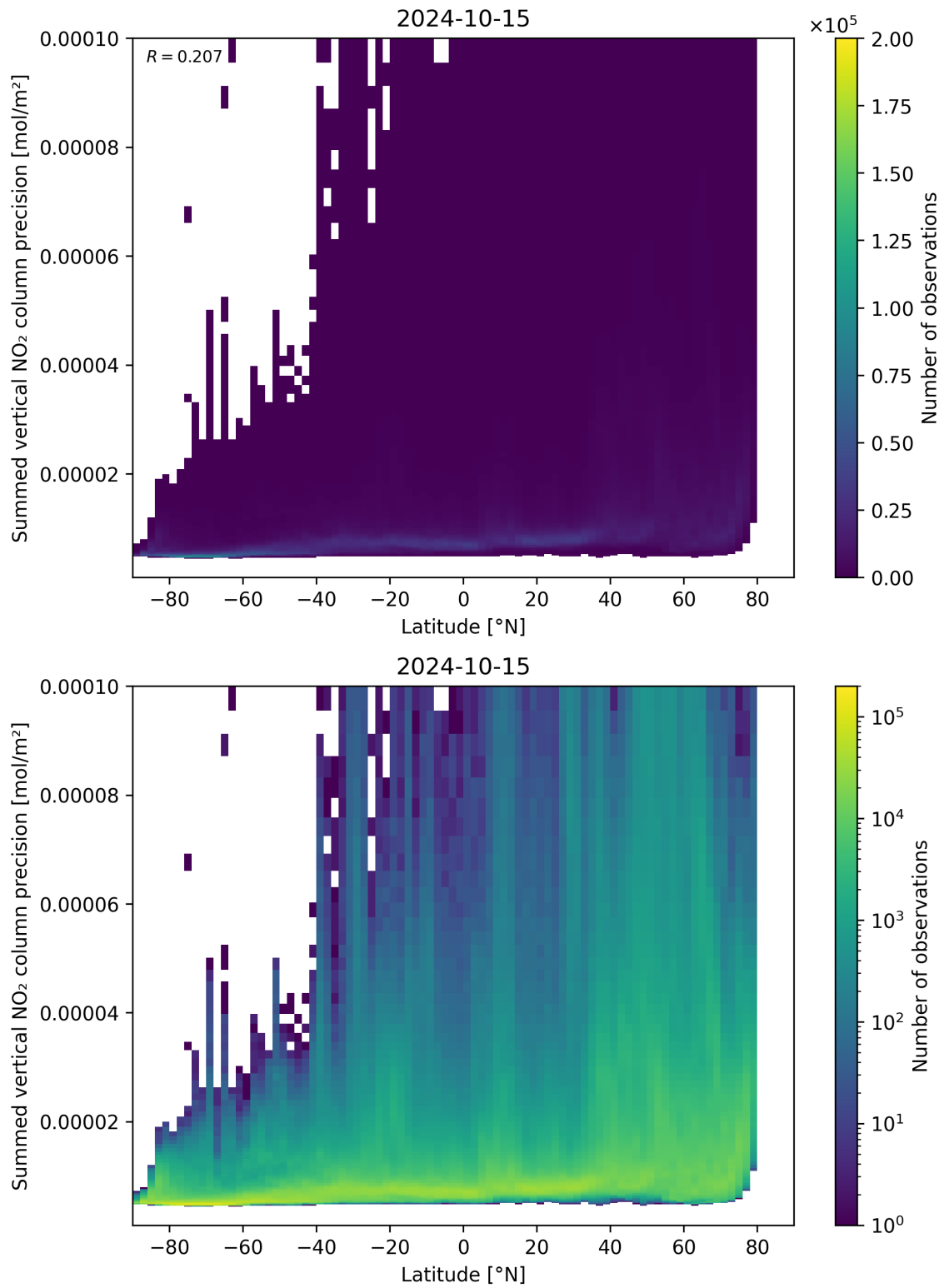
Figure 89: Scatter density plot of “Latitude” against “Summed vertical NO 2 column precision” for 2024-10-14 to 2024-10-16.
