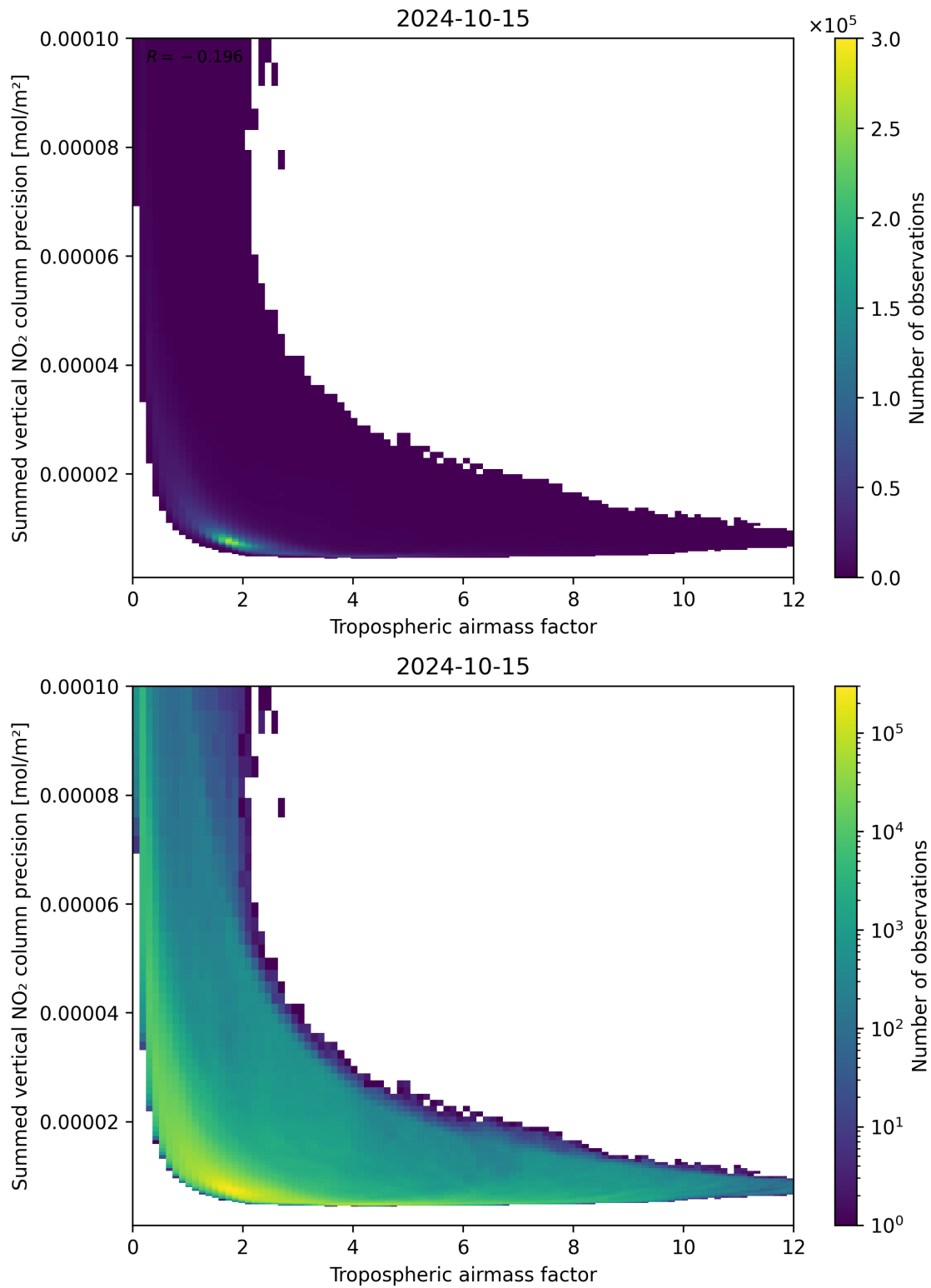
Figure 76: Scatter density plot of “Tropospheric air mass factor” against “Summed vertical NO 2 column precision” for 2024-10-14 to 2024-10-16.
