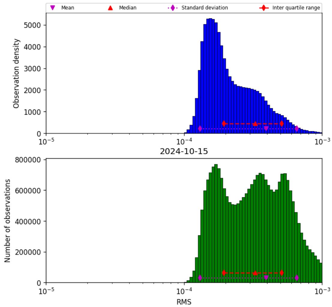
Figure 43: Histogram of “RMS” for 2024-10-14 to 2024-10-16
