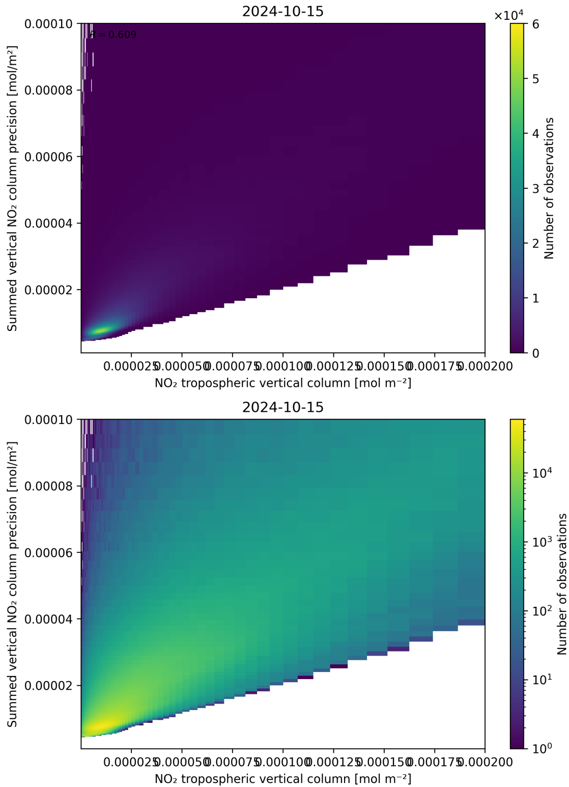
Figure 127: Scatter density plot of “NO 2 tropospheric vertical column” against “Summed vertical NO 2 column precision” for 2024-10-14 to 2024-10-16.
