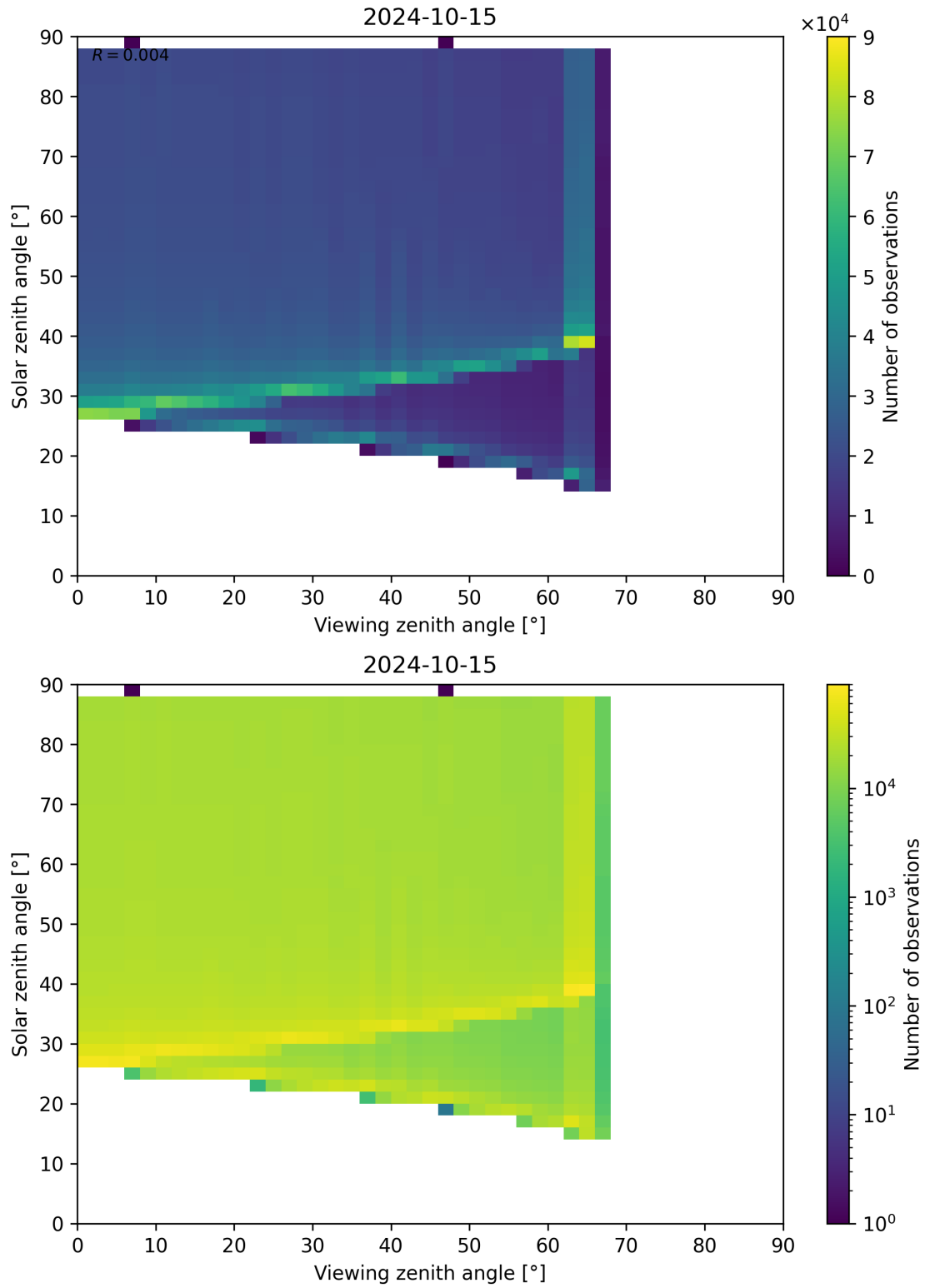
Figure 172: Scatter density plot of “Viewing zenith angle” against “Solar zenith angle” for 2024-10-14 to 2024-10-16.
