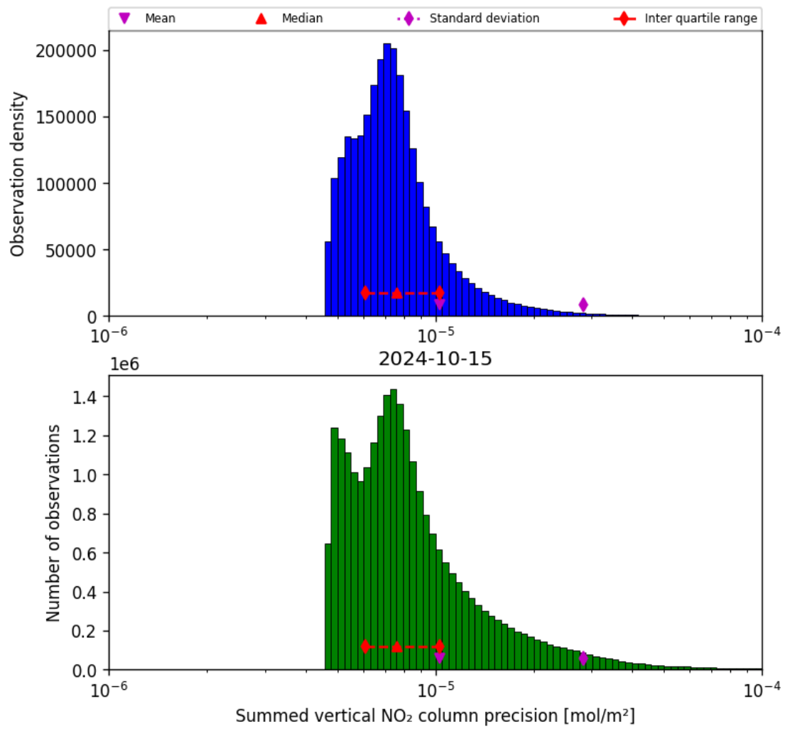
Figure 41: Histogram of "Summed vertical NO 2 column precision" for 2024-10-14 to 2024-10-16
