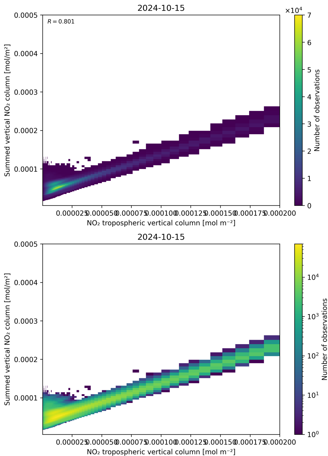
Figure 126: Scatter density plot of “NO 2 tropospheric vertical column” against “Summed vertical NO 2 column” for 2024-10-14 to 2024-10-16.
