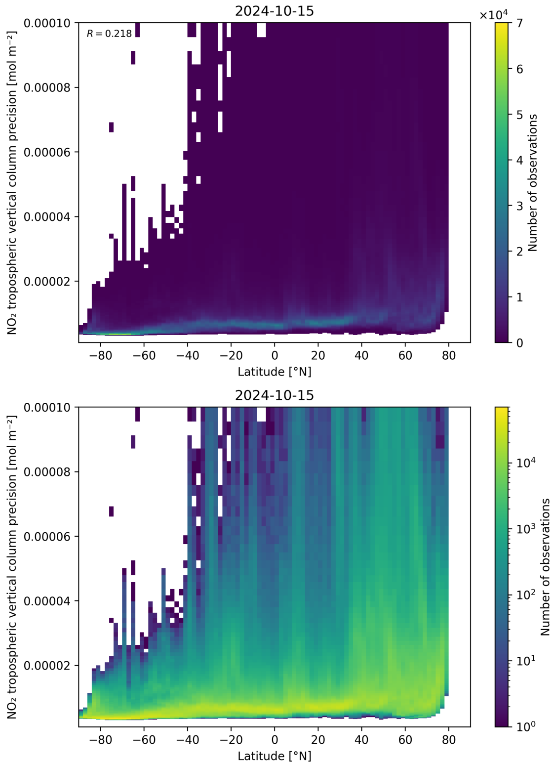
Figure 93: Scatter density plot of “Latitude” against “NO 2 tropospheric vertical column precision” for 2024-10-14 to 2024-10-16.
