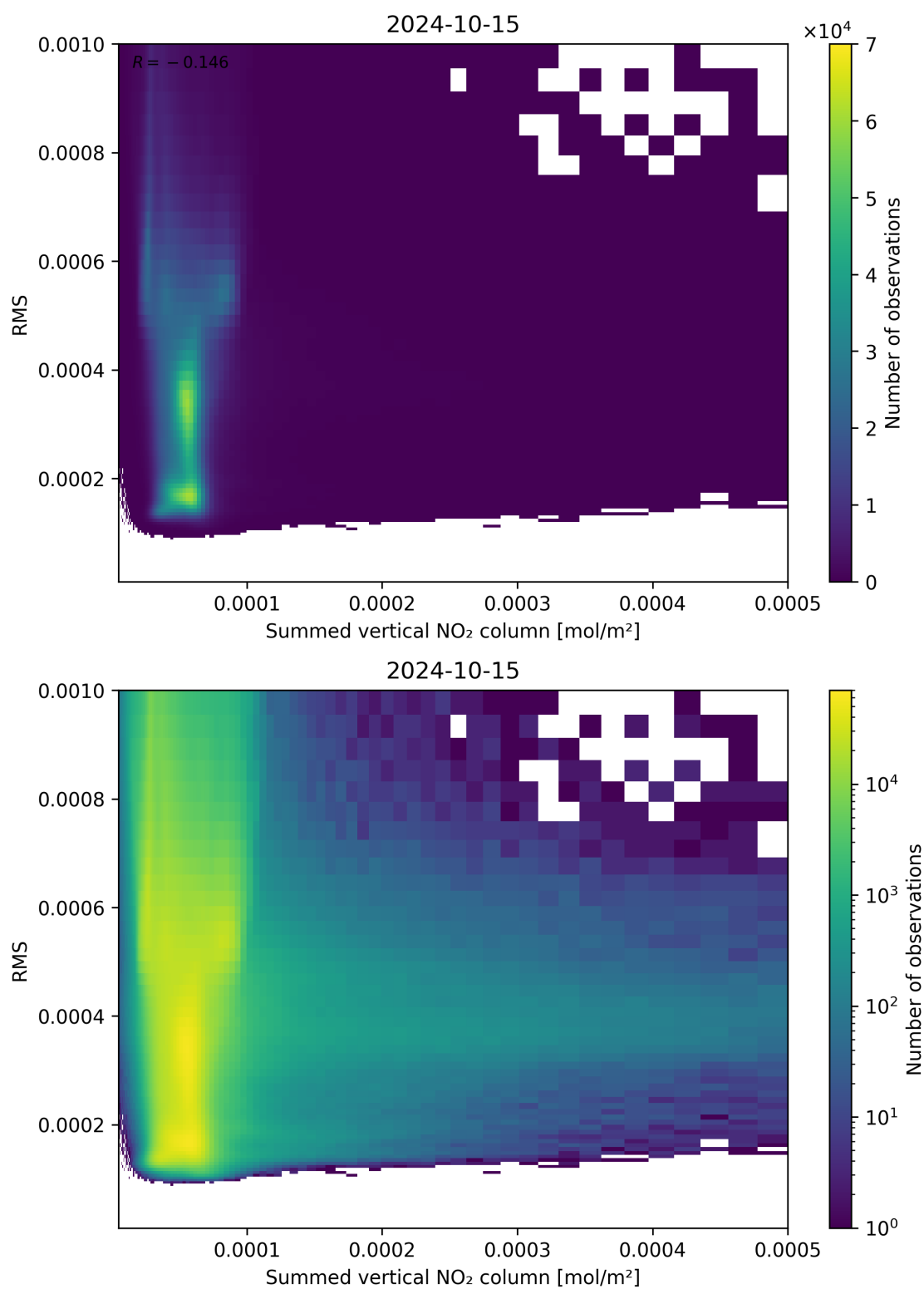
Figure 109: Scatter density plot of “Summed vertical NO 2 column” against “RMS” for 2024-10-14 to 2024-10-16.
