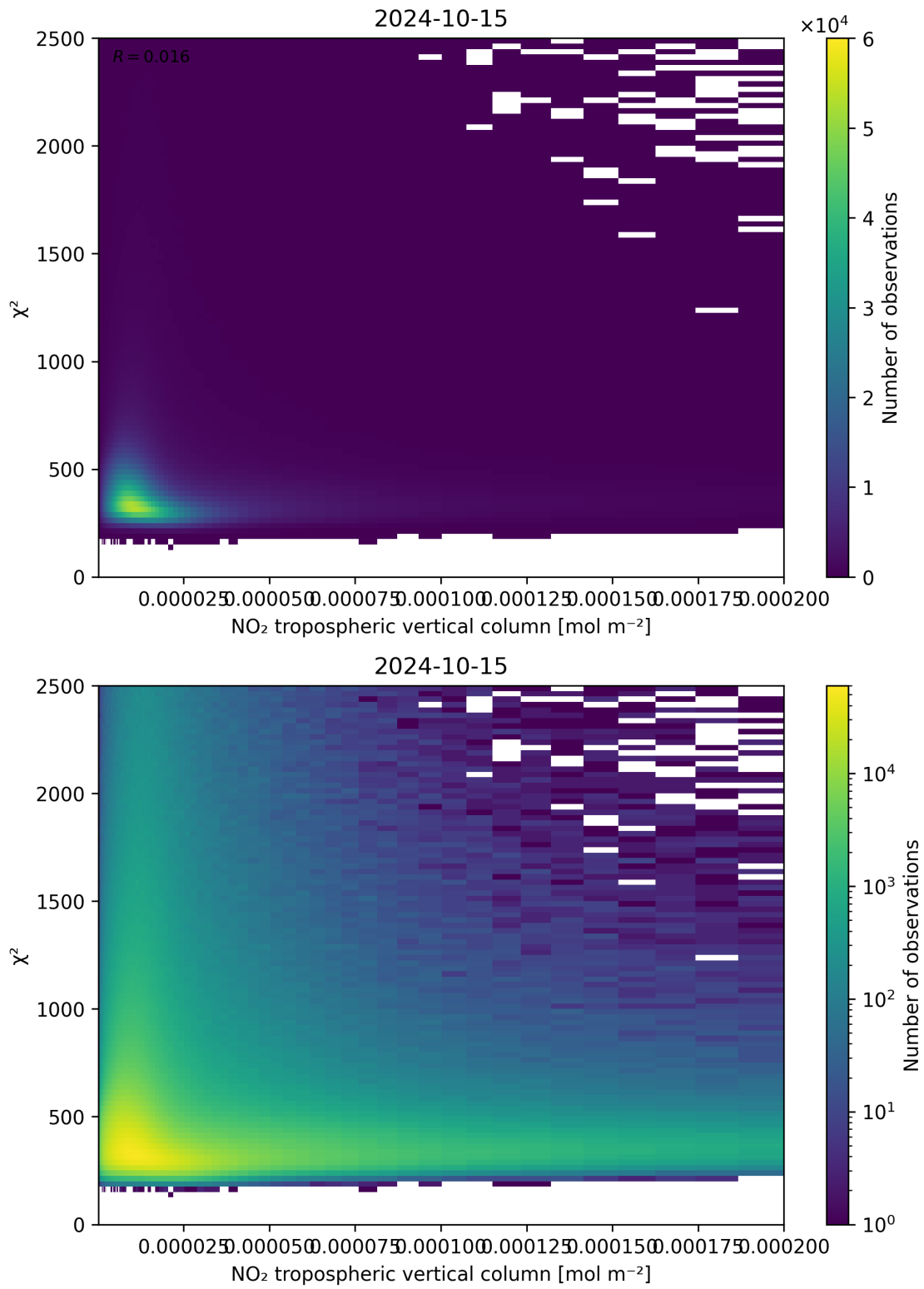
Figure 124: Scatter density plot of “NO 2 tropospheric vertical column” against “ \chi^2 ” for 2024-10-14 to 2024-10-16.
