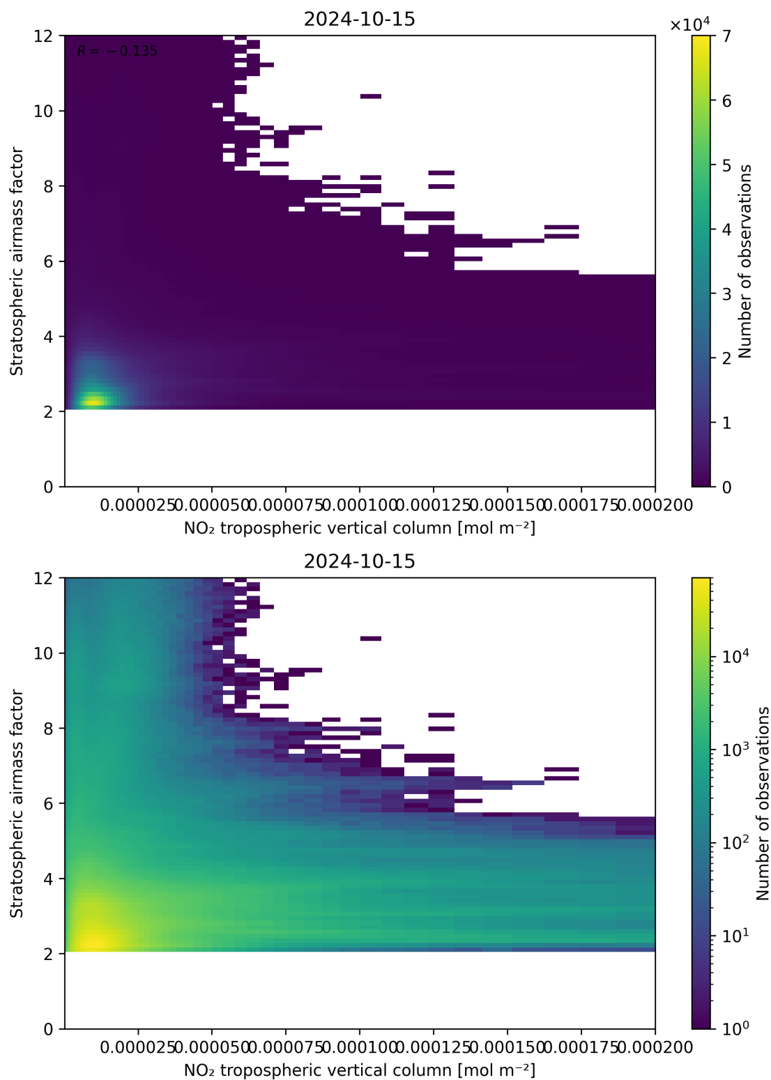
Figure 121: Scatter density plot of “NO 2 tropospheric vertical column” against “Stratospheric air mass factor” for 2024-10-14 to 2024-10-16.
