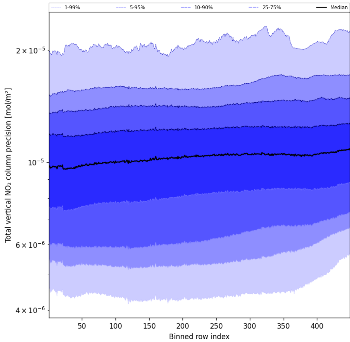
Figure 56: Along track statistics of “Total vertical NO 2 column precision” for 2024-10-14 to 2024-10-16
