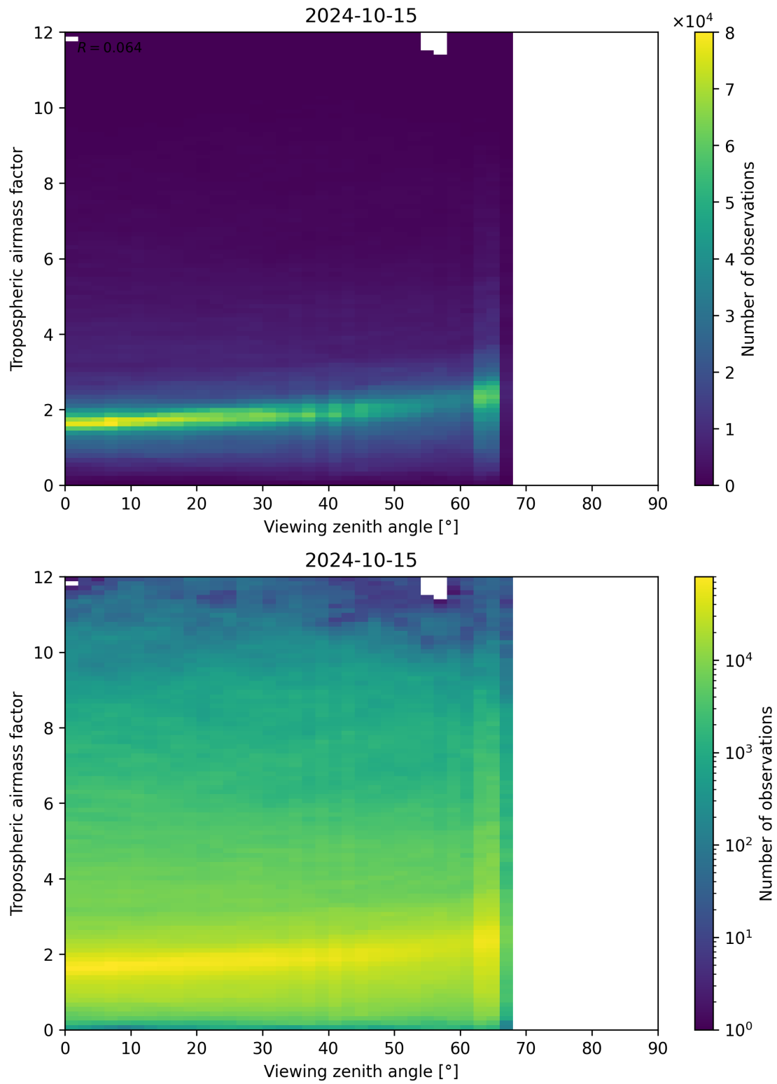
Figure 161: Scatter density plot of “Viewing zenith angle” against “Tropospheric airmass factor” for 2024-10-14 to 2024-10-16.
