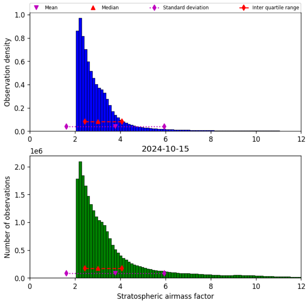
Figure 44: Histogram of “Stratospheric airmass factor” for 2024-10-14 to 2024-10-16
