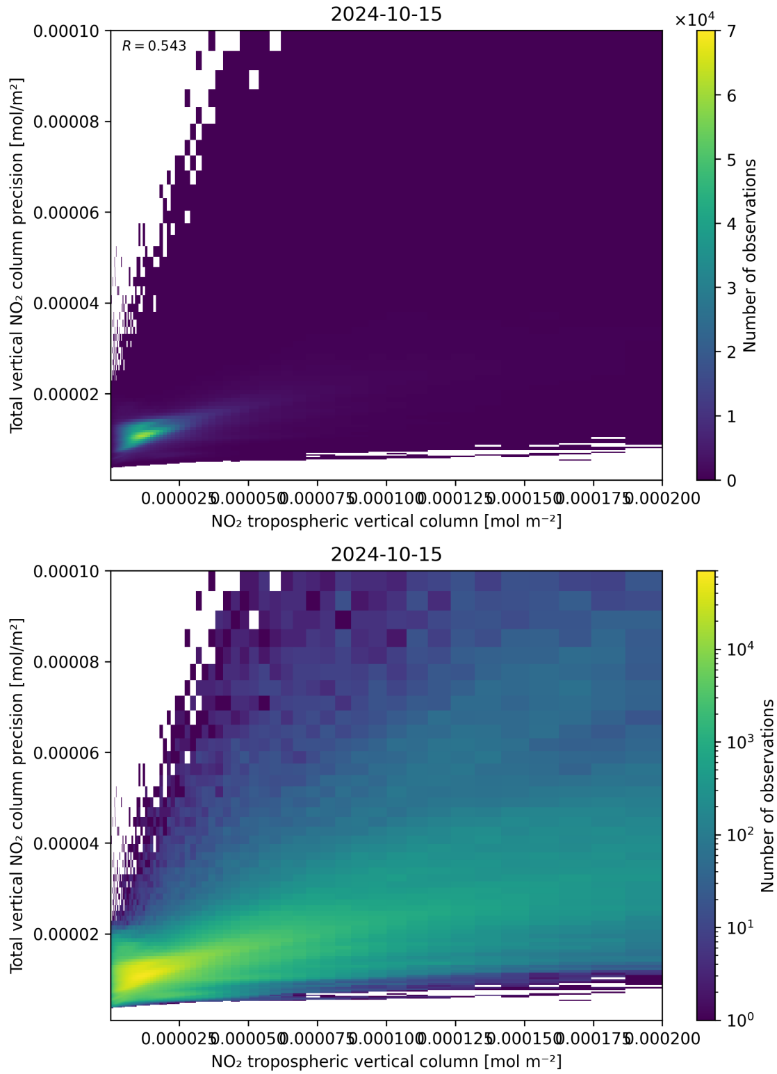
Figure 129: Scatter density plot of “NO 2 tropospheric vertical column” against “Total vertical NO 2 column precision” for 2024-10-14 to 2024-10-16.
