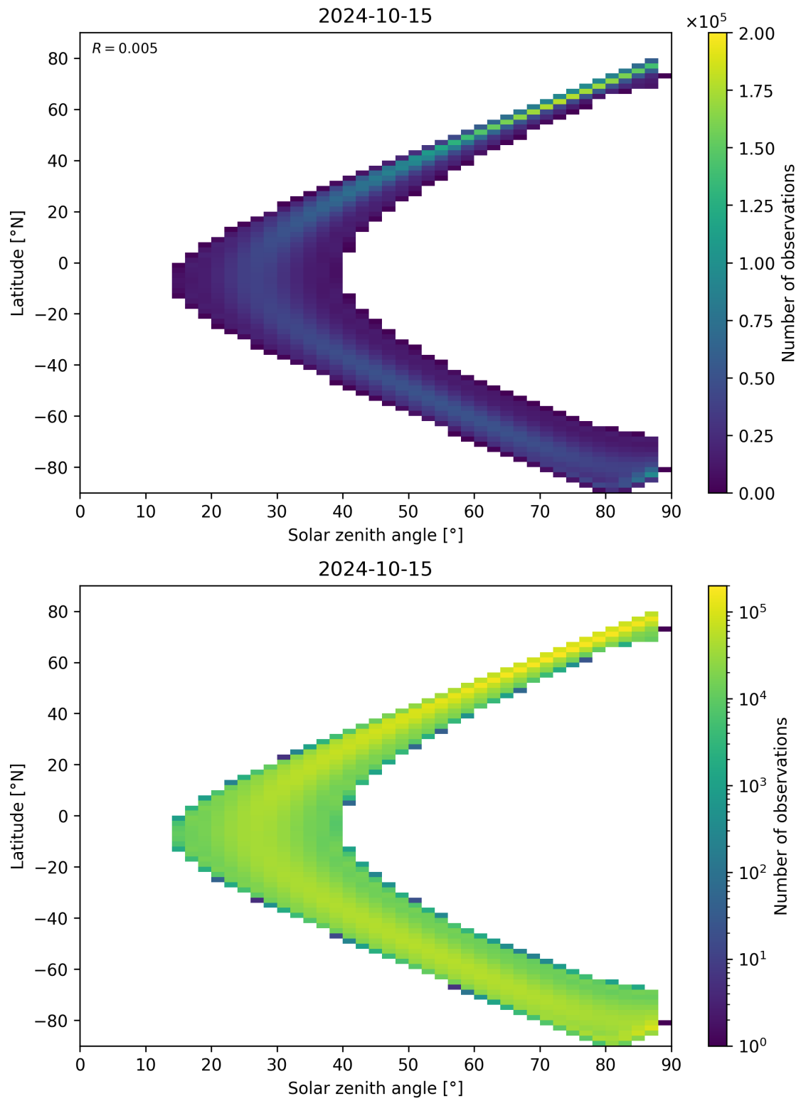
Figure 149: Scatter density plot of “Solar zenith angle” against “Latitude” for 2024-10-14 to 2024-10-16.
