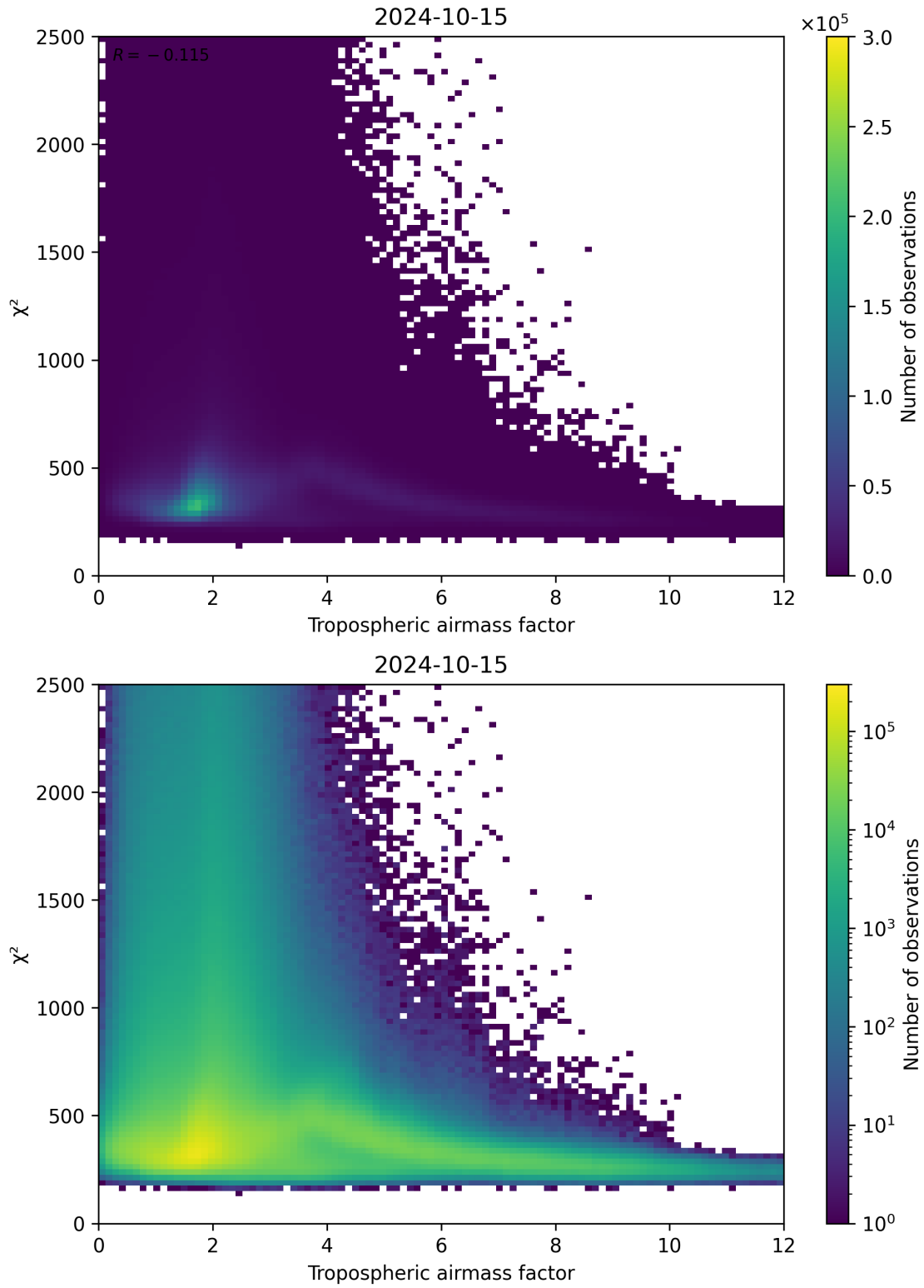
Figure 73: Scatter density plot of “Tropospheric airmass factor” against “ \chi^2 ” for 2024-10-14 to 2024-10-16.
