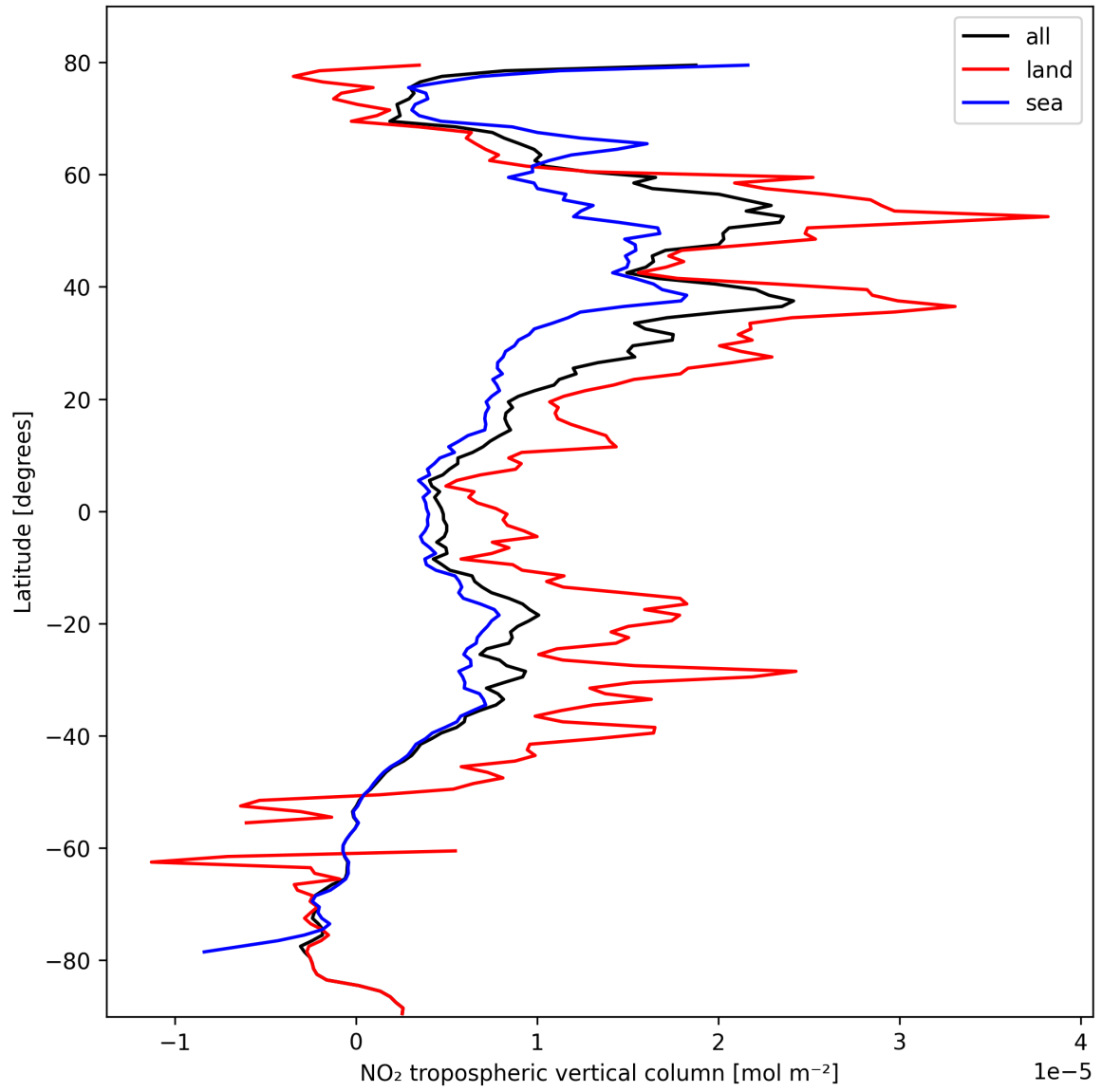
Figure 12: Zonal average of “NO 2 tropospheric vertical column” for 2024-10-14 to 2024-10-16.
