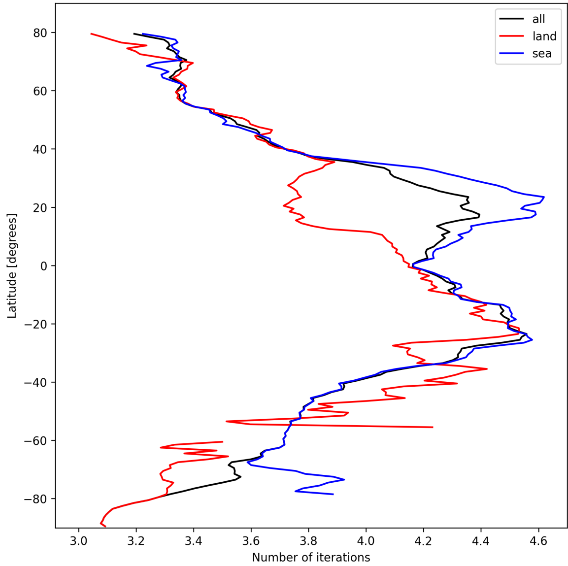
Figure 17: Zonal average of “Number of iterations” for 2024-10-14 to 2024-10-16.
