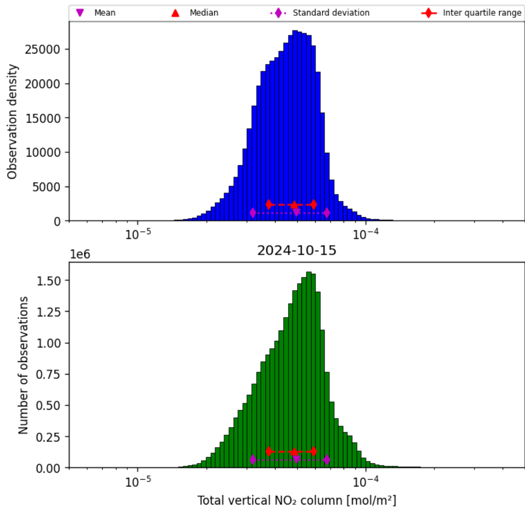
Figure 38: Histogram of “Total vertical NO 2 column” for 2024-10-14 to 2024-10-16
