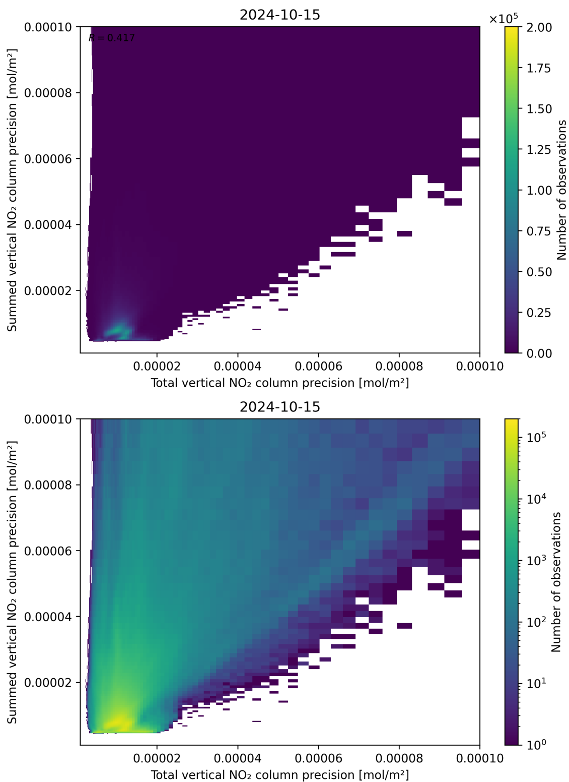
Figure 118: Scatter density plot of “Total vertical NO 2 column precision” against “Summed vertical NO 2 column precision” for 2024-10-14 to 2024-10-16.
