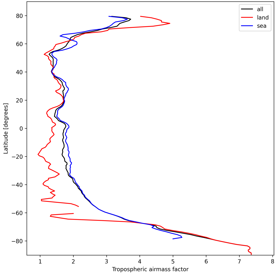
Figure 14: Zonal average of “Tropospheric airmass factor” for 2024-10-14 to 2024-10-16.
