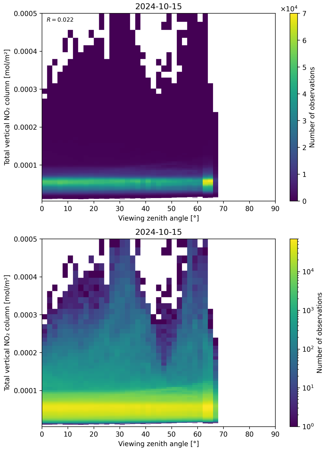
Figure 167: Scatter density plot of “Viewing zenith angle” against “Total vertical NO 2 column” for 2024-10-14 to 2024-10-16.
