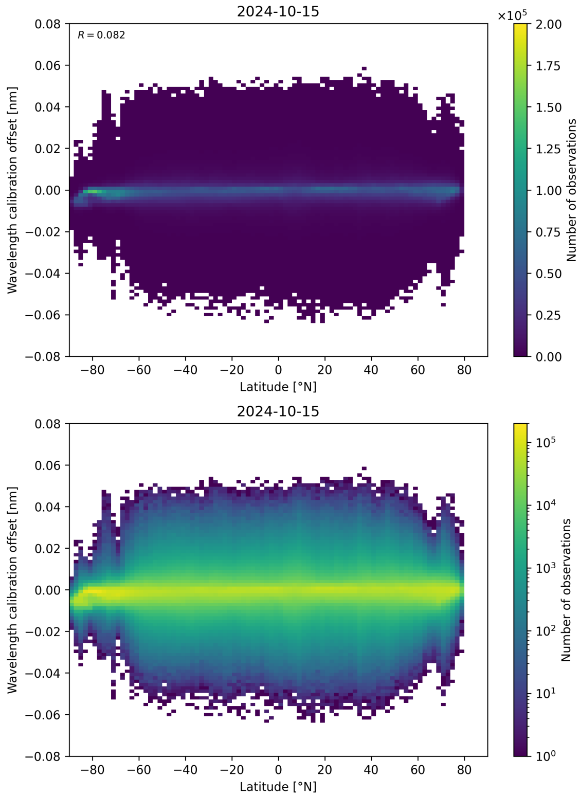
Figure 95: Scatter density plot of “Latitude” against “Wavelength calibration offset” for 2024-10-14 to 2024-10-16.
