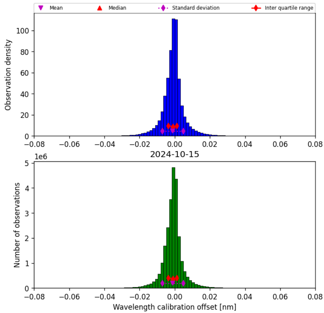
Figure 35: Histogram of “Wavelength calibration offset” for 2024-10-14 to 2024-10-16
