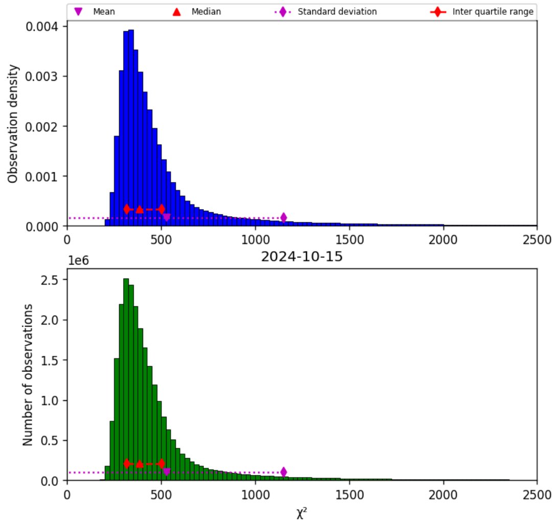
Figure 42: Histogram of “ \chi^2 ” for 2024-10-14 to 2024-10-16
