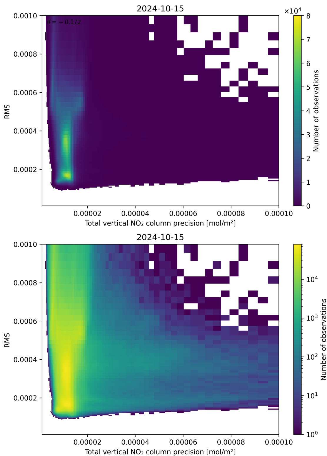
Figure 119: Scatter density plot of “Total vertical NO 2 column precision” against “RMS” for 2024-10-14 to 2024-10-16.
