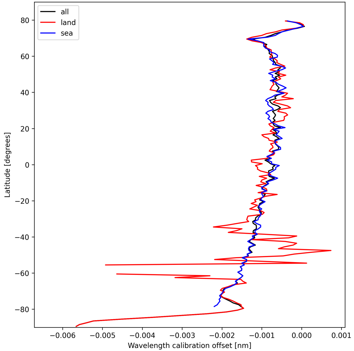
Figure 18: Zonal average of “Wavelength calibration offset” for 2024-10-14 to 2024-10-16.
