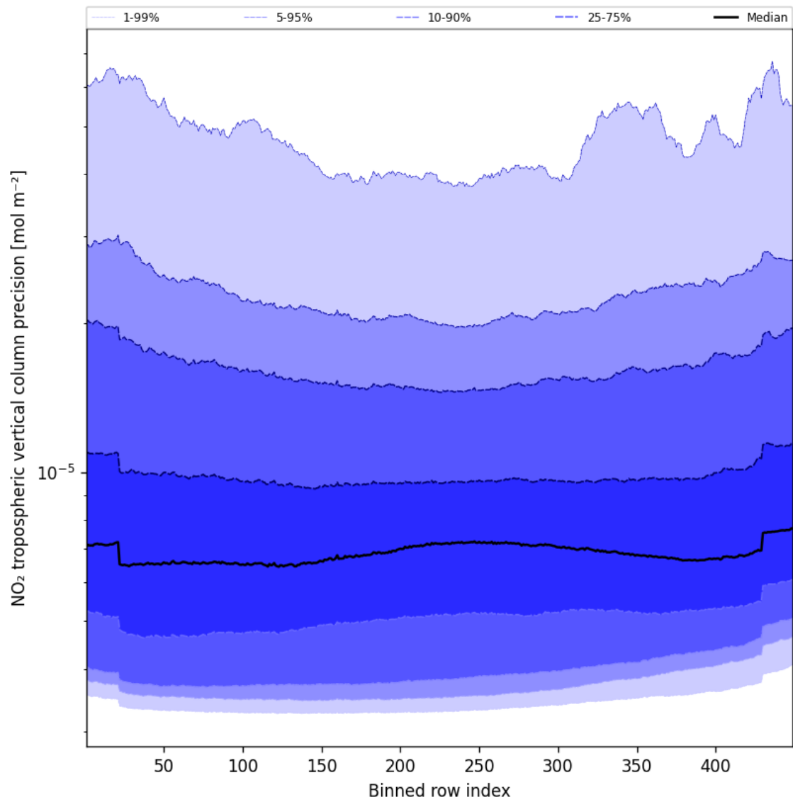
Figure 47: Along track statistics of “NO 2 tropospheric vertical column precision” for 2024-10-14 to 2024-10-16
