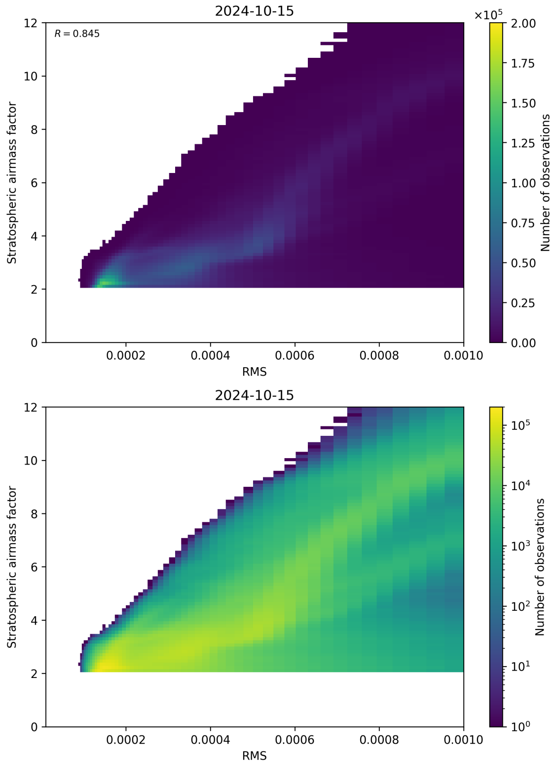
Figure 144: Scatter density plot of “RMS” against “Stratospheric airmass factor” for 2024-10-14 to 2024-10-16.
