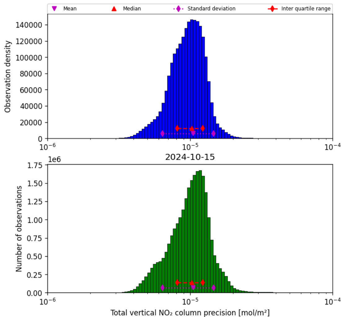
Figure 39: Histogram of “Total vertical NO 2 column precision” for 2024-10-14 to 2024-10-16
