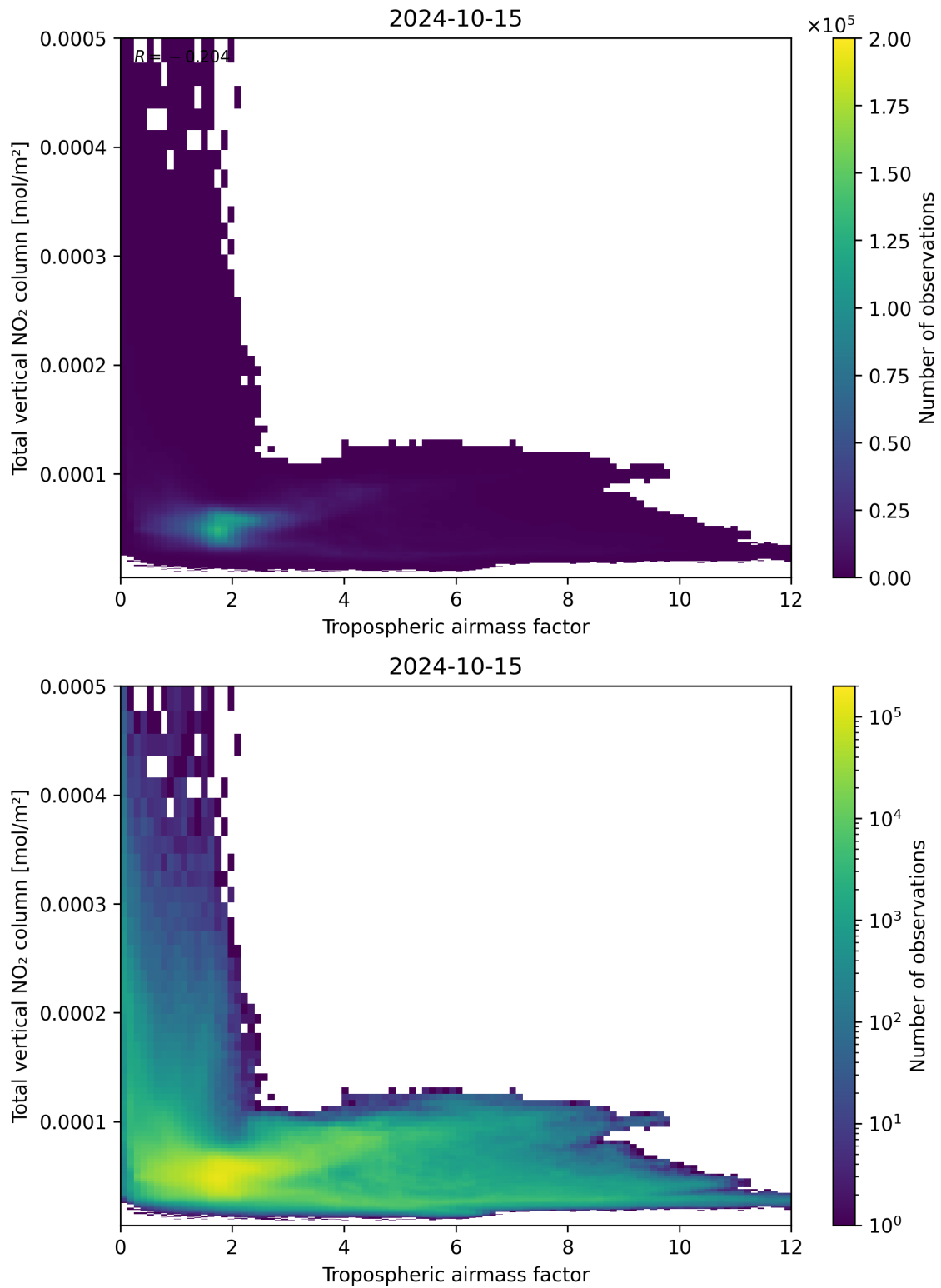
Figure 77: Scatter density plot of “Tropospheric airmass factor” against “Total vertical NO 2 column” for 2024-10-14 to 2024-10-16.
