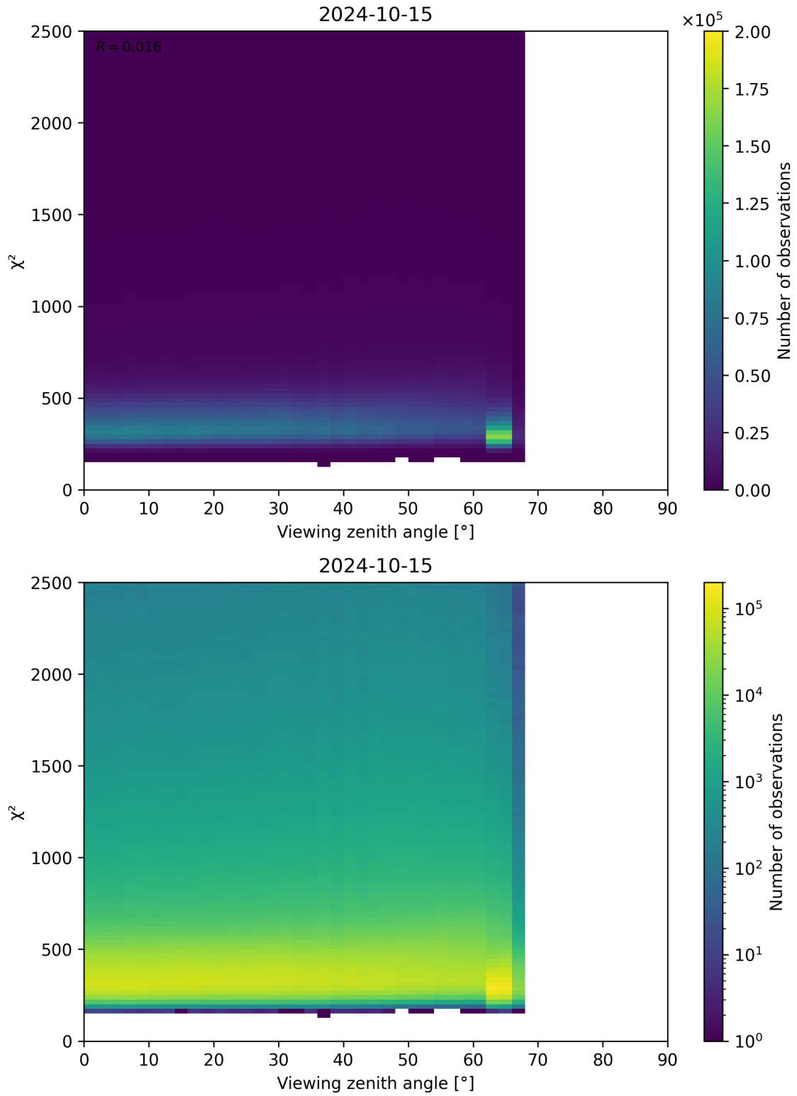
Figure 162: Scatter density plot of “Viewing zenith angle” against “ \chi^2 ” for 2024-10-14 to 2024-10-16.
