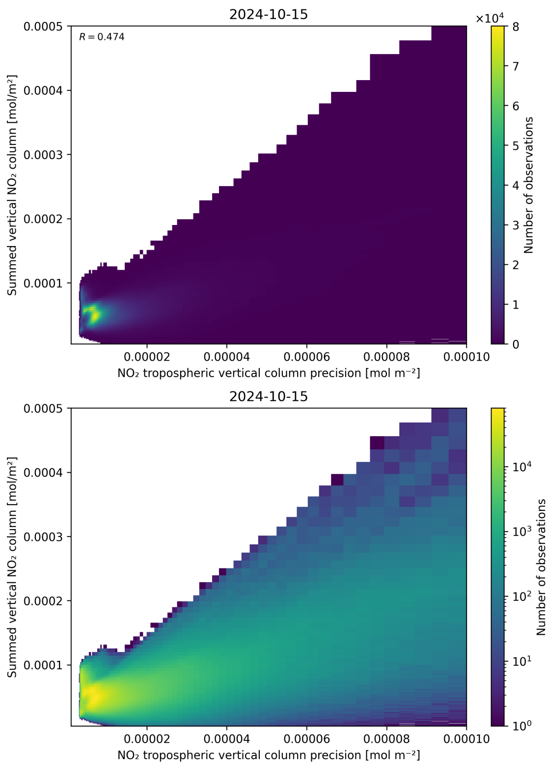
Figure 136: Scatter density plot of “NO 2 tropospheric vertical column precision” against “Summed vertical NO 2 column” for 2024-10-14 to 2024-10-16.
