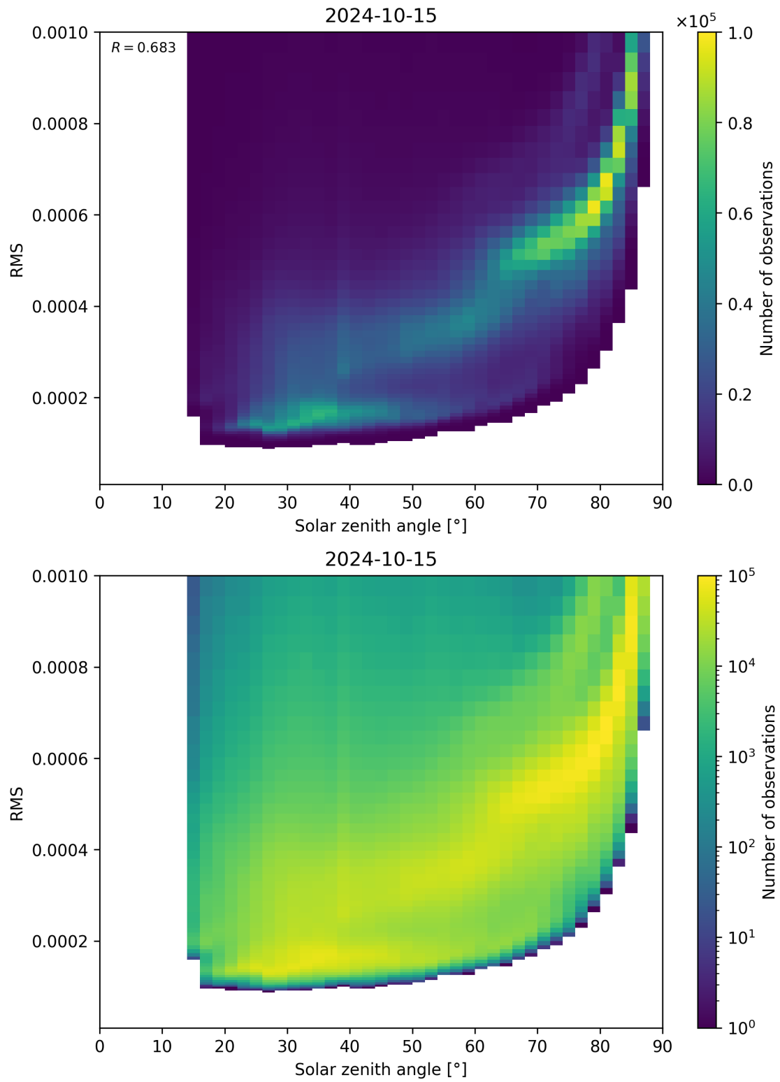
Figure 157: Scatter density plot of “Solar zenith angle” against “RMS” for 2024-10-14 to 2024-10-16.
