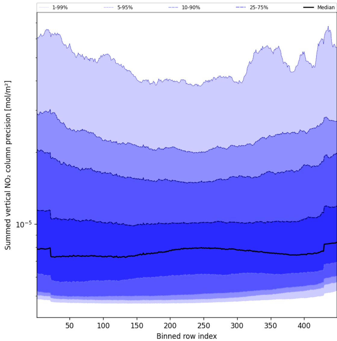
Figure 58: Along track statistics of “Summed vertical NO 2 column precision” for 2024-10-14 to 2024-10-16
