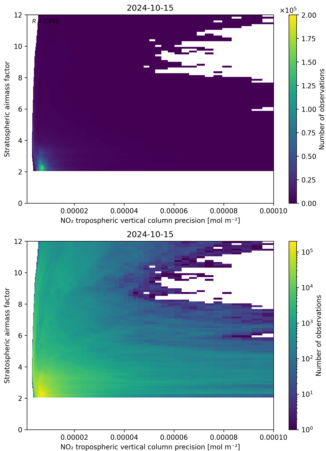
Figure 131: Scatter density plot of “NO 2 tropospheric vertical column precision” against “Stratospheric airmass factor” for 2024-10-14 to 2024-10-16.
