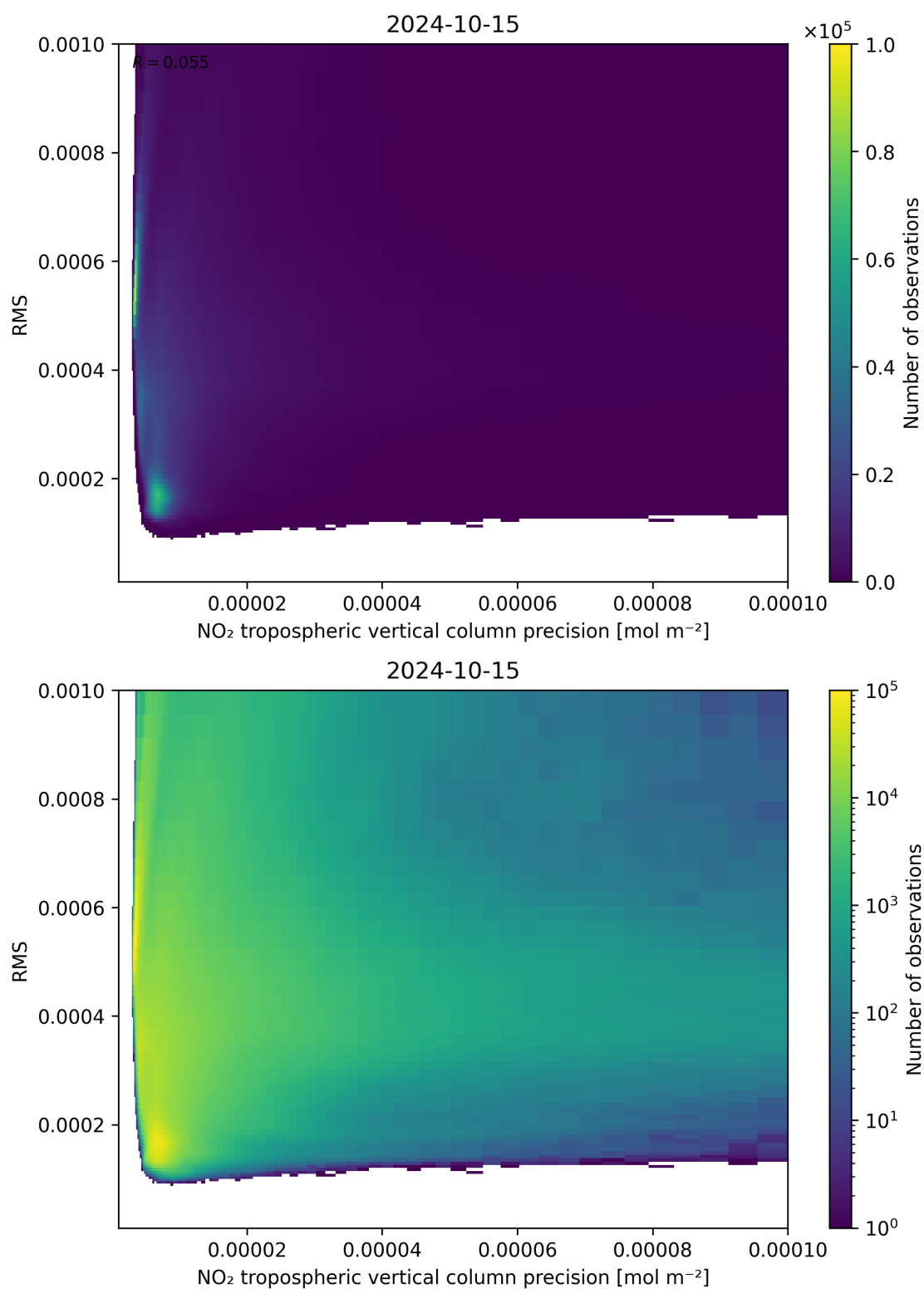
Figure 140: Scatter density plot of “NO 2 tropospheric vertical column precision” against “RMS” for 2024-10-14 to 2024-10-16.
