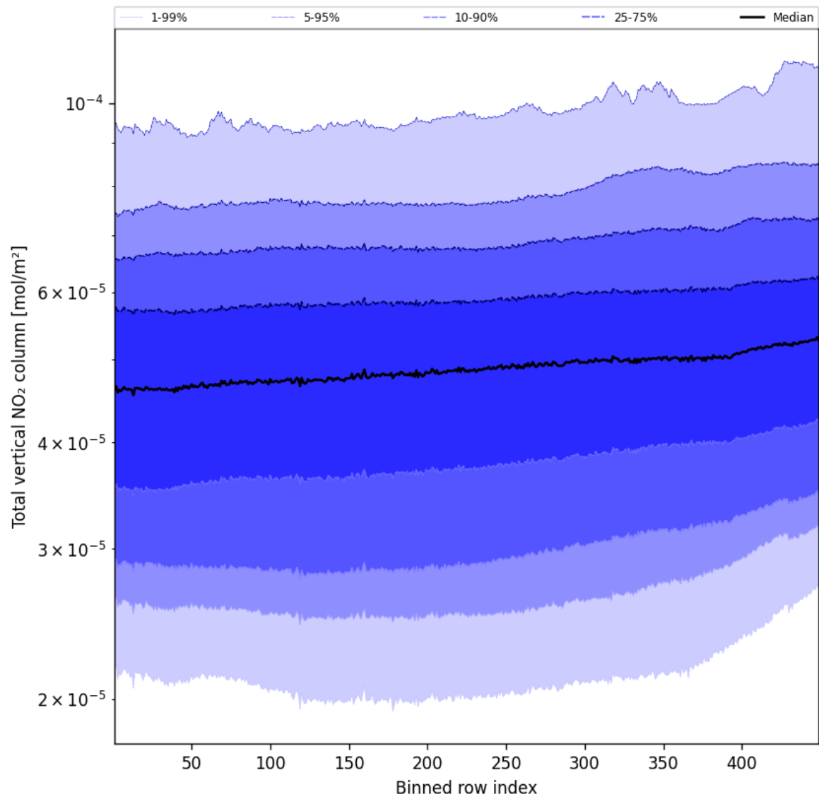
Figure 55: Along track statistics of “Total vertical NO 2 column” for 2024-10-14 to 2024-10-16
