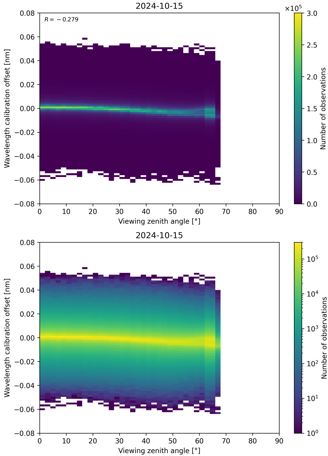
Figure 173: Scatter density plot of “Viewing zenith angle” against “Wavelength calibration offset” for 2024-10-14 to 2024-10-16.
