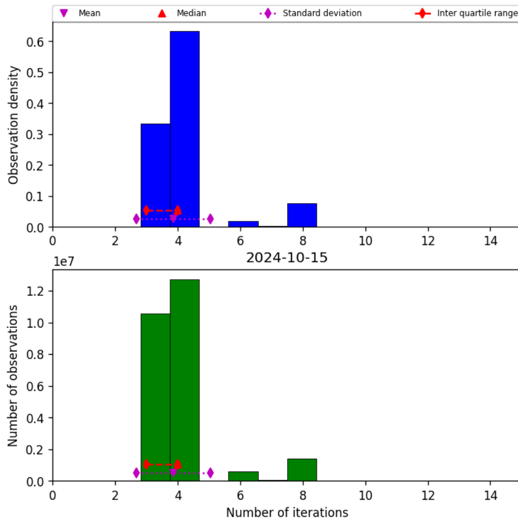
Figure 34: Histogram of “Number of iterations” for 2024-10-14 to 2024-10-16
