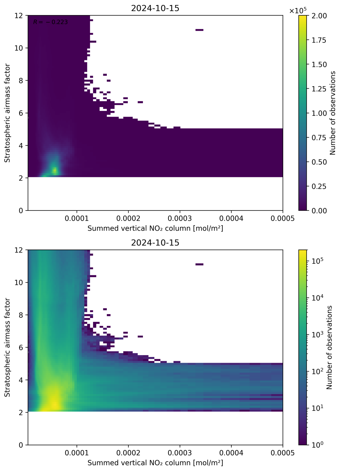
Figure 103: Scatter density plot of “Summed vertical NO 2 column” against “Stratospheric air mass factor” for 2024-10-14 to 2024-10-16.
