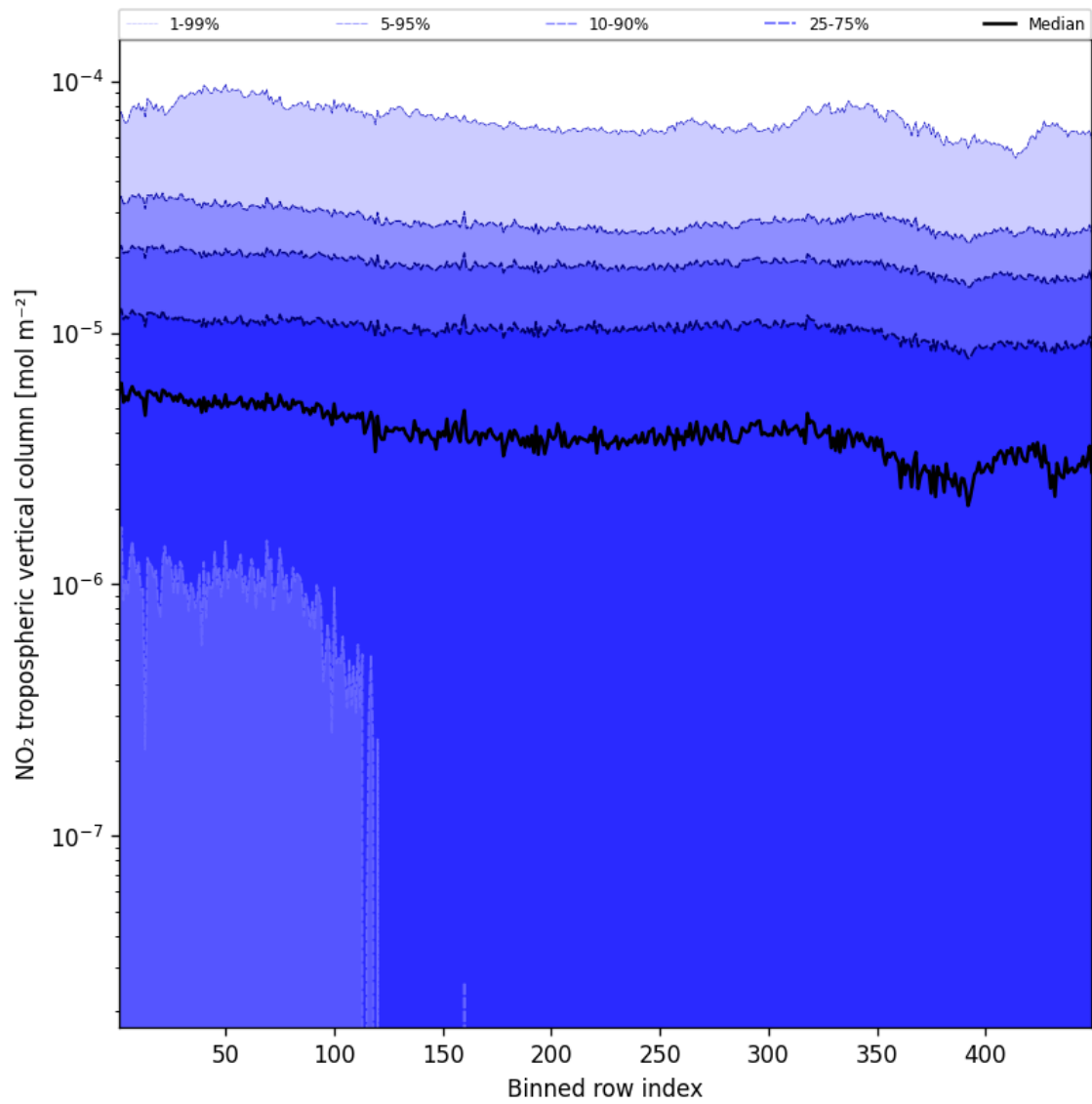
Figure 46: Along track statistics of “NO 2 tropospheric vertical column” for 2024-10-14 to 2024-10-16
