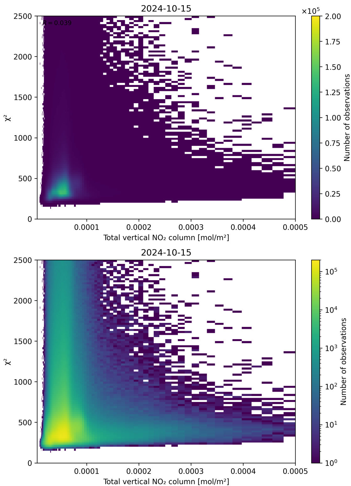
Figure 111: Scatter density plot of “Total vertical NO 2 column” against “ \chi^2 ” for 2024-10-14 to 2024-10-16.
