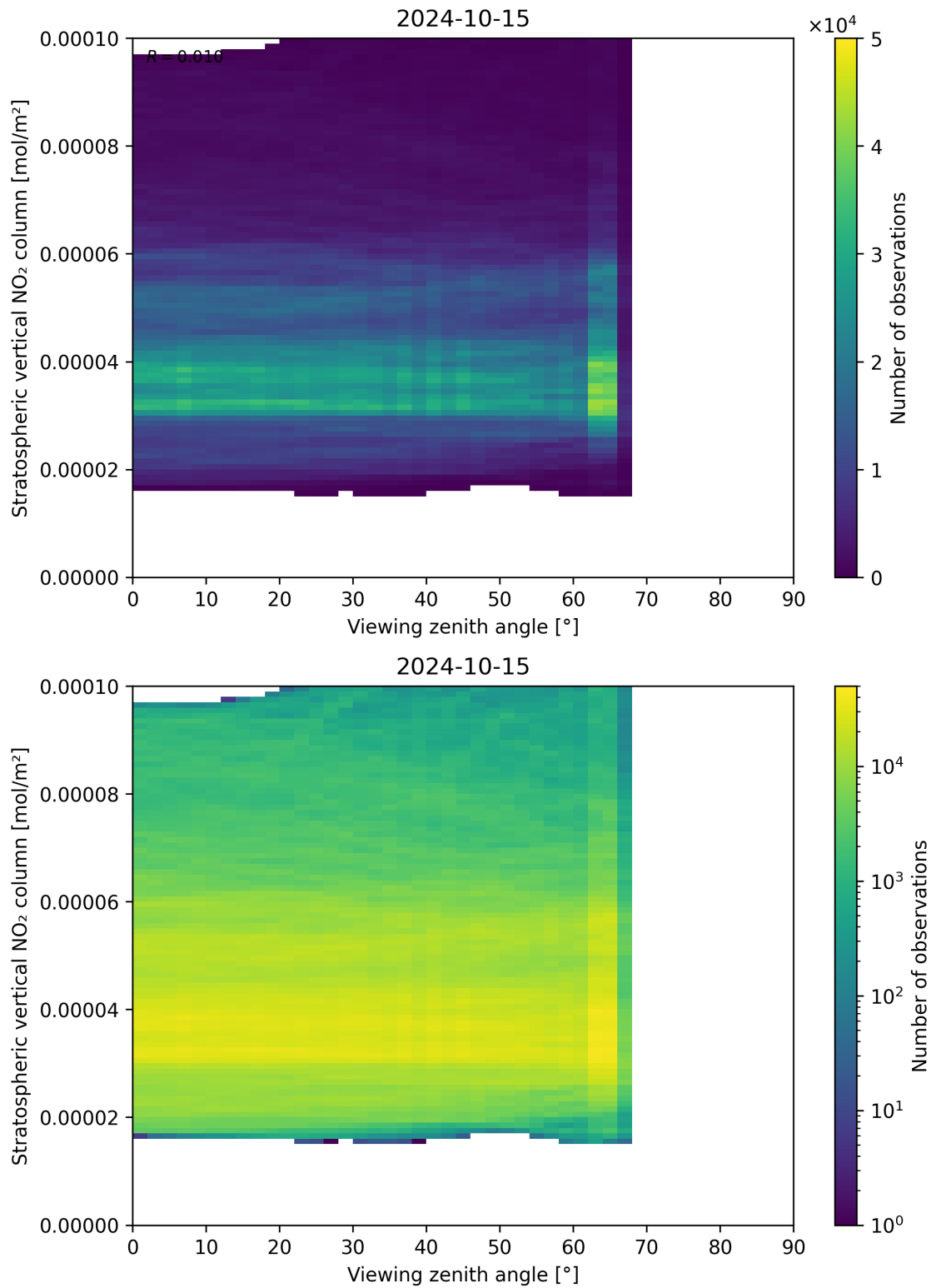
Figure 164: Scatter density plot of “Viewing zenith angle” against “Stratospheric vertical NO 2 column” for 2024-10-14 to 2024-10-16.
