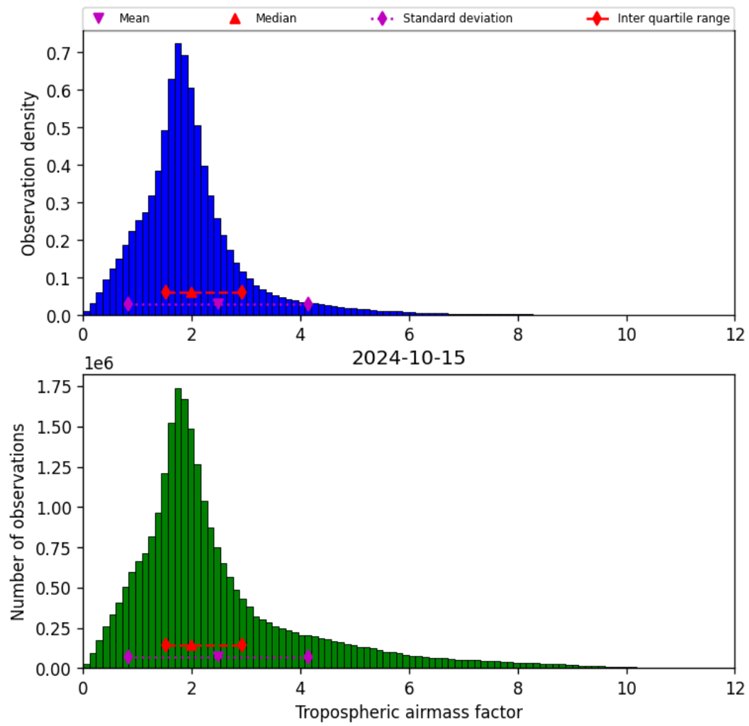
Figure 31: Histogram of “Tropospheric airmass factor” for 2024-10-14 to 2024-10-16
