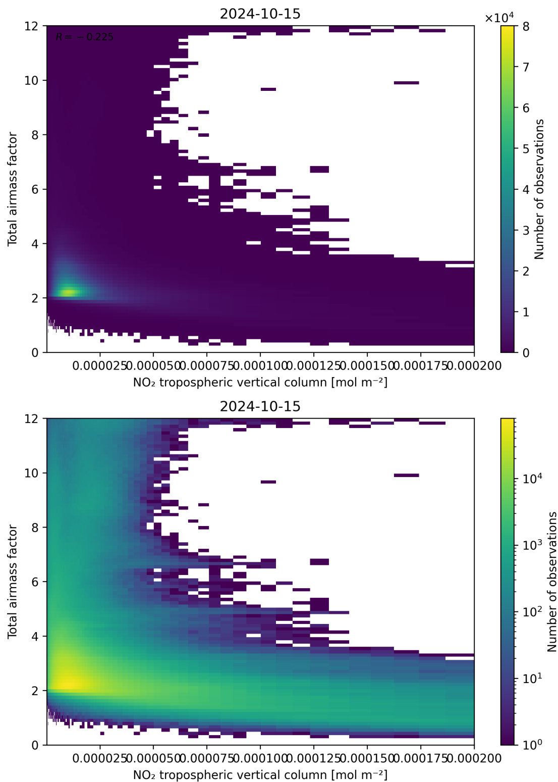
Figure 122: Scatter density plot of “NO 2 tropospheric vertical column” against “Total air mass factor” for 2024-10-14 to 2024-10-16.
