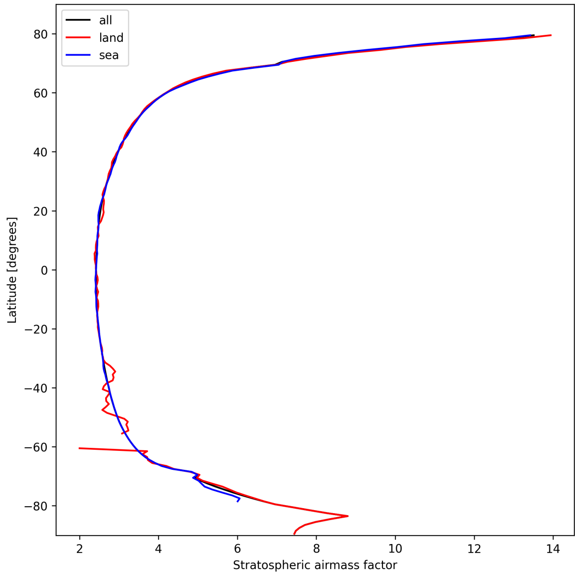
Figure 27: Zonal average of “Stratospheric airmass factor” for 2024-10-14 to 2024-10-16.
