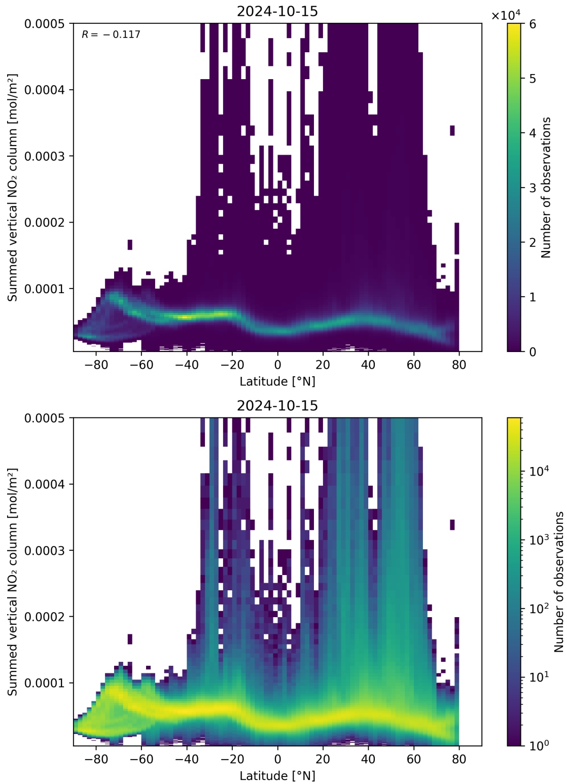
Figure 88: Scatter density plot of “Latitude” against “Summed vertical NO 2 column” for 2024-10-14 to 2024-10-16.
