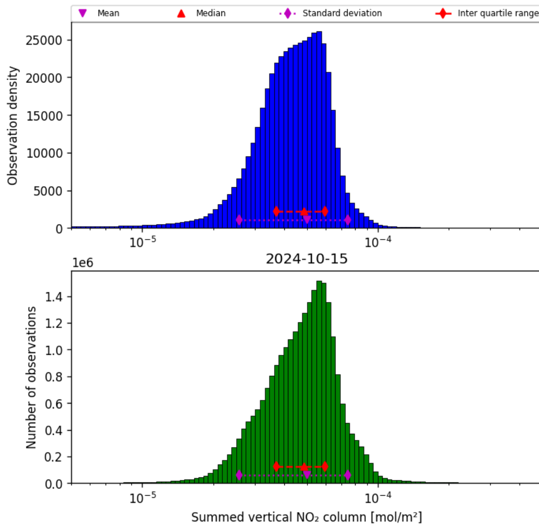
Figure 40: Histogram of “Summed vertical NO 2 column” for 2024-10-14 to 2024-10-16
