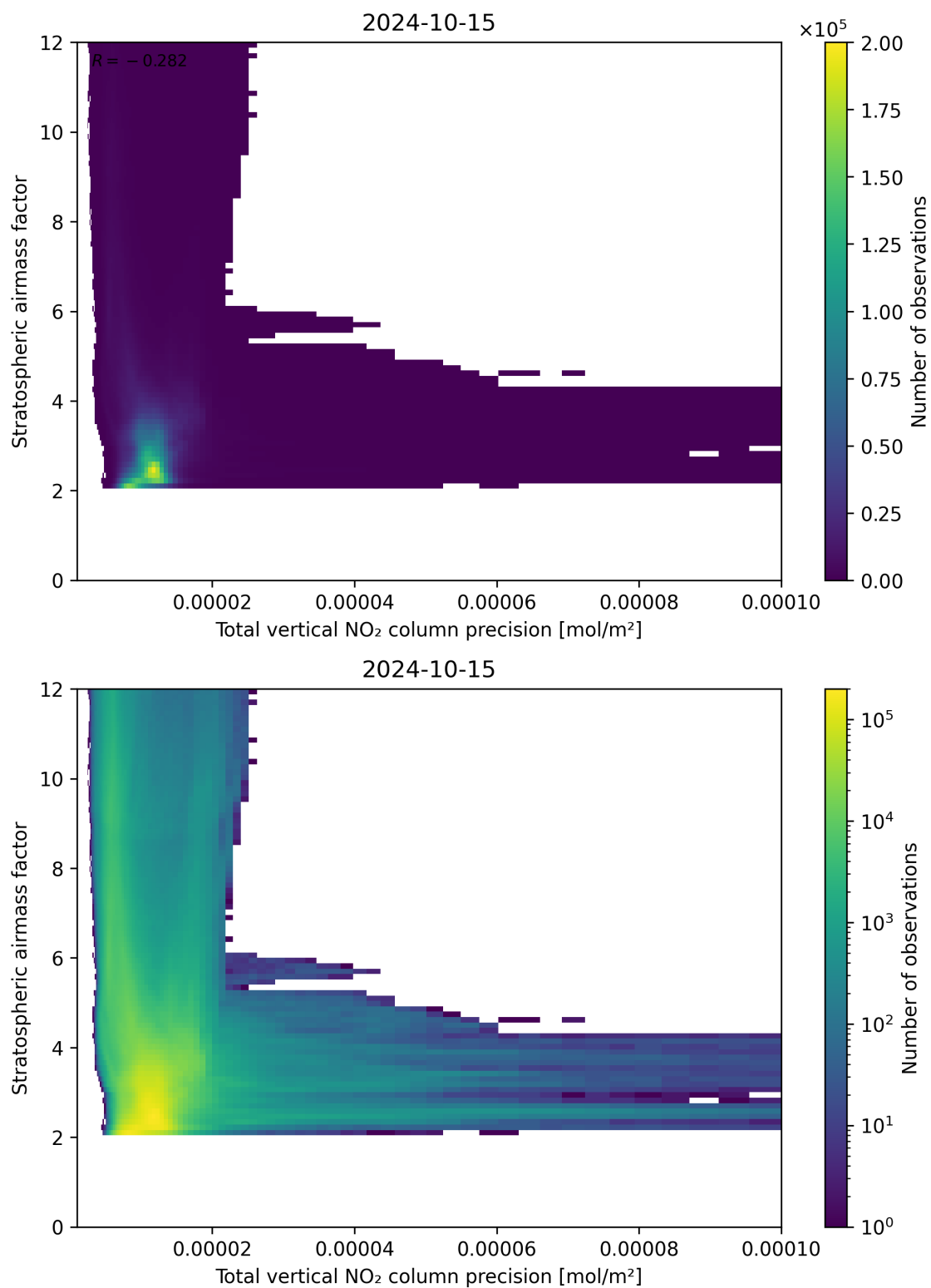
Figure 115: Scatter density plot of “Total vertical NO 2 column precision” against “Stratospheric air mass factor” for 2024-10-14 to 2024-10-16.
