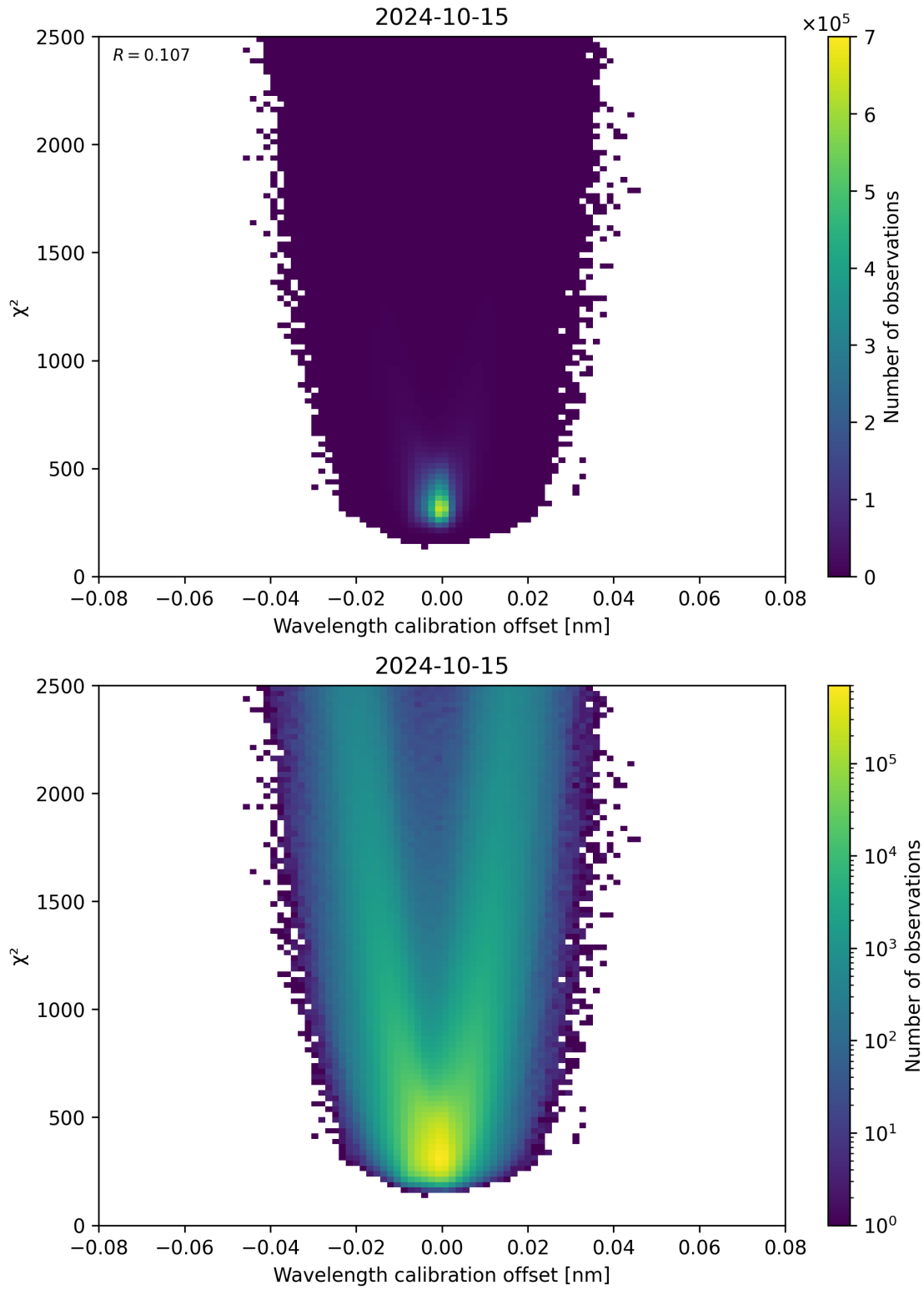
Figure 175: Scatter density plot of “Wavelength calibration offset” against “ \chi^2 ” for 2024-10-14 to 2024-10-16.
