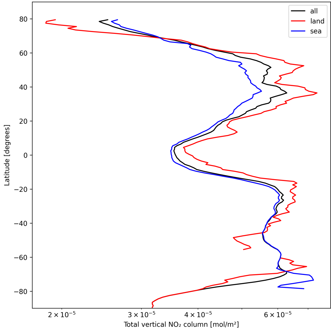
Figure 21: Zonal average of “Total vertical NO 2 column” for 2024-10-14 to 2024-10-16.
