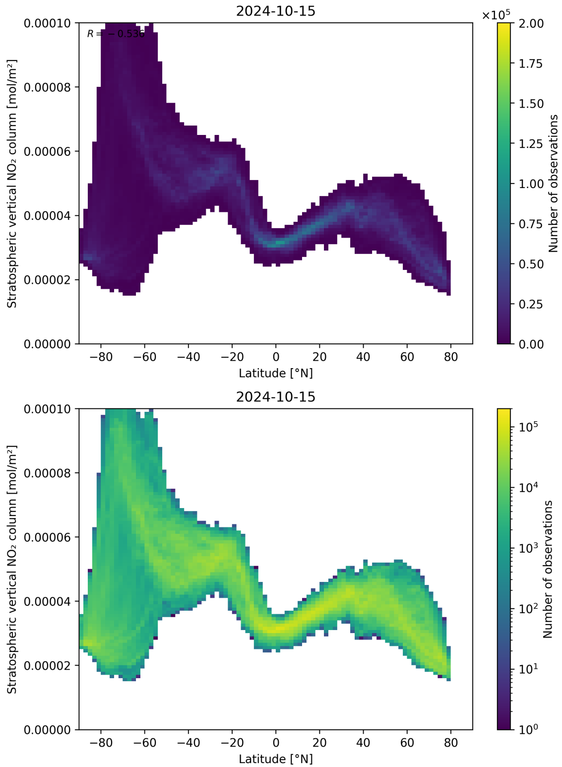
Figure 87: Scatter density plot of “Latitude” against “Stratospheric vertical NO 2 column” for 2024-10-14 to 2024-10-16.
