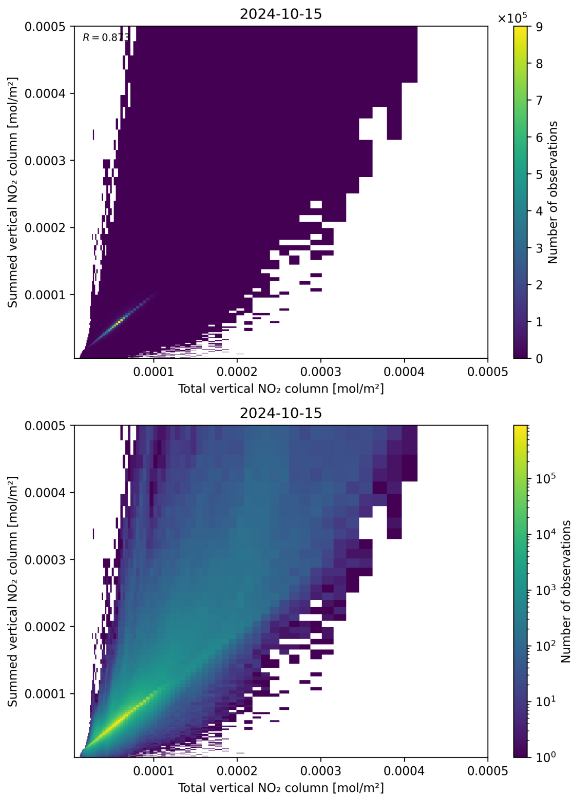
Figure 112: Scatter density plot of “Total vertical NO 2 column” against “Summed vertical NO 2 column” for 2024-10-14 to 2024-10-16.
