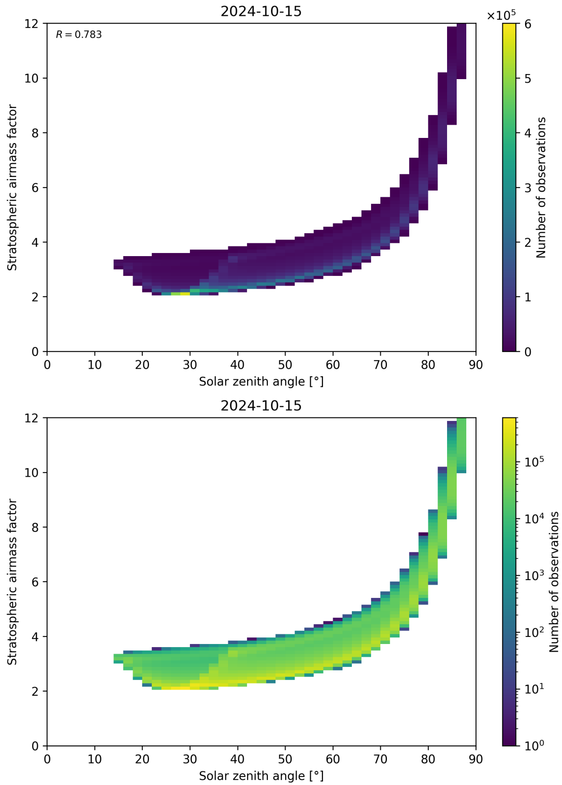
Figure 145: Scatter density plot of “Solar zenith angle” against “Stratospheric airmass factor” for 2024-10-14 to 2024-10-16.
