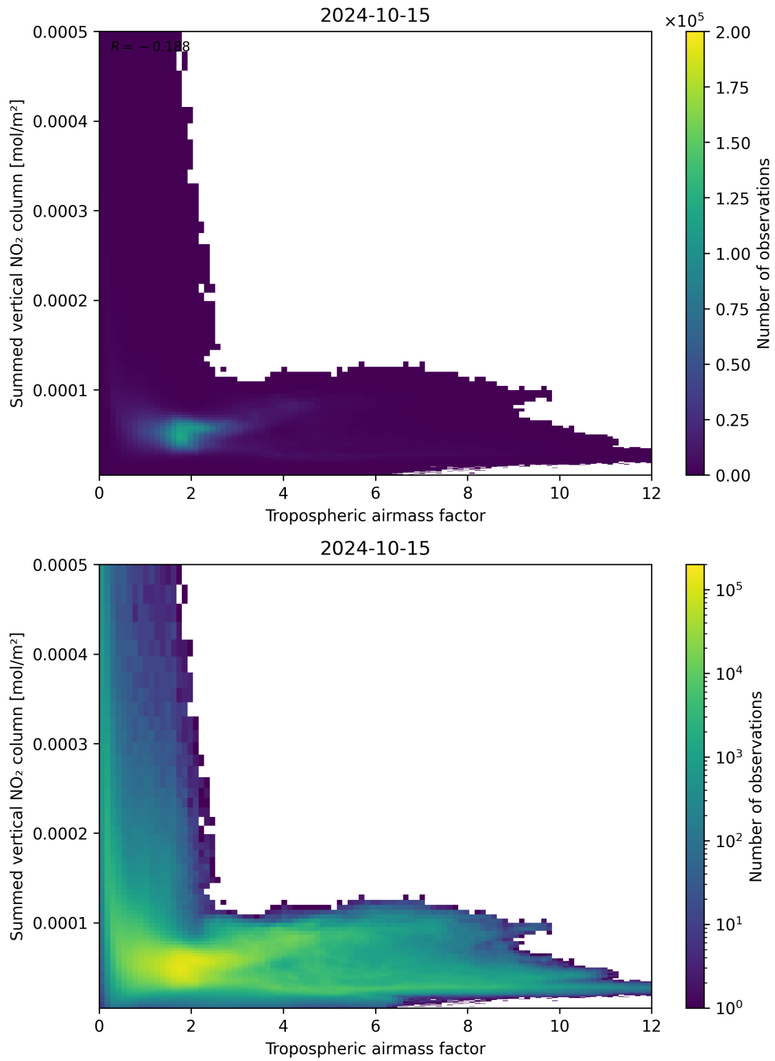
Figure 75: Scatter density plot of “Tropospheric airmass factor” against “Summed vertical NO 2 column” for 2024-10-14 to 2024-10-16.
