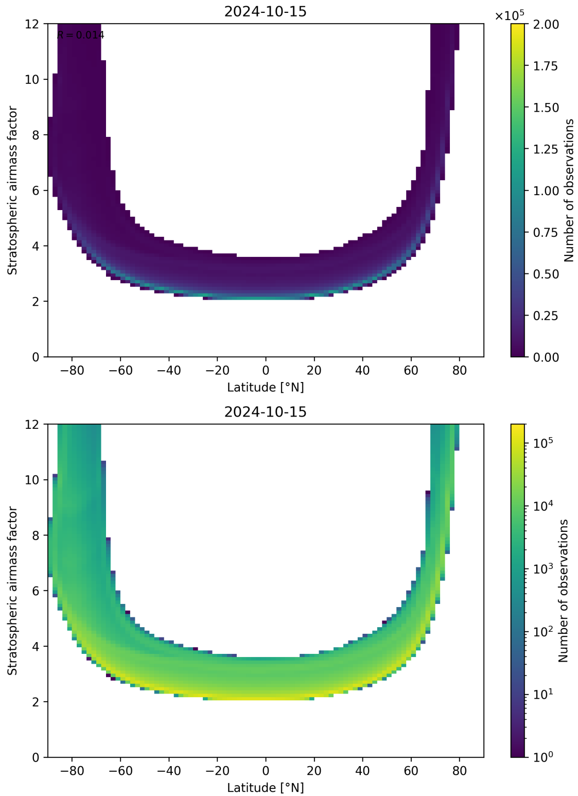
Figure 83: Scatter density plot of “Latitude” against “Stratospheric airmass factor” for 2024-10-14 to 2024-10-16.
