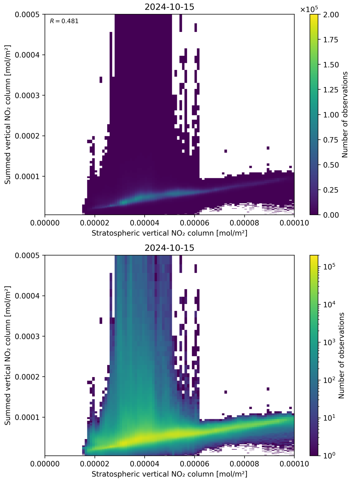
Figure 98: Scatter density plot of “Stratospheric vertical NO 2 column” against “Summed vertical NO 2 column” for 2024-10-14 to 2024-10-16.
