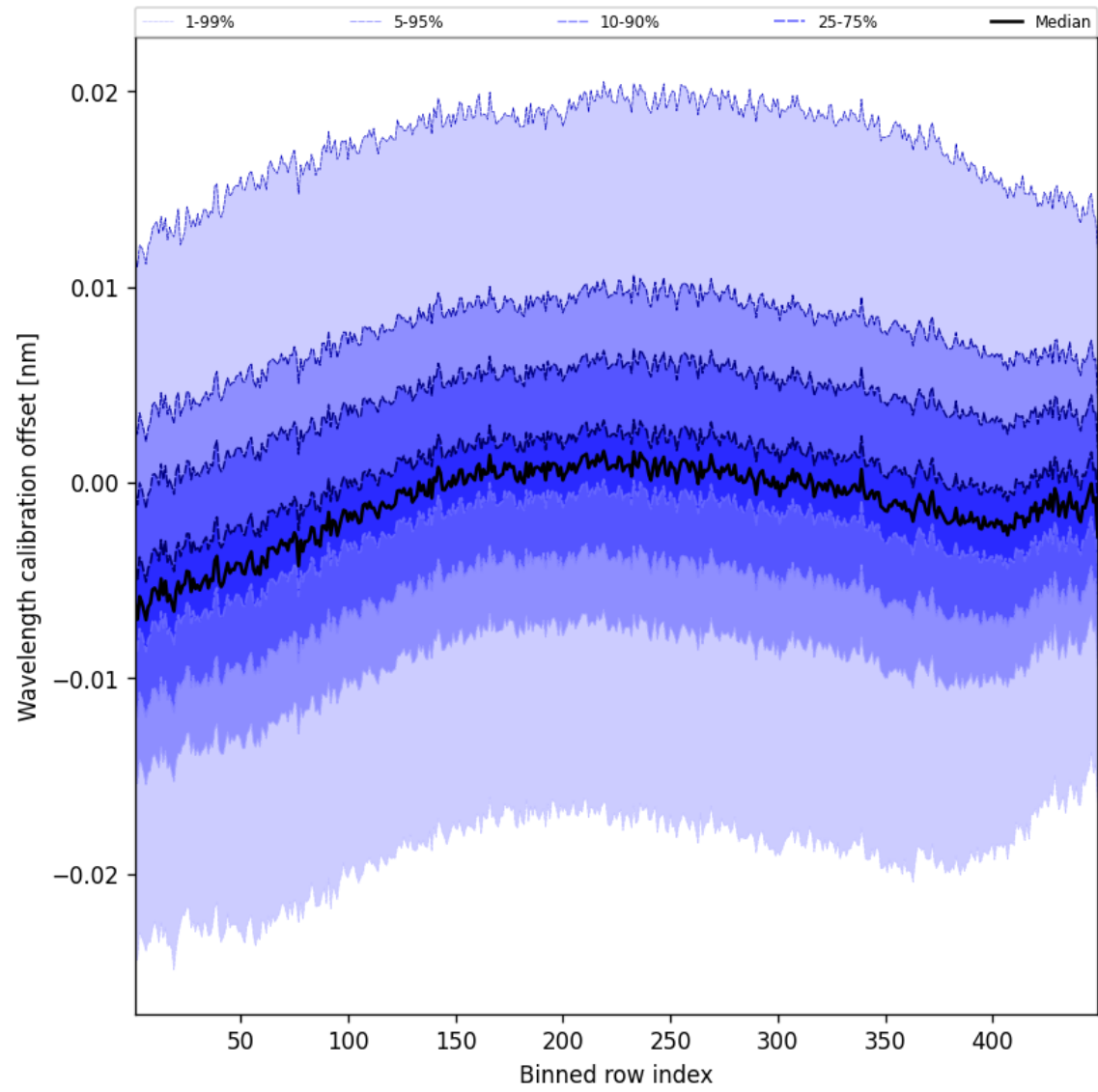
Figure 52: Along track statistics of “Wavelength calibration offset” for 2024-10-14 to 2024-10-16
