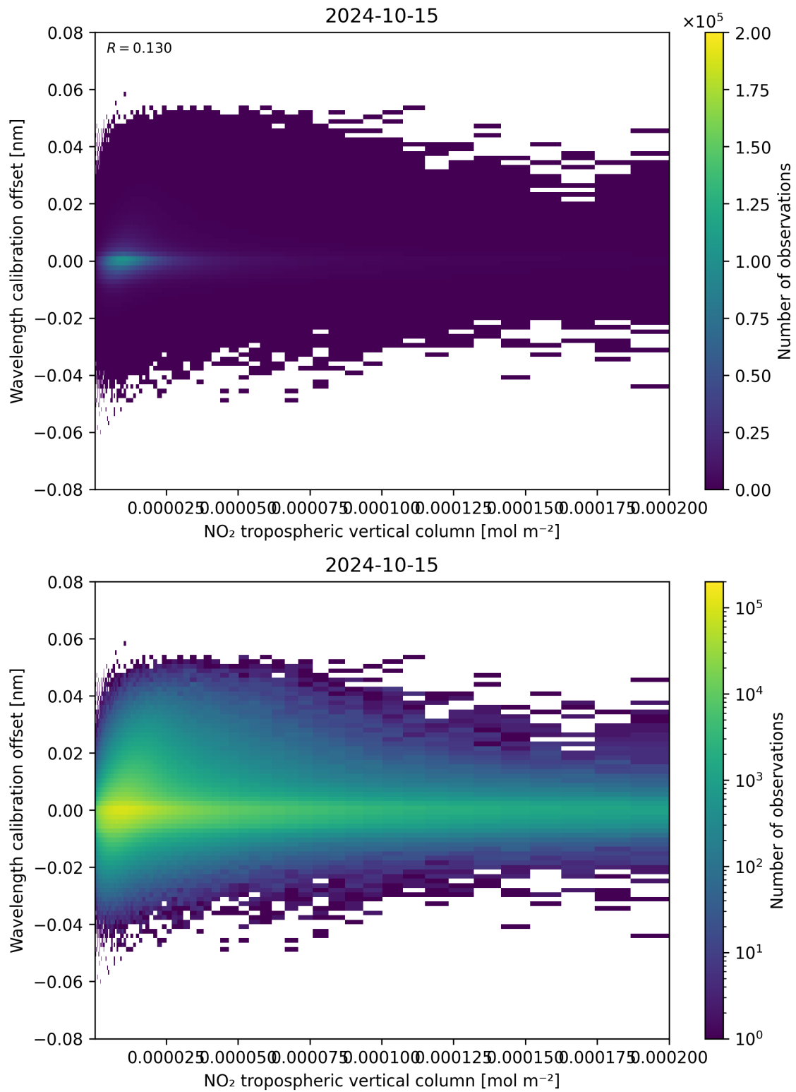
Figure 143: Scatter density plot of “NO 2 tropospheric vertical column” against “Wavelength calibration offset” for 2024-10-14 to 2024-10-16.
