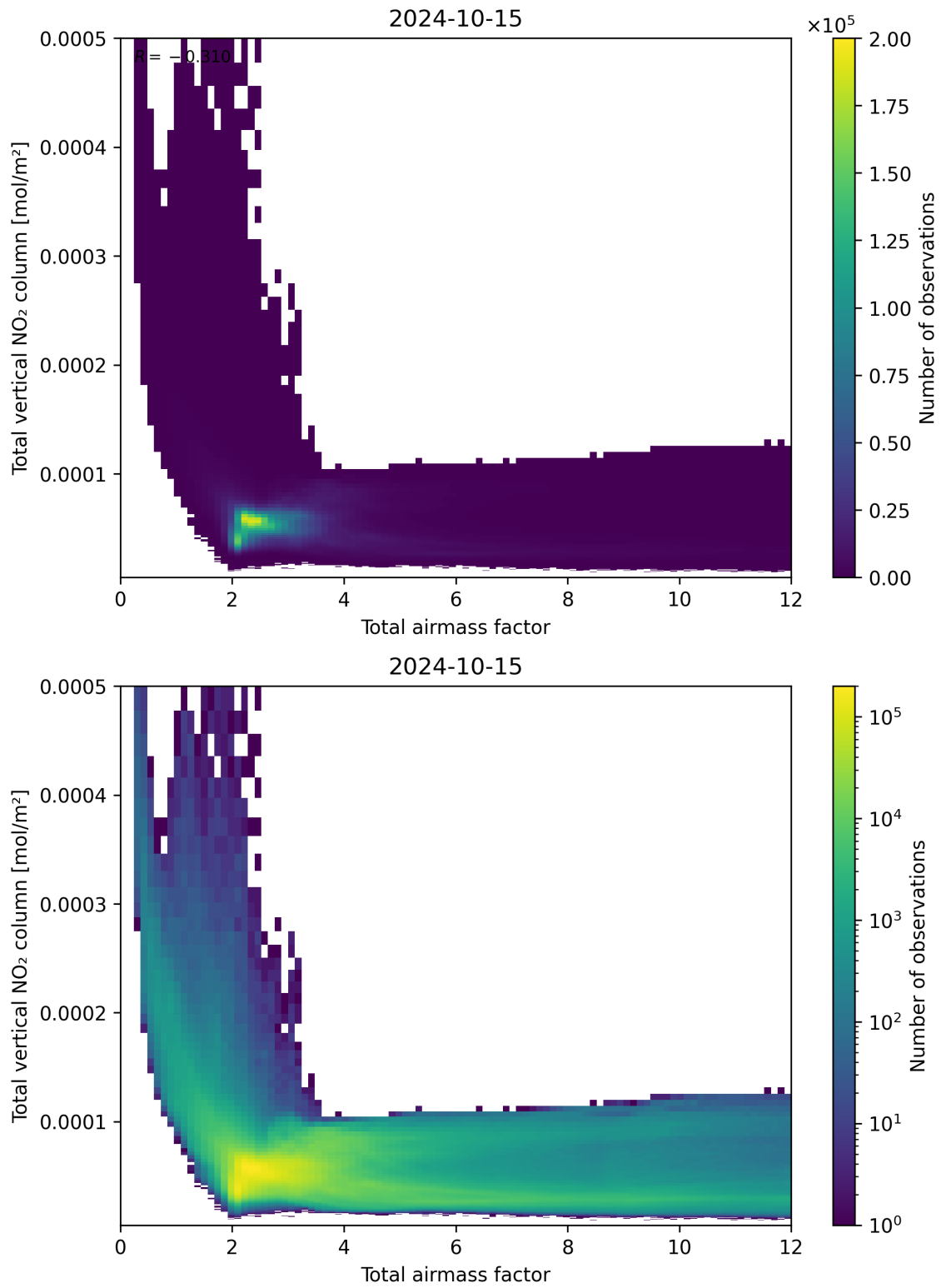
Figure 67: Scatter density plot of “Total airmass factor” against “Total vertical NO 2 column” for 2024-10-14 to 2024-10-16.
