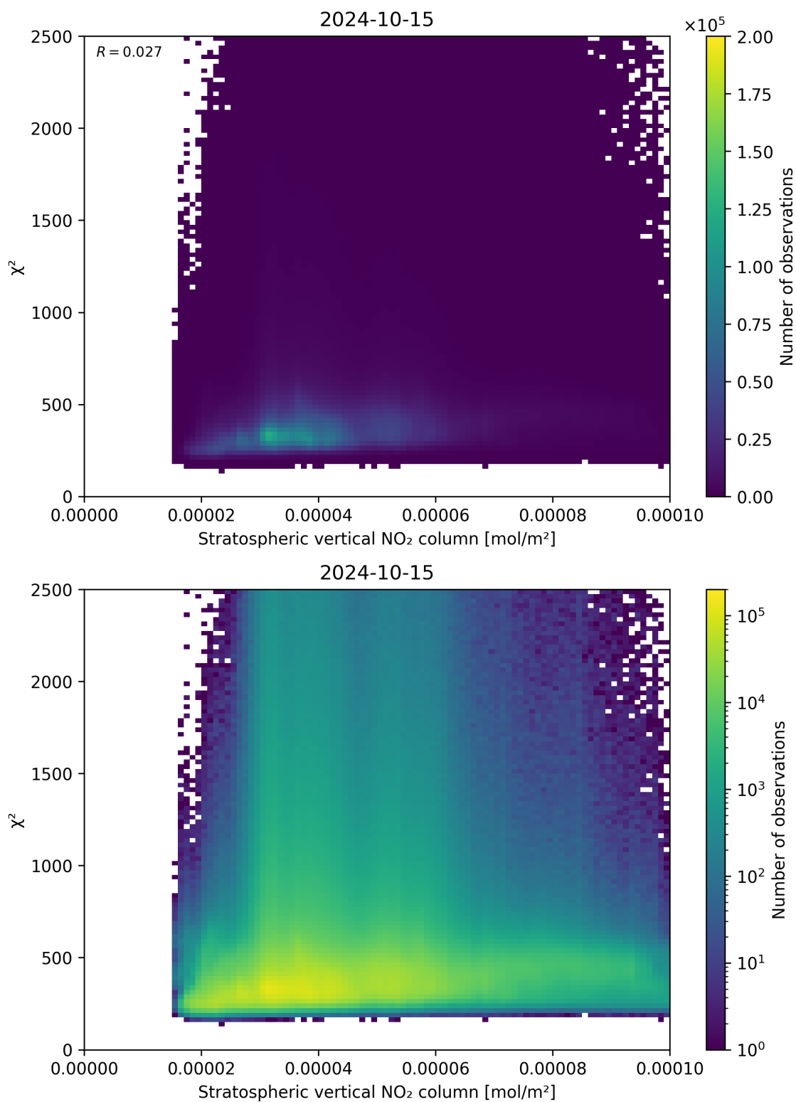
Figure 97: Scatter density plot of “Stratospheric vertical NO 2 column” against “ \chi^2 ” for 2024-10-14 to 2024-10-16.
