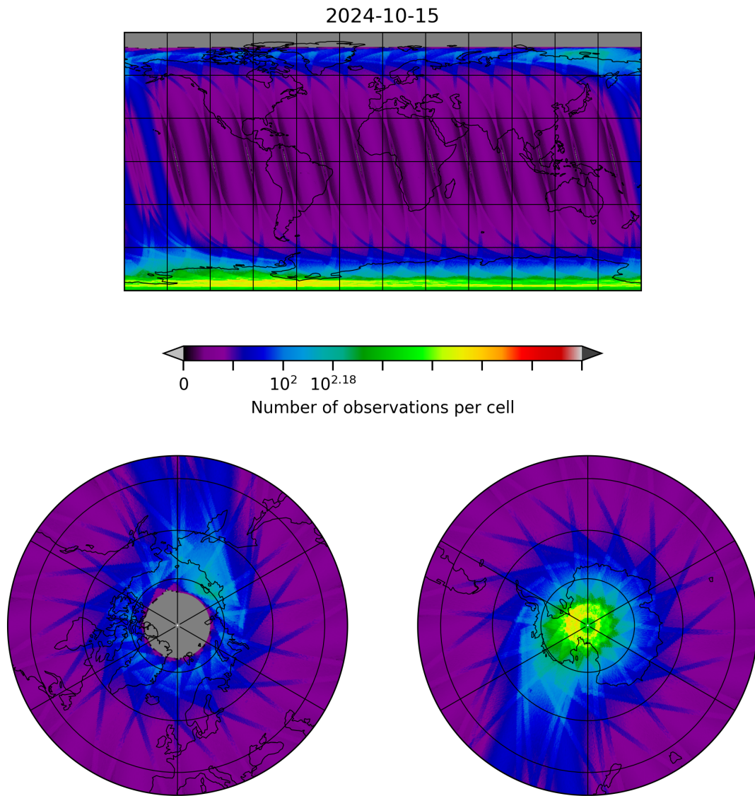
Figure 10: Map of the number of observations for 2024-10-14 to 2024-10-16
