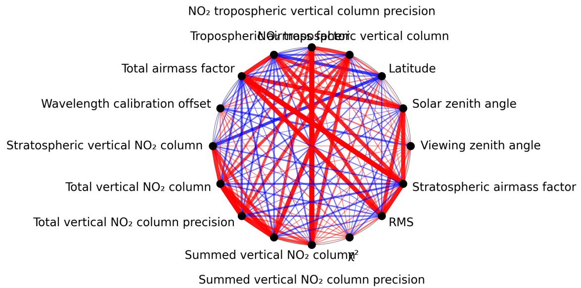
Figure 1: Map of correlation graph for 2024-10-14 to 2024-10-16.
