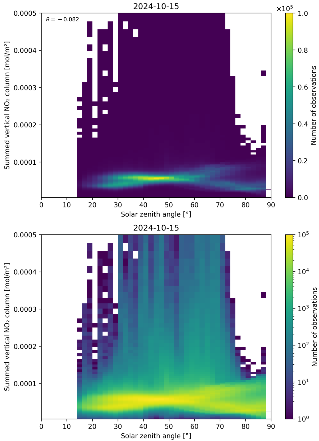
Figure 151: Scatter density plot of “Solar zenith angle” against “Summed vertical NO 2 column” for 2024-10-14 to 2024-10-16.
