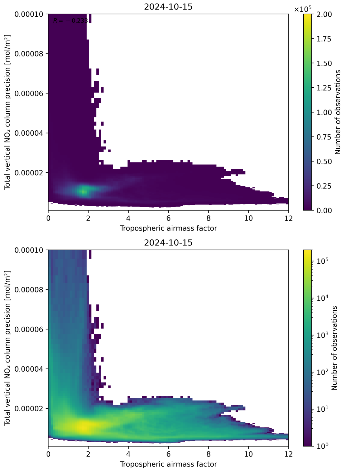
Figure 78: Scatter density plot of “Tropospheric air mass factor” against “Total vertical NO 2 column precision” for 2024-10-14 to 2024-10-16.
