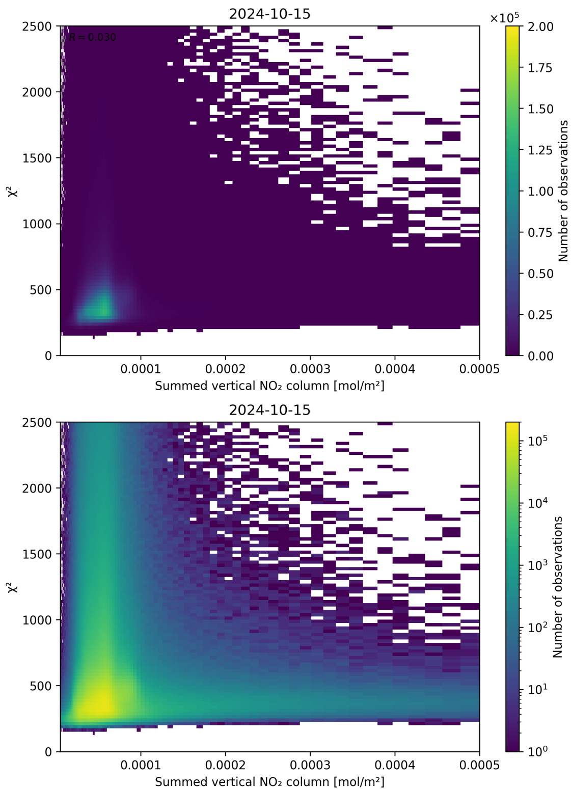
Figure 104: Scatter density plot of “Summed vertical NO 2 column” against “ \chi^2 ” for 2024-10-14 to 2024-10-16.
