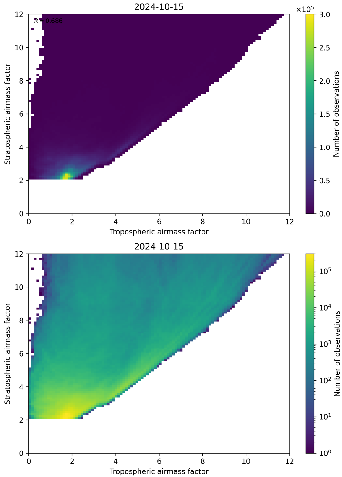
Figure 71: Scatter density plot of “Tropospheric airmass factor” against “Stratospheric airmass factor” for 2024-10-14 to 2024-10-16.
