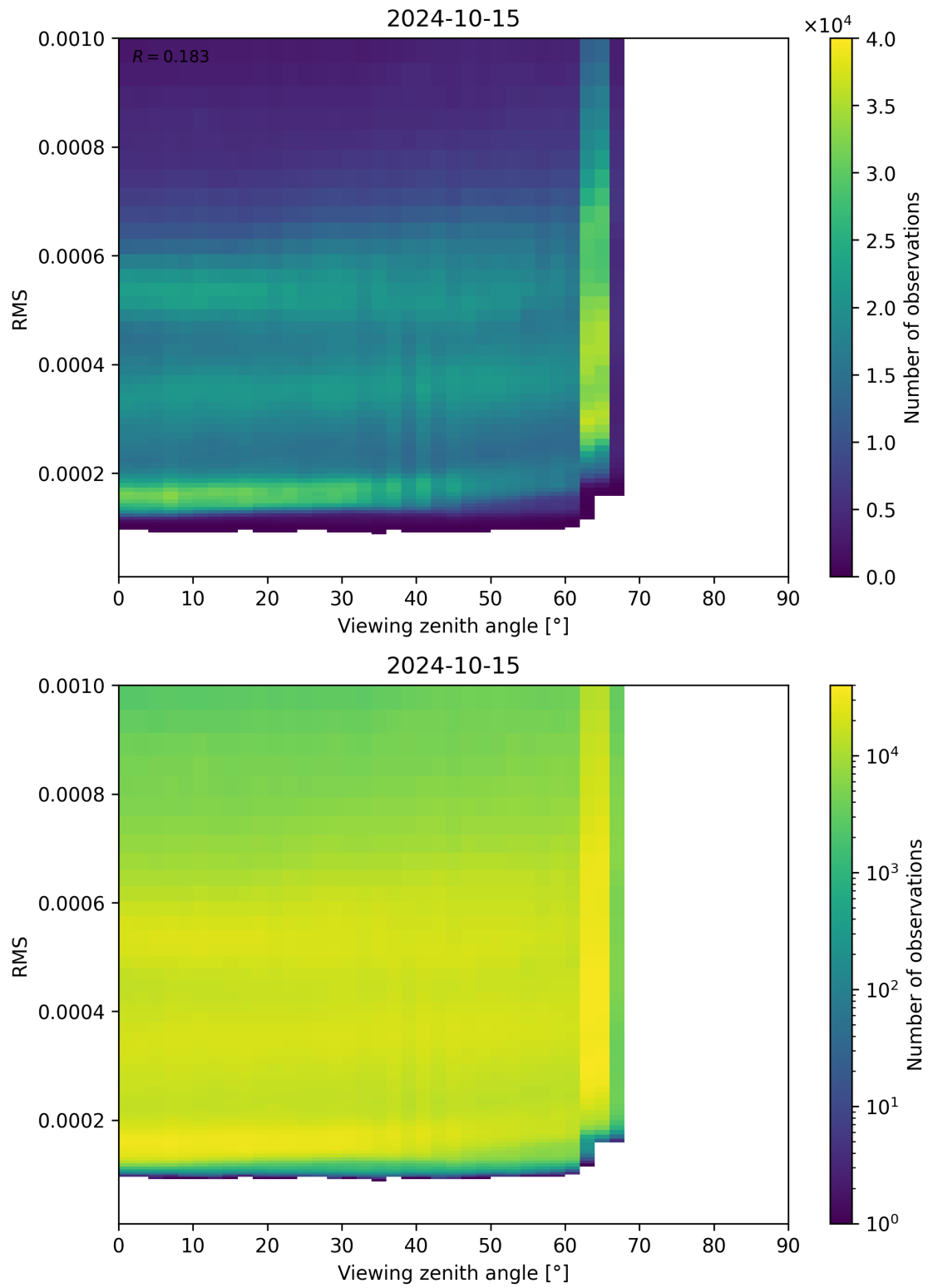
Figure 171: Scatter density plot of “Viewing zenith angle” against “RMS” for 2024-10-14 to 2024-10-16.
