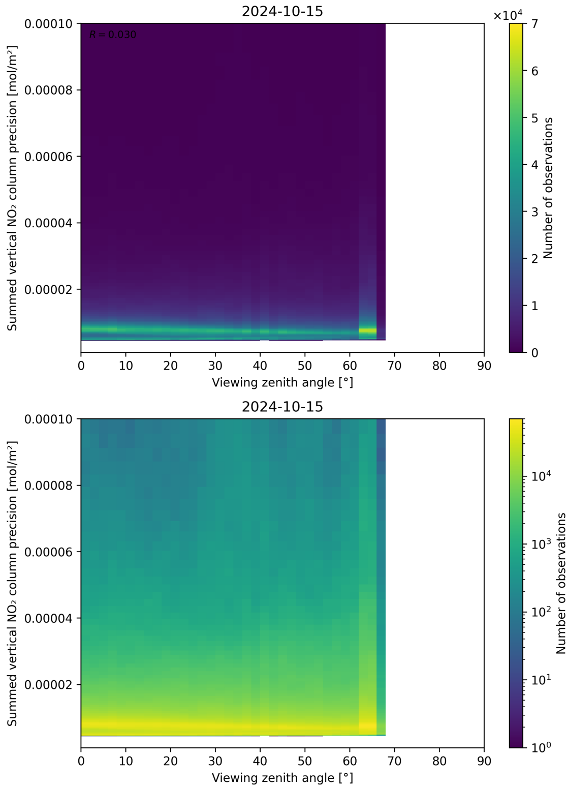
Figure 166: Scatter density plot of “Viewing zenith angle” against “Summed vertical NO 2 column precision” for 2024-10-14 to 2024-10-16.
