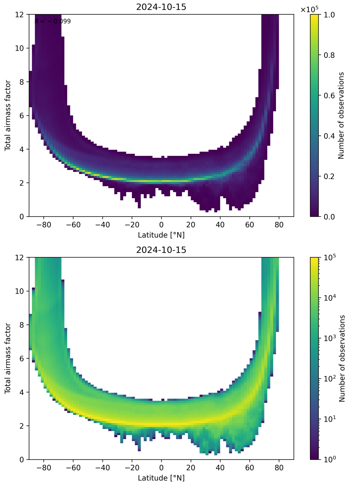
Figure 84: Scatter density plot of “Latitude” against “Total airmass factor” for 2024-10-14 to 2024-10-16.
