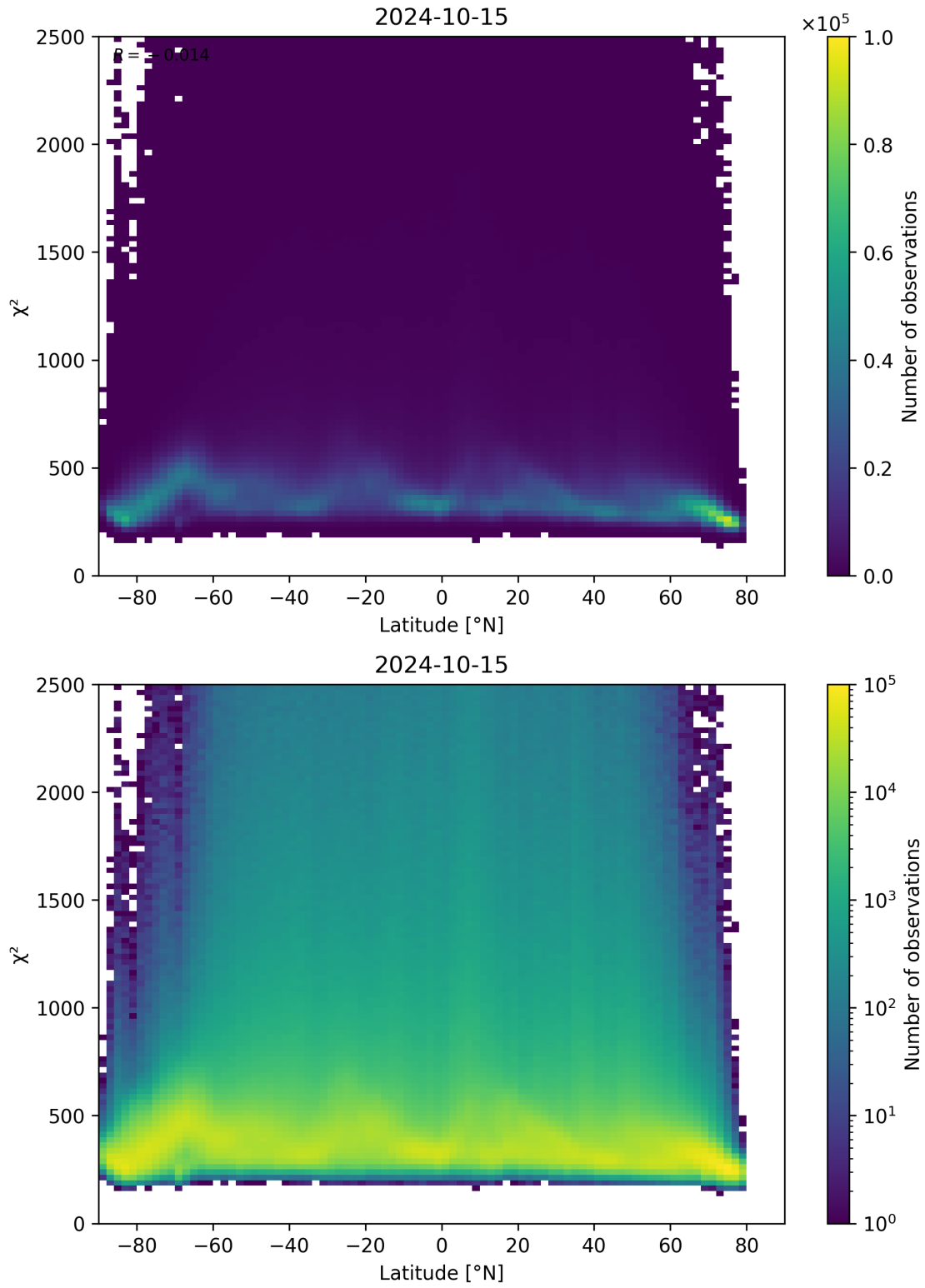
Figure 86: Scatter density plot of “Latitude” against “ \chi^2 ” for 2024-10-14 to 2024-10-16.
