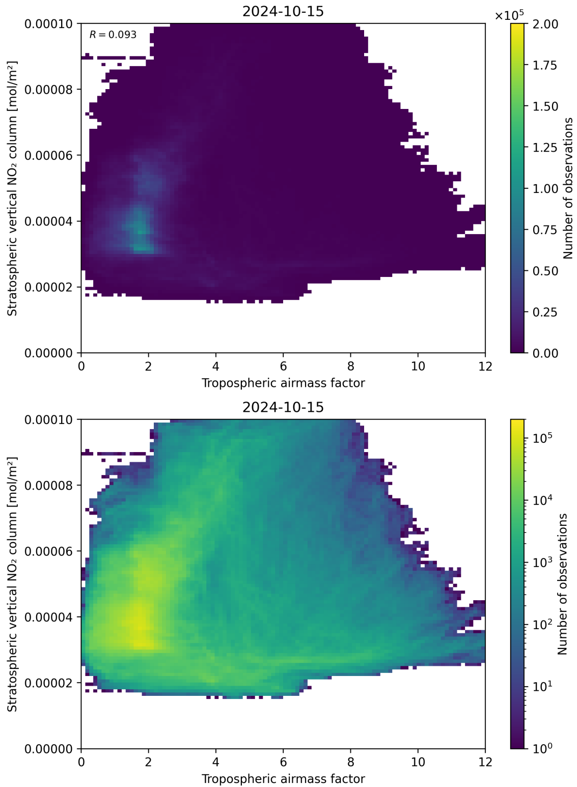
Figure 74: Scatter density plot of “Tropospheric airmass factor” against “Stratospheric vertical NO 2 column” for 2024-10-14 to 2024-10-16.
