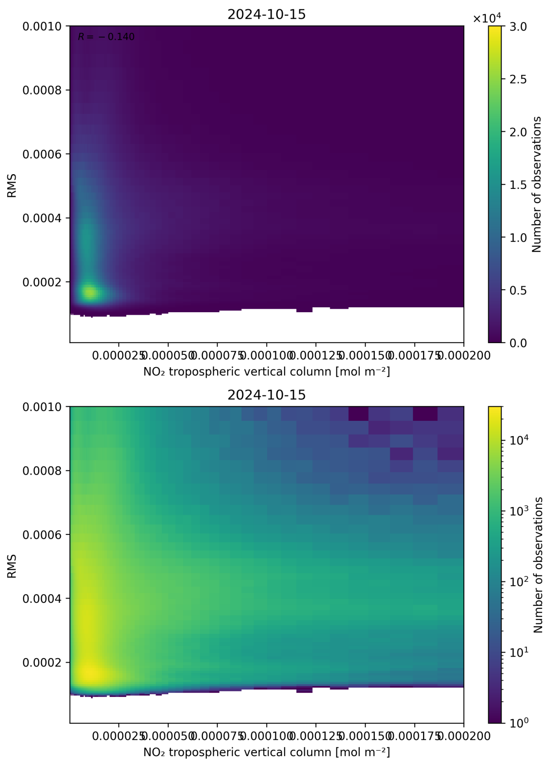
Figure 142: Scatter density plot of “NO 2 tropospheric vertical column” against “RMS” for 2024-10-14 to 2024-10-16.
