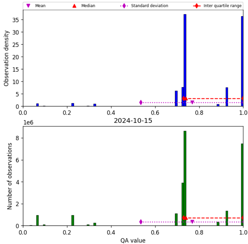
Figure 28: Histogram of “QA value” for 2024-10-14 to 2024-10-16
