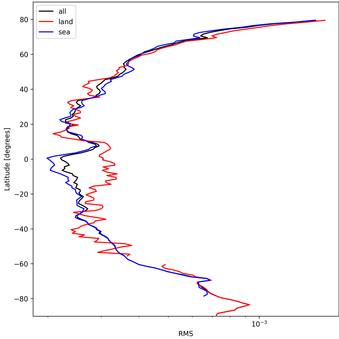
Figure 26: Zonal average of “RMS” for 2024-10-14 to 2024-10-16.
