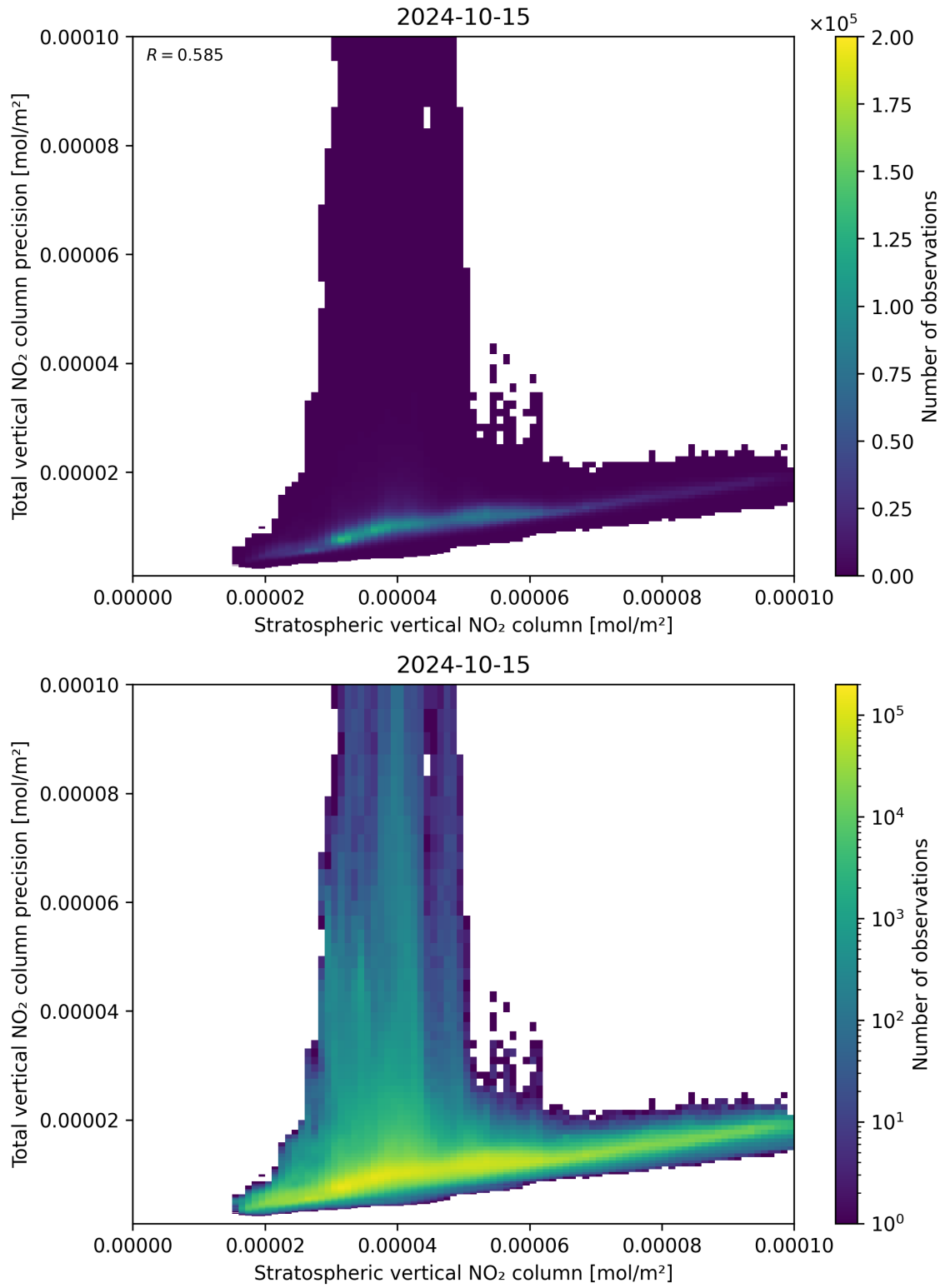
Figure 101: Scatter density plot of “Stratospheric vertical NO 2 column” against “Total vertical NO 2 column precision” for 2024-10-14 to 2024-10-16.
