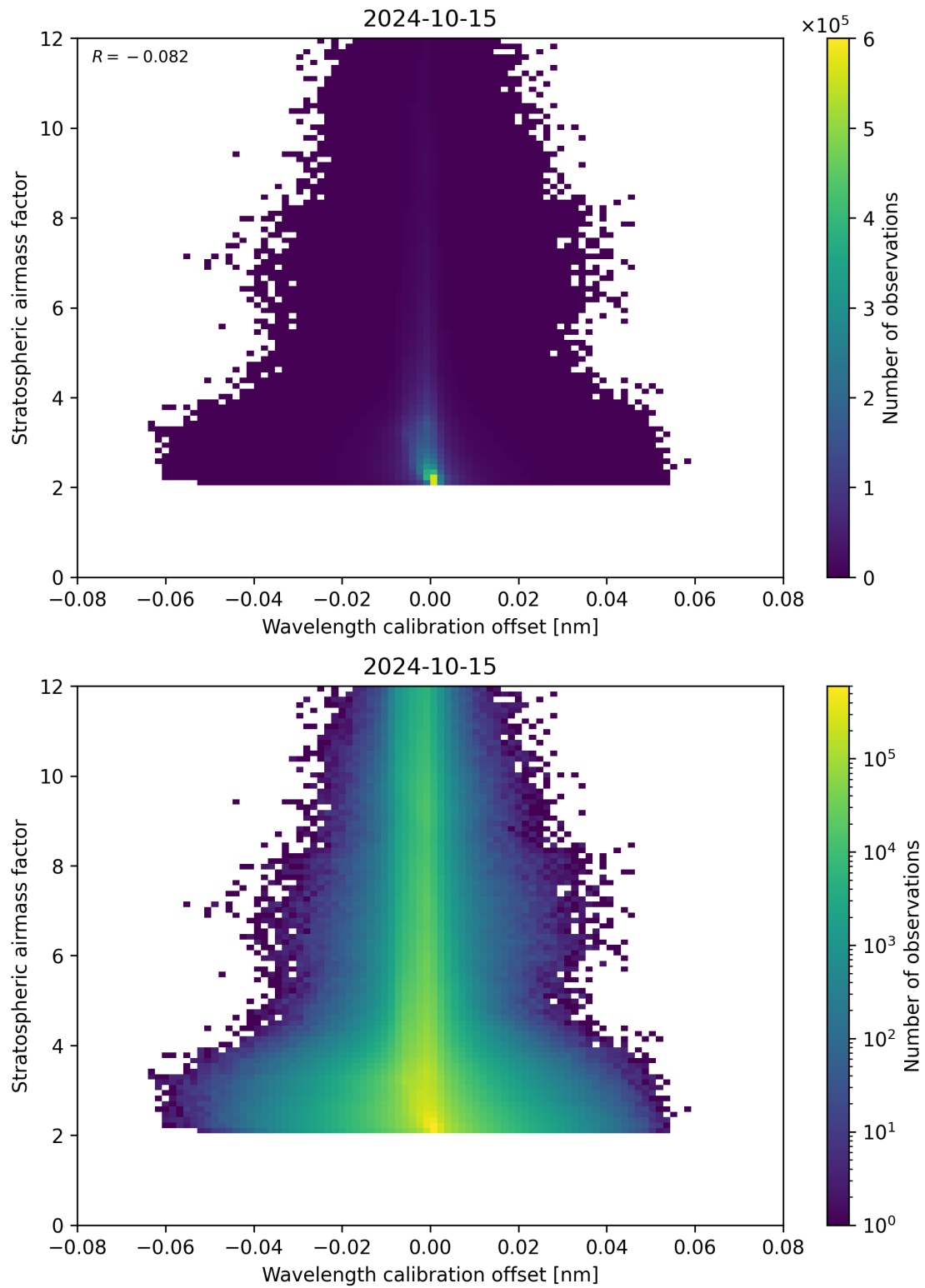
Figure 174: Scatter density plot of “Wavelength calibration offset” against “Stratospheric airmass factor” for 2024-10-14 to 2024-10-16.
