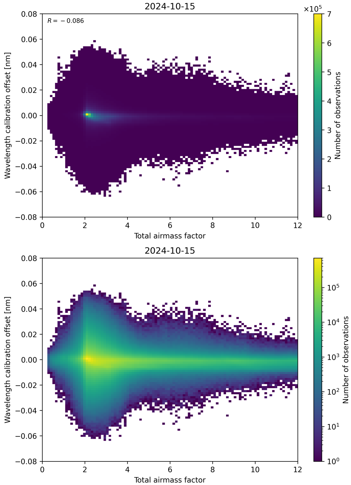
Figure 70: Scatter density plot of “Total airmass factor” against “Wavelength calibration offset” for 2024-10-14 to 2024-10-16.
