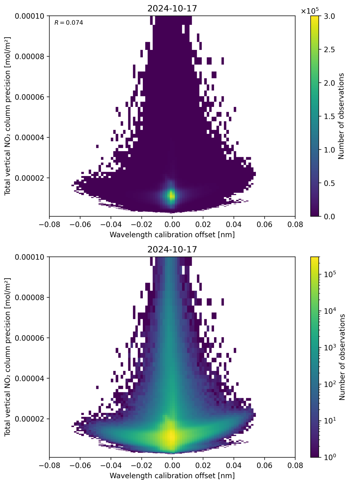
Figure 180: Scatter density plot of “Wavelength calibration offset” against “Total vertical NO 2 column precision” for 2024-10-16 to 2024-10-18.
