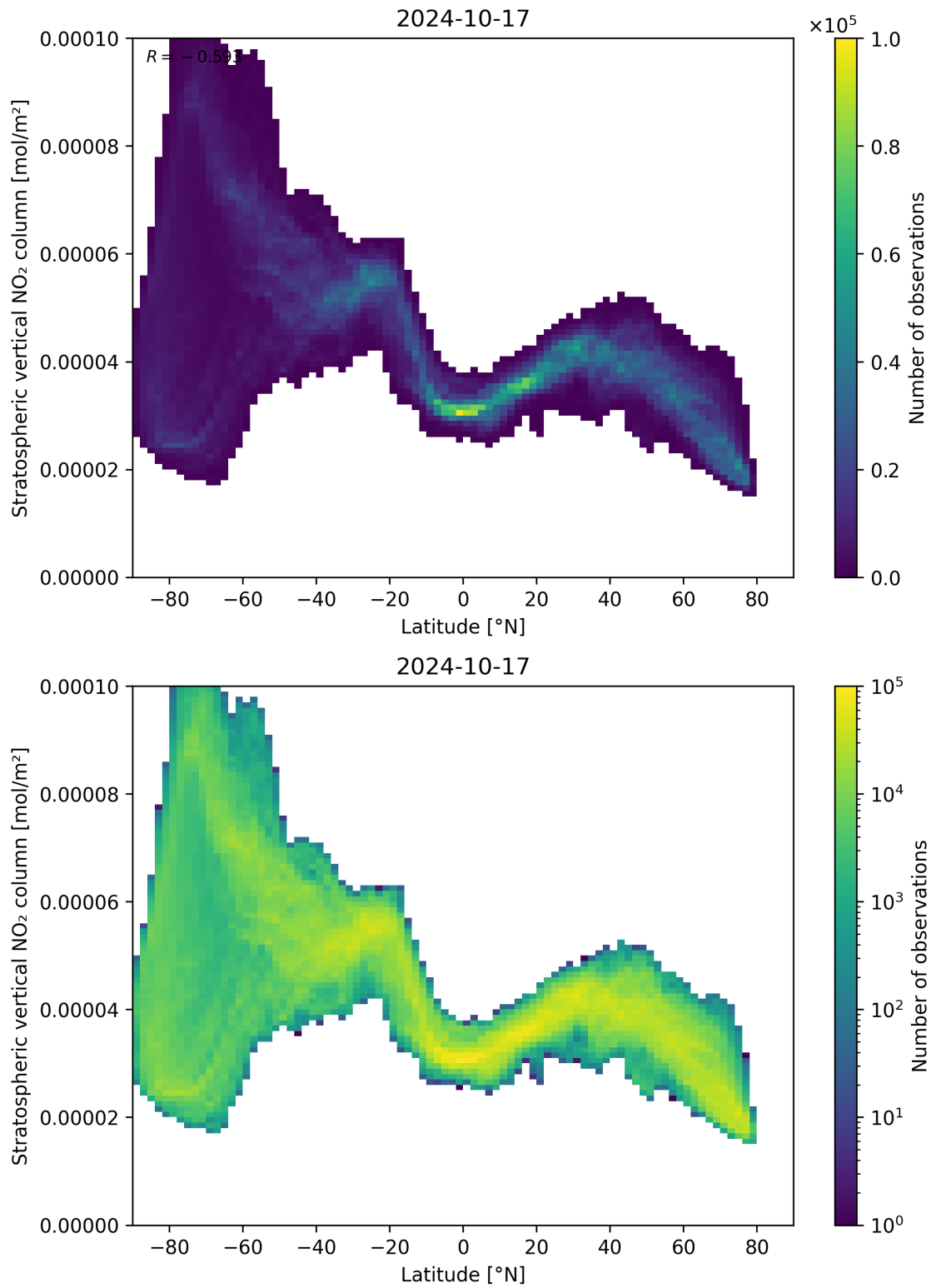
Figure 87: Scatter density plot of “Latitude” against “Stratospheric vertical NO 2 column” for 2024-10-16 to 2024-10-18.
