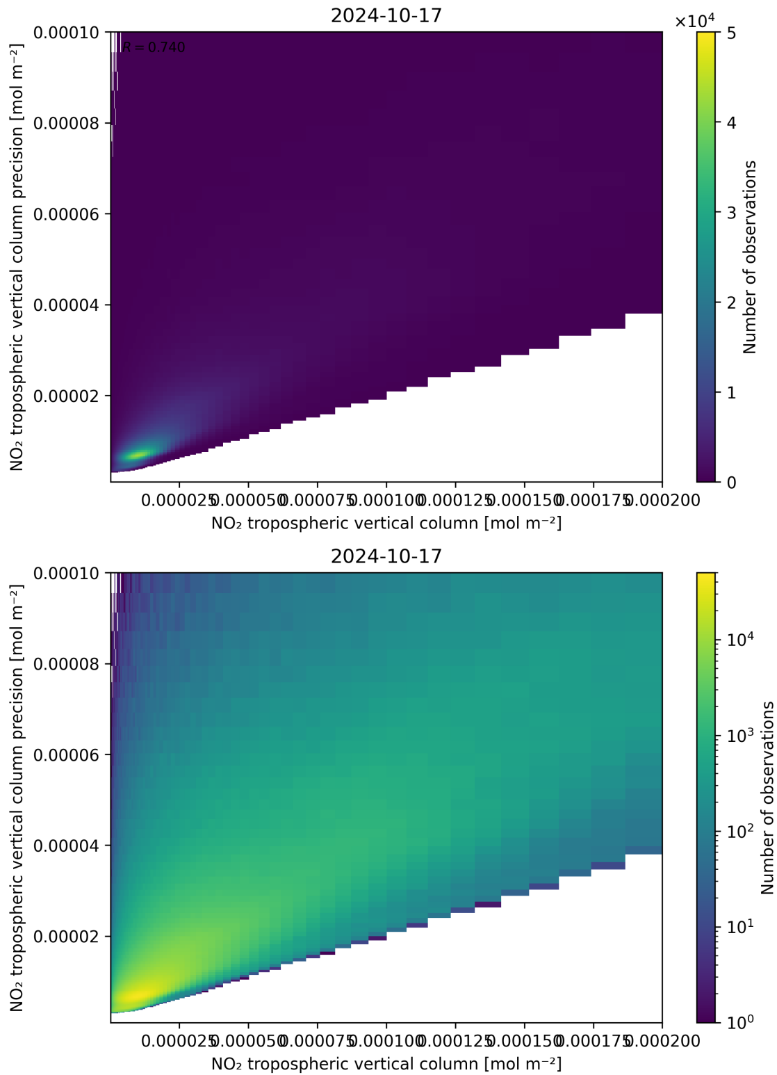
Figure 130: Scatter density plot of “NO 2 tropospheric vertical column” against “NO 2 tropospheric vertical column precision” for 2024-10-16 to 2024-10-18.
