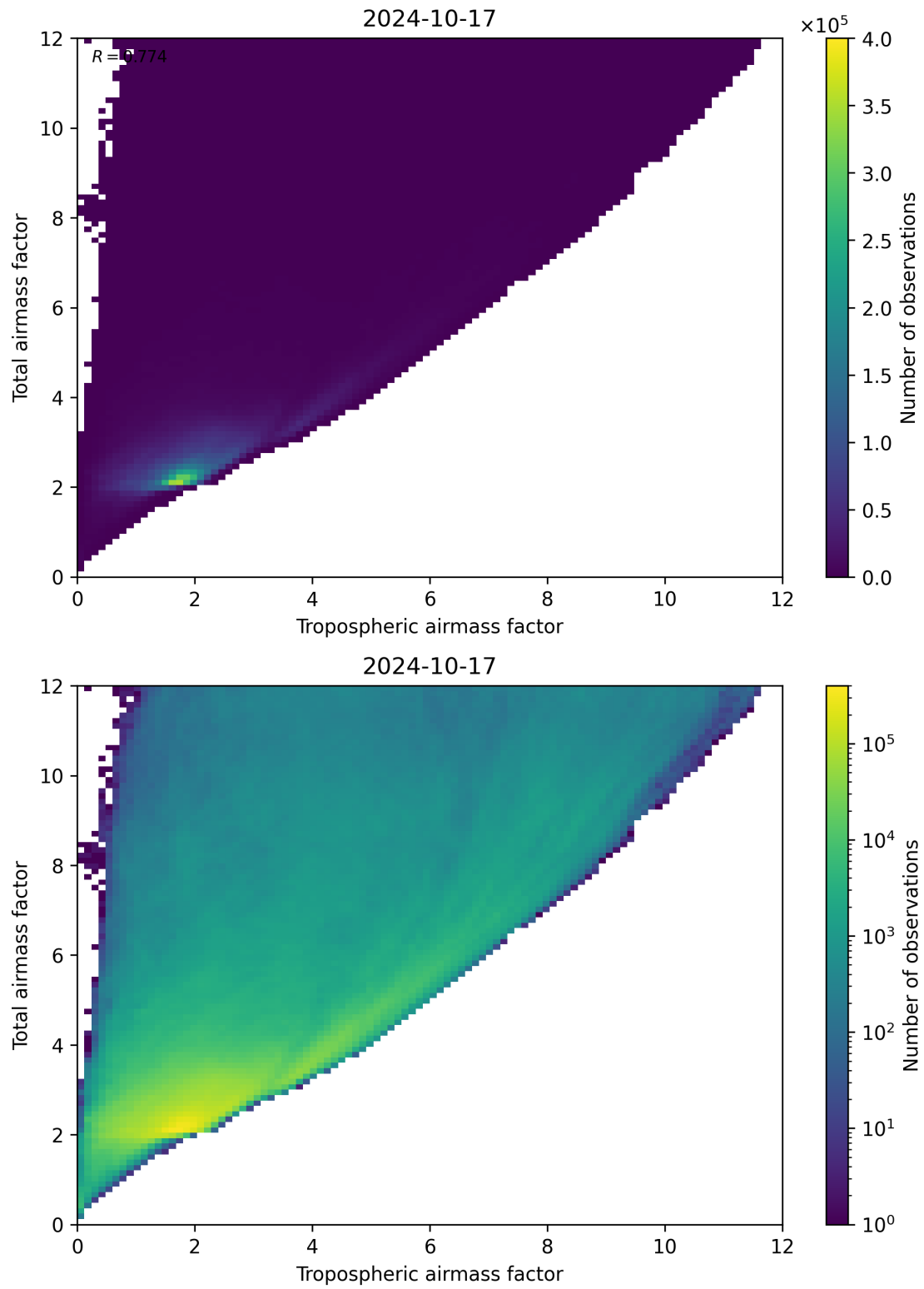
Figure 72: Scatter density plot of “Tropospheric airmass factor” against “Total airmass factor” for 2024-10-16 to 2024-10-18.
