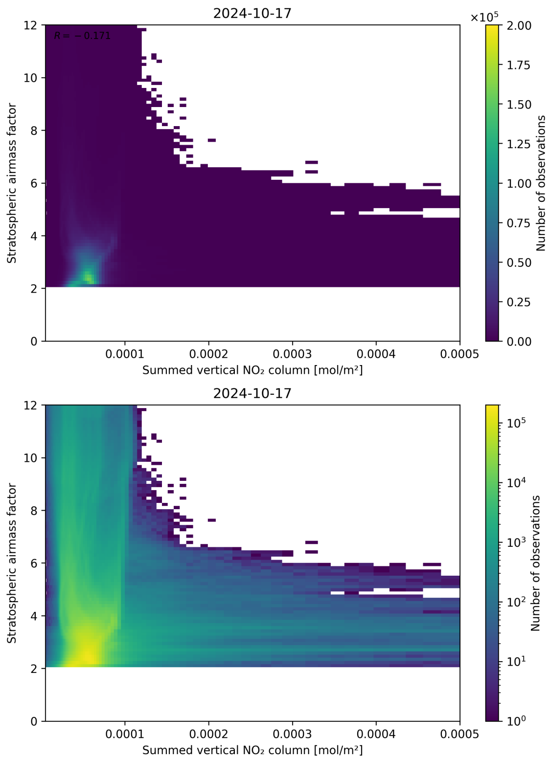
Figure 103: Scatter density plot of “Summed vertical NO 2 column” against “Stratospheric airmass factor” for 2024-10-16 to 2024-10-18.
