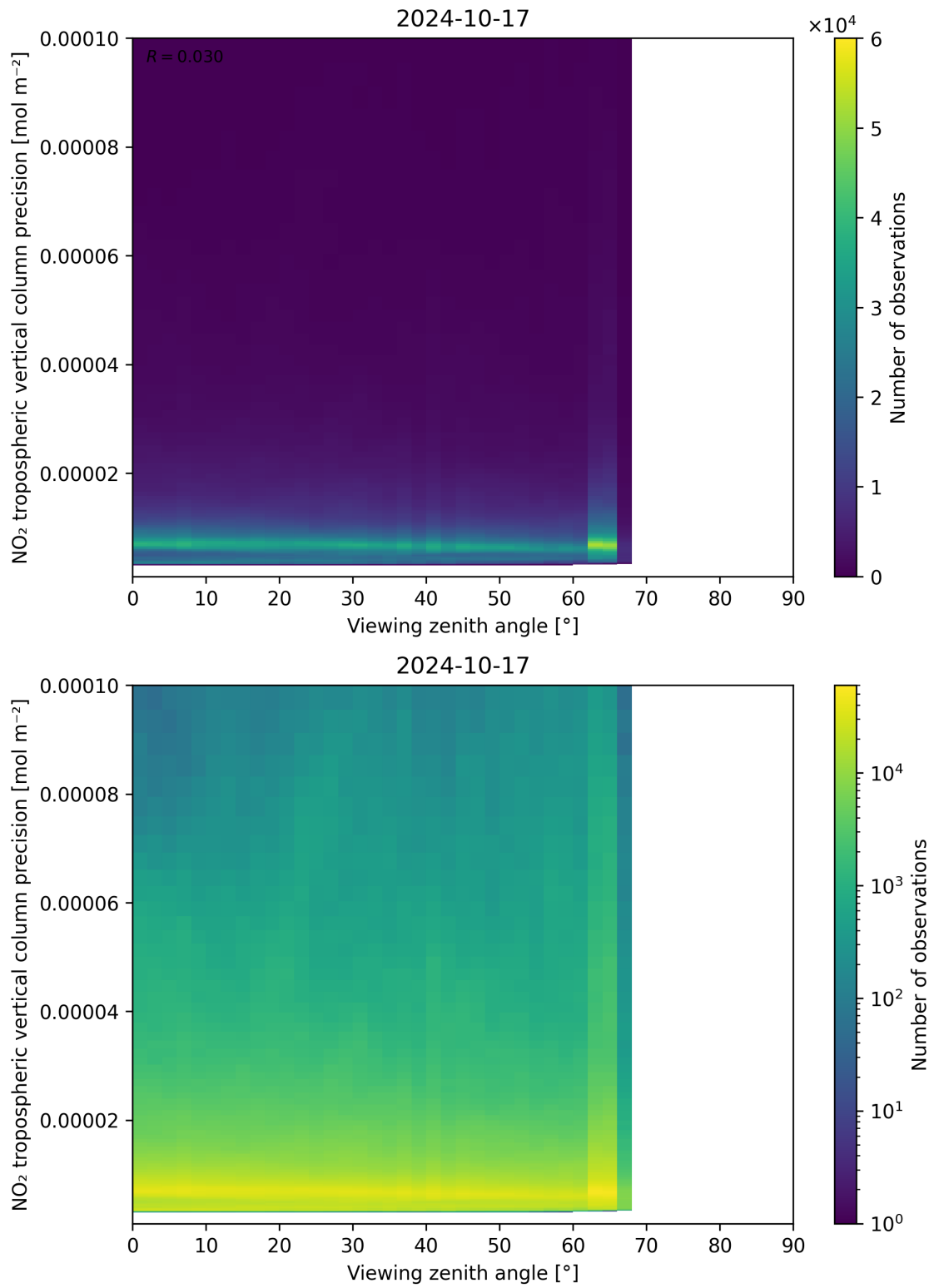
Figure 170: Scatter density plot of “Viewing zenith angle” against “NO 2 tropospheric vertical column precision” for 2024-10-16 to 2024-10-18.
