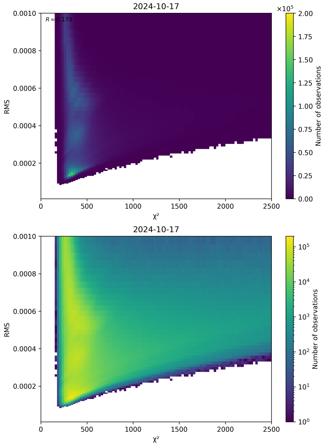
Figure 82: Scatter density plot of “ \chi^2 ” against “RMS” for 2024-10-16 to 2024-10-18.
