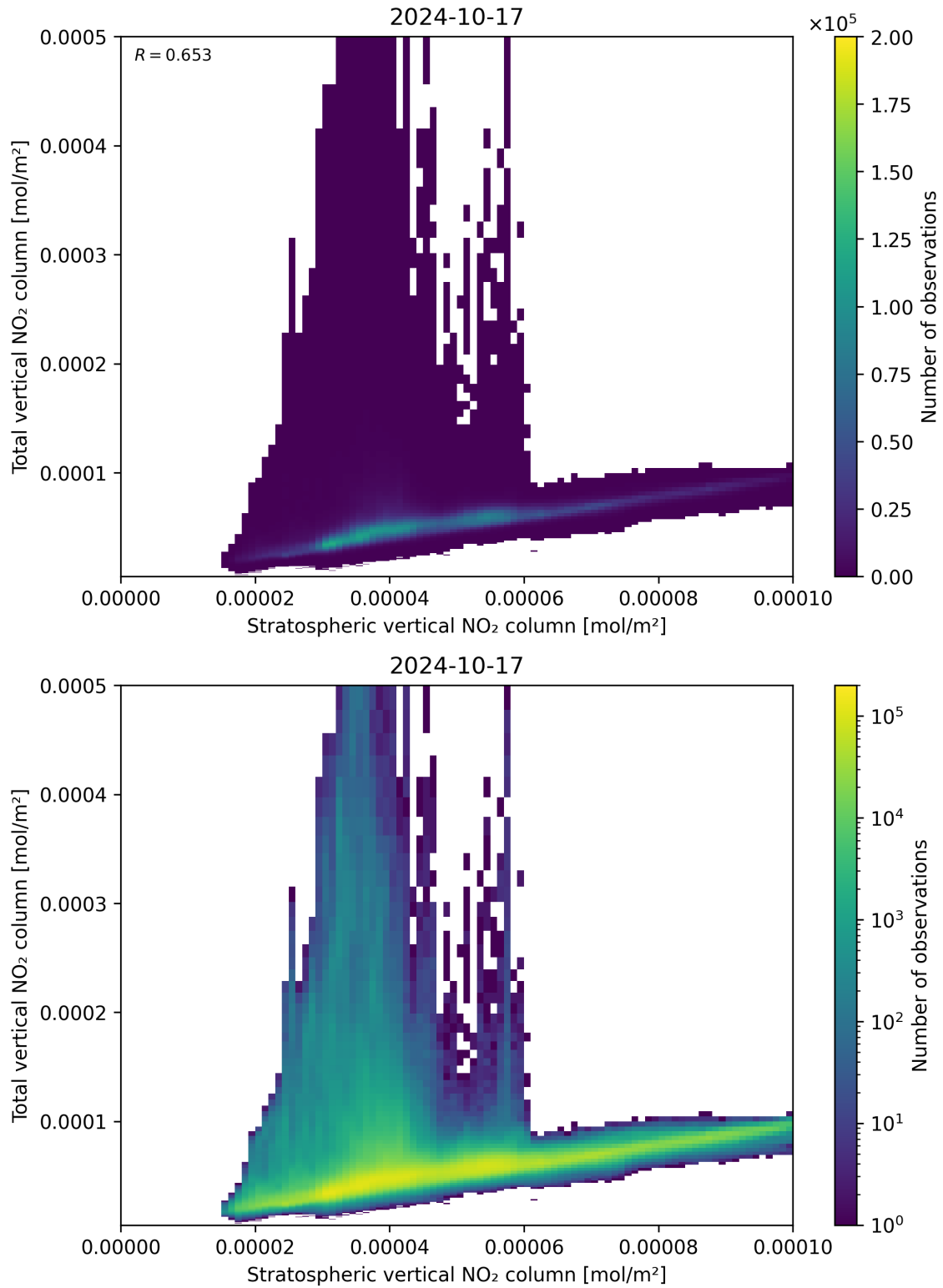
Figure 100: Scatter density plot of “Stratospheric vertical NO 2 column” against “Total vertical NO 2 column” for 2024-10-16 to 2024-10-18.
