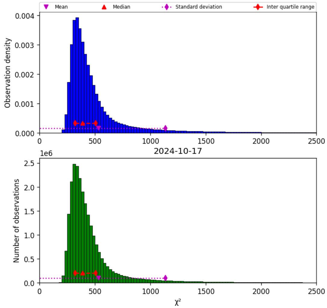
Figure 42: Histogram of “ \chi^2 ” for 2024-10-16 to 2024-10-18
