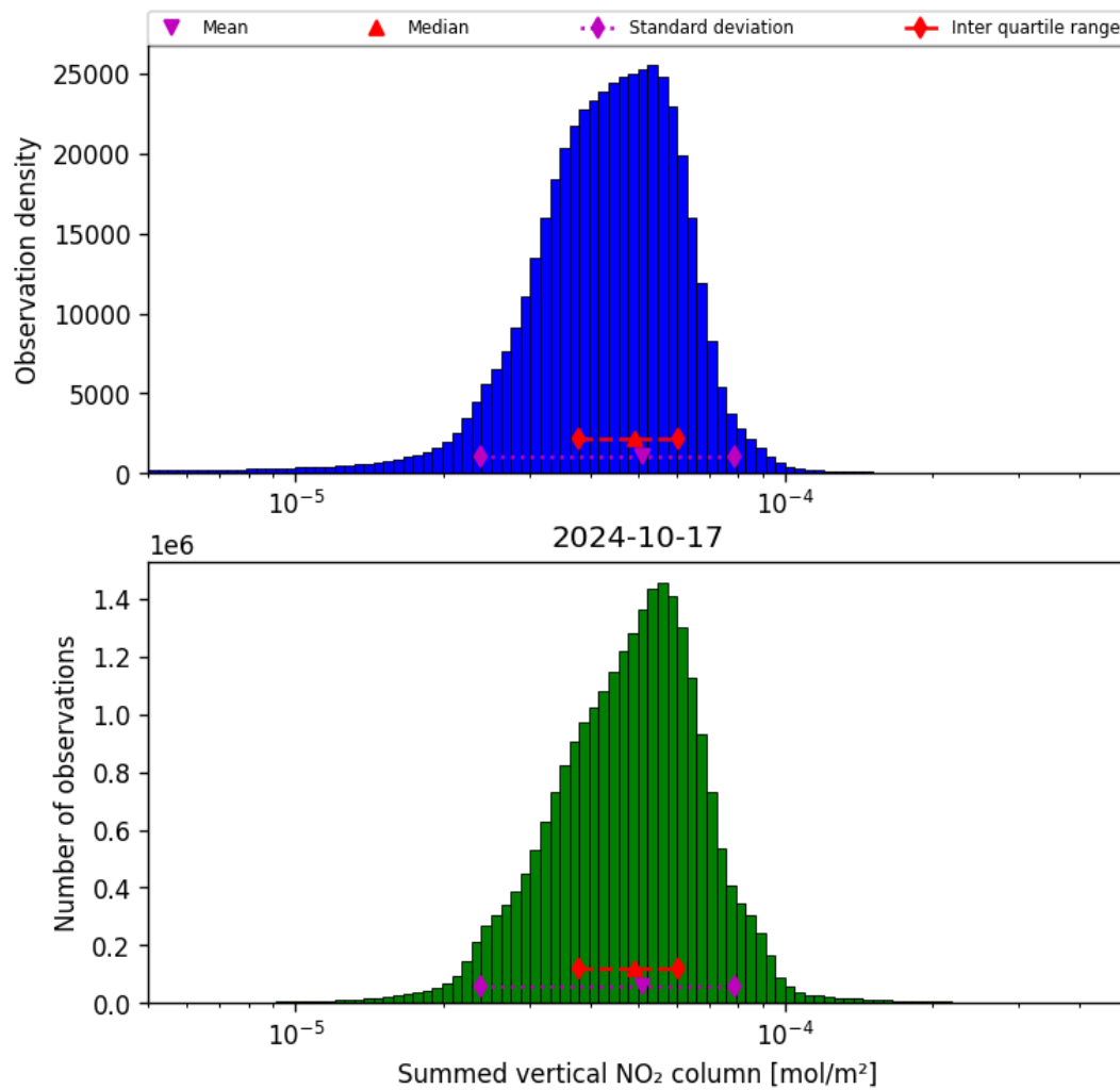
Figure 40: Histogram of “Summed vertical NO 2 column” for 2024-10-16 to 2024-10-18
