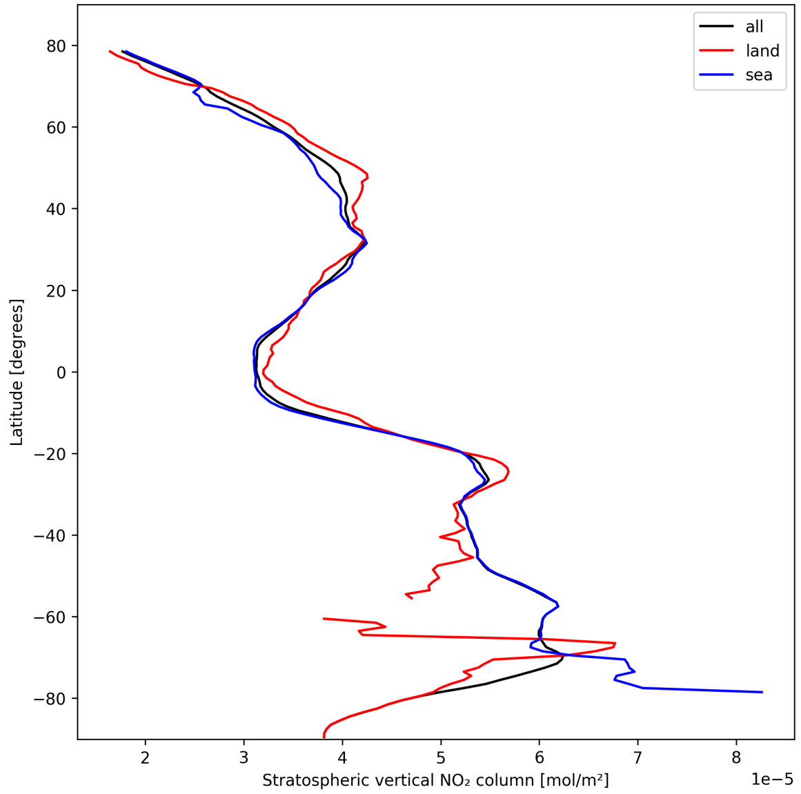
Figure 19: Zonal average of “Stratospheric vertical NO 2 column” for 2024-10-16 to 2024-10-18.
