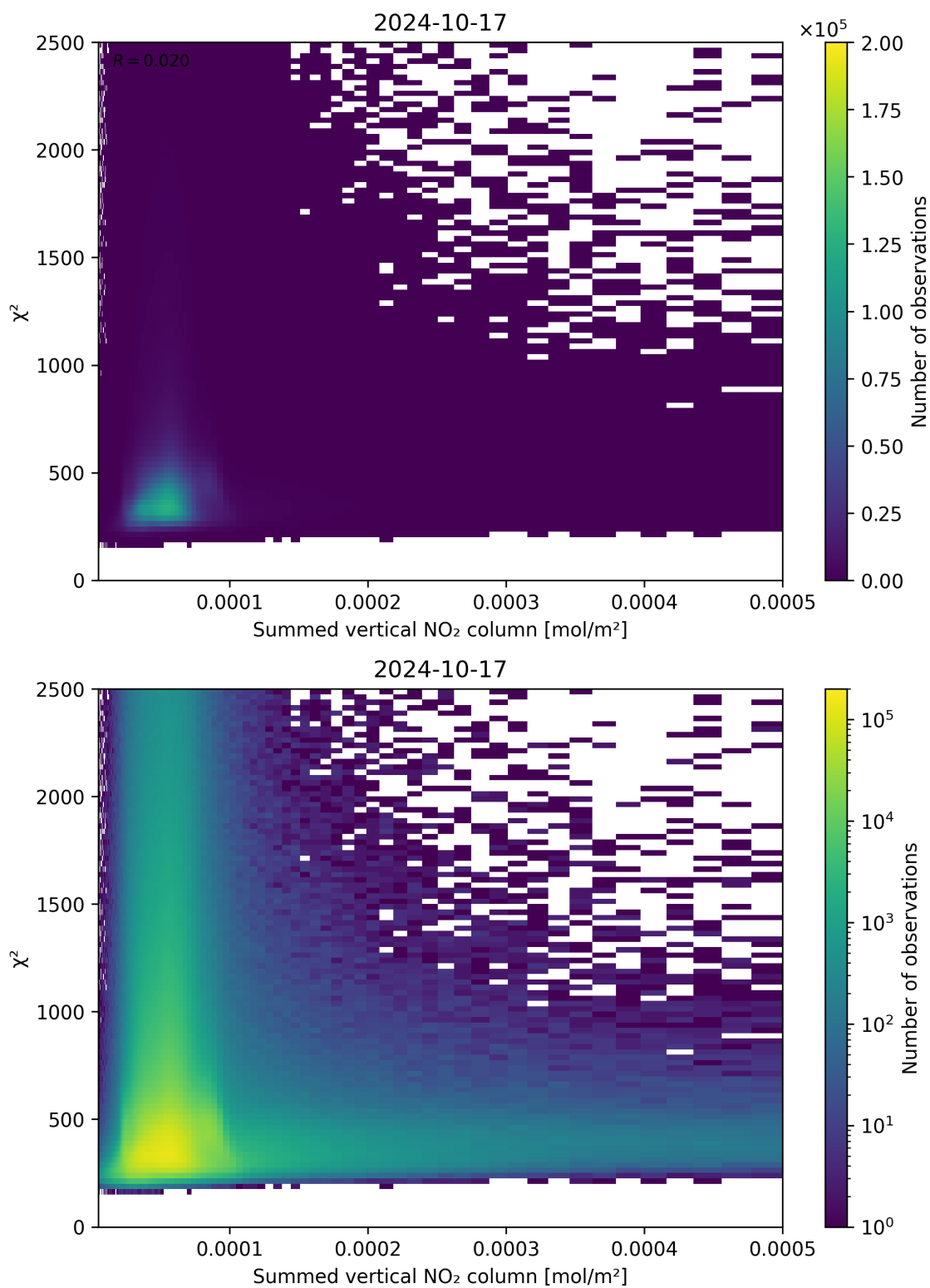
Figure 104: Scatter density plot of “Summed vertical NO 2 column” against “ \chi^2 ” for 2024-10-16 to 2024-10-18.
