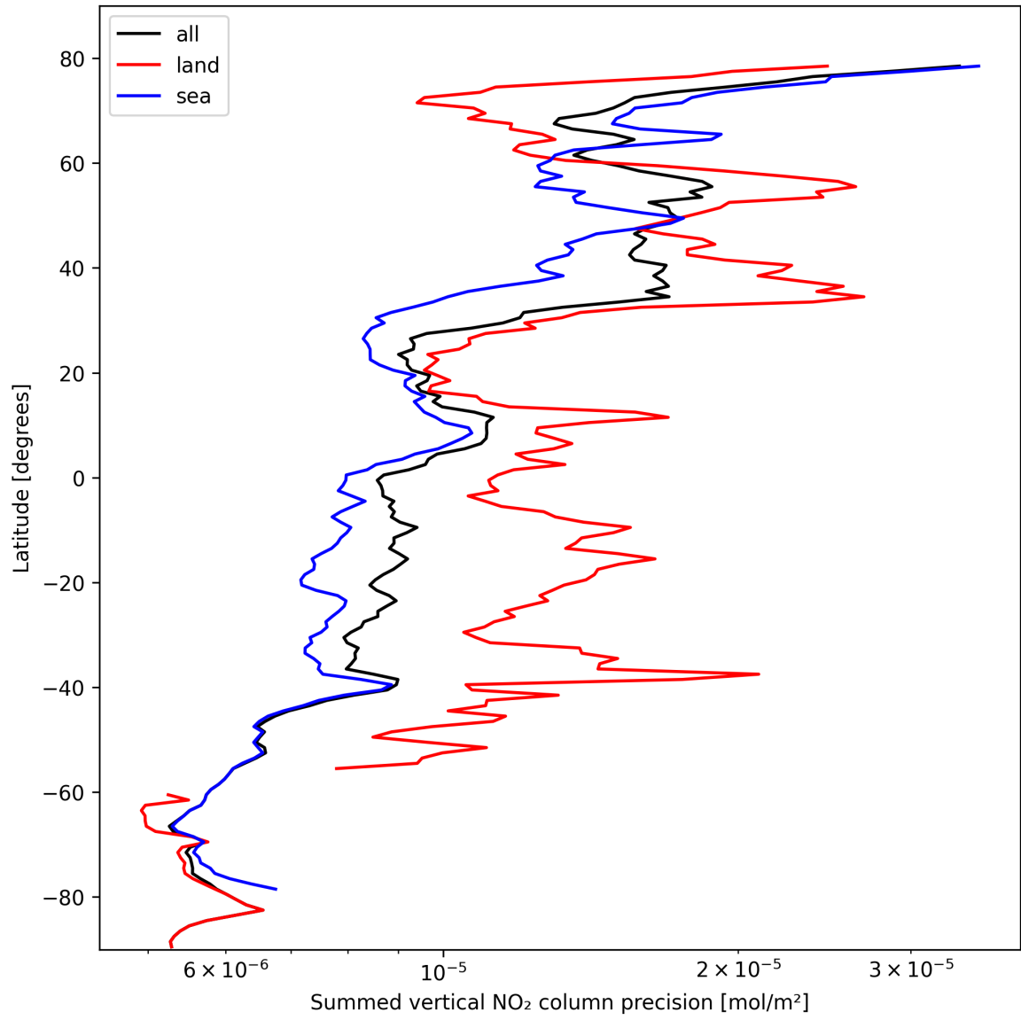
Figure 24: Zonal average of “Summed vertical NO 2 column precision” for 2024-10-16 to 2024-10-18.
