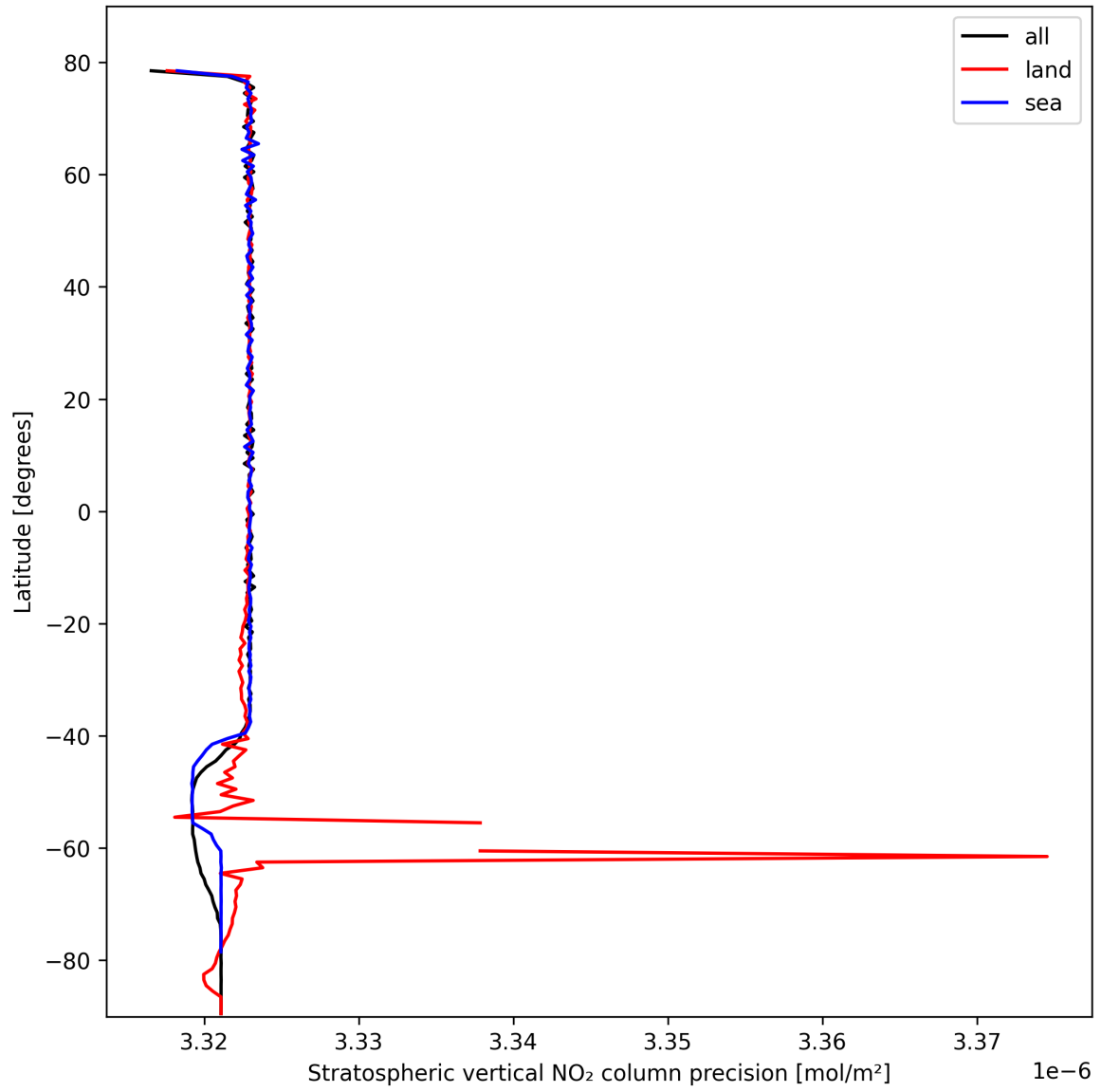
Figure 20: Zonal average of “Stratospheric vertical NO 2 column precision” for 2024-10-16 to 2024-10-18.
