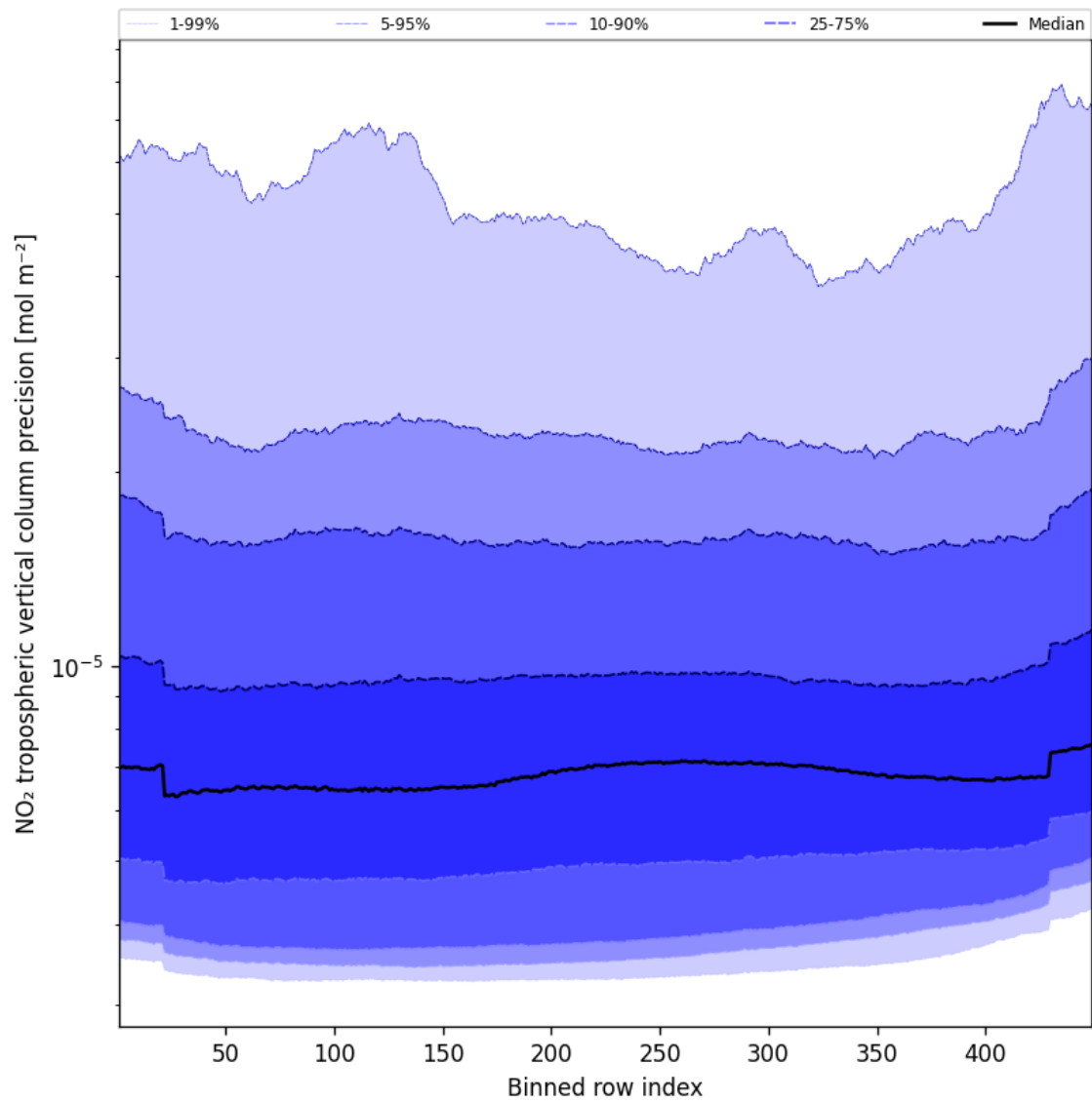
Figure 47: Along track statistics of “NO 2 tropospheric vertical column precision” for 2024-10-16 to 2024-10-18
