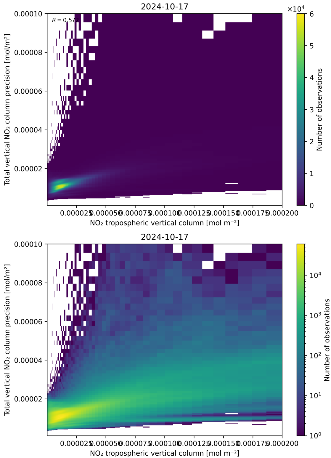
Figure 129: Scatter density plot of “NO 2 tropospheric vertical column” against “Total vertical NO 2 column precision” for 2024-10-16 to 2024-10-18.
