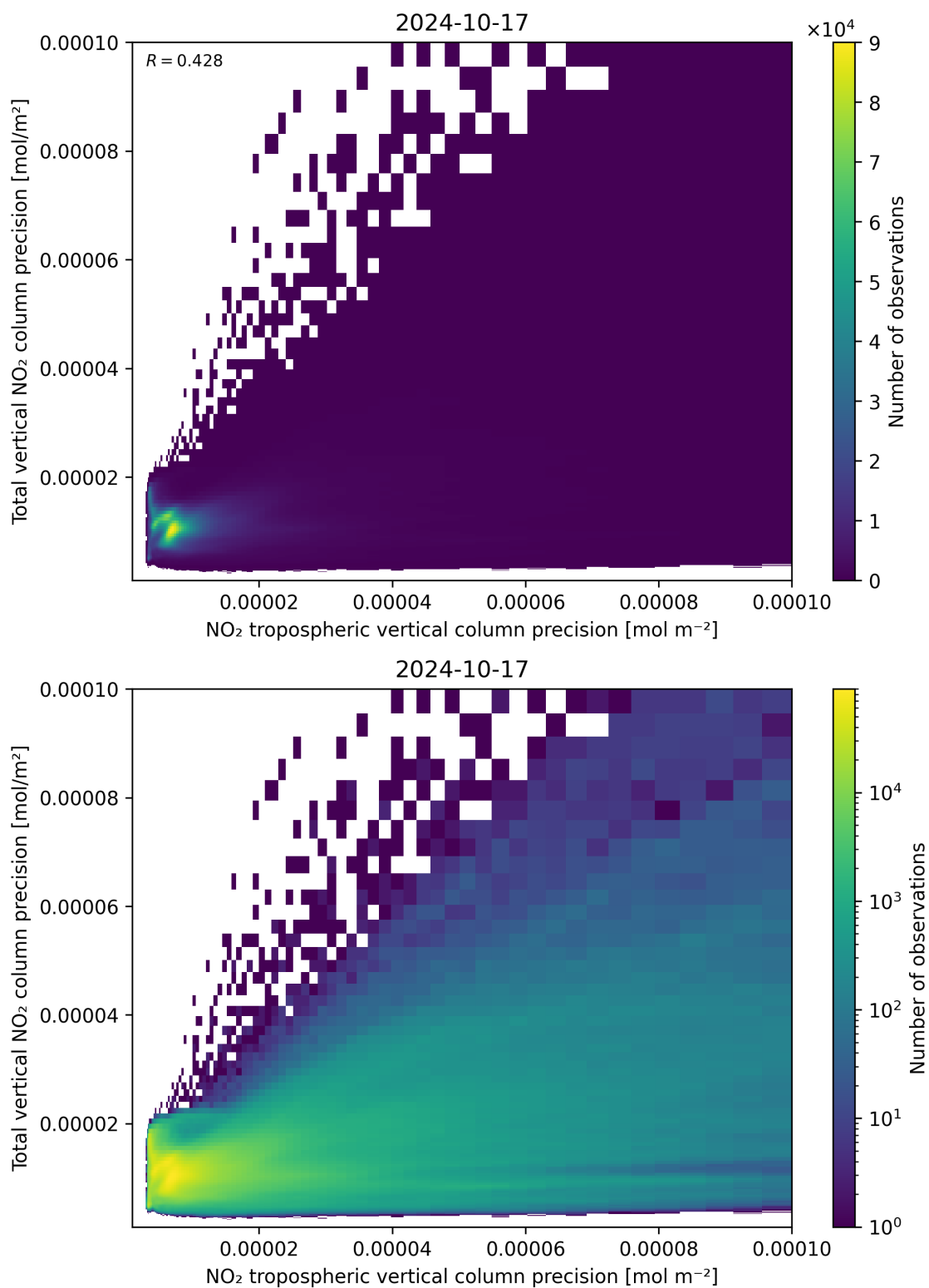
Figure 139: Scatter density plot of “NO 2 tropospheric vertical column precision” against “Total vertical NO 2 column precision” for 2024-10-16 to 2024-10-18.
