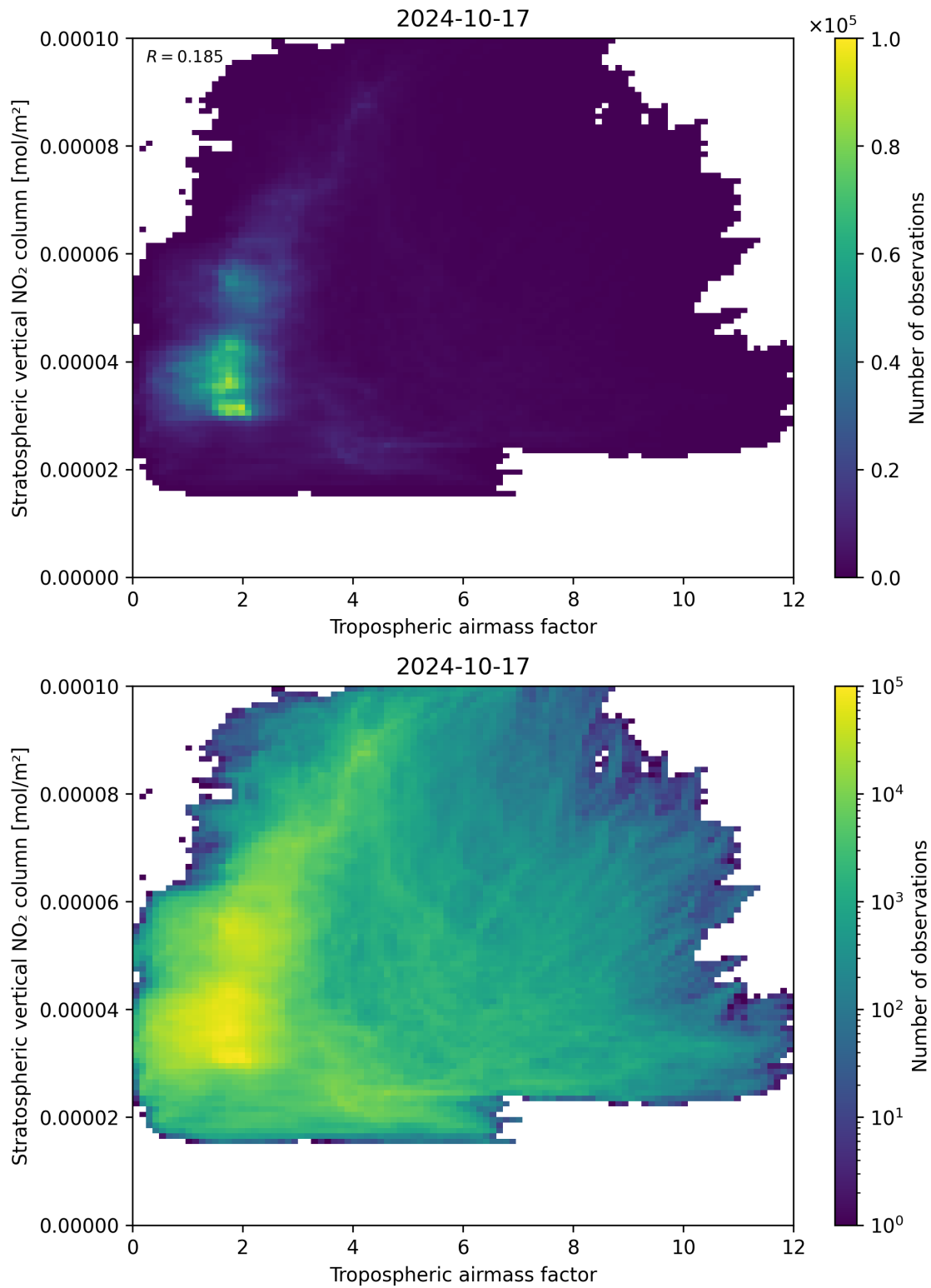
Figure 74: Scatter density plot of “Tropospheric air mass factor” against “Stratospheric vertical NO 2 column” for 2024-10-16 to 2024-10-18.
