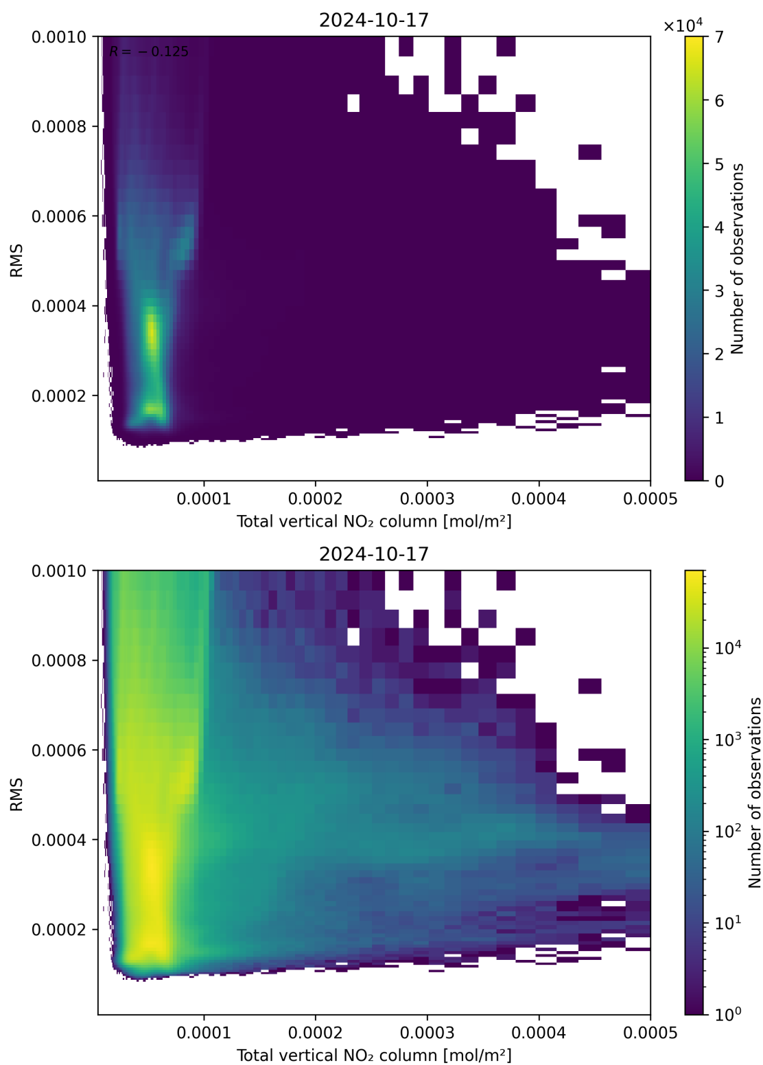
Figure 120: Scatter density plot of “Total vertical NO 2 column” against “RMS” for 2024-10-16 to 2024-10-18.
