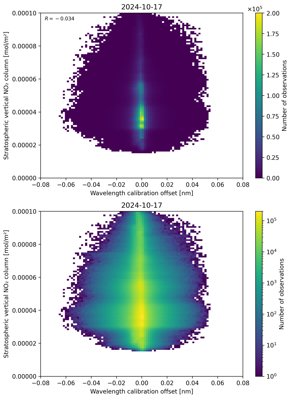
Figure 176: Scatter density plot of “Wavelength calibration offset” against “Stratospheric vertical NO 2 column” for 2024-10-16 to 2024-10-18.
