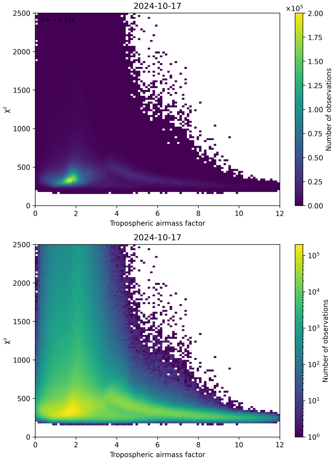
Figure 73: Scatter density plot of “Tropospheric airmass factor” against “ \chi^2 ” for 2024-10-16 to 2024-10-18.
