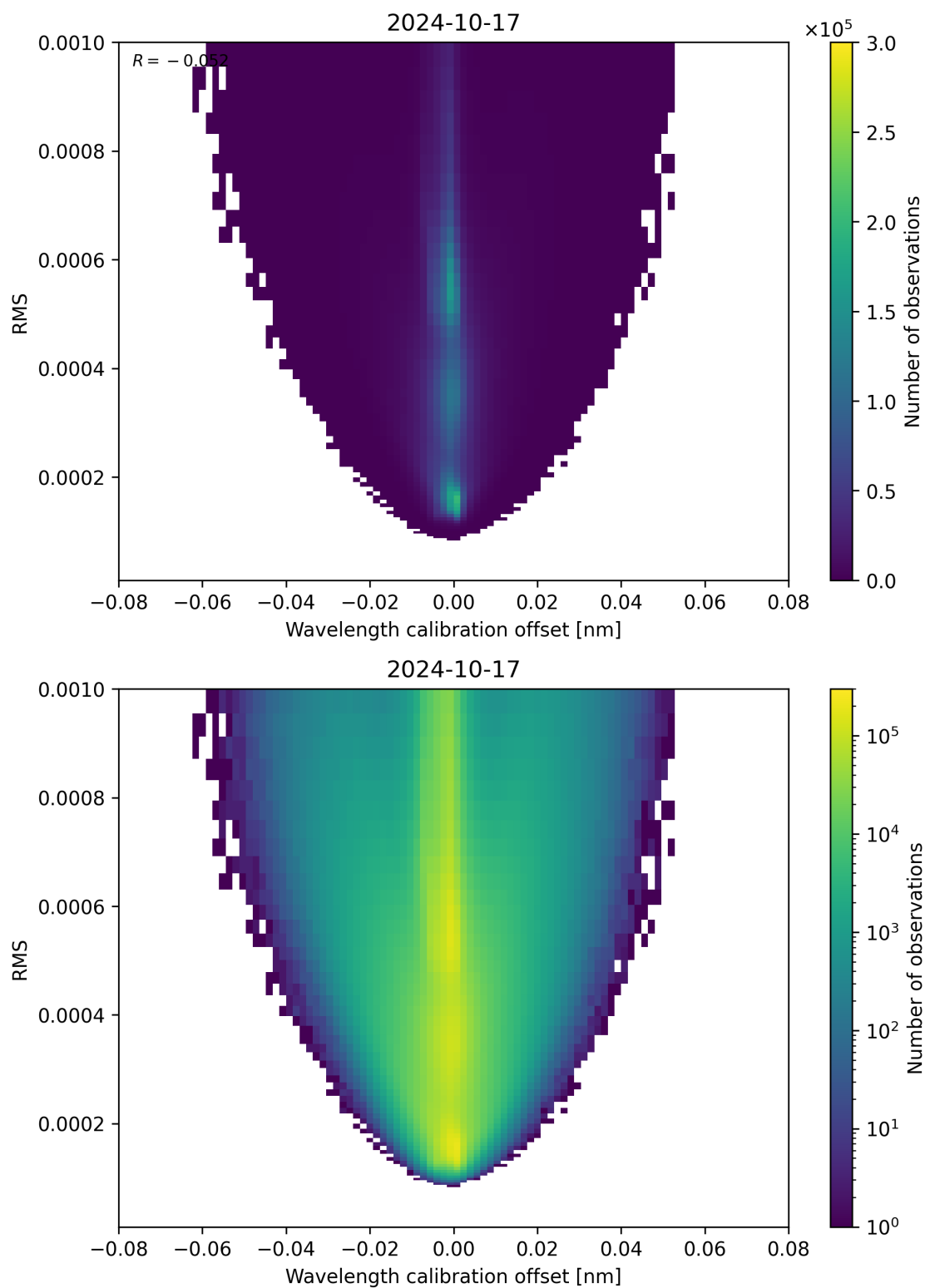
Figure 181: Scatter density plot of “Wavelength calibration offset” against “RMS” for 2024-10-16 to 2024-10-18.
