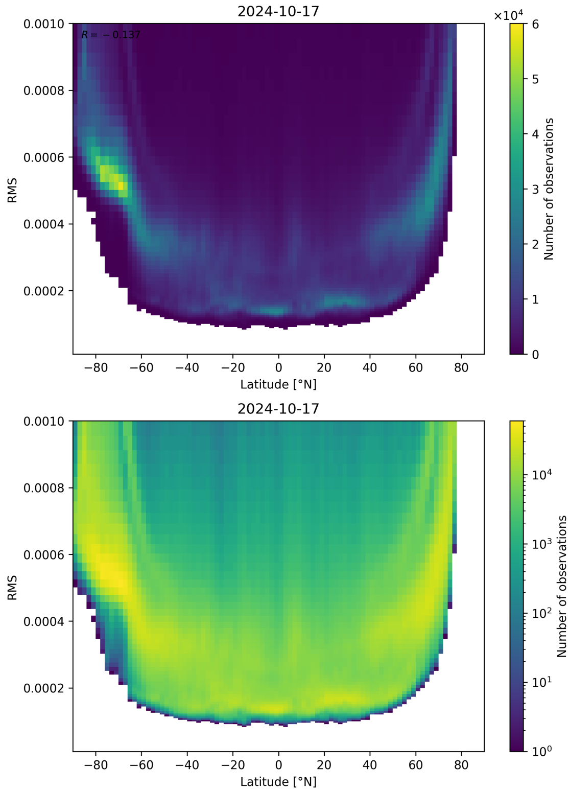
Figure 94: Scatter density plot of “Latitude” against “RMS” for 2024-10-16 to 2024-10-18.
