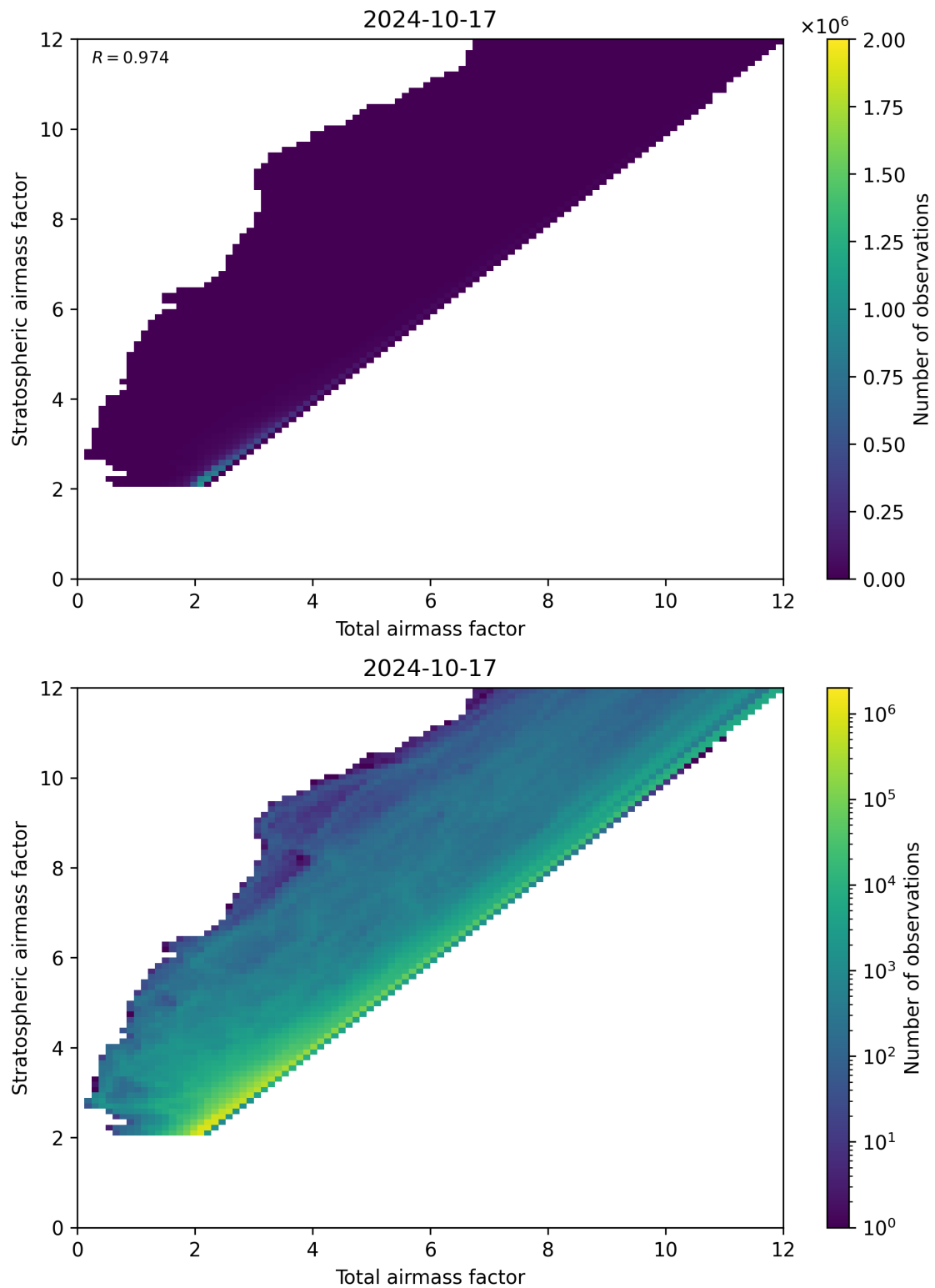
Figure 62: Scatter density plot of “Total airmass factor” against “Stratospheric airmass factor” for 2024-10-16 to 2024-10-18.
