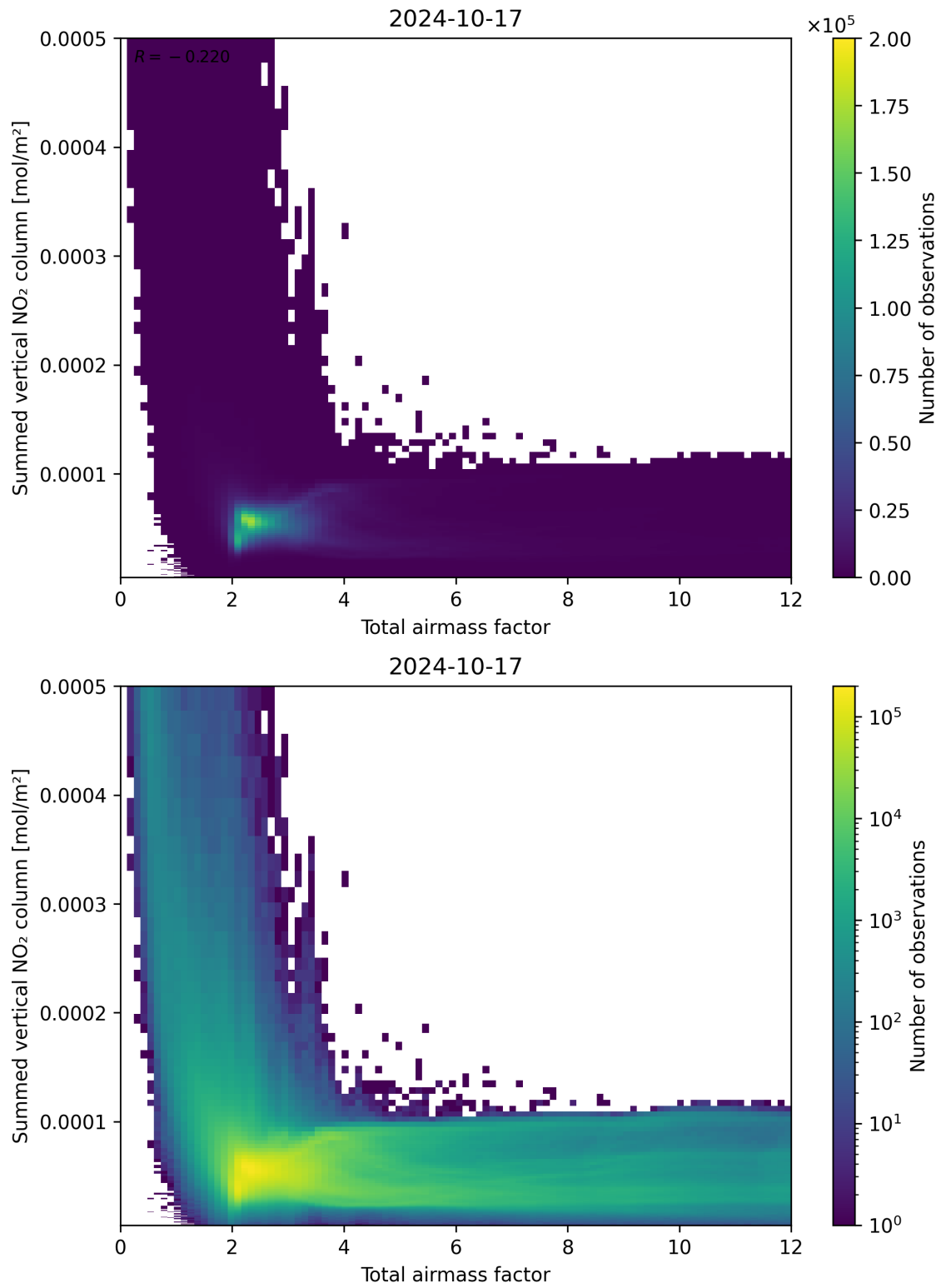
Figure 65: Scatter density plot of “Total airmass factor” against “Summed vertical NO 2 column” for 2024-10-16 to 2024-10-18.
