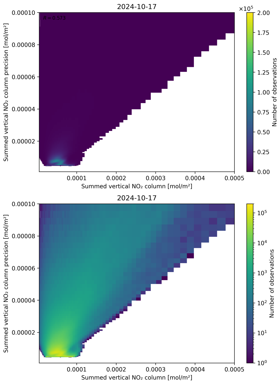
Figure 105: Scatter density plot of “Summed vertical NO 2 column” against “Summed vertical NO 2 column precision” for 2024-10-16 to 2024-10-18.
