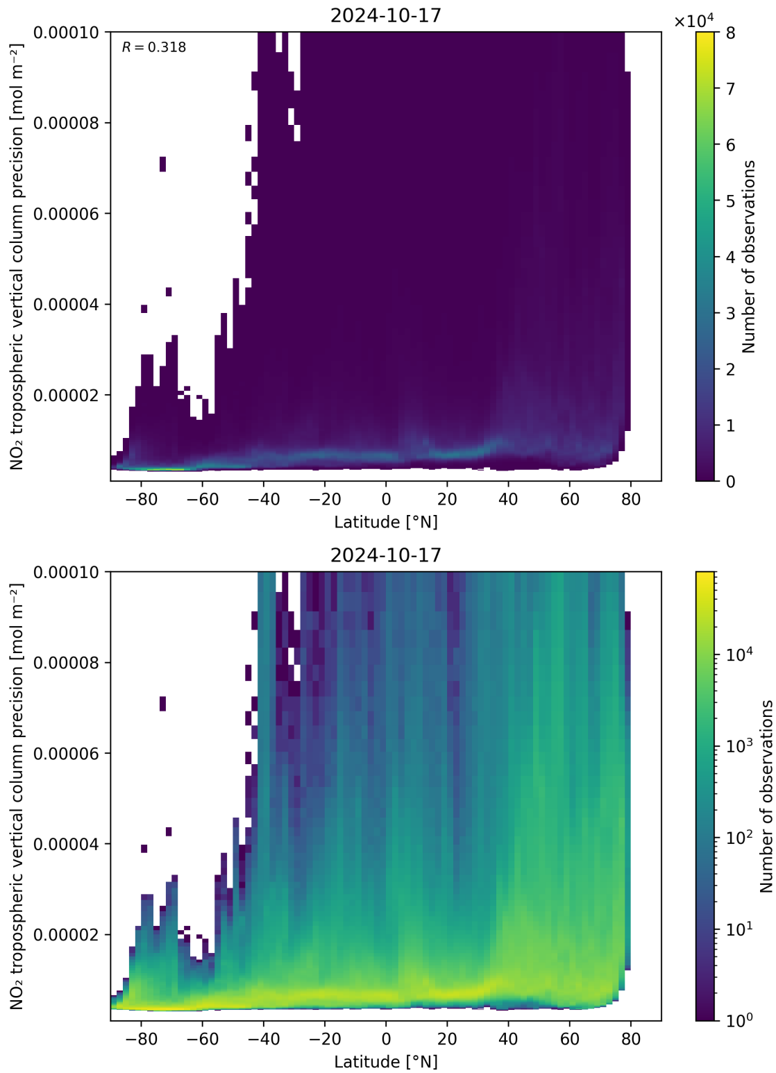
Figure 93: Scatter density plot of “Latitude” against “NO 2 tropospheric vertical column precision” for 2024-10-16 to 2024-10-18.
