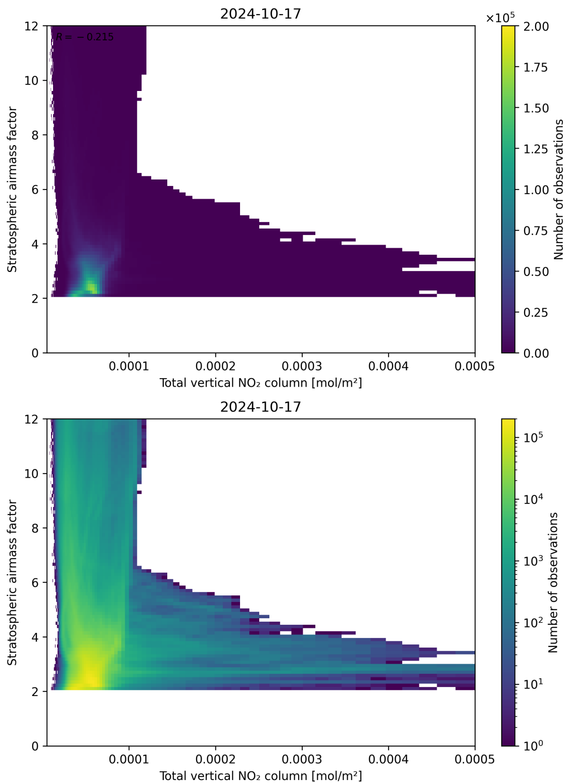
Figure 110: Scatter density plot of “Total vertical NO 2 column” against “Stratospheric airmass factor” for 2024-10-16 to 2024-10-18.
