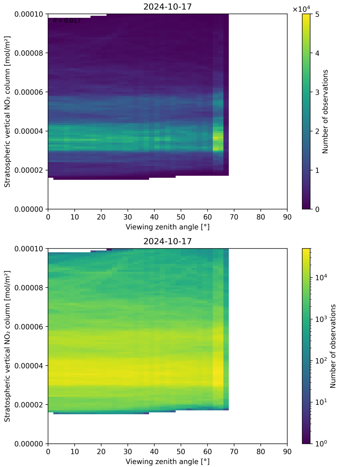
Figure 164: Scatter density plot of “Viewing zenith angle” against “Stratospheric vertical NO 2 column” for 2024-10-16 to 2024-10-18.
