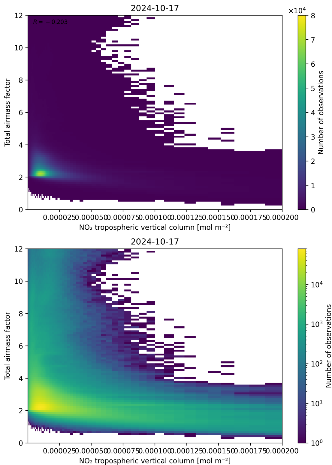
Figure 122: Scatter density plot of “NO 2 tropospheric vertical column” against “Total air mass factor” for 2024-10-16 to 2024-10-18.
