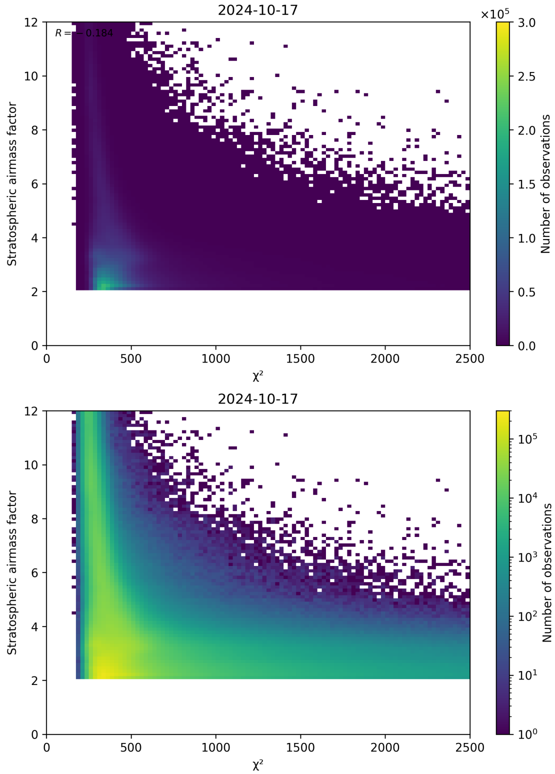
Figure 81: Scatter density plot of “ \chi^2 ” against “Stratospheric airmass factor” for 2024-10-16 to 2024-10-18.
