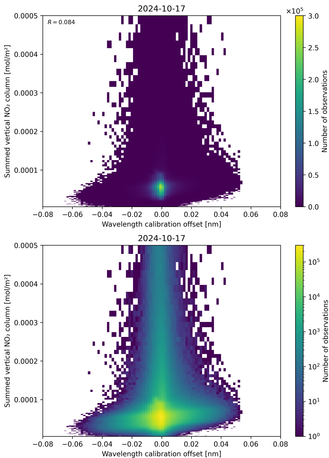
Figure 177: Scatter density plot of “Wavelength calibration offset” against “Summed vertical NO 2 column” for 2024-10-16 to 2024-10-18.
