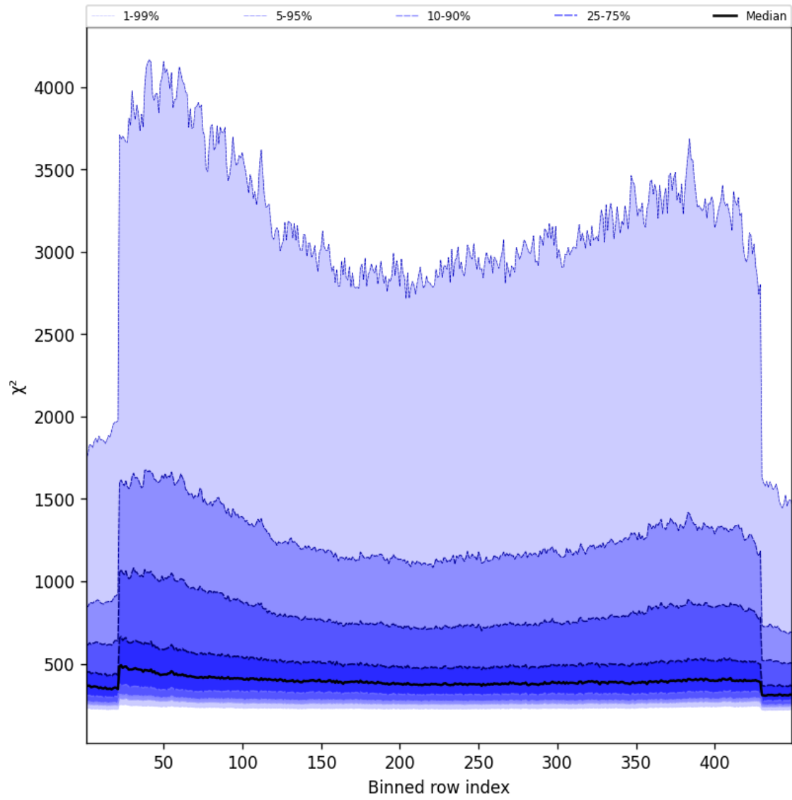
Figure 59: Along track statistics of “ \chi^2 ” for 2024-10-16 to 2024-10-18
