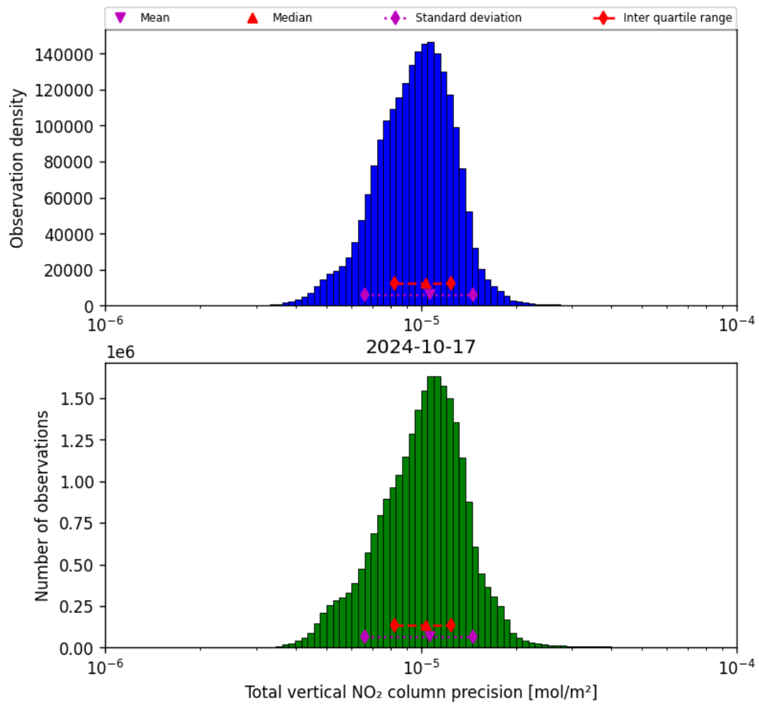
Figure 39: Histogram of “Total vertical NO 2 column precision” for 2024-10-16 to 2024-10-18
