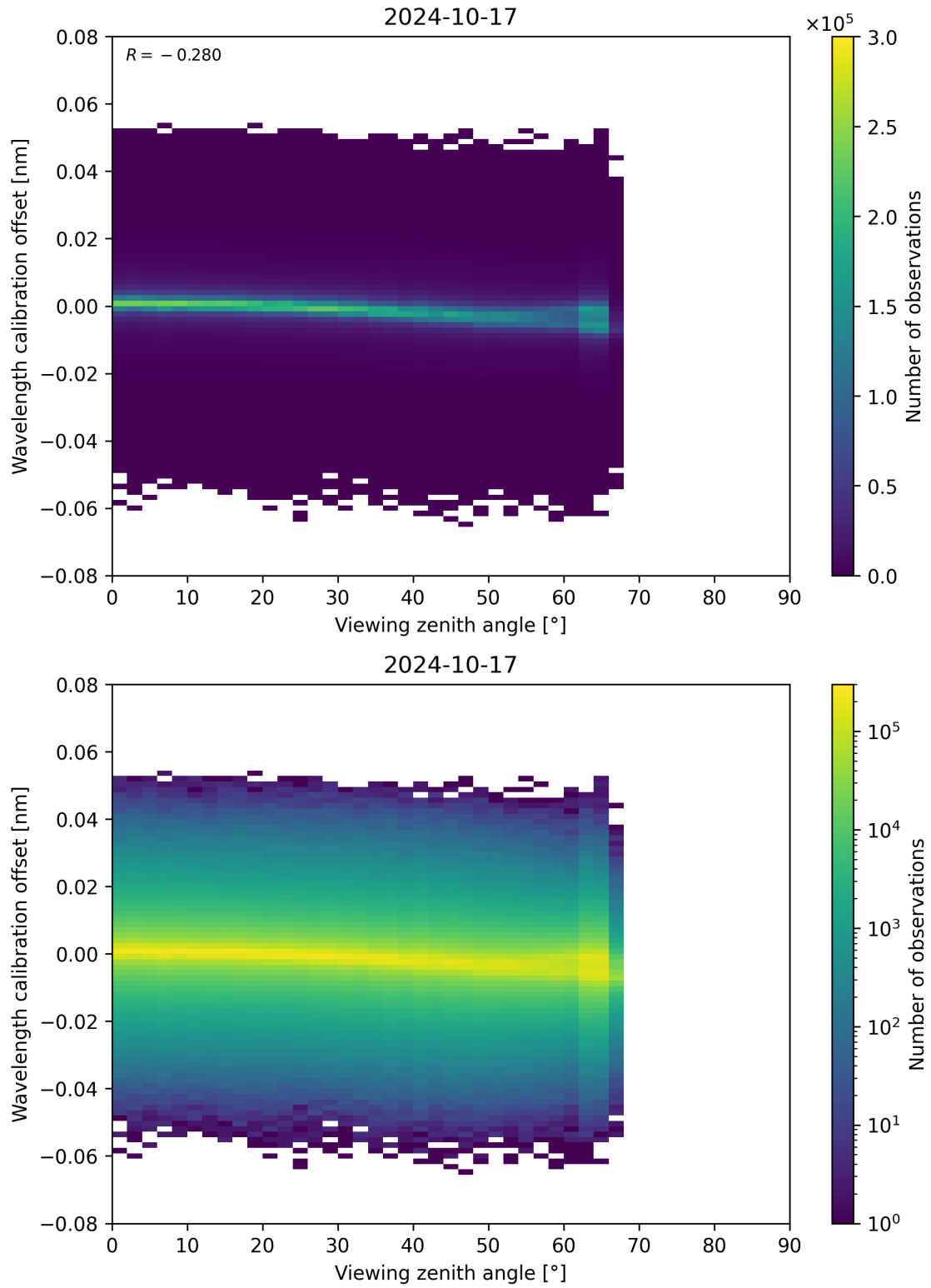
Figure 173: Scatter density plot of “Viewing zenith angle” against “Wavelength calibration offset” for 2024-10-16 to 2024-10-18.
