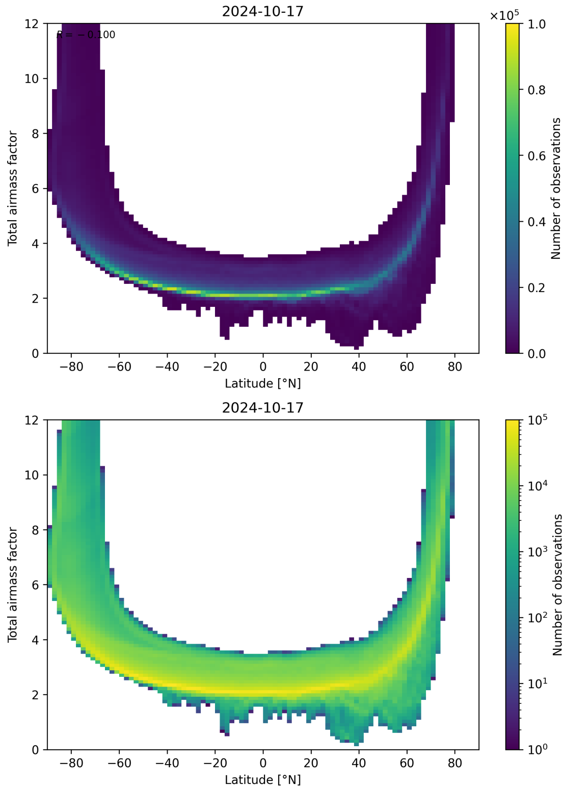
Figure 84: Scatter density plot of “Latitude” against “Total airmass factor” for 2024-10-16 to 2024-10-18.
