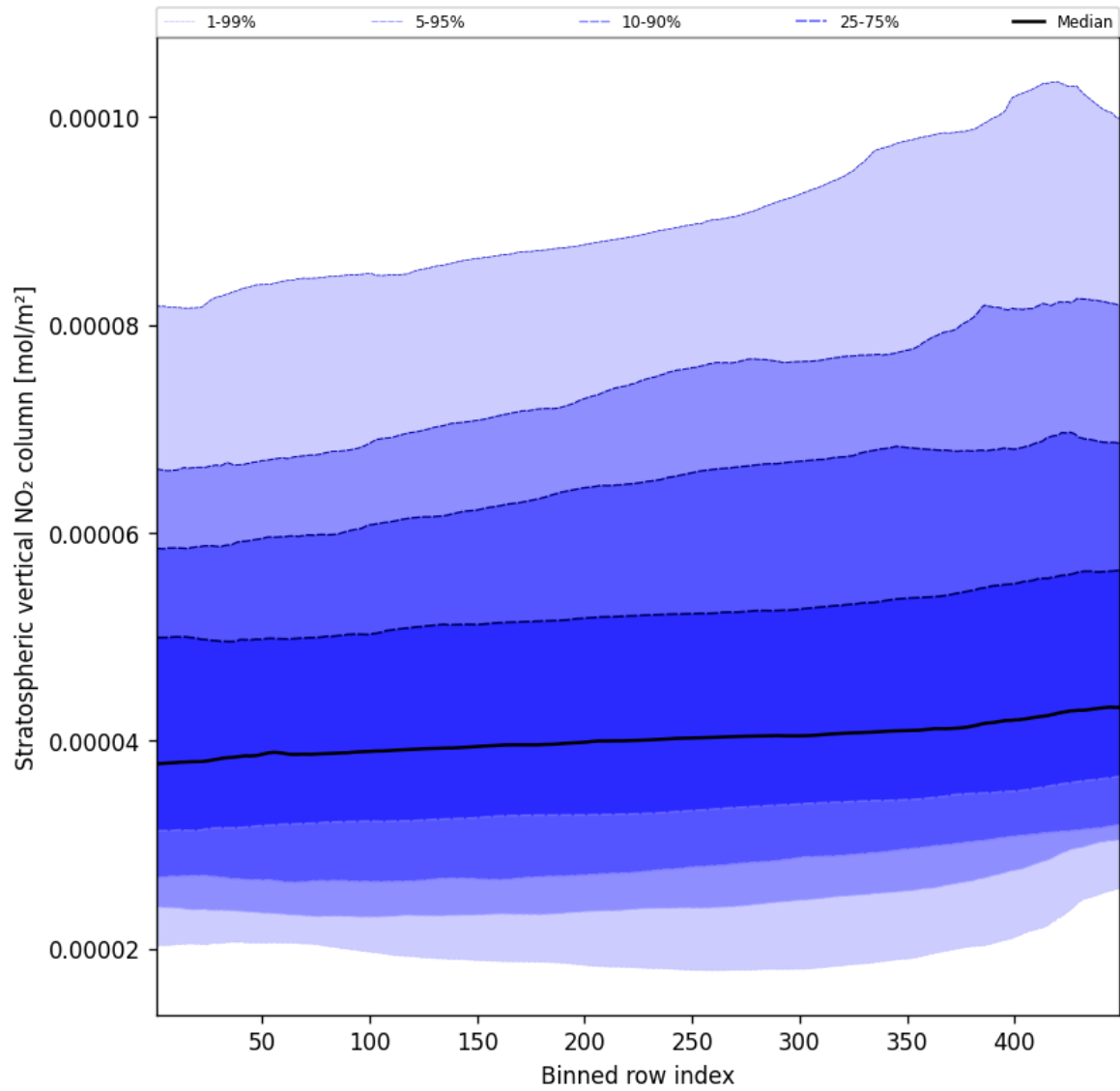
Figure 53: Along track statistics of “Stratospheric vertical NO 2 column” for 2024-10-16 to 2024-10-18
