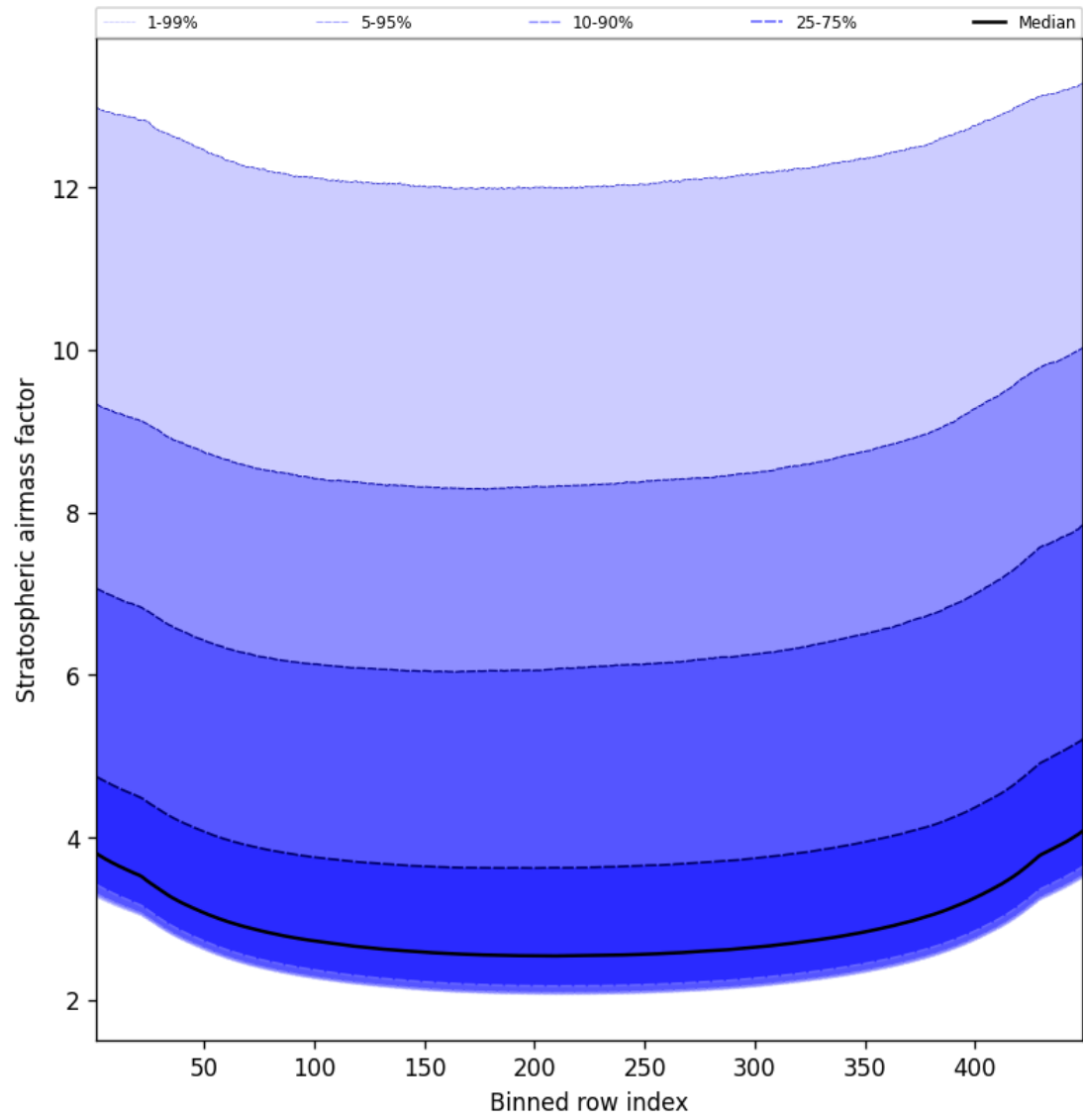
Figure 61: Along track statistics of “Stratospheric airmass factor” for 2024-10-16 to 2024-10-18
