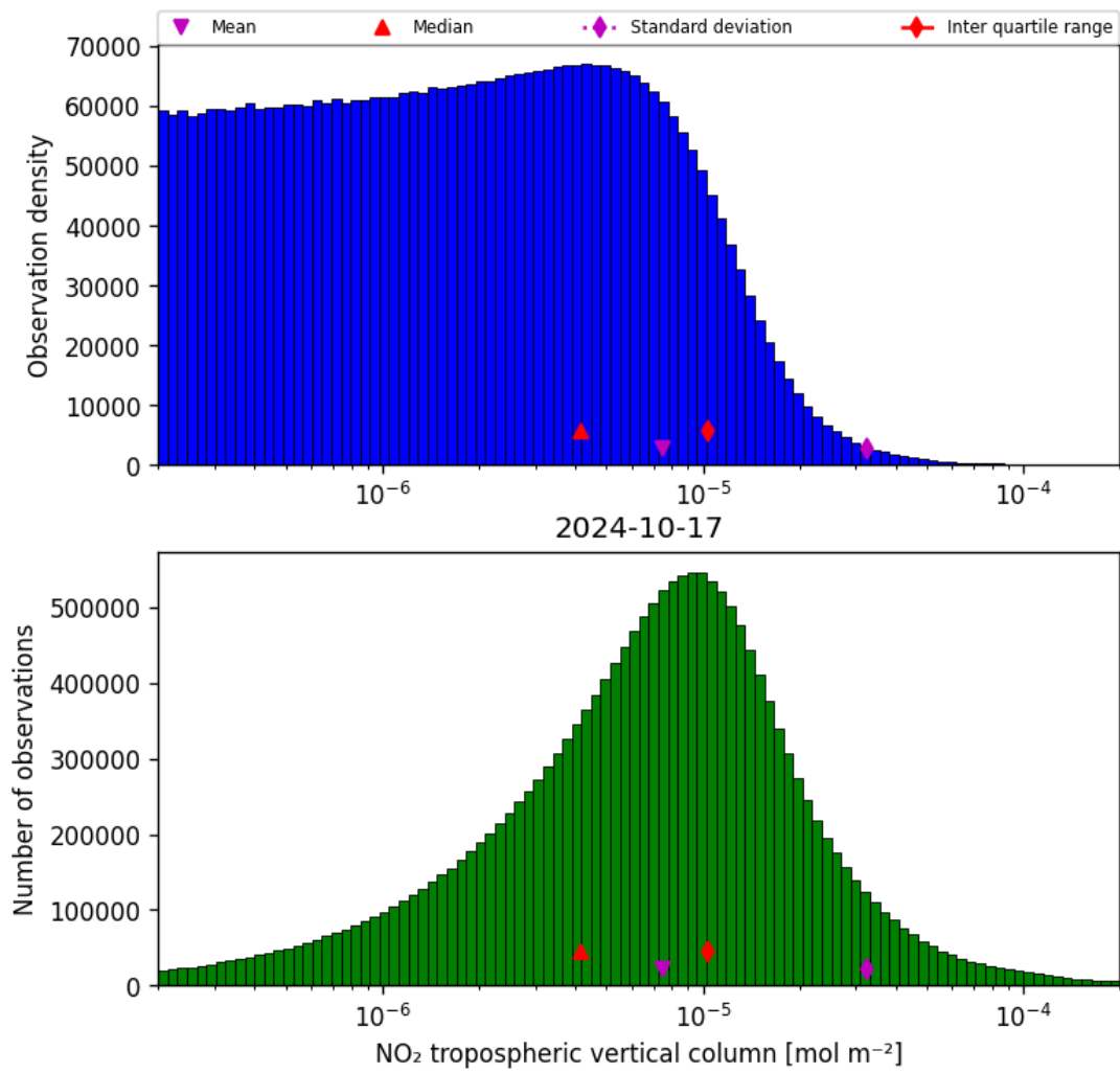
Figure 29: Histogram of “NO 2 tropospheric vertical column” for 2024-10-16 to 2024-10-18
