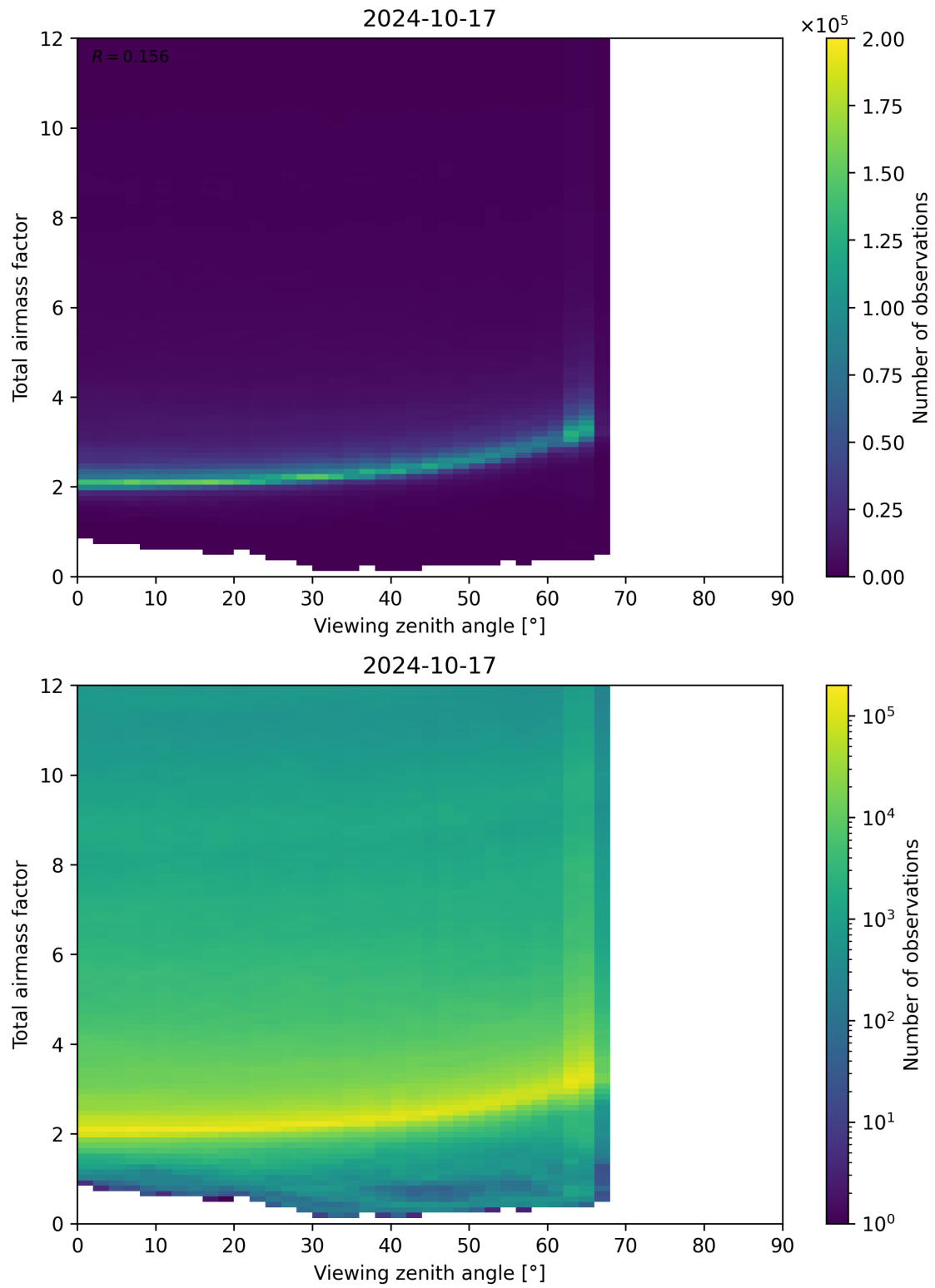
Figure 160: Scatter density plot of “Viewing zenith angle” against “Total airmass factor” for 2024-10-16 to 2024-10-18.
