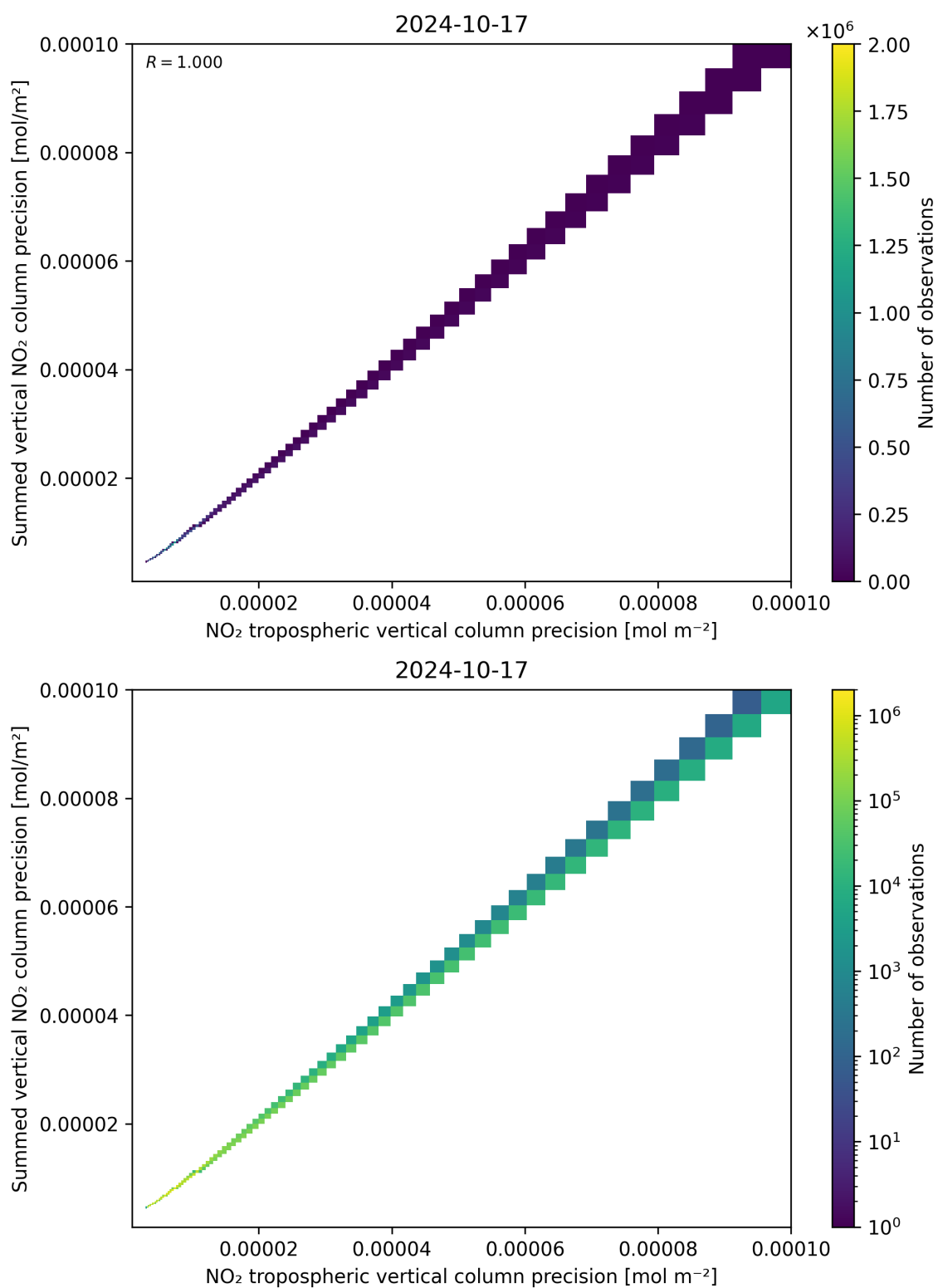
Figure 137: Scatter density plot of “NO 2 tropospheric vertical column precision” against “Summed vertical NO 2 column precision” for 2024-10-16 to 2024-10-18.
