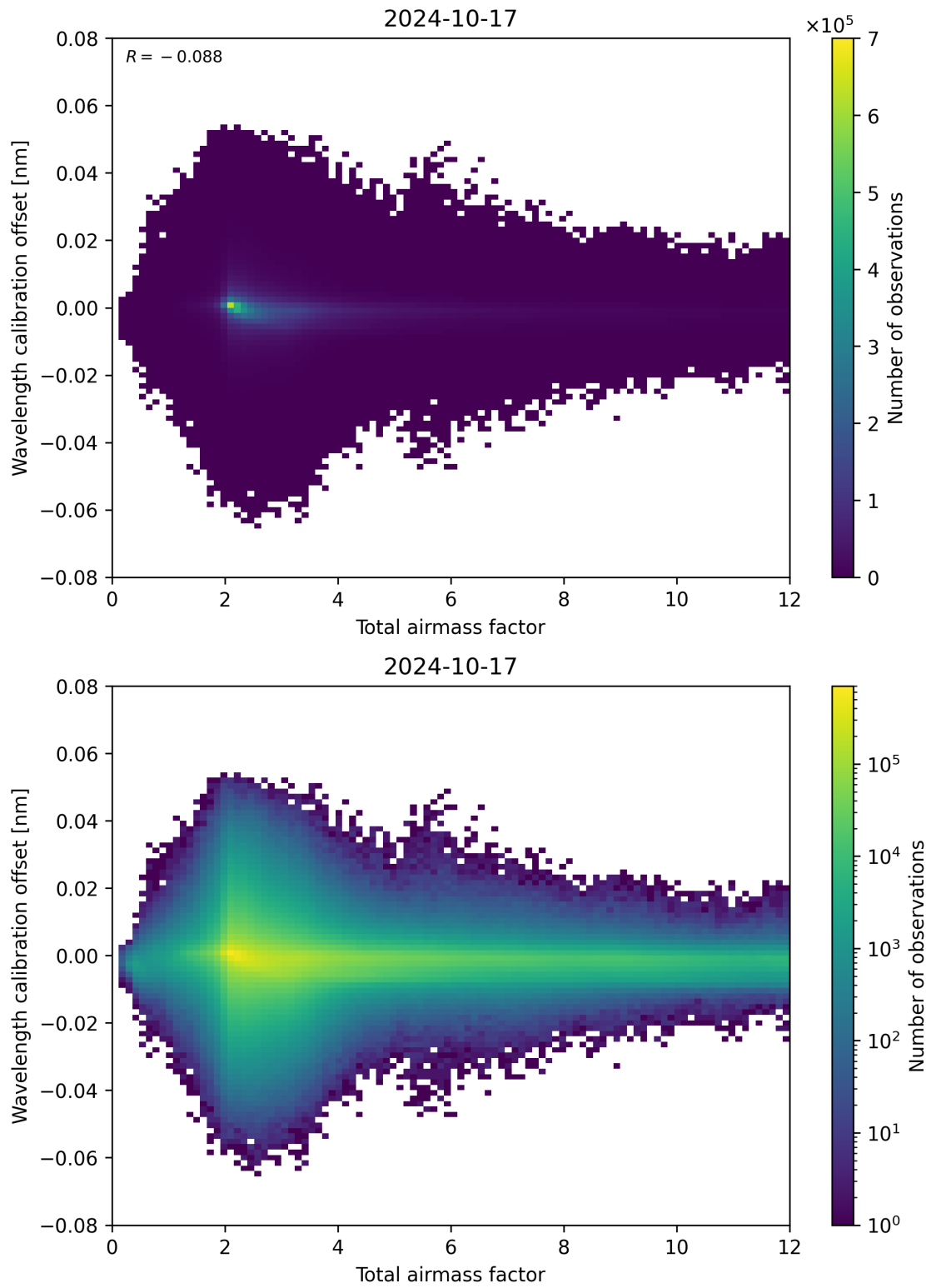
Figure 70: Scatter density plot of “Total airmass factor” against “Wavelength calibration offset” for 2024-10-16 to 2024-10-18.
