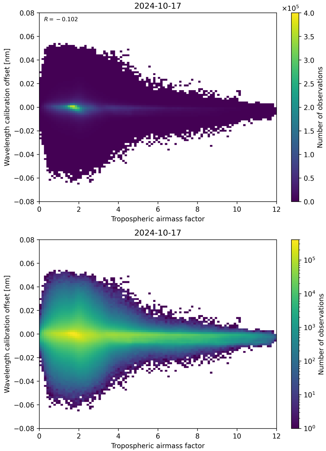
Figure 80: Scatter density plot of “Tropospheric airmass factor” against “Wavelength calibration offset” for 2024-10-16 to 2024-10-18.
