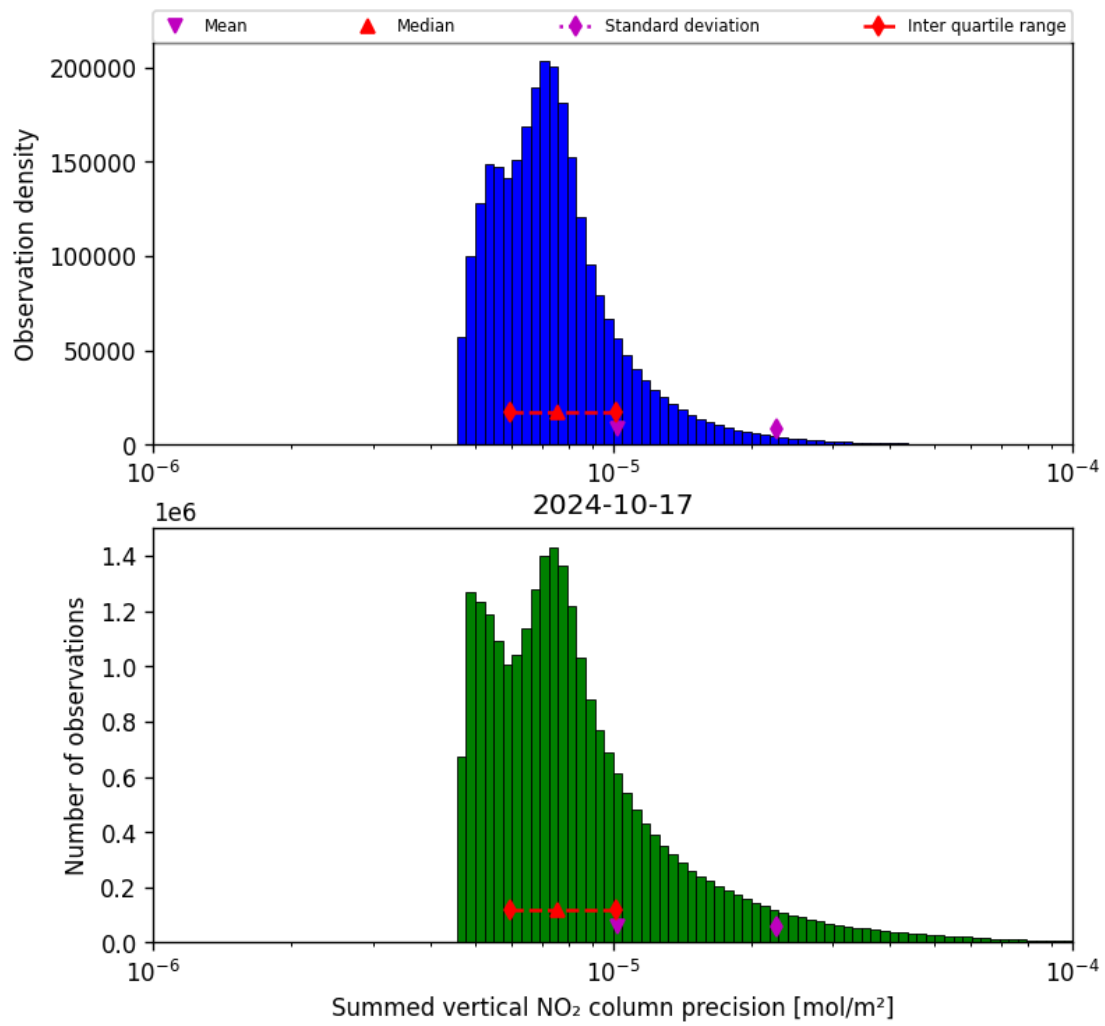
Figure 41: Histogram of "Summed vertical NO 2 column precision" for 2024-10-16 to 2024-10-18
