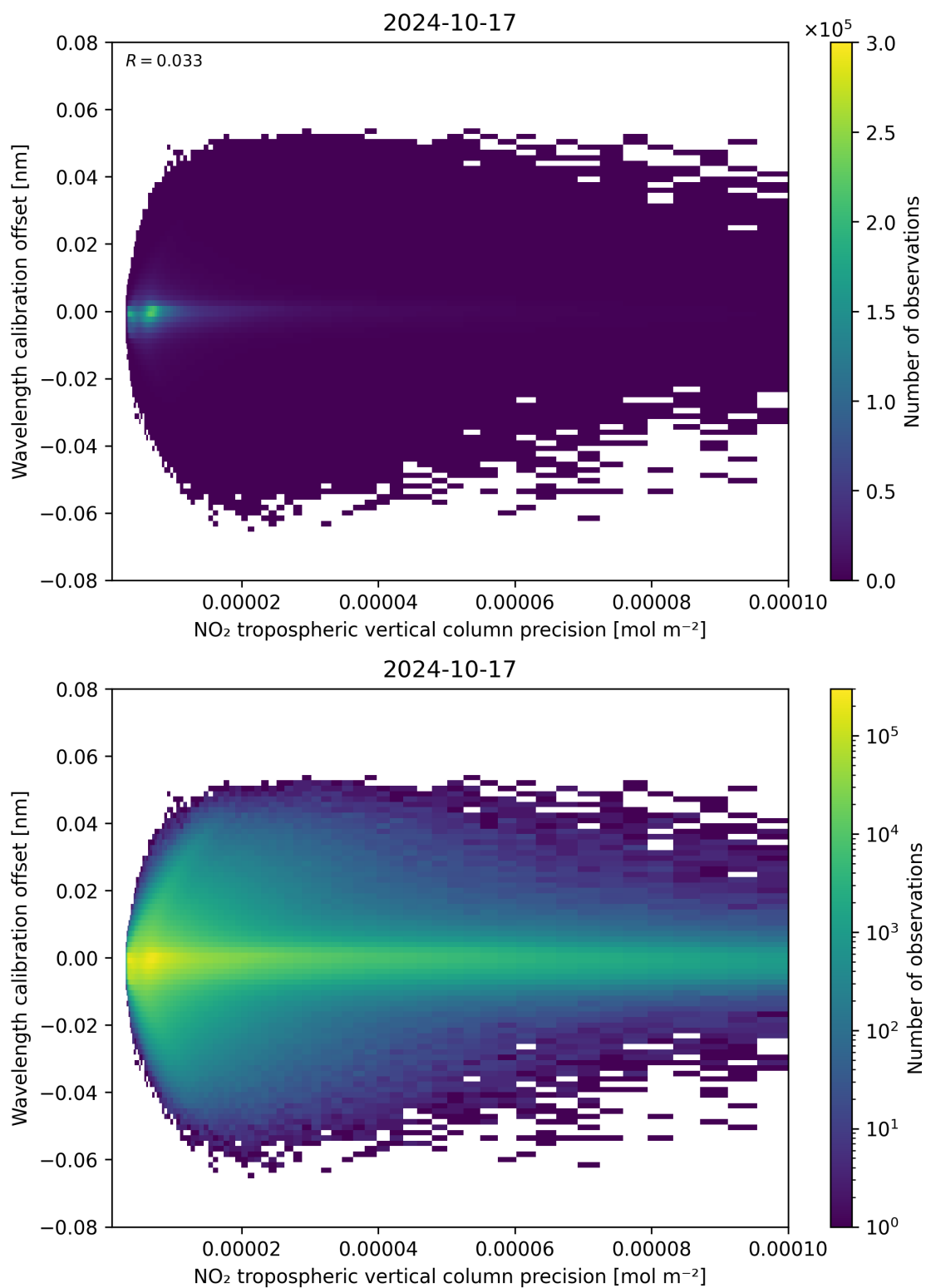
Figure 141: Scatter density plot of “NO 2 tropospheric vertical column precision” against “Wavelength calibration offset” for 2024-10-16 to 2024-10-18.
