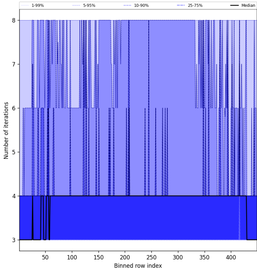
Figure 51: Along track statistics of “Number of iterations” for 2024-10-16 to 2024-10-18
