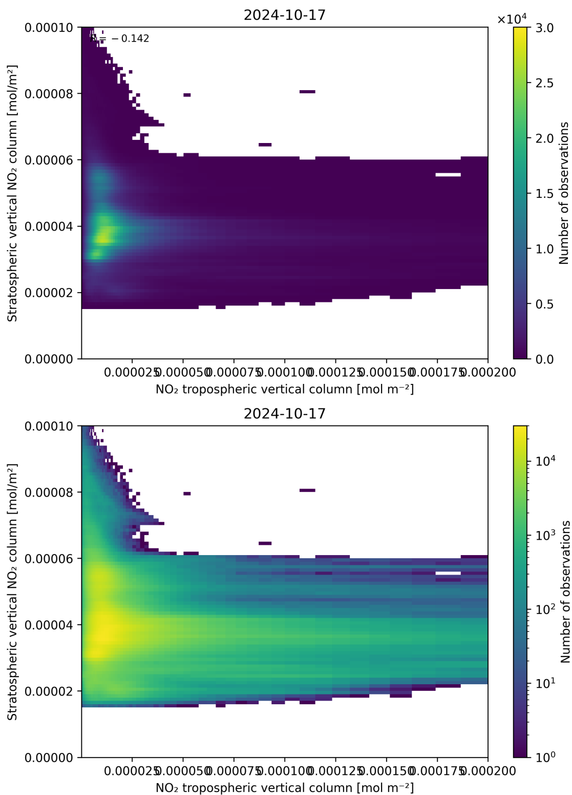
Figure 125: Scatter density plot of “NO 2 tropospheric vertical column” against “Stratospheric vertical NO 2 column” for 2024-10-16 to 2024-10-18.
