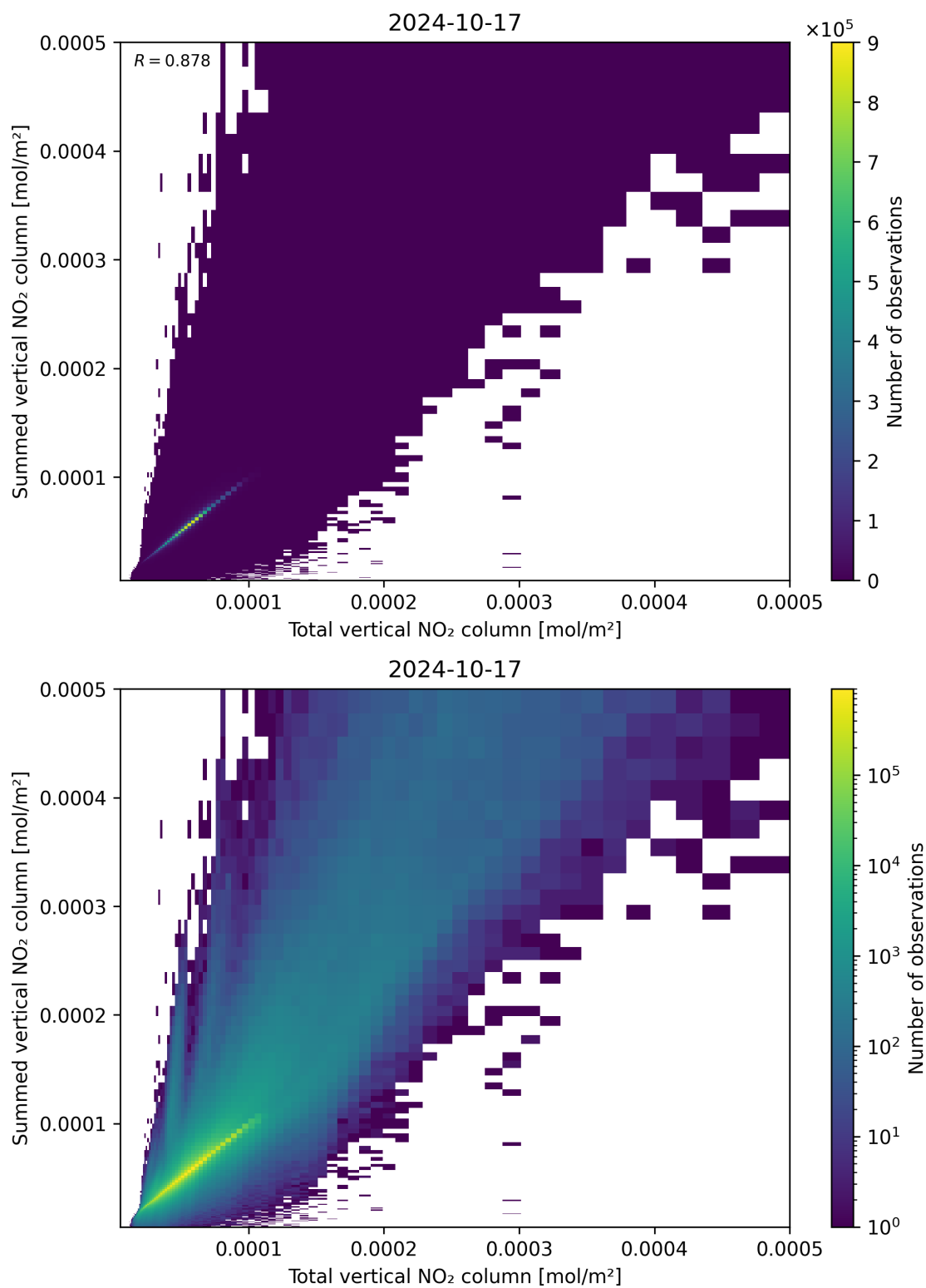
Figure 112: Scatter density plot of “Total vertical NO 2 column” against “Summed vertical NO 2 column” for 2024-10-16 to 2024-10-18.
