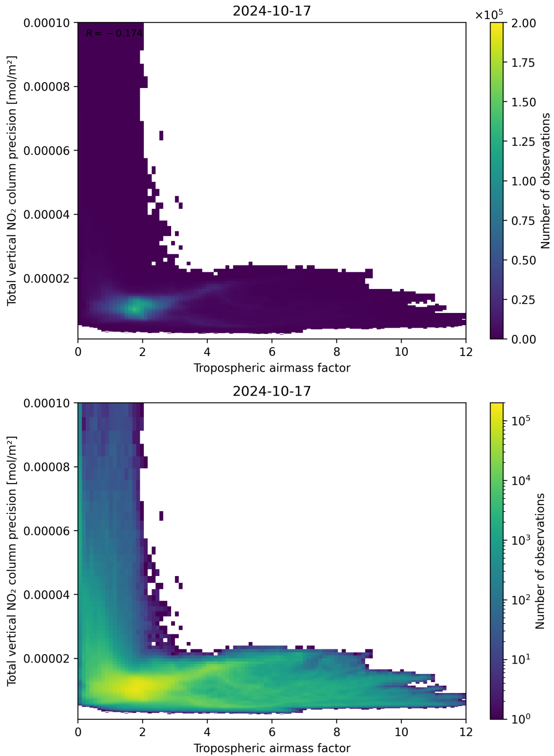
Figure 78: Scatter density plot of “Tropospheric air mass factor” against “Total vertical NO 2 column precision” for 2024-10-16 to 2024-10-18.
