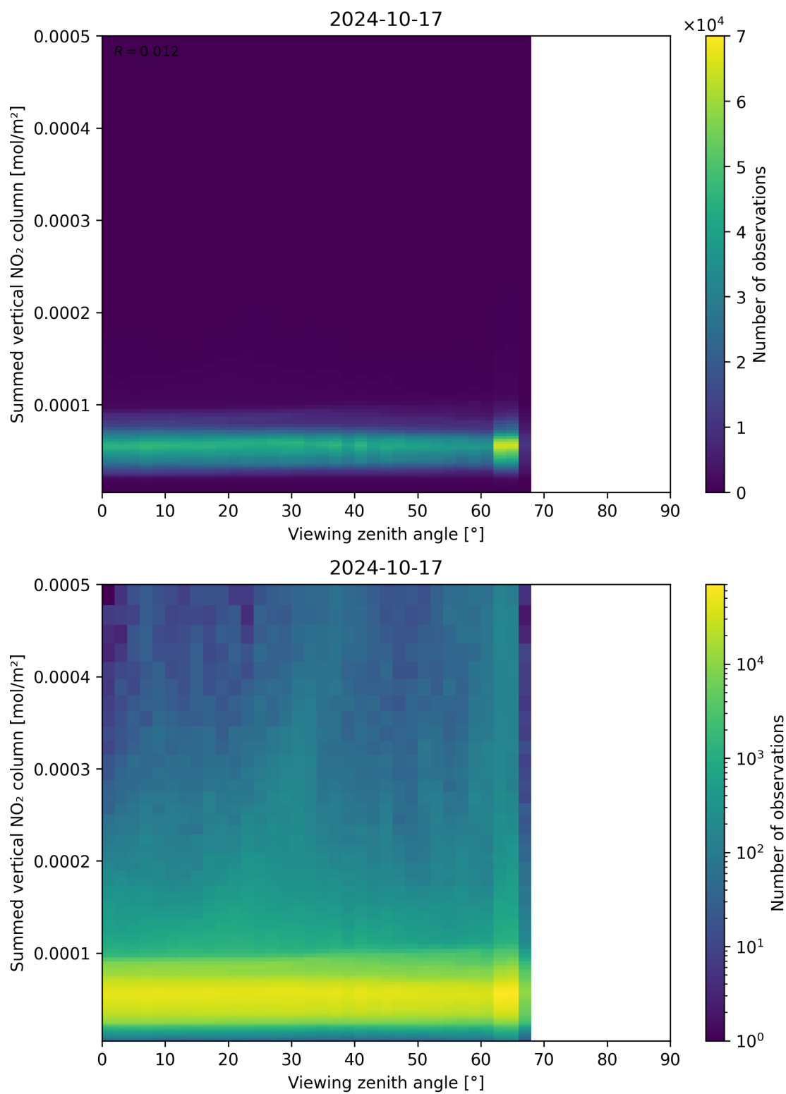
Figure 165: Scatter density plot of “Viewing zenith angle” against “Summed vertical NO 2 column” for 2024-10-16 to 2024-10-18.
