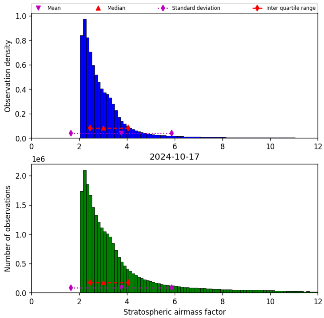
Figure 44: Histogram of “Stratospheric airmass factor” for 2024-10-16 to 2024-10-18
