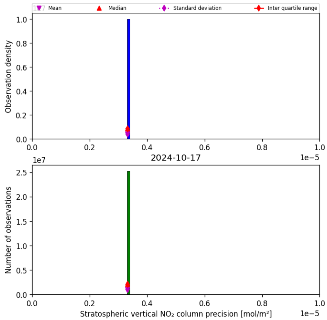
Figure 37: Histogram of “Stratospheric vertical NO 2 column precision” for 2024-10-16 to 2024-10-18
