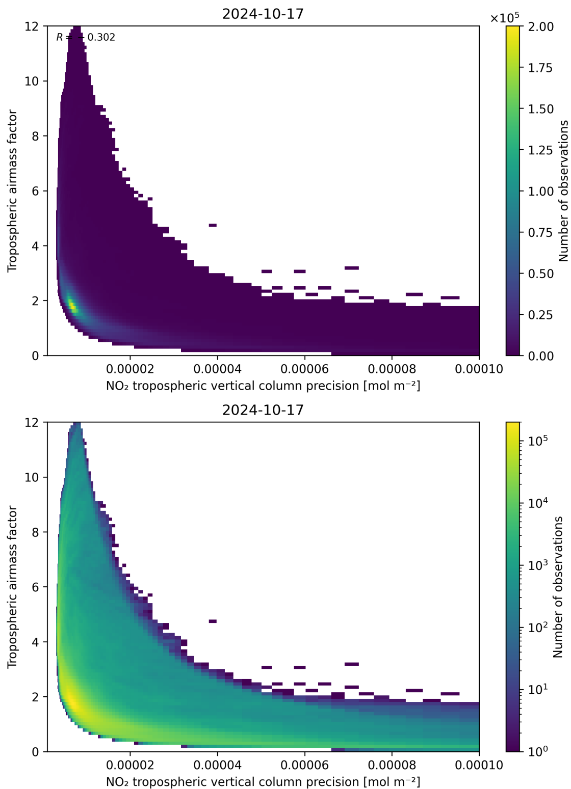
Figure 133: Scatter density plot of “NO 2 tropospheric vertical column precision” against “Tropospheric air mass factor” for 2024-10-16 to 2024-10-18.
