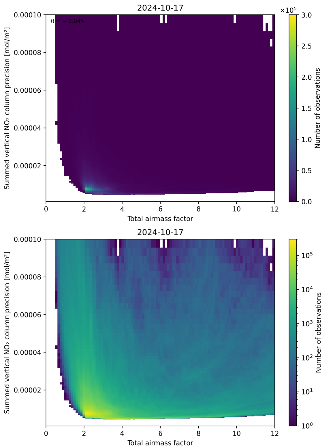
Figure 66: Scatter density plot of “Total airmass factor” against “Summed vertical NO 2 column precision” for 2024-10-16 to 2024-10-18.
