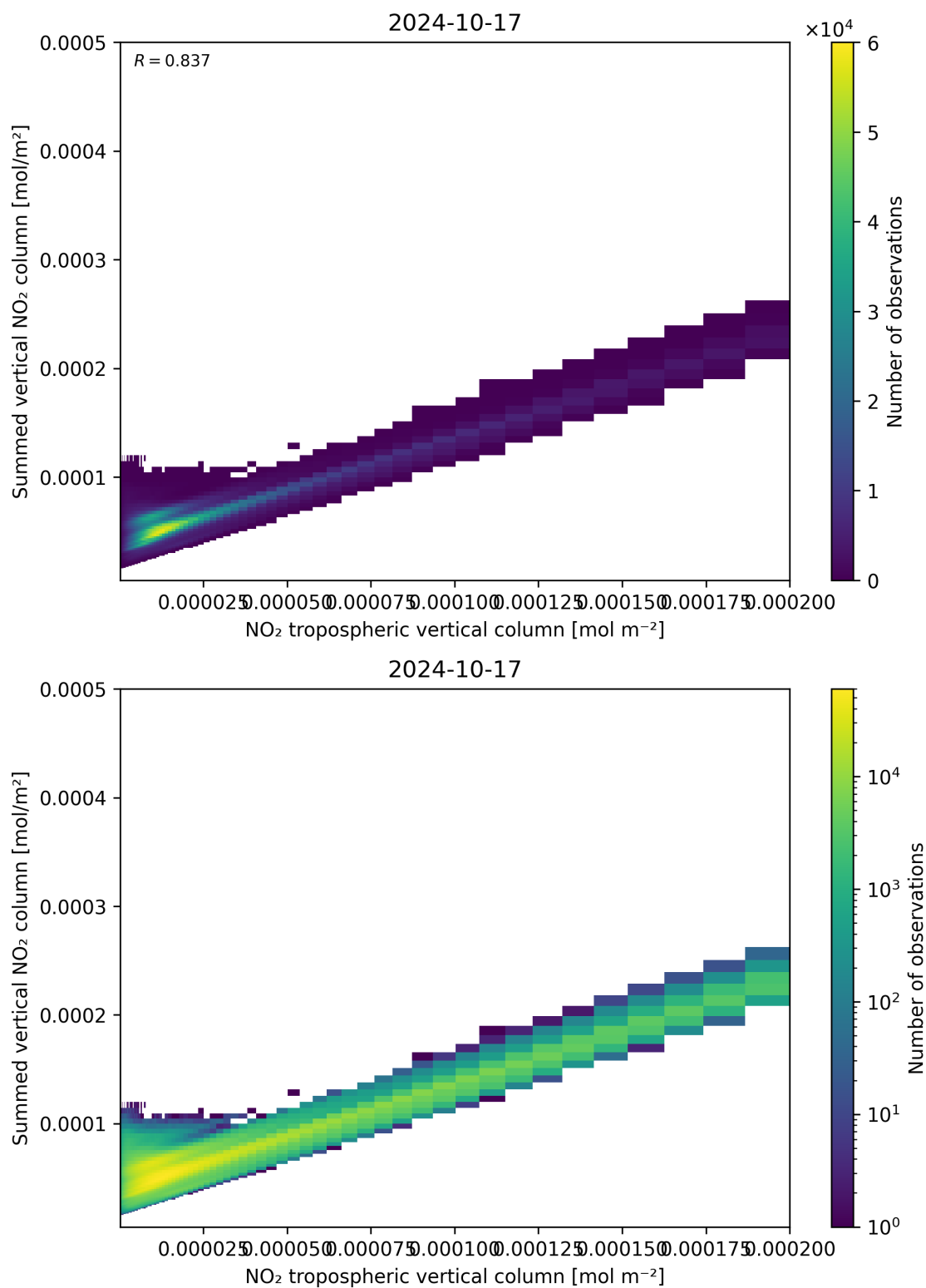
Figure 126: Scatter density plot of “NO 2 tropospheric vertical column” against “Summed vertical NO 2 column” for 2024-10-16 to 2024-10-18.
