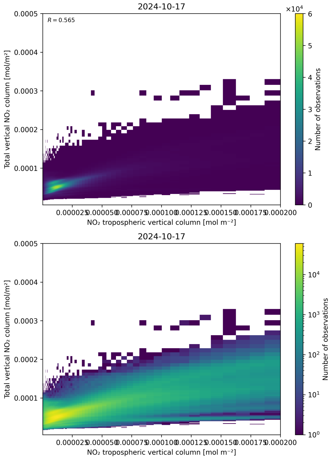
Figure 128: Scatter density plot of “NO 2 tropospheric vertical column” against “Total vertical NO 2 column” for 2024-10-16 to 2024-10-18.
