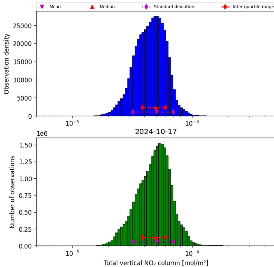
Figure 38: Histogram of “Total vertical NO 2 column” for 2024-10-16 to 2024-10-18
