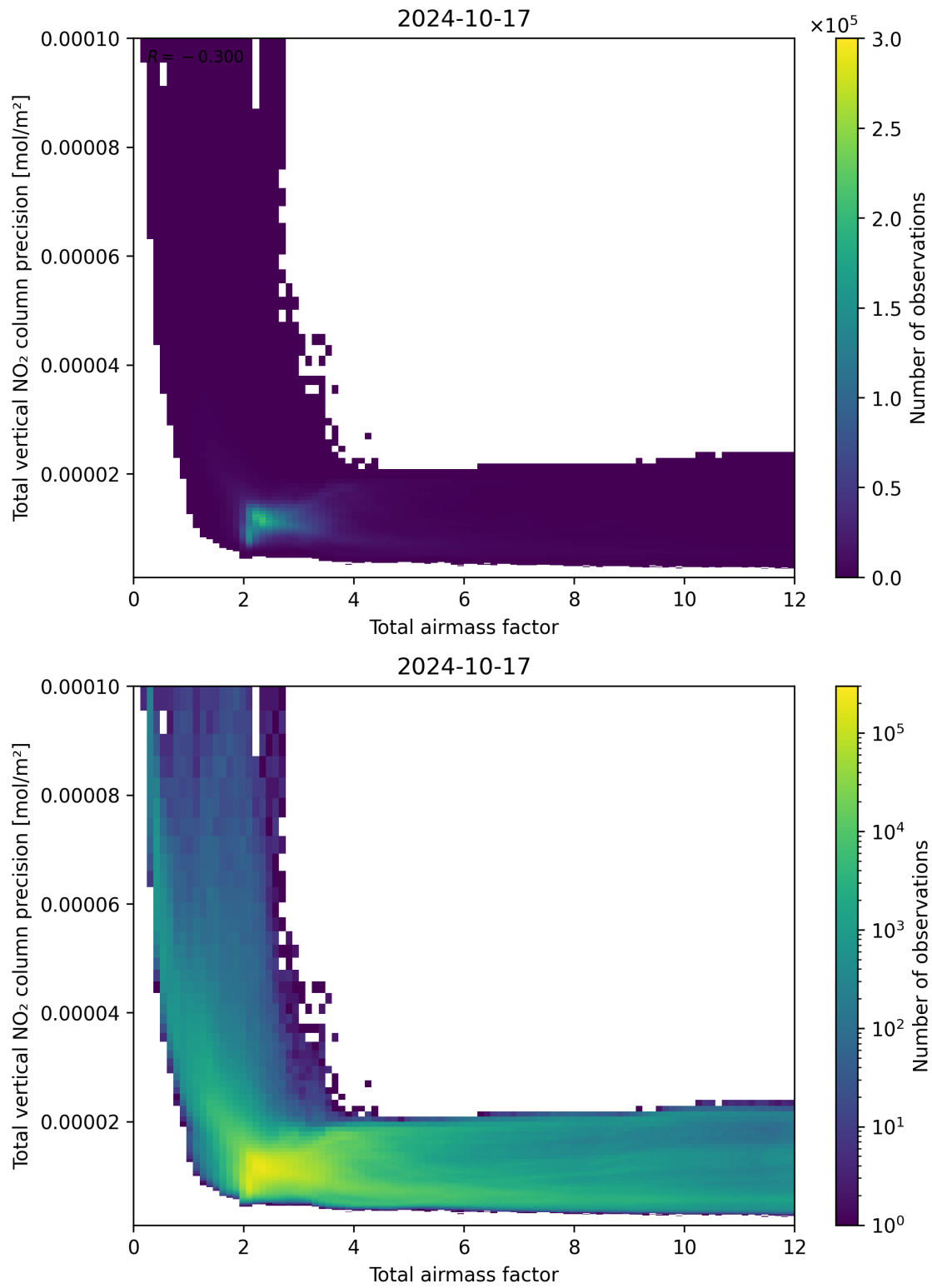
Figure 68: Scatter density plot of “Total airmass factor” against “Total vertical NO 2 column precision” for 2024-10-16 to 2024-10-18.
