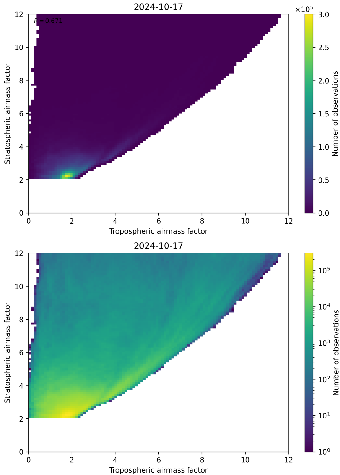
Figure 71: Scatter density plot of “Tropospheric airmass factor” against “Stratospheric airmass factor” for 2024-10-16 to 2024-10-18.
