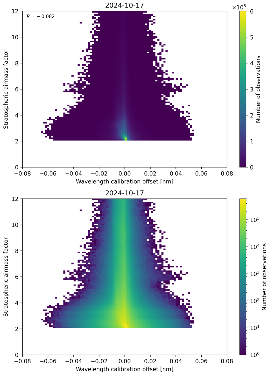
Figure 174: Scatter density plot of “Wavelength calibration offset” against “Stratospheric air mass factor” for 2024-10-16 to 2024-10-18.
