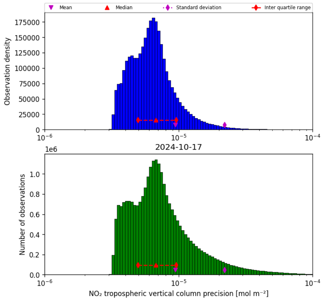
Figure 30: Histogram of “NO 2 tropospheric vertical column precision” for 2024-10-16 to 2024-10-18
