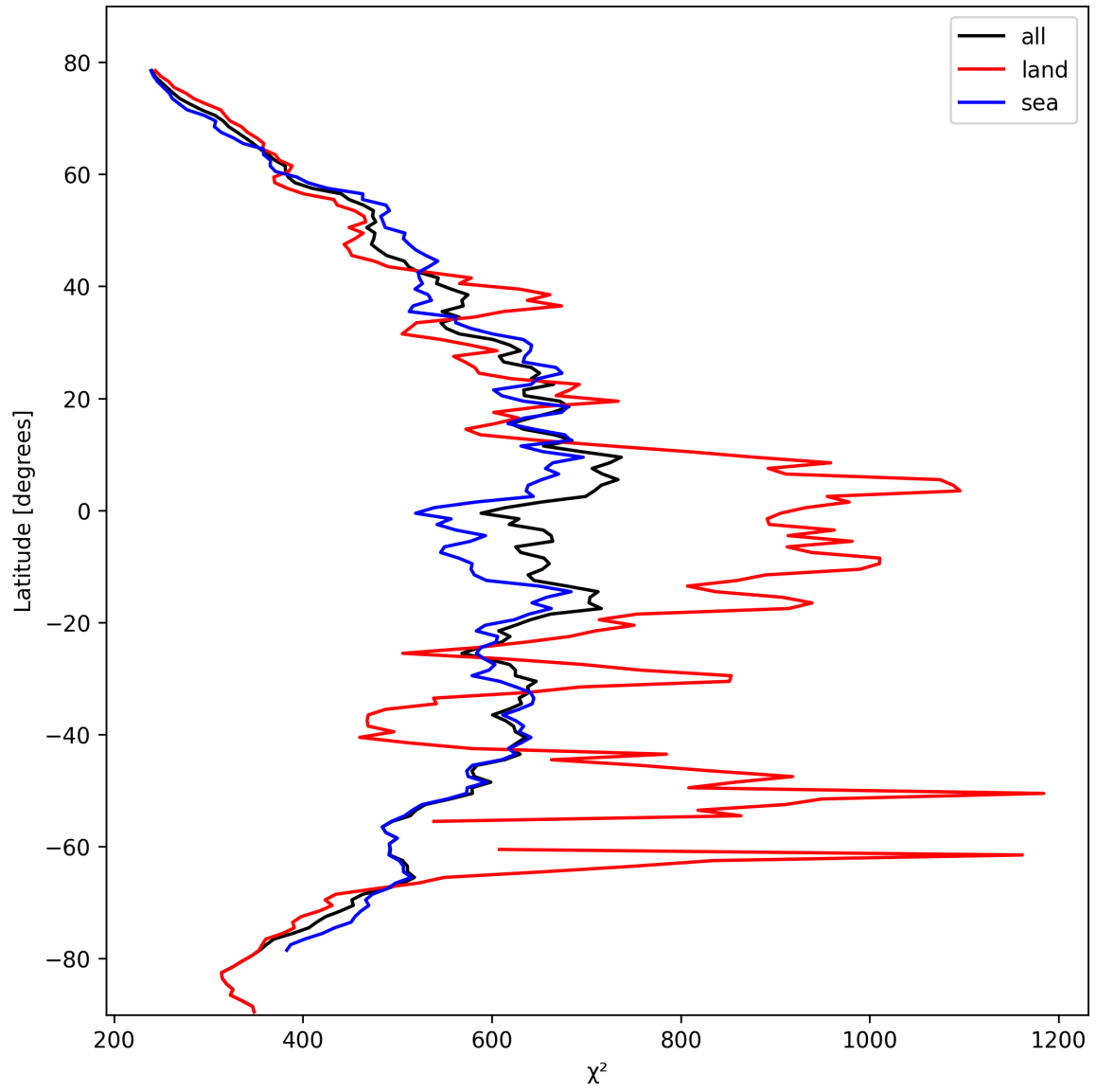
Figure 25: Zonal average of “ \chi^2 ” for 2024-10-16 to 2024-10-18.
