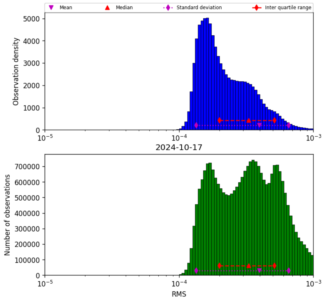
Figure 43: Histogram of “RMS” for 2024-10-16 to 2024-10-18
