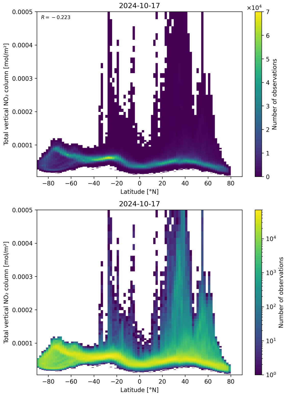
Figure 90: Scatter density plot of “Latitude” against “Total vertical NO 2 column” for 2024-10-16 to 2024-10-18.
