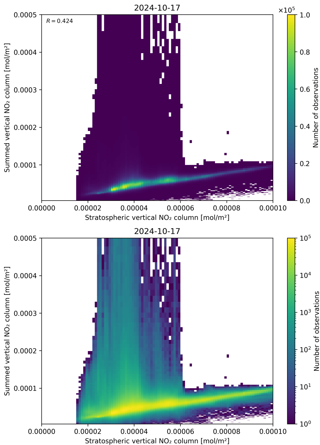
Figure 98: Scatter density plot of “Stratospheric vertical NO 2 column” against “Summed vertical NO 2 column” for 2024-10-16 to 2024-10-18.
