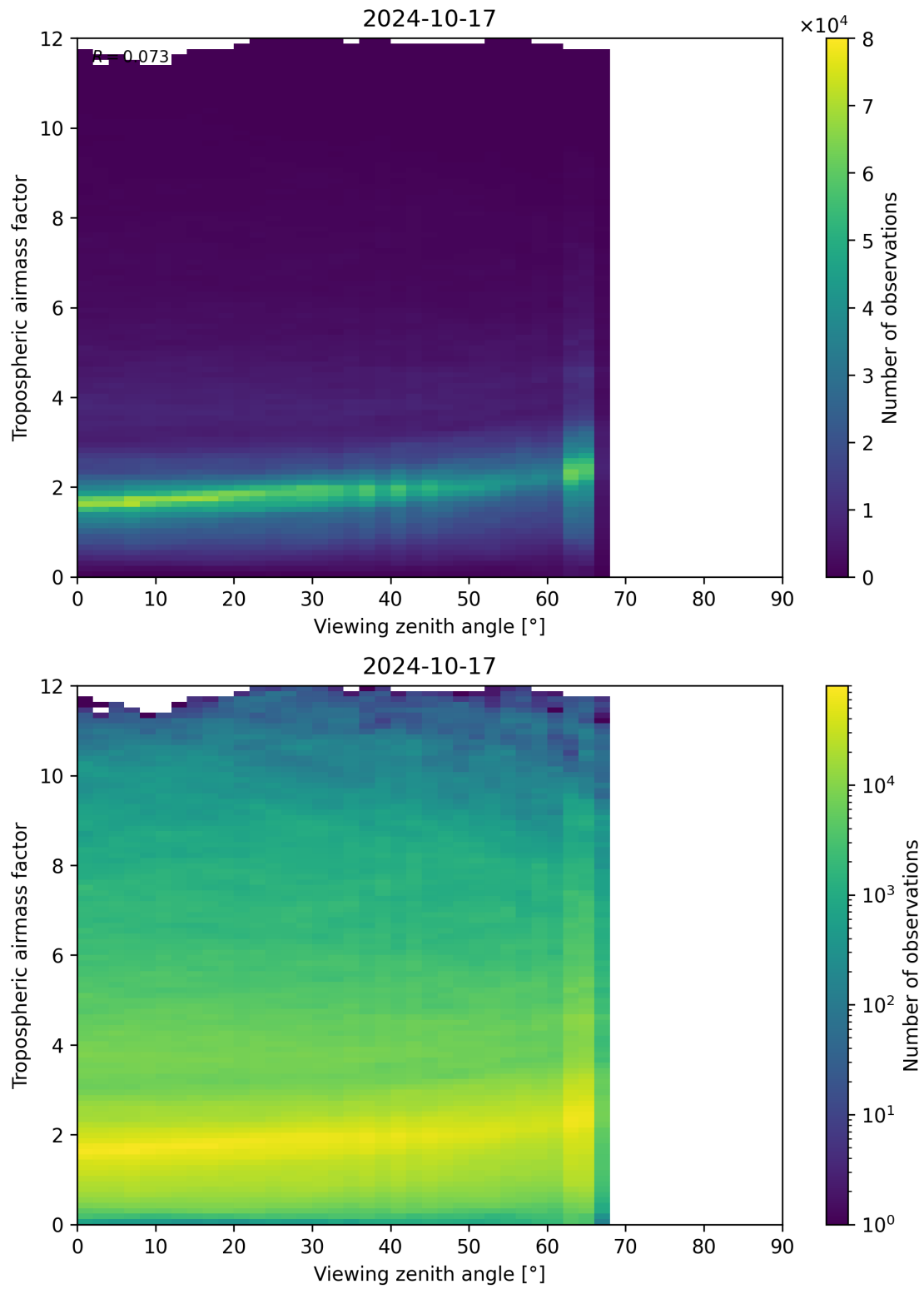
Figure 161: Scatter density plot of “Viewing zenith angle” against “Tropospheric airmass factor” for 2024-10-16 to 2024-10-18.
