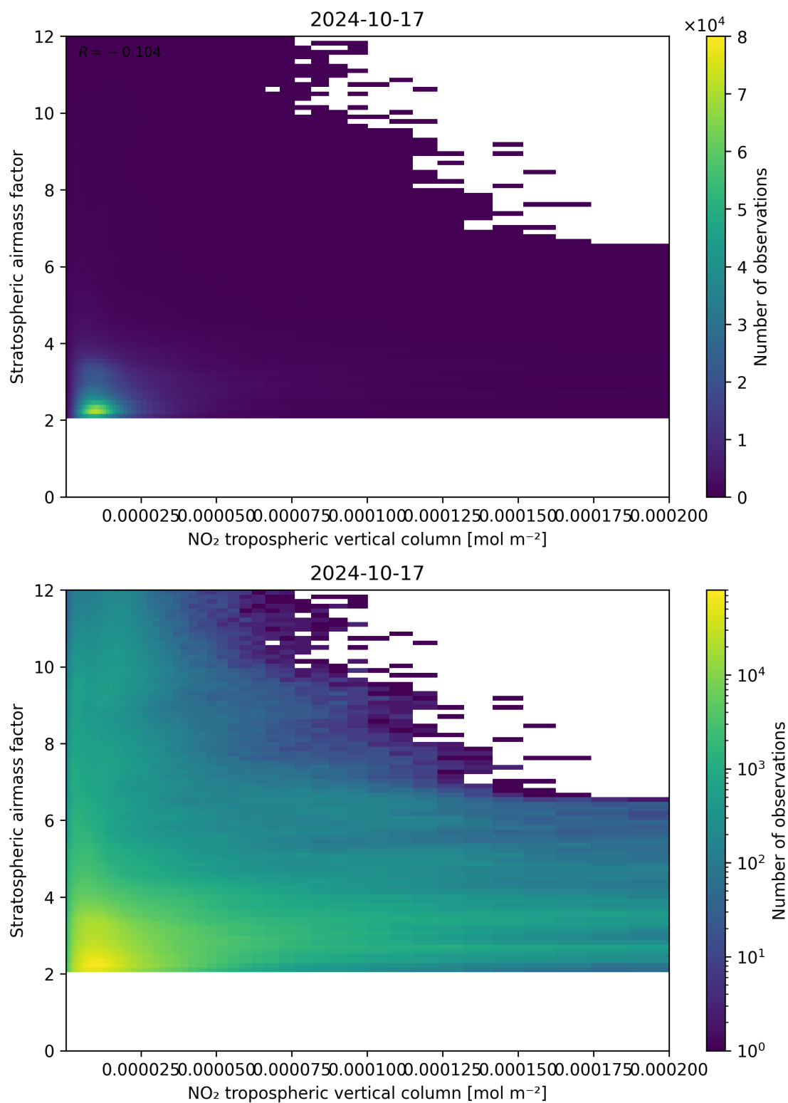
Figure 121: Scatter density plot of “NO 2 tropospheric vertical column” against “Stratospheric air mass factor” for 2024-10-16 to 2024-10-18.
