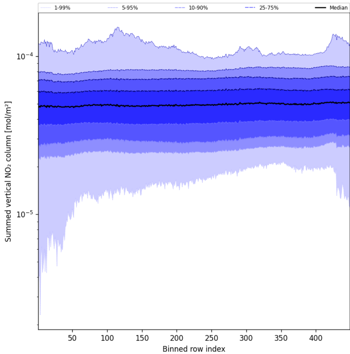
Figure 57: Along track statistics of “Summed vertical NO 2 column” for 2024-10-16 to 2024-10-18
