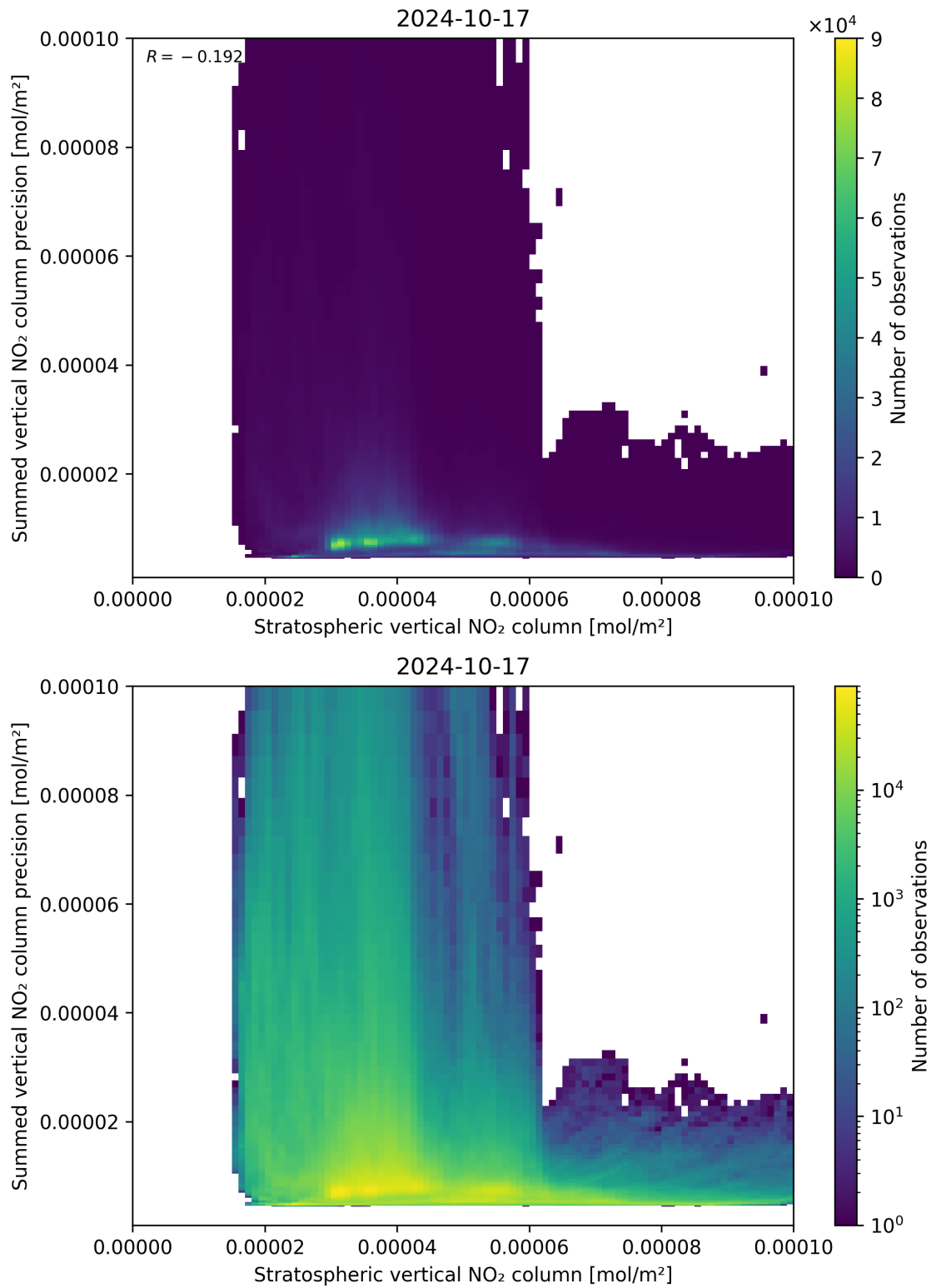
Figure 99: Scatter density plot of “Stratospheric vertical NO 2 column” against “Summed vertical NO 2 column precision” for 2024-10-16 to 2024-10-18.
