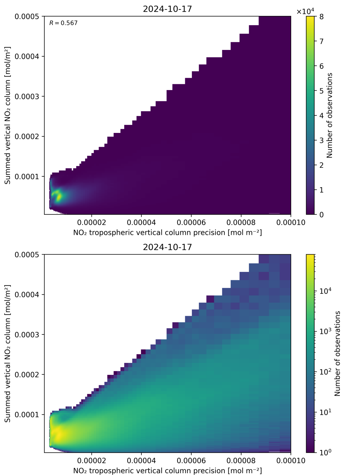
Figure 136: Scatter density plot of “NO 2 tropospheric vertical column precision” against “Summed vertical NO 2 column” for 2024-10-16 to 2024-10-18.
