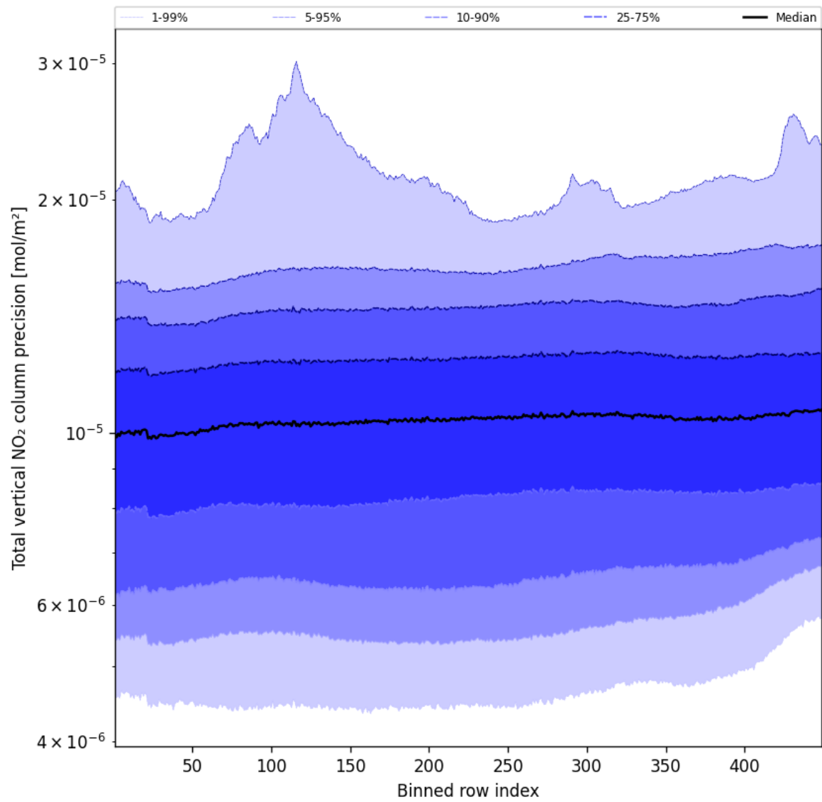
Figure 56: Along track statistics of “Total vertical NO 2 column precision” for 2024-10-16 to 2024-10-18
