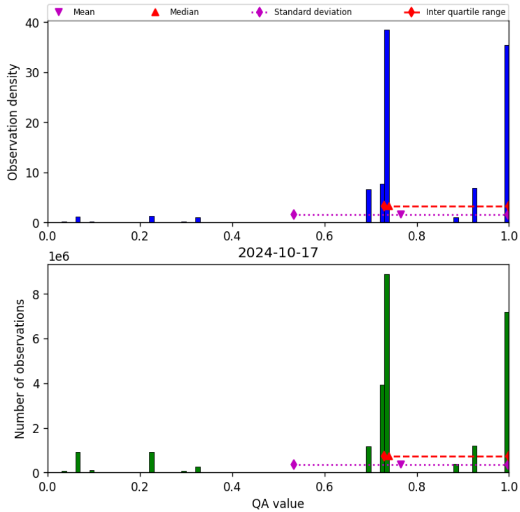
Figure 28: Histogram of “QA value” for 2024-10-16 to 2024-10-18
