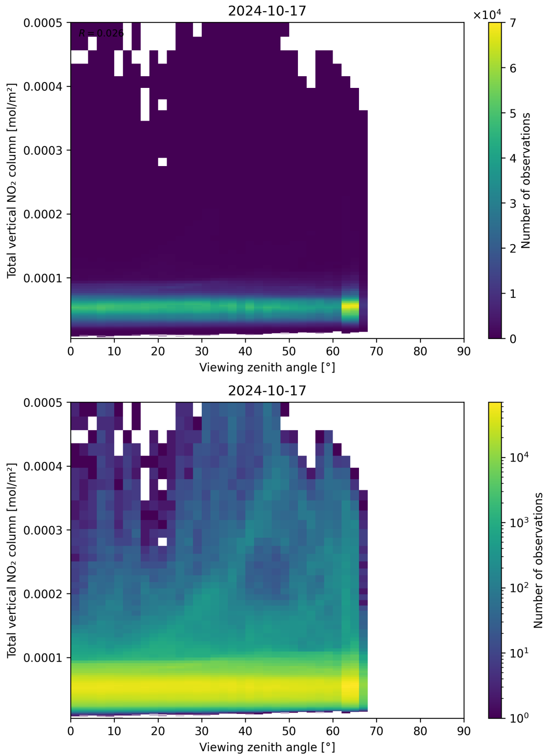
Figure 167: Scatter density plot of “Viewing zenith angle” against “Total vertical NO 2 column” for 2024-10-16 to 2024-10-18.
