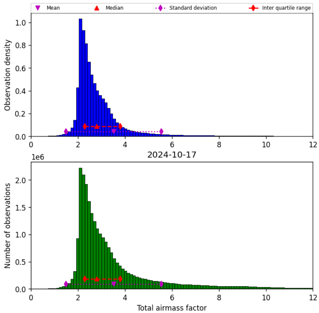
Figure 32: Histogram of “Total airmass factor” for 2024-10-16 to 2024-10-18
