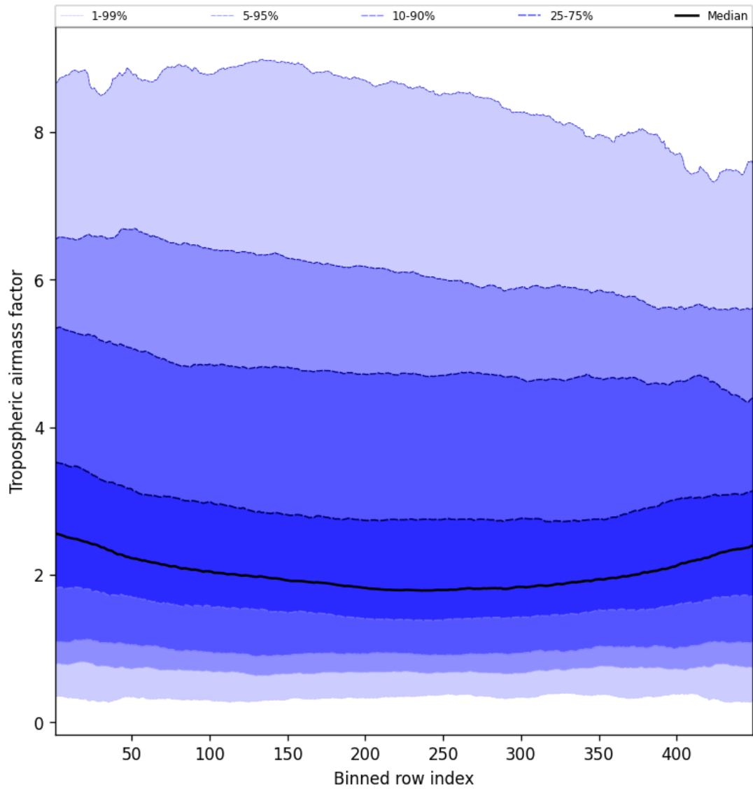
Figure 48: Along track statistics of “Tropospheric air mass factor” for 2024-10-16 to 2024-10-18
