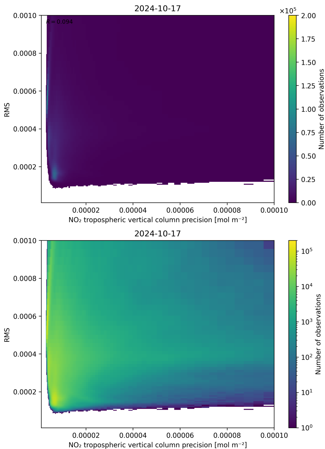
Figure 140: Scatter density plot of “NO 2 tropospheric vertical column precision” against “RMS” for 2024-10-16 to 2024-10-18.
