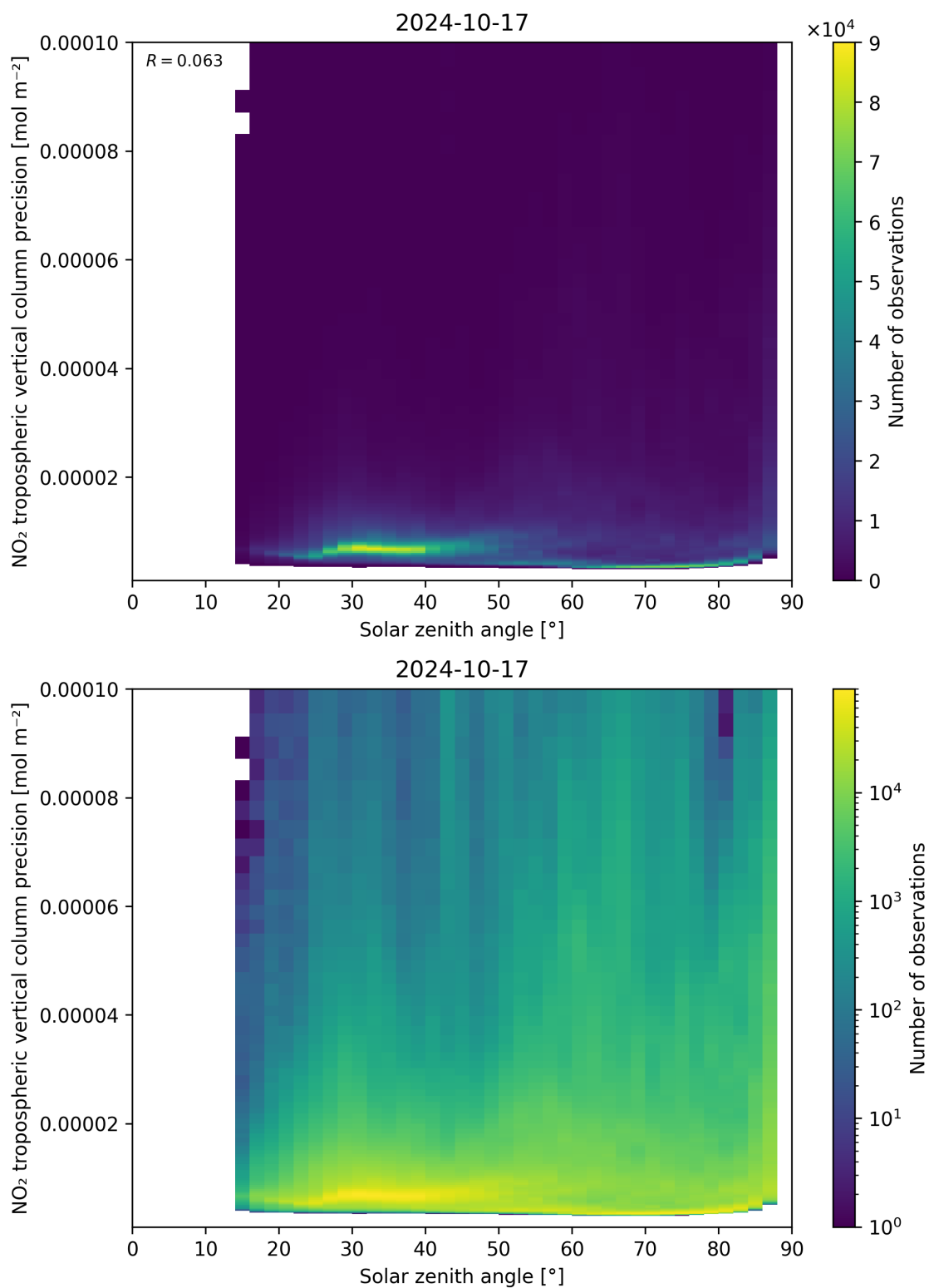
Figure 156: Scatter density plot of “Solar zenith angle” against “NO 2 tropospheric vertical column precision” for 2024-10-16 to 2024-10-18.
