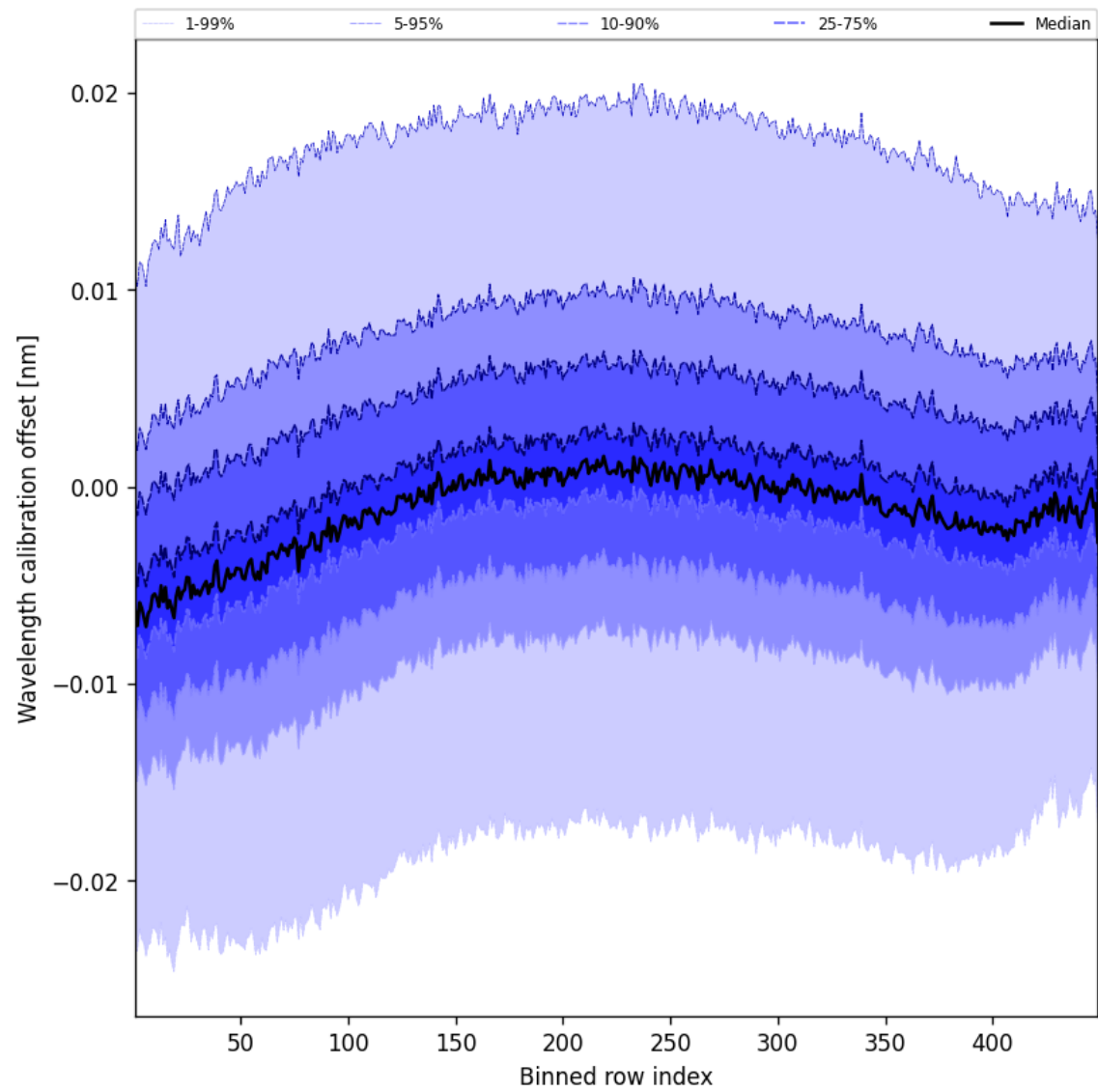
Figure 52: Along track statistics of “Wavelength calibration offset” for 2024-10-16 to 2024-10-18
