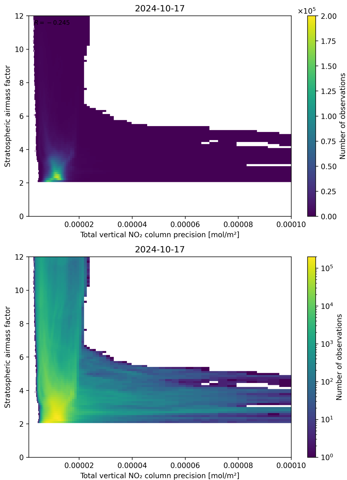
Figure 115: Scatter density plot of “Total vertical NO 2 column precision” against “Stratospheric air mass factor” for 2024-10-16 to 2024-10-18.
