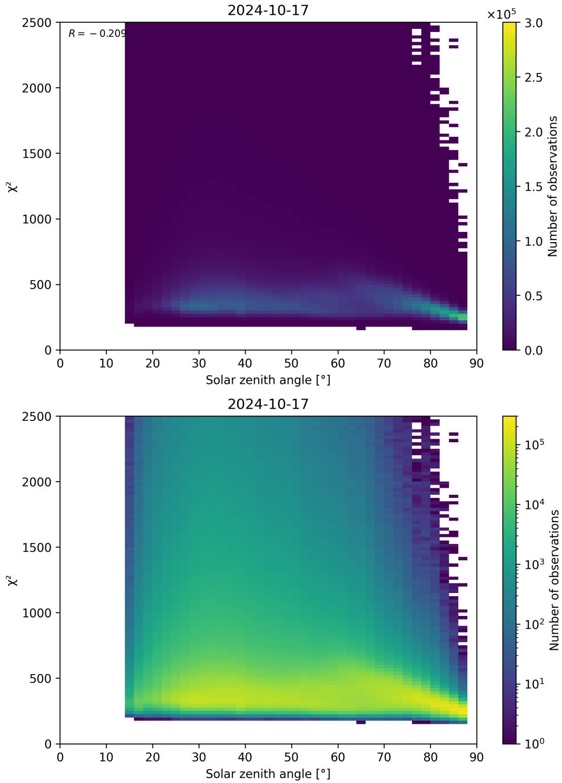
Figure 148: Scatter density plot of “Solar zenith angle” against “ \chi^2 ” for 2024-10-16 to 2024-10-18.
