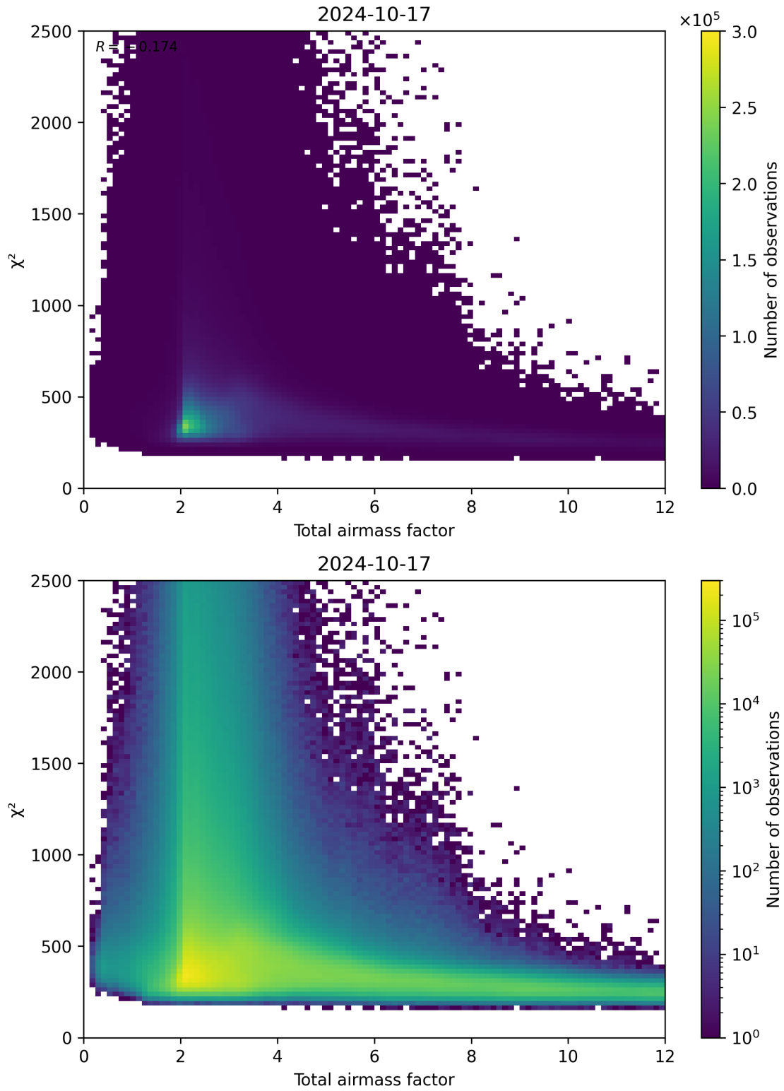
Figure 63: Scatter density plot of “Total airmass factor” against “ \chi^2 ” for 2024-10-16 to 2024-10-18.
