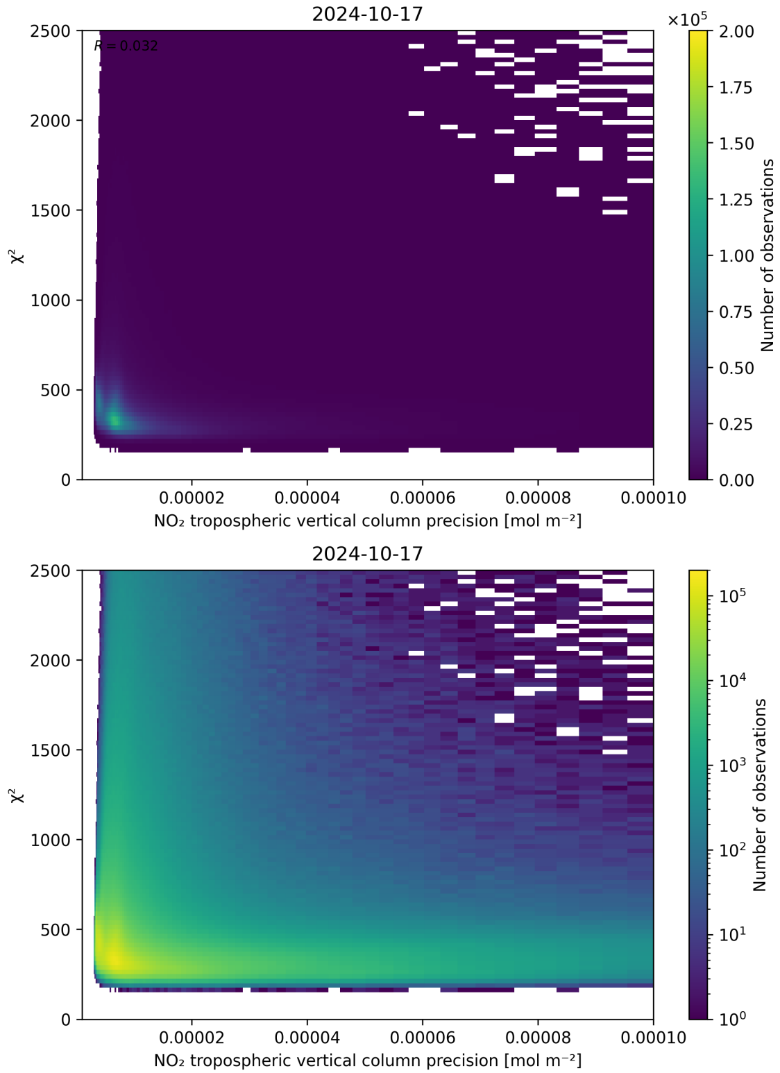
Figure 134: Scatter density plot of “NO 2 tropospheric vertical column precision” against “ \chi^2 ” for 2024-10-16 to 2024-10-18.
