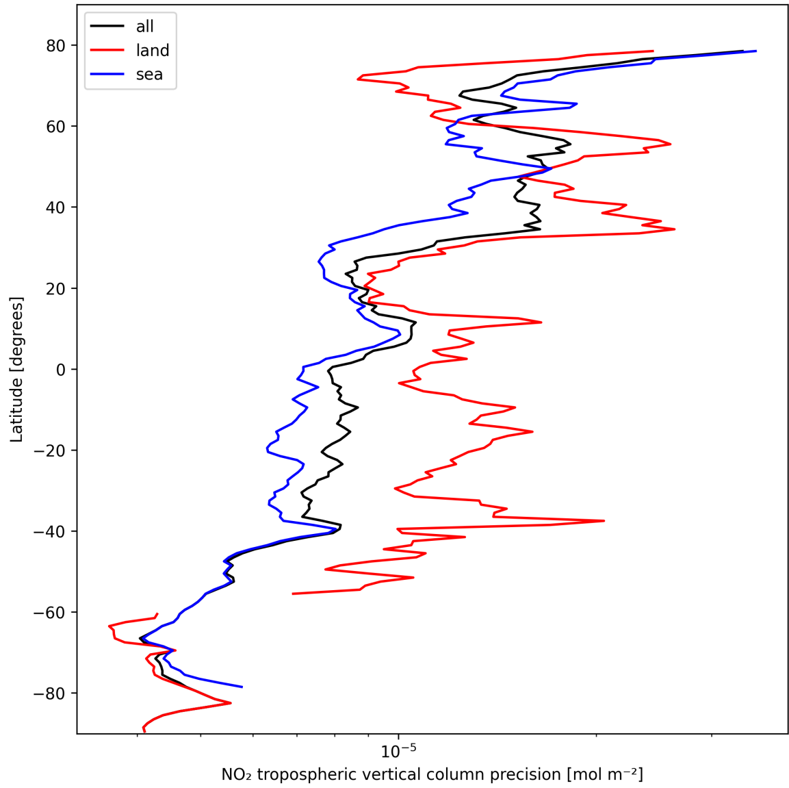
Figure 13: Zonal average of “NO 2 tropospheric vertical column precision” for 2024-10-16 to 2024-10-18.
