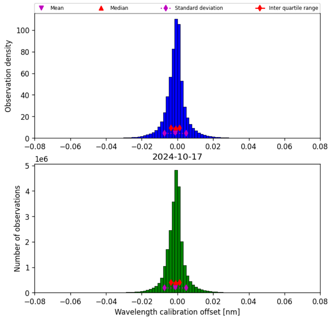
Figure 35: Histogram of “Wavelength calibration offset” for 2024-10-16 to 2024-10-18
