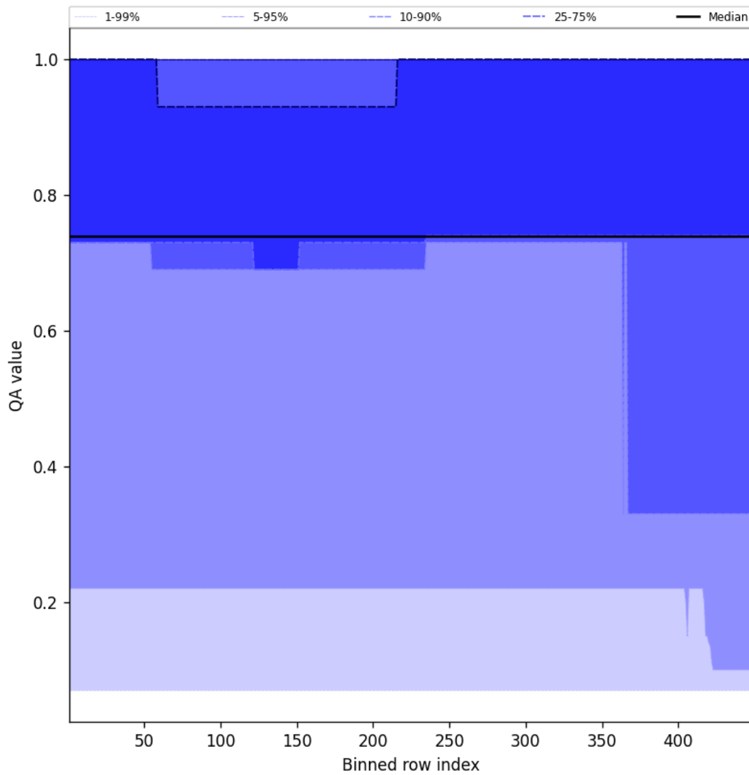
Figure 45: Along track statistics of “QA value” for 2024-10-16 to 2024-10-18
