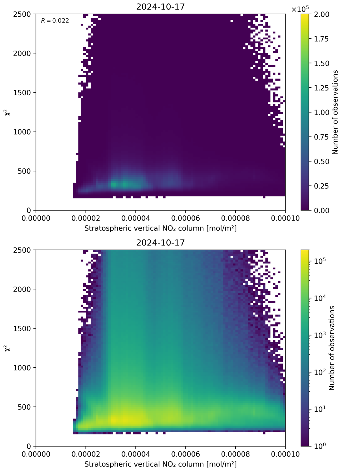
Figure 97: Scatter density plot of “Stratospheric vertical NO 2 column” against “ \chi^2 ” for 2024-10-16 to 2024-10-18.
