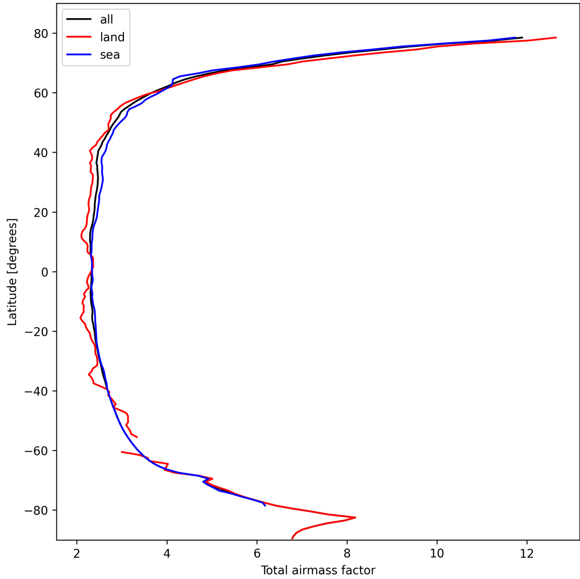
Figure 15: Zonal average of “Total airmass factor” for 2024-10-16 to 2024-10-18.
