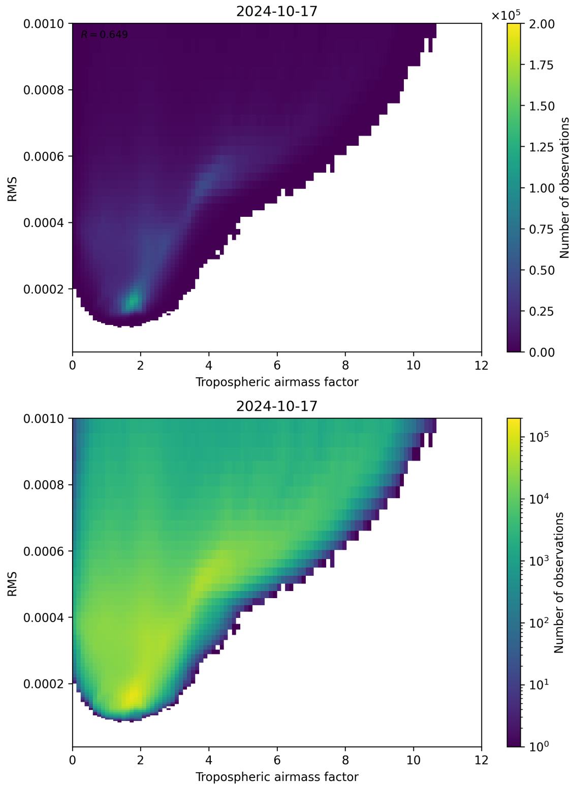
Figure 79: Scatter density plot of “Tropospheric airmass factor” against “RMS” for 2024-10-16 to 2024-10-18.
