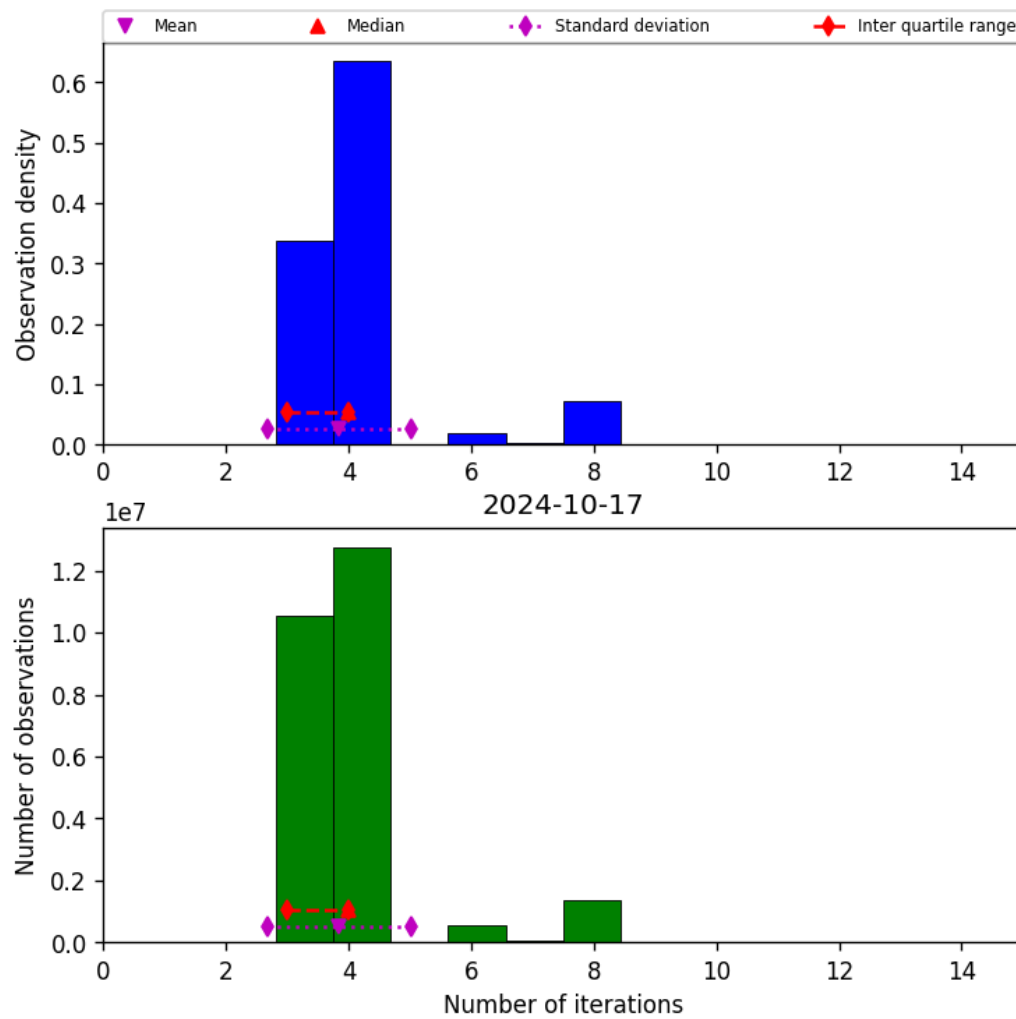
Figure 34: Histogram of “Number of iterations” for 2024-10-16 to 2024-10-18
