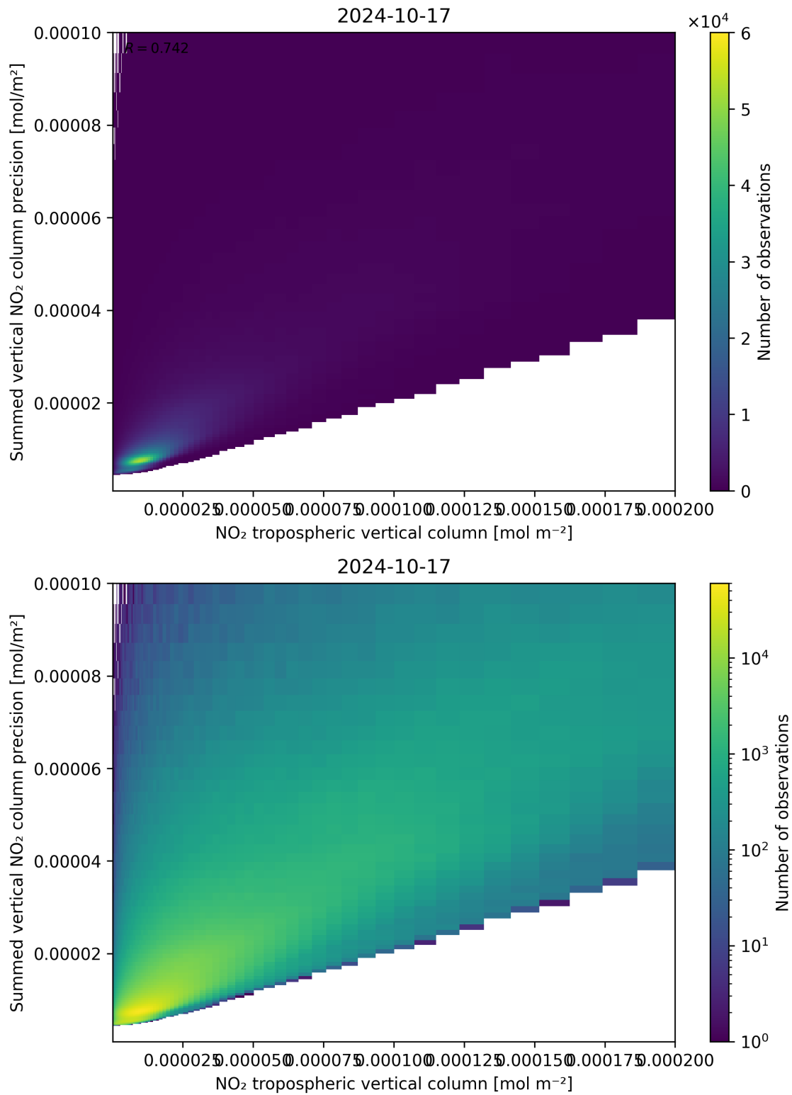
Figure 127: Scatter density plot of “NO 2 tropospheric vertical column” against “Summed vertical NO 2 column precision” for 2024-10-16 to 2024-10-18.
