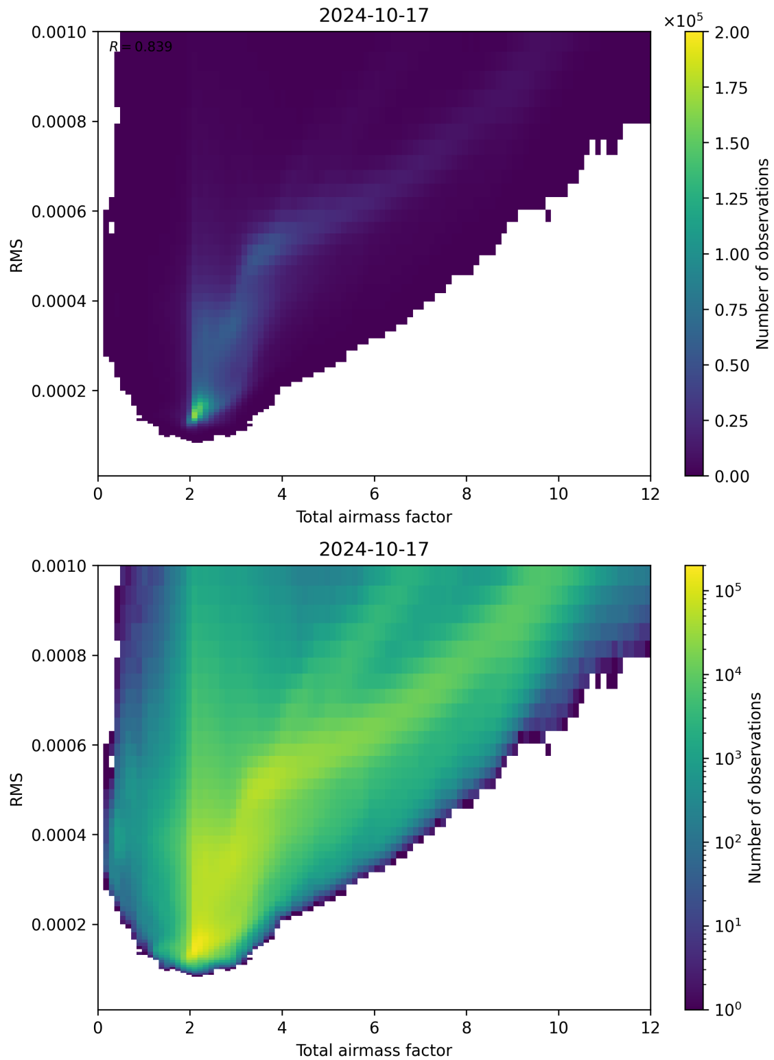
Figure 69: Scatter density plot of “Total airmass factor” against “RMS” for 2024-10-16 to 2024-10-18.
