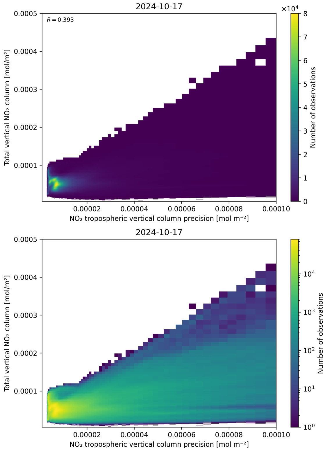
Figure 138: Scatter density plot of “NO 2 tropospheric vertical column precision” against “Total vertical NO 2 column” for 2024-10-16 to 2024-10-18.
