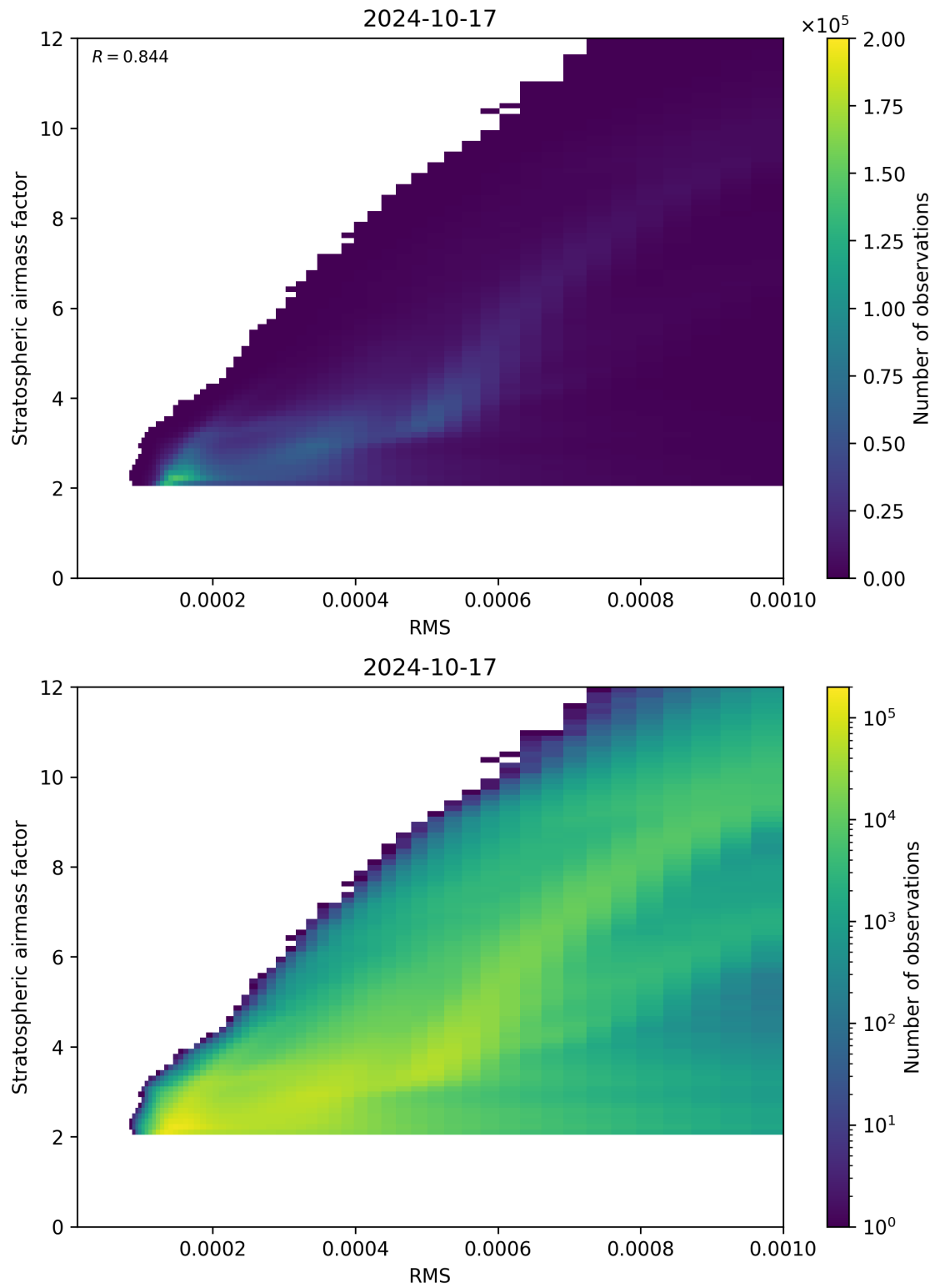
Figure 144: Scatter density plot of “RMS” against “Stratospheric airmass factor” for 2024-10-16 to 2024-10-18.
