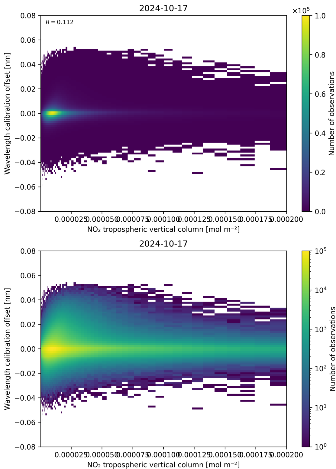
Figure 143: Scatter density plot of “NO 2 tropospheric vertical column” against “Wavelength calibration offset” for 2024-10-16 to 2024-10-18.
