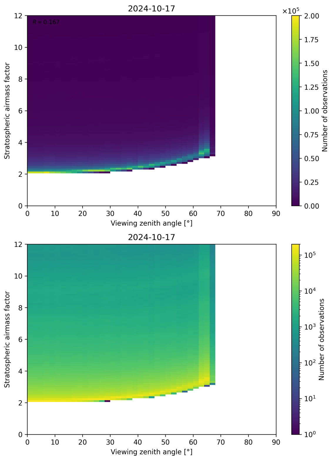
Figure 159: Scatter density plot of “Viewing zenith angle” against “Stratospheric airmass factor” for 2024-10-16 to 2024-10-18.
