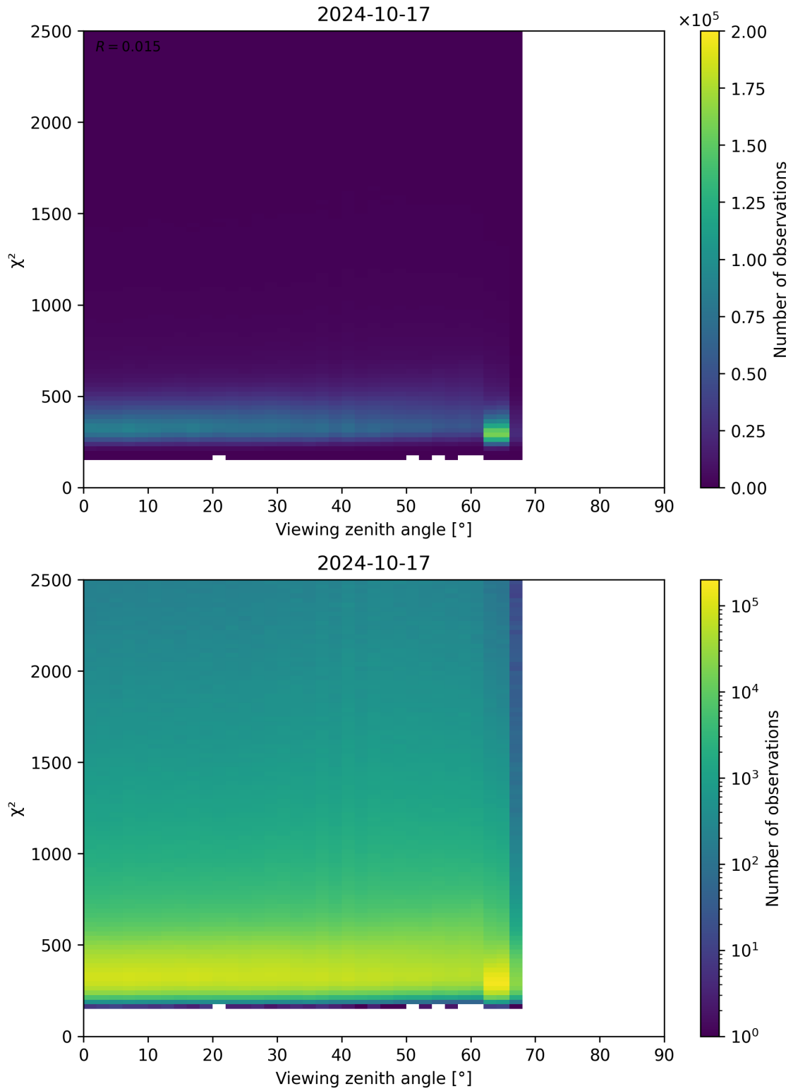
Figure 162: Scatter density plot of “Viewing zenith angle” against “ \chi^2 ” for 2024-10-16 to 2024-10-18.
