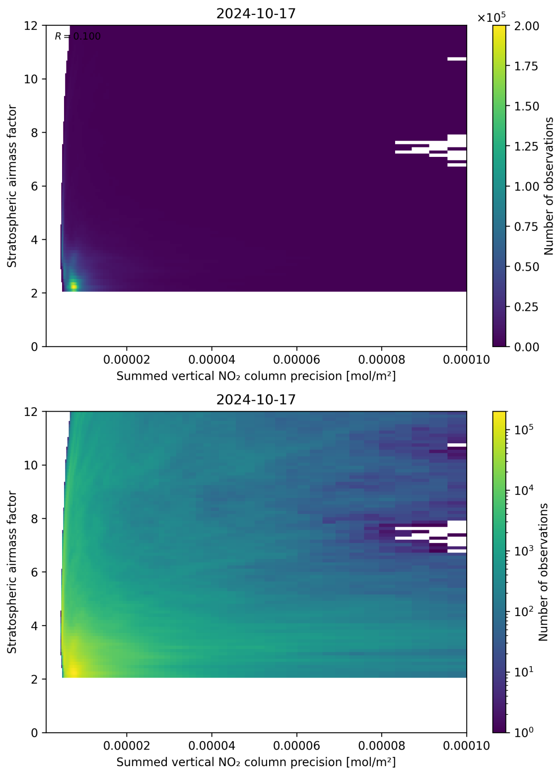
Figure 106: Scatter density plot of “Summed vertical NO 2 column precision” against “Stratospheric airmass factor” for 2024-10-16 to 2024-10-18.
