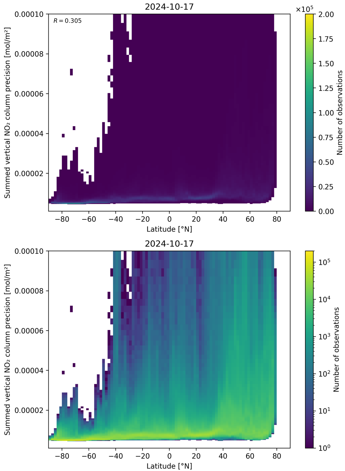
Figure 89: Scatter density plot of “Latitude” against “Summed vertical NO 2 column precision” for 2024-10-16 to 2024-10-18.
