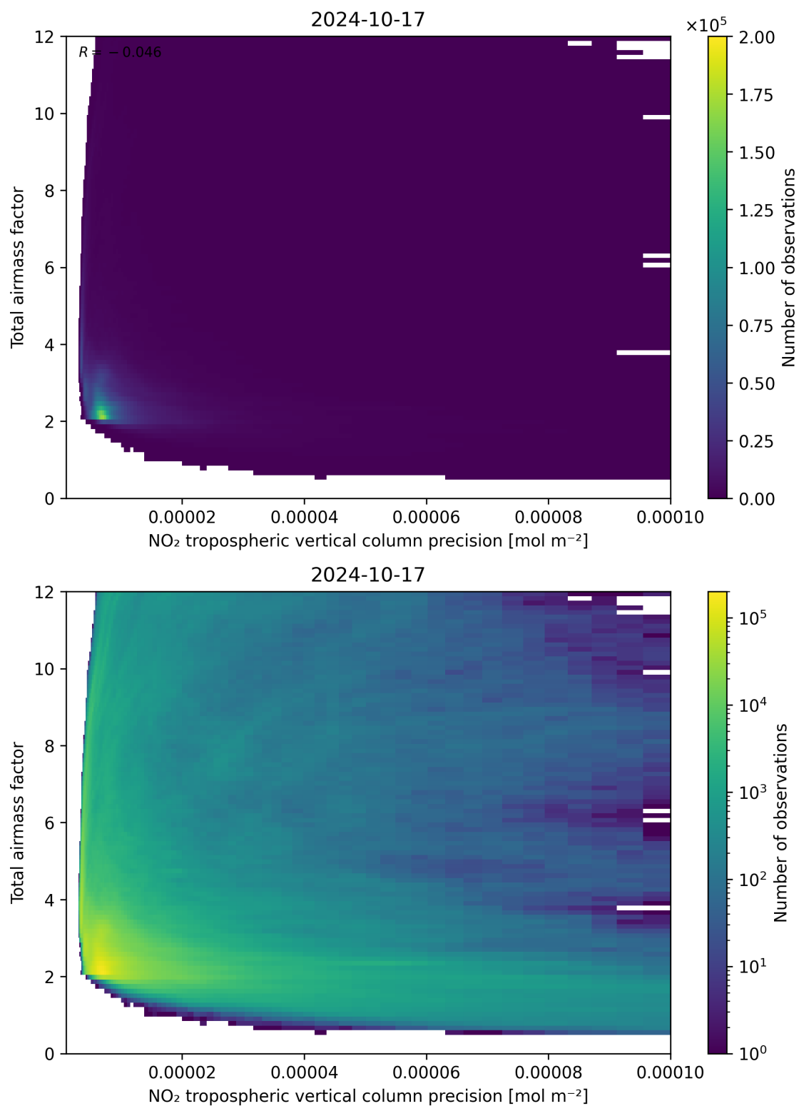
Figure 132: Scatter density plot of “NO 2 tropospheric vertical column precision” against “Total air mass factor” for 2024-10-16 to 2024-10-18.
