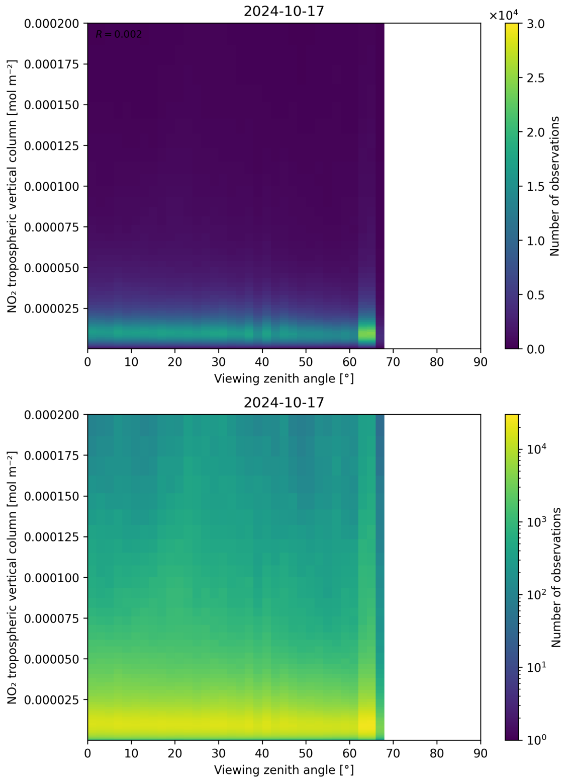
Figure 169: Scatter density plot of “Viewing zenith angle” against “NO 2 tropospheric vertical column” for 2024-10-16 to 2024-10-18.
