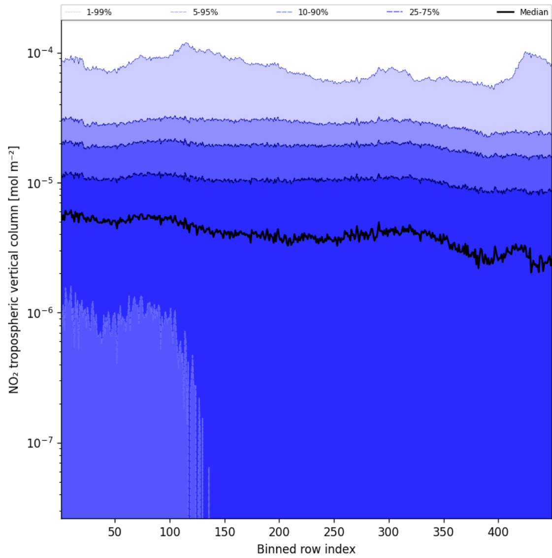
Figure 46: Along track statistics of “NO 2 tropospheric vertical column” for 2024-10-16 to 2024-10-18
