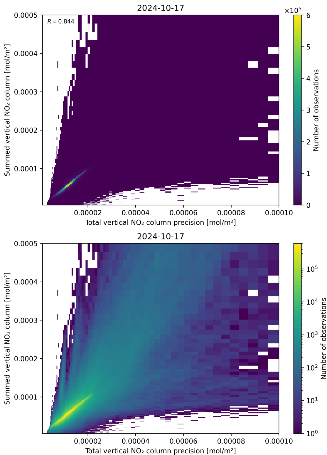
Figure 117: Scatter density plot of “Total vertical NO 2 column precision” against “Summed vertical NO 2 column” for 2024-10-16 to 2024-10-18.
