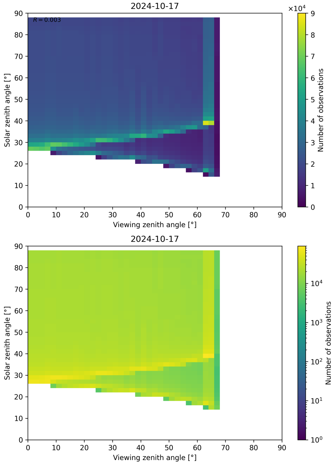
Figure 172: Scatter density plot of “Viewing zenith angle” against “Solar zenith angle” for 2024-10-16 to 2024-10-18.
