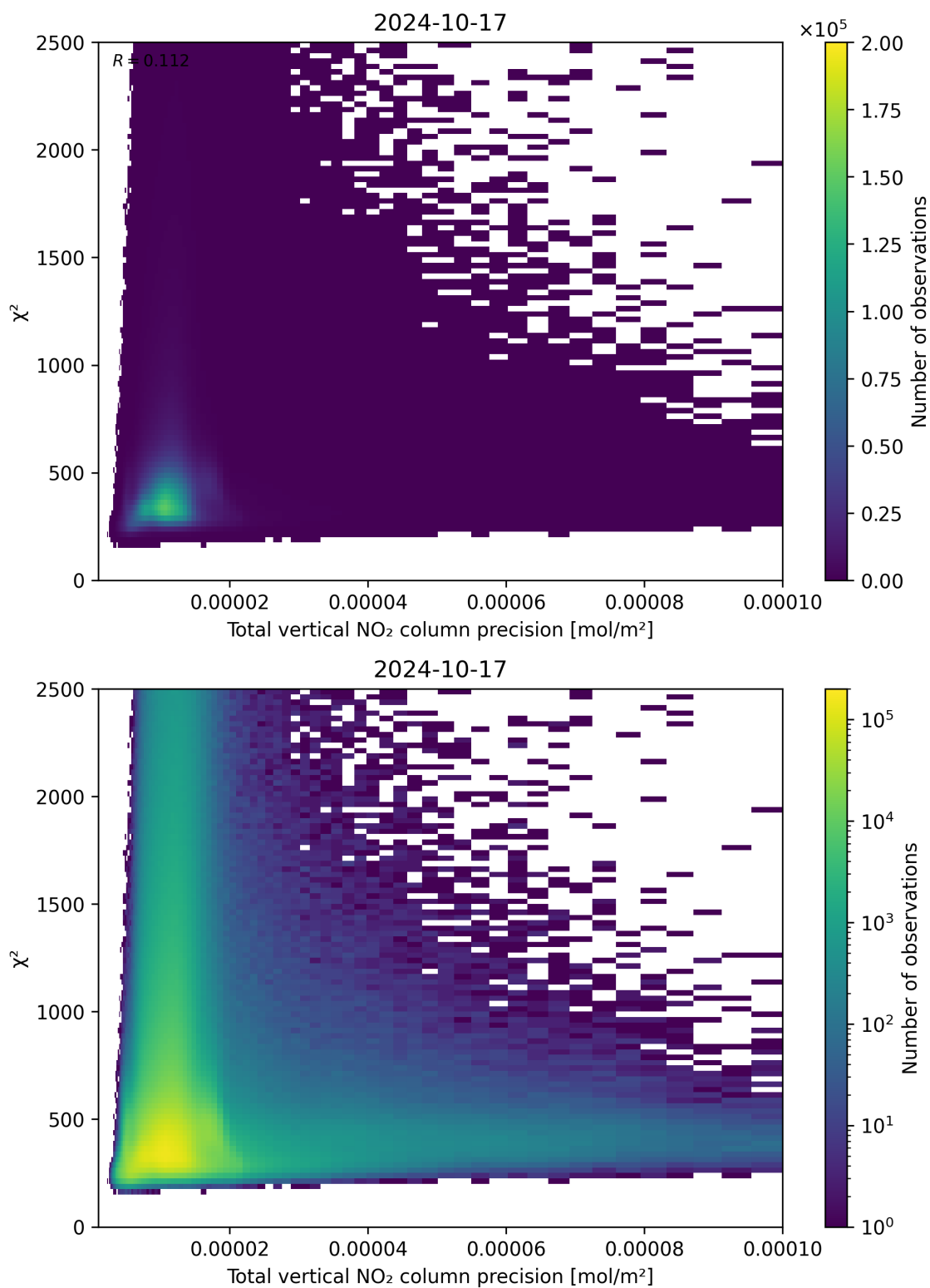
Figure 116: Scatter density plot of “Total vertical NO 2 column precision” against “ \chi^2 ” for 2024-10-16 to 2024-10-18.
