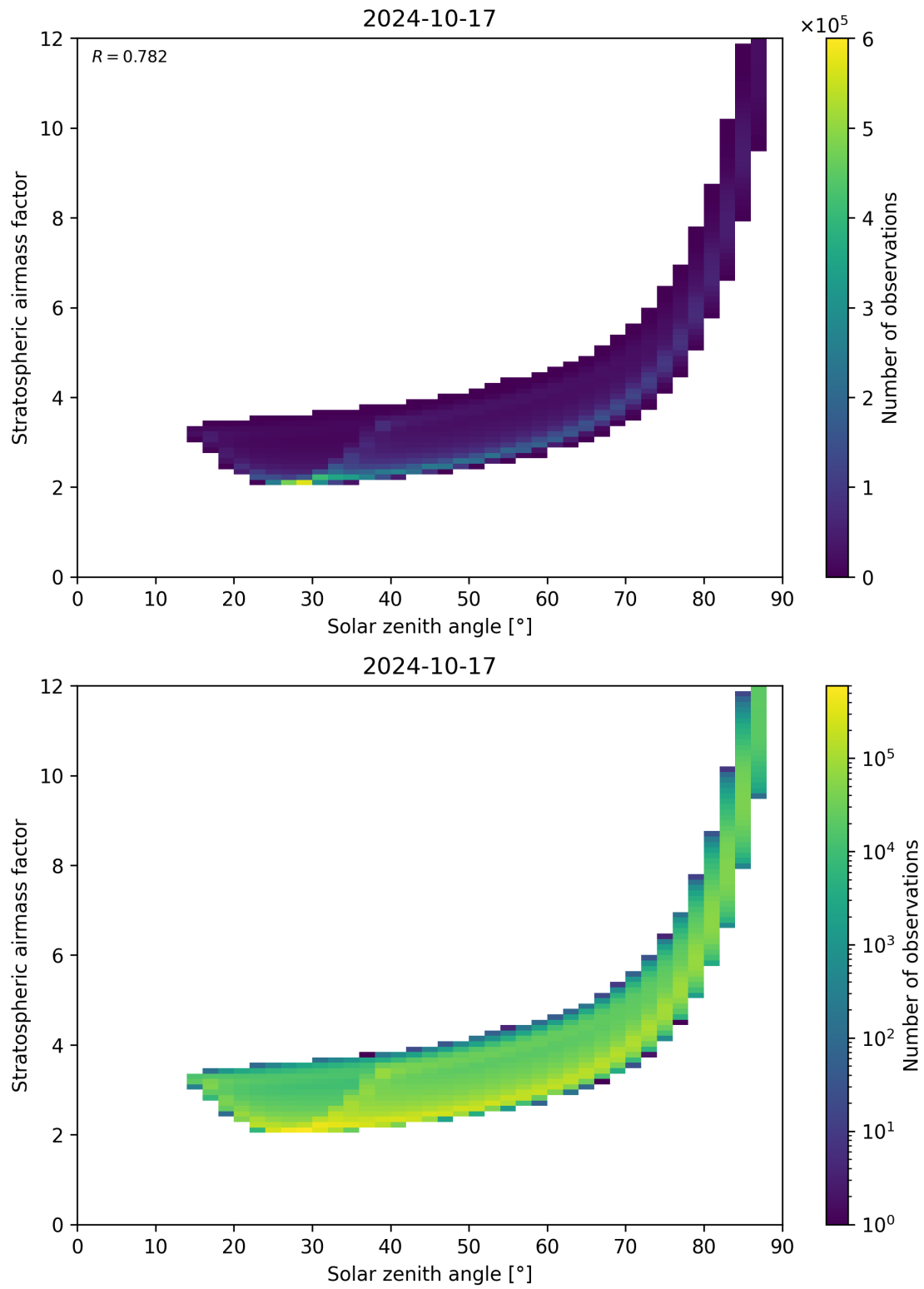
Figure 145: Scatter density plot of “Solar zenith angle” against “Stratospheric airmass factor” for 2024-10-16 to 2024-10-18.
