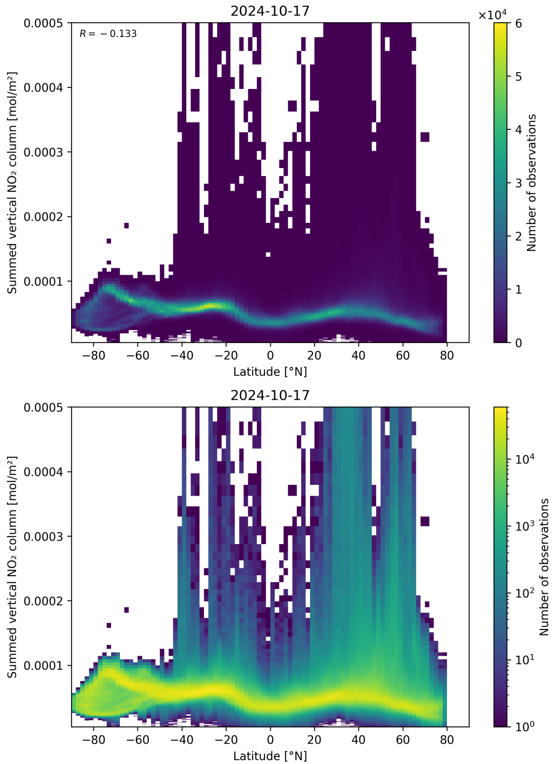
Figure 88: Scatter density plot of “Latitude” against “Summed vertical NO 2 column” for 2024-10-16 to 2024-10-18.
