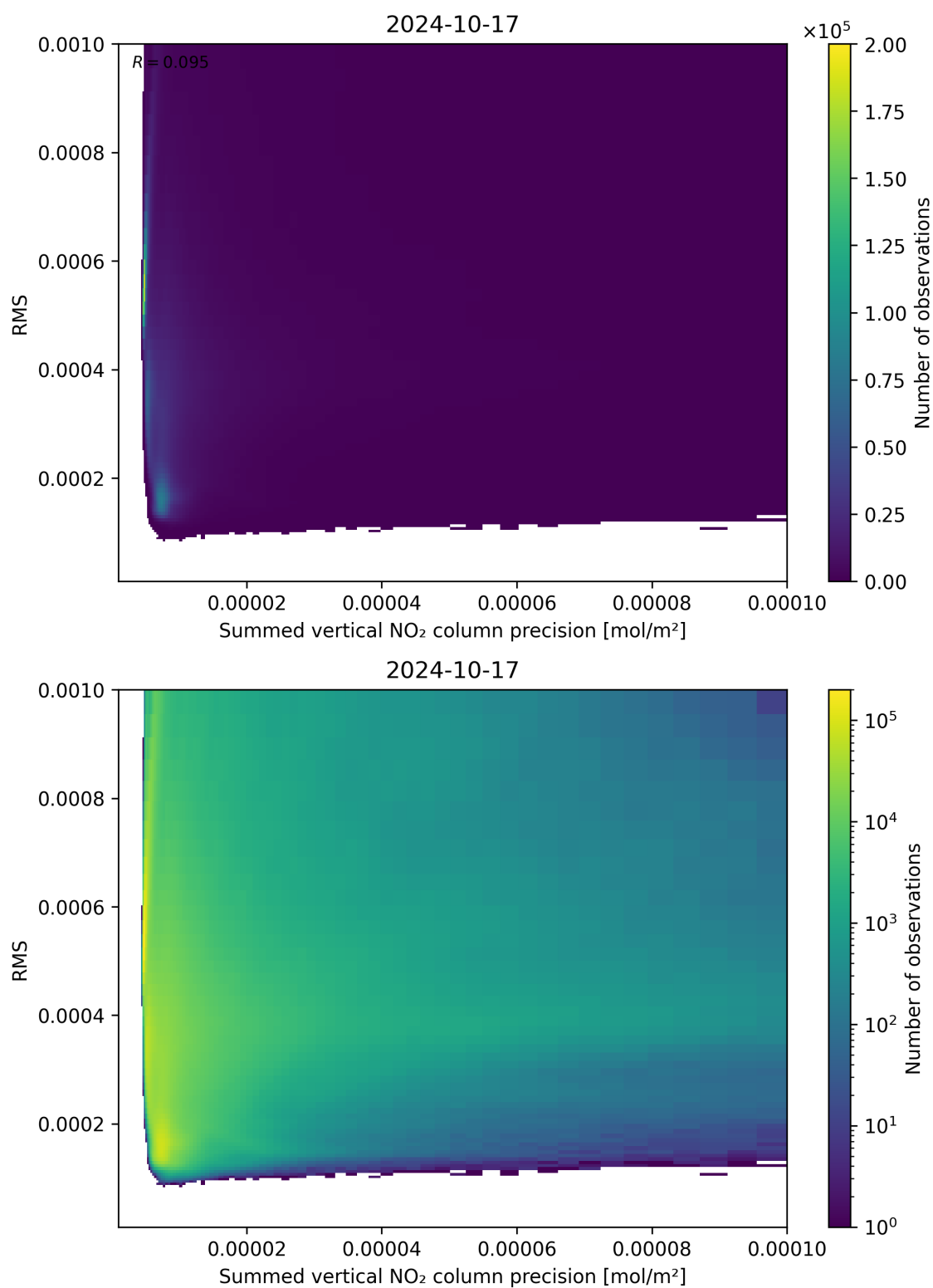
Figure 108: Scatter density plot of “Summed vertical NO 2 column precision” against “RMS” for 2024-10-16 to 2024-10-18.
