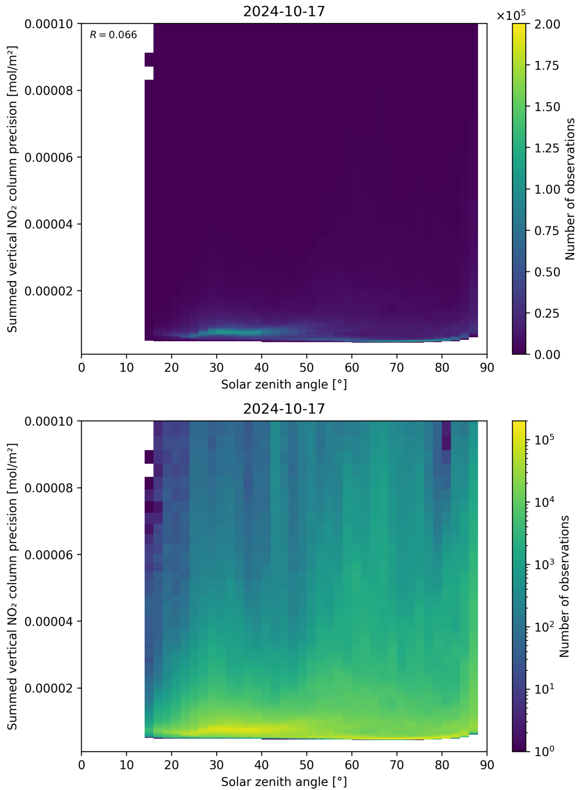
Figure 152: Scatter density plot of “Solar zenith angle” against “Summed vertical NO 2 column precision” for 2024-10-16 to 2024-10-18.
