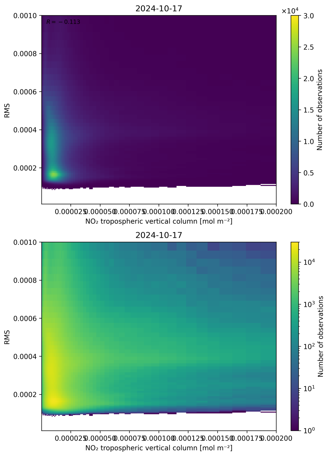
Figure 142: Scatter density plot of “NO 2 tropospheric vertical column” against “RMS” for 2024-10-16 to 2024-10-18.
