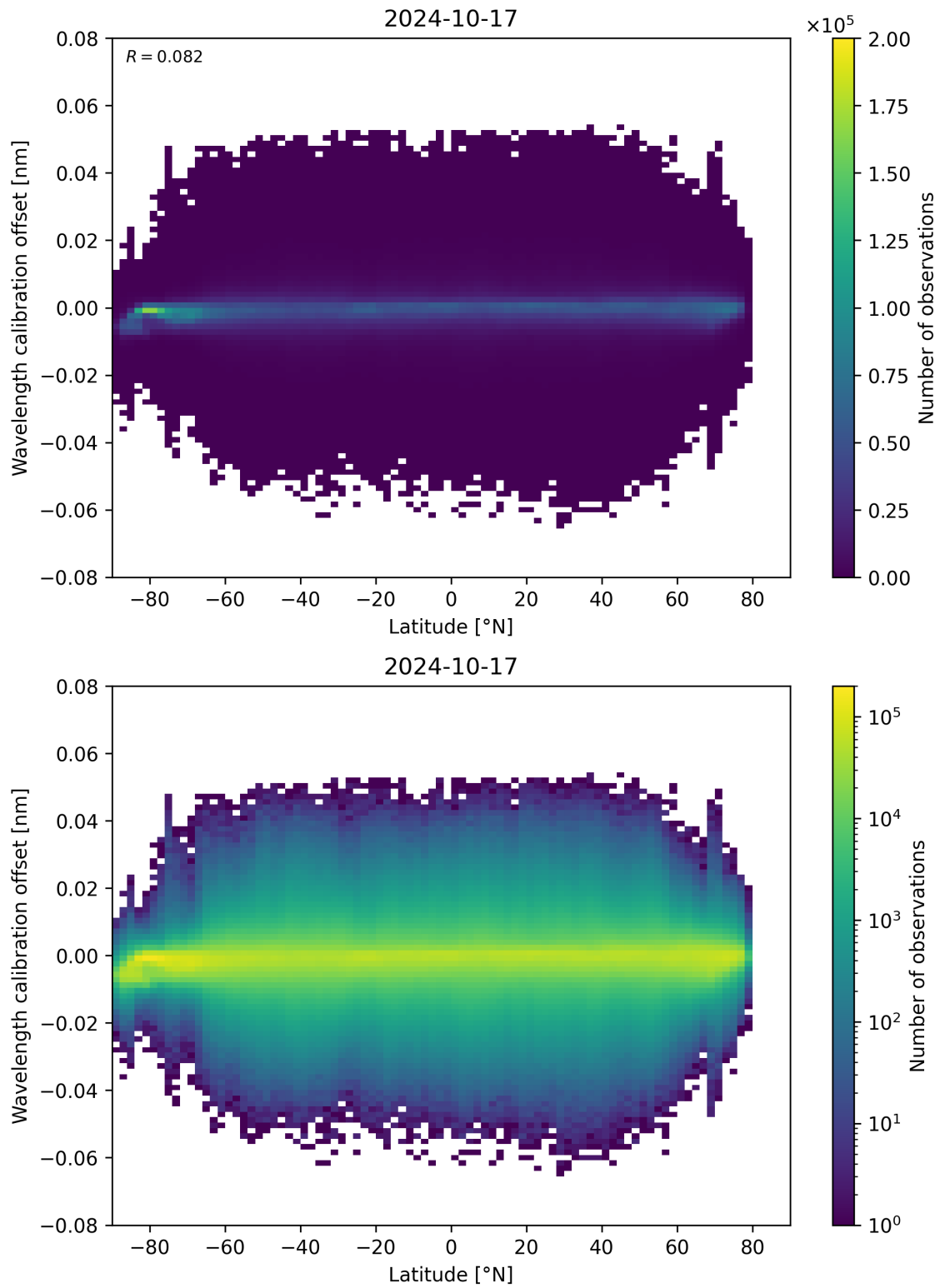
Figure 95: Scatter density plot of “Latitude” against “Wavelength calibration offset” for 2024-10-16 to 2024-10-18.
