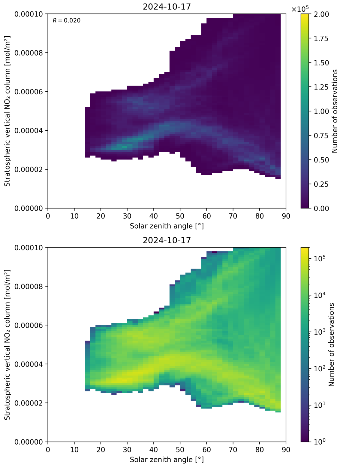
Figure 150: Scatter density plot of “Solar zenith angle” against “Stratospheric vertical NO 2 column” for 2024-10-16 to 2024-10-18.
