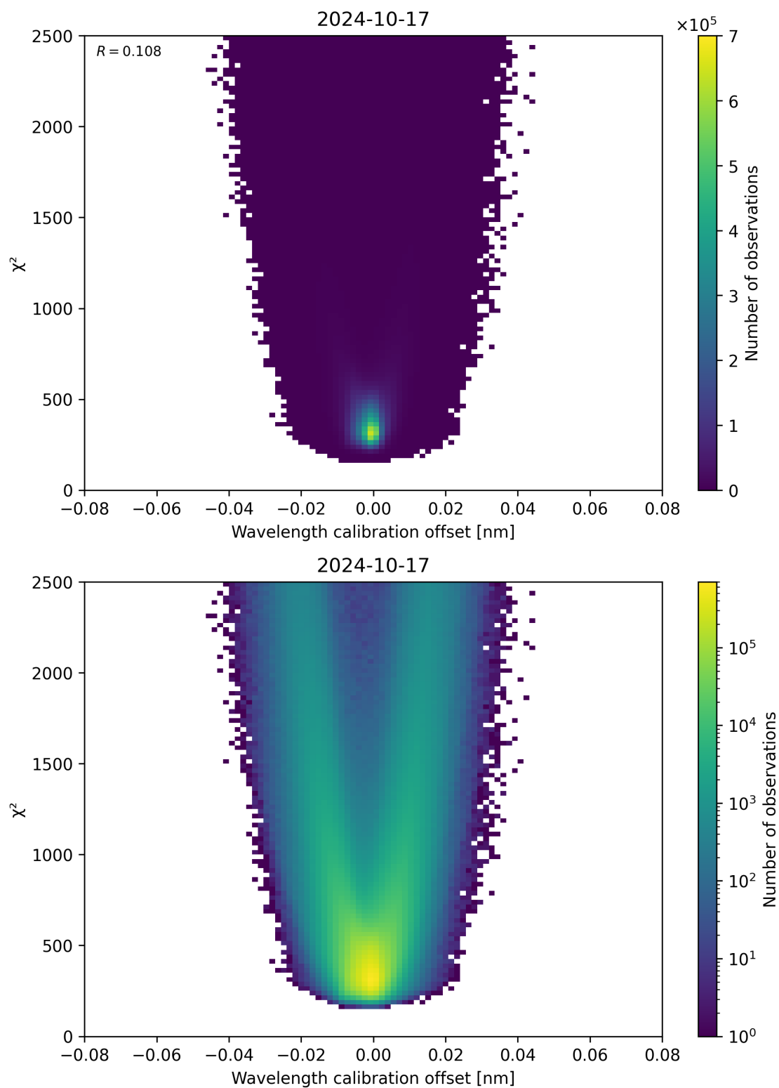
Figure 175: Scatter density plot of “Wavelength calibration offset” against “ \chi^2 ” for 2024-10-16 to 2024-10-18.
