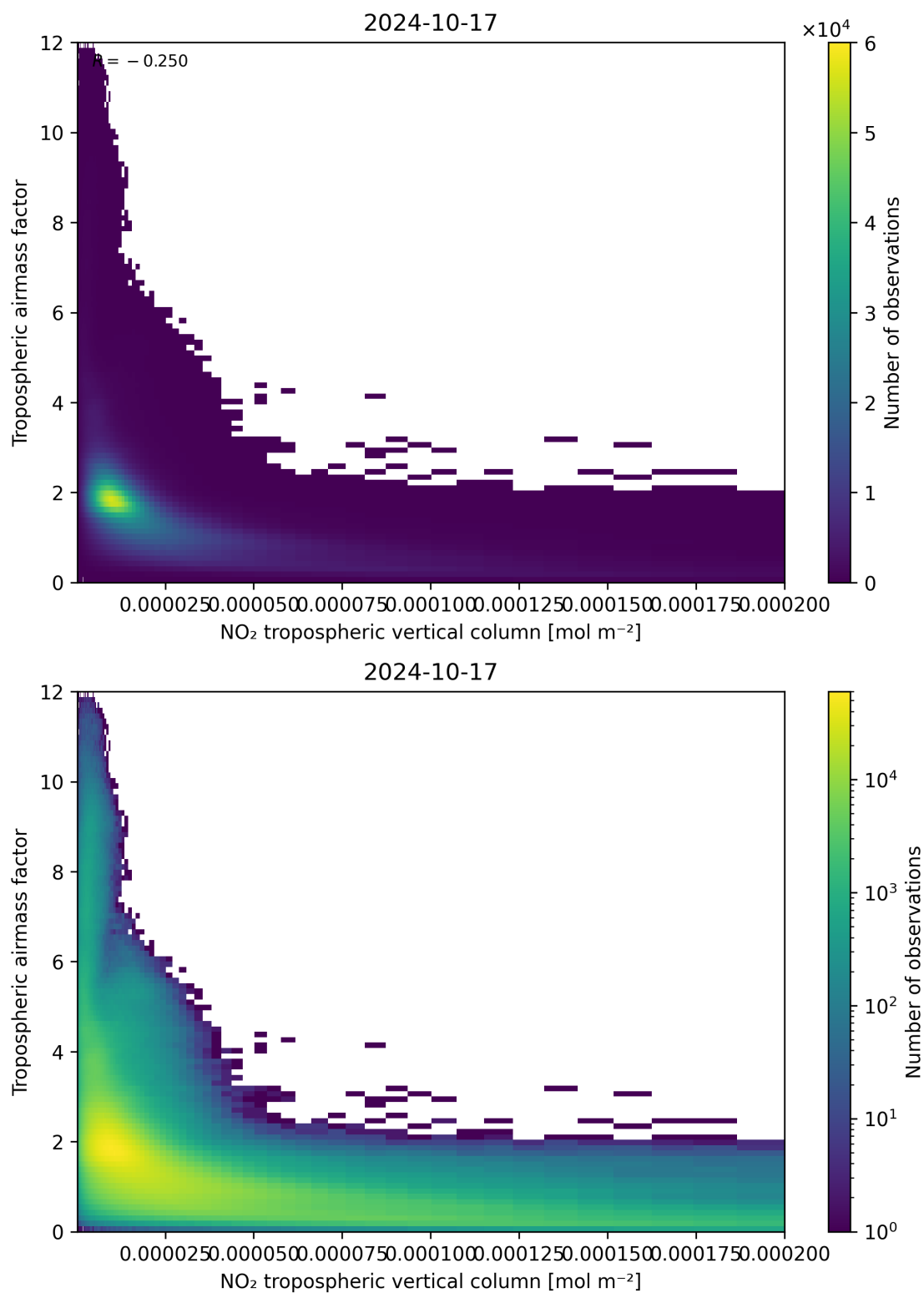
Figure 123: Scatter density plot of “NO 2 tropospheric vertical column” against “Tropospheric air mass factor” for 2024-10-16 to 2024-10-18.
