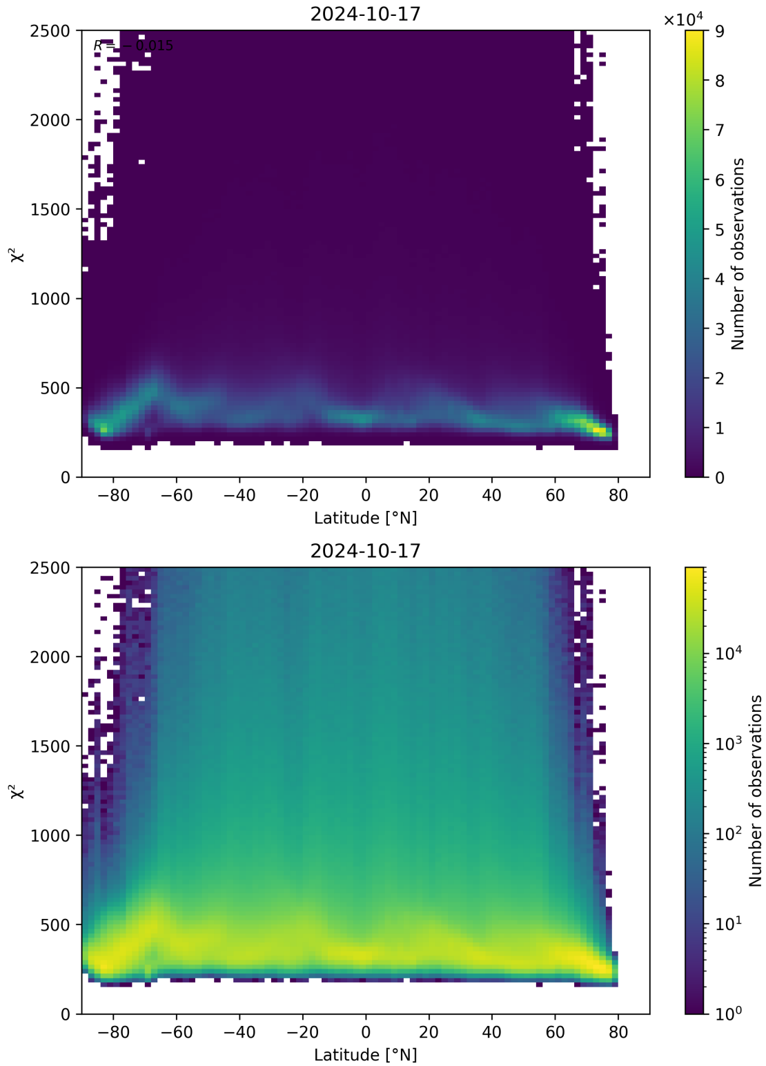
Figure 86: Scatter density plot of “Latitude” against “ \chi^2 ” for 2024-10-16 to 2024-10-18.
