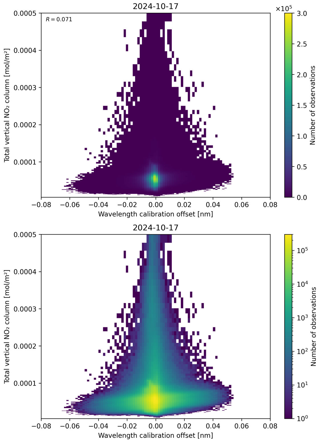
Figure 179: Scatter density plot of “Wavelength calibration offset” against “Total vertical NO 2 column” for 2024-10-16 to 2024-10-18.
