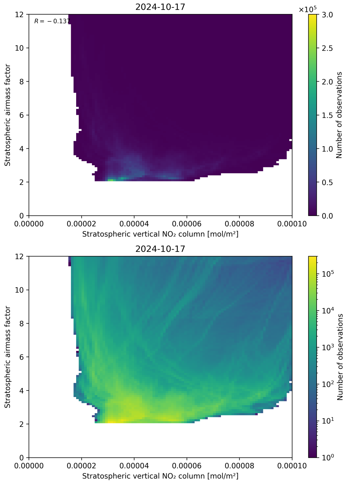
Figure 96: Scatter density plot of “Stratospheric vertical NO 2 column” against “Stratospheric airmass factor” for 2024-10-16 to 2024-10-18.
