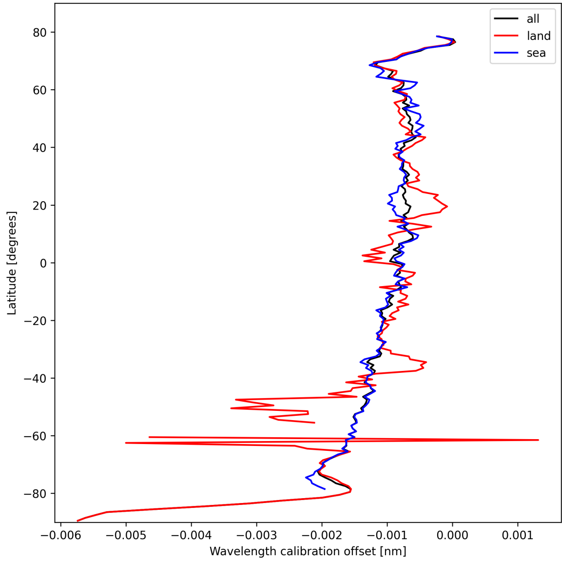
Figure 18: Zonal average of “Wavelength calibration offset” for 2024-10-16 to 2024-10-18.
