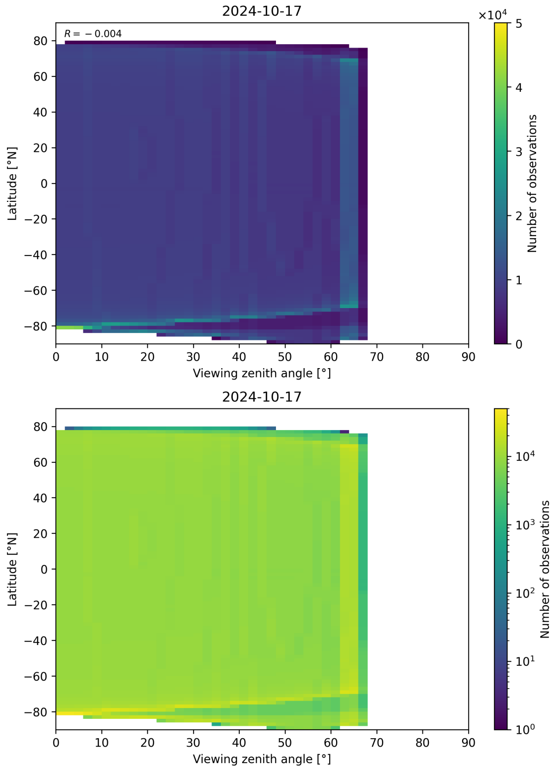
Figure 163: Scatter density plot of “Viewing zenith angle” against “Latitude” for 2024-10-16 to 2024-10-18.
