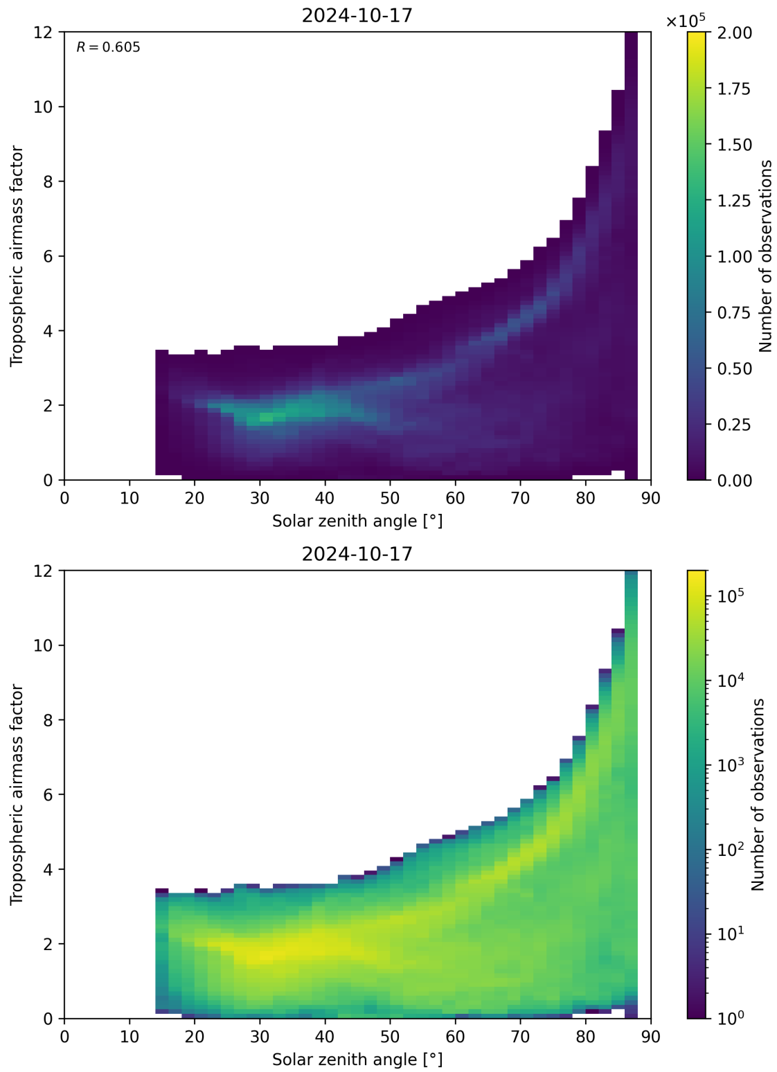
Figure 147: Scatter density plot of “Solar zenith angle” against “Tropospheric airmass factor” for 2024-10-16 to 2024-10-18.
