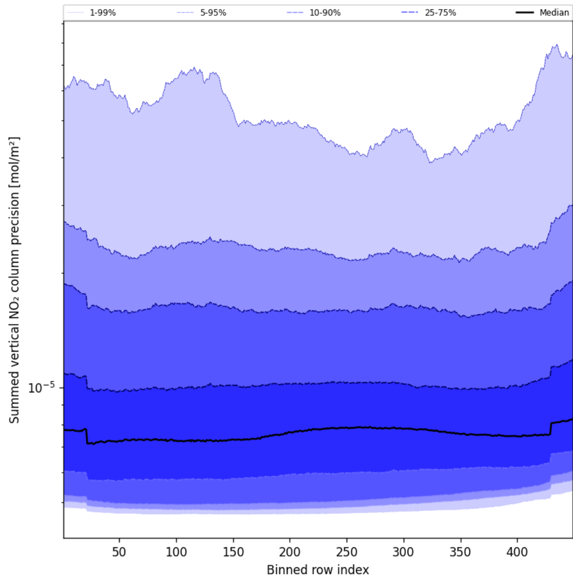
Figure 58: Along track statistics of “Summed vertical NO 2 column precision” for 2024-10-16 to 2024-10-18
