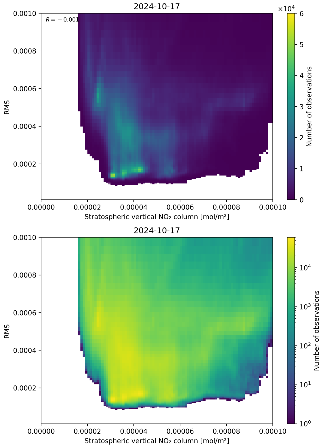
Figure 102: Scatter density plot of “Stratospheric vertical NO 2 column” against “RMS” for 2024-10-16 to 2024-10-18.
