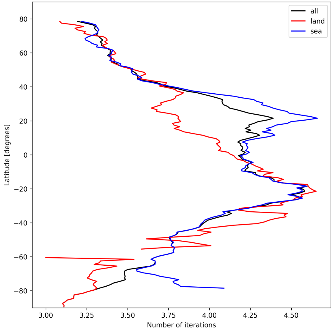
Figure 17: Zonal average of “Number of iterations” for 2024-10-16 to 2024-10-18.
