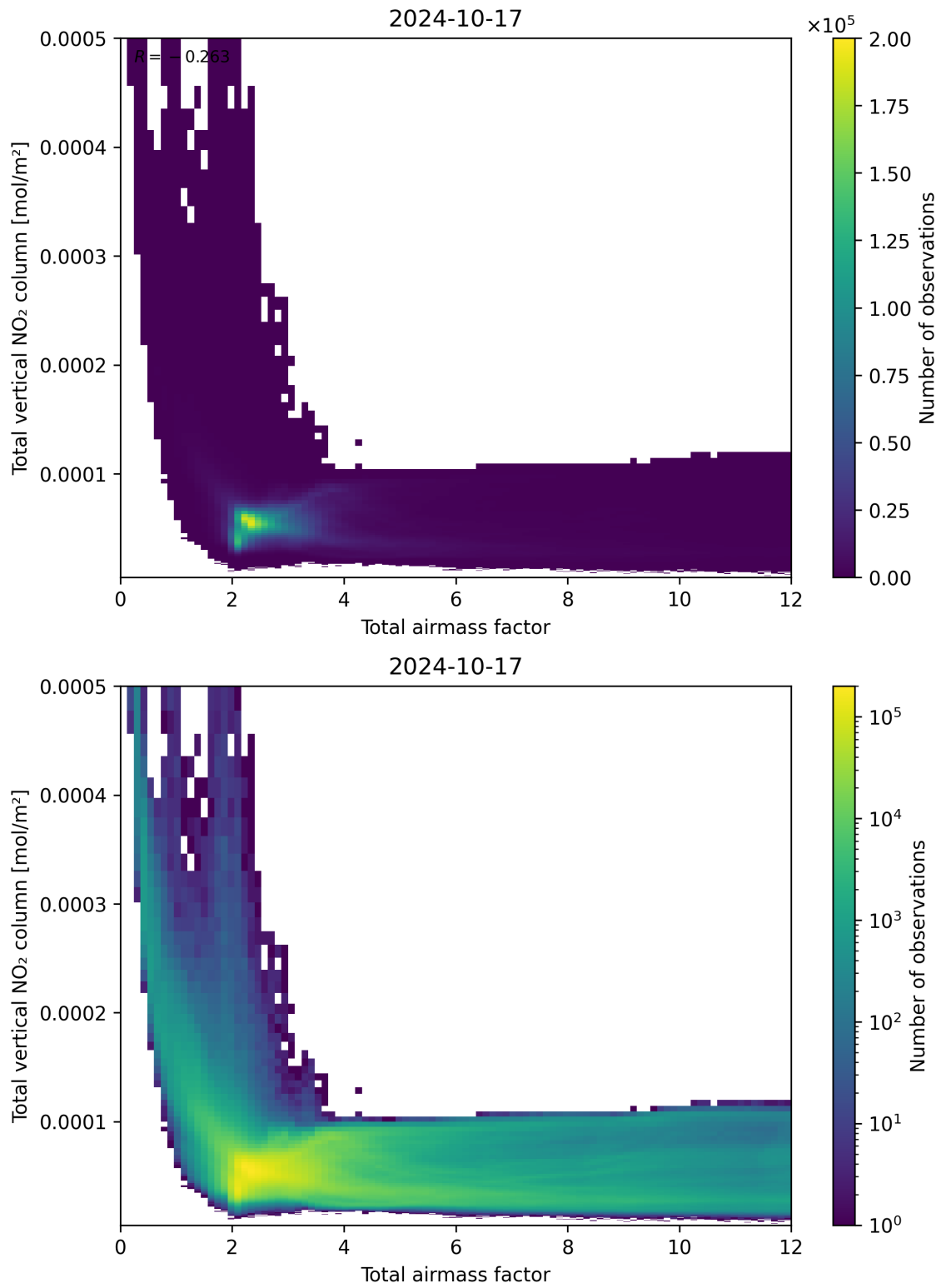
Figure 67: Scatter density plot of “Total airmass factor” against “Total vertical NO 2 column” for 2024-10-16 to 2024-10-18.
