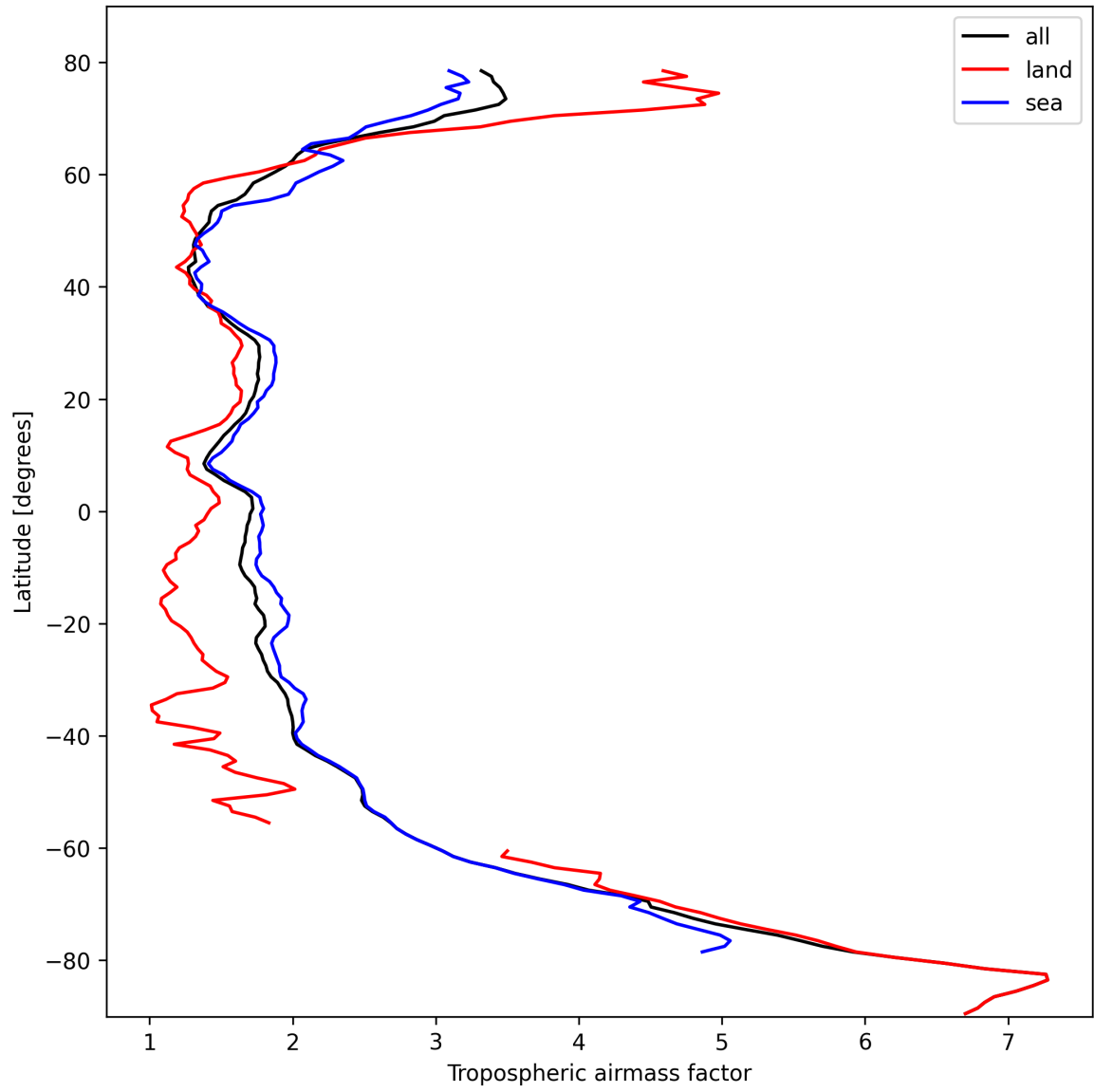
Figure 14: Zonal average of “Tropospheric airmass factor” for 2024-10-16 to 2024-10-18.
