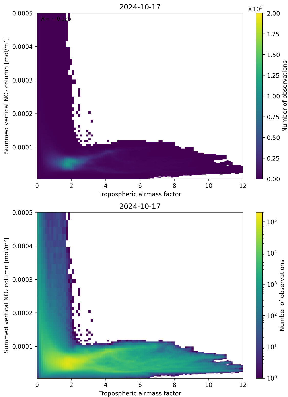
Figure 75: Scatter density plot of “Tropospheric airmass factor” against “Summed vertical NO 2 column” for 2024-10-16 to 2024-10-18.
