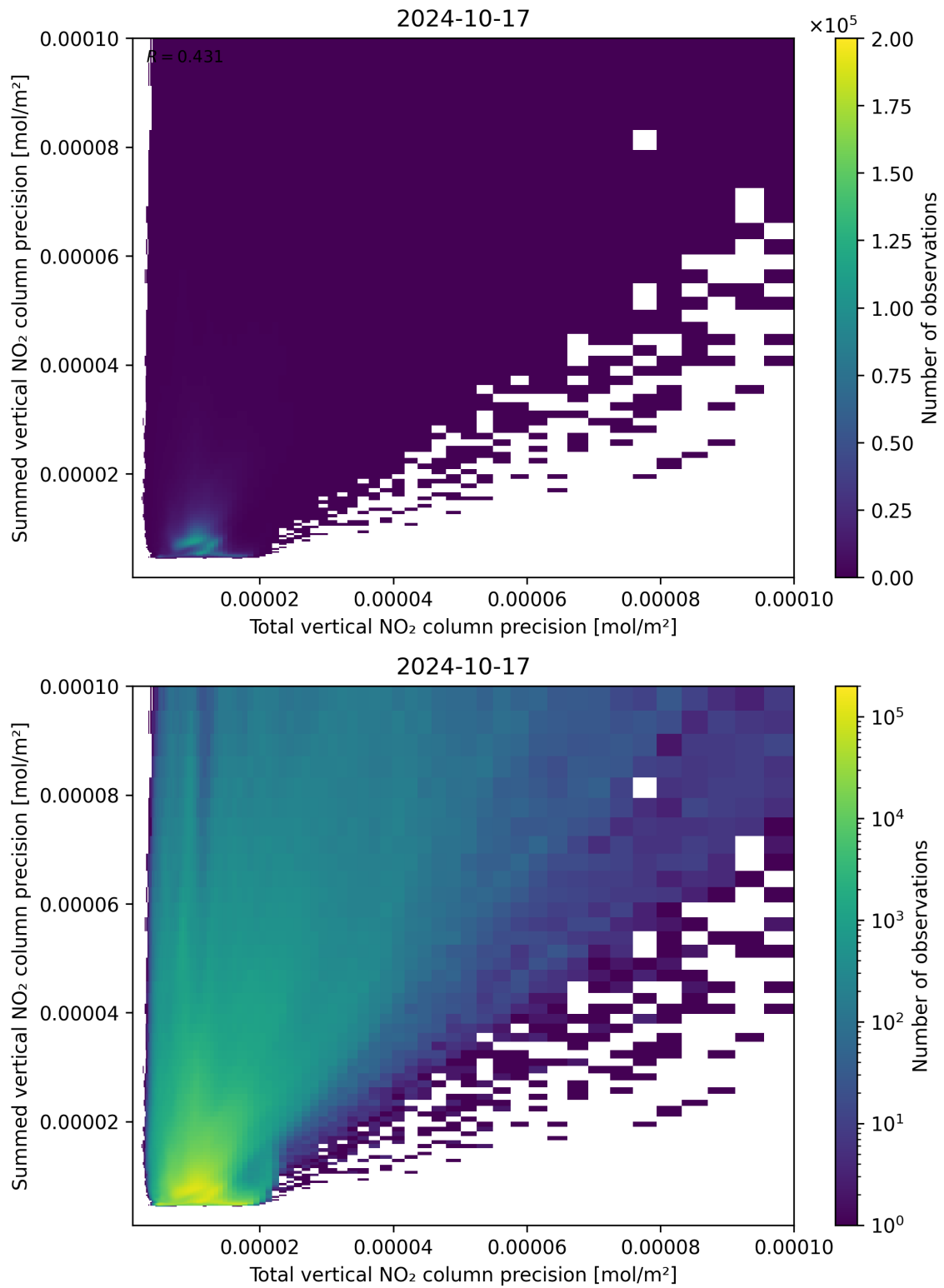
Figure 118: Scatter density plot of “Total vertical NO 2 column precision” against “Summed vertical NO 2 column precision” for 2024-10-16 to 2024-10-18.
