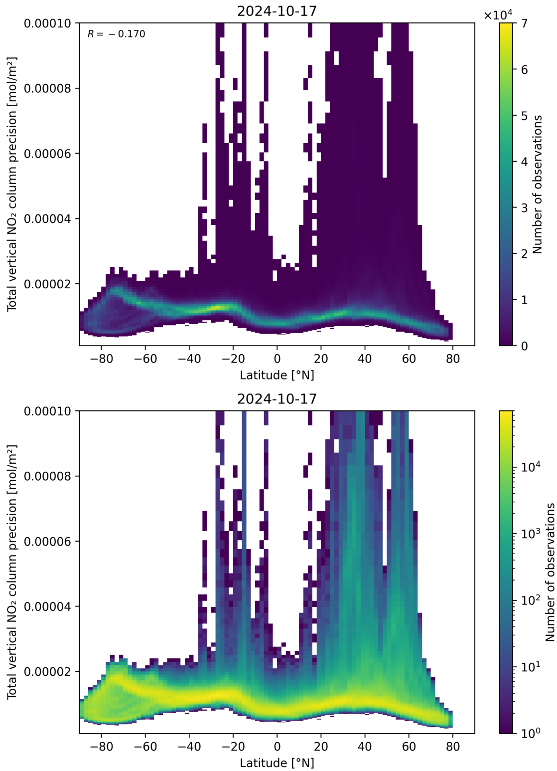
Figure 91: Scatter density plot of “Latitude” against “Total vertical NO 2 column precision” for 2024-10-16 to 2024-10-18.
