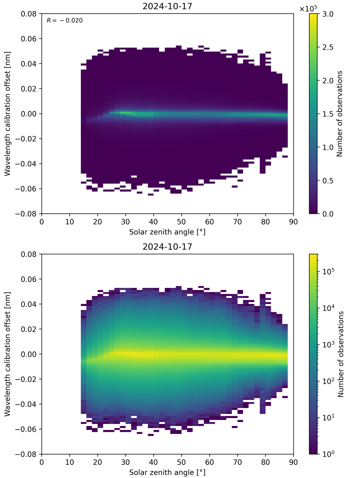
Figure 158: Scatter density plot of “Solar zenith angle” against “Wavelength calibration offset” for 2024-10-16 to 2024-10-18.
