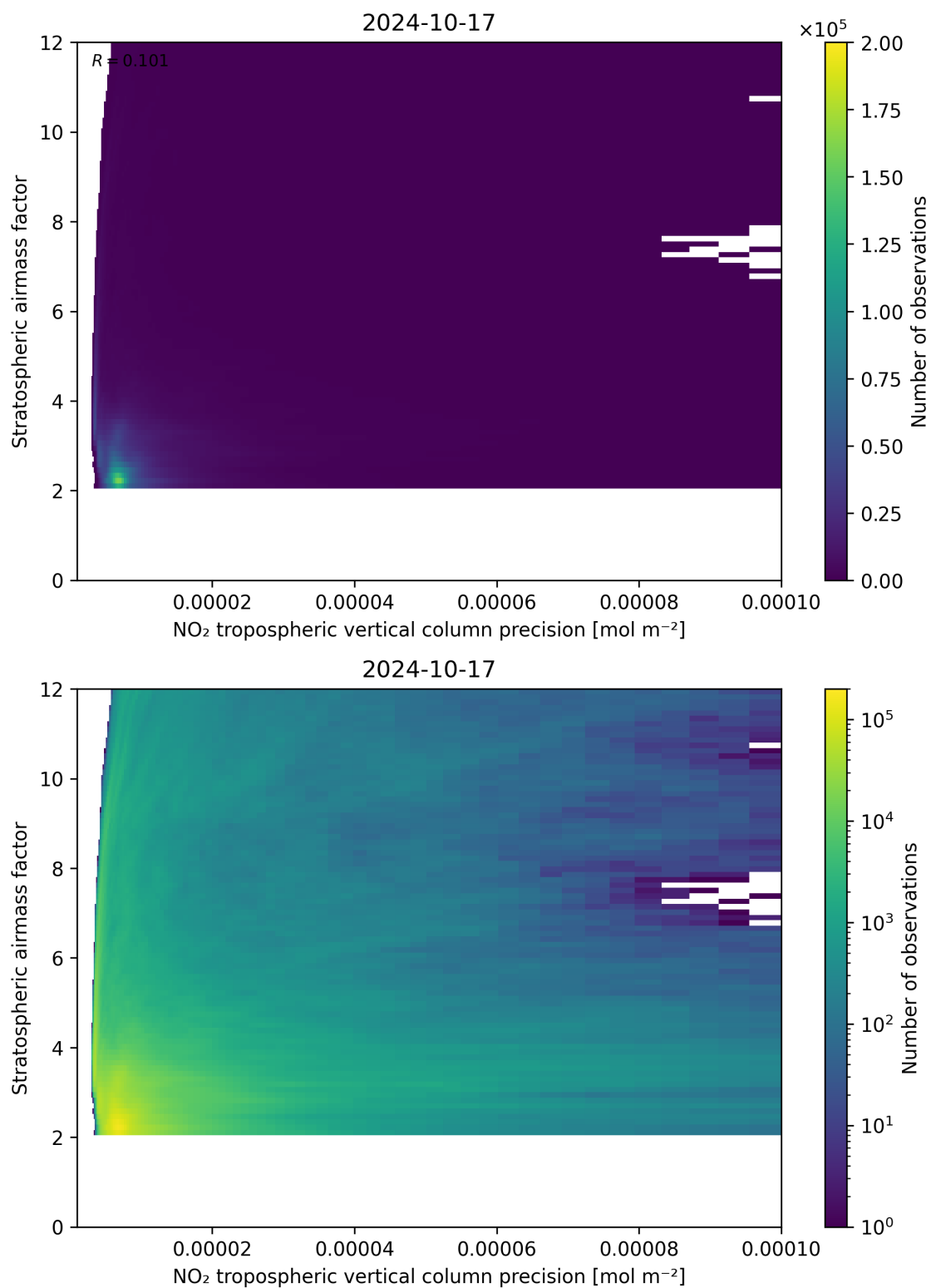
Figure 131: Scatter density plot of “NO 2 tropospheric vertical column precision” against “Stratospheric airmass factor” for 2024-10-16 to 2024-10-18.
