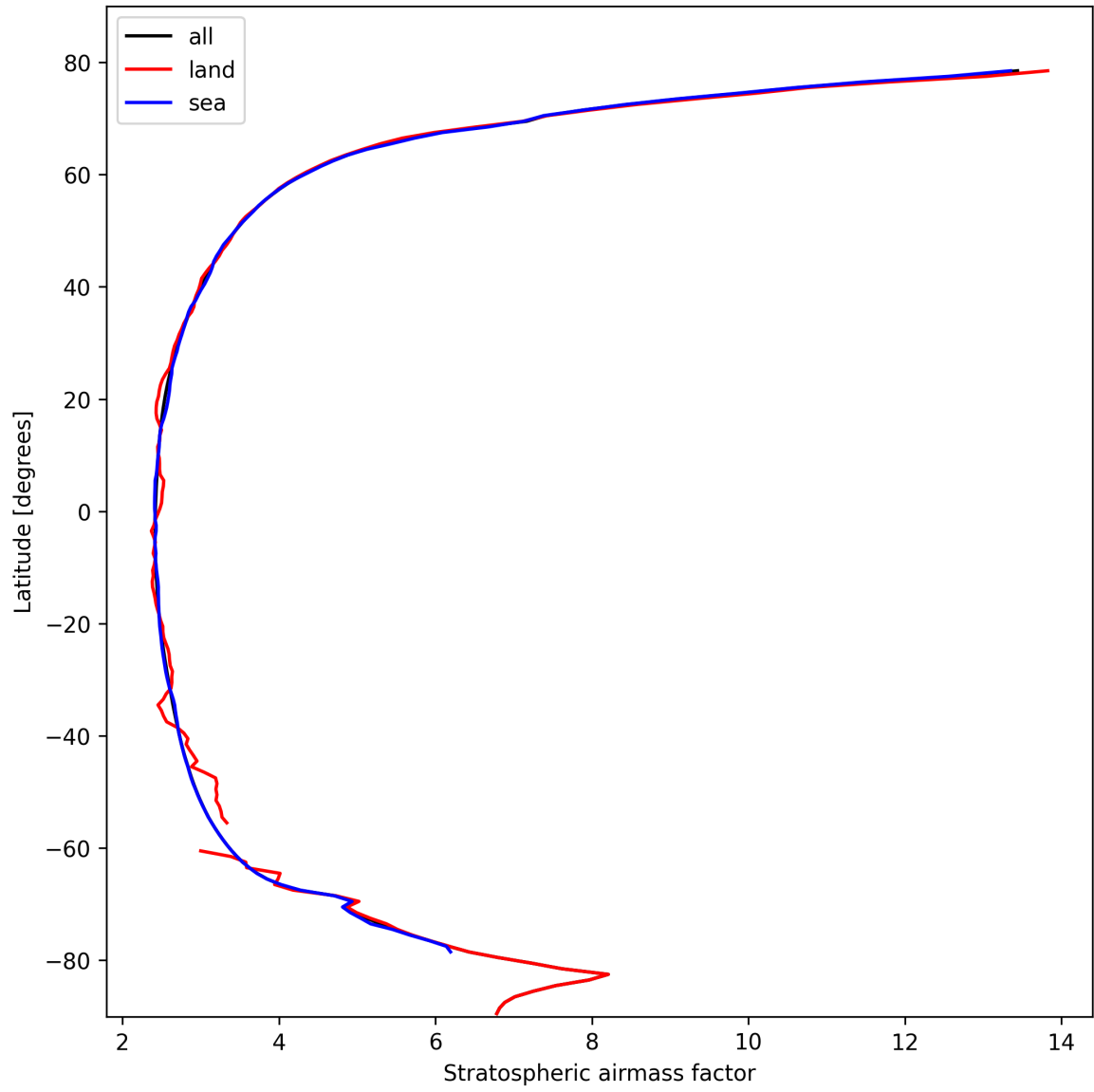
Figure 27: Zonal average of “Stratospheric air mass factor” for 2024-10-16 to 2024-10-18.
