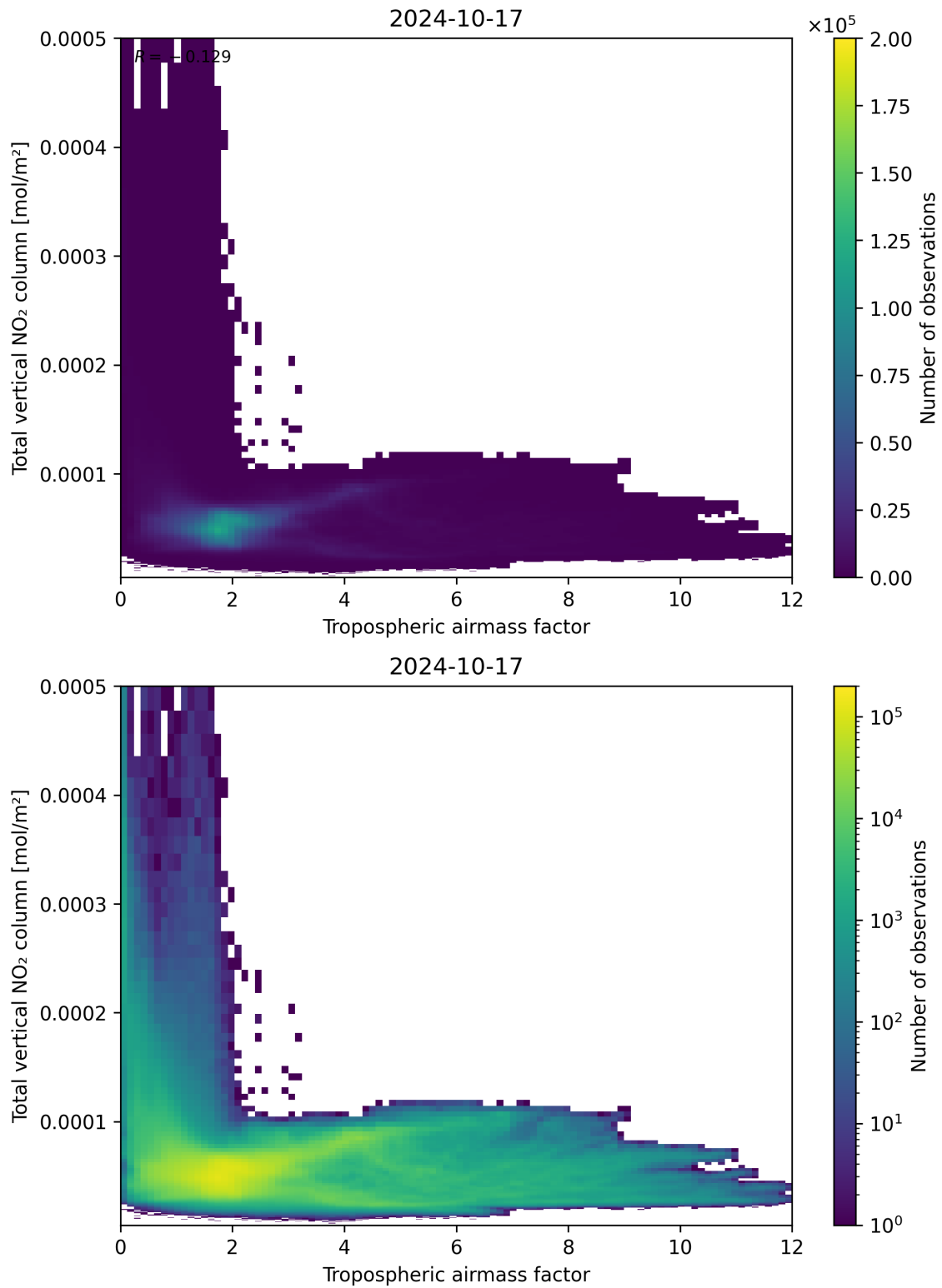
Figure 77: Scatter density plot of “Tropospheric airmass factor” against “Total vertical NO 2 column” for 2024-10-16 to 2024-10-18.
