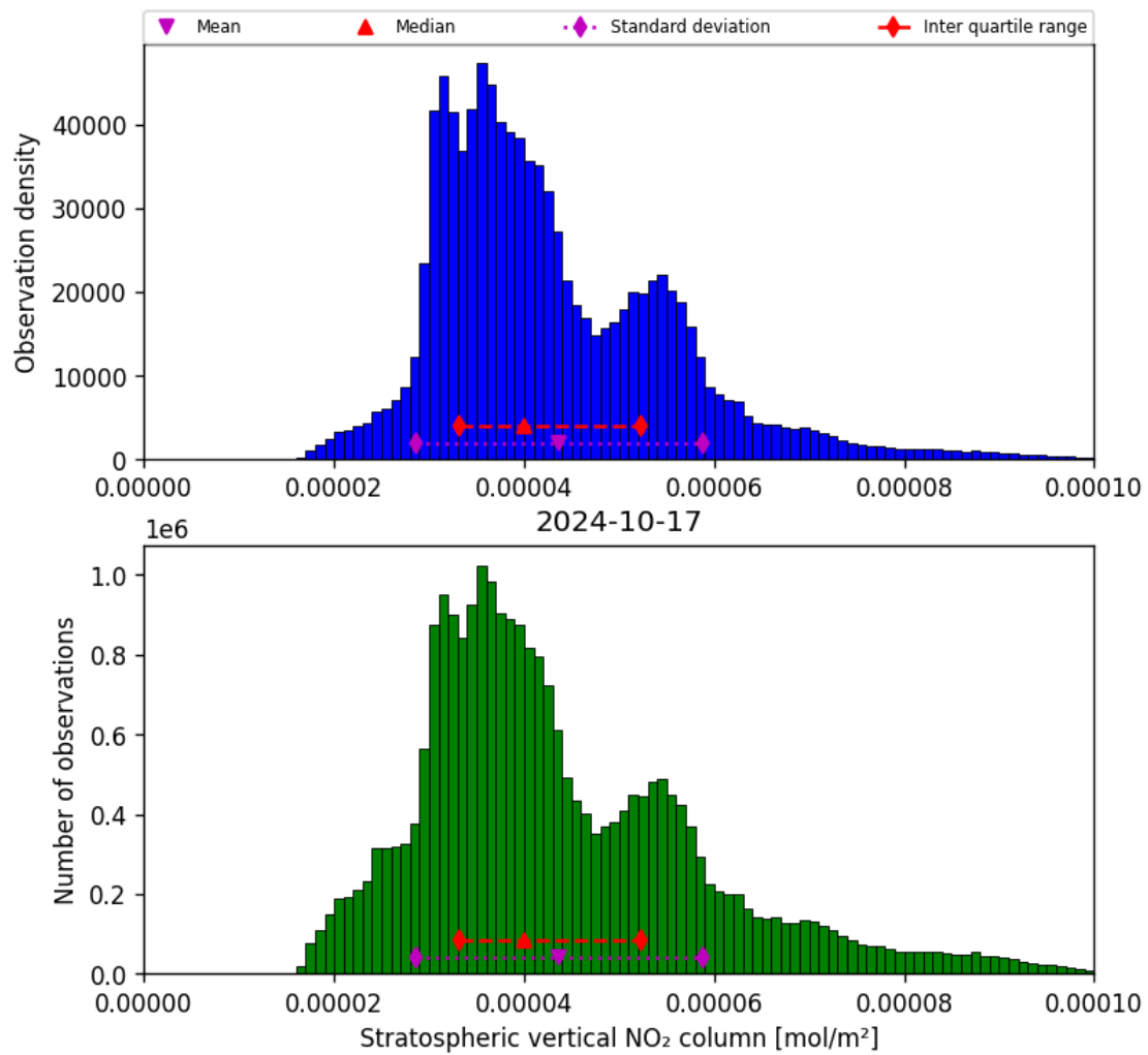
Figure 36: Histogram of “Stratospheric vertical NO 2 column” for 2024-10-16 to 2024-10-18
