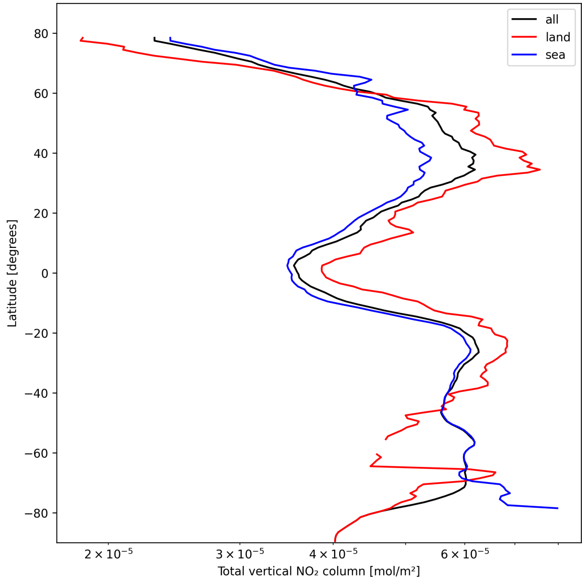
Figure 21: Zonal average of “Total vertical NO 2 column” for 2024-10-16 to 2024-10-18.
