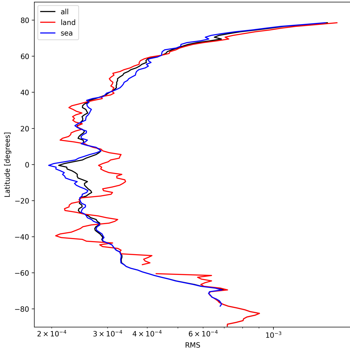
Figure 26: Zonal average of “RMS” for 2024-10-16 to 2024-10-18.
