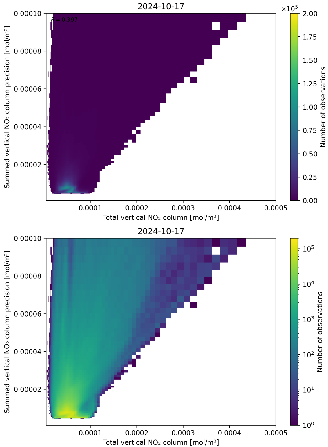
Figure 113: Scatter density plot of “Total vertical NO 2 column” against “Summed vertical NO 2 column precision” for 2024-10-16 to 2024-10-18.
