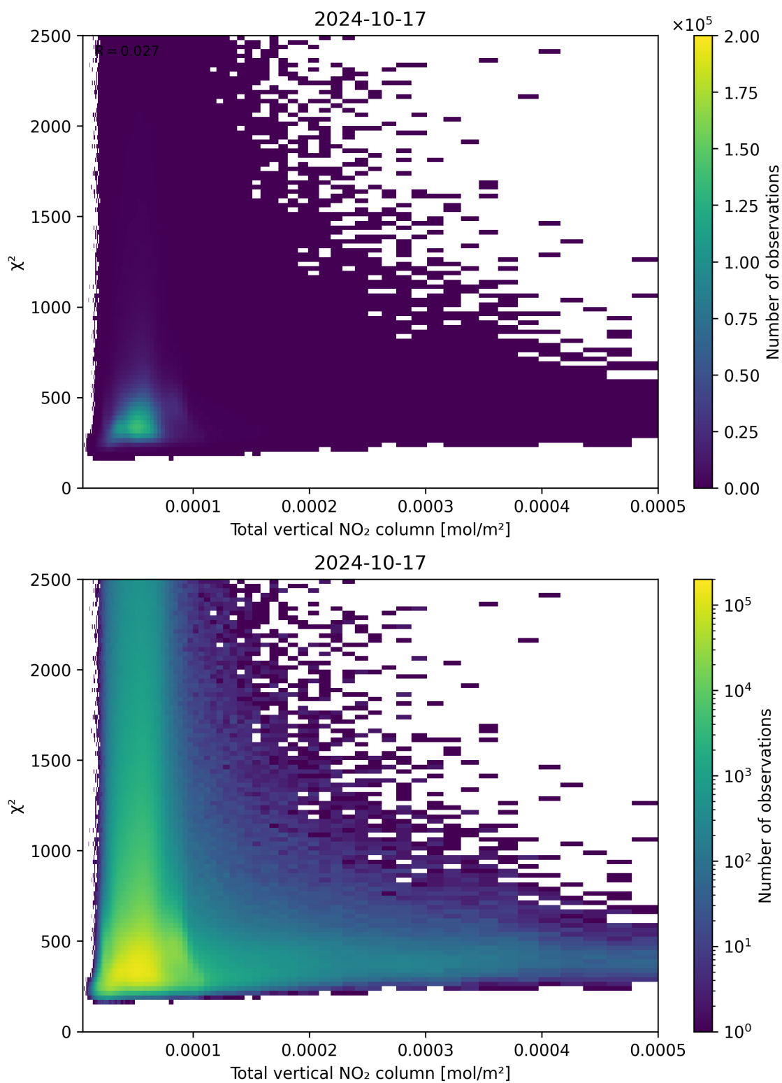
Figure 111: Scatter density plot of “Total vertical NO 2 column” against “ \chi^2 ” for 2024-10-16 to 2024-10-18.
