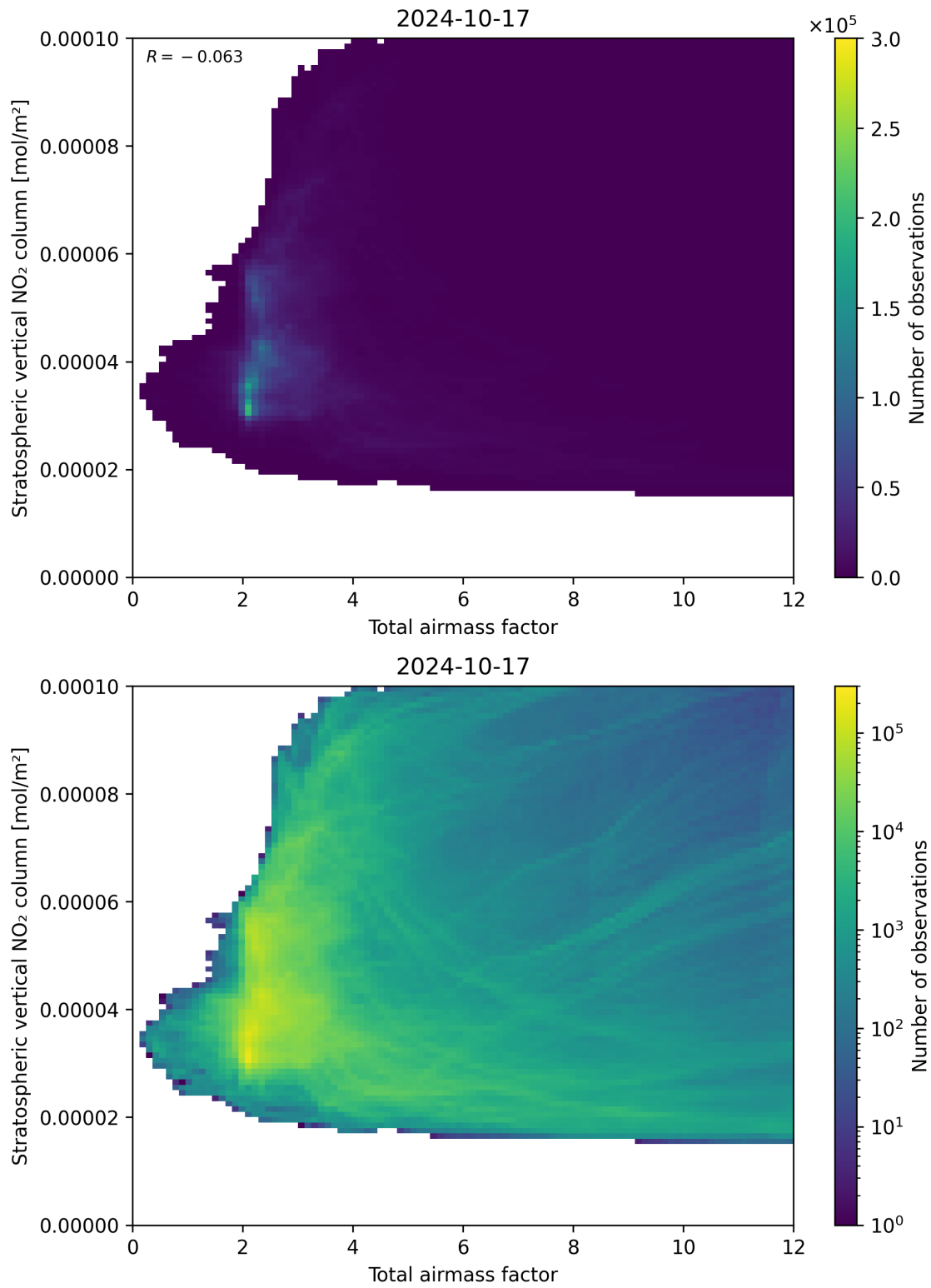
Figure 64: Scatter density plot of “Total airmass factor” against “Stratospheric vertical NO 2 column” for 2024-10-16 to 2024-10-18.
