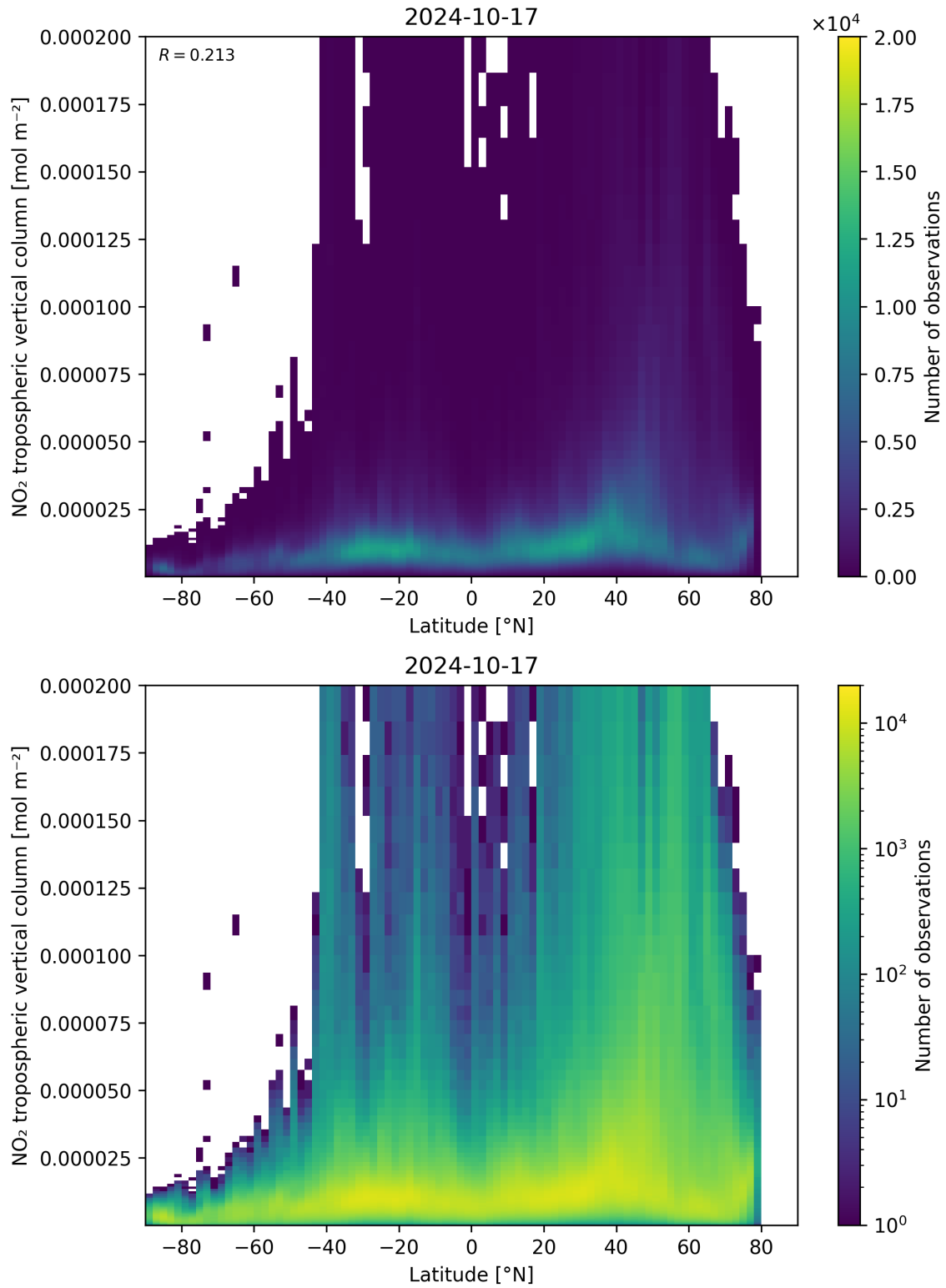
Figure 92: Scatter density plot of “Latitude” against “NO 2 tropospheric vertical column” for 2024-10-16 to 2024-10-18.
