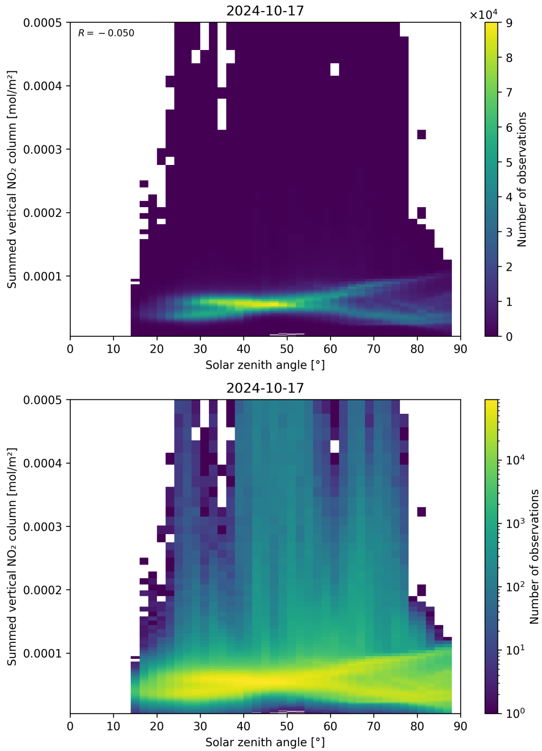
Figure 151: Scatter density plot of “Solar zenith angle” against “Summed vertical NO 2 column” for 2024-10-16 to 2024-10-18.
