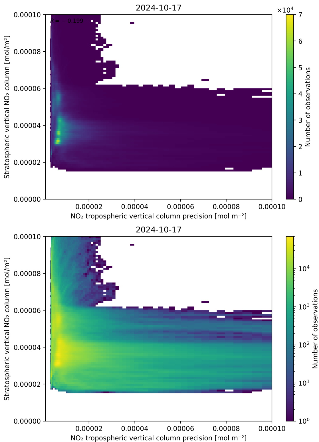
Figure 135: Scatter density plot of “NO 2 tropospheric vertical column precision” against “Stratospheric vertical NO 2 column” for 2024-10-16 to 2024-10-18.
