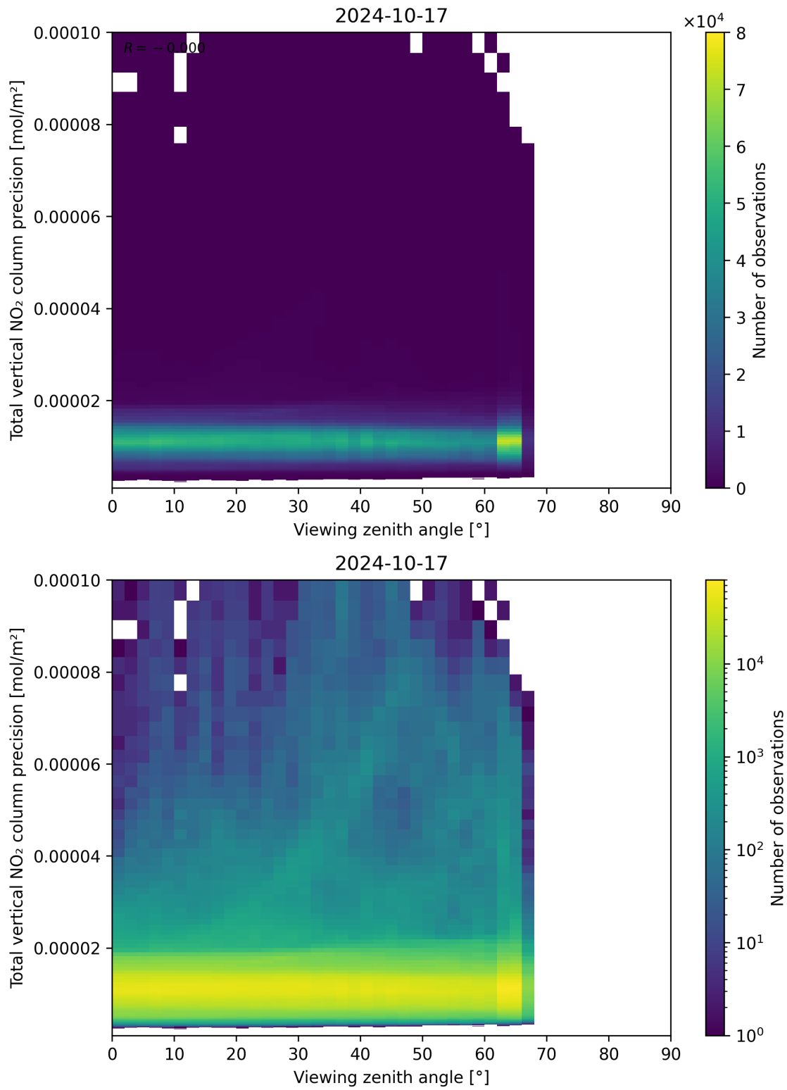
Figure 168: Scatter density plot of “Viewing zenith angle” against “Total vertical NO 2 column precision” for 2024-10-16 to 2024-10-18.
