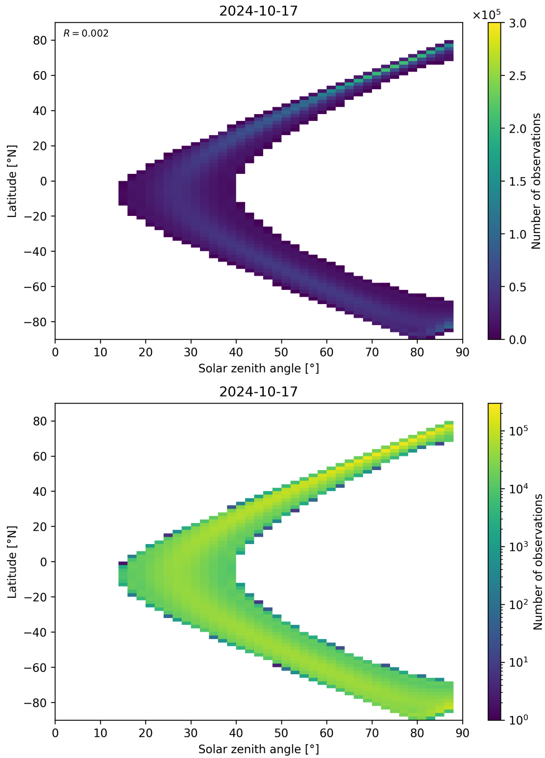
Figure 149: Scatter density plot of “Solar zenith angle” against “Latitude” for 2024-10-16 to 2024-10-18.
