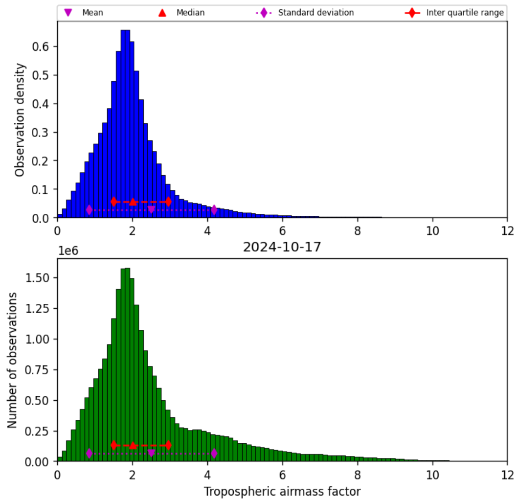
Figure 31: Histogram of “Tropospheric airmass factor” for 2024-10-16 to 2024-10-18
