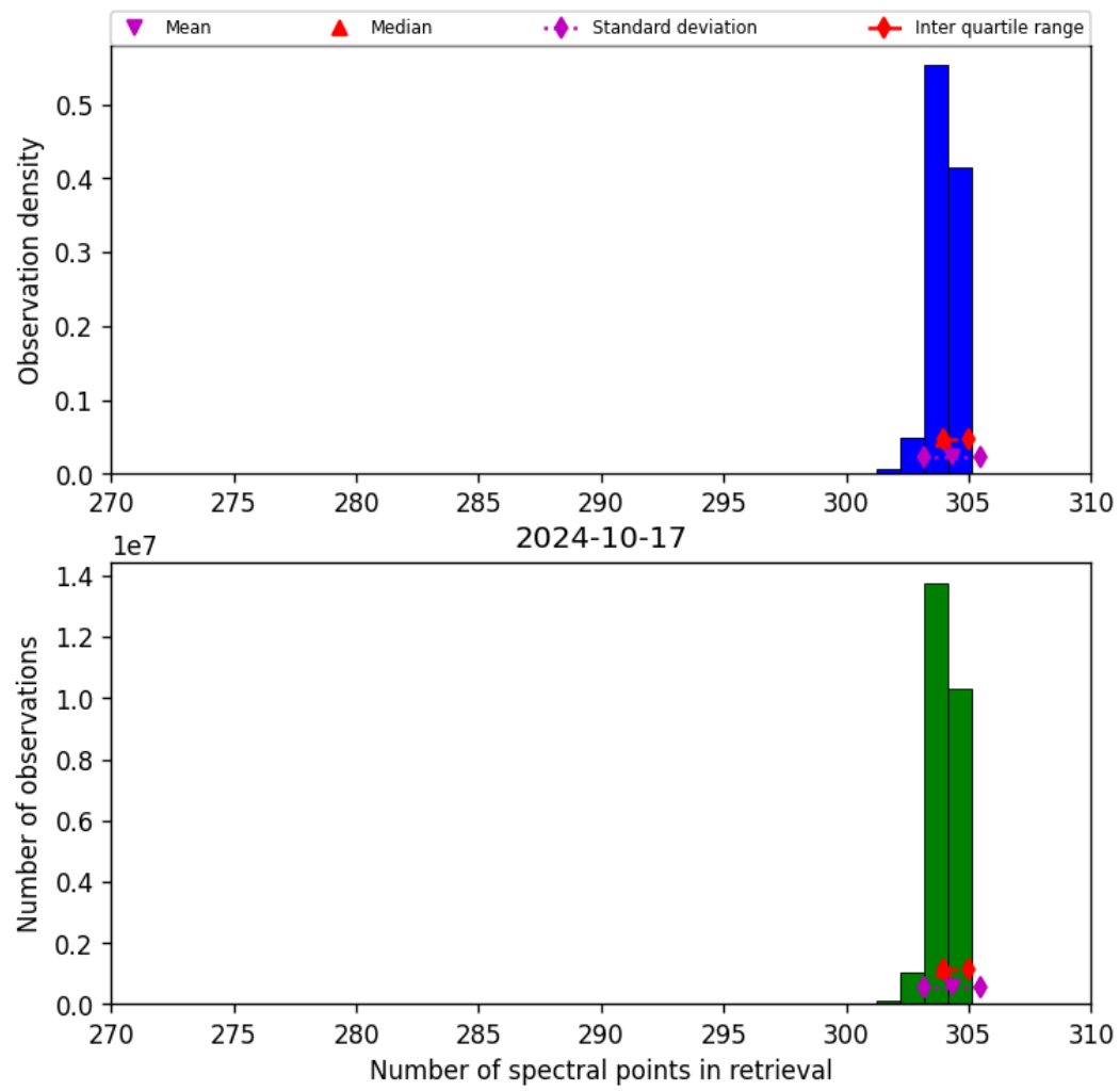
Figure 33: Histogram of “Number of spectral points in retrieval” for 2024-10-16 to 2024-10-18
