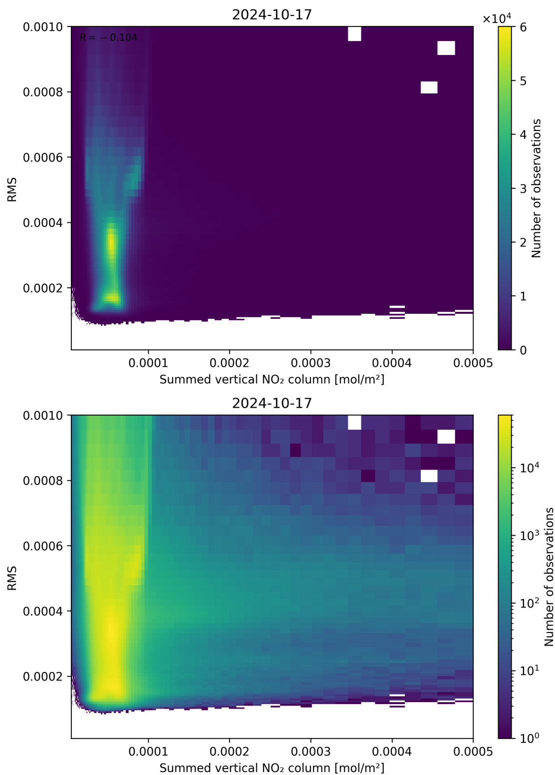
Figure 109: Scatter density plot of “Summed vertical NO 2 column” against “RMS” for 2024-10-16 to 2024-10-18.
