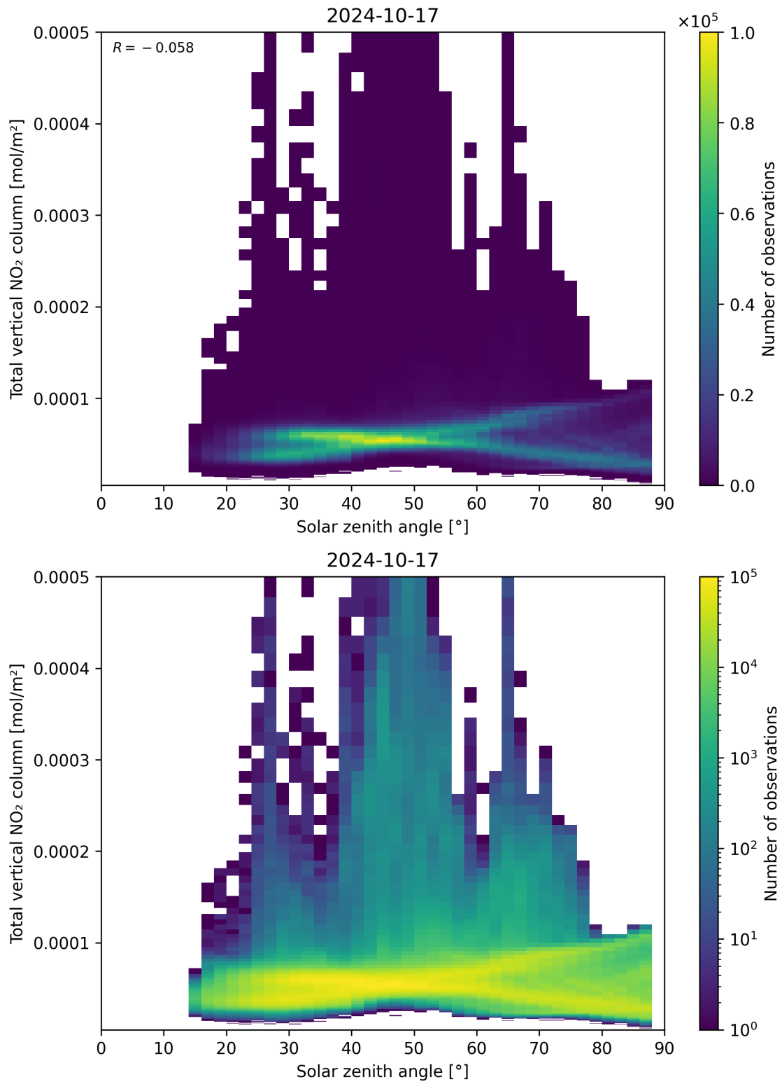
Figure 153: Scatter density plot of “Solar zenith angle” against “Total vertical NO 2 column” for 2024-10-16 to 2024-10-18.
