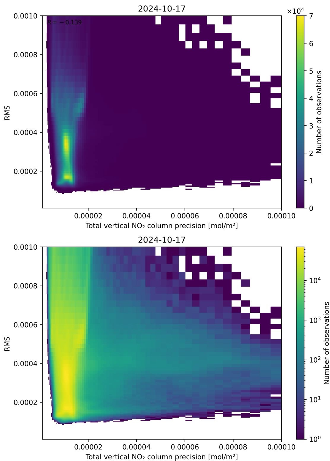
Figure 119: Scatter density plot of “Total vertical NO 2 column precision” against “RMS” for 2024-10-16 to 2024-10-18.
