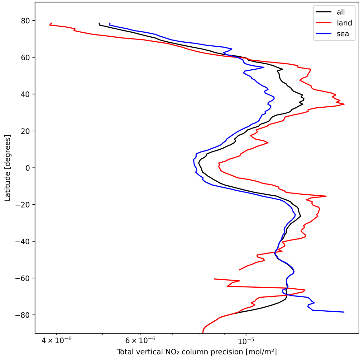
Figure 22: Zonal average of “Total vertical NO 2 column precision” for 2024-10-16 to 2024-10-18.
