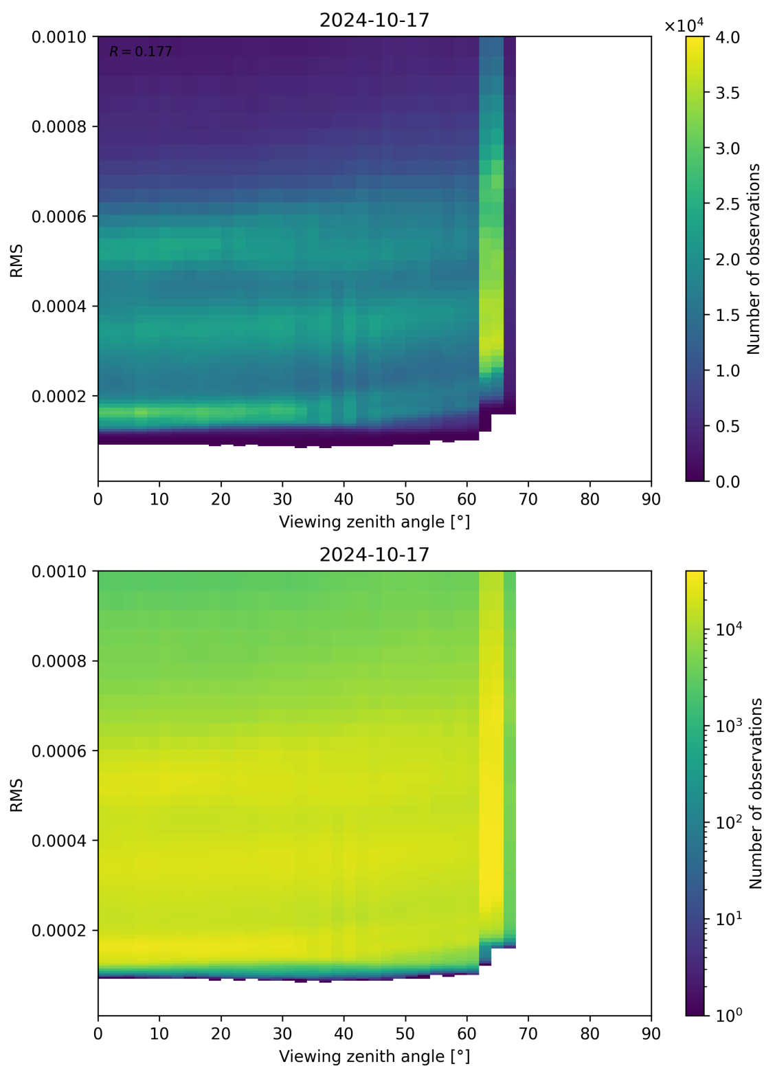
Figure 171: Scatter density plot of “Viewing zenith angle” against “RMS” for 2024-10-16 to 2024-10-18.
