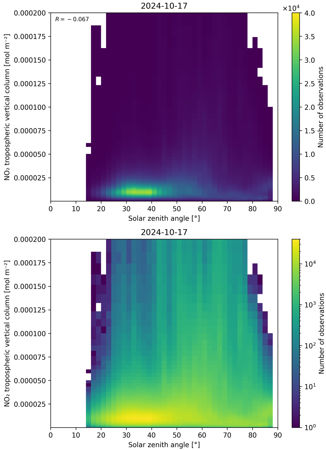
Figure 155: Scatter density plot of “Solar zenith angle” against “NO 2 tropospheric vertical column” for 2024-10-16 to 2024-10-18.
