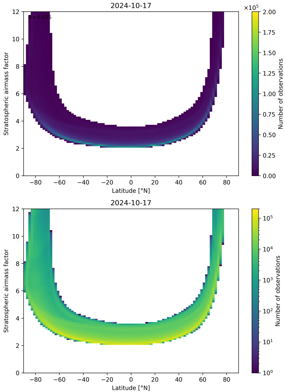
Figure 83: Scatter density plot of “Latitude” against “Stratospheric airmass factor” for 2024-10-16 to 2024-10-18.
