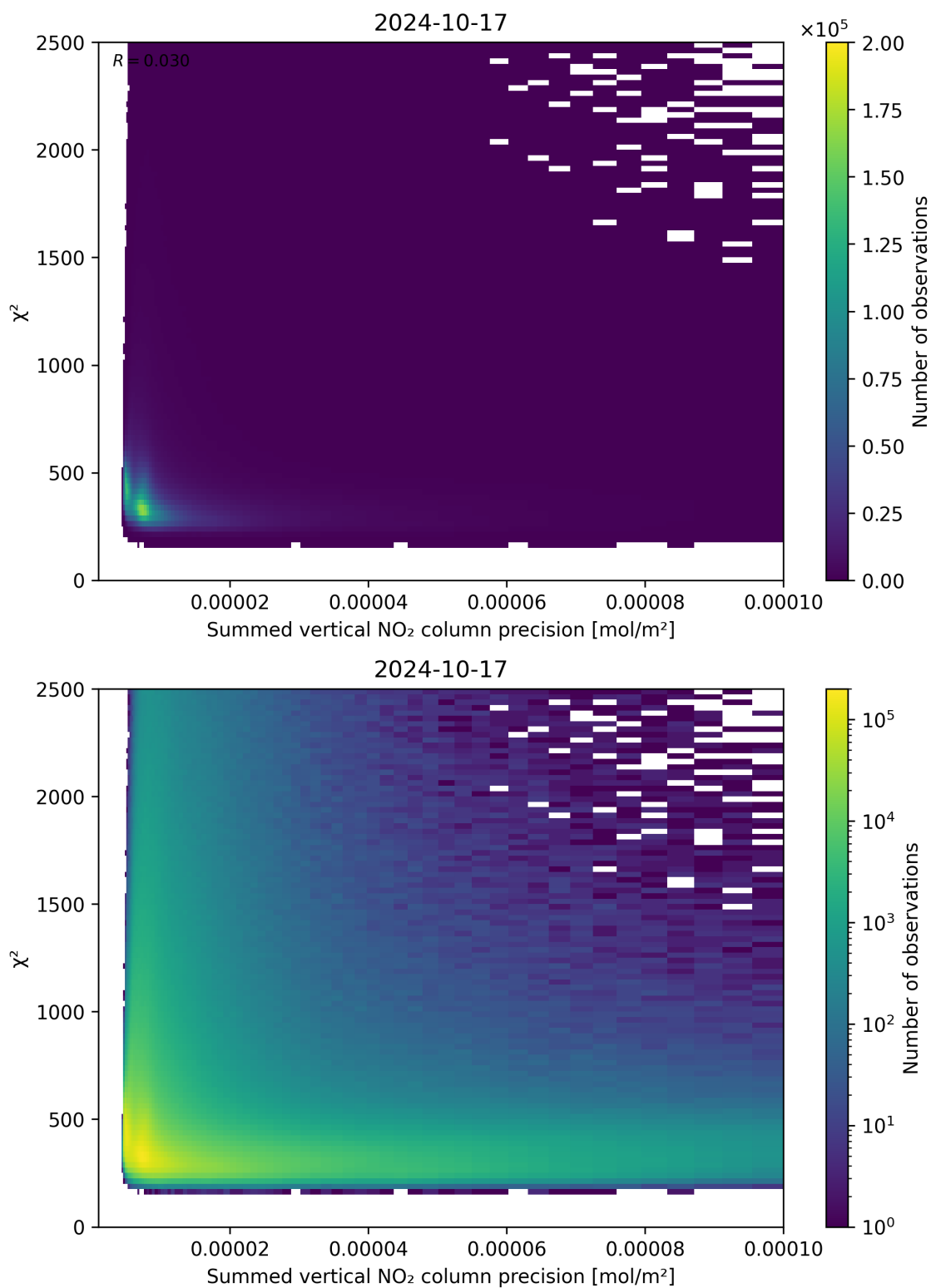
Figure 107: Scatter density plot of “Summed vertical NO 2 column precision” against “ \chi^2 ” for 2024-10-16 to 2024-10-18.
