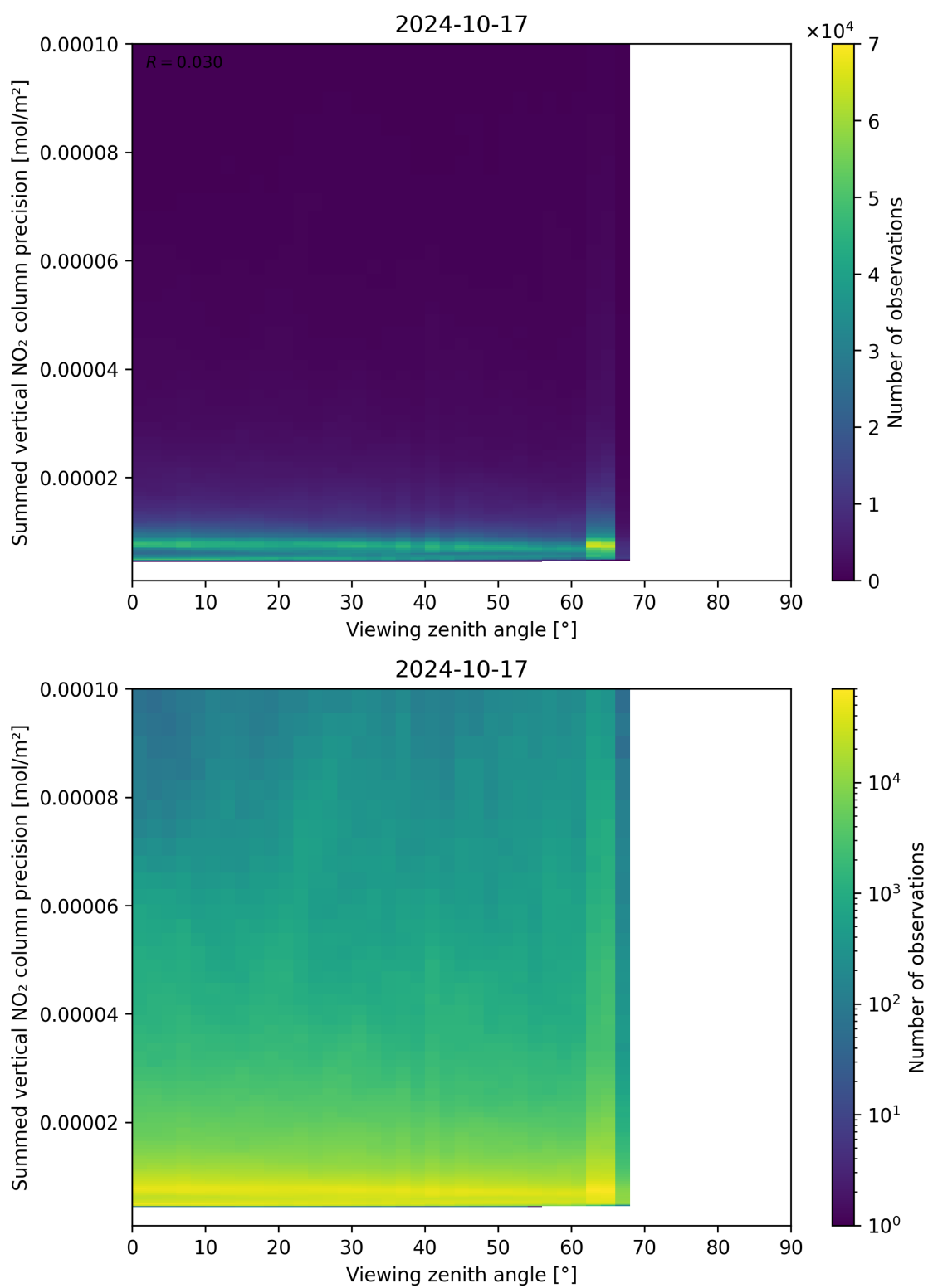
Figure 166: Scatter density plot of “Viewing zenith angle” against “Summed vertical NO 2 column precision” for 2024-10-16 to 2024-10-18.
