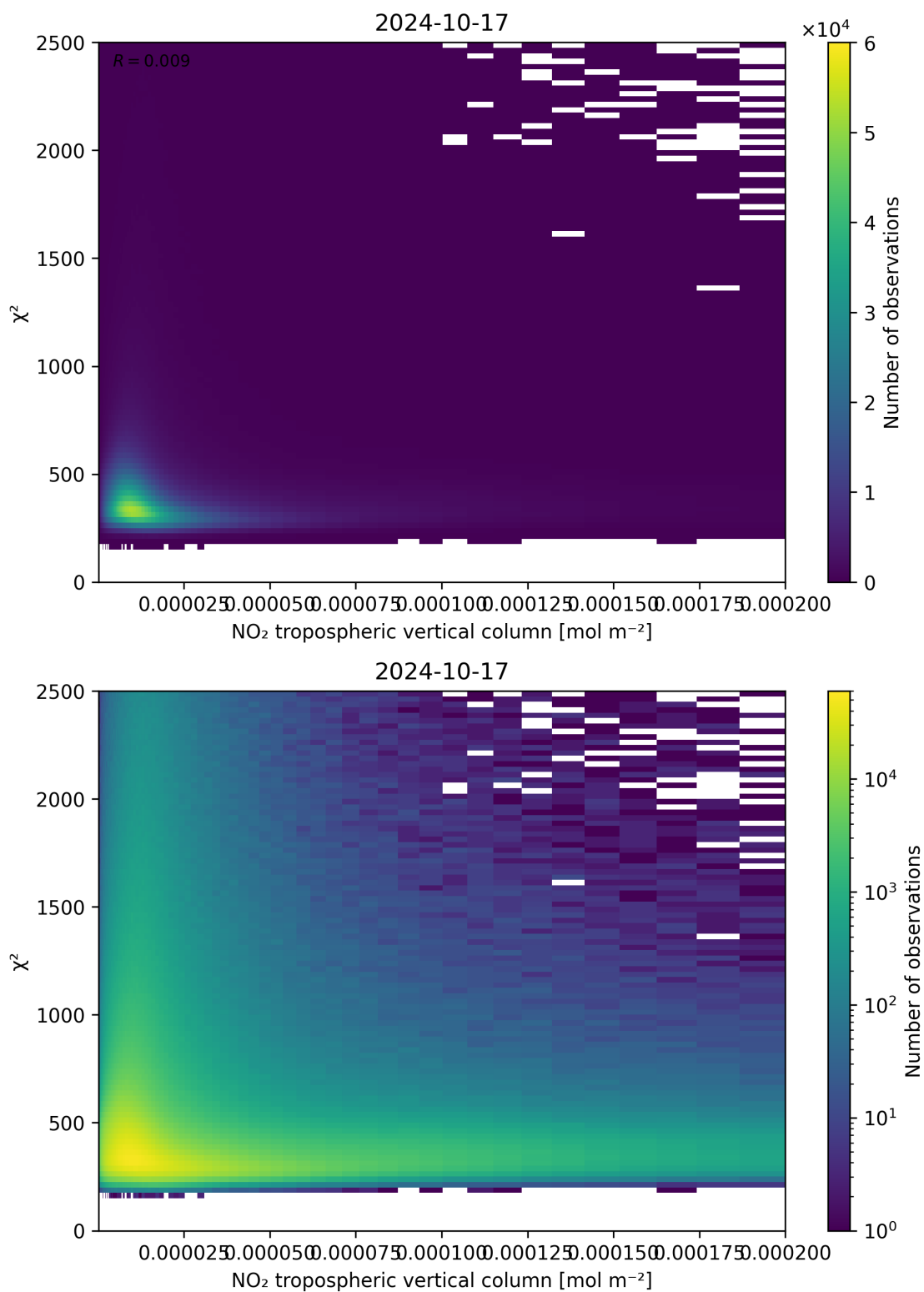
Figure 124: Scatter density plot of “NO 2 tropospheric vertical column” against “ \chi^2 ” for 2024-10-16 to 2024-10-18.
