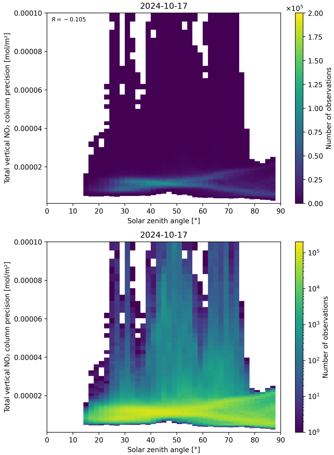
Figure 154: Scatter density plot of “Solar zenith angle” against “Total vertical NO 2 column precision” for 2024-10-16 to 2024-10-18.
