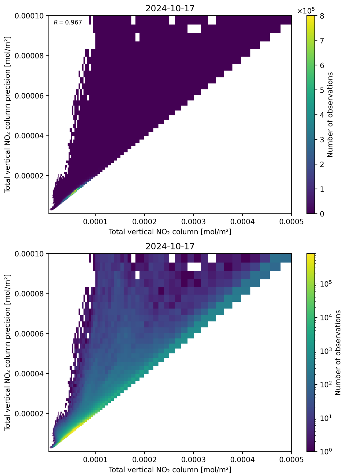
Figure 114: Scatter density plot of “Total vertical NO 2 column” against “Total vertical NO 2 column precision” for 2024-10-16 to 2024-10-18.
