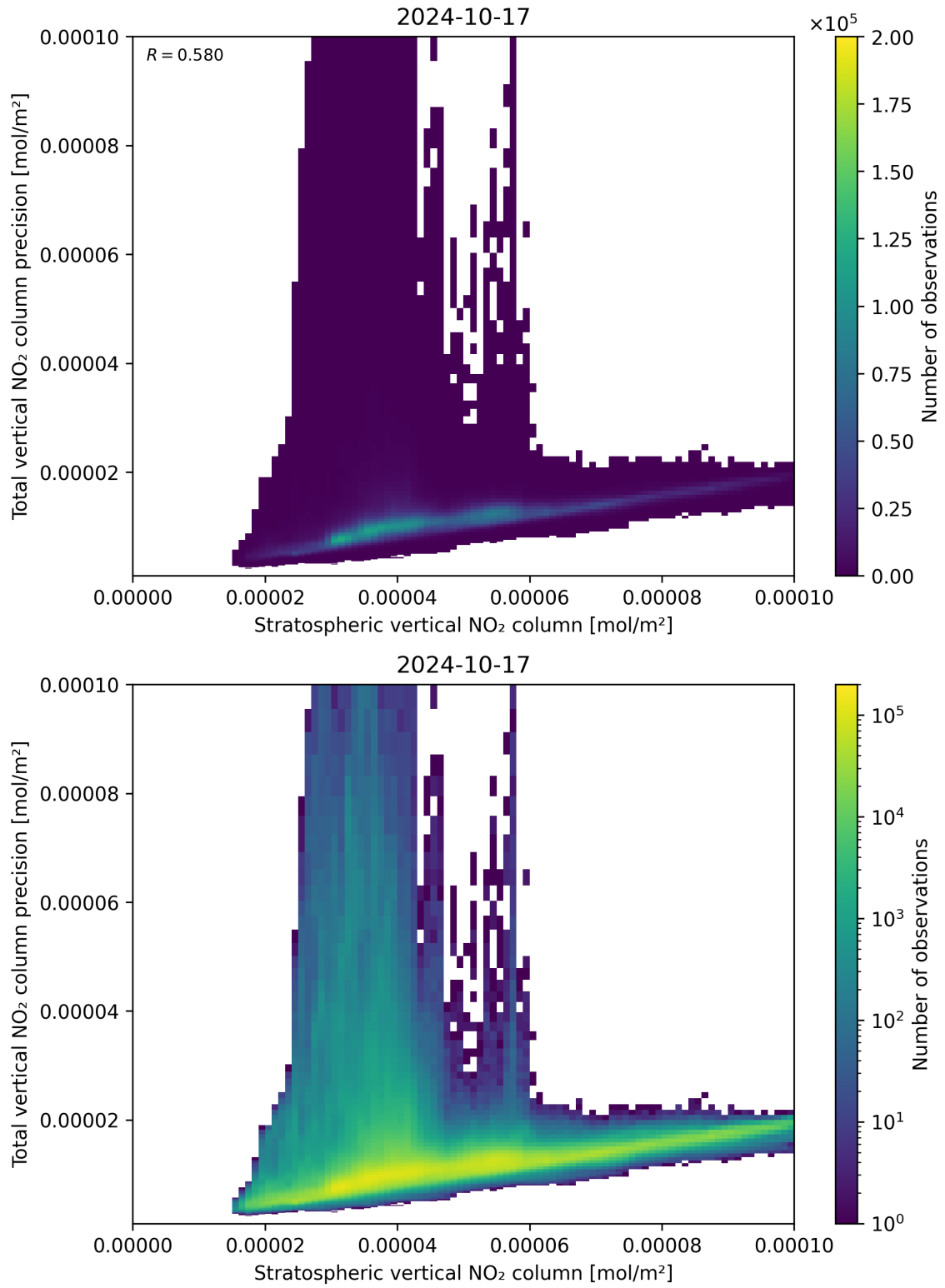
Figure 101: Scatter density plot of “Stratospheric vertical NO 2 column” against “Total vertical NO 2 column precision” for 2024-10-16 to 2024-10-18.
