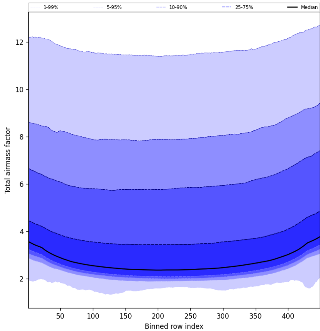
Figure 49: Along track statistics of “Total airmass factor” for 2024-10-16 to 2024-10-18
