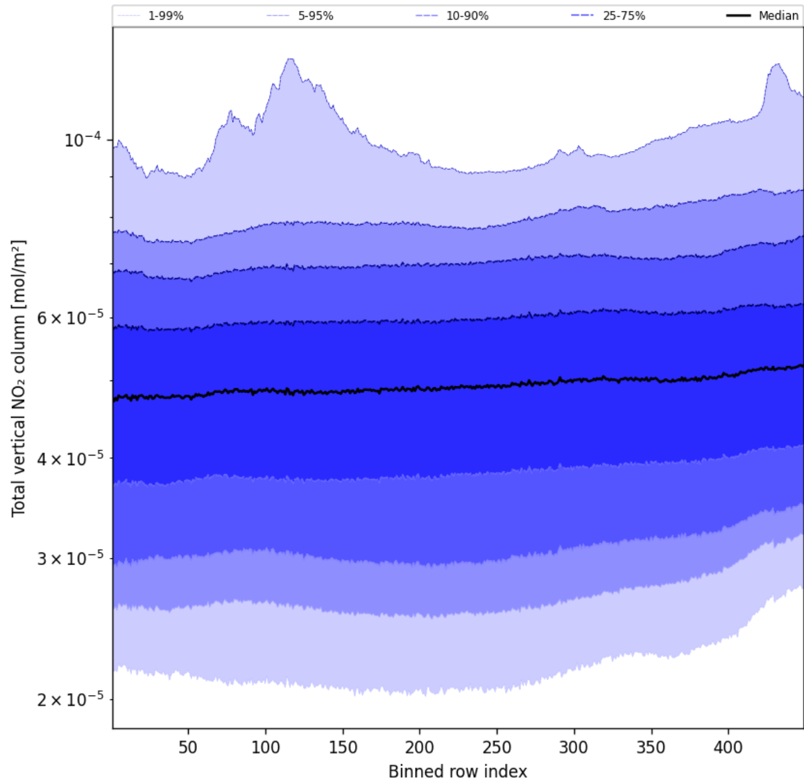
Figure 55: Along track statistics of “Total vertical NO 2 column” for 2024-10-16 to 2024-10-18
