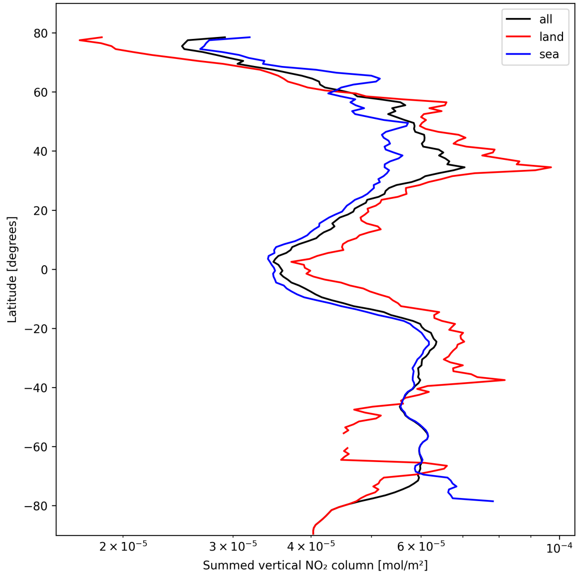
Figure 23: Zonal average of “Summed vertical NO 2 column” for 2024-10-16 to 2024-10-18.
