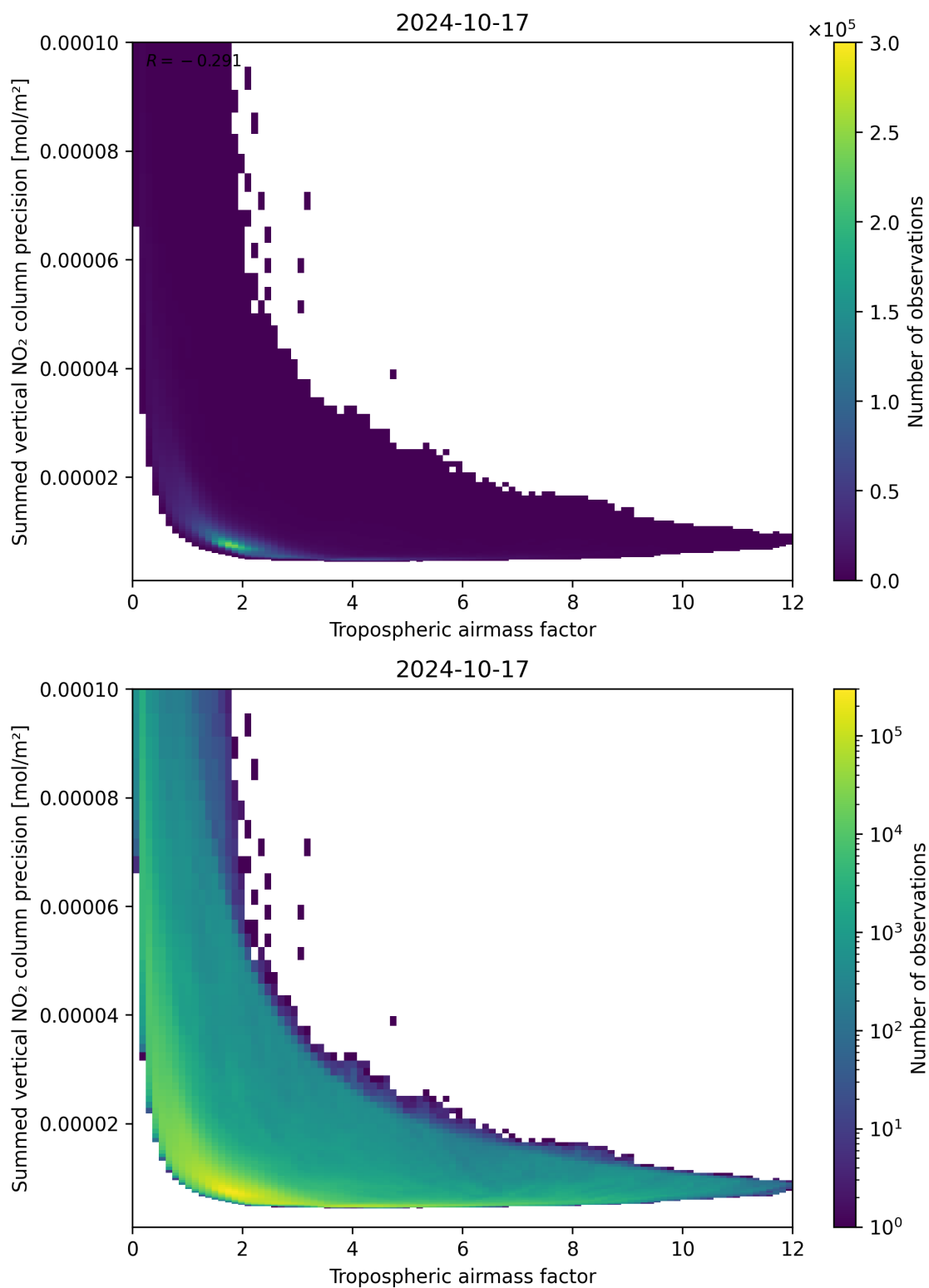
Figure 76: Scatter density plot of “Tropospheric airmass factor” against “Summed vertical NO 2 column precision” for 2024-10-16 to 2024-10-18.
