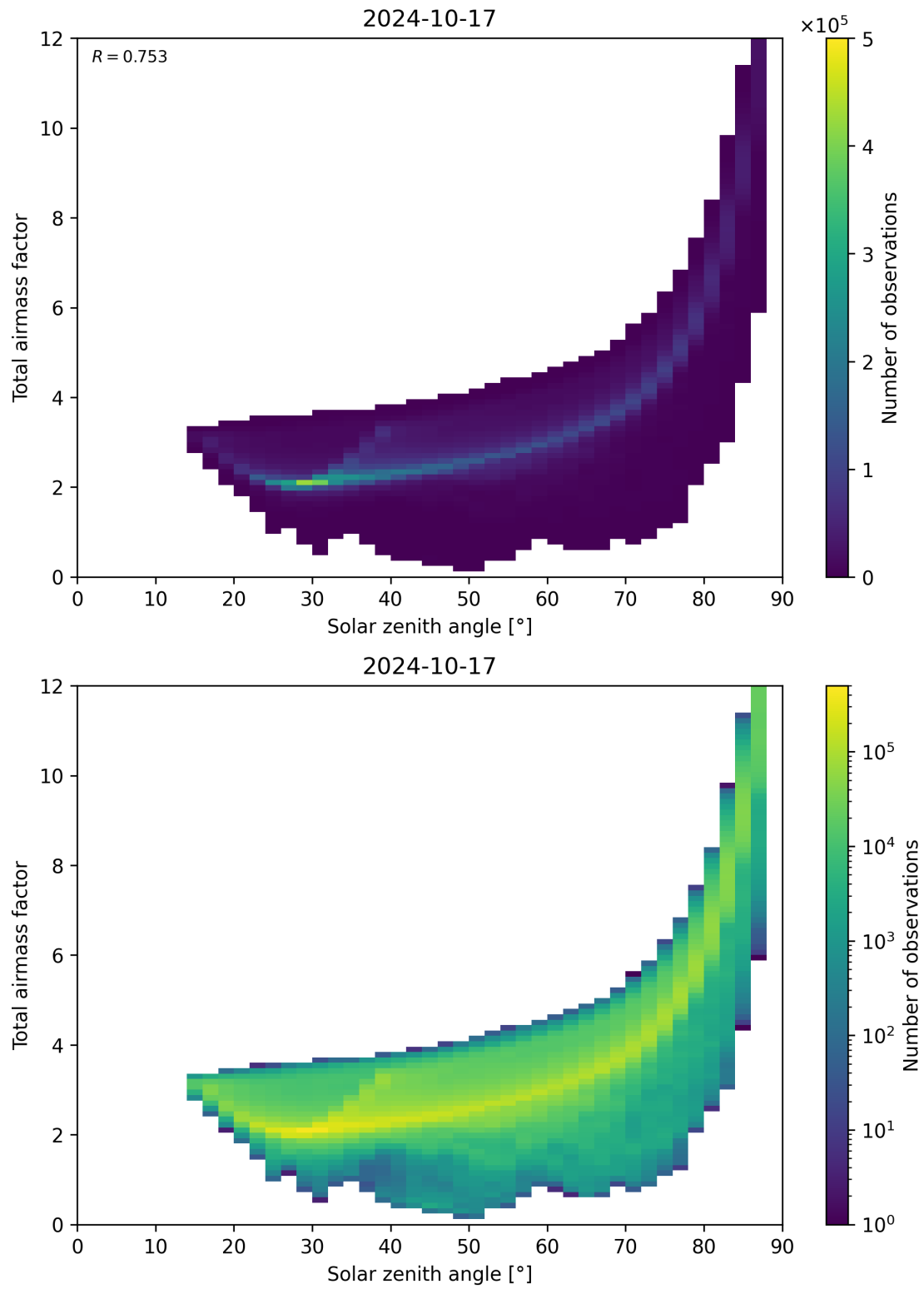
Figure 146: Scatter density plot of “Solar zenith angle” against “Total airmass factor” for 2024-10-16 to 2024-10-18.
