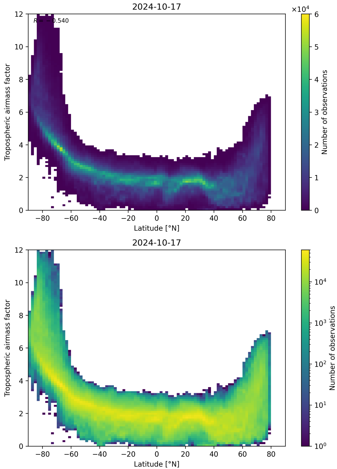
Figure 85: Scatter density plot of “Latitude” against “Tropospheric air mass factor” for 2024-10-16 to 2024-10-18.
