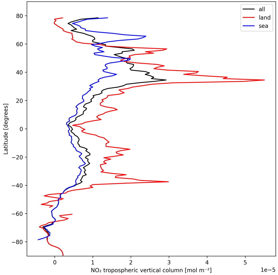
Figure 12: Zonal average of “NO 2 tropospheric vertical column” for 2024-10-16 to 2024-10-18.
