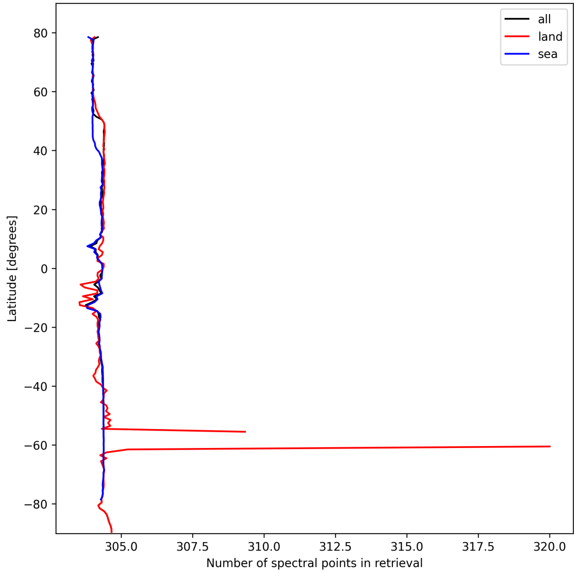
Figure 16: Zonal average of “Number of spectral points in retrieval” for 2024-10-16 to 2024-10-18.
