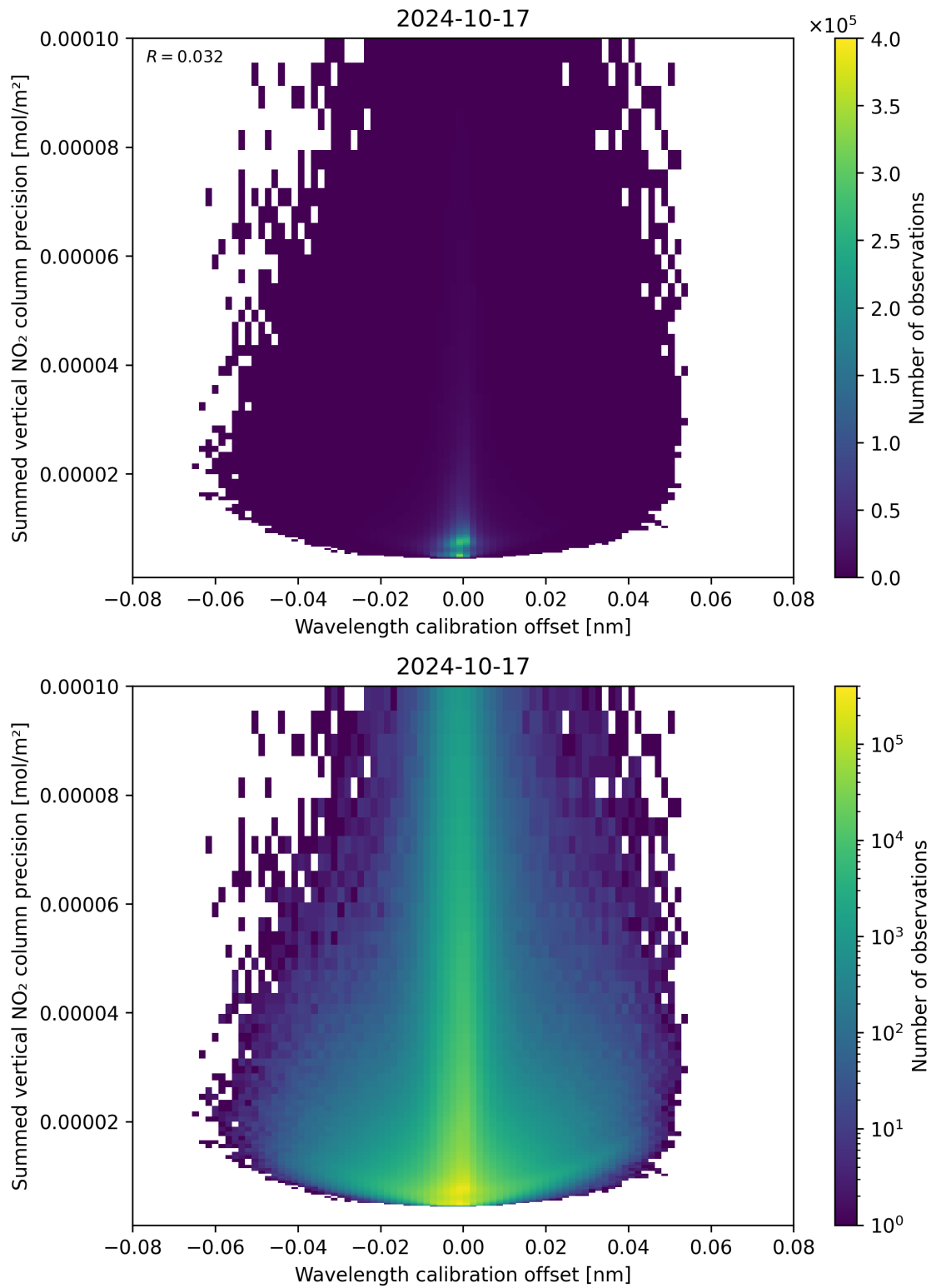
Figure 178: Scatter density plot of “Wavelength calibration offset” against “Summed vertical NO 2 column precision” for 2024-10-16 to 2024-10-18.
