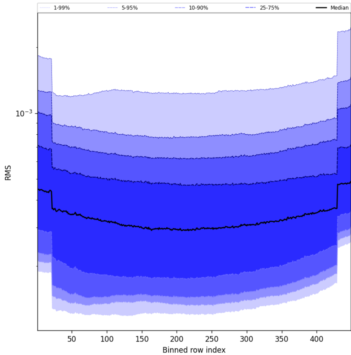
Figure 60: Along track statistics of “RMS” for 2024-10-16 to 2024-10-18
