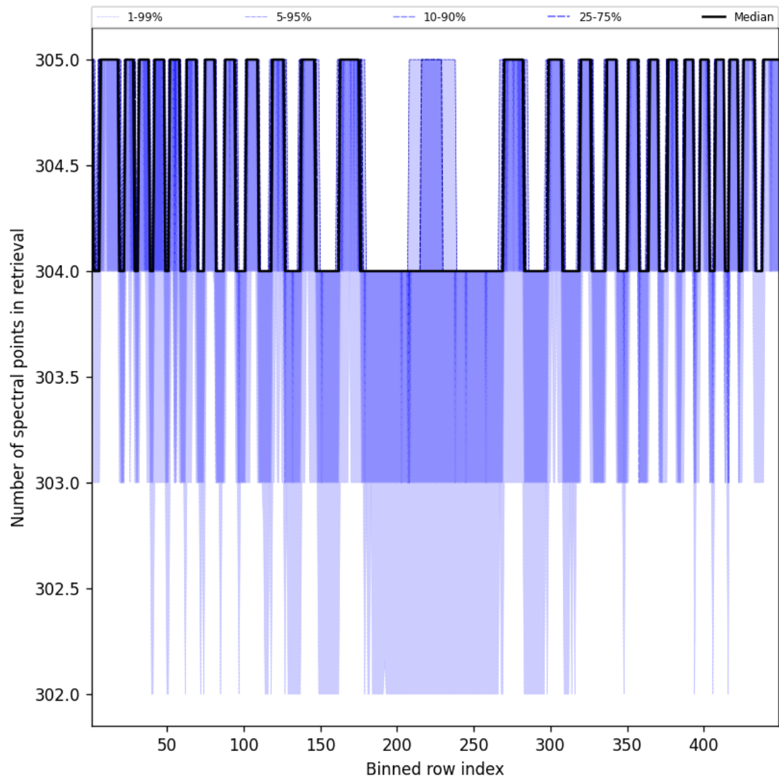
Figure 50: Along track statistics of “Number of spectral points in retrieval” for 2024-10-16 to 2024-10-18
