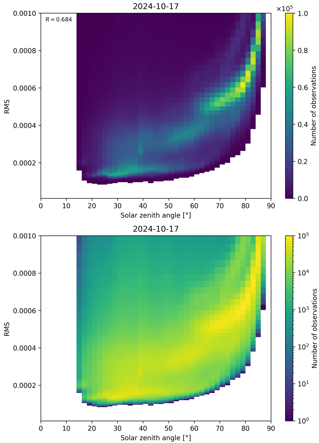
Figure 157: Scatter density plot of “Solar zenith angle” against “RMS” for 2024-10-16 to 2024-10-18.
