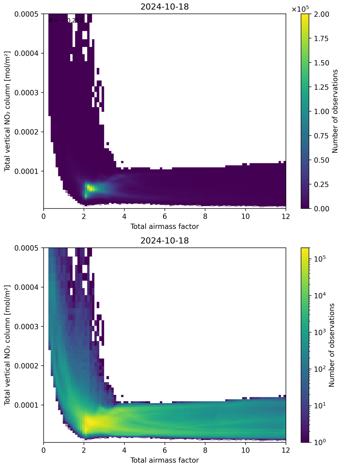
Figure 67: Scatter density plot of “Total airmass factor” against “Total vertical NO 2 column” for 2024-10-17 to 2024-10-19.
