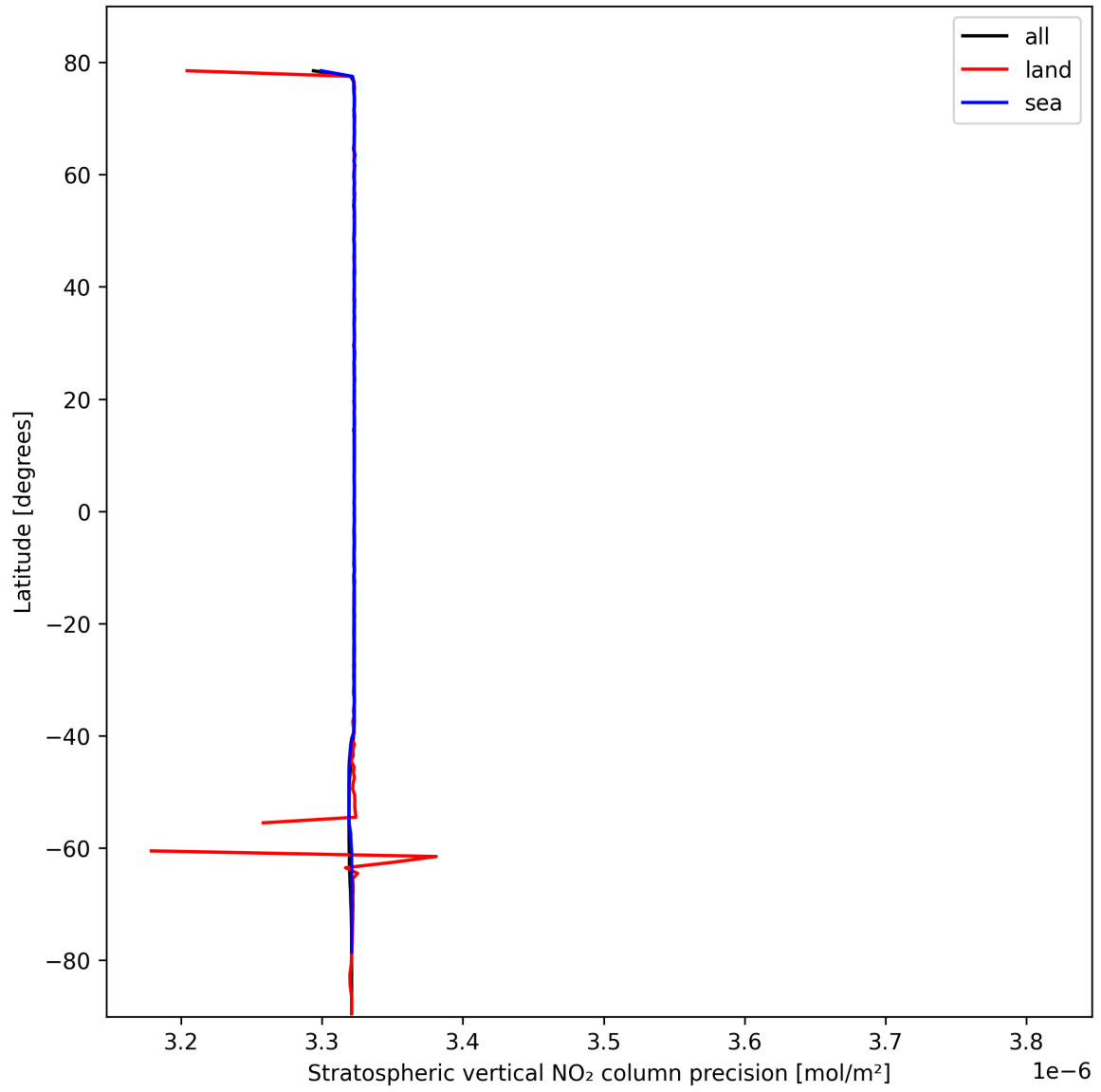
Figure 20: Zonal average of “Stratospheric vertical NO 2 column precision” for 2024-10-17 to 2024-10-19.
