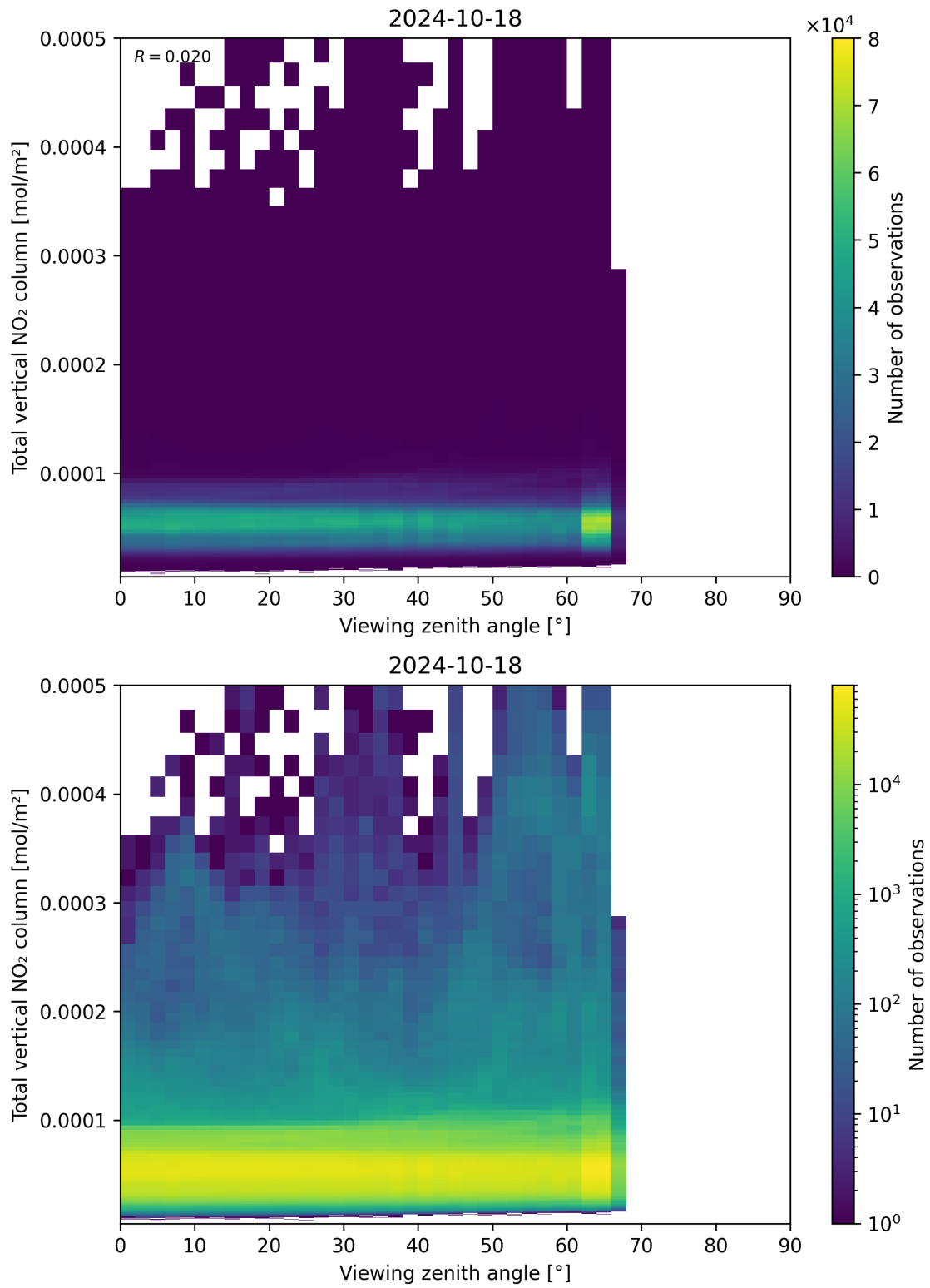
Figure 167: Scatter density plot of “Viewing zenith angle” against “Total vertical NO 2 column” for 2024-10-17 to 2024-10-19.
