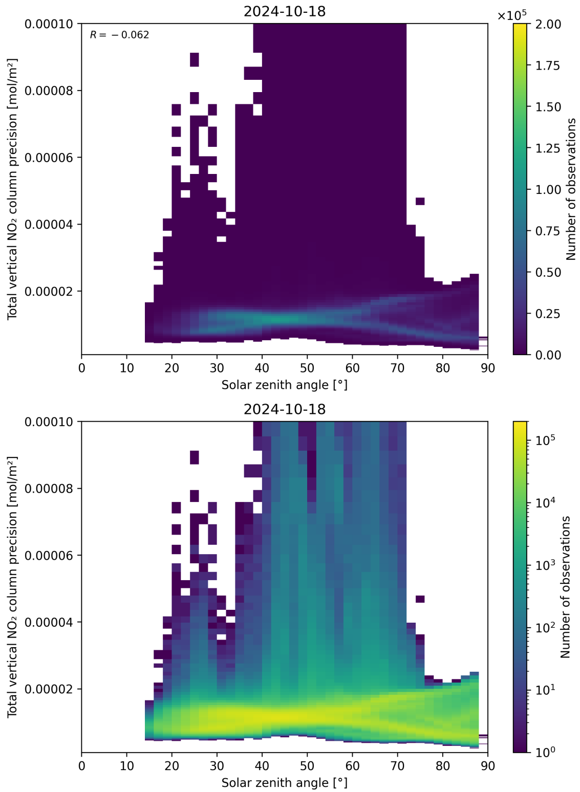
Figure 154: Scatter density plot of “Solar zenith angle” against “Total vertical NO 2 column precision” for 2024-10-17 to 2024-10-19.
