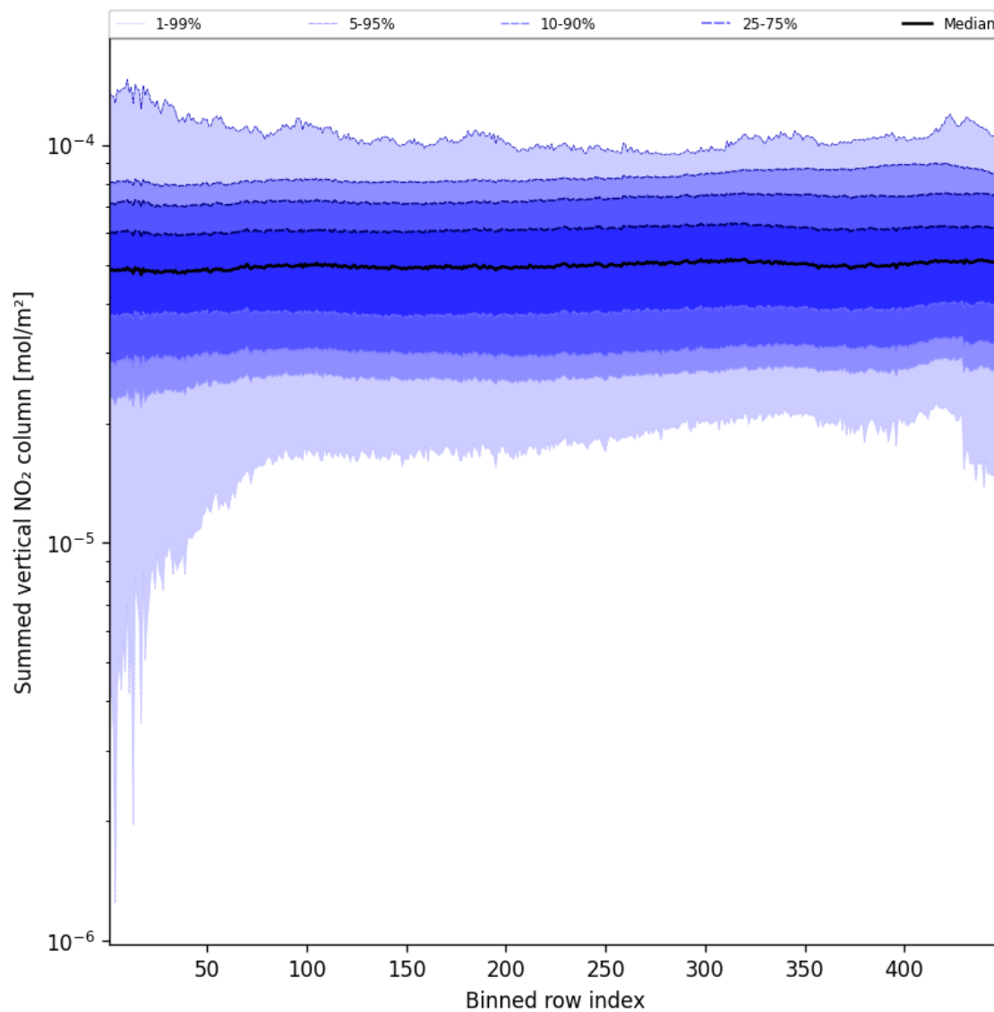
Figure 57: Along track statistics of “Summed vertical NO 2 column” for 2024-10-17 to 2024-10-19
