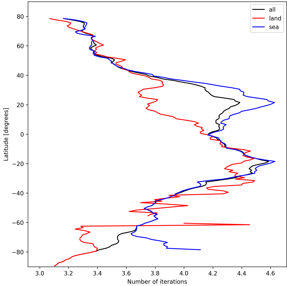
Figure 17: Zonal average of “Number of iterations” for 2024-10-17 to 2024-10-19.
