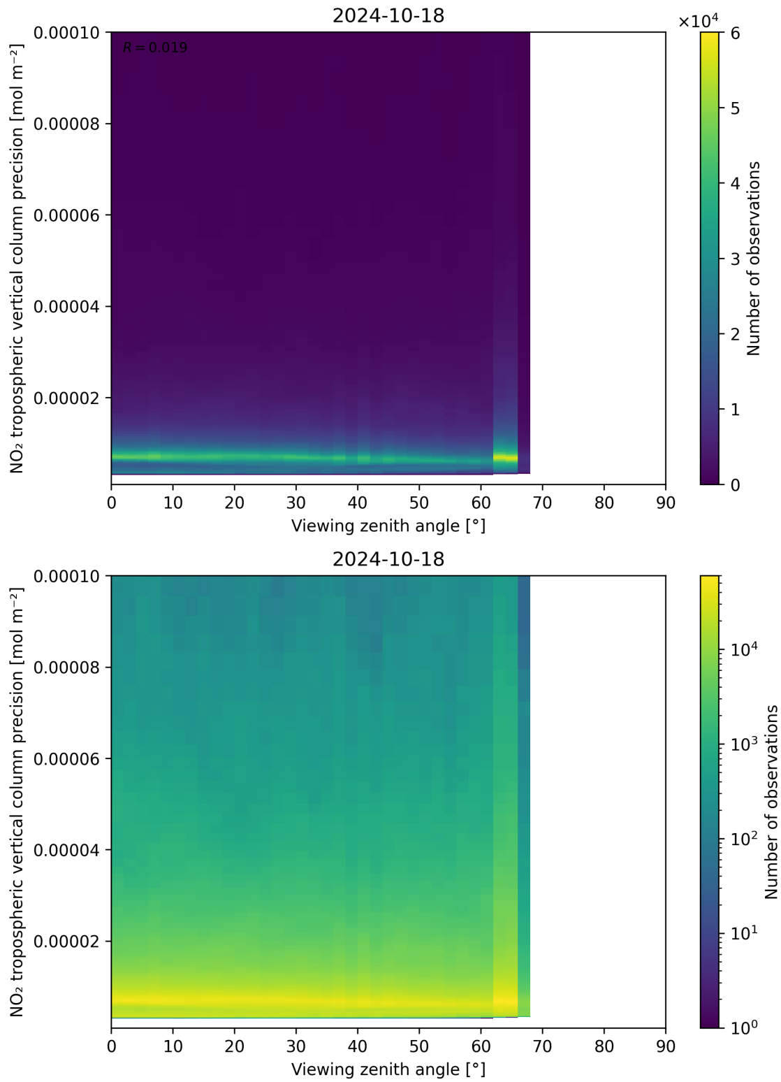
Figure 170: Scatter density plot of “Viewing zenith angle” against “NO 2 tropospheric vertical column precision” for 2024-10-17 to 2024-10-19.
