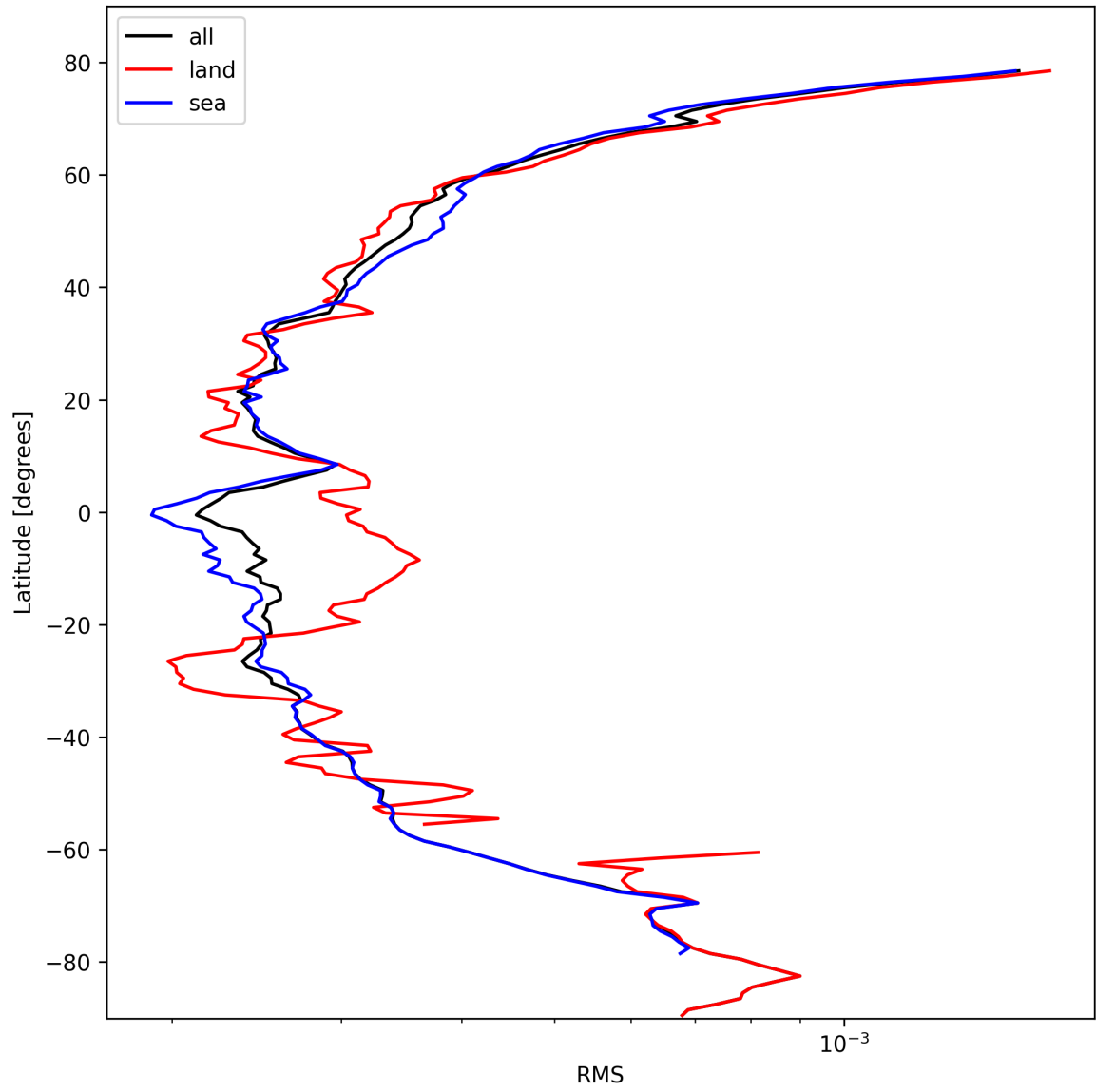
Figure 26: Zonal average of “RMS” for 2024-10-17 to 2024-10-19.
