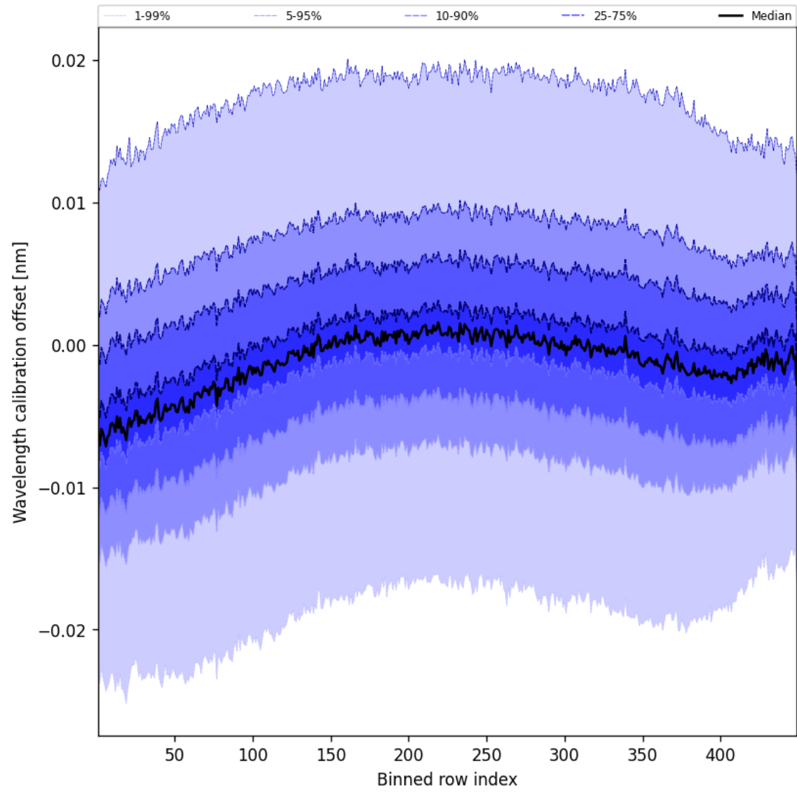
Figure 52: Along track statistics of “Wavelength calibration offset” for 2024-10-17 to 2024-10-19
