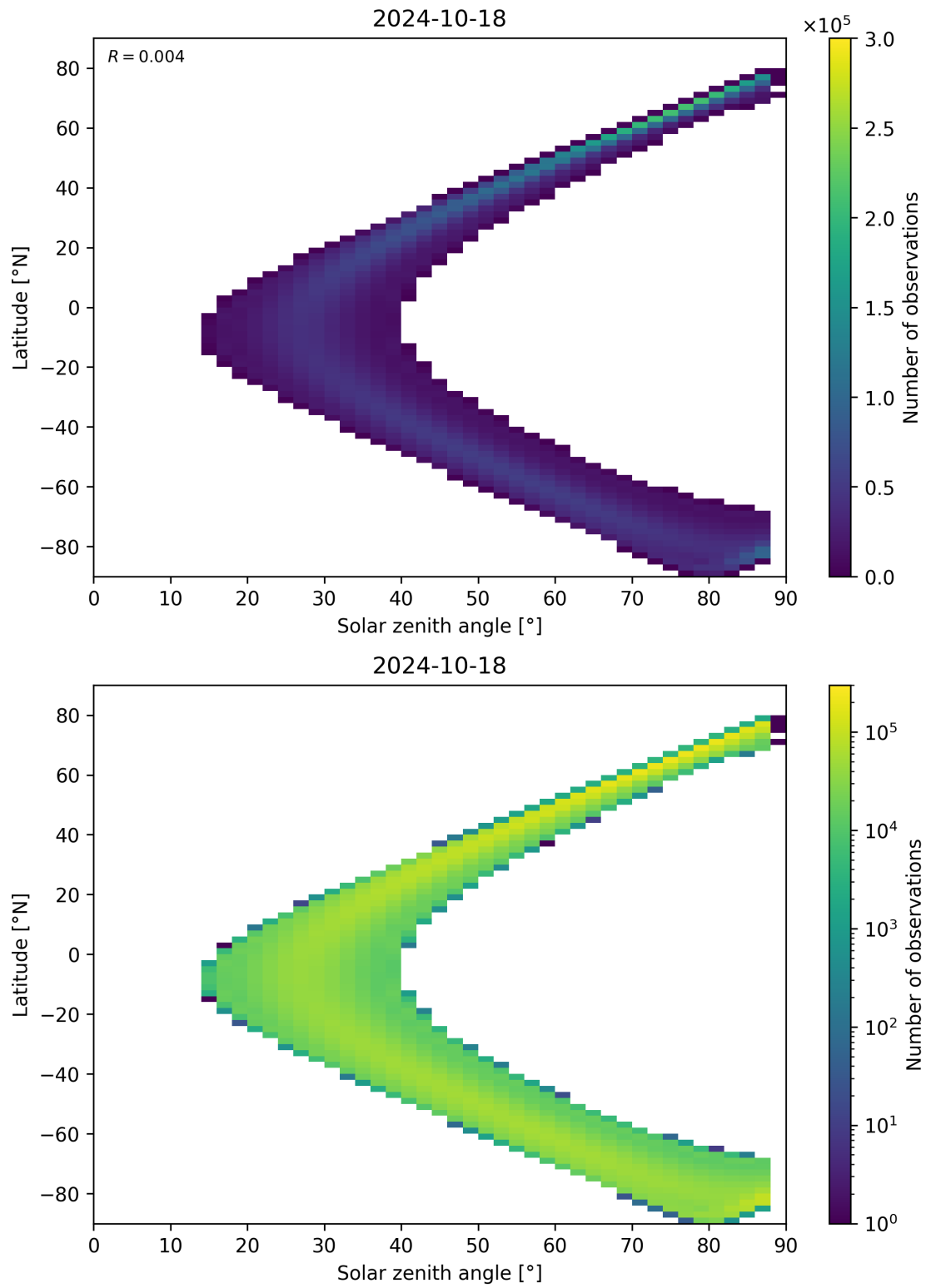
Figure 149: Scatter density plot of “Solar zenith angle” against “Latitude” for 2024-10-17 to 2024-10-19.
