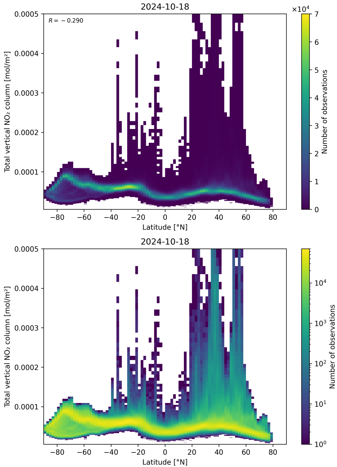
Figure 90: Scatter density plot of “Latitude” against “Total vertical NO 2 column” for 2024-10-17 to 2024-10-19.
