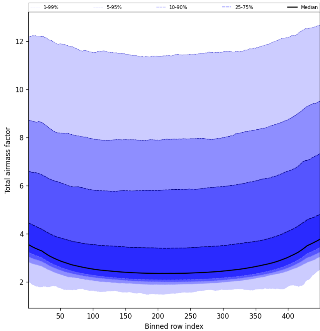
Figure 49: Along track statistics of “Total airmass factor” for 2024-10-17 to 2024-10-19
