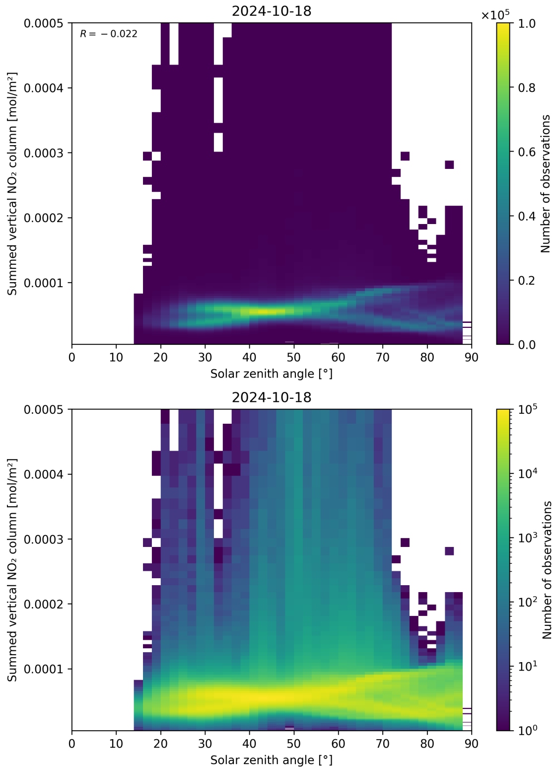
Figure 151: Scatter density plot of “Solar zenith angle” against “Summed vertical NO 2 column” for 2024-10-17 to 2024-10-19.
