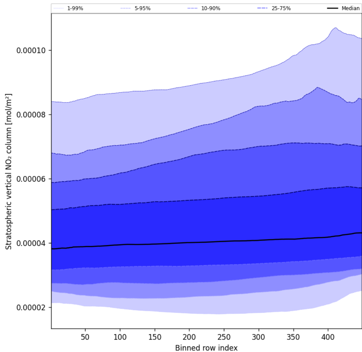
Figure 53: Along track statistics of “Stratospheric vertical NO 2 column” for 2024-10-17 to 2024-10-19
