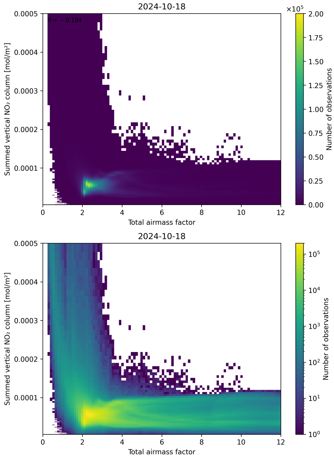
Figure 65: Scatter density plot of “Total airmass factor” against “Summed vertical NO 2 column” for 2024-10-17 to 2024-10-19.
