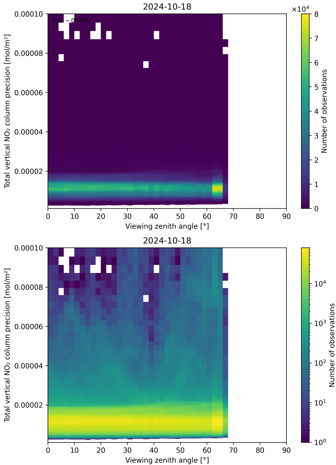
Figure 168: Scatter density plot of “Viewing zenith angle” against “Total vertical NO 2 column precision” for 2024-10-17 to 2024-10-19.
