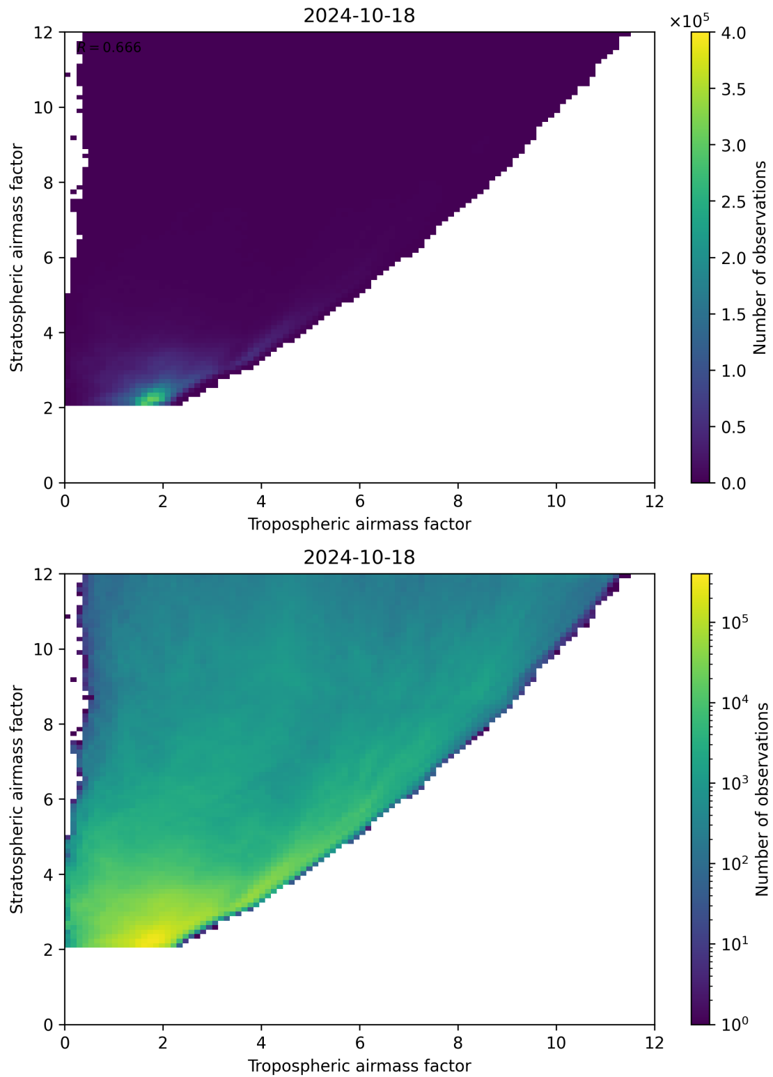
Figure 71: Scatter density plot of “Tropospheric airmass factor” against “Stratospheric airmass factor” for 2024-10-17 to 2024-10-19.
