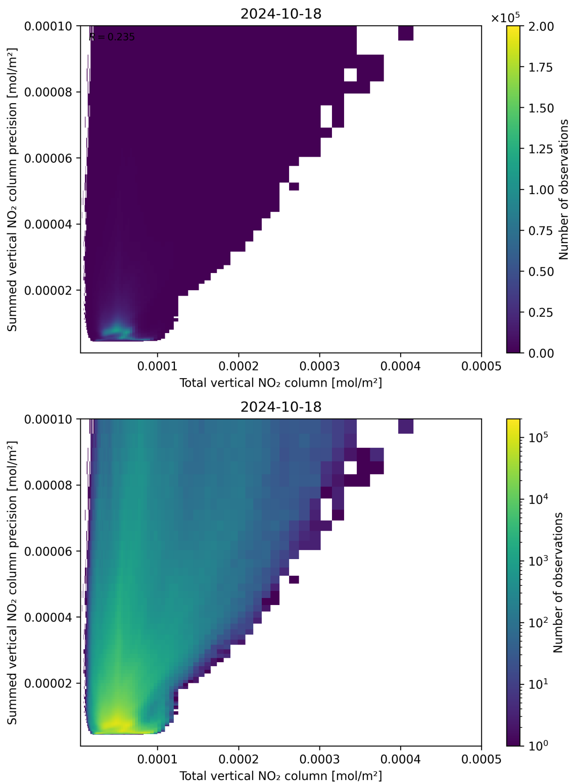
Figure 113: Scatter density plot of “Total vertical NO 2 column” against “Summed vertical NO 2 column precision” for 2024-10-17 to 2024-10-19.
