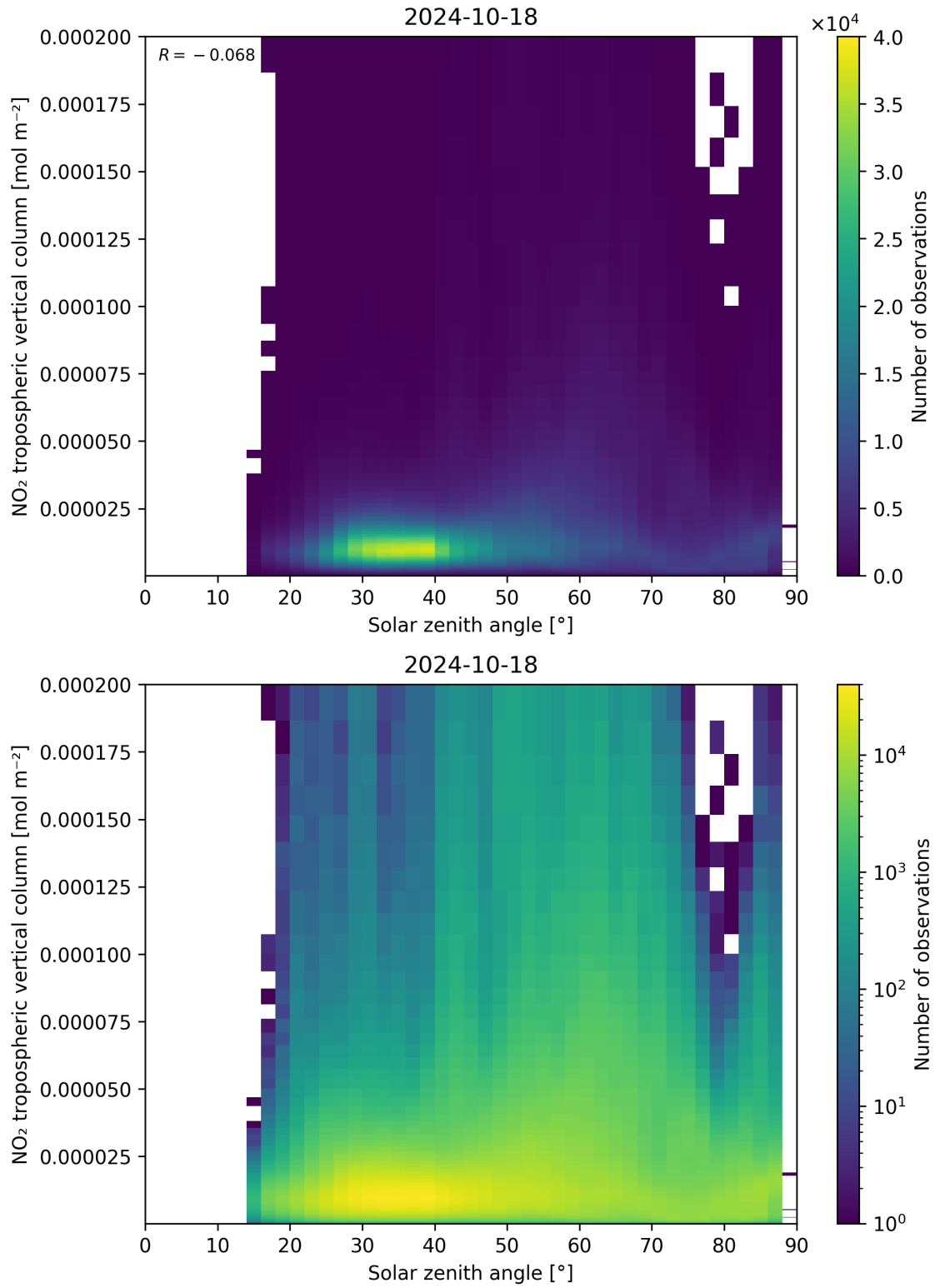
Figure 155: Scatter density plot of “Solar zenith angle” against “NO 2 tropospheric vertical column” for 2024-10-17 to 2024-10-19.
