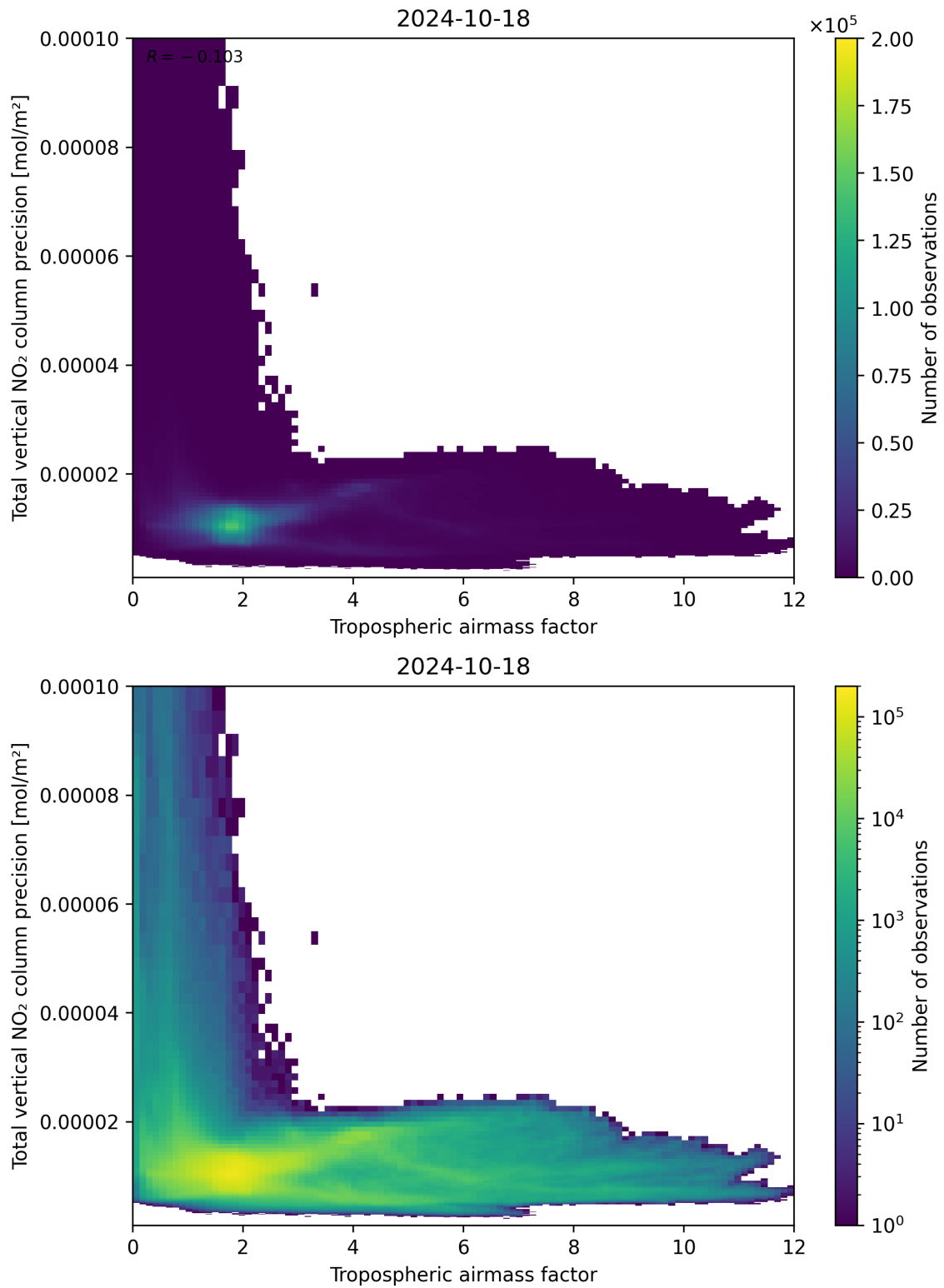
Figure 78: Scatter density plot of “Tropospheric airmass factor” against “Total vertical NO 2 column precision” for 2024-10-17 to 2024-10-19.
