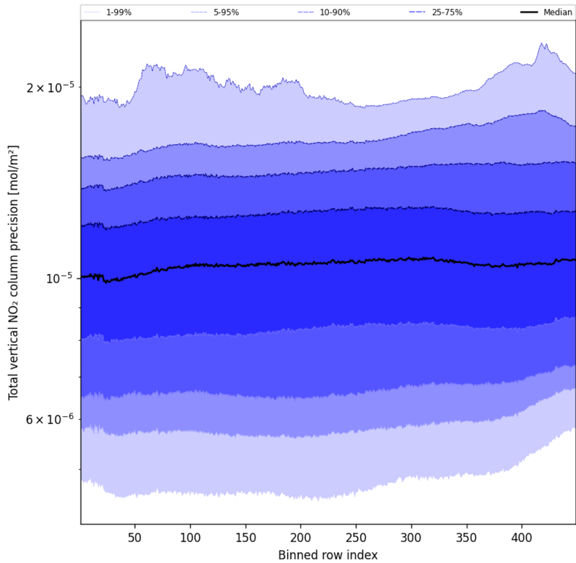
Figure 56: Along track statistics of “Total vertical NO 2 column precision” for 2024-10-17 to 2024-10-19
