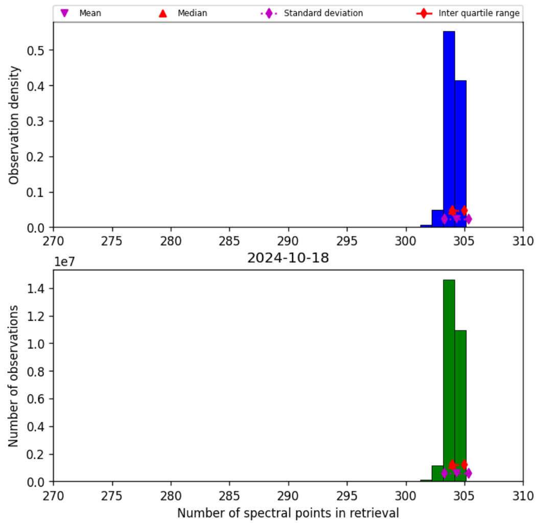
Figure 33: Histogram of “Number of spectral points in retrieval” for 2024-10-17 to 2024-10-19
