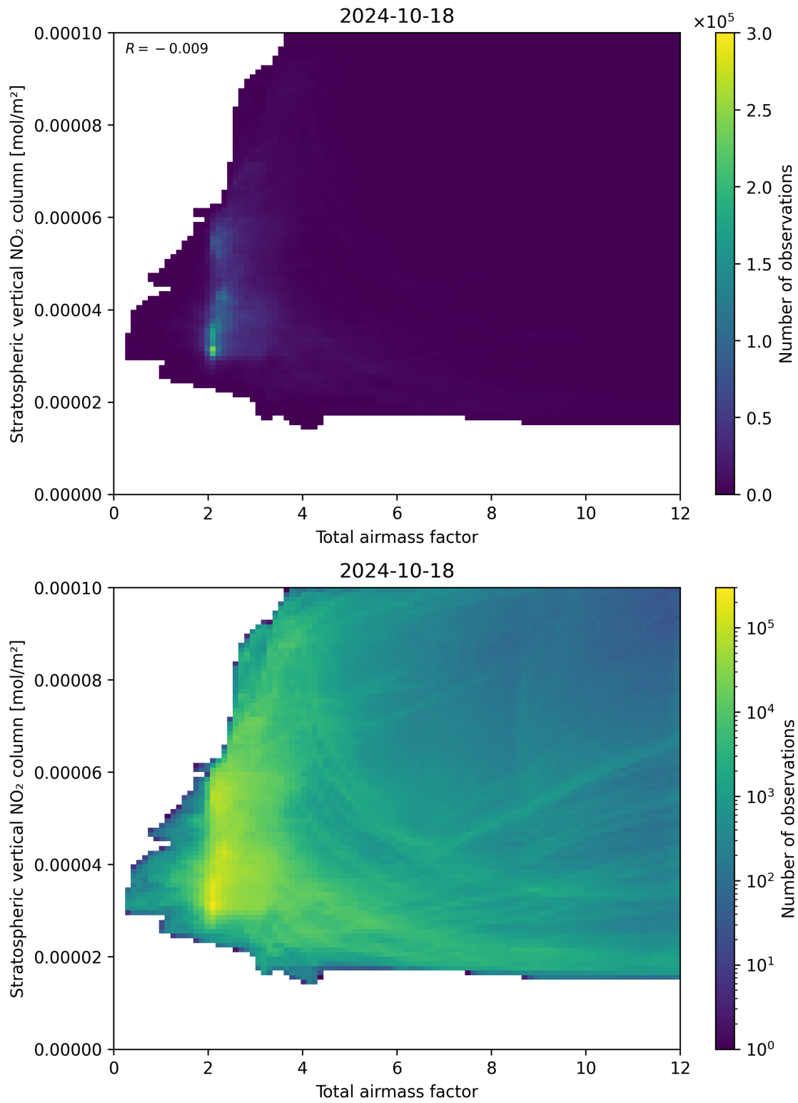
Figure 64: Scatter density plot of “Total airmass factor” against “Stratospheric vertical NO 2 column” for 2024-10-17 to 2024-10-19.
