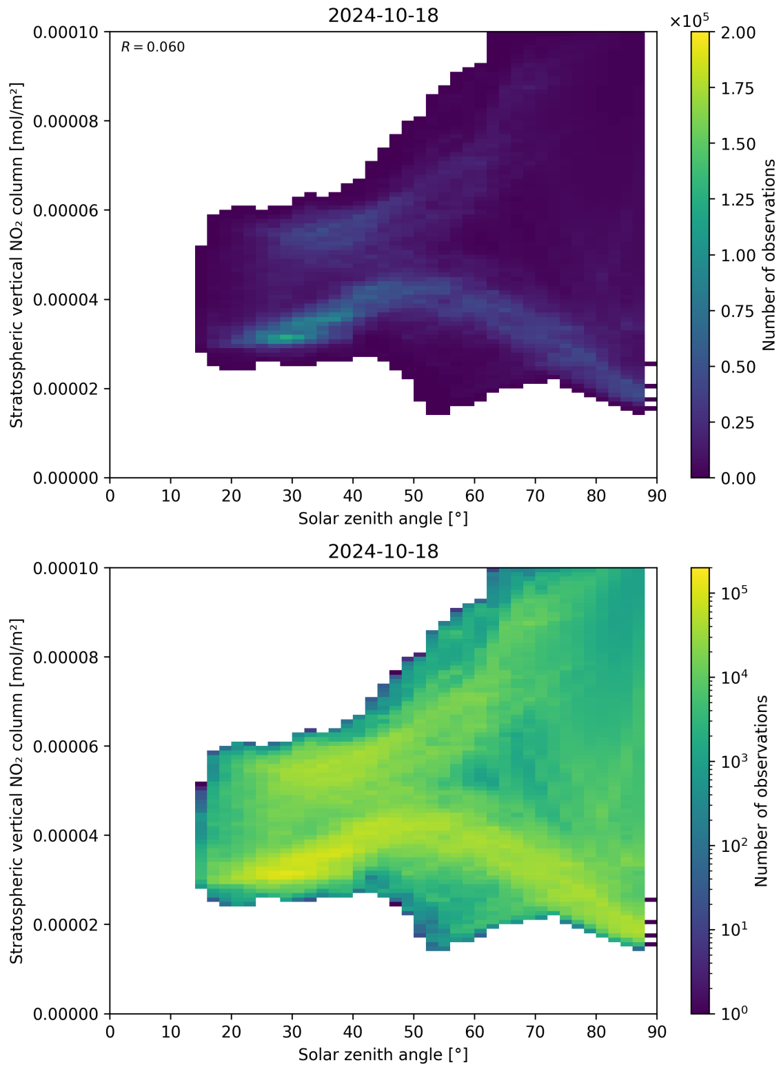
Figure 150: Scatter density plot of “Solar zenith angle” against “Stratospheric vertical NO 2 column” for 2024-10-17 to 2024-10-19.
