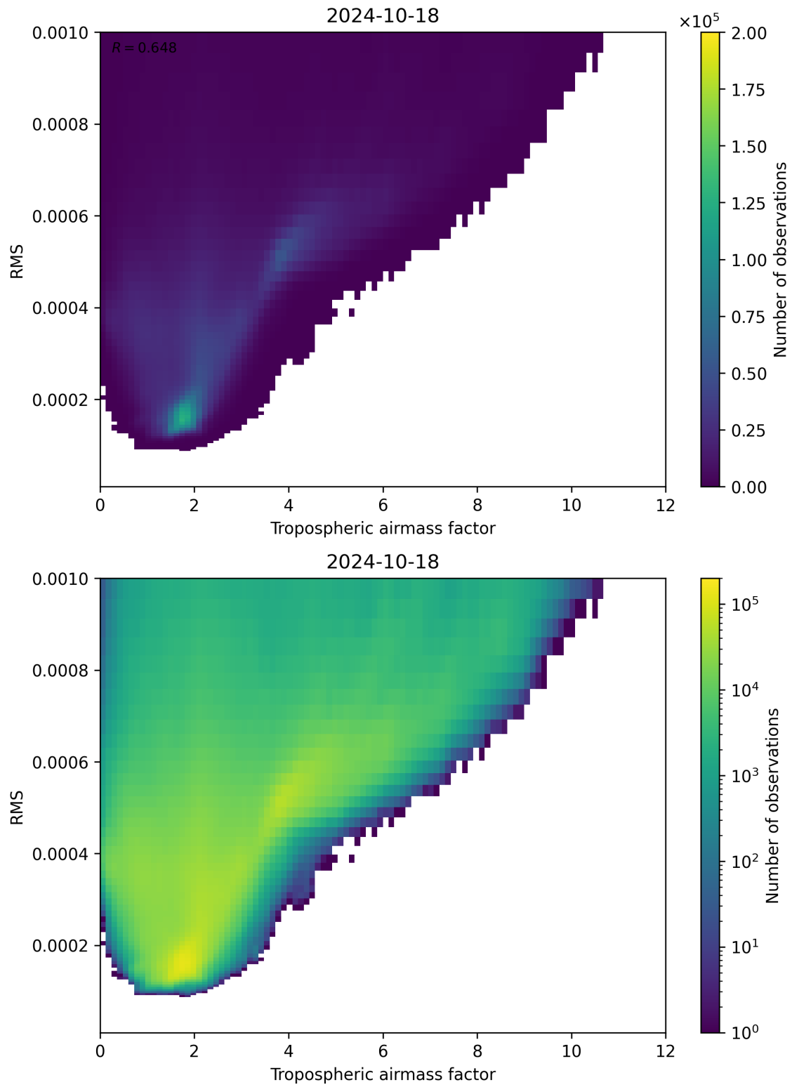
Figure 79: Scatter density plot of “Tropospheric airmass factor” against “RMS” for 2024-10-17 to 2024-10-19.
