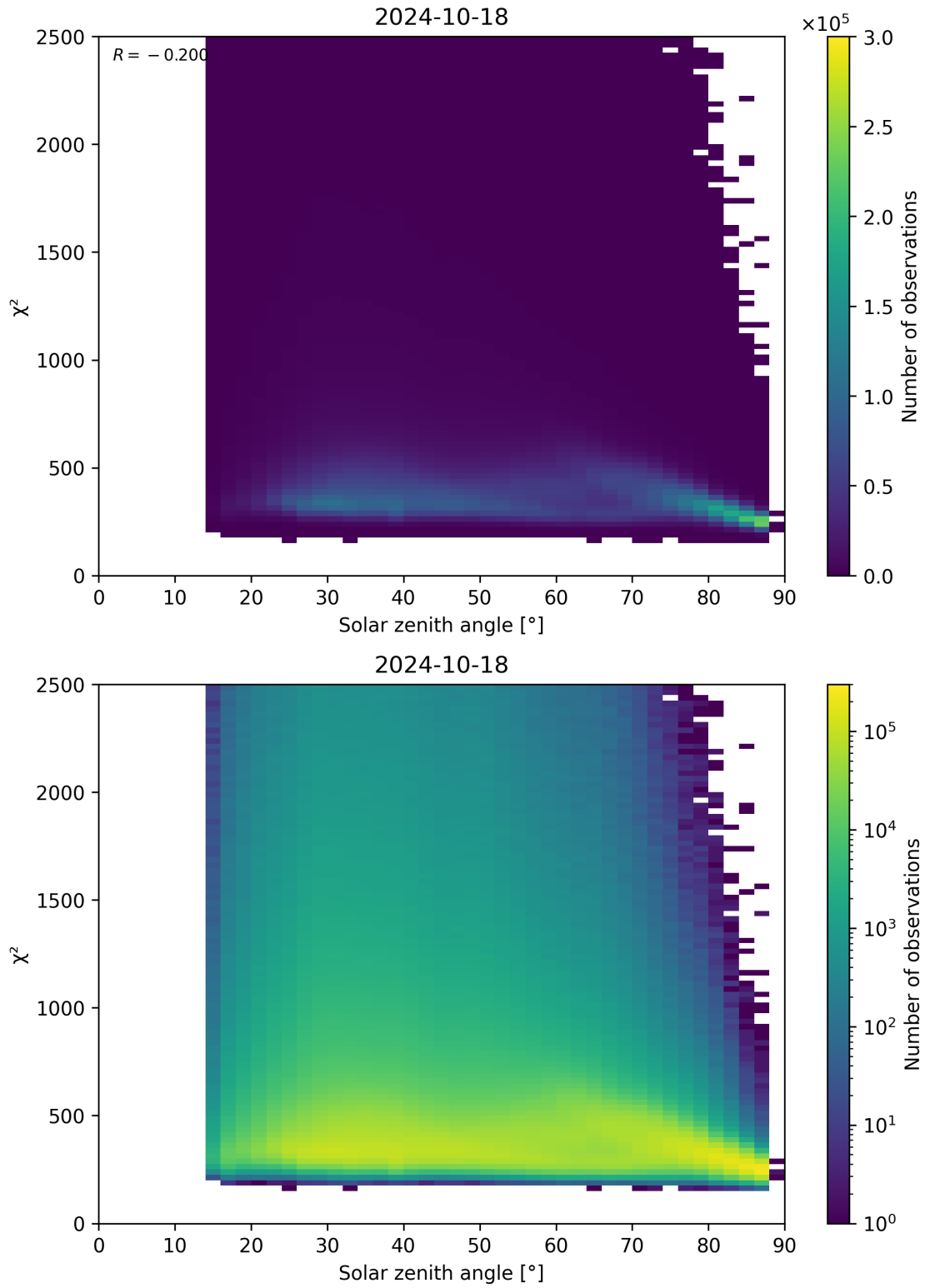
Figure 148: Scatter density plot of “Solar zenith angle” against “ \chi^2 ” for 2024-10-17 to 2024-10-19.
