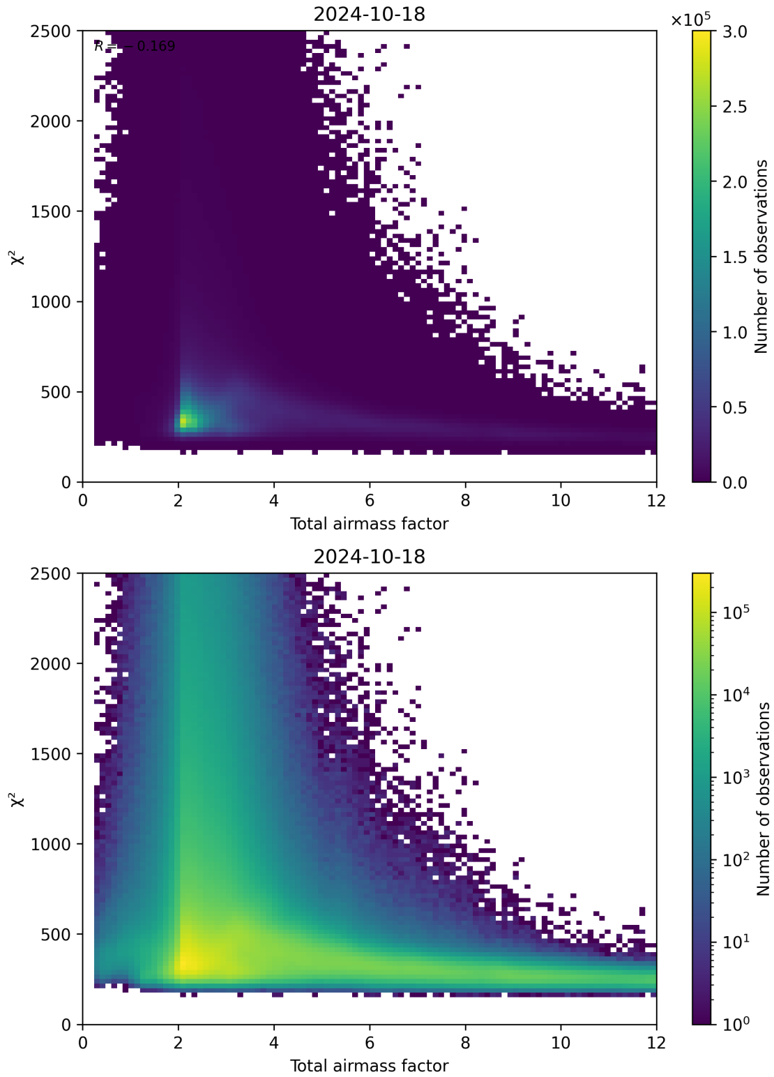
Figure 63: Scatter density plot of “Total airmass factor” against “ \chi^2 ” for 2024-10-17 to 2024-10-19.
