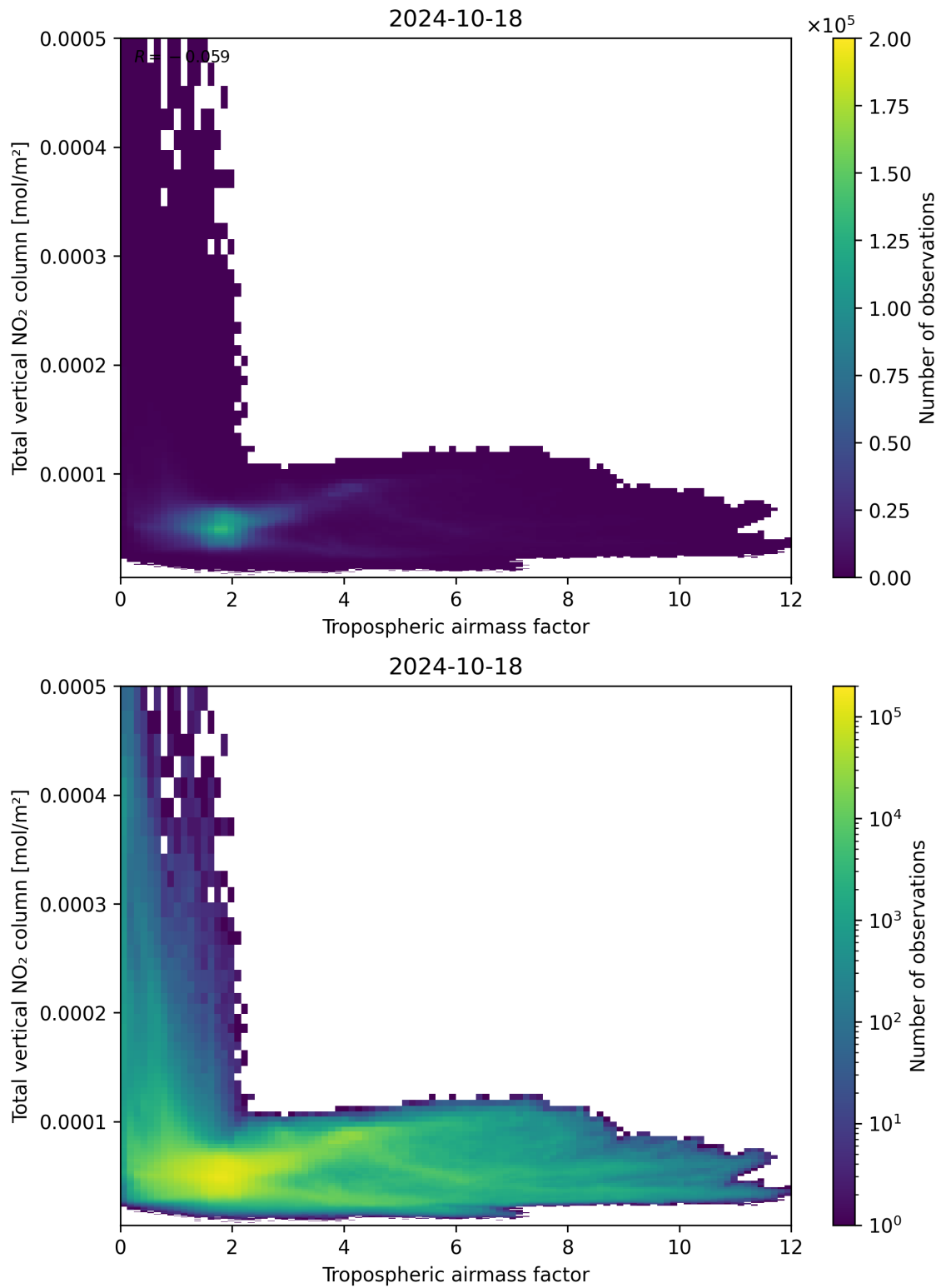
Figure 77: Scatter density plot of “Tropospheric airmass factor” against “Total vertical NO 2 column” for 2024-10-17 to 2024-10-19.
