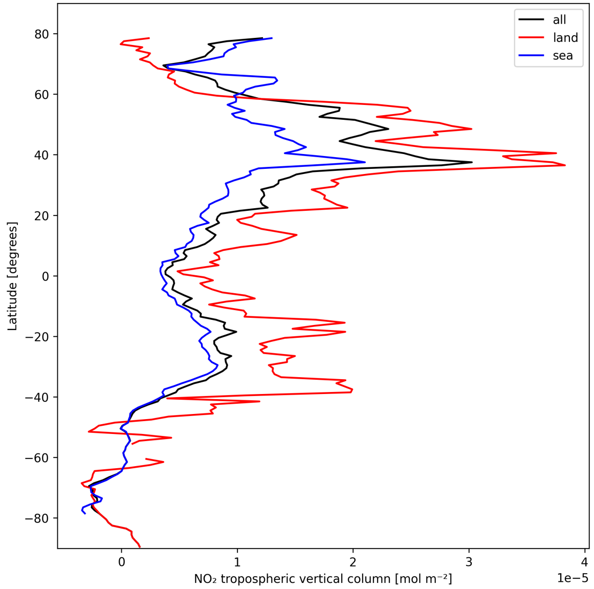
Figure 12: Zonal average of “NO 2 tropospheric vertical column” for 2024-10-17 to 2024-10-19.
