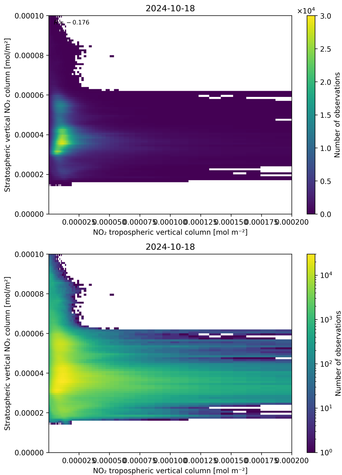
Figure 125: Scatter density plot of “NO 2 tropospheric vertical column” against “Stratospheric vertical NO 2 column” for 2024-10-17 to 2024-10-19.
