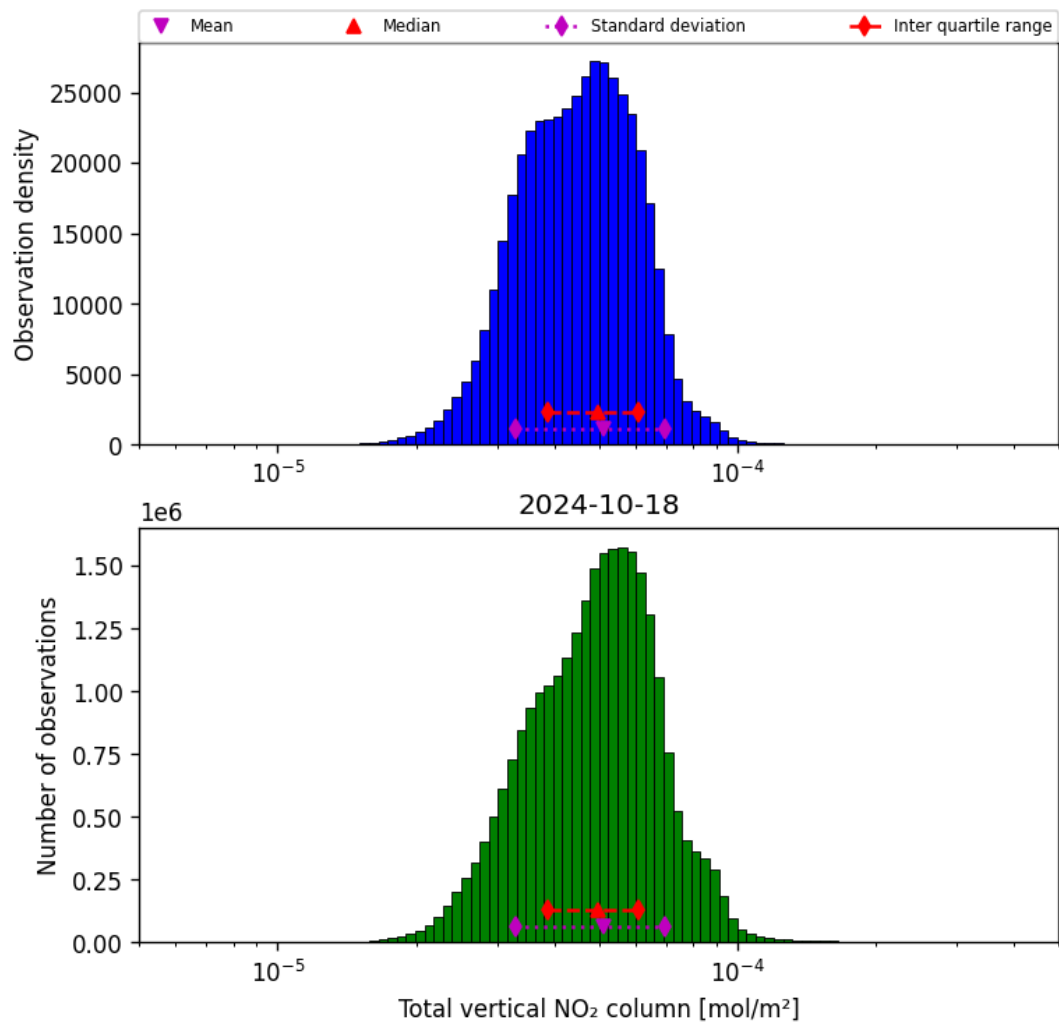
Figure 38: Histogram of “Total vertical NO 2 column” for 2024-10-17 to 2024-10-19
