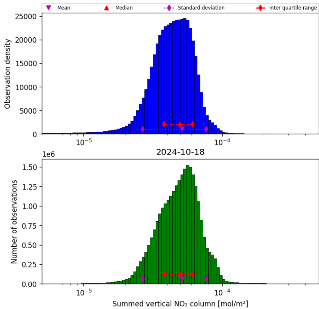
Figure 40: Histogram of “Summed vertical NO 2 column” for 2024-10-17 to 2024-10-19
