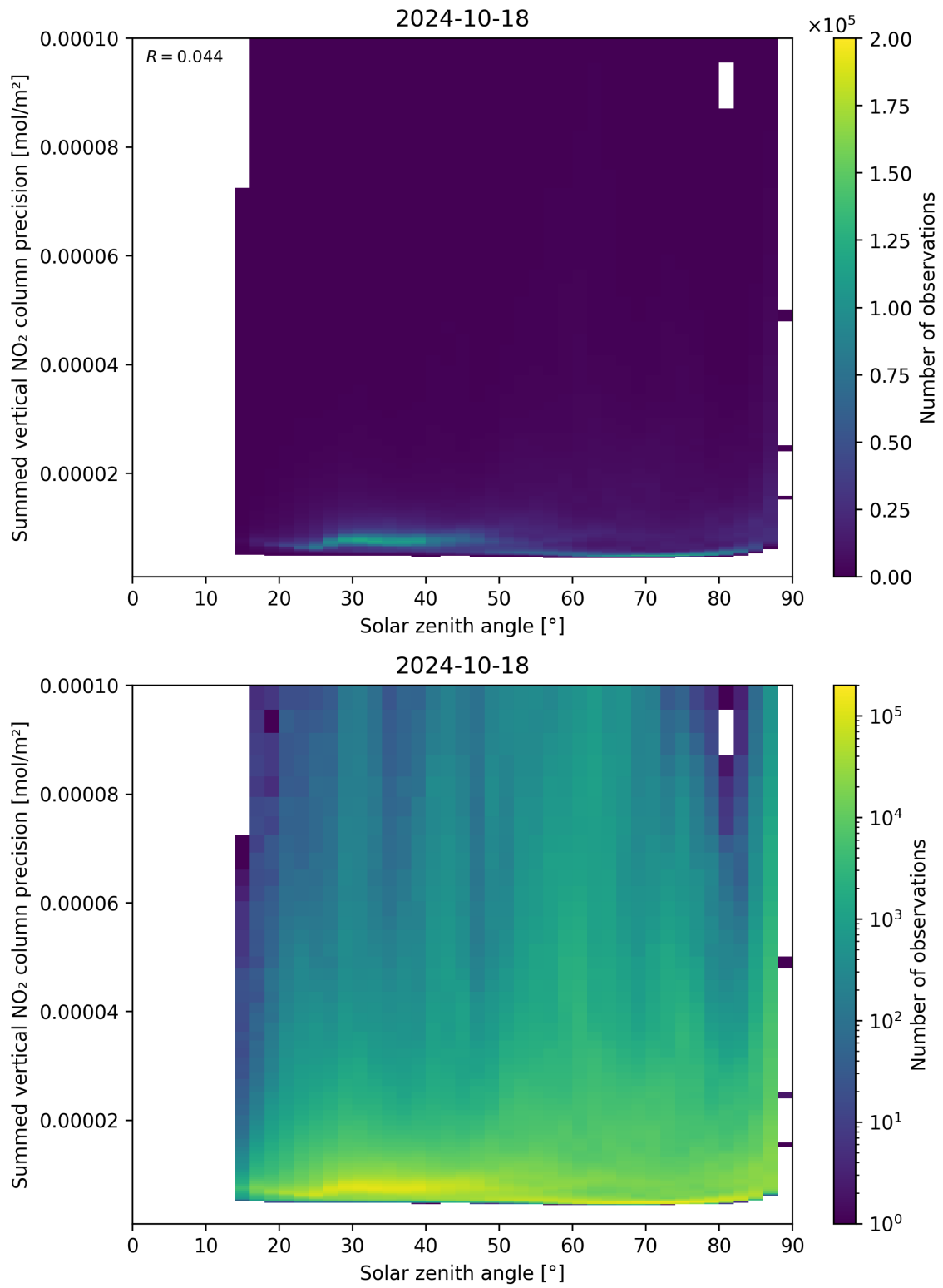
Figure 152: Scatter density plot of “Solar zenith angle” against “Summed vertical NO 2 column precision” for 2024-10-17 to 2024-10-19.
