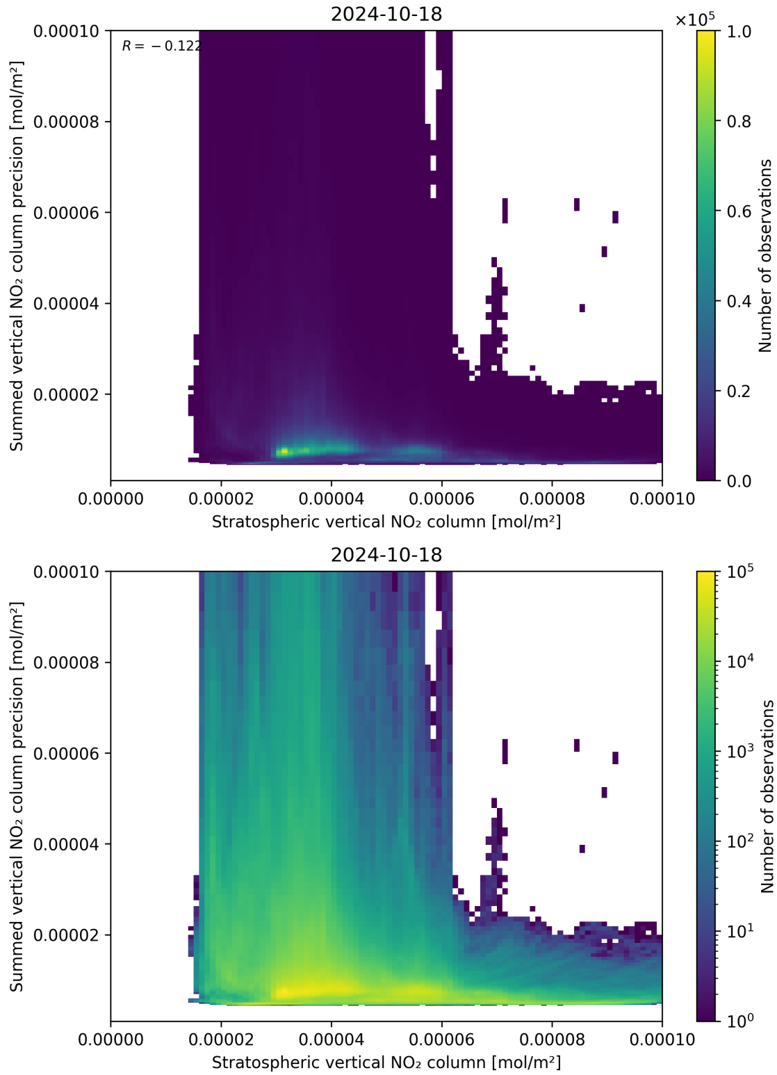
Figure 99: Scatter density plot of “Stratospheric vertical NO 2 column” against “Summed vertical NO 2 column precision” for 2024-10-17 to 2024-10-19.
