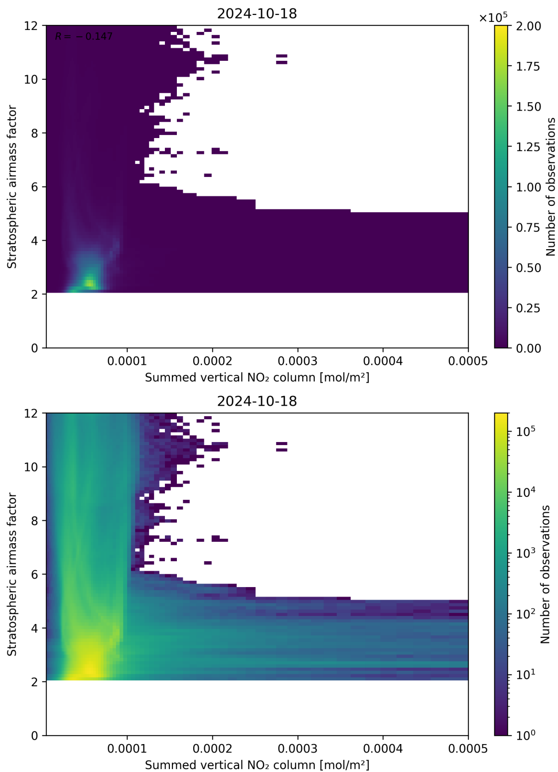
Figure 103: Scatter density plot of “Summed vertical NO 2 column” against “Stratospheric airmass factor” for 2024-10-17 to 2024-10-19.
