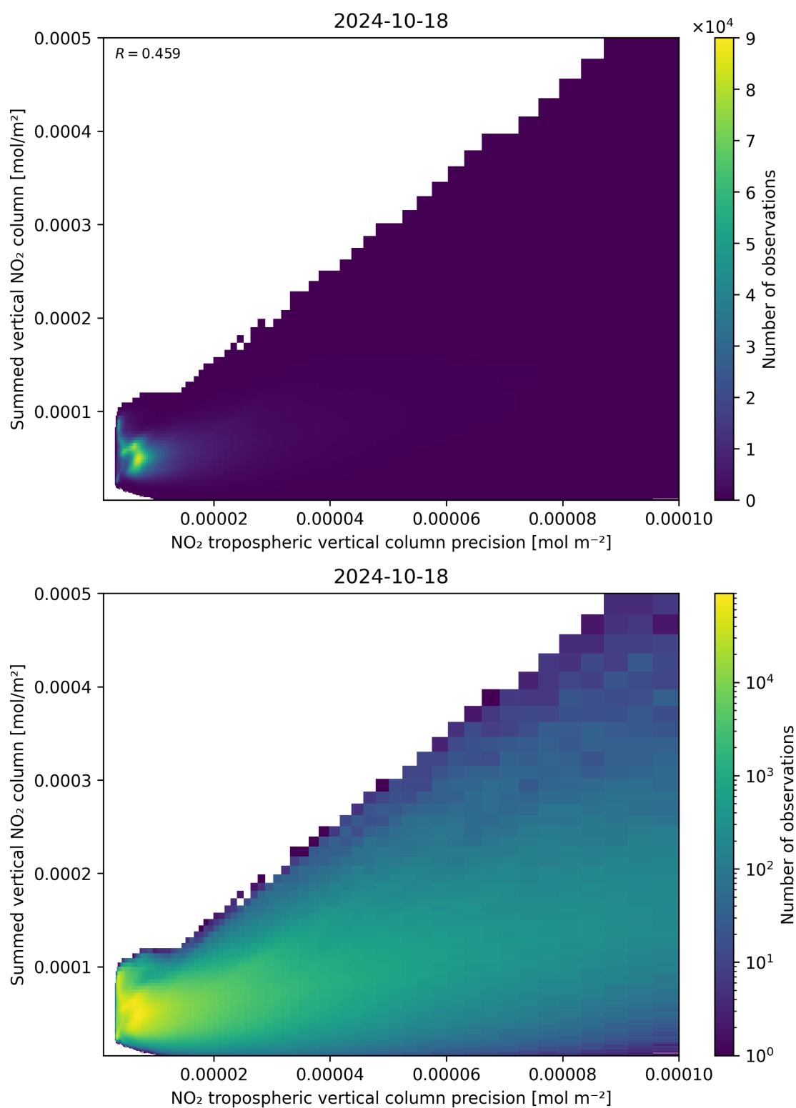
Figure 136: Scatter density plot of “NO 2 tropospheric vertical column precision” against “Summed vertical NO 2 column” for 2024-10-17 to 2024-10-19.
