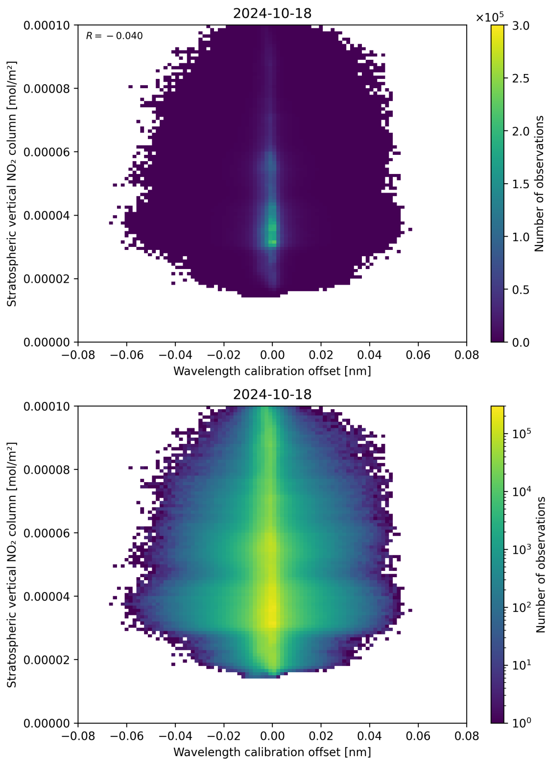
Figure 176: Scatter density plot of “Wavelength calibration offset” against “Stratospheric vertical NO 2 column” for 2024-10-17 to 2024-10-19.
