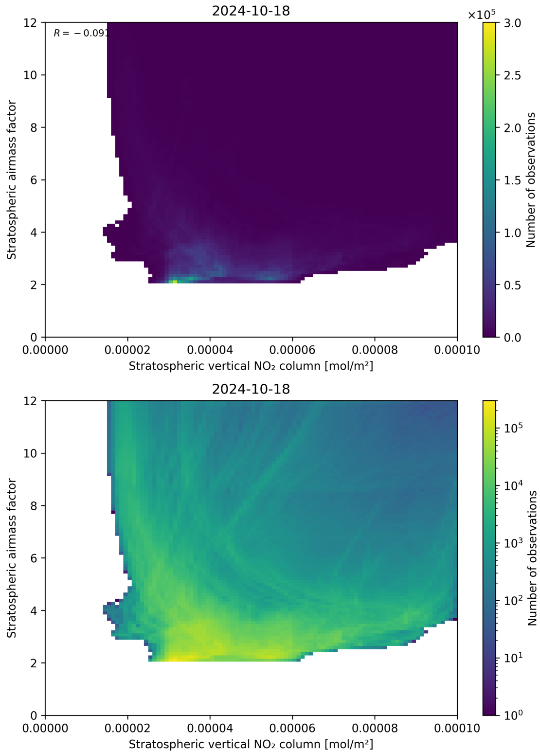
Figure 96: Scatter density plot of “Stratospheric vertical NO 2 column” against “Stratospheric airmass factor” for 2024-10-17 to 2024-10-19.
