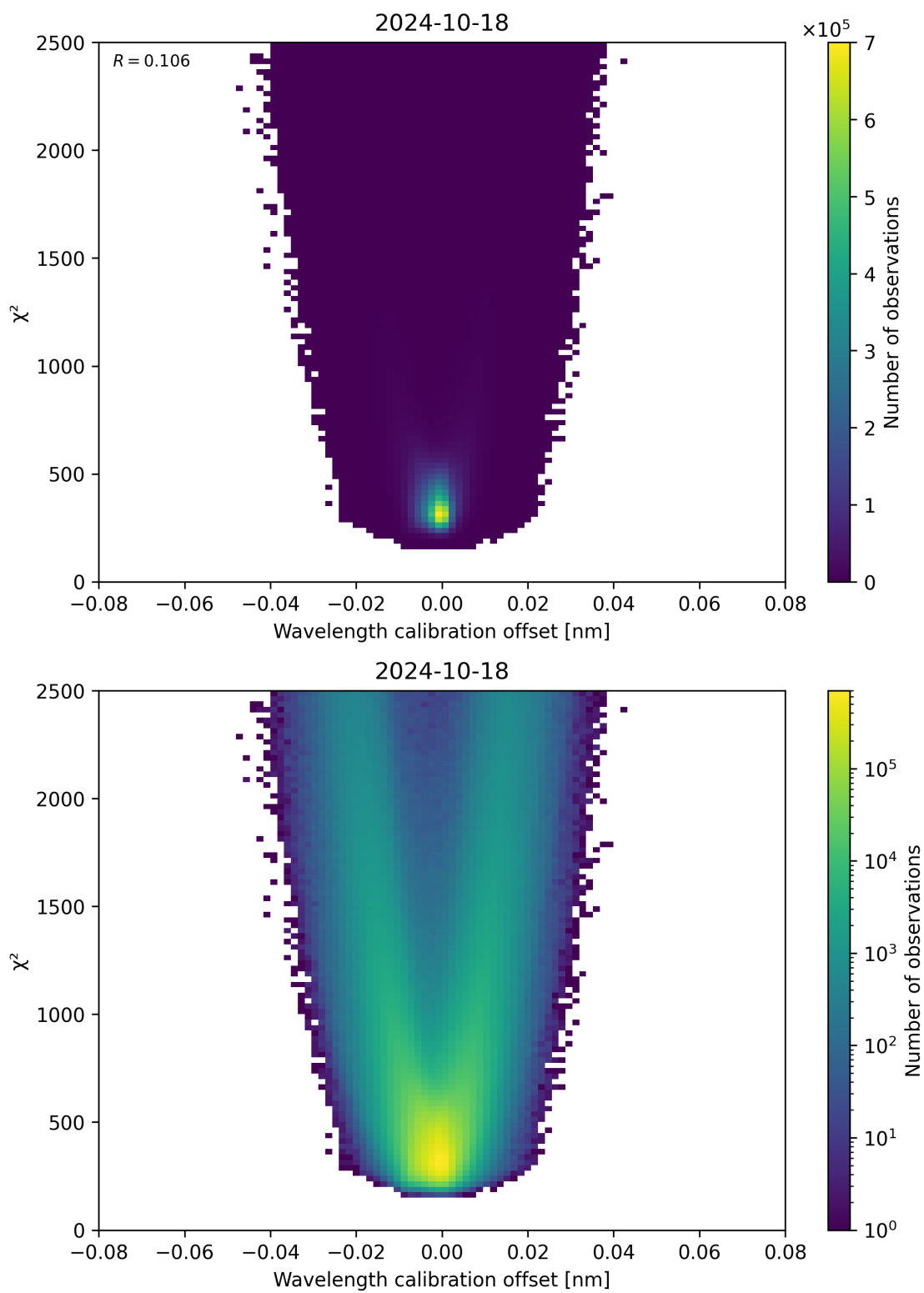
Figure 175: Scatter density plot of “Wavelength calibration offset” against “ \chi^2 ” for 2024-10-17 to 2024-10-19.
