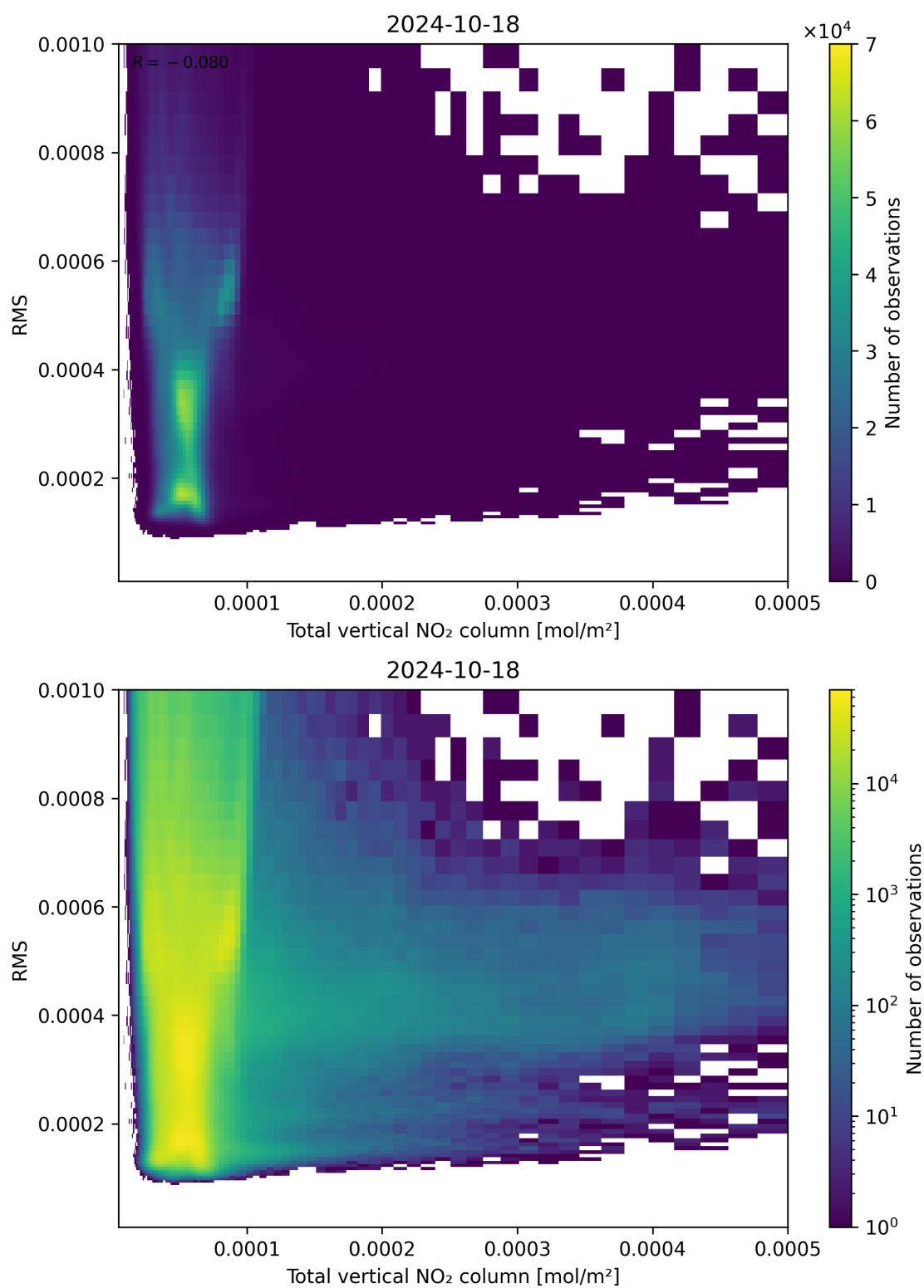
Figure 120: Scatter density plot of “Total vertical NO 2 column” against “RMS” for 2024-10-17 to 2024-10-19.
