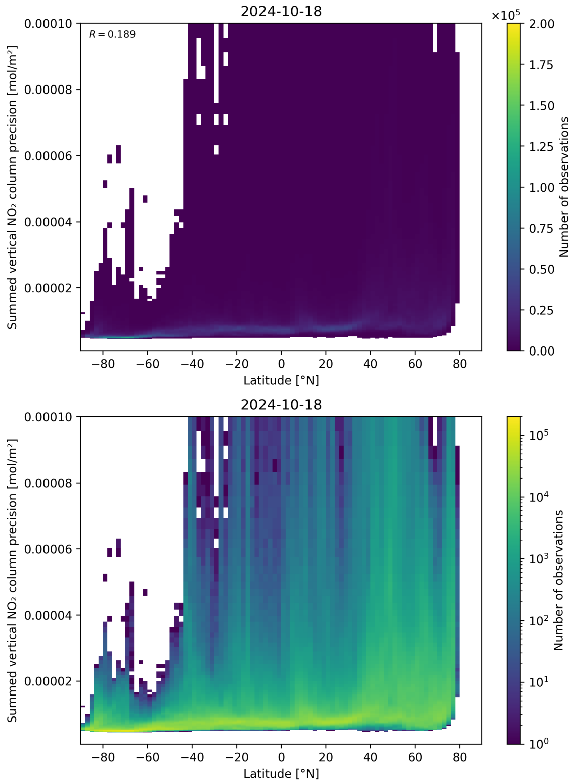
Figure 89: Scatter density plot of “Latitude” against “Summed vertical NO 2 column precision” for 2024-10-17 to 2024-10-19.
