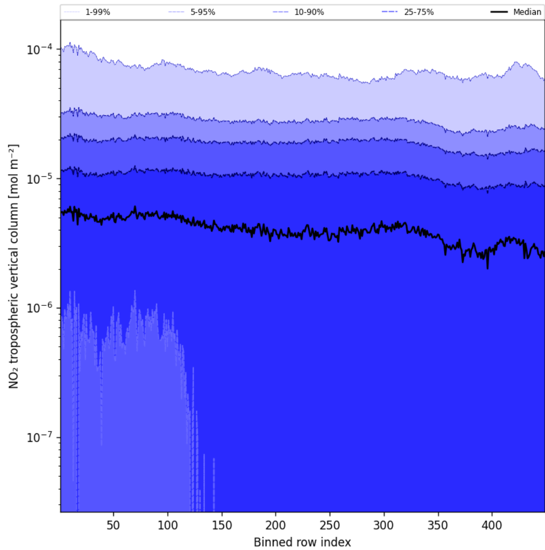
Figure 46: Along track statistics of “NO 2 tropospheric vertical column” for 2024-10-17 to 2024-10-19
