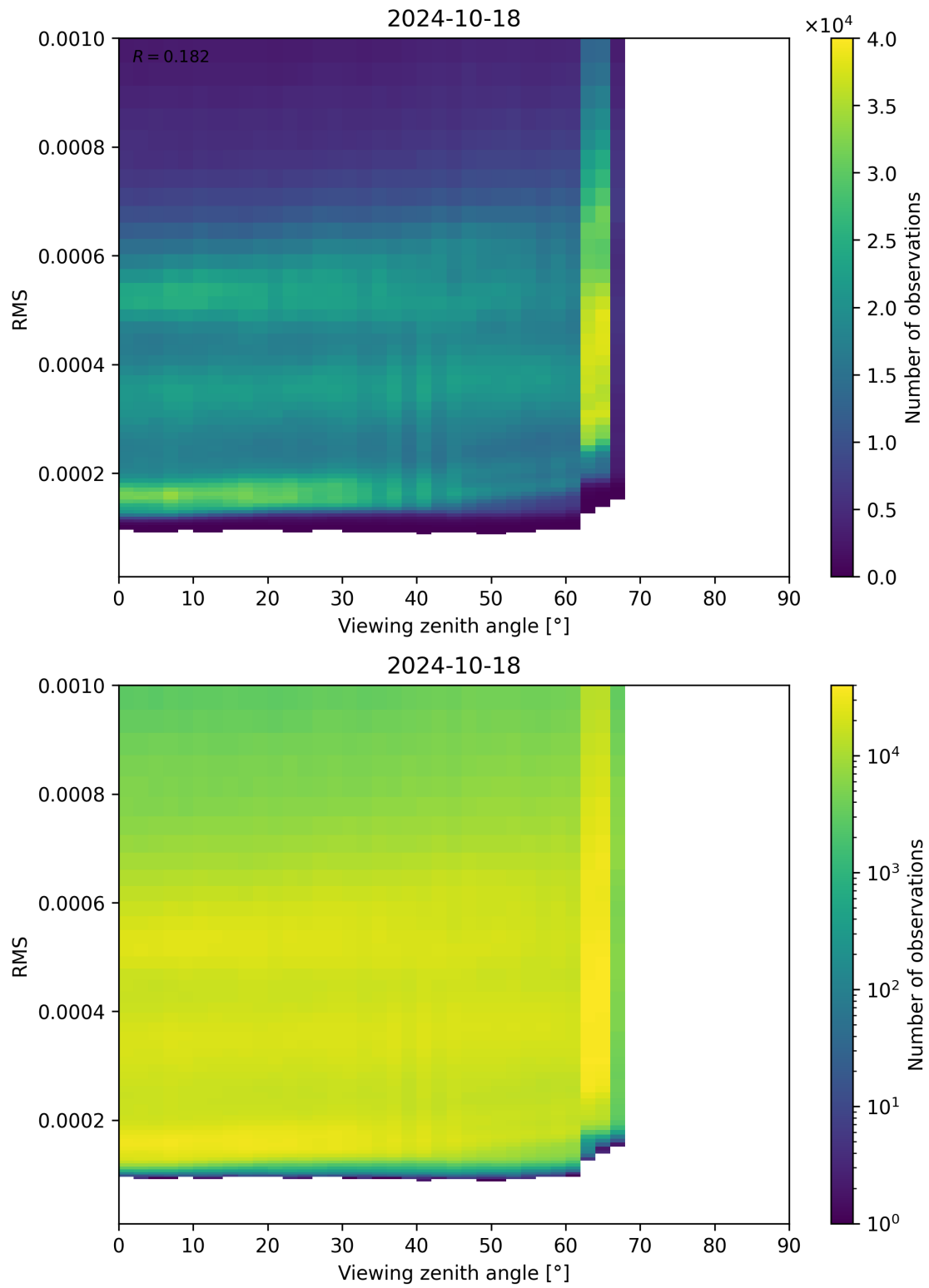
Figure 171: Scatter density plot of “Viewing zenith angle” against “RMS” for 2024-10-17 to 2024-10-19.
