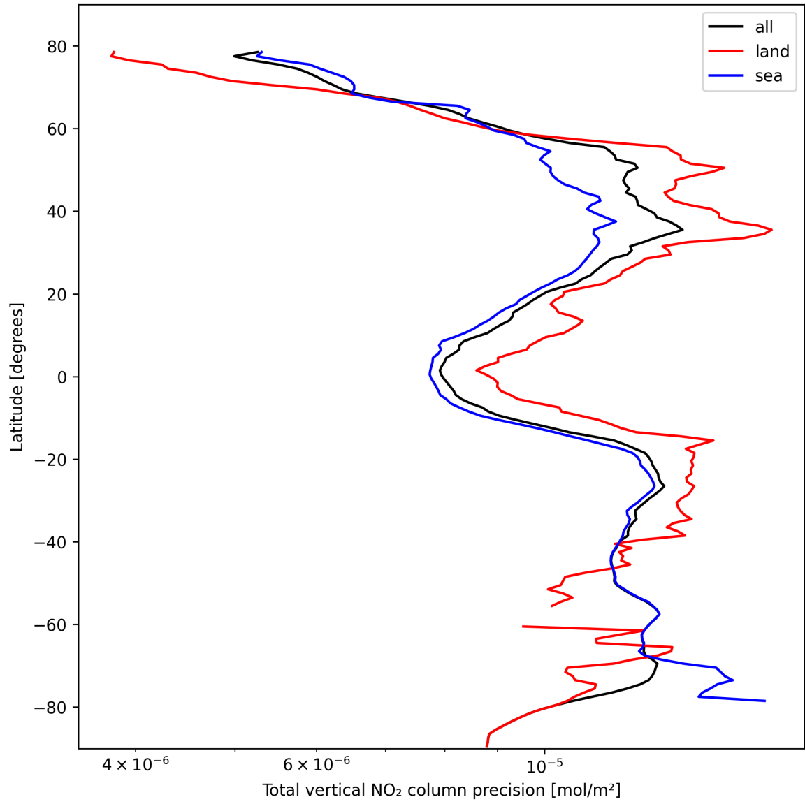
Figure 22: Zonal average of “Total vertical NO 2 column precision” for 2024-10-17 to 2024-10-19.
