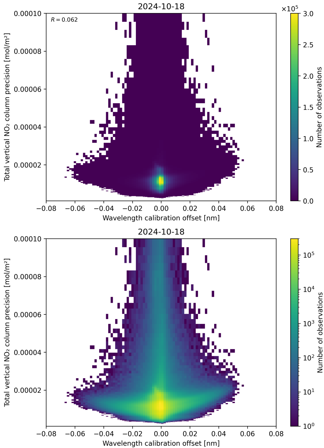
Figure 180: Scatter density plot of “Wavelength calibration offset” against “Total vertical NO 2 column precision” for 2024-10-17 to 2024-10-19.
