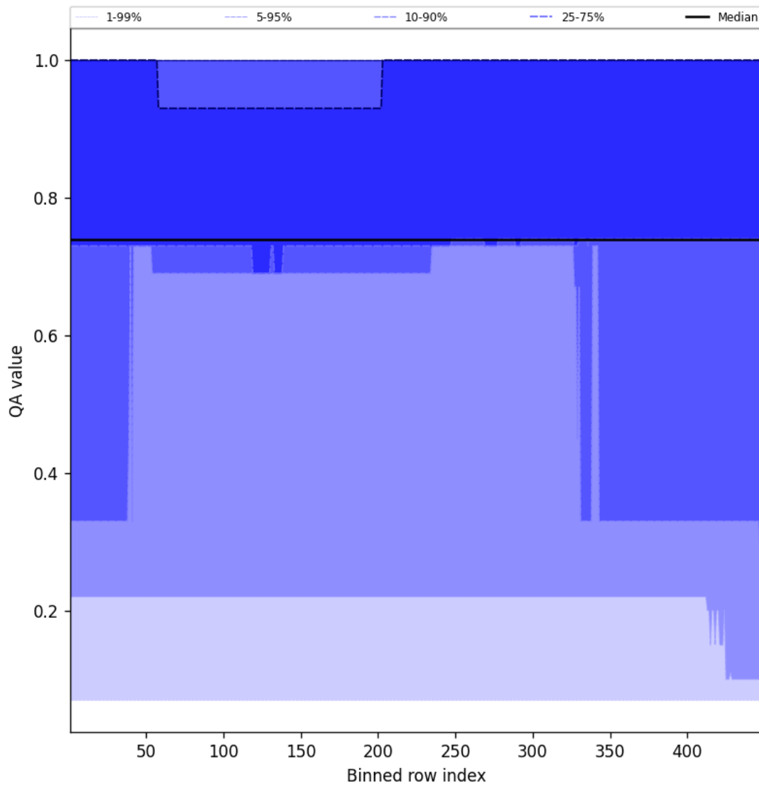
Figure 45: Along track statistics of “QA value” for 2024-10-17 to 2024-10-19
