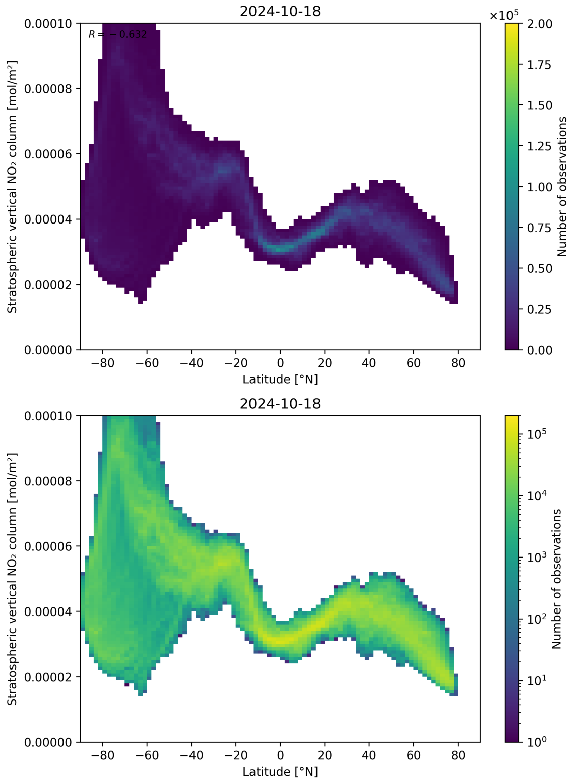
Figure 87: Scatter density plot of “Latitude” against “Stratospheric vertical NO 2 column” for 2024-10-17 to 2024-10-19.
