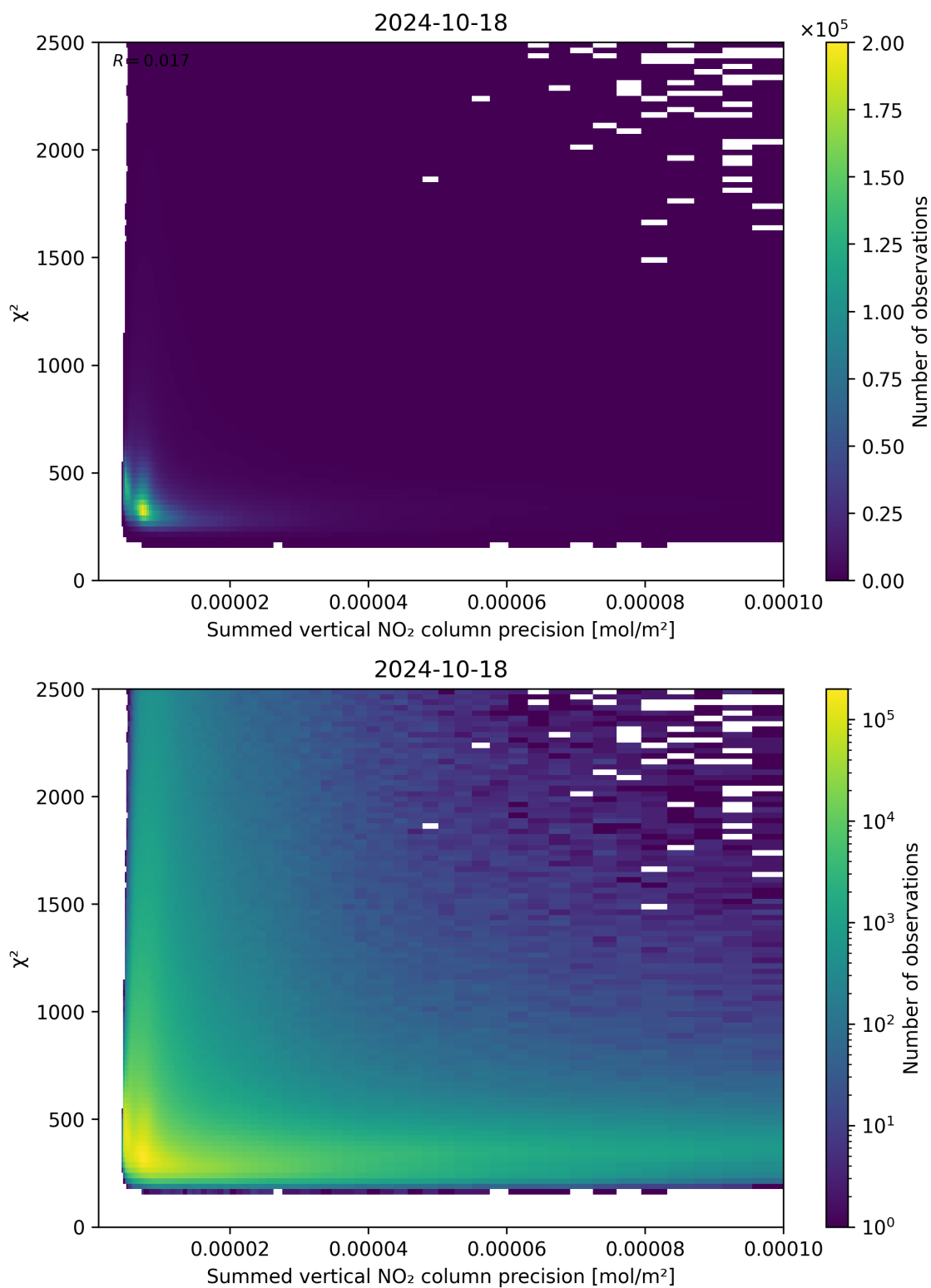
Figure 107: Scatter density plot of “Summed vertical NO 2 column precision” against “ \chi^2 ” for 2024-10-17 to 2024-10-19.
