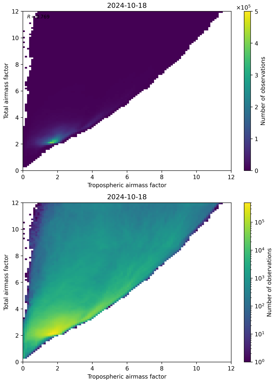
Figure 72: Scatter density plot of “Tropospheric airmass factor” against “Total airmass factor” for 2024-10-17 to 2024-10-19.
