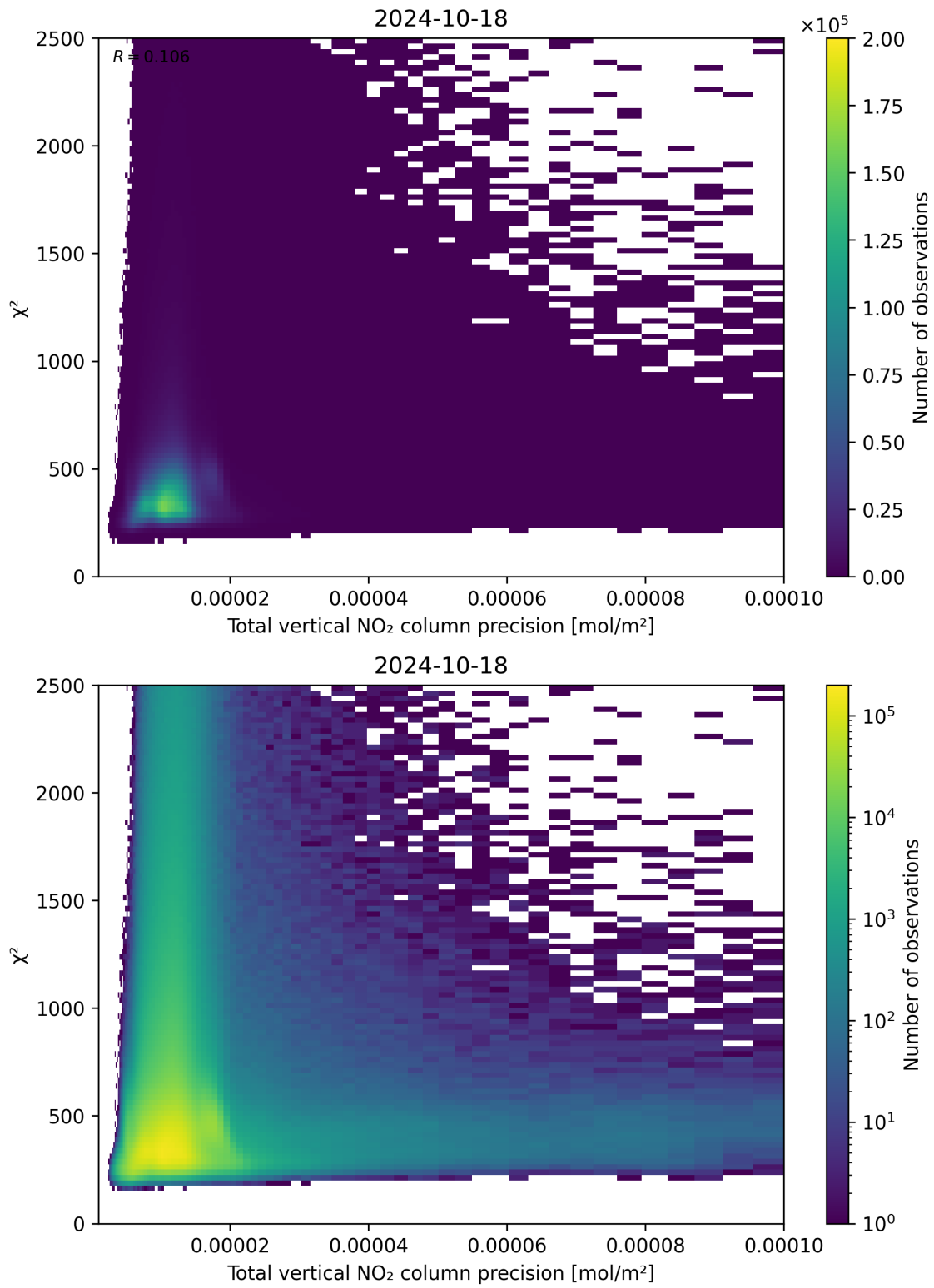
Figure 116: Scatter density plot of “Total vertical NO 2 column precision” against “ \chi^2 ” for 2024-10-17 to 2024-10-19.
