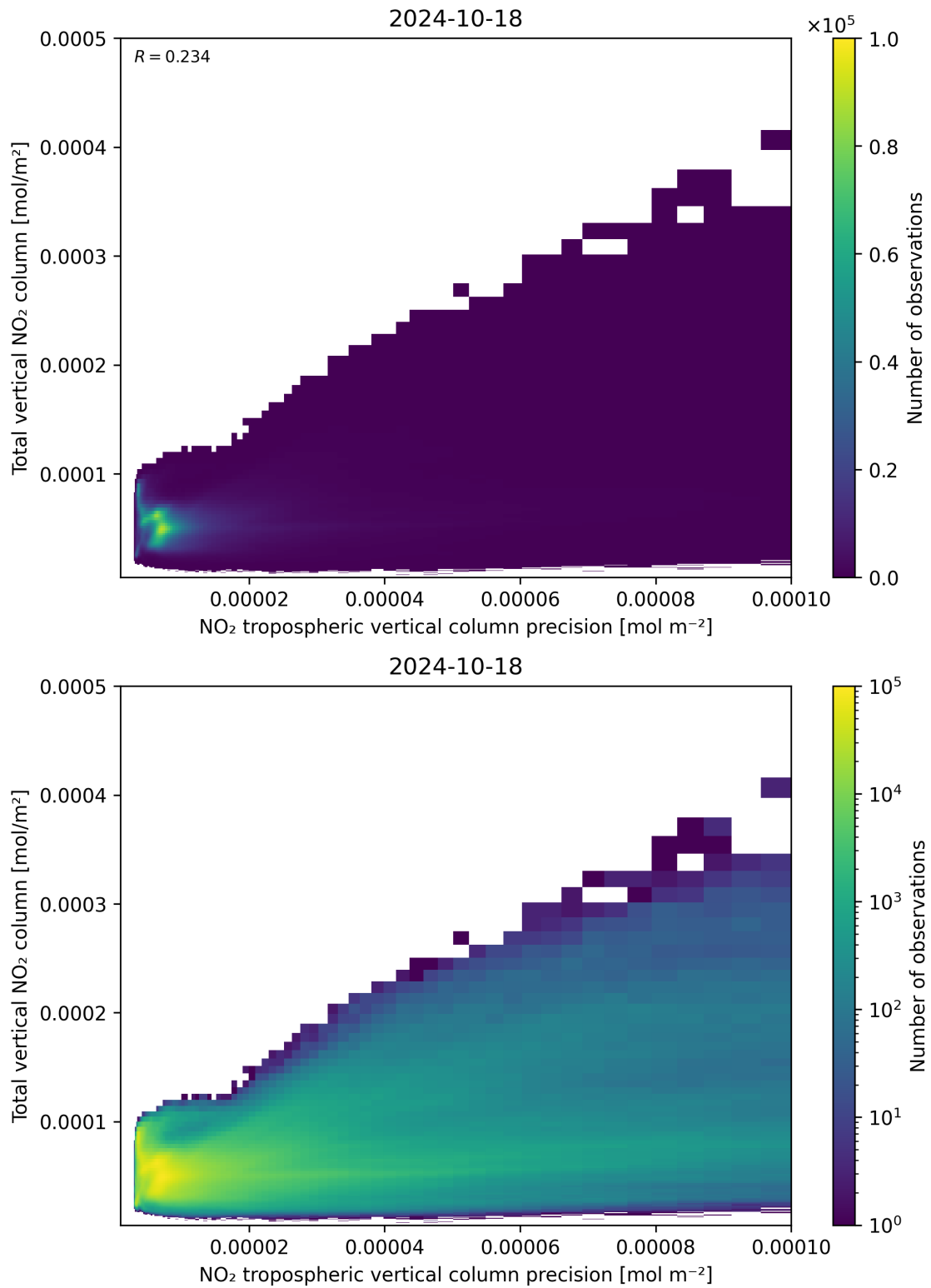
Figure 138: Scatter density plot of “NO 2 tropospheric vertical column precision” against “Total vertical NO 2 column” for 2024-10-17 to 2024-10-19.
