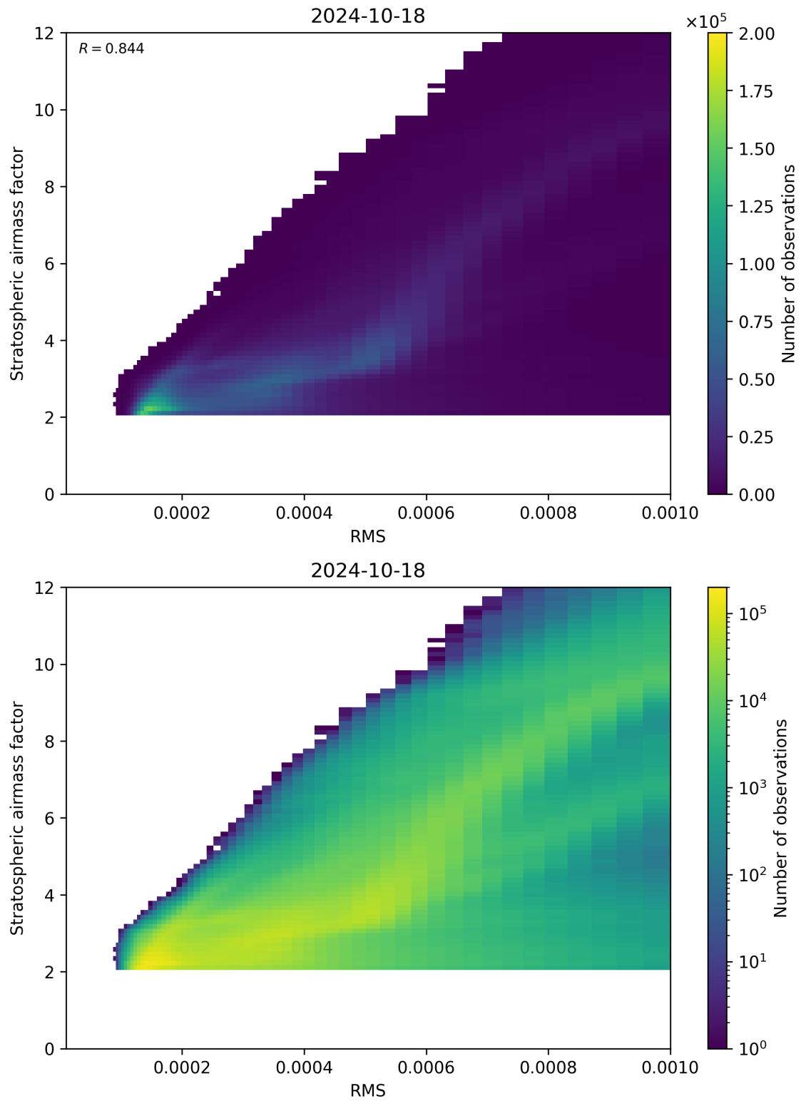
Figure 144: Scatter density plot of “RMS” against “Stratospheric airmass factor” for 2024-10-17 to 2024-10-19.
