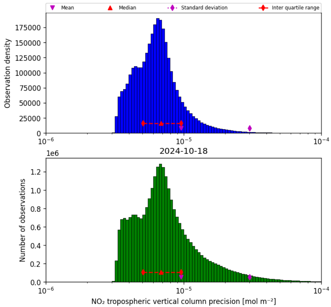
Figure 30: Histogram of “NO 2 tropospheric vertical column precision” for 2024-10-17 to 2024-10-19
