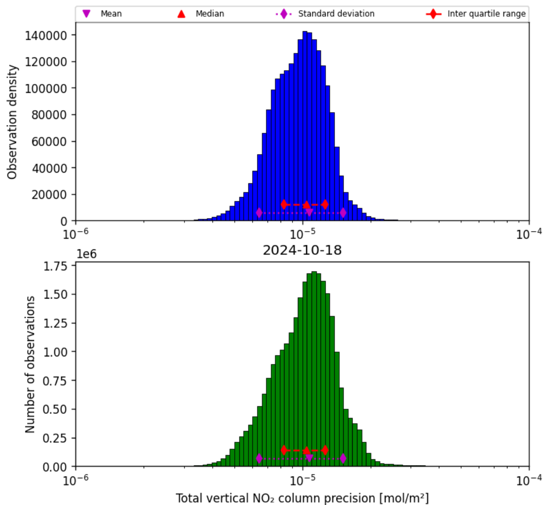
Figure 39: Histogram of “Total vertical NO 2 column precision” for 2024-10-17 to 2024-10-19
