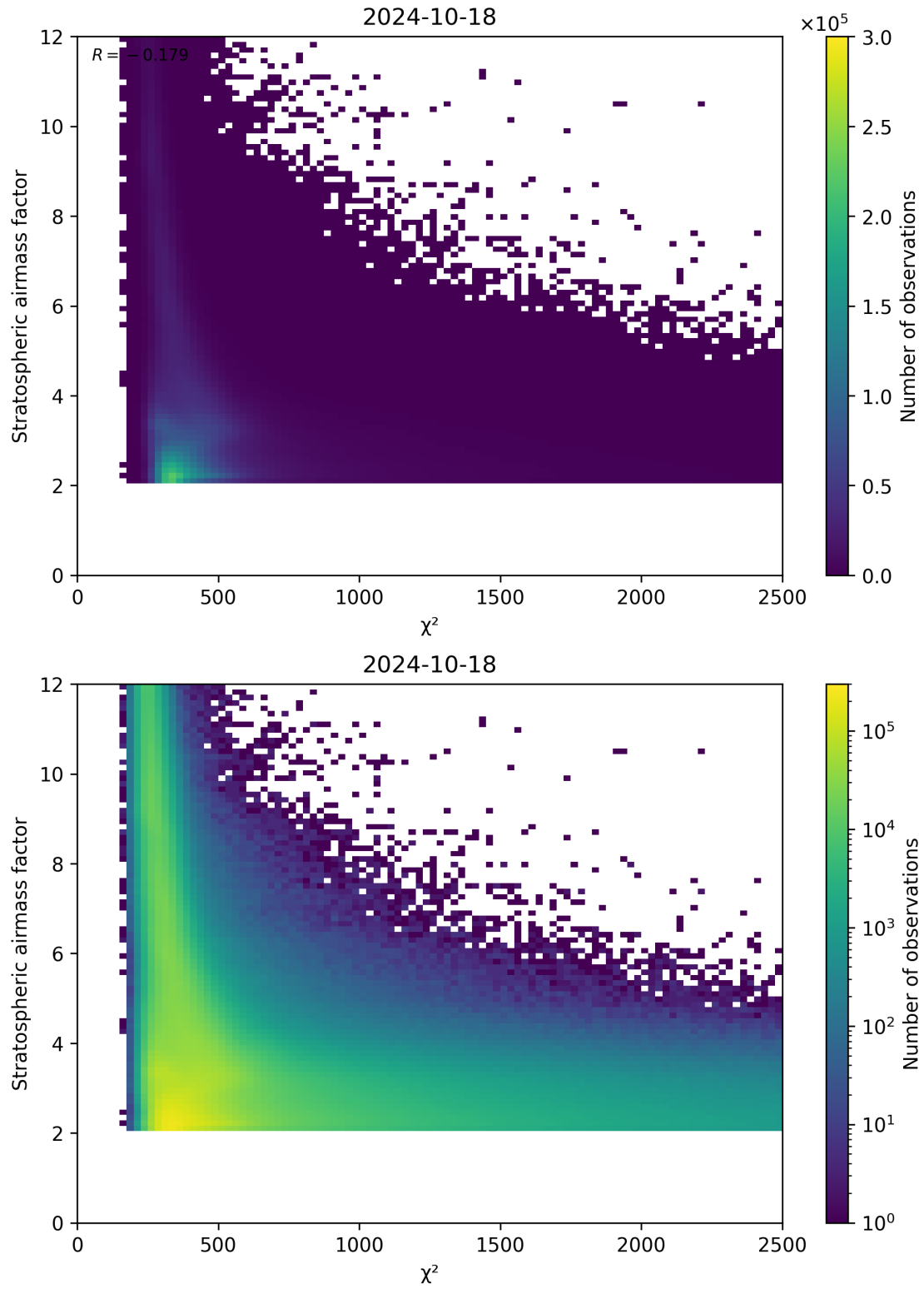
Figure 81: Scatter density plot of “ \chi^2 ” against “Stratospheric airmass factor” for 2024-10-17 to 2024-10-19.
