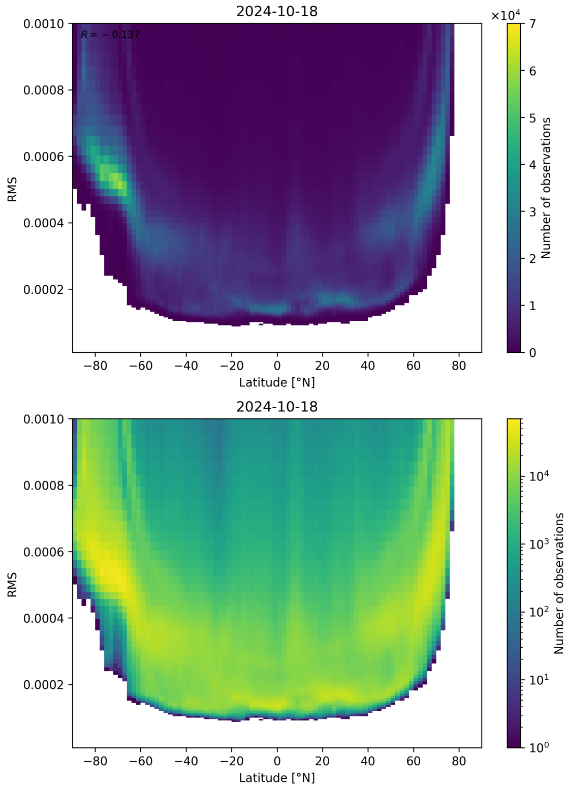
Figure 94: Scatter density plot of “Latitude” against “RMS” for 2024-10-17 to 2024-10-19.
