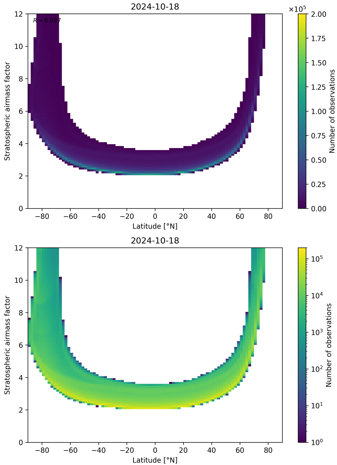
Figure 83: Scatter density plot of “Latitude” against “Stratospheric airmass factor” for 2024-10-17 to 2024-10-19.
