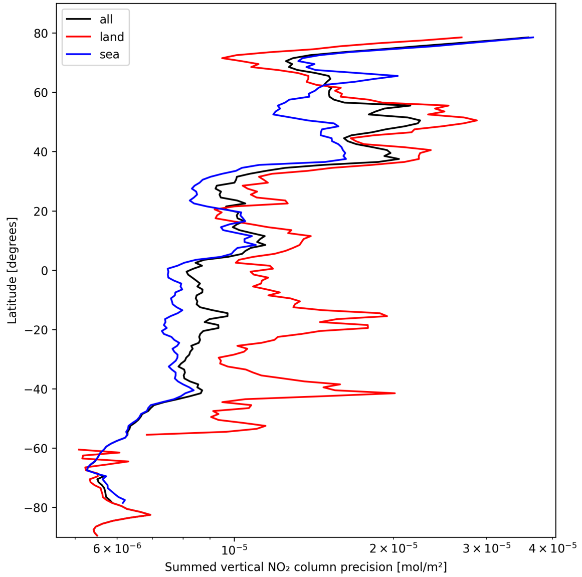
Figure 24: Zonal average of “Summed vertical NO 2 column precision” for 2024-10-17 to 2024-10-19.
