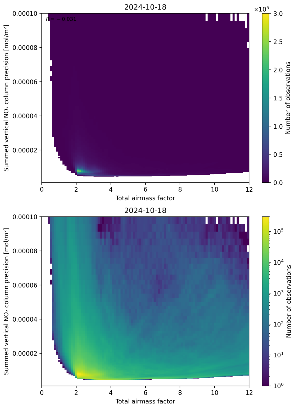
Figure 66: Scatter density plot of “Total airmass factor” against “Summed vertical NO 2 column precision” for 2024-10-17 to 2024-10-19.
