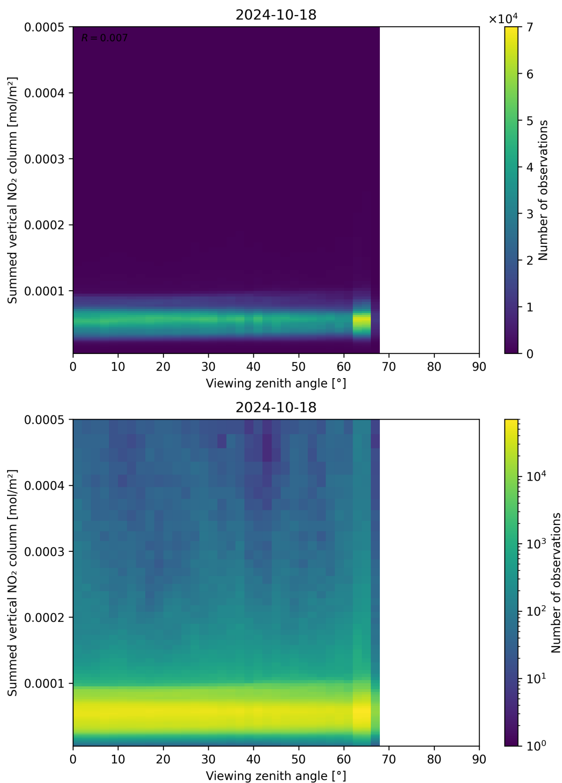
Figure 165: Scatter density plot of “Viewing zenith angle” against “Summed vertical NO 2 column” for 2024-10-17 to 2024-10-19.
