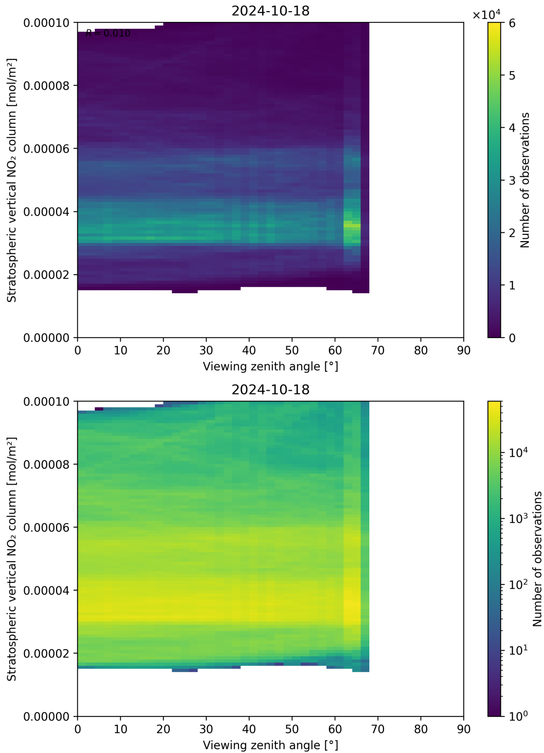
Figure 164: Scatter density plot of “Viewing zenith angle” against “Stratospheric vertical NO 2 column” for 2024-10-17 to 2024-10-19.
