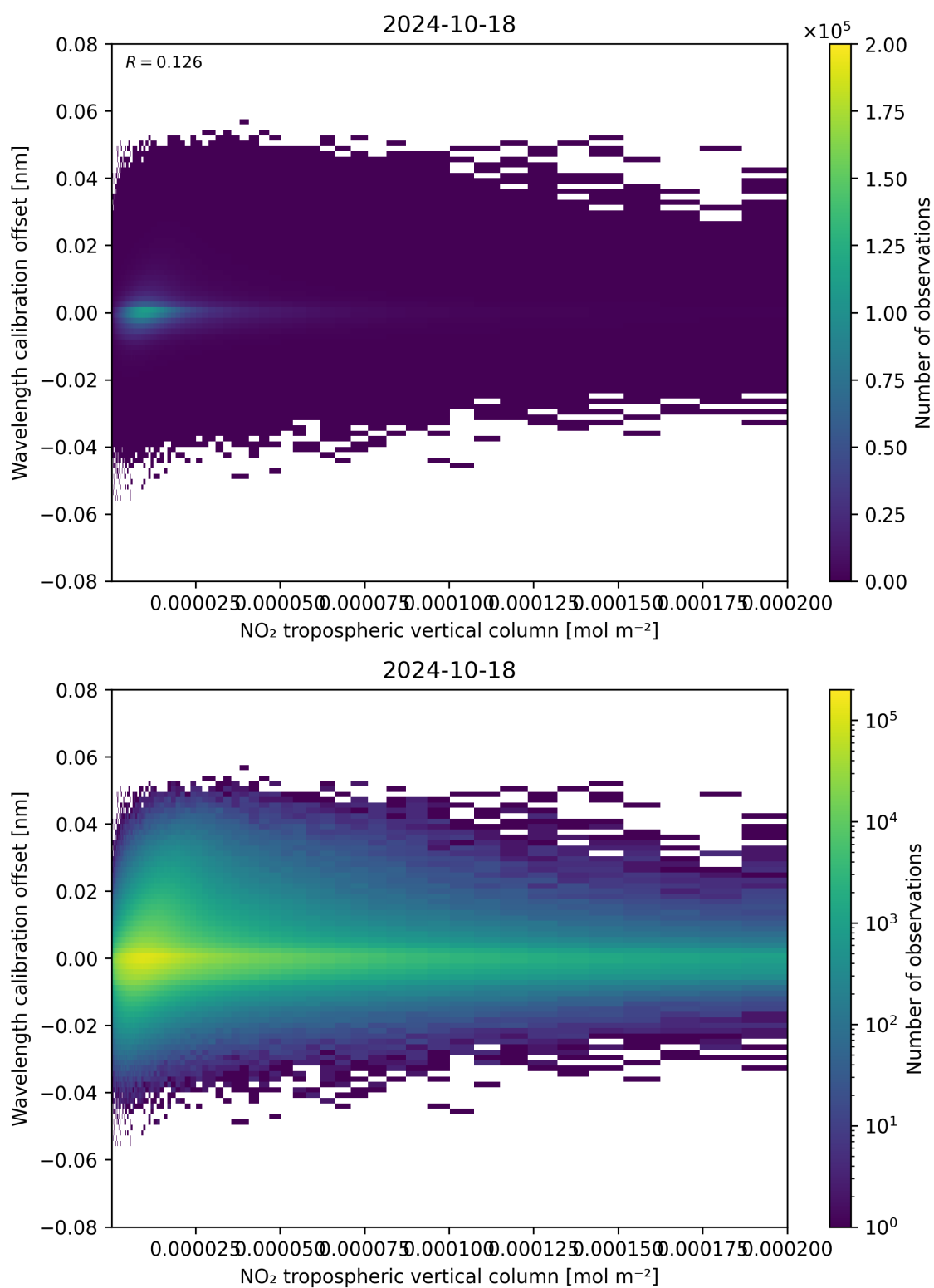
Figure 143: Scatter density plot of “NO 2 tropospheric vertical column” against “Wavelength calibration offset” for 2024-10-17 to 2024-10-19.
