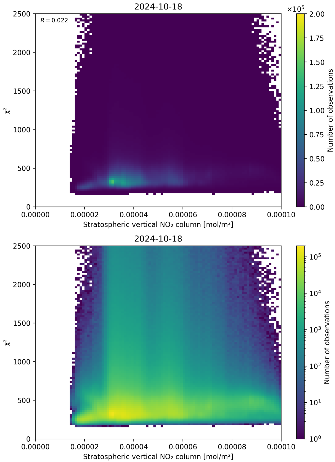
Figure 97: Scatter density plot of “Stratospheric vertical NO 2 column” against “ \chi^2 ” for 2024-10-17 to 2024-10-19.
