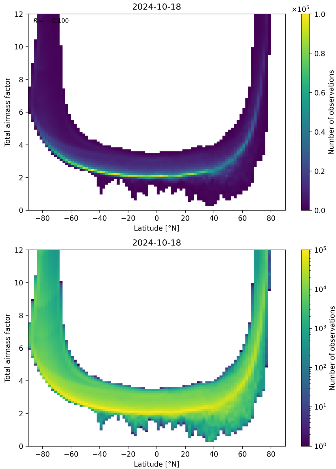
Figure 84: Scatter density plot of “Latitude” against “Total airmass factor” for 2024-10-17 to 2024-10-19.
