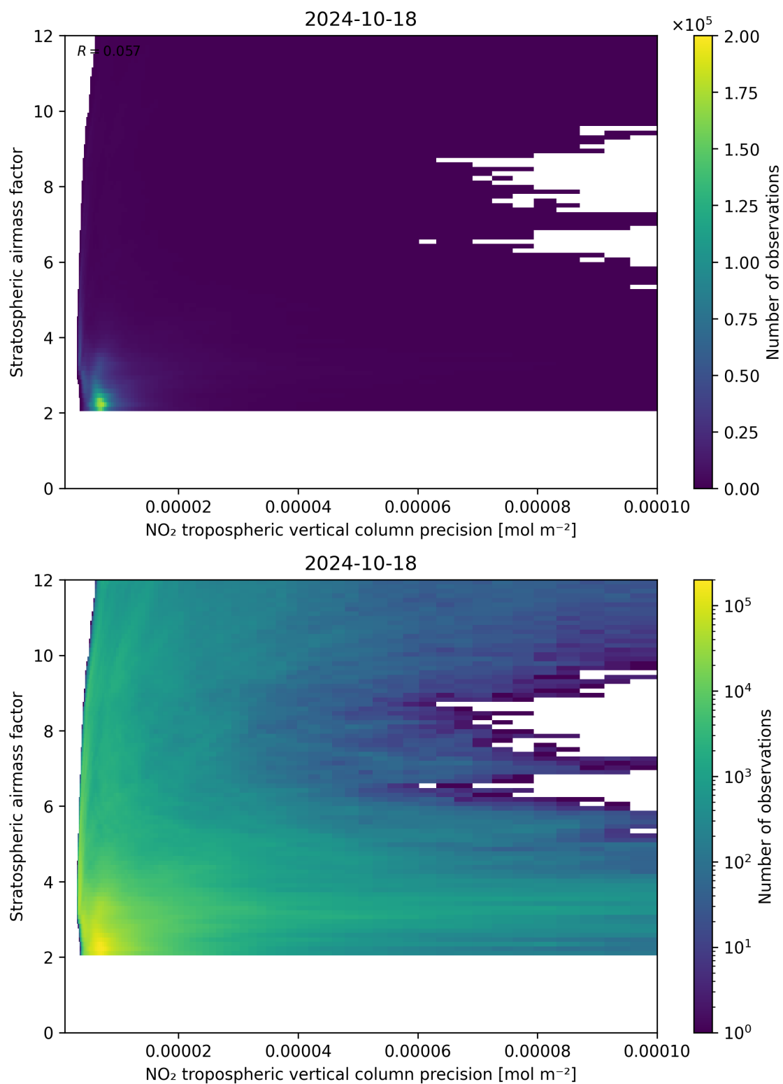
Figure 131: Scatter density plot of “NO 2 tropospheric vertical column precision” against “Stratospheric airmass factor” for 2024-10-17 to 2024-10-19.
