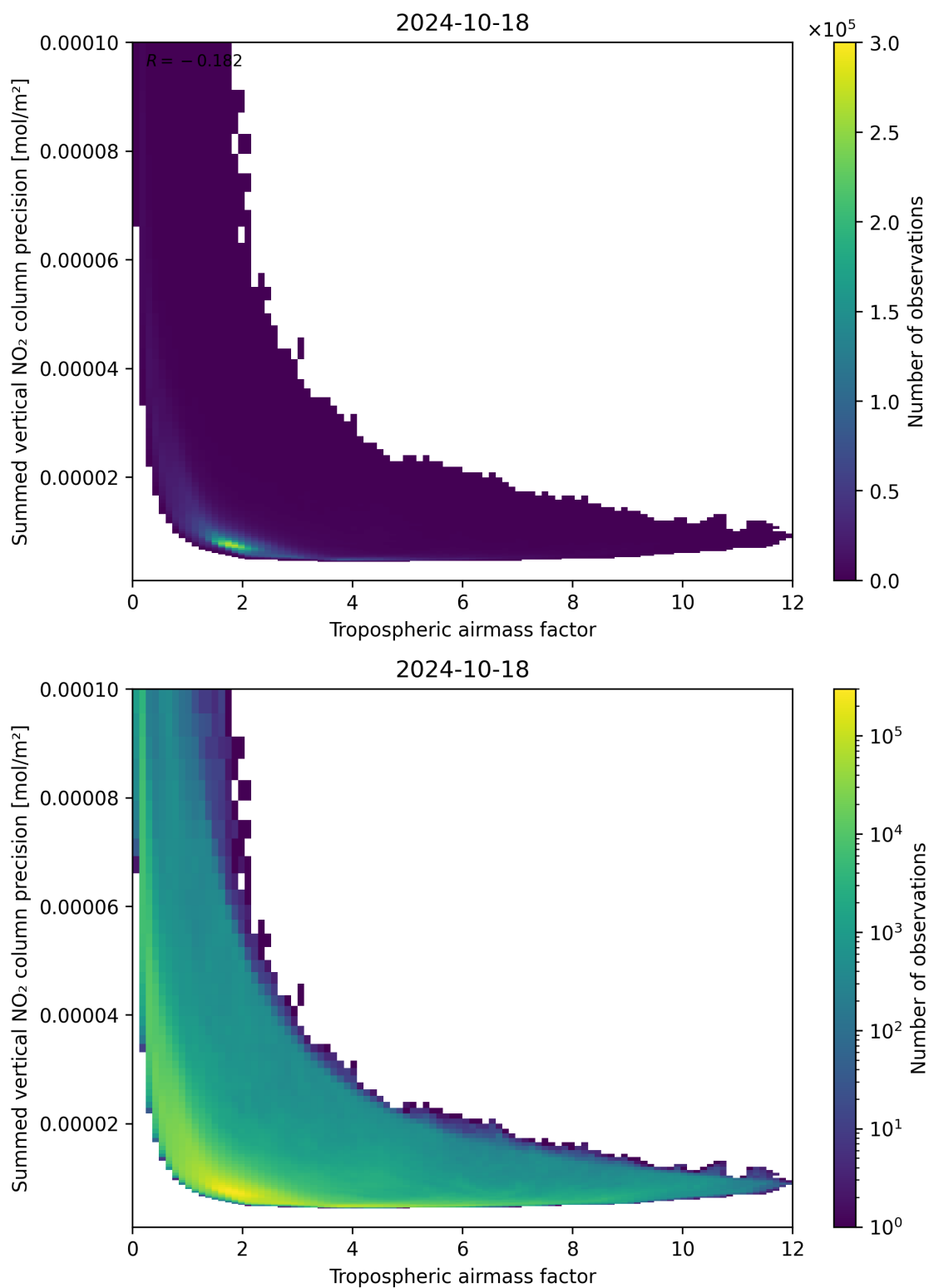
Figure 76: Scatter density plot of “Tropospheric airmass factor” against “Summed vertical NO 2 column precision” for 2024-10-17 to 2024-10-19.
