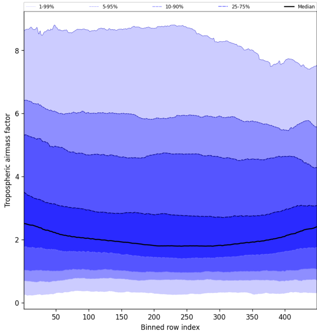
Figure 48: Along track statistics of “Tropospheric air mass factor” for 2024-10-17 to 2024-10-19
