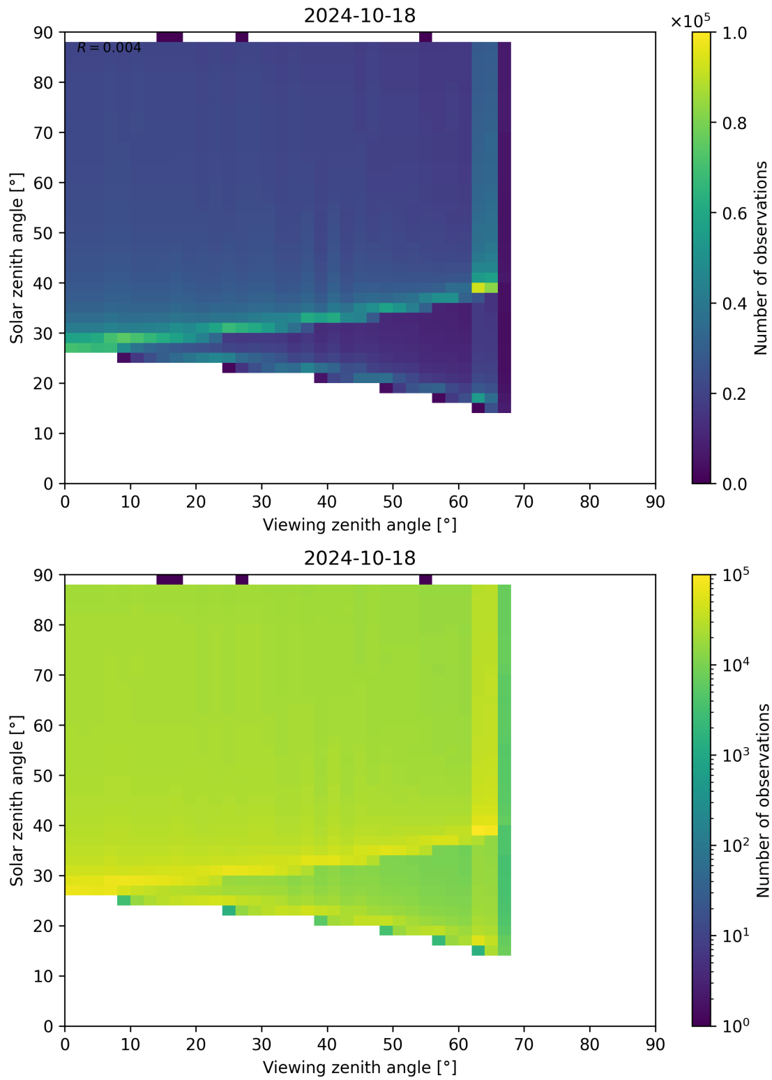
Figure 172: Scatter density plot of “Viewing zenith angle” against “Solar zenith angle” for 2024-10-17 to 2024-10-19.
