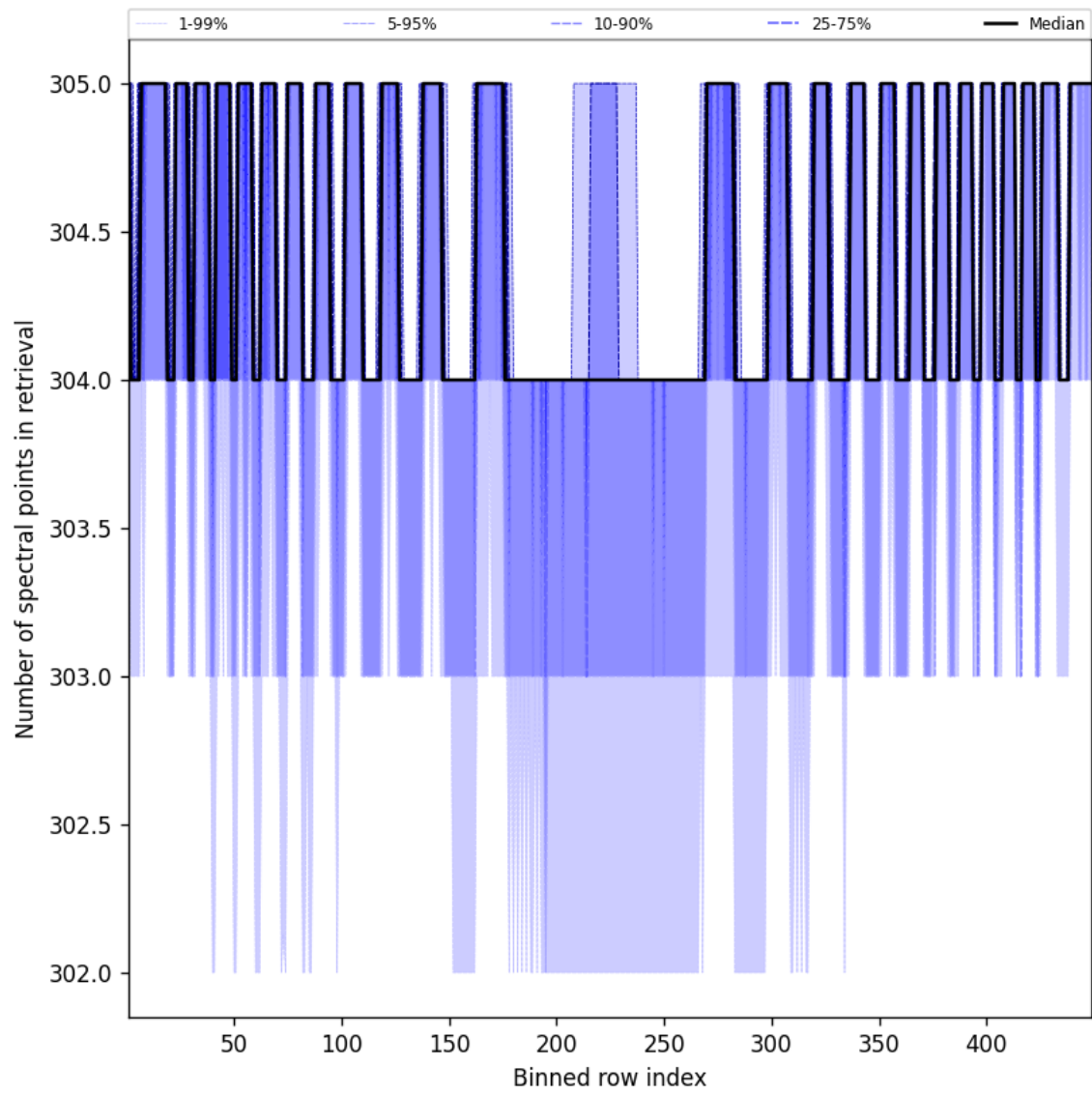
Figure 50: Along track statistics of “Number of spectral points in retrieval” for 2024-10-17 to 2024-10-19
