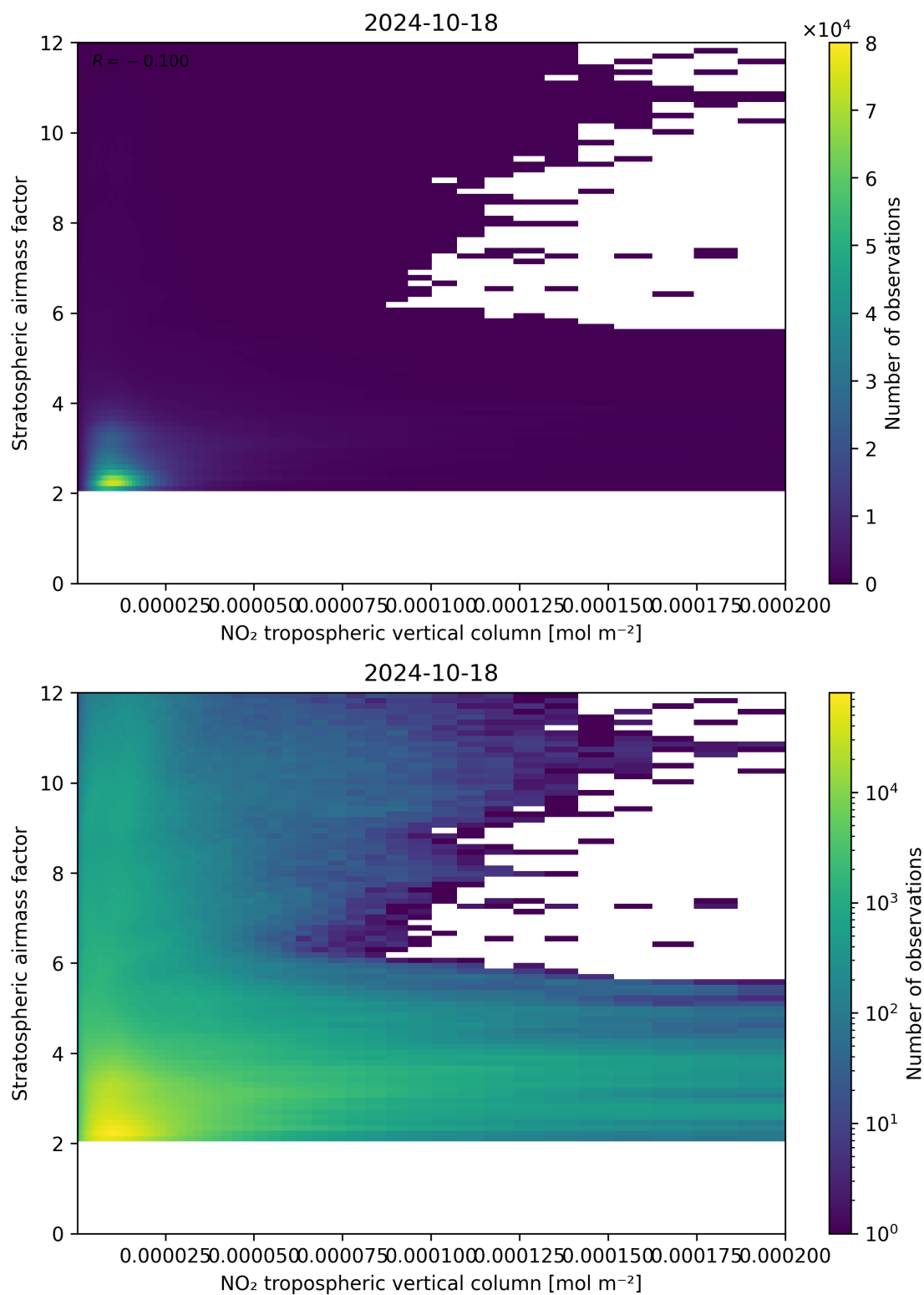
Figure 121: Scatter density plot of “NO 2 tropospheric vertical column” against “Stratospheric air mass factor” for 2024-10-17 to 2024-10-19.
