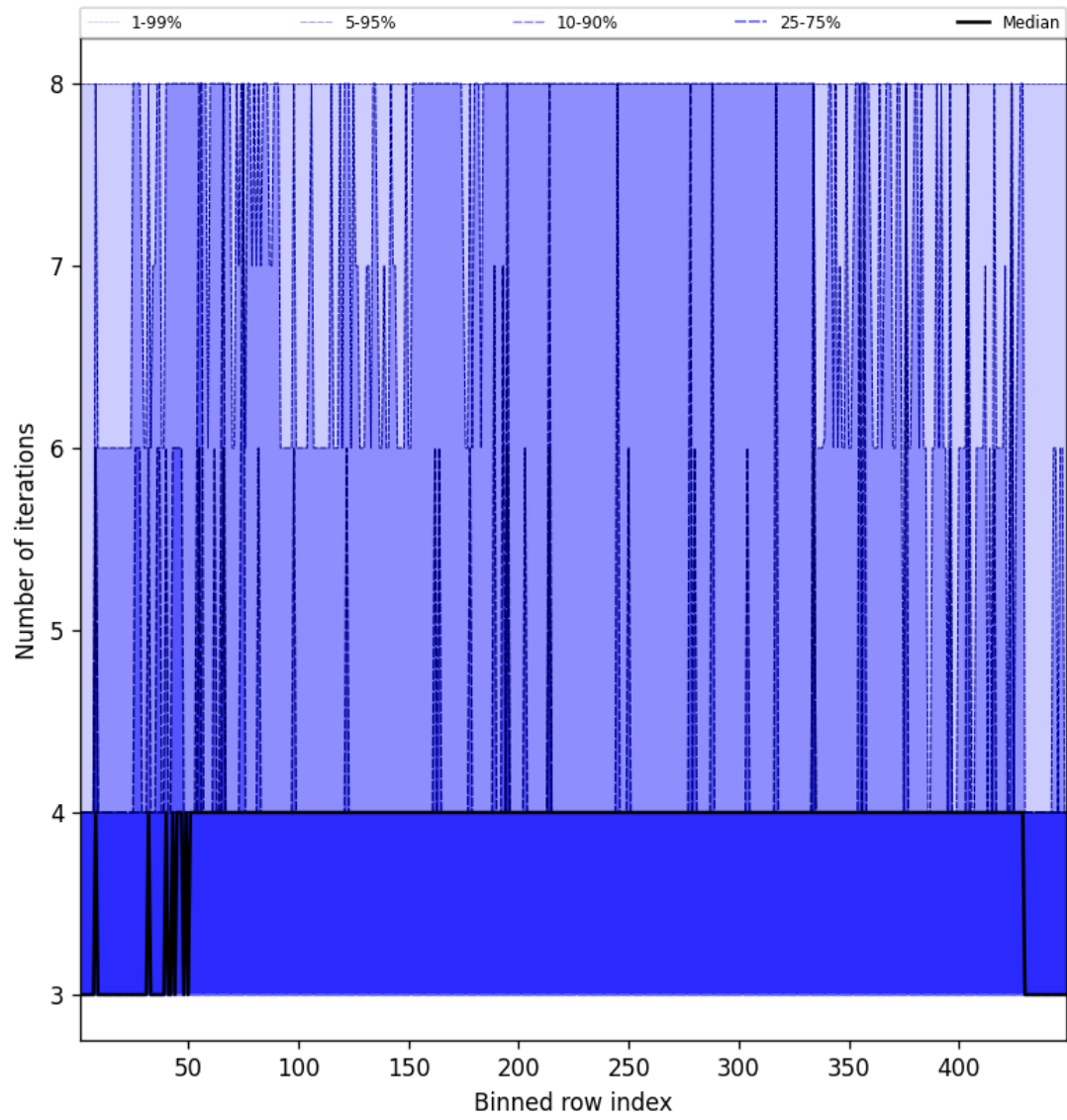
Figure 51: Along track statistics of “Number of iterations” for 2024-10-17 to 2024-10-19
