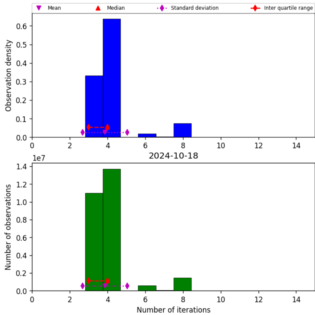
Figure 34: Histogram of “Number of iterations” for 2024-10-17 to 2024-10-19
