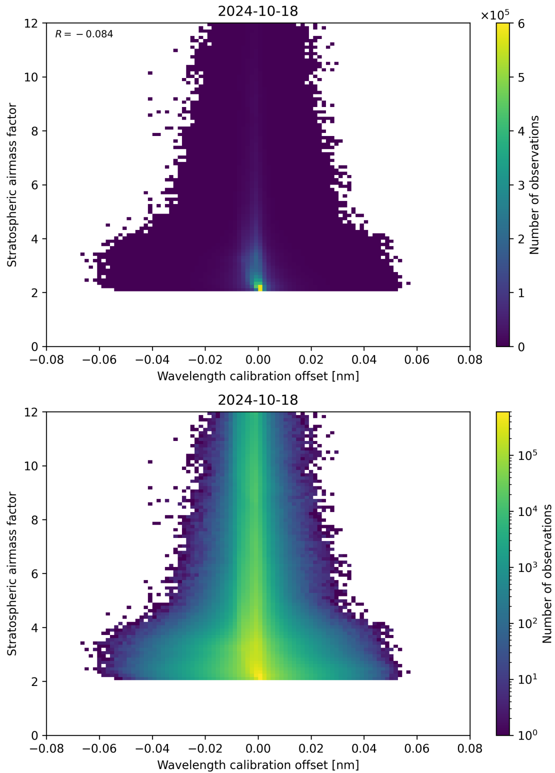
Figure 174: Scatter density plot of “Wavelength calibration offset” against “Stratospheric airmass factor” for 2024-10-17 to 2024-10-19.
