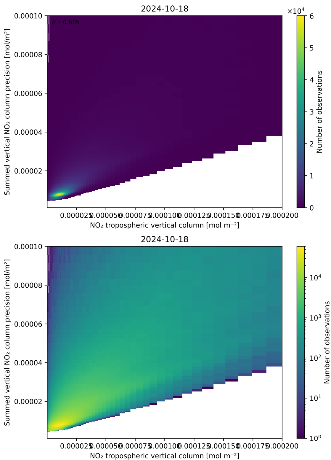
Figure 127: Scatter density plot of “NO 2 tropospheric vertical column” against “Summed vertical NO 2 column precision” for 2024-10-17 to 2024-10-19.
