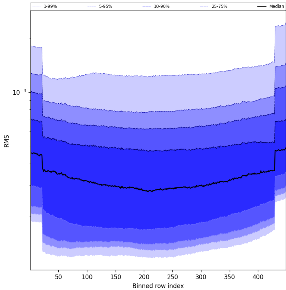
Figure 60: Along track statistics of “RMS” for 2024-10-17 to 2024-10-19
