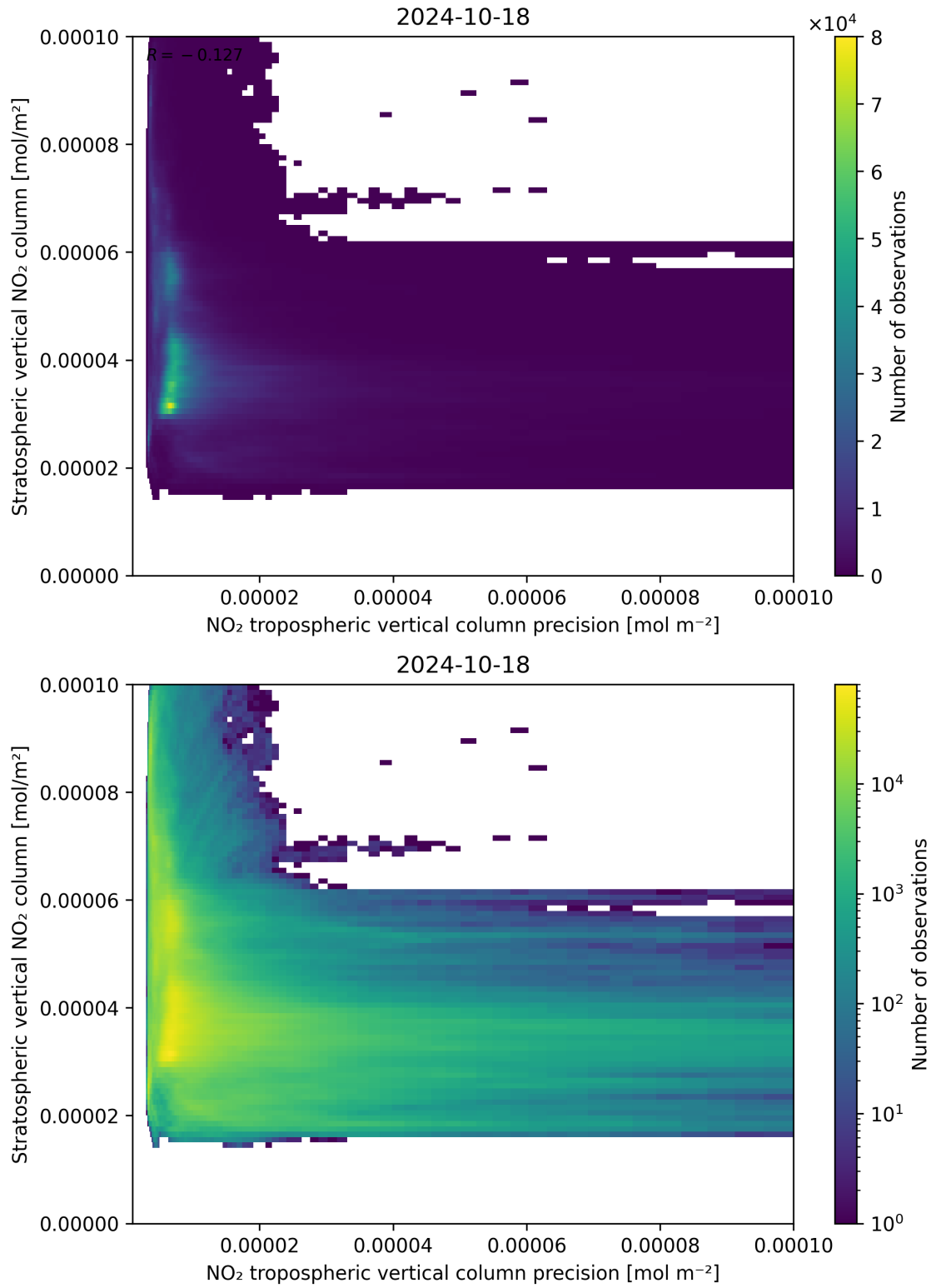
Figure 135: Scatter density plot of “NO 2 tropospheric vertical column precision” against “Stratospheric vertical NO 2 column” for 2024-10-17 to 2024-10-19.
