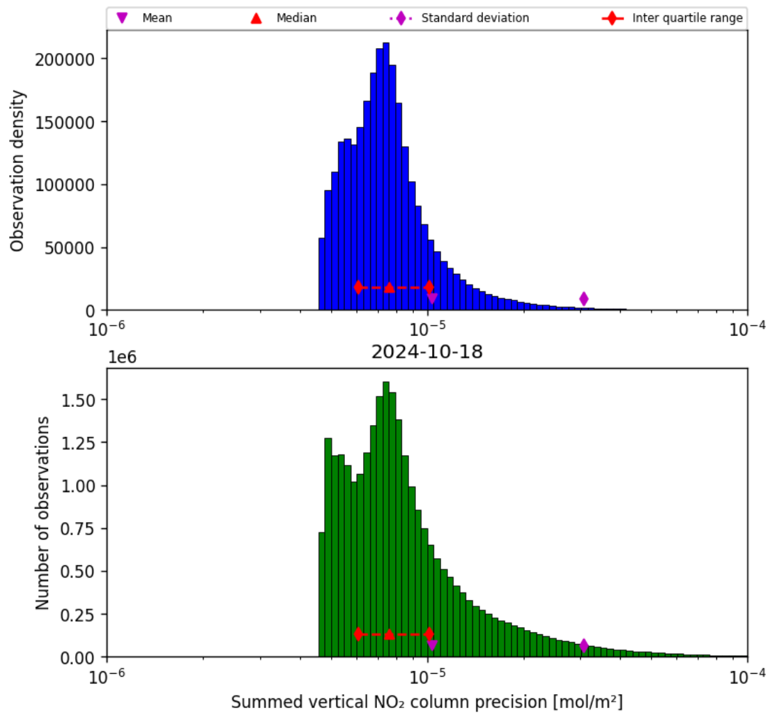
Figure 41: Histogram of "Summed vertical NO 2 column precision" for 2024-10-17 to 2024-10-19
