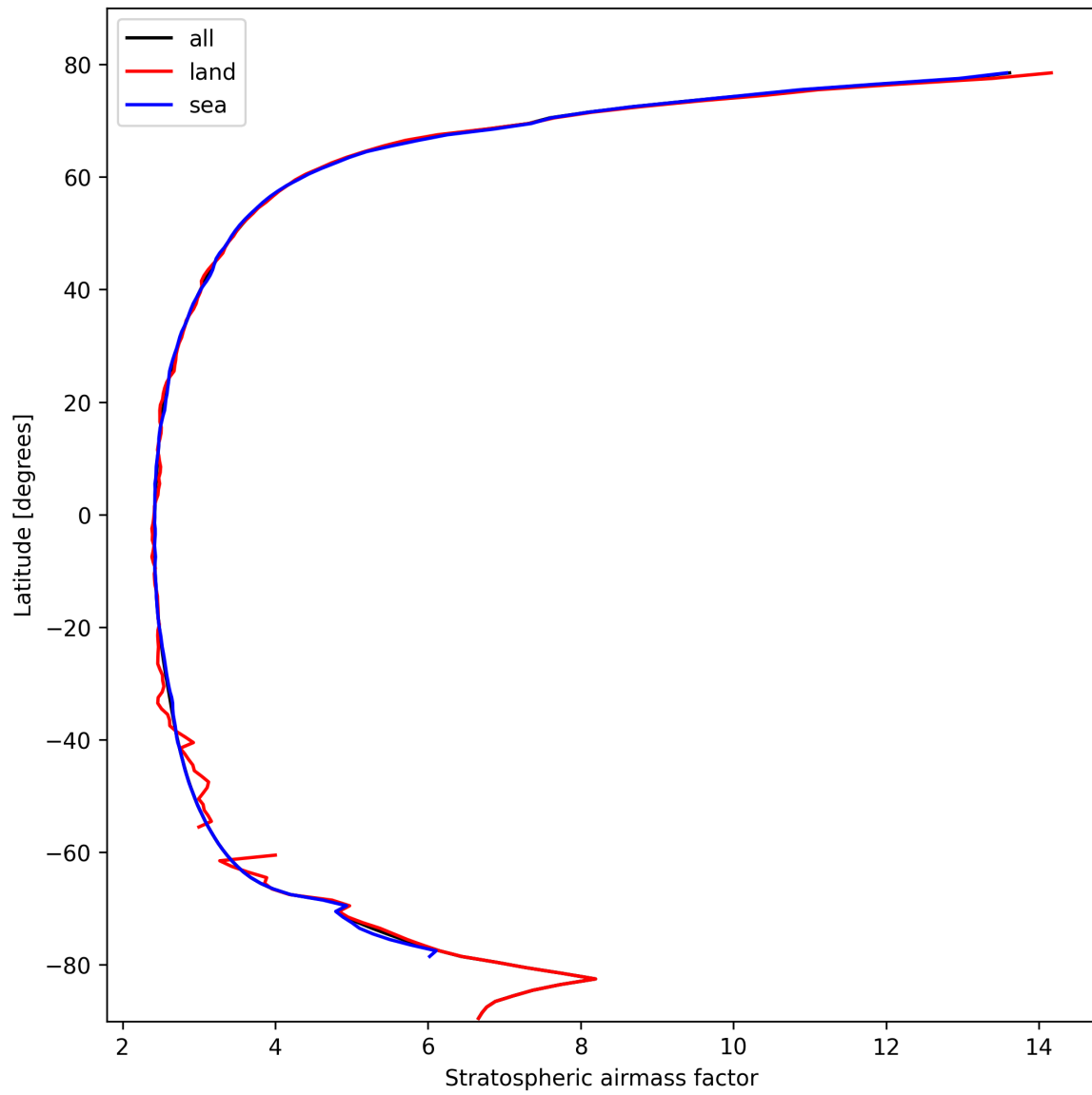
Figure 27: Zonal average of “Stratospheric air mass factor” for 2024-10-17 to 2024-10-19.
