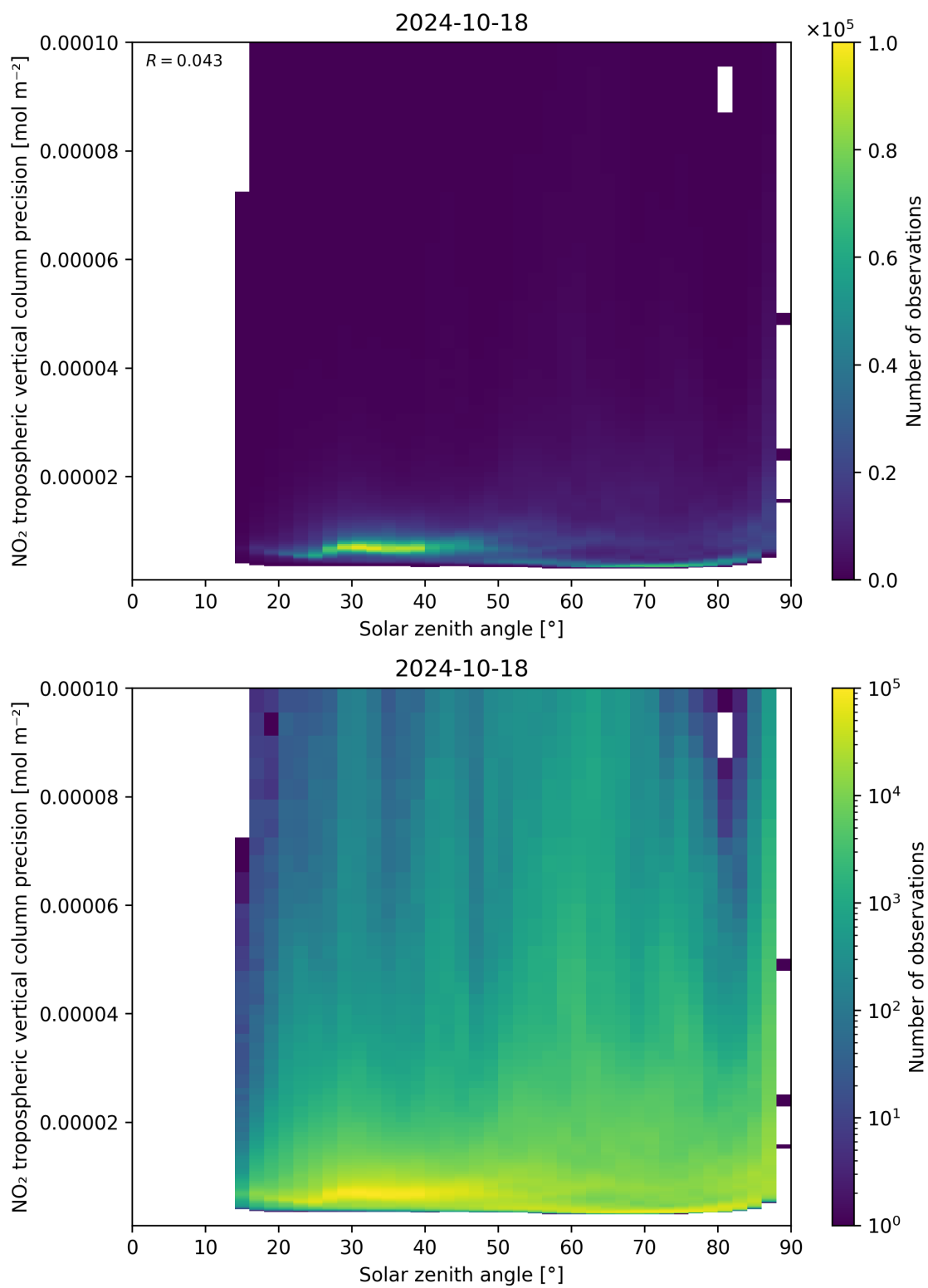
Figure 156: Scatter density plot of “Solar zenith angle” against “NO 2 tropospheric vertical column precision” for 2024-10-17 to 2024-10-19.
