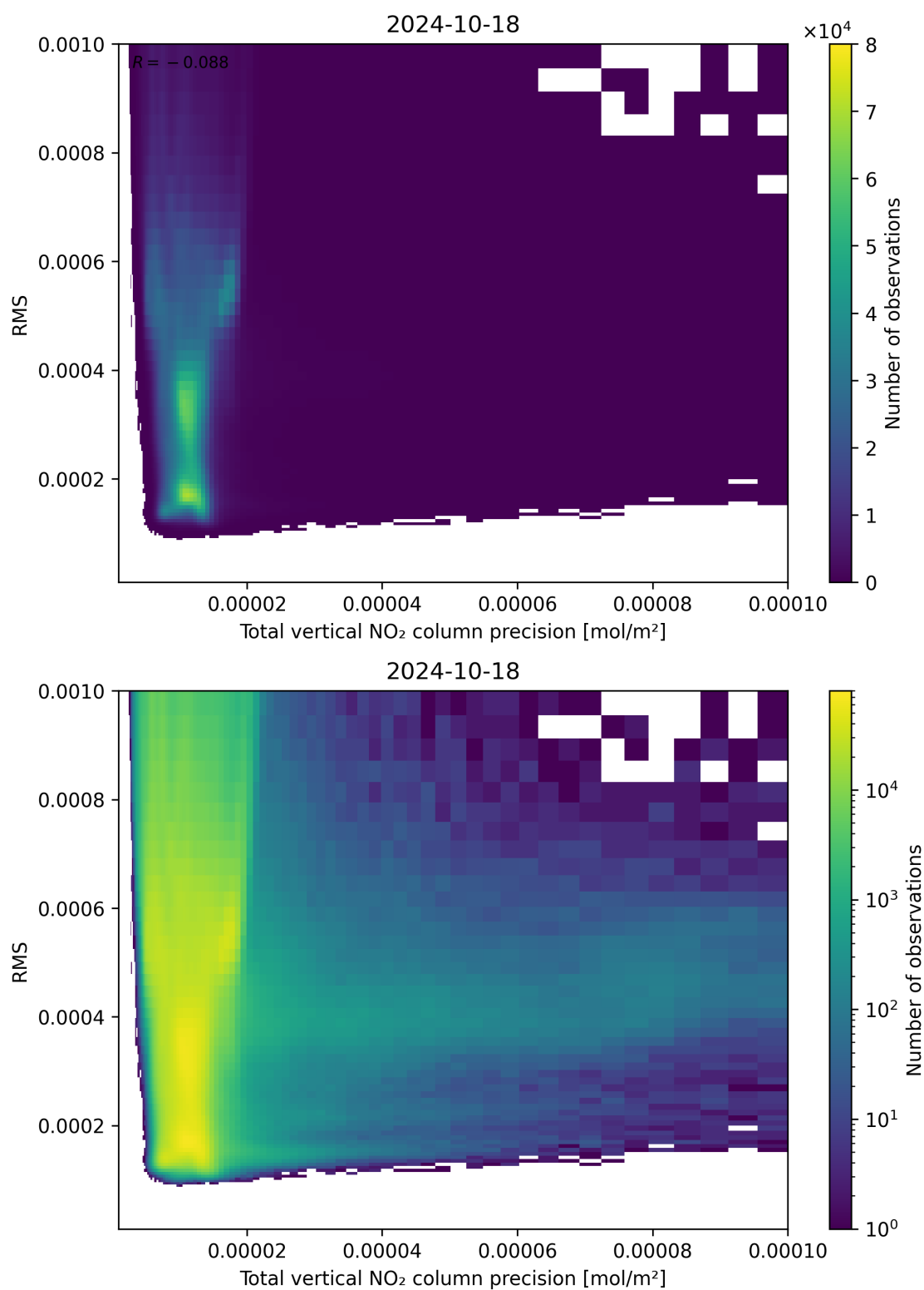
Figure 119: Scatter density plot of “Total vertical NO 2 column precision” against “RMS” for 2024-10-17 to 2024-10-19.
