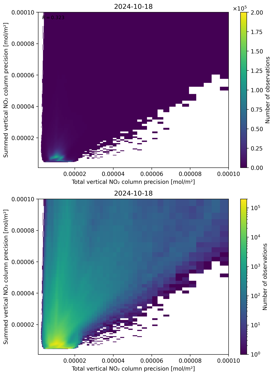
Figure 118: Scatter density plot of “Total vertical NO 2 column precision” against “Summed vertical NO 2 column precision” for 2024-10-17 to 2024-10-19.
