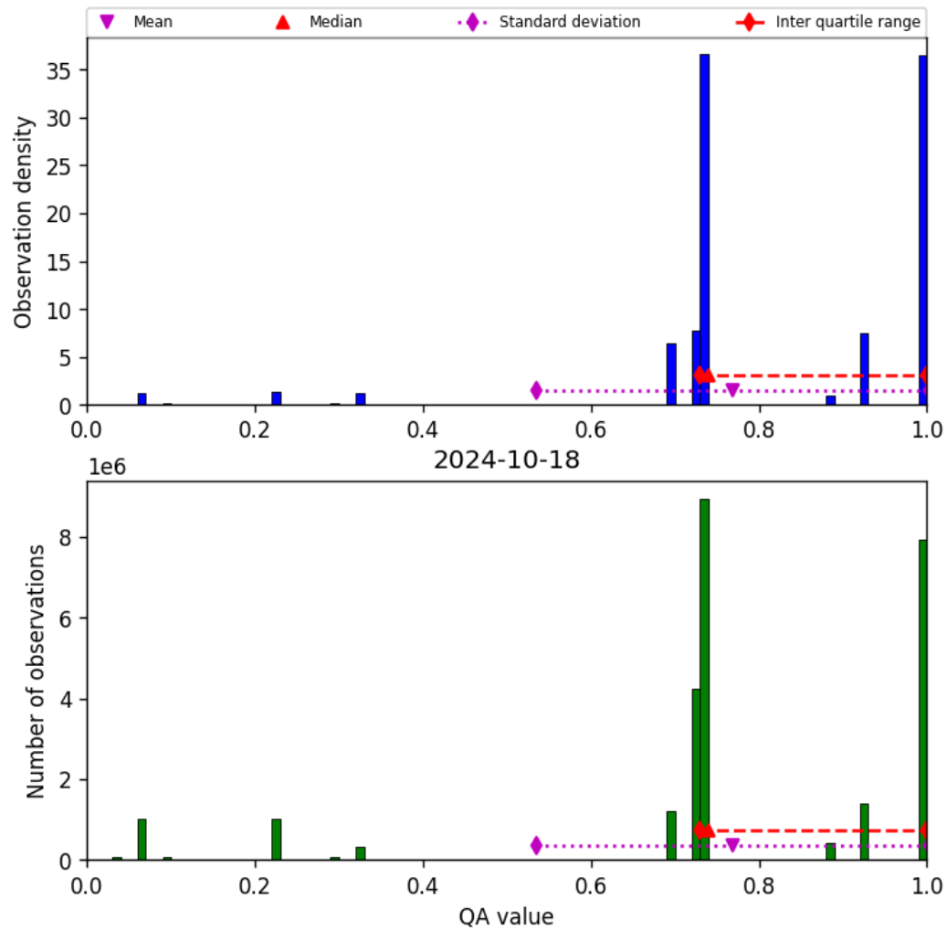
Figure 28: Histogram of “QA value” for 2024-10-17 to 2024-10-19
