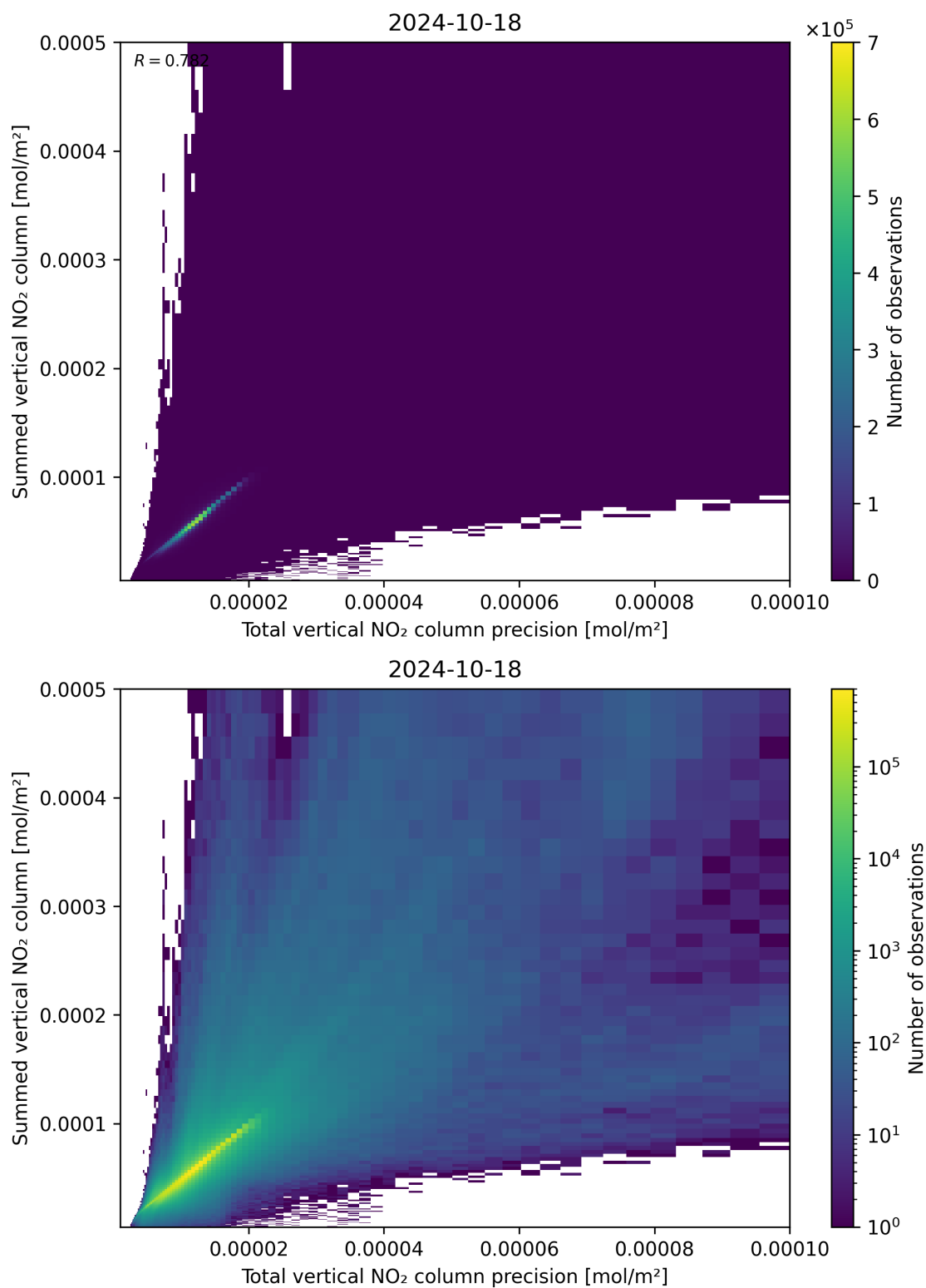
Figure 117: Scatter density plot of “Total vertical NO 2 column precision” against “Summed vertical NO 2 column” for 2024-10-17 to 2024-10-19.
