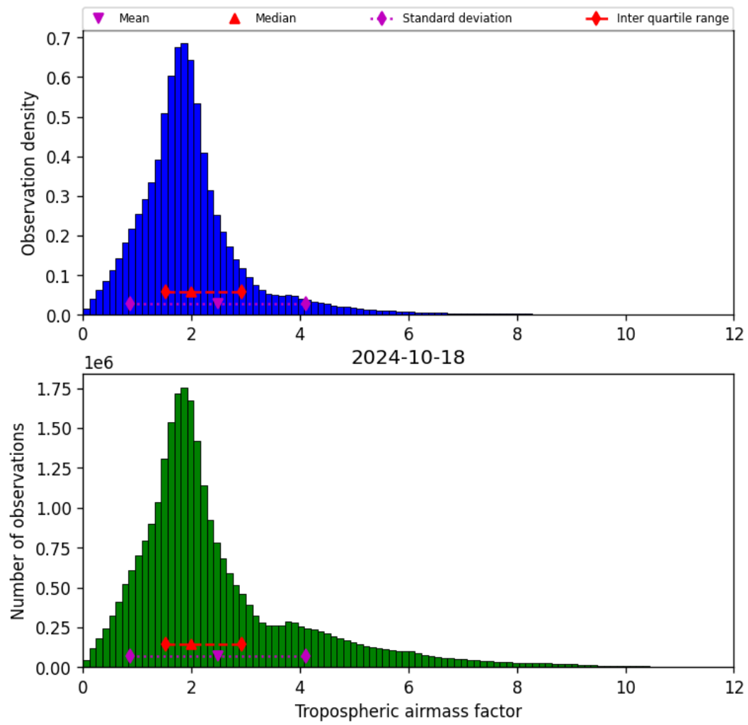
Figure 31: Histogram of “Tropospheric airmass factor” for 2024-10-17 to 2024-10-19
