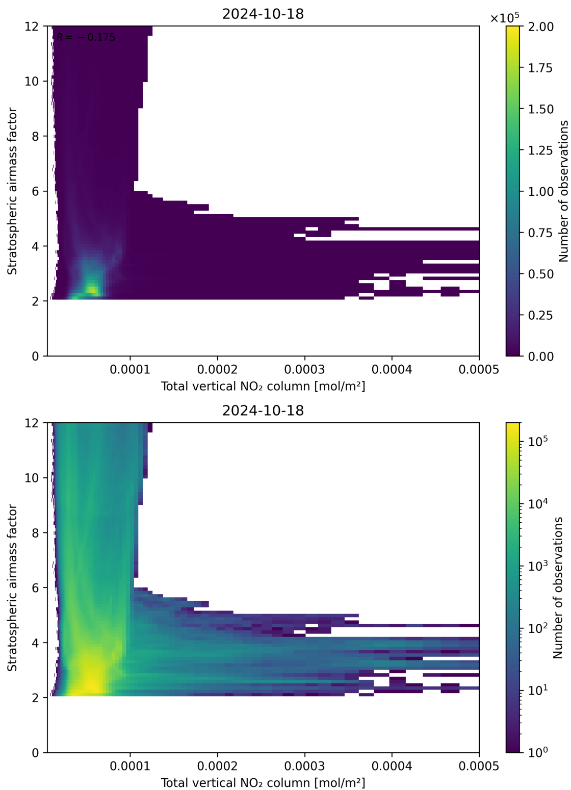
Figure 110: Scatter density plot of “Total vertical NO 2 column” against “Stratospheric airmass factor” for 2024-10-17 to 2024-10-19.
