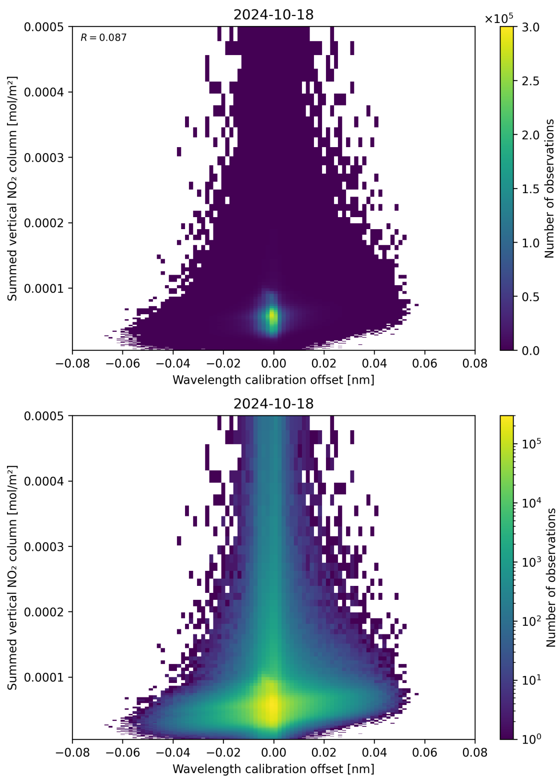
Figure 177: Scatter density plot of “Wavelength calibration offset” against “Summed vertical NO 2 column” for 2024-10-17 to 2024-10-19.
