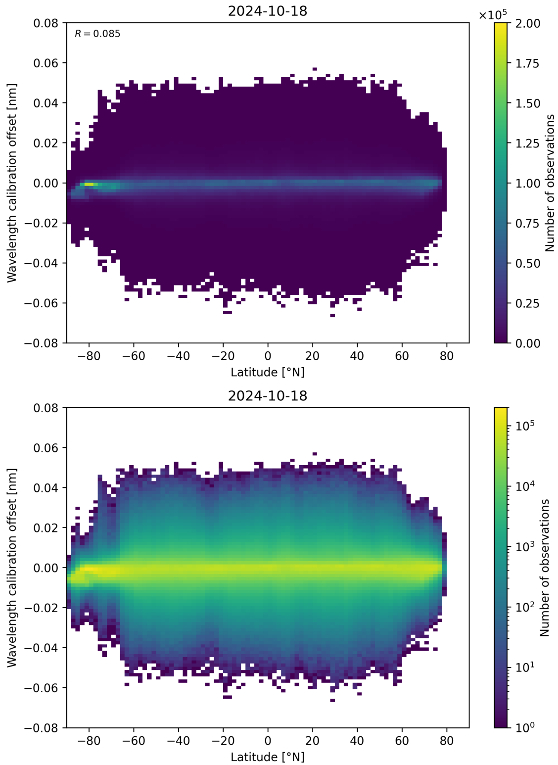
Figure 95: Scatter density plot of “Latitude” against “Wavelength calibration offset” for 2024-10-17 to 2024-10-19.
