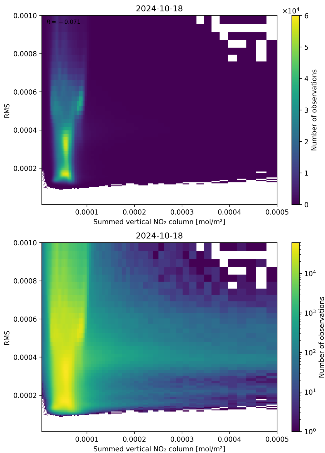
Figure 109: Scatter density plot of “Summed vertical NO 2 column” against “RMS” for 2024-10-17 to 2024-10-19.
