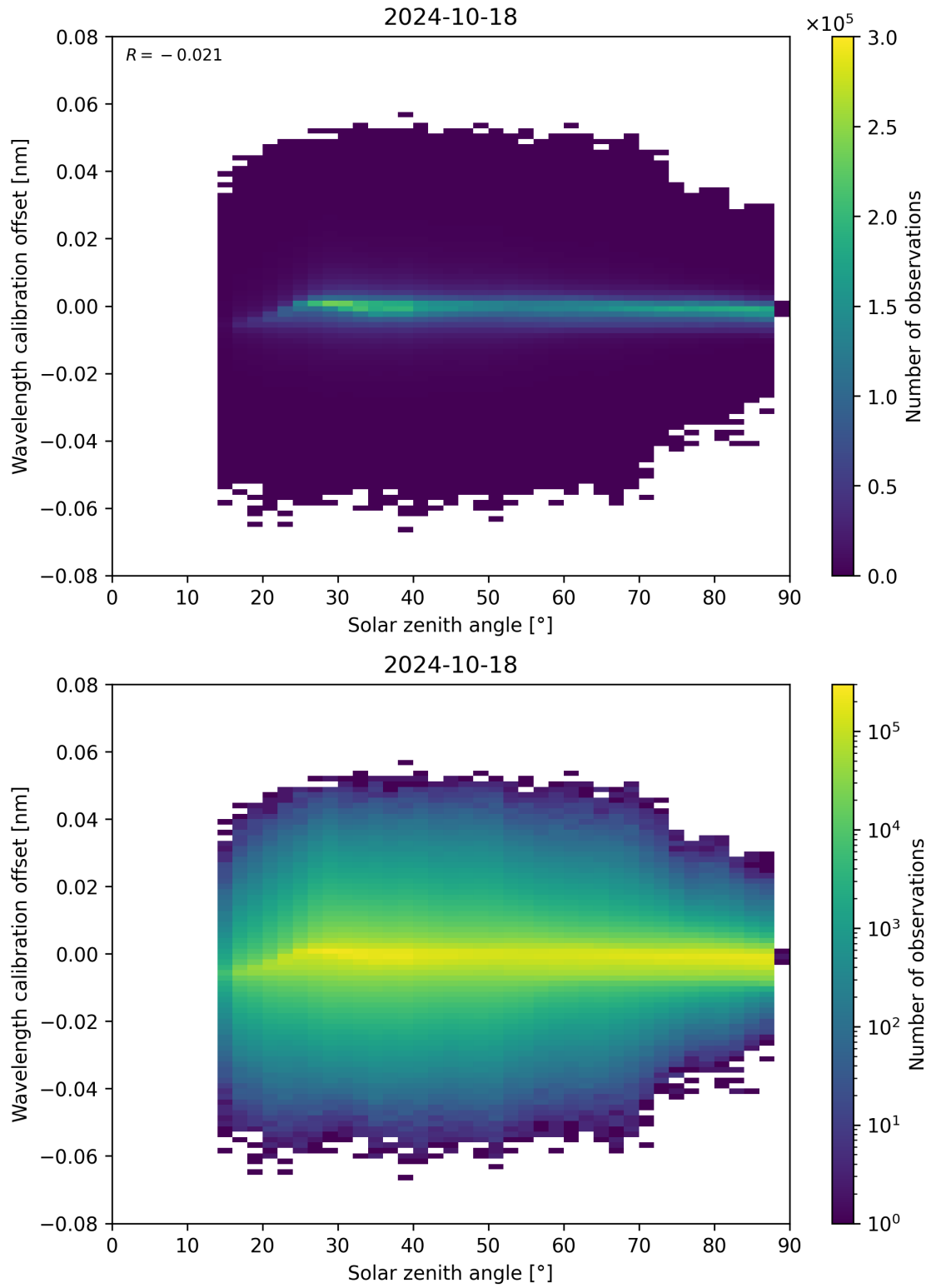
Figure 158: Scatter density plot of “Solar zenith angle” against “Wavelength calibration offset” for 2024-10-17 to 2024-10-19.
