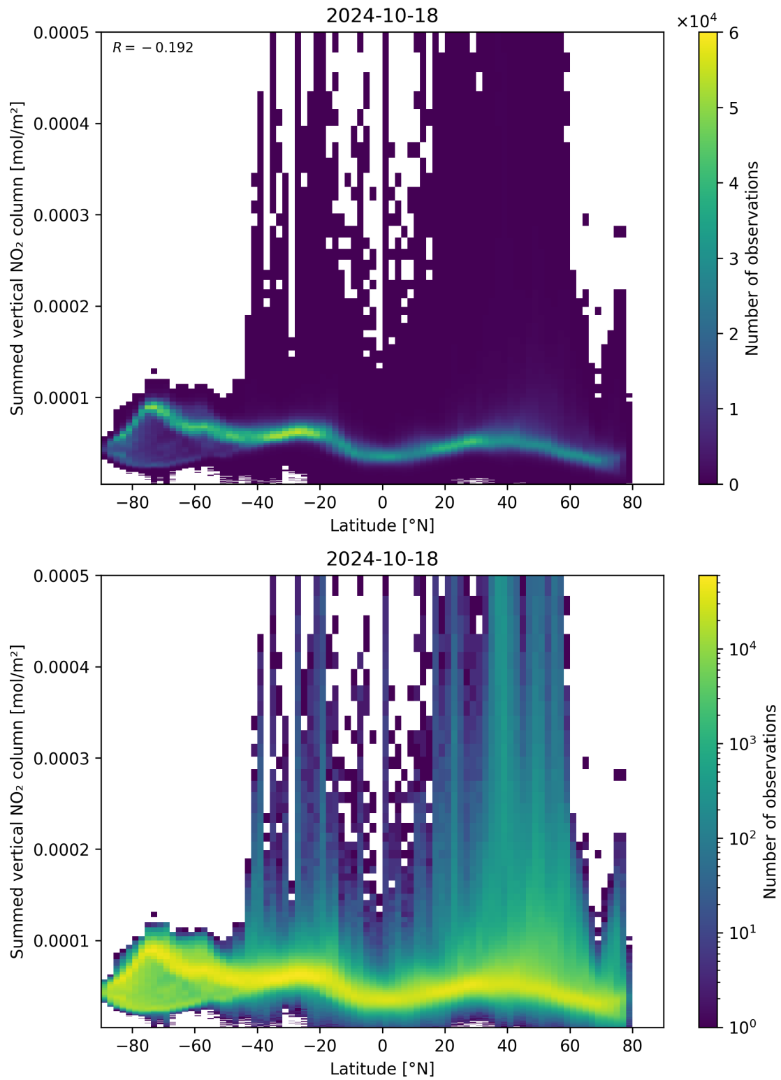
Figure 88: Scatter density plot of “Latitude” against “Summed vertical NO 2 column” for 2024-10-17 to 2024-10-19.
