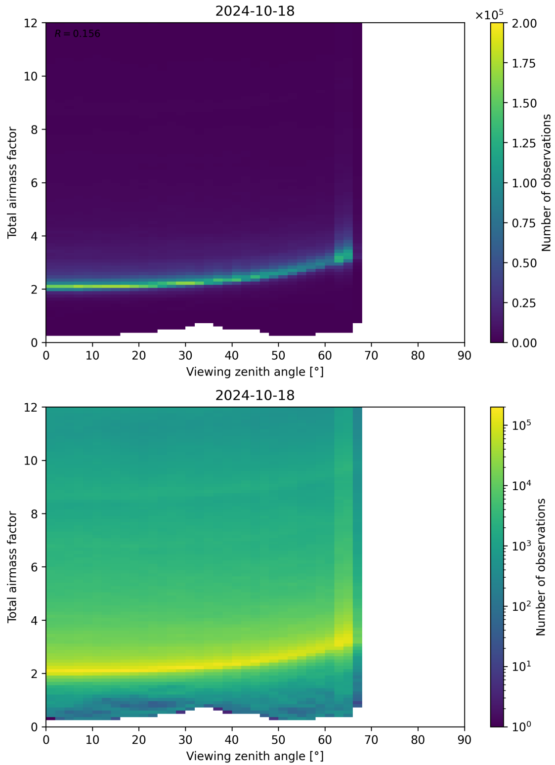
Figure 160: Scatter density plot of “Viewing zenith angle” against “Total airmass factor” for 2024-10-17 to 2024-10-19.
