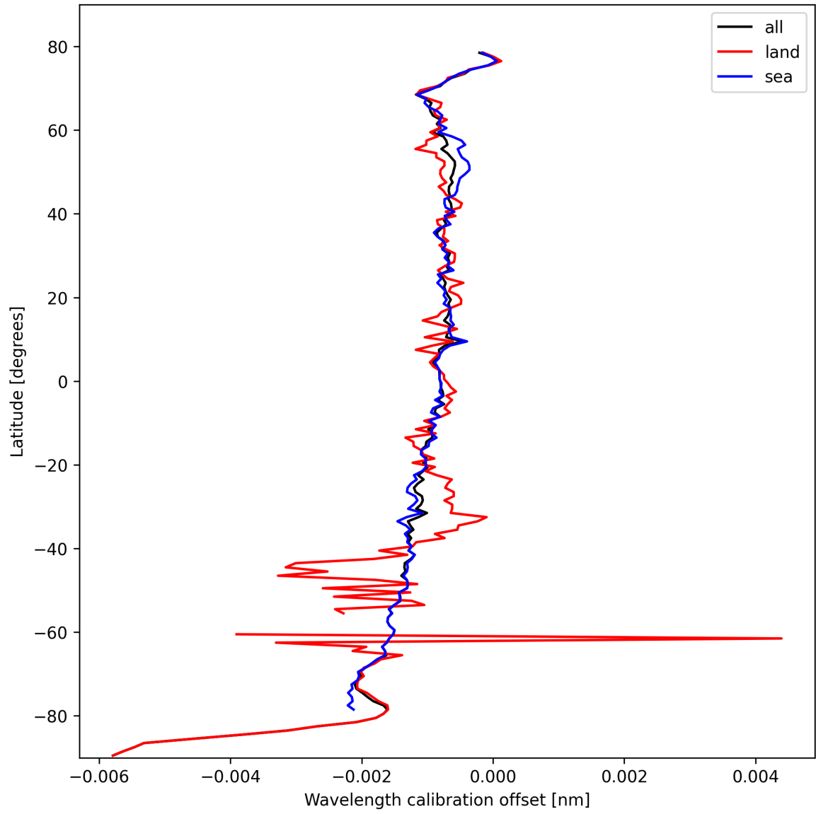
Figure 18: Zonal average of “Wavelength calibration offset” for 2024-10-17 to 2024-10-19.
