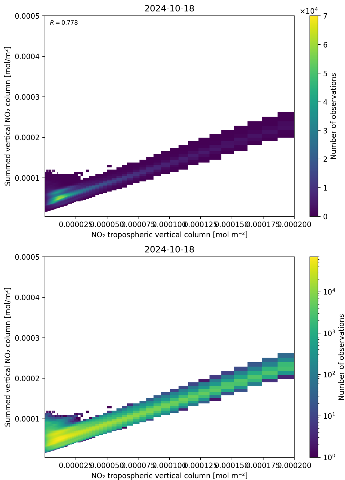
Figure 126: Scatter density plot of “NO 2 tropospheric vertical column” against “Summed vertical NO 2 column” for 2024-10-17 to 2024-10-19.
