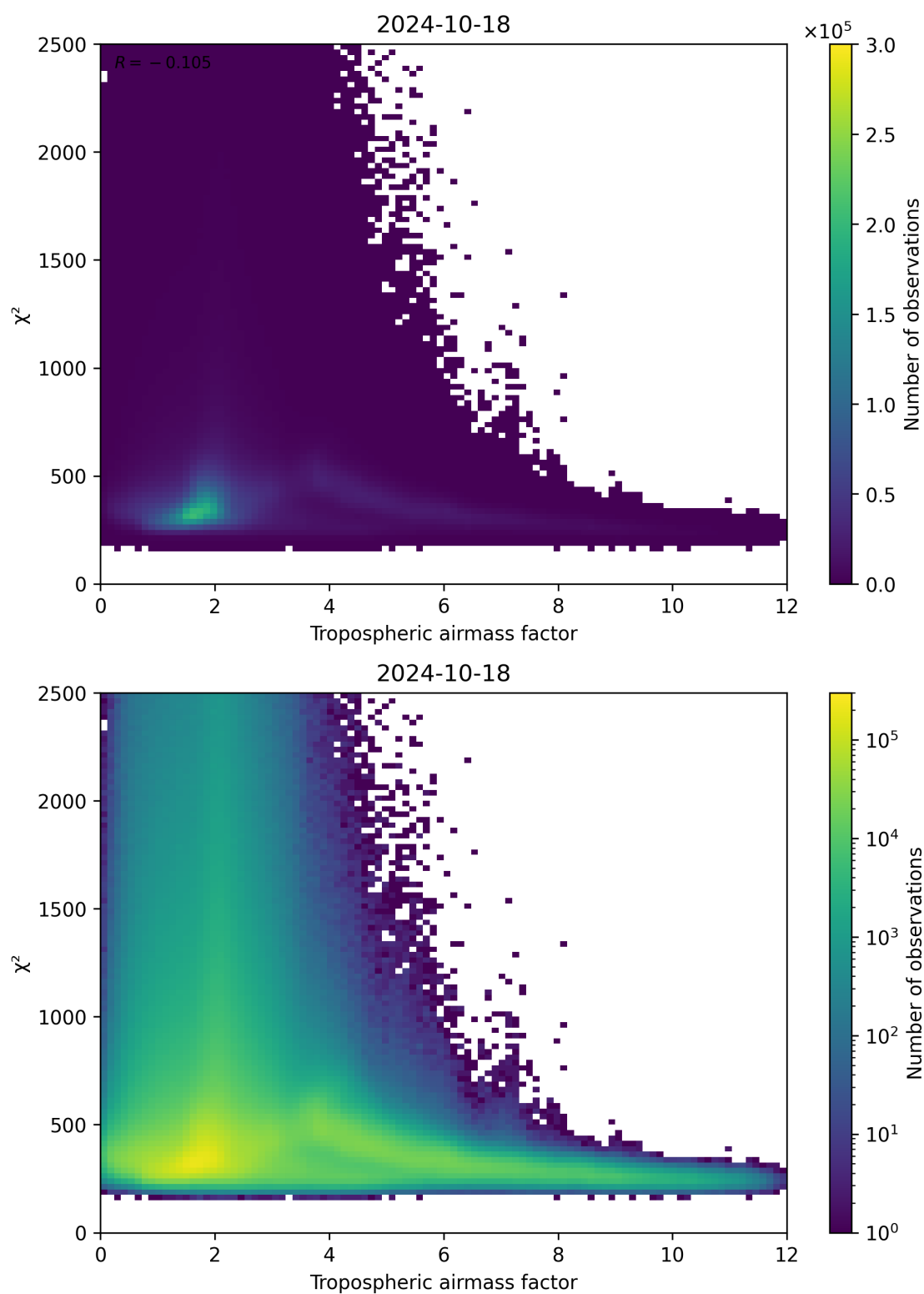
Figure 73: Scatter density plot of “Tropospheric airmass factor” against “ \chi^2 ” for 2024-10-17 to 2024-10-19.
