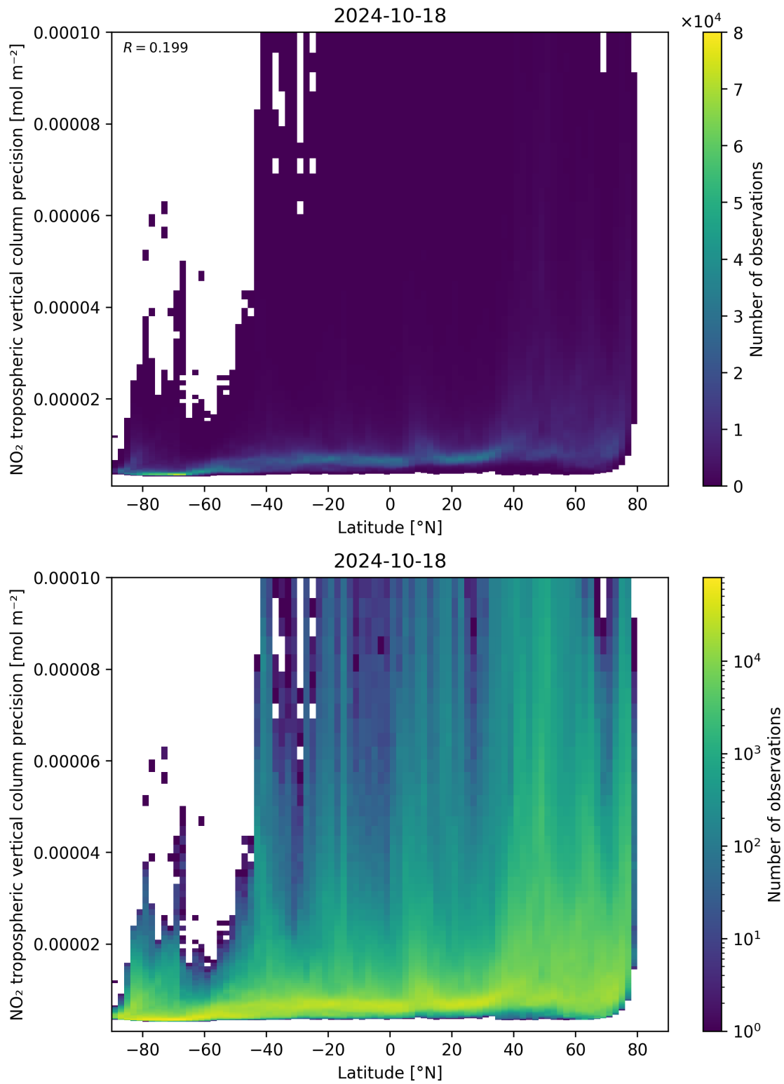
Figure 93: Scatter density plot of “Latitude” against “NO 2 tropospheric vertical column precision” for 2024-10-17 to 2024-10-19.
