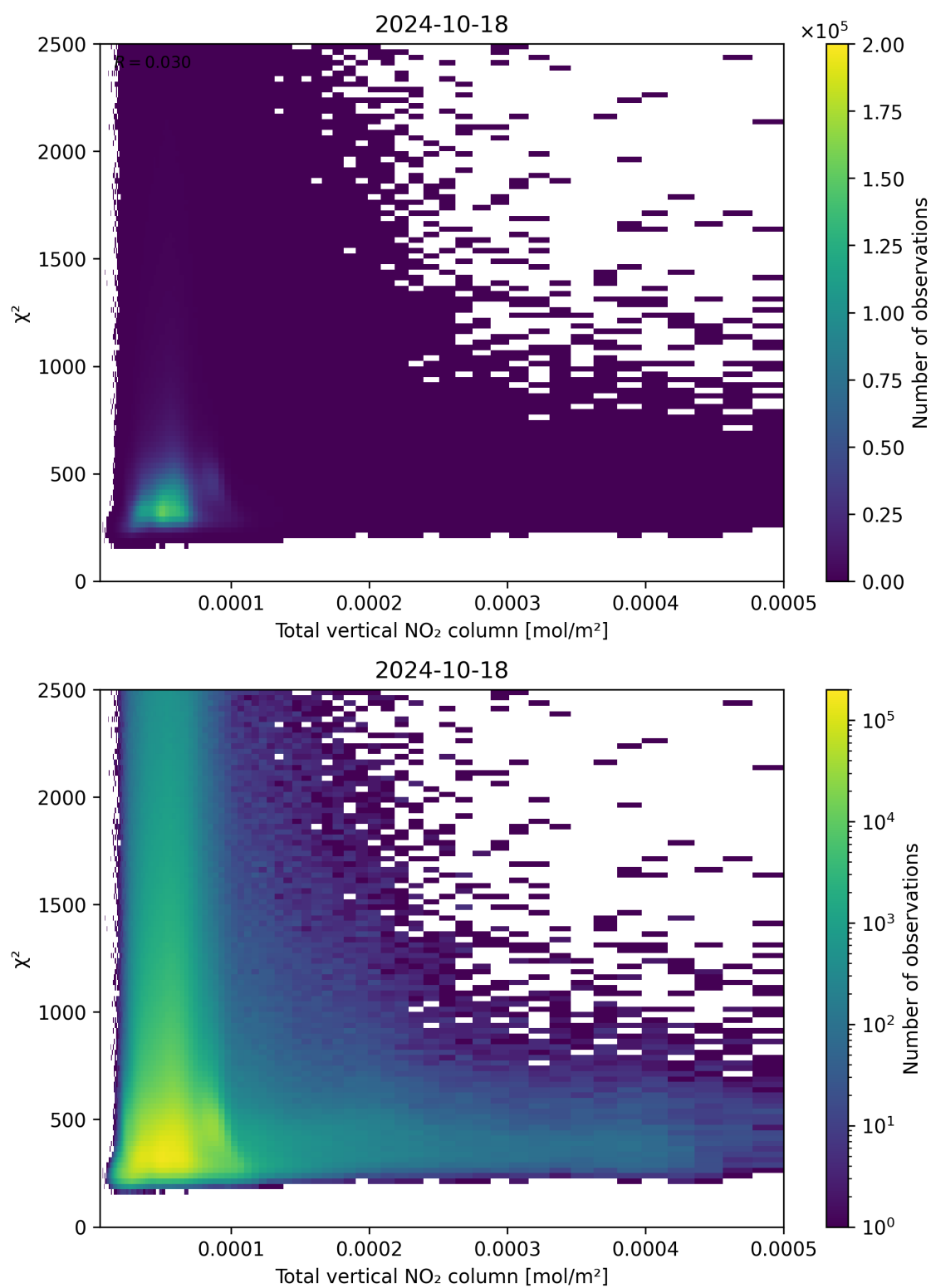
Figure 111: Scatter density plot of “Total vertical NO 2 column” against “ \chi^2 ” for 2024-10-17 to 2024-10-19.
