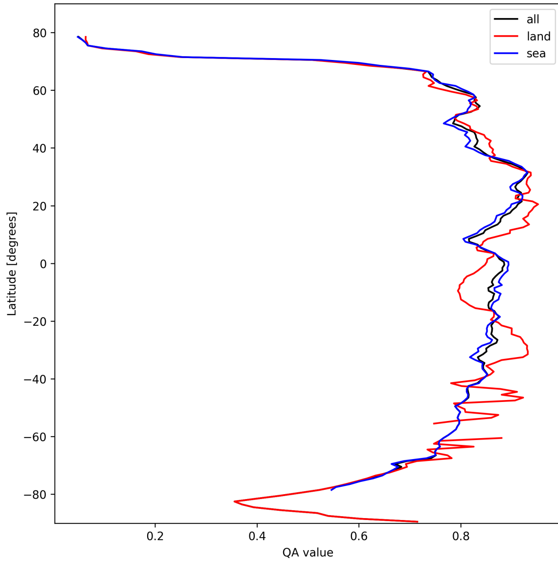
Figure 11: Zonal average of “QA value” for 2024-10-17 to 2024-10-19.
