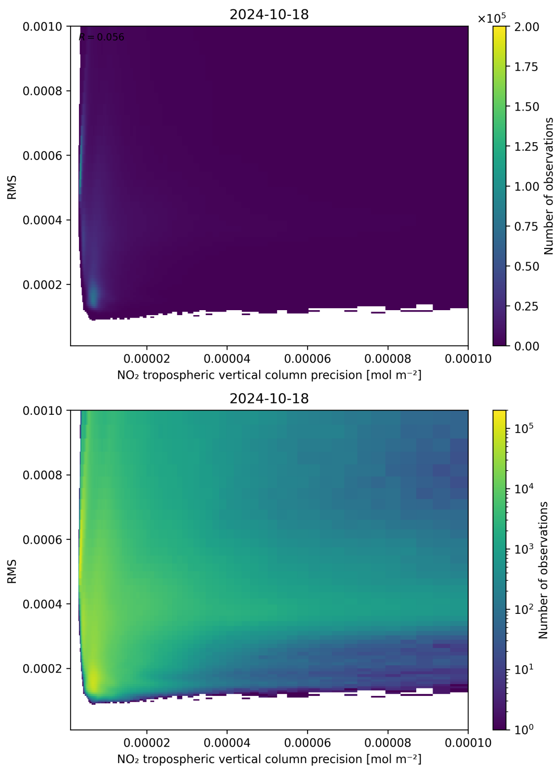
Figure 140: Scatter density plot of “NO 2 tropospheric vertical column precision” against “RMS” for 2024-10-17 to 2024-10-19.
