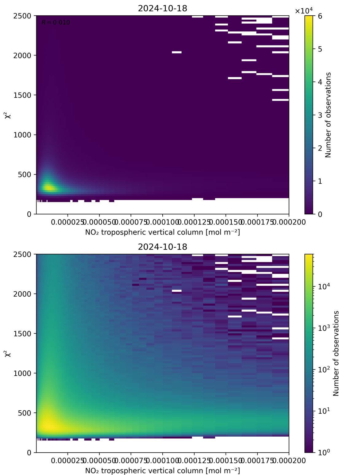
Figure 124: Scatter density plot of “NO 2 tropospheric vertical column” against “ \chi^2 ” for 2024-10-17 to 2024-10-19.
