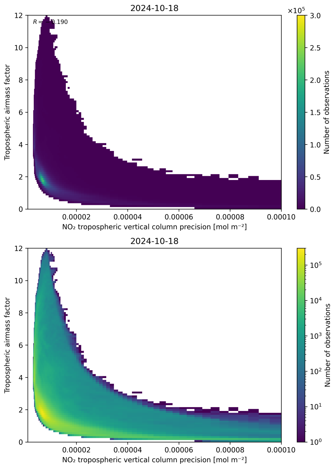
Figure 133: Scatter density plot of “NO 2 tropospheric vertical column precision” against “Tropospheric airmass factor” for 2024-10-17 to 2024-10-19.
