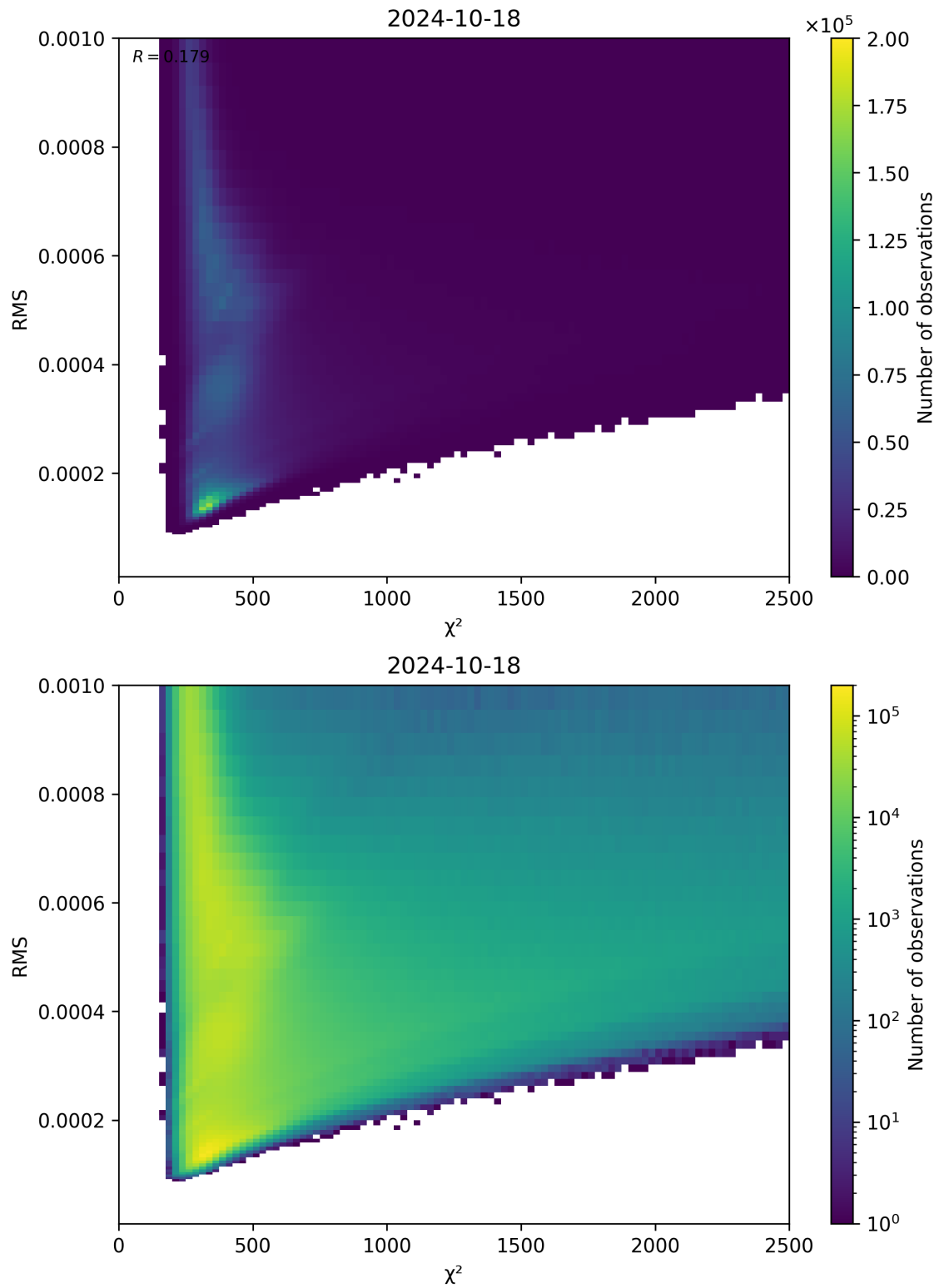
Figure 82: Scatter density plot of “ \chi^2 ” against “RMS” for 2024-10-17 to 2024-10-19.
