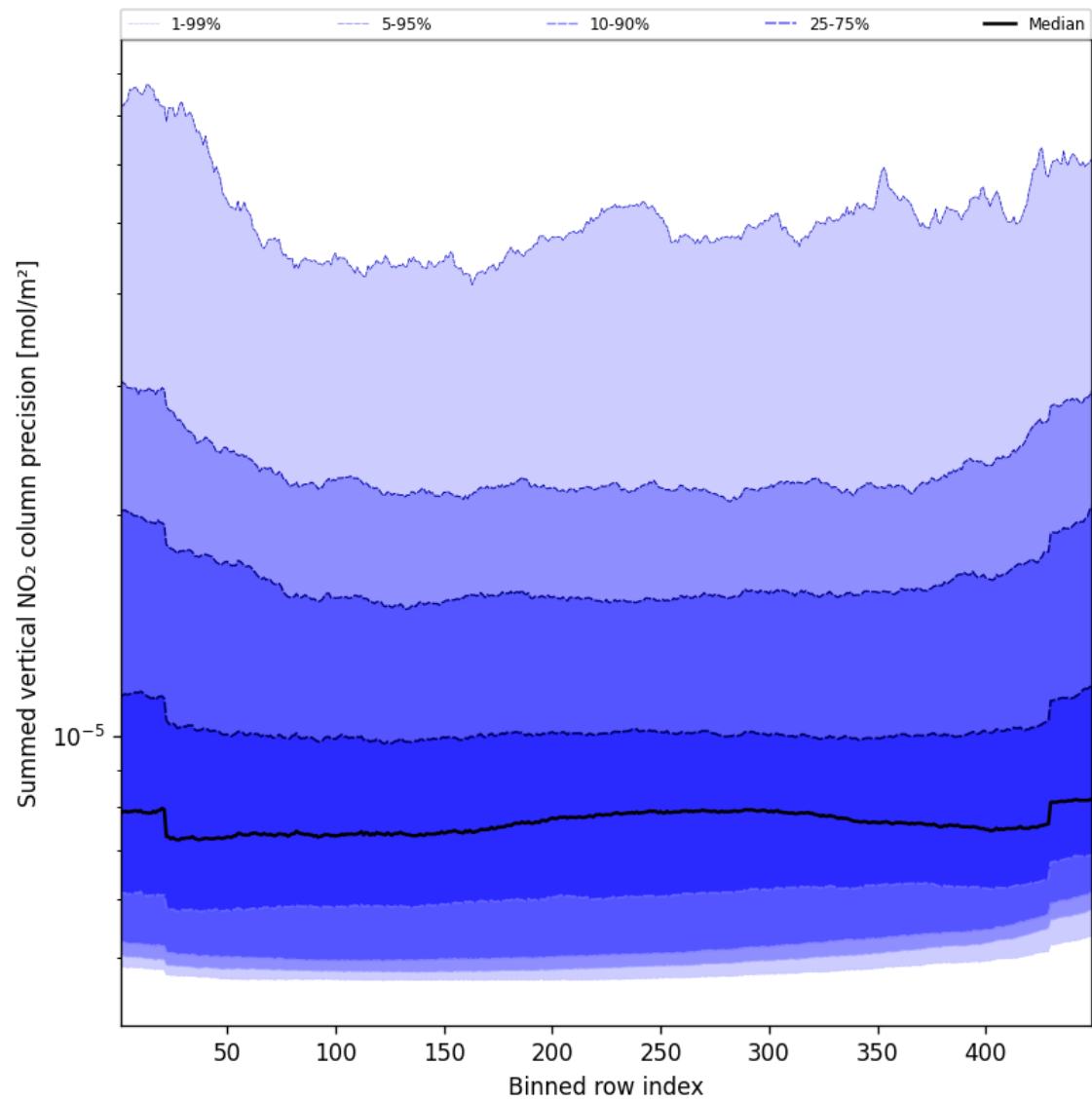
Figure 58: Along track statistics of “Summed vertical NO 2 column precision” for 2024-10-17 to 2024-10-19
