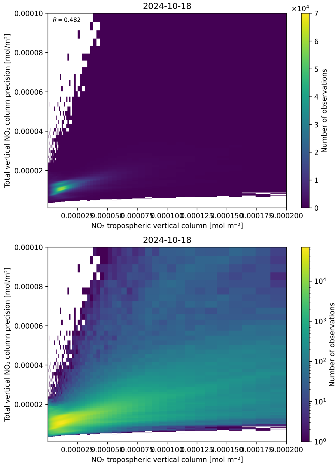
Figure 129: Scatter density plot of “NO 2 tropospheric vertical column” against “Total vertical NO 2 column precision” for 2024-10-17 to 2024-10-19.
