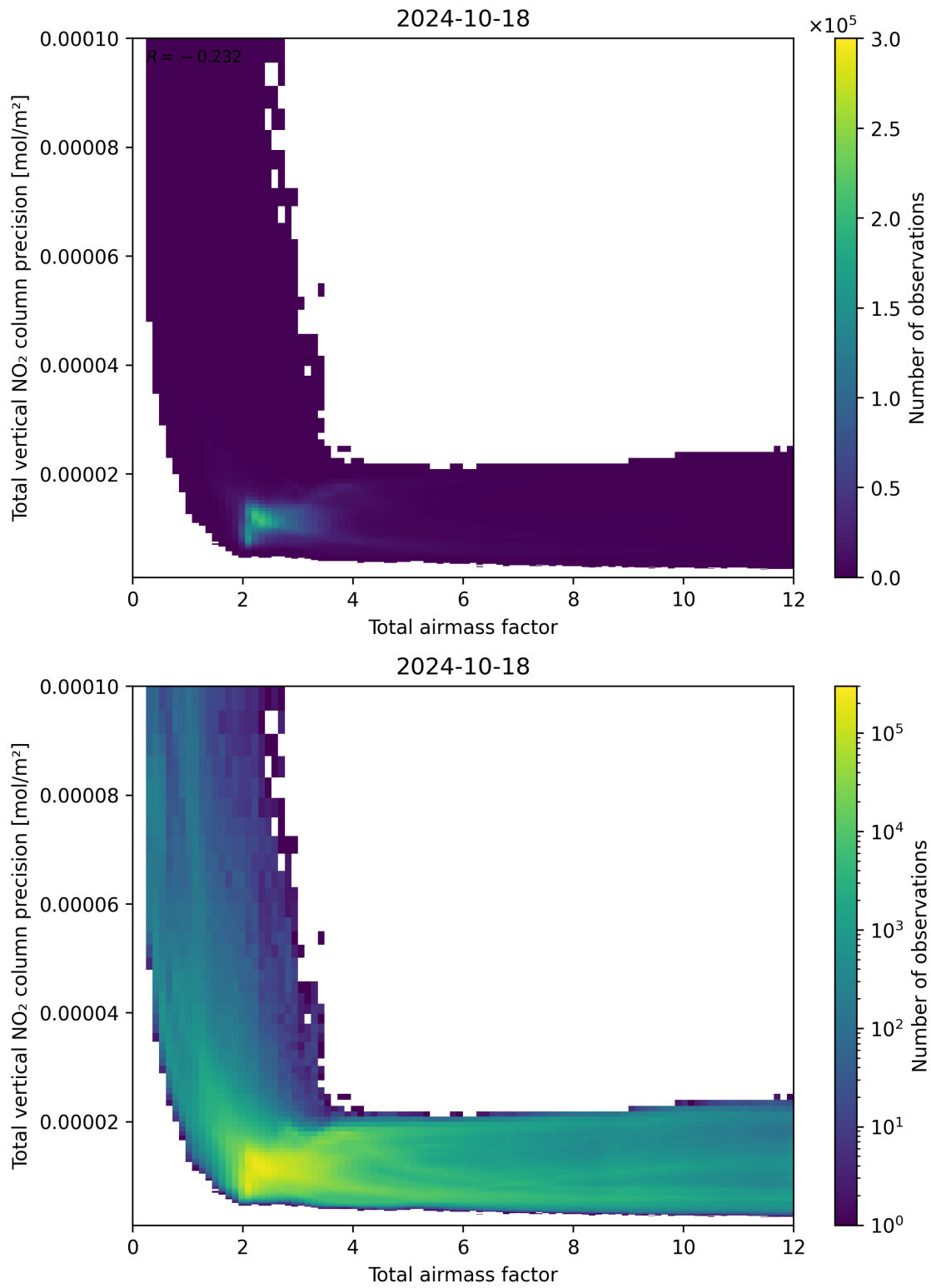
Figure 68: Scatter density plot of “Total airmass factor” against “Total vertical NO 2 column precision” for 2024-10-17 to 2024-10-19.
