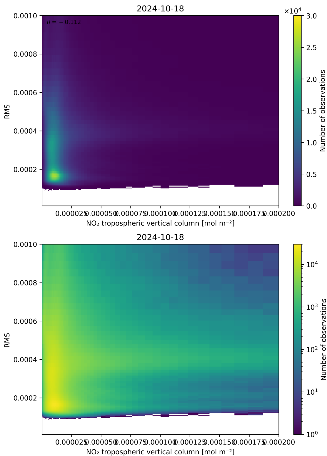
Figure 142: Scatter density plot of “NO 2 tropospheric vertical column” against “RMS” for 2024-10-17 to 2024-10-19.
