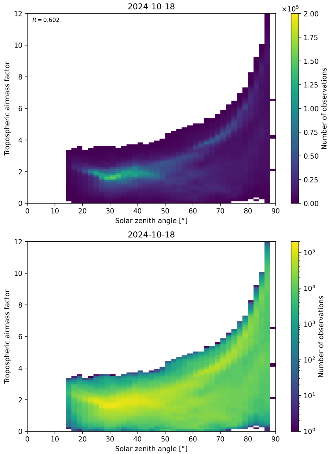
Figure 147: Scatter density plot of “Solar zenith angle” against “Tropospheric airmass factor” for 2024-10-17 to 2024-10-19.
