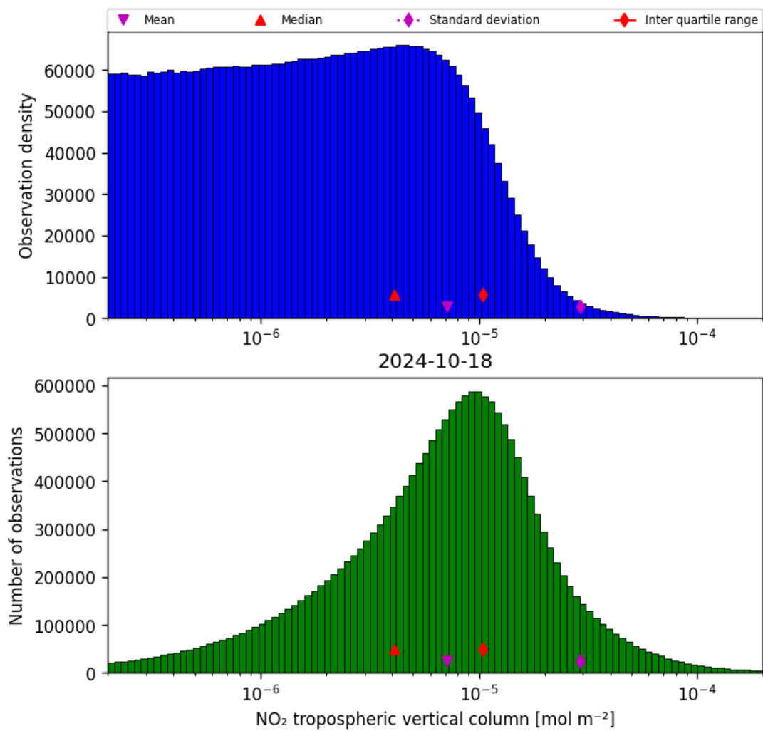
Figure 29: Histogram of “NO 2 tropospheric vertical column” for 2024-10-17 to 2024-10-19
