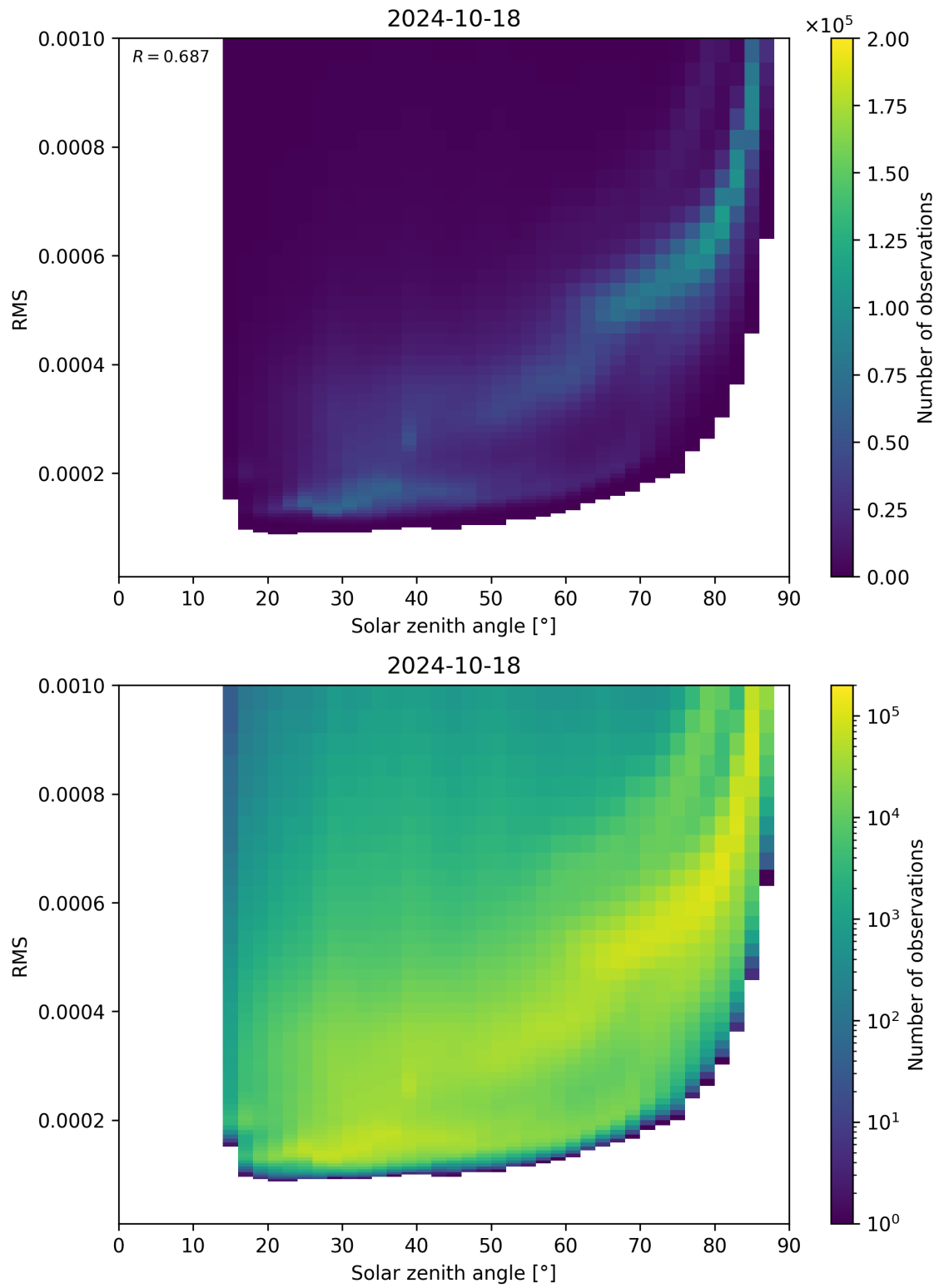
Figure 157: Scatter density plot of “Solar zenith angle” against “RMS” for 2024-10-17 to 2024-10-19.
