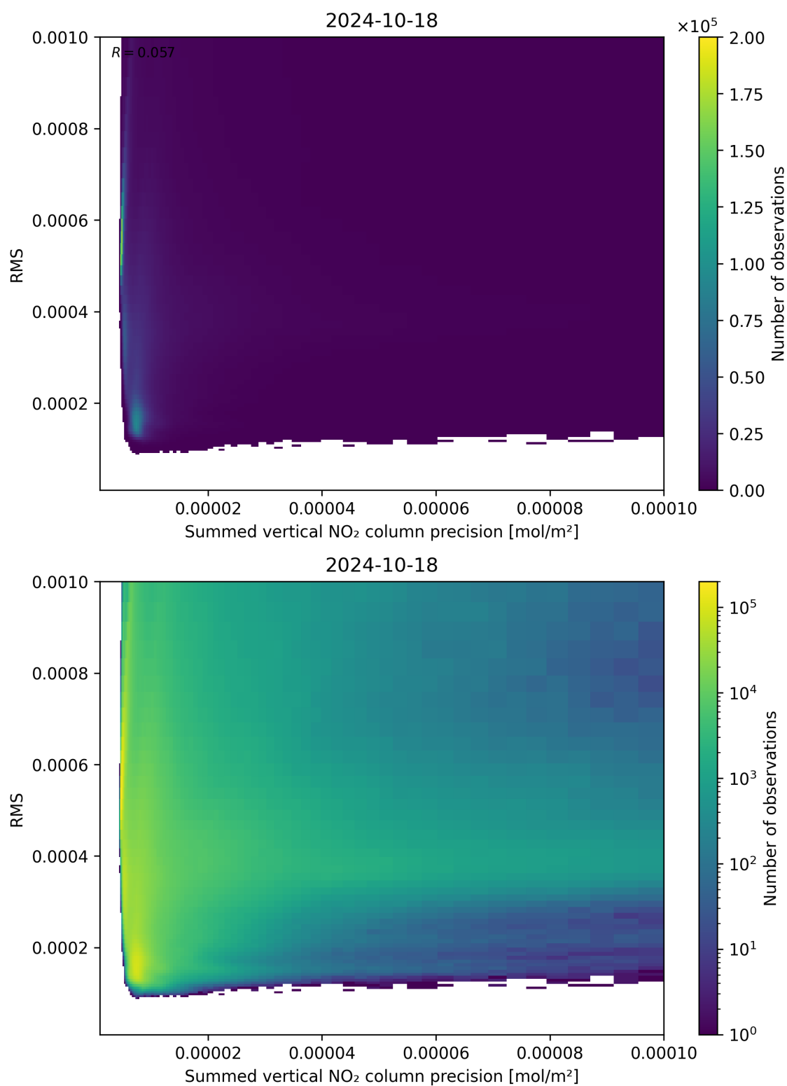
Figure 108: Scatter density plot of “Summed vertical NO 2 column precision” against “RMS” for 2024-10-17 to 2024-10-19.
