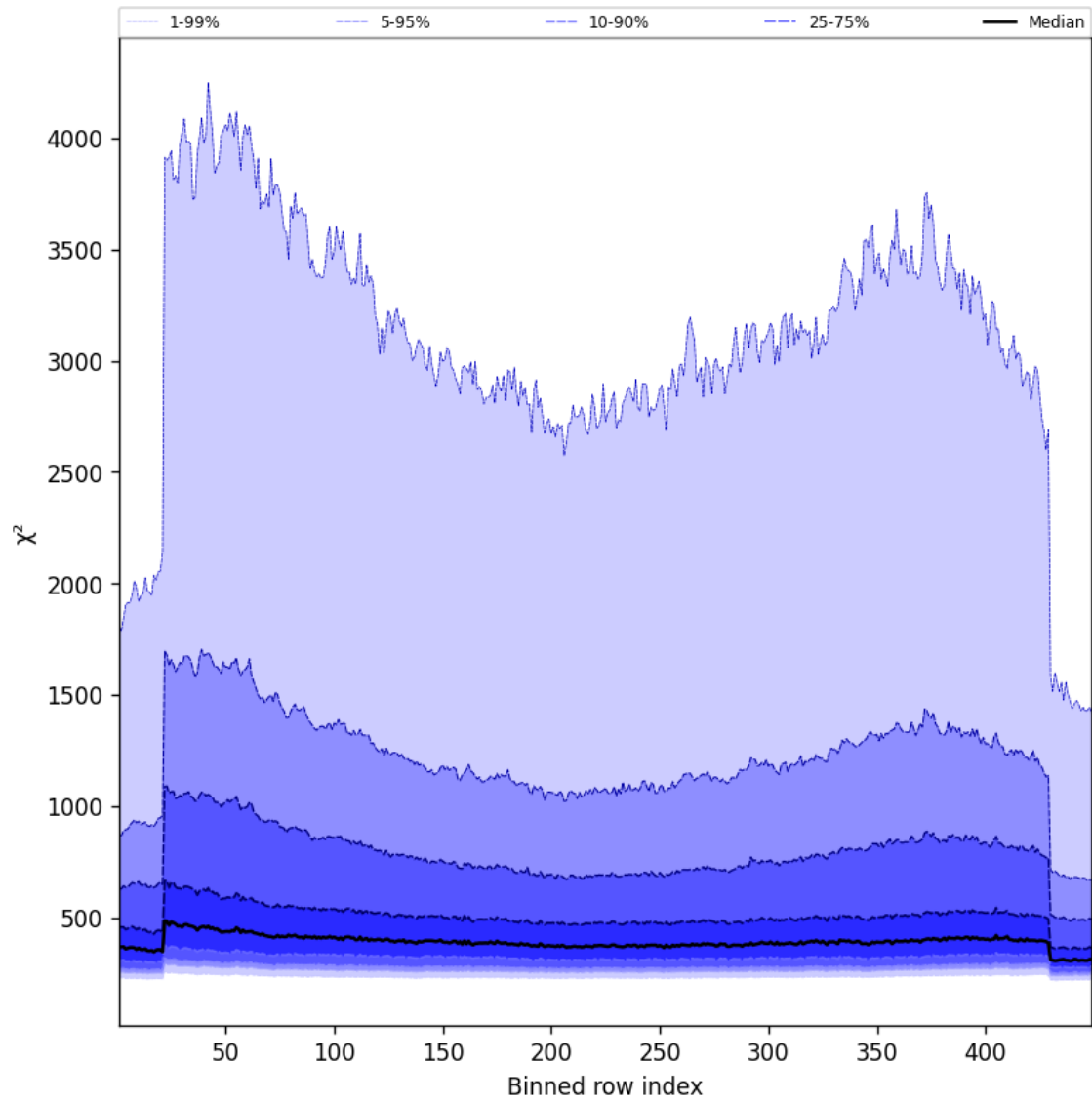
Figure 59: Along track statistics of “ \chi^2 ” for 2024-10-17 to 2024-10-19
