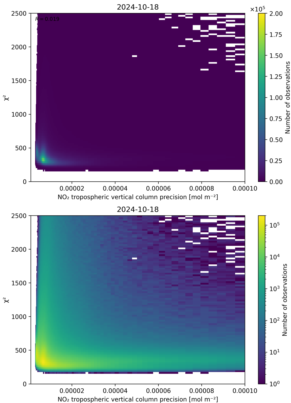
Figure 134: Scatter density plot of “NO 2 tropospheric vertical column precision” against “ \chi^2 ” for 2024-10-17 to 2024-10-19.
