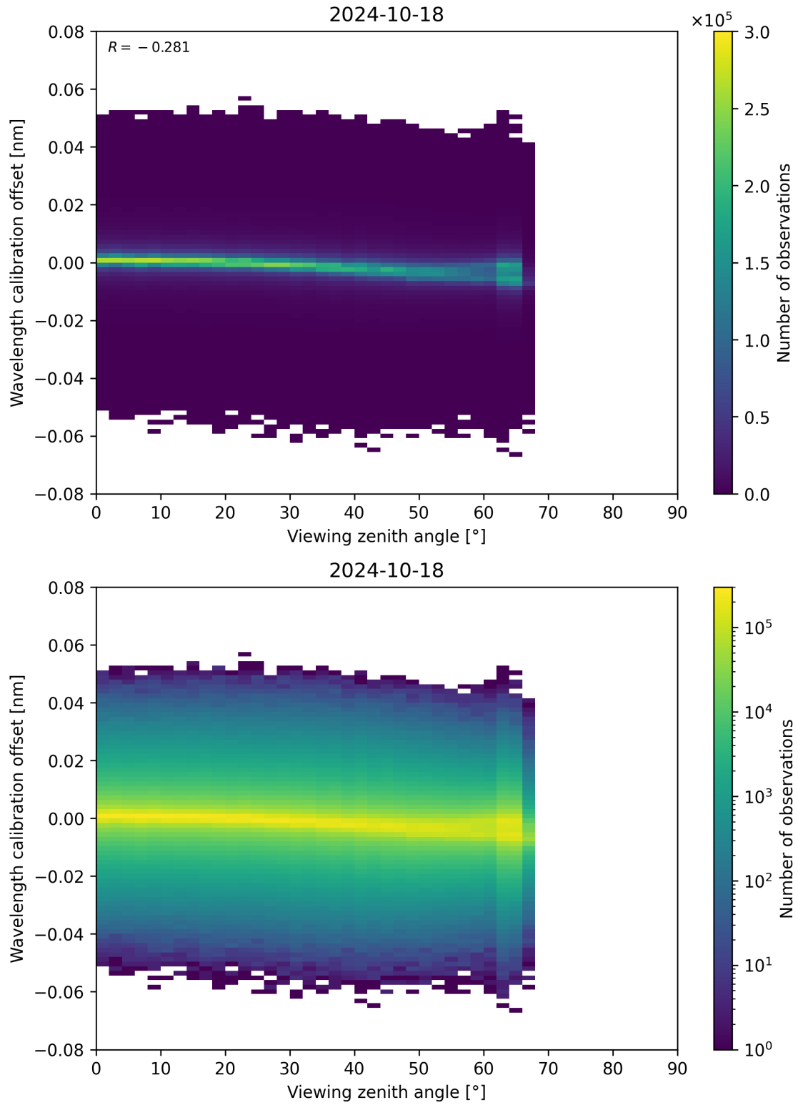
Figure 173: Scatter density plot of “Viewing zenith angle” against “Wavelength calibration offset” for 2024-10-17 to 2024-10-19.
