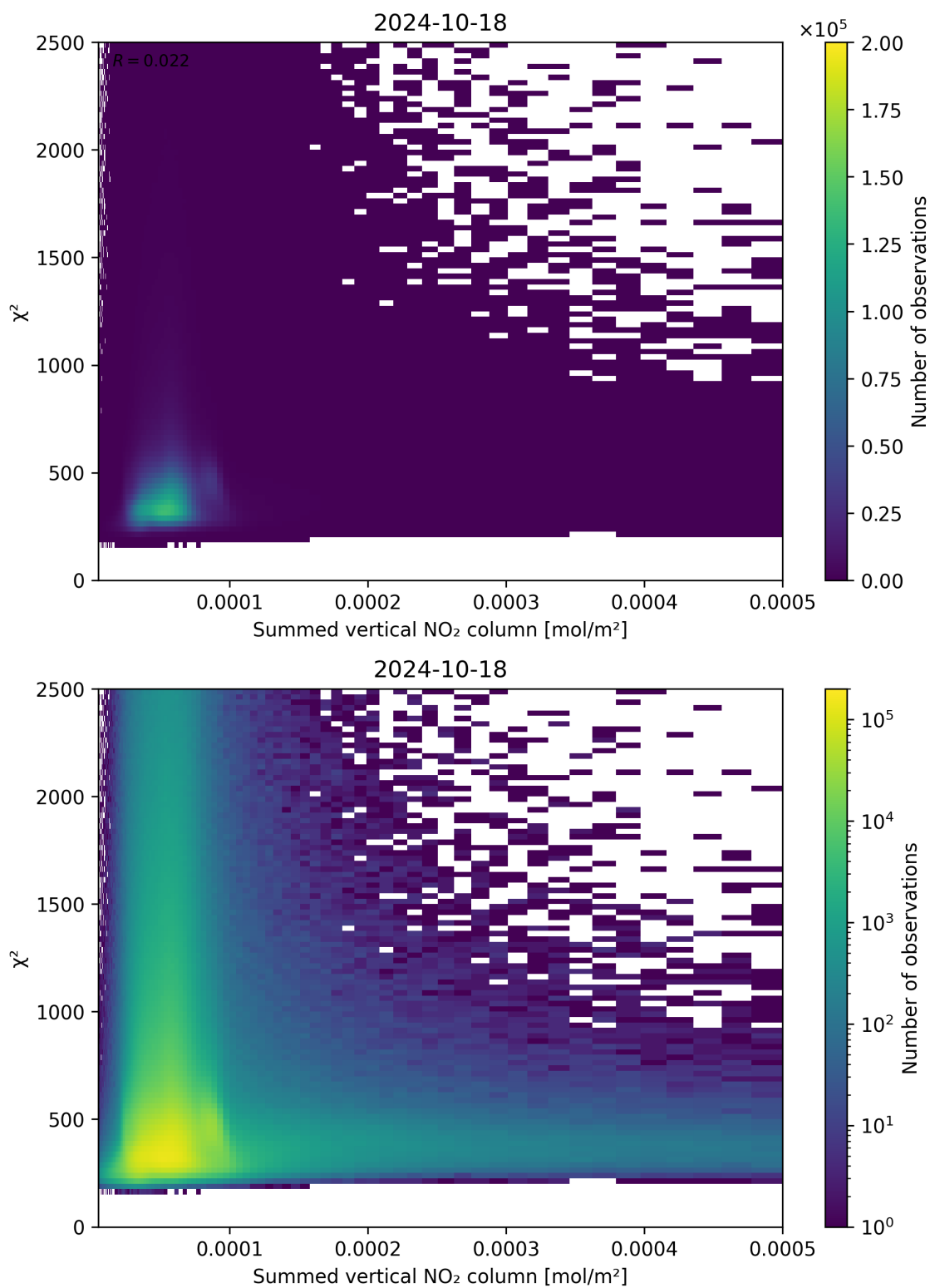
Figure 104: Scatter density plot of “Summed vertical NO 2 column” against “ \chi^2 ” for 2024-10-17 to 2024-10-19.
