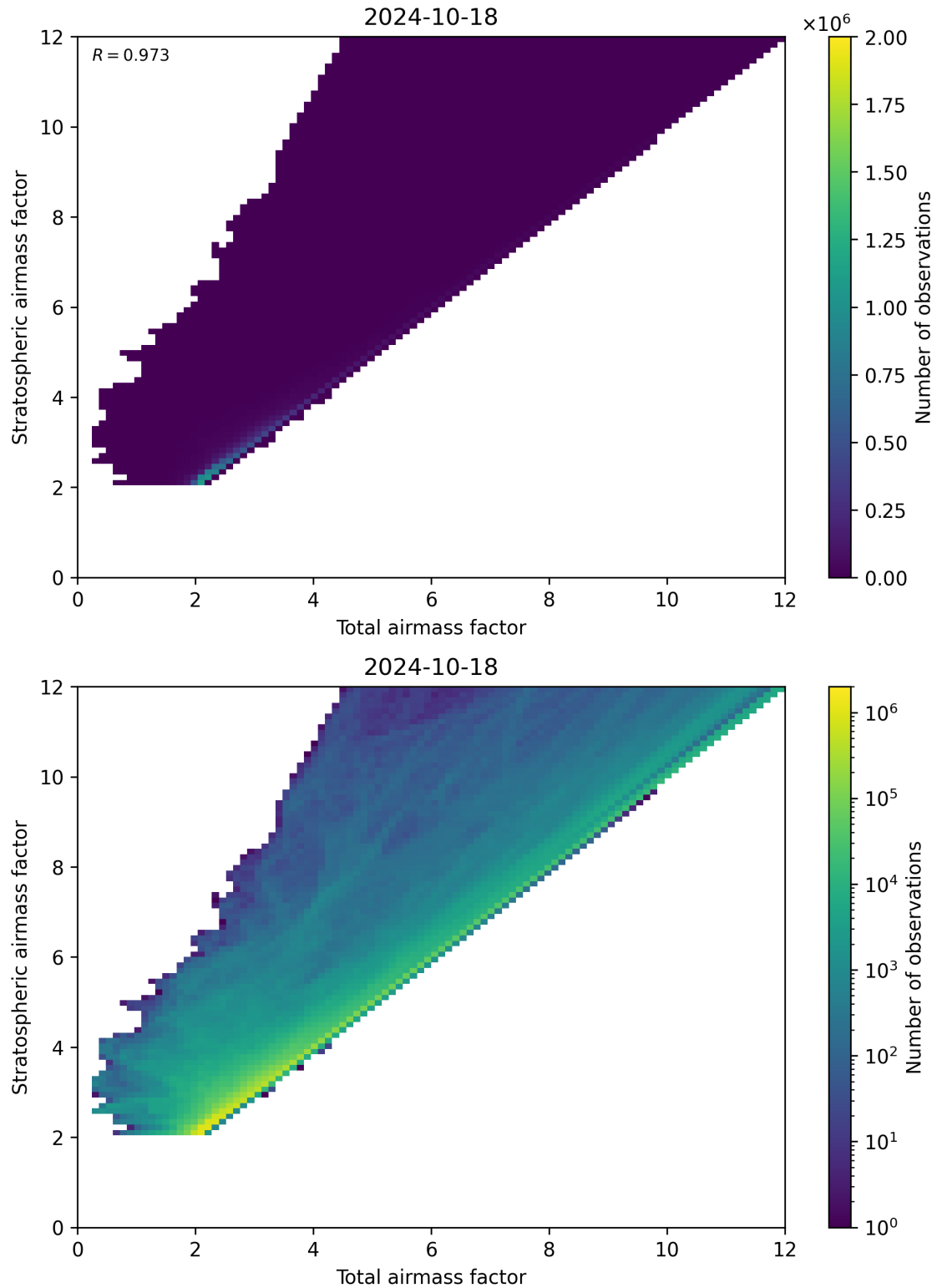
Figure 62: Scatter density plot of “Total airmass factor” against “Stratospheric airmass factor” for 2024-10-17 to 2024-10-19.
