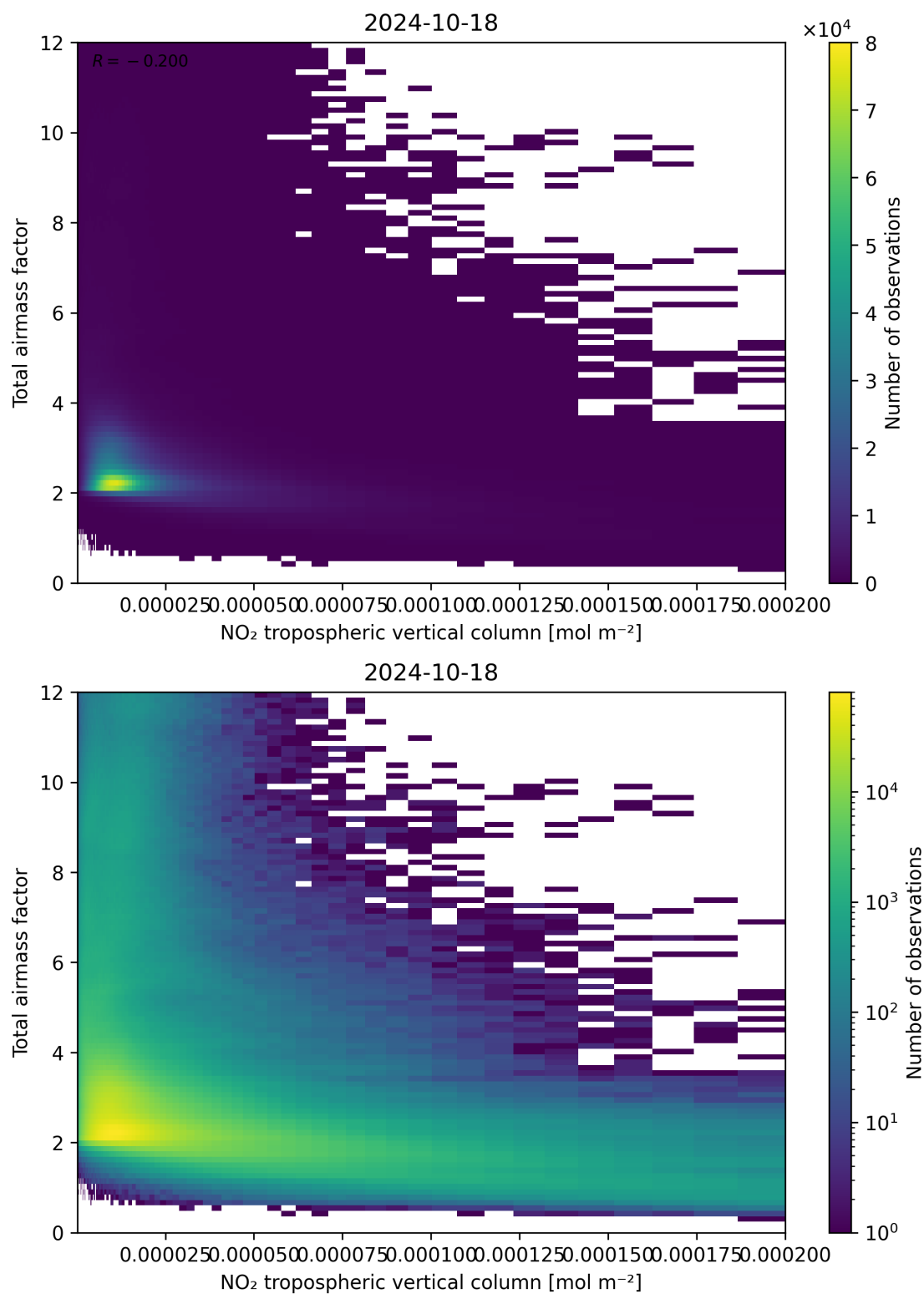
Figure 122: Scatter density plot of “NO 2 tropospheric vertical column” against “Total air mass factor” for 2024-10-17 to 2024-10-19.
