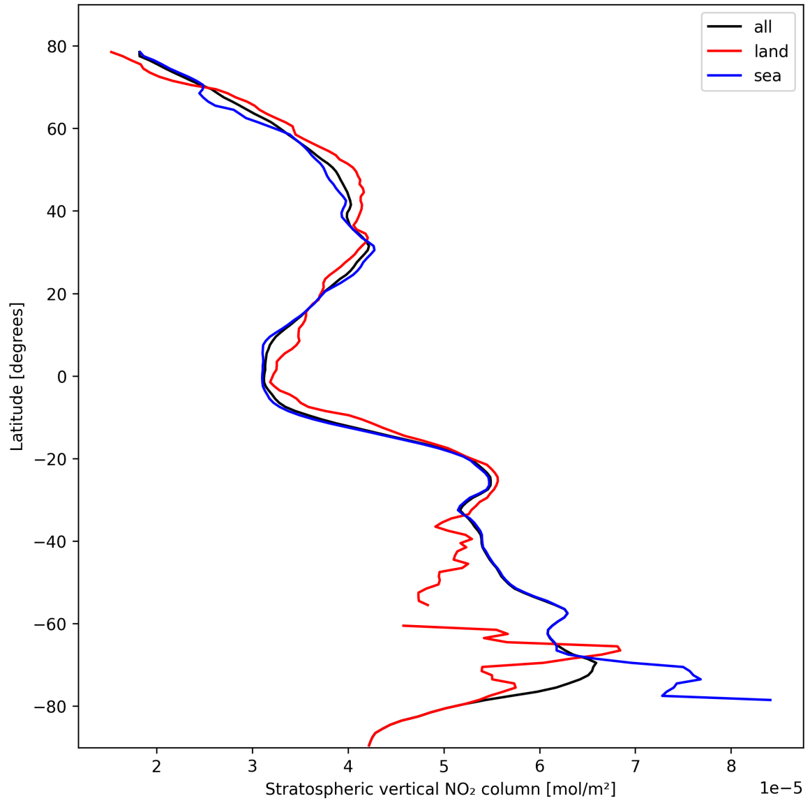
Figure 19: Zonal average of “Stratospheric vertical NO 2 column” for 2024-10-17 to 2024-10-19.
