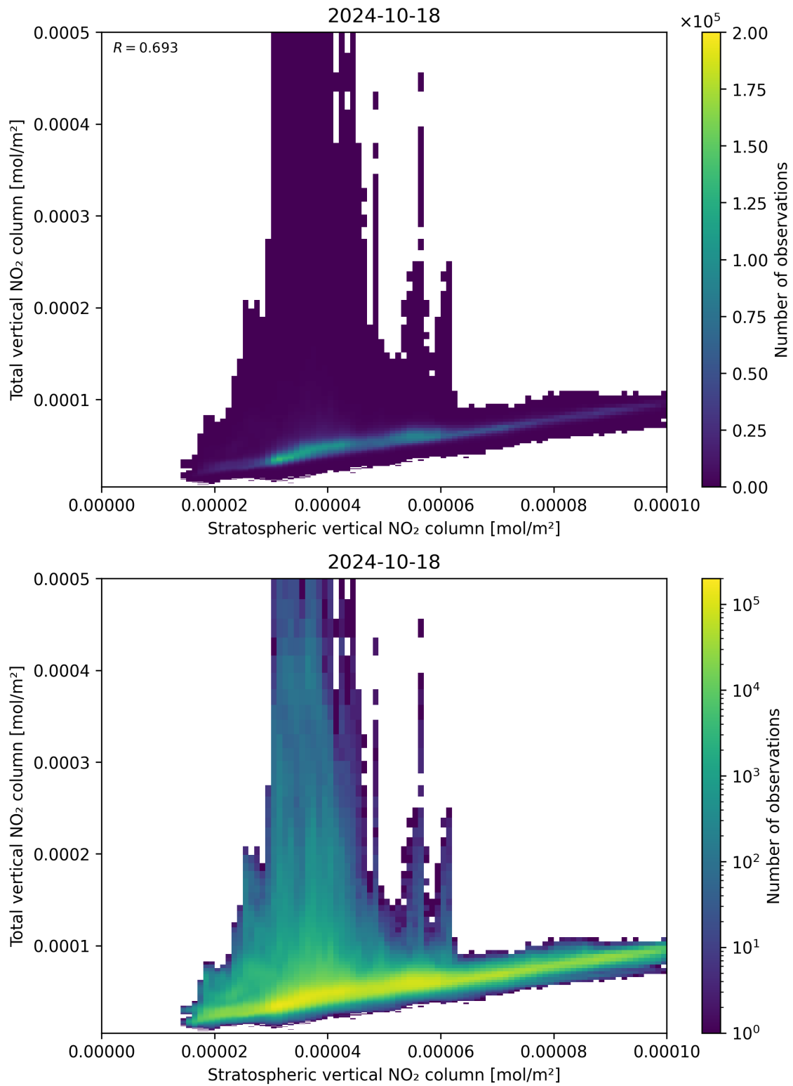
Figure 100: Scatter density plot of “Stratospheric vertical NO 2 column” against “Total vertical NO 2 column” for 2024-10-17 to 2024-10-19.
