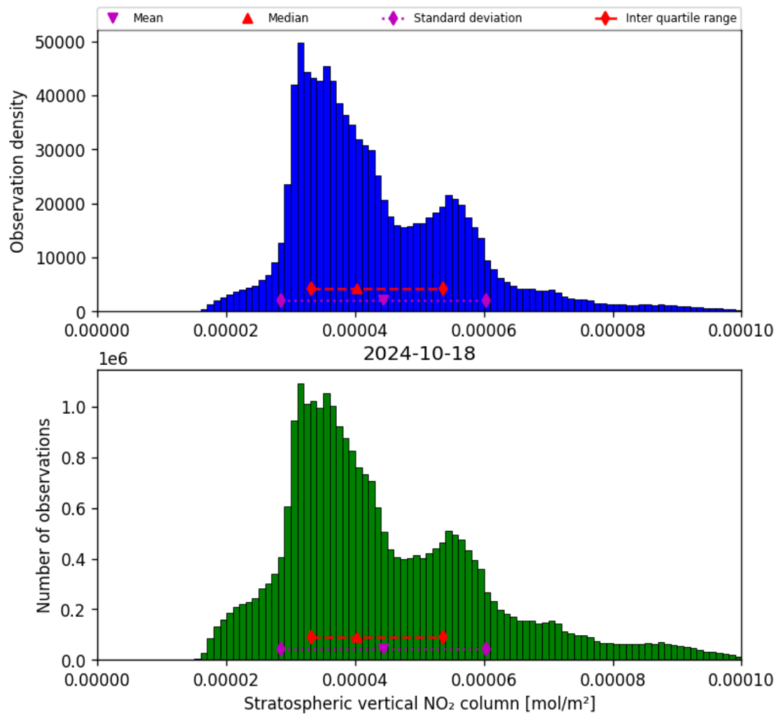
Figure 36: Histogram of “Stratospheric vertical NO 2 column” for 2024-10-17 to 2024-10-19
