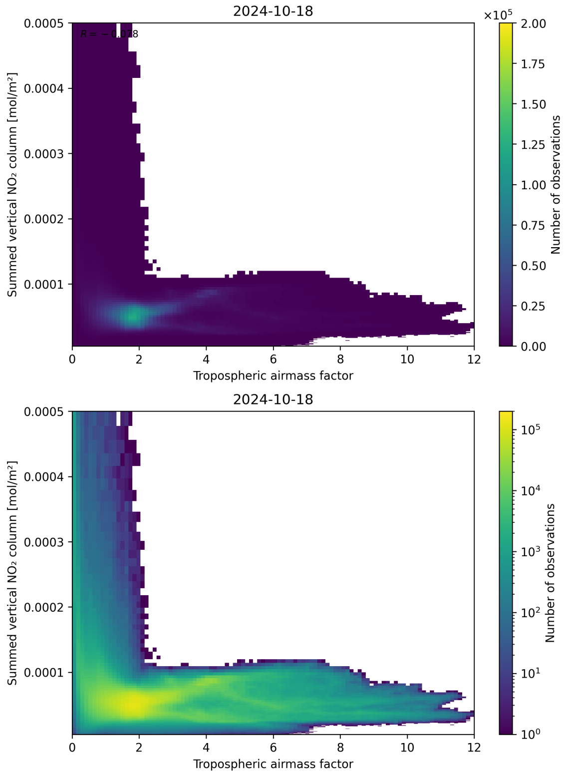
Figure 75: Scatter density plot of “Tropospheric airmass factor” against “Summed vertical NO 2 column” for 2024-10-17 to 2024-10-19.
