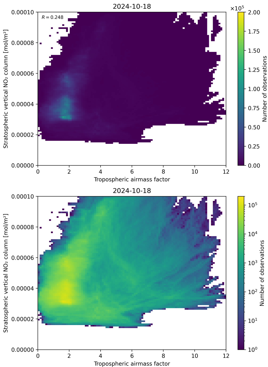
Figure 74: Scatter density plot of “Tropospheric airmass factor” against “Stratospheric vertical NO 2 column” for 2024-10-17 to 2024-10-19.
