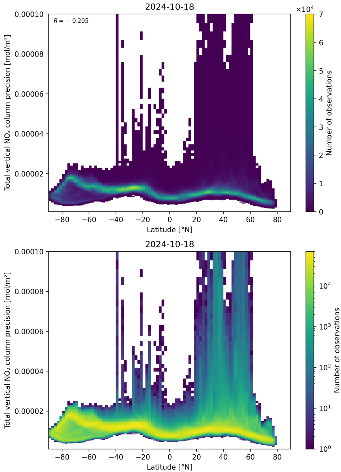
Figure 91: Scatter density plot of “Latitude” against “Total vertical NO 2 column precision” for 2024-10-17 to 2024-10-19.
