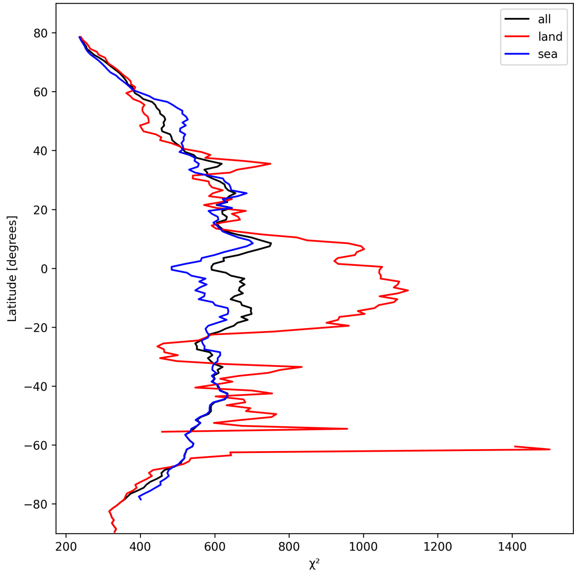
Figure 25: Zonal average of “ \chi^2 ” for 2024-10-17 to 2024-10-19.
