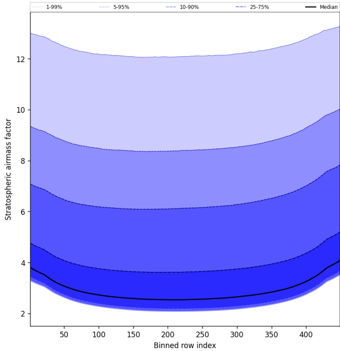
Figure 61: Along track statistics of “Stratospheric air mass factor” for 2024-10-17 to 2024-10-19
