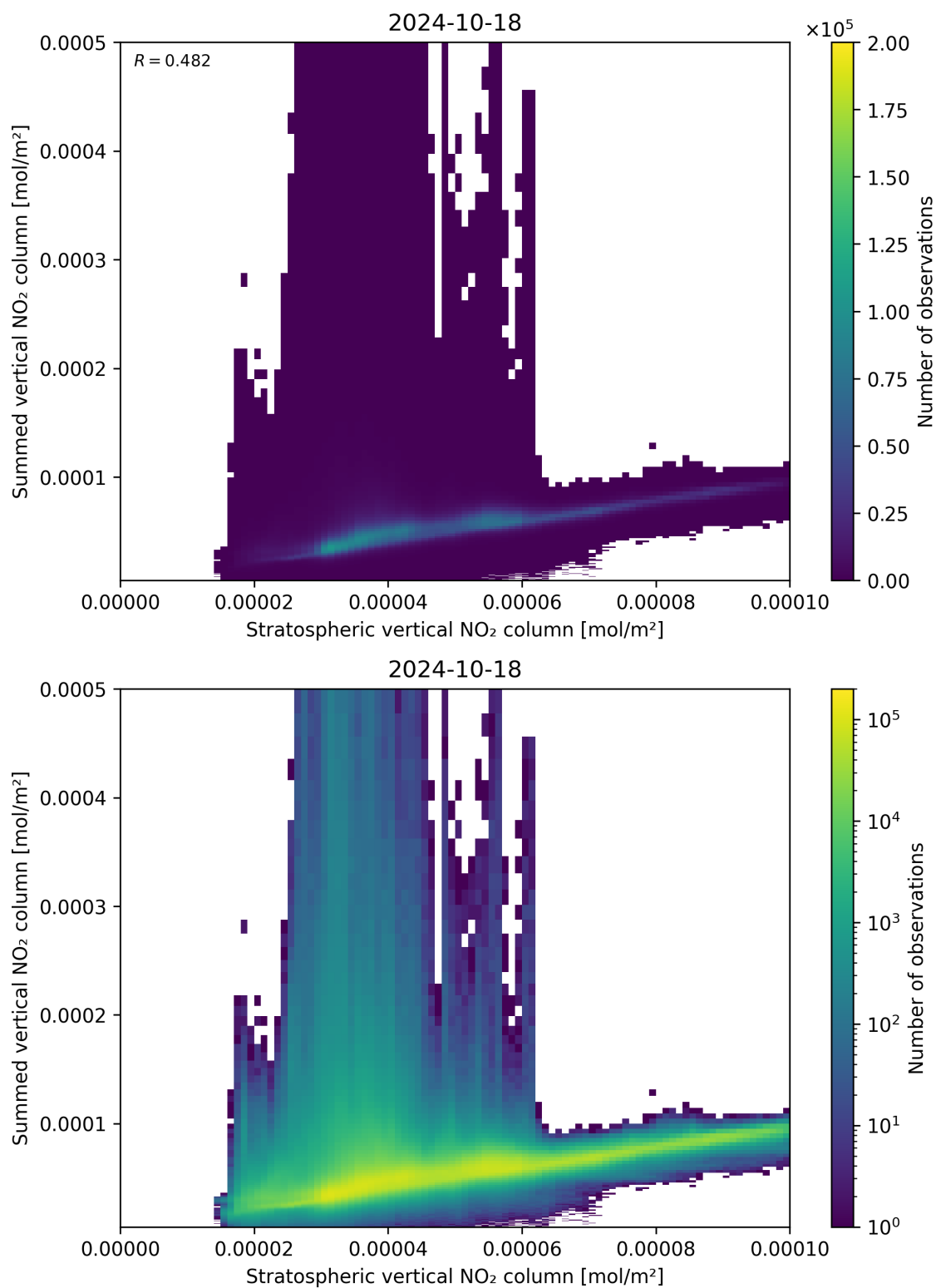
Figure 98: Scatter density plot of “Stratospheric vertical NO 2 column” against “Summed vertical NO 2 column” for 2024-10-17 to 2024-10-19.
