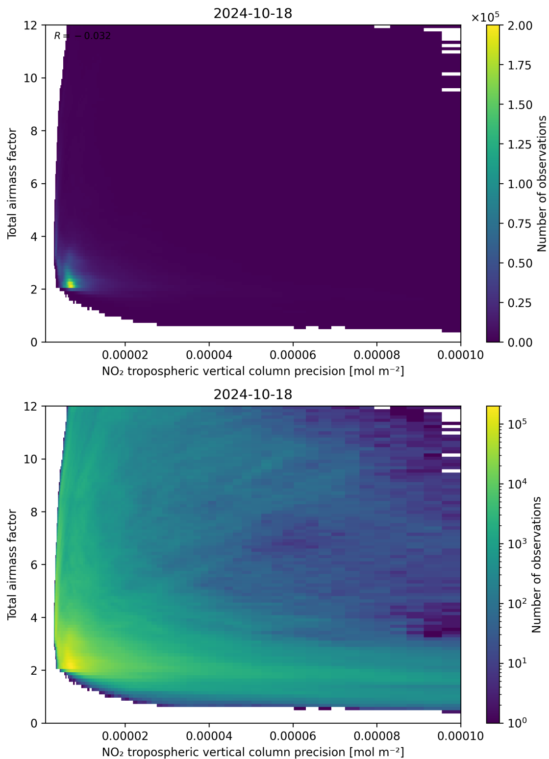
Figure 132: Scatter density plot of “NO 2 tropospheric vertical column precision” against “Total airmass factor” for 2024-10-17 to 2024-10-19.
