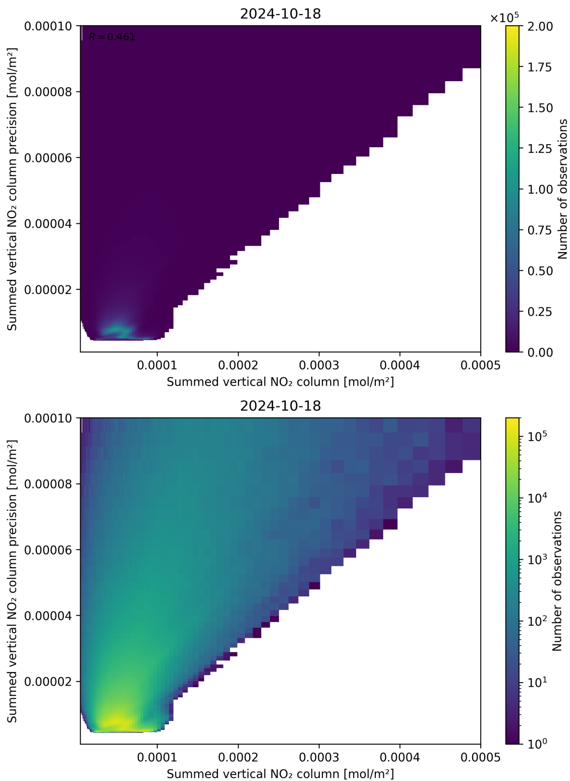
Figure 105: Scatter density plot of “Summed vertical NO 2 column” against “Summed vertical NO 2 column precision” for 2024-10-17 to 2024-10-19.
