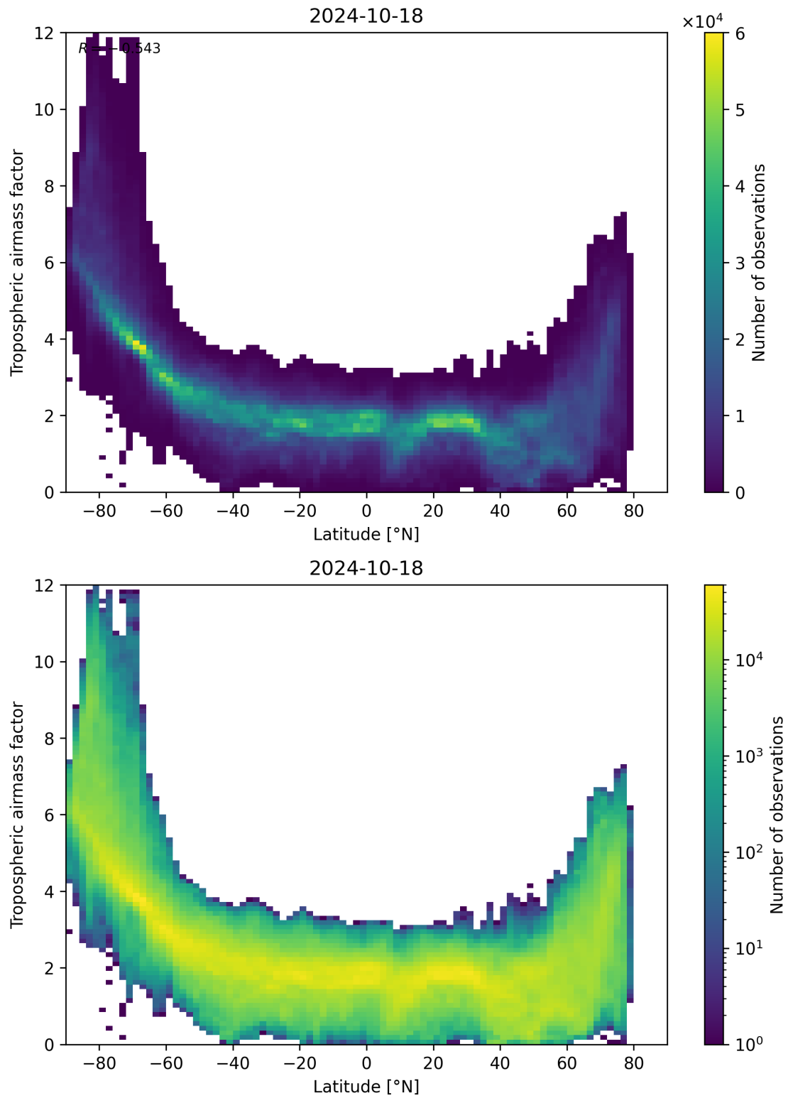
Figure 85: Scatter density plot of “Latitude” against “Tropospheric air mass factor” for 2024-10-17 to 2024-10-19.
