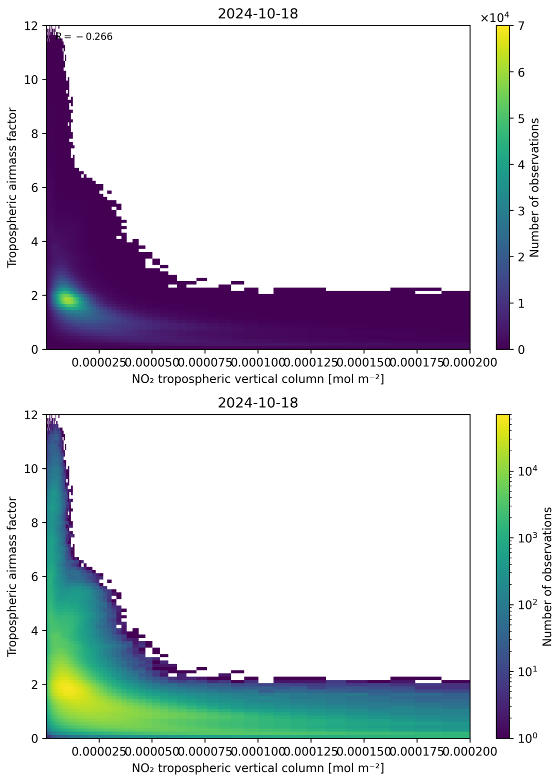
Figure 123: Scatter density plot of “NO 2 tropospheric vertical column” against “Tropospheric air mass factor” for 2024-10-17 to 2024-10-19.
