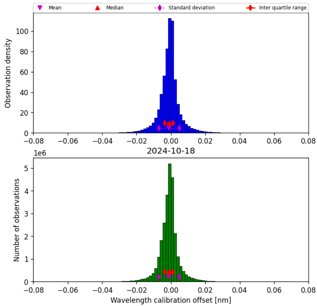
Figure 35: Histogram of “Wavelength calibration offset” for 2024-10-17 to 2024-10-19
