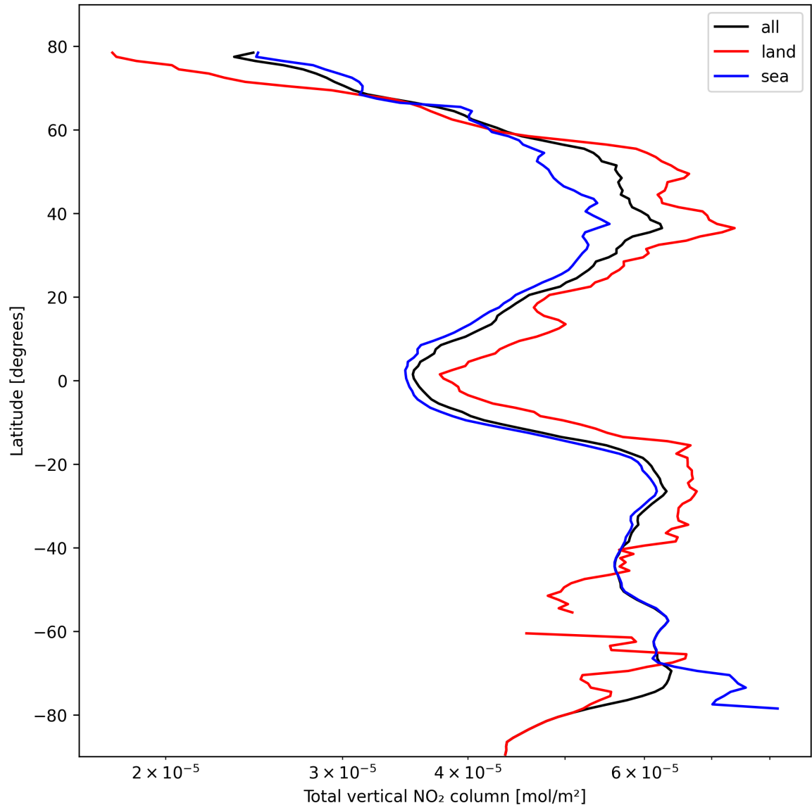
Figure 21: Zonal average of “Total vertical NO 2 column” for 2024-10-17 to 2024-10-19.
