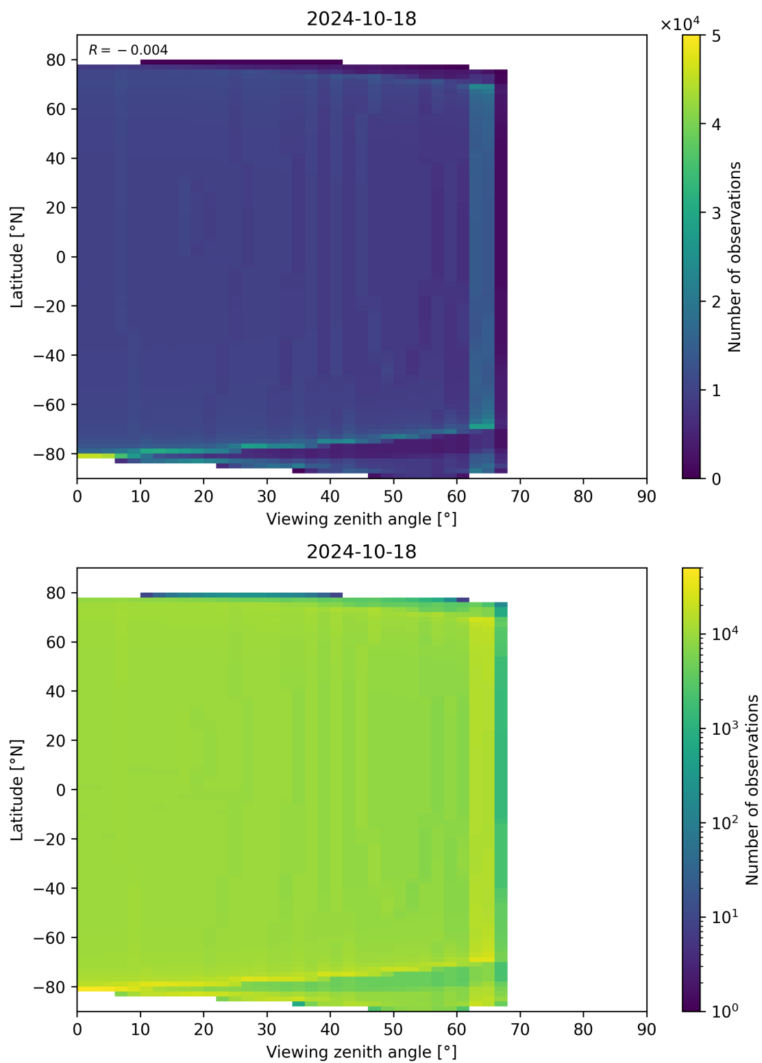
Figure 163: Scatter density plot of “Viewing zenith angle” against “Latitude” for 2024-10-17 to 2024-10-19.
