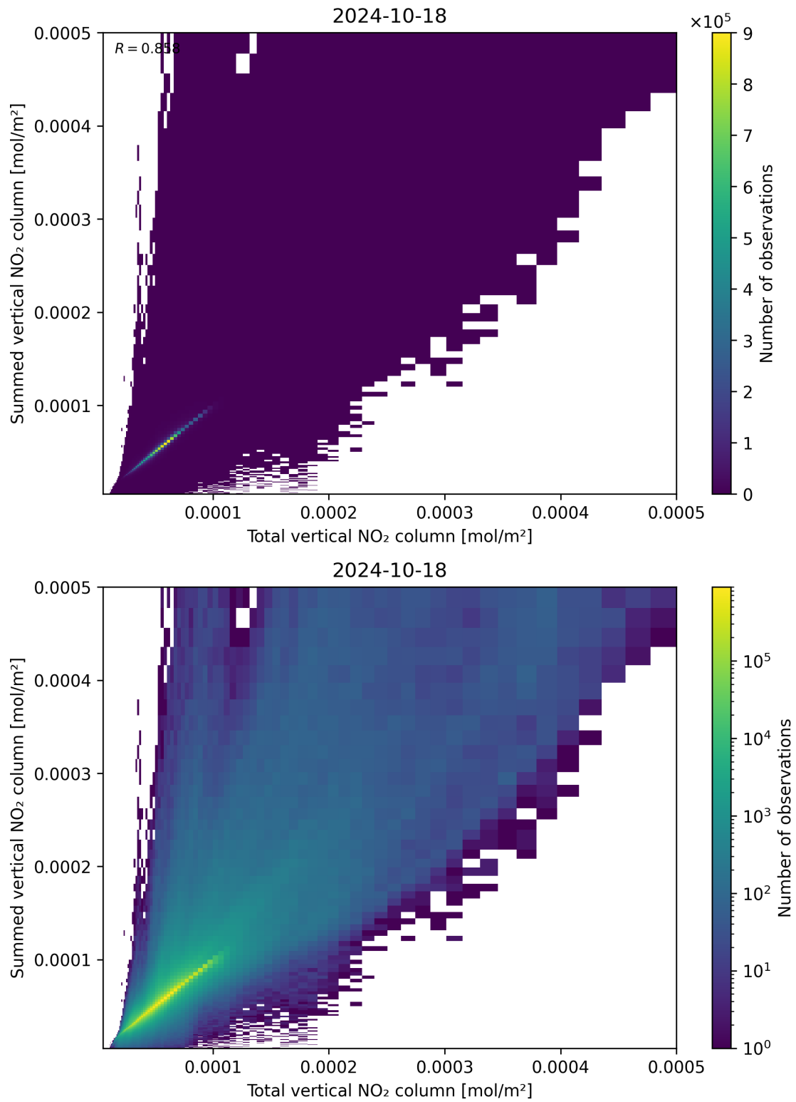
Figure 112: Scatter density plot of “Total vertical NO 2 column” against “Summed vertical NO 2 column” for 2024-10-17 to 2024-10-19.
