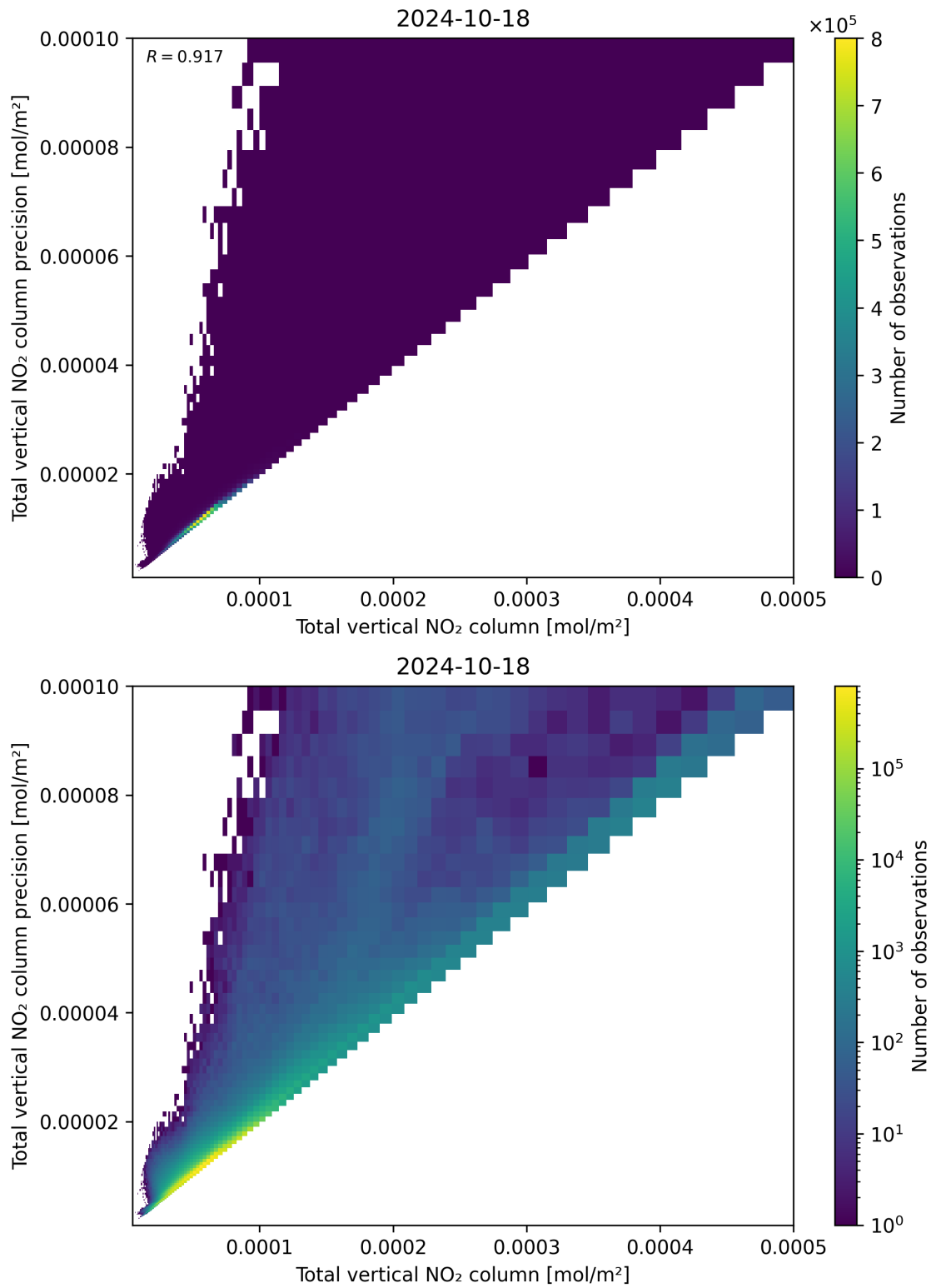
Figure 114: Scatter density plot of “Total vertical NO 2 column” against “Total vertical NO 2 column precision” for 2024-10-17 to 2024-10-19.
