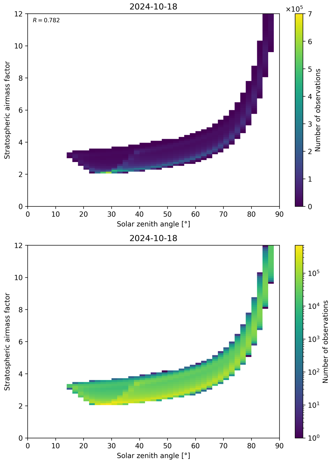
Figure 145: Scatter density plot of “Solar zenith angle” against “Stratospheric airmass factor” for 2024-10-17 to 2024-10-19.
