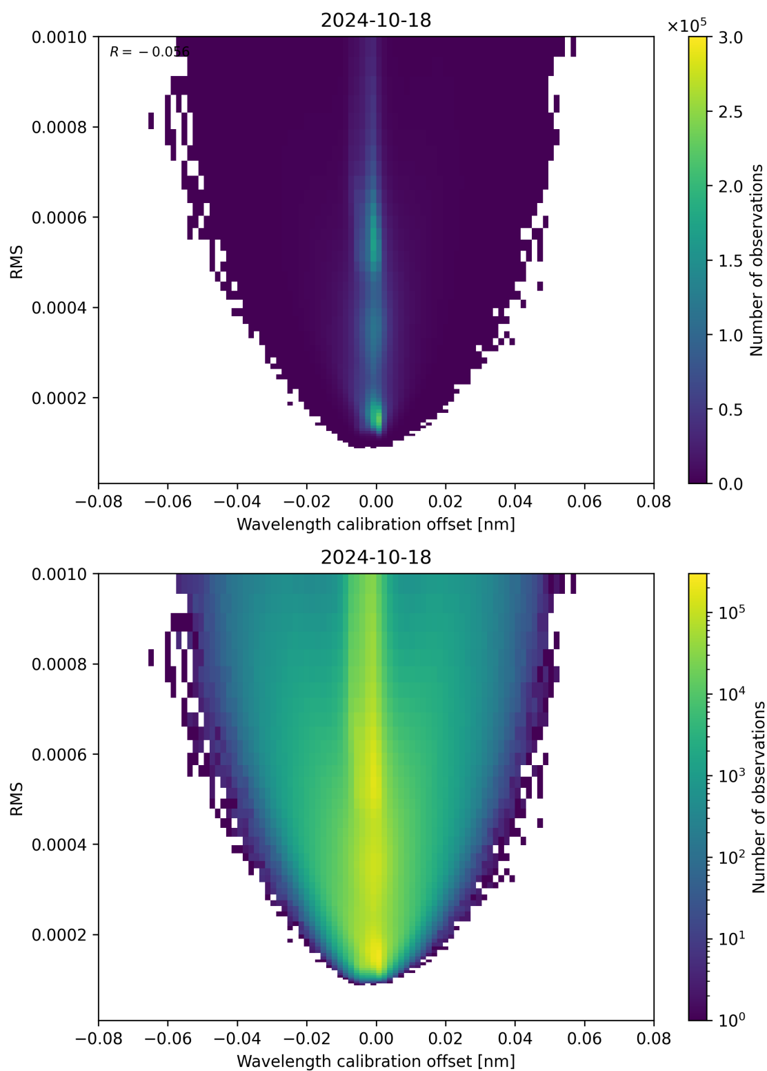
Figure 181: Scatter density plot of “Wavelength calibration offset” against “RMS” for 2024-10-17 to 2024-10-19.
