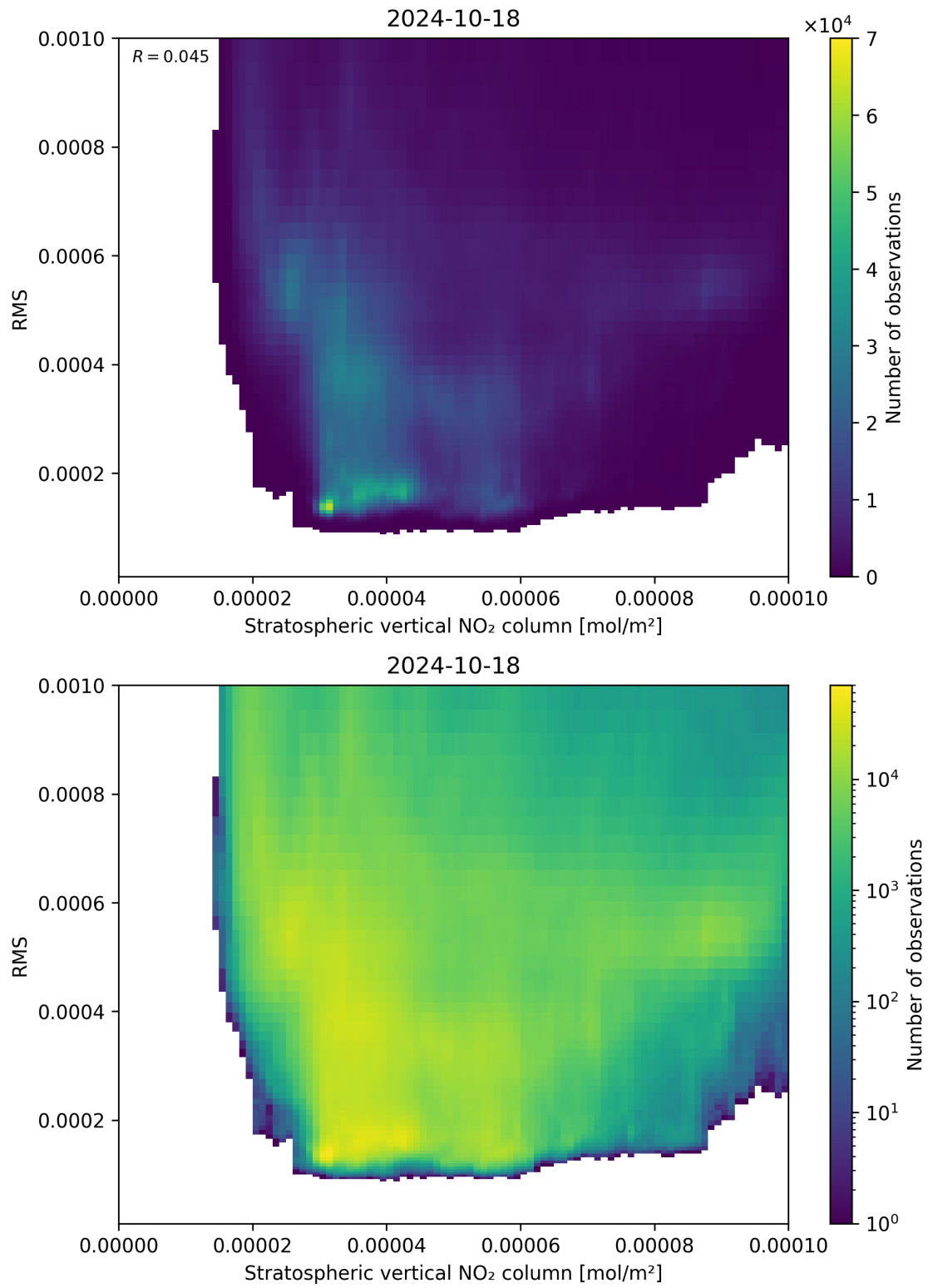
Figure 102: Scatter density plot of “Stratospheric vertical NO 2 column” against “RMS” for 2024-10-17 to 2024-10-19.
