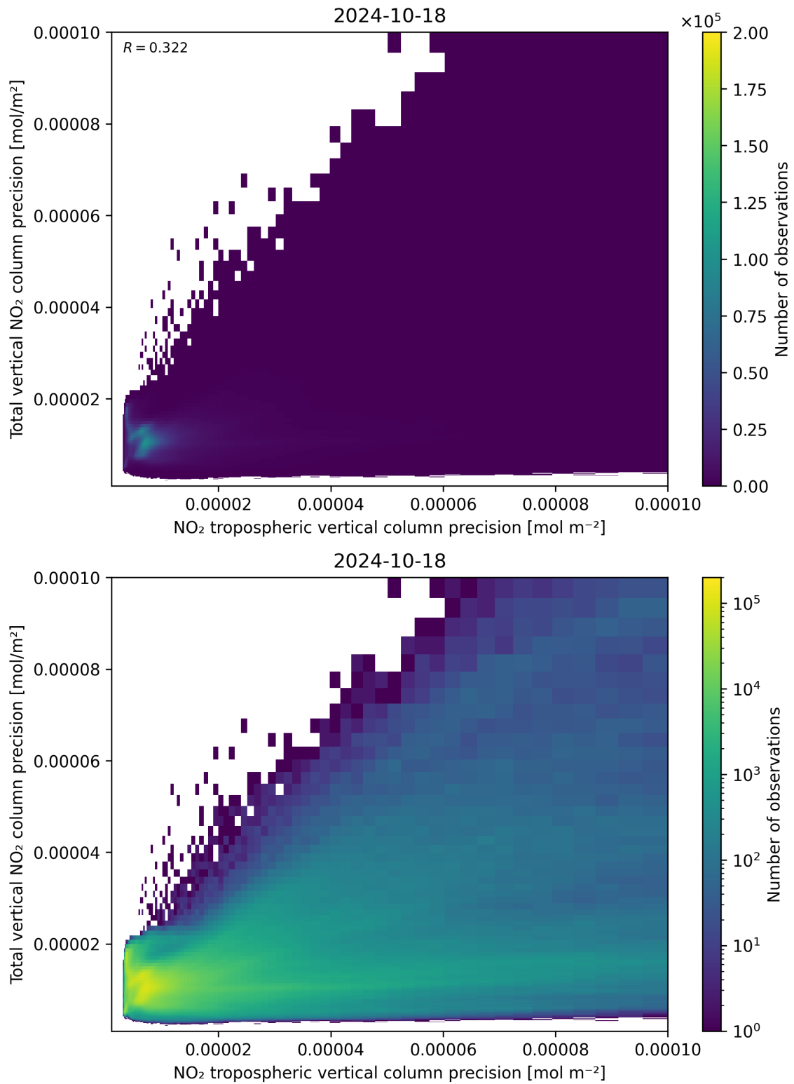
Figure 139: Scatter density plot of “NO 2 tropospheric vertical column precision” against “Total vertical NO 2 column precision” for 2024-10-17 to 2024-10-19.
