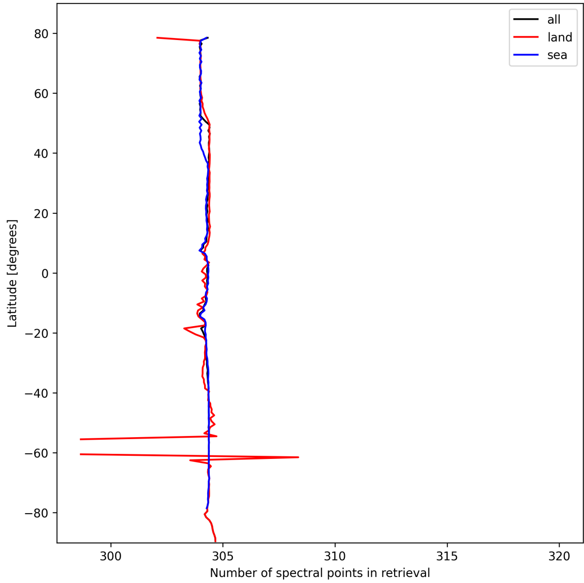
Figure 16: Zonal average of “Number of spectral points in retrieval” for 2024-10-17 to 2024-10-19.
