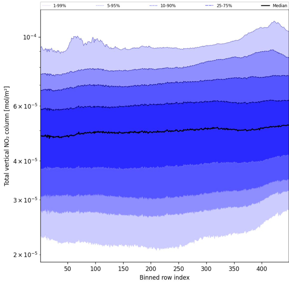
Figure 55: Along track statistics of “Total vertical NO 2 column” for 2024-10-17 to 2024-10-19
