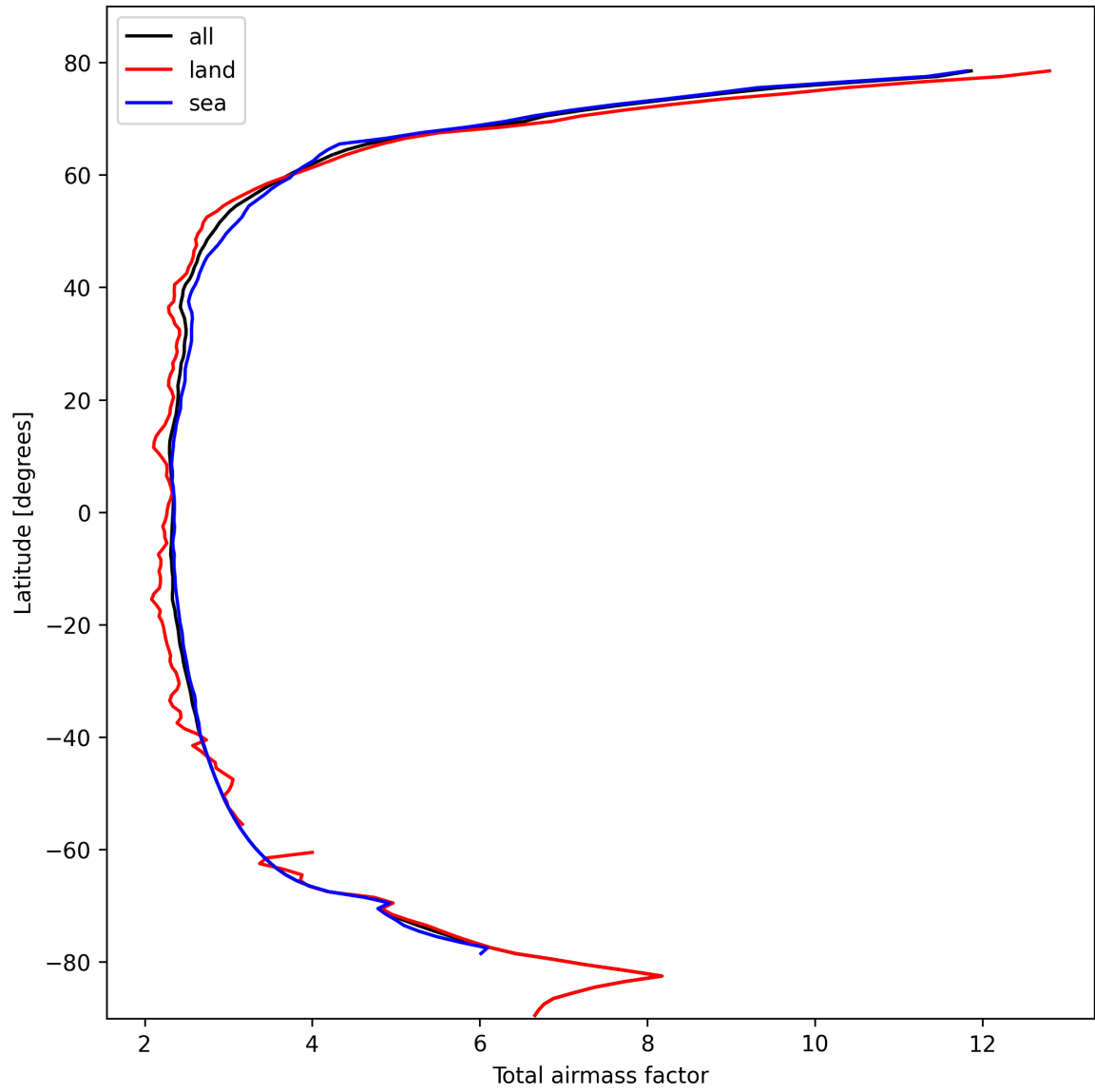
Figure 15: Zonal average of “Total airmass factor” for 2024-10-17 to 2024-10-19.
