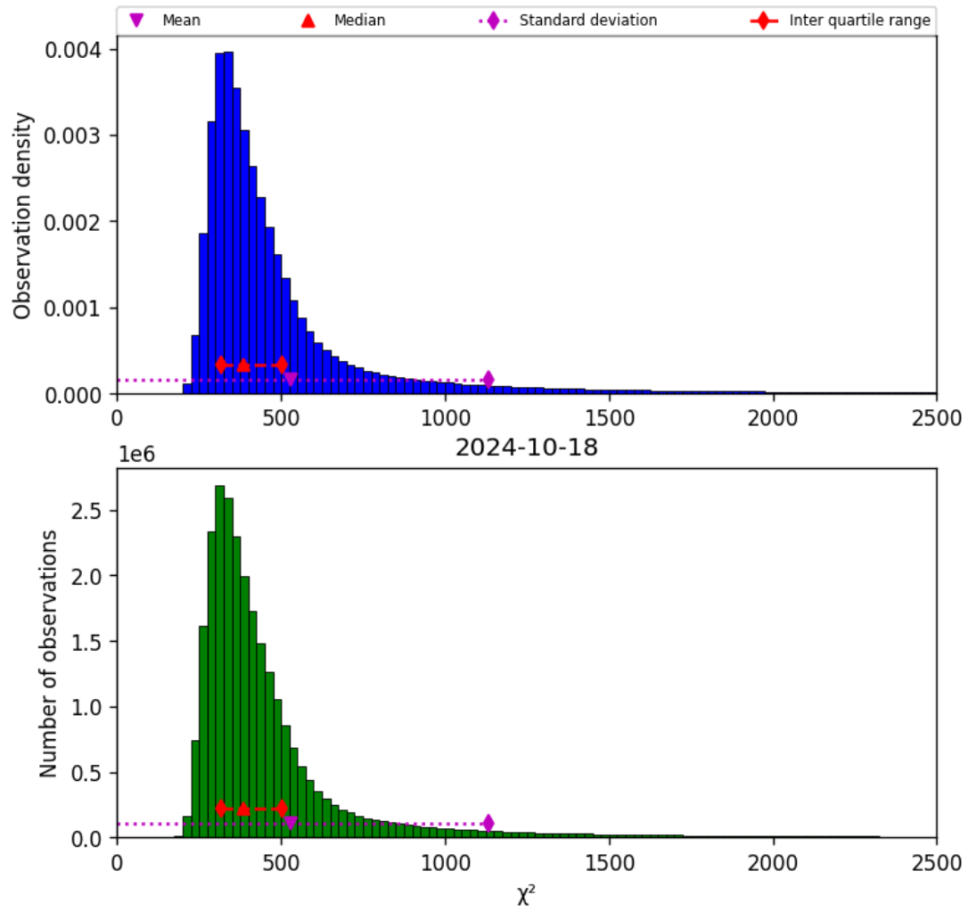
Figure 42: Histogram of “ \chi^2 ” for 2024-10-17 to 2024-10-19
