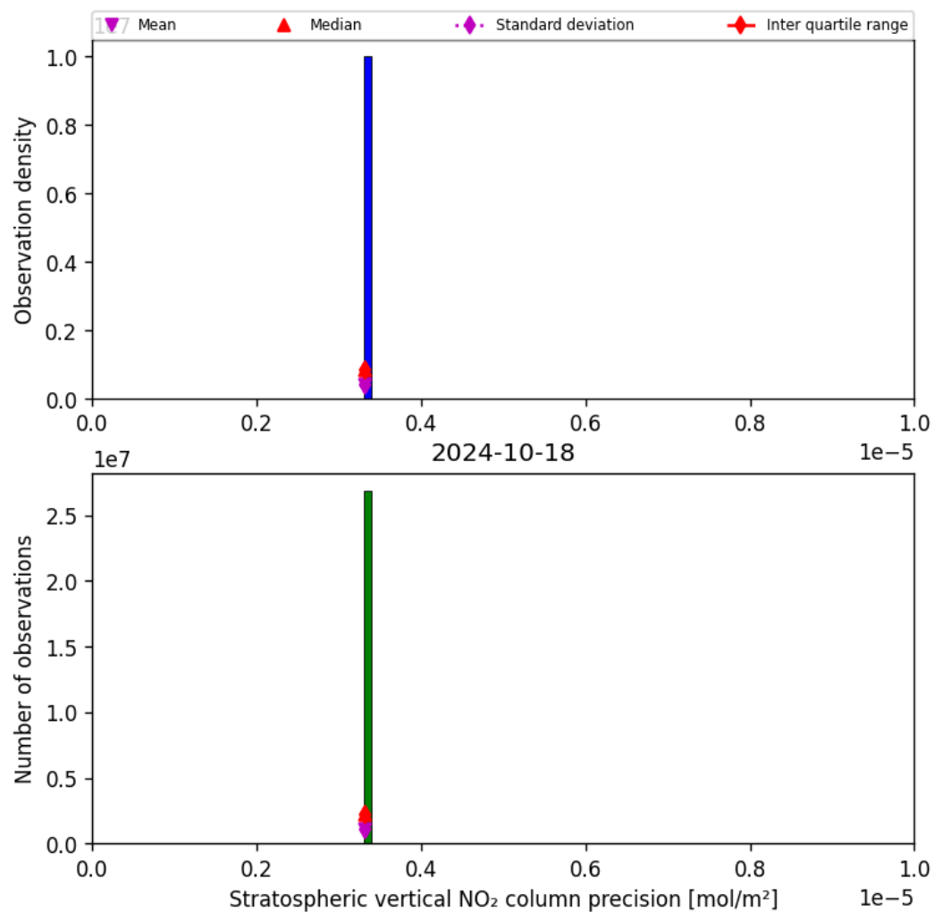
Figure 37: Histogram of “Stratospheric vertical NO 2 column precision” for 2024-10-17 to 2024-10-19
