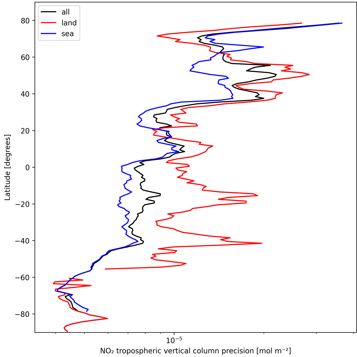
Figure 13: Zonal average of “NO 2 tropospheric vertical column precision” for 2024-10-17 to 2024-10-19.
