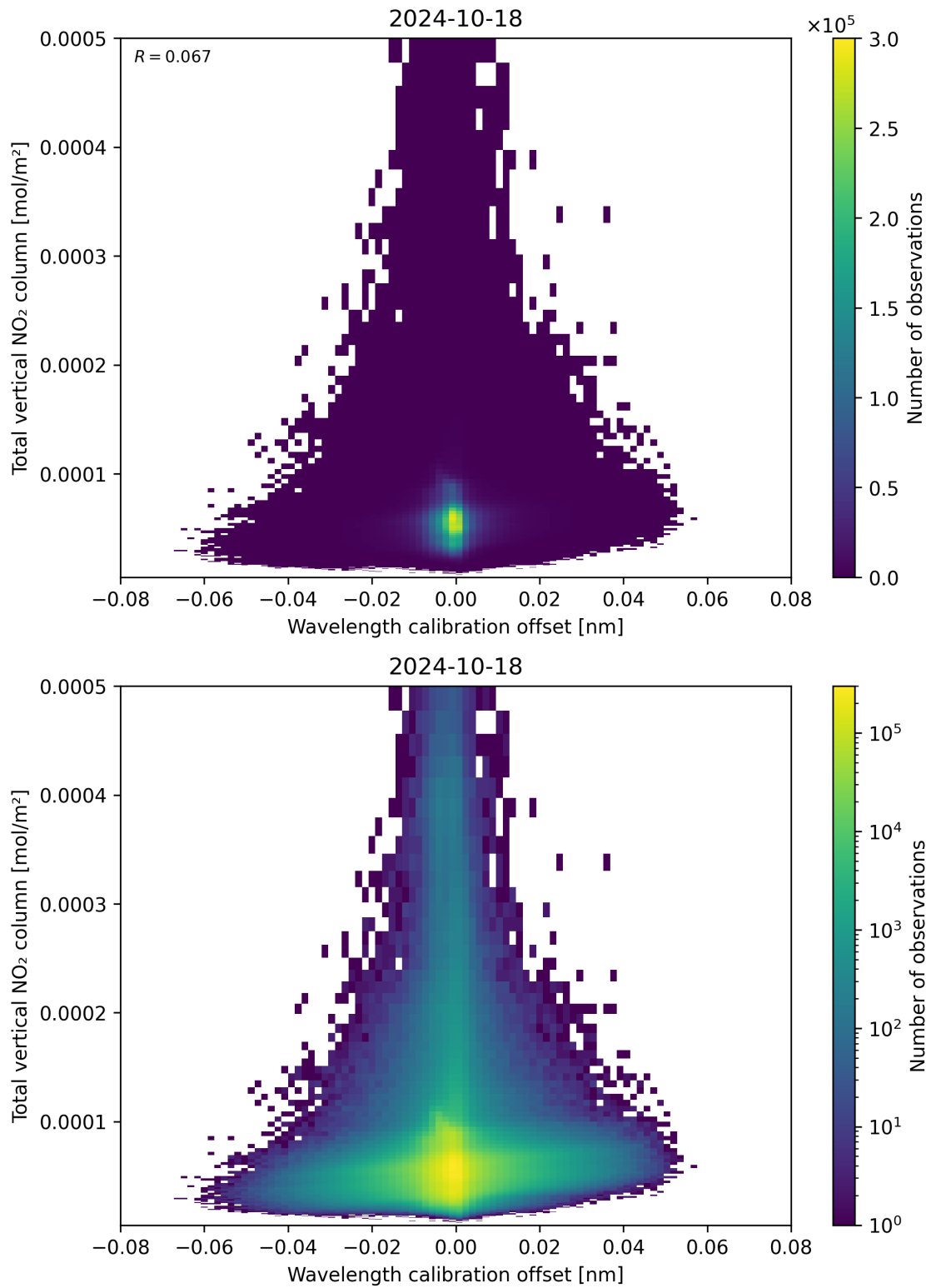
Figure 179: Scatter density plot of “Wavelength calibration offset” against “Total vertical NO 2 column” for 2024-10-17 to 2024-10-19.
