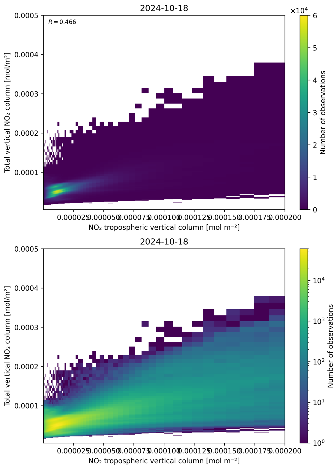
Figure 128: Scatter density plot of “NO 2 tropospheric vertical column” against “Total vertical NO 2 column” for 2024-10-17 to 2024-10-19.
