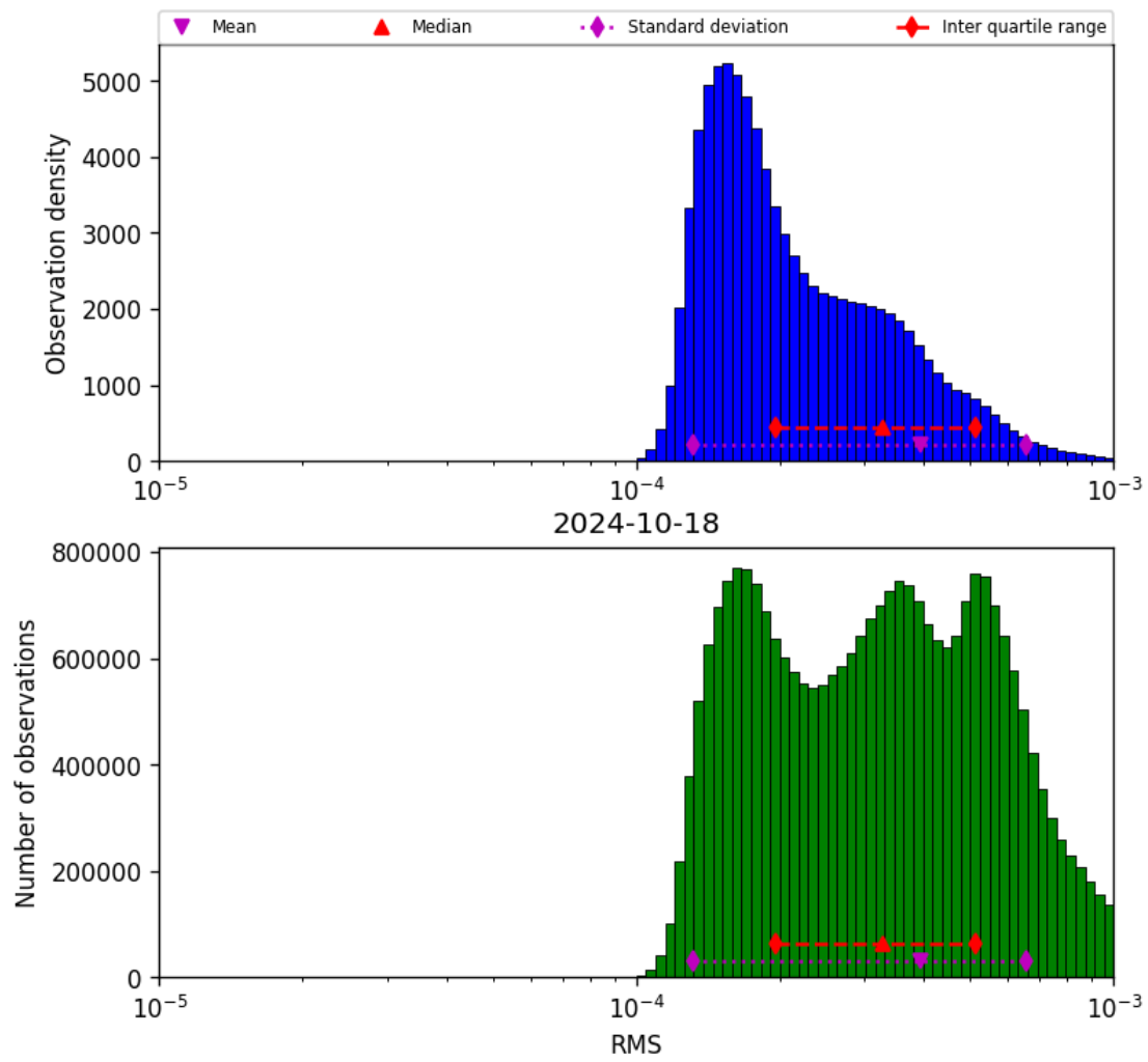
Figure 43: Histogram of “RMS” for 2024-10-17 to 2024-10-19
