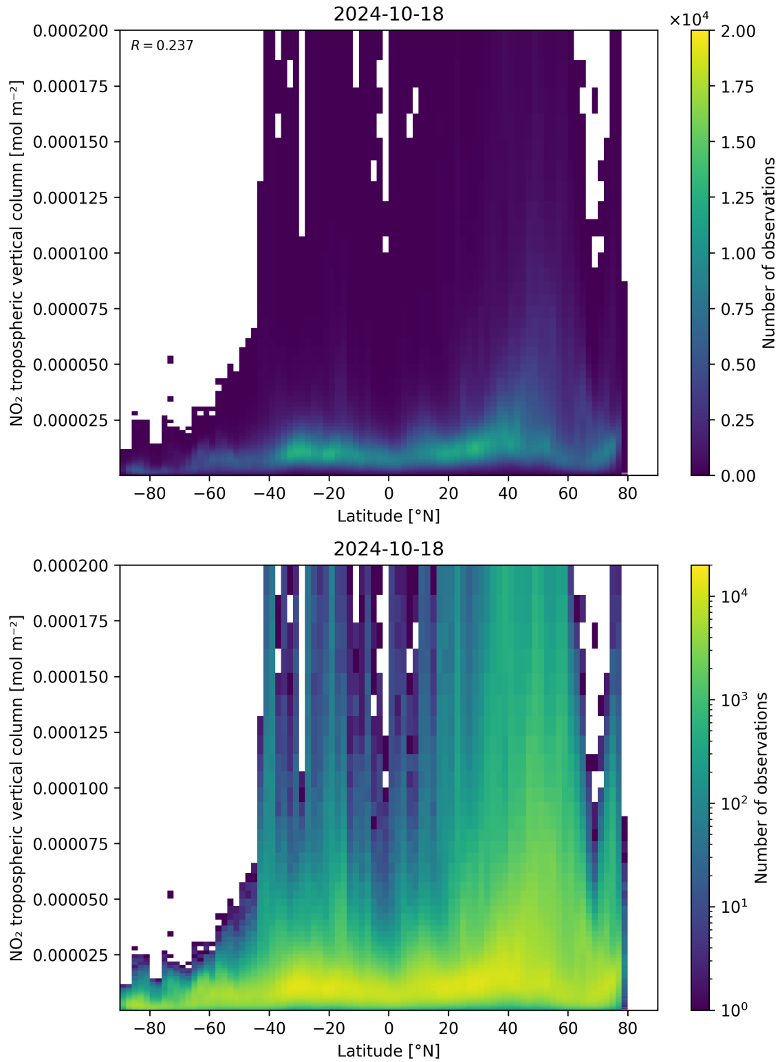
Figure 92: Scatter density plot of “Latitude” against “NO 2 tropospheric vertical column” for 2024-10-17 to 2024-10-19.
