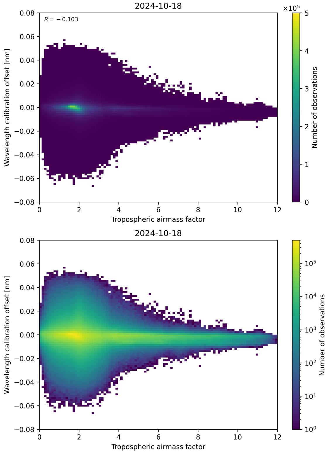
Figure 80: Scatter density plot of “Tropospheric airmass factor” against “Wavelength calibration offset” for 2024-10-17 to 2024-10-19.
