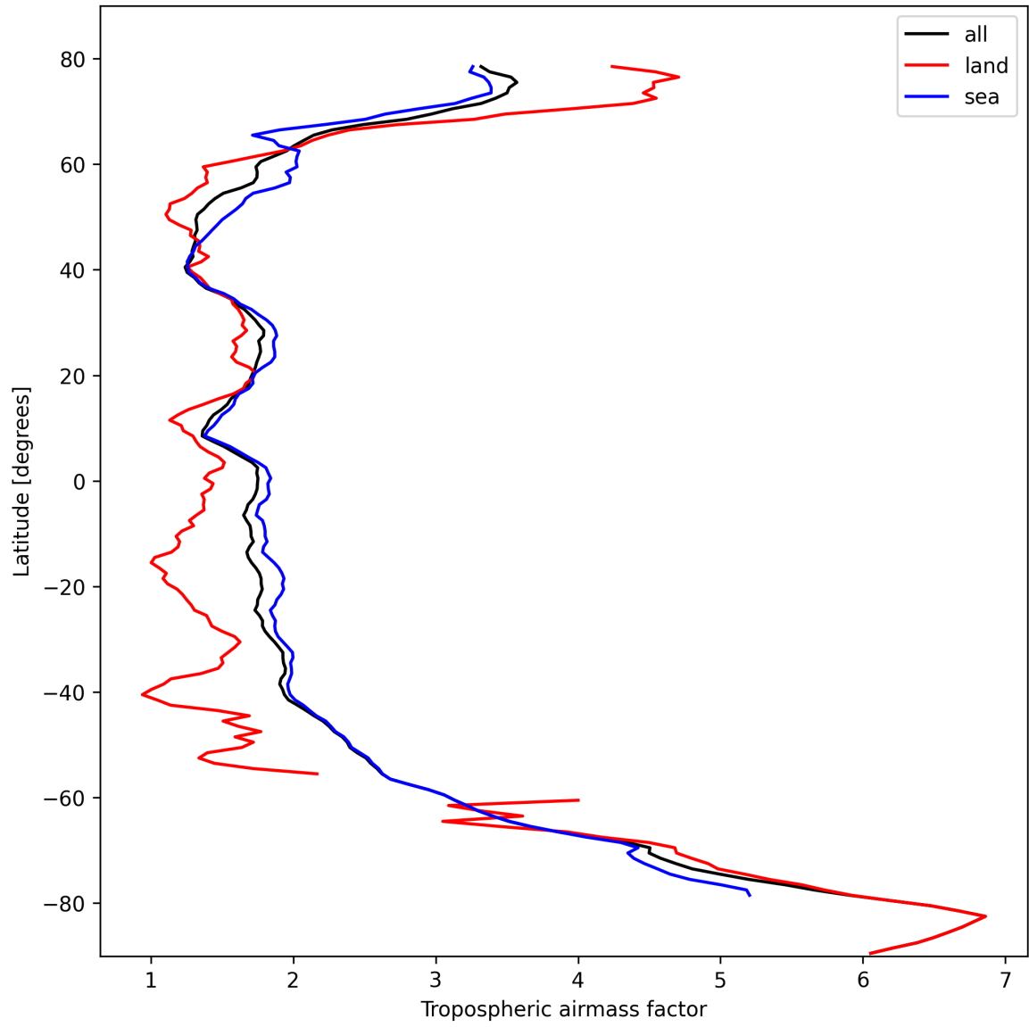
Figure 14: Zonal average of “Tropospheric air mass factor” for 2024-10-17 to 2024-10-19.
