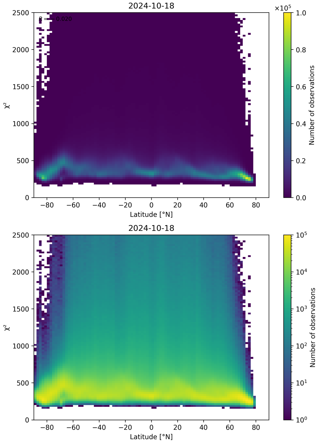
Figure 86: Scatter density plot of “Latitude” against “ \chi^2 ” for 2024-10-17 to 2024-10-19.
