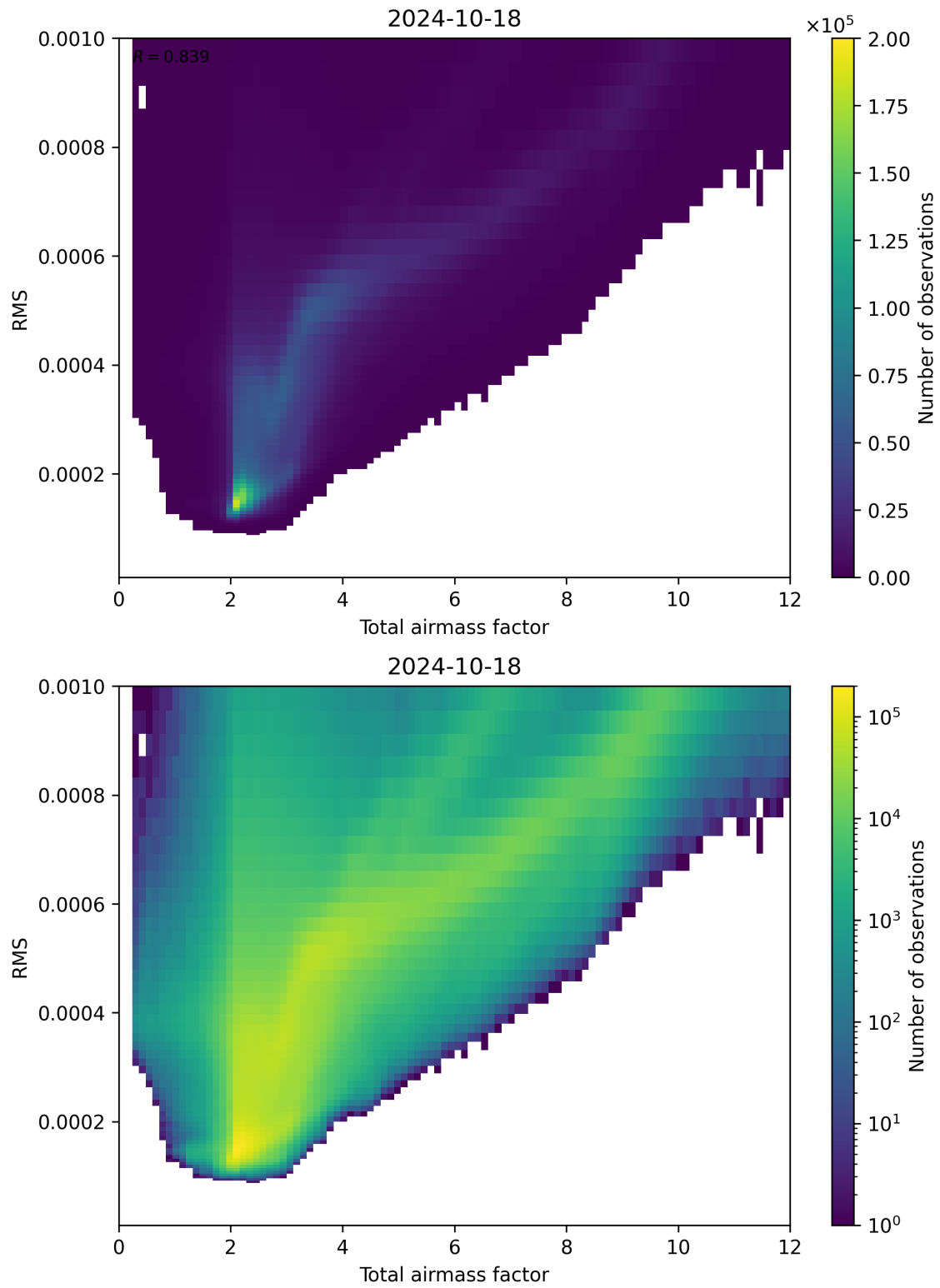
Figure 69: Scatter density plot of “Total airmass factor” against “RMS” for 2024-10-17 to 2024-10-19.
