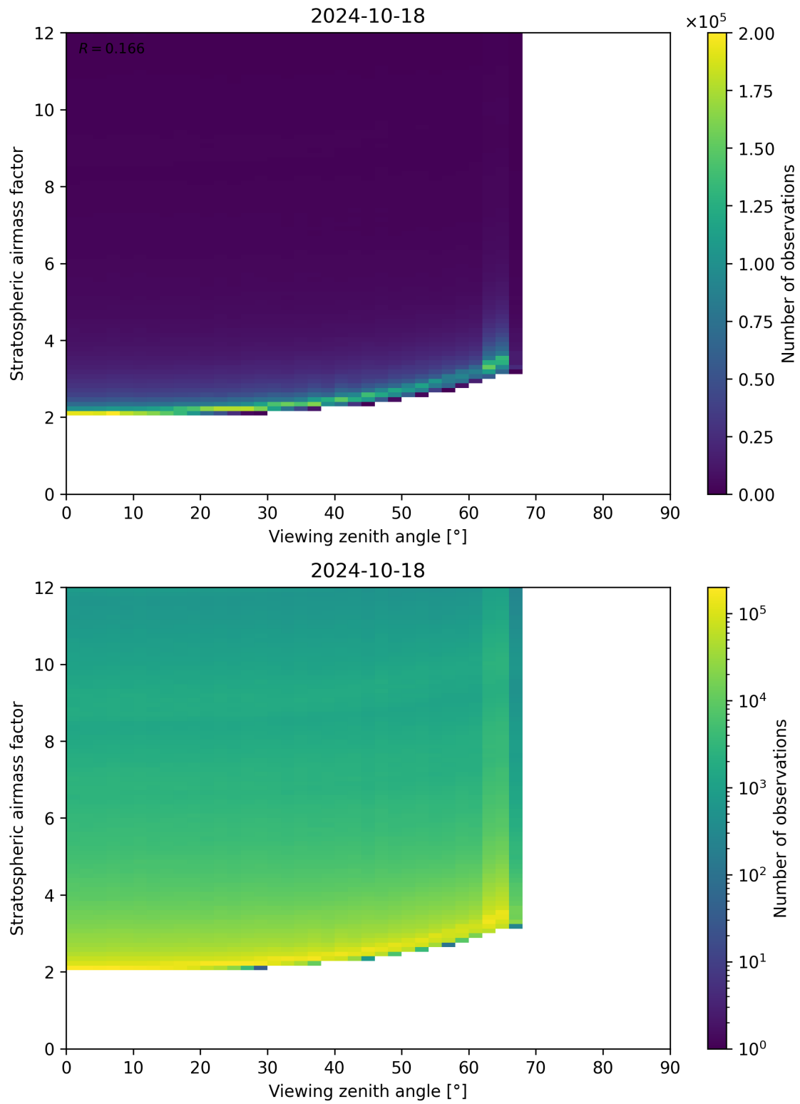
Figure 159: Scatter density plot of “Viewing zenith angle” against “Stratospheric airmass factor” for 2024-10-17 to 2024-10-19.
