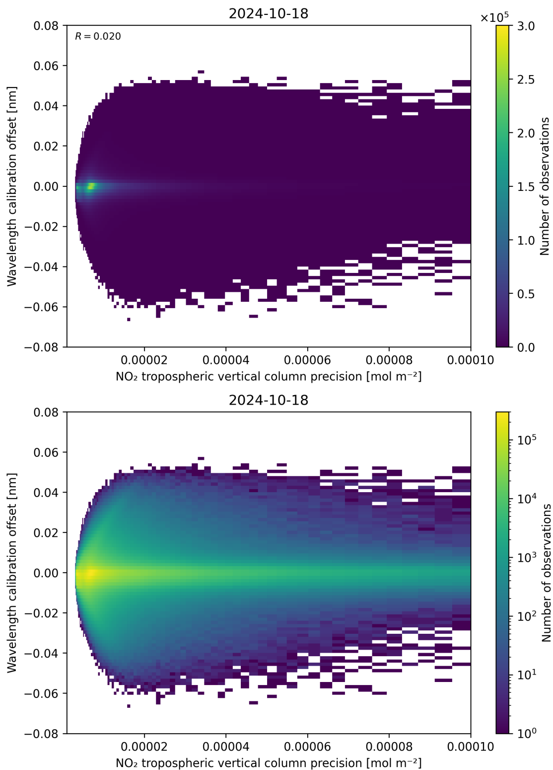
Figure 141: Scatter density plot of “NO 2 tropospheric vertical column precision” against “Wavelength calibration offset” for 2024-10-17 to 2024-10-19.
