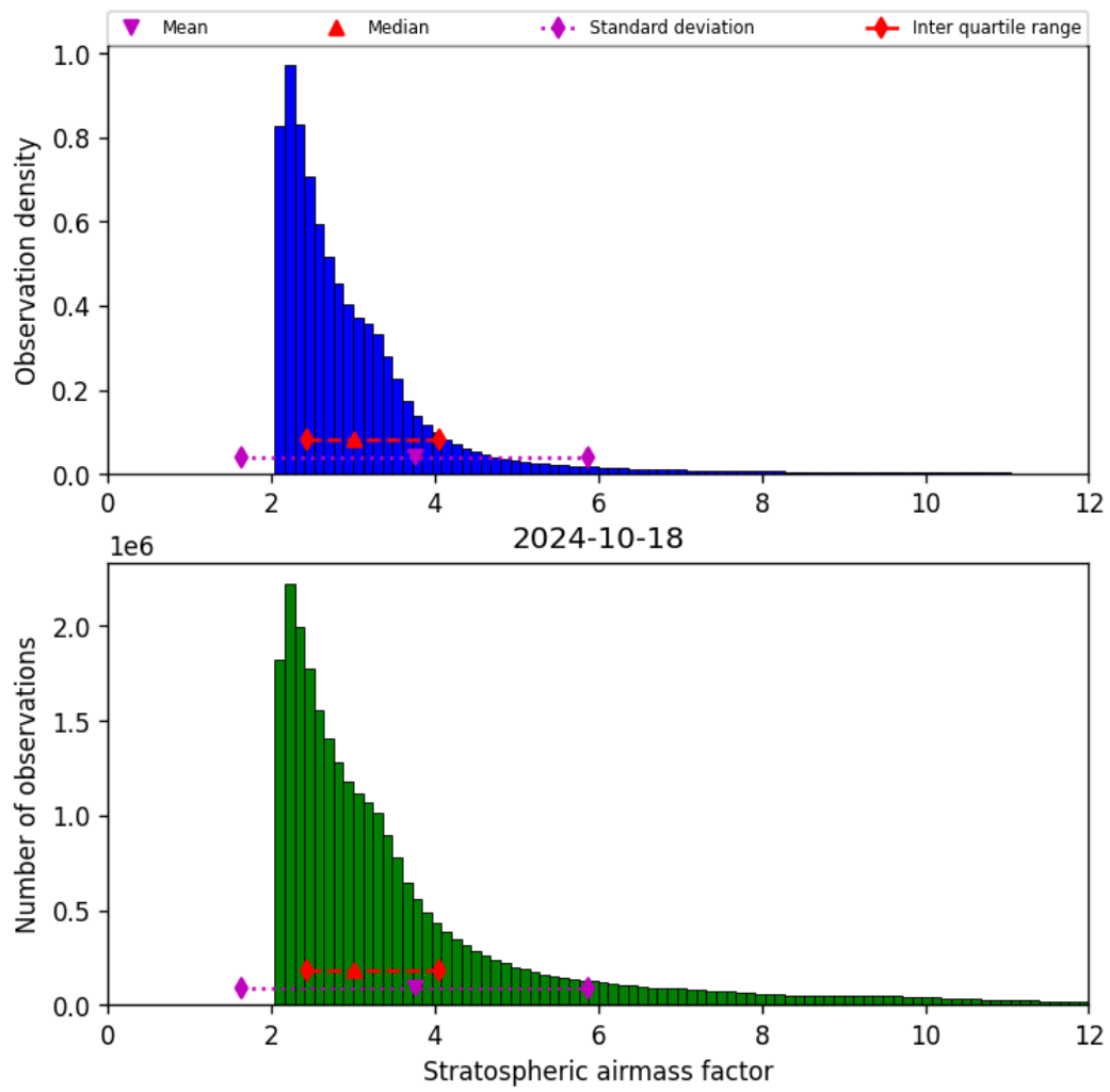
Figure 44: Histogram of “Stratospheric airmass factor” for 2024-10-17 to 2024-10-19
