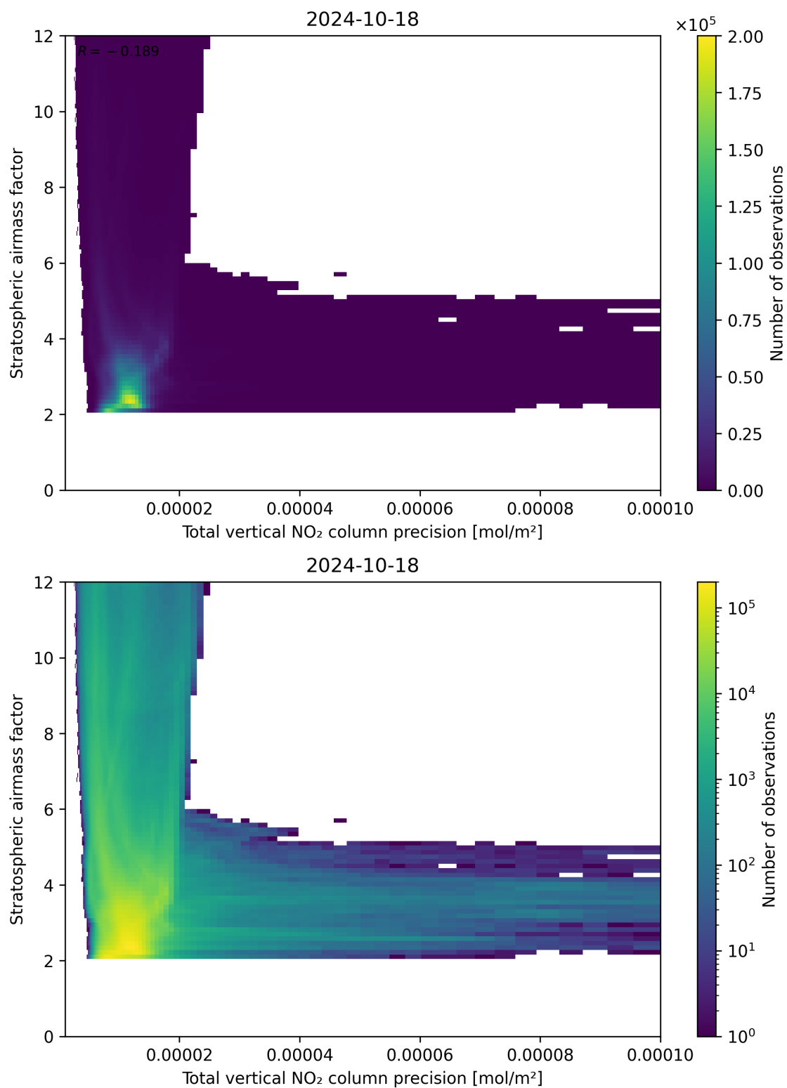
Figure 115: Scatter density plot of “Total vertical NO 2 column precision” against “Stratospheric air mass factor” for 2024-10-17 to 2024-10-19.
