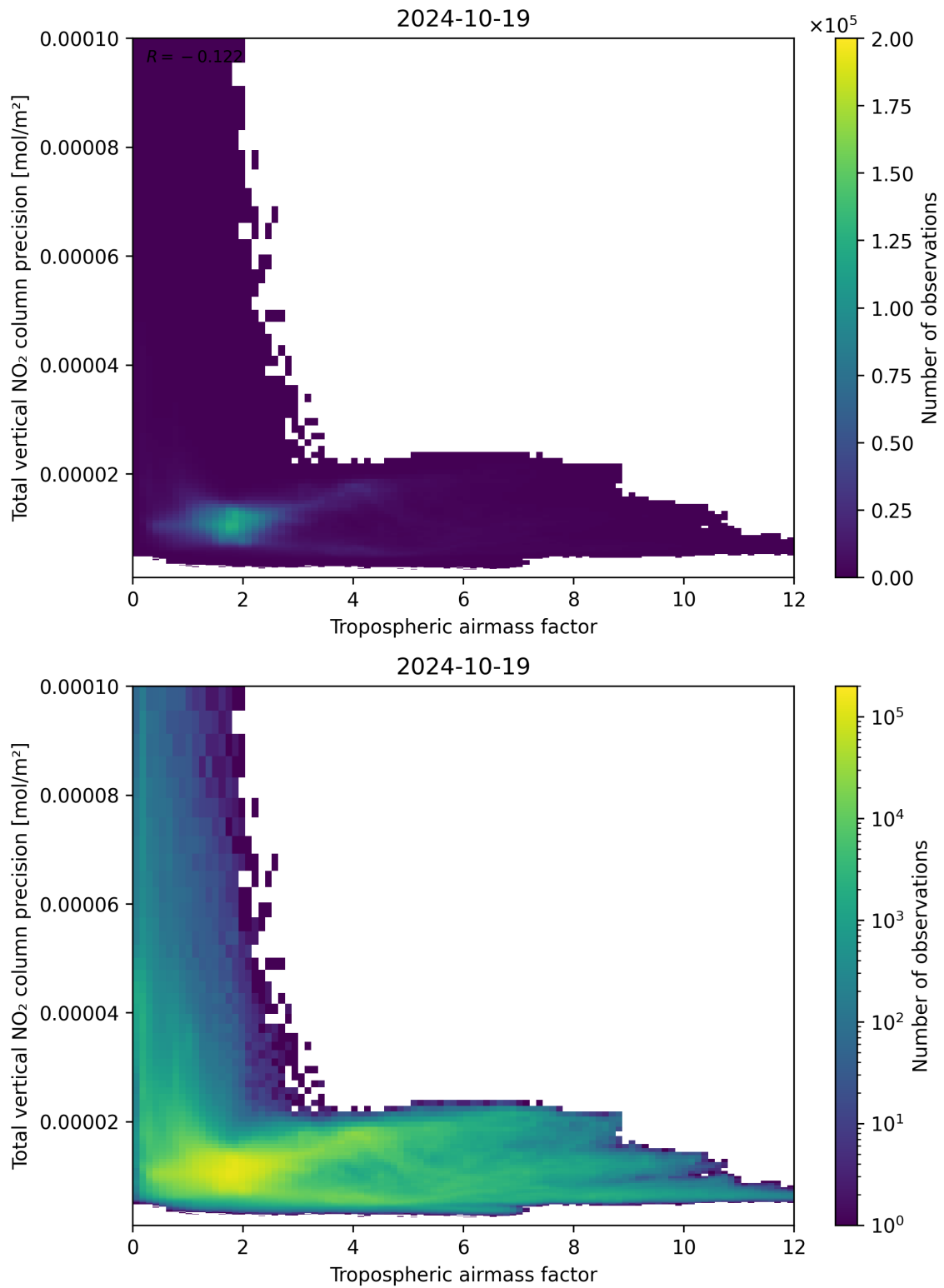
Figure 78: Scatter density plot of “Tropospheric air mass factor” against “Total vertical NO 2 column precision” for 2024-10-19 to 2024-10-20.
