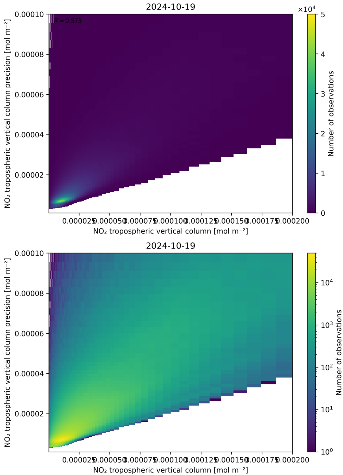
Figure 130: Scatter density plot of “NO 2 tropospheric vertical column” against “NO 2 tropospheric vertical column precision” for 2024-10-19 to 2024-10-20.
