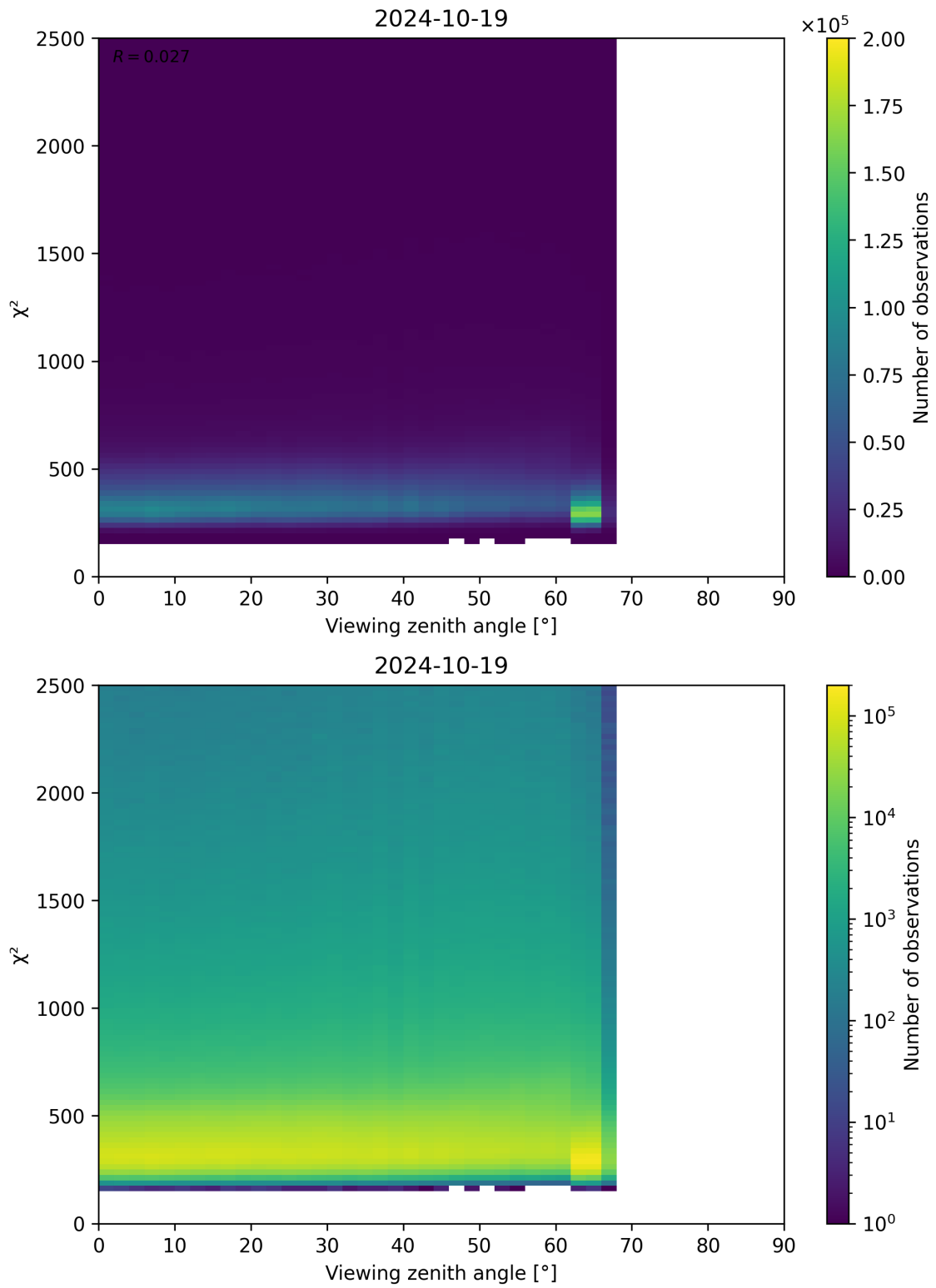
Figure 162: Scatter density plot of “Viewing zenith angle” against “ \chi^2 ” for 2024-10-19 to 2024-10-20.
