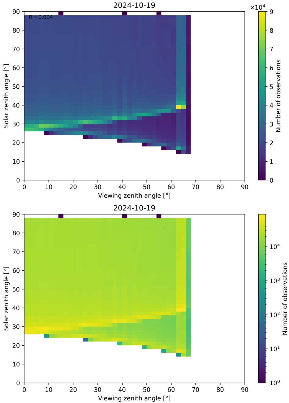
Figure 172: Scatter density plot of “Viewing zenith angle” against “Solar zenith angle” for 2024-10-19 to 2024-10-20.
