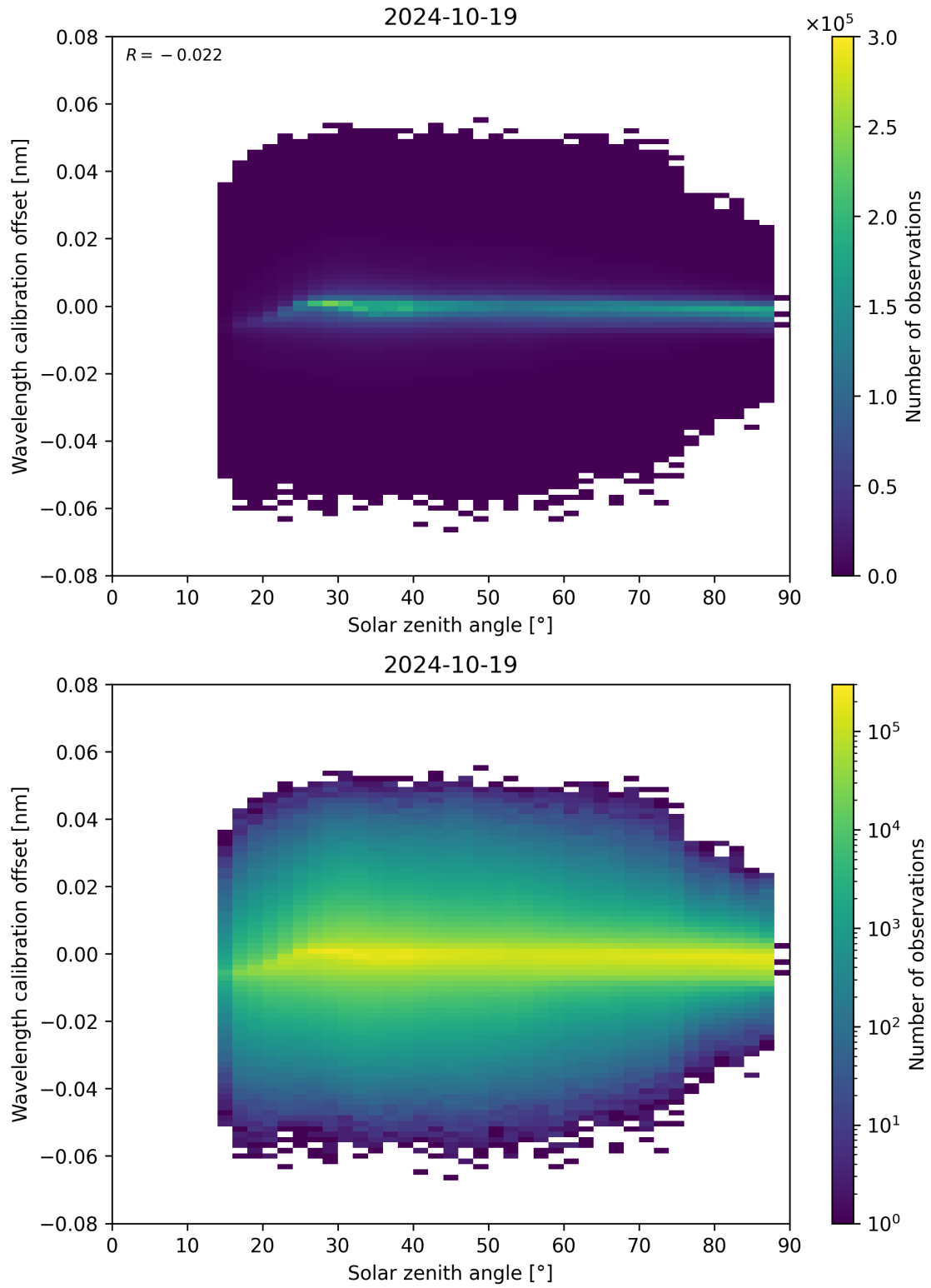
Figure 158: Scatter density plot of “Solar zenith angle” against “Wavelength calibration offset” for 2024-10-19 to 2024-10-20.
