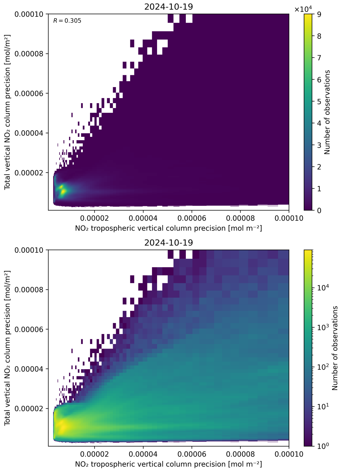
Figure 139: Scatter density plot of “NO 2 tropospheric vertical column precision” against “Total vertical NO 2 column precision” for 2024-10-19 to 2024-10-20.
