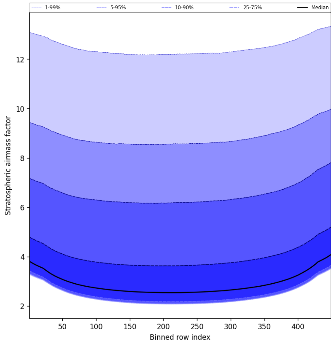
Figure 61: Along track statistics of “Stratospheric air mass factor” for 2024-10-19 to 2024-10-20
