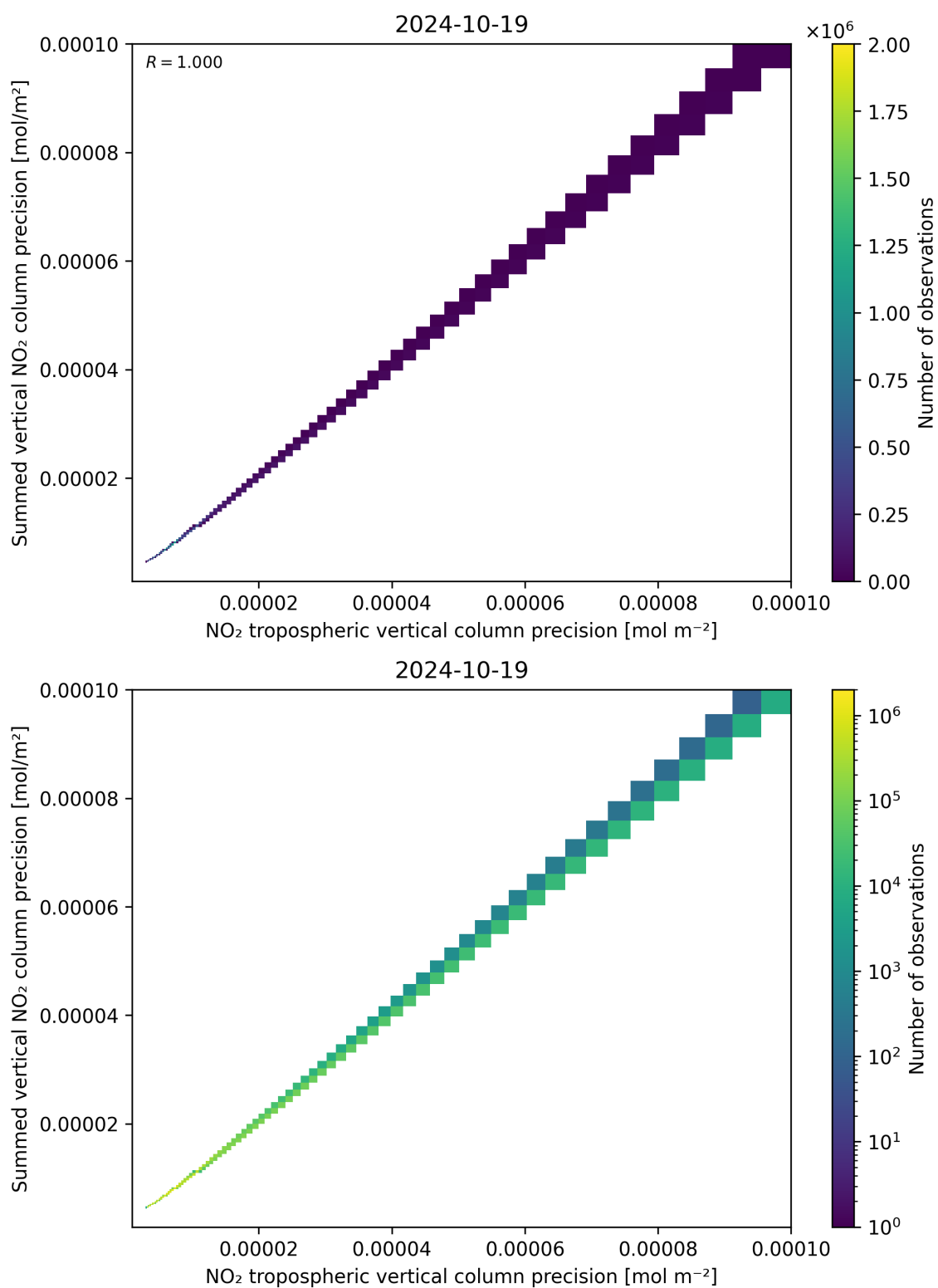
Figure 137: Scatter density plot of “NO 2 tropospheric vertical column precision” against “Summed vertical NO 2 column precision” for 2024-10-19 to 2024-10-20.
