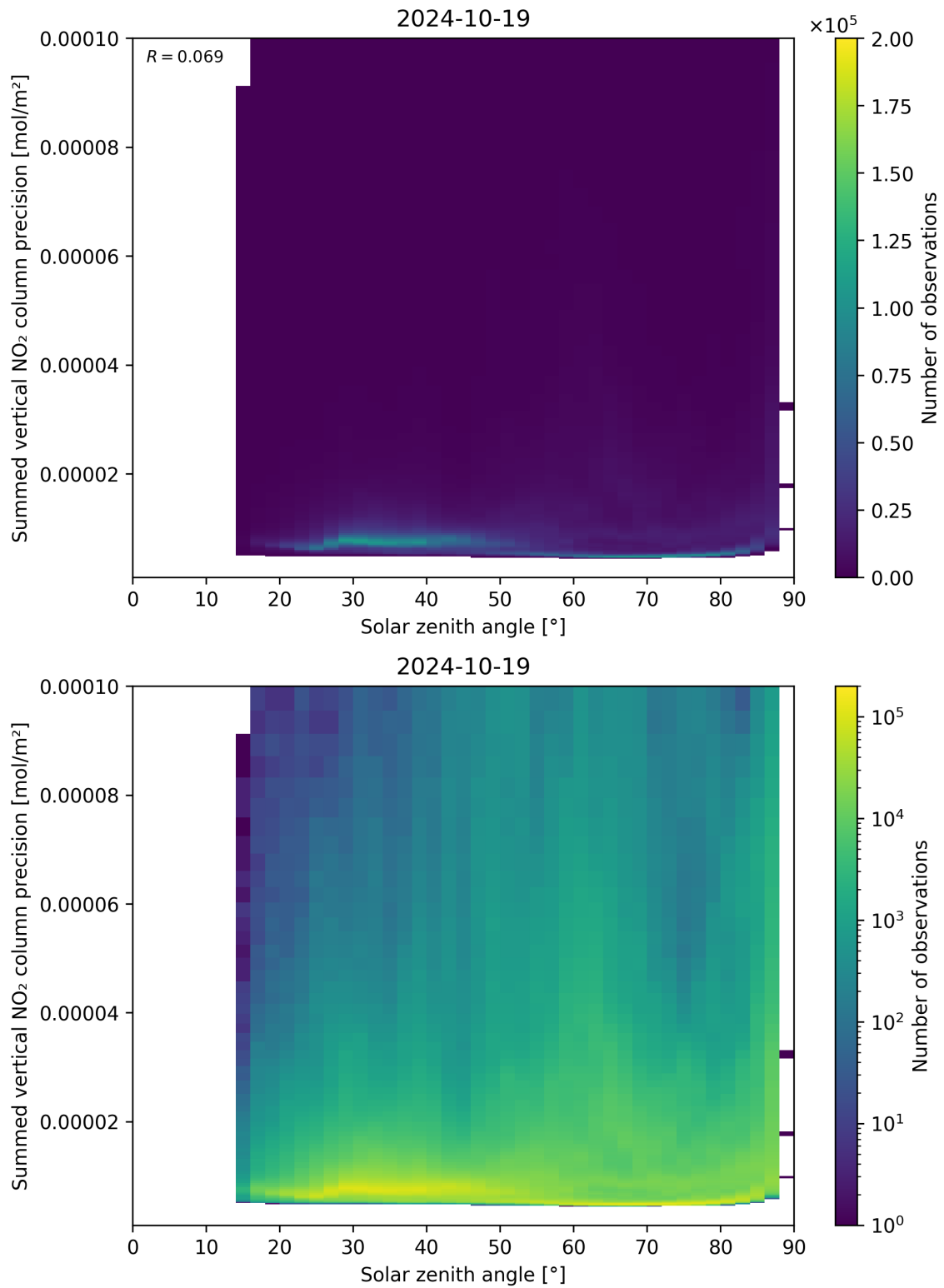
Figure 152: Scatter density plot of “Solar zenith angle” against “Summed vertical NO 2 column precision” for 2024-10-19 to 2024-10-20.
