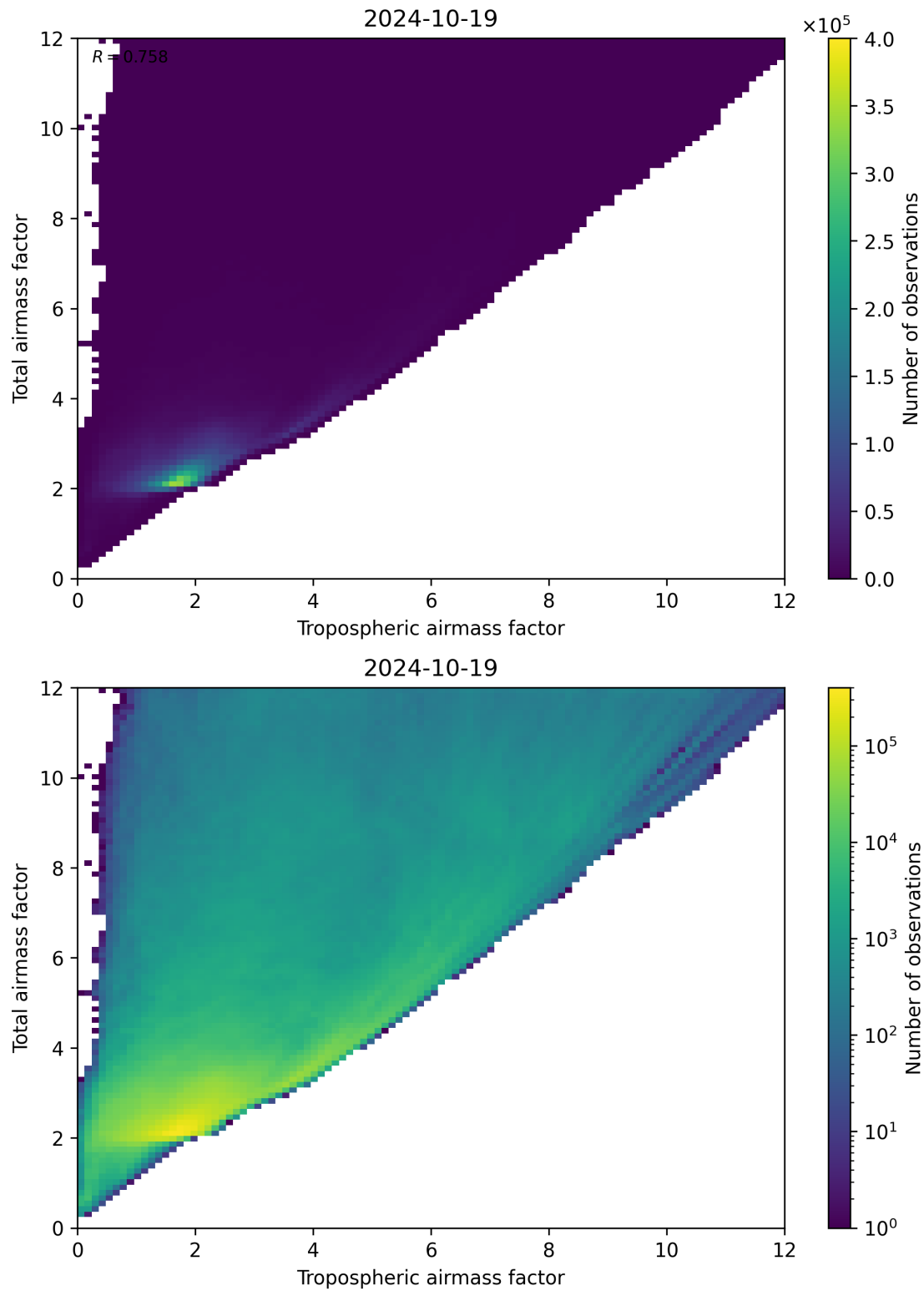
Figure 72: Scatter density plot of “Tropospheric airmass factor” against “Total airmass factor” for 2024-10-19 to 2024-10-20.
