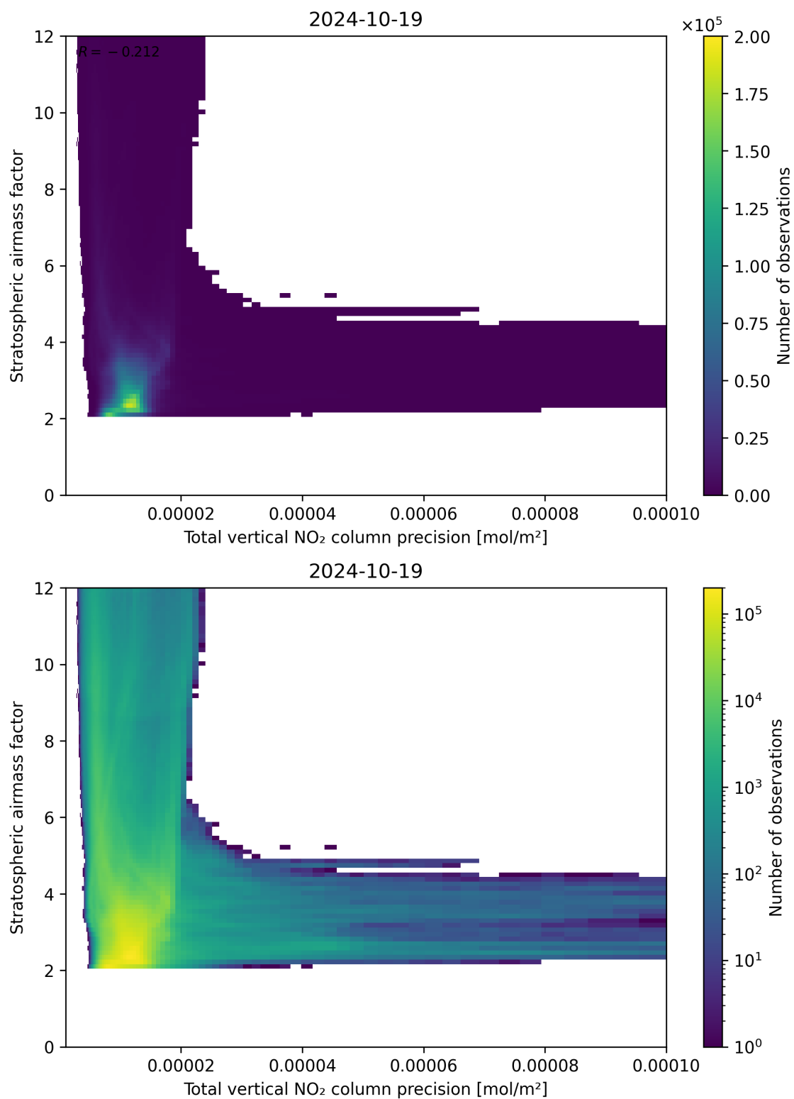
Figure 115: Scatter density plot of “Total vertical NO 2 column precision” against “Stratospheric air mass factor” for 2024-10-19 to 2024-10-20.
