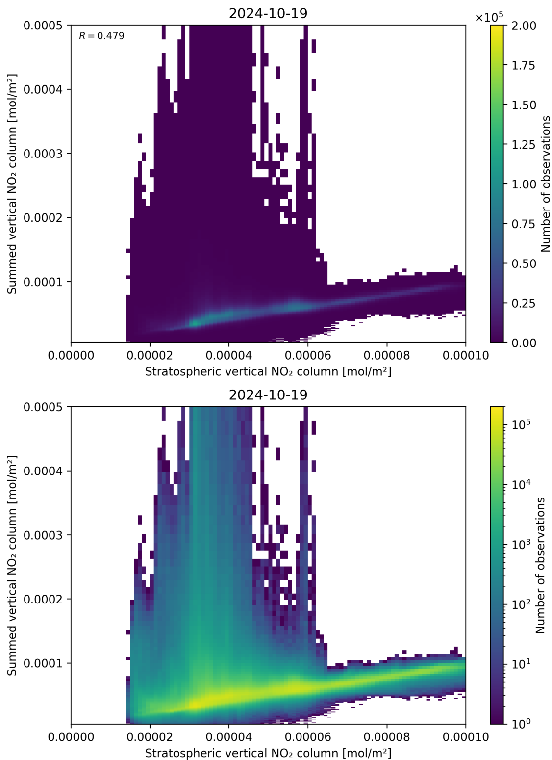
Figure 98: Scatter density plot of “Stratospheric vertical NO 2 column” against “Summed vertical NO 2 column” for 2024-10-19 to 2024-10-20.
