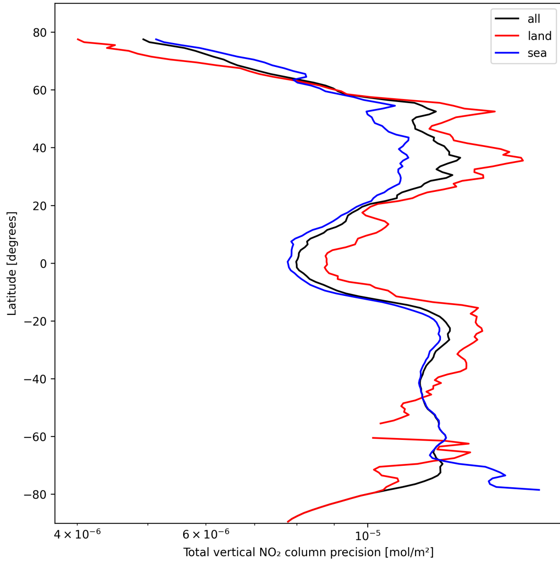
Figure 22: Zonal average of “Total vertical NO 2 column precision” for 2024-10-19 to 2024-10-20.
