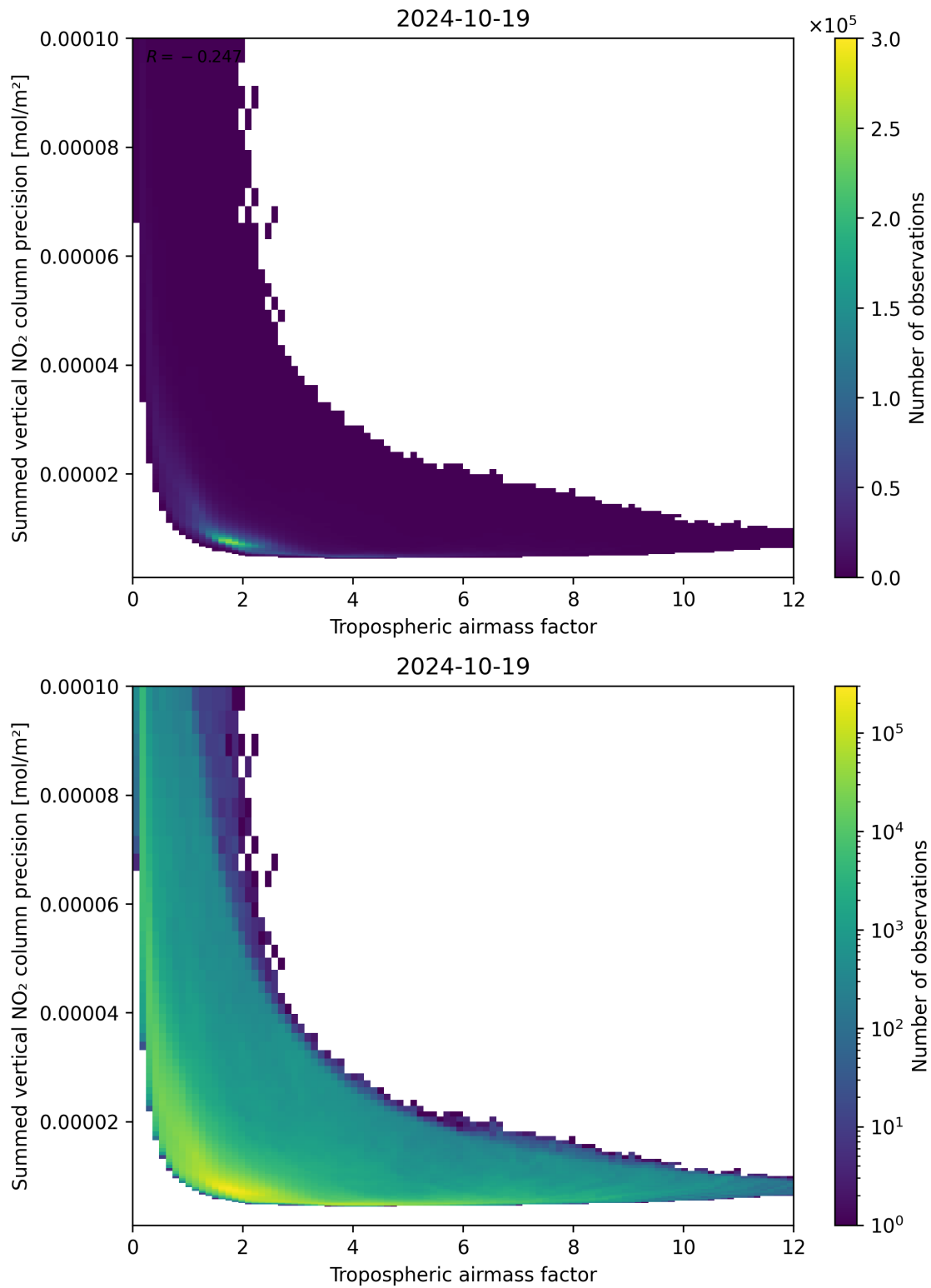
Figure 76: Scatter density plot of “Tropospheric air mass factor” against “Summed vertical NO 2 column precision” for 2024-10-19 to 2024-10-20.
