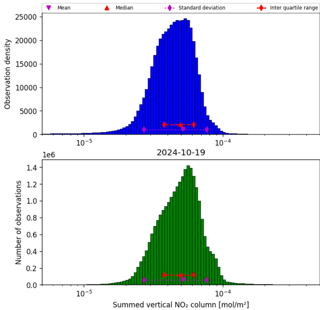
Figure 40: Histogram of “Summed vertical NO 2 column” for 2024-10-19 to 2024-10-20
