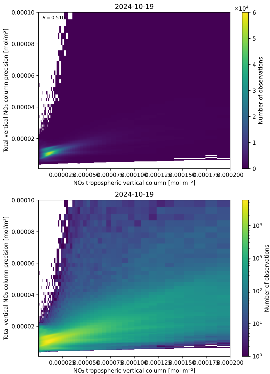
Figure 129: Scatter density plot of “NO 2 tropospheric vertical column” against “Total vertical NO 2 column precision” for 2024-10-19 to 2024-10-20.
