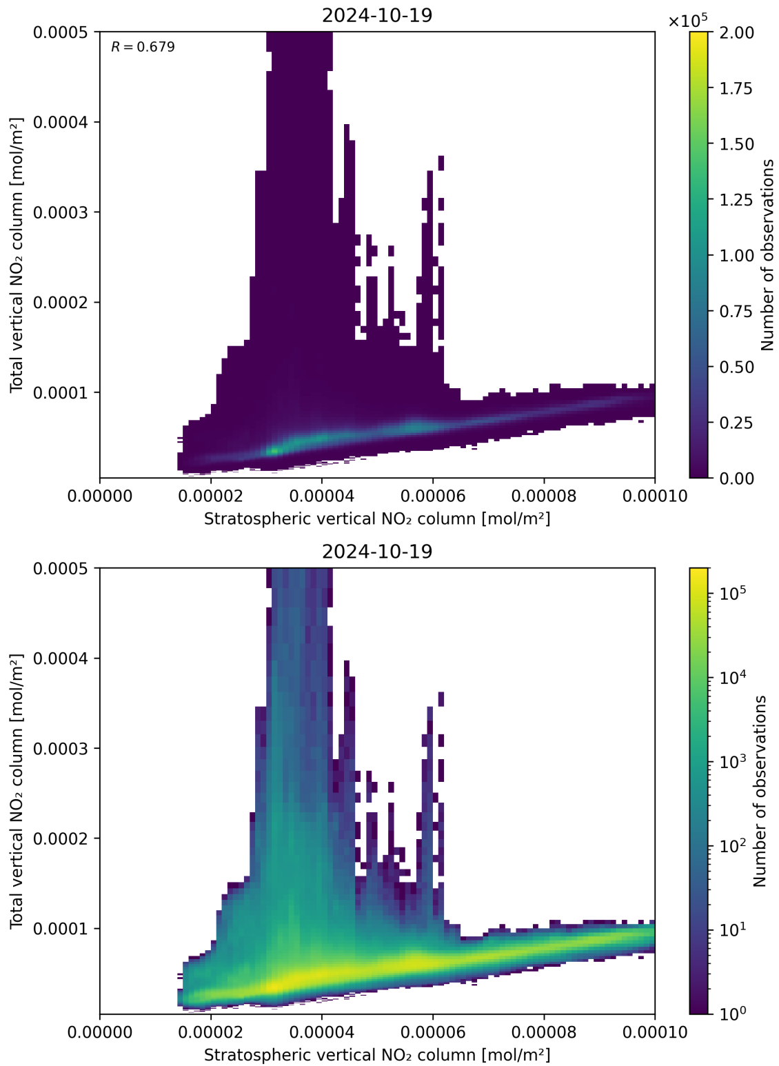
Figure 100: Scatter density plot of “Stratospheric vertical NO 2 column” against “Total vertical NO 2 column” for 2024-10-19 to 2024-10-20.
