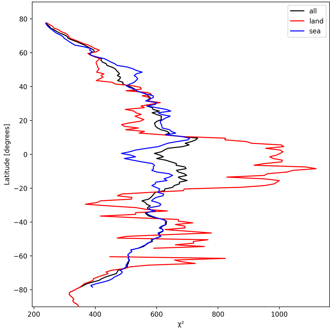
Figure 25: Zonal average of “ \chi^2 ” for 2024-10-19 to 2024-10-20.
