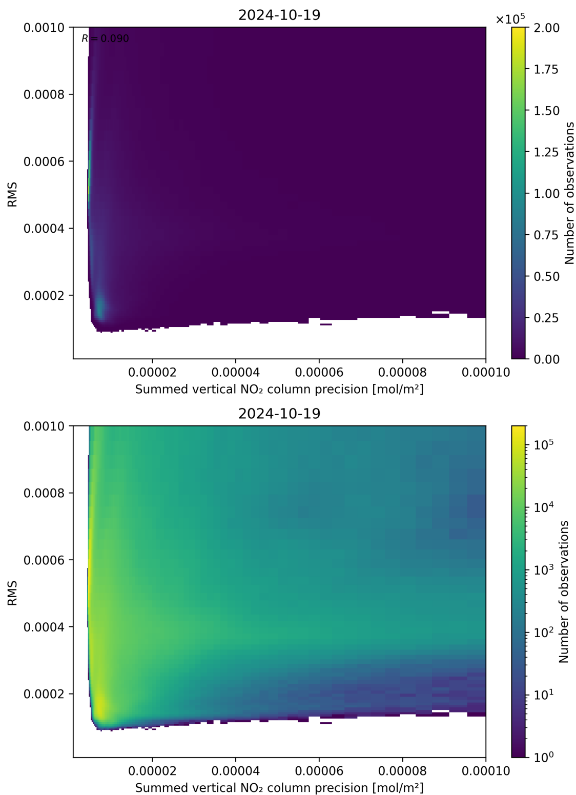
Figure 108: Scatter density plot of “Summed vertical NO 2 column precision” against “RMS” for 2024-10-19 to 2024-10-20.
