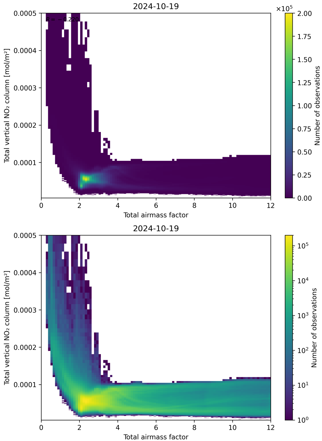
Figure 67: Scatter density plot of “Total airmass factor” against “Total vertical NO 2 column” for 2024-10-19 to 2024-10-20.
