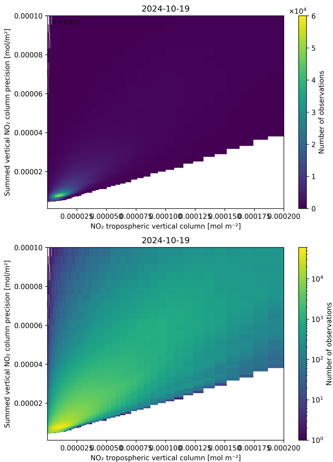
Figure 127: Scatter density plot of “NO 2 tropospheric vertical column” against “Summed vertical NO 2 column precision” for 2024-10-19 to 2024-10-20.
