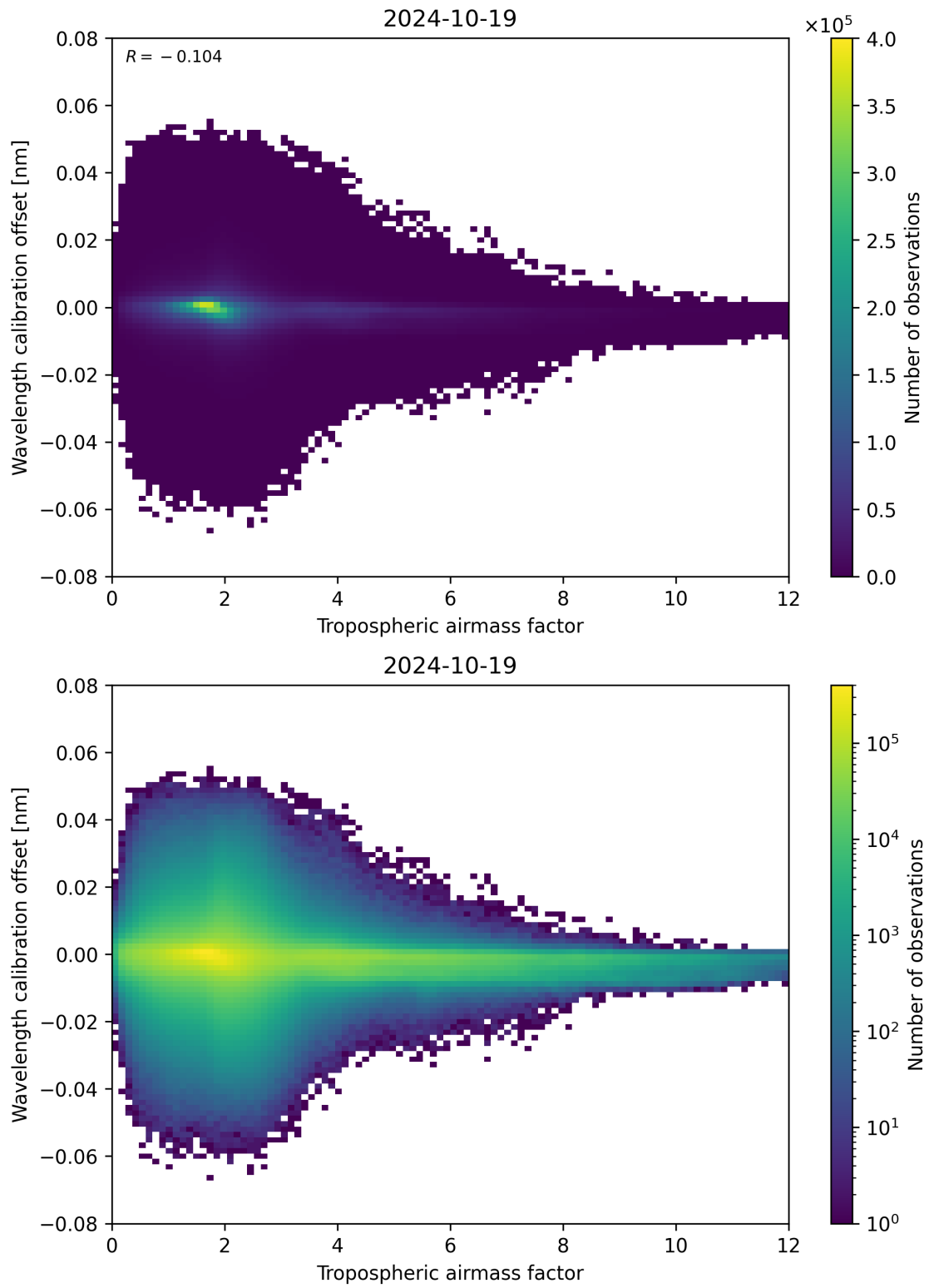
Figure 80: Scatter density plot of “Tropospheric airmass factor” against “Wavelength calibration offset” for 2024-10-19 to 2024-10-20.
