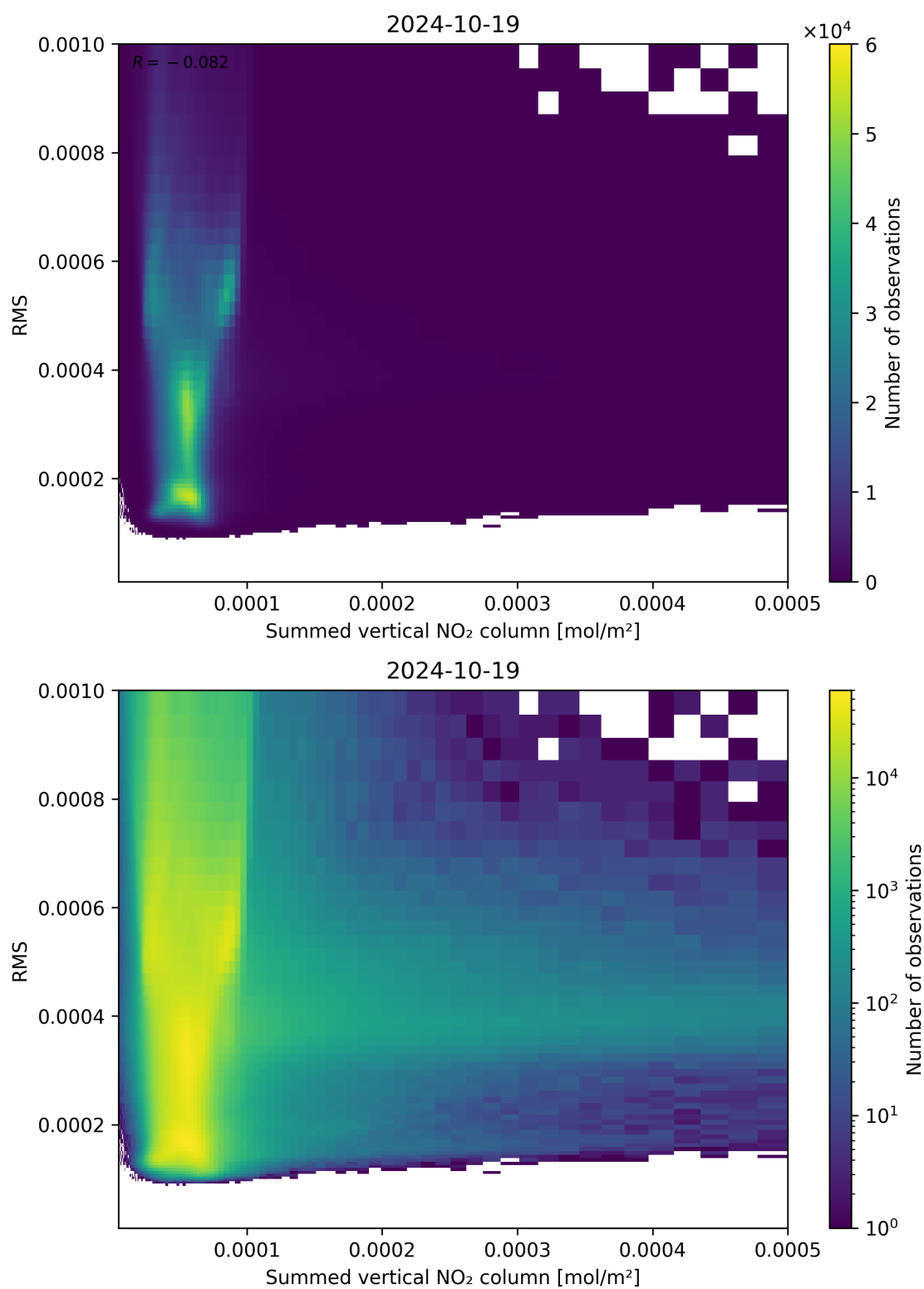
Figure 109: Scatter density plot of “Summed vertical NO 2 column” against “RMS” for 2024-10-19 to 2024-10-20.
