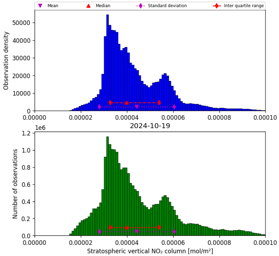
Figure 36: Histogram of “Stratospheric vertical NO 2 column” for 2024-10-19 to 2024-10-20
