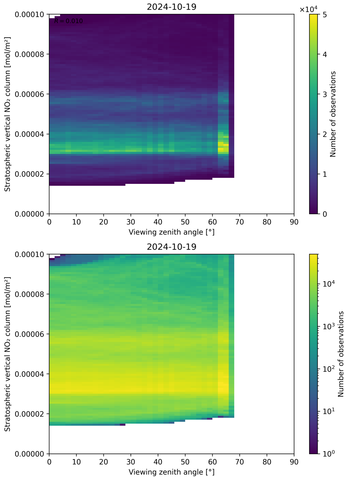
Figure 164: Scatter density plot of “Viewing zenith angle” against “Stratospheric vertical NO 2 column” for 2024-10-19 to 2024-10-20.
