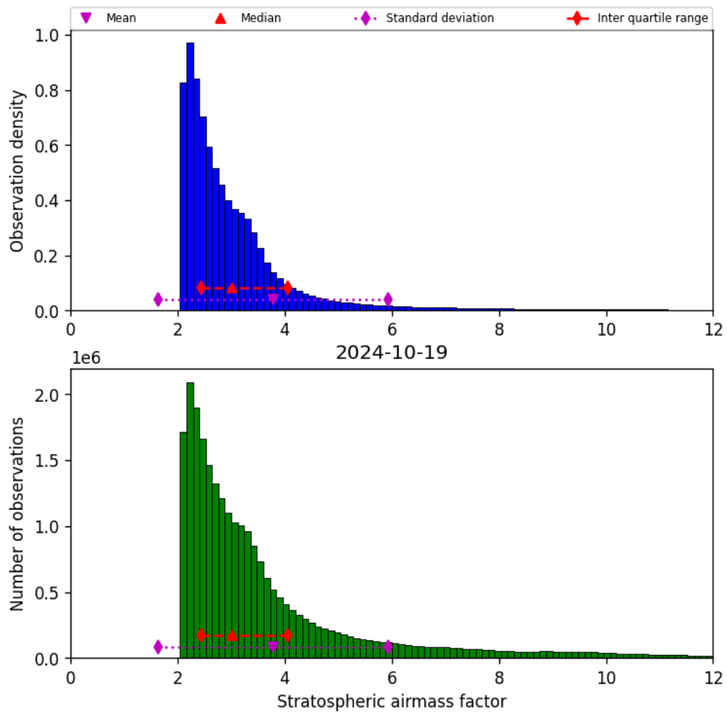
Figure 44: Histogram of “Stratospheric airmass factor” for 2024-10-19 to 2024-10-20
