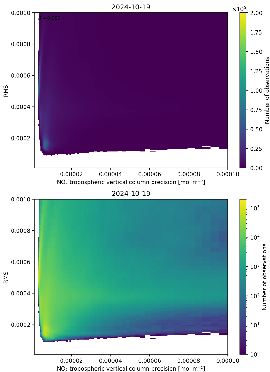
Figure 140: Scatter density plot of “NO 2 tropospheric vertical column precision” against “RMS” for 2024-10-19 to 2024-10-20.
