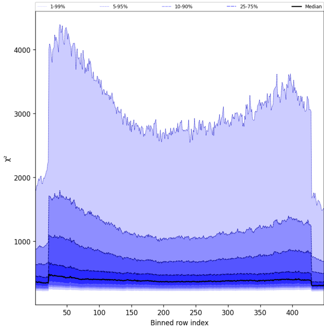
Figure 59: Along track statistics of “ \chi^2 ” for 2024-10-19 to 2024-10-20
