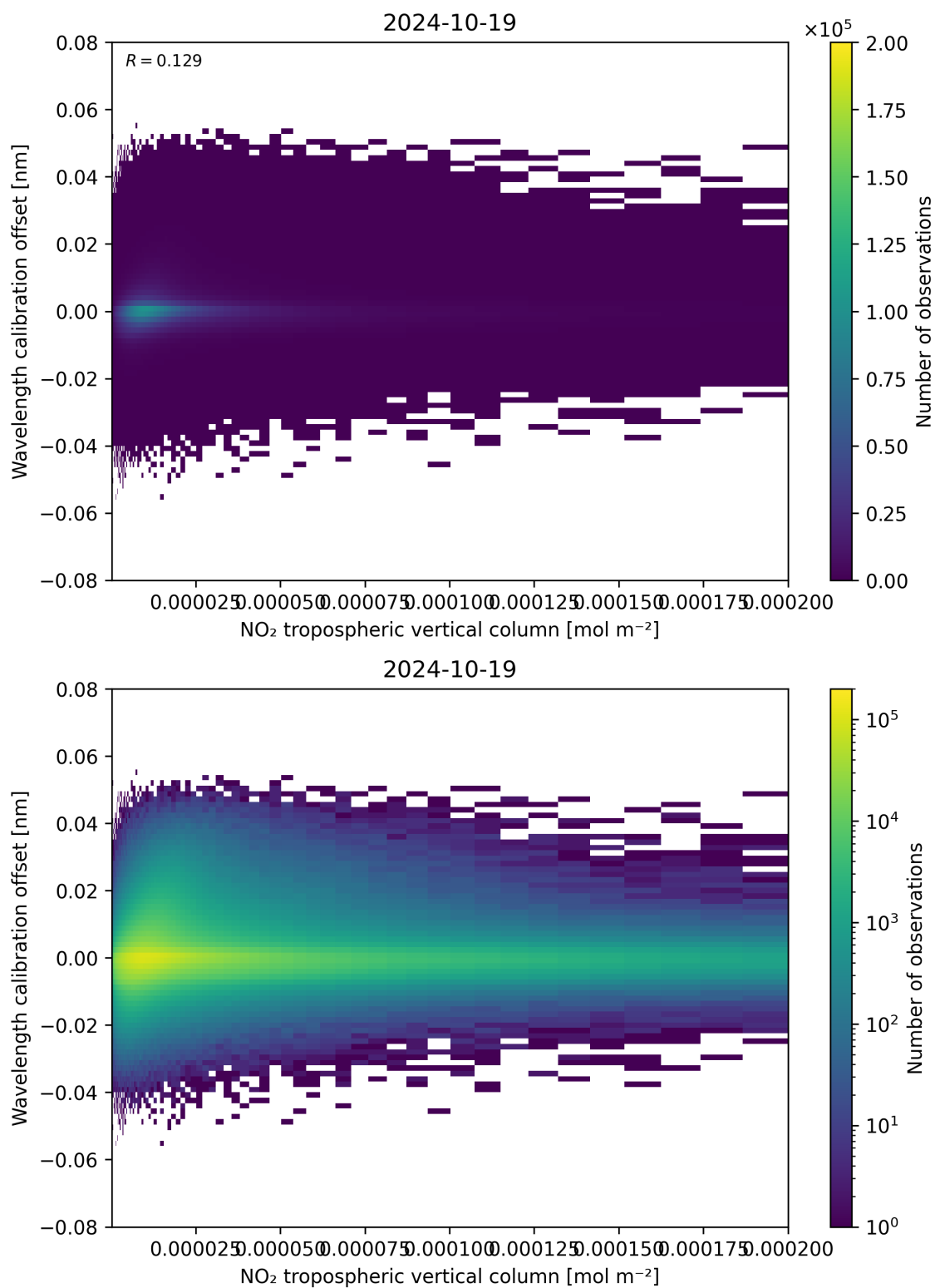
Figure 143: Scatter density plot of “NO 2 tropospheric vertical column” against “Wavelength calibration offset” for 2024-10-19 to 2024-10-20.
