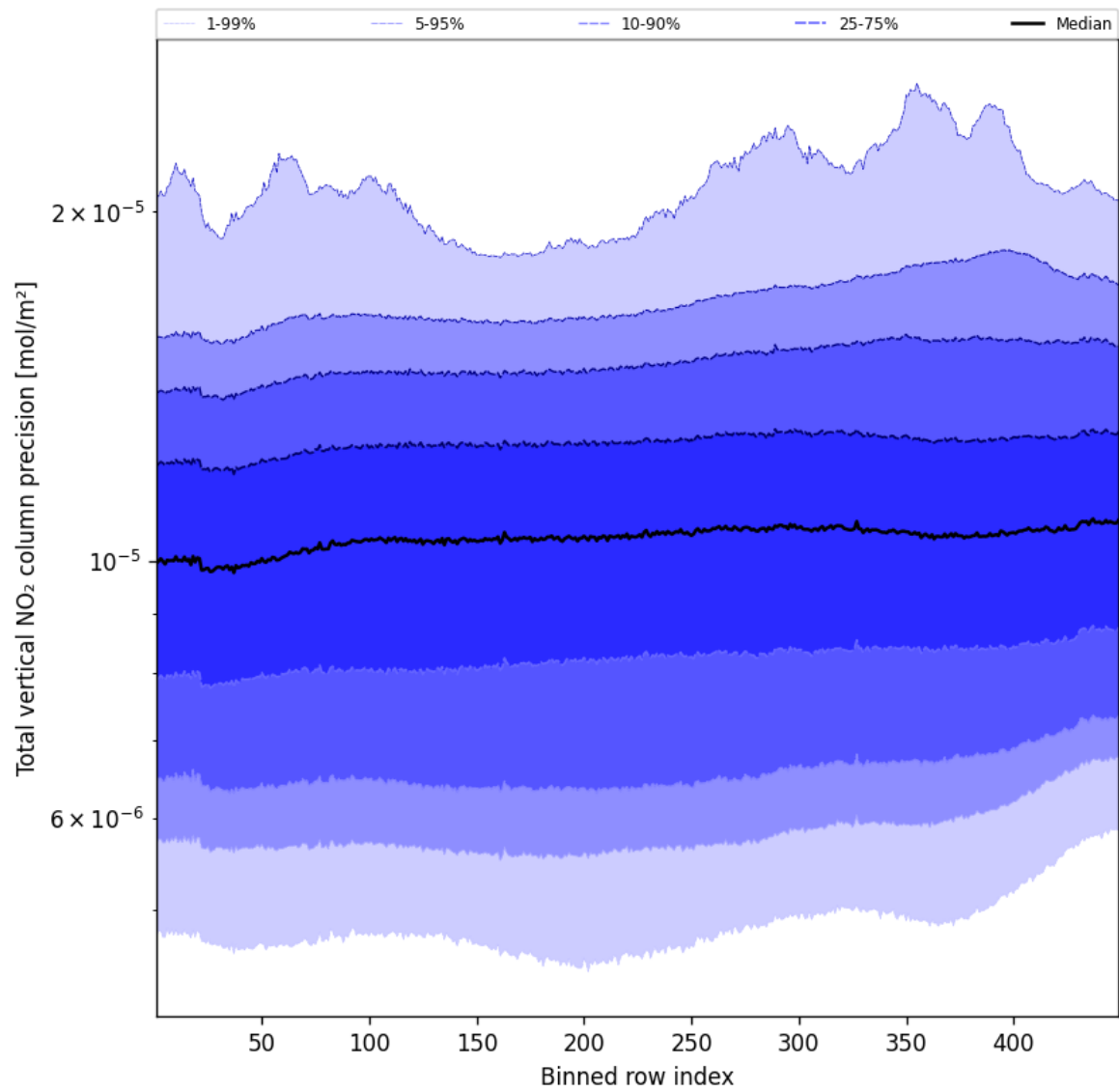
Figure 56: Along track statistics of “Total vertical NO 2 column precision” for 2024-10-19 to 2024-10-20
