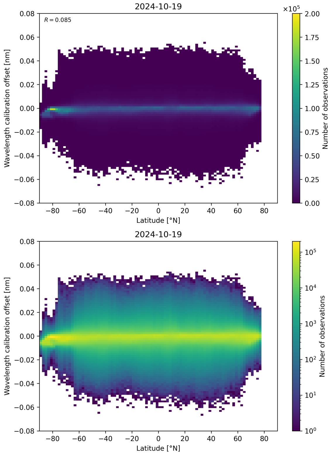
Figure 95: Scatter density plot of “Latitude” against “Wavelength calibration offset” for 2024-10-19 to 2024-10-20.
