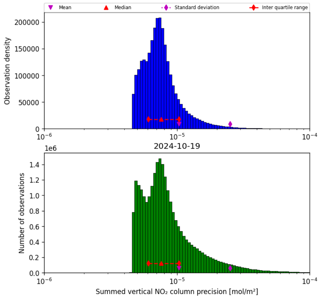
Figure 41: Histogram of "Summed vertical NO 2 column precision" for 2024-10-19 to 2024-10-20
