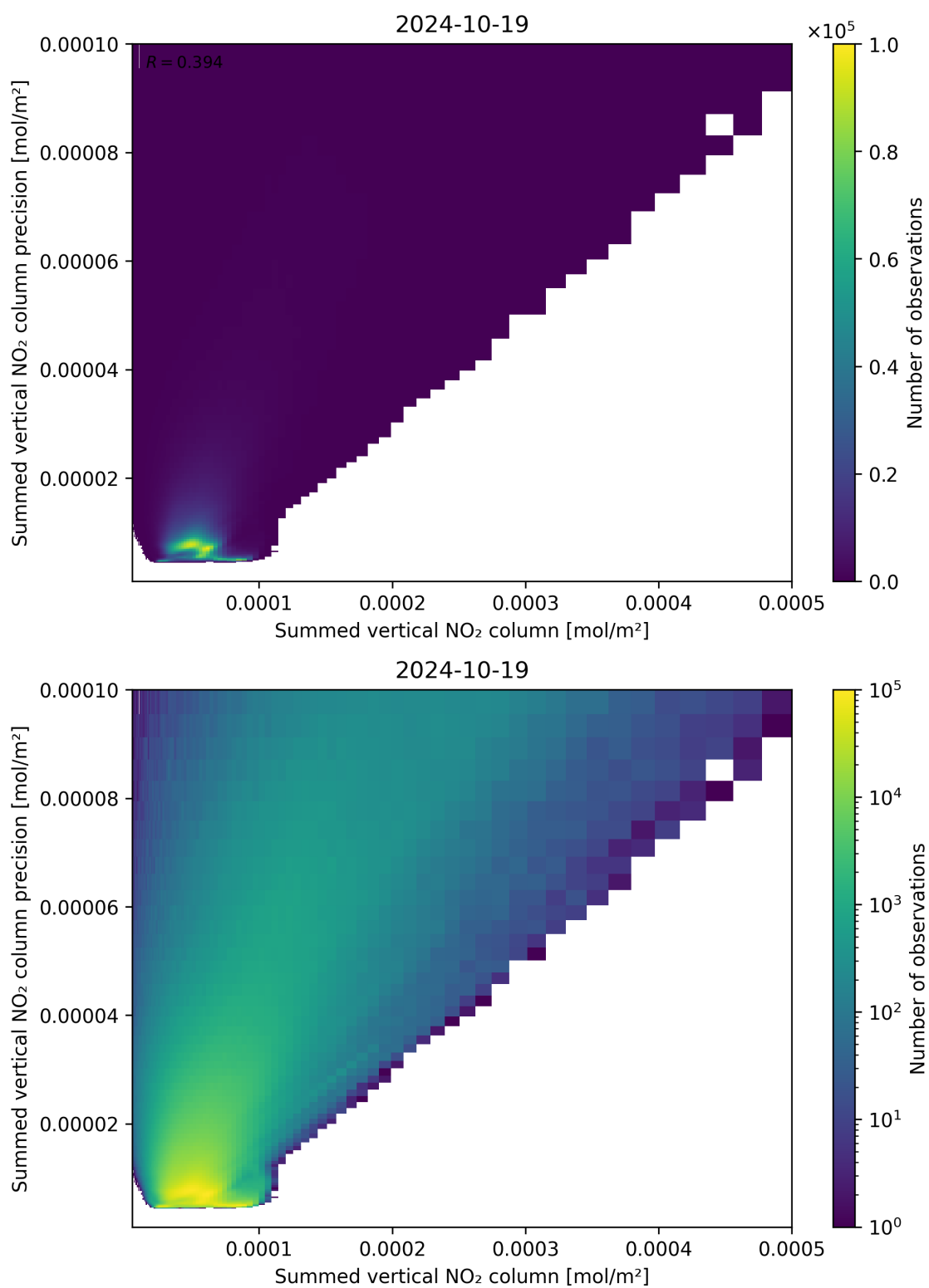
Figure 105: Scatter density plot of “Summed vertical NO 2 column” against “Summed vertical NO 2 column precision” for 2024-10-19 to 2024-10-20.
