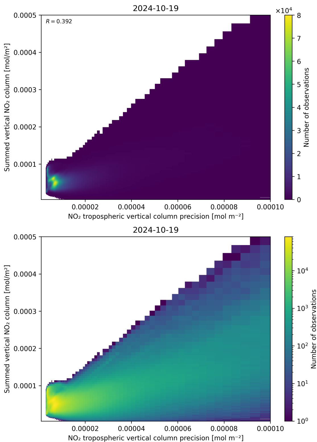
Figure 136: Scatter density plot of “NO 2 tropospheric vertical column precision” against “Summed vertical NO 2 column” for 2024-10-19 to 2024-10-20.
