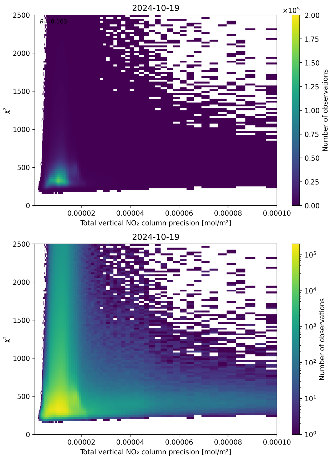
Figure 116: Scatter density plot of “Total vertical NO 2 column precision” against “ \chi^2 ” for 2024-10-19 to 2024-10-20.
