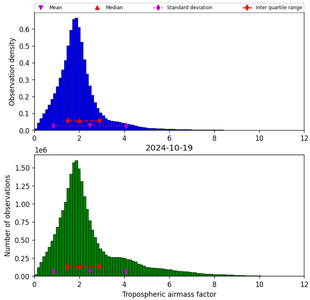
Figure 31: Histogram of “Tropospheric airmass factor” for 2024-10-19 to 2024-10-20
