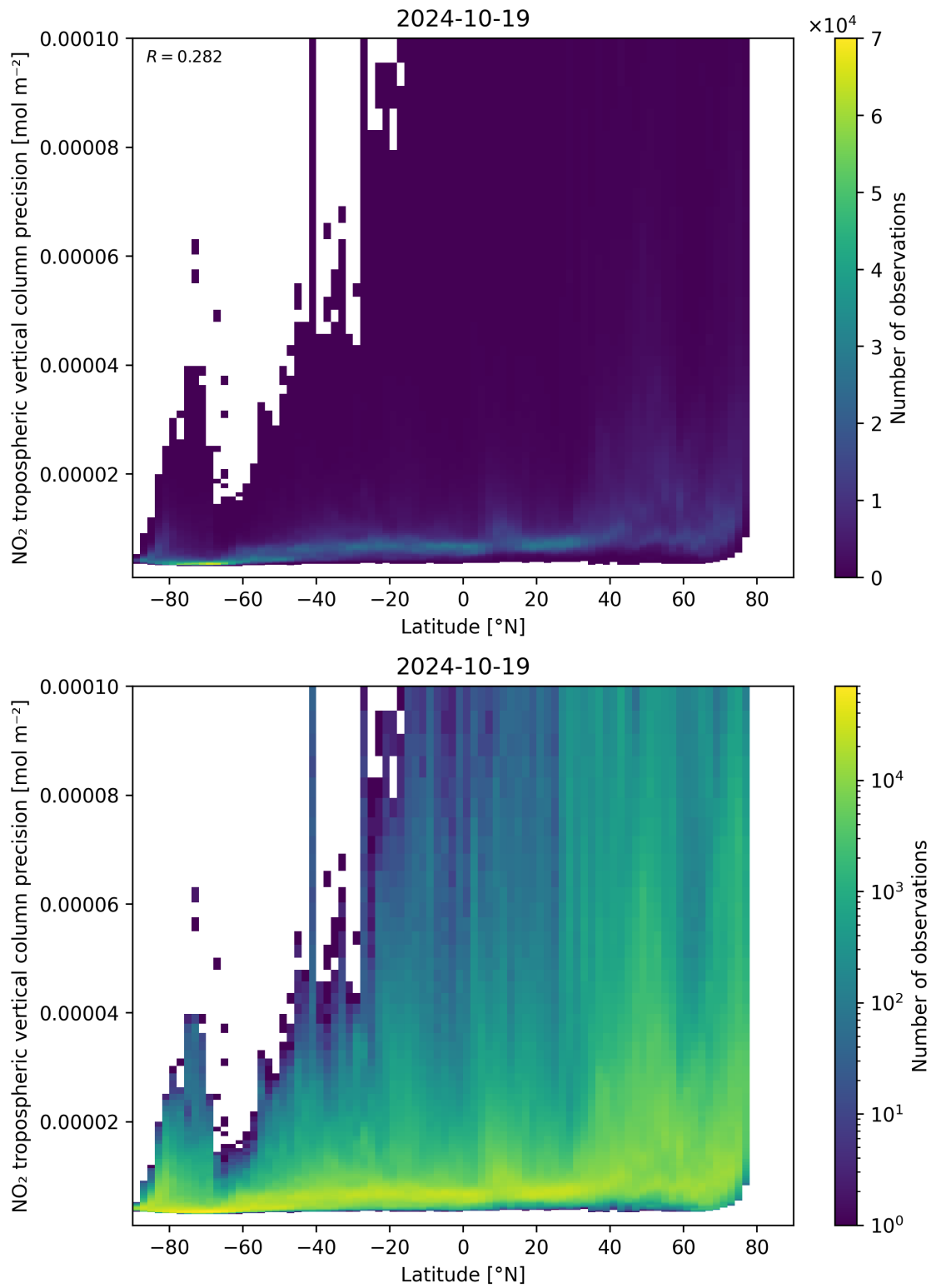
Figure 93: Scatter density plot of “Latitude” against “NO 2 tropospheric vertical column precision” for 2024-10-19 to 2024-10-20.
