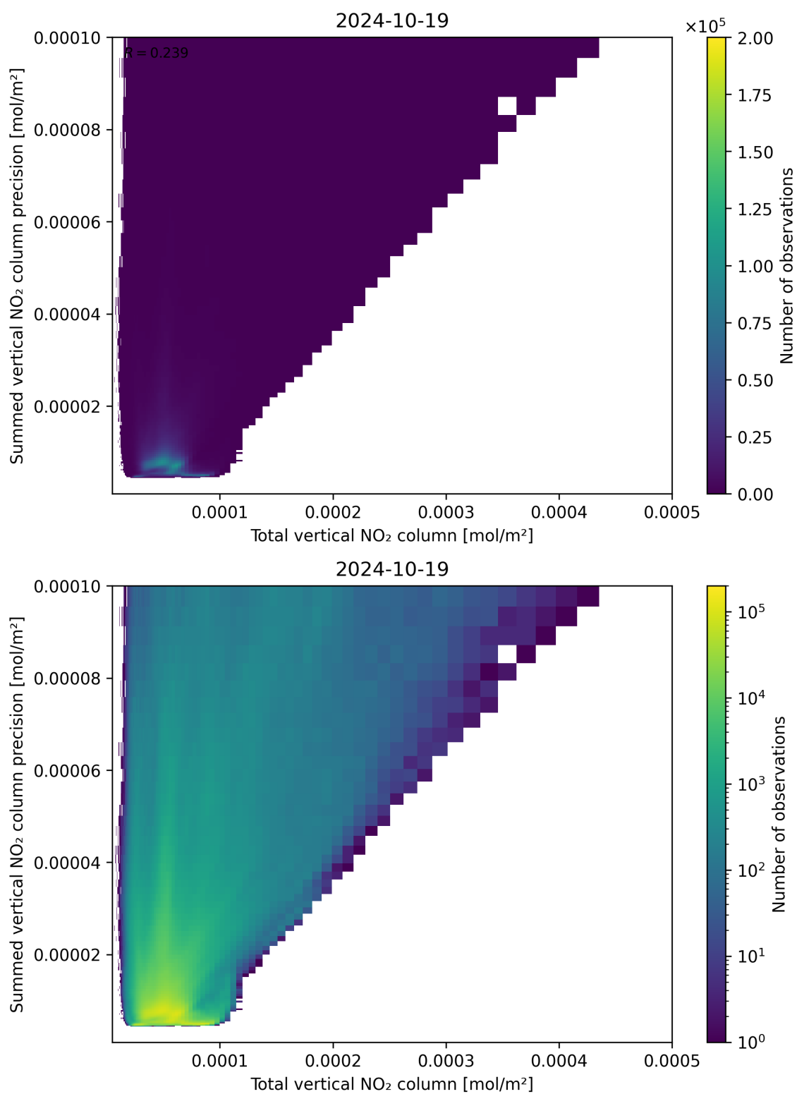
Figure 113: Scatter density plot of “Total vertical NO 2 column” against “Summed vertical NO 2 column precision” for 2024-10-19 to 2024-10-20.
