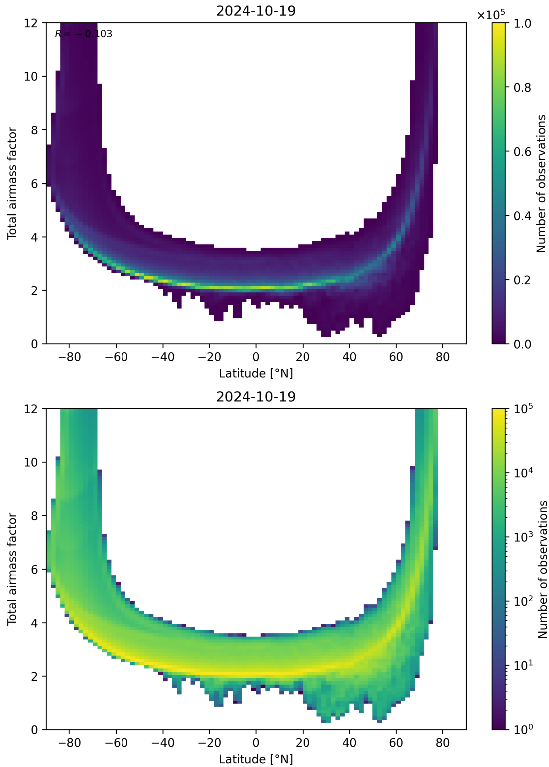
Figure 84: Scatter density plot of “Latitude” against “Total airmass factor” for 2024-10-19 to 2024-10-20.
