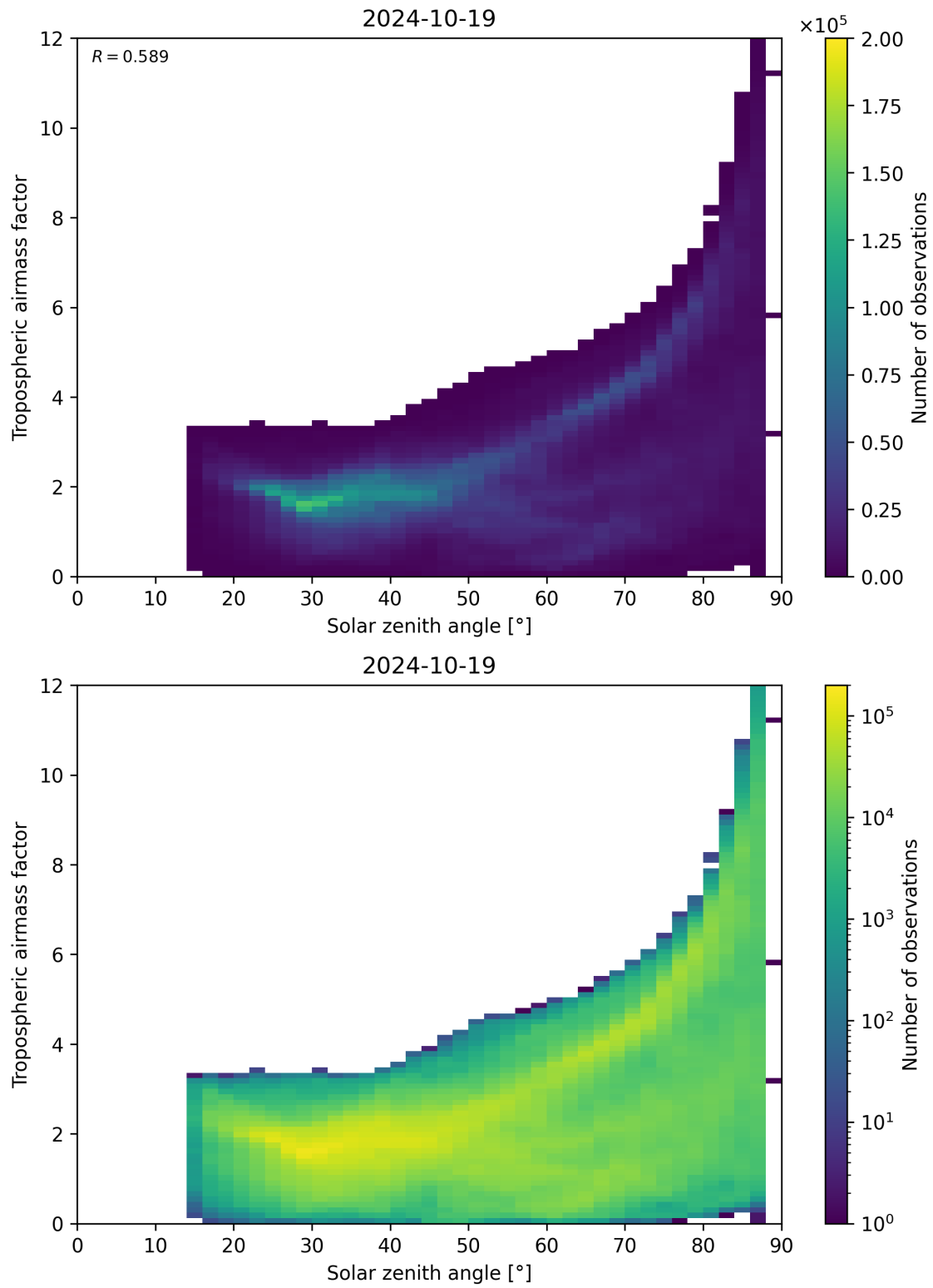
Figure 147: Scatter density plot of “Solar zenith angle” against “Tropospheric airmass factor” for 2024-10-19 to 2024-10-20.
