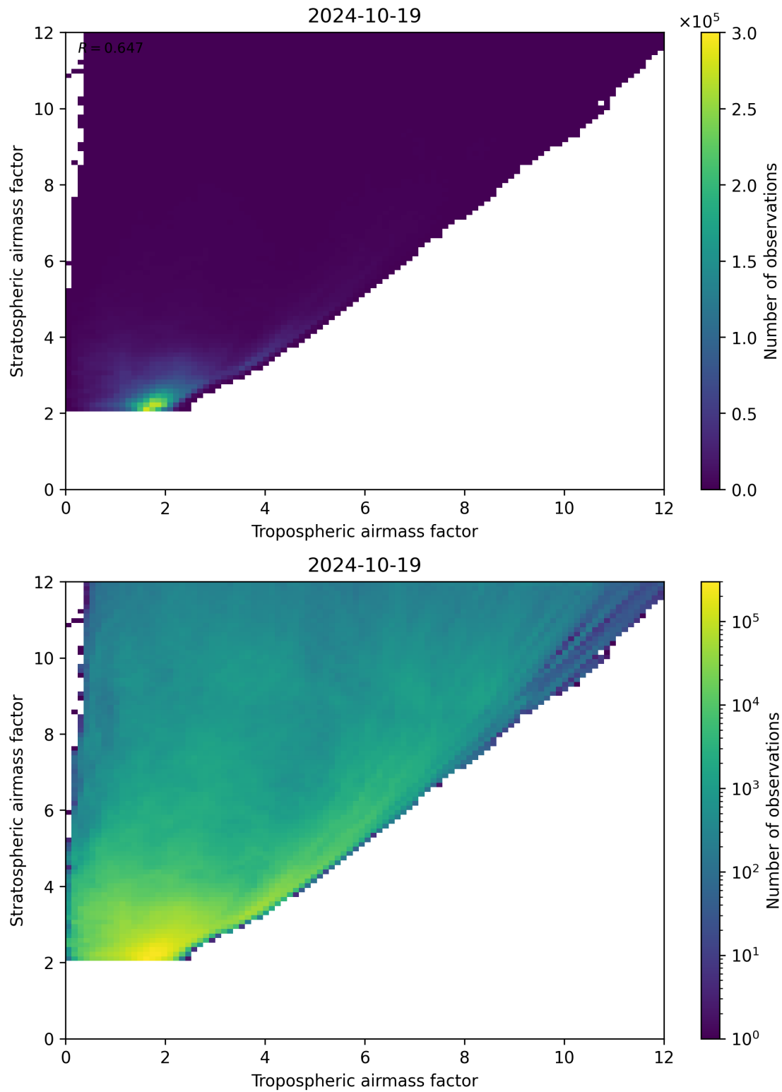
Figure 71: Scatter density plot of “Tropospheric airmass factor” against “Stratospheric airmass factor” for 2024-10-19 to 2024-10-20.
