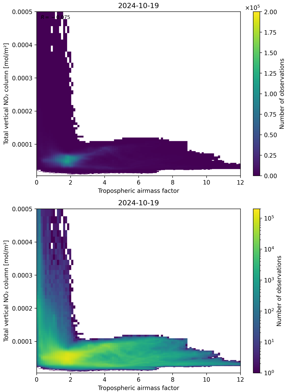
Figure 77: Scatter density plot of “Tropospheric airmass factor” against “Total vertical NO 2 column” for 2024-10-19 to 2024-10-20.
