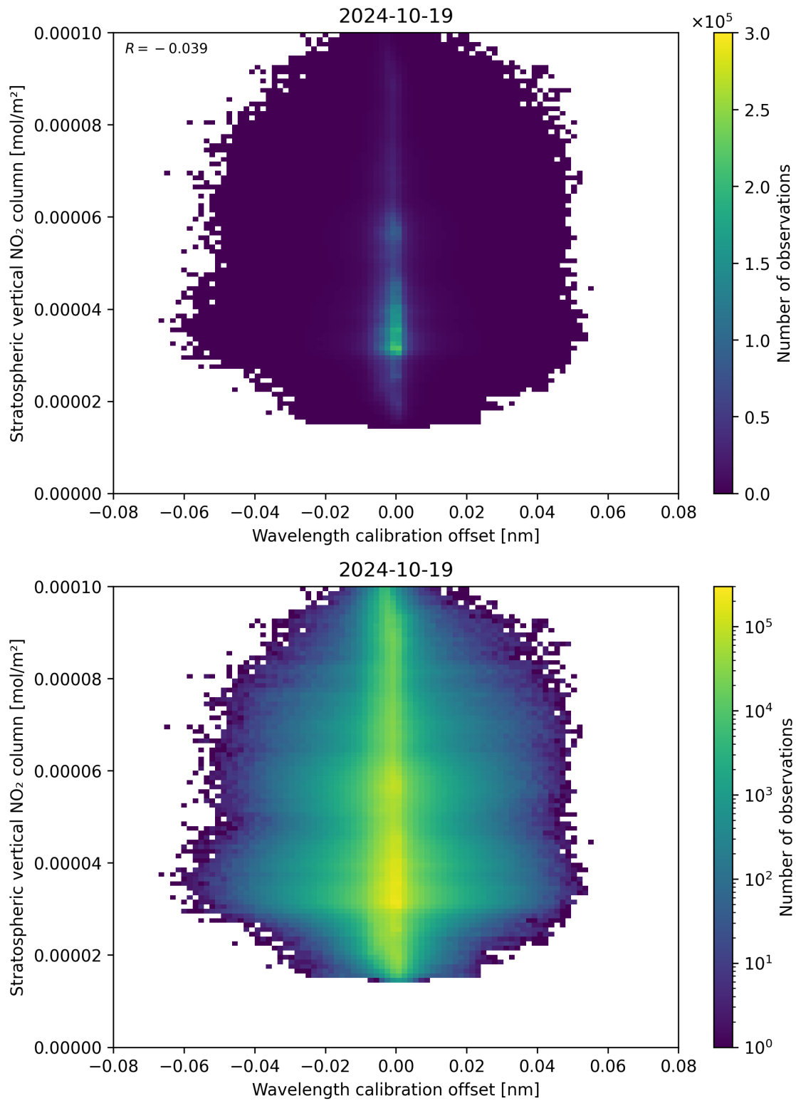
Figure 176: Scatter density plot of “Wavelength calibration offset” against “Stratospheric vertical NO 2 column” for 2024-10-19 to 2024-10-20.
