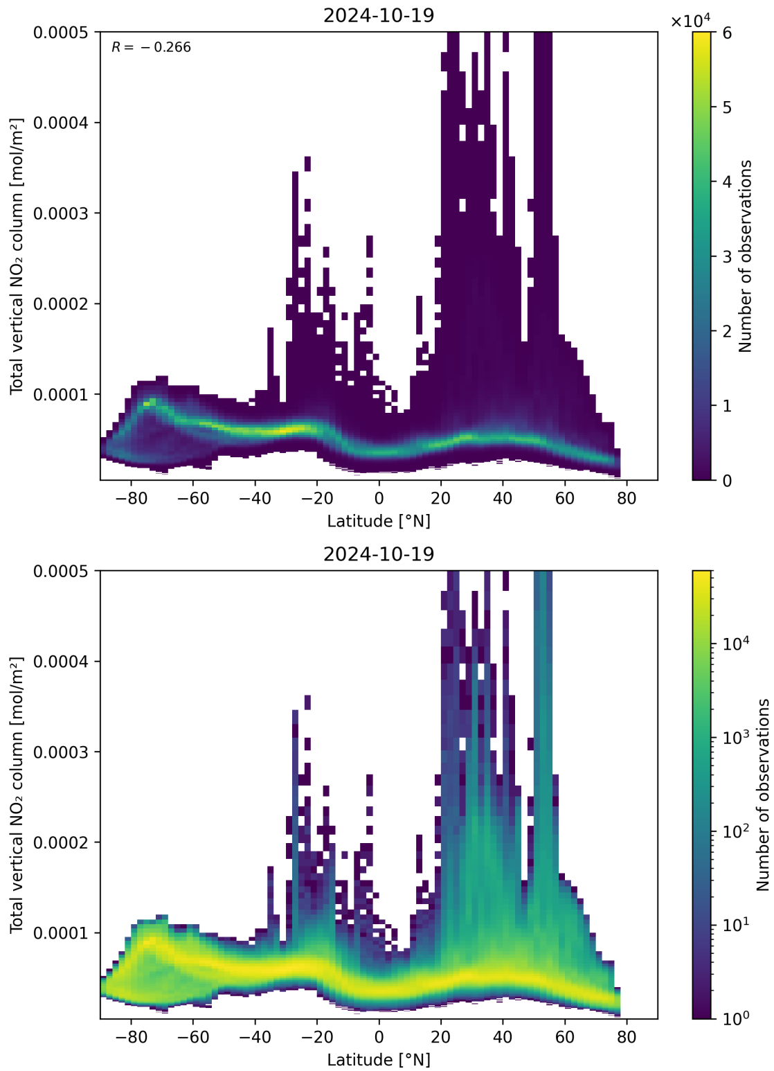
Figure 90: Scatter density plot of “Latitude” against “Total vertical NO 2 column” for 2024-10-19 to 2024-10-20.
