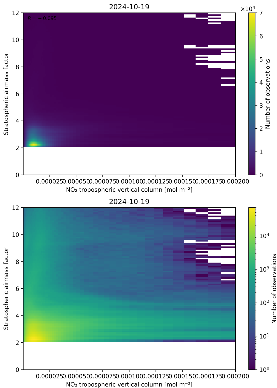
Figure 121: Scatter density plot of “NO 2 tropospheric vertical column” against “Stratospheric airmass factor” for 2024-10-19 to 2024-10-20.
