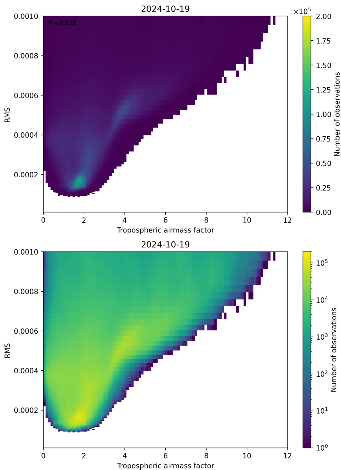
Figure 79: Scatter density plot of “Tropospheric airmass factor” against “RMS” for 2024-10-19 to 2024-10-20.
