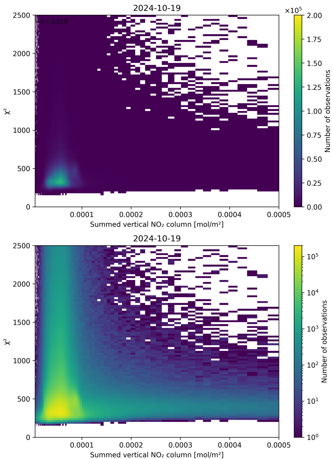
Figure 104: Scatter density plot of “Summed vertical NO 2 column” against “ \chi^2 ” for 2024-10-19 to 2024-10-20.
