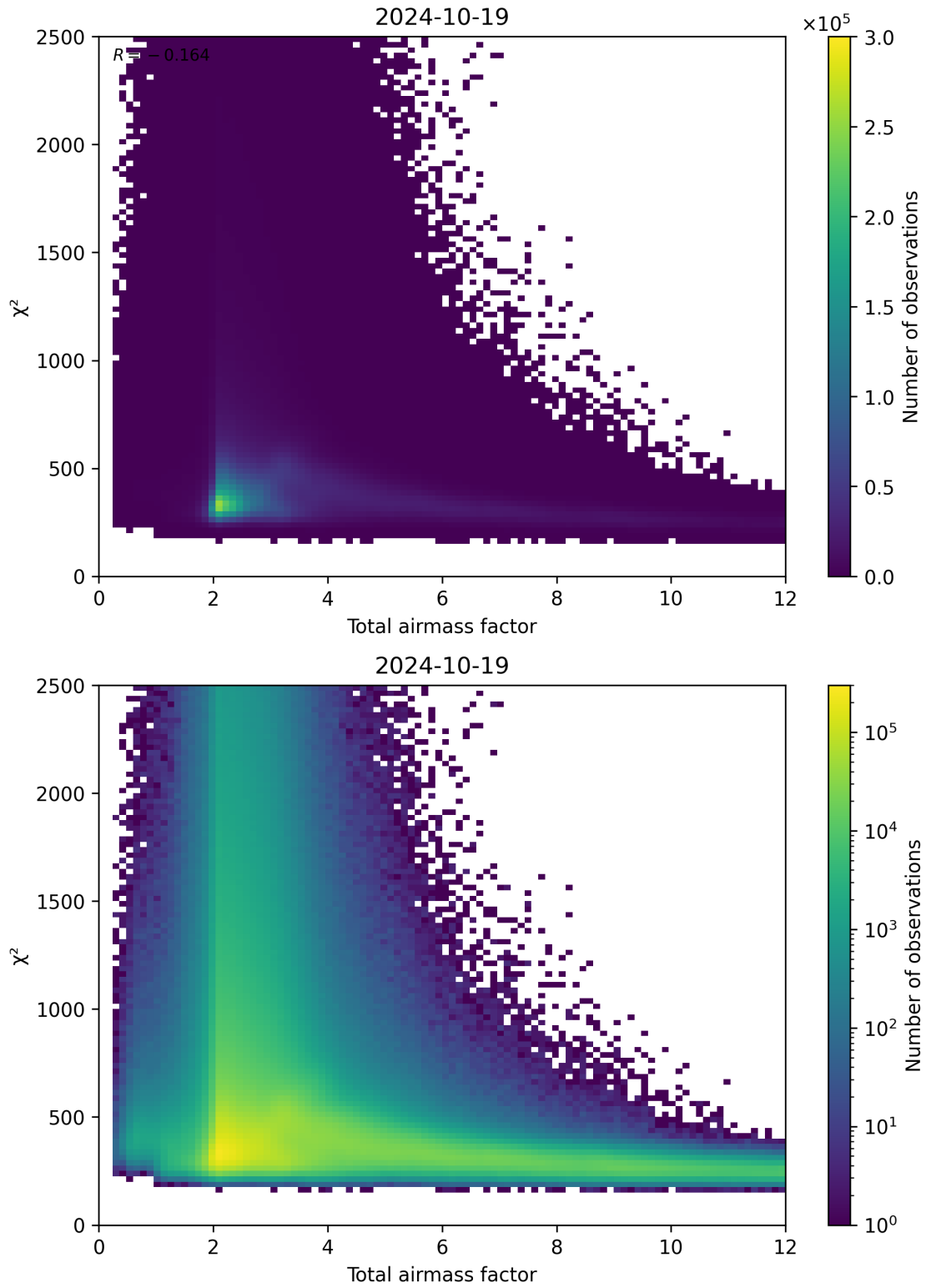
Figure 63: Scatter density plot of “Total airmass factor” against “ \chi^2 ” for 2024-10-19 to 2024-10-20.
