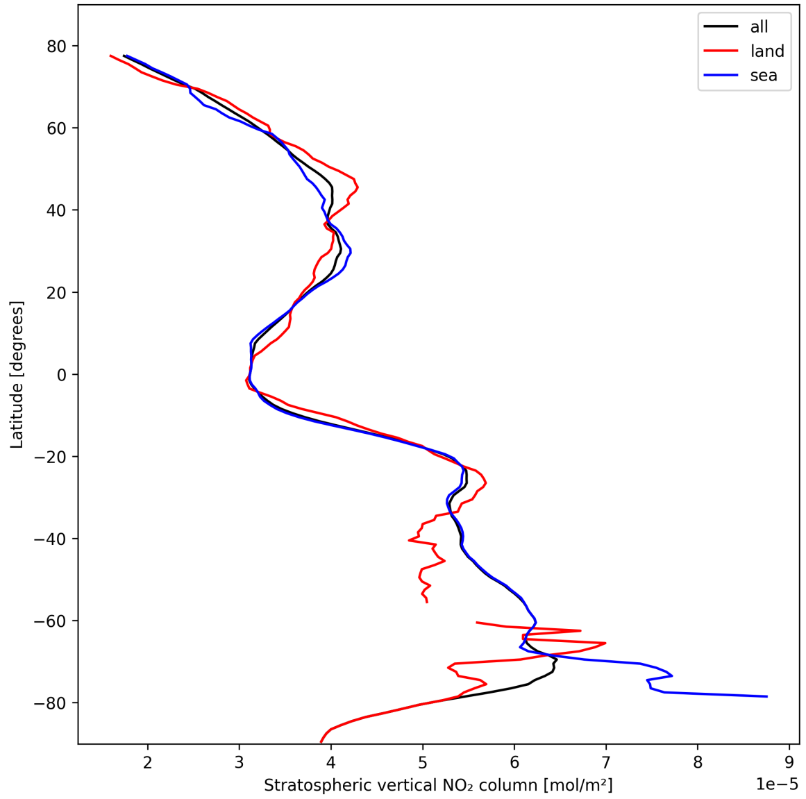
Figure 19: Zonal average of “Stratospheric vertical NO 2 column” for 2024-10-19 to 2024-10-20.
