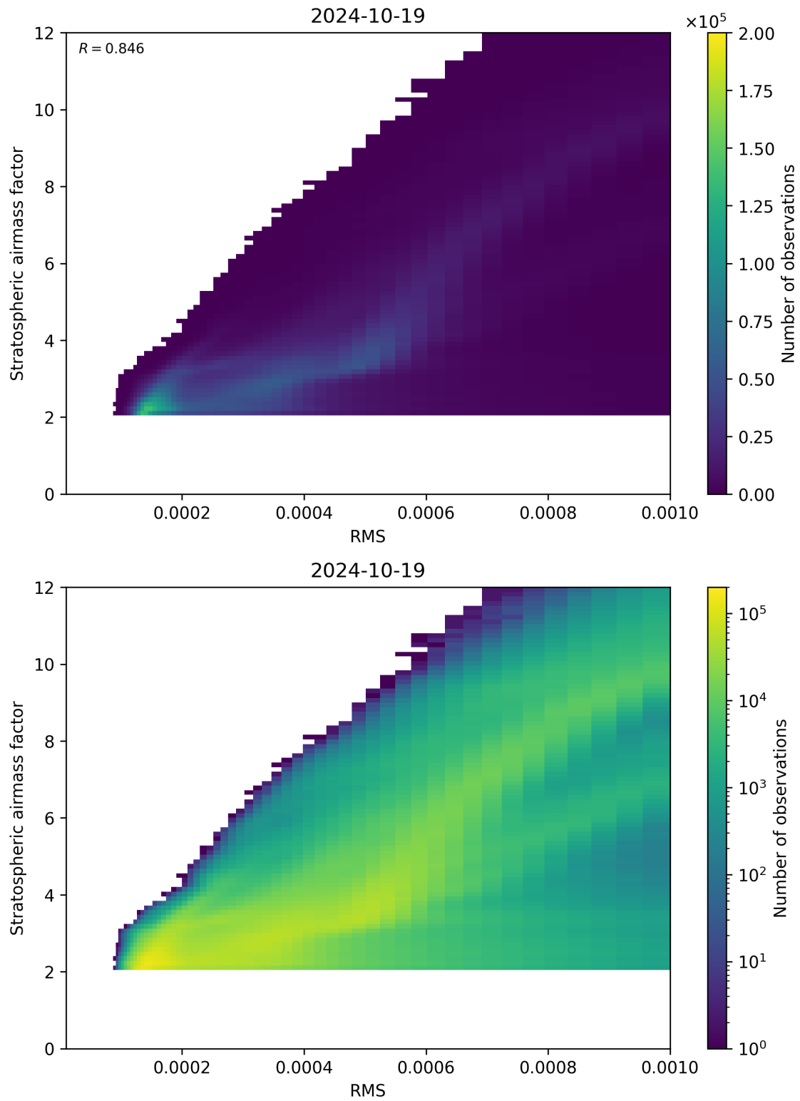
Figure 144: Scatter density plot of “RMS” against “Stratospheric airmass factor” for 2024-10-19 to 2024-10-20.
