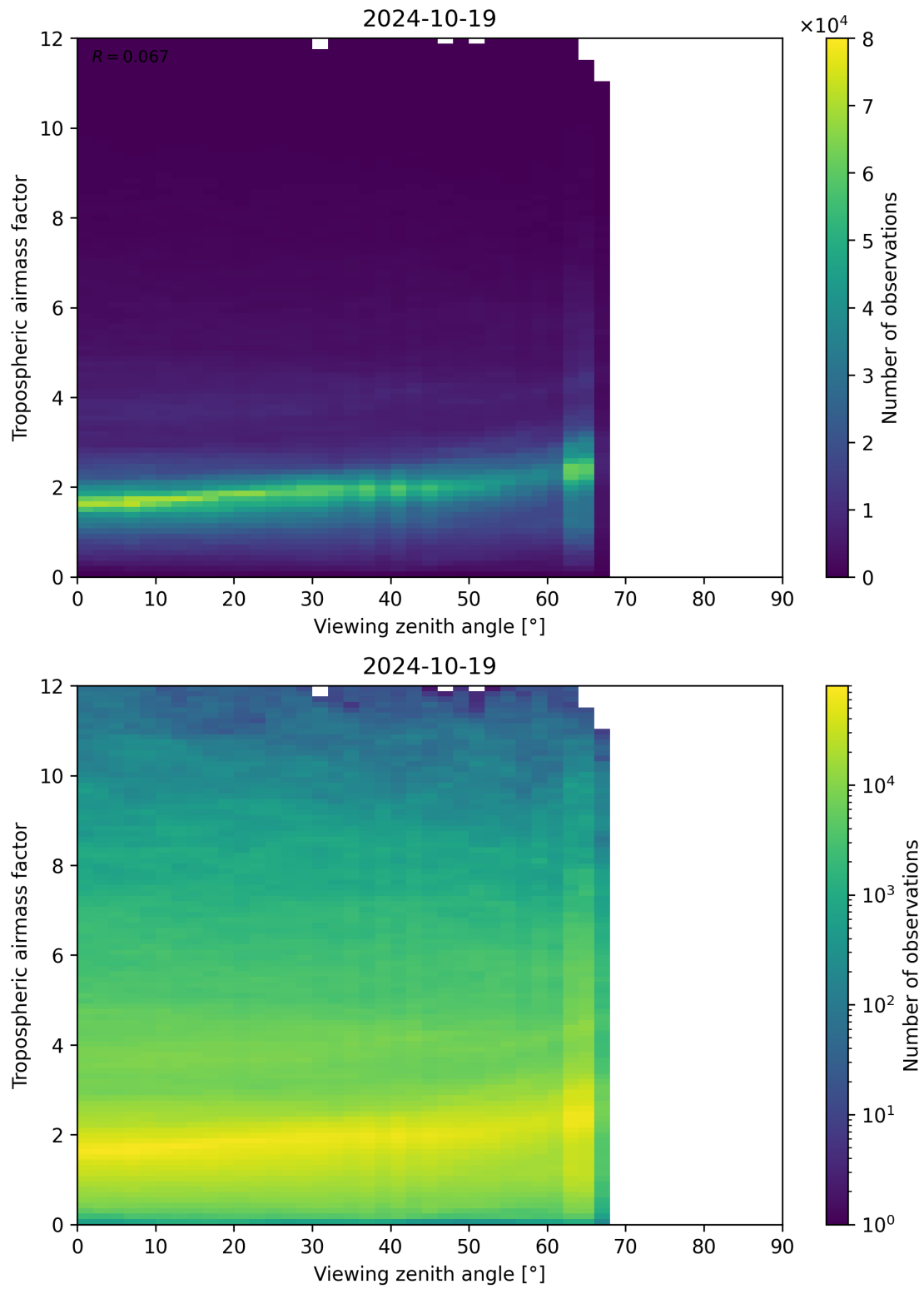
Figure 161: Scatter density plot of “Viewing zenith angle” against “Tropospheric airmass factor” for 2024-10-19 to 2024-10-20.
