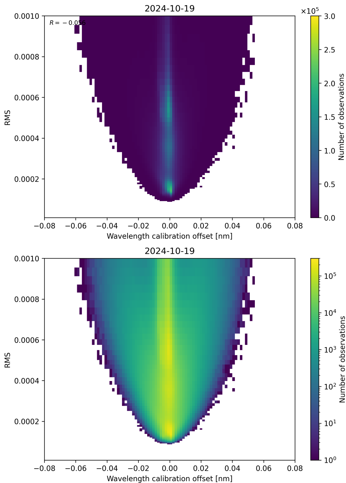
Figure 181: Scatter density plot of “Wavelength calibration offset” against “RMS” for 2024-10-19 to 2024-10-20.
