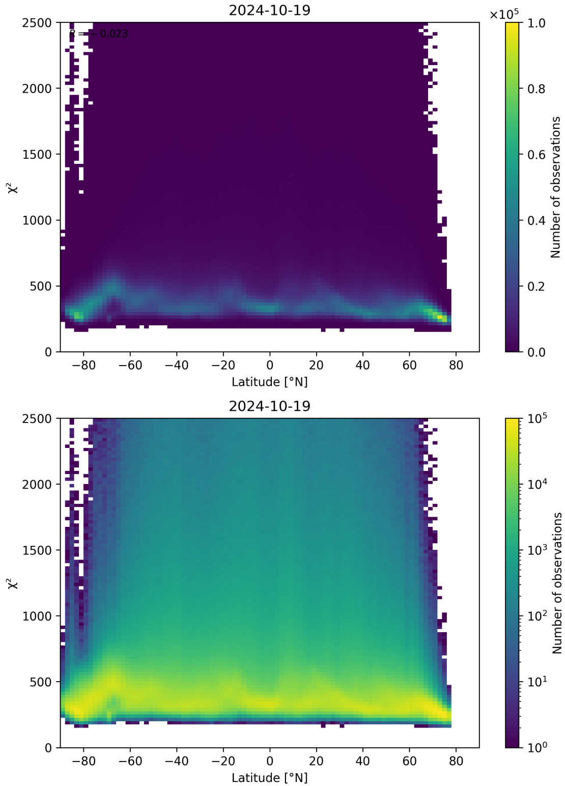
Figure 86: Scatter density plot of “Latitude” against “ \chi^2 ” for 2024-10-19 to 2024-10-20.
