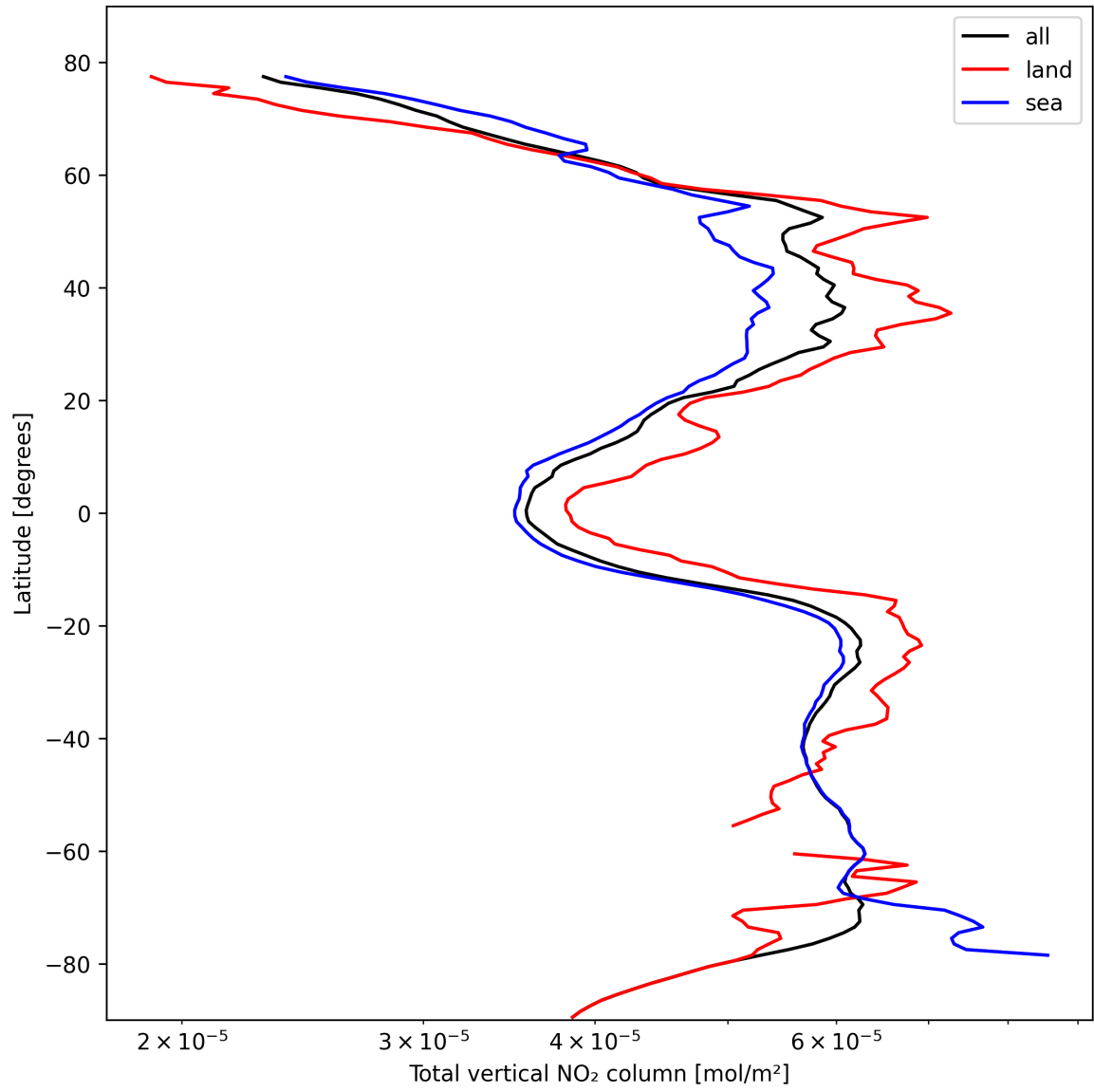
Figure 21: Zonal average of “Total vertical NO 2 column” for 2024-10-19 to 2024-10-20.
