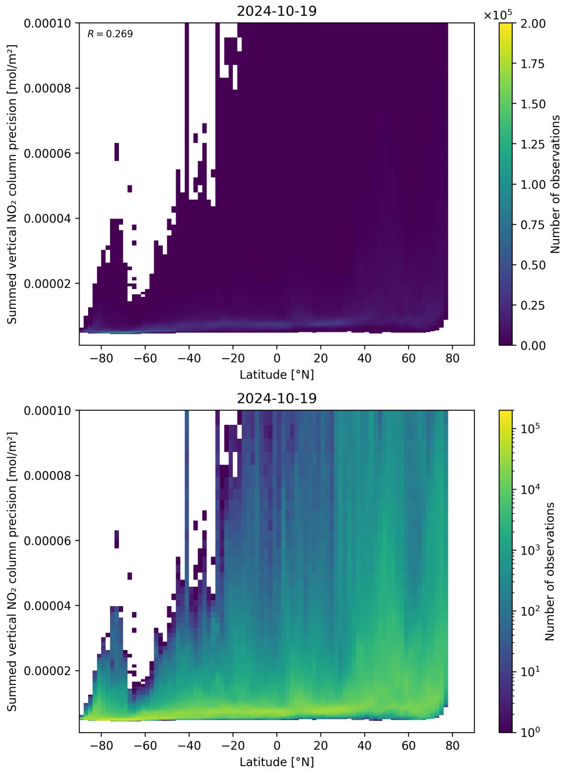
Figure 89: Scatter density plot of “Latitude” against “Summed vertical NO 2 column precision” for 2024-10-19 to 2024-10-20.
