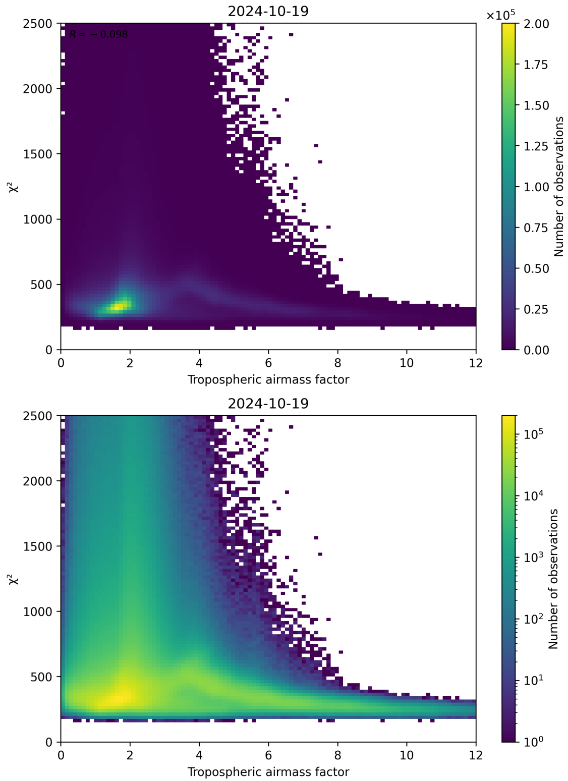
Figure 73: Scatter density plot of “Tropospheric airmass factor” against “ \chi^2 ” for 2024-10-19 to 2024-10-20.
