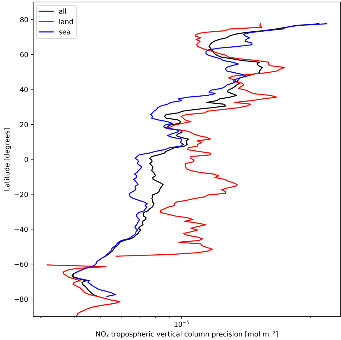
Figure 13: Zonal average of “NO 2 tropospheric vertical column precision” for 2024-10-19 to 2024-10-20.
