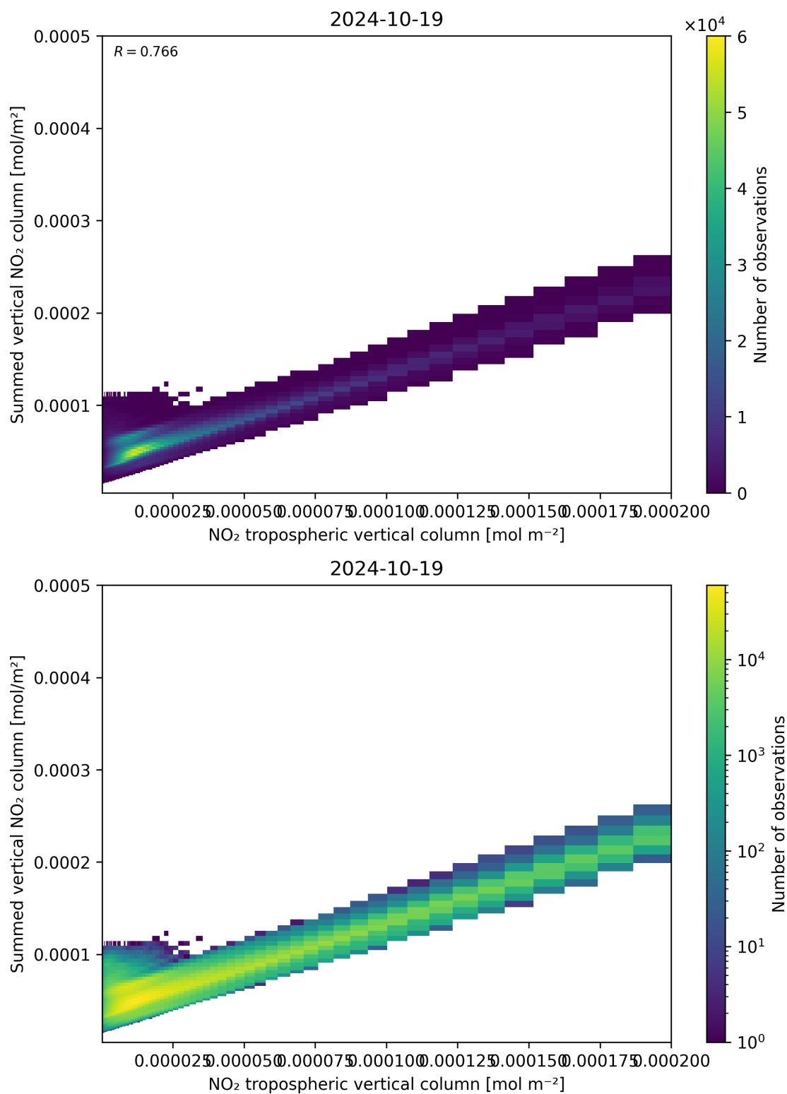
Figure 126: Scatter density plot of “NO 2 tropospheric vertical column” against “Summed vertical NO 2 column” for 2024-10-19 to 2024-10-20.
