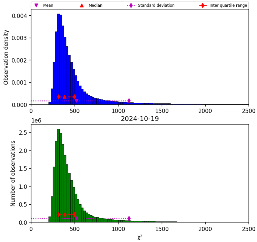
Figure 42: Histogram of “ \chi^2 ” for 2024-10-19 to 2024-10-20
