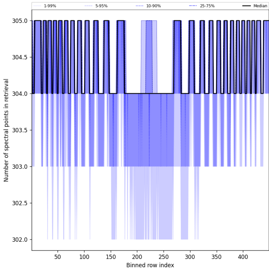
Figure 50: Along track statistics of “Number of spectral points in retrieval” for 2024-10-19 to 2024-10-20
