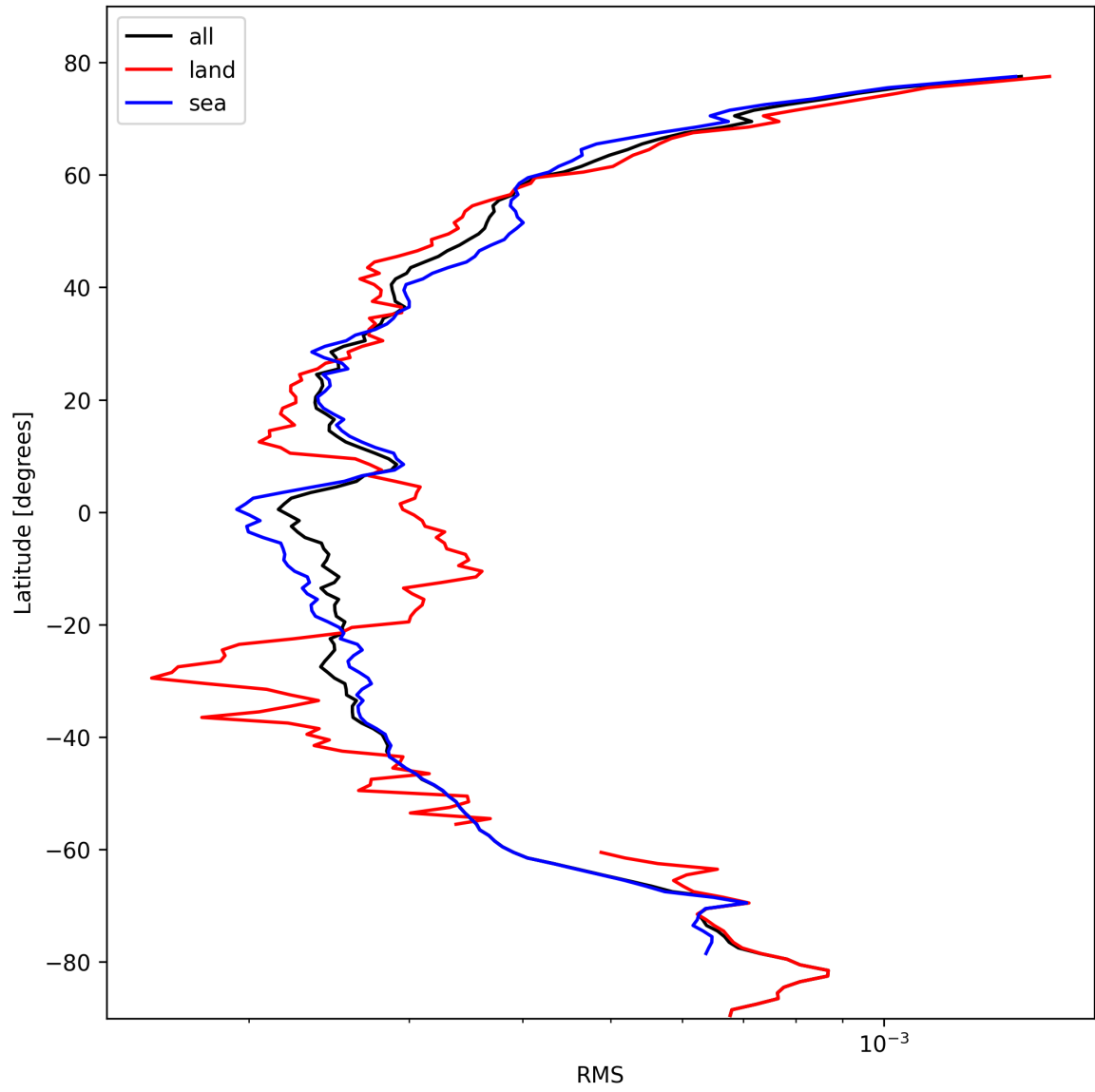
Figure 26: Zonal average of “RMS” for 2024-10-19 to 2024-10-20.
