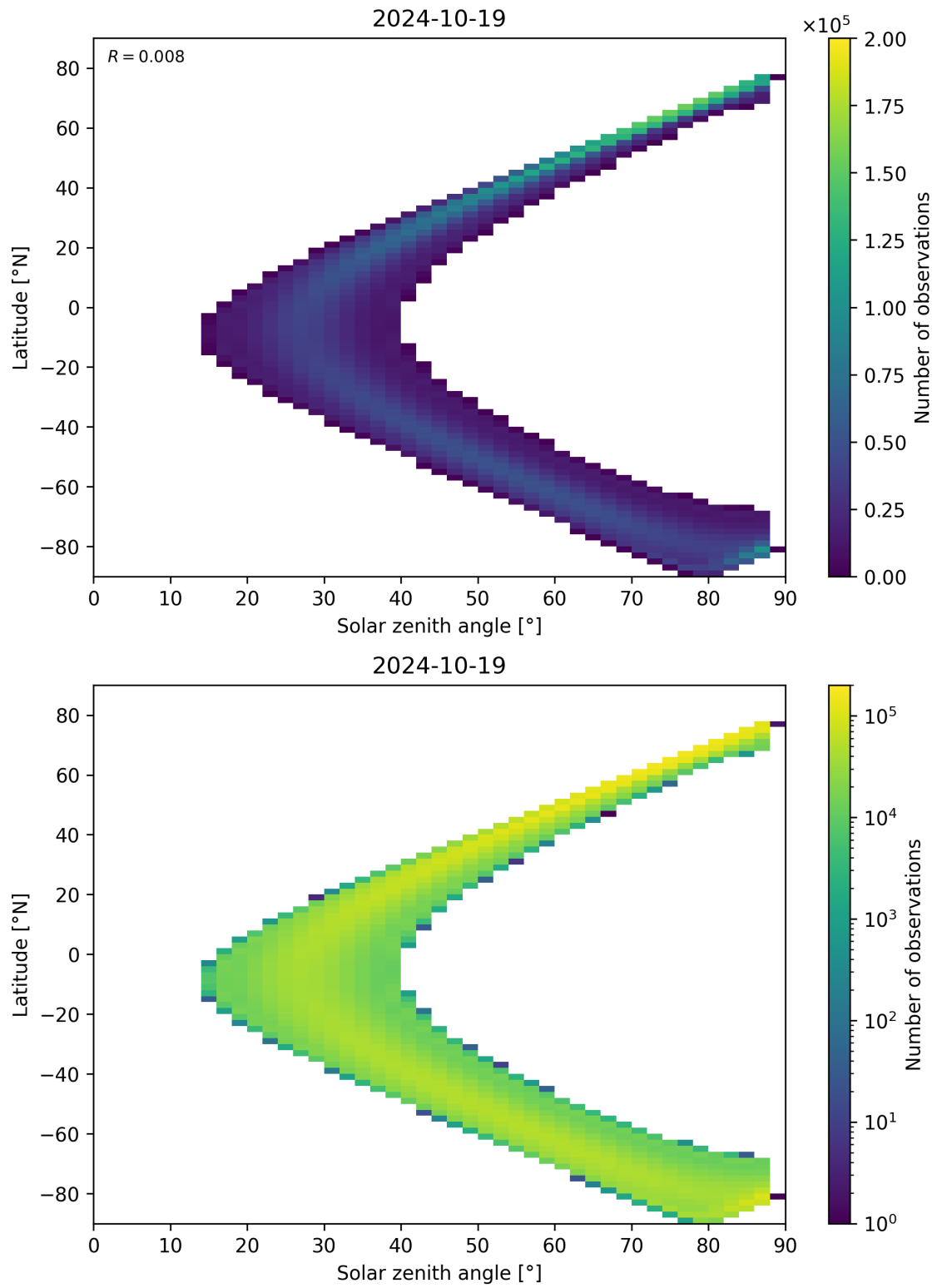
Figure 149: Scatter density plot of “Solar zenith angle” against “Latitude” for 2024-10-19 to 2024-10-20.
