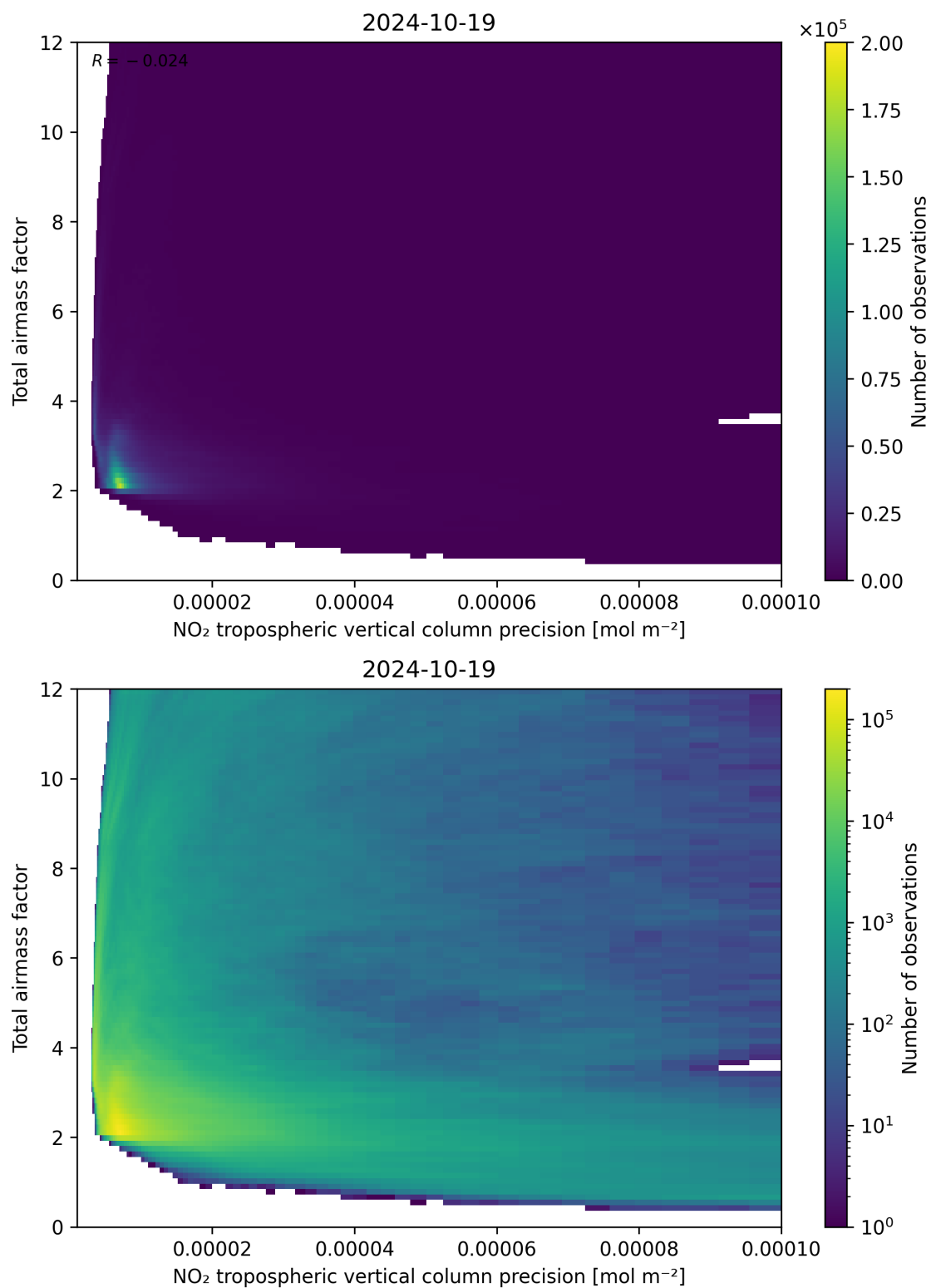
Figure 132: Scatter density plot of “NO 2 tropospheric vertical column precision” against “Total air mass factor” for 2024-10-19 to 2024-10-20.
