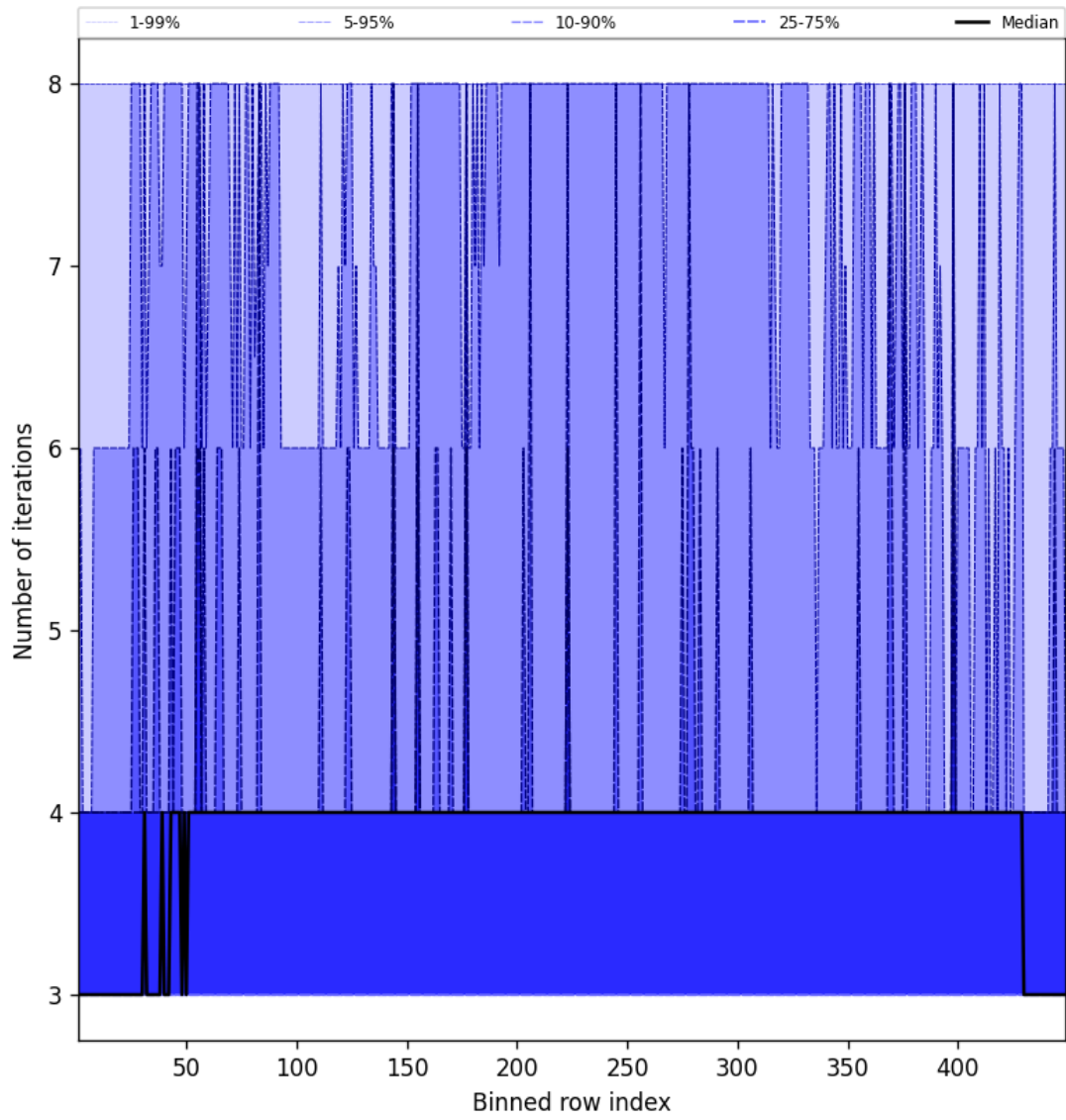
Figure 51: Along track statistics of “Number of iterations” for 2024-10-19 to 2024-10-20
