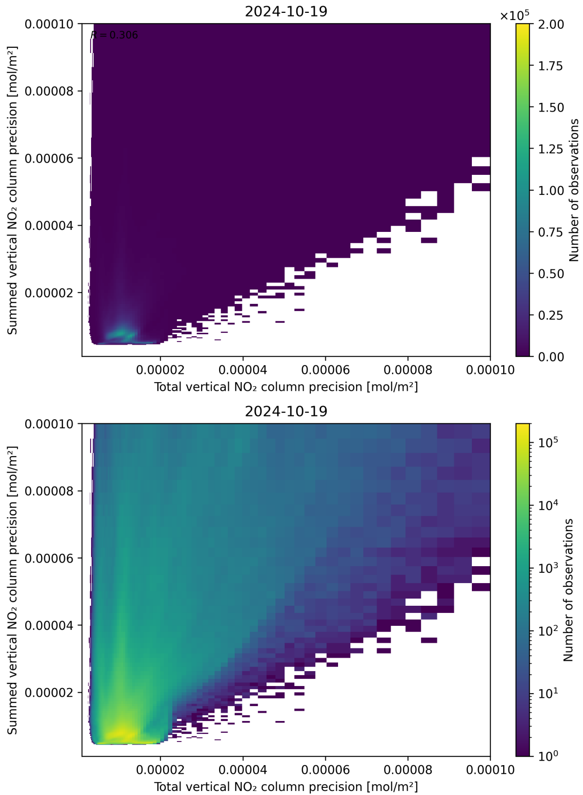
Figure 118: Scatter density plot of “Total vertical NO 2 column precision” against “Summed vertical NO 2 column precision” for 2024-10-19 to 2024-10-20.
