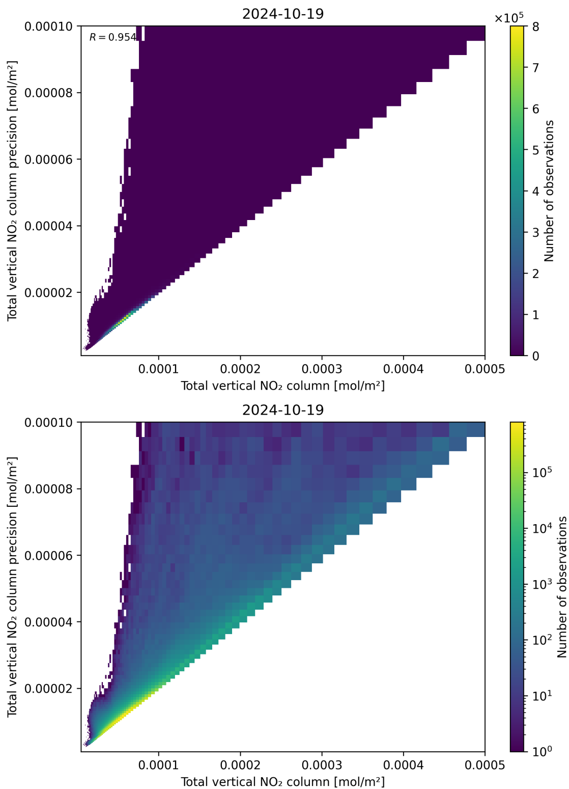
Figure 114: Scatter density plot of “Total vertical NO 2 column” against “Total vertical NO 2 column precision” for 2024-10-19 to 2024-10-20.
