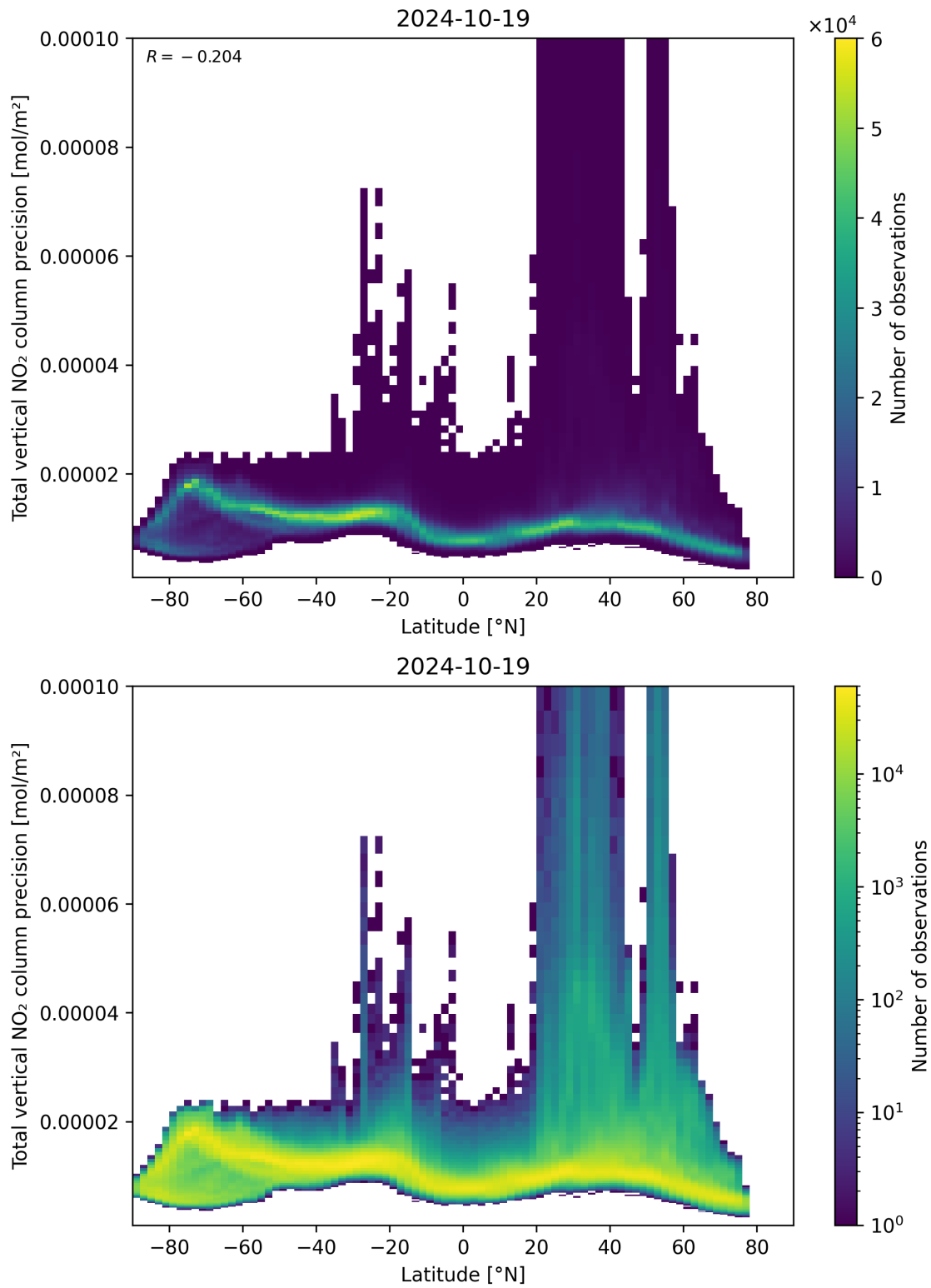
Figure 91: Scatter density plot of “Latitude” against “Total vertical NO 2 column precision” for 2024-10-19 to 2024-10-20.
