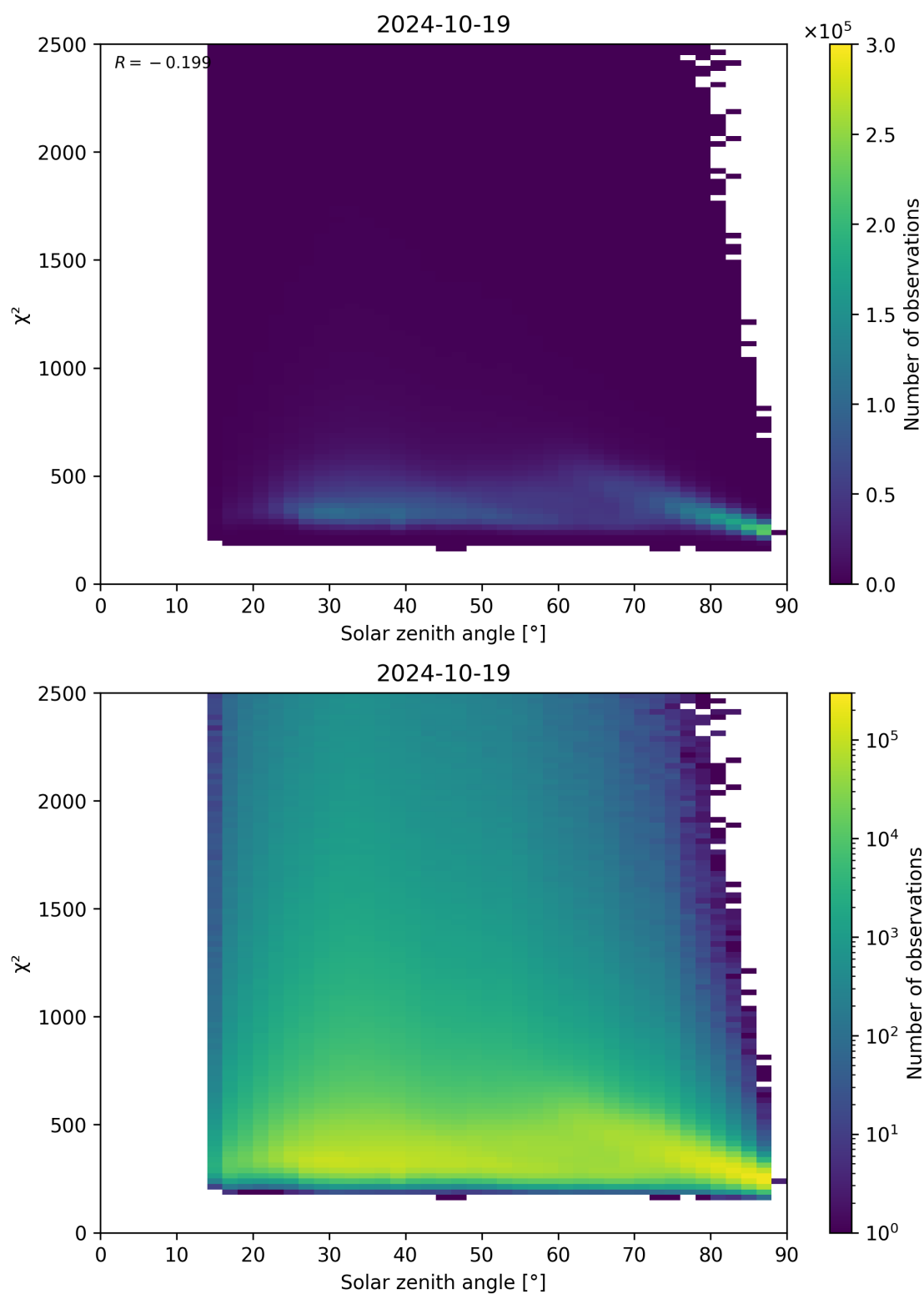
Figure 148: Scatter density plot of “Solar zenith angle” against “ \chi^2 ” for 2024-10-19 to 2024-10-20.
