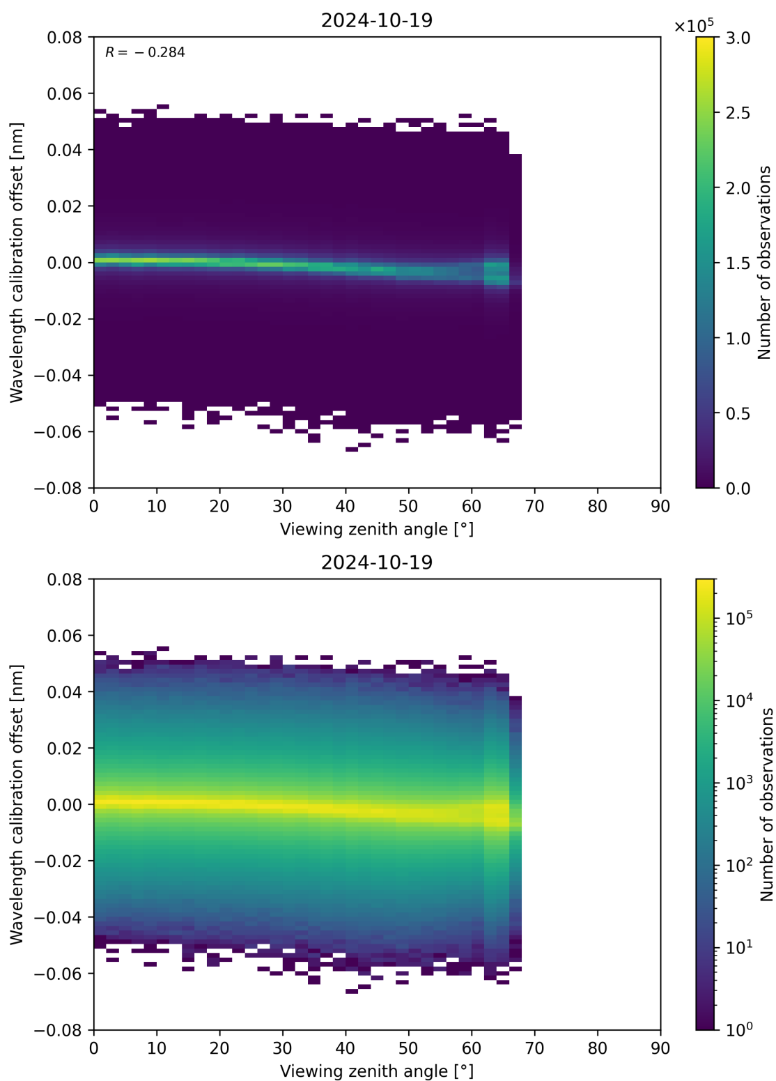
Figure 173: Scatter density plot of “Viewing zenith angle” against “Wavelength calibration offset” for 2024-10-19 to 2024-10-20.
