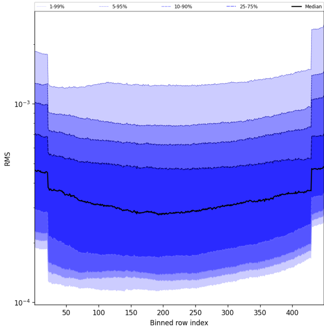
Figure 60: Along track statistics of “RMS” for 2024-10-19 to 2024-10-20
