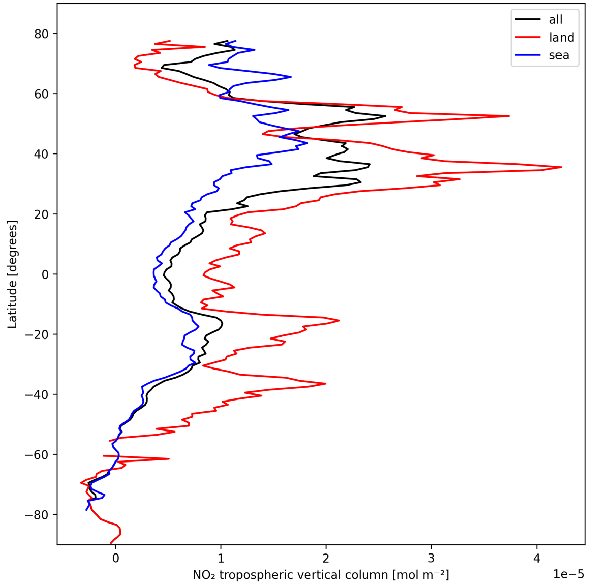
Figure 12: Zonal average of “NO 2 tropospheric vertical column” for 2024-10-19 to 2024-10-20.
