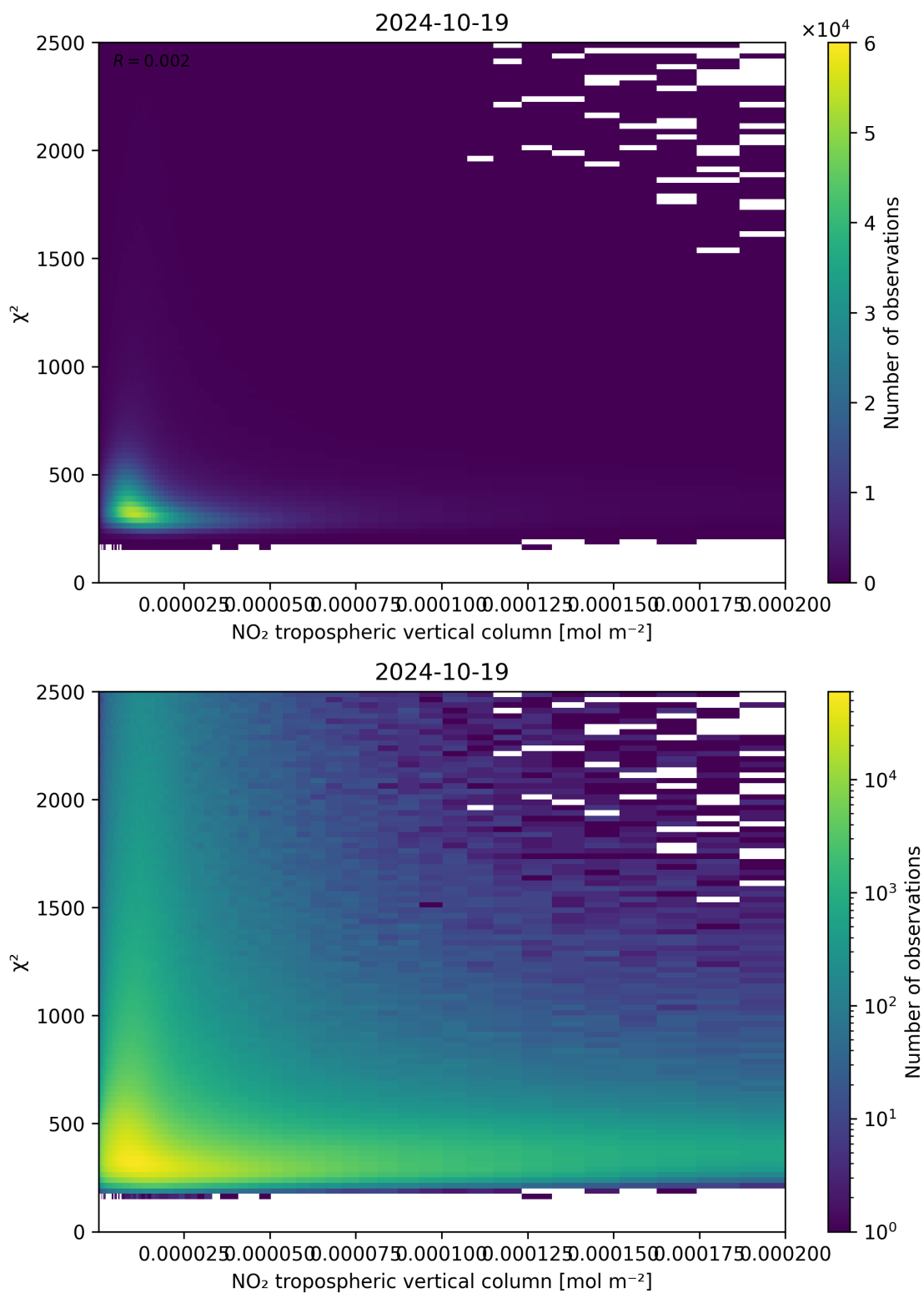
Figure 124: Scatter density plot of “NO 2 tropospheric vertical column” against “ \chi^2 ” for 2024-10-19 to 2024-10-20.
