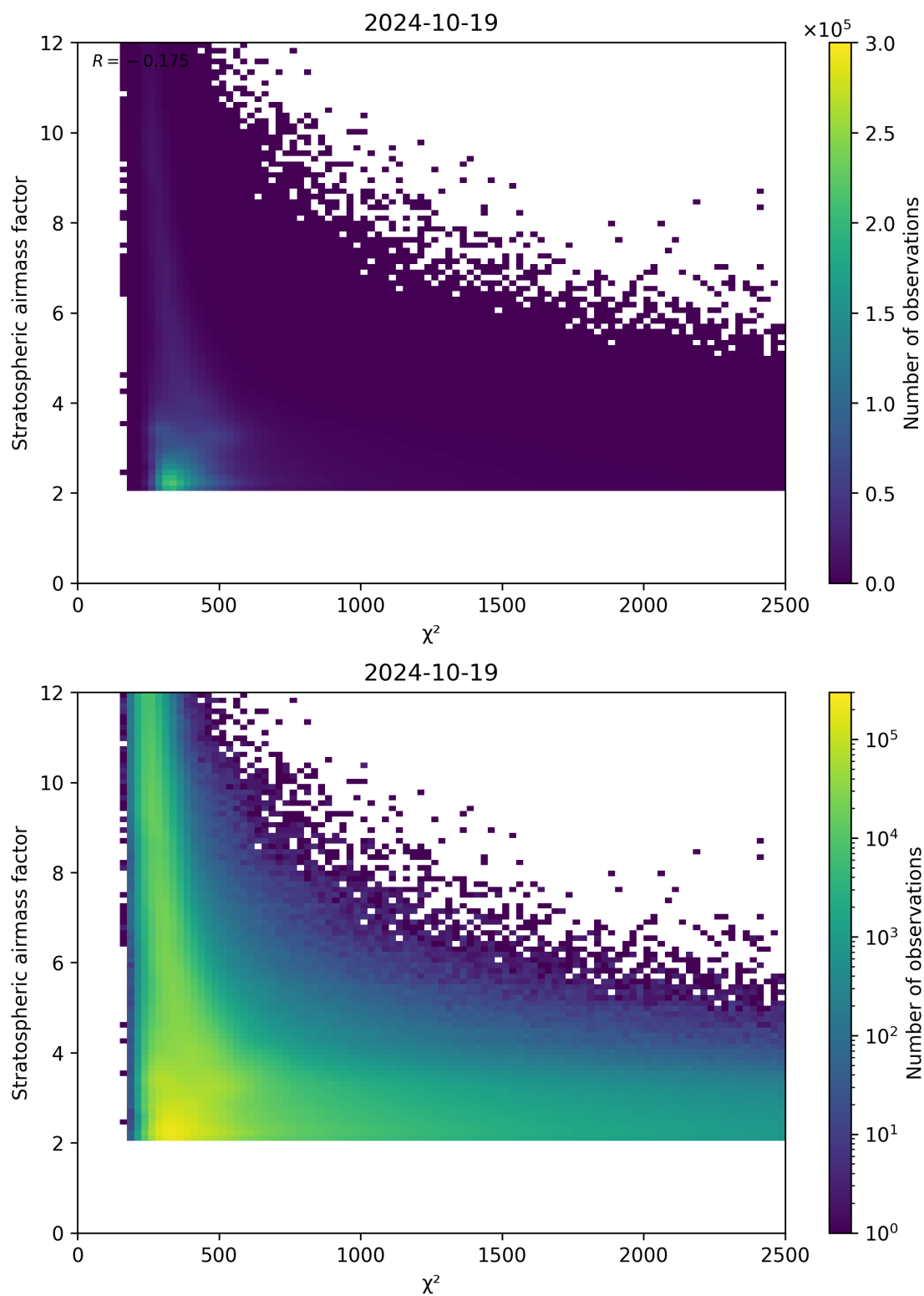
Figure 81: Scatter density plot of “ \chi^2 ” against “Stratospheric airmass factor” for 2024-10-19 to 2024-10-20.
