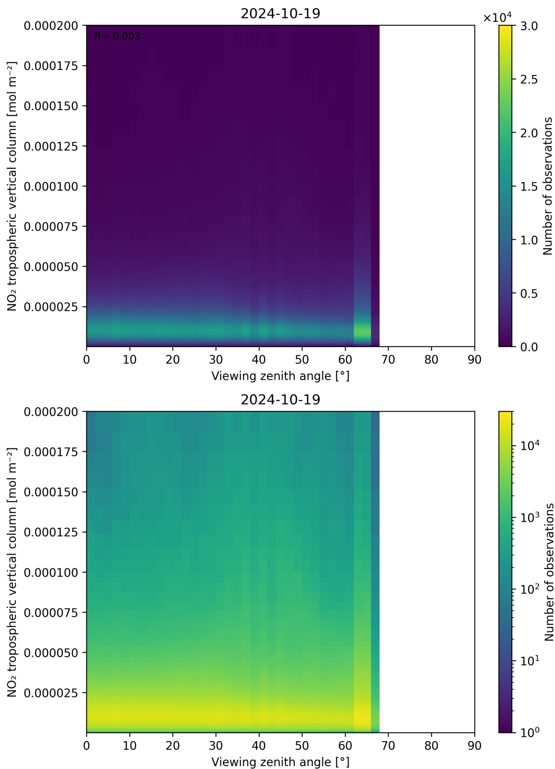
Figure 169: Scatter density plot of “Viewing zenith angle” against “NO 2 tropospheric vertical column” for 2024-10-19 to 2024-10-20.
