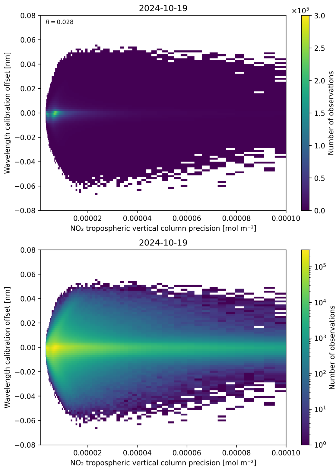
Figure 141: Scatter density plot of “NO 2 tropospheric vertical column precision” against “Wavelength calibration offset” for 2024-10-19 to 2024-10-20.
