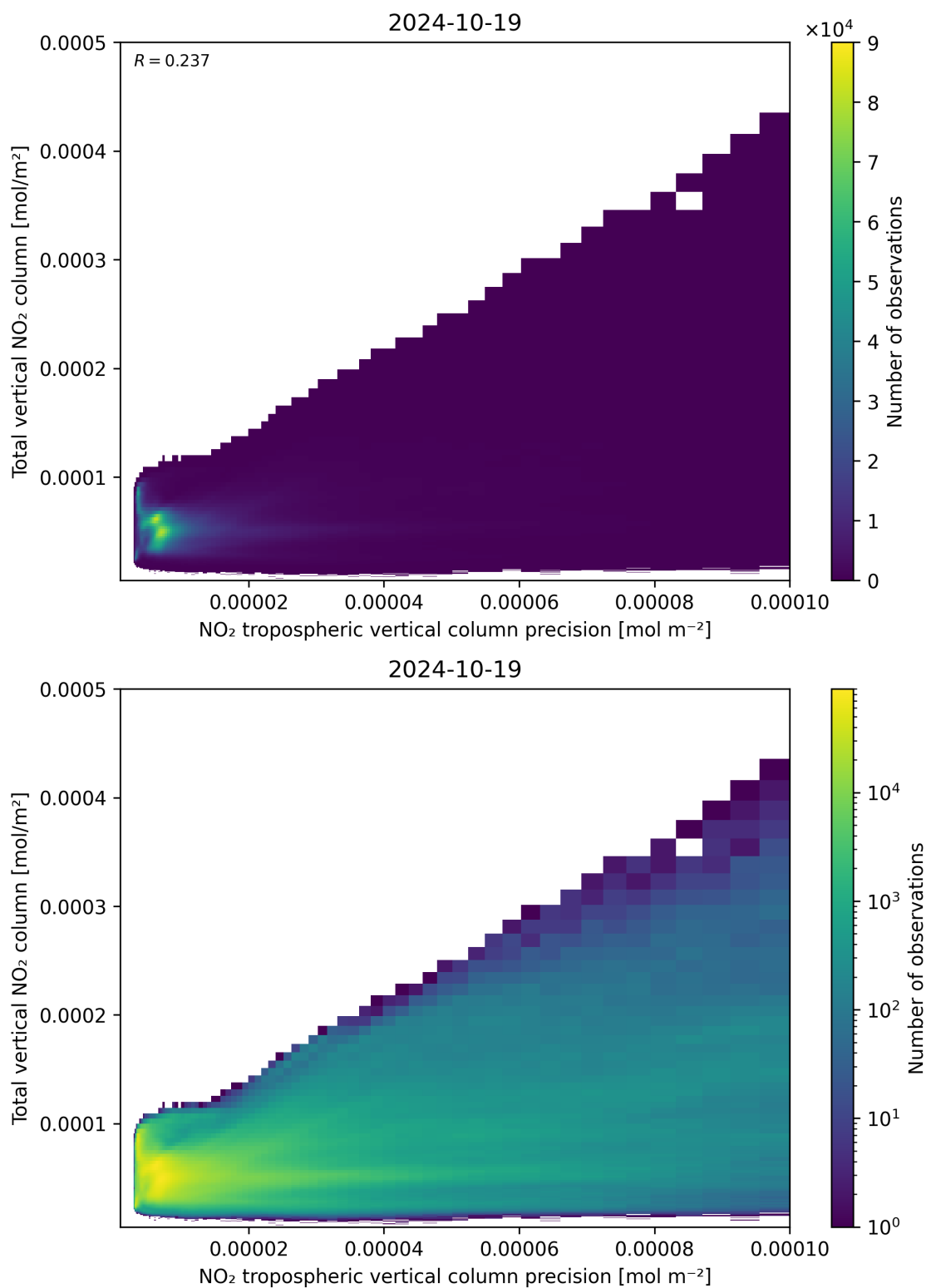
Figure 138: Scatter density plot of “NO 2 tropospheric vertical column precision” against “Total vertical NO 2 column” for 2024-10-19 to 2024-10-20.
