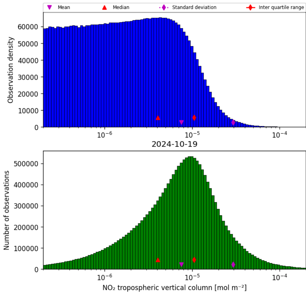
Figure 29: Histogram of “NO 2 tropospheric vertical column” for 2024-10-19 to 2024-10-20
