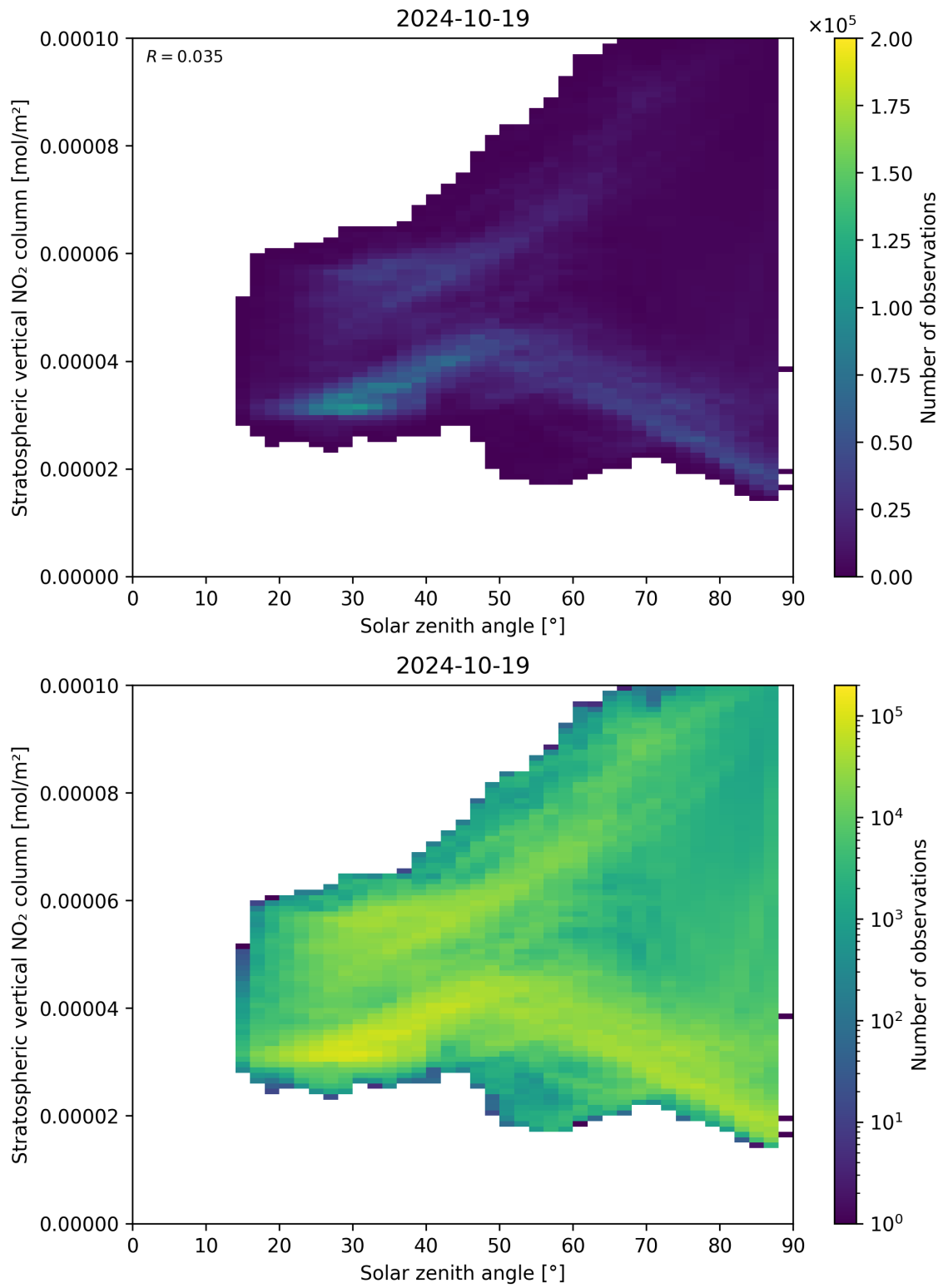
Figure 150: Scatter density plot of “Solar zenith angle” against “Stratospheric vertical NO 2 column” for 2024-10-19 to 2024-10-20.
