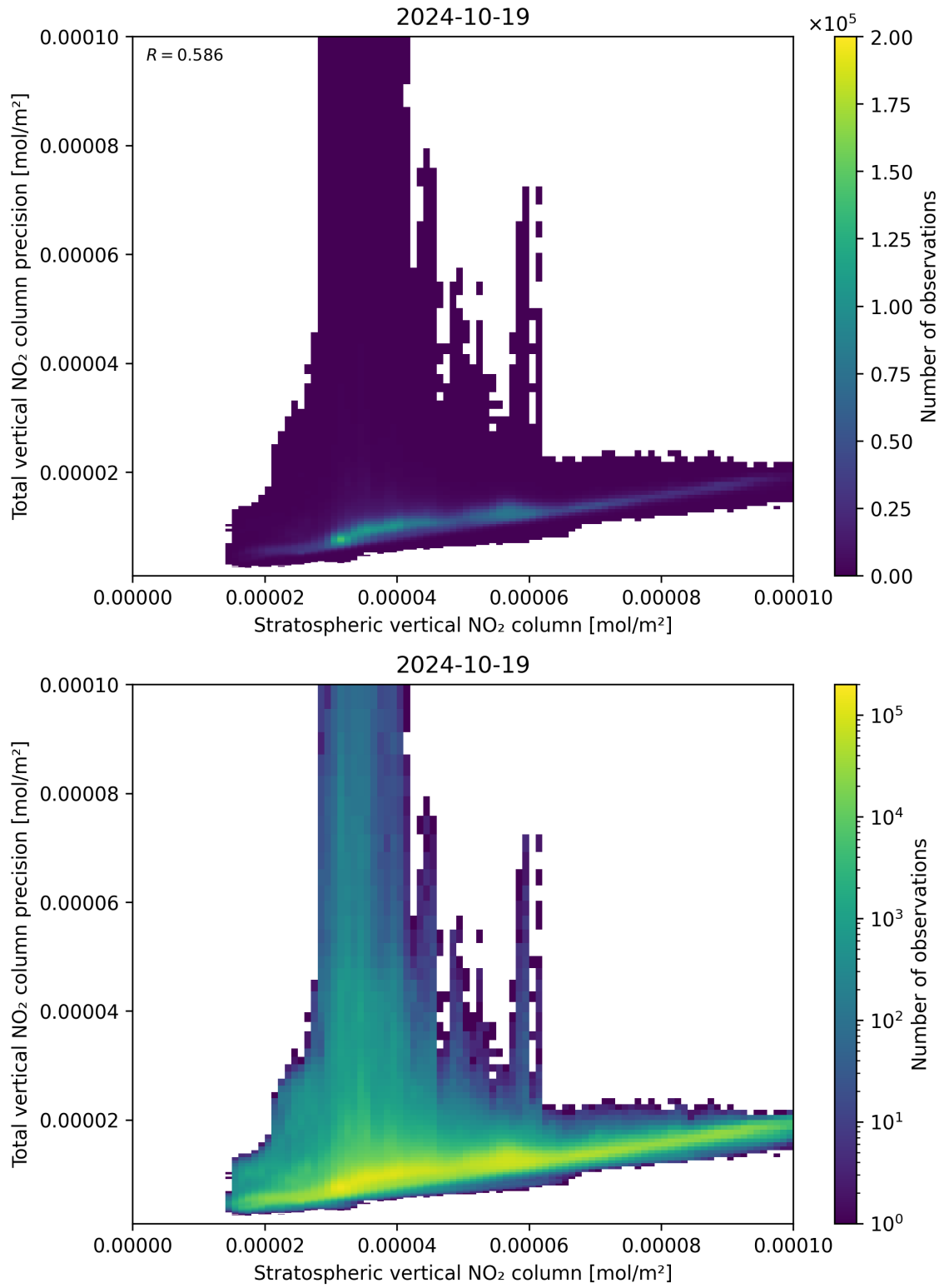
Figure 101: Scatter density plot of “Stratospheric vertical NO 2 column” against “Total vertical NO 2 column precision” for 2024-10-19 to 2024-10-20.
