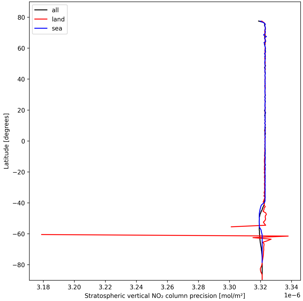
Figure 20: Zonal average of “Stratospheric vertical NO 2 column precision” for 2024-10-19 to 2024-10-20.
