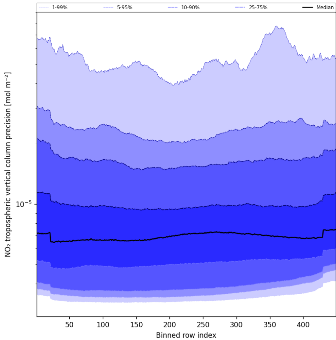
Figure 47: Along track statistics of “NO 2 tropospheric vertical column precision” for 2024-10-19 to 2024-10-20
