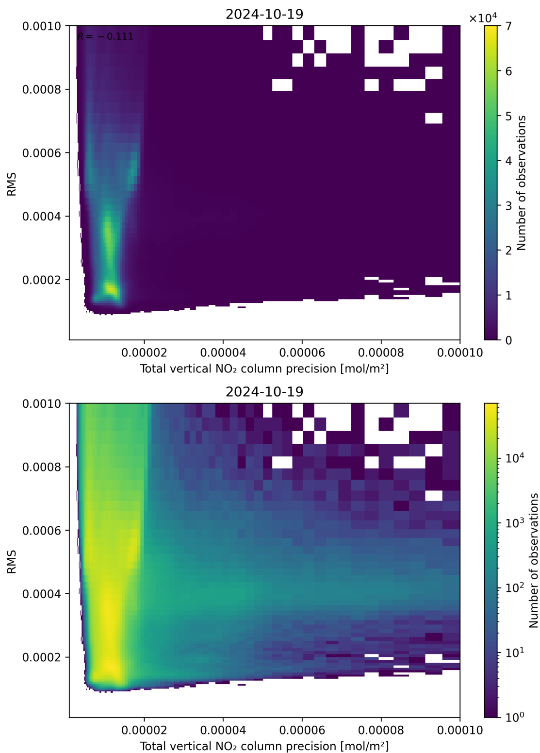
Figure 119: Scatter density plot of “Total vertical NO 2 column precision” against “RMS” for 2024-10-19 to 2024-10-20.
