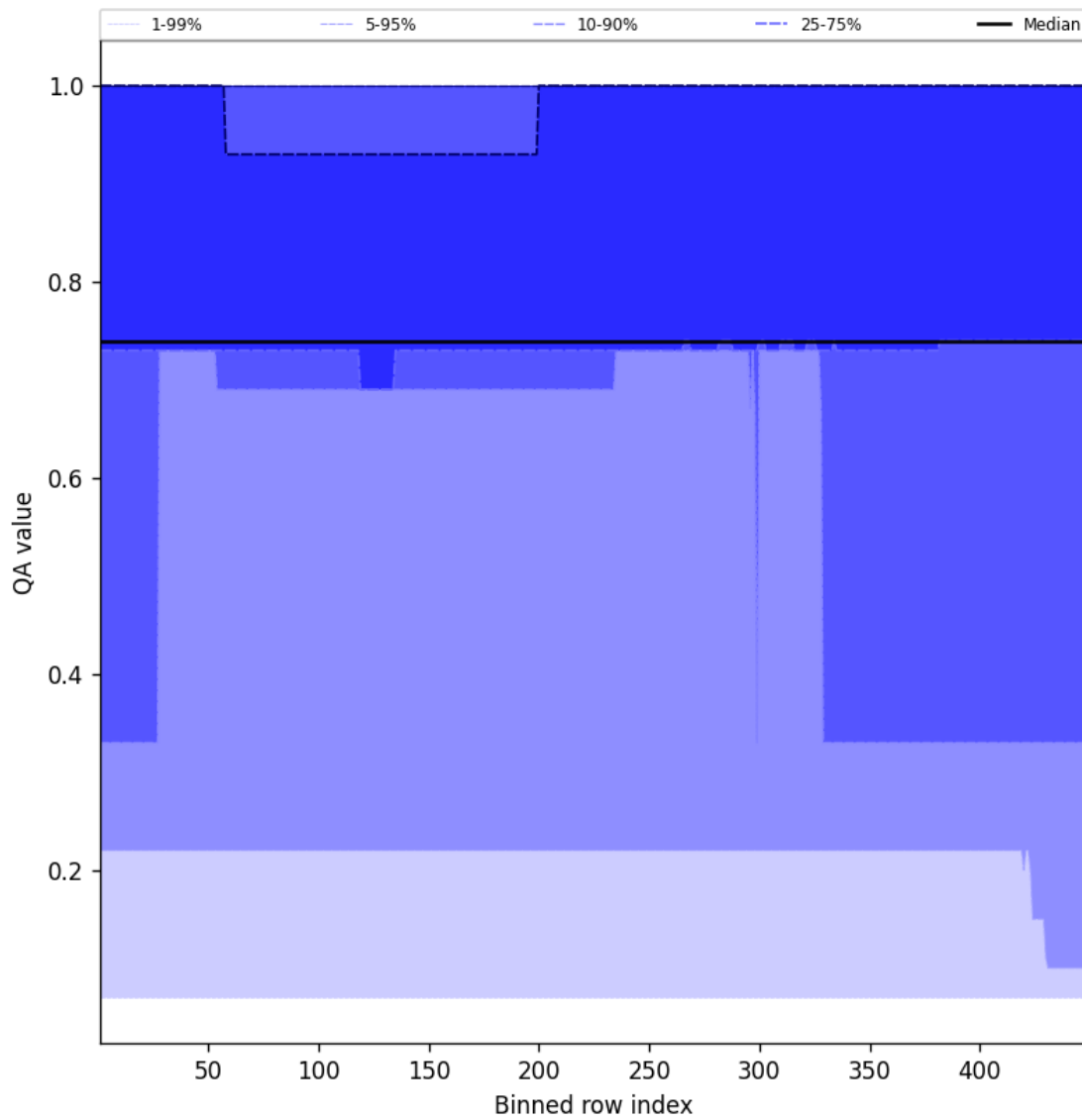
Figure 45: Along track statistics of “QA value” for 2024-10-19 to 2024-10-20
