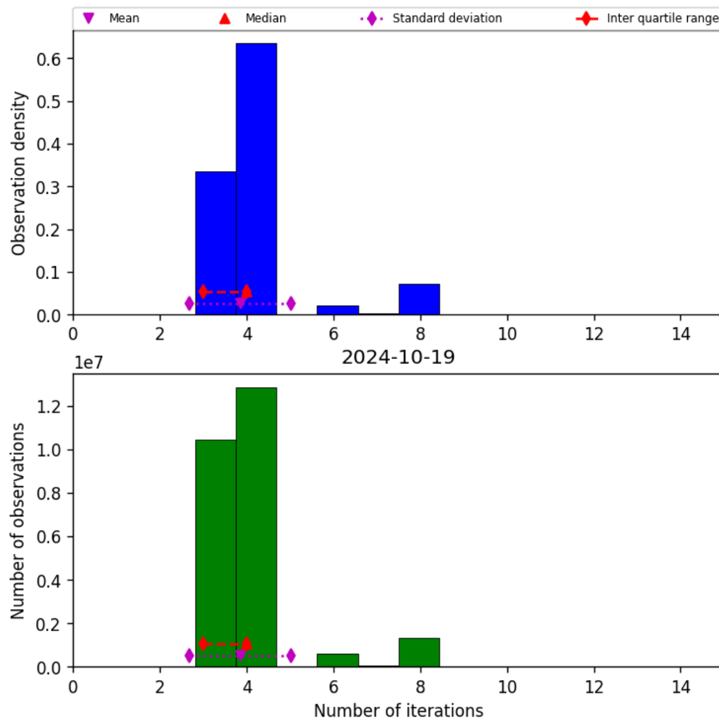
Figure 34: Histogram of “Number of iterations” for 2024-10-19 to 2024-10-20
