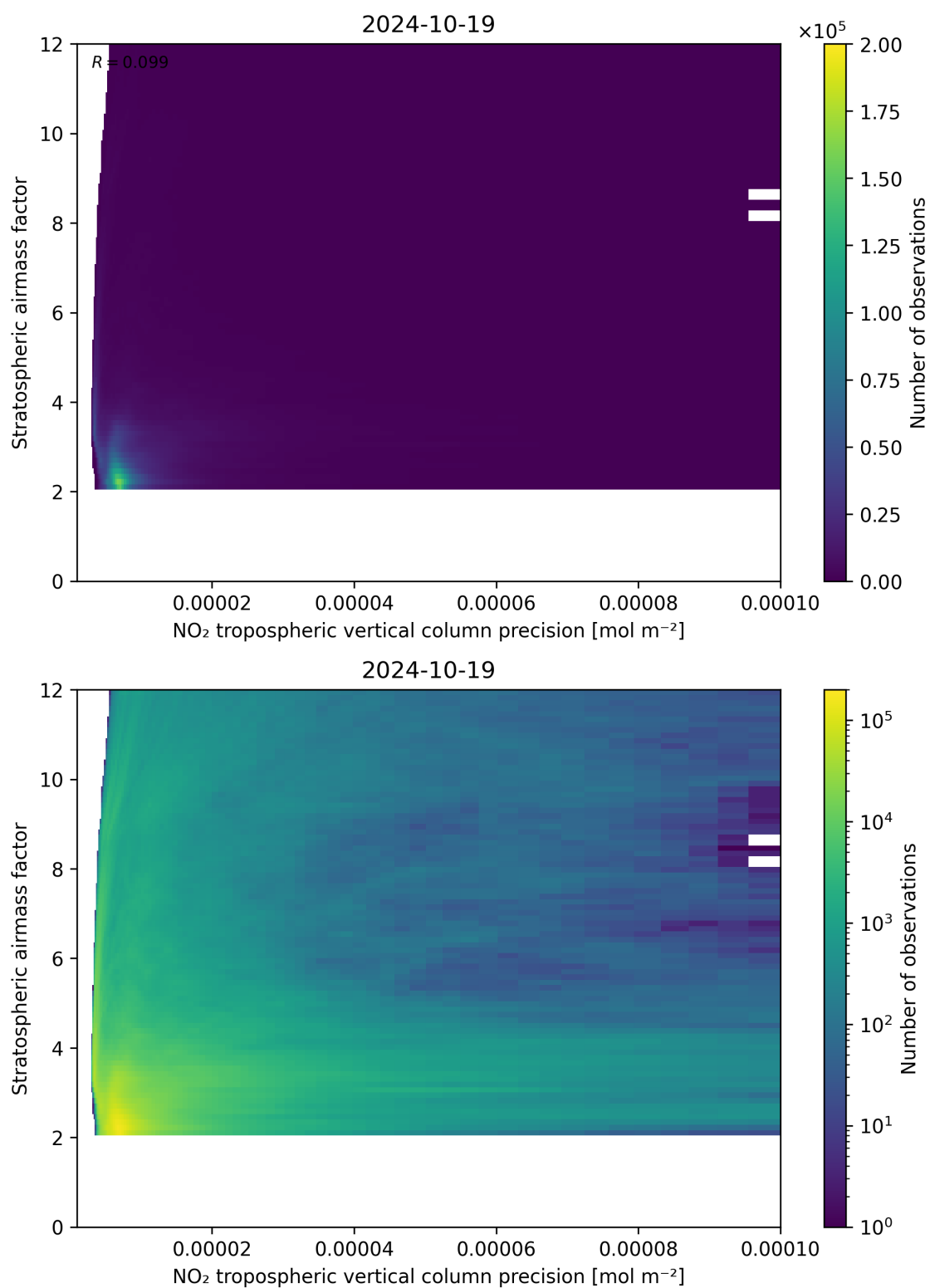
Figure 131: Scatter density plot of “NO 2 tropospheric vertical column precision” against “Stratospheric airmass factor” for 2024-10-19 to 2024-10-20.
