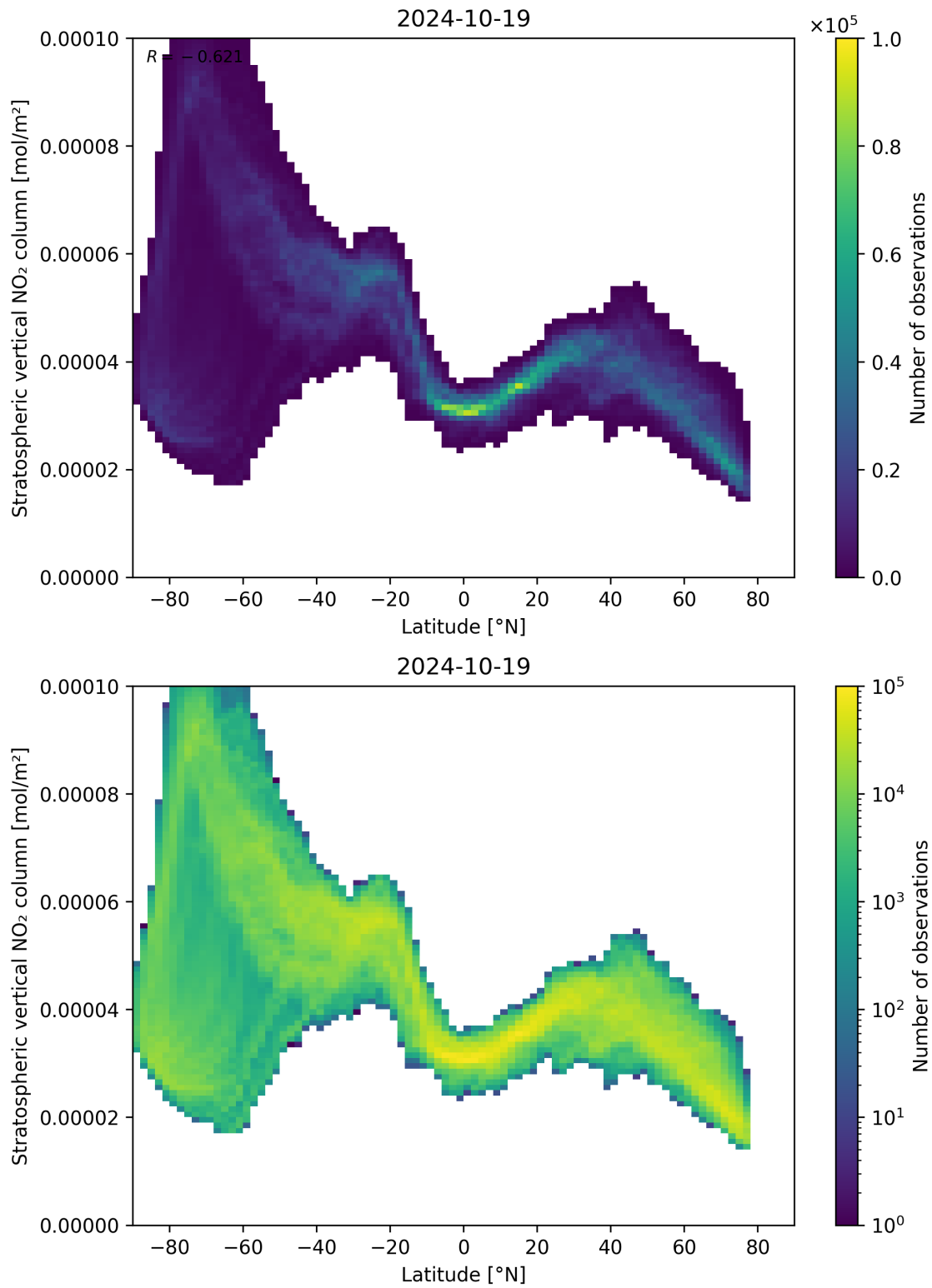
Figure 87: Scatter density plot of “Latitude” against “Stratospheric vertical NO 2 column” for 2024-10-19 to 2024-10-20.
