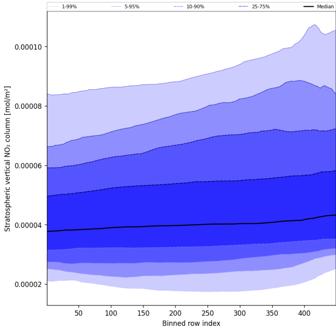
Figure 53: Along track statistics of “Stratospheric vertical NO 2 column” for 2024-10-19 to 2024-10-20
