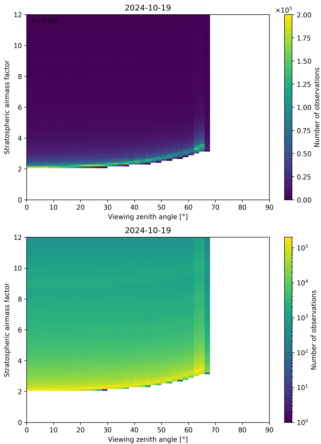
Figure 159: Scatter density plot of “Viewing zenith angle” against “Stratospheric airmass factor” for 2024-10-19 to 2024-10-20.
