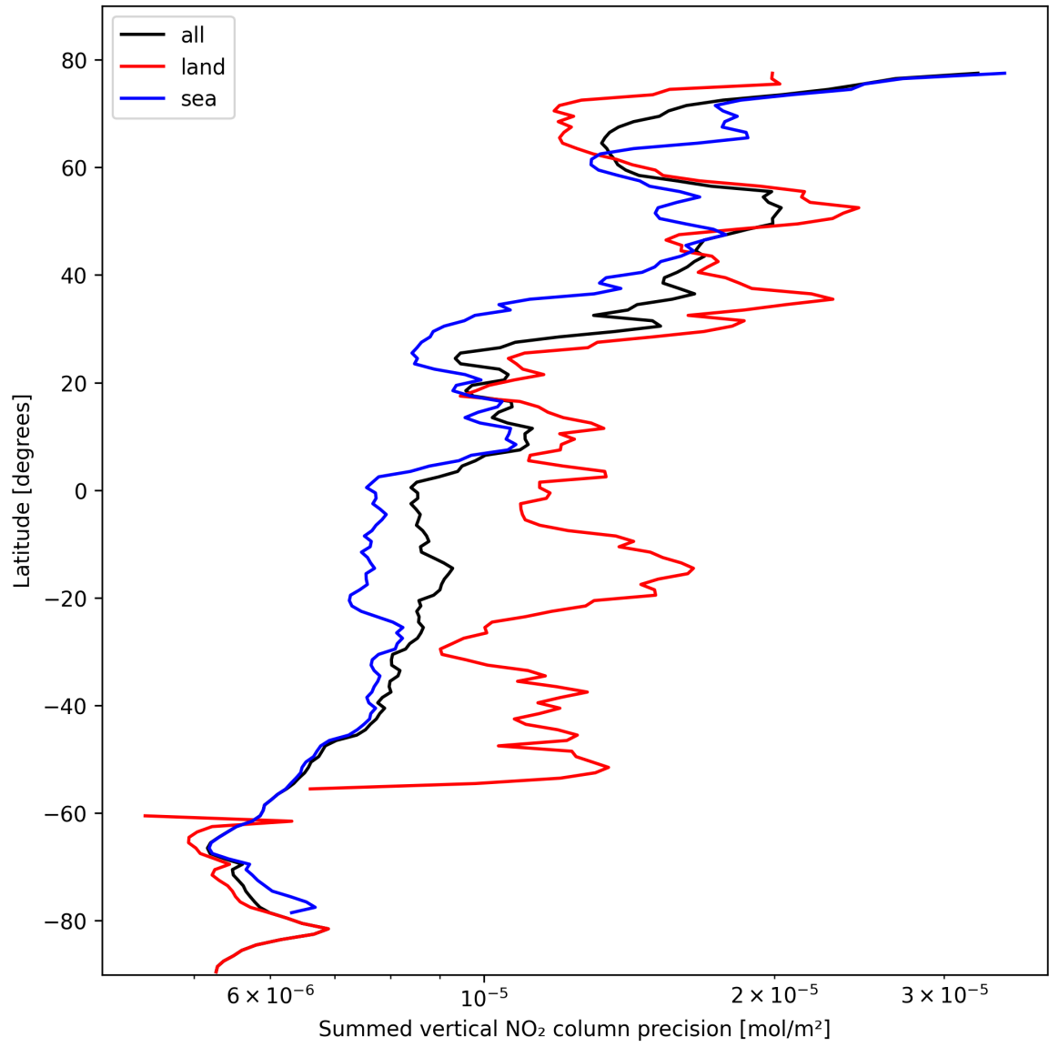
Figure 24: Zonal average of “Summed vertical NO 2 column precision” for 2024-10-19 to 2024-10-20.
