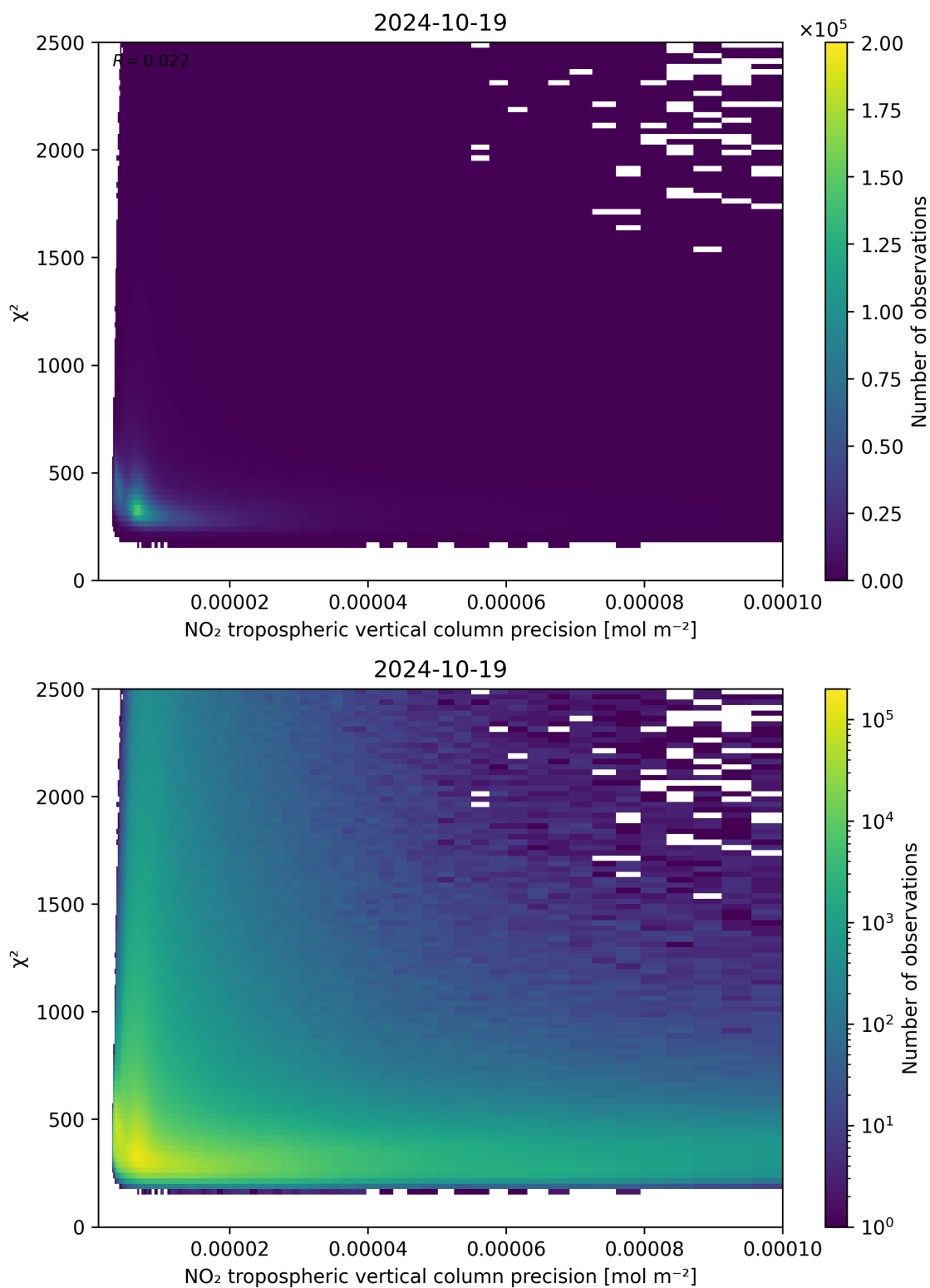
Figure 134: Scatter density plot of “NO 2 tropospheric vertical column precision” against “ \chi^2 ” for 2024-10-19 to 2024-10-20.
