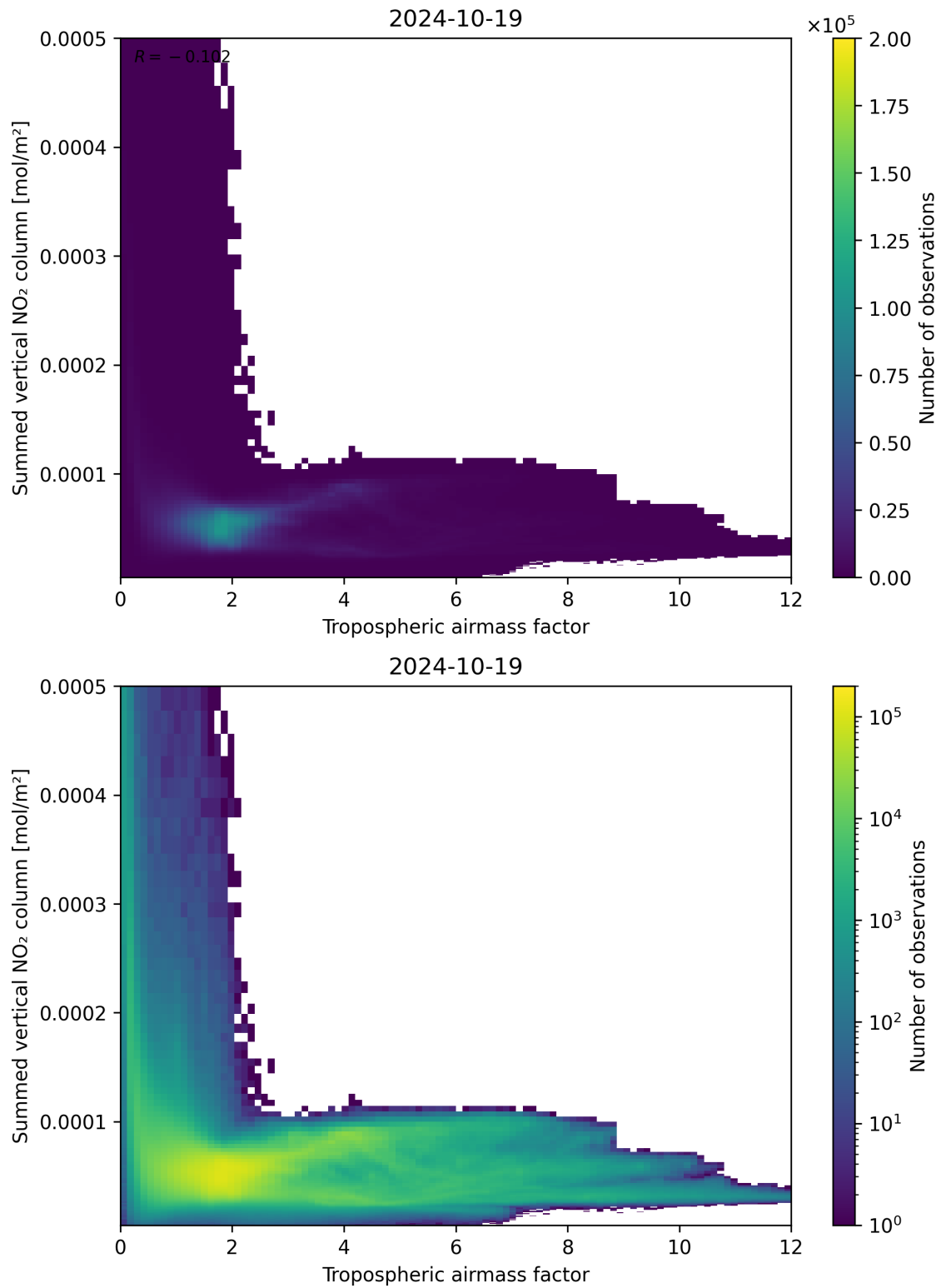
Figure 75: Scatter density plot of “Tropospheric airmass factor” against “Summed vertical NO 2 column” for 2024-10-19 to 2024-10-20.
