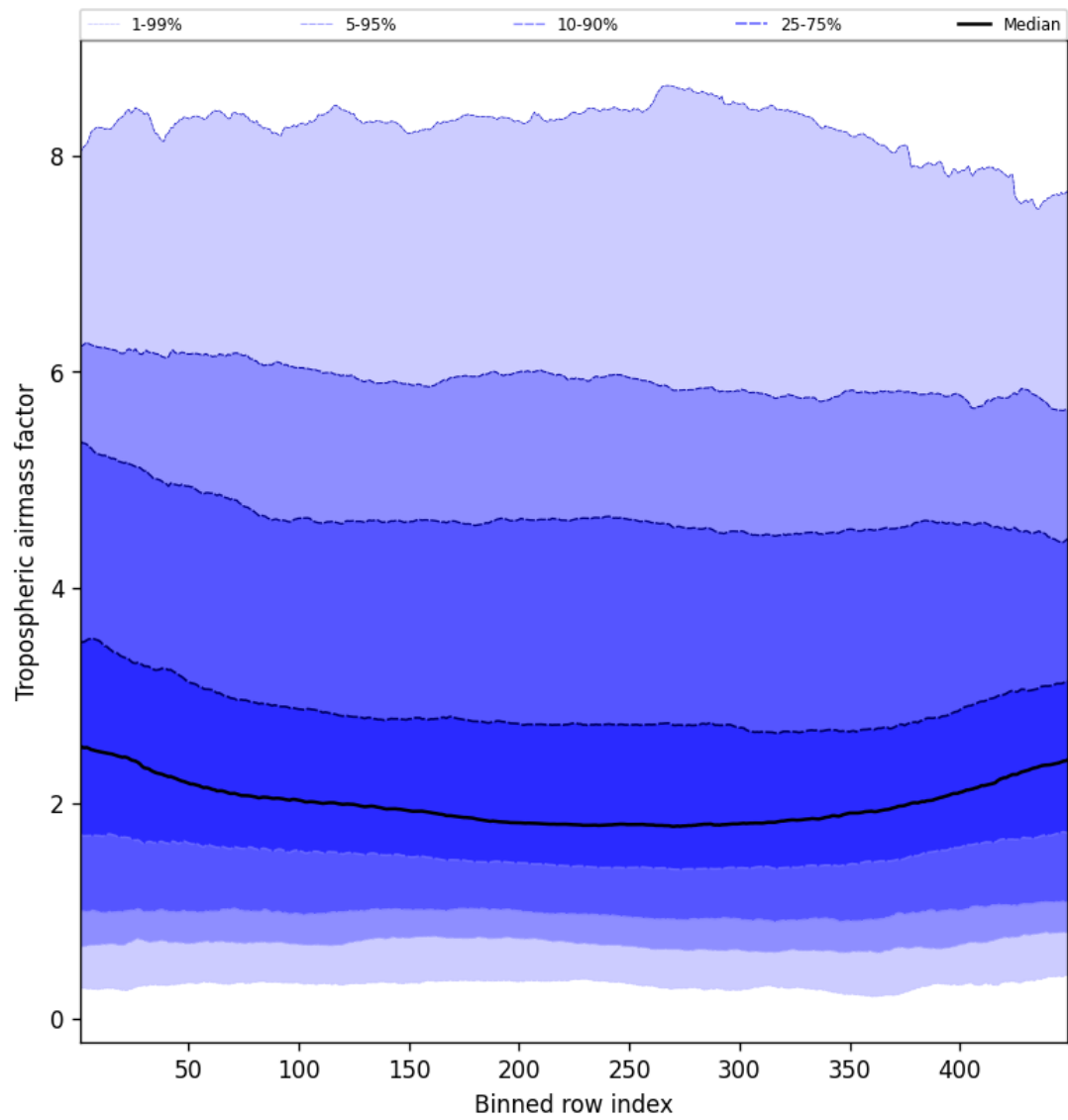
Figure 48: Along track statistics of “Tropospheric air mass factor” for 2024-10-19 to 2024-10-20
