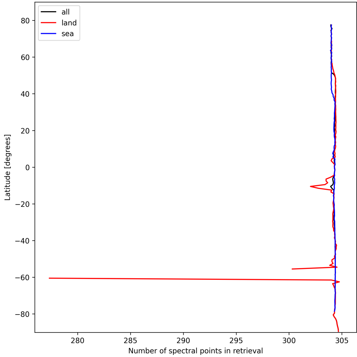
Figure 16: Zonal average of “Number of spectral points in retrieval” for 2024-10-19 to 2024-10-20.
