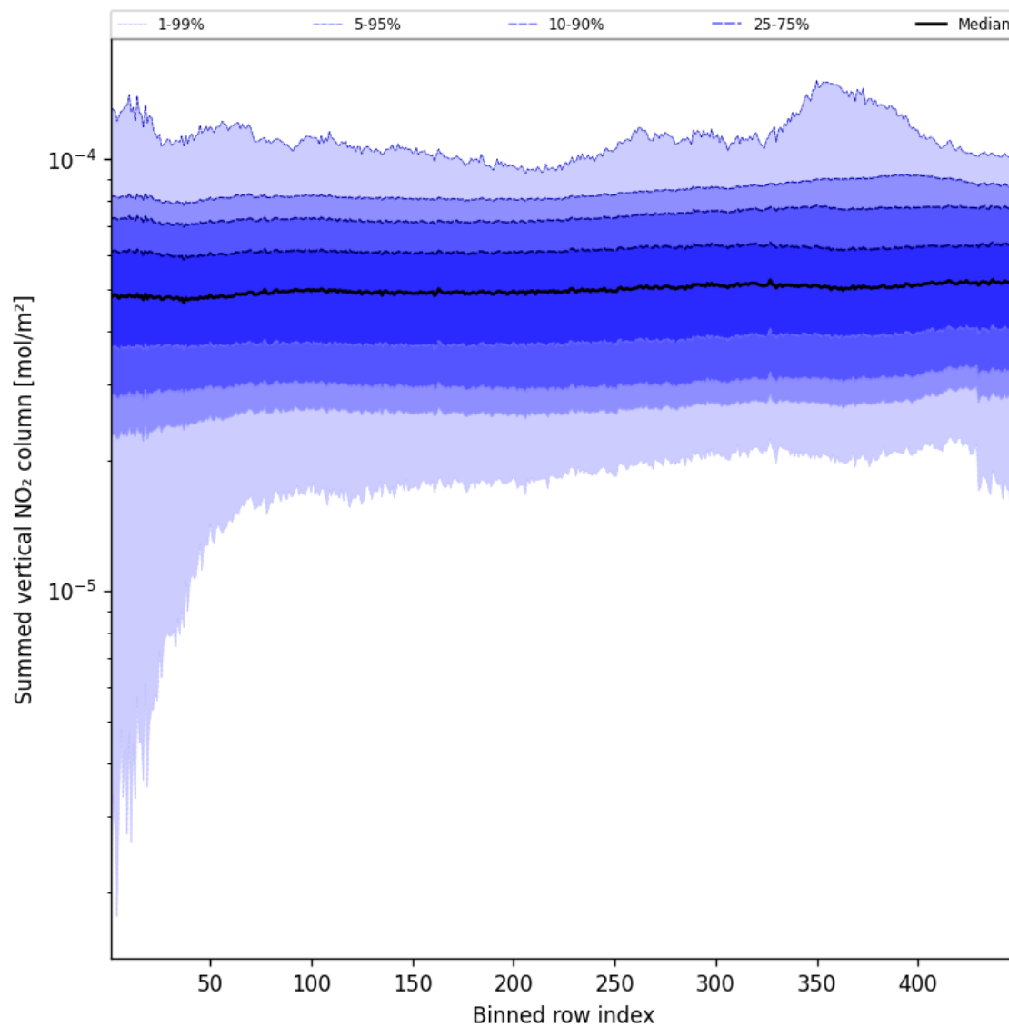
Figure 57: Along track statistics of “Summed vertical NO 2 column” for 2024-10-19 to 2024-10-20
