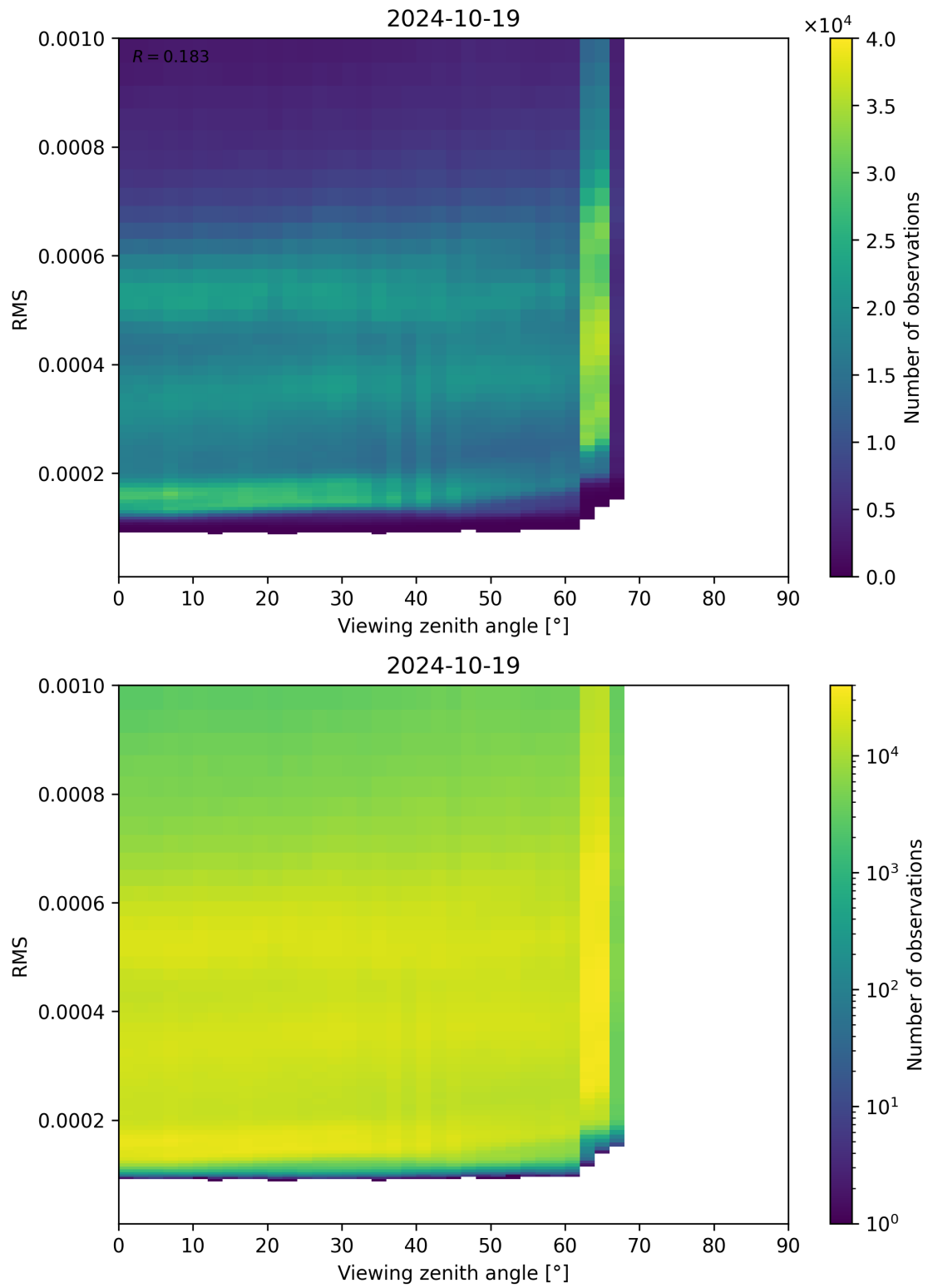
Figure 171: Scatter density plot of “Viewing zenith angle” against “RMS” for 2024-10-19 to 2024-10-20.
