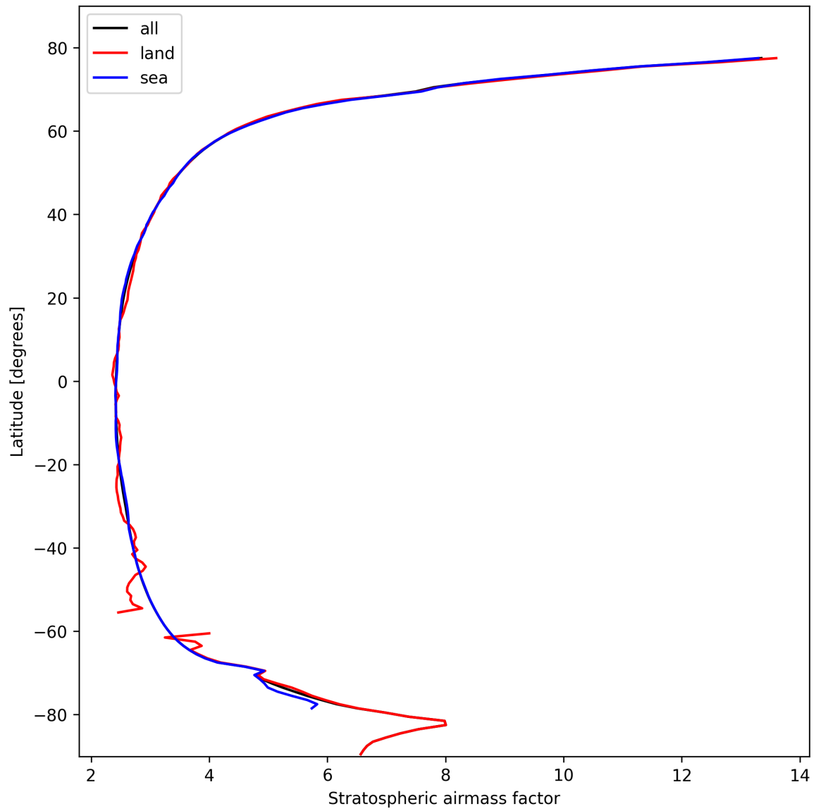
Figure 27: Zonal average of “Stratospheric airmass factor” for 2024-10-19 to 2024-10-20.
