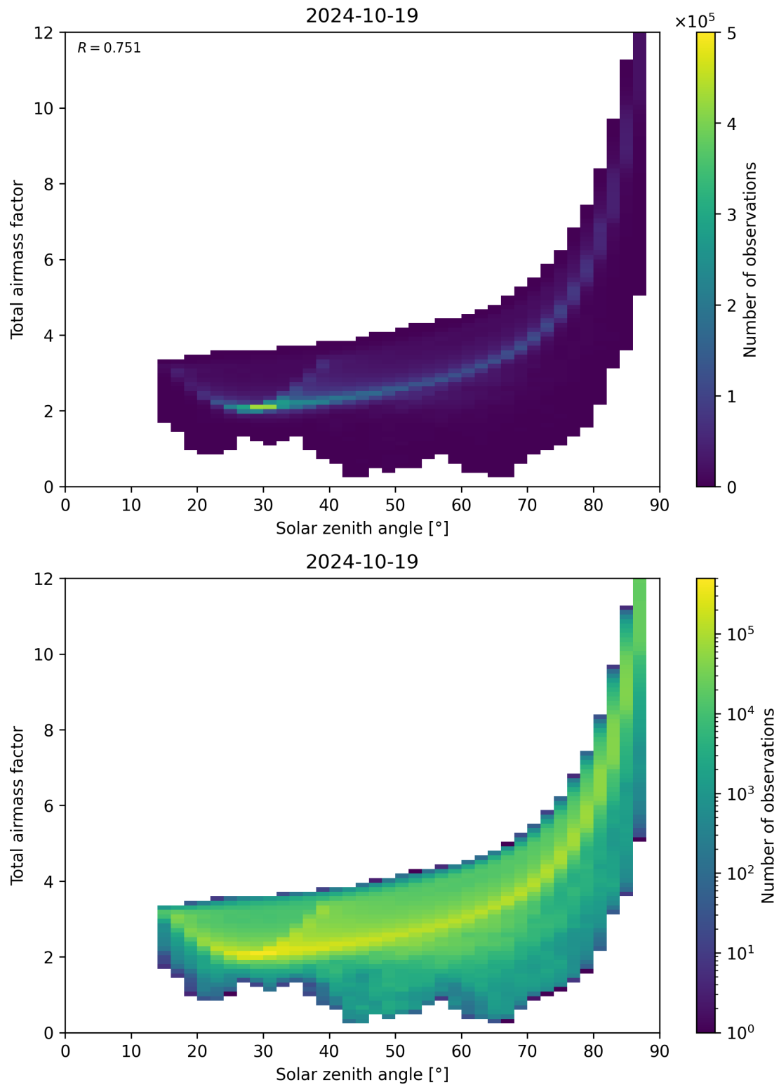
Figure 146: Scatter density plot of “Solar zenith angle” against “Total air mass factor” for 2024-10-19 to 2024-10-20.
