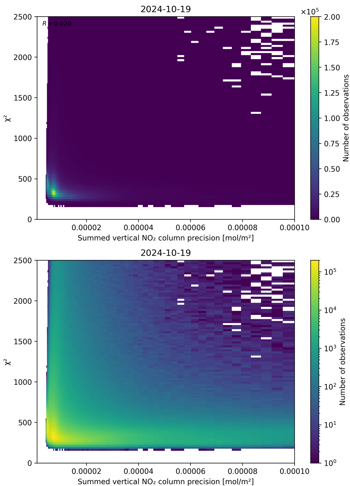
Figure 107: Scatter density plot of “Summed vertical NO 2 column precision” against “ \chi^2 ” for 2024-10-19 to 2024-10-20.
