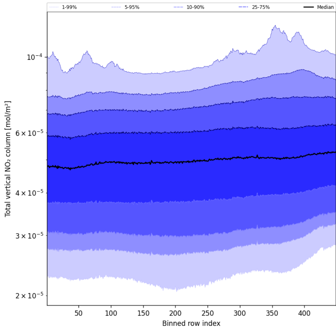
Figure 55: Along track statistics of “Total vertical NO 2 column” for 2024-10-19 to 2024-10-20
