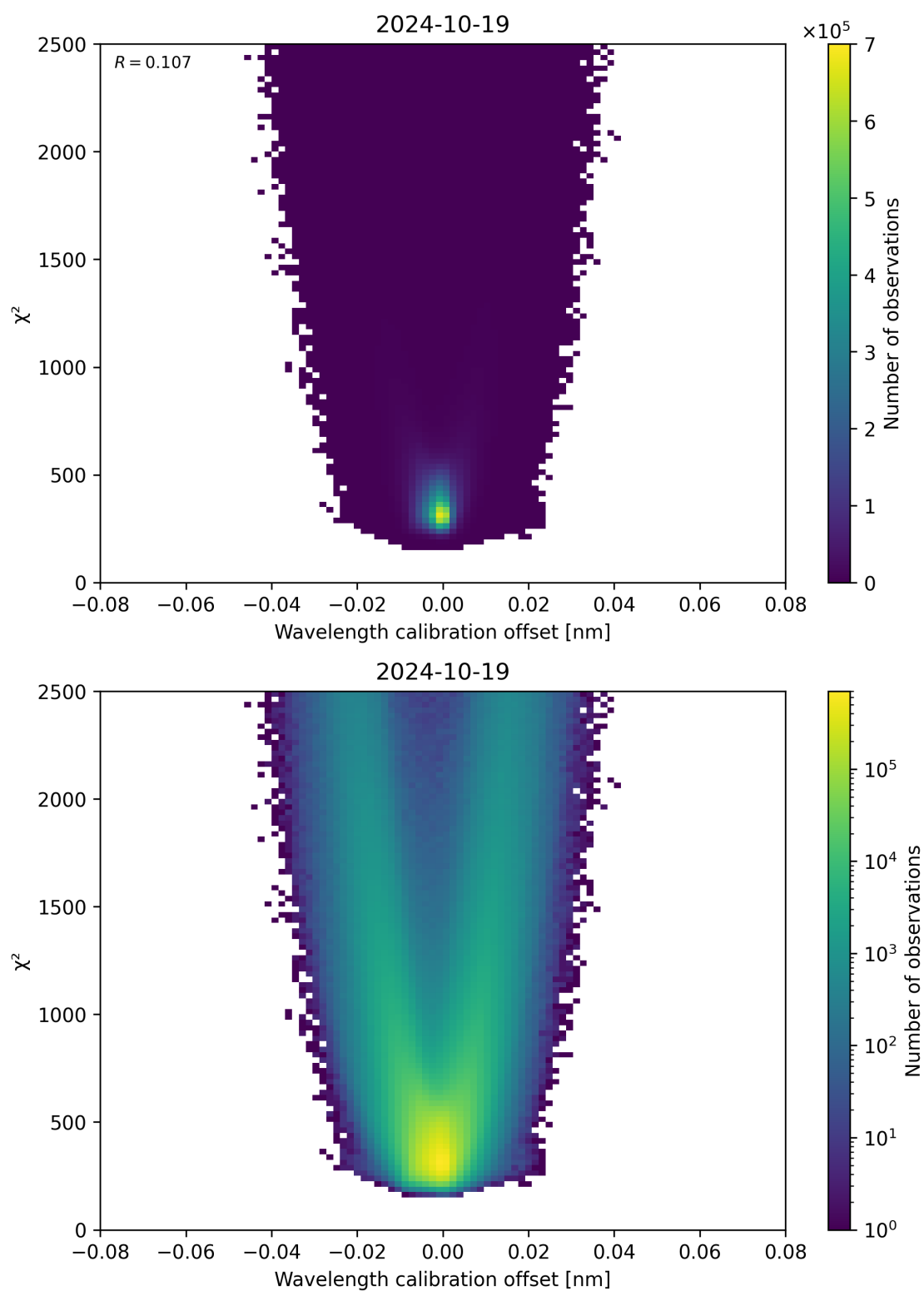
Figure 175: Scatter density plot of “Wavelength calibration offset” against “ \chi^2 ” for 2024-10-19 to 2024-10-20.
