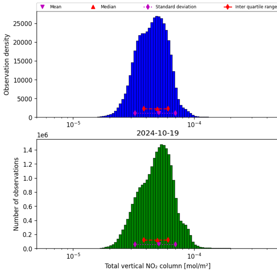
Figure 38: Histogram of “Total vertical NO 2 column” for 2024-10-19 to 2024-10-20
