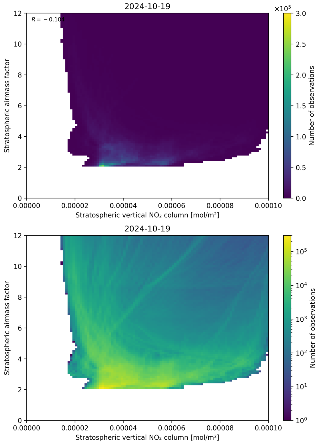
Figure 96: Scatter density plot of “Stratospheric vertical NO 2 column” against “Stratospheric airmass factor” for 2024-10-19 to 2024-10-20.
