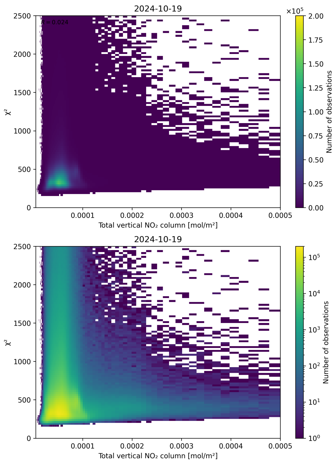
Figure 111: Scatter density plot of “Total vertical NO 2 column” against “ \chi^2 ” for 2024-10-19 to 2024-10-20.
