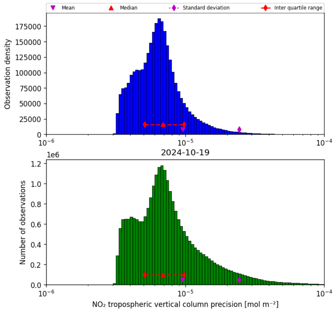
Figure 30: Histogram of “NO 2 tropospheric vertical column precision” for 2024-10-19 to 2024-10-20
