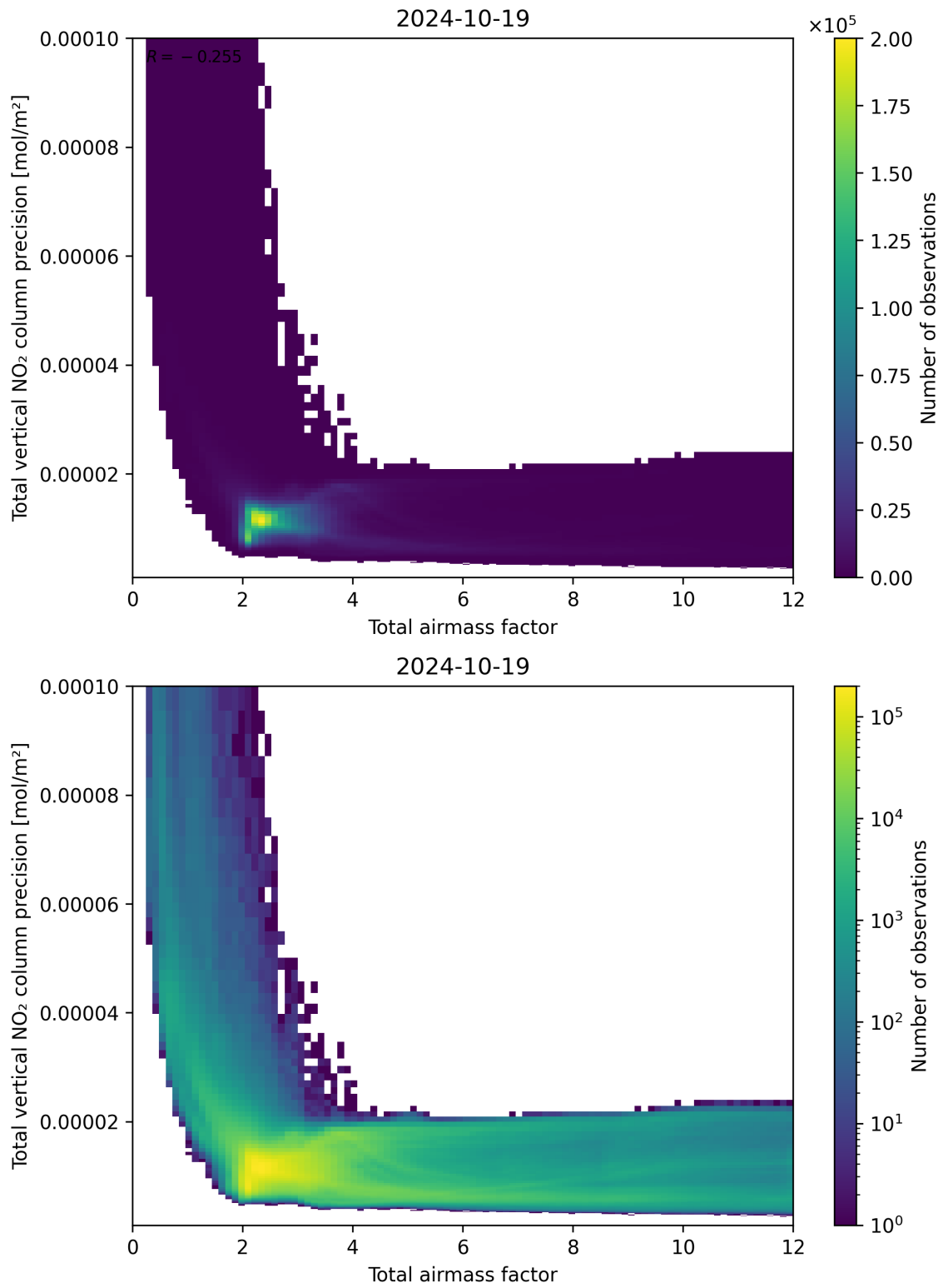
Figure 68: Scatter density plot of “Total airmass factor” against “Total vertical NO 2 column precision” for 2024-10-19 to 2024-10-20.
