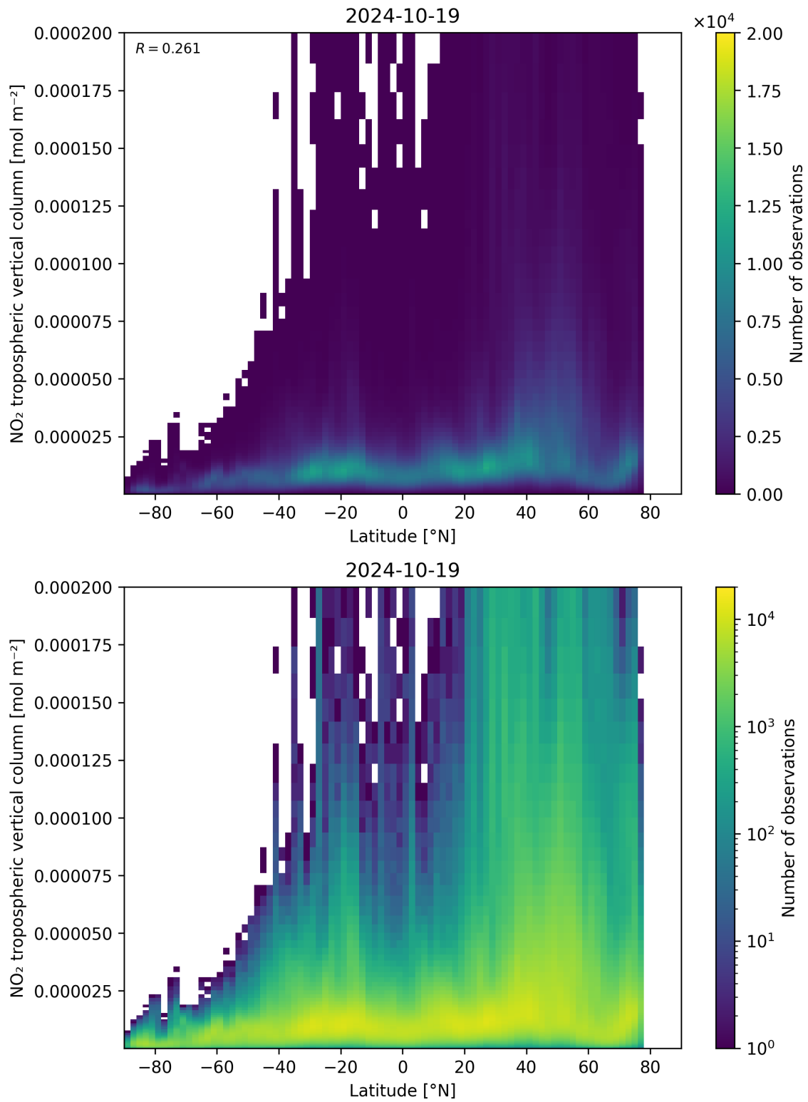
Figure 92: Scatter density plot of “Latitude” against “NO 2 tropospheric vertical column” for 2024-10-19 to 2024-10-20.
