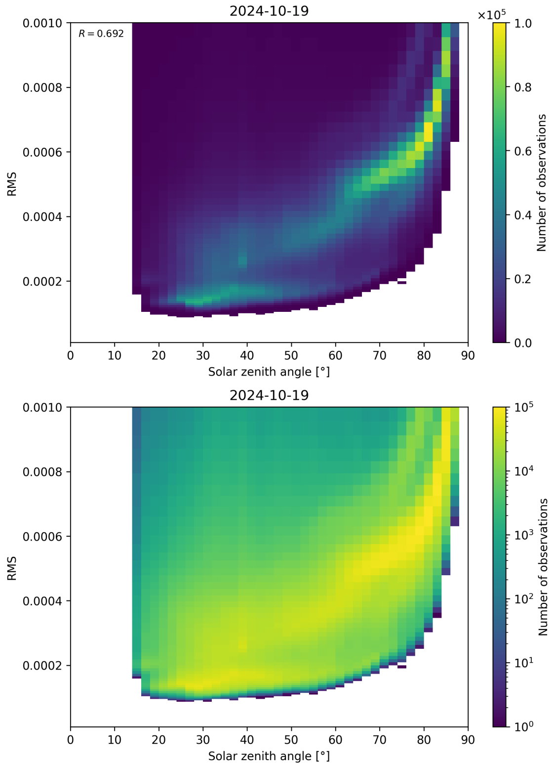
Figure 157: Scatter density plot of “Solar zenith angle” against “RMS” for 2024-10-19 to 2024-10-20.
