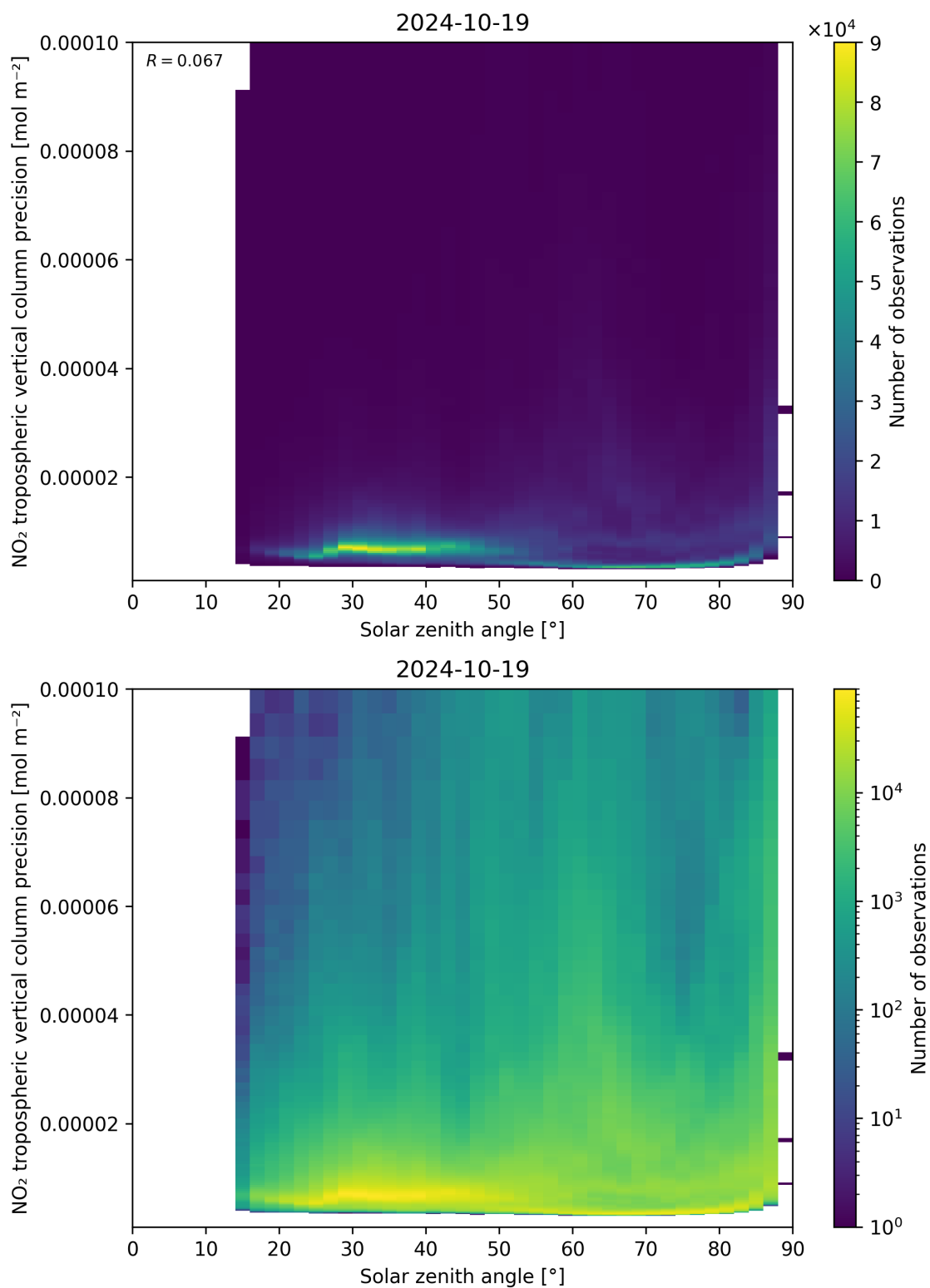
Figure 156: Scatter density plot of “Solar zenith angle” against “NO 2 tropospheric vertical column precision” for 2024-10-19 to 2024-10-20.
