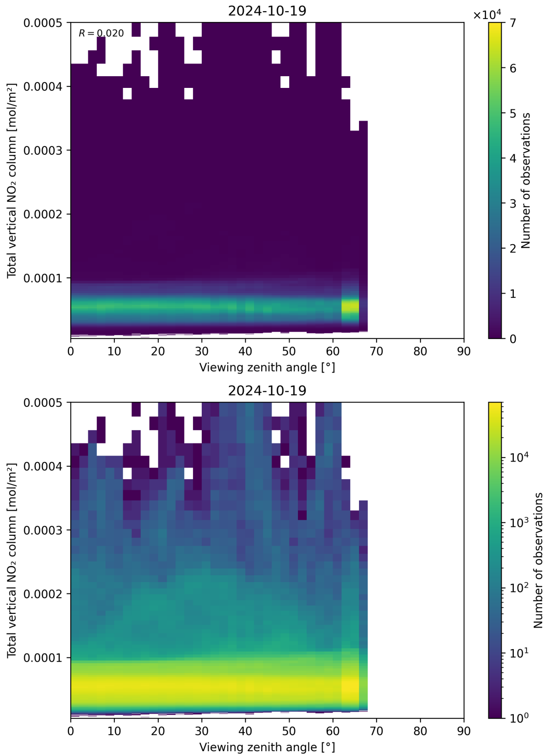
Figure 167: Scatter density plot of “Viewing zenith angle” against “Total vertical NO 2 column” for 2024-10-19 to 2024-10-20.
