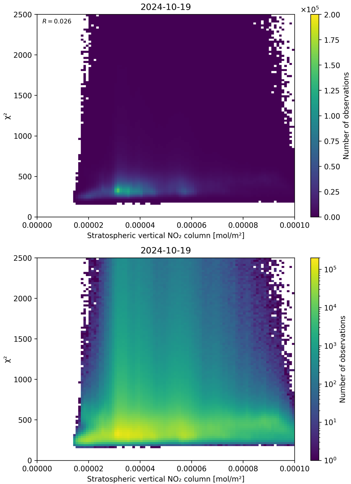
Figure 97: Scatter density plot of “Stratospheric vertical NO 2 column” against “ \chi^2 ” for 2024-10-19 to 2024-10-20.
