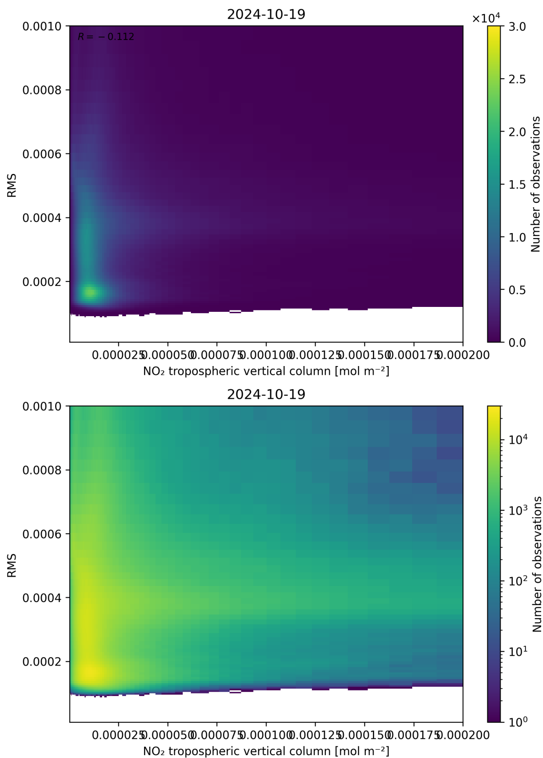
Figure 142: Scatter density plot of “NO 2 tropospheric vertical column” against “RMS” for 2024-10-19 to 2024-10-20.
