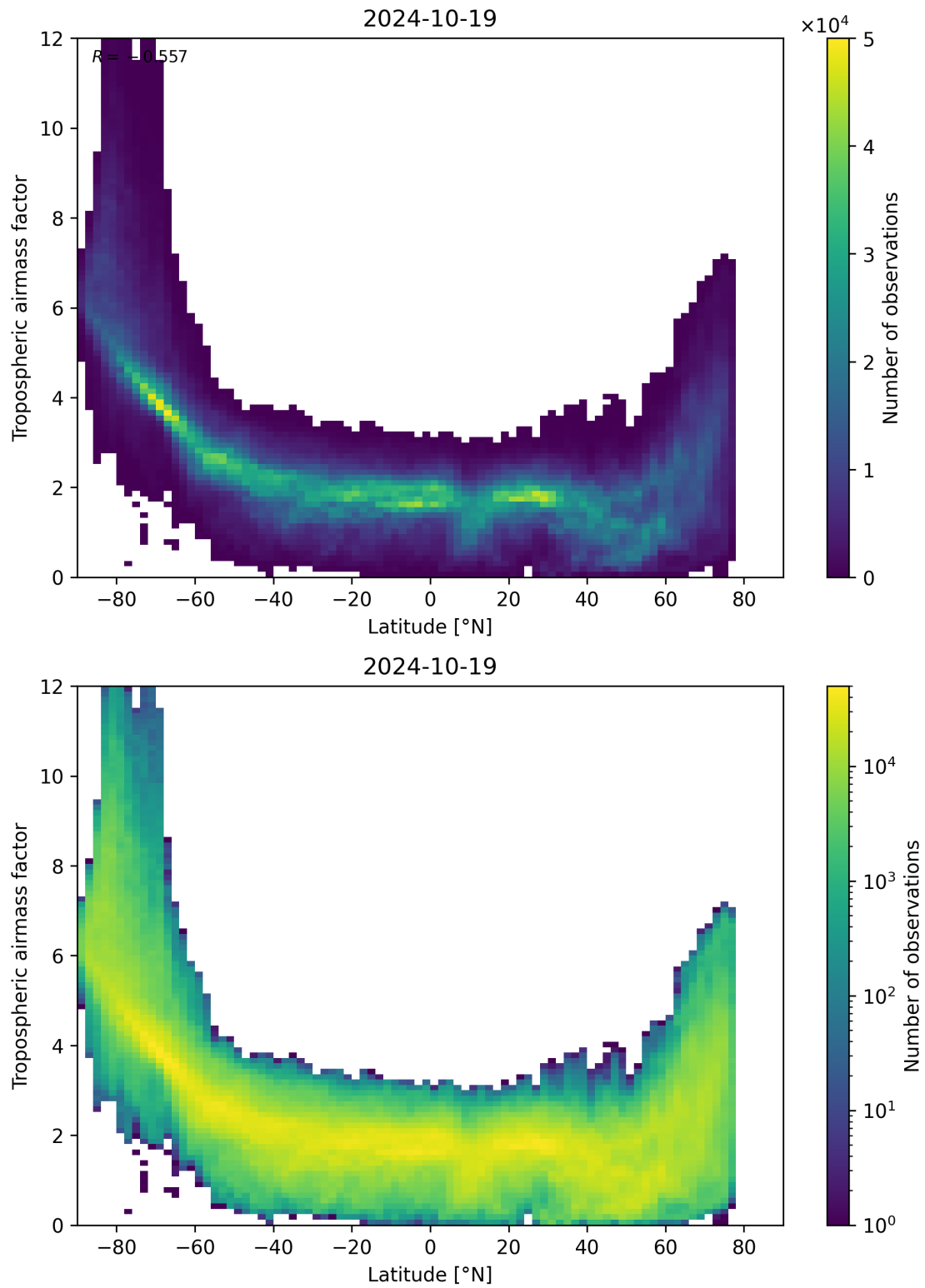
Figure 85: Scatter density plot of “Latitude” against “Tropospheric airmass factor” for 2024-10-19 to 2024-10-20.
