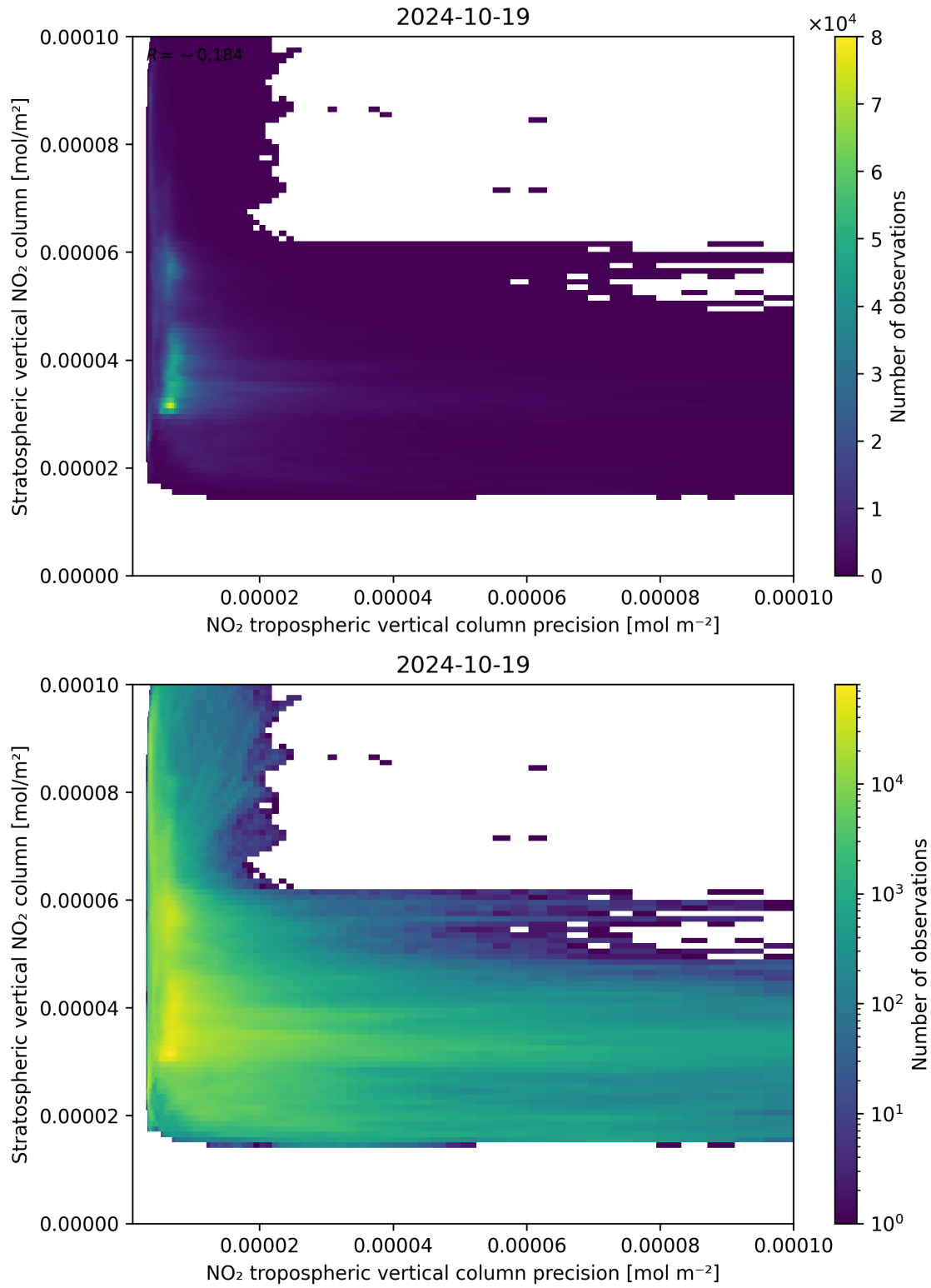
Figure 135: Scatter density plot of “NO 2 tropospheric vertical column precision” against “Stratospheric vertical NO 2 column” for 2024-10-19 to 2024-10-20.
