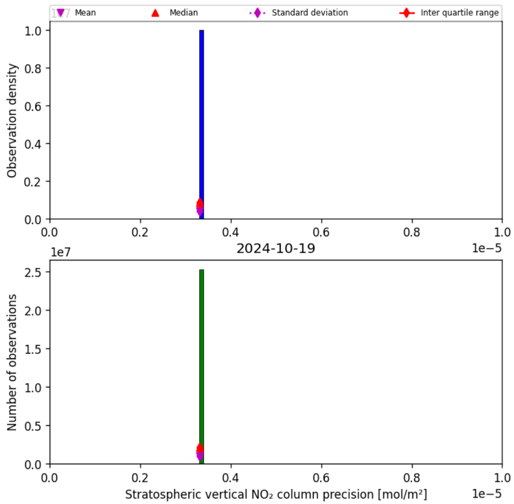
Figure 37: Histogram of “Stratospheric vertical NO 2 column precision” for 2024-10-19 to 2024-10-20
