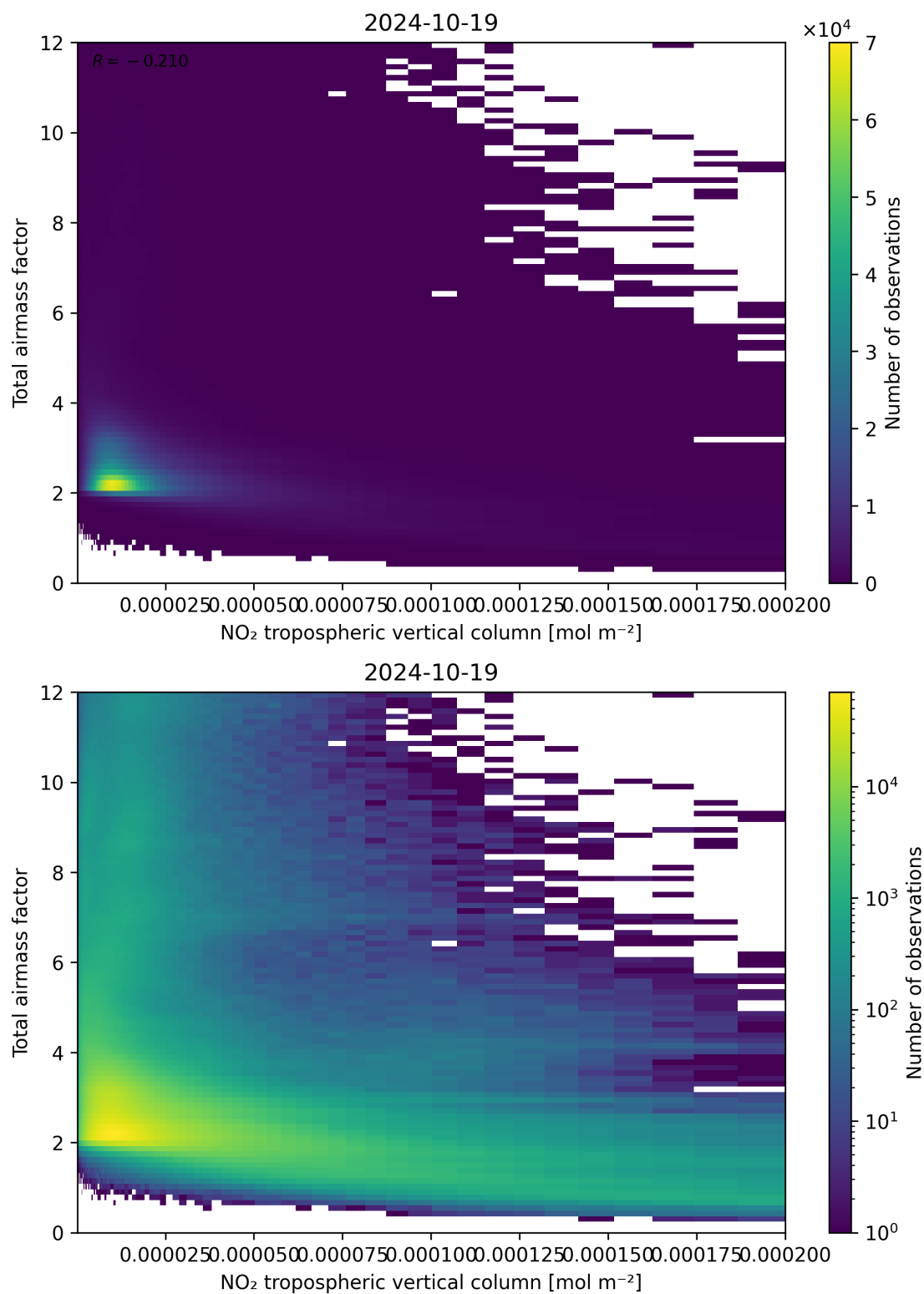
Figure 122: Scatter density plot of “NO 2 tropospheric vertical column” against “Total air mass factor” for 2024-10-19 to 2024-10-20.
