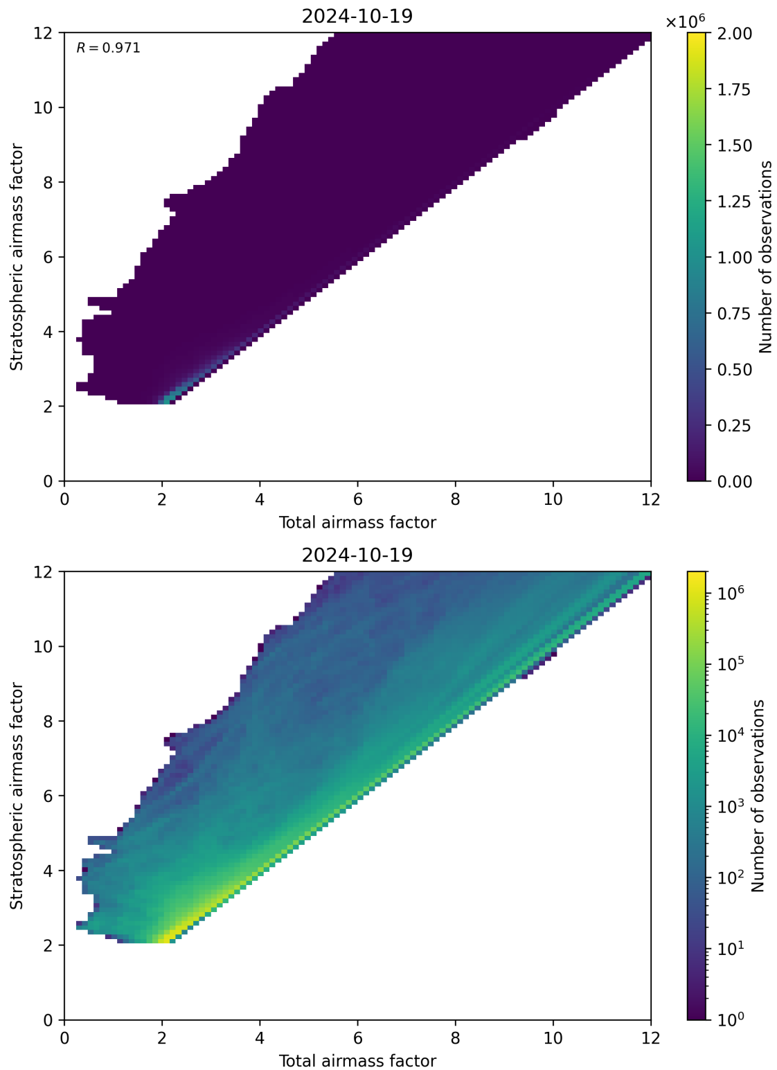
Figure 62: Scatter density plot of “Total airmass factor” against “Stratospheric airmass factor” for 2024-10-19 to 2024-10-20.
