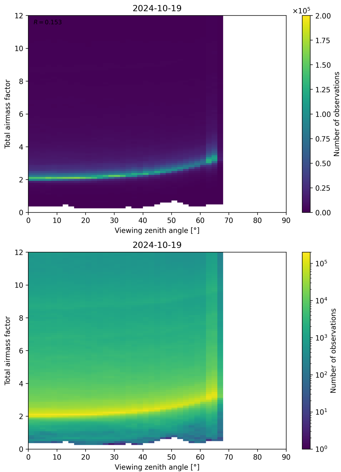
Figure 160: Scatter density plot of “Viewing zenith angle” against “Total airmass factor” for 2024-10-19 to 2024-10-20.
