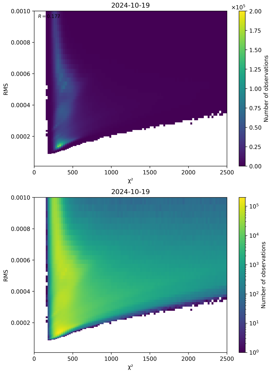
Figure 82: Scatter density plot of “ \chi^2 ” against “RMS” for 2024-10-19 to 2024-10-20.
