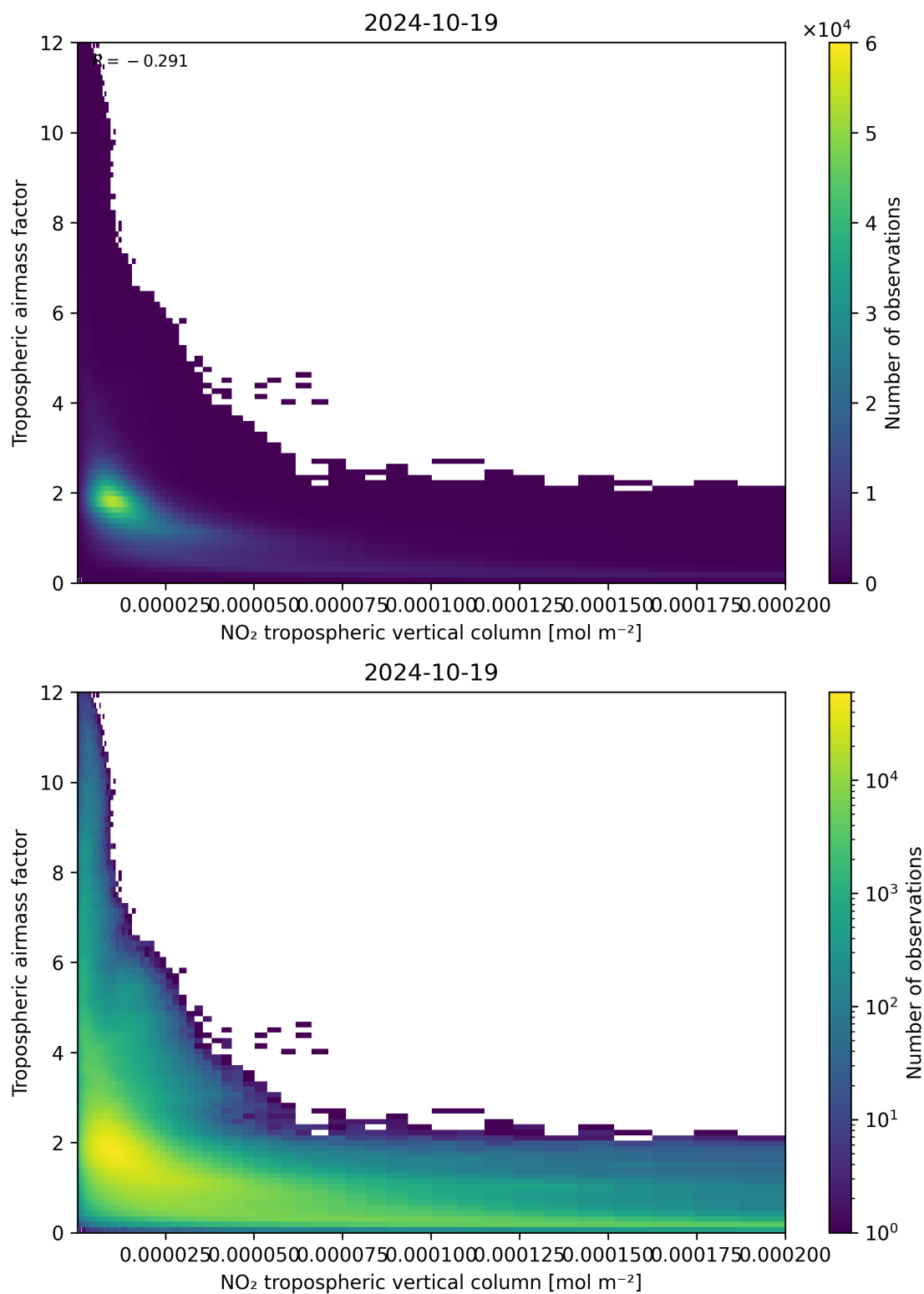
Figure 123: Scatter density plot of “NO 2 tropospheric vertical column” against “Tropospheric air mass factor” for 2024-10-19 to 2024-10-20.
