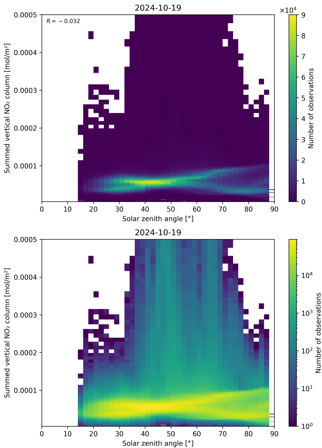
Figure 151: Scatter density plot of “Solar zenith angle” against “Summed vertical NO 2 column” for 2024-10-19 to 2024-10-20.
