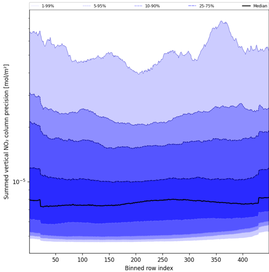
Figure 58: Along track statistics of “Summed vertical NO 2 column precision” for 2024-10-19 to 2024-10-20
