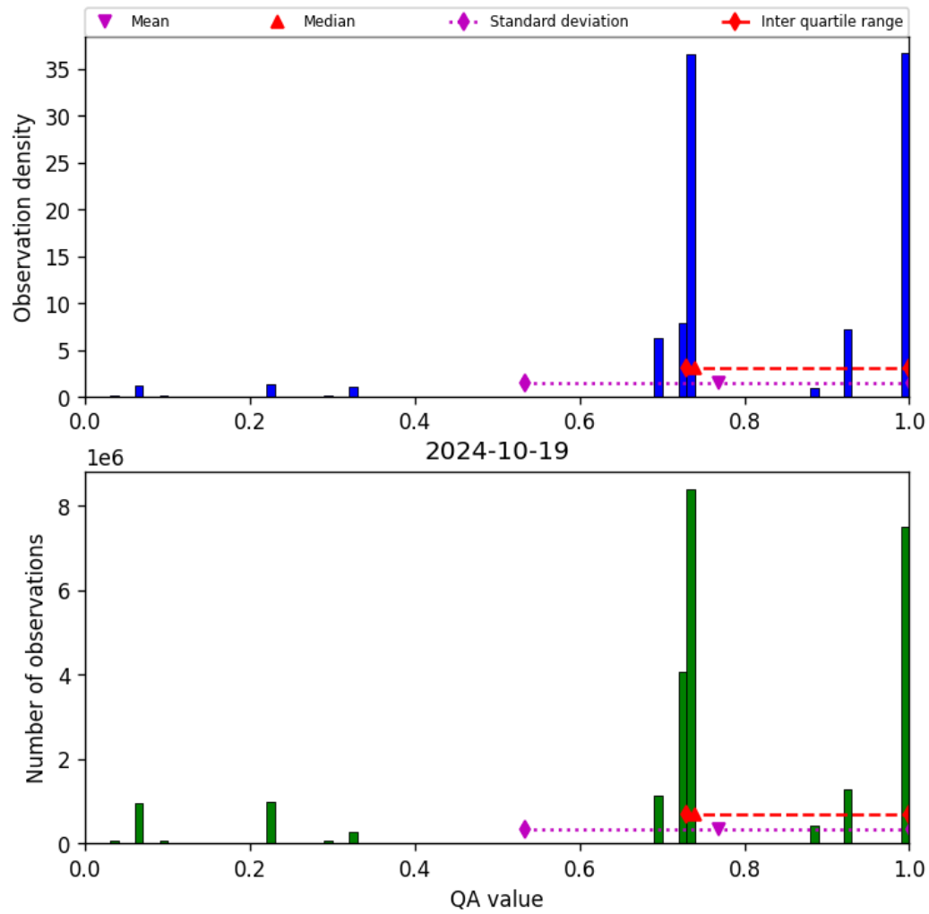
Figure 28: Histogram of “QA value” for 2024-10-19 to 2024-10-20
