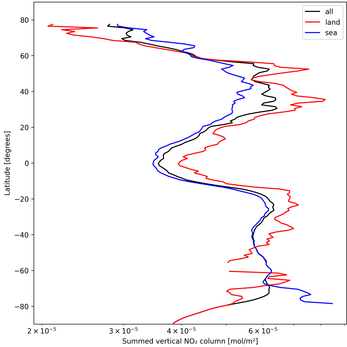
Figure 23: Zonal average of “Summed vertical NO 2 column” for 2024-10-19 to 2024-10-20.
