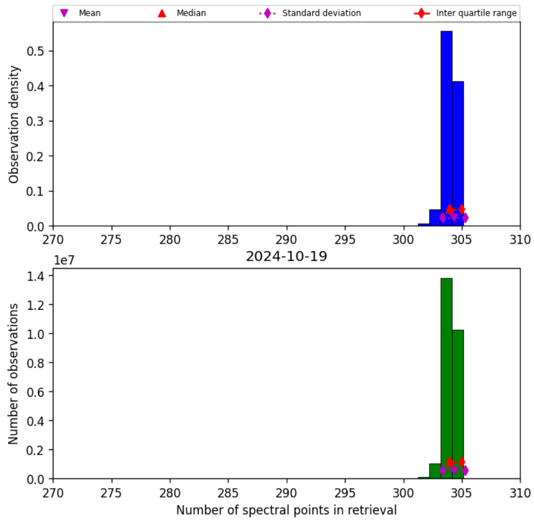
Figure 33: Histogram of “Number of spectral points in retrieval” for 2024-10-19 to 2024-10-20
