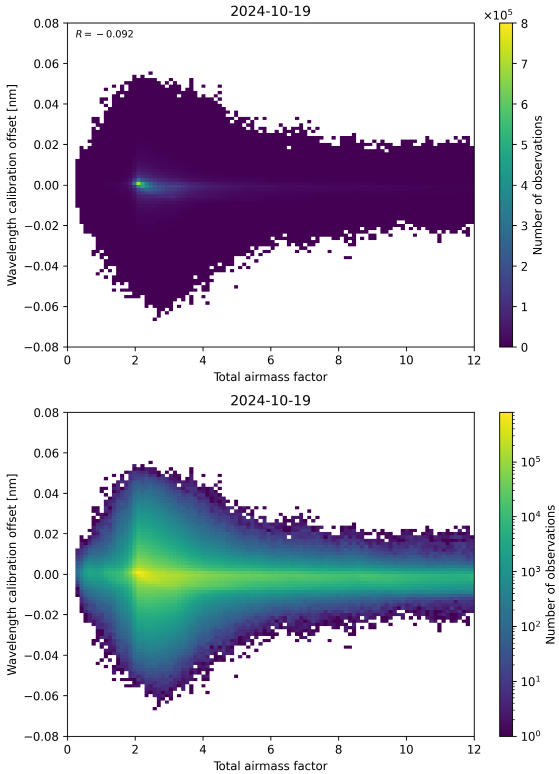
Figure 70: Scatter density plot of “Total airmass factor” against “Wavelength calibration offset” for 2024-10-19 to 2024-10-20.
