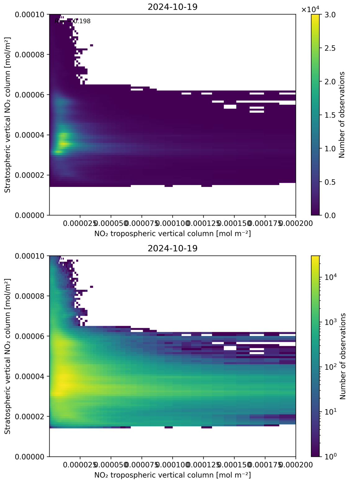
Figure 125: Scatter density plot of “NO 2 tropospheric vertical column” against “Stratospheric vertical NO 2 column” for 2024-10-19 to 2024-10-20.
