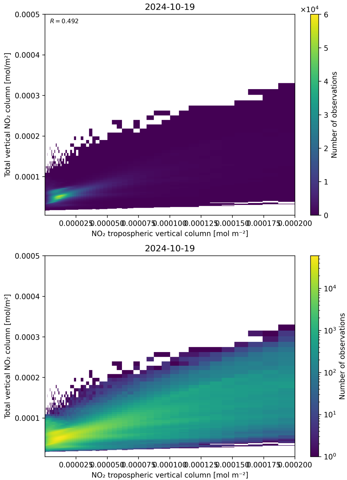
Figure 128: Scatter density plot of “NO 2 tropospheric vertical column” against “Total vertical NO 2 column” for 2024-10-19 to 2024-10-20.
