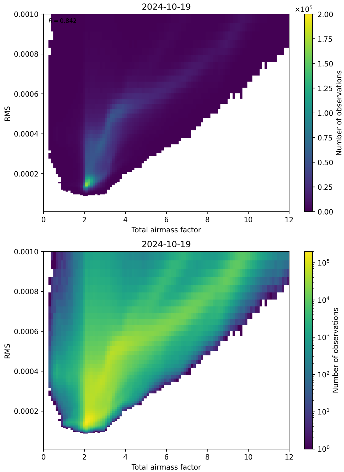
Figure 69: Scatter density plot of “Total airmass factor” against “RMS” for 2024-10-19 to 2024-10-20.
