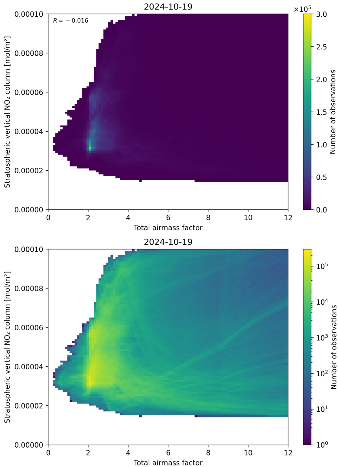
Figure 64: Scatter density plot of “Total airmass factor” against “Stratospheric vertical NO 2 column” for 2024-10-19 to 2024-10-20.
