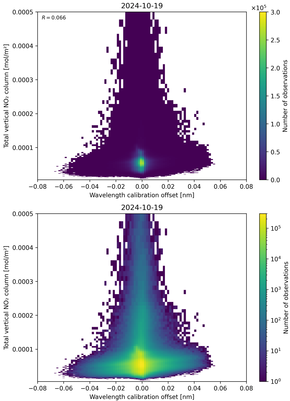
Figure 179: Scatter density plot of “Wavelength calibration offset” against “Total vertical NO 2 column” for 2024-10-19 to 2024-10-20.
