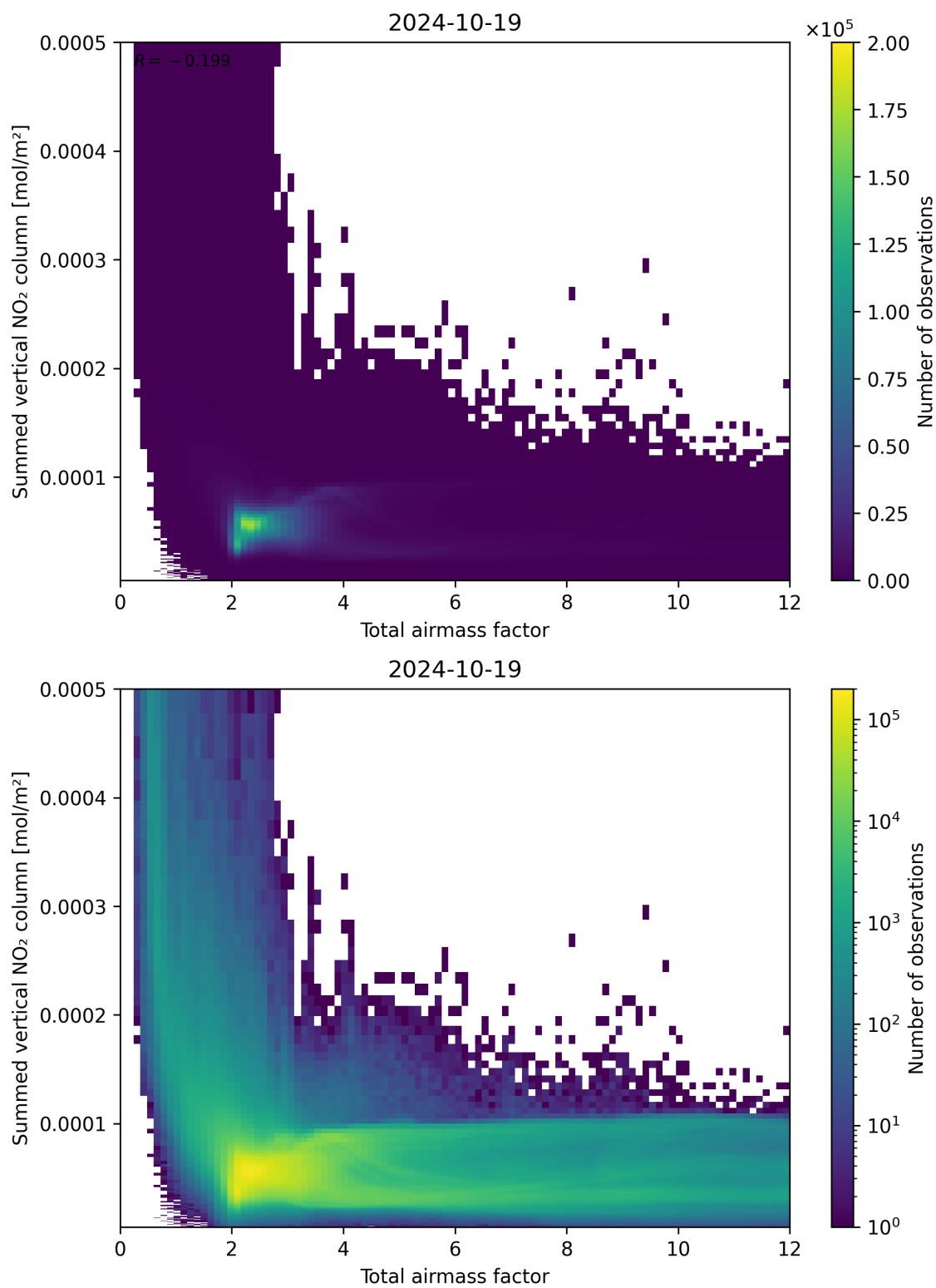
Figure 65: Scatter density plot of “Total airmass factor” against “Summed vertical NO 2 column” for 2024-10-19 to 2024-10-20.
