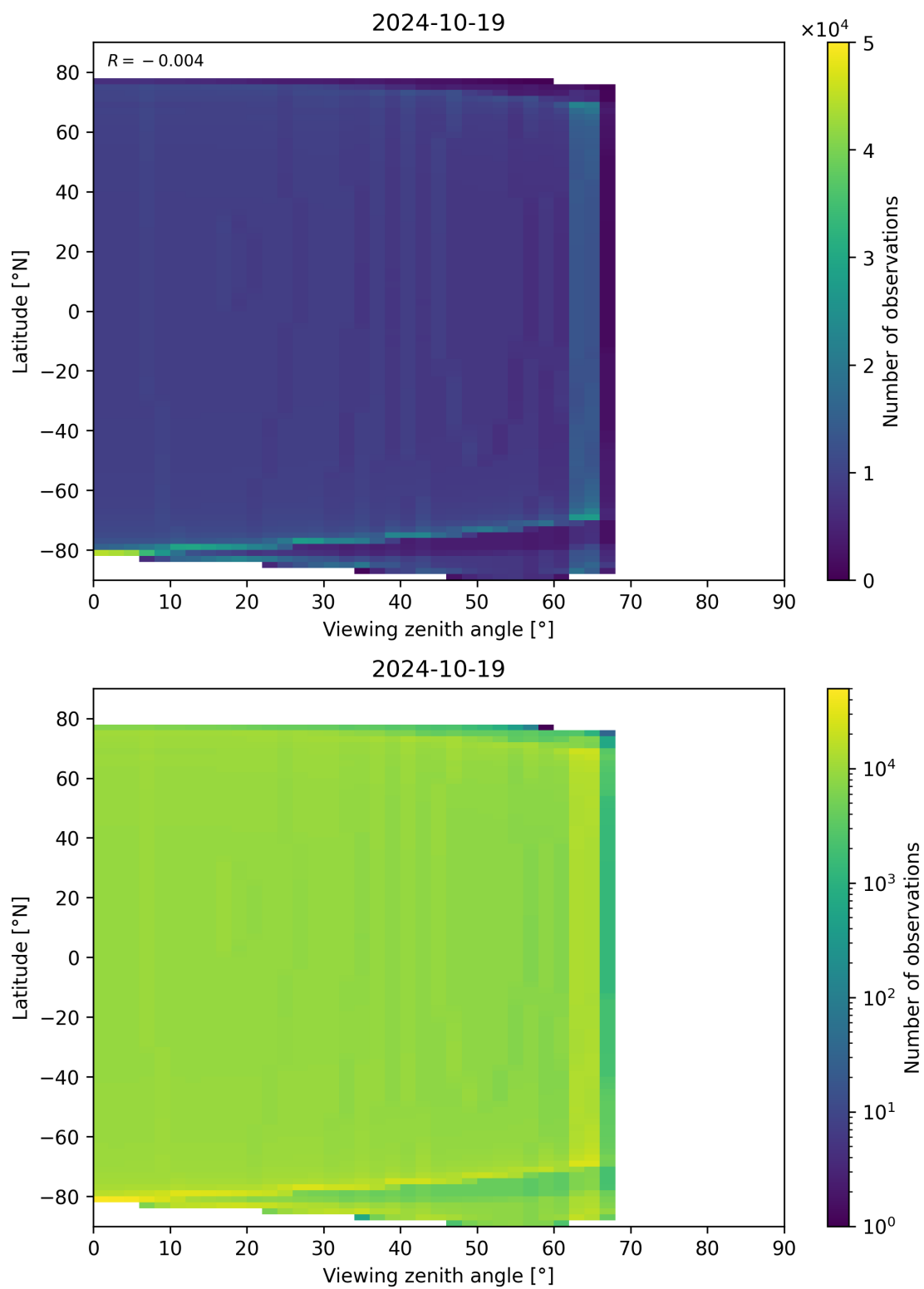
Figure 163: Scatter density plot of “Viewing zenith angle” against “Latitude” for 2024-10-19 to 2024-10-20.
