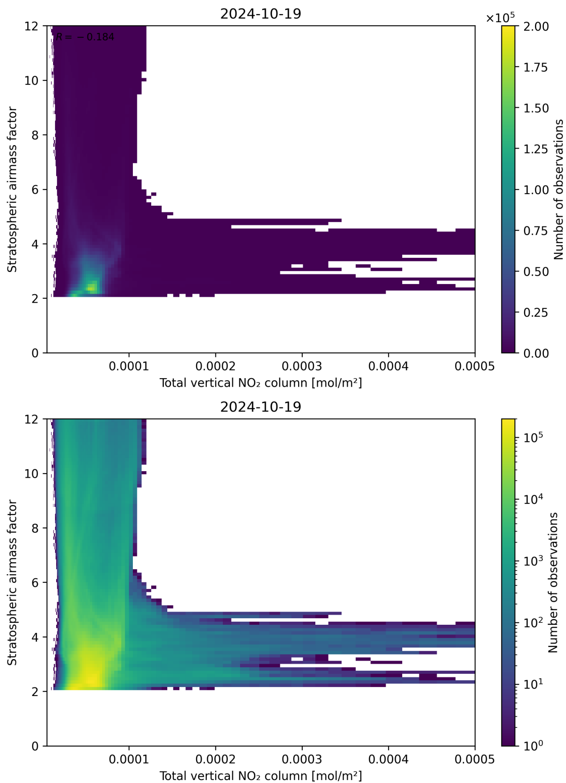
Figure 110: Scatter density plot of “Total vertical NO 2 column” against “Stratospheric airmass factor” for 2024-10-19 to 2024-10-20.
