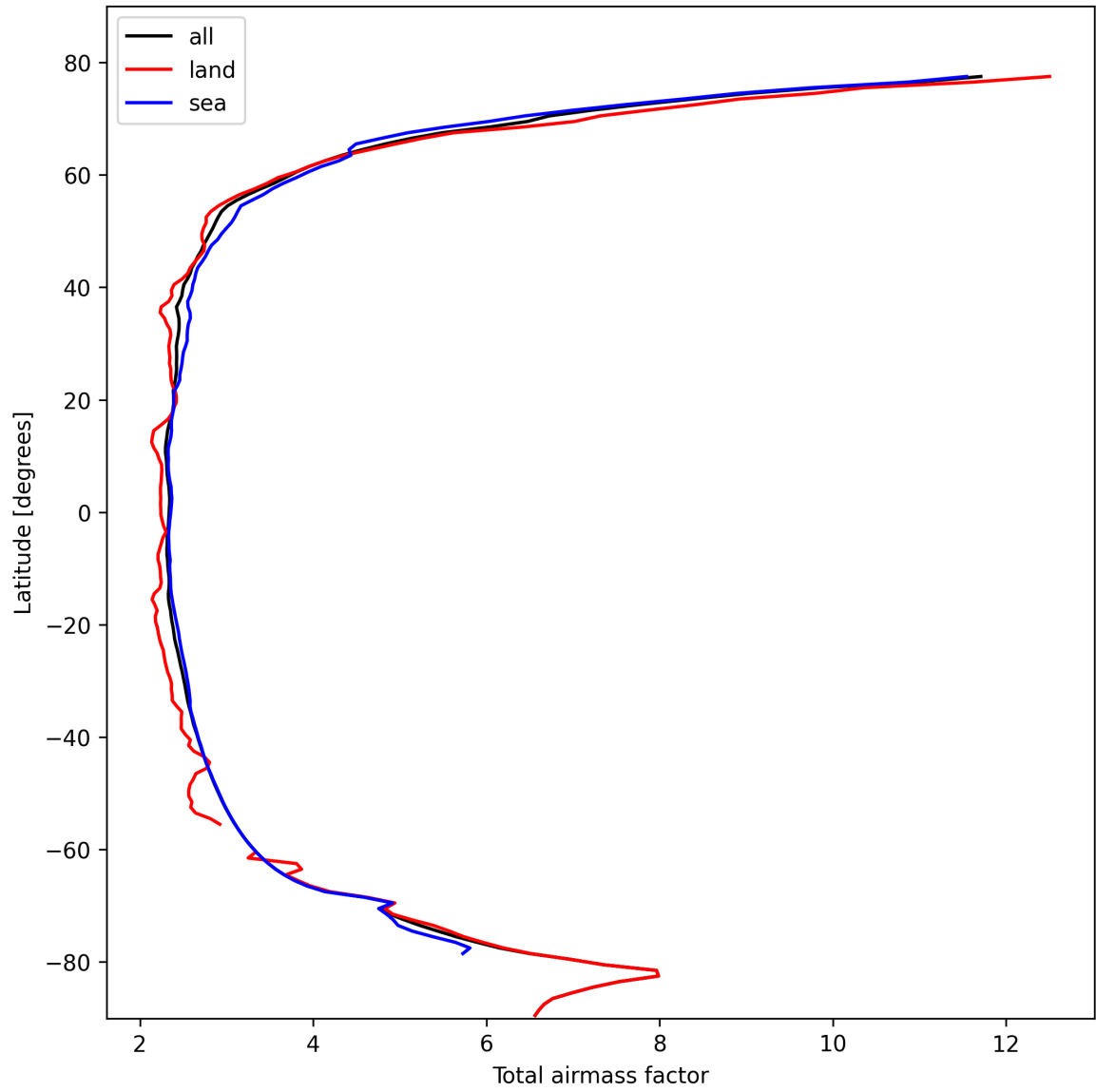
Figure 15: Zonal average of “Total airmass factor” for 2024-10-19 to 2024-10-20.
