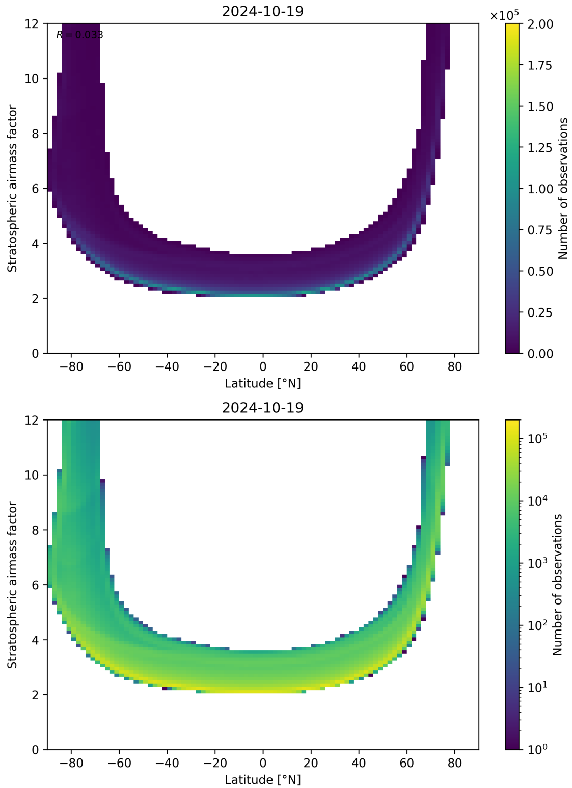
Figure 83: Scatter density plot of “Latitude” against “Stratospheric airmass factor” for 2024-10-19 to 2024-10-20.
