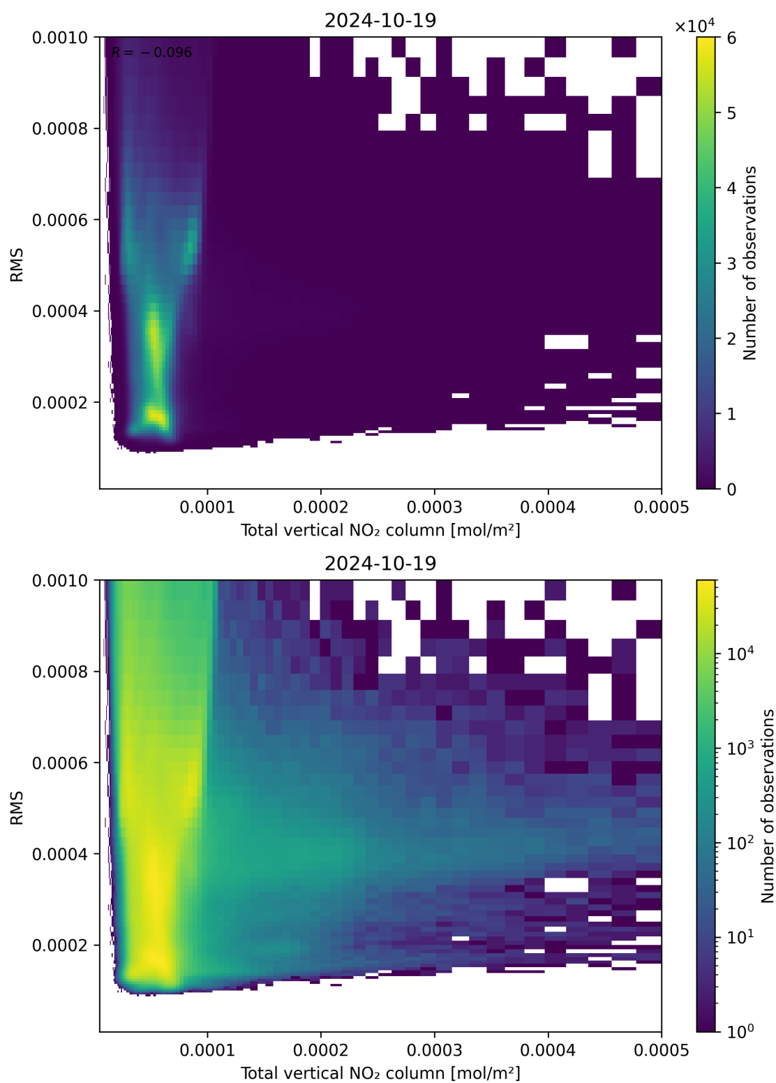
Figure 120: Scatter density plot of “Total vertical NO 2 column” against “RMS” for 2024-10-19 to 2024-10-20.
