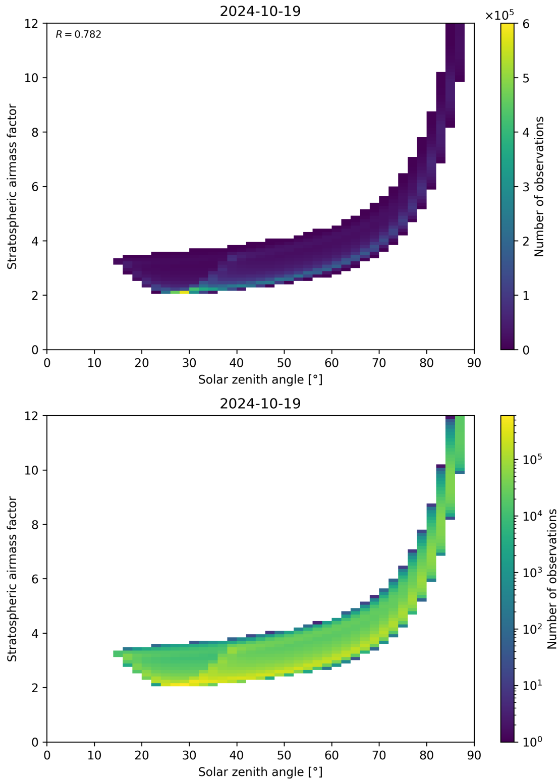
Figure 145: Scatter density plot of “Solar zenith angle” against “Stratospheric airmass factor” for 2024-10-19 to 2024-10-20.
