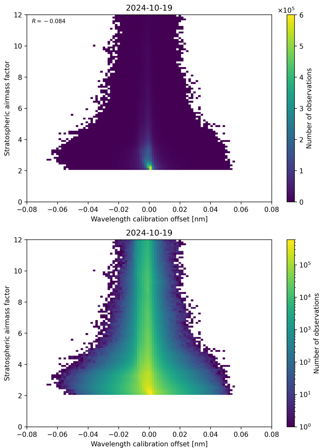
Figure 174: Scatter density plot of “Wavelength calibration offset” against “Stratospheric airmass factor” for 2024-10-19 to 2024-10-20.
