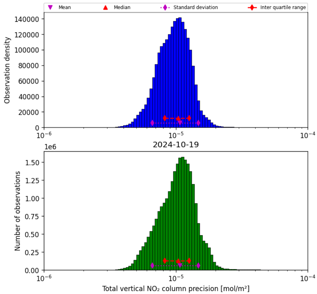
Figure 39: Histogram of “Total vertical NO 2 column precision” for 2024-10-19 to 2024-10-20
