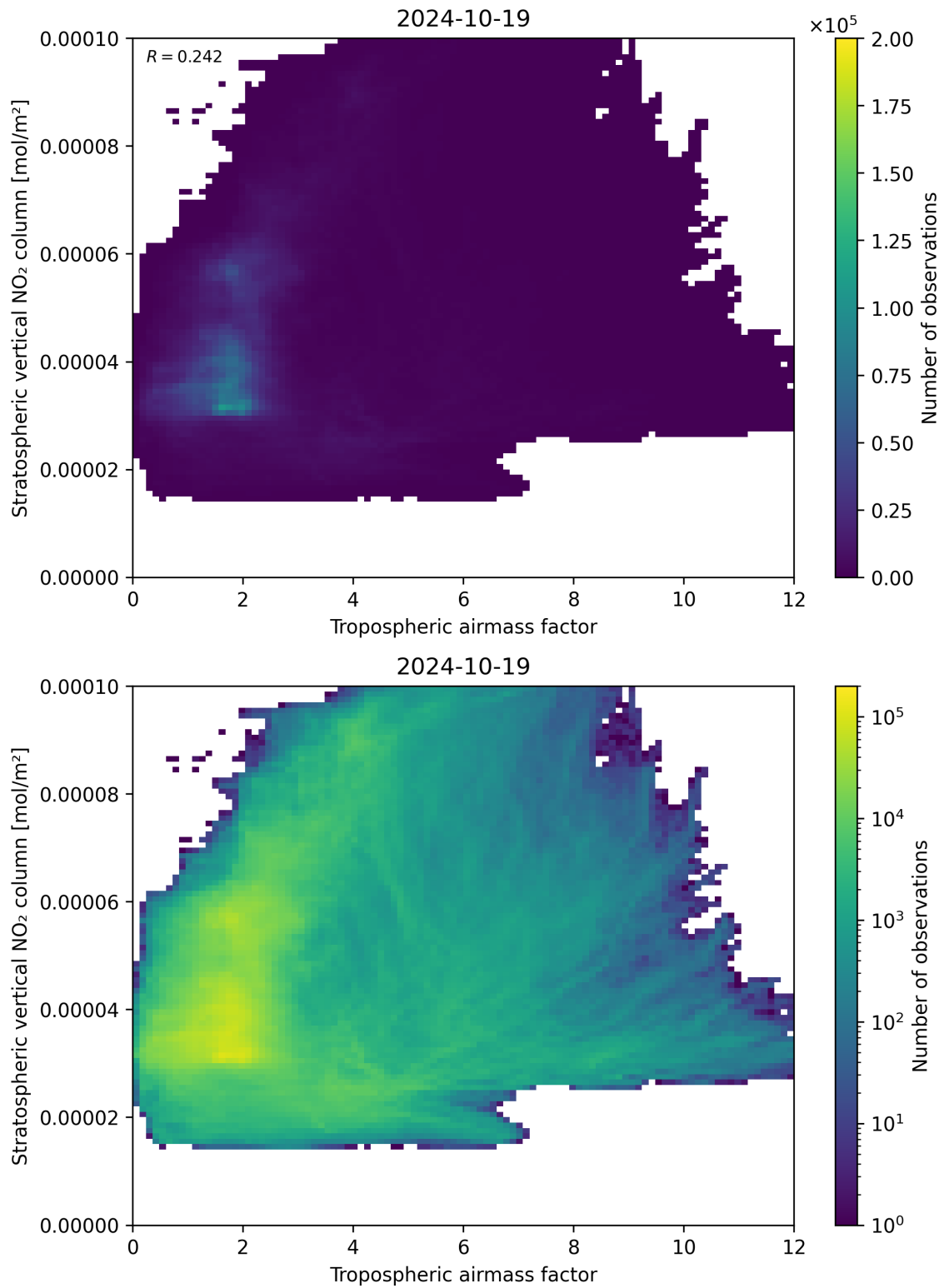
Figure 74: Scatter density plot of “Tropospheric air mass factor” against “Stratospheric vertical NO 2 column” for 2024-10-19 to 2024-10-20.
