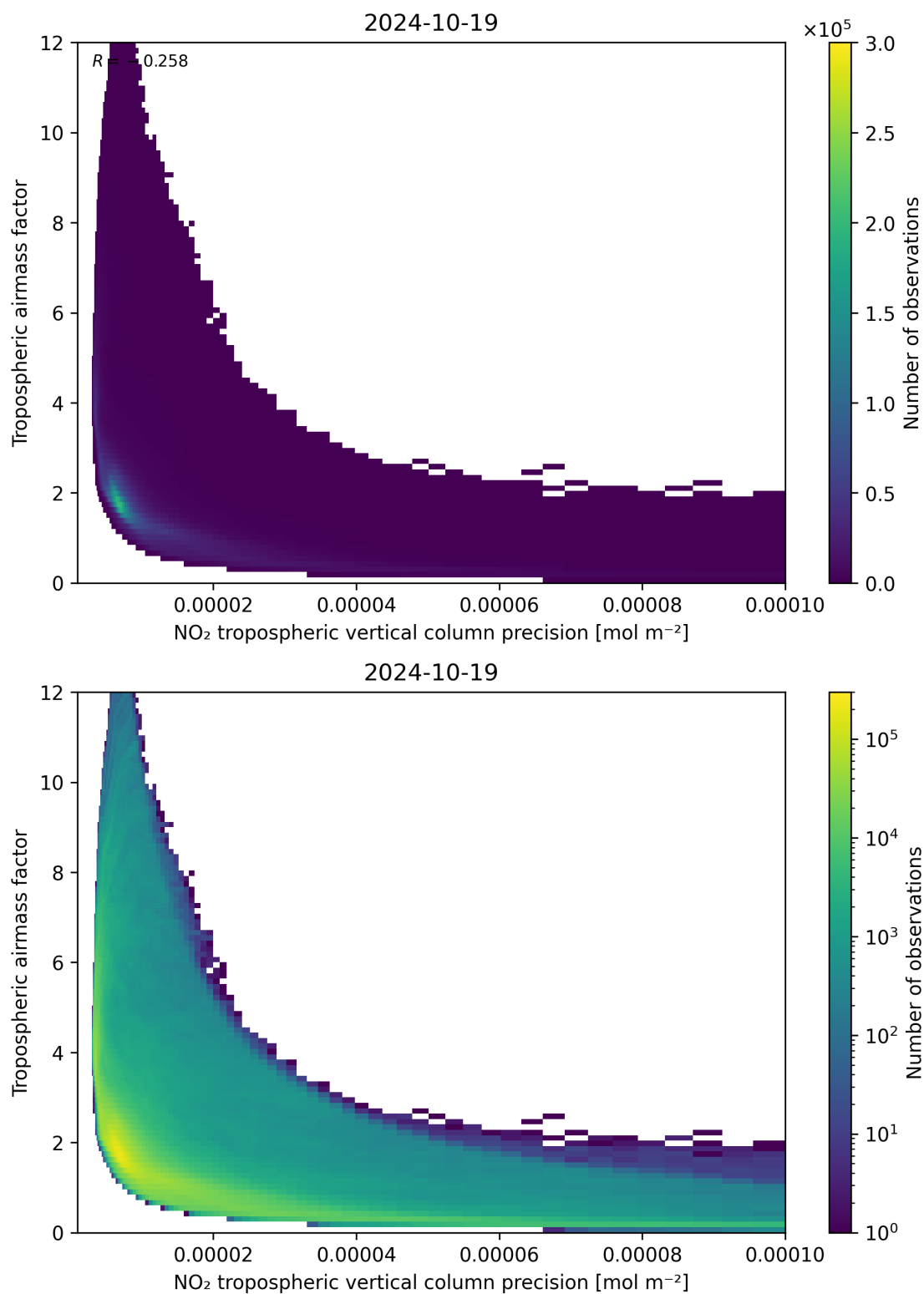
Figure 133: Scatter density plot of “NO 2 tropospheric vertical column precision” against “Tropospheric airmass factor” for 2024-10-19 to 2024-10-20.
