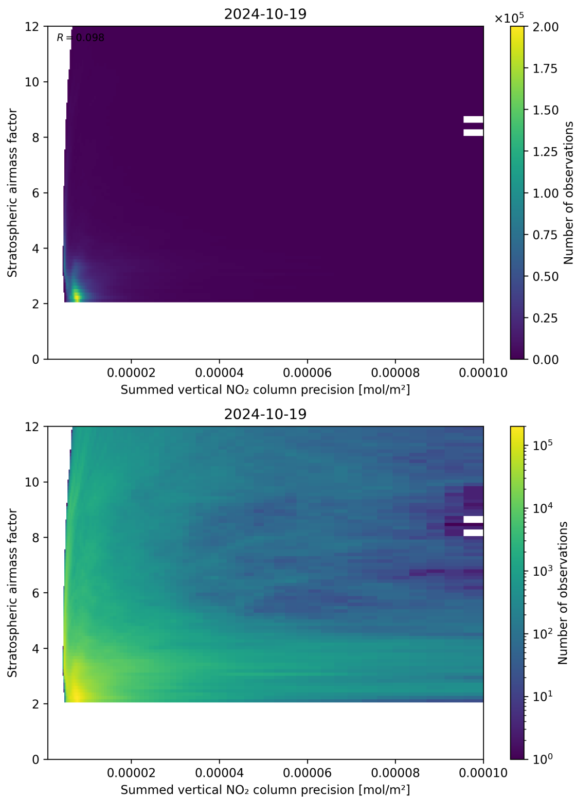
Figure 106: Scatter density plot of “Summed vertical NO 2 column precision” against “Stratospheric airmass factor” for 2024-10-19 to 2024-10-20.
