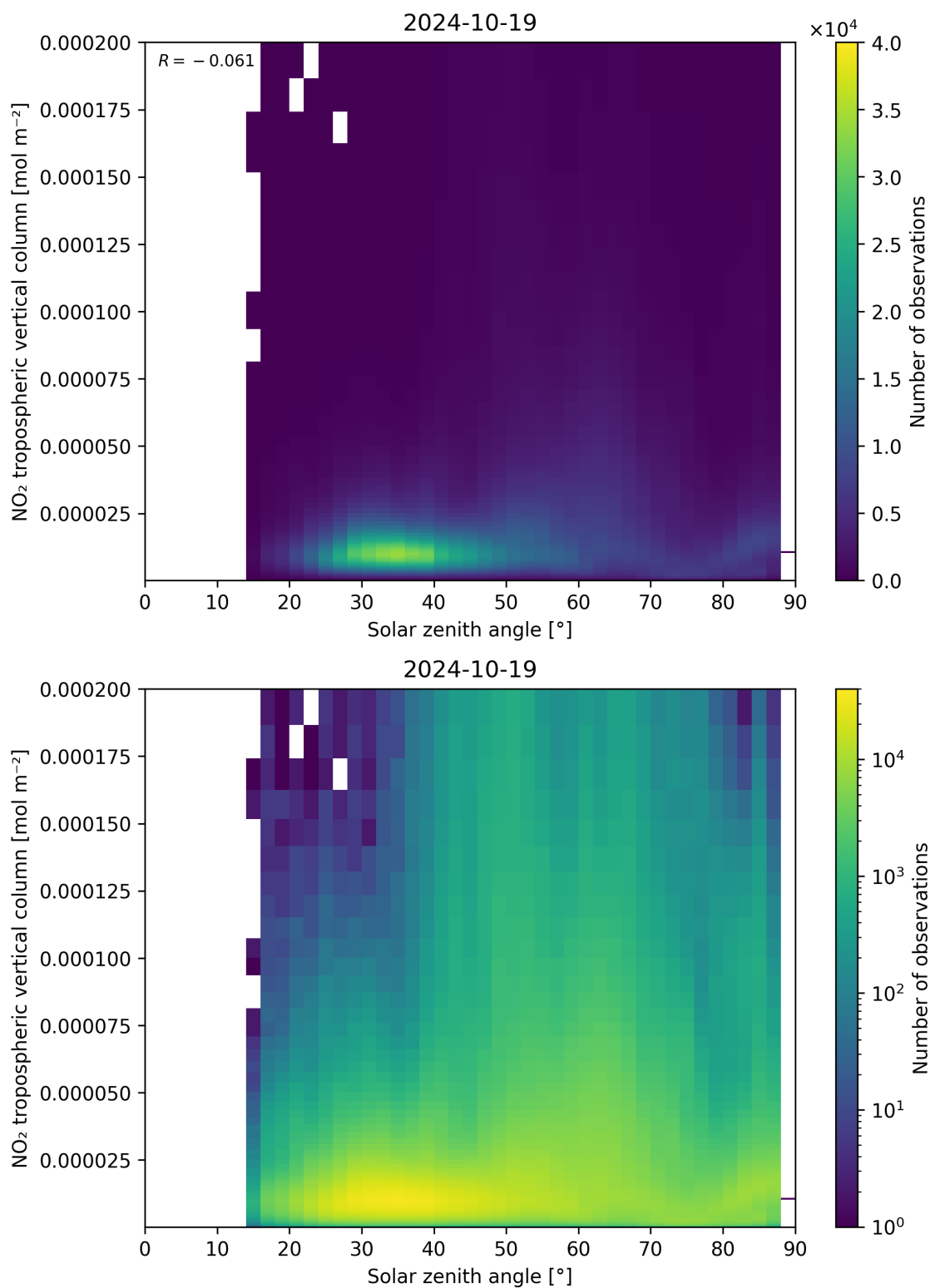
Figure 155: Scatter density plot of “Solar zenith angle” against “NO 2 tropospheric vertical column” for 2024-10-19 to 2024-10-20.
