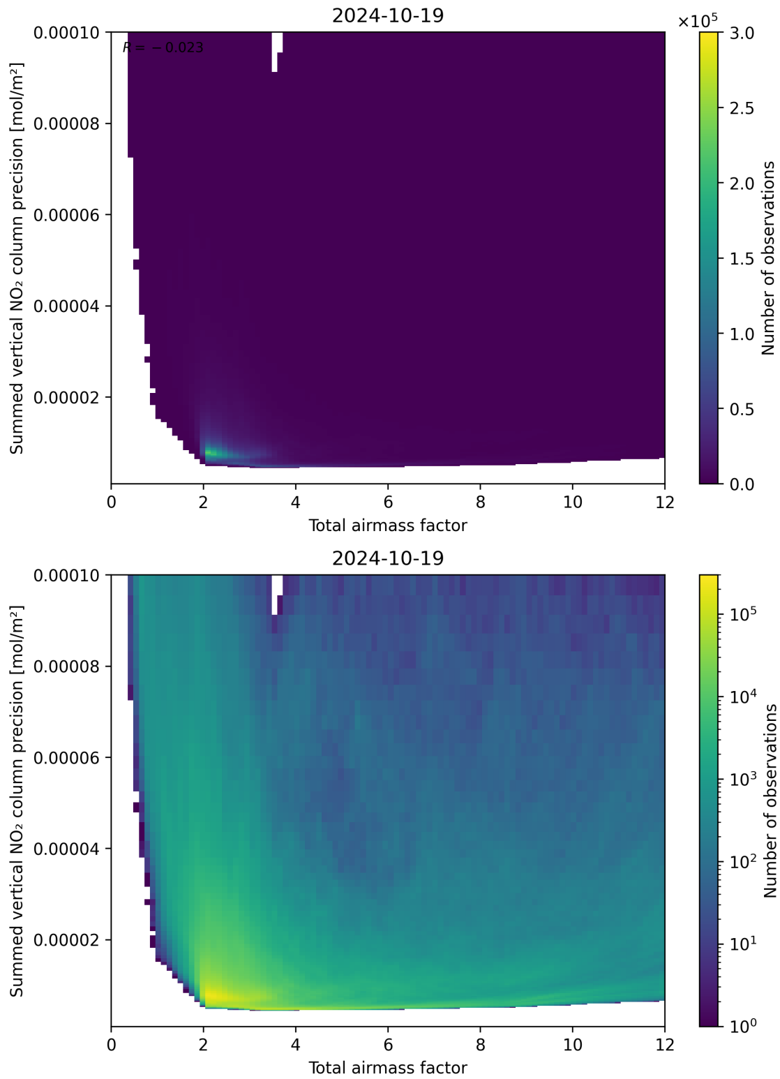
Figure 66: Scatter density plot of “Total airmass factor” against “Summed vertical NO 2 column precision” for 2024-10-19 to 2024-10-20.
