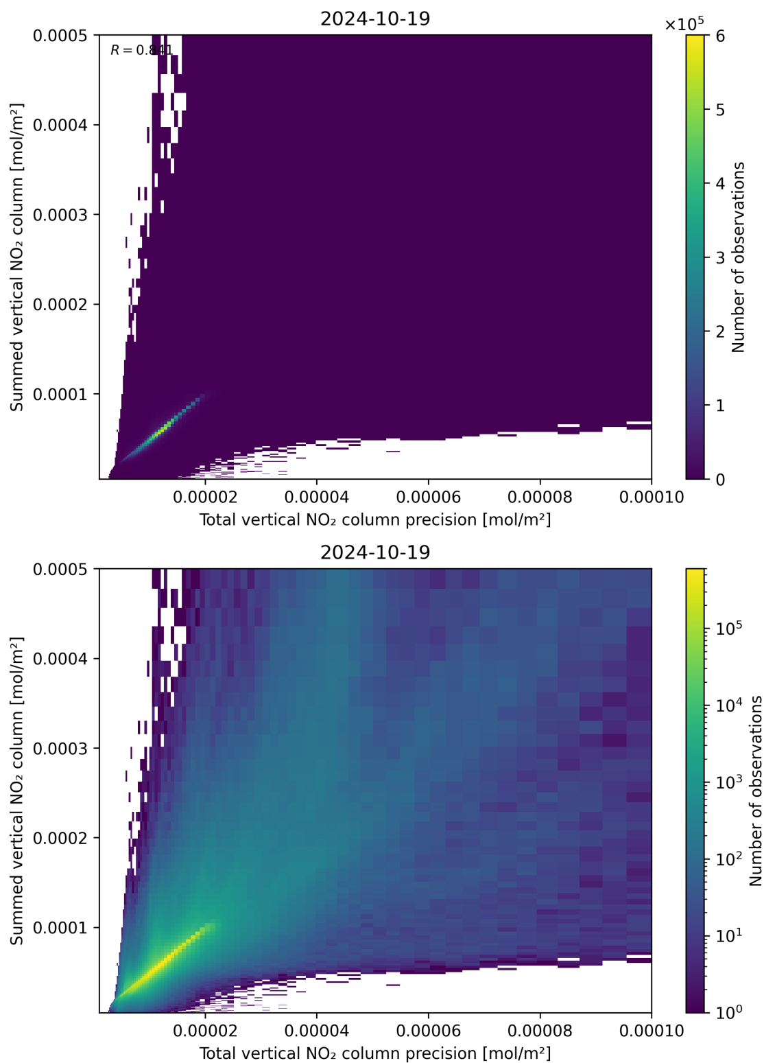
Figure 117: Scatter density plot of “Total vertical NO 2 column precision” against “Summed vertical NO 2 column” for 2024-10-19 to 2024-10-20.
