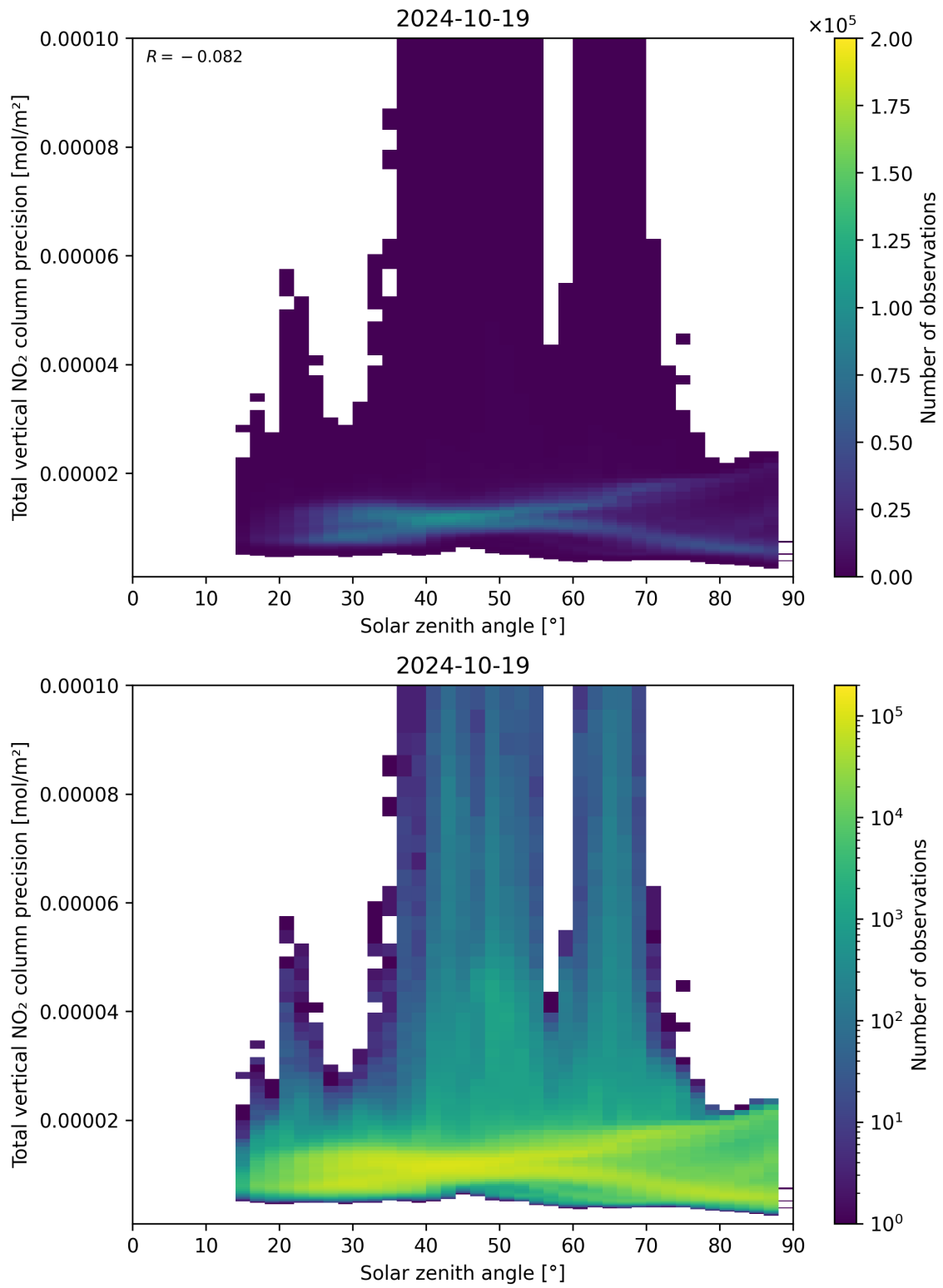
Figure 154: Scatter density plot of “Solar zenith angle” against “Total vertical NO 2 column precision” for 2024-10-19 to 2024-10-20.
