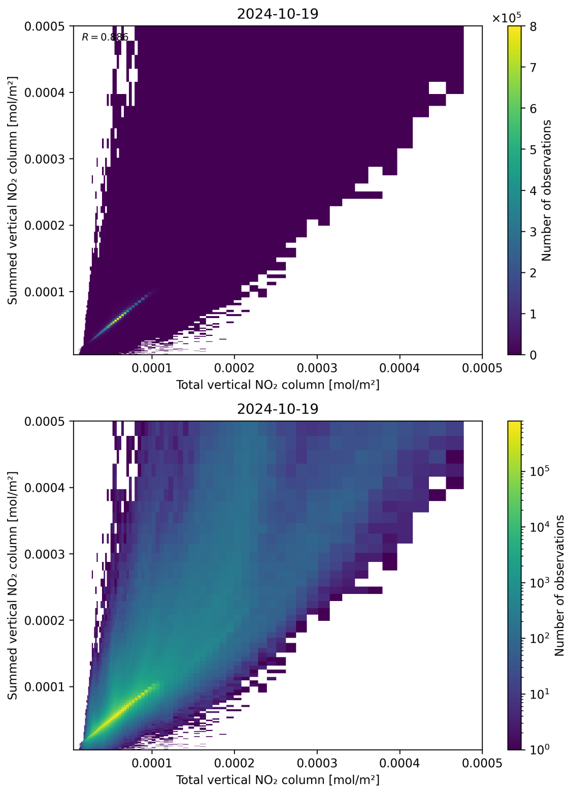
Figure 112: Scatter density plot of “Total vertical NO 2 column” against “Summed vertical NO 2 column” for 2024-10-19 to 2024-10-20.
