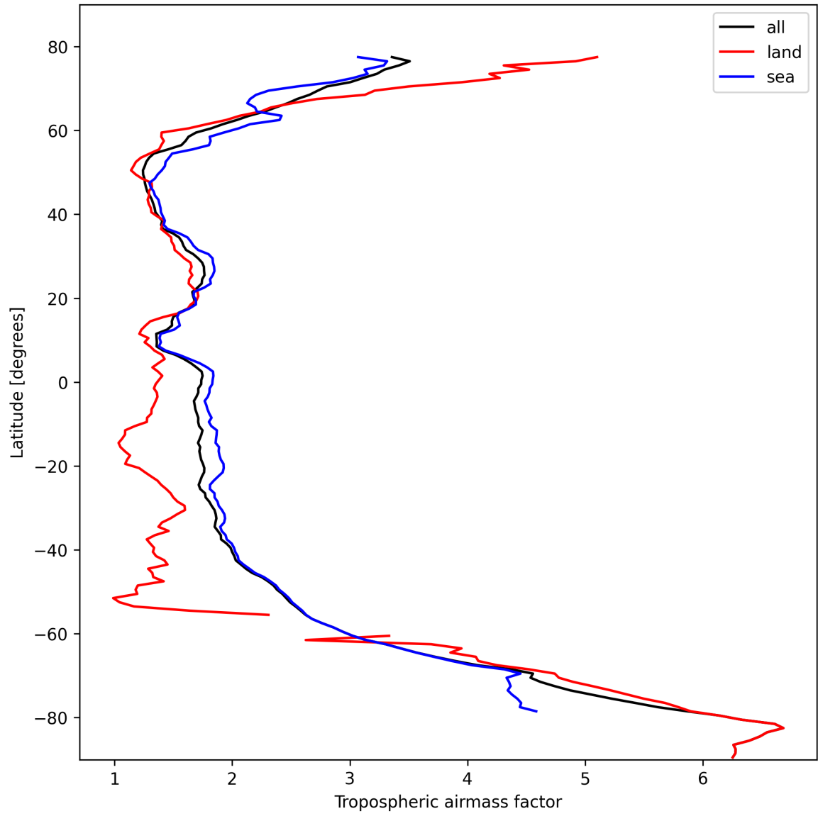
Figure 14: Zonal average of “Tropospheric airmass factor” for 2024-10-19 to 2024-10-20.
