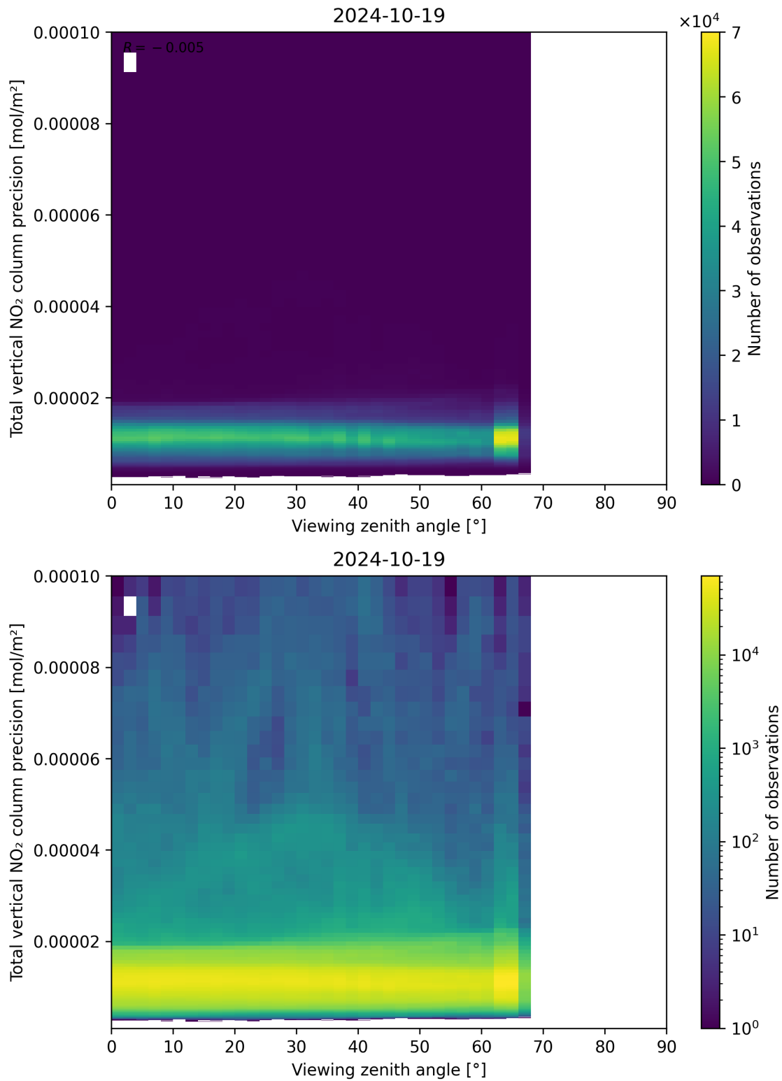
Figure 168: Scatter density plot of “Viewing zenith angle” against “Total vertical NO 2 column precision” for 2024-10-19 to 2024-10-20.
