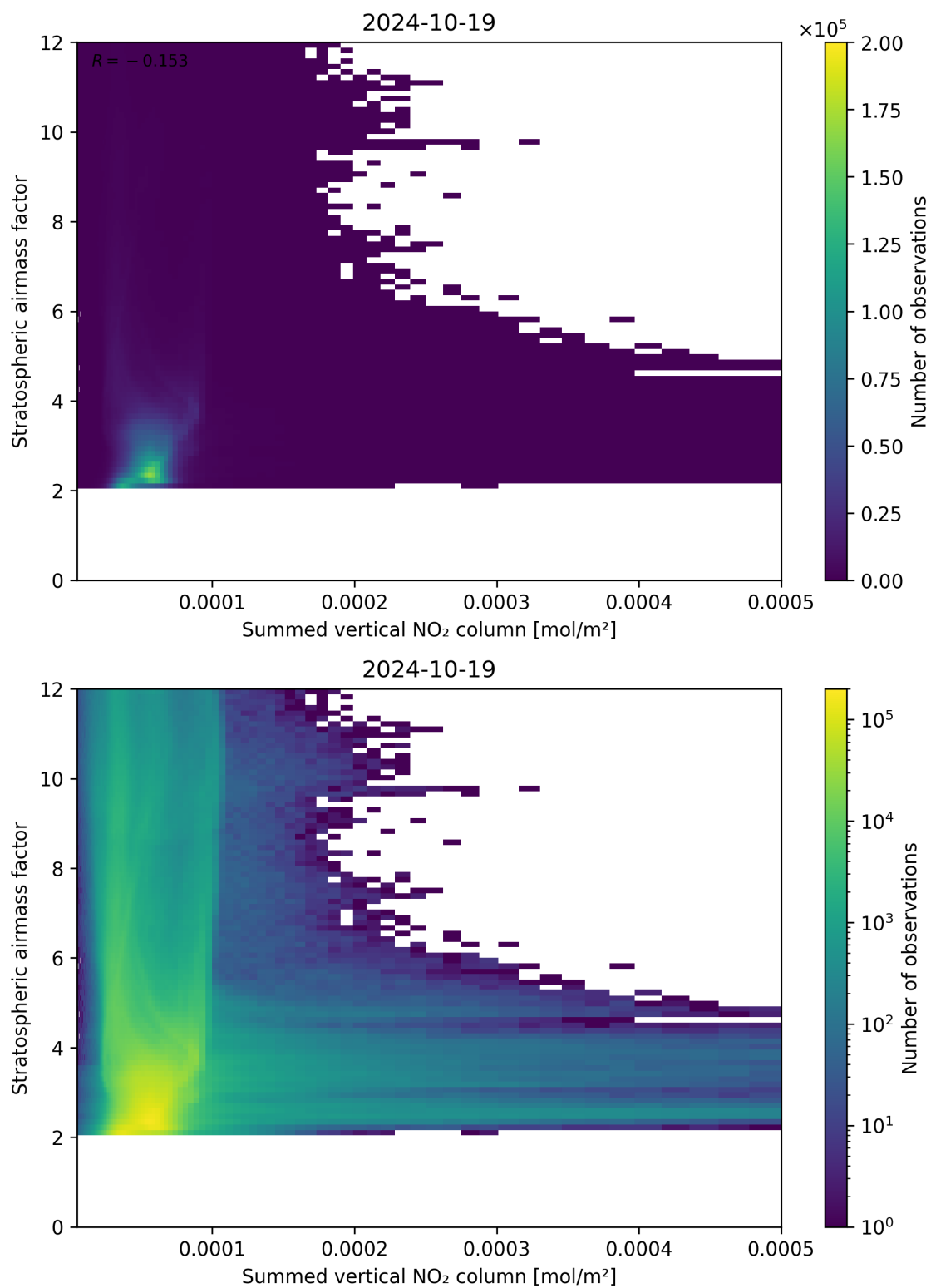
Figure 103: Scatter density plot of “Summed vertical NO 2 column” against “Stratospheric air mass factor” for 2024-10-19 to 2024-10-20.
