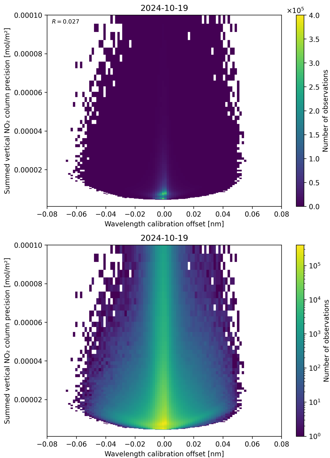
Figure 178: Scatter density plot of “Wavelength calibration offset” against “Summed vertical NO 2 column precision” for 2024-10-19 to 2024-10-20.
