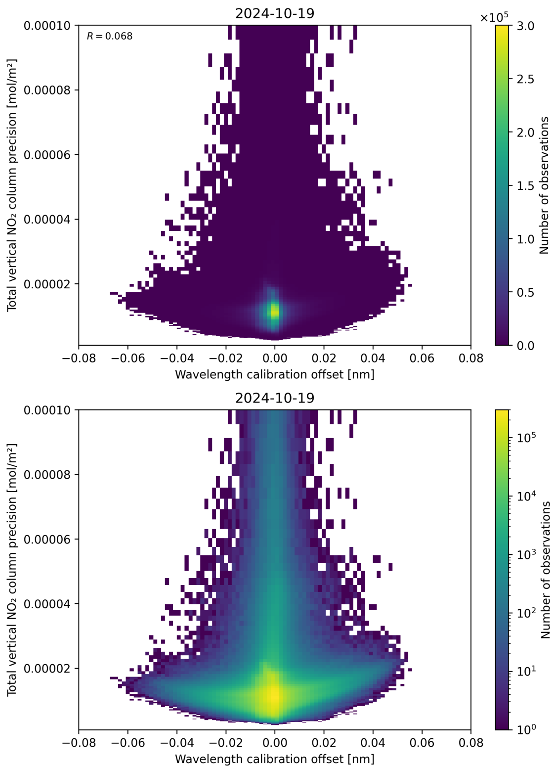
Figure 180: Scatter density plot of “Wavelength calibration offset” against “Total vertical NO 2 column precision” for 2024-10-19 to 2024-10-20.
