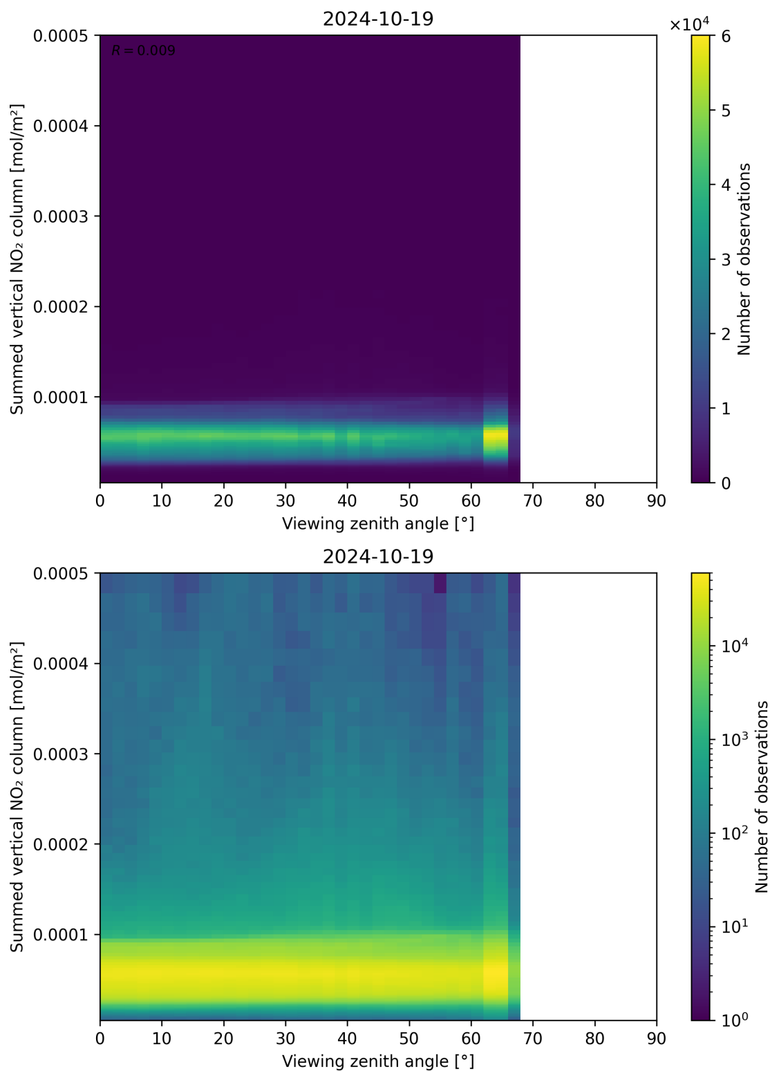
Figure 165: Scatter density plot of “Viewing zenith angle” against “Summed vertical NO 2 column” for 2024-10-19 to 2024-10-20.
