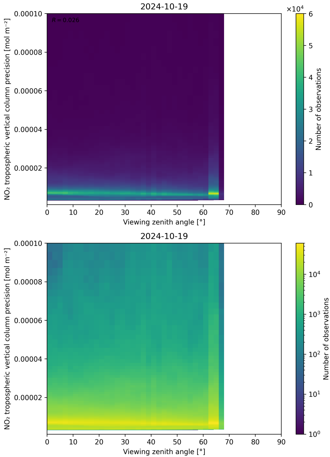
Figure 170: Scatter density plot of “Viewing zenith angle” against “NO 2 tropospheric vertical column precision” for 2024-10-19 to 2024-10-20.
