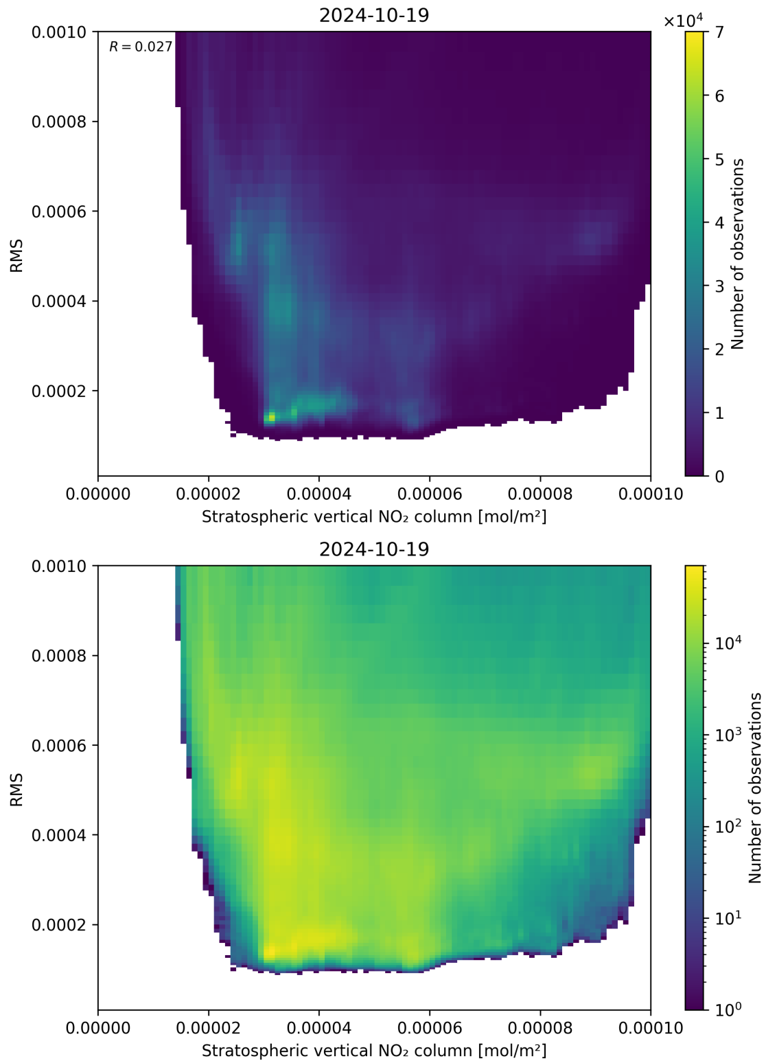
Figure 102: Scatter density plot of “Stratospheric vertical NO 2 column” against “RMS” for 2024-10-19 to 2024-10-20.
