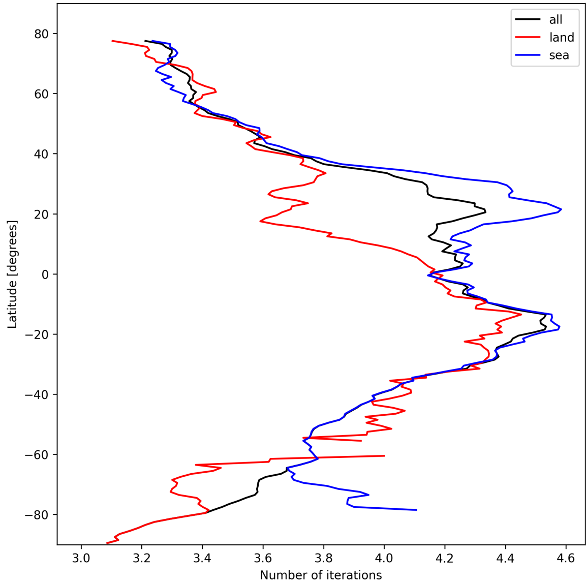
Figure 17: Zonal average of “Number of iterations” for 2024-10-19 to 2024-10-20.
