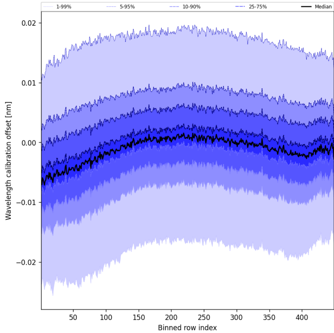
Figure 52: Along track statistics of “Wavelength calibration offset” for 2024-10-19 to 2024-10-20
