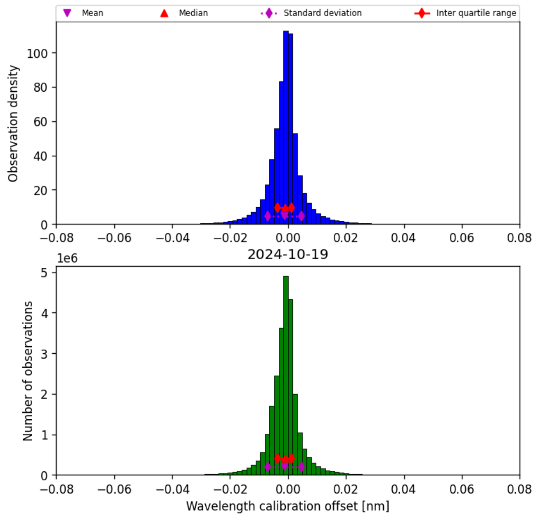
Figure 35: Histogram of “Wavelength calibration offset” for 2024-10-19 to 2024-10-20
