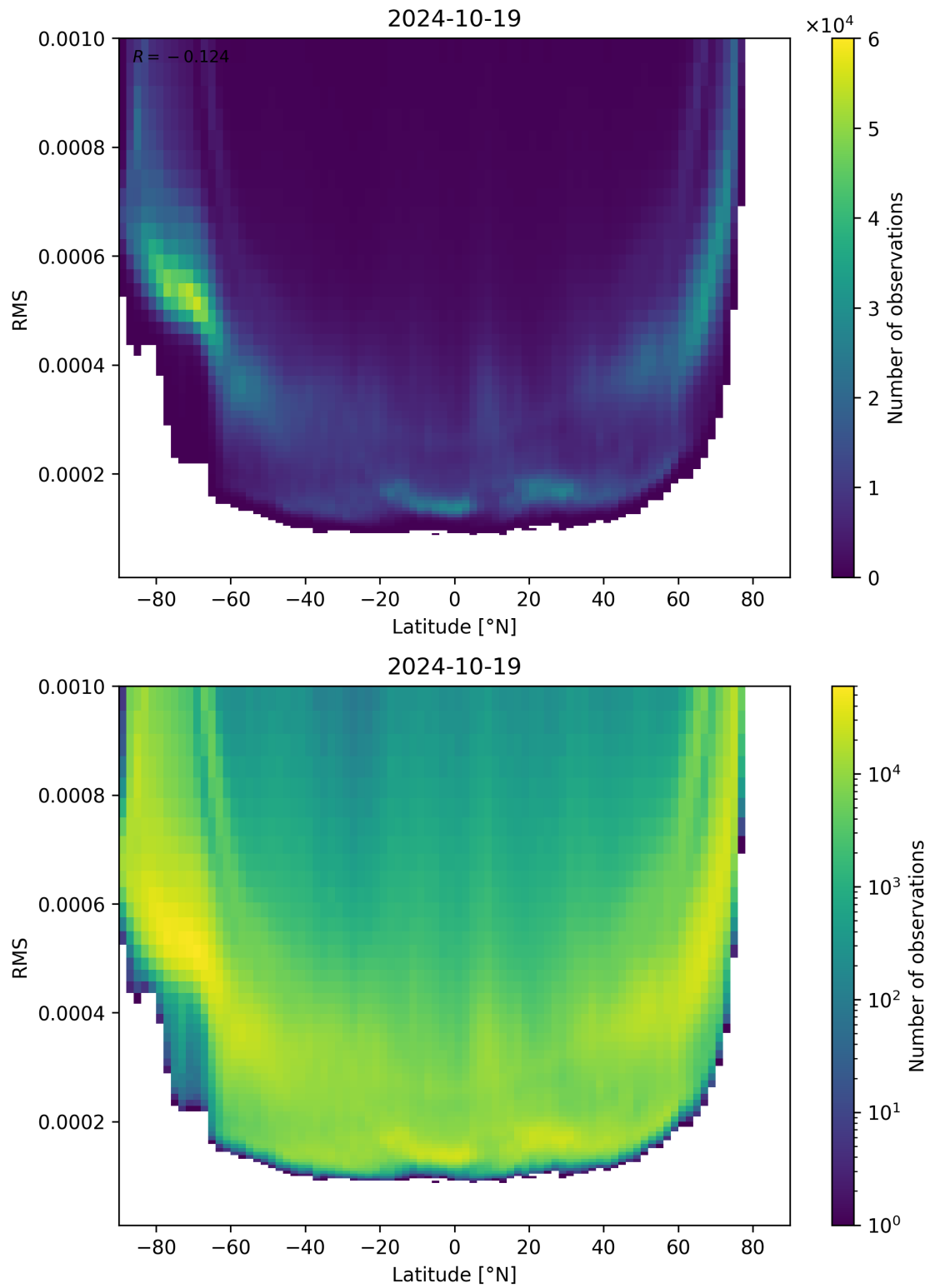
Figure 94: Scatter density plot of “Latitude” against “RMS” for 2024-10-19 to 2024-10-20.
