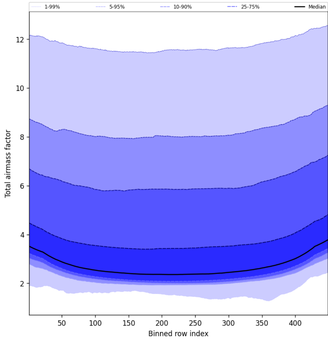
Figure 49: Along track statistics of “Total airmass factor” for 2024-10-19 to 2024-10-20
