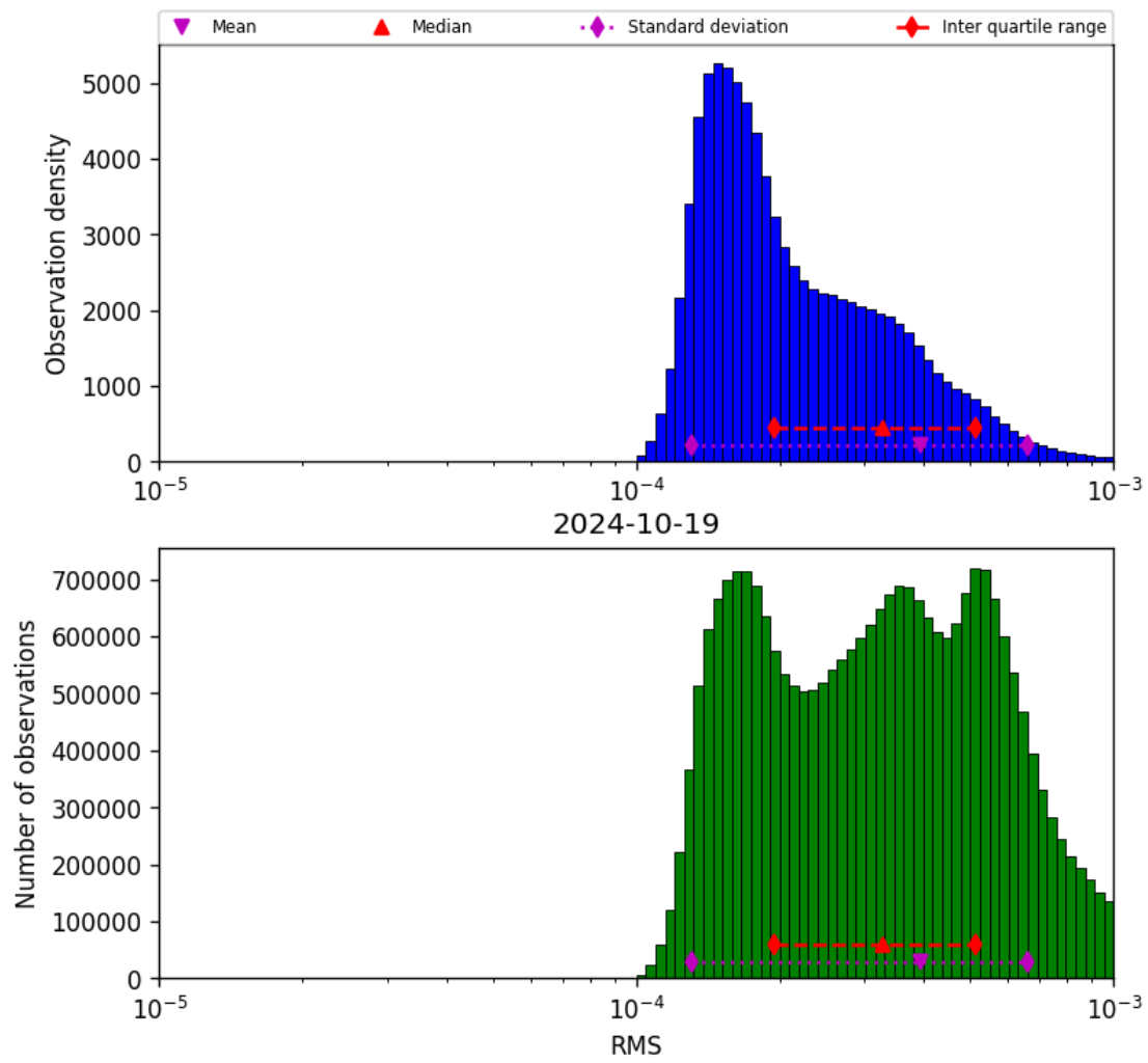
Figure 43: Histogram of “RMS” for 2024-10-19 to 2024-10-20
