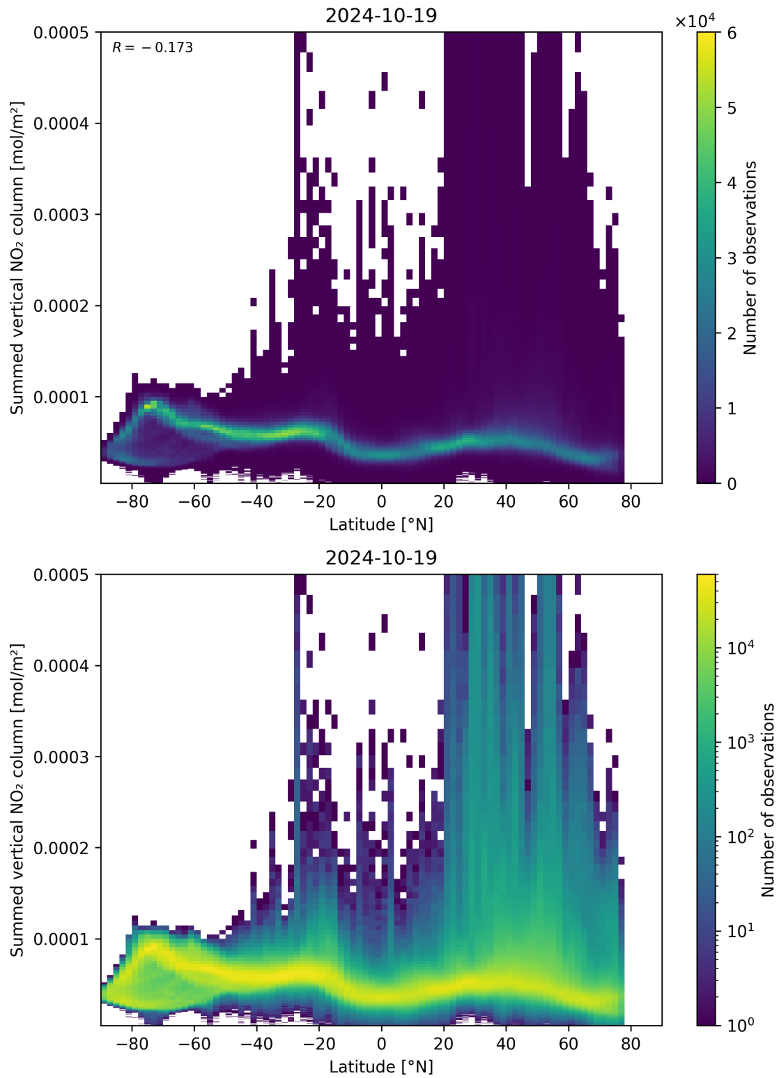
Figure 88: Scatter density plot of “Latitude” against “Summed vertical NO 2 column” for 2024-10-19 to 2024-10-20.
