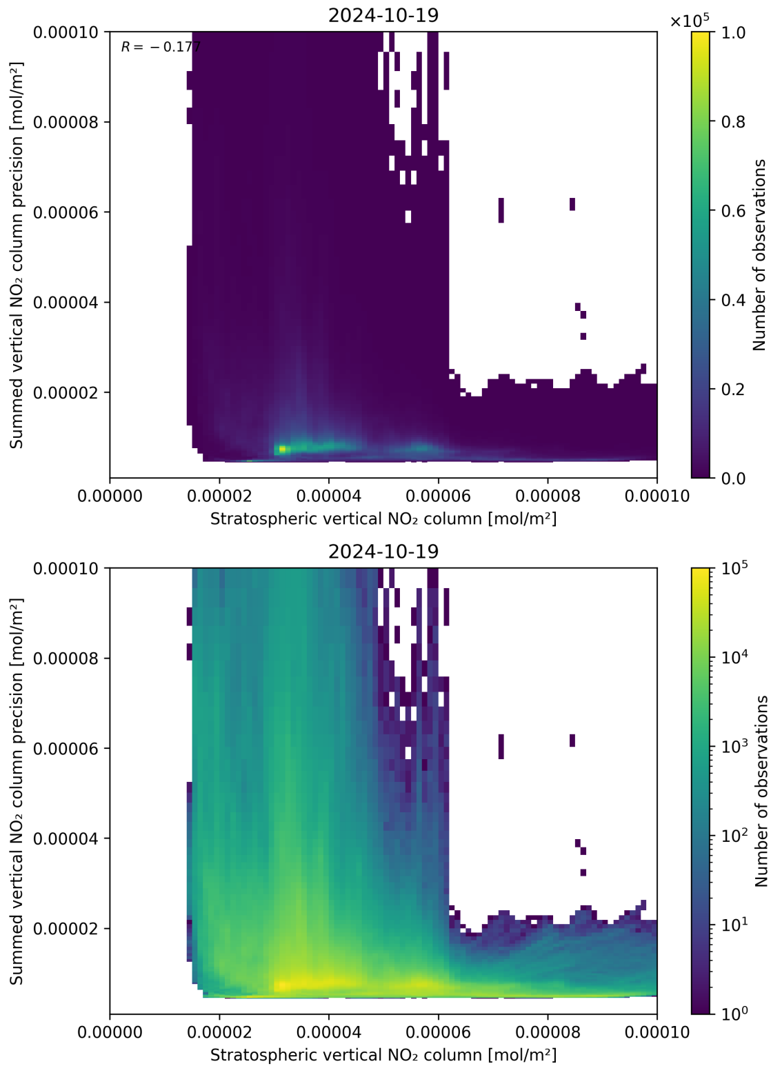
Figure 99: Scatter density plot of “Stratospheric vertical NO 2 column” against “Summed vertical NO 2 column precision” for 2024-10-19 to 2024-10-20.
