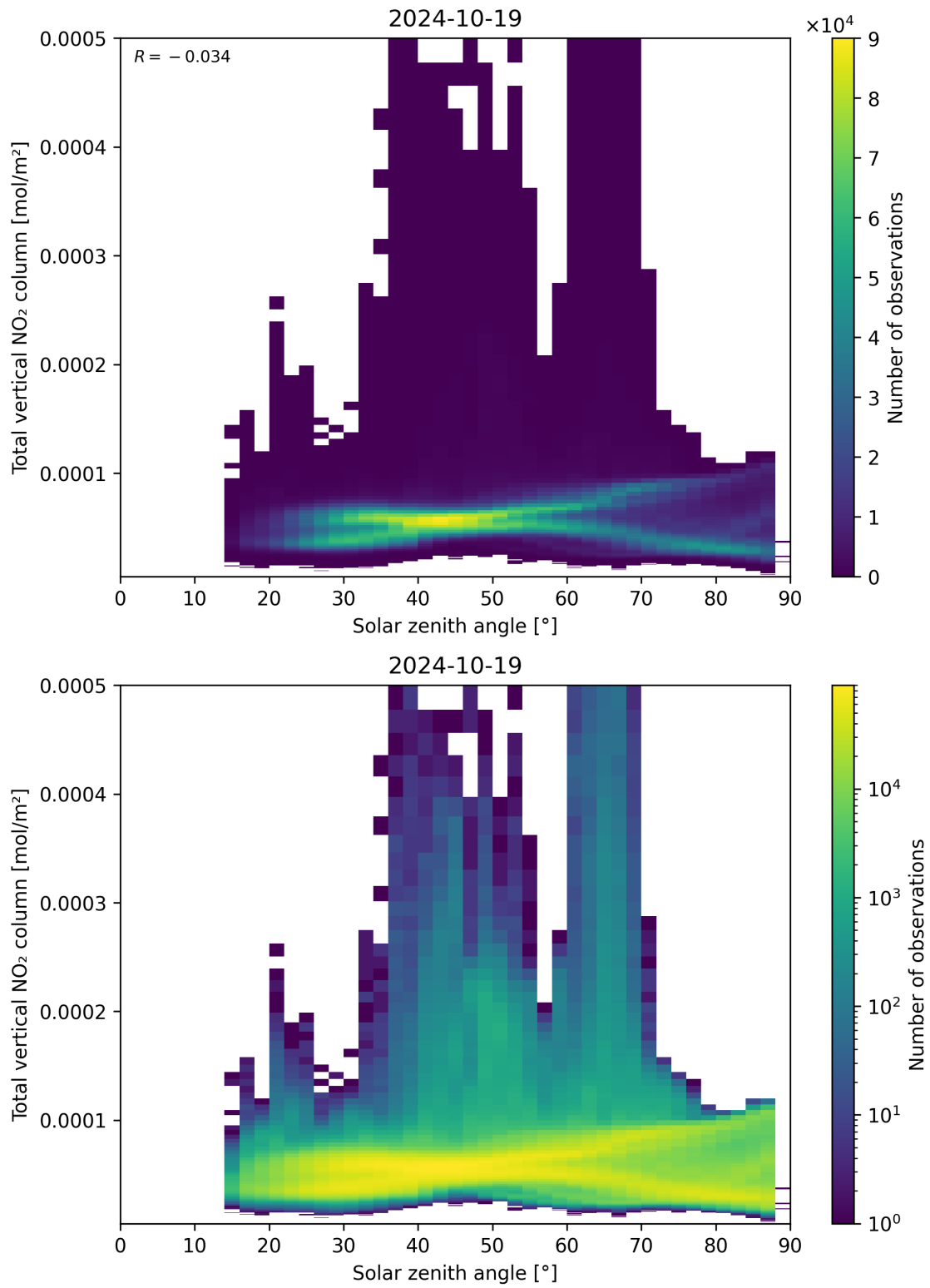
Figure 153: Scatter density plot of “Solar zenith angle” against “Total vertical NO 2 column” for 2024-10-19 to 2024-10-20.
