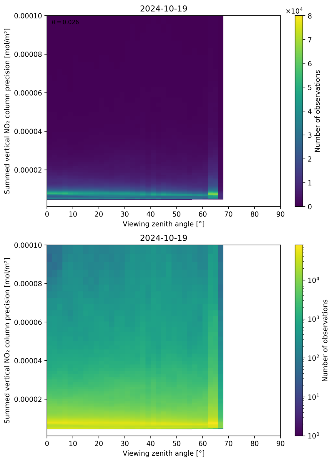
Figure 166: Scatter density plot of “Viewing zenith angle” against “Summed vertical NO 2 column precision” for 2024-10-19 to 2024-10-20.
