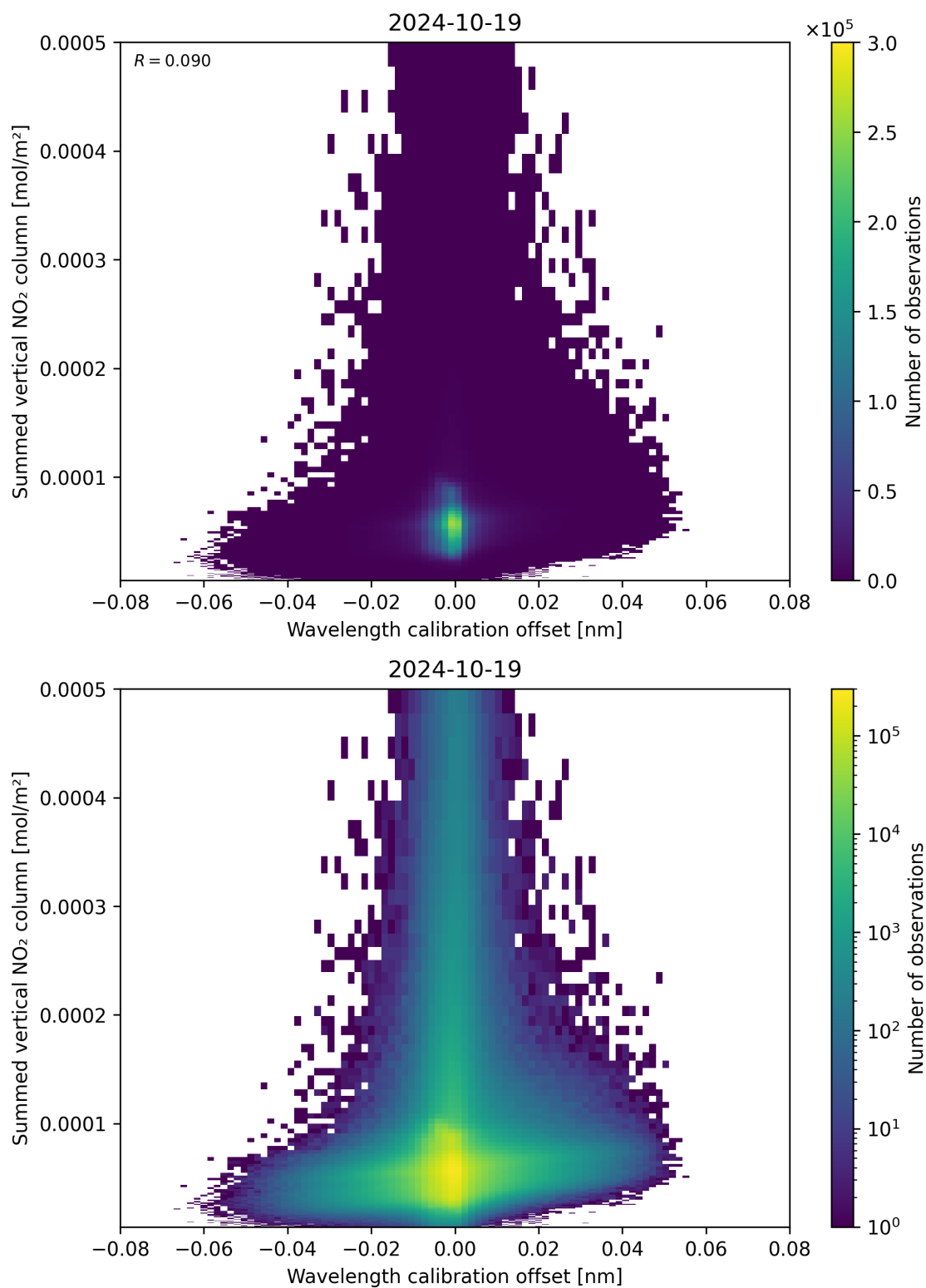
Figure 177: Scatter density plot of “Wavelength calibration offset” against “Summed vertical NO 2 column” for 2024-10-19 to 2024-10-20.
