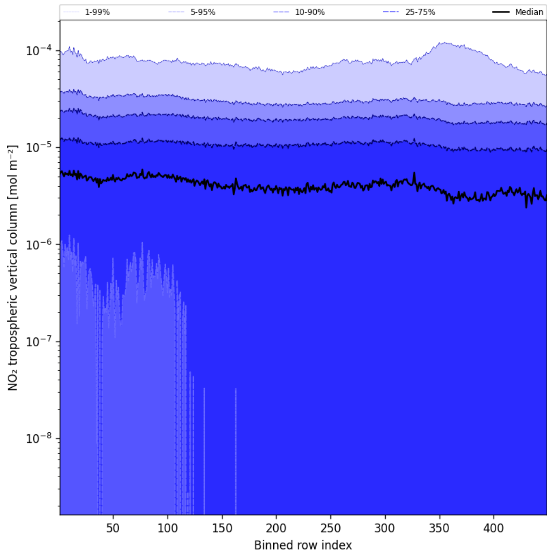
Figure 46: Along track statistics of “NO 2 tropospheric vertical column” for 2024-10-19 to 2024-10-20
