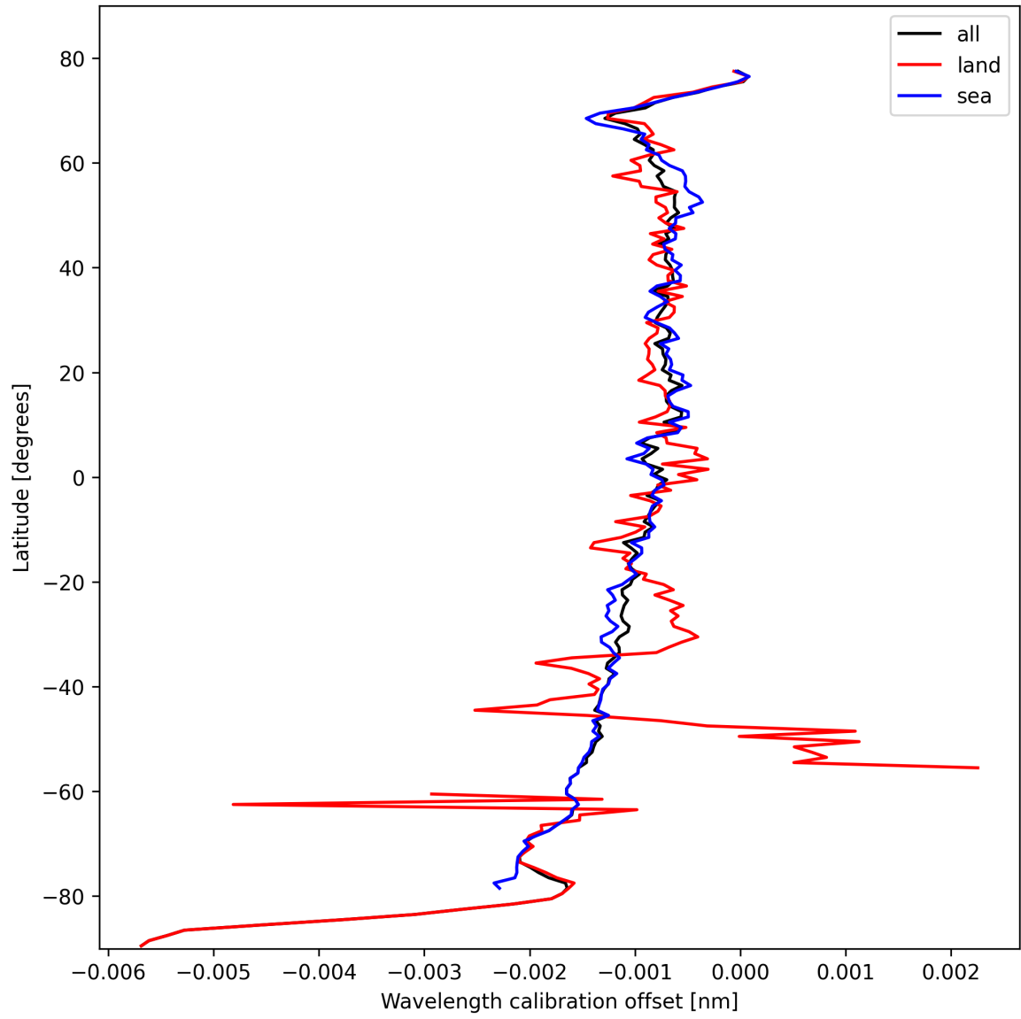
Figure 18: Zonal average of “Wavelength calibration offset” for 2024-10-19 to 2024-10-20.
