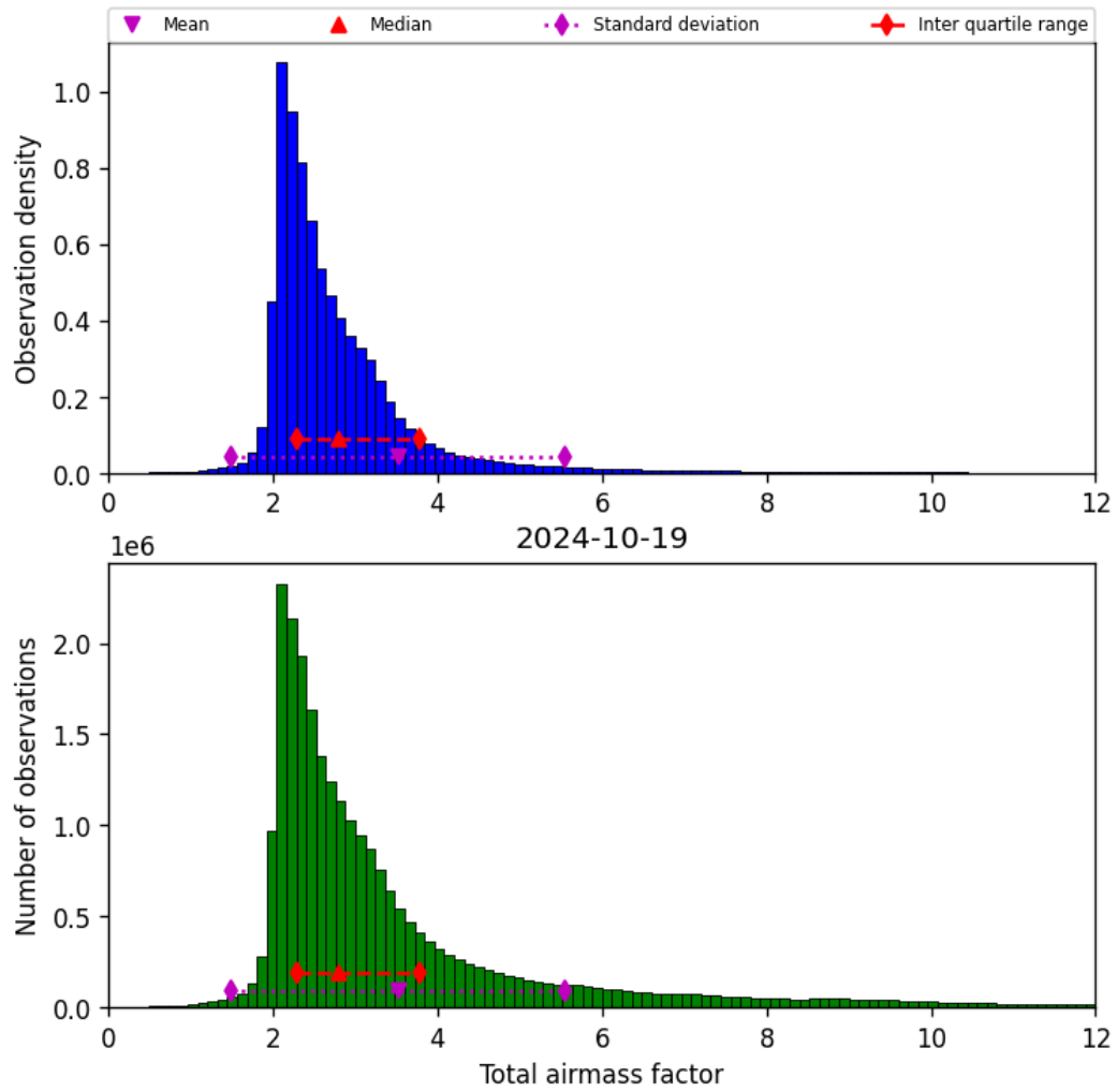
Figure 32: Histogram of “Total airmass factor” for 2024-10-19 to 2024-10-20
