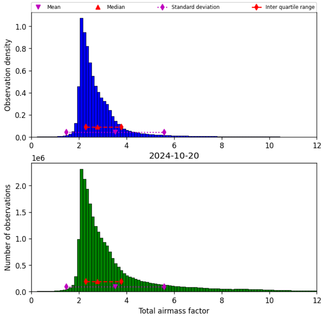
Figure 32: Histogram of “Total airmass factor” for 2024-10-19 to 2024-10-21
