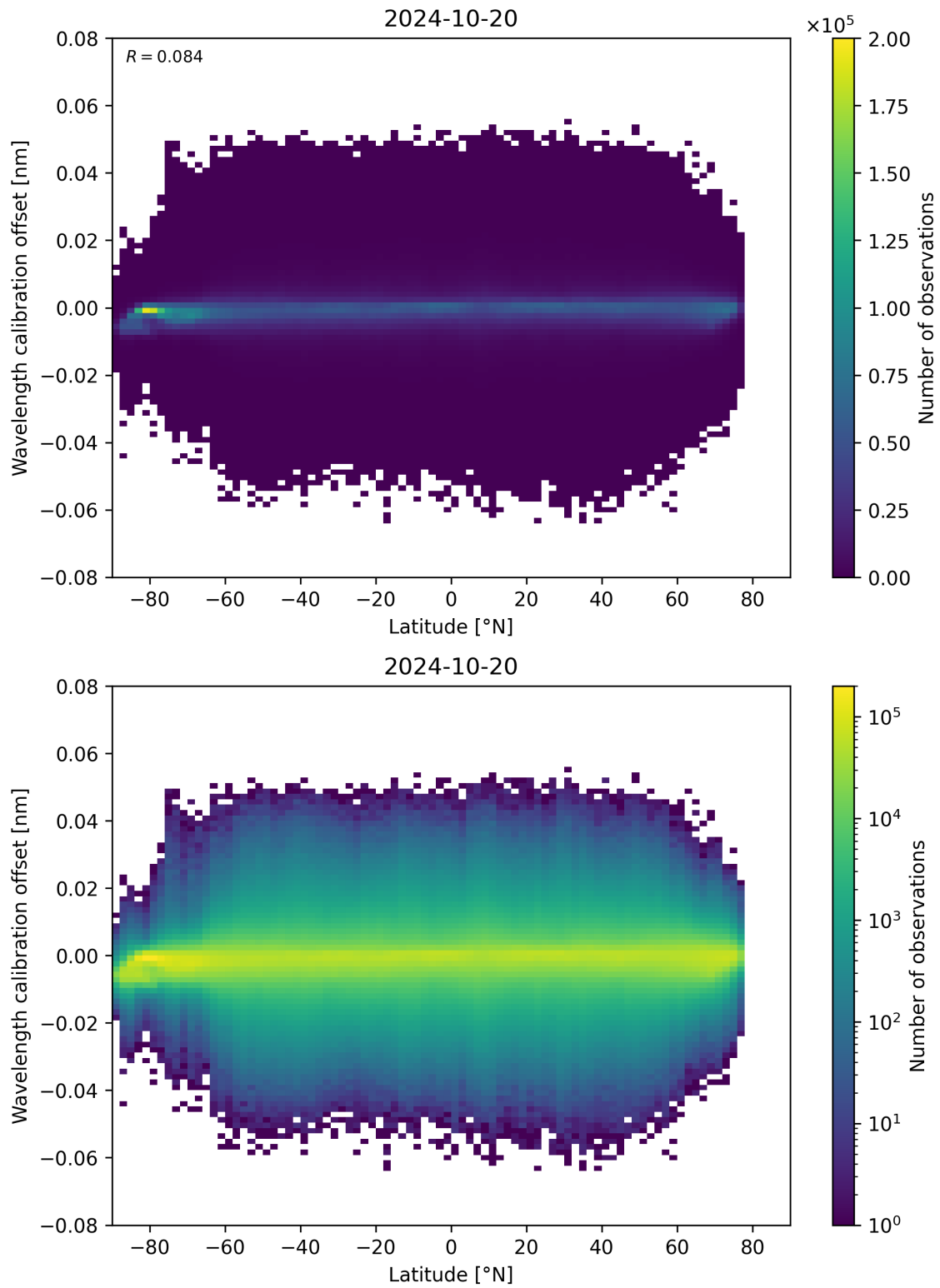
Figure 95: Scatter density plot of “Latitude” against “Wavelength calibration offset” for 2024-10-19 to 2024-10-21.
