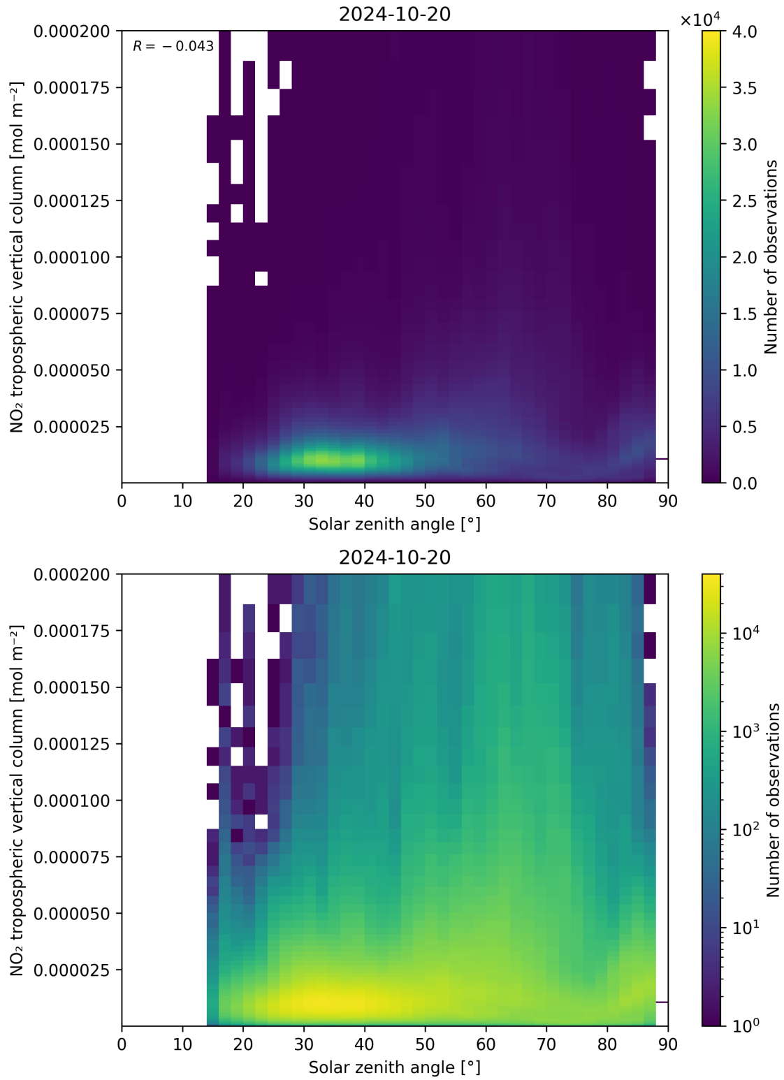
Figure 155: Scatter density plot of “Solar zenith angle” against “NO 2 tropospheric vertical column” for 2024-10-19 to 2024-10-21.
