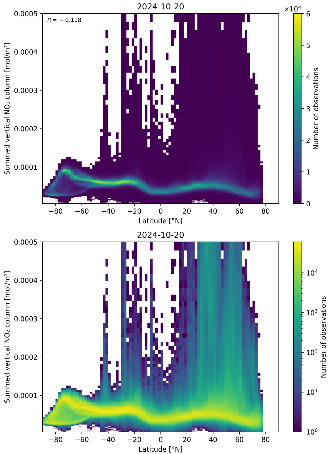
Figure 88: Scatter density plot of “Latitude” against “Summed vertical NO 2 column” for 2024-10-19 to 2024-10-21.
