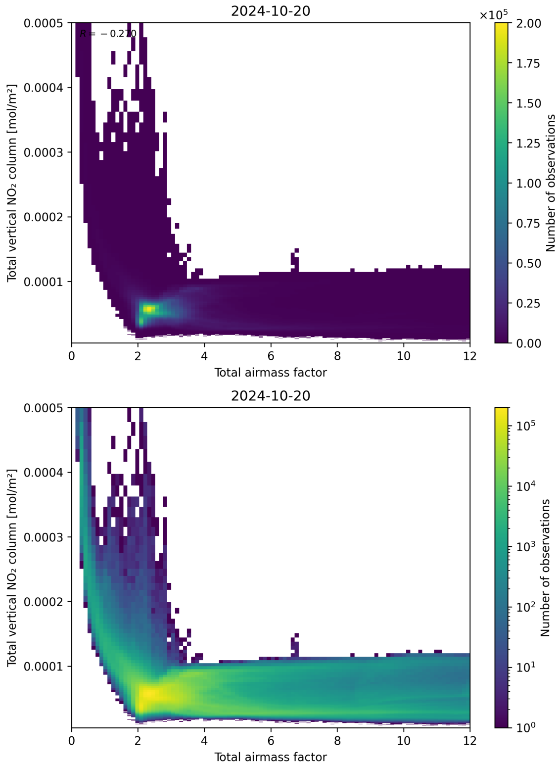
Figure 67: Scatter density plot of “Total airmass factor” against “Total vertical NO 2 column” for 2024-10-19 to 2024-10-21.
