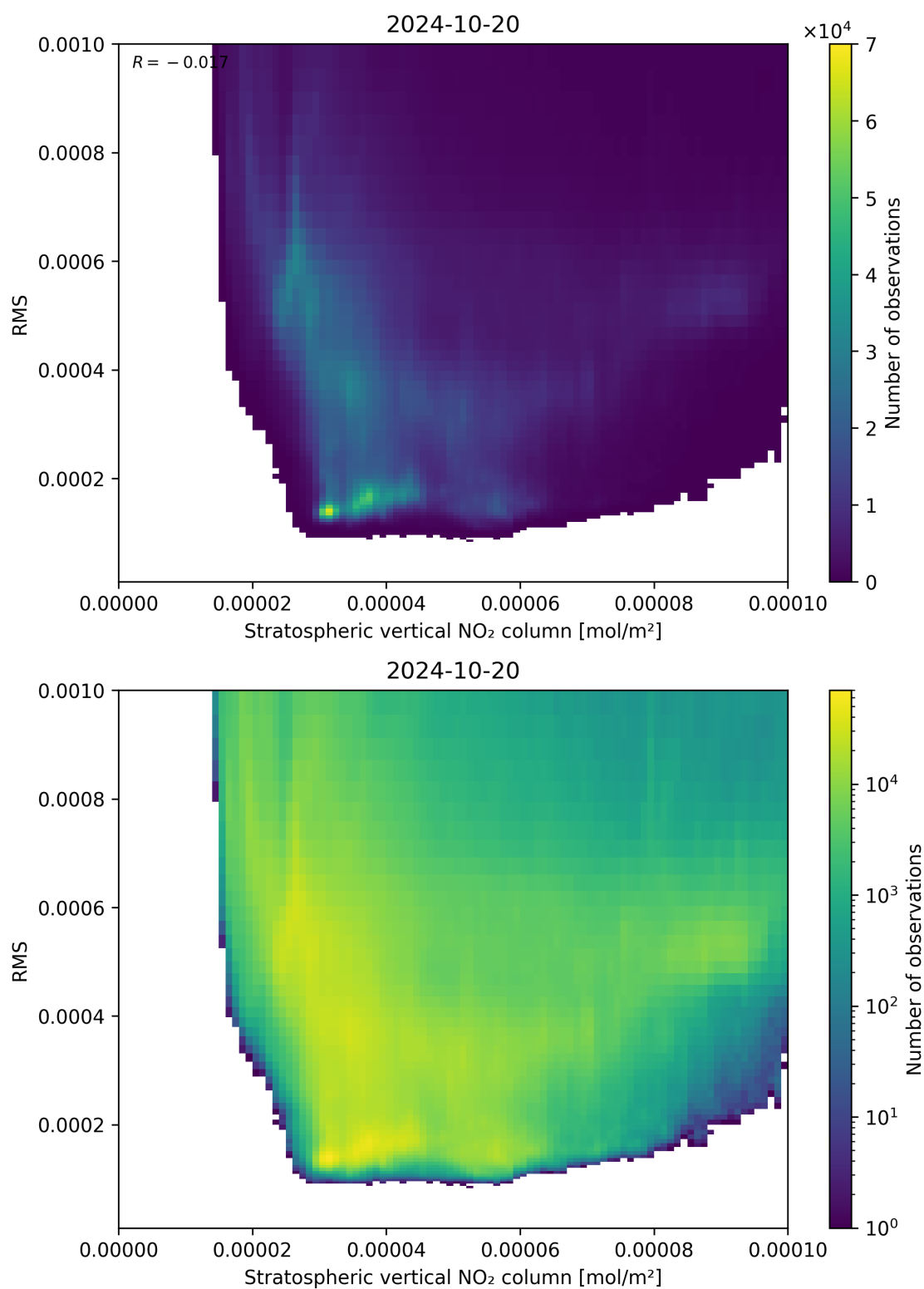
Figure 102: Scatter density plot of “Stratospheric vertical NO 2 column” against “RMS” for 2024-10-19 to 2024-10-21.
