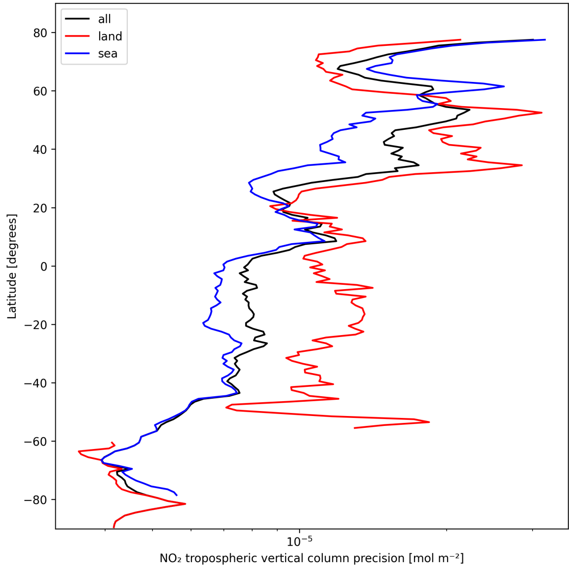
Figure 13: Zonal average of “NO 2 tropospheric vertical column precision” for 2024-10-19 to 2024-10-21.
