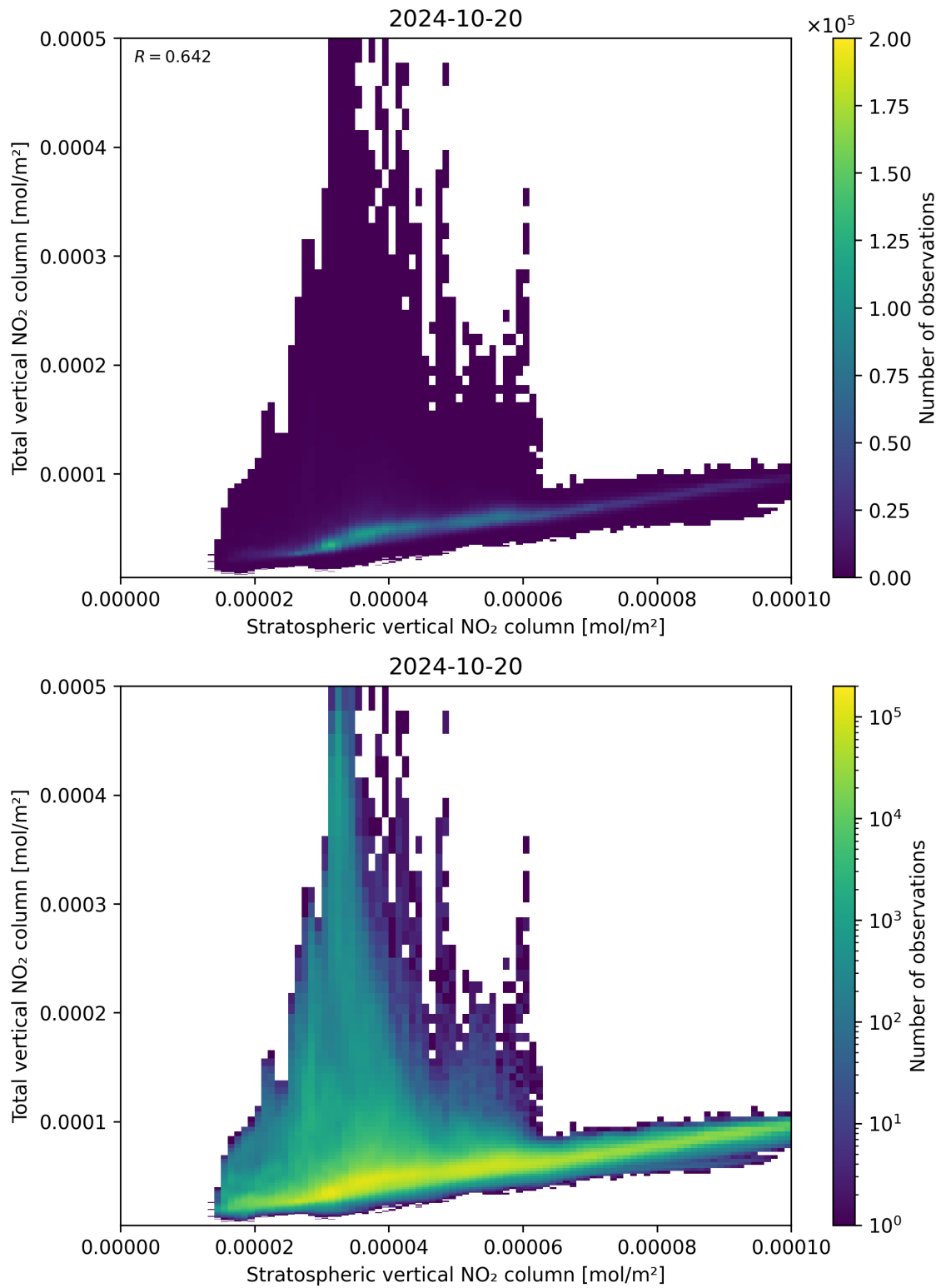
Figure 100: Scatter density plot of “Stratospheric vertical NO 2 column” against “Total vertical NO 2 column” for 2024-10-19 to 2024-10-21.
