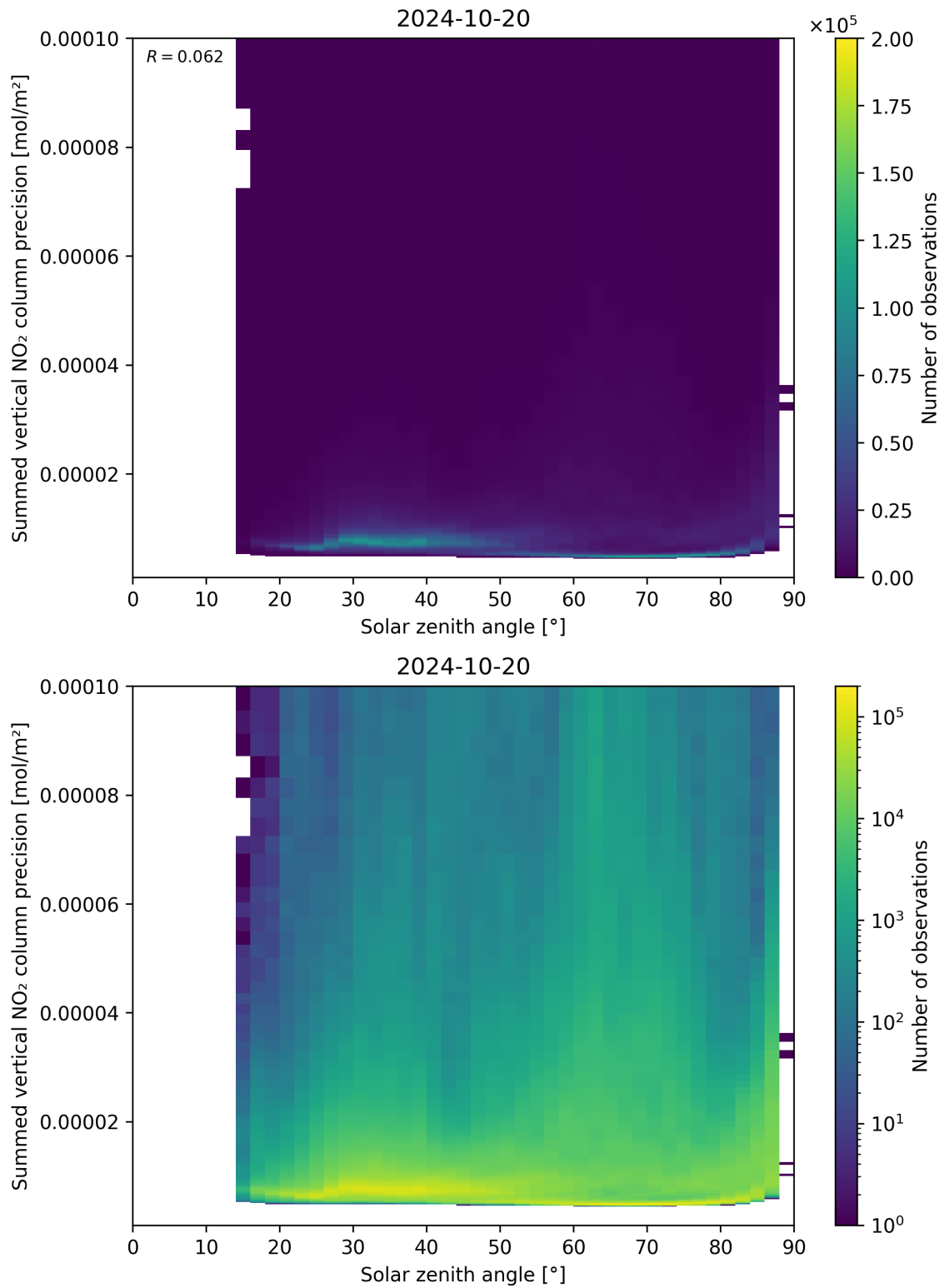
Figure 152: Scatter density plot of “Solar zenith angle” against “Summed vertical NO 2 column precision” for 2024-10-19 to 2024-10-21.
