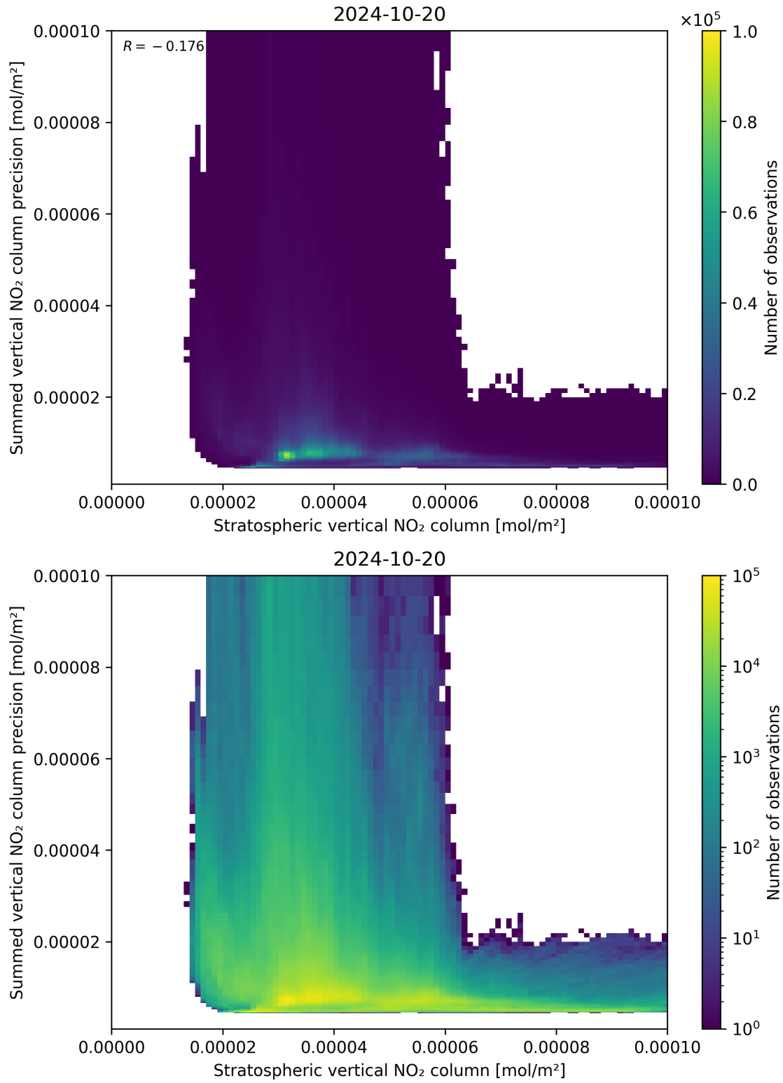
Figure 99: Scatter density plot of “Stratospheric vertical NO 2 column” against “Summed vertical NO 2 column precision” for 2024-10-19 to 2024-10-21.
