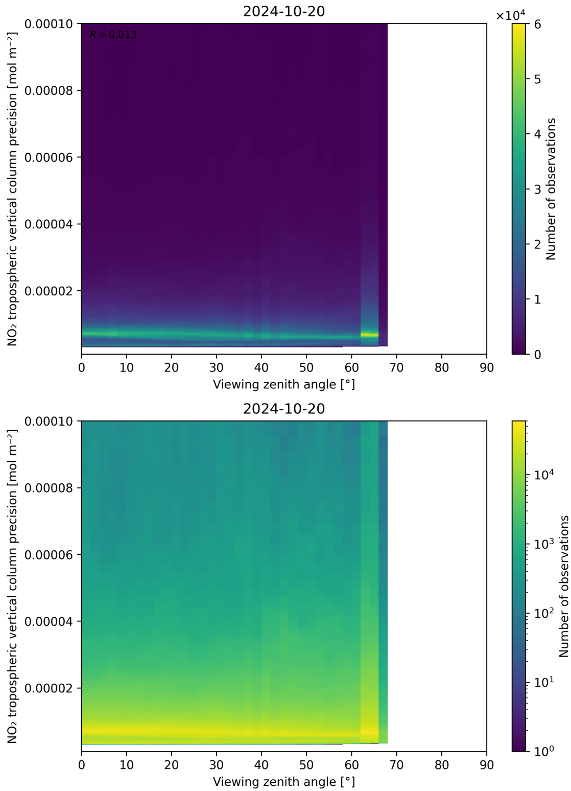
Figure 170: Scatter density plot of “Viewing zenith angle” against “NO 2 tropospheric vertical column precision” for 2024-10-19 to 2024-10-21.
