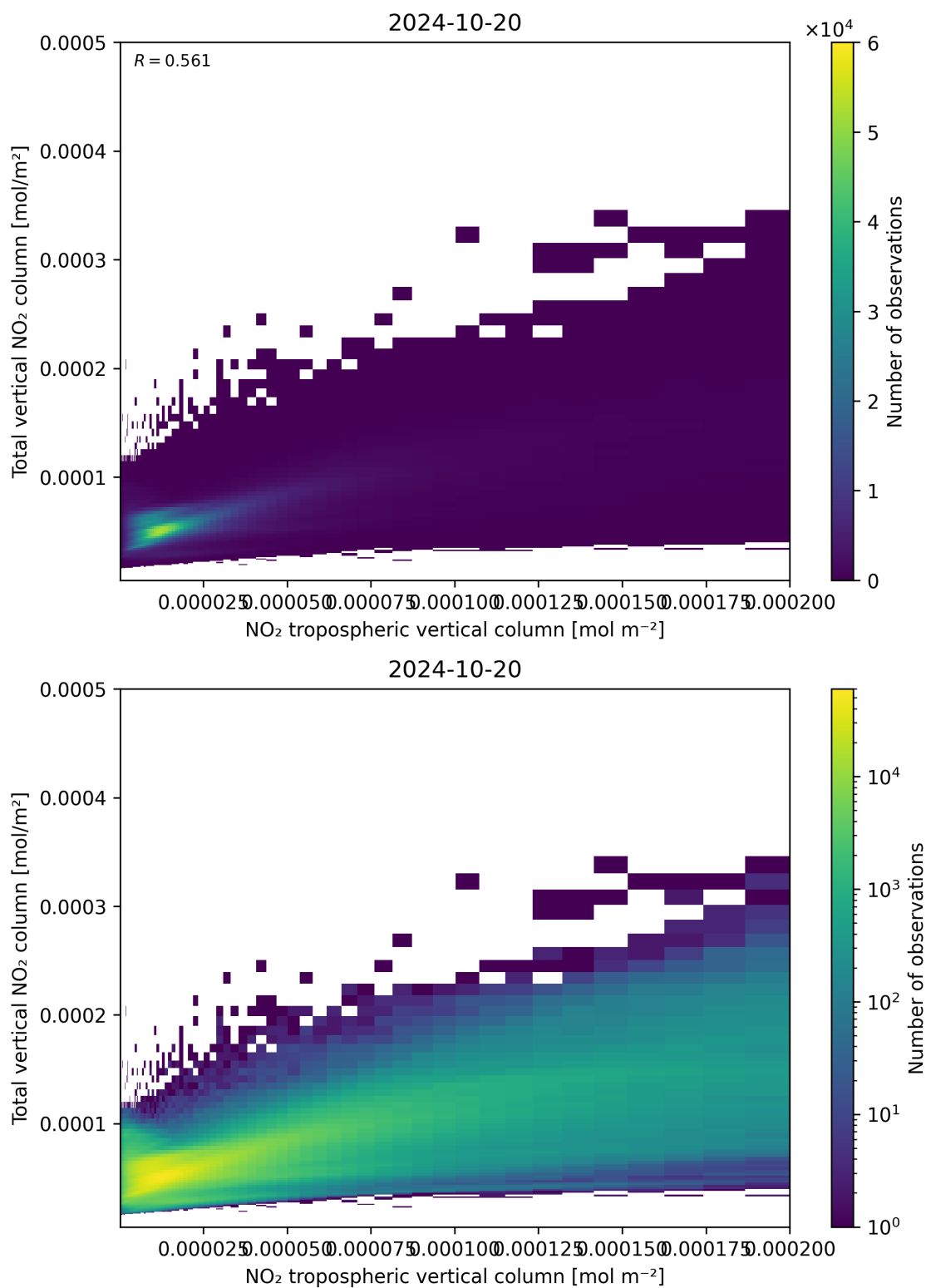
Figure 128: Scatter density plot of “NO 2 tropospheric vertical column” against “Total vertical NO 2 column” for 2024-10-19 to 2024-10-21.
