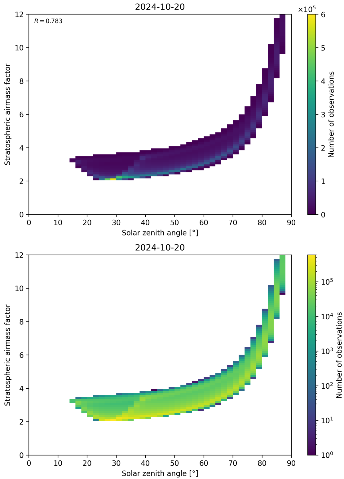
Figure 145: Scatter density plot of “Solar zenith angle” against “Stratospheric airmass factor” for 2024-10-19 to 2024-10-21.
