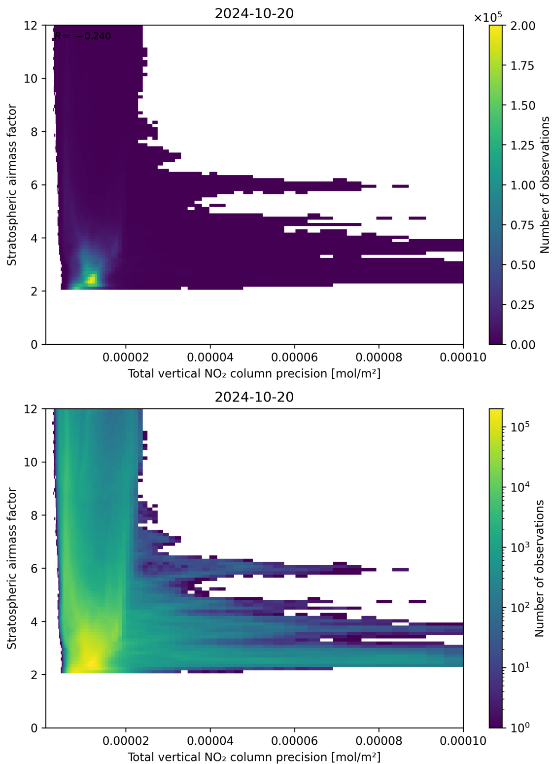
Figure 115: Scatter density plot of “Total vertical NO 2 column precision” against “Stratospheric air mass factor” for 2024-10-19 to 2024-10-21.
