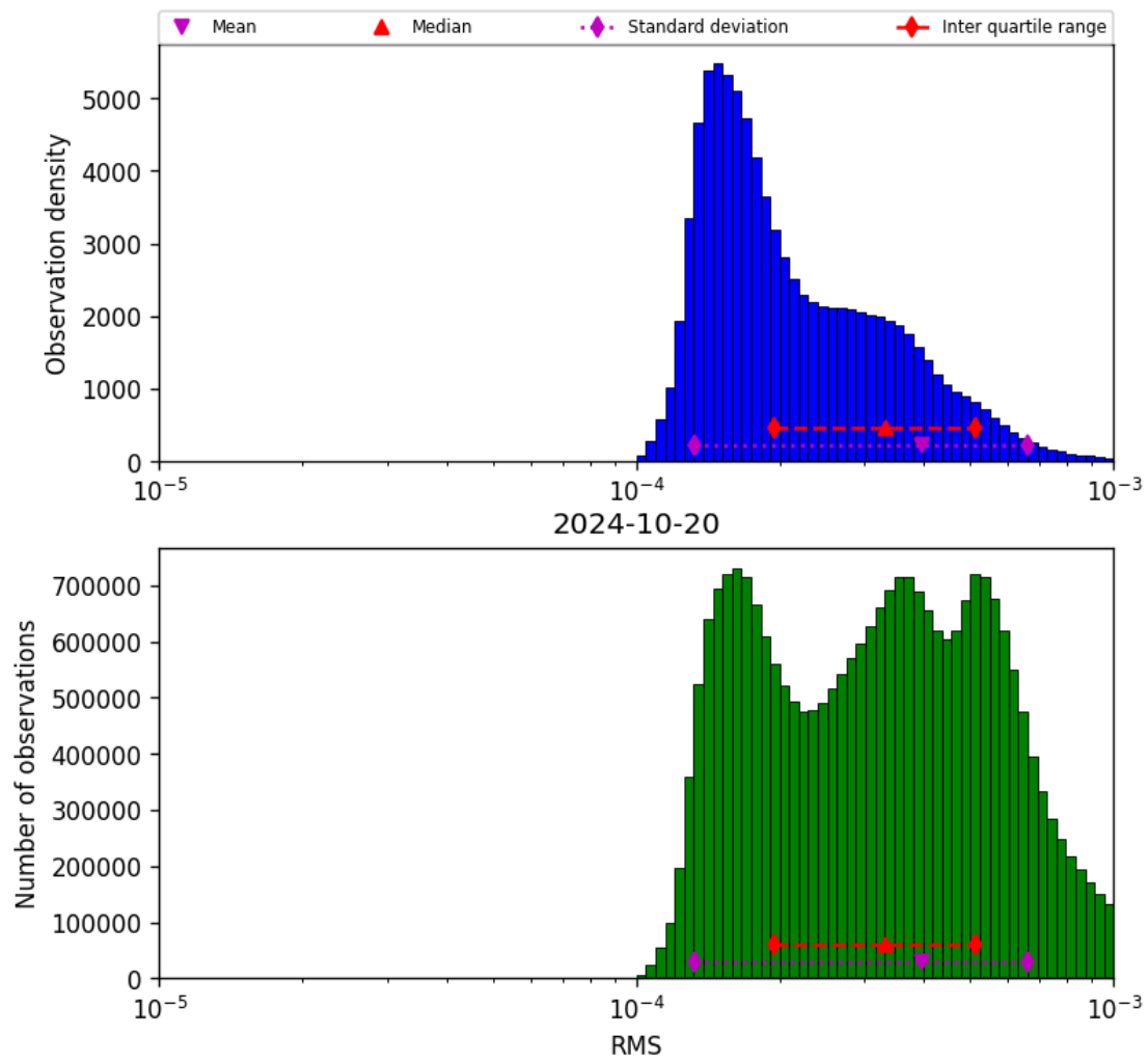
Figure 43: Histogram of “RMS” for 2024-10-19 to 2024-10-21
