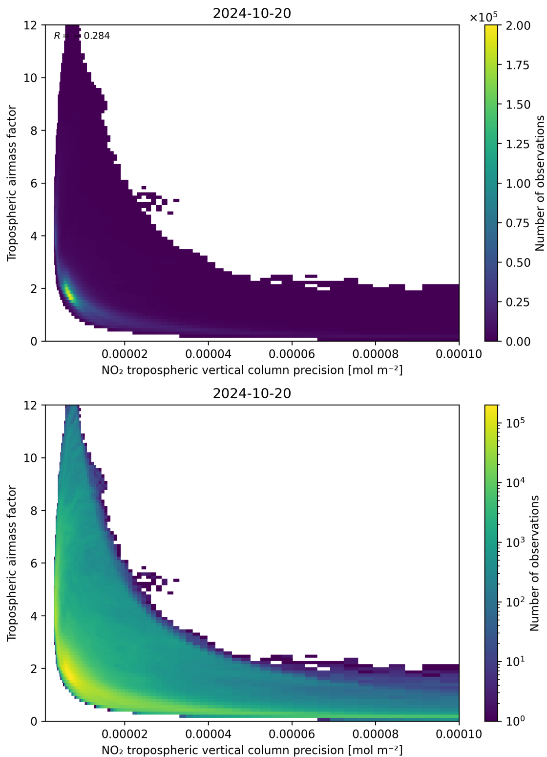
Figure 133: Scatter density plot of “NO 2 tropospheric vertical column precision” against “Tropospheric air mass factor” for 2024-10-19 to 2024-10-21.
