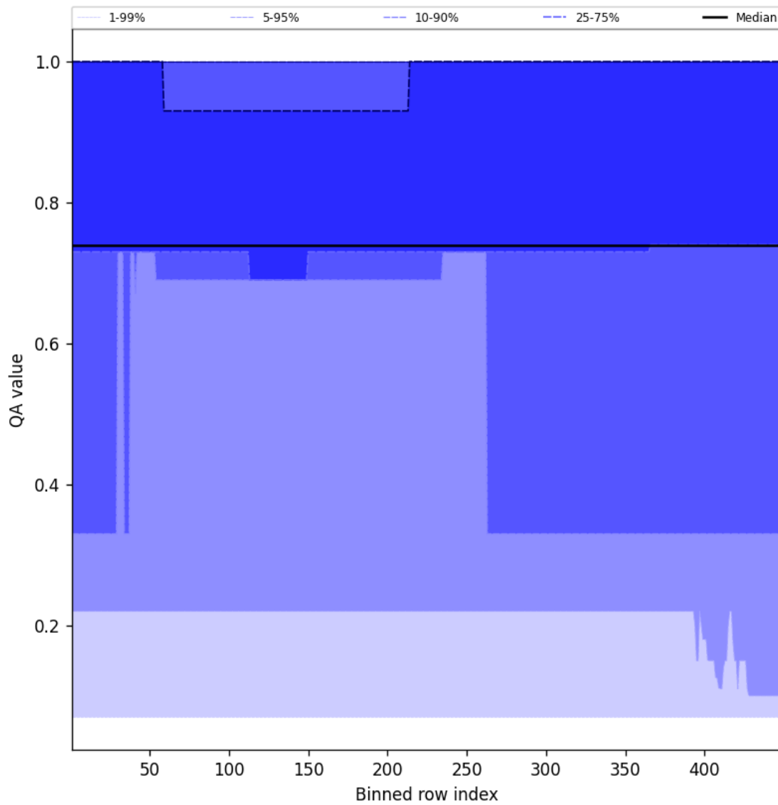
Figure 45: Along track statistics of “QA value” for 2024-10-19 to 2024-10-21
