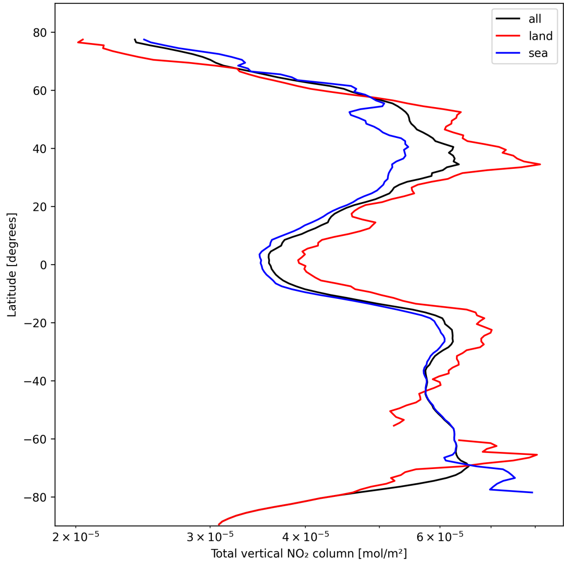
Figure 21: Zonal average of “Total vertical NO 2 column” for 2024-10-19 to 2024-10-21.
