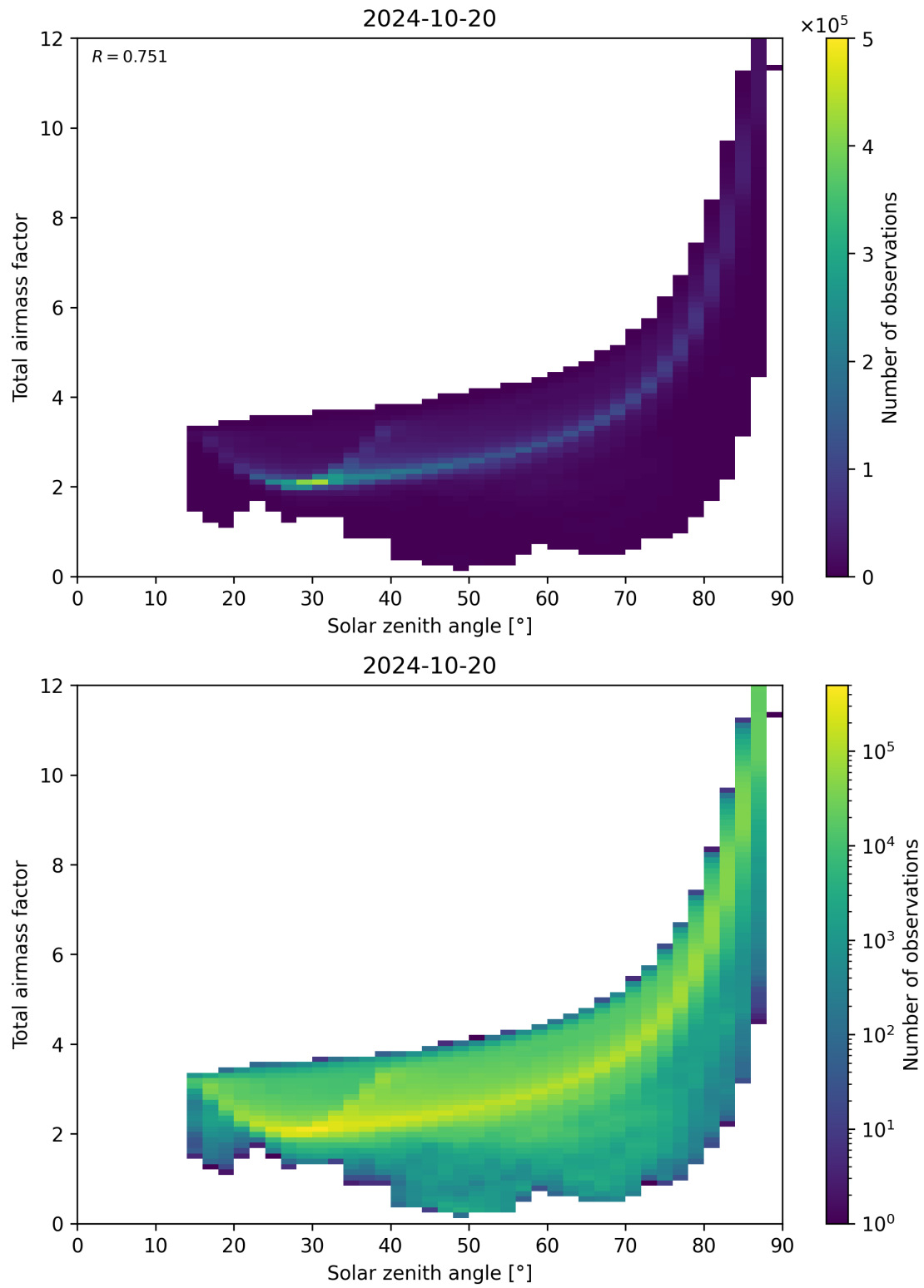
Figure 146: Scatter density plot of “Solar zenith angle” against “Total air mass factor” for 2024-10-19 to 2024-10-21.
