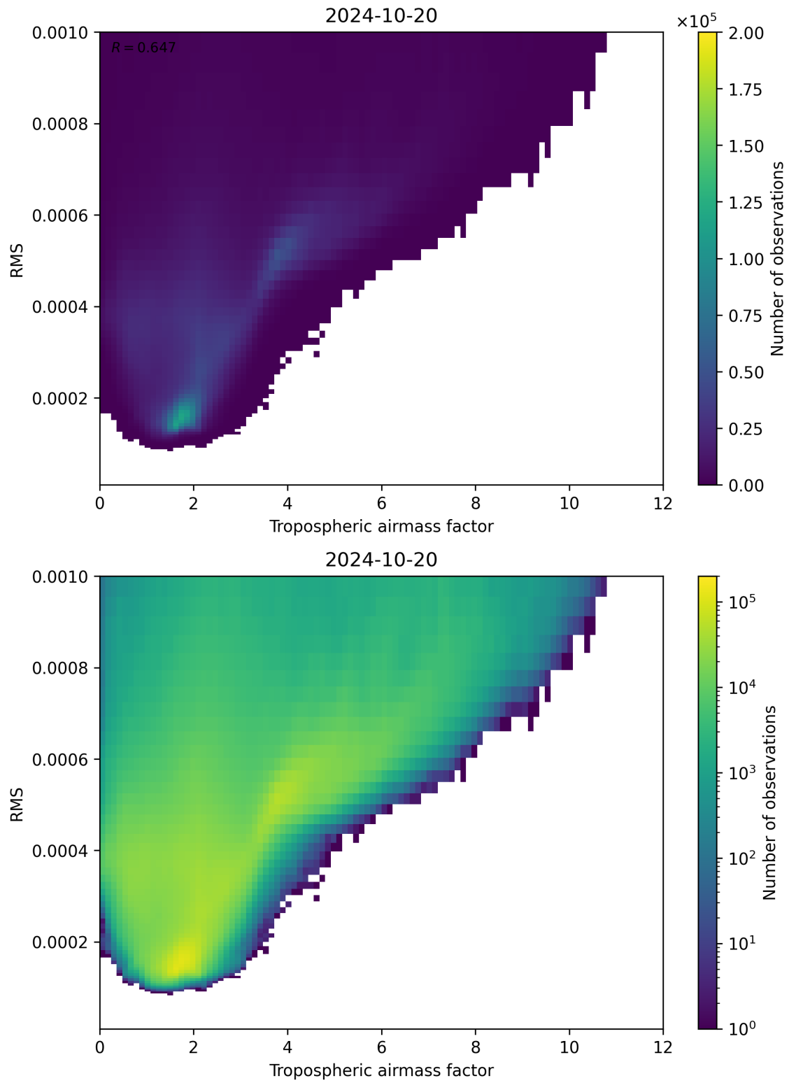
Figure 79: Scatter density plot of “Tropospheric airmass factor” against “RMS” for 2024-10-19 to 2024-10-21.
