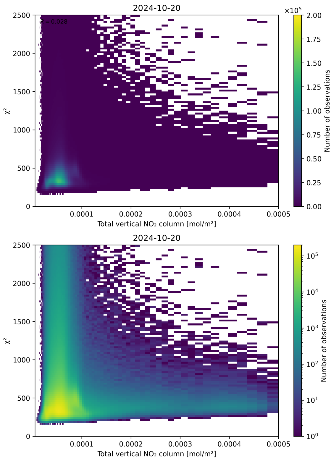
Figure 111: Scatter density plot of “Total vertical NO 2 column” against “ \chi^2 ” for 2024-10-19 to 2024-10-21.
