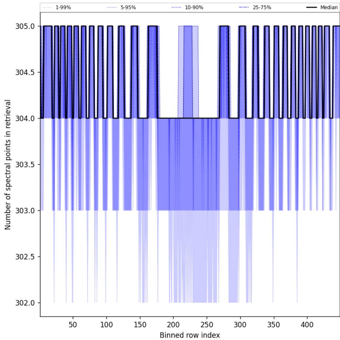
Figure 50: Along track statistics of “Number of spectral points in retrieval” for 2024-10-19 to 2024-10-21
