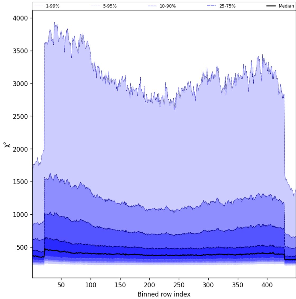
Figure 59: Along track statistics of “ \chi^2 ” for 2024-10-19 to 2024-10-21
