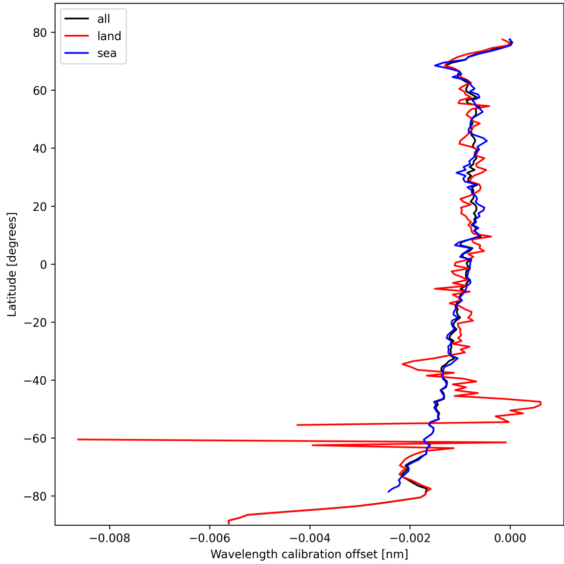
Figure 18: Zonal average of “Wavelength calibration offset” for 2024-10-19 to 2024-10-21.
