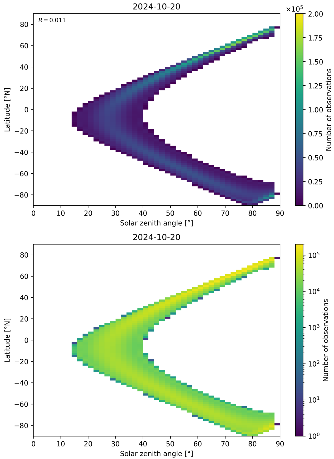
Figure 149: Scatter density plot of “Solar zenith angle” against “Latitude” for 2024-10-19 to 2024-10-21.
