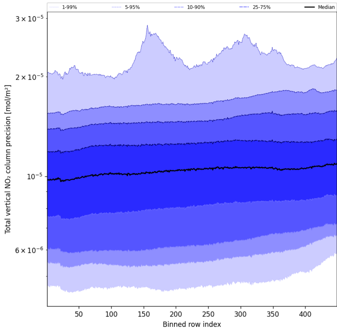
Figure 56: Along track statistics of “Total vertical NO 2 column precision” for 2024-10-19 to 2024-10-21
