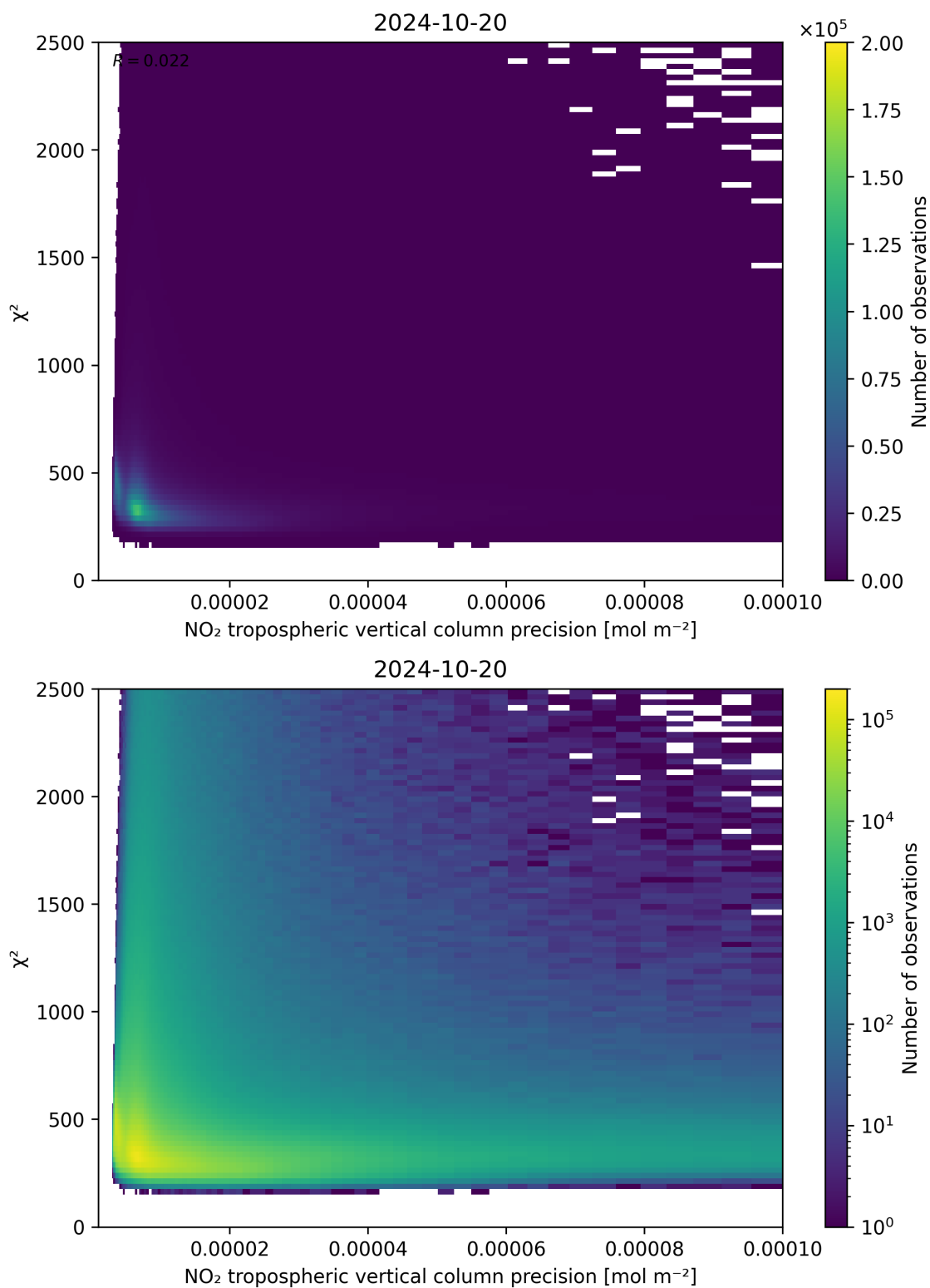
Figure 134: Scatter density plot of “NO 2 tropospheric vertical column precision” against “ \chi^2 ” for 2024-10-19 to 2024-10-21.
