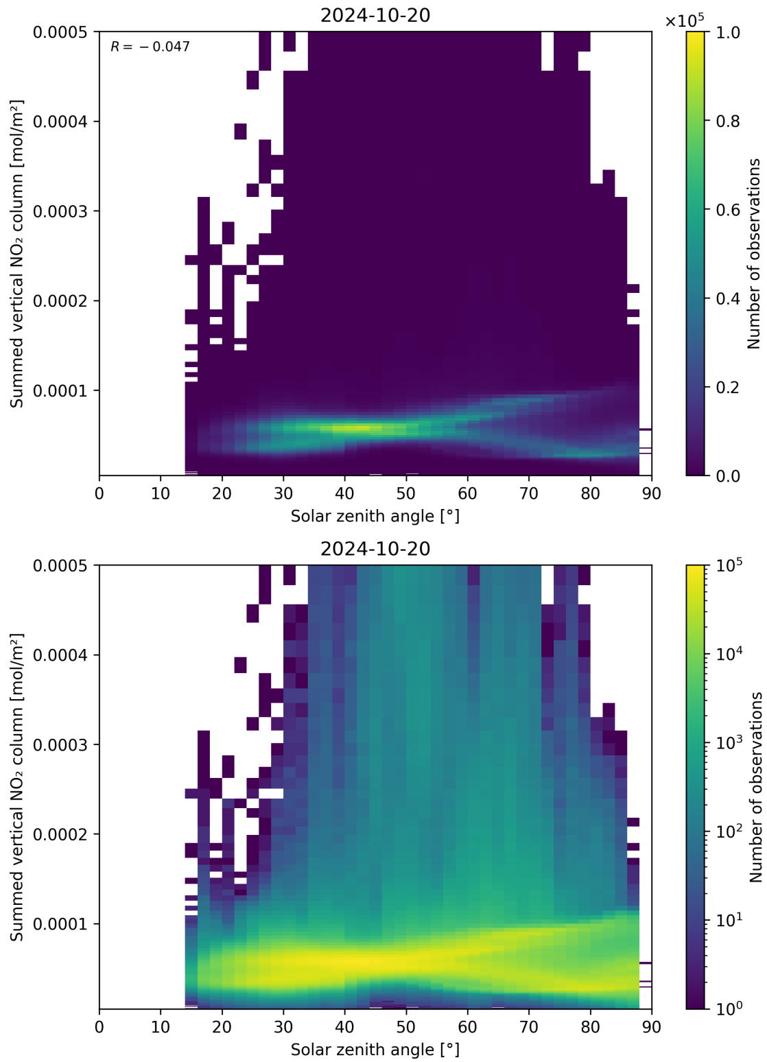
Figure 151: Scatter density plot of “Solar zenith angle” against “Summed vertical NO 2 column” for 2024-10-19 to 2024-10-21.
