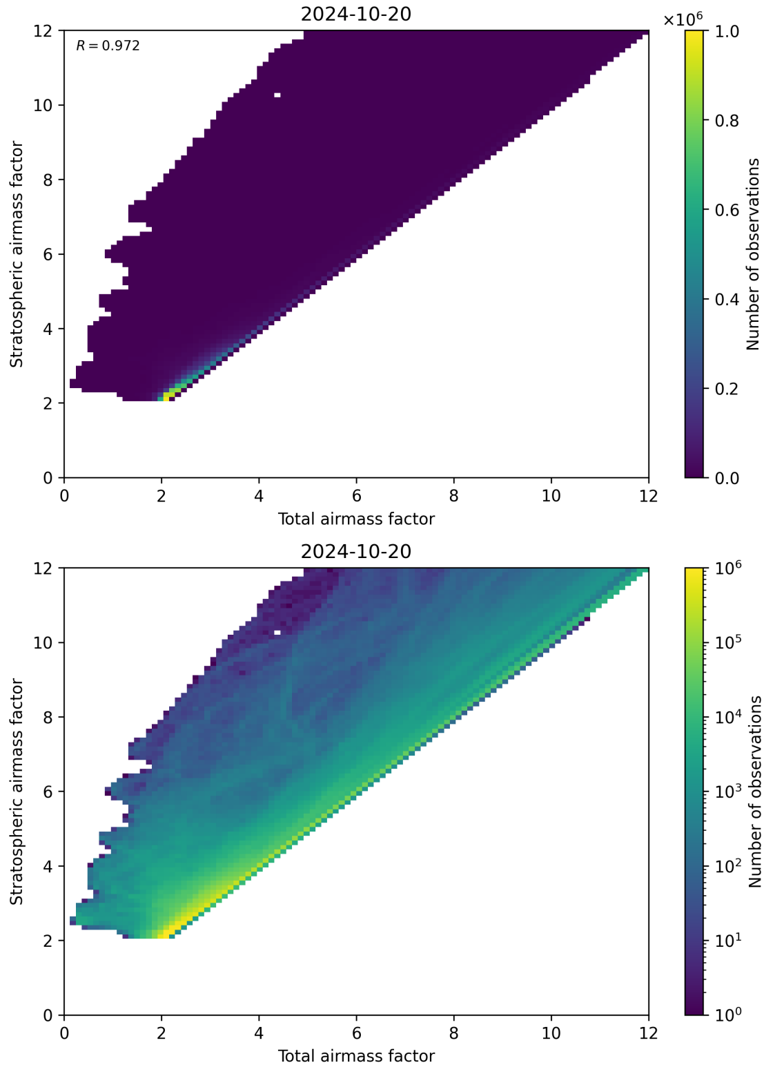
Figure 62: Scatter density plot of “Total airmass factor” against “Stratospheric airmass factor” for 2024-10-19 to 2024-10-21.
