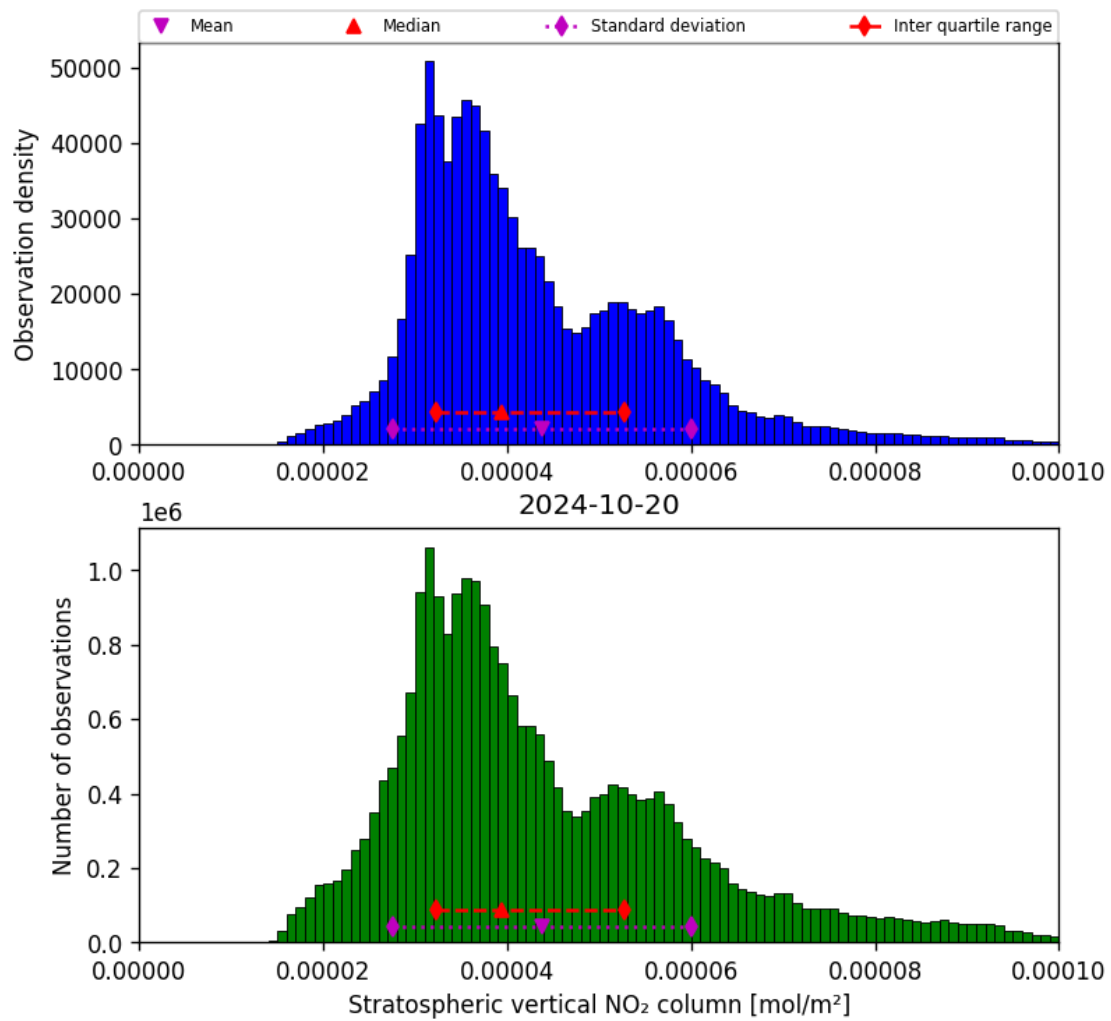
Figure 36: Histogram of “Stratospheric vertical NO 2 column” for 2024-10-19 to 2024-10-21
