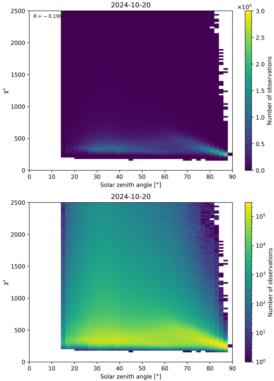
Figure 148: Scatter density plot of “Solar zenith angle” against “ \chi^2 ” for 2024-10-19 to 2024-10-21.
