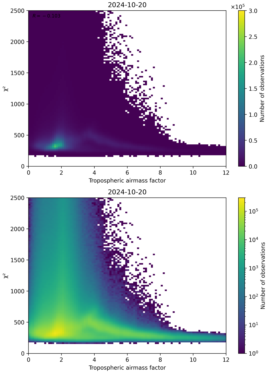
Figure 73: Scatter density plot of “Tropospheric airmass factor” against “ \chi^2 ” for 2024-10-19 to 2024-10-21.
