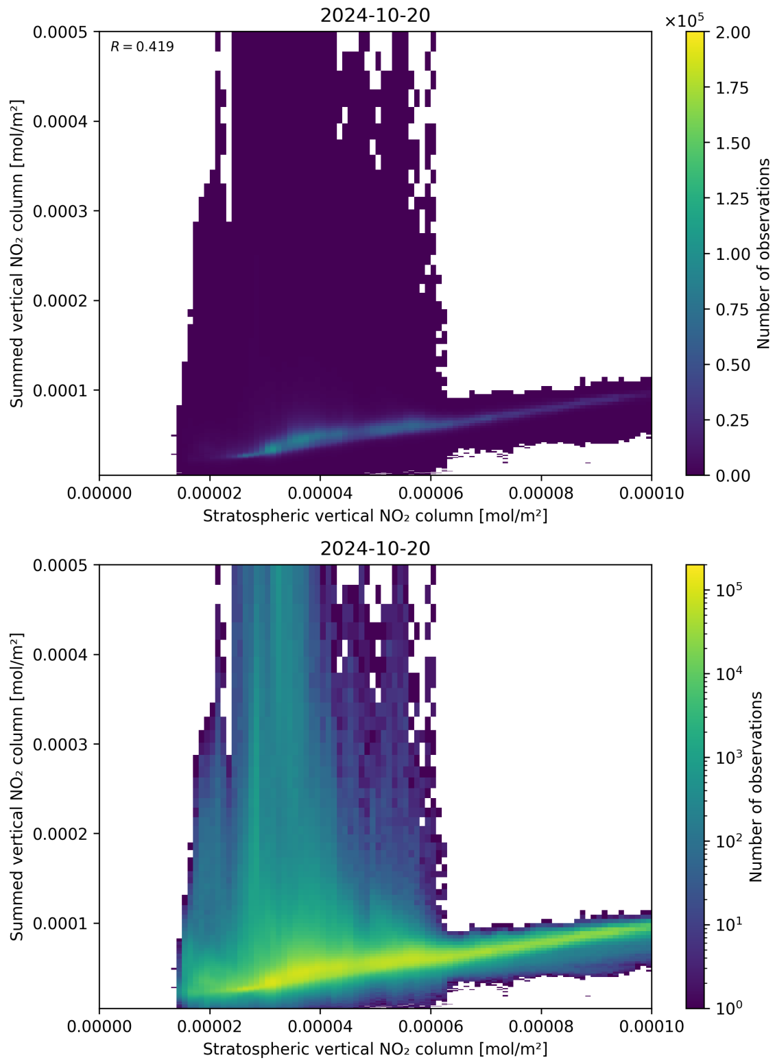
Figure 98: Scatter density plot of “Stratospheric vertical NO 2 column” against “Summed vertical NO 2 column” for 2024-10-19 to 2024-10-21.
