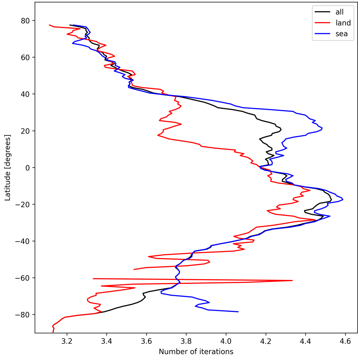
Figure 17: Zonal average of “Number of iterations” for 2024-10-19 to 2024-10-21.
