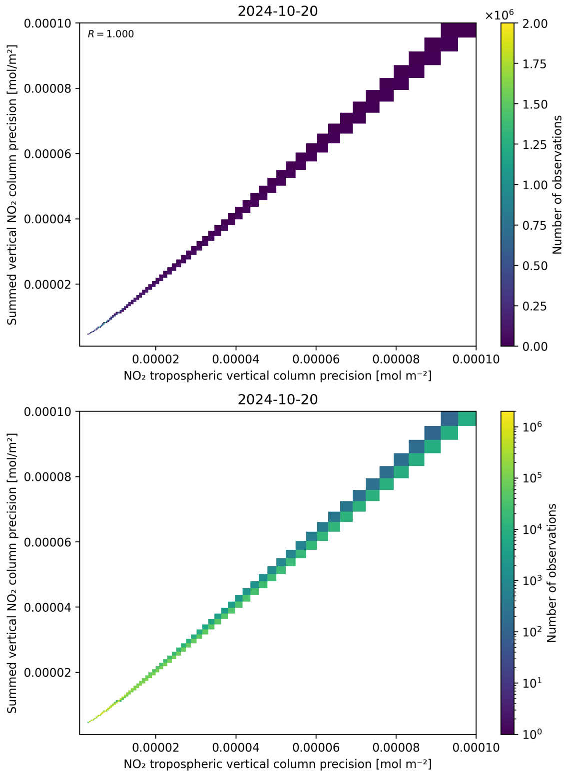
Figure 137: Scatter density plot of “NO 2 tropospheric vertical column precision” against “Summed vertical NO 2 column precision” for 2024-10-19 to 2024-10-21.
