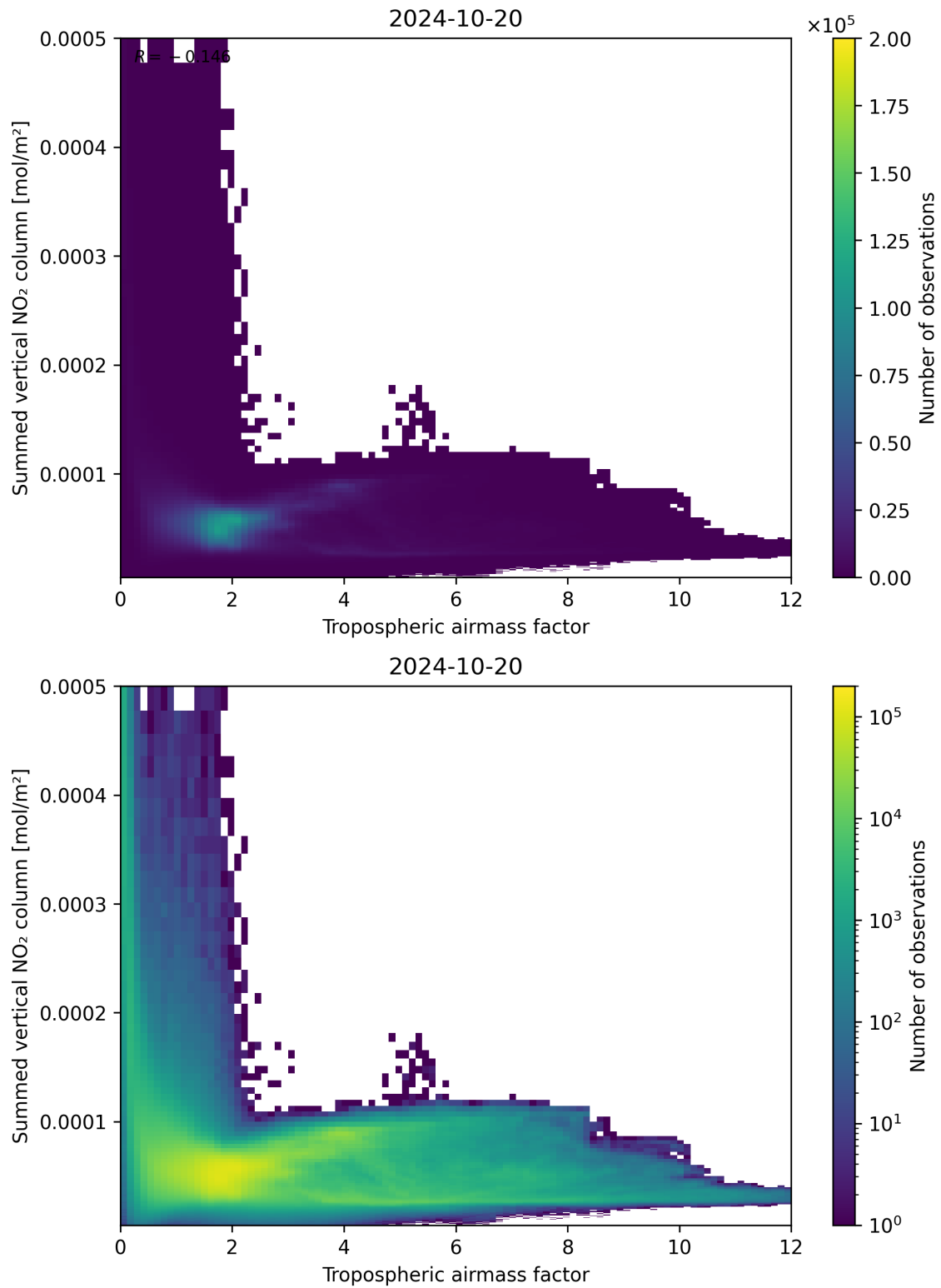
Figure 75: Scatter density plot of “Tropospheric airmass factor” against “Summed vertical NO 2 column” for 2024-10-19 to 2024-10-21.
