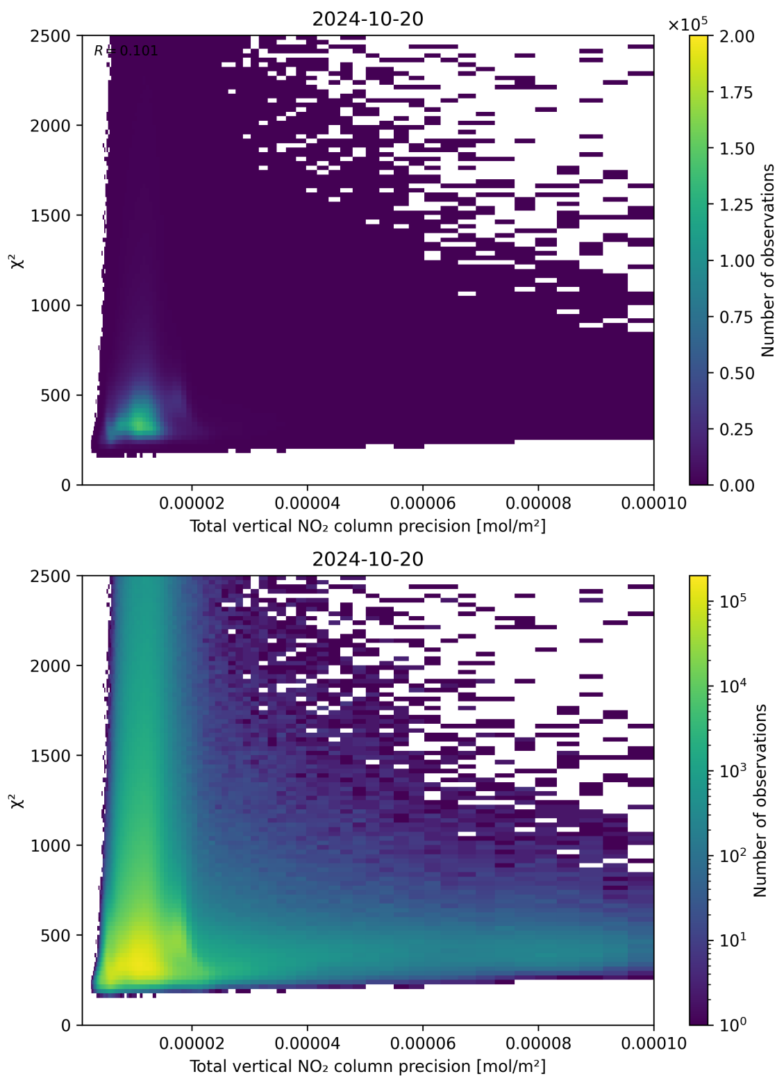
Figure 116: Scatter density plot of “Total vertical NO 2 column precision” against “ \chi^2 ” for 2024-10-19 to 2024-10-21.
