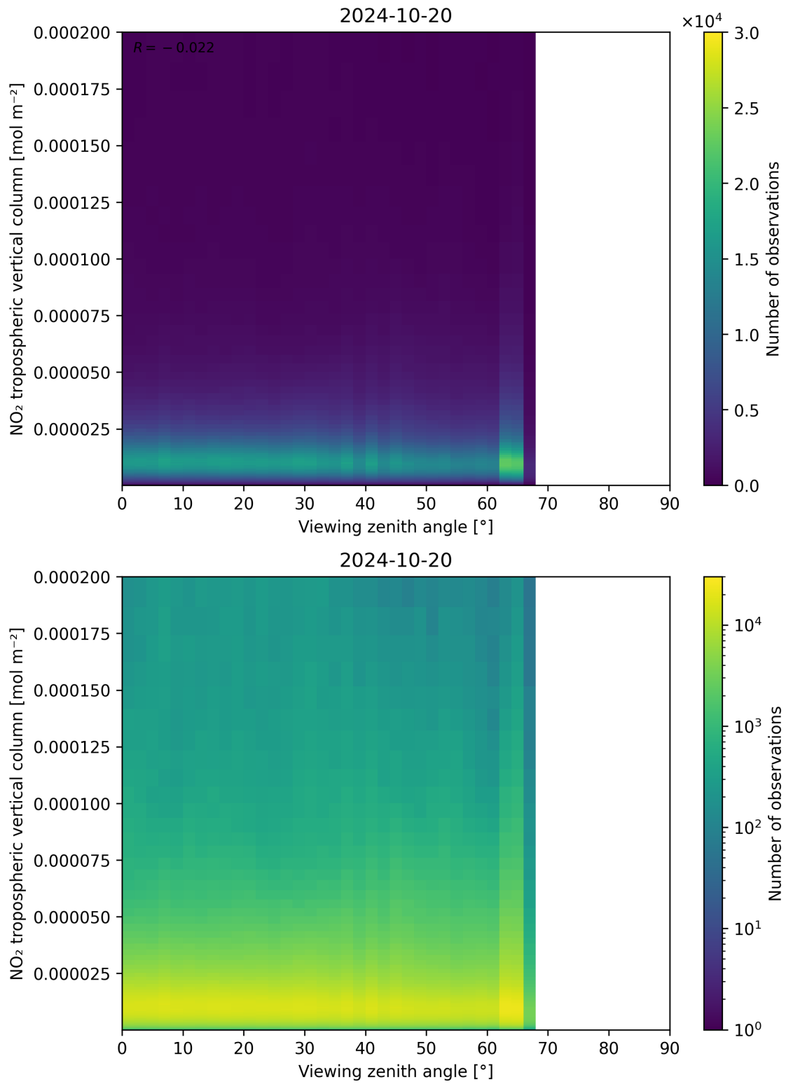
Figure 169: Scatter density plot of “Viewing zenith angle” against “NO 2 tropospheric vertical column” for 2024-10-19 to 2024-10-21.
