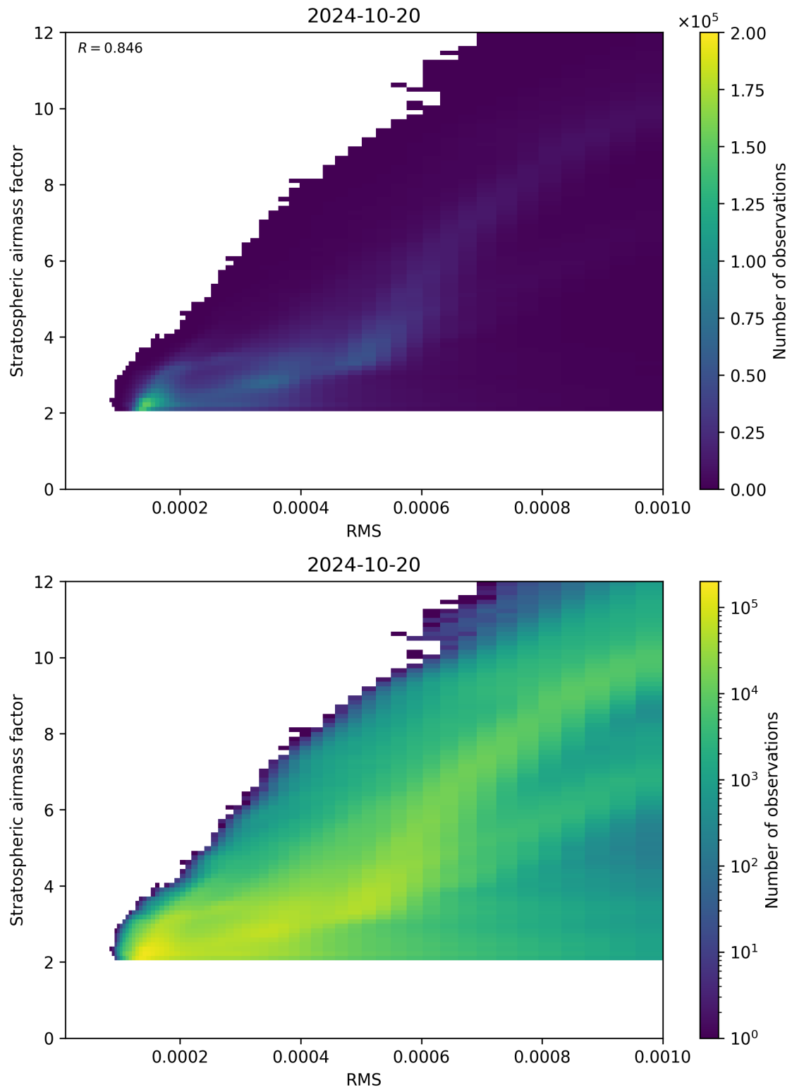
Figure 144: Scatter density plot of “RMS” against “Stratospheric airmass factor” for 2024-10-19 to 2024-10-21.
