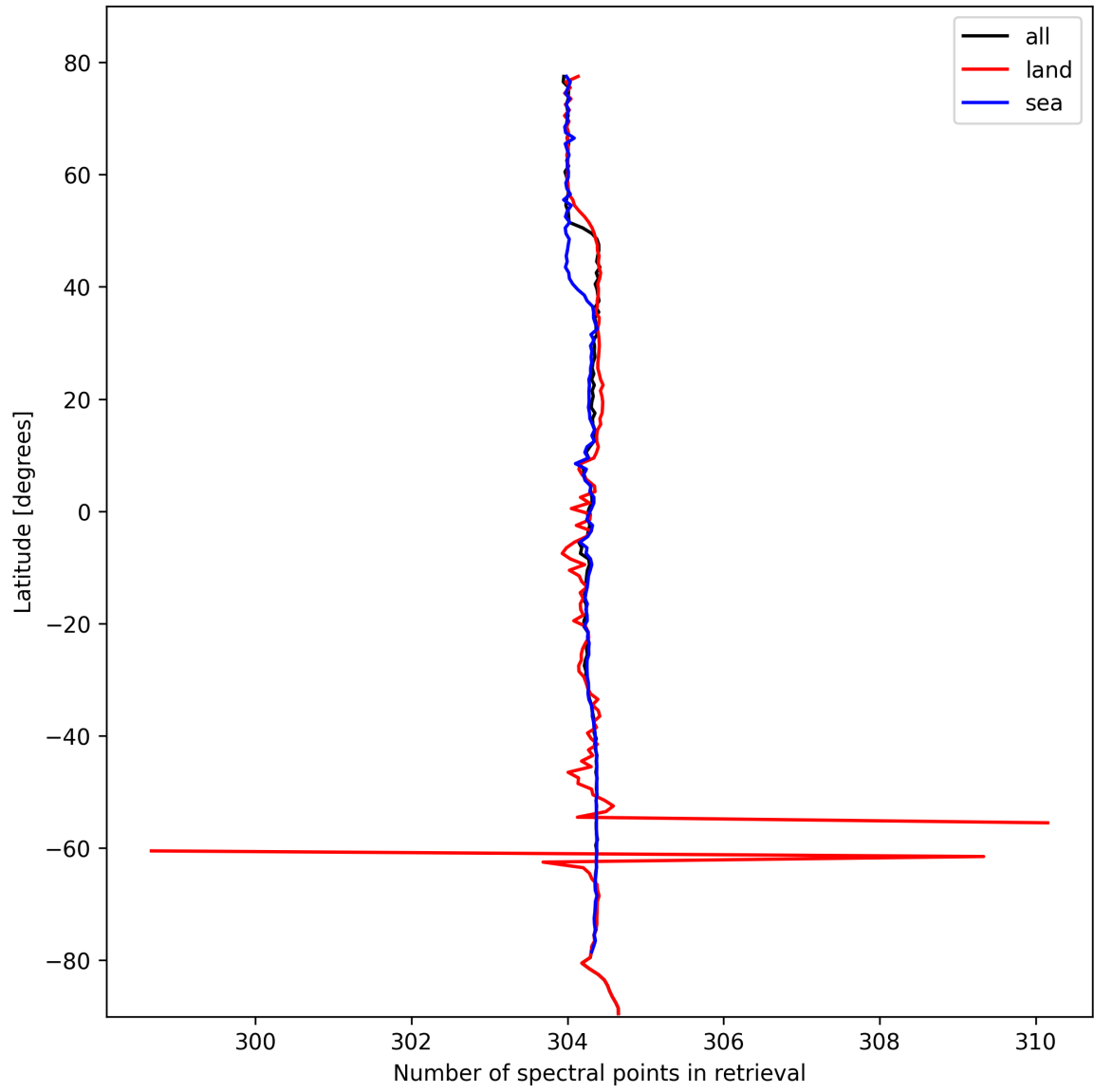
Figure 16: Zonal average of “Number of spectral points in retrieval” for 2024-10-19 to 2024-10-21.
