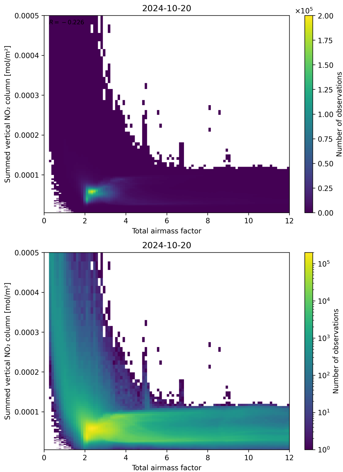
Figure 65: Scatter density plot of “Total airmass factor” against “Summed vertical NO 2 column” for 2024-10-19 to 2024-10-21.
