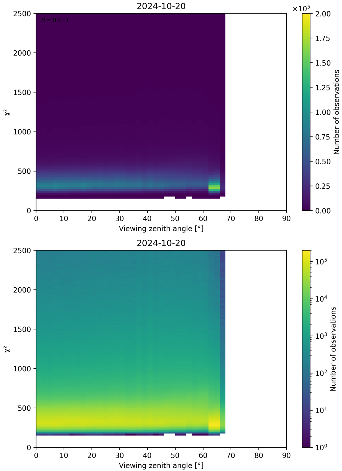
Figure 162: Scatter density plot of “Viewing zenith angle” against “ \chi^2 ” for 2024-10-19 to 2024-10-21.
