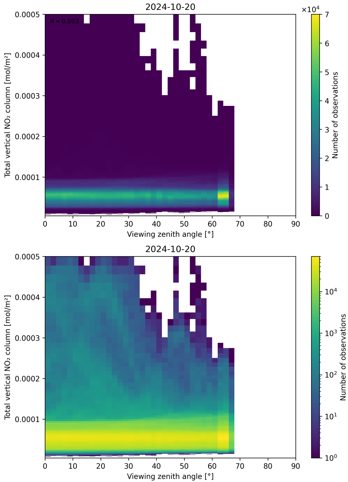
Figure 167: Scatter density plot of “Viewing zenith angle” against “Total vertical NO 2 column” for 2024-10-19 to 2024-10-21.
