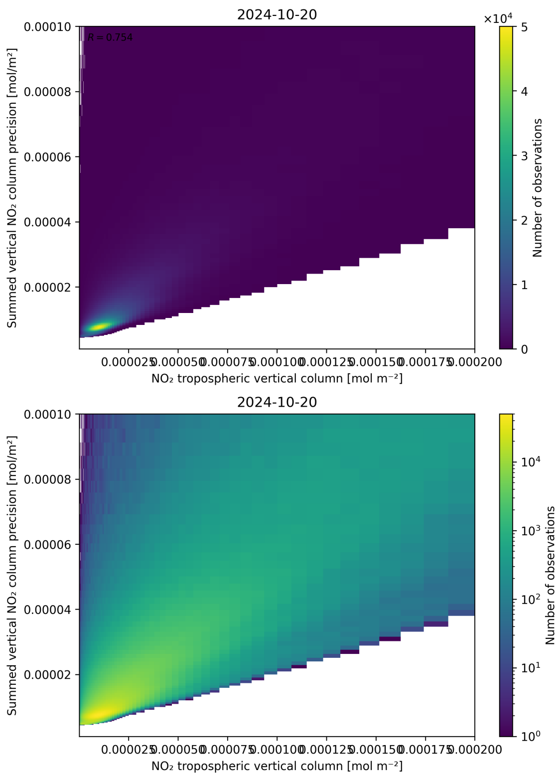
Figure 127: Scatter density plot of “NO 2 tropospheric vertical column” against “Summed vertical NO 2 column precision” for 2024-10-19 to 2024-10-21.
