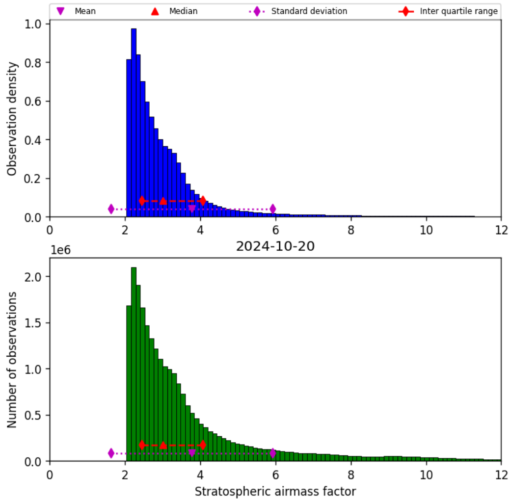
Figure 44: Histogram of “Stratospheric airmass factor” for 2024-10-19 to 2024-10-21
