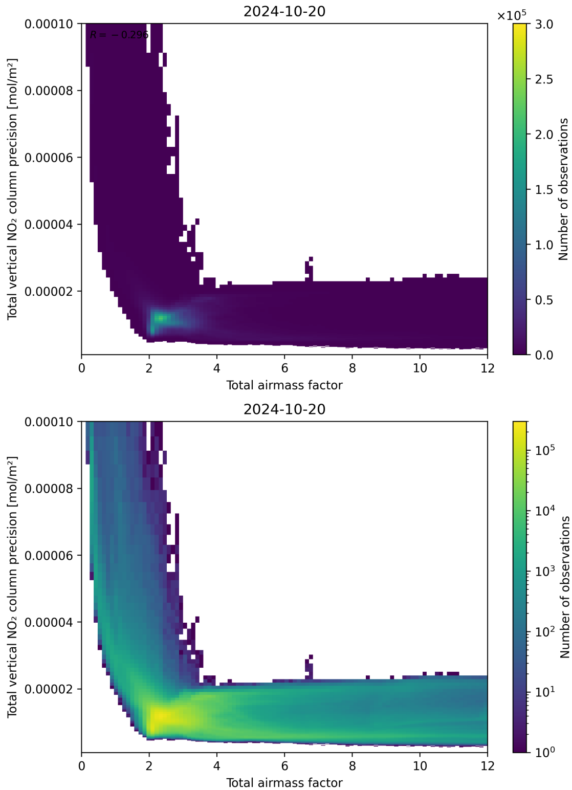
Figure 68: Scatter density plot of “Total airmass factor” against “Total vertical NO 2 column precision” for 2024-10-19 to 2024-10-21.
