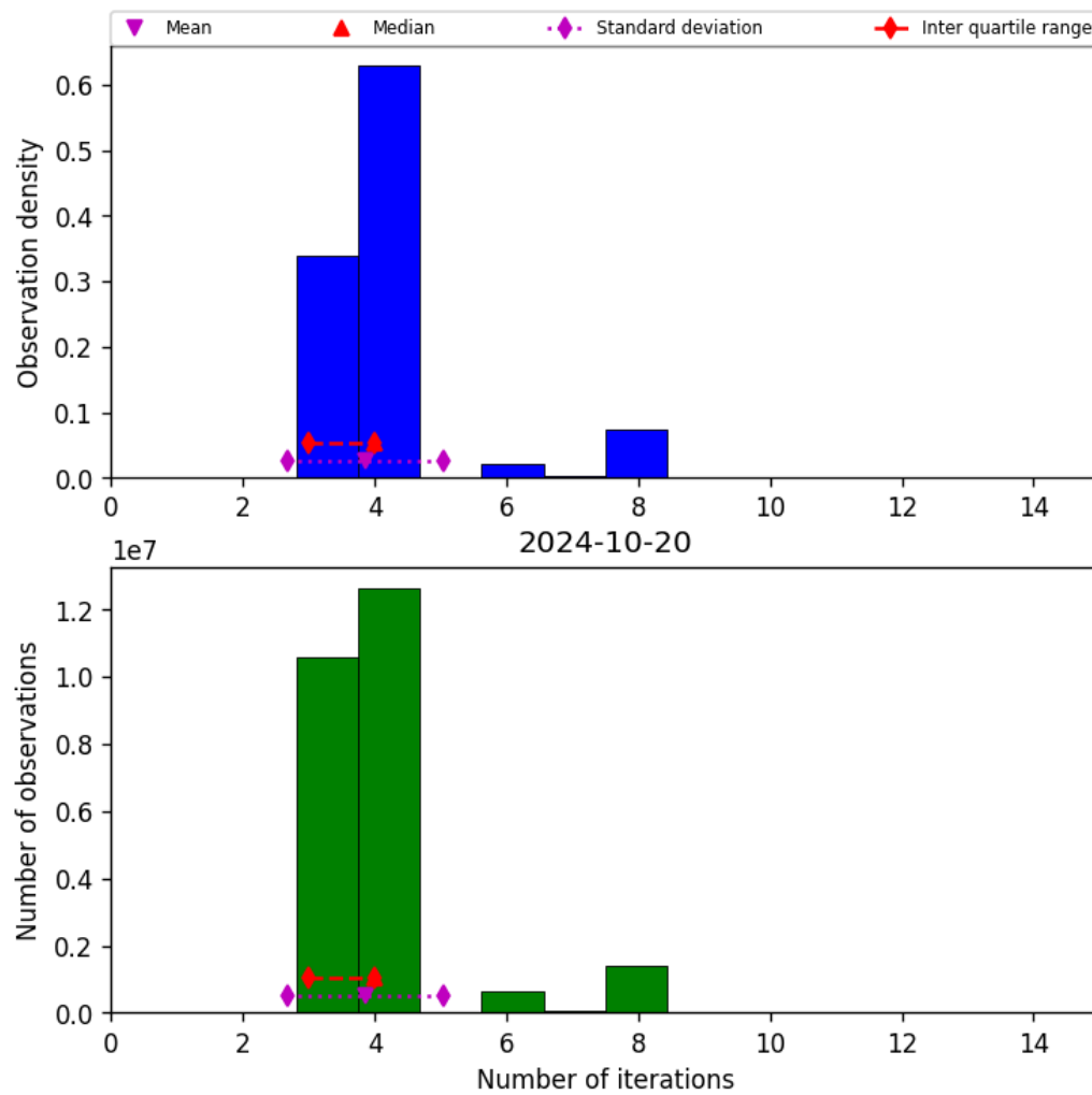
Figure 34: Histogram of “Number of iterations” for 2024-10-19 to 2024-10-21
