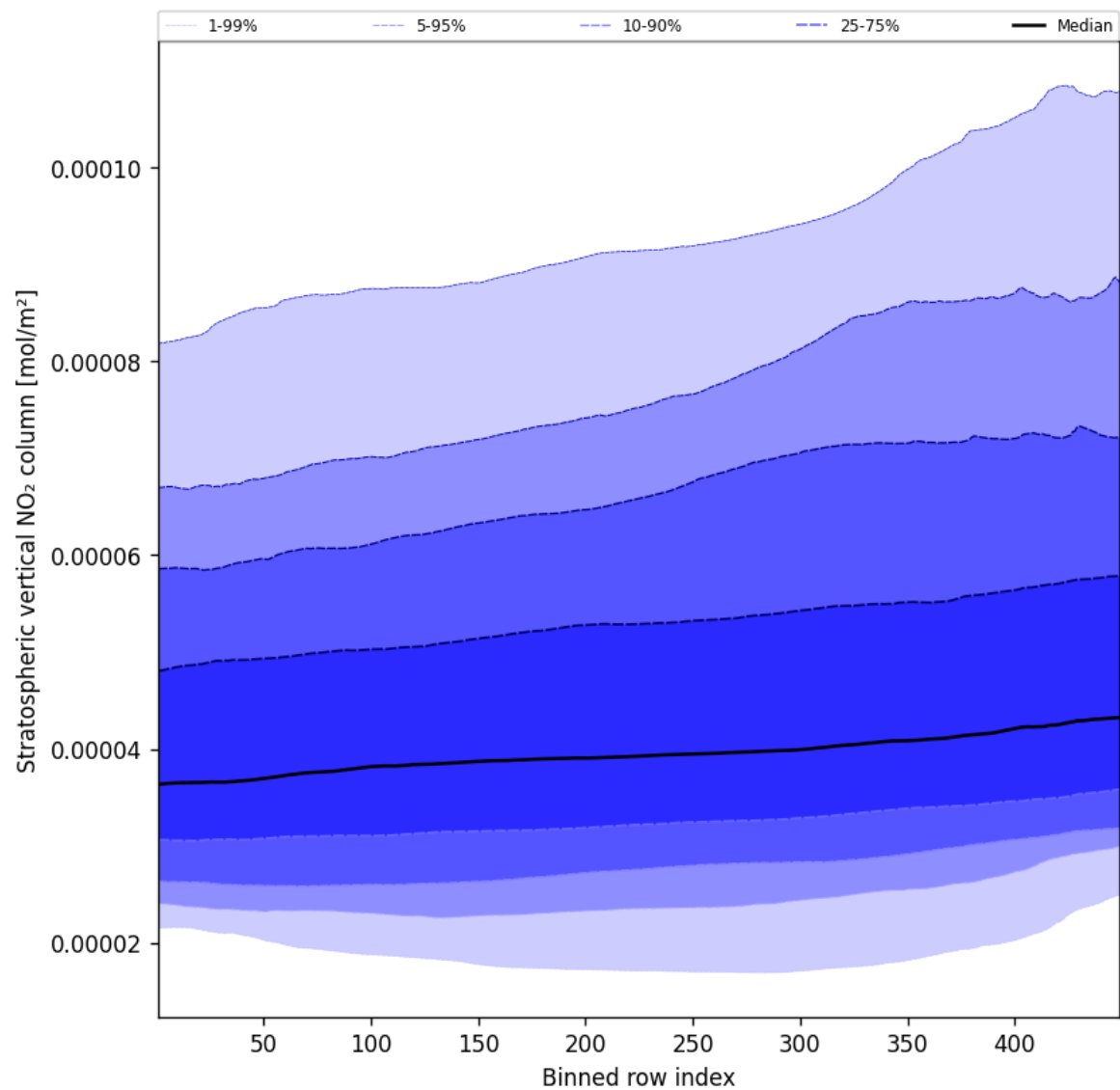
Figure 53: Along track statistics of “Stratospheric vertical NO 2 column” for 2024-10-19 to 2024-10-21
