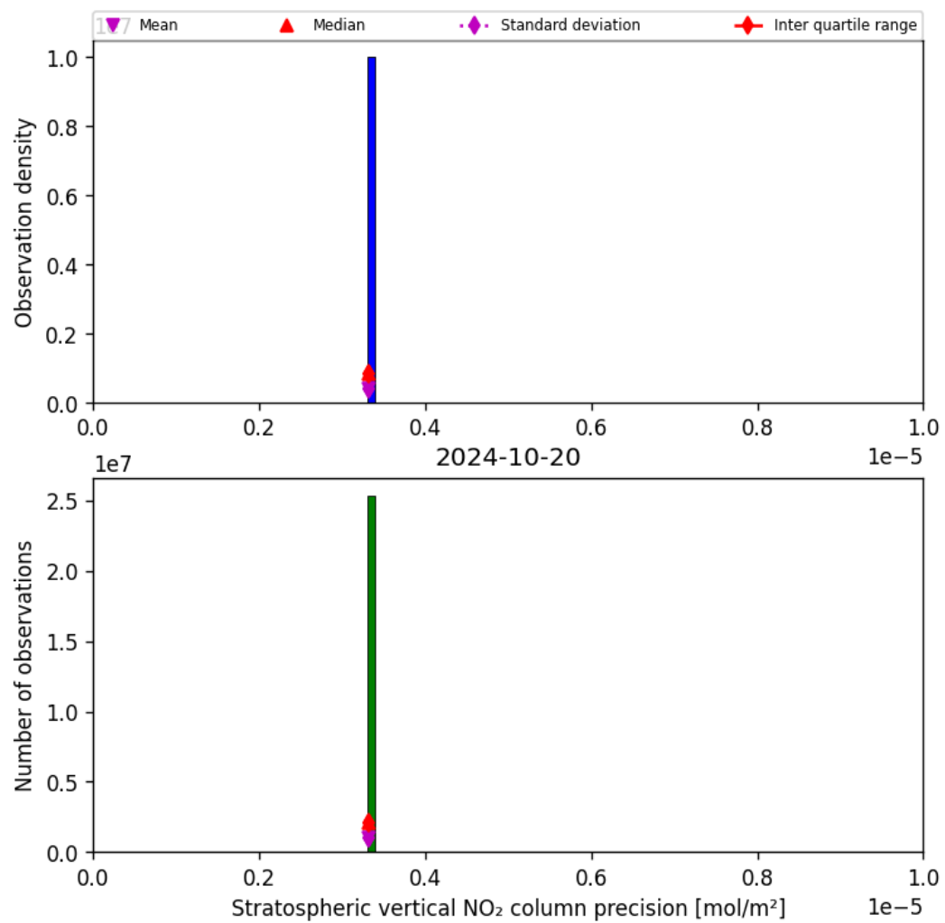
Figure 37: Histogram of “Stratospheric vertical NO 2 column precision” for 2024-10-19 to 2024-10-21
