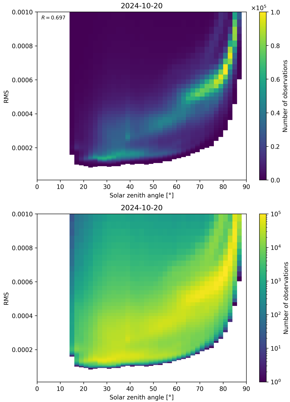
Figure 157: Scatter density plot of “Solar zenith angle” against “RMS” for 2024-10-19 to 2024-10-21.
