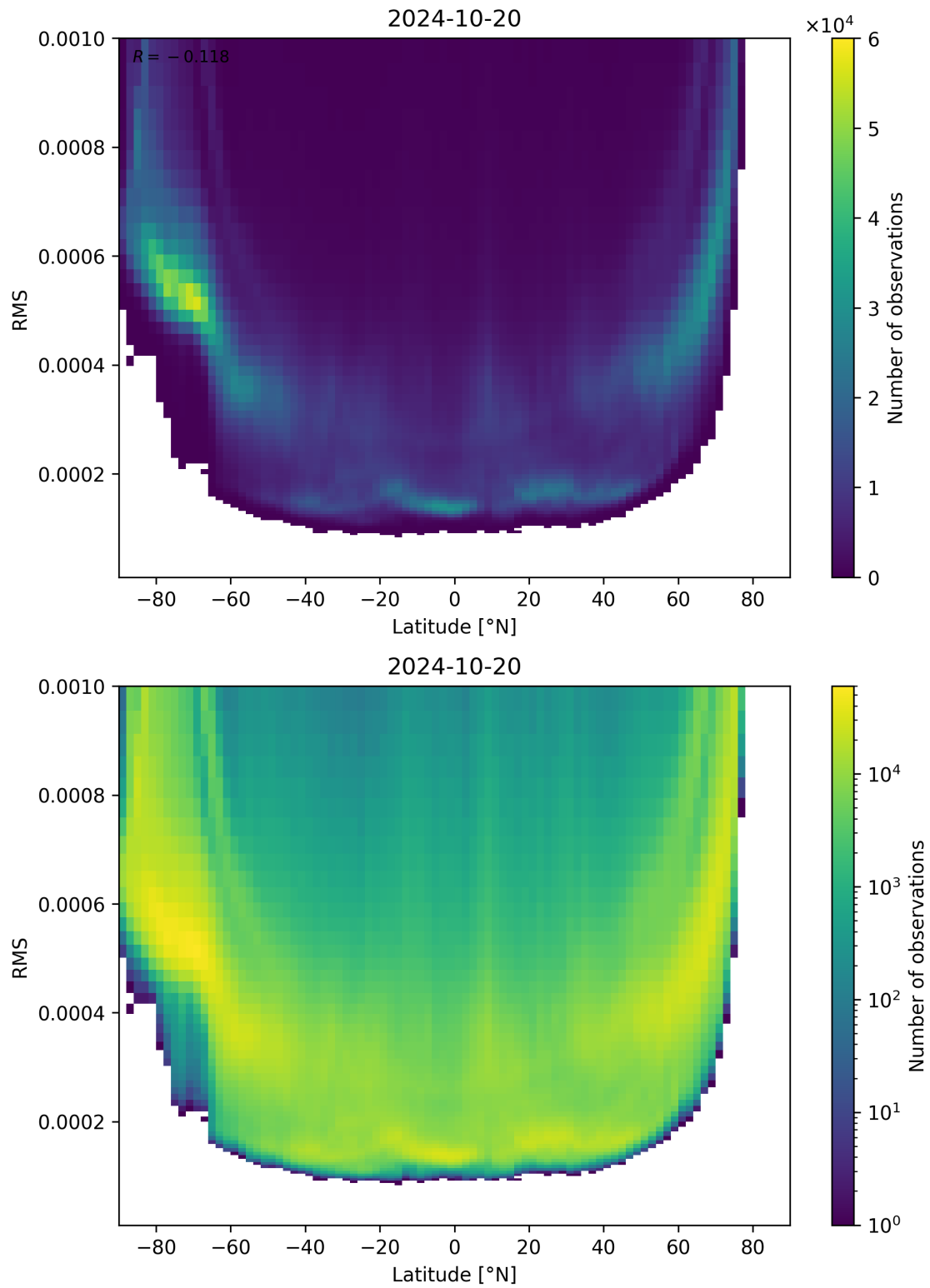
Figure 94: Scatter density plot of “Latitude” against “RMS” for 2024-10-19 to 2024-10-21.
