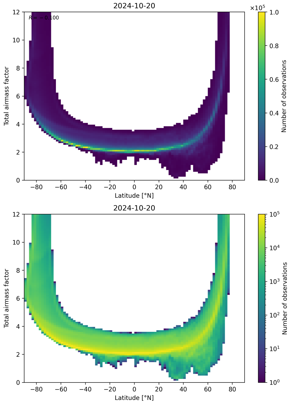
Figure 84: Scatter density plot of “Latitude” against “Total airmass factor” for 2024-10-19 to 2024-10-21.
