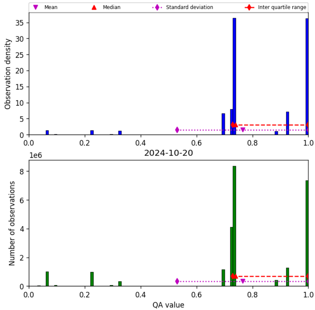
Figure 28: Histogram of “QA value” for 2024-10-19 to 2024-10-21
