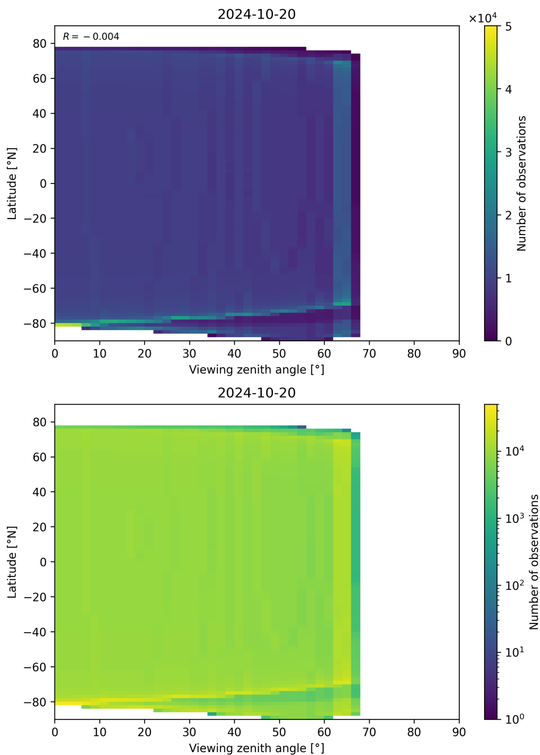
Figure 163: Scatter density plot of “Viewing zenith angle” against “Latitude” for 2024-10-19 to 2024-10-21.
