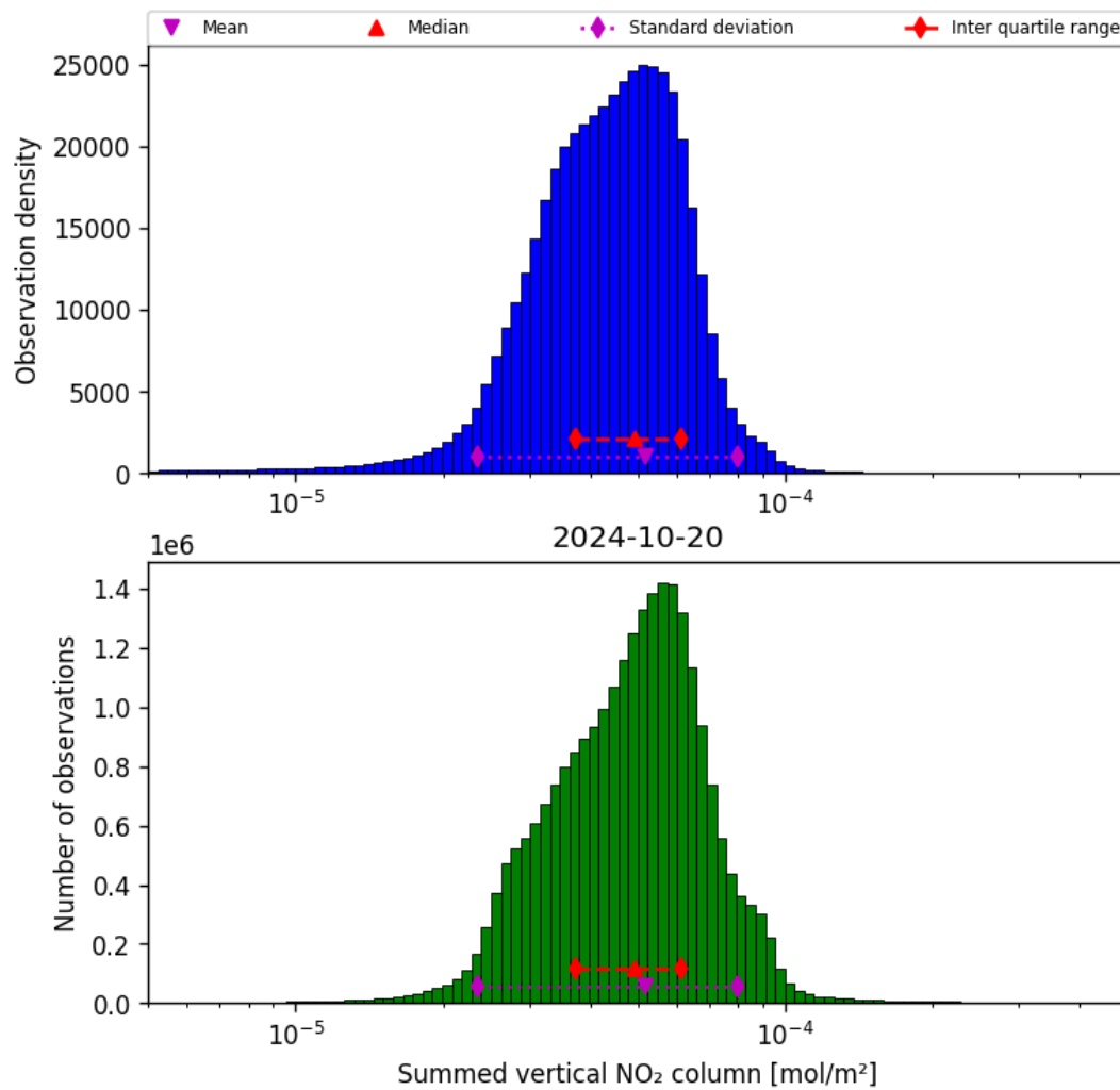
Figure 40: Histogram of "Summed vertical NO 2 column" for 2024-10-19 to 2024-10-21
