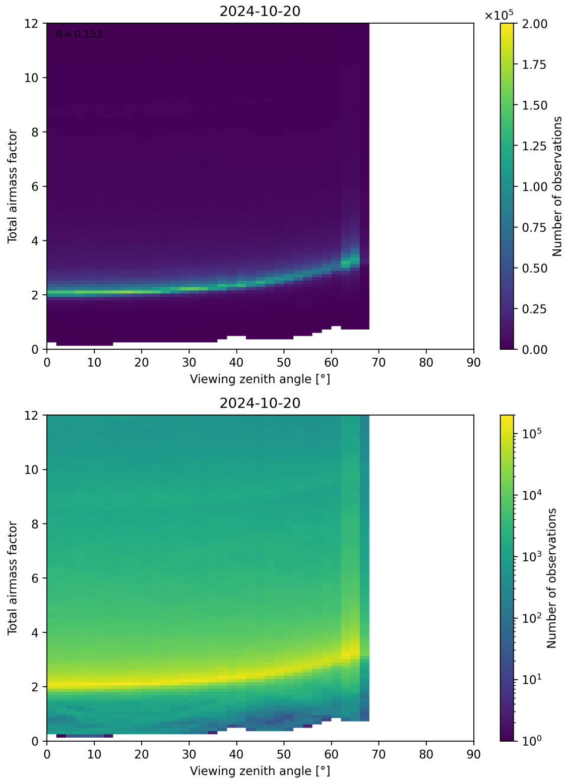
Figure 160: Scatter density plot of “Viewing zenith angle” against “Total airmass factor” for 2024-10-19 to 2024-10-21.
