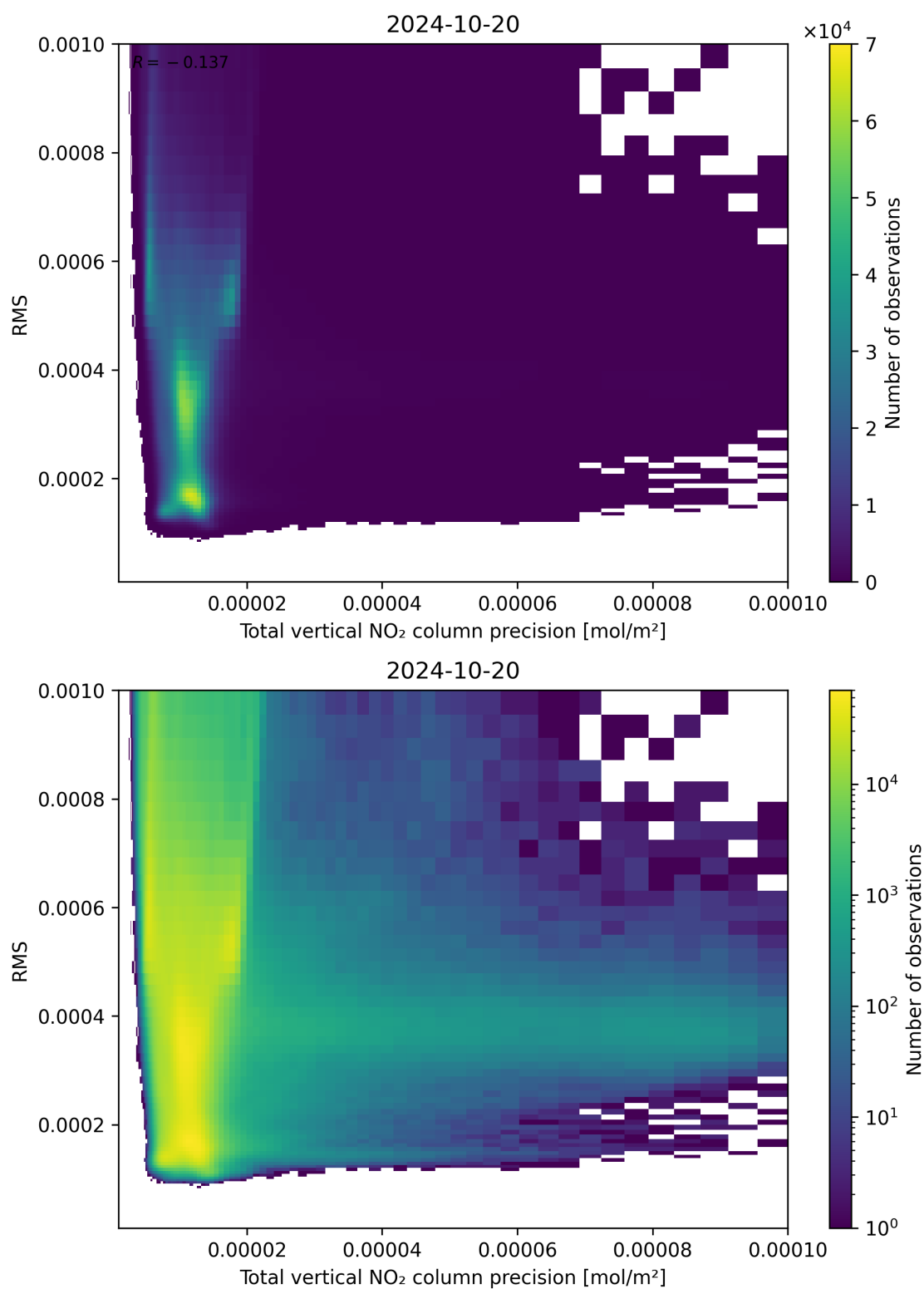
Figure 119: Scatter density plot of “Total vertical NO 2 column precision” against “RMS” for 2024-10-19 to 2024-10-21.
