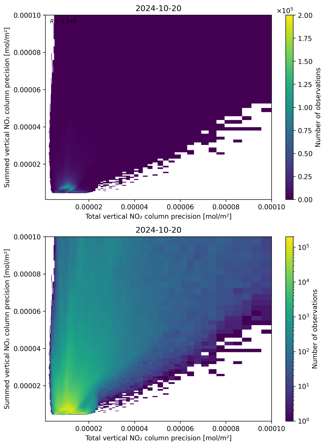
Figure 118: Scatter density plot of “Total vertical NO 2 column precision” against “Summed vertical NO 2 column precision” for 2024-10-19 to 2024-10-21.
