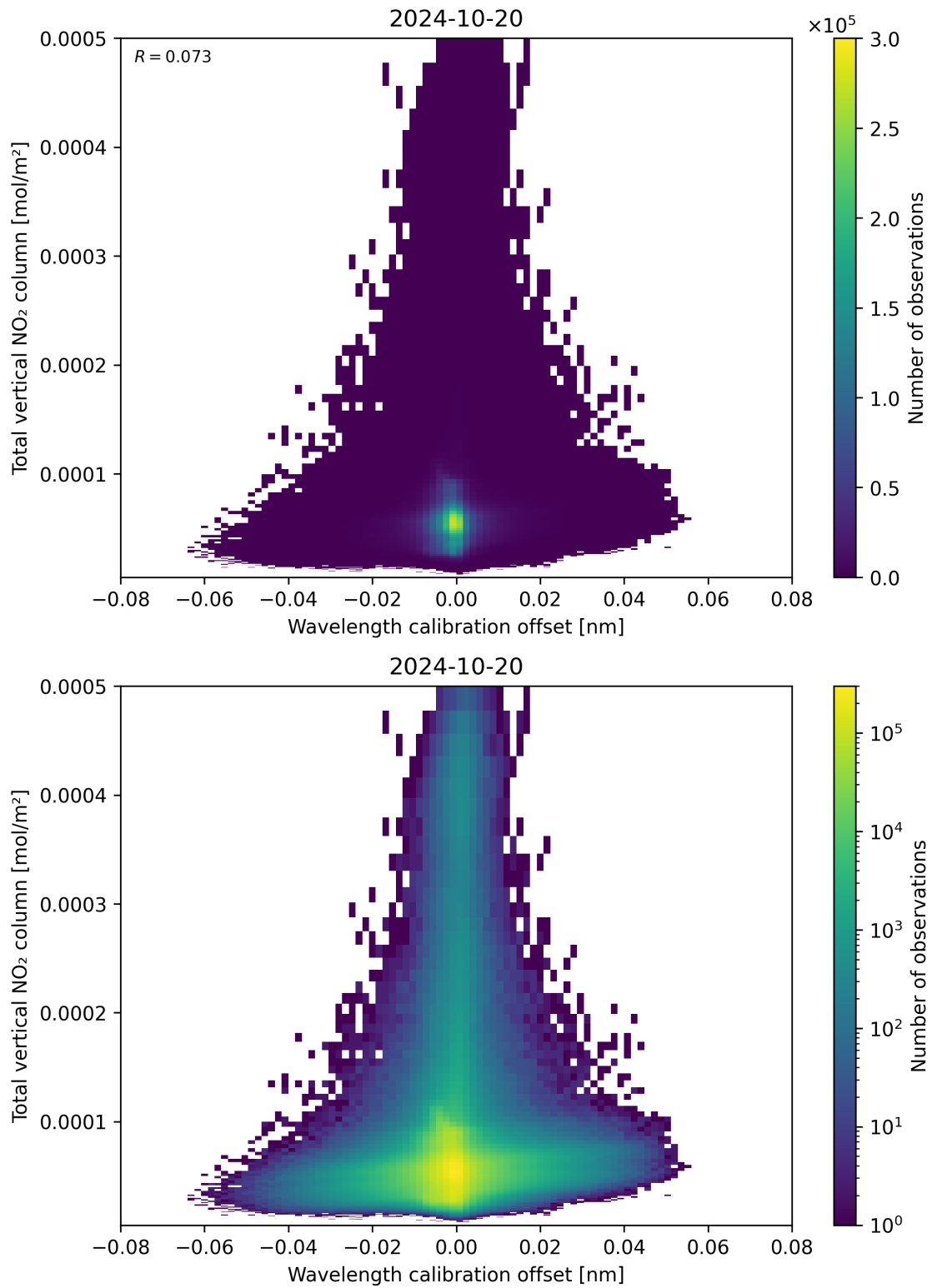
Figure 179: Scatter density plot of “Wavelength calibration offset” against “Total vertical NO 2 column” for 2024-10-19 to 2024-10-21.
