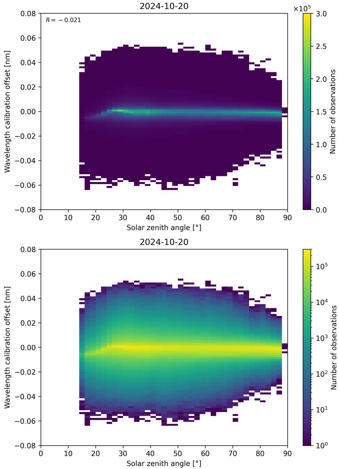
Figure 158: Scatter density plot of “Solar zenith angle” against “Wavelength calibration offset” for 2024-10-19 to 2024-10-21.
