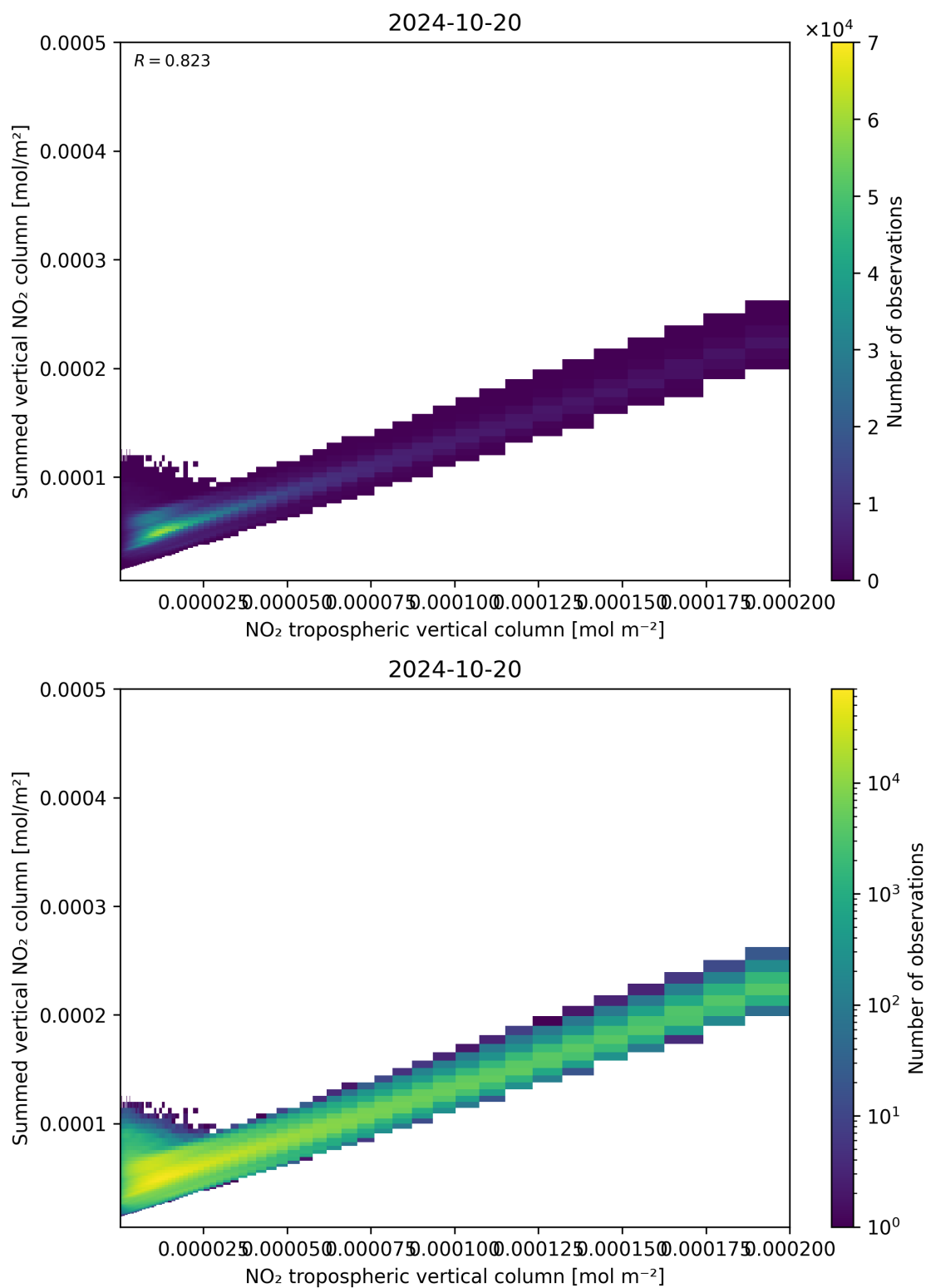
Figure 126: Scatter density plot of “NO 2 tropospheric vertical column” against “Summed vertical NO 2 column” for 2024-10-19 to 2024-10-21.
