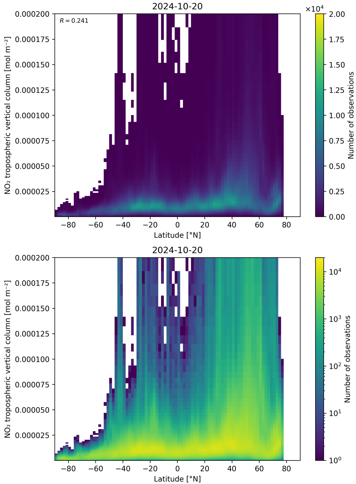
Figure 92: Scatter density plot of “Latitude” against “NO 2 tropospheric vertical column” for 2024-10-19 to 2024-10-21.
