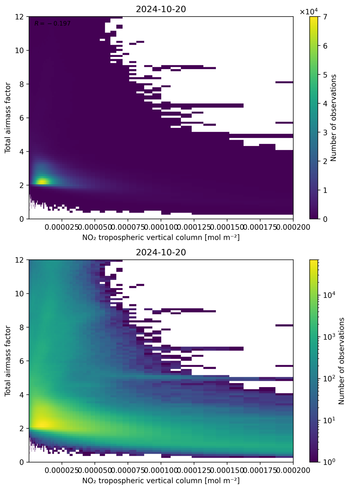
Figure 122: Scatter density plot of “NO 2 tropospheric vertical column” against “Total air mass factor” for 2024-10-19 to 2024-10-21.
