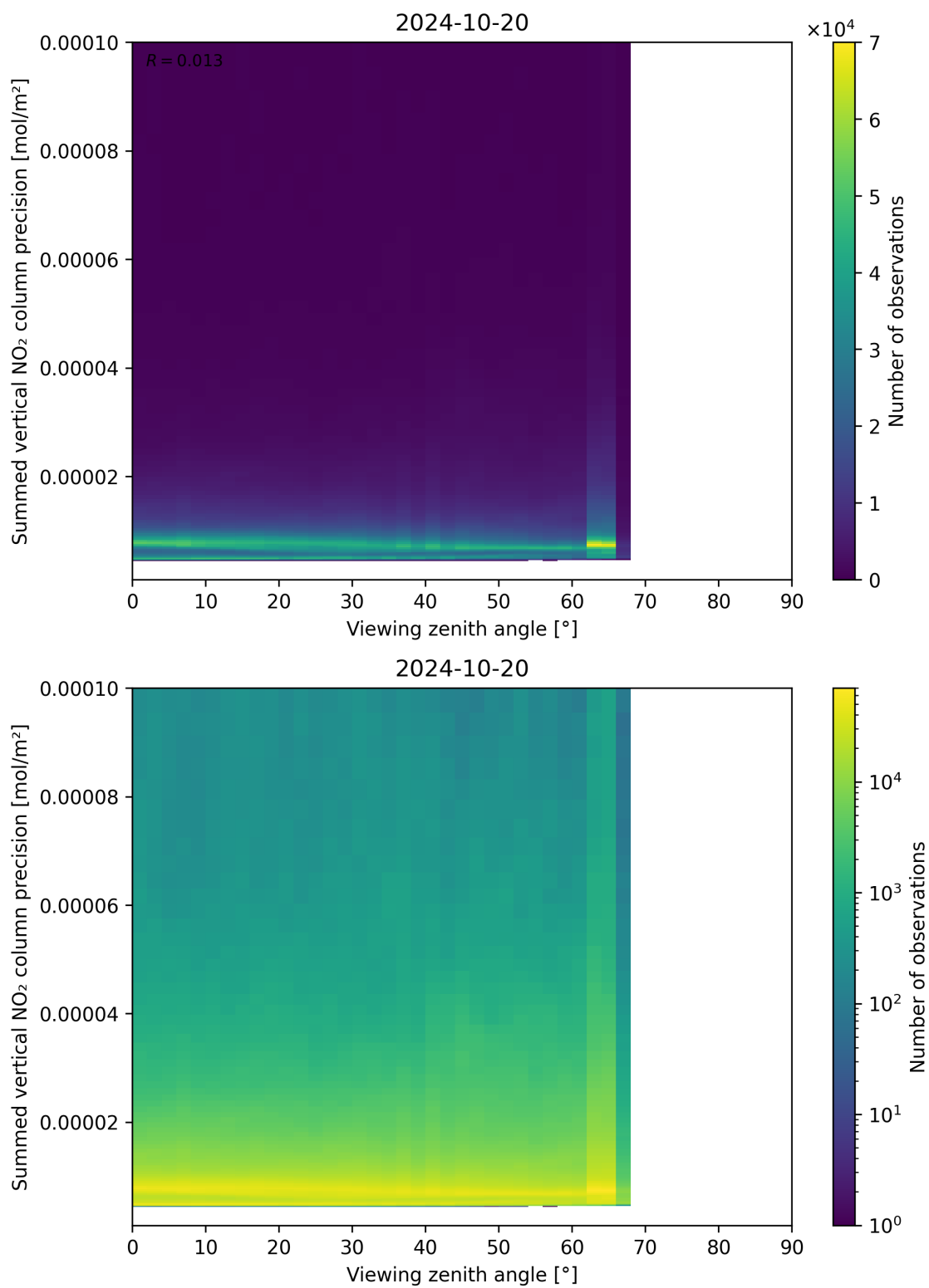
Figure 166: Scatter density plot of “Viewing zenith angle” against “Summed vertical NO 2 column precision” for 2024-10-19 to 2024-10-21.
