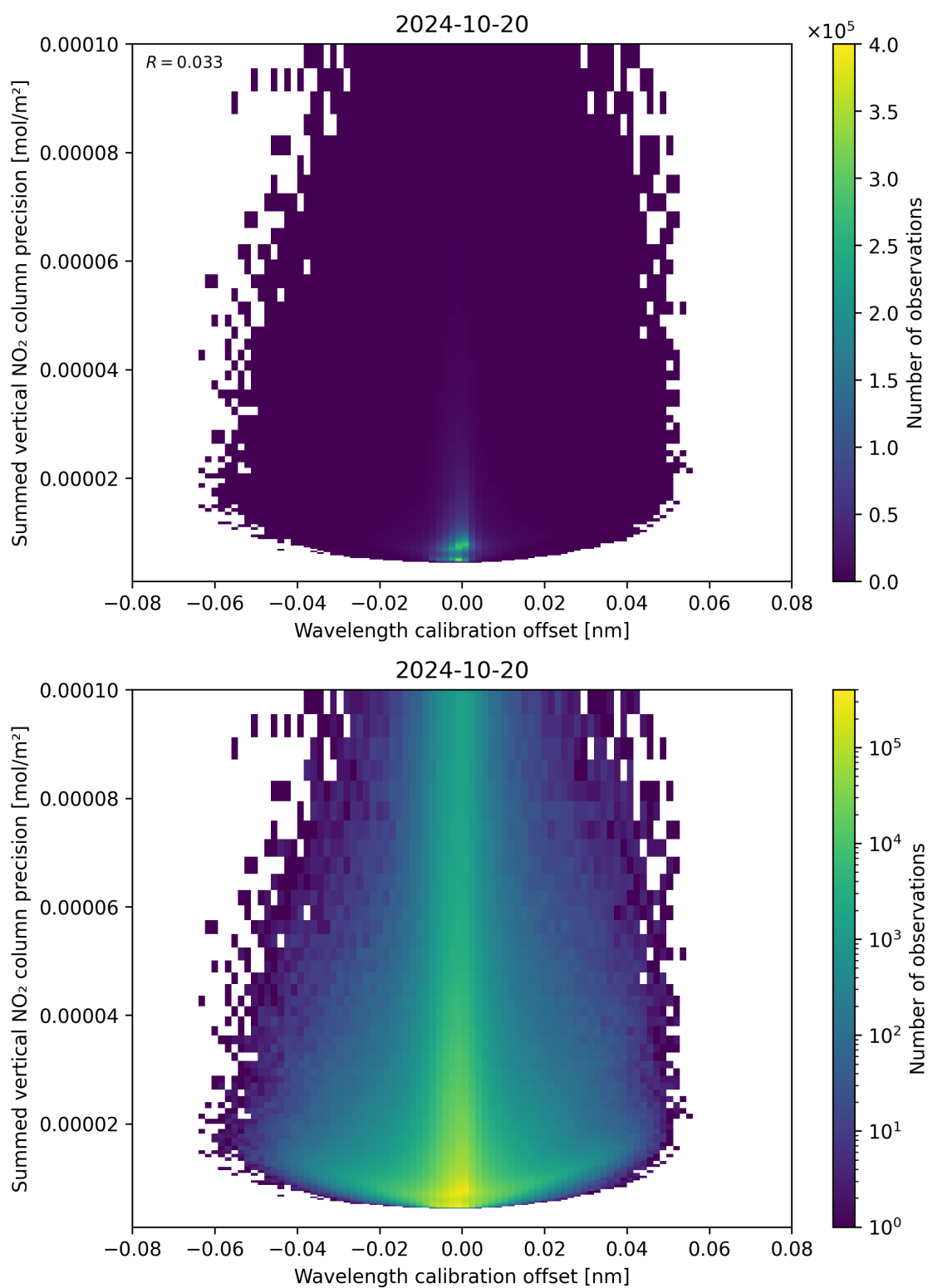
Figure 178: Scatter density plot of “Wavelength calibration offset” against “Summed vertical NO 2 column precision” for 2024-10-19 to 2024-10-21.
