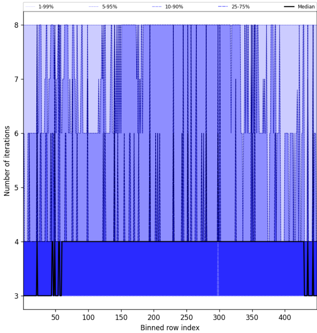
Figure 51: Along track statistics of “Number of iterations” for 2024-10-19 to 2024-10-21
