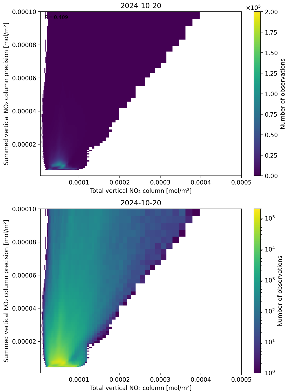
Figure 113: Scatter density plot of “Total vertical NO 2 column” against “Summed vertical NO 2 column precision” for 2024-10-19 to 2024-10-21.
