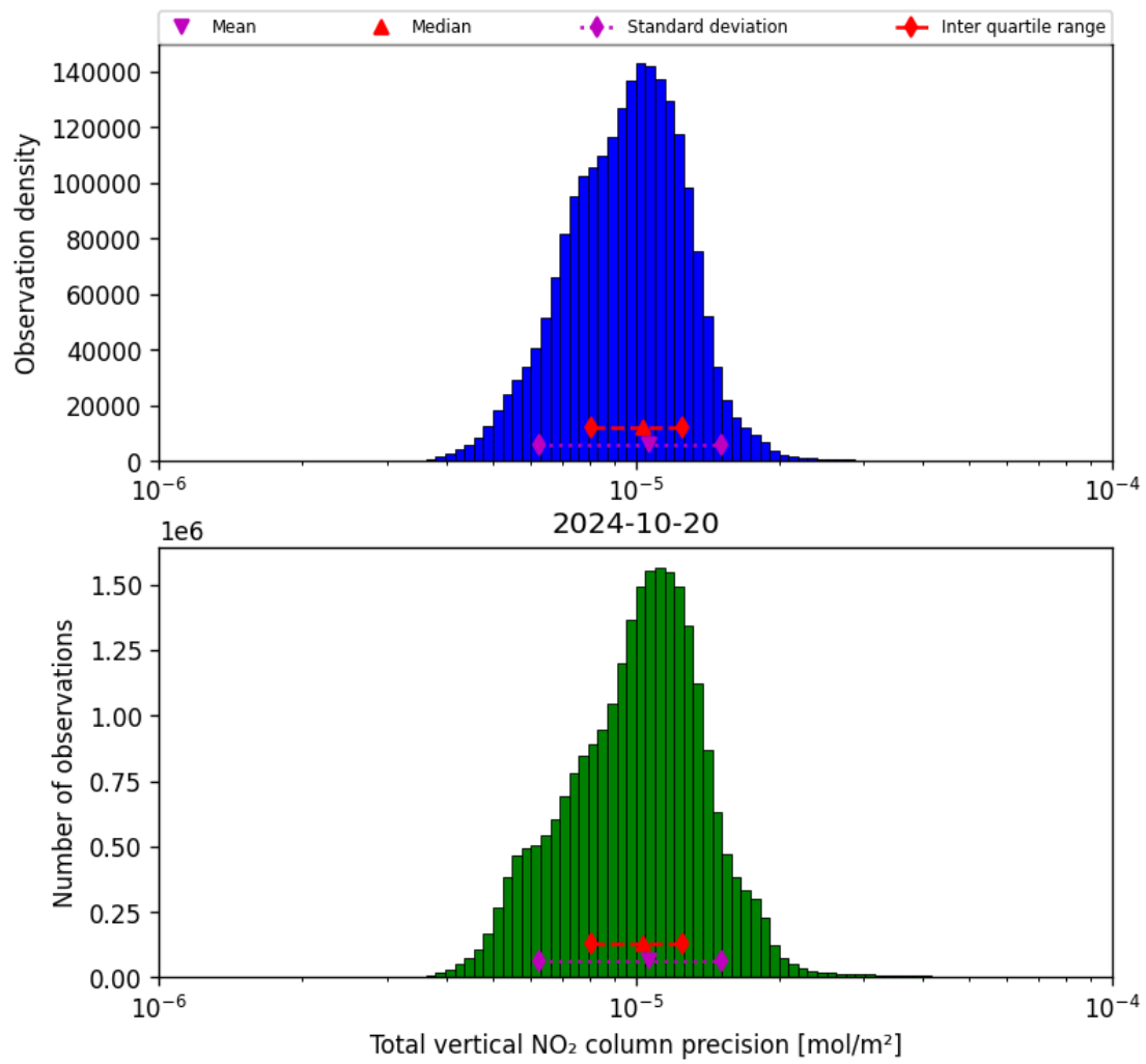
Figure 39: Histogram of “Total vertical NO 2 column precision” for 2024-10-19 to 2024-10-21
