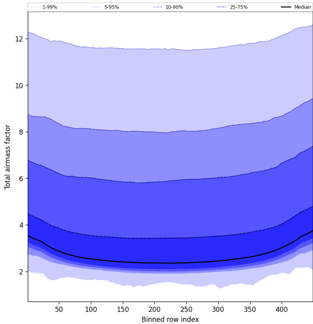
Figure 49: Along track statistics of “Total airmass factor” for 2024-10-19 to 2024-10-21
