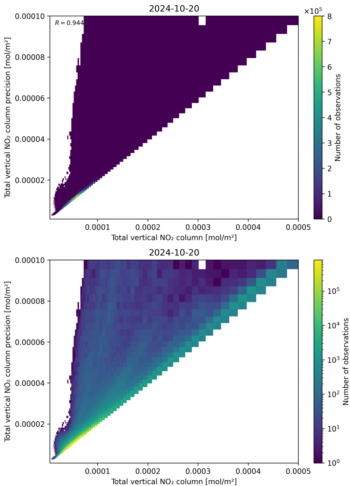
Figure 114: Scatter density plot of “Total vertical NO 2 column” against “Total vertical NO 2 column precision” for 2024-10-19 to 2024-10-21.
