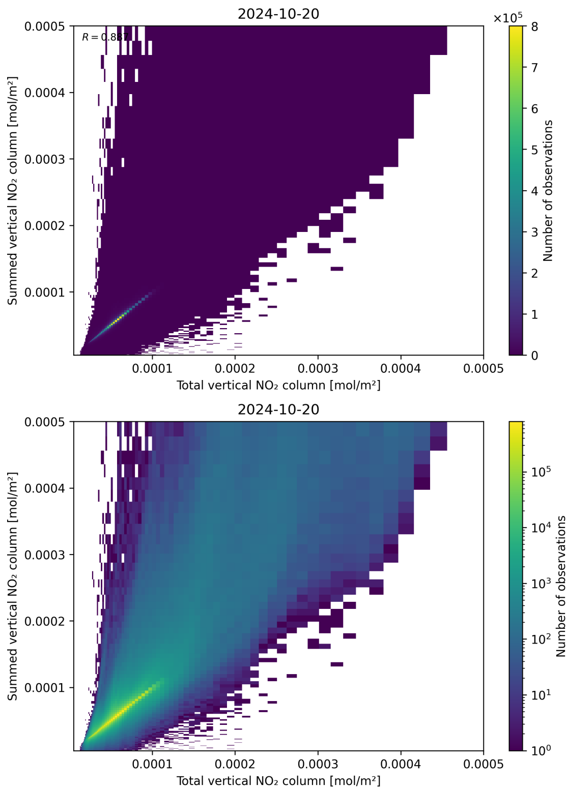
Figure 112: Scatter density plot of “Total vertical NO 2 column” against “Summed vertical NO 2 column” for 2024-10-19 to 2024-10-21.
