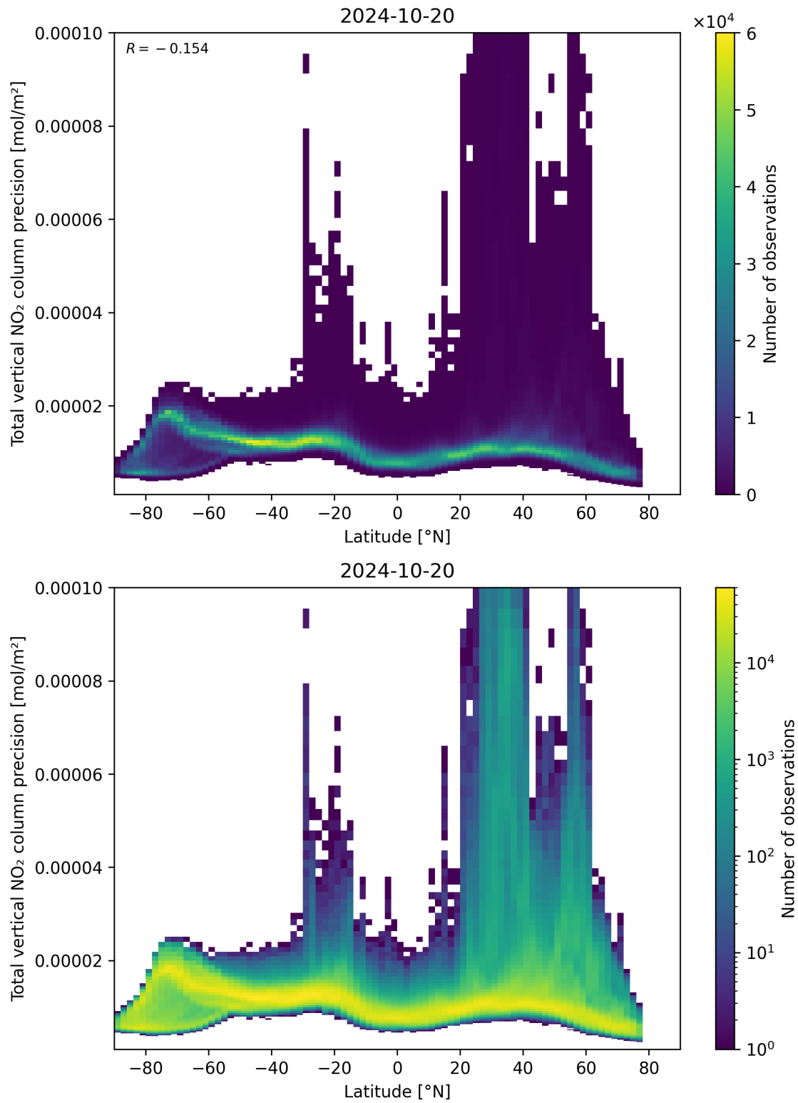
Figure 91: Scatter density plot of “Latitude” against “Total vertical NO 2 column precision” for 2024-10-19 to 2024-10-21.
