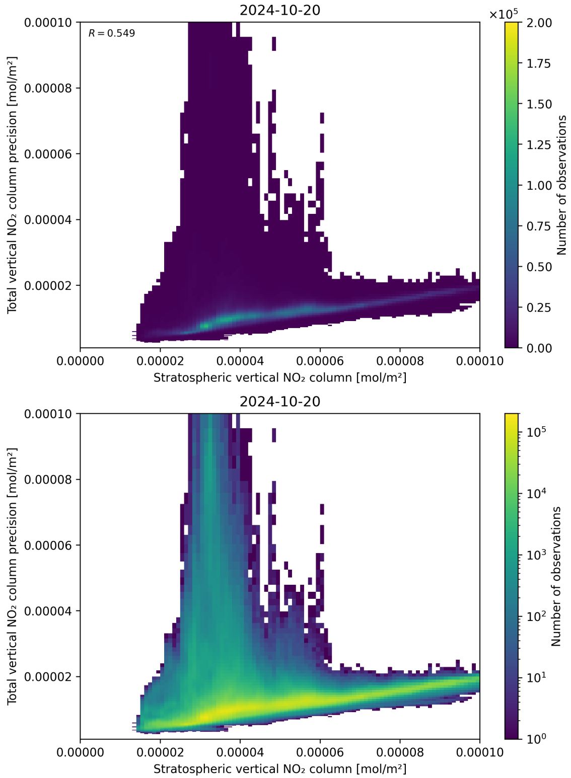
Figure 101: Scatter density plot of “Stratospheric vertical NO 2 column” against “Total vertical NO 2 column precision” for 2024-10-19 to 2024-10-21.
