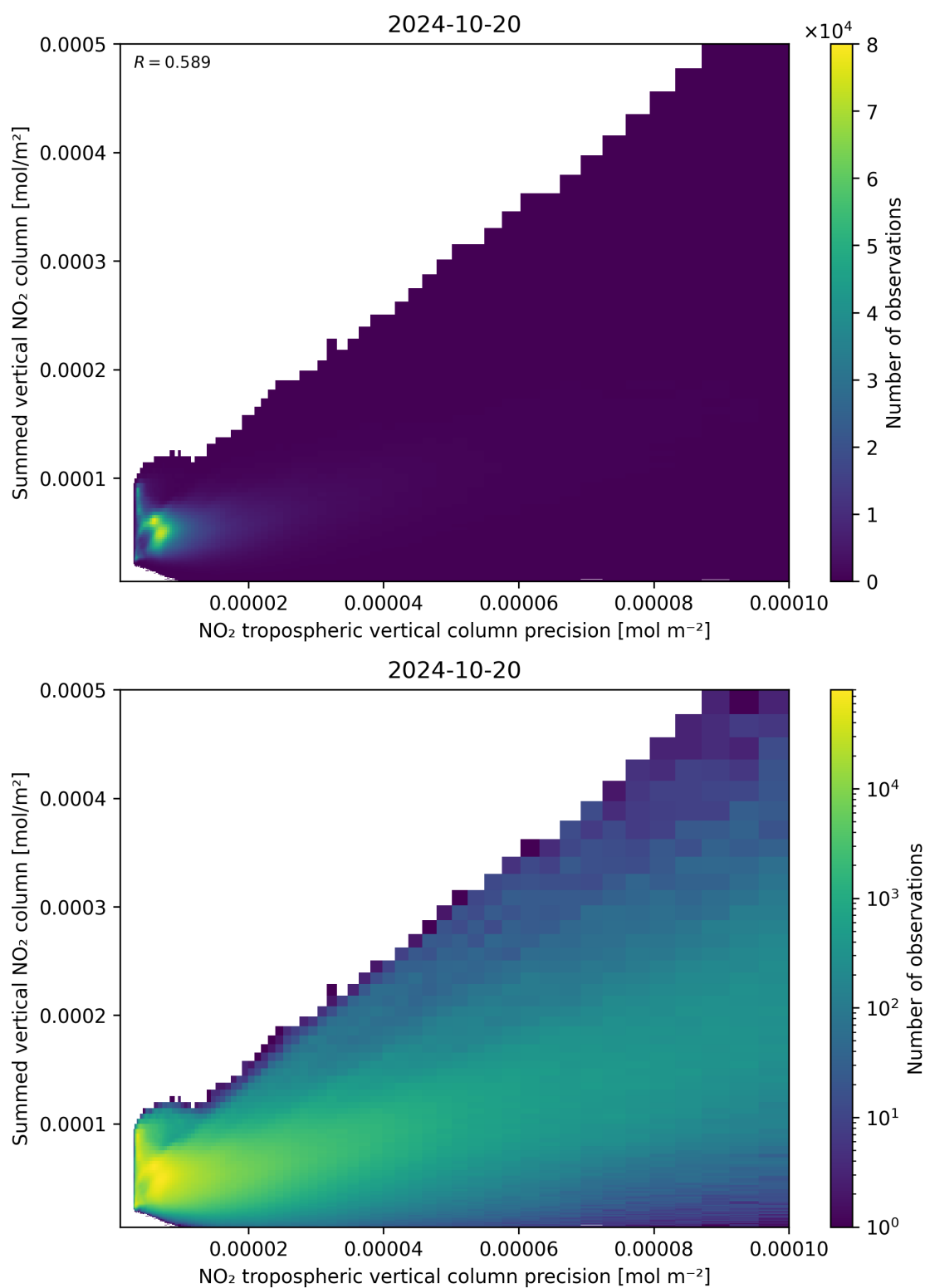
Figure 136: Scatter density plot of “NO 2 tropospheric vertical column precision” against “Summed vertical NO 2 column” for 2024-10-19 to 2024-10-21.
