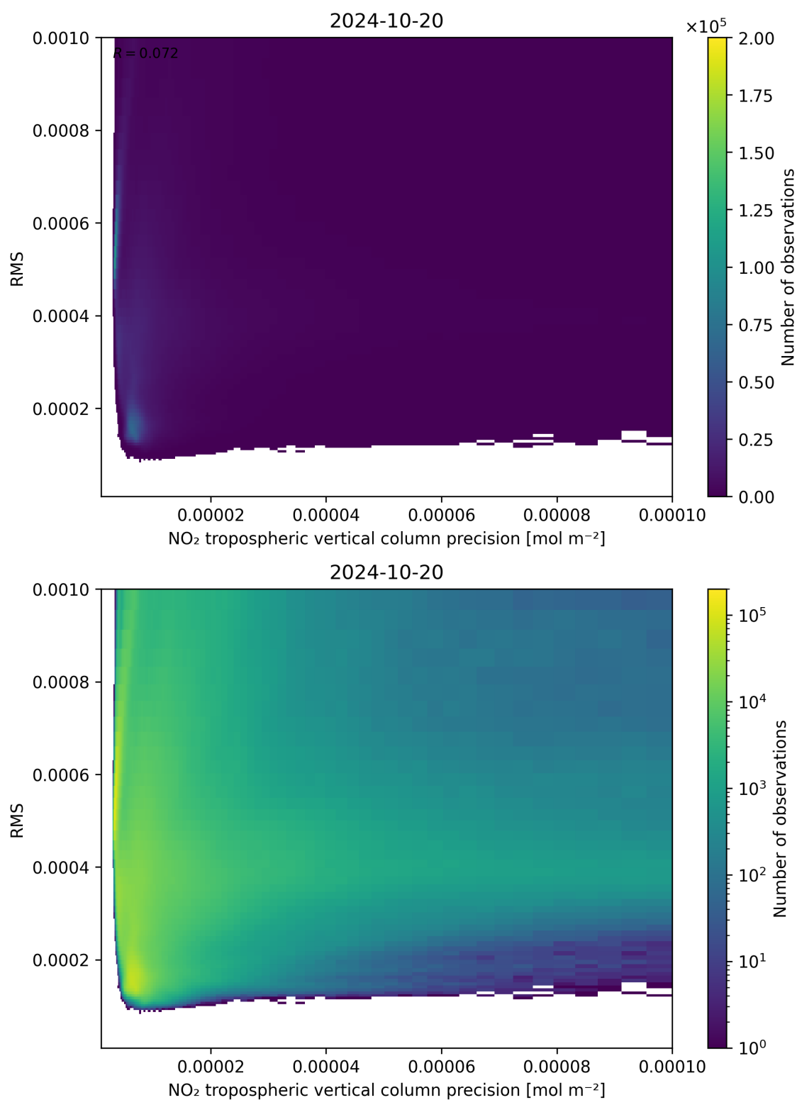
Figure 140: Scatter density plot of “NO 2 tropospheric vertical column precision” against “RMS” for 2024-10-19 to 2024-10-21.
