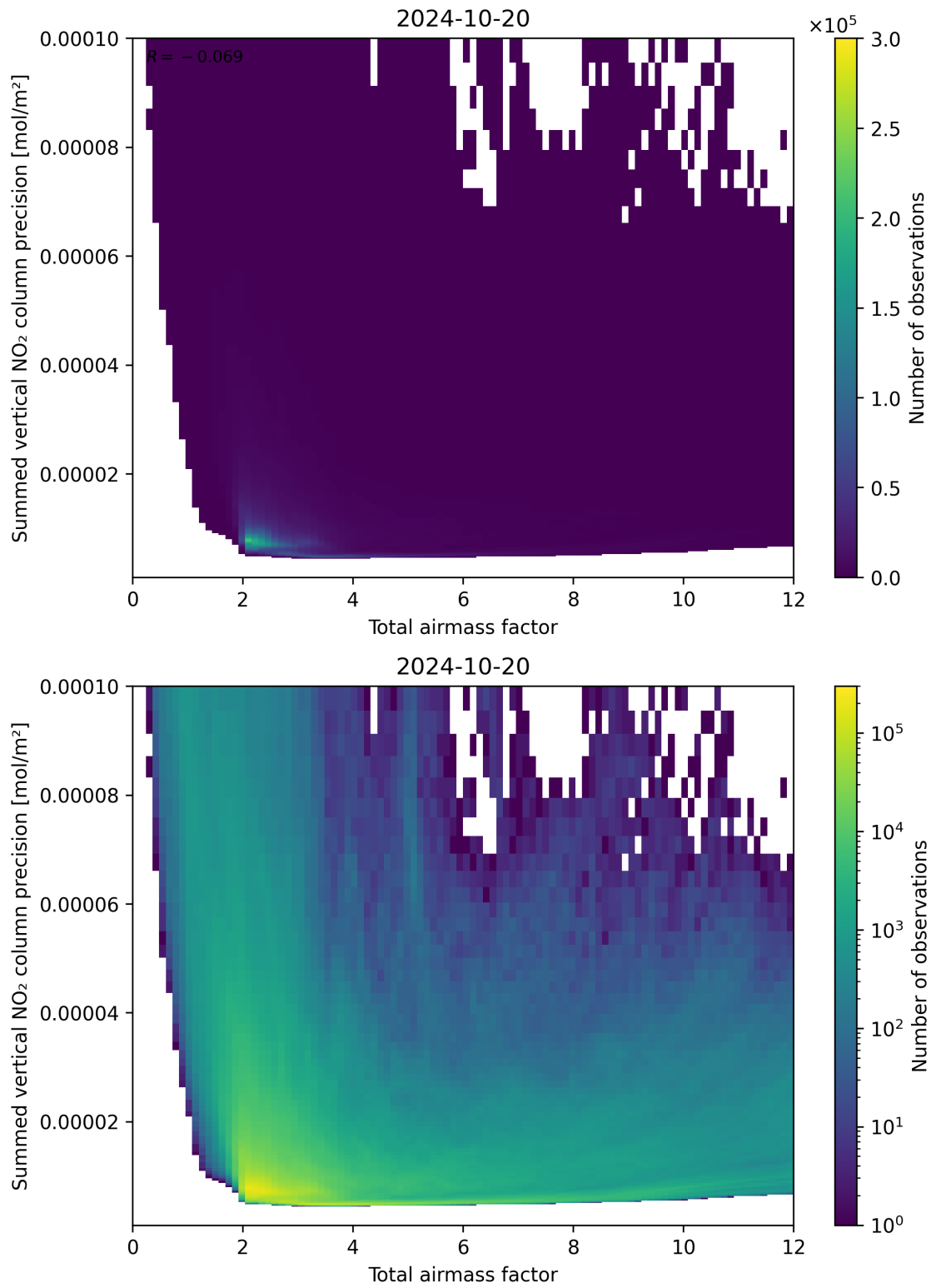
Figure 66: Scatter density plot of “Total airmass factor” against “Summed vertical NO 2 column precision” for 2024-10-19 to 2024-10-21.
