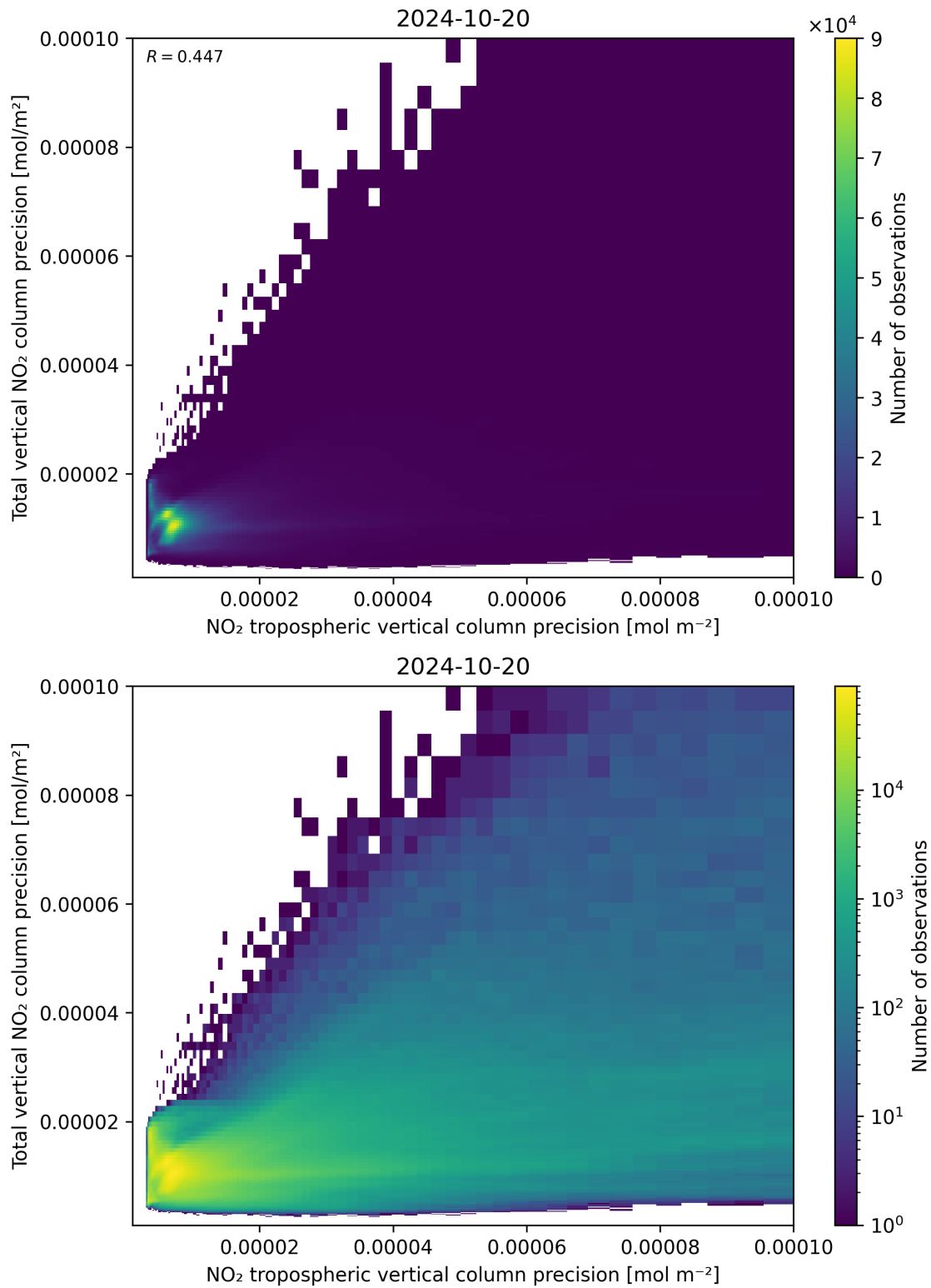
Figure 139: Scatter density plot of “NO 2 tropospheric vertical column precision” against “Total vertical NO 2 column precision” for 2024-10-19 to 2024-10-21.
