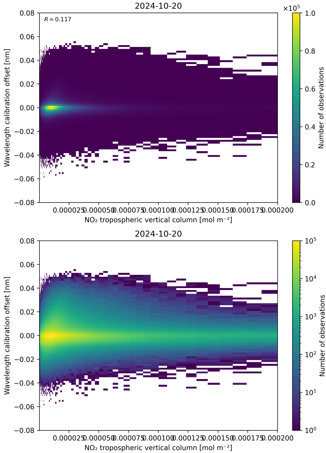
Figure 143: Scatter density plot of “NO 2 tropospheric vertical column” against “Wavelength calibration offset” for 2024-10-19 to 2024-10-21.
