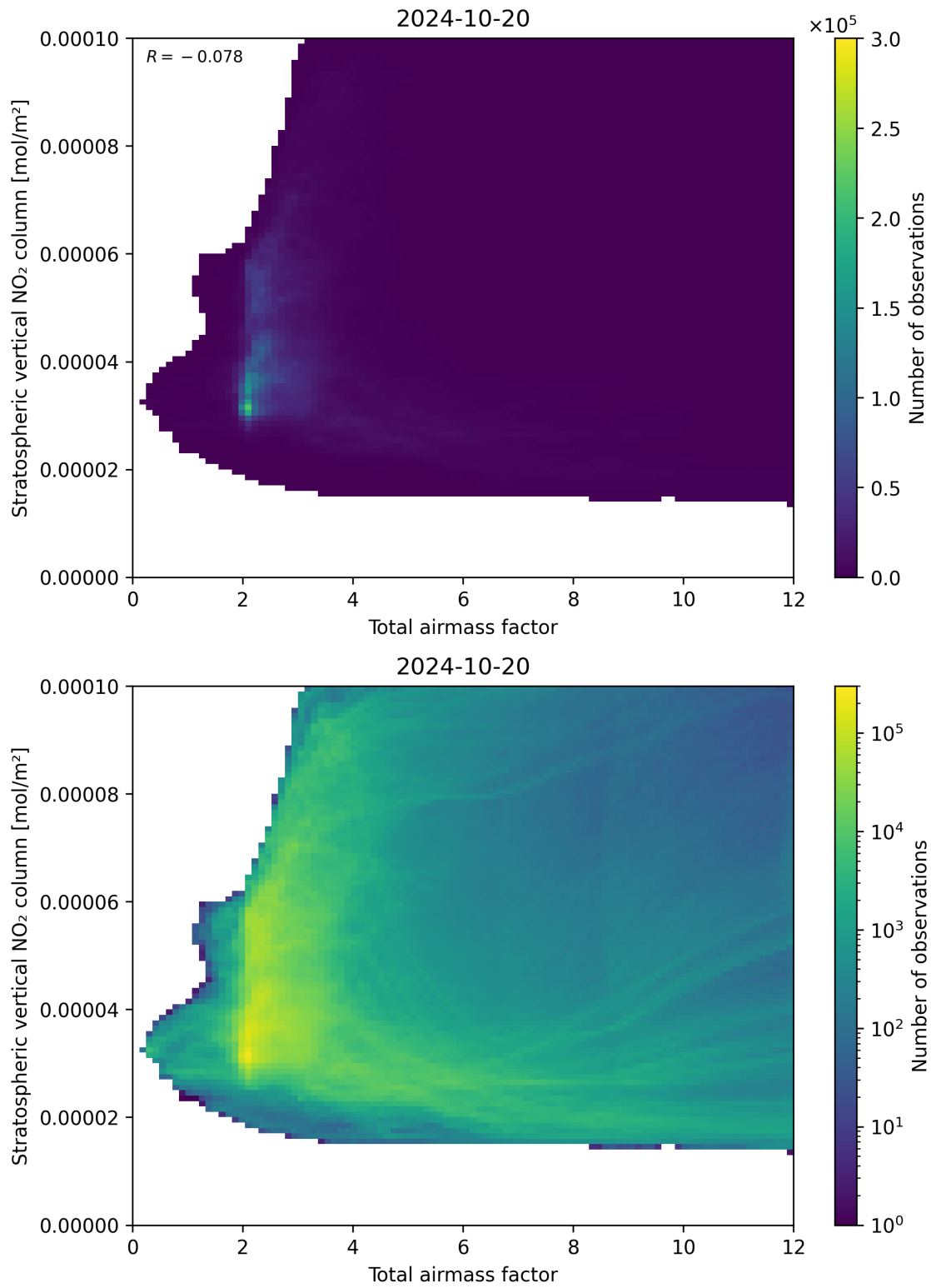
Figure 64: Scatter density plot of “Total airmass factor” against “Stratospheric vertical NO 2 column” for 2024-10-19 to 2024-10-21.
