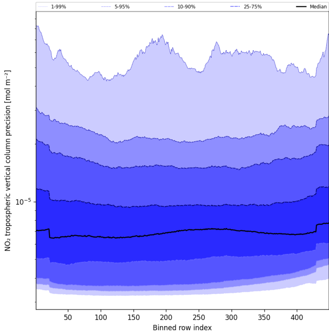
Figure 47: Along track statistics of “NO 2 tropospheric vertical column precision” for 2024-10-19 to 2024-10-21
