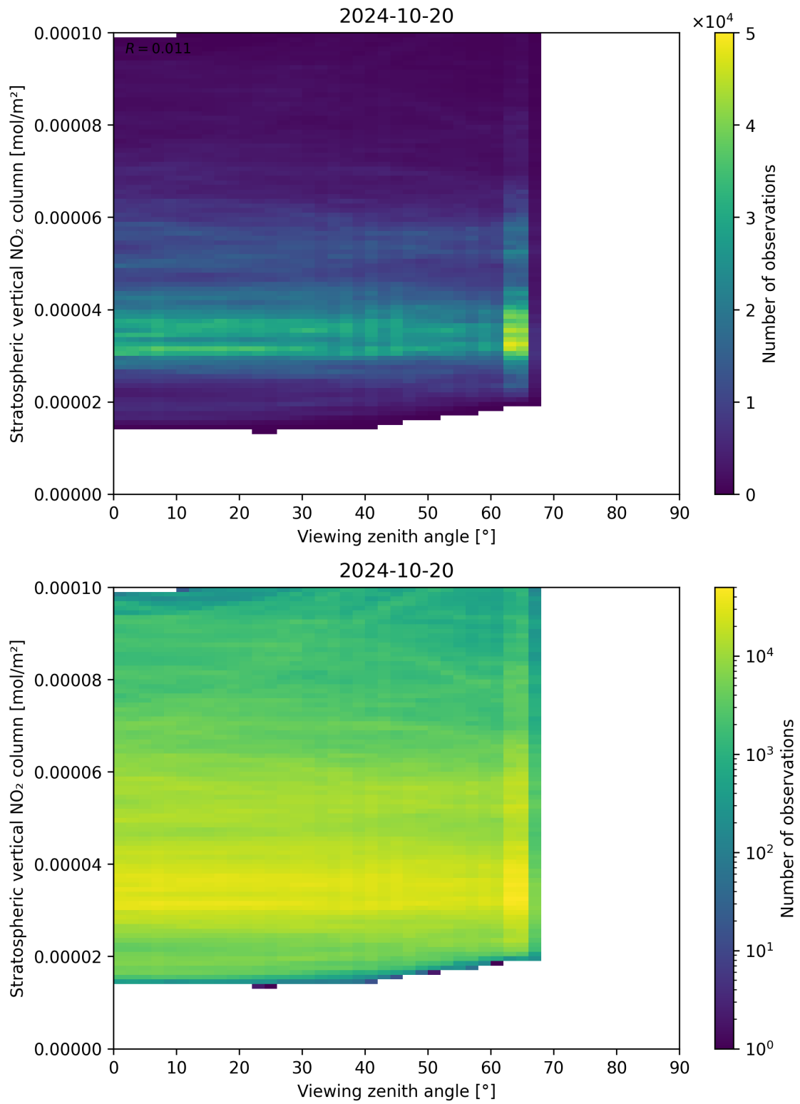
Figure 164: Scatter density plot of “Viewing zenith angle” against “Stratospheric vertical NO 2 column” for 2024-10-19 to 2024-10-21.
