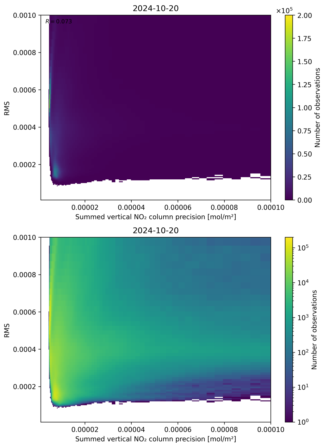
Figure 108: Scatter density plot of “Summed vertical NO 2 column precision” against “RMS” for 2024-10-19 to 2024-10-21.
