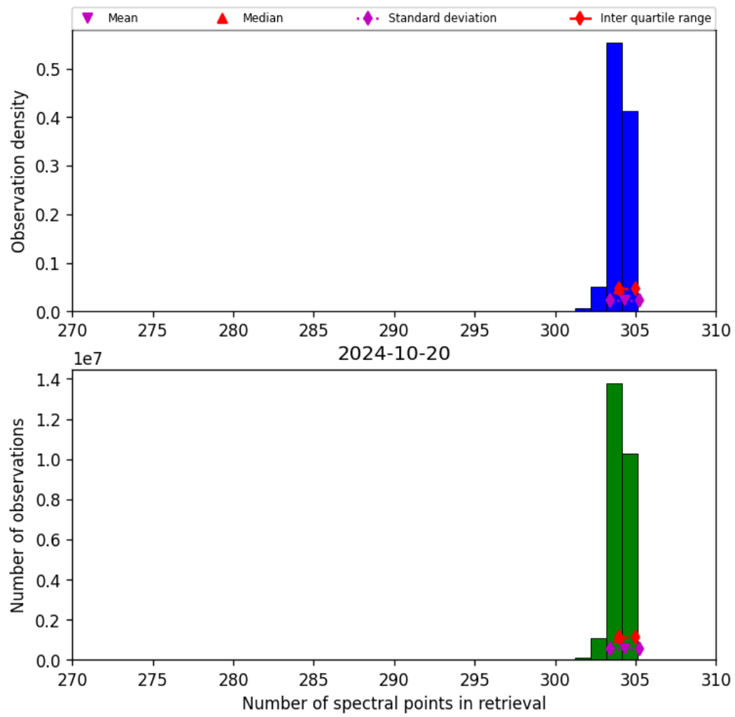
Figure 33: Histogram of “Number of spectral points in retrieval” for 2024-10-19 to 2024-10-21
