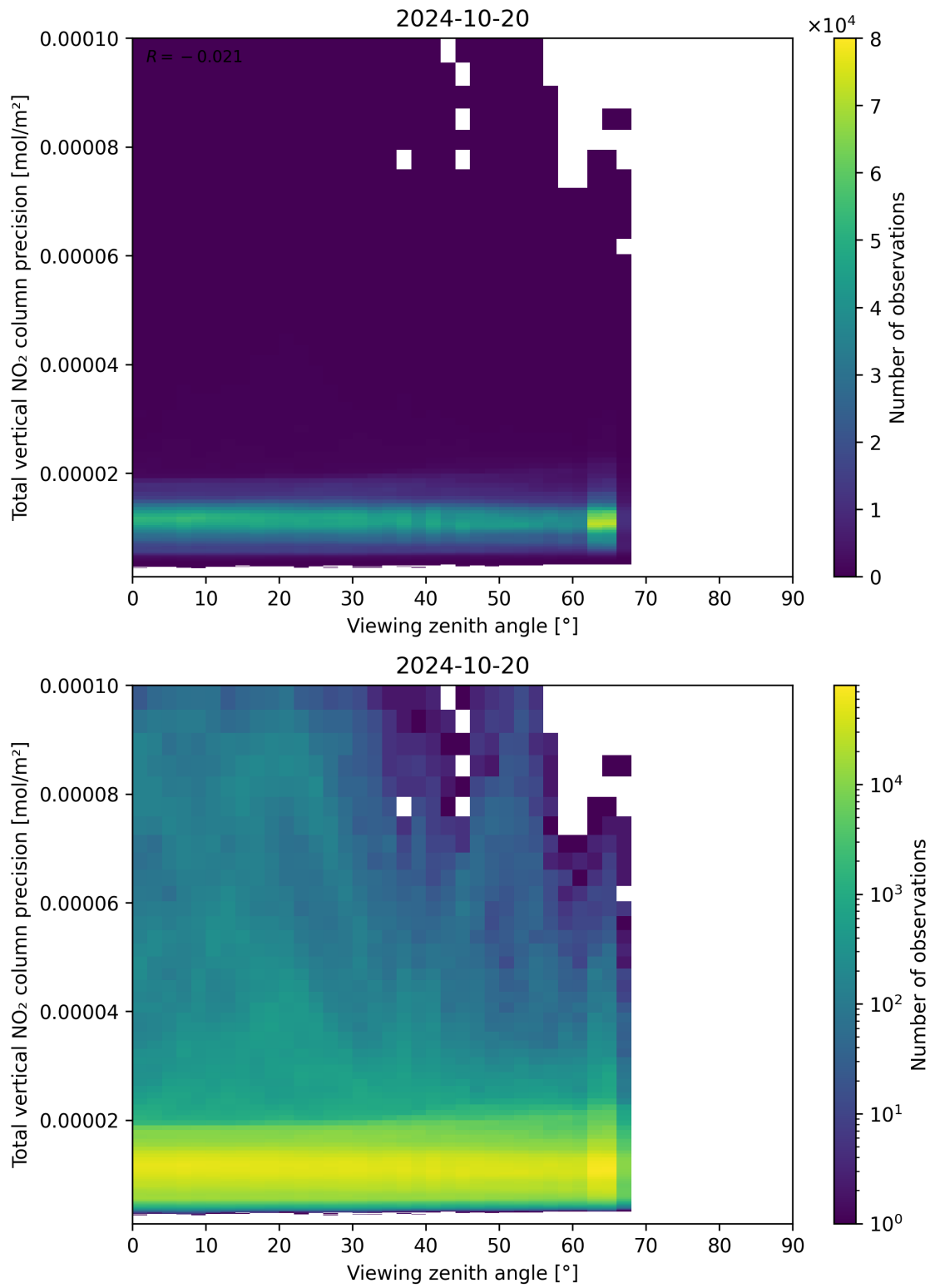
Figure 168: Scatter density plot of “Viewing zenith angle” against “Total vertical NO 2 column precision” for 2024-10-19 to 2024-10-21.
