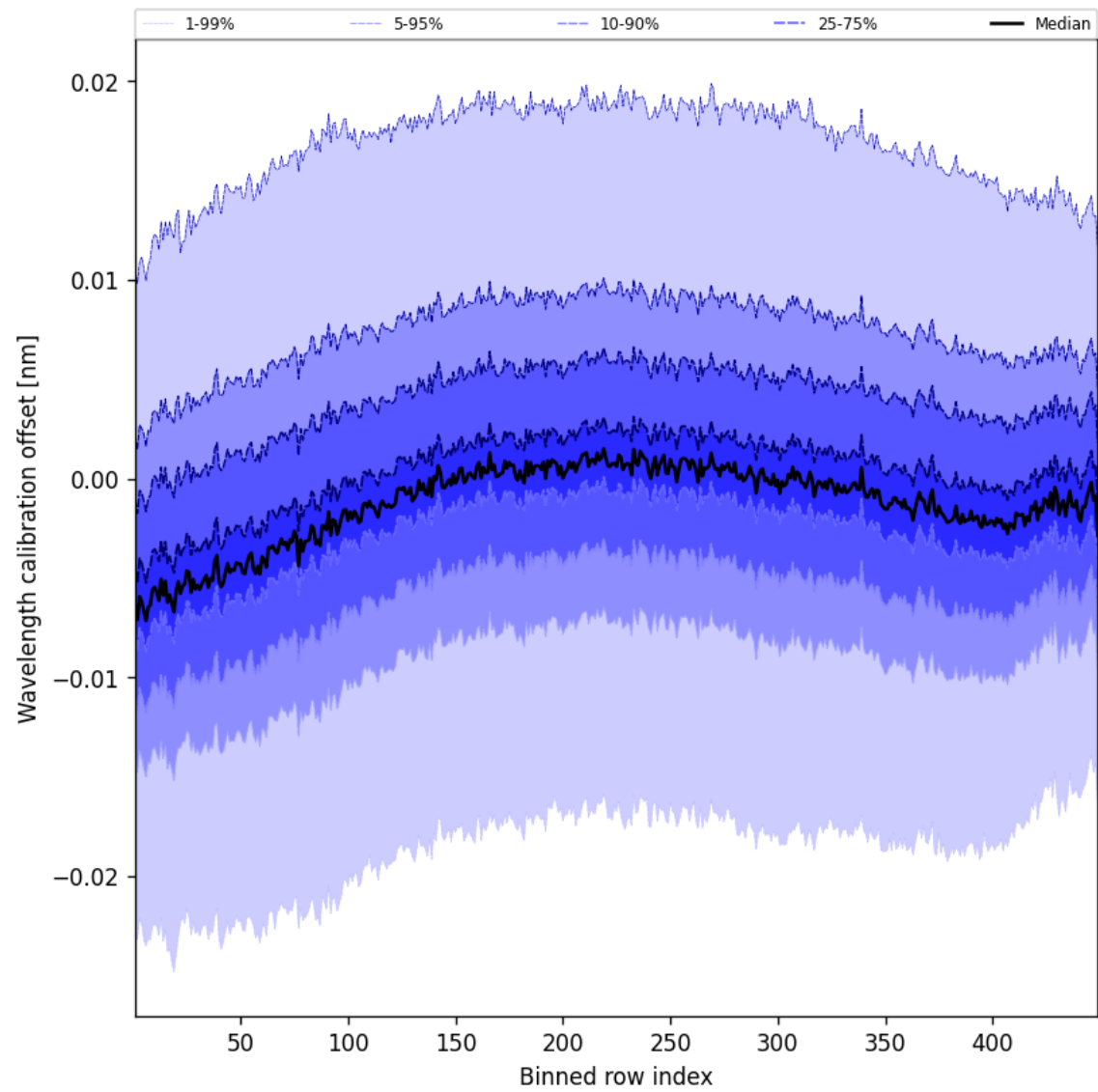
Figure 52: Along track statistics of “Wavelength calibration offset” for 2024-10-19 to 2024-10-21
