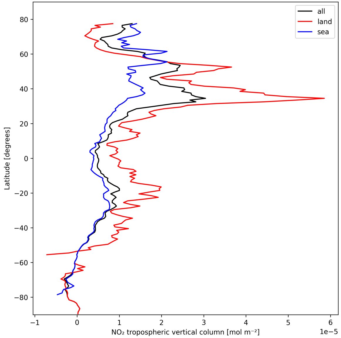
Figure 12: Zonal average of “NO 2 tropospheric vertical column” for 2024-10-19 to 2024-10-21.
