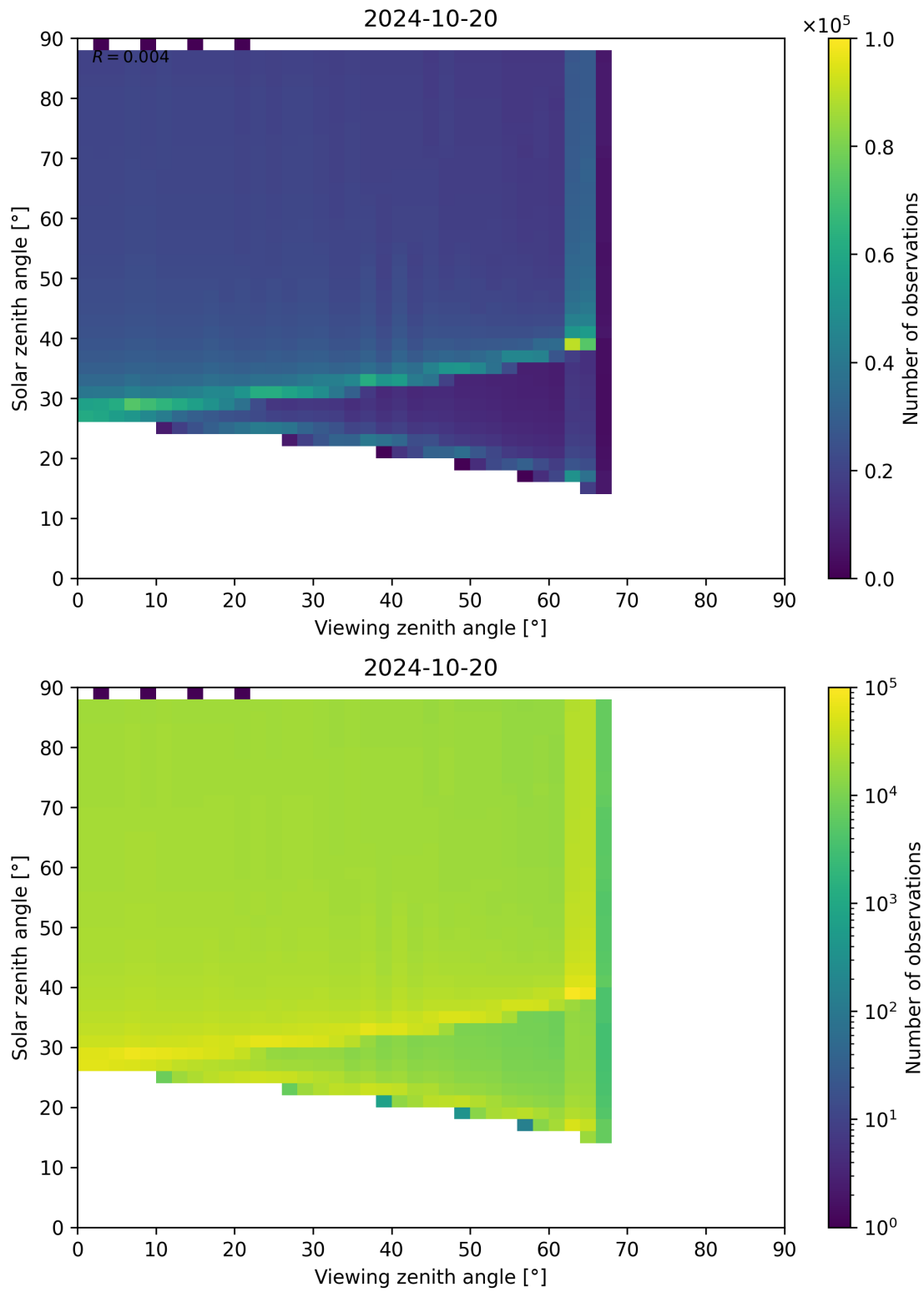
Figure 172: Scatter density plot of “Viewing zenith angle” against “Solar zenith angle” for 2024-10-19 to 2024-10-21.
