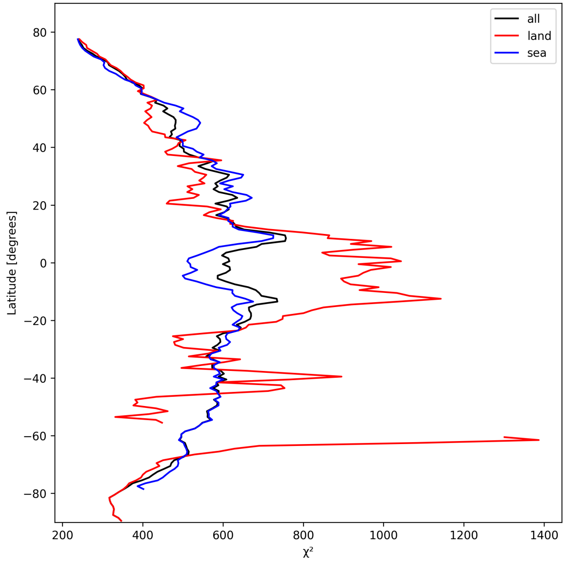
Figure 25: Zonal average of “ \chi^2 ” for 2024-10-19 to 2024-10-21.
