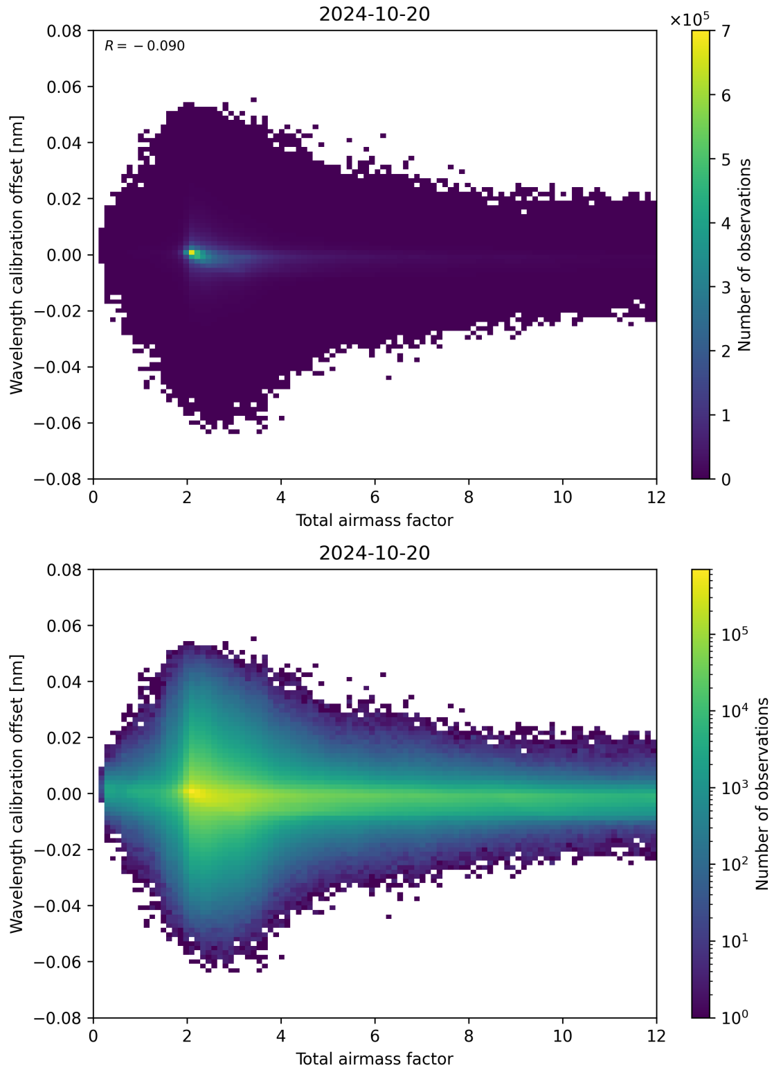
Figure 70: Scatter density plot of “Total airmass factor” against “Wavelength calibration offset” for 2024-10-19 to 2024-10-21.
