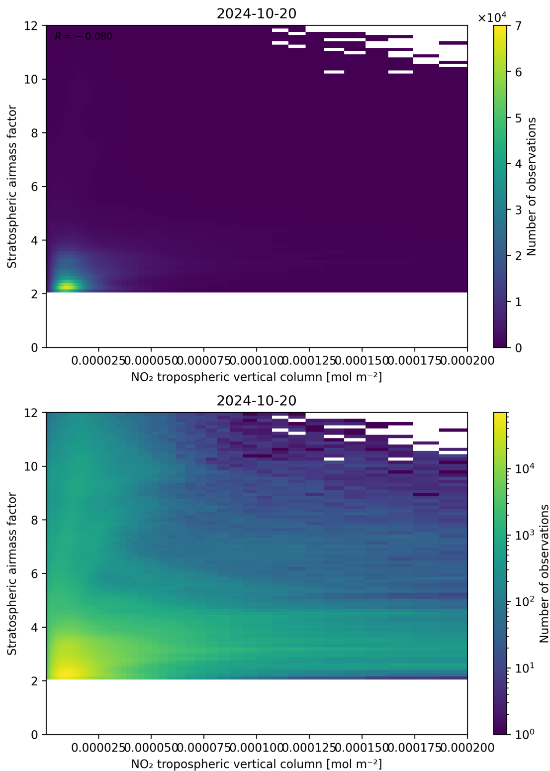
Figure 121: Scatter density plot of “NO 2 tropospheric vertical column” against “Stratospheric airmass factor” for 2024-10-19 to 2024-10-21.
