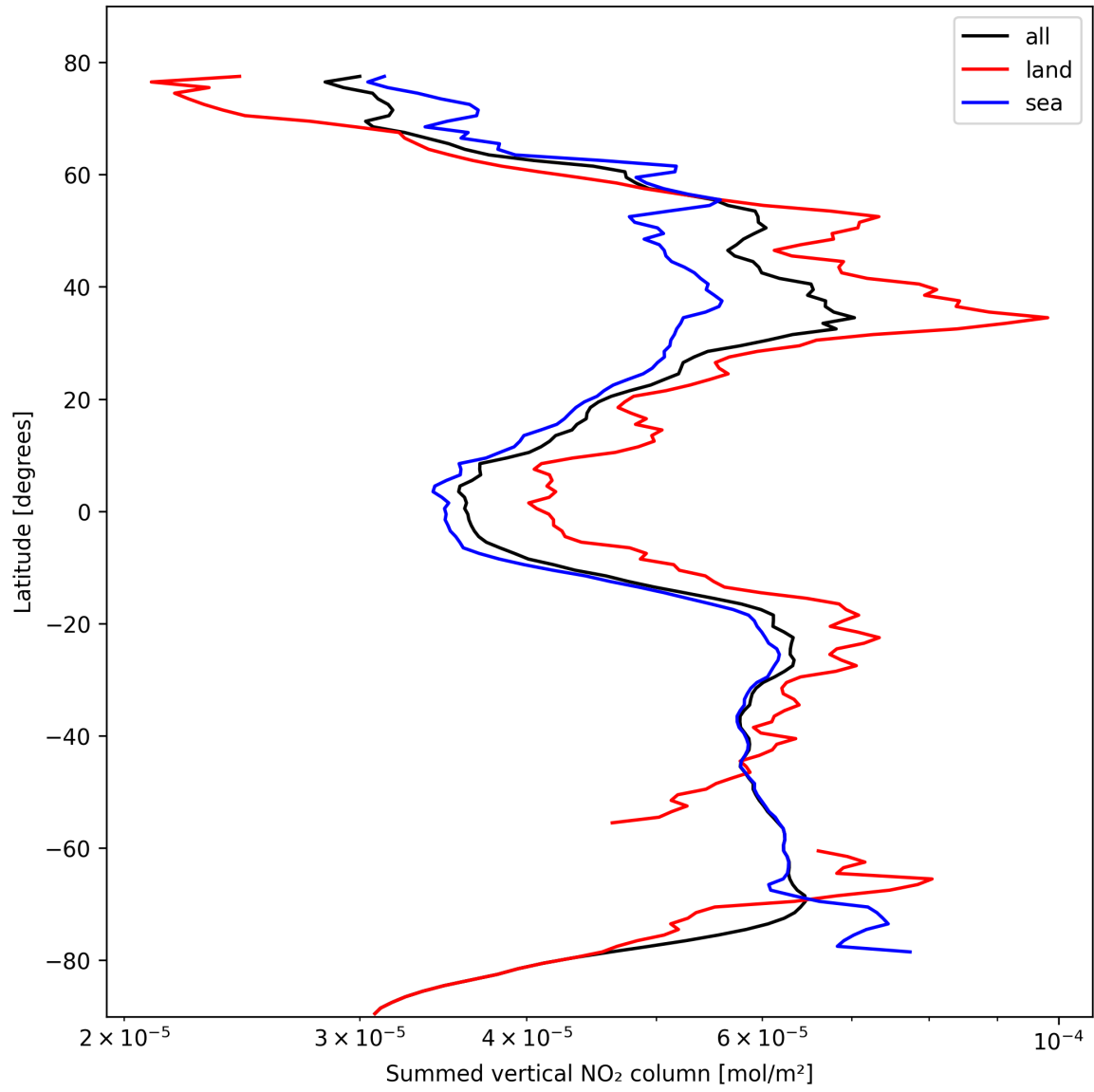
Figure 23: Zonal average of “Summed vertical NO 2 column” for 2024-10-19 to 2024-10-21.
