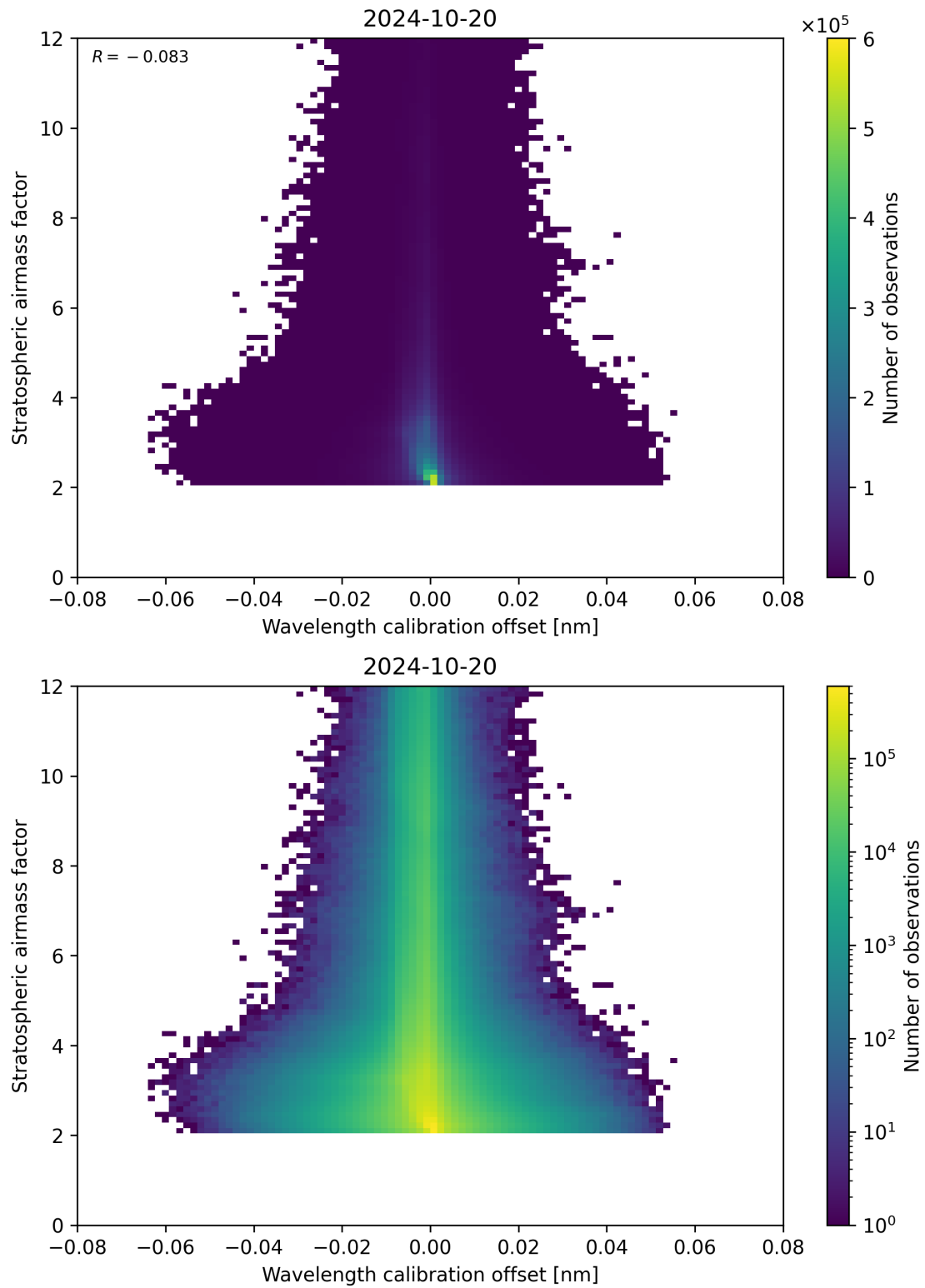
Figure 174: Scatter density plot of “Wavelength calibration offset” against “Stratospheric air mass factor” for 2024-10-19 to 2024-10-21.
