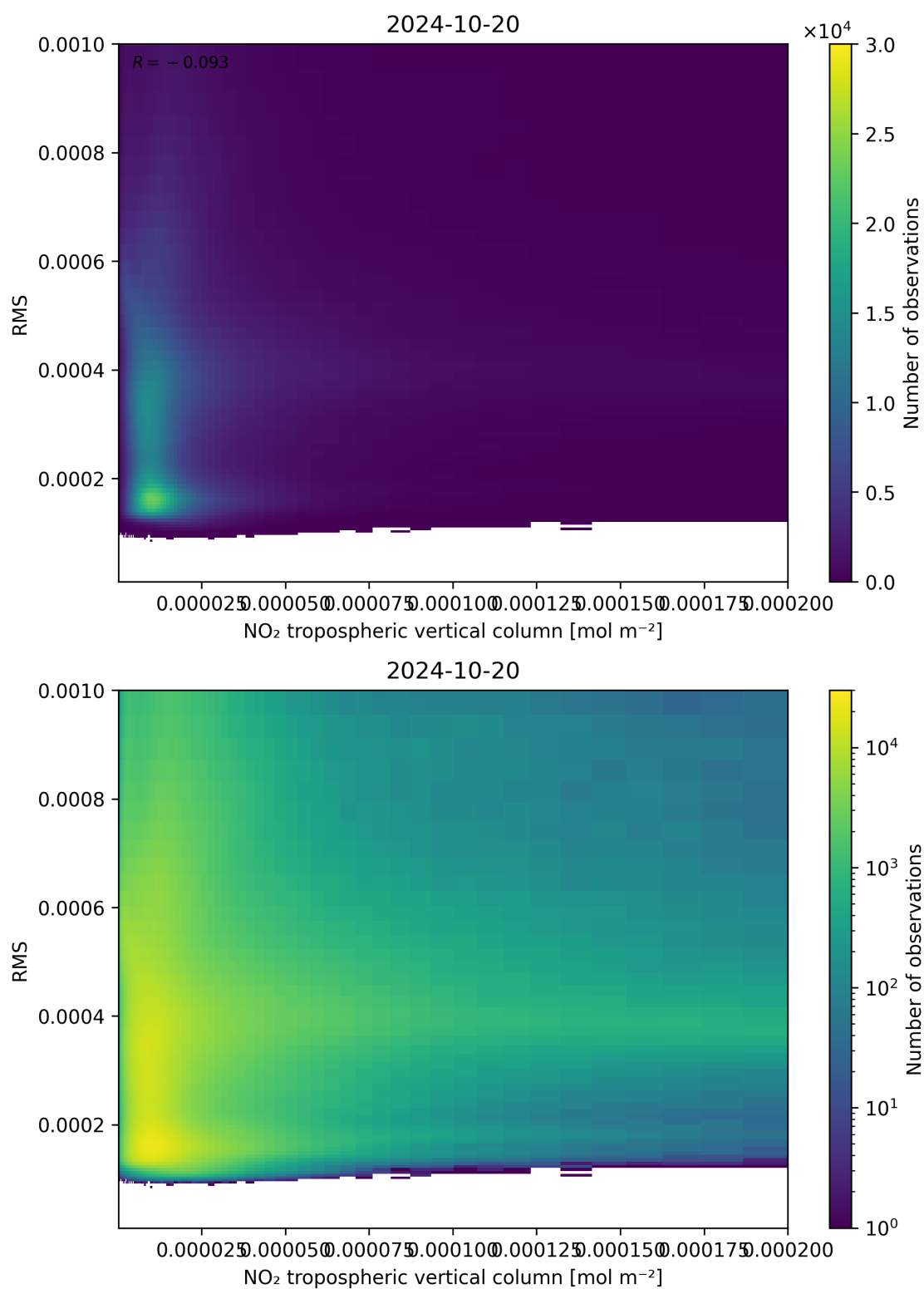
Figure 142: Scatter density plot of “NO 2 tropospheric vertical column” against “RMS” for 2024-10-19 to 2024-10-21.
