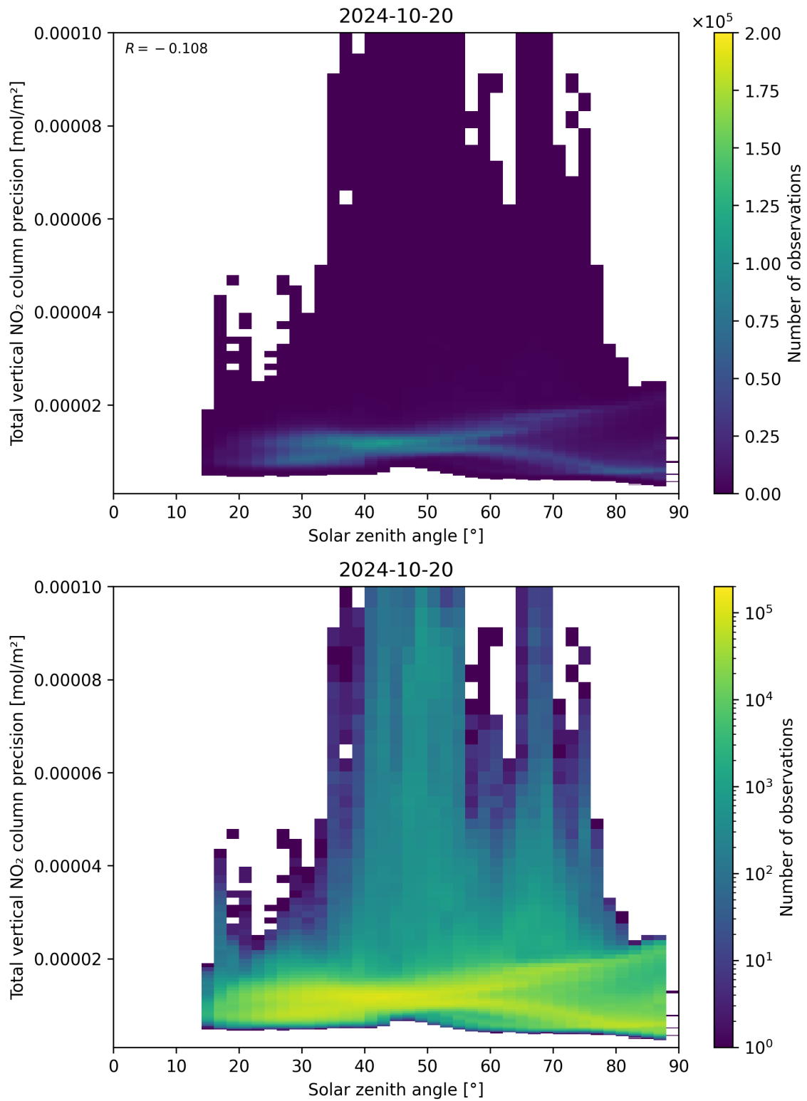
Figure 154: Scatter density plot of “Solar zenith angle” against “Total vertical NO 2 column precision” for 2024-10-19 to 2024-10-21.
