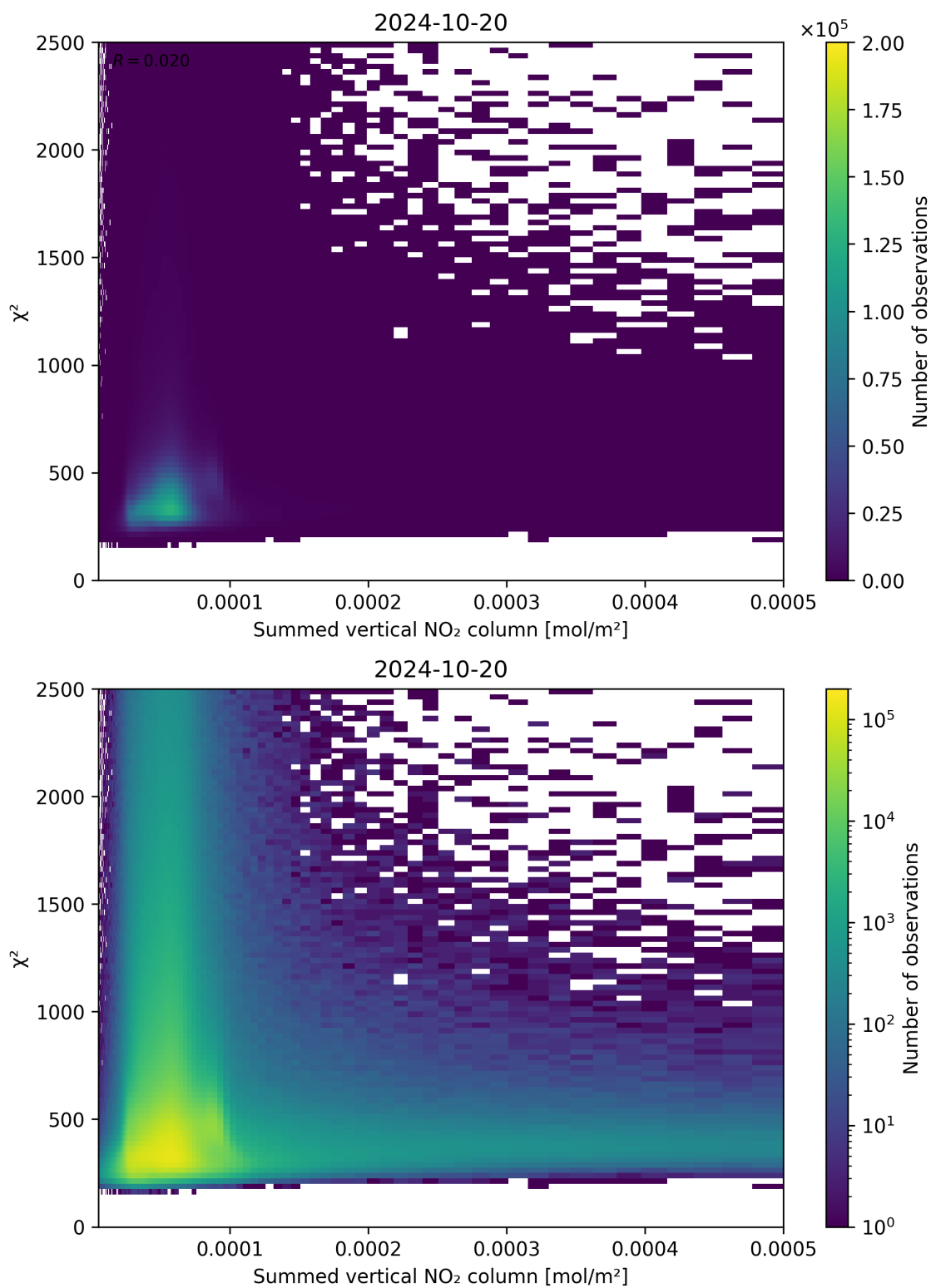
Figure 104: Scatter density plot of “Summed vertical NO 2 column” against “ \chi^2 ” for 2024-10-19 to 2024-10-21.
