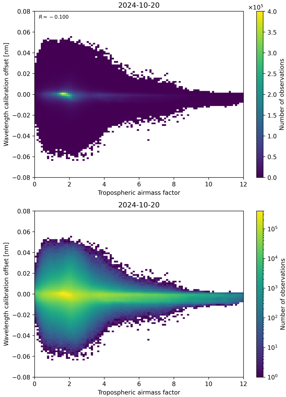
Figure 80: Scatter density plot of “Tropospheric airmass factor” against “Wavelength calibration offset” for 2024-10-19 to 2024-10-21.
