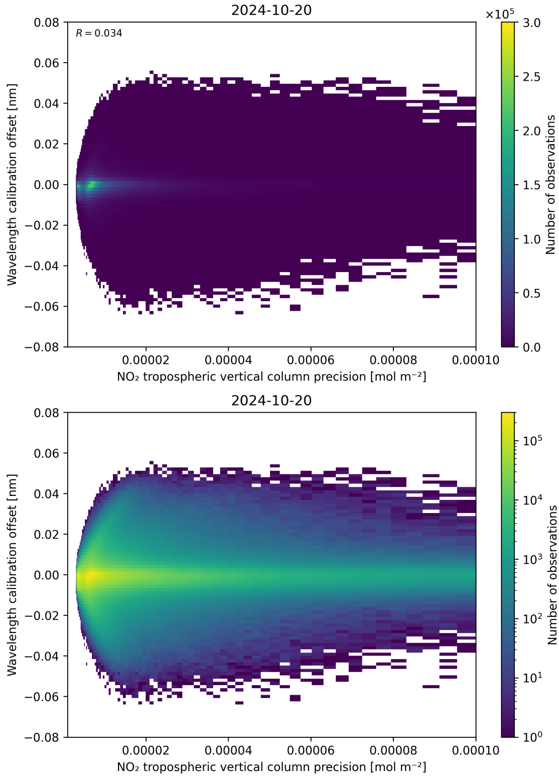
Figure 141: Scatter density plot of “NO 2 tropospheric vertical column precision” against “Wavelength calibration offset” for 2024-10-19 to 2024-10-21.
