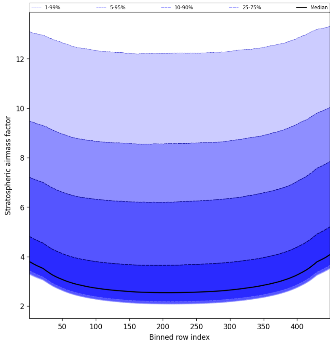
Figure 61: Along track statistics of “Stratospheric air mass factor” for 2024-10-19 to 2024-10-21
