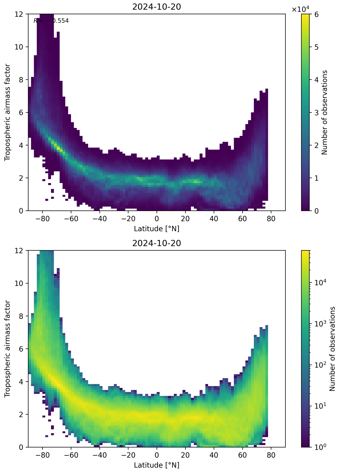
Figure 85: Scatter density plot of “Latitude” against “Tropospheric air mass factor” for 2024-10-19 to 2024-10-21.
