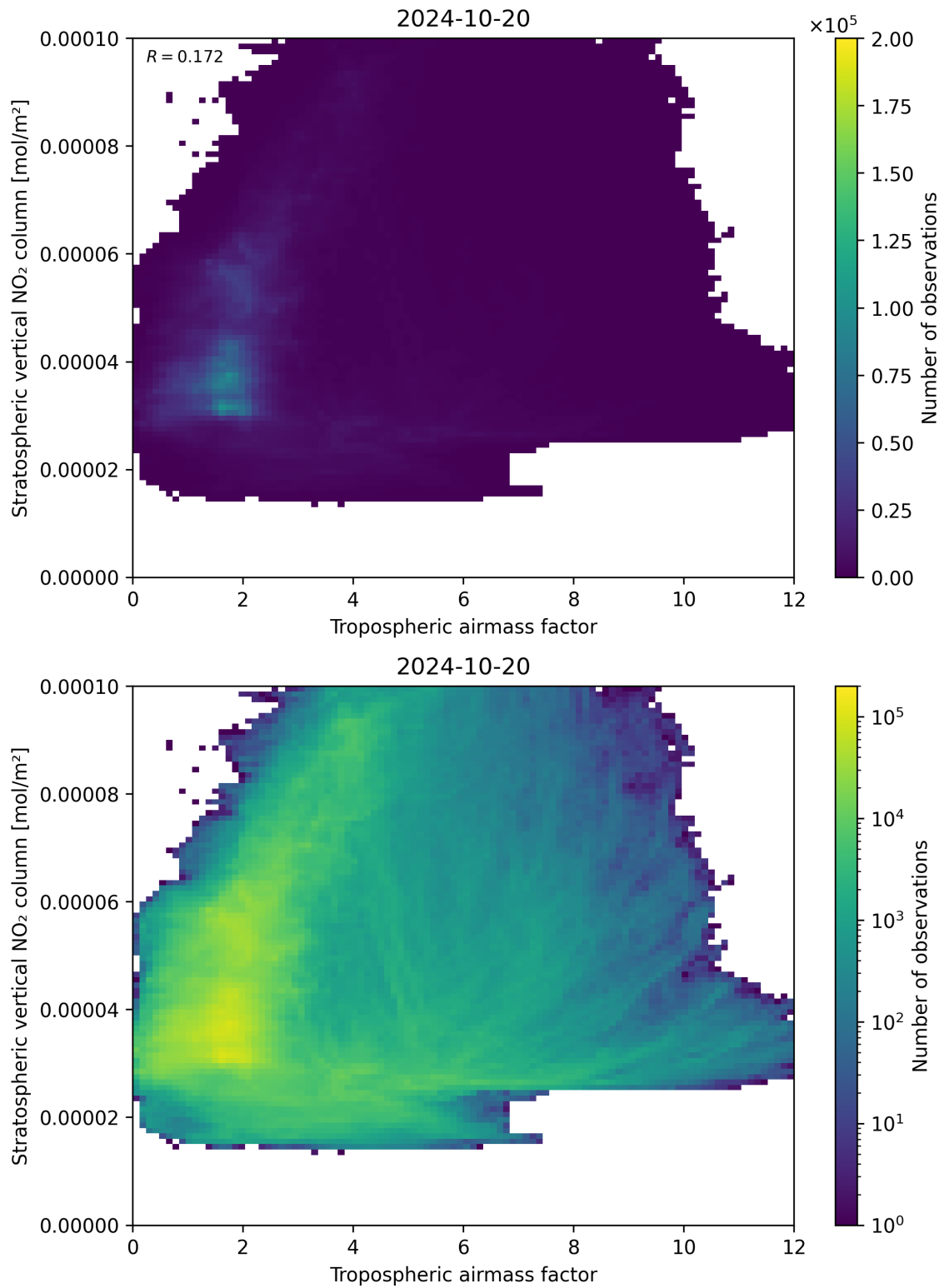
Figure 74: Scatter density plot of “Tropospheric air mass factor” against “Stratospheric vertical NO 2 column” for 2024-10-19 to 2024-10-21.
