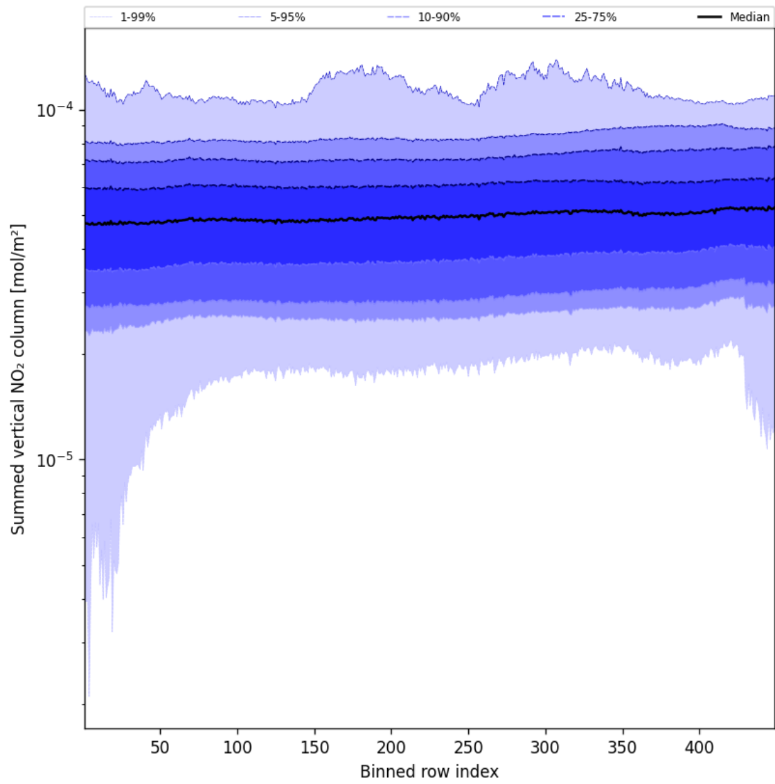
Figure 57: Along track statistics of “Summed vertical NO 2 column” for 2024-10-19 to 2024-10-21
