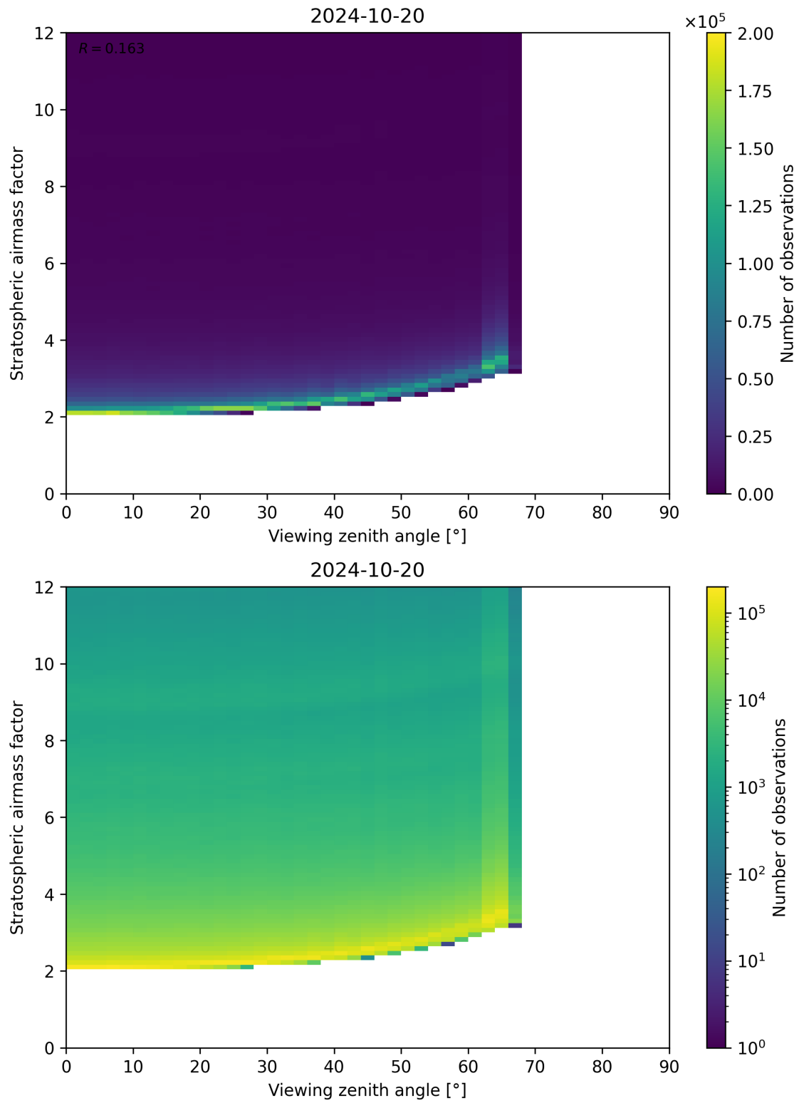
Figure 159: Scatter density plot of “Viewing zenith angle” against “Stratospheric airmass factor” for 2024-10-19 to 2024-10-21.
