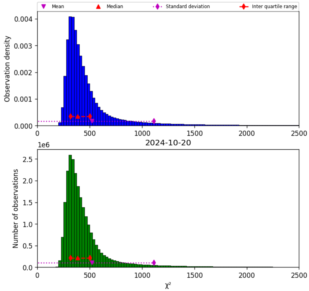
Figure 42: Histogram of “ \chi^2 ” for 2024-10-19 to 2024-10-21
