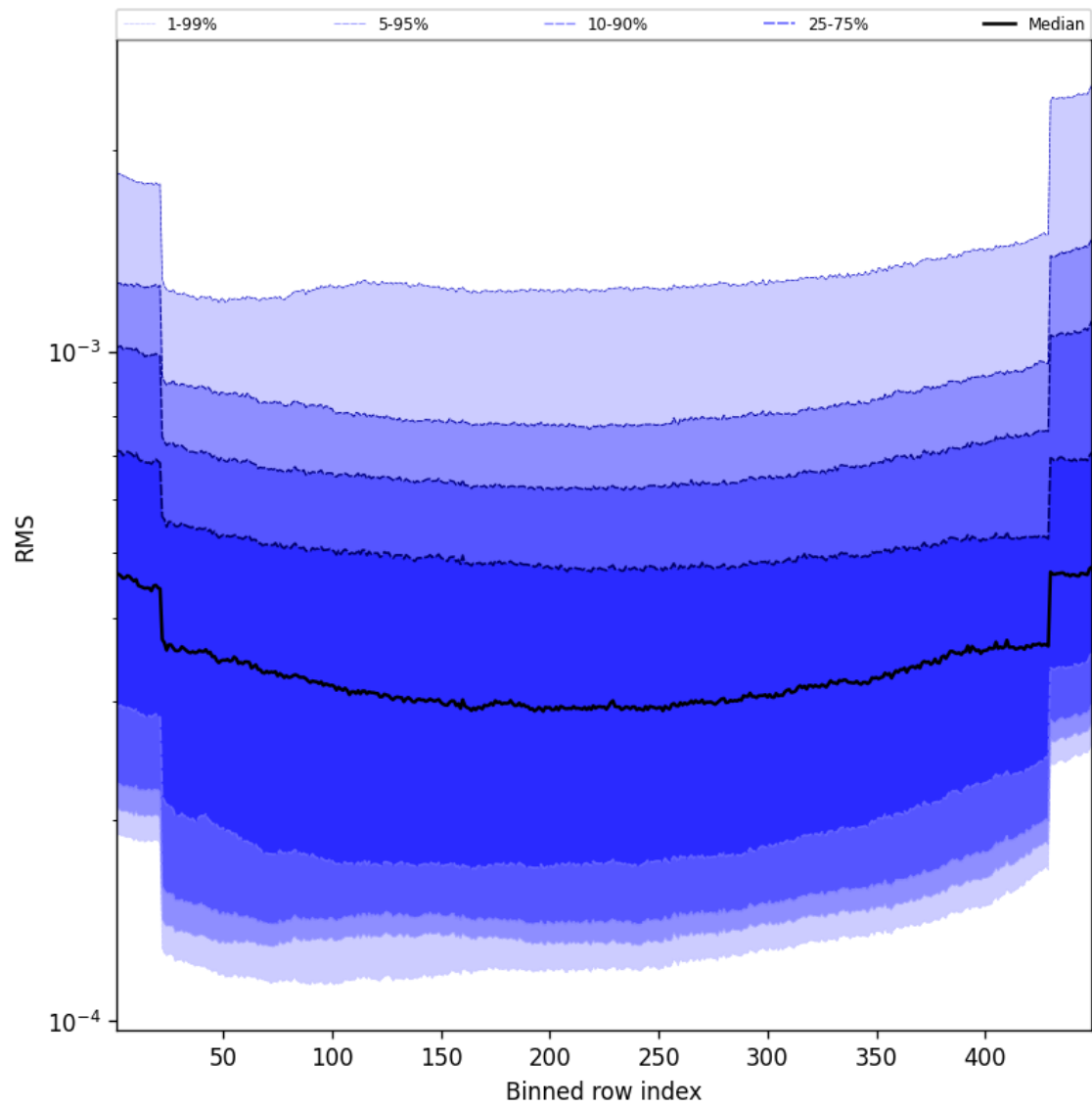
Figure 60: Along track statistics of “RMS” for 2024-10-19 to 2024-10-21
