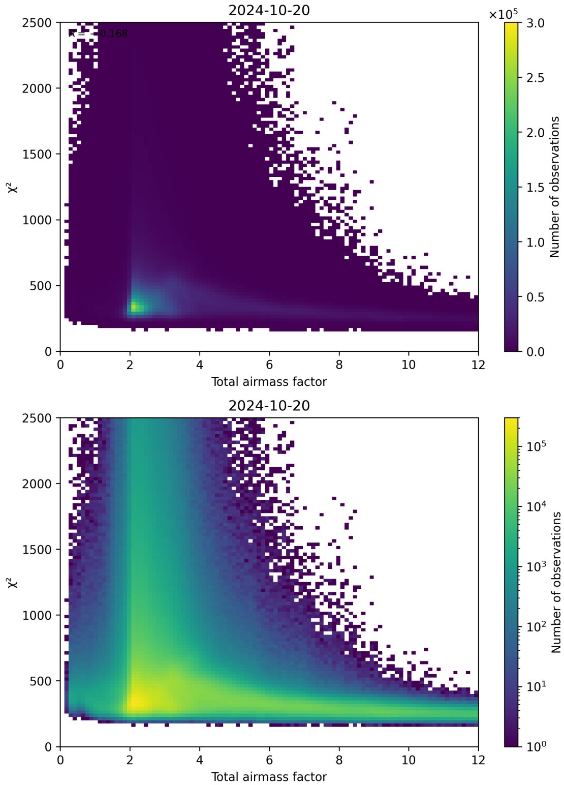
Figure 63: Scatter density plot of “Total airmass factor” against “ \chi^2 ” for 2024-10-19 to 2024-10-21.
