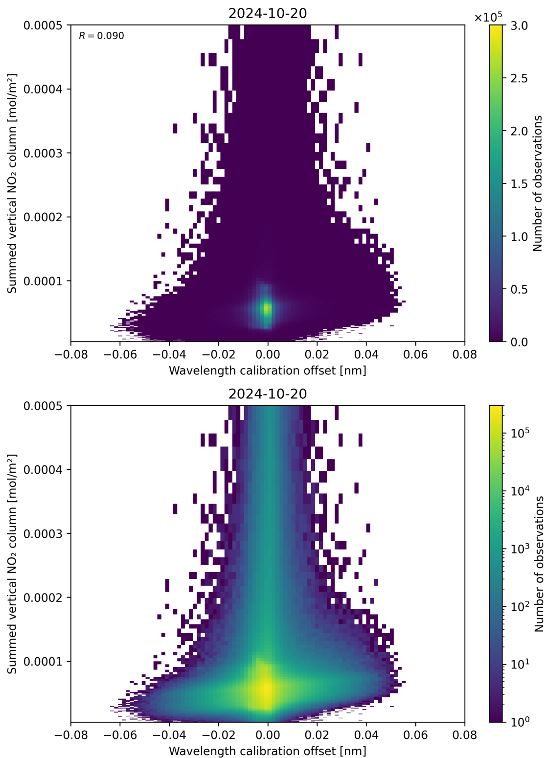
Figure 177: Scatter density plot of “Wavelength calibration offset” against “Summed vertical NO 2 column” for 2024-10-19 to 2024-10-21.
