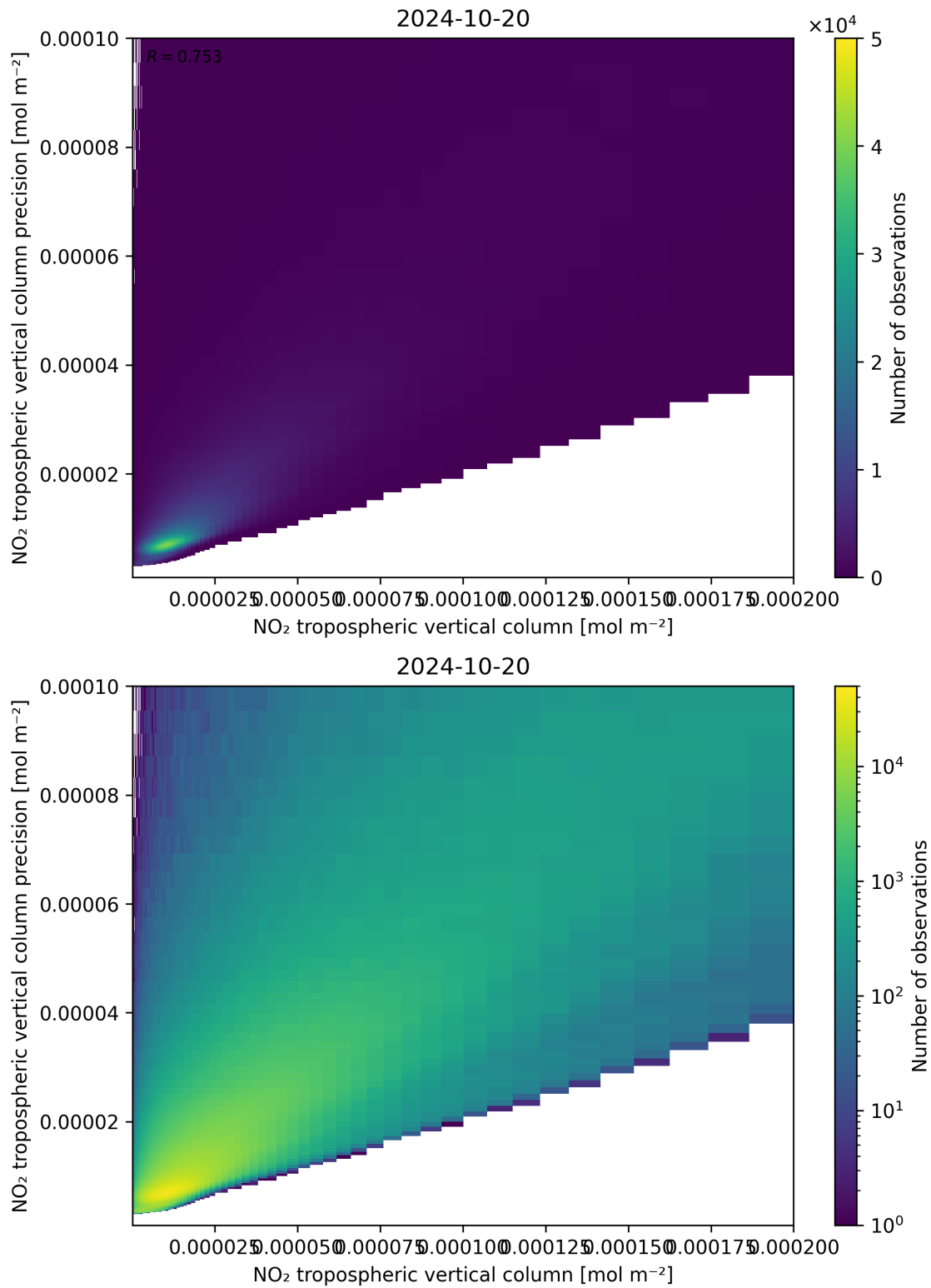
Figure 130: Scatter density plot of “NO 2 tropospheric vertical column” against “NO 2 tropospheric vertical column precision” for 2024-10-19 to 2024-10-21.
