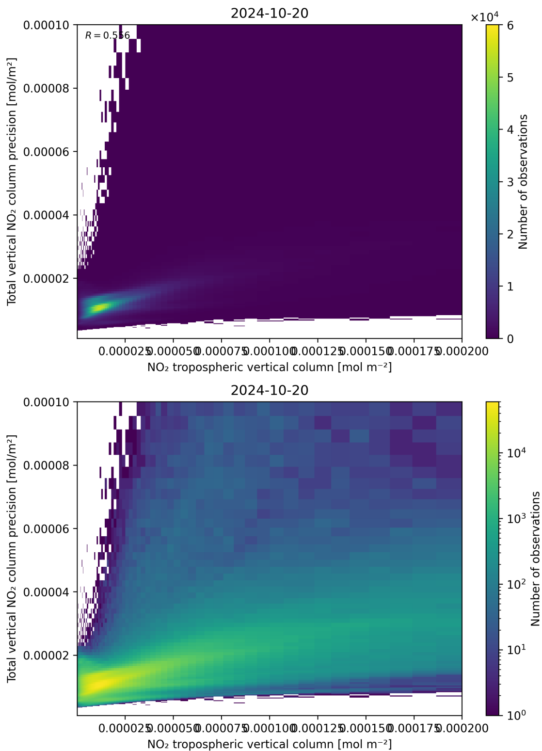
Figure 129: Scatter density plot of “NO 2 tropospheric vertical column” against “Total vertical NO 2 column precision” for 2024-10-19 to 2024-10-21.
