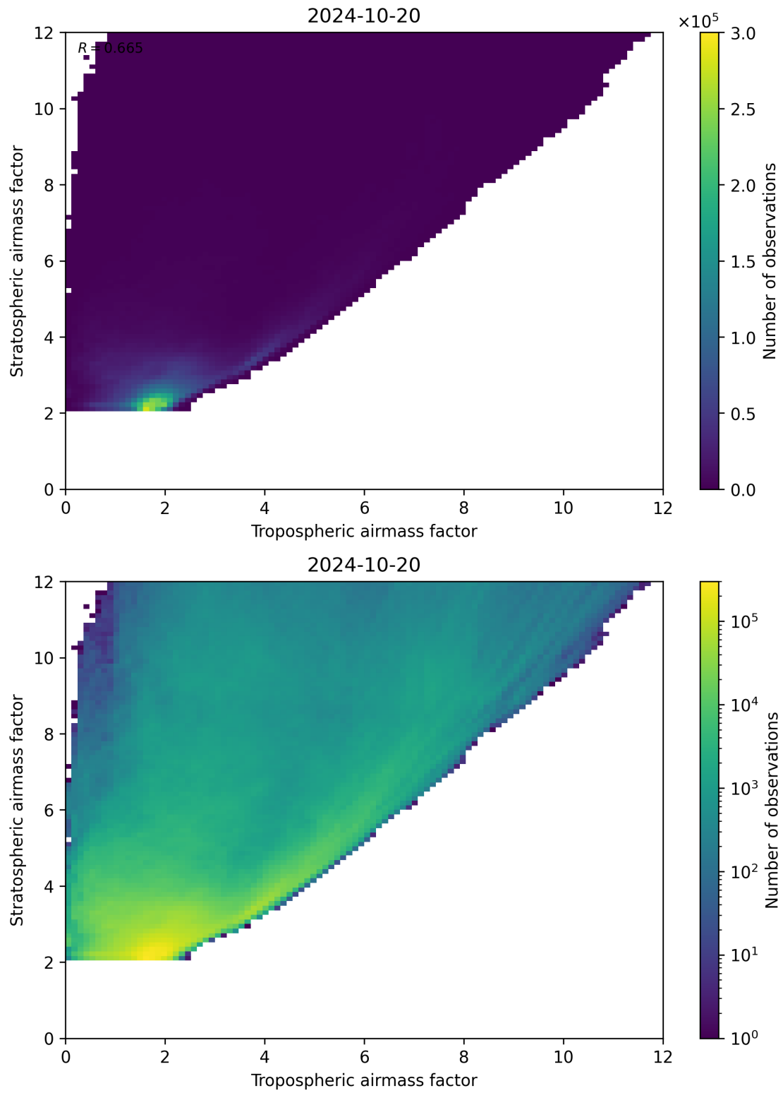
Figure 71: Scatter density plot of “Tropospheric airmass factor” against “Stratospheric airmass factor” for 2024-10-19 to 2024-10-21.
