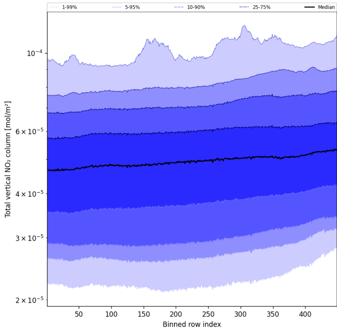
Figure 55: Along track statistics of “Total vertical NO 2 column” for 2024-10-19 to 2024-10-21
