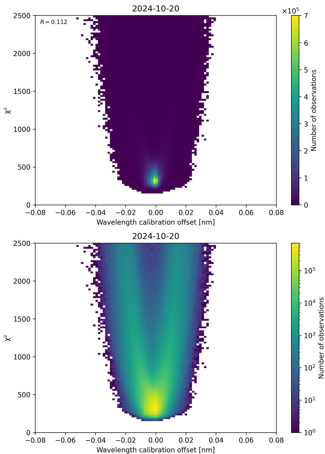
Figure 175: Scatter density plot of “Wavelength calibration offset” against “ \chi^2 ” for 2024-10-19 to 2024-10-21.
