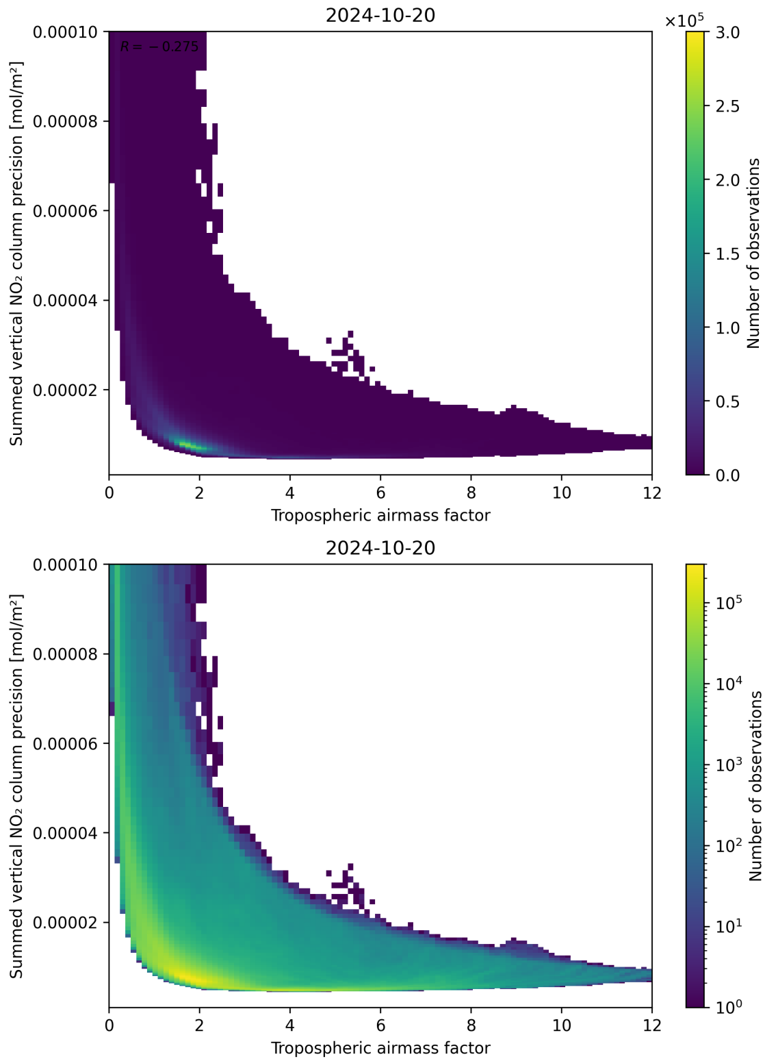
Figure 76: Scatter density plot of “Tropospheric airmass factor” against “Summed vertical NO 2 column precision” for 2024-10-19 to 2024-10-21.
