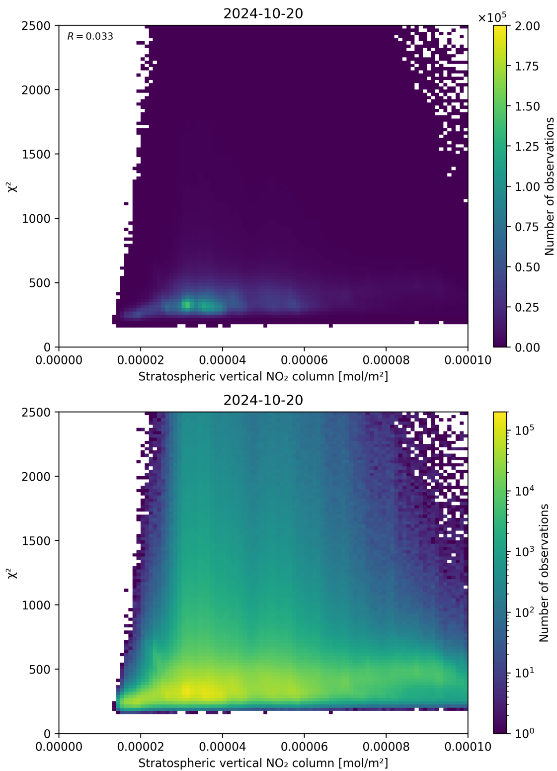
Figure 97: Scatter density plot of “Stratospheric vertical NO 2 column” against “ \chi^2 ” for 2024-10-19 to 2024-10-21.
