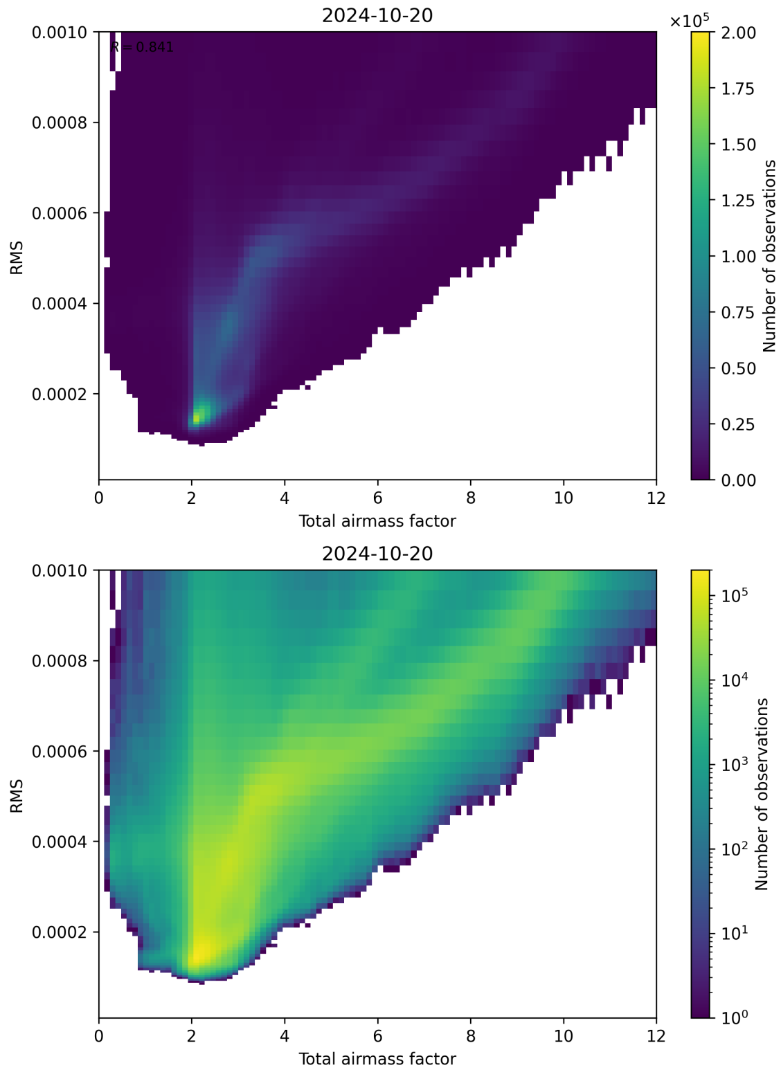
Figure 69: Scatter density plot of “Total airmass factor” against “RMS” for 2024-10-19 to 2024-10-21.
