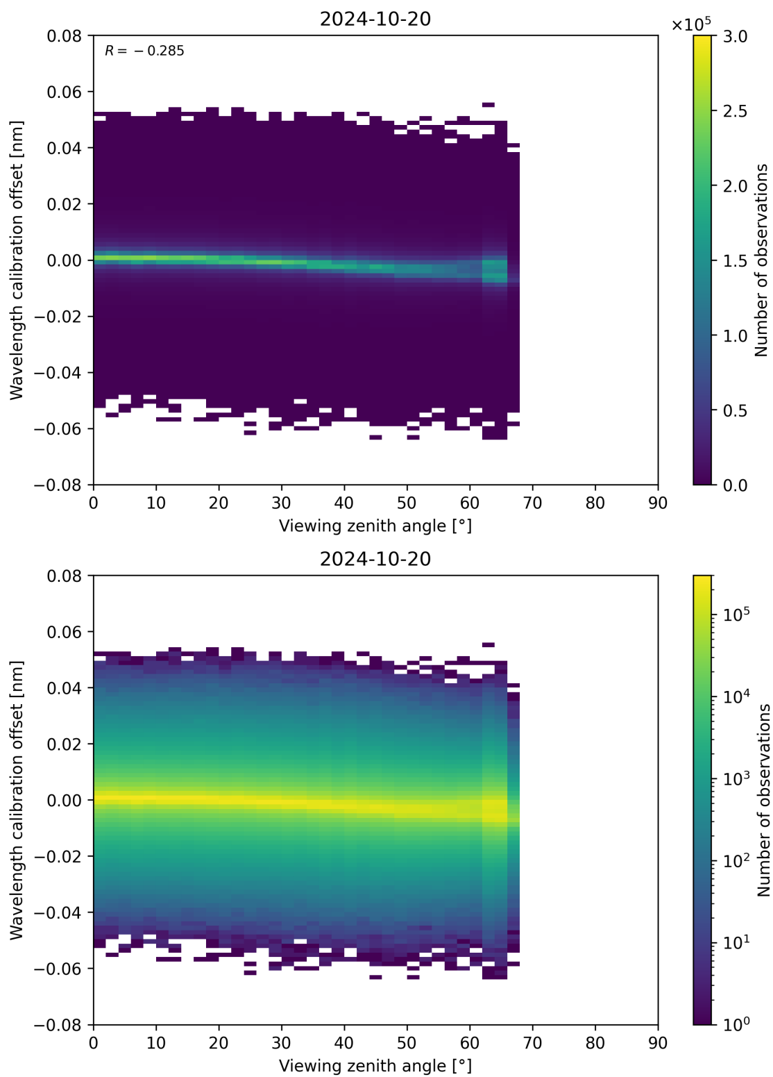
Figure 173: Scatter density plot of “Viewing zenith angle” against “Wavelength calibration offset” for 2024-10-19 to 2024-10-21.
