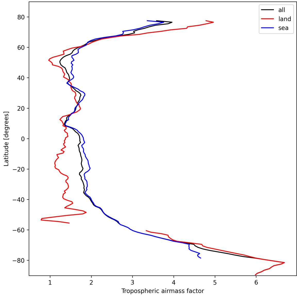
Figure 14: Zonal average of “Tropospheric airmass factor” for 2024-10-19 to 2024-10-21.
