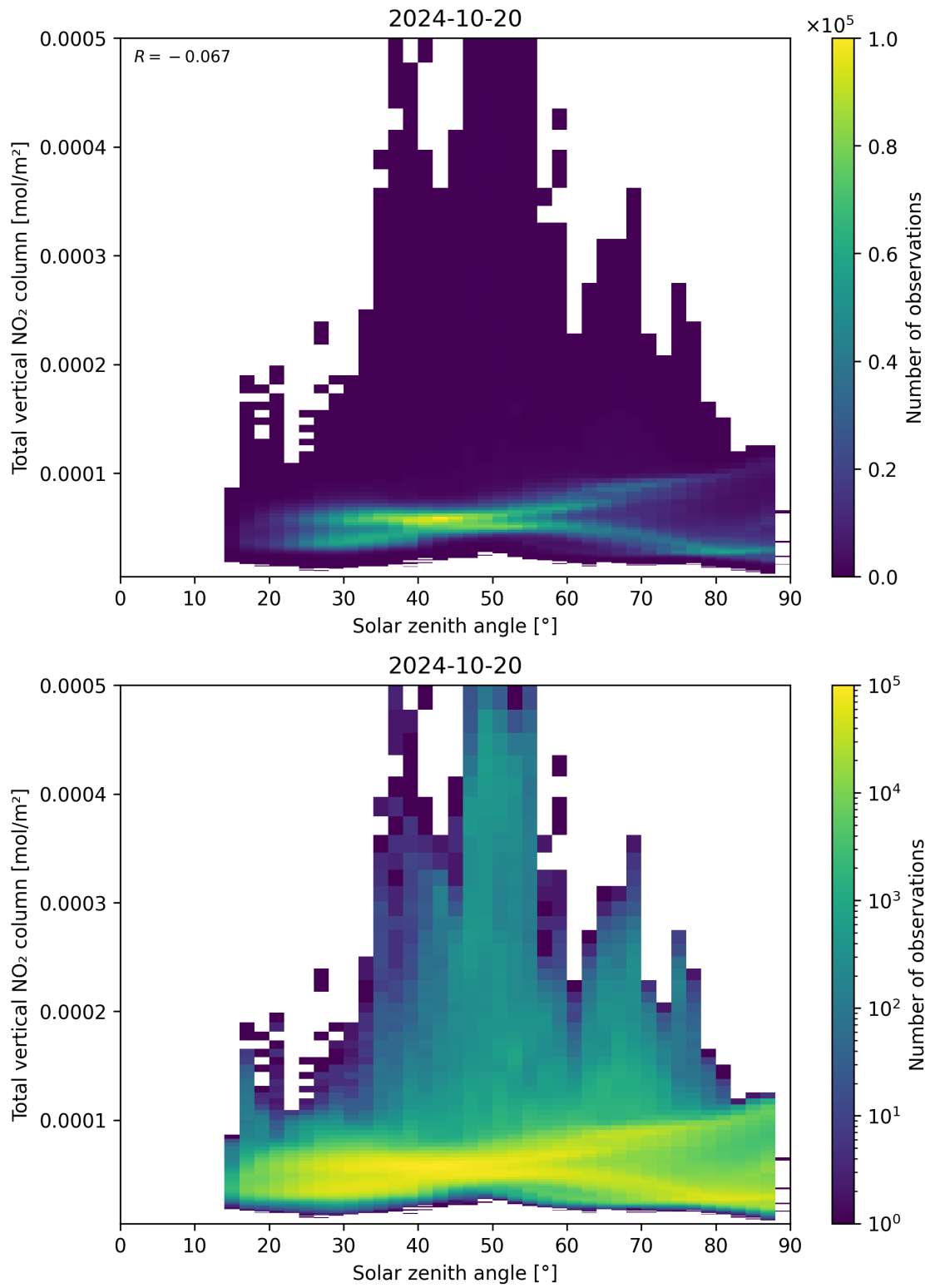
Figure 153: Scatter density plot of “Solar zenith angle” against “Total vertical NO 2 column” for 2024-10-19 to 2024-10-21.
