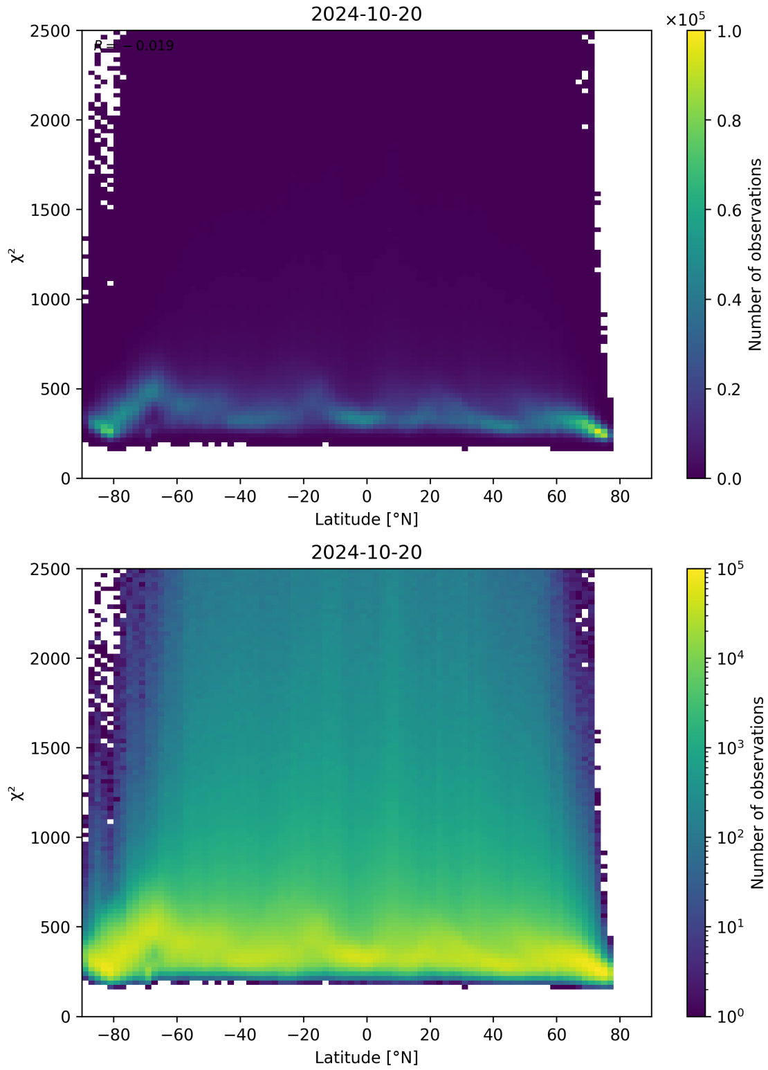
Figure 86: Scatter density plot of “Latitude” against “ \chi^2 ” for 2024-10-19 to 2024-10-21.
