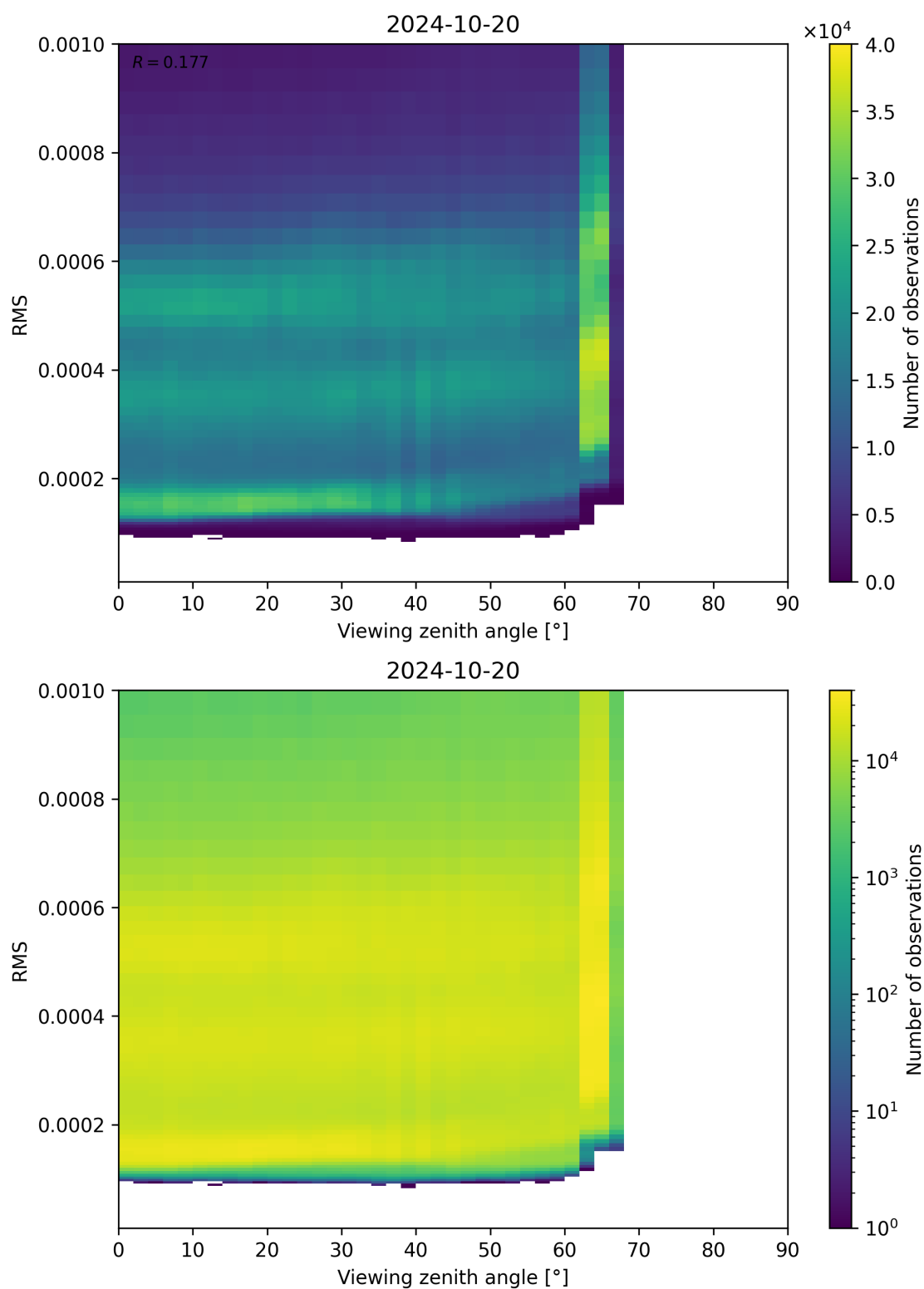
Figure 171: Scatter density plot of “Viewing zenith angle” against “RMS” for 2024-10-19 to 2024-10-21.
