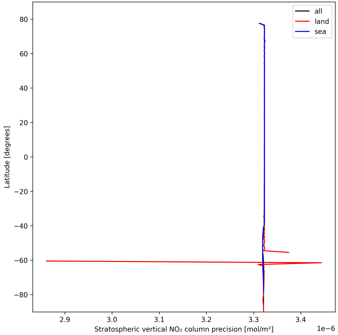
Figure 20: Zonal average of “Stratospheric vertical NO 2 column precision” for 2024-10-19 to 2024-10-21.
