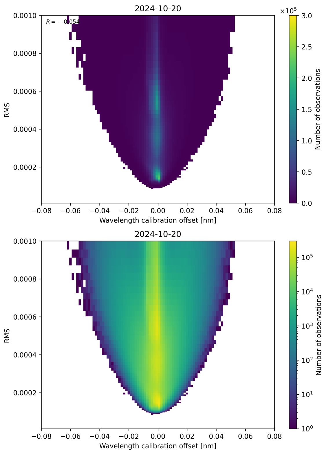
Figure 181: Scatter density plot of “Wavelength calibration offset” against “RMS” for 2024-10-19 to 2024-10-21.
