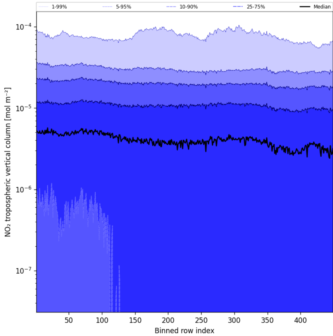
Figure 46: Along track statistics of “NO 2 tropospheric vertical column” for 2024-10-19 to 2024-10-21
