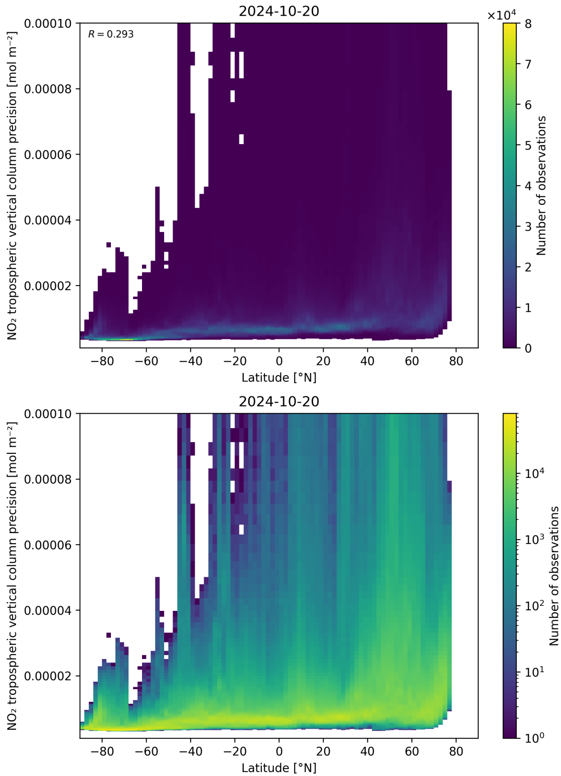
Figure 93: Scatter density plot of “Latitude” against “NO 2 tropospheric vertical column precision” for 2024-10-19 to 2024-10-21.
