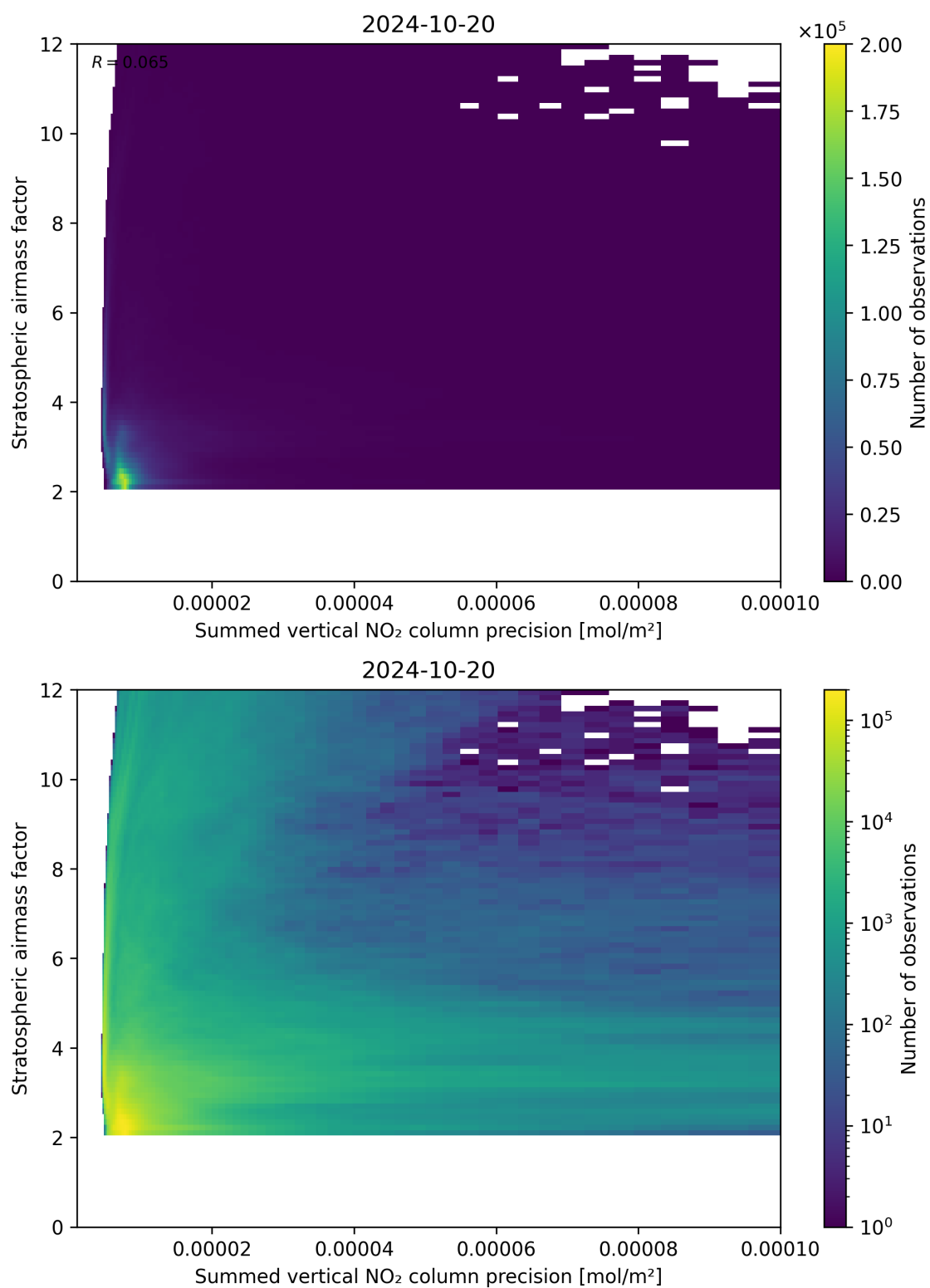
Figure 106: Scatter density plot of “Summed vertical NO 2 column precision” against “Stratospheric airmass factor” for 2024-10-19 to 2024-10-21.
