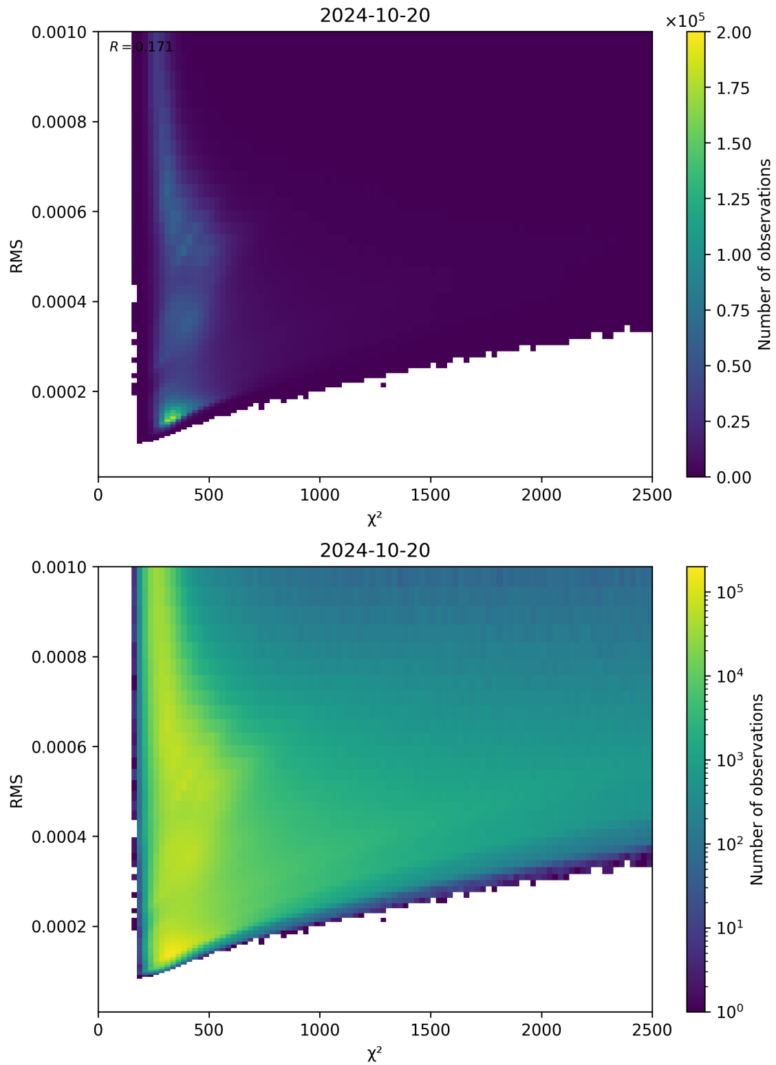
Figure 82: Scatter density plot of “ \chi^2 ” against “RMS” for 2024-10-19 to 2024-10-21.
