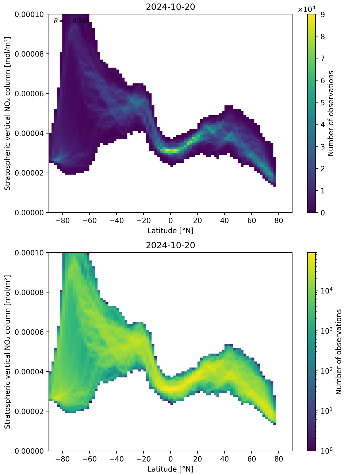
Figure 87: Scatter density plot of “Latitude” against “Stratospheric vertical NO 2 column” for 2024-10-19 to 2024-10-21.
