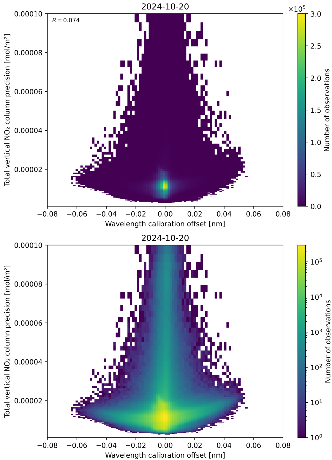
Figure 180: Scatter density plot of “Wavelength calibration offset” against “Total vertical NO 2 column precision” for 2024-10-19 to 2024-10-21.
