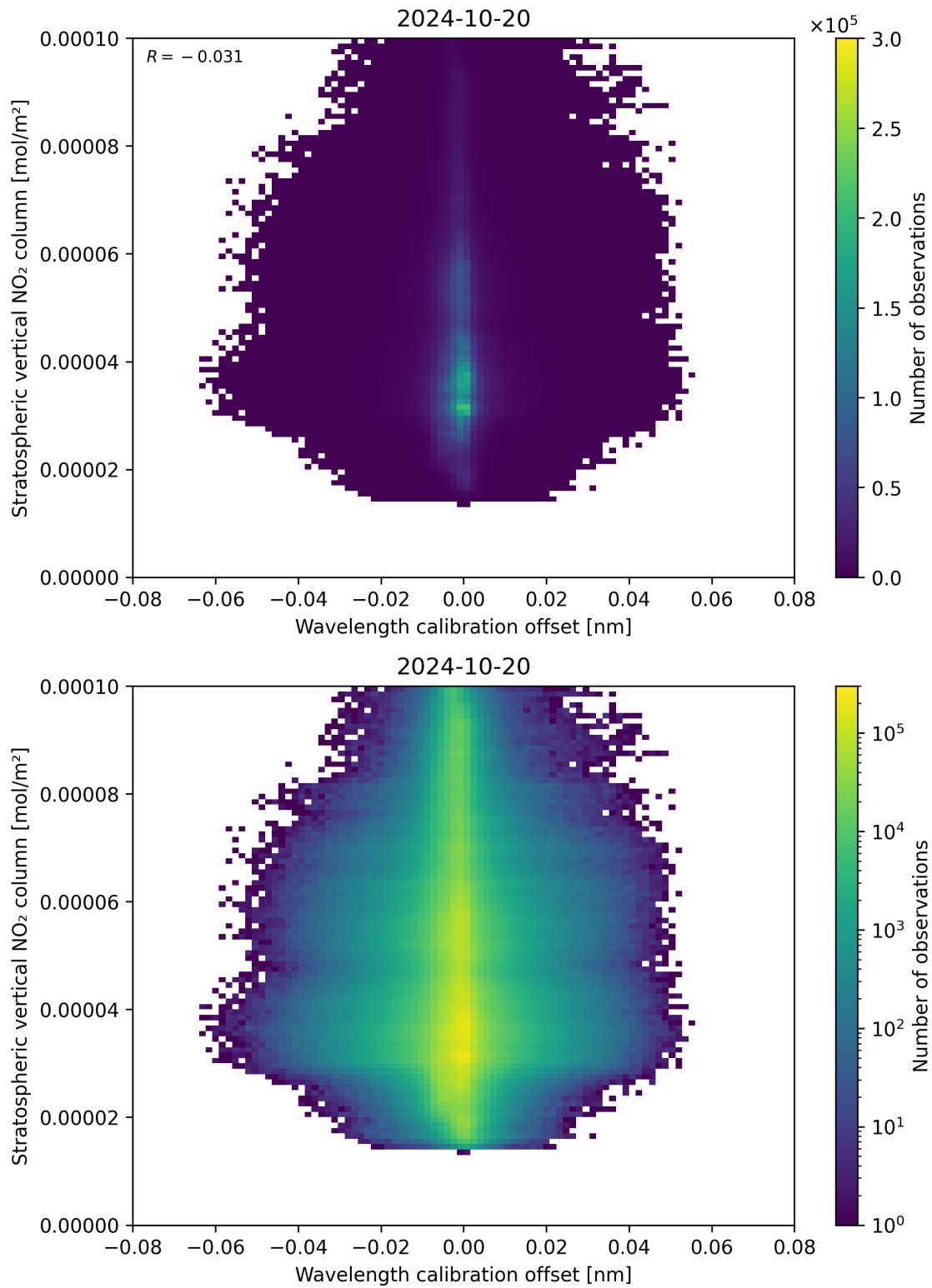
Figure 176: Scatter density plot of “Wavelength calibration offset” against “Stratospheric vertical NO 2 column” for 2024-10-19 to 2024-10-21.
