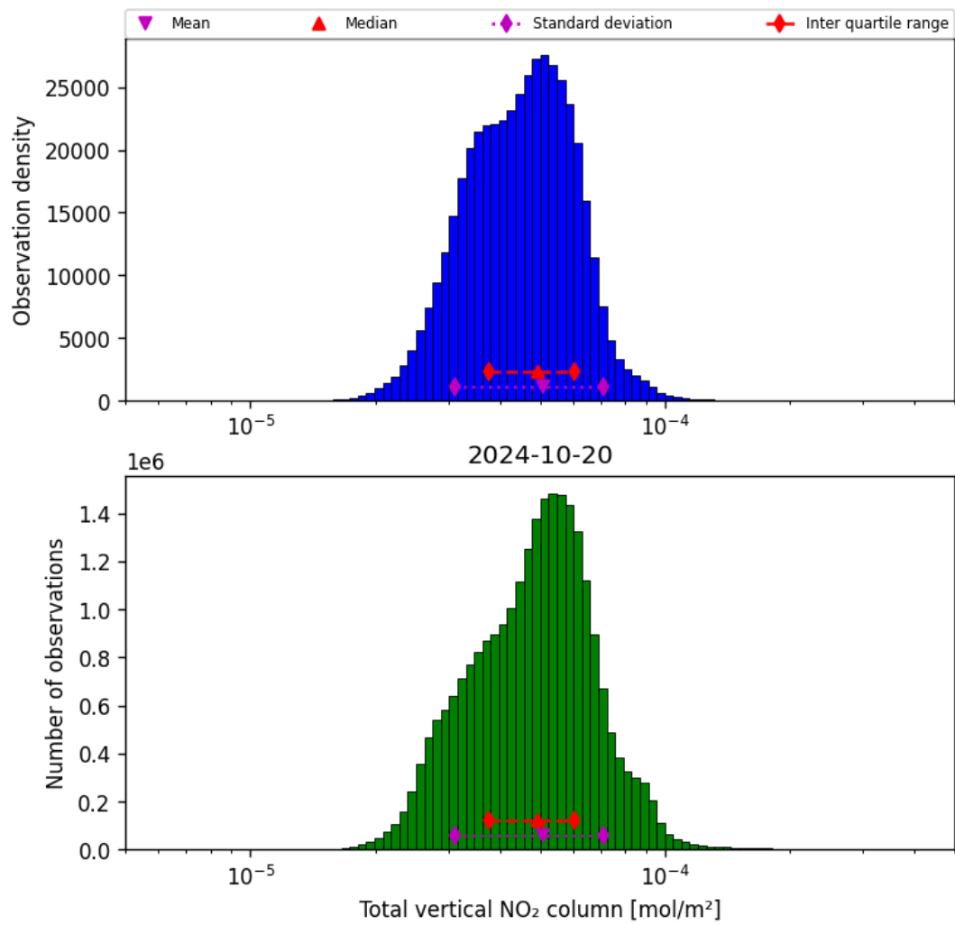
Figure 38: Histogram of “Total vertical NO 2 column” for 2024-10-19 to 2024-10-21
