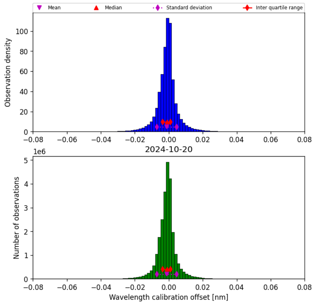
Figure 35: Histogram of “Wavelength calibration offset” for 2024-10-19 to 2024-10-21
