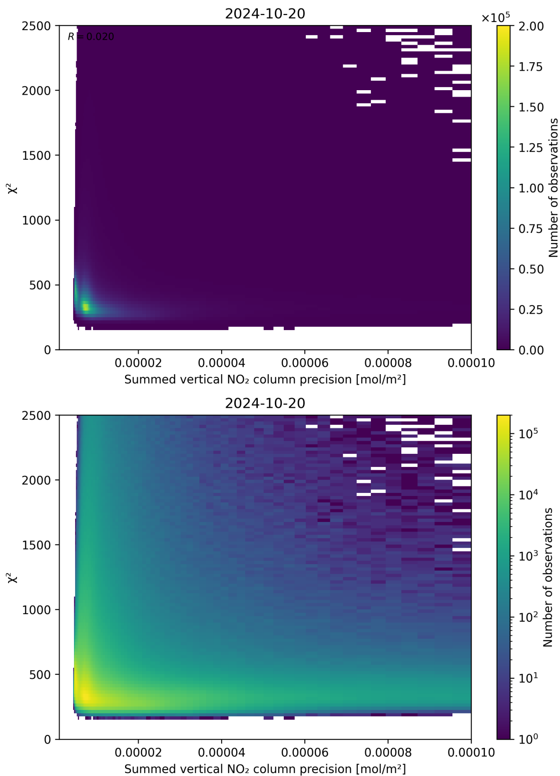
Figure 107: Scatter density plot of “Summed vertical NO 2 column precision” against “ \chi^2 ” for 2024-10-19 to 2024-10-21.
