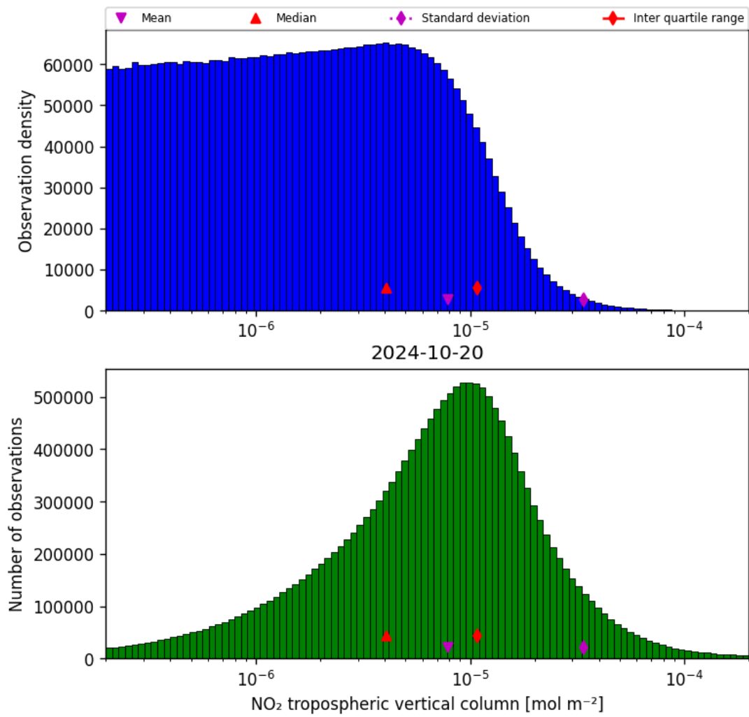
Figure 29: Histogram of “NO 2 tropospheric vertical column” for 2024-10-19 to 2024-10-21
