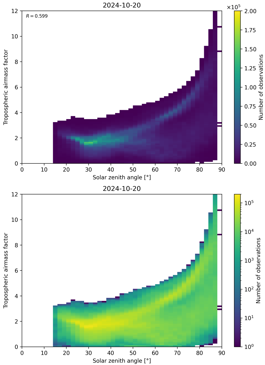
Figure 147: Scatter density plot of “Solar zenith angle” against “Tropospheric airmass factor” for 2024-10-19 to 2024-10-21.
