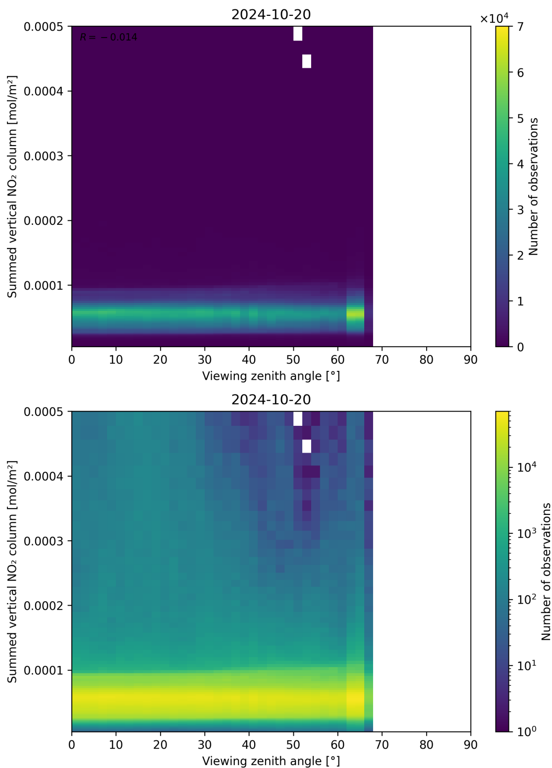
Figure 165: Scatter density plot of “Viewing zenith angle” against “Summed vertical NO 2 column” for 2024-10-19 to 2024-10-21.
