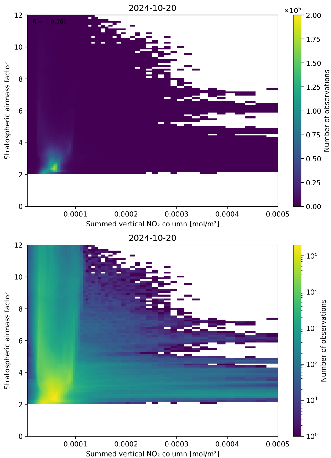
Figure 103: Scatter density plot of “Summed vertical NO 2 column” against “Stratospheric airmass factor” for 2024-10-19 to 2024-10-21.
