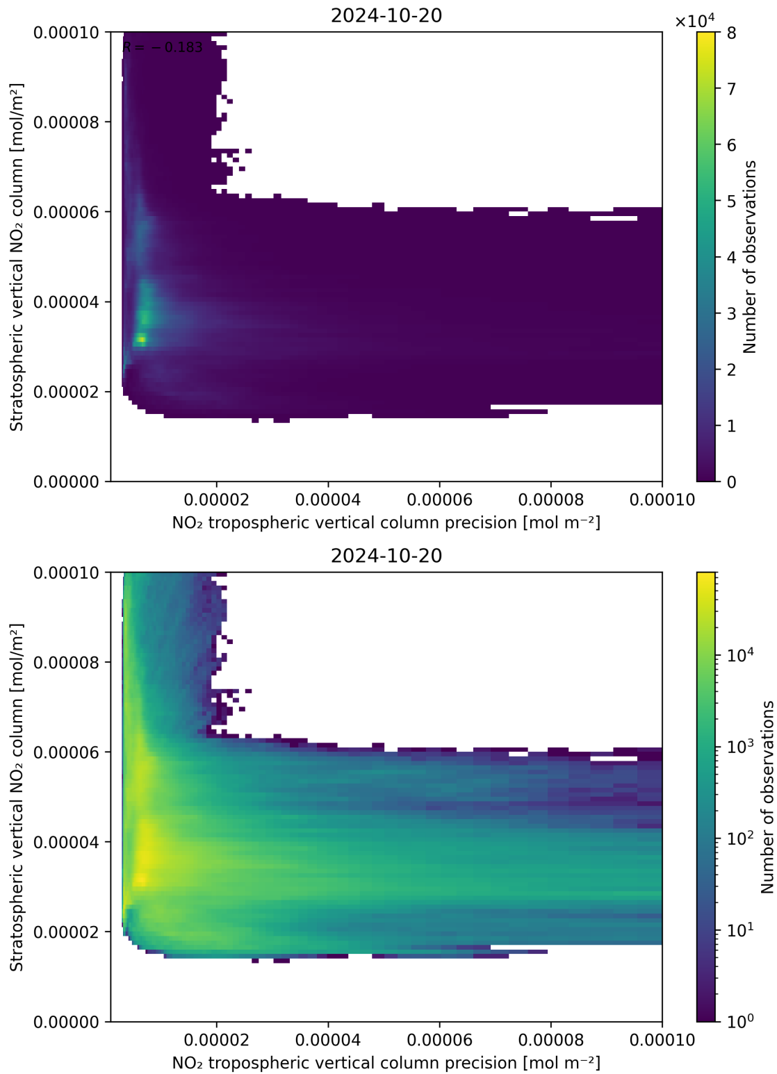
Figure 135: Scatter density plot of “NO 2 tropospheric vertical column precision” against “Stratospheric vertical NO 2 column” for 2024-10-19 to 2024-10-21.
