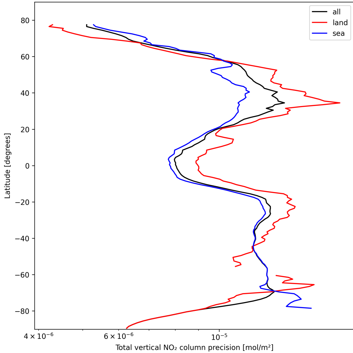
Figure 22: Zonal average of “Total vertical NO 2 column precision” for 2024-10-19 to 2024-10-21.
