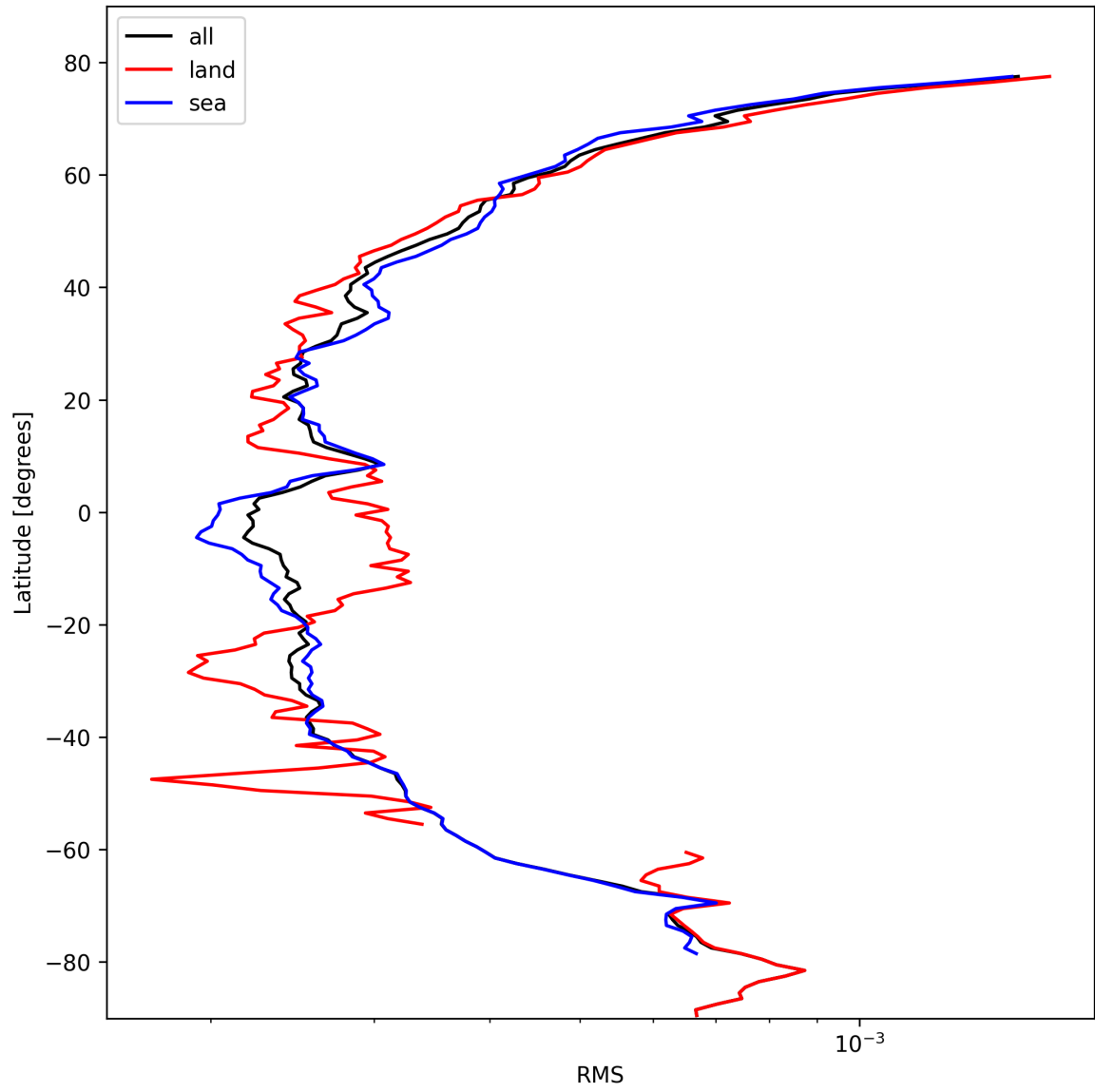
Figure 26: Zonal average of “RMS” for 2024-10-19 to 2024-10-21.
