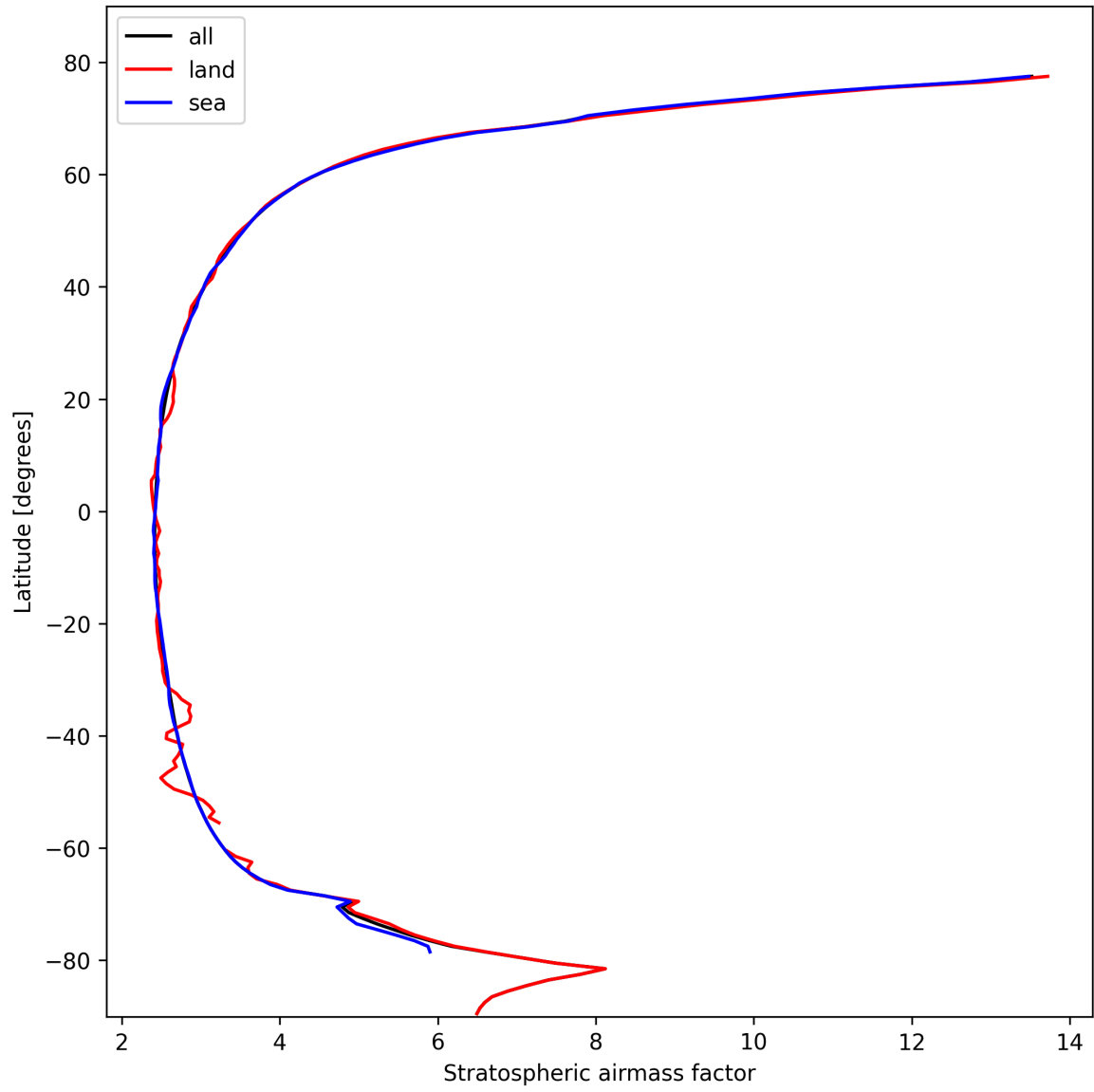
Figure 27: Zonal average of “Stratospheric airmass factor” for 2024-10-19 to 2024-10-21.
