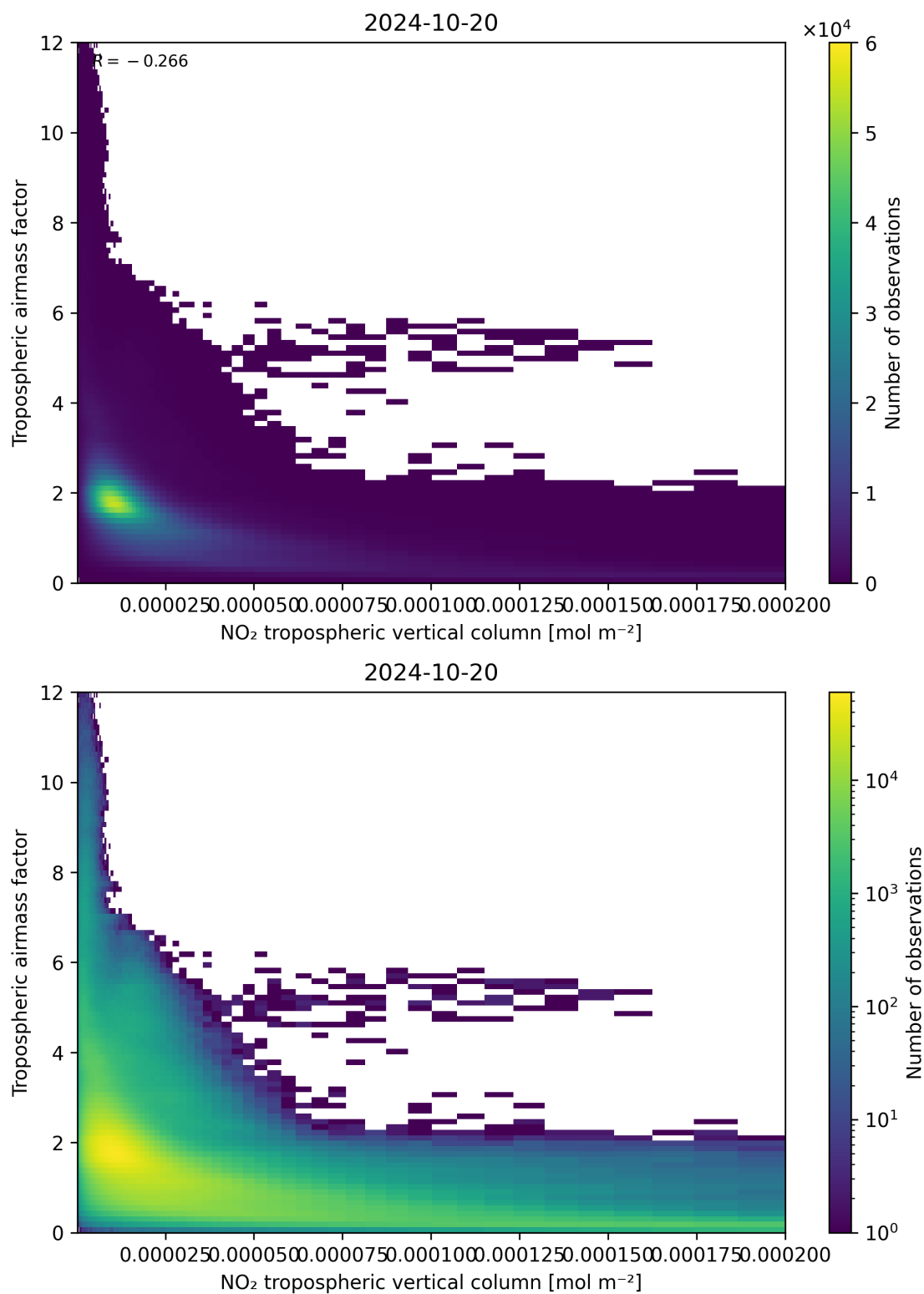
Figure 123: Scatter density plot of “NO 2 tropospheric vertical column” against “Tropospheric air mass factor” for 2024-10-19 to 2024-10-21.
