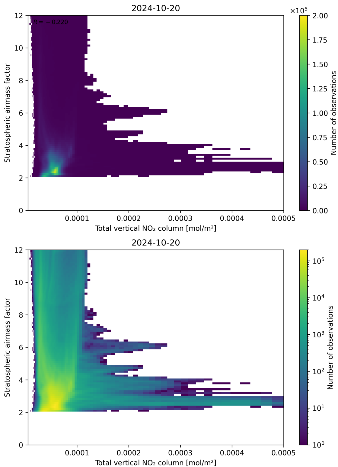
Figure 110: Scatter density plot of “Total vertical NO 2 column” against “Stratospheric airmass factor” for 2024-10-19 to 2024-10-21.
