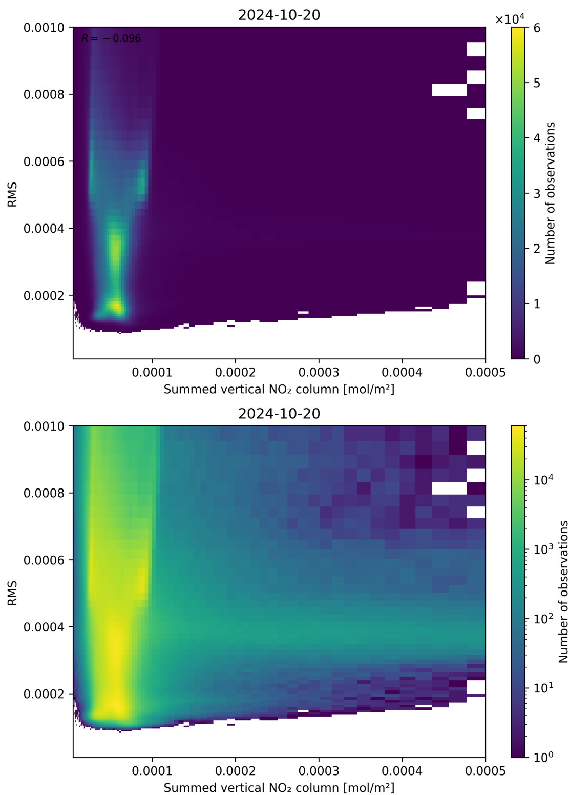
Figure 109: Scatter density plot of “Summed vertical NO 2 column” against “RMS” for 2024-10-19 to 2024-10-21.
