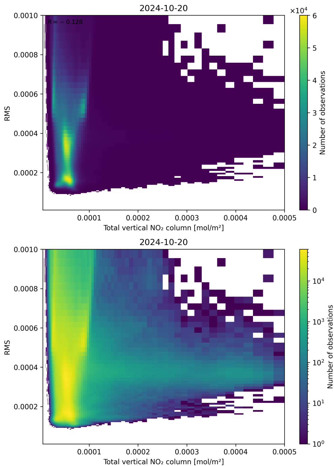
Figure 120: Scatter density plot of “Total vertical NO 2 column” against “RMS” for 2024-10-19 to 2024-10-21.
