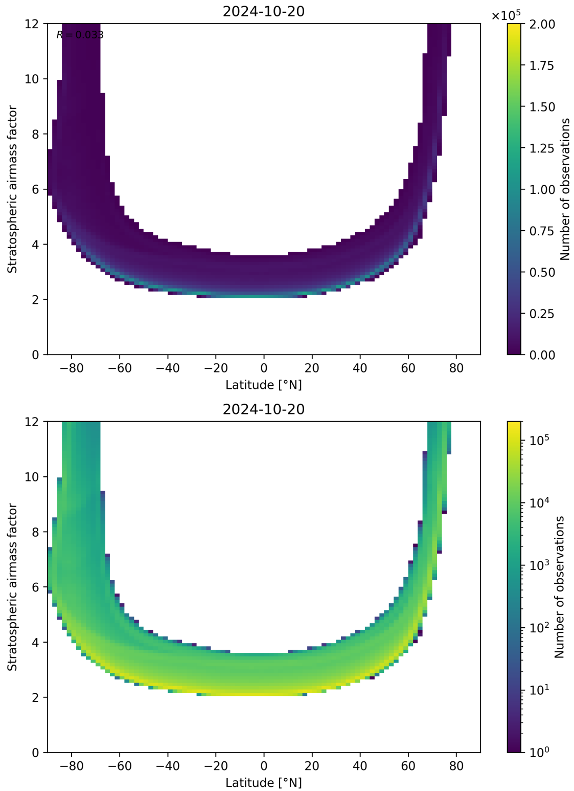
Figure 83: Scatter density plot of “Latitude” against “Stratospheric air mass factor” for 2024-10-19 to 2024-10-21.
