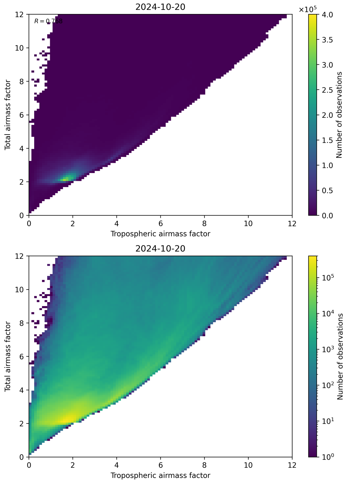
Figure 72: Scatter density plot of “Tropospheric airmass factor” against “Total airmass factor” for 2024-10-19 to 2024-10-21.
