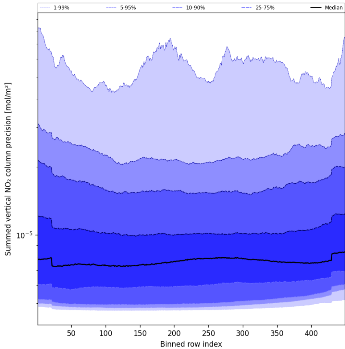
Figure 58: Along track statistics of “Summed vertical NO 2 column precision” for 2024-10-19 to 2024-10-21
