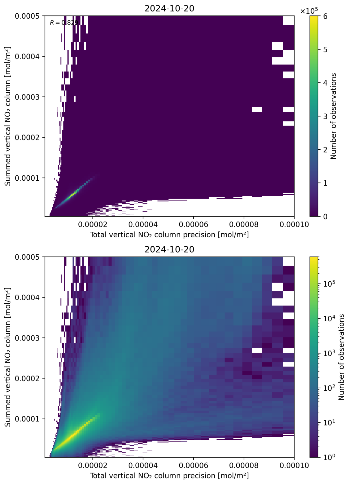
Figure 117: Scatter density plot of “Total vertical NO 2 column precision” against “Summed vertical NO 2 column” for 2024-10-19 to 2024-10-21.
