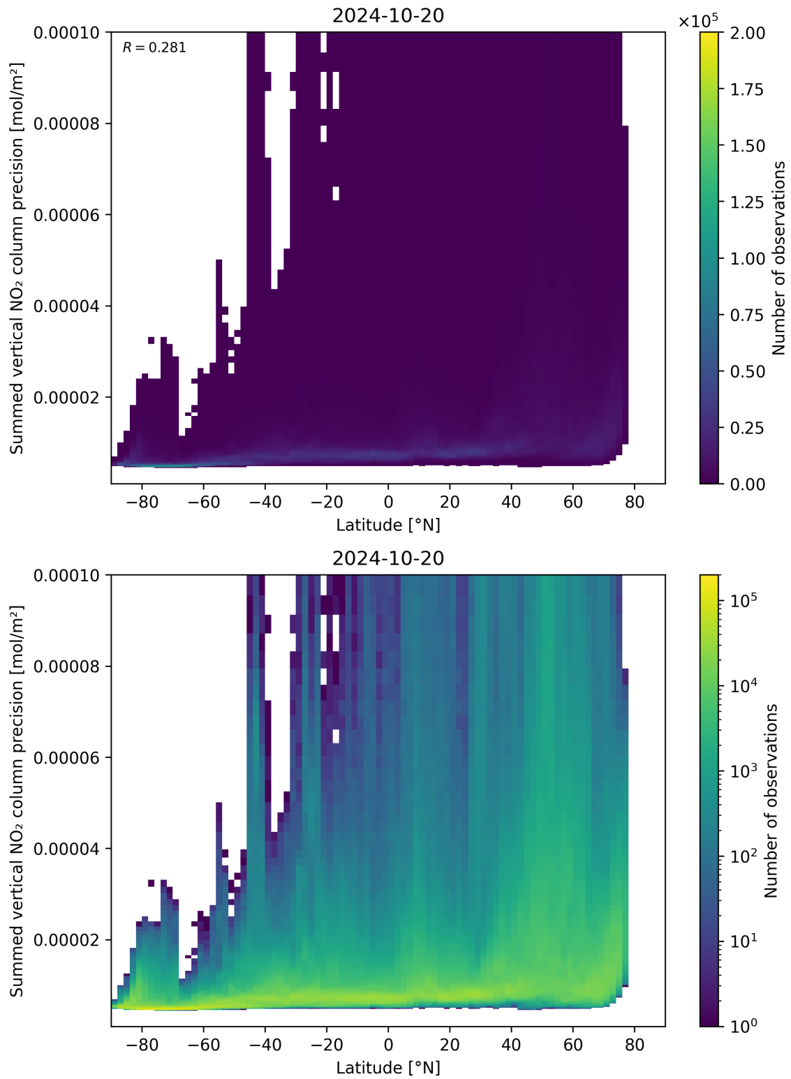
Figure 89: Scatter density plot of “Latitude” against “Summed vertical NO 2 column precision” for 2024-10-19 to 2024-10-21.
