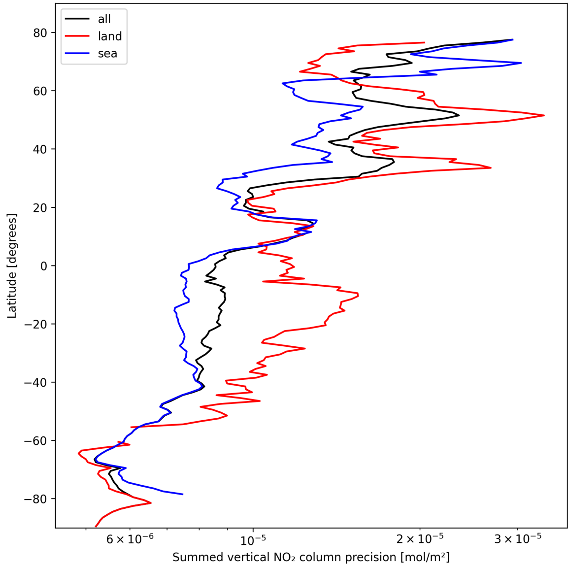
Figure 24: Zonal average of "Summed vertical NO 2 column precision" for 2024-10-20 to 2024-10-22.
