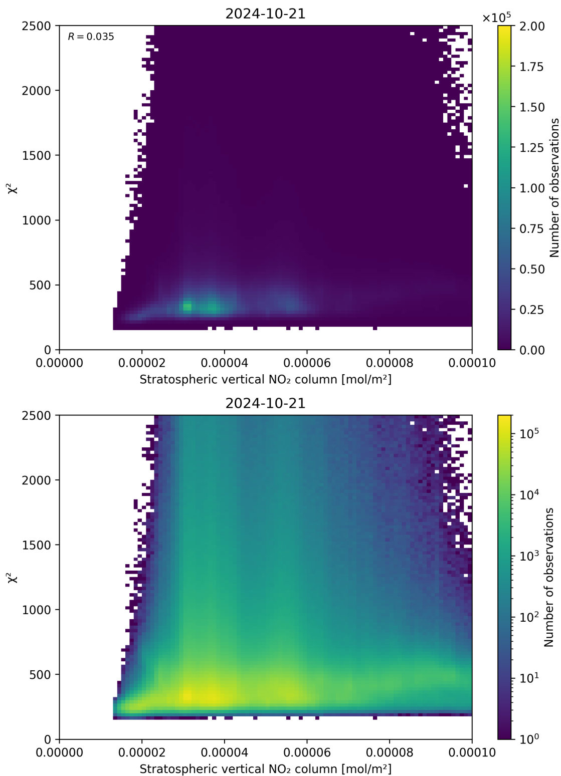
Figure 97: Scatter density plot of “Stratospheric vertical NO 2 column” against “ \chi^2 ” for 2024-10-20 to 2024-10-22.
