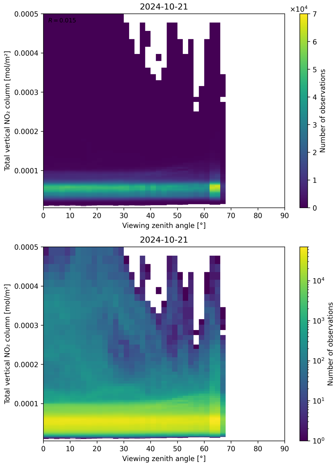
Figure 167: Scatter density plot of “Viewing zenith angle” against “Total vertical NO 2 column” for 2024-10-20 to 2024-10-22.
