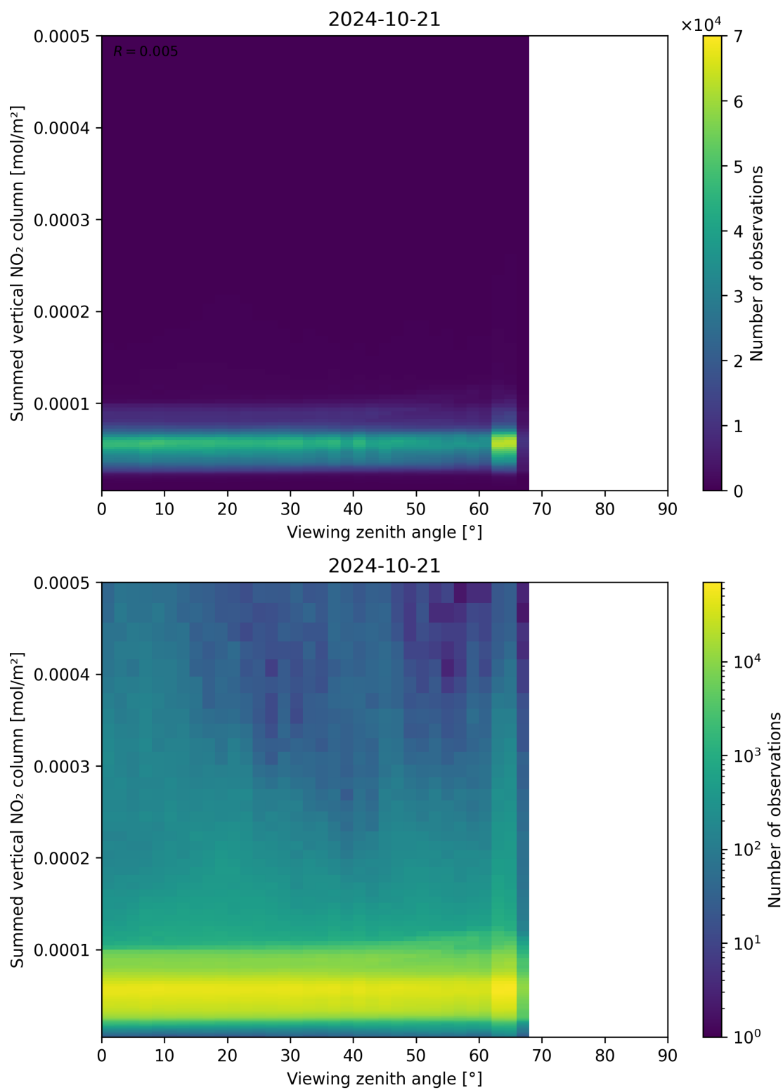
Figure 165: Scatter density plot of “Viewing zenith angle” against “Summed vertical NO 2 column” for 2024-10-20 to 2024-10-22.
