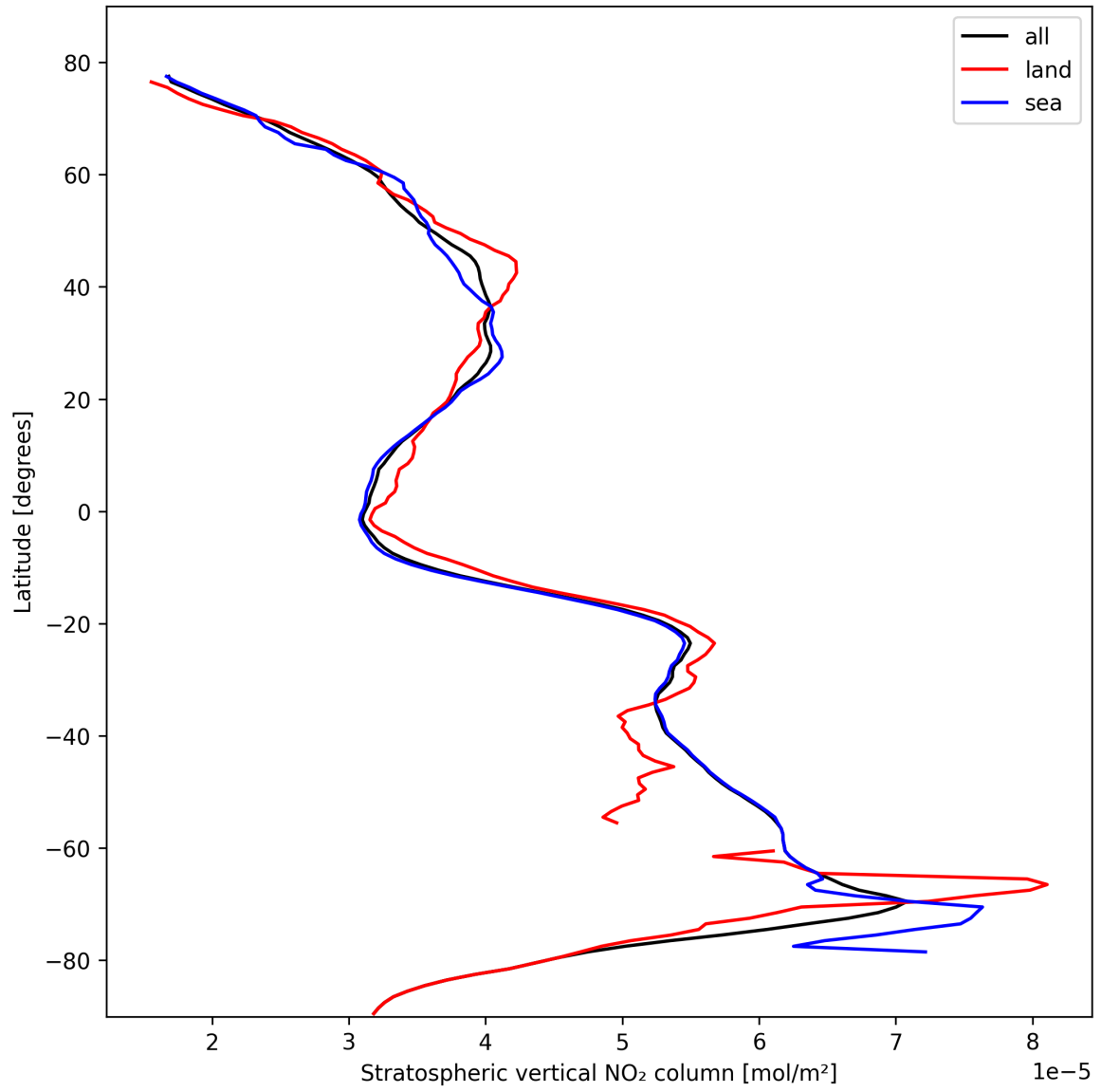
Figure 19: Zonal average of “Stratospheric vertical NO 2 column” for 2024-10-20 to 2024-10-22.
