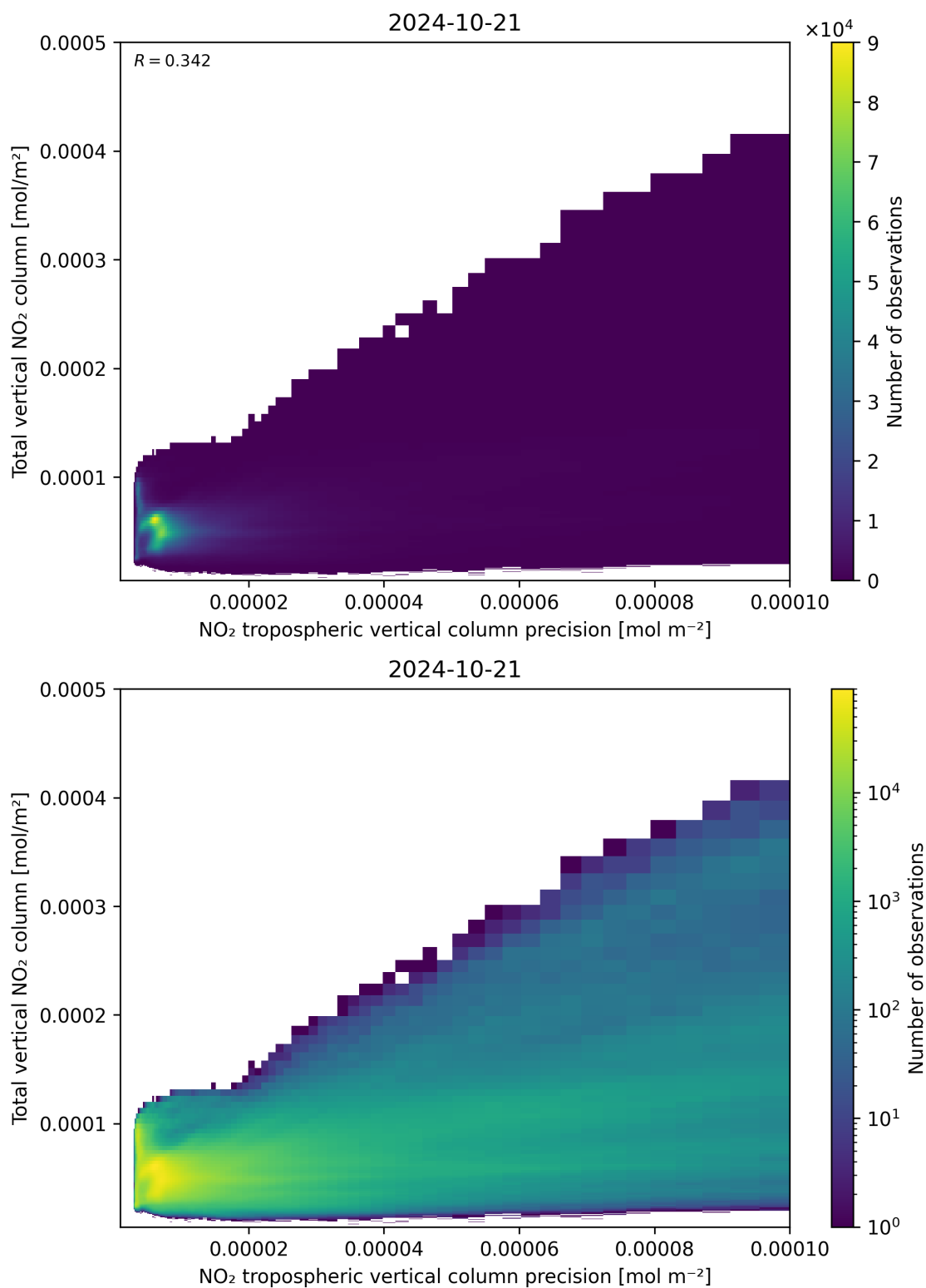
Figure 138: Scatter density plot of “NO 2 tropospheric vertical column precision” against “Total vertical NO 2 column” for 2024-10-20 to 2024-10-22.
