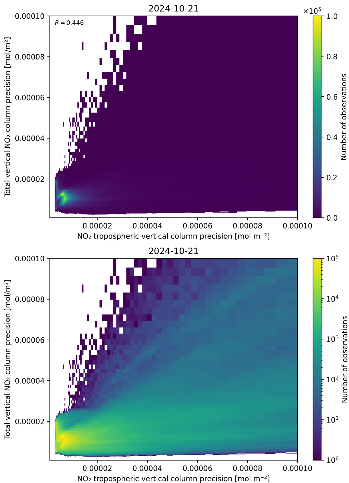
Figure 139: Scatter density plot of “NO 2 tropospheric vertical column precision” against “Total vertical NO 2 column precision” for 2024-10-20 to 2024-10-22.
