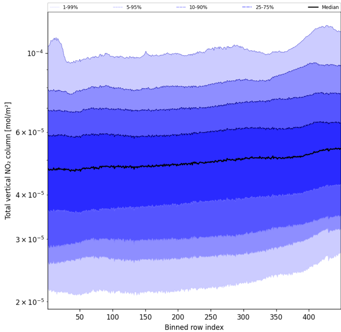
Figure 55: Along track statistics of "Total vertical NO 2 column" for 2024-10-20 to 2024-10-22
