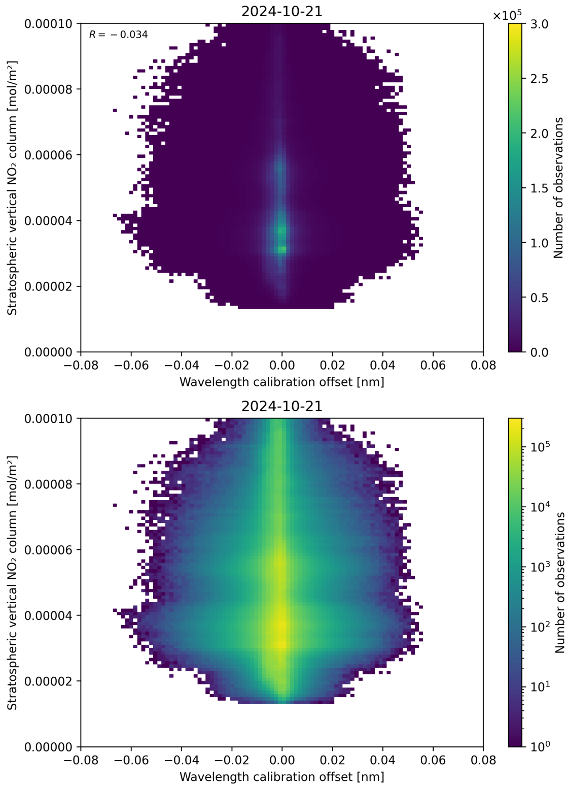
Figure 176: Scatter density plot of “Wavelength calibration offset” against “Stratospheric vertical NO 2 column” for 2024-10-20 to 2024-10-22.
