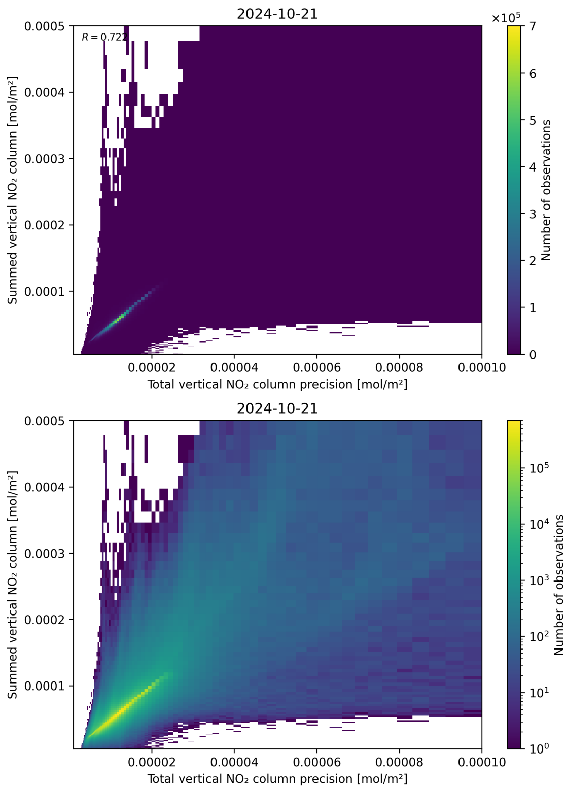
Figure 117: Scatter density plot of “Total vertical NO 2 column precision” against “Summed vertical NO 2 column” for 2024-10-20 to 2024-10-22.
