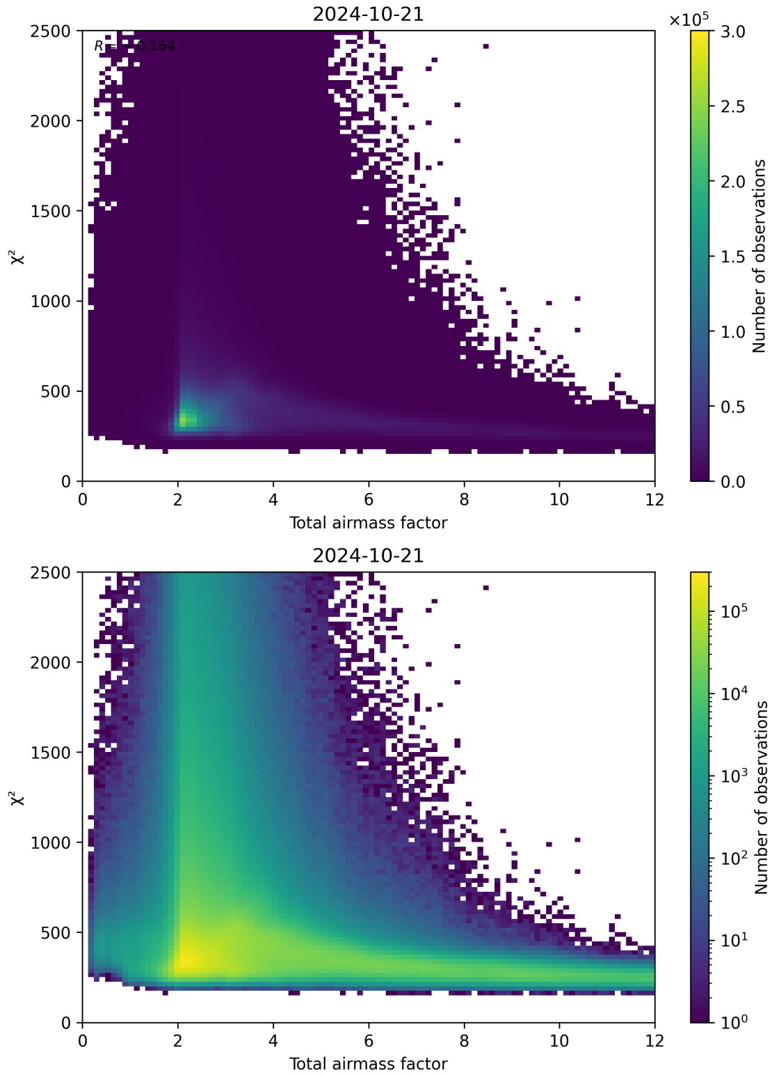
Figure 63: Scatter density plot of “Total airmass factor” against “ \chi^2 ” for 2024-10-20 to 2024-10-22.
