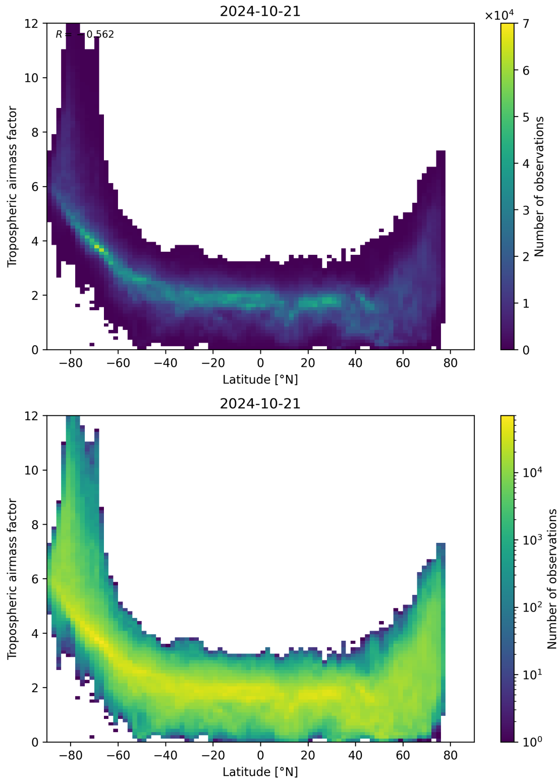
Figure 85: Scatter density plot of “Latitude” against “Tropospheric air mass factor” for 2024-10-20 to 2024-10-22.
