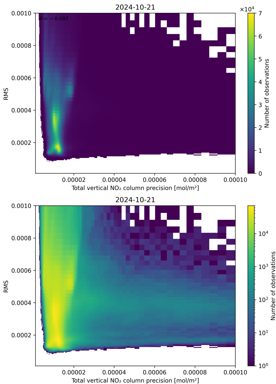
Figure 119: Scatter density plot of “Total vertical NO 2 column precision” against “RMS” for 2024-10-20 to 2024-10-22.
