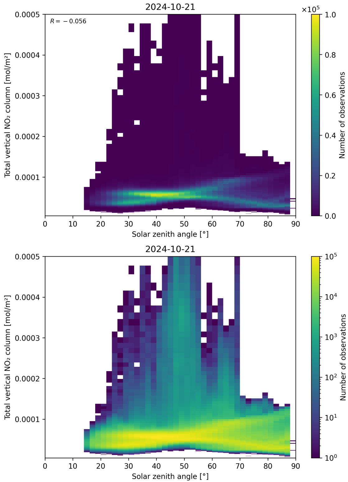
Figure 153: Scatter density plot of “Solar zenith angle” against “Total vertical NO 2 column” for 2024-10-20 to 2024-10-22.
