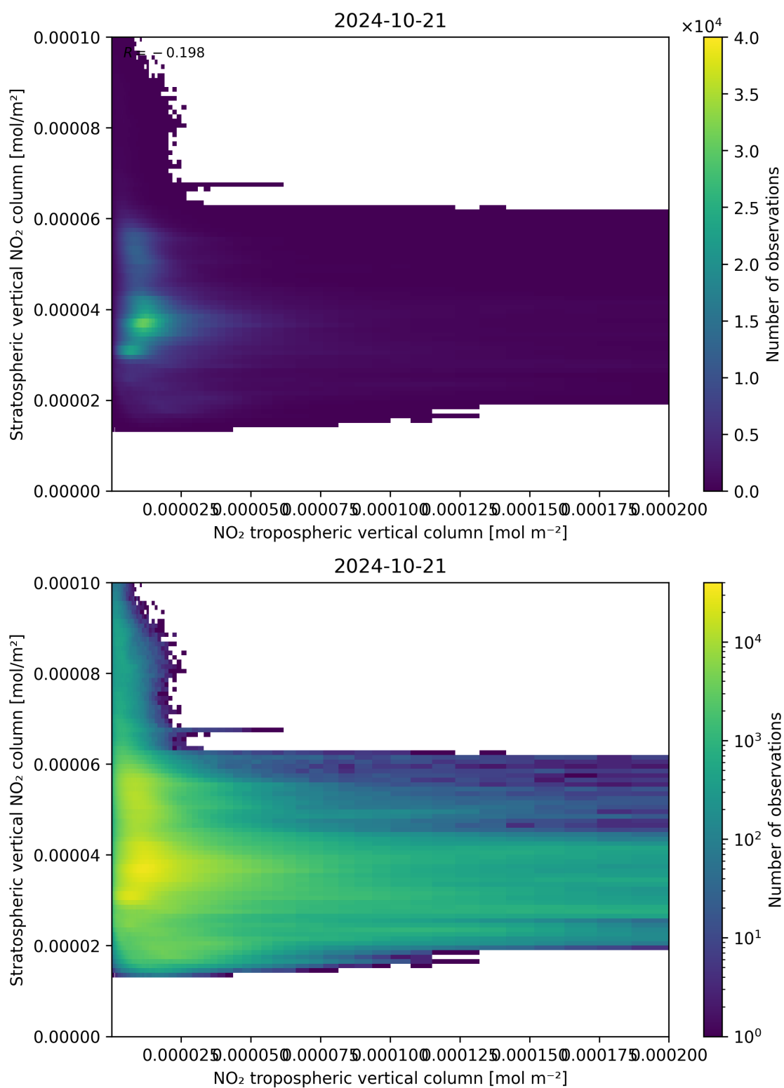
Figure 125: Scatter density plot of “NO 2 tropospheric vertical column” against “Stratospheric vertical NO 2 column” for 2024-10-20 to 2024-10-22.
