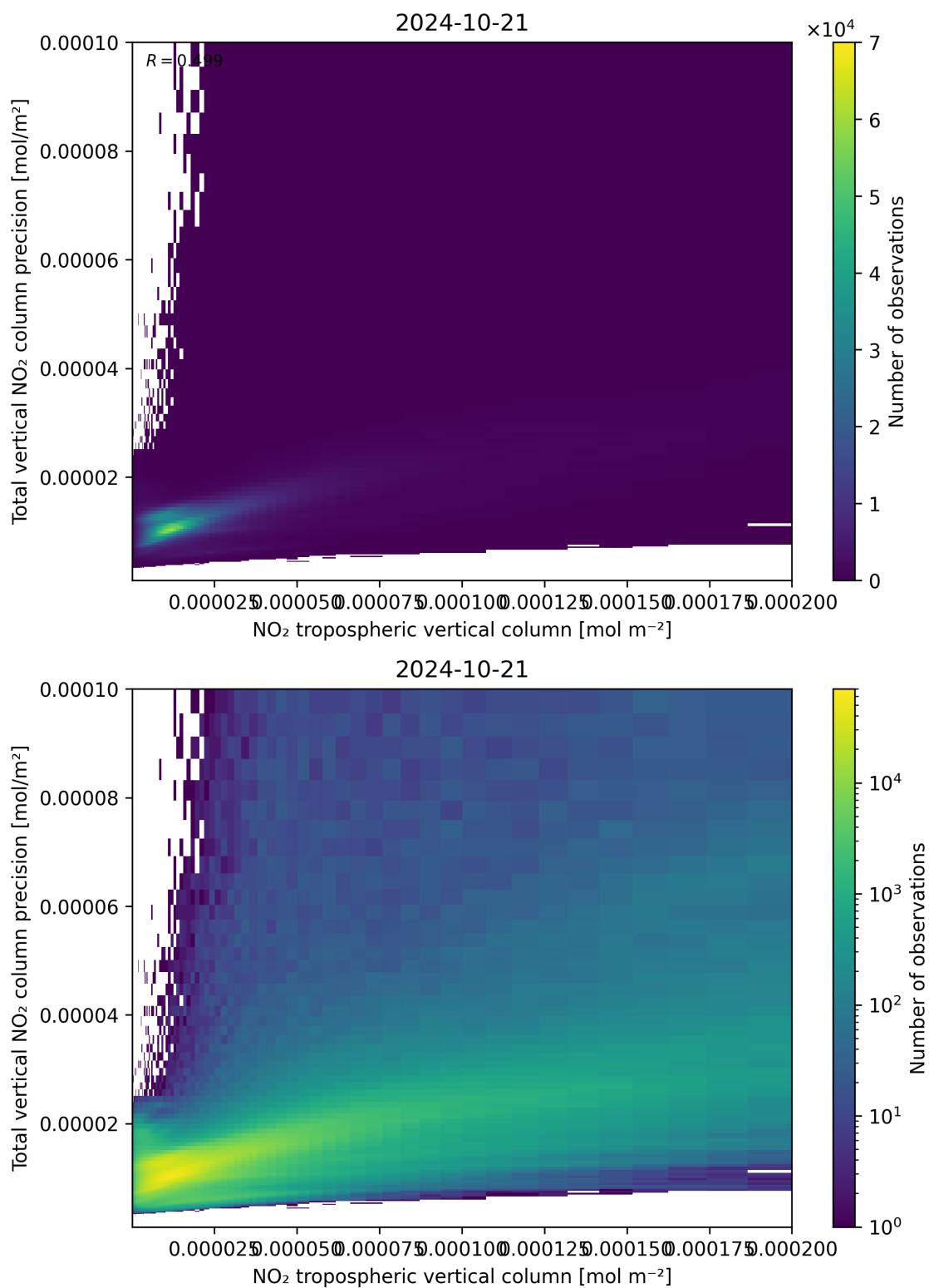
Figure 129: Scatter density plot of “NO 2 tropospheric vertical column” against “Total vertical NO 2 column precision” for 2024-10-20 to 2024-10-22.
