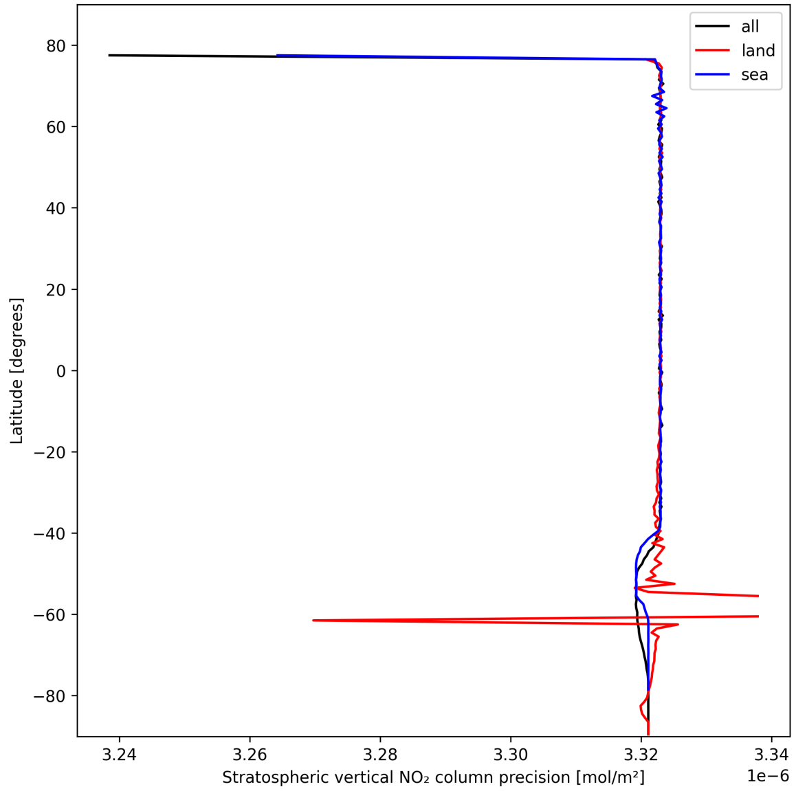
Figure 20: Zonal average of “Stratospheric vertical NO 2 column precision” for 2024-10-20 to 2024-10-22.
