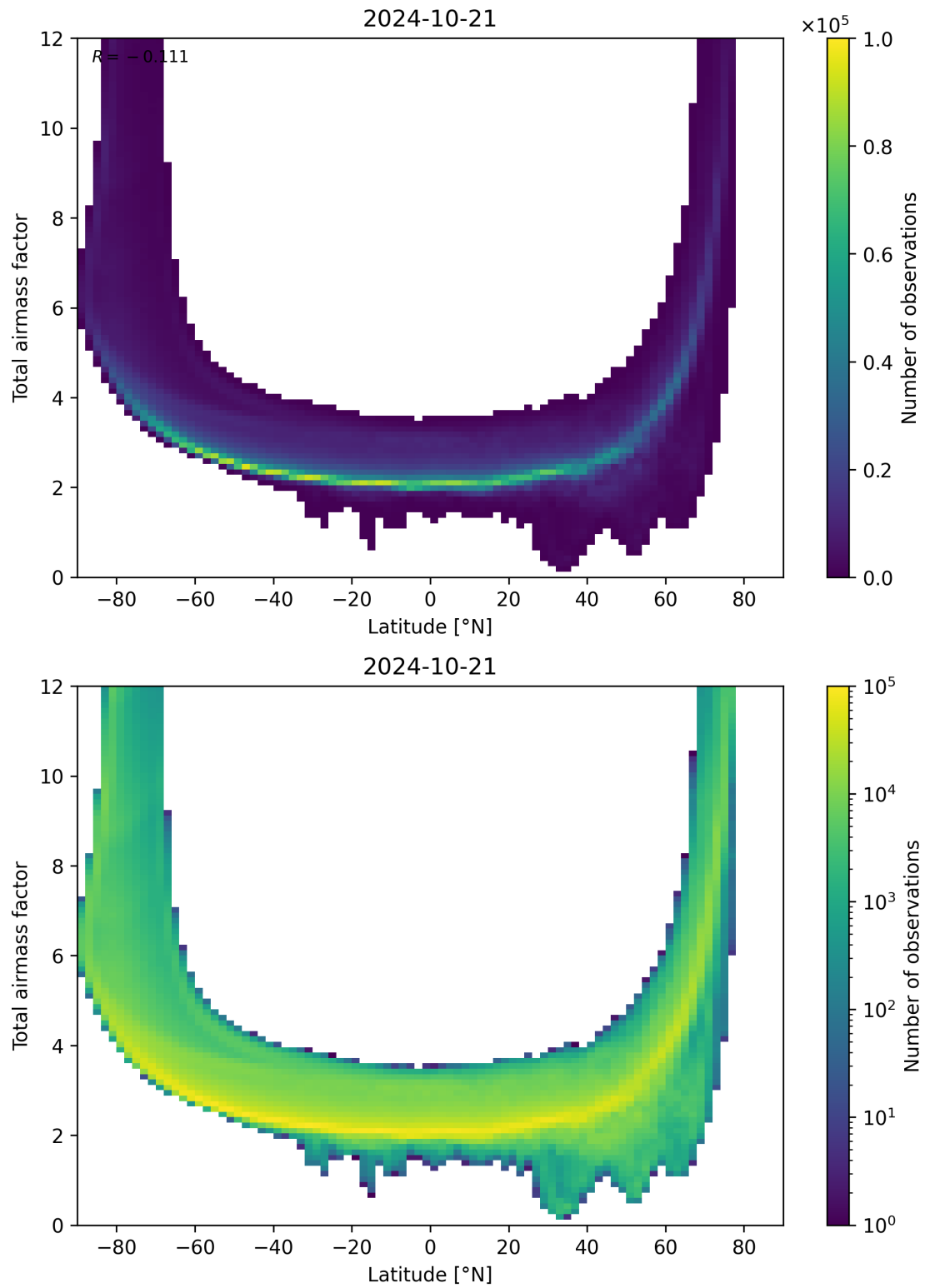
Figure 84: Scatter density plot of “Latitude” against “Total airmass factor” for 2024-10-20 to 2024-10-22.
