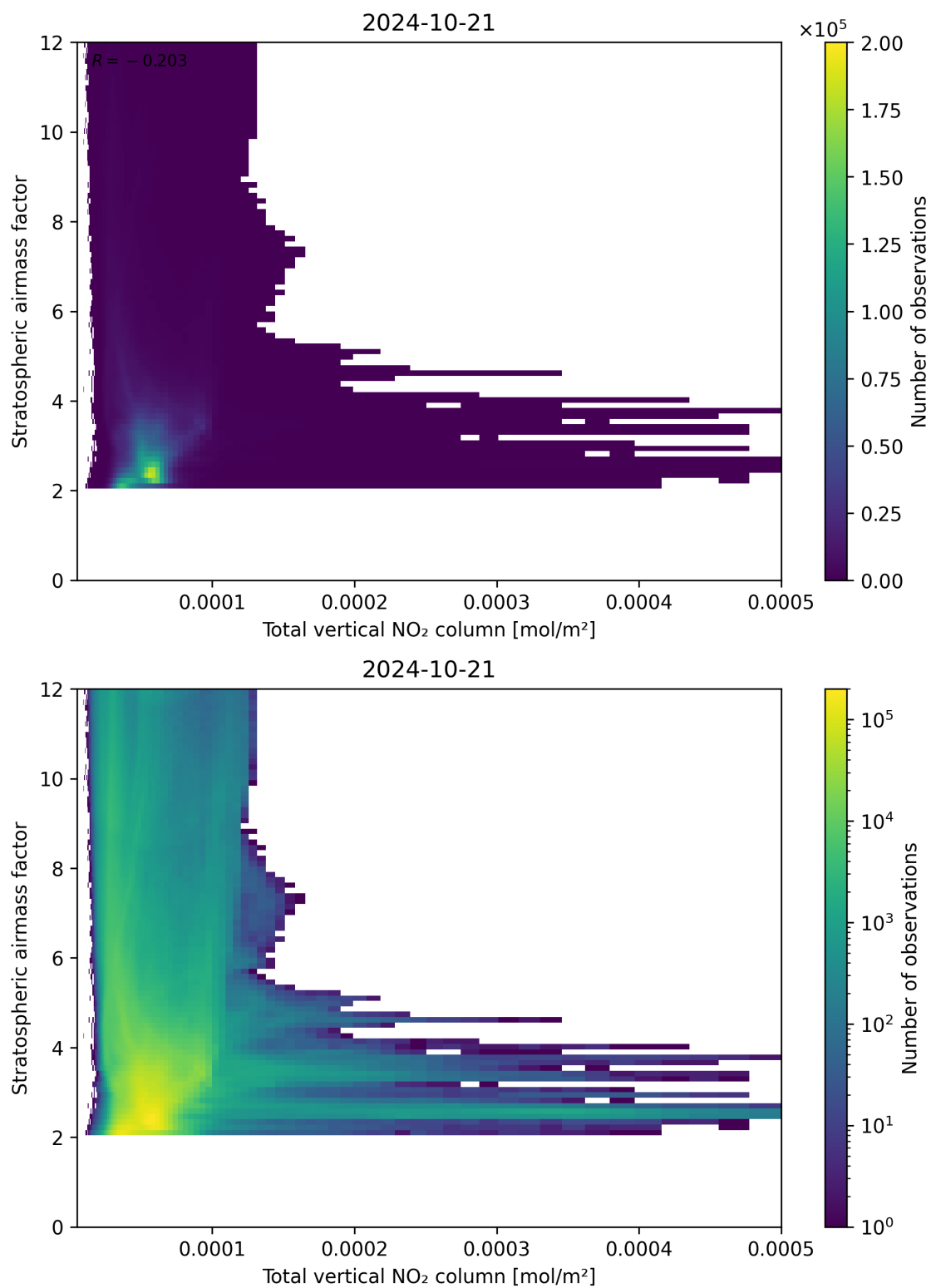
Figure 110: Scatter density plot of “Total vertical NO 2 column” against “Stratospheric airmass factor” for 2024-10-20 to 2024-10-22.
