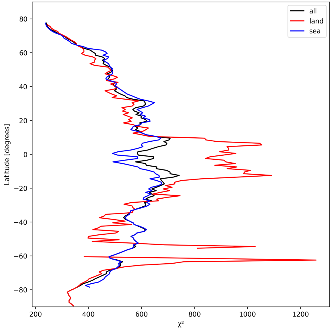
Figure 25: Zonal average of “ \chi^2 ” for 2024-10-20 to 2024-10-22.
