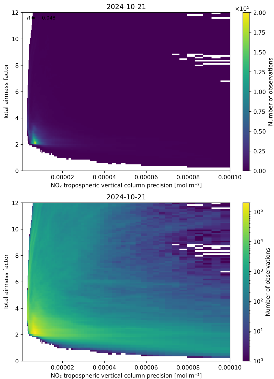
Figure 132: Scatter density plot of “NO 2 tropospheric vertical column precision” against “Total air mass factor” for 2024-10-20 to 2024-10-22.
