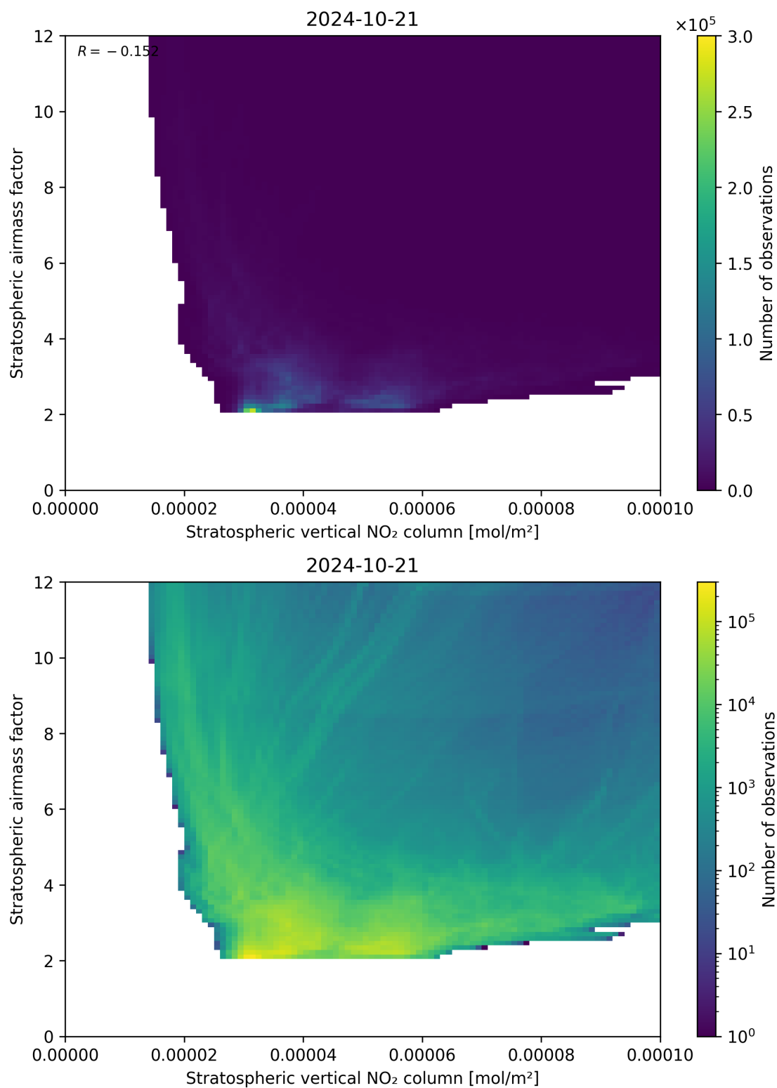
Figure 96: Scatter density plot of “Stratospheric vertical NO 2 column” against “Stratospheric airmass factor” for 2024-10-20 to 2024-10-22.
