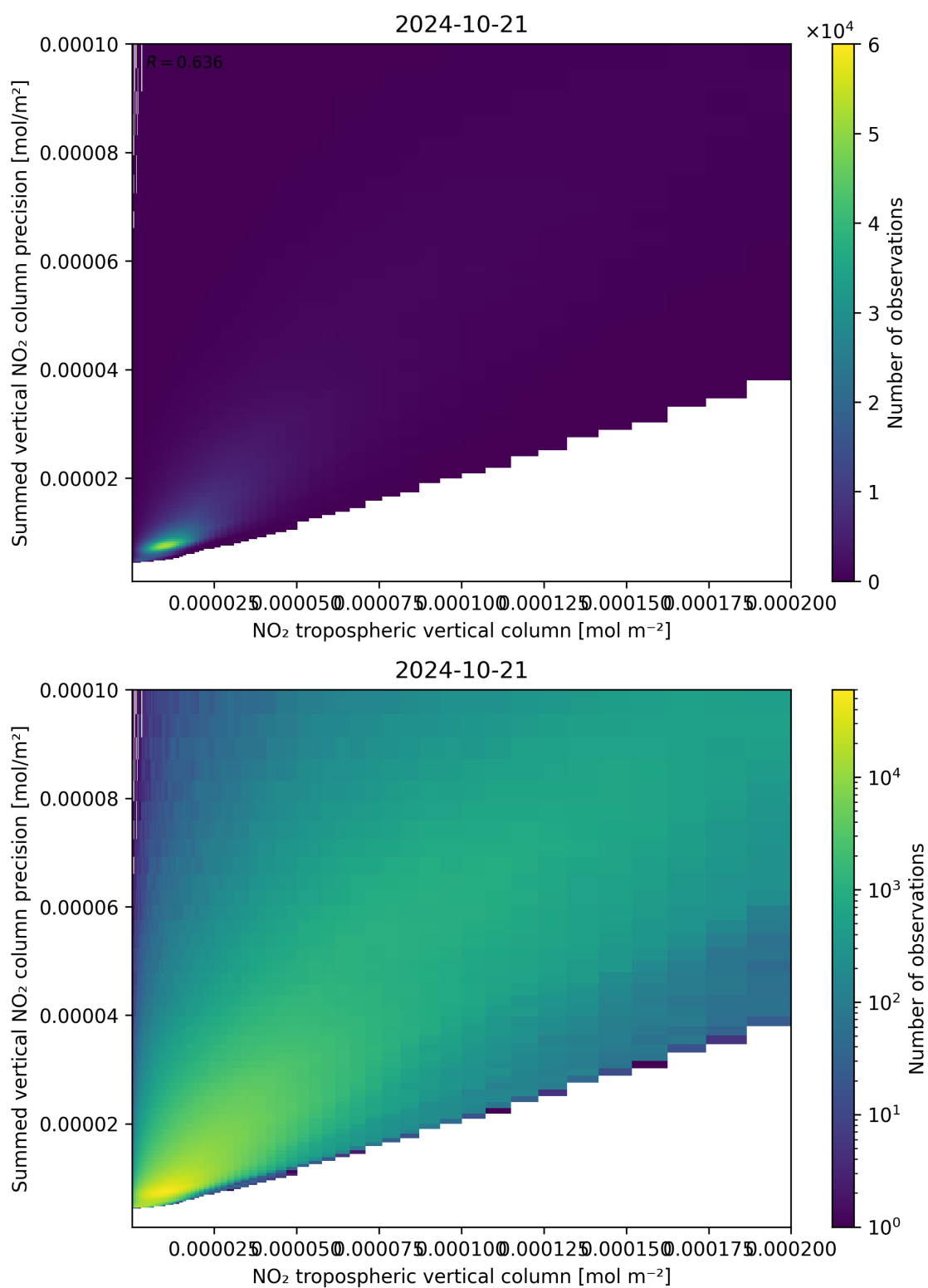
Figure 127: Scatter density plot of “NO 2 tropospheric vertical column” against “Summed vertical NO 2 column precision” for 2024-10-20 to 2024-10-22.
