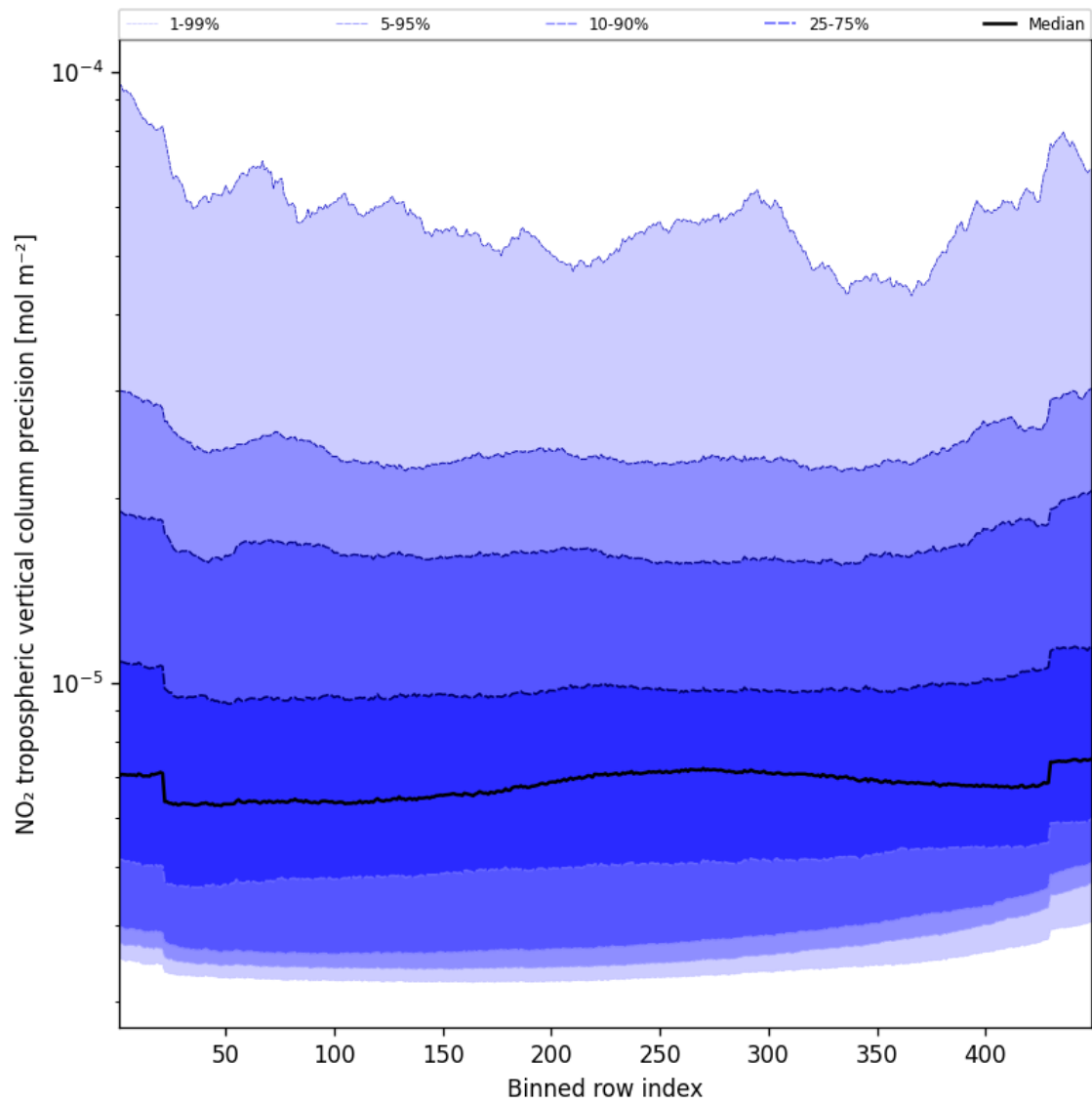
Figure 47: Along track statistics of “NO 2 tropospheric vertical column precision” for 2024-10-20 to 2024-10-22
