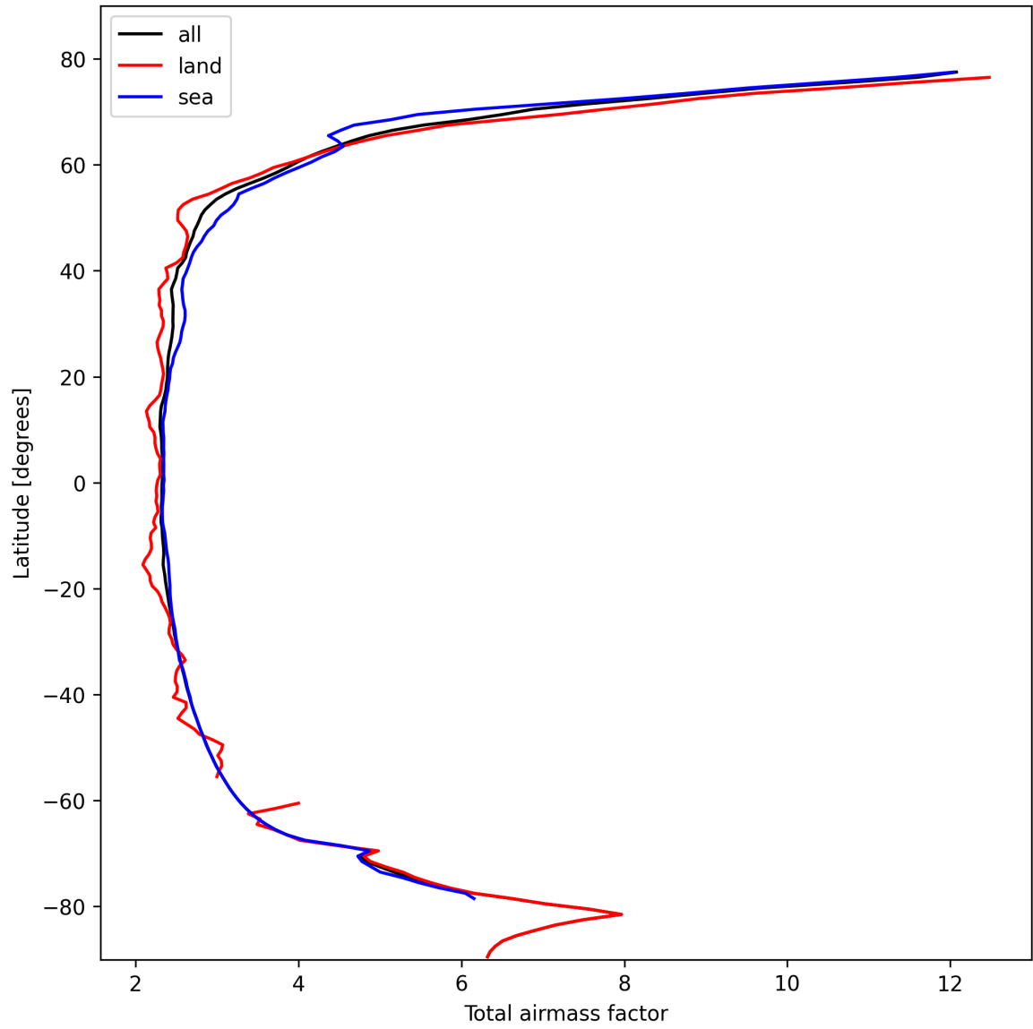
Figure 15: Zonal average of “Total airmass factor” for 2024-10-20 to 2024-10-22.
