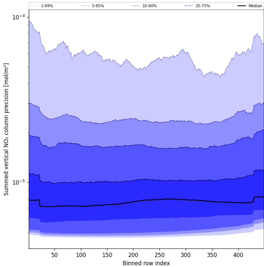
Figure 58: Along track statistics of “Summed vertical NO 2 column precision” for 2024-10-20 to 2024-10-22
