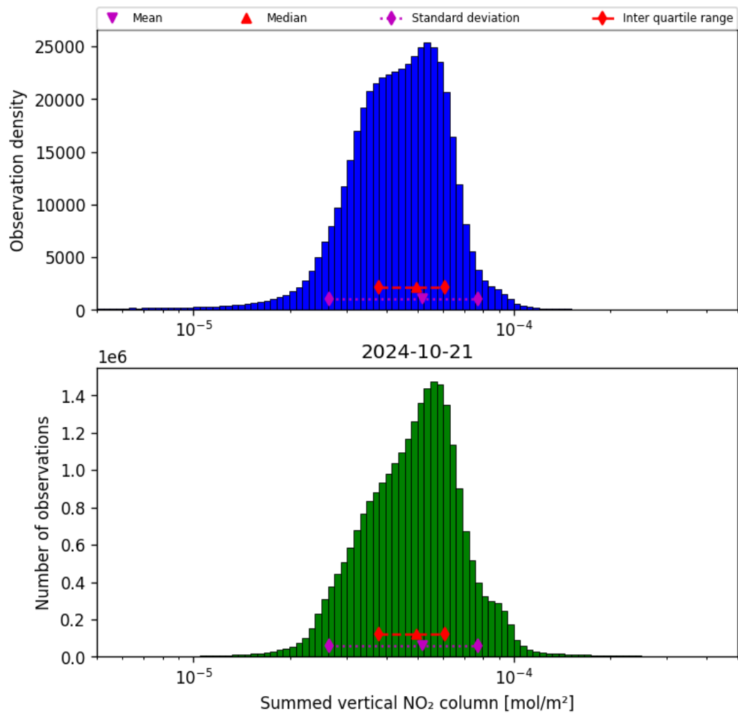
Figure 40: Histogram of “Summed vertical NO 2 column” for 2024-10-20 to 2024-10-22
