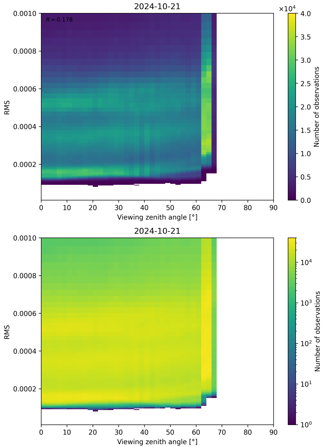
Figure 171: Scatter density plot of “Viewing zenith angle” against “RMS” for 2024-10-20 to 2024-10-22.
