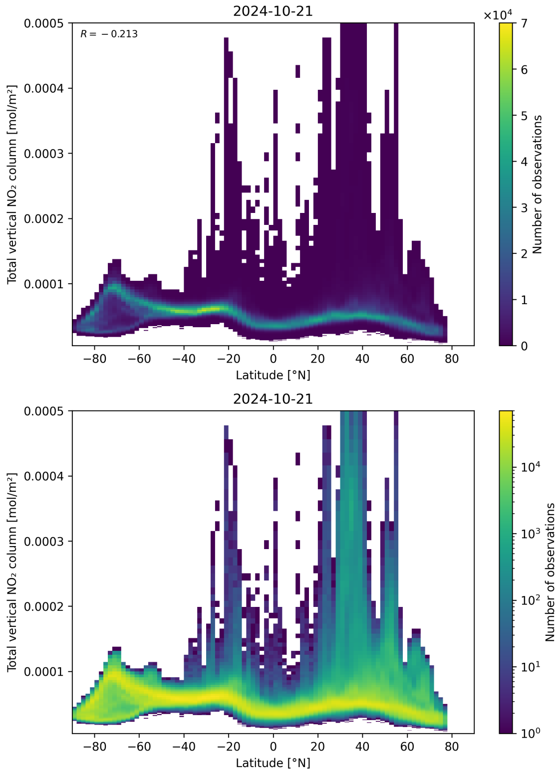
Figure 90: Scatter density plot of “Latitude” against “Total vertical NO 2 column” for 2024-10-20 to 2024-10-22.
