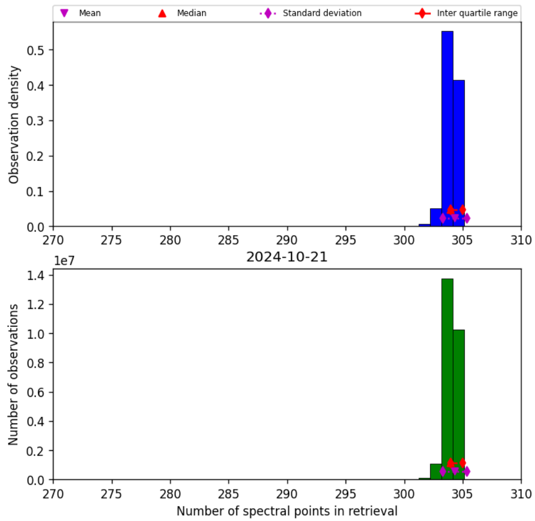
Figure 33: Histogram of “Number of spectral points in retrieval” for 2024-10-20 to 2024-10-22
