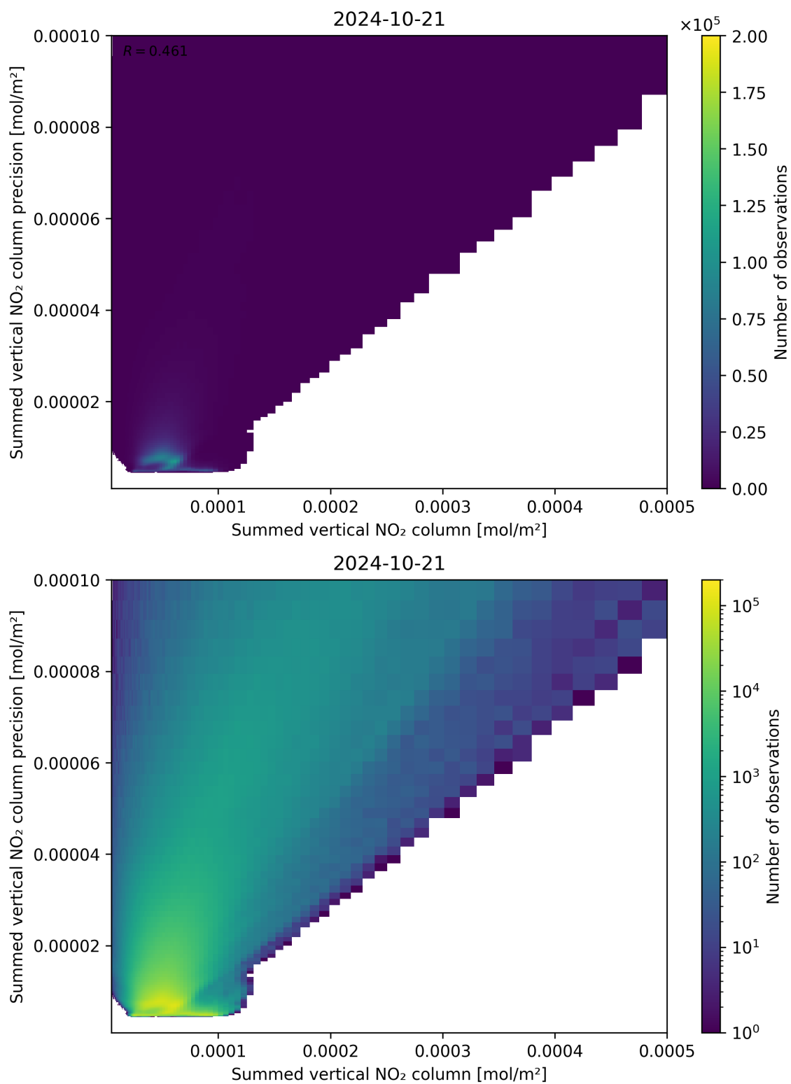
Figure 105: Scatter density plot of “Summed vertical NO 2 column” against “Summed vertical NO 2 column precision” for 2024-10-20 to 2024-10-22.
