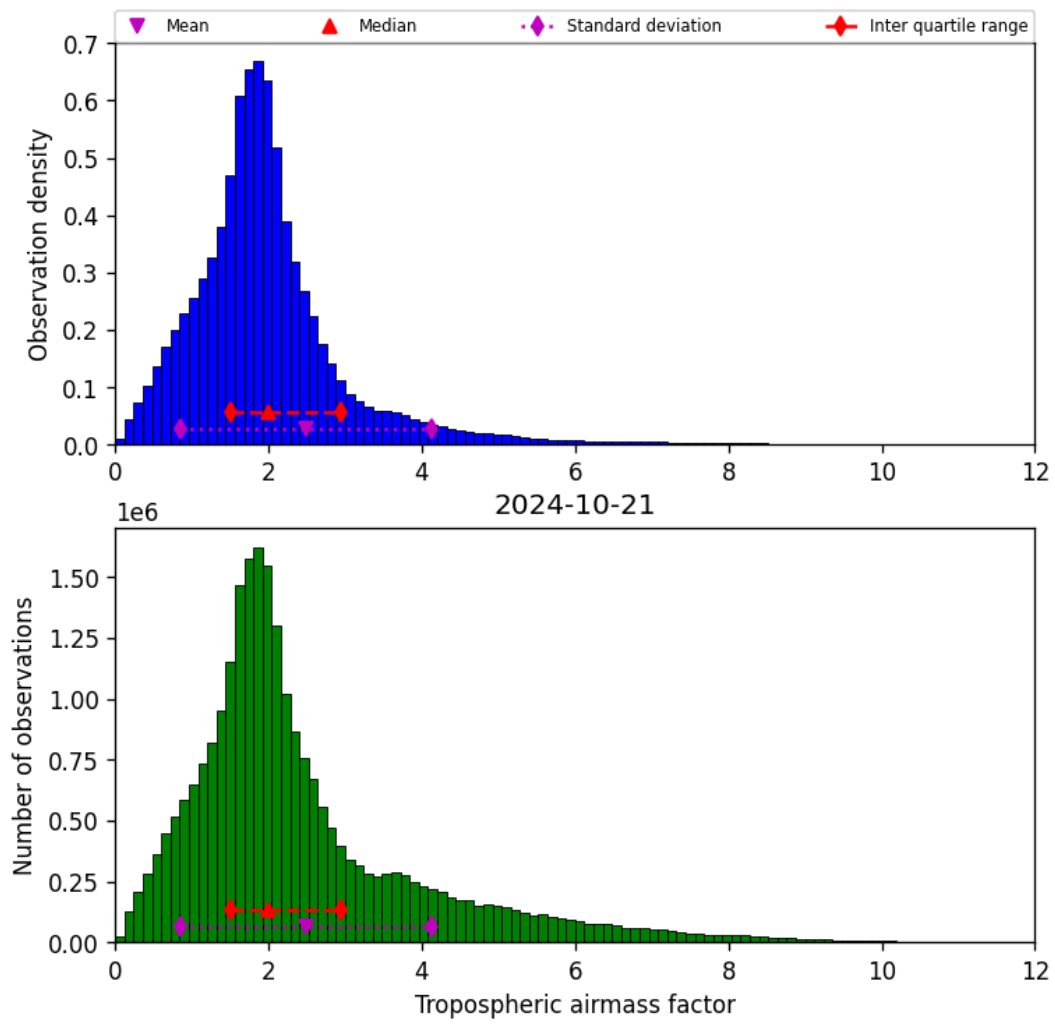
Figure 31: Histogram of “Tropospheric airmass factor” for 2024-10-20 to 2024-10-22
