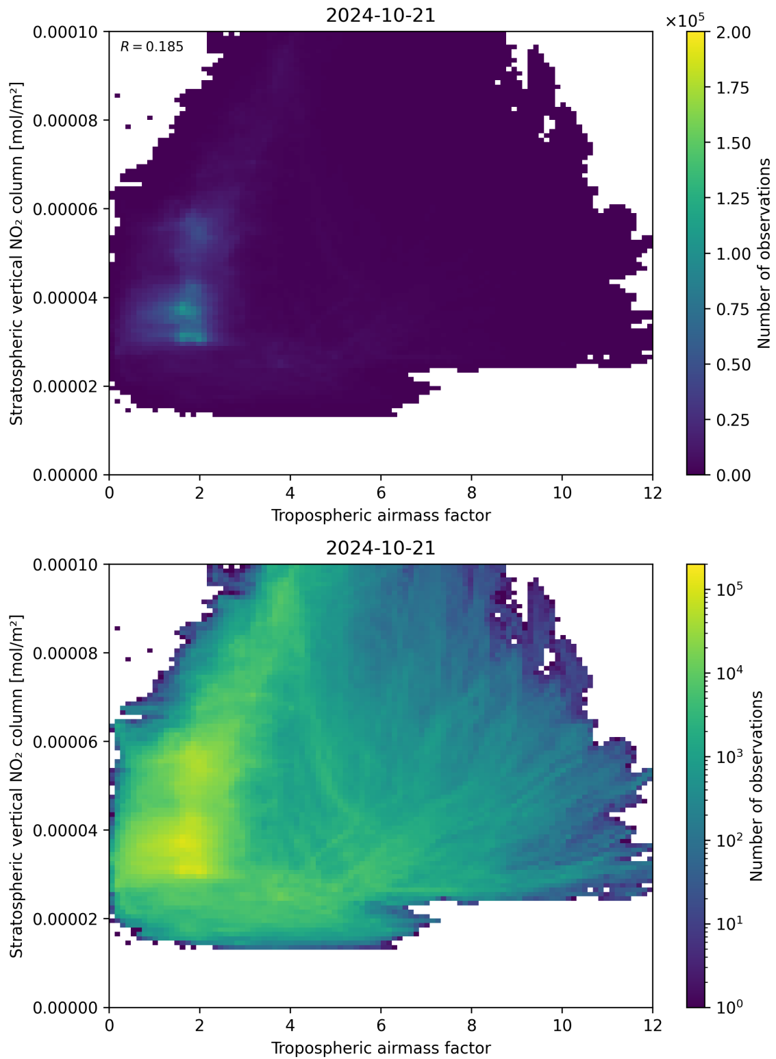
Figure 74: Scatter density plot of “Tropospheric air mass factor” against “Stratospheric vertical NO 2 column” for 2024-10-20 to 2024-10-22.
