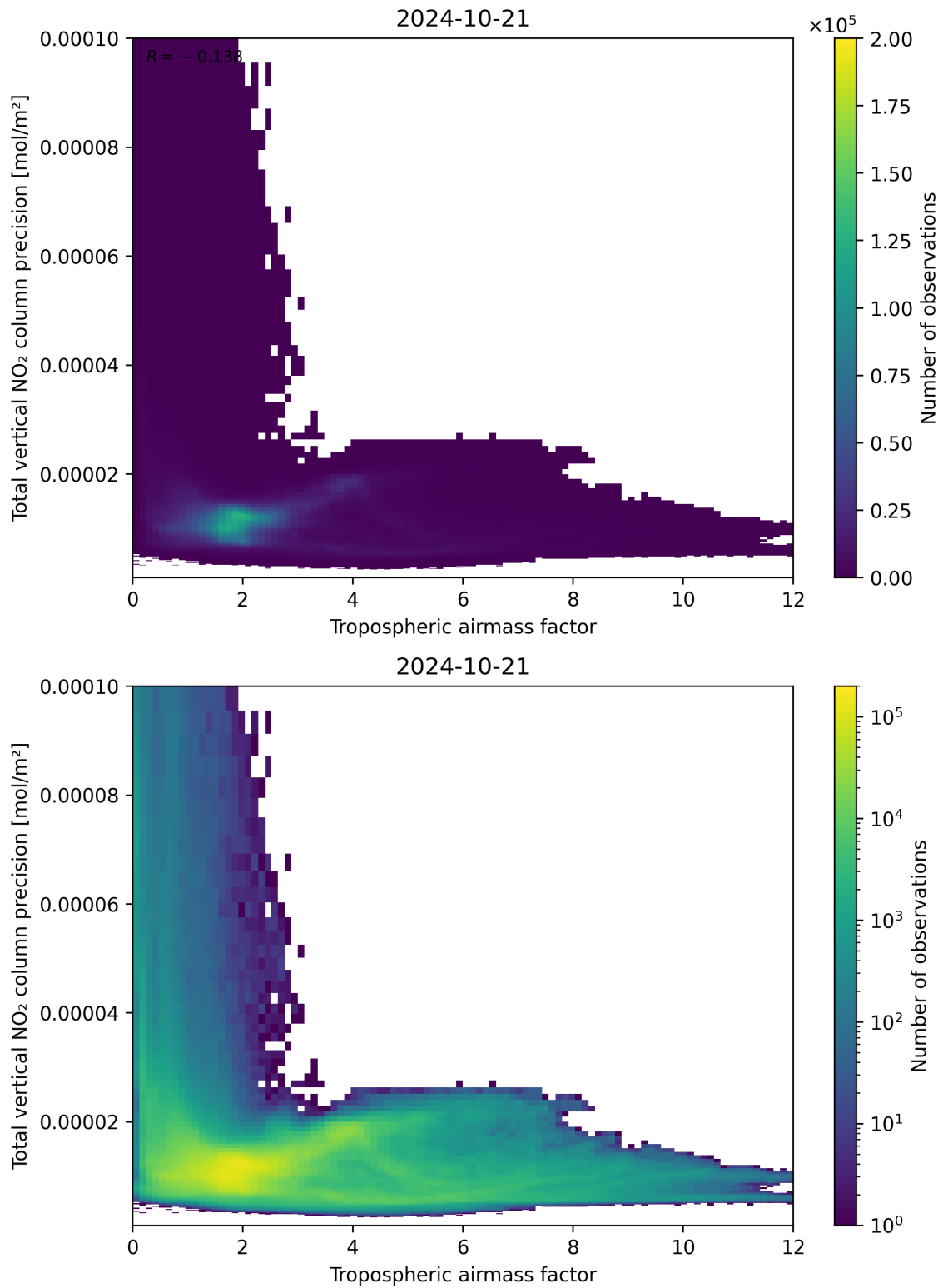
Figure 78: Scatter density plot of “Tropospheric air mass factor” against “Total vertical NO 2 column precision” for 2024-10-20 to 2024-10-22.
