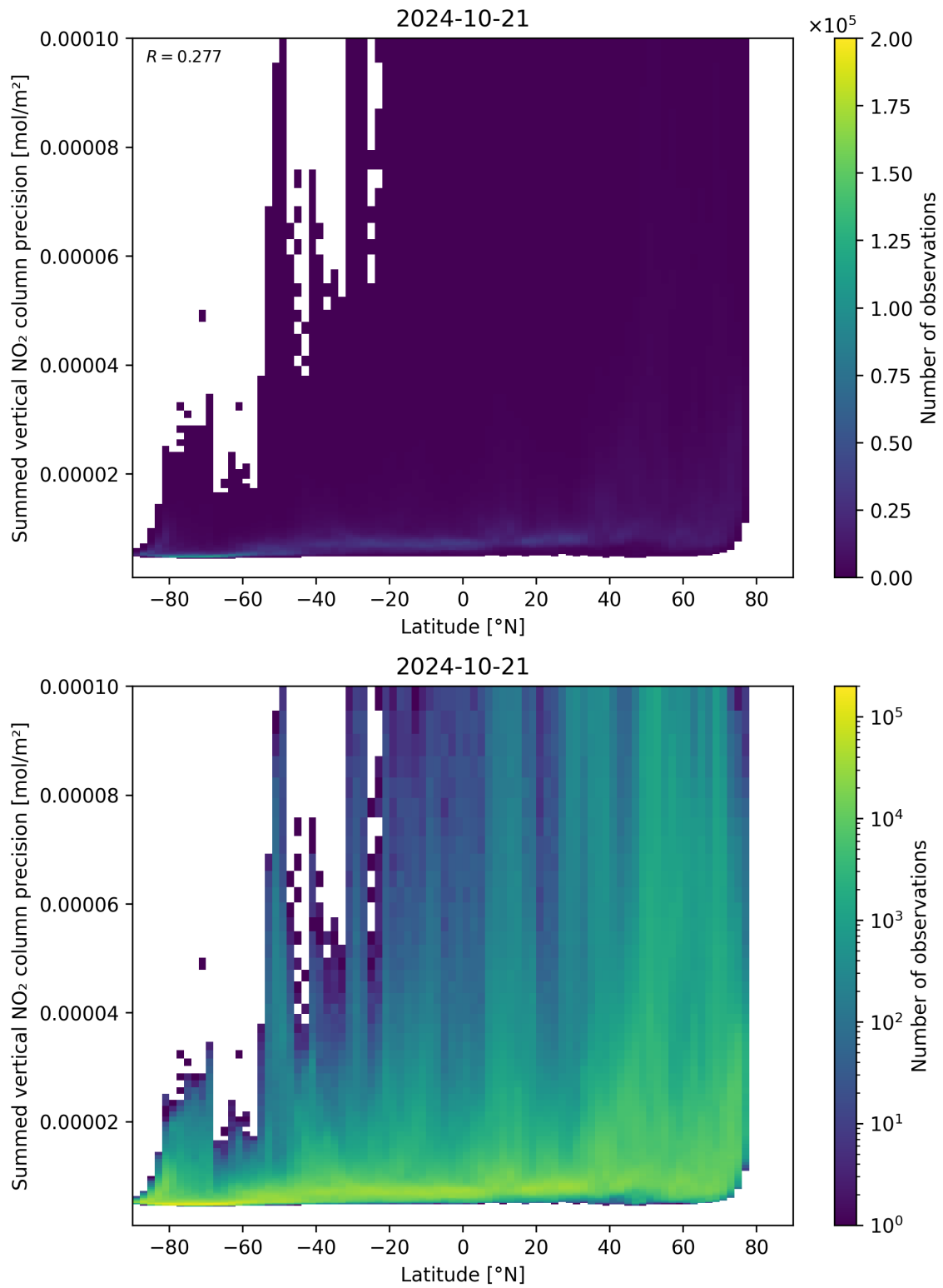
Figure 89: Scatter density plot of “Latitude” against “Summed vertical NO 2 column precision” for 2024-10-20 to 2024-10-22.
