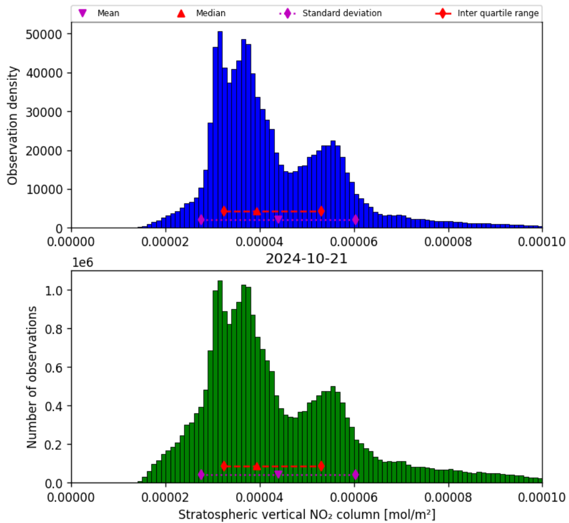
Figure 36: Histogram of “Stratospheric vertical NO 2 column” for 2024-10-20 to 2024-10-22
