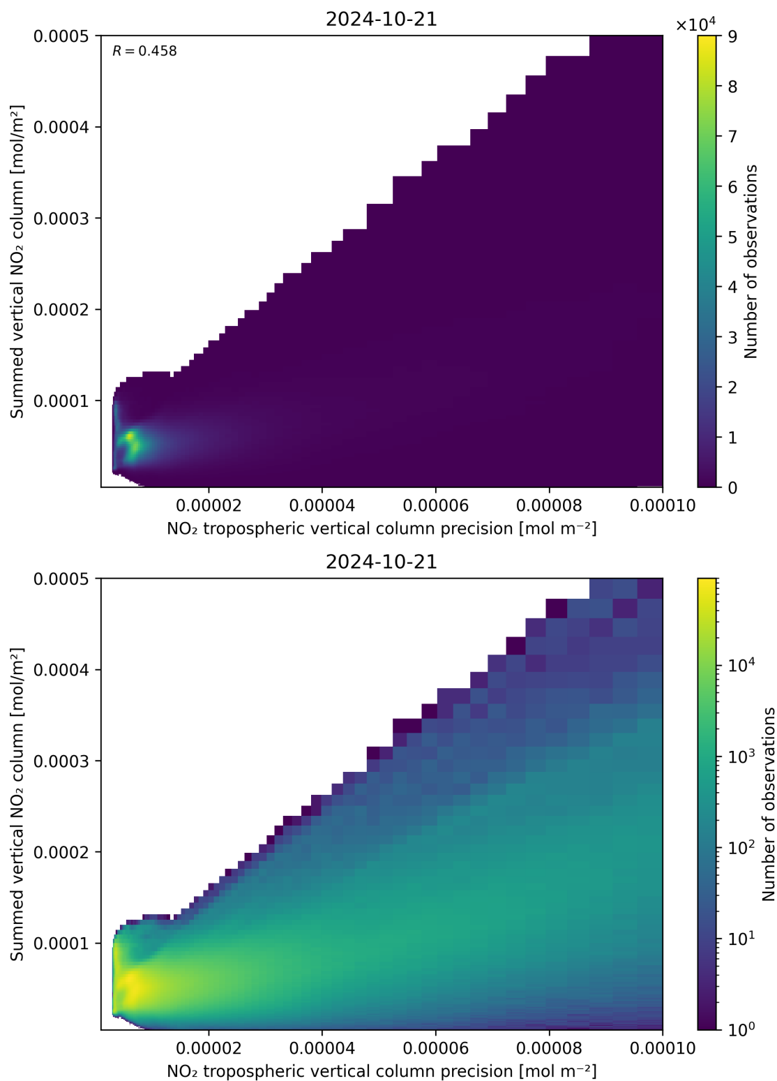
Figure 136: Scatter density plot of “NO 2 tropospheric vertical column precision” against “Summed vertical NO 2 column” for 2024-10-20 to 2024-10-22.
