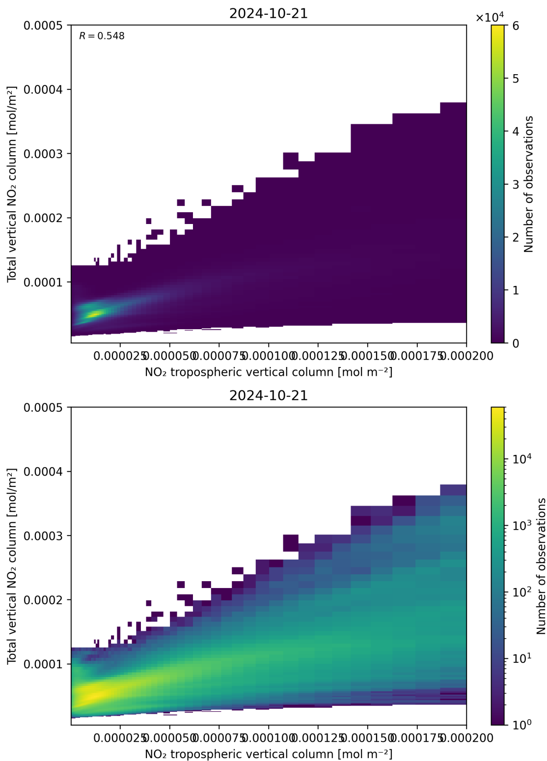
Figure 128: Scatter density plot of “NO 2 tropospheric vertical column” against “Total vertical NO 2 column” for 2024-10-20 to 2024-10-22.
