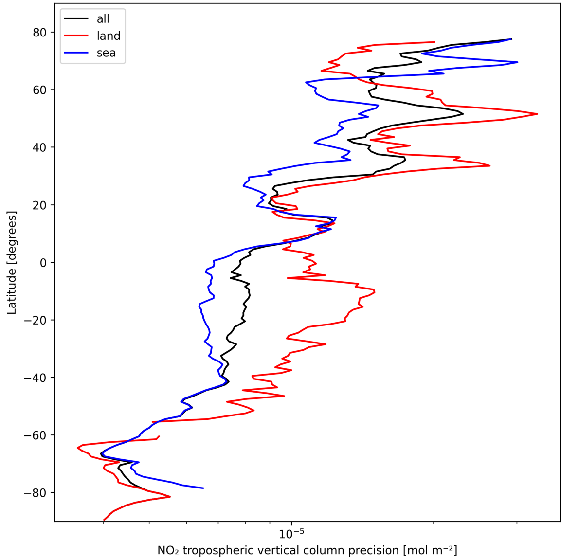
Figure 13: Zonal average of “NO 2 tropospheric vertical column precision” for 2024-10-20 to 2024-10-22.
