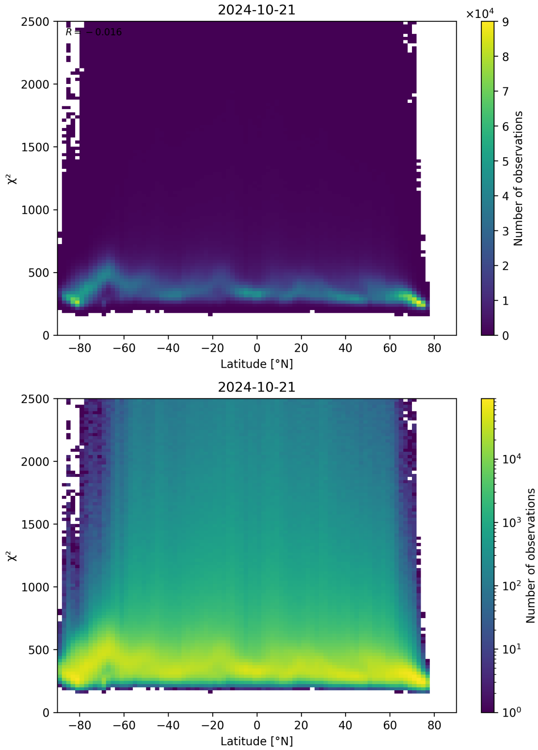
Figure 86: Scatter density plot of “Latitude” against “ \chi^2 ” for 2024-10-20 to 2024-10-22.
