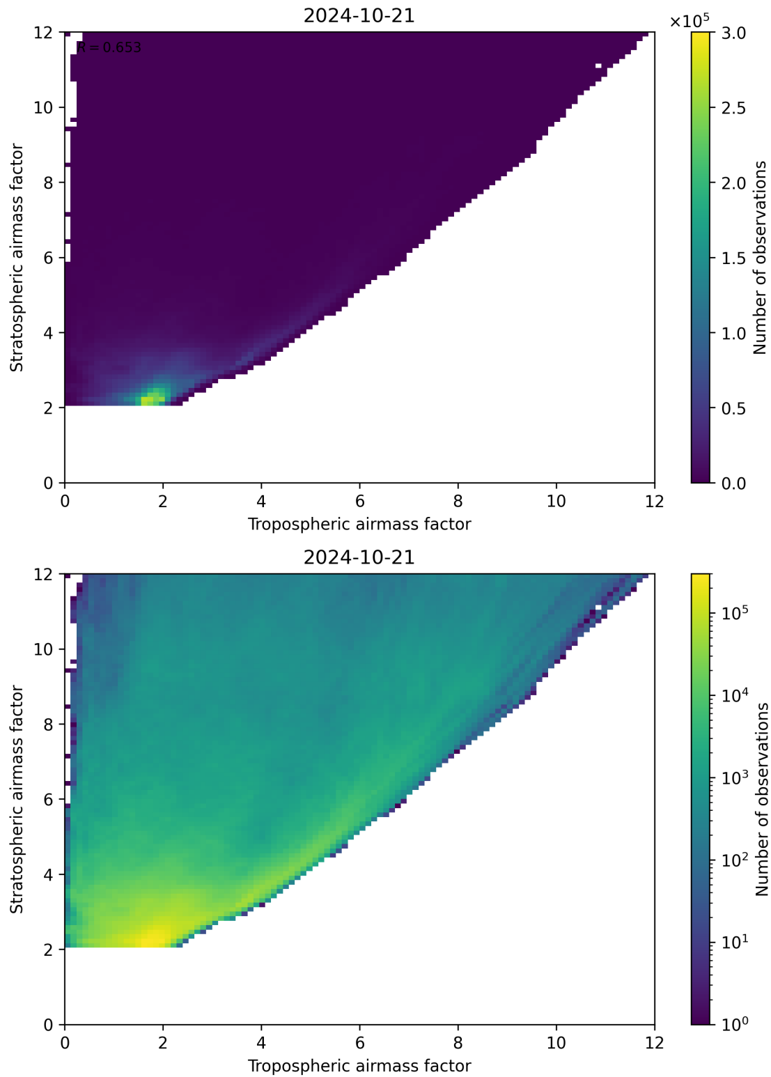
Figure 71: Scatter density plot of “Tropospheric airmass factor” against “Stratospheric airmass factor” for 2024-10-20 to 2024-10-22.
