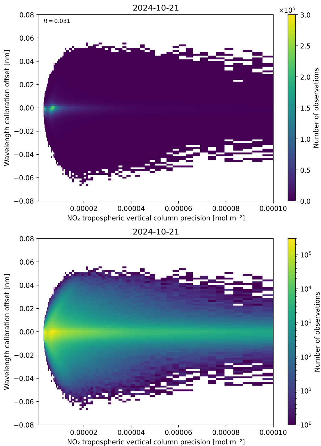
Figure 141: Scatter density plot of “NO 2 tropospheric vertical column precision” against “Wavelength calibration offset” for 2024-10-20 to 2024-10-22.
