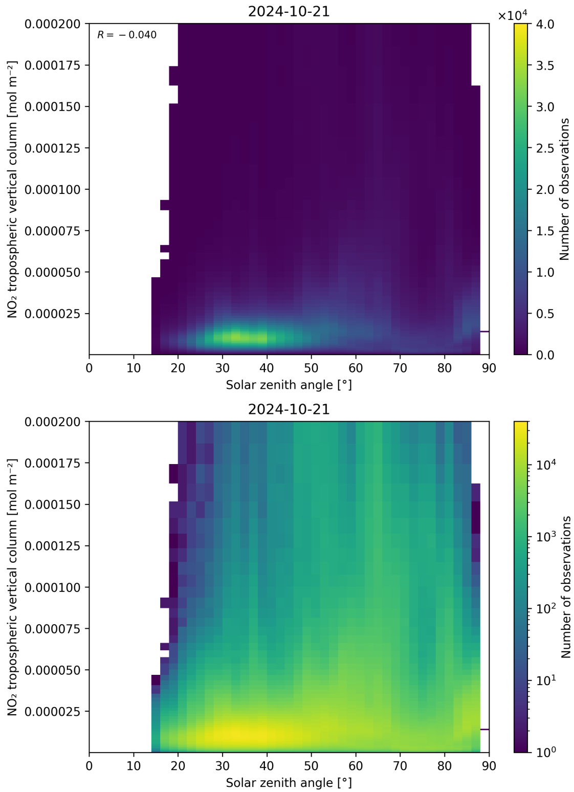
Figure 155: Scatter density plot of “Solar zenith angle” against “NO 2 tropospheric vertical column” for 2024-10-20 to 2024-10-22.
