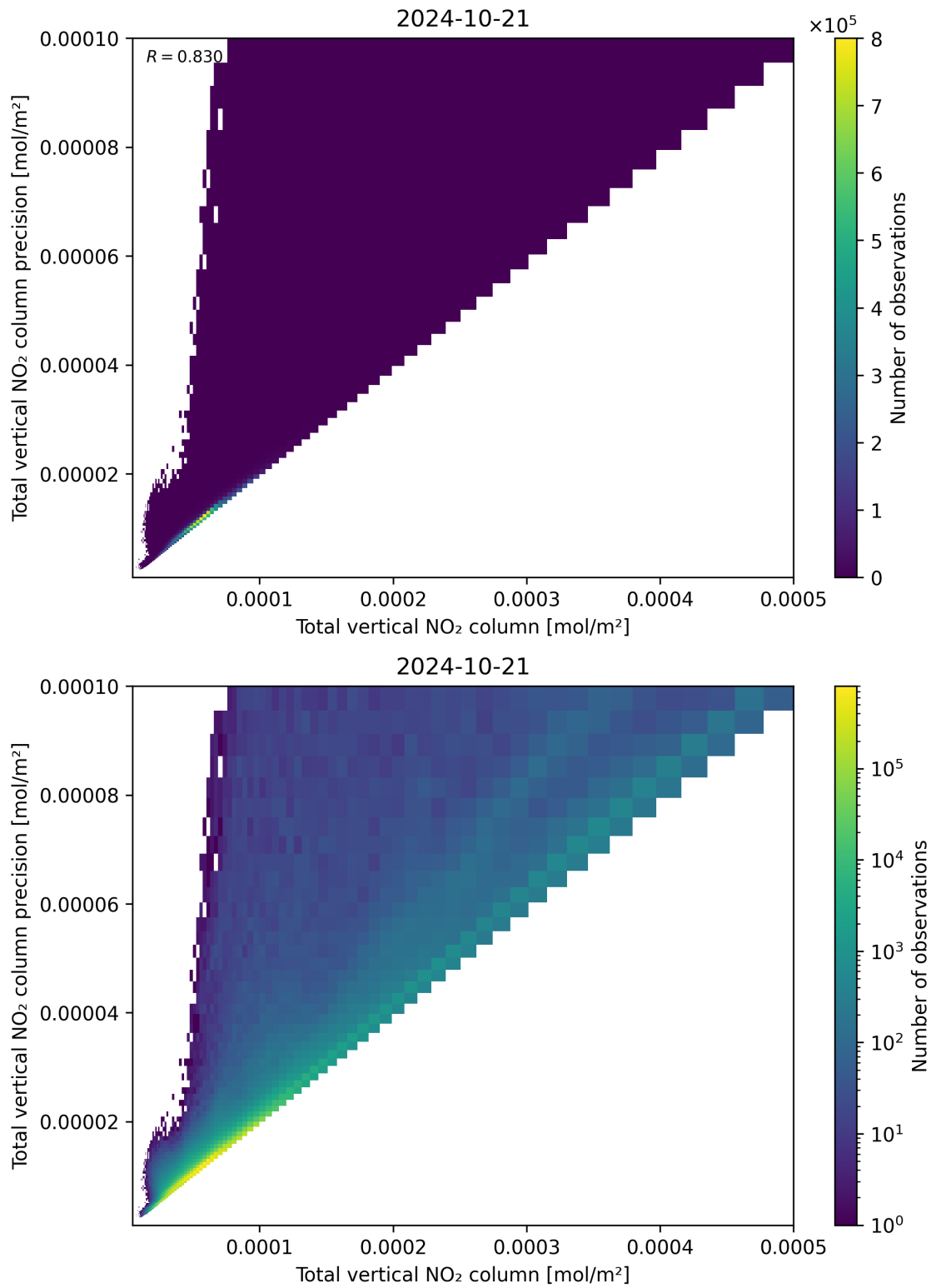
Figure 114: Scatter density plot of “Total vertical NO 2 column” against “Total vertical NO 2 column precision” for 2024-10-20 to 2024-10-22.
