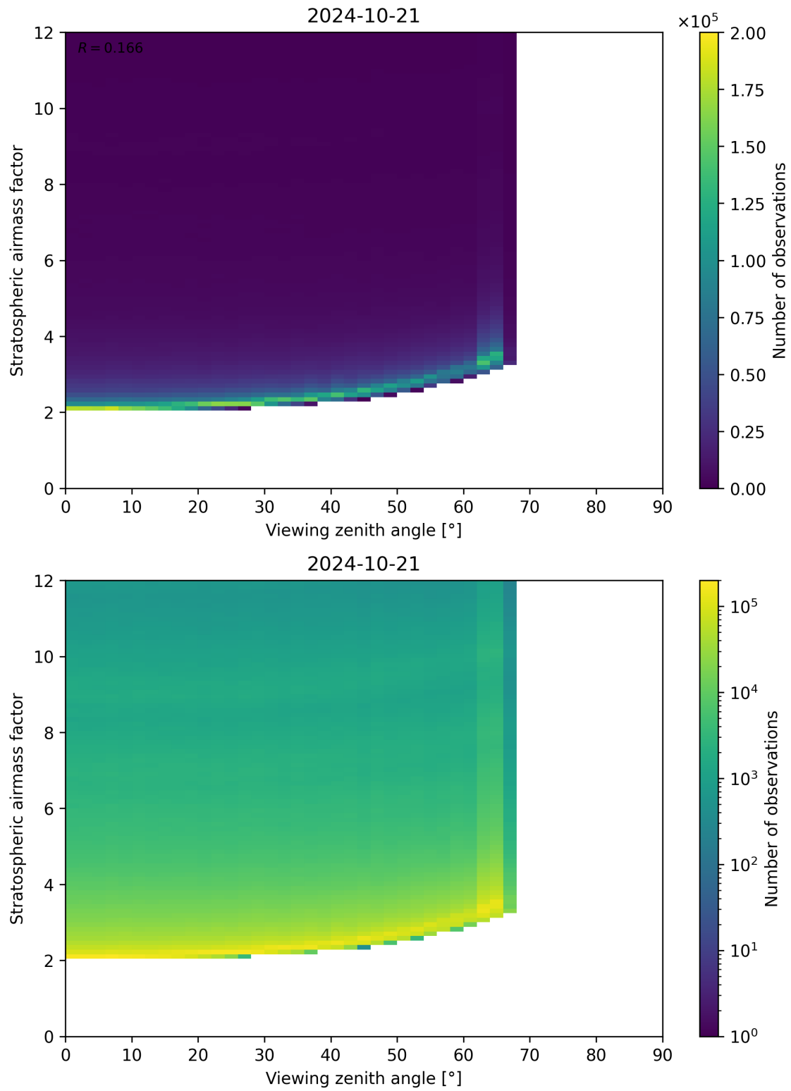
Figure 159: Scatter density plot of “Viewing zenith angle” against “Stratospheric airmass factor” for 2024-10-20 to 2024-10-22.
