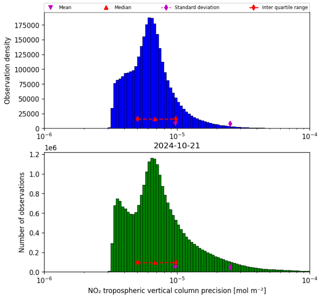
Figure 30: Histogram of “NO 2 tropospheric vertical column precision” for 2024-10-20 to 2024-10-22
