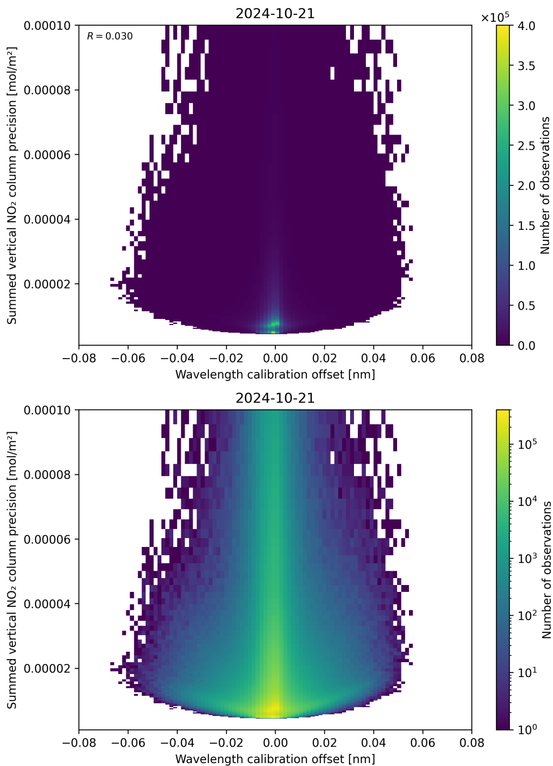
Figure 178: Scatter density plot of “Wavelength calibration offset” against “Summed vertical NO 2 column precision” for 2024-10-20 to 2024-10-22.
