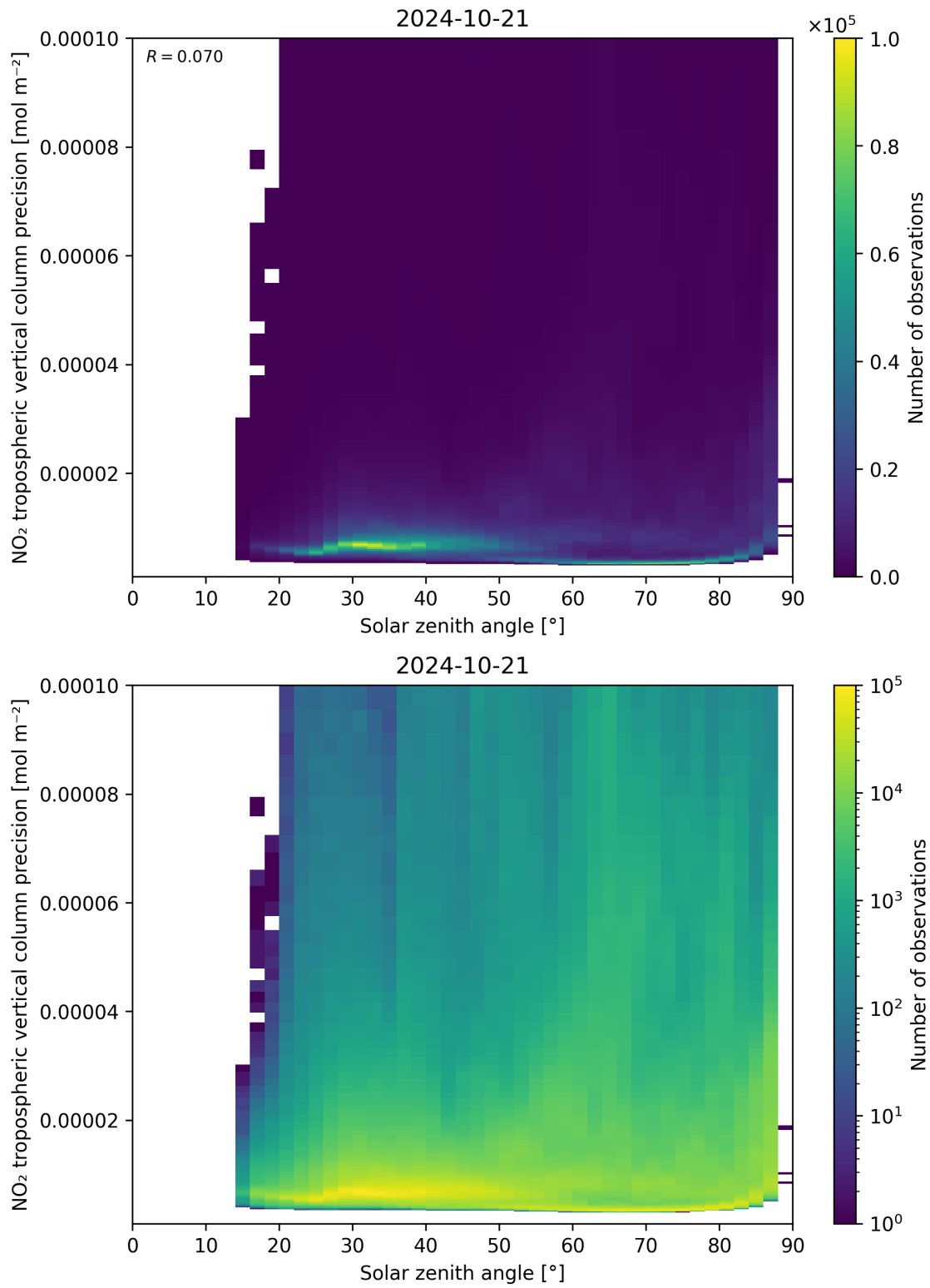
Figure 156: Scatter density plot of “Solar zenith angle” against “NO 2 tropospheric vertical column precision” for 2024-10-20 to 2024-10-22.
