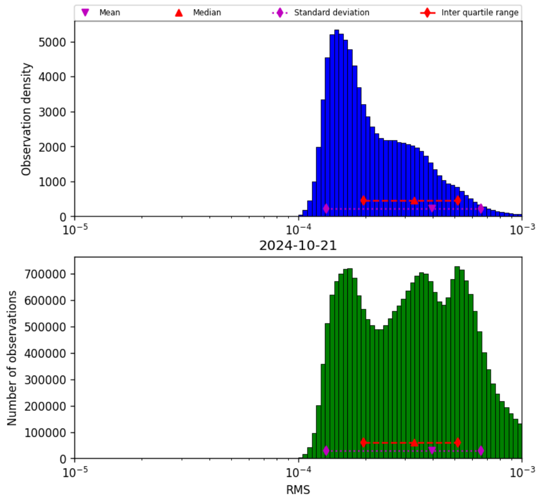
Figure 43: Histogram of “RMS” for 2024-10-20 to 2024-10-22
