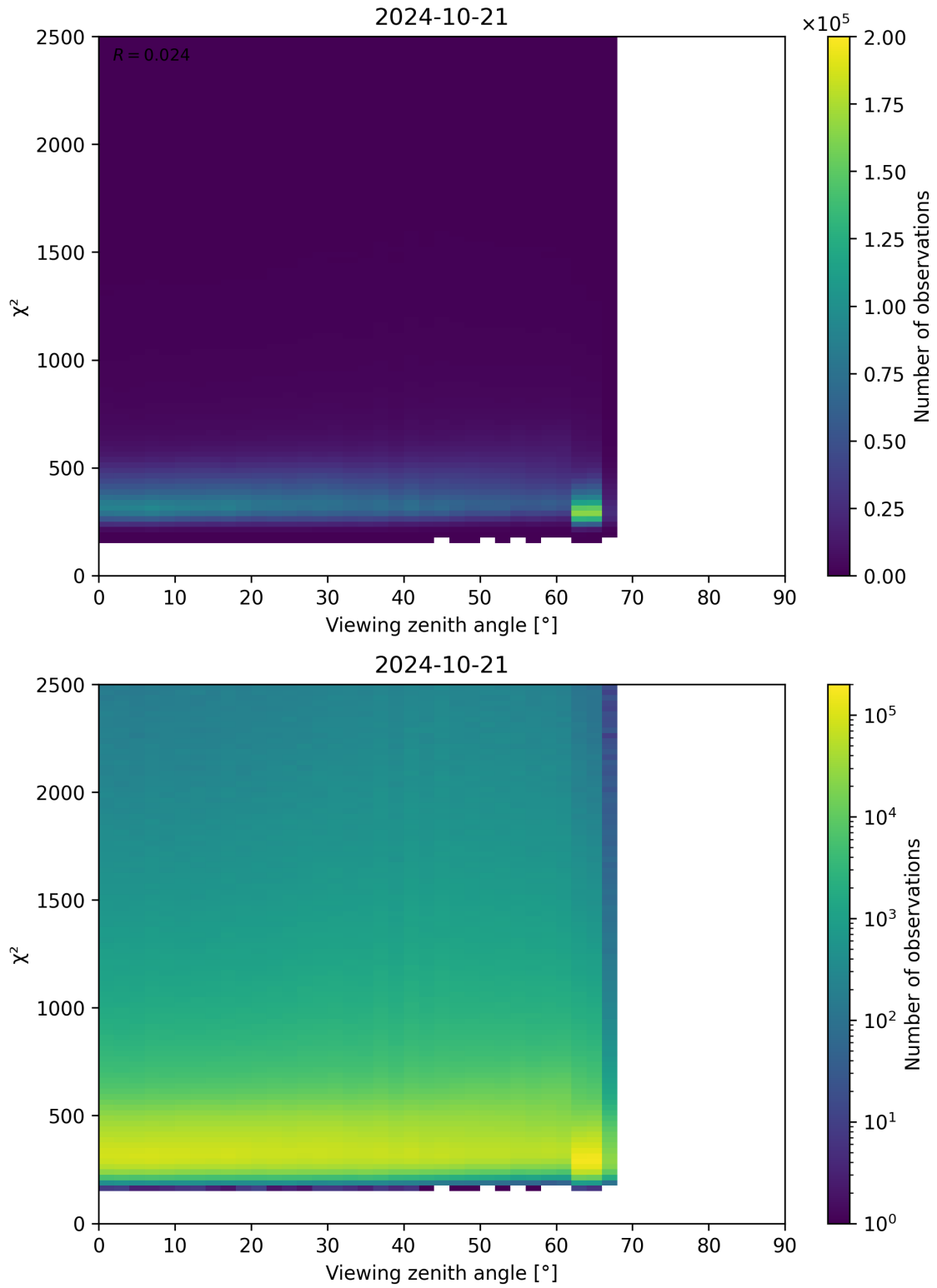
Figure 162: Scatter density plot of “Viewing zenith angle” against “ \chi^2 ” for 2024-10-20 to 2024-10-22.
