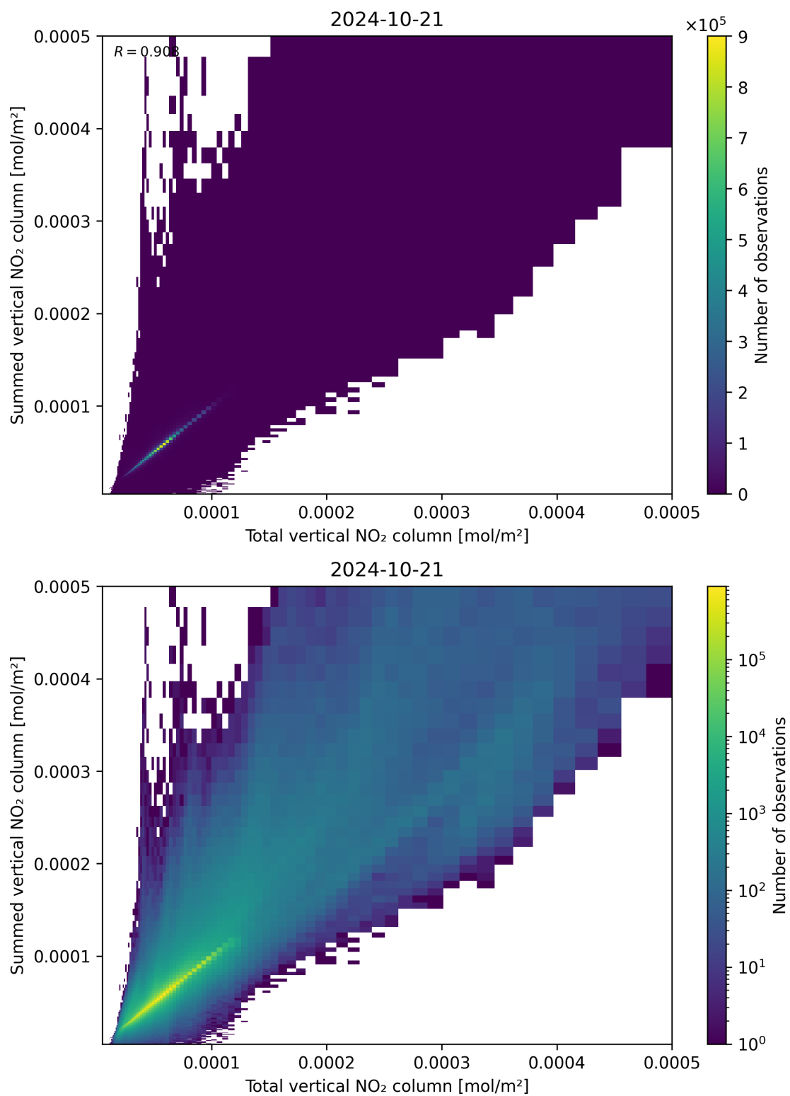
Figure 112: Scatter density plot of “Total vertical NO 2 column” against “Summed vertical NO 2 column” for 2024-10-20 to 2024-10-22.
