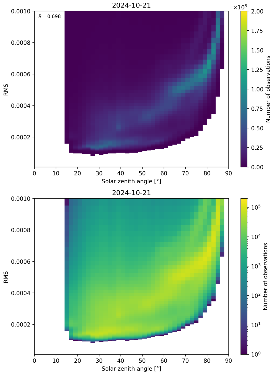
Figure 157: Scatter density plot of “Solar zenith angle” against “RMS” for 2024-10-20 to 2024-10-22.
