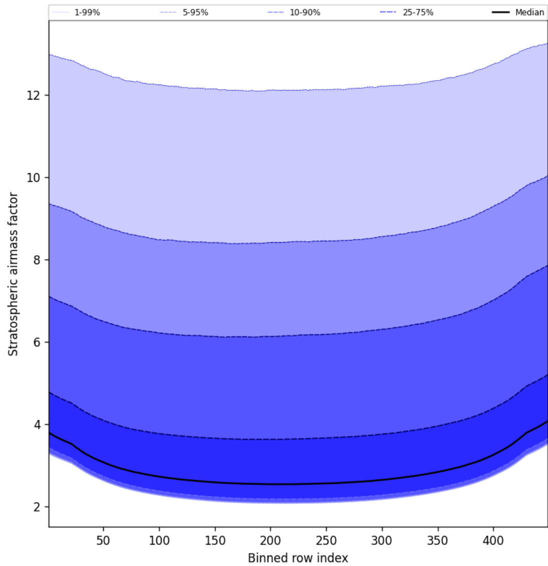
Figure 61: Along track statistics of “Stratospheric airmass factor” for 2024-10-20 to 2024-10-22
