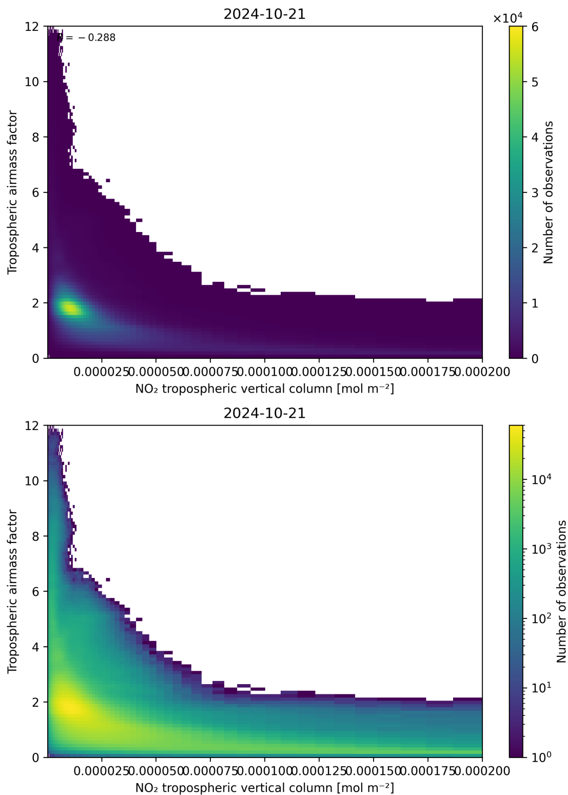
Figure 123: Scatter density plot of “NO 2 tropospheric vertical column” against “Tropospheric air mass factor” for 2024-10-20 to 2024-10-22.
