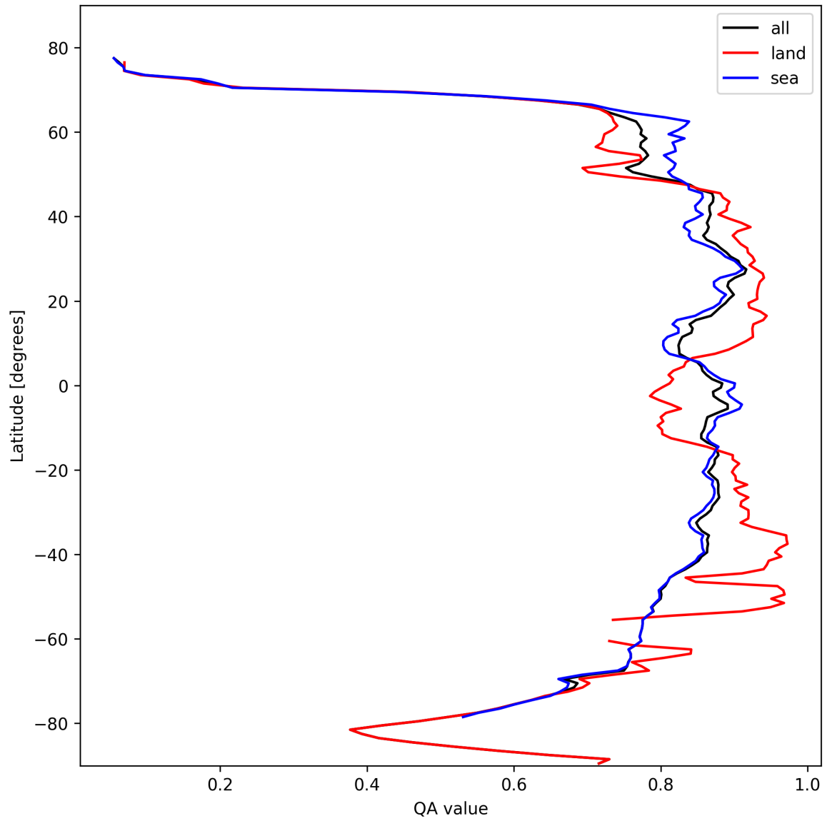
Figure 11: Zonal average of “QA value” for 2024-10-20 to 2024-10-22.
