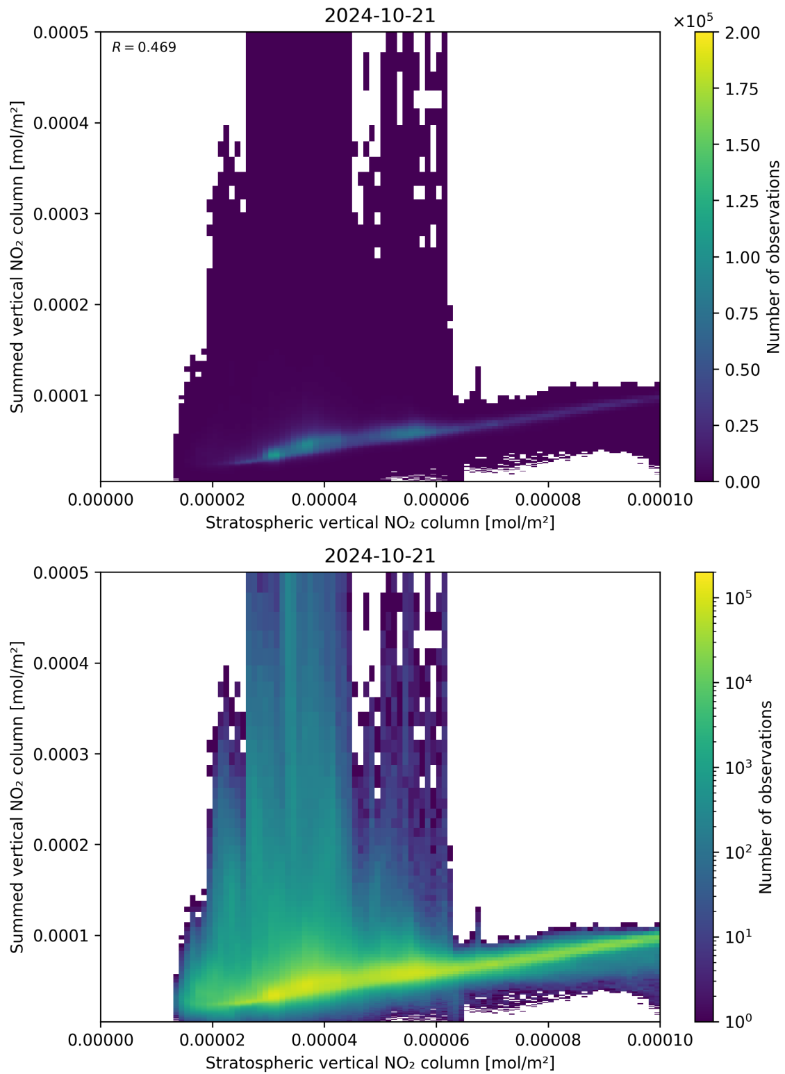
Figure 98: Scatter density plot of “Stratospheric vertical NO 2 column” against “Summed vertical NO 2 column” for 2024-10-20 to 2024-10-22.
