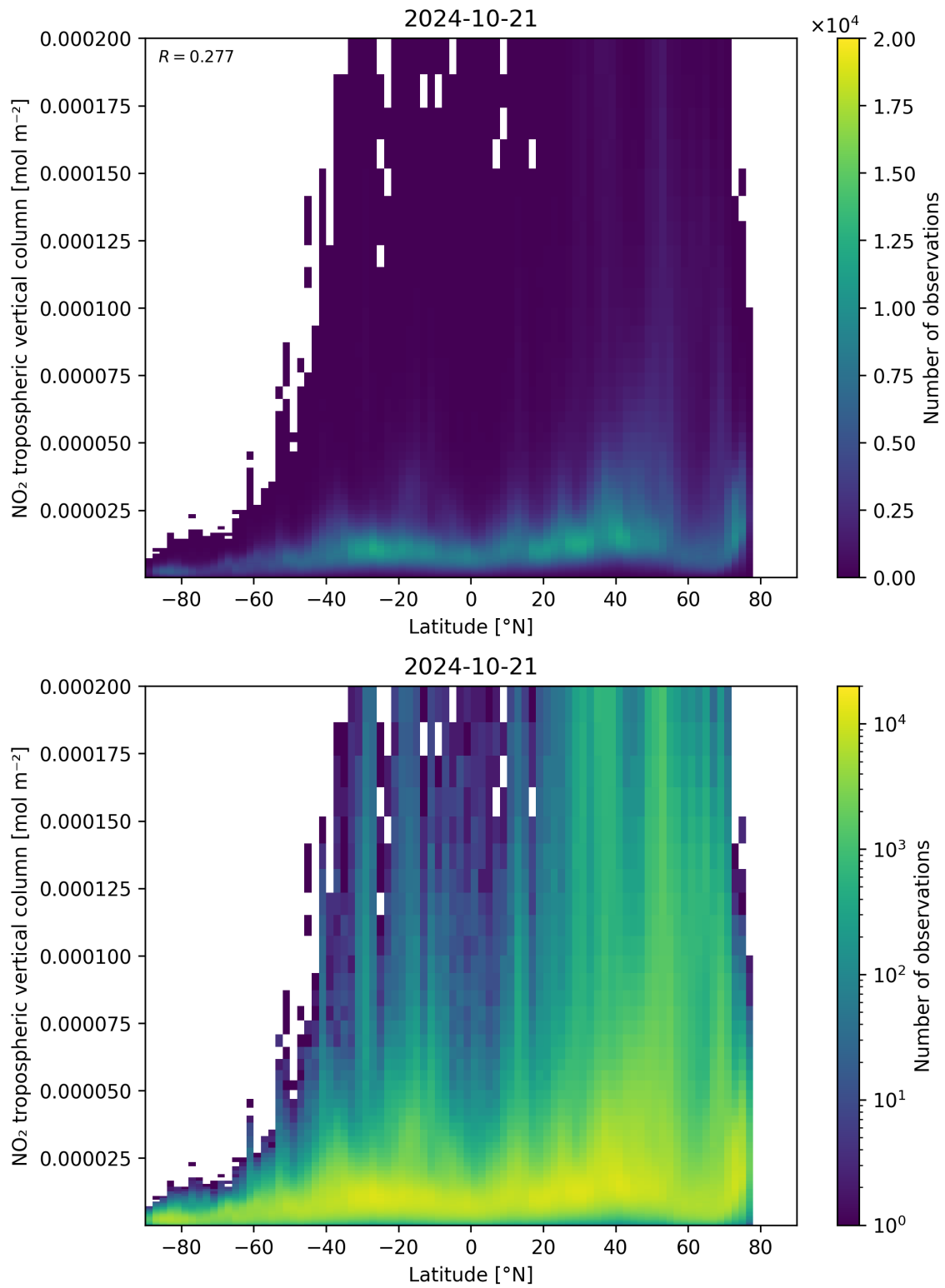
Figure 92: Scatter density plot of “Latitude” against “NO 2 tropospheric vertical column” for 2024-10-20 to 2024-10-22.
