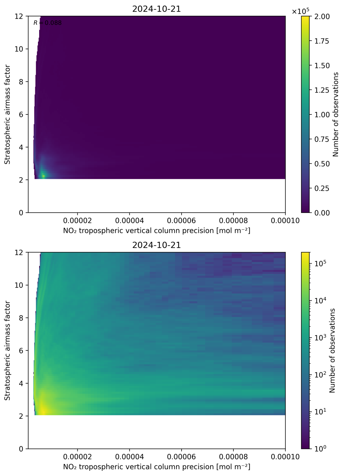
Figure 131: Scatter density plot of “NO 2 tropospheric vertical column precision” against “Stratospheric airmass factor” for 2024-10-20 to 2024-10-22.
