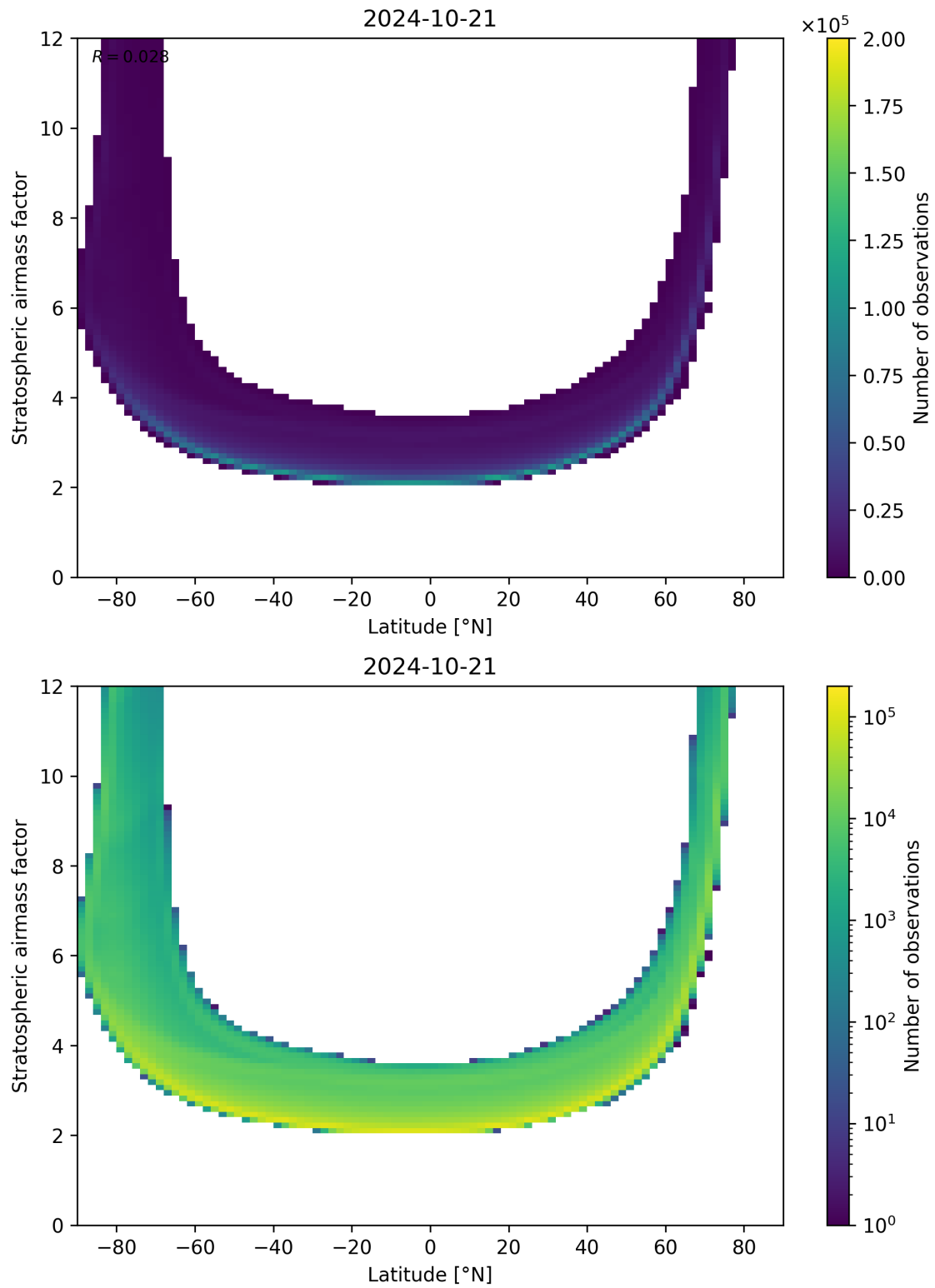
Figure 83: Scatter density plot of “Latitude” against “Stratospheric airmass factor” for 2024-10-20 to 2024-10-22.
