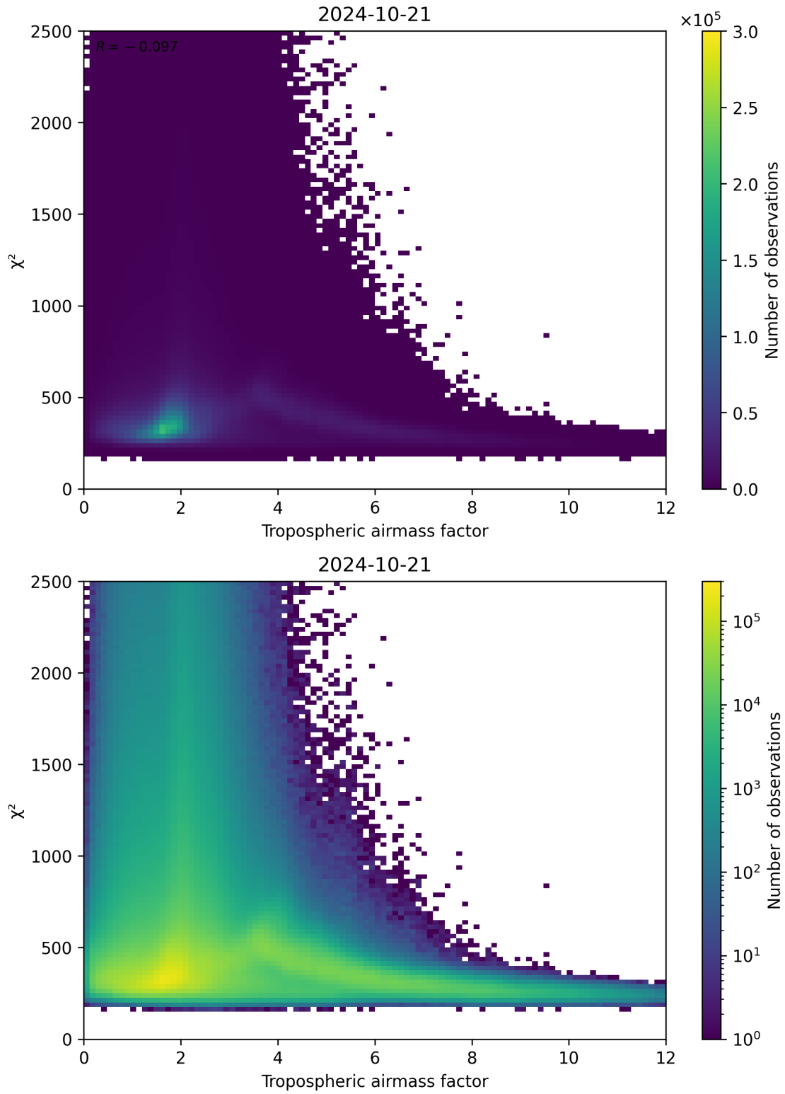
Figure 73: Scatter density plot of “Tropospheric airmass factor” against “ \chi^2 ” for 2024-10-20 to 2024-10-22.
