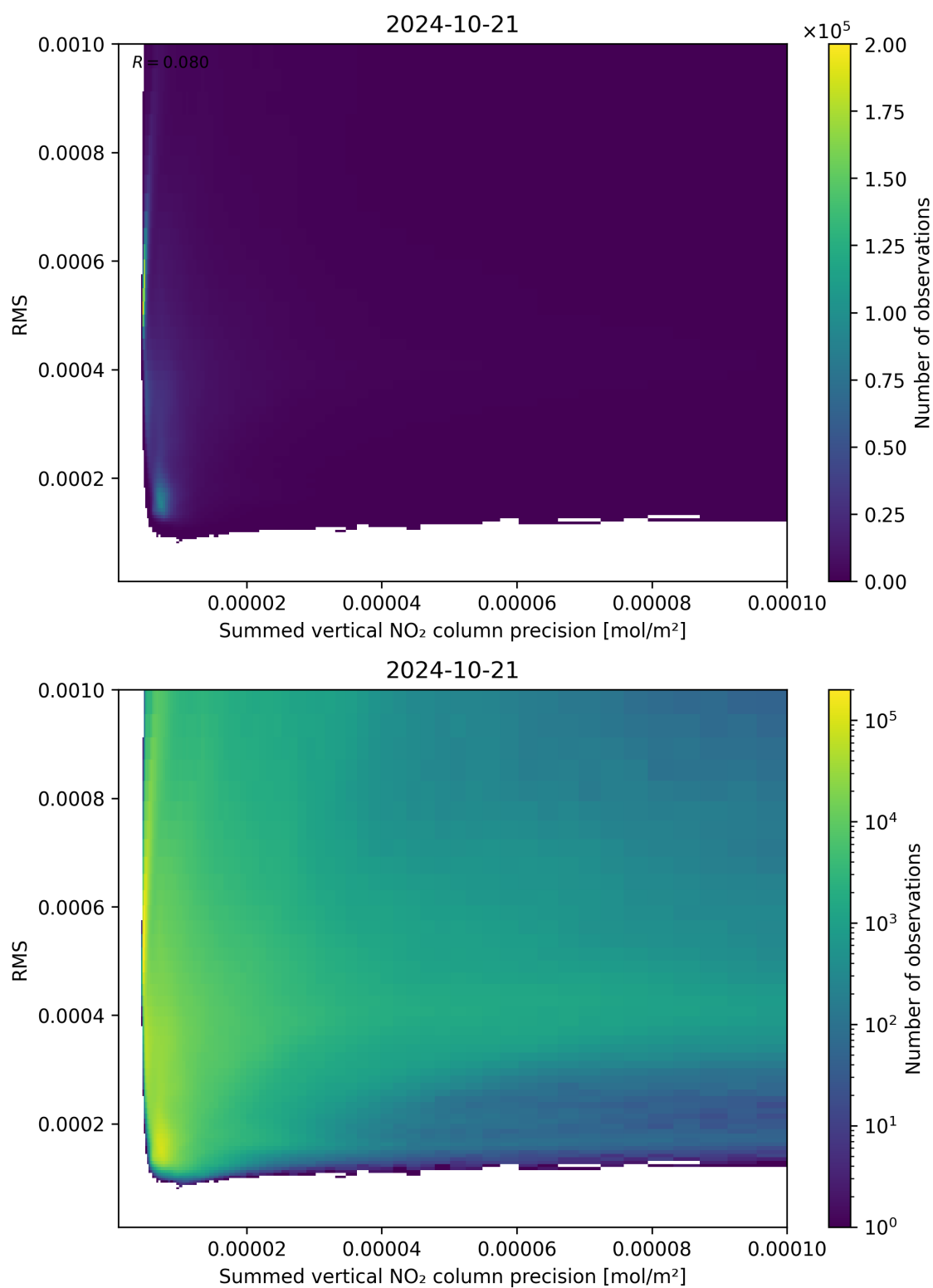
Figure 108: Scatter density plot of “Summed vertical NO 2 column precision” against “RMS” for 2024-10-20 to 2024-10-22.
