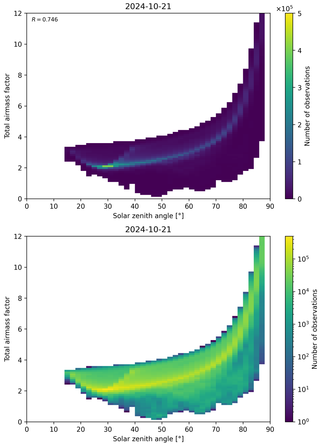
Figure 146: Scatter density plot of “Solar zenith angle” against “Total air mass factor” for 2024-10-20 to 2024-10-22.
