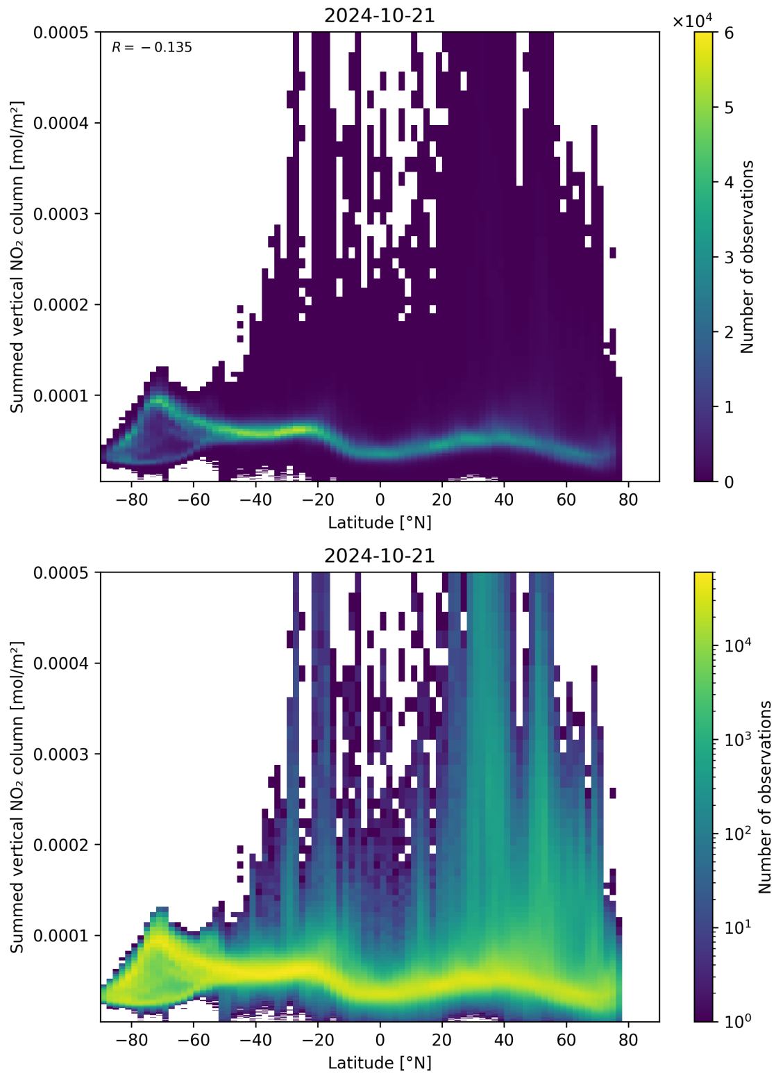
Figure 88: Scatter density plot of “Latitude” against “Summed vertical NO 2 column” for 2024-10-20 to 2024-10-22.
