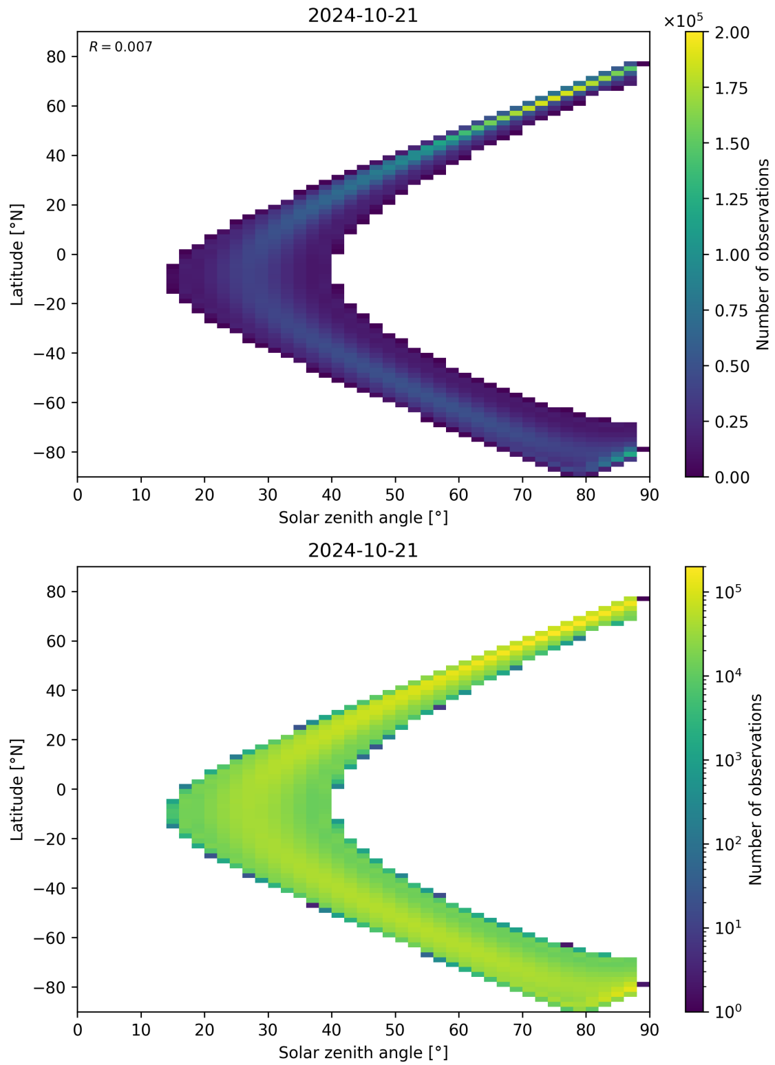
Figure 149: Scatter density plot of “Solar zenith angle” against “Latitude” for 2024-10-20 to 2024-10-22.
