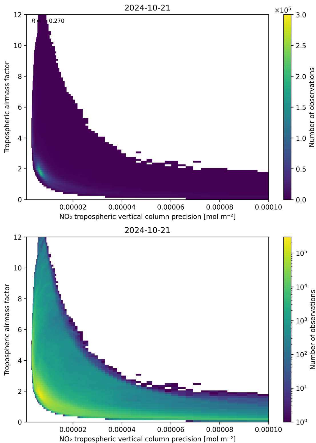
Figure 133: Scatter density plot of “NO 2 tropospheric vertical column precision” against “Tropospheric airmass factor” for 2024-10-20 to 2024-10-22.
