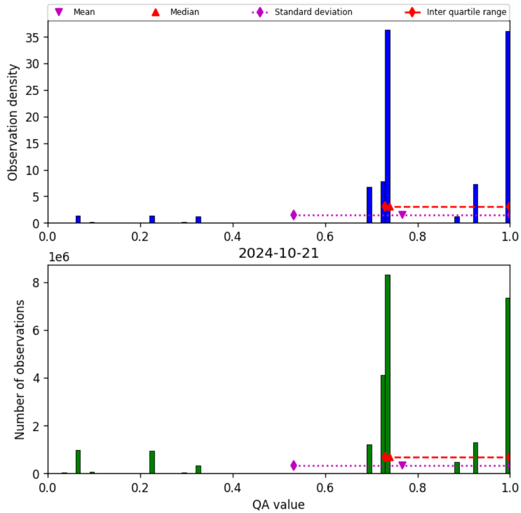
Figure 28: Histogram of “QA value” for 2024-10-20 to 2024-10-22
