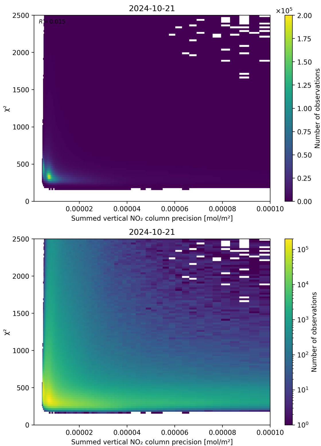
Figure 107: Scatter density plot of “Summed vertical NO 2 column precision” against “ \chi^2 ” for 2024-10-20 to 2024-10-22.
