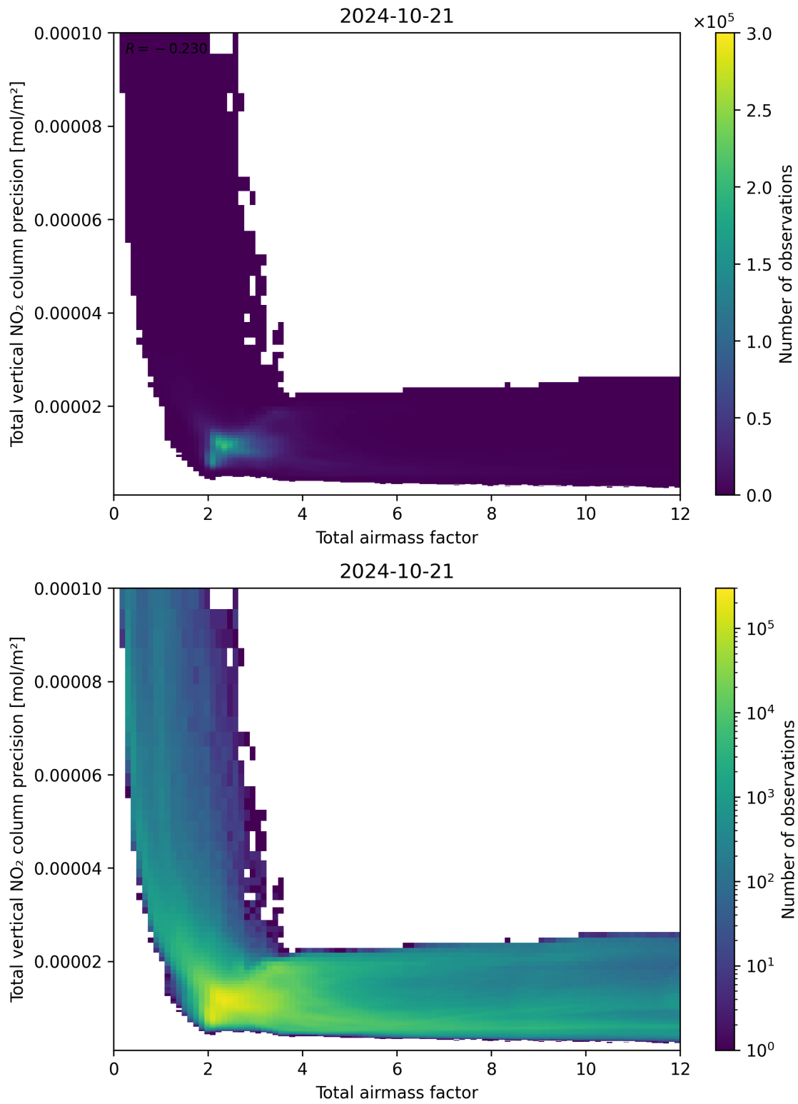
Figure 68: Scatter density plot of “Total airmass factor” against “Total vertical NO 2 column precision” for 2024-10-20 to 2024-10-22.
