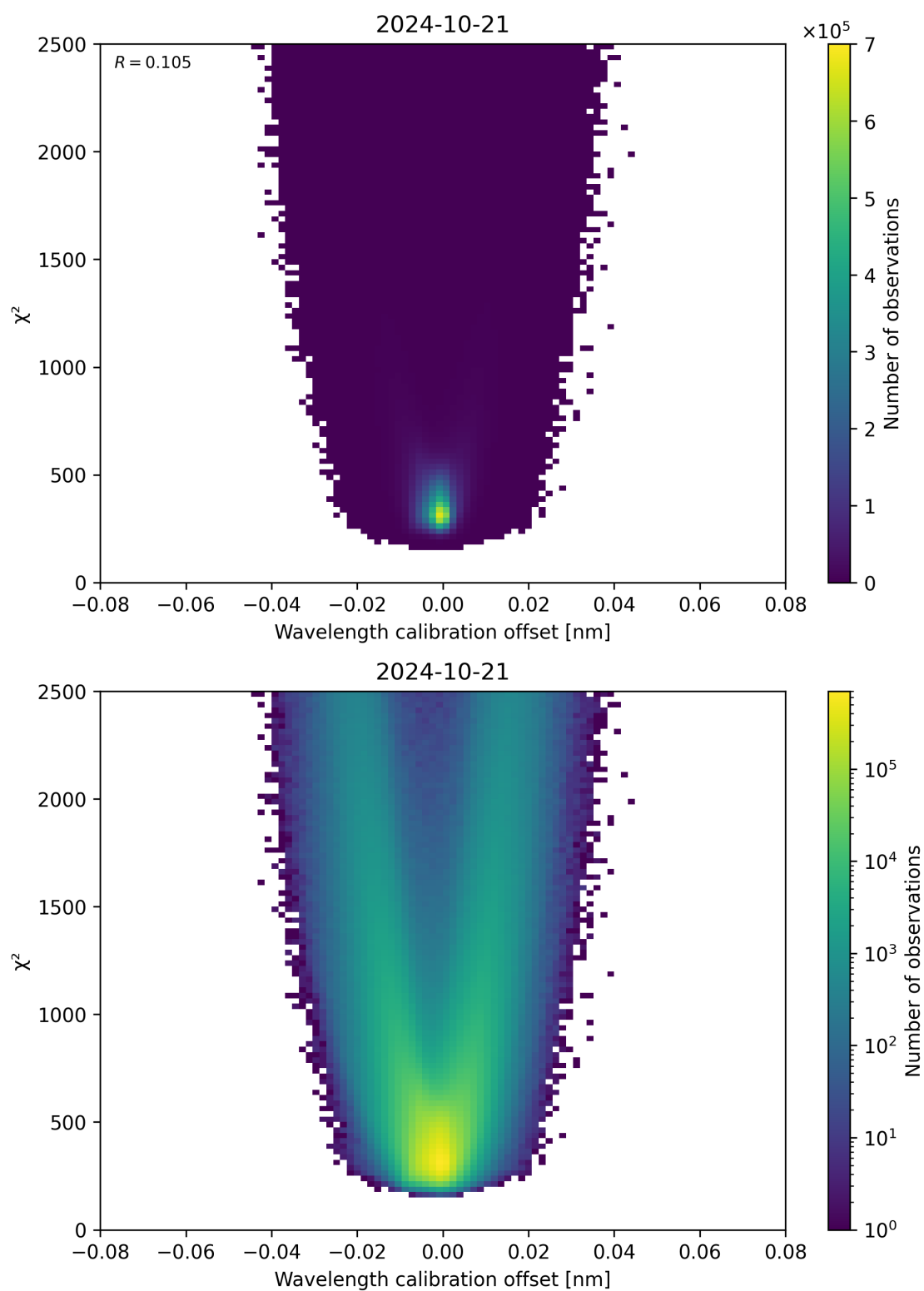
Figure 175: Scatter density plot of “Wavelength calibration offset” against “ \chi^2 ” for 2024-10-20 to 2024-10-22.
