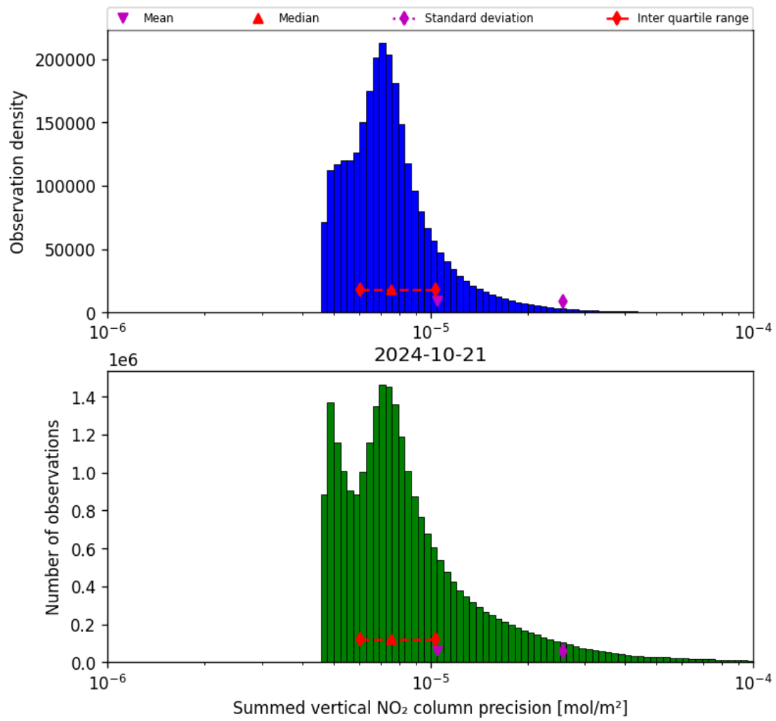
Figure 41: Histogram of "Summed vertical NO 2 column precision" for 2024-10-20 to 2024-10-22
