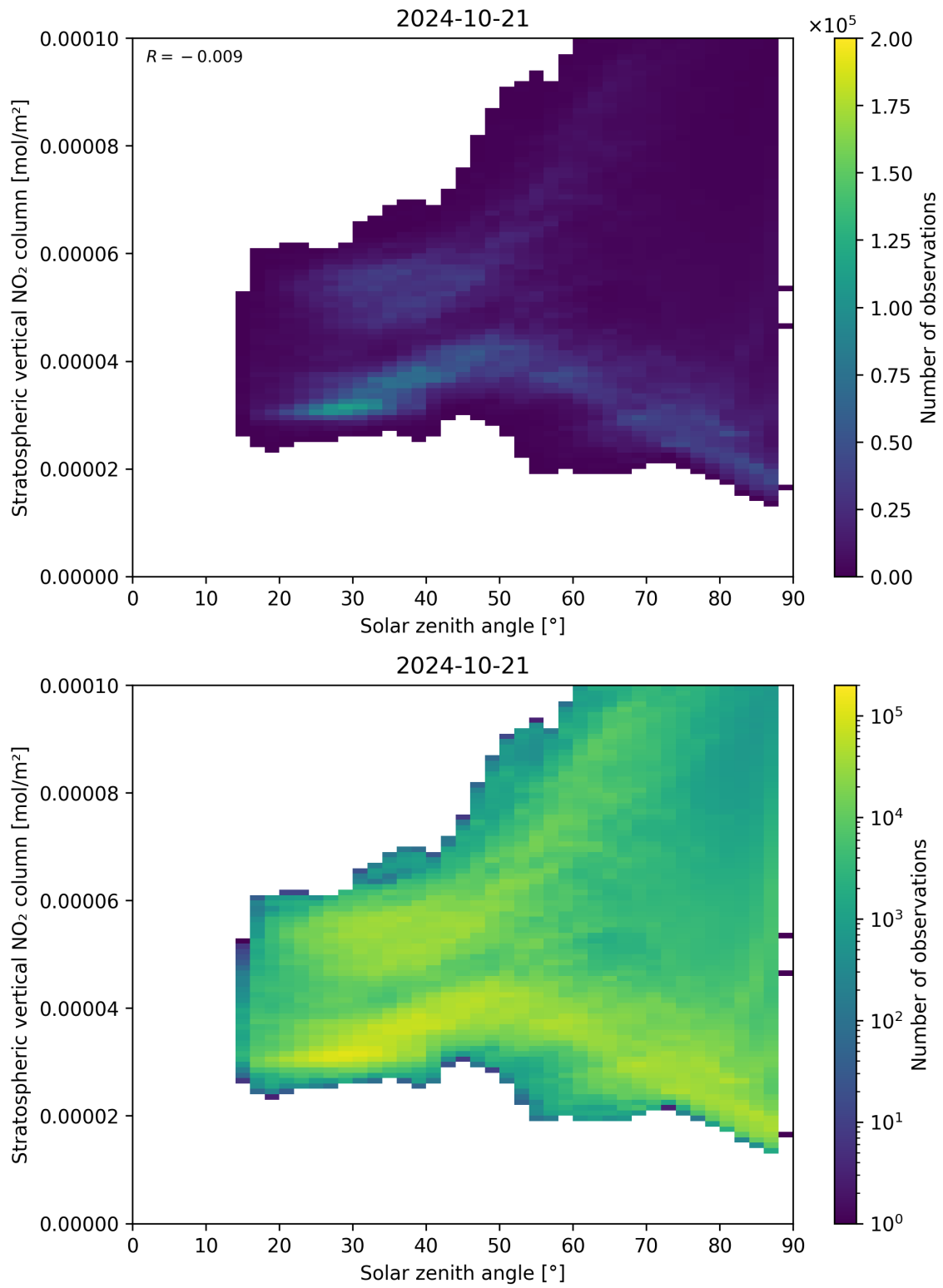
Figure 150: Scatter density plot of “Solar zenith angle” against “Stratospheric vertical NO 2 column” for 2024-10-20 to 2024-10-22.
