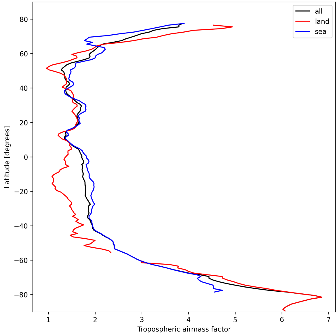
Figure 14: Zonal average of “Tropospheric airmass factor” for 2024-10-20 to 2024-10-22.
