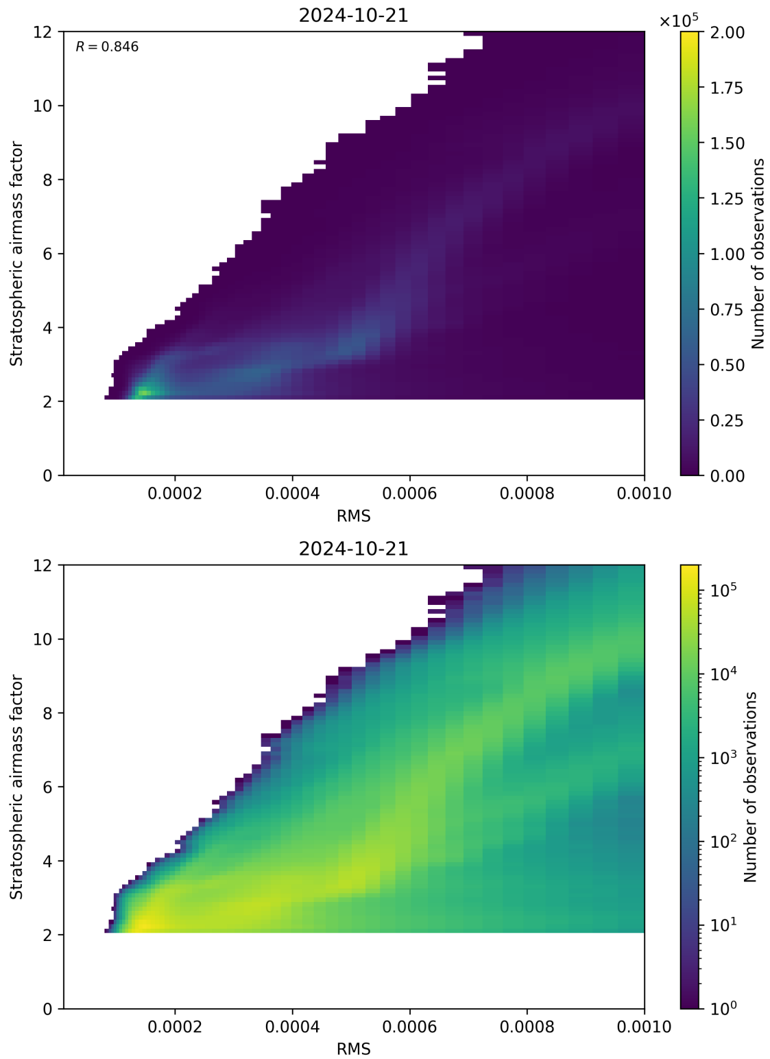
Figure 144: Scatter density plot of “RMS” against “Stratospheric airmass factor” for 2024-10-20 to 2024-10-22.
