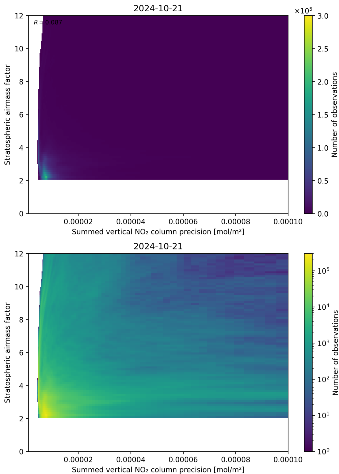
Figure 106: Scatter density plot of “Summed vertical NO 2 column precision” against “Stratospheric airmass factor” for 2024-10-20 to 2024-10-22.
