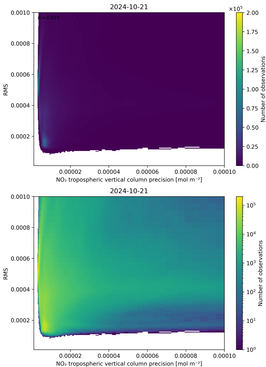
Figure 140: Scatter density plot of “NO 2 tropospheric vertical column precision” against “RMS” for 2024-10-20 to 2024-10-22.
