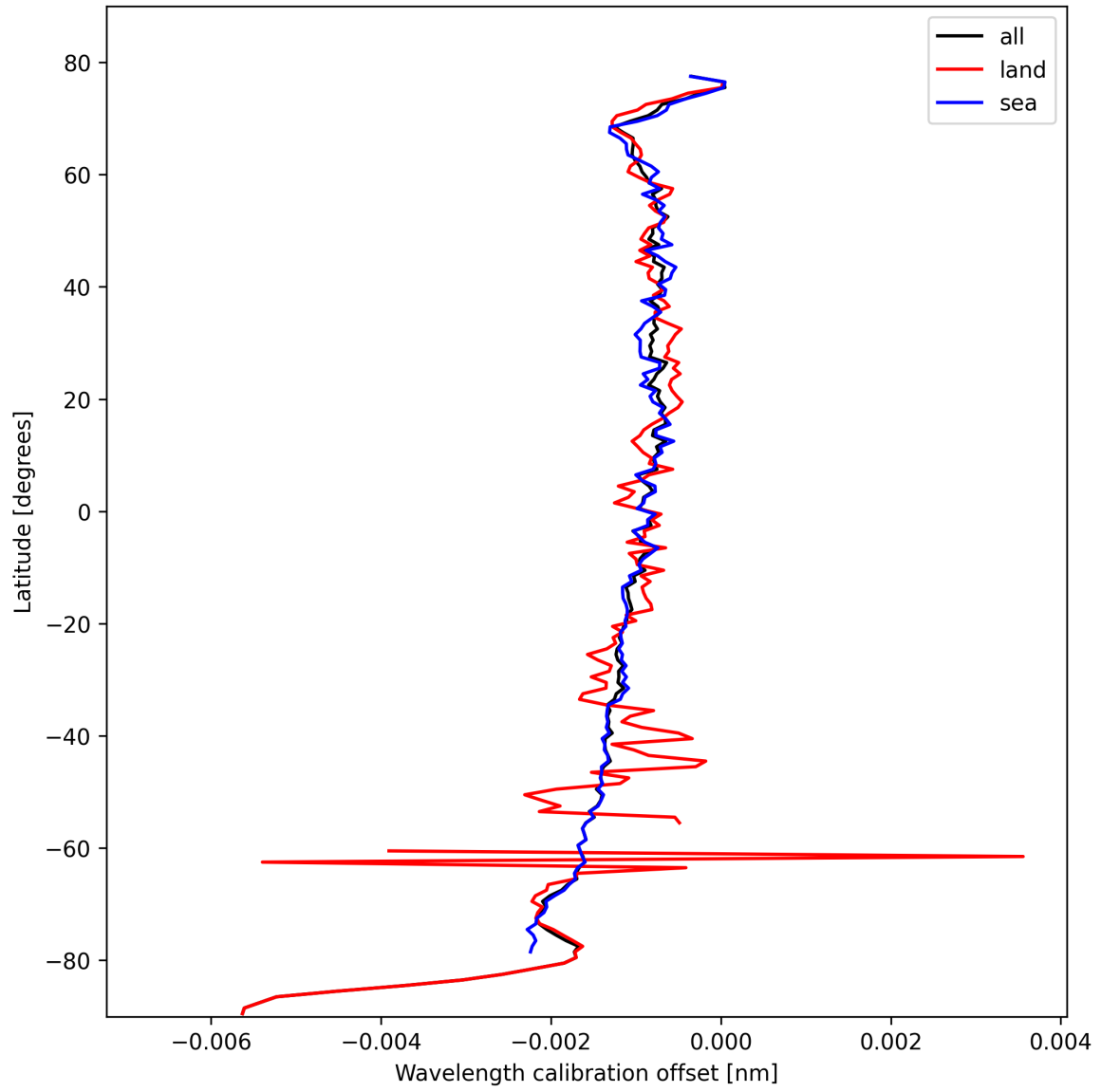
Figure 18: Zonal average of “Wavelength calibration offset” for 2024-10-20 to 2024-10-22.
