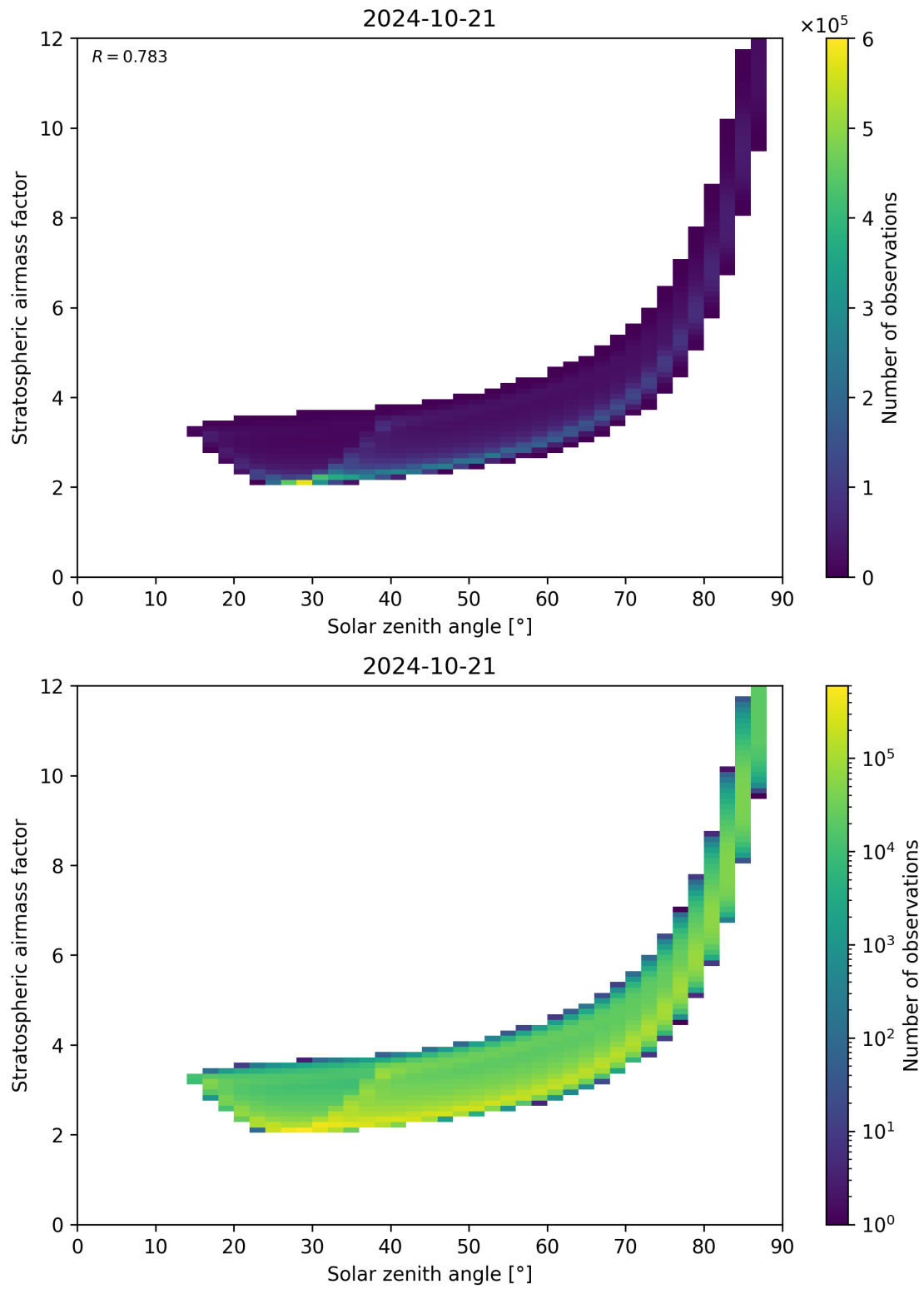
Figure 145: Scatter density plot of “Solar zenith angle” against “Stratospheric airmass factor” for 2024-10-20 to 2024-10-22.
