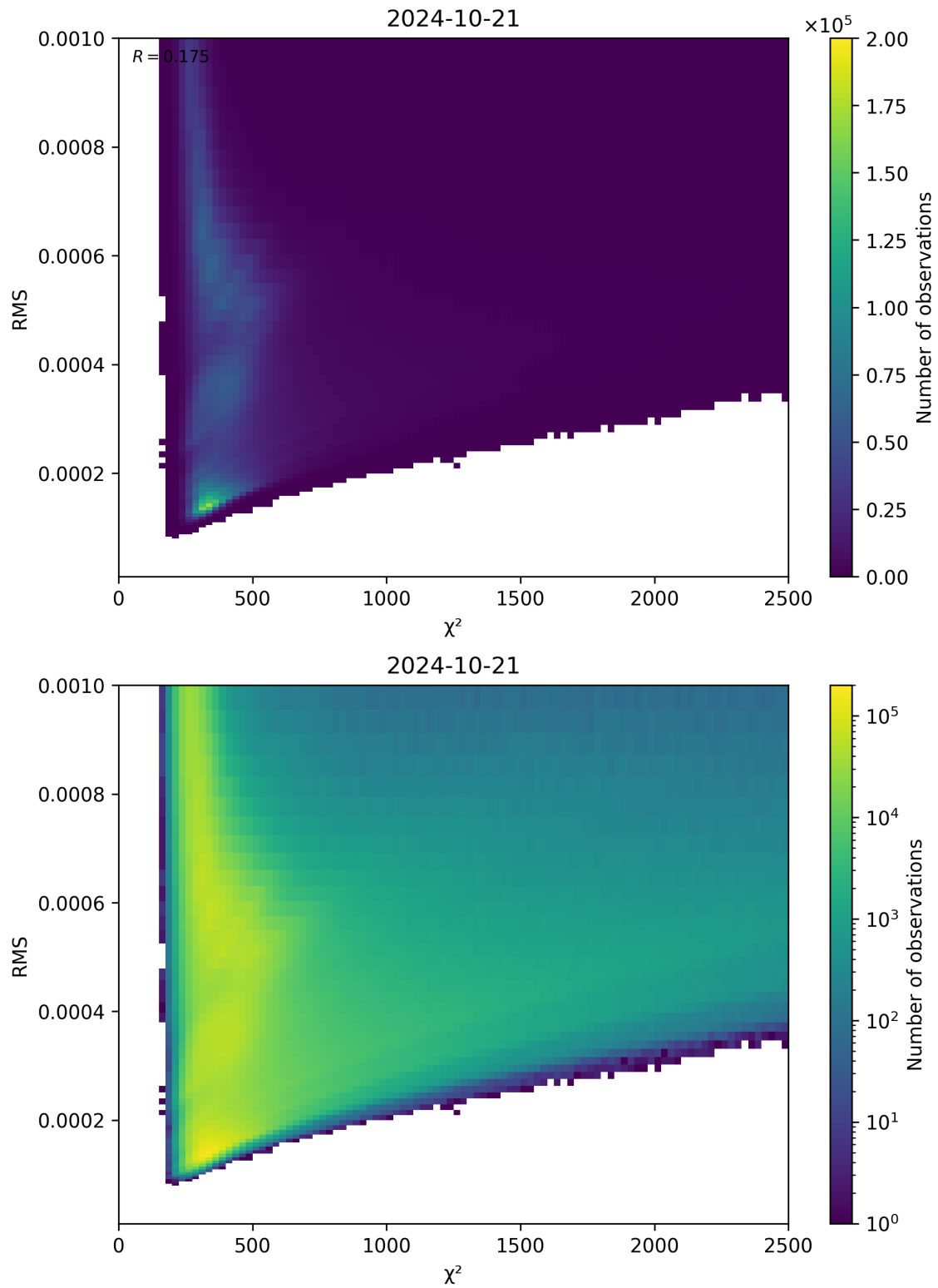
Figure 82: Scatter density plot of “ \chi^2 ” against “RMS” for 2024-10-20 to 2024-10-22.
