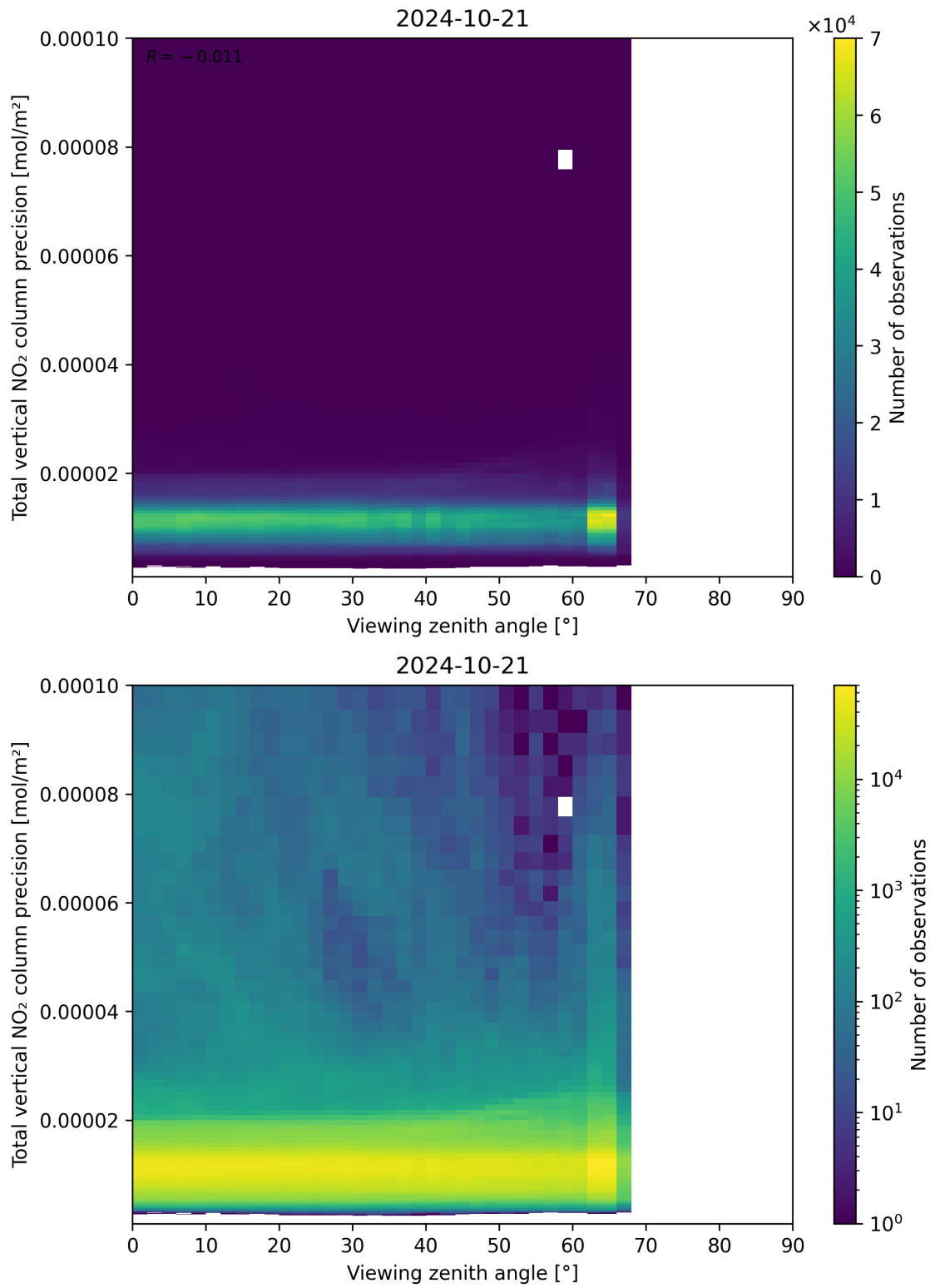
Figure 168: Scatter density plot of “Viewing zenith angle” against “Total vertical NO 2 column precision” for 2024-10-20 to 2024-10-22.
