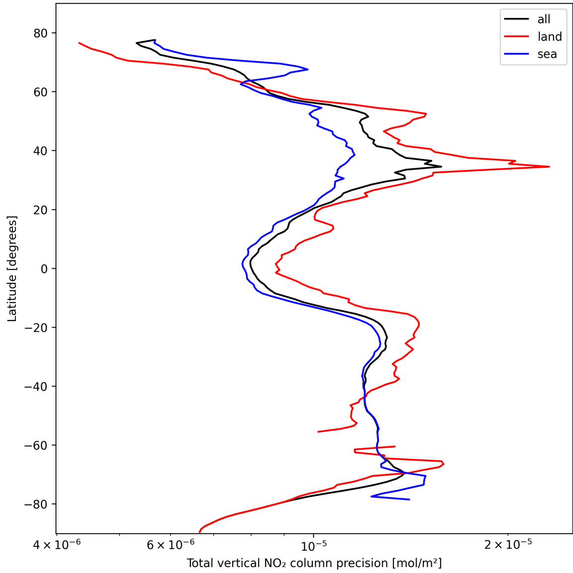
Figure 22: Zonal average of “Total vertical NO 2 column precision” for 2024-10-20 to 2024-10-22.
