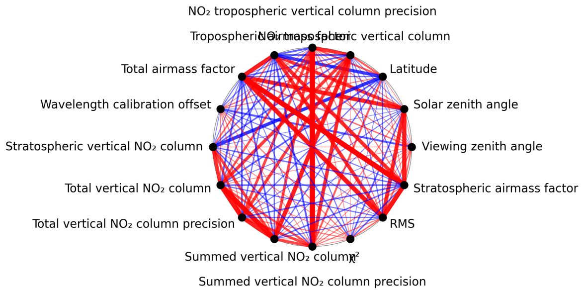
Figure 1: Map of correlation graph for 2024-10-20 to 2024-10-22.
