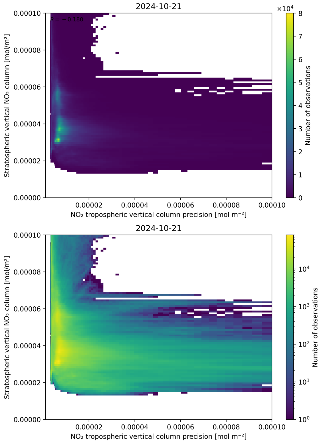
Figure 135: Scatter density plot of “NO 2 tropospheric vertical column precision” against “Stratospheric vertical NO 2 column” for 2024-10-20 to 2024-10-22.
