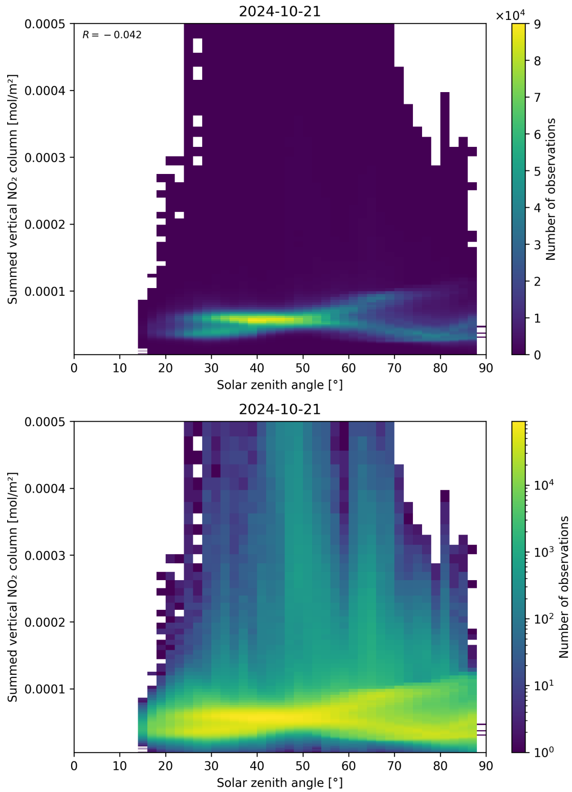
Figure 151: Scatter density plot of “Solar zenith angle” against “Summed vertical NO 2 column” for 2024-10-20 to 2024-10-22.
