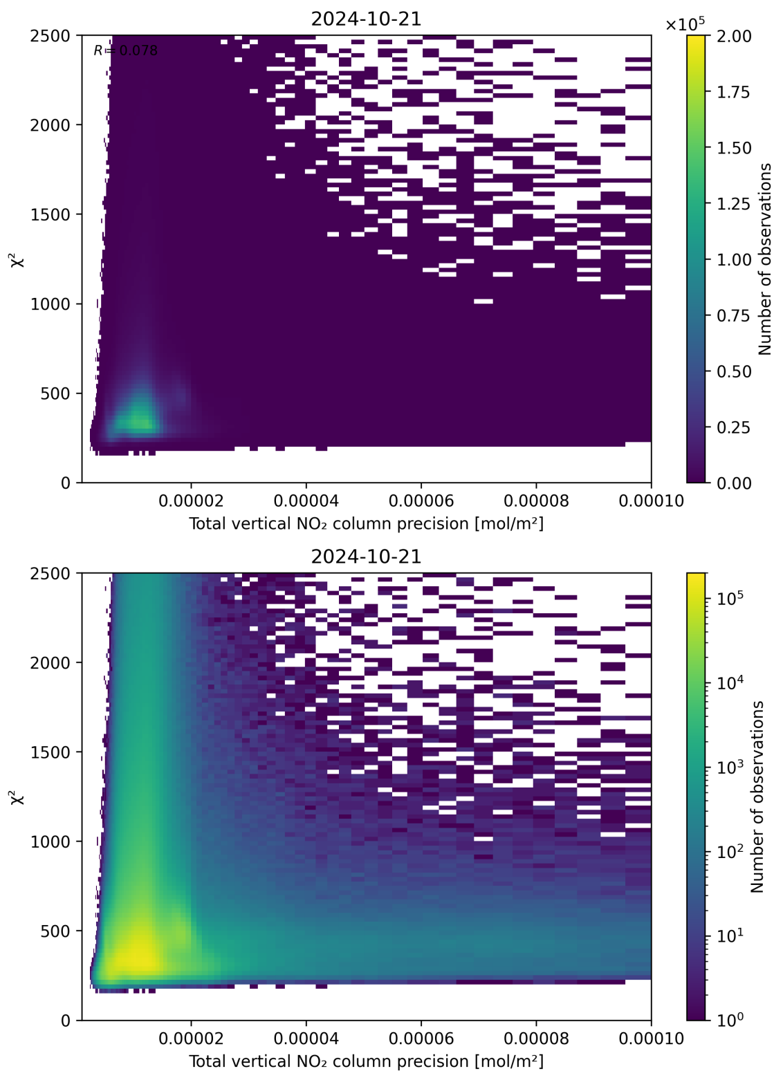
Figure 116: Scatter density plot of “Total vertical NO 2 column precision” against “ \chi^2 ” for 2024-10-20 to 2024-10-22.
