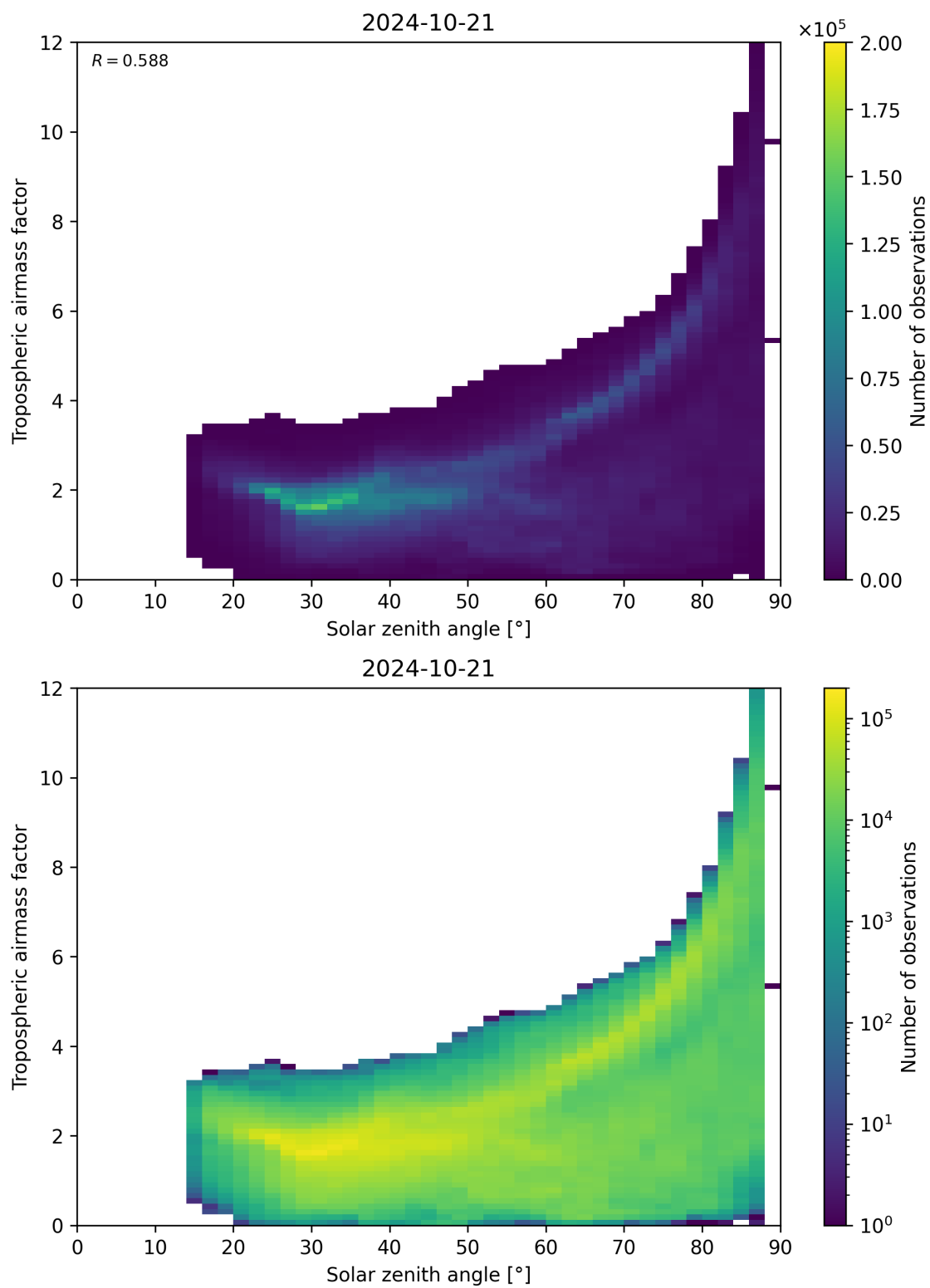
Figure 147: Scatter density plot of “Solar zenith angle” against “Tropospheric airmass factor” for 2024-10-20 to 2024-10-22.
