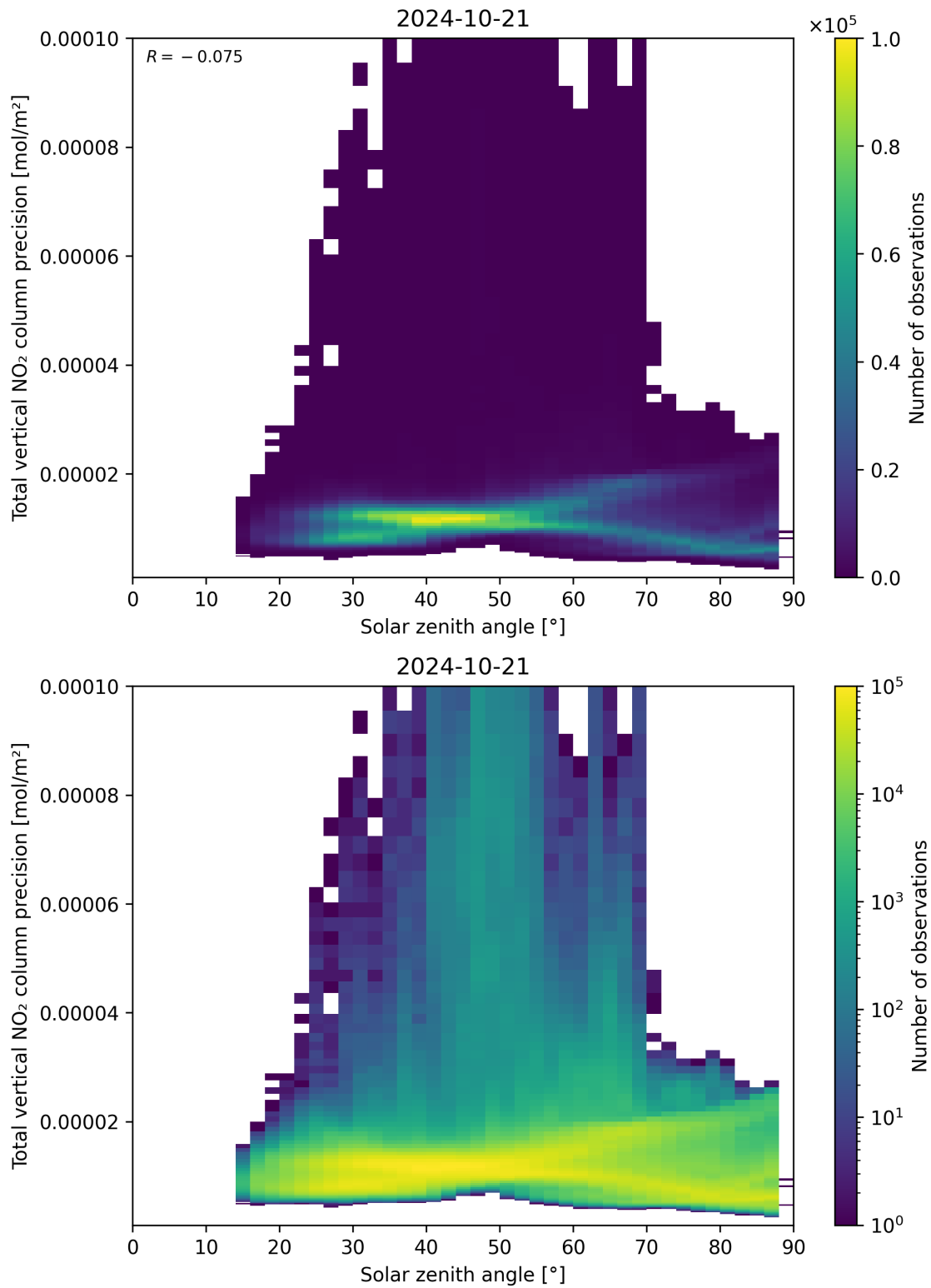
Figure 154: Scatter density plot of “Solar zenith angle” against “Total vertical NO 2 column precision” for 2024-10-20 to 2024-10-22.
