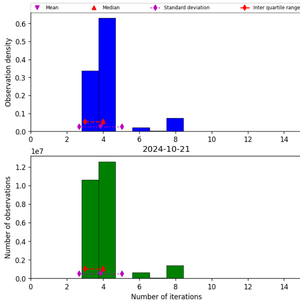
Figure 34: Histogram of “Number of iterations” for 2024-10-20 to 2024-10-22
