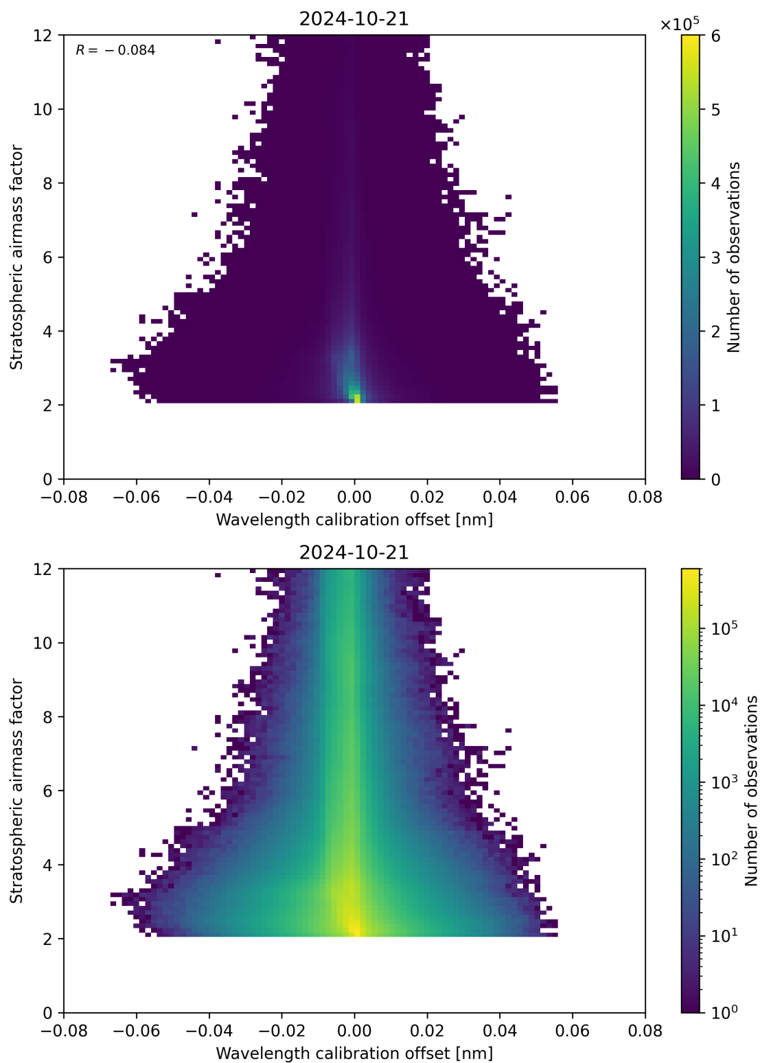
Figure 174: Scatter density plot of “Wavelength calibration offset” against “Stratospheric airmass factor” for 2024-10-20 to 2024-10-22.
