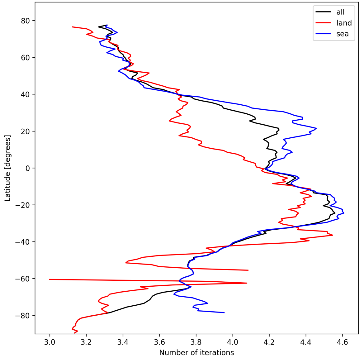
Figure 17: Zonal average of “Number of iterations” for 2024-10-20 to 2024-10-22.
