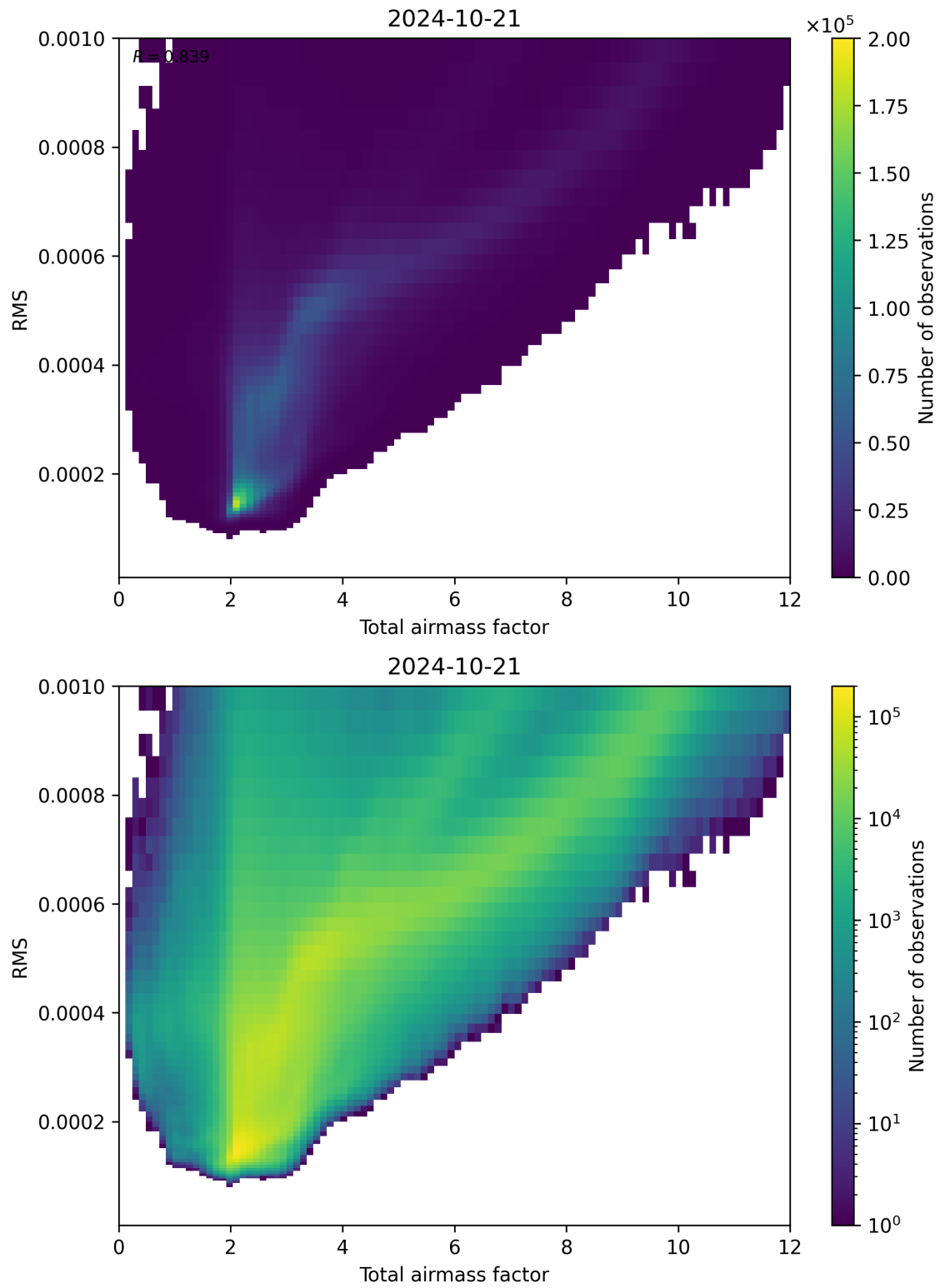
Figure 69: Scatter density plot of “Total airmass factor” against “RMS” for 2024-10-20 to 2024-10-22.
