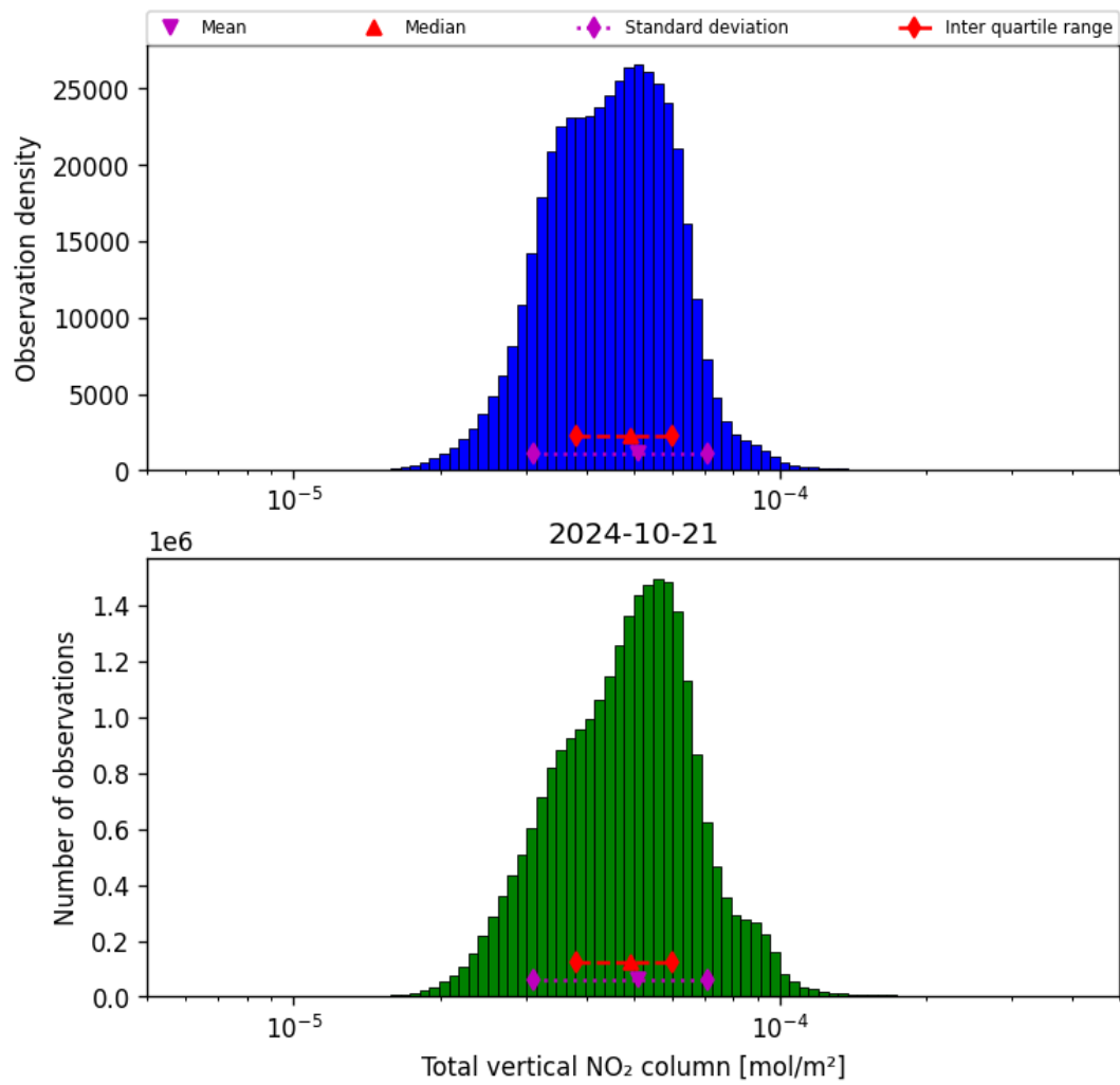
Figure 38: Histogram of “Total vertical NO 2 column” for 2024-10-20 to 2024-10-22
