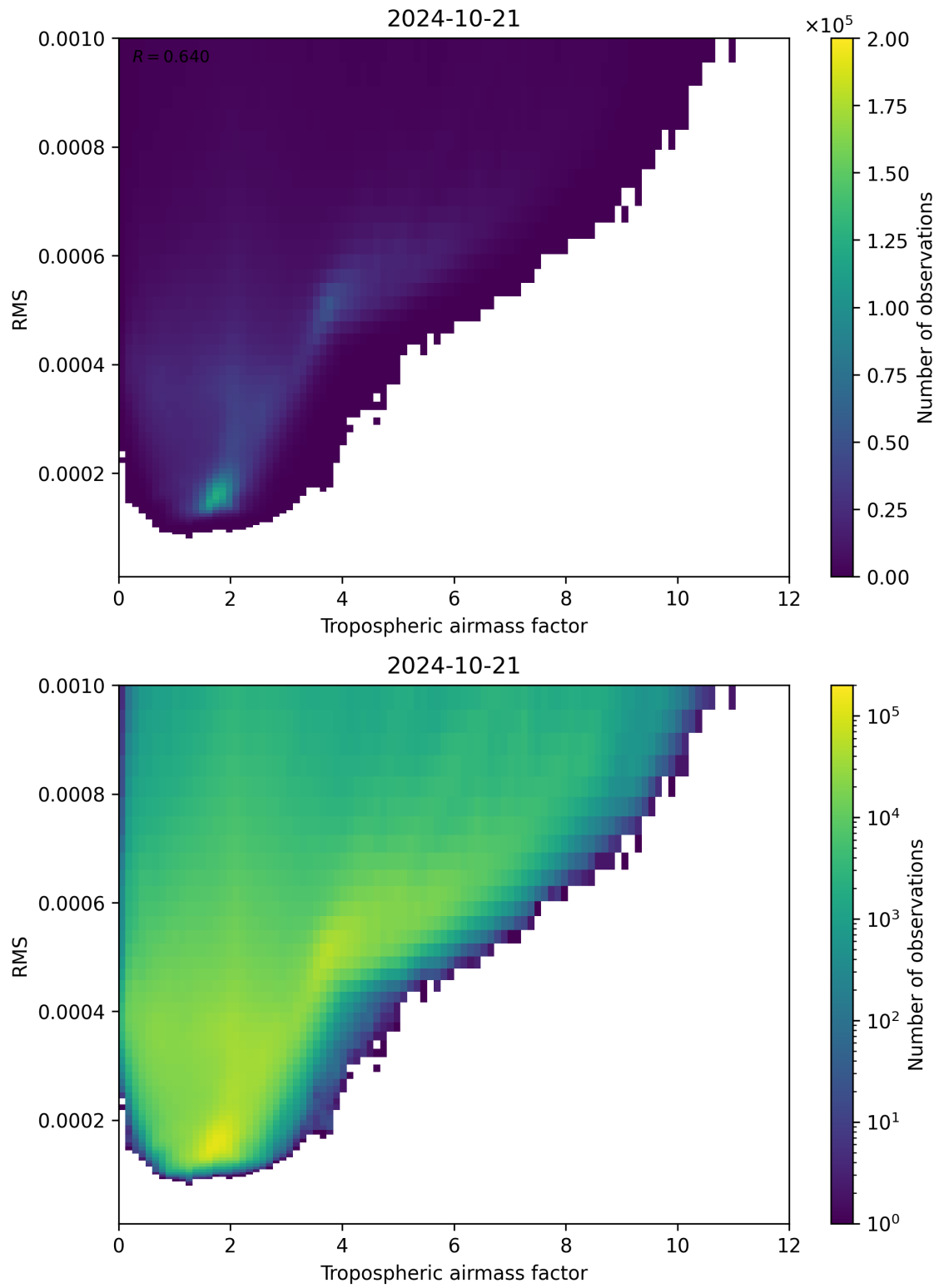
Figure 79: Scatter density plot of “Tropospheric airmass factor” against “RMS” for 2024-10-20 to 2024-10-22.
