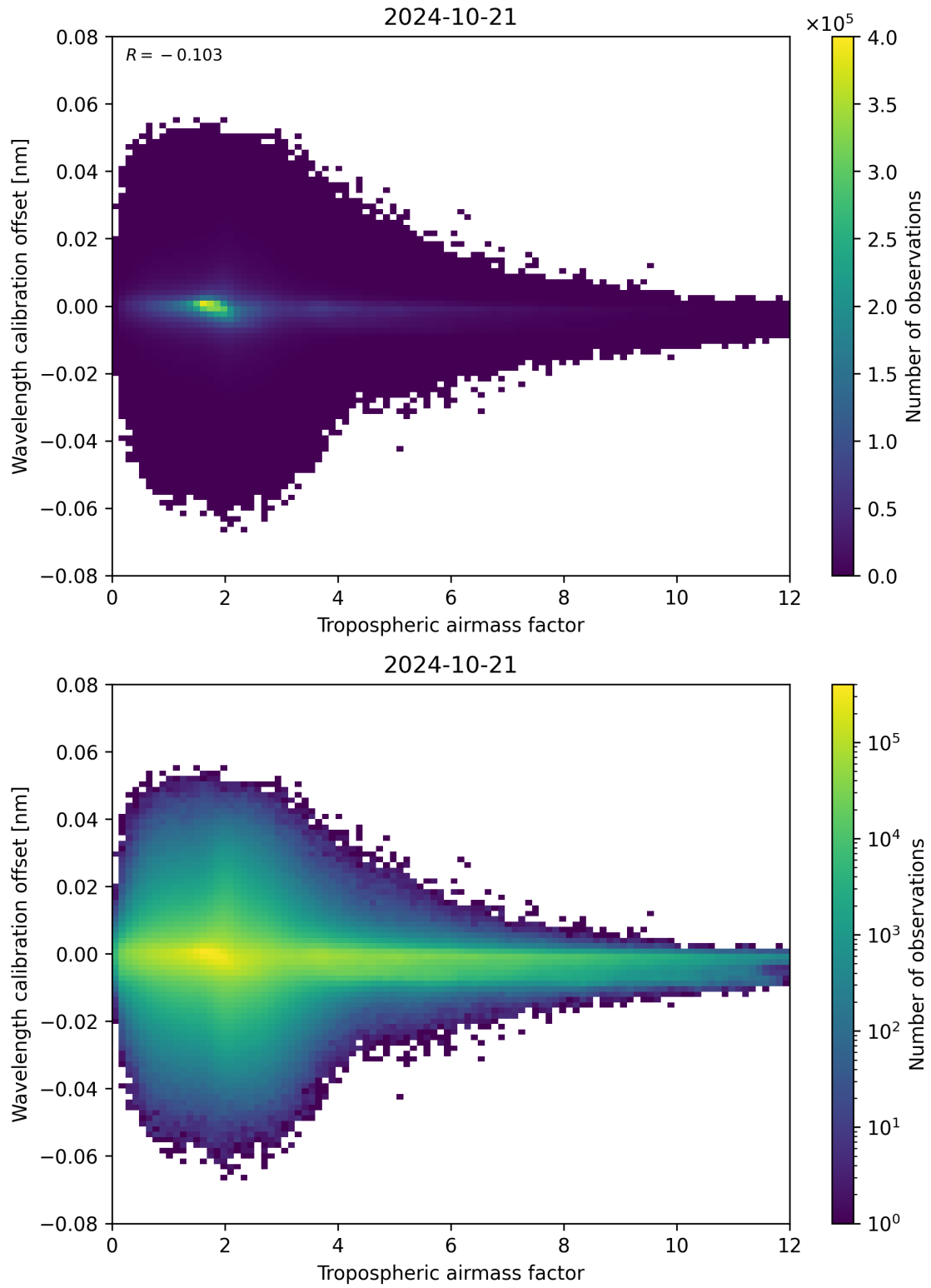
Figure 80: Scatter density plot of “Tropospheric airmass factor” against “Wavelength calibration offset” for 2024-10-20 to 2024-10-22.
