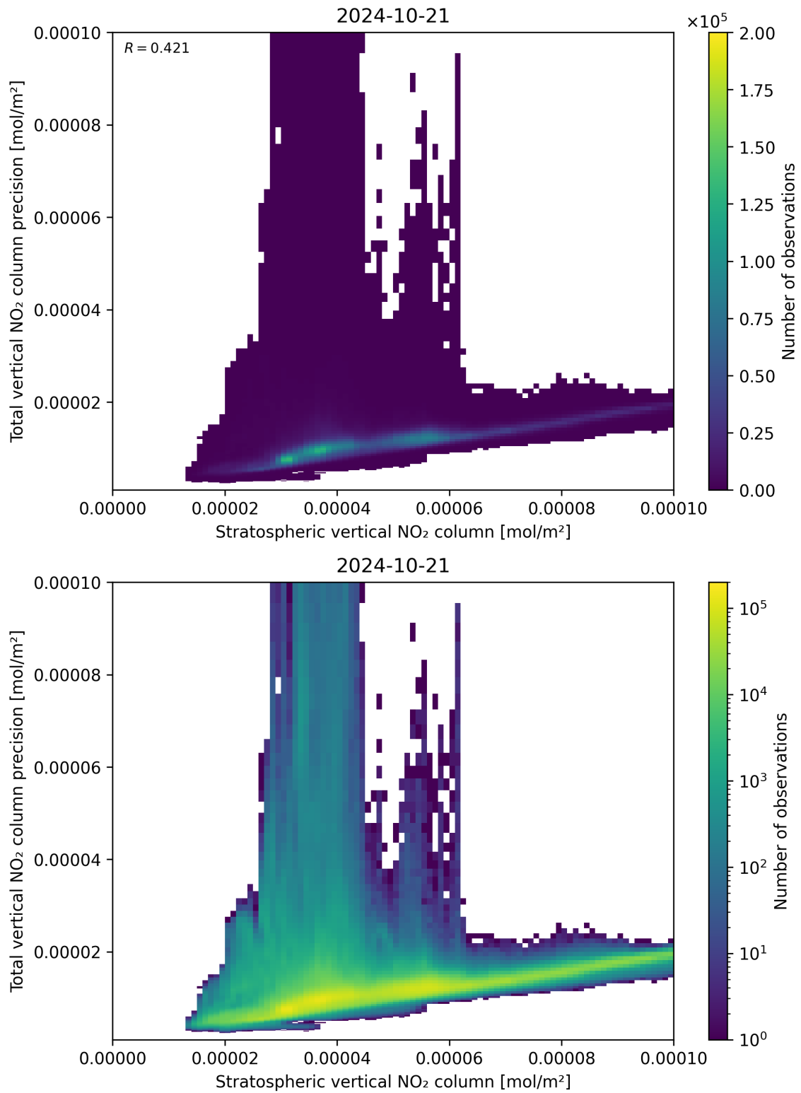
Figure 101: Scatter density plot of “Stratospheric vertical NO 2 column” against “Total vertical NO 2 column precision” for 2024-10-20 to 2024-10-22.
