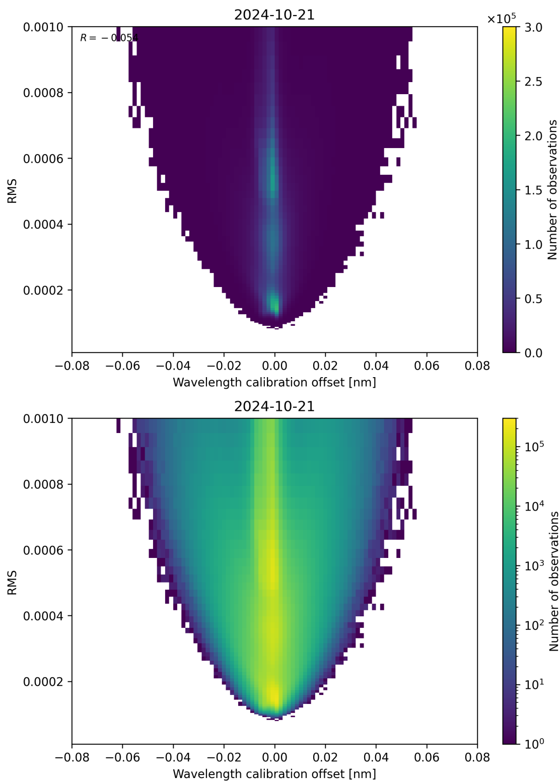
Figure 181: Scatter density plot of “Wavelength calibration offset” against “RMS” for 2024-10-20 to 2024-10-22.
