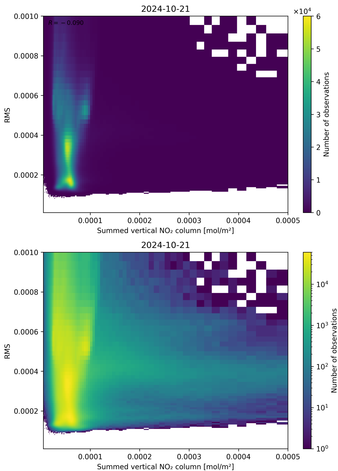
Figure 109: Scatter density plot of “Summed vertical NO 2 column” against “RMS” for 2024-10-20 to 2024-10-22.
