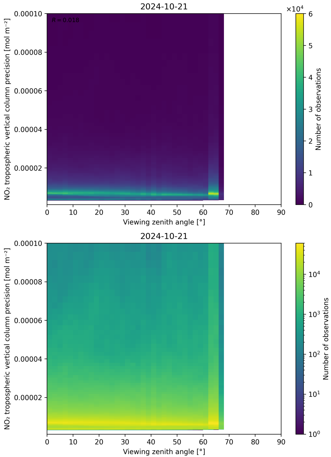
Figure 170: Scatter density plot of “Viewing zenith angle” against “NO 2 tropospheric vertical column precision” for 2024-10-20 to 2024-10-22.
