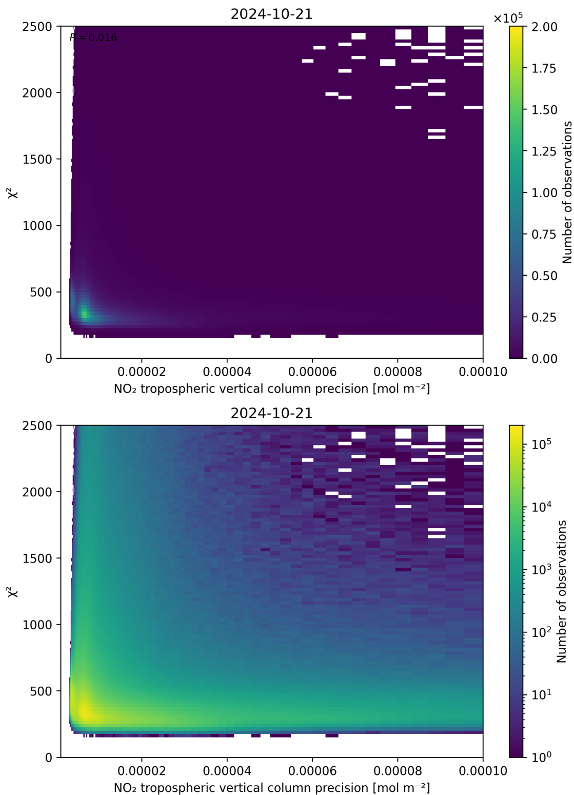
Figure 134: Scatter density plot of “NO 2 tropospheric vertical column precision” against “ \chi^2 ” for 2024-10-20 to 2024-10-22.
