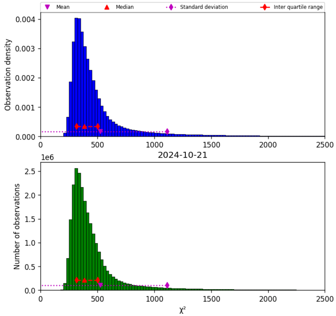
Figure 42: Histogram of “ \chi^2 ” for 2024-10-20 to 2024-10-22
