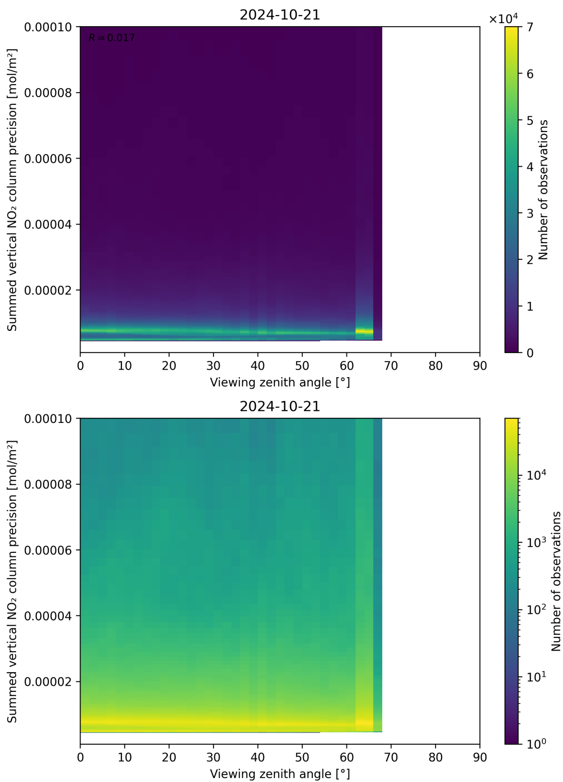
Figure 166: Scatter density plot of “Viewing zenith angle” against “Summed vertical NO 2 column precision” for 2024-10-20 to 2024-10-22.
