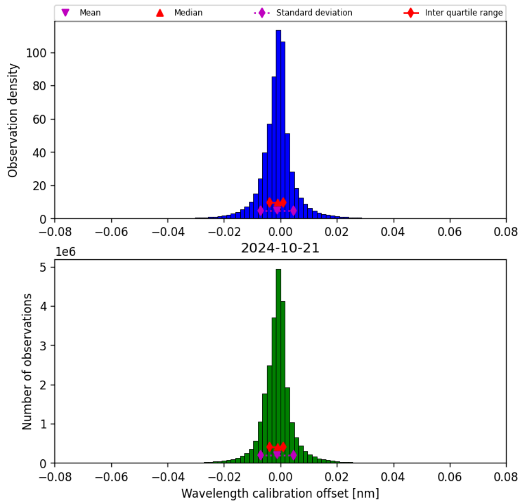
Figure 35: Histogram of “Wavelength calibration offset” for 2024-10-20 to 2024-10-22
