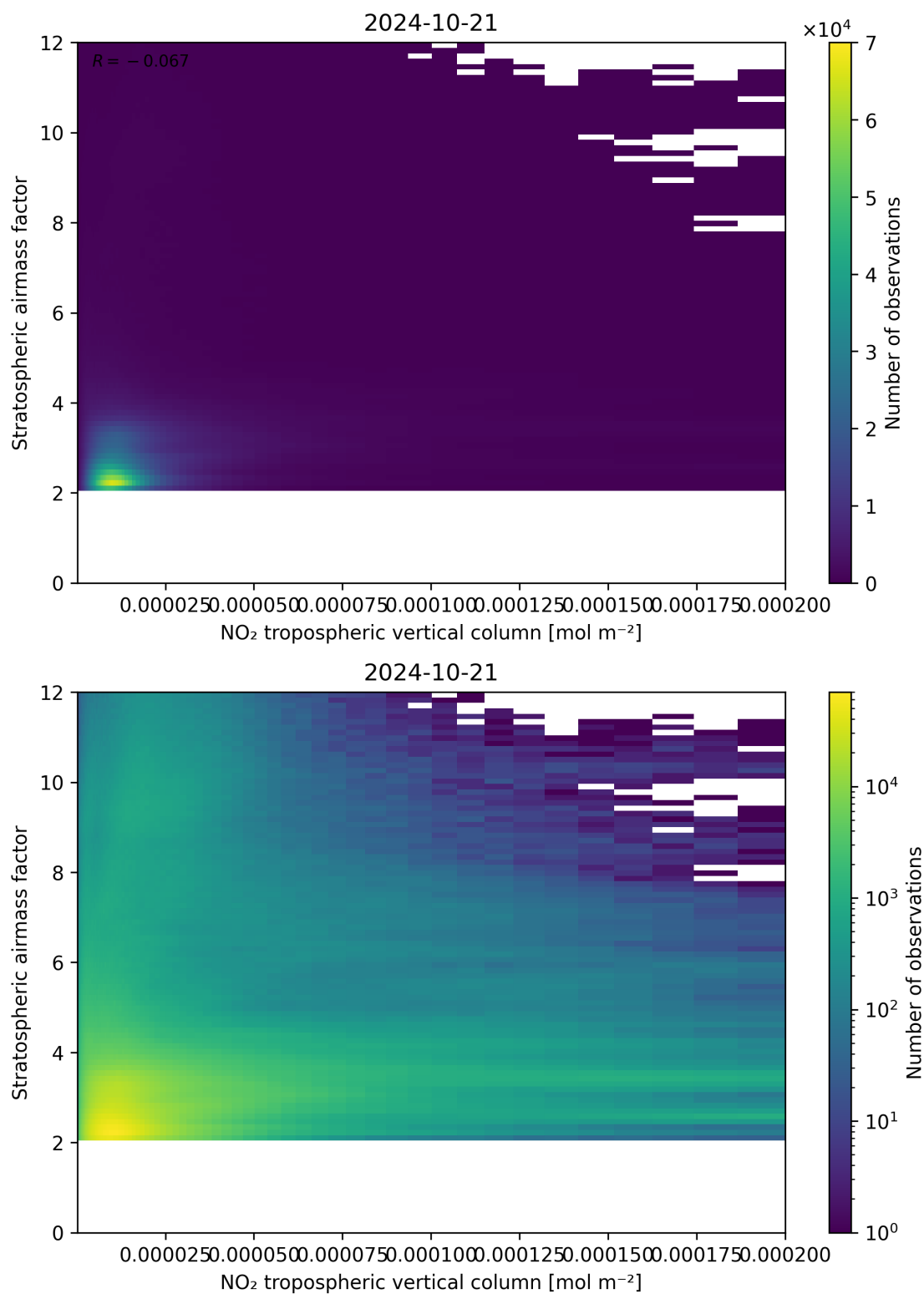
Figure 121: Scatter density plot of “NO 2 tropospheric vertical column” against “Stratospheric airmass factor” for 2024-10-20 to 2024-10-22.
