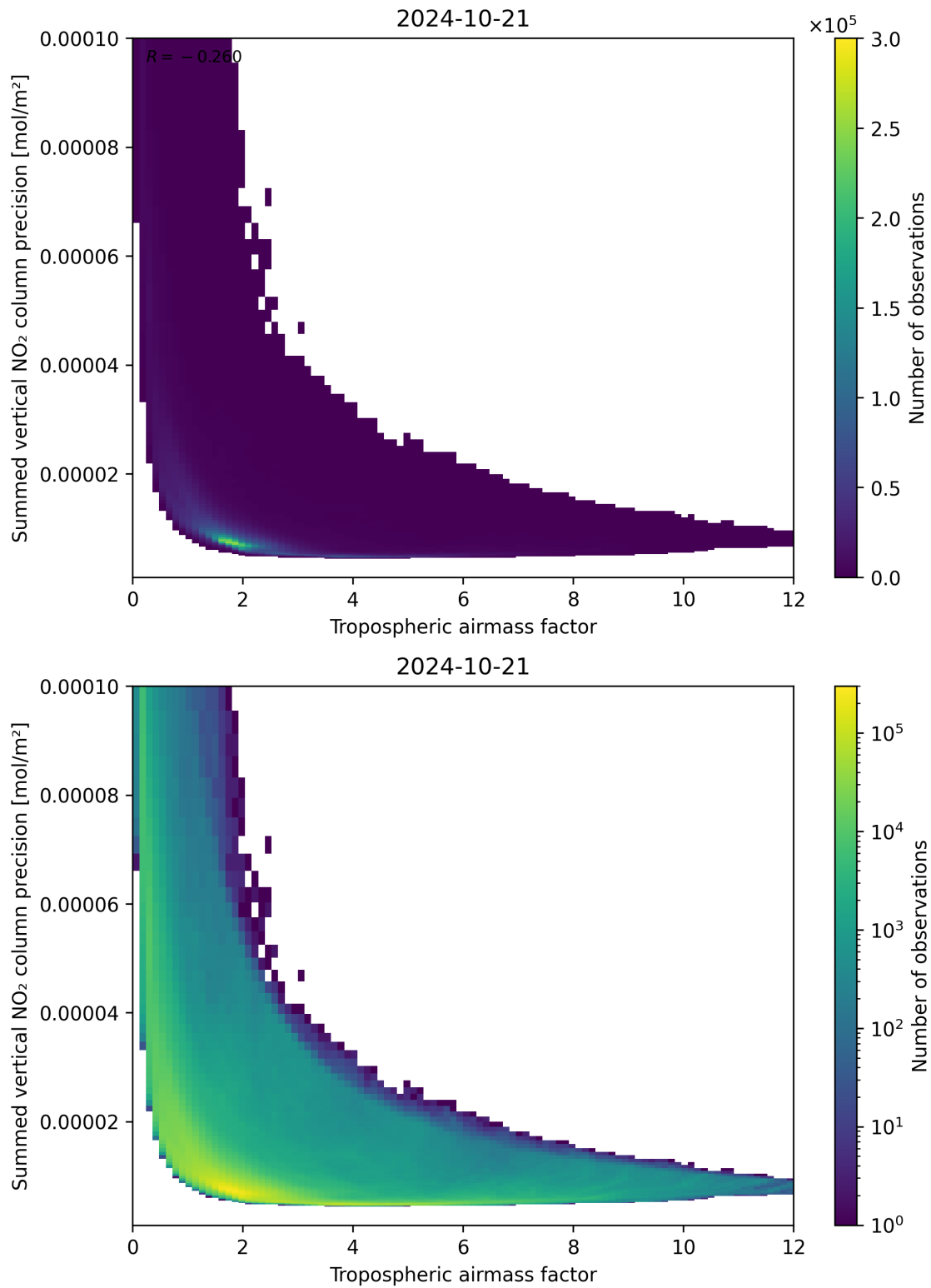
Figure 76: Scatter density plot of “Tropospheric airmass factor” against “Summed vertical NO 2 column precision” for 2024-10-20 to 2024-10-22.
