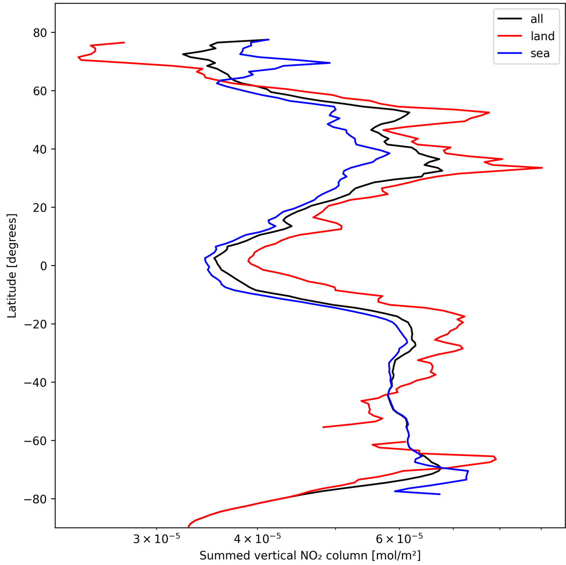
Figure 23: Zonal average of “Summed vertical NO 2 column” for 2024-10-20 to 2024-10-22.
