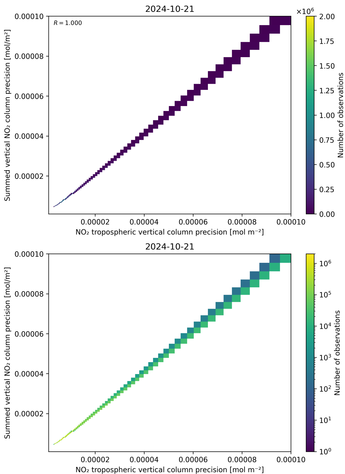
Figure 137: Scatter density plot of “NO 2 tropospheric vertical column precision” against “Summed vertical NO 2 column precision” for 2024-10-20 to 2024-10-22.
