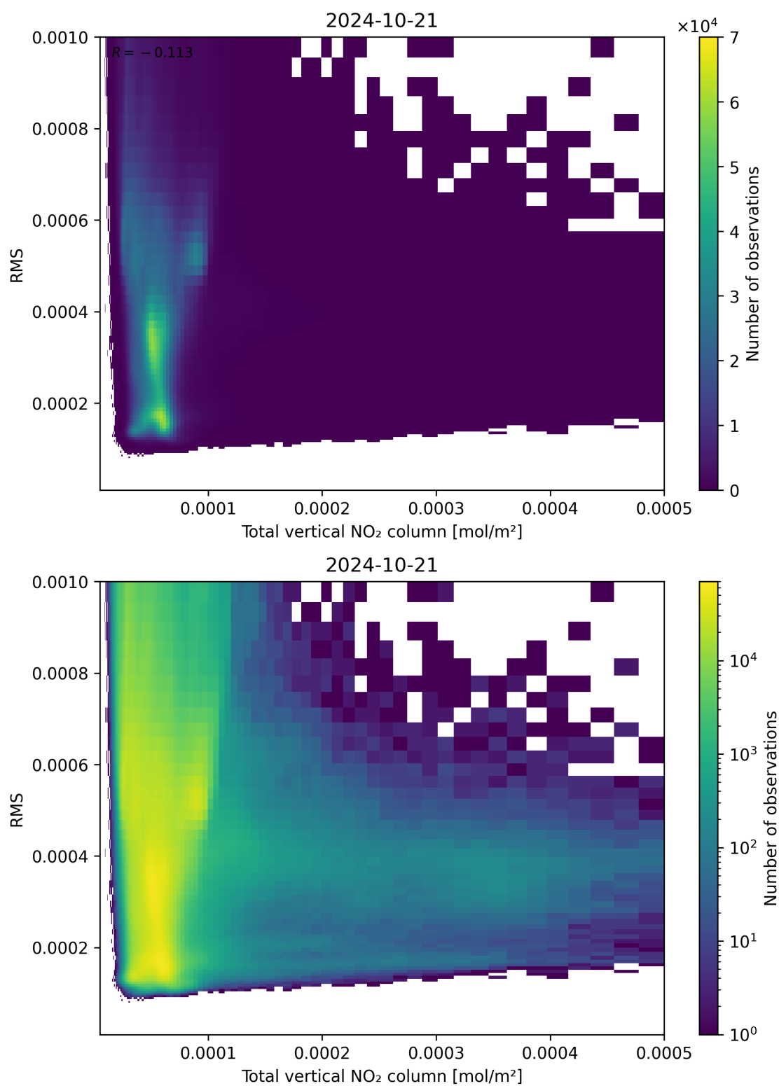
Figure 120: Scatter density plot of “Total vertical NO 2 column” against “RMS” for 2024-10-20 to 2024-10-22.
