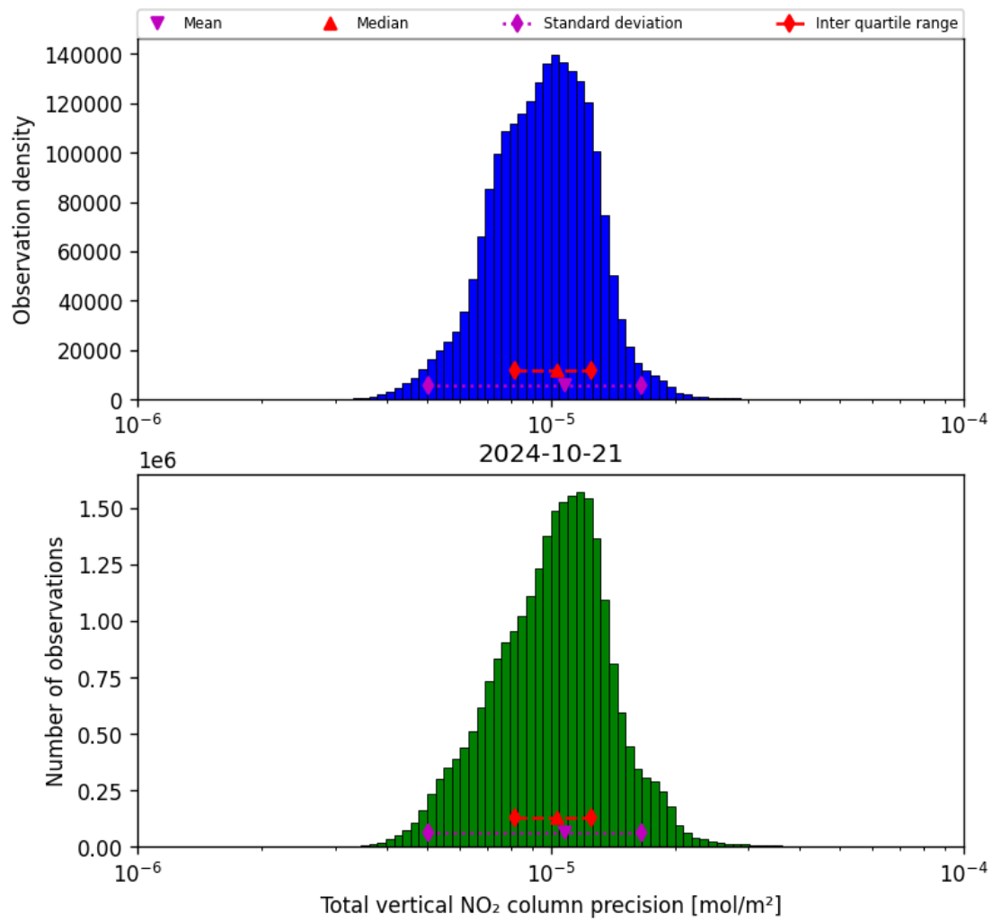
Figure 39: Histogram of “Total vertical NO 2 column precision” for 2024-10-20 to 2024-10-22
