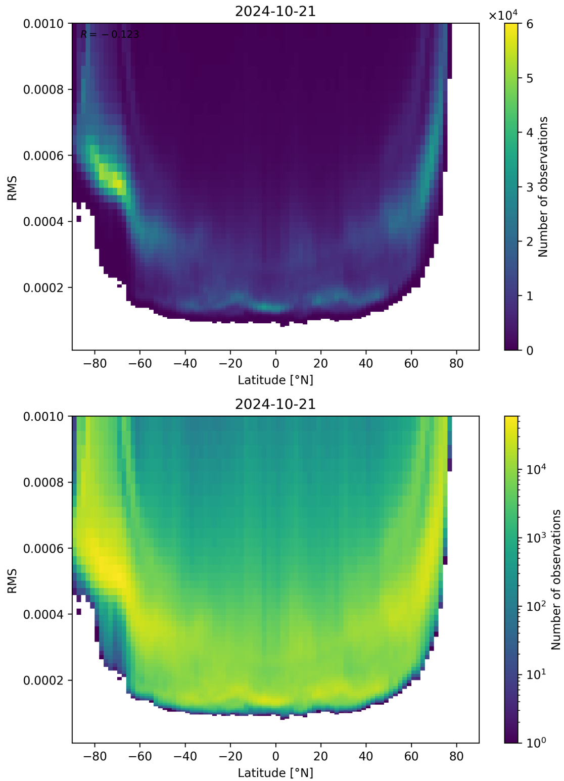
Figure 94: Scatter density plot of “Latitude” against “RMS” for 2024-10-20 to 2024-10-22.
