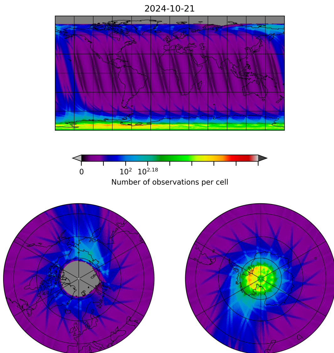
Figure 10: Map of the number of observations for 2024-10-20 to 2024-10-22
