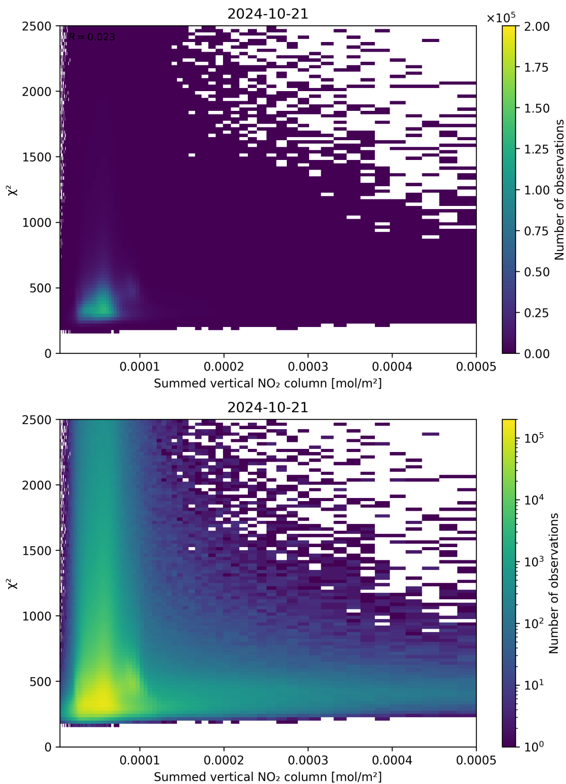
Figure 104: Scatter density plot of “Summed vertical NO 2 column” against “ \chi^2 ” for 2024-10-20 to 2024-10-22.
