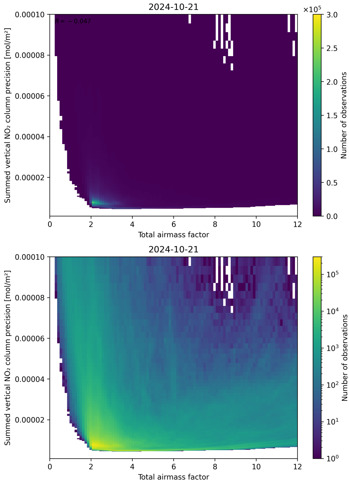
Figure 66: Scatter density plot of “Total airmass factor” against “Summed vertical NO 2 column precision” for 2024-10-20 to 2024-10-22.
