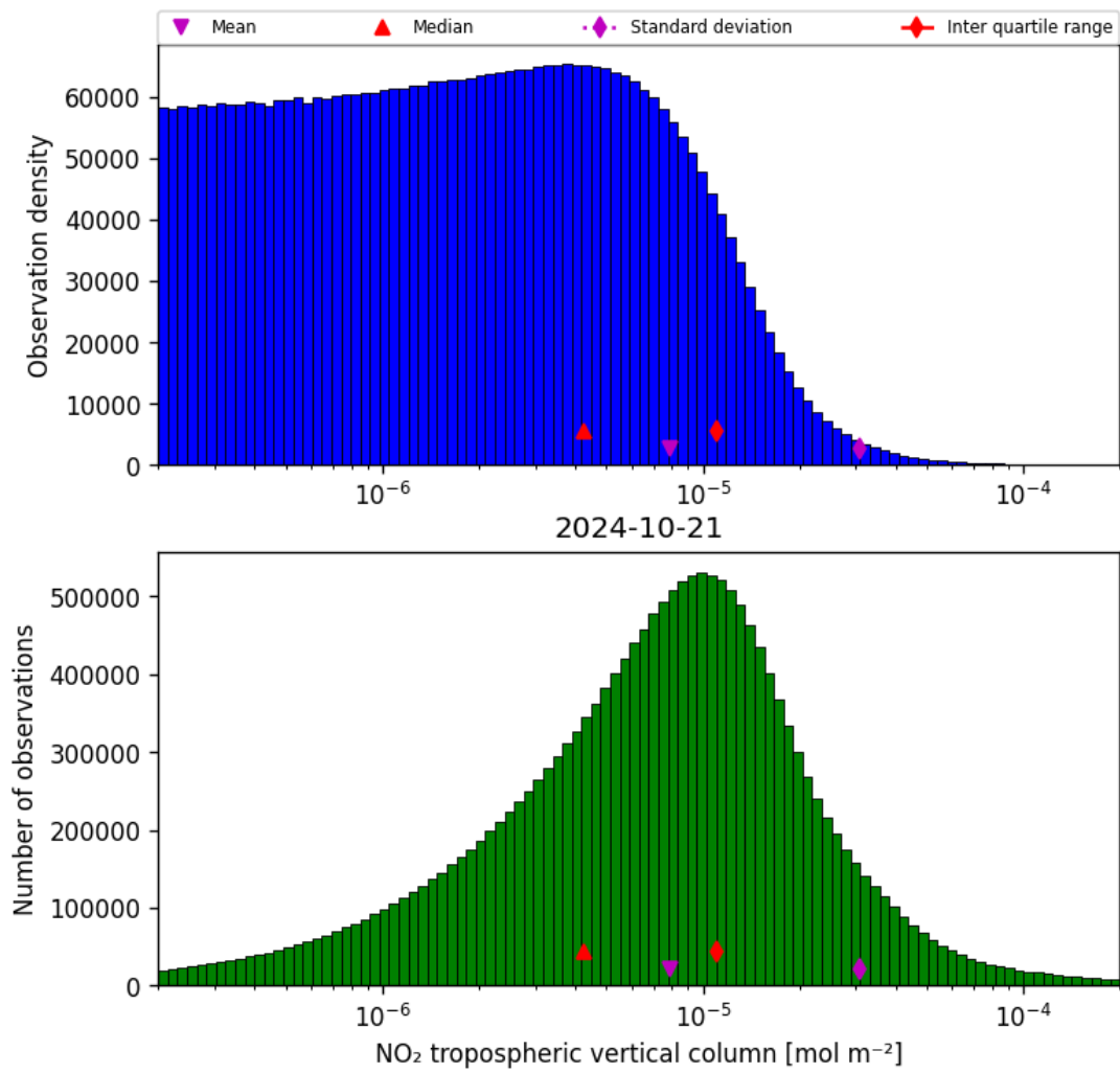
Figure 29: Histogram of “NO 2 tropospheric vertical column” for 2024-10-20 to 2024-10-22
