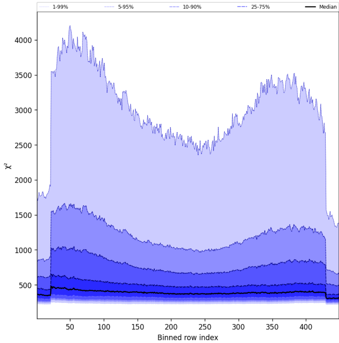
Figure 59: Along track statistics of “ \chi^2 ” for 2024-10-20 to 2024-10-22
