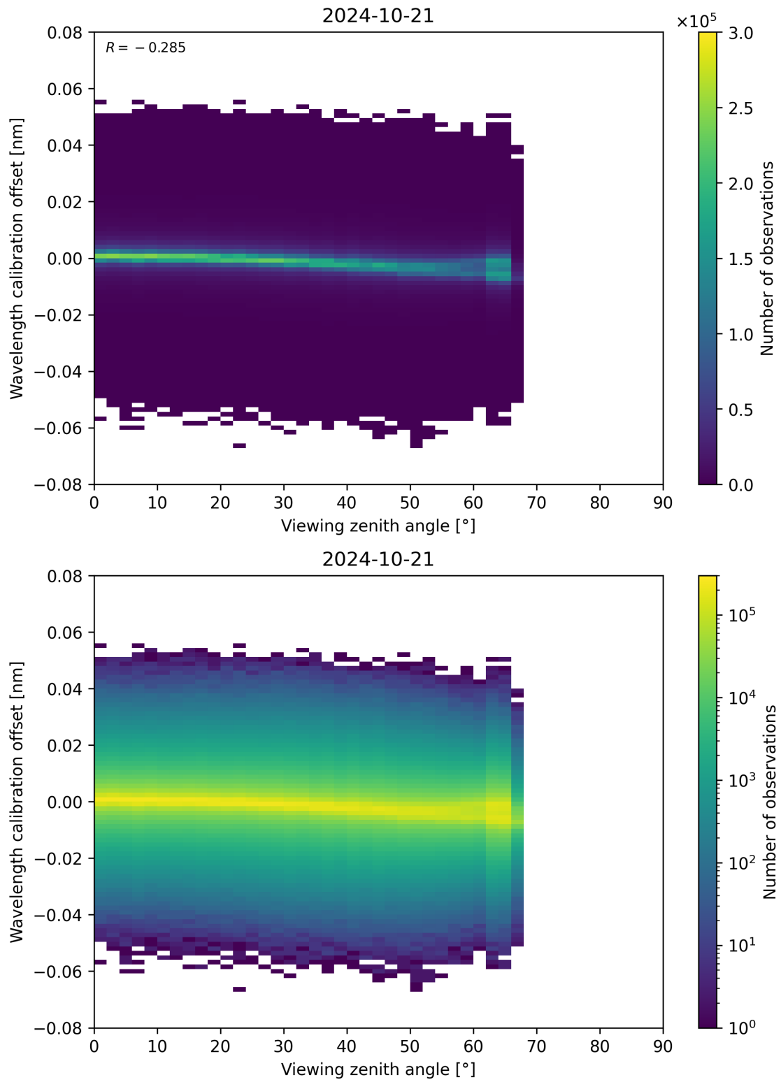
Figure 173: Scatter density plot of “Viewing zenith angle” against “Wavelength calibration offset” for 2024-10-20 to 2024-10-22.
