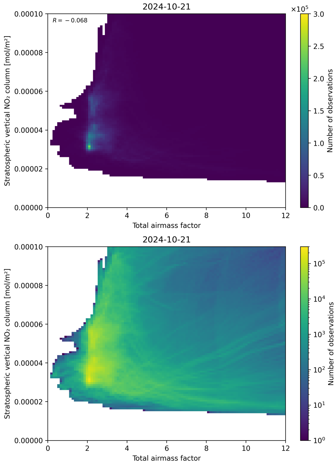
Figure 64: Scatter density plot of “Total airmass factor” against “Stratospheric vertical NO 2 column” for 2024-10-20 to 2024-10-22.
