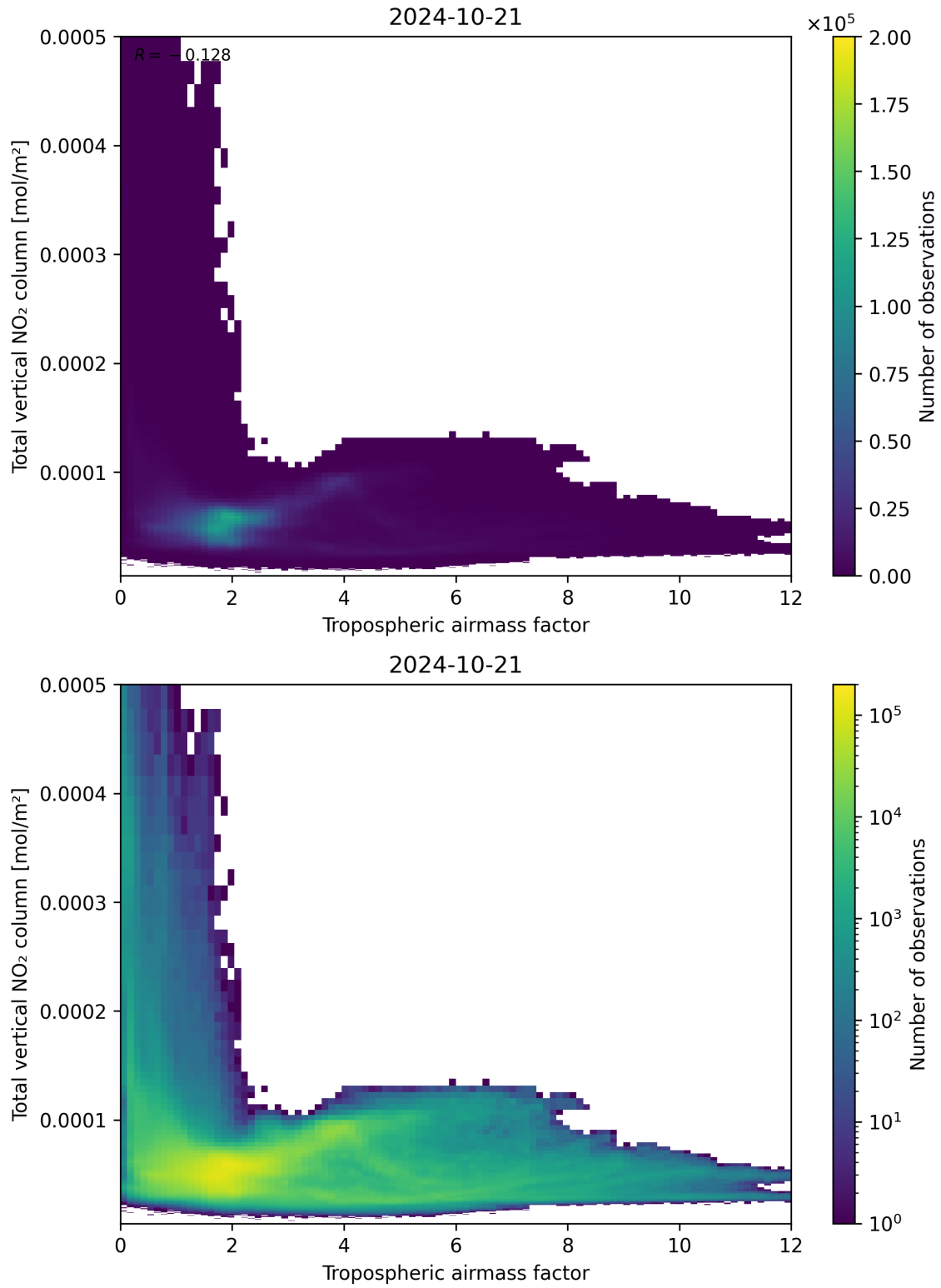
Figure 77: Scatter density plot of “Tropospheric airmass factor” against “Total vertical NO 2 column” for 2024-10-20 to 2024-10-22.
