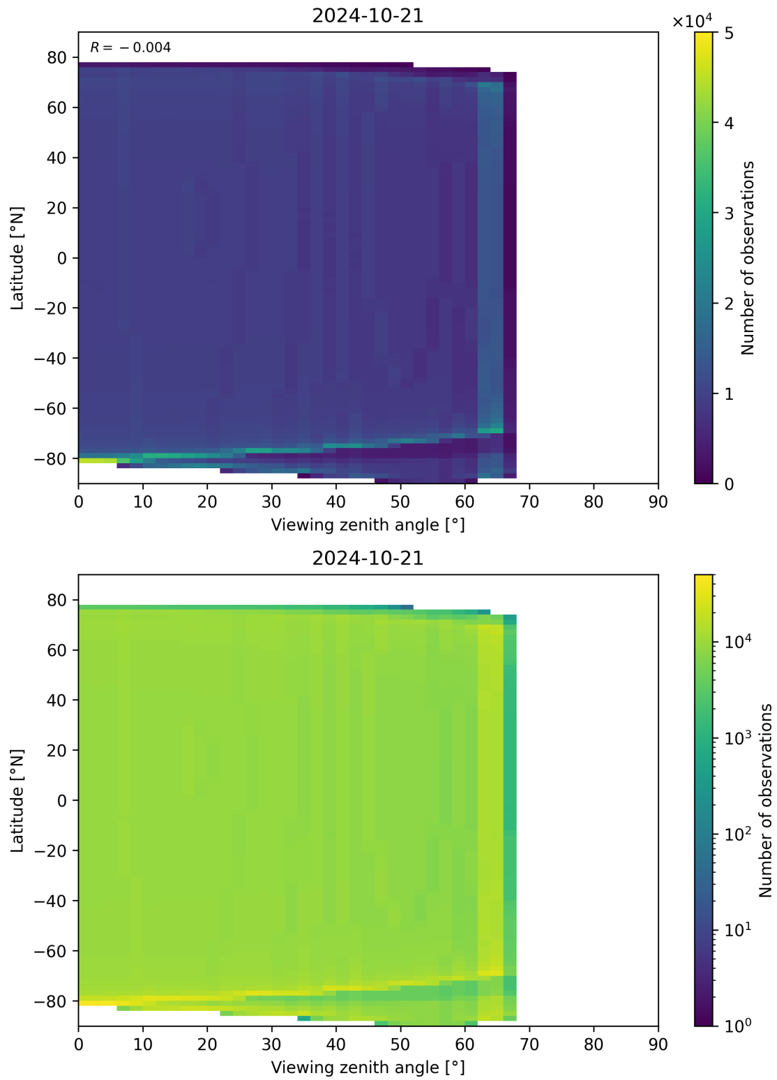
Figure 163: Scatter density plot of “Viewing zenith angle” against “Latitude” for 2024-10-20 to 2024-10-22.
