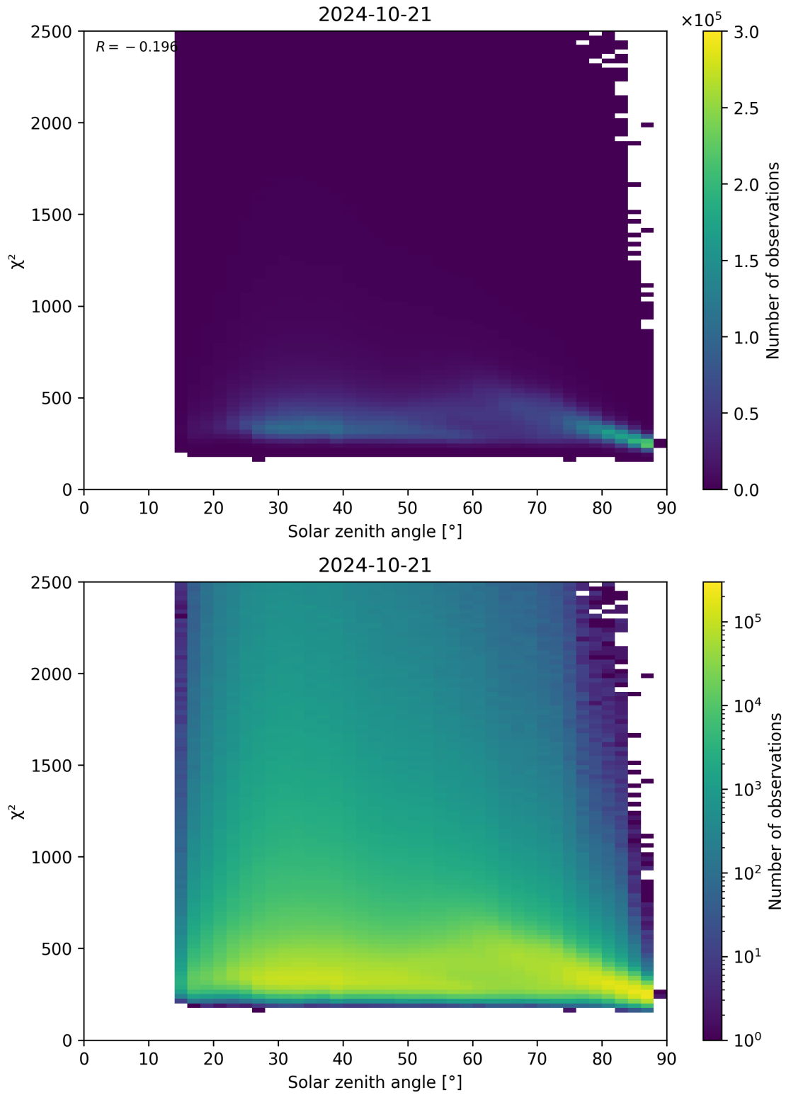
Figure 148: Scatter density plot of “Solar zenith angle” against “ \chi^2 ” for 2024-10-20 to 2024-10-22.
