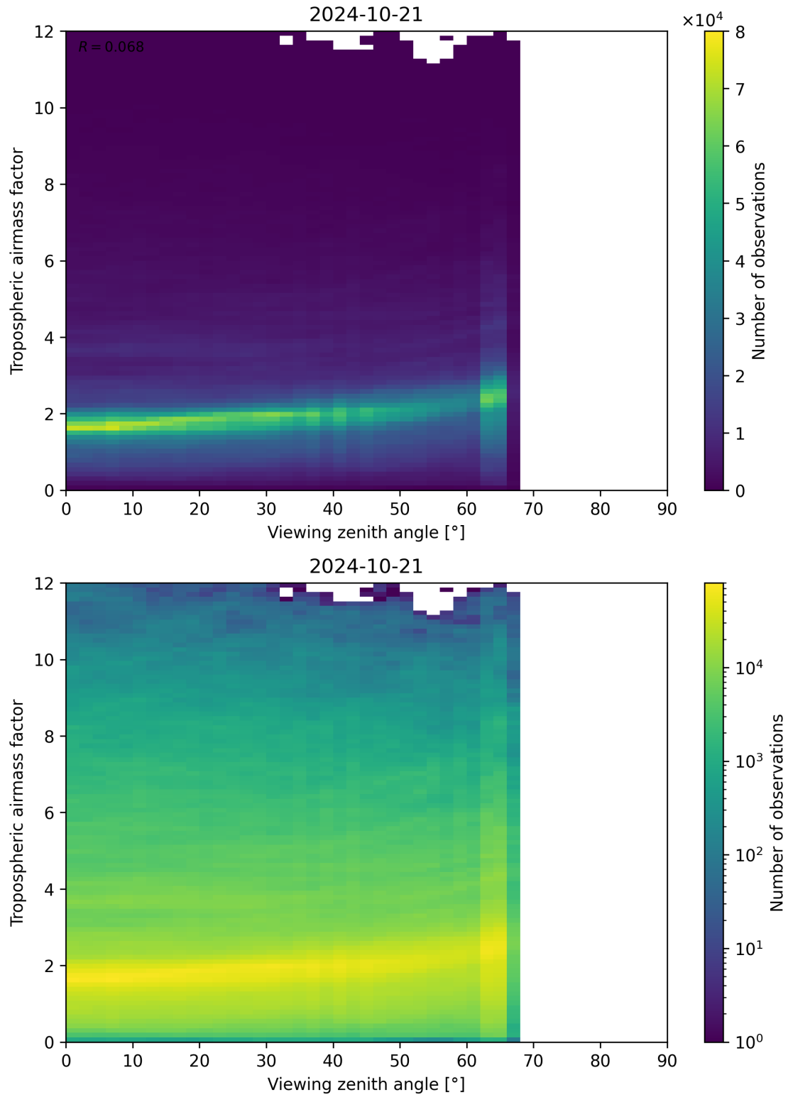
Figure 161: Scatter density plot of “Viewing zenith angle” against “Tropospheric airmass factor” for 2024-10-20 to 2024-10-22.
