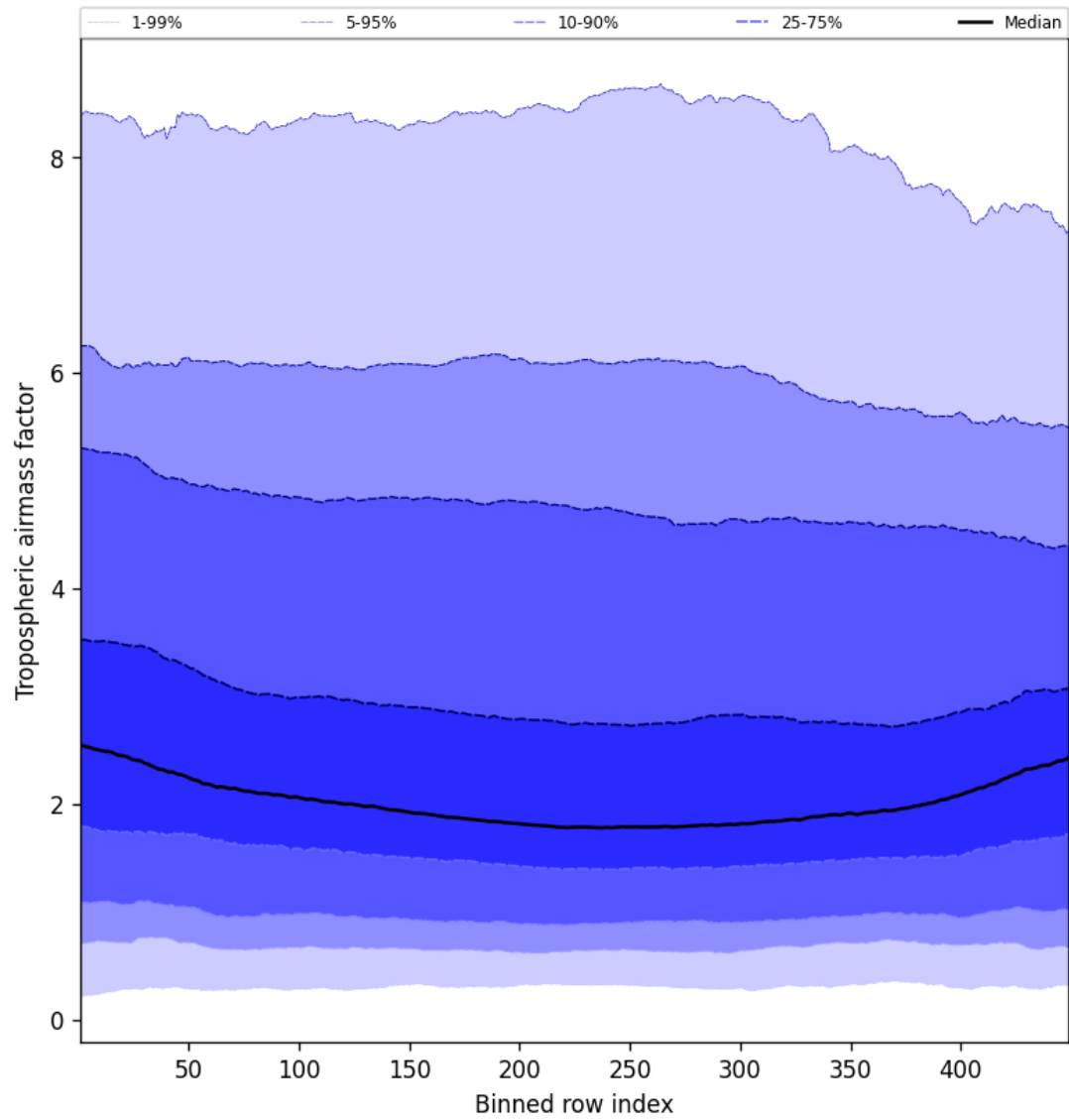
Figure 48: Along track statistics of “Tropospheric air mass factor” for 2024-10-20 to 2024-10-22
