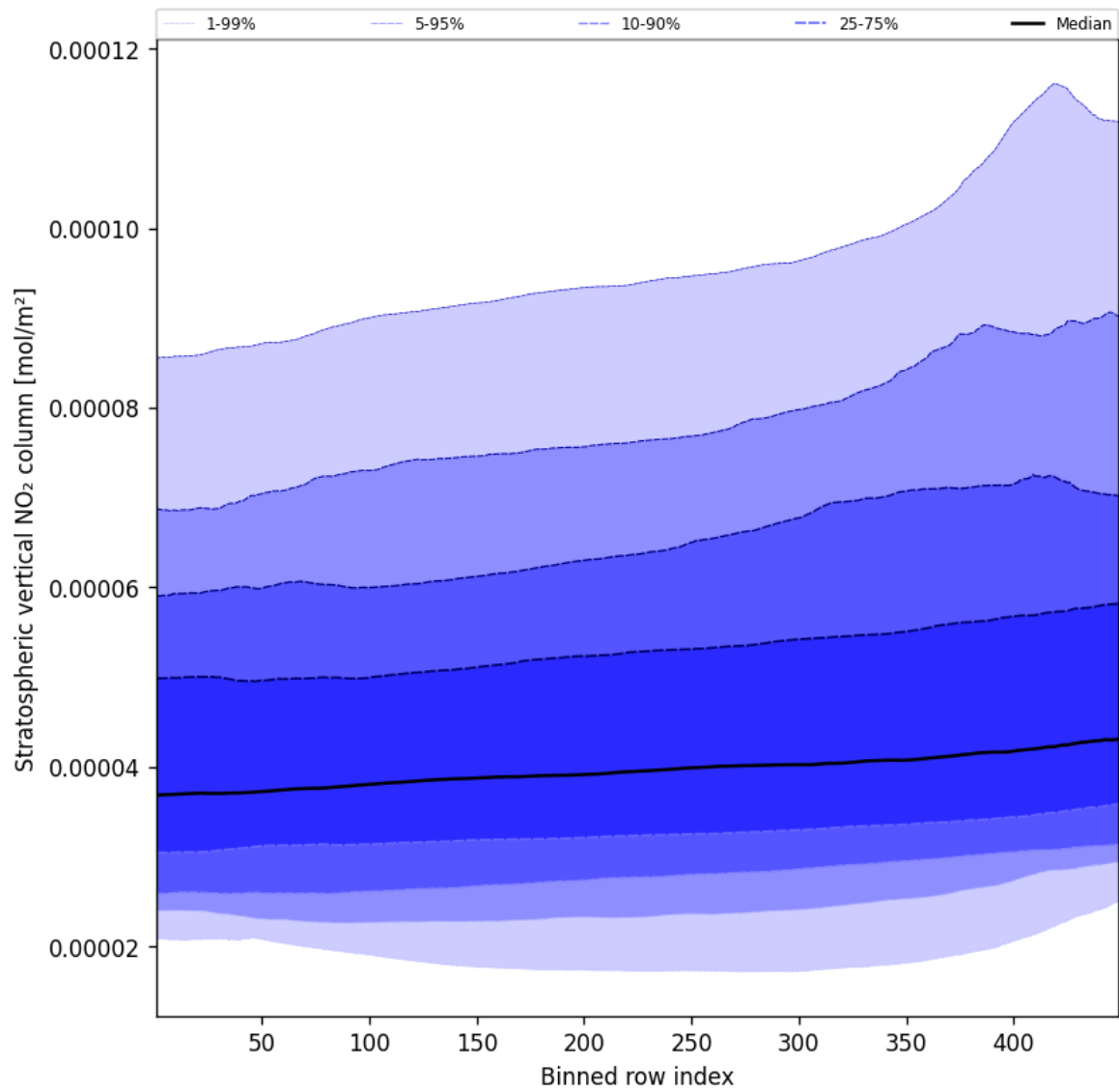
Figure 53: Along track statistics of “Stratospheric vertical NO 2 column” for 2024-10-20 to 2024-10-22
