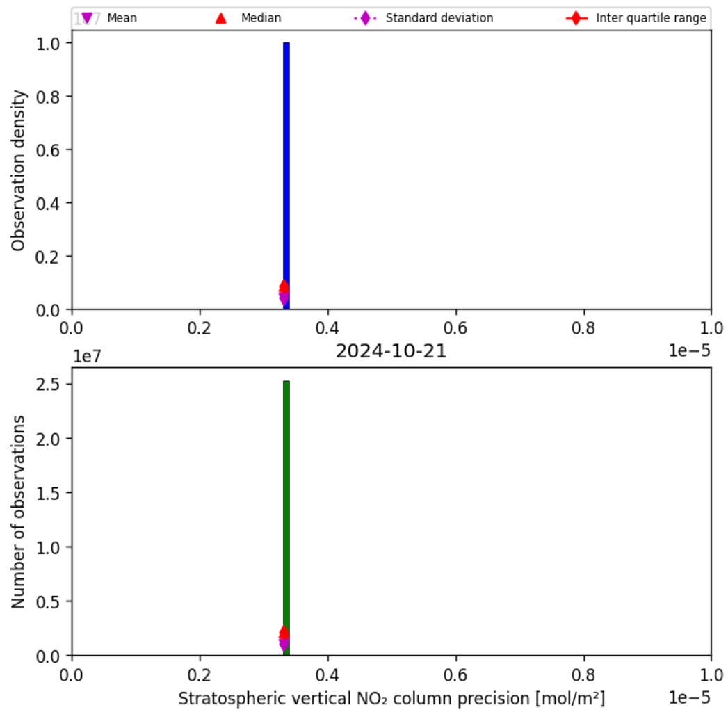
Figure 37: Histogram of “Stratospheric vertical NO 2 column precision” for 2024-10-20 to 2024-10-22
