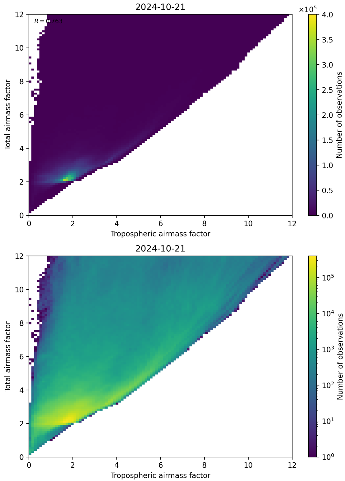
Figure 72: Scatter density plot of “Tropospheric airmass factor” against “Total airmass factor” for 2024-10-20 to 2024-10-22.
