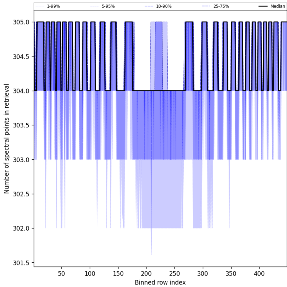
Figure 50: Along track statistics of “Number of spectral points in retrieval” for 2024-10-20 to 2024-10-22
