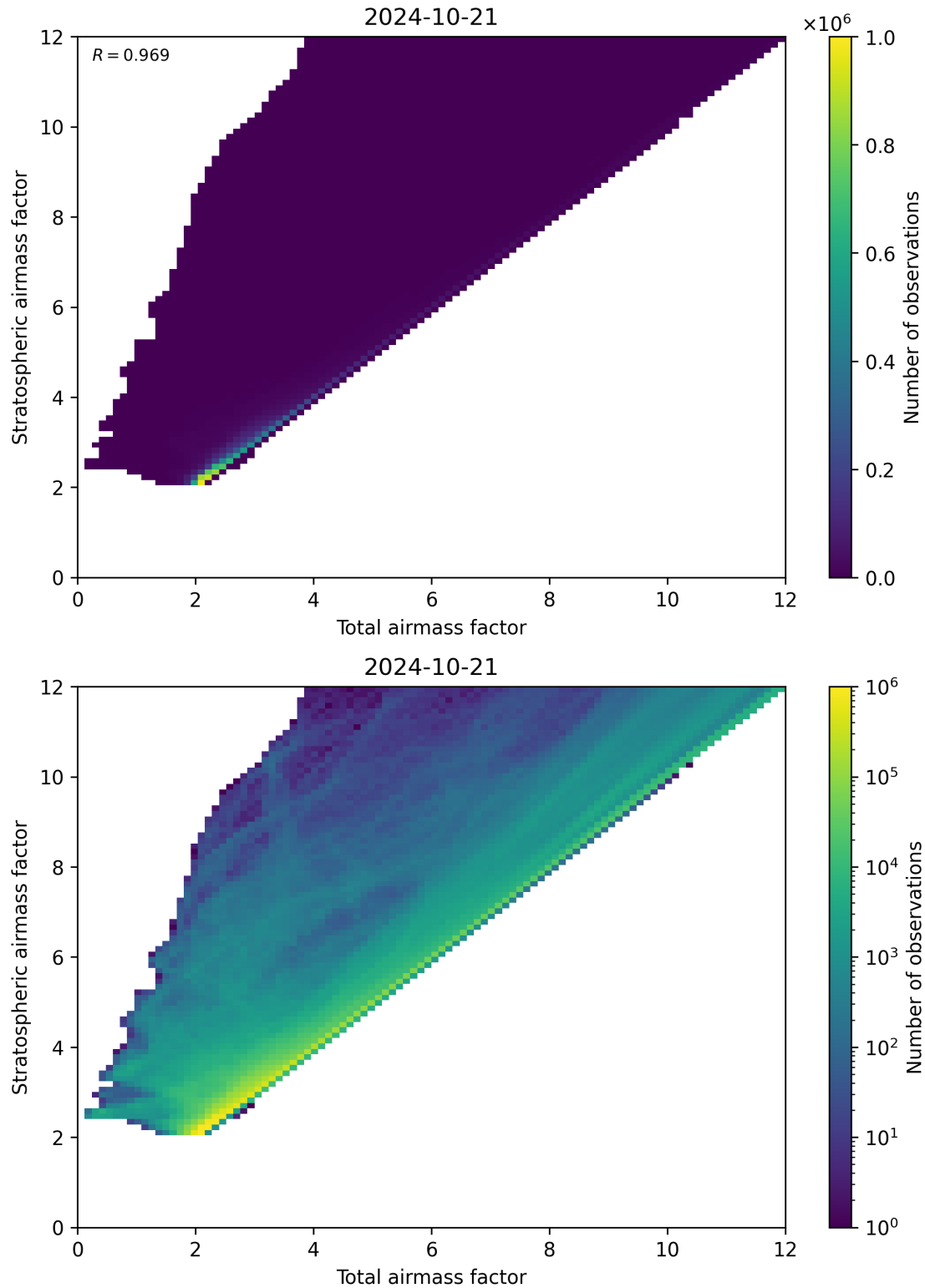
Figure 62: Scatter density plot of “Total airmass factor” against “Stratospheric airmass factor” for 2024-10-20 to 2024-10-22.
