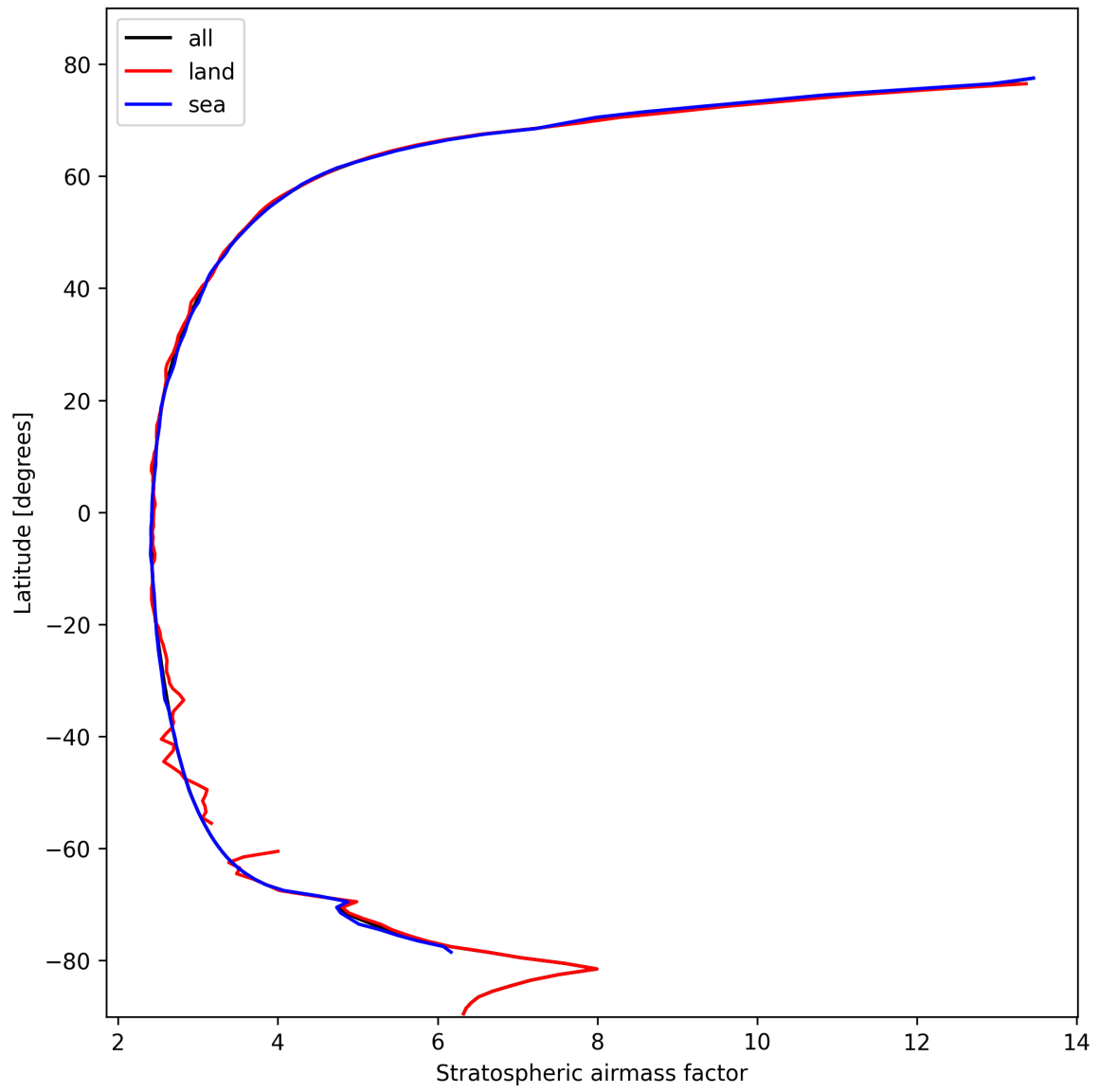
Figure 27: Zonal average of “Stratospheric airmass factor” for 2024-10-20 to 2024-10-22.
