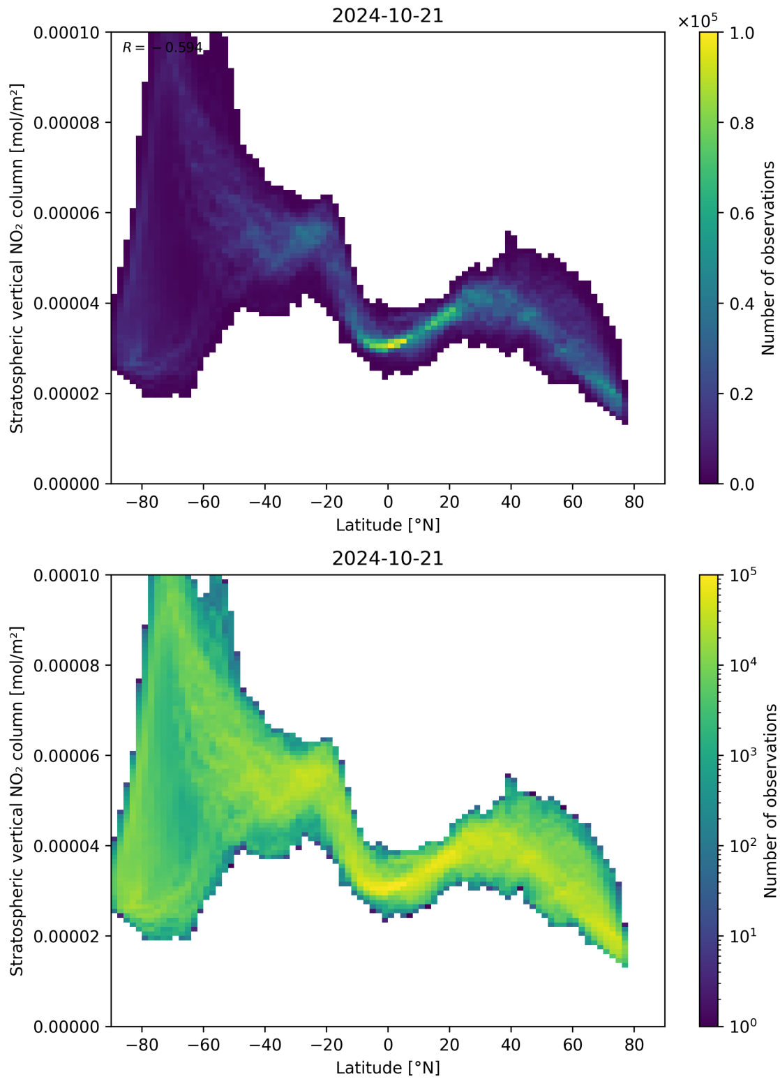
Figure 87: Scatter density plot of “Latitude” against “Stratospheric vertical NO 2 column” for 2024-10-20 to 2024-10-22.
