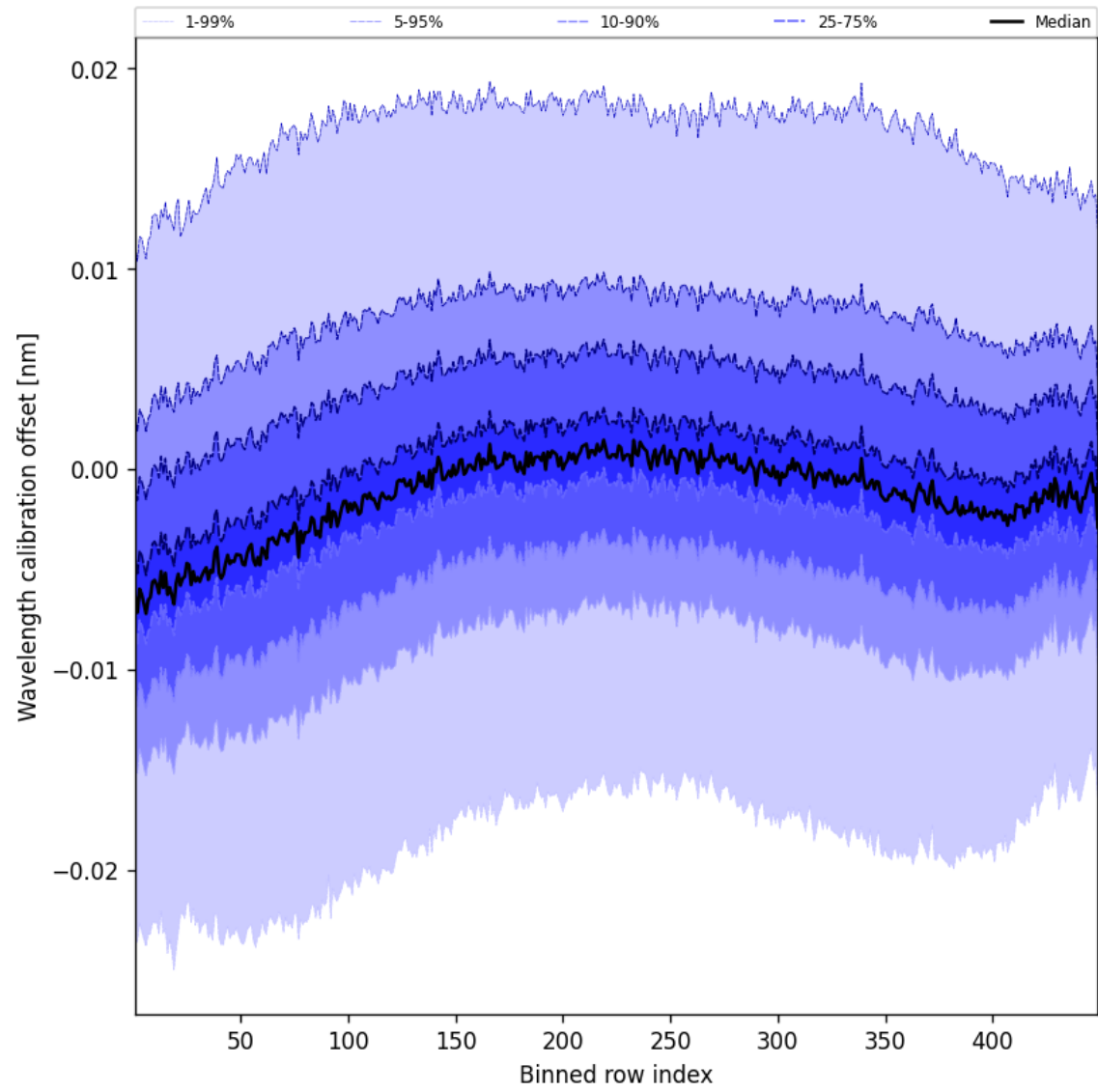
Figure 52: Along track statistics of “Wavelength calibration offset” for 2024-10-20 to 2024-10-22
