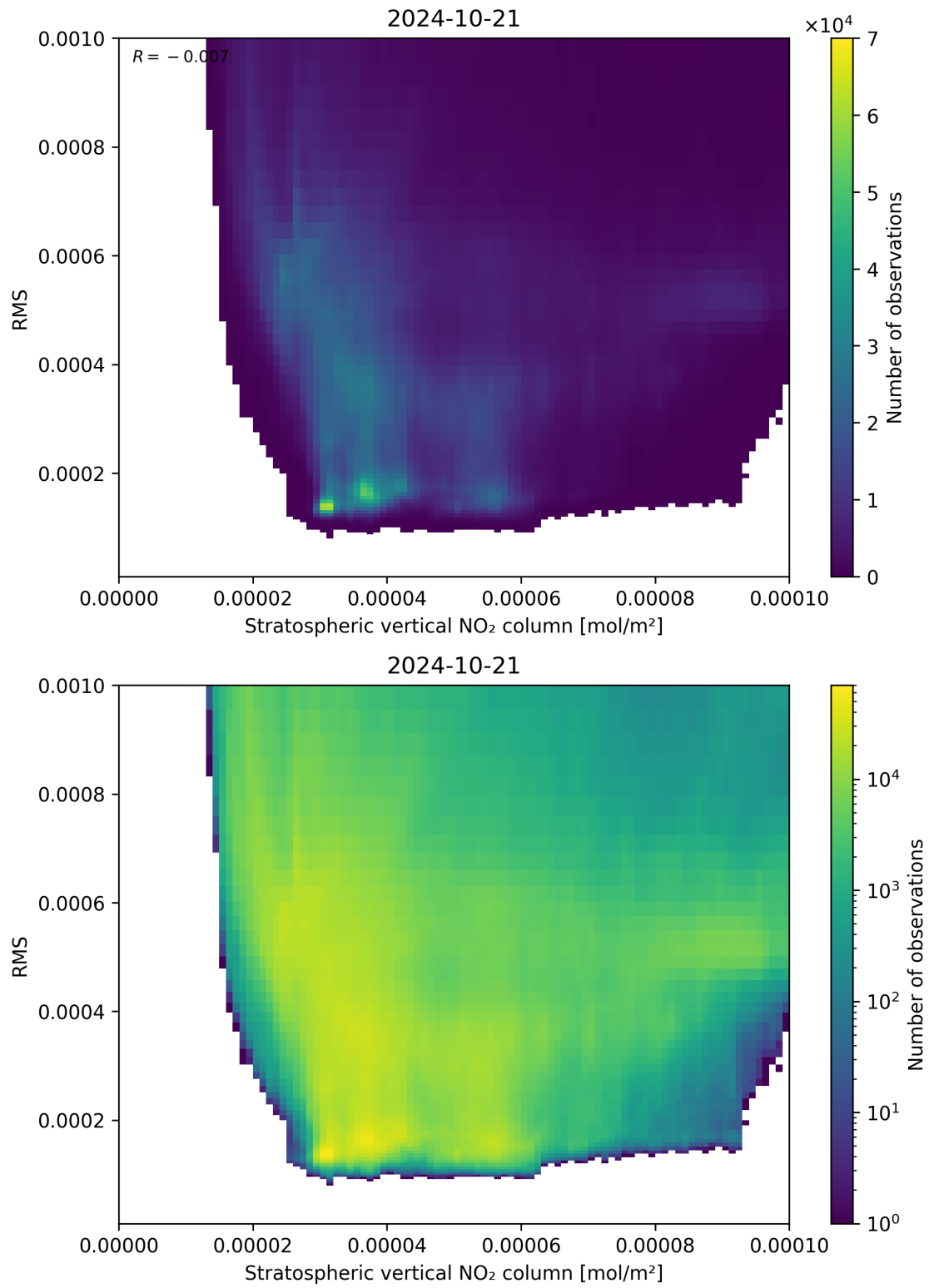
Figure 102: Scatter density plot of “Stratospheric vertical NO 2 column” against “RMS” for 2024-10-20 to 2024-10-22.
