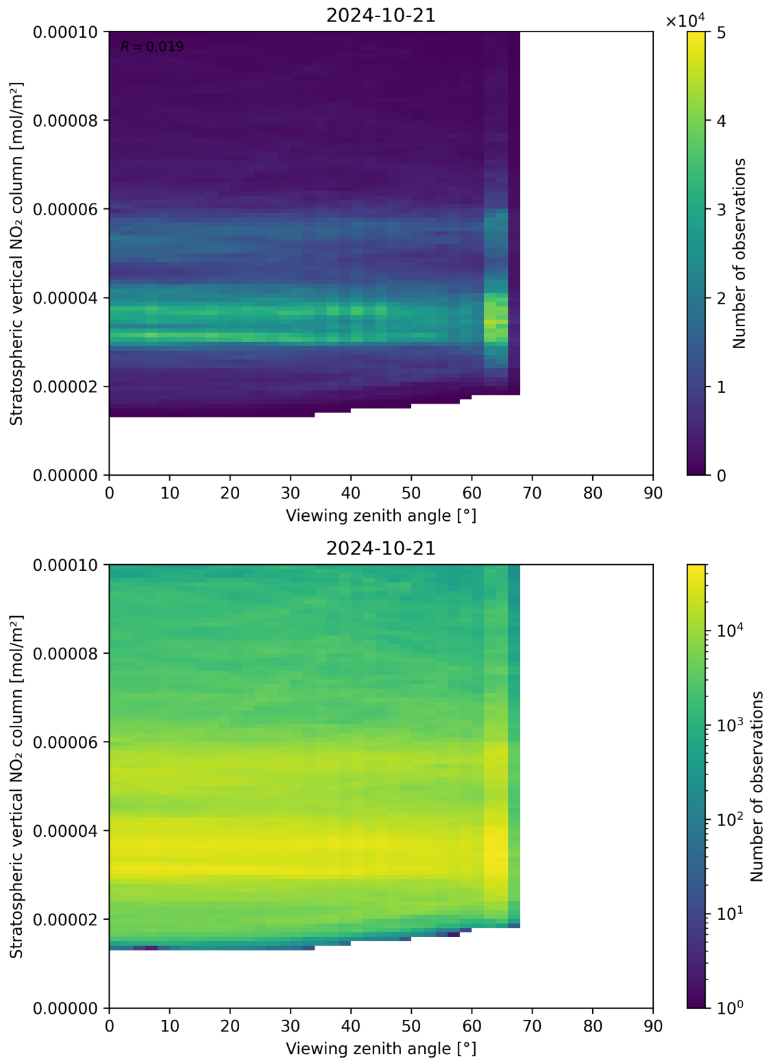
Figure 164: Scatter density plot of “Viewing zenith angle” against “Stratospheric vertical NO 2 column” for 2024-10-20 to 2024-10-22.
