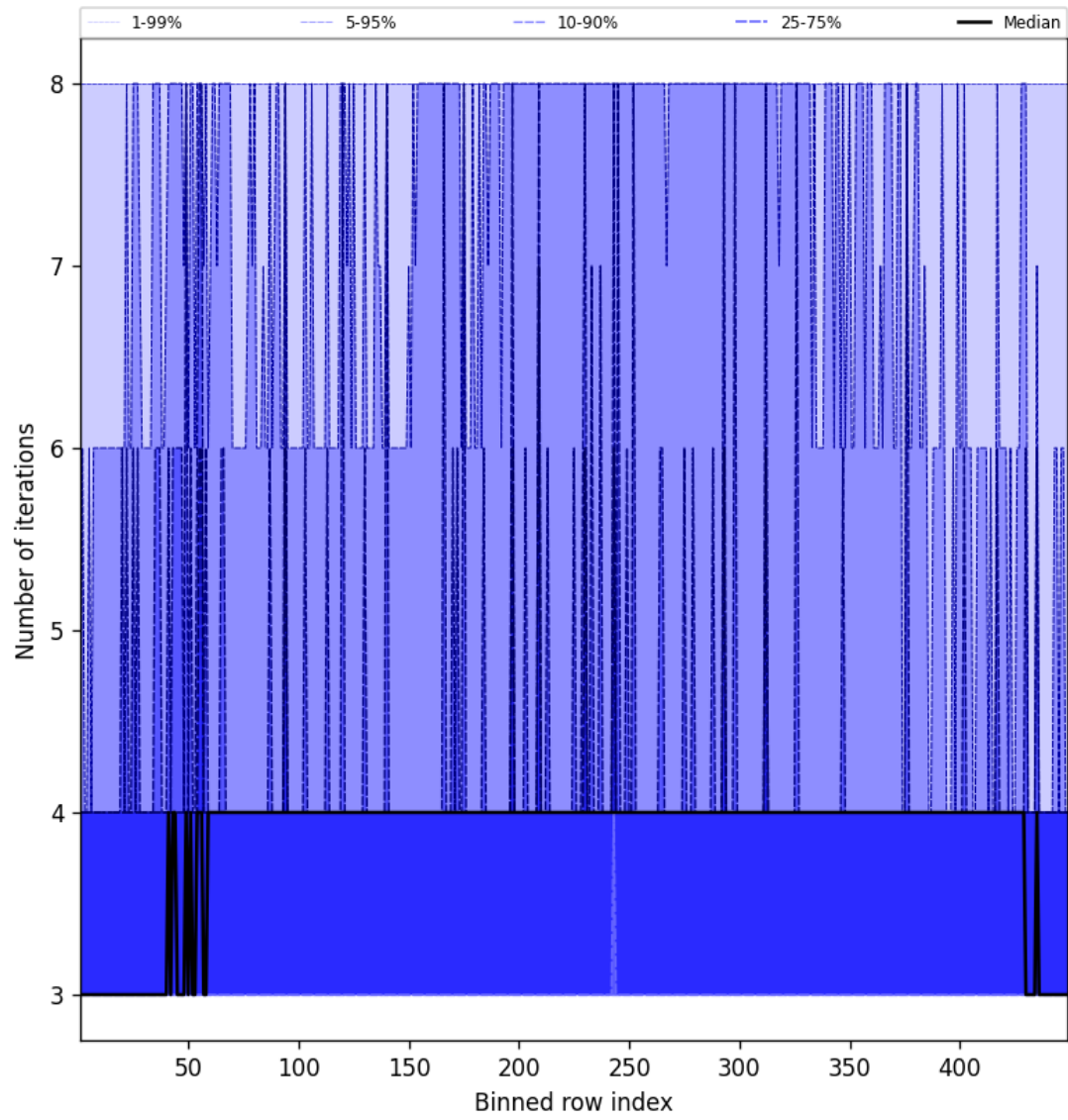
Figure 51: Along track statistics of “Number of iterations” for 2024-10-20 to 2024-10-22
