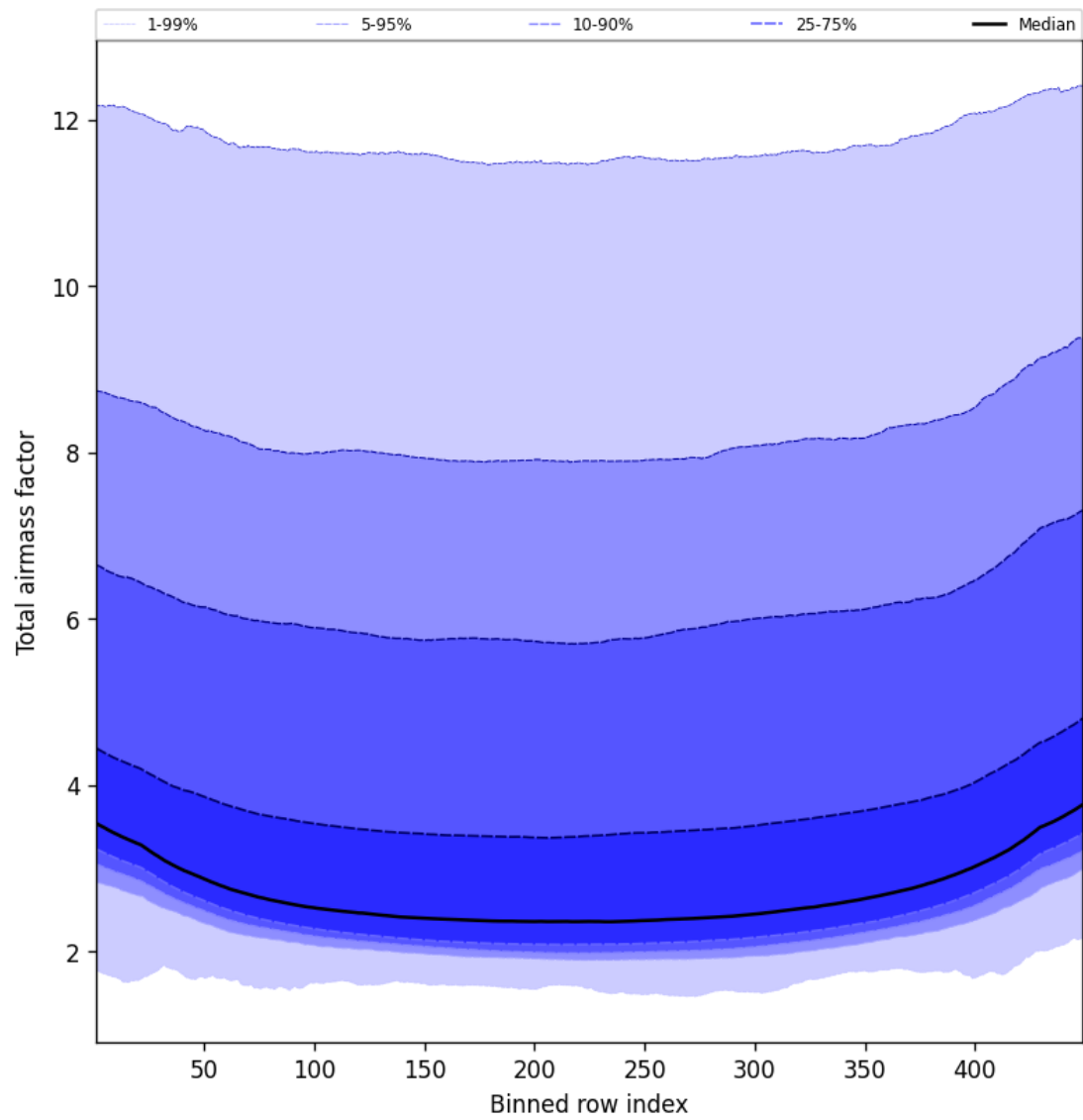
Figure 49: Along track statistics of “Total airmass factor” for 2024-10-20 to 2024-10-22
