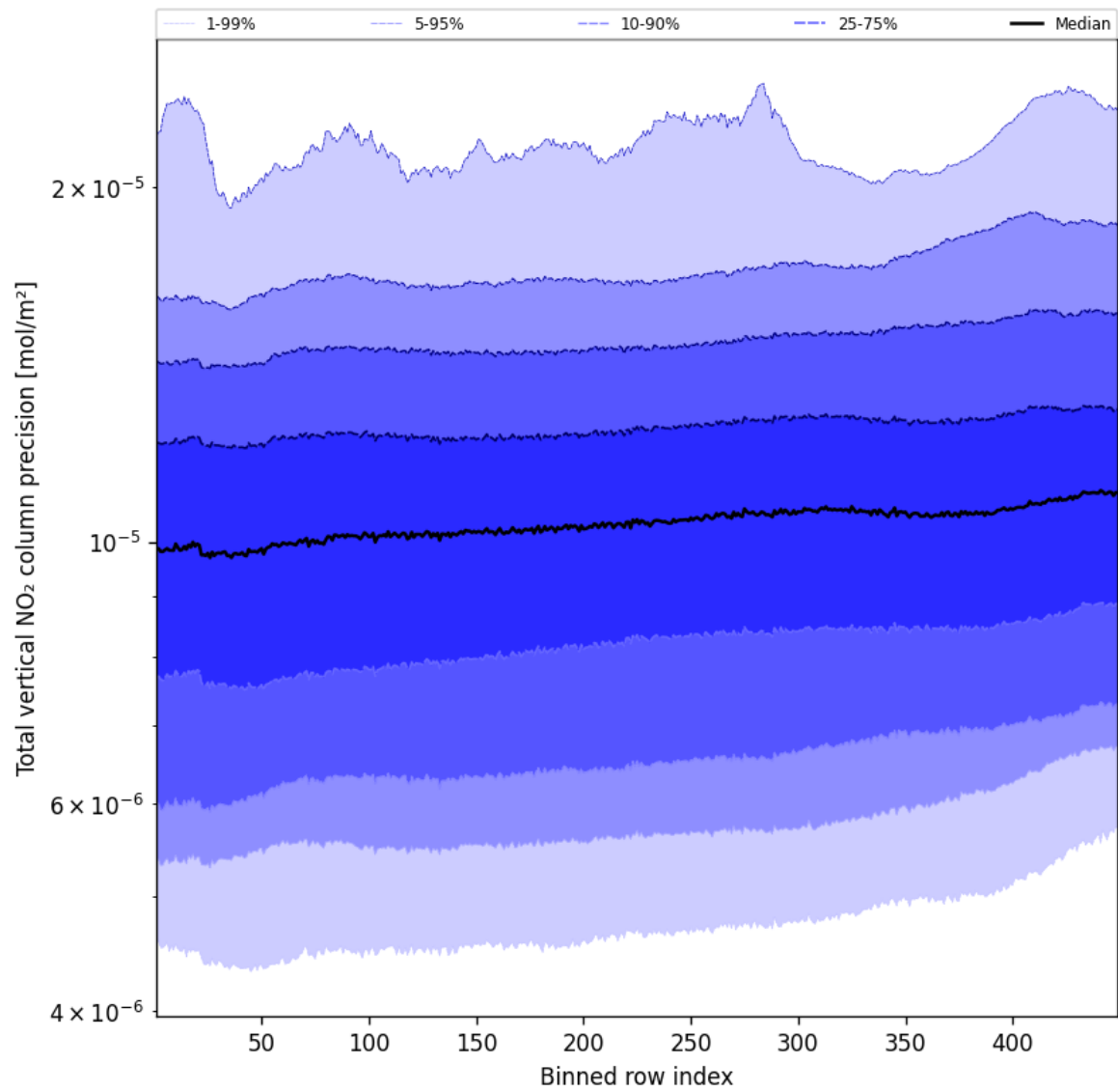
Figure 56: Along track statistics of "Total vertical NO 2 column precision" for 2024-10-20 to 2024-10-22
