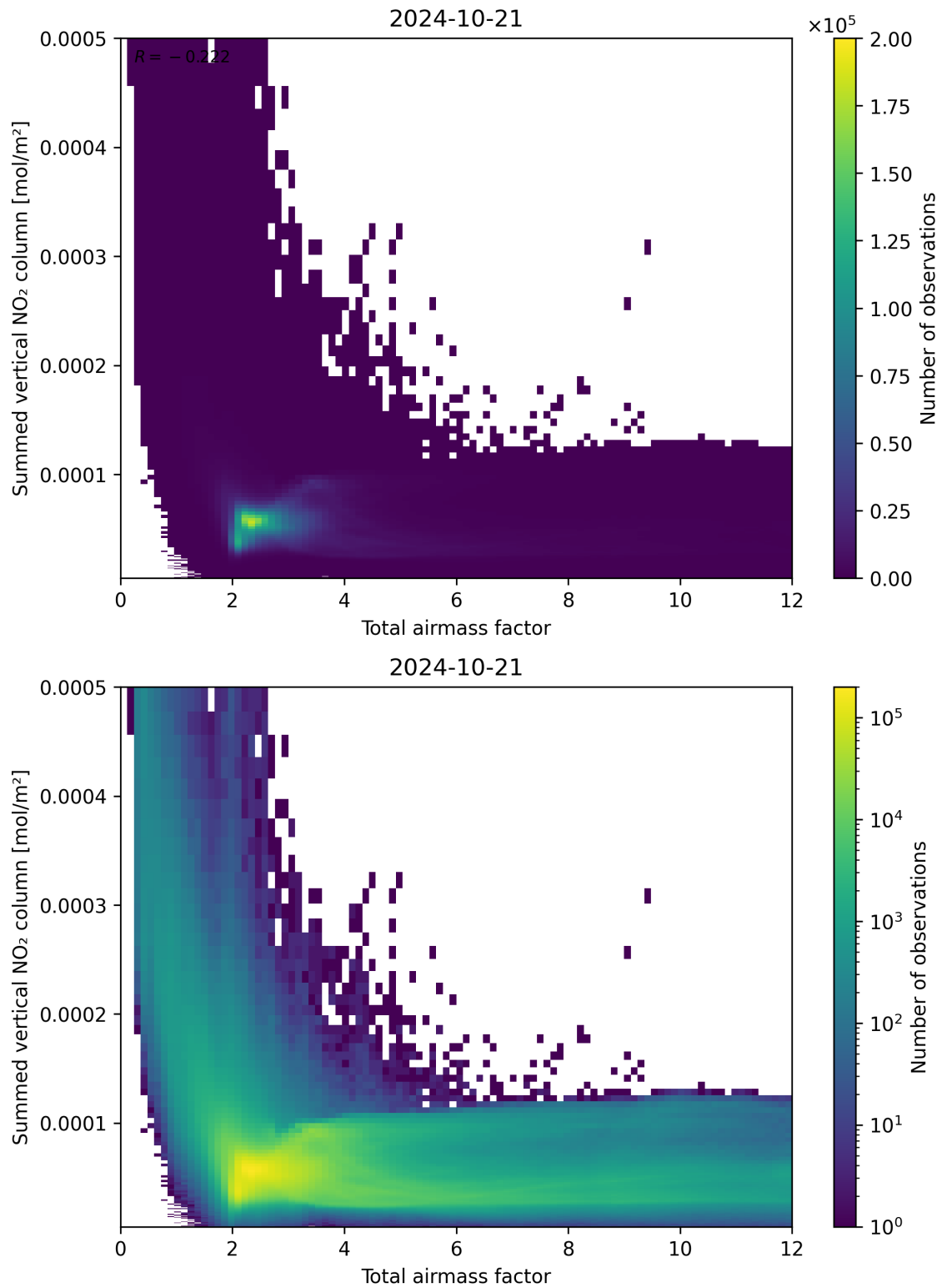
Figure 65: Scatter density plot of “Total airmass factor” against “Summed vertical NO 2 column” for 2024-10-20 to 2024-10-22.
