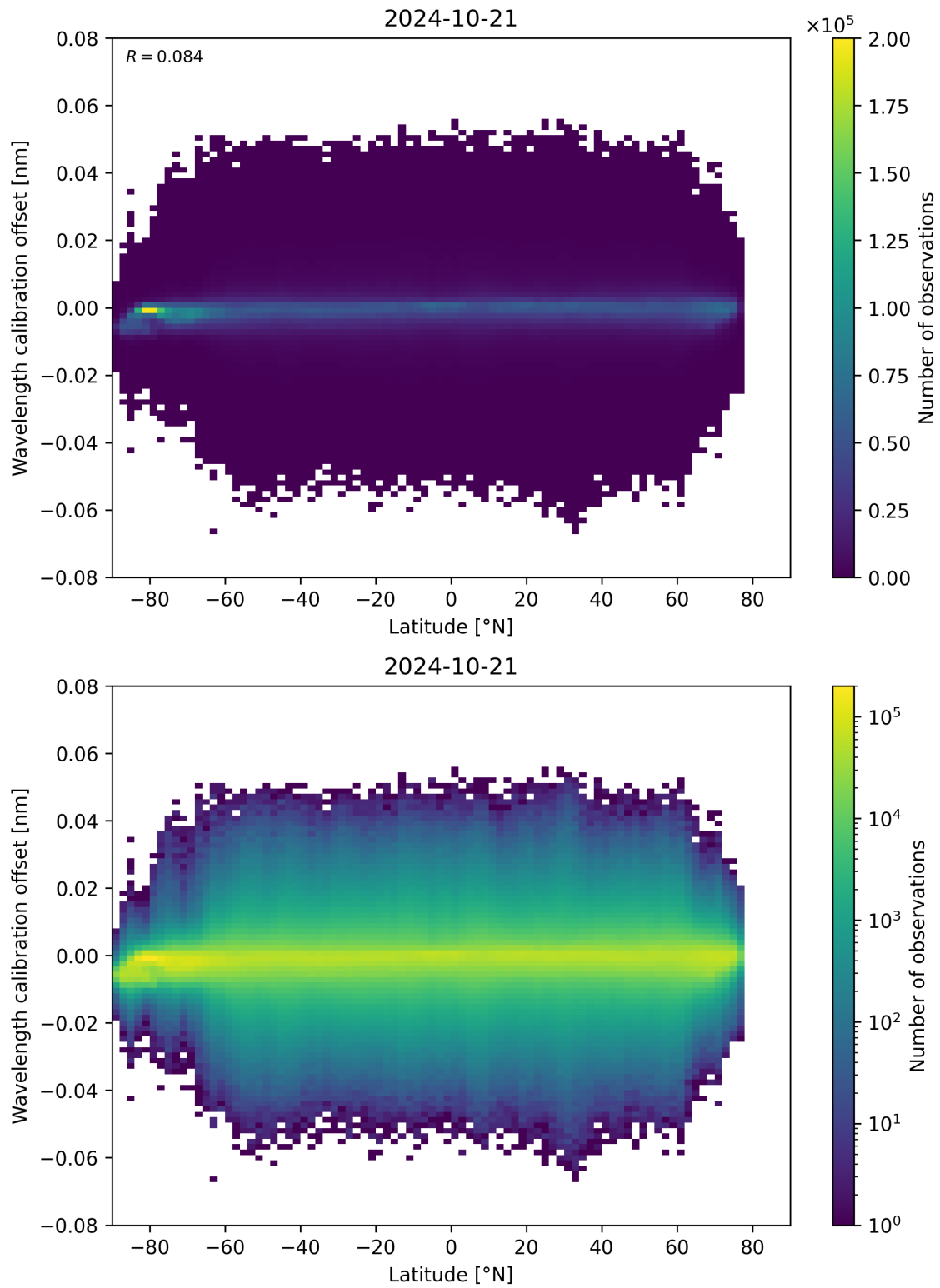
Figure 95: Scatter density plot of “Latitude” against “Wavelength calibration offset” for 2024-10-20 to 2024-10-22.
