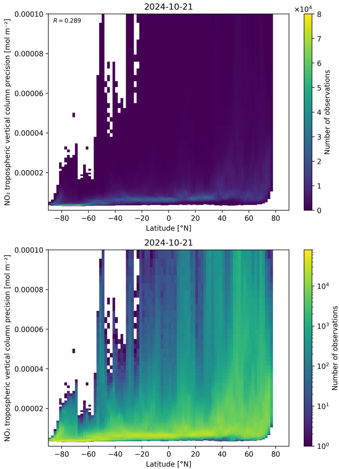
Figure 93: Scatter density plot of “Latitude” against “NO 2 tropospheric vertical column precision” for 2024-10-20 to 2024-10-22.
