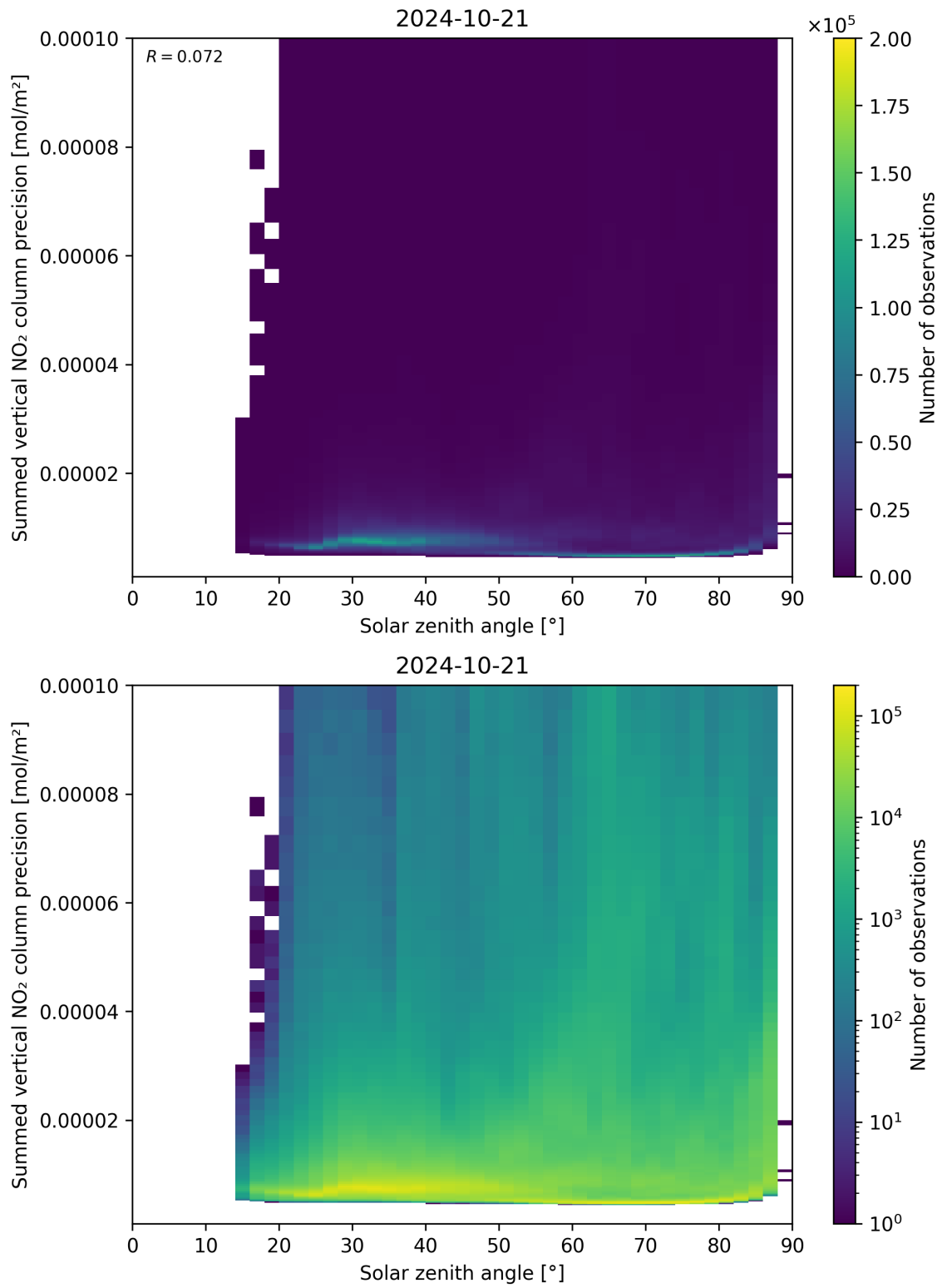
Figure 152: Scatter density plot of “Solar zenith angle” against “Summed vertical NO 2 column precision” for 2024-10-20 to 2024-10-22.
