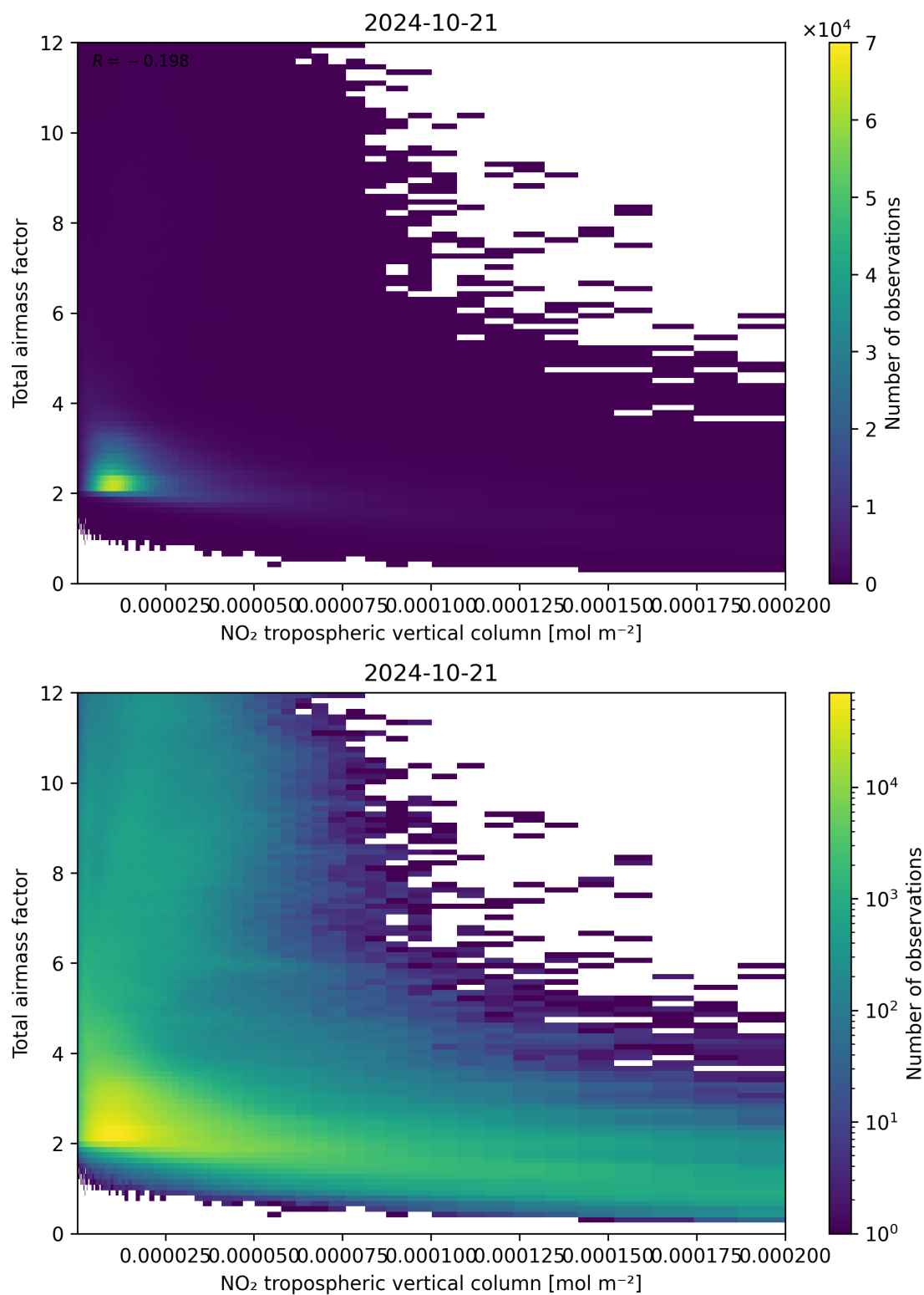
Figure 122: Scatter density plot of “NO 2 tropospheric vertical column” against “Total air mass factor” for 2024-10-20 to 2024-10-22.
