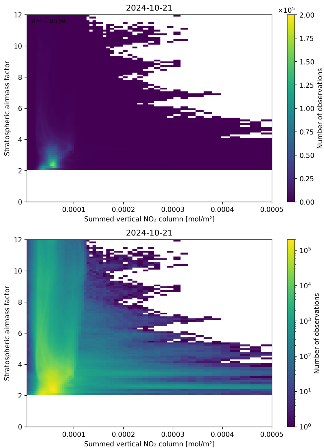
Figure 103: Scatter density plot of “Summed vertical NO 2 column” against “Stratospheric airmass factor” for 2024-10-20 to 2024-10-22.
