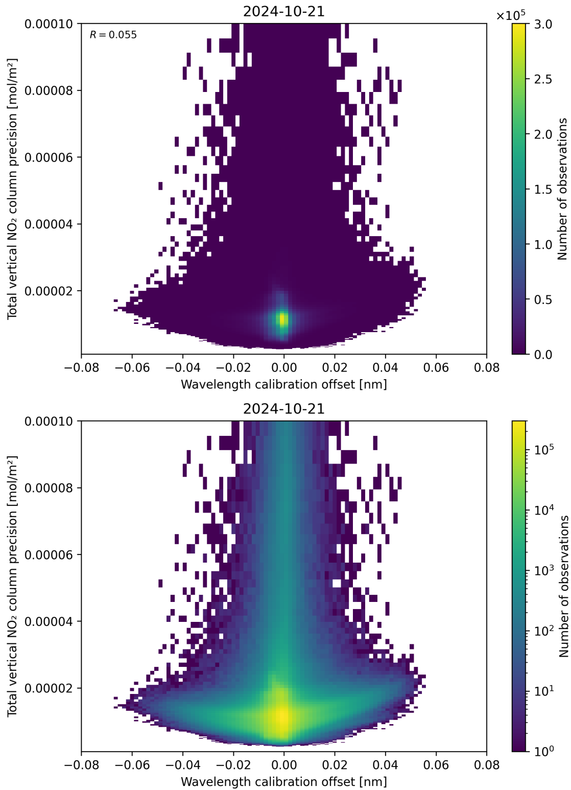
Figure 180: Scatter density plot of “Wavelength calibration offset” against “Total vertical NO 2 column precision” for 2024-10-20 to 2024-10-22.
