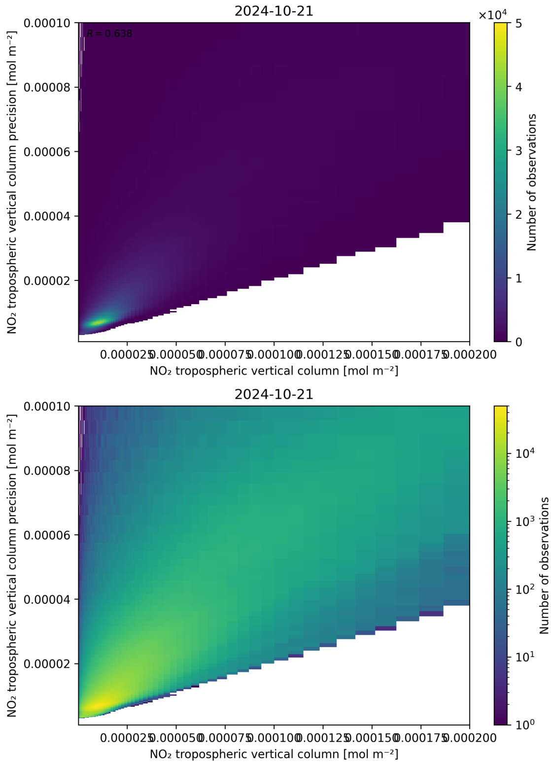
Figure 130: Scatter density plot of “NO 2 tropospheric vertical column” against “NO 2 tropospheric vertical column precision” for 2024-10-20 to 2024-10-22.
