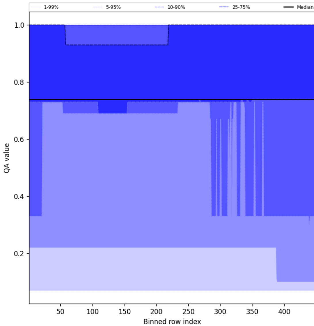
Figure 45: Along track statistics of “QA value” for 2024-10-20 to 2024-10-22
