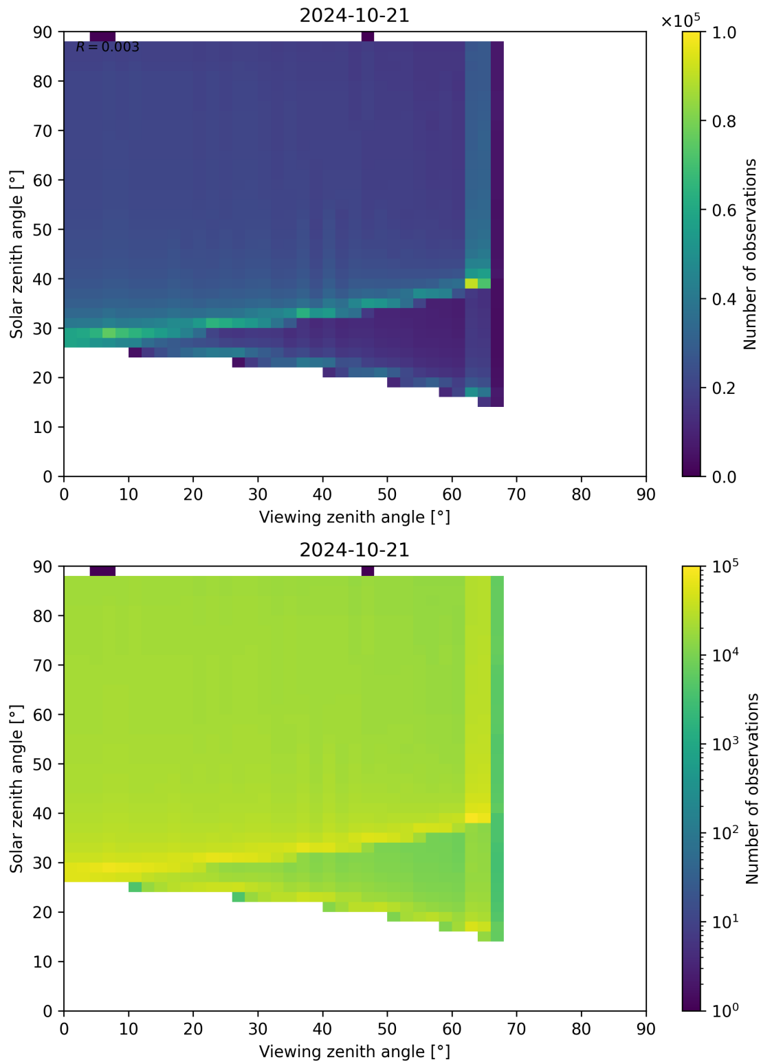
Figure 172: Scatter density plot of “Viewing zenith angle” against “Solar zenith angle” for 2024-10-20 to 2024-10-22.
