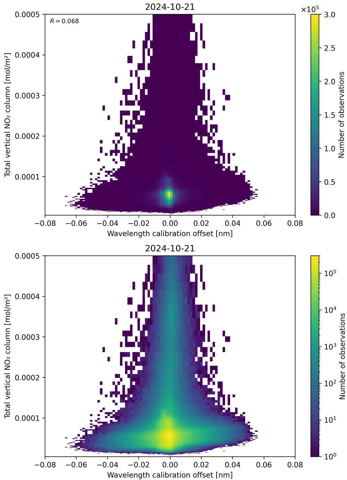
Figure 179: Scatter density plot of “Wavelength calibration offset” against “Total vertical NO 2 column” for 2024-10-20 to 2024-10-22.
