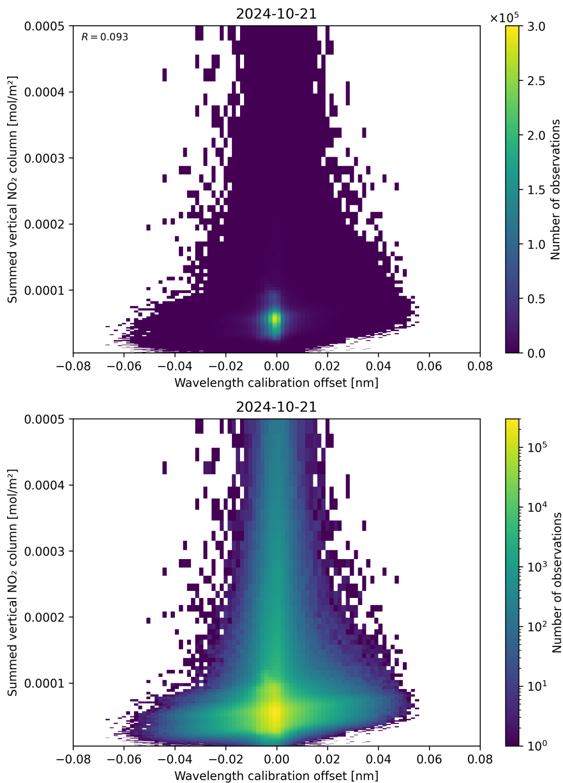
Figure 177: Scatter density plot of “Wavelength calibration offset” against “Summed vertical NO 2 column” for 2024-10-20 to 2024-10-22.
