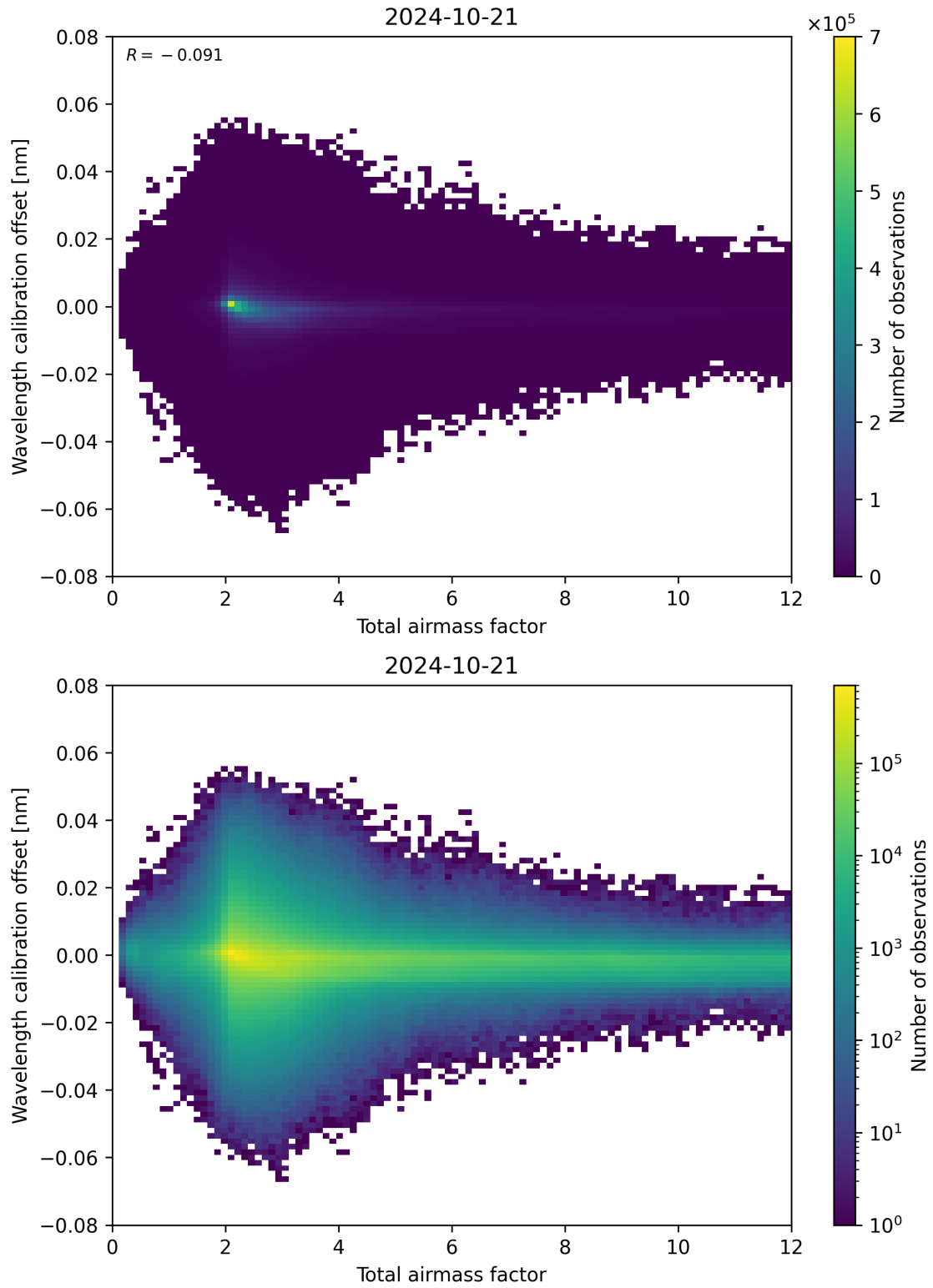
Figure 70: Scatter density plot of “Total airmass factor” against “Wavelength calibration offset” for 2024-10-20 to 2024-10-22.
