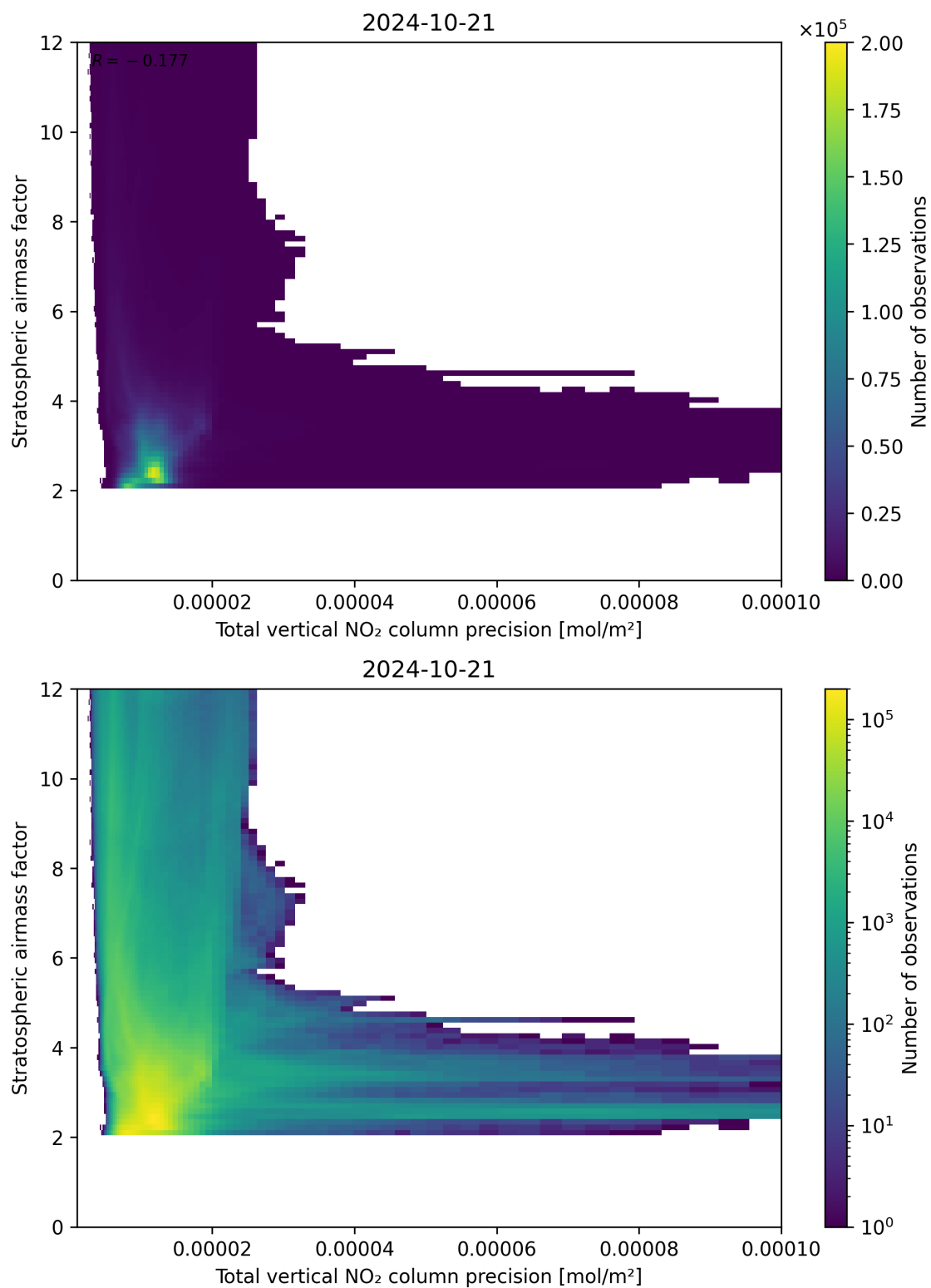
Figure 115: Scatter density plot of “Total vertical NO 2 column precision” against “Stratospheric air mass factor” for 2024-10-20 to 2024-10-22.
