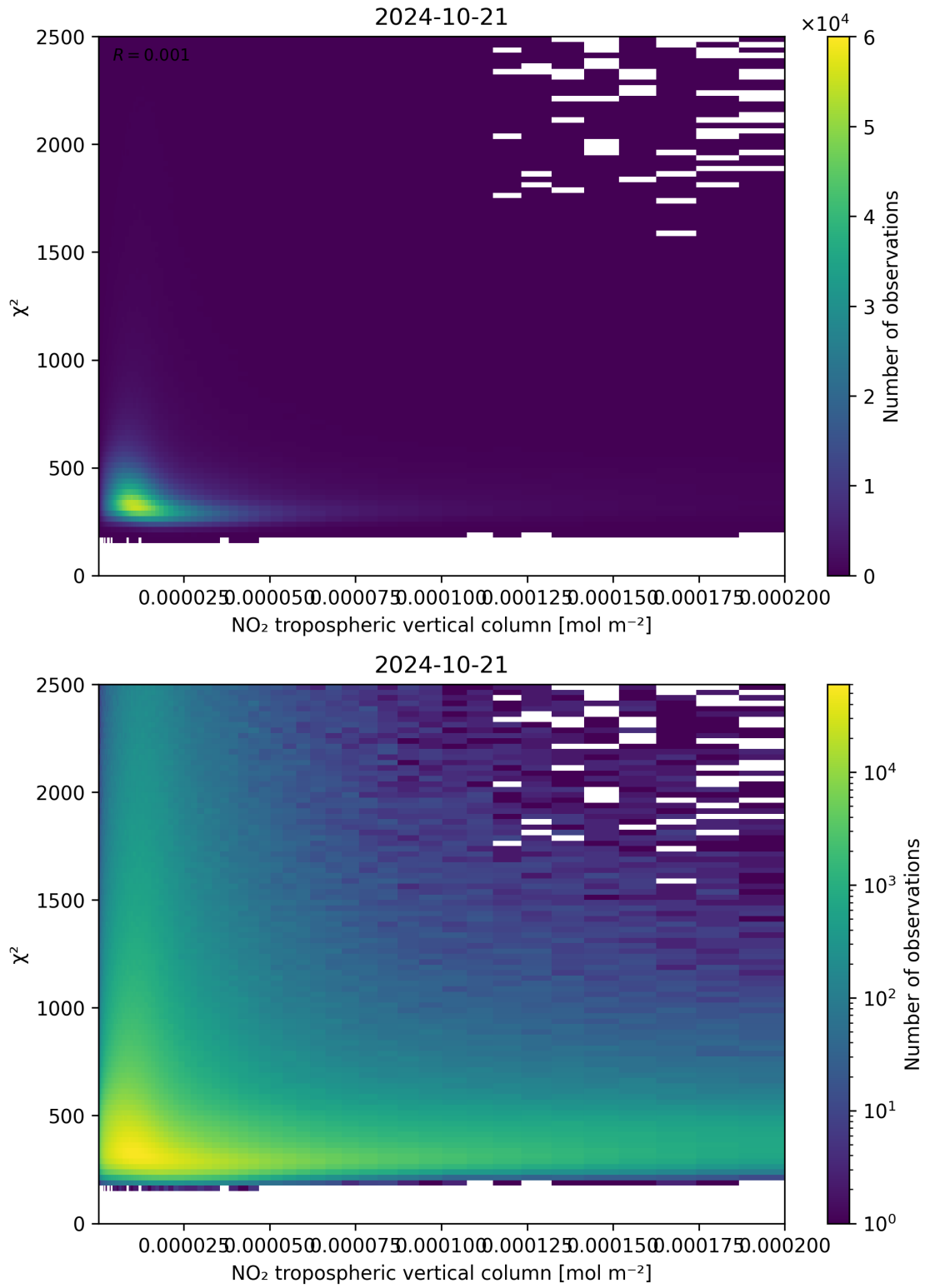
Figure 124: Scatter density plot of “NO 2 tropospheric vertical column” against “ \chi^2 ” for 2024-10-20 to 2024-10-22.
