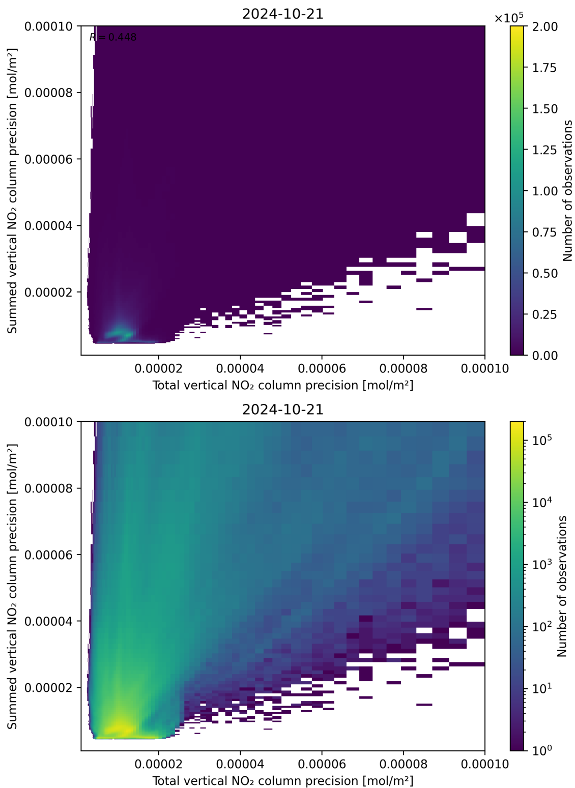
Figure 118: Scatter density plot of “Total vertical NO 2 column precision” against “Summed vertical NO 2 column precision” for 2024-10-20 to 2024-10-22.
