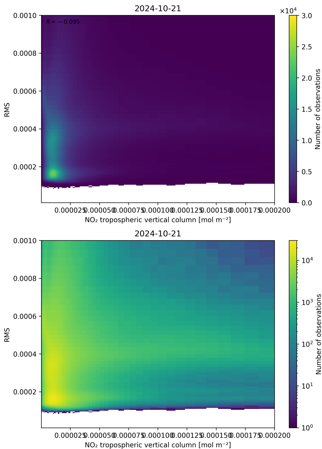
Figure 142: Scatter density plot of “NO 2 tropospheric vertical column” against “RMS” for 2024-10-20 to 2024-10-22.
