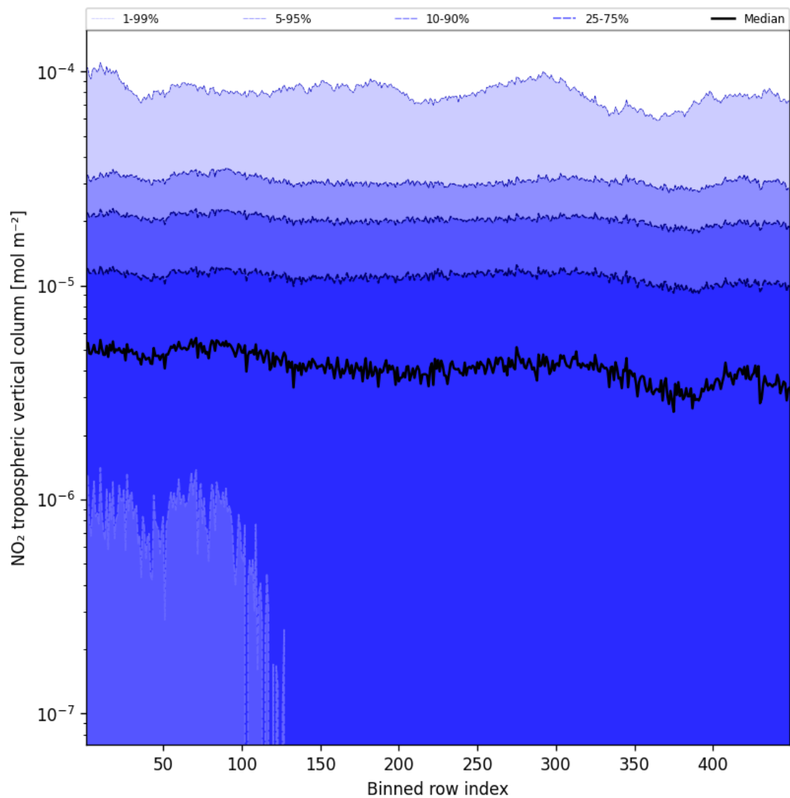
Figure 46: Along track statistics of “NO 2 tropospheric vertical column” for 2024-10-20 to 2024-10-22
