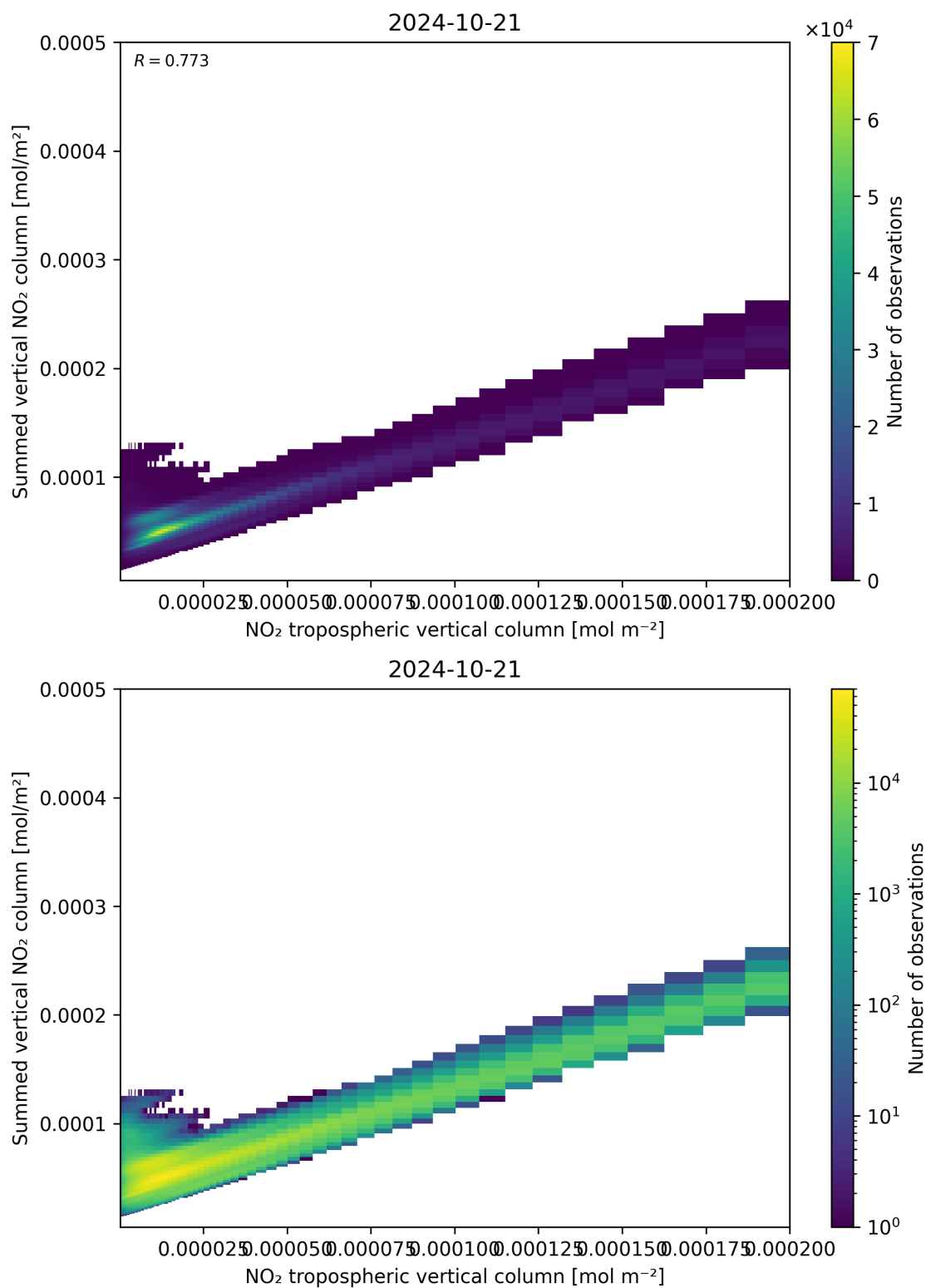
Figure 126: Scatter density plot of “NO 2 tropospheric vertical column” against “Summed vertical NO 2 column” for 2024-10-20 to 2024-10-22.
