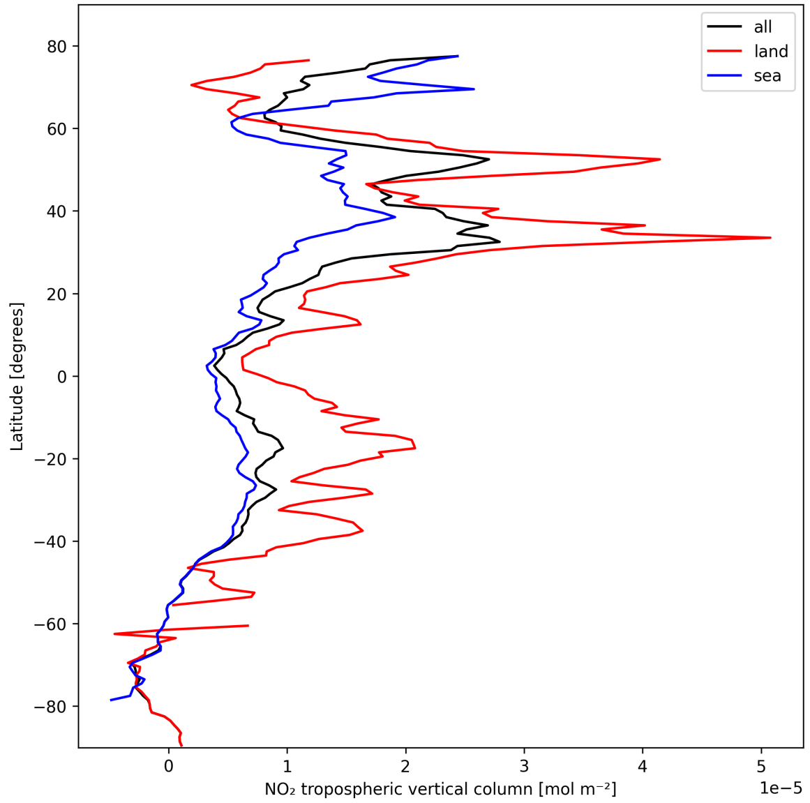
Figure 12: Zonal average of “NO 2 tropospheric vertical column” for 2024-10-20 to 2024-10-22.
