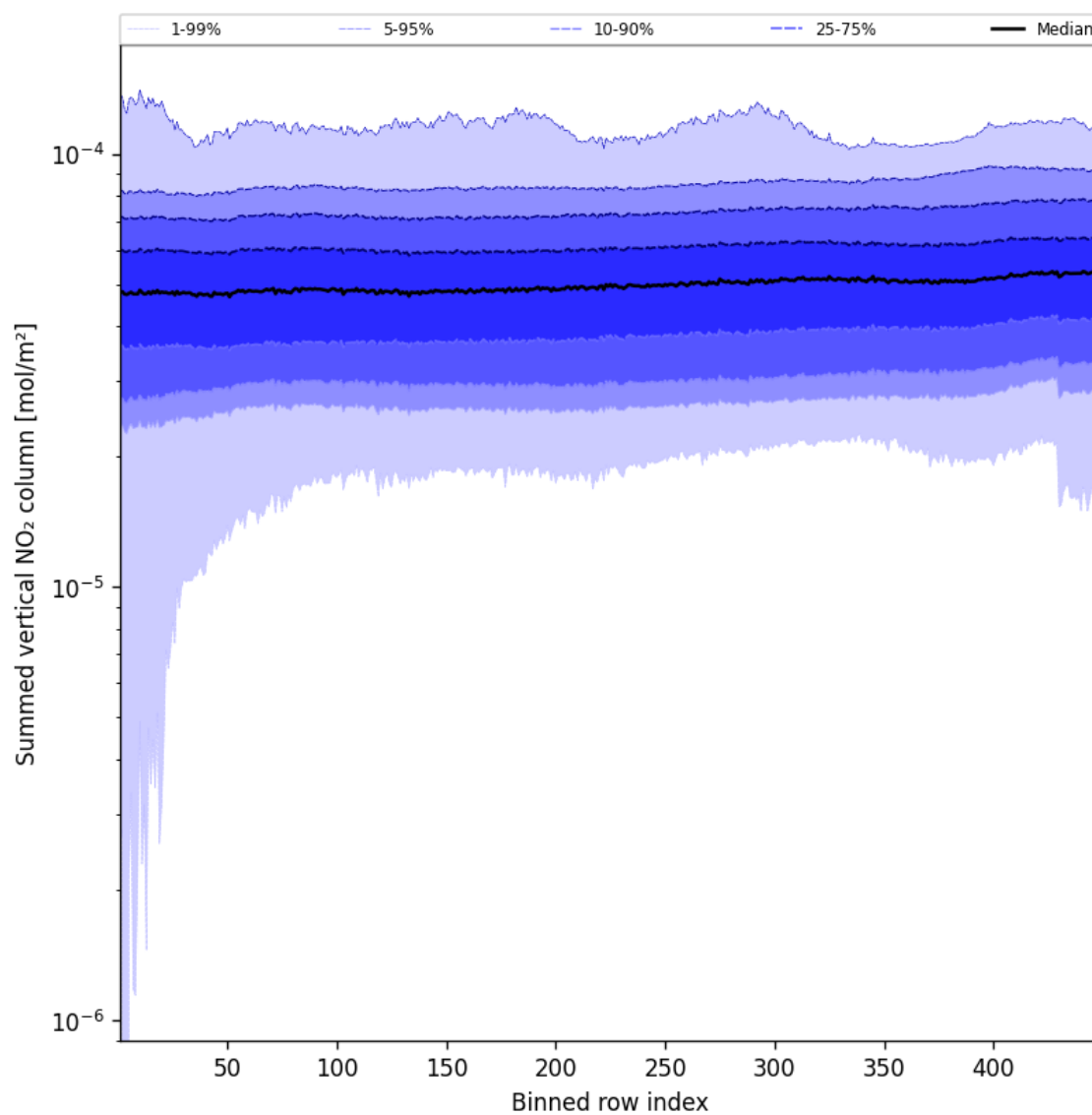
Figure 57: Along track statistics of “Summed vertical NO 2 column” for 2024-10-20 to 2024-10-22
