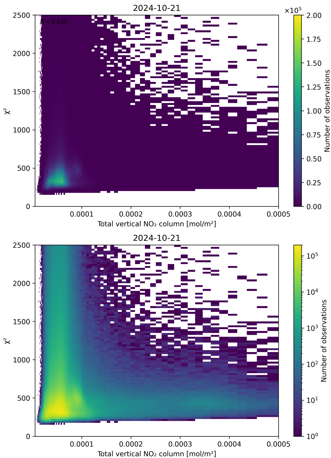
Figure 111: Scatter density plot of “Total vertical NO 2 column” against “ \chi^2 ” for 2024-10-20 to 2024-10-22.
