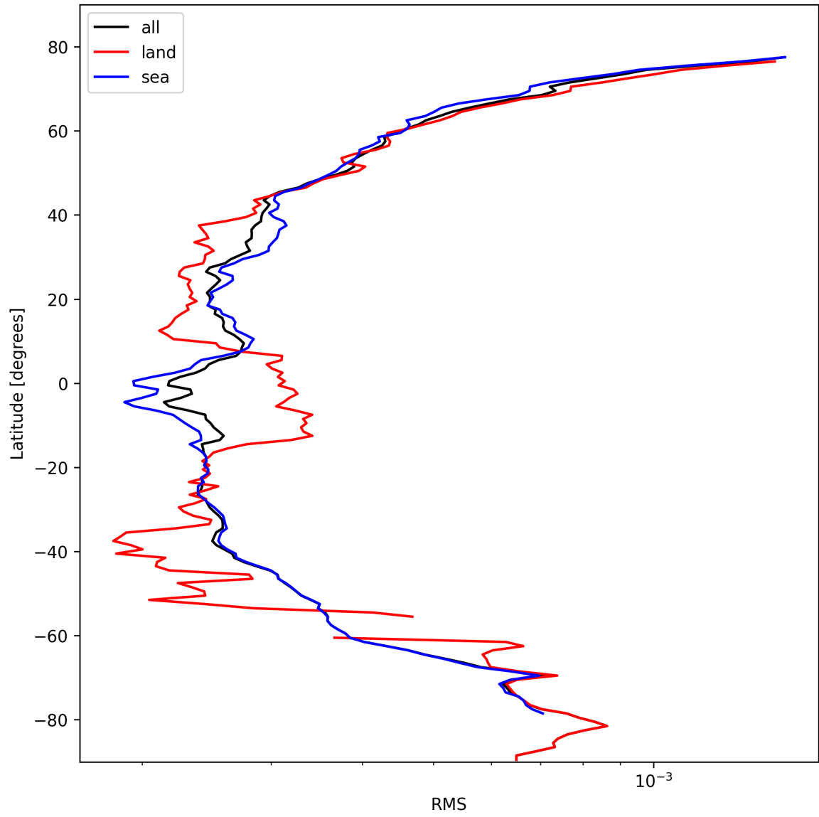
Figure 26: Zonal average of “RMS” for 2024-10-20 to 2024-10-22.
