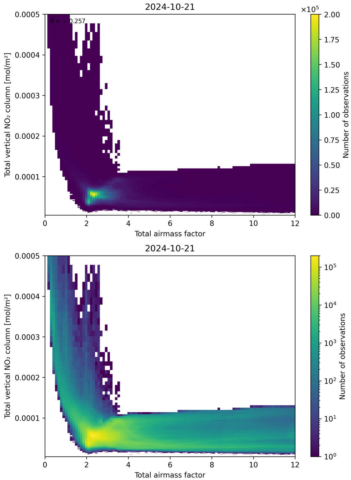
Figure 67: Scatter density plot of “Total airmass factor” against “Total vertical NO 2 column” for 2024-10-20 to 2024-10-22.
