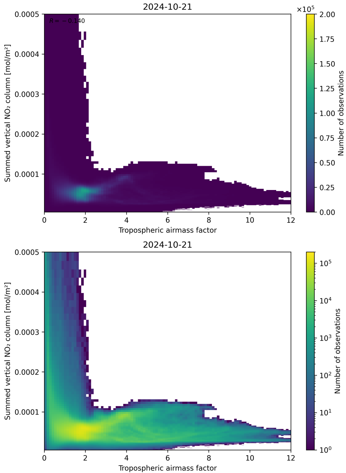
Figure 75: Scatter density plot of “Tropospheric airmass factor” against “Summed vertical NO 2 column” for 2024-10-20 to 2024-10-22.
