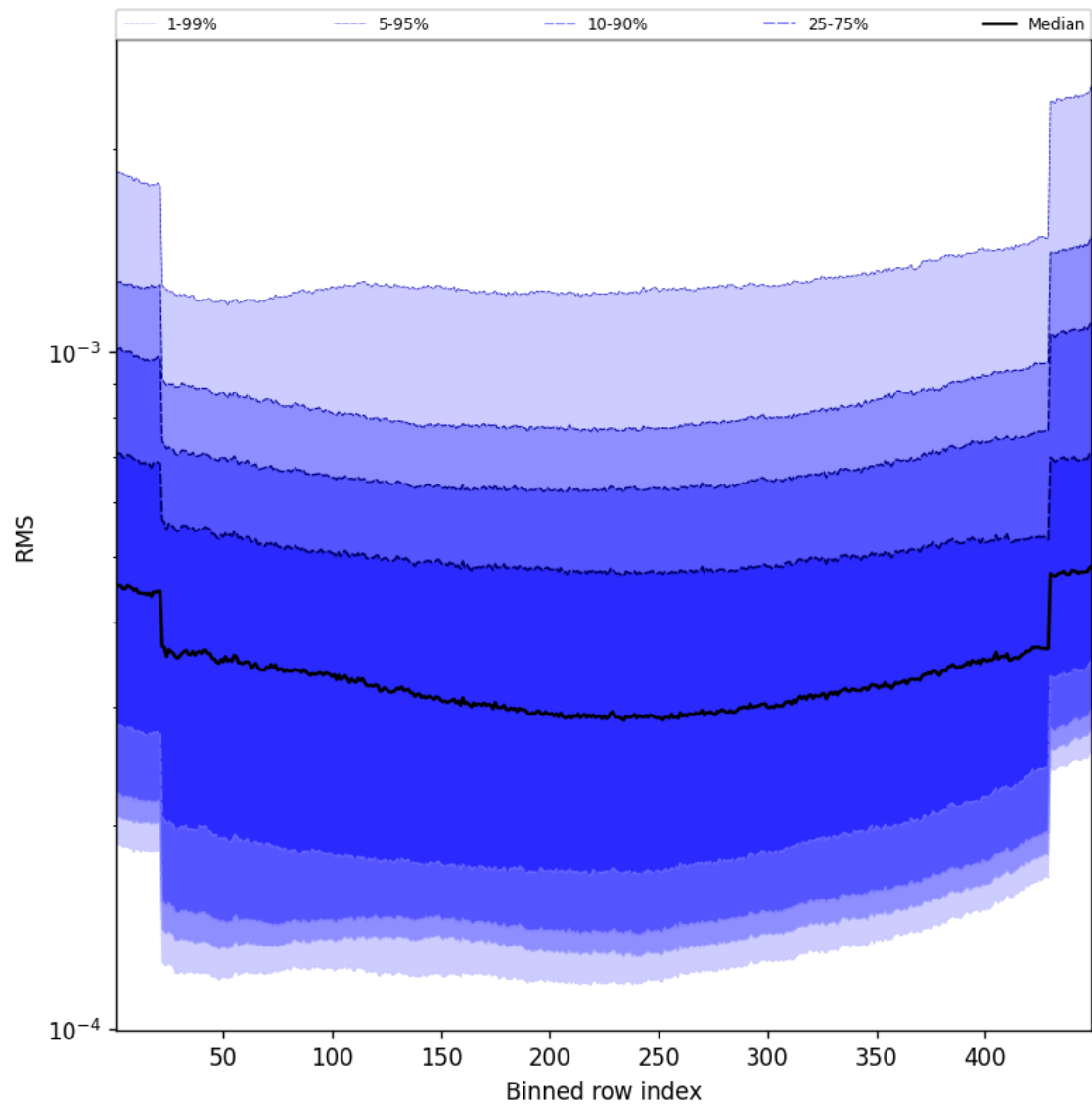
Figure 60: Along track statistics of “RMS” for 2024-10-20 to 2024-10-22
