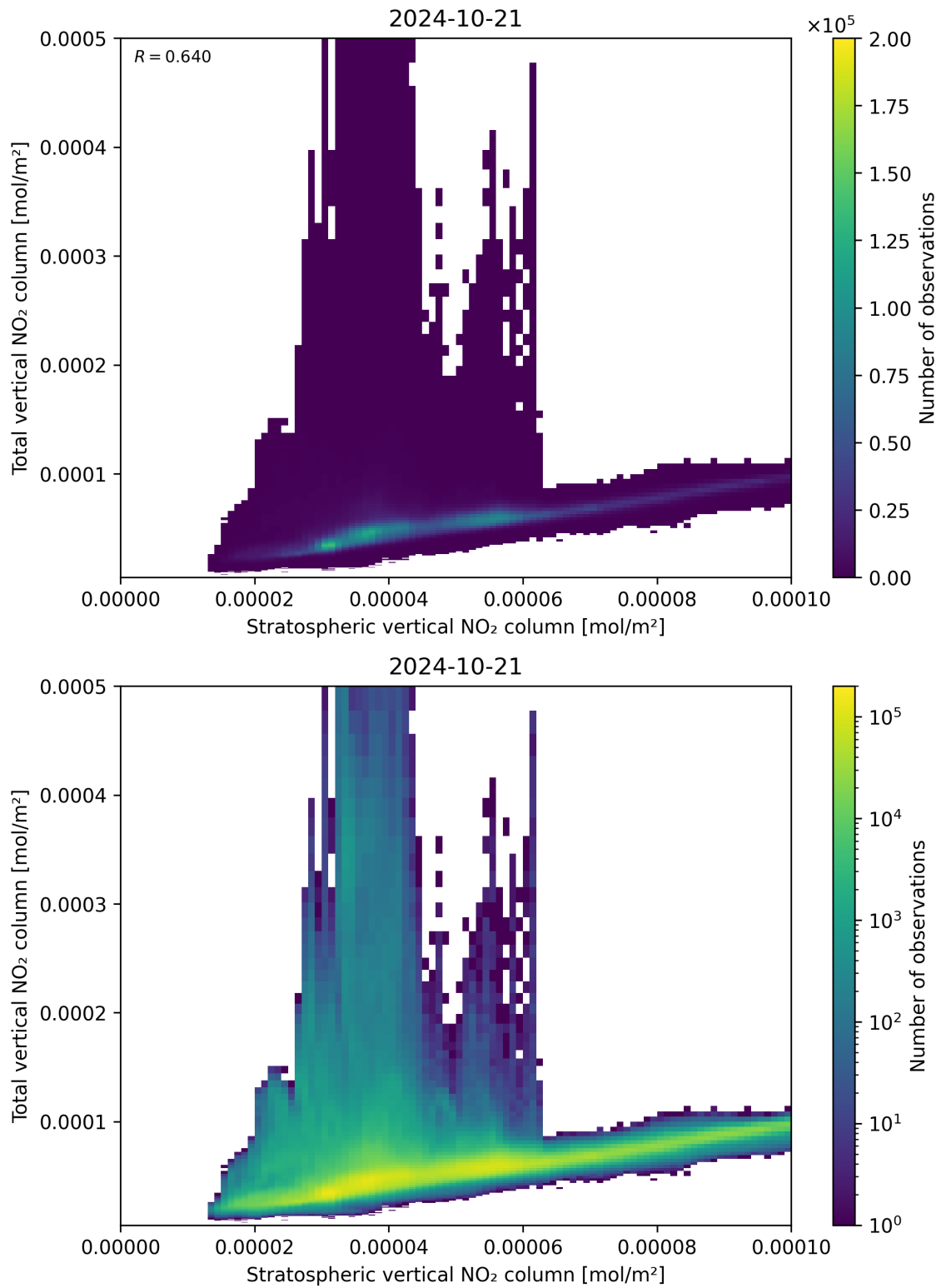
Figure 100: Scatter density plot of “Stratospheric vertical NO 2 column” against “Total vertical NO 2 column” for 2024-10-20 to 2024-10-22.
