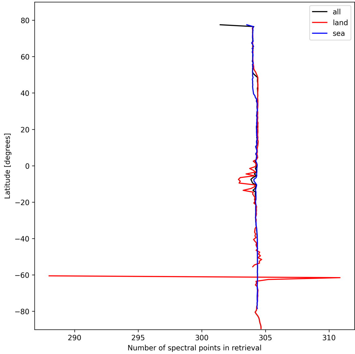
Figure 16: Zonal average of “Number of spectral points in retrieval” for 2024-10-20 to 2024-10-22.
