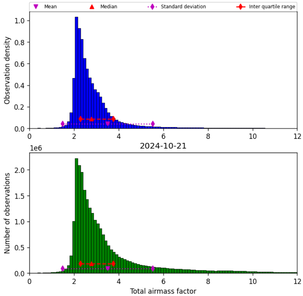
Figure 32: Histogram of “Total airmass factor” for 2024-10-20 to 2024-10-22
