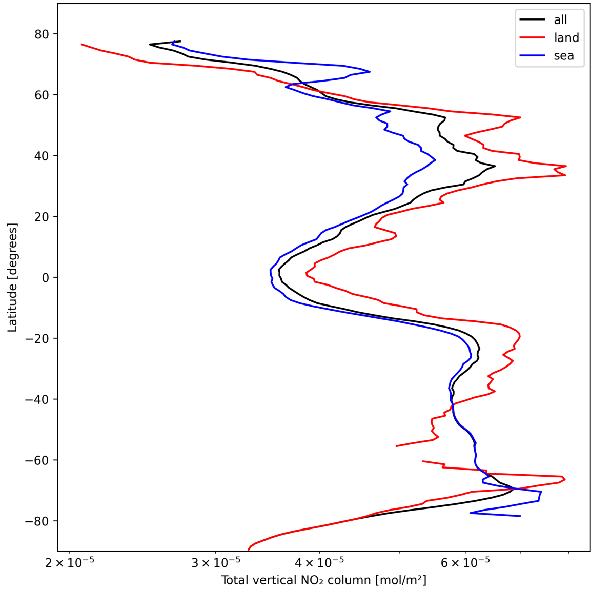
Figure 21: Zonal average of “Total vertical NO 2 column” for 2024-10-20 to 2024-10-22.
