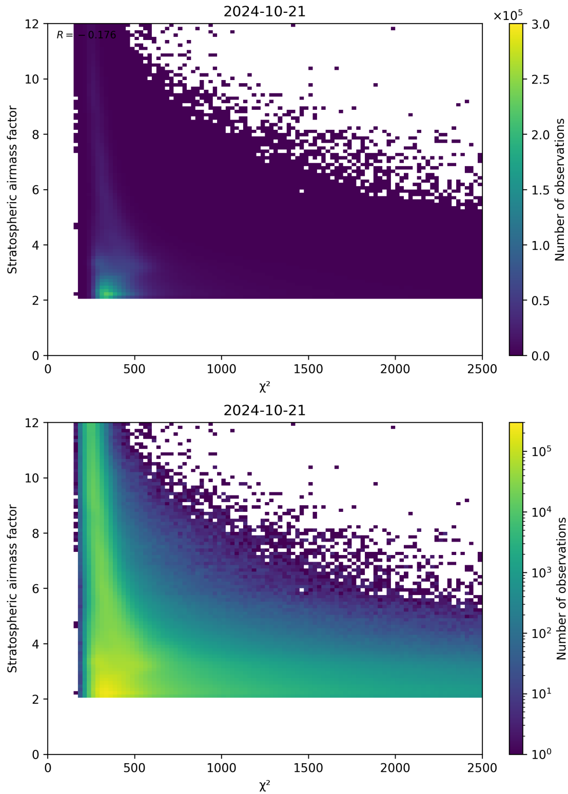
Figure 81: Scatter density plot of “ \chi^2 ” against “Stratospheric airmass factor” for 2024-10-20 to 2024-10-22.
