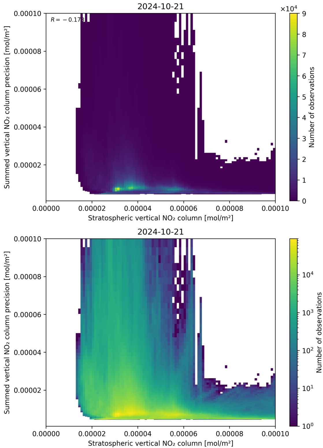
Figure 99: Scatter density plot of “Stratospheric vertical NO 2 column” against “Summed vertical NO 2 column precision” for 2024-10-20 to 2024-10-22.
