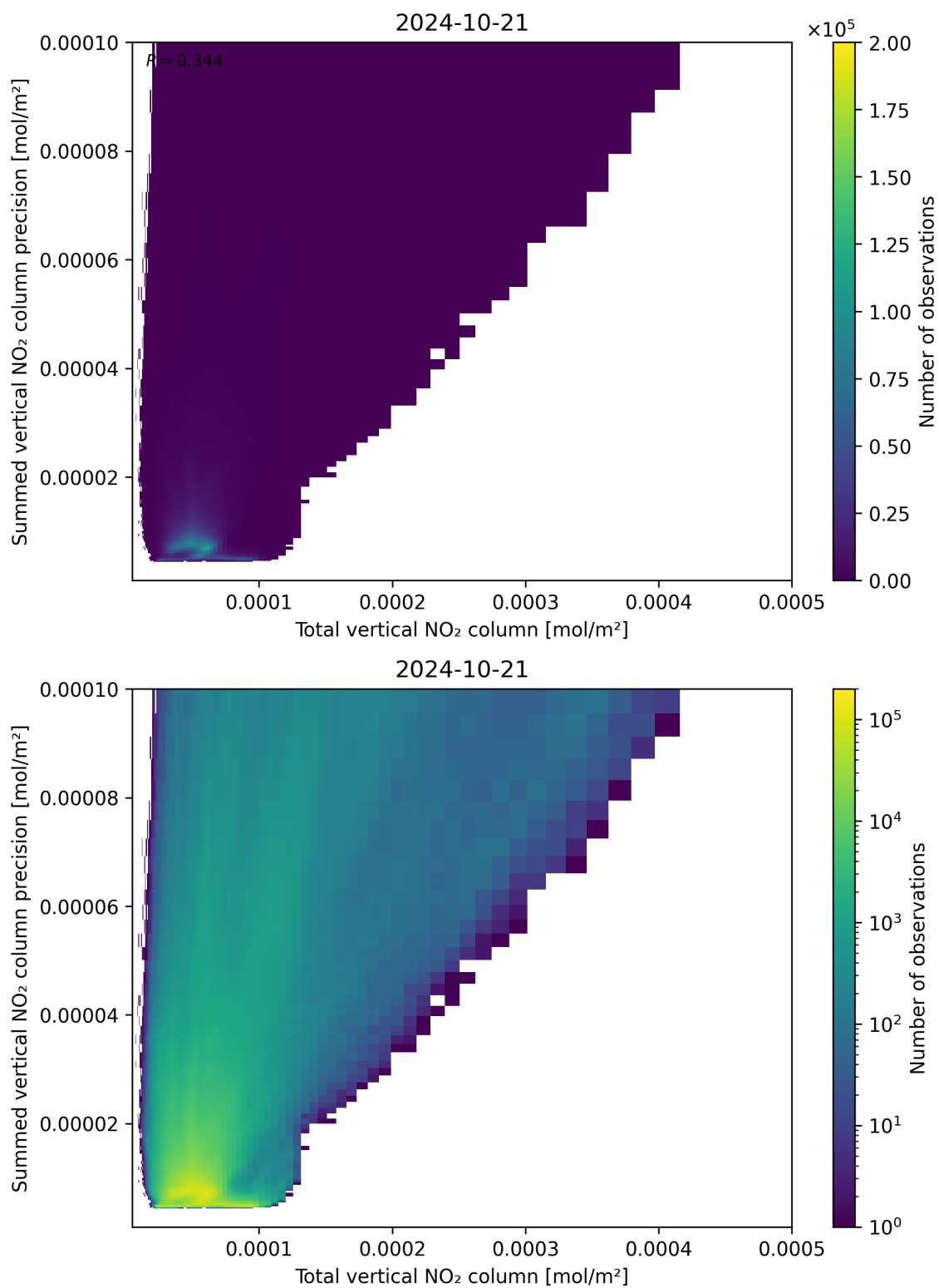
Figure 113: Scatter density plot of “Total vertical NO 2 column” against “Summed vertical NO 2 column precision” for 2024-10-20 to 2024-10-22.
