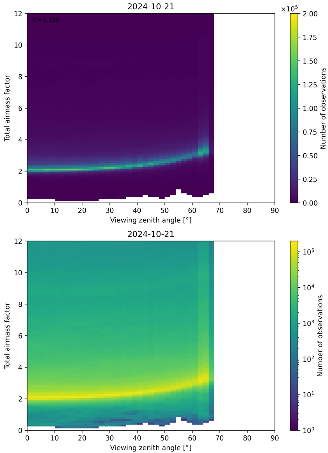
Figure 160: Scatter density plot of “Viewing zenith angle” against “Total airmass factor” for 2024-10-20 to 2024-10-22.
