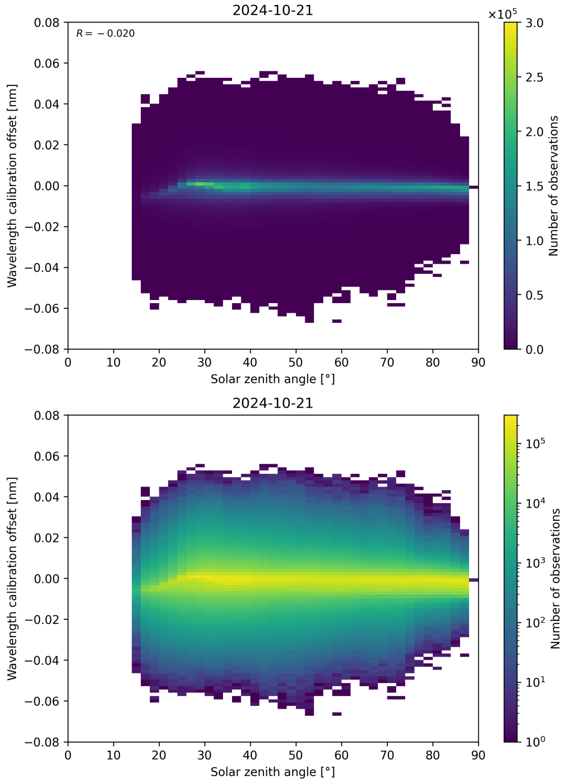
Figure 158: Scatter density plot of “Solar zenith angle” against “Wavelength calibration offset” for 2024-10-20 to 2024-10-22.
