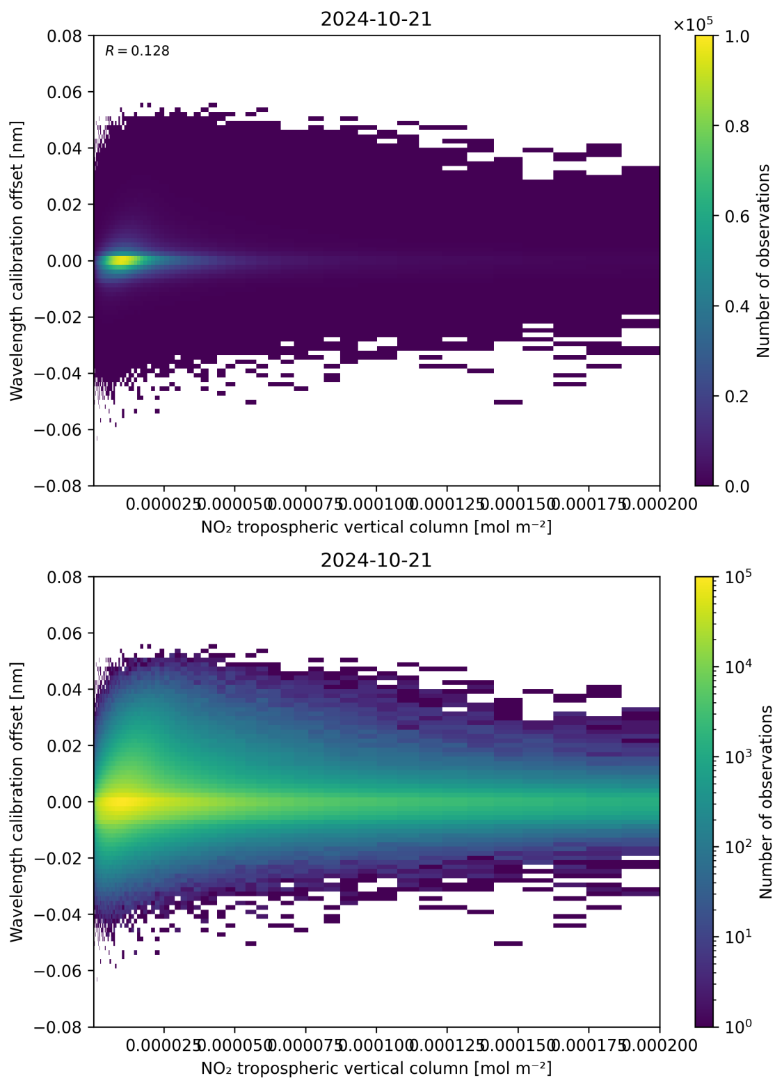
Figure 143: Scatter density plot of “NO 2 tropospheric vertical column” against “Wavelength calibration offset” for 2024-10-20 to 2024-10-22.
