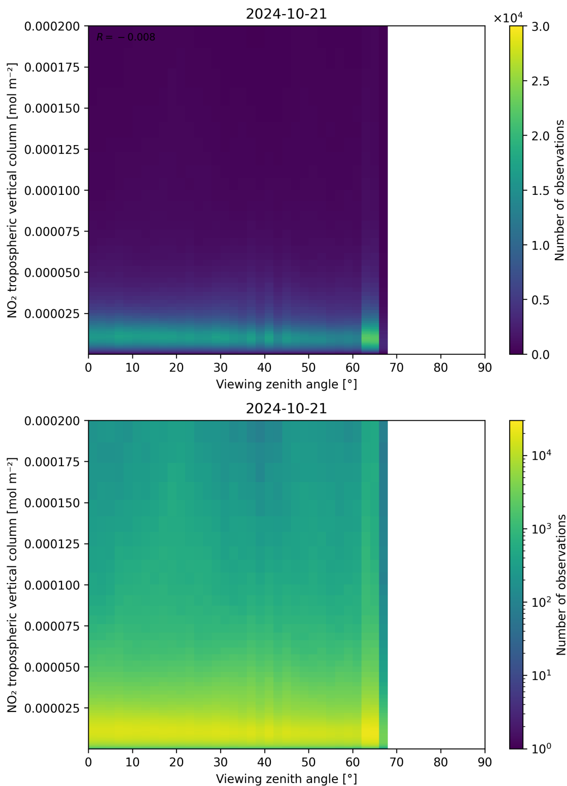
Figure 169: Scatter density plot of “Viewing zenith angle” against “NO 2 tropospheric vertical column” for 2024-10-20 to 2024-10-22.
