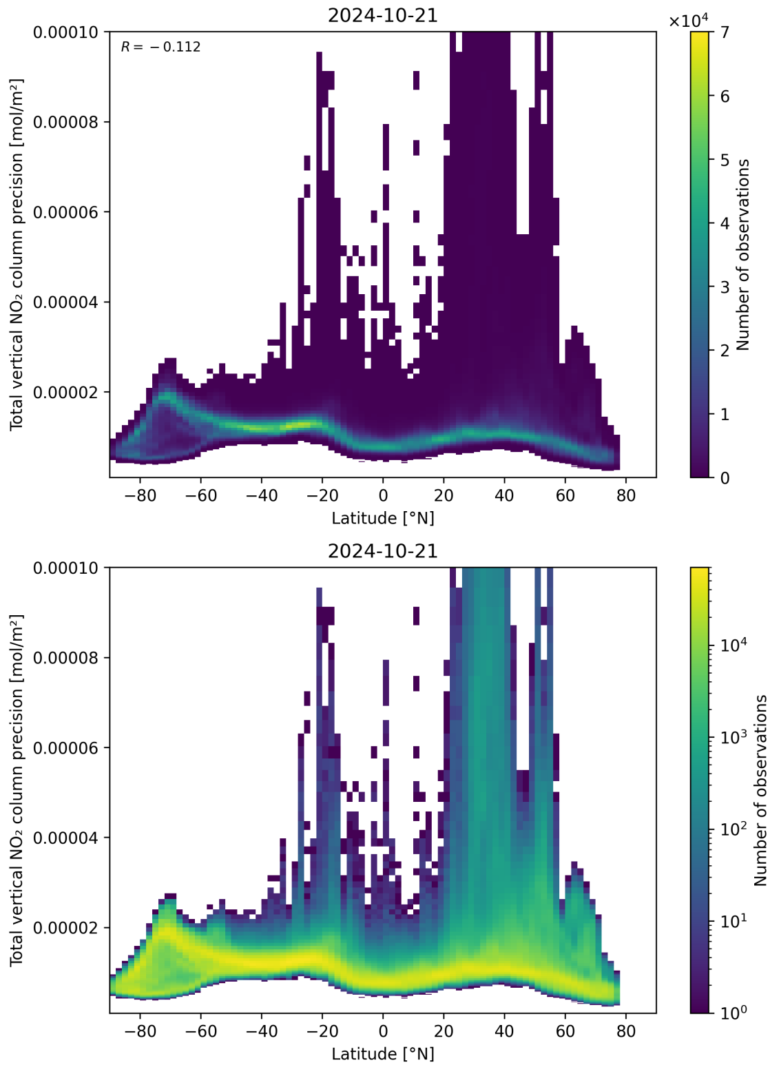
Figure 91: Scatter density plot of “Latitude” against “Total vertical NO 2 column precision” for 2024-10-20 to 2024-10-22.
