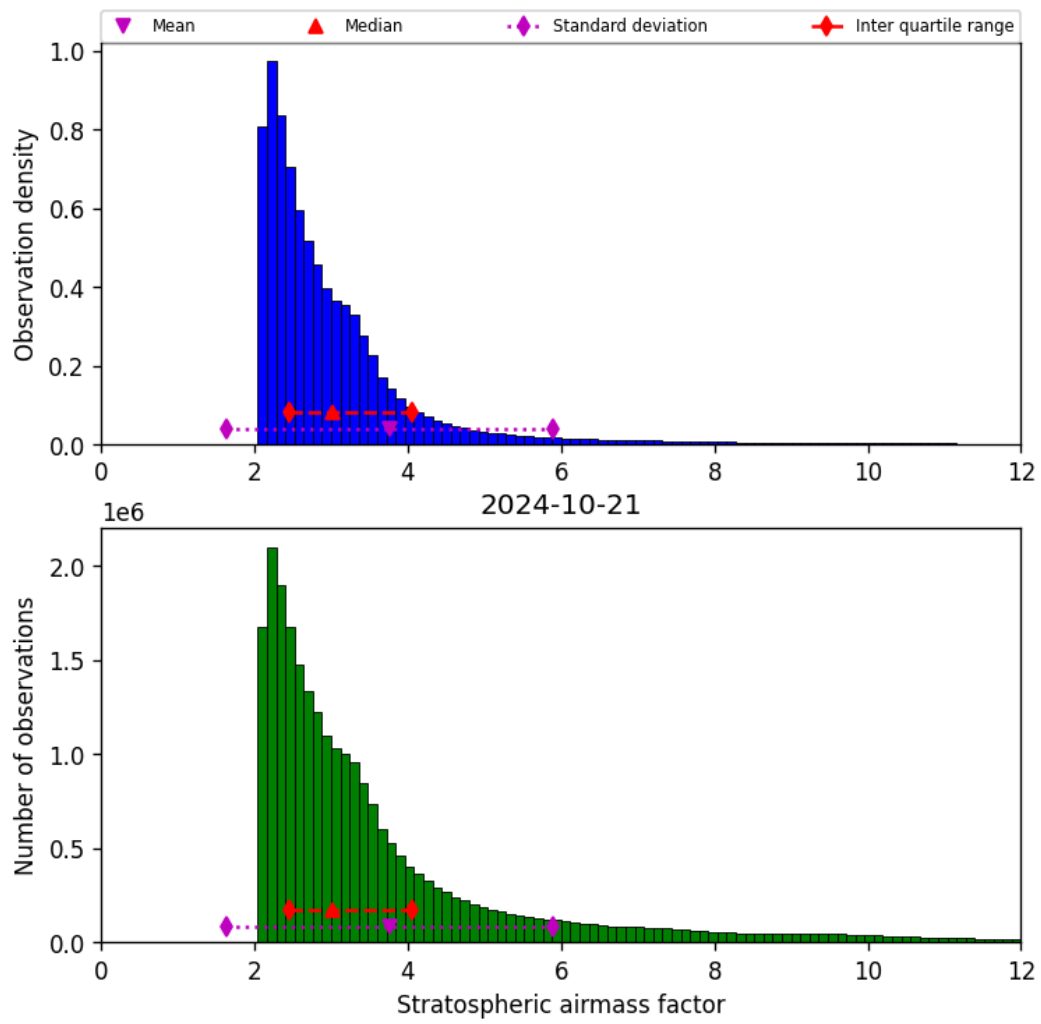
Figure 44: Histogram of “Stratospheric airmass factor” for 2024-10-20 to 2024-10-22
