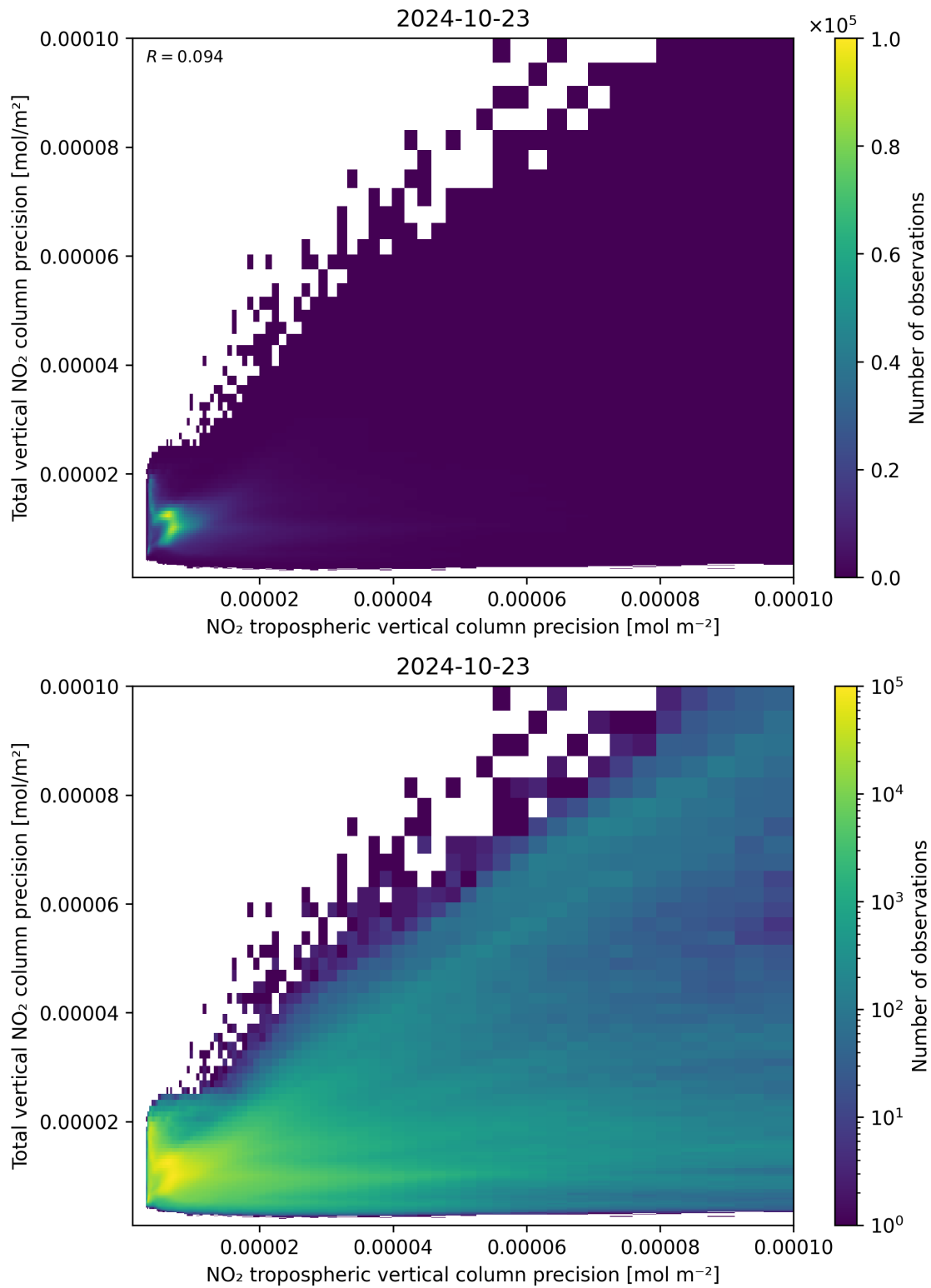
Figure 139: Scatter density plot of “NO 2 tropospheric vertical column precision” against “Total vertical NO 2 column precision” for 2024-10-22 to 2024-10-24.
