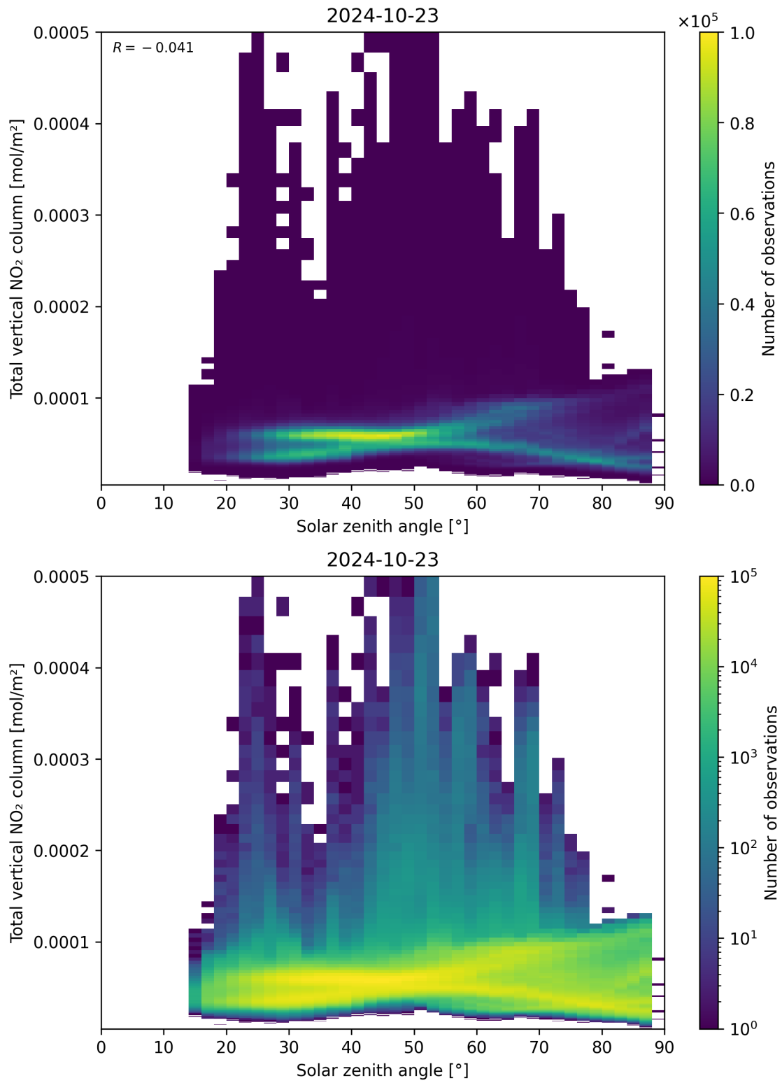
Figure 153: Scatter density plot of “Solar zenith angle” against “Total vertical NO 2 column” for 2024-10-22 to 2024-10-24.
