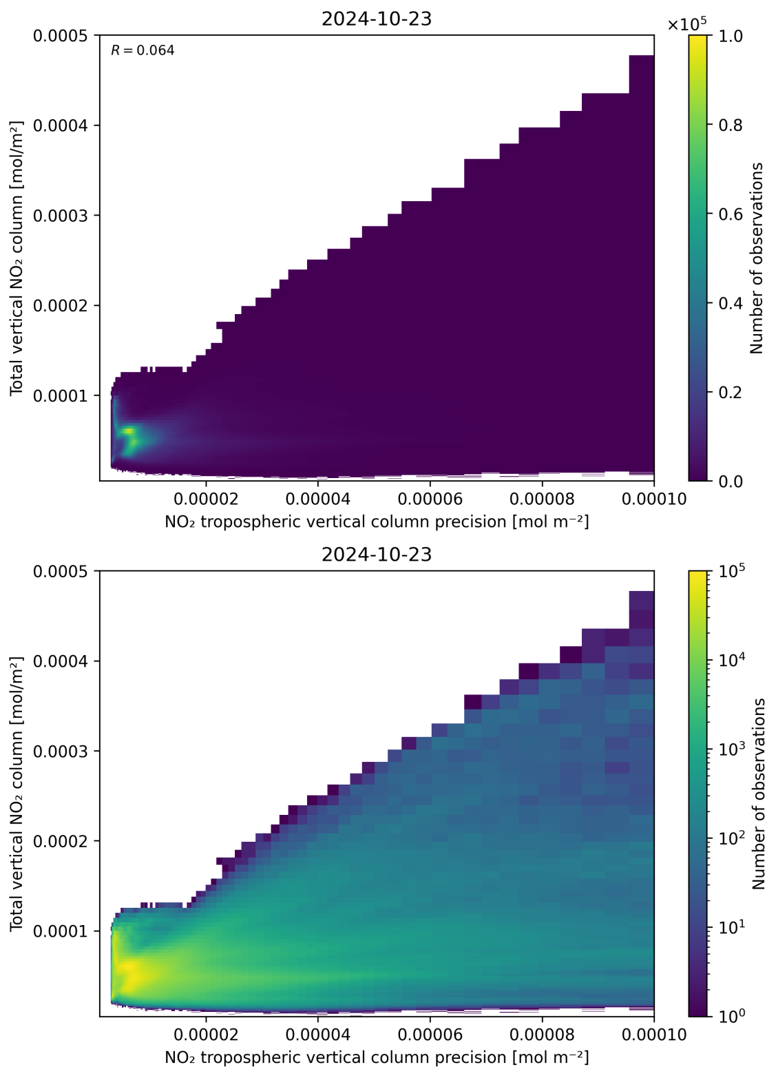
Figure 138: Scatter density plot of “NO 2 tropospheric vertical column precision” against “Total vertical NO 2 column” for 2024-10-22 to 2024-10-24.
