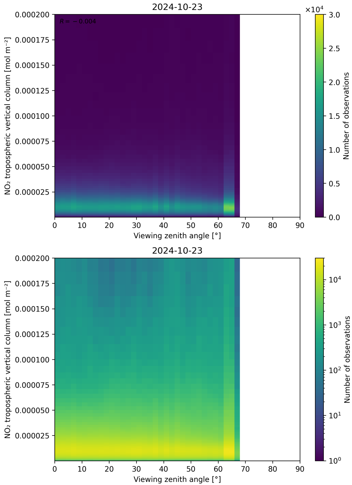
Figure 169: Scatter density plot of “Viewing zenith angle” against “NO 2 tropospheric vertical column” for 2024-10-22 to 2024-10-24.
