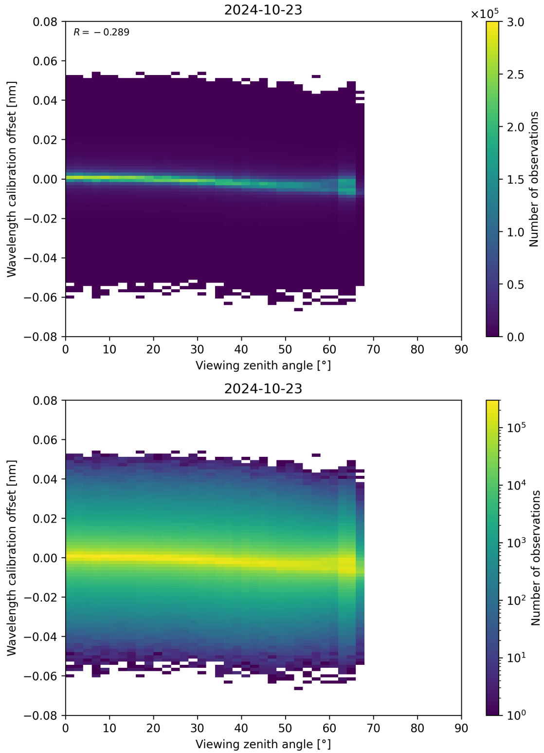
Figure 173: Scatter density plot of “Viewing zenith angle” against “Wavelength calibration offset” for 2024-10-22 to 2024-10-24.
