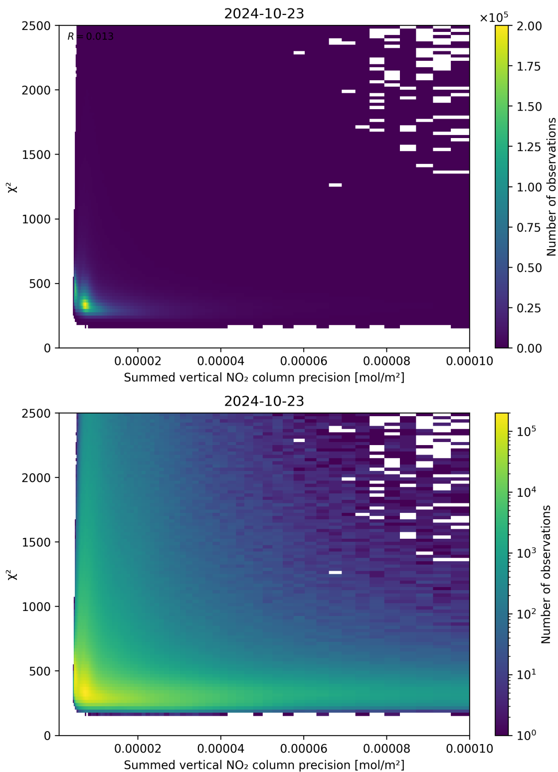
Figure 107: Scatter density plot of “Summed vertical NO 2 column precision” against “ \chi^2 ” for 2024-10-22 to 2024-10-24.
