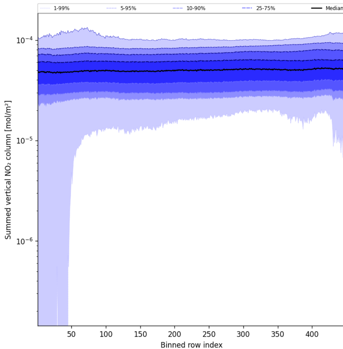
Figure 57: Along track statistics of “Summed vertical NO 2 column” for 2024-10-22 to 2024-10-24
