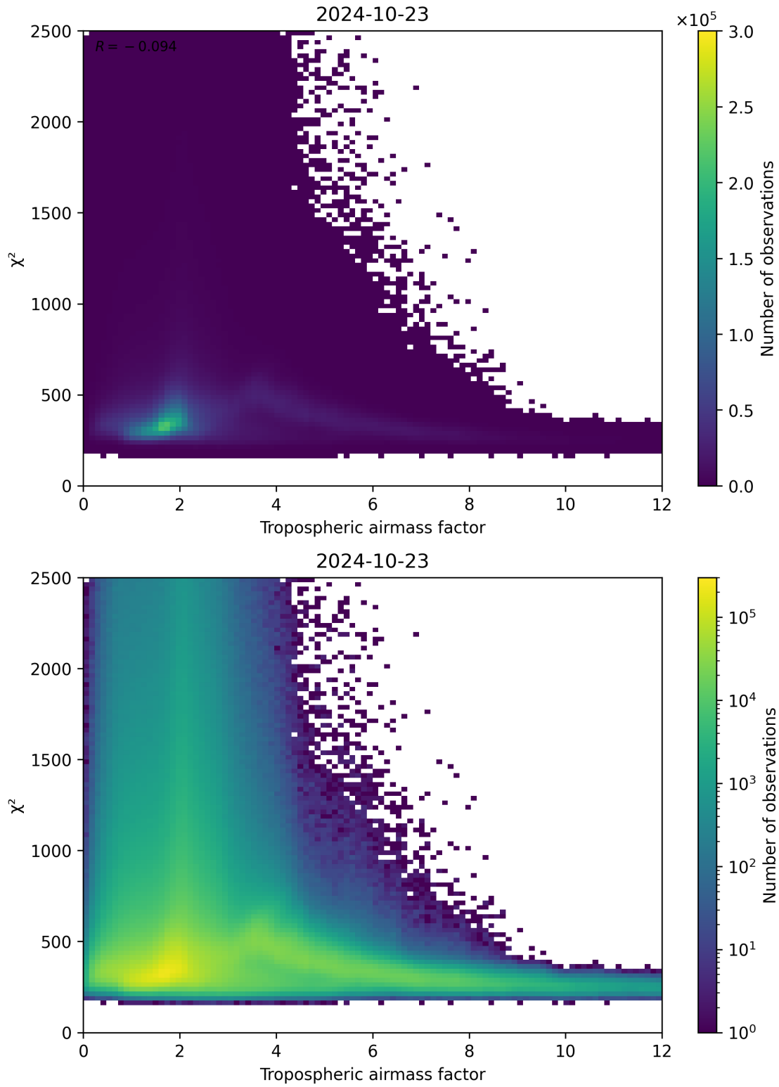
Figure 73: Scatter density plot of “Tropospheric airmass factor” against “ \chi^2 ” for 2024-10-22 to 2024-10-24.
