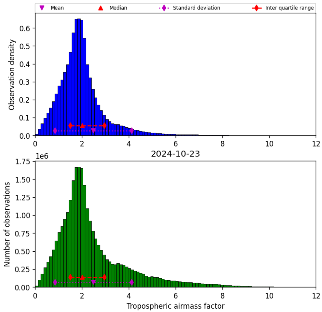
Figure 31: Histogram of “Tropospheric airmass factor” for 2024-10-22 to 2024-10-24
