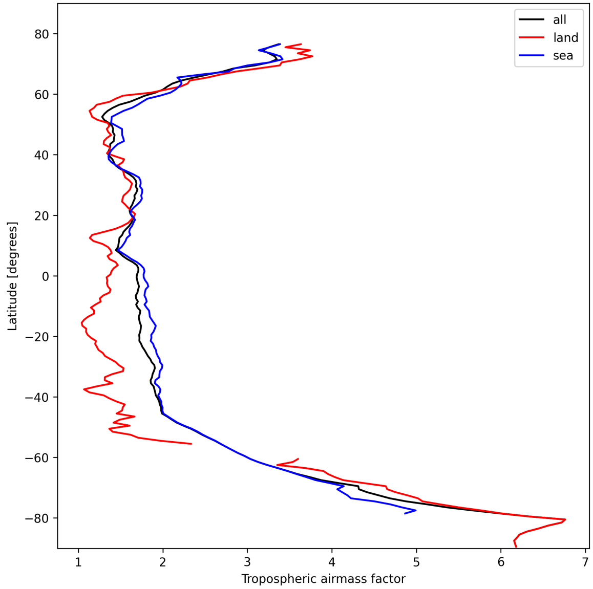
Figure 14: Zonal average of “Tropospheric air mass factor” for 2024-10-22 to 2024-10-24.
