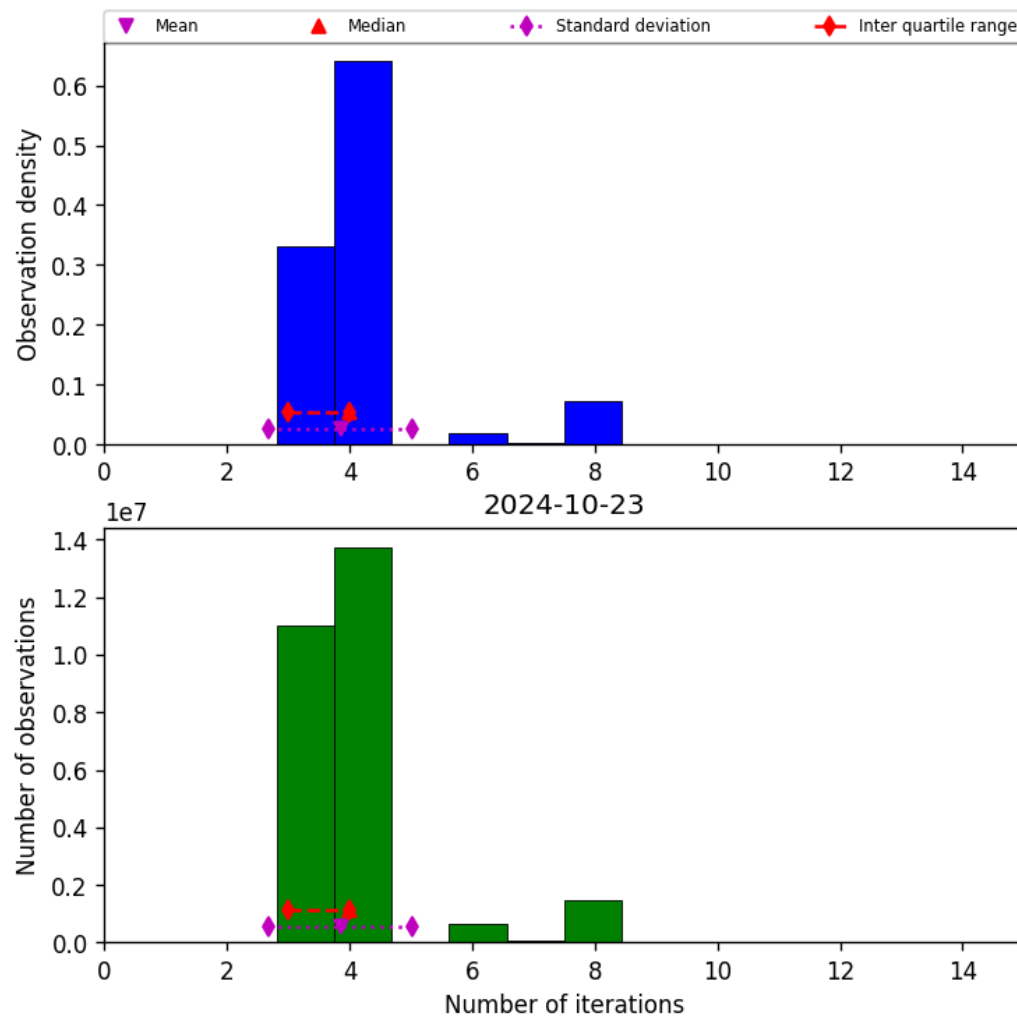
Figure 34: Histogram of “Number of iterations” for 2024-10-22 to 2024-10-24
