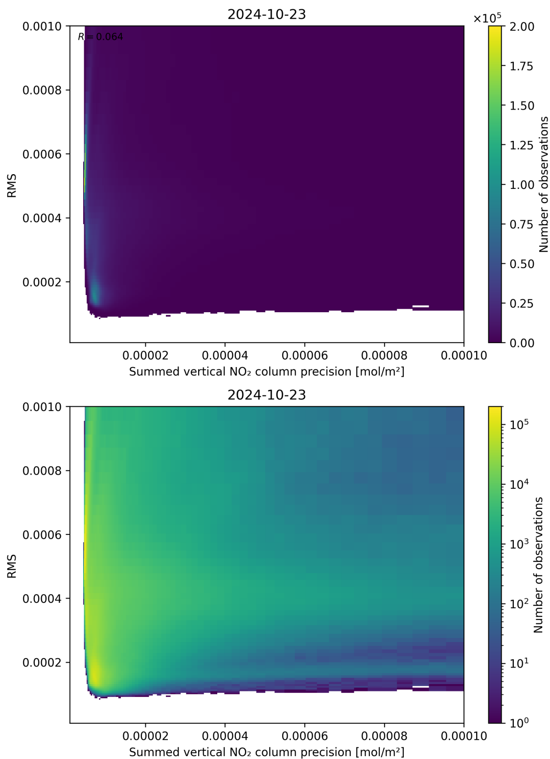
Figure 108: Scatter density plot of “Summed vertical NO 2 column precision” against “RMS” for 2024-10-22 to 2024-10-24.
