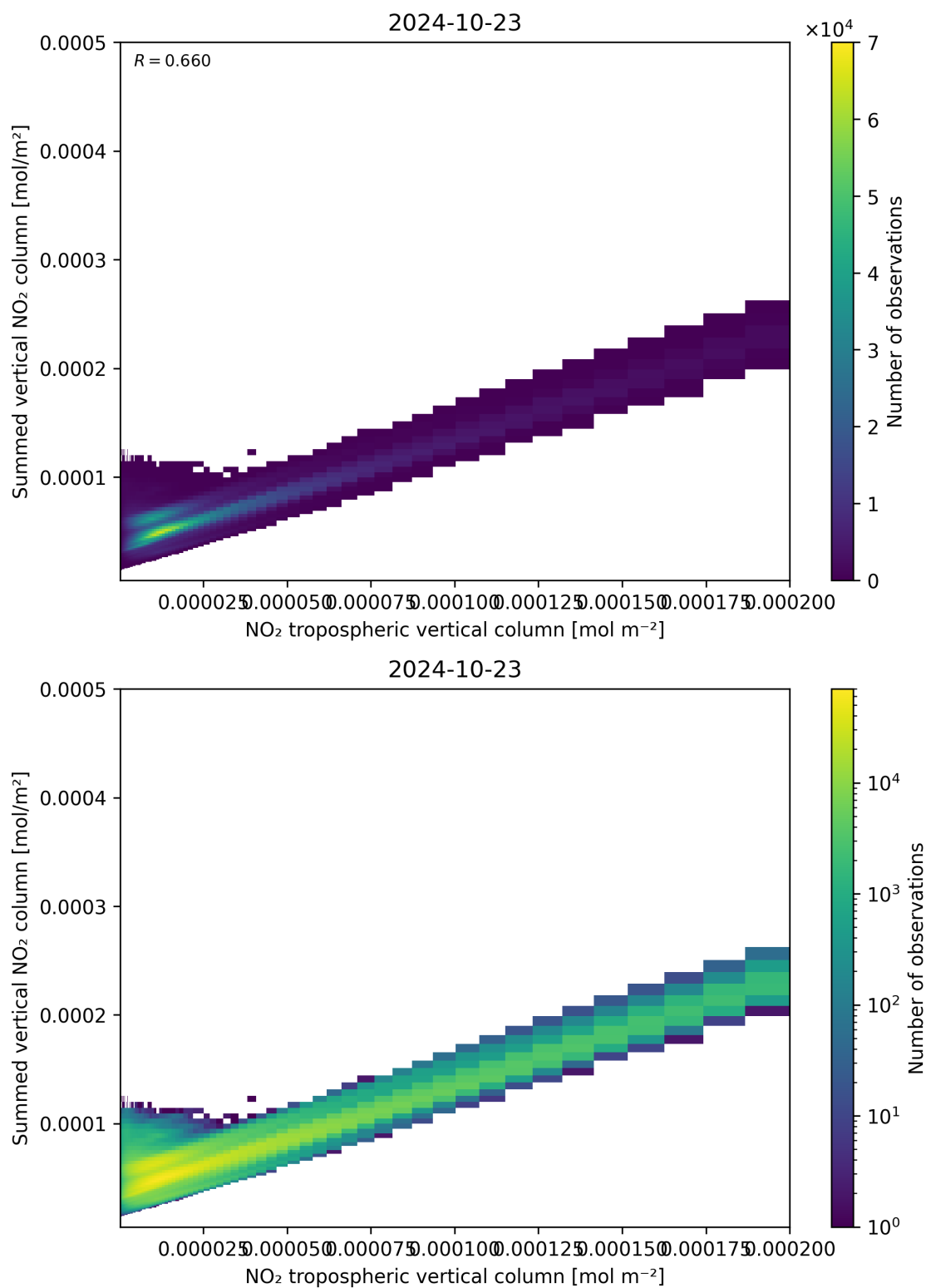
Figure 126: Scatter density plot of “NO 2 tropospheric vertical column” against “Summed vertical NO 2 column” for 2024-10-22 to 2024-10-24.
