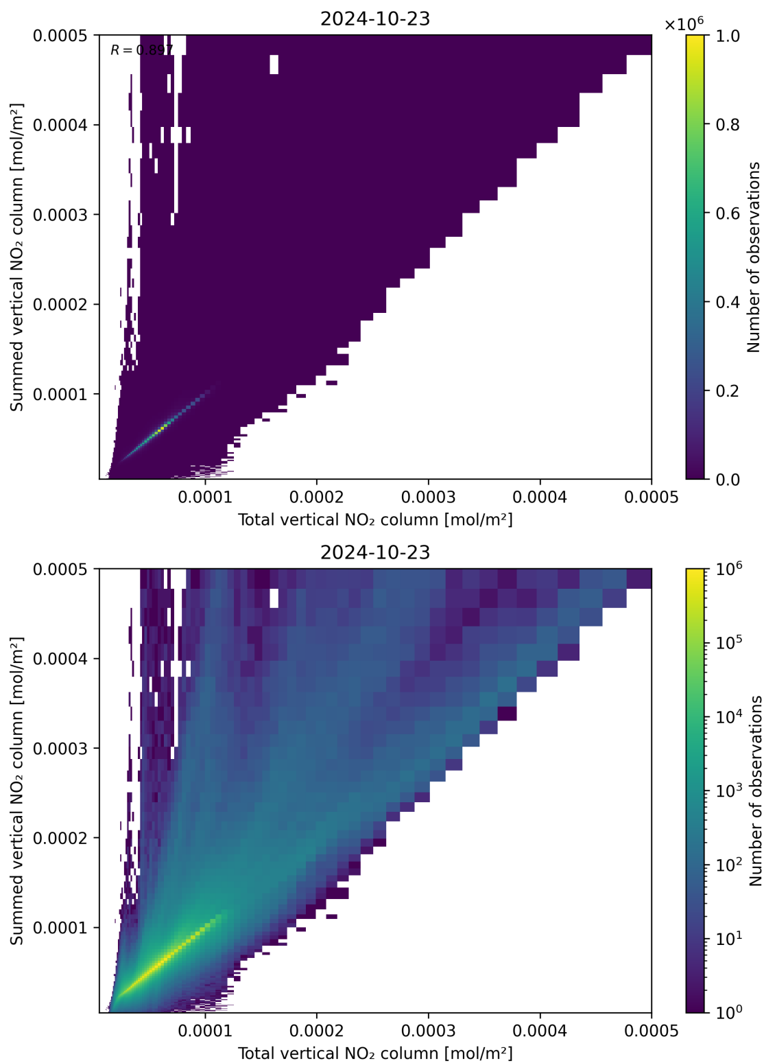
Figure 112: Scatter density plot of “Total vertical NO 2 column” against “Summed vertical NO 2 column” for 2024-10-22 to 2024-10-24.
