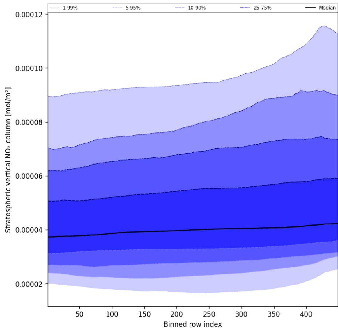
Figure 53: Along track statistics of “Stratospheric vertical NO 2 column” for 2024-10-22 to 2024-10-24
