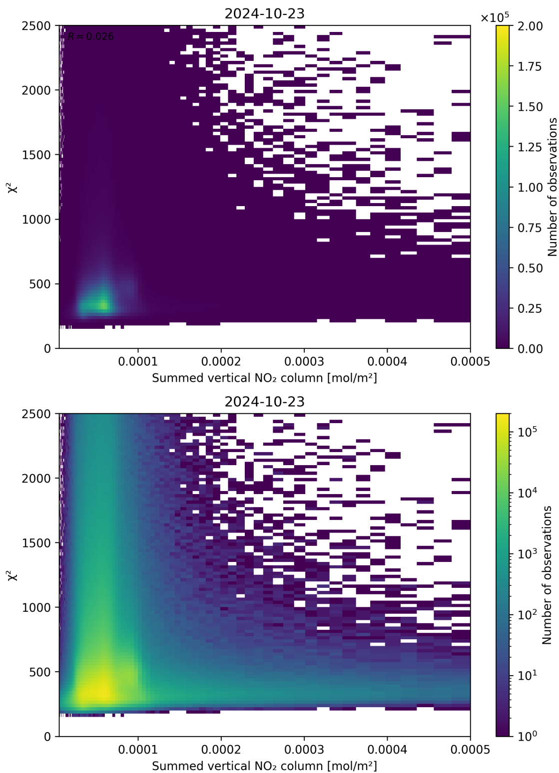
Figure 104: Scatter density plot of “Summed vertical NO 2 column” against “ \chi^2 ” for 2024-10-22 to 2024-10-24.
