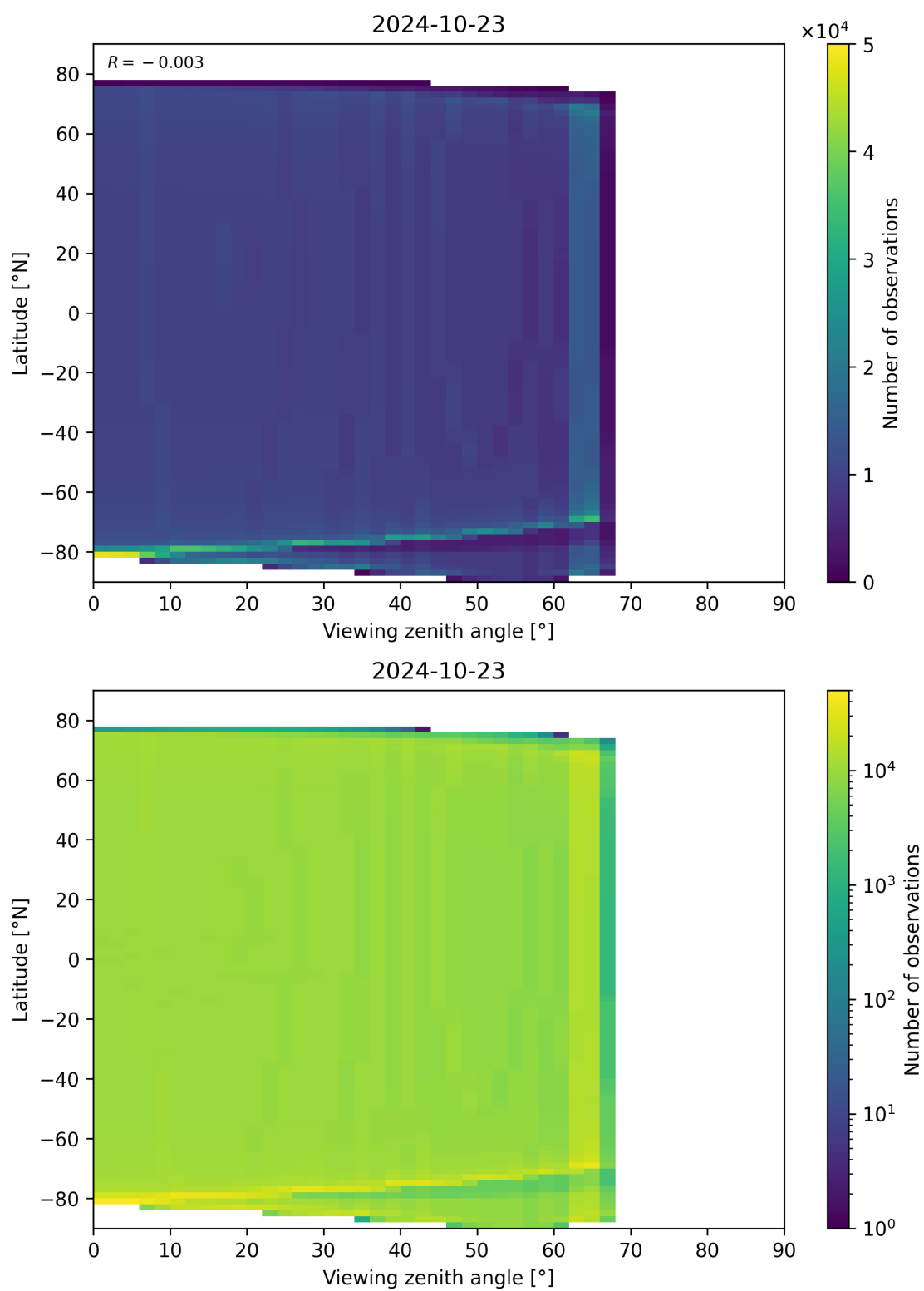
Figure 163: Scatter density plot of “Viewing zenith angle” against “Latitude” for 2024-10-22 to 2024-10-24.
