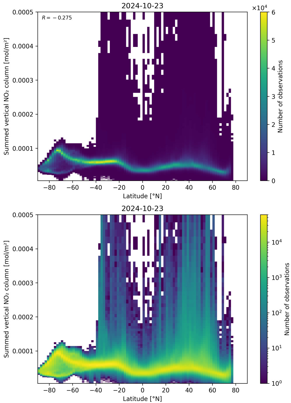
Figure 88: Scatter density plot of “Latitude” against “Summed vertical NO 2 column” for 2024-10-22 to 2024-10-24.
