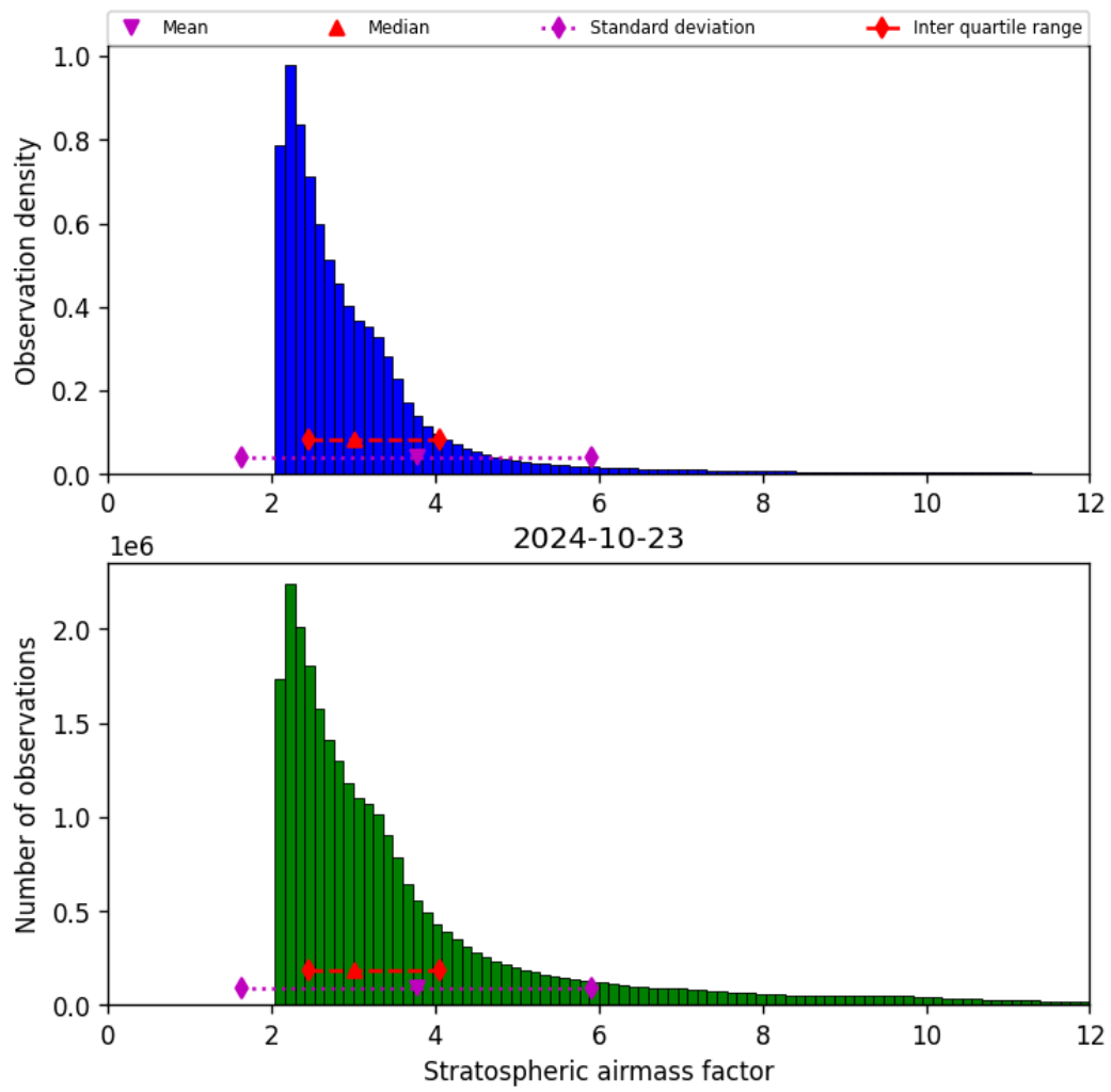
Figure 44: Histogram of “Stratospheric airmass factor” for 2024-10-22 to 2024-10-24
