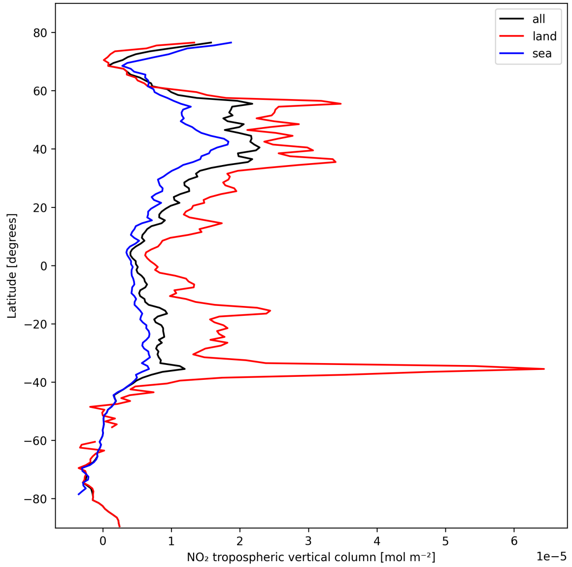
Figure 12: Zonal average of “NO 2 tropospheric vertical column” for 2024-10-22 to 2024-10-24.
