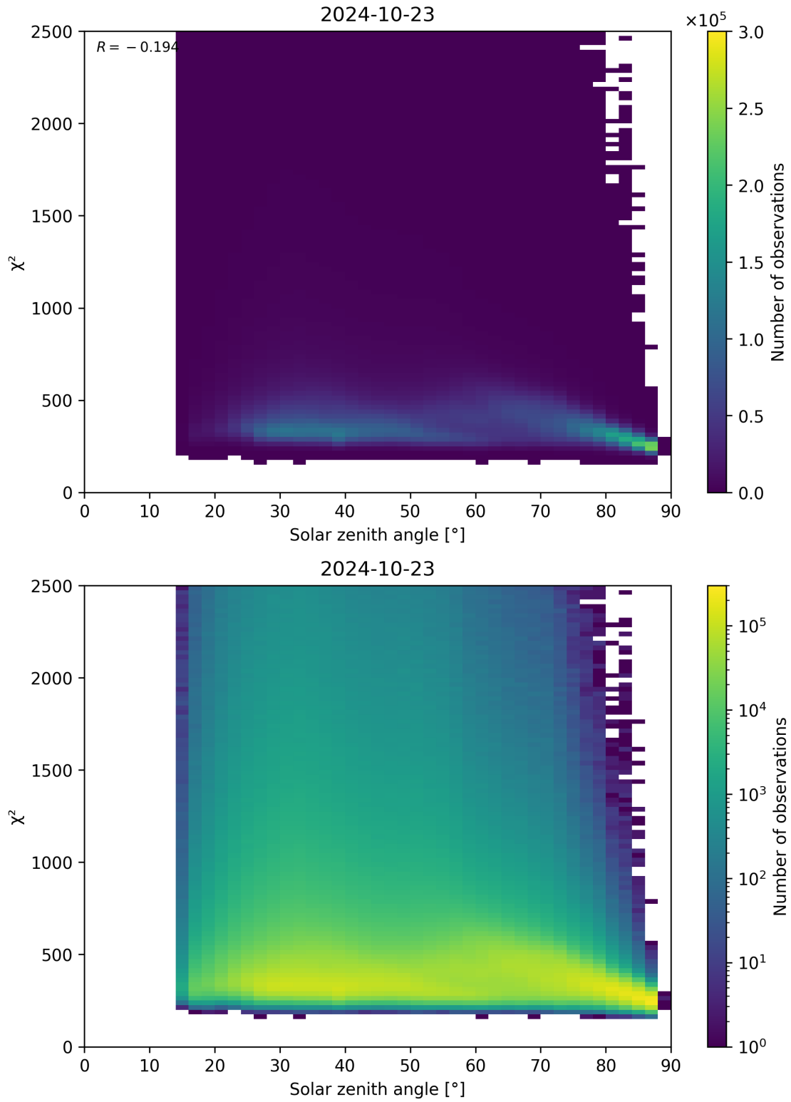
Figure 148: Scatter density plot of “Solar zenith angle” against “ \chi^2 ” for 2024-10-22 to 2024-10-24.
