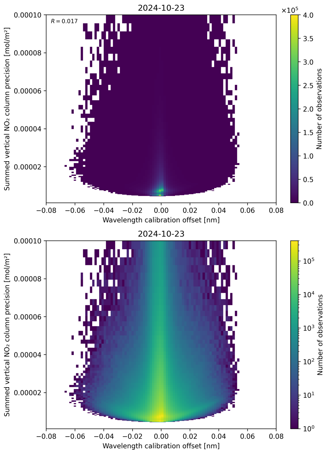
Figure 178: Scatter density plot of “Wavelength calibration offset” against “Summed vertical NO 2 column precision” for 2024-10-22 to 2024-10-24.
