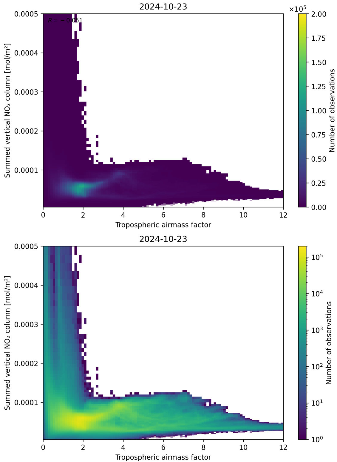
Figure 75: Scatter density plot of “Tropospheric airmass factor” against “Summed vertical NO 2 column” for 2024-10-22 to 2024-10-24.
