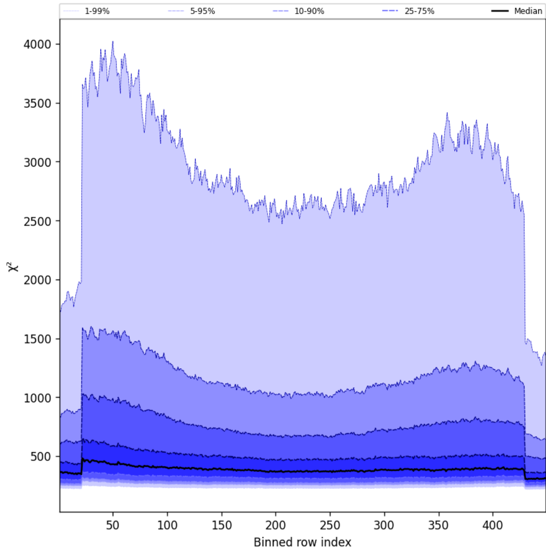
Figure 59: Along track statistics of “ \chi^2 ” for 2024-10-22 to 2024-10-24
