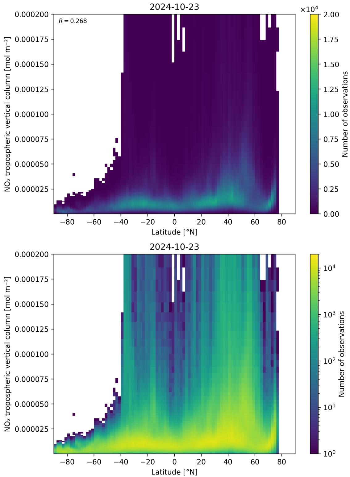
Figure 92: Scatter density plot of “Latitude” against “NO 2 tropospheric vertical column” for 2024-10-22 to 2024-10-24.
