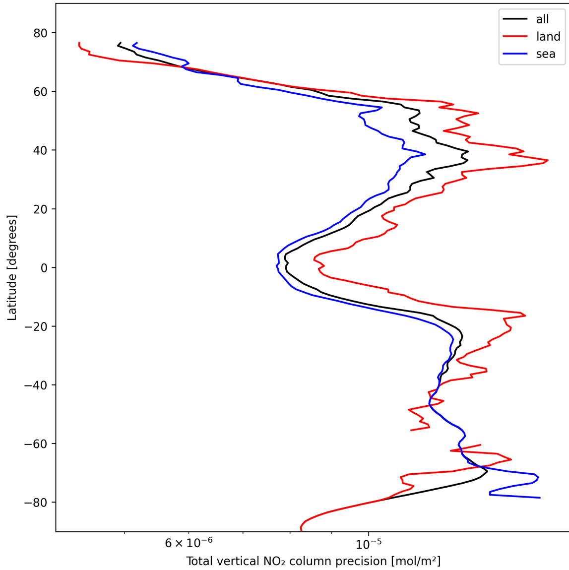
Figure 22: Zonal average of “Total vertical NO 2 column precision” for 2024-10-22 to 2024-10-24.
