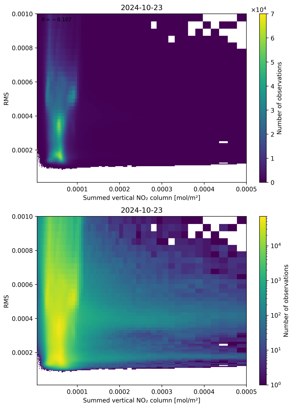
Figure 109: Scatter density plot of “Summed vertical NO 2 column” against “RMS” for 2024-10-22 to 2024-10-24.
