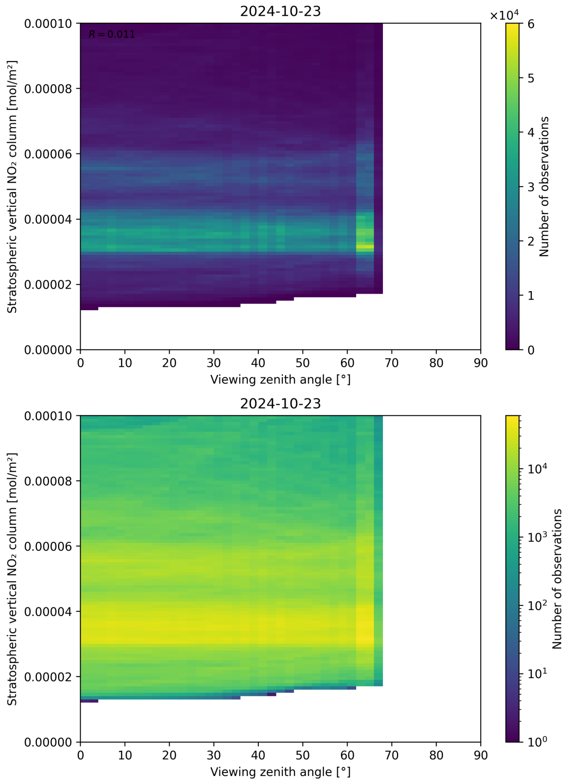
Figure 164: Scatter density plot of “Viewing zenith angle” against “Stratospheric vertical NO 2 column” for 2024-10-22 to 2024-10-24.
