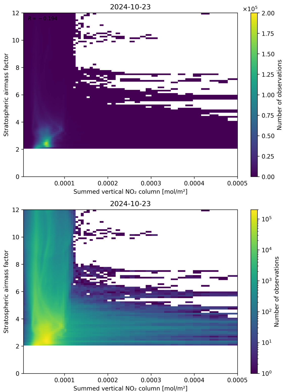
Figure 103: Scatter density plot of “Summed vertical NO 2 column” against “Stratospheric airmass factor” for 2024-10-22 to 2024-10-24.
