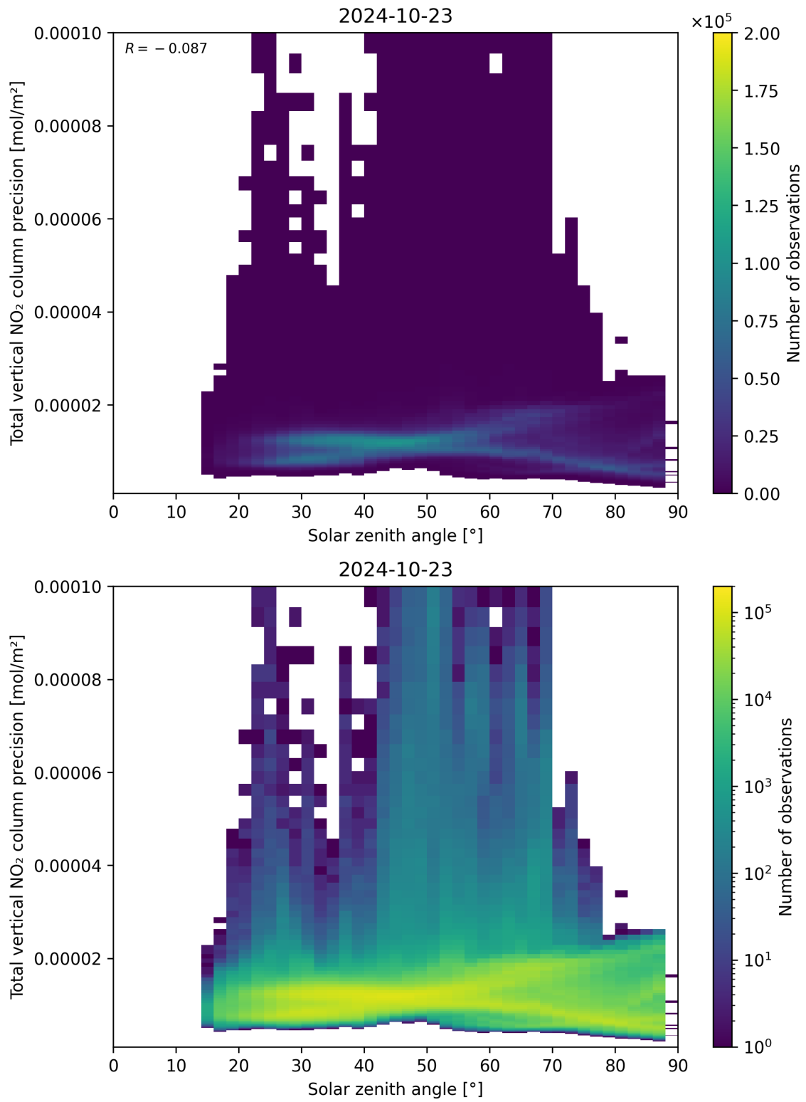
Figure 154: Scatter density plot of “Solar zenith angle” against “Total vertical NO 2 column precision” for 2024-10-22 to 2024-10-24.
