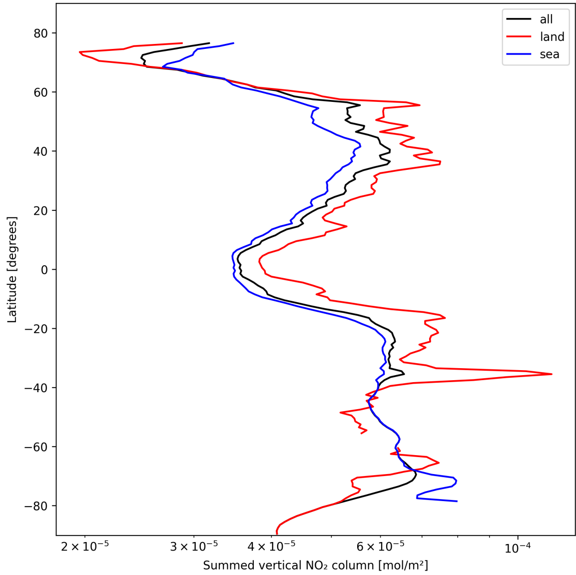
Figure 23: Zonal average of “Summed vertical NO 2 column” for 2024-10-22 to 2024-10-24.
