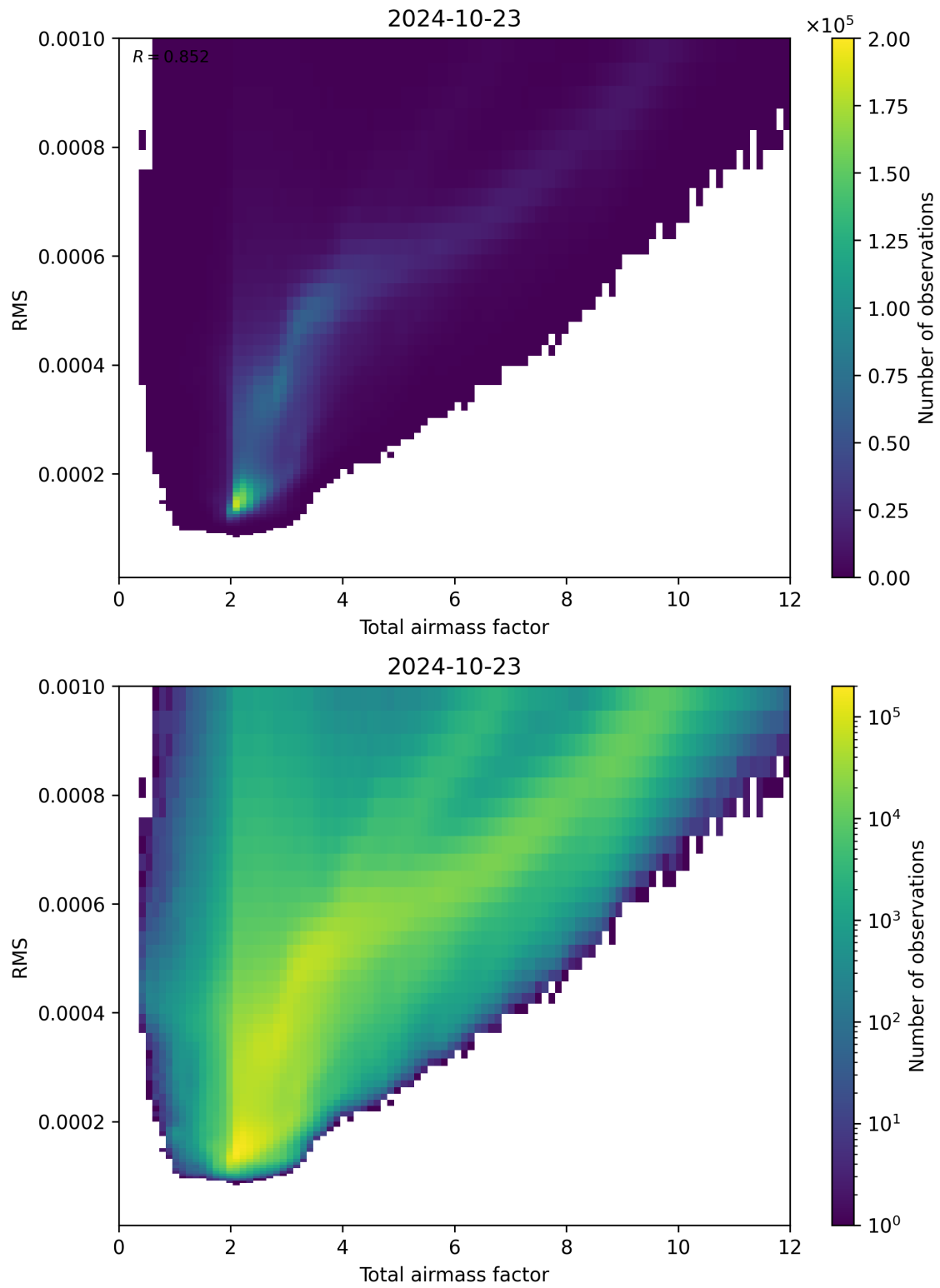
Figure 69: Scatter density plot of “Total airmass factor” against “RMS” for 2024-10-22 to 2024-10-24.
