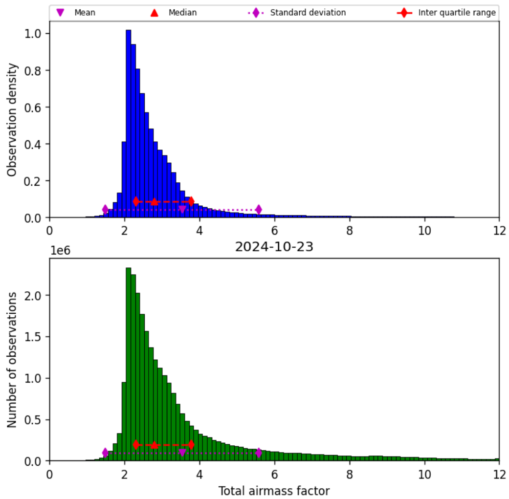
Figure 32: Histogram of “Total airmass factor” for 2024-10-22 to 2024-10-24
