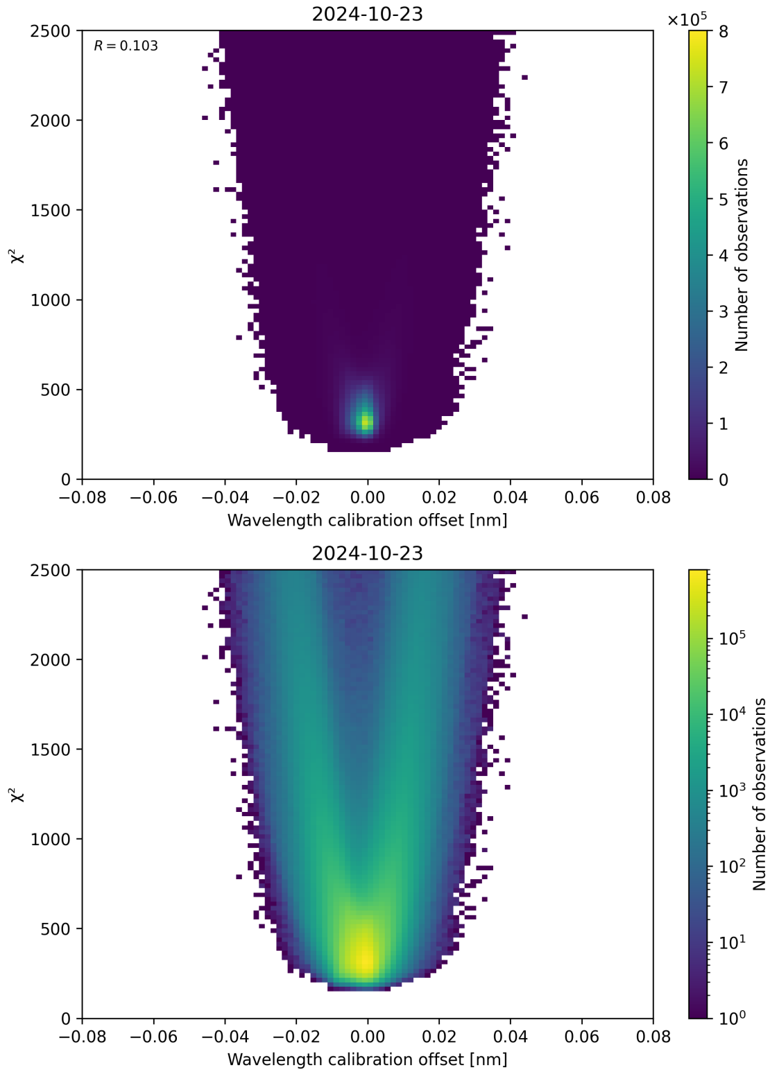
Figure 175: Scatter density plot of “Wavelength calibration offset” against “ \chi^2 ” for 2024-10-22 to 2024-10-24.
