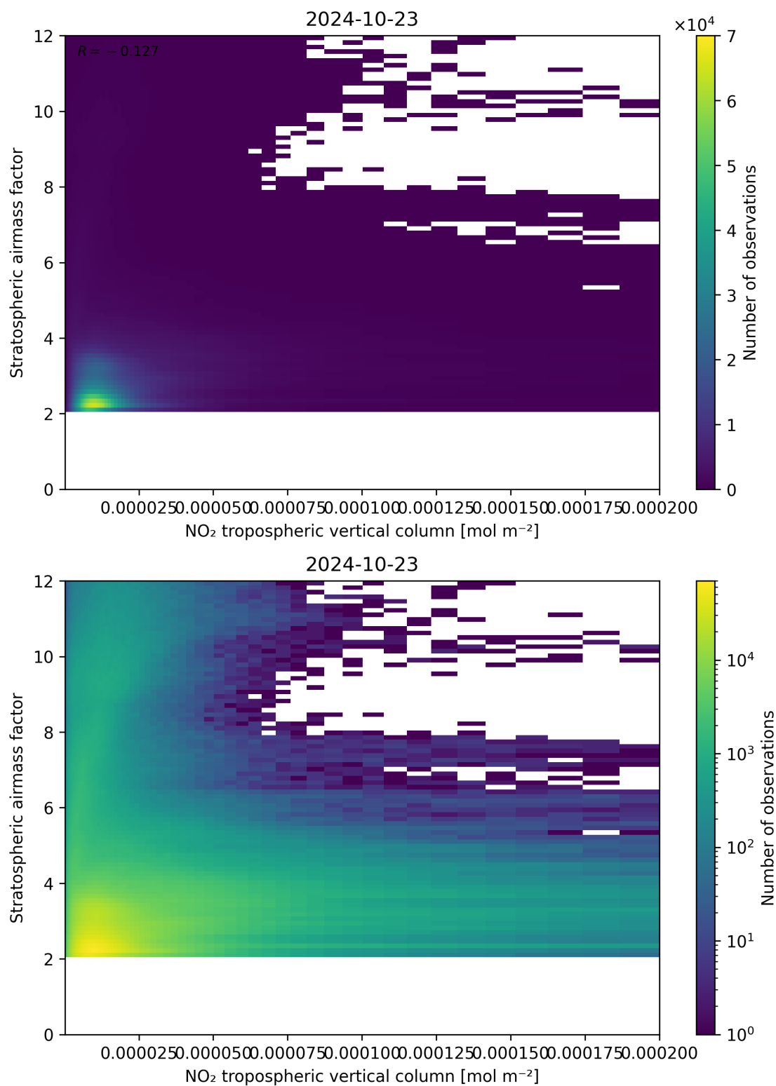
Figure 121: Scatter density plot of “NO 2 tropospheric vertical column” against “Stratospheric airmass factor” for 2024-10-22 to 2024-10-24.
