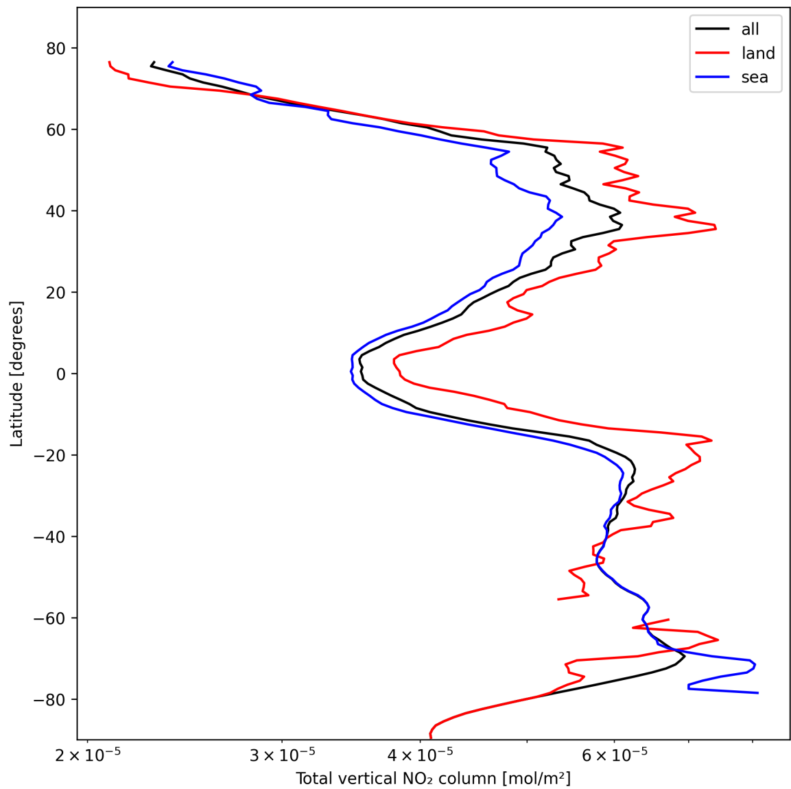
Figure 21: Zonal average of “Total vertical NO 2 column” for 2024-10-22 to 2024-10-24.
