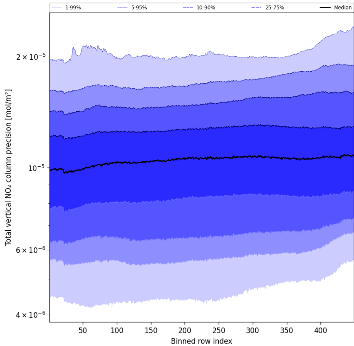
Figure 56: Along track statistics of “Total vertical NO 2 column precision” for 2024-10-22 to 2024-10-24
