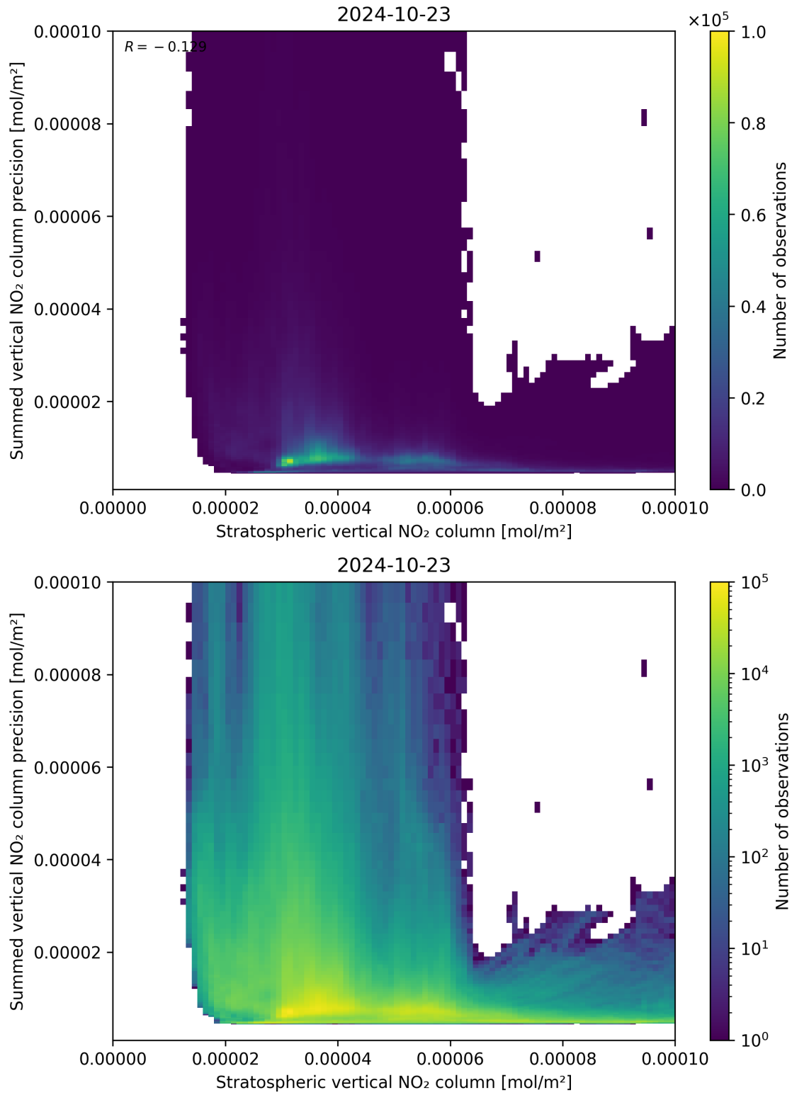
Figure 99: Scatter density plot of “Stratospheric vertical NO 2 column” against “Summed vertical NO 2 column precision” for 2024-10-22 to 2024-10-24.
