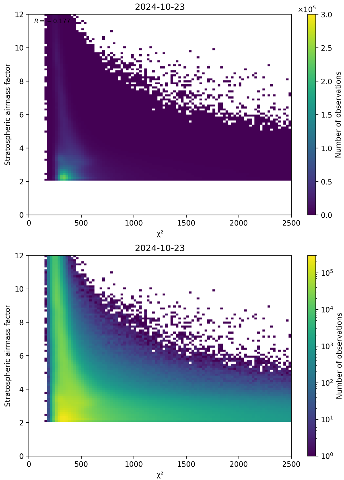
Figure 81: Scatter density plot of “ \chi^2 ” against “Stratospheric airmass factor” for 2024-10-22 to 2024-10-24.
