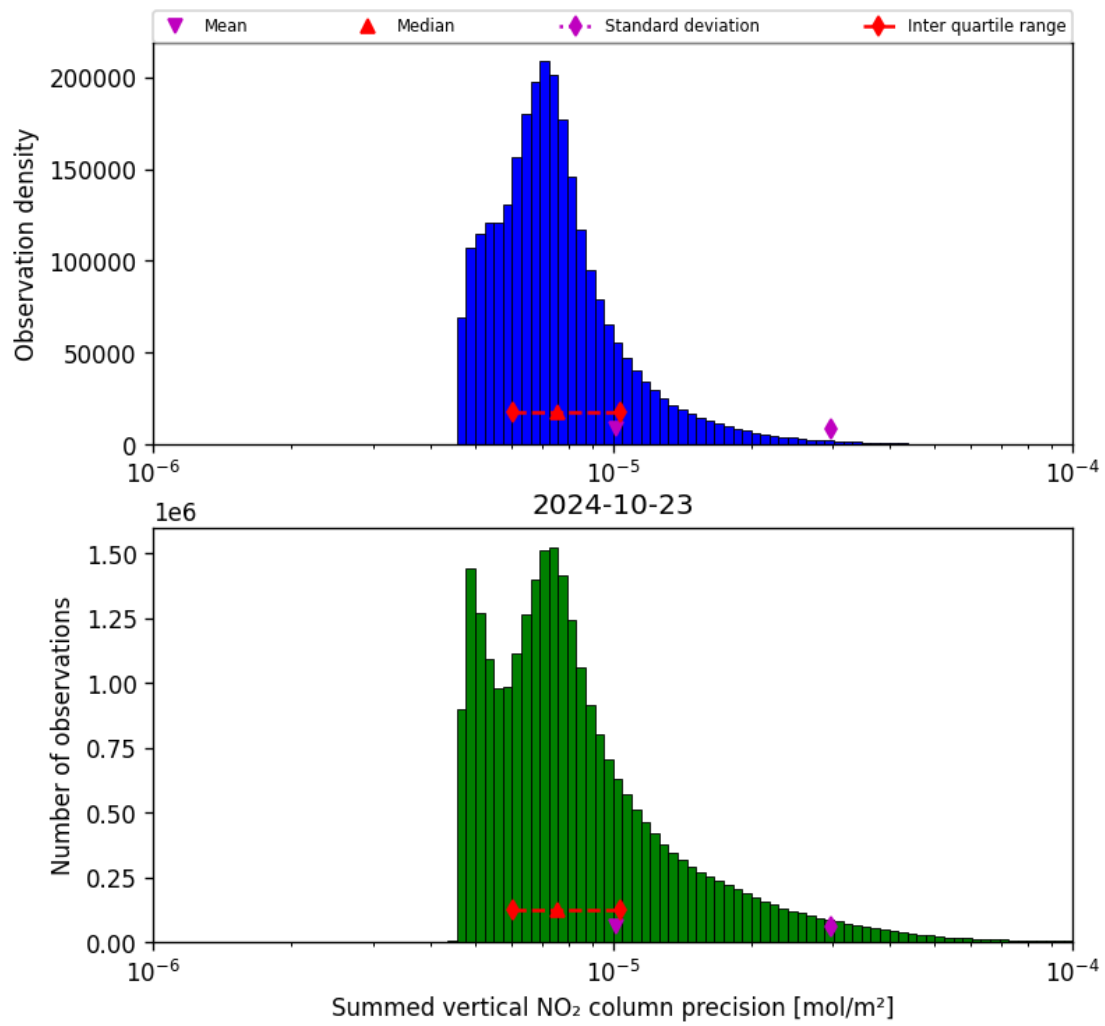
Figure 41: Histogram of "Summed vertical NO 2 column precision" for 2024-10-22 to 2024-10-24
