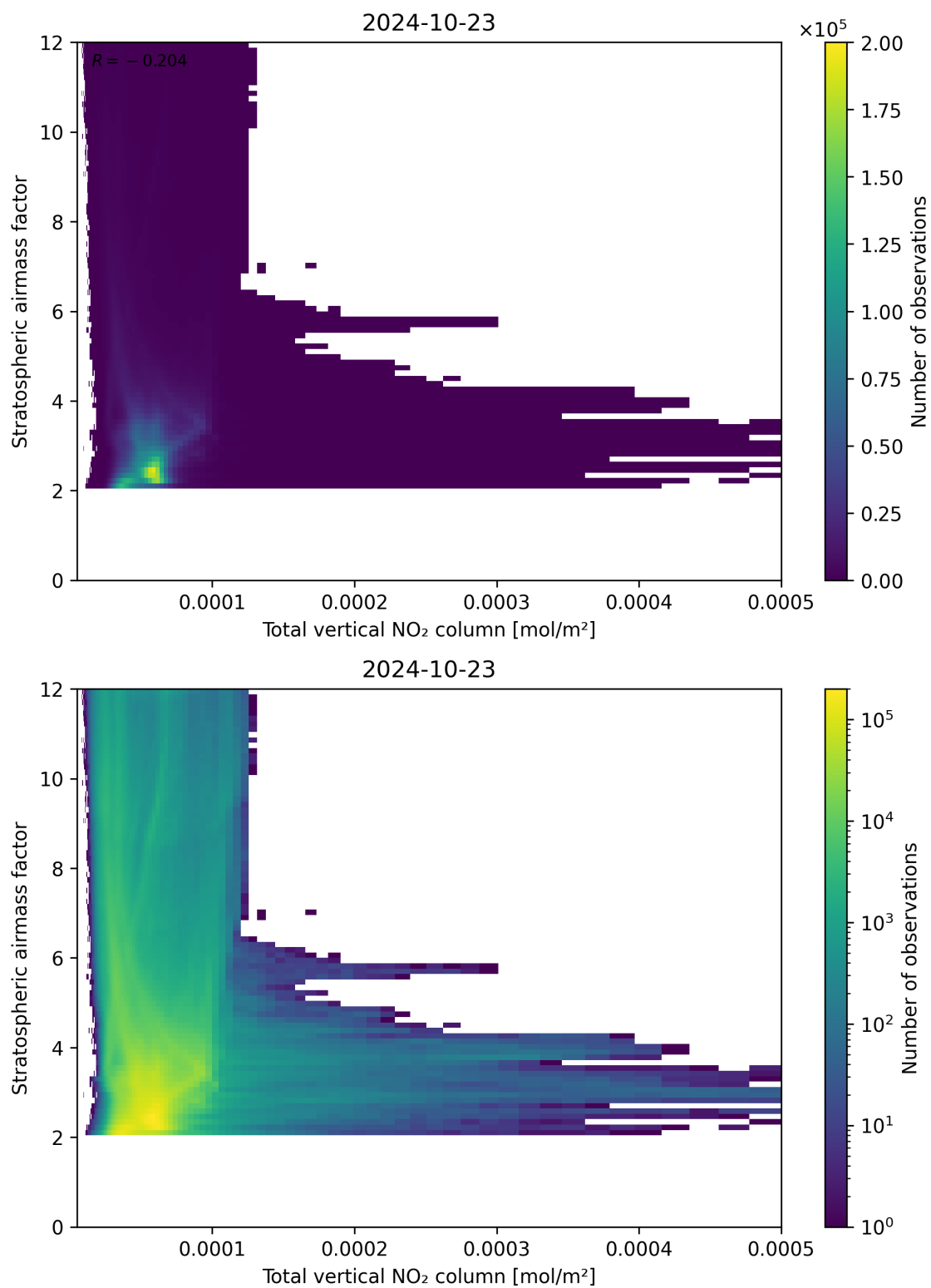
Figure 110: Scatter density plot of “Total vertical NO 2 column” against “Stratospheric airmass factor” for 2024-10-22 to 2024-10-24.
