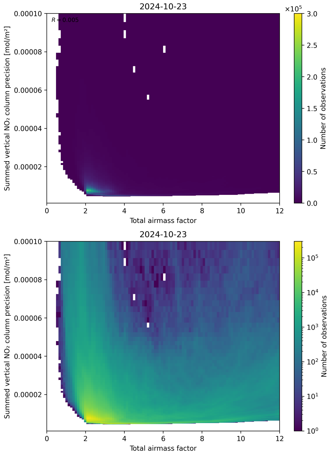
Figure 66: Scatter density plot of “Total airmass factor” against “Summed vertical NO 2 column precision” for 2024-10-22 to 2024-10-24.
