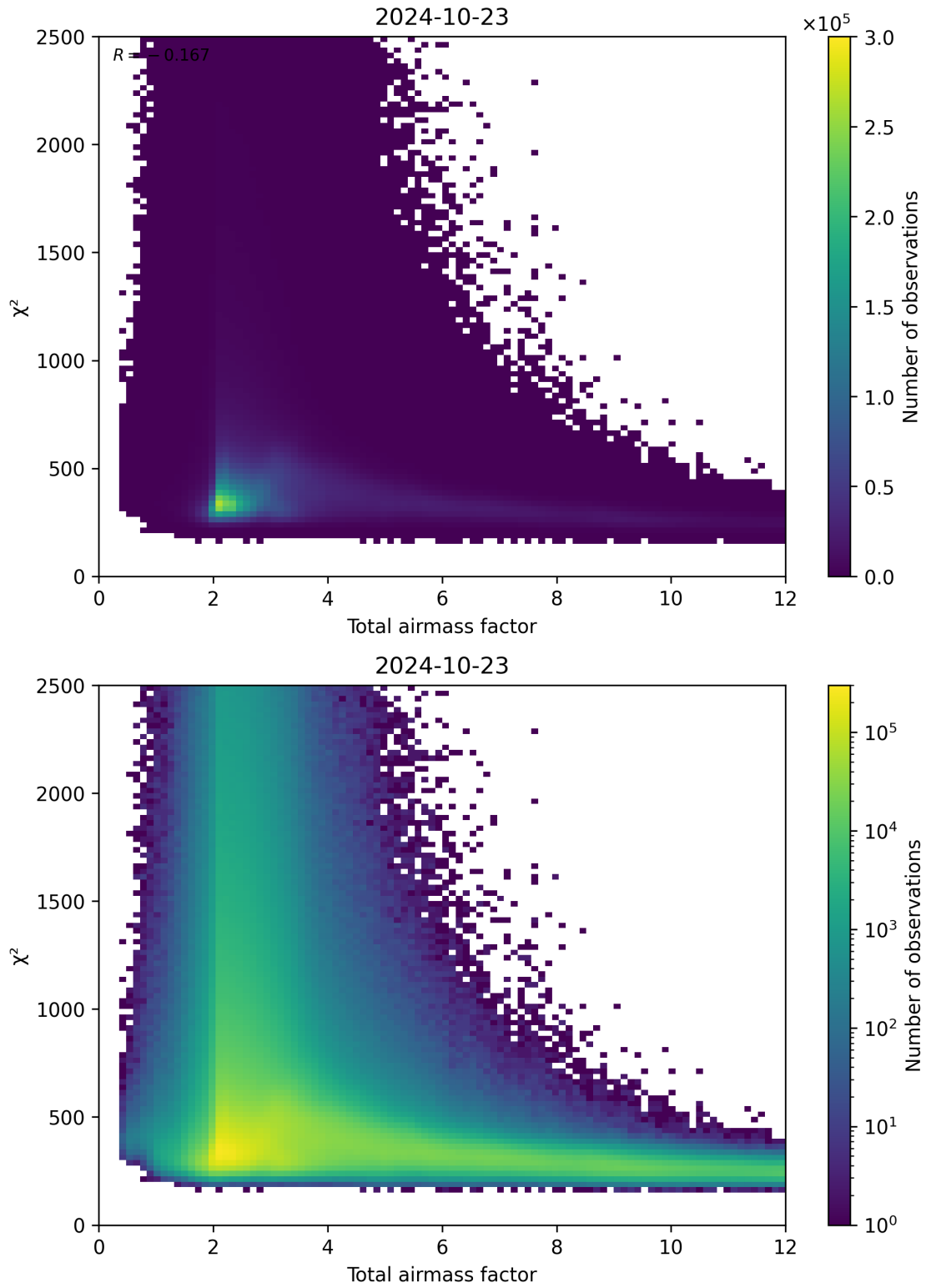
Figure 63: Scatter density plot of “Total airmass factor” against “ \chi^2 ” for 2024-10-22 to 2024-10-24.
