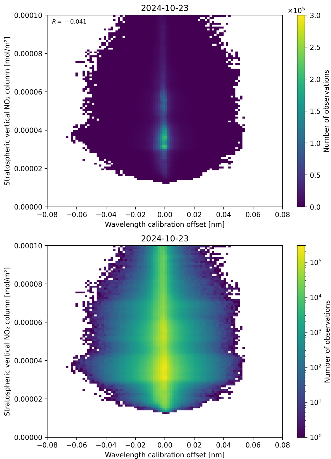
Figure 176: Scatter density plot of “Wavelength calibration offset” against “Stratospheric vertical NO 2 column” for 2024-10-22 to 2024-10-24.
