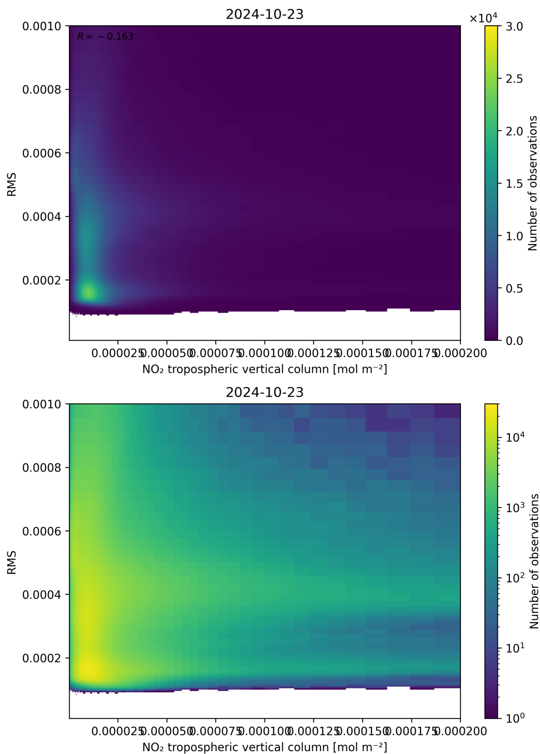
Figure 142: Scatter density plot of “NO 2 tropospheric vertical column” against “RMS” for 2024-10-22 to 2024-10-24.
