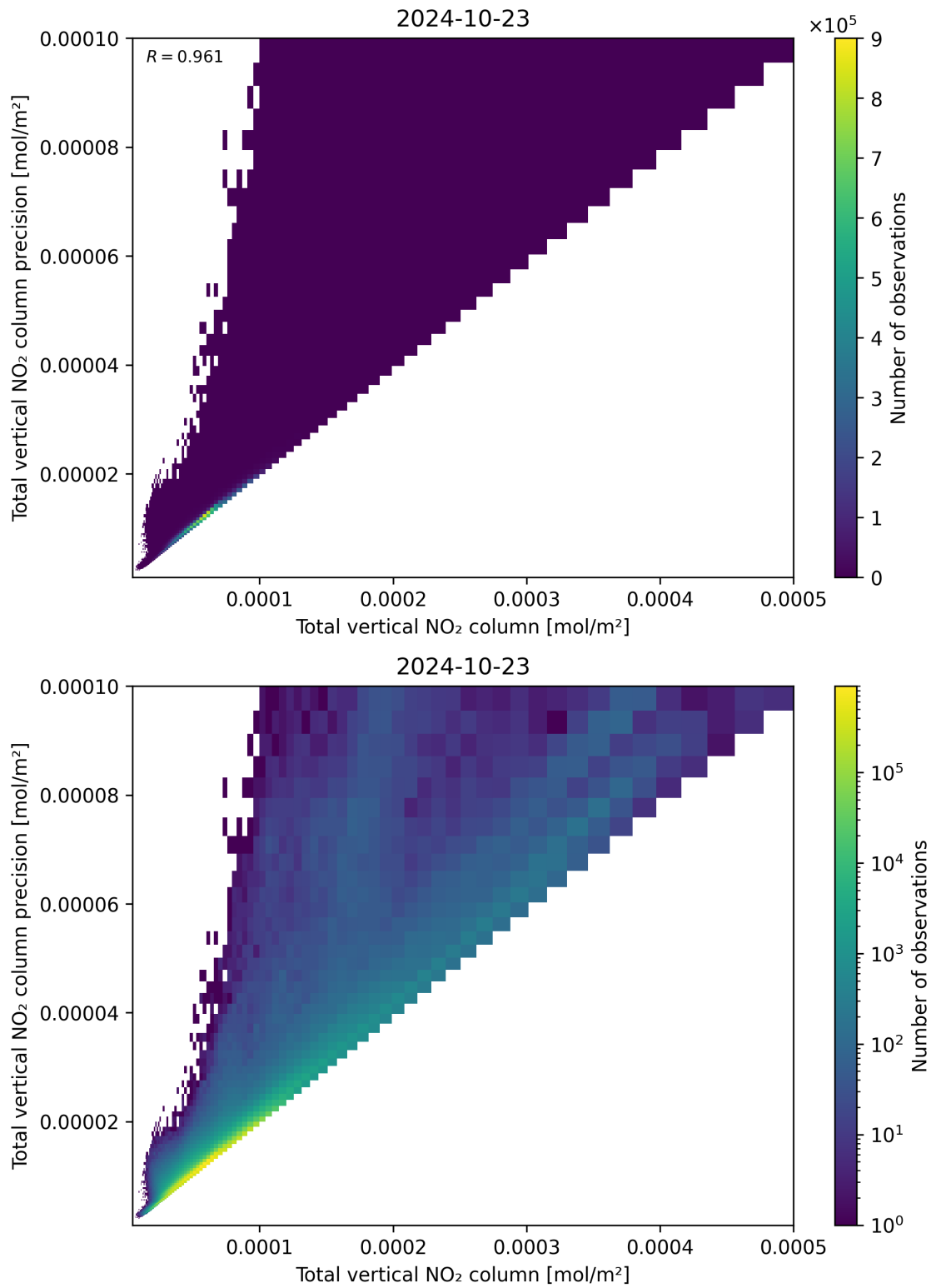
Figure 114: Scatter density plot of “Total vertical NO 2 column” against “Total vertical NO 2 column precision” for 2024-10-22 to 2024-10-24.
