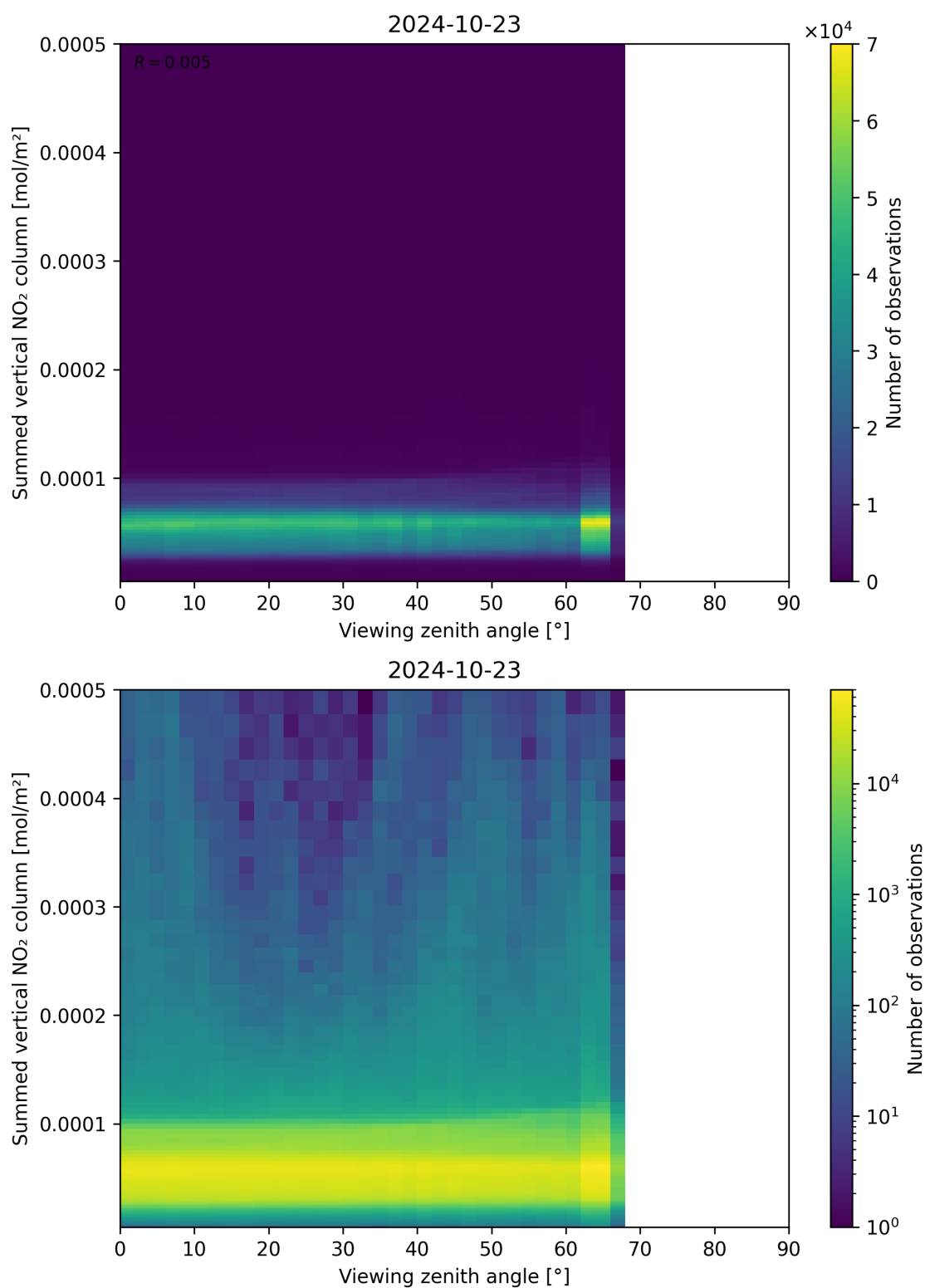
Figure 165: Scatter density plot of “Viewing zenith angle” against “Summed vertical NO 2 column” for 2024-10-22 to 2024-10-24.
