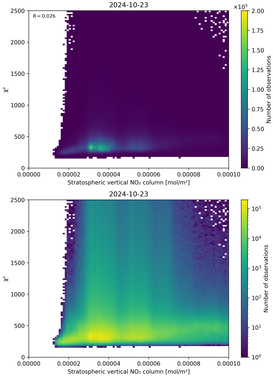
Figure 97: Scatter density plot of “Stratospheric vertical NO 2 column” against “ \chi^2 ” for 2024-10-22 to 2024-10-24.
