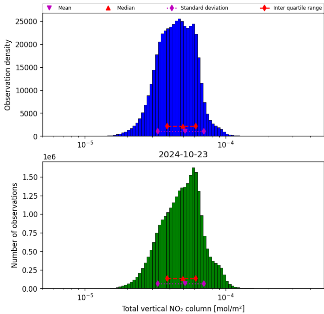
Figure 38: Histogram of “Total vertical NO 2 column” for 2024-10-22 to 2024-10-24
