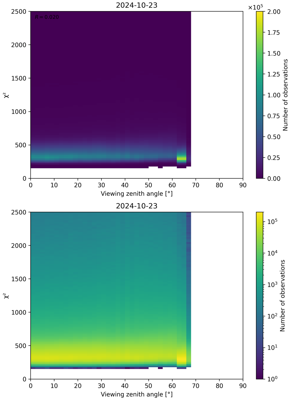
Figure 162: Scatter density plot of “Viewing zenith angle” against “ \chi^2 ” for 2024-10-22 to 2024-10-24.
