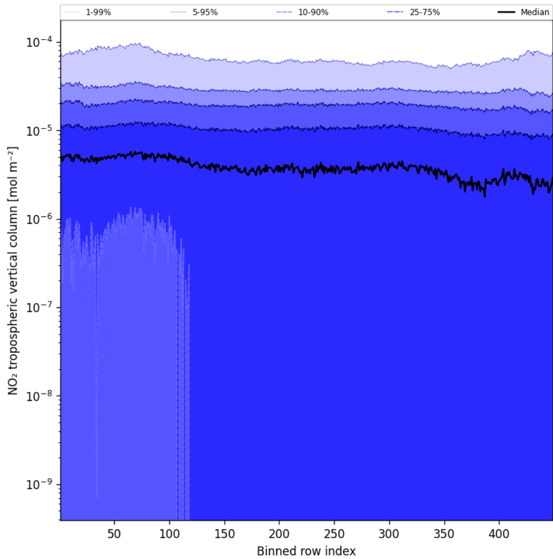
Figure 46: Along track statistics of “NO 2 tropospheric vertical column” for 2024-10-22 to 2024-10-24
