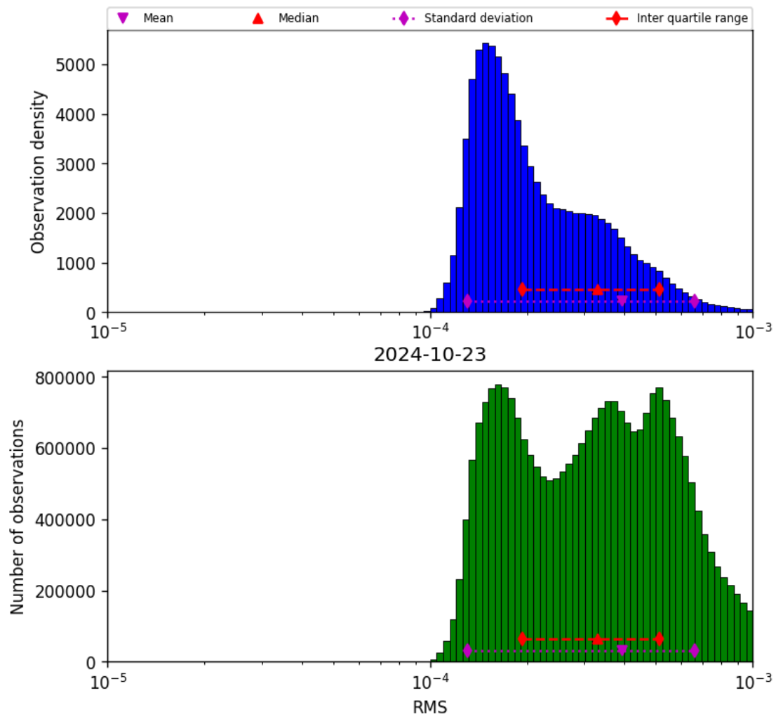
Figure 43: Histogram of “RMS” for 2024-10-22 to 2024-10-24
