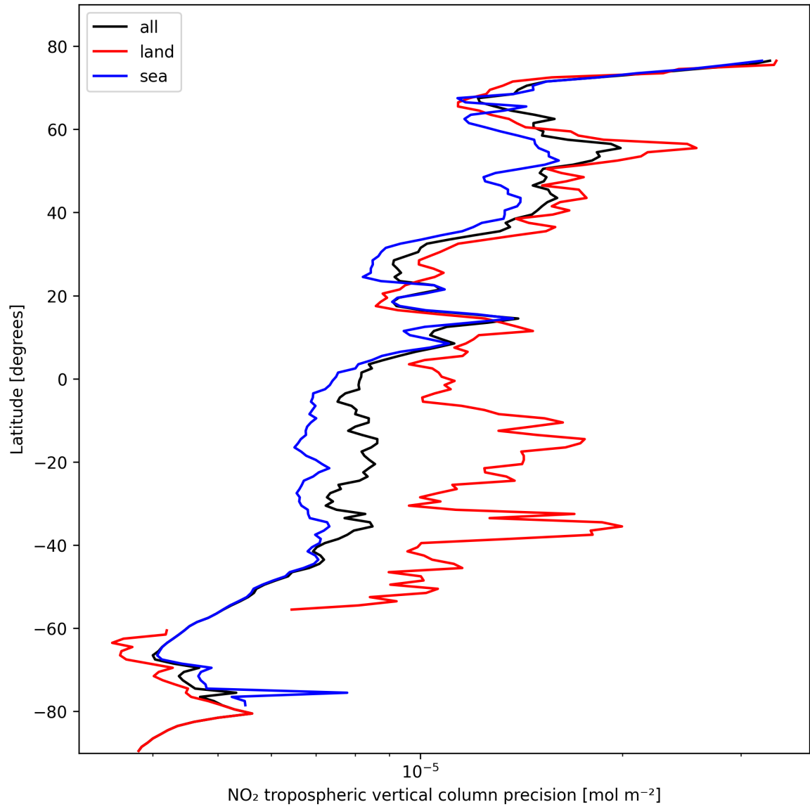
Figure 13: Zonal average of “NO 2 tropospheric vertical column precision” for 2024-10-22 to 2024-10-24.
