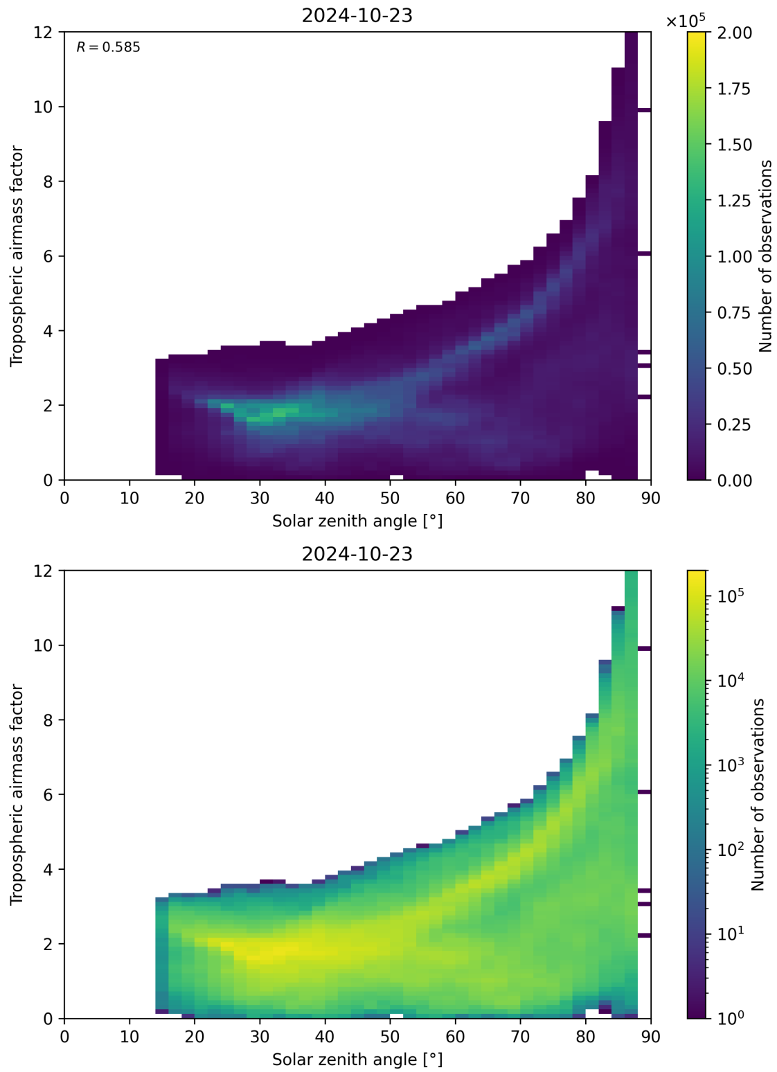
Figure 147: Scatter density plot of “Solar zenith angle” against “Tropospheric airmass factor” for 2024-10-22 to 2024-10-24.
