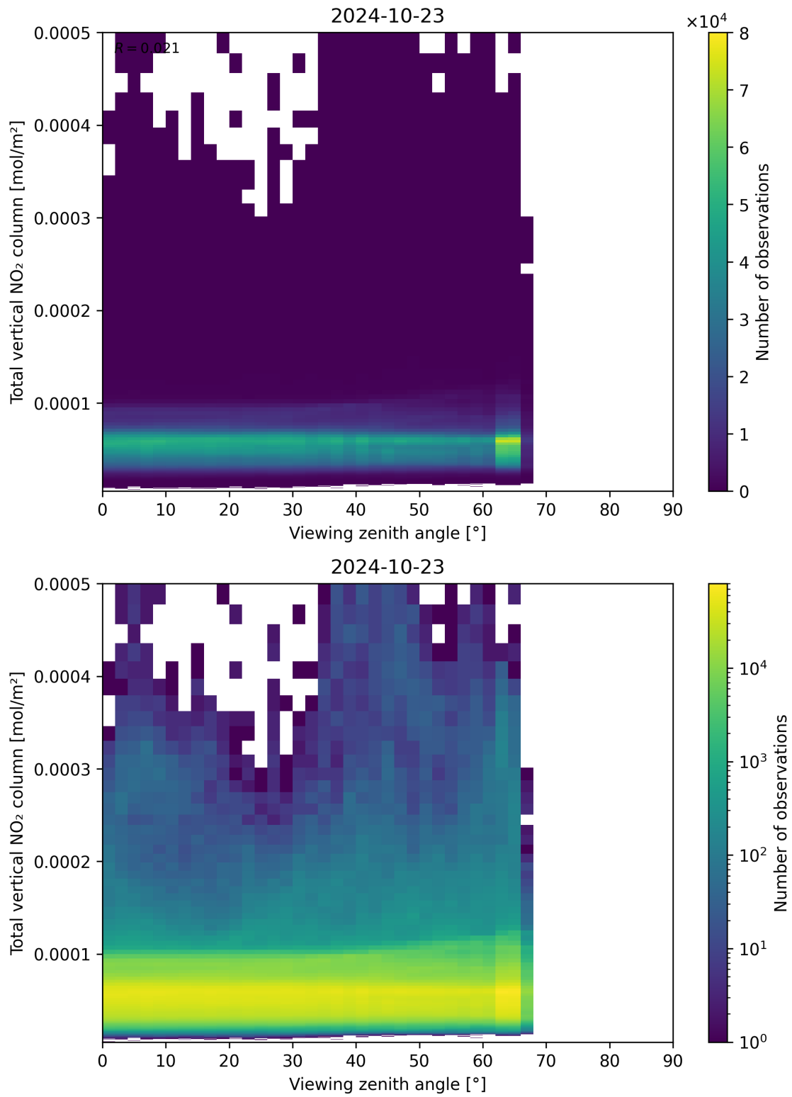
Figure 167: Scatter density plot of “Viewing zenith angle” against “Total vertical NO 2 column” for 2024-10-22 to 2024-10-24.
