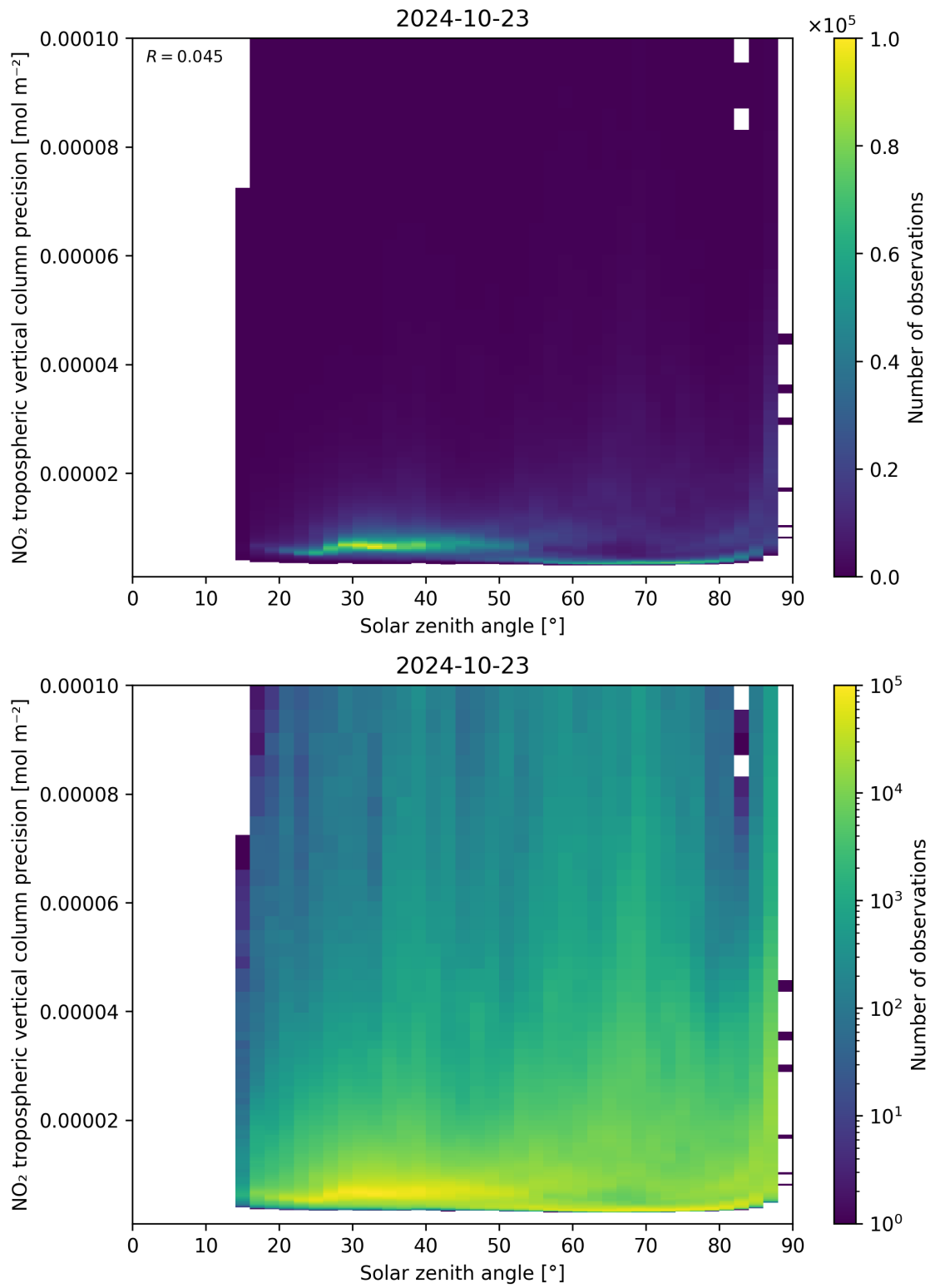
Figure 156: Scatter density plot of “Solar zenith angle” against “NO 2 tropospheric vertical column precision” for 2024-10-22 to 2024-10-24.
