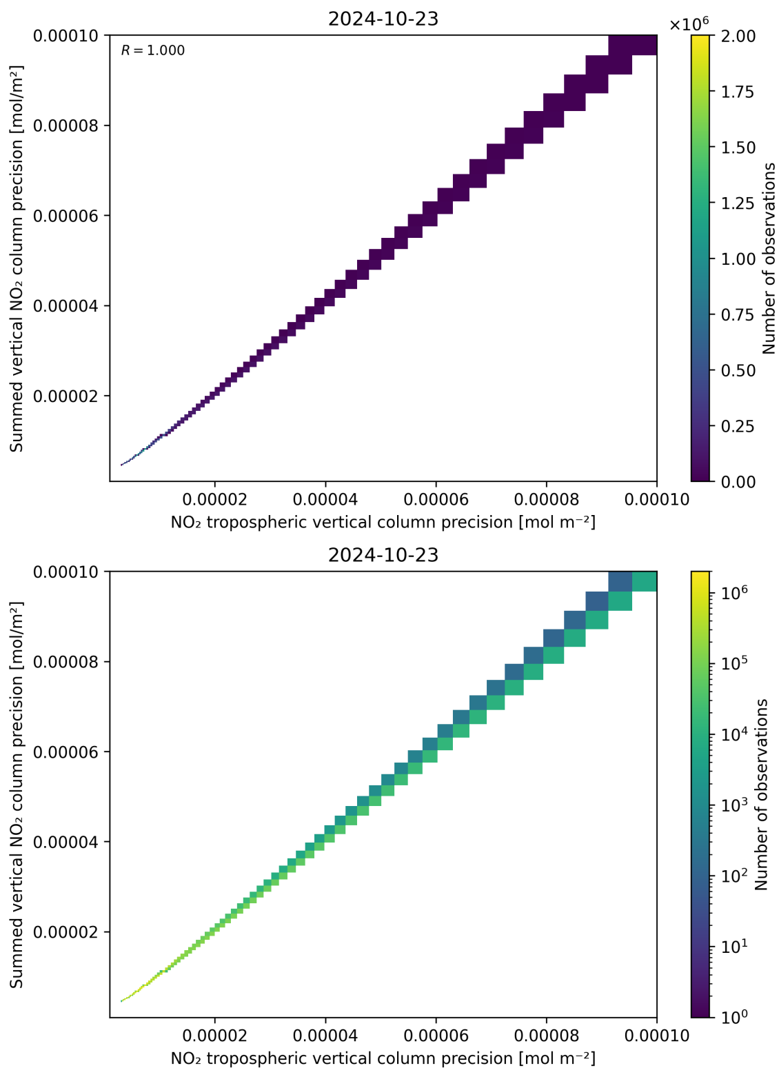
Figure 137: Scatter density plot of “NO 2 tropospheric vertical column precision” against “Summed vertical NO 2 column precision” for 2024-10-22 to 2024-10-24.
