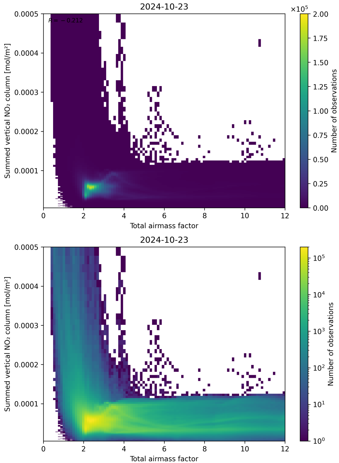
Figure 65: Scatter density plot of “Total airmass factor” against “Summed vertical NO 2 column” for 2024-10-22 to 2024-10-24.
