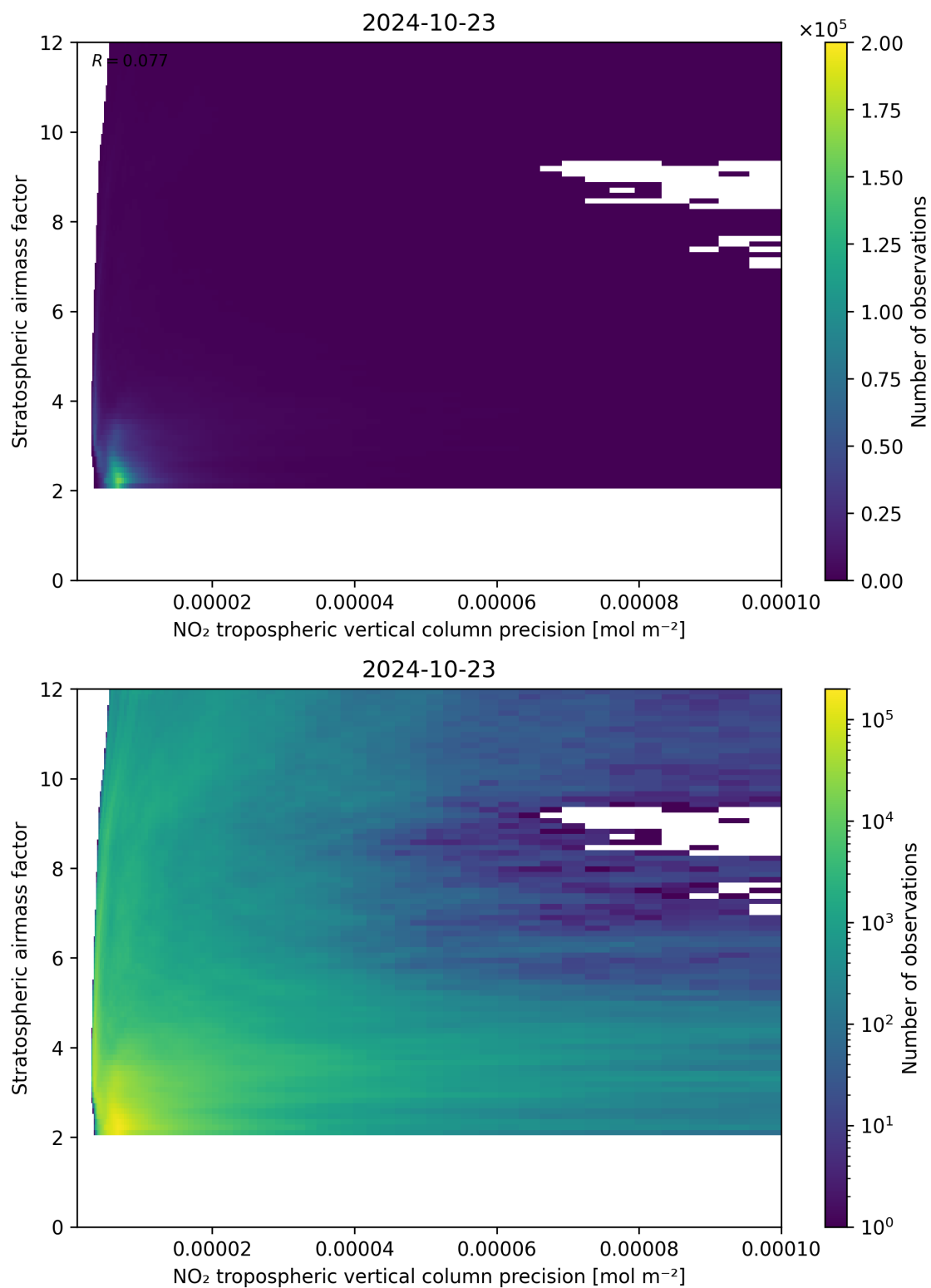
Figure 131: Scatter density plot of “NO 2 tropospheric vertical column precision” against “Stratospheric airmass factor” for 2024-10-22 to 2024-10-24.
