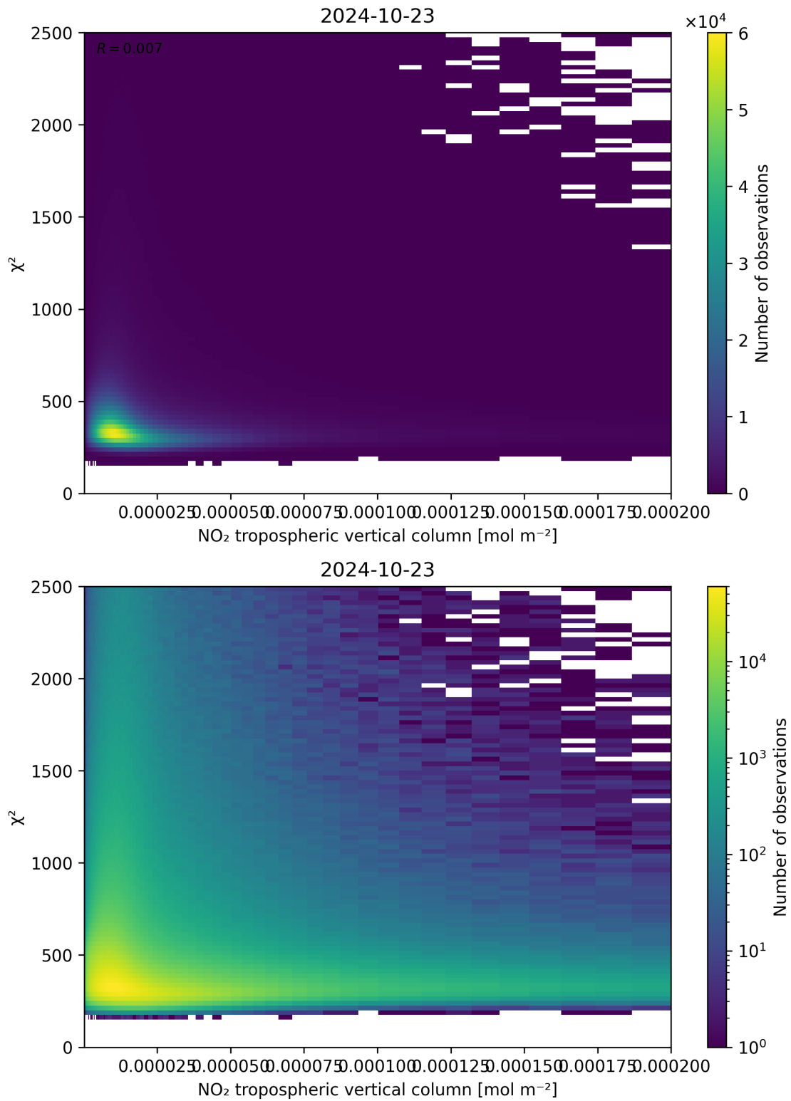
Figure 124: Scatter density plot of “NO 2 tropospheric vertical column” against “ \chi^2 ” for 2024-10-22 to 2024-10-24.
