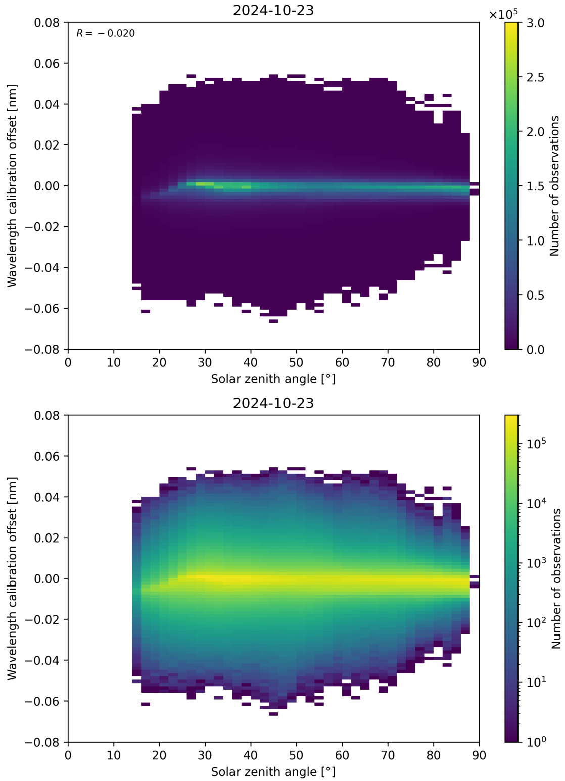
Figure 158: Scatter density plot of “Solar zenith angle” against “Wavelength calibration offset” for 2024-10-22 to 2024-10-24.
