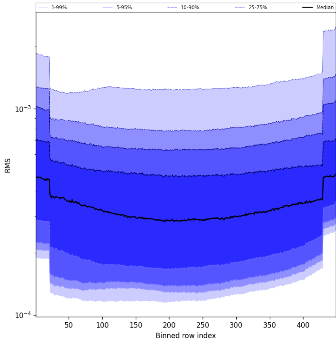
Figure 60: Along track statistics of “RMS” for 2024-10-22 to 2024-10-24
