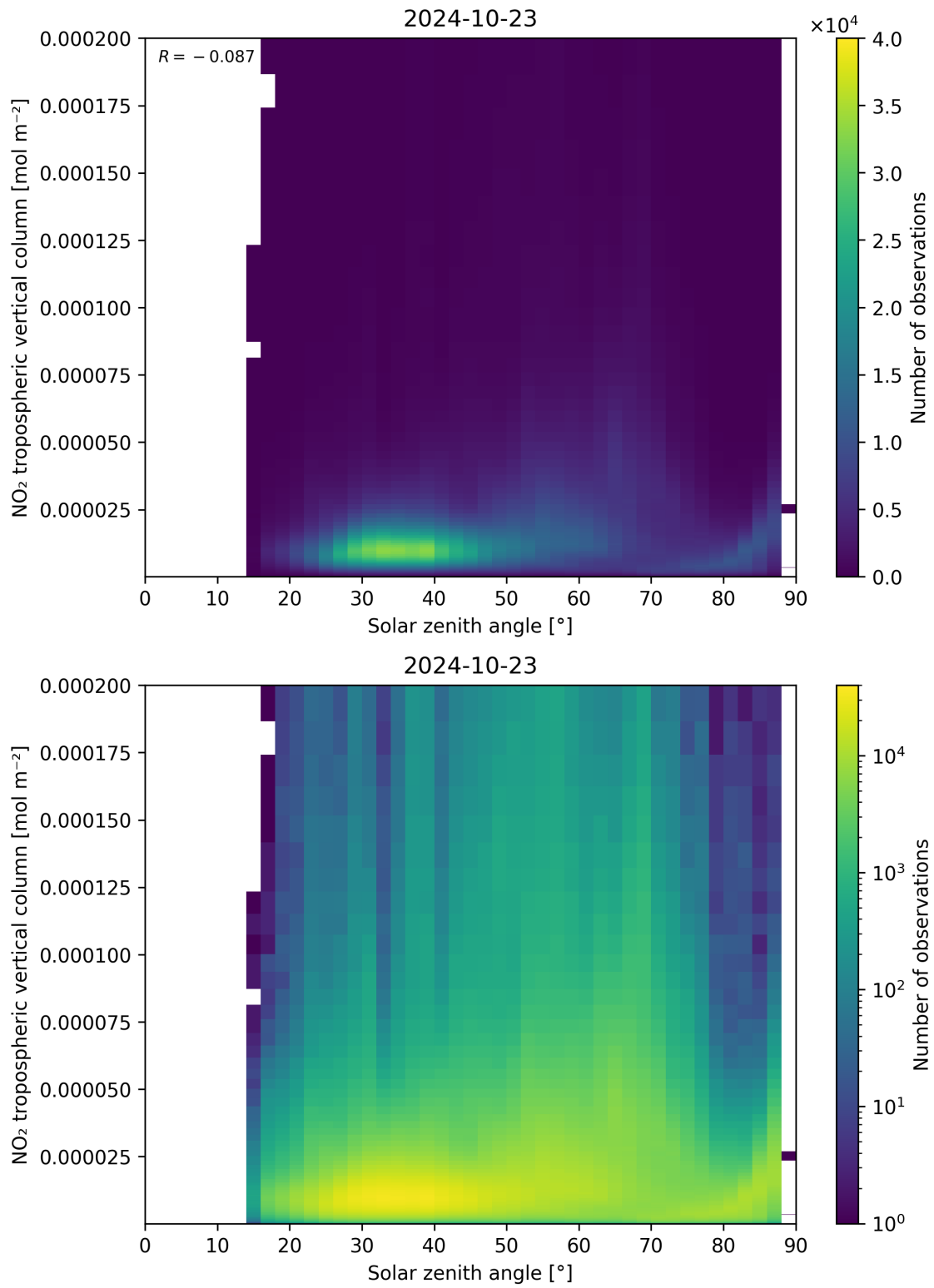
Figure 155: Scatter density plot of “Solar zenith angle” against “NO 2 tropospheric vertical column” for 2024-10-22 to 2024-10-24.
