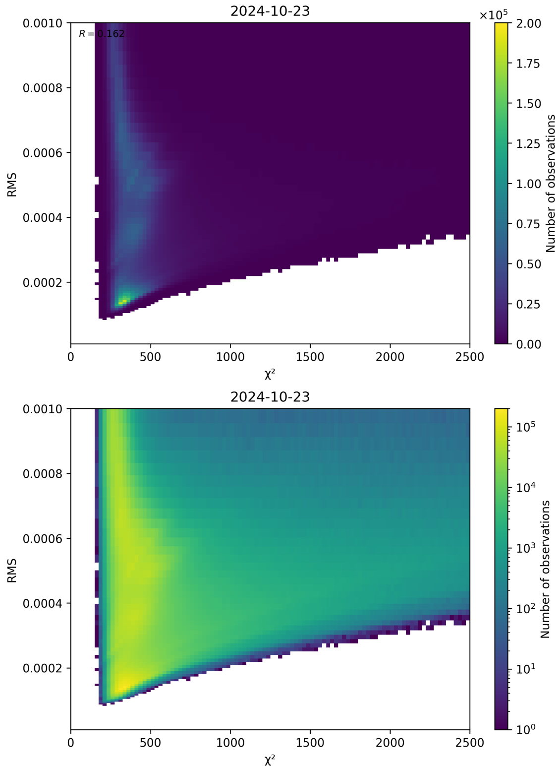
Figure 82: Scatter density plot of “ \chi^2 ” against “RMS” for 2024-10-22 to 2024-10-24.
