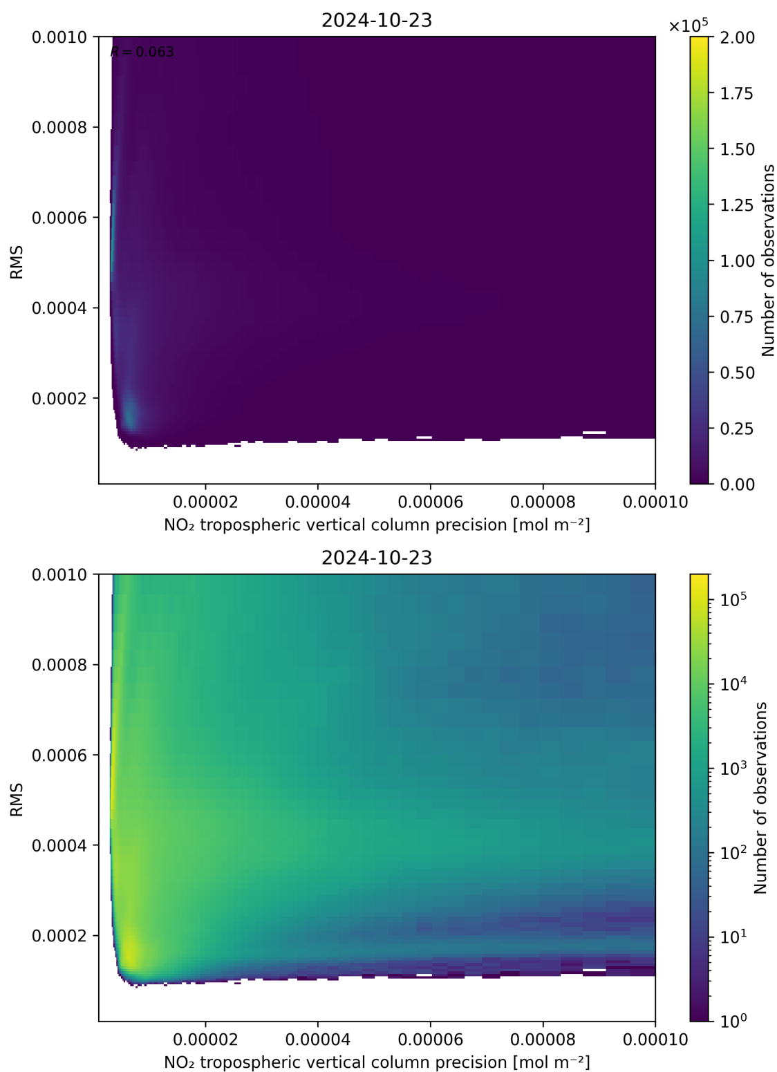
Figure 140: Scatter density plot of “NO 2 tropospheric vertical column precision” against “RMS” for 2024-10-22 to 2024-10-24.
