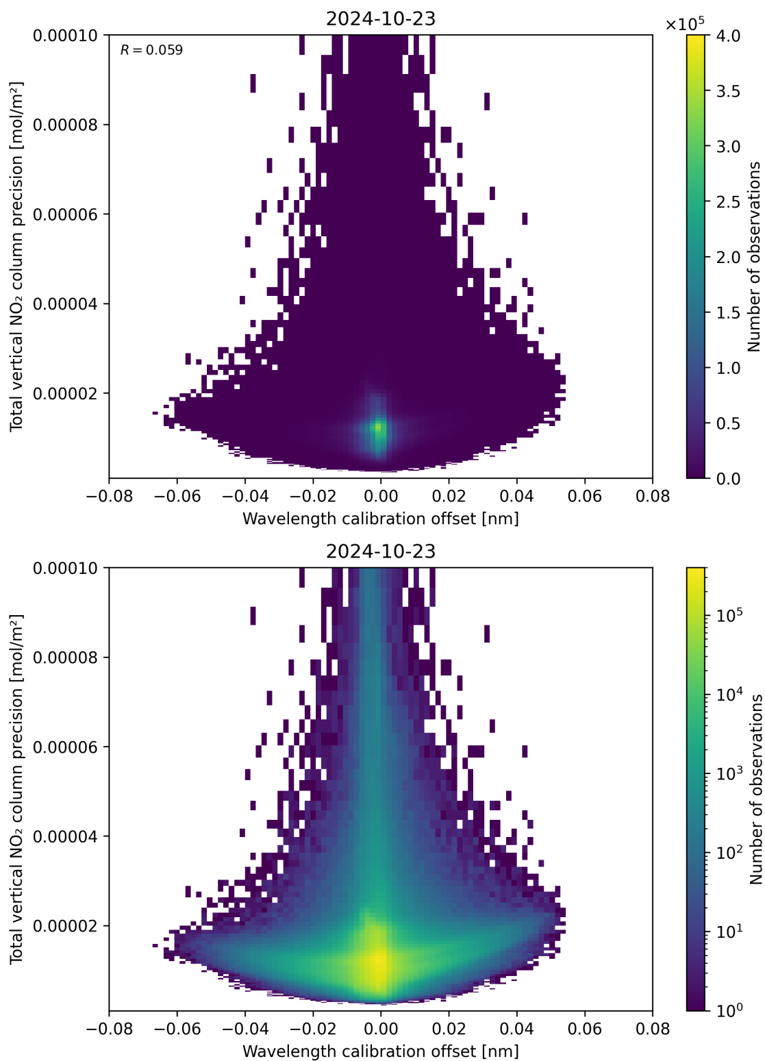
Figure 180: Scatter density plot of “Wavelength calibration offset” against “Total vertical NO 2 column precision” for 2024-10-22 to 2024-10-24.
