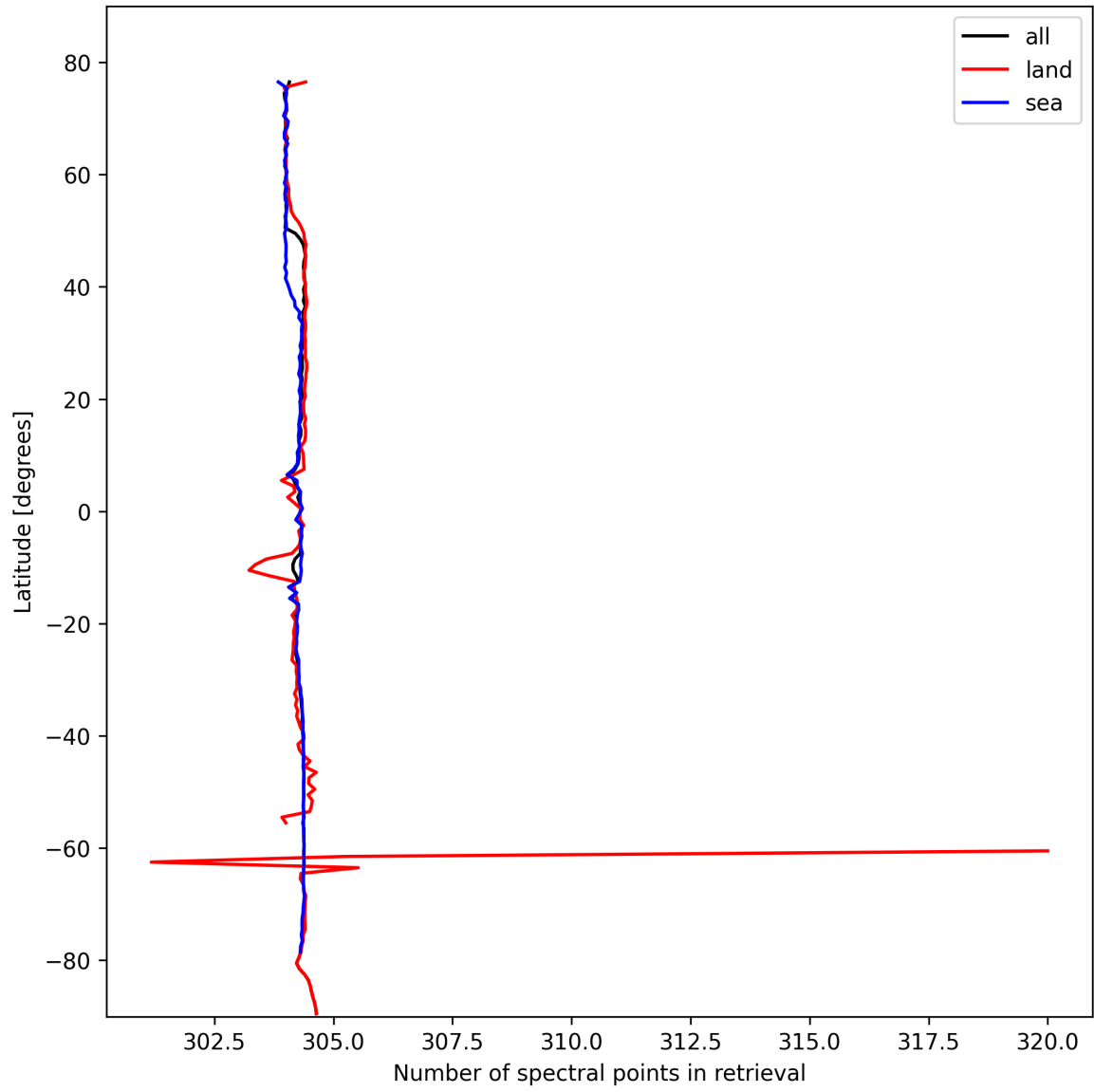
Figure 16: Zonal average of “Number of spectral points in retrieval” for 2024-10-22 to 2024-10-24.
