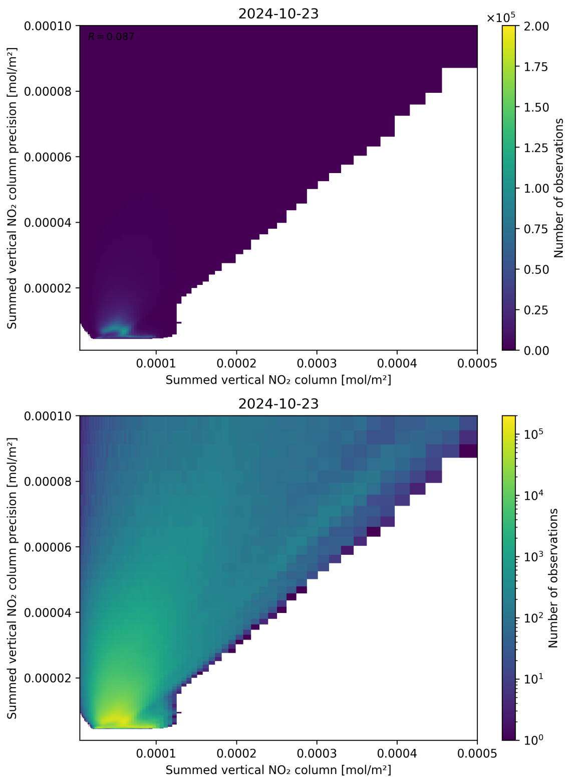
Figure 105: Scatter density plot of “Summed vertical NO 2 column” against “Summed vertical NO 2 column precision” for 2024-10-22 to 2024-10-24.
