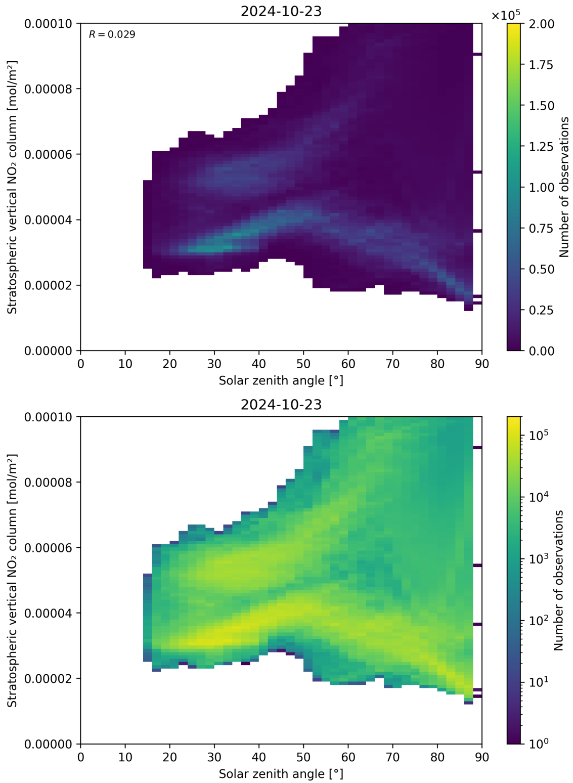
Figure 150: Scatter density plot of “Solar zenith angle” against “Stratospheric vertical NO 2 column” for 2024-10-22 to 2024-10-24.
