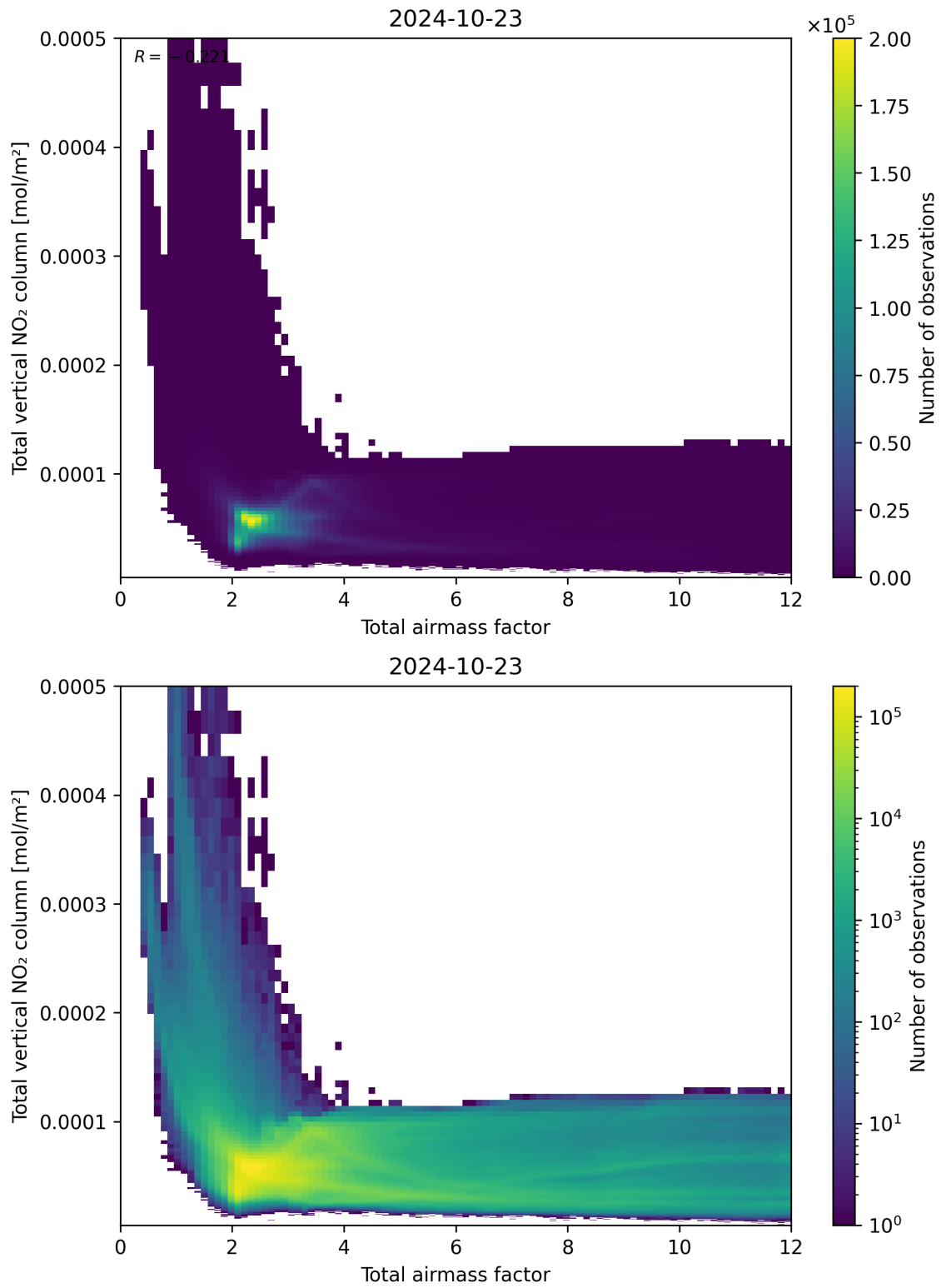
Figure 67: Scatter density plot of “Total air mass factor” against “Total vertical NO 2 column” for 2024-10-22 to 2024-10-24.
