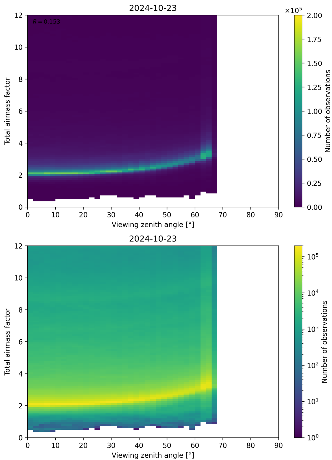
Figure 160: Scatter density plot of “Viewing zenith angle” against “Total airmass factor” for 2024-10-22 to 2024-10-24.
