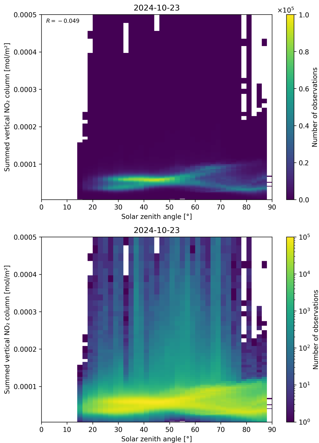
Figure 151: Scatter density plot of “Solar zenith angle” against “Summed vertical NO 2 column” for 2024-10-22 to 2024-10-24.
