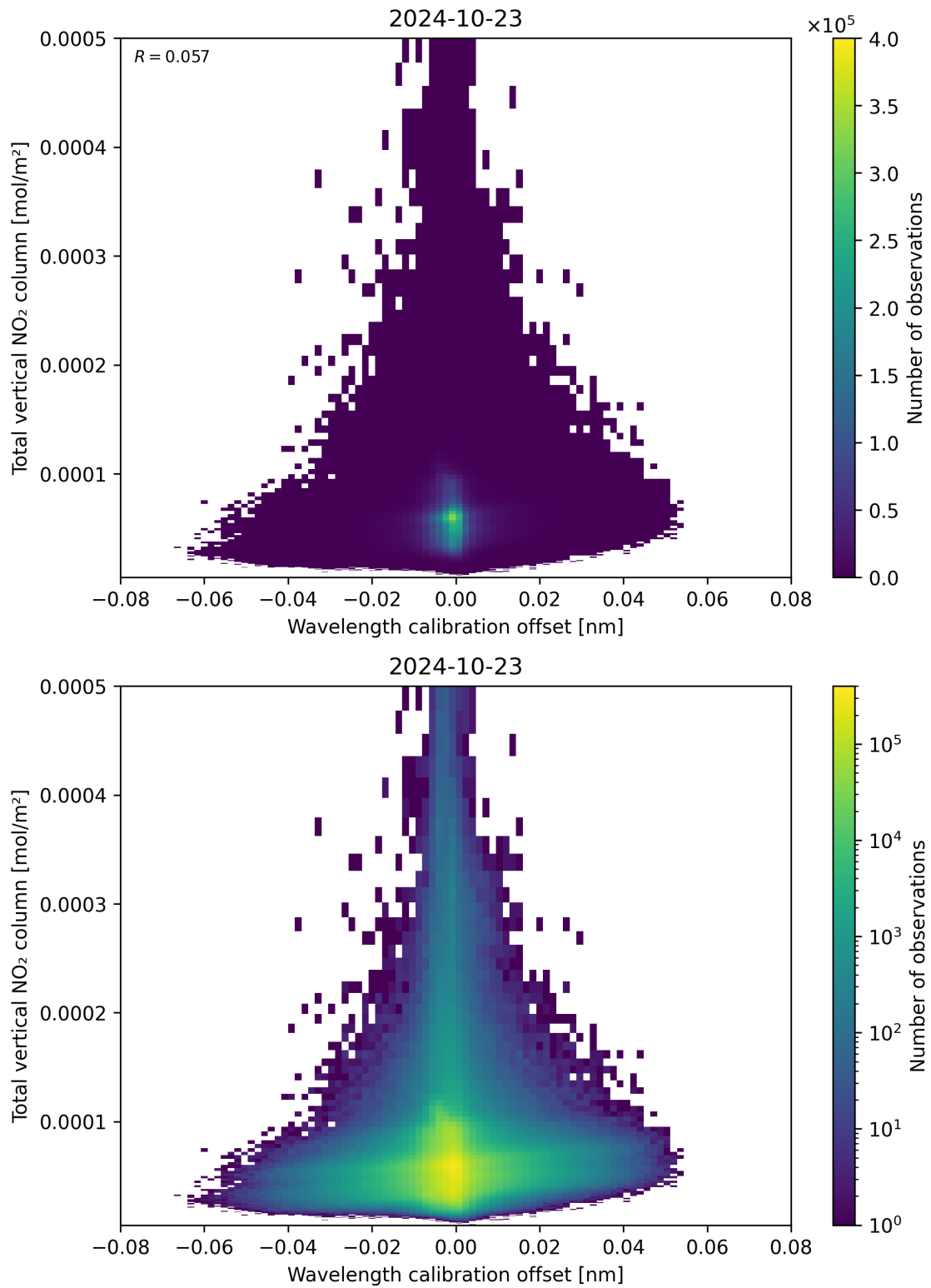
Figure 179: Scatter density plot of “Wavelength calibration offset” against “Total vertical NO 2 column” for 2024-10-22 to 2024-10-24.
