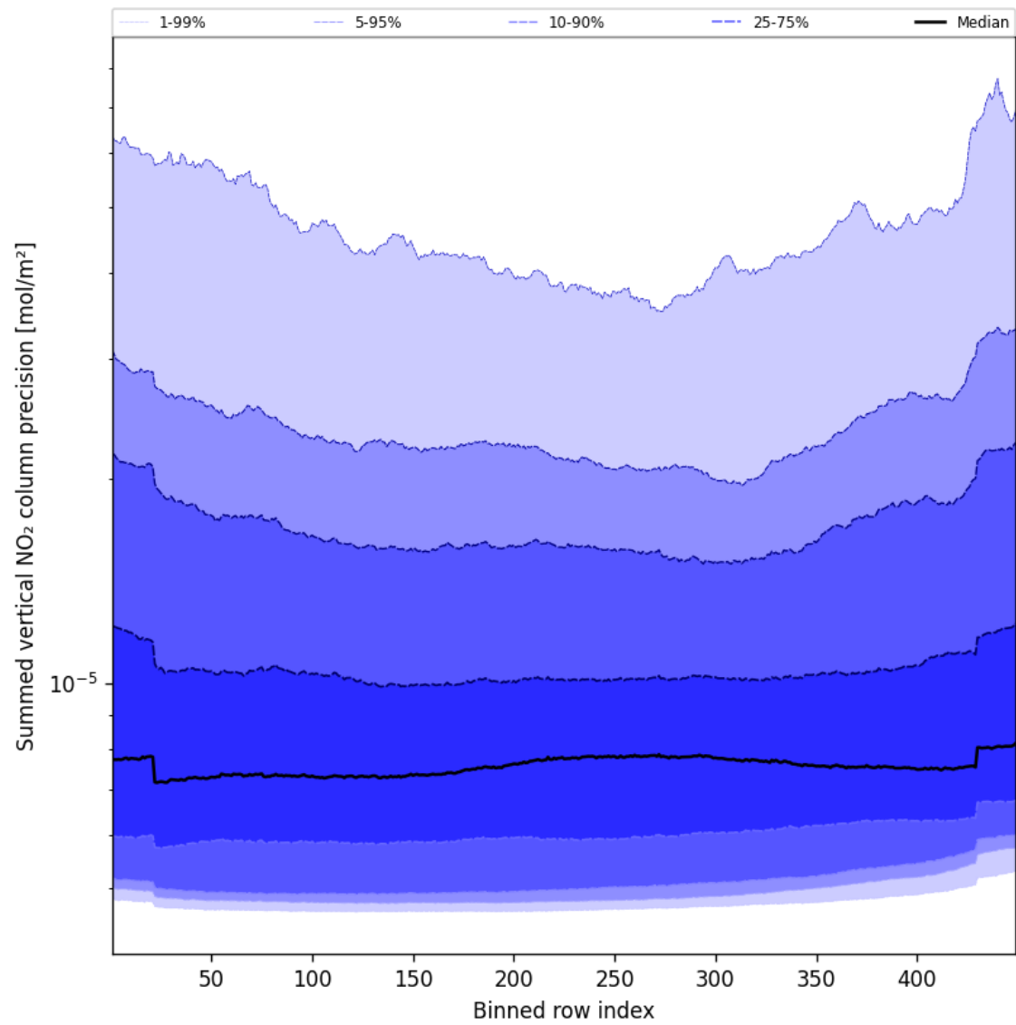
Figure 58: Along track statistics of “Summed vertical NO 2 column precision” for 2024-10-22 to 2024-10-24
