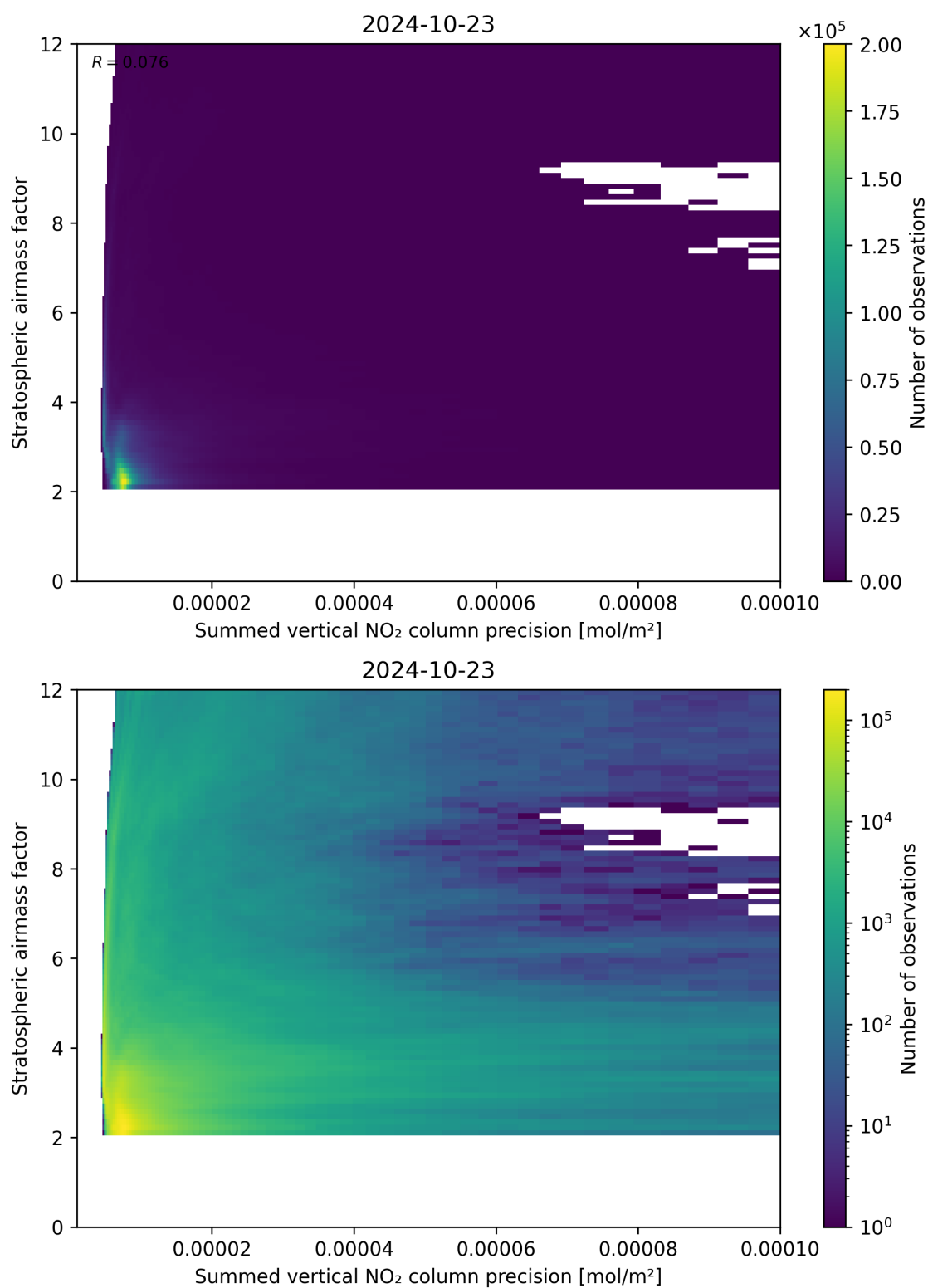
Figure 106: Scatter density plot of “Summed vertical NO 2 column precision” against “Stratospheric airmass factor” for 2024-10-22 to 2024-10-24.
