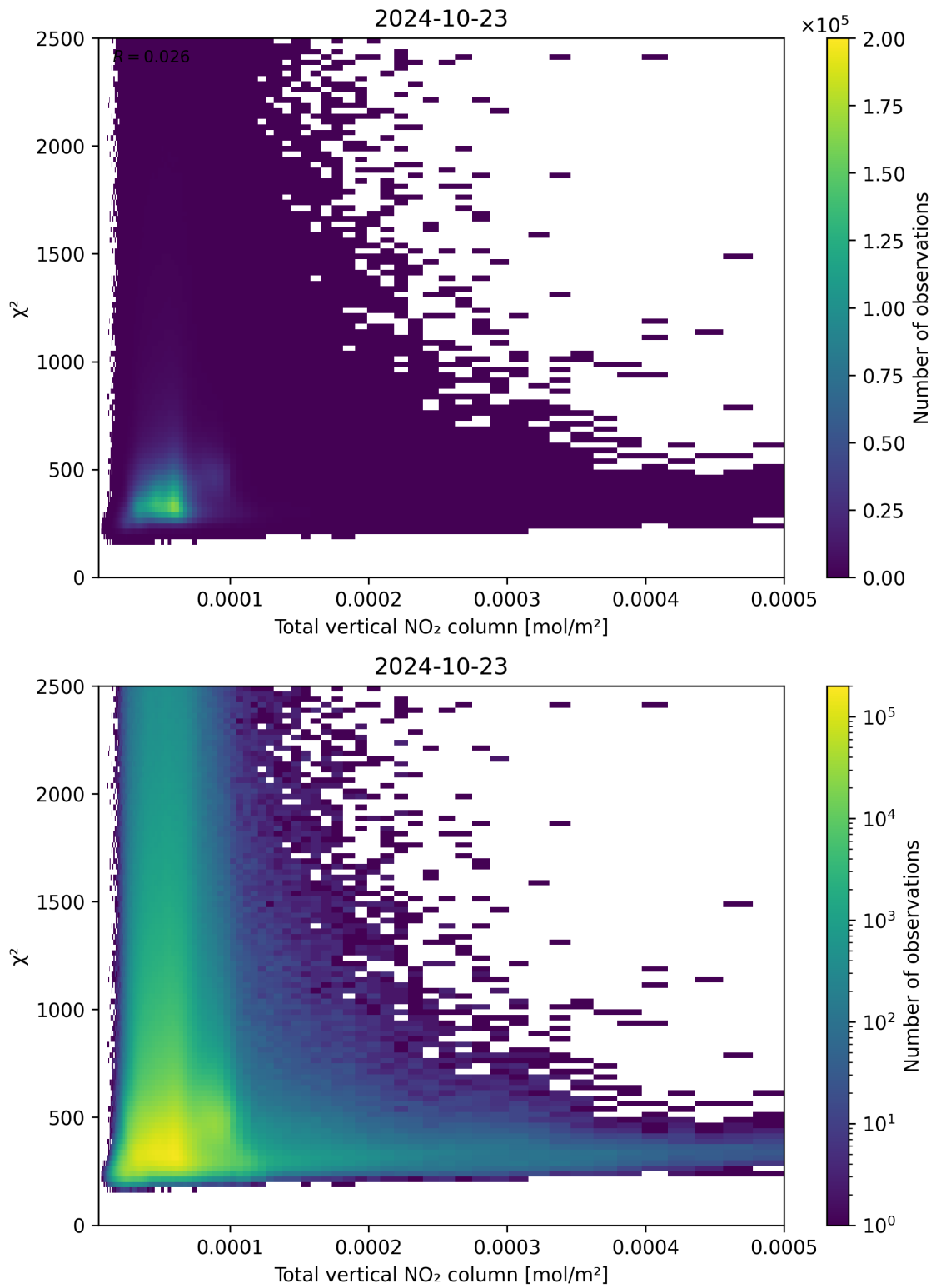
Figure 111: Scatter density plot of “Total vertical NO 2 column” against “ \chi^2 ” for 2024-10-22 to 2024-10-24.
