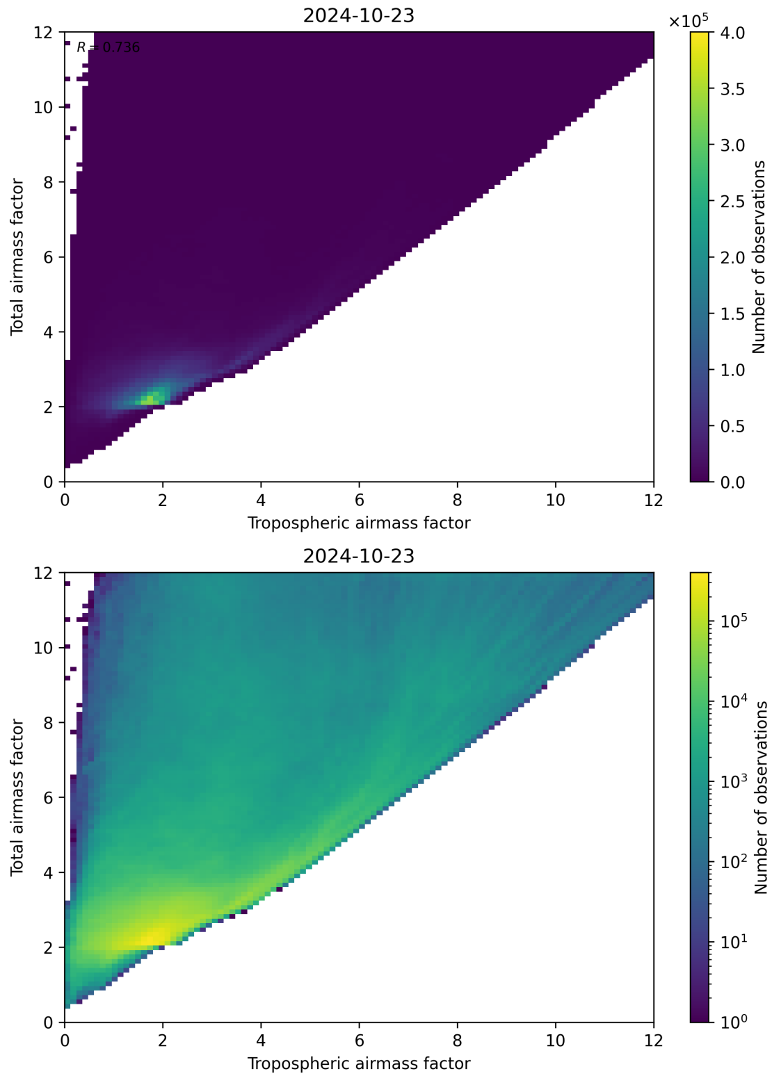
Figure 72: Scatter density plot of “Tropospheric airmass factor” against “Total airmass factor” for 2024-10-22 to 2024-10-24.
