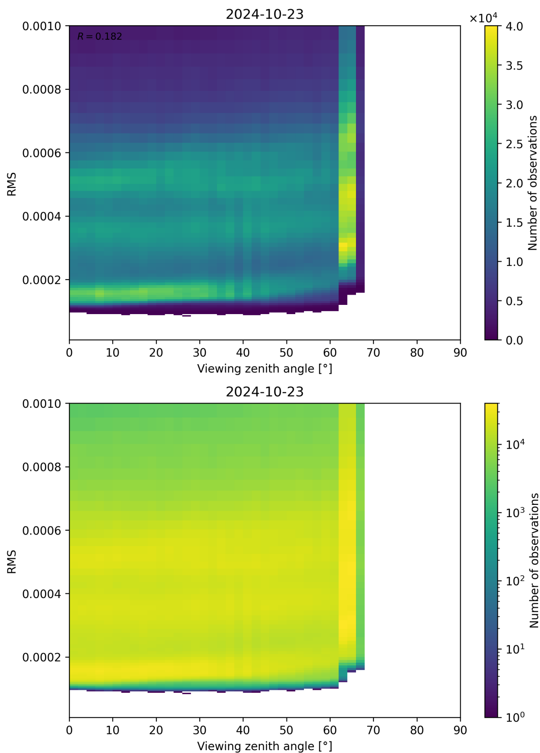
Figure 171: Scatter density plot of “Viewing zenith angle” against “RMS” for 2024-10-22 to 2024-10-24.
