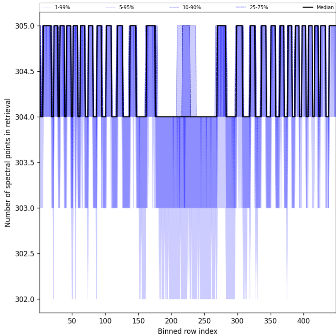
Figure 50: Along track statistics of “Number of spectral points in retrieval” for 2024-10-22 to 2024-10-24
