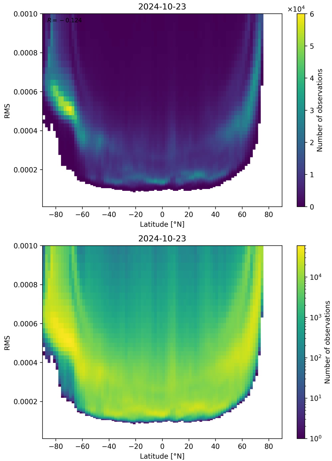
Figure 94: Scatter density plot of “Latitude” against “RMS” for 2024-10-22 to 2024-10-24.
