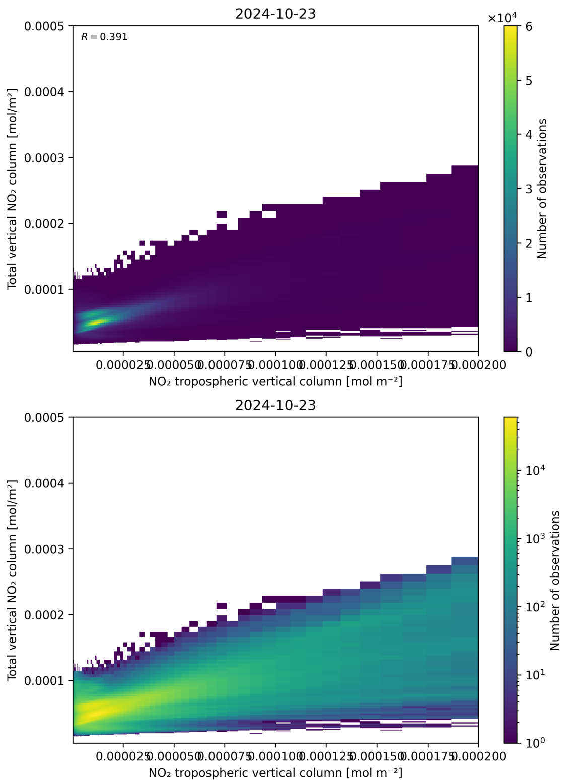
Figure 128: Scatter density plot of “NO 2 tropospheric vertical column” against “Total vertical NO 2 column” for 2024-10-22 to 2024-10-24.
