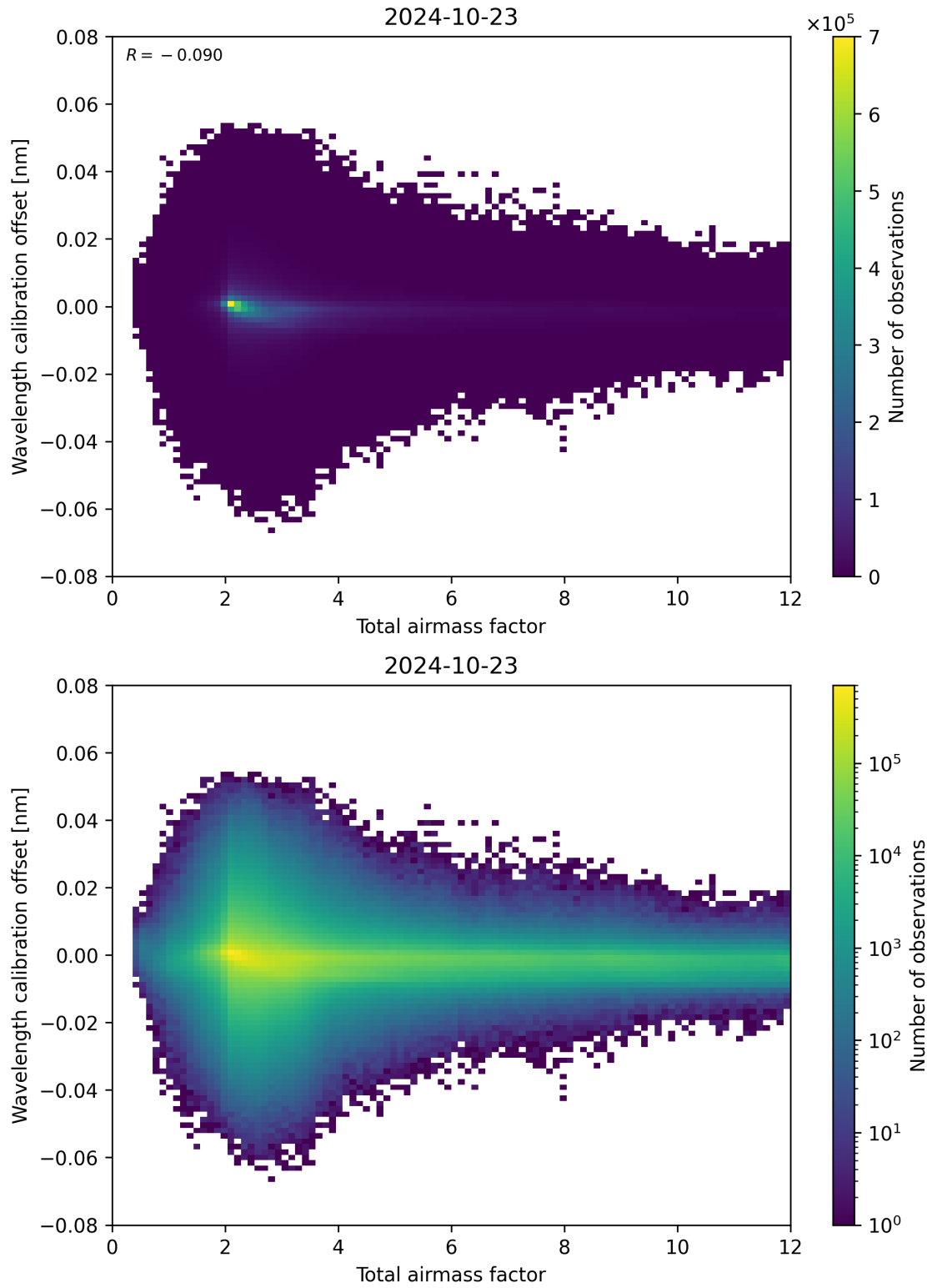
Figure 70: Scatter density plot of “Total airmass factor” against “Wavelength calibration offset” for 2024-10-22 to 2024-10-24.
