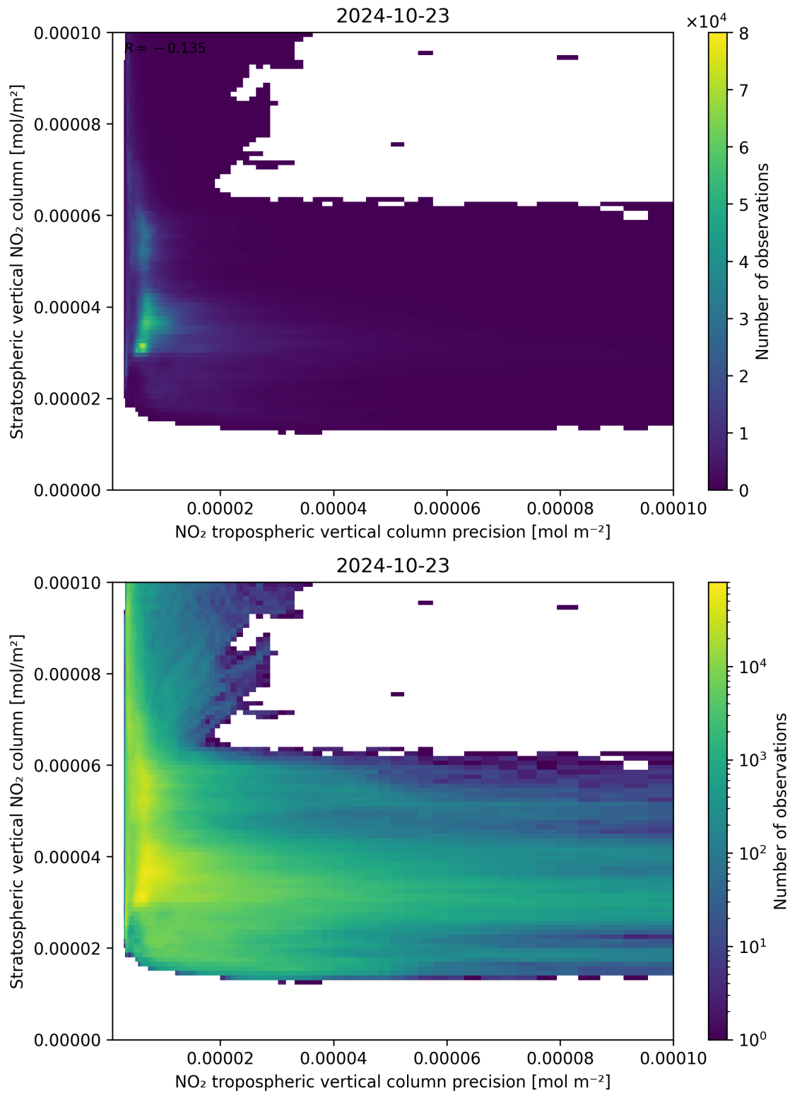
Figure 135: Scatter density plot of “NO 2 tropospheric vertical column precision” against “Stratospheric vertical NO 2 column” for 2024-10-22 to 2024-10-24.
