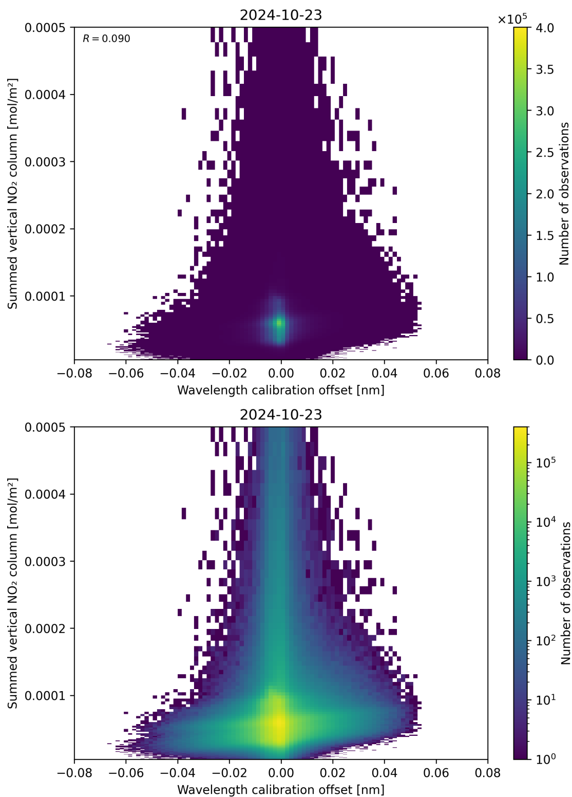
Figure 177: Scatter density plot of “Wavelength calibration offset” against “Summed vertical NO 2 column” for 2024-10-22 to 2024-10-24.
