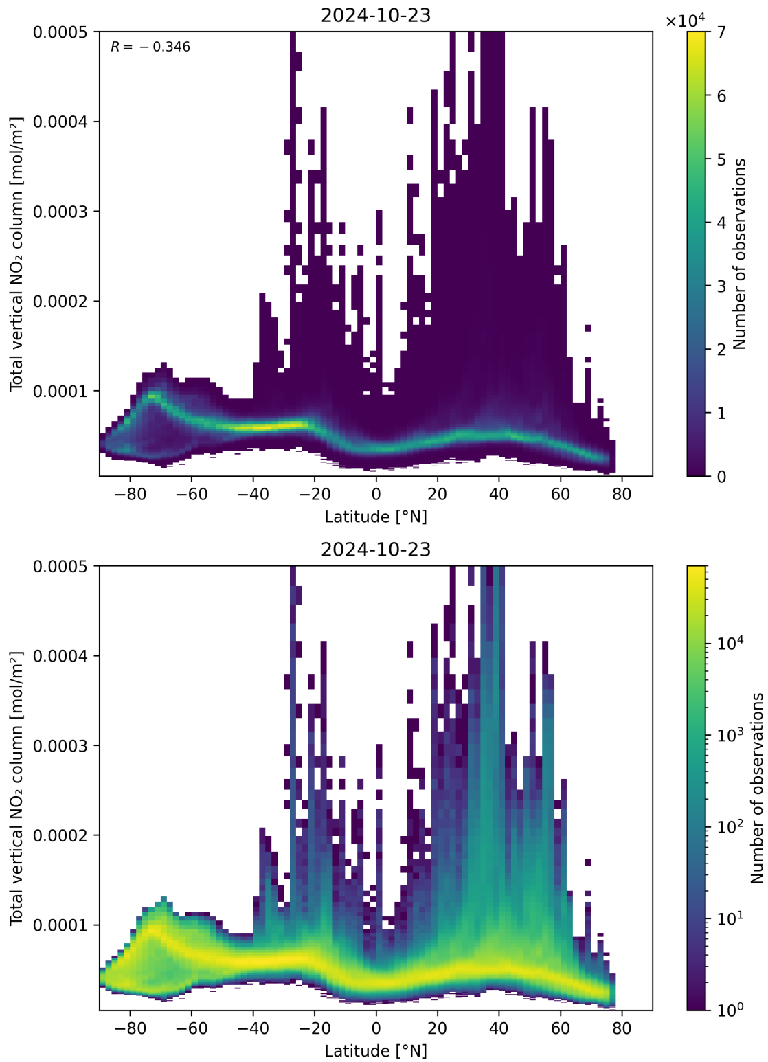
Figure 90: Scatter density plot of “Latitude” against “Total vertical NO 2 column” for 2024-10-22 to 2024-10-24.
