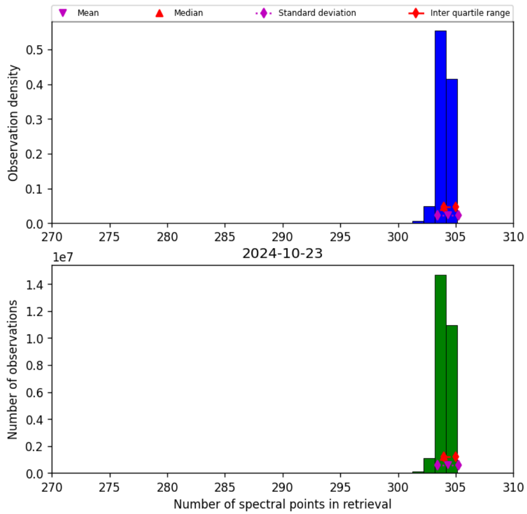
Figure 33: Histogram of “Number of spectral points in retrieval” for 2024-10-22 to 2024-10-24
