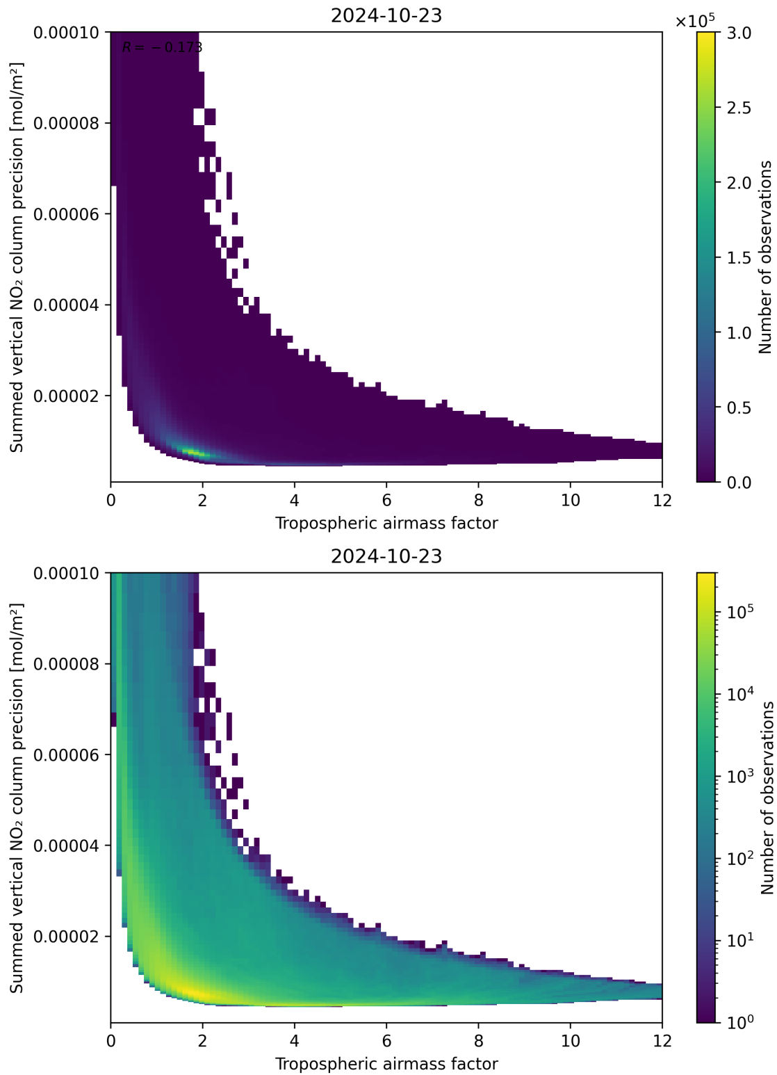
Figure 76: Scatter density plot of “Tropospheric air mass factor” against “Summed vertical NO 2 column precision” for 2024-10-22 to 2024-10-24.
