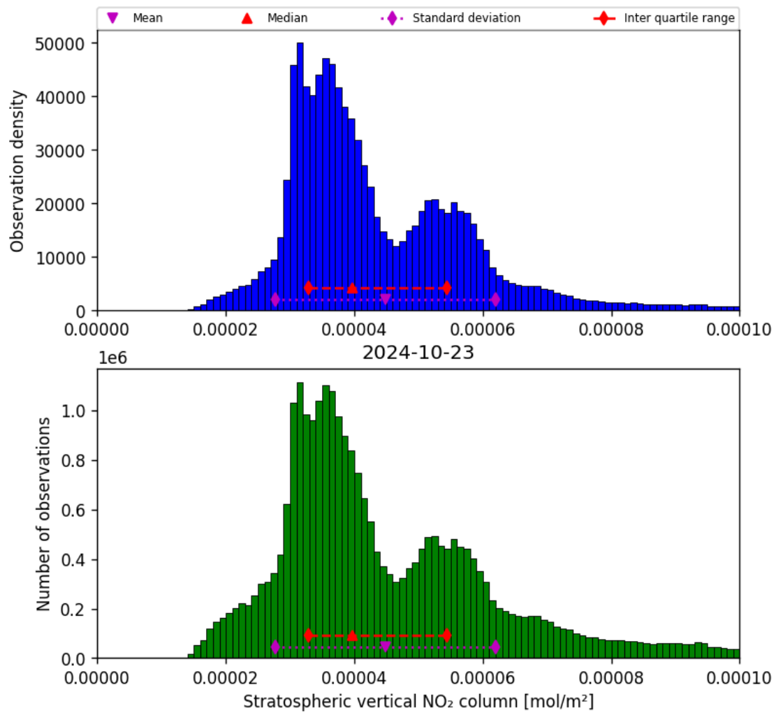
Figure 36: Histogram of “Stratospheric vertical NO 2 column” for 2024-10-22 to 2024-10-24
