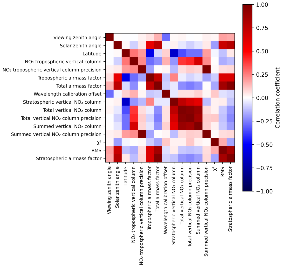
Figure 2: Map of correlation matrix for 2024-10-22 to 2024-10-24.
