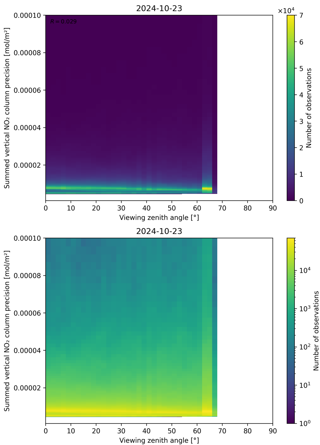
Figure 166: Scatter density plot of “Viewing zenith angle” against “Summed vertical NO 2 column precision” for 2024-10-22 to 2024-10-24.
