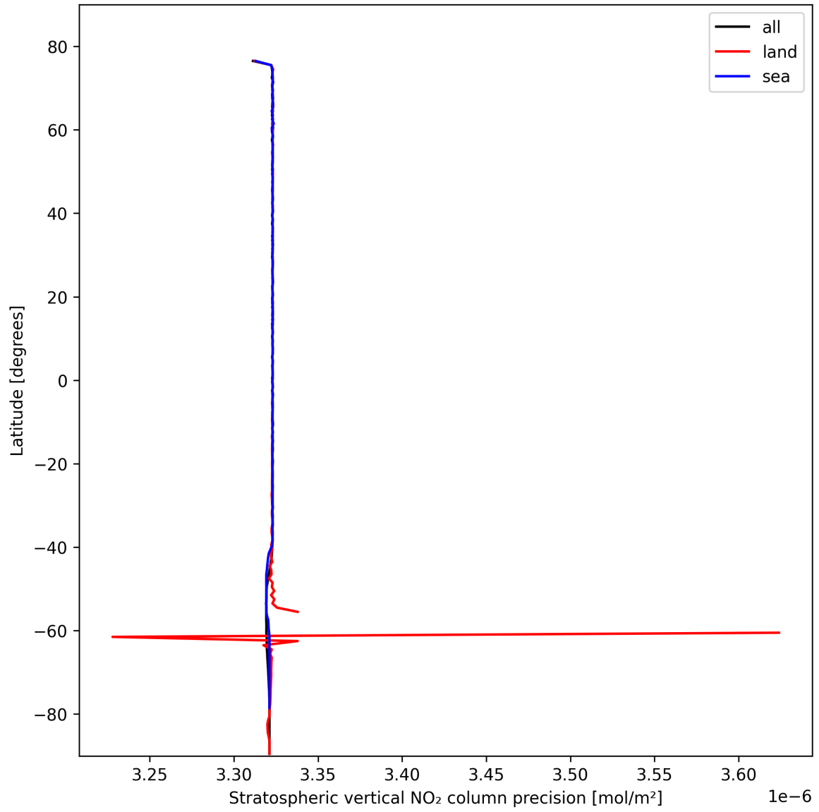
Figure 20: Zonal average of “Stratospheric vertical NO 2 column precision” for 2024-10-22 to 2024-10-24.
