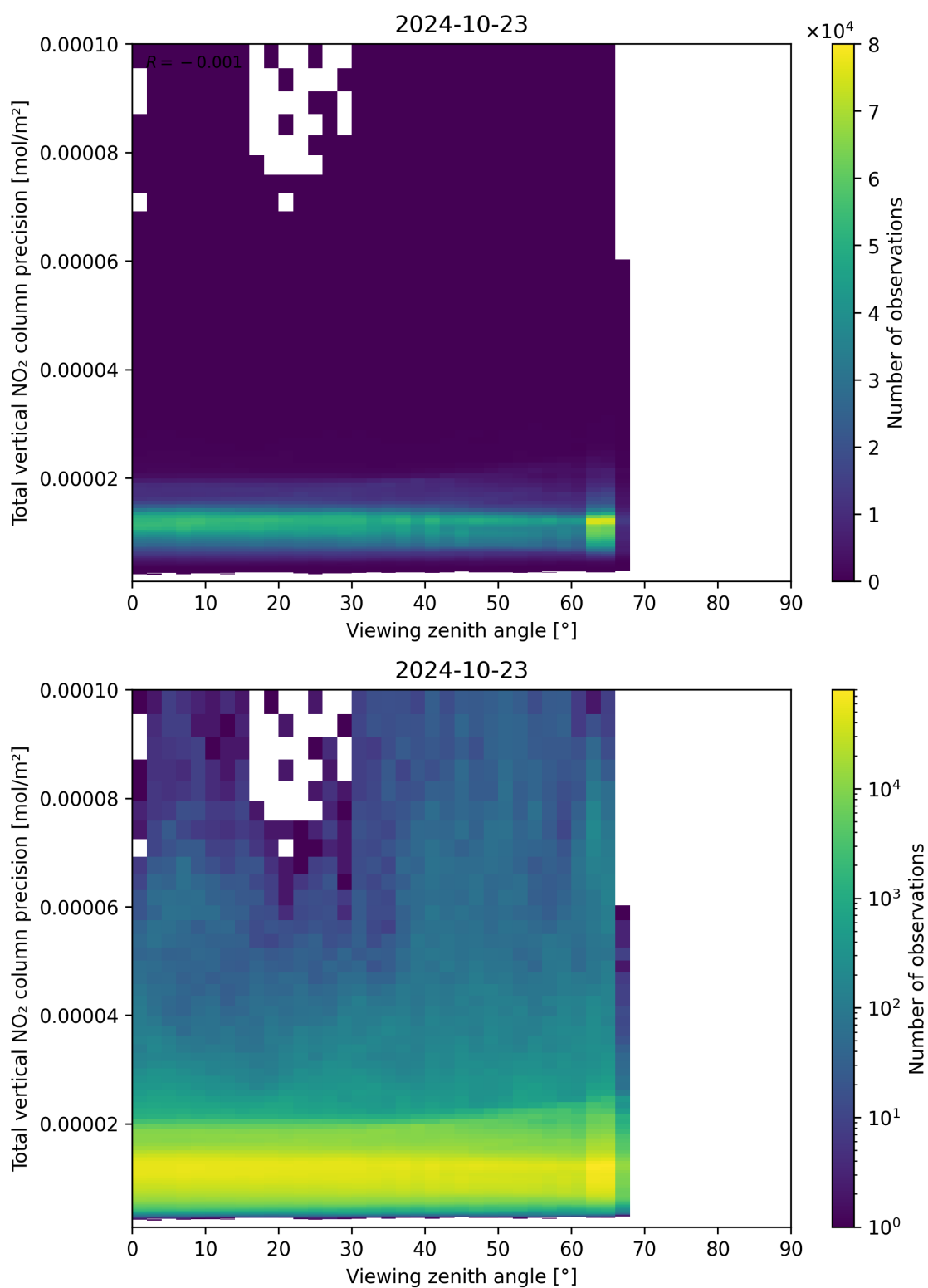
Figure 168: Scatter density plot of “Viewing zenith angle” against “Total vertical NO 2 column precision” for 2024-10-22 to 2024-10-24.
