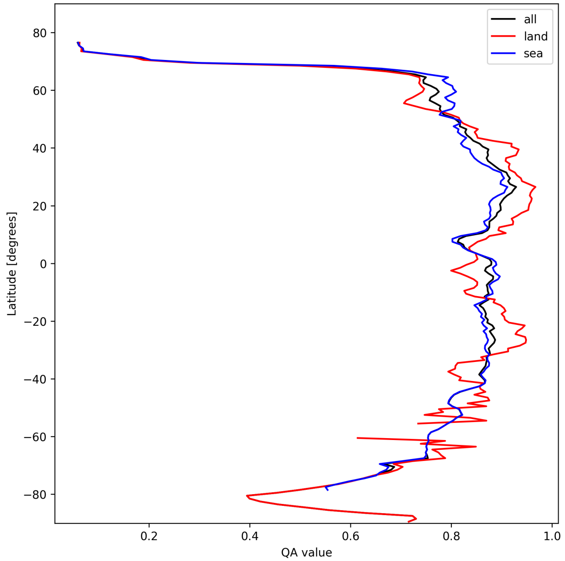
Figure 11: Zonal average of “QA value” for 2024-10-22 to 2024-10-24.
