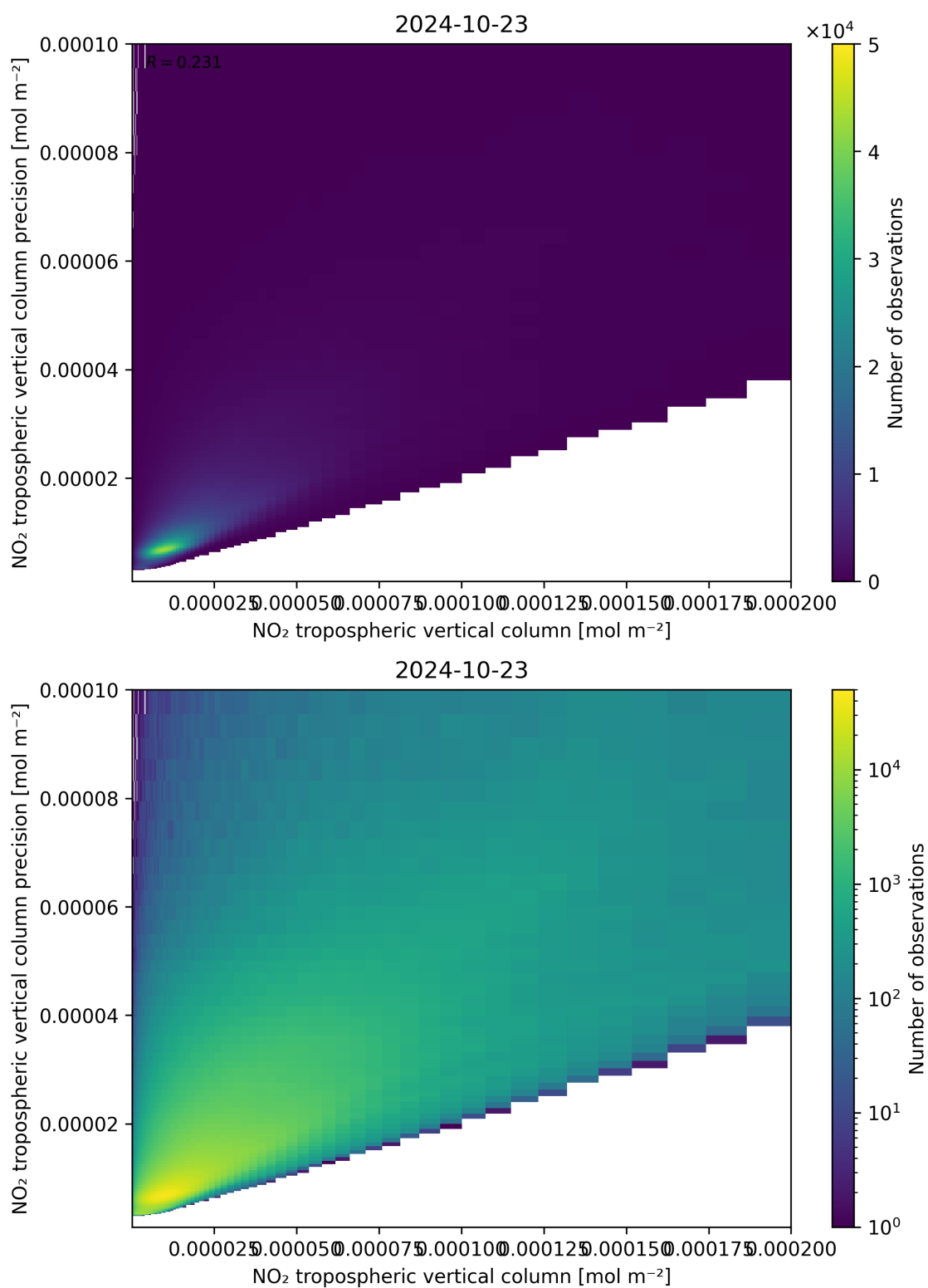
Figure 130: Scatter density plot of “NO 2 tropospheric vertical column” against “NO 2 tropospheric vertical column precision” for 2024-10-22 to 2024-10-24.
