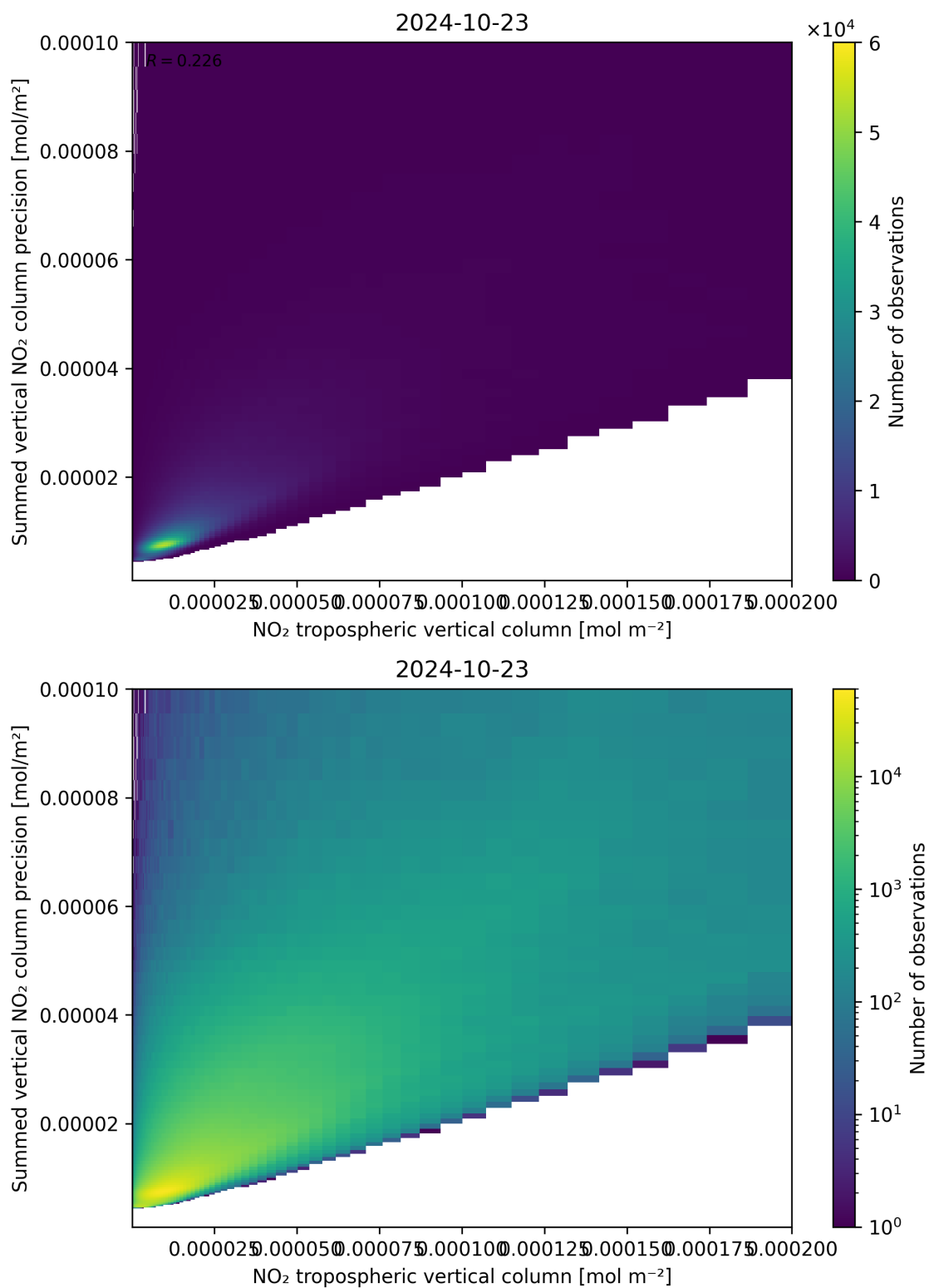
Figure 127: Scatter density plot of “NO 2 tropospheric vertical column” against “Summed vertical NO 2 column precision” for 2024-10-22 to 2024-10-24.
