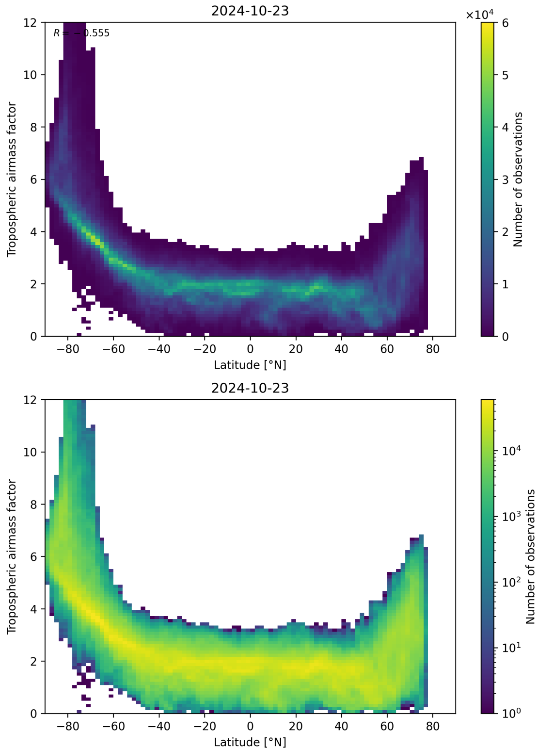
Figure 85: Scatter density plot of “Latitude” against “Tropospheric air mass factor” for 2024-10-22 to 2024-10-24.
