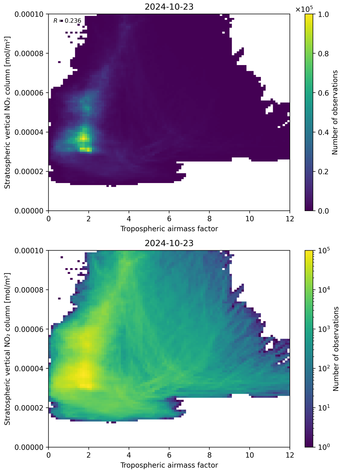
Figure 74: Scatter density plot of “Tropospheric air mass factor” against “Stratospheric vertical NO 2 column” for 2024-10-22 to 2024-10-24.
