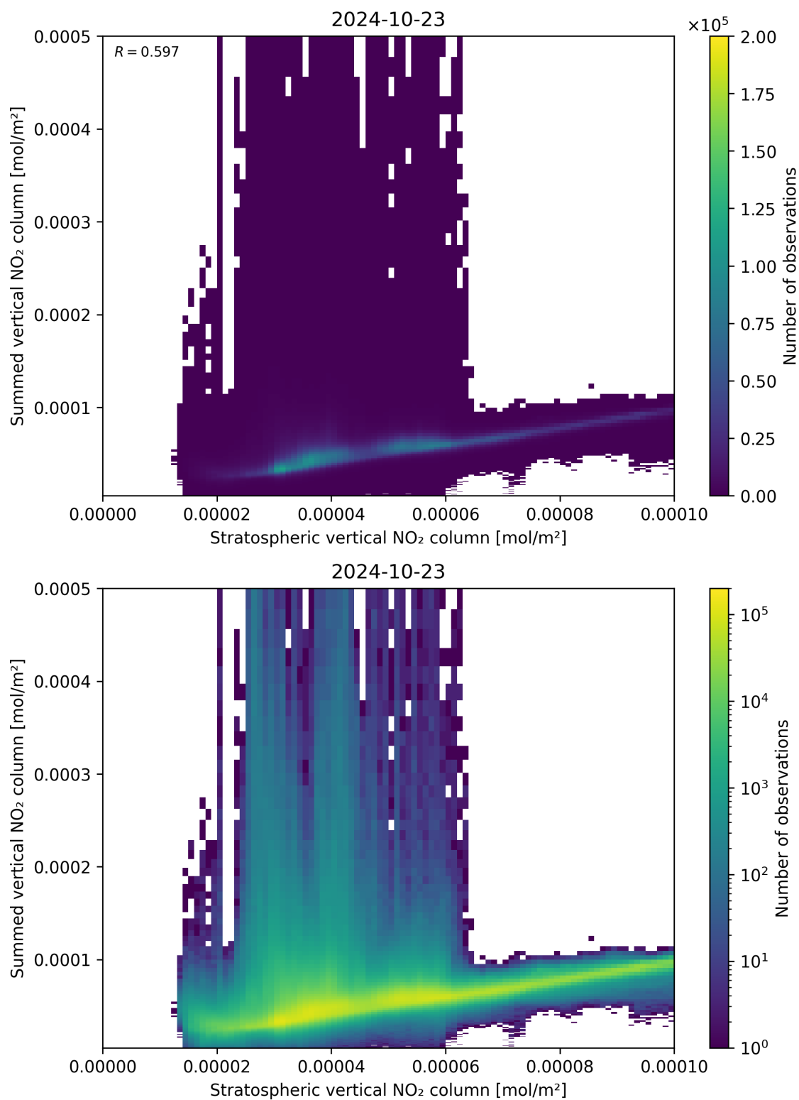
Figure 98: Scatter density plot of “Stratospheric vertical NO 2 column” against “Summed vertical NO 2 column” for 2024-10-22 to 2024-10-24.
