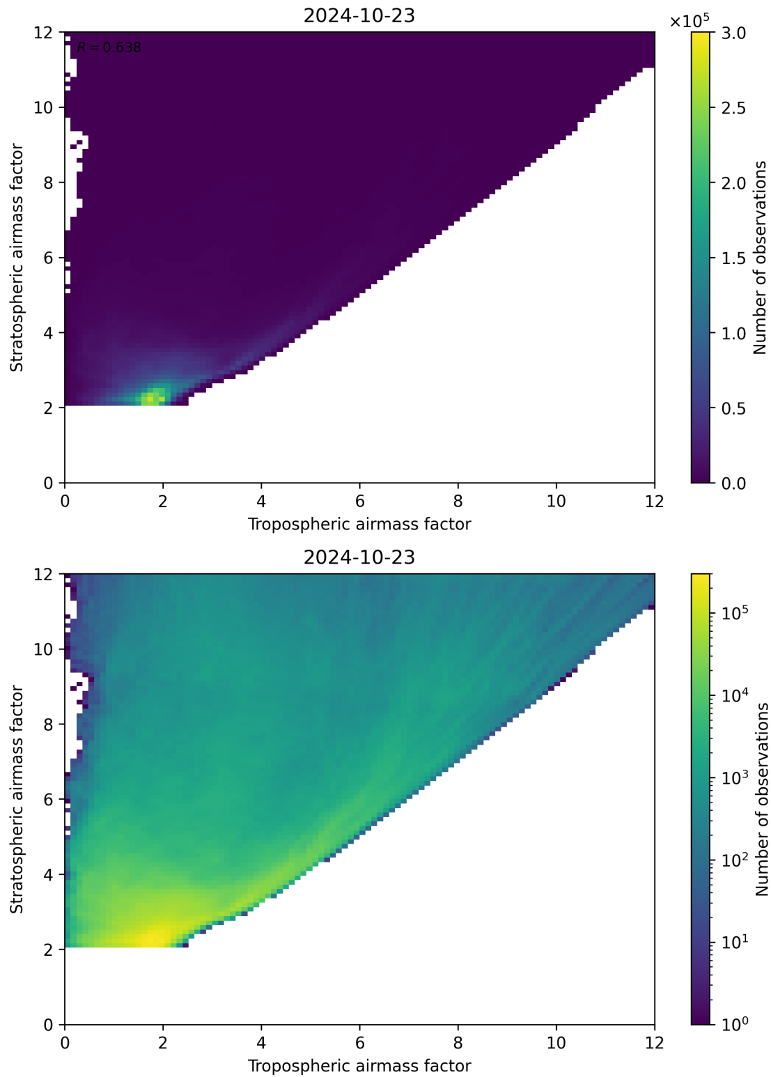
Figure 71: Scatter density plot of “Tropospheric airmass factor” against “Stratospheric airmass factor” for 2024-10-22 to 2024-10-24.
