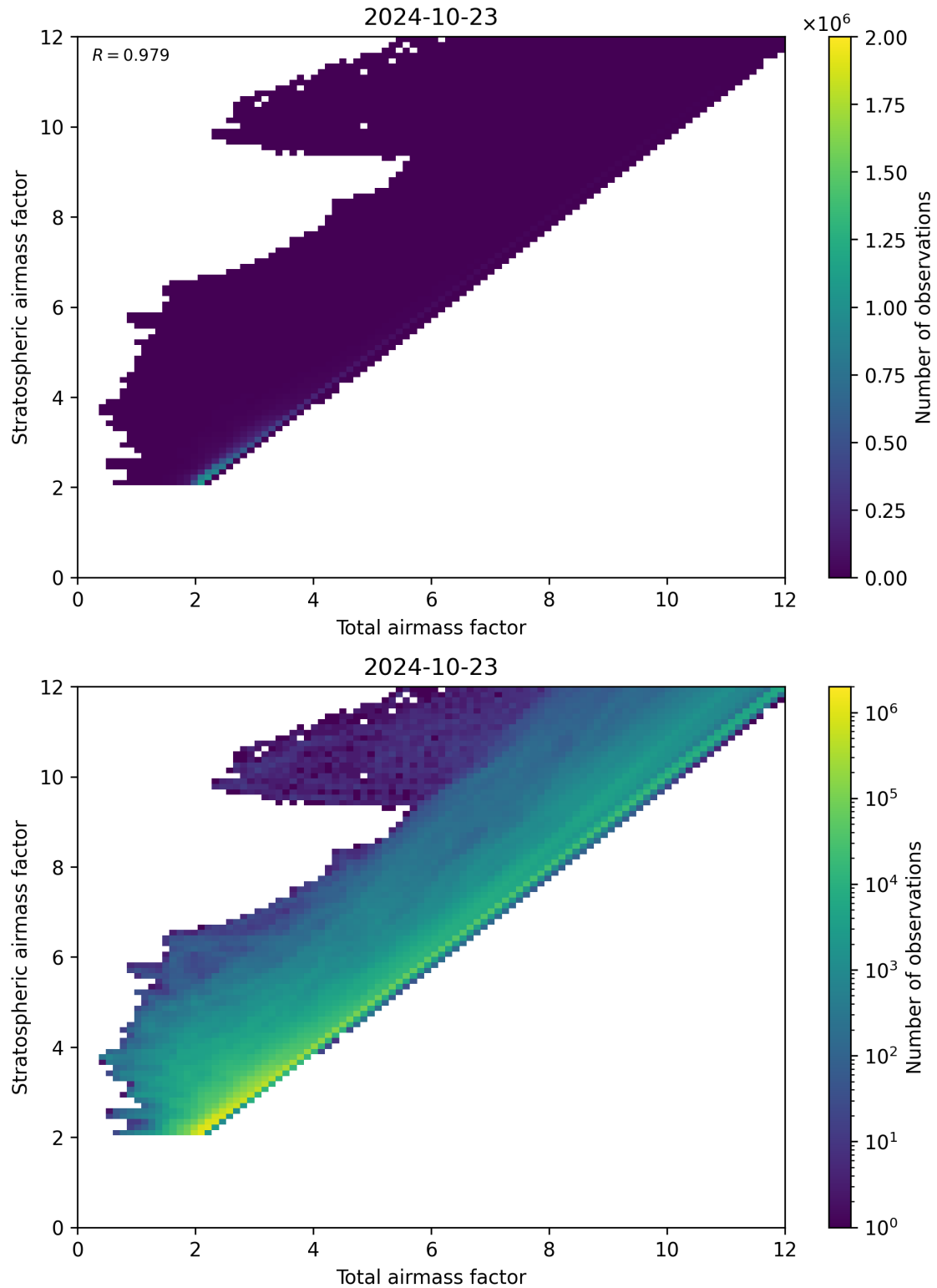
Figure 62: Scatter density plot of “Total airmass factor” against “Stratospheric airmass factor” for 2024-10-22 to 2024-10-24.
