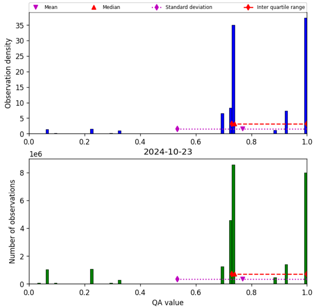
Figure 28: Histogram of “QA value” for 2024-10-22 to 2024-10-24
