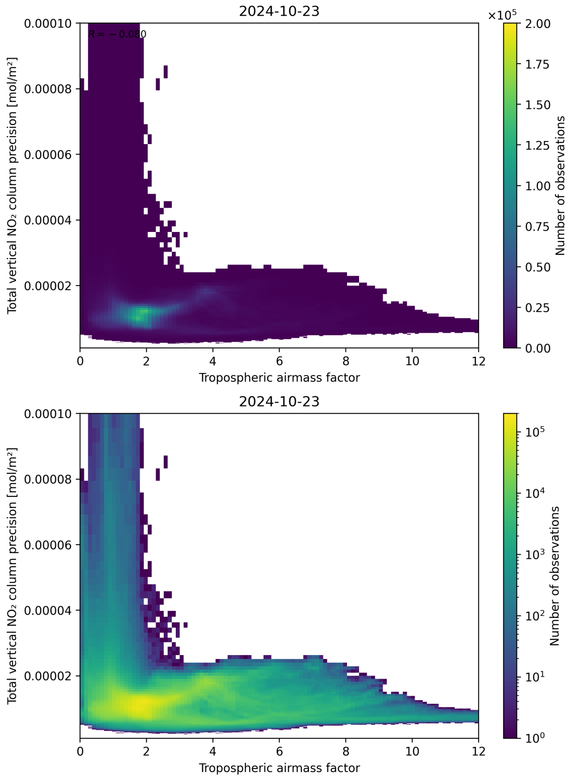
Figure 78: Scatter density plot of “Tropospheric air mass factor” against “Total vertical NO 2 column precision” for 2024-10-22 to 2024-10-24.
