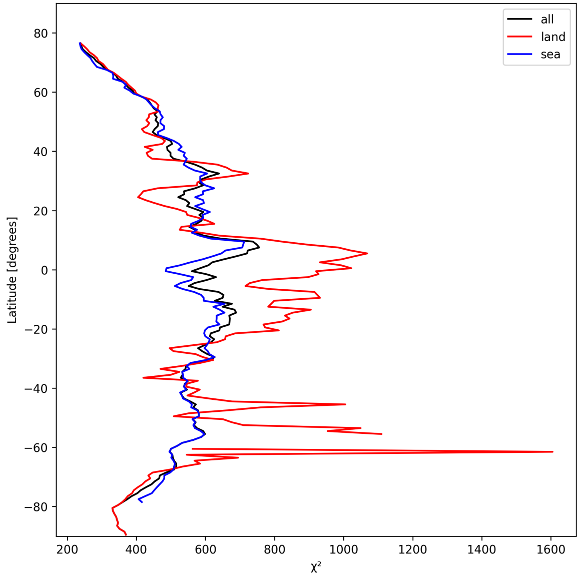
Figure 25: Zonal average of “ \chi^2 ” for 2024-10-22 to 2024-10-24.
