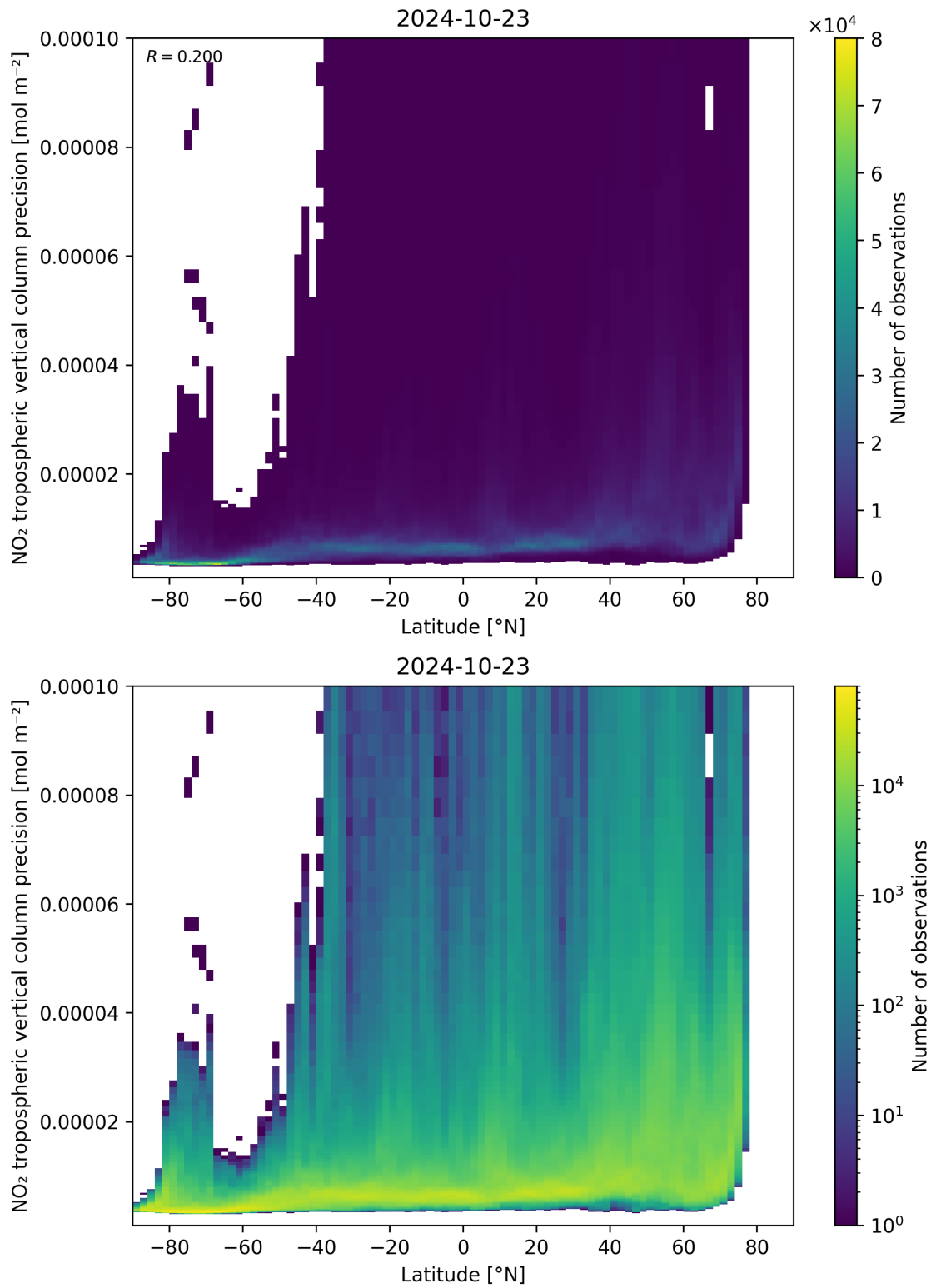
Figure 93: Scatter density plot of “Latitude” against “NO 2 tropospheric vertical column precision” for 2024-10-22 to 2024-10-24.
