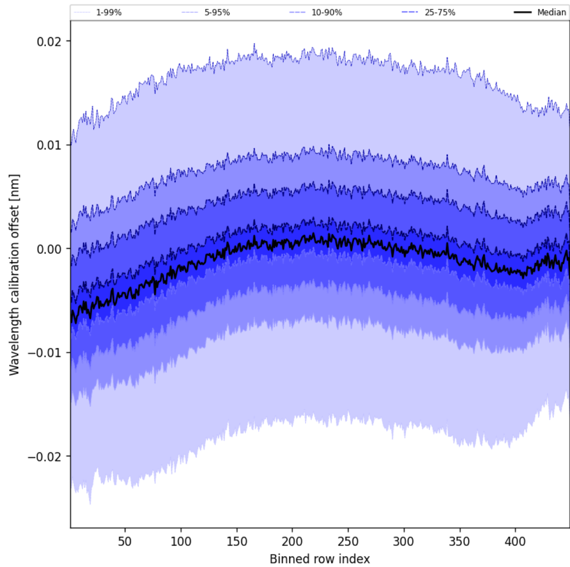
Figure 52: Along track statistics of “Wavelength calibration offset” for 2024-10-22 to 2024-10-24
