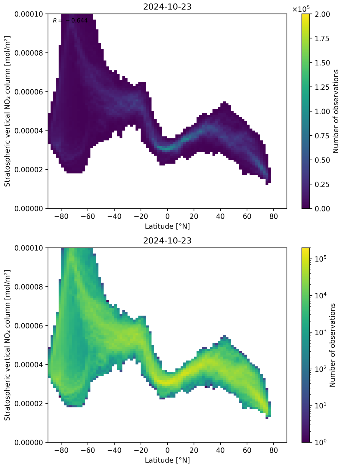
Figure 87: Scatter density plot of “Latitude” against “Stratospheric vertical NO 2 column” for 2024-10-22 to 2024-10-24.
