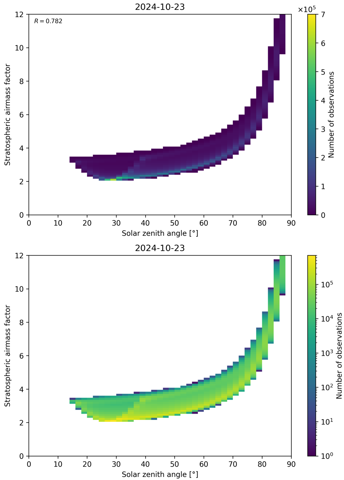
Figure 145: Scatter density plot of “Solar zenith angle” against “Stratospheric airmass factor” for 2024-10-22 to 2024-10-24.
