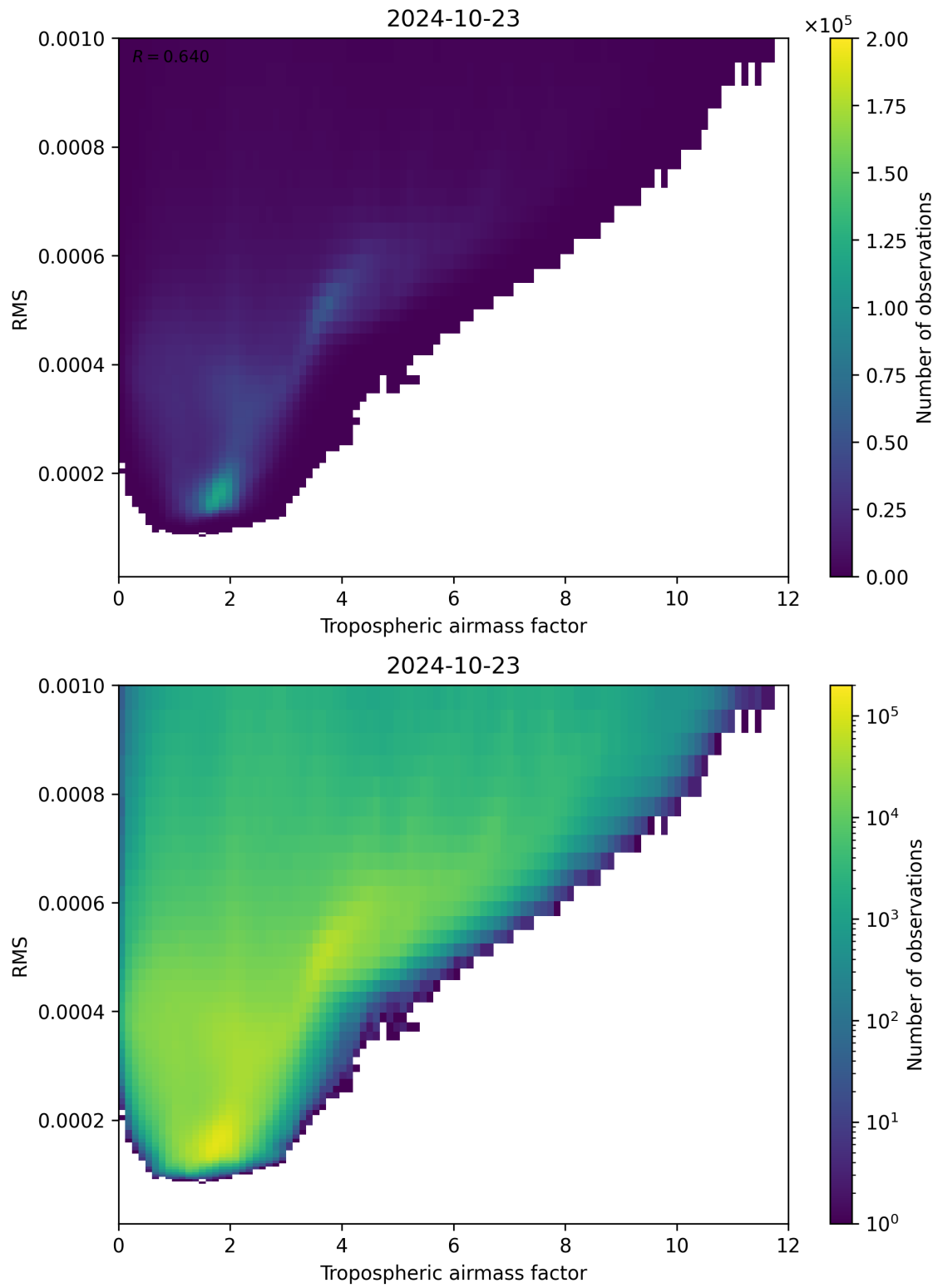
Figure 79: Scatter density plot of “Tropospheric airmass factor” against “RMS” for 2024-10-22 to 2024-10-24.
