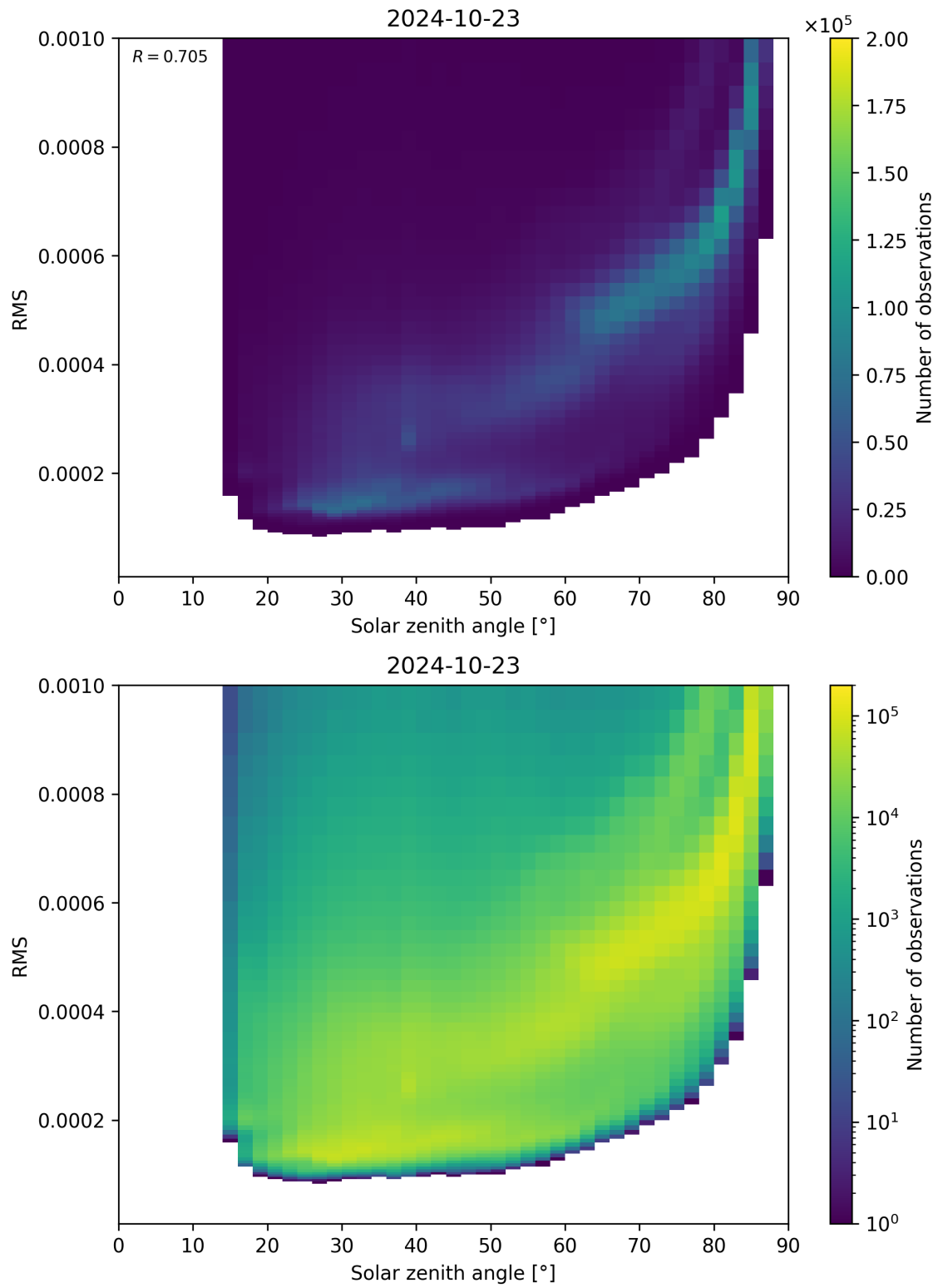
Figure 157: Scatter density plot of “Solar zenith angle” against “RMS” for 2024-10-22 to 2024-10-24.
