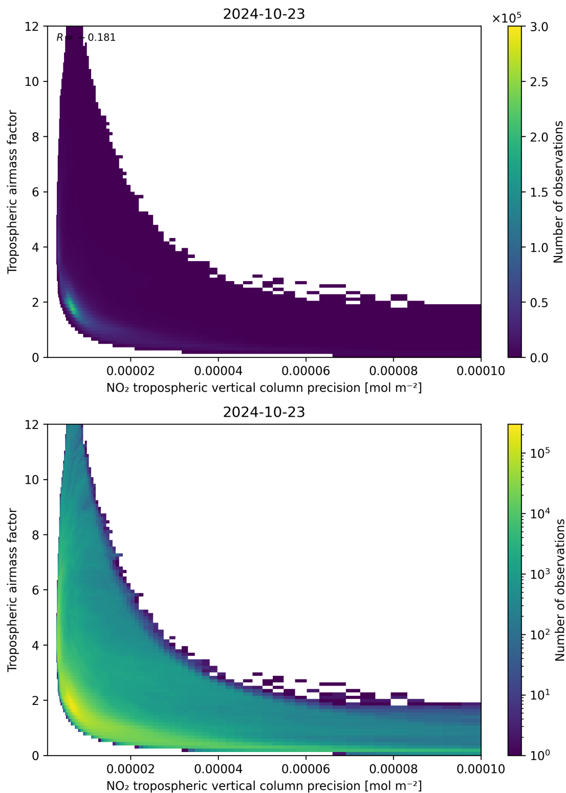
Figure 133: Scatter density plot of “NO 2 tropospheric vertical column precision” against “Tropospheric airmass factor” for 2024-10-22 to 2024-10-24.
