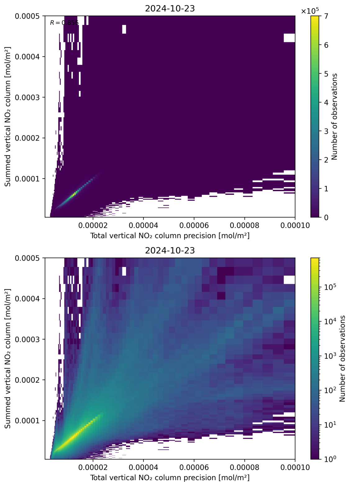
Figure 117: Scatter density plot of “Total vertical NO 2 column precision” against “Summed vertical NO 2 column” for 2024-10-22 to 2024-10-24.
