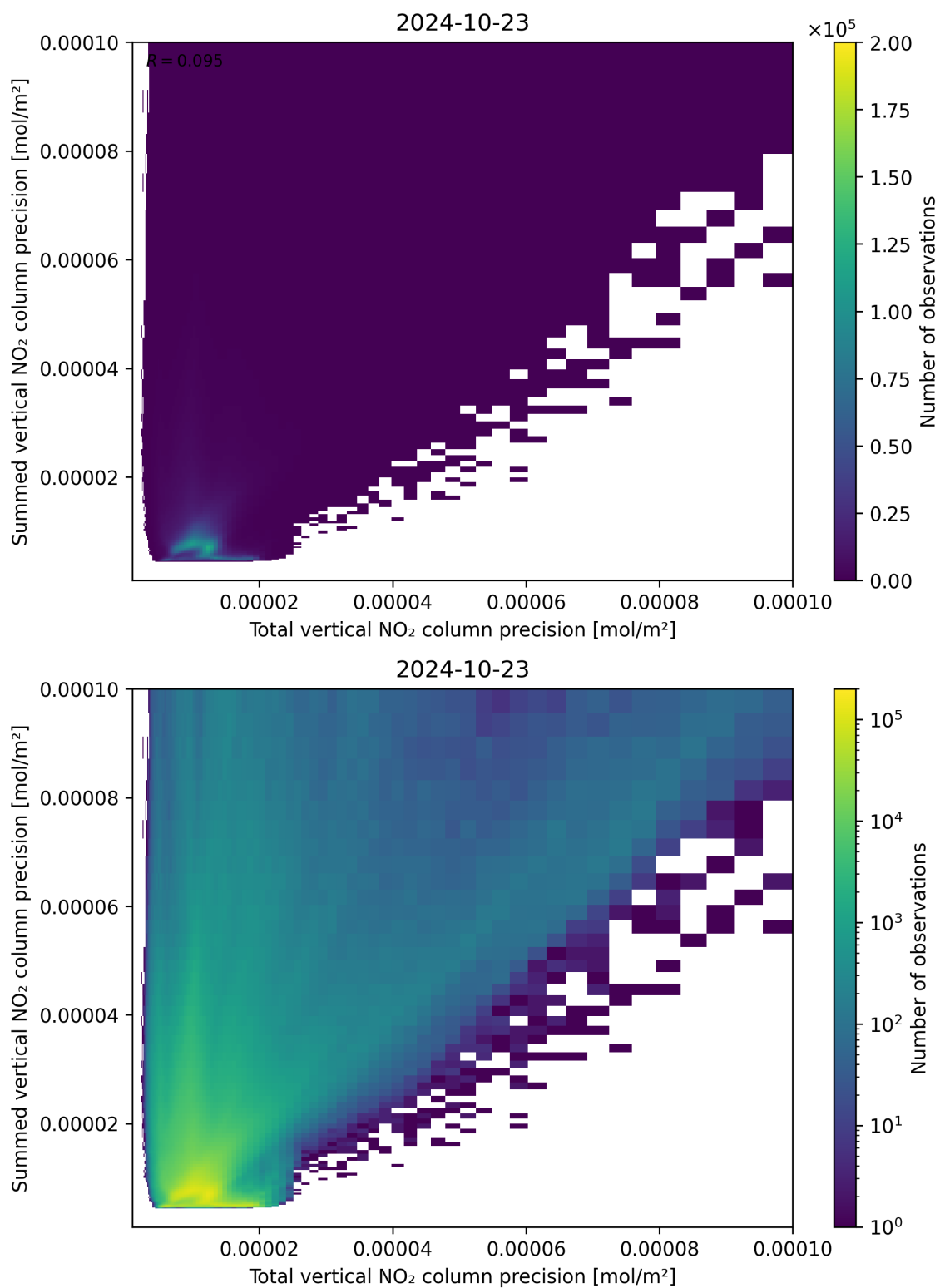
Figure 118: Scatter density plot of “Total vertical NO 2 column precision” against “Summed vertical NO 2 column precision” for 2024-10-22 to 2024-10-24.
