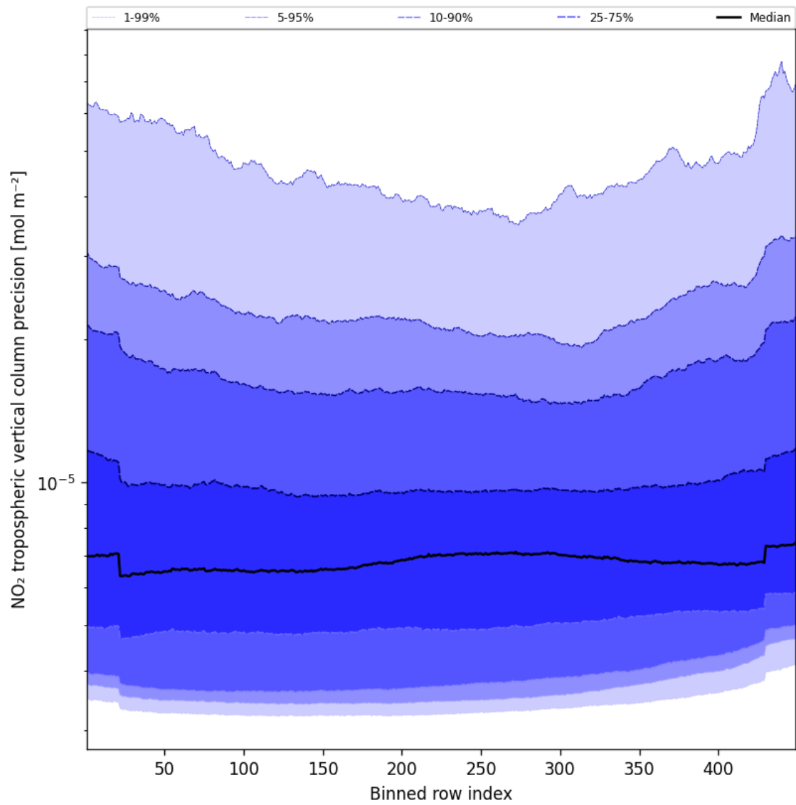
Figure 47: Along track statistics of “NO 2 tropospheric vertical column precision” for 2024-10-22 to 2024-10-24
