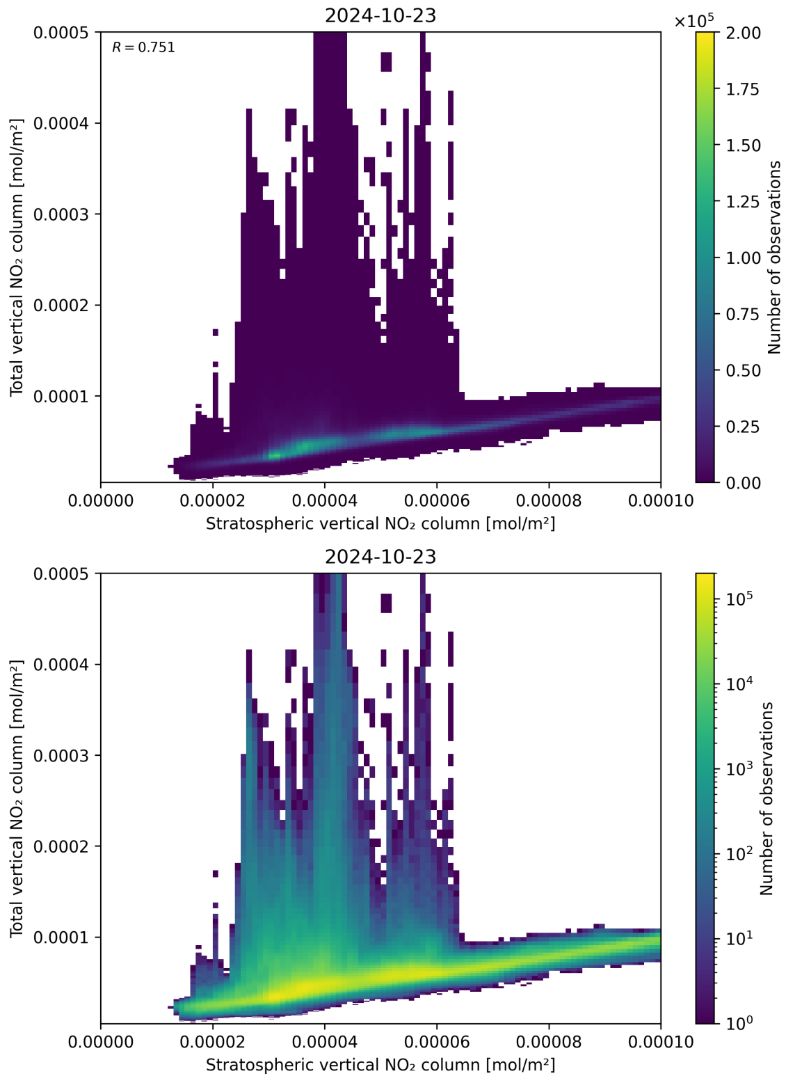
Figure 100: Scatter density plot of “Stratospheric vertical NO 2 column” against “Total vertical NO 2 column” for 2024-10-22 to 2024-10-24.
