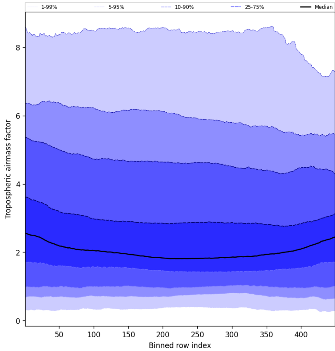
Figure 48: Along track statistics of “Tropospheric air mass factor” for 2024-10-22 to 2024-10-24
