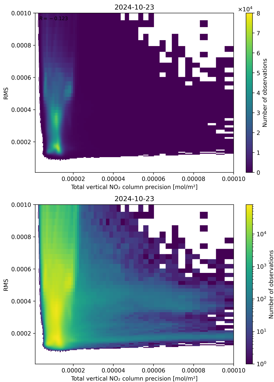
Figure 119: Scatter density plot of “Total vertical NO 2 column precision” against “RMS” for 2024-10-22 to 2024-10-24.
