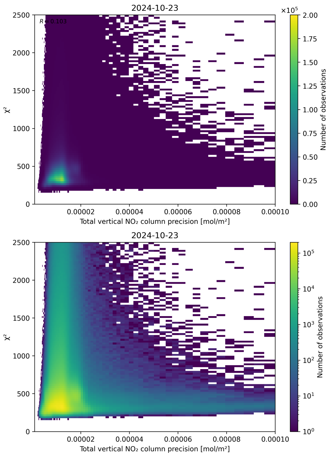
Figure 116: Scatter density plot of “Total vertical NO 2 column precision” against “ \chi^2 ” for 2024-10-22 to 2024-10-24.
