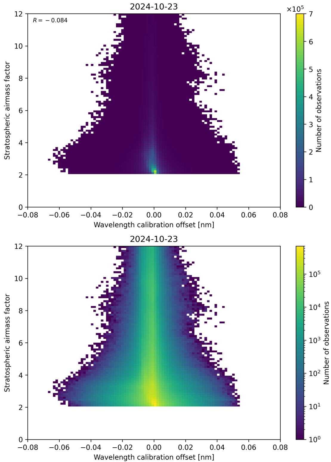
Figure 174: Scatter density plot of “Wavelength calibration offset” against “Stratospheric air mass factor” for 2024-10-22 to 2024-10-24.
