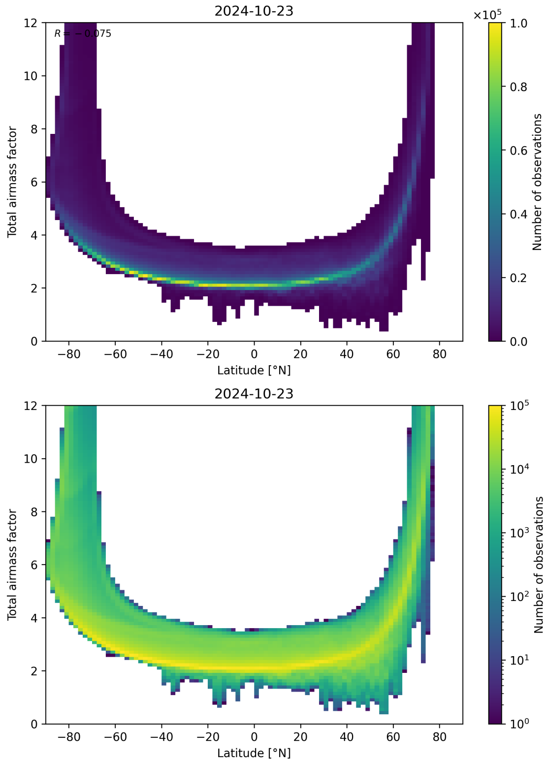
Figure 84: Scatter density plot of “Latitude” against “Total airmass factor” for 2024-10-22 to 2024-10-24.
