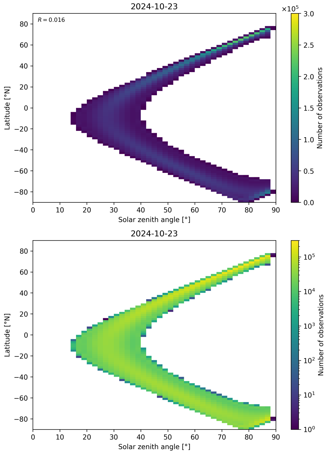
Figure 149: Scatter density plot of “Solar zenith angle” against “Latitude” for 2024-10-22 to 2024-10-24.
