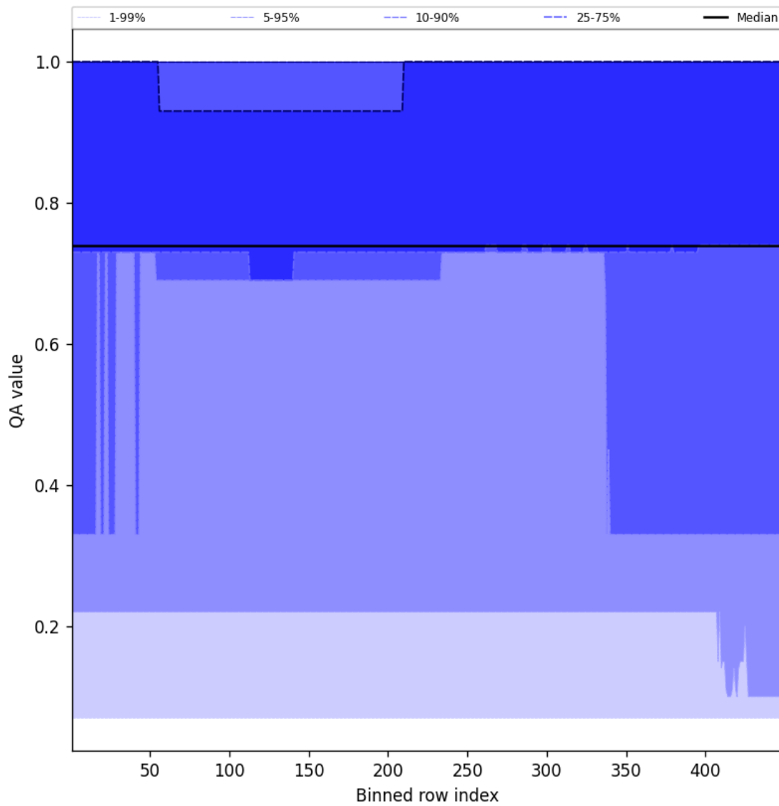
Figure 45: Along track statistics of “QA value” for 2024-10-22 to 2024-10-24
