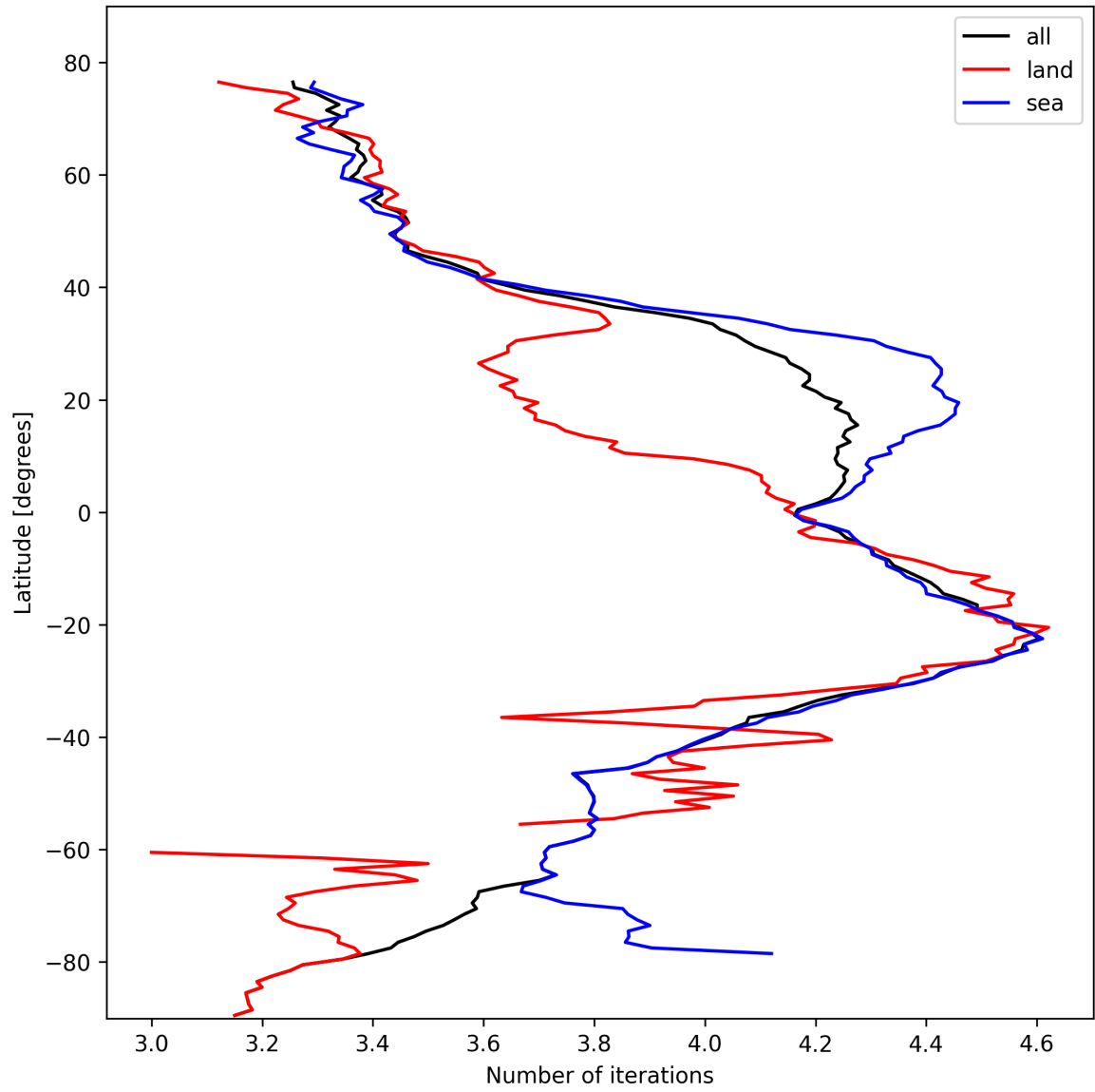
Figure 17: Zonal average of “Number of iterations” for 2024-10-22 to 2024-10-24.
