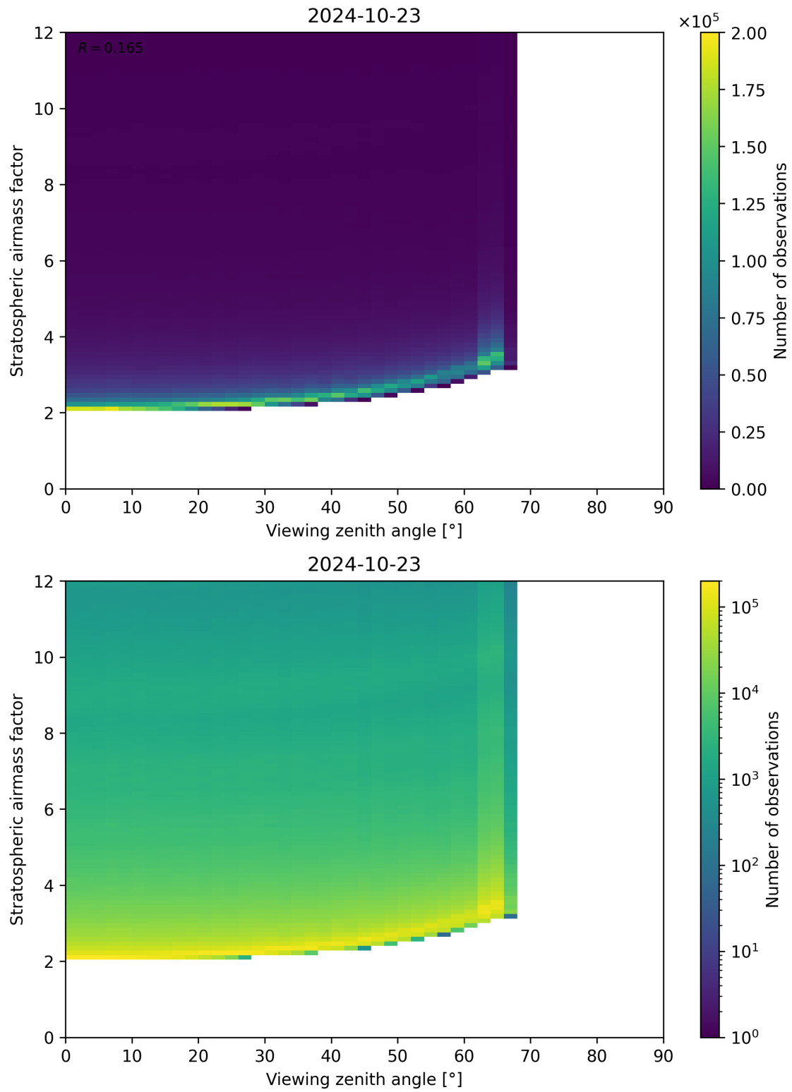
Figure 159: Scatter density plot of “Viewing zenith angle” against “Stratospheric airmass factor” for 2024-10-22 to 2024-10-24.
