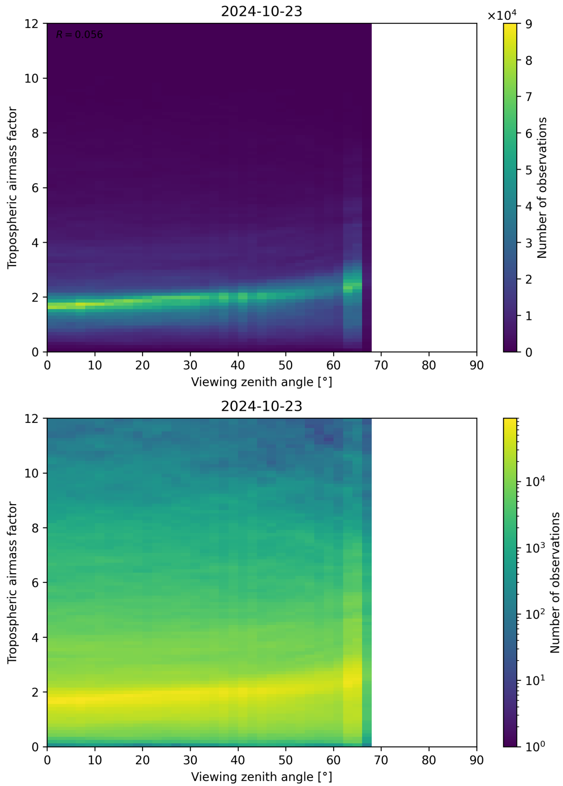
Figure 161: Scatter density plot of “Viewing zenith angle” against “Tropospheric airmass factor” for 2024-10-22 to 2024-10-24.
