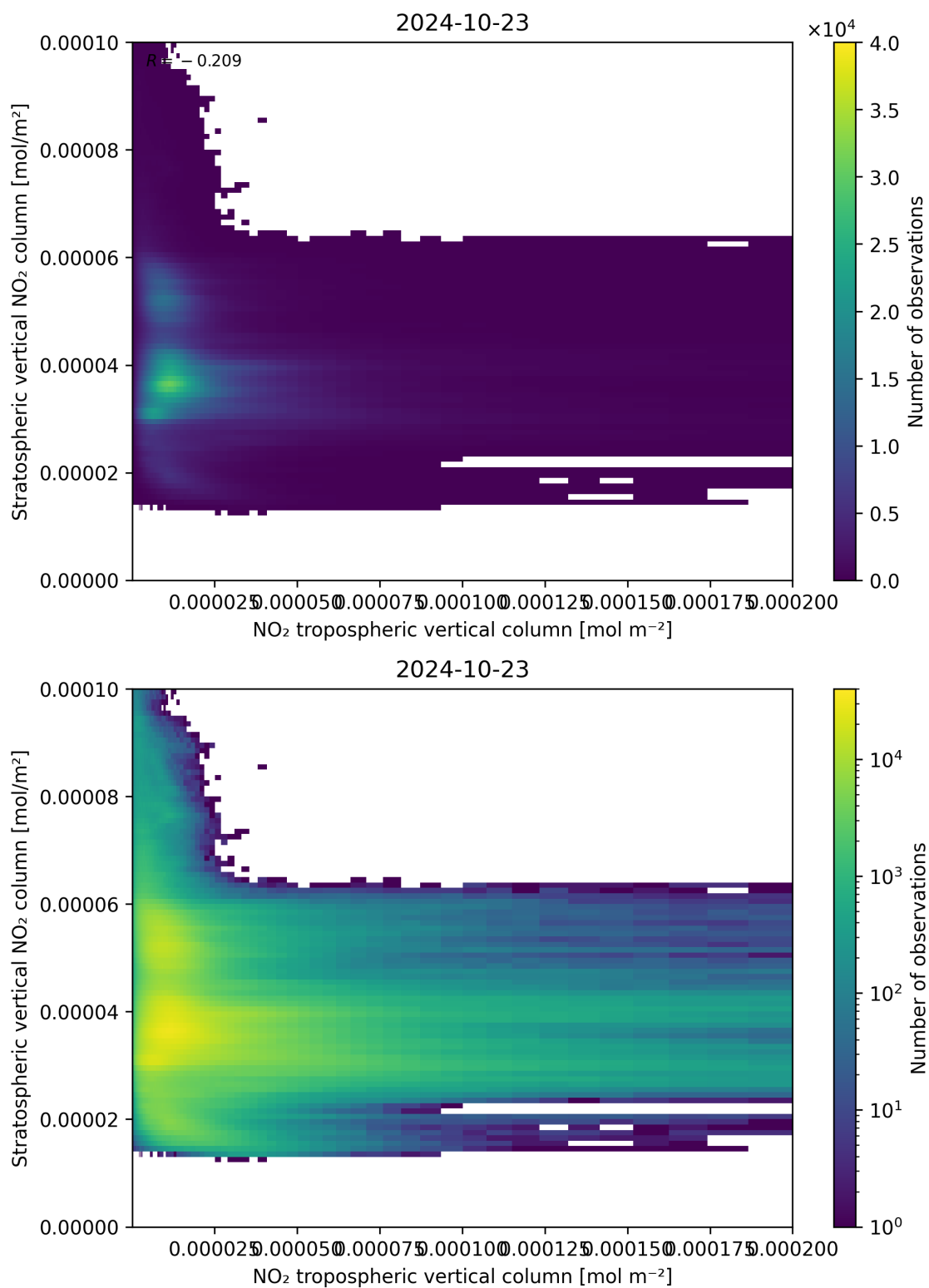
Figure 125: Scatter density plot of “NO 2 tropospheric vertical column” against “Stratospheric vertical NO 2 column” for 2024-10-22 to 2024-10-24.
