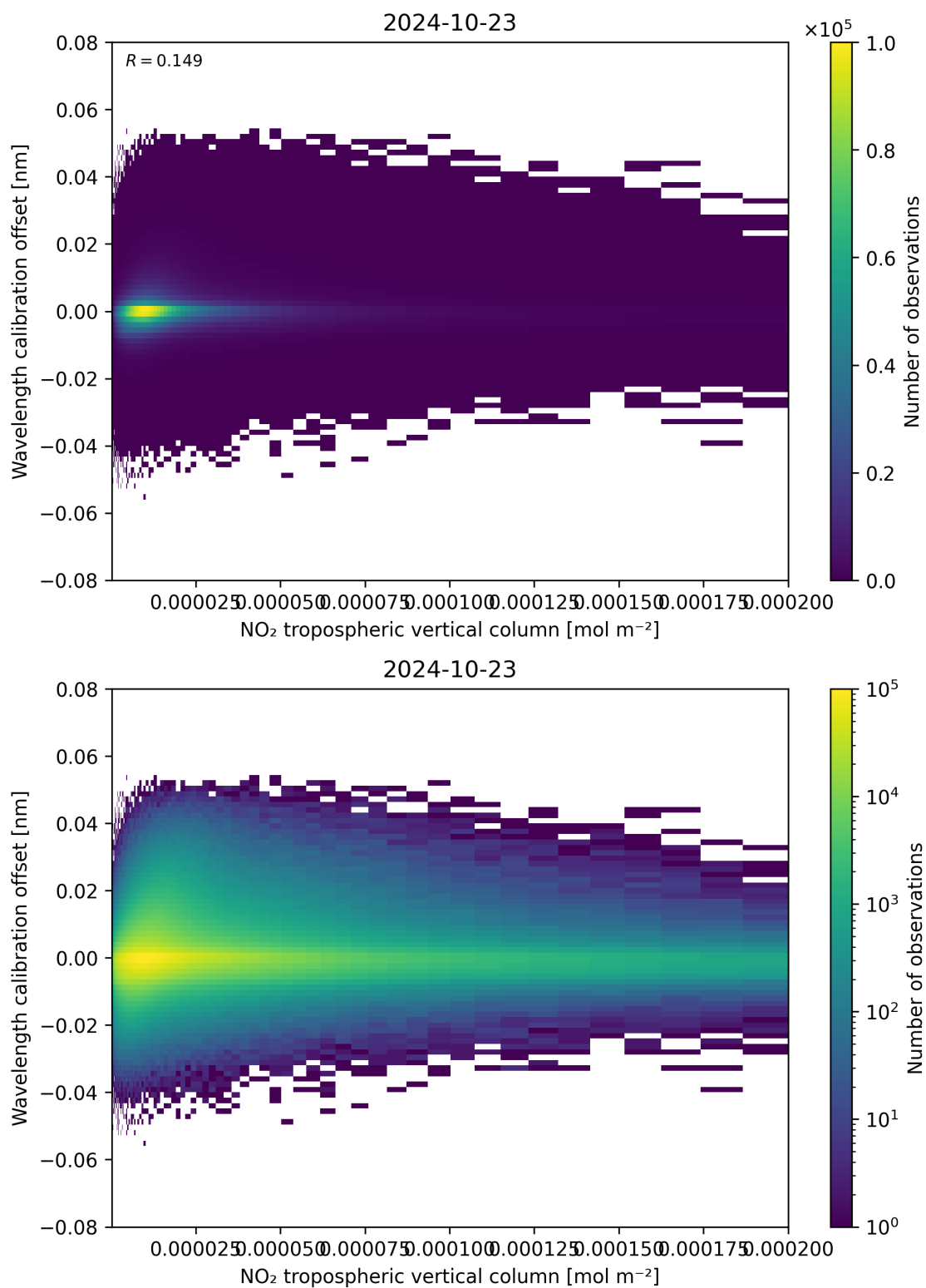
Figure 143: Scatter density plot of “NO 2 tropospheric vertical column” against “Wavelength calibration offset” for 2024-10-22 to 2024-10-24.
