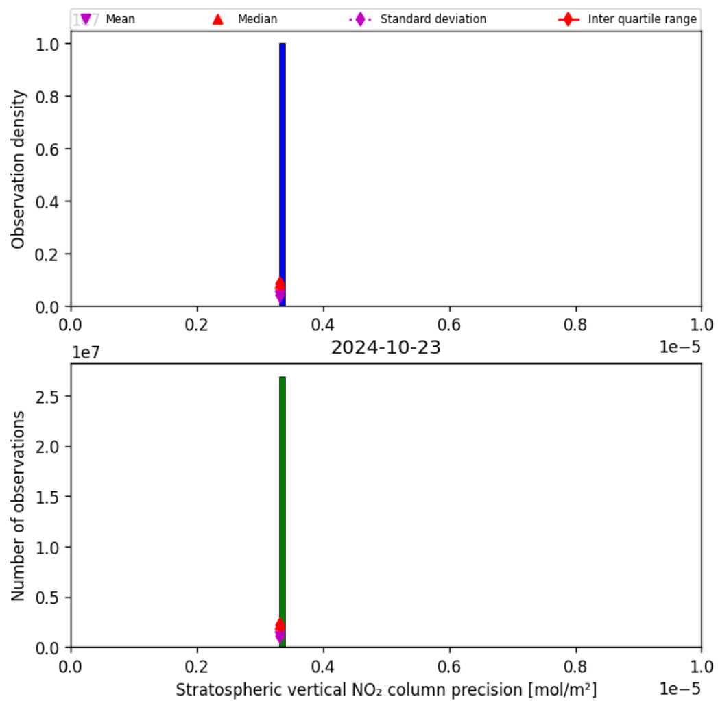
Figure 37: Histogram of “Stratospheric vertical NO 2 column precision” for 2024-10-22 to 2024-10-24
