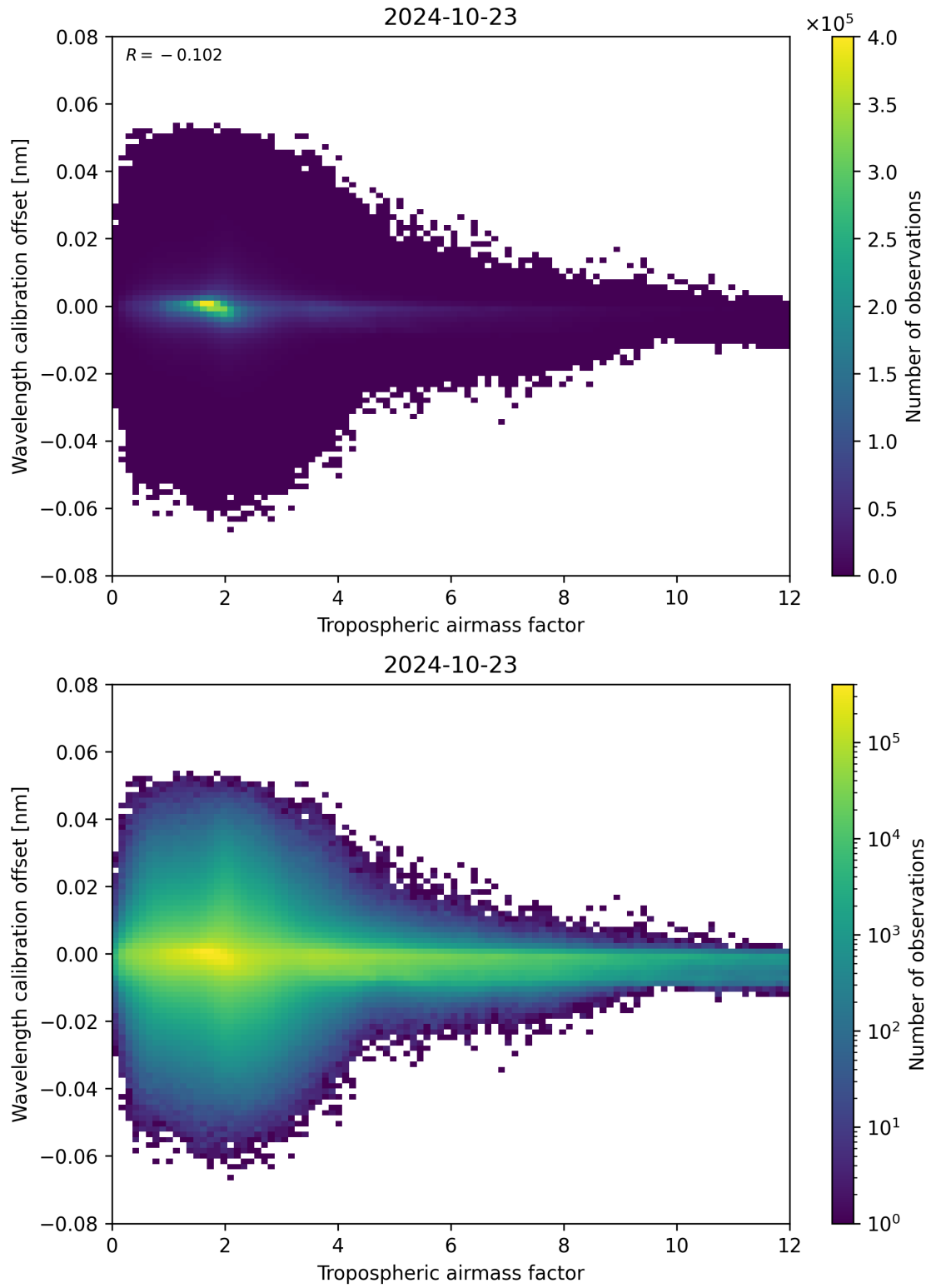
Figure 80: Scatter density plot of “Tropospheric airmass factor” against “Wavelength calibration offset” for 2024-10-22 to 2024-10-24.
