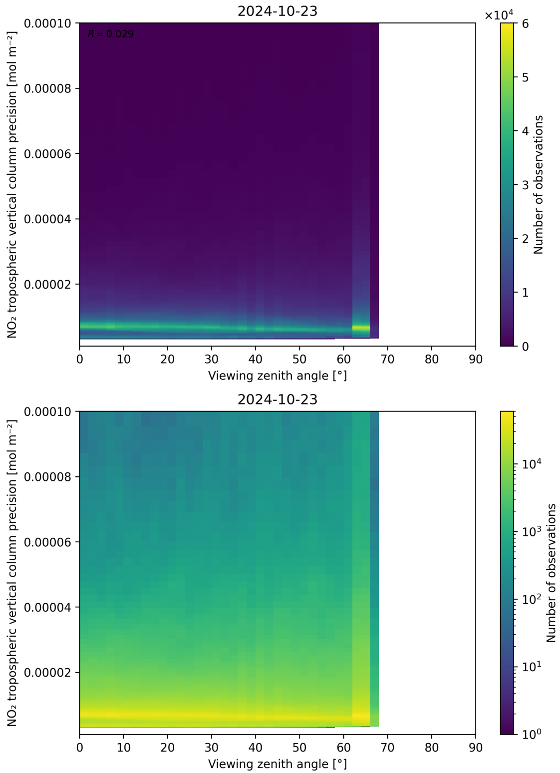
Figure 170: Scatter density plot of “Viewing zenith angle” against “NO 2 tropospheric vertical column precision” for 2024-10-22 to 2024-10-24.
