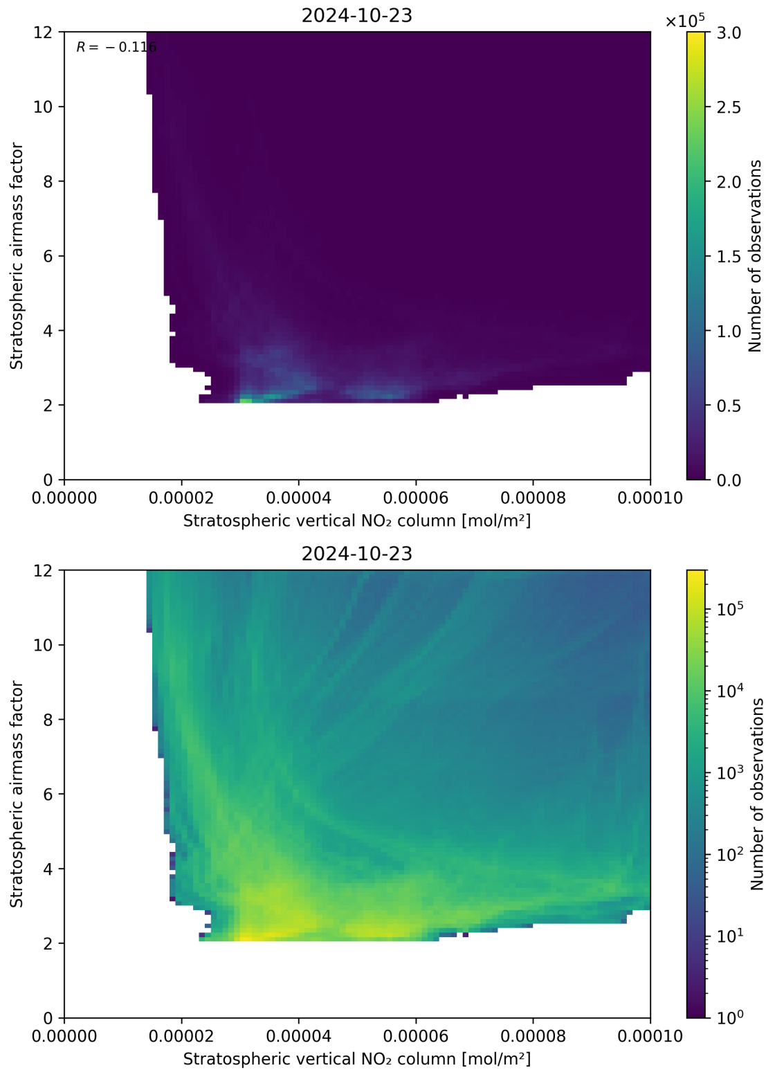
Figure 96: Scatter density plot of “Stratospheric vertical NO 2 column” against “Stratospheric airmass factor” for 2024-10-22 to 2024-10-24.
