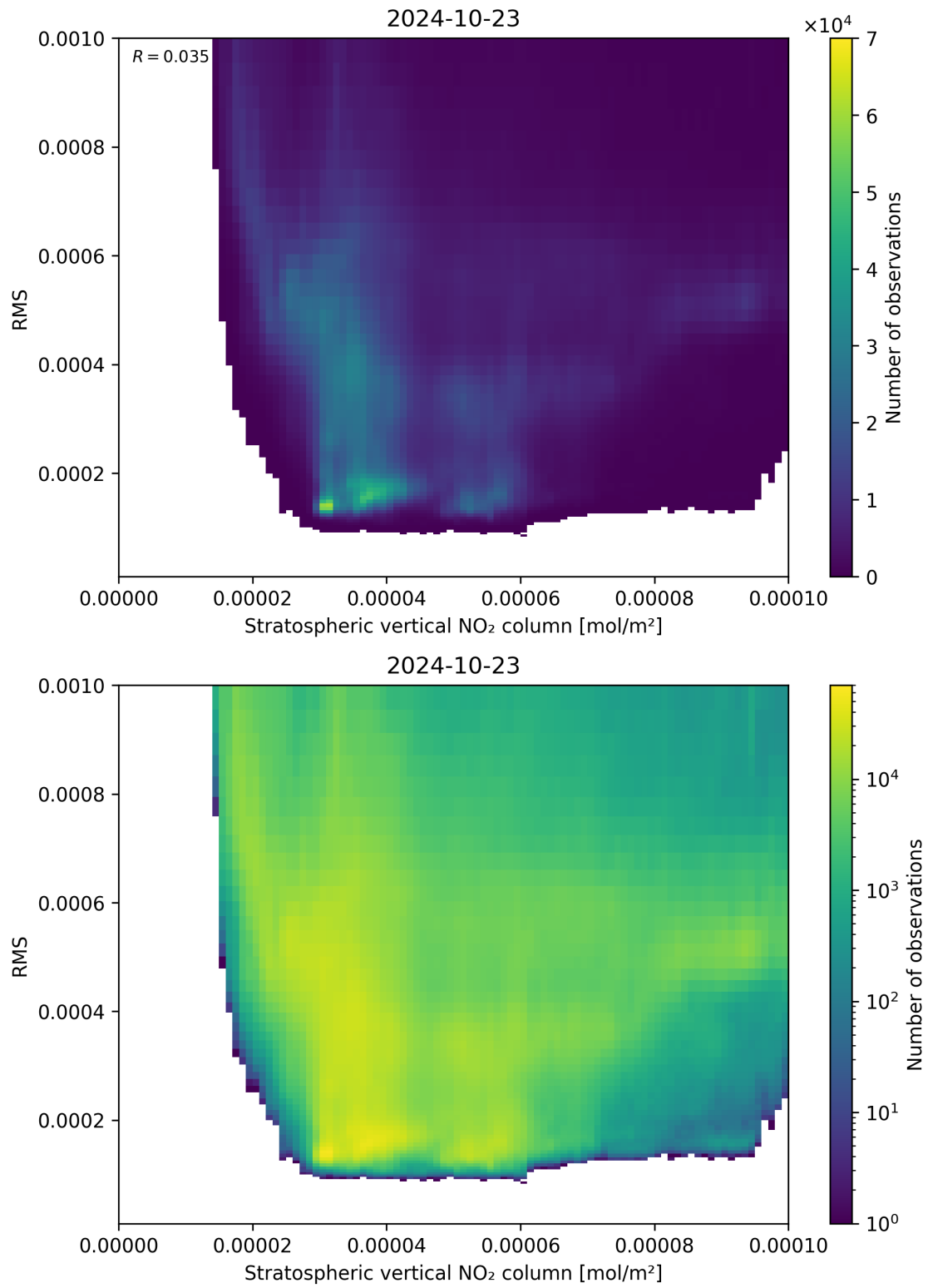
Figure 102: Scatter density plot of “Stratospheric vertical NO 2 column” against “RMS” for 2024-10-22 to 2024-10-24.
