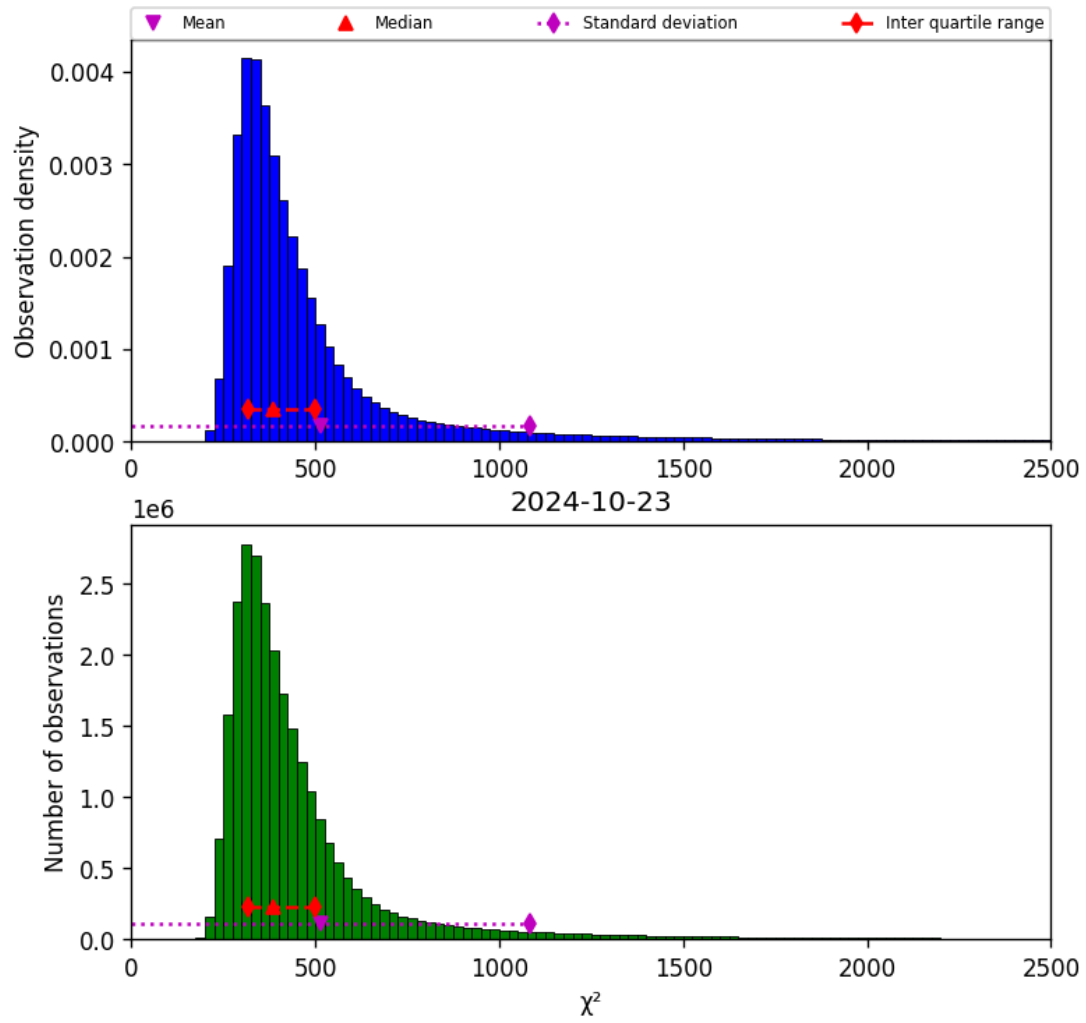
Figure 42: Histogram of “ \chi^2 ” for 2024-10-22 to 2024-10-24
