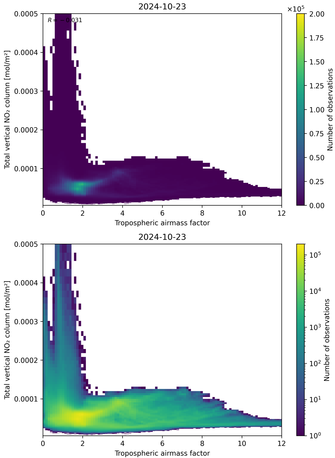
Figure 77: Scatter density plot of “Tropospheric airmass factor” against “Total vertical NO 2 column” for 2024-10-22 to 2024-10-24.
