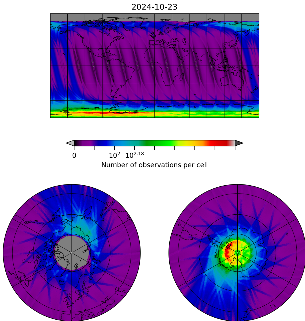
Figure 10: Map of the number of observations for 2024-10-22 to 2024-10-24
