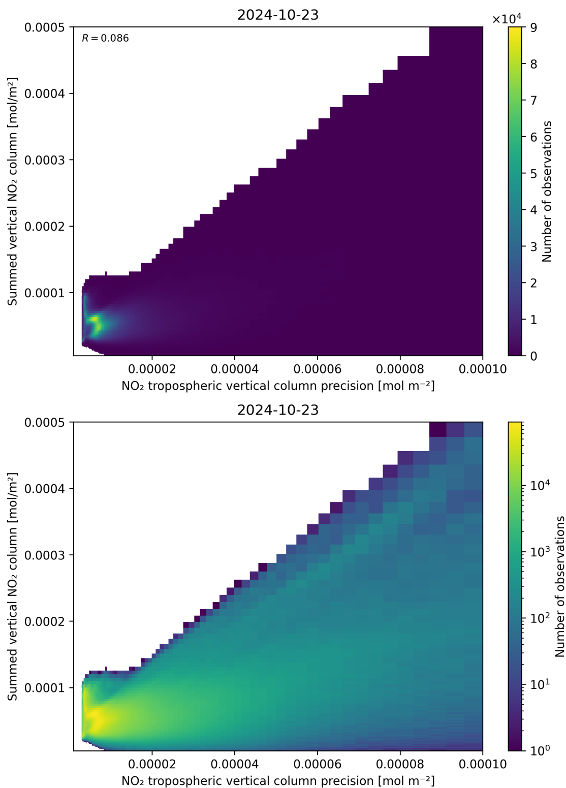
Figure 136: Scatter density plot of “NO 2 tropospheric vertical column precision” against “Summed vertical NO 2 column” for 2024-10-22 to 2024-10-24.
