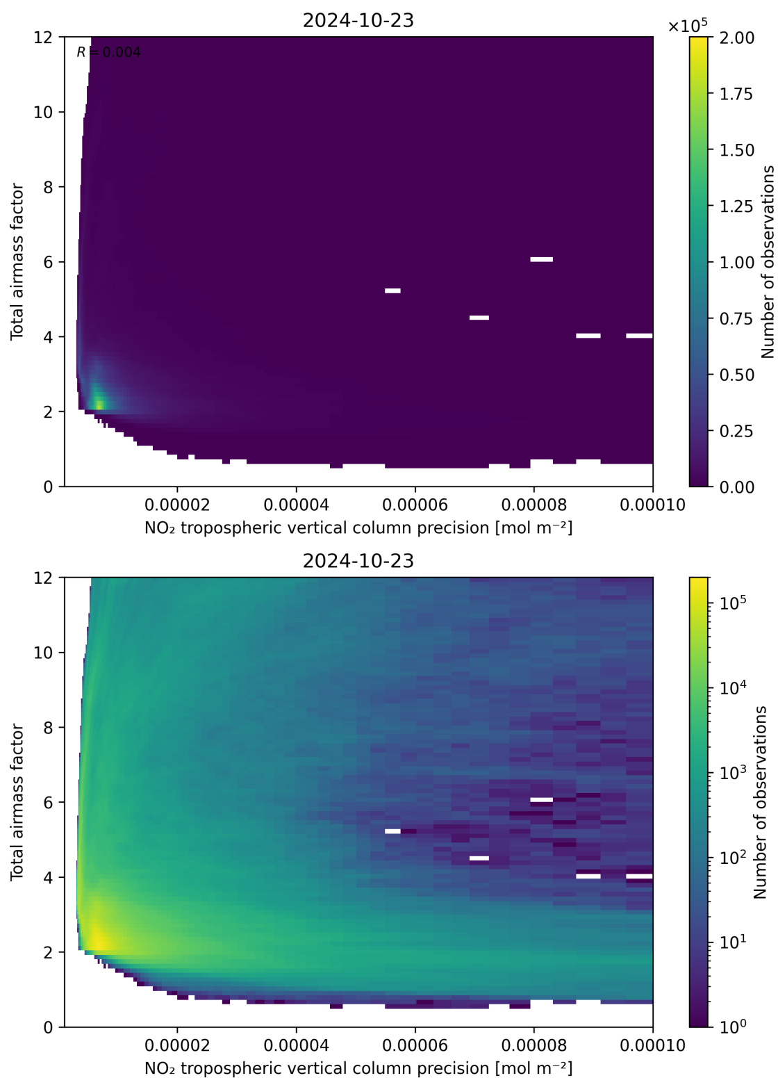
Figure 132: Scatter density plot of “NO 2 tropospheric vertical column precision” against “Total air mass factor” for 2024-10-22 to 2024-10-24.
