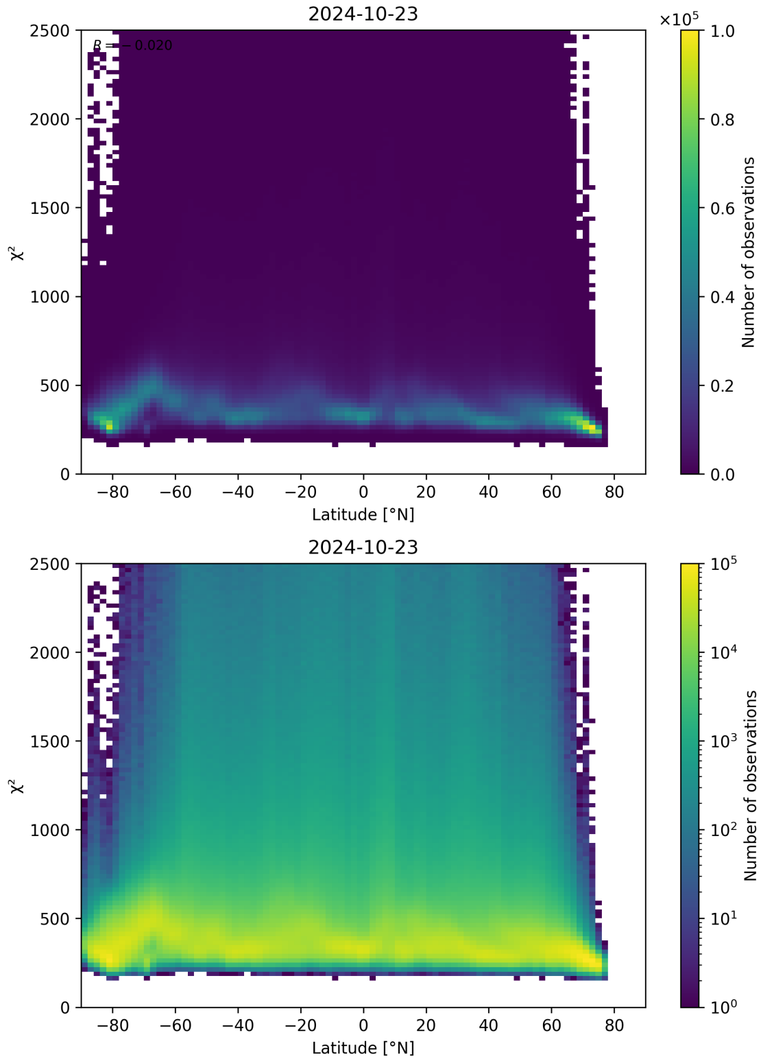
Figure 86: Scatter density plot of “Latitude” against “ \chi^2 ” for 2024-10-22 to 2024-10-24.
