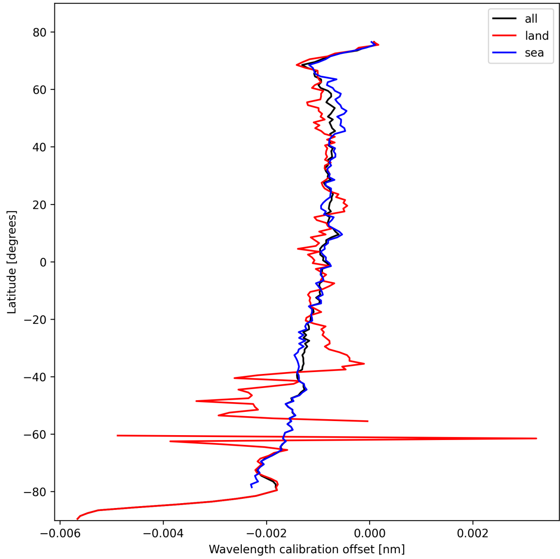
Figure 18: Zonal average of “Wavelength calibration offset” for 2024-10-22 to 2024-10-24.
