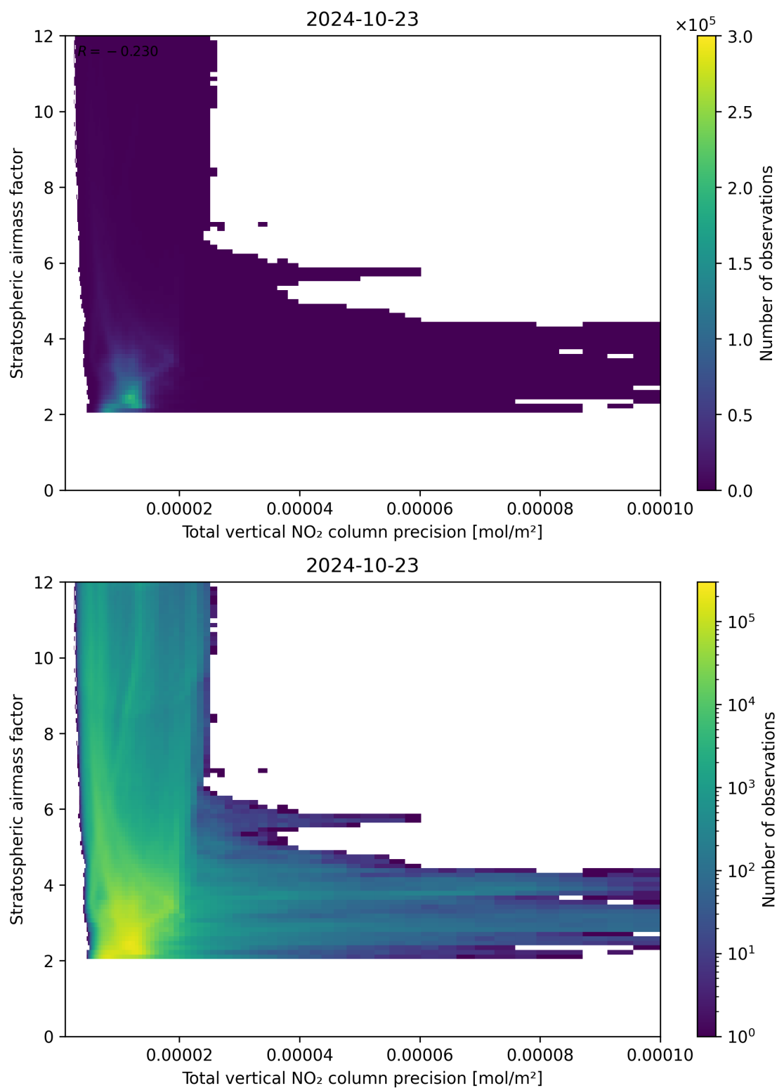
Figure 115: Scatter density plot of “Total vertical NO 2 column precision” against “Stratospheric air mass factor” for 2024-10-22 to 2024-10-24.
