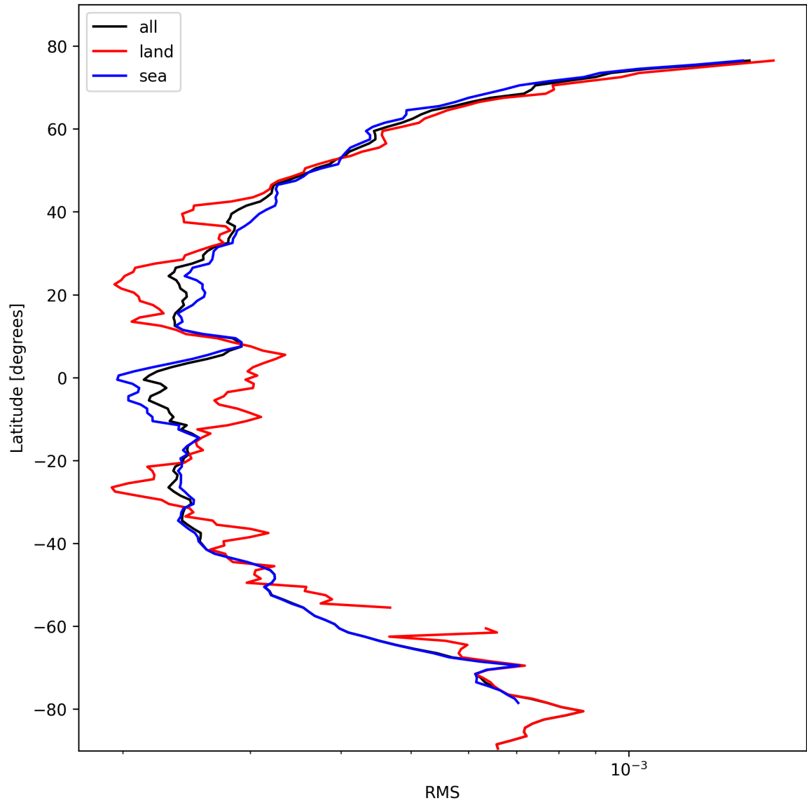
Figure 26: Zonal average of “RMS” for 2024-10-22 to 2024-10-24.
