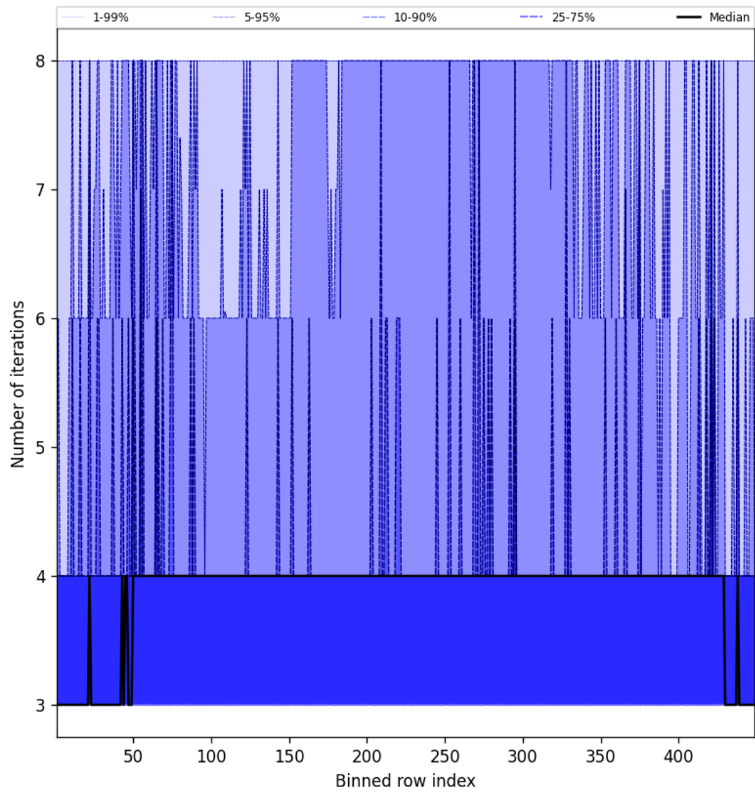
Figure 51: Along track statistics of “Number of iterations” for 2024-10-22 to 2024-10-24
