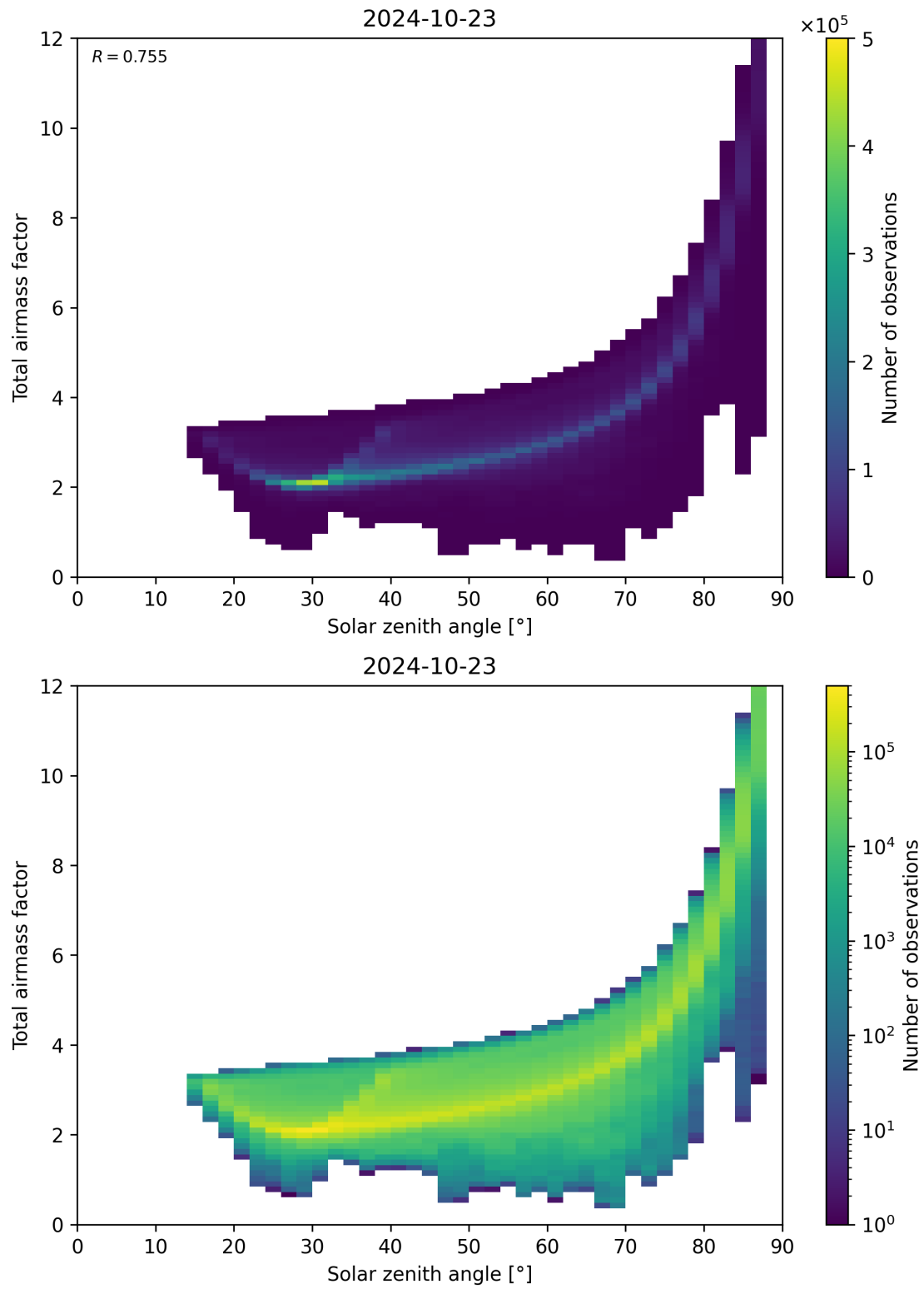
Figure 146: Scatter density plot of “Solar zenith angle” against “Total air mass factor” for 2024-10-22 to 2024-10-24.
