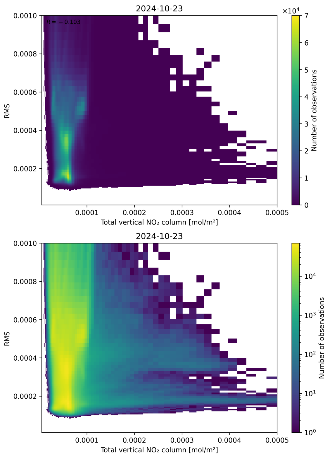
Figure 120: Scatter density plot of “Total vertical NO 2 column” against “RMS” for 2024-10-22 to 2024-10-24.
