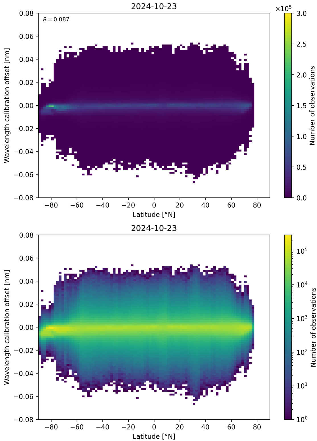
Figure 95: Scatter density plot of “Latitude” against “Wavelength calibration offset” for 2024-10-22 to 2024-10-24.
