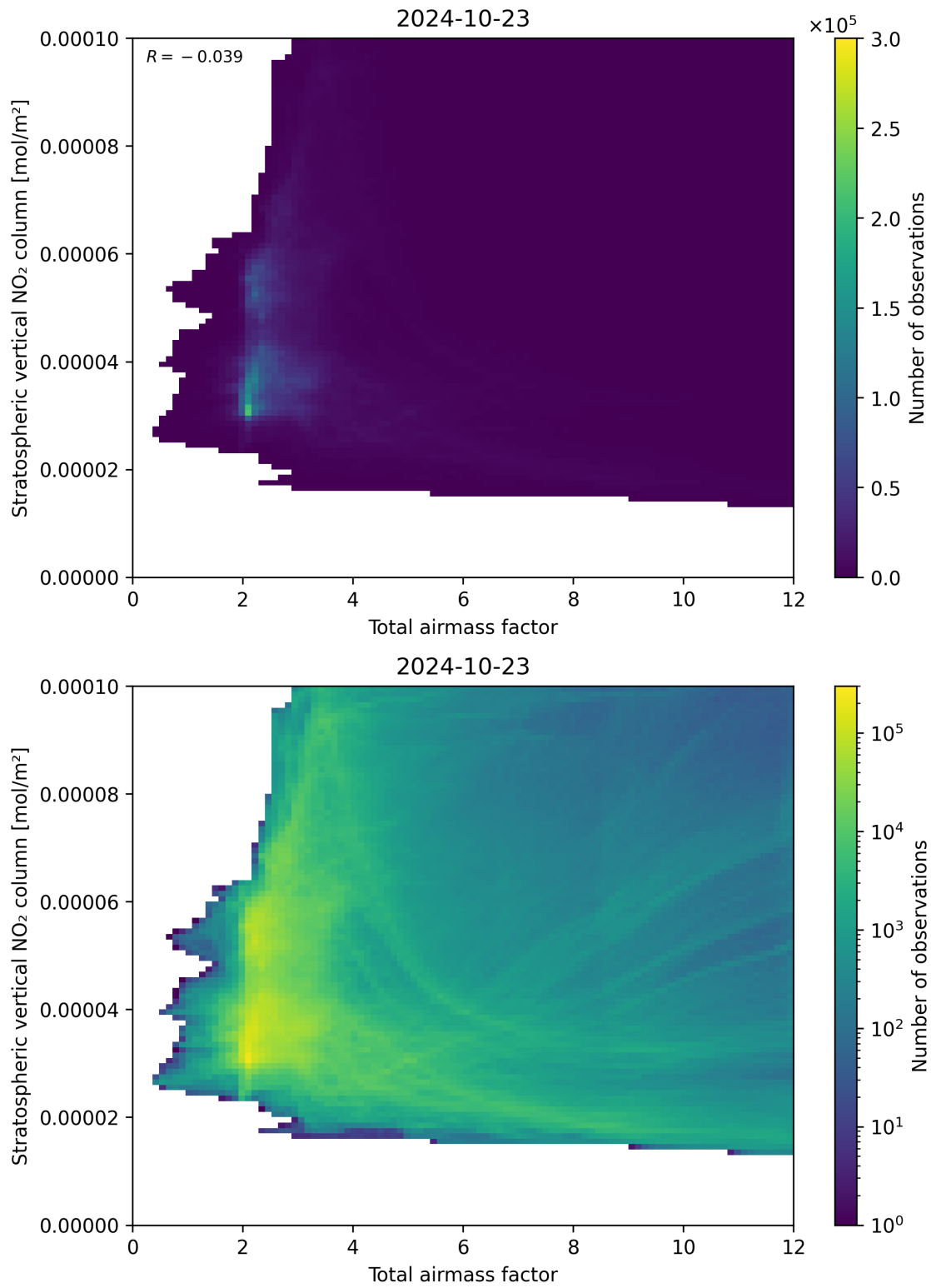
Figure 64: Scatter density plot of “Total airmass factor” against “Stratospheric vertical NO 2 column” for 2024-10-22 to 2024-10-24.
