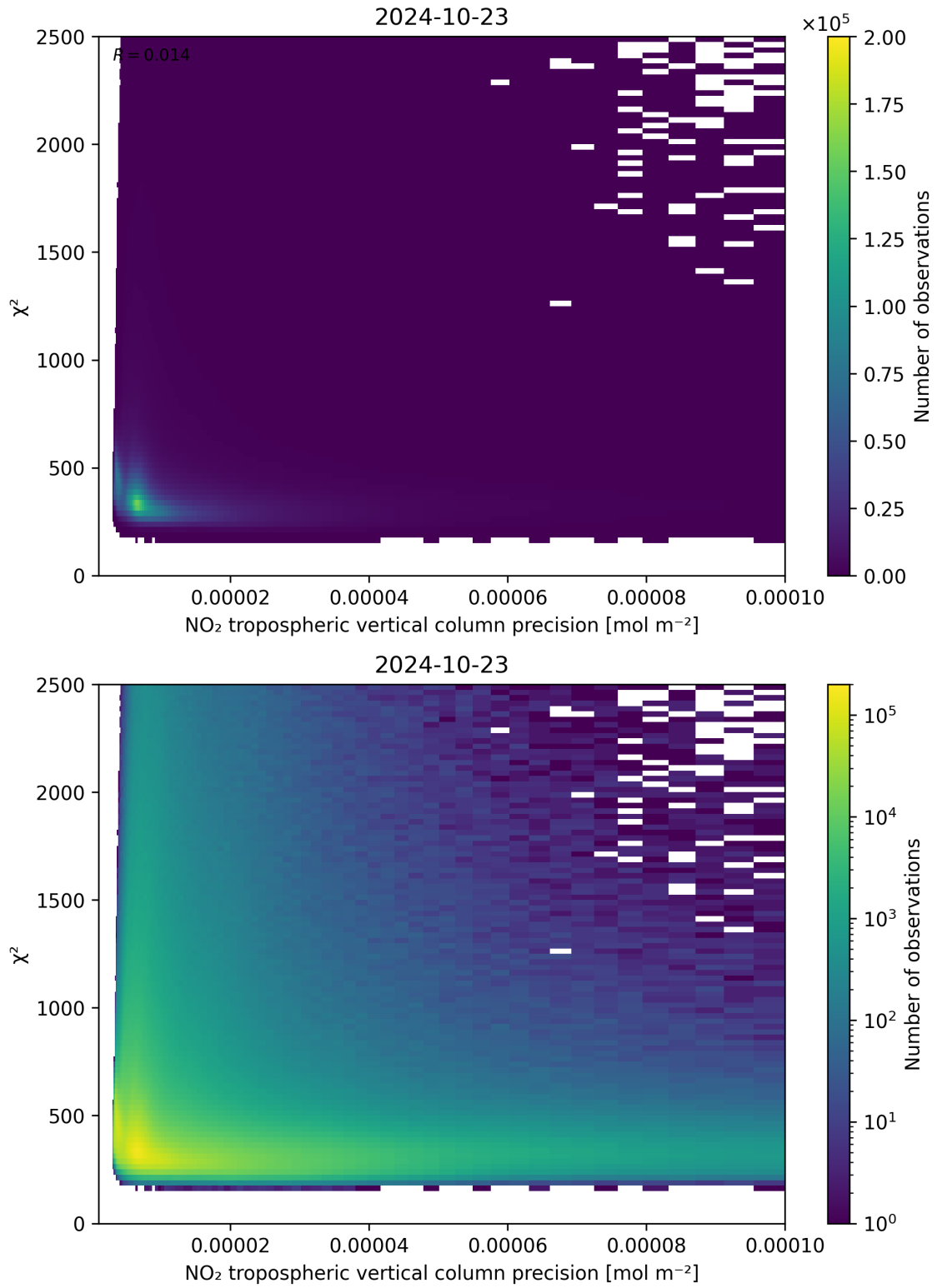
Figure 134: Scatter density plot of “NO 2 tropospheric vertical column precision” against “ \chi^2 ” for 2024-10-22 to 2024-10-24.
