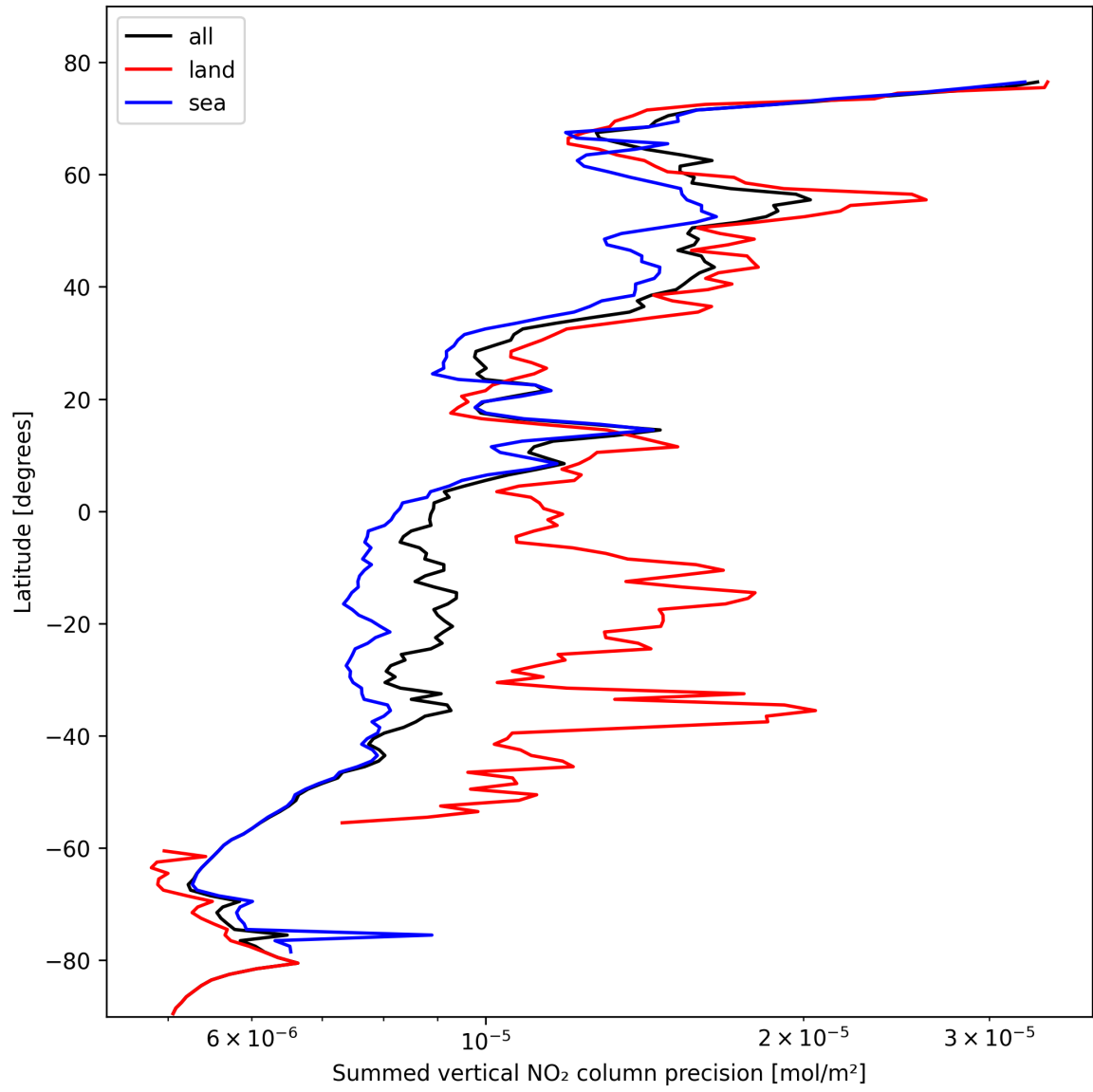
Figure 24: Zonal average of “Summed vertical NO 2 column precision” for 2024-10-22 to 2024-10-24.
