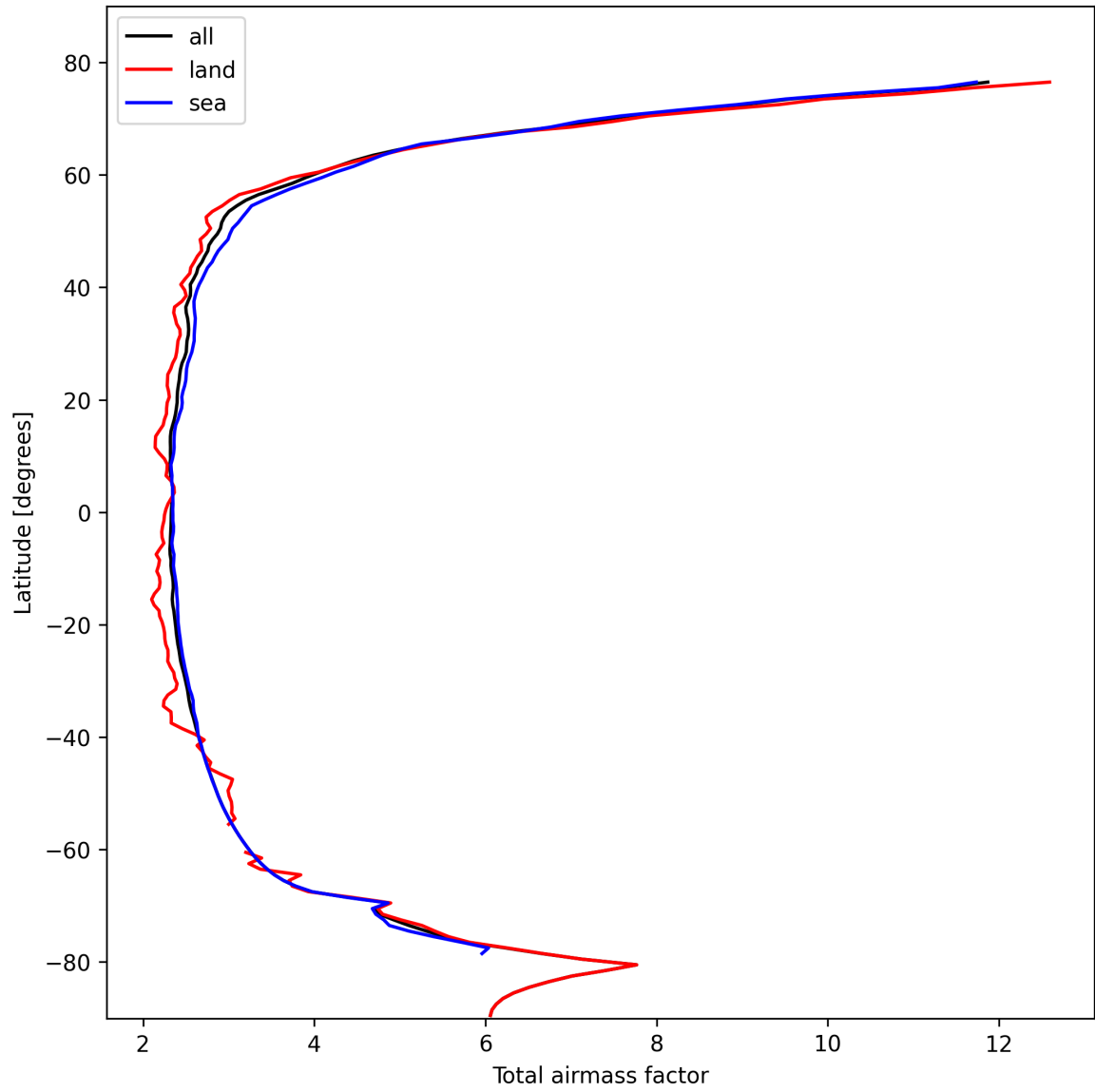
Figure 15: Zonal average of “Total airmass factor” for 2024-10-22 to 2024-10-24.
