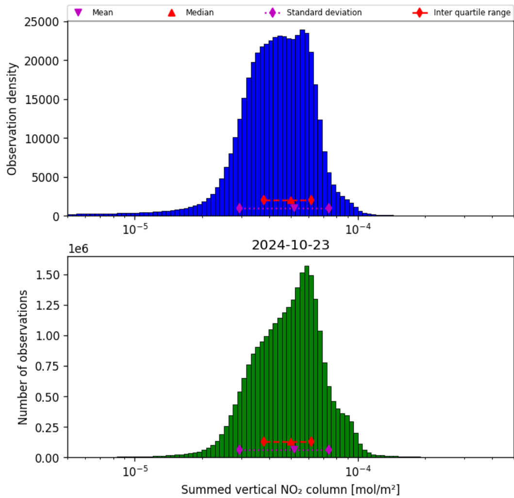
Figure 40: Histogram of “Summed vertical NO 2 column” for 2024-10-22 to 2024-10-24
