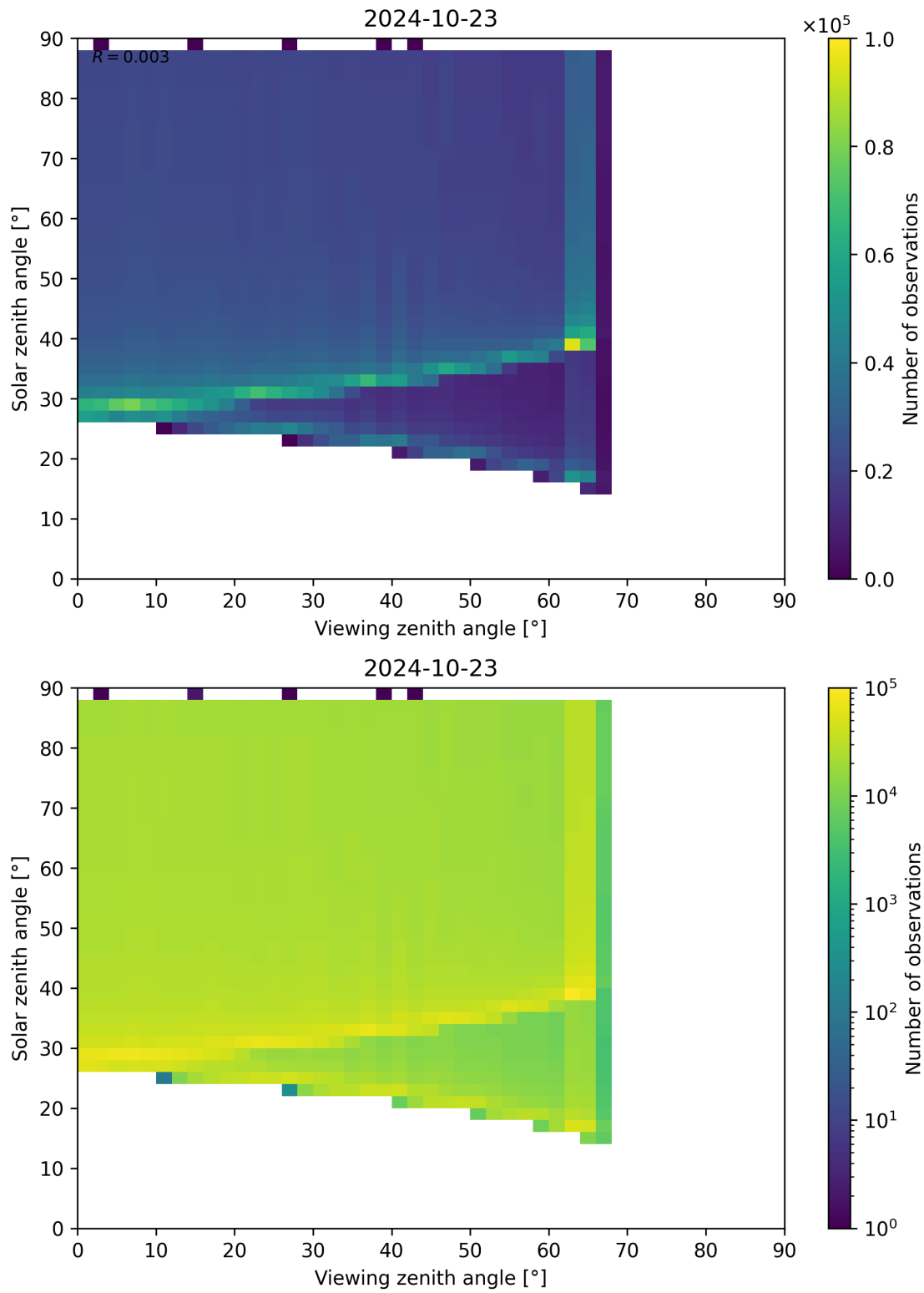
Figure 172: Scatter density plot of “Viewing zenith angle” against “Solar zenith angle” for 2024-10-22 to 2024-10-24.
