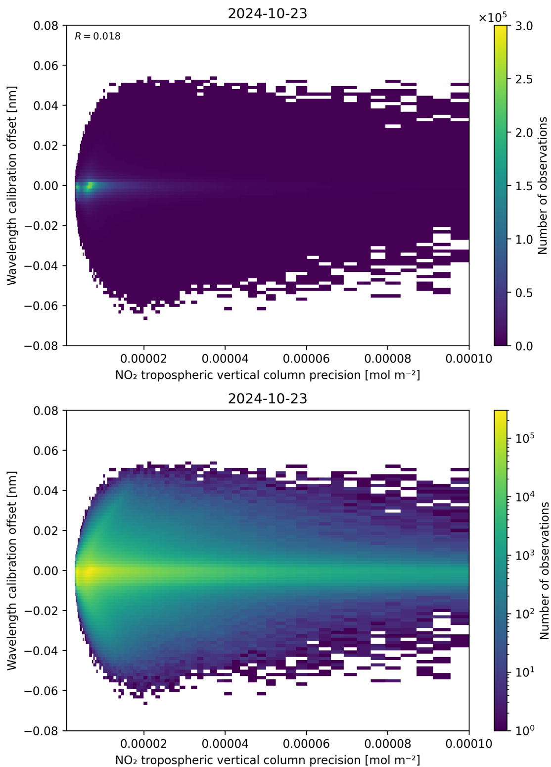
Figure 141: Scatter density plot of “NO 2 tropospheric vertical column precision” against “Wavelength calibration offset” for 2024-10-22 to 2024-10-24.
