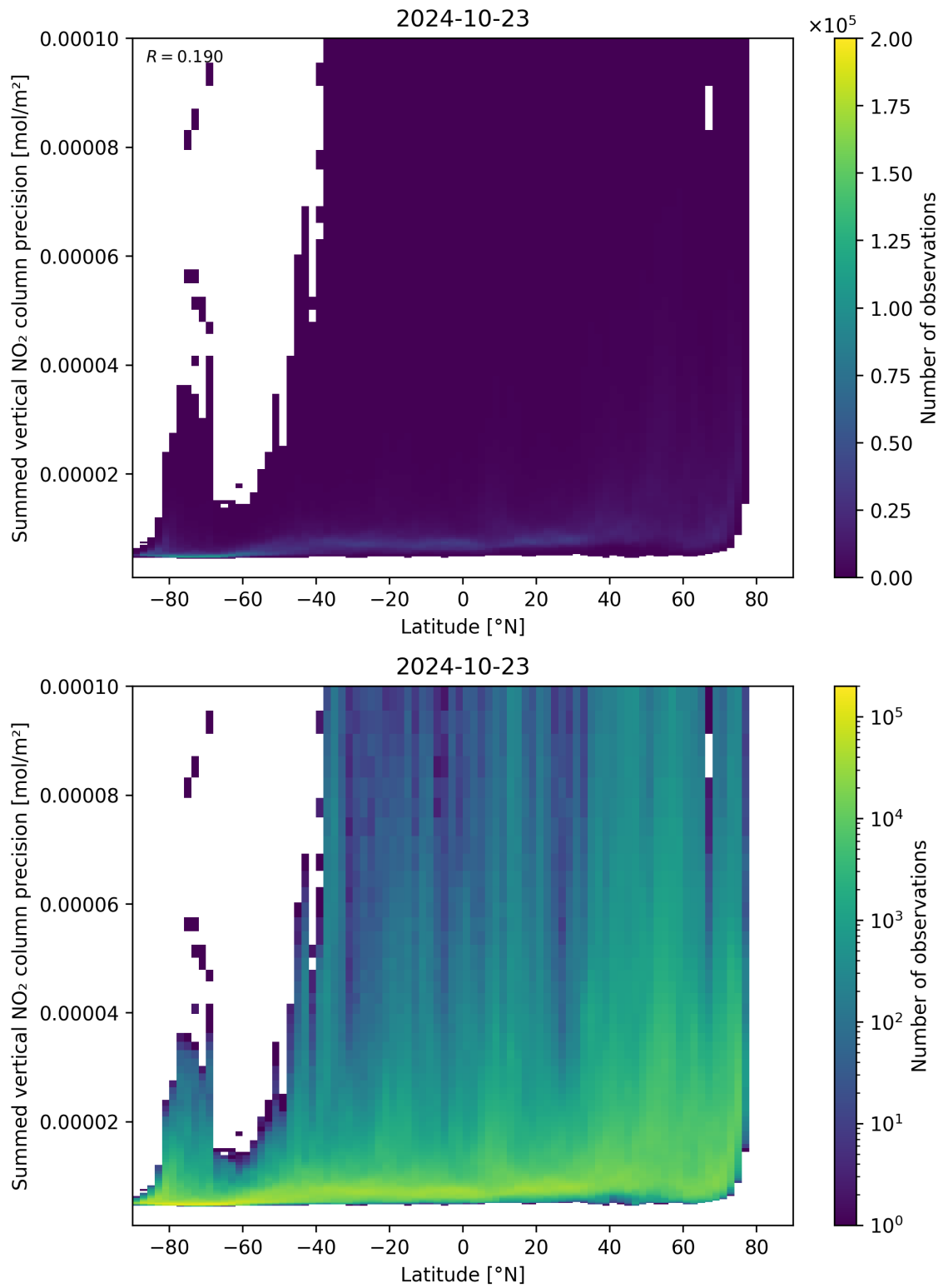
Figure 89: Scatter density plot of “Latitude” against “Summed vertical NO 2 column precision” for 2024-10-22 to 2024-10-24.
