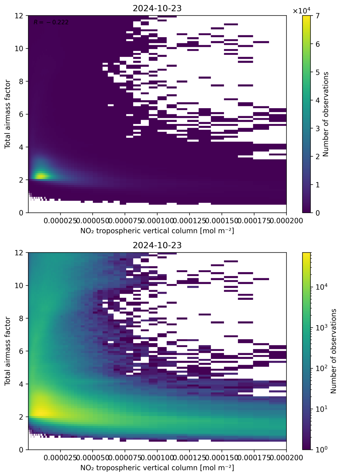
Figure 122: Scatter density plot of “NO 2 tropospheric vertical column” against “Total airmass factor” for 2024-10-22 to 2024-10-24.
