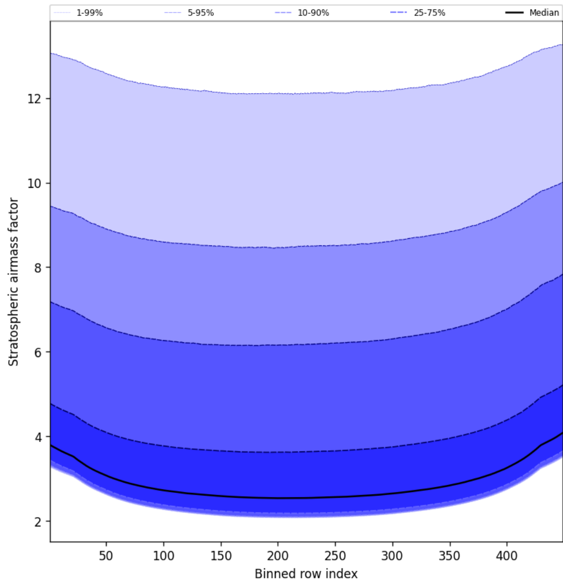
Figure 61: Along track statistics of “Stratospheric airmass factor” for 2024-10-22 to 2024-10-24
