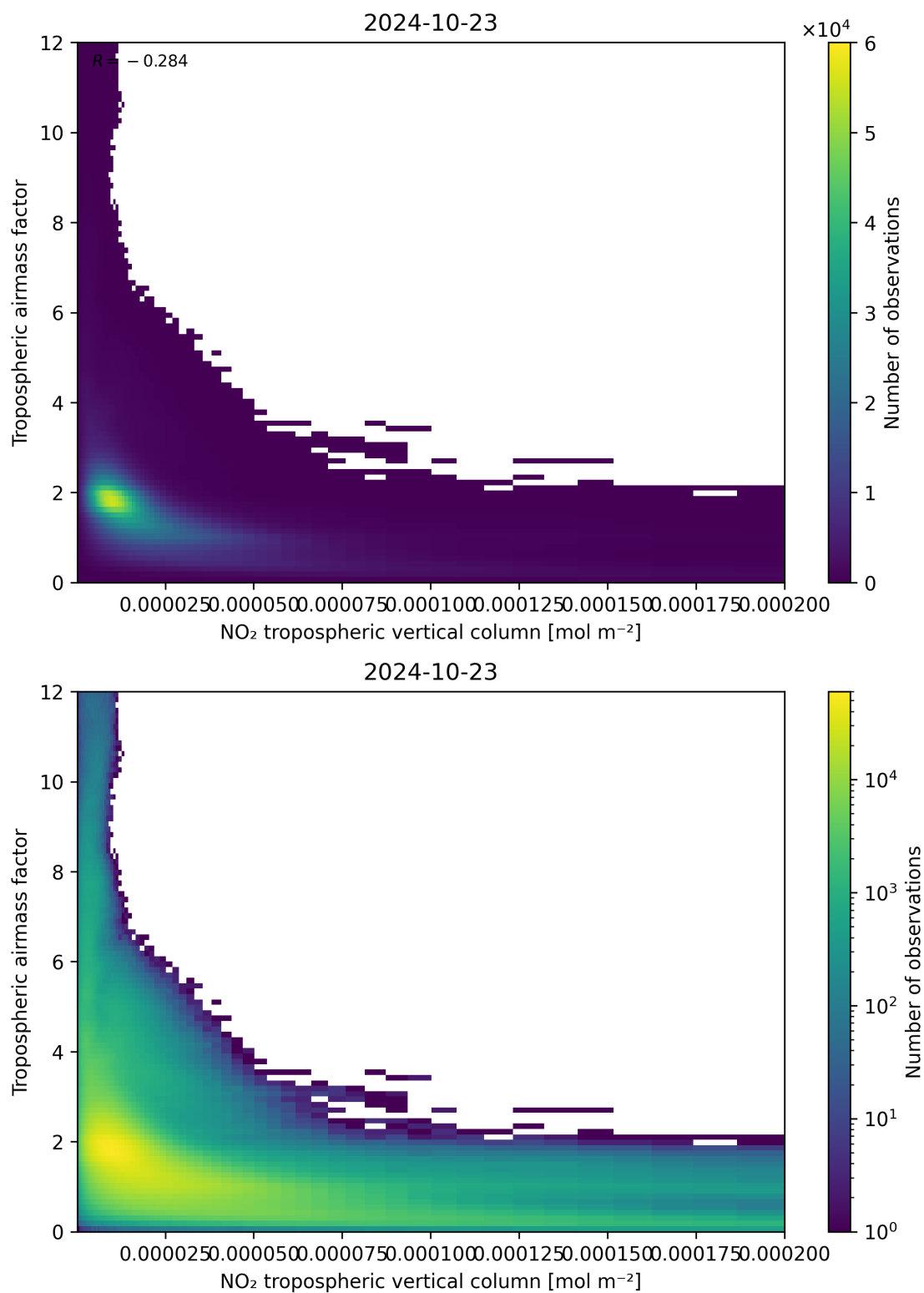
Figure 123: Scatter density plot of “NO 2 tropospheric vertical column” against “Tropospheric airmass factor” for 2024-10-22 to 2024-10-24.
