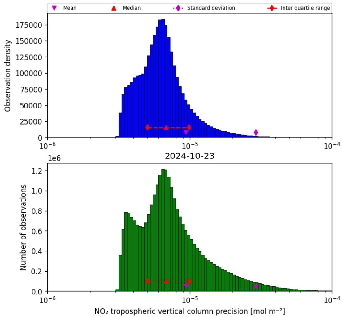
Figure 30: Histogram of “NO 2 tropospheric vertical column precision” for 2024-10-22 to 2024-10-24
