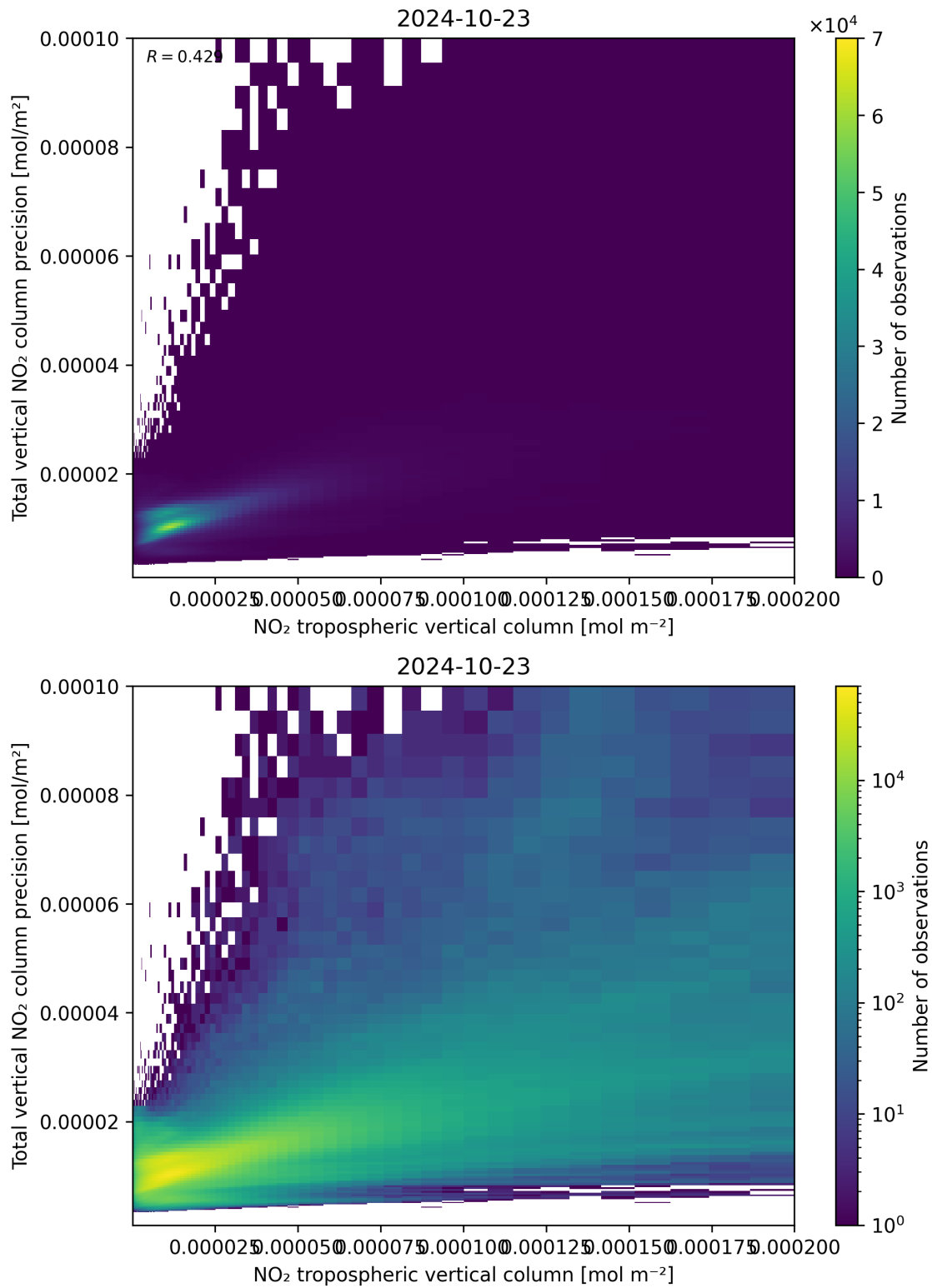
Figure 129: Scatter density plot of “NO 2 tropospheric vertical column” against “Total vertical NO 2 column precision” for 2024-10-22 to 2024-10-24.
