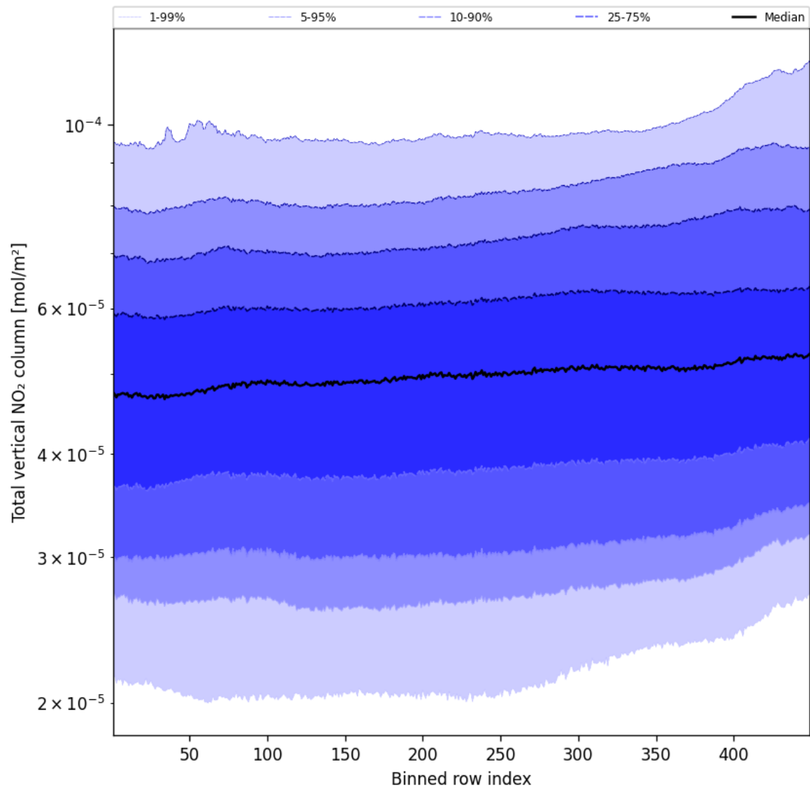
Figure 55: Along track statistics of “Total vertical NO 2 column” for 2024-10-22 to 2024-10-24
