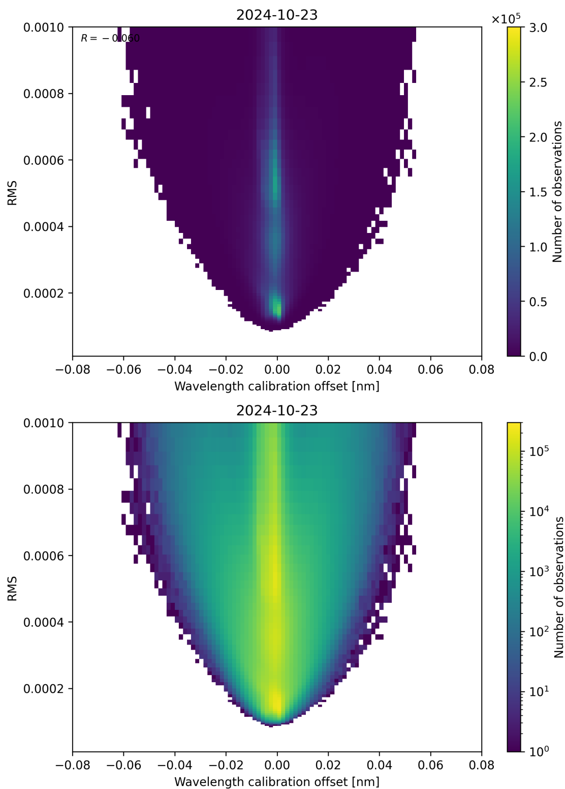
Figure 181: Scatter density plot of “Wavelength calibration offset” against “RMS” for 2024-10-22 to 2024-10-24.
