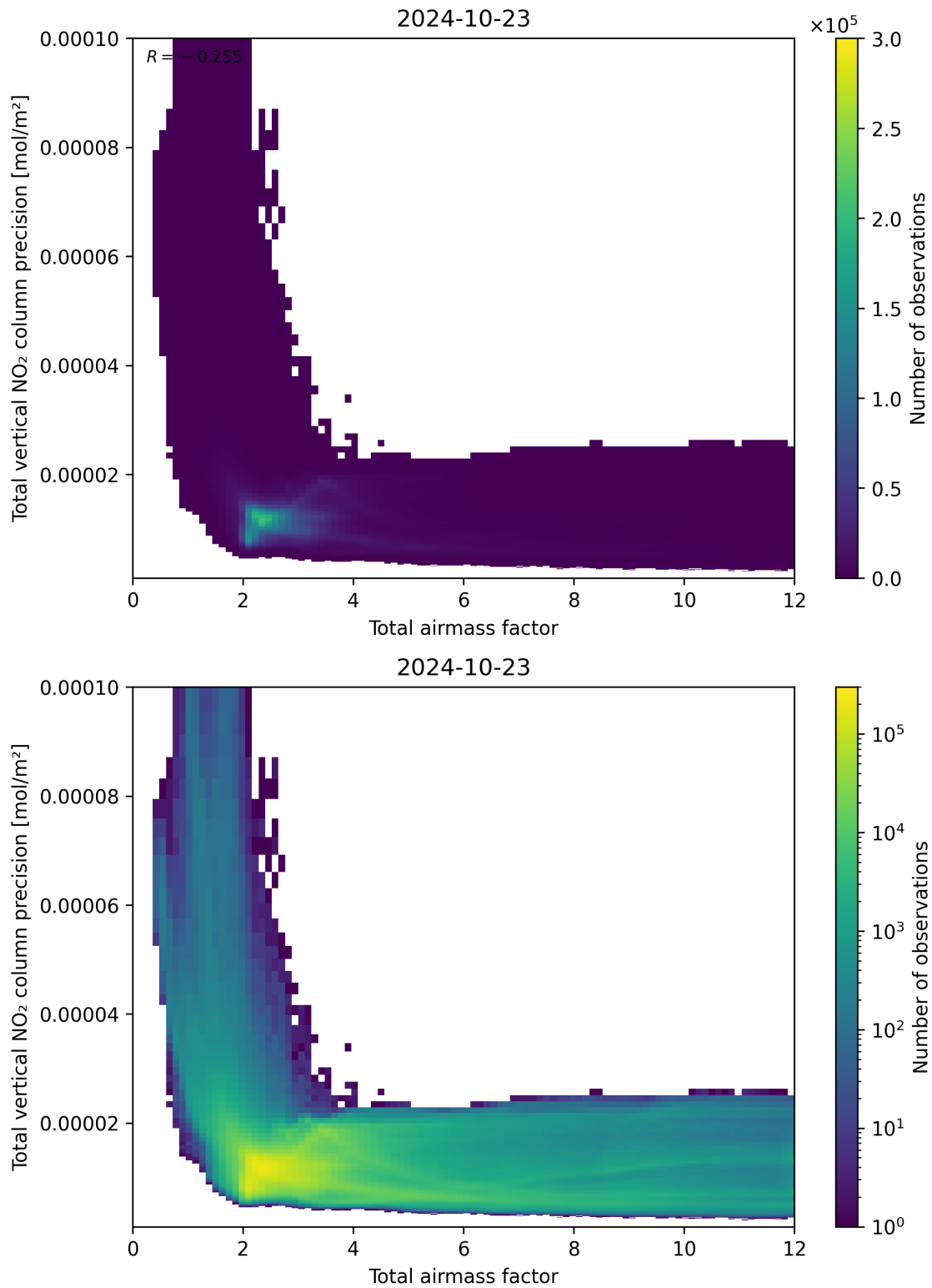
Figure 68: Scatter density plot of “Total airmass factor” against “Total vertical NO 2 column precision” for 2024-10-22 to 2024-10-24.
