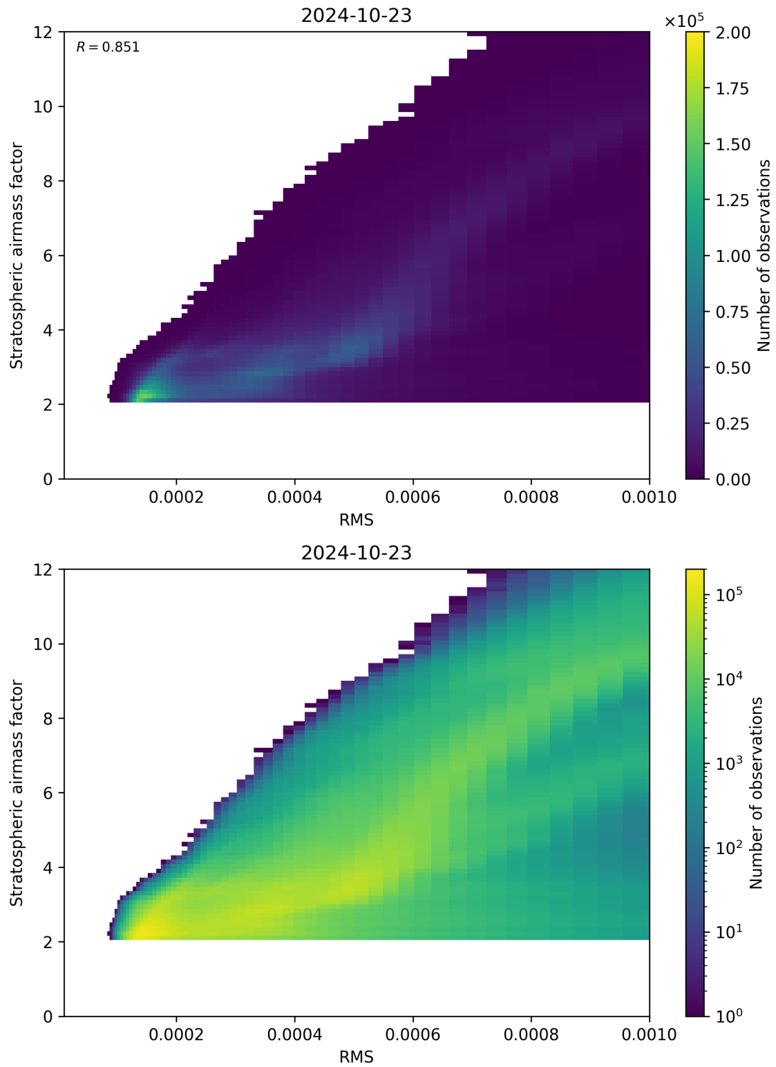
Figure 144: Scatter density plot of “RMS” against “Stratospheric airmass factor” for 2024-10-22 to 2024-10-24.
