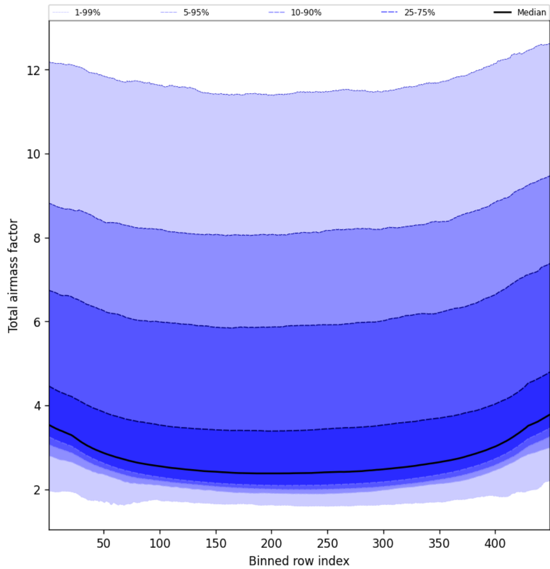
Figure 49: Along track statistics of “Total airmass factor” for 2024-10-22 to 2024-10-24
