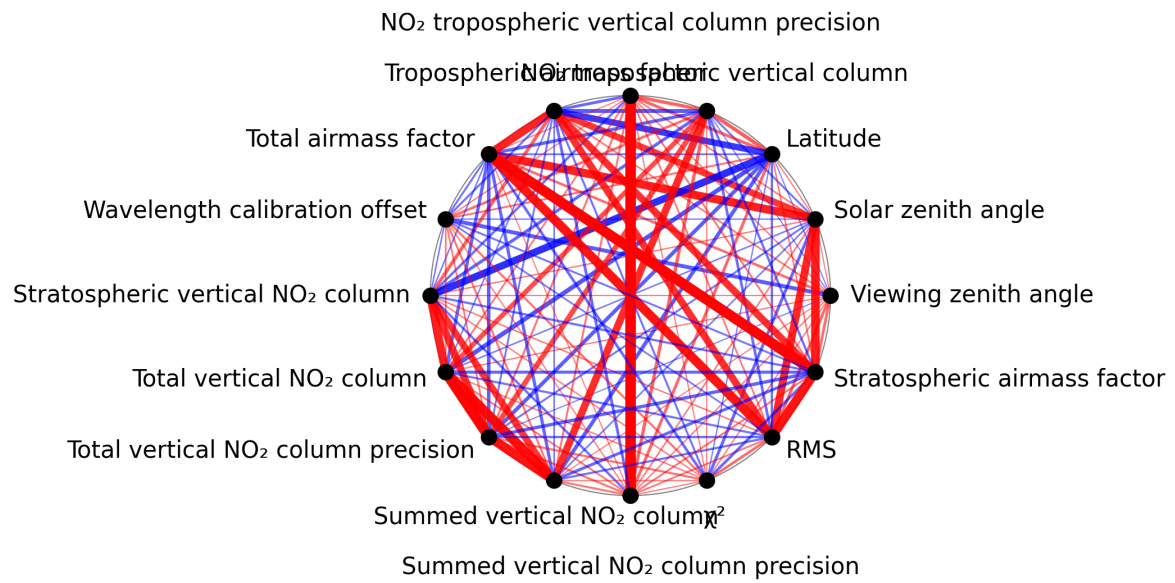
Figure 1: Map of correlation graph for 2024-10-22 to 2024-10-24.
