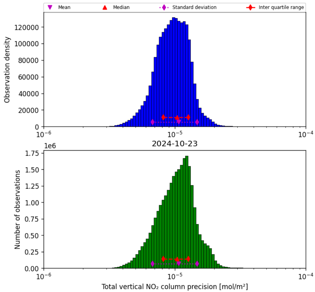
Figure 39: Histogram of “Total vertical NO 2 column precision” for 2024-10-22 to 2024-10-24
