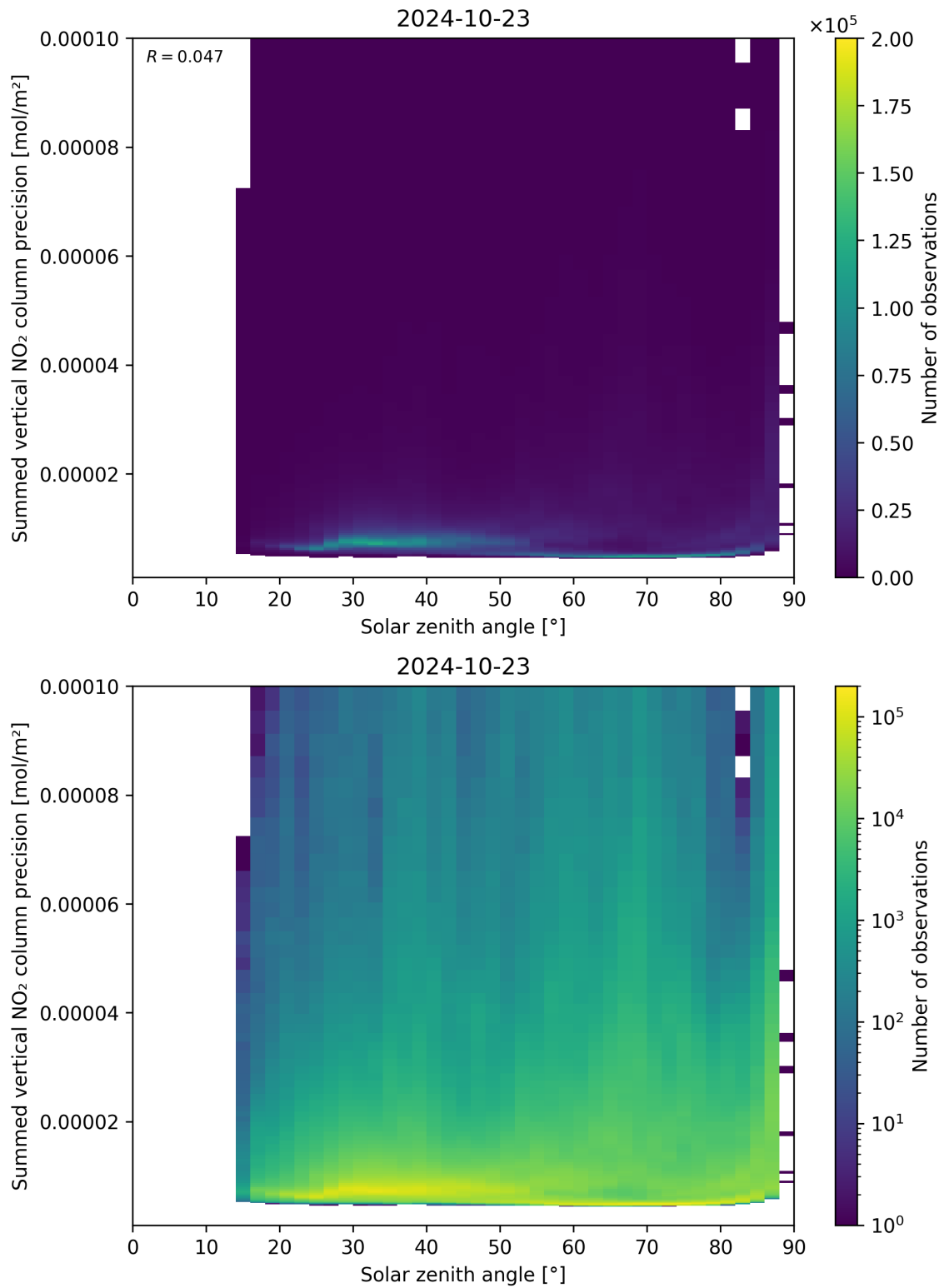
Figure 152: Scatter density plot of “Solar zenith angle” against “Summed vertical NO 2 column precision” for 2024-10-22 to 2024-10-24.
