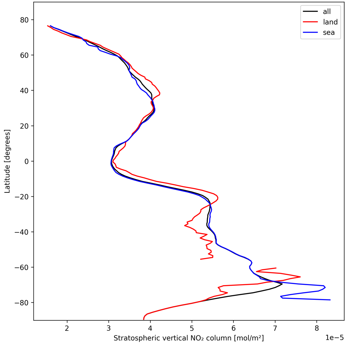
Figure 19: Zonal average of “Stratospheric vertical NO 2 column” for 2024-10-22 to 2024-10-24.
