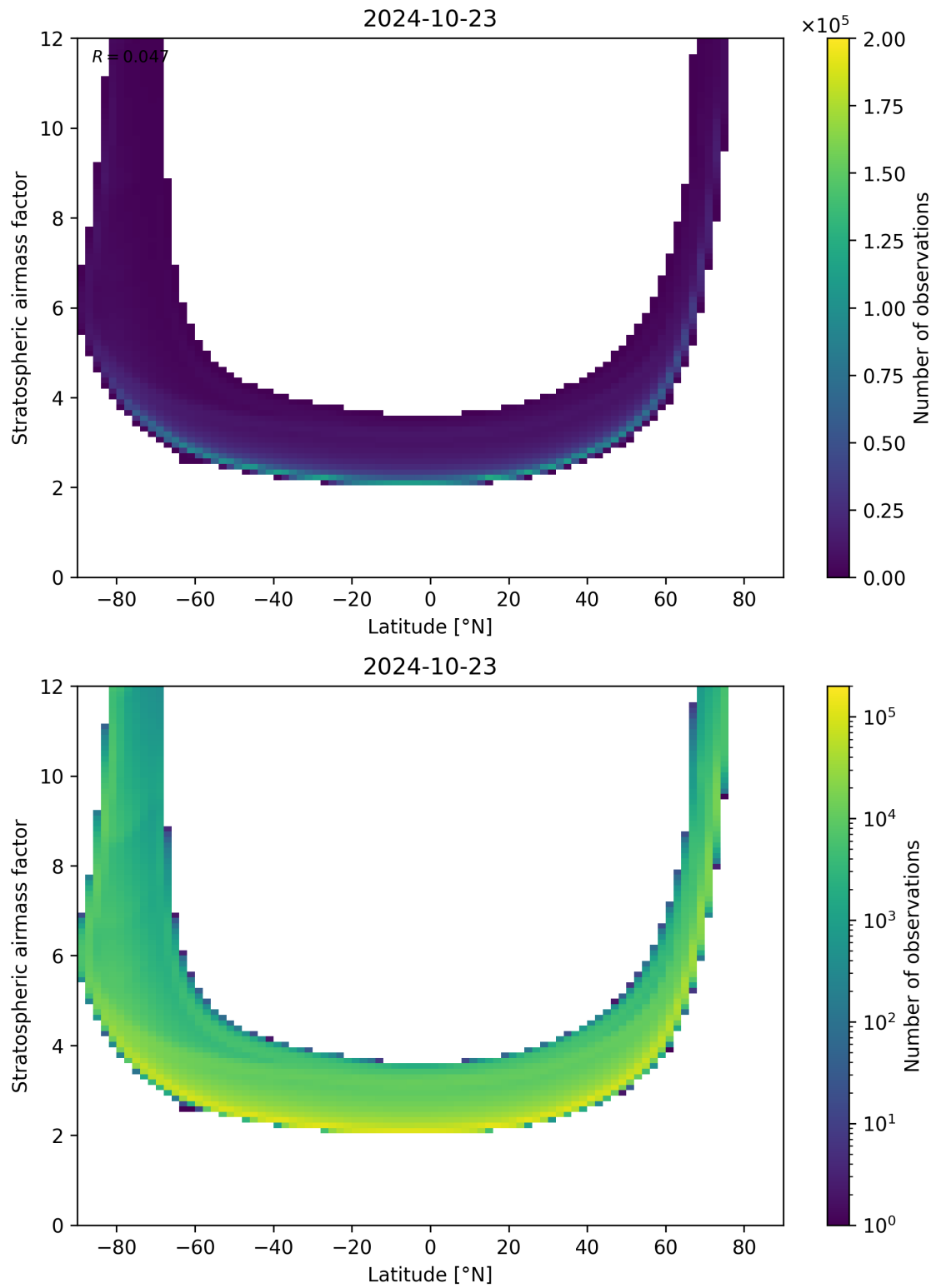
Figure 83: Scatter density plot of “Latitude” against “Stratospheric airmass factor” for 2024-10-22 to 2024-10-24.
