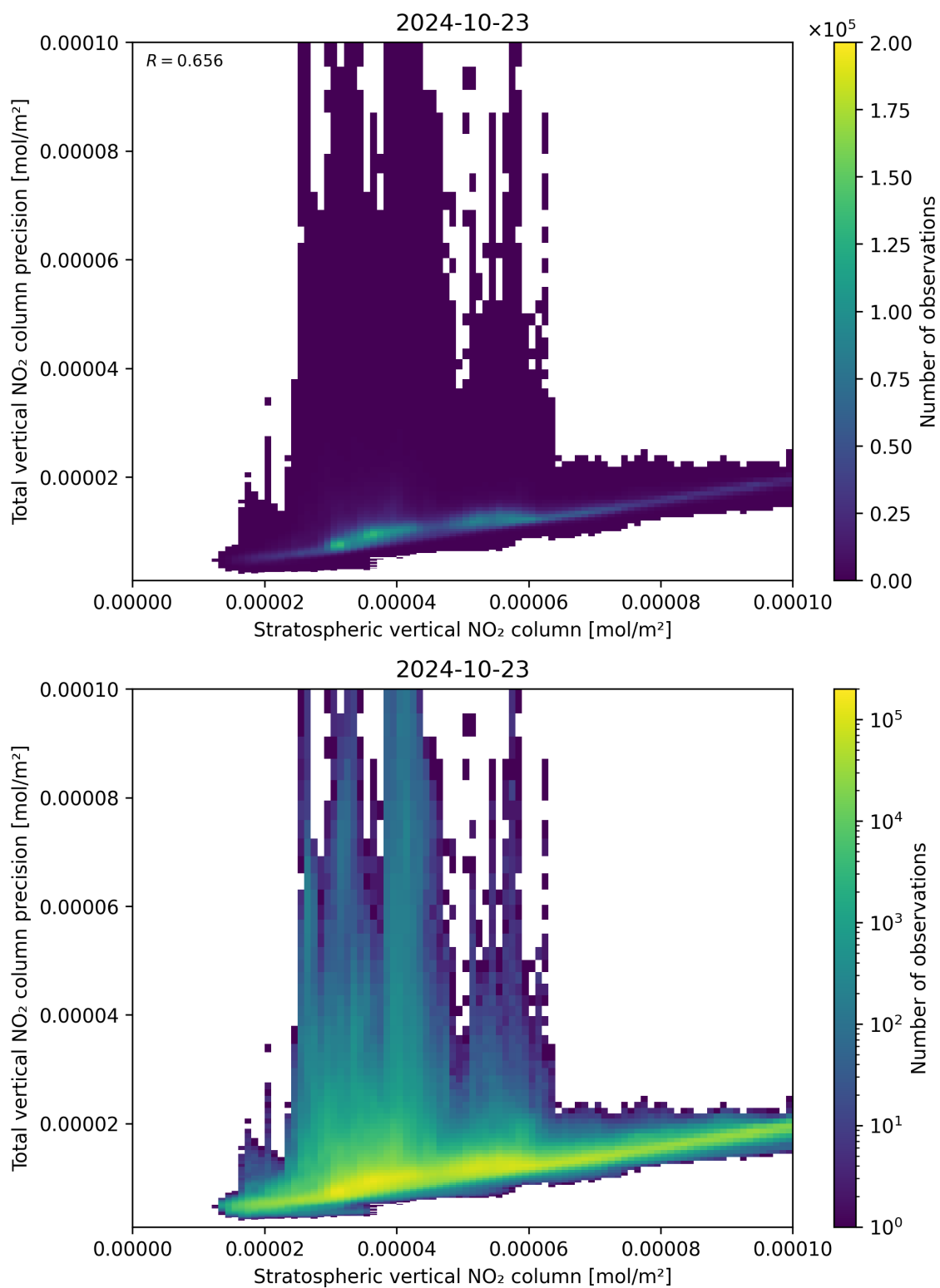
Figure 101: Scatter density plot of “Stratospheric vertical NO 2 column” against “Total vertical NO 2 column precision” for 2024-10-22 to 2024-10-24.
