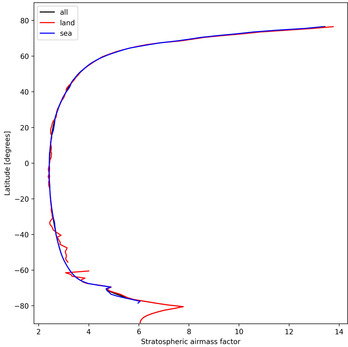
Figure 27: Zonal average of “Stratospheric air mass factor” for 2024-10-22 to 2024-10-24.
