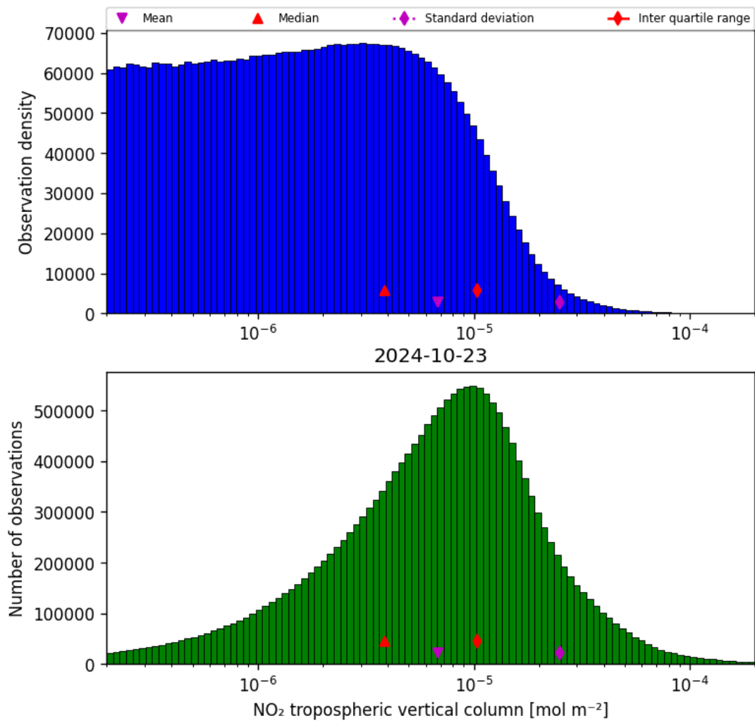
Figure 29: Histogram of “NO 2 tropospheric vertical column” for 2024-10-22 to 2024-10-24
