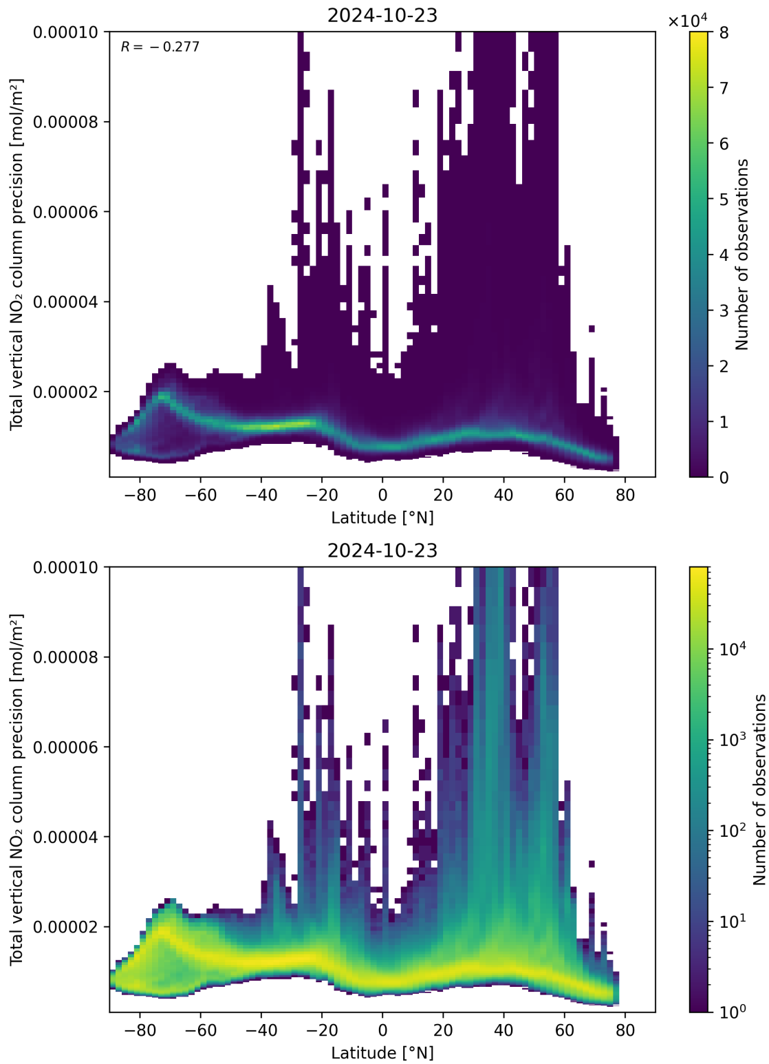
Figure 91: Scatter density plot of “Latitude” against “Total vertical NO 2 column precision” for 2024-10-22 to 2024-10-24.
