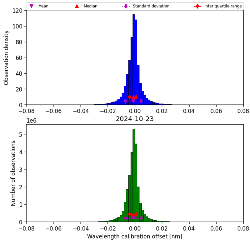
Figure 35: Histogram of “Wavelength calibration offset” for 2024-10-22 to 2024-10-24
