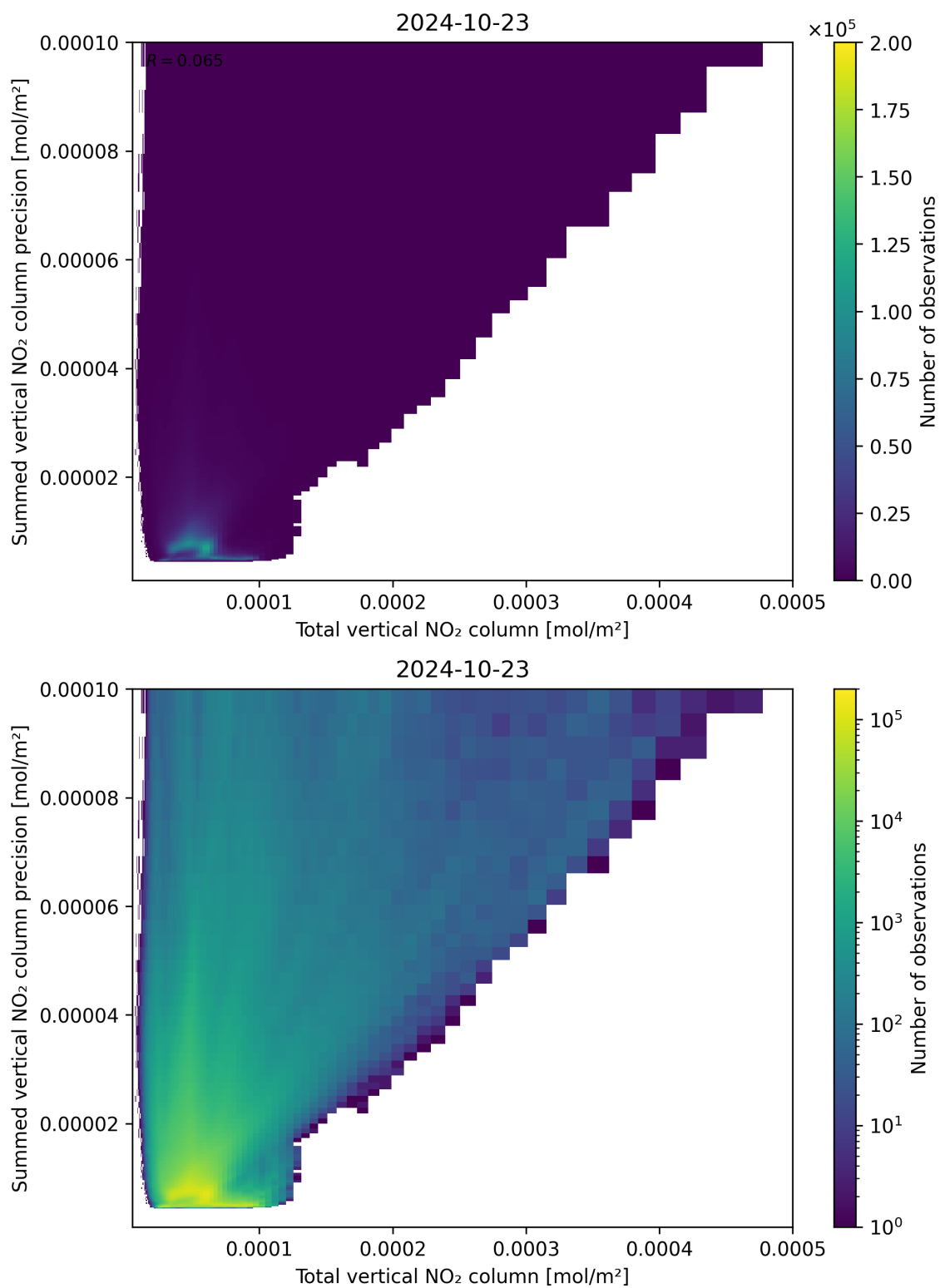
Figure 113: Scatter density plot of “Total vertical NO 2 column” against “Summed vertical NO 2 column precision” for 2024-10-22 to 2024-10-24.
