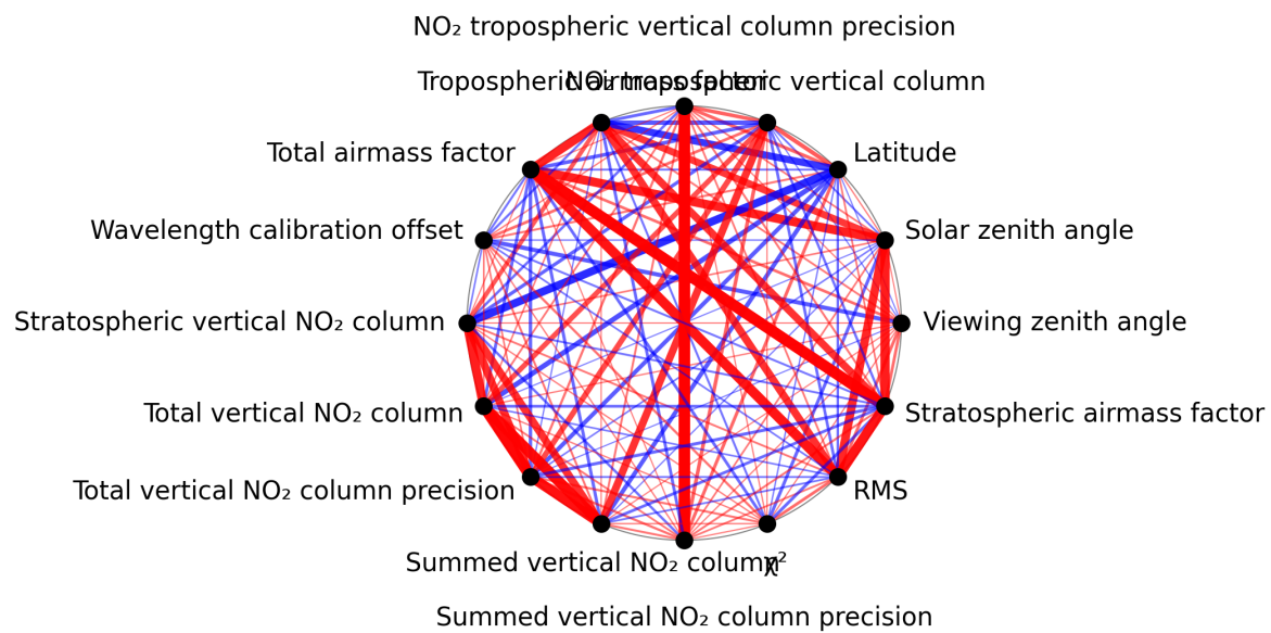
Figure 1: Map of correlation graph for 2024-10-24 to 2024-10-26.
