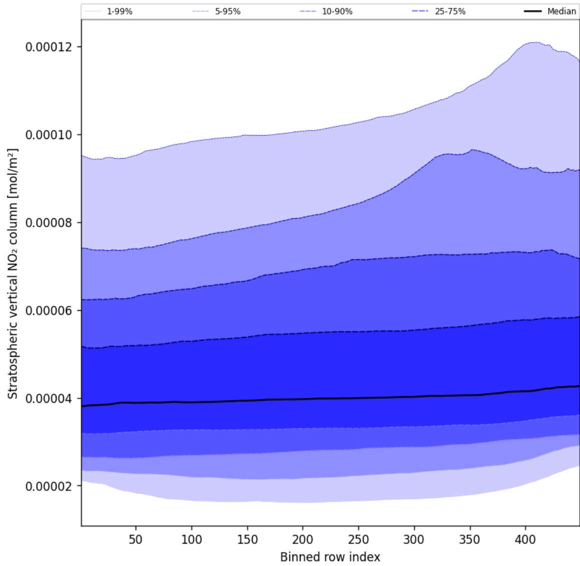
Figure 53: Along track statistics of “Stratospheric vertical NO 2 column” for 2024-10-24 to 2024-10-26
