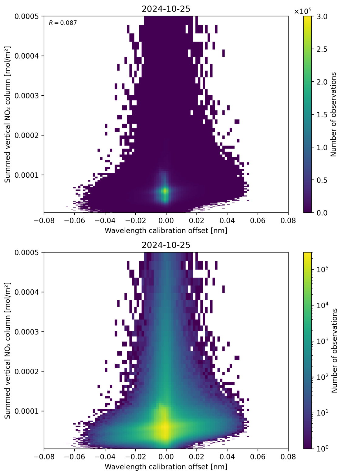
Figure 177: Scatter density plot of “Wavelength calibration offset” against “Summed vertical NO 2 column” for 2024-10-24 to 2024-10-26.
