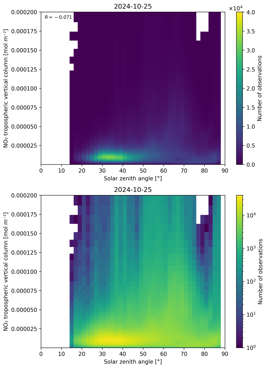
Figure 155: Scatter density plot of “Solar zenith angle” against “NO 2 tropospheric vertical column” for 2024-10-24 to 2024-10-26.
