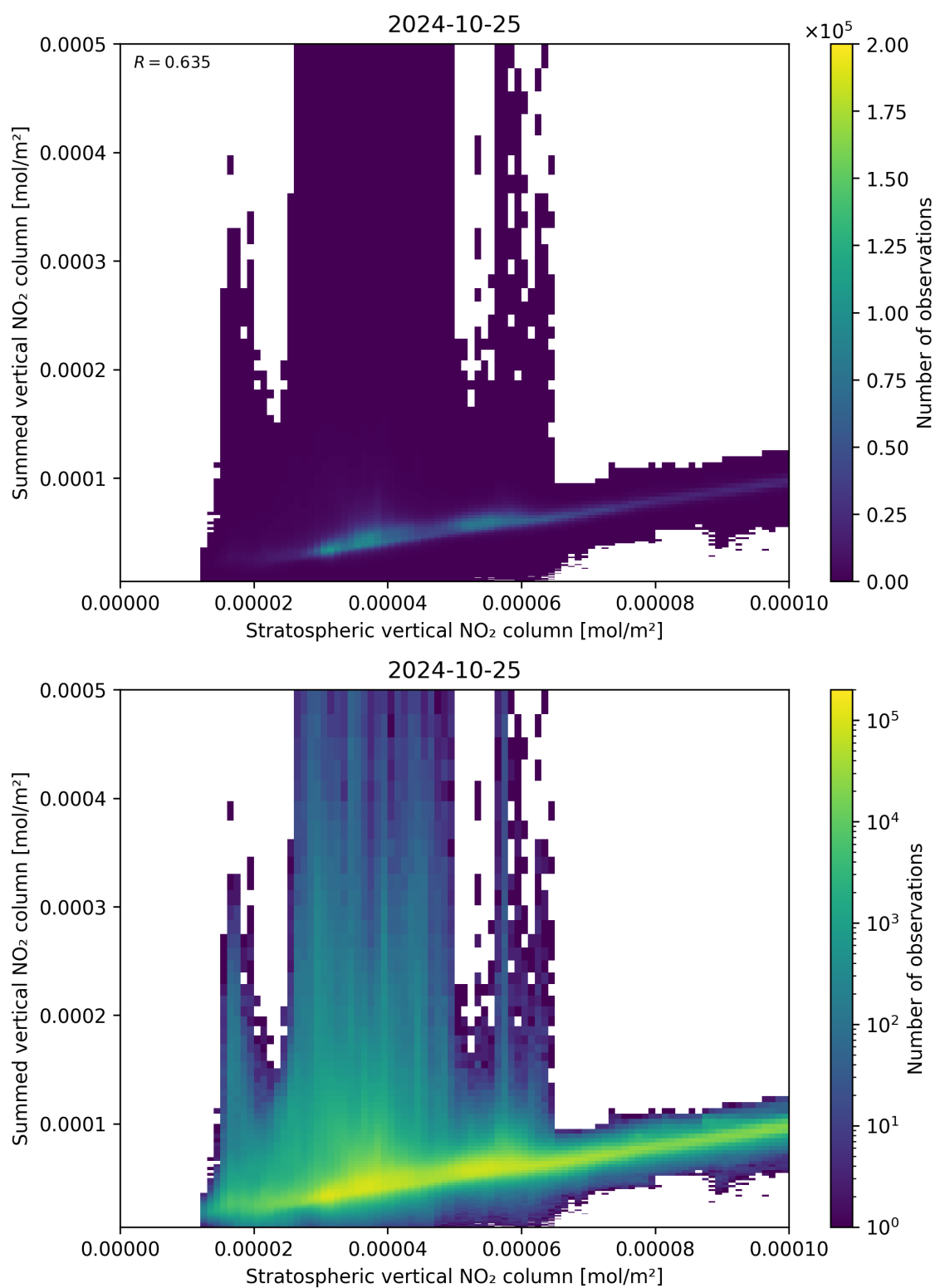
Figure 98: Scatter density plot of “Stratospheric vertical NO 2 column” against “Summed vertical NO 2 column” for 2024-10-24 to 2024-10-26.
