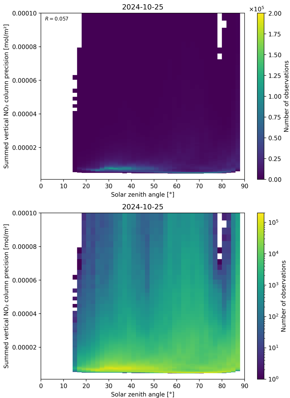
Figure 152: Scatter density plot of “Solar zenith angle” against “Summed vertical NO 2 column precision” for 2024-10-24 to 2024-10-26.
