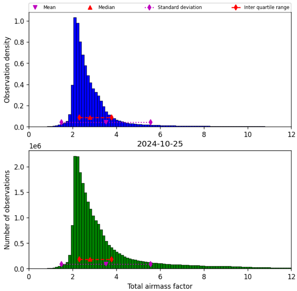
Figure 32: Histogram of “Total airmass factor” for 2024-10-24 to 2024-10-26
