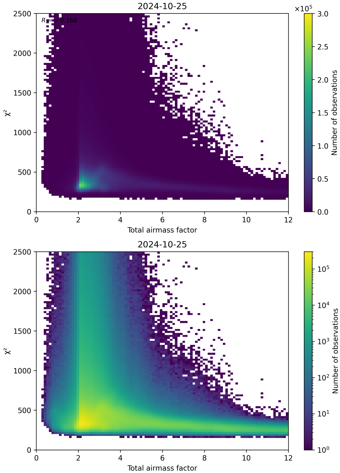
Figure 63: Scatter density plot of “Total airmass factor” against “ \chi^2 ” for 2024-10-24 to 2024-10-26.
