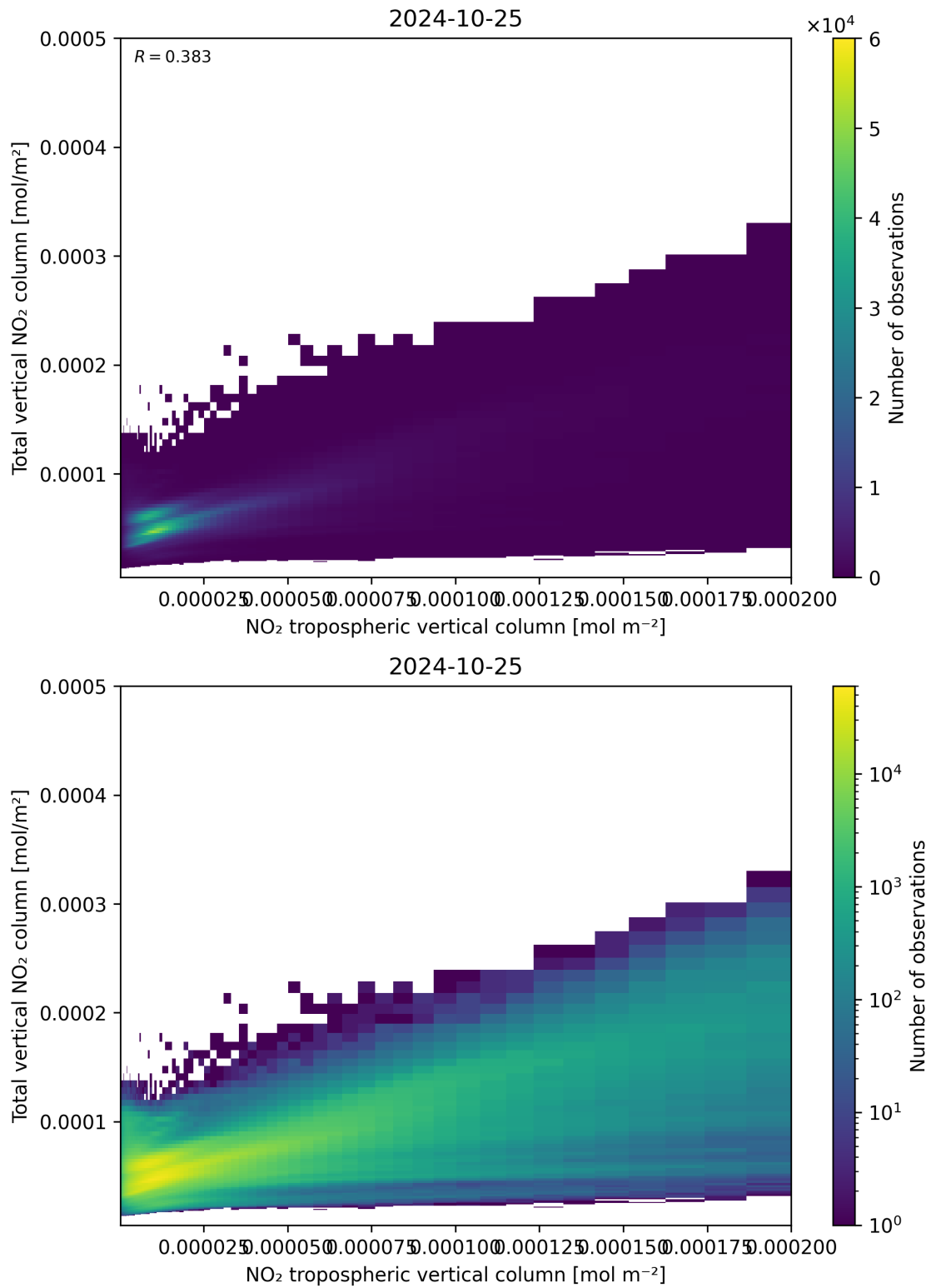
Figure 128: Scatter density plot of “NO 2 tropospheric vertical column” against “Total vertical NO 2 column” for 2024-10-24 to 2024-10-26.
