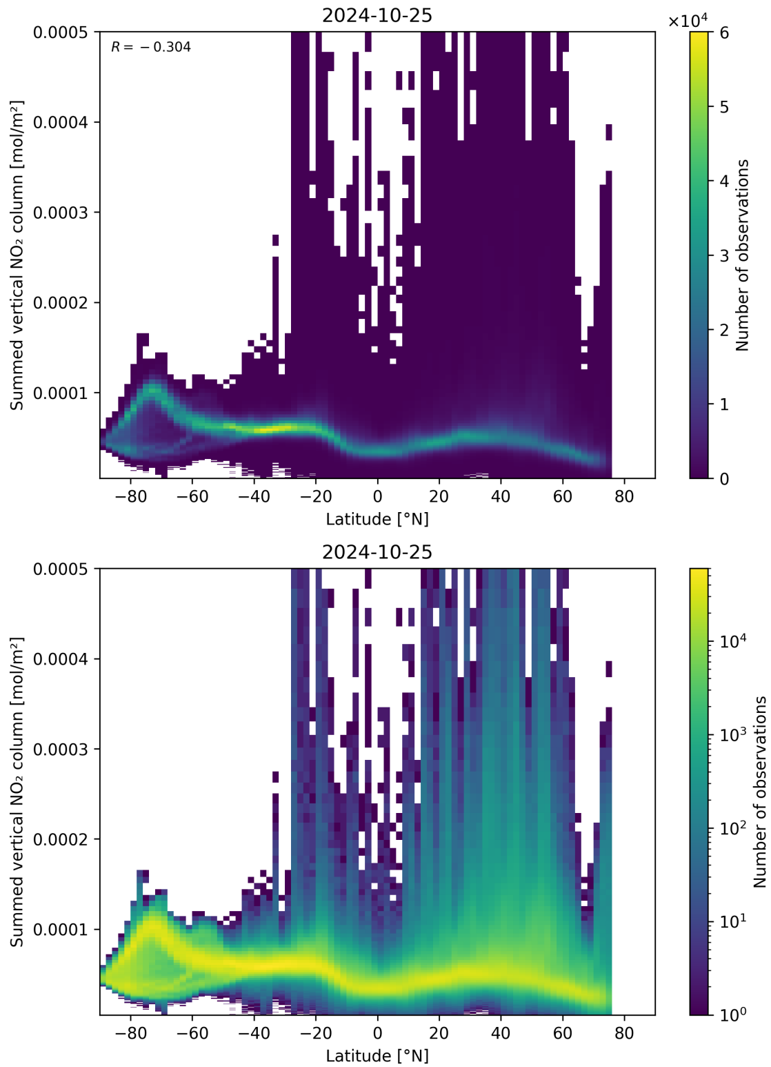
Figure 88: Scatter density plot of “Latitude” against “Summed vertical NO 2 column” for 2024-10-24 to 2024-10-26.
