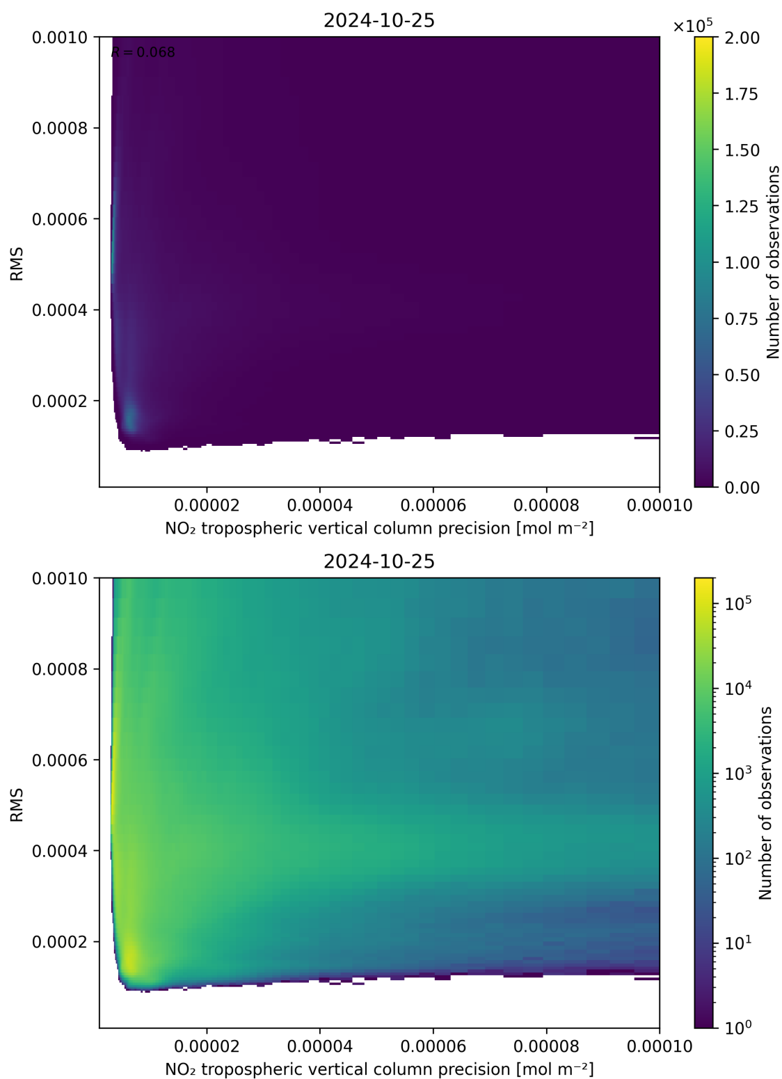
Figure 140: Scatter density plot of “NO 2 tropospheric vertical column precision” against “RMS” for 2024-10-24 to 2024-10-26.
