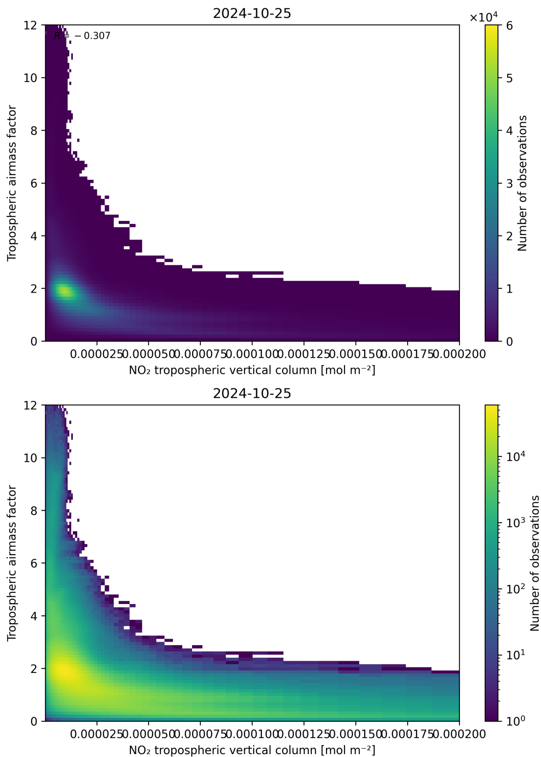
Figure 123: Scatter density plot of “NO 2 tropospheric vertical column” against “Tropospheric air mass factor” for 2024-10-24 to 2024-10-26.
