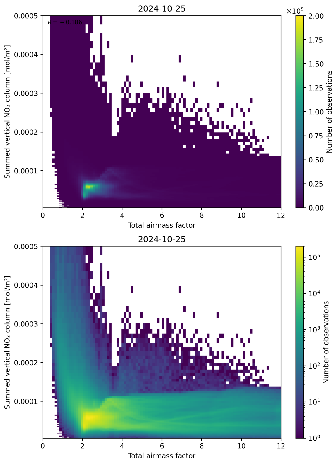
Figure 65: Scatter density plot of “Total airmass factor” against “Summed vertical NO 2 column” for 2024-10-24 to 2024-10-26.
