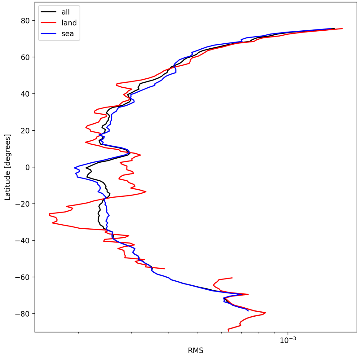
Figure 26: Zonal average of “RMS” for 2024-10-24 to 2024-10-26.
