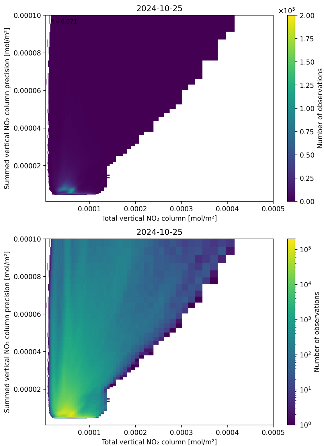
Figure 113: Scatter density plot of “Total vertical NO 2 column” against “Summed vertical NO 2 column precision” for 2024-10-24 to 2024-10-26.
