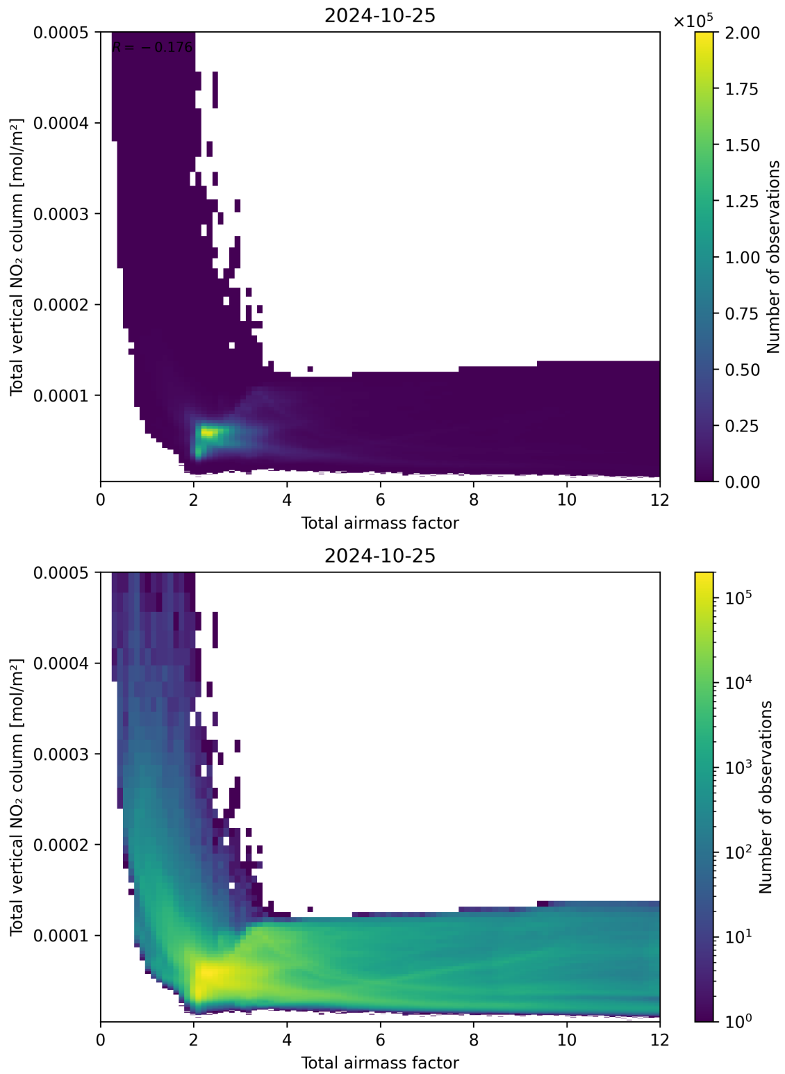
Figure 67: Scatter density plot of “Total airmass factor” against “Total vertical NO 2 column” for 2024-10-24 to 2024-10-26.
