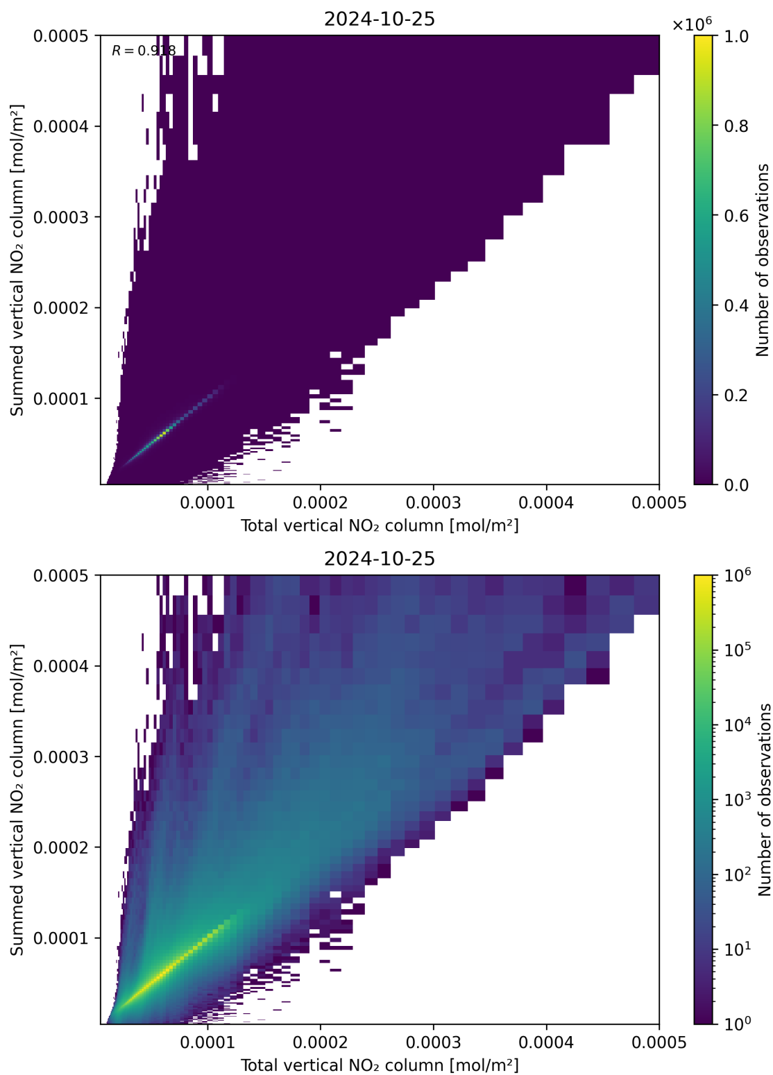
Figure 112: Scatter density plot of “Total vertical NO 2 column” against “Summed vertical NO 2 column” for 2024-10-24 to 2024-10-26.
