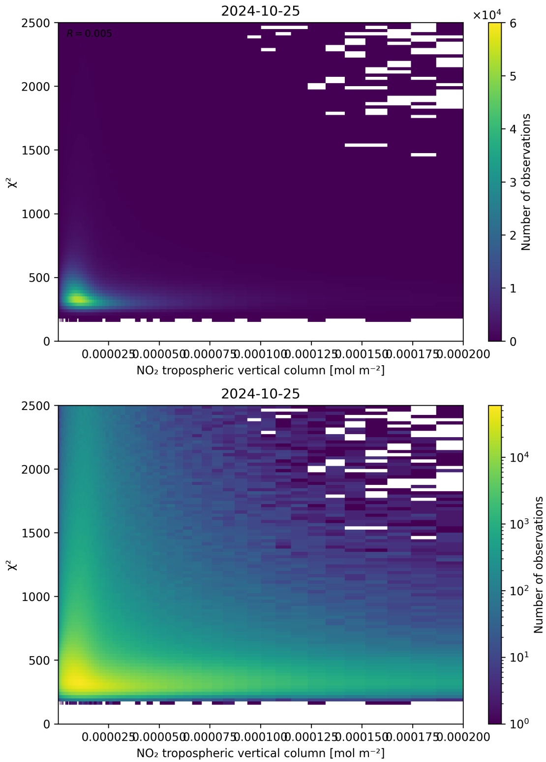
Figure 124: Scatter density plot of “NO 2 tropospheric vertical column” against “ \chi^2 ” for 2024-10-24 to 2024-10-26.
