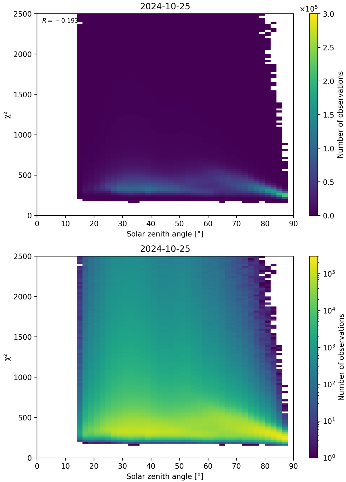
Figure 148: Scatter density plot of “Solar zenith angle” against “ \chi^2 ” for 2024-10-24 to 2024-10-26.
