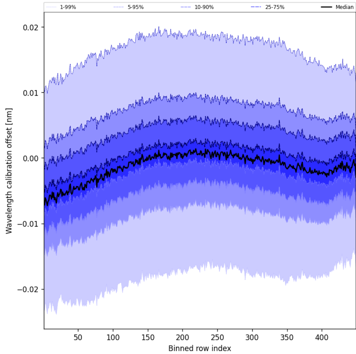
Figure 52: Along track statistics of “Wavelength calibration offset” for 2024-10-24 to 2024-10-26
