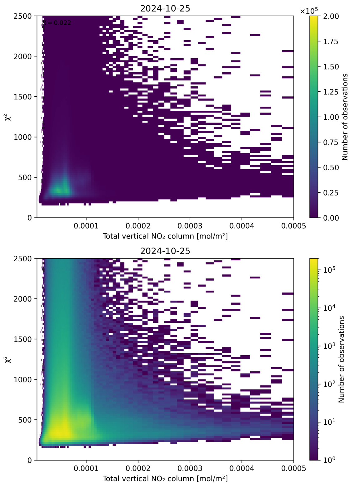
Figure 111: Scatter density plot of “Total vertical NO 2 column” against “ \chi^2 ” for 2024-10-24 to 2024-10-26.
