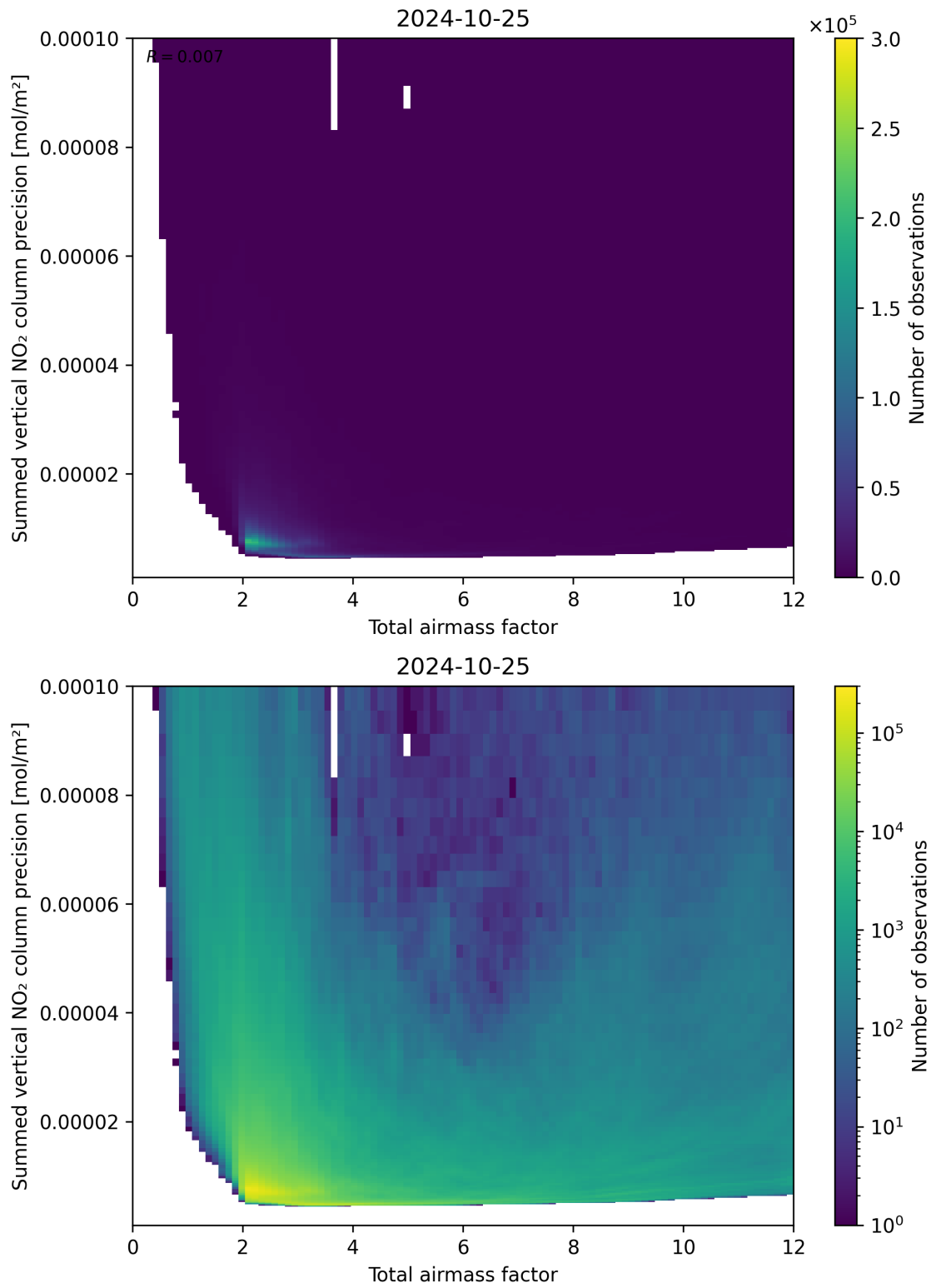
Figure 66: Scatter density plot of “Total airmass factor” against “Summed vertical NO 2 column precision” for 2024-10-24 to 2024-10-26.
