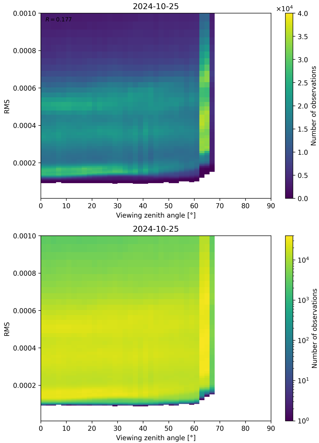
Figure 171: Scatter density plot of “Viewing zenith angle” against “RMS” for 2024-10-24 to 2024-10-26.
