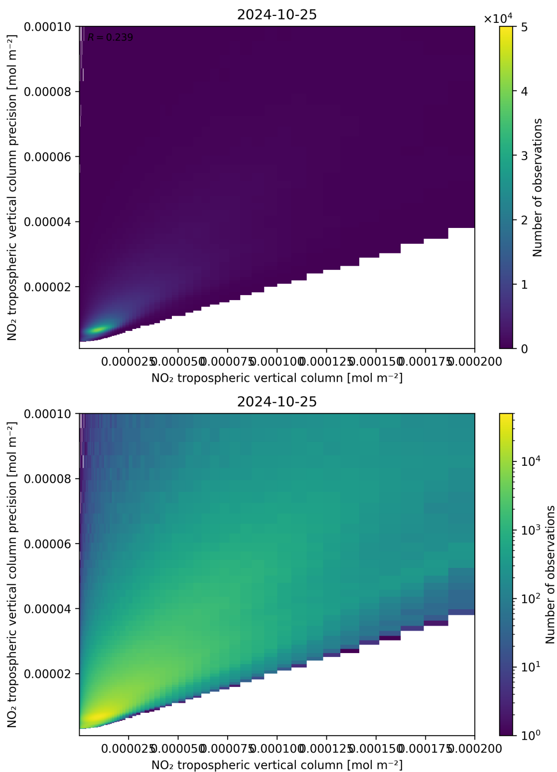
Figure 130: Scatter density plot of “NO 2 tropospheric vertical column” against “NO 2 tropospheric vertical column precision” for 2024-10-24 to 2024-10-26.
