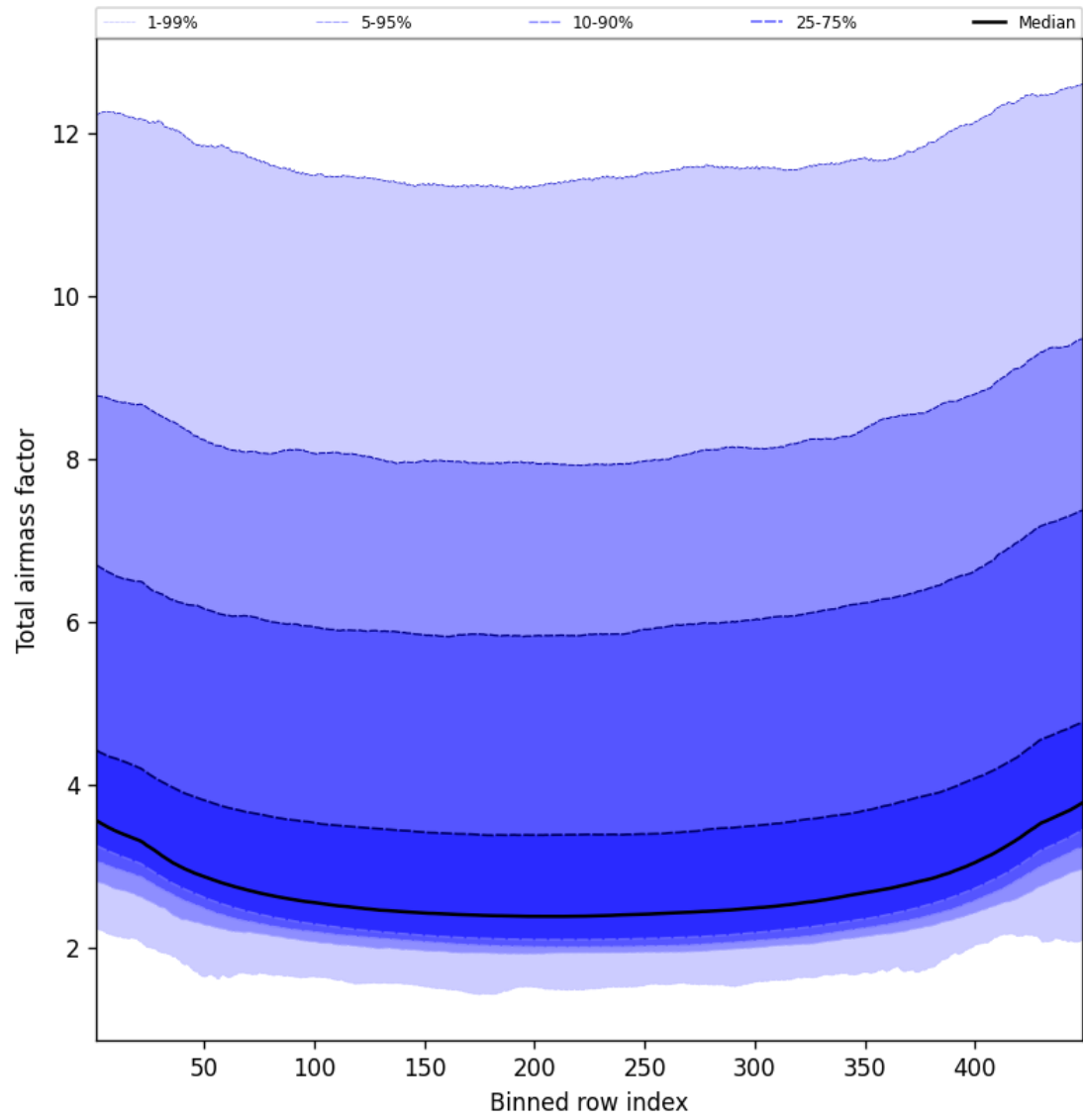
Figure 49: Along track statistics of “Total airmass factor” for 2024-10-24 to 2024-10-26
