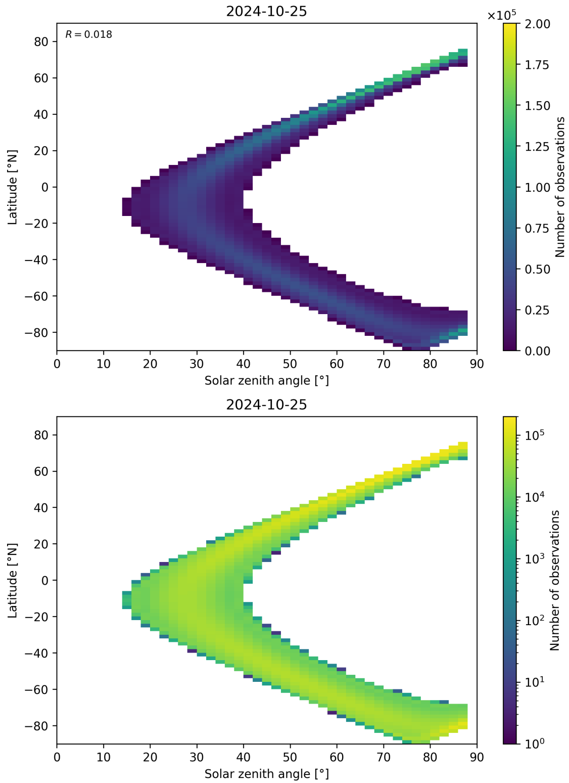
Figure 149: Scatter density plot of “Solar zenith angle” against “Latitude” for 2024-10-24 to 2024-10-26.
