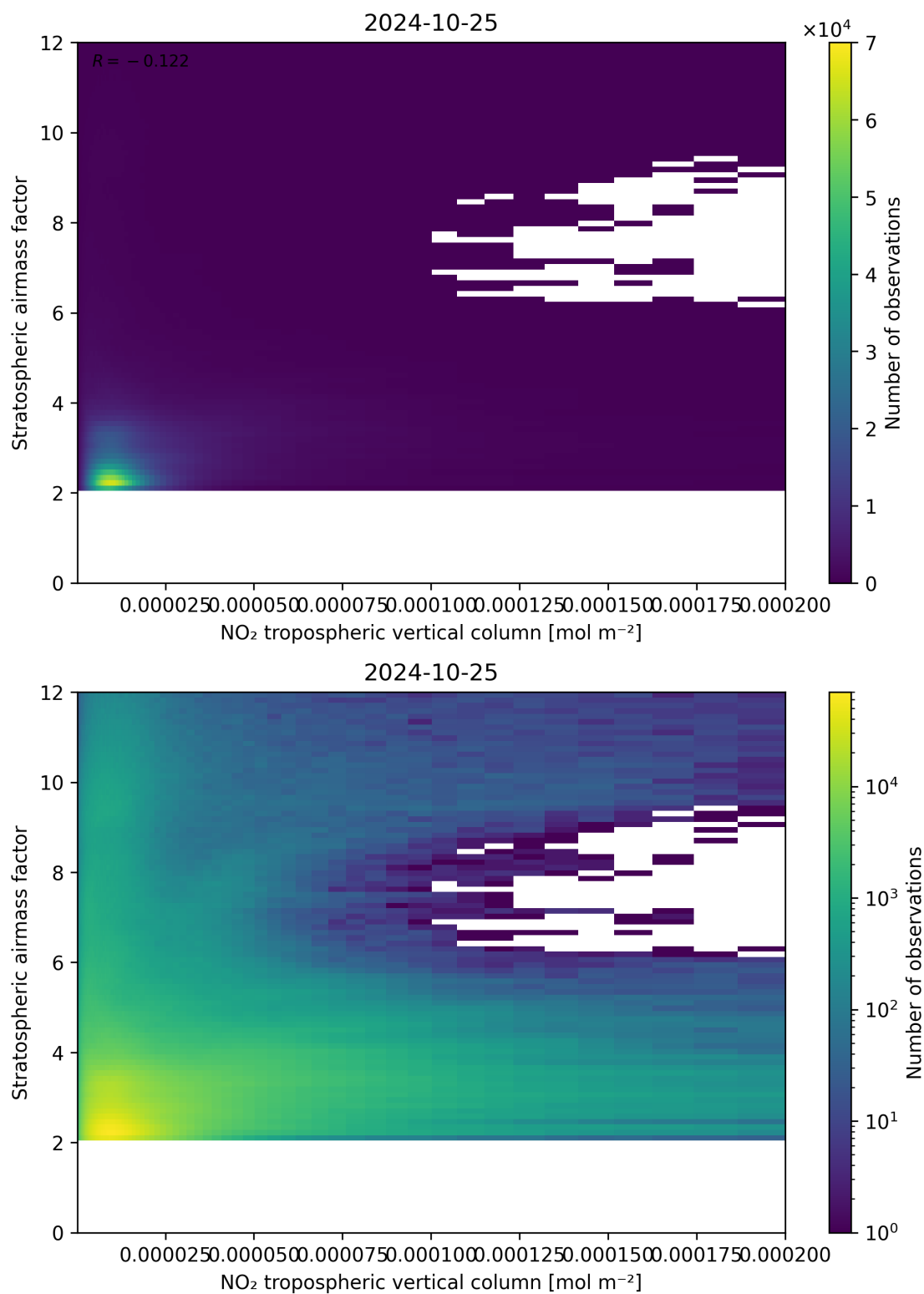
Figure 121: Scatter density plot of “NO 2 tropospheric vertical column” against “Stratospheric air mass factor” for 2024-10-24 to 2024-10-26.
