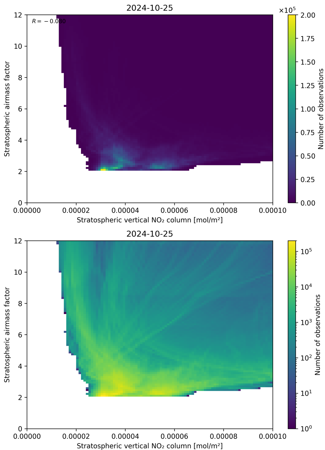
Figure 96: Scatter density plot of “Stratospheric vertical NO 2 column” against “Stratospheric airmass factor” for 2024-10-24 to 2024-10-26.
