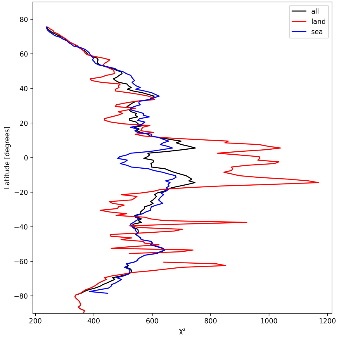
Figure 25: Zonal average of “ \chi^2 ” for 2024-10-24 to 2024-10-26.
