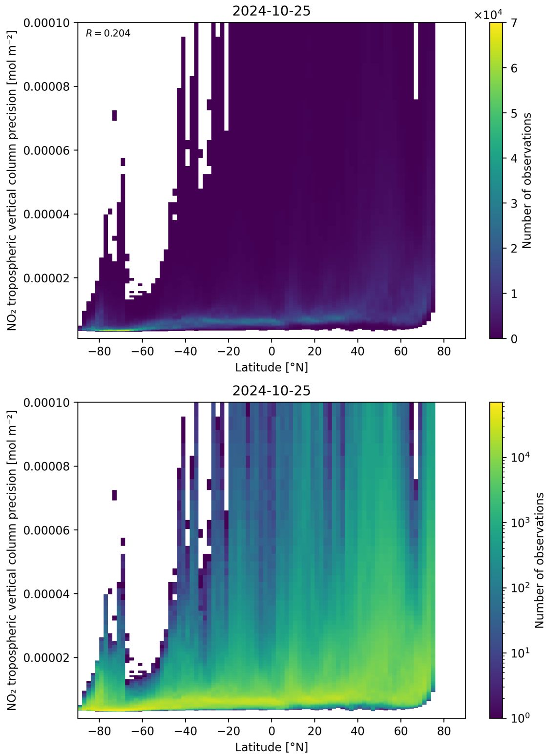
Figure 93: Scatter density plot of “Latitude” against “NO 2 tropospheric vertical column precision” for 2024-10-24 to 2024-10-26.
