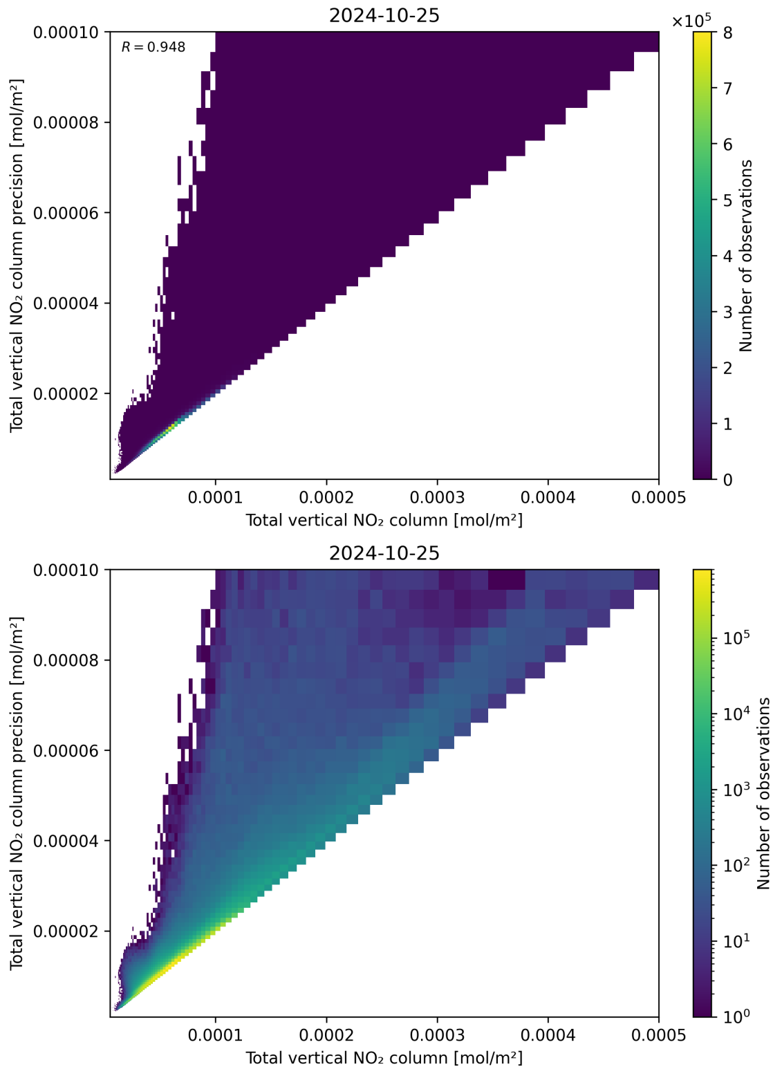
Figure 114: Scatter density plot of “Total vertical NO 2 column” against “Total vertical NO 2 column precision” for 2024-10-24 to 2024-10-26.
