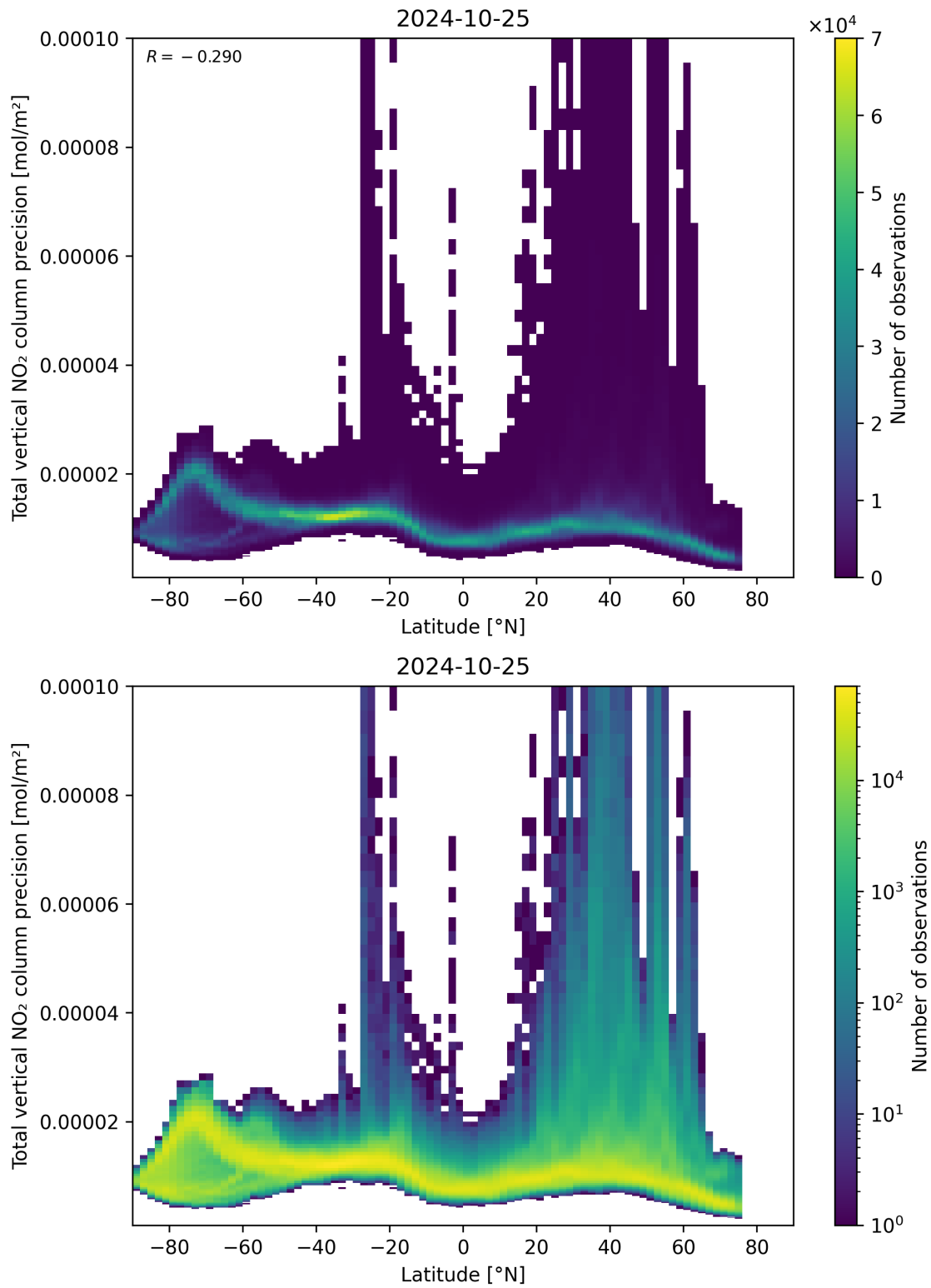
Figure 91: Scatter density plot of “Latitude” against “Total vertical NO 2 column precision” for 2024-10-24 to 2024-10-26.
