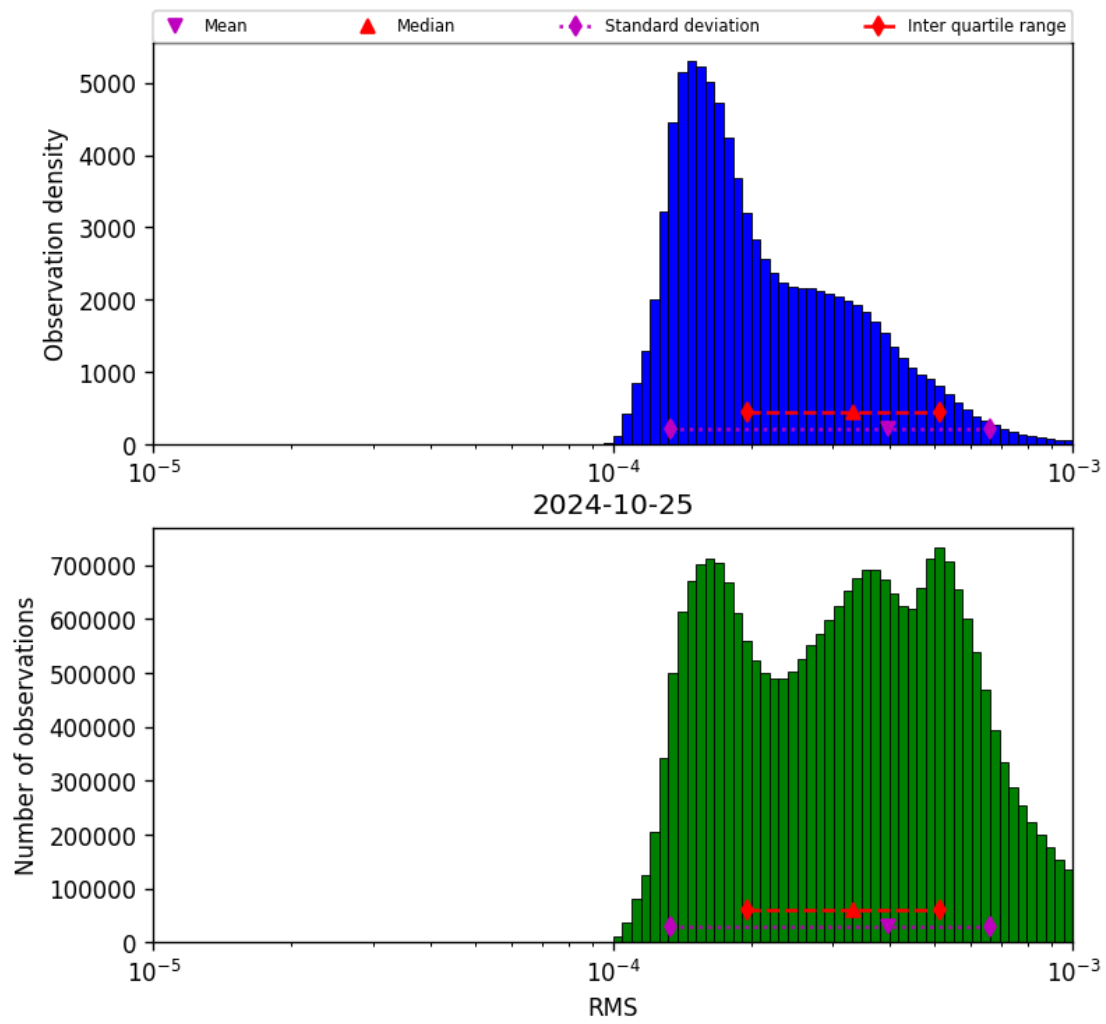
Figure 43: Histogram of “RMS” for 2024-10-24 to 2024-10-26
