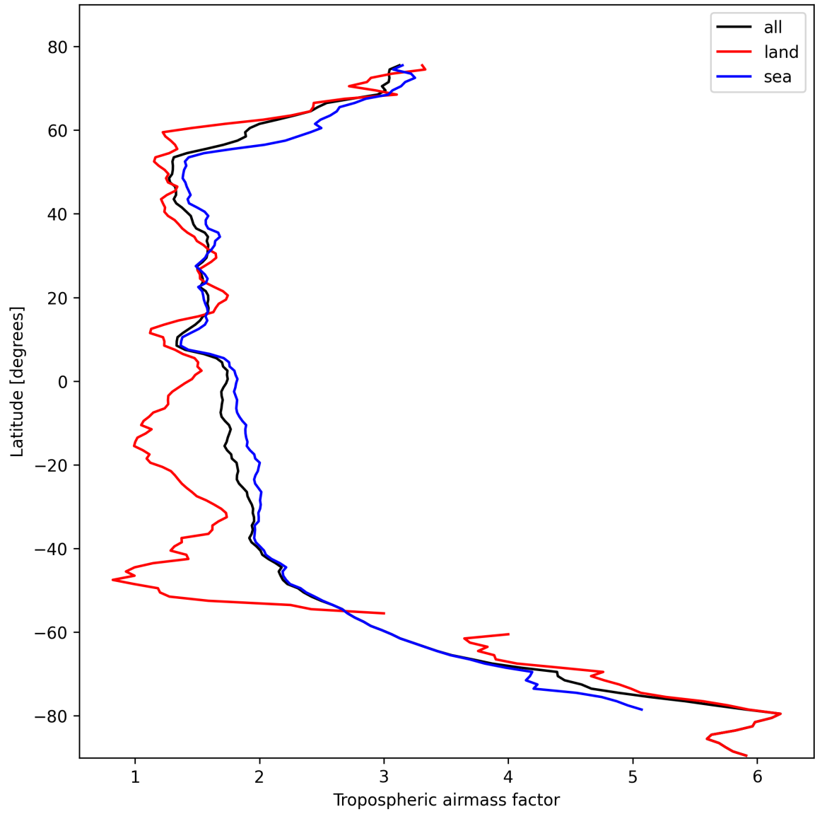
Figure 14: Zonal average of “Tropospheric airmass factor” for 2024-10-24 to 2024-10-26.
