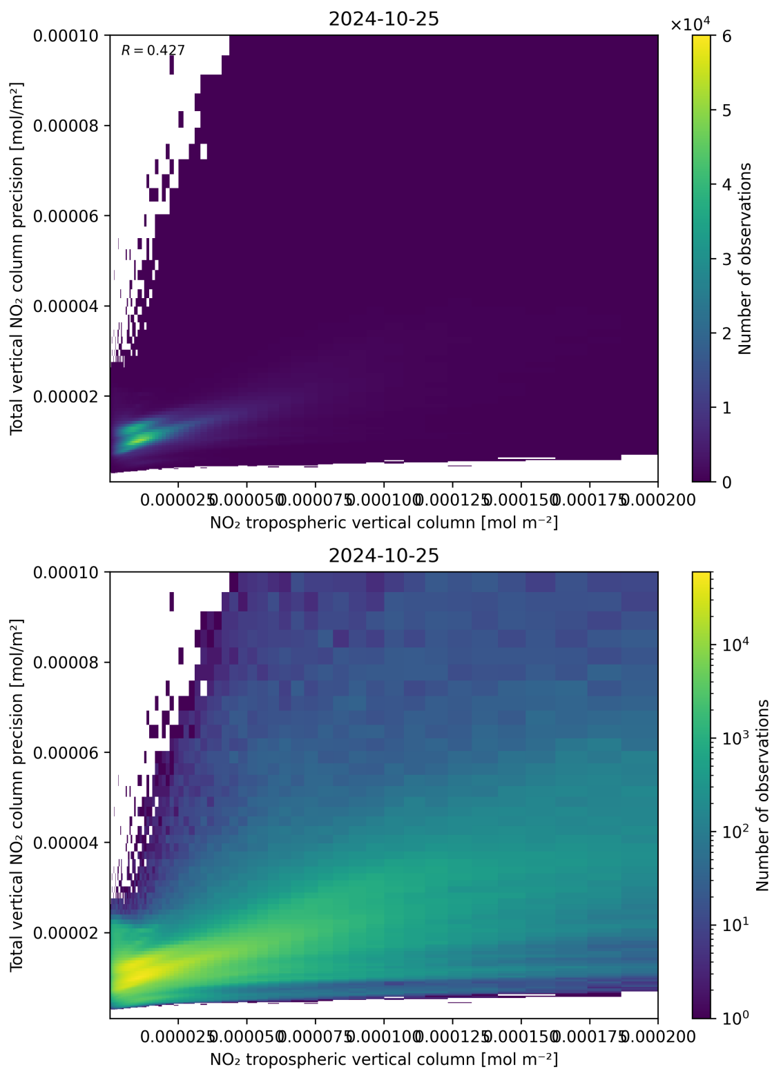
Figure 129: Scatter density plot of “NO 2 tropospheric vertical column” against “Total vertical NO 2 column precision” for 2024-10-24 to 2024-10-26.
