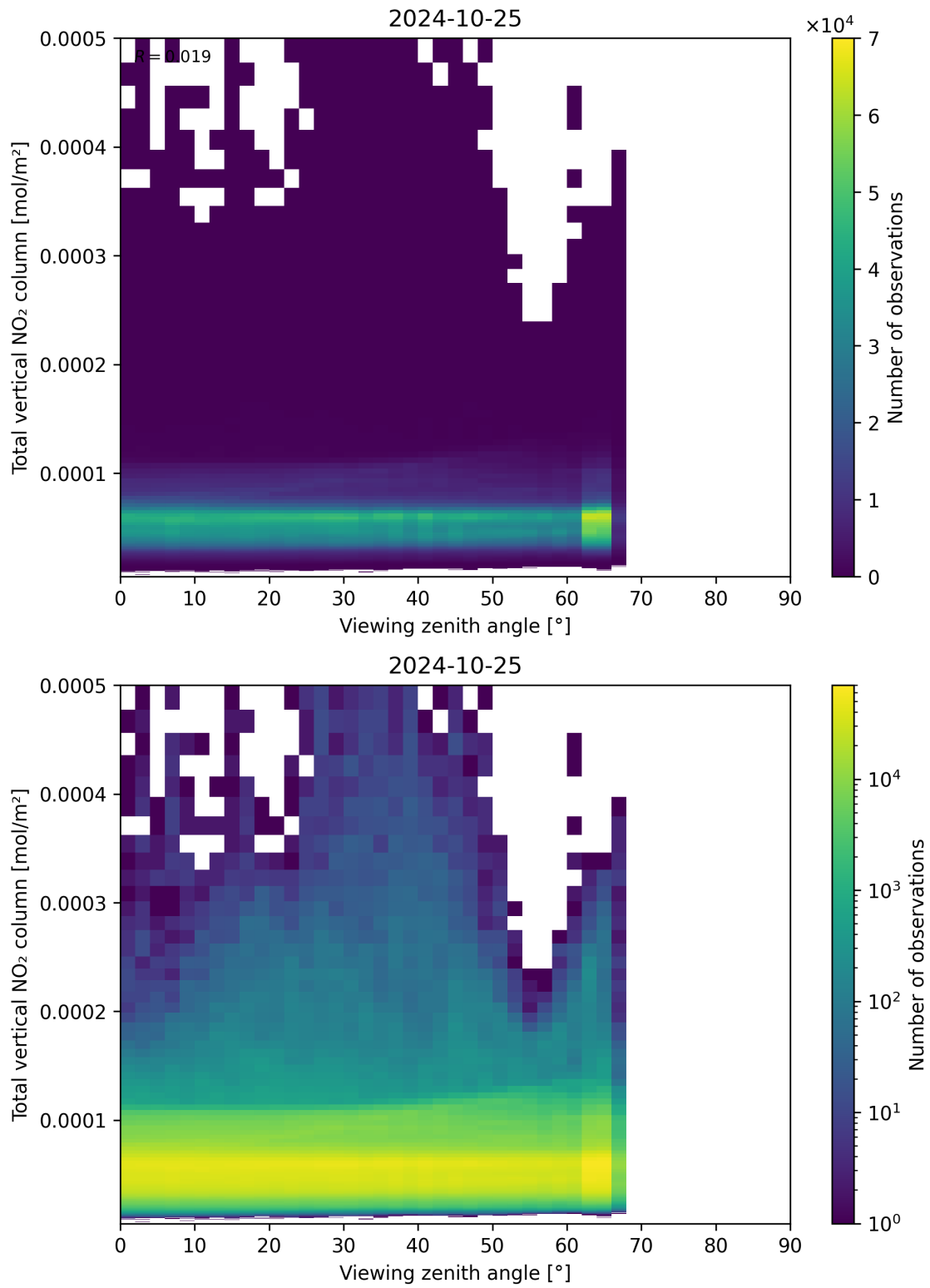
Figure 167: Scatter density plot of “Viewing zenith angle” against “Total vertical NO 2 column” for 2024-10-24 to 2024-10-26.
