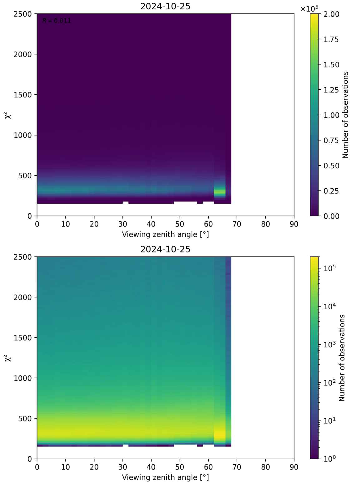
Figure 162: Scatter density plot of “Viewing zenith angle” against “ \chi^2 ” for 2024-10-24 to 2024-10-26.
