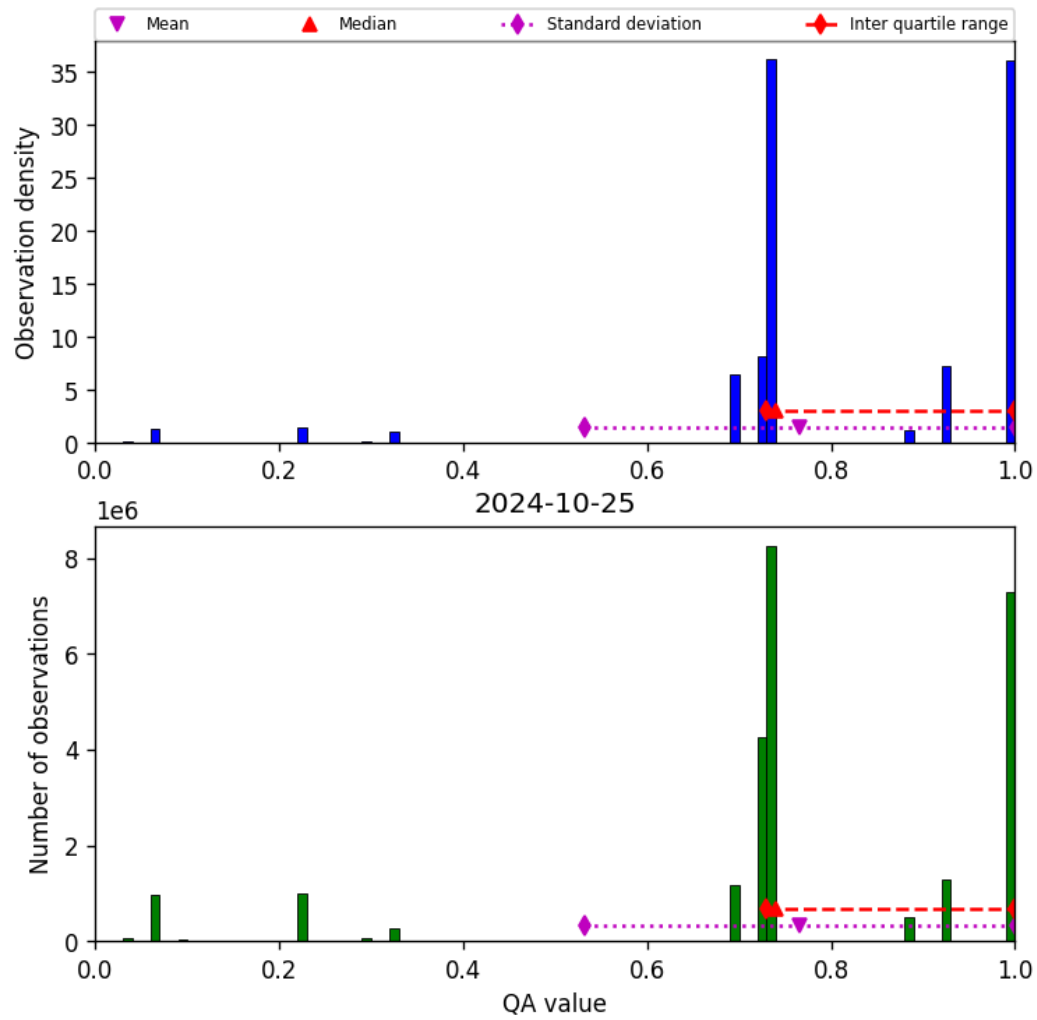
Figure 28: Histogram of “QA value” for 2024-10-24 to 2024-10-26
