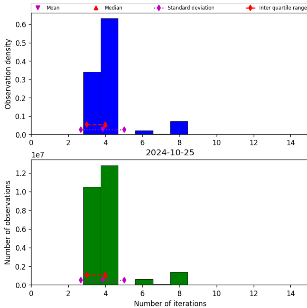
Figure 34: Histogram of “Number of iterations” for 2024-10-24 to 2024-10-26
