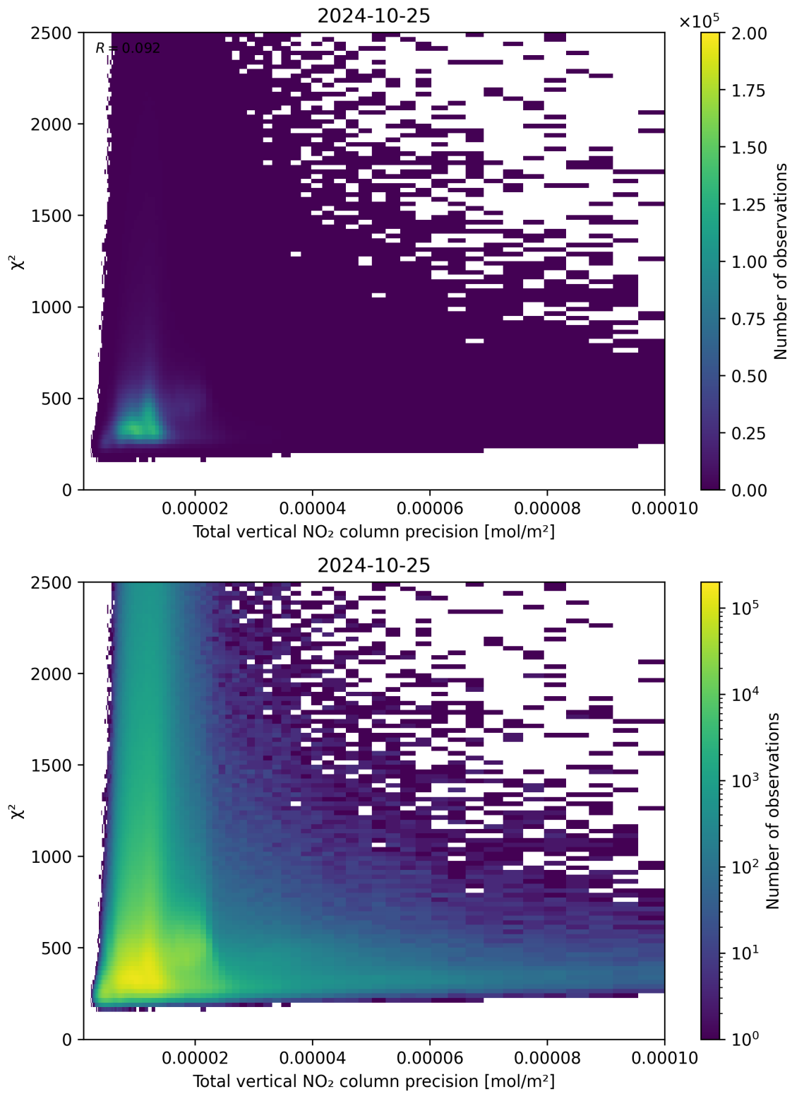
Figure 116: Scatter density plot of "Total vertical NO 2 column precision" against " \chi^2 " for 2024-10-24 to 2024-10-26.
