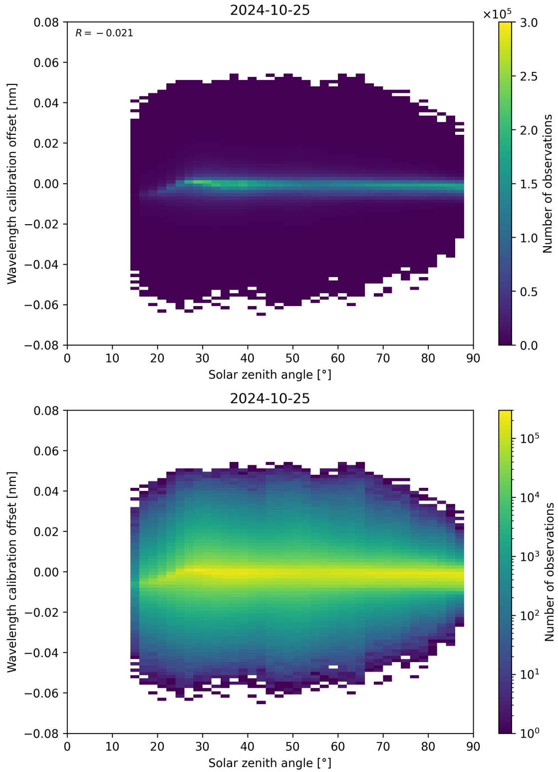
Figure 158: Scatter density plot of “Solar zenith angle” against “Wavelength calibration offset” for 2024-10-24 to 2024-10-26.
