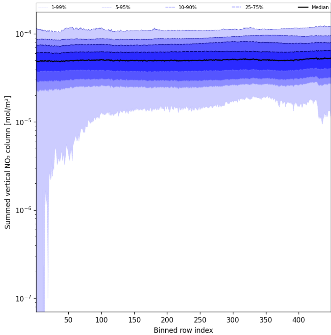
Figure 57: Along track statistics of “Summed vertical NO 2 column” for 2024-10-24 to 2024-10-26
