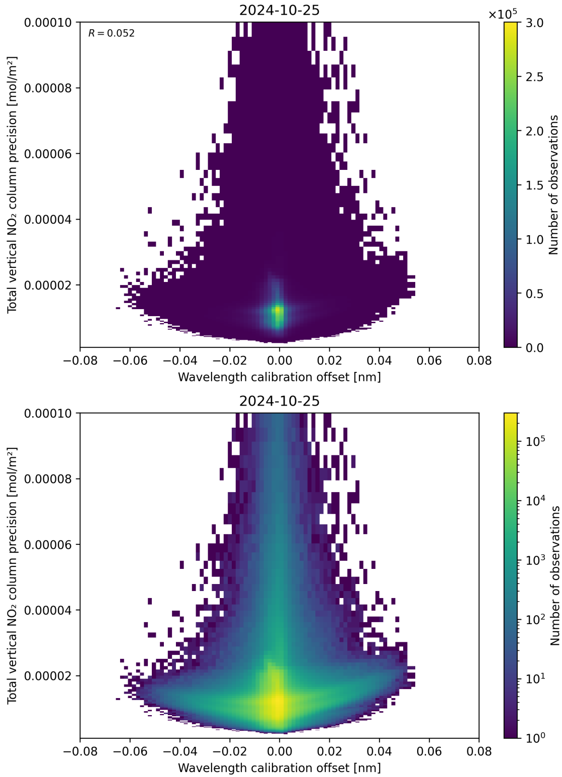
Figure 180: Scatter density plot of “Wavelength calibration offset” against “Total vertical NO 2 column precision” for 2024-10-24 to 2024-10-26.
