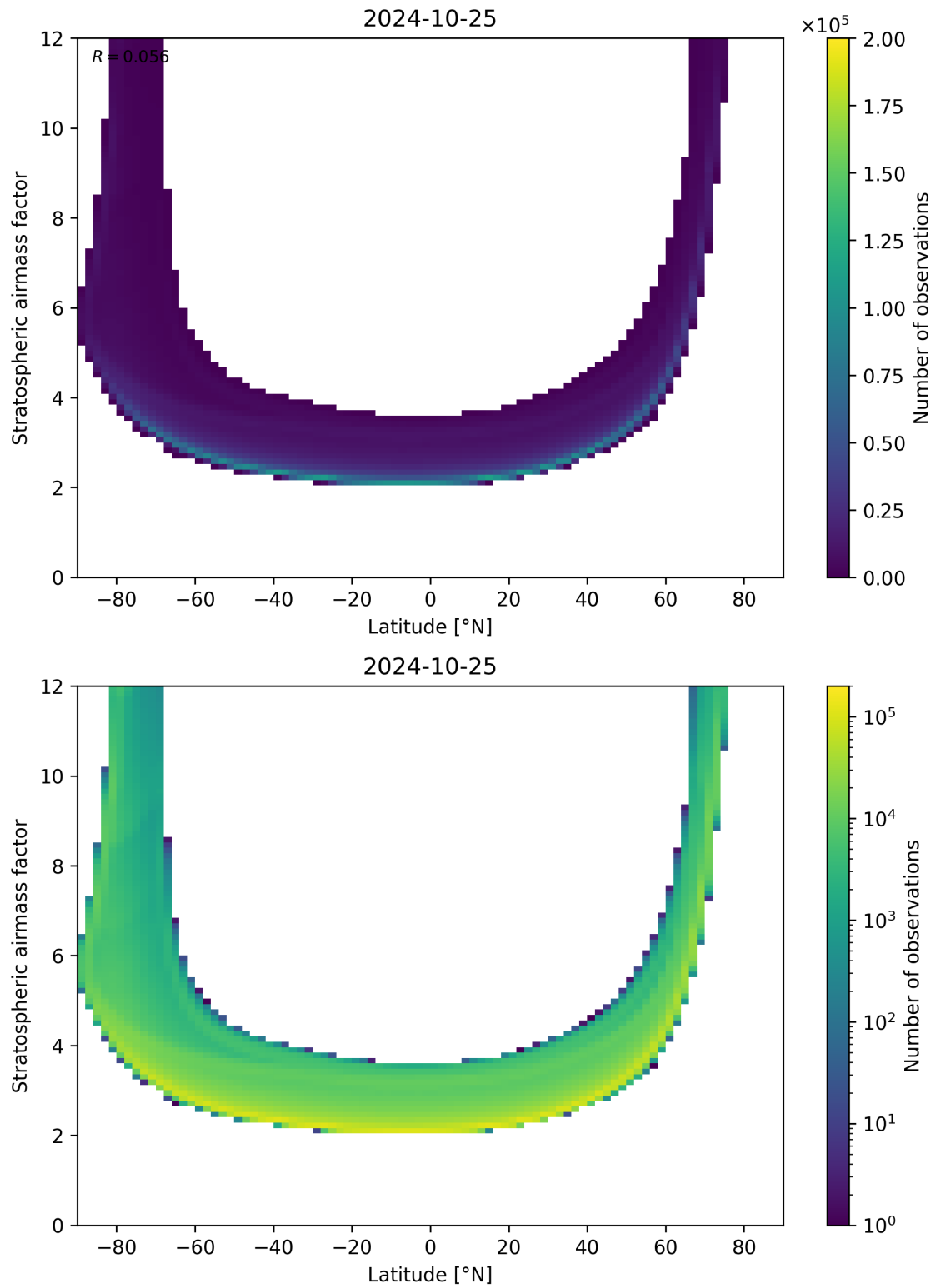
Figure 83: Scatter density plot of “Latitude” against “Stratospheric airmass factor” for 2024-10-24 to 2024-10-26.
