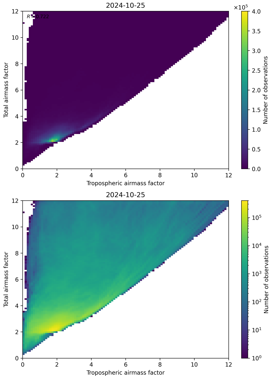
Figure 72: Scatter density plot of “Tropospheric airmass factor” against “Total airmass factor” for 2024-10-24 to 2024-10-26.
