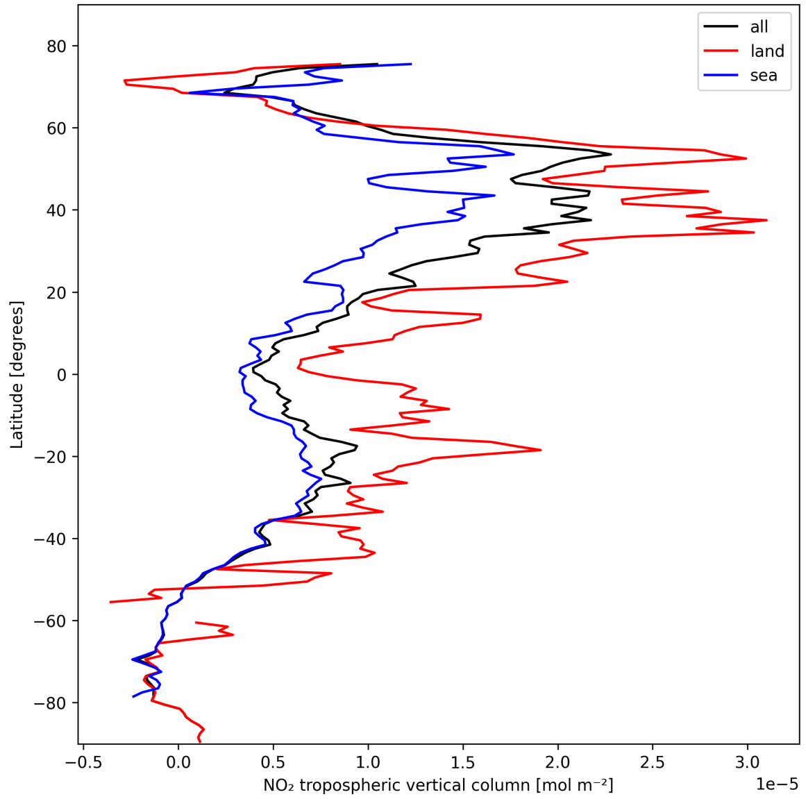
Figure 12: Zonal average of “NO 2 tropospheric vertical column” for 2024-10-24 to 2024-10-26.
