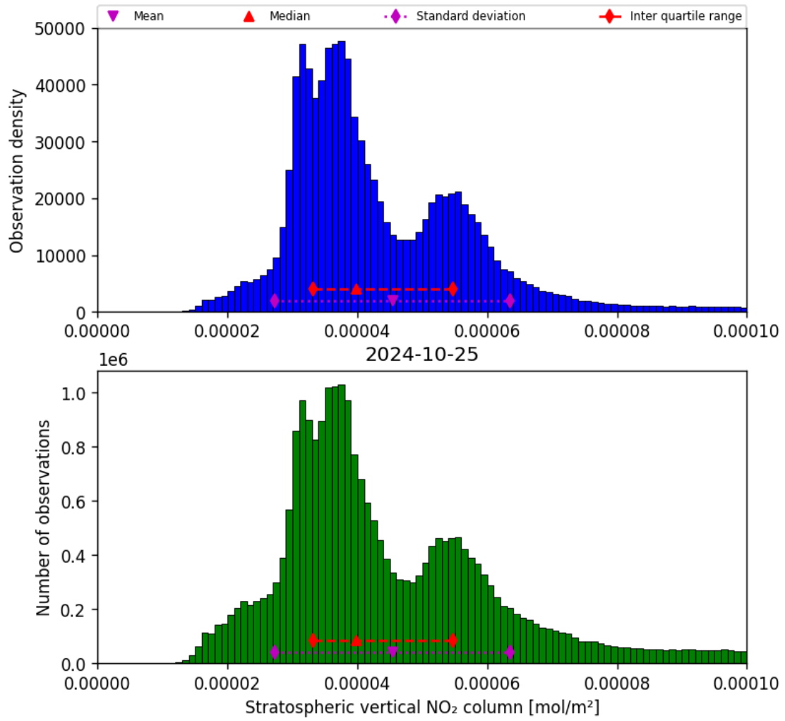
Figure 36: Histogram of “Stratospheric vertical NO 2 column” for 2024-10-24 to 2024-10-26
