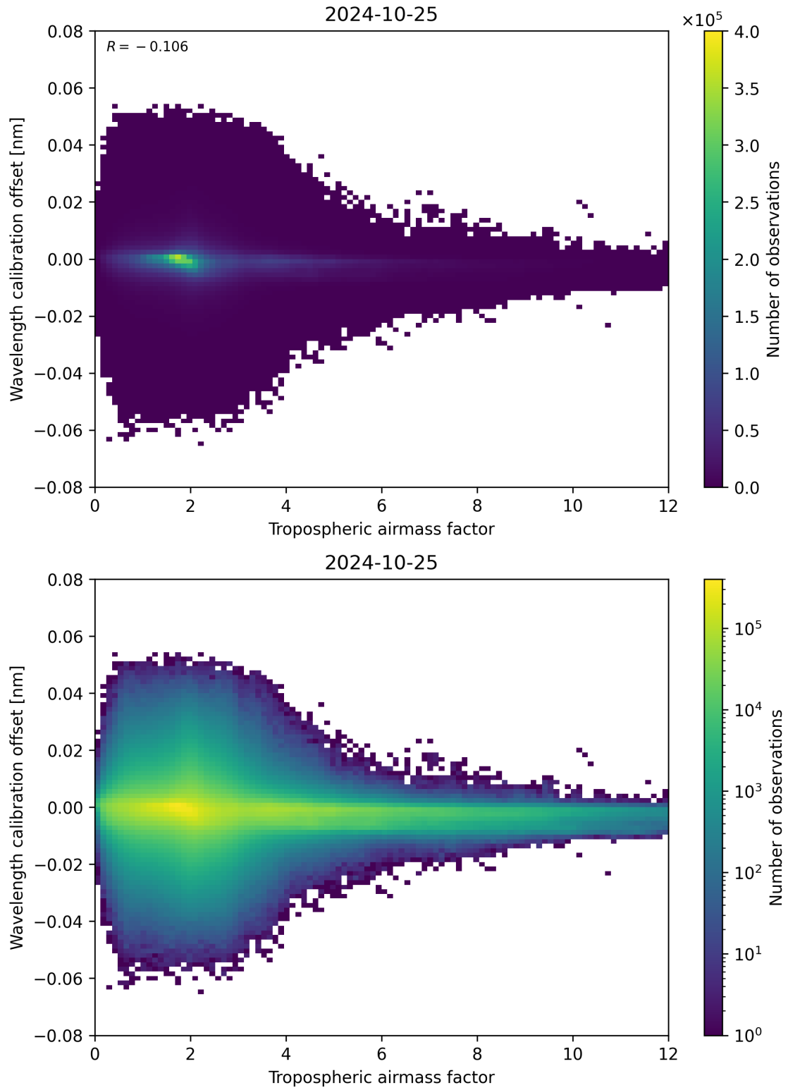
Figure 80: Scatter density plot of “Tropospheric airmass factor” against “Wavelength calibration offset” for 2024-10-24 to 2024-10-26.
