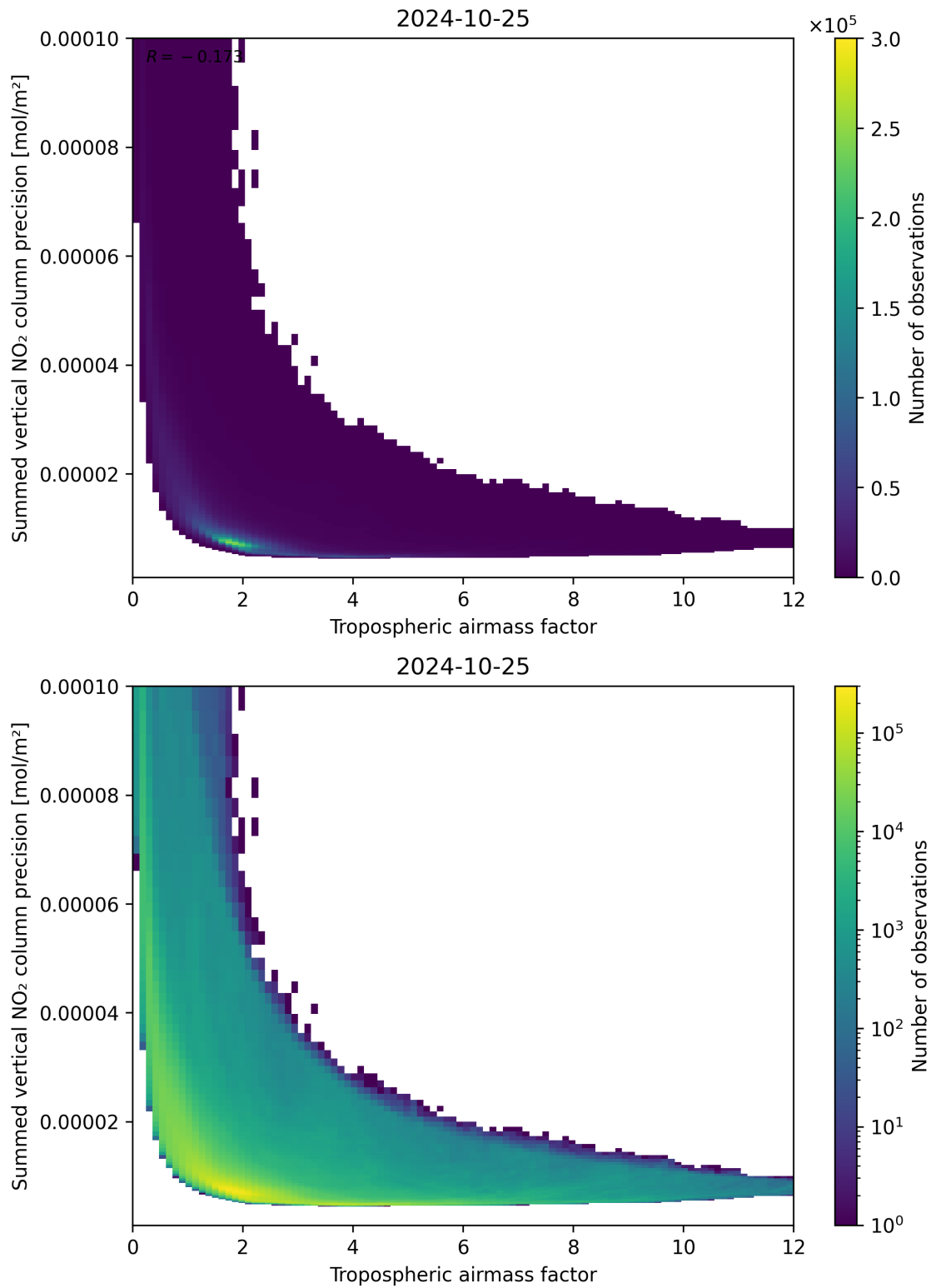
Figure 76: Scatter density plot of “Tropospheric air mass factor” against “Summed vertical NO 2 column precision” for 2024-10-24 to 2024-10-26.
