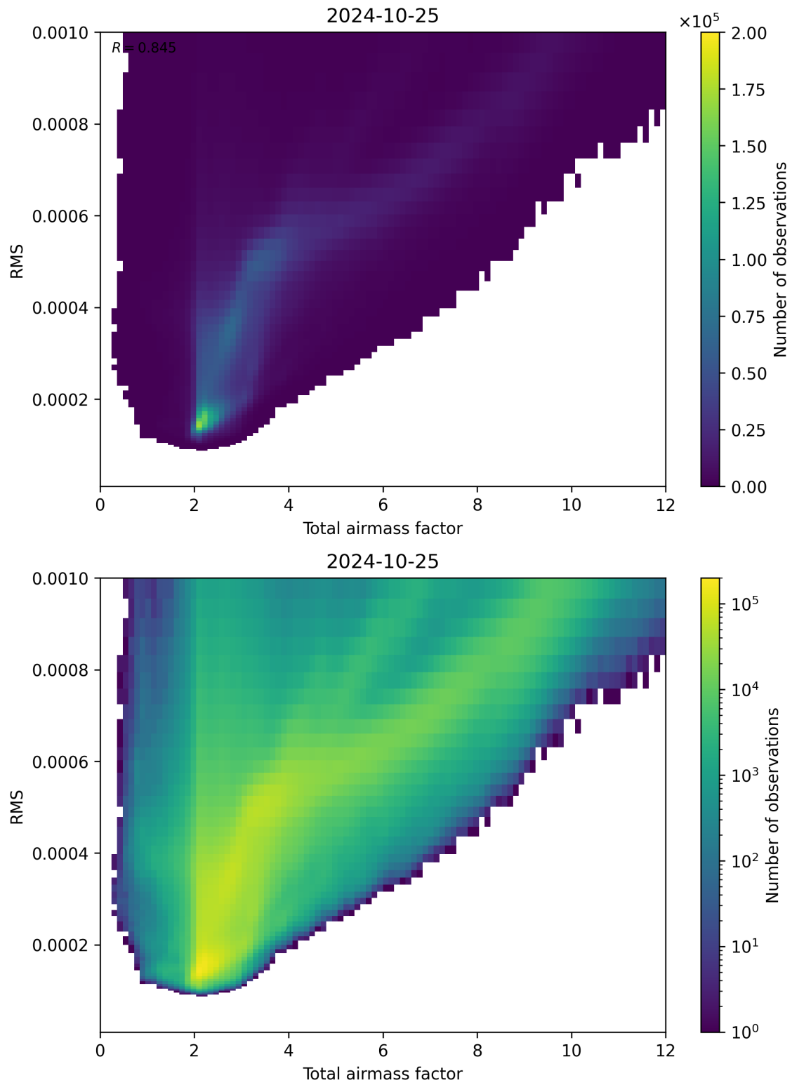
Figure 69: Scatter density plot of “Total airmass factor” against “RMS” for 2024-10-24 to 2024-10-26.
