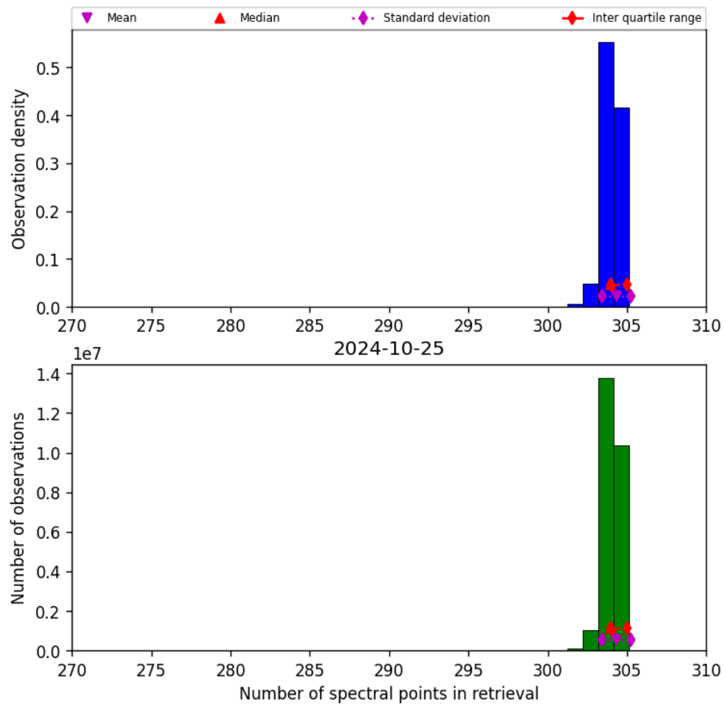
Figure 33: Histogram of “Number of spectral points in retrieval” for 2024-10-24 to 2024-10-26
