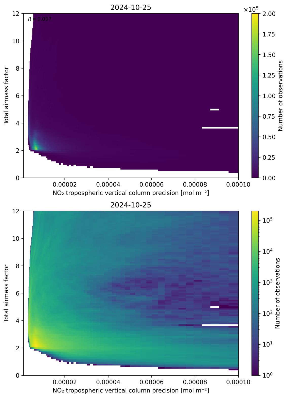
Figure 132: Scatter density plot of “NO 2 tropospheric vertical column precision” against “Total air mass factor” for 2024-10-24 to 2024-10-26.
