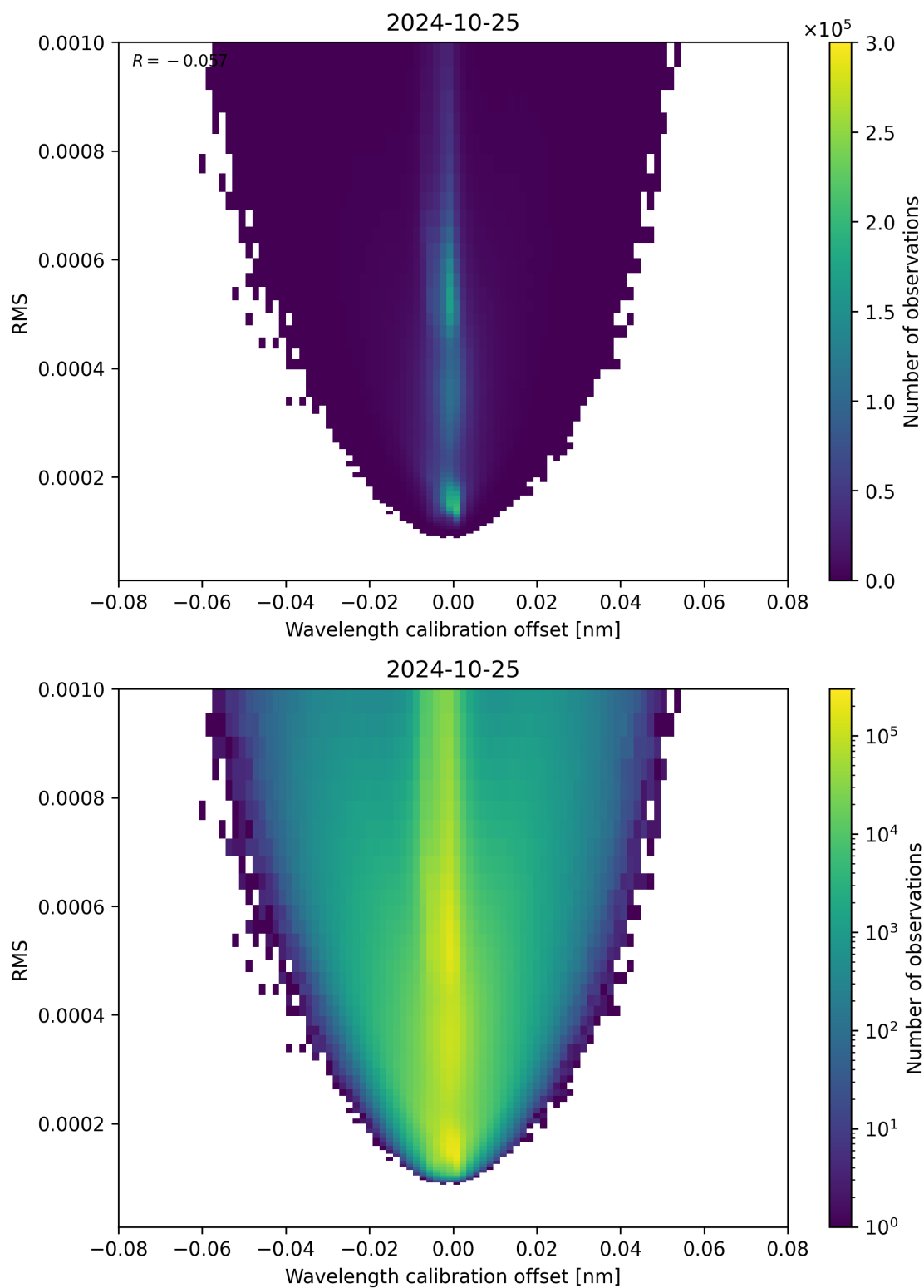
Figure 181: Scatter density plot of “Wavelength calibration offset” against “RMS” for 2024-10-24 to 2024-10-26.
