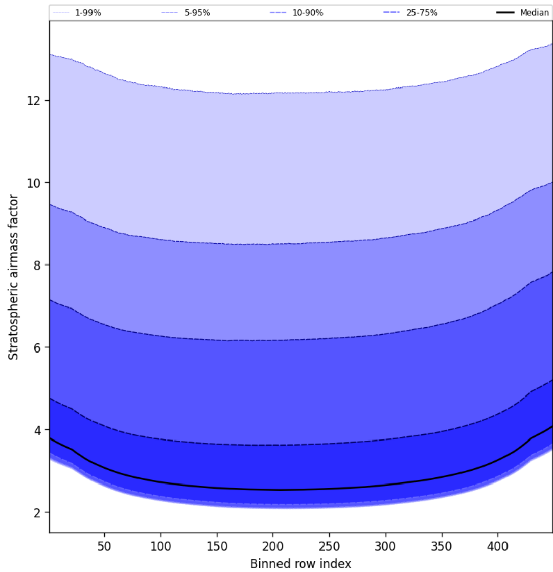
Figure 61: Along track statistics of “Stratospheric airmass factor” for 2024-10-24 to 2024-10-26
