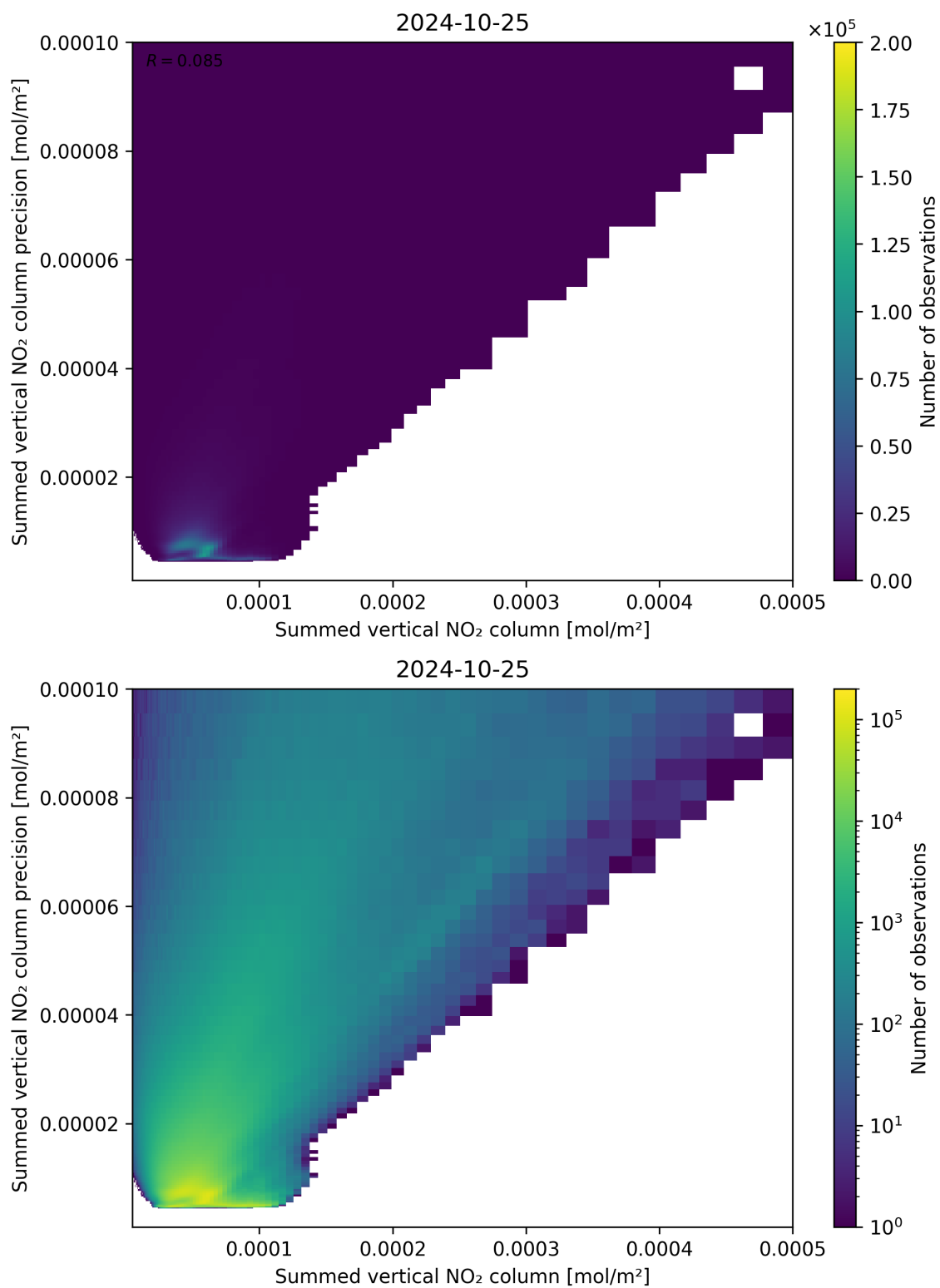
Figure 105: Scatter density plot of “Summed vertical NO 2 column” against “Summed vertical NO 2 column precision” for 2024-10-24 to 2024-10-26.
