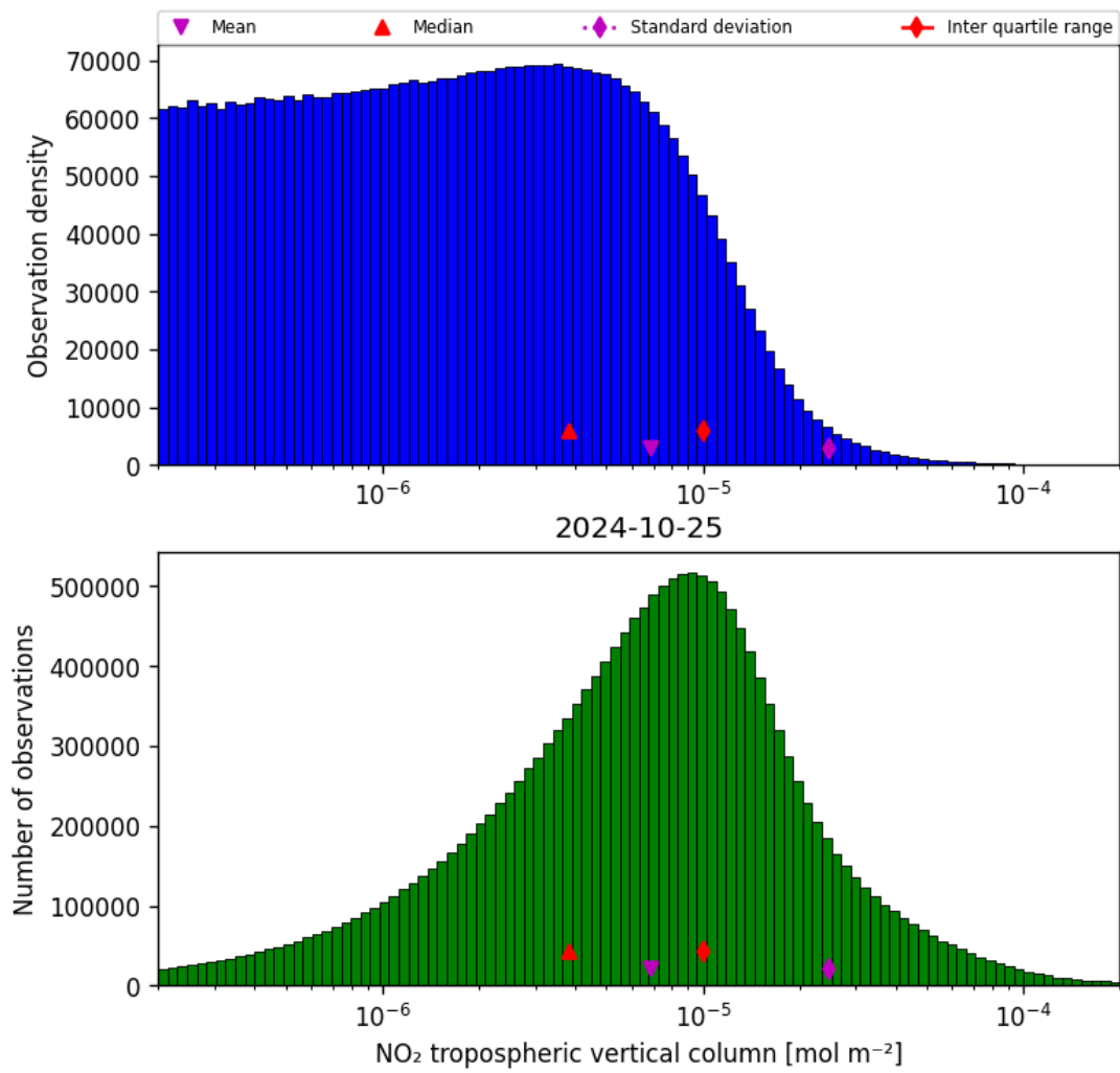
Figure 29: Histogram of “NO 2 tropospheric vertical column” for 2024-10-24 to 2024-10-26
