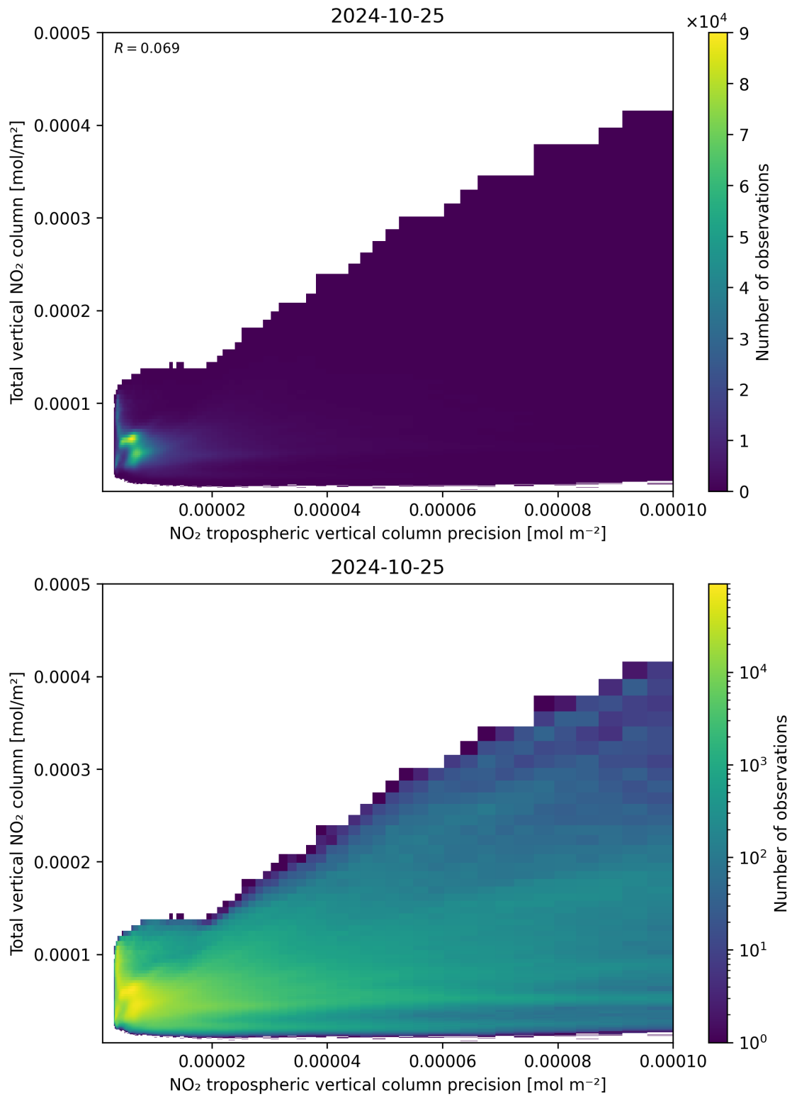
Figure 138: Scatter density plot of “NO 2 tropospheric vertical column precision” against “Total vertical NO 2 column” for 2024-10-24 to 2024-10-26.
