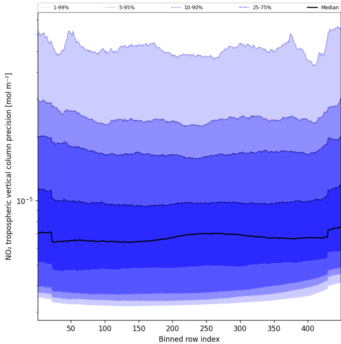
Figure 47: Along track statistics of “NO 2 tropospheric vertical column precision” for 2024-10-24 to 2024-10-26
