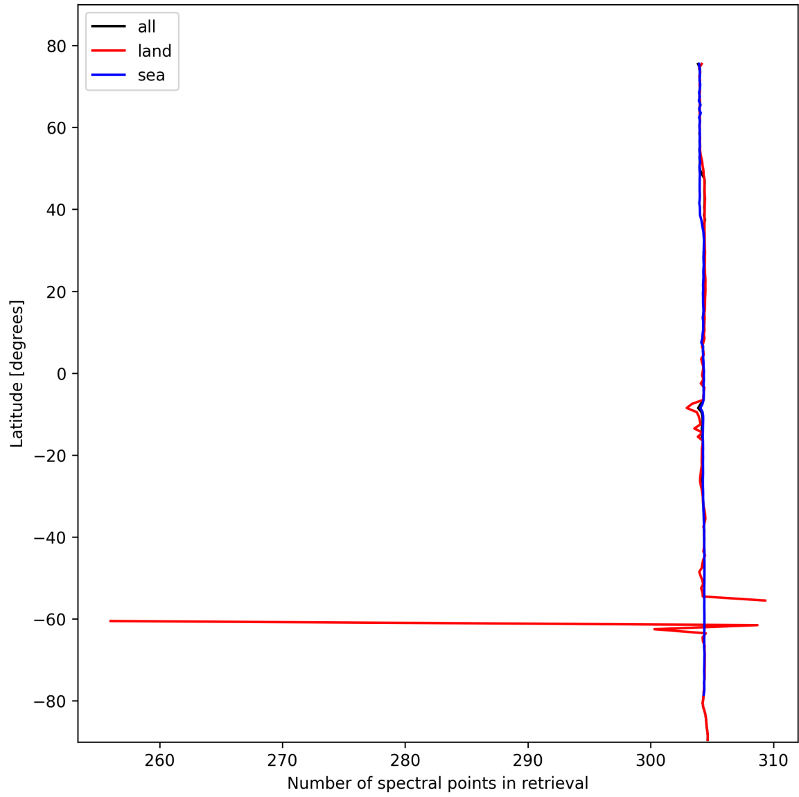
Figure 16: Zonal average of “Number of spectral points in retrieval” for 2024-10-24 to 2024-10-26.
