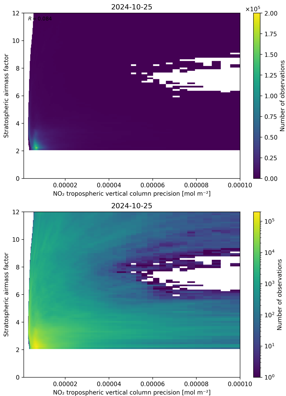
Figure 131: Scatter density plot of “NO 2 tropospheric vertical column precision” against “Stratospheric airmass factor” for 2024-10-24 to 2024-10-26.
