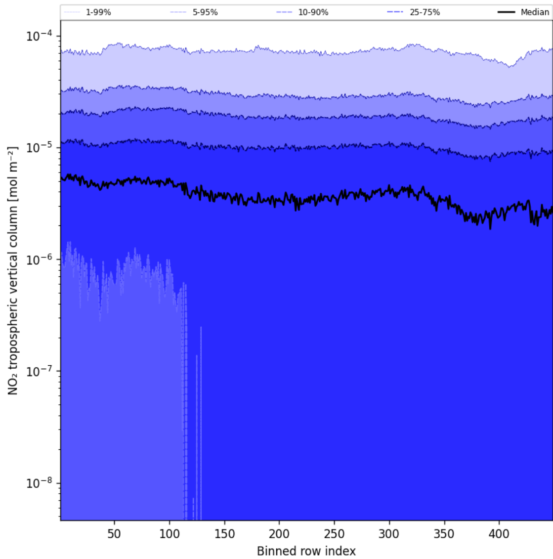
Figure 46: Along track statistics of “NO 2 tropospheric vertical column” for 2024-10-24 to 2024-10-26
