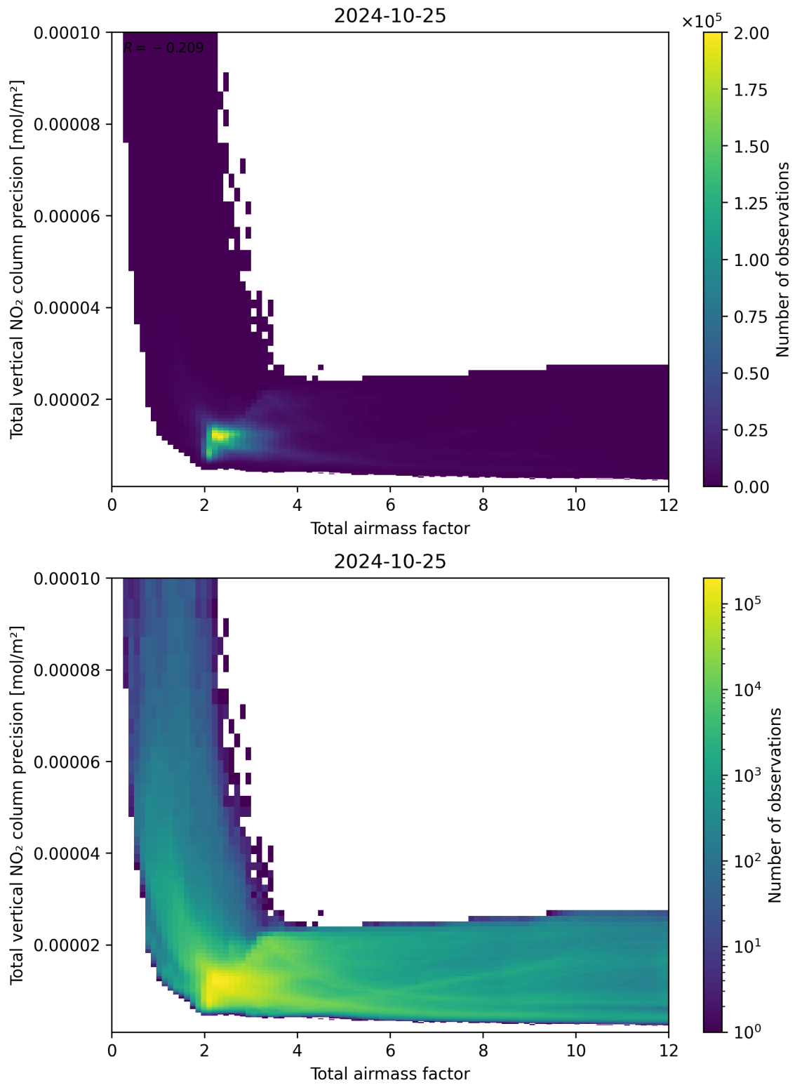
Figure 68: Scatter density plot of “Total airmass factor” against “Total vertical NO 2 column precision” for 2024-10-24 to 2024-10-26.
