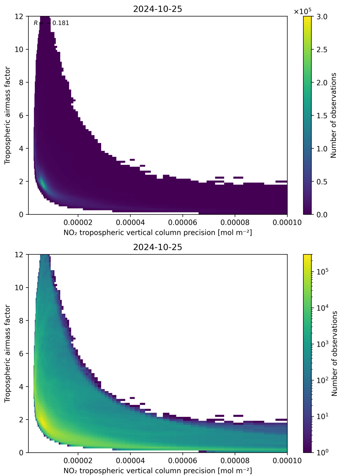
Figure 133: Scatter density plot of “NO 2 tropospheric vertical column precision” against “Tropospheric airmass factor” for 2024-10-24 to 2024-10-26.
