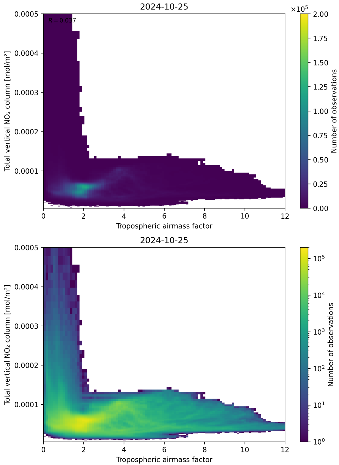
Figure 77: Scatter density plot of “Tropospheric airmass factor” against “Total vertical NO 2 column” for 2024-10-24 to 2024-10-26.
