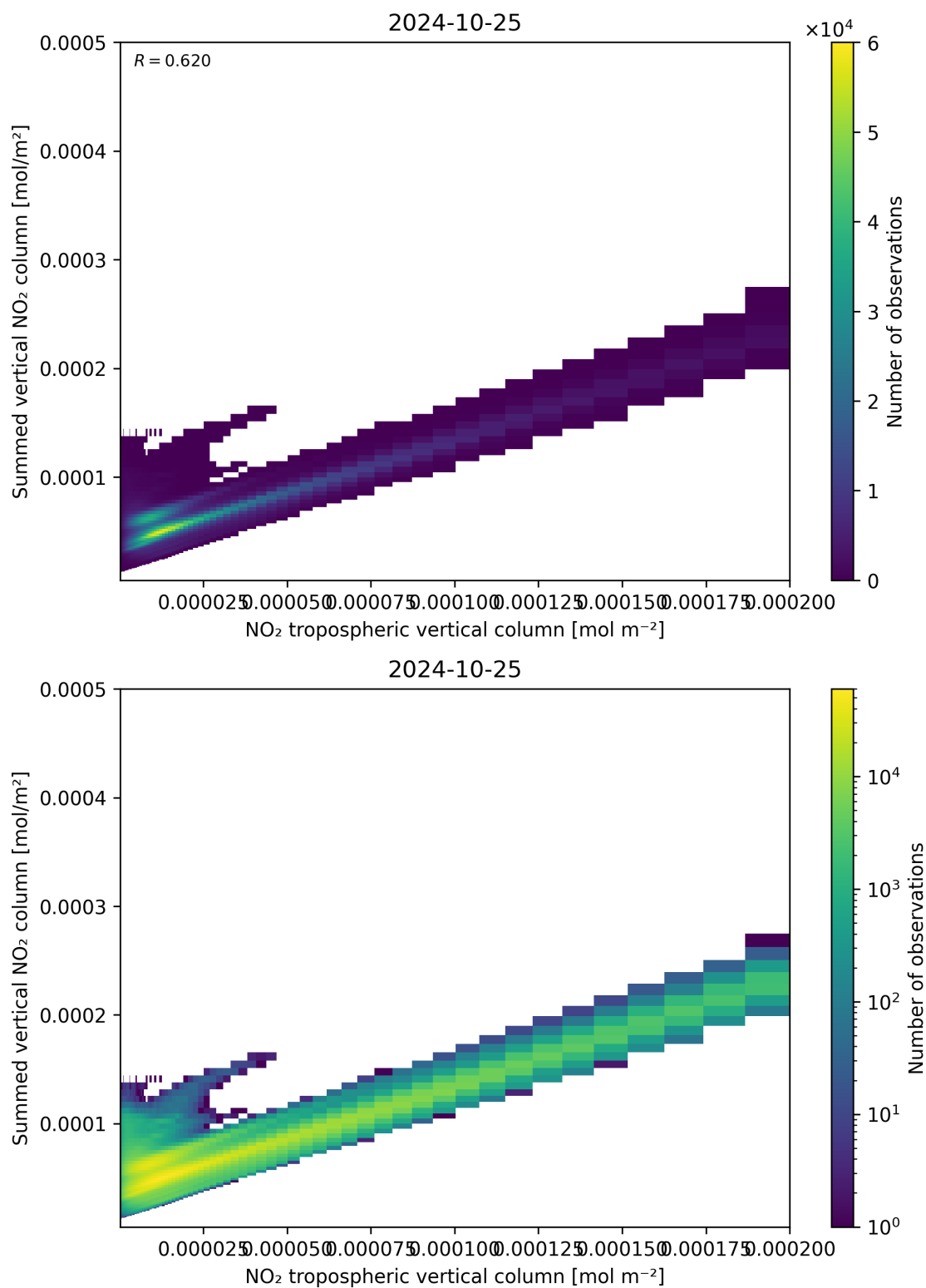
Figure 126: Scatter density plot of “NO 2 tropospheric vertical column” against “Summed vertical NO 2 column” for 2024-10-24 to 2024-10-26.
