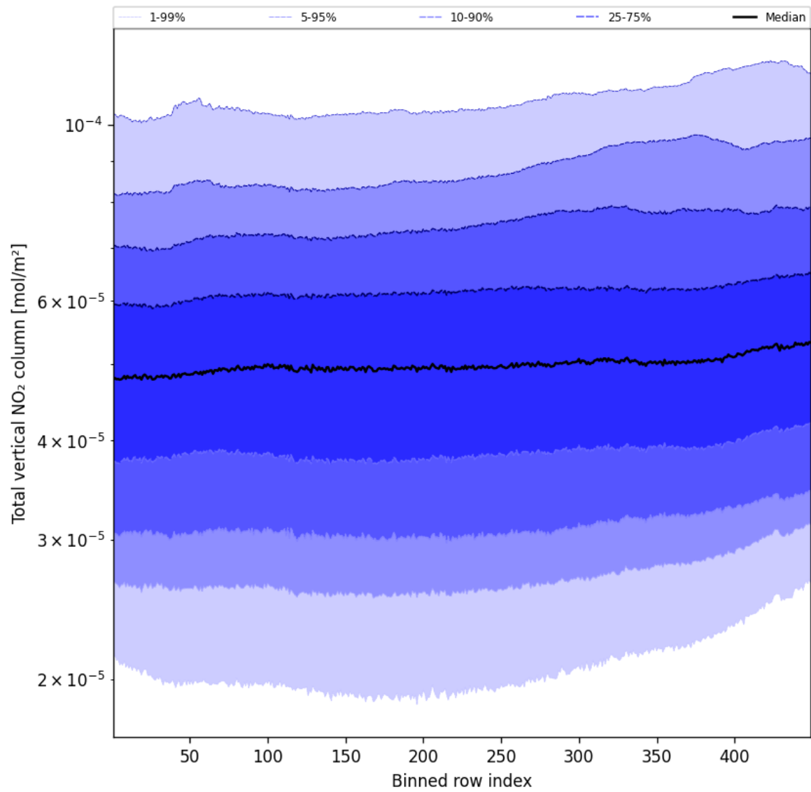
Figure 55: Along track statistics of “Total vertical NO 2 column” for 2024-10-24 to 2024-10-26
