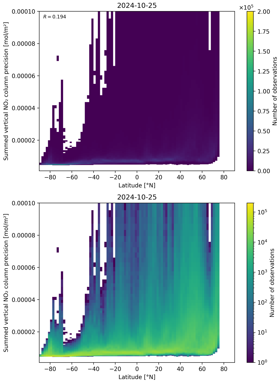
Figure 89: Scatter density plot of “Latitude” against “Summed vertical NO 2 column precision” for 2024-10-24 to 2024-10-26.
