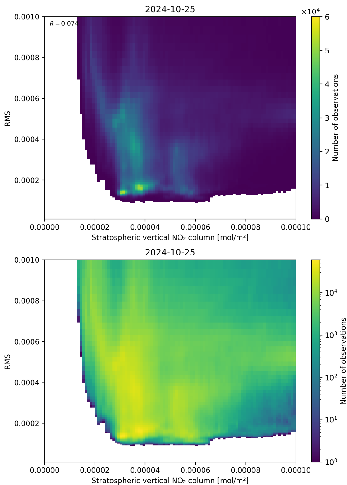
Figure 102: Scatter density plot of “Stratospheric vertical NO 2 column” against “RMS” for 2024-10-24 to 2024-10-26.
