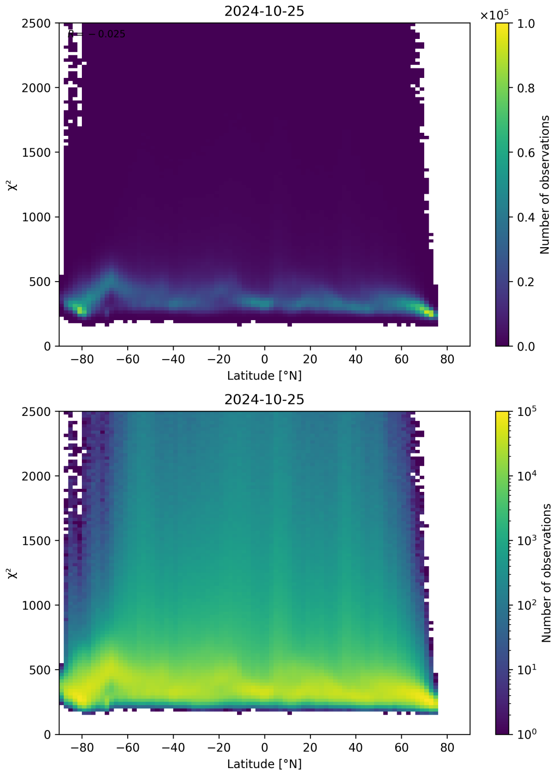
Figure 86: Scatter density plot of “Latitude” against “ \chi^2 ” for 2024-10-24 to 2024-10-26.
