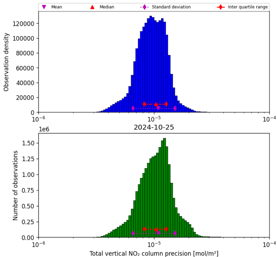
Figure 39: Histogram of “Total vertical NO 2 column precision” for 2024-10-24 to 2024-10-26
