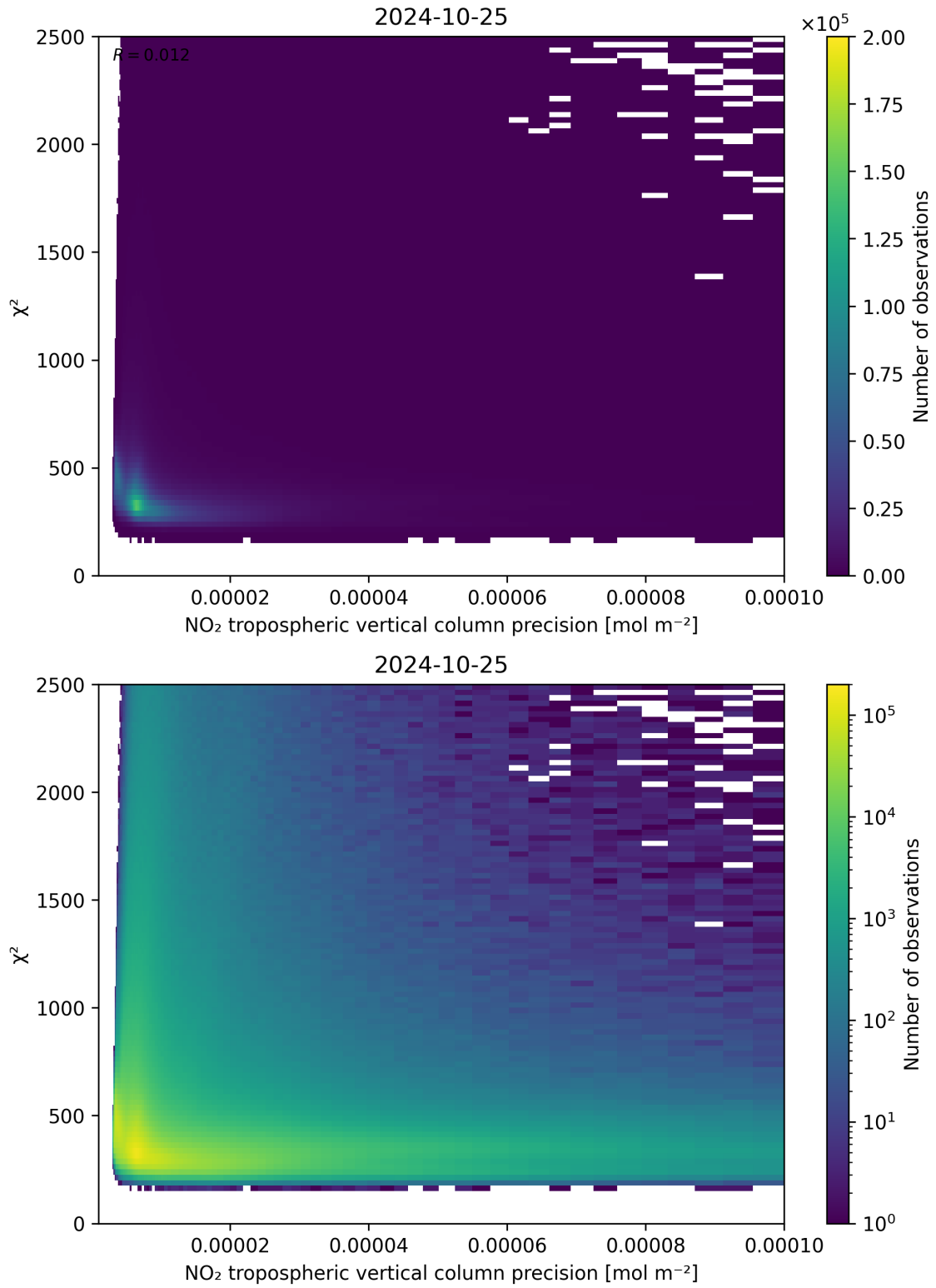
Figure 134: Scatter density plot of “NO 2 tropospheric vertical column precision” against “ \chi^2 ” for 2024-10-24 to 2024-10-26.
