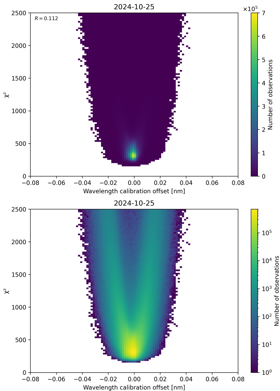
Figure 175: Scatter density plot of “Wavelength calibration offset” against “ \chi^2 ” for 2024-10-24 to 2024-10-26.
