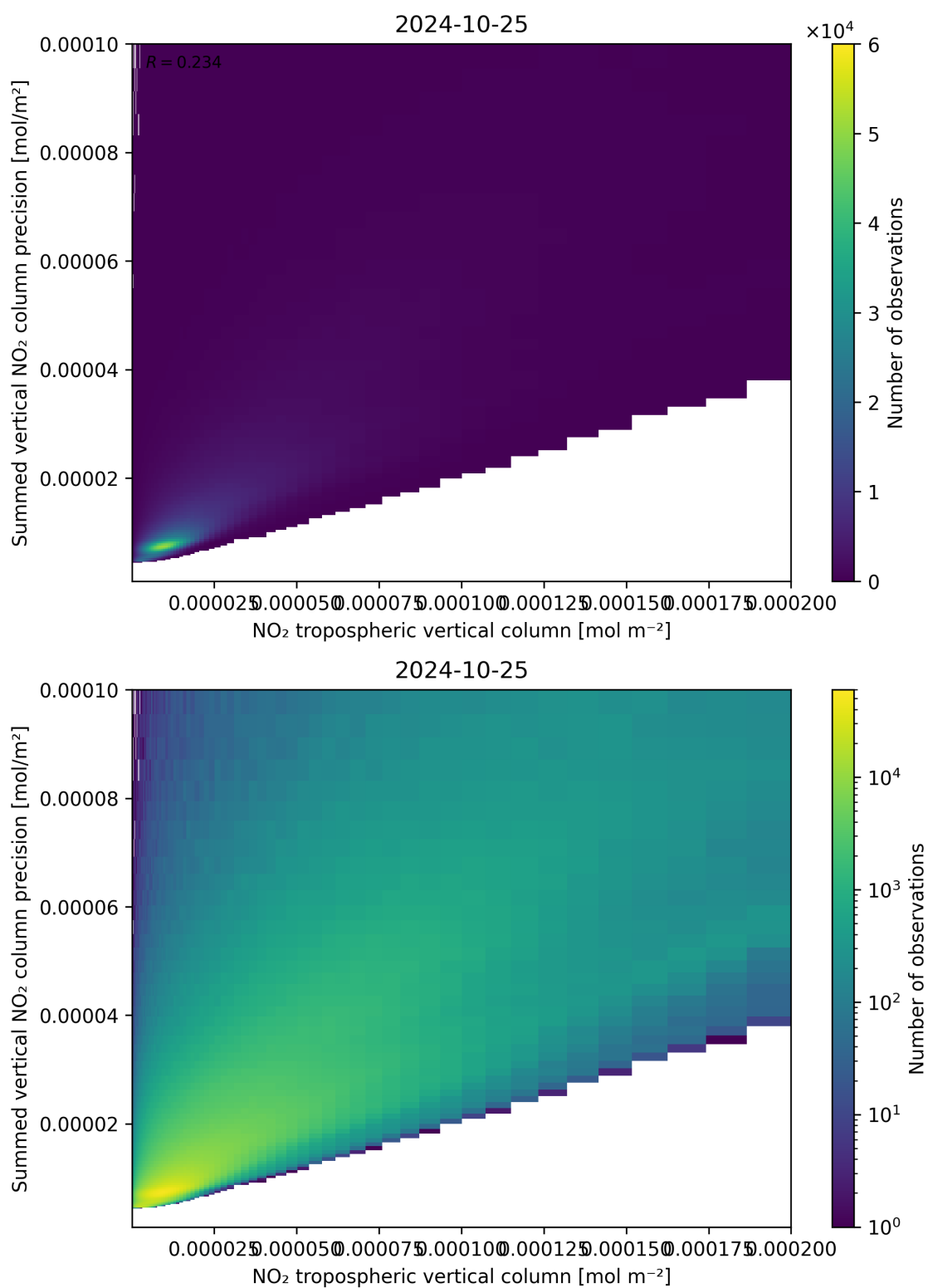
Figure 127: Scatter density plot of “NO 2 tropospheric vertical column” against “Summed vertical NO 2 column precision” for 2024-10-24 to 2024-10-26.
