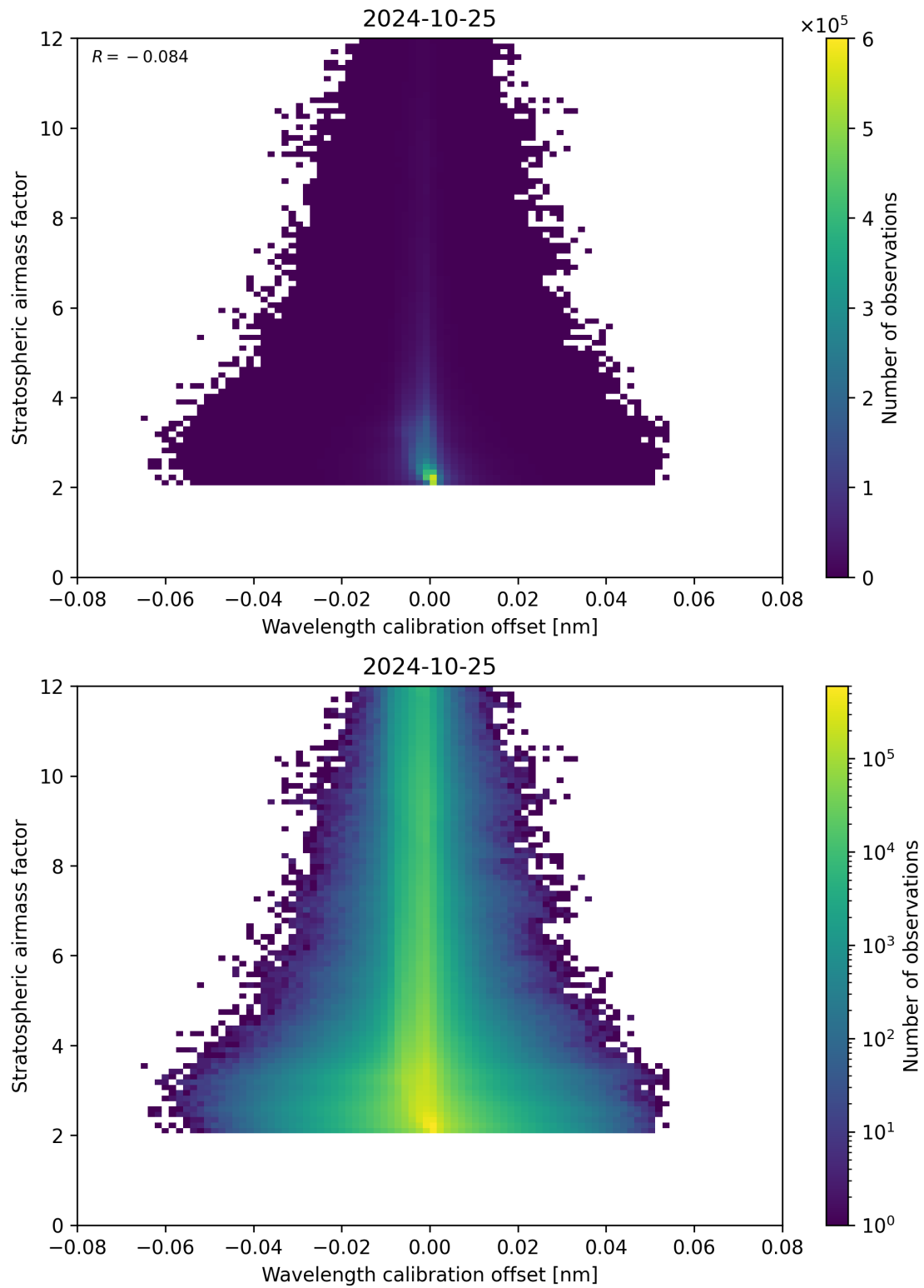
Figure 174: Scatter density plot of “Wavelength calibration offset” against “Stratospheric airmass factor” for 2024-10-24 to 2024-10-26.
