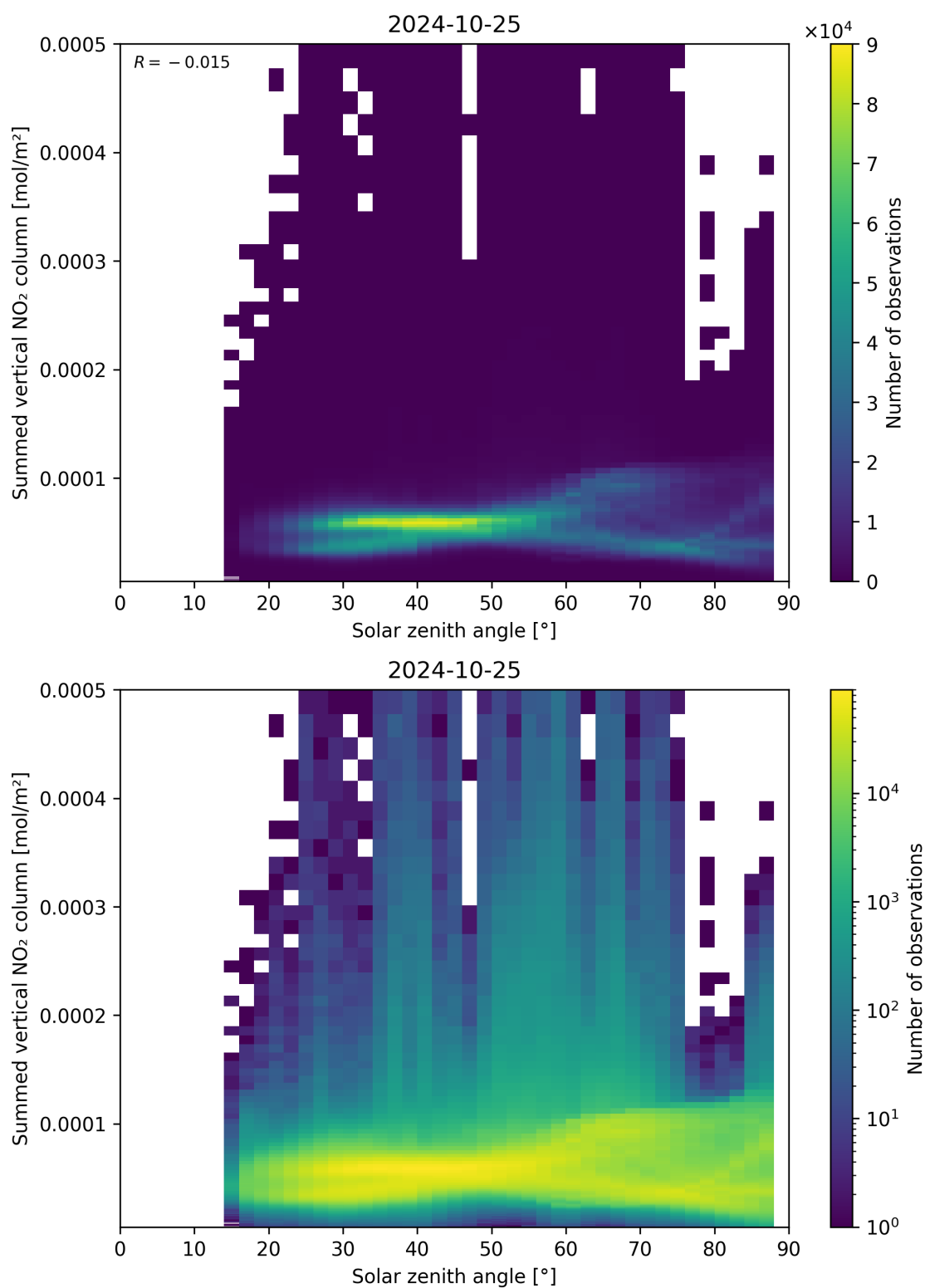
Figure 151: Scatter density plot of “Solar zenith angle” against “Summed vertical NO 2 column” for 2024-10-24 to 2024-10-26.
