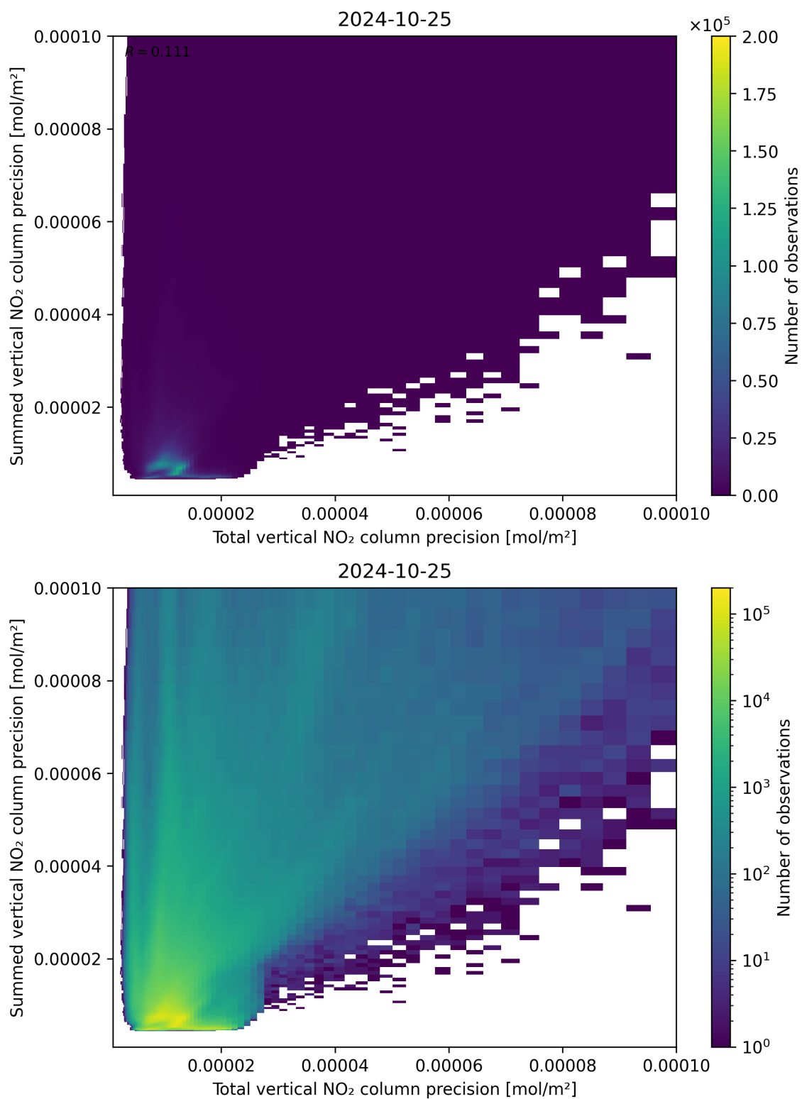
Figure 118: Scatter density plot of “Total vertical NO 2 column precision” against “Summed vertical NO 2 column precision” for 2024-10-24 to 2024-10-26.
