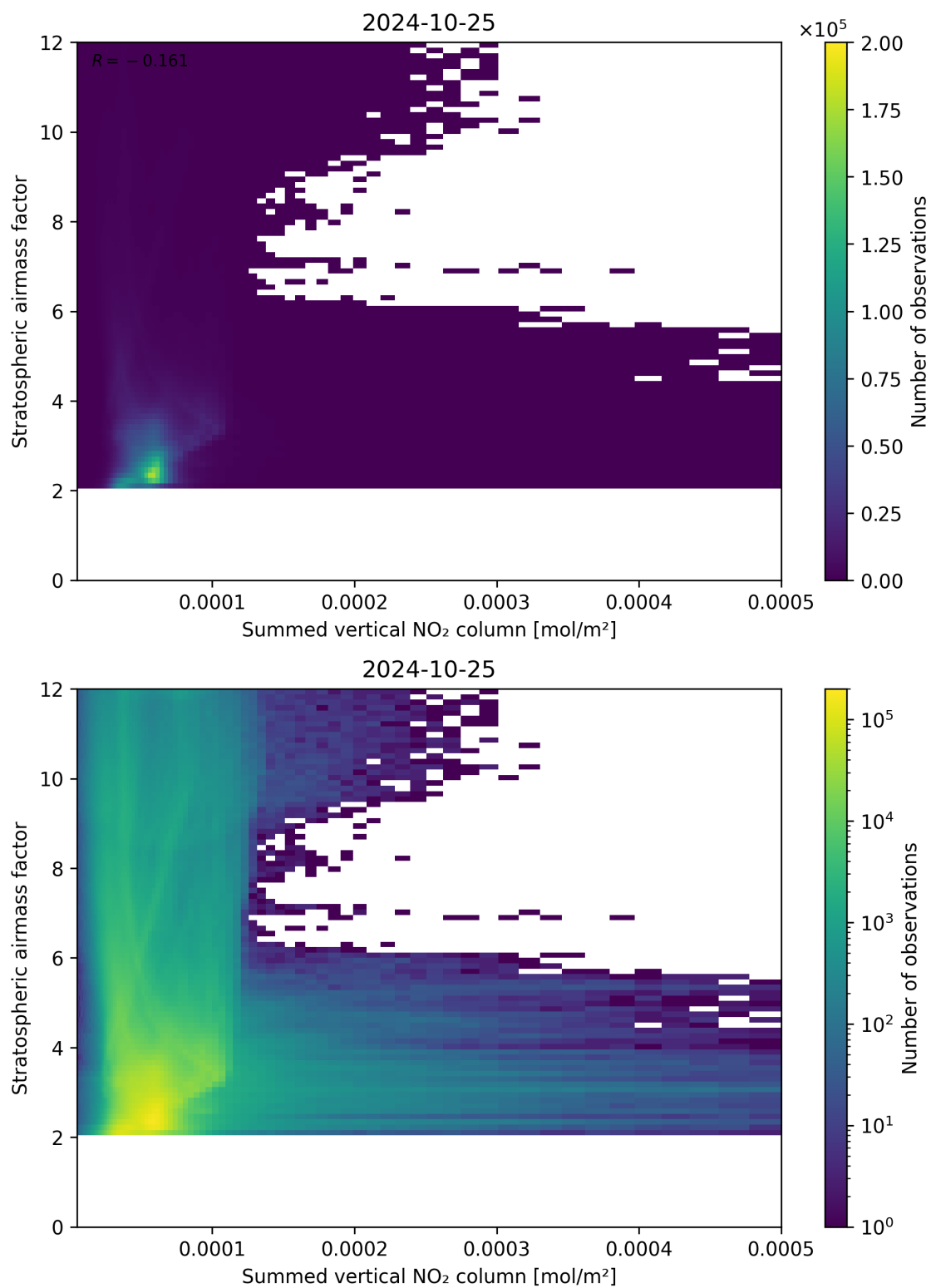
Figure 103: Scatter density plot of “Summed vertical NO 2 column” against “Stratospheric air mass factor” for 2024-10-24 to 2024-10-26.
