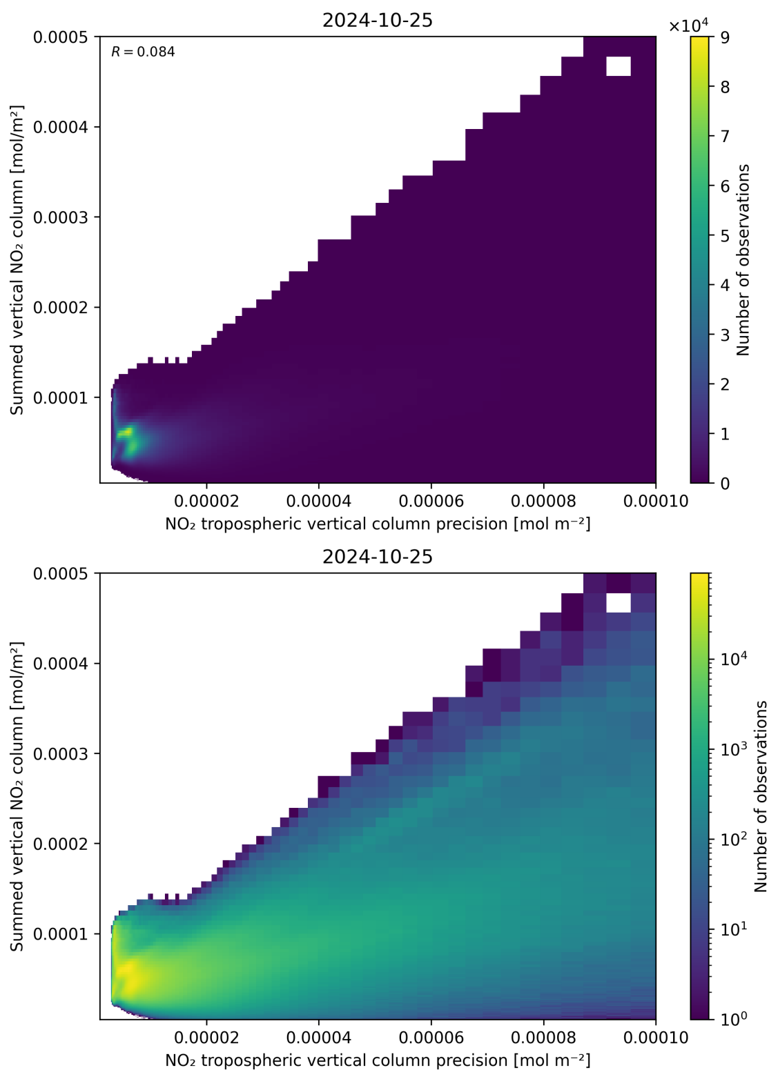
Figure 136: Scatter density plot of “NO 2 tropospheric vertical column precision” against “Summed vertical NO 2 column” for 2024-10-24 to 2024-10-26.
