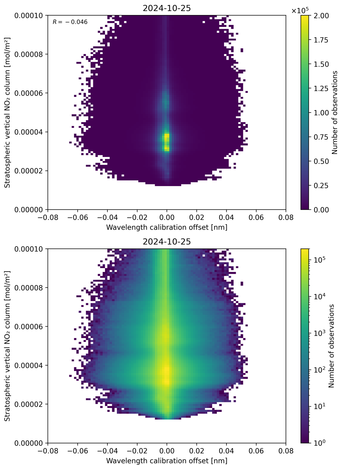
Figure 176: Scatter density plot of “Wavelength calibration offset” against “Stratospheric vertical NO 2 column” for 2024-10-24 to 2024-10-26.
