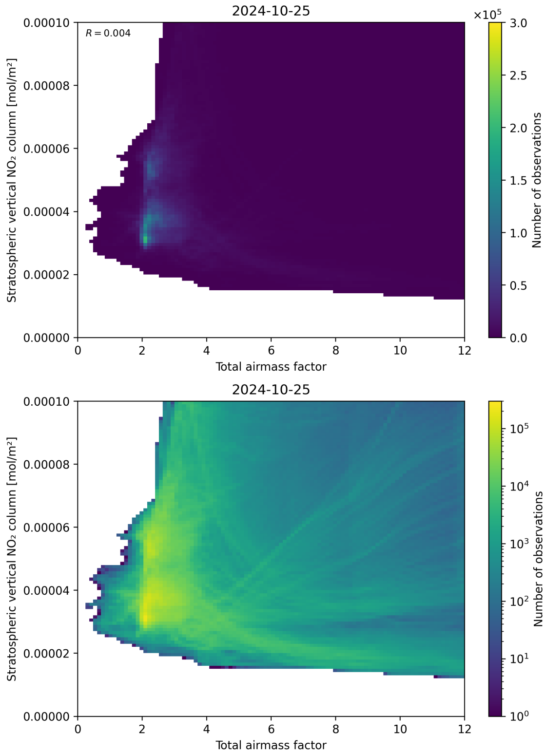
Figure 64: Scatter density plot of “Total airmass factor” against “Stratospheric vertical NO 2 column” for 2024-10-24 to 2024-10-26.
