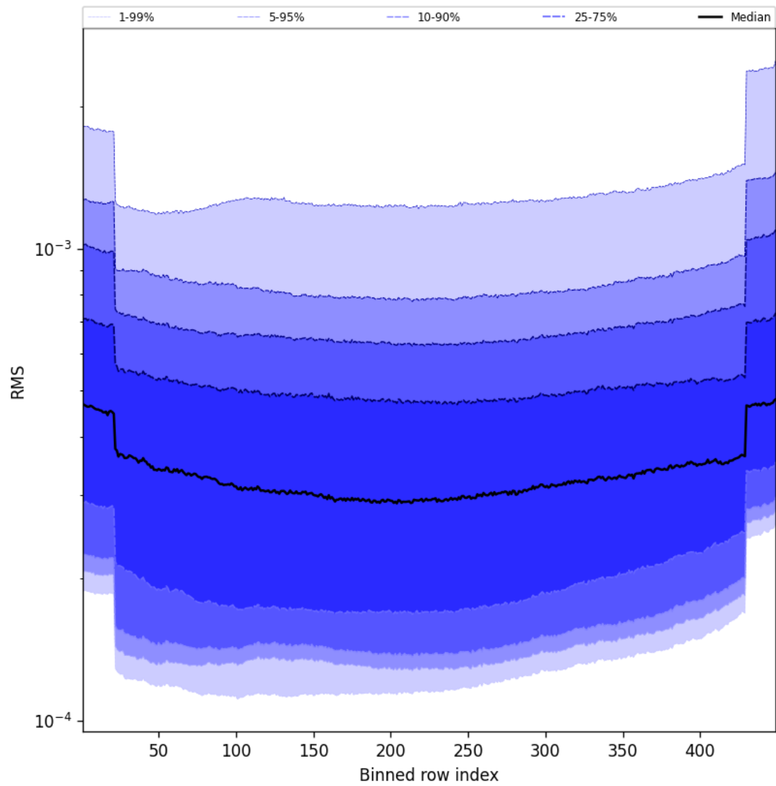
Figure 60: Along track statistics of “RMS” for 2024-10-24 to 2024-10-26
