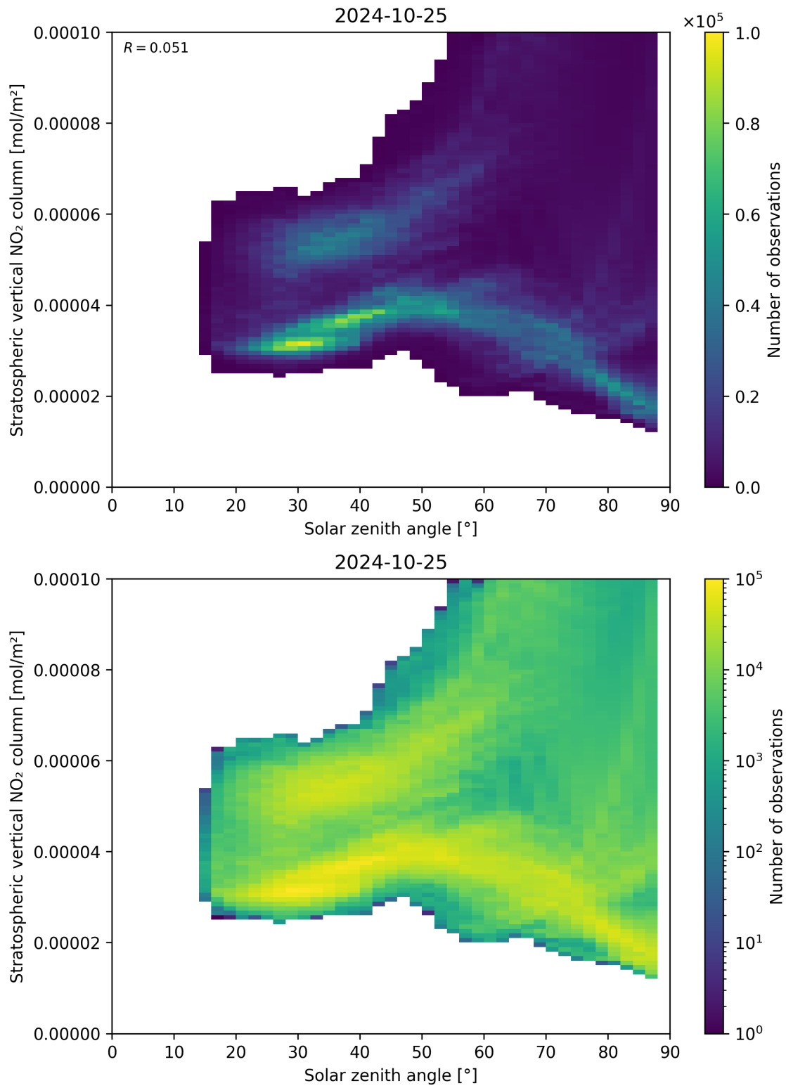
Figure 150: Scatter density plot of “Solar zenith angle” against “Stratospheric vertical NO 2 column” for 2024-10-24 to 2024-10-26.
