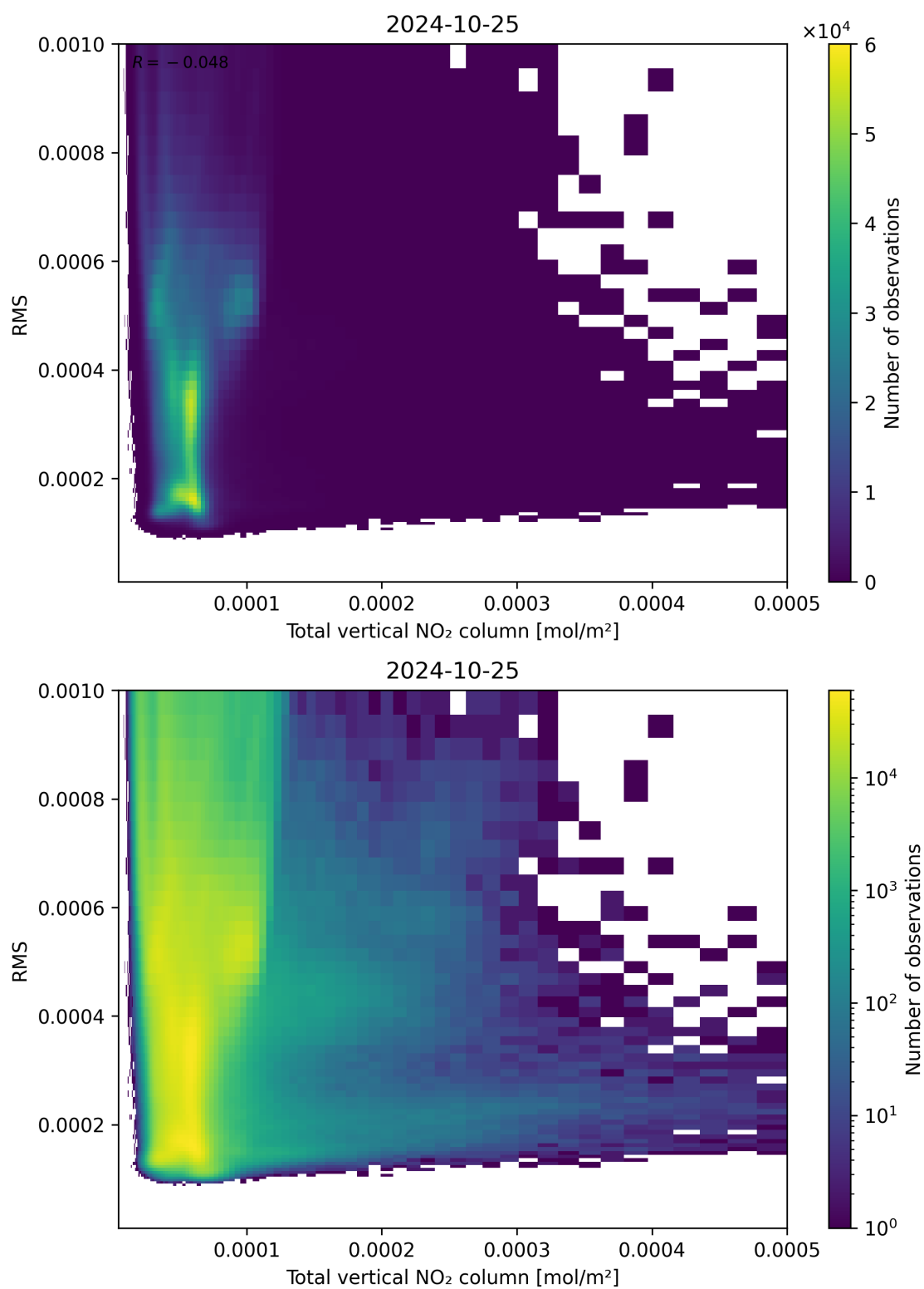
Figure 120: Scatter density plot of “Total vertical NO 2 column” against “RMS” for 2024-10-24 to 2024-10-26.
