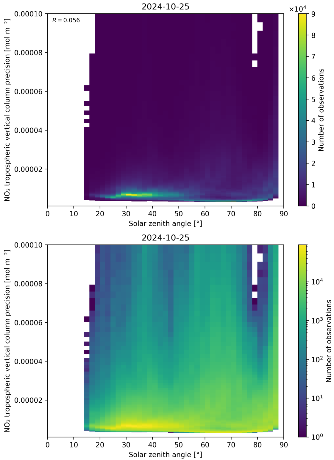
Figure 156: Scatter density plot of “Solar zenith angle” against “NO 2 tropospheric vertical column precision” for 2024-10-24 to 2024-10-26.
