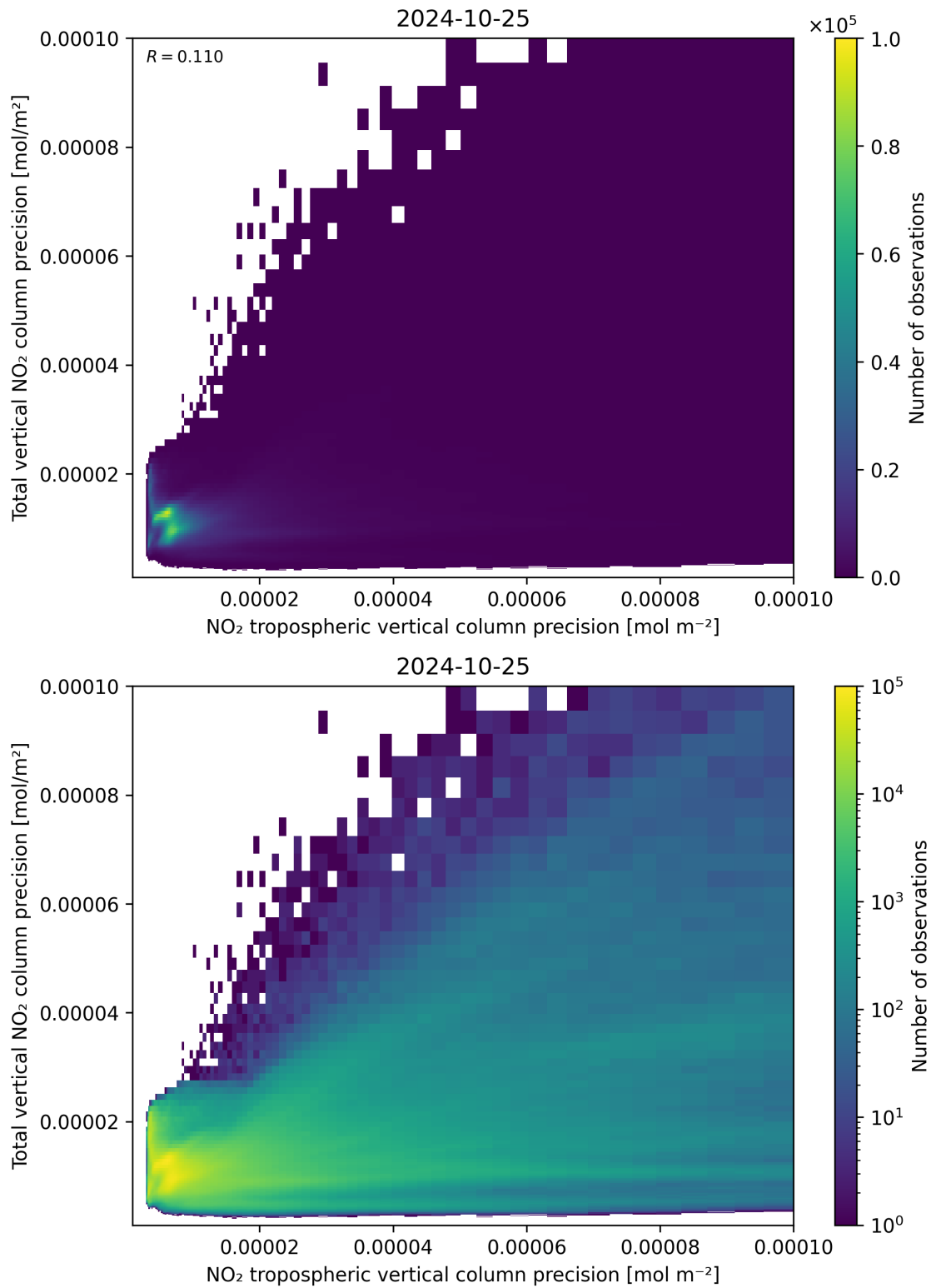
Figure 139: Scatter density plot of “NO 2 tropospheric vertical column precision” against “Total vertical NO 2 column precision” for 2024-10-24 to 2024-10-26.
