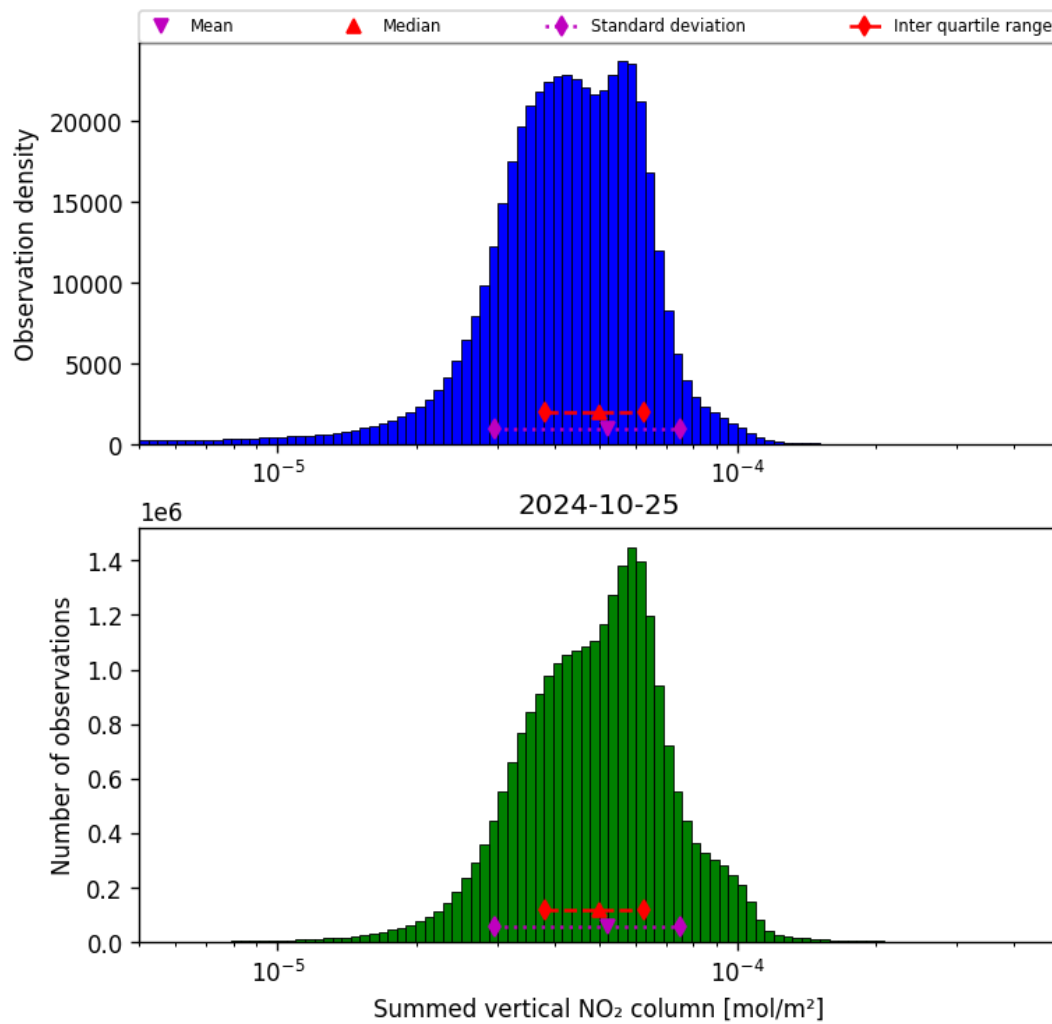
Figure 40: Histogram of “Summed vertical NO 2 column” for 2024-10-24 to 2024-10-26
