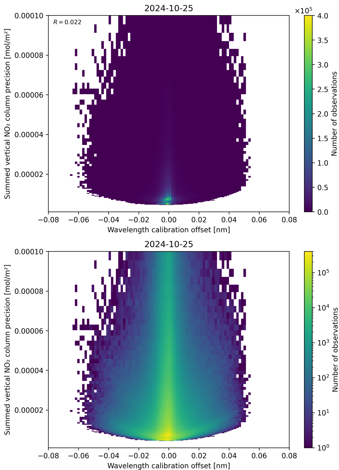
Figure 178: Scatter density plot of “Wavelength calibration offset” against “Summed vertical NO 2 column precision” for 2024-10-24 to 2024-10-26.
