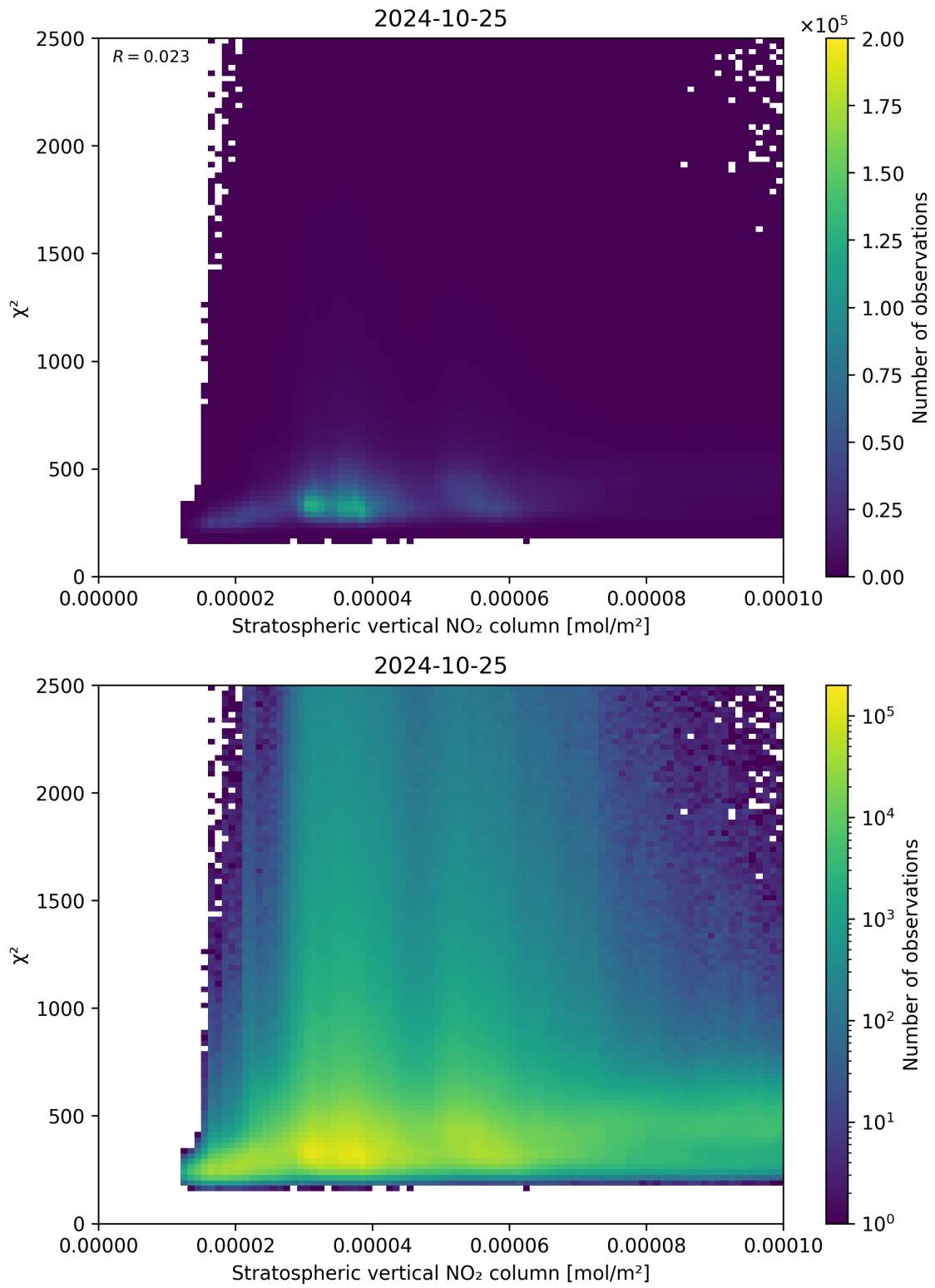
Figure 97: Scatter density plot of “Stratospheric vertical NO 2 column” against “ \chi^2 ” for 2024-10-24 to 2024-10-26.
