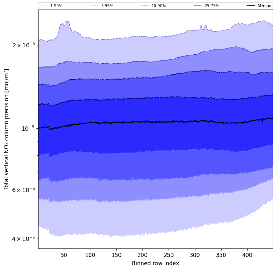
Figure 56: Along track statistics of "Total vertical NO 2 column precision" for 2024-10-24 to 2024-10-26
