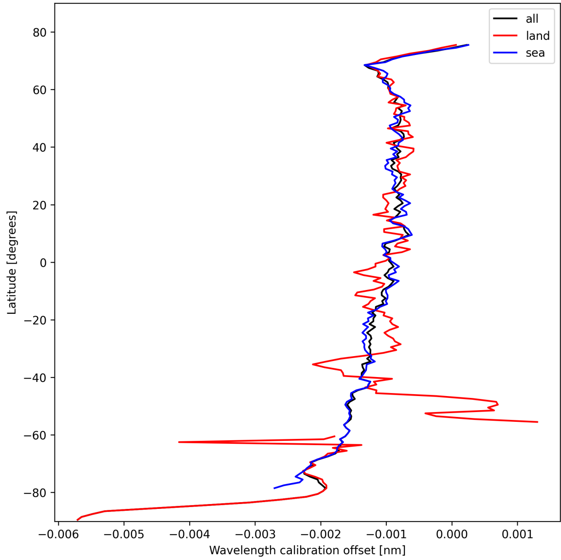
Figure 18: Zonal average of “Wavelength calibration offset” for 2024-10-24 to 2024-10-26.
