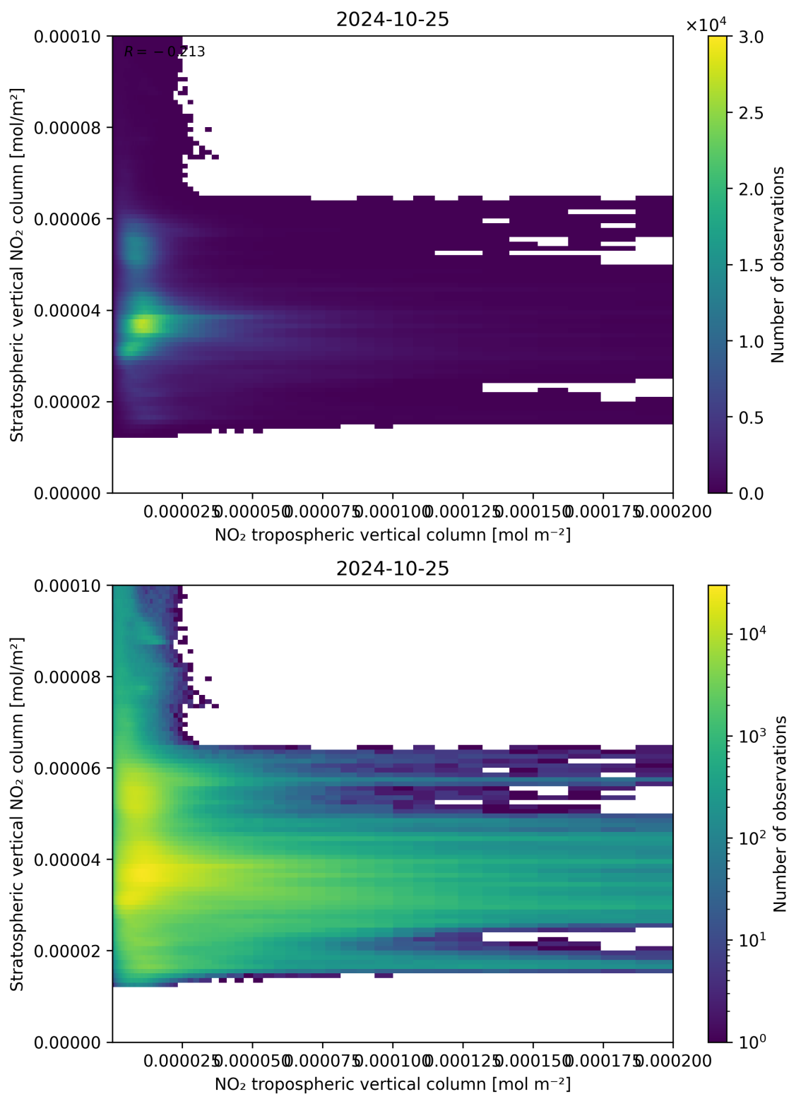
Figure 125: Scatter density plot of “NO 2 tropospheric vertical column” against “Stratospheric vertical NO 2 column” for 2024-10-24 to 2024-10-26.
