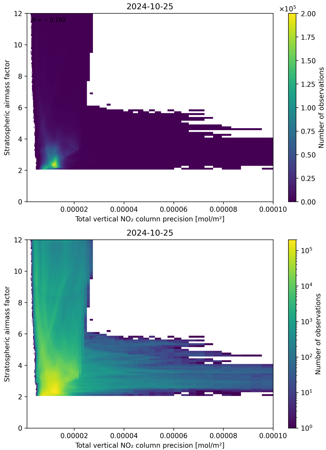
Figure 115: Scatter density plot of “Total vertical NO 2 column precision” against “Stratospheric air mass factor” for 2024-10-24 to 2024-10-26.
