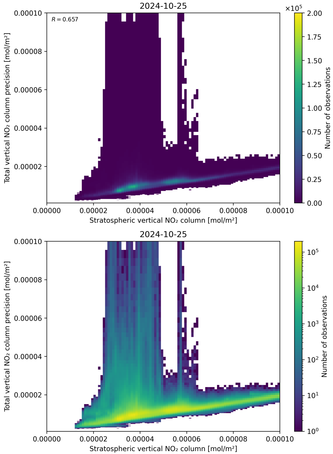
Figure 101: Scatter density plot of “Stratospheric vertical NO 2 column” against “Total vertical NO 2 column precision” for 2024-10-24 to 2024-10-26.
