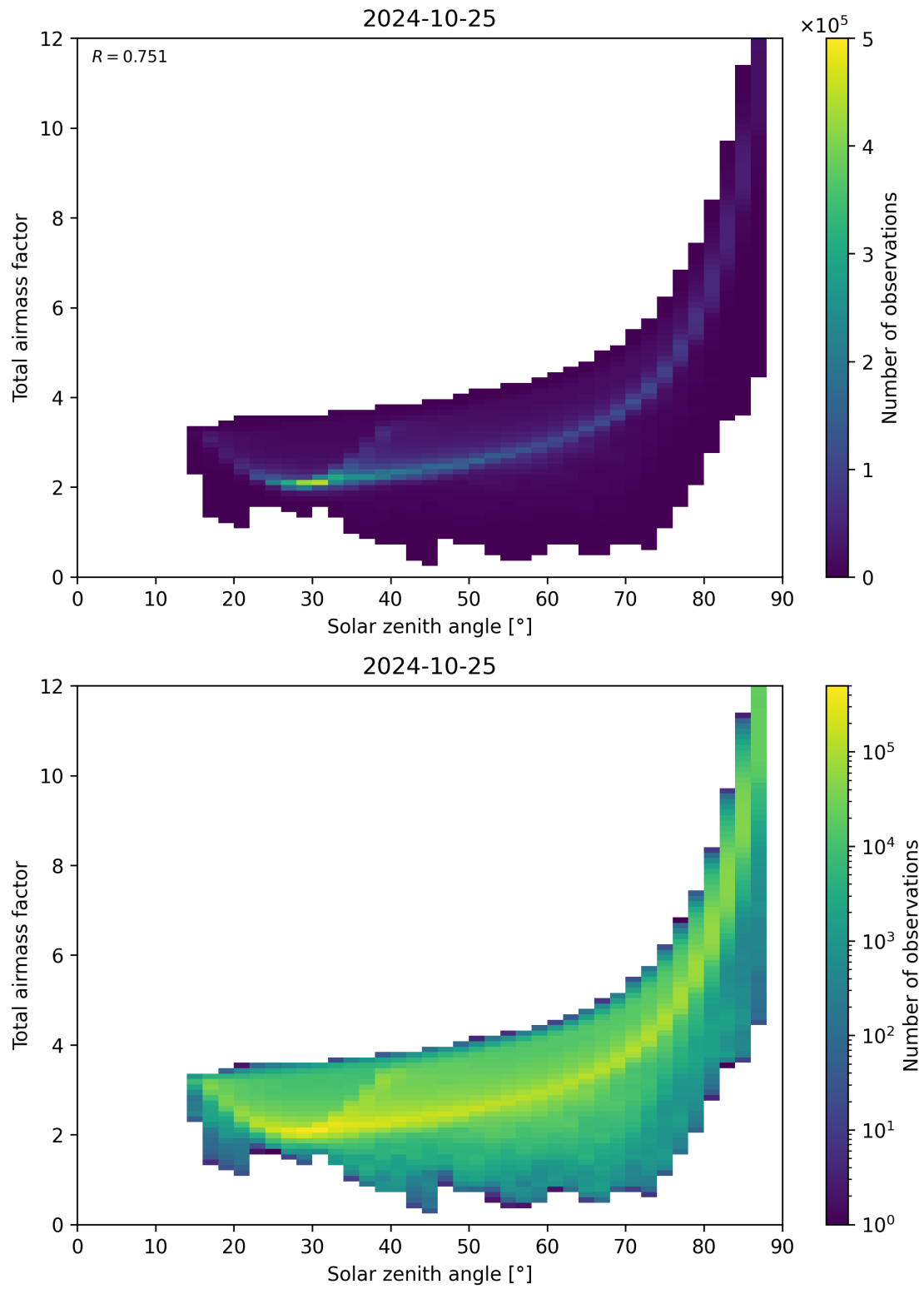
Figure 146: Scatter density plot of “Solar zenith angle” against “Total air mass factor” for 2024-10-24 to 2024-10-26.
