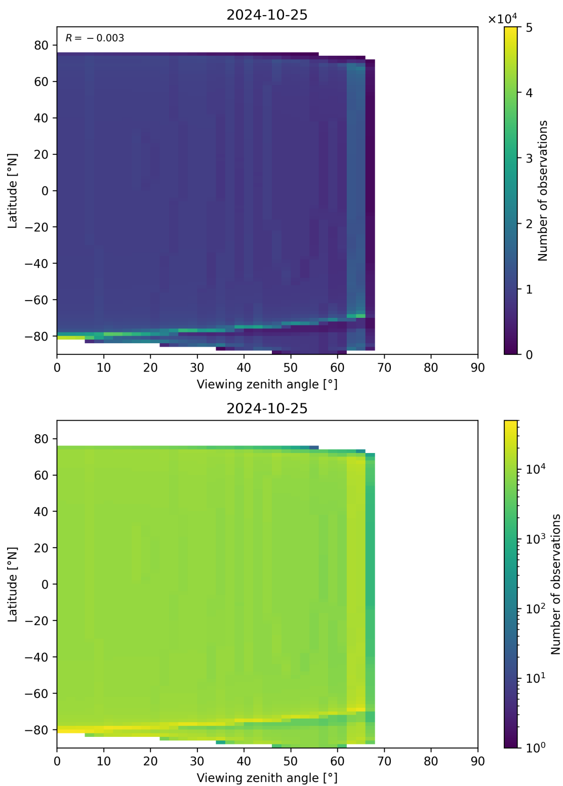
Figure 163: Scatter density plot of “Viewing zenith angle” against “Latitude” for 2024-10-24 to 2024-10-26.
