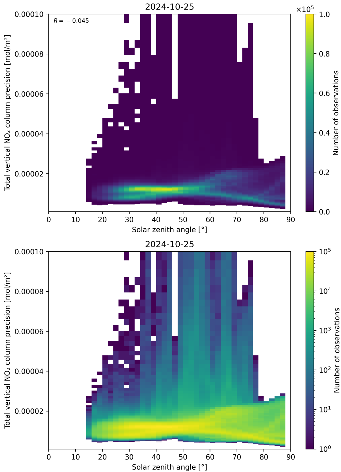
Figure 154: Scatter density plot of “Solar zenith angle” against “Total vertical NO 2 column precision” for 2024-10-24 to 2024-10-26.
