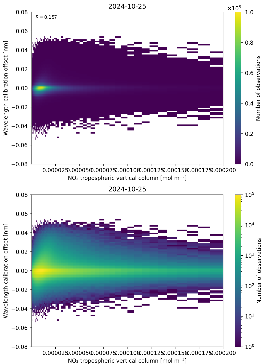
Figure 143: Scatter density plot of “NO 2 tropospheric vertical column” against “Wavelength calibration offset” for 2024-10-24 to 2024-10-26.
