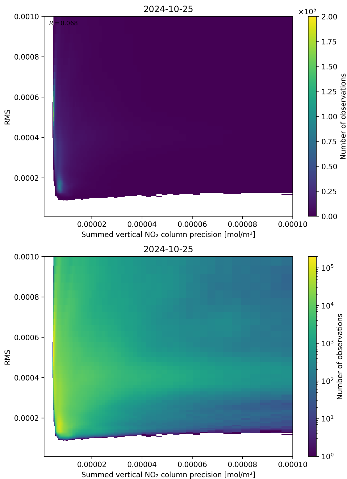
Figure 108: Scatter density plot of “Summed vertical NO 2 column precision” against “RMS” for 2024-10-24 to 2024-10-26.
