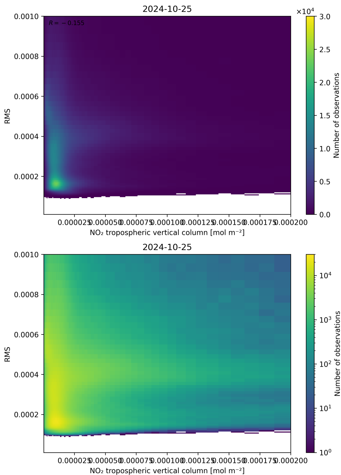
Figure 142: Scatter density plot of “NO 2 tropospheric vertical column” against “RMS” for 2024-10-24 to 2024-10-26.
