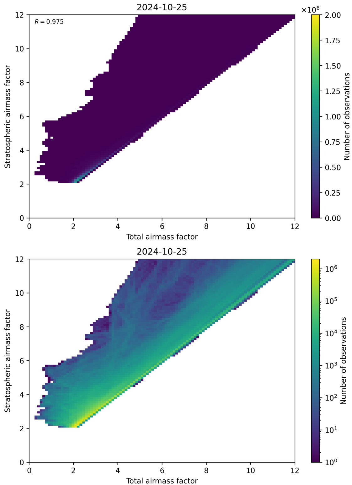
Figure 62: Scatter density plot of “Total airmass factor” against “Stratospheric airmass factor” for 2024-10-24 to 2024-10-26.
