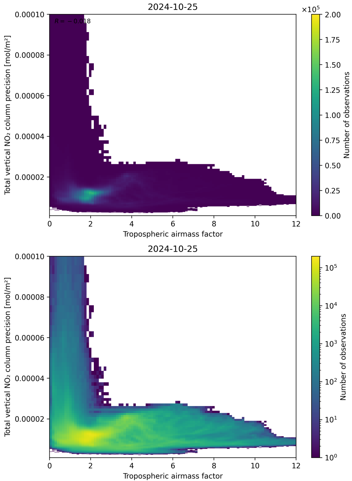
Figure 78: Scatter density plot of “Tropospheric air mass factor” against “Total vertical NO 2 column precision” for 2024-10-24 to 2024-10-26.
