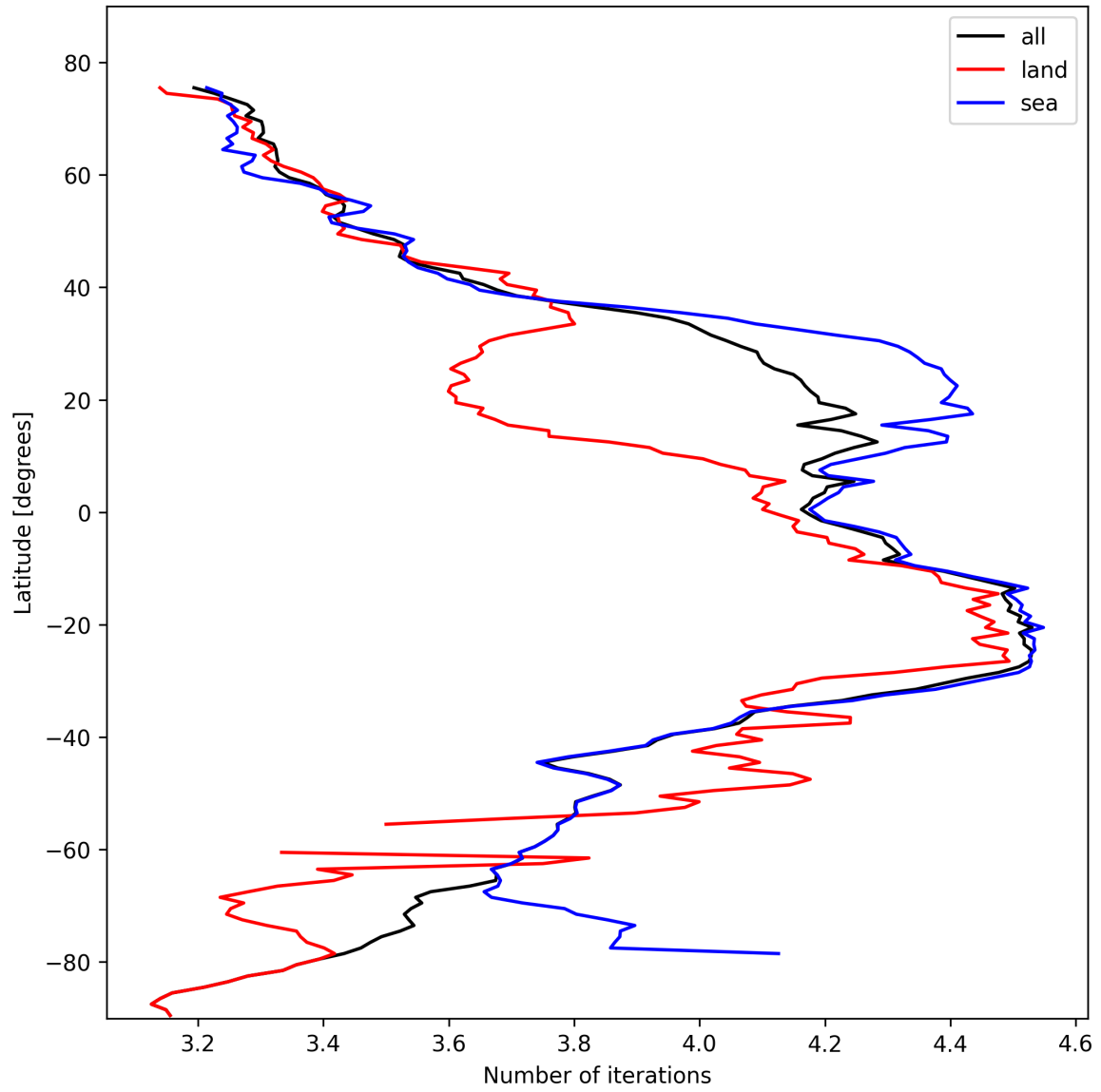
Figure 17: Zonal average of “Number of iterations” for 2024-10-24 to 2024-10-26.
