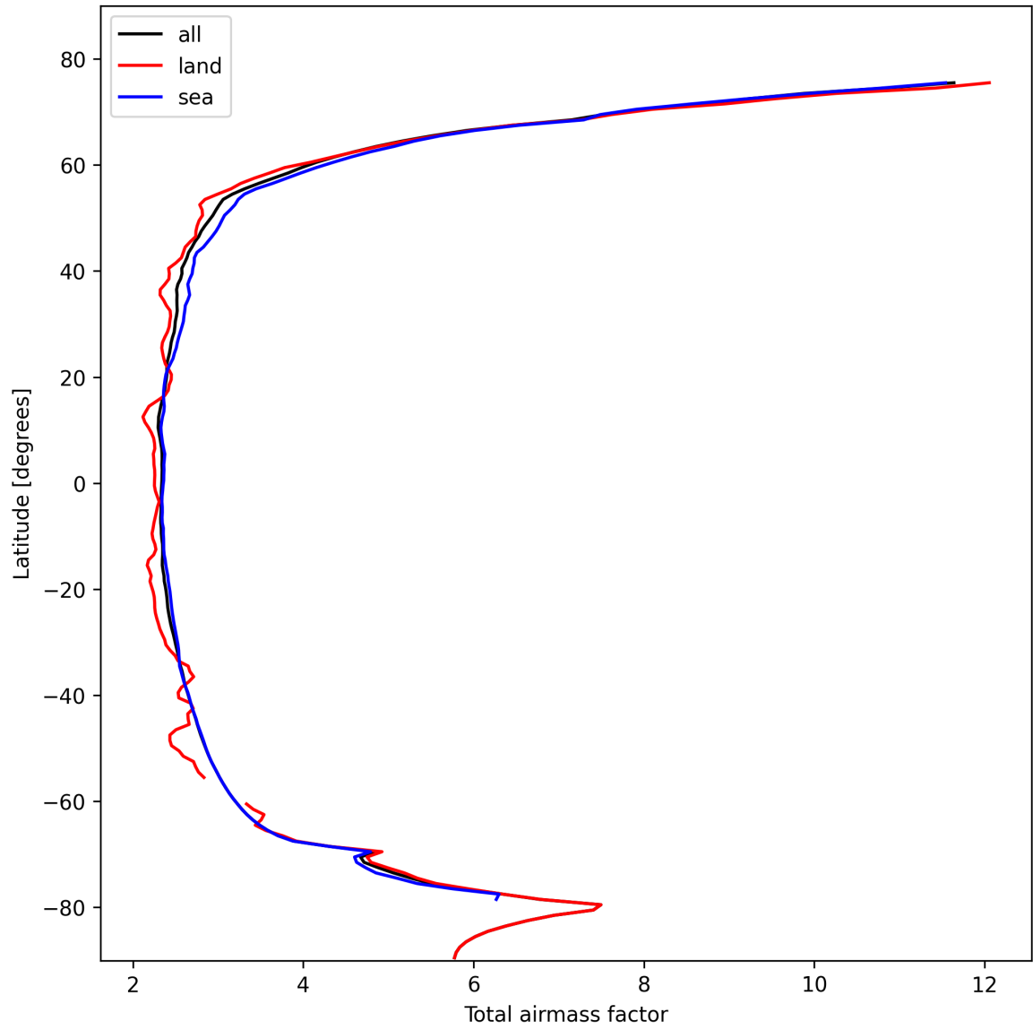
Figure 15: Zonal average of “Total airmass factor” for 2024-10-24 to 2024-10-26.
