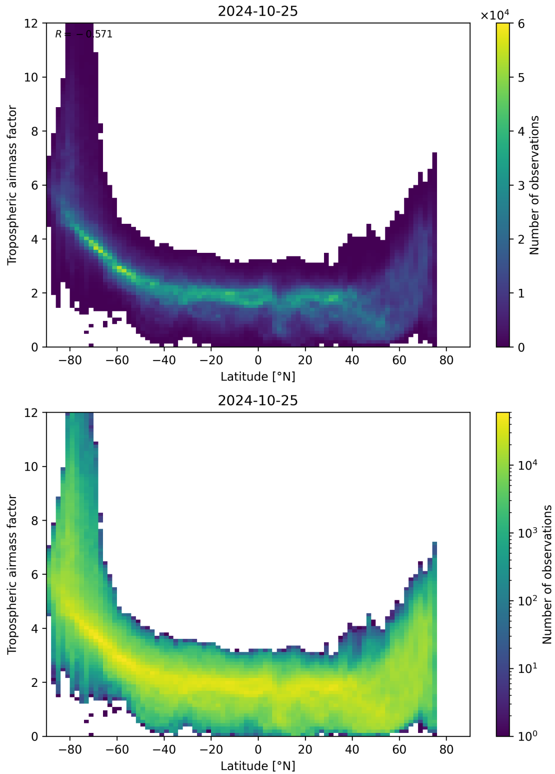
Figure 85: Scatter density plot of “Latitude” against “Tropospheric airmass factor” for 2024-10-24 to 2024-10-26.
