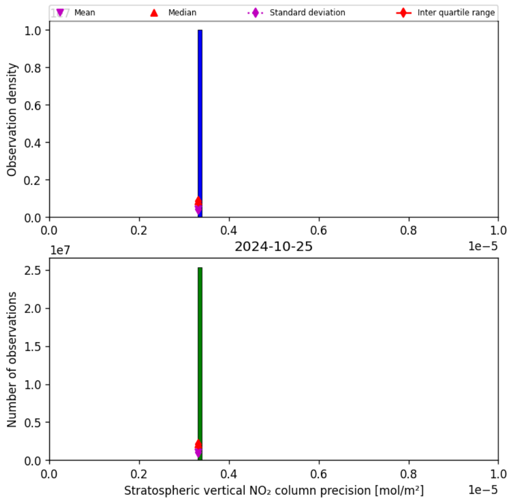
Figure 37: Histogram of “Stratospheric vertical NO 2 column precision” for 2024-10-24 to 2024-10-26
