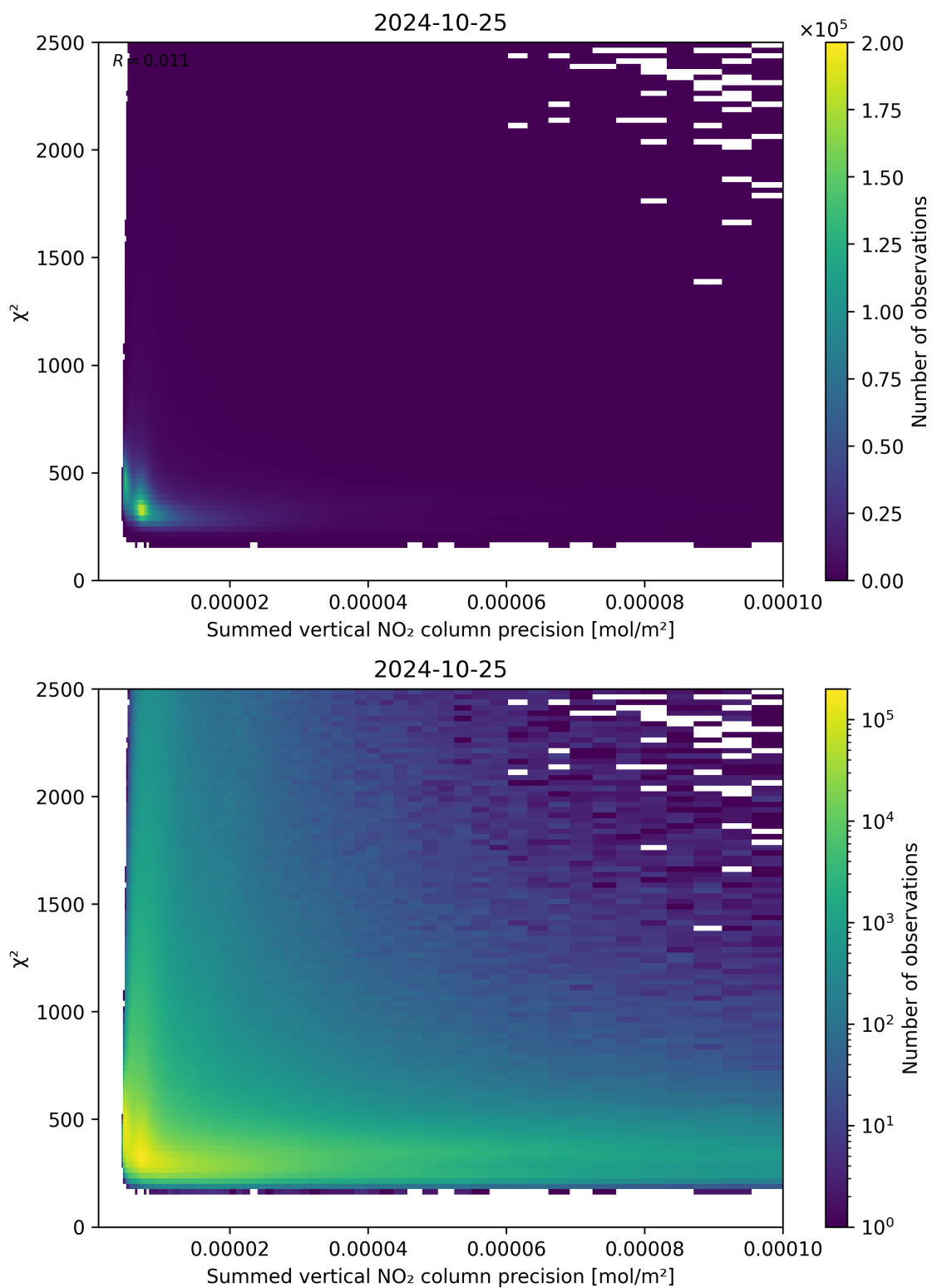
Figure 107: Scatter density plot of “Summed vertical NO 2 column precision” against “ \chi^2 ” for 2024-10-24 to 2024-10-26.
