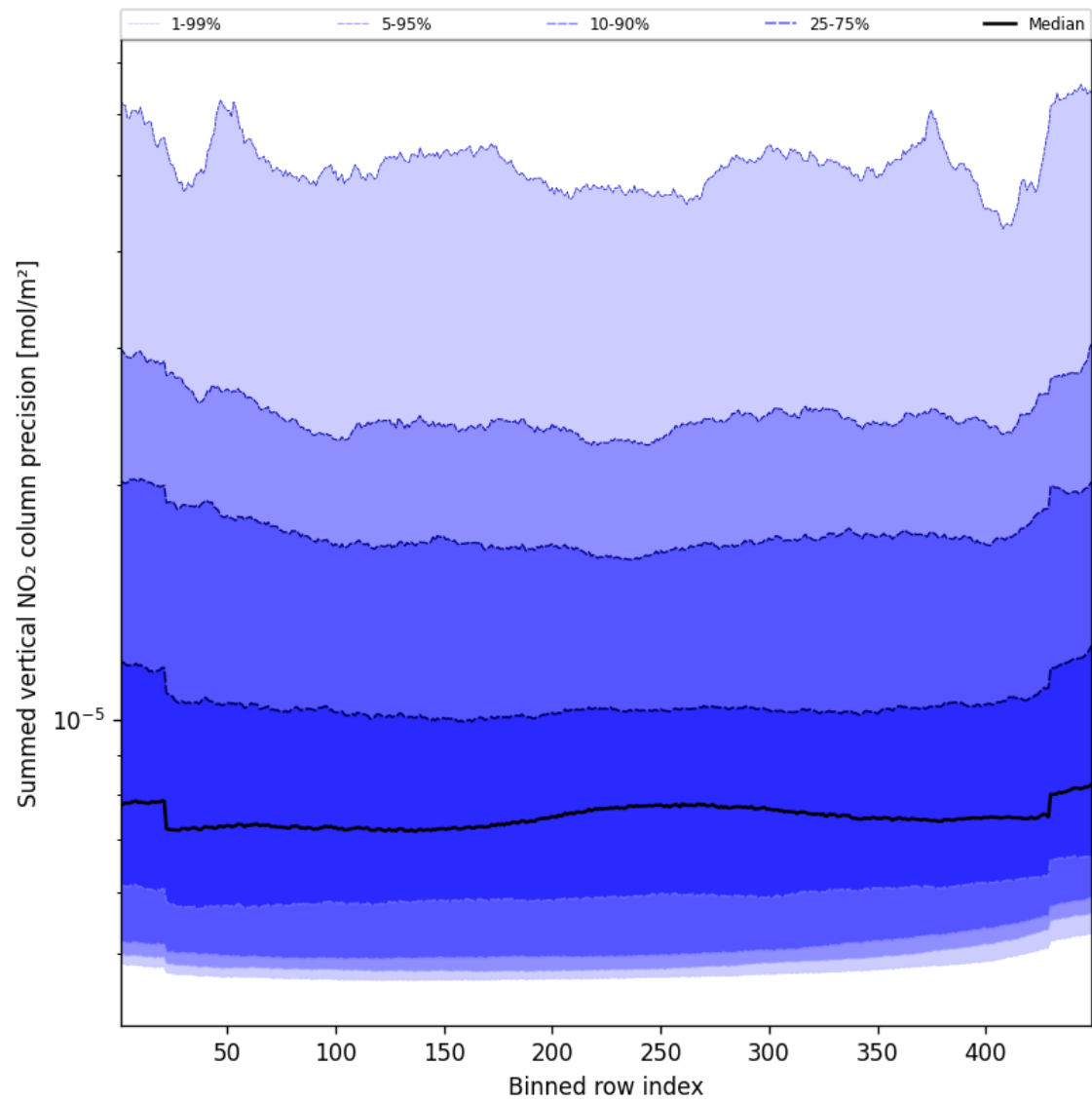
Figure 58: Along track statistics of “Summed vertical NO 2 column precision” for 2024-10-24 to 2024-10-26
