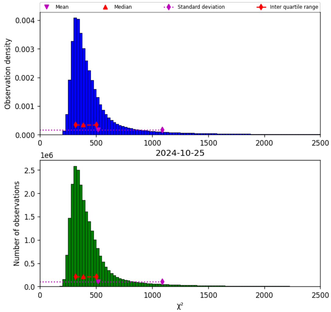
Figure 42: Histogram of “ \chi^2 ” for 2024-10-24 to 2024-10-26
