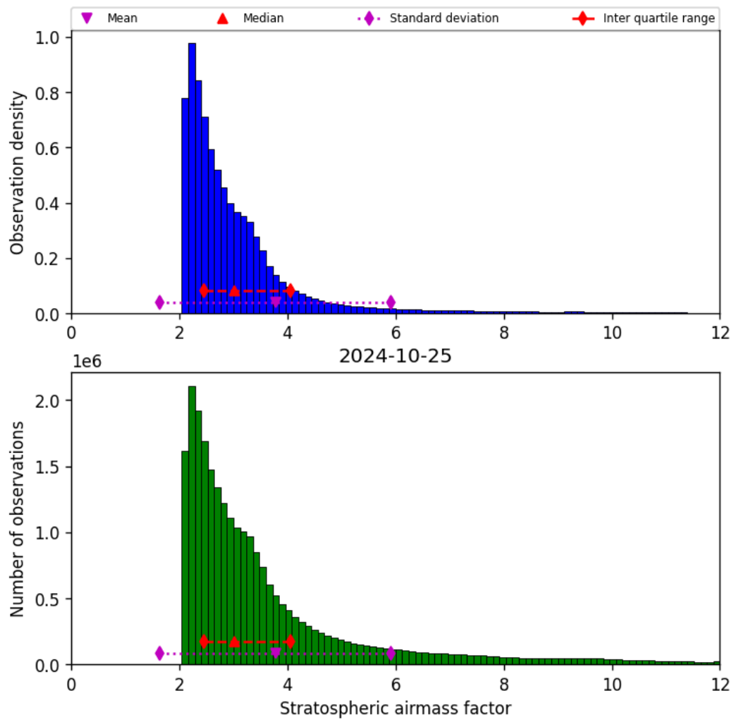
Figure 44: Histogram of “Stratospheric airmass factor” for 2024-10-24 to 2024-10-26
