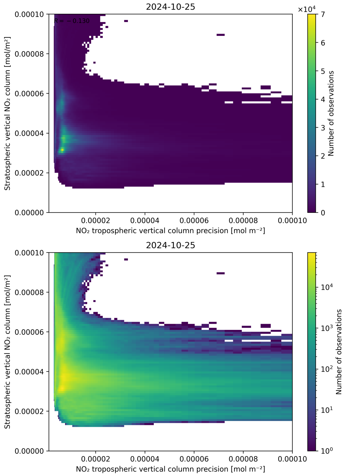
Figure 135: Scatter density plot of “NO 2 tropospheric vertical column precision” against “Stratospheric vertical NO 2 column” for 2024-10-24 to 2024-10-26.
