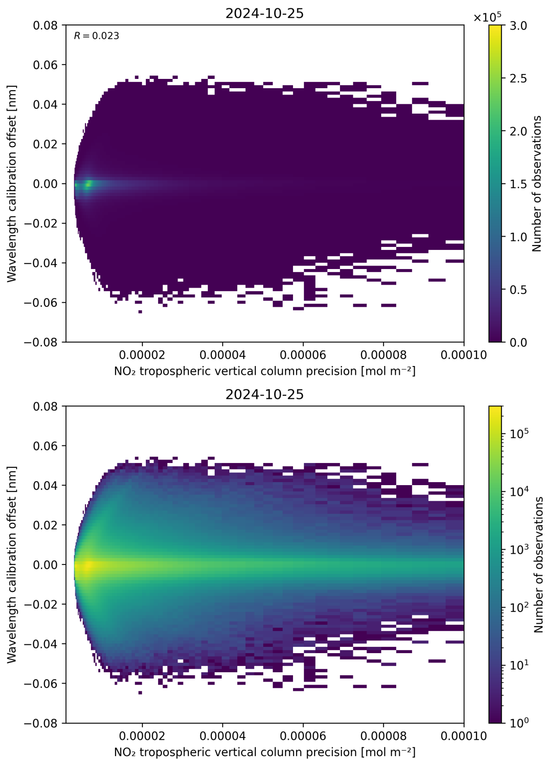
Figure 141: Scatter density plot of “NO 2 tropospheric vertical column precision” against “Wavelength calibration offset” for 2024-10-24 to 2024-10-26.
