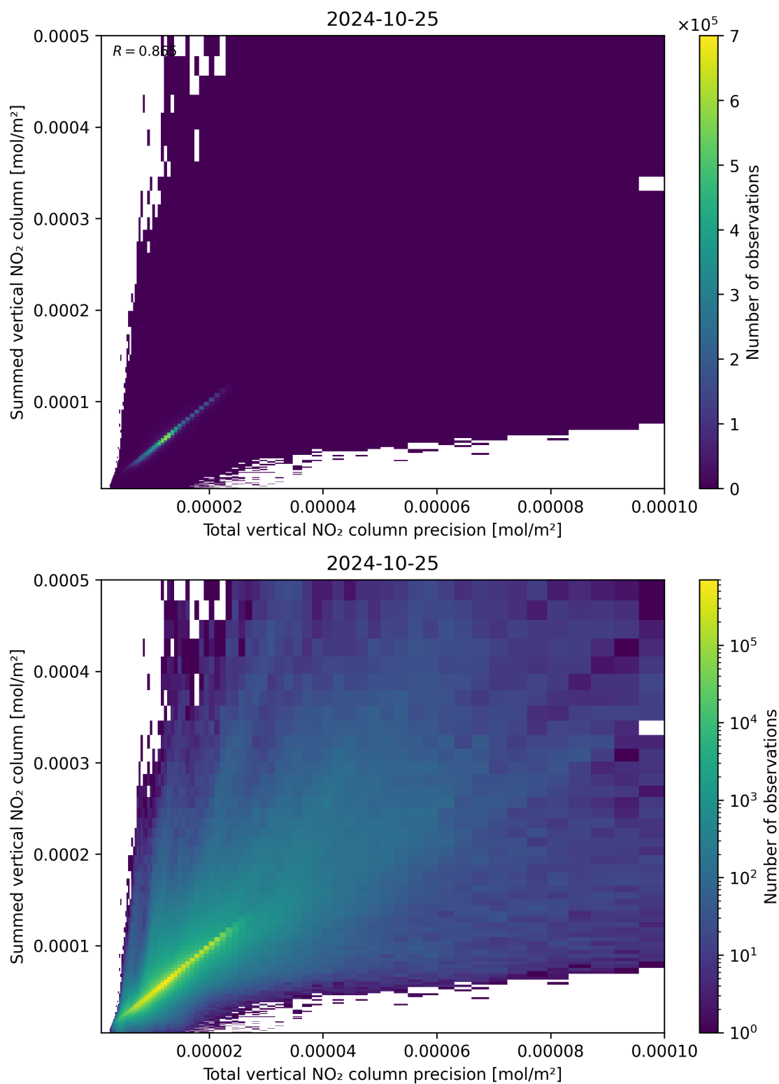
Figure 117: Scatter density plot of “Total vertical NO 2 column precision” against “Summed vertical NO 2 column” for 2024-10-24 to 2024-10-26.
