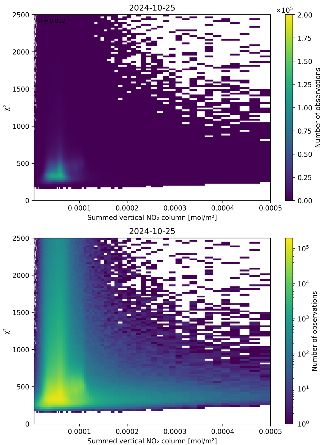
Figure 104: Scatter density plot of “Summed vertical NO 2 column” against “ \chi^2 ” for 2024-10-24 to 2024-10-26.
