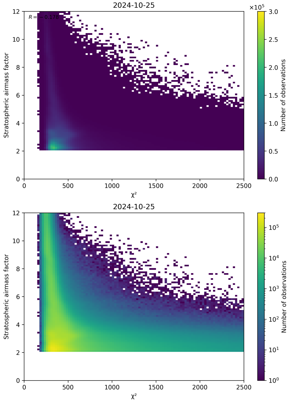
Figure 81: Scatter density plot of “ \chi^2 ” against “Stratospheric airmass factor” for 2024-10-24 to 2024-10-26.
