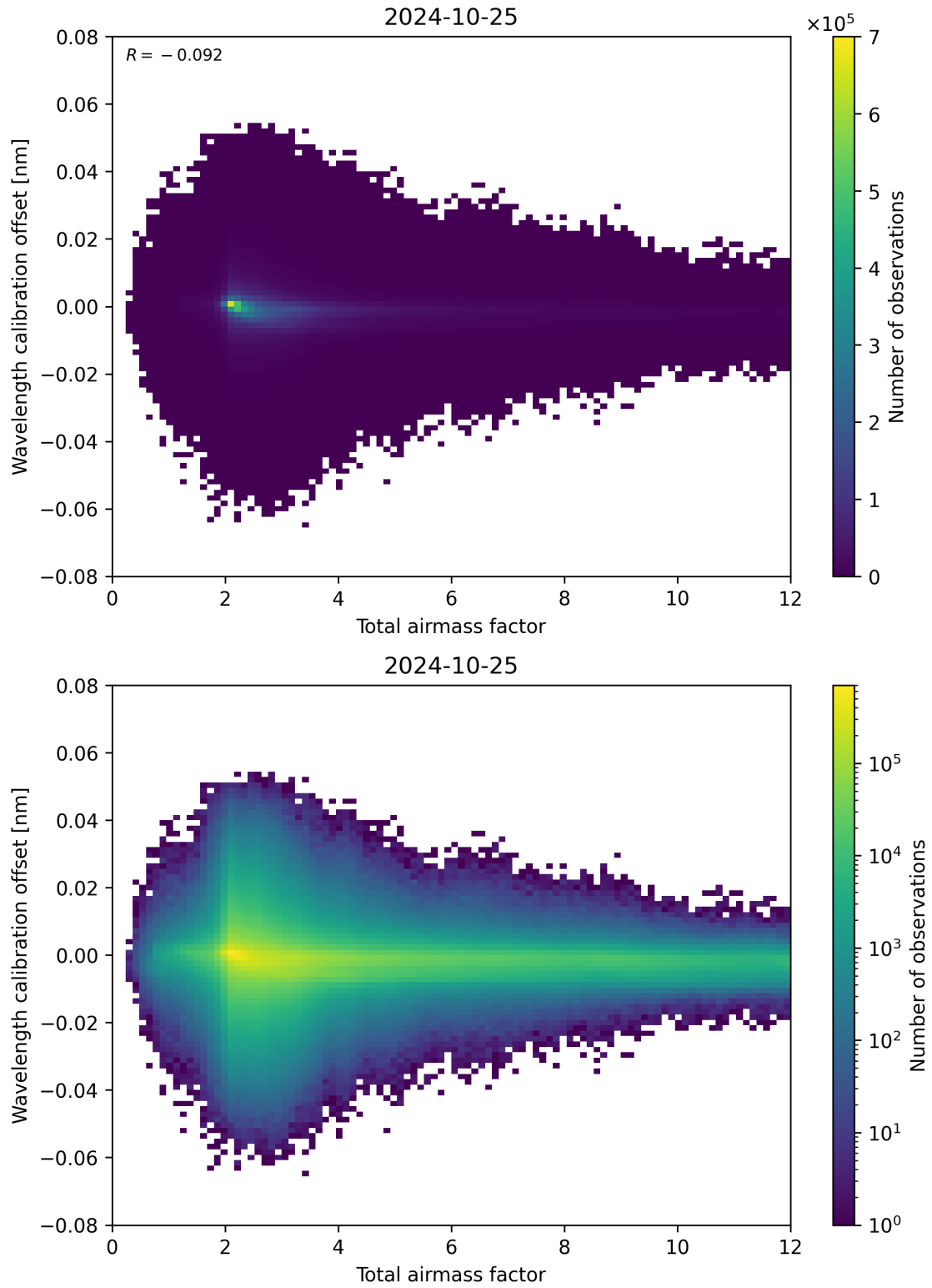
Figure 70: Scatter density plot of “Total airmass factor” against “Wavelength calibration offset” for 2024-10-24 to 2024-10-26.
