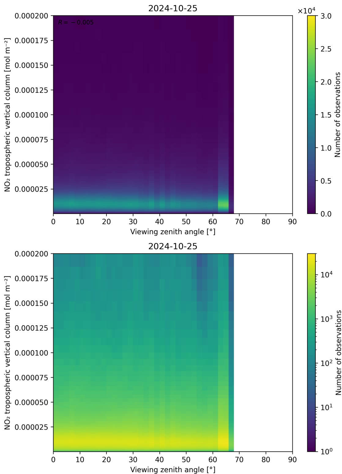
Figure 169: Scatter density plot of “Viewing zenith angle” against “NO 2 tropospheric vertical column” for 2024-10-24 to 2024-10-26.
