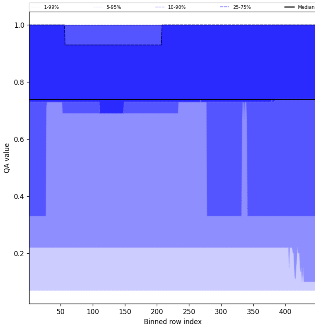
Figure 45: Along track statistics of “QA value” for 2024-10-24 to 2024-10-26
