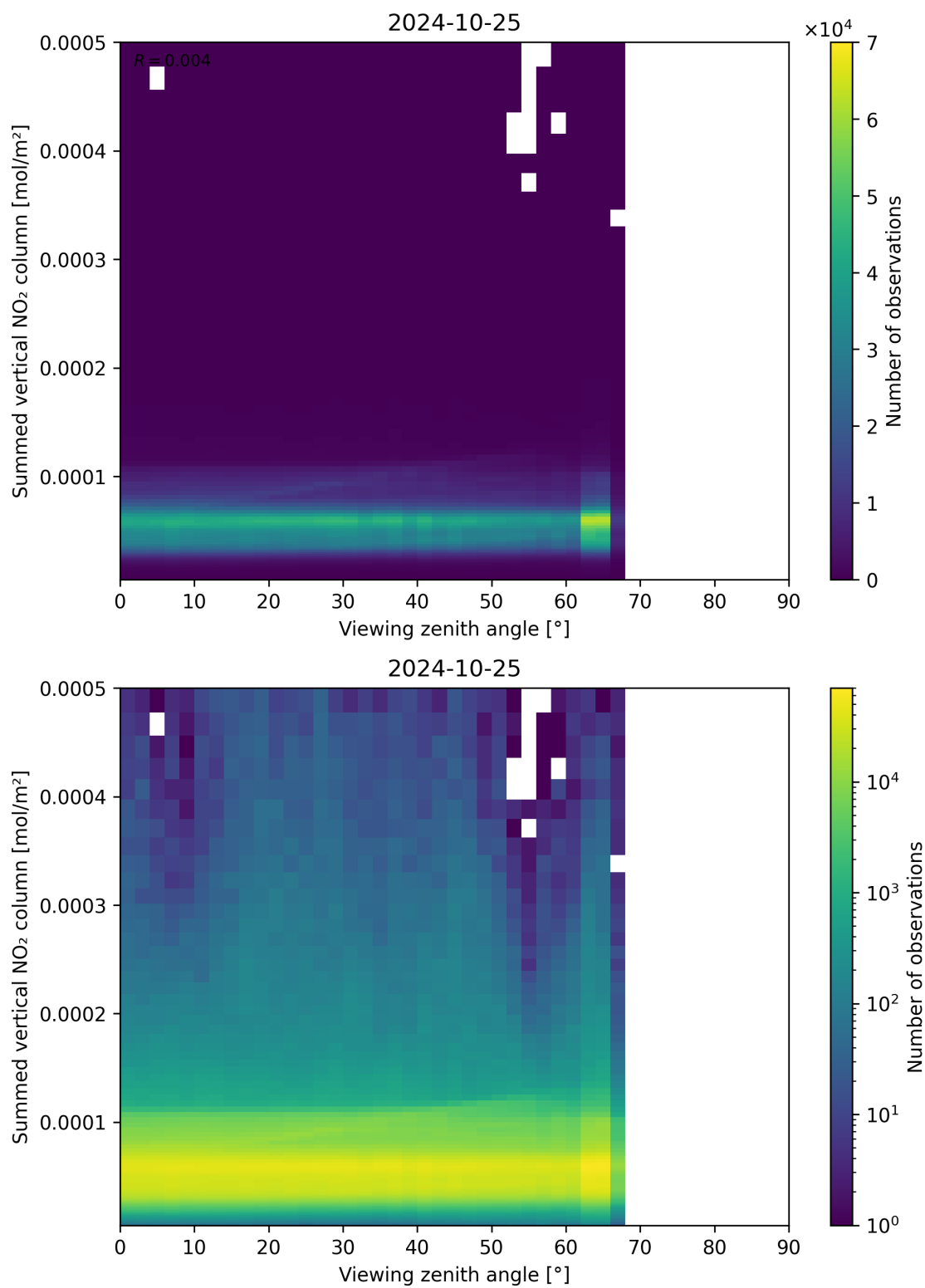
Figure 165: Scatter density plot of “Viewing zenith angle” against “Summed vertical NO 2 column” for 2024-10-24 to 2024-10-26.
