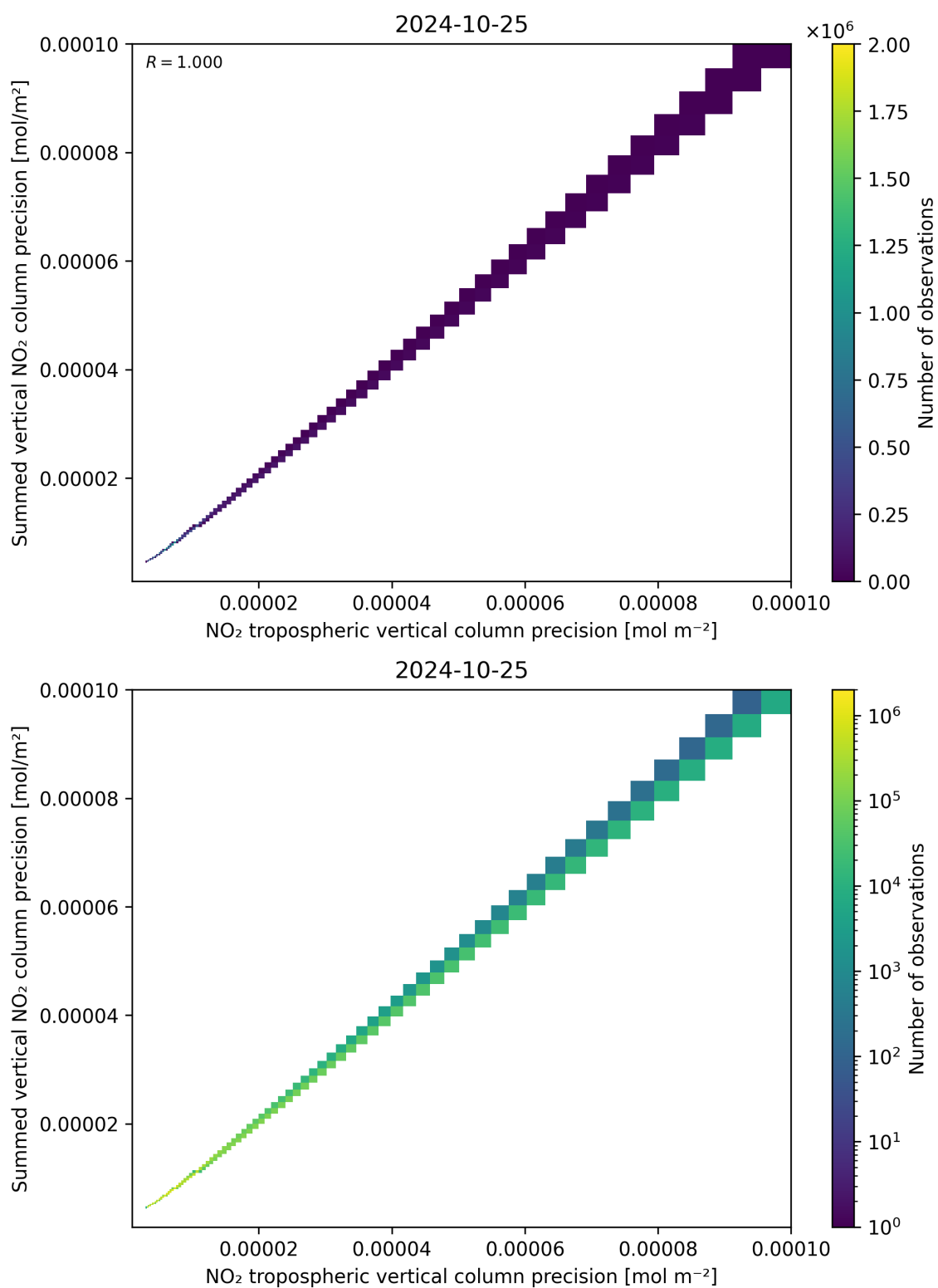
Figure 137: Scatter density plot of “NO 2 tropospheric vertical column precision” against “Summed vertical NO 2 column precision” for 2024-10-24 to 2024-10-26.
