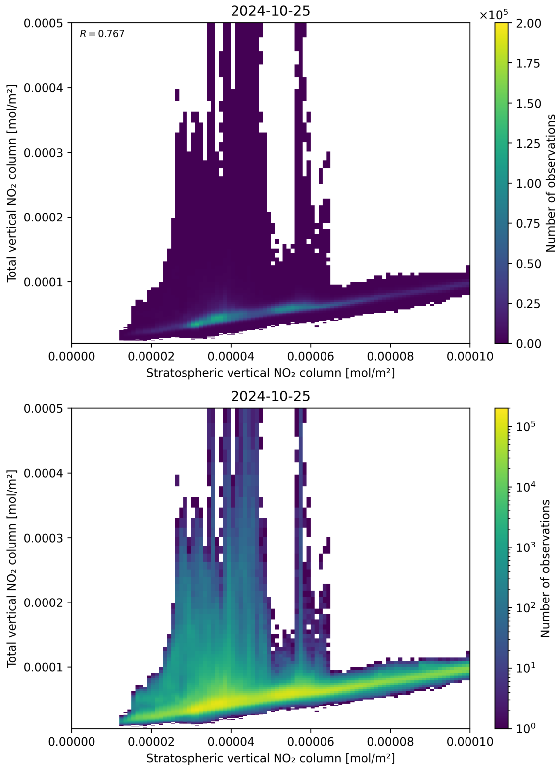
Figure 100: Scatter density plot of “Stratospheric vertical NO 2 column” against “Total vertical NO 2 column” for 2024-10-24 to 2024-10-26.
