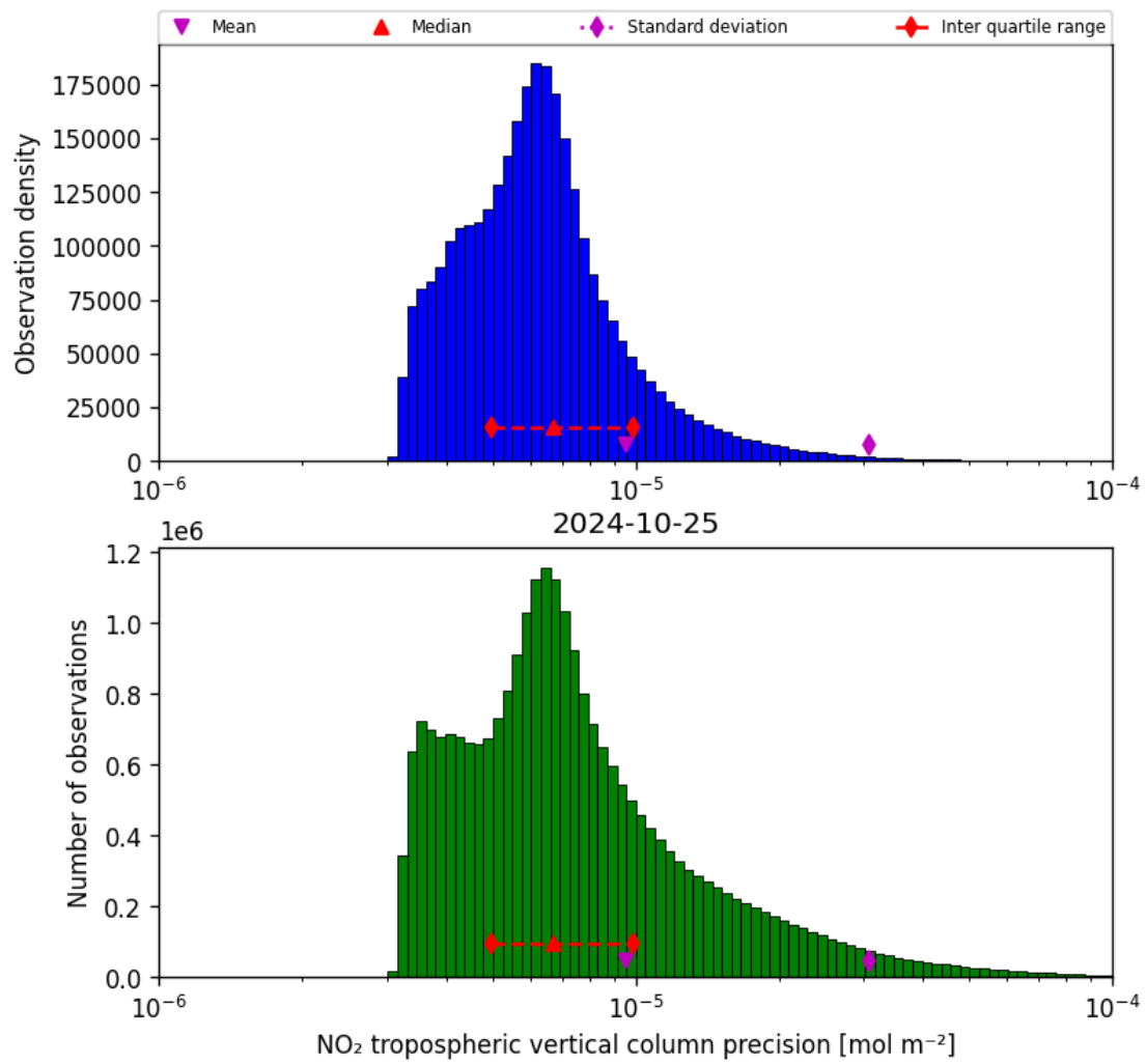
Figure 30: Histogram of “NO 2 tropospheric vertical column precision” for 2024-10-24 to 2024-10-26
