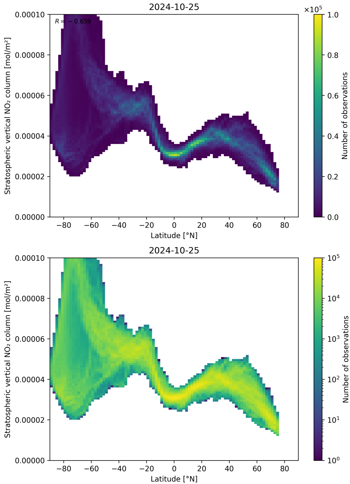
Figure 87: Scatter density plot of “Latitude” against “Stratospheric vertical NO 2 column” for 2024-10-24 to 2024-10-26.
