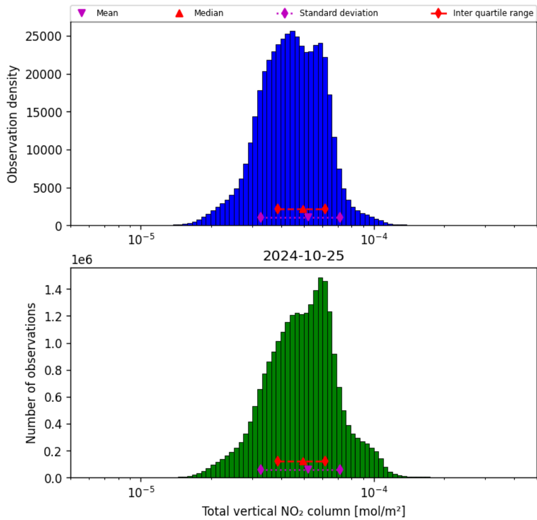
Figure 38: Histogram of “Total vertical NO 2 column” for 2024-10-24 to 2024-10-26
