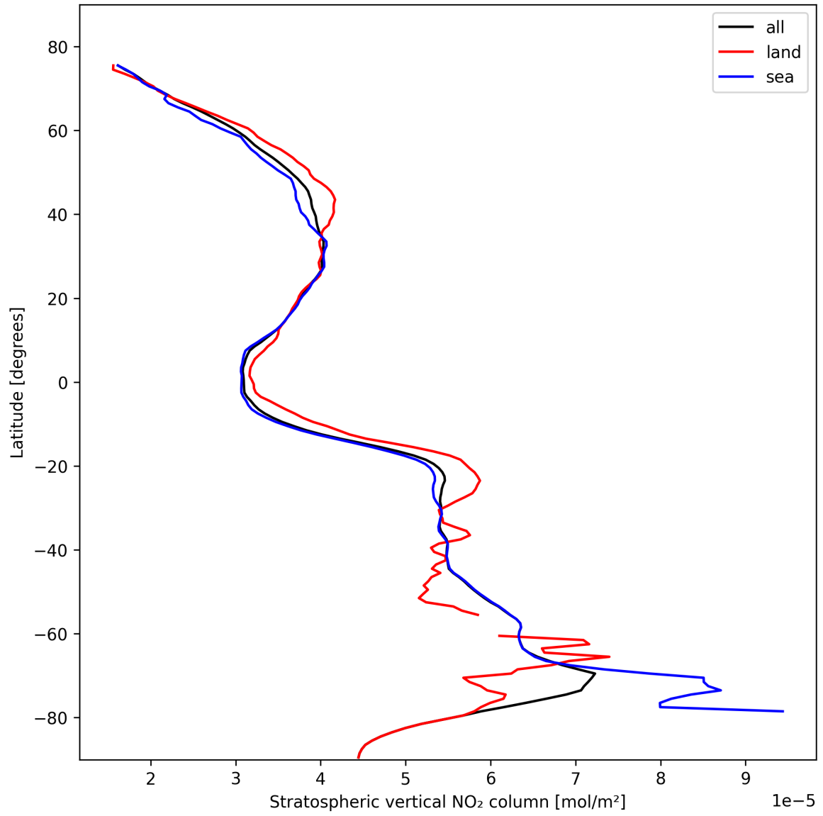
Figure 19: Zonal average of “Stratospheric vertical NO 2 column” for 2024-10-24 to 2024-10-26.
