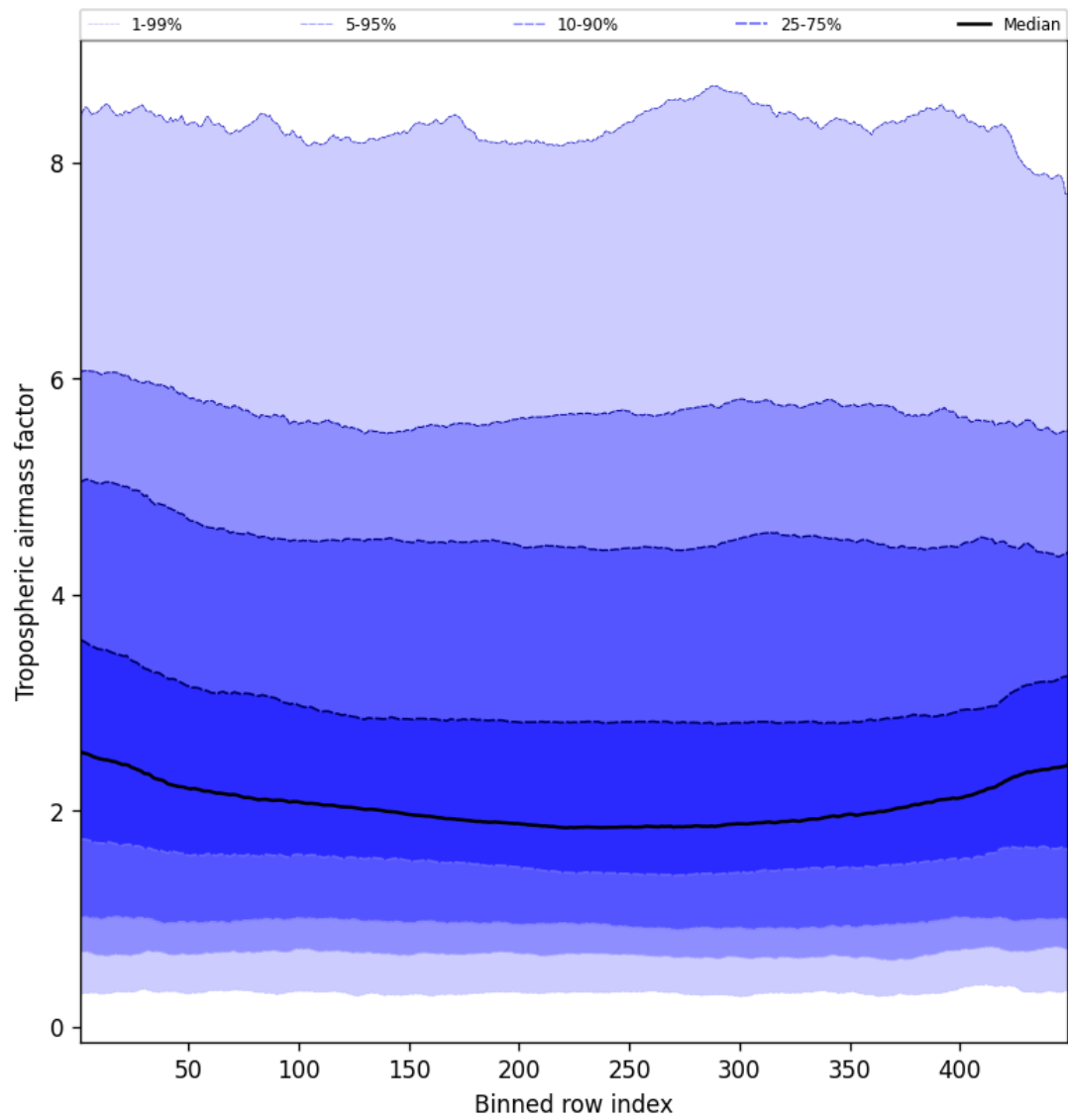
Figure 48: Along track statistics of “Tropospheric air mass factor” for 2024-10-24 to 2024-10-26
