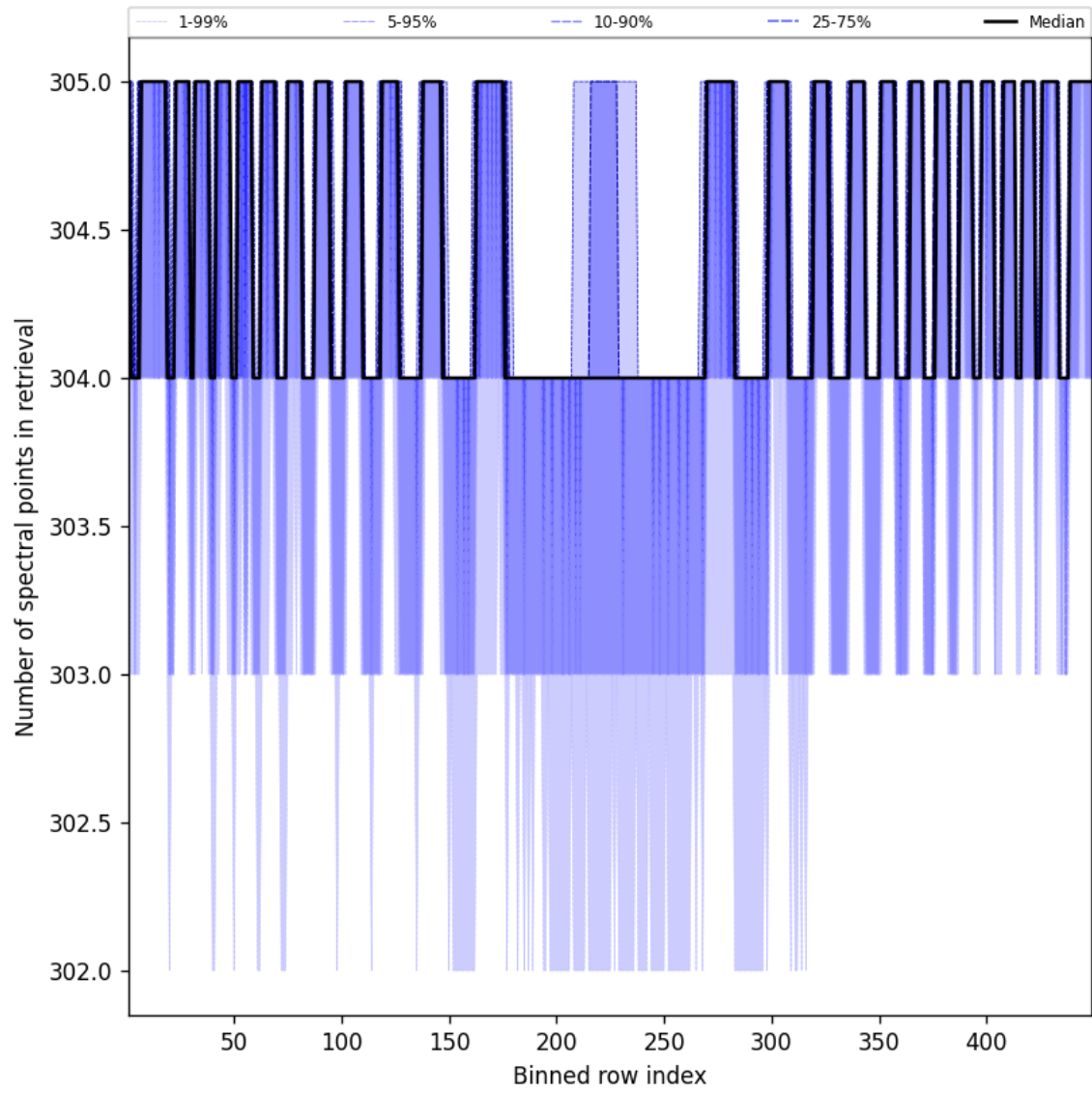
Figure 50: Along track statistics of “Number of spectral points in retrieval” for 2024-10-24 to 2024-10-26
