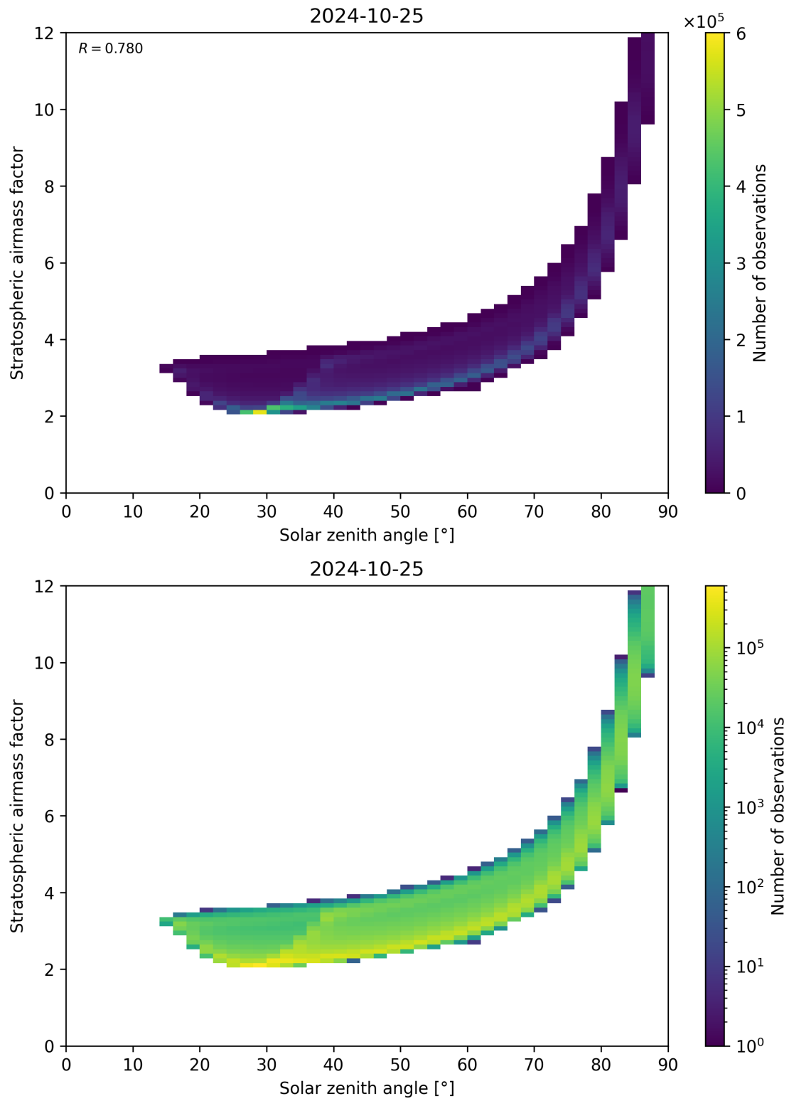
Figure 145: Scatter density plot of “Solar zenith angle” against “Stratospheric airmass factor” for 2024-10-24 to 2024-10-26.
