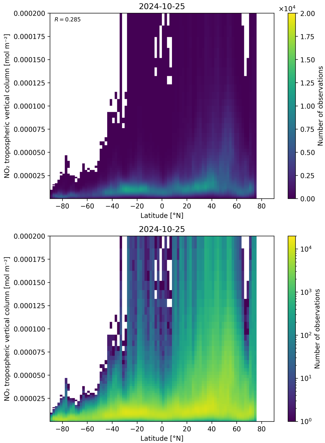
Figure 92: Scatter density plot of “Latitude” against “NO 2 tropospheric vertical column” for 2024-10-24 to 2024-10-26.
