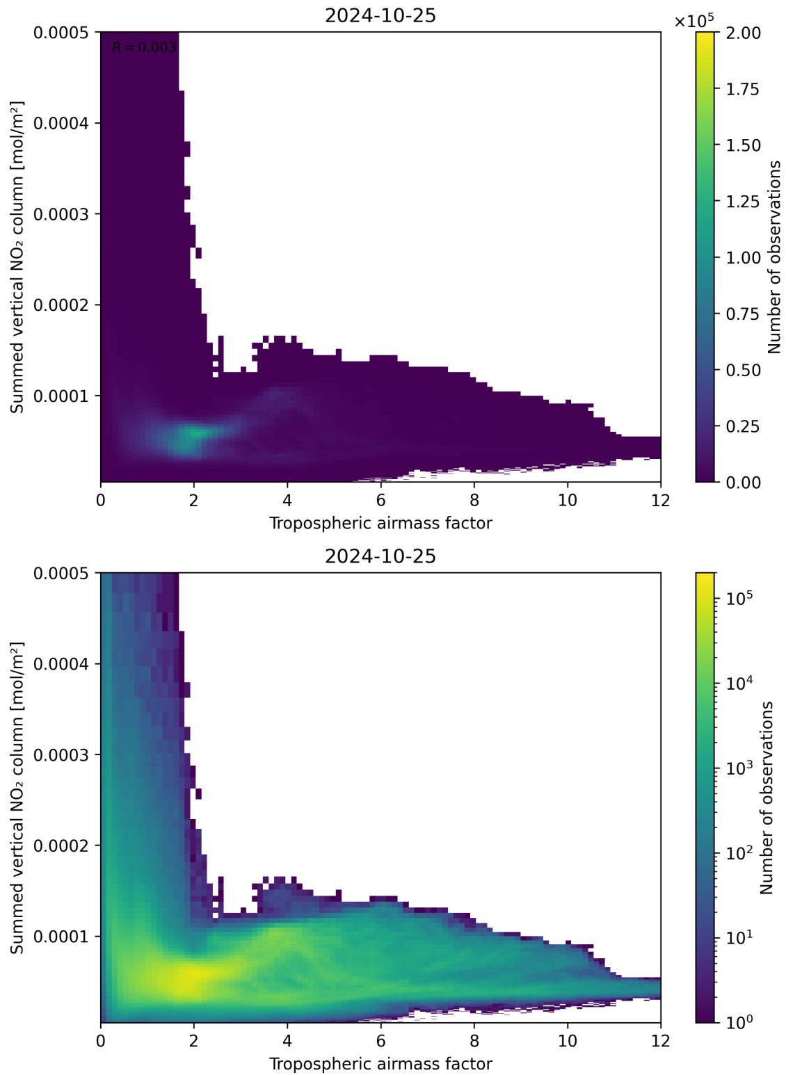
Figure 75: Scatter density plot of “Tropospheric air mass factor” against “Summed vertical NO 2 column” for 2024-10-24 to 2024-10-26.
