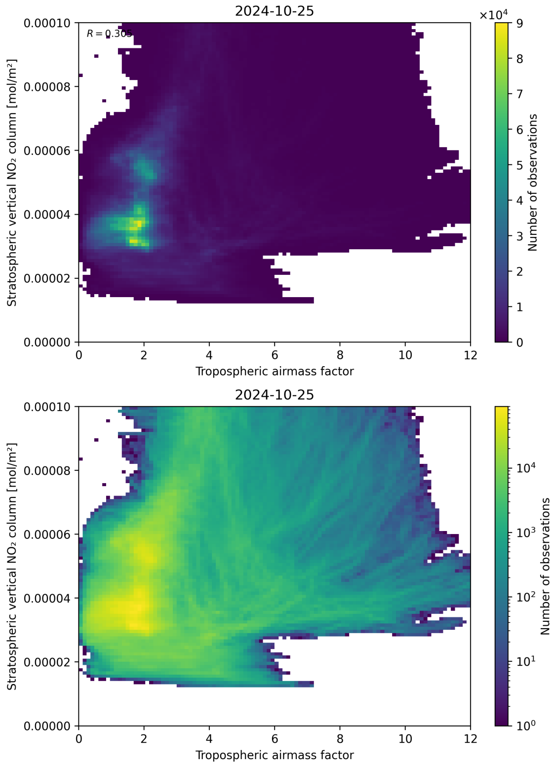
Figure 74: Scatter density plot of “Tropospheric air mass factor” against “Stratospheric vertical NO 2 column” for 2024-10-24 to 2024-10-26.
