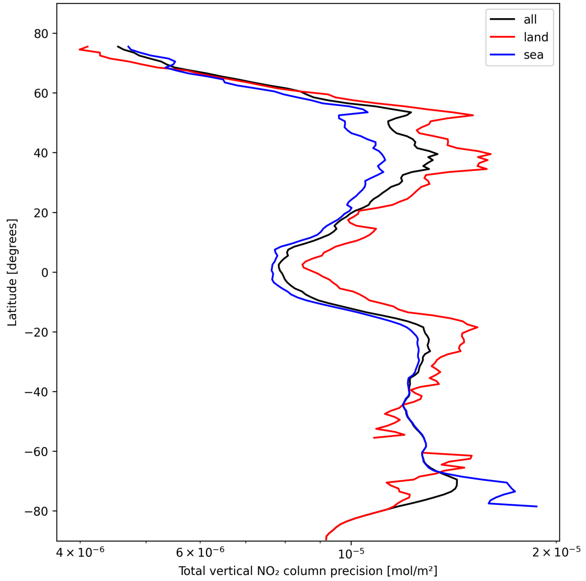
Figure 22: Zonal average of "Total vertical NO 2 column precision" for 2024-10-24 to 2024-10-26.
