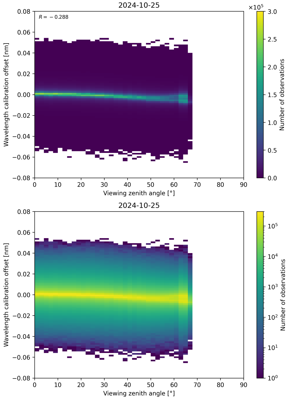
Figure 173: Scatter density plot of “Viewing zenith angle” against “Wavelength calibration offset” for 2024-10-24 to 2024-10-26.
