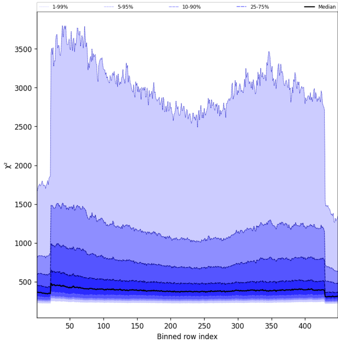
Figure 59: Along track statistics of “ \chi^2 ” for 2024-10-24 to 2024-10-26
