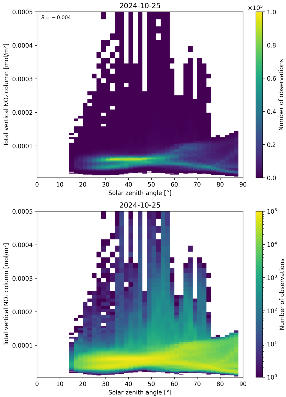
Figure 153: Scatter density plot of “Solar zenith angle” against “Total vertical NO 2 column” for 2024-10-24 to 2024-10-26.
