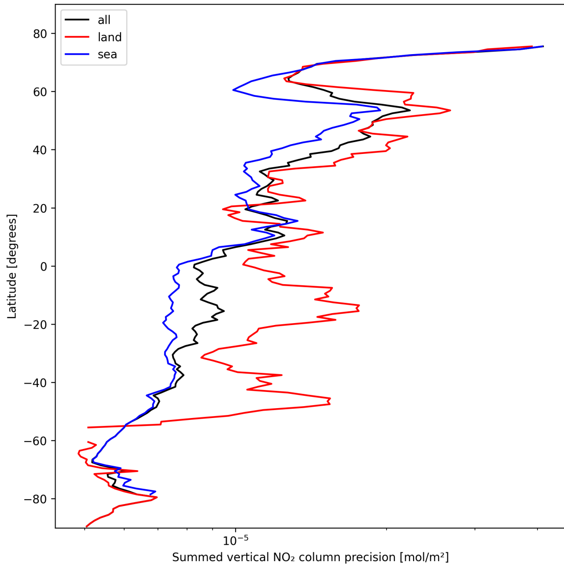
Figure 24: Zonal average of “Summed vertical NO 2 column precision” for 2024-10-24 to 2024-10-26.
