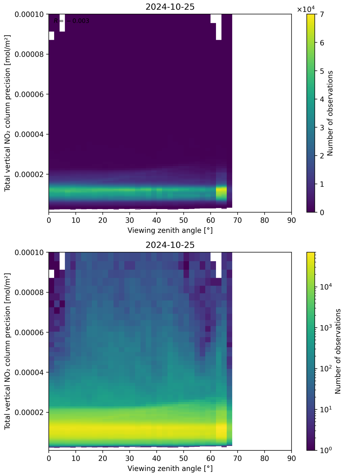
Figure 168: Scatter density plot of “Viewing zenith angle” against “Total vertical NO 2 column precision” for 2024-10-24 to 2024-10-26.
