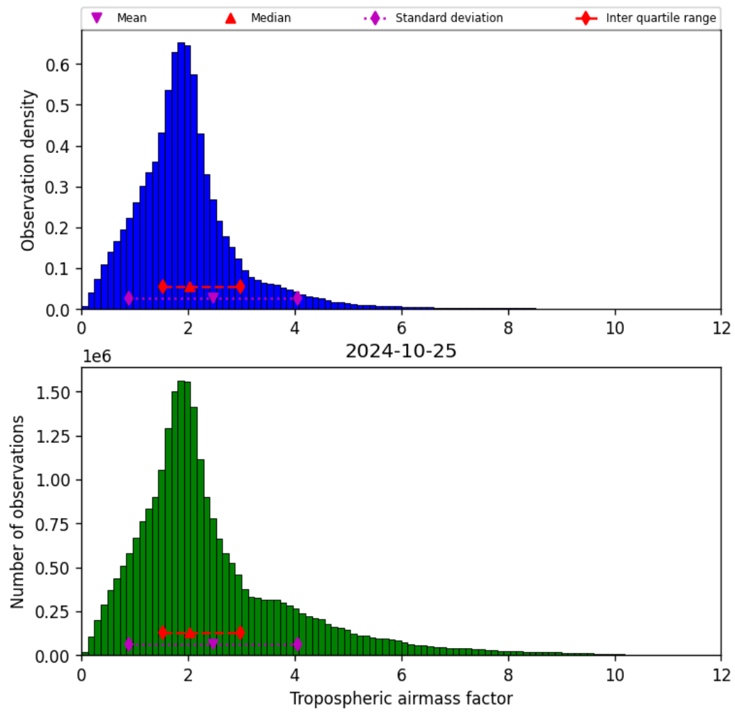
Figure 31: Histogram of “Tropospheric airmass factor” for 2024-10-24 to 2024-10-26
