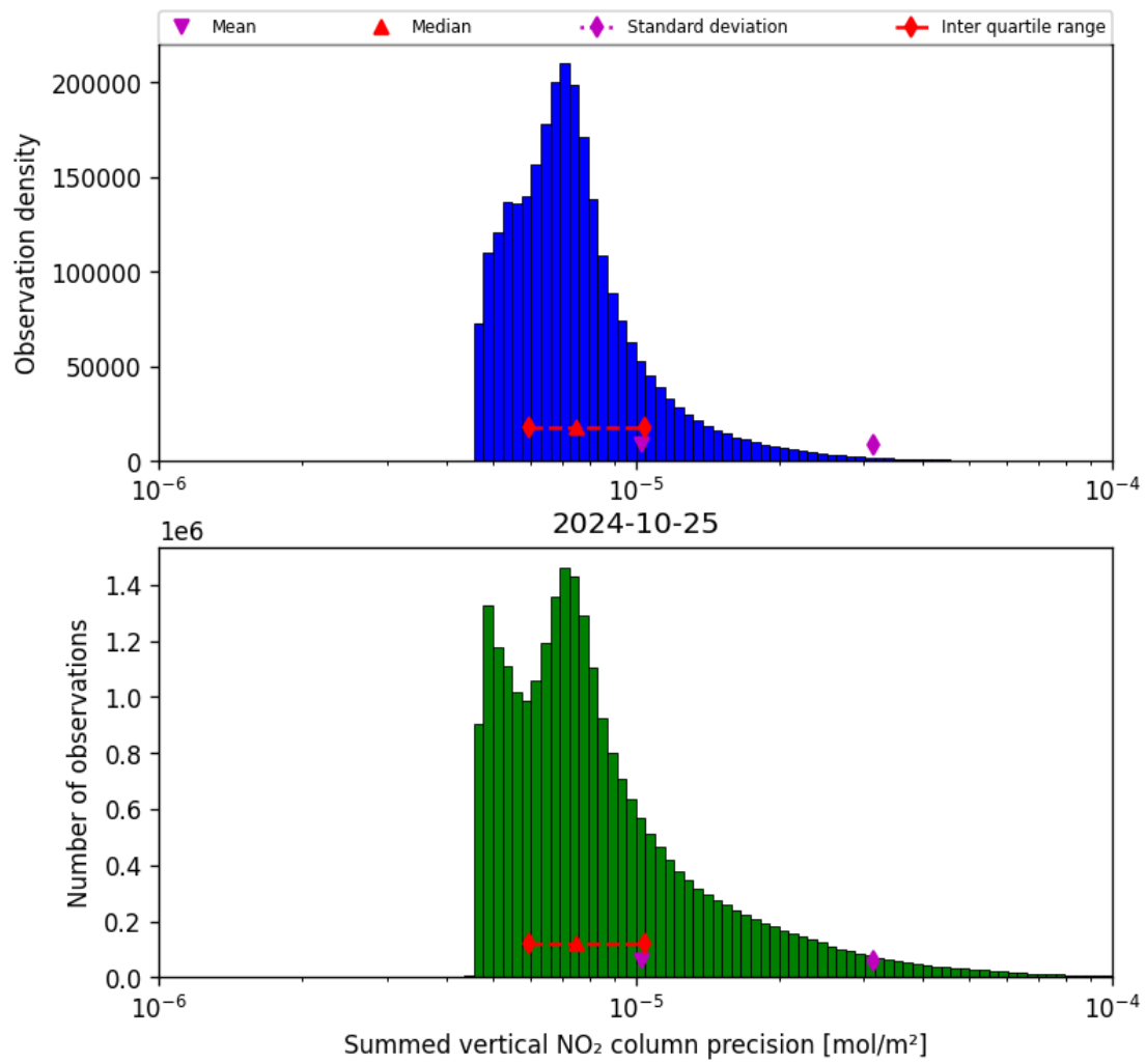
Figure 41: Histogram of "Summed vertical NO 2 column precision" for 2024-10-24 to 2024-10-26
