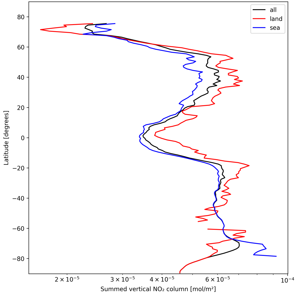
Figure 23: Zonal average of “Summed vertical NO 2 column” for 2024-10-24 to 2024-10-26.
