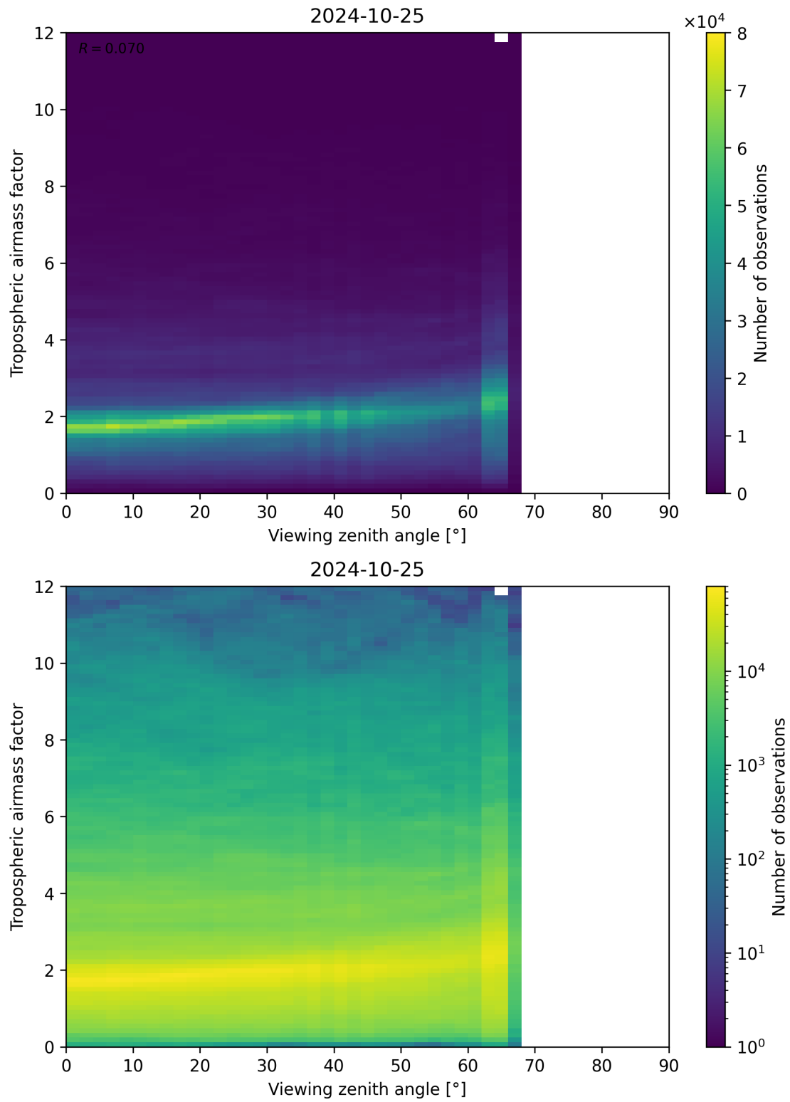
Figure 161: Scatter density plot of “Viewing zenith angle” against “Tropospheric airmass factor” for 2024-10-24 to 2024-10-26.
