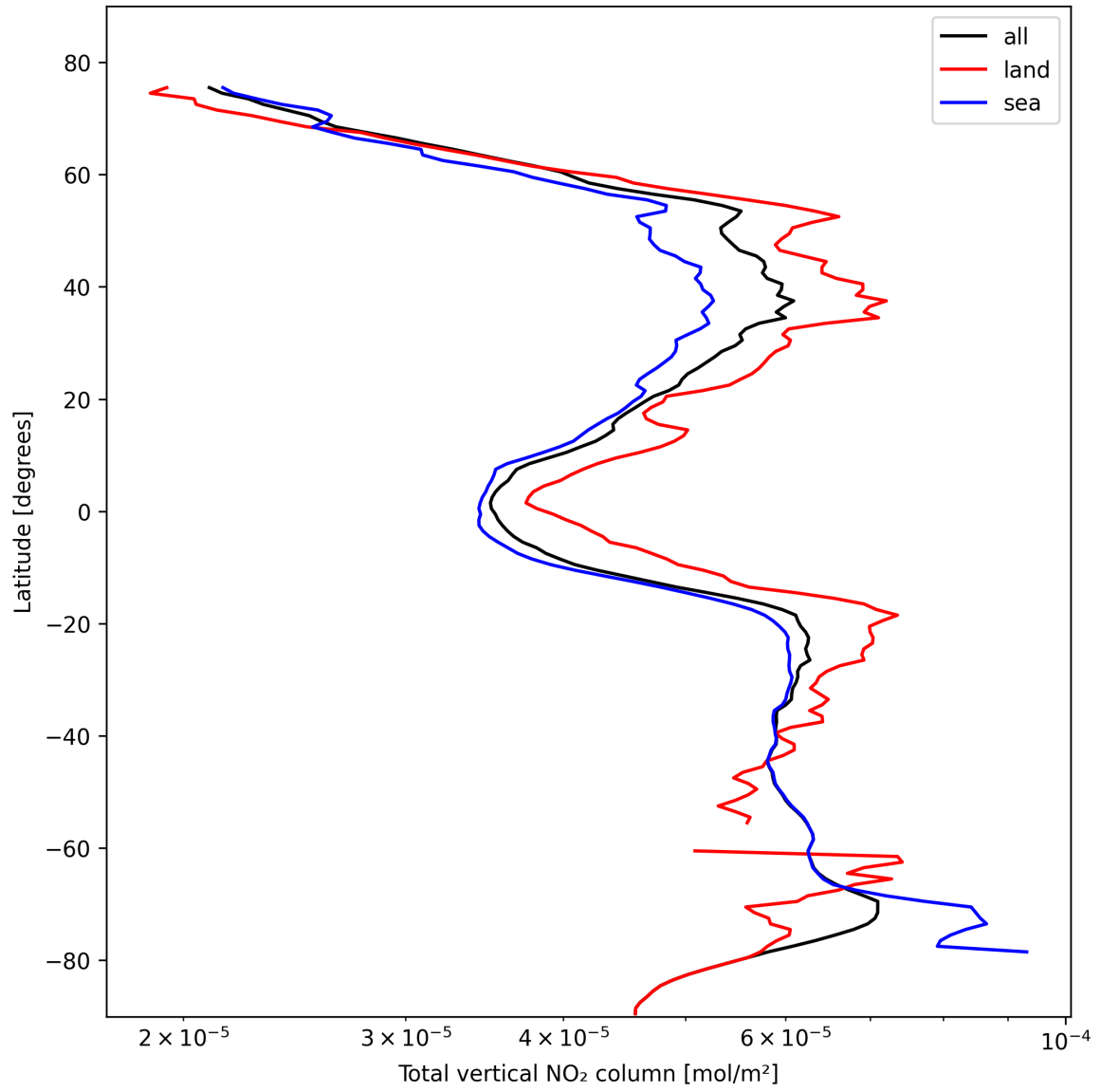
Figure 21: Zonal average of “Total vertical NO 2 column” for 2024-10-24 to 2024-10-26.
