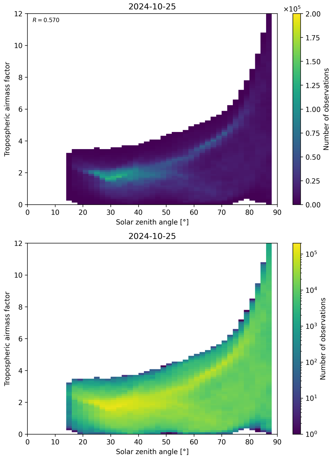
Figure 147: Scatter density plot of “Solar zenith angle” against “Tropospheric airmass factor” for 2024-10-24 to 2024-10-26.
