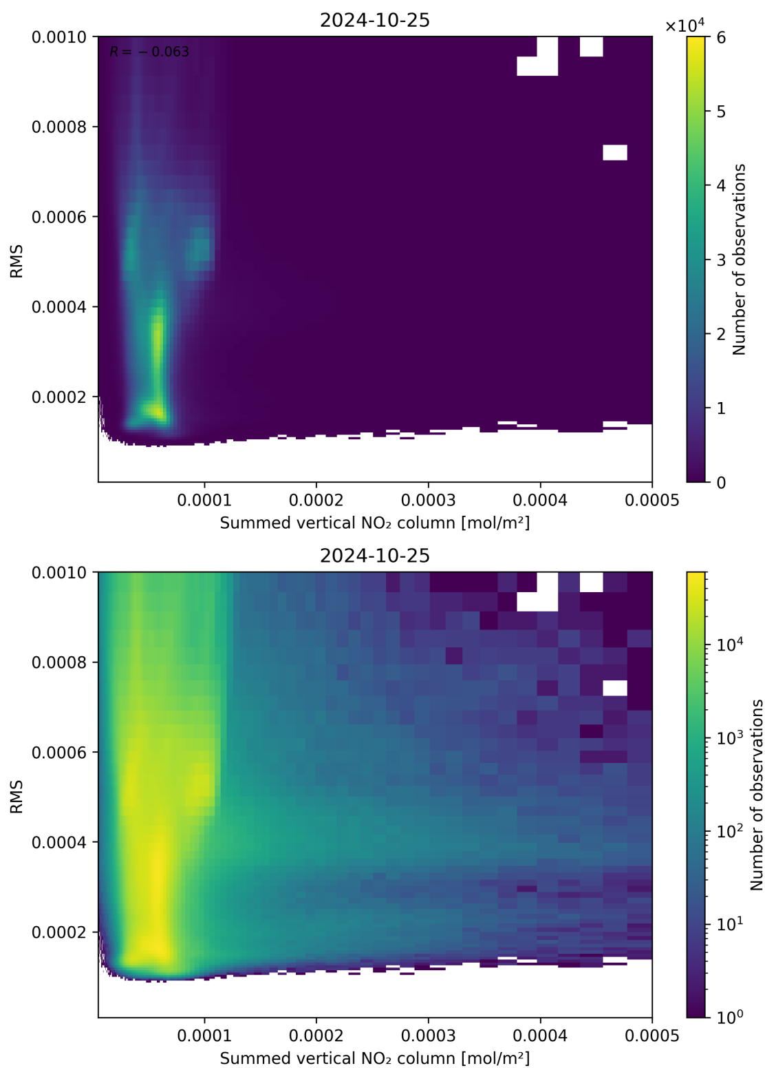
Figure 109: Scatter density plot of “Summed vertical NO 2 column” against “RMS” for 2024-10-24 to 2024-10-26.
