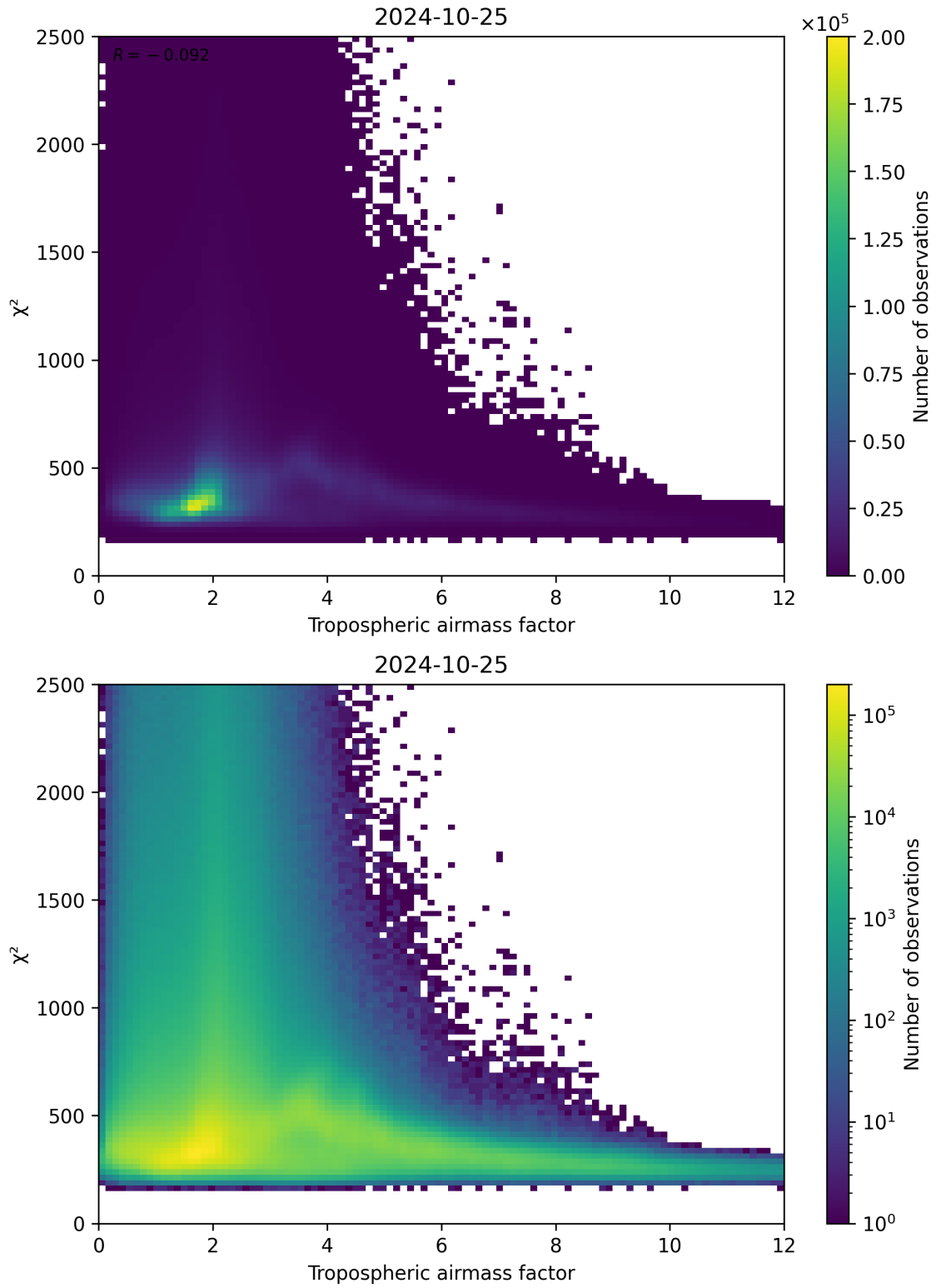
Figure 73: Scatter density plot of “Tropospheric airmass factor” against “ \chi^2 ” for 2024-10-24 to 2024-10-26.
