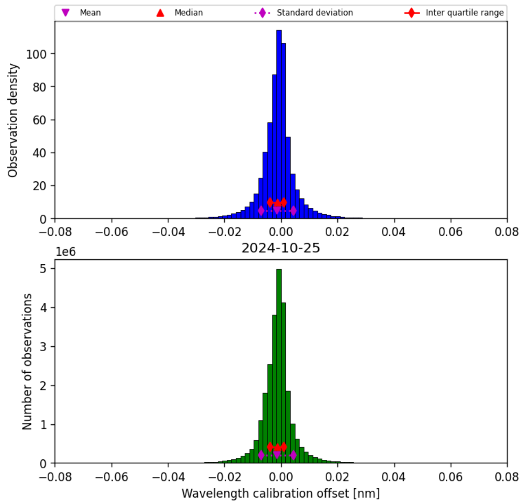
Figure 35: Histogram of “Wavelength calibration offset” for 2024-10-24 to 2024-10-26
