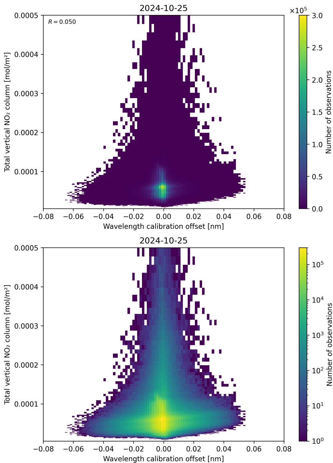
Figure 179: Scatter density plot of “Wavelength calibration offset” against “Total vertical NO 2 column” for 2024-10-24 to 2024-10-26.
