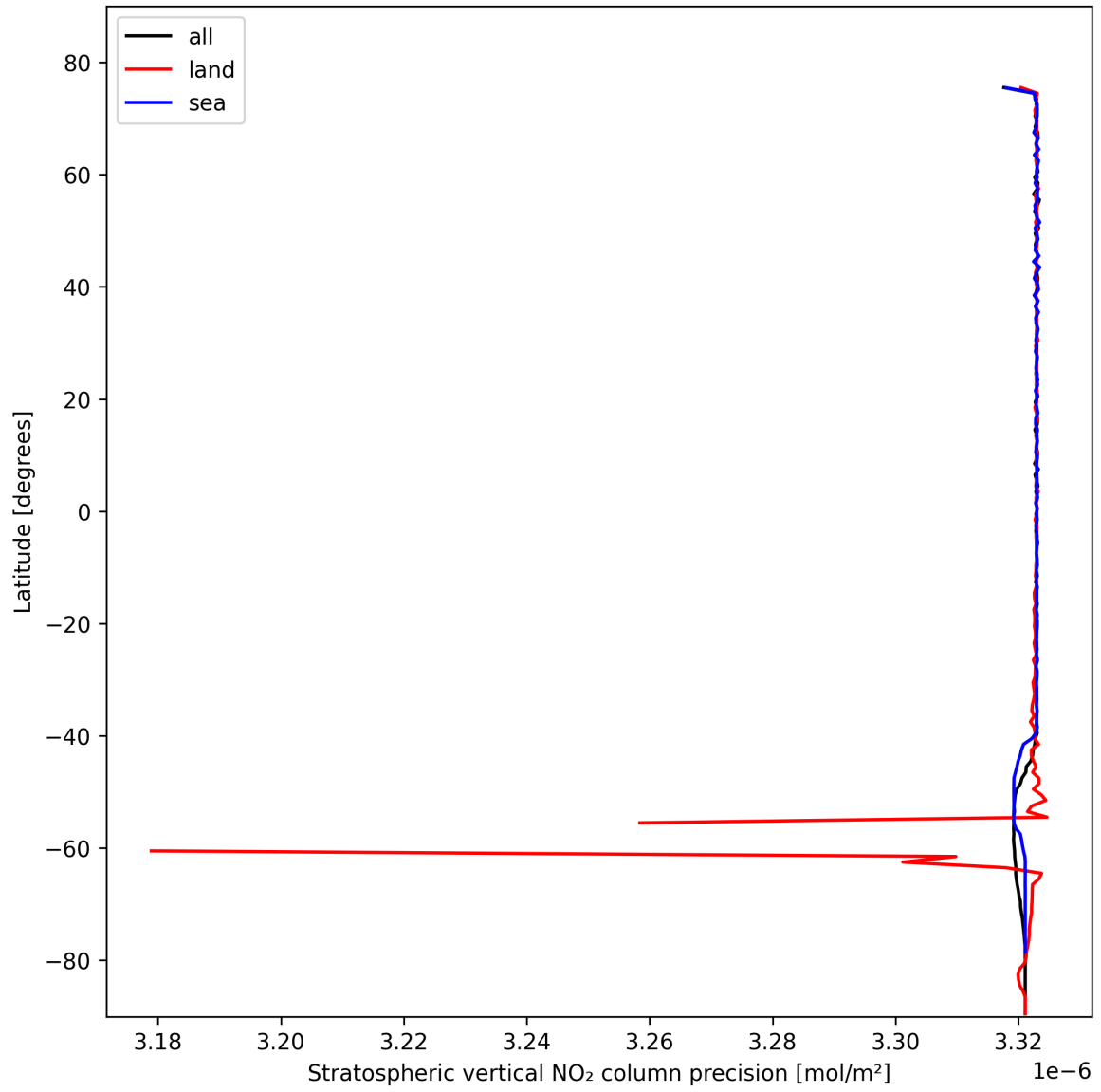
Figure 20: Zonal average of “Stratospheric vertical NO 2 column precision” for 2024-10-24 to 2024-10-26.
