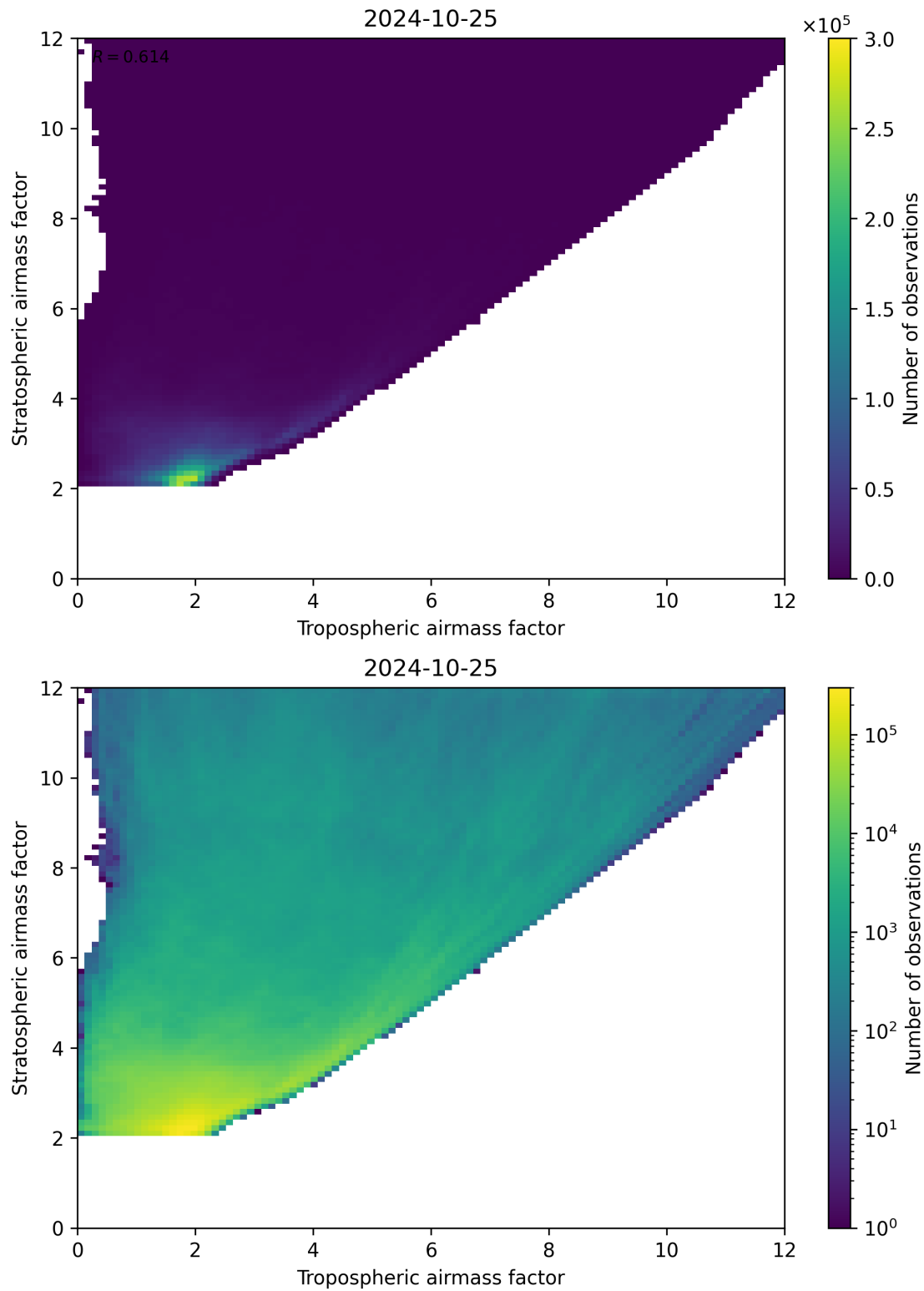
Figure 71: Scatter density plot of “Tropospheric airmass factor” against “Stratospheric airmass factor” for 2024-10-24 to 2024-10-26.
