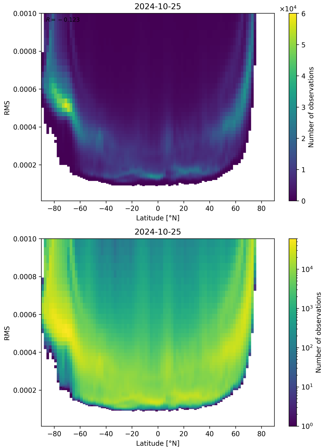
Figure 94: Scatter density plot of “Latitude” against “RMS” for 2024-10-24 to 2024-10-26.
