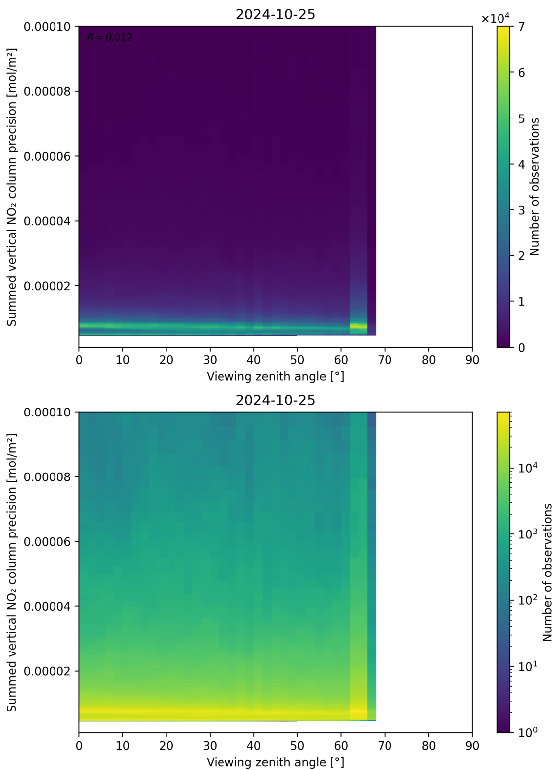
Figure 166: Scatter density plot of “Viewing zenith angle” against “Summed vertical NO 2 column precision” for 2024-10-24 to 2024-10-26.
