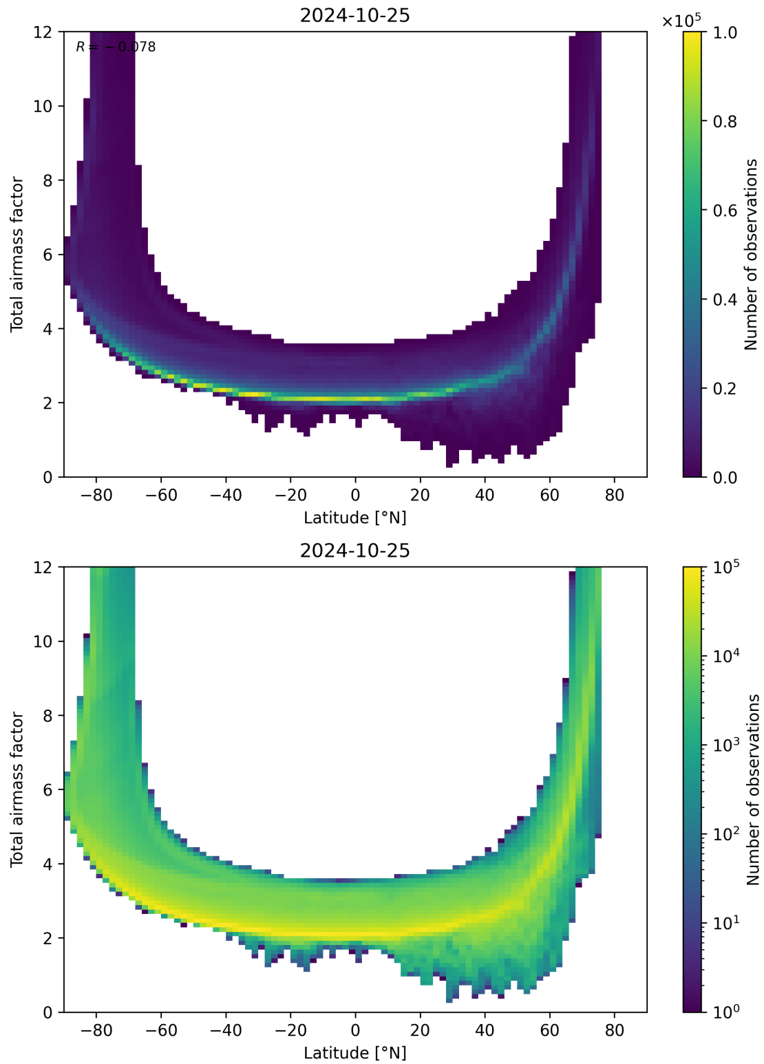
Figure 84: Scatter density plot of “Latitude” against “Total airmass factor” for 2024-10-24 to 2024-10-26.
