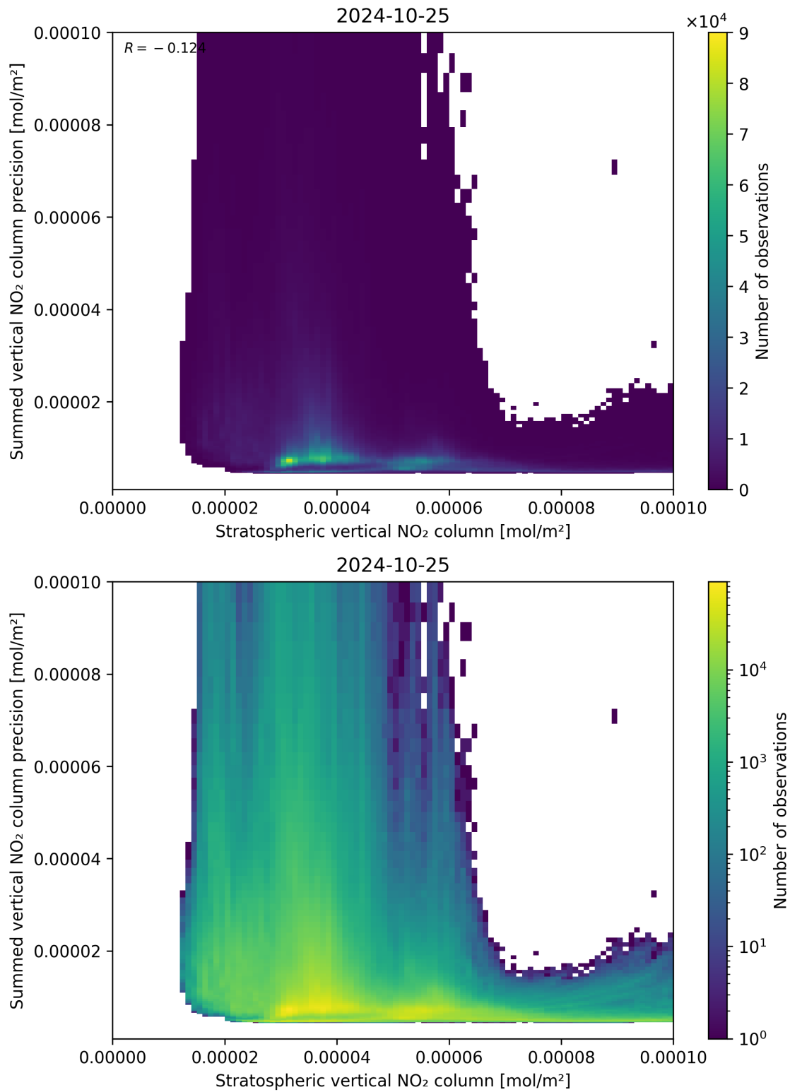
Figure 99: Scatter density plot of “Stratospheric vertical NO 2 column” against “Summed vertical NO 2 column precision” for 2024-10-24 to 2024-10-26.
