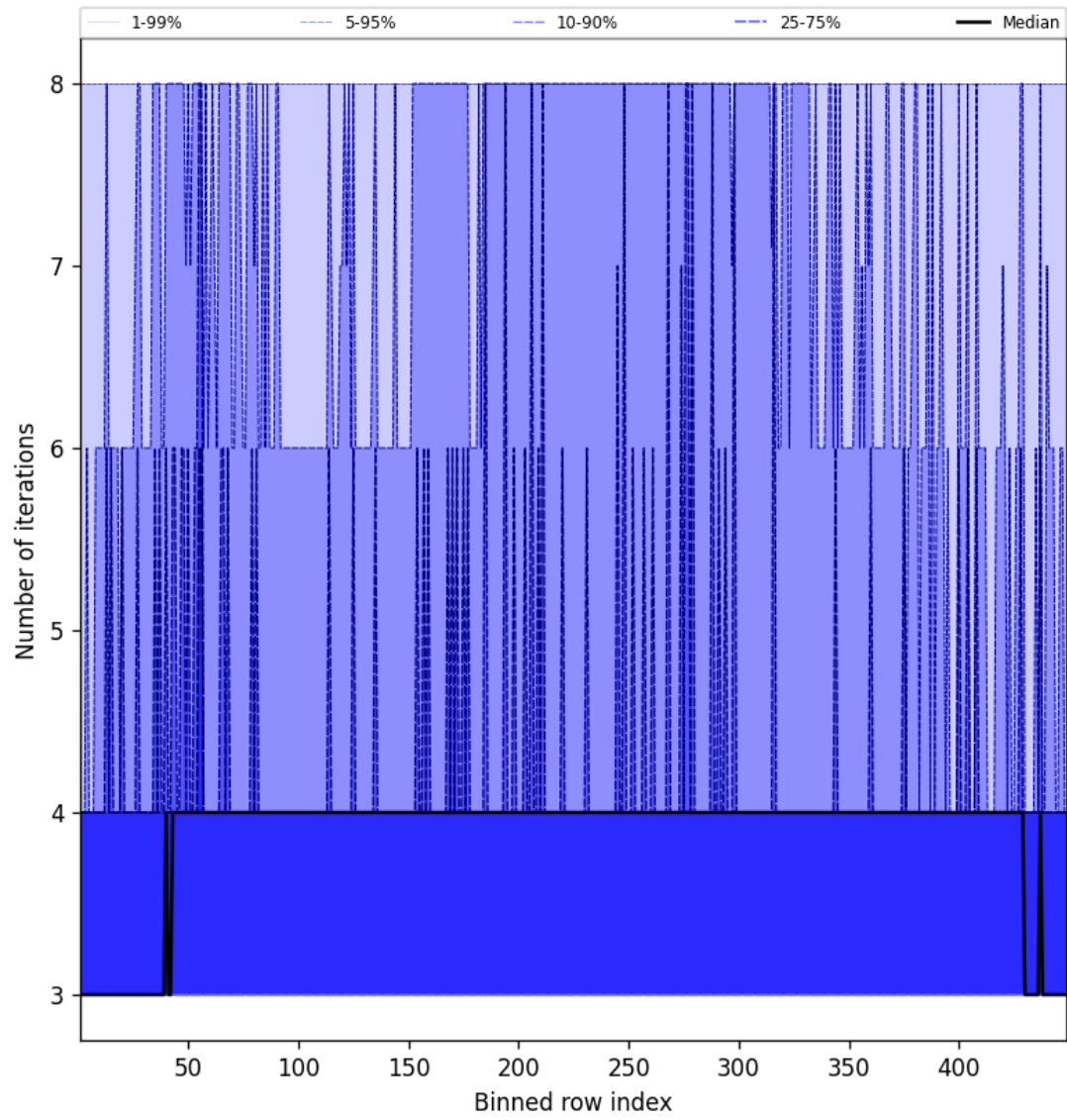
Figure 51: Along track statistics of “Number of iterations” for 2024-10-24 to 2024-10-26
