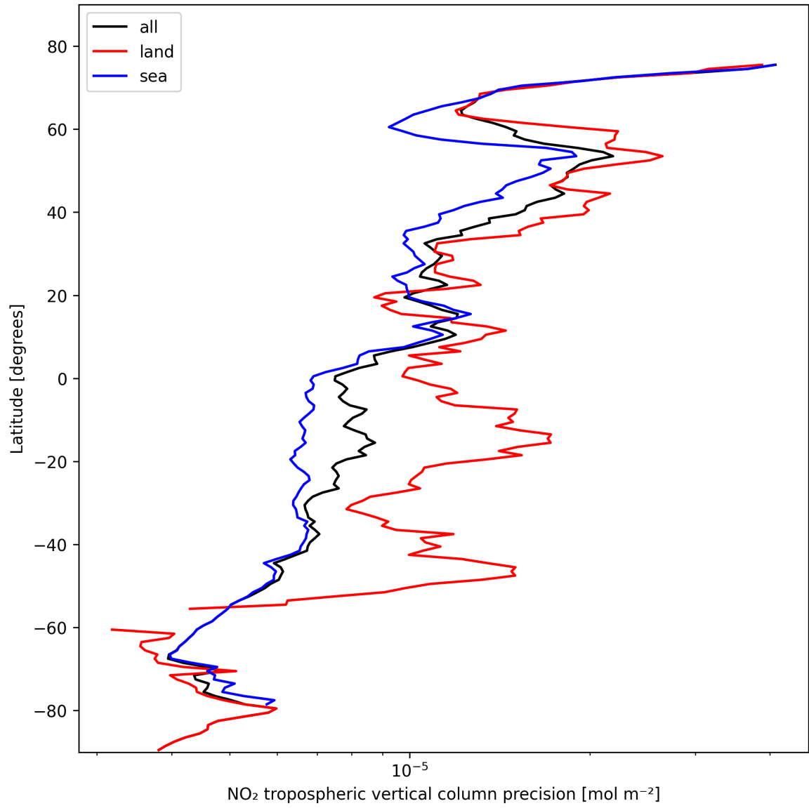
Figure 13: Zonal average of “NO 2 tropospheric vertical column precision” for 2024-10-24 to 2024-10-26.
