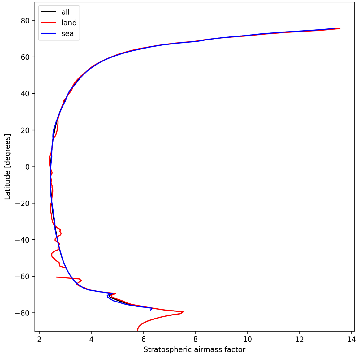
Figure 27: Zonal average of “Stratospheric air mass factor” for 2024-10-24 to 2024-10-26.
