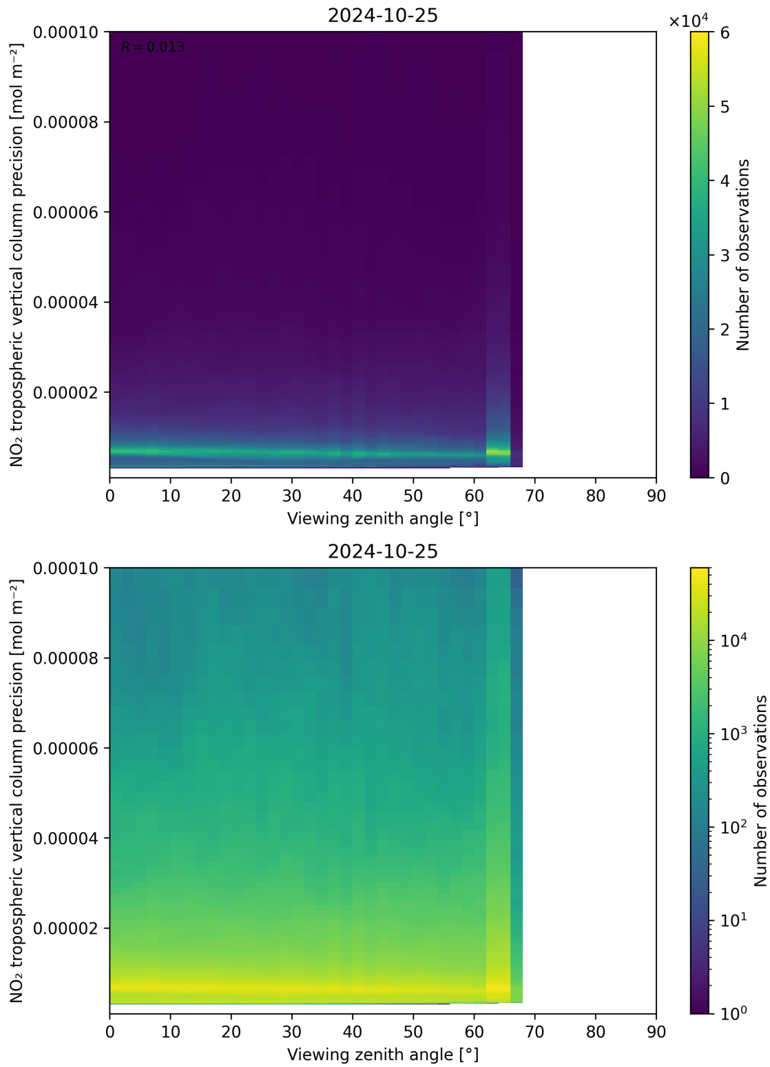
Figure 170: Scatter density plot of “Viewing zenith angle” against “NO 2 tropospheric vertical column precision” for 2024-10-24 to 2024-10-26.
