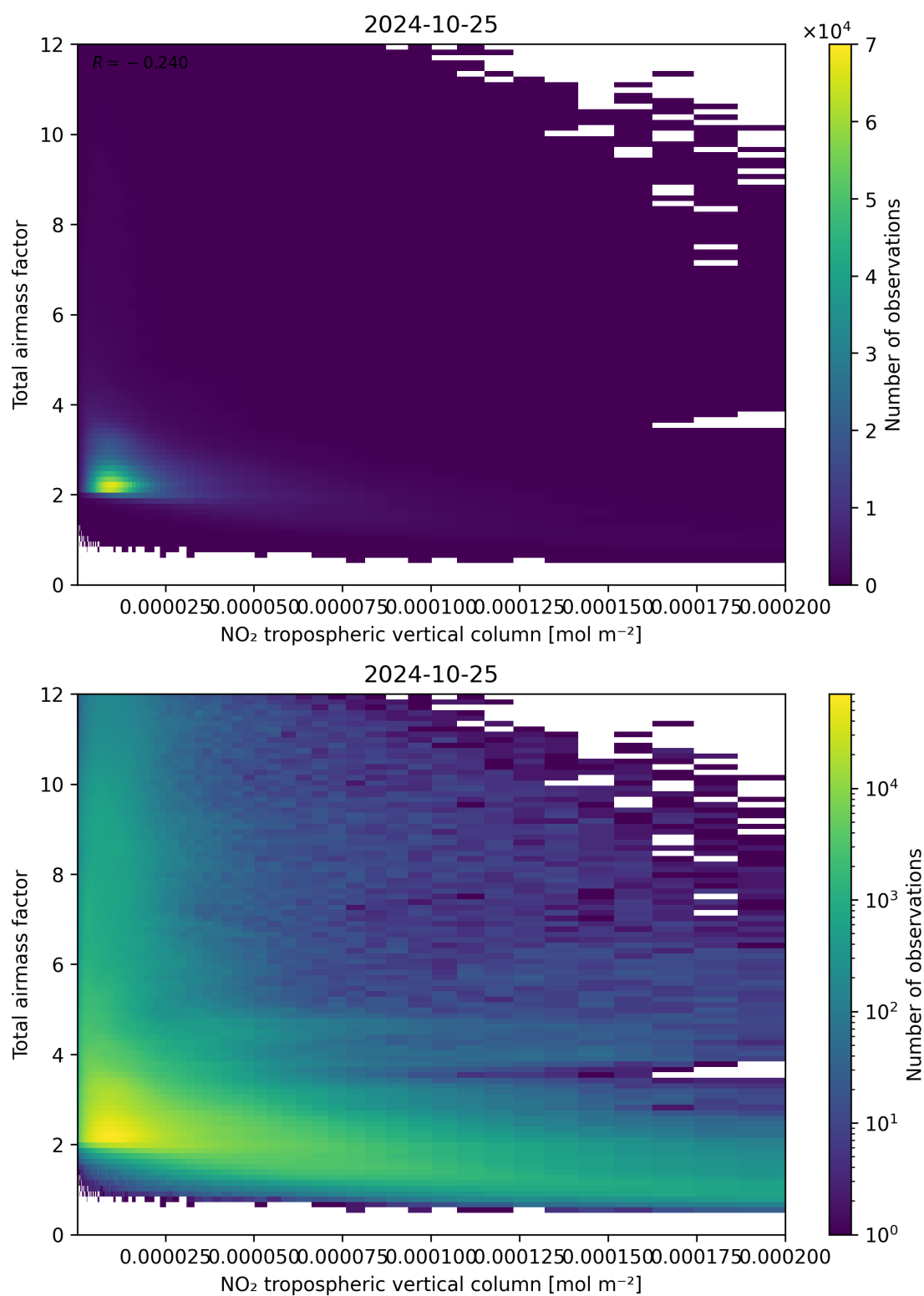
Figure 122: Scatter density plot of “NO 2 tropospheric vertical column” against “Total air mass factor” for 2024-10-24 to 2024-10-26.
