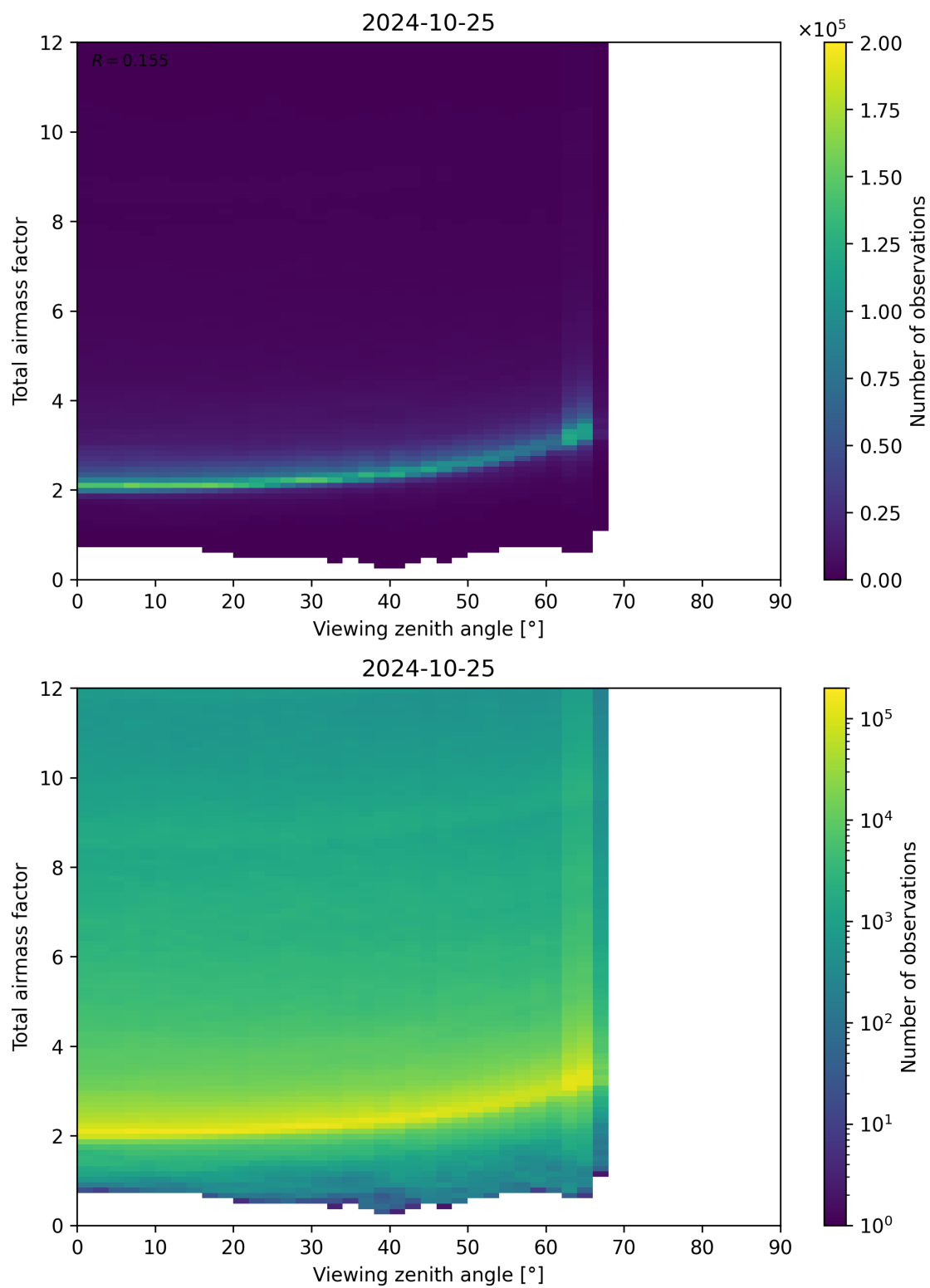
Figure 160: Scatter density plot of “Viewing zenith angle” against “Total airmass factor” for 2024-10-24 to 2024-10-26.
