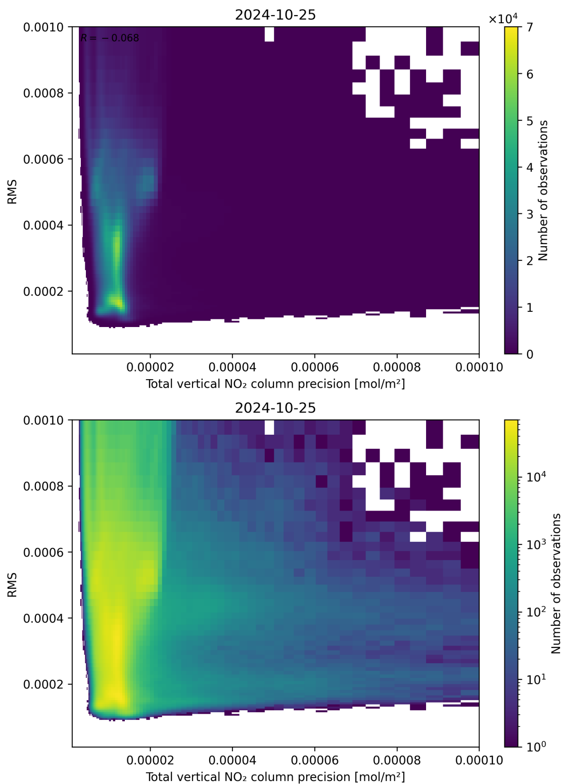
Figure 119: Scatter density plot of “Total vertical NO 2 column precision” against “RMS” for 2024-10-24 to 2024-10-26.
