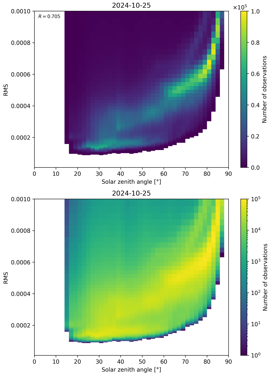
Figure 157: Scatter density plot of “Solar zenith angle” against “RMS” for 2024-10-24 to 2024-10-26.
