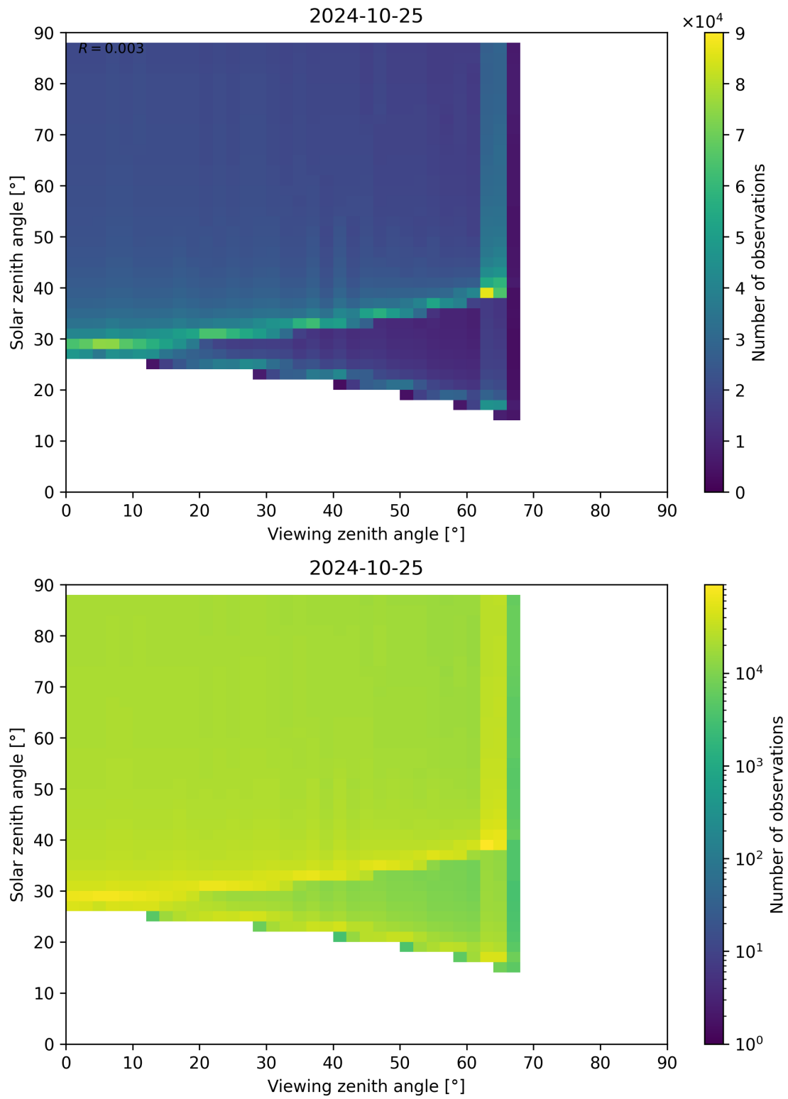
Figure 172: Scatter density plot of “Viewing zenith angle” against “Solar zenith angle” for 2024-10-24 to 2024-10-26.
