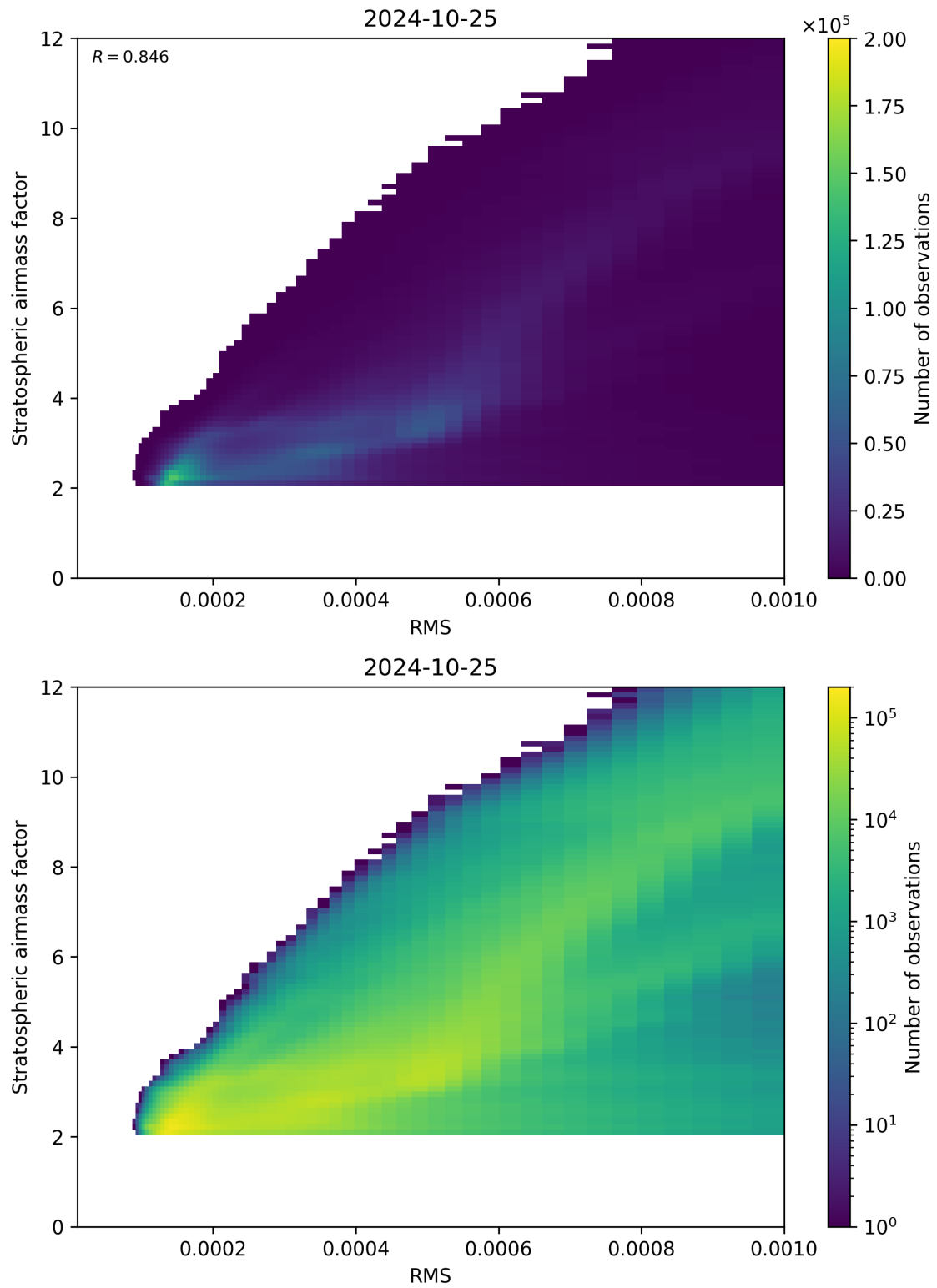
Figure 144: Scatter density plot of “RMS” against “Stratospheric airmass factor” for 2024-10-24 to 2024-10-26.
