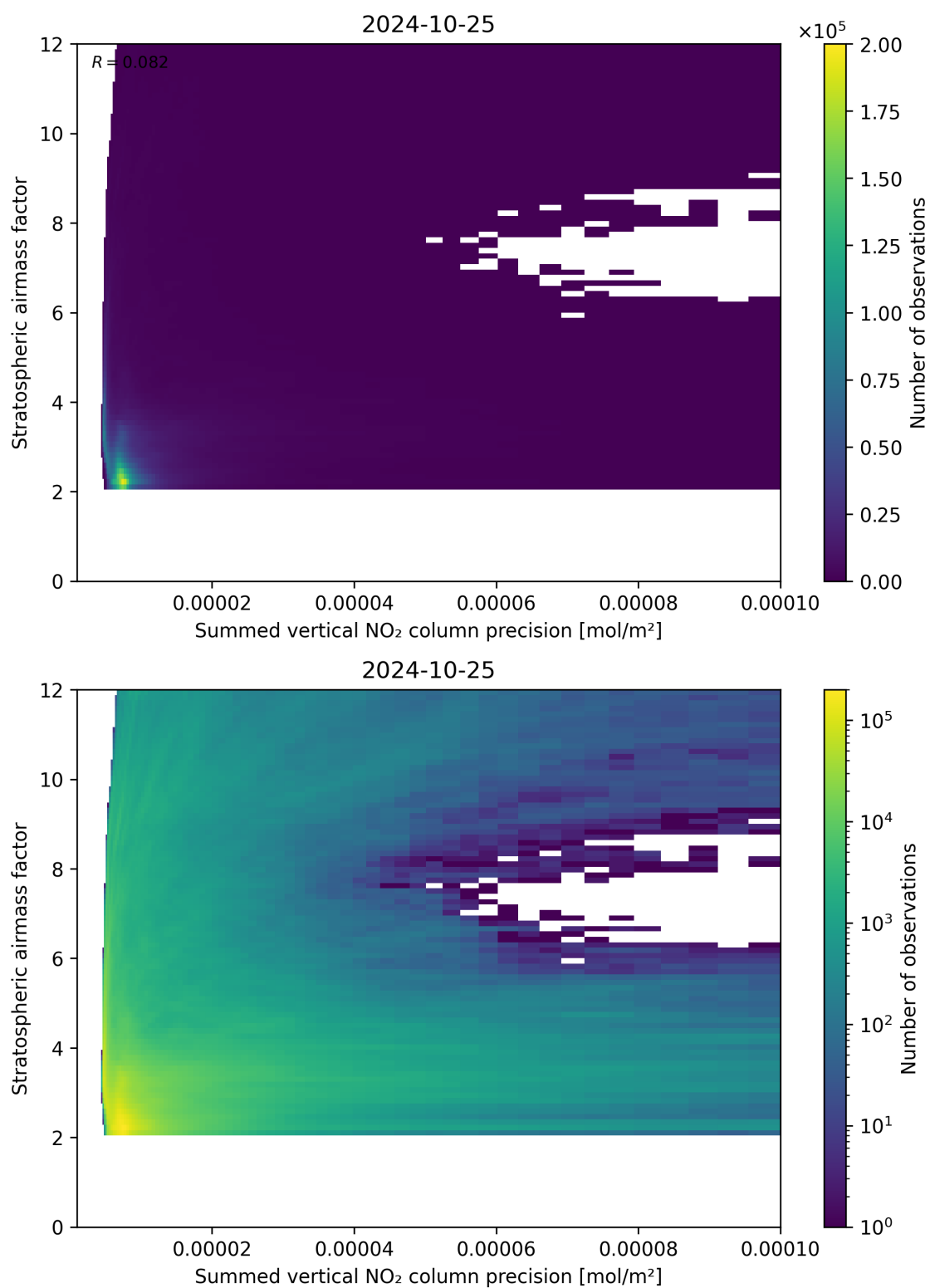
Figure 106: Scatter density plot of “Summed vertical NO 2 column precision” against “Stratospheric airmass factor” for 2024-10-24 to 2024-10-26.
