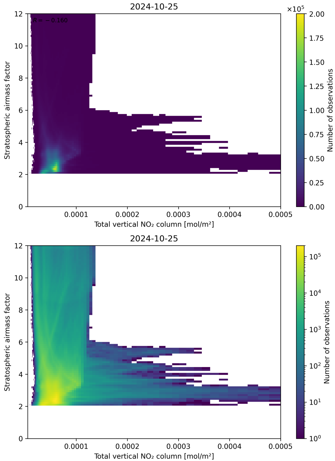
Figure 110: Scatter density plot of “Total vertical NO 2 column” against “Stratospheric airmass factor” for 2024-10-24 to 2024-10-26.
