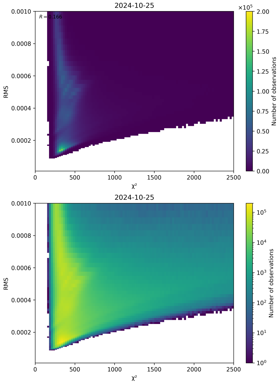
Figure 82: Scatter density plot of “ \chi^2 ” against “RMS” for 2024-10-24 to 2024-10-26.
