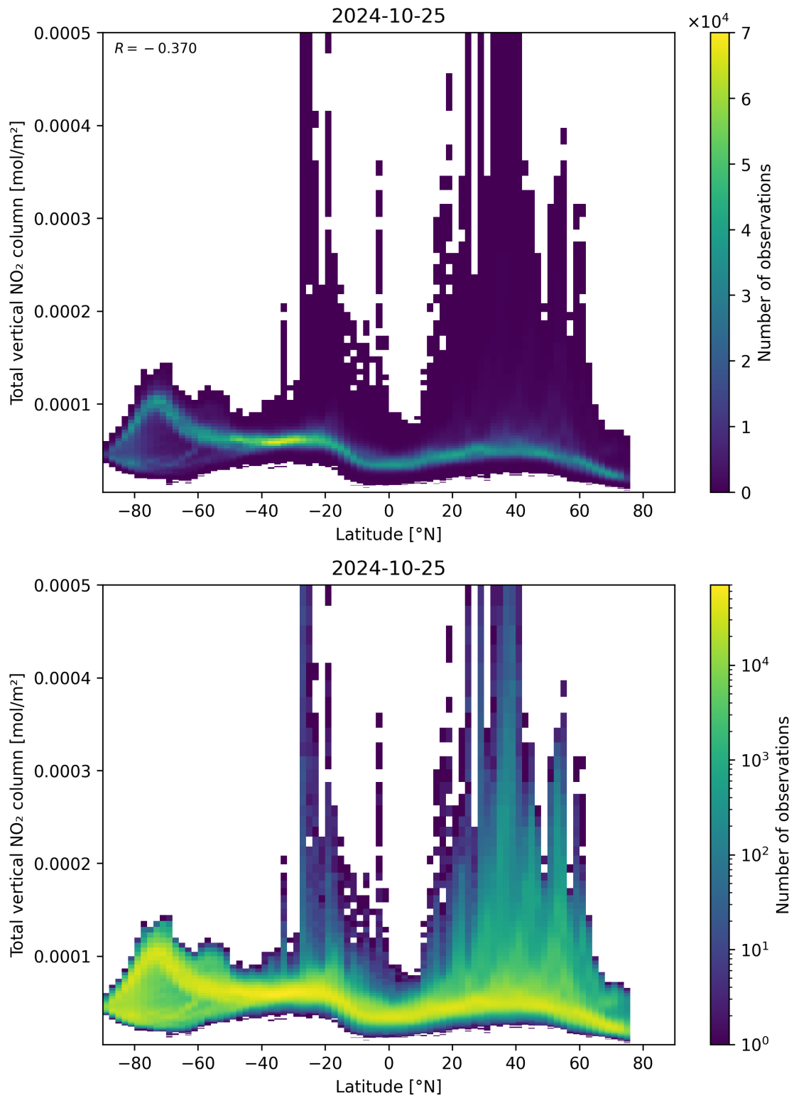
Figure 90: Scatter density plot of “Latitude” against “Total vertical NO 2 column” for 2024-10-24 to 2024-10-26.
