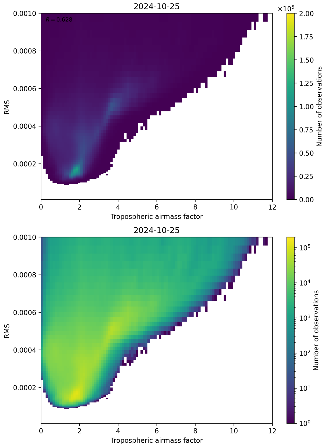
Figure 79: Scatter density plot of “Tropospheric airmass factor” against “RMS” for 2024-10-24 to 2024-10-26.
