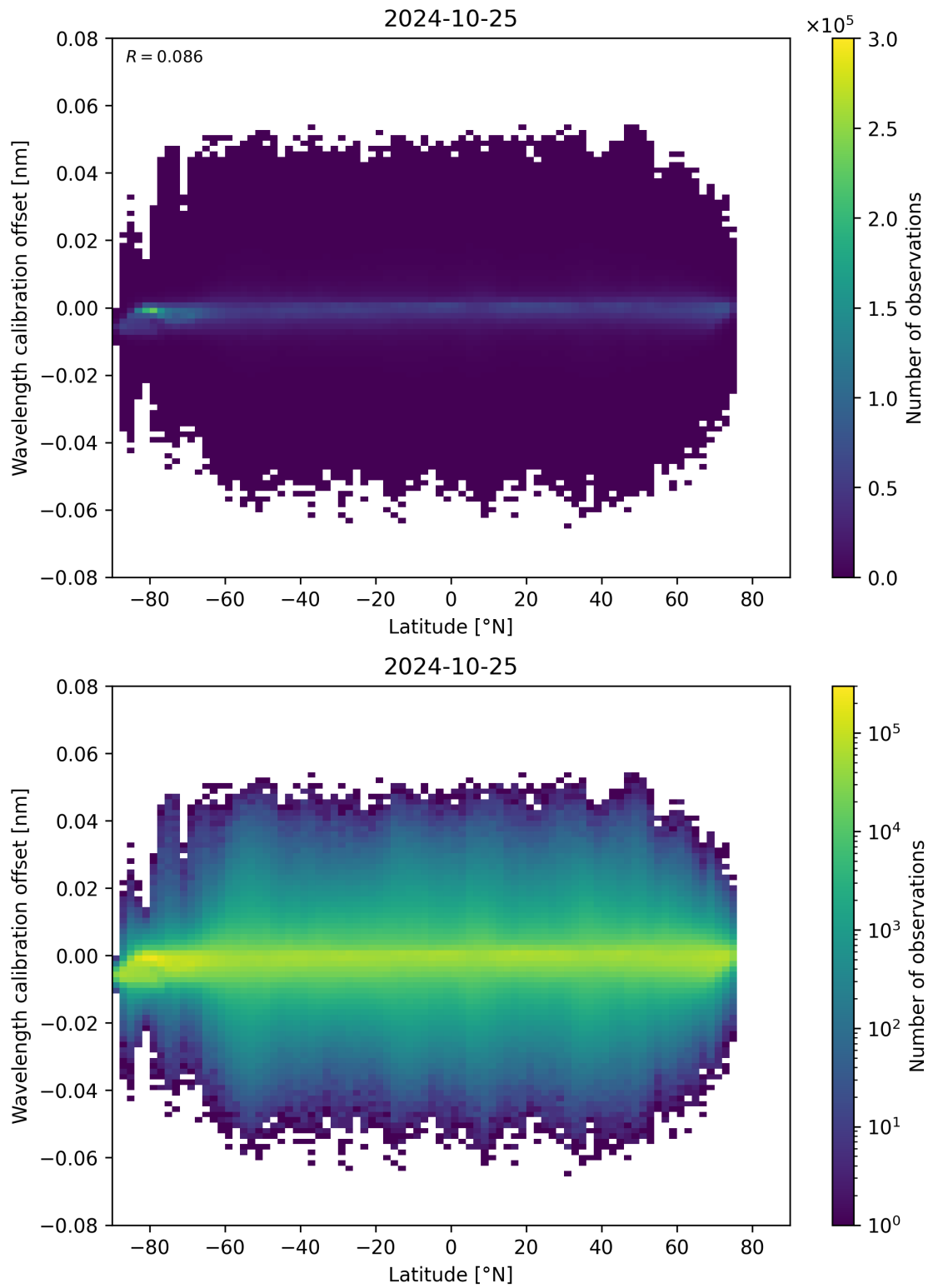
Figure 95: Scatter density plot of “Latitude” against “Wavelength calibration offset” for 2024-10-24 to 2024-10-26.
