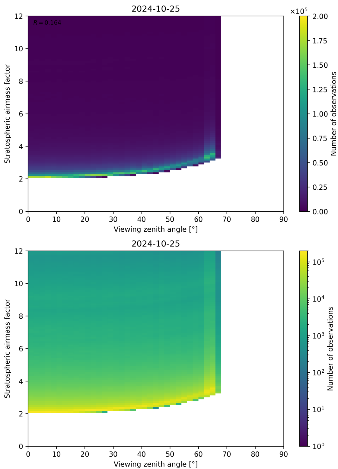
Figure 159: Scatter density plot of “Viewing zenith angle” against “Stratospheric airmass factor” for 2024-10-24 to 2024-10-26.
