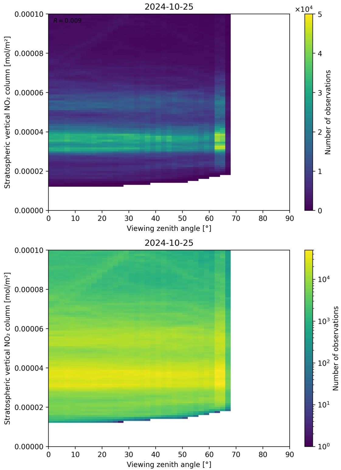
Figure 164: Scatter density plot of “Viewing zenith angle” against “Stratospheric vertical NO 2 column” for 2024-10-24 to 2024-10-26.
