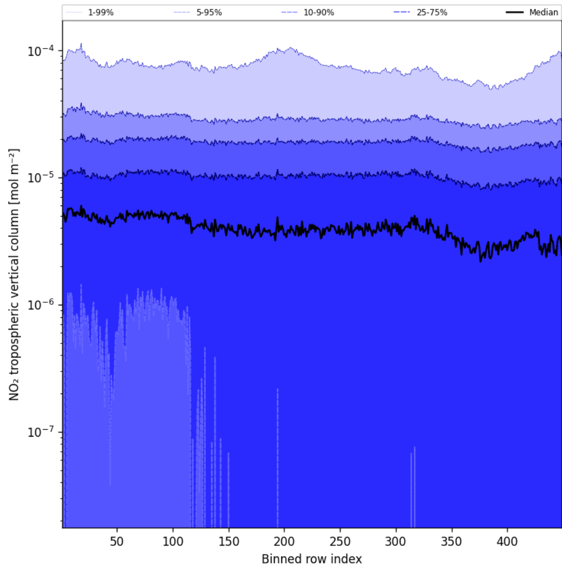
Figure 46: Along track statistics of “NO 2 tropospheric vertical column” for 2024-10-25 to 2024-10-27
