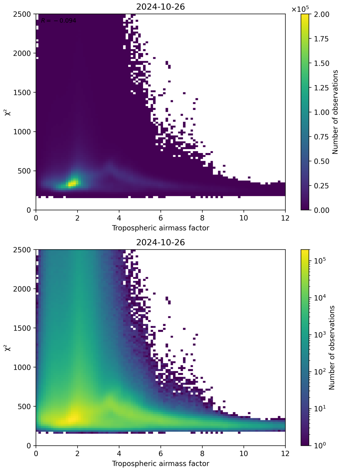
Figure 73: Scatter density plot of “Tropospheric airmass factor” against “ \chi^2 ” for 2024-10-25 to 2024-10-27.
