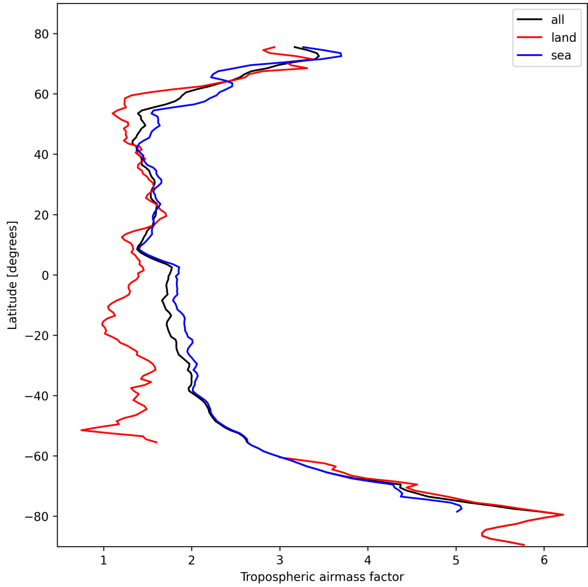
Figure 14: Zonal average of “Tropospheric airmass factor” for 2024-10-25 to 2024-10-27.
