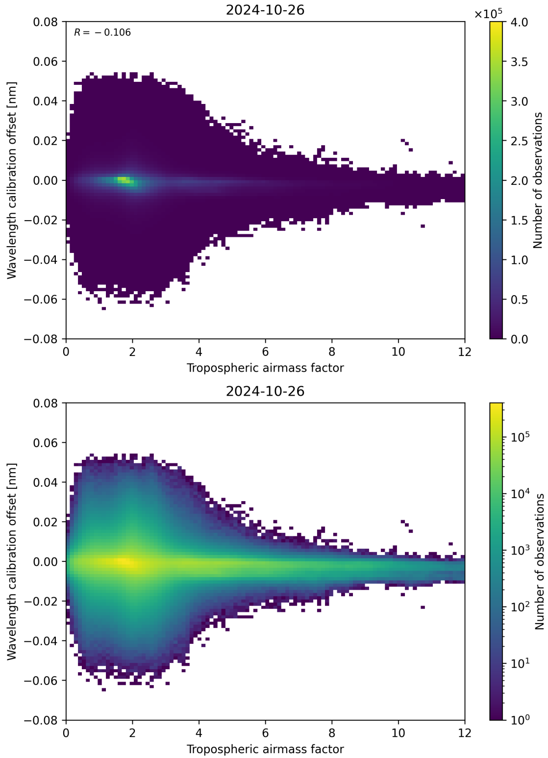
Figure 80: Scatter density plot of “Tropospheric airmass factor” against “Wavelength calibration offset” for 2024-10-25 to 2024-10-27.
