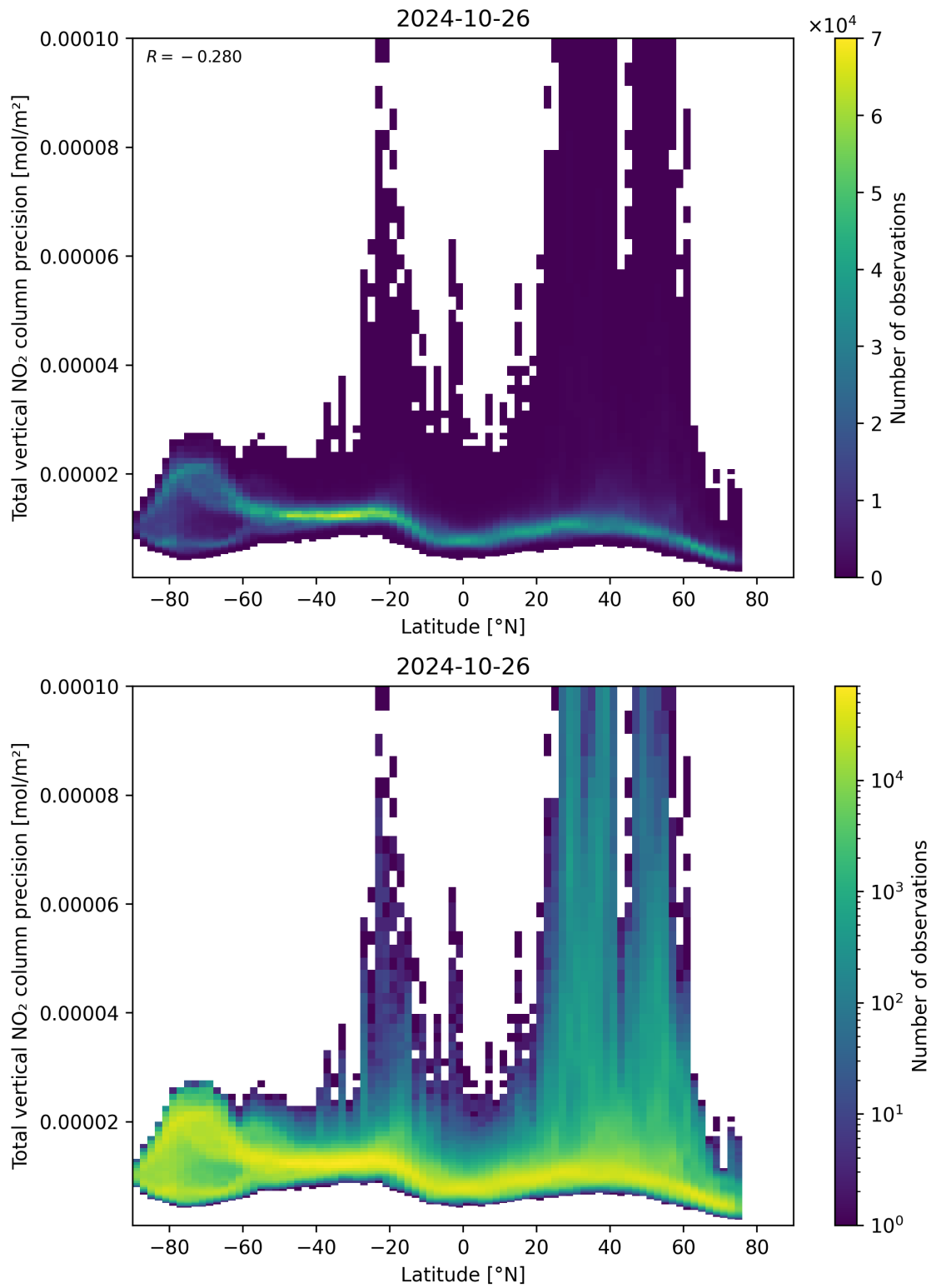
Figure 91: Scatter density plot of “Latitude” against “Total vertical NO 2 column precision” for 2024-10-25 to 2024-10-27.
