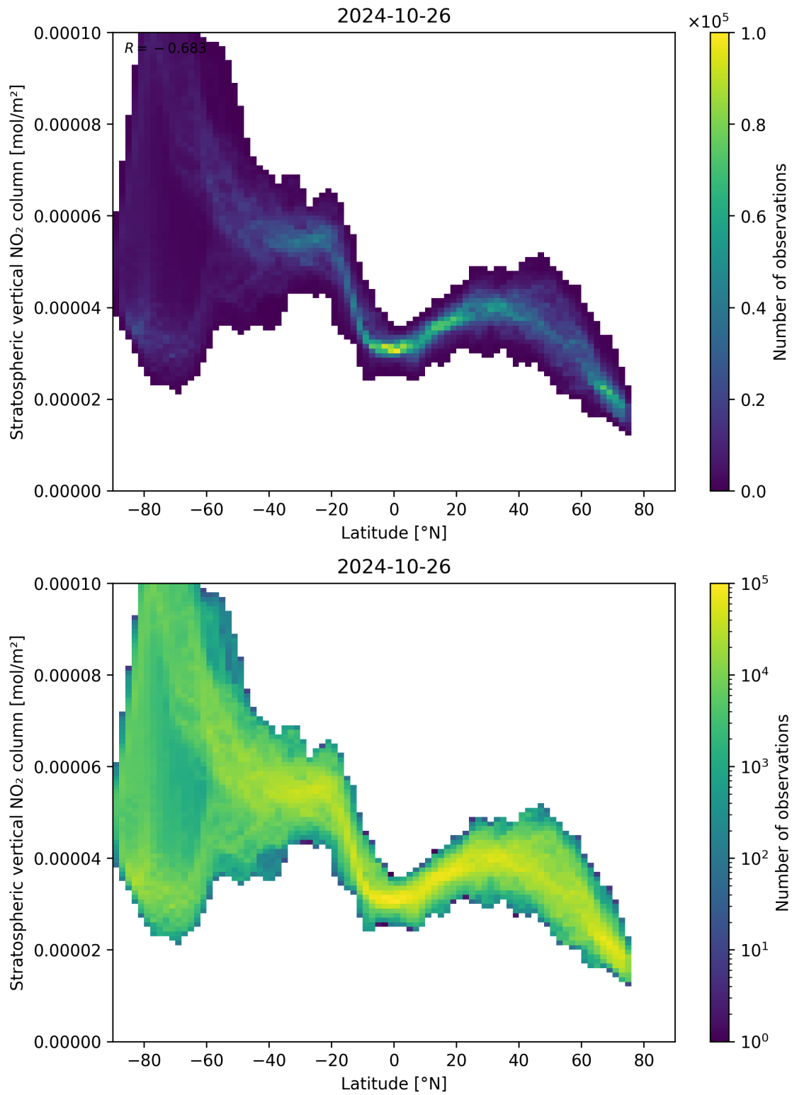
Figure 87: Scatter density plot of “Latitude” against “Stratospheric vertical NO 2 column” for 2024-10-25 to 2024-10-27.
