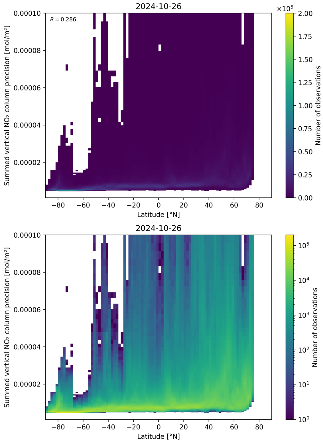
Figure 89: Scatter density plot of “Latitude” against “Summed vertical NO 2 column precision” for 2024-10-25 to 2024-10-27.
