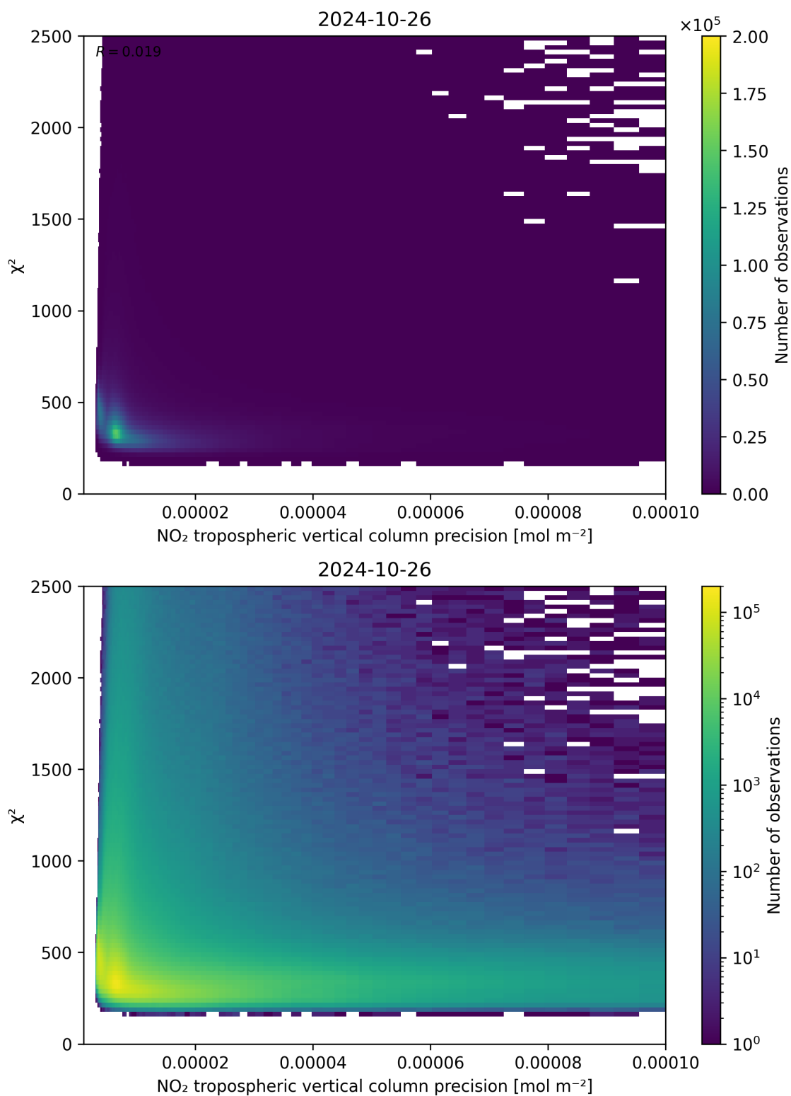
Figure 134: Scatter density plot of “NO 2 tropospheric vertical column precision” against “ \chi^2 ” for 2024-10-25 to 2024-10-27.
