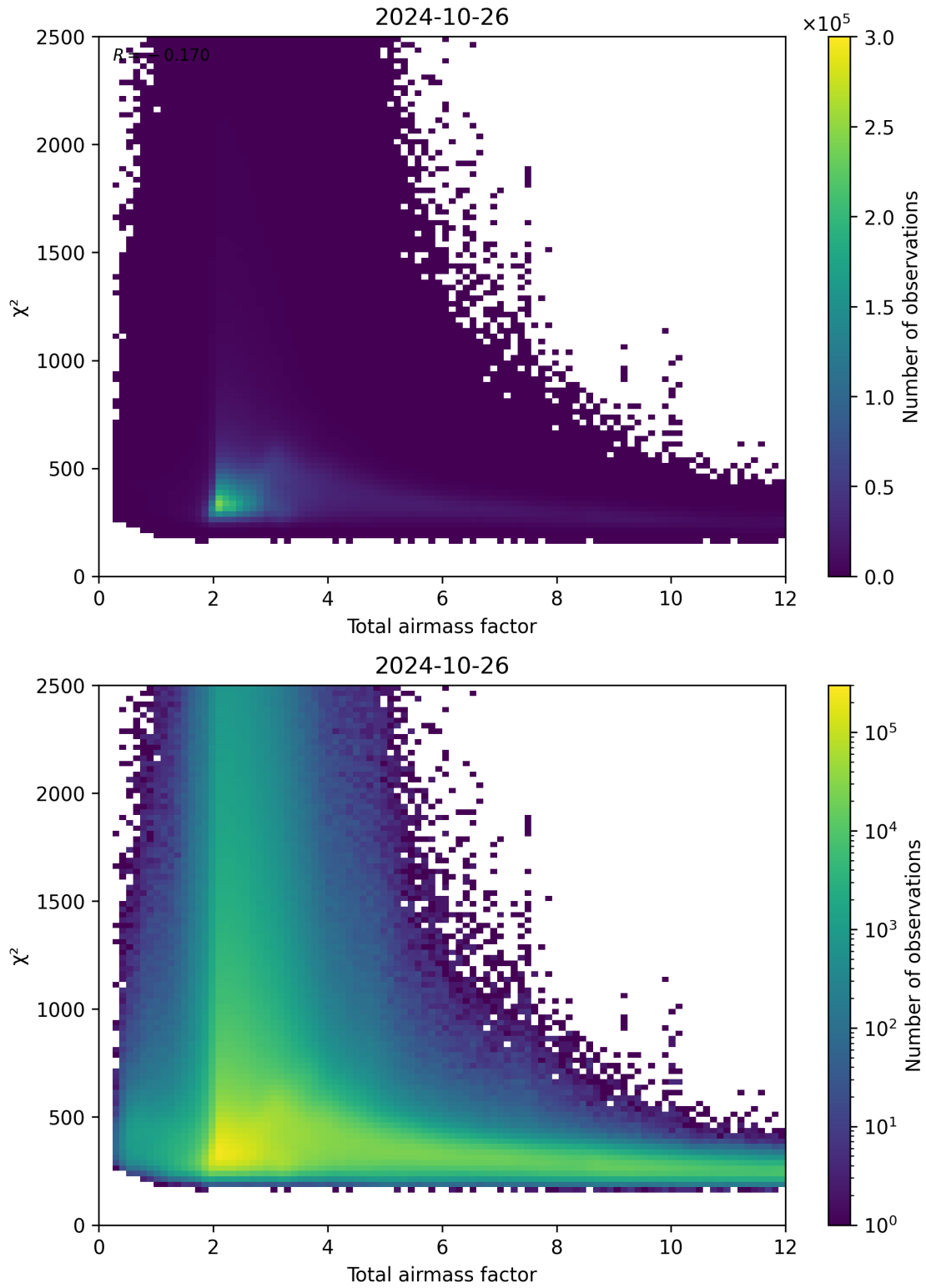
Figure 63: Scatter density plot of “Total airmass factor” against “ \chi^2 ” for 2024-10-25 to 2024-10-27.
