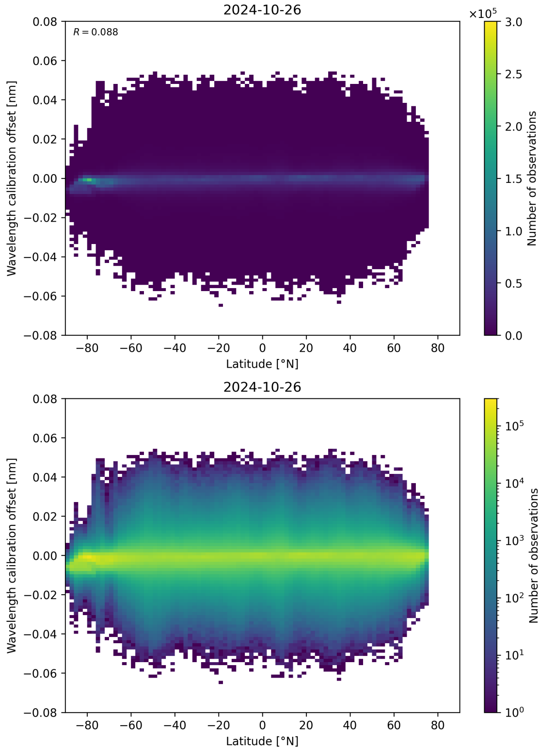
Figure 95: Scatter density plot of “Latitude” against “Wavelength calibration offset” for 2024-10-25 to 2024-10-27.
