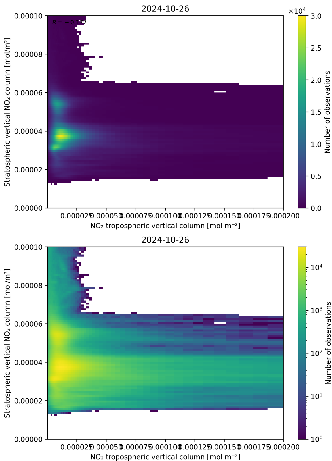
Figure 125: Scatter density plot of “NO 2 tropospheric vertical column” against “Stratospheric vertical NO 2 column” for 2024-10-25 to 2024-10-27.
