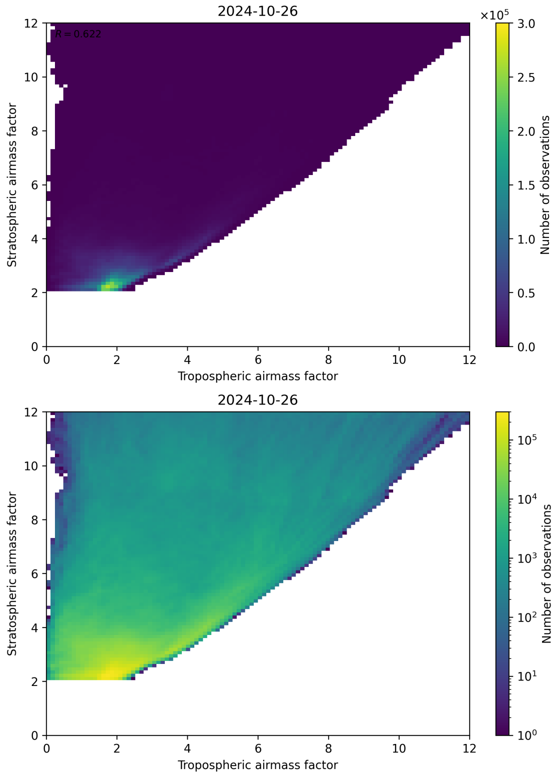
Figure 71: Scatter density plot of “Tropospheric airmass factor” against “Stratospheric airmass factor” for 2024-10-25 to 2024-10-27.
