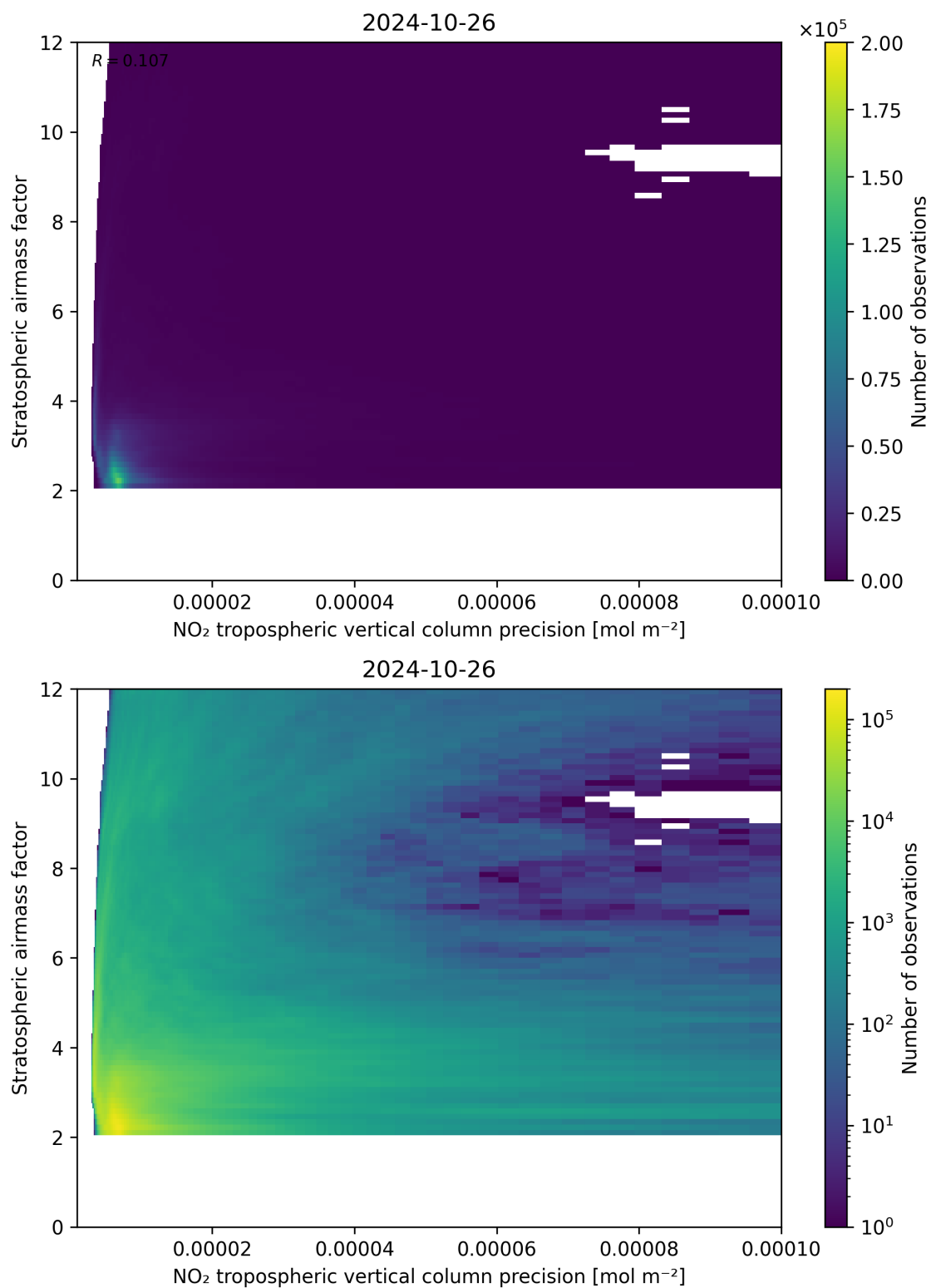
Figure 131: Scatter density plot of “NO 2 tropospheric vertical column precision” against “Stratospheric airmass factor” for 2024-10-25 to 2024-10-27.
