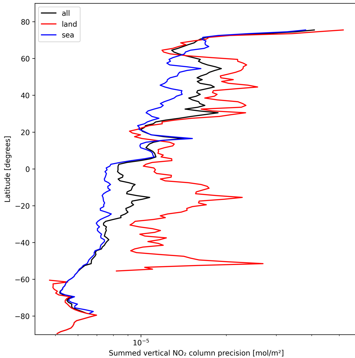
Figure 24: Zonal average of “Summed vertical NO 2 column precision” for 2024-10-25 to 2024-10-27.
