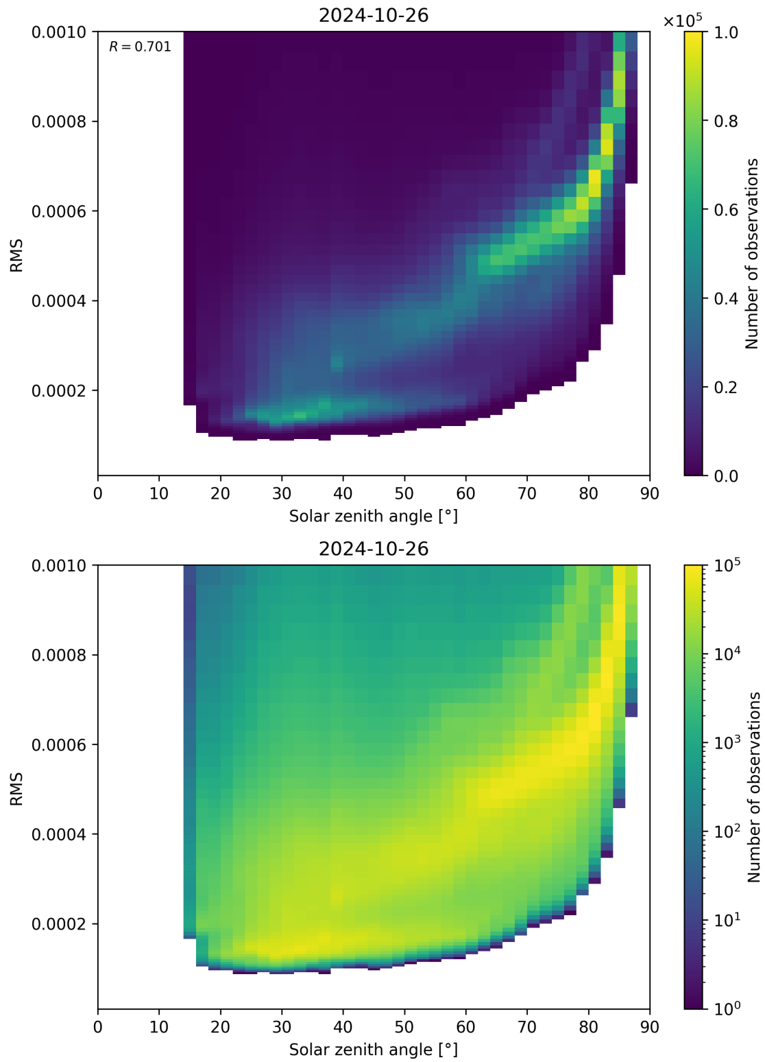
Figure 157: Scatter density plot of “Solar zenith angle” against “RMS” for 2024-10-25 to 2024-10-27.
