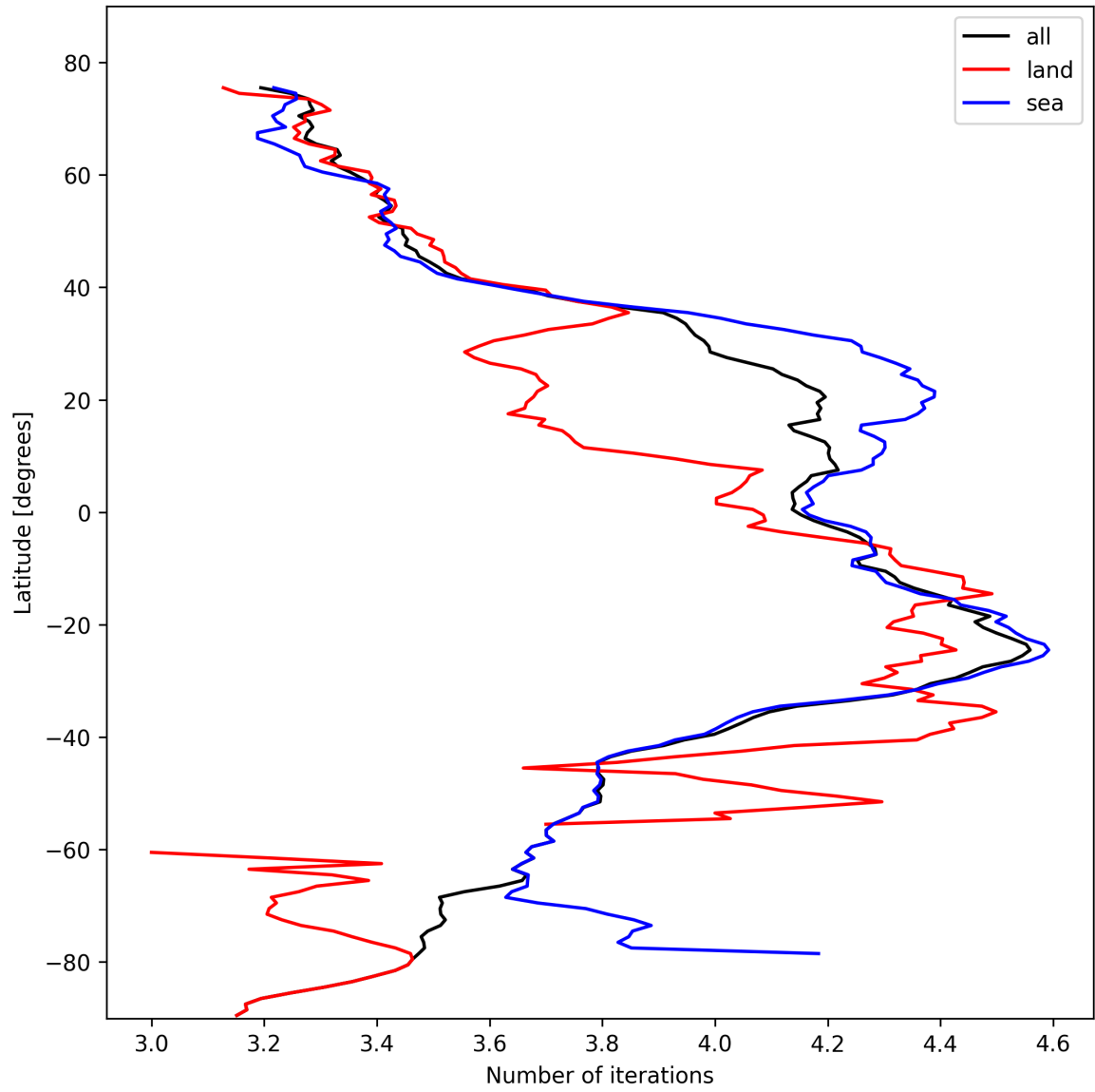
Figure 17: Zonal average of “Number of iterations” for 2024-10-25 to 2024-10-27.
