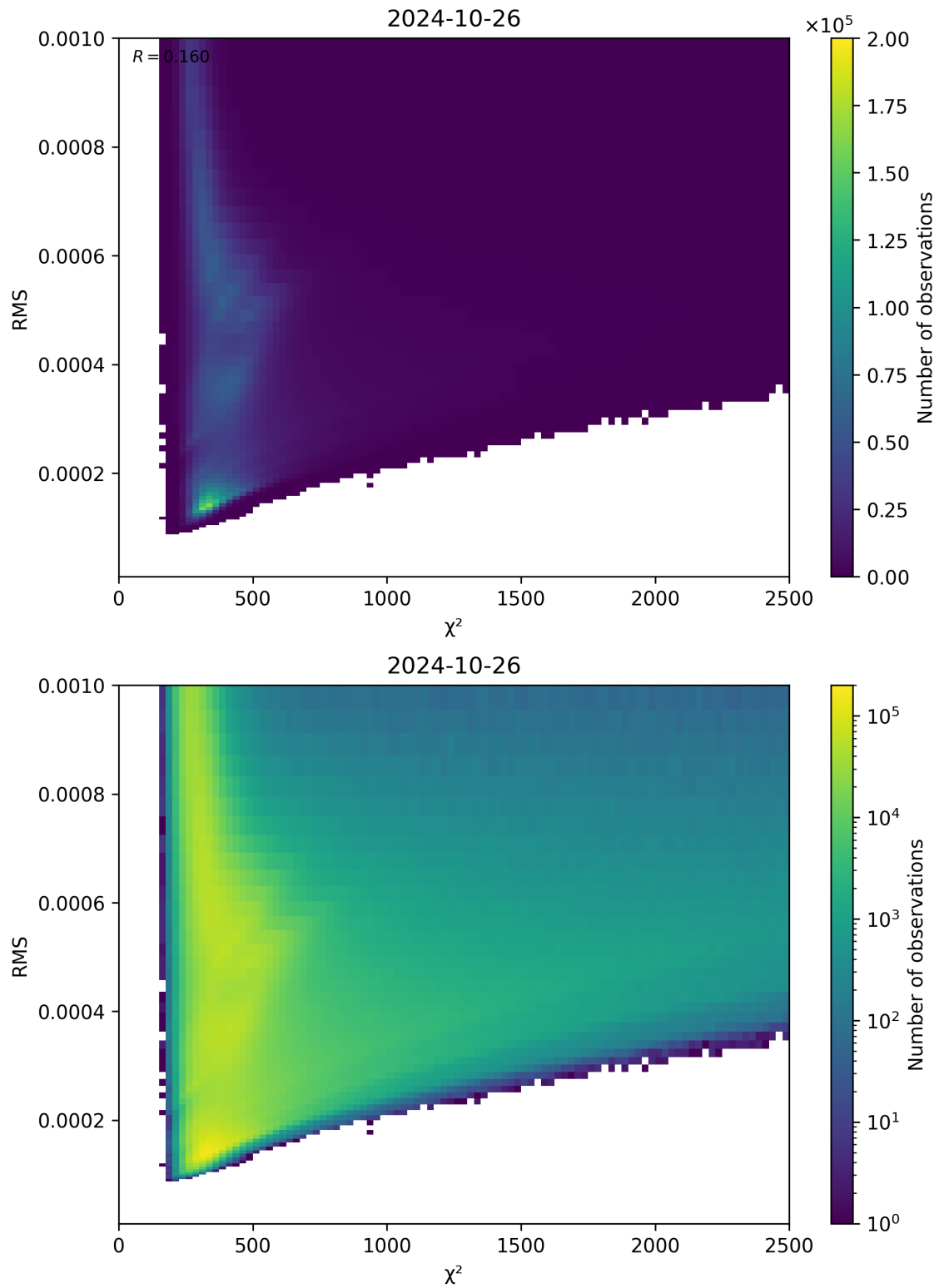
Figure 82: Scatter density plot of “ \chi^2 ” against “RMS” for 2024-10-25 to 2024-10-27.
