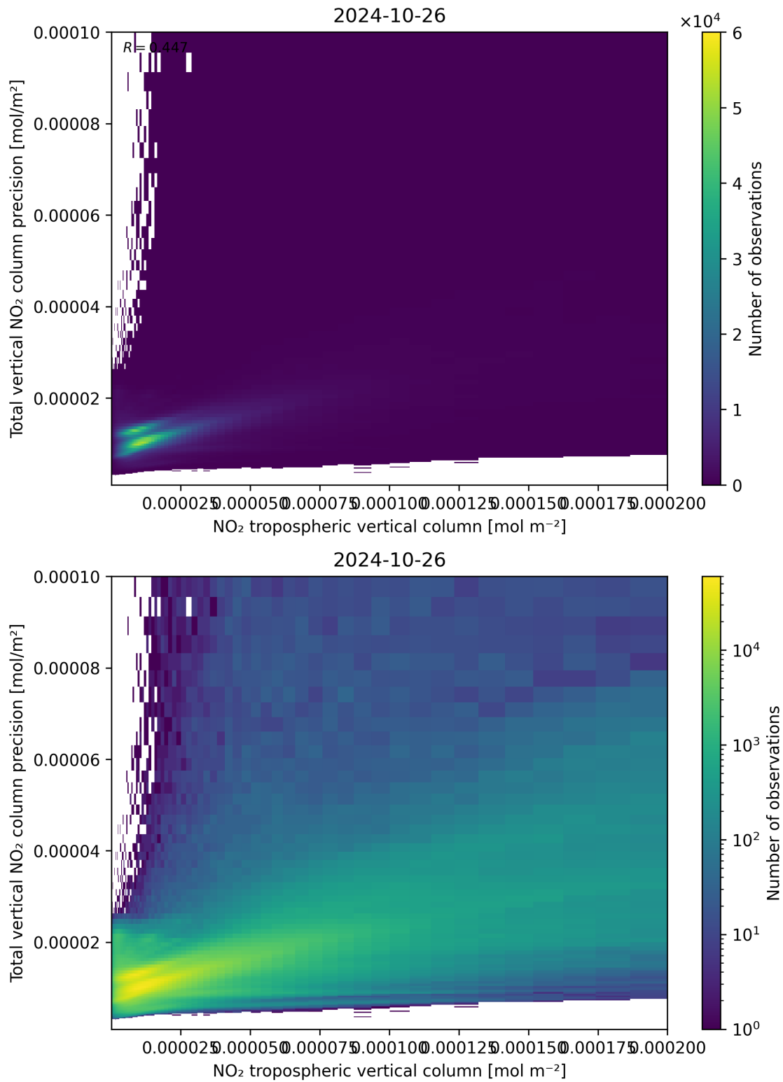
Figure 129: Scatter density plot of “NO 2 tropospheric vertical column” against “Total vertical NO 2 column precision” for 2024-10-25 to 2024-10-27.
