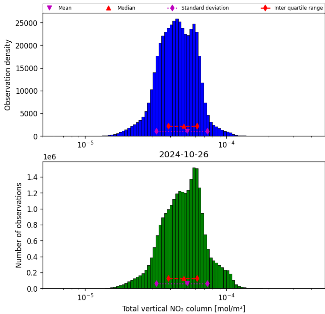
Figure 38: Histogram of “Total vertical NO 2 column” for 2024-10-25 to 2024-10-27
