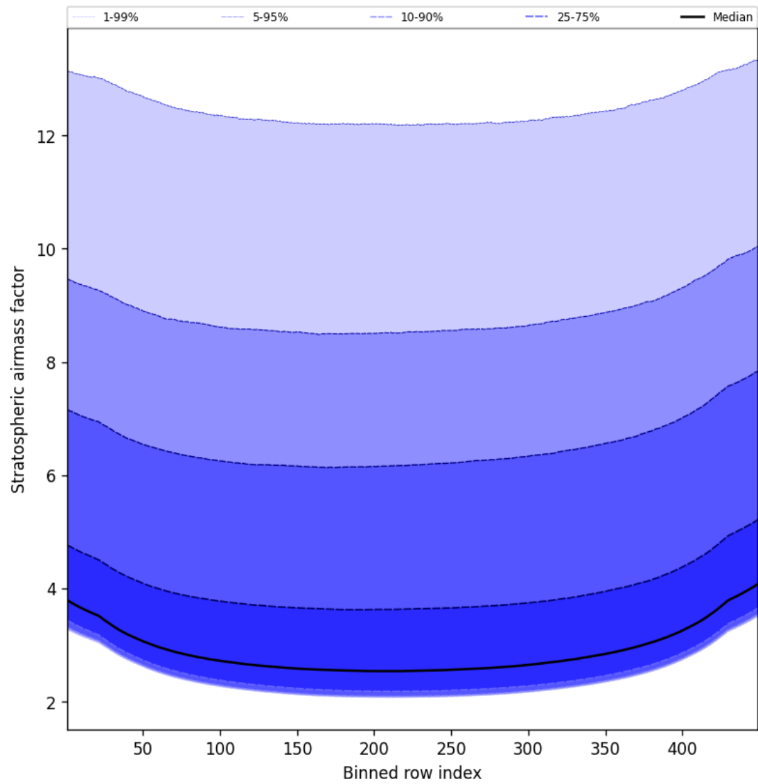
Figure 61: Along track statistics of “Stratospheric airmass factor” for 2024-10-25 to 2024-10-27
