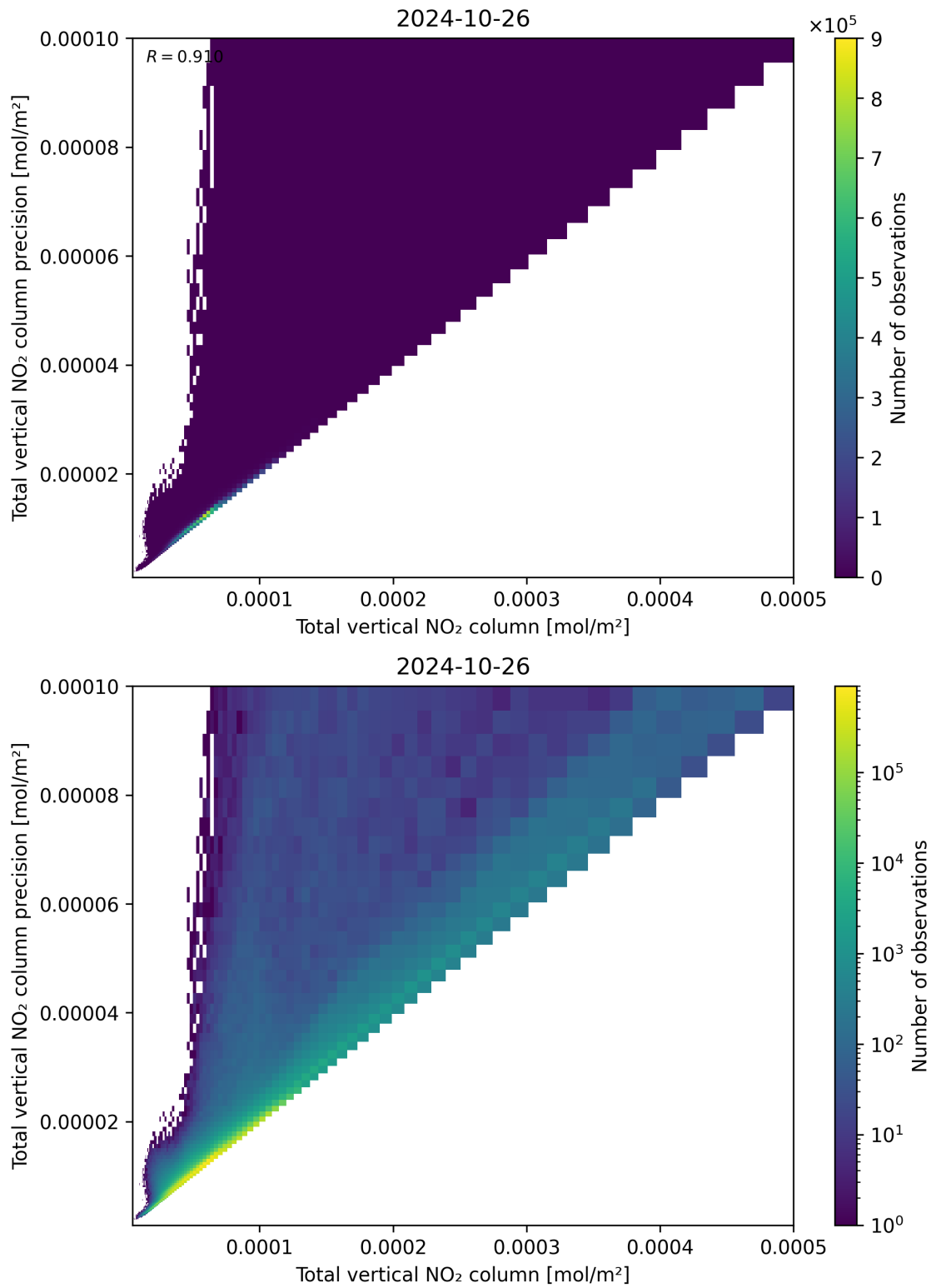
Figure 114: Scatter density plot of “Total vertical NO 2 column” against “Total vertical NO 2 column precision” for 2024-10-25 to 2024-10-27.
