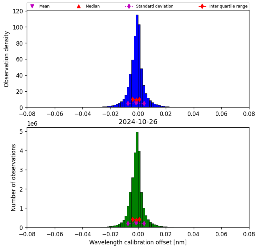
Figure 35: Histogram of “Wavelength calibration offset” for 2024-10-25 to 2024-10-27
