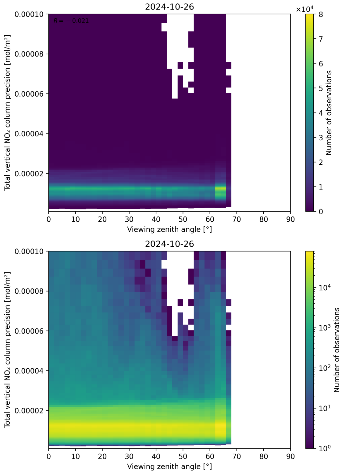
Figure 168: Scatter density plot of “Viewing zenith angle” against “Total vertical NO 2 column precision” for 2024-10-25 to 2024-10-27.
