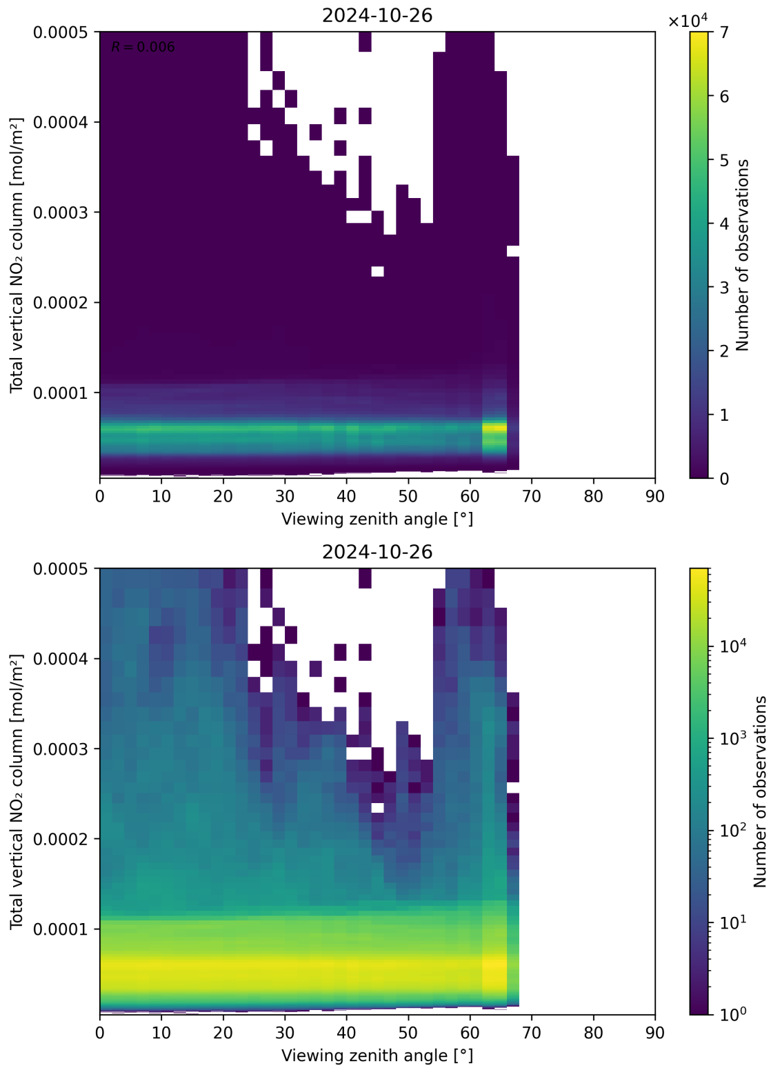
Figure 167: Scatter density plot of “Viewing zenith angle” against “Total vertical NO 2 column” for 2024-10-25 to 2024-10-27.
