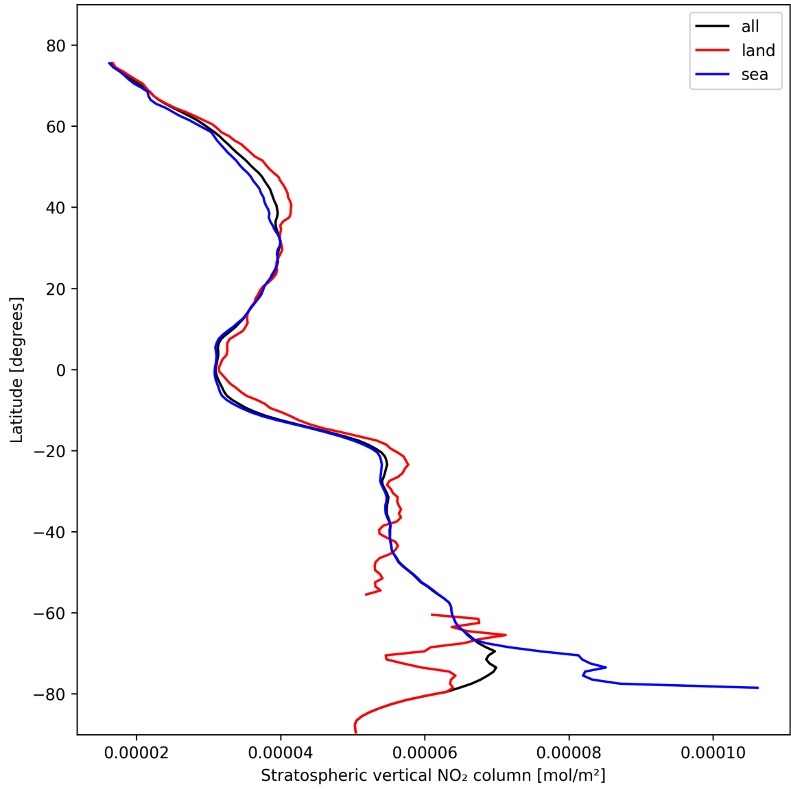
Figure 19: Zonal average of “Stratospheric vertical NO 2 column” for 2024-10-25 to 2024-10-27.
