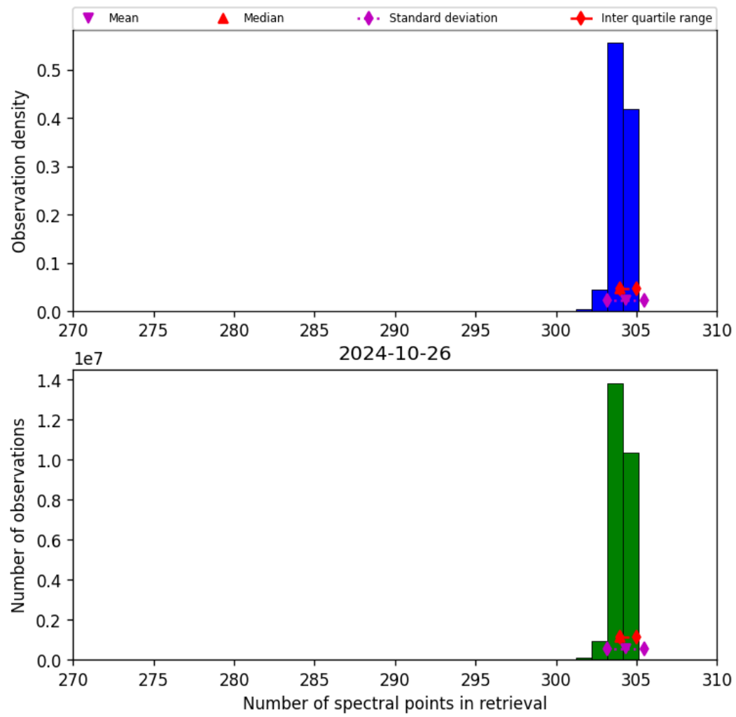
Figure 33: Histogram of “Number of spectral points in retrieval” for 2024-10-25 to 2024-10-27
