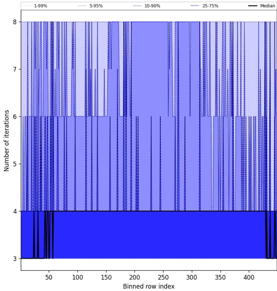
Figure 51: Along track statistics of “Number of iterations” for 2024-10-25 to 2024-10-27
