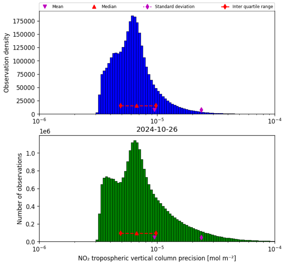
Figure 30: Histogram of “NO 2 tropospheric vertical column precision” for 2024-10-25 to 2024-10-27
