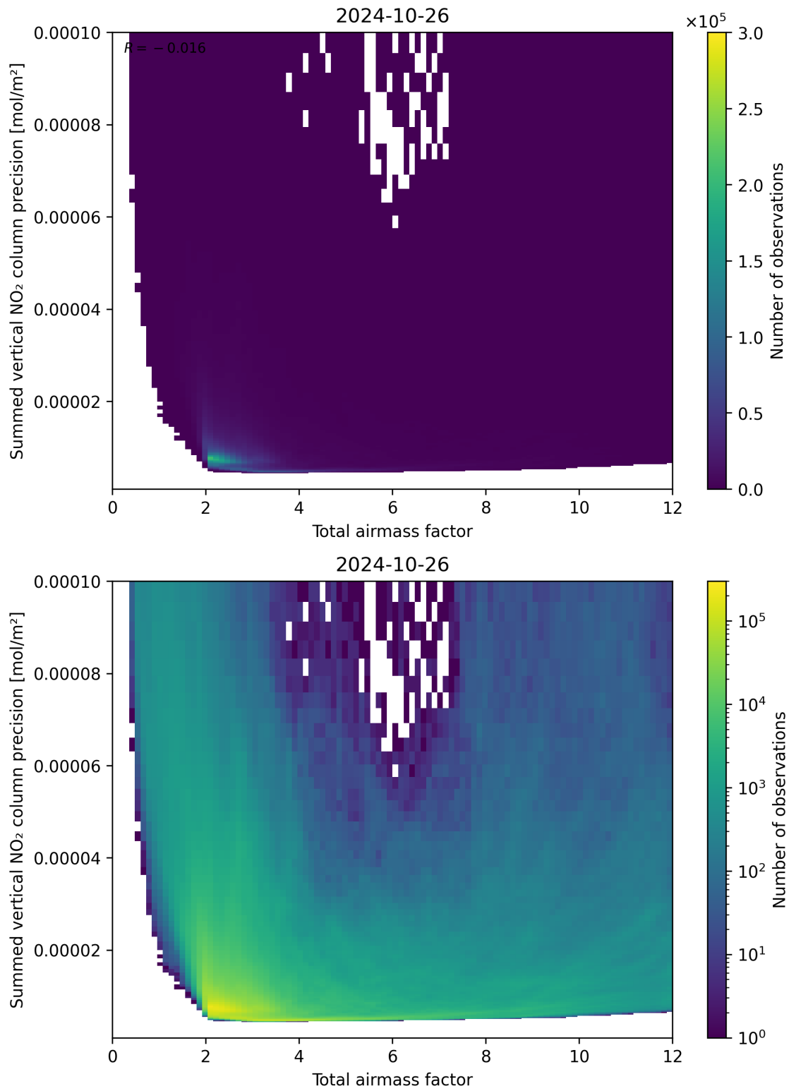
Figure 66: Scatter density plot of “Total airmass factor” against “Summed vertical NO 2 column precision” for 2024-10-25 to 2024-10-27.
