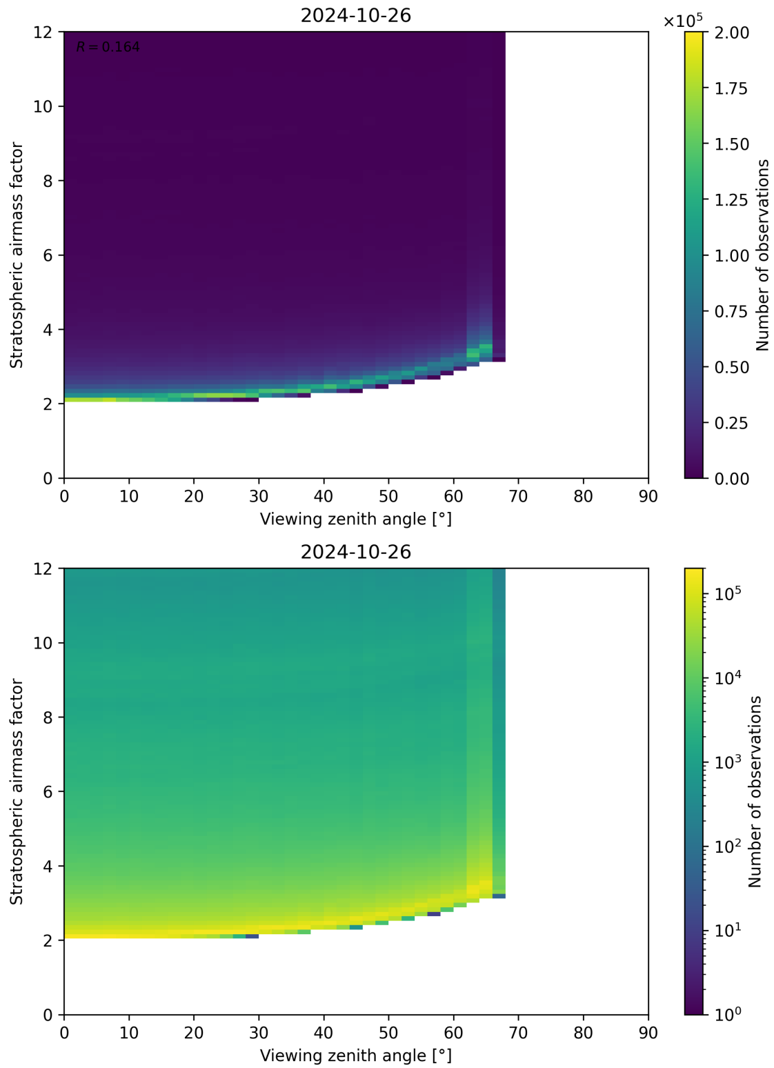
Figure 159: Scatter density plot of “Viewing zenith angle” against “Stratospheric airmass factor” for 2024-10-25 to 2024-10-27.
