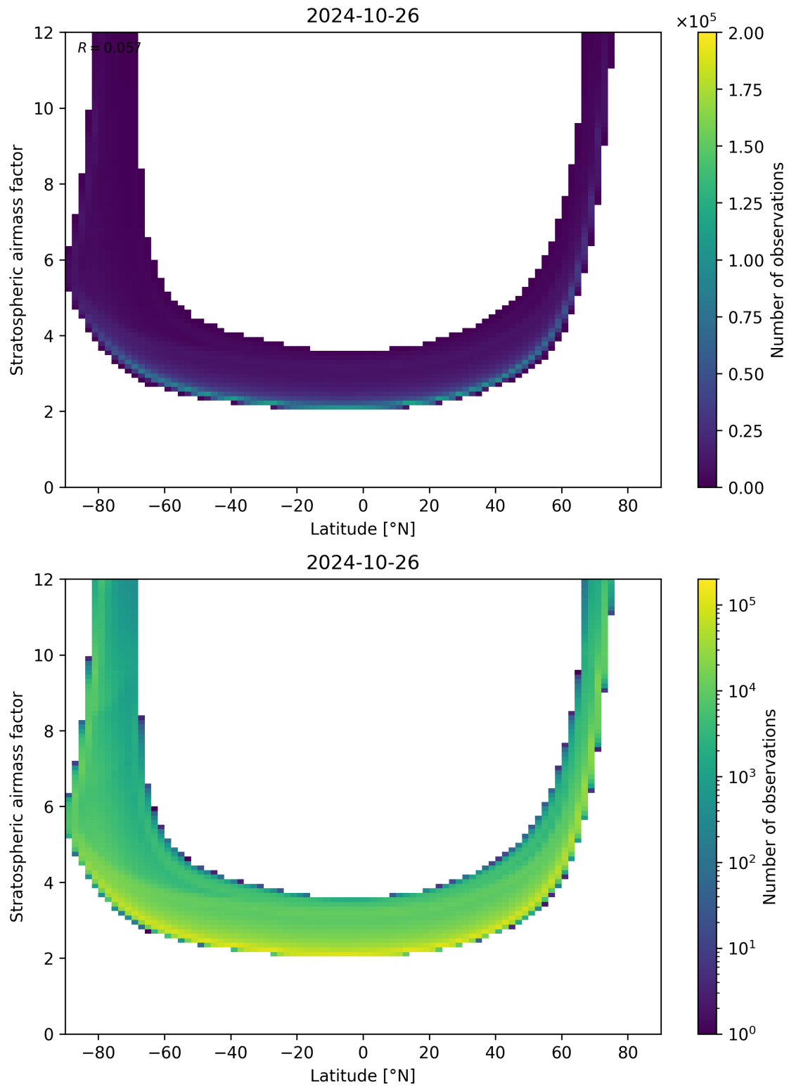
Figure 83: Scatter density plot of “Latitude” against “Stratospheric airmass factor” for 2024-10-25 to 2024-10-27.
