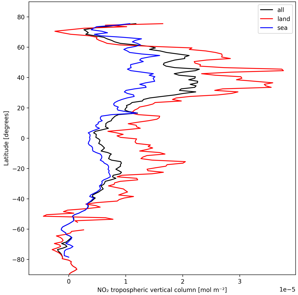
Figure 12: Zonal average of “NO 2 tropospheric vertical column” for 2024-10-25 to 2024-10-27.
