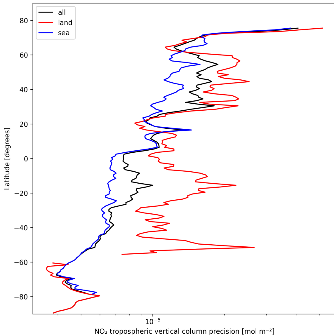
Figure 13: Zonal average of “NO 2 tropospheric vertical column precision” for 2024-10-25 to 2024-10-27.
