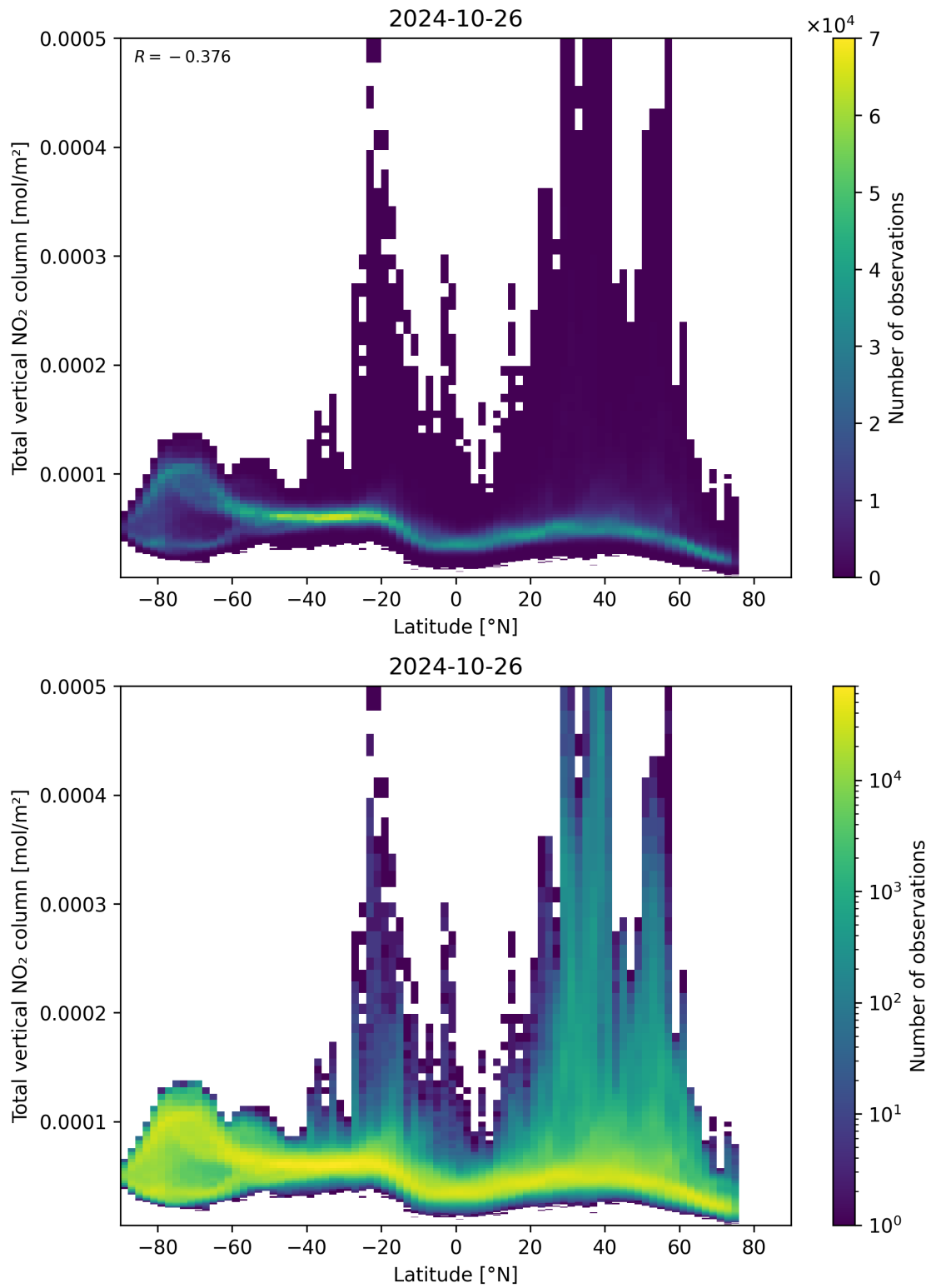
Figure 90: Scatter density plot of “Latitude” against “Total vertical NO 2 column” for 2024-10-25 to 2024-10-27.
