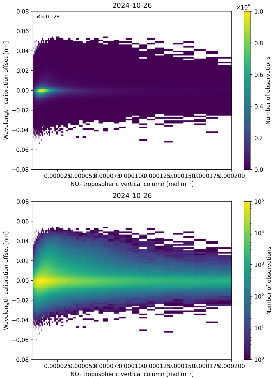
Figure 143: Scatter density plot of “NO 2 tropospheric vertical column” against “Wavelength calibration offset” for 2024-10-25 to 2024-10-27.
