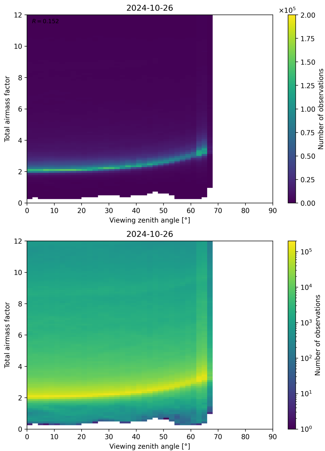
Figure 160: Scatter density plot of “Viewing zenith angle” against “Total airmass factor” for 2024-10-25 to 2024-10-27.
