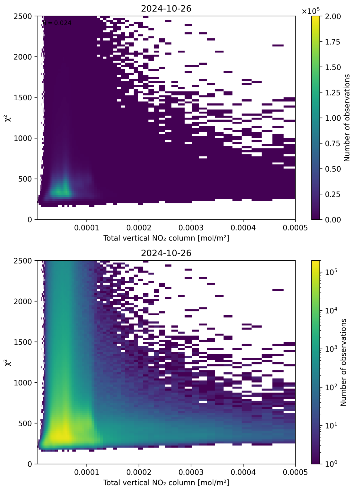
Figure 111: Scatter density plot of “Total vertical NO 2 column” against “ \chi^2 ” for 2024-10-25 to 2024-10-27.
