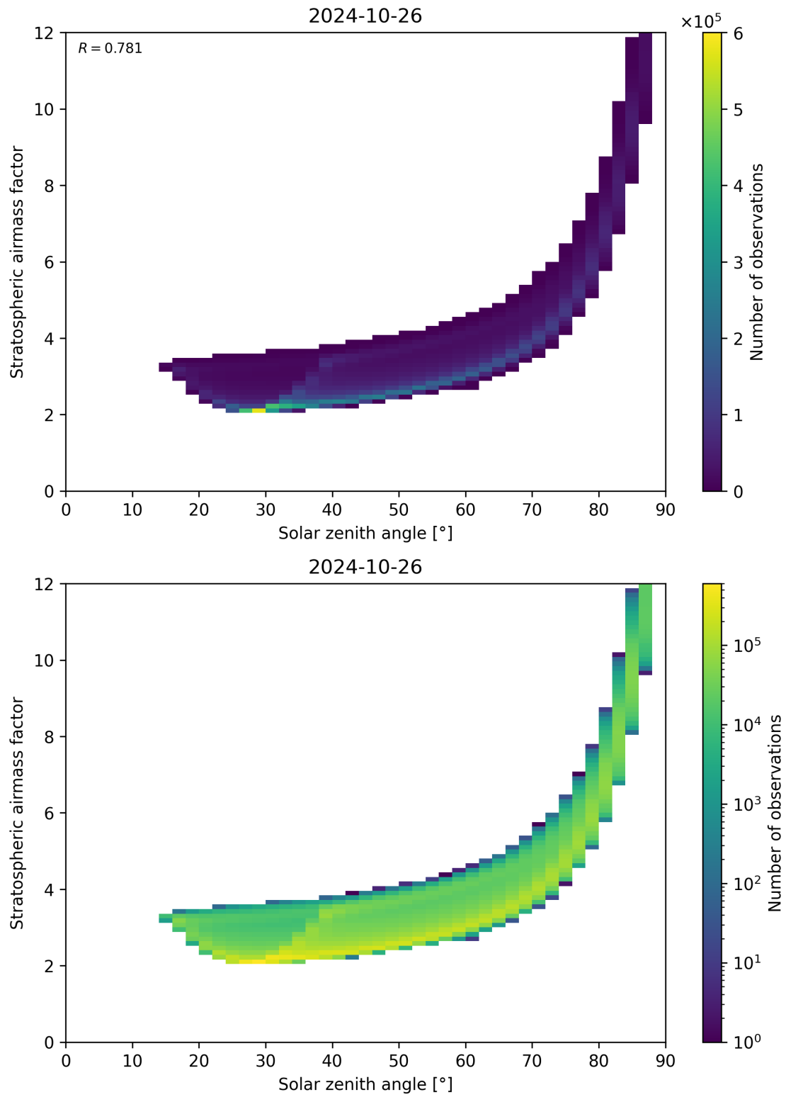
Figure 145: Scatter density plot of “Solar zenith angle” against “Stratospheric airmass factor” for 2024-10-25 to 2024-10-27.
