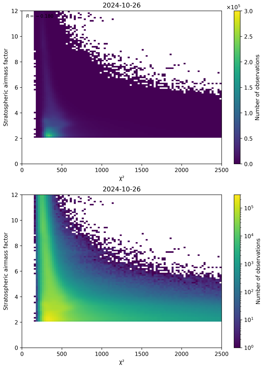
Figure 81: Scatter density plot of “ \chi^2 ” against “Stratospheric airmass factor” for 2024-10-25 to 2024-10-27.
