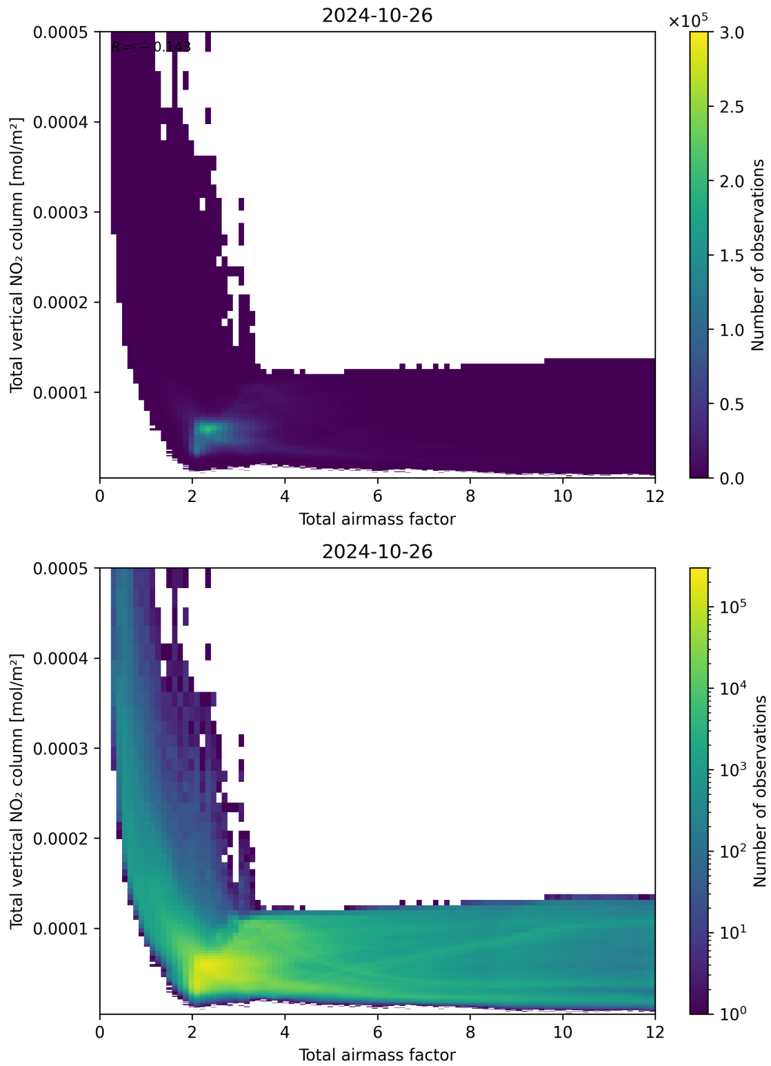
Figure 67: Scatter density plot of “Total airmass factor” against “Total vertical NO 2 column” for 2024-10-25 to 2024-10-27.
