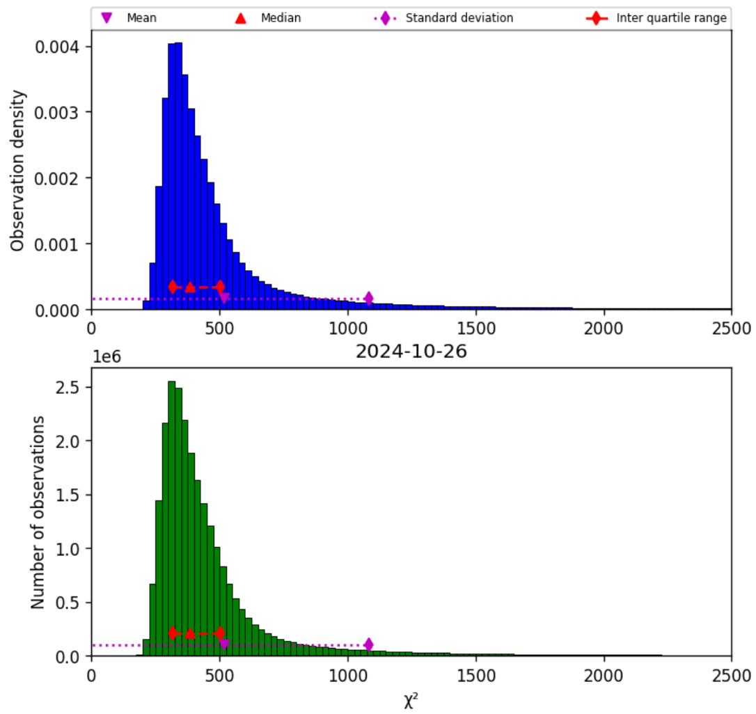
Figure 42: Histogram of “ \chi^2 ” for 2024-10-25 to 2024-10-27
