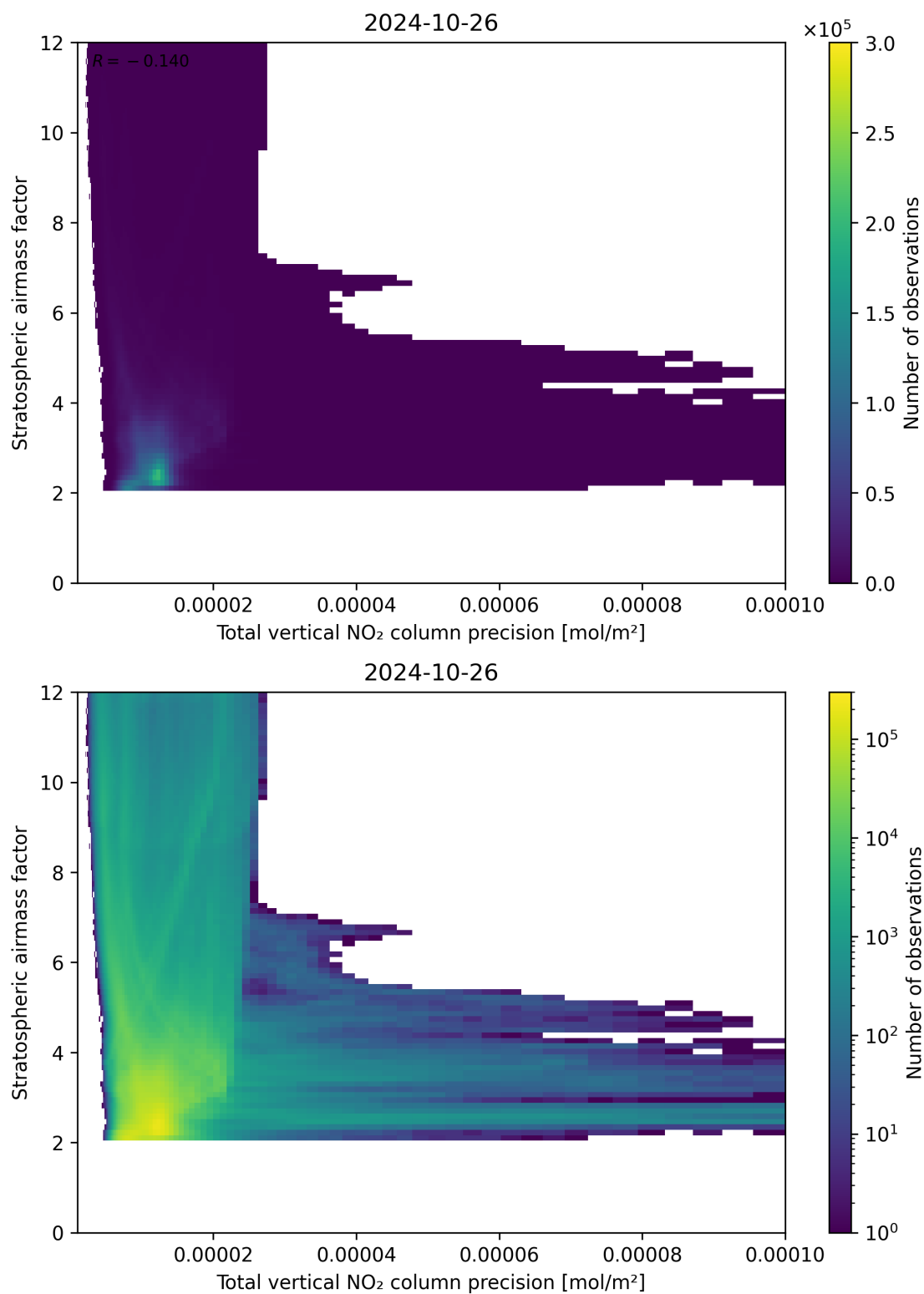
Figure 115: Scatter density plot of “Total vertical NO 2 column precision” against “Stratospheric air mass factor” for 2024-10-25 to 2024-10-27.
