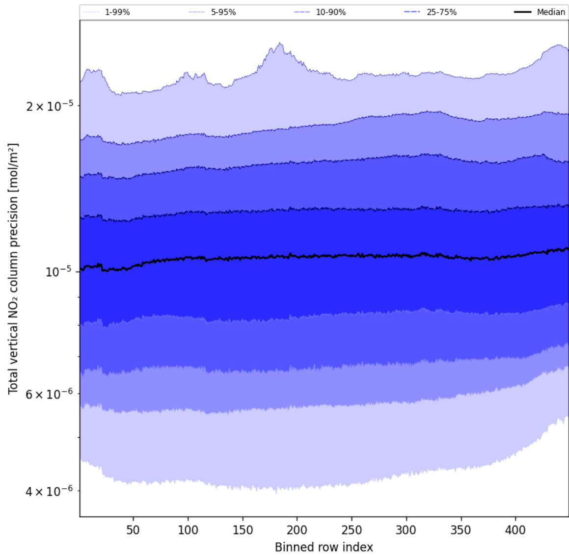
Figure 56: Along track statistics of “Total vertical NO 2 column precision” for 2024-10-25 to 2024-10-27
