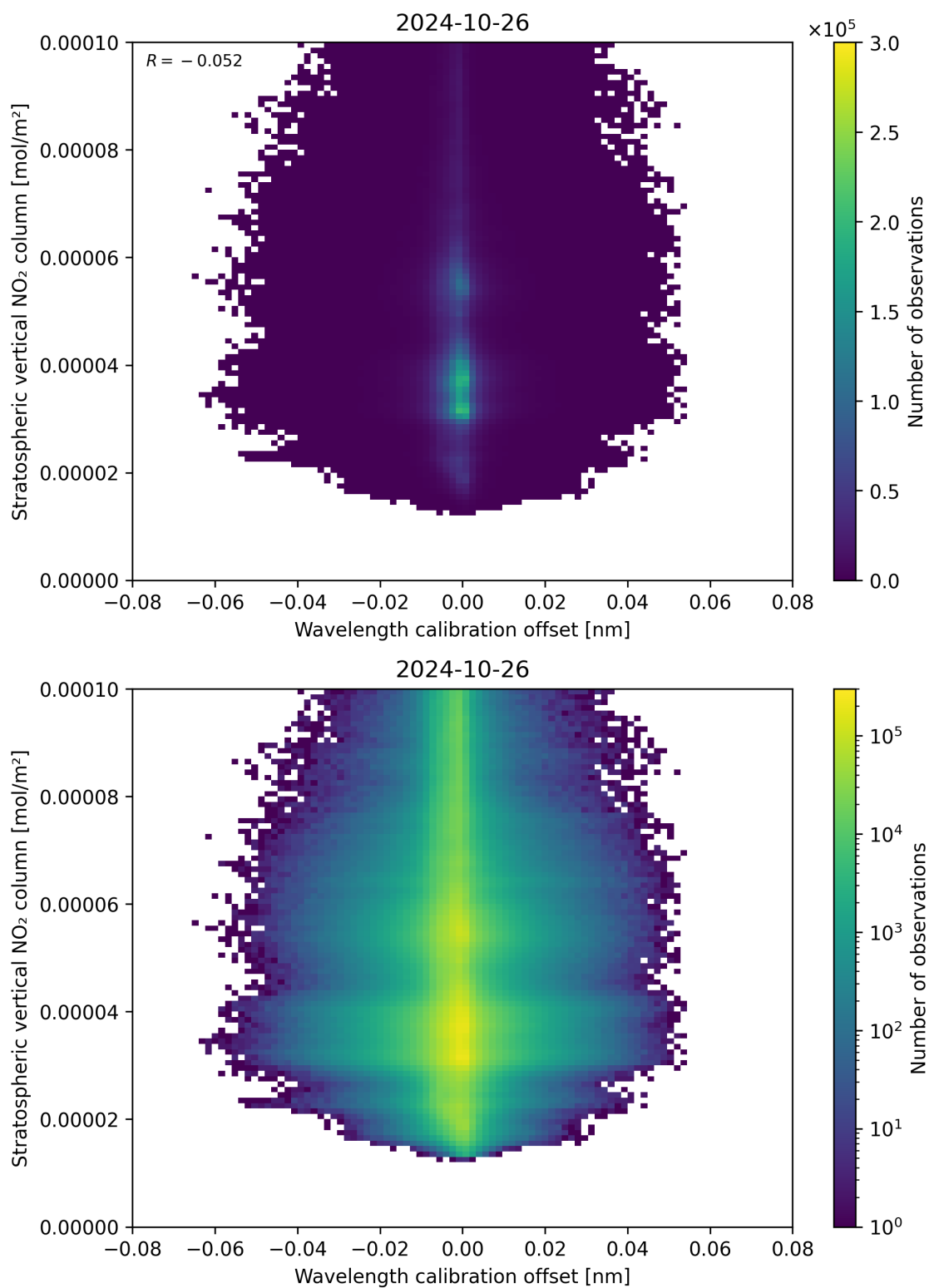
Figure 176: Scatter density plot of “Wavelength calibration offset” against “Stratospheric vertical NO 2 column” for 2024-10-25 to 2024-10-27.
