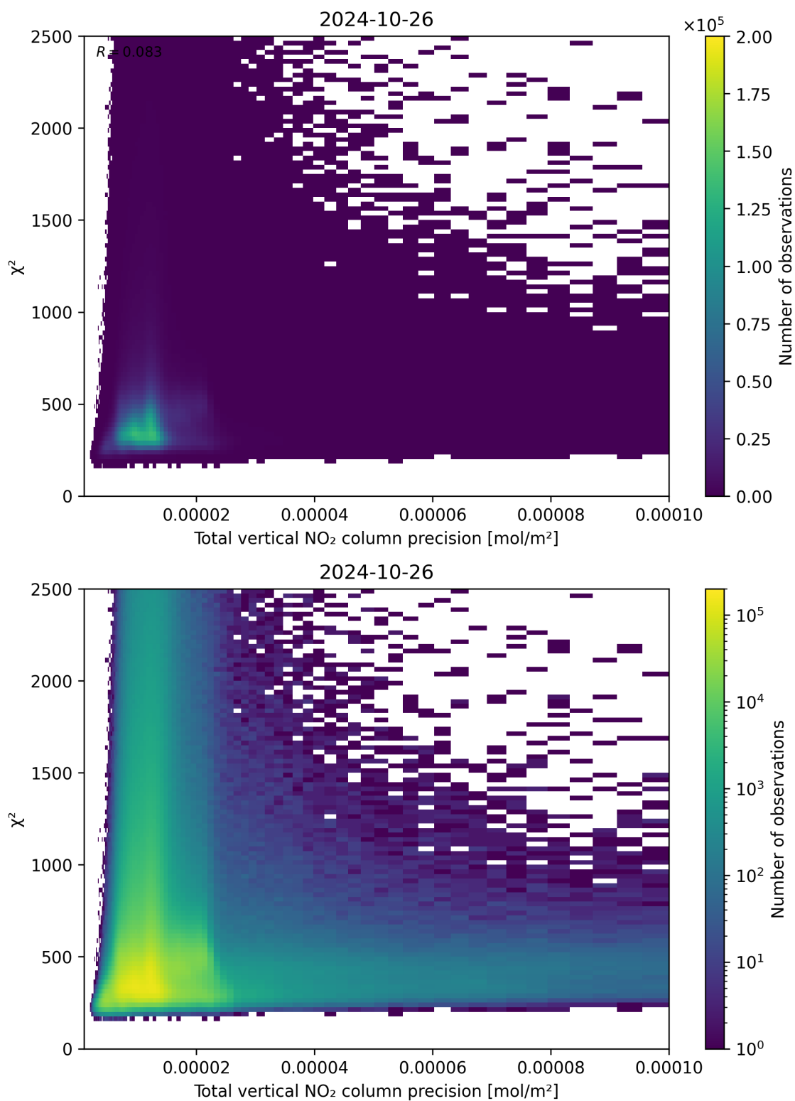
Figure 116: Scatter density plot of “Total vertical NO 2 column precision” against “ \chi^2 ” for 2024-10-25 to 2024-10-27.
