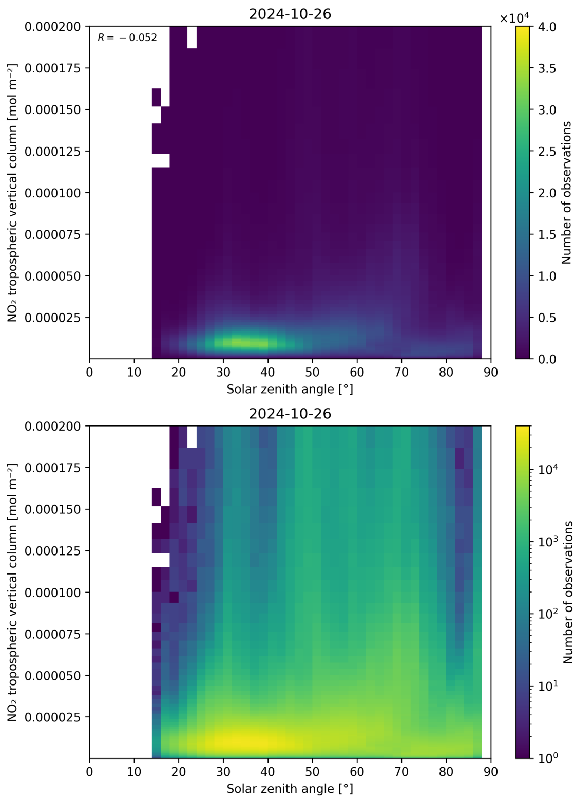
Figure 155: Scatter density plot of “Solar zenith angle” against “NO 2 tropospheric vertical column” for 2024-10-25 to 2024-10-27.
