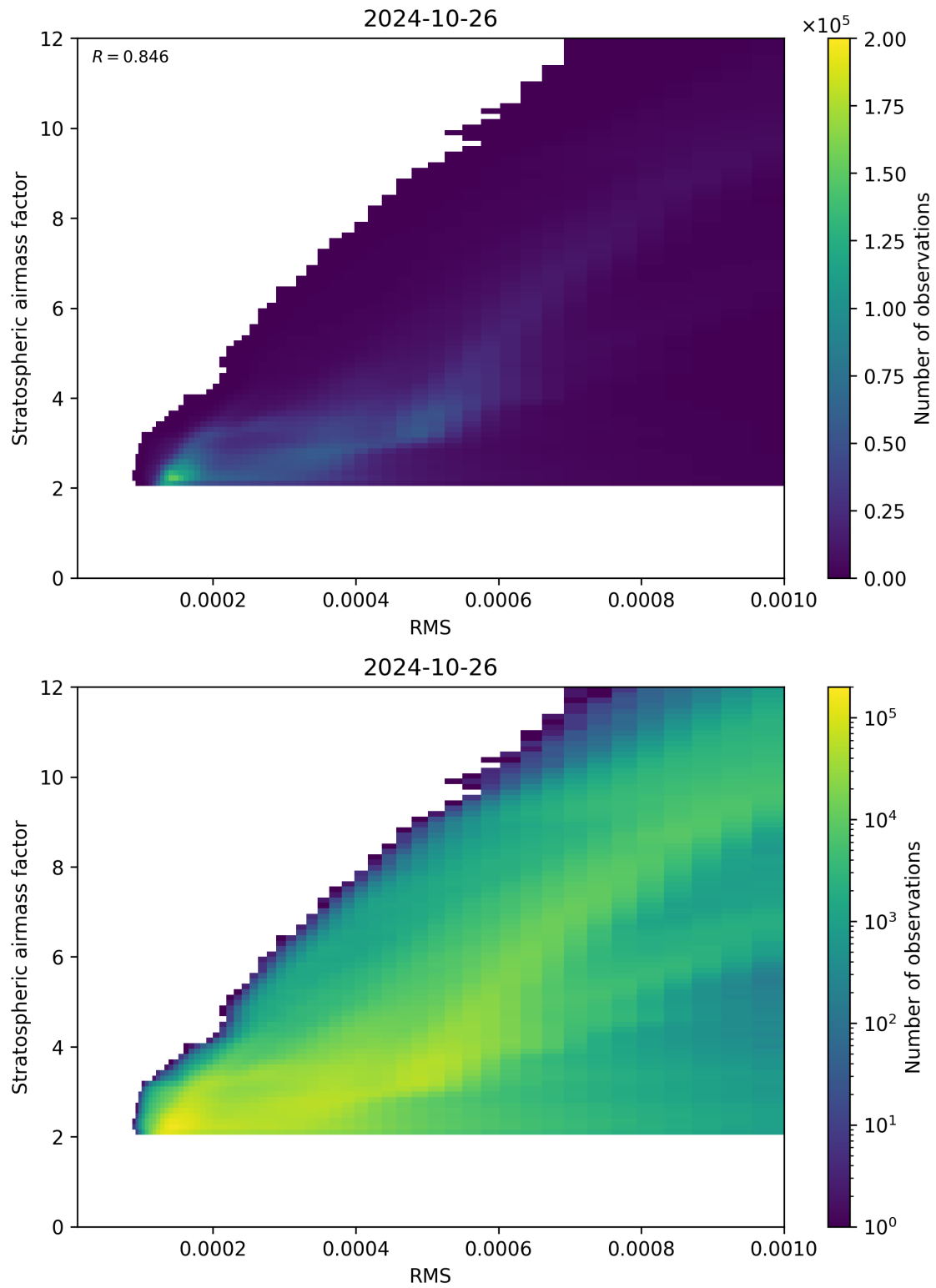
Figure 144: Scatter density plot of “RMS” against “Stratospheric airmass factor” for 2024-10-25 to 2024-10-27.
