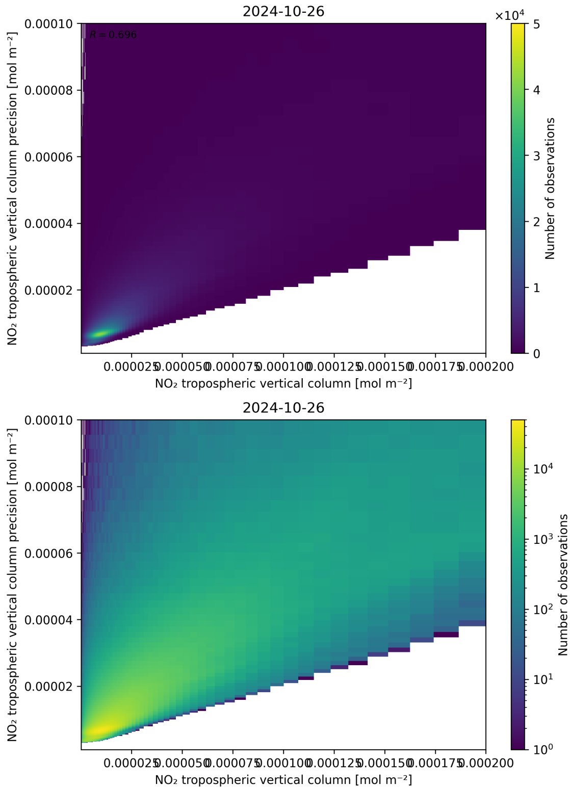
Figure 130: Scatter density plot of “NO 2 tropospheric vertical column” against “NO 2 tropospheric vertical column precision” for 2024-10-25 to 2024-10-27.
