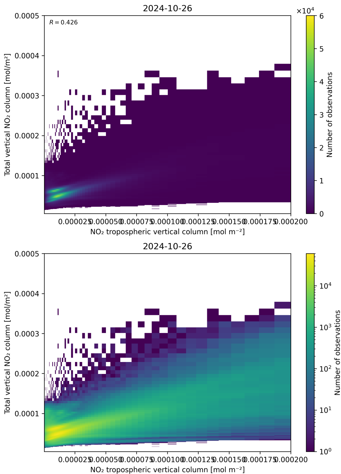
Figure 128: Scatter density plot of “NO 2 tropospheric vertical column” against “Total vertical NO 2 column” for 2024-10-25 to 2024-10-27.
