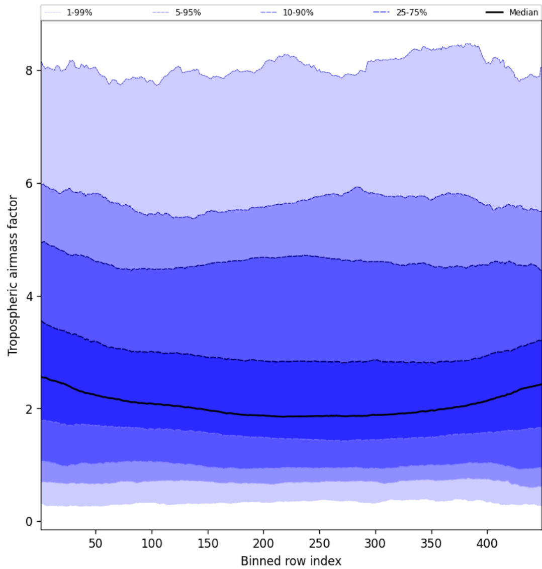
Figure 48: Along track statistics of “Tropospheric airmass factor” for 2024-10-25 to 2024-10-27
