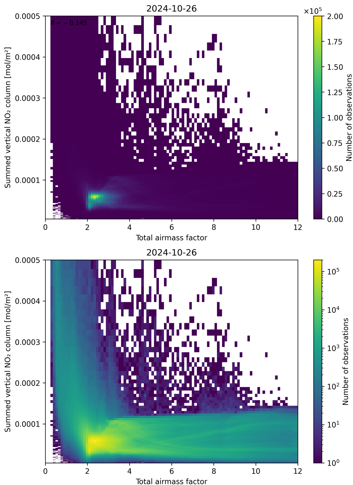
Figure 65: Scatter density plot of “Total airmass factor” against “Summed vertical NO 2 column” for 2024-10-25 to 2024-10-27.
