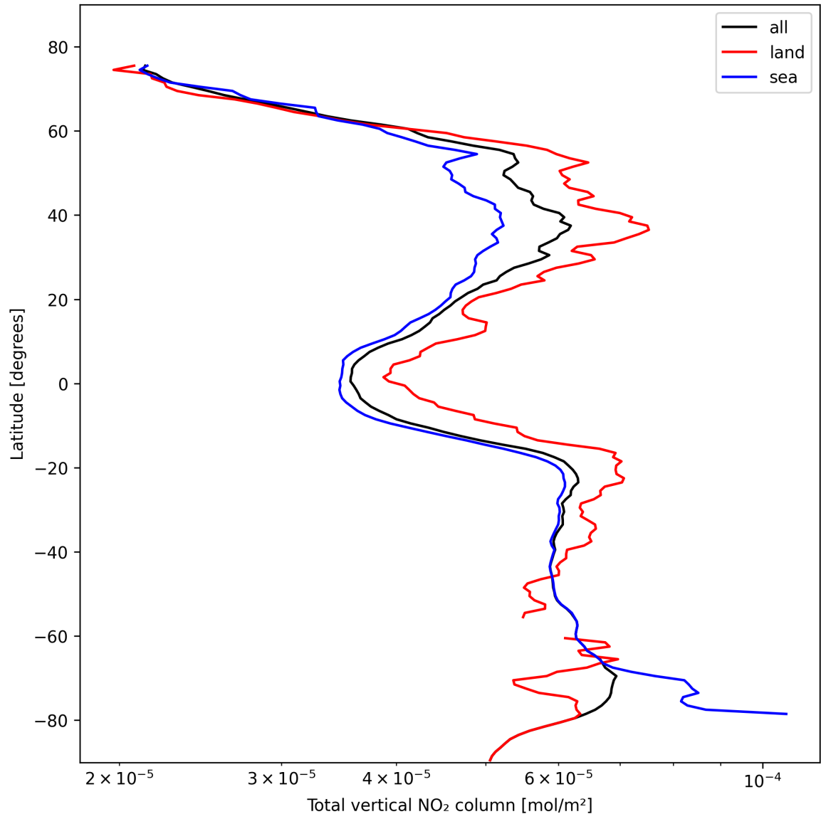
Figure 21: Zonal average of “Total vertical NO 2 column” for 2024-10-25 to 2024-10-27.
