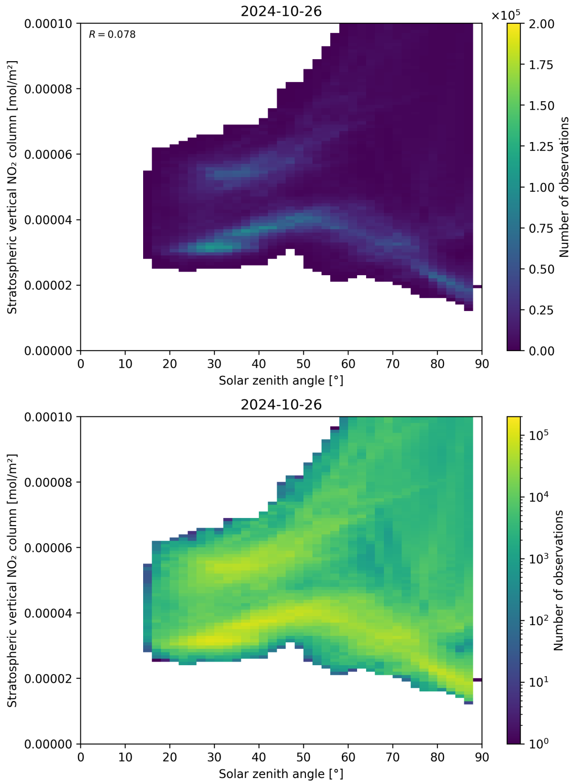
Figure 150: Scatter density plot of “Solar zenith angle” against “Stratospheric vertical NO 2 column” for 2024-10-25 to 2024-10-27.
