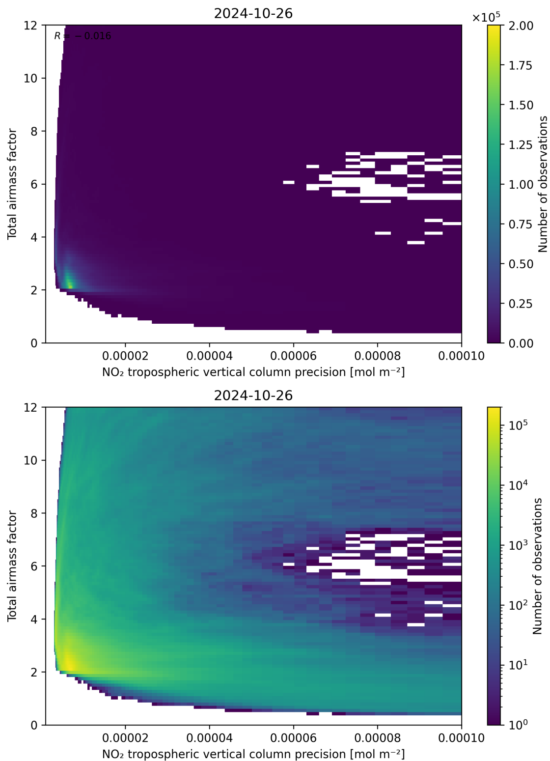
Figure 132: Scatter density plot of “NO 2 tropospheric vertical column precision” against “Total air mass factor” for 2024-10-25 to 2024-10-27.
