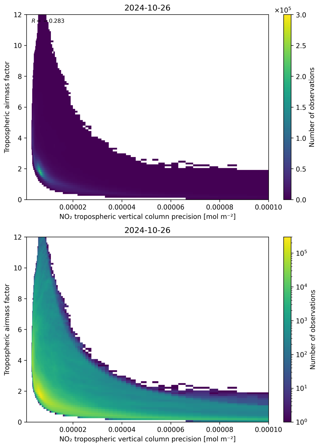
Figure 133: Scatter density plot of “NO 2 tropospheric vertical column precision” against “Tropospheric airmass factor” for 2024-10-25 to 2024-10-27.
