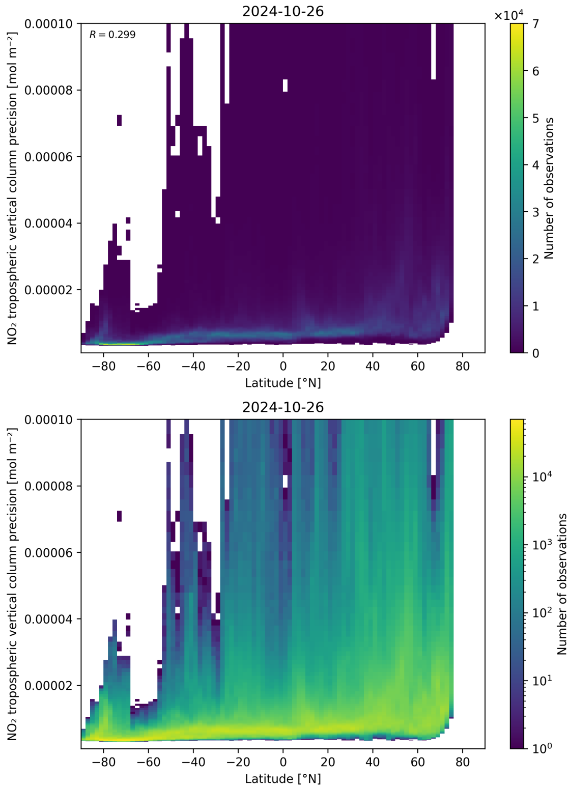
Figure 93: Scatter density plot of “Latitude” against “NO 2 tropospheric vertical column precision” for 2024-10-25 to 2024-10-27.
