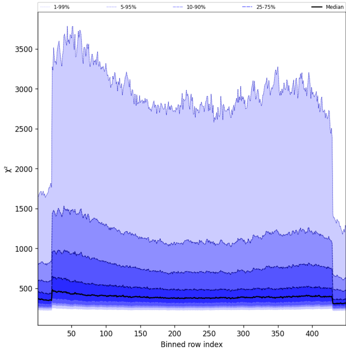
Figure 59: Along track statistics of “ \chi^2 ” for 2024-10-25 to 2024-10-27
