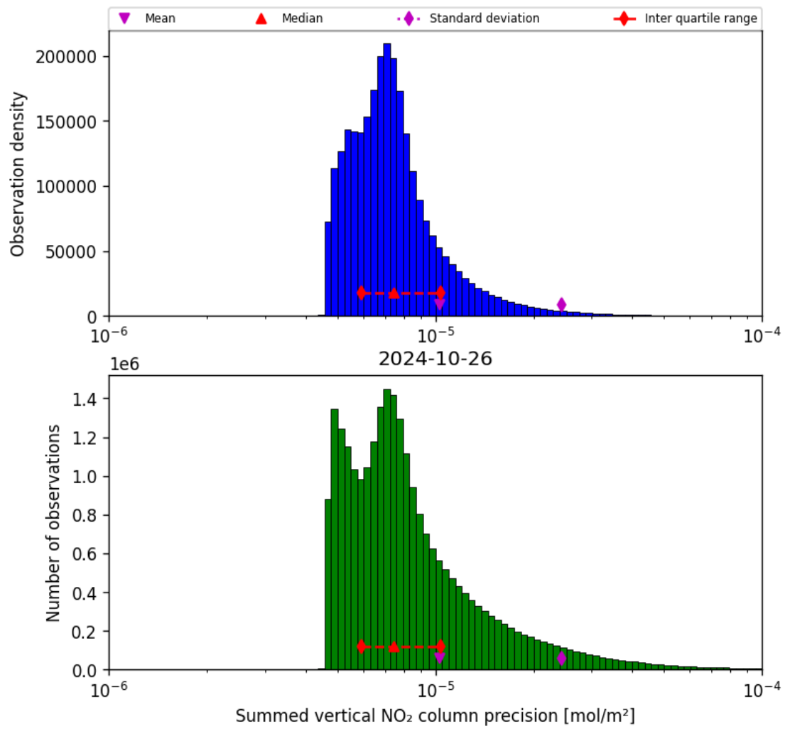
Figure 41: Histogram of "Summed vertical NO 2 column precision" for 2024-10-25 to 2024-10-27
