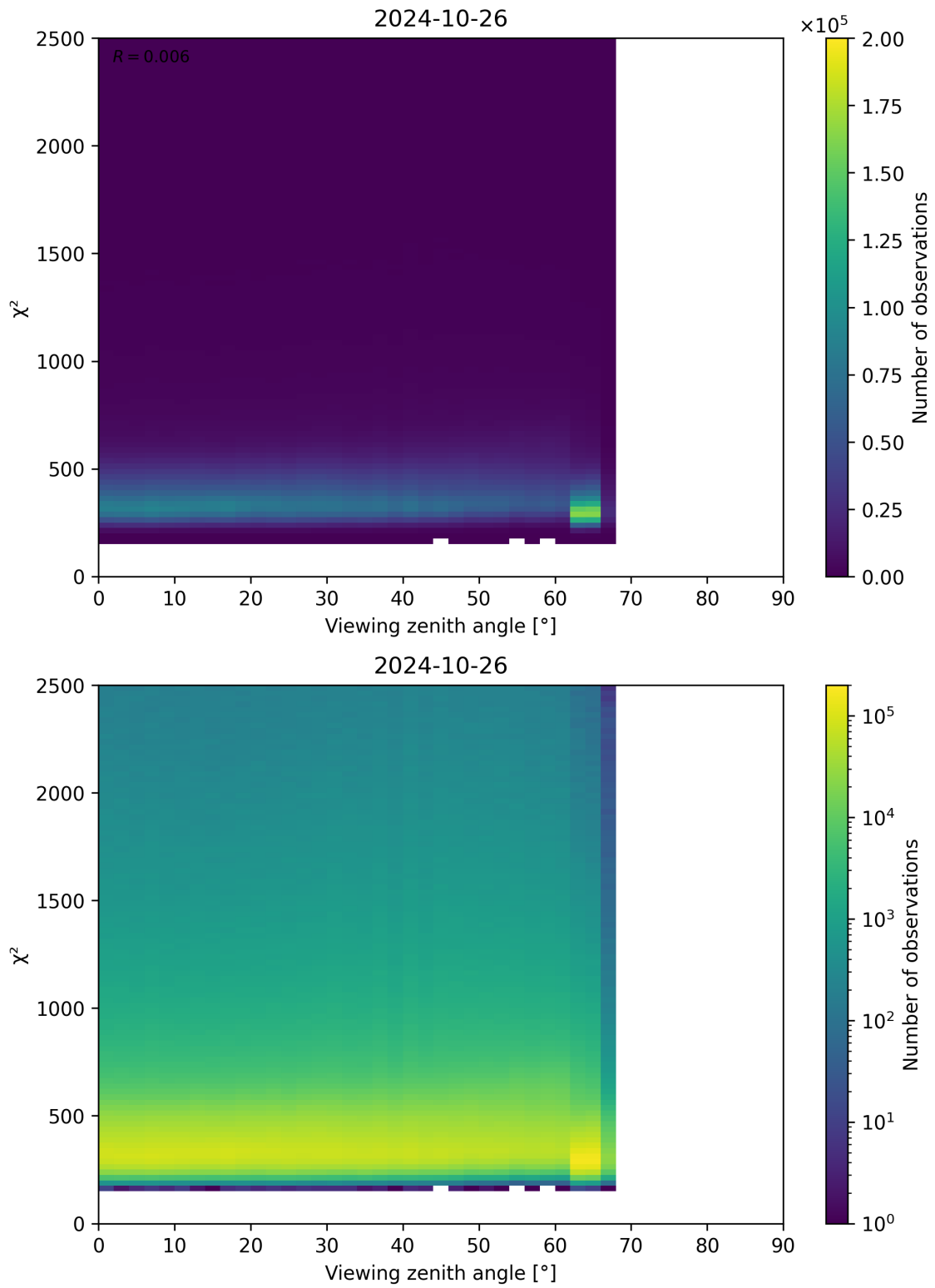
Figure 162: Scatter density plot of “Viewing zenith angle” against “ \chi^2 ” for 2024-10-25 to 2024-10-27.
