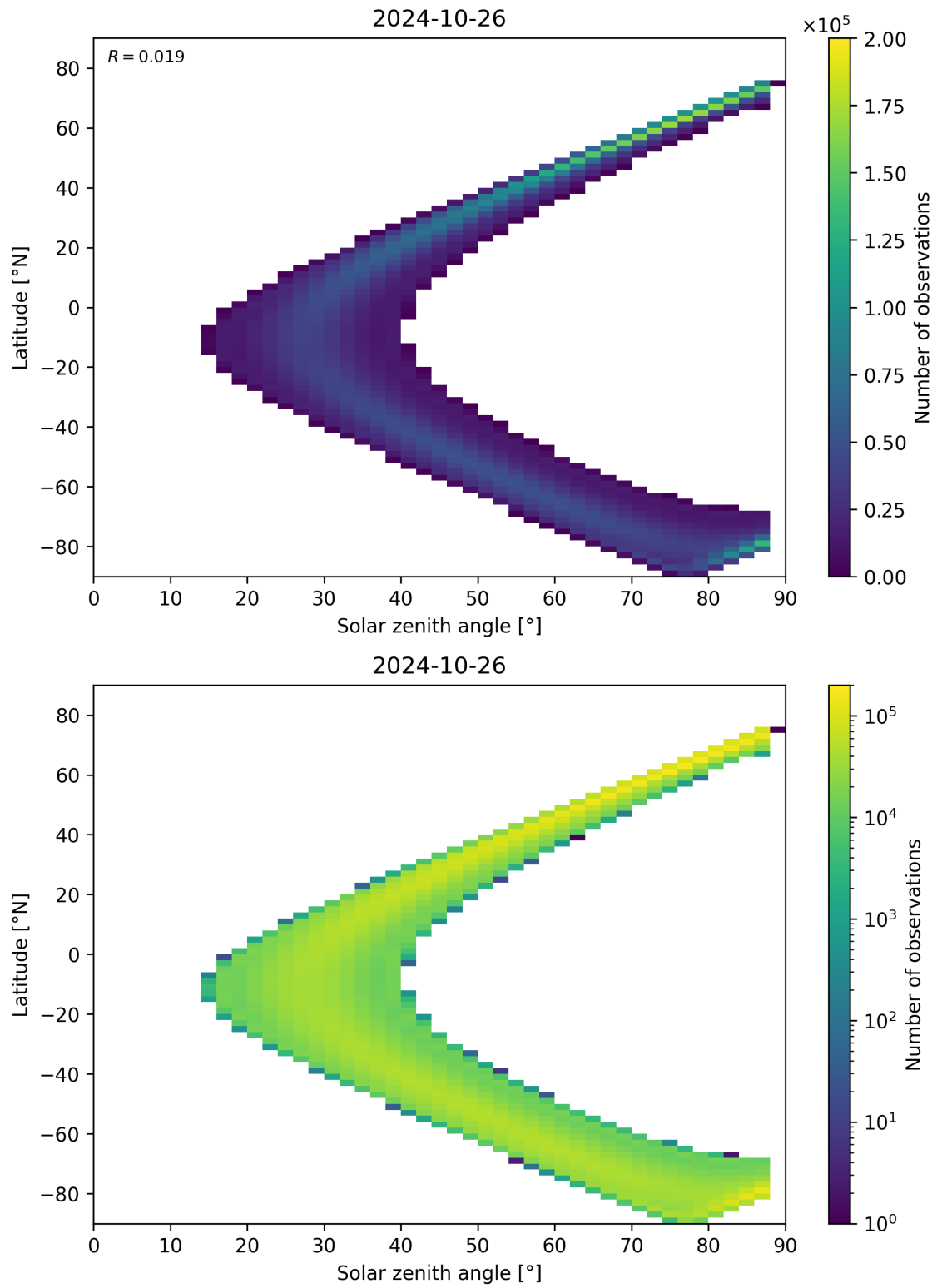
Figure 149: Scatter density plot of “Solar zenith angle” against “Latitude” for 2024-10-25 to 2024-10-27.
