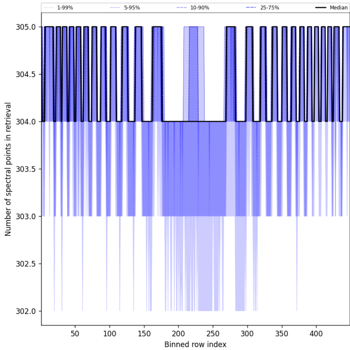
Figure 50: Along track statistics of “Number of spectral points in retrieval” for 2024-10-25 to 2024-10-27
