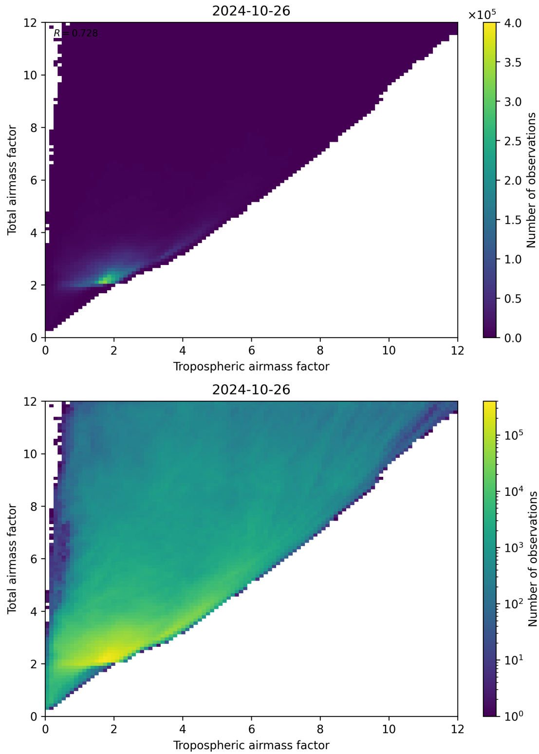
Figure 72: Scatter density plot of “Tropospheric airmass factor” against “Total airmass factor” for 2024-10-25 to 2024-10-27.
