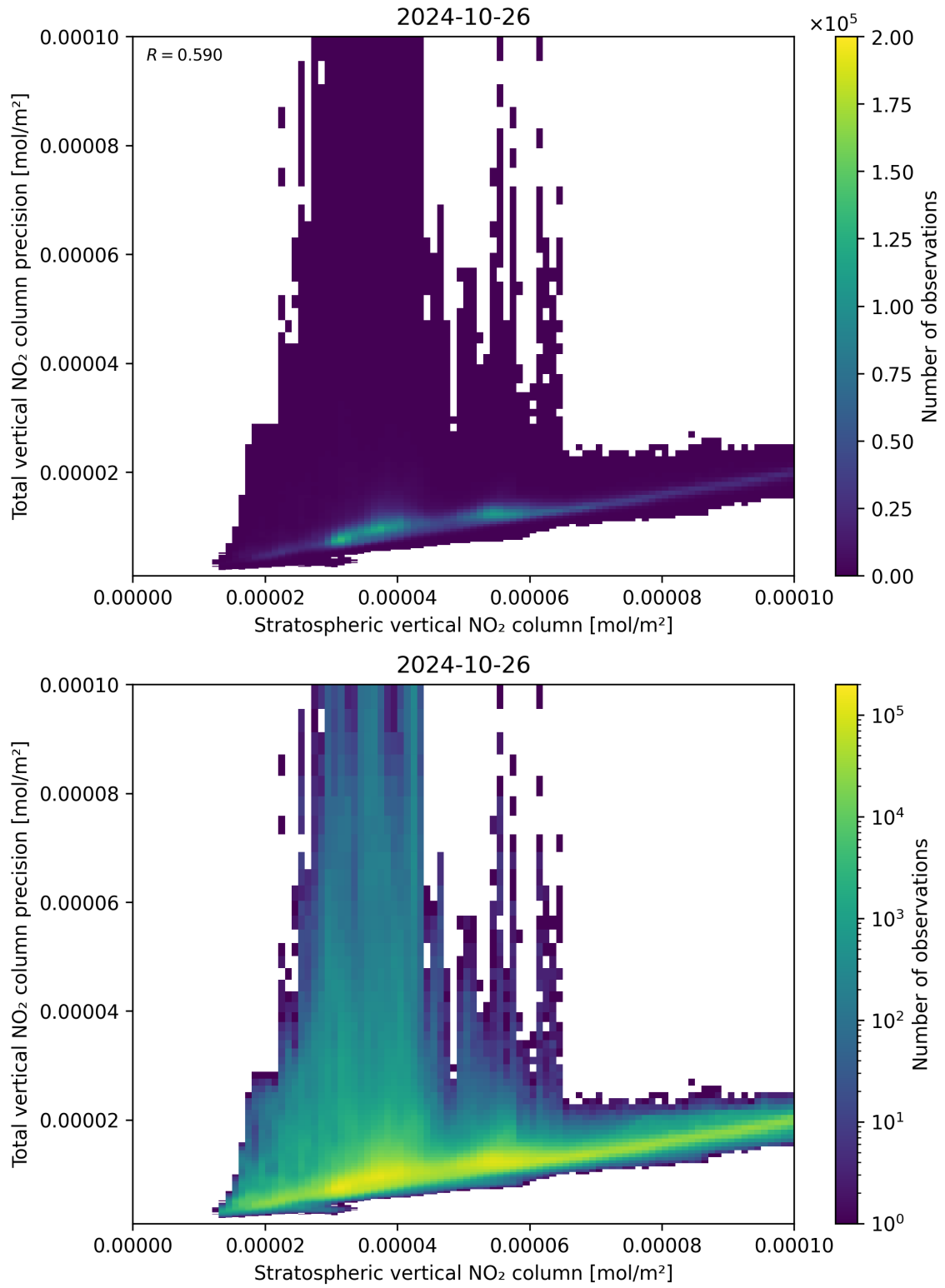
Figure 101: Scatter density plot of “Stratospheric vertical NO 2 column” against “Total vertical NO 2 column precision” for 2024-10-25 to 2024-10-27.
