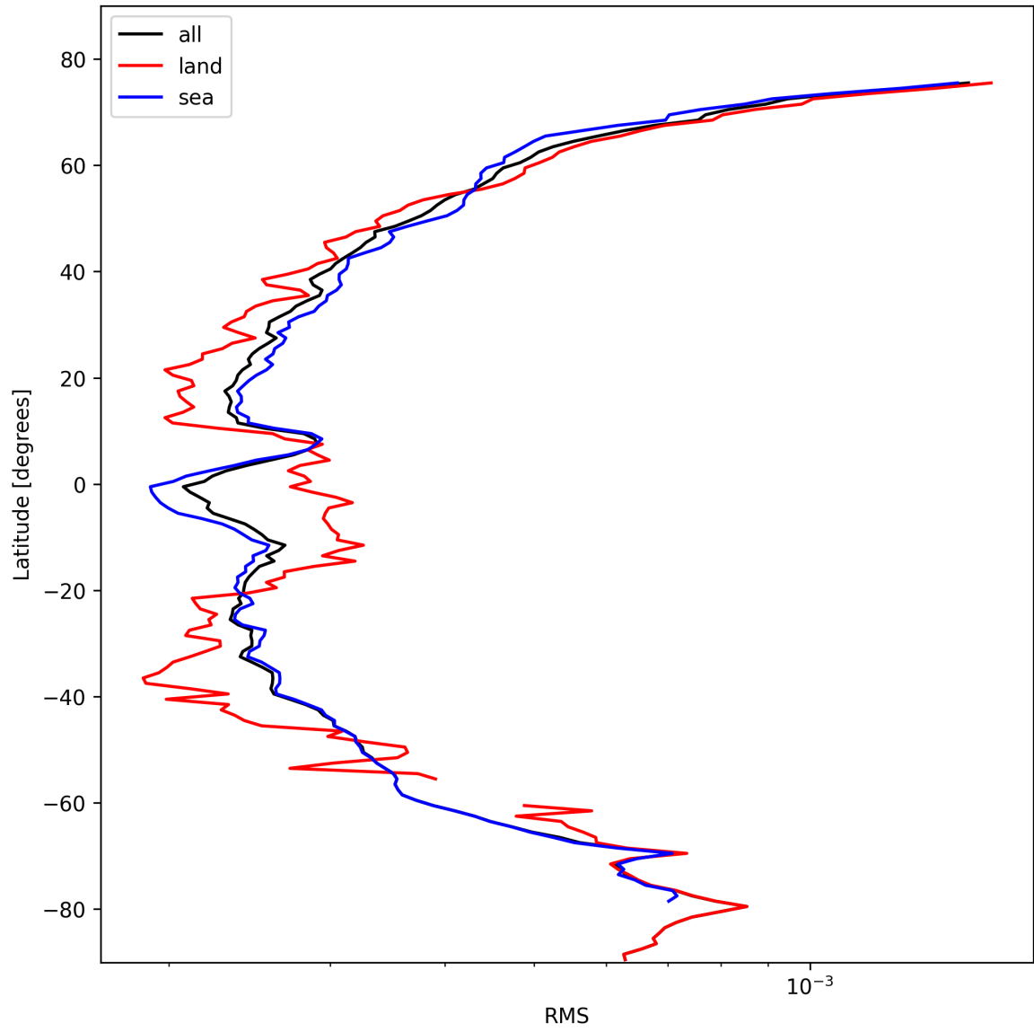
Figure 26: Zonal average of “RMS” for 2024-10-25 to 2024-10-27.
