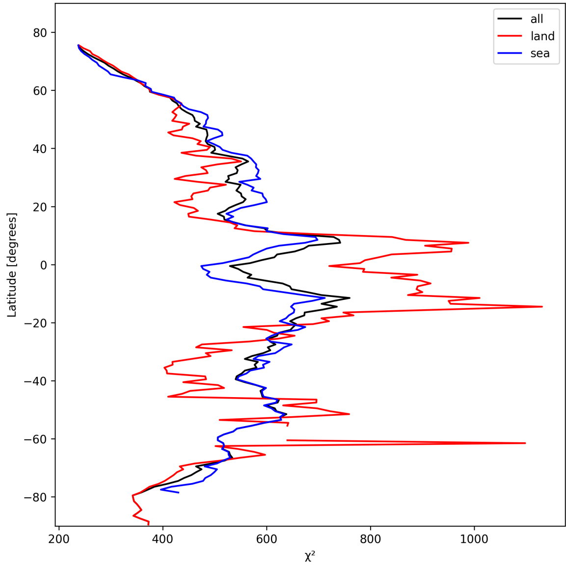
Figure 25: Zonal average of “ \chi^2 ” for 2024-10-25 to 2024-10-27.
