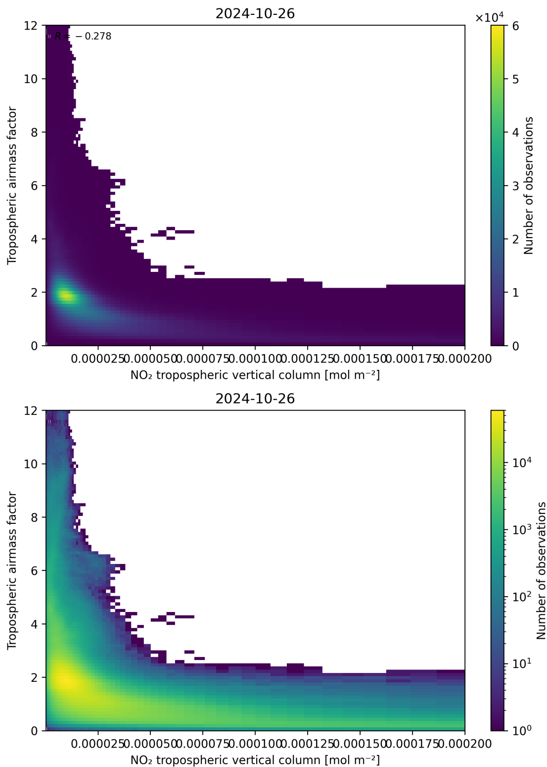
Figure 123: Scatter density plot of “NO 2 tropospheric vertical column” against “Tropospheric air mass factor” for 2024-10-25 to 2024-10-27.
