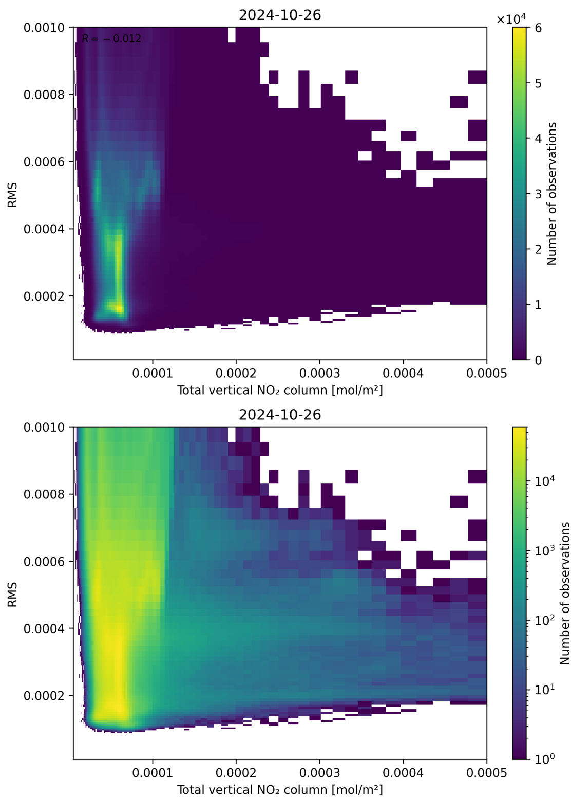
Figure 120: Scatter density plot of “Total vertical NO 2 column” against “RMS” for 2024-10-25 to 2024-10-27.
