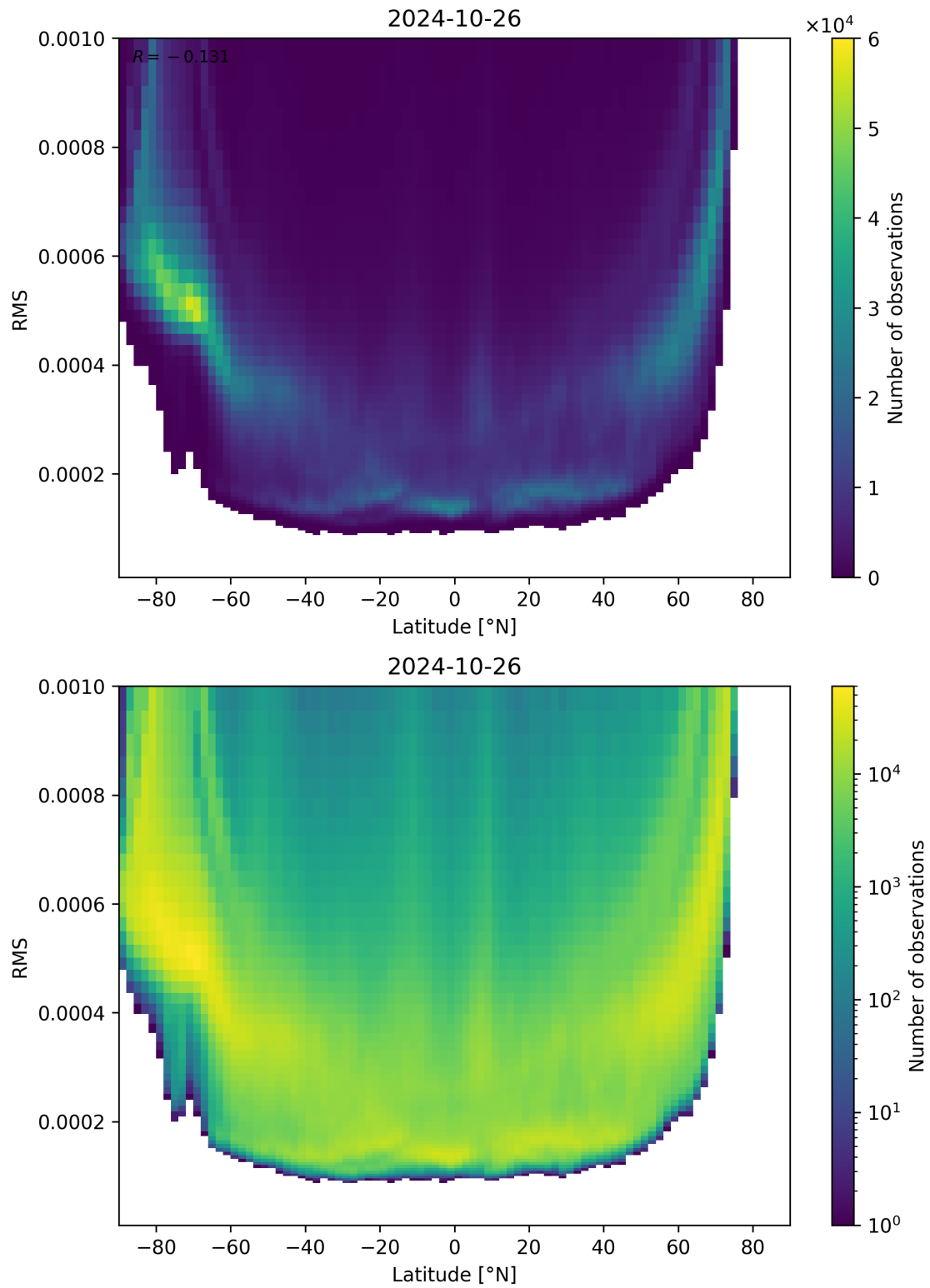
Figure 94: Scatter density plot of “Latitude” against “RMS” for 2024-10-25 to 2024-10-27.
