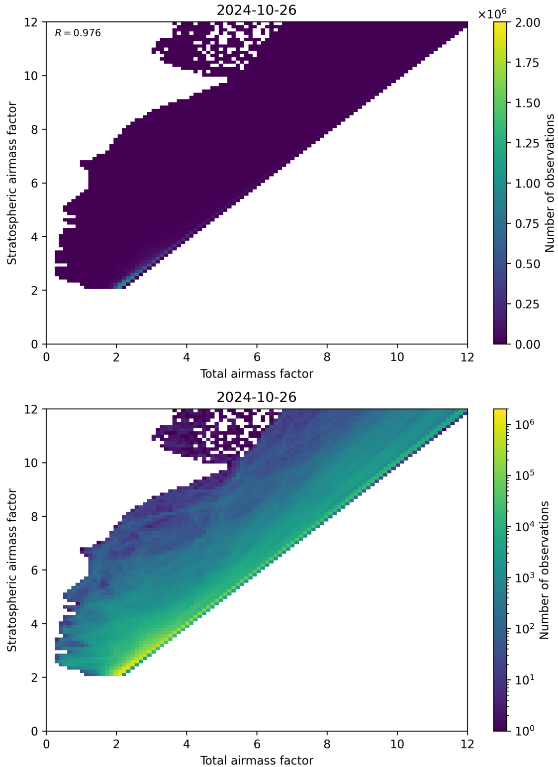
Figure 62: Scatter density plot of “Total air mass factor” against “Stratospheric air mass factor” for 2024-10-25 to 2024-10-27.
