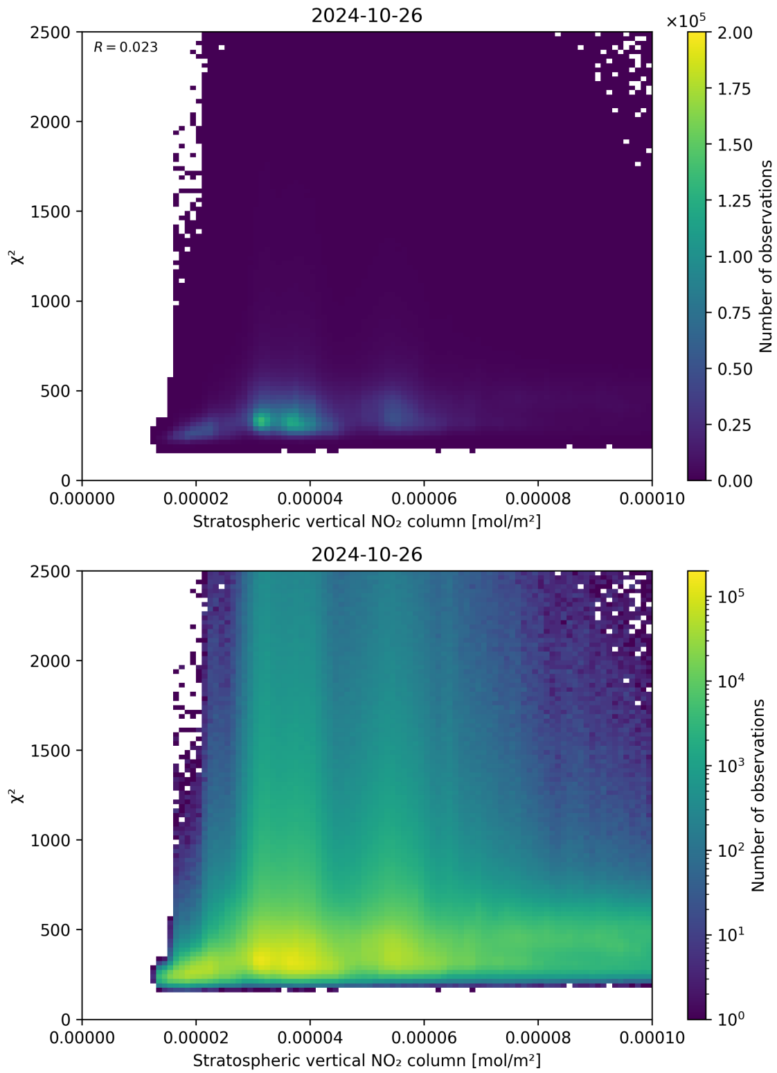
Figure 97: Scatter density plot of “Stratospheric vertical NO 2 column” against “ \chi^2 ” for 2024-10-25 to 2024-10-27.
