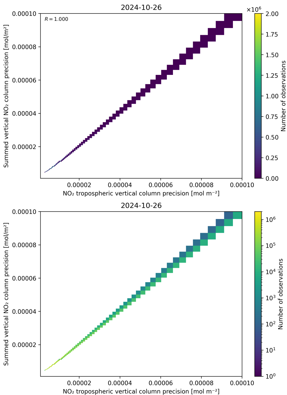
Figure 137: Scatter density plot of “NO 2 tropospheric vertical column precision” against “Summed vertical NO 2 column precision” for 2024-10-25 to 2024-10-27.
