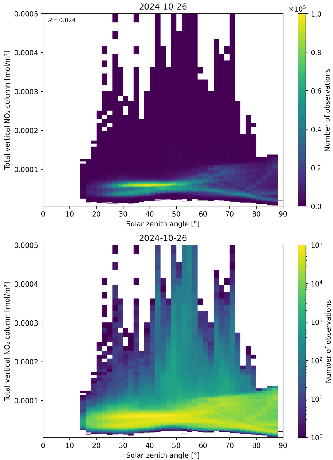
Figure 153: Scatter density plot of “Solar zenith angle” against “Total vertical NO 2 column” for 2024-10-25 to 2024-10-27.
