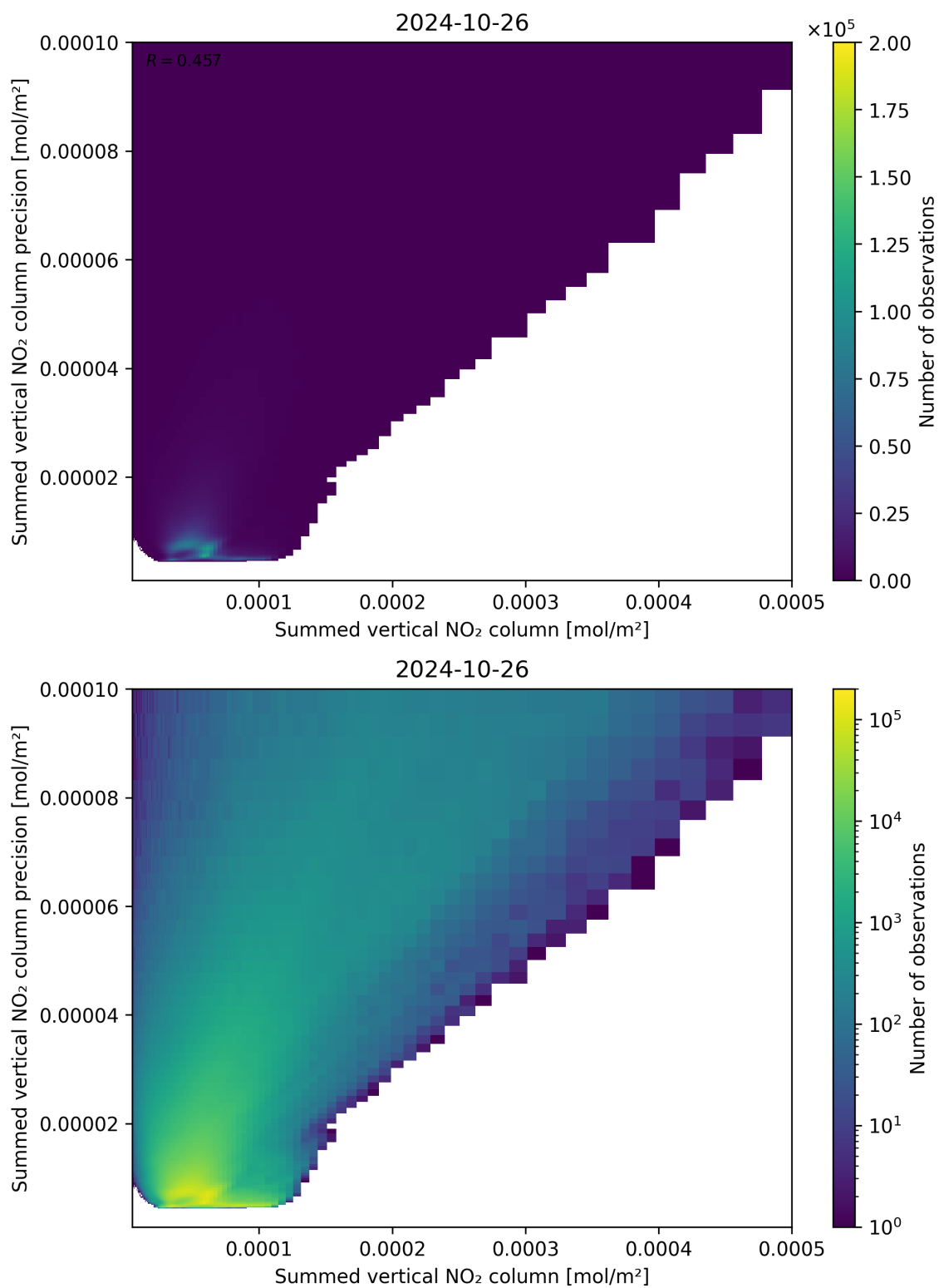
Figure 105: Scatter density plot of “Summed vertical NO 2 column” against “Summed vertical NO 2 column precision” for 2024-10-25 to 2024-10-27.
