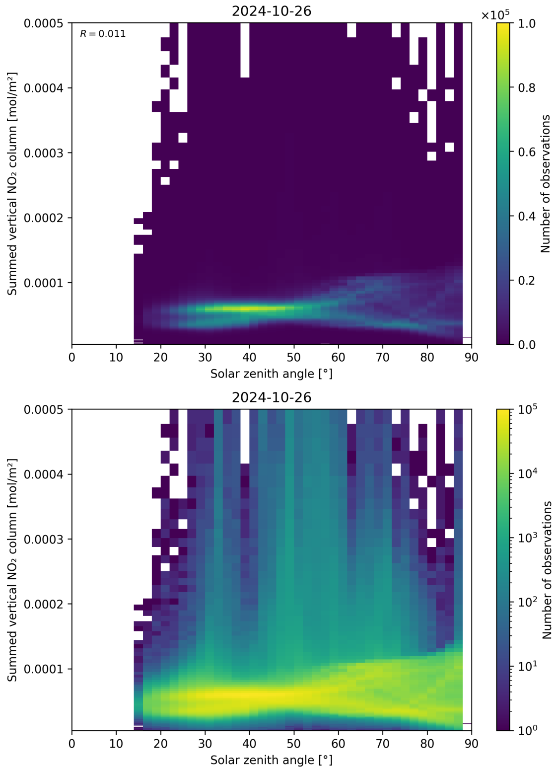
Figure 151: Scatter density plot of “Solar zenith angle” against “Summed vertical NO 2 column” for 2024-10-25 to 2024-10-27.
