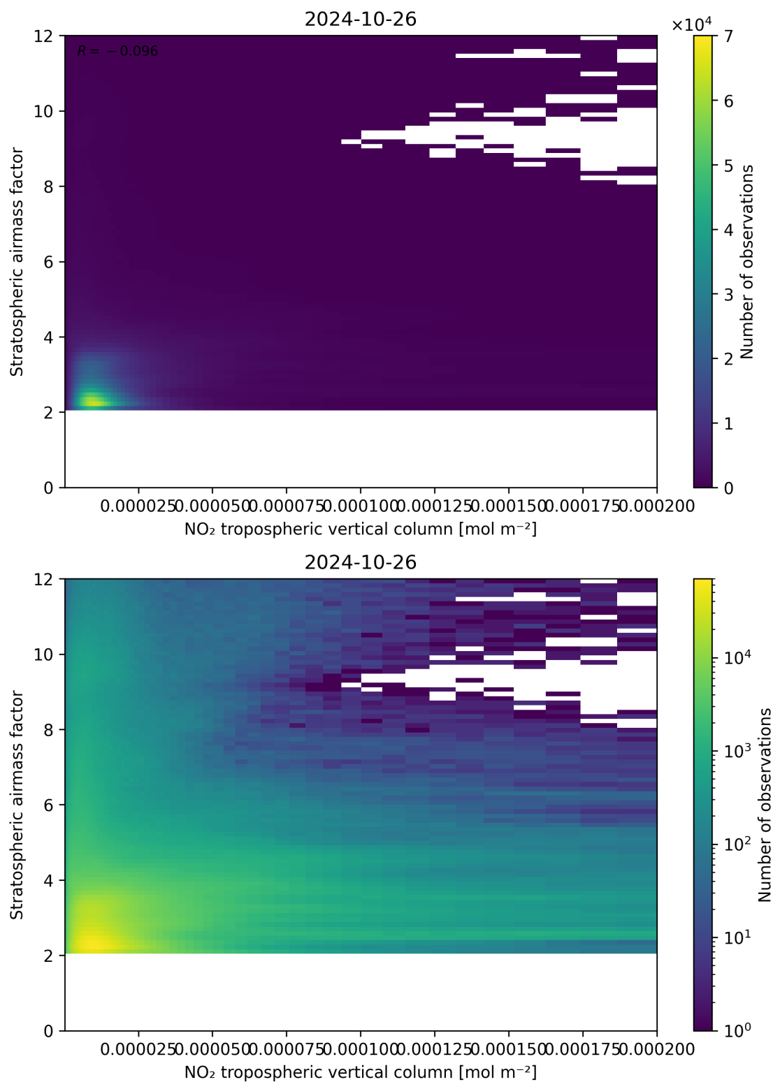
Figure 121: Scatter density plot of “NO 2 tropospheric vertical column” against “Stratospheric airmass factor” for 2024-10-25 to 2024-10-27.
