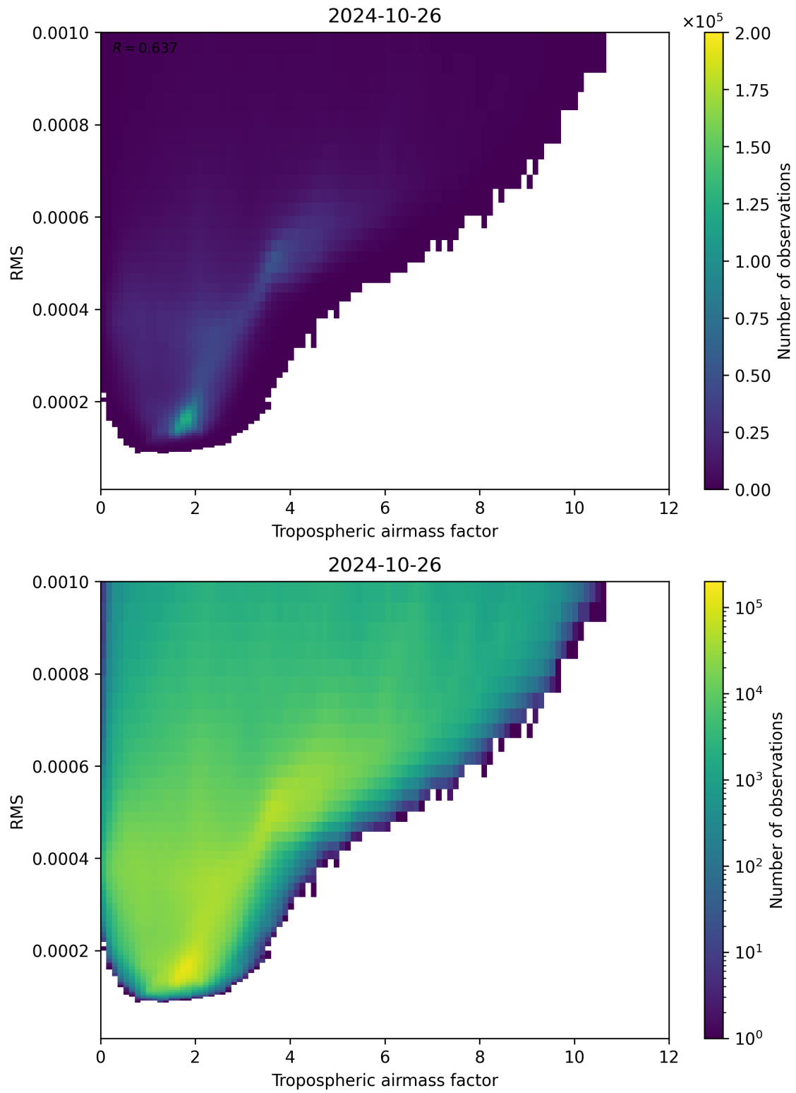
Figure 79: Scatter density plot of “Tropospheric airmass factor” against “RMS” for 2024-10-25 to 2024-10-27.
