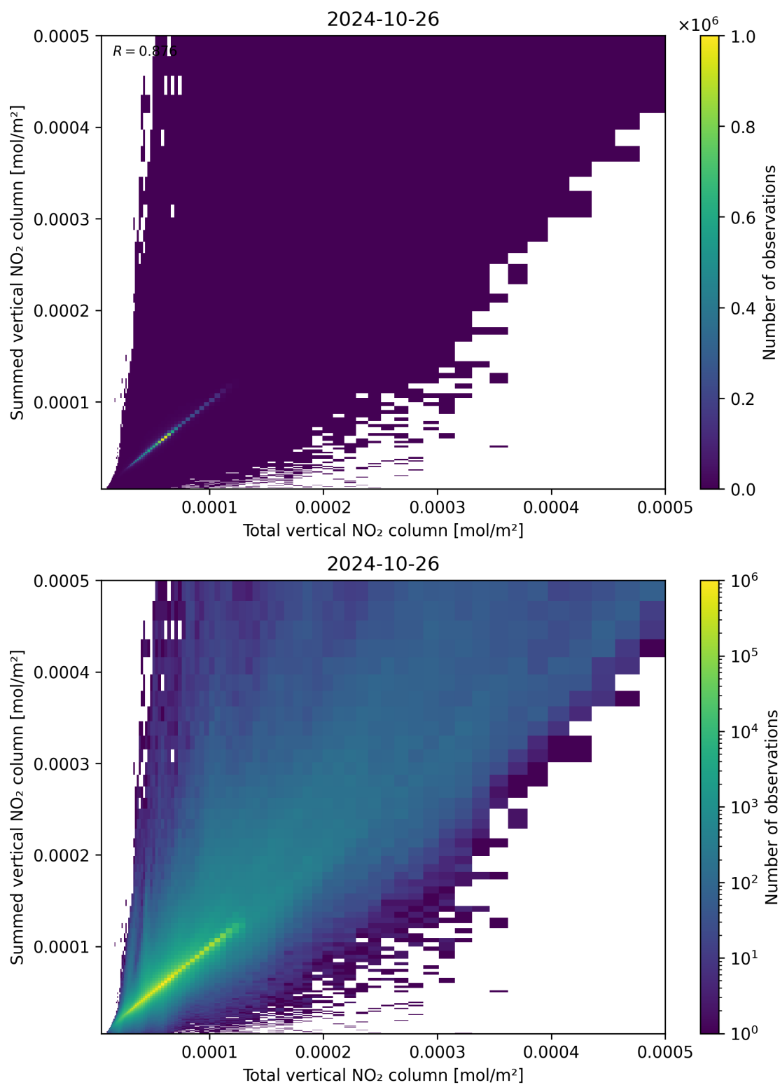
Figure 112: Scatter density plot of “Total vertical NO 2 column” against “Summed vertical NO 2 column” for 2024-10-25 to 2024-10-27.
