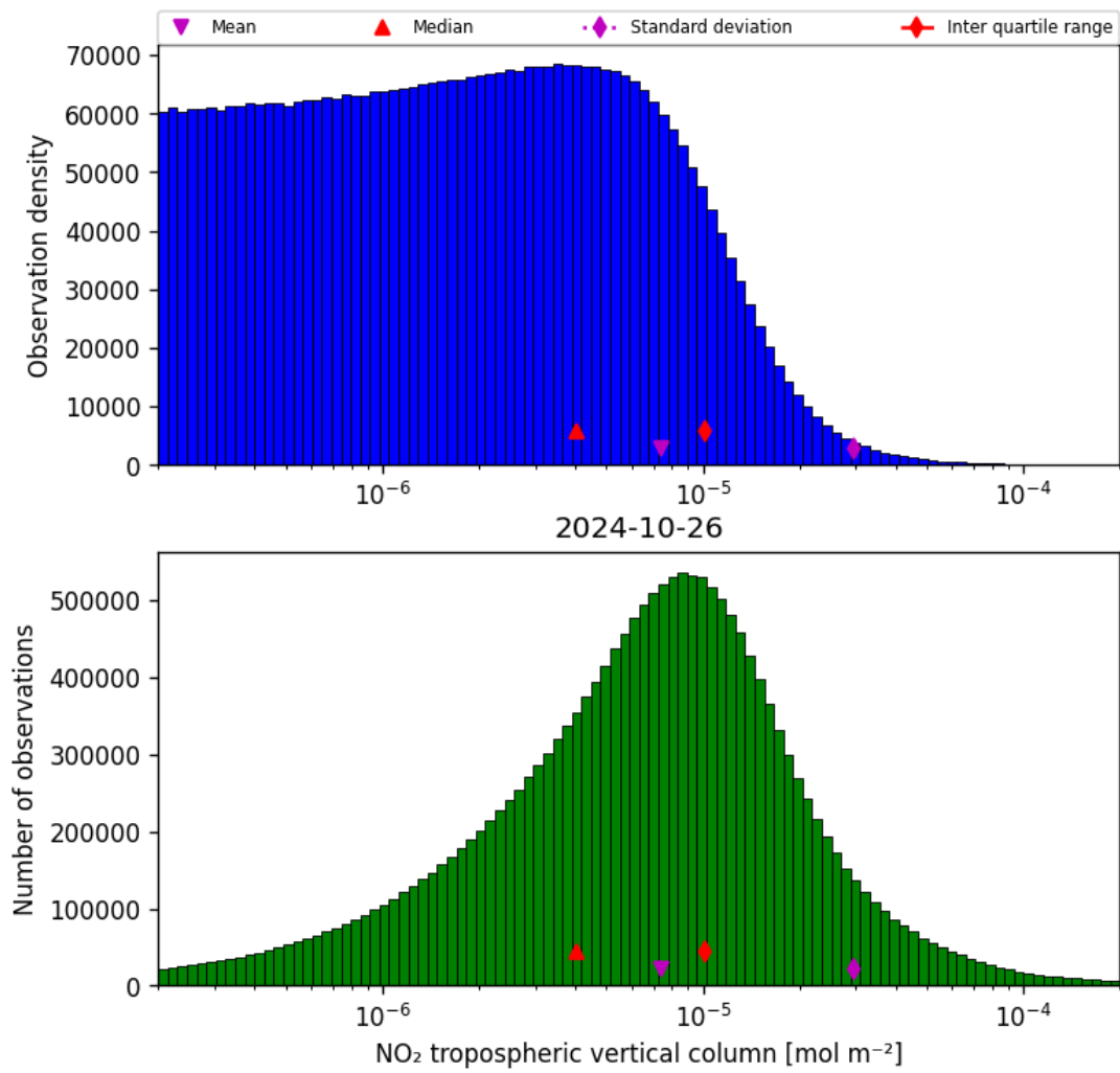
Figure 29: Histogram of “NO 2 tropospheric vertical column” for 2024-10-25 to 2024-10-27
