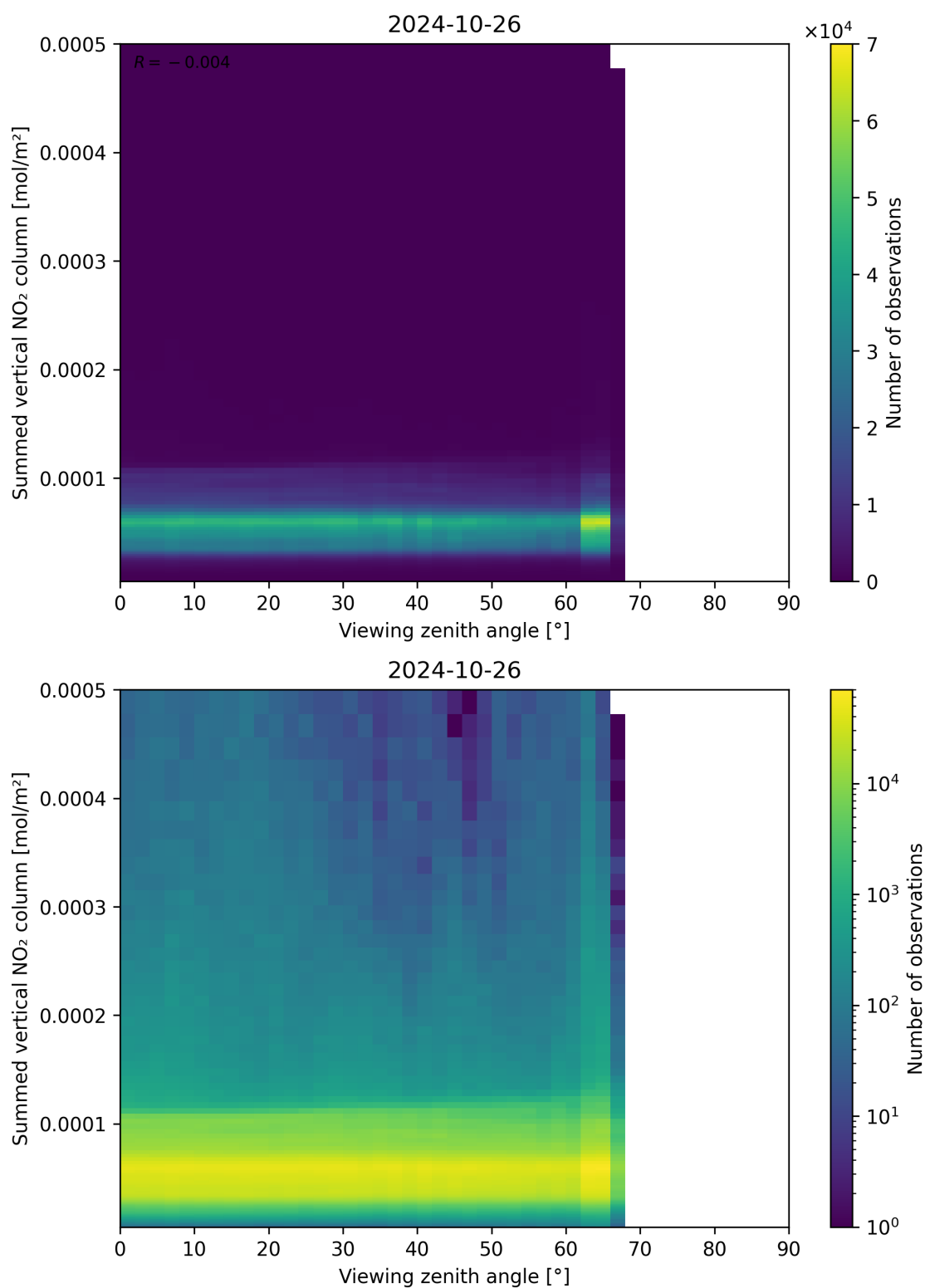
Figure 165: Scatter density plot of “Viewing zenith angle” against “Summed vertical NO 2 column” for 2024-10-25 to 2024-10-27.
