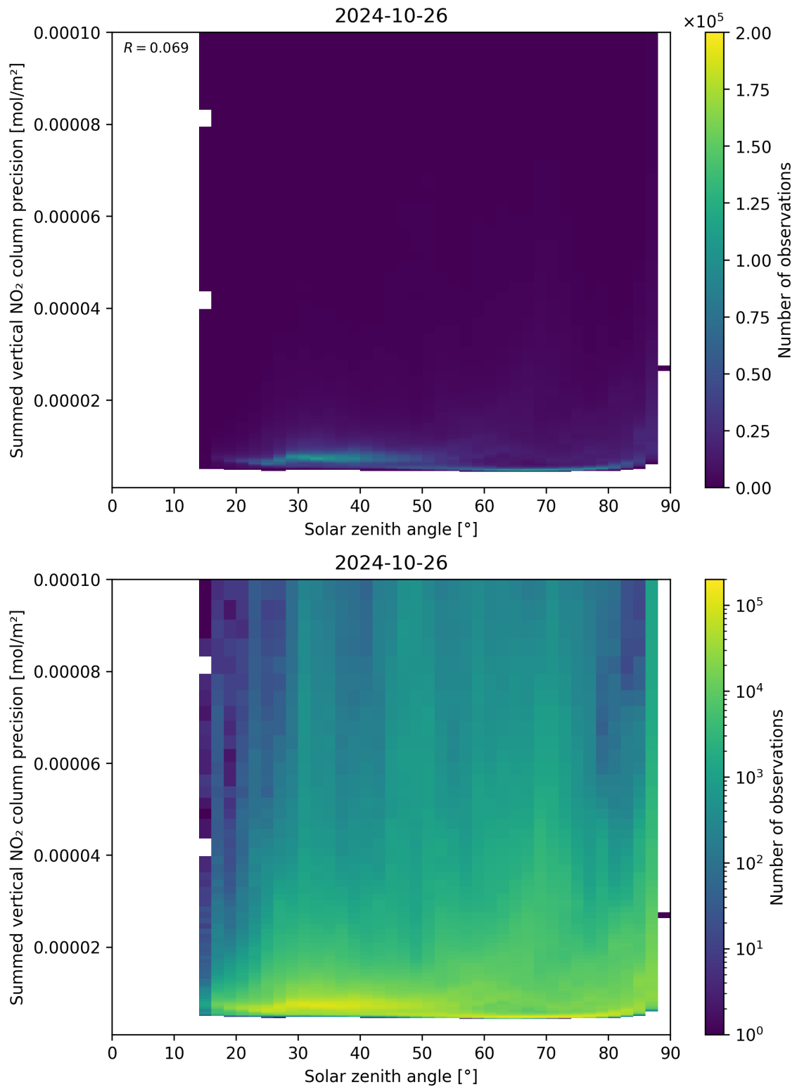
Figure 152: Scatter density plot of “Solar zenith angle” against “Summed vertical NO 2 column precision” for 2024-10-25 to 2024-10-27.
