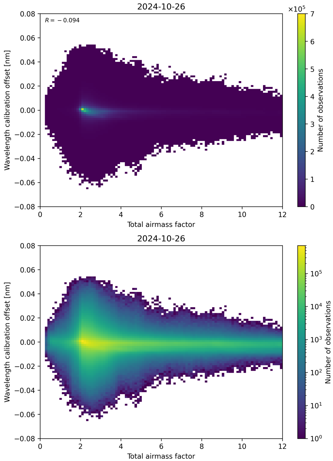
Figure 70: Scatter density plot of “Total airmass factor” against “Wavelength calibration offset” for 2024-10-25 to 2024-10-27.
