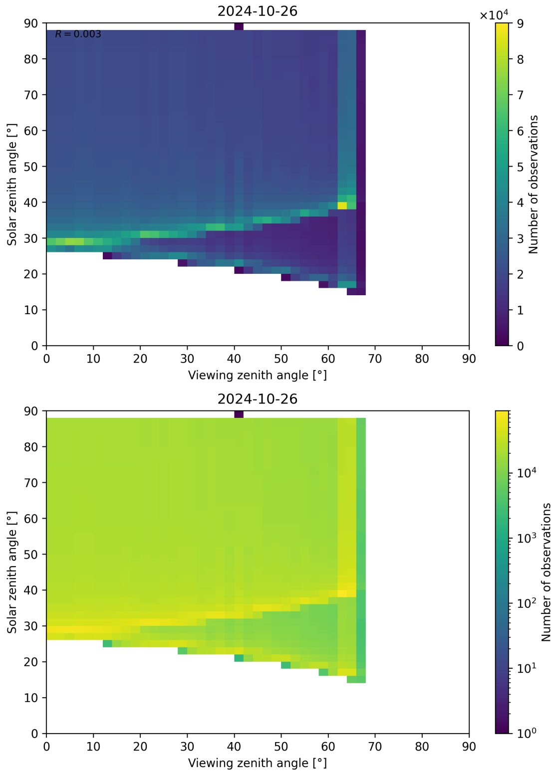
Figure 172: Scatter density plot of “Viewing zenith angle” against “Solar zenith angle” for 2024-10-25 to 2024-10-27.
