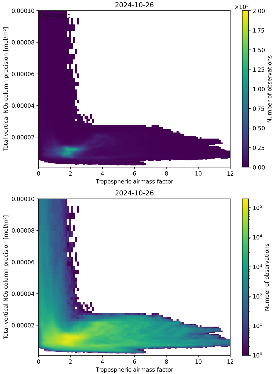
Figure 78: Scatter density plot of “Tropospheric airmass factor” against “Total vertical NO 2 column precision” for 2024-10-25 to 2024-10-27.
