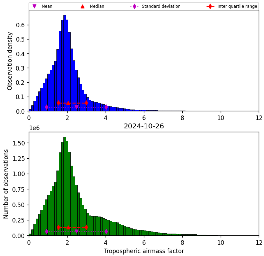
Figure 31: Histogram of “Tropospheric airmass factor” for 2024-10-25 to 2024-10-27
