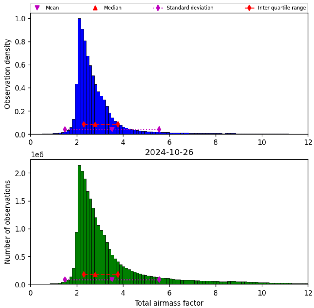
Figure 32: Histogram of “Total airmass factor” for 2024-10-25 to 2024-10-27
