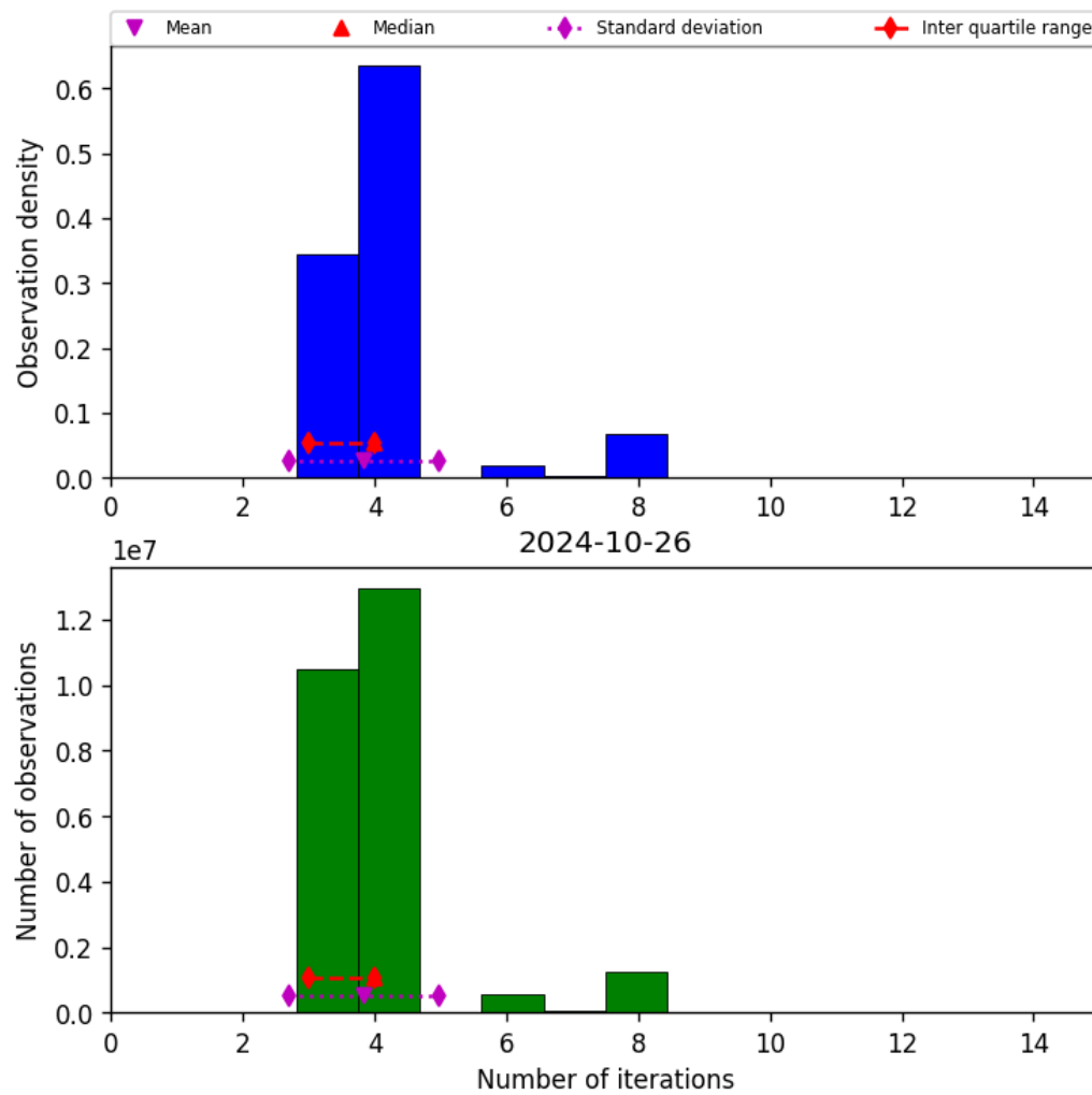
Figure 34: Histogram of “Number of iterations” for 2024-10-25 to 2024-10-27
