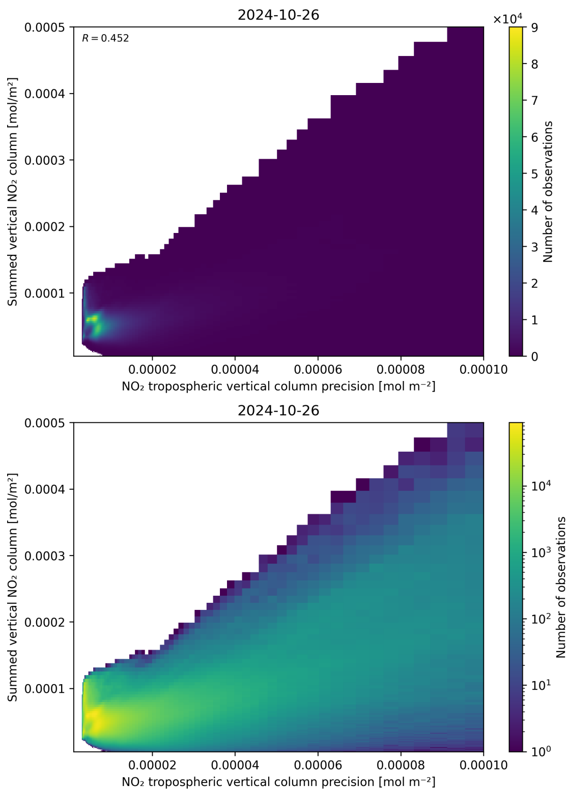
Figure 136: Scatter density plot of “NO 2 tropospheric vertical column precision” against “Summed vertical NO 2 column” for 2024-10-25 to 2024-10-27.
