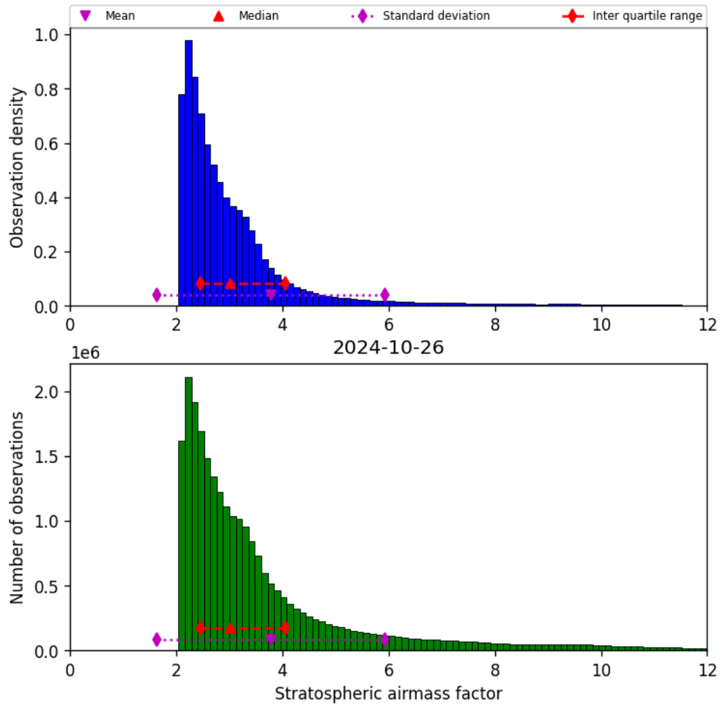
Figure 44: Histogram of “Stratospheric airmass factor” for 2024-10-25 to 2024-10-27
