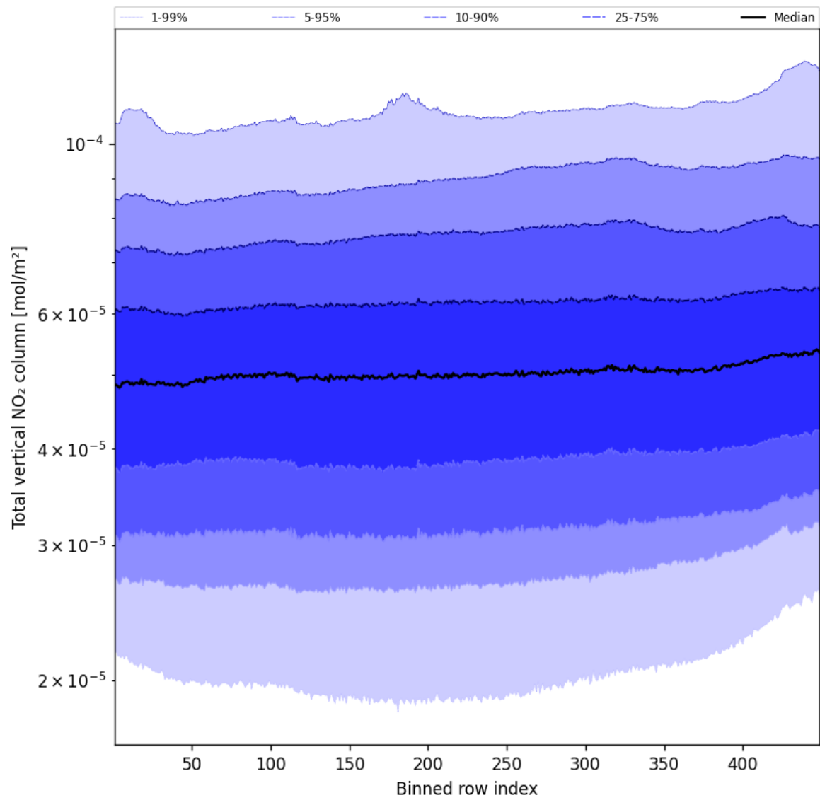
Figure 55: Along track statistics of “Total vertical NO 2 column” for 2024-10-25 to 2024-10-27
