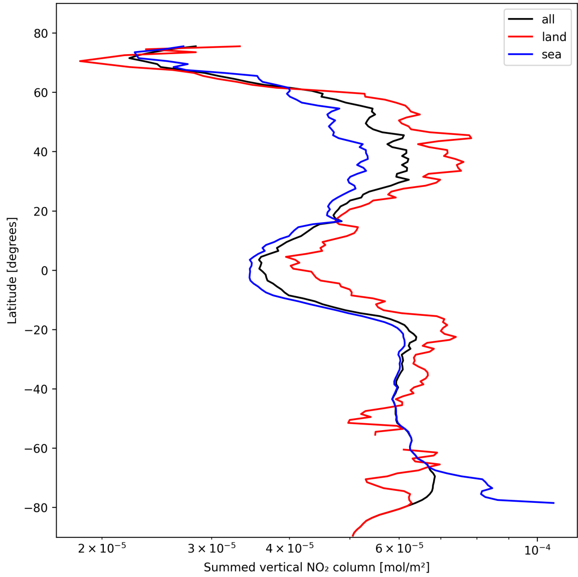
Figure 23: Zonal average of “Summed vertical NO 2 column” for 2024-10-25 to 2024-10-27.
