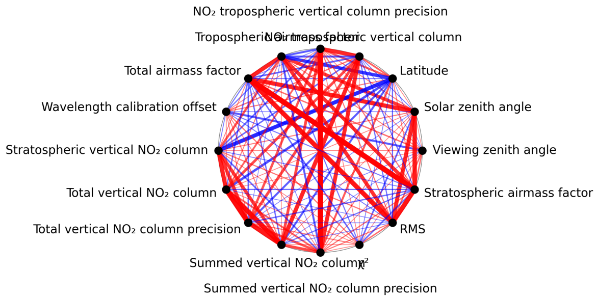
Figure 1: Map of correlation graph for 2024-10-25 to 2024-10-27.
