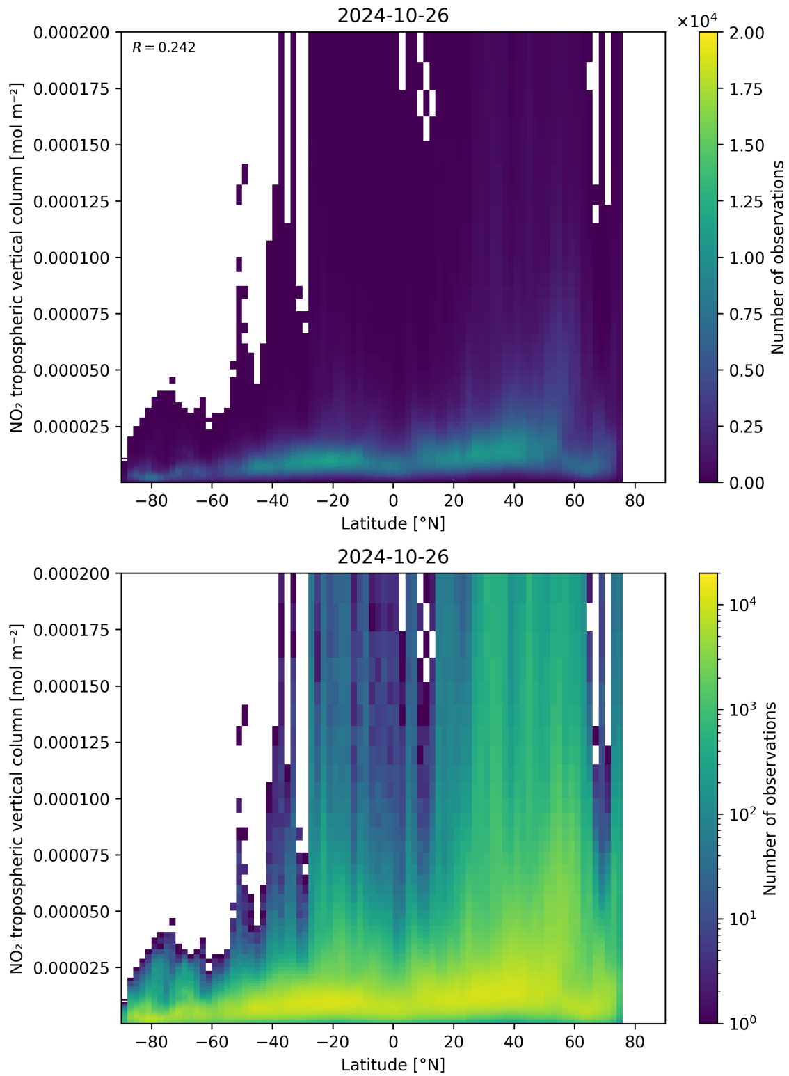
Figure 92: Scatter density plot of “Latitude” against “NO 2 tropospheric vertical column” for 2024-10-25 to 2024-10-27.
