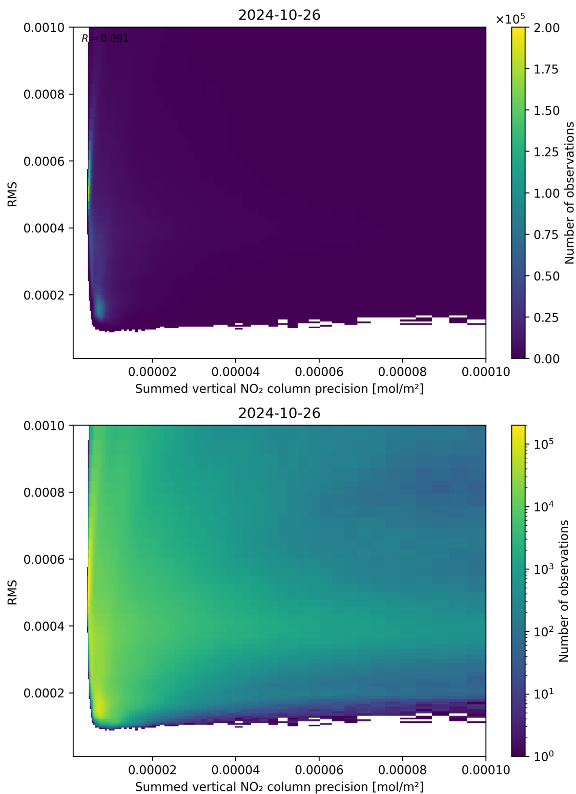
Figure 108: Scatter density plot of “Summed vertical NO 2 column precision” against “RMS” for 2024-10-25 to 2024-10-27.
