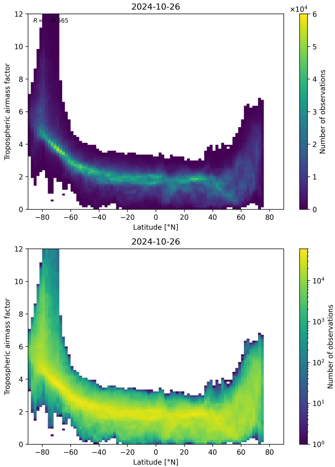
Figure 85: Scatter density plot of “Latitude” against “Tropospheric air mass factor” for 2024-10-25 to 2024-10-27.
