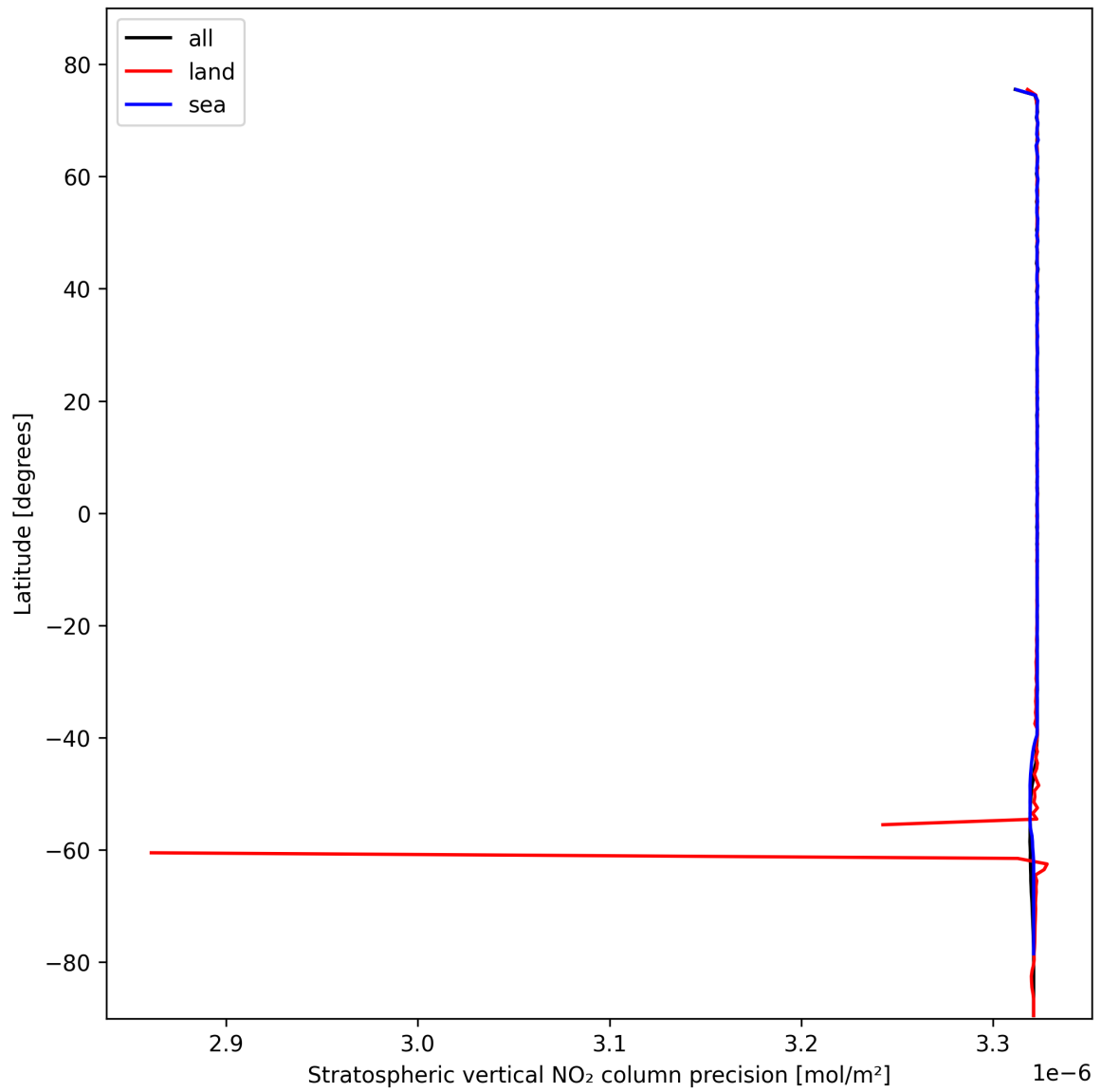
Figure 20: Zonal average of “Stratospheric vertical NO 2 column precision” for 2024-10-25 to 2024-10-27.
