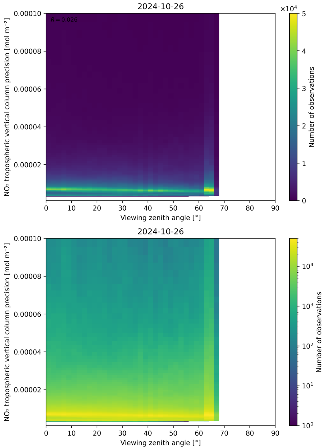
Figure 170: Scatter density plot of “Viewing zenith angle” against “NO 2 tropospheric vertical column precision” for 2024-10-25 to 2024-10-27.
