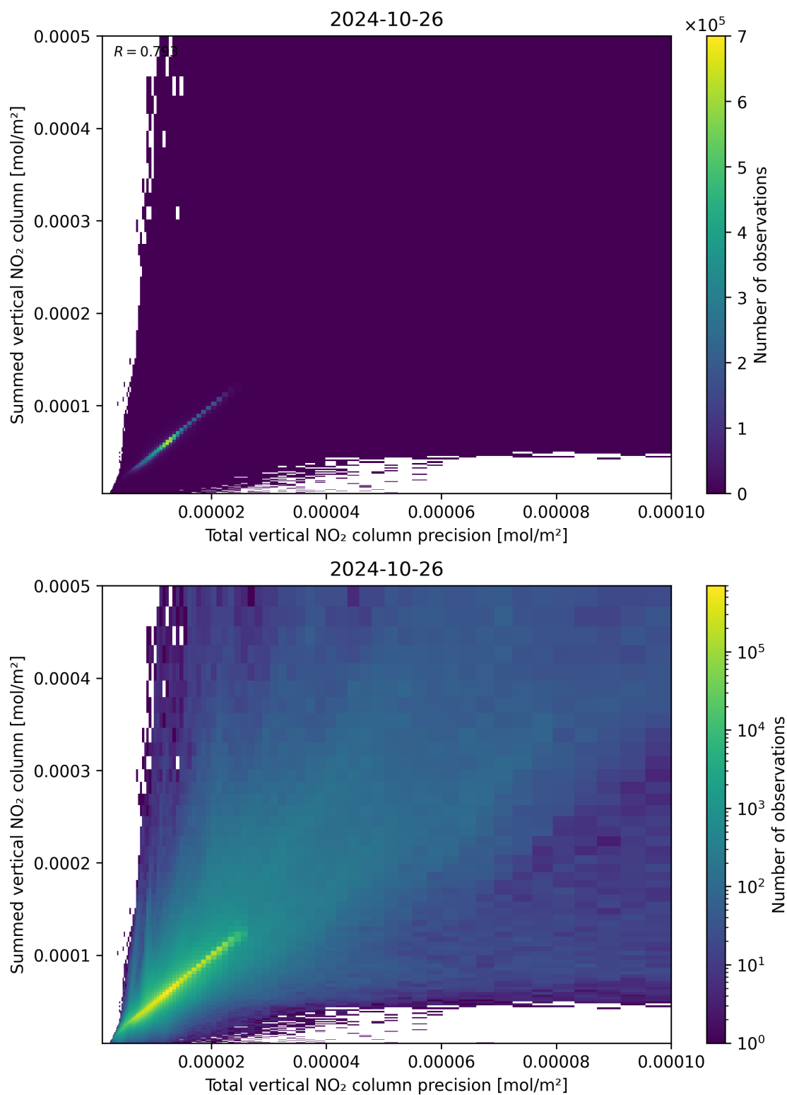
Figure 117: Scatter density plot of “Total vertical NO 2 column precision” against “Summed vertical NO 2 column” for 2024-10-25 to 2024-10-27.
