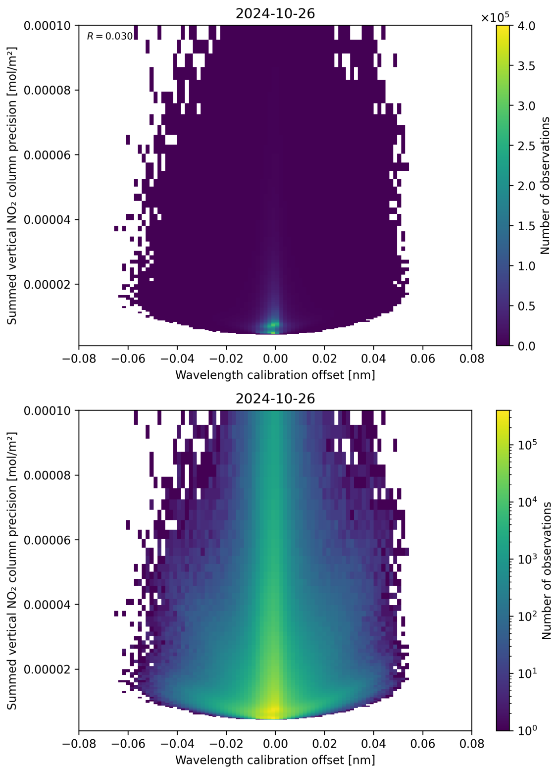
Figure 178: Scatter density plot of “Wavelength calibration offset” against “Summed vertical NO 2 column precision” for 2024-10-25 to 2024-10-27.
