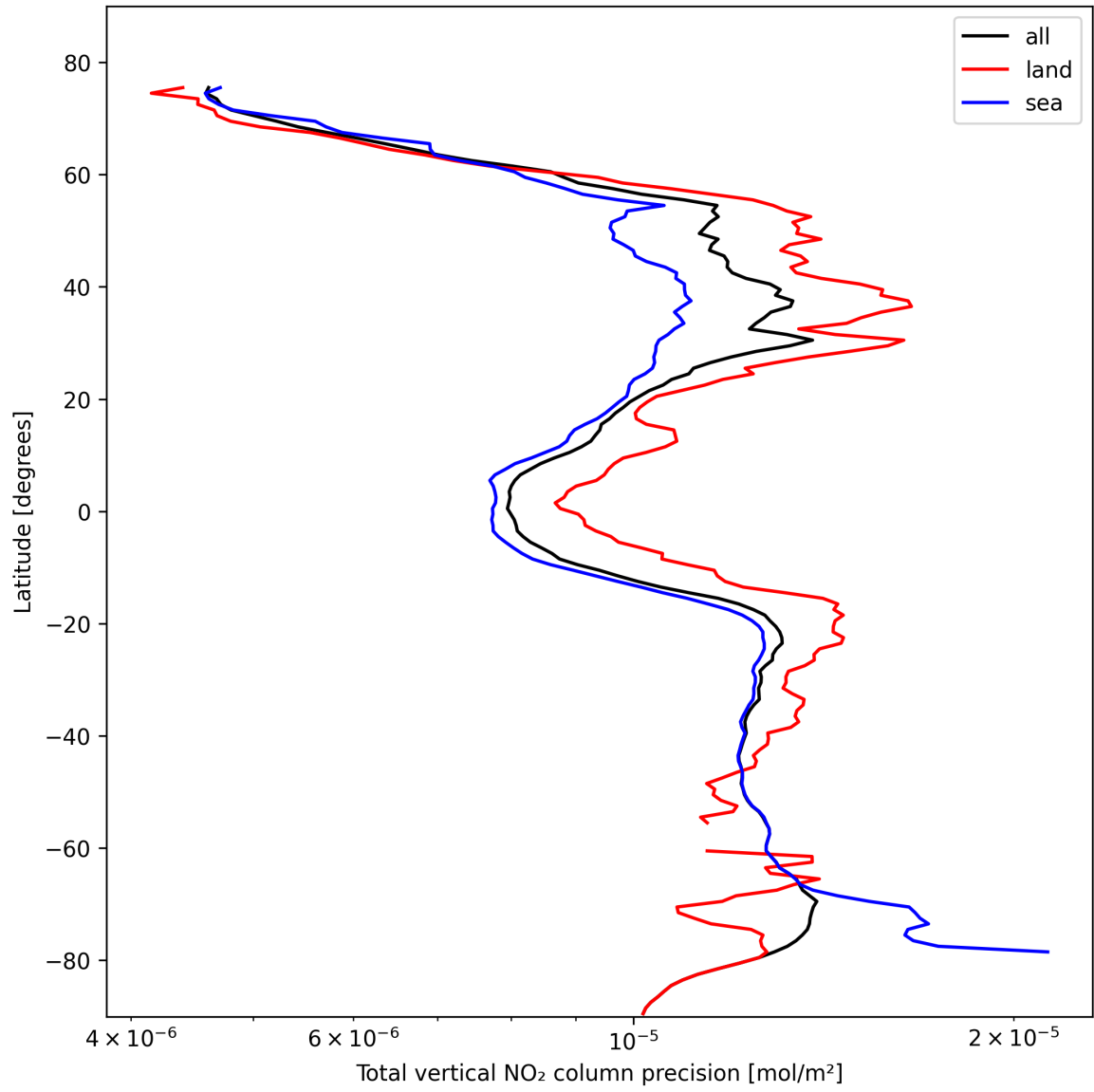
Figure 22: Zonal average of "Total vertical NO 2 column precision" for 2024-10-25 to 2024-10-27.
