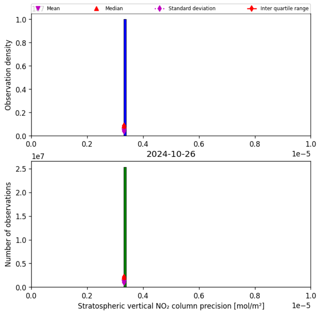
Figure 37: Histogram of “Stratospheric vertical NO 2 column precision” for 2024-10-25 to 2024-10-27
