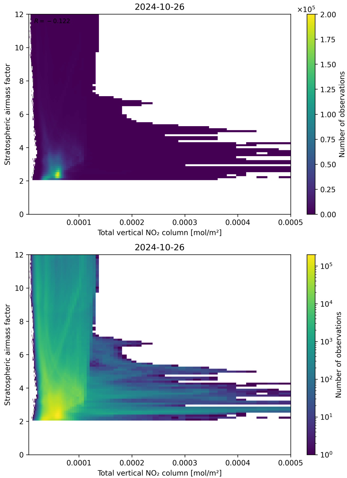
Figure 110: Scatter density plot of “Total vertical NO 2 column” against “Stratospheric airmass factor” for 2024-10-25 to 2024-10-27.
