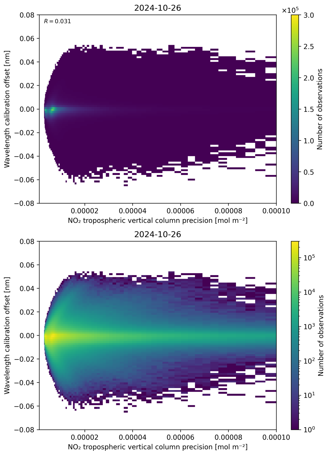
Figure 141: Scatter density plot of “NO 2 tropospheric vertical column precision” against “Wavelength calibration offset” for 2024-10-25 to 2024-10-27.
