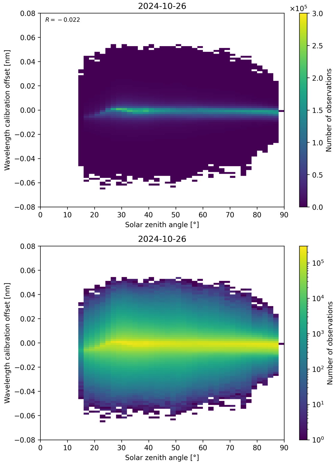
Figure 158: Scatter density plot of “Solar zenith angle” against “Wavelength calibration offset” for 2024-10-25 to 2024-10-27.
