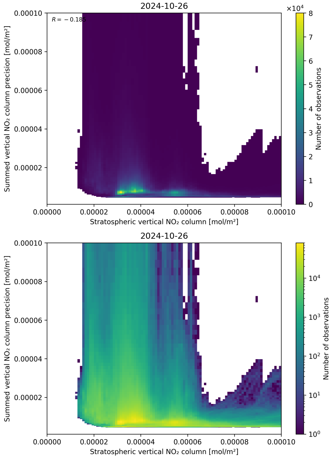
Figure 99: Scatter density plot of “Stratospheric vertical NO 2 column” against “Summed vertical NO 2 column precision” for 2024-10-25 to 2024-10-27.
