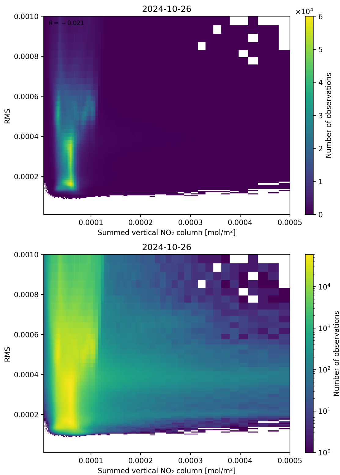
Figure 109: Scatter density plot of “Summed vertical NO 2 column” against “RMS” for 2024-10-25 to 2024-10-27.
