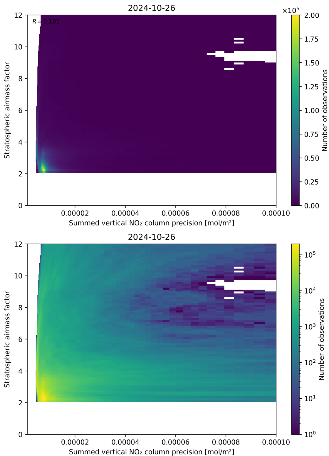
Figure 106: Scatter density plot of “Summed vertical NO 2 column precision” against “Stratospheric airmass factor” for 2024-10-25 to 2024-10-27.
