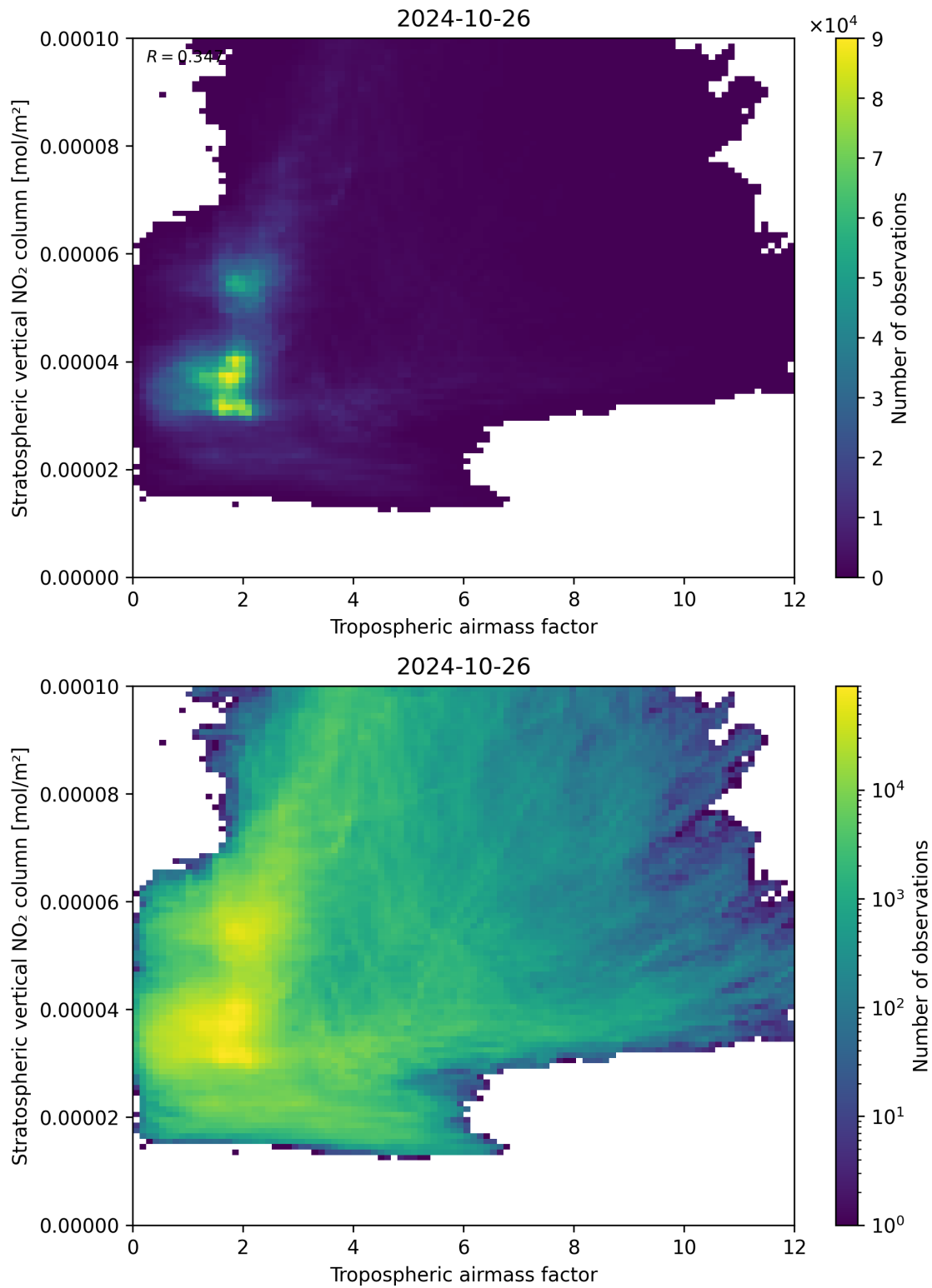
Figure 74: Scatter density plot of “Tropospheric air mass factor” against “Stratospheric vertical NO 2 column” for 2024-10-25 to 2024-10-27.
