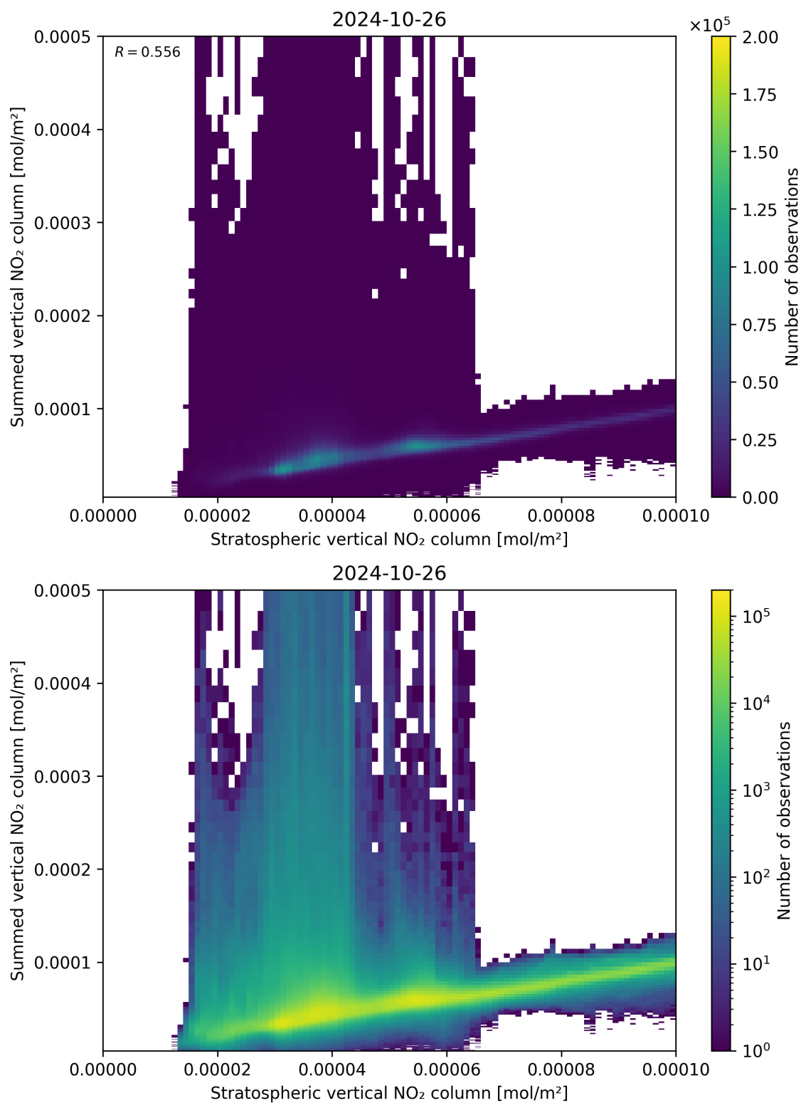
Figure 98: Scatter density plot of “Stratospheric vertical NO 2 column” against “Summed vertical NO 2 column” for 2024-10-25 to 2024-10-27.
