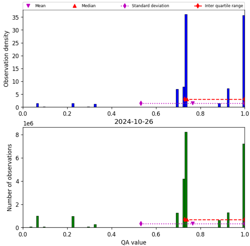
Figure 28: Histogram of “QA value” for 2024-10-25 to 2024-10-27
