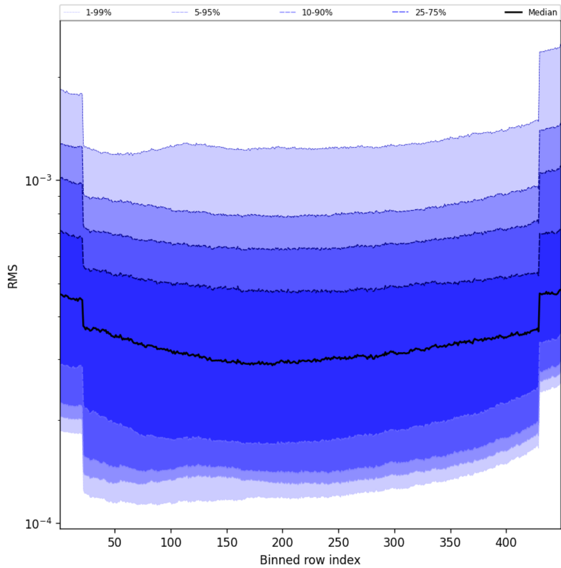
Figure 60: Along track statistics of “RMS” for 2024-10-25 to 2024-10-27
