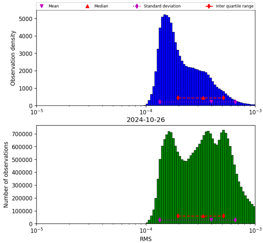
Figure 43: Histogram of “RMS” for 2024-10-25 to 2024-10-27
