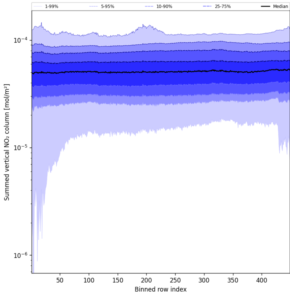
Figure 57: Along track statistics of “Summed vertical NO 2 column” for 2024-10-25 to 2024-10-27
