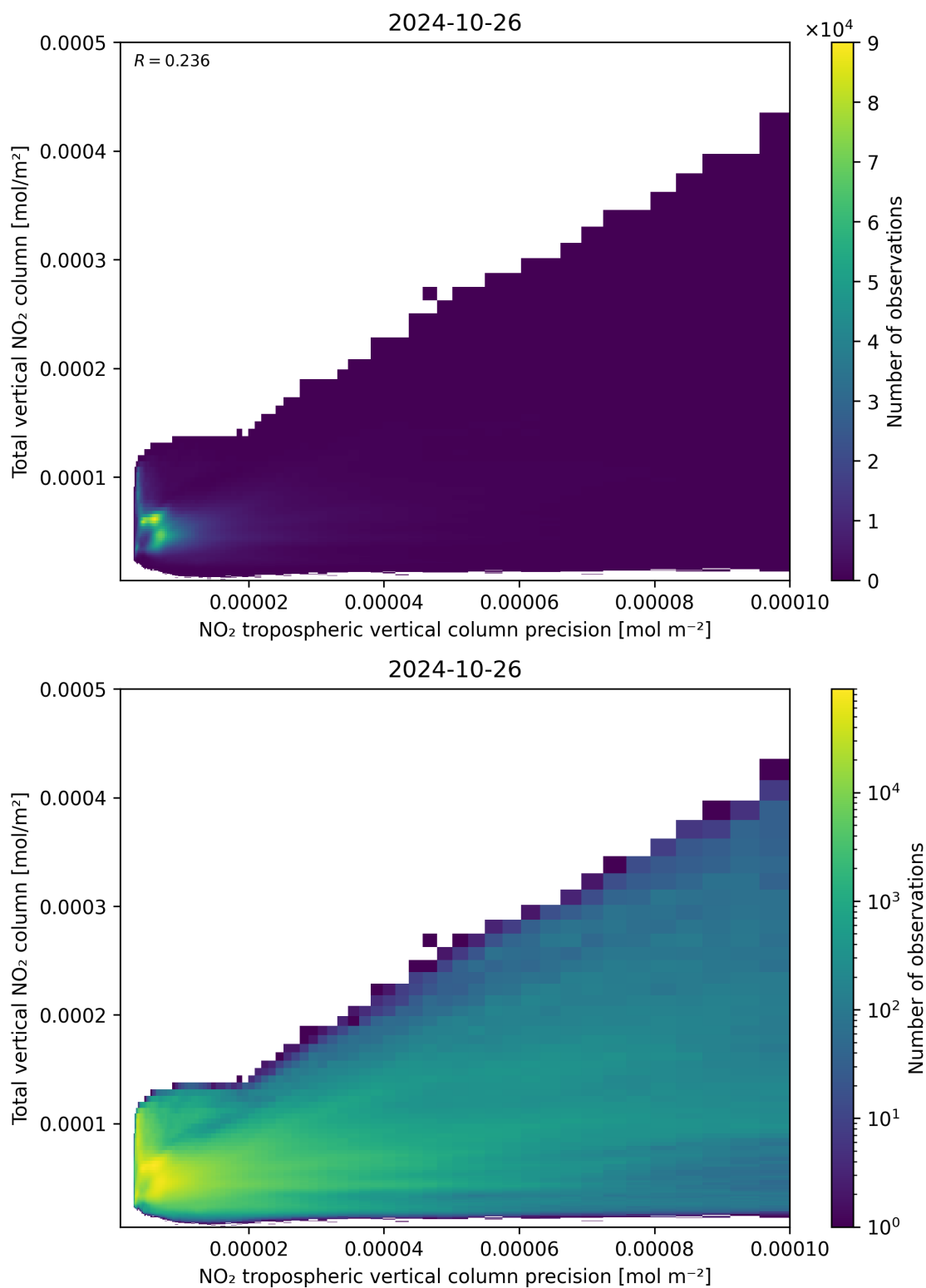
Figure 138: Scatter density plot of “NO 2 tropospheric vertical column precision” against “Total vertical NO 2 column” for 2024-10-25 to 2024-10-27.
