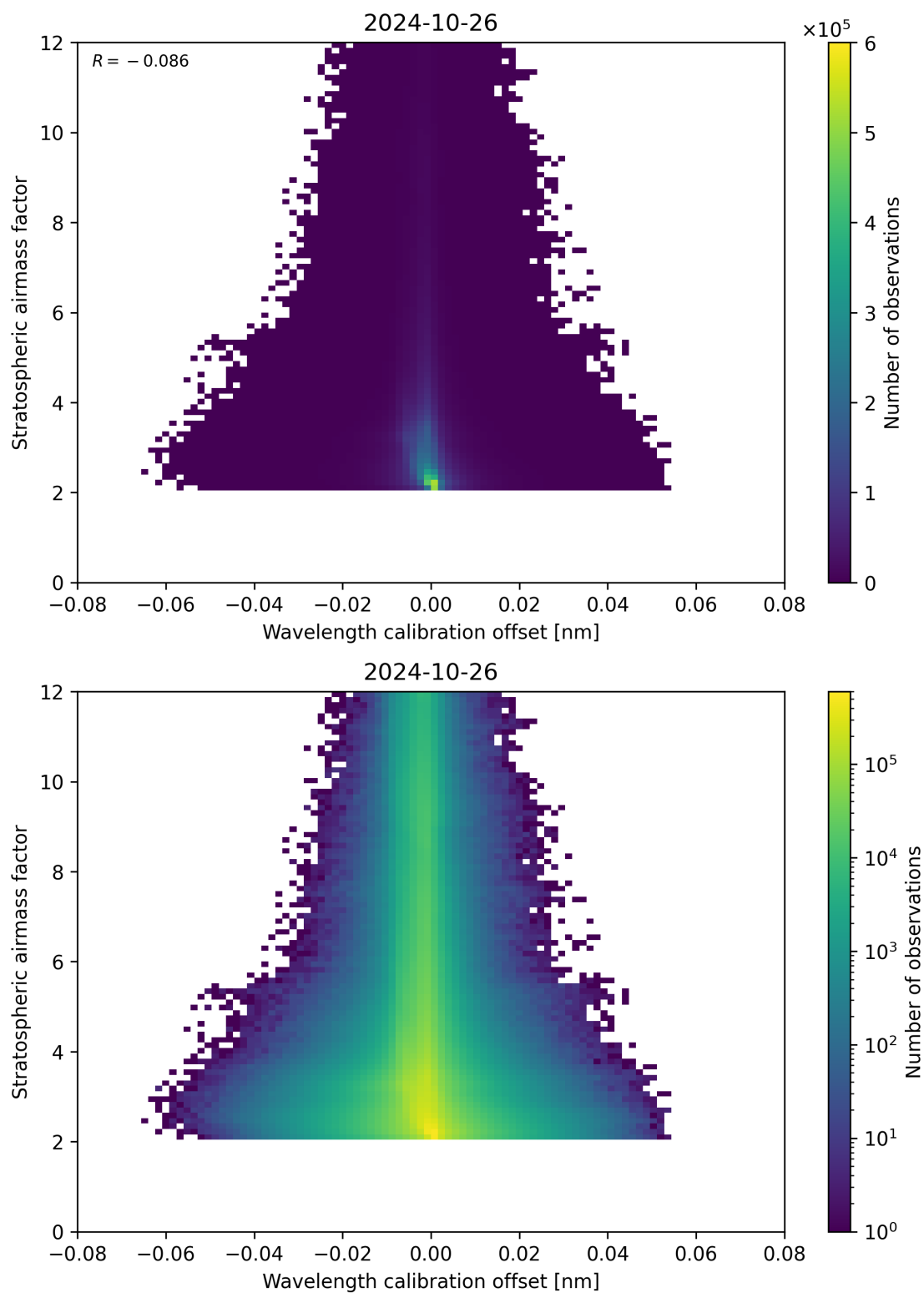
Figure 174: Scatter density plot of “Wavelength calibration offset” against “Stratospheric air mass factor” for 2024-10-25 to 2024-10-27.
