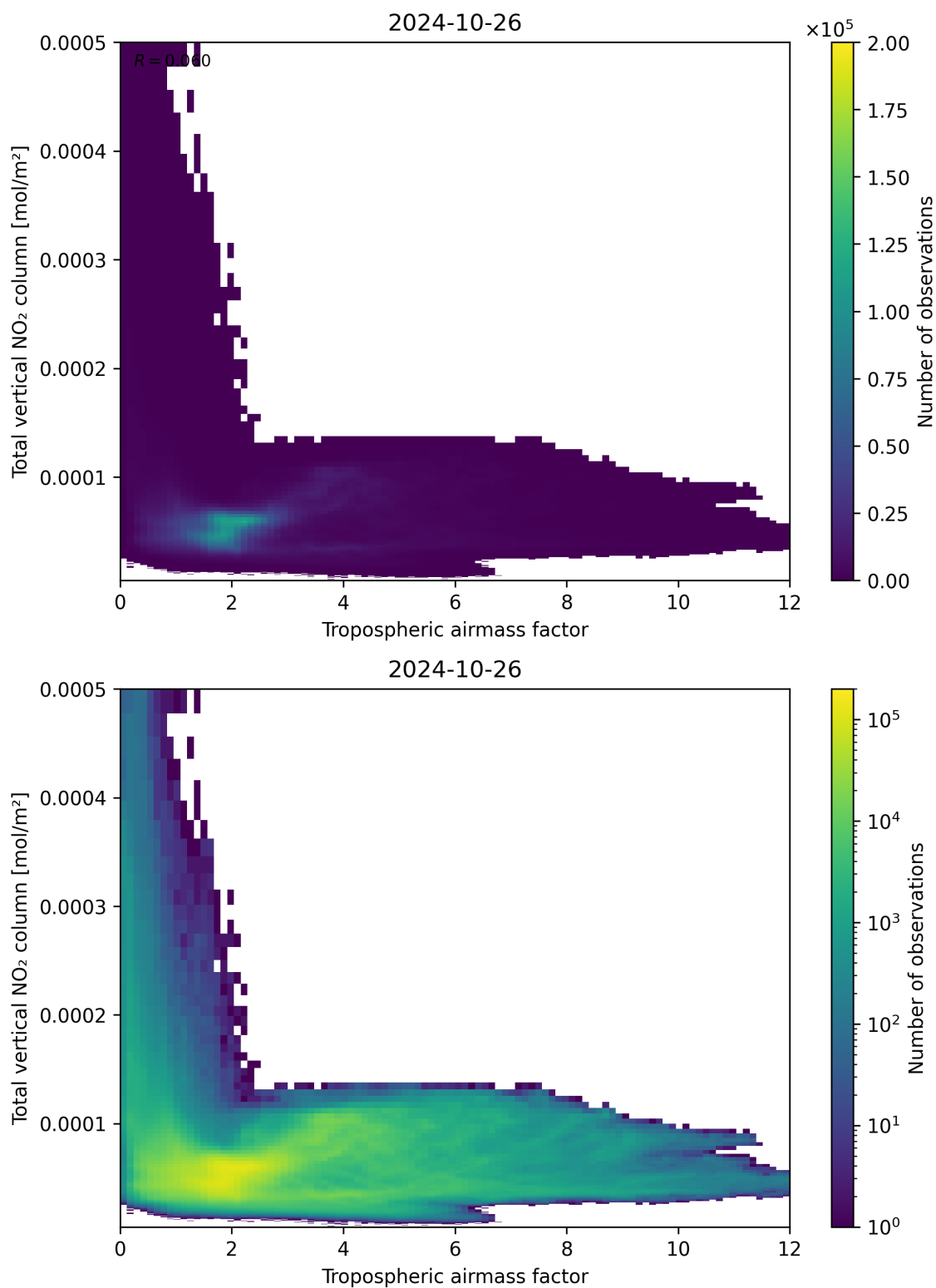
Figure 77: Scatter density plot of “Tropospheric airmass factor” against “Total vertical NO 2 column” for 2024-10-25 to 2024-10-27.
