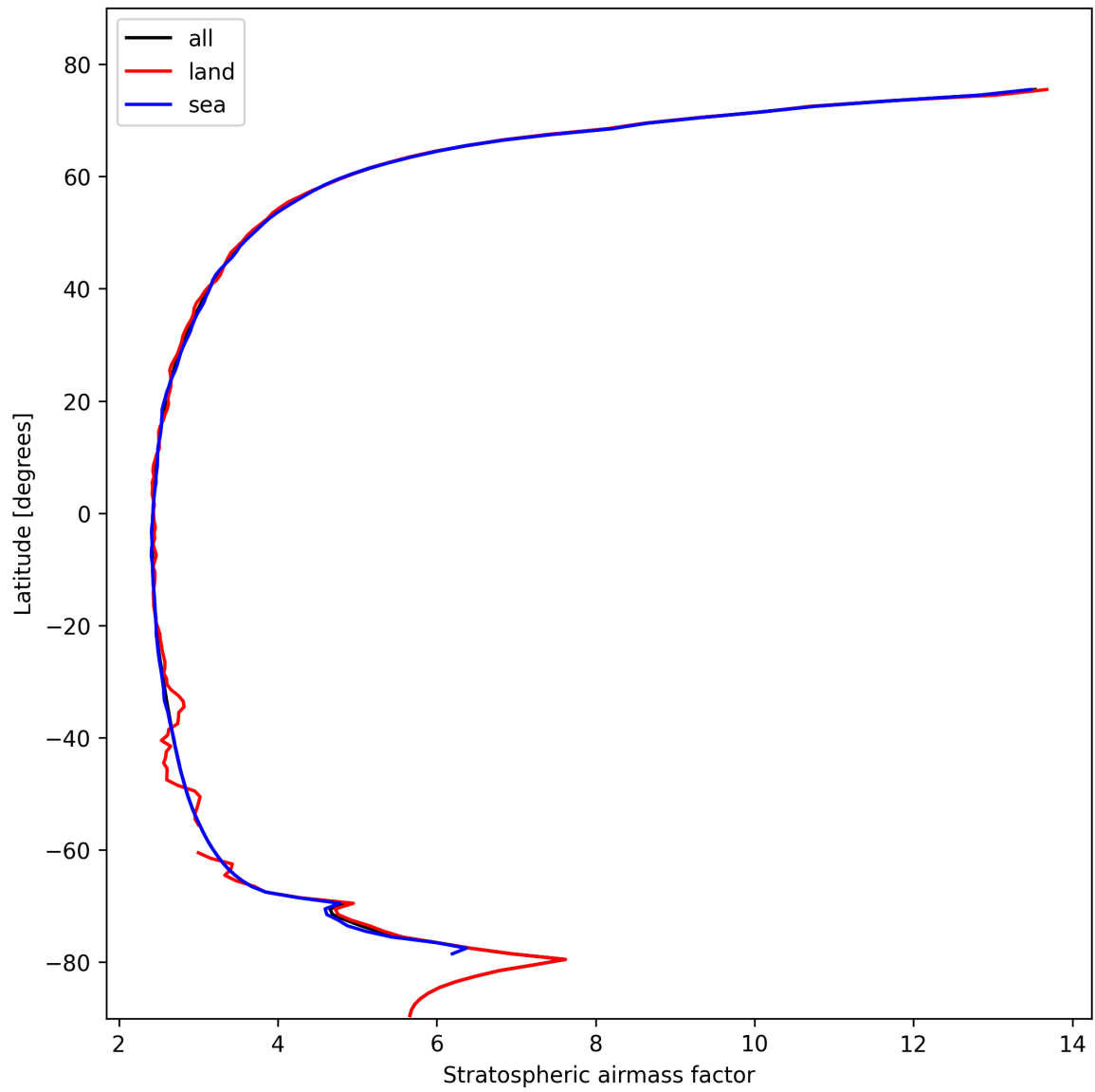
Figure 27: Zonal average of “Stratospheric airmass factor” for 2024-10-25 to 2024-10-27.
