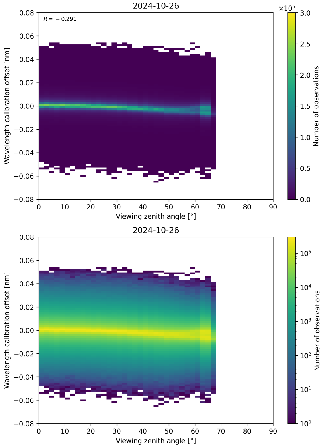
Figure 173: Scatter density plot of “Viewing zenith angle” against “Wavelength calibration offset” for 2024-10-25 to 2024-10-27.
