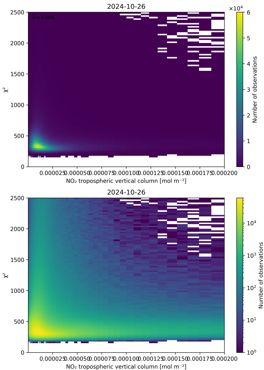
Figure 124: Scatter density plot of “NO 2 tropospheric vertical column” against “ \chi^2 ” for 2024-10-25 to 2024-10-27.
