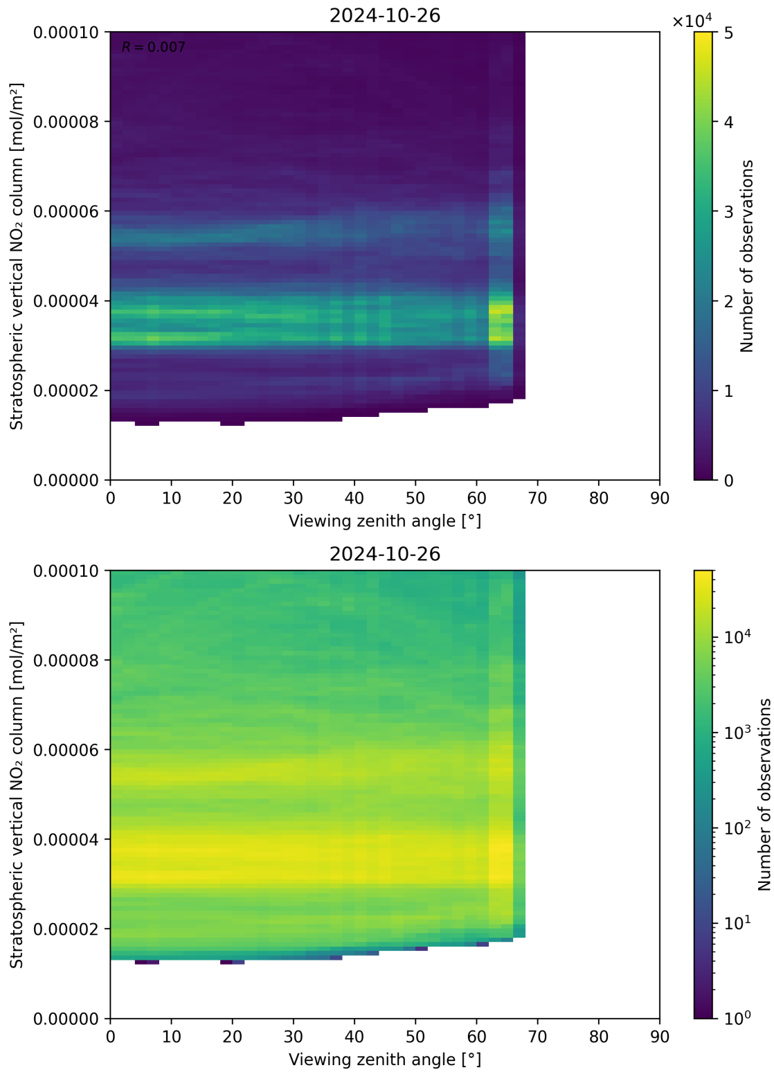
Figure 164: Scatter density plot of “Viewing zenith angle” against “Stratospheric vertical NO 2 column” for 2024-10-25 to 2024-10-27.
