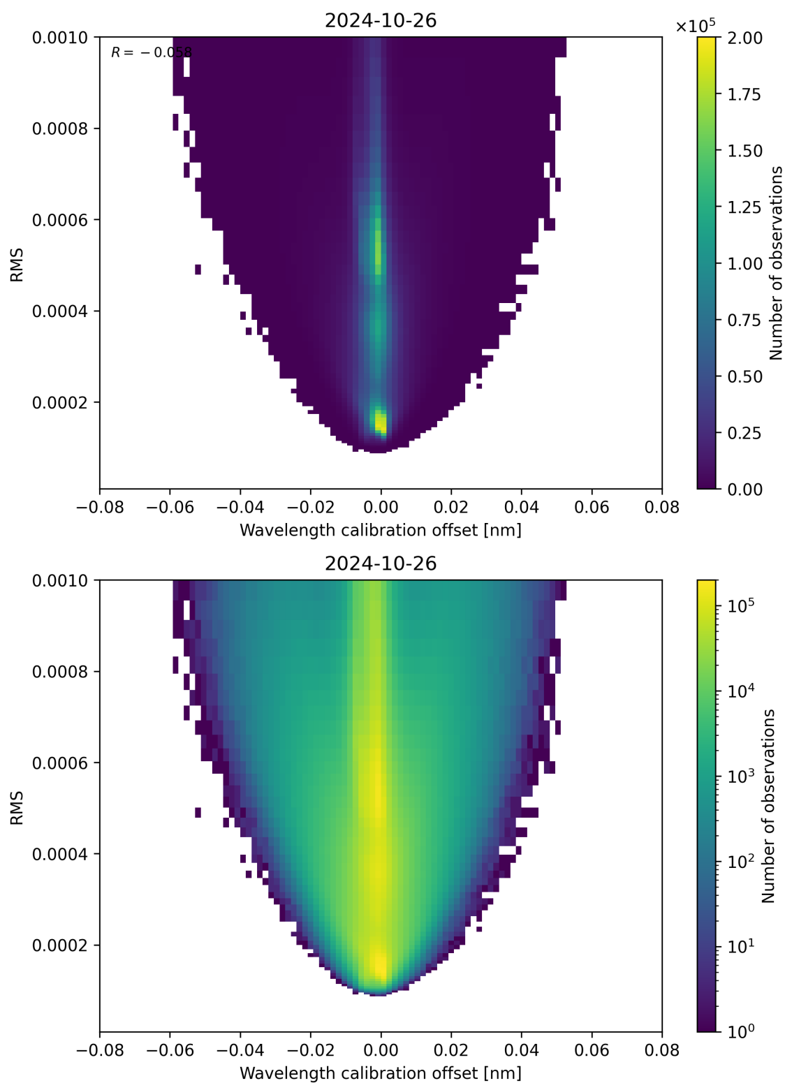
Figure 181: Scatter density plot of “Wavelength calibration offset” against “RMS” for 2024-10-25 to 2024-10-27.
