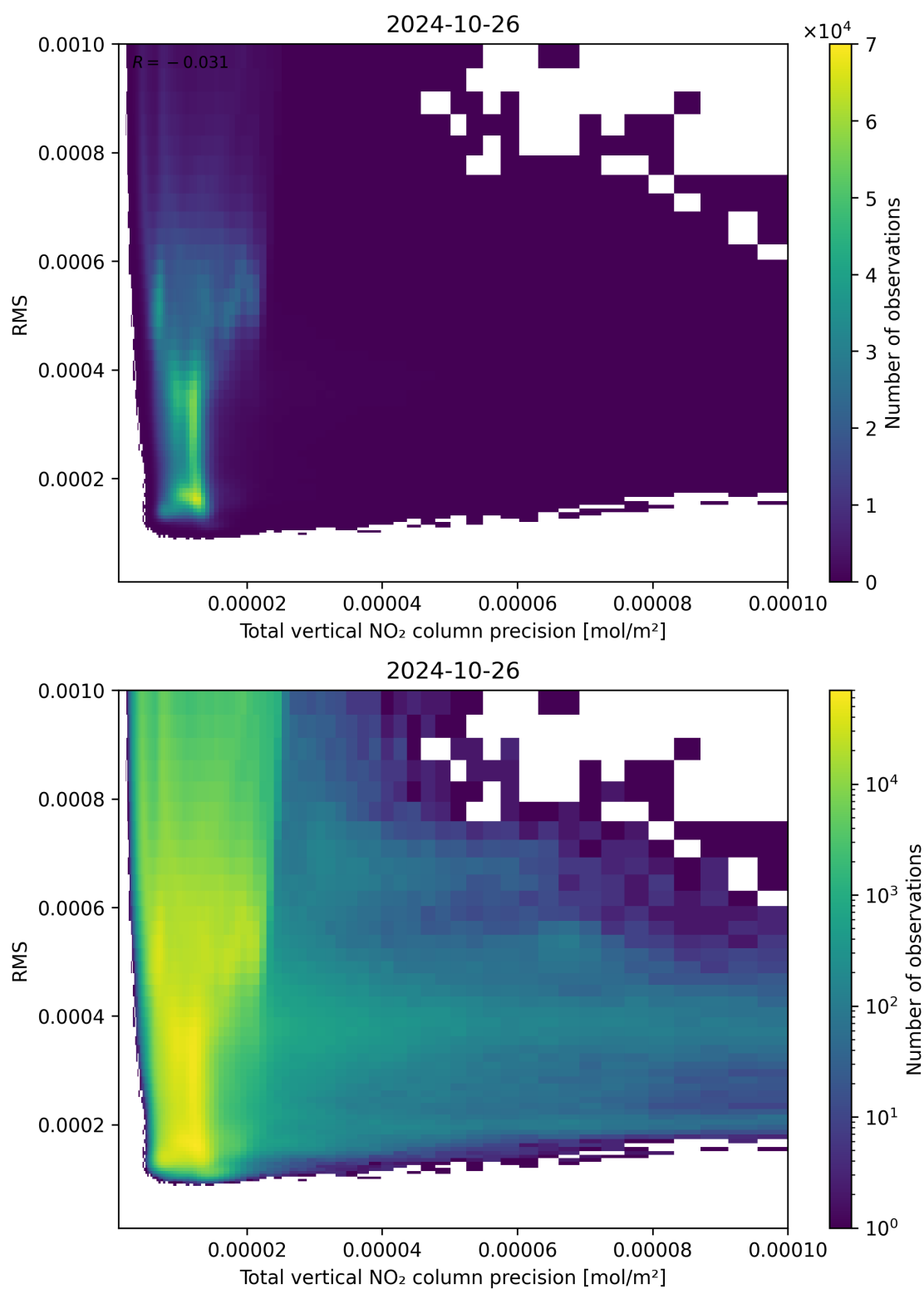
Figure 119: Scatter density plot of “Total vertical NO 2 column precision” against “RMS” for 2024-10-25 to 2024-10-27.
