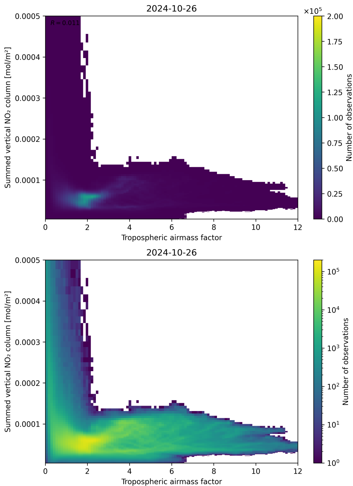
Figure 75: Scatter density plot of “Tropospheric airmass factor” against “Summed vertical NO 2 column” for 2024-10-25 to 2024-10-27.
