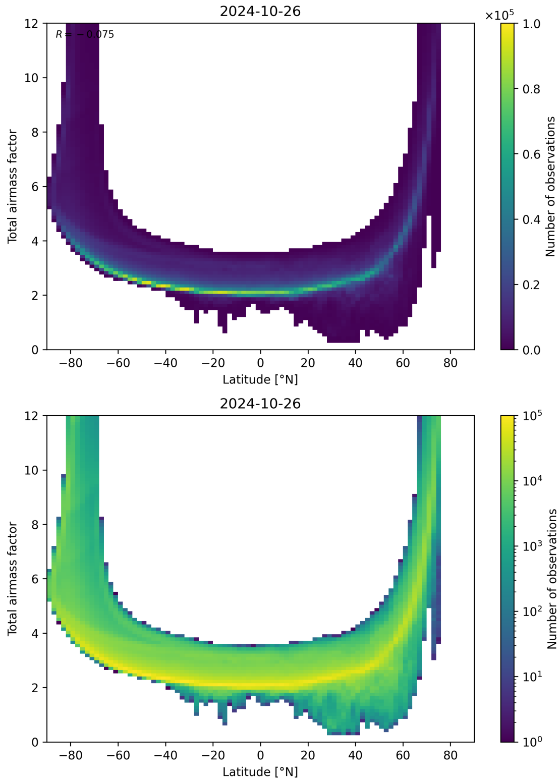
Figure 84: Scatter density plot of “Latitude” against “Total airmass factor” for 2024-10-25 to 2024-10-27.
