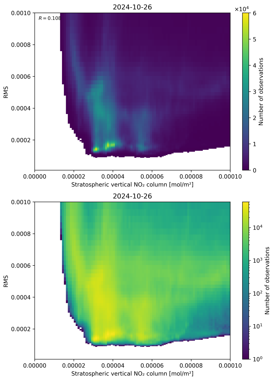
Figure 102: Scatter density plot of “Stratospheric vertical NO 2 column” against “RMS” for 2024-10-25 to 2024-10-27.
