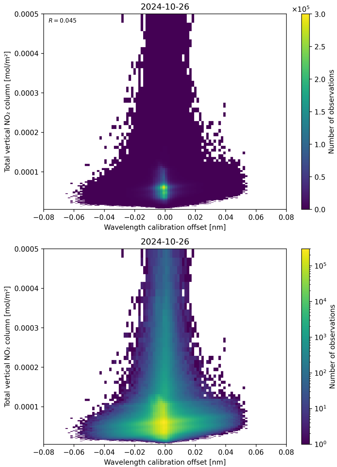
Figure 179: Scatter density plot of “Wavelength calibration offset” against “Total vertical NO 2 column” for 2024-10-25 to 2024-10-27.
