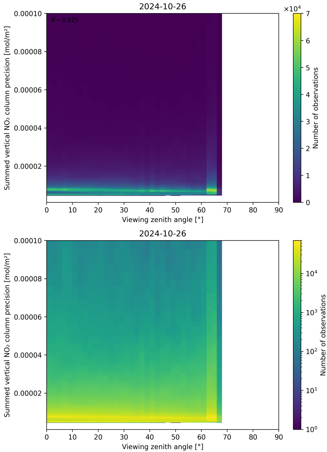
Figure 166: Scatter density plot of “Viewing zenith angle” against “Summed vertical NO 2 column precision” for 2024-10-25 to 2024-10-27.
