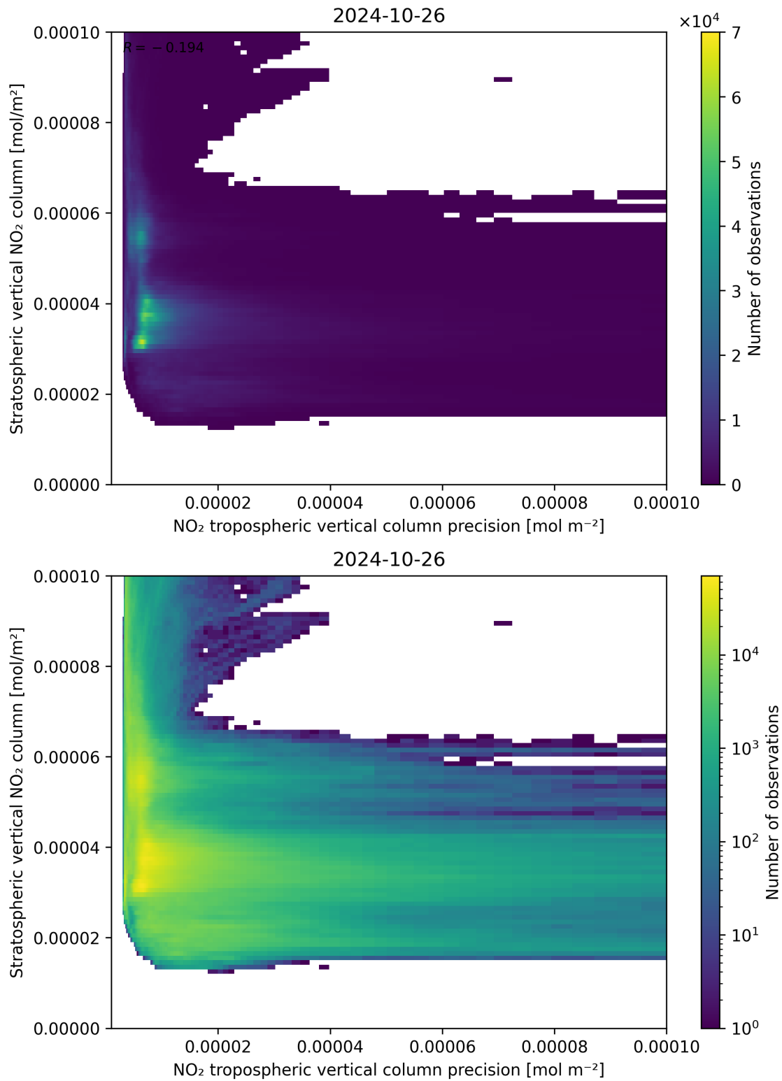
Figure 135: Scatter density plot of “NO 2 tropospheric vertical column precision” against “Stratospheric vertical NO 2 column” for 2024-10-25 to 2024-10-27.
