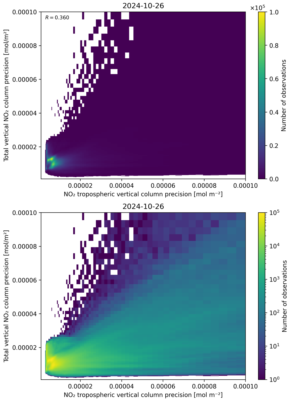
Figure 139: Scatter density plot of “NO 2 tropospheric vertical column precision” against “Total vertical NO 2 column precision” for 2024-10-25 to 2024-10-27.
