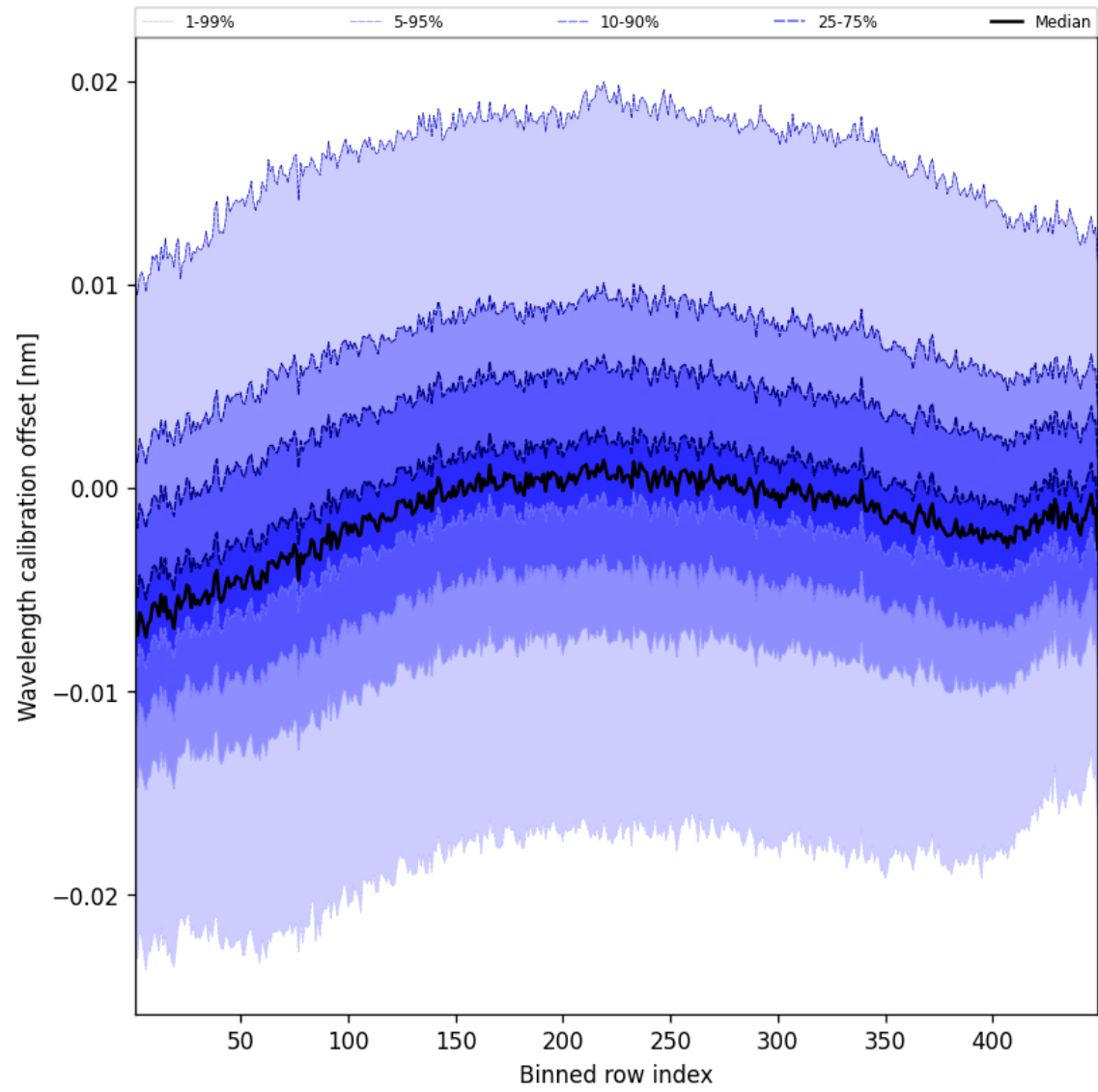
Figure 52: Along track statistics of “Wavelength calibration offset” for 2024-10-25 to 2024-10-27
