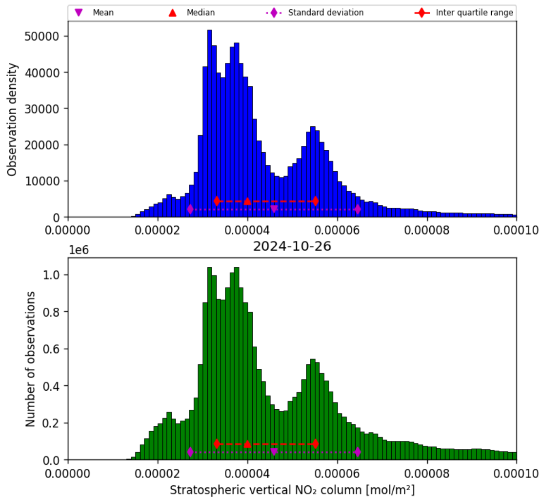
Figure 36: Histogram of “Stratospheric vertical NO 2 column” for 2024-10-25 to 2024-10-27
