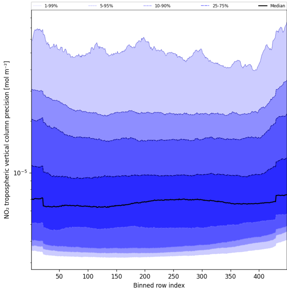
Figure 47: Along track statistics of “NO 2 tropospheric vertical column precision” for 2024-10-25 to 2024-10-27
