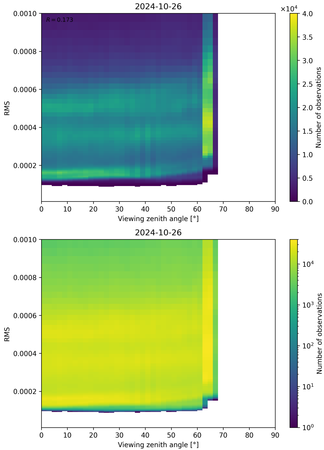
Figure 171: Scatter density plot of “Viewing zenith angle” against “RMS” for 2024-10-25 to 2024-10-27.
