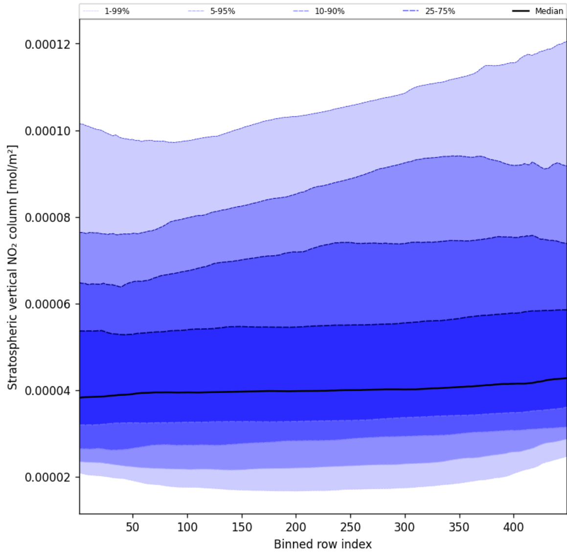
Figure 53: Along track statistics of “Stratospheric vertical NO 2 column” for 2024-10-25 to 2024-10-27
