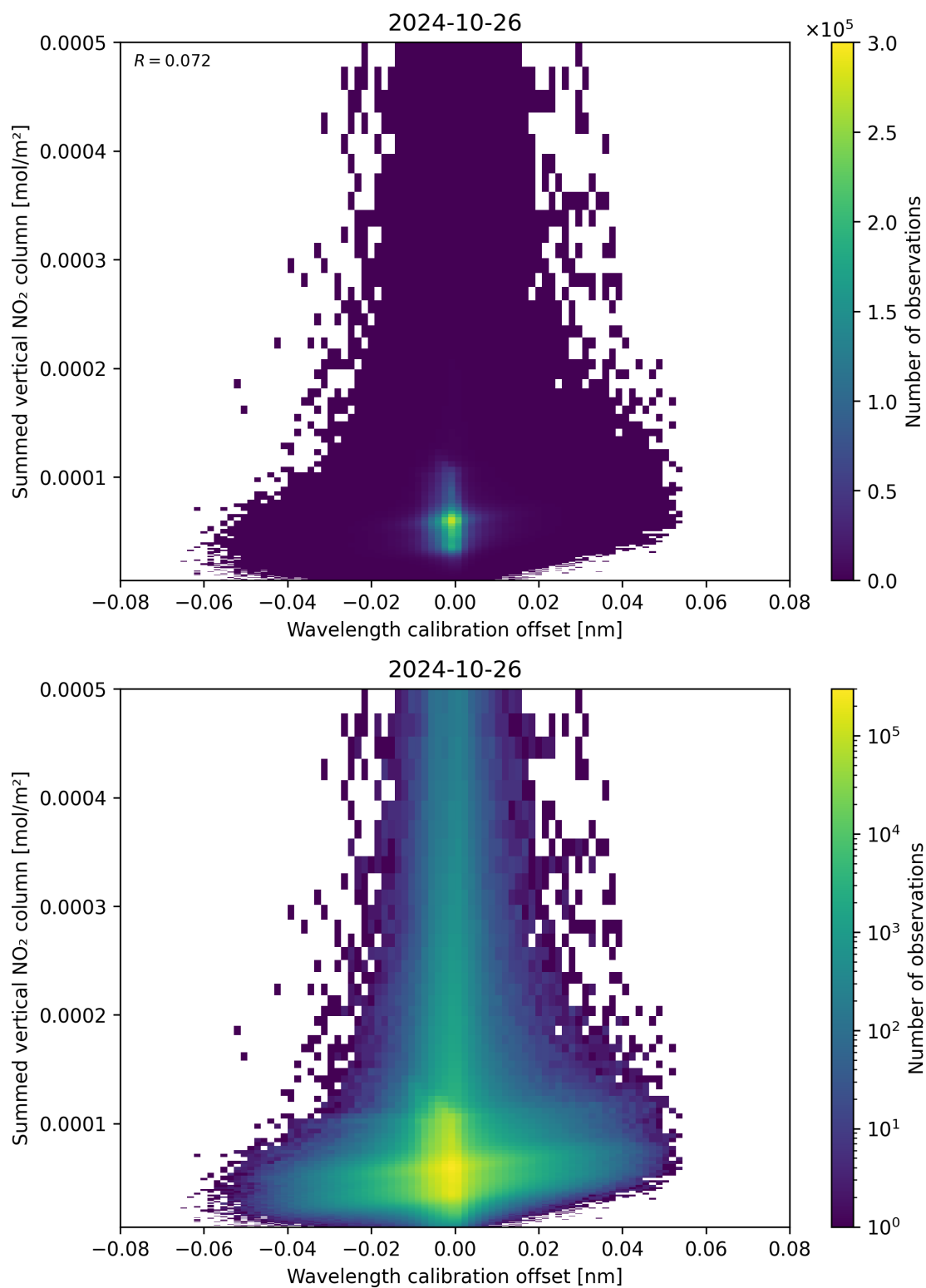
Figure 177: Scatter density plot of “Wavelength calibration offset” against “Summed vertical NO 2 column” for 2024-10-25 to 2024-10-27.
