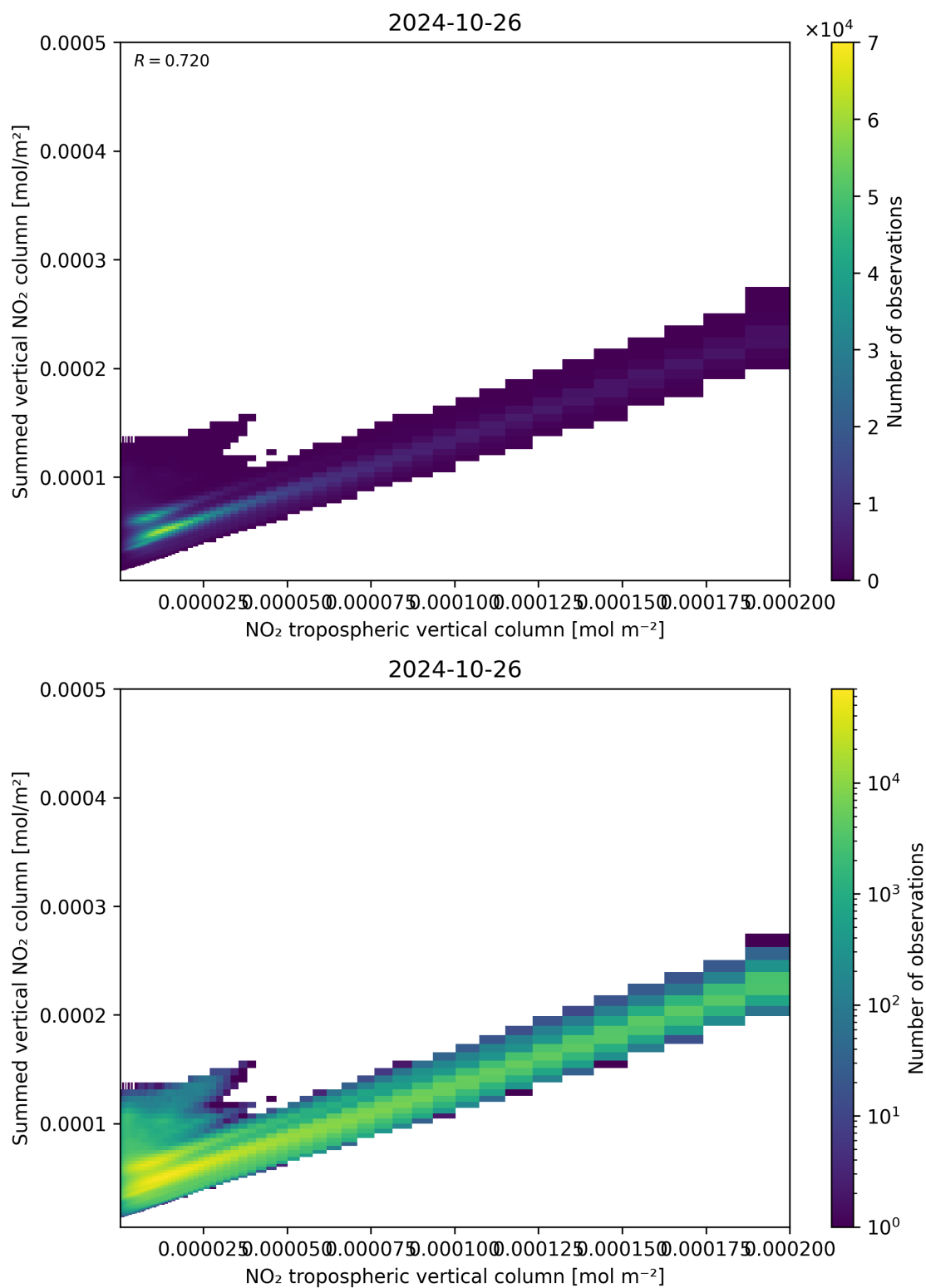
Figure 126: Scatter density plot of “NO 2 tropospheric vertical column” against “Summed vertical NO 2 column” for 2024-10-25 to 2024-10-27.
