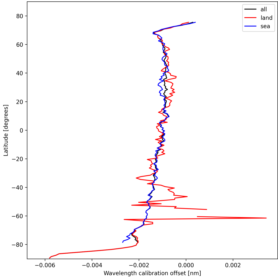
Figure 18: Zonal average of “Wavelength calibration offset” for 2024-10-25 to 2024-10-27.
