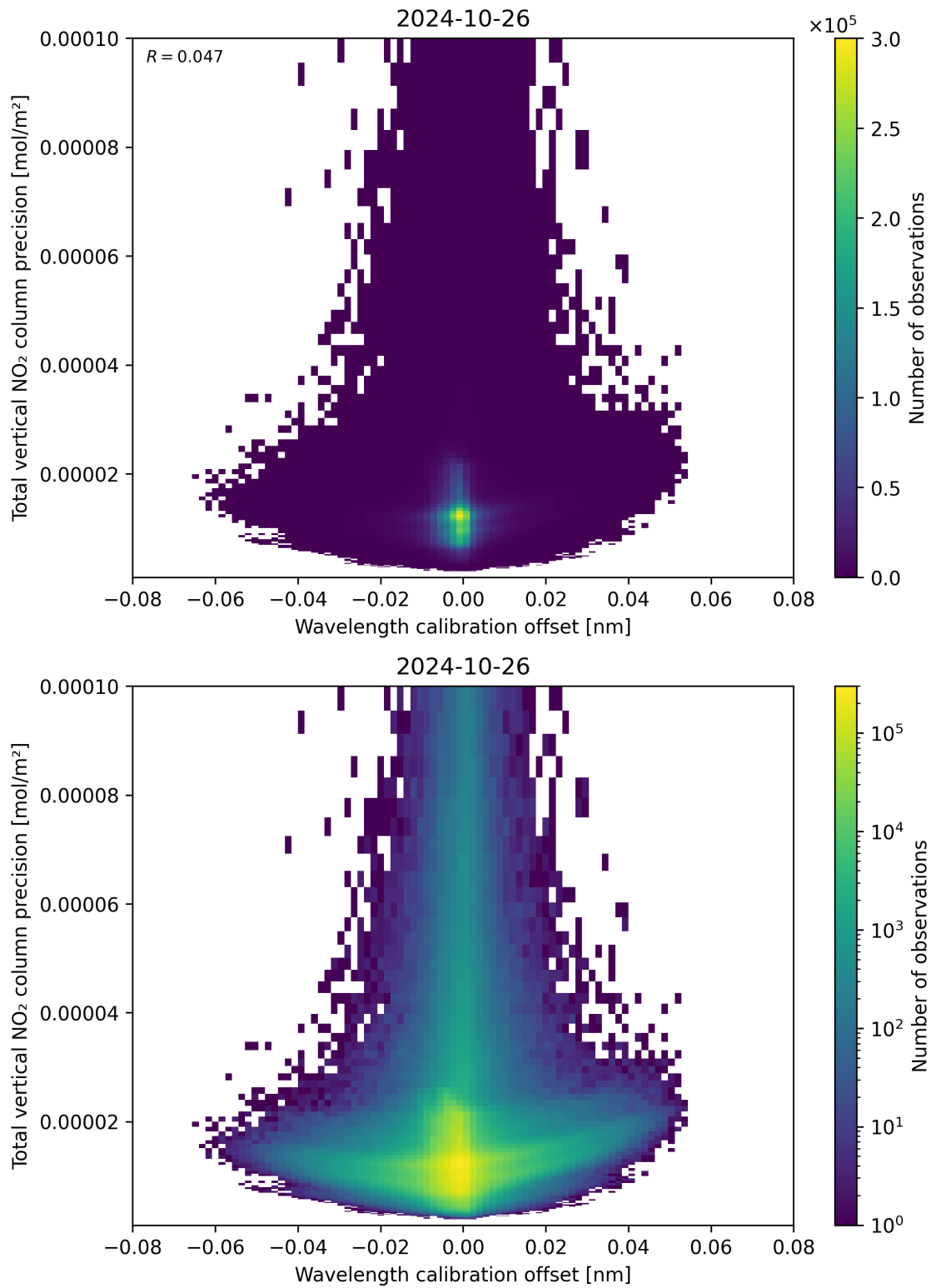
Figure 180: Scatter density plot of “Wavelength calibration offset” against “Total vertical NO 2 column precision” for 2024-10-25 to 2024-10-27.
