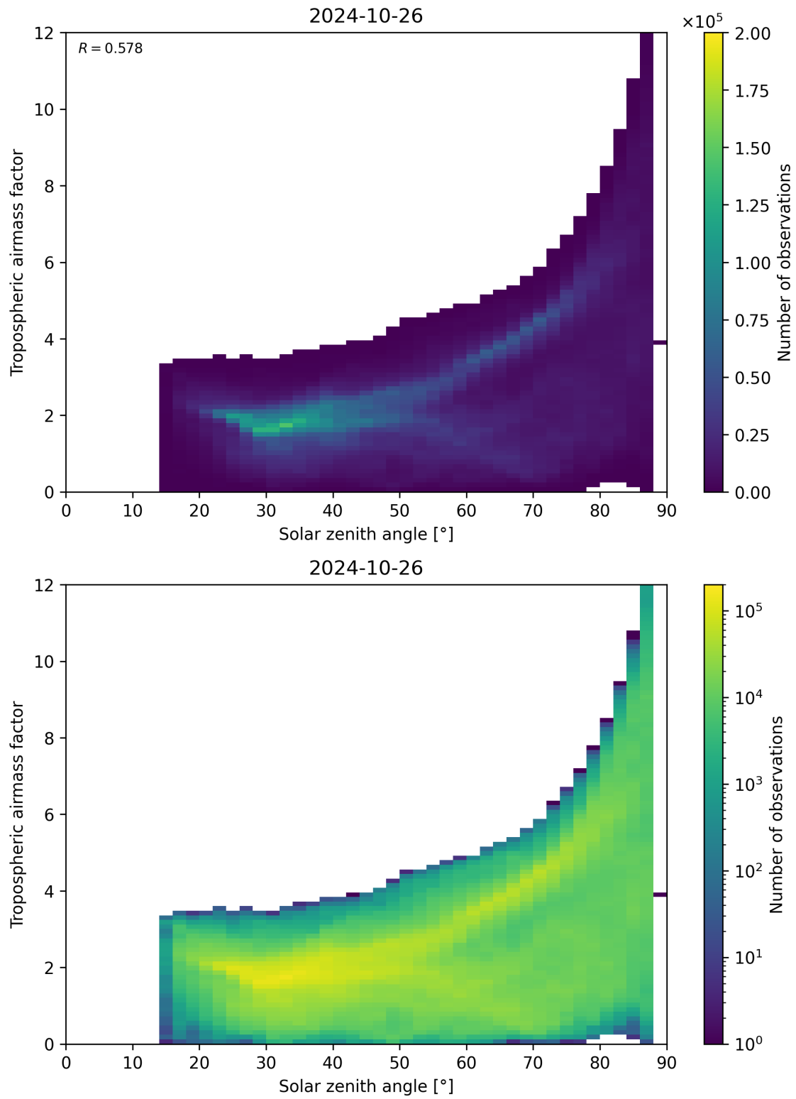
Figure 147: Scatter density plot of “Solar zenith angle” against “Tropospheric airmass factor” for 2024-10-25 to 2024-10-27.
