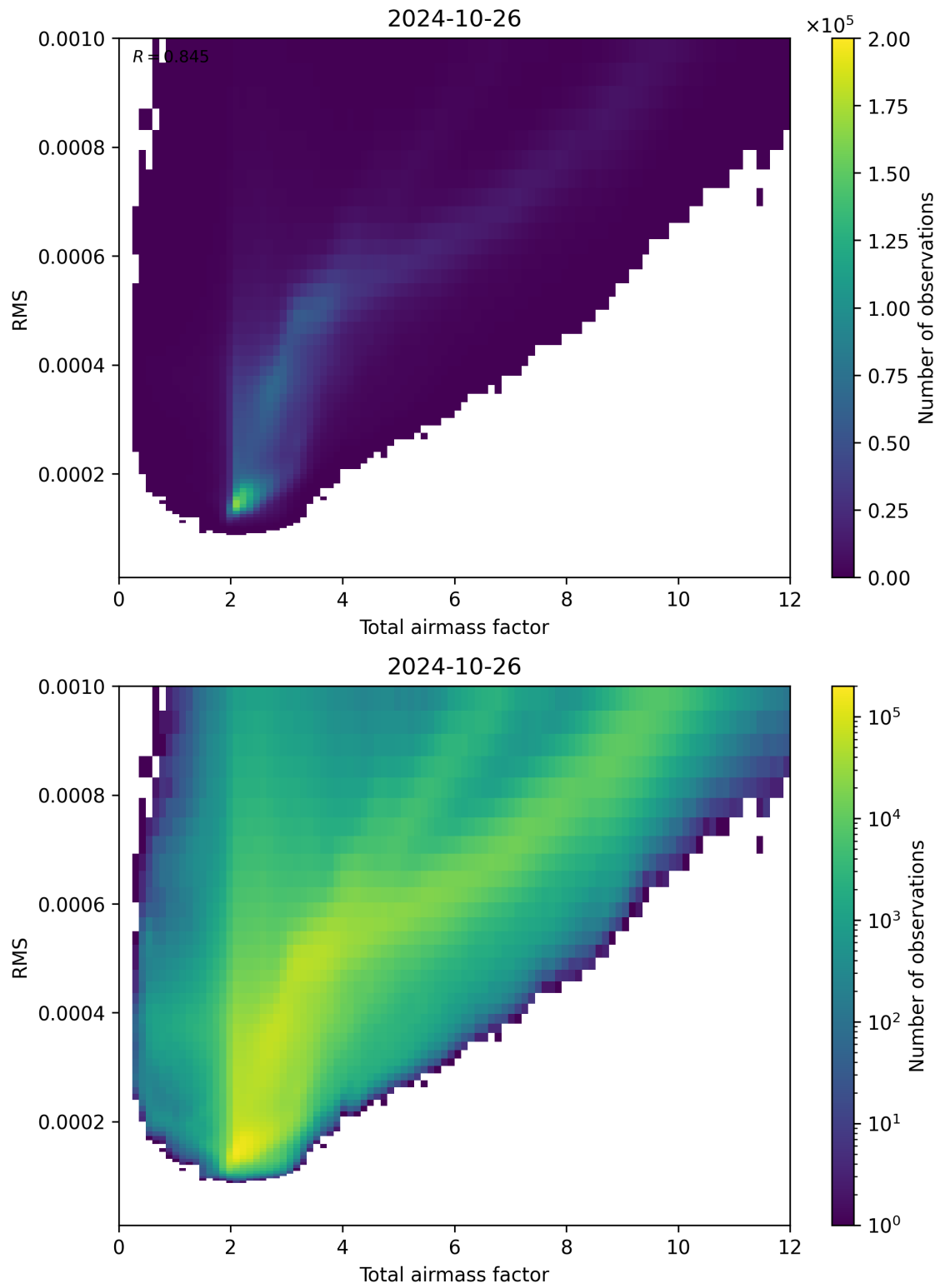
Figure 69: Scatter density plot of “Total airmass factor” against “RMS” for 2024-10-25 to 2024-10-27.
