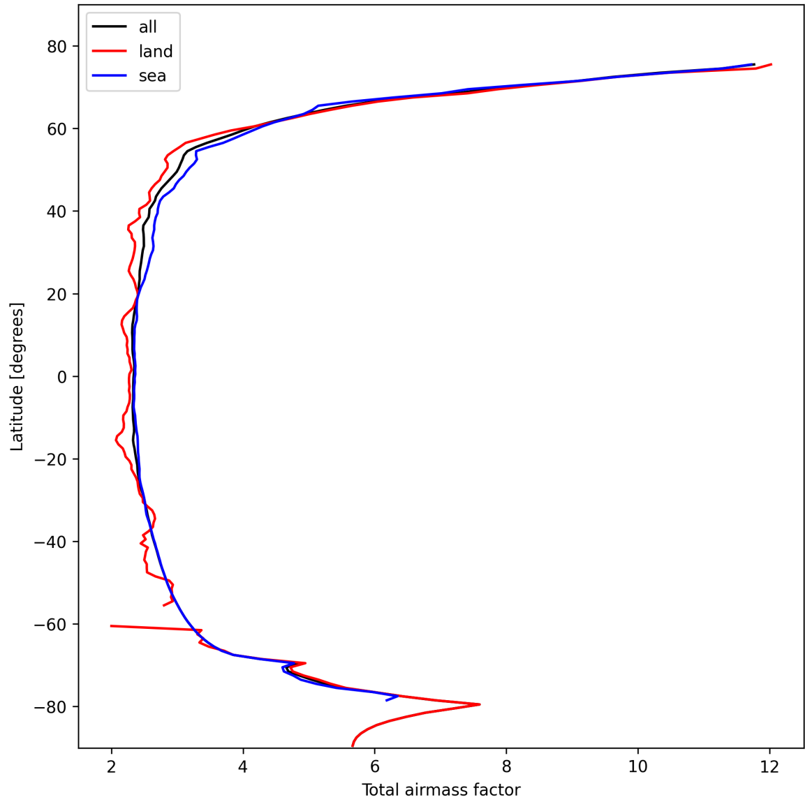
Figure 15: Zonal average of “Total airmass factor” for 2024-10-25 to 2024-10-27.
