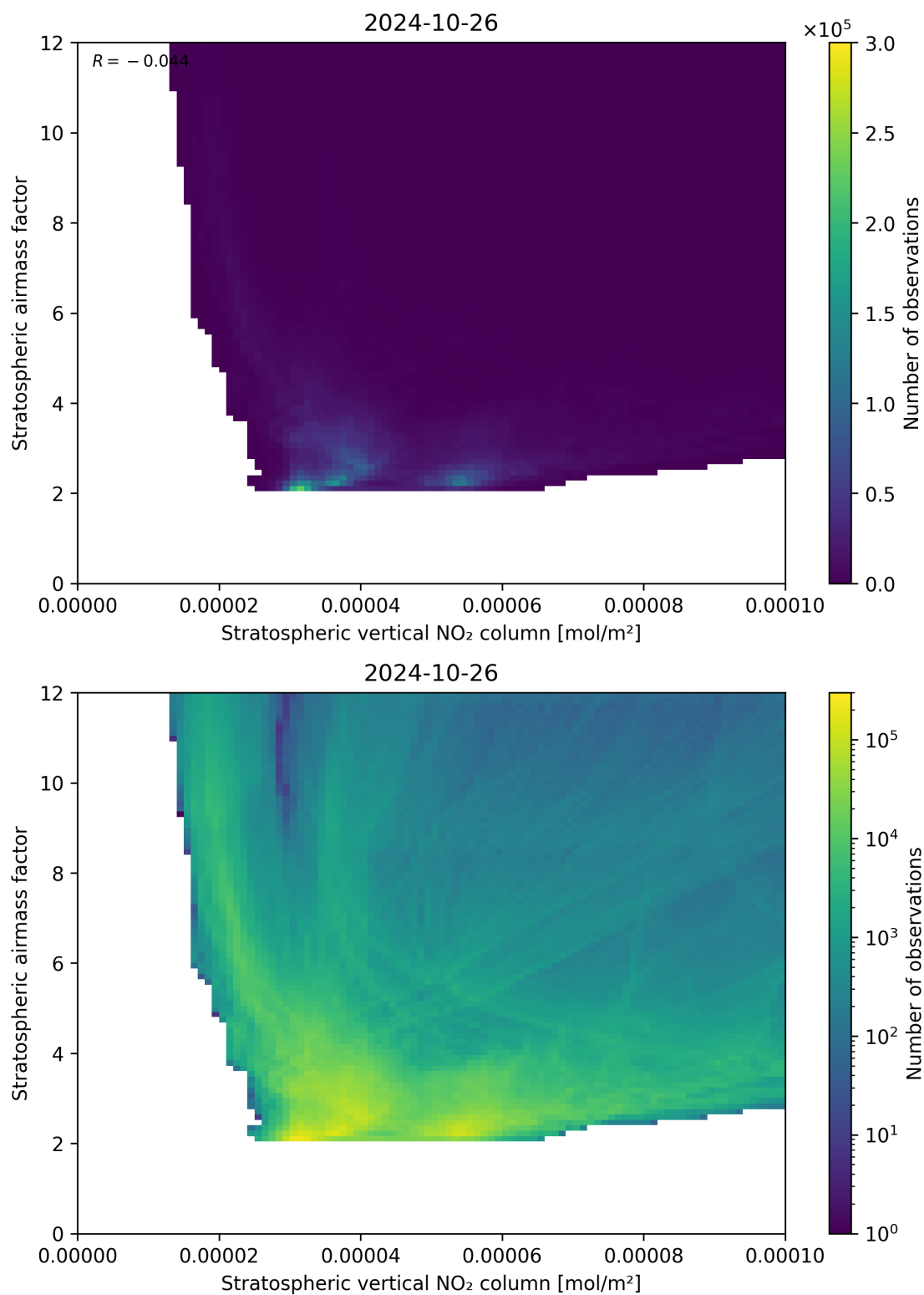
Figure 96: Scatter density plot of “Stratospheric vertical NO 2 column” against “Stratospheric airmass factor” for 2024-10-25 to 2024-10-27.
