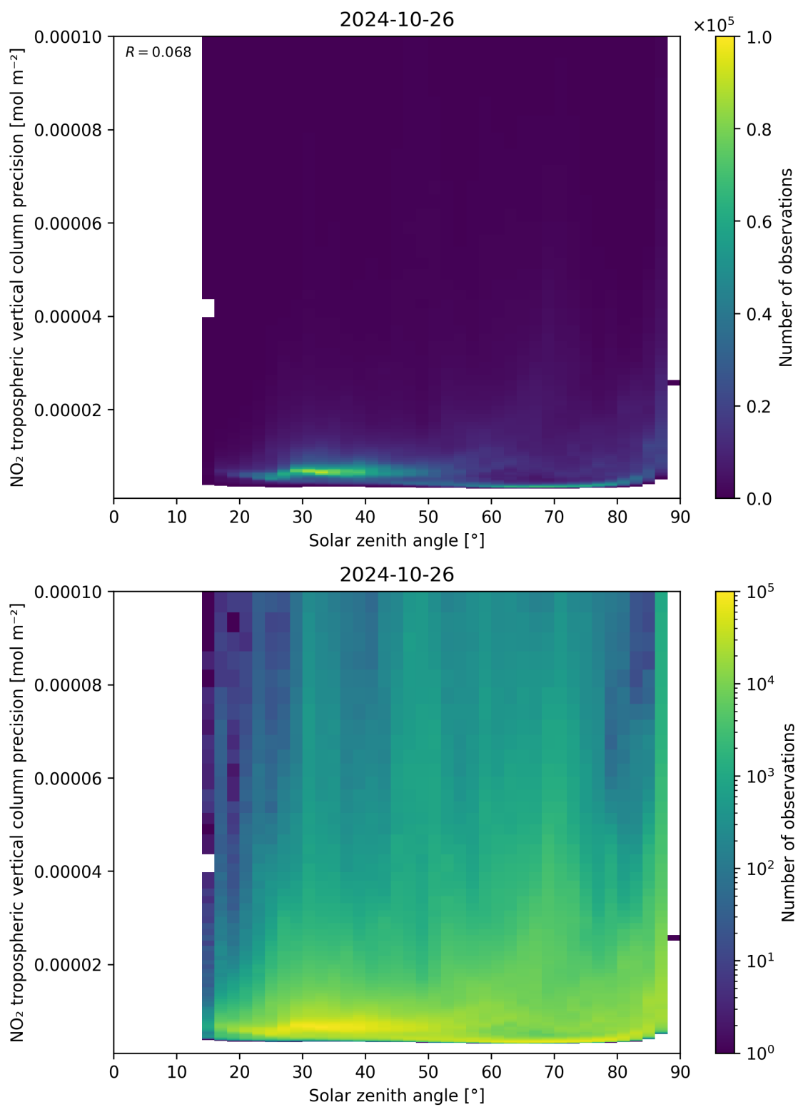
Figure 156: Scatter density plot of “Solar zenith angle” against “NO 2 tropospheric vertical column precision” for 2024-10-25 to 2024-10-27.
