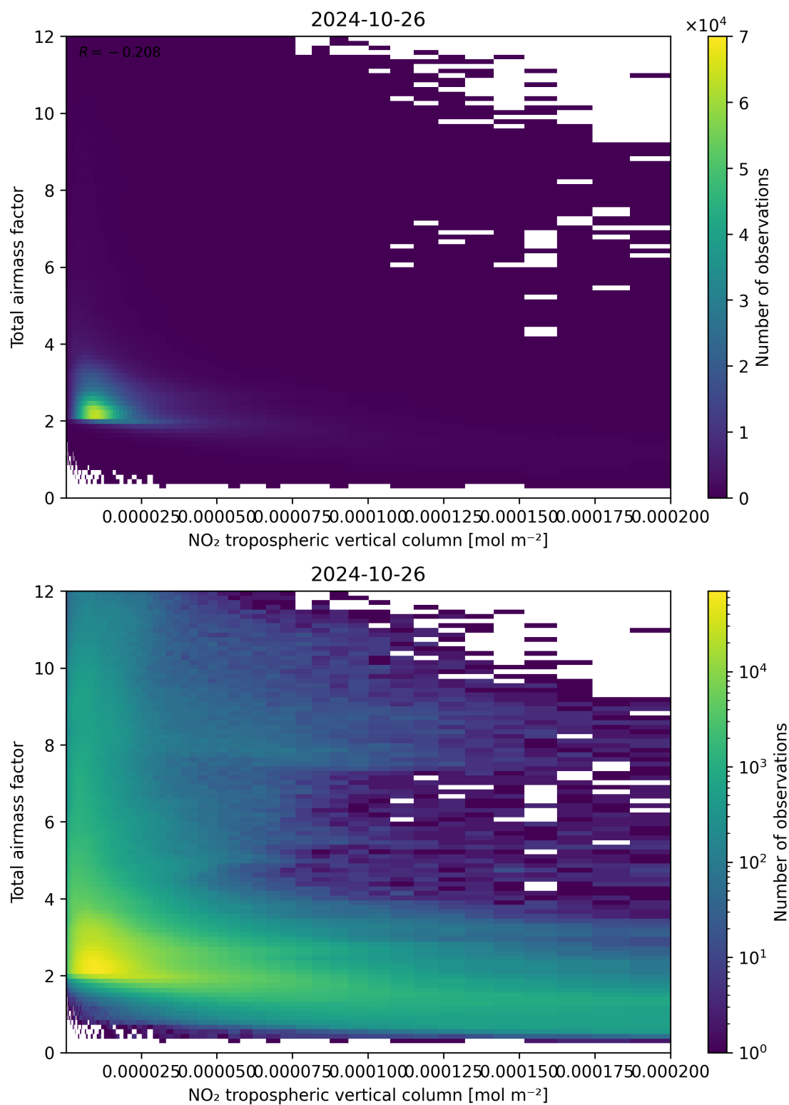
Figure 122: Scatter density plot of “NO 2 tropospheric vertical column” against “Total air mass factor” for 2024-10-25 to 2024-10-27.
