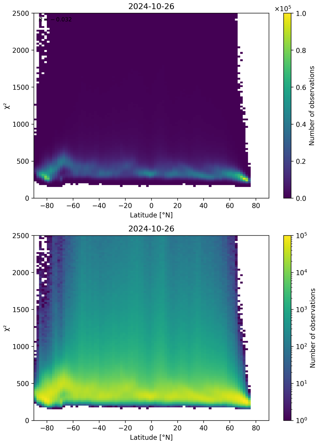
Figure 86: Scatter density plot of “Latitude” against “ \chi^2 ” for 2024-10-25 to 2024-10-27.
