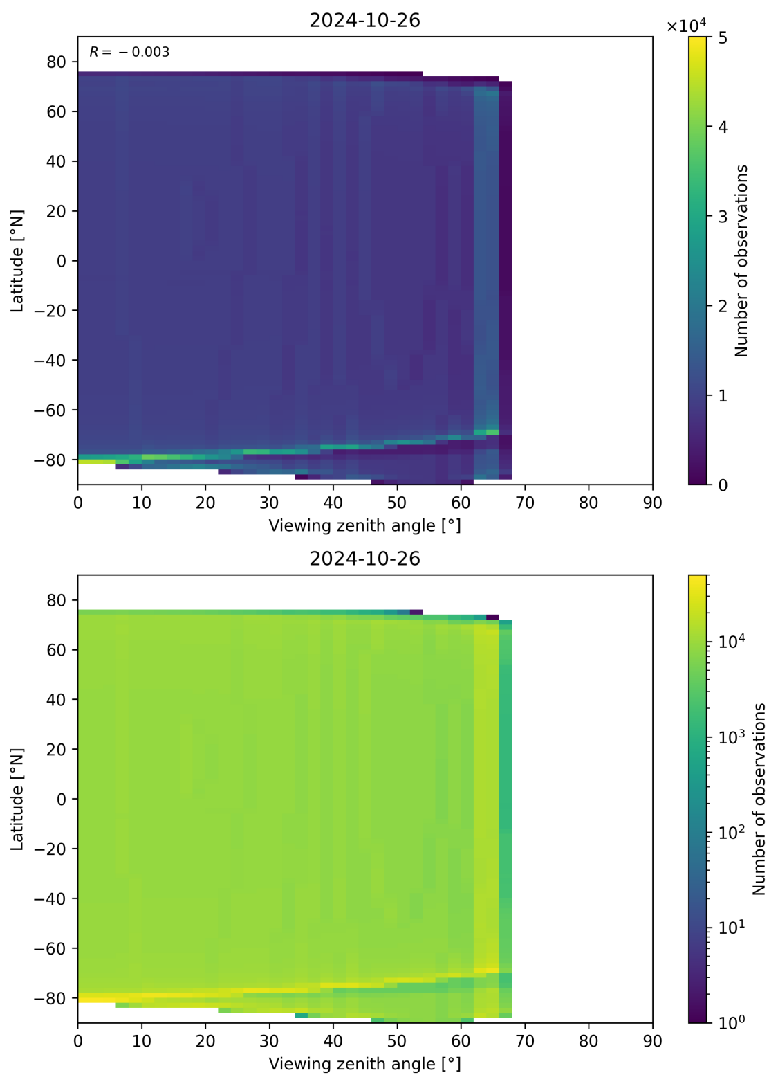
Figure 163: Scatter density plot of “Viewing zenith angle” against “Latitude” for 2024-10-25 to 2024-10-27.
