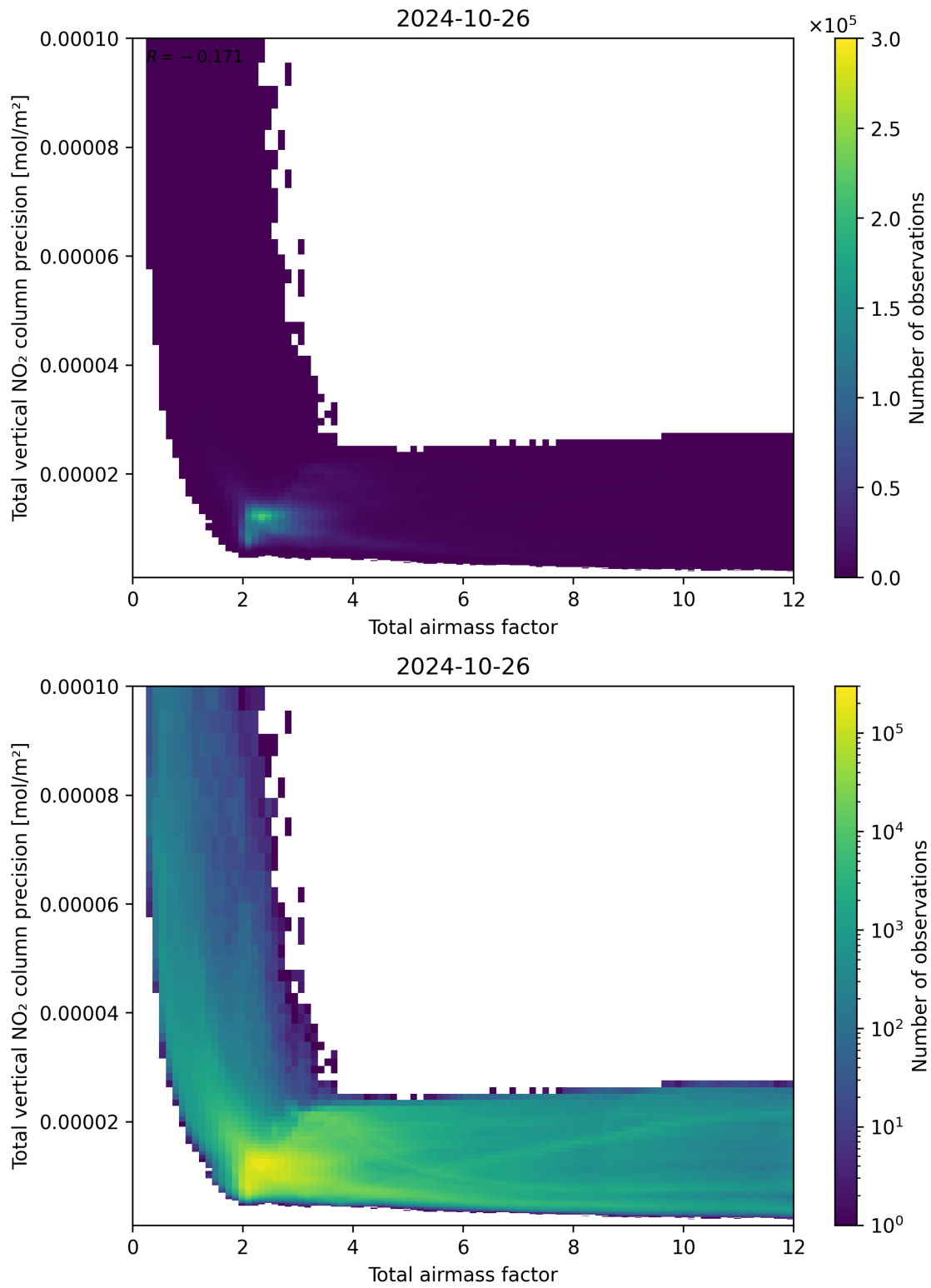
Figure 68: Scatter density plot of “Total airmass factor” against “Total vertical NO 2 column precision” for 2024-10-25 to 2024-10-27.
