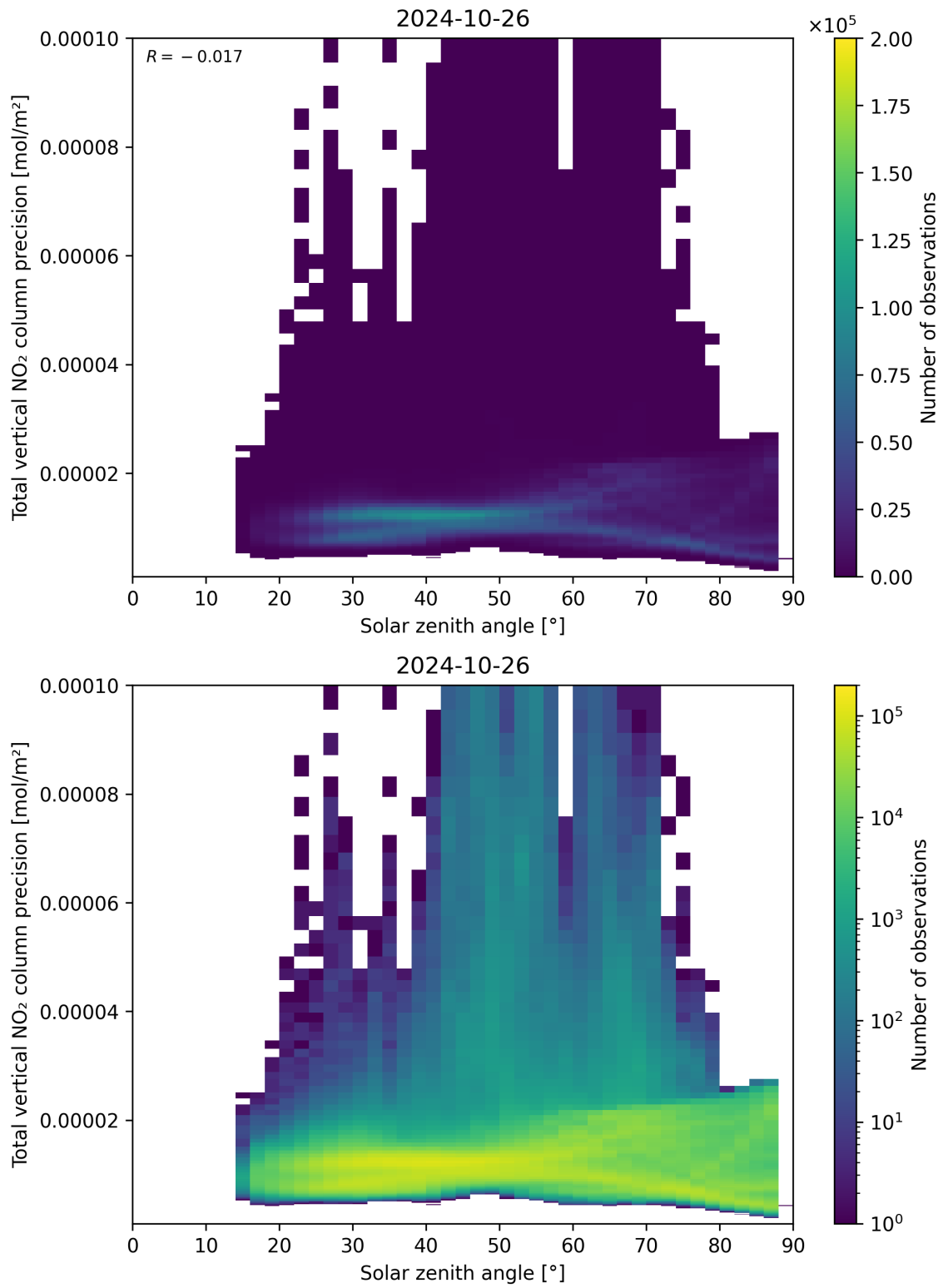
Figure 154: Scatter density plot of “Solar zenith angle” against “Total vertical NO 2 column precision” for 2024-10-25 to 2024-10-27.
