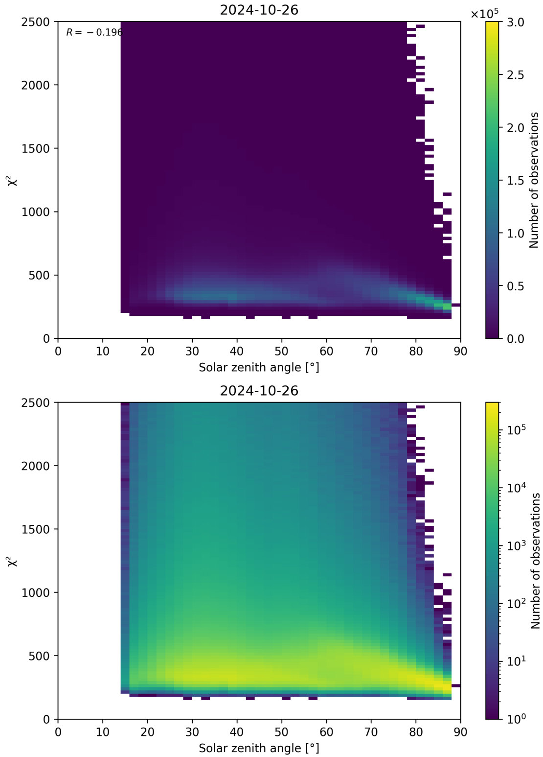
Figure 148: Scatter density plot of “Solar zenith angle” against “ \chi^2 ” for 2024-10-25 to 2024-10-27.
