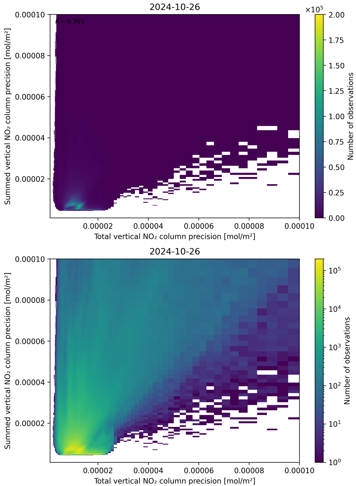
Figure 118: Scatter density plot of “Total vertical NO 2 column precision” against “Summed vertical NO 2 column precision” for 2024-10-25 to 2024-10-27.
