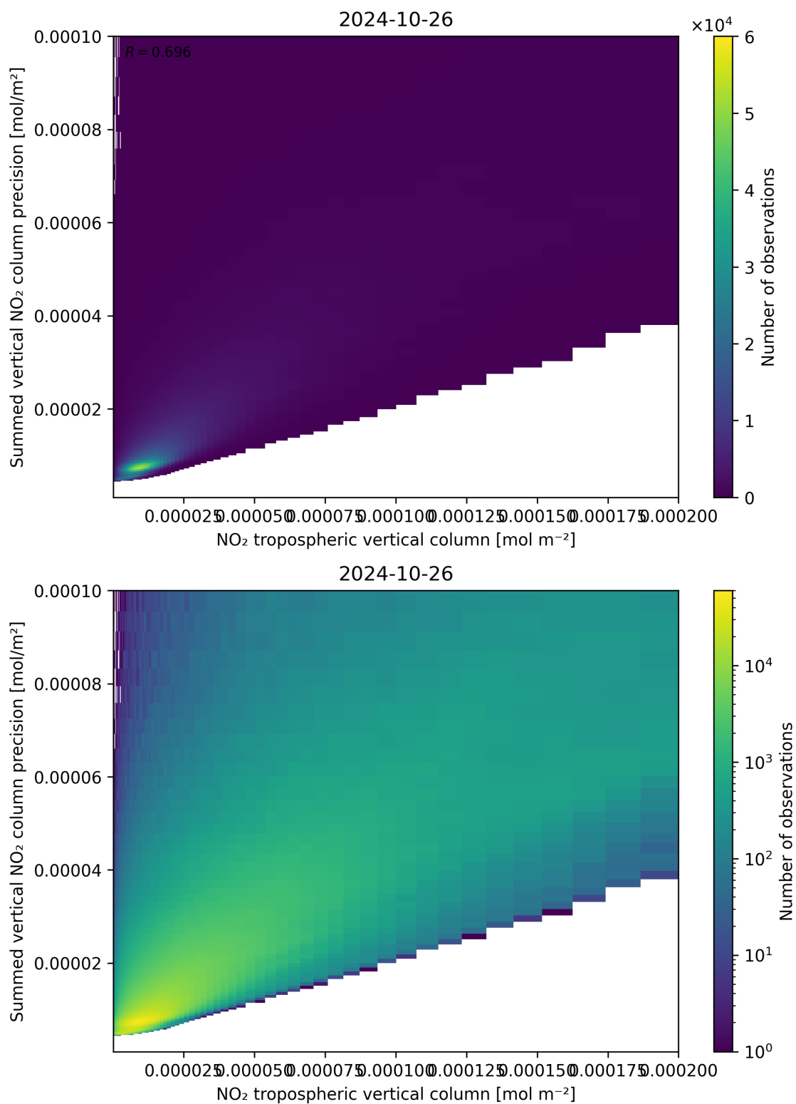
Figure 127: Scatter density plot of “NO 2 tropospheric vertical column” against “Summed vertical NO 2 column precision” for 2024-10-25 to 2024-10-27.
