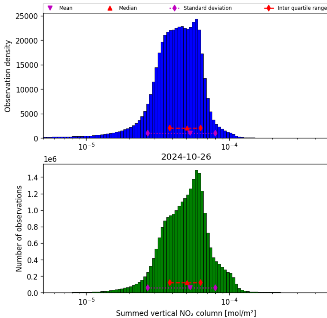
Figure 40: Histogram of “Summed vertical NO 2 column” for 2024-10-25 to 2024-10-27
