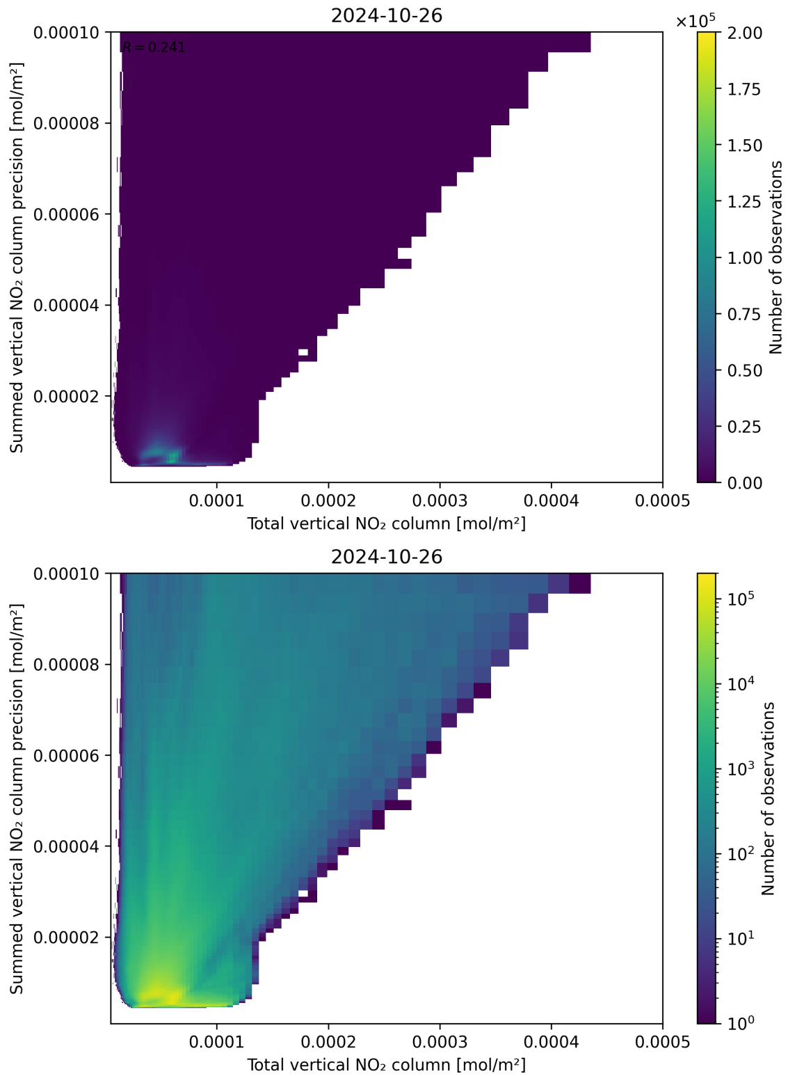
Figure 113: Scatter density plot of “Total vertical NO 2 column” against “Summed vertical NO 2 column precision” for 2024-10-25 to 2024-10-27.
