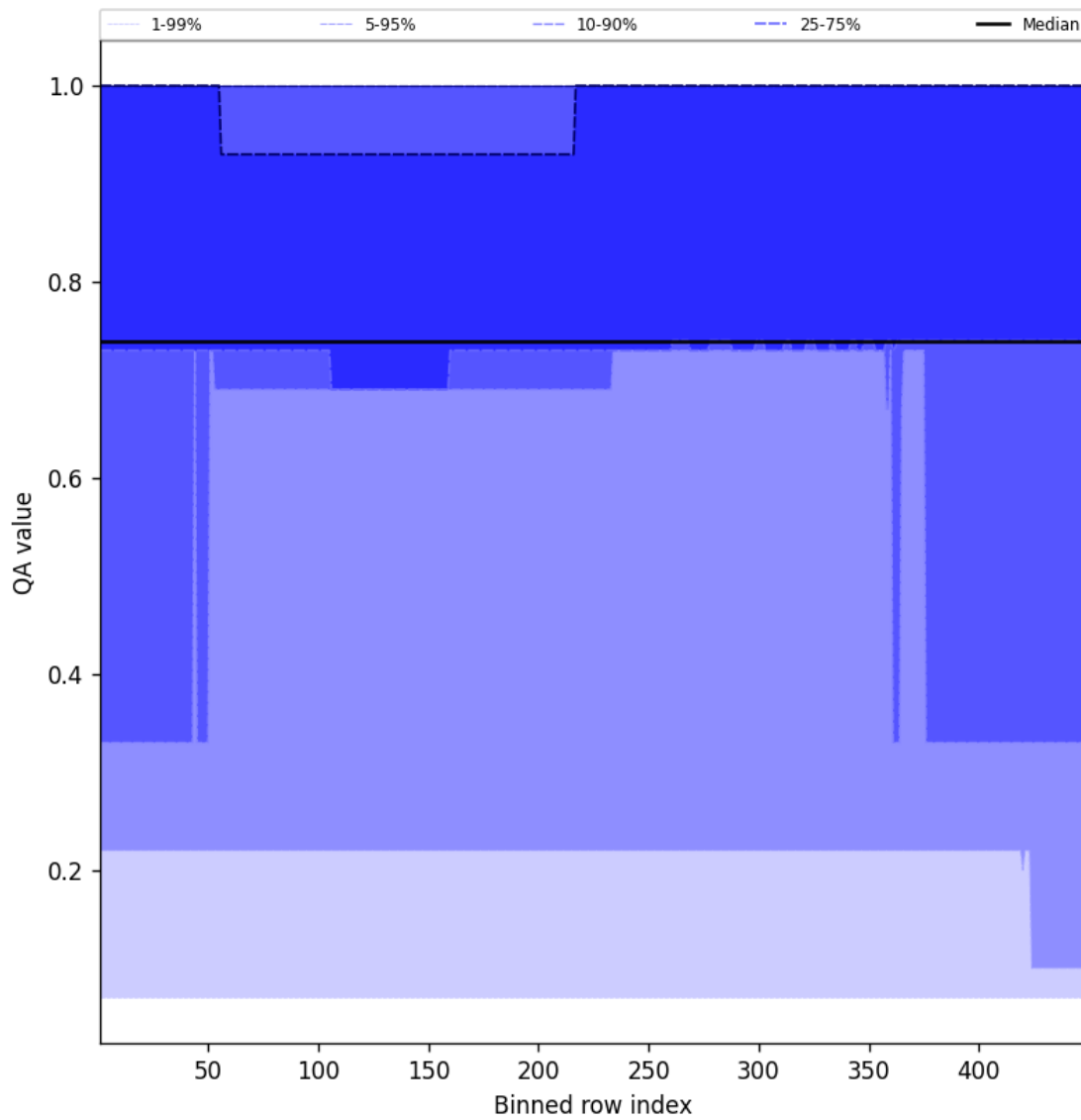
Figure 45: Along track statistics of “QA value” for 2024-10-25 to 2024-10-27
