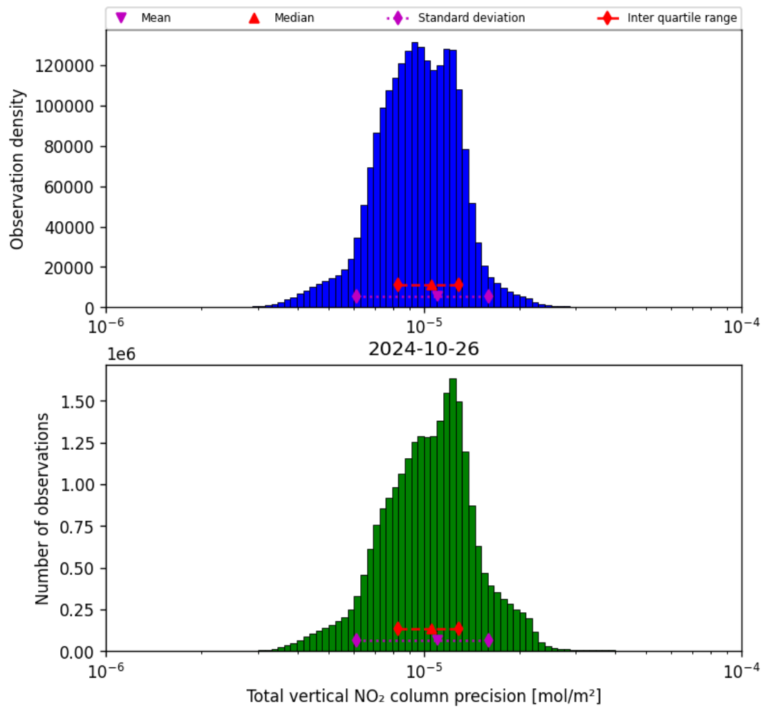
Figure 39: Histogram of “Total vertical NO 2 column precision” for 2024-10-25 to 2024-10-27
