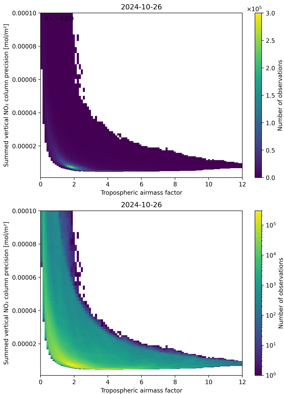
Figure 76: Scatter density plot of “Tropospheric airmass factor” against “Summed vertical NO 2 column precision” for 2024-10-25 to 2024-10-27.
