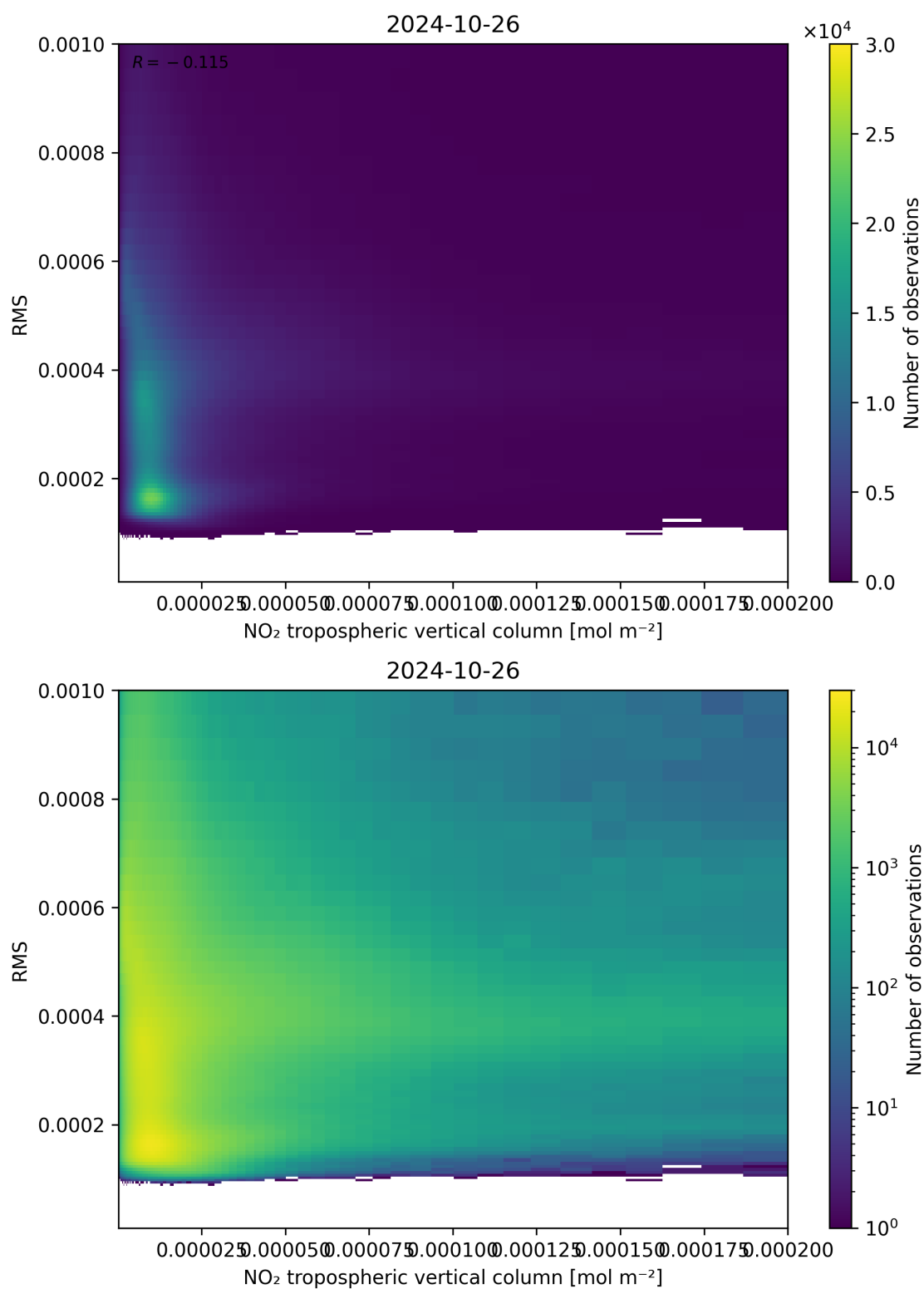
Figure 142: Scatter density plot of “NO 2 tropospheric vertical column” against “RMS” for 2024-10-25 to 2024-10-27.
