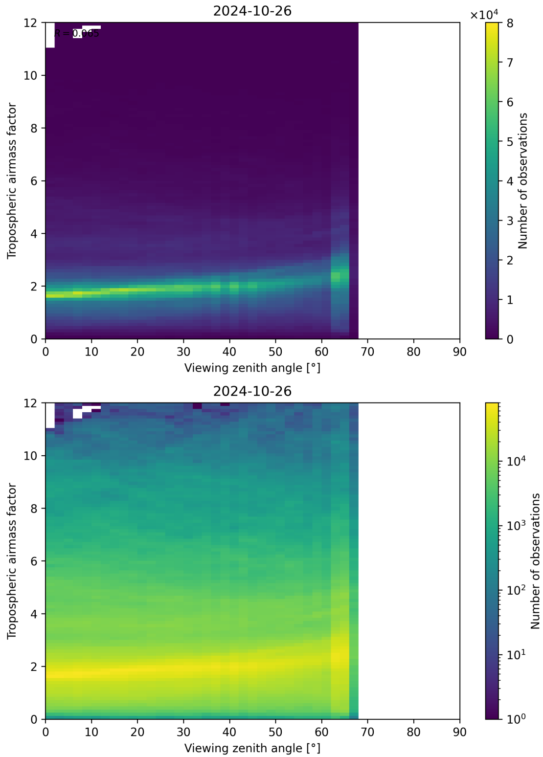
Figure 161: Scatter density plot of “Viewing zenith angle” against “Tropospheric airmass factor” for 2024-10-25 to 2024-10-27.
