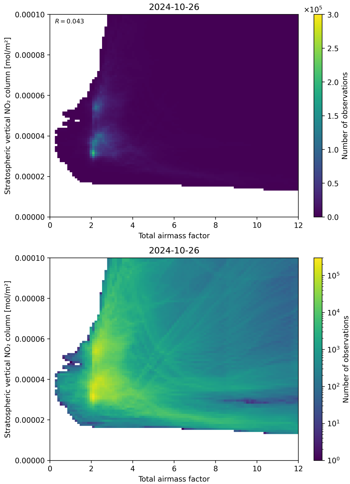
Figure 64: Scatter density plot of “Total airmass factor” against “Stratospheric vertical \text{NO}_2 column” for 2024-10-25 to 2024-10-27.
