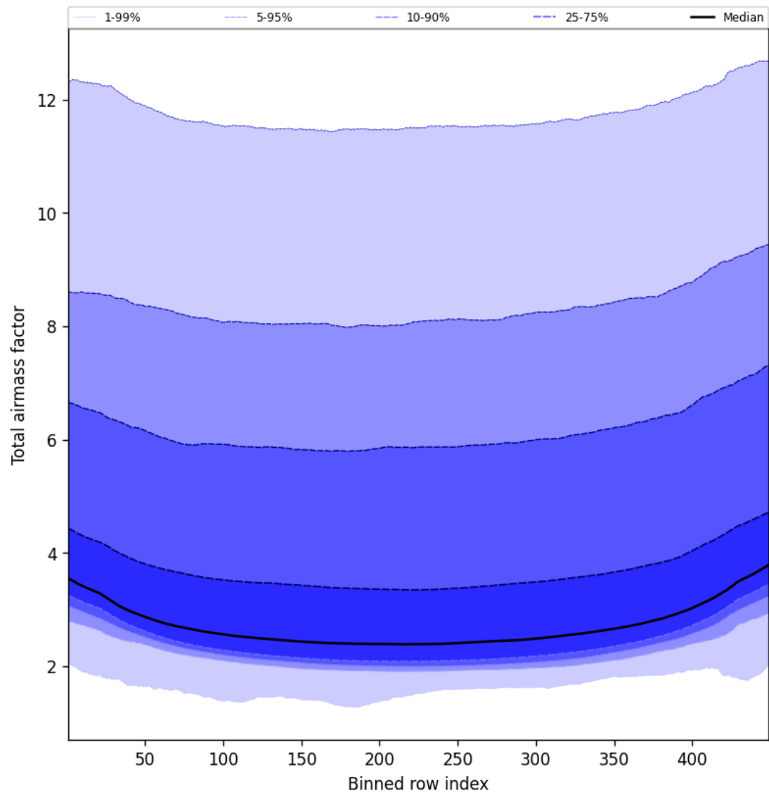
Figure 49: Along track statistics of “Total airmass factor” for 2024-10-25 to 2024-10-27
