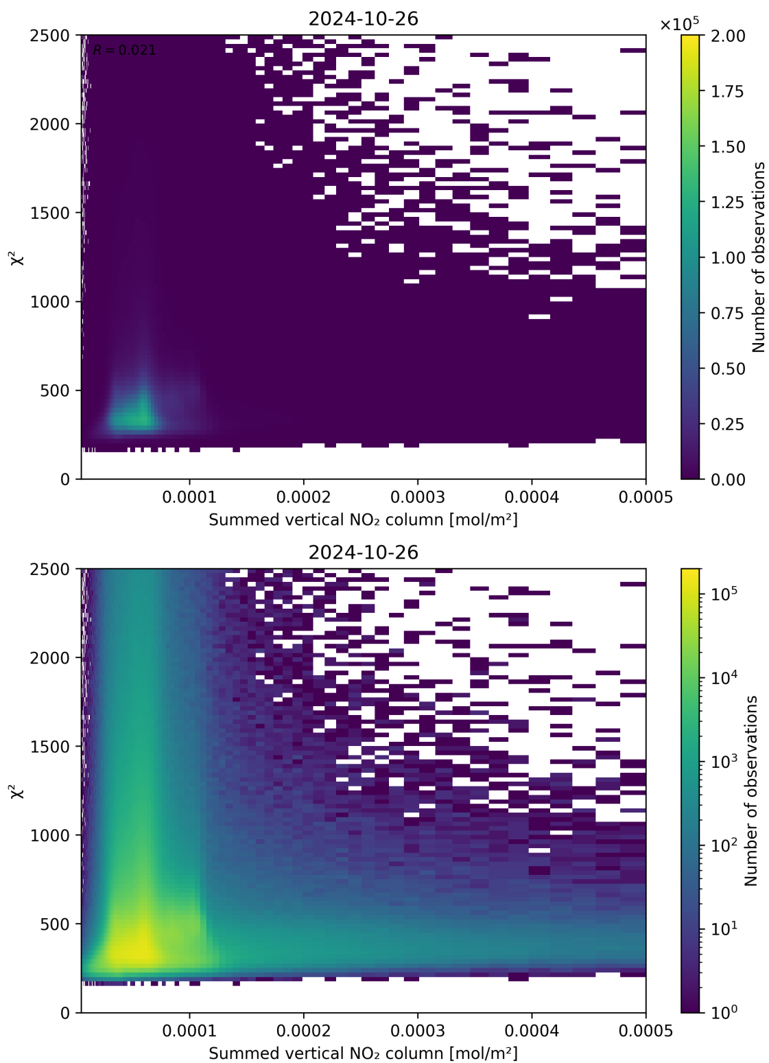
Figure 104: Scatter density plot of “Summed vertical NO 2 column” against “ \chi^2 ” for 2024-10-25 to 2024-10-27.
