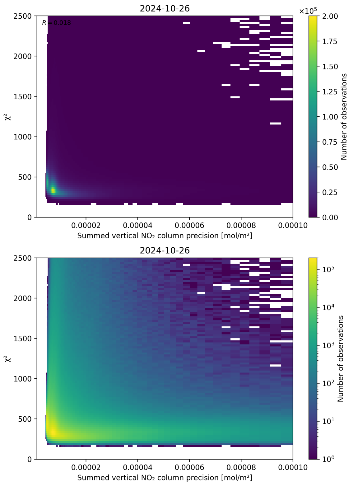
Figure 107: Scatter density plot of “Summed vertical NO 2 column precision” against “ \chi^2 ” for 2024-10-25 to 2024-10-27.
