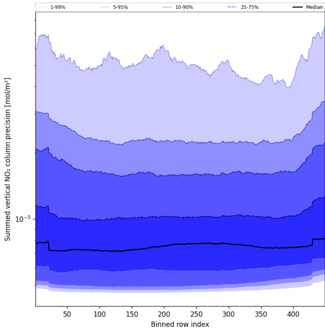
Figure 58: Along track statistics of “Summed vertical NO 2 column precision” for 2024-10-25 to 2024-10-27
