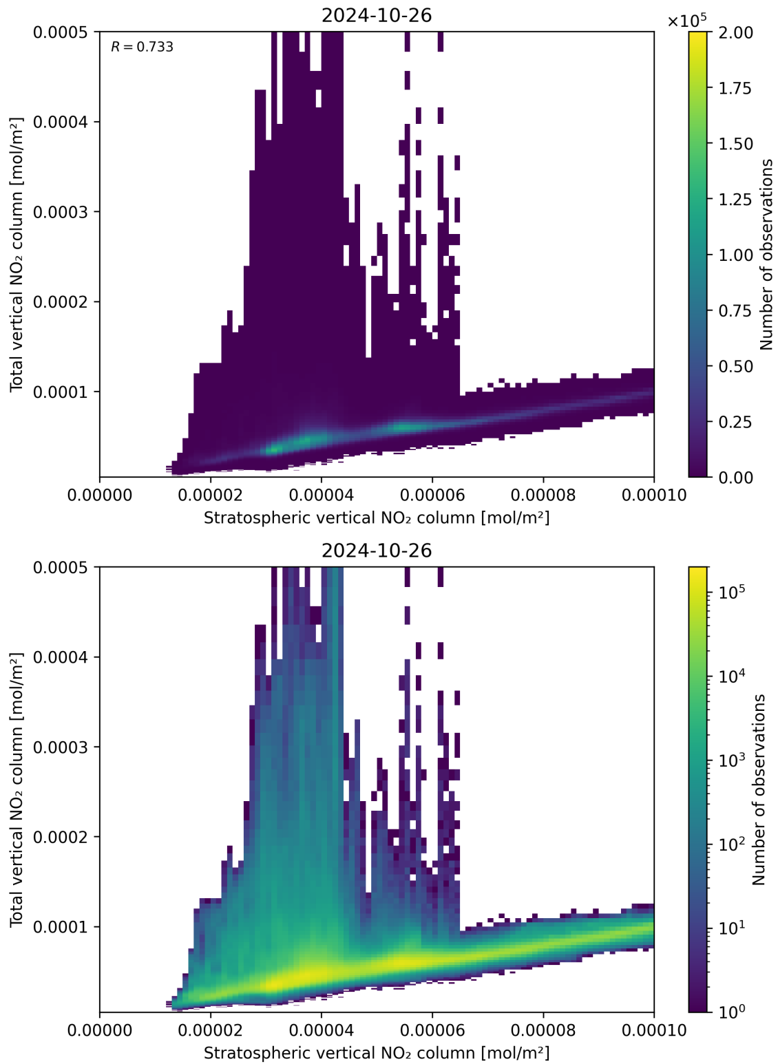
Figure 100: Scatter density plot of “Stratospheric vertical NO 2 column” against “Total vertical NO 2 column” for 2024-10-25 to 2024-10-27.
