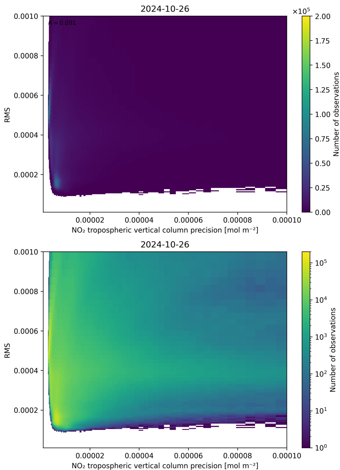
Figure 140: Scatter density plot of “NO 2 tropospheric vertical column precision” against “RMS” for 2024-10-25 to 2024-10-27.
