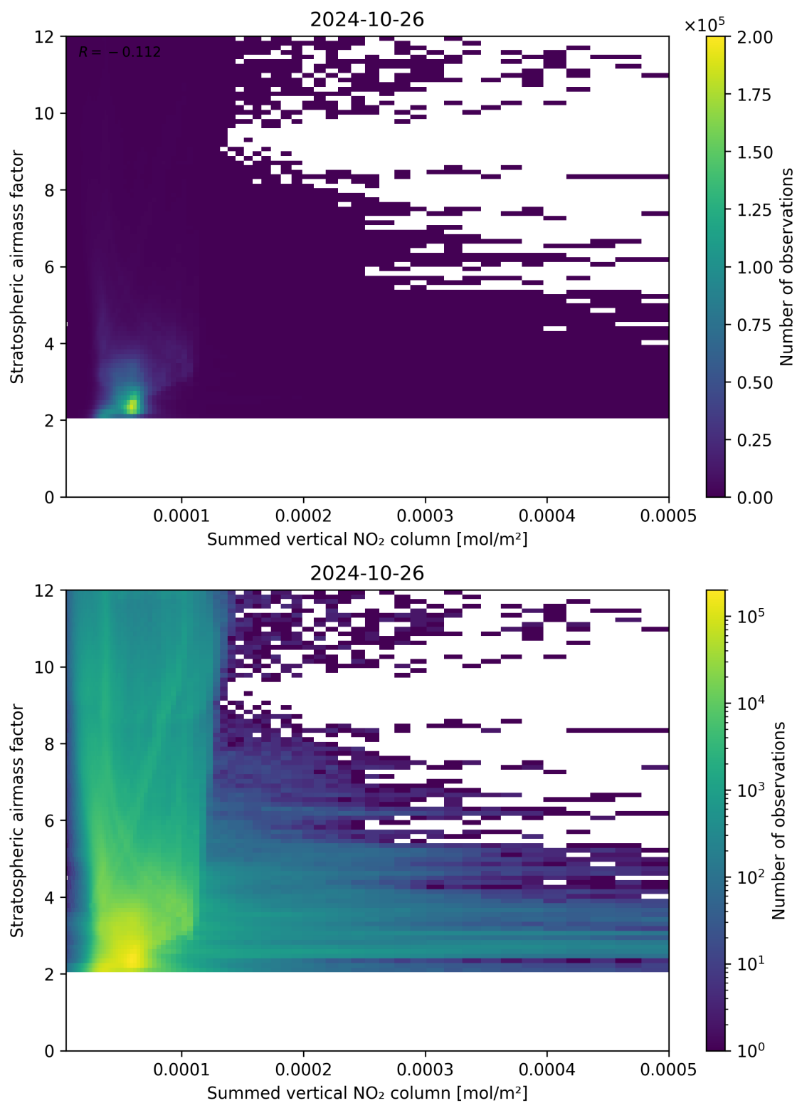
Figure 103: Scatter density plot of “Summed vertical NO 2 column” against “Stratospheric airmass factor” for 2024-10-25 to 2024-10-27.
