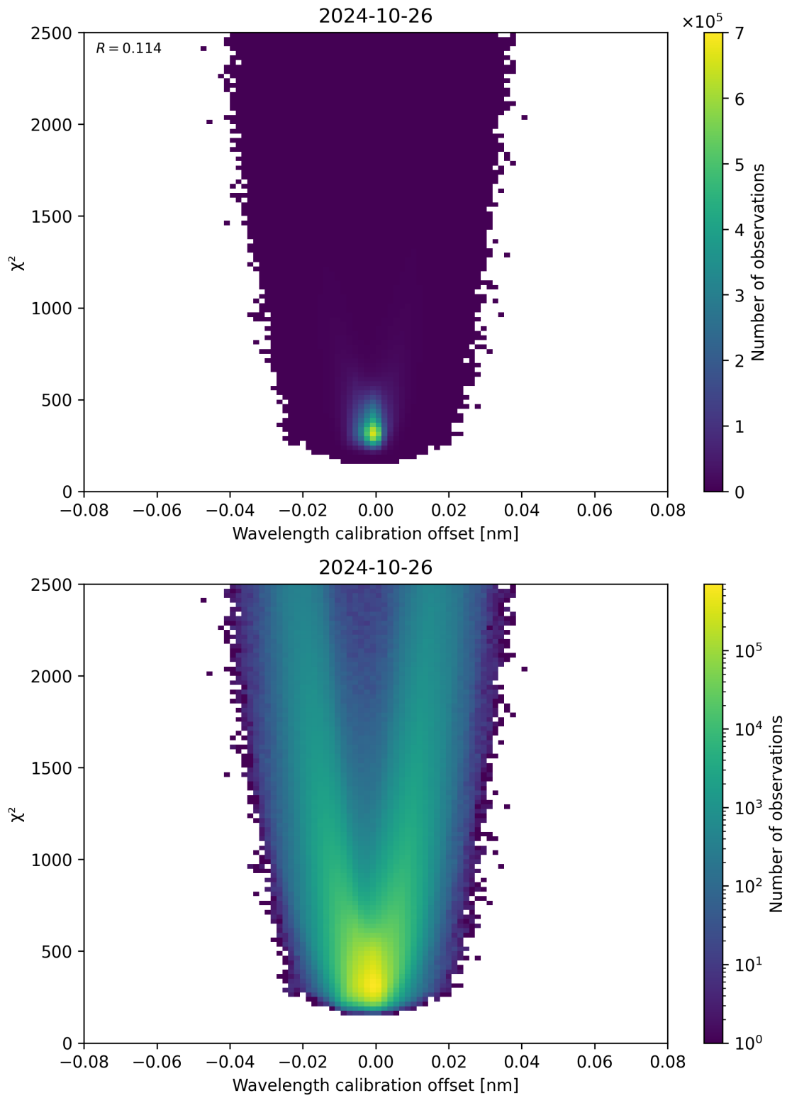
Figure 175: Scatter density plot of “Wavelength calibration offset” against “ \chi^2 ” for 2024-10-25 to 2024-10-27.
