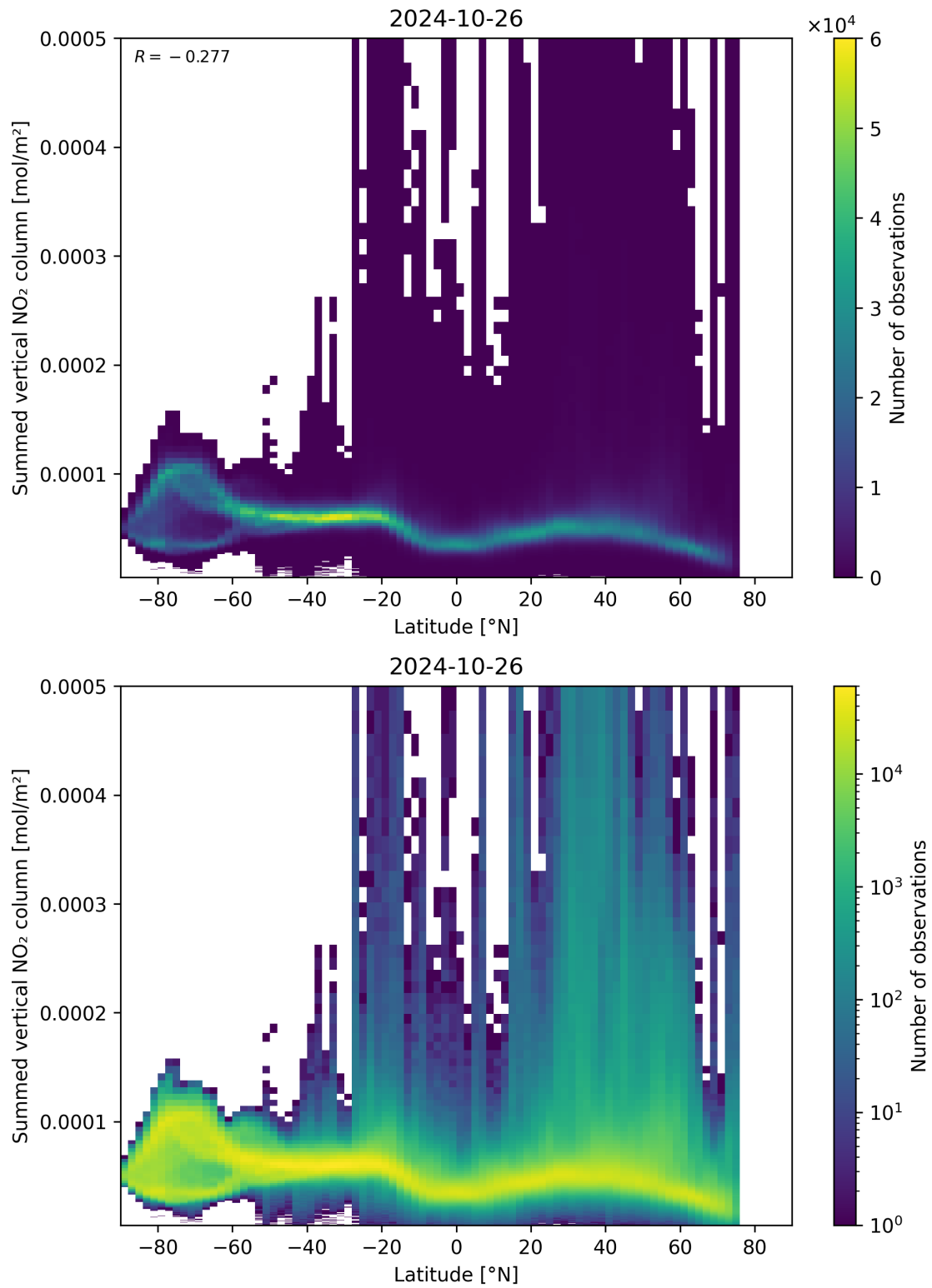
Figure 88: Scatter density plot of “Latitude” against “Summed vertical NO 2 column” for 2024-10-25 to 2024-10-27.
