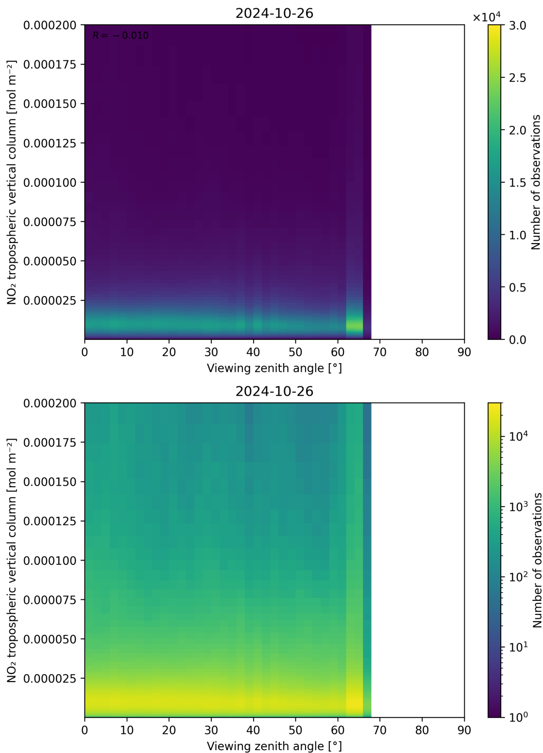
Figure 169: Scatter density plot of “Viewing zenith angle” against “NO 2 tropospheric vertical column” for 2024-10-25 to 2024-10-27.
