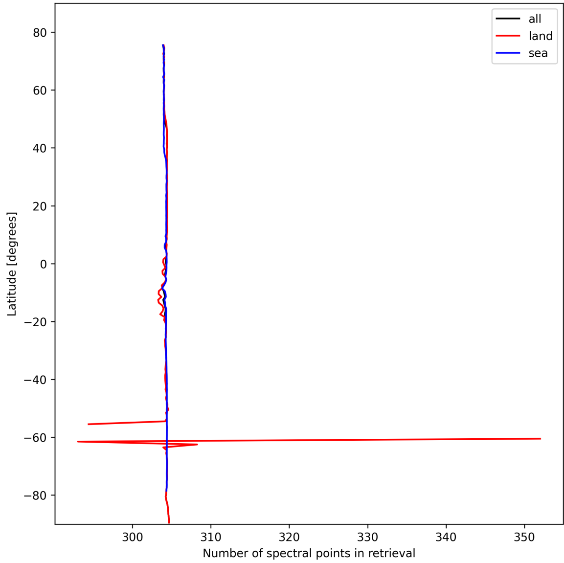
Figure 16: Zonal average of “Number of spectral points in retrieval” for 2024-10-25 to 2024-10-27.
