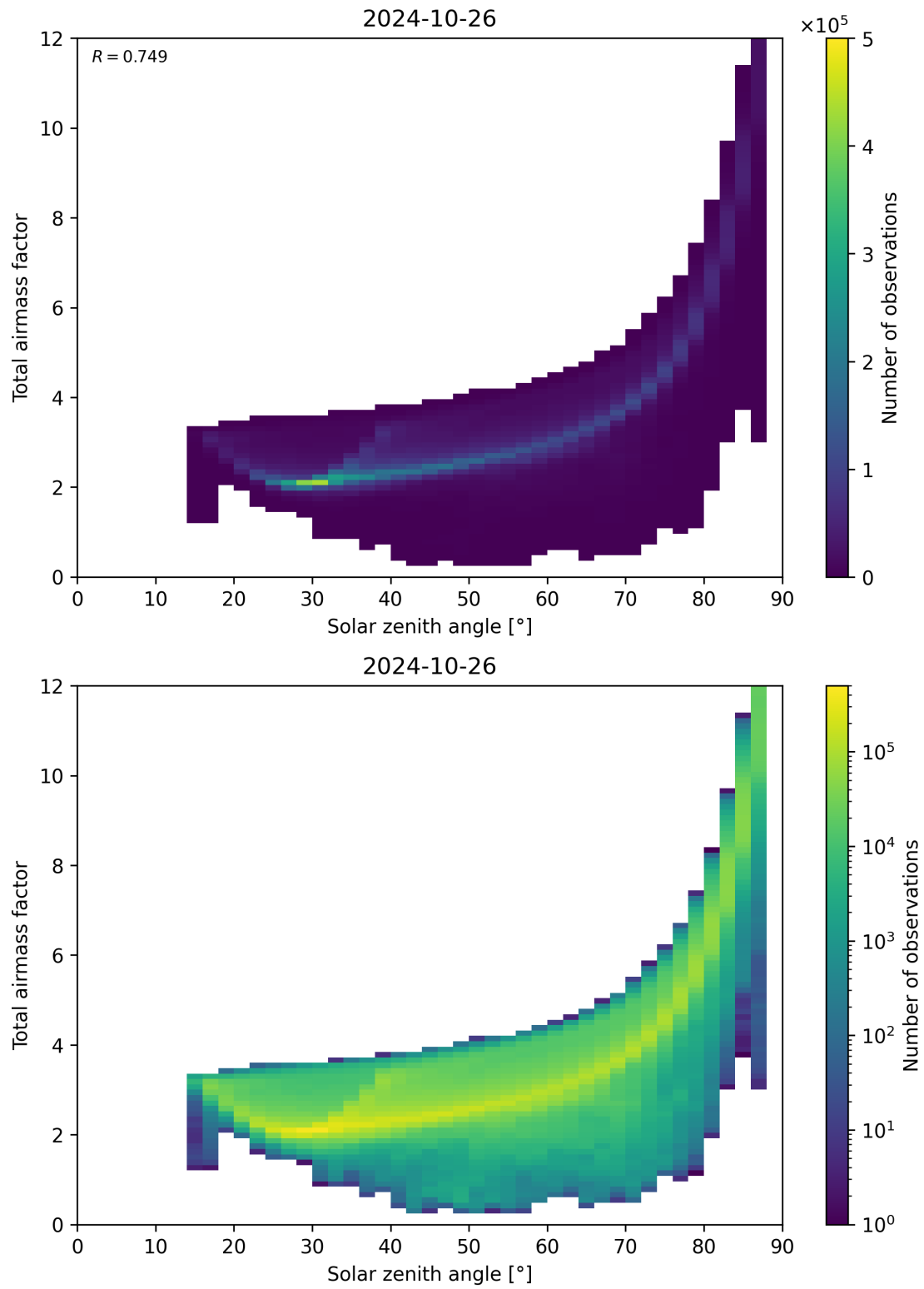
Figure 146: Scatter density plot of “Solar zenith angle” against “Total airmass factor” for 2024-10-25 to 2024-10-27.
